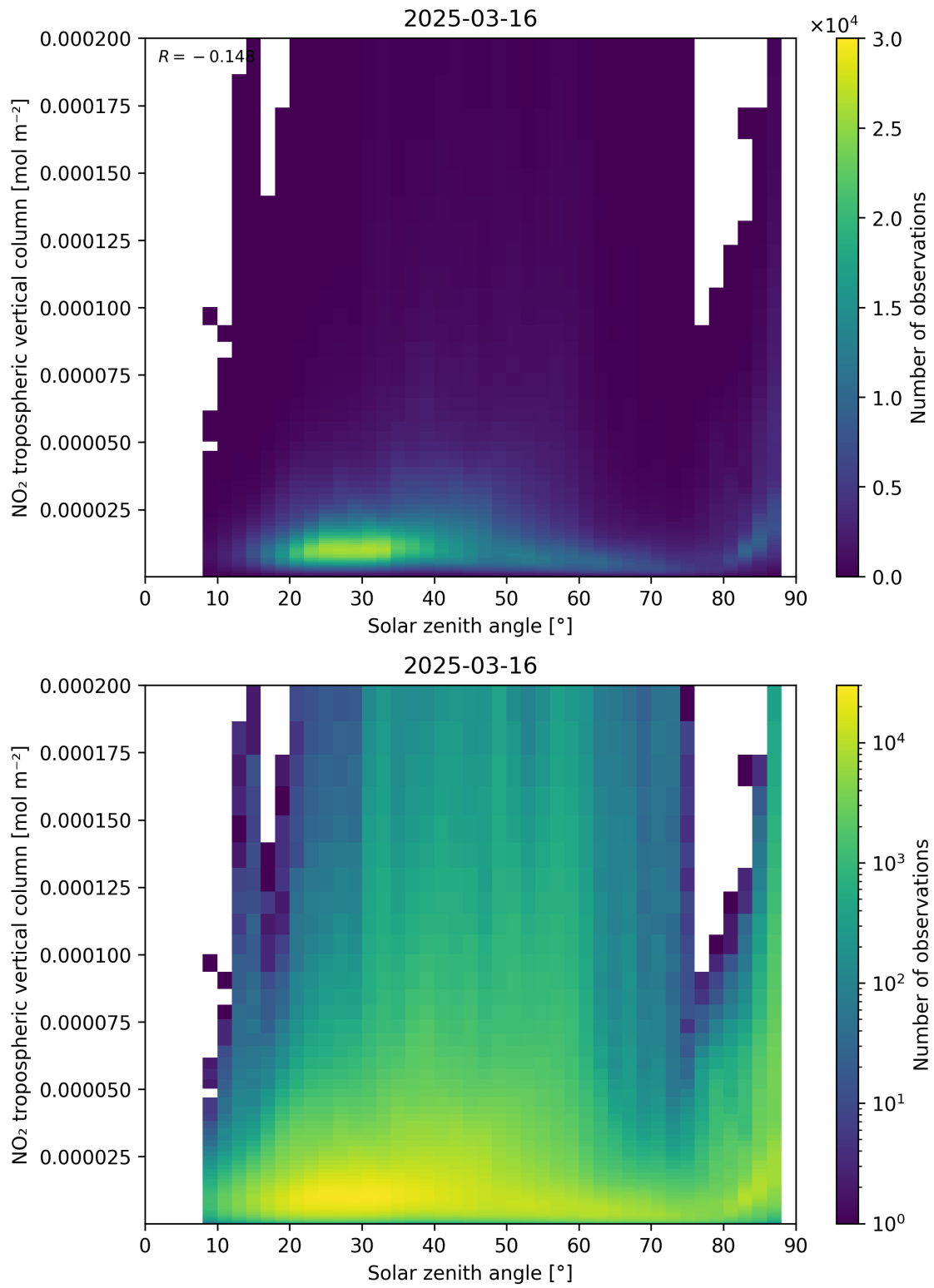
Figure 155: Scatter density plot of “Solar zenith angle” against “NO 2 tropospheric vertical column” for 2025-03-16 to 2025-03-17.
