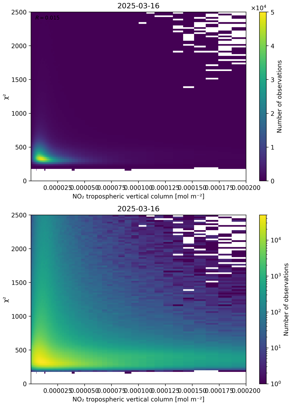
Figure 124: Scatter density plot of “NO 2 tropospheric vertical column” against “ \chi^2 ” for 2025-03-16 to 2025-03-17.
