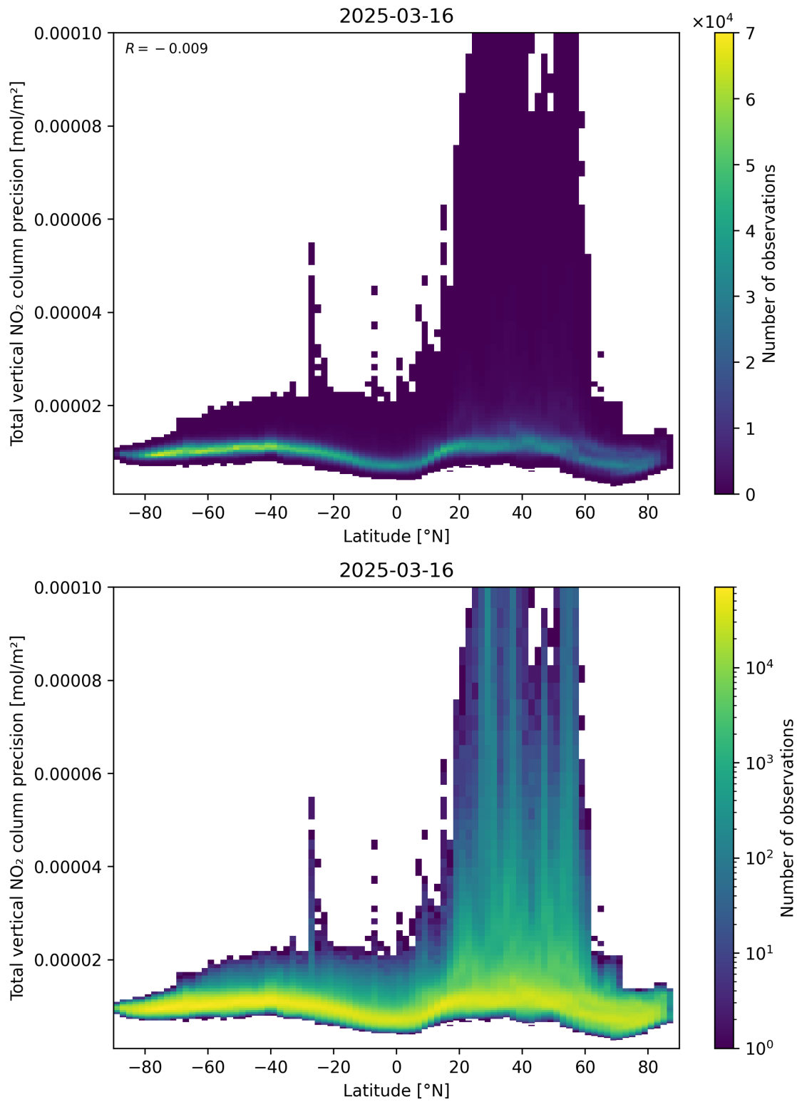
Figure 91: Scatter density plot of “Latitude” against “Total vertical NO 2 column precision” for 2025-03-16 to 2025-03-17.
