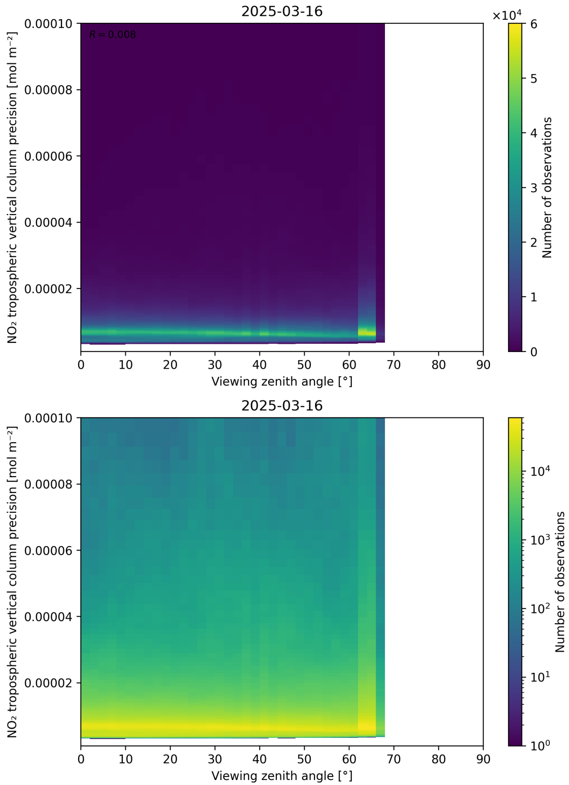
Figure 170: Scatter density plot of “Viewing zenith angle” against “NO 2 tropospheric vertical column precision” for 2025-03-16 to 2025-03-17.
