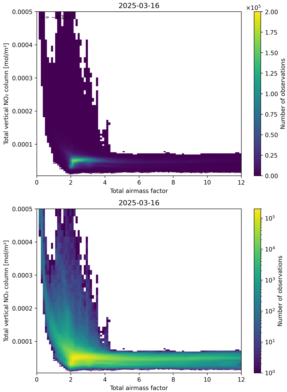
Figure 67: Scatter density plot of “Total airmass factor” against “Total vertical NO 2 column” for 2025-03-16 to 2025-03-17.
