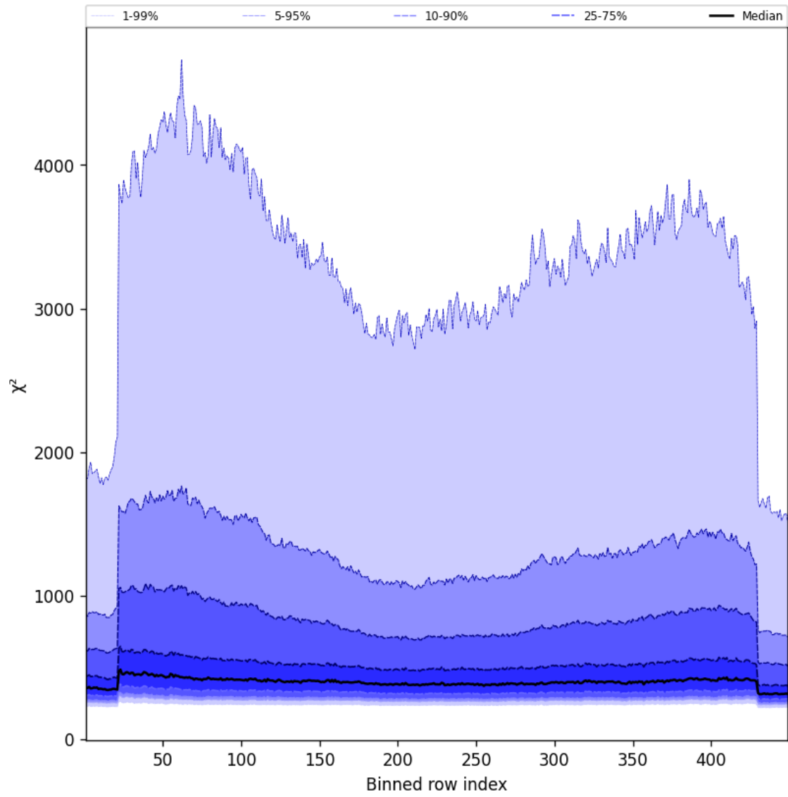
Figure 59: Along track statistics of “ \chi^2 ” for 2025-03-16 to 2025-03-17
