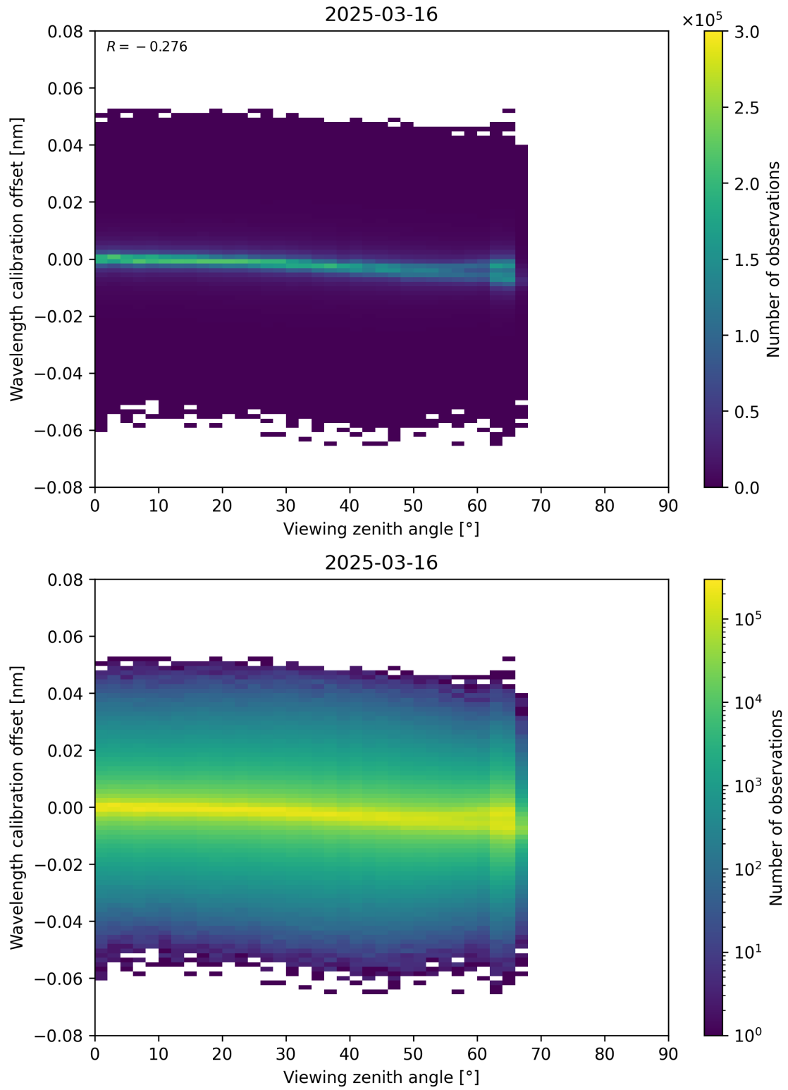
Figure 173: Scatter density plot of “Viewing zenith angle” against “Wavelength calibration offset” for 2025-03-16 to 2025-03-17.
