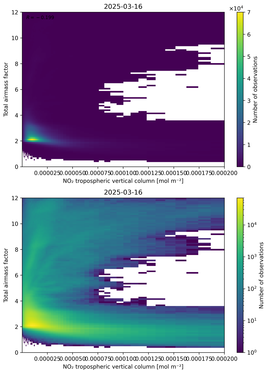
Figure 122: Scatter density plot of “NO 2 tropospheric vertical column” against “Total air mass factor” for 2025-03-16 to 2025-03-17.
