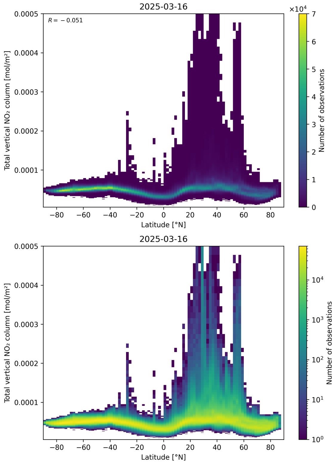
Figure 90: Scatter density plot of “Latitude” against “Total vertical NO 2 column” for 2025-03-16 to 2025-03-17.
