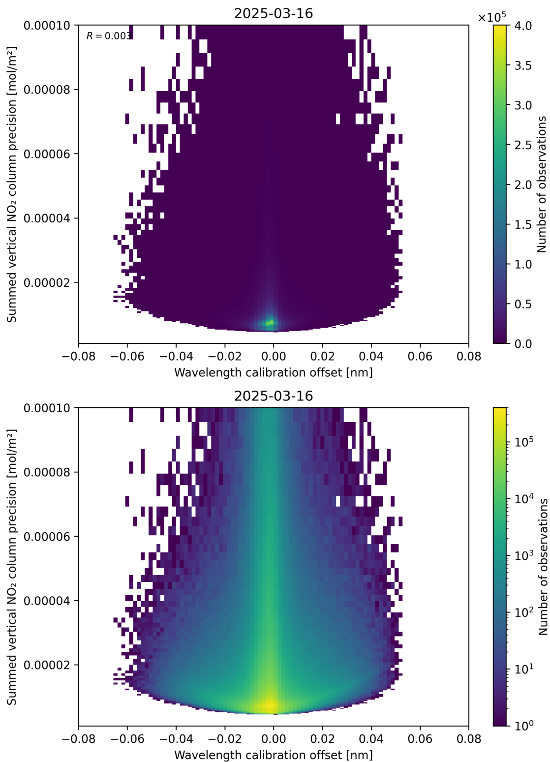
Figure 178: Scatter density plot of “Wavelength calibration offset” against “Summed vertical NO 2 column precision” for 2025-03-16 to 2025-03-17.
