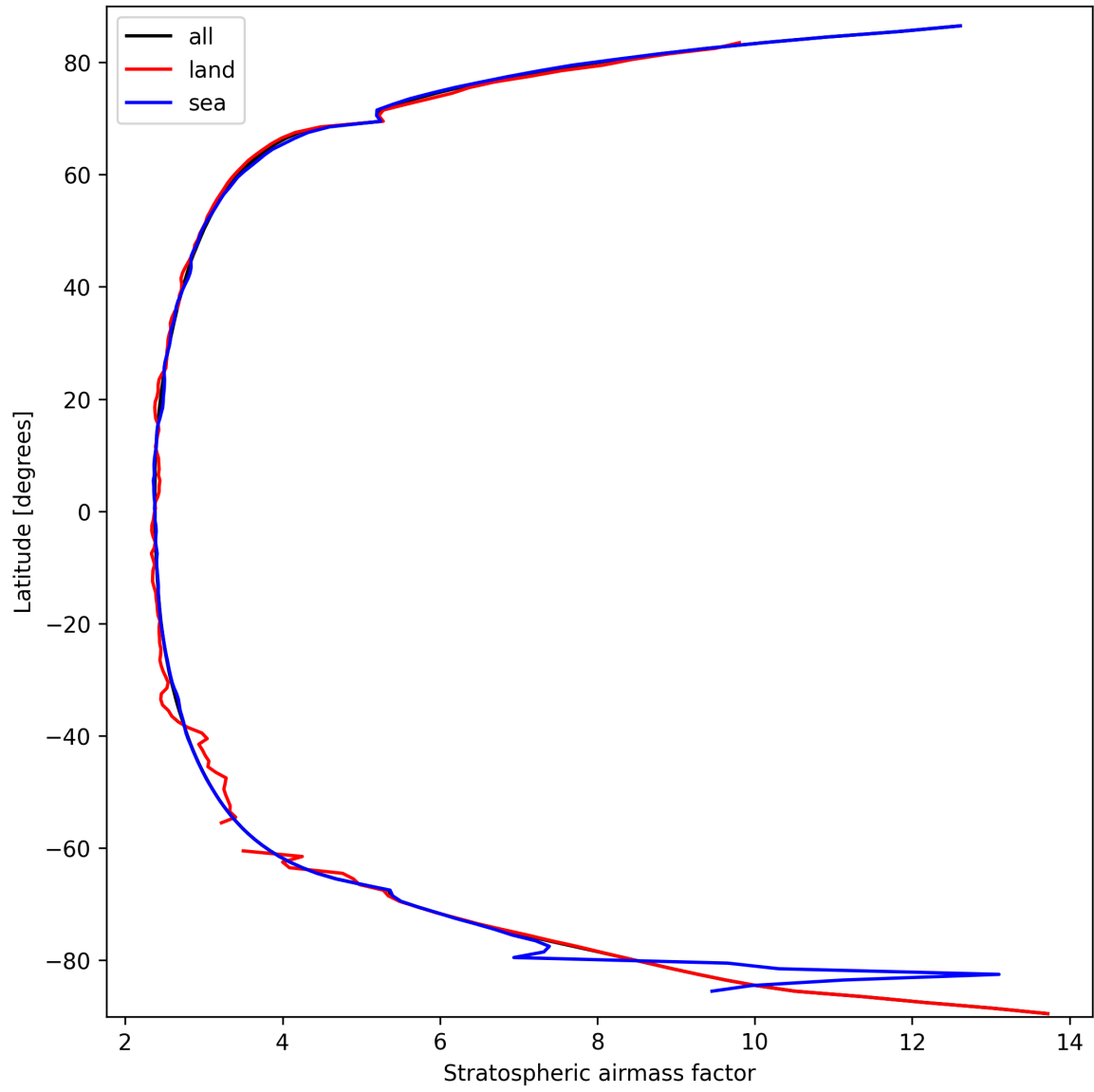
Figure 27: Zonal average of “Stratospheric air mass factor” for 2025-03-16 to 2025-03-17.
