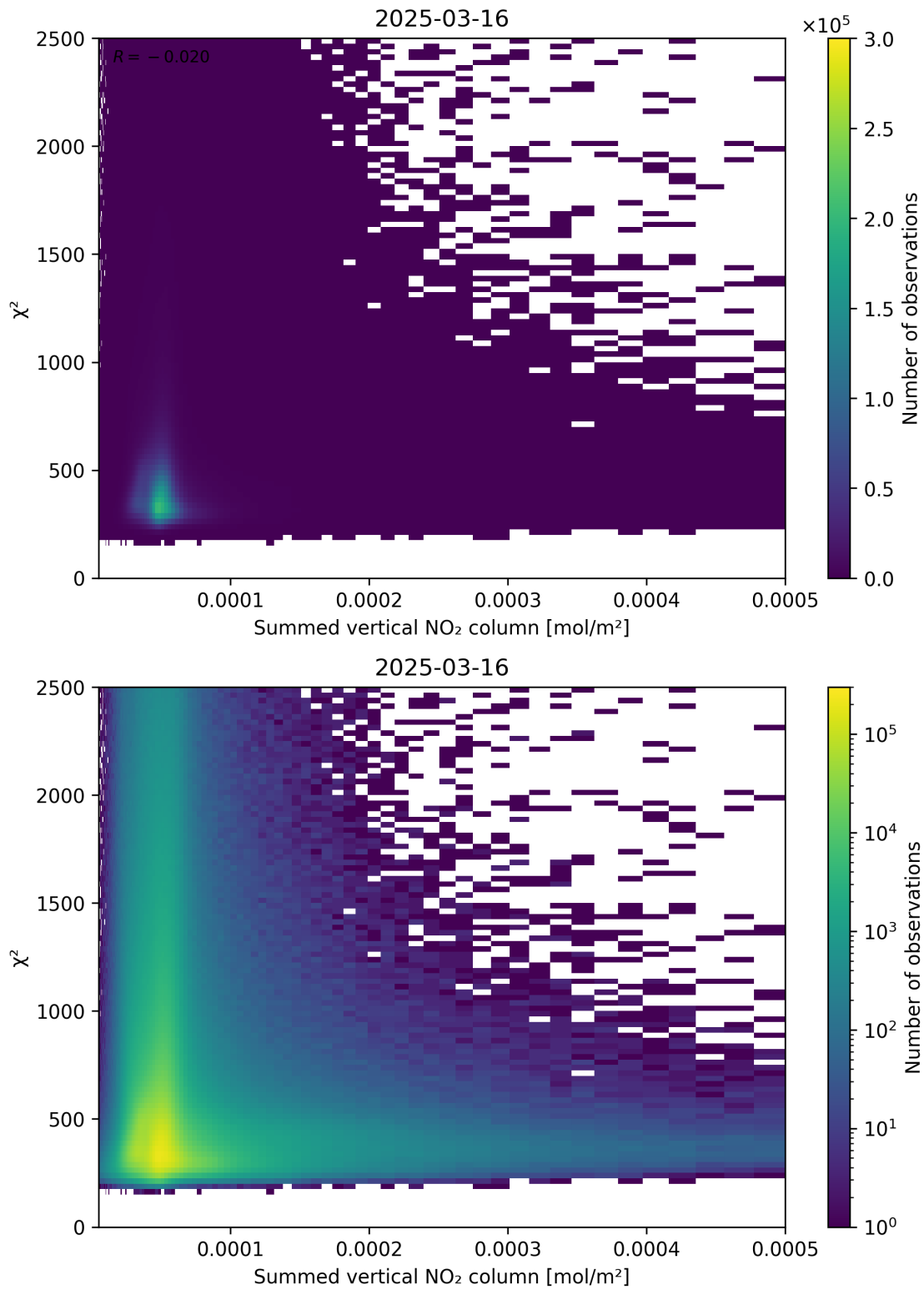
Figure 104: Scatter density plot of “Summed vertical NO 2 column” against “ \chi^2 ” for 2025-03-16 to 2025-03-17.
