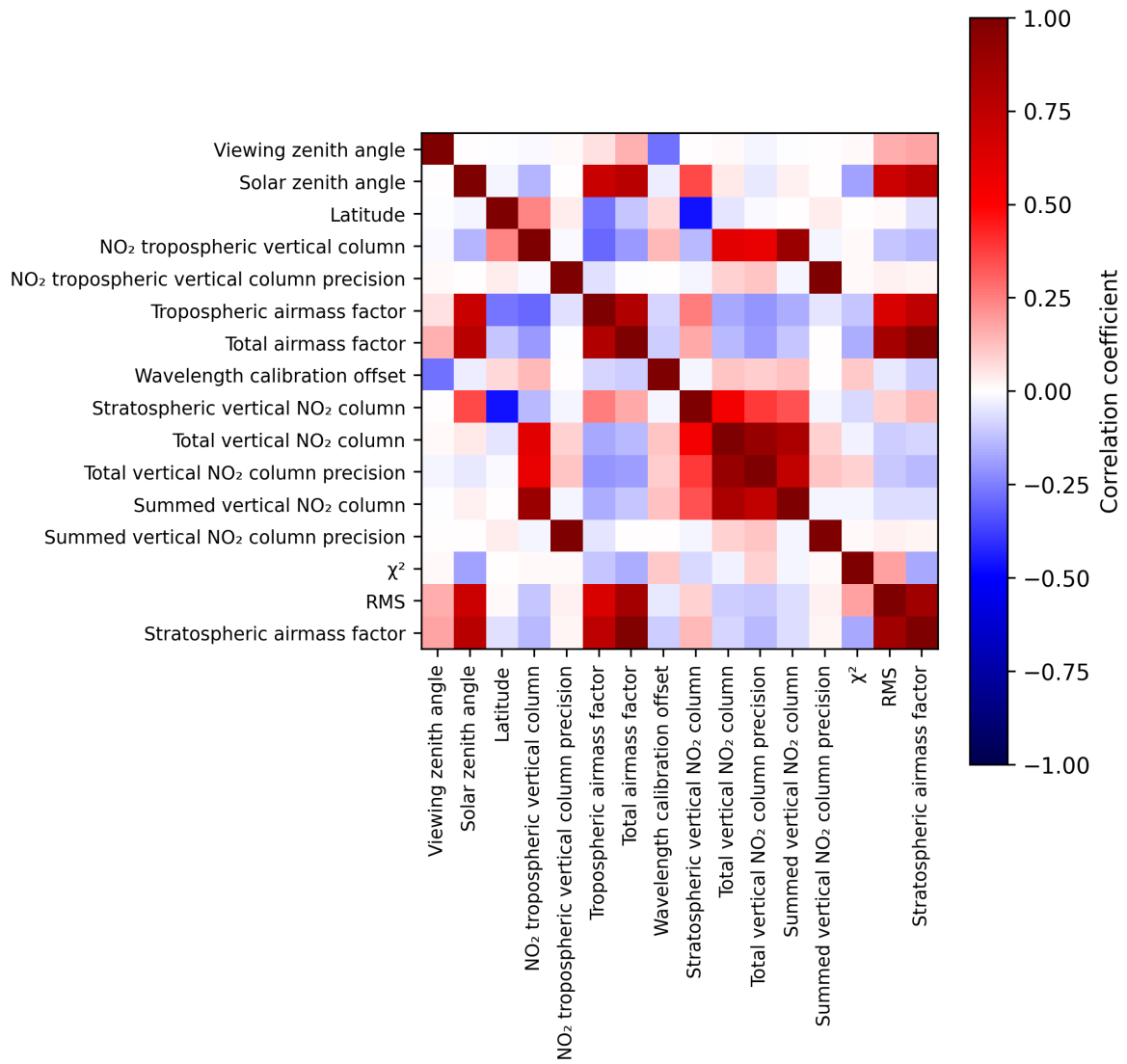
Figure 2: Map of correlation matrix for 2025-03-16 to 2025-03-17.
