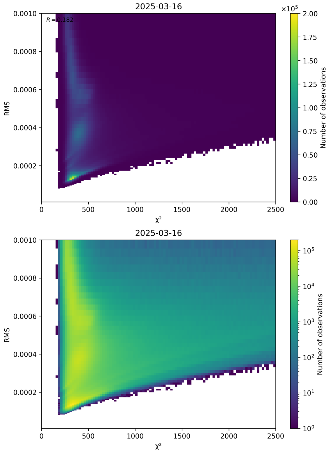
Figure 82: Scatter density plot of “ \chi^2 ” against “RMS” for 2025-03-16 to 2025-03-17.
