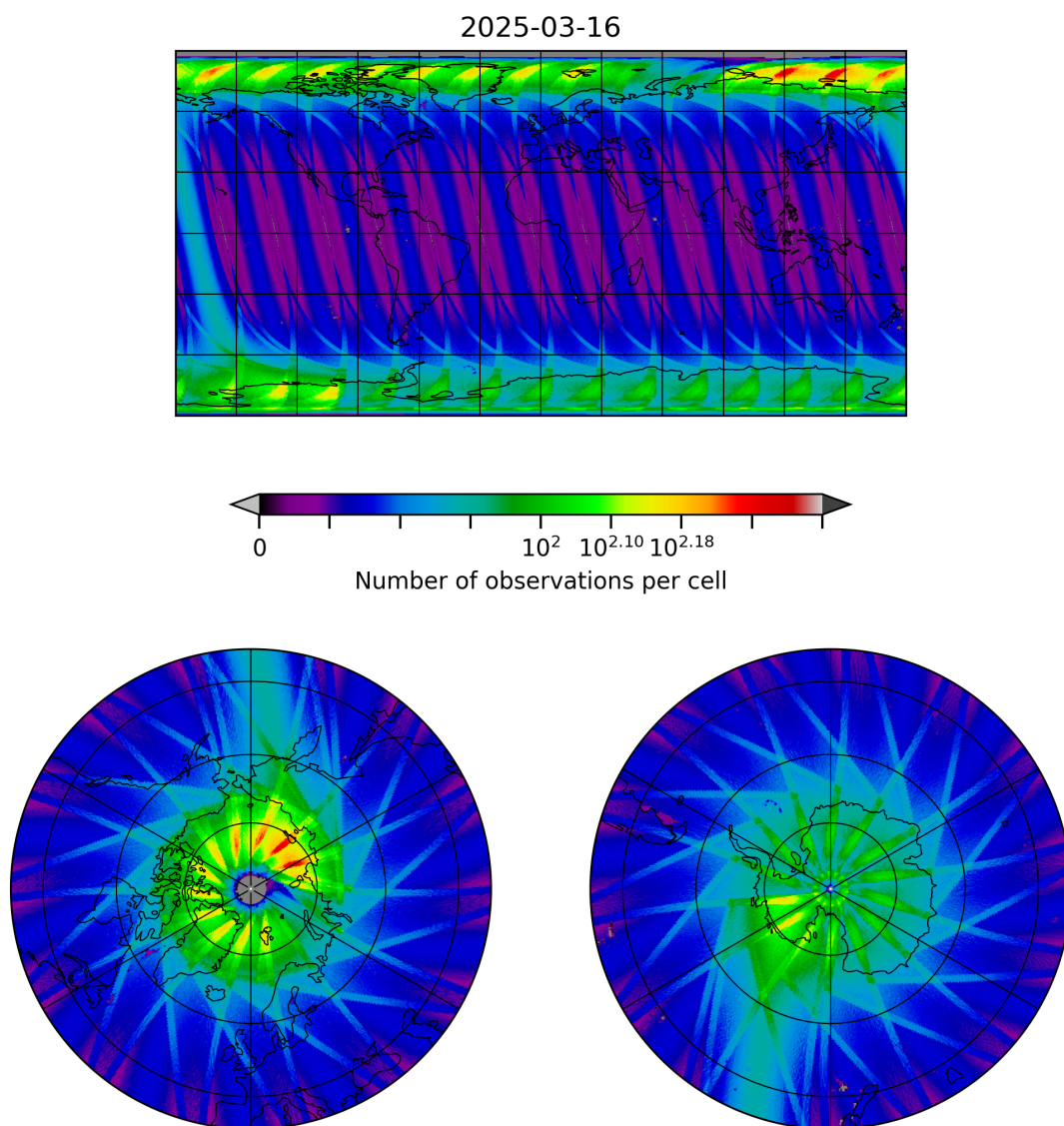
Figure 10: Map of the number of observations for 2025-03-16 to 2025-03-17
