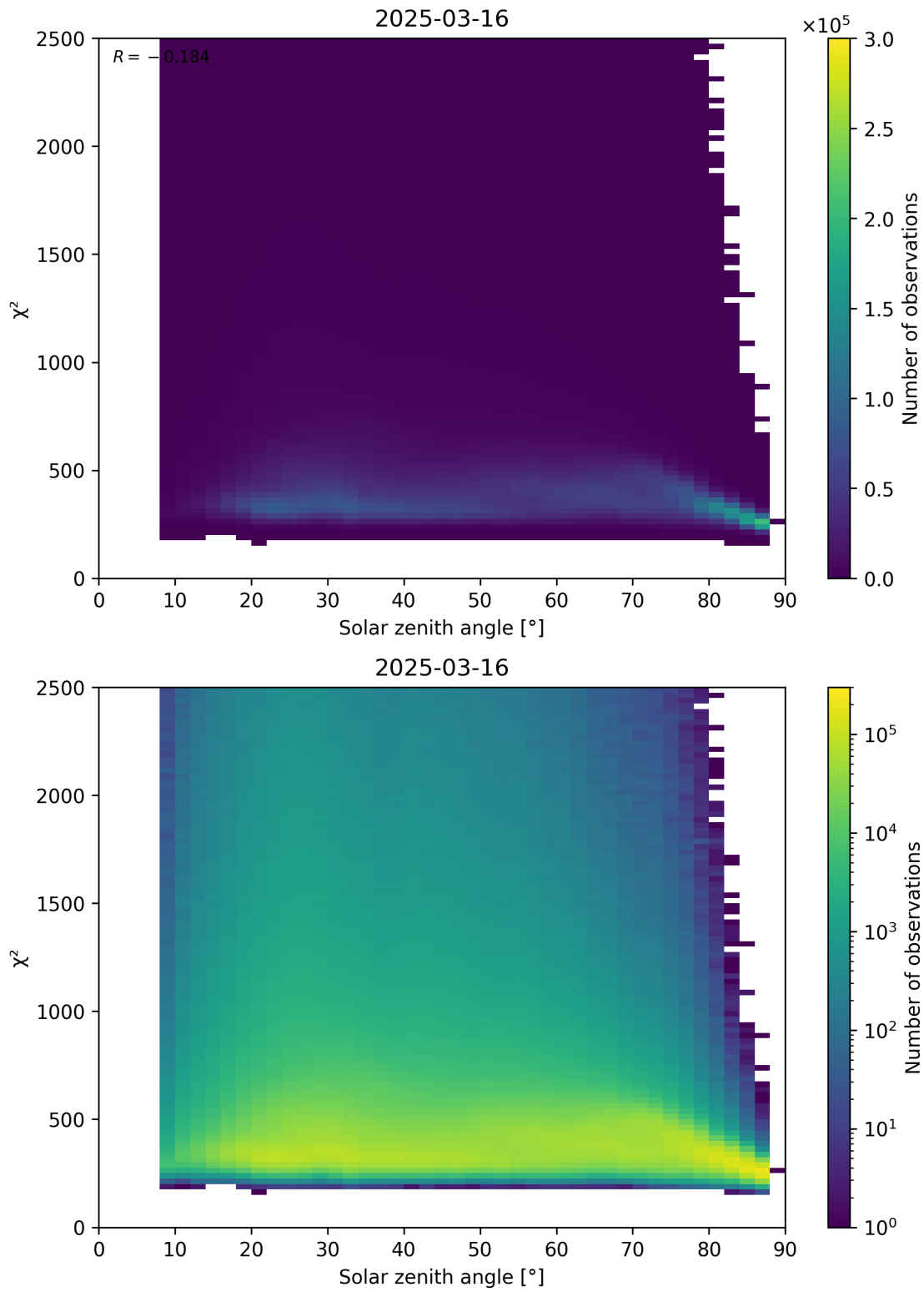
Figure 148: Scatter density plot of “Solar zenith angle” against “ \chi^2 ” for 2025-03-16 to 2025-03-17.
