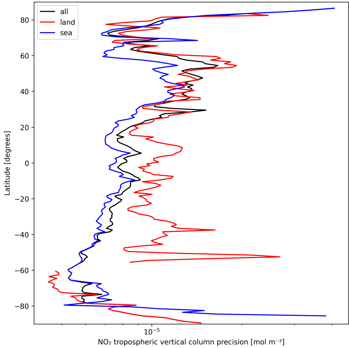
Figure 13: Zonal average of “NO 2 tropospheric vertical column precision” for 2025-03-16 to 2025-03-17.
