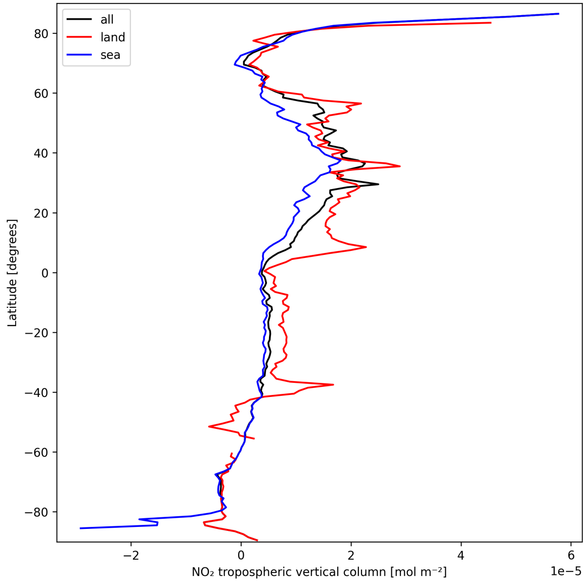
Figure 12: Zonal average of “NO 2 tropospheric vertical column” for 2025-03-16 to 2025-03-17.
