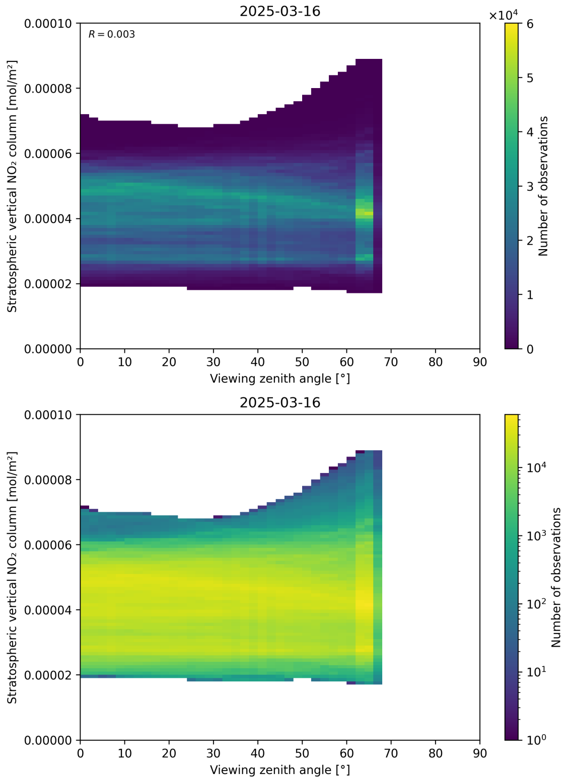
Figure 164: Scatter density plot of “Viewing zenith angle” against “Stratospheric vertical NO 2 column” for 2025-03-16 to 2025-03-17.
