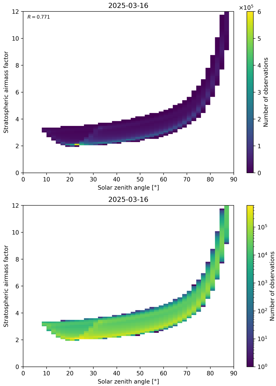
Figure 145: Scatter density plot of “Solar zenith angle” against “Stratospheric airmass factor” for 2025-03-16 to 2025-03-17.
