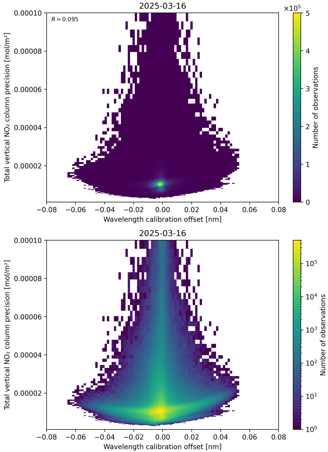
Figure 180: Scatter density plot of “Wavelength calibration offset” against “Total vertical NO 2 column precision” for 2025-03-16 to 2025-03-17.
