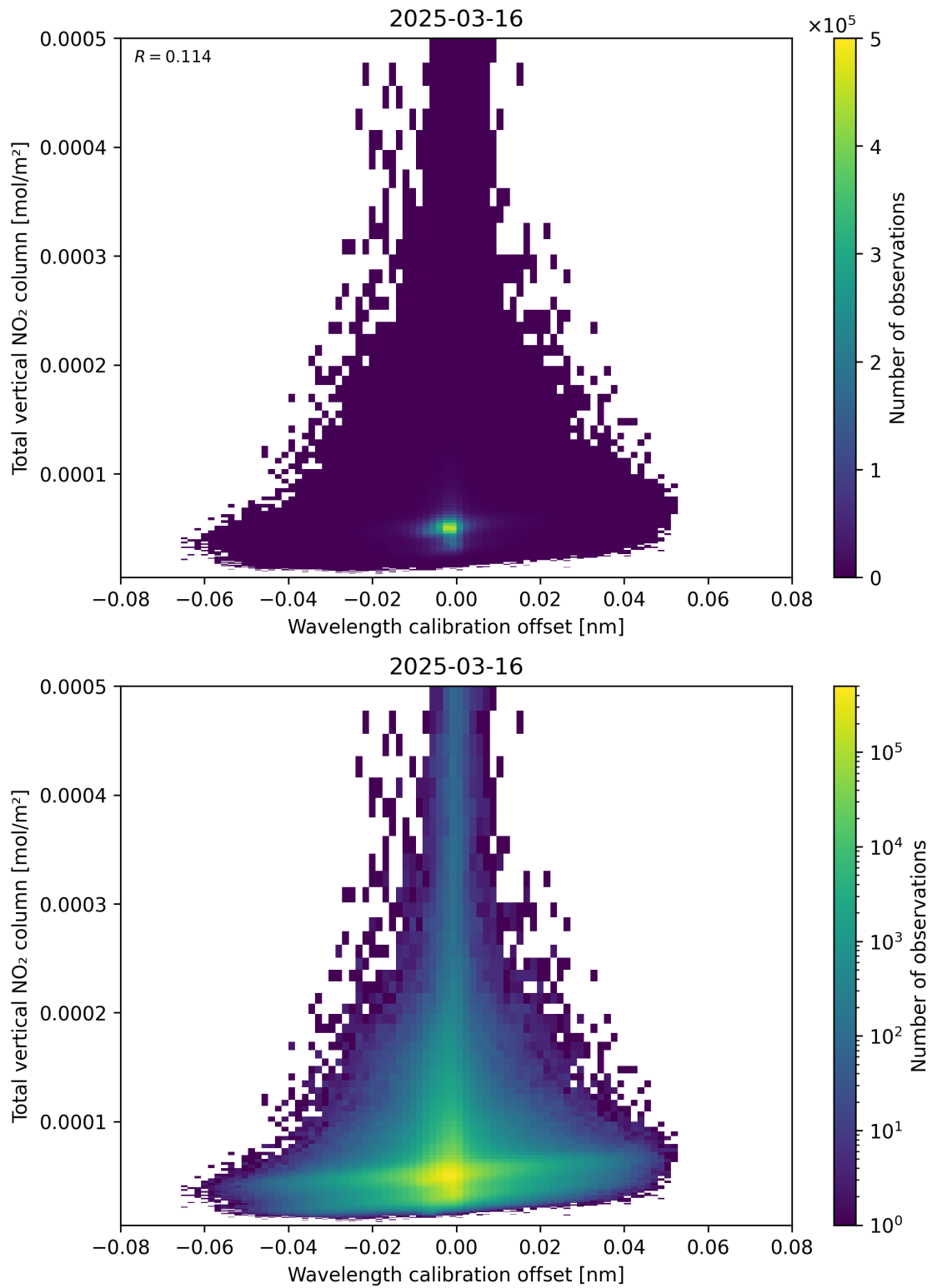
Figure 179: Scatter density plot of “Wavelength calibration offset” against “Total vertical NO 2 column” for 2025-03-16 to 2025-03-17.
