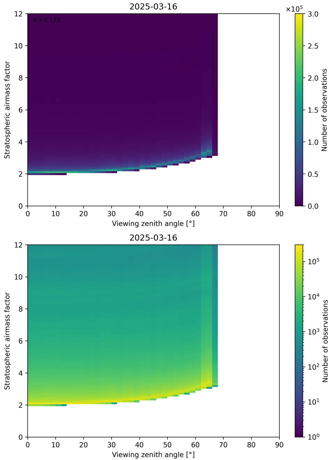
Figure 159: Scatter density plot of “Viewing zenith angle” against “Stratospheric airmass factor” for 2025-03-16 to 2025-03-17.
