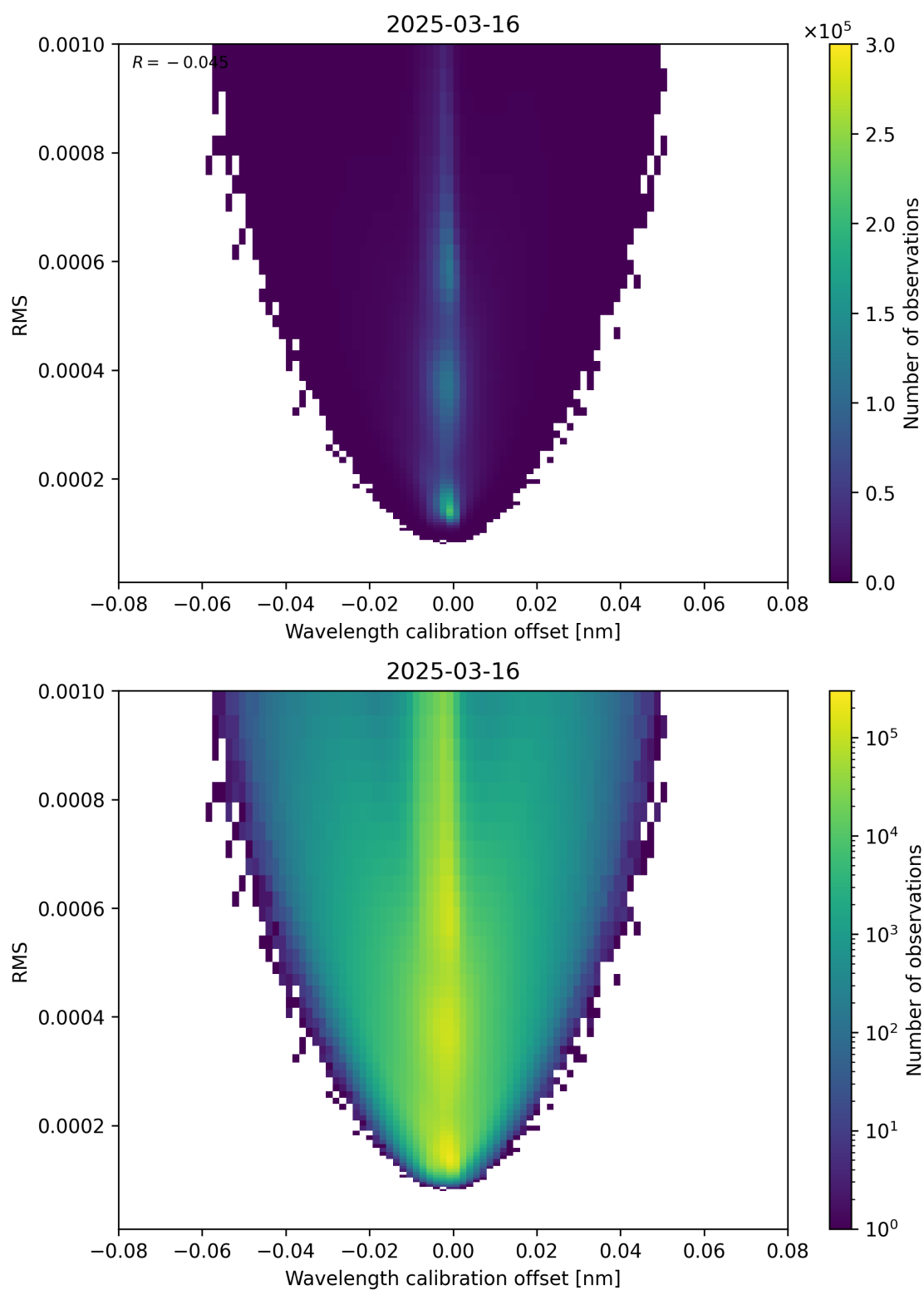
Figure 181: Scatter density plot of “Wavelength calibration offset” against “RMS” for 2025-03-16 to 2025-03-17.
