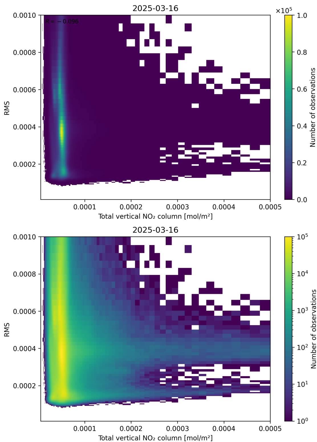
Figure 120: Scatter density plot of “Total vertical NO 2 column” against “RMS” for 2025-03-16 to 2025-03-17.
