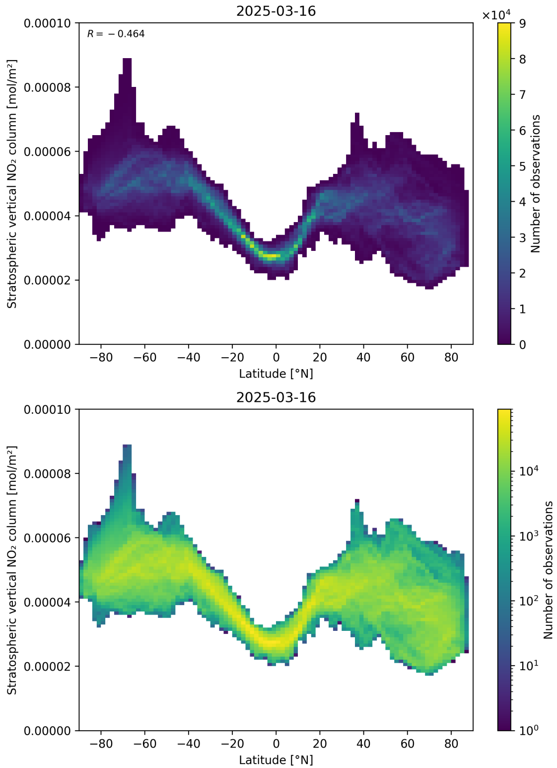
Figure 87: Scatter density plot of “Latitude” against “Stratospheric vertical NO 2 column” for 2025-03-16 to 2025-03-17.
