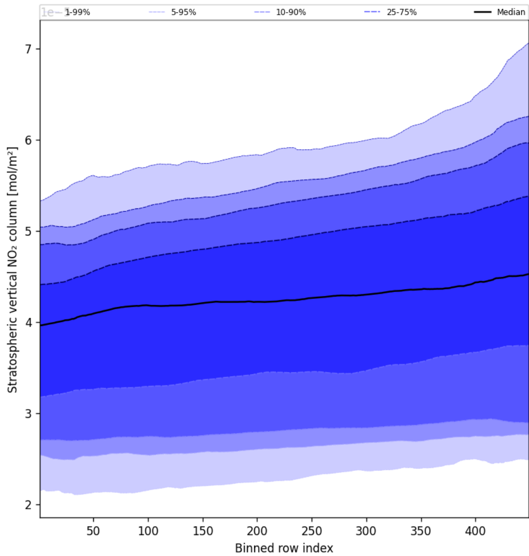
Figure 53: Along track statistics of “Stratospheric vertical NO 2 column” for 2025-03-16 to 2025-03-17
