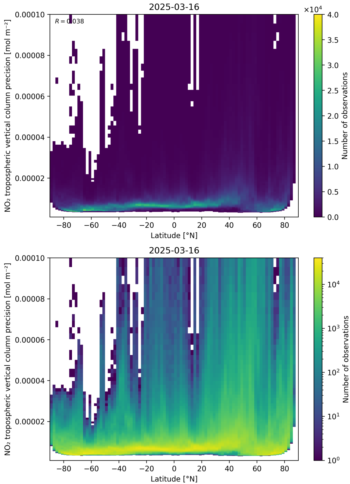
Figure 93: Scatter density plot of “Latitude” against “NO 2 tropospheric vertical column precision” for 2025-03-16 to 2025-03-17.
