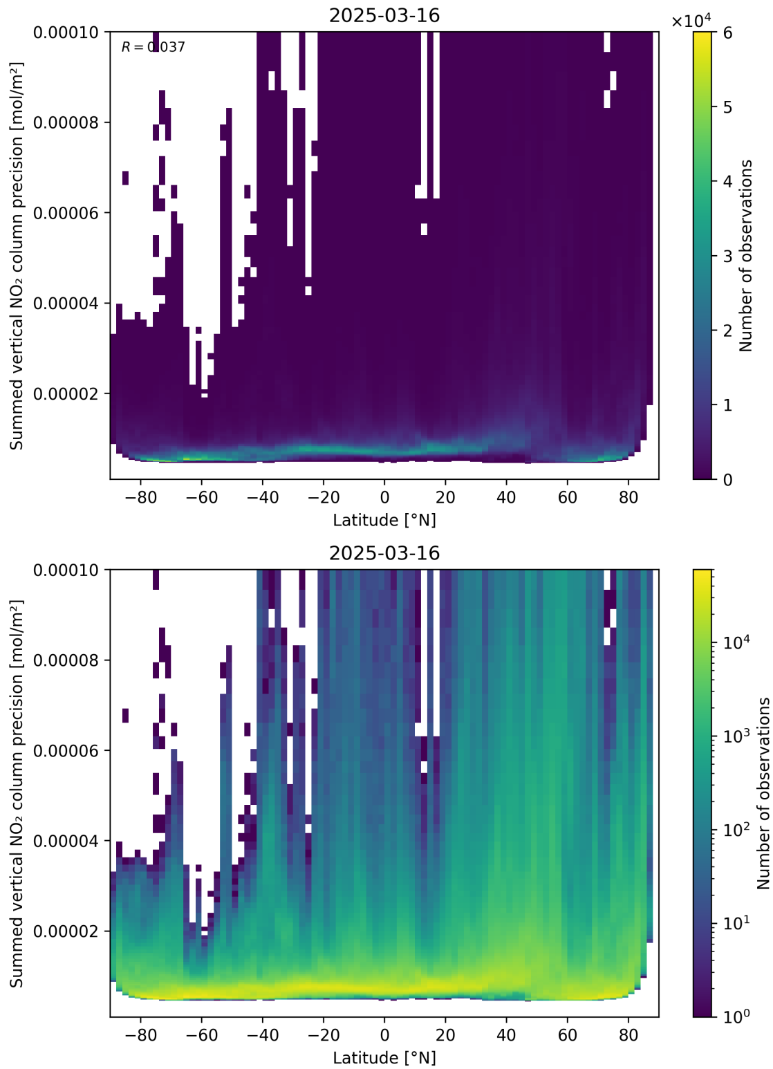
Figure 89: Scatter density plot of “Latitude” against “Summed vertical NO 2 column precision” for 2025-03-16 to 2025-03-17.
