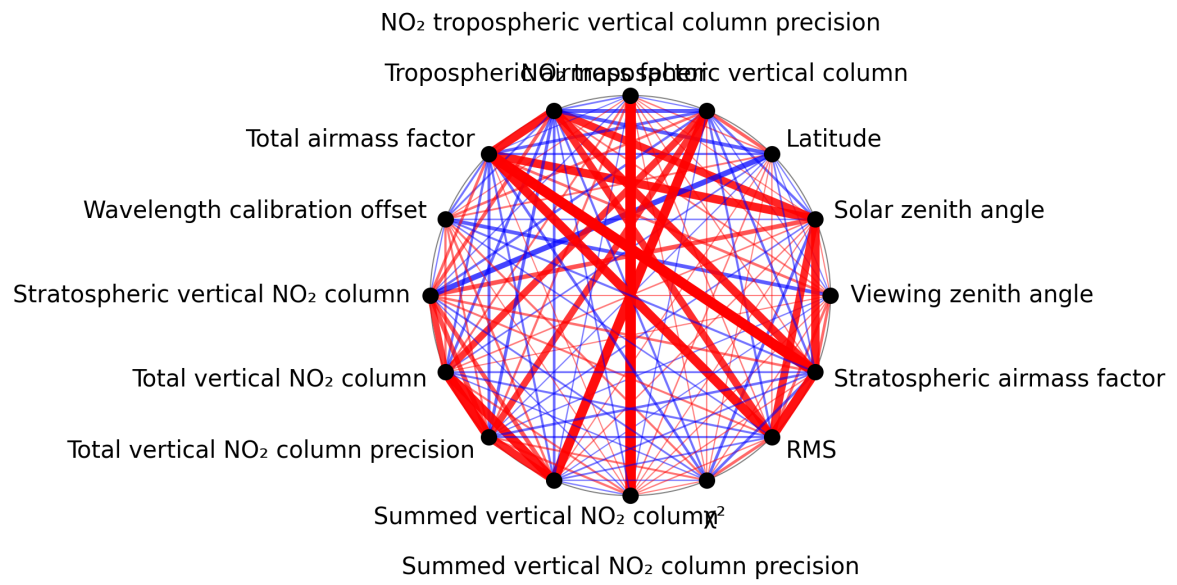
Figure 1: Map of correlation graph for 2025-03-16 to 2025-03-17.
