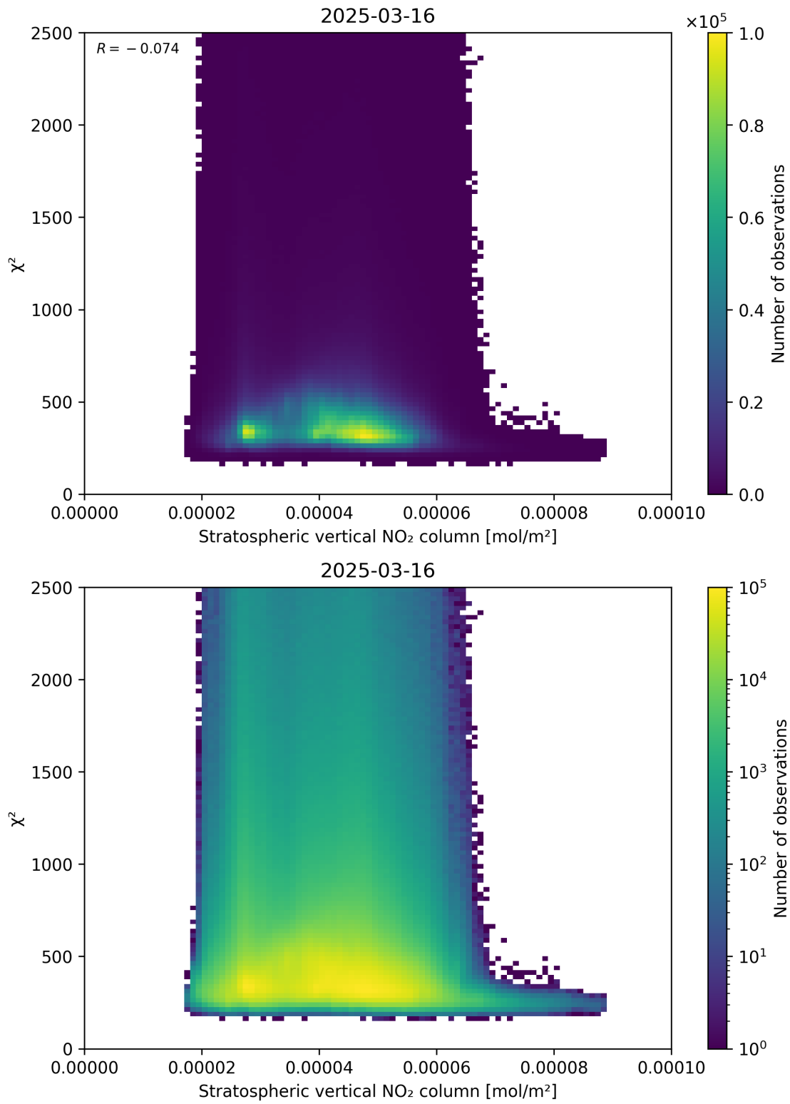
Figure 97: Scatter density plot of “Stratospheric vertical NO 2 column” against “ \chi^2 ” for 2025-03-16 to 2025-03-17.
