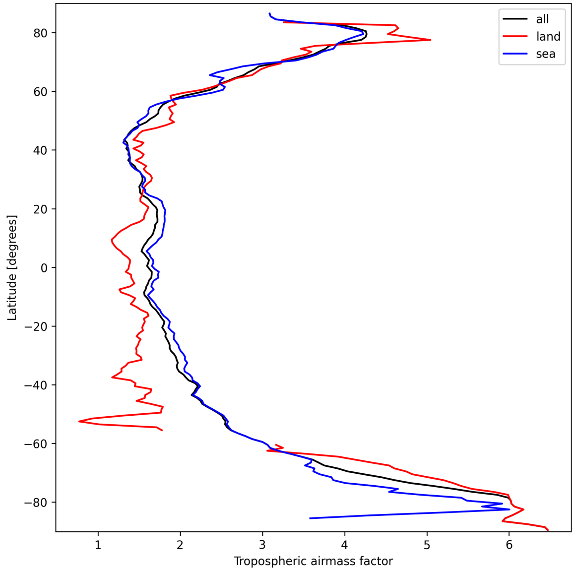
Figure 14: Zonal average of “Tropospheric airmass factor” for 2025-03-16 to 2025-03-17.
