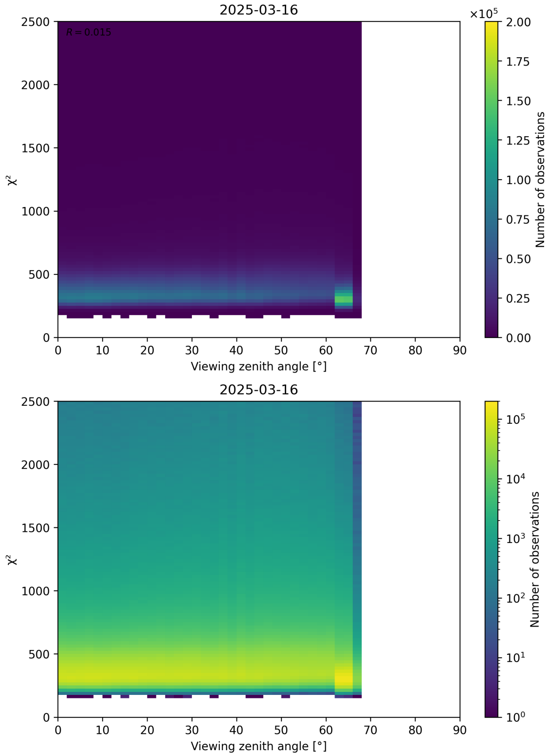
Figure 162: Scatter density plot of “Viewing zenith angle” against “ \chi^2 ” for 2025-03-16 to 2025-03-17.
