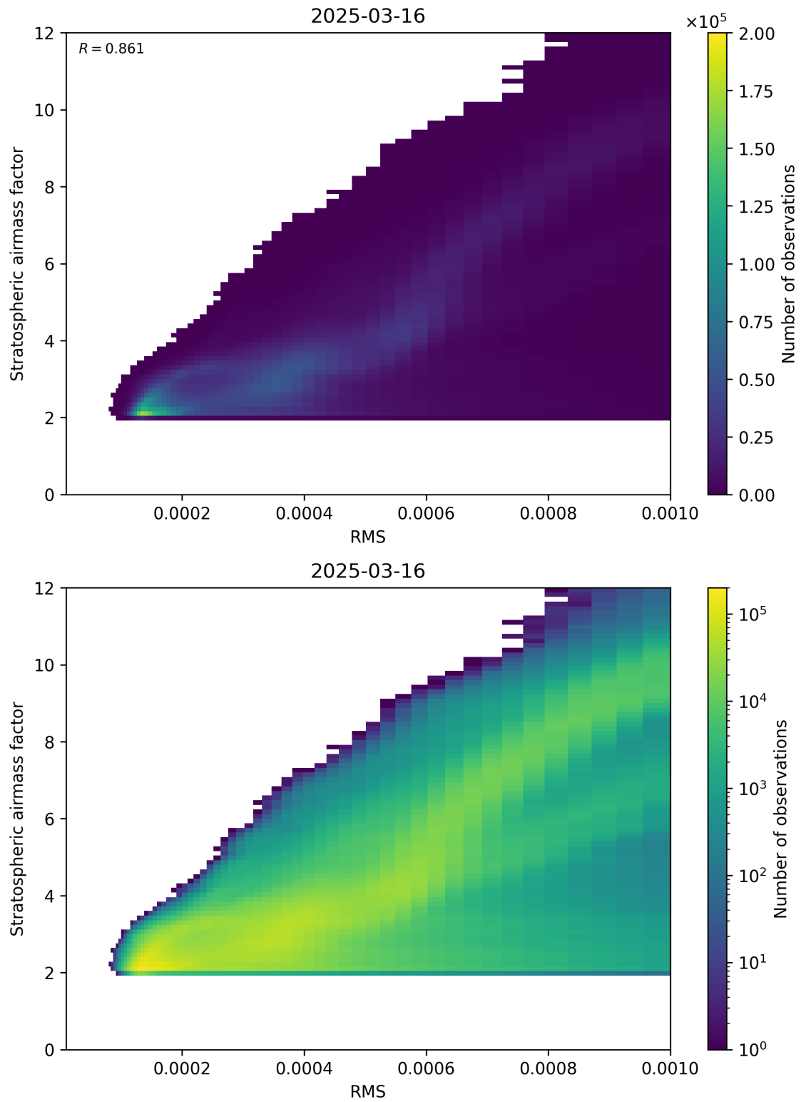
Figure 144: Scatter density plot of “RMS” against “Stratospheric airmass factor” for 2025-03-16 to 2025-03-17.
