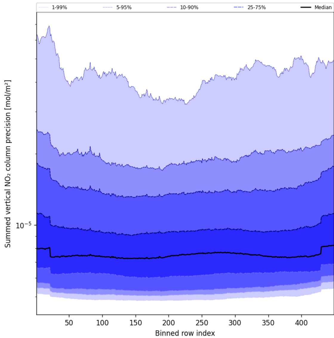
Figure 58: Along track statistics of “Summed vertical NO 2 column precision” for 2025-03-16 to 2025-03-17
