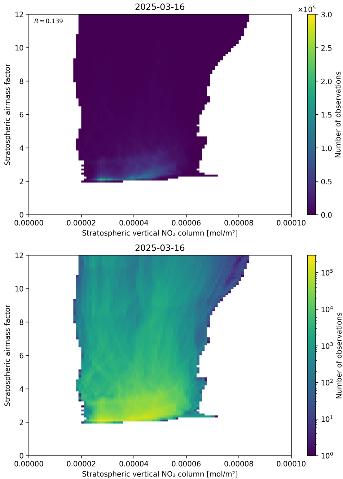
Figure 96: Scatter density plot of “Stratospheric vertical NO 2 column” against “Stratospheric airmass factor” for 2025-03-16 to 2025-03-17.
