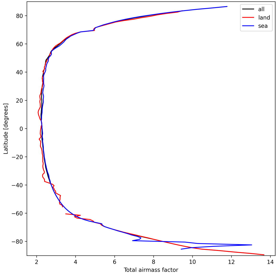
Figure 15: Zonal average of “Total airmass factor” for 2025-03-16 to 2025-03-17.
