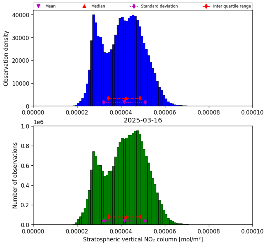
Figure 36: Histogram of “Stratospheric vertical NO 2 column” for 2025-03-16 to 2025-03-17
