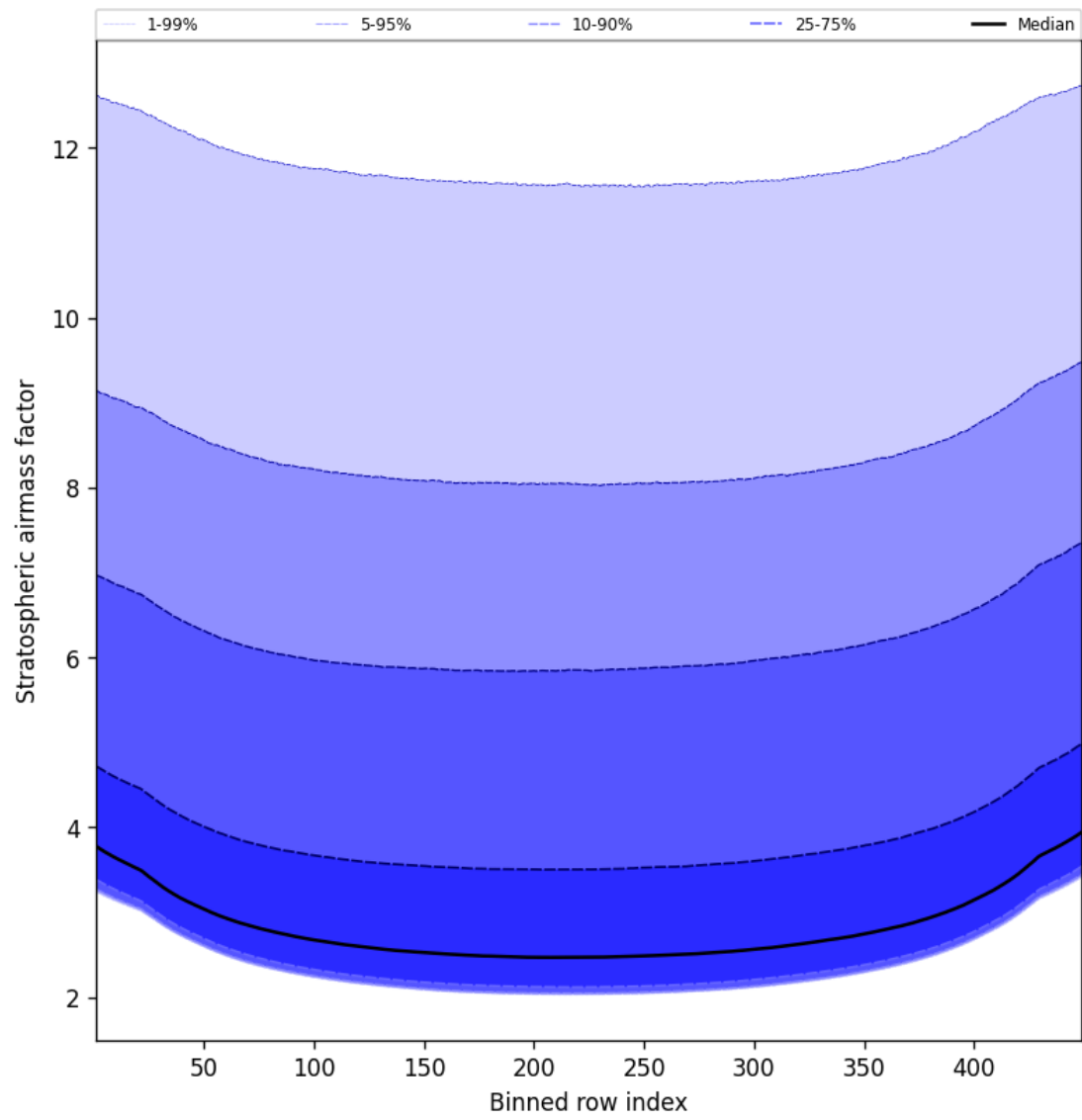
Figure 61: Along track statistics of “Stratospheric airmass factor” for 2025-03-16 to 2025-03-17
