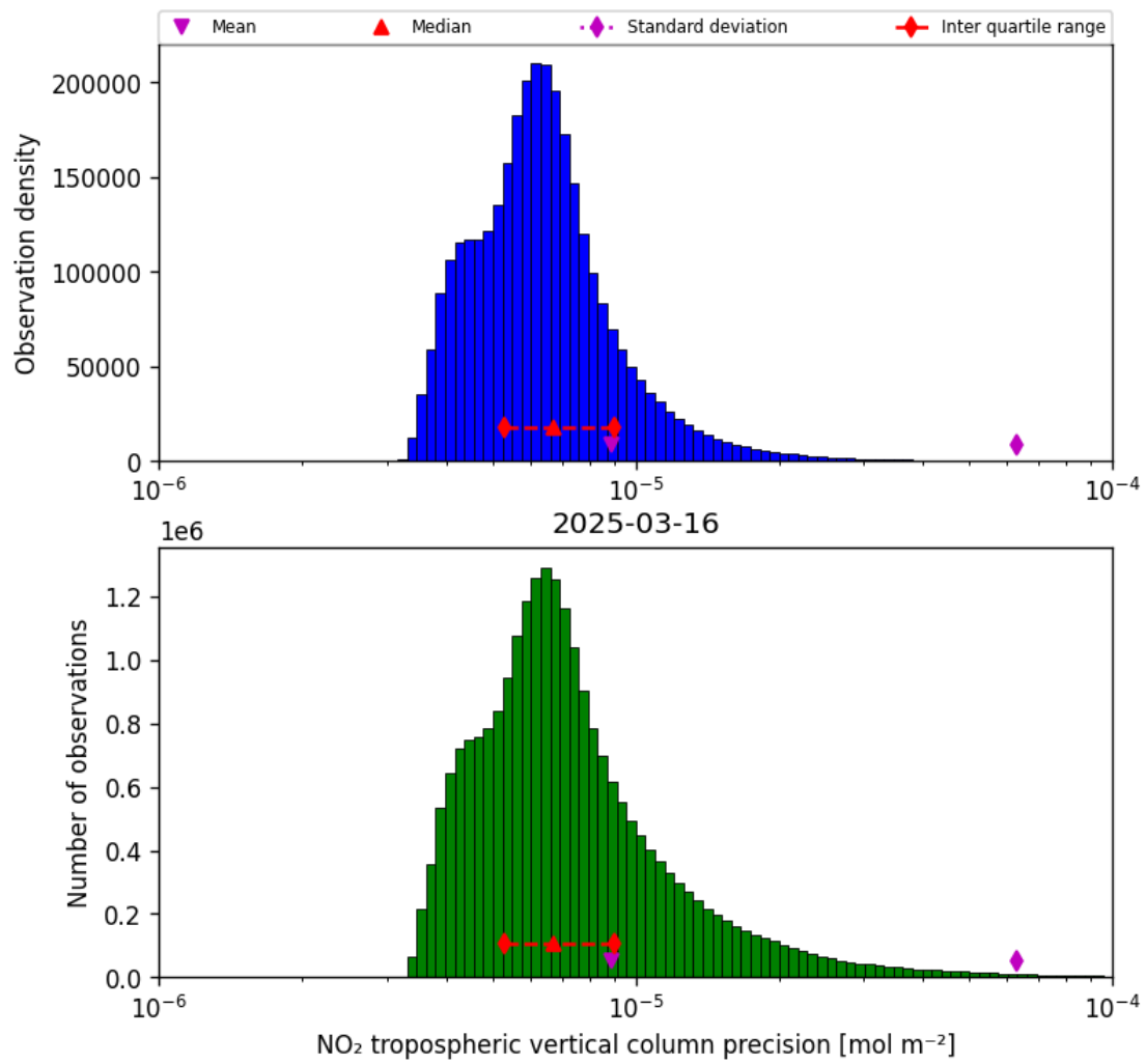
Figure 30: Histogram of “NO 2 tropospheric vertical column precision” for 2025-03-16 to 2025-03-17
