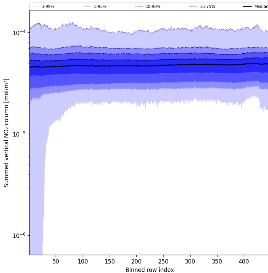
Figure 57: Along track statistics of “Summed vertical NO 2 column” for 2025-03-16 to 2025-03-17
