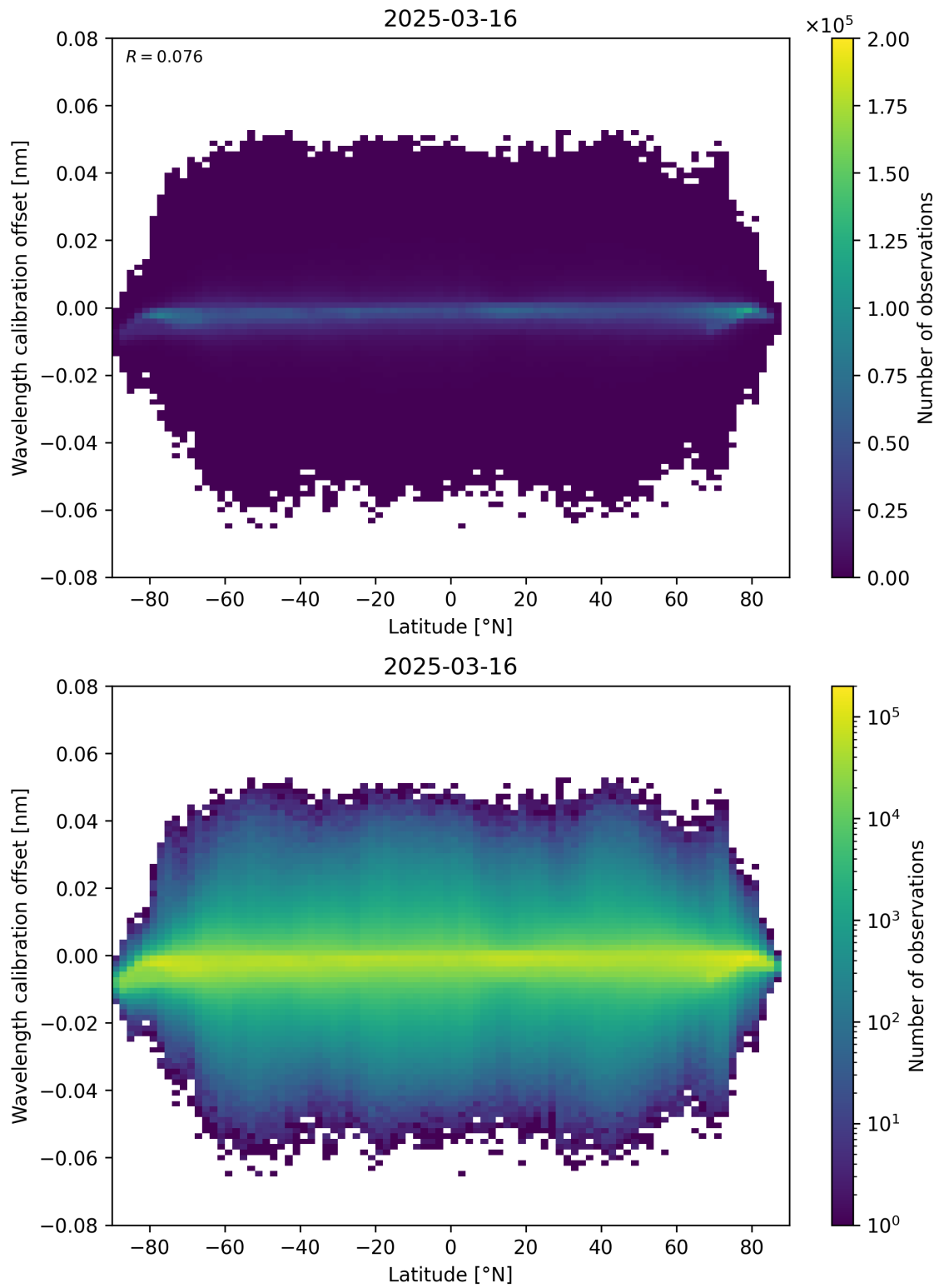
Figure 95: Scatter density plot of “Latitude” against “Wavelength calibration offset” for 2025-03-16 to 2025-03-17.
