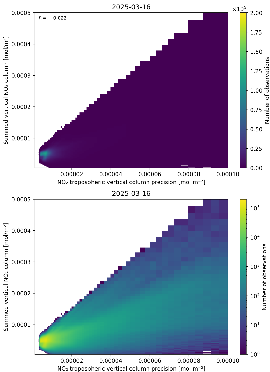
Figure 136: Scatter density plot of “NO 2 tropospheric vertical column precision” against “Summed vertical NO 2 column” for 2025-03-16 to 2025-03-17.
