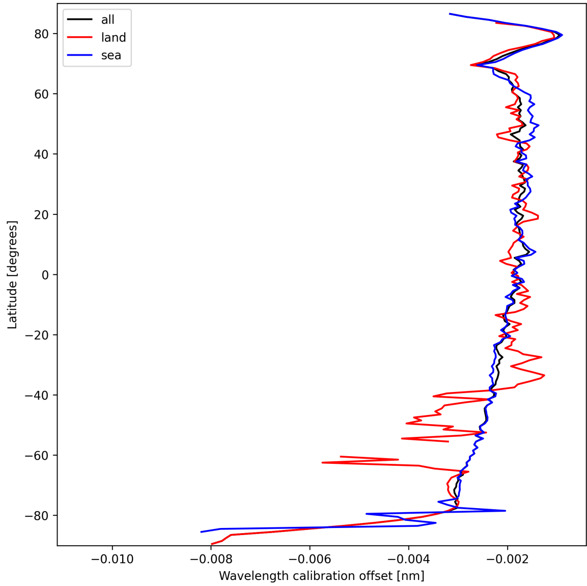
Figure 18: Zonal average of “Wavelength calibration offset” for 2025-03-16 to 2025-03-17.
