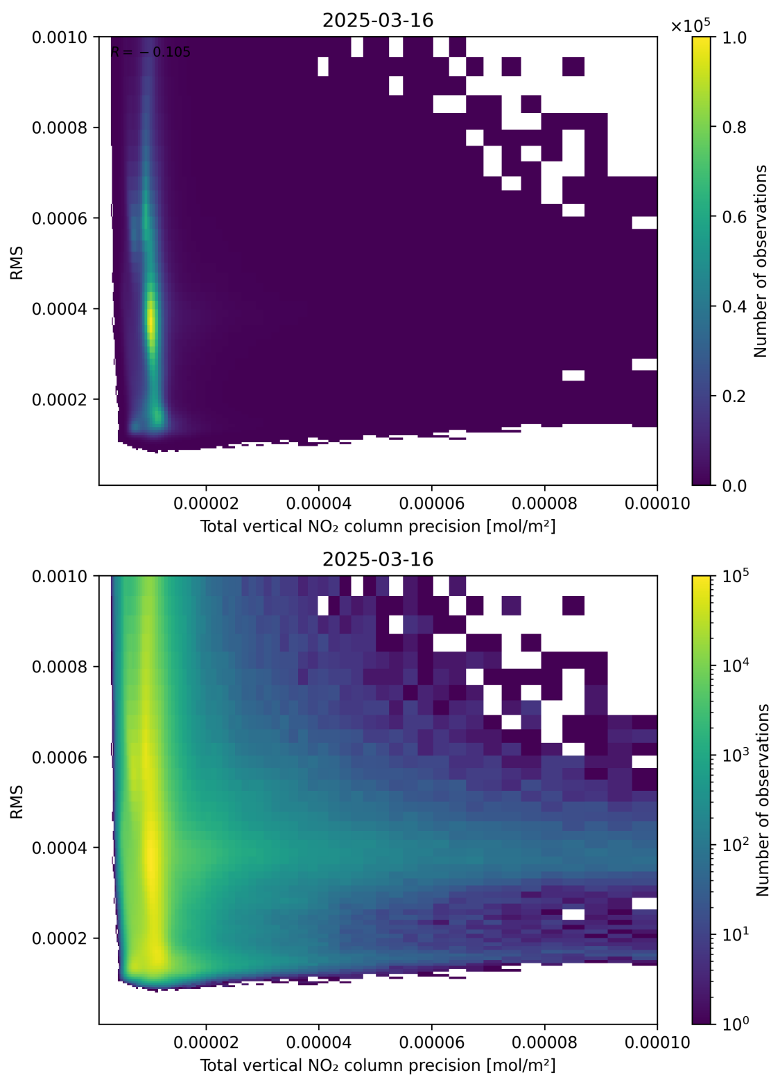
Figure 119: Scatter density plot of “Total vertical NO 2 column precision” against “RMS” for 2025-03-16 to 2025-03-17.
