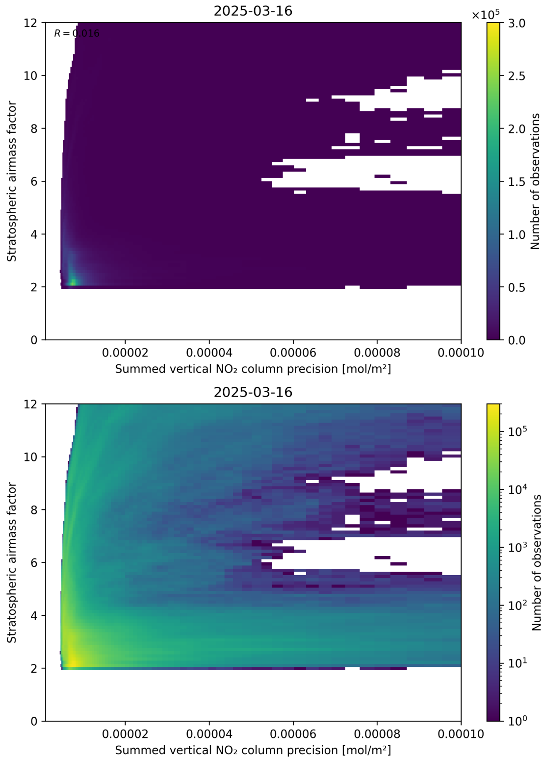
Figure 106: Scatter density plot of “Summed vertical NO 2 column precision” against “Stratospheric airmass factor” for 2025-03-16 to 2025-03-17.
