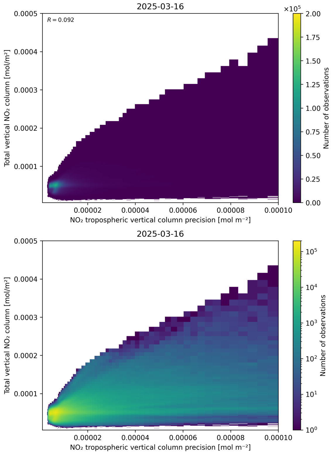
Figure 138: Scatter density plot of “NO 2 tropospheric vertical column precision” against “Total vertical NO 2 column” for 2025-03-16 to 2025-03-17.
