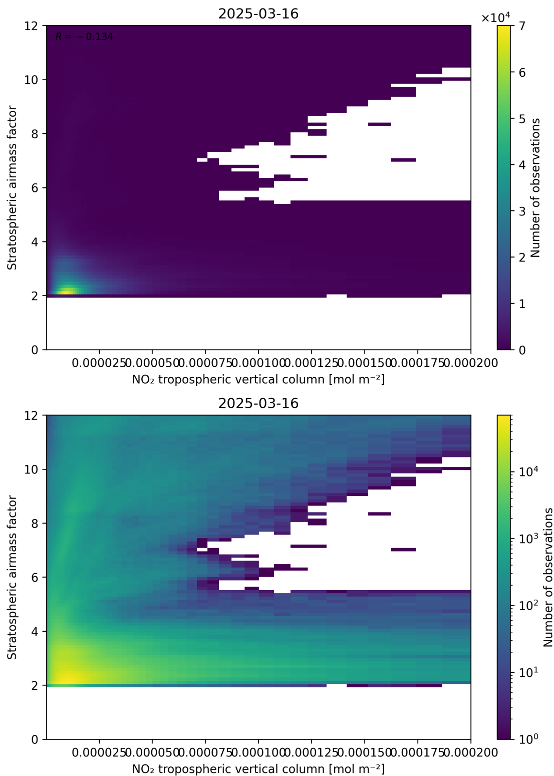
Figure 121: Scatter density plot of “NO 2 tropospheric vertical column” against “Stratospheric air mass factor” for 2025-03-16 to 2025-03-17.
