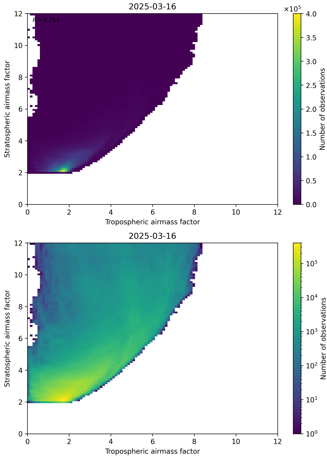
Figure 71: Scatter density plot of “Tropospheric airmass factor” against “Stratospheric airmass factor” for 2025-03-16 to 2025-03-17.
