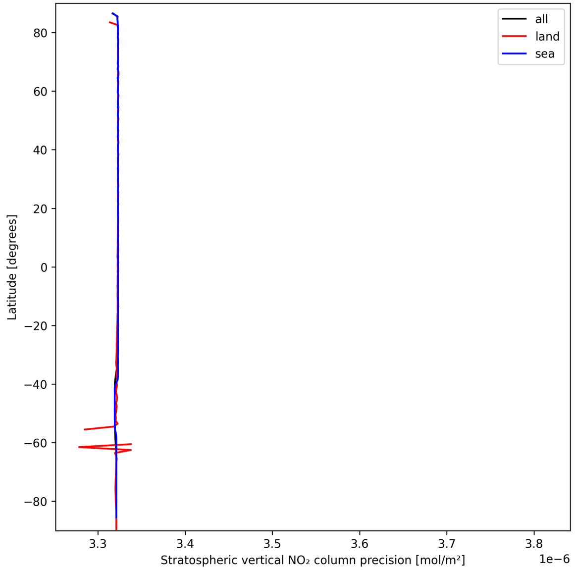
Figure 20: Zonal average of “Stratospheric vertical NO 2 column precision” for 2025-03-16 to 2025-03-17.
