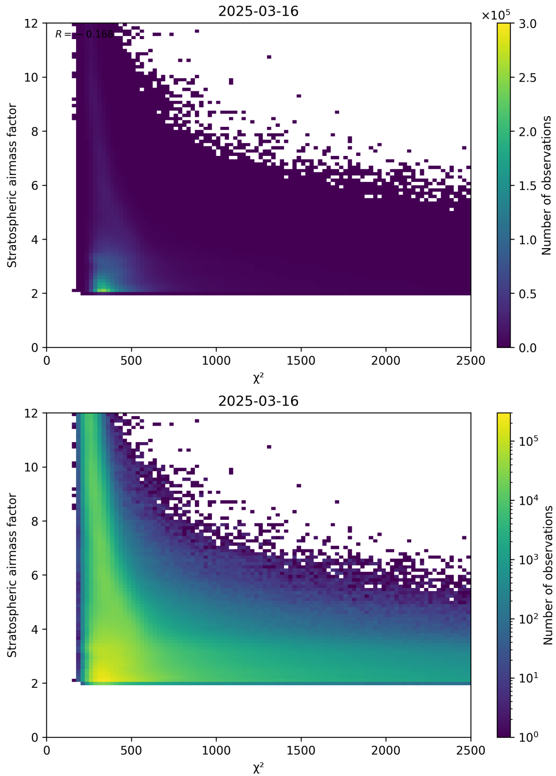
Figure 81: Scatter density plot of “ \chi^2 ” against “Stratospheric airmass factor” for 2025-03-16 to 2025-03-17.
