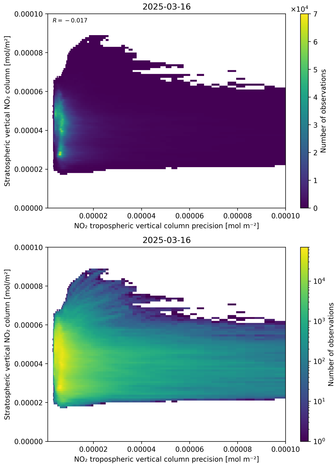
Figure 135: Scatter density plot of “NO 2 tropospheric vertical column precision” against “Stratospheric vertical NO 2 column” for 2025-03-16 to 2025-03-17.
