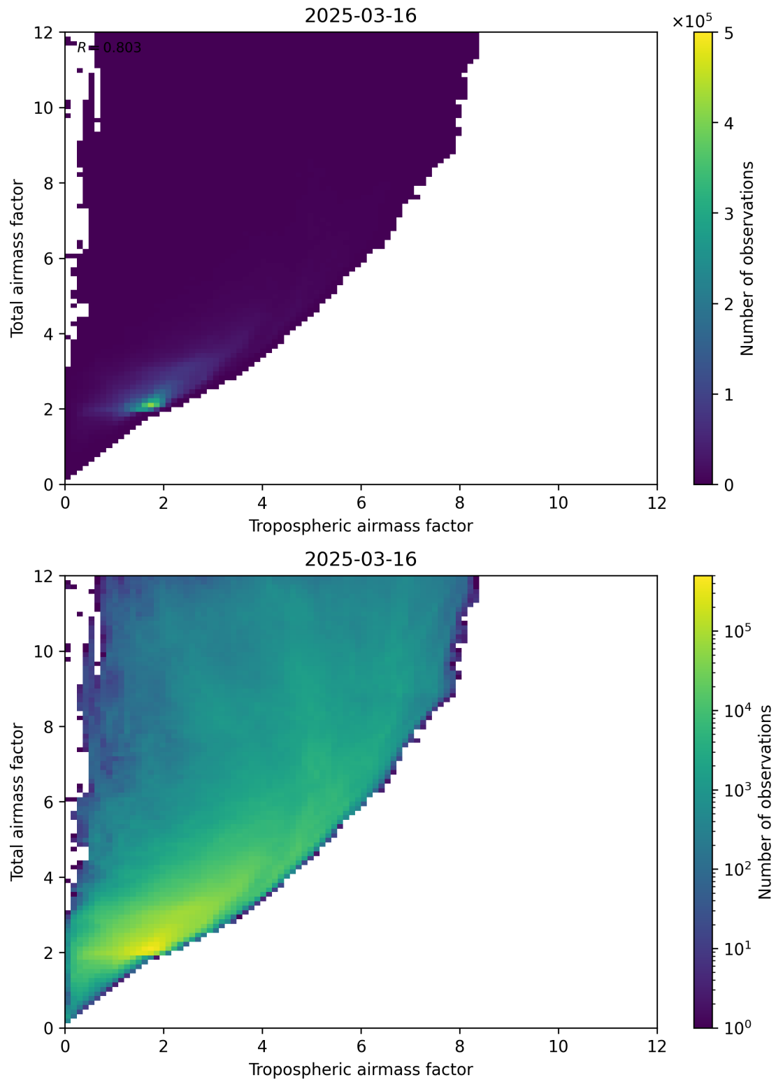
Figure 72: Scatter density plot of “Tropospheric airmass factor” against “Total airmass factor” for 2025-03-16 to 2025-03-17.
