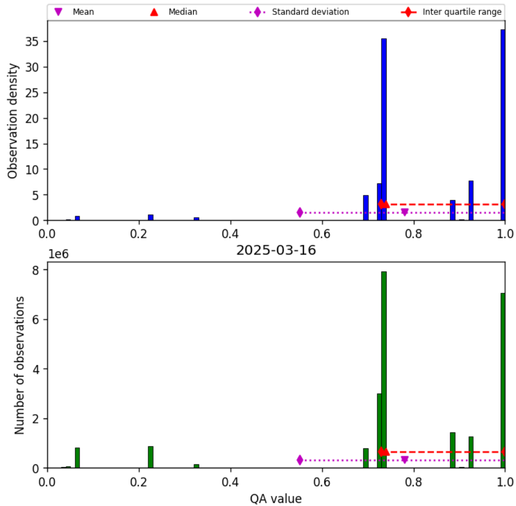
Figure 28: Histogram of “QA value” for 2025-03-16 to 2025-03-17
