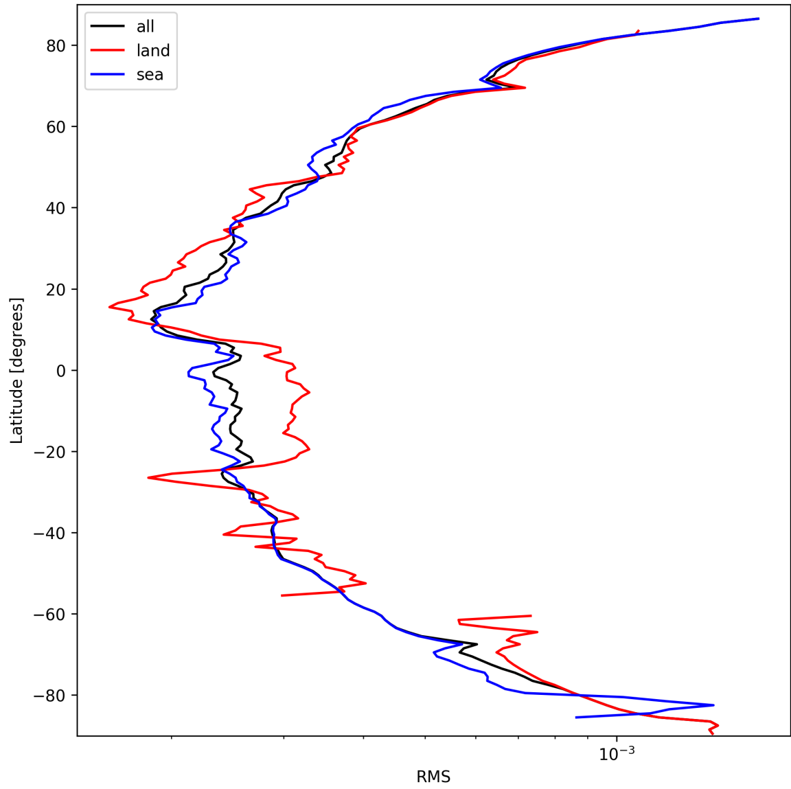
Figure 26: Zonal average of “RMS” for 2025-03-16 to 2025-03-17.
