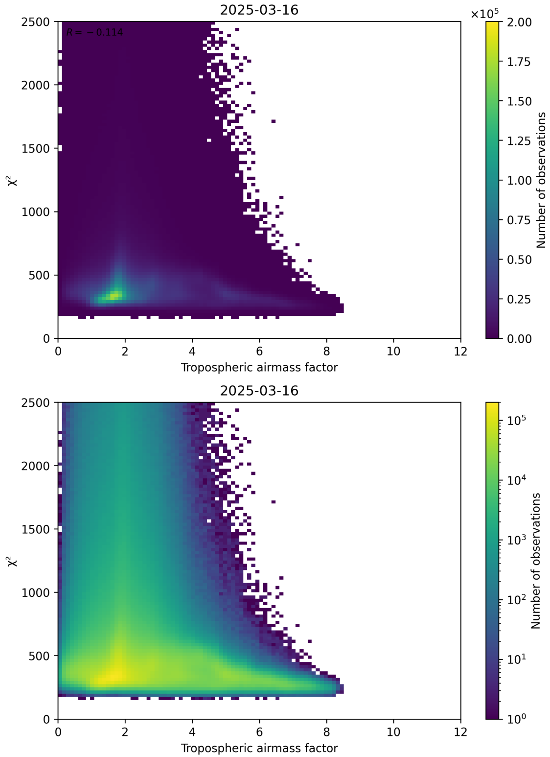
Figure 73: Scatter density plot of “Tropospheric airmass factor” against “ \chi^2 ” for 2025-03-16 to 2025-03-17.
