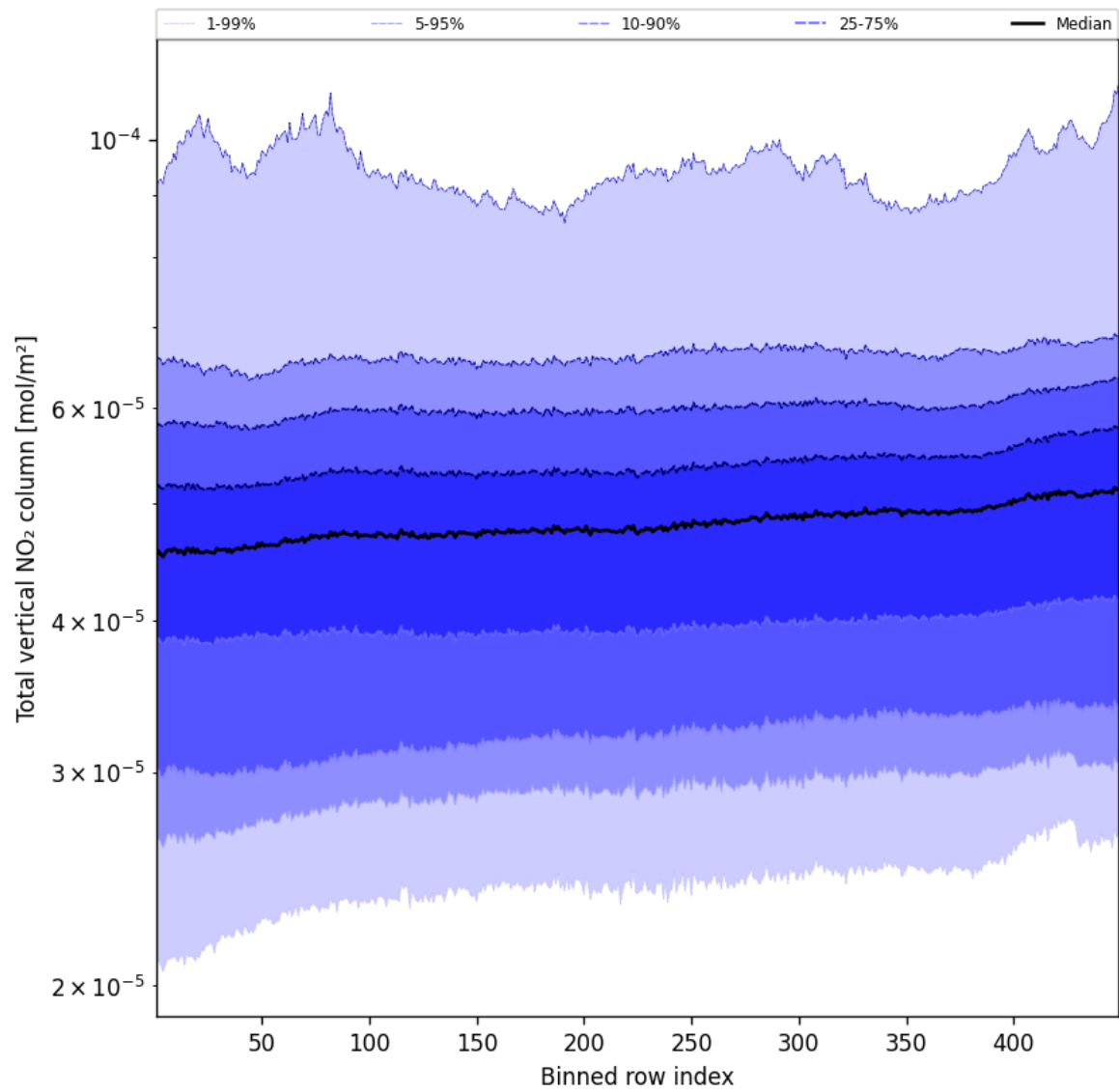
Figure 55: Along track statistics of “Total vertical NO 2 column” for 2025-03-16 to 2025-03-17
