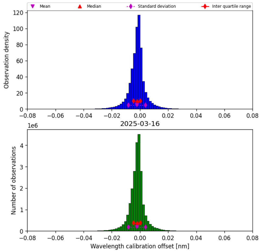
Figure 35: Histogram of “Wavelength calibration offset” for 2025-03-16 to 2025-03-17
