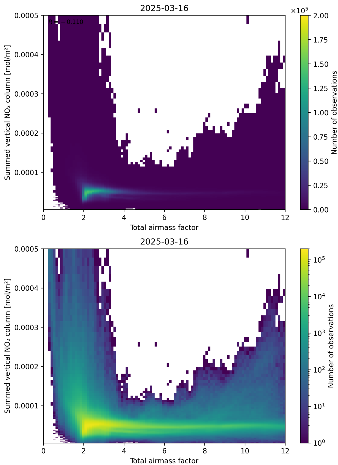
Figure 65: Scatter density plot of “Total airmass factor” against “Summed vertical NO 2 column” for 2025-03-16 to 2025-03-17.
