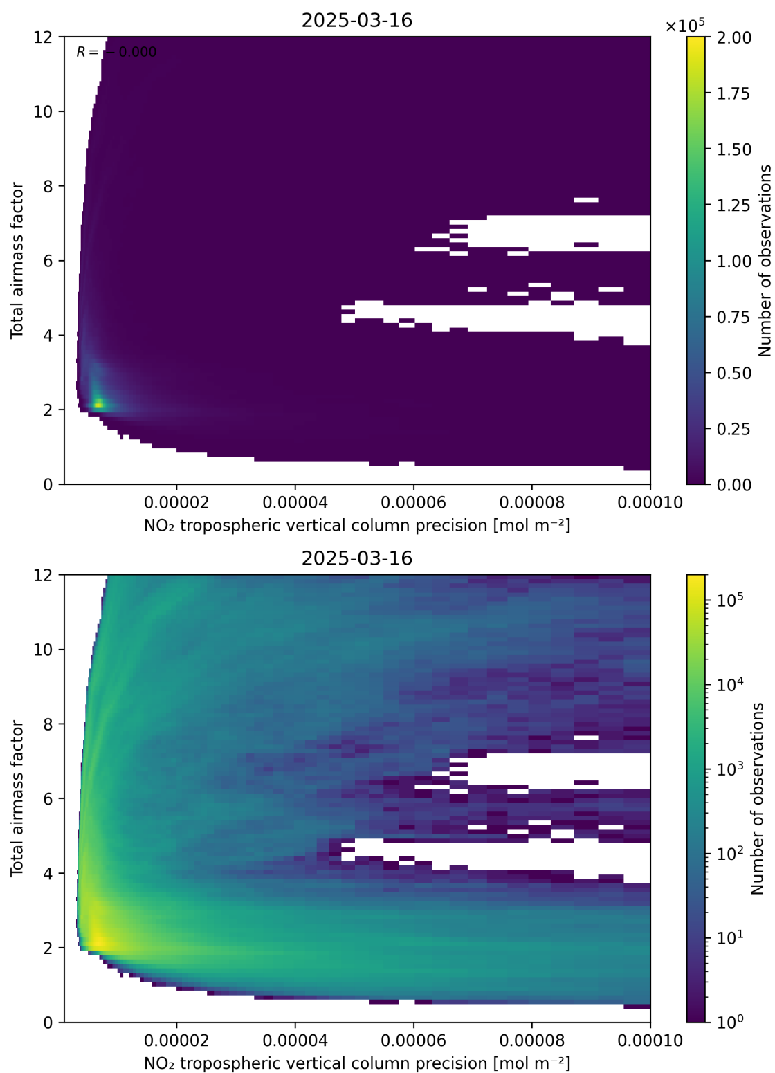
Figure 132: Scatter density plot of “NO 2 tropospheric vertical column precision” against “Total air mass factor” for 2025-03-16 to 2025-03-17.
