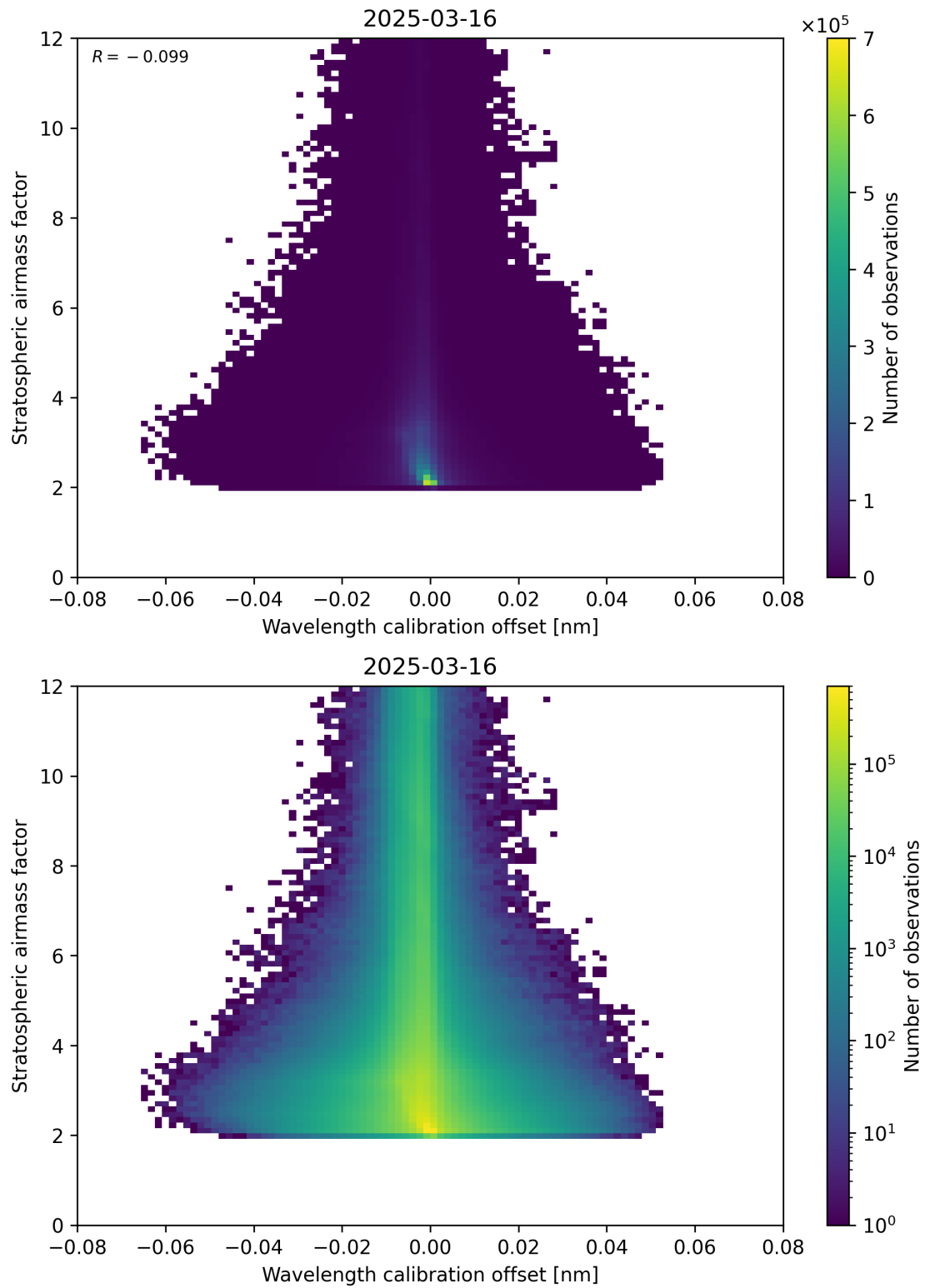
Figure 174: Scatter density plot of “Wavelength calibration offset” against “Stratospheric airmass factor” for 2025-03-16 to 2025-03-17.
