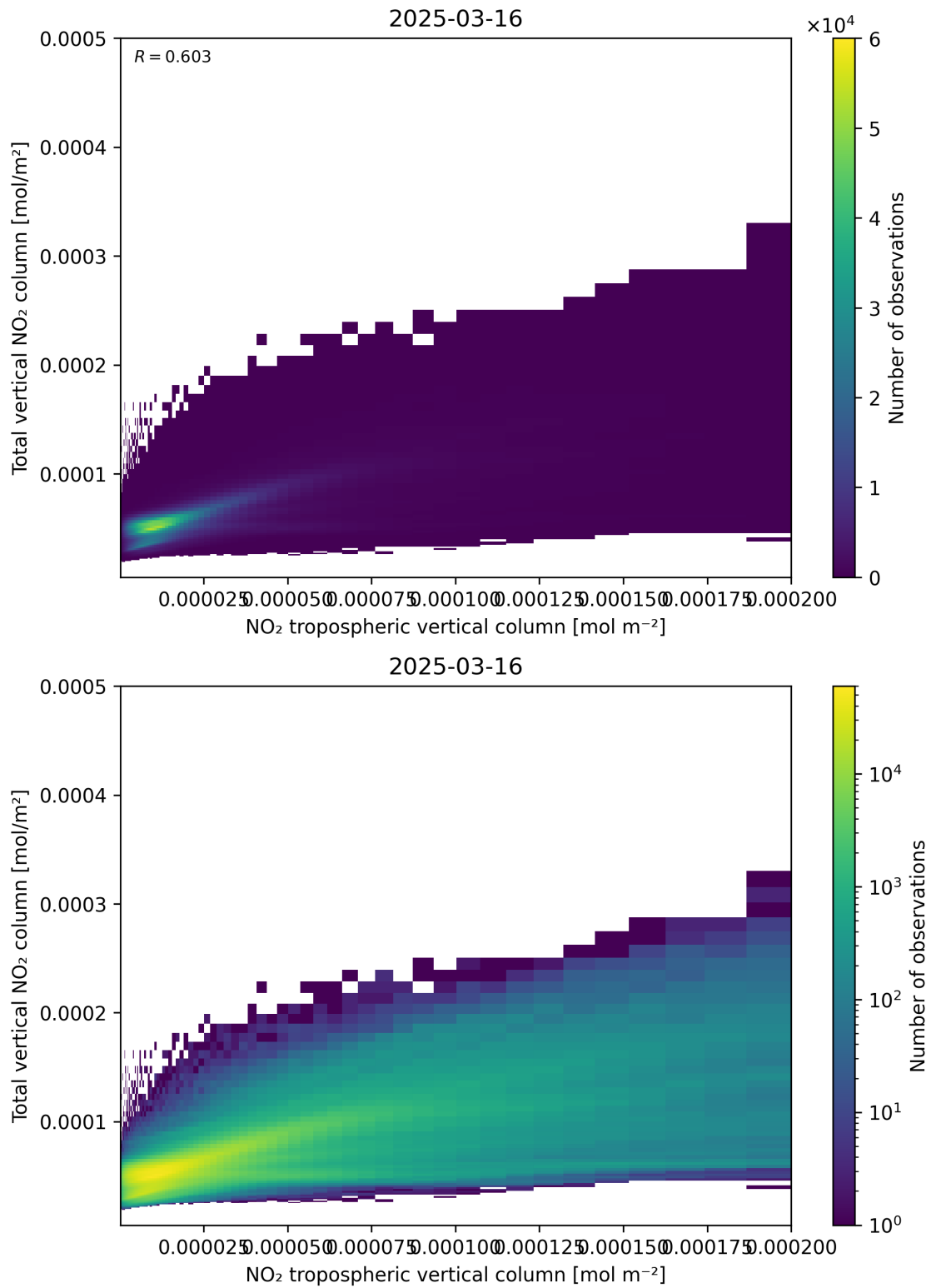
Figure 128: Scatter density plot of “NO 2 tropospheric vertical column” against “Total vertical NO 2 column” for 2025-03-16 to 2025-03-17.
