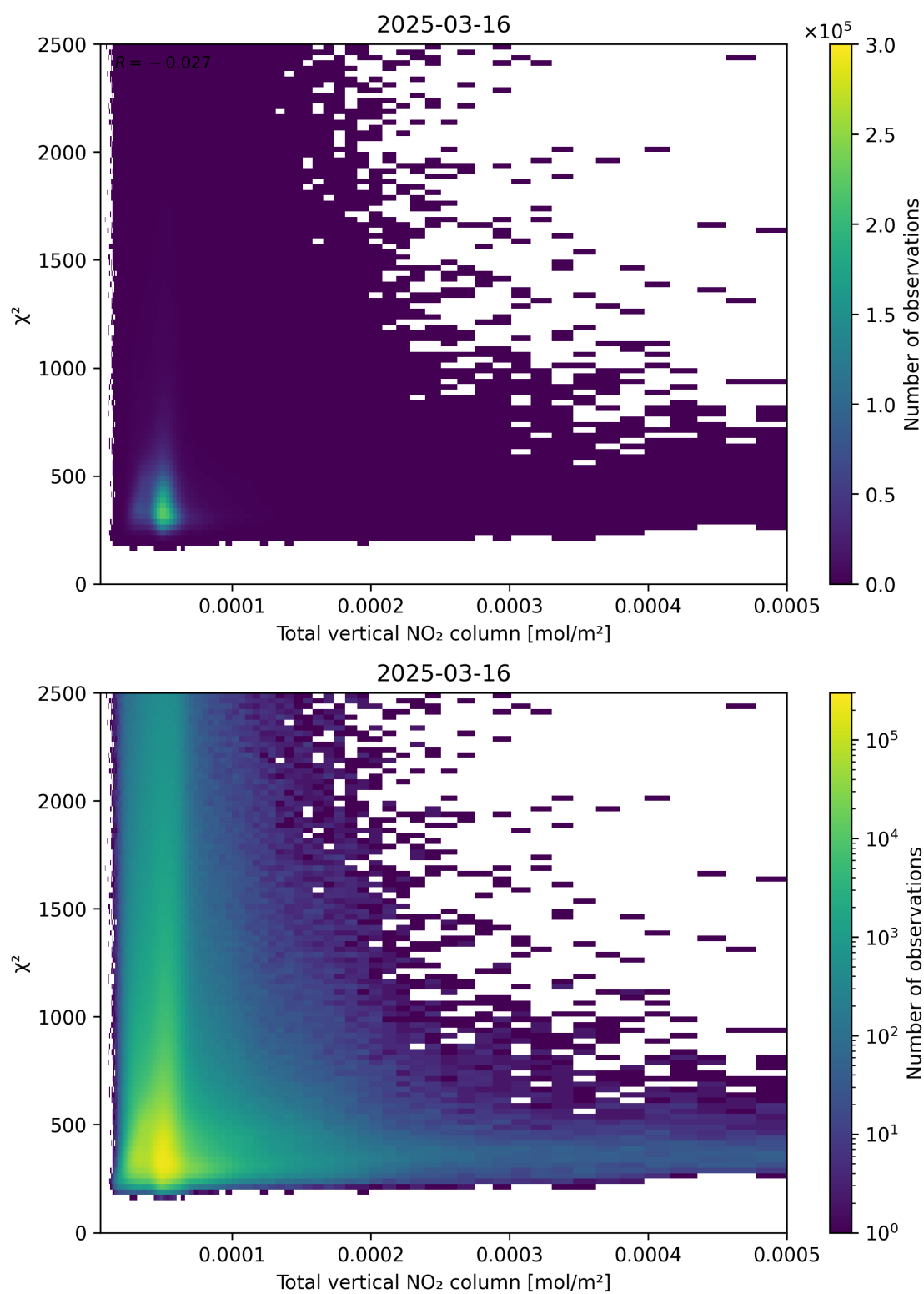
Figure 111: Scatter density plot of “Total vertical NO 2 column” against “ \chi^2 ” for 2025-03-16 to 2025-03-17.
