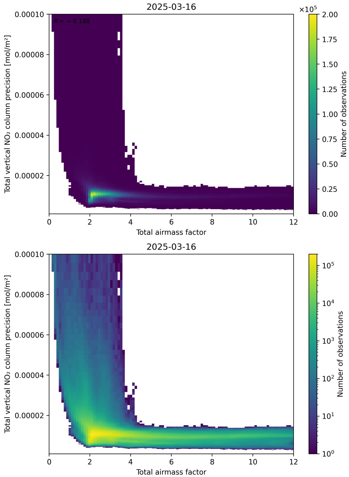
Figure 68: Scatter density plot of “Total airmass factor” against “Total vertical NO 2 column precision” for 2025-03-16 to 2025-03-17.
