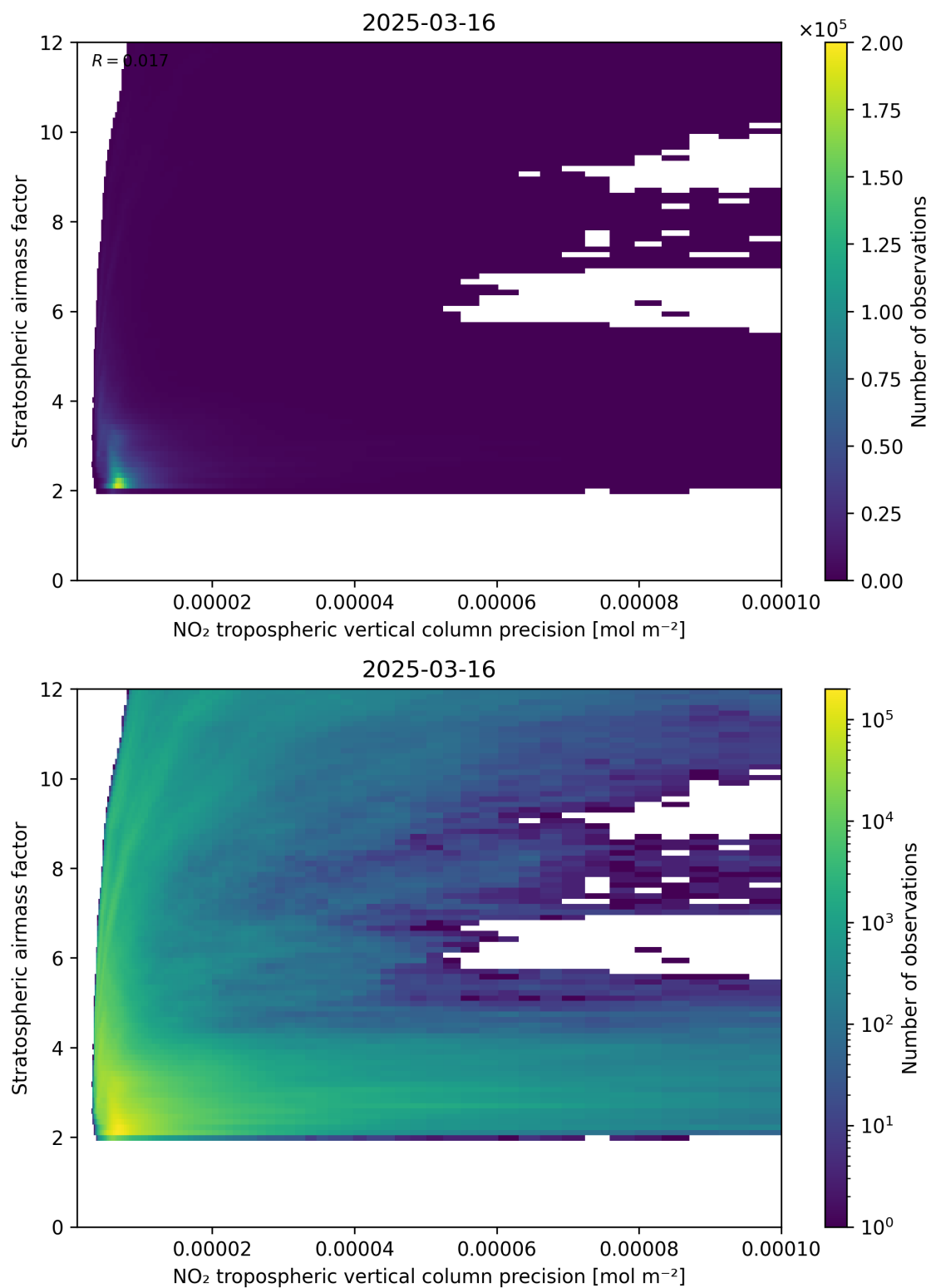
Figure 131: Scatter density plot of “NO 2 tropospheric vertical column precision” against “Stratospheric airmass factor” for 2025-03-16 to 2025-03-17.
