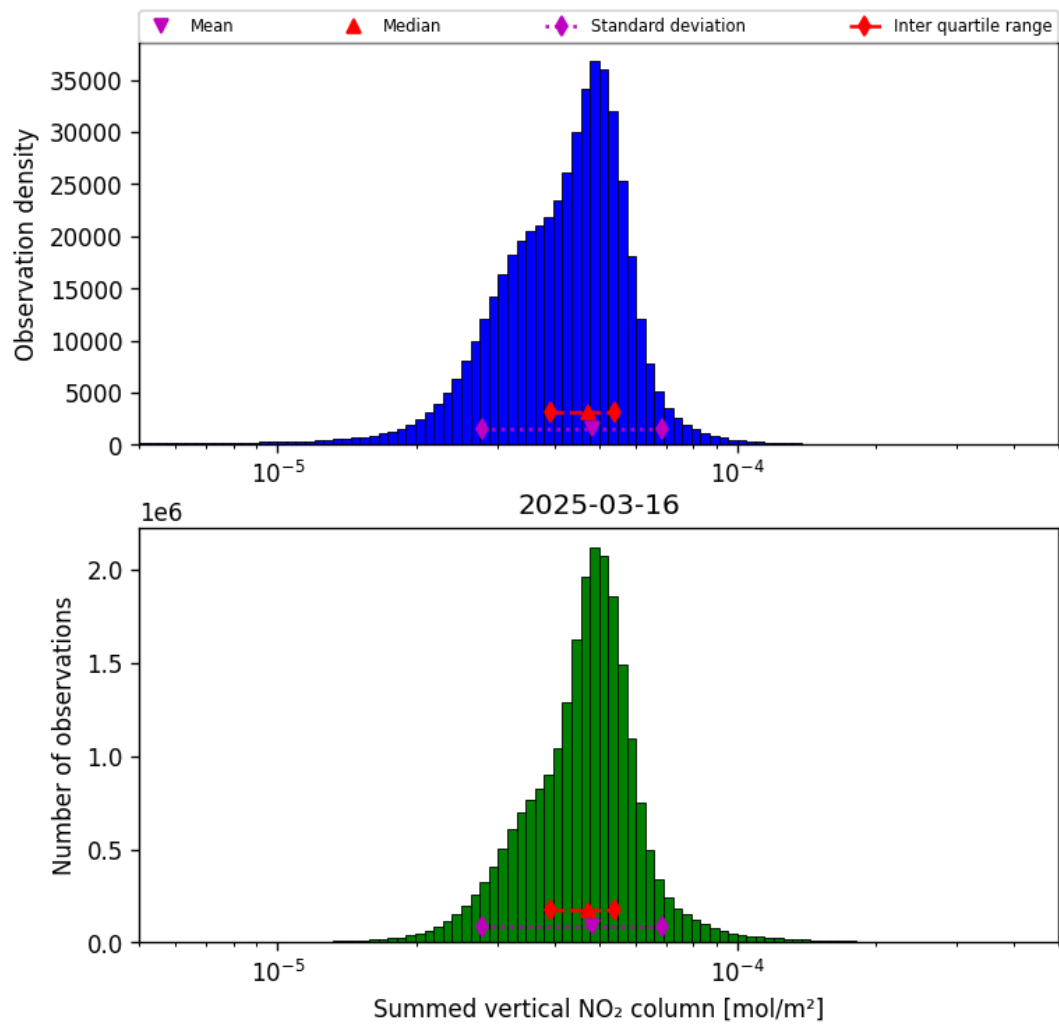
Figure 40: Histogram of “Summed vertical NO 2 column” for 2025-03-16 to 2025-03-17
