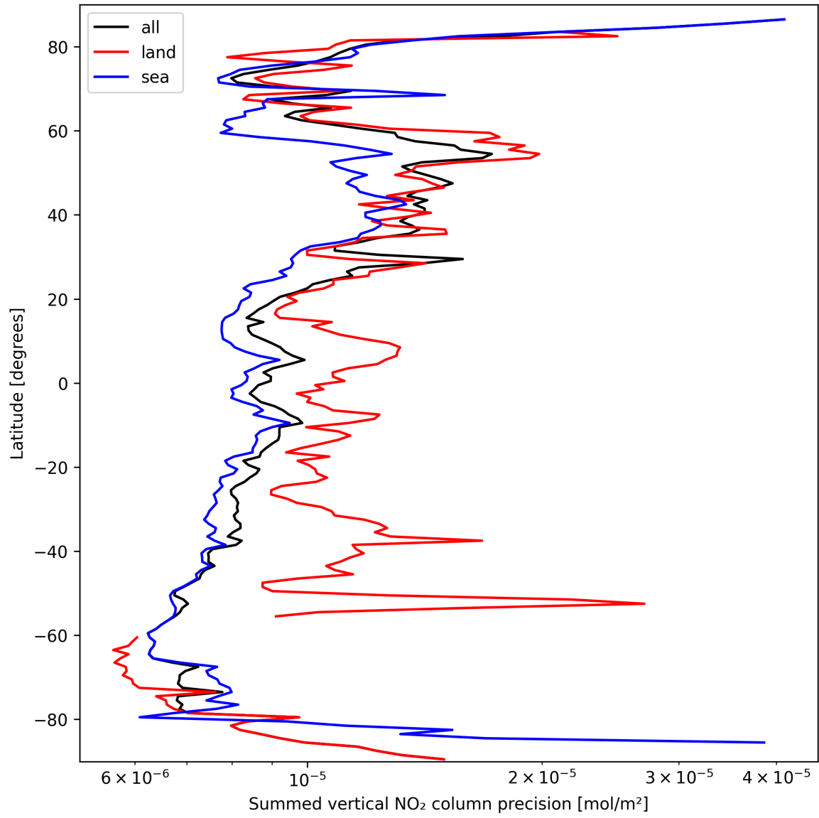
Figure 24: Zonal average of “Summed vertical NO 2 column precision” for 2025-03-16 to 2025-03-17.
