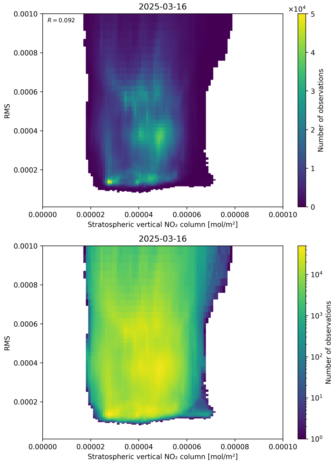
Figure 102: Scatter density plot of “Stratospheric vertical NO 2 column” against “RMS” for 2025-03-16 to 2025-03-17.
