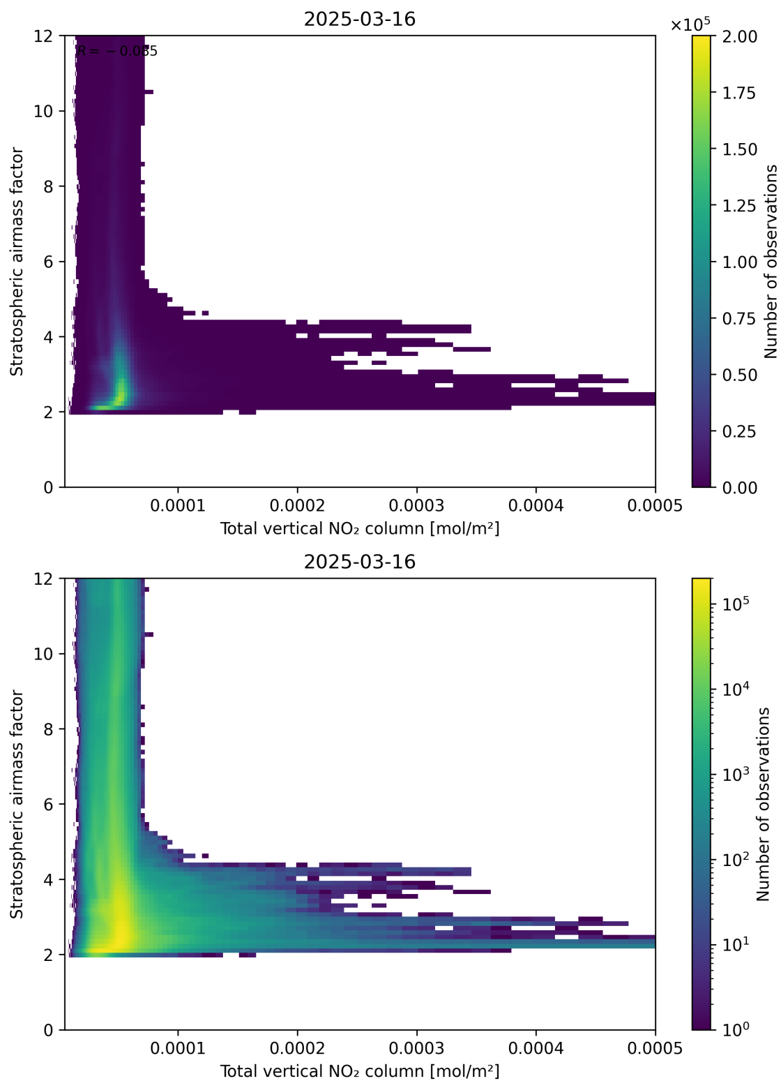
Figure 110: Scatter density plot of “Total vertical NO 2 column” against “Stratospheric airmass factor” for 2025-03-16 to 2025-03-17.
