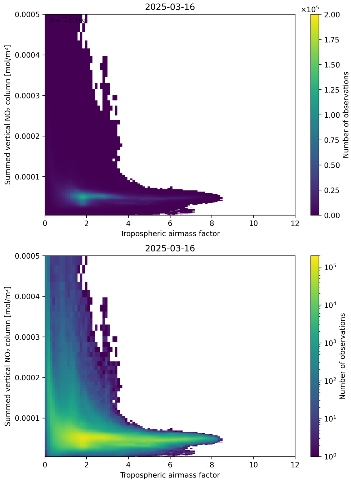
Figure 75: Scatter density plot of “Tropospheric air mass factor” against “Summed vertical NO 2 column” for 2025-03-16 to 2025-03-17.
