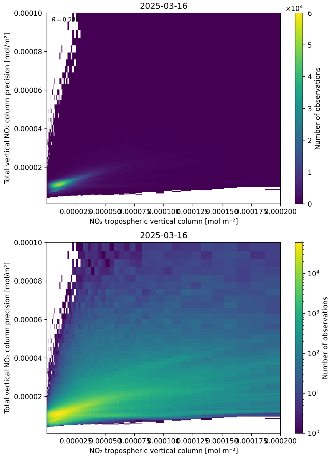
Figure 129: Scatter density plot of “NO 2 tropospheric vertical column” against “Total vertical NO 2 column precision” for 2025-03-16 to 2025-03-17.
