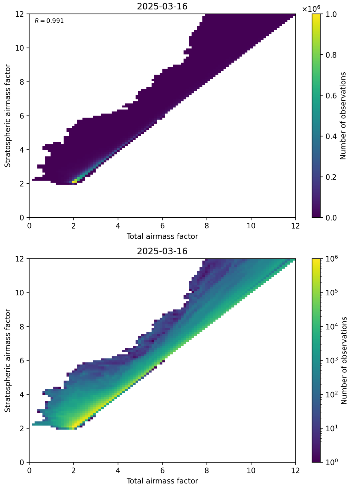
Figure 62: Scatter density plot of “Total airmass factor” against “Stratospheric airmass factor” for 2025-03-16 to 2025-03-17.
