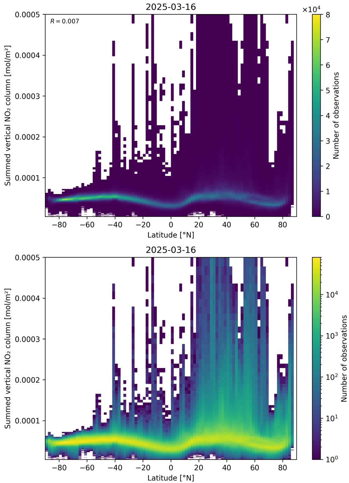
Figure 88: Scatter density plot of “Latitude” against “Summed vertical NO 2 column” for 2025-03-16 to 2025-03-17.
