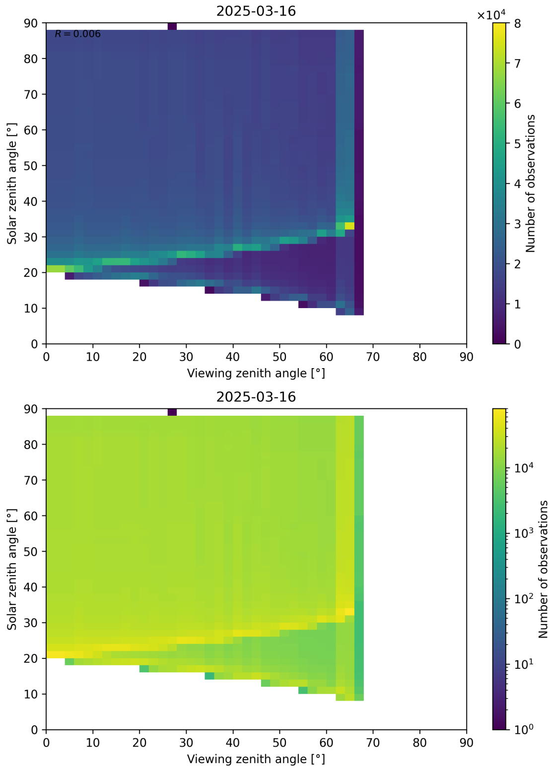
Figure 172: Scatter density plot of “Viewing zenith angle” against “Solar zenith angle” for 2025-03-16 to 2025-03-17.
