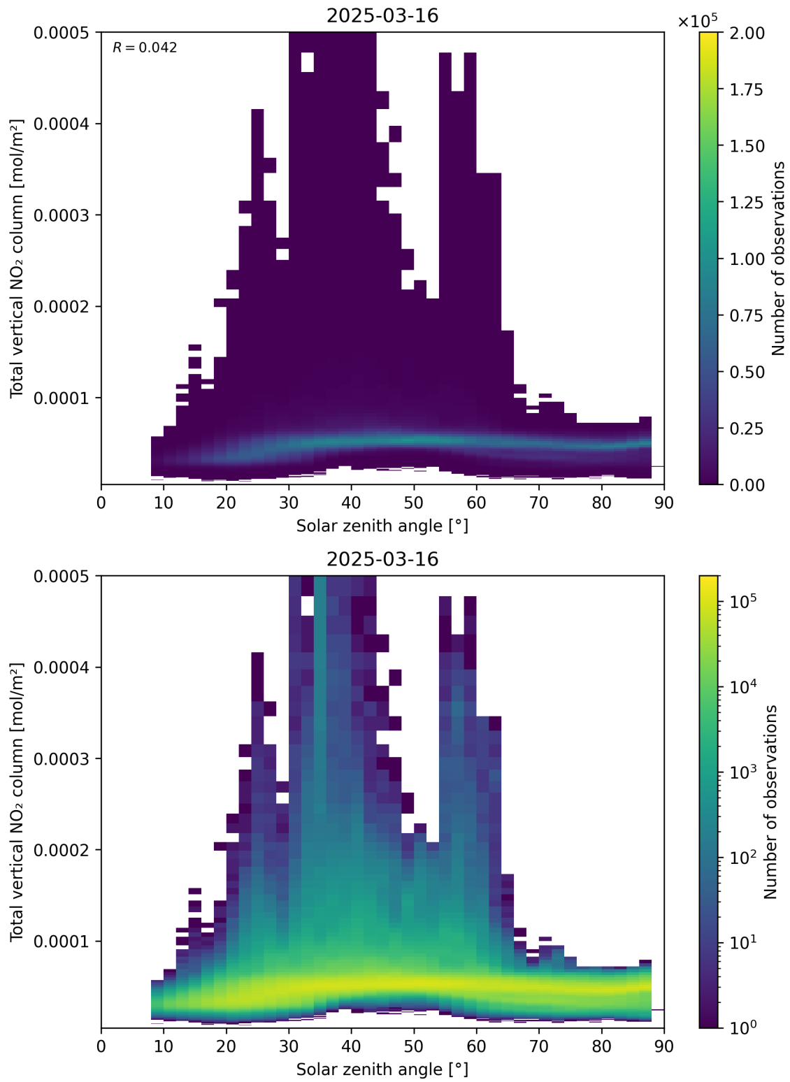
Figure 153: Scatter density plot of “Solar zenith angle” against “Total vertical NO 2 column” for 2025-03-16 to 2025-03-17.
