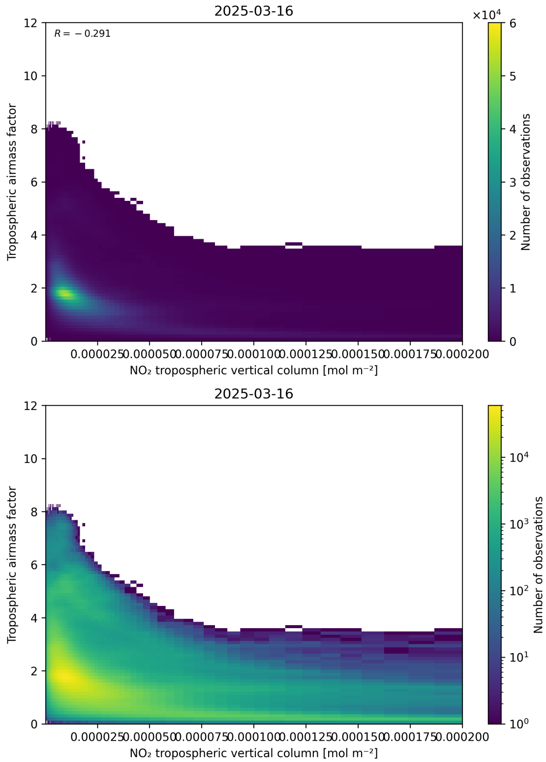
Figure 123: Scatter density plot of “NO 2 tropospheric vertical column” against “Tropospheric air mass factor” for 2025-03-16 to 2025-03-17.
