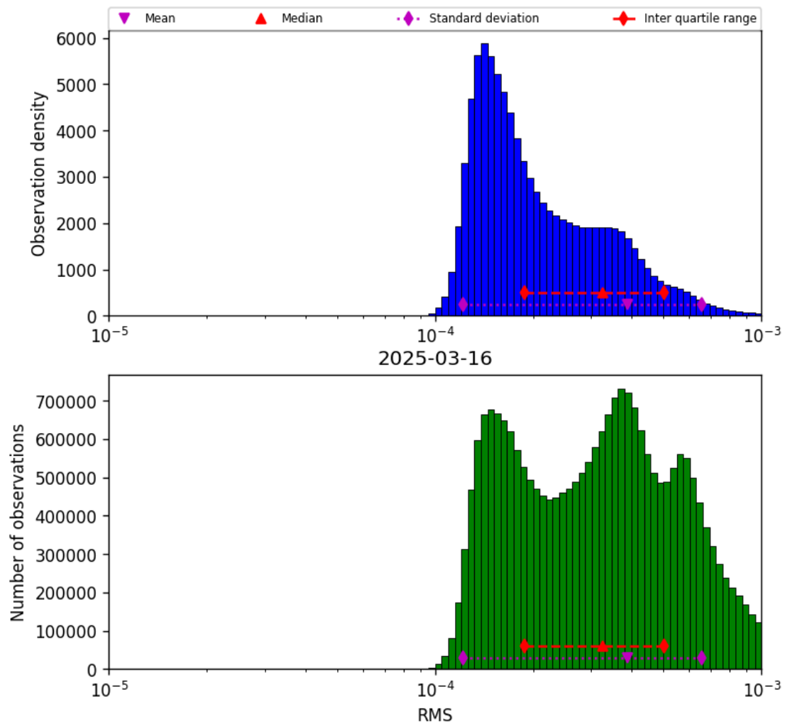
Figure 43: Histogram of “RMS” for 2025-03-16 to 2025-03-17
