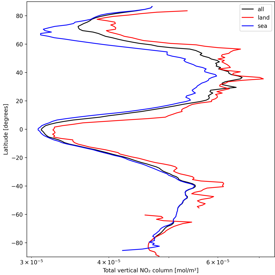
Figure 21: Zonal average of “Total vertical NO 2 column” for 2025-03-16 to 2025-03-17.
