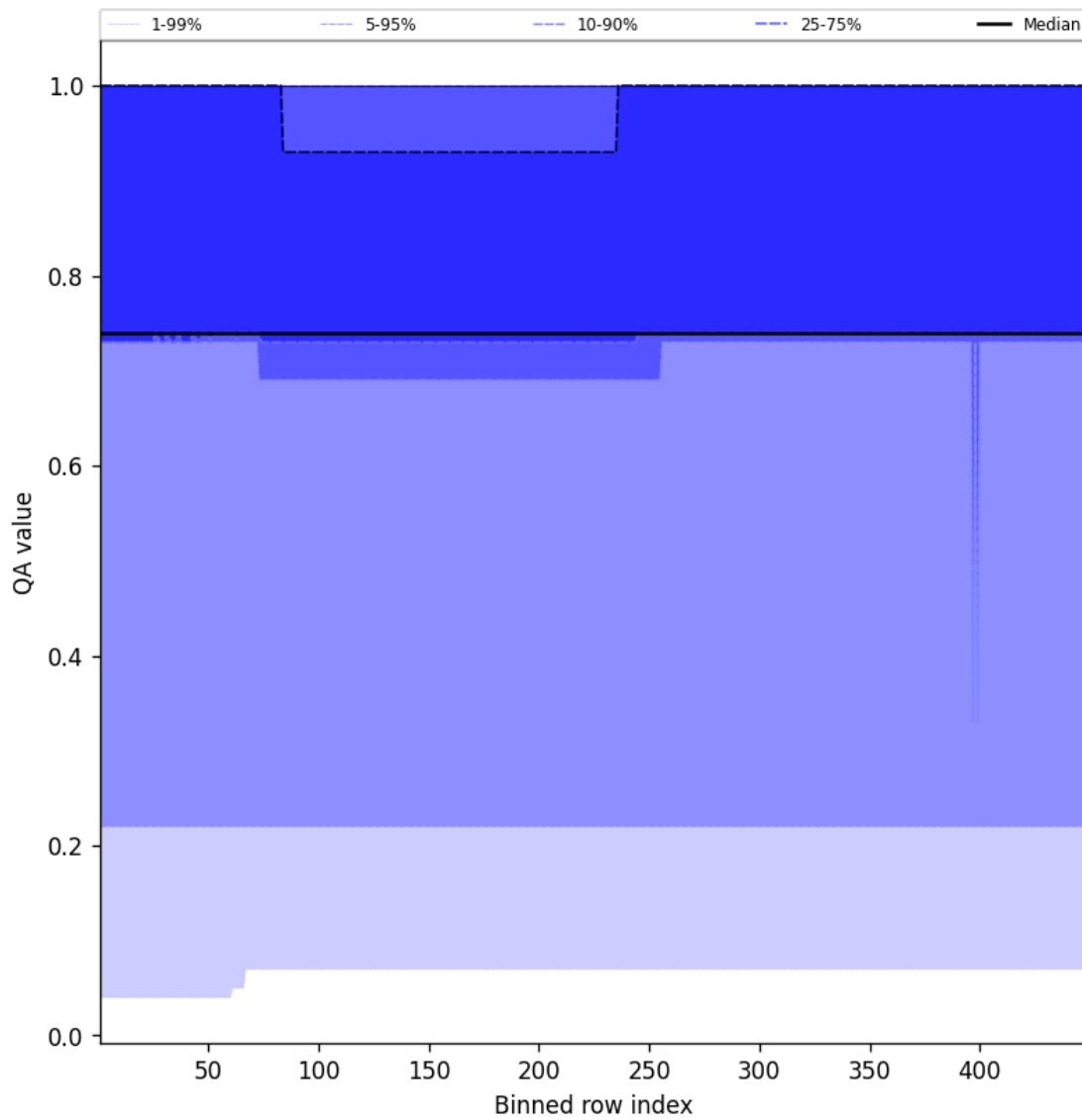
Figure 45: Along track statistics of “QA value” for 2025-03-16 to 2025-03-17
