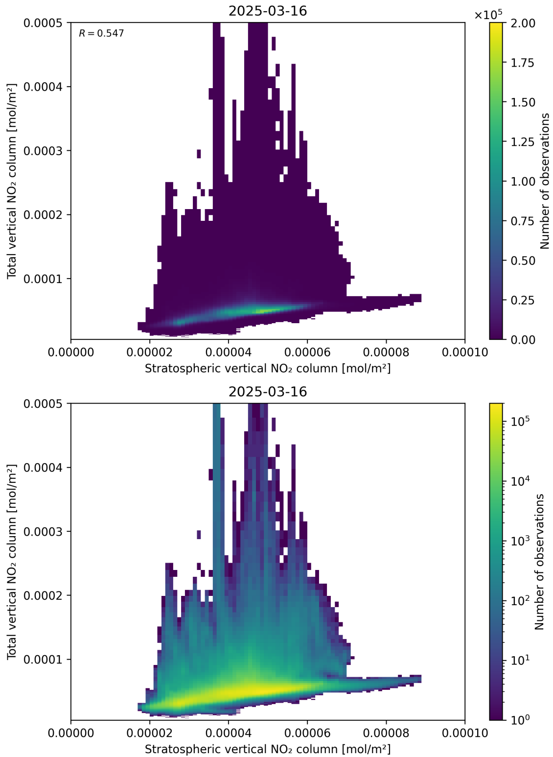
Figure 100: Scatter density plot of “Stratospheric vertical NO 2 column” against “Total vertical NO 2 column” for 2025-03-16 to 2025-03-17.
