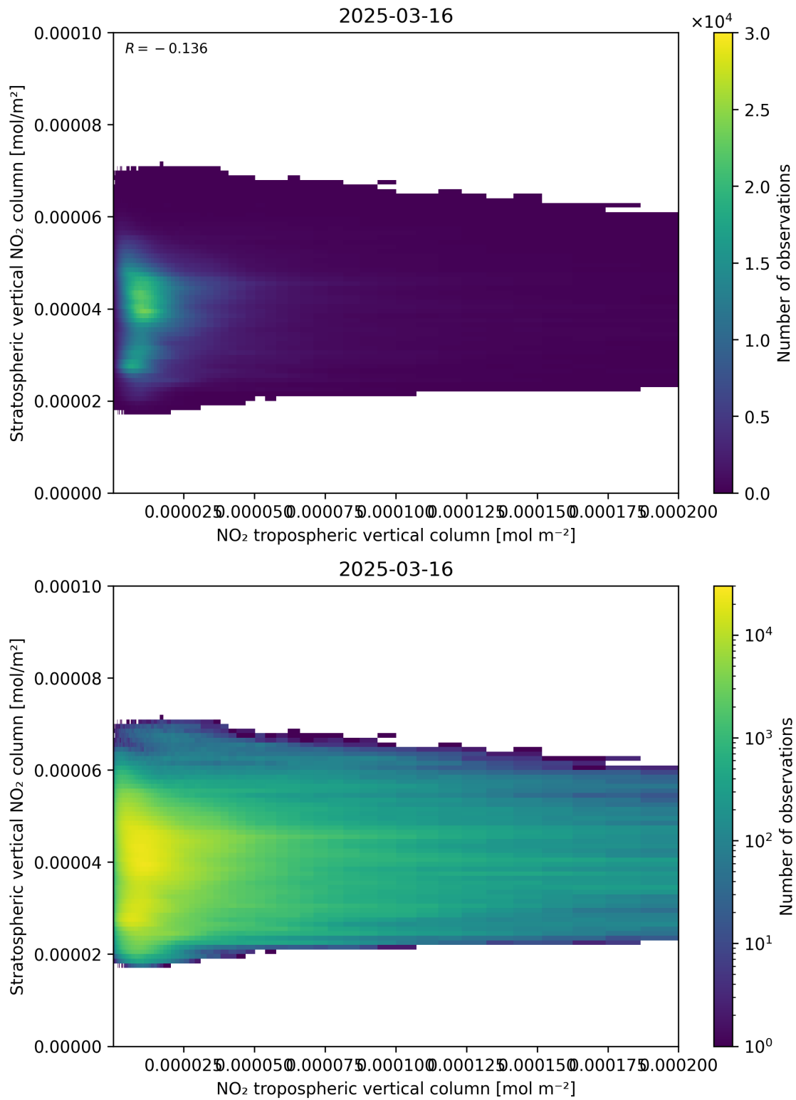
Figure 125: Scatter density plot of “NO 2 tropospheric vertical column” against “Stratospheric vertical NO 2 column” for 2025-03-16 to 2025-03-17.
