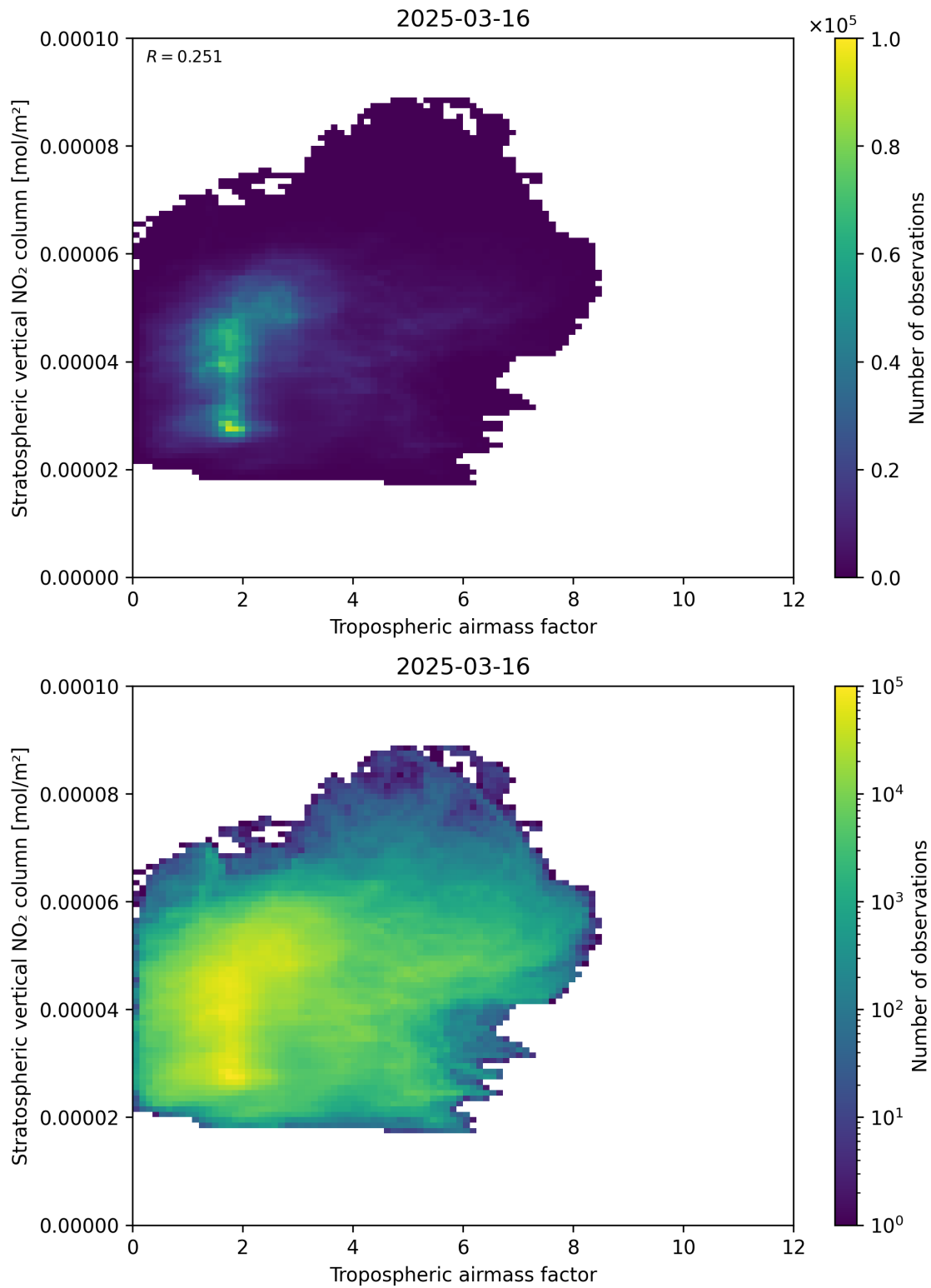
Figure 74: Scatter density plot of “Tropospheric air mass factor” against “Stratospheric vertical NO 2 column” for 2025-03-16 to 2025-03-17.
