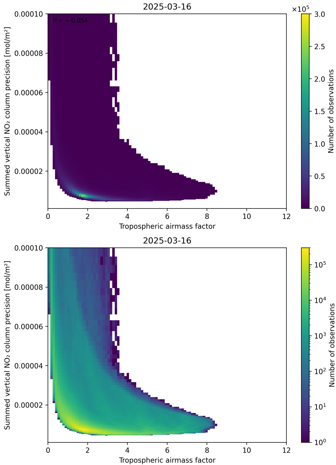
Figure 76: Scatter density plot of “Tropospheric air mass factor” against “Summed vertical NO 2 column precision” for 2025-03-16 to 2025-03-17.
