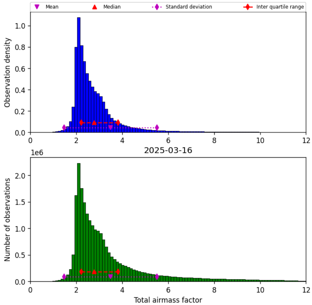
Figure 32: Histogram of “Total airmass factor” for 2025-03-16 to 2025-03-17
