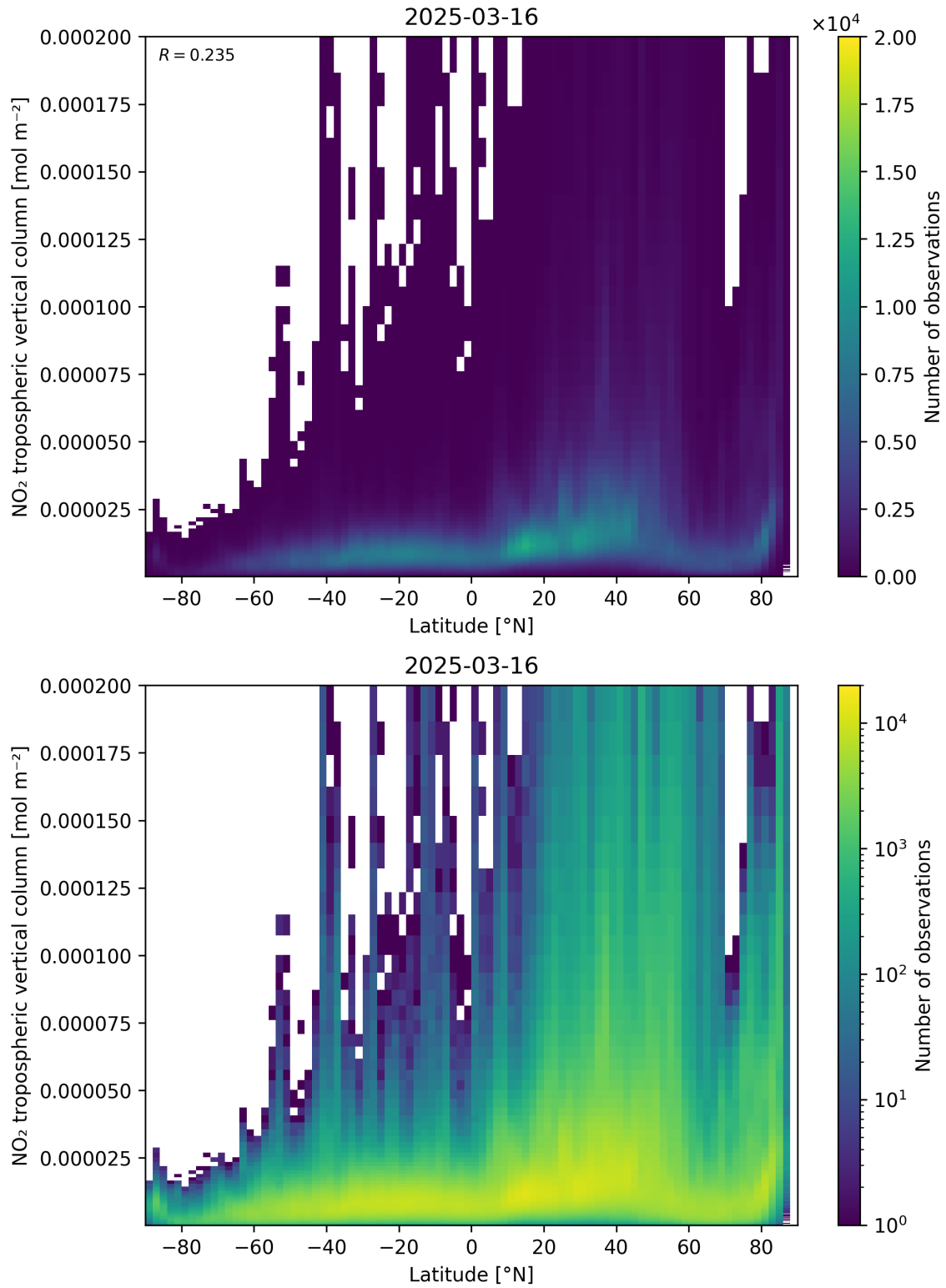
Figure 92: Scatter density plot of “Latitude” against “NO 2 tropospheric vertical column” for 2025-03-16 to 2025-03-17.
