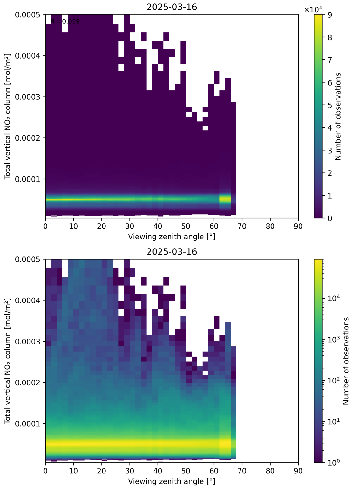
Figure 167: Scatter density plot of “Viewing zenith angle” against “Total vertical NO 2 column” for 2025-03-16 to 2025-03-17.
