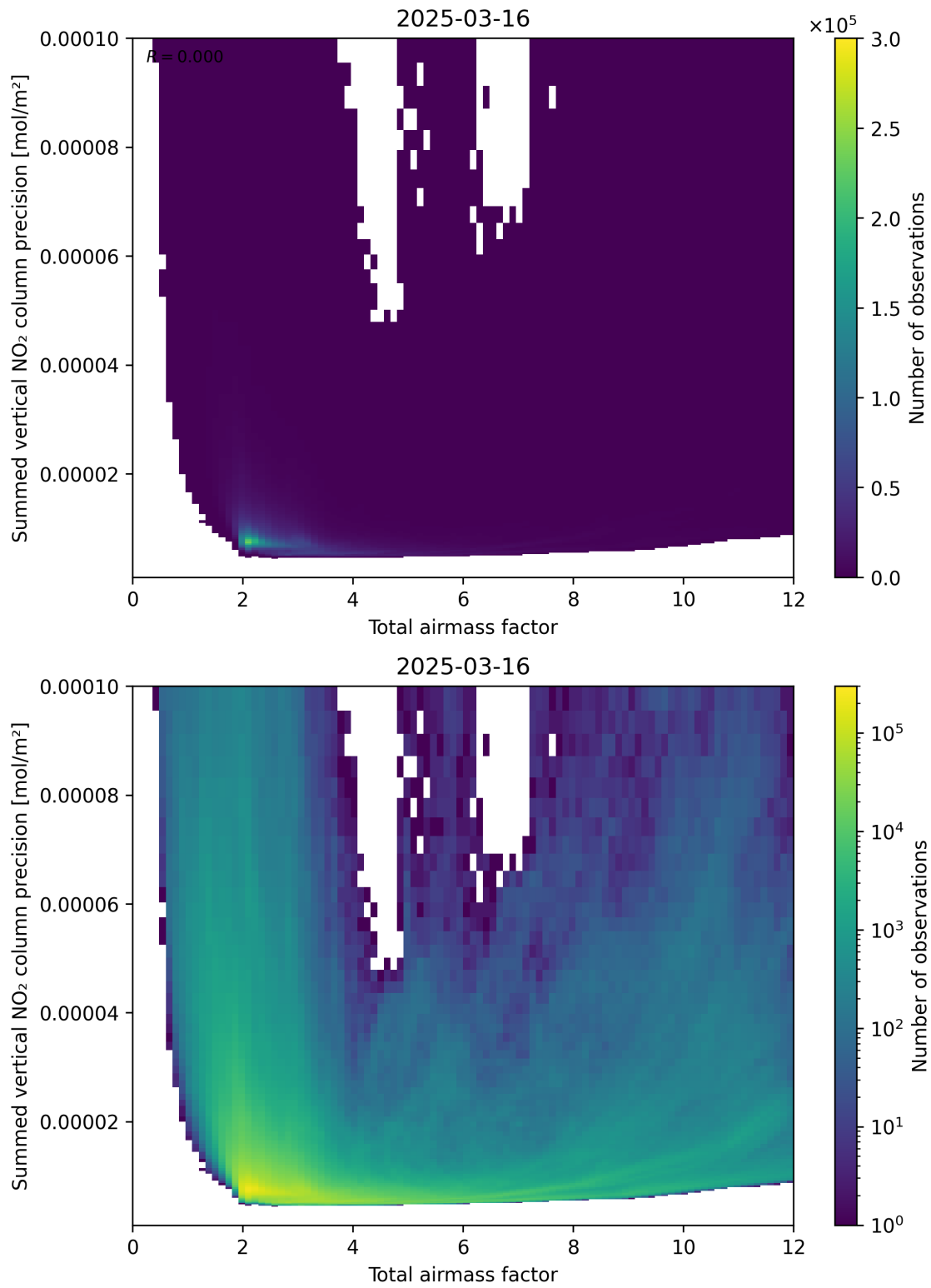
Figure 66: Scatter density plot of “Total airmass factor” against “Summed vertical NO 2 column precision” for 2025-03-16 to 2025-03-17.
