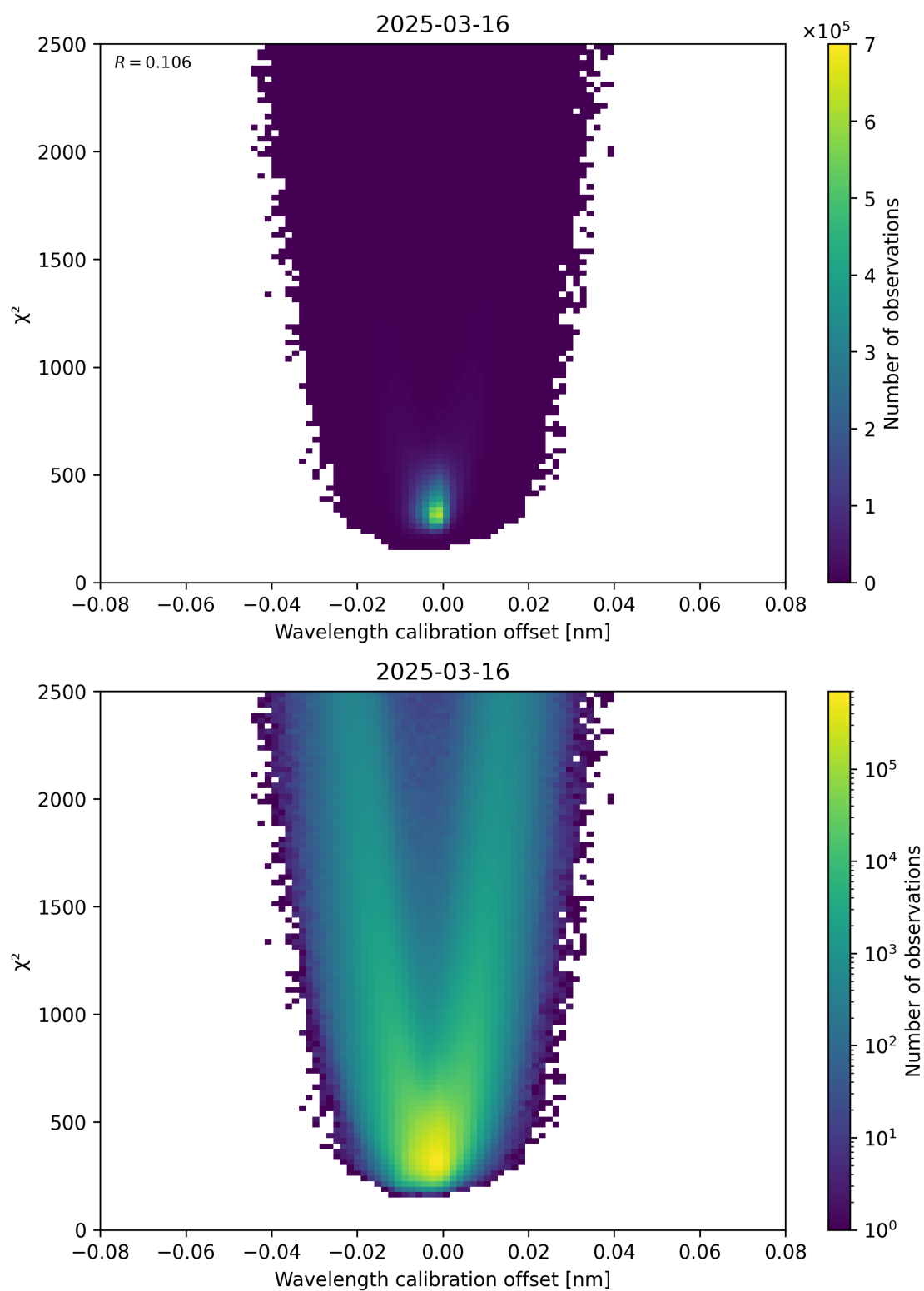
Figure 175: Scatter density plot of “Wavelength calibration offset” against “ \chi^2 ” for 2025-03-16 to 2025-03-17.
