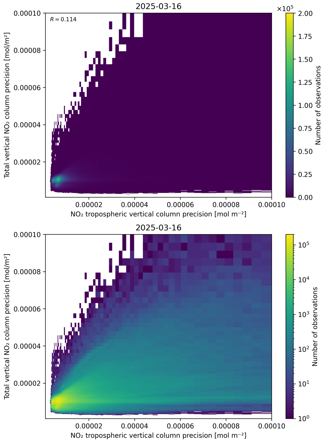
Figure 139: Scatter density plot of “NO 2 tropospheric vertical column precision” against “Total vertical NO 2 column precision” for 2025-03-16 to 2025-03-17.
