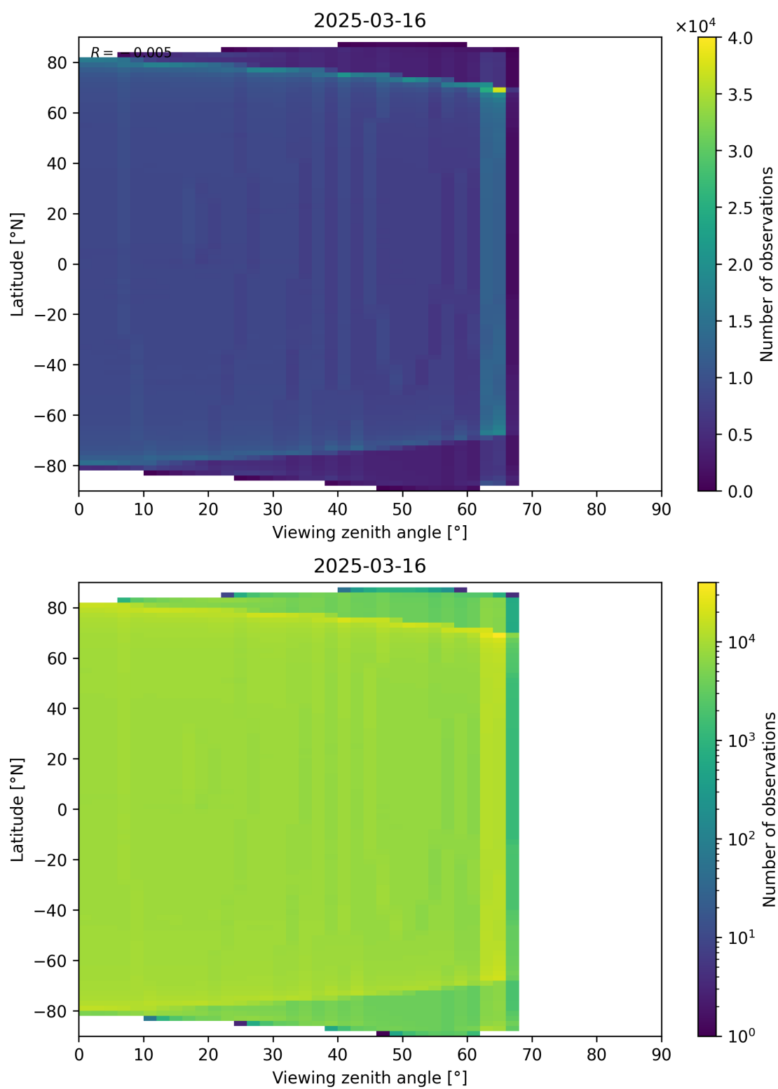
Figure 163: Scatter density plot of “Viewing zenith angle” against “Latitude” for 2025-03-16 to 2025-03-17.
