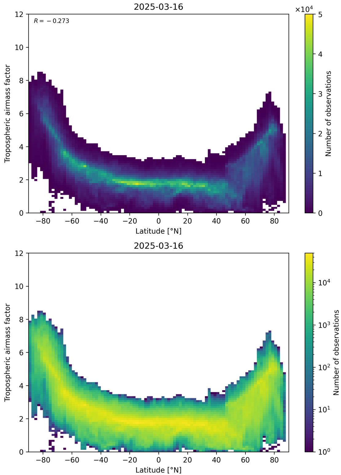
Figure 85: Scatter density plot of “Latitude” against “Tropospheric airmass factor” for 2025-03-16 to 2025-03-17.
