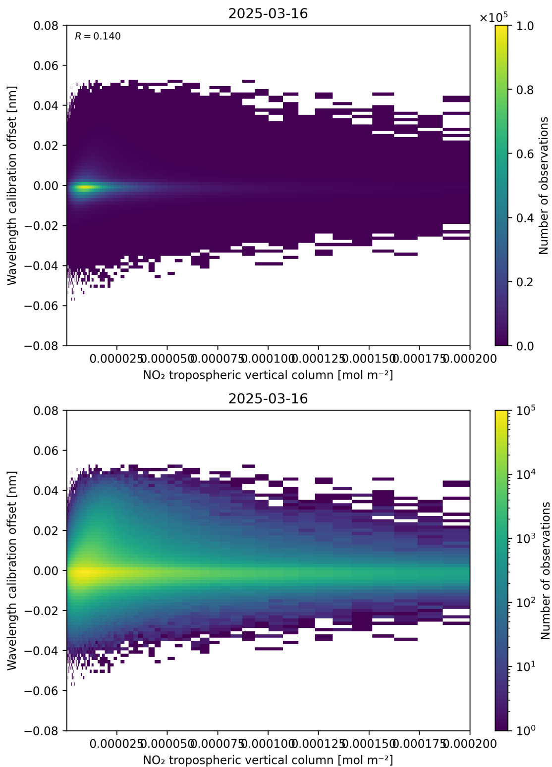
Figure 143: Scatter density plot of “NO 2 tropospheric vertical column” against “Wavelength calibration offset” for 2025-03-16 to 2025-03-17.
