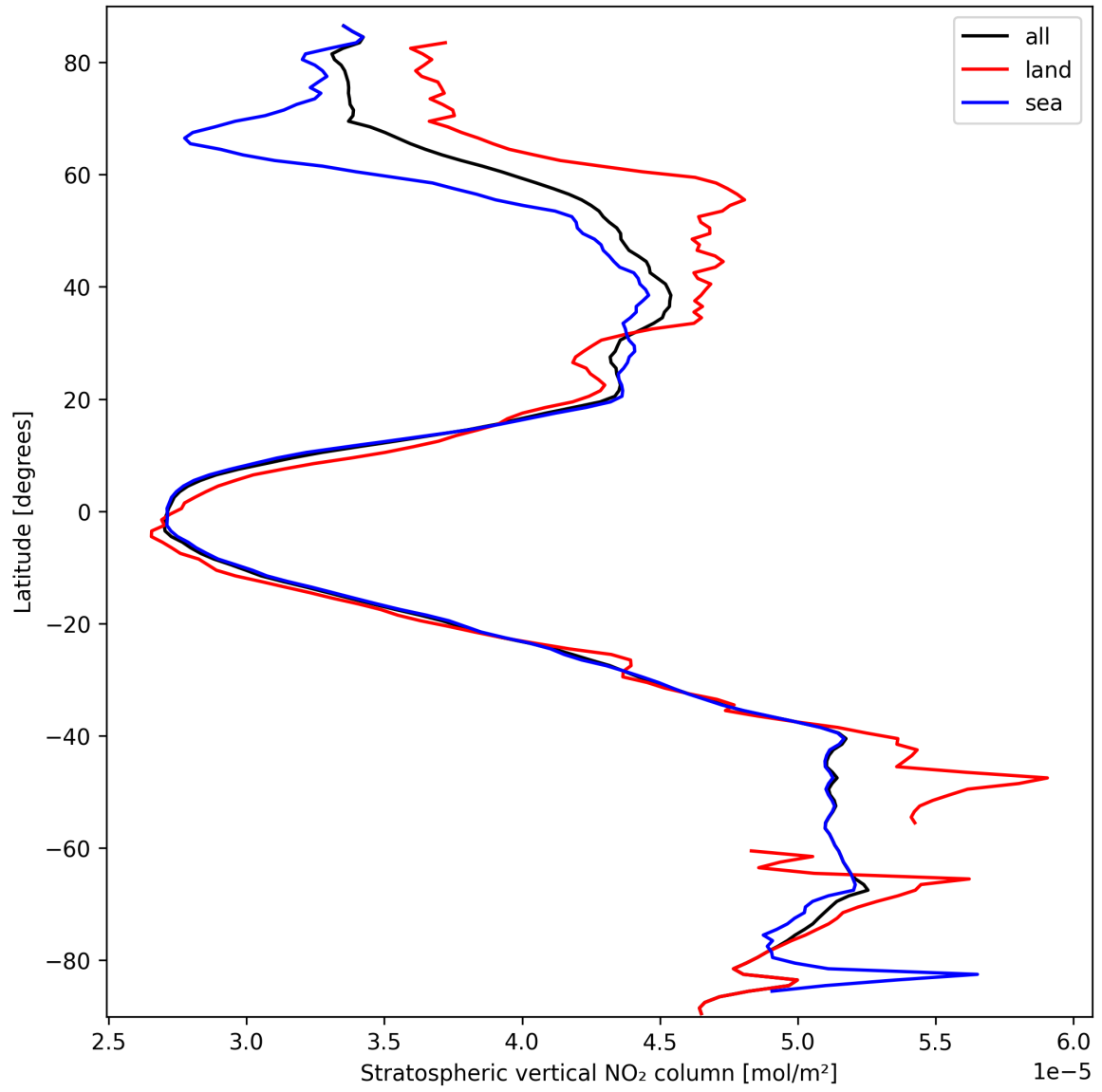
Figure 19: Zonal average of “Stratospheric vertical NO 2 column” for 2025-03-16 to 2025-03-17.
