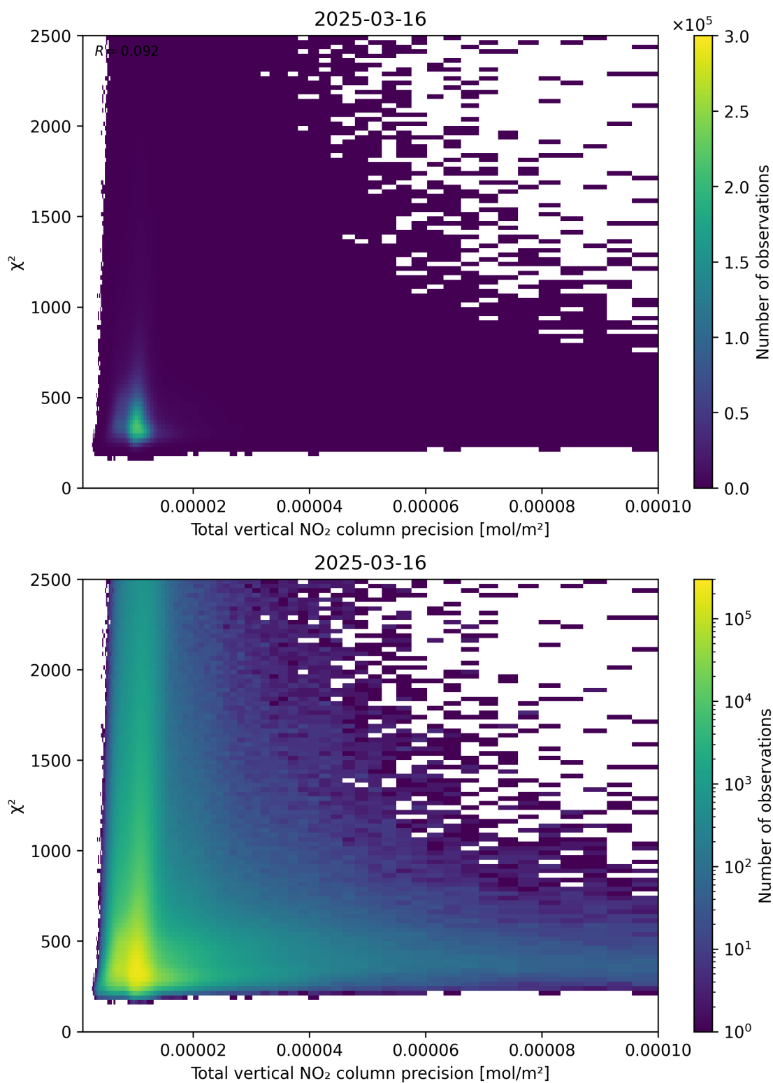
Figure 116: Scatter density plot of “Total vertical NO 2 column precision” against “ \chi^2 ” for 2025-03-16 to 2025-03-17.
