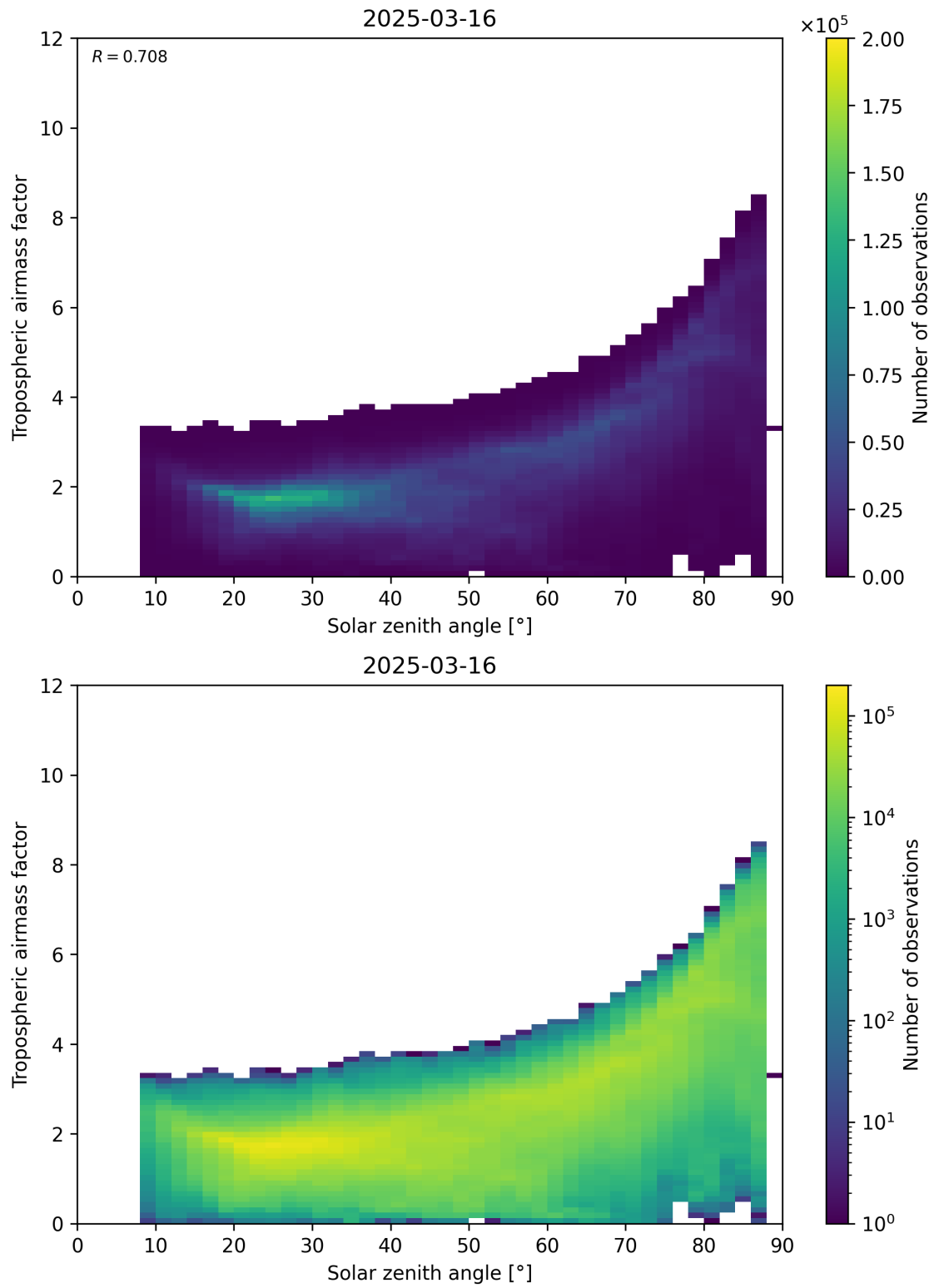
Figure 147: Scatter density plot of “Solar zenith angle” against “Tropospheric airmass factor” for 2025-03-16 to 2025-03-17.
