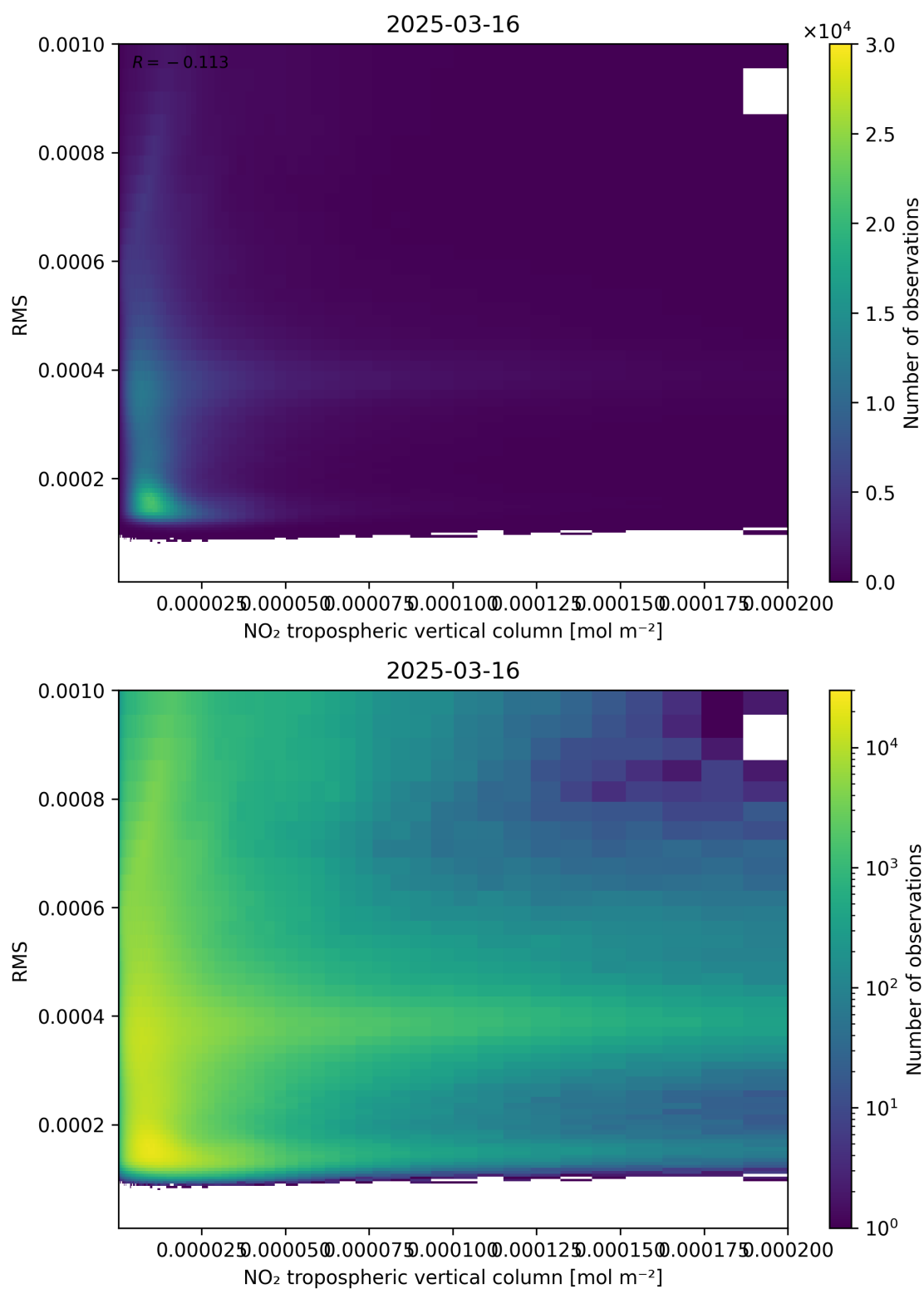
Figure 142: Scatter density plot of “NO 2 tropospheric vertical column” against “RMS” for 2025-03-16 to 2025-03-17.
