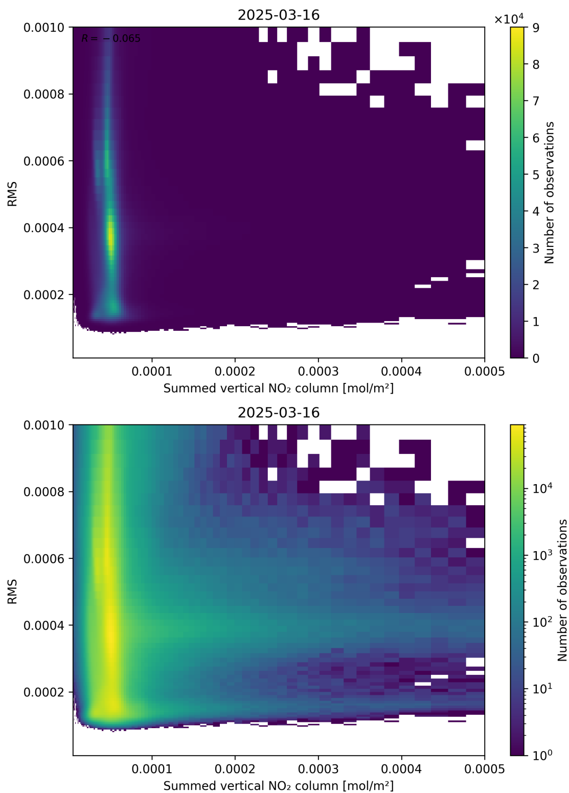
Figure 109: Scatter density plot of “Summed vertical NO 2 column” against “RMS” for 2025-03-16 to 2025-03-17.
