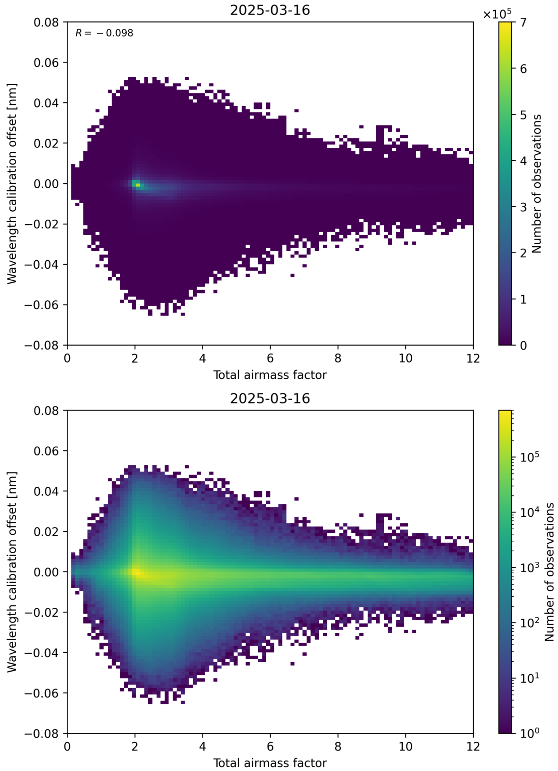
Figure 70: Scatter density plot of “Total airmass factor” against “Wavelength calibration offset” for 2025-03-16 to 2025-03-17.
