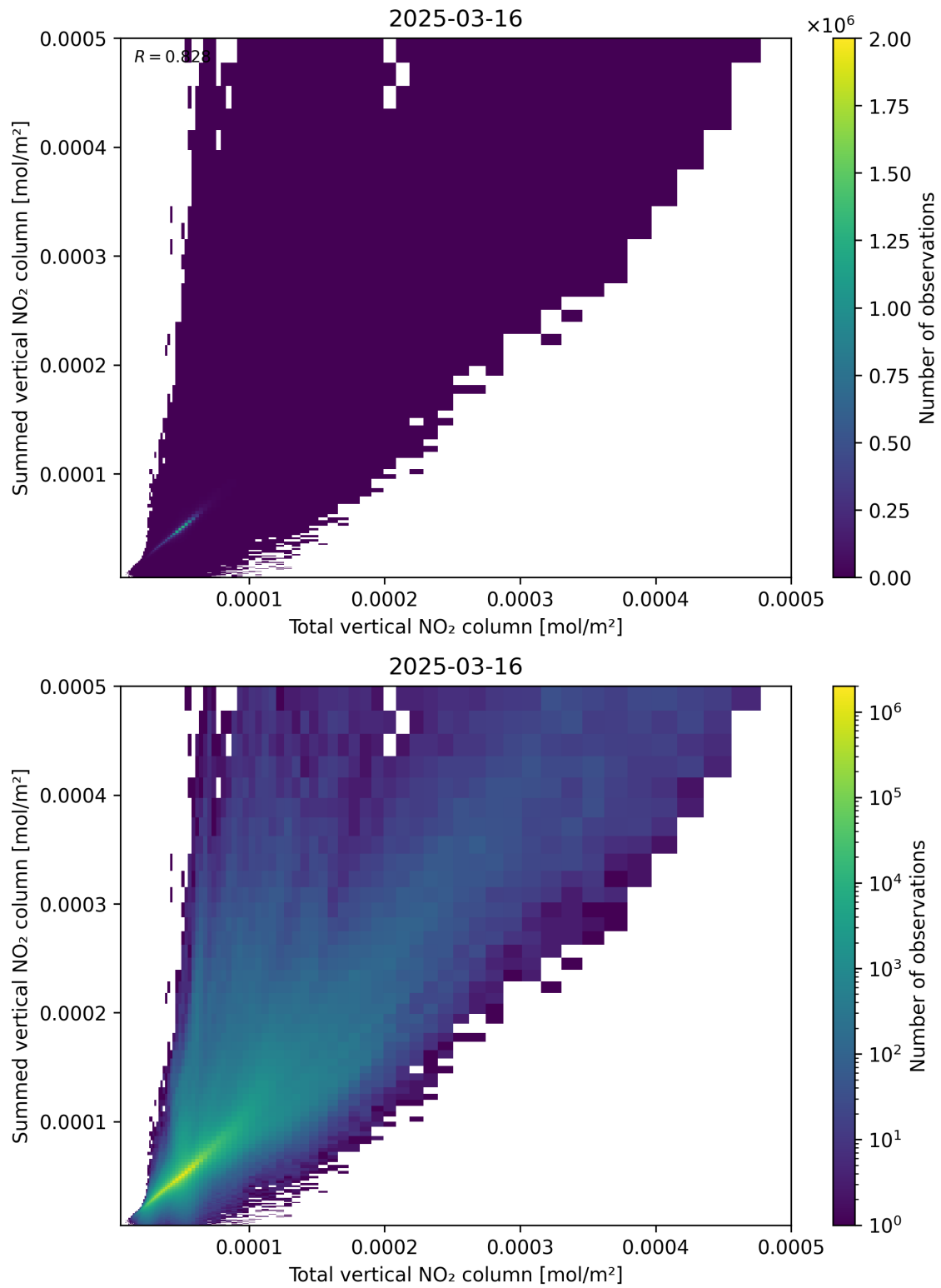
Figure 112: Scatter density plot of “Total vertical NO 2 column” against “Summed vertical NO 2 column” for 2025-03-16 to 2025-03-17.
