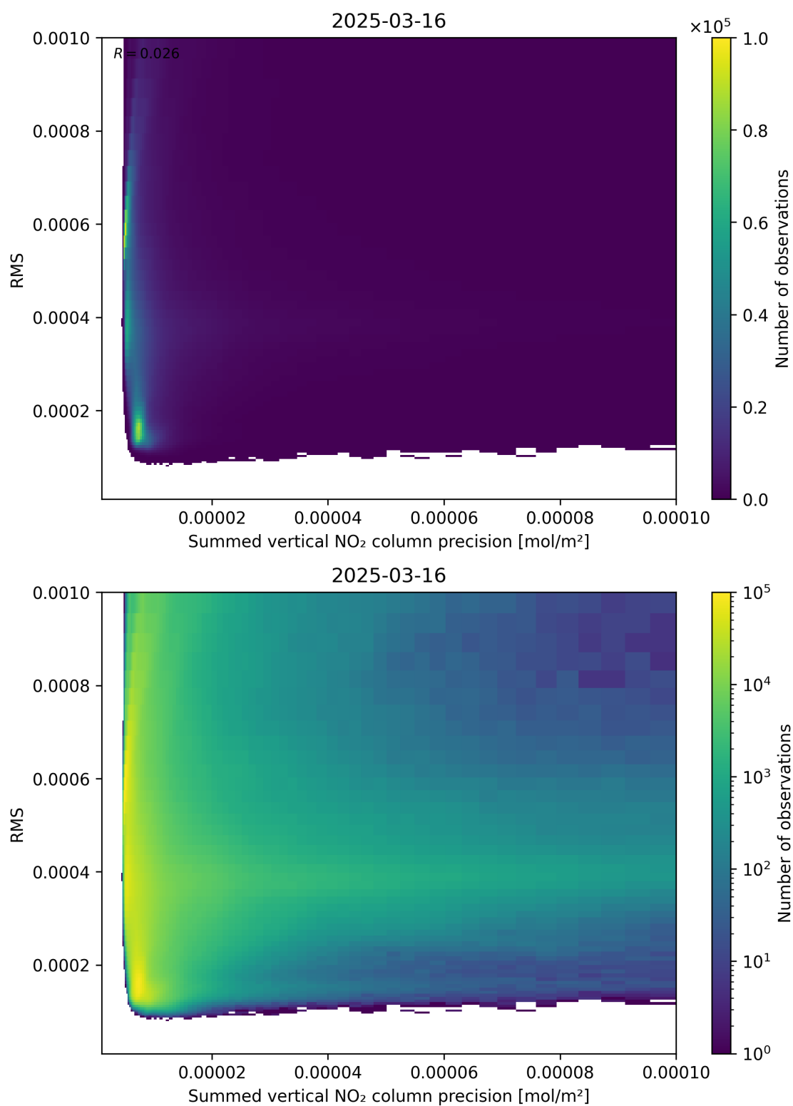
Figure 108: Scatter density plot of “Summed vertical NO 2 column precision” against “RMS” for 2025-03-16 to 2025-03-17.
