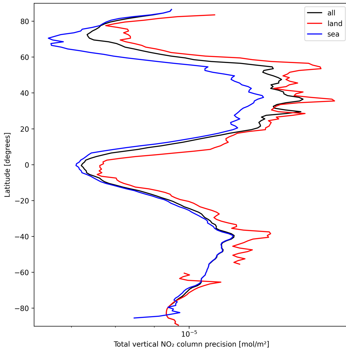
Figure 22: Zonal average of “Total vertical NO 2 column precision” for 2025-03-16 to 2025-03-17.
