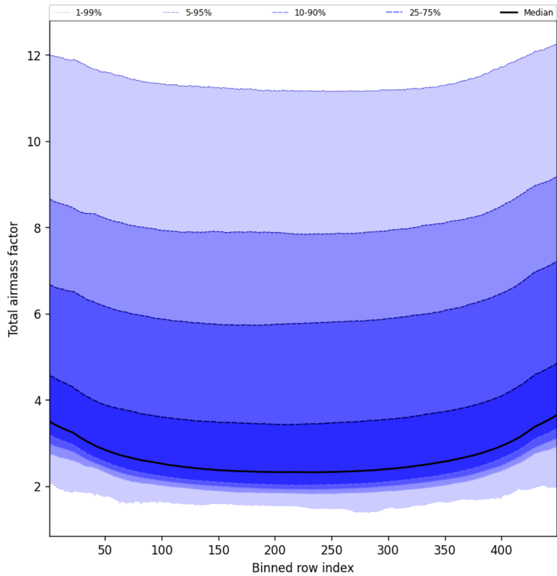
Figure 49: Along track statistics of “Total airmass factor” for 2025-03-16 to 2025-03-17
