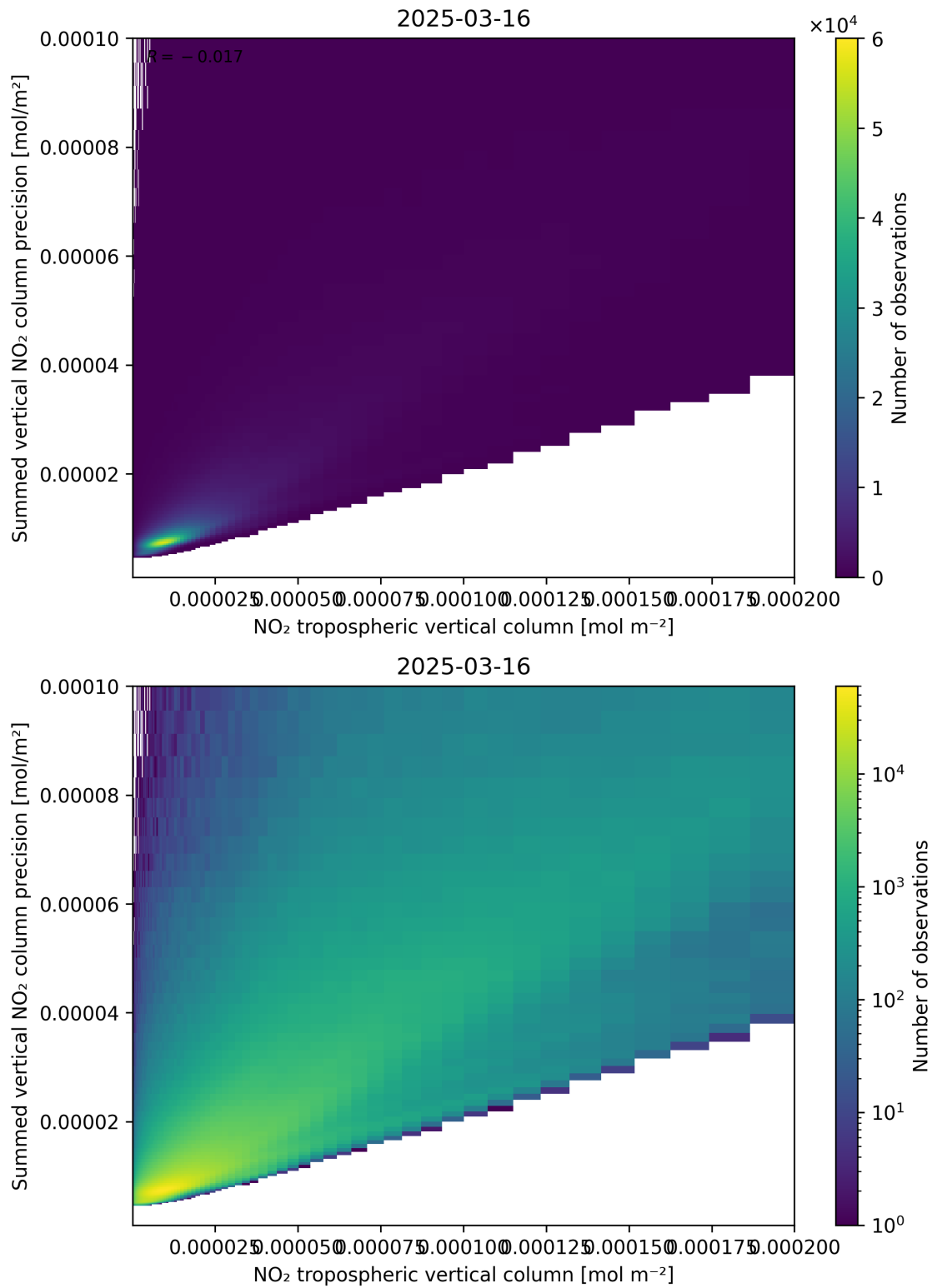
Figure 127: Scatter density plot of “NO 2 tropospheric vertical column” against “Summed vertical NO 2 column precision” for 2025-03-16 to 2025-03-17.
