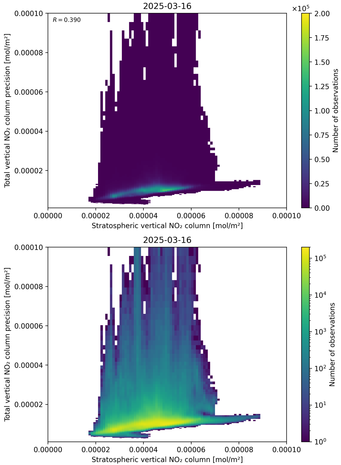
Figure 101: Scatter density plot of “Stratospheric vertical NO 2 column” against “Total vertical NO 2 column precision” for 2025-03-16 to 2025-03-17.
