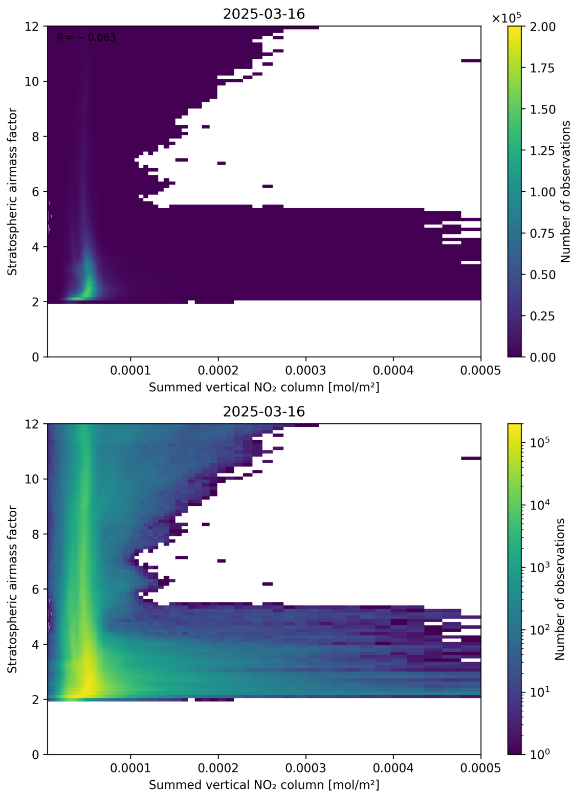
Figure 103: Scatter density plot of “Summed vertical NO 2 column” against “Stratospheric air mass factor” for 2025-03-16 to 2025-03-17.
