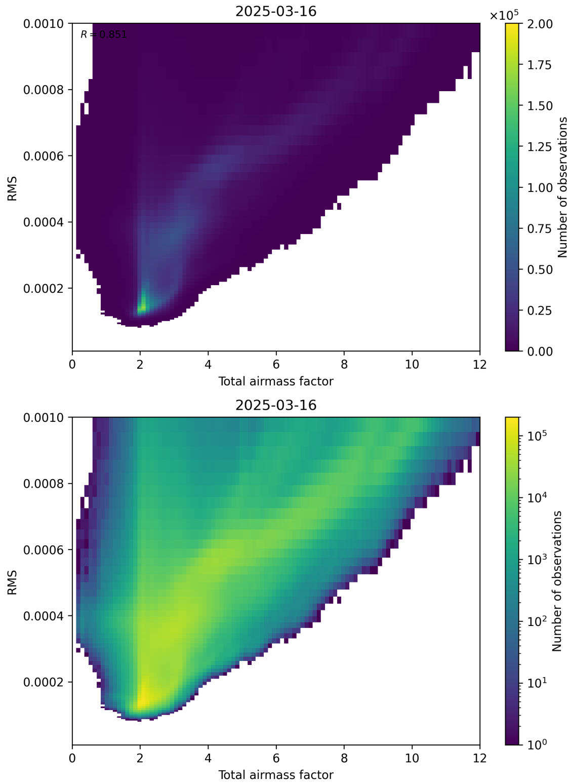
Figure 69: Scatter density plot of “Total airmass factor” against “RMS” for 2025-03-16 to 2025-03-17.
