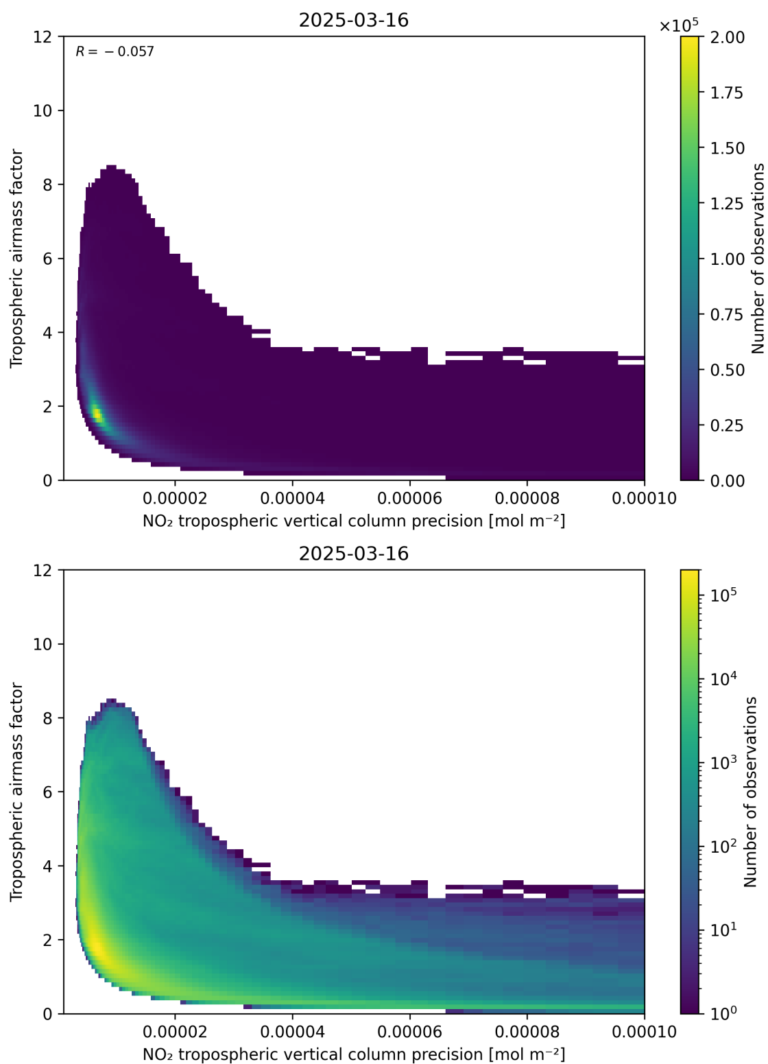
Figure 133: Scatter density plot of “NO 2 tropospheric vertical column precision” against “Tropospheric air mass factor” for 2025-03-16 to 2025-03-17.
