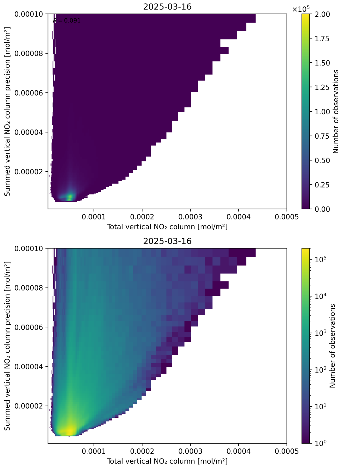
Figure 113: Scatter density plot of “Total vertical NO 2 column” against “Summed vertical NO 2 column precision” for 2025-03-16 to 2025-03-17.
