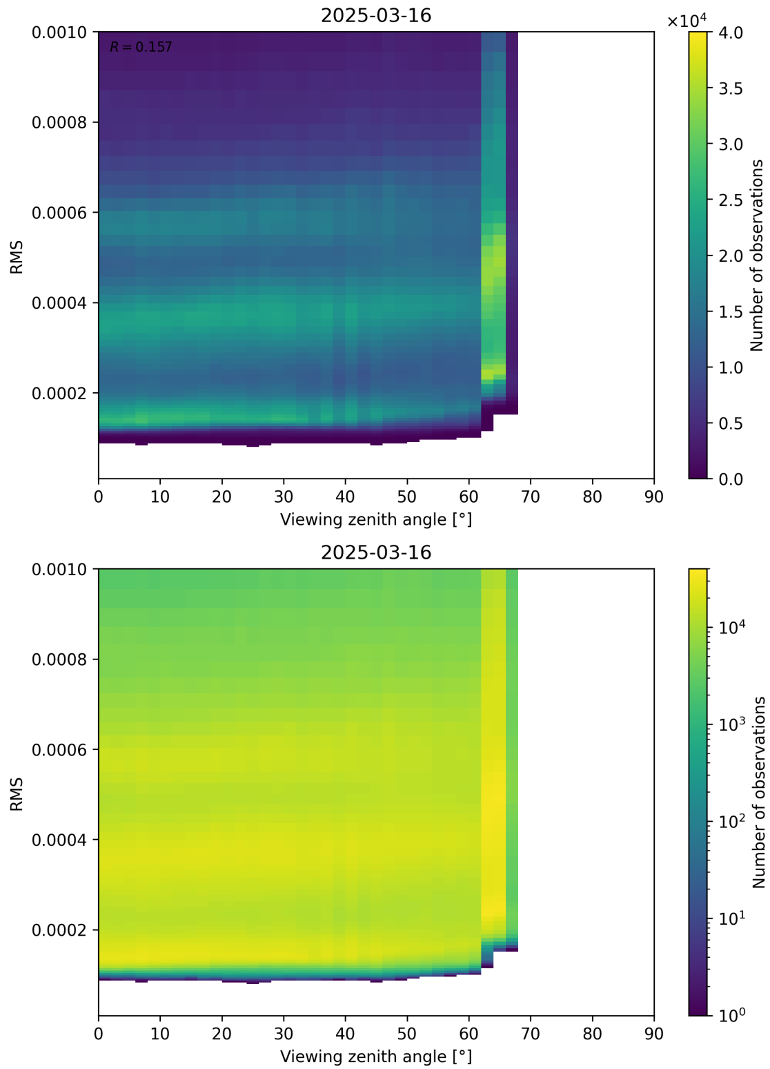
Figure 171: Scatter density plot of “Viewing zenith angle” against “RMS” for 2025-03-16 to 2025-03-17.
