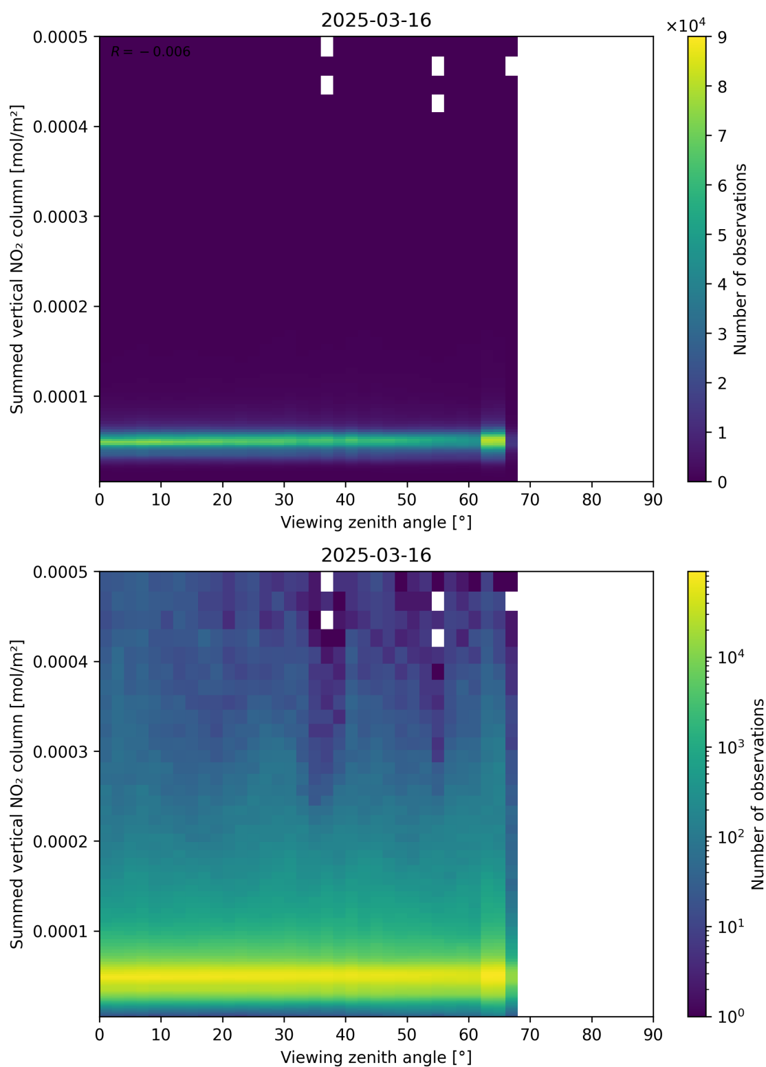
Figure 165: Scatter density plot of “Viewing zenith angle” against “Summed vertical NO 2 column” for 2025-03-16 to 2025-03-17.
