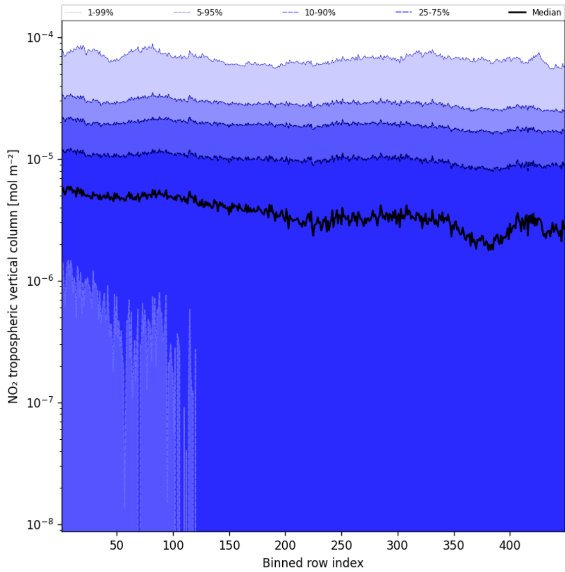
Figure 46: Along track statistics of “NO 2 tropospheric vertical column” for 2025-03-16 to 2025-03-17
