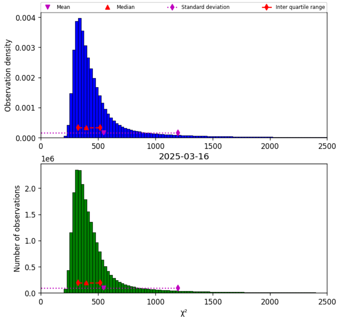
Figure 42: Histogram of “ \chi^2 ” for 2025-03-16 to 2025-03-17
