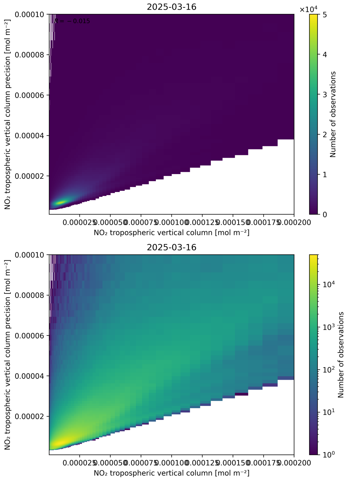
Figure 130: Scatter density plot of “NO 2 tropospheric vertical column” against “NO 2 tropospheric vertical column precision” for 2025-03-16 to 2025-03-17.
