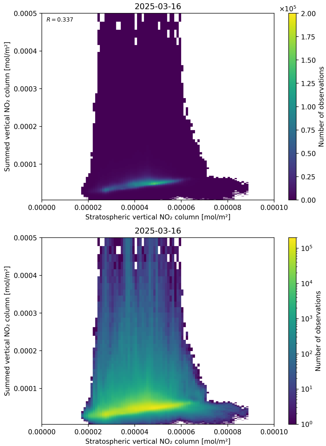
Figure 98: Scatter density plot of “Stratospheric vertical NO 2 column” against “Summed vertical NO 2 column” for 2025-03-16 to 2025-03-17.
