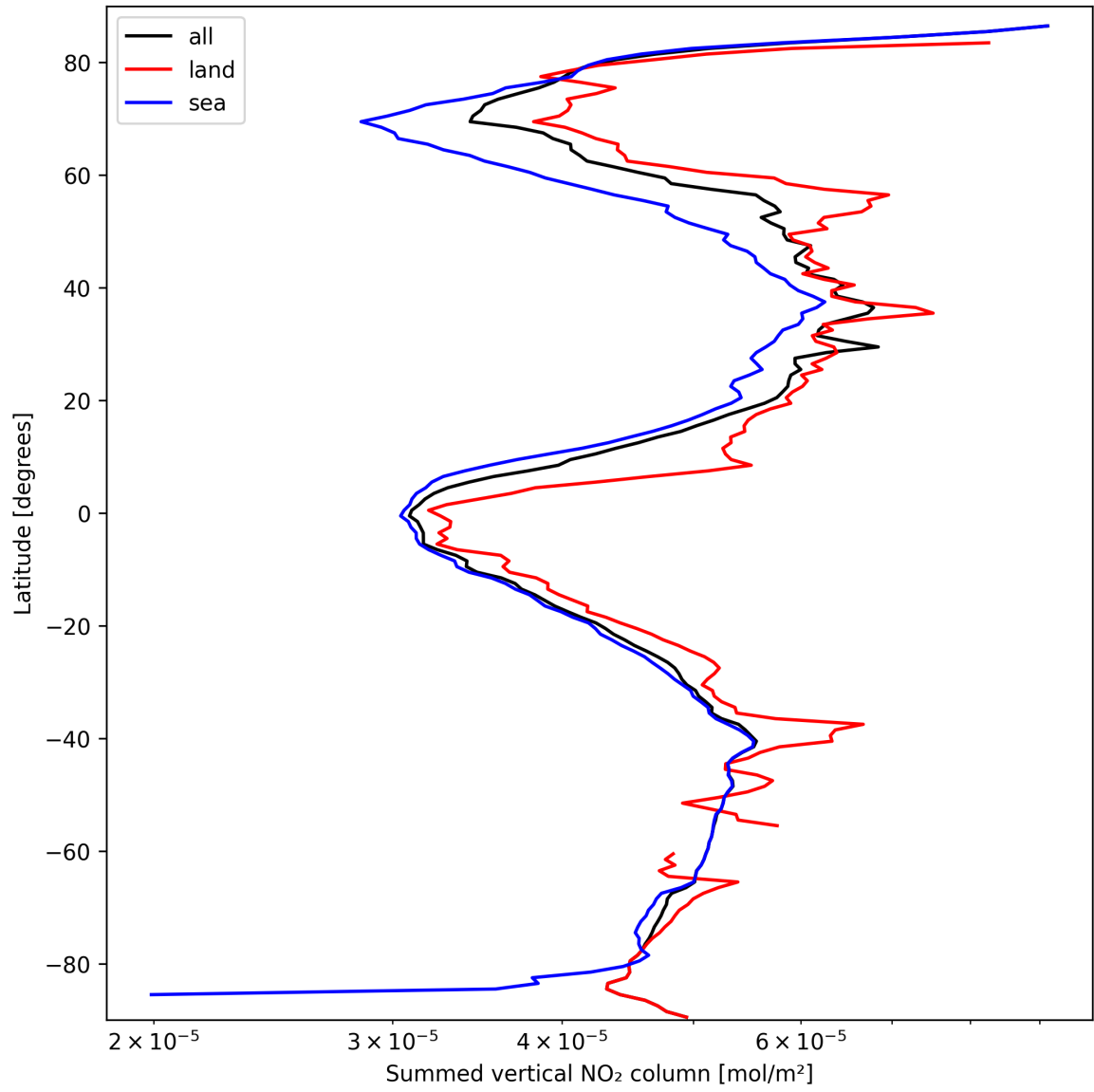
Figure 23: Zonal average of “Summed vertical NO 2 column” for 2025-03-16 to 2025-03-17.
