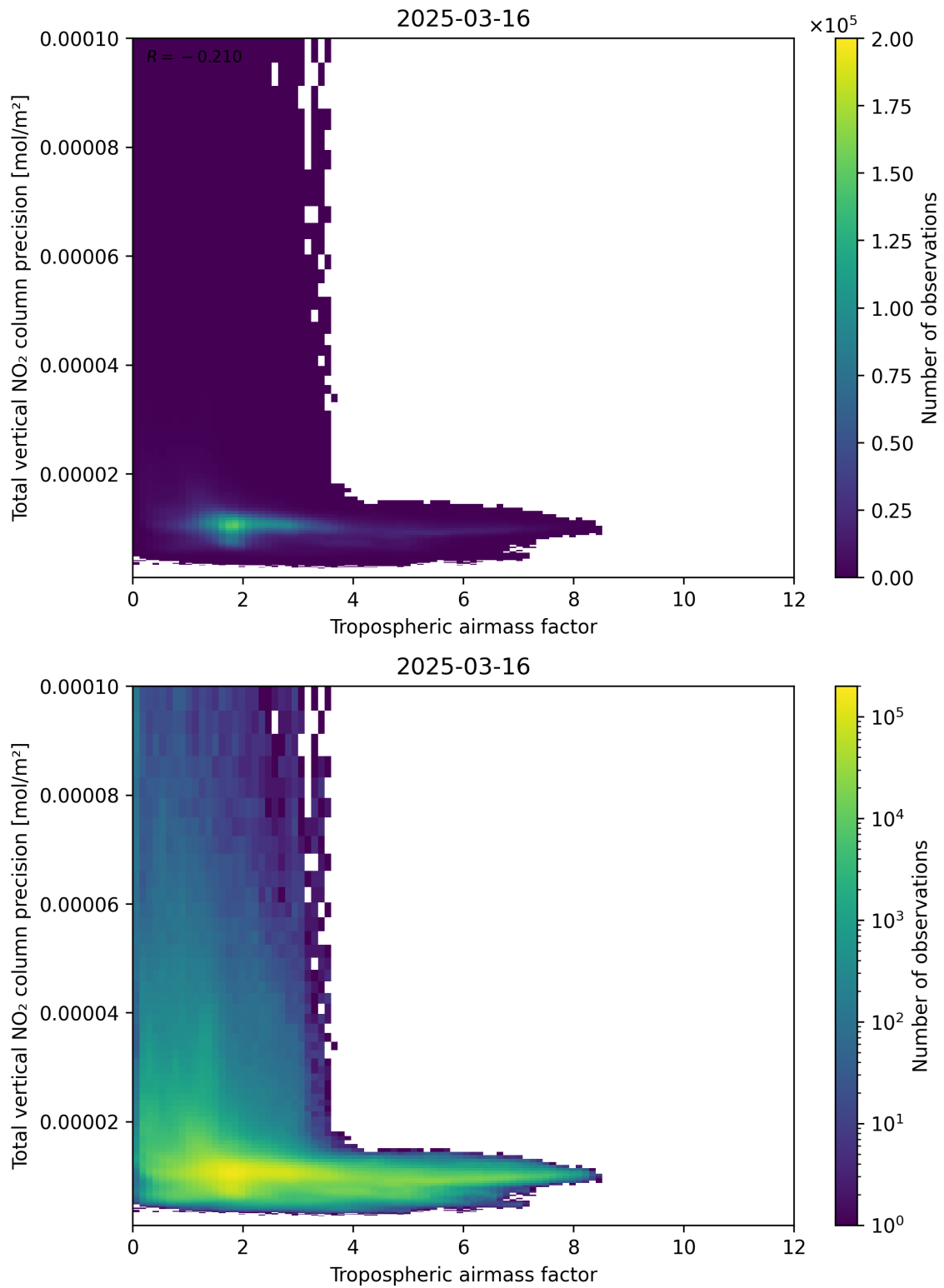
Figure 78: Scatter density plot of “Tropospheric air mass factor” against “Total vertical NO 2 column precision” for 2025-03-16 to 2025-03-17.
