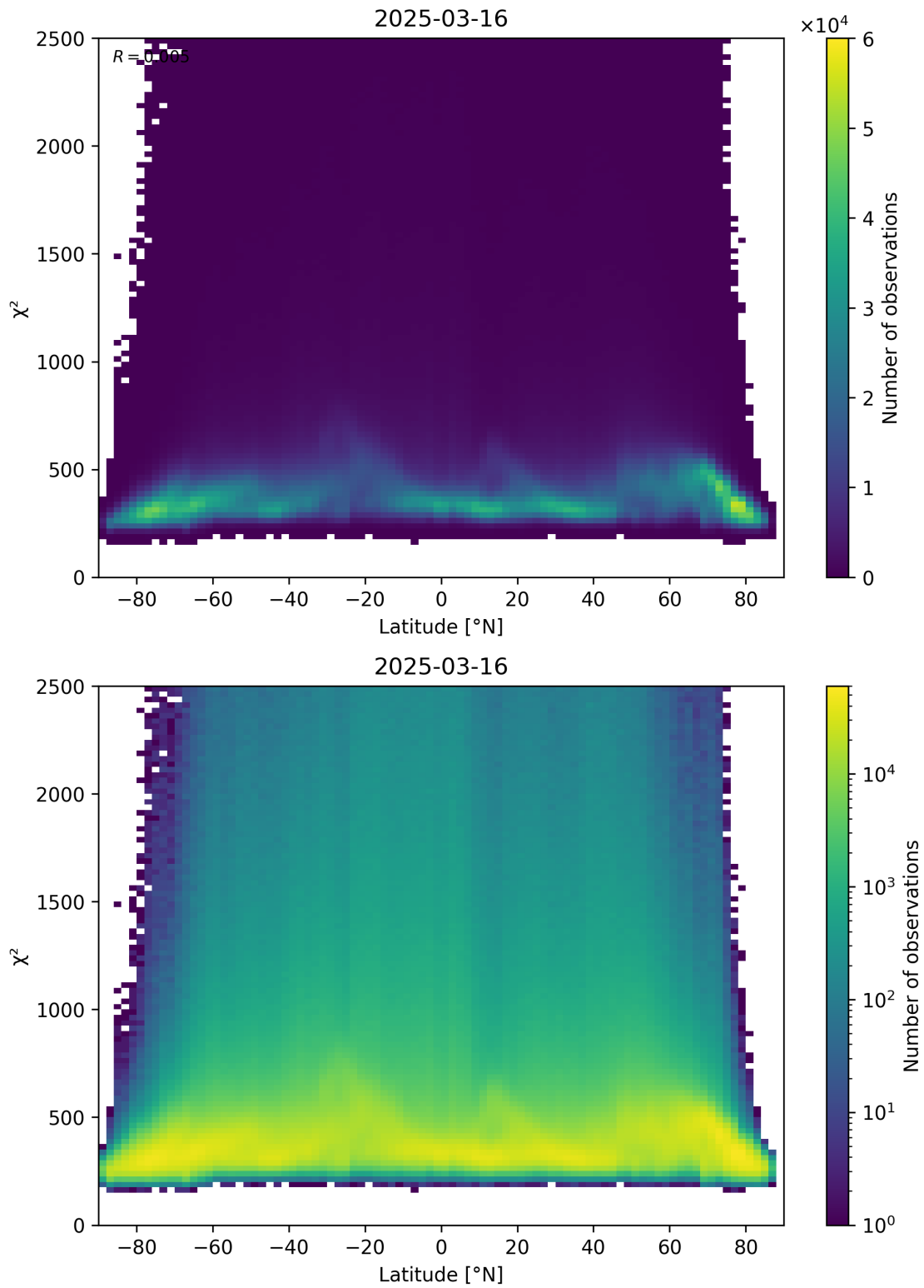
Figure 86: Scatter density plot of “Latitude” against “ \chi^2 ” for 2025-03-16 to 2025-03-17.
