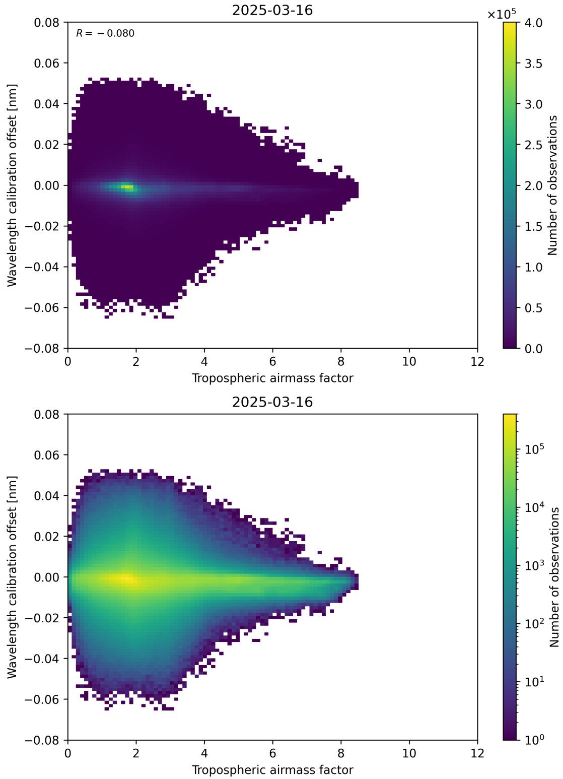
Figure 80: Scatter density plot of “Tropospheric airmass factor” against “Wavelength calibration offset” for 2025-03-16 to 2025-03-17.
