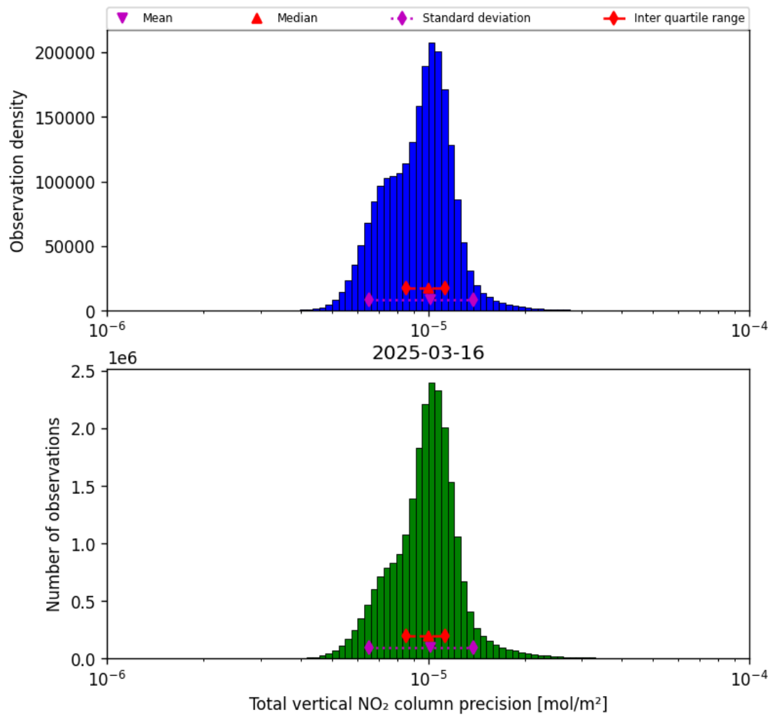
Figure 39: Histogram of “Total vertical NO 2 column precision” for 2025-03-16 to 2025-03-17
