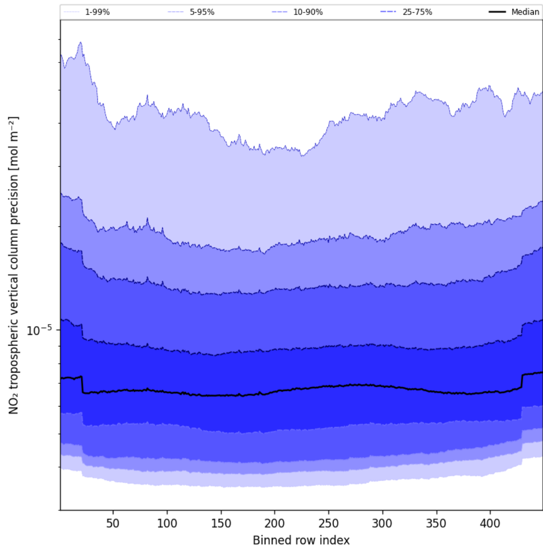
Figure 47: Along track statistics of “NO 2 tropospheric vertical column precision” for 2025-03-16 to 2025-03-17
