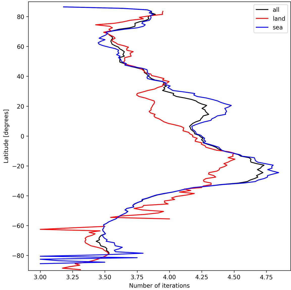
Figure 17: Zonal average of “Number of iterations” for 2025-03-16 to 2025-03-17.
