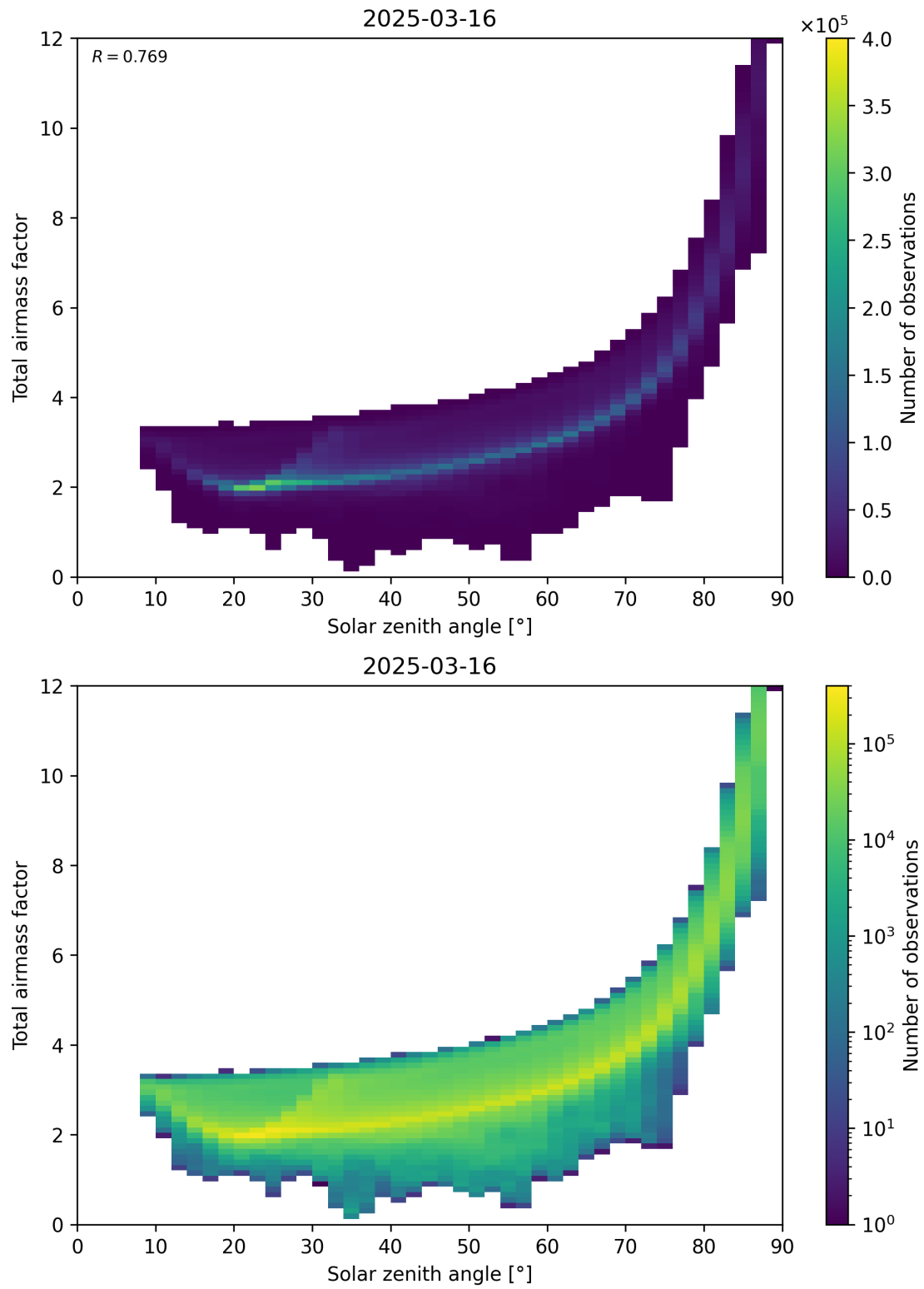
Figure 146: Scatter density plot of “Solar zenith angle” against “Total airmass factor” for 2025-03-16 to 2025-03-17.
