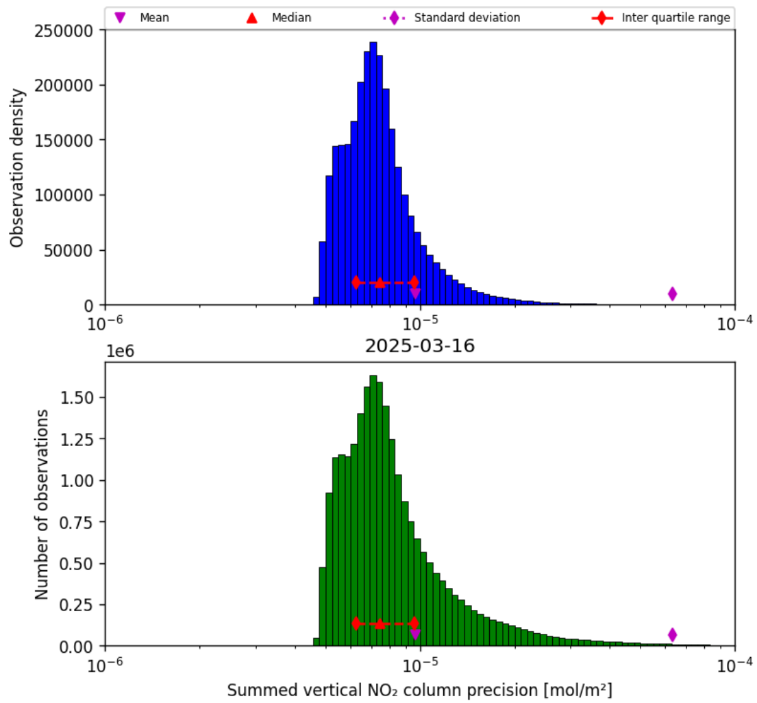
Figure 41: Histogram of “Summed vertical NO 2 column precision” for 2025-03-16 to 2025-03-17
