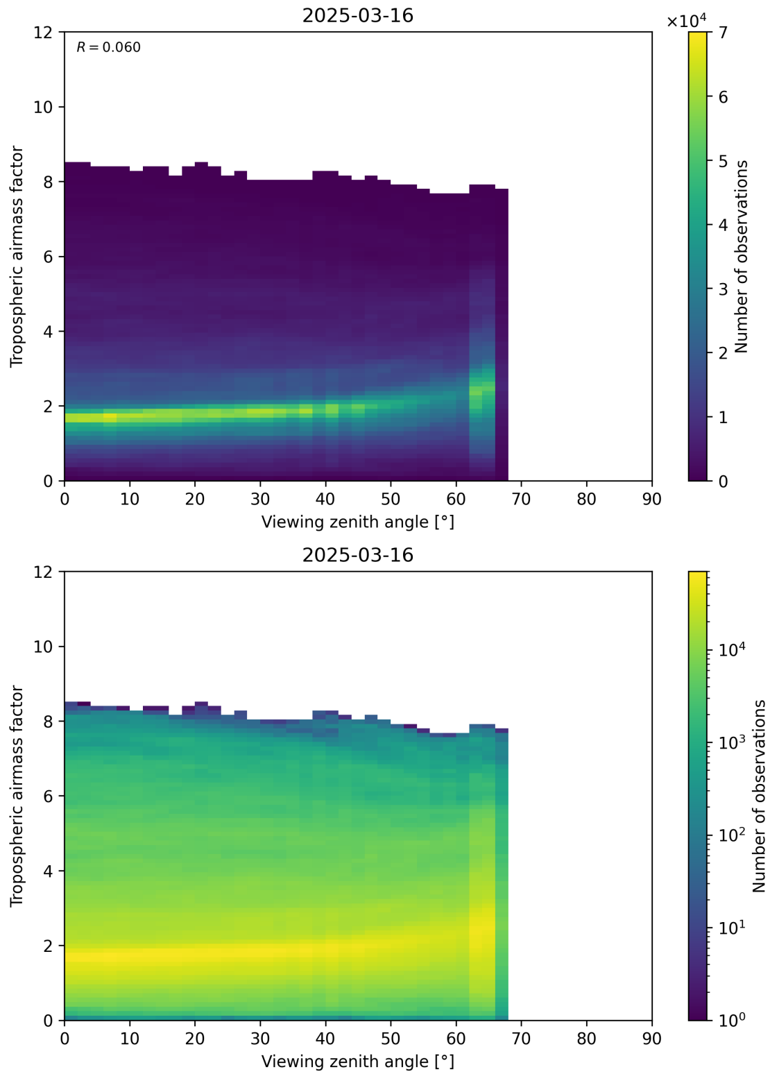
Figure 161: Scatter density plot of “Viewing zenith angle” against “Tropospheric airmass factor” for 2025-03-16 to 2025-03-17.
