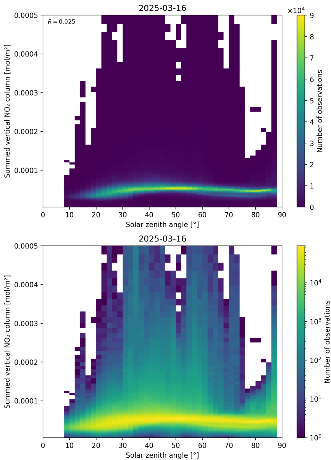
Figure 151: Scatter density plot of “Solar zenith angle” against “Summed vertical NO 2 column” for 2025-03-16 to 2025-03-17.
