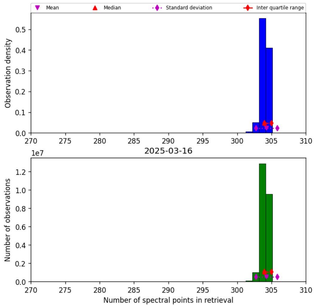
Figure 33: Histogram of “Number of spectral points in retrieval” for 2025-03-16 to 2025-03-17
