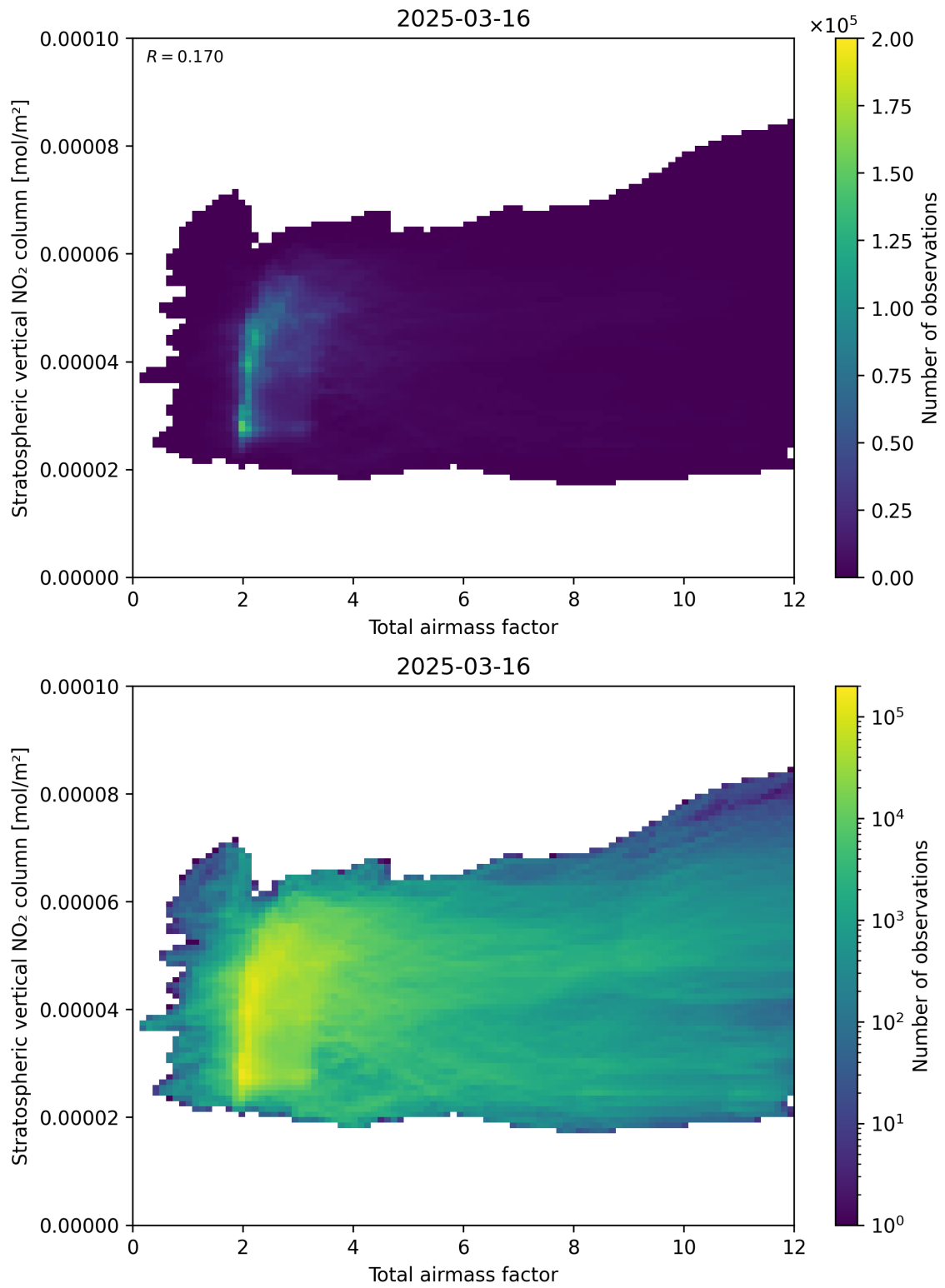
Figure 64: Scatter density plot of “Total airmass factor” against “Stratospheric vertical NO 2 column” for 2025-03-16 to 2025-03-17.
