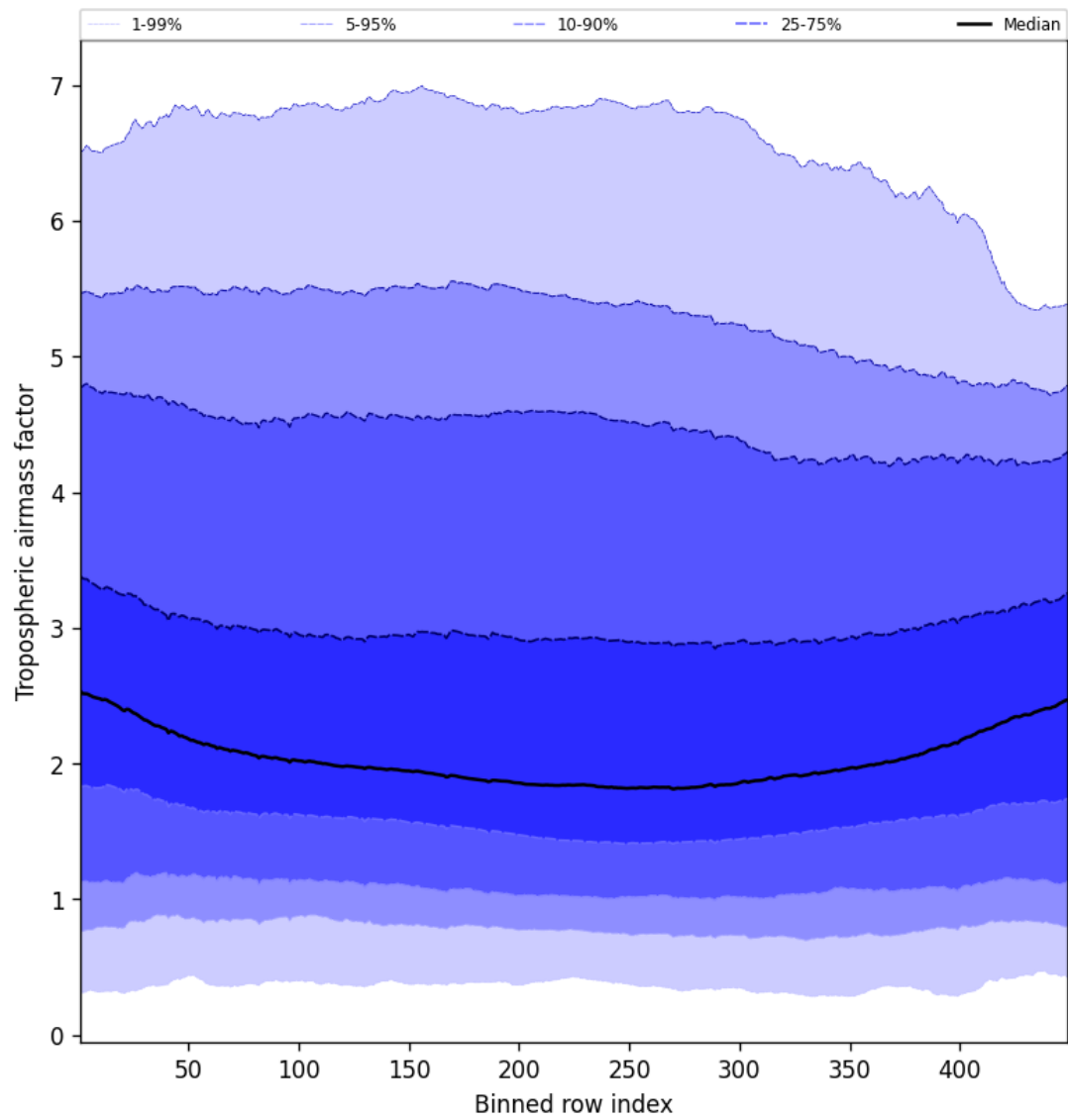
Figure 48: Along track statistics of “Tropospheric air mass factor” for 2025-03-16 to 2025-03-17
