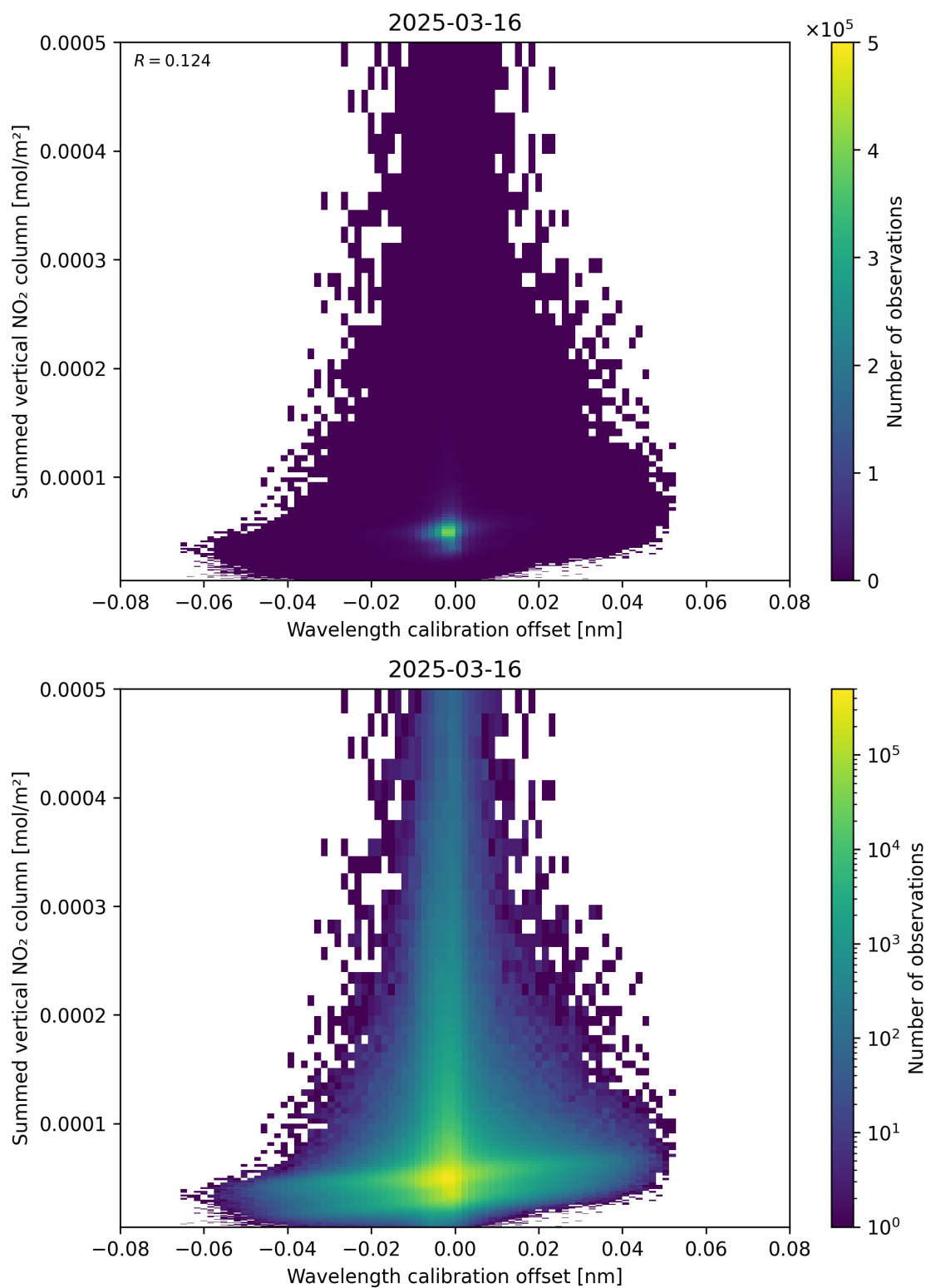
Figure 177: Scatter density plot of “Wavelength calibration offset” against “Summed vertical NO 2 column” for 2025-03-16 to 2025-03-17.
