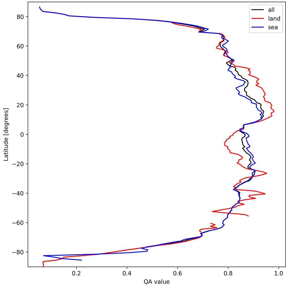
Figure 11: Zonal average of “QA value” for 2025-03-16 to 2025-03-17.
