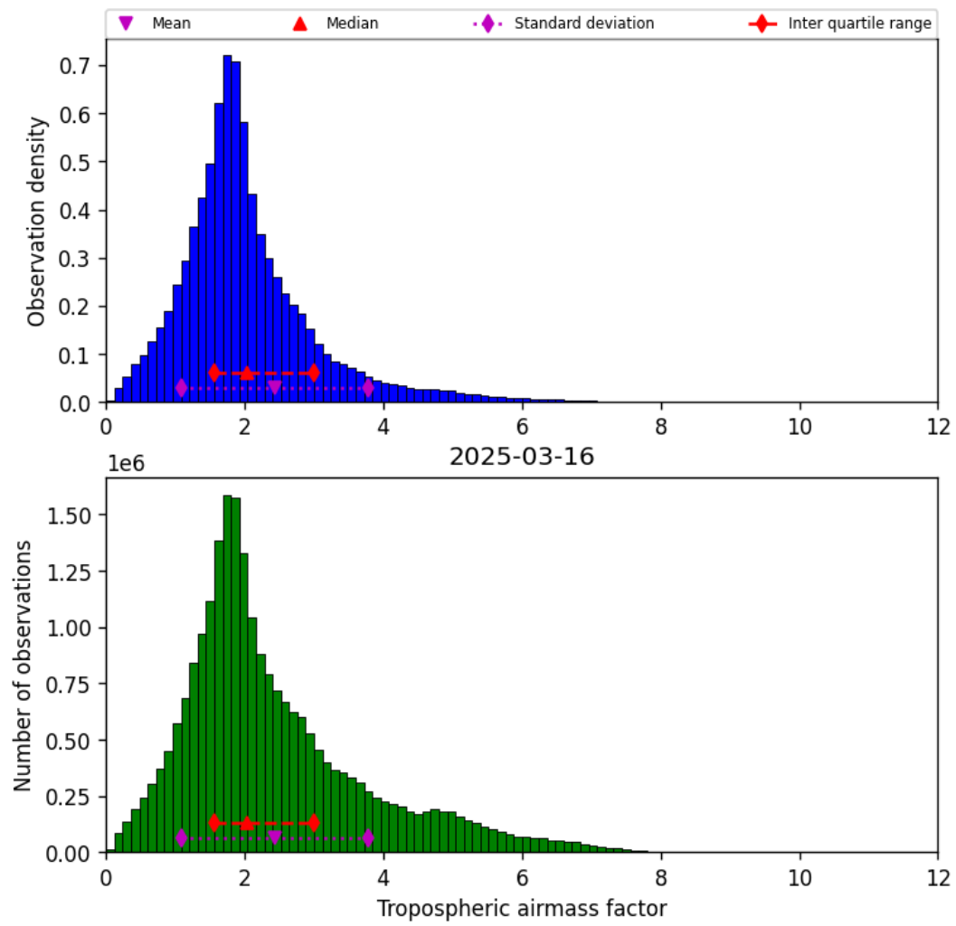
Figure 31: Histogram of “Tropospheric airmass factor” for 2025-03-16 to 2025-03-17
