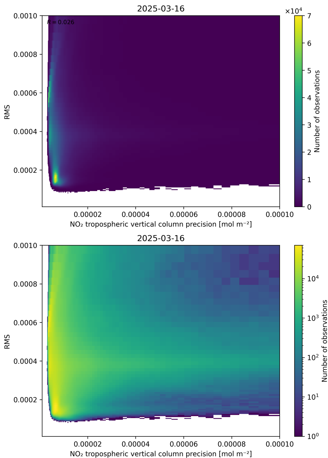
Figure 140: Scatter density plot of “NO 2 tropospheric vertical column precision” against “RMS” for 2025-03-16 to 2025-03-17.
