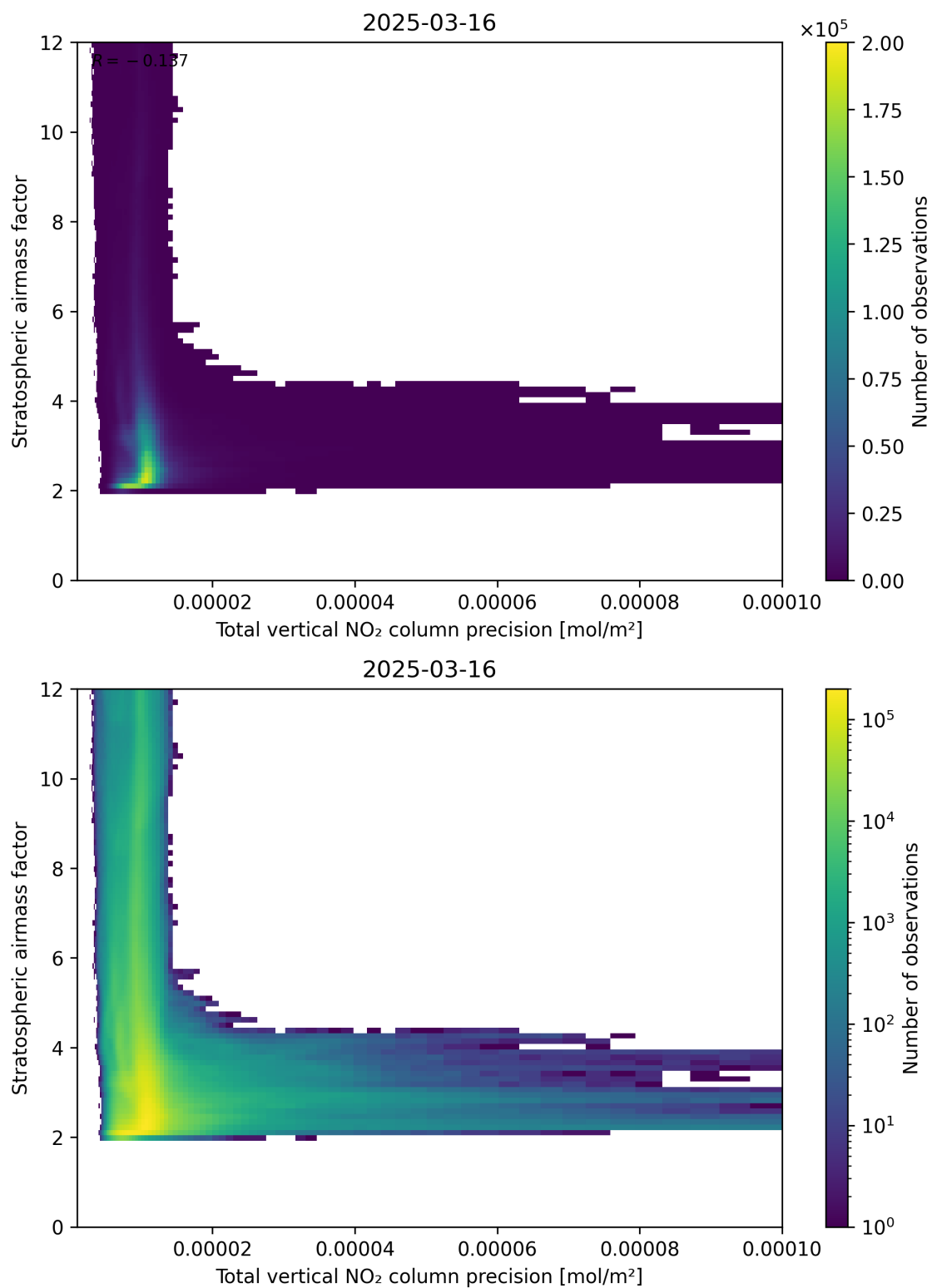
Figure 115: Scatter density plot of “Total vertical NO 2 column precision” against “Stratospheric airmass factor” for 2025-03-16 to 2025-03-17.
