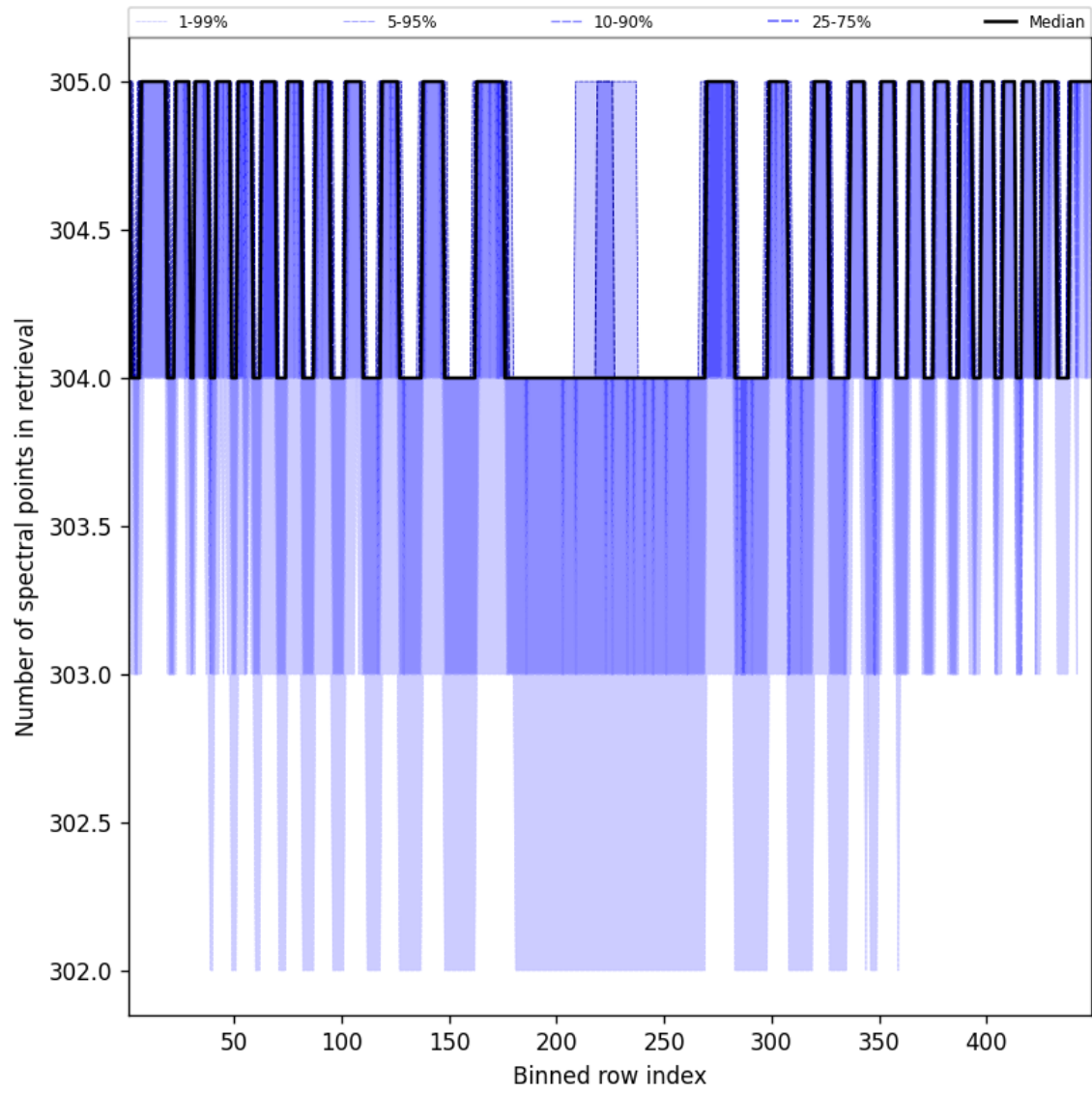
Figure 50: Along track statistics of “Number of spectral points in retrieval” for 2025-03-16 to 2025-03-17
