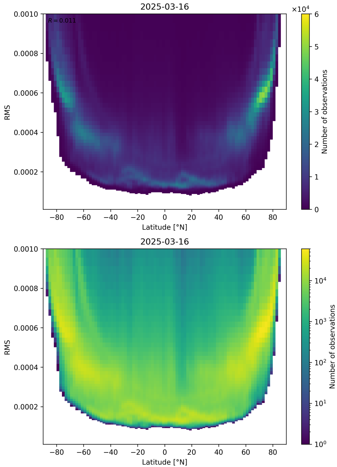
Figure 94: Scatter density plot of “Latitude” against “RMS” for 2025-03-16 to 2025-03-17.
