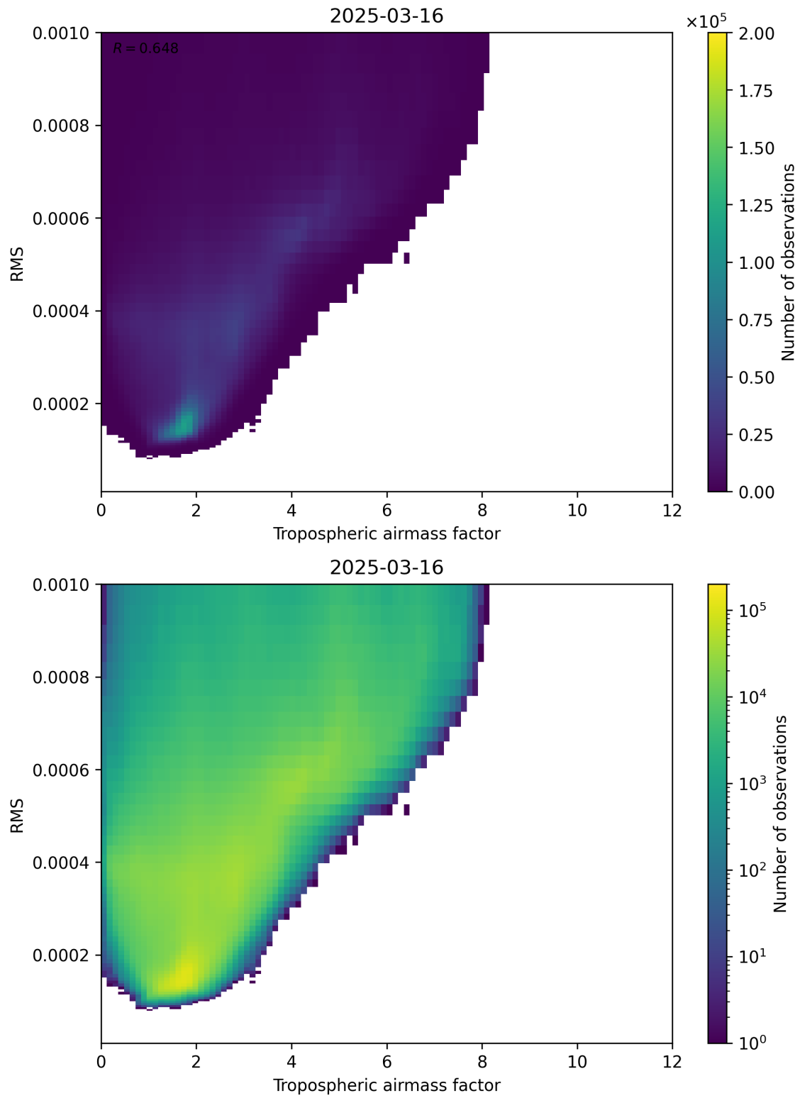
Figure 79: Scatter density plot of “Tropospheric airmass factor” against “RMS” for 2025-03-16 to 2025-03-17.
