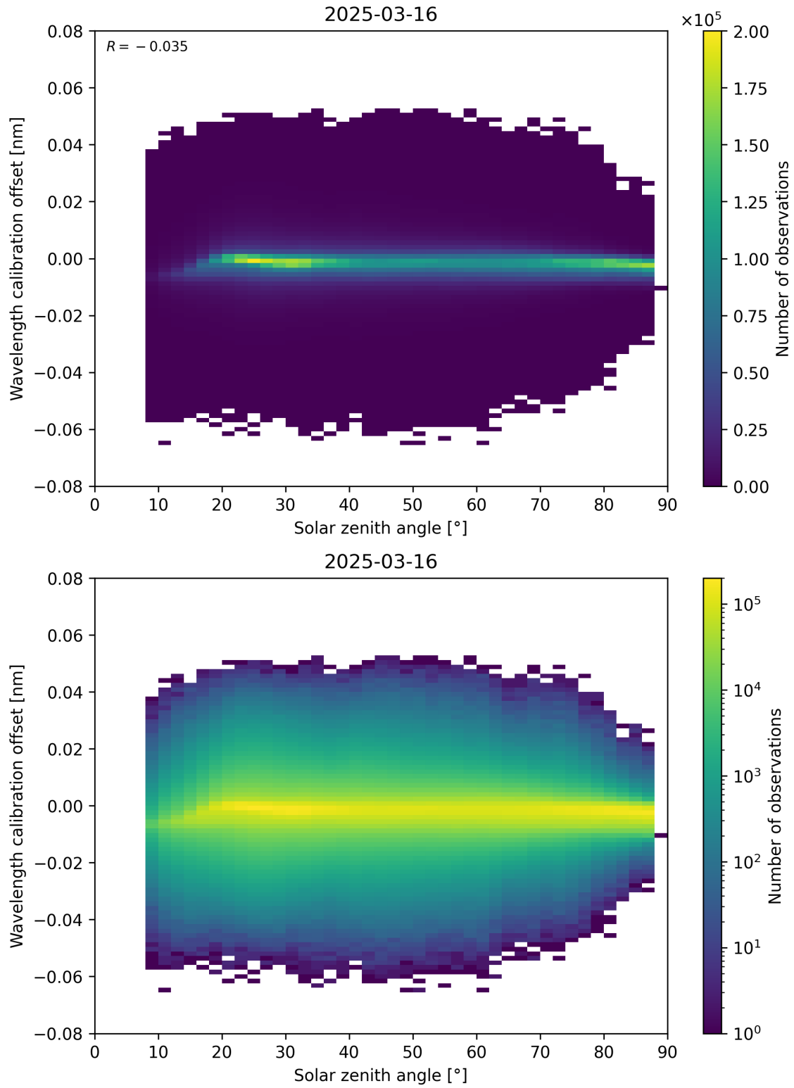
Figure 158: Scatter density plot of “Solar zenith angle” against “Wavelength calibration offset” for 2025-03-16 to 2025-03-17.
