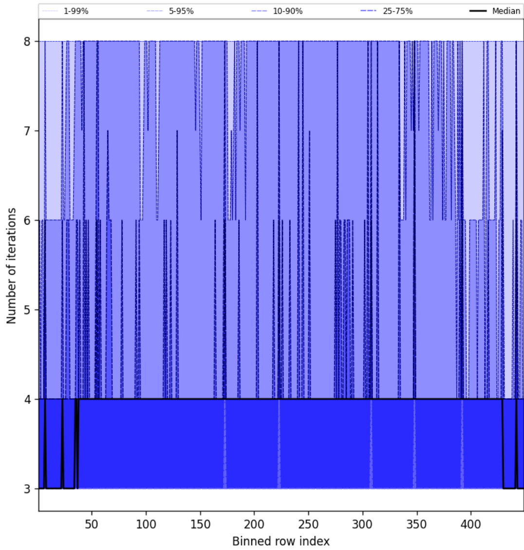
Figure 51: Along track statistics of “Number of iterations” for 2025-03-16 to 2025-03-17
