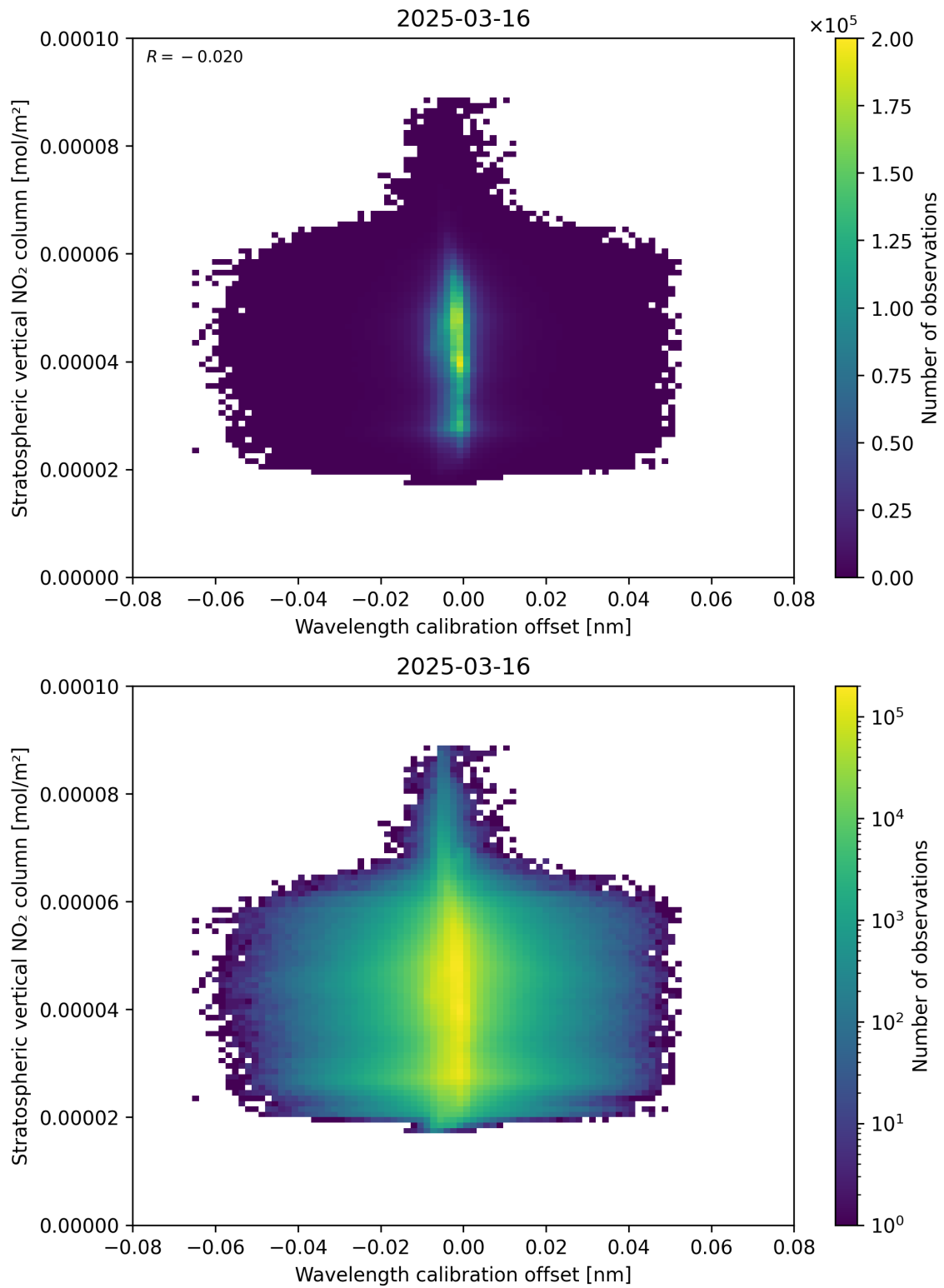
Figure 176: Scatter density plot of “Wavelength calibration offset” against “Stratospheric vertical NO 2 column” for 2025-03-16 to 2025-03-17.
