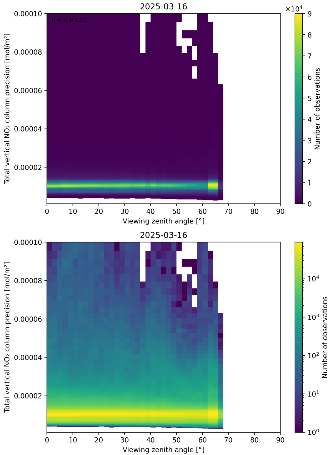
Figure 168: Scatter density plot of “Viewing zenith angle” against “Total vertical NO 2 column precision” for 2025-03-16 to 2025-03-17.
