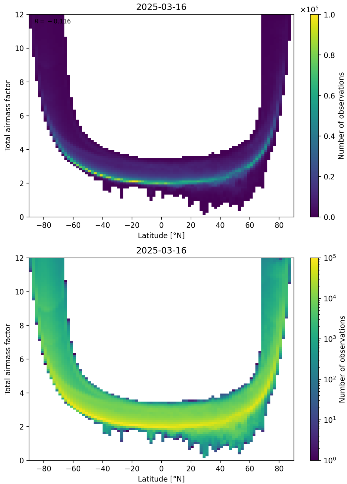
Figure 84: Scatter density plot of “Latitude” against “Total airmass factor” for 2025-03-16 to 2025-03-17.
