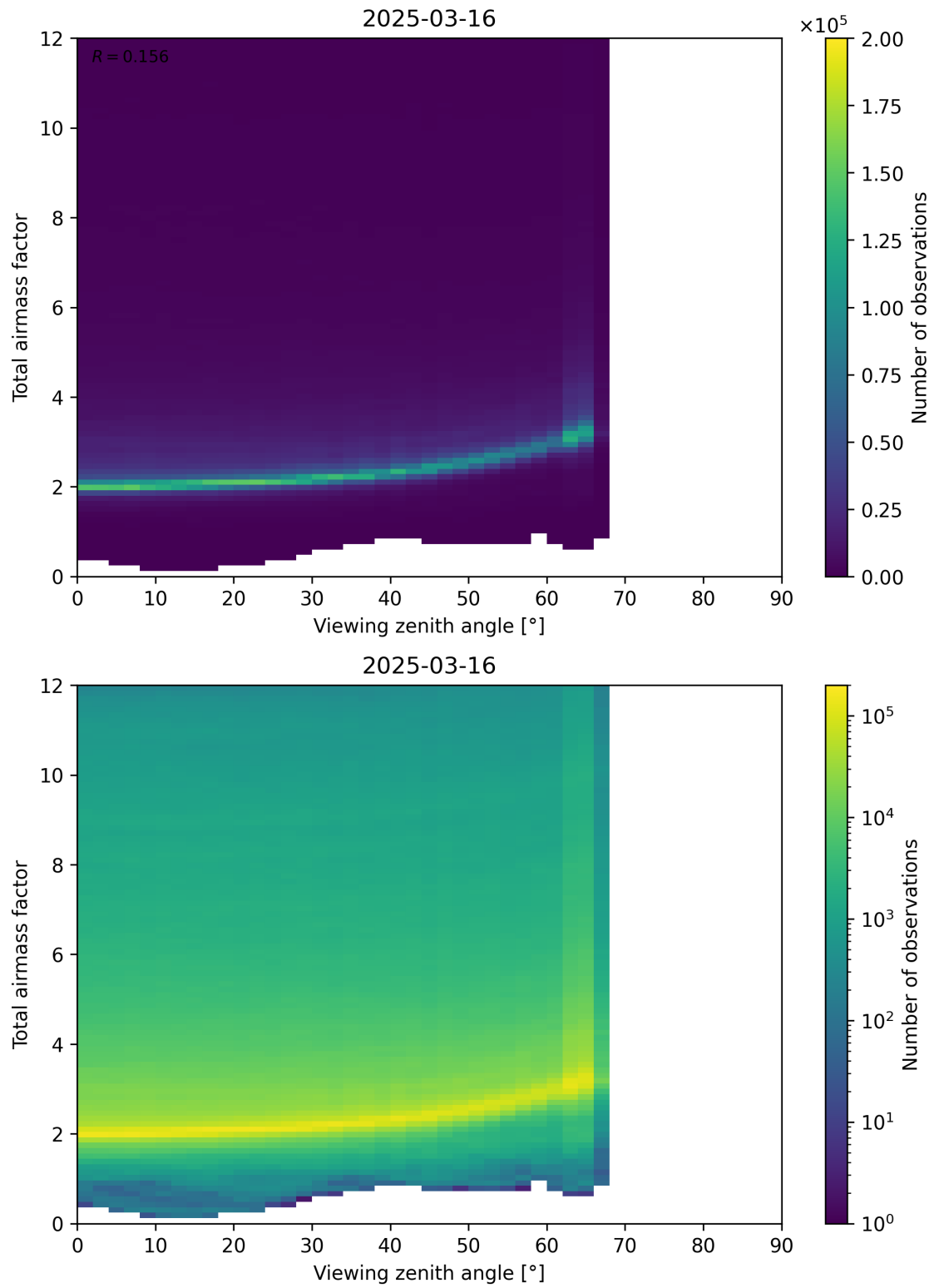
Figure 160: Scatter density plot of “Viewing zenith angle” against “Total airmass factor” for 2025-03-16 to 2025-03-17.
