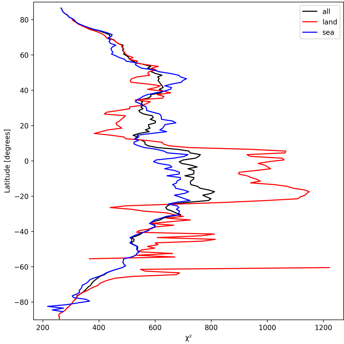
Figure 25: Zonal average of “ \chi^2 ” for 2025-03-16 to 2025-03-17.
