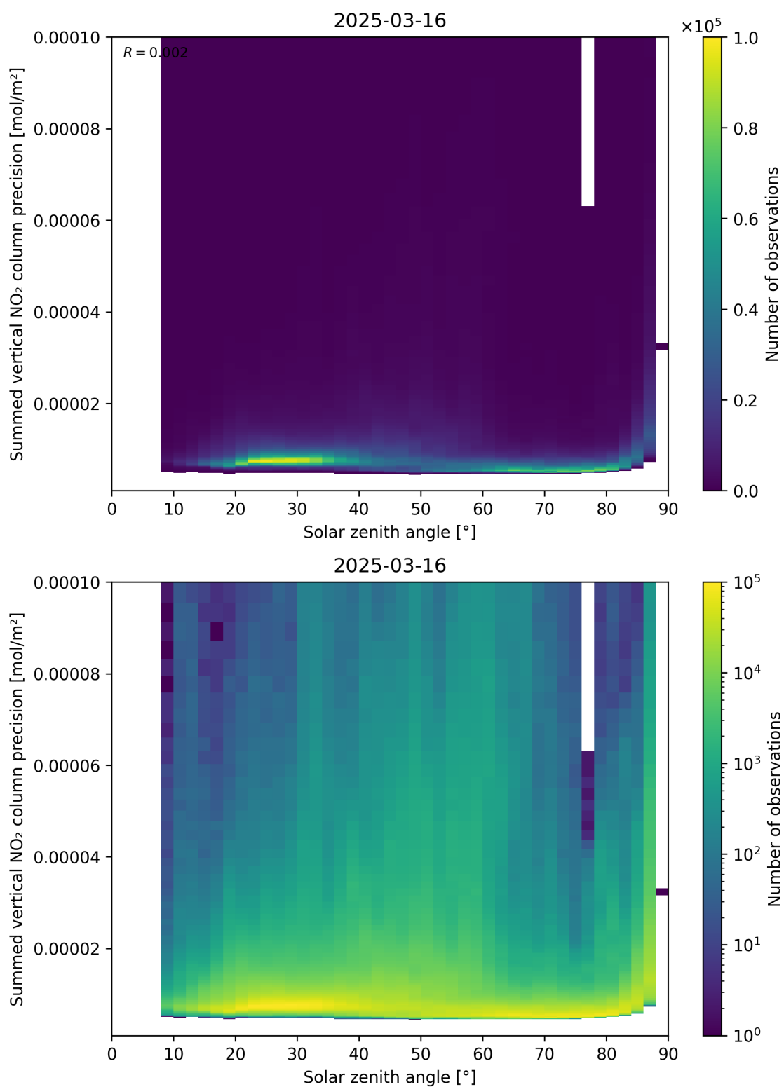
Figure 152: Scatter density plot of “Solar zenith angle” against “Summed vertical NO 2 column precision” for 2025-03-16 to 2025-03-17.
