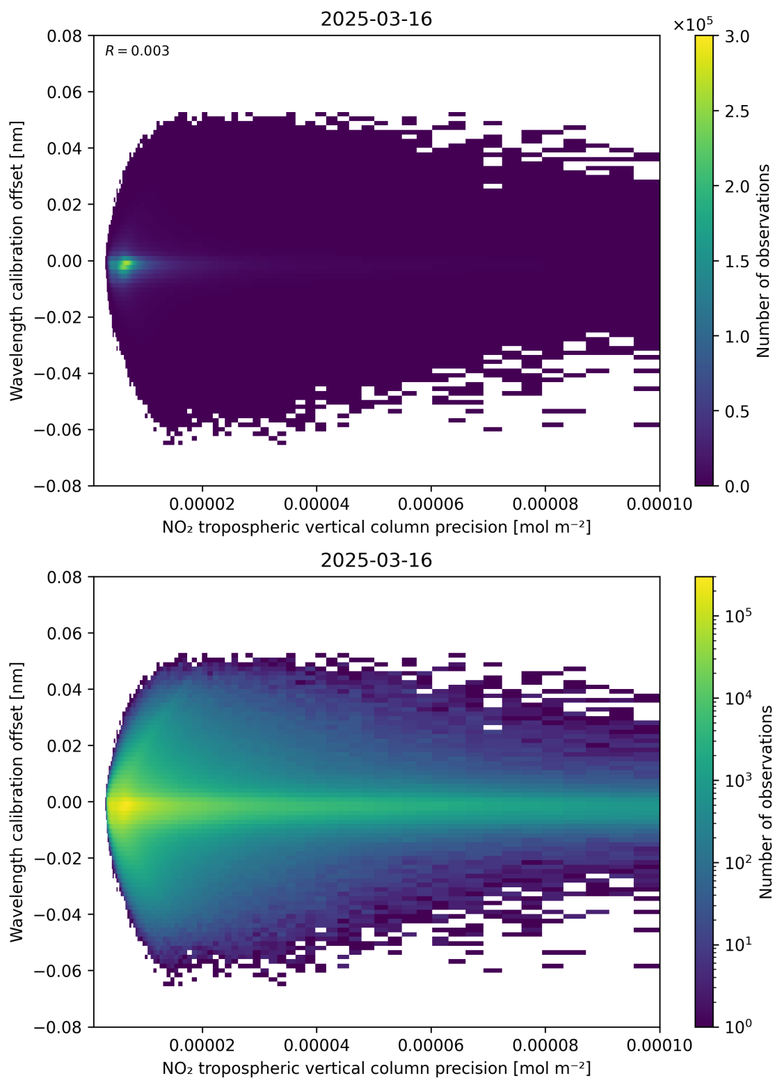
Figure 141: Scatter density plot of “NO 2 tropospheric vertical column precision” against “Wavelength calibration offset” for 2025-03-16 to 2025-03-17.
