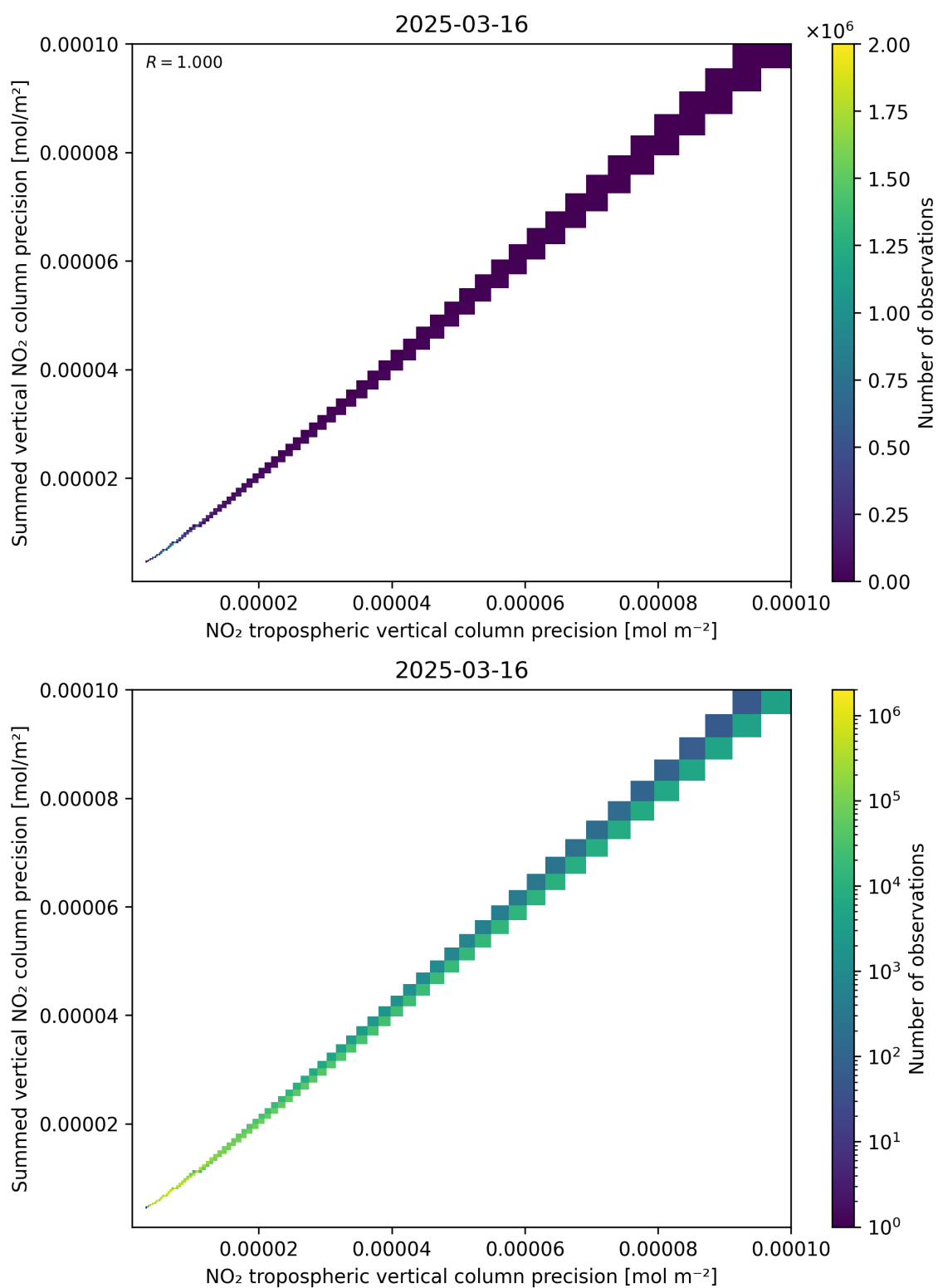
Figure 137: Scatter density plot of “NO 2 tropospheric vertical column precision” against “Summed vertical NO 2 column precision” for 2025-03-16 to 2025-03-17.
