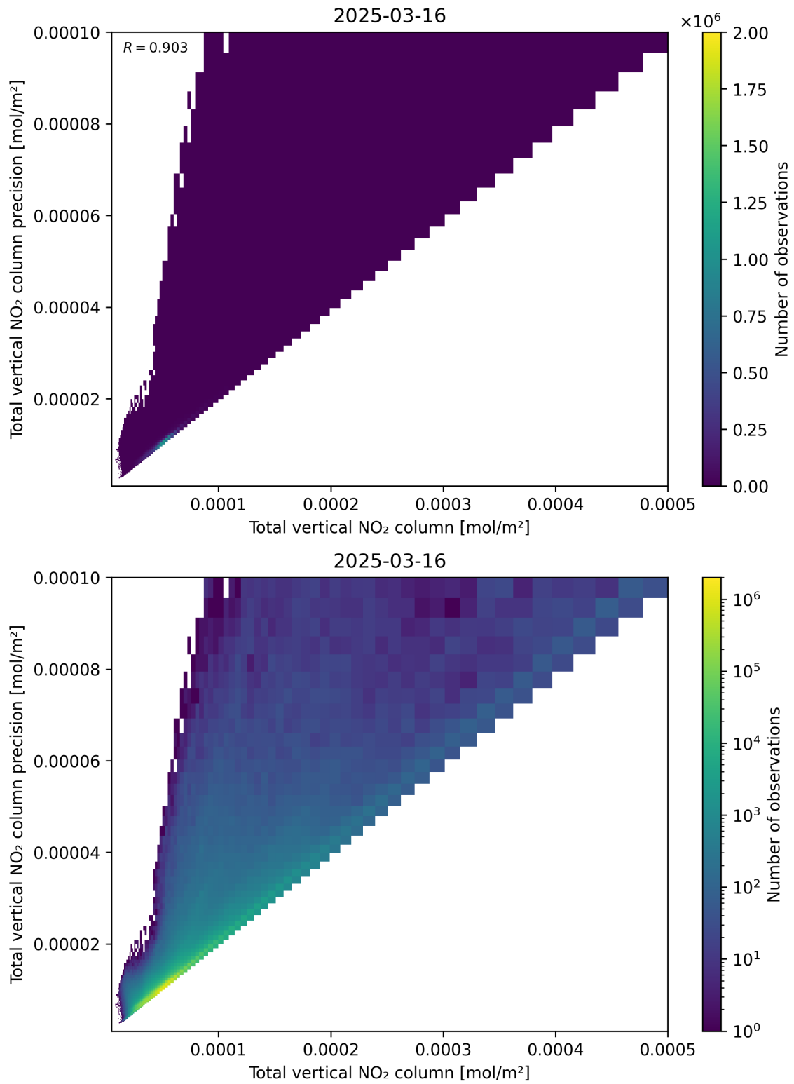
Figure 114: Scatter density plot of “Total vertical NO 2 column” against “Total vertical NO 2 column precision” for 2025-03-16 to 2025-03-17.
