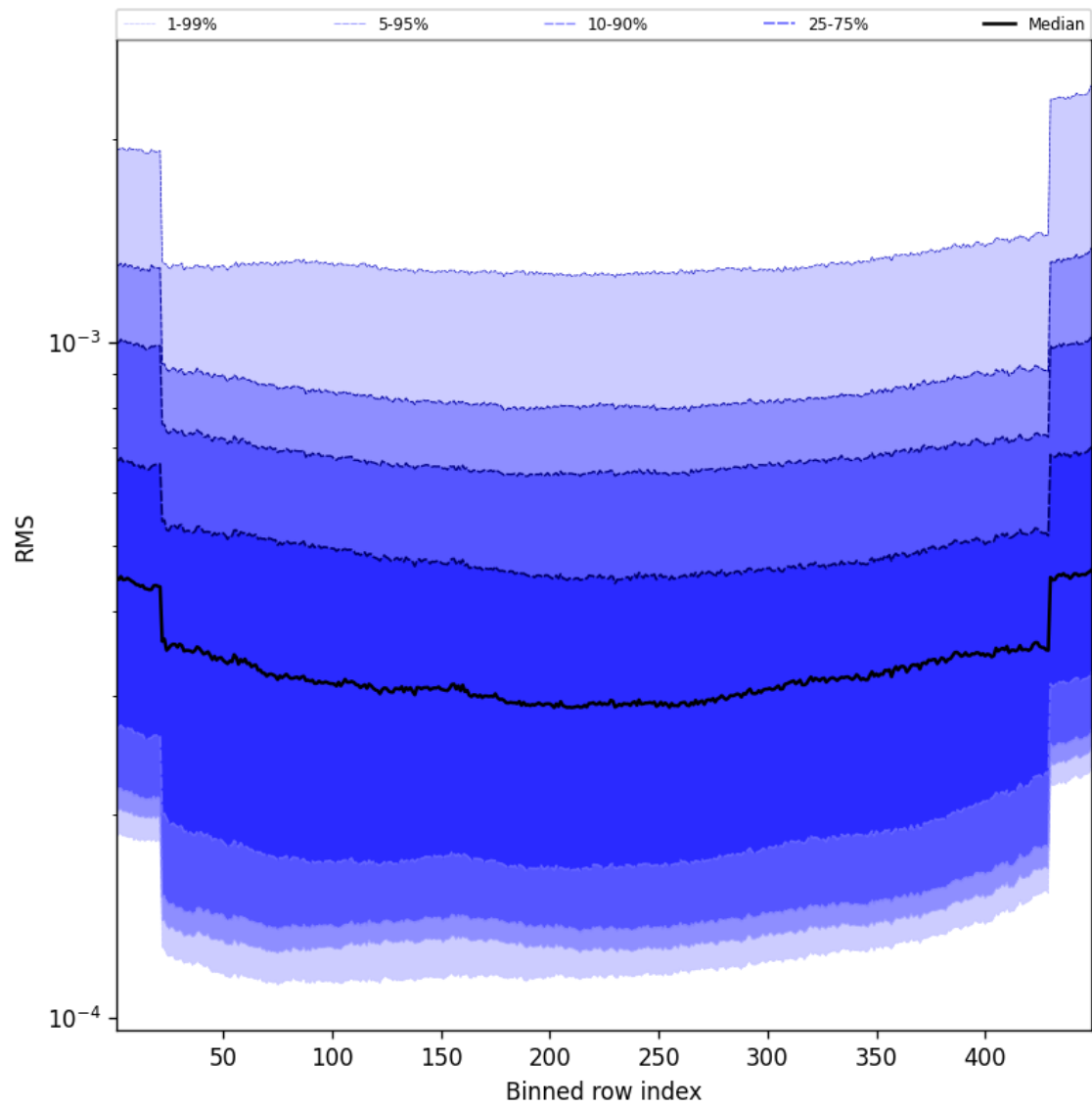
Figure 60: Along track statistics of “RMS” for 2025-03-16 to 2025-03-17
