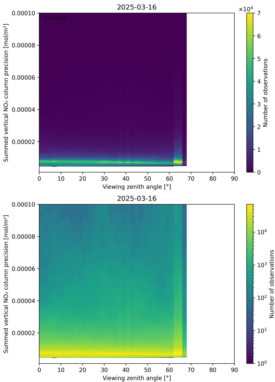
Figure 166: Scatter density plot of “Viewing zenith angle” against “Summed vertical NO 2 column precision” for 2025-03-16 to 2025-03-17.
