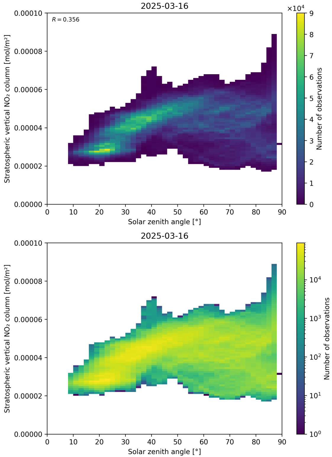
Figure 150: Scatter density plot of “Solar zenith angle” against “Stratospheric vertical NO 2 column” for 2025-03-16 to 2025-03-17.
