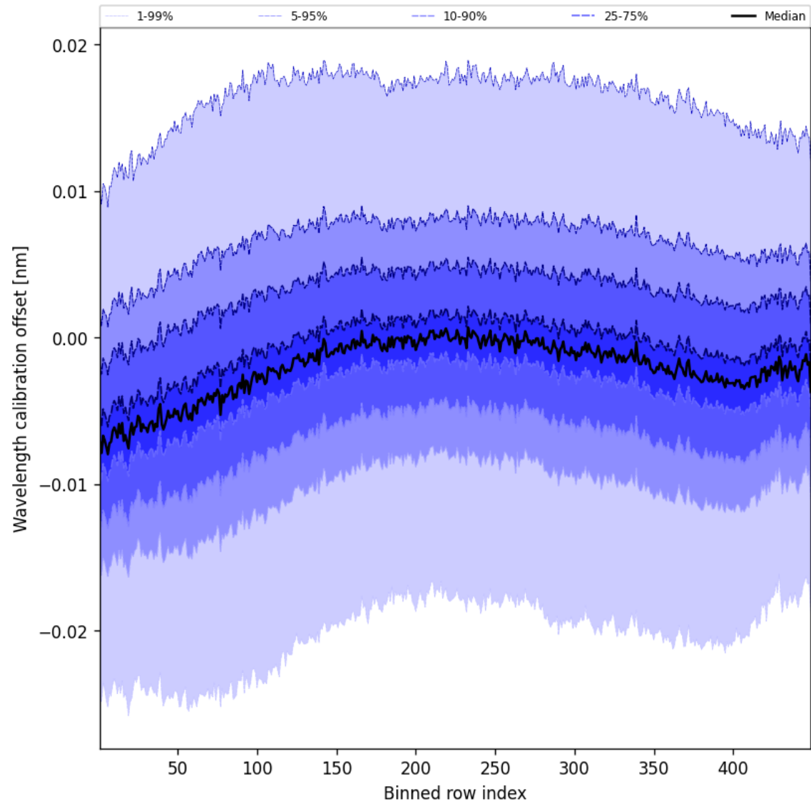
Figure 52: Along track statistics of “Wavelength calibration offset” for 2025-03-16 to 2025-03-17
