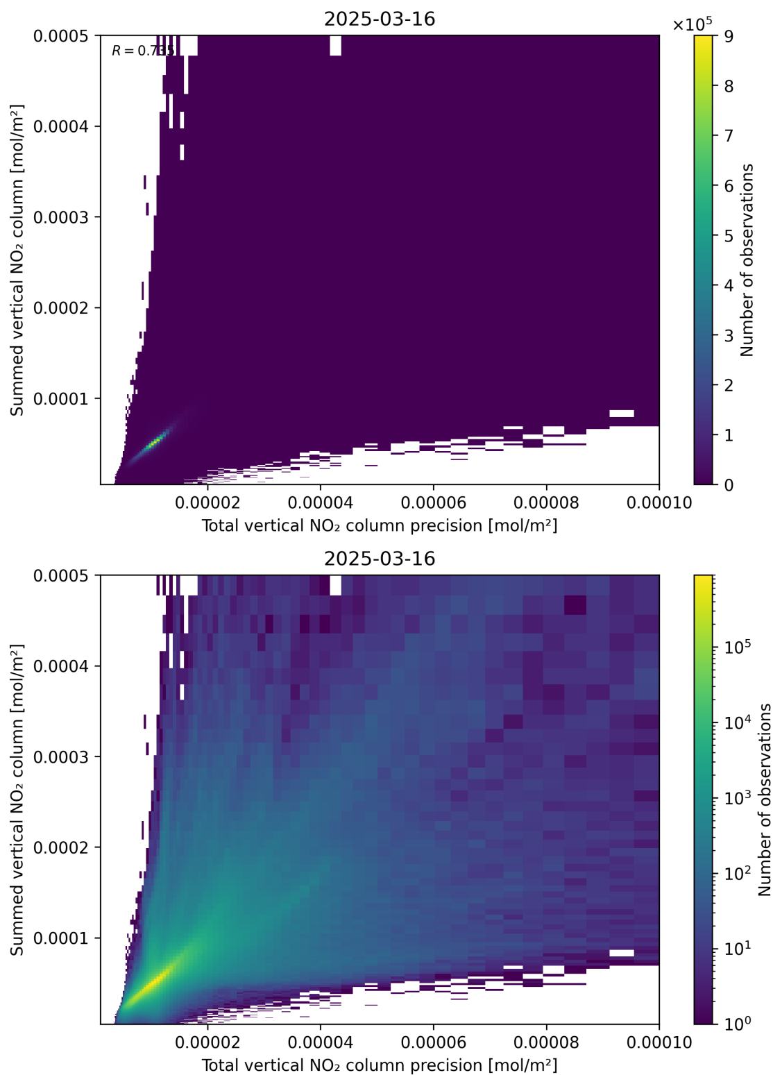
Figure 117: Scatter density plot of “Total vertical NO 2 column precision” against “Summed vertical NO 2 column” for 2025-03-16 to 2025-03-17.
