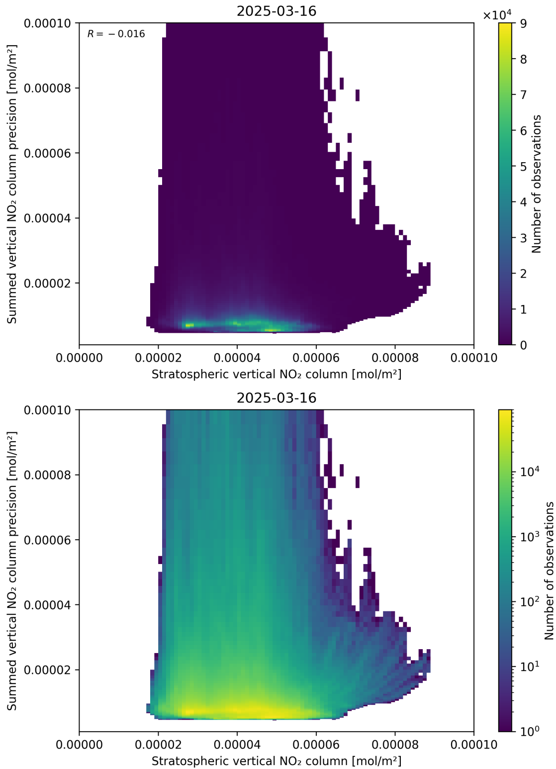
Figure 99: Scatter density plot of “Stratospheric vertical NO 2 column” against “Summed vertical NO 2 column precision” for 2025-03-16 to 2025-03-17.
