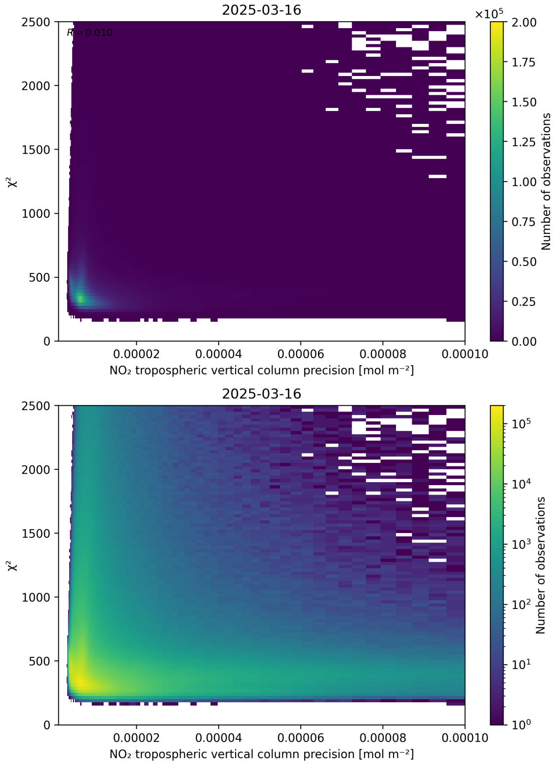
Figure 134: Scatter density plot of “NO 2 tropospheric vertical column precision” against “ \chi^2 ” for 2025-03-16 to 2025-03-17.
