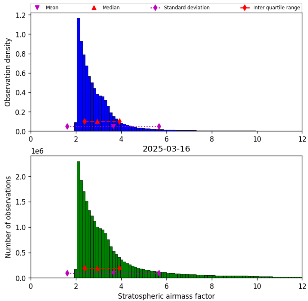
Figure 44: Histogram of “Stratospheric airmass factor” for 2025-03-16 to 2025-03-17
