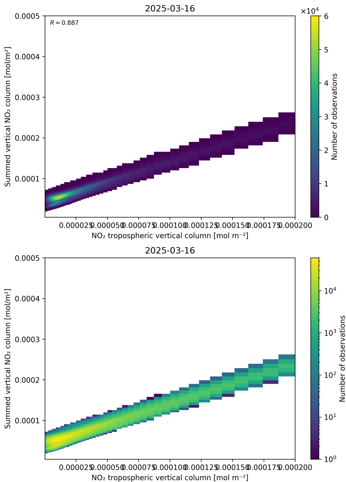
Figure 126: Scatter density plot of “NO 2 tropospheric vertical column” against “Summed vertical NO 2 column” for 2025-03-16 to 2025-03-17.
