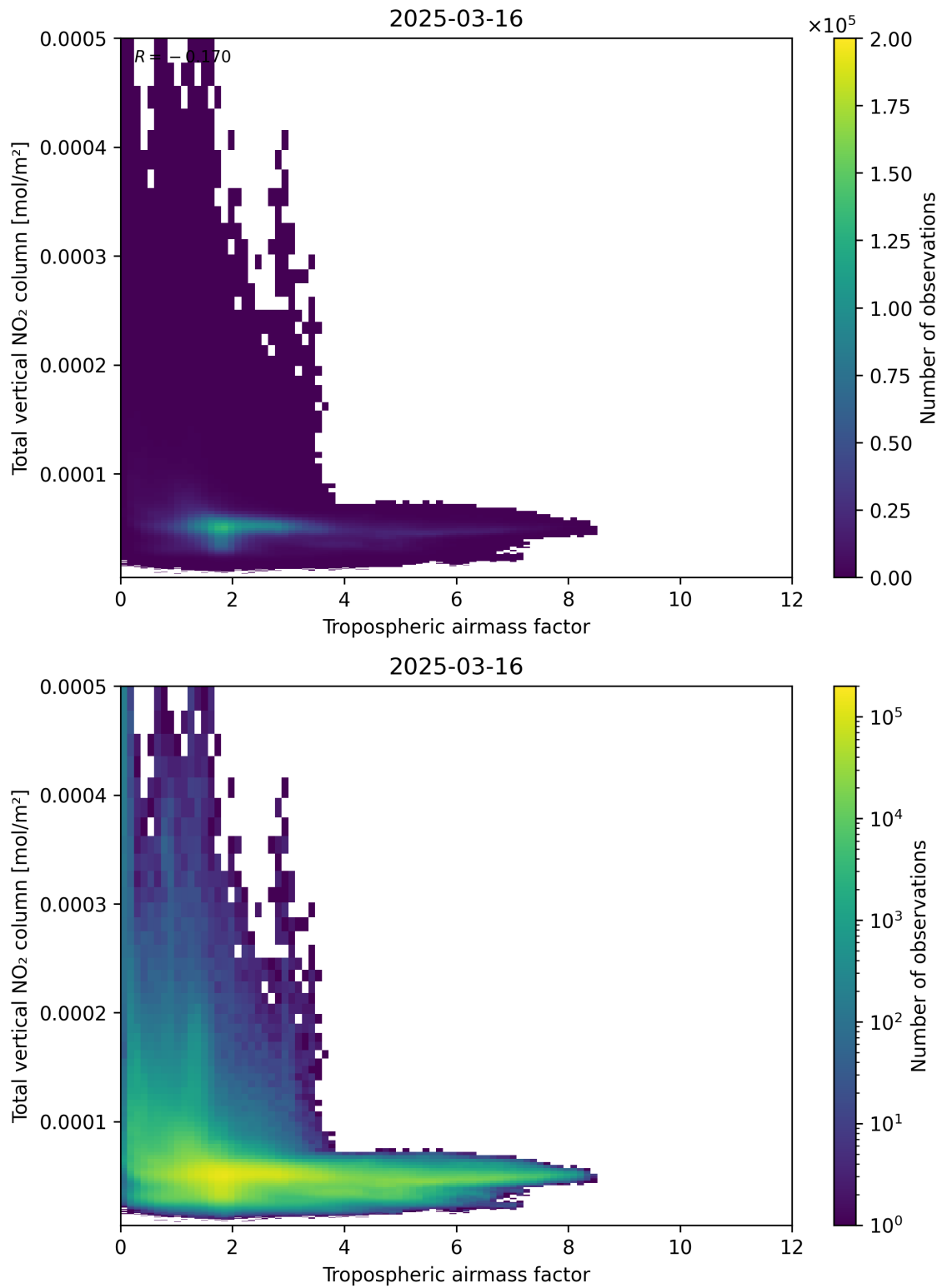
Figure 77: Scatter density plot of “Tropospheric airmass factor” against “Total vertical NO 2 column” for 2025-03-16 to 2025-03-17.
