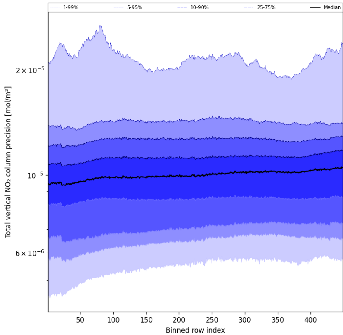
Figure 56: Along track statistics of “Total vertical NO 2 column precision” for 2025-03-16 to 2025-03-17
