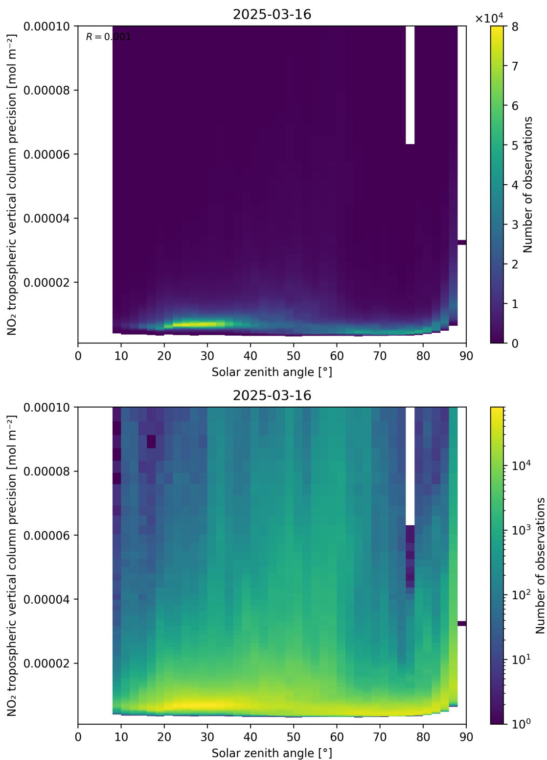
Figure 156: Scatter density plot of “Solar zenith angle” against “NO 2 tropospheric vertical column precision” for 2025-03-16 to 2025-03-17.
