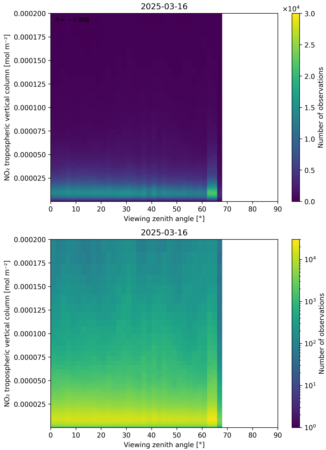
Figure 169: Scatter density plot of “Viewing zenith angle” against “NO 2 tropospheric vertical column” for 2025-03-16 to 2025-03-17.
