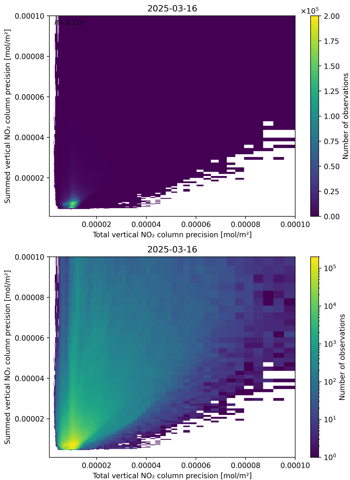
Figure 118: Scatter density plot of “Total vertical NO 2 column precision” against “Summed vertical NO 2 column precision” for 2025-03-16 to 2025-03-17.
