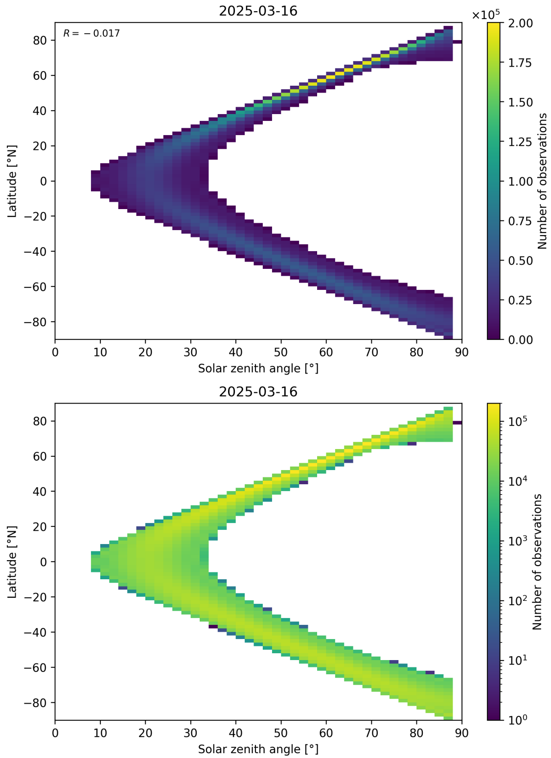
Figure 149: Scatter density plot of “Solar zenith angle” against “Latitude” for 2025-03-16 to 2025-03-17.
