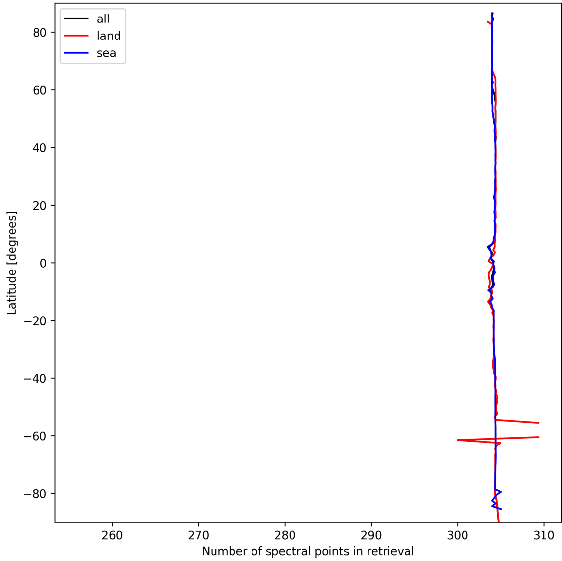
Figure 16: Zonal average of “Number of spectral points in retrieval” for 2025-03-16 to 2025-03-17.
