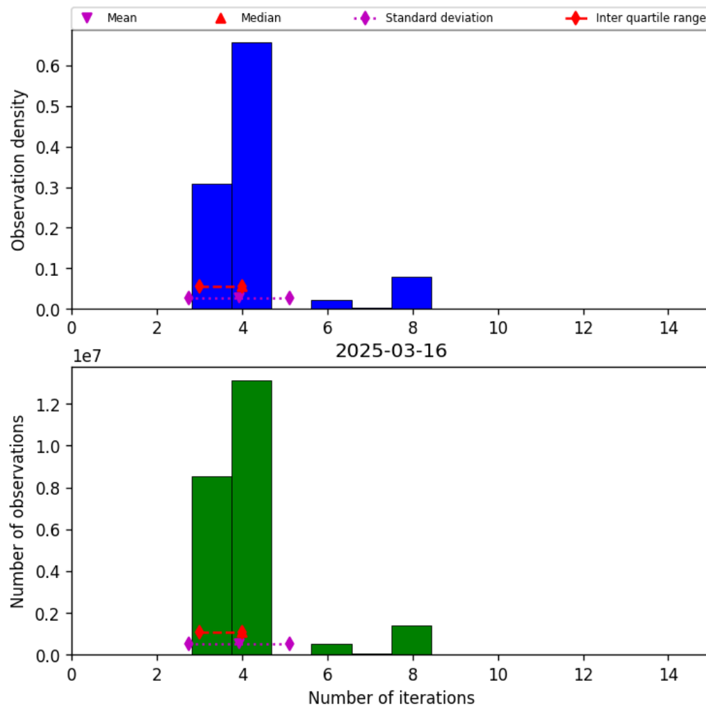
Figure 34: Histogram of “Number of iterations” for 2025-03-16 to 2025-03-17
