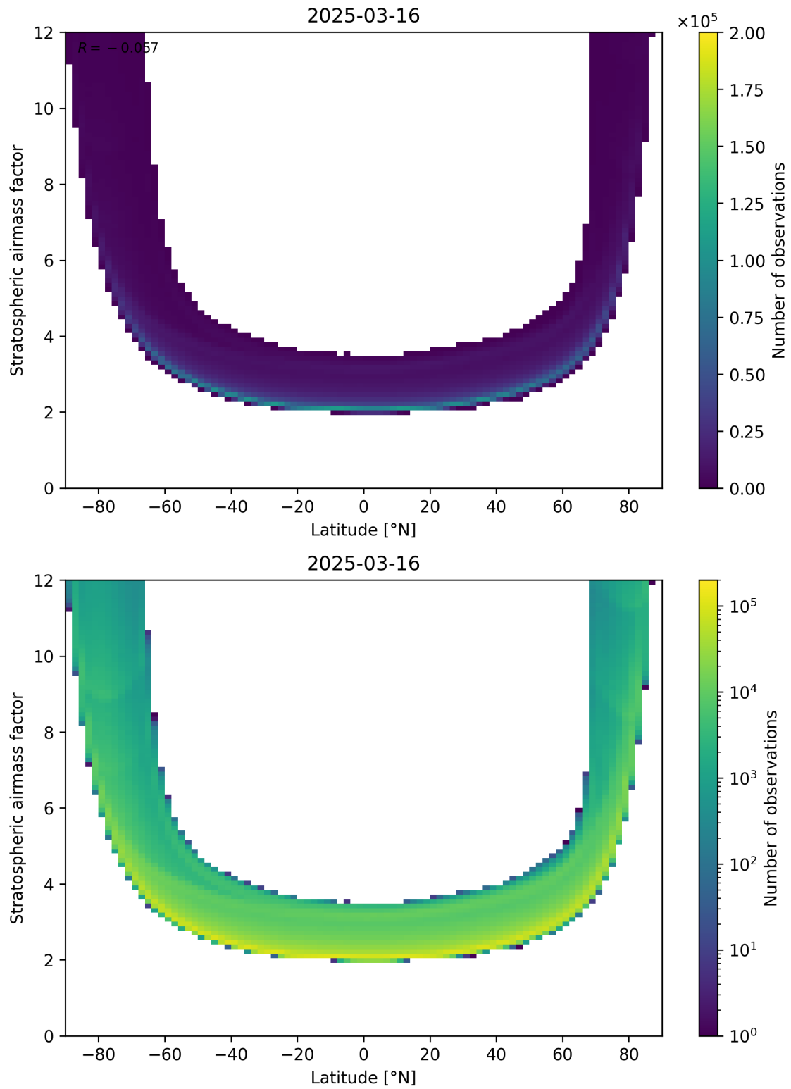
Figure 83: Scatter density plot of “Latitude” against “Stratospheric air mass factor” for 2025-03-16 to 2025-03-17.
