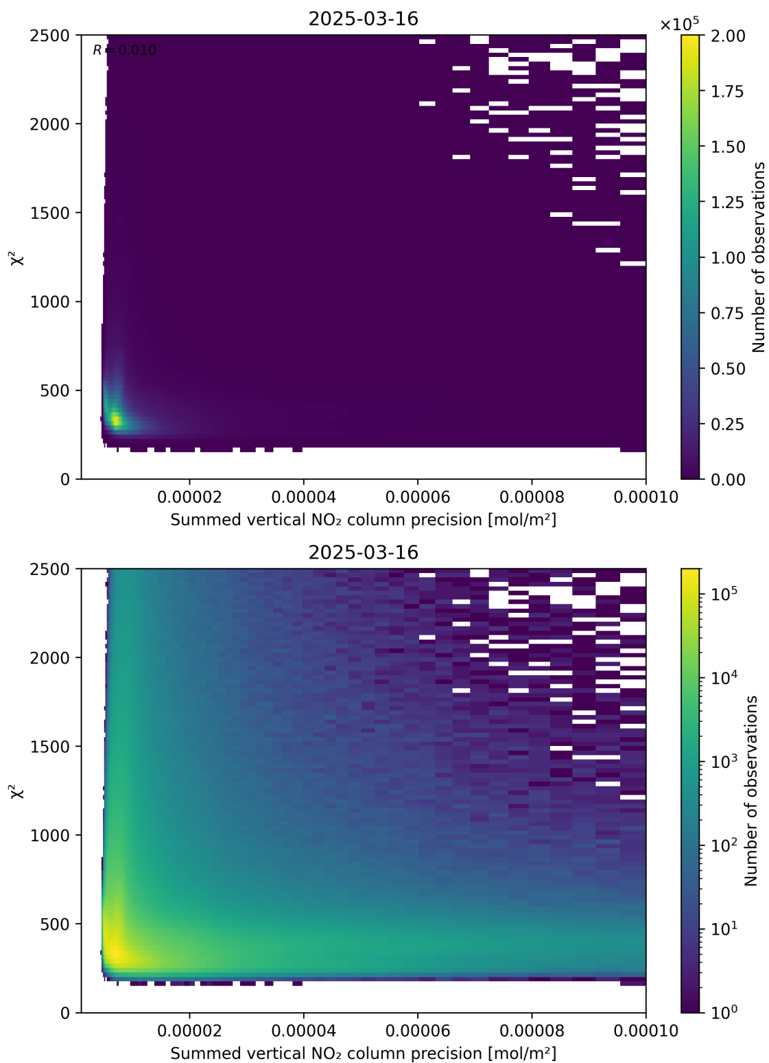
Figure 107: Scatter density plot of “Summed vertical NO 2 column precision” against “ \chi^2 ” for 2025-03-16 to 2025-03-17.
