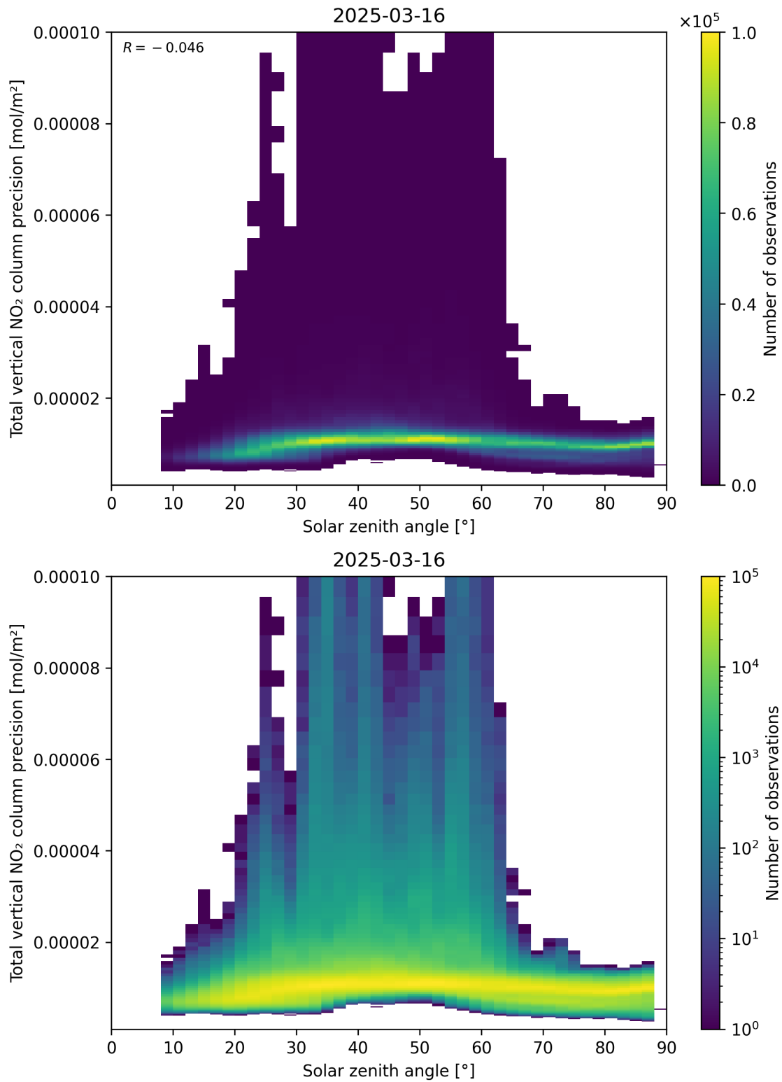
Figure 154: Scatter density plot of “Solar zenith angle” against “Total vertical NO 2 column precision” for 2025-03-16 to 2025-03-17.
