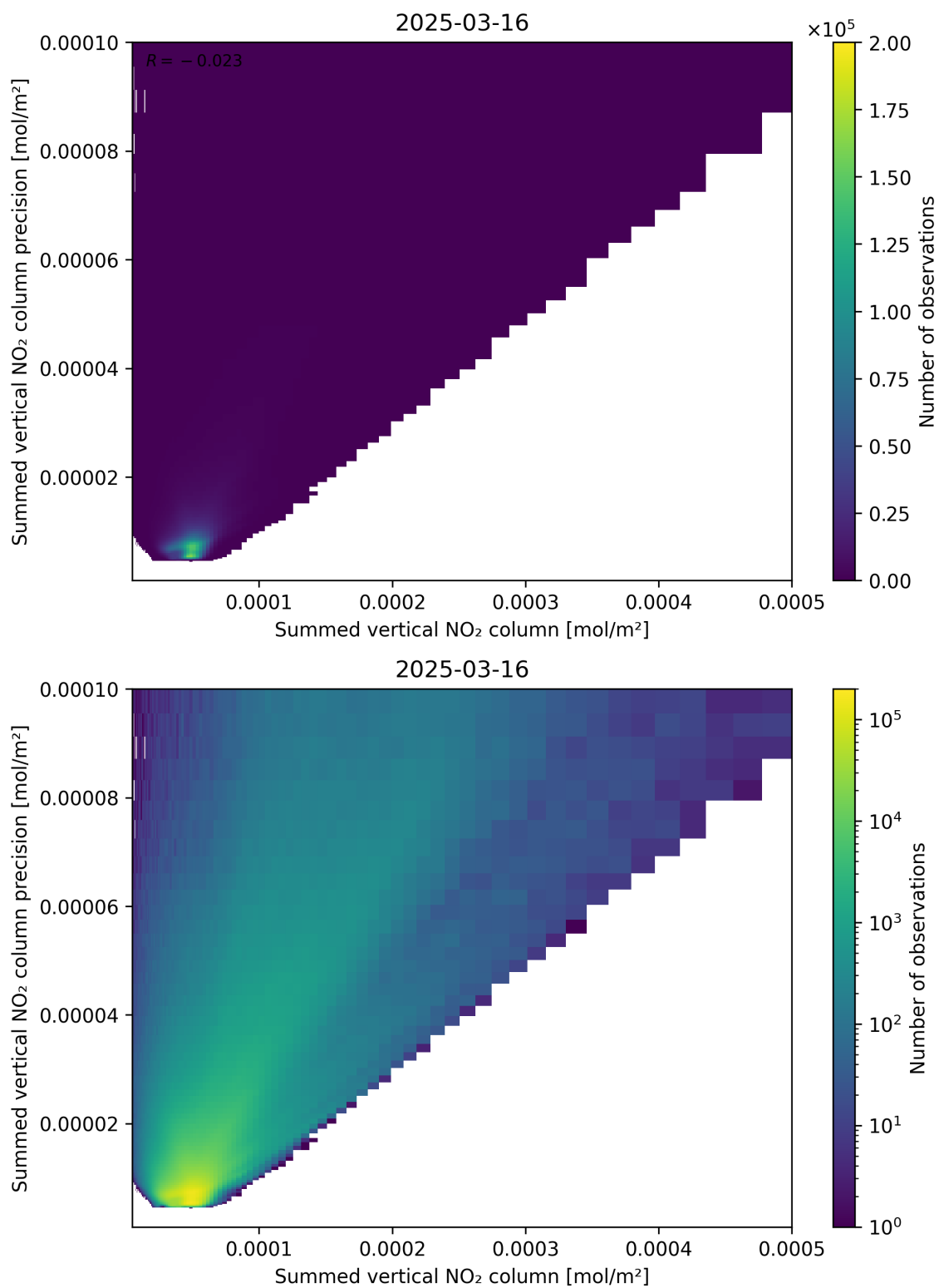
Figure 105: Scatter density plot of “Summed vertical NO 2 column” against “Summed vertical NO 2 column precision” for 2025-03-16 to 2025-03-17.
