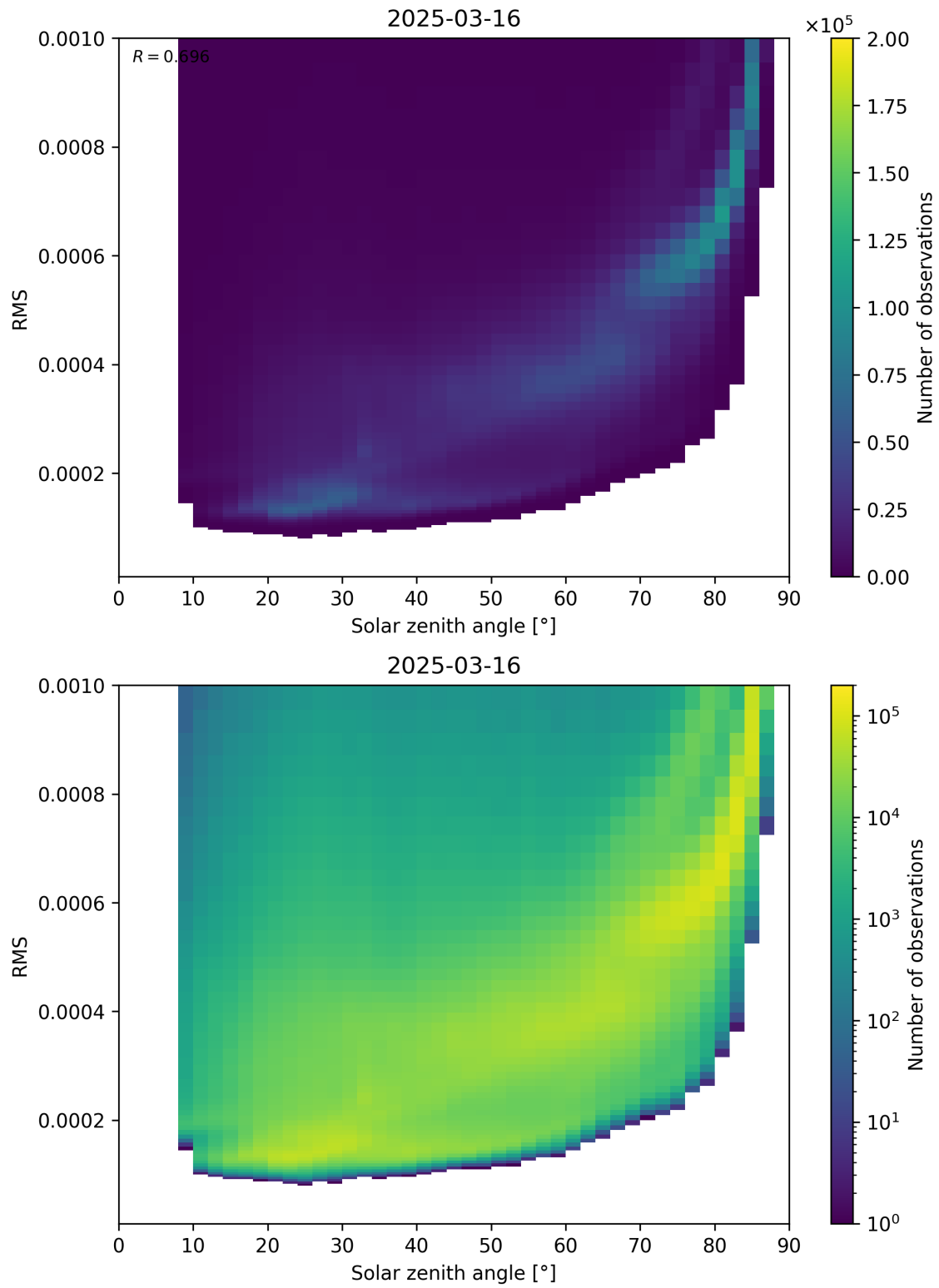
Figure 157: Scatter density plot of “Solar zenith angle” against “RMS” for 2025-03-16 to 2025-03-17.
