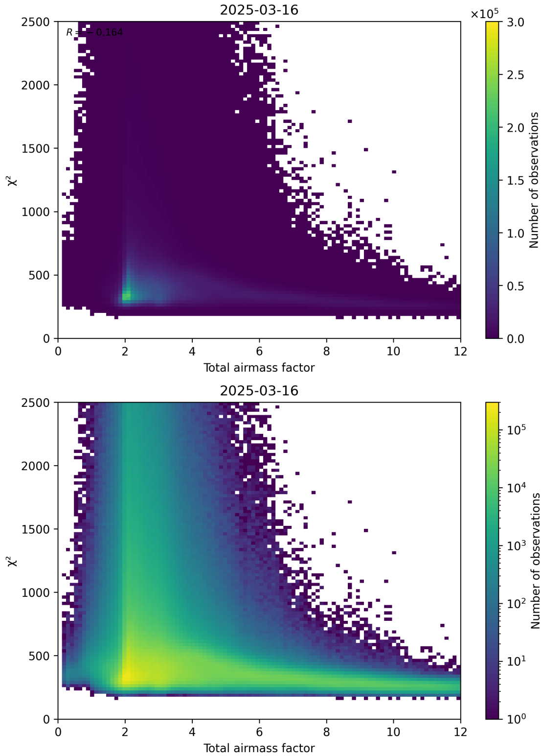
Figure 63: Scatter density plot of “Total airmass factor” against “ \chi^2 ” for 2025-03-16 to 2025-03-17.
