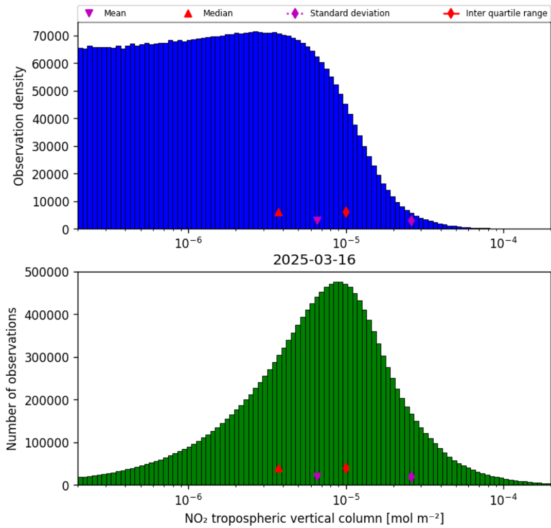
Figure 29: Histogram of “NO 2 tropospheric vertical column” for 2025-03-16 to 2025-03-17
