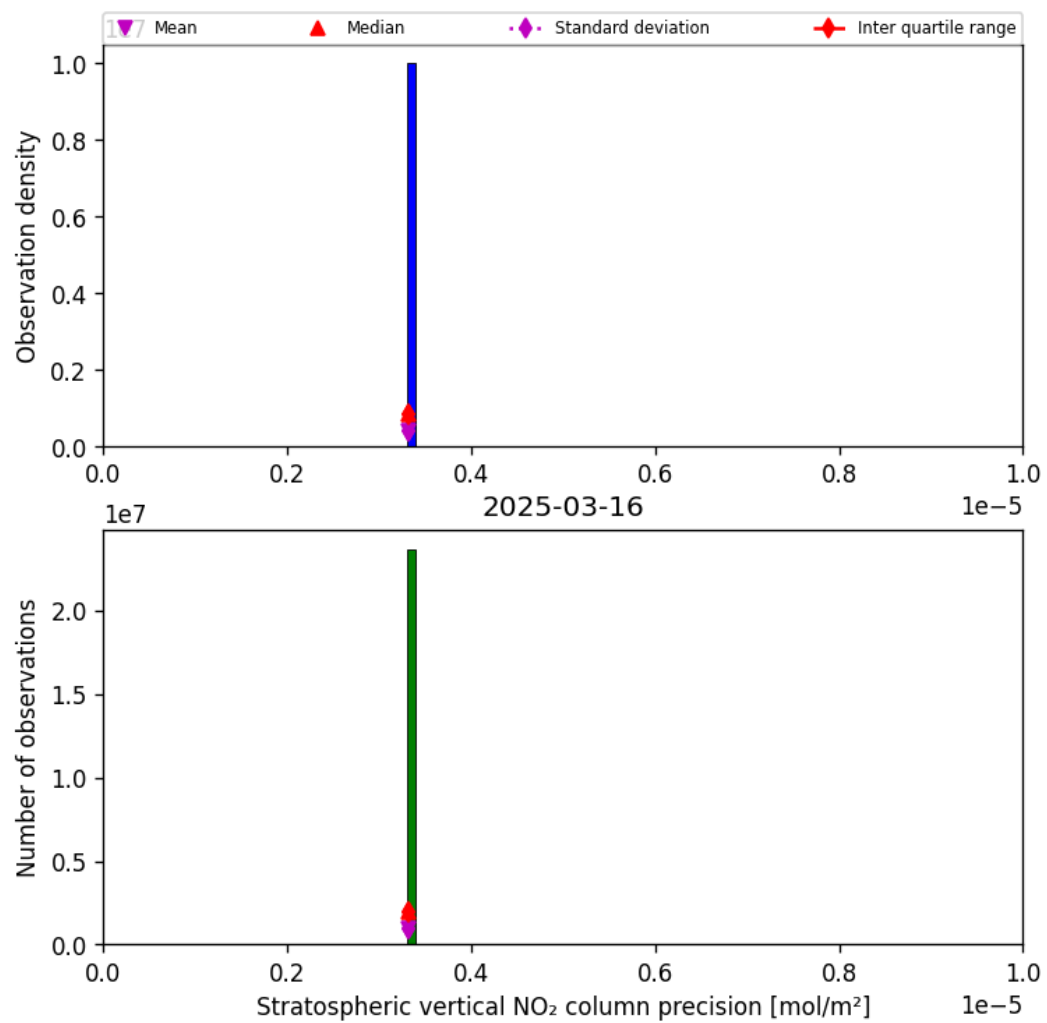
Figure 37: Histogram of “Stratospheric vertical NO 2 column precision” for 2025-03-16 to 2025-03-17
