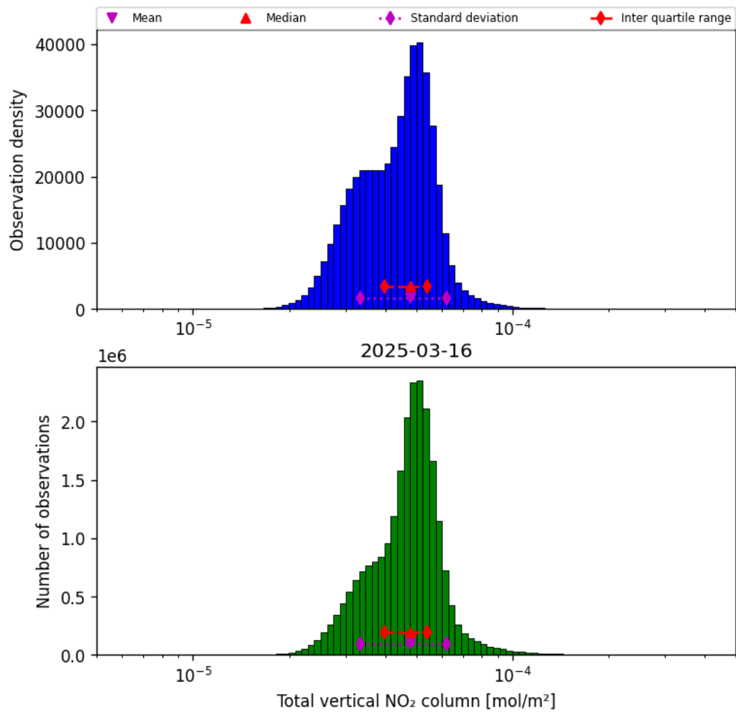
Figure 38: Histogram of “Total vertical NO 2 column” for 2025-03-16 to 2025-03-17
