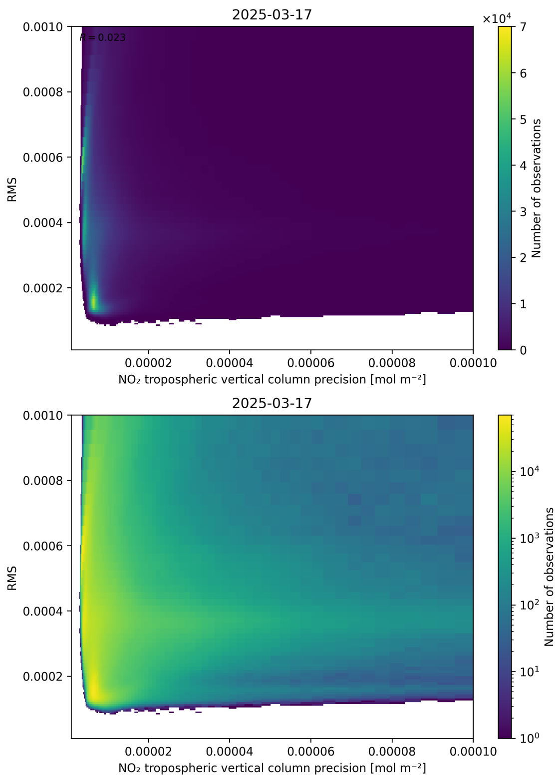
Figure 140: Scatter density plot of “NO 2 tropospheric vertical column precision” against “RMS” for 2025-03-17 to 2025-03-18.
