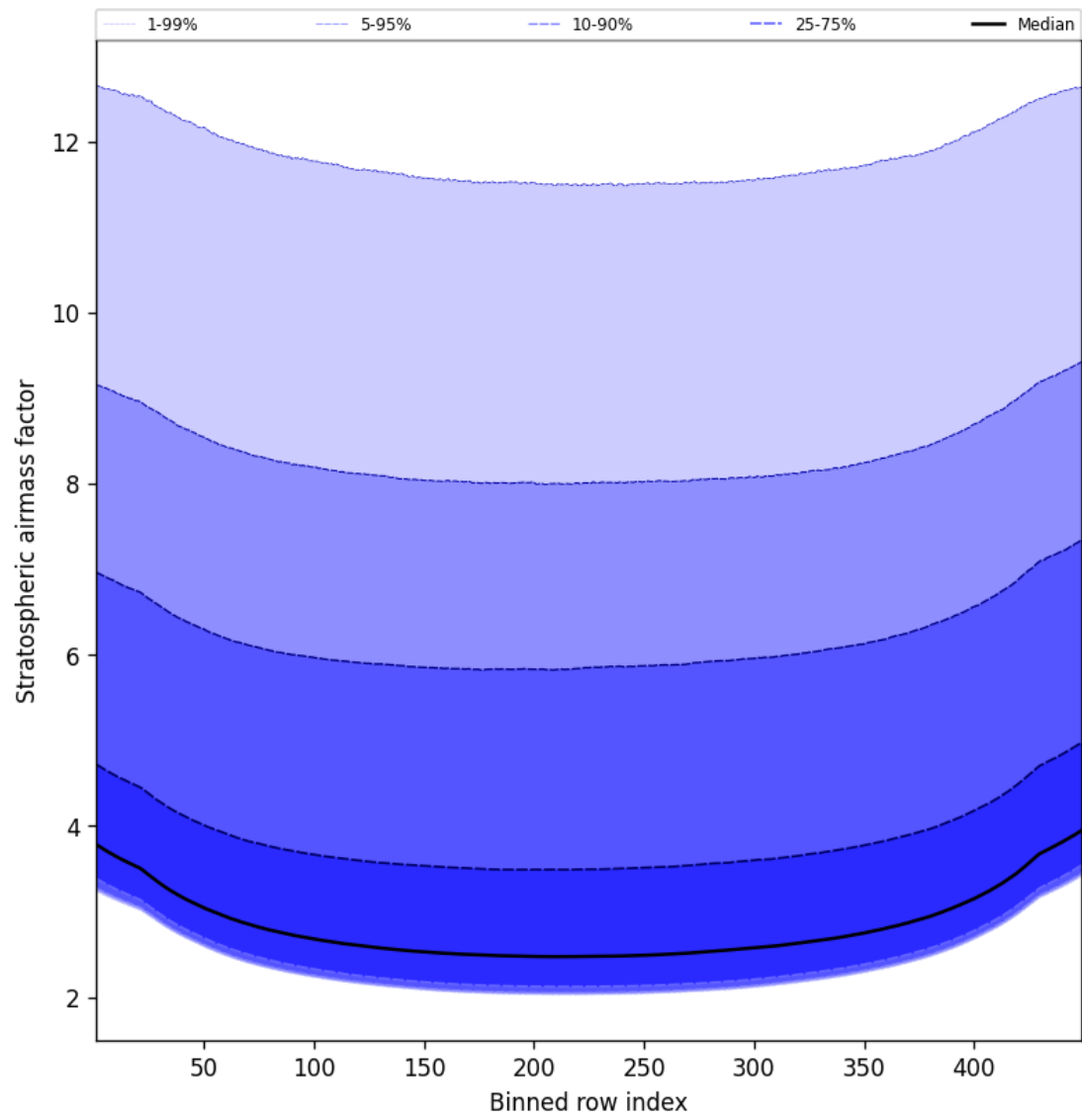
Figure 61: Along track statistics of “Stratospheric airmass factor” for 2025-03-17 to 2025-03-18
