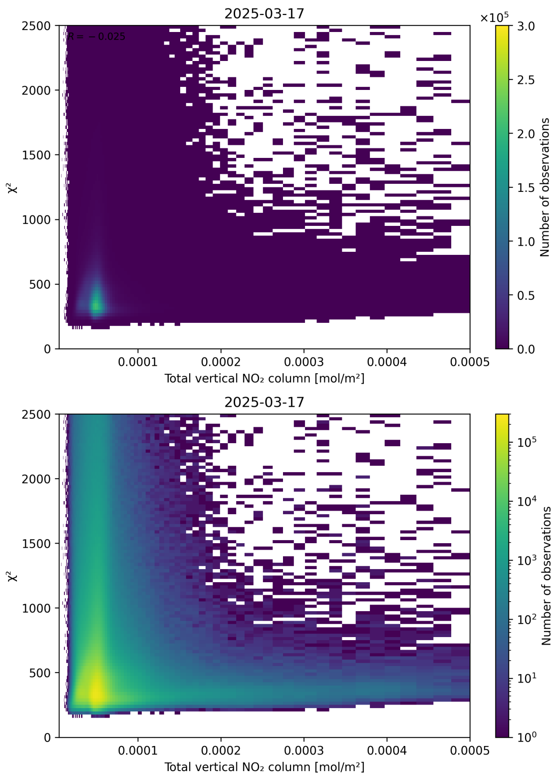
Figure 111: Scatter density plot of “Total vertical NO 2 column” against “ \chi^2 ” for 2025-03-17 to 2025-03-18.
