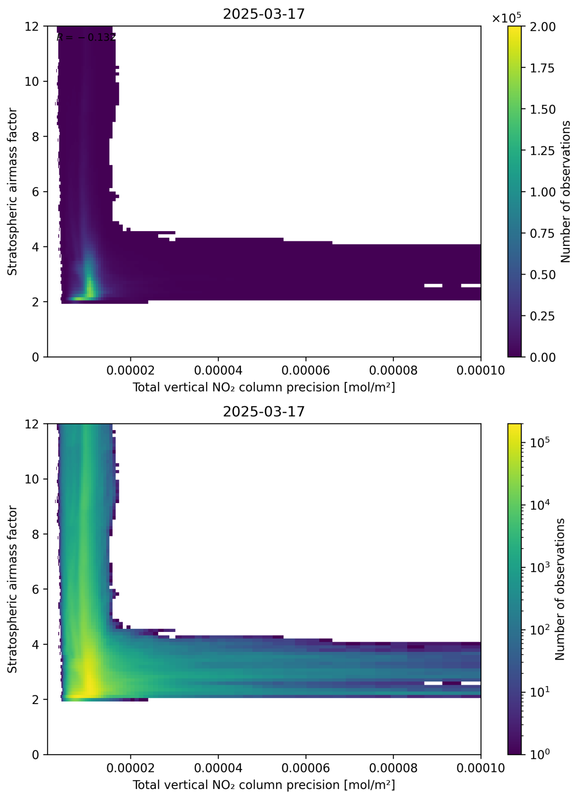
Figure 115: Scatter density plot of “Total vertical NO 2 column precision” against “Stratospheric air mass factor” for 2025-03-17 to 2025-03-18.
