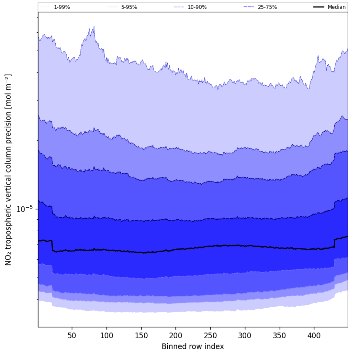
Figure 47: Along track statistics of “NO 2 tropospheric vertical column precision” for 2025-03-17 to 2025-03-18
