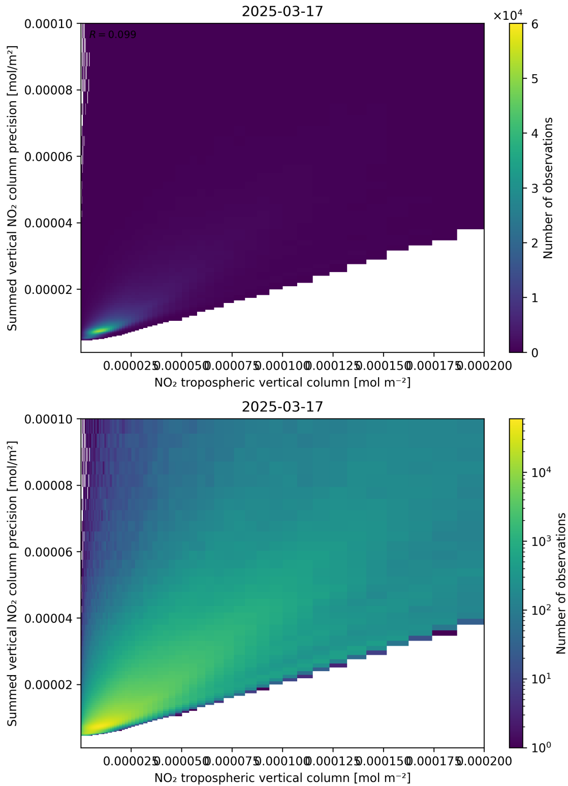
Figure 127: Scatter density plot of “NO 2 tropospheric vertical column” against “Summed vertical NO 2 column precision” for 2025-03-17 to 2025-03-18.
