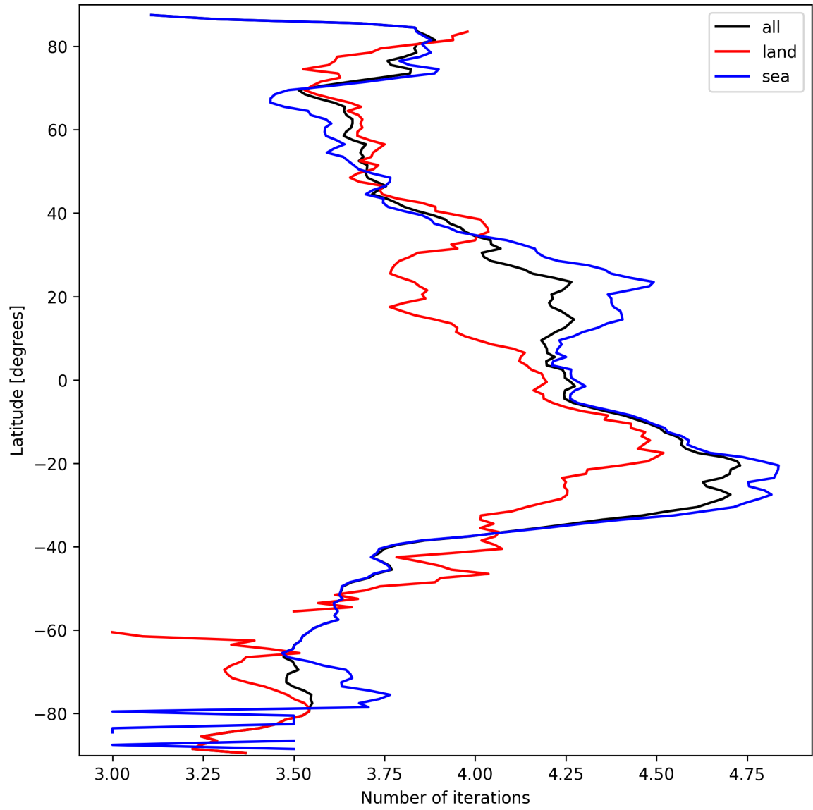
Figure 17: Zonal average of “Number of iterations” for 2025-03-17 to 2025-03-18.
