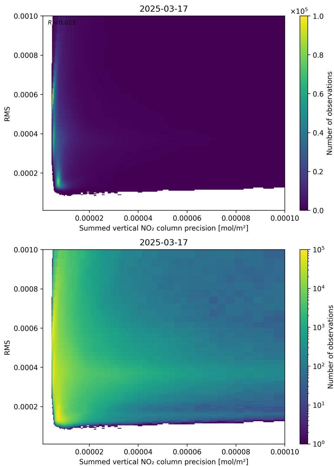
Figure 108: Scatter density plot of “Summed vertical NO 2 column precision” against “RMS” for 2025-03-17 to 2025-03-18.
