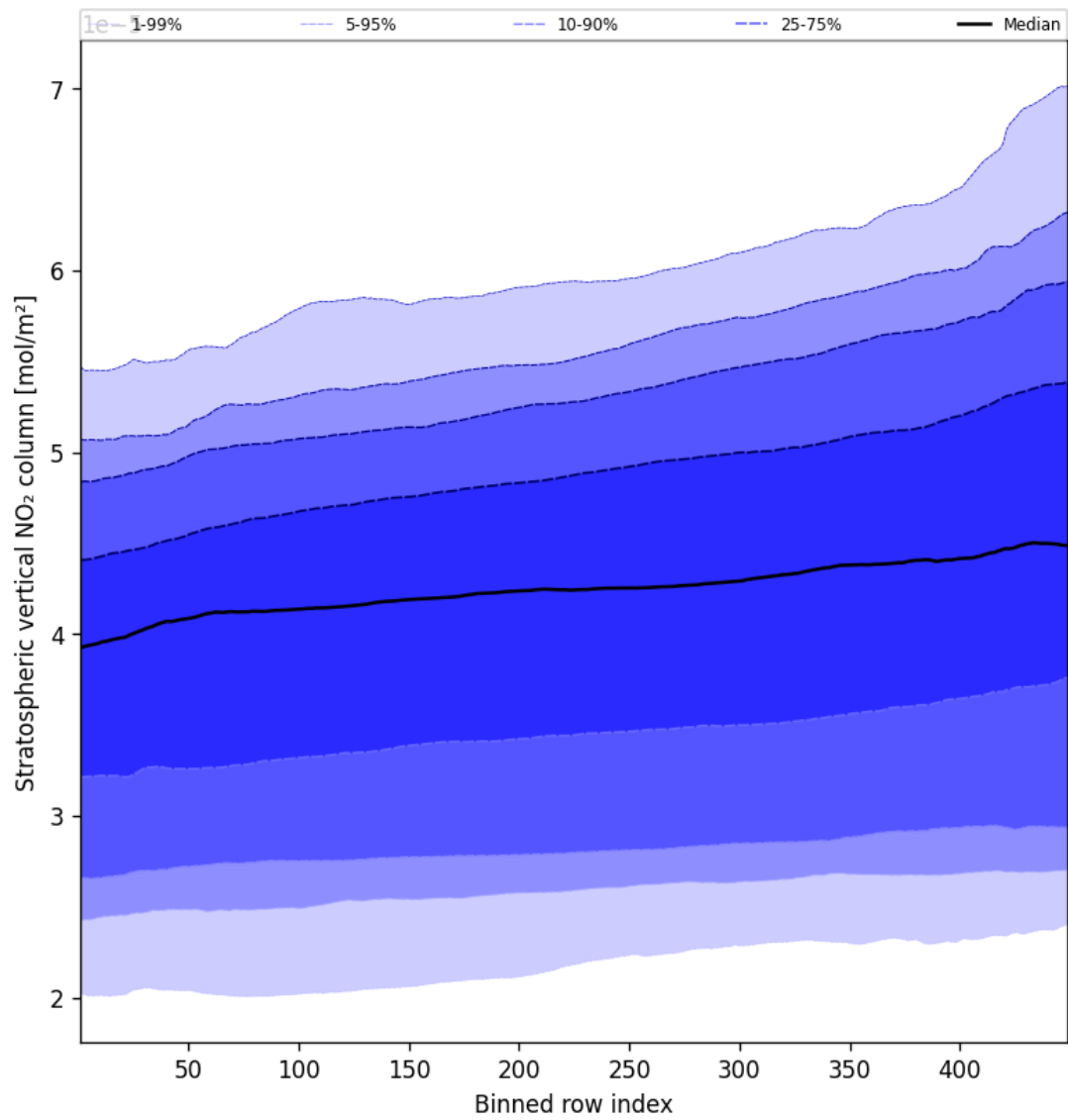
Figure 53: Along track statistics of “Stratospheric vertical NO 2 column” for 2025-03-17 to 2025-03-18
