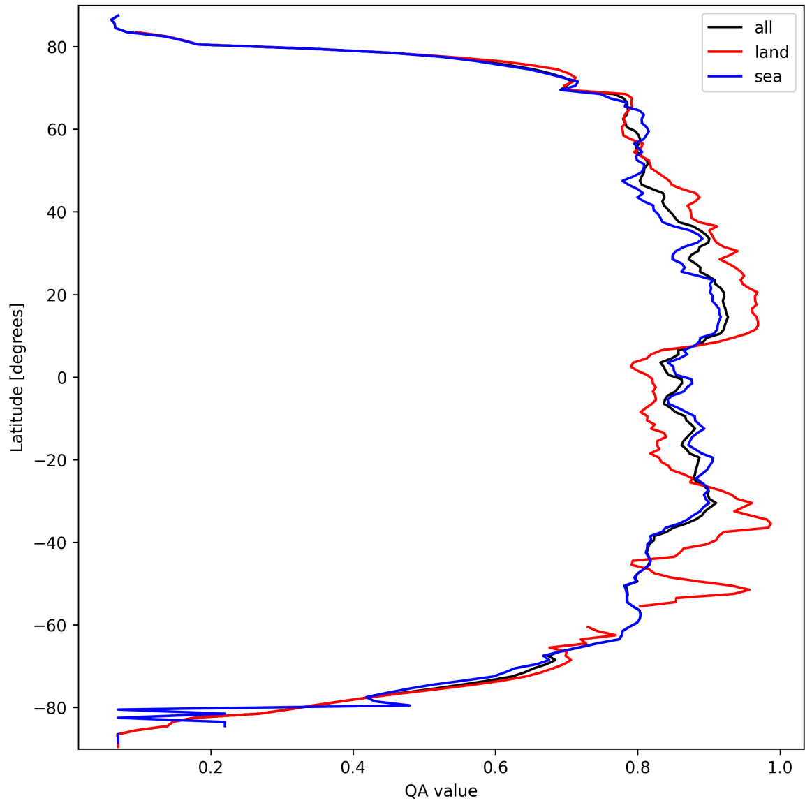
Figure 11: Zonal average of “QA value” for 2025-03-17 to 2025-03-18.
