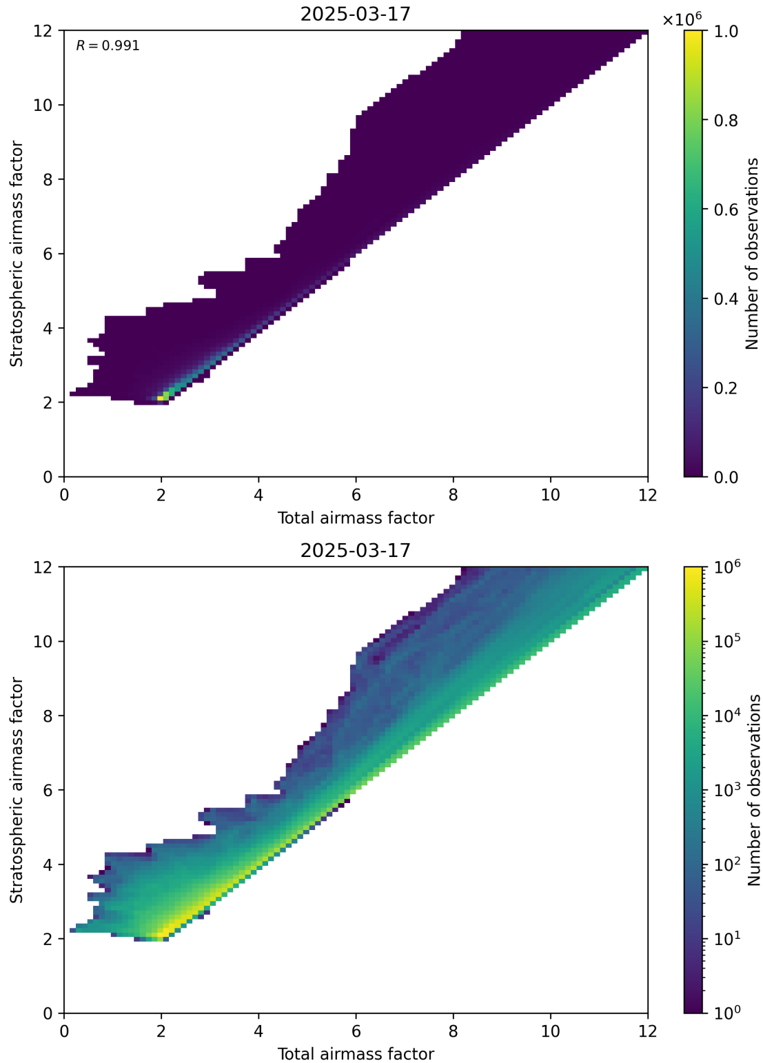
Figure 62: Scatter density plot of “Total airmass factor” against “Stratospheric airmass factor” for 2025-03-17 to 2025-03-18.
