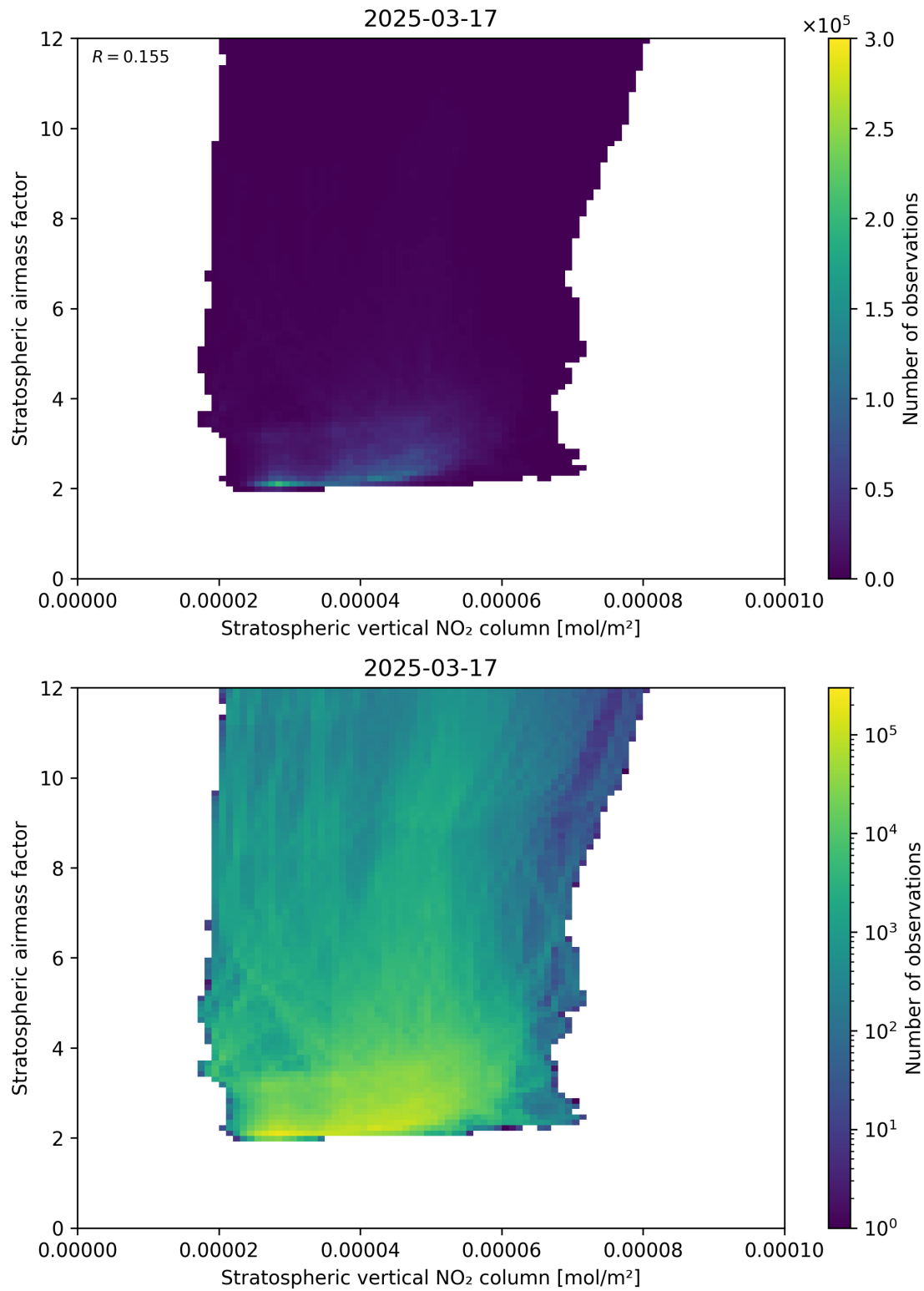
Figure 96: Scatter density plot of “Stratospheric vertical NO 2 column” against “Stratospheric airmass factor” for 2025-03-17 to 2025-03-18.
