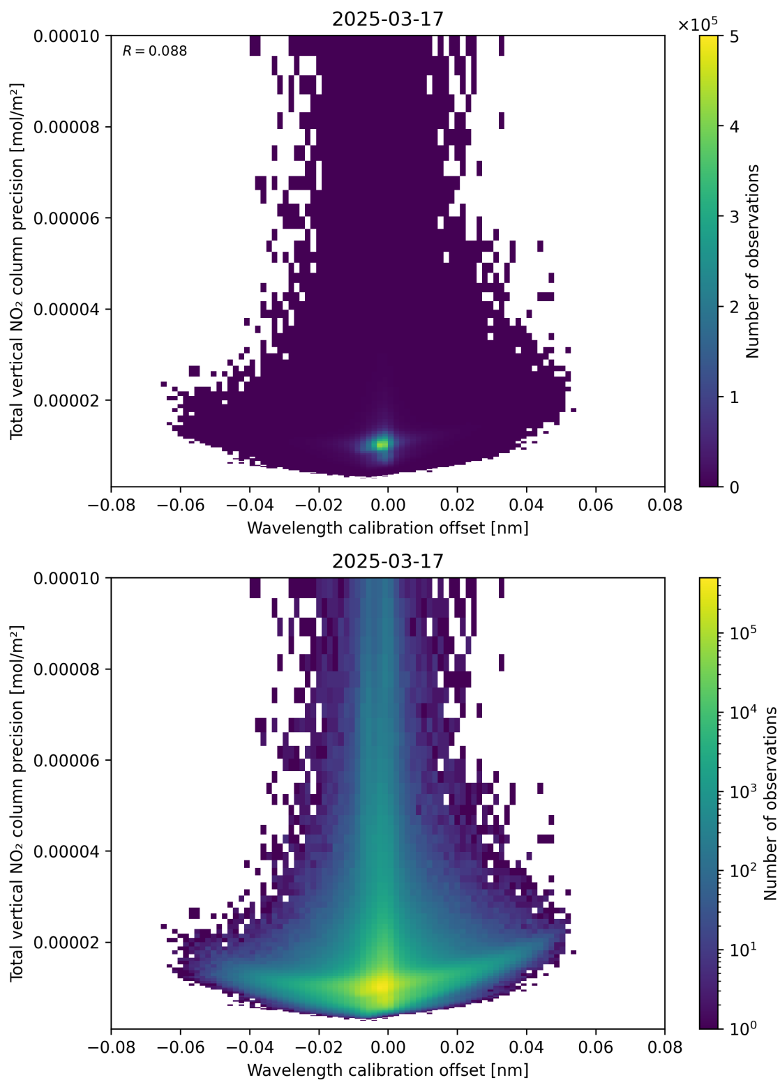
Figure 180: Scatter density plot of “Wavelength calibration offset” against “Total vertical NO 2 column precision” for 2025-03-17 to 2025-03-18.
