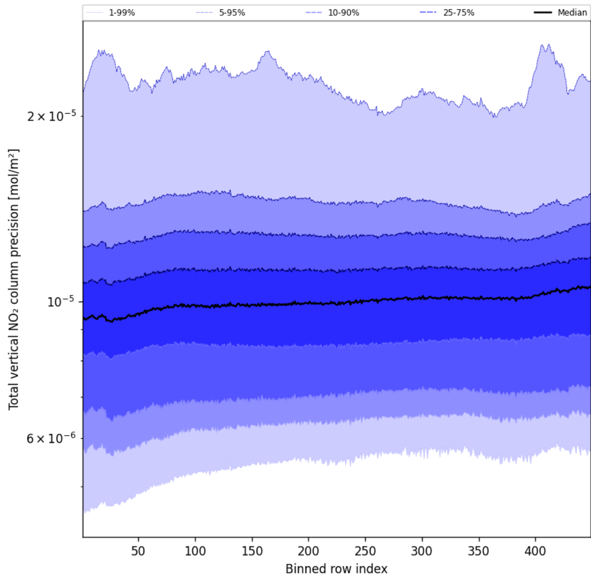
Figure 56: Along track statistics of “Total vertical NO 2 column precision” for 2025-03-17 to 2025-03-18
