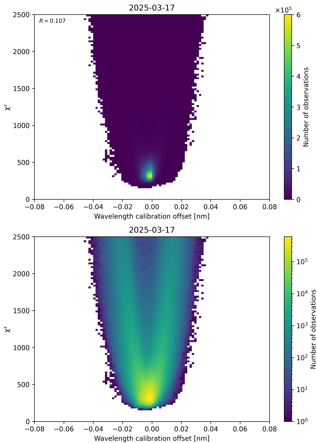
Figure 175: Scatter density plot of “Wavelength calibration offset” against “ \chi^2 ” for 2025-03-17 to 2025-03-18.
