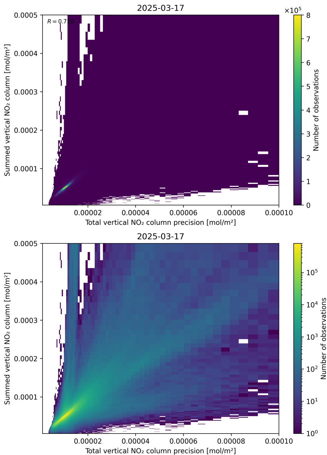
Figure 117: Scatter density plot of “Total vertical NO 2 column precision” against “Summed vertical NO 2 column” for 2025-03-17 to 2025-03-18.
