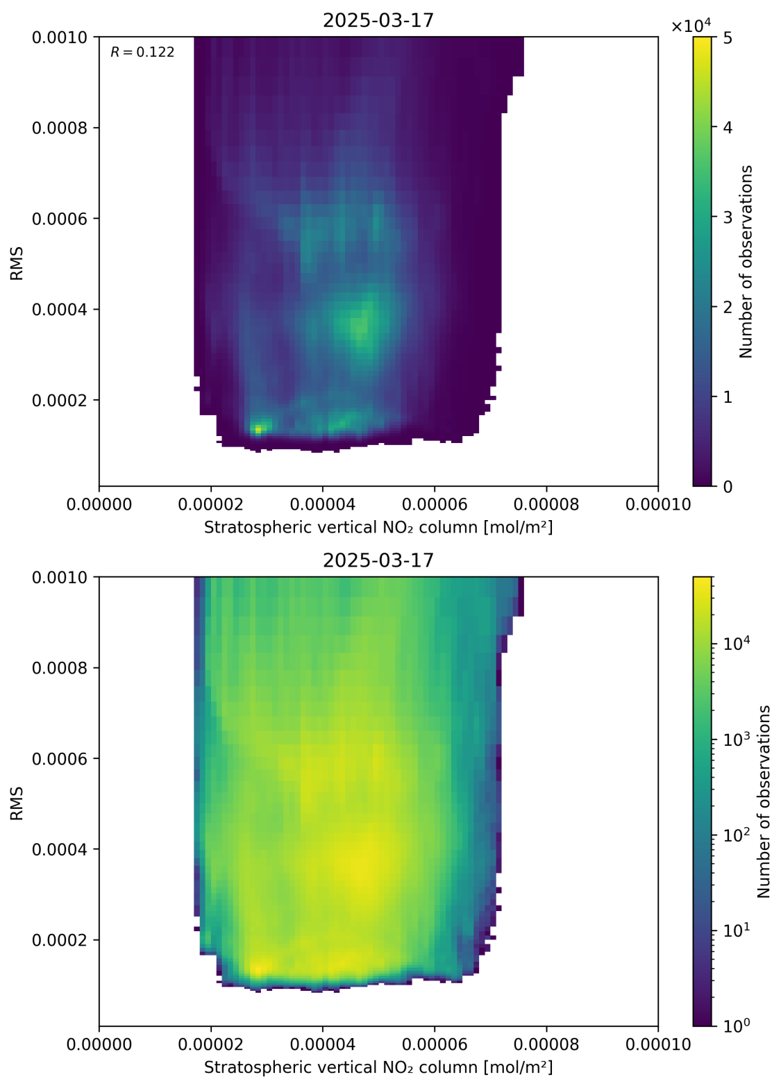
Figure 102: Scatter density plot of “Stratospheric vertical NO 2 column” against “RMS” for 2025-03-17 to 2025-03-18.
