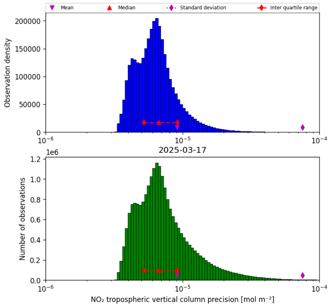
Figure 30: Histogram of “NO 2 tropospheric vertical column precision” for 2025-03-17 to 2025-03-18
