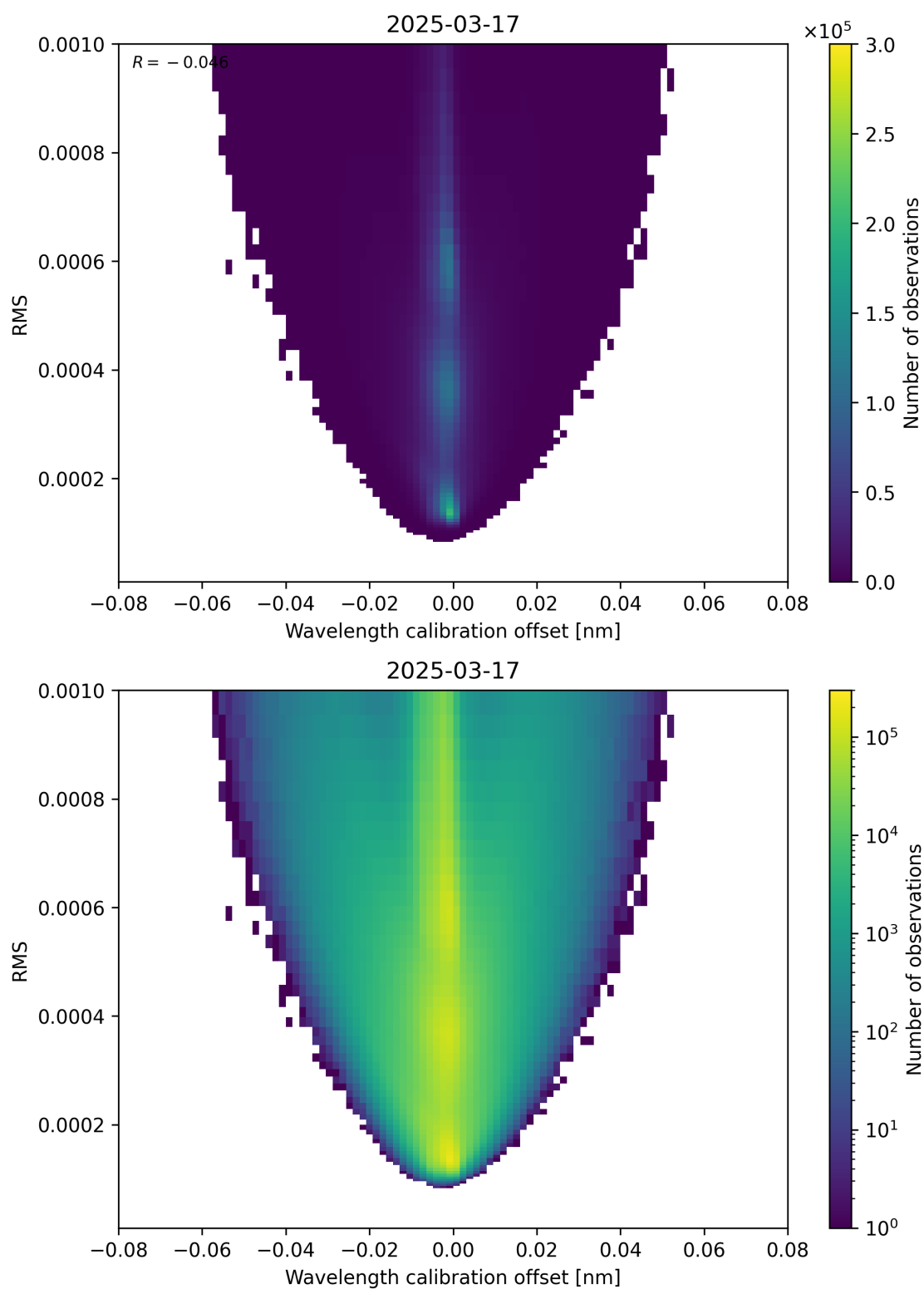
Figure 181: Scatter density plot of “Wavelength calibration offset” against “RMS” for 2025-03-17 to 2025-03-18.
