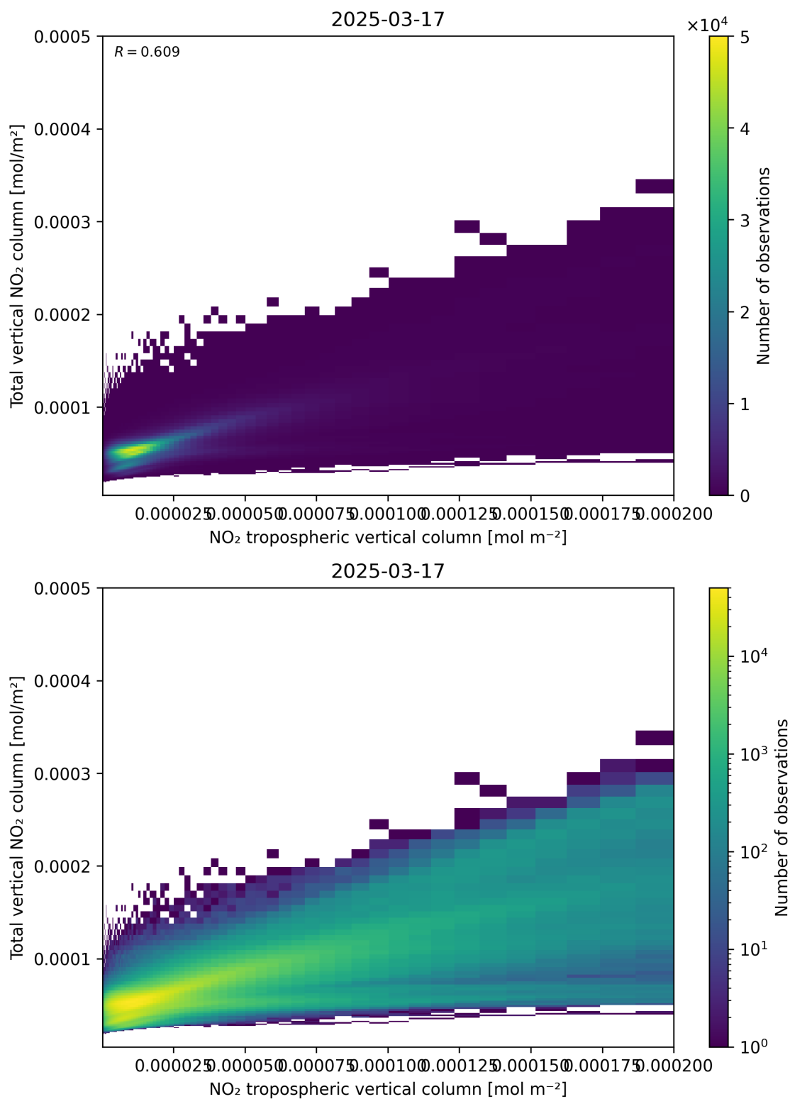
Figure 128: Scatter density plot of “NO 2 tropospheric vertical column” against “Total vertical NO 2 column” for 2025-03-17 to 2025-03-18.
