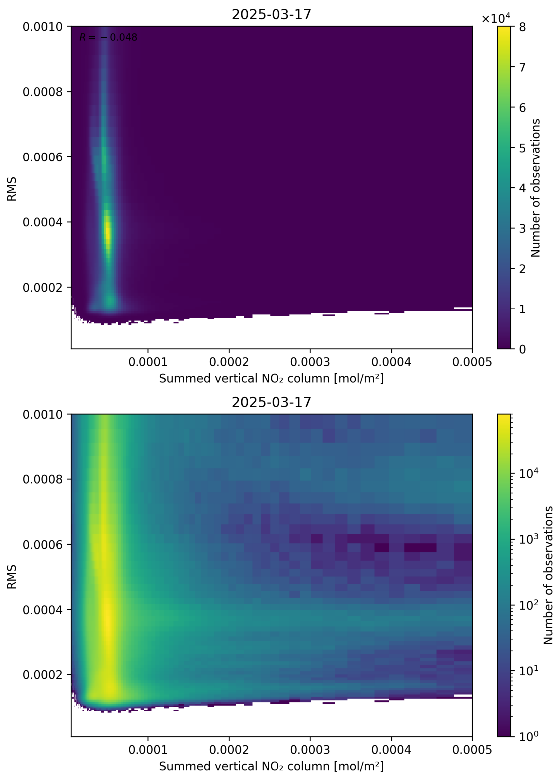
Figure 109: Scatter density plot of “Summed vertical NO 2 column” against “RMS” for 2025-03-17 to 2025-03-18.
