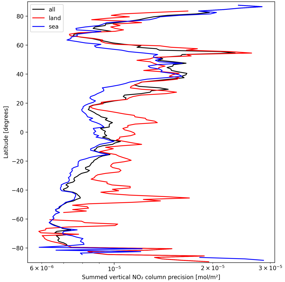
Figure 24: Zonal average of “Summed vertical NO 2 column precision” for 2025-03-17 to 2025-03-18.
