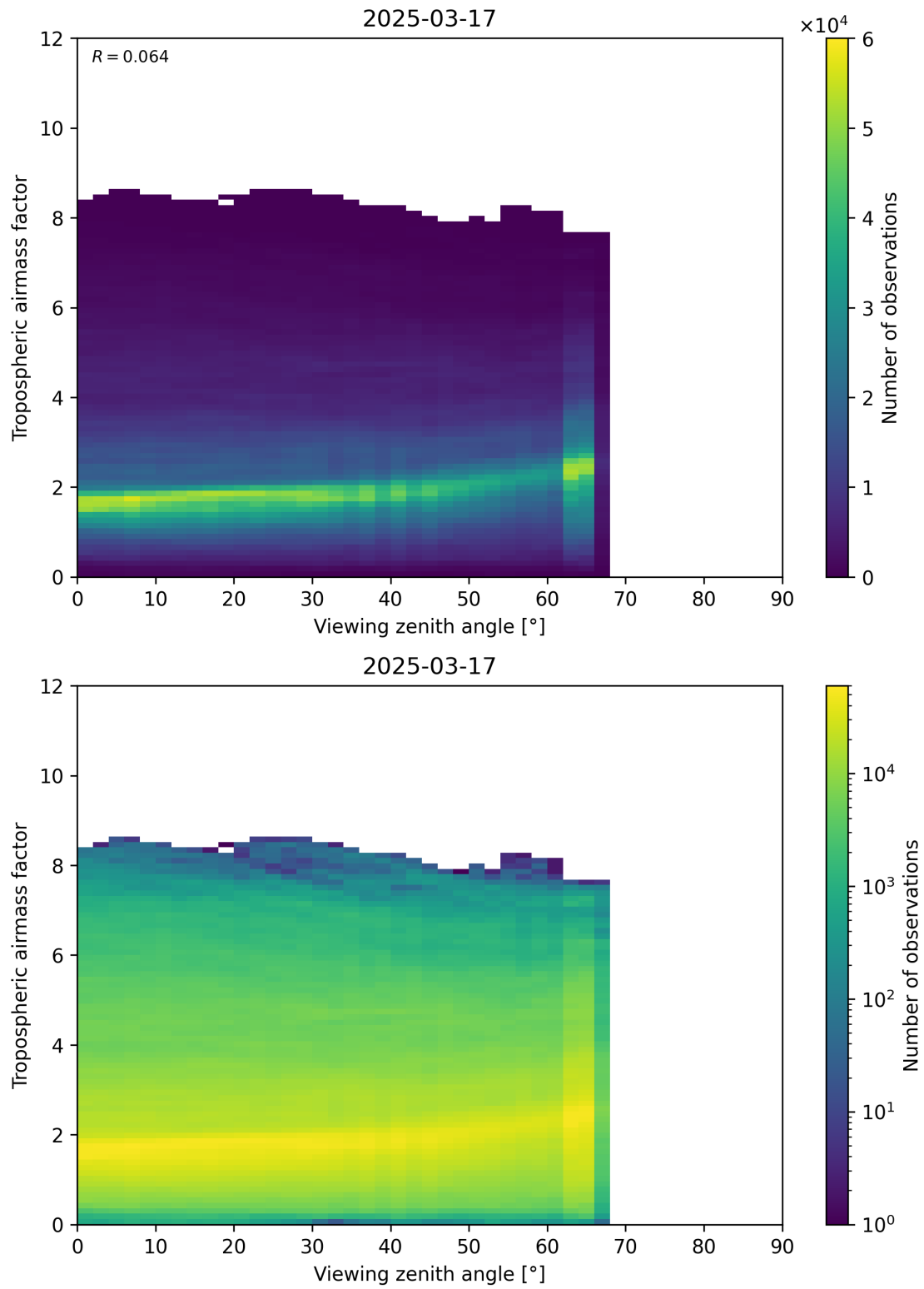
Figure 161: Scatter density plot of “Viewing zenith angle” against “Tropospheric airmass factor” for 2025-03-17 to 2025-03-18.
