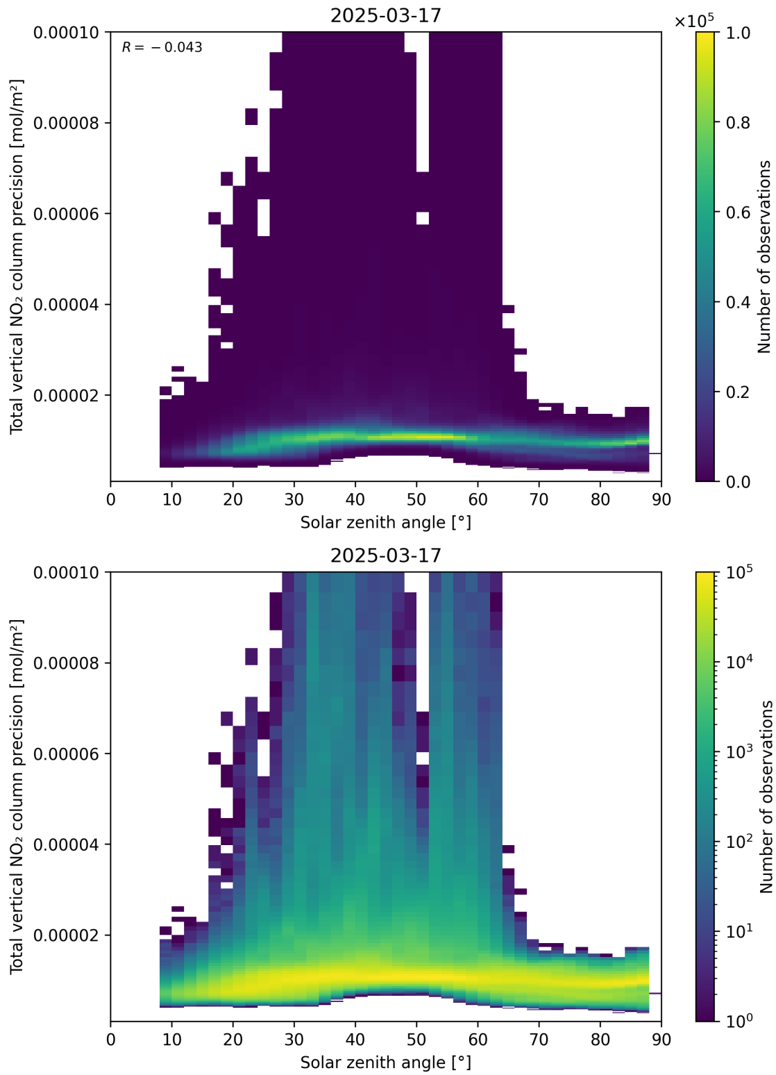
Figure 154: Scatter density plot of “Solar zenith angle” against “Total vertical NO 2 column precision” for 2025-03-17 to 2025-03-18.
