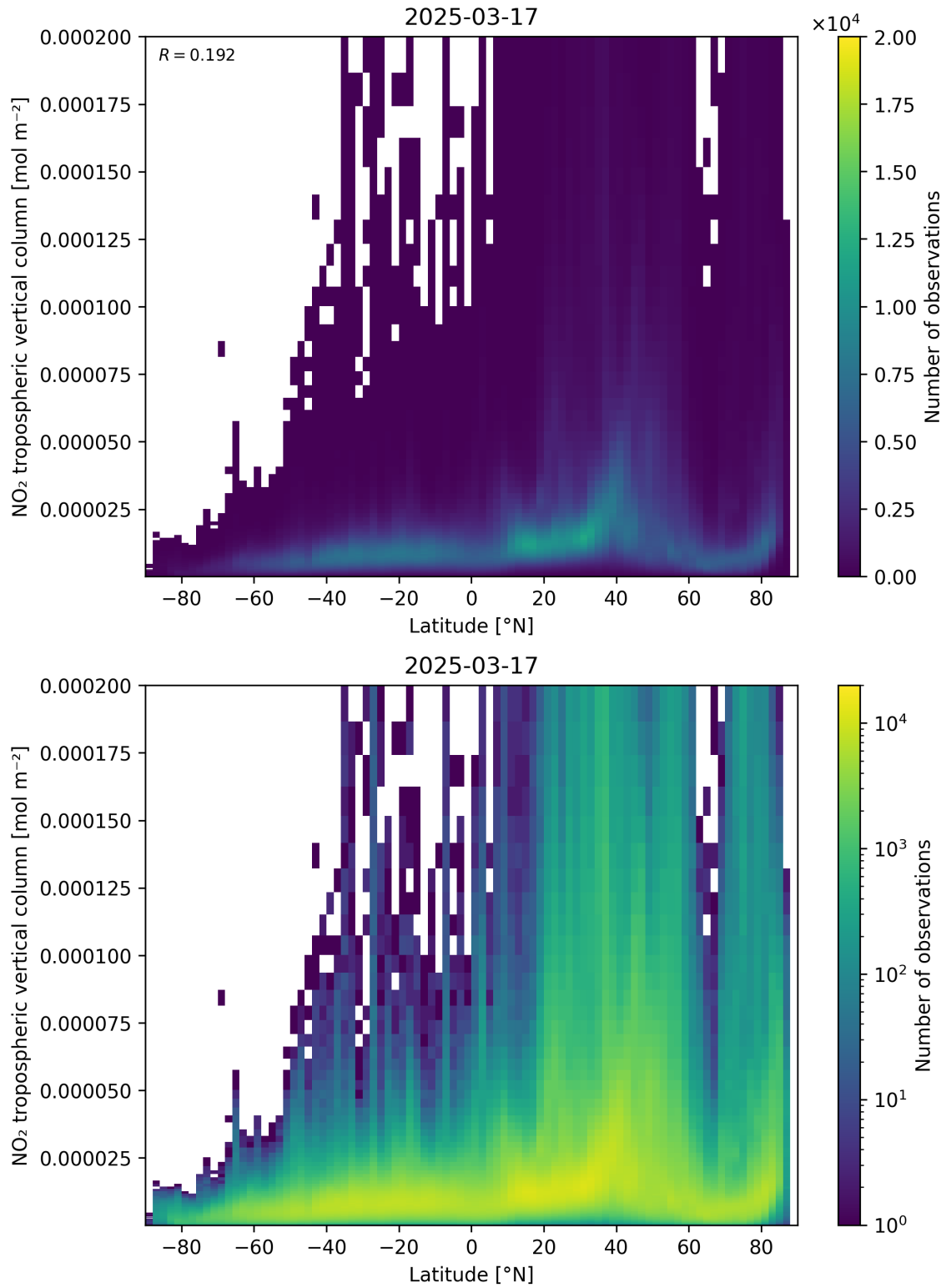
Figure 92: Scatter density plot of “Latitude” against “NO 2 tropospheric vertical column” for 2025-03-17 to 2025-03-18.
