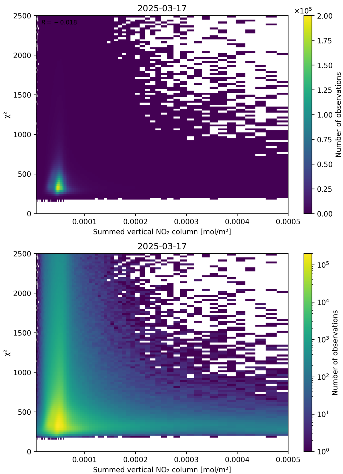
Figure 104: Scatter density plot of “Summed vertical NO 2 column” against “ \chi^2 ” for 2025-03-17 to 2025-03-18.
