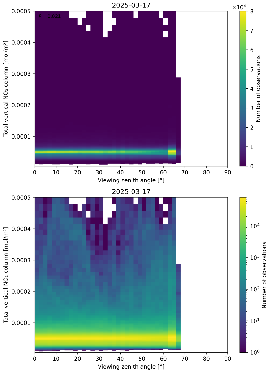
Figure 167: Scatter density plot of “Viewing zenith angle” against “Total vertical NO 2 column” for 2025-03-17 to 2025-03-18.
