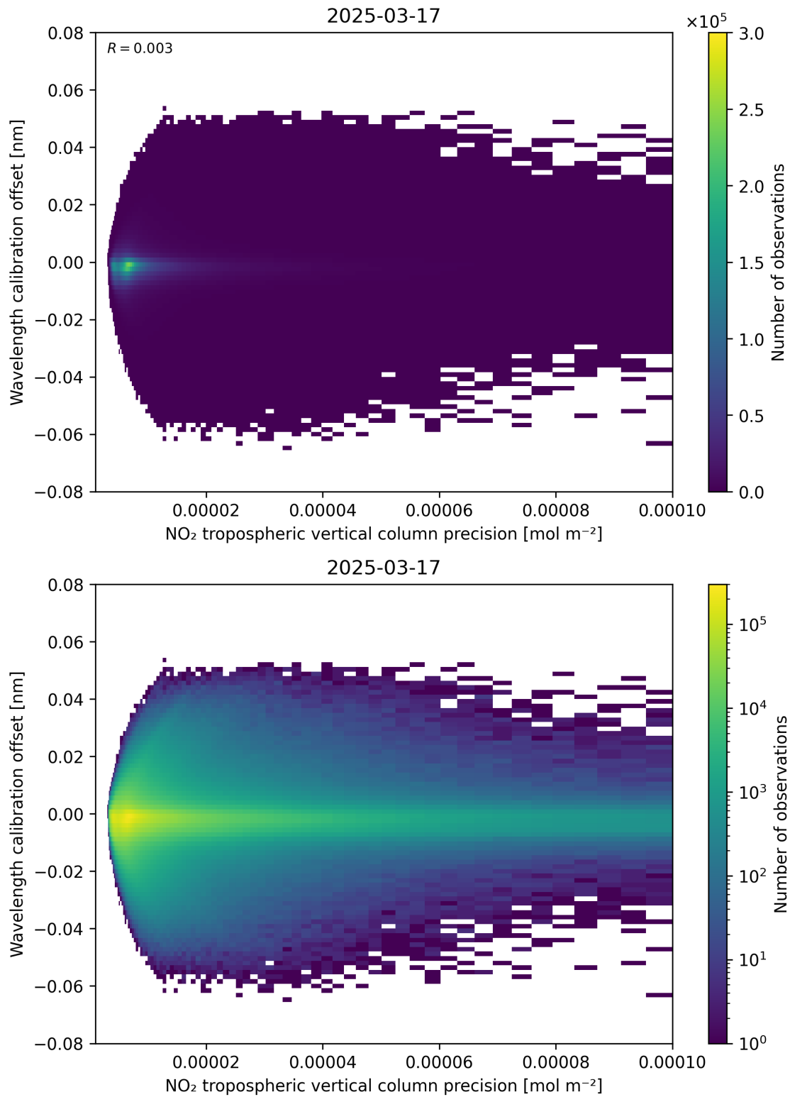
Figure 141: Scatter density plot of “NO 2 tropospheric vertical column precision” against “Wavelength calibration offset” for 2025-03-17 to 2025-03-18.
