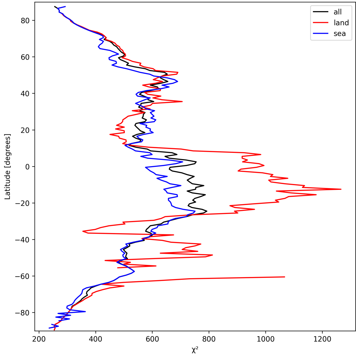
Figure 25: Zonal average of “ \chi^2 ” for 2025-03-17 to 2025-03-18.
