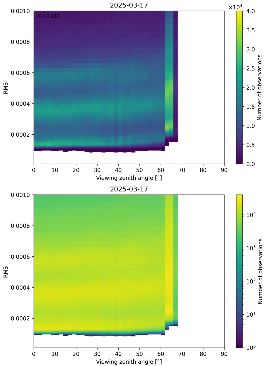
Figure 171: Scatter density plot of “Viewing zenith angle” against “RMS” for 2025-03-17 to 2025-03-18.
