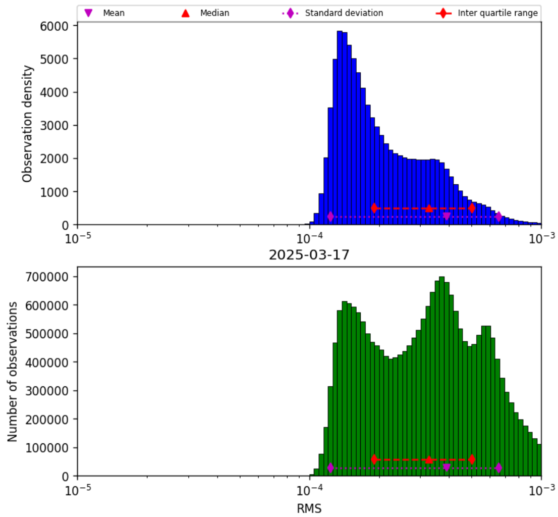
Figure 43: Histogram of “RMS” for 2025-03-17 to 2025-03-18
