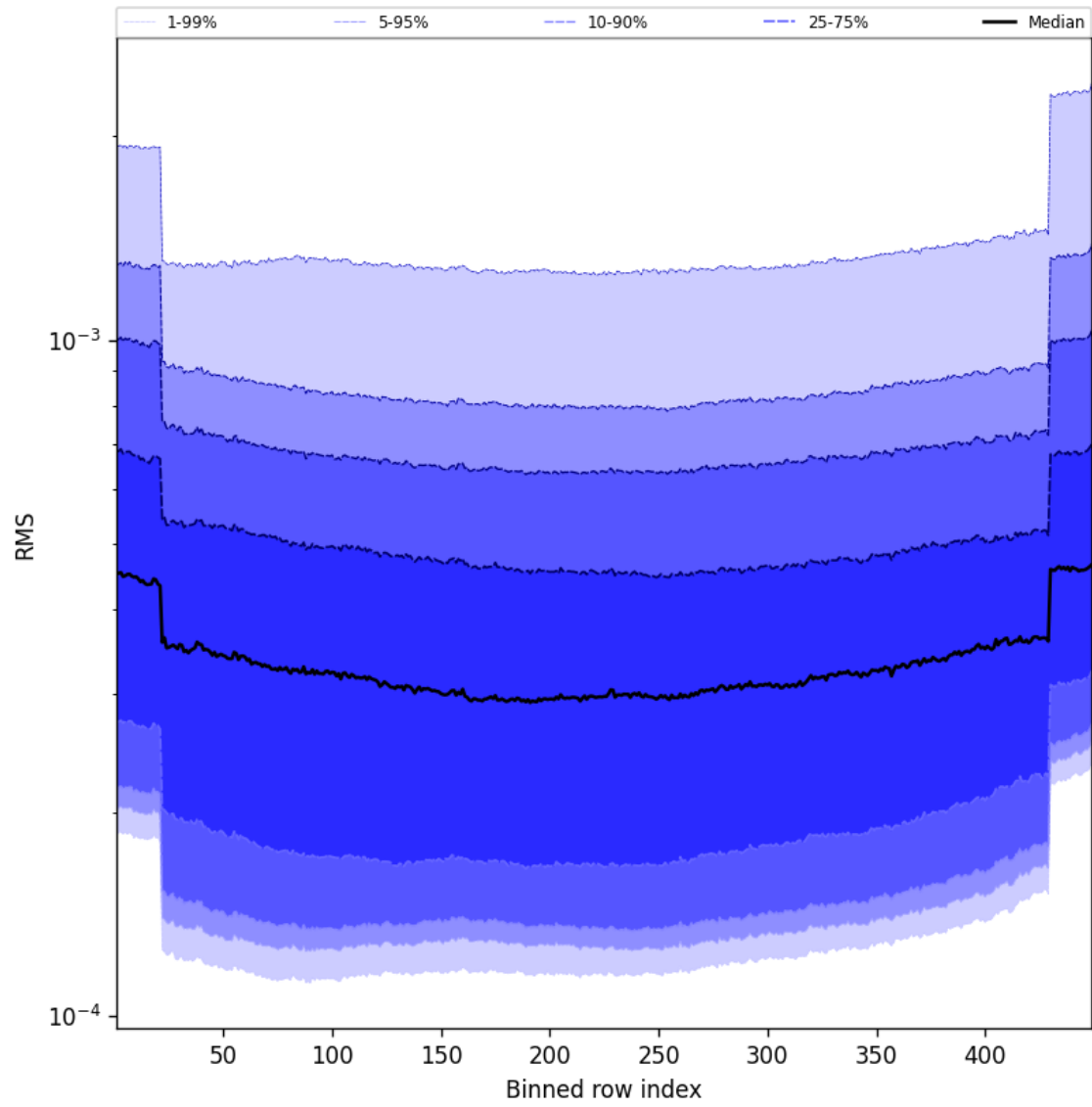
Figure 60: Along track statistics of “RMS” for 2025-03-17 to 2025-03-18
