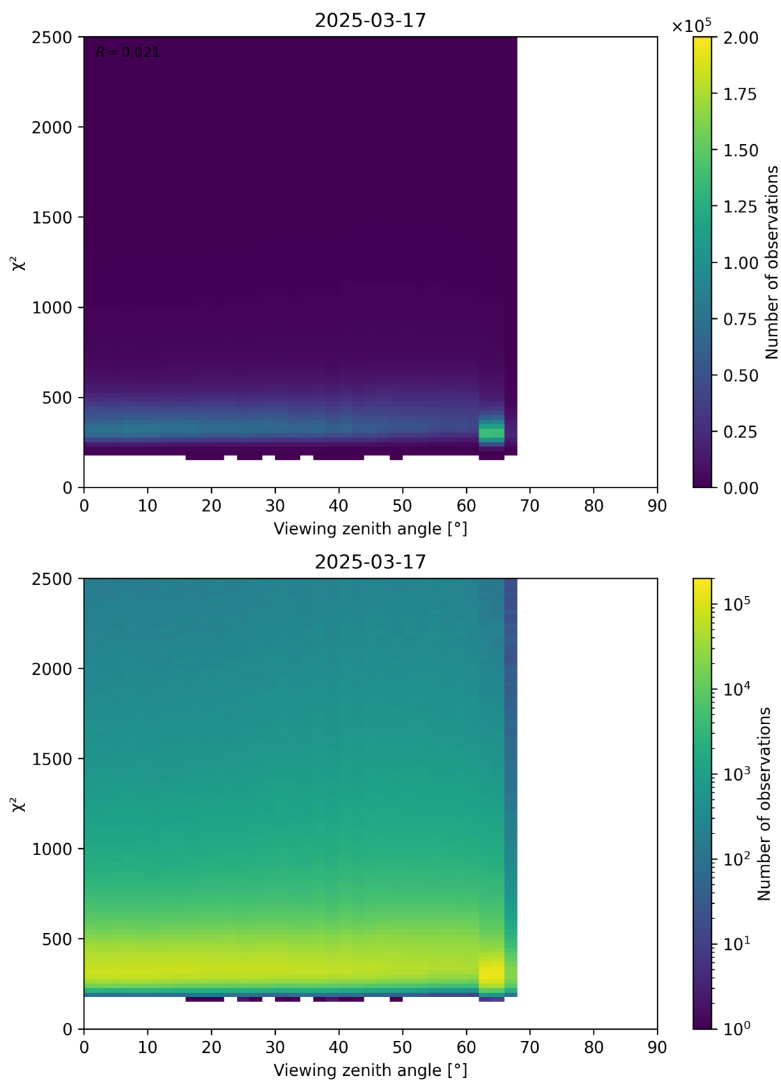
Figure 162: Scatter density plot of “Viewing zenith angle” against “ \chi^2 ” for 2025-03-17 to 2025-03-18.
