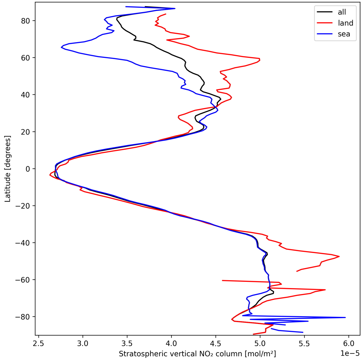
Figure 19: Zonal average of “Stratospheric vertical NO 2 column” for 2025-03-17 to 2025-03-18.
