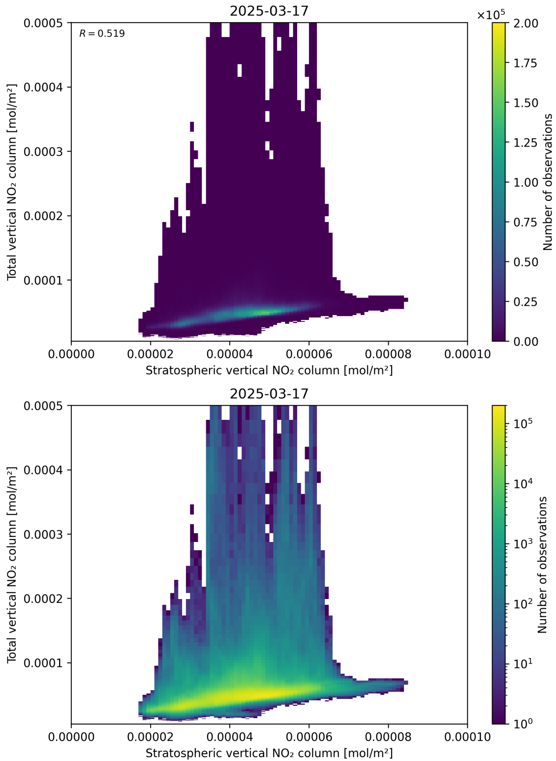
Figure 100: Scatter density plot of “Stratospheric vertical NO 2 column” against “Total vertical NO 2 column” for 2025-03-17 to 2025-03-18.
