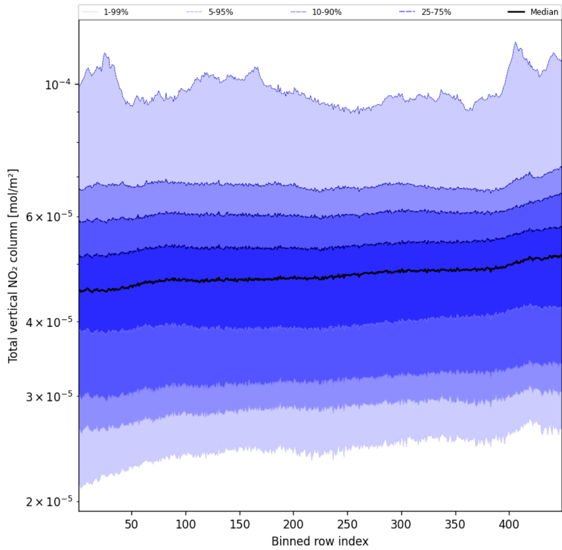
Figure 55: Along track statistics of “Total vertical NO 2 column” for 2025-03-17 to 2025-03-18
