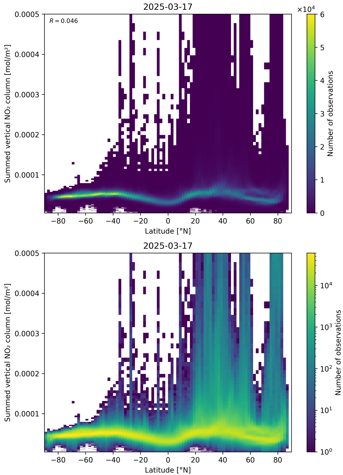
Figure 88: Scatter density plot of “Latitude” against “Summed vertical NO 2 column” for 2025-03-17 to 2025-03-18.
