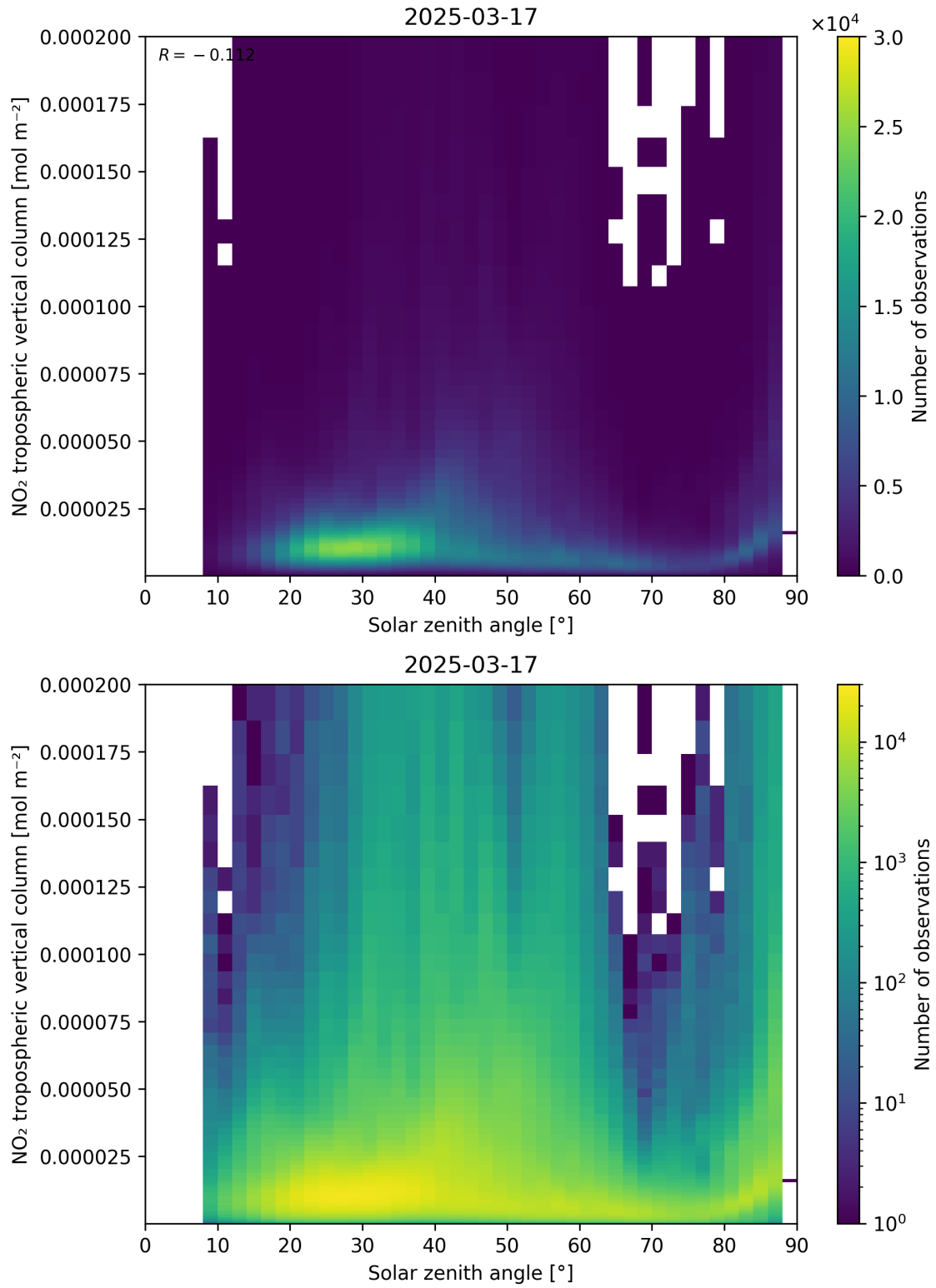
Figure 155: Scatter density plot of “Solar zenith angle” against “NO 2 tropospheric vertical column” for 2025-03-17 to 2025-03-18.
