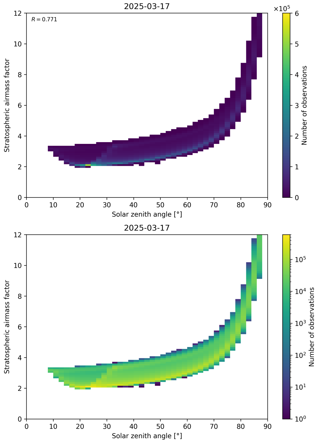
Figure 145: Scatter density plot of “Solar zenith angle” against “Stratospheric airmass factor” for 2025-03-17 to 2025-03-18.
