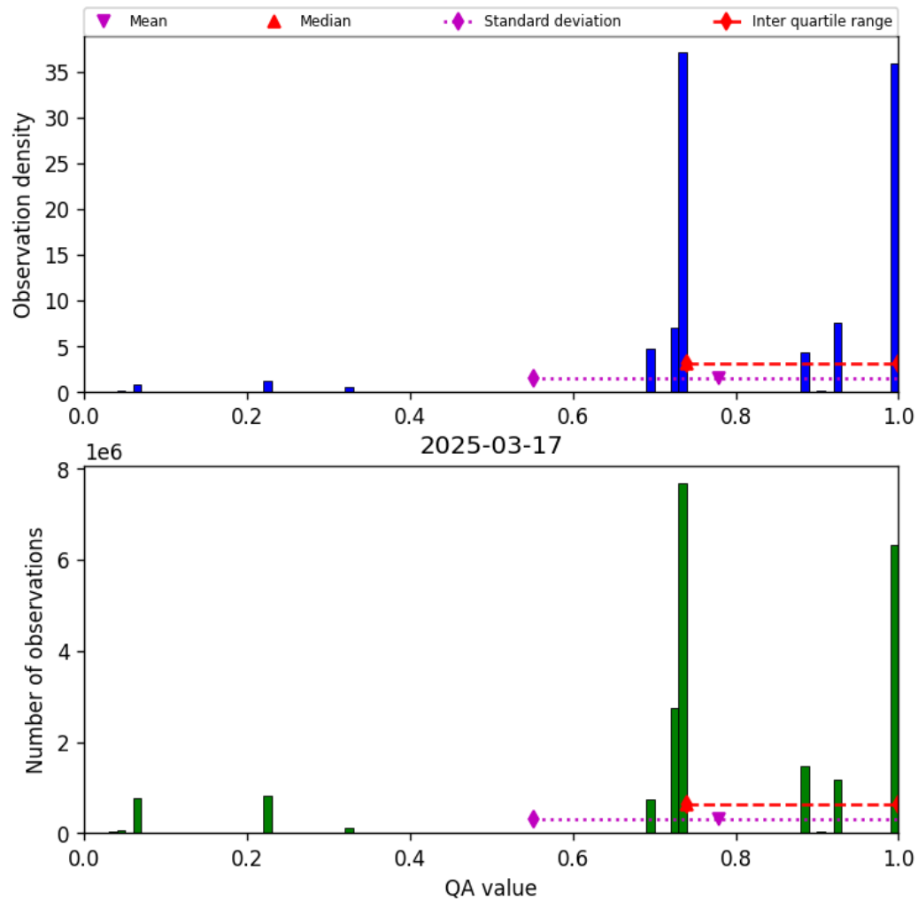
Figure 28: Histogram of “QA value” for 2025-03-17 to 2025-03-18
