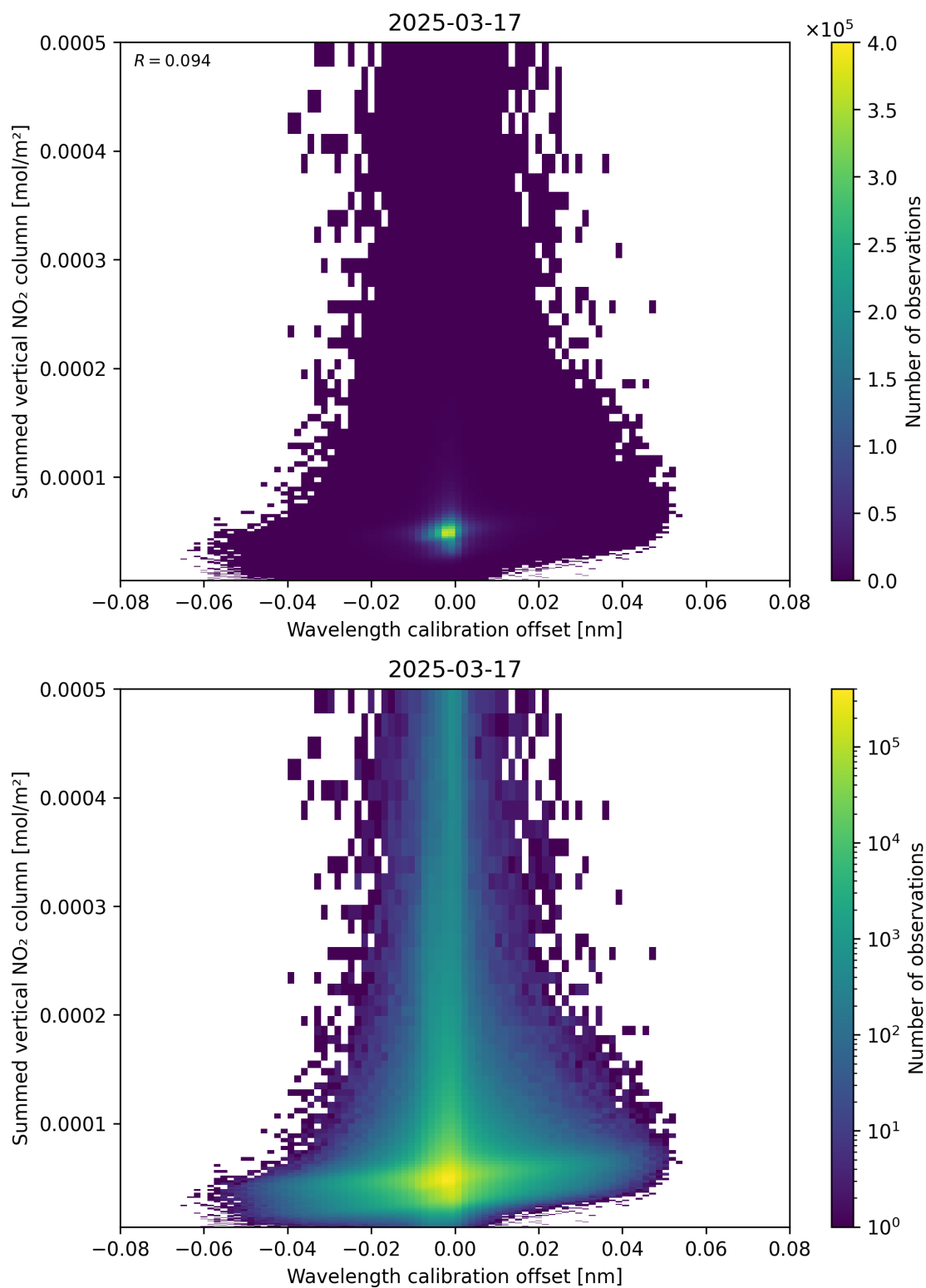
Figure 177: Scatter density plot of “Wavelength calibration offset” against “Summed vertical NO 2 column” for 2025-03-17 to 2025-03-18.
