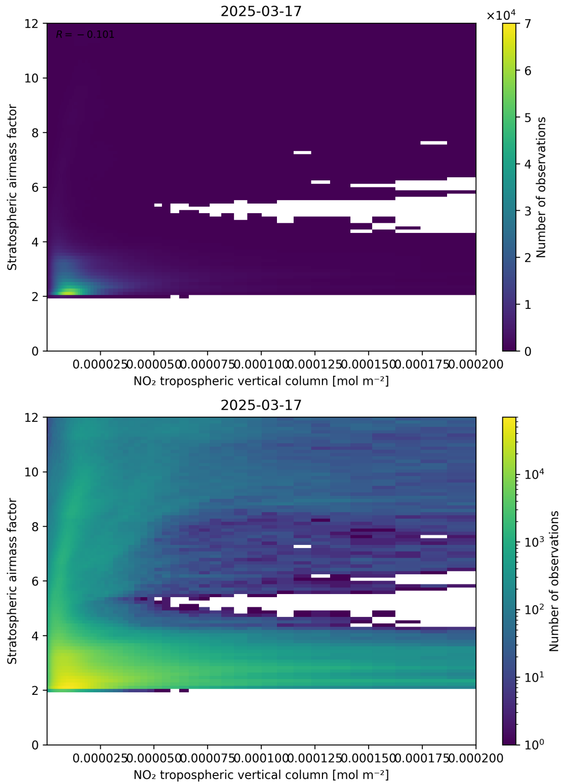
Figure 121: Scatter density plot of “NO 2 tropospheric vertical column” against “Stratospheric air mass factor” for 2025-03-17 to 2025-03-18.
