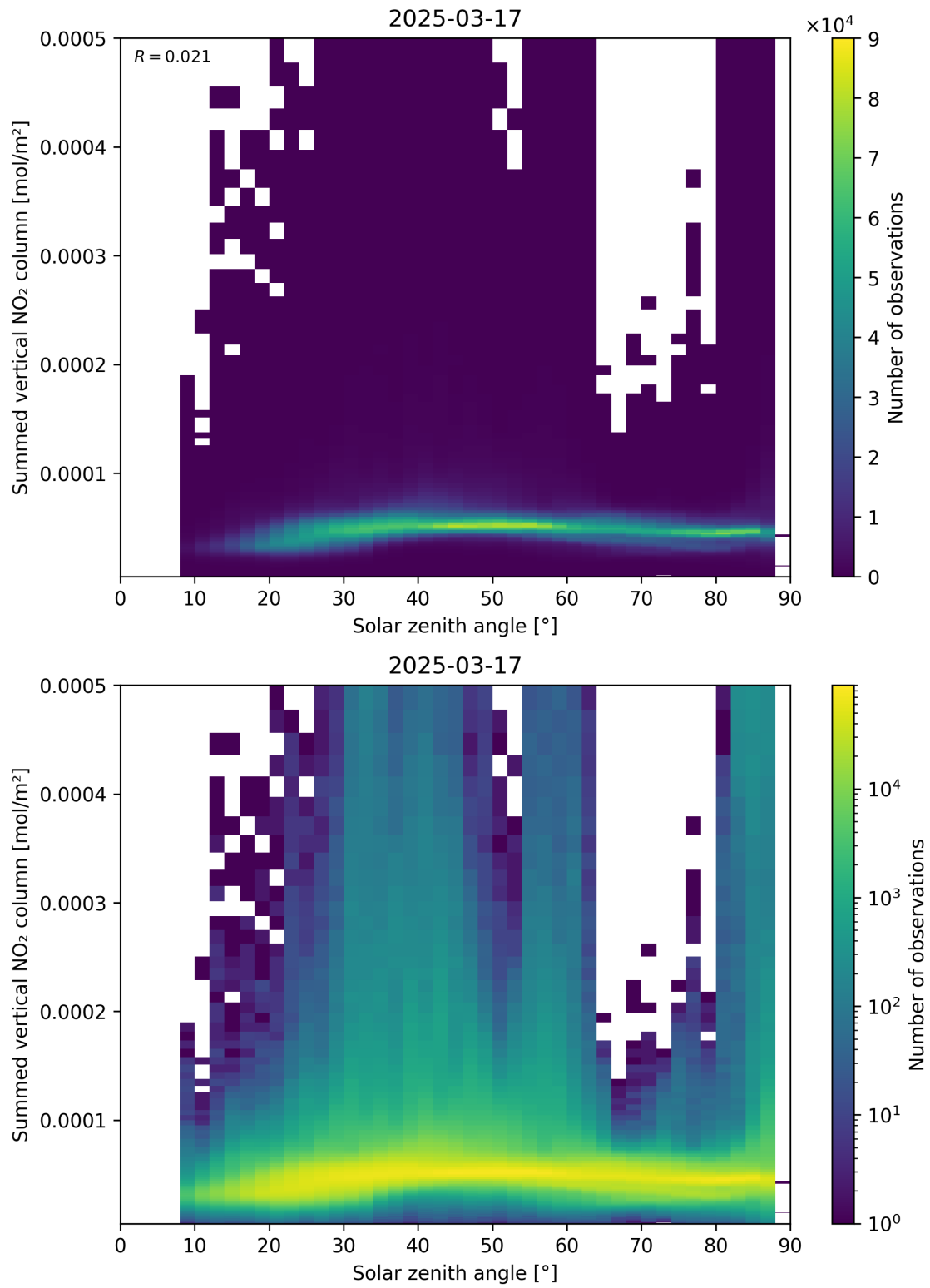
Figure 151: Scatter density plot of “Solar zenith angle” against “Summed vertical NO 2 column” for 2025-03-17 to 2025-03-18.
