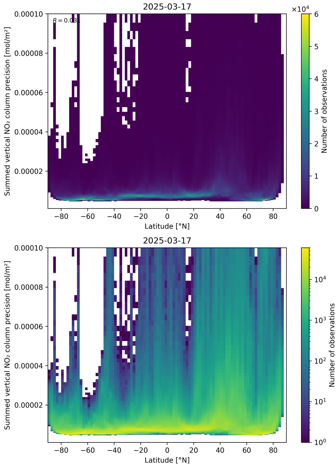
Figure 89: Scatter density plot of “Latitude” against “Summed vertical NO 2 column precision” for 2025-03-17 to 2025-03-18.
