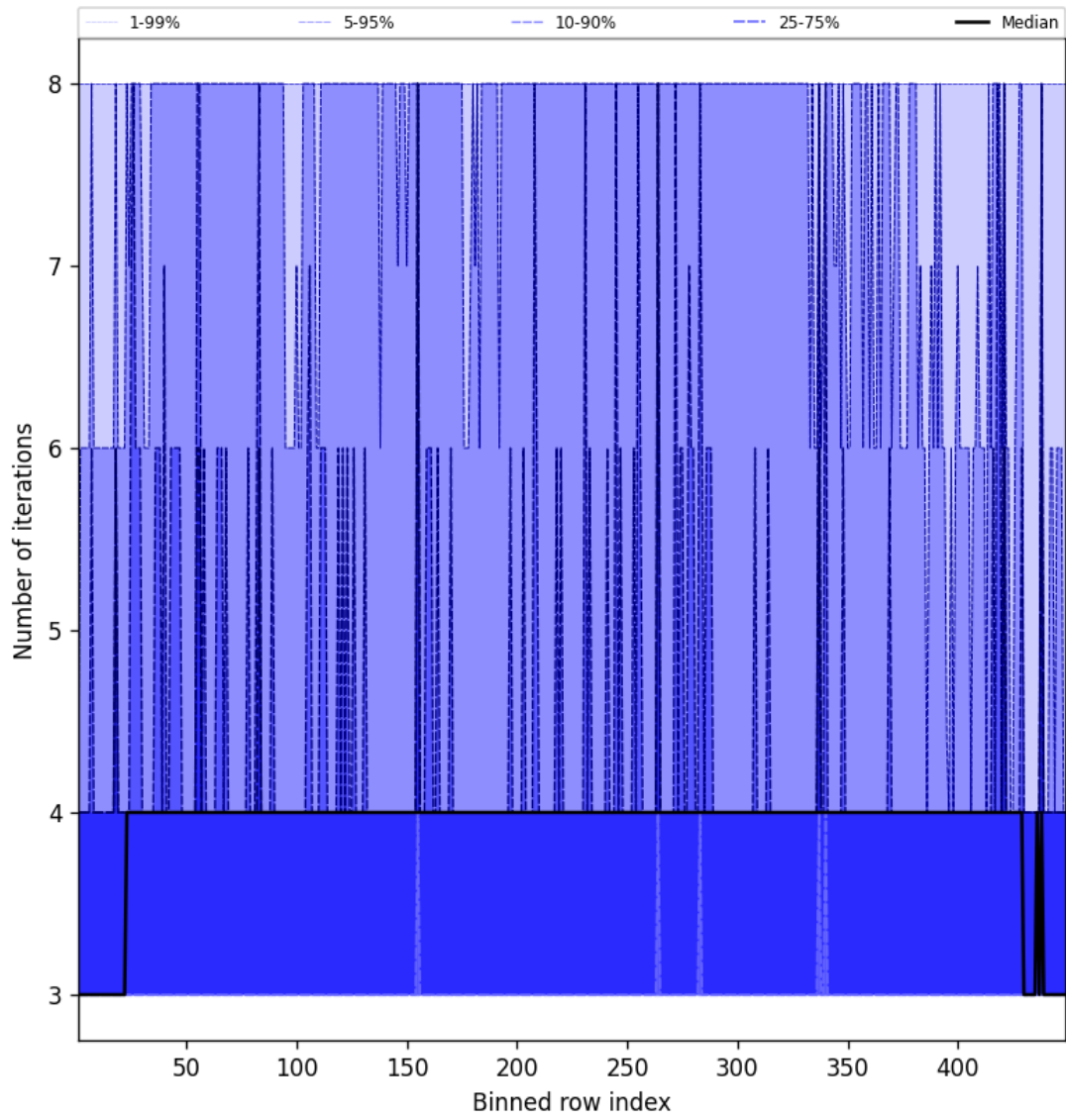
Figure 51: Along track statistics of “Number of iterations” for 2025-03-17 to 2025-03-18
