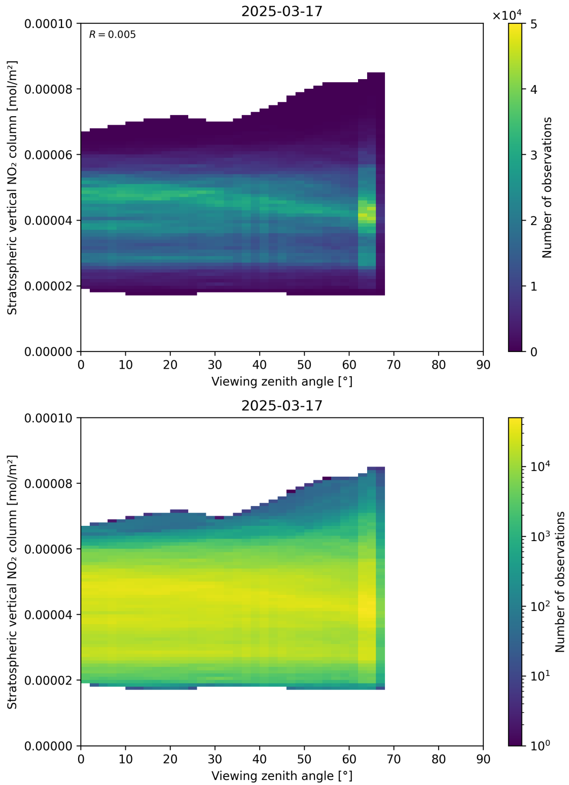
Figure 164: Scatter density plot of “Viewing zenith angle” against “Stratospheric vertical NO 2 column” for 2025-03-17 to 2025-03-18.
