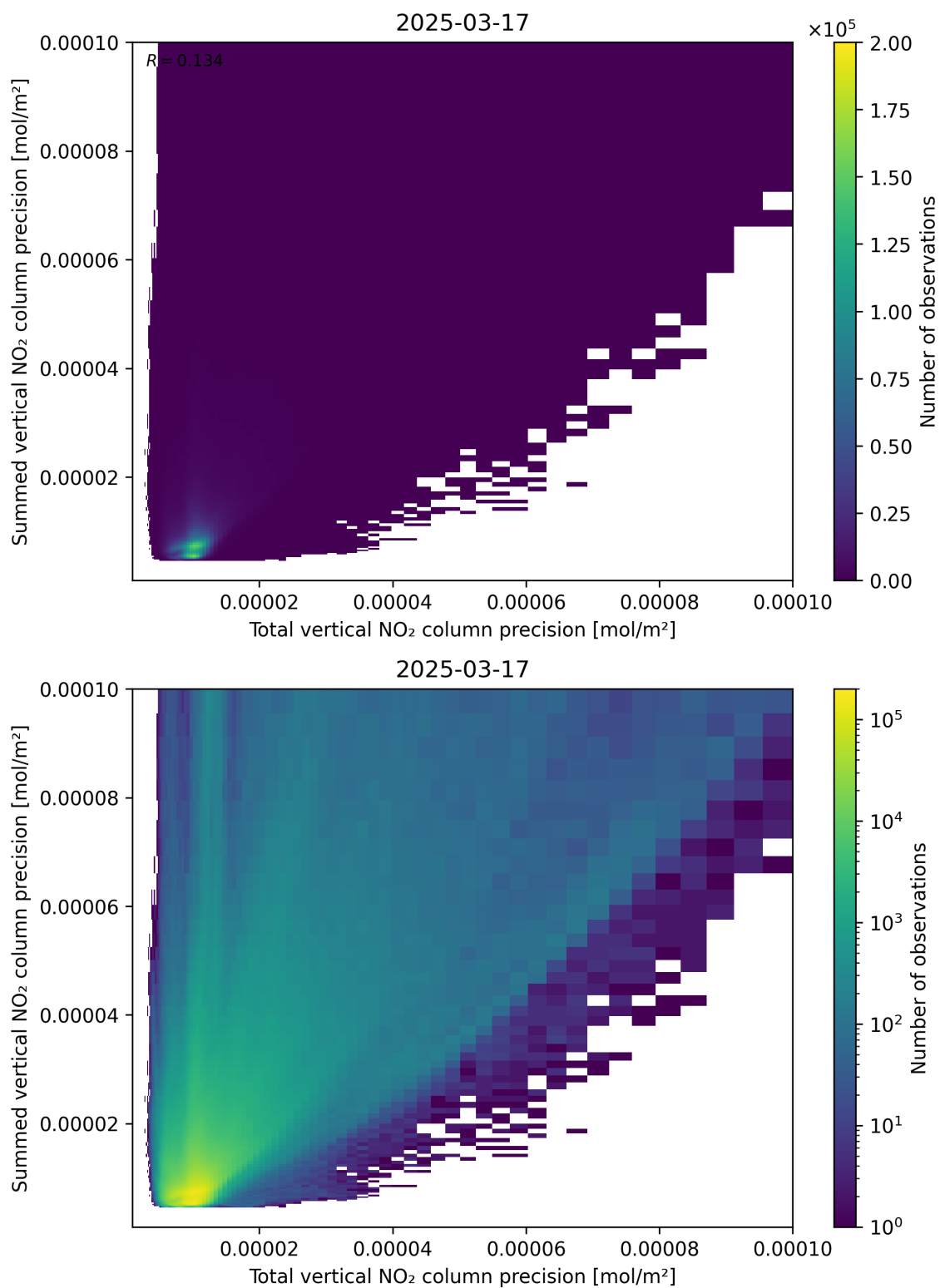
Figure 118: Scatter density plot of “Total vertical NO 2 column precision” against “Summed vertical NO 2 column precision” for 2025-03-17 to 2025-03-18.
