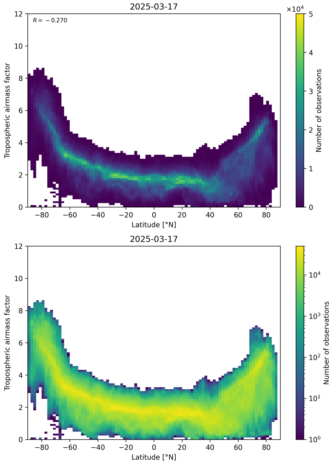
Figure 85: Scatter density plot of “Latitude” against “Tropospheric airmass factor” for 2025-03-17 to 2025-03-18.
