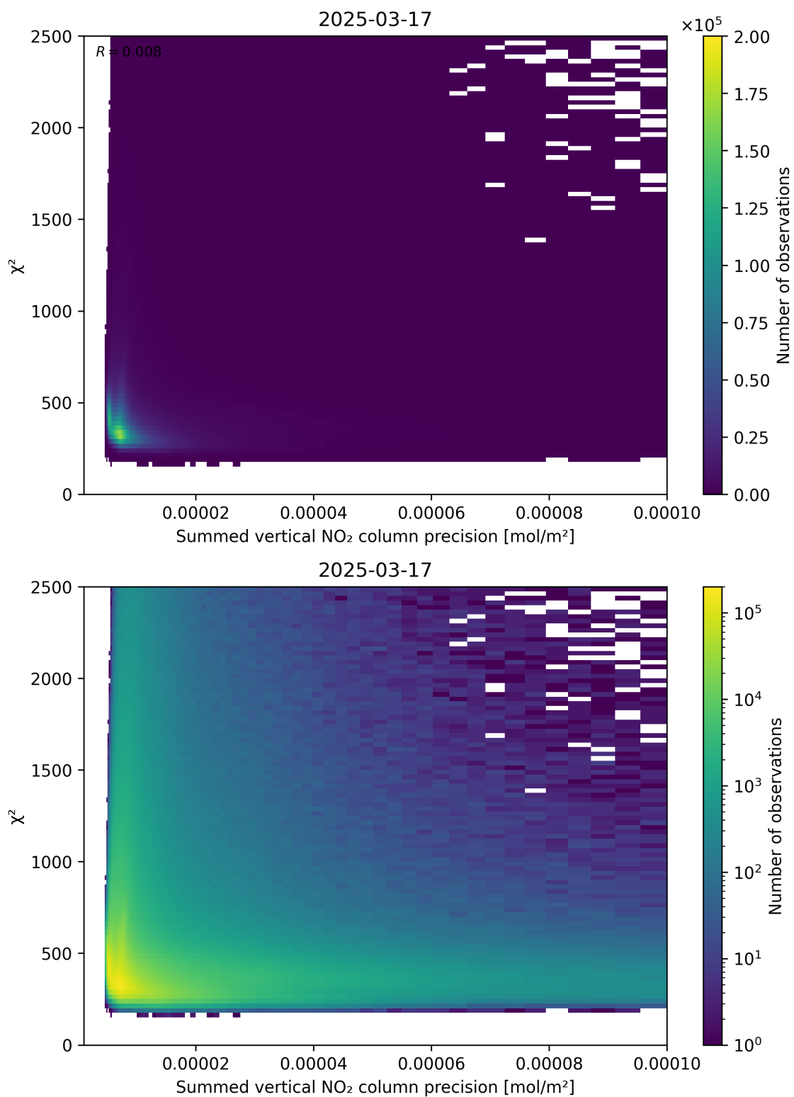
Figure 107: Scatter density plot of “Summed vertical NO 2 column precision” against “ \chi^2 ” for 2025-03-17 to 2025-03-18.
