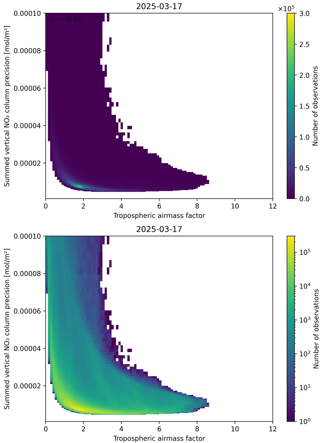
Figure 76: Scatter density plot of “Tropospheric air mass factor” against “Summed vertical NO 2 column precision” for 2025-03-17 to 2025-03-18.
