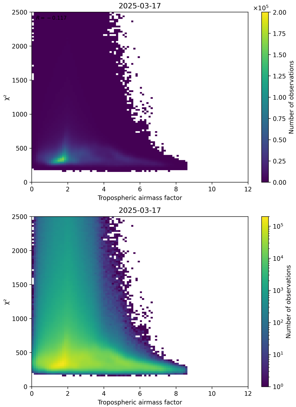
Figure 73: Scatter density plot of “Tropospheric airmass factor” against “ \chi^2 ” for 2025-03-17 to 2025-03-18.
