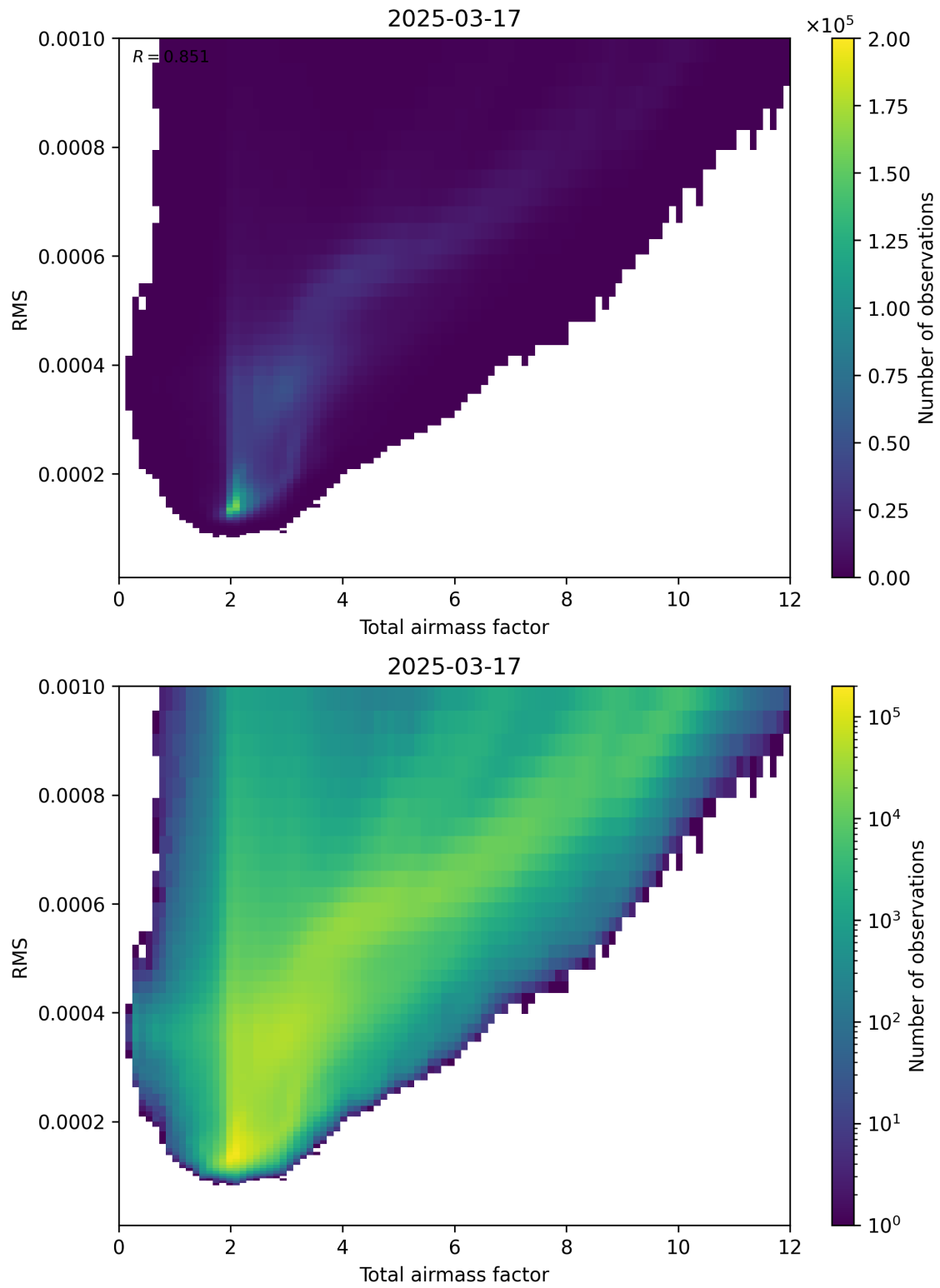
Figure 69: Scatter density plot of “Total airmass factor” against “RMS” for 2025-03-17 to 2025-03-18.
