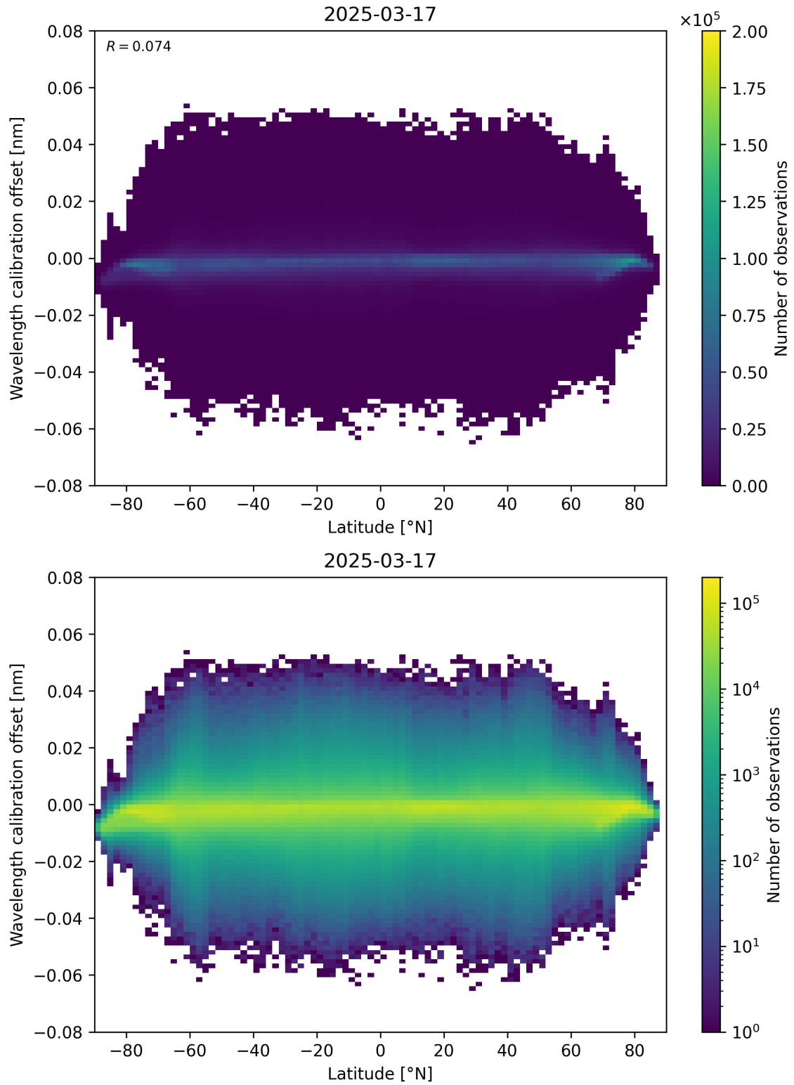
Figure 95: Scatter density plot of “Latitude” against “Wavelength calibration offset” for 2025-03-17 to 2025-03-18.
