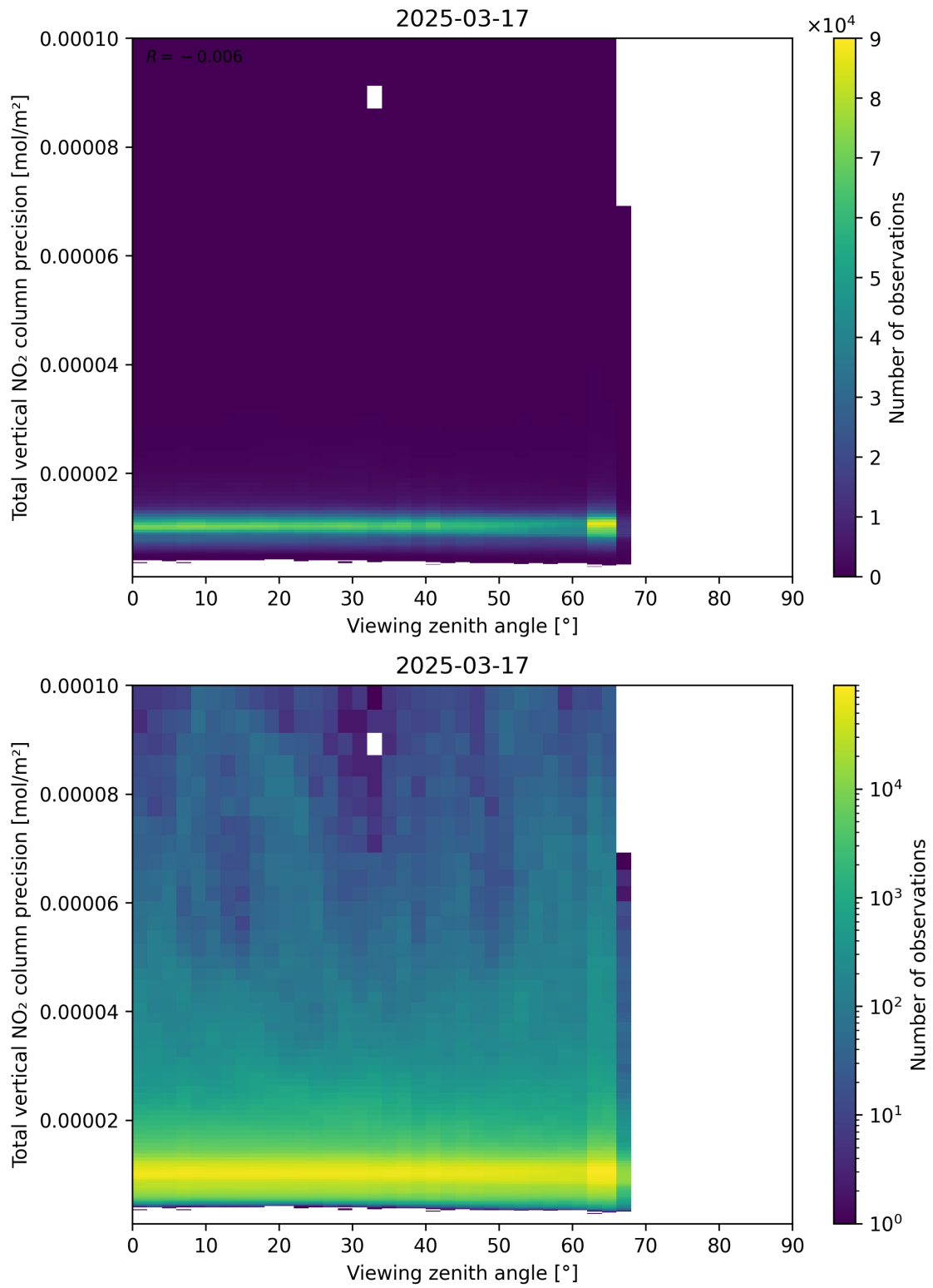
Figure 168: Scatter density plot of “Viewing zenith angle” against “Total vertical NO 2 column precision” for 2025-03-17 to 2025-03-18.
