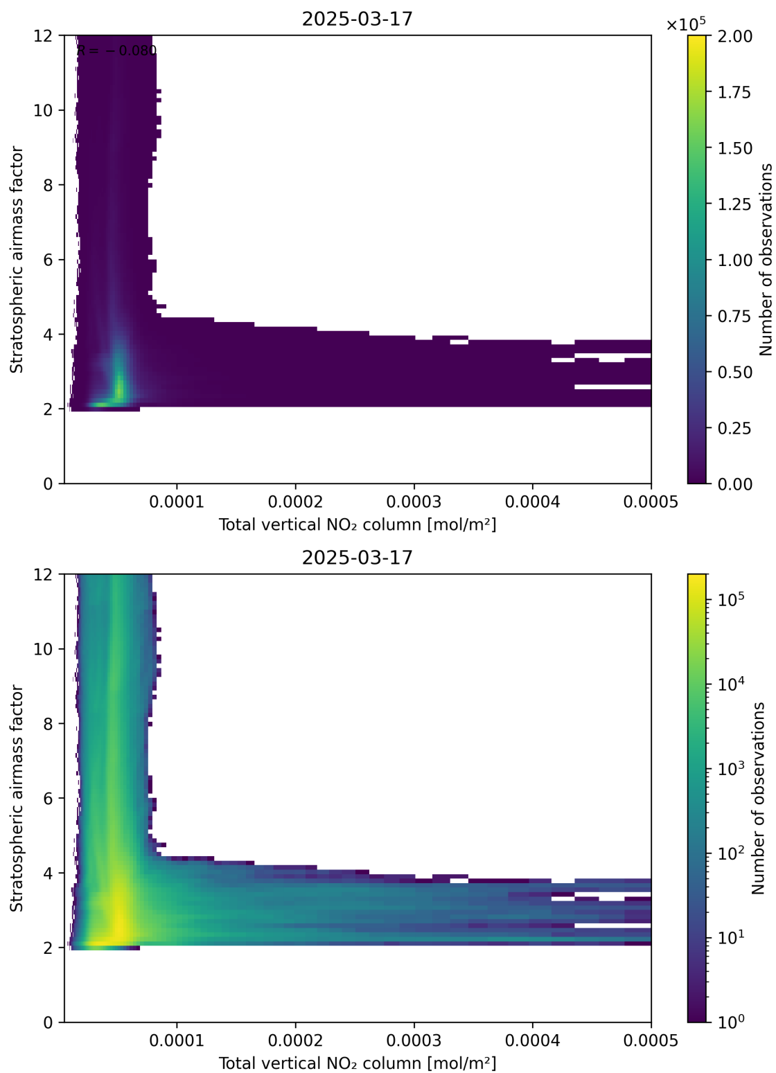
Figure 110: Scatter density plot of “Total vertical NO 2 column” against “Stratospheric airmass factor” for 2025-03-17 to 2025-03-18.
