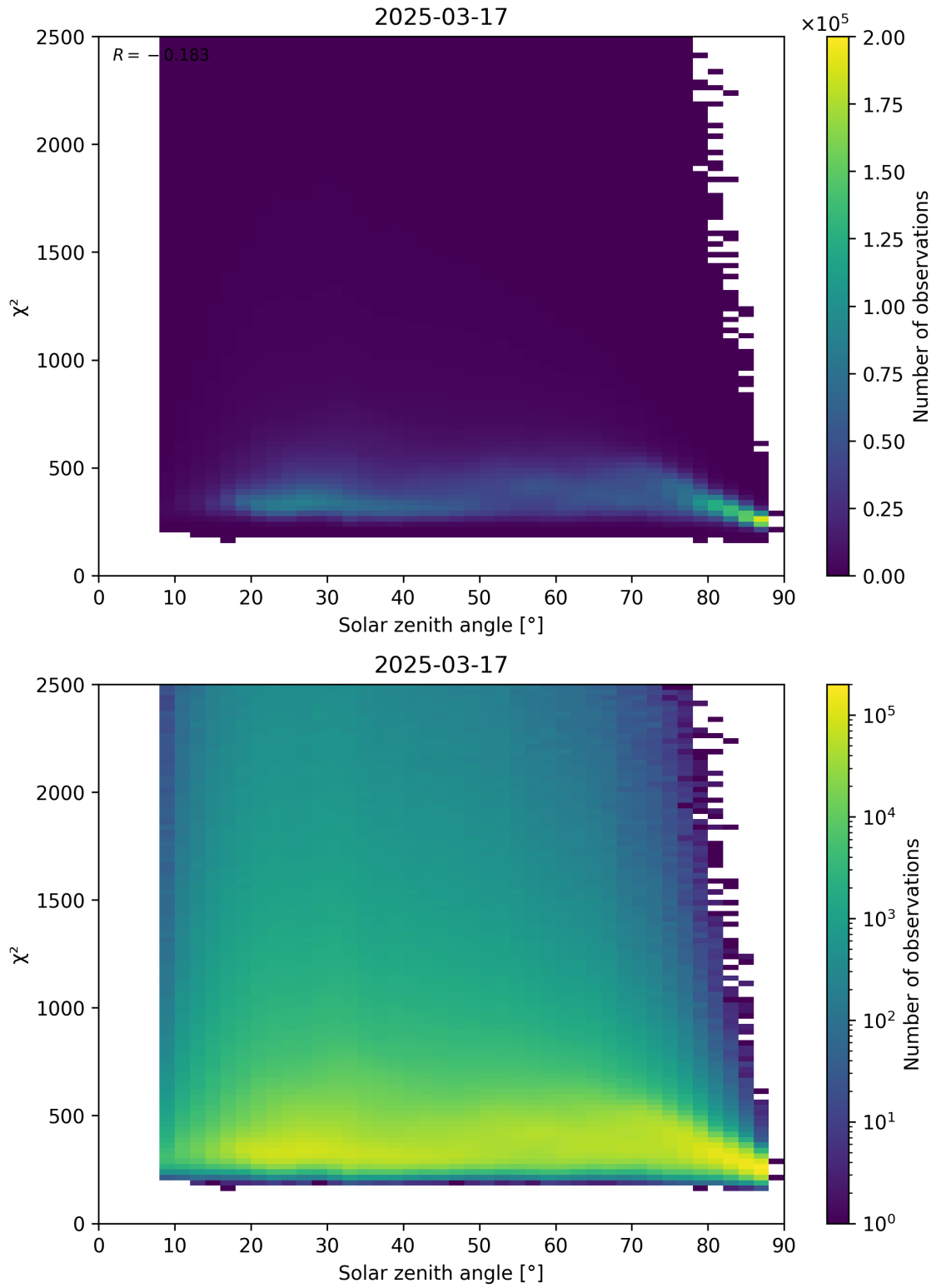
Figure 148: Scatter density plot of “Solar zenith angle” against “ \chi^2 ” for 2025-03-17 to 2025-03-18.
