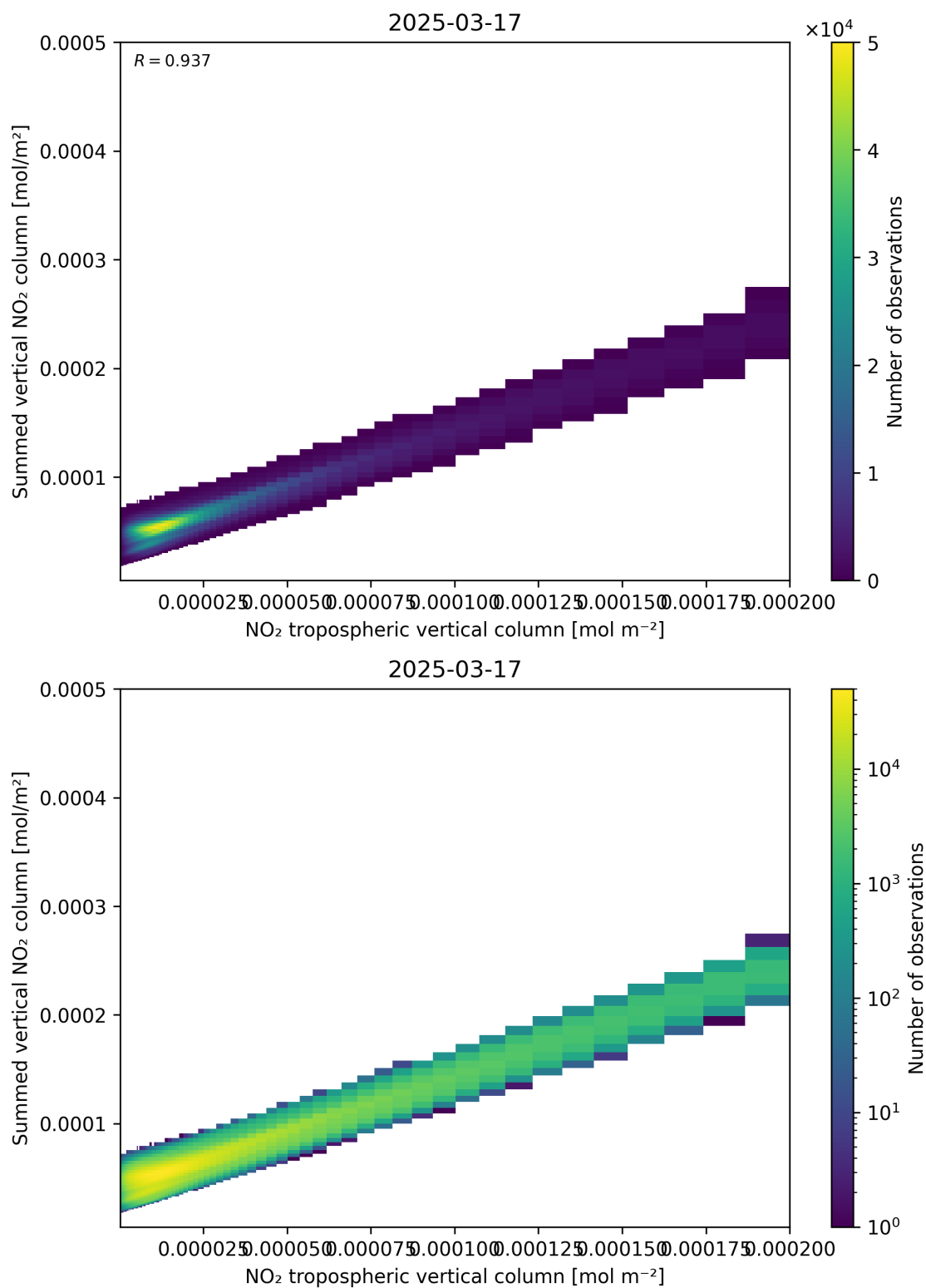
Figure 126: Scatter density plot of “NO 2 tropospheric vertical column” against “Summed vertical NO 2 column” for 2025-03-17 to 2025-03-18.
