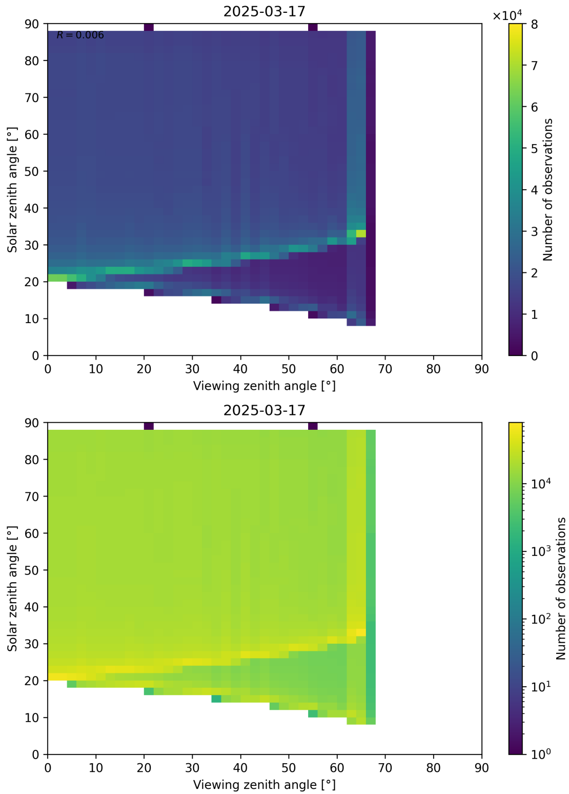
Figure 172: Scatter density plot of “Viewing zenith angle” against “Solar zenith angle” for 2025-03-17 to 2025-03-18.
