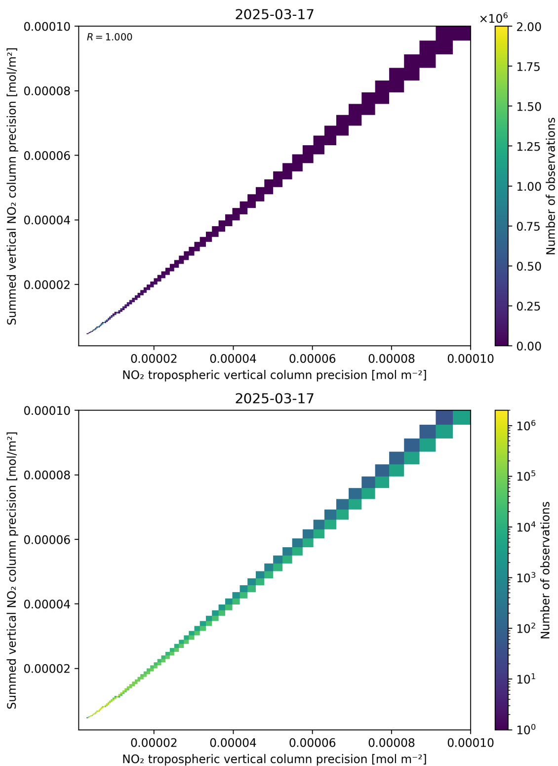
Figure 137: Scatter density plot of “NO 2 tropospheric vertical column precision” against “Summed vertical NO 2 column precision” for 2025-03-17 to 2025-03-18.
