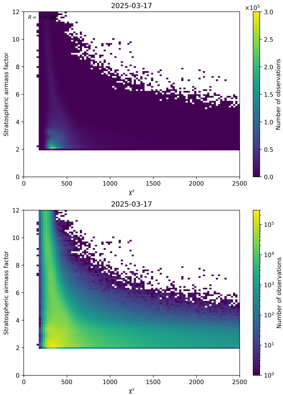
Figure 81: Scatter density plot of “ \chi^2 ” against “Stratospheric airmass factor” for 2025-03-17 to 2025-03-18.
