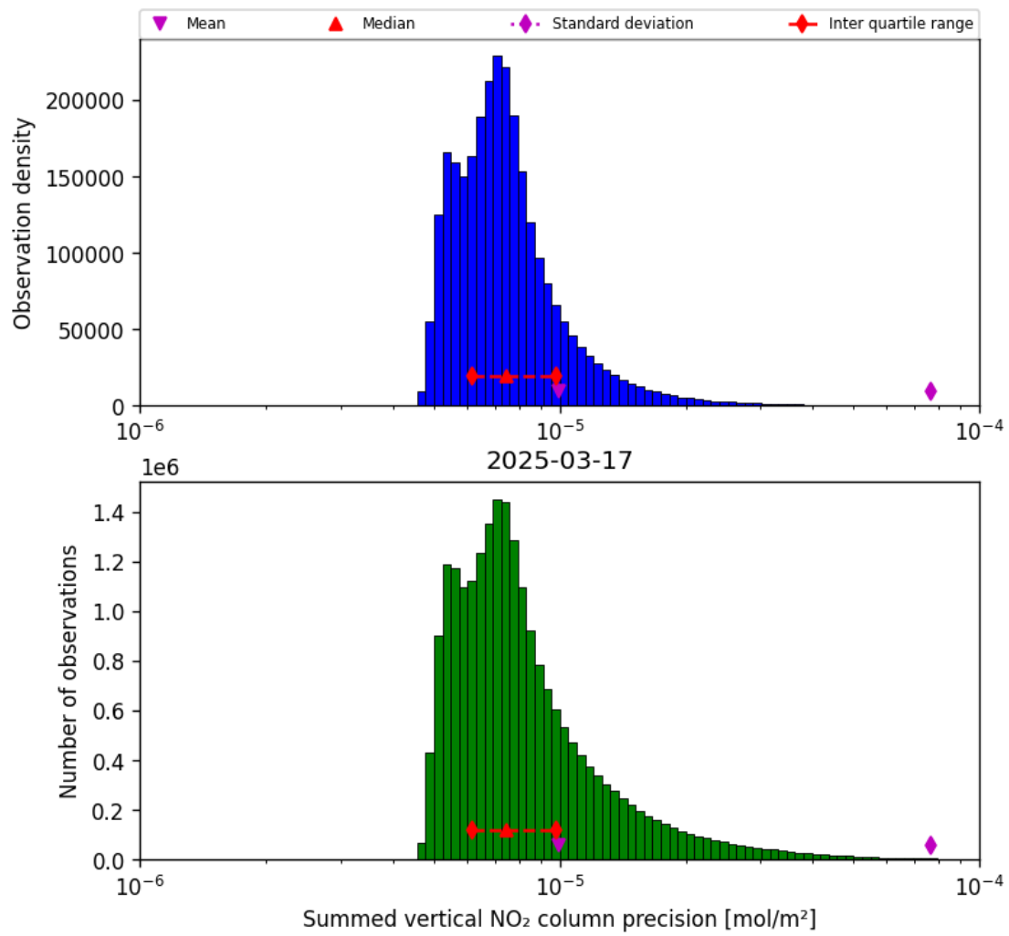
Figure 41: Histogram of "Summed vertical NO 2 column precision" for 2025-03-17 to 2025-03-18
