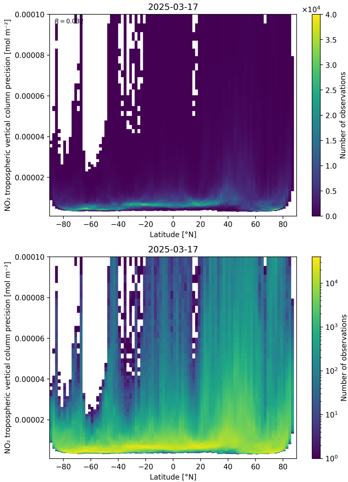
Figure 93: Scatter density plot of “Latitude” against “NO 2 tropospheric vertical column precision” for 2025-03-17 to 2025-03-18.
