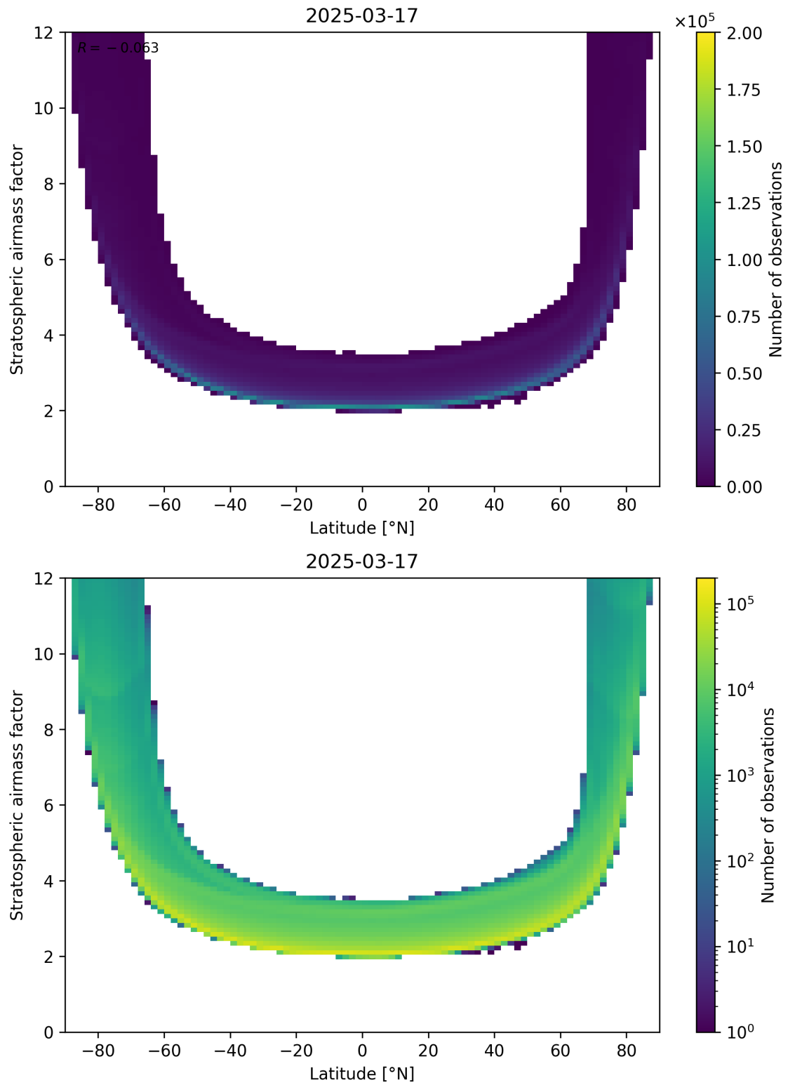
Figure 83: Scatter density plot of “Latitude” against “Stratospheric air mass factor” for 2025-03-17 to 2025-03-18.
