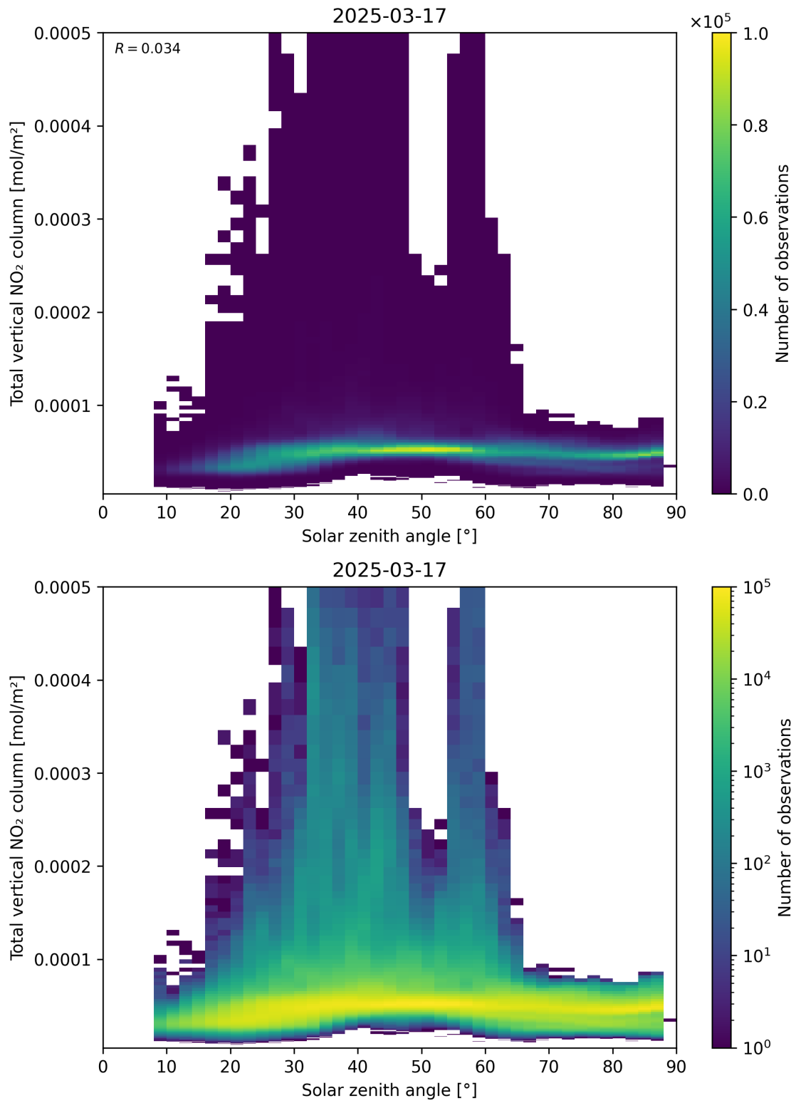
Figure 153: Scatter density plot of “Solar zenith angle” against “Total vertical NO 2 column” for 2025-03-17 to 2025-03-18.
