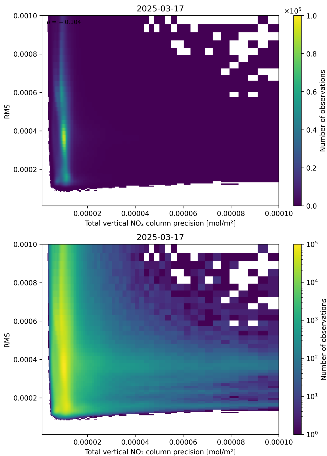
Figure 119: Scatter density plot of “Total vertical NO 2 column precision” against “RMS” for 2025-03-17 to 2025-03-18.
