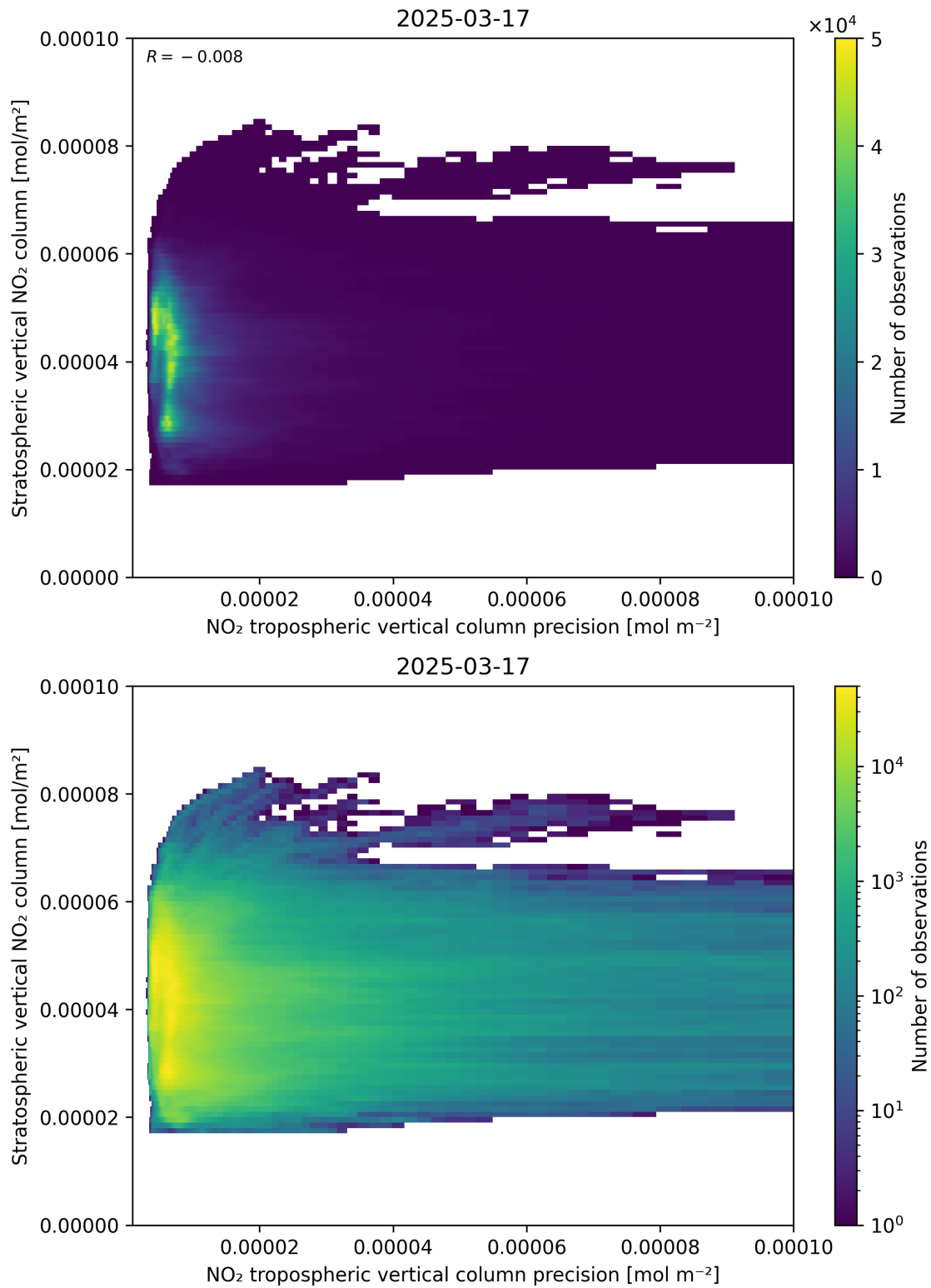
Figure 135: Scatter density plot of “NO 2 tropospheric vertical column precision” against “Stratospheric vertical NO 2 column” for 2025-03-17 to 2025-03-18.
