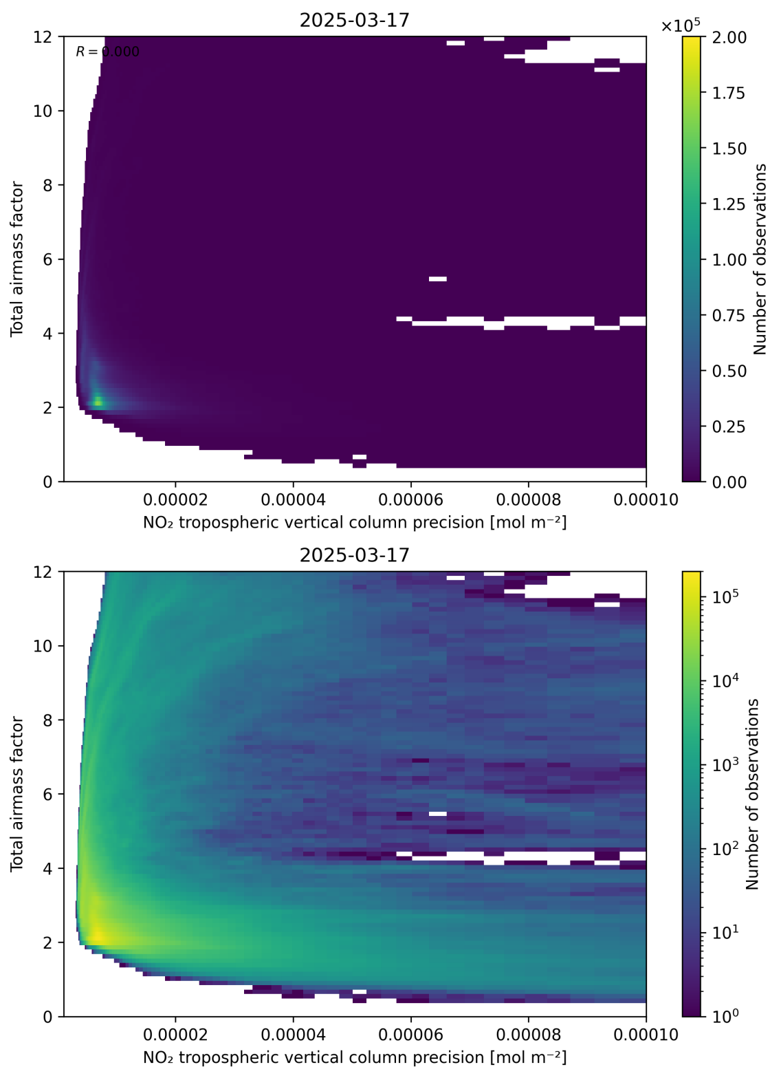
Figure 132: Scatter density plot of “NO 2 tropospheric vertical column precision” against “Total air mass factor” for 2025-03-17 to 2025-03-18.
