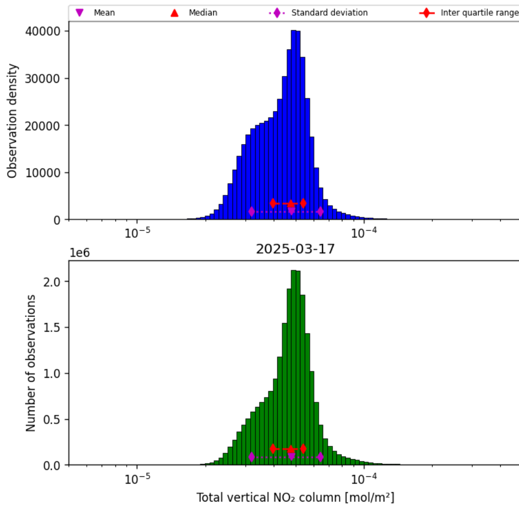
Figure 38: Histogram of “Total vertical NO 2 column” for 2025-03-17 to 2025-03-18
