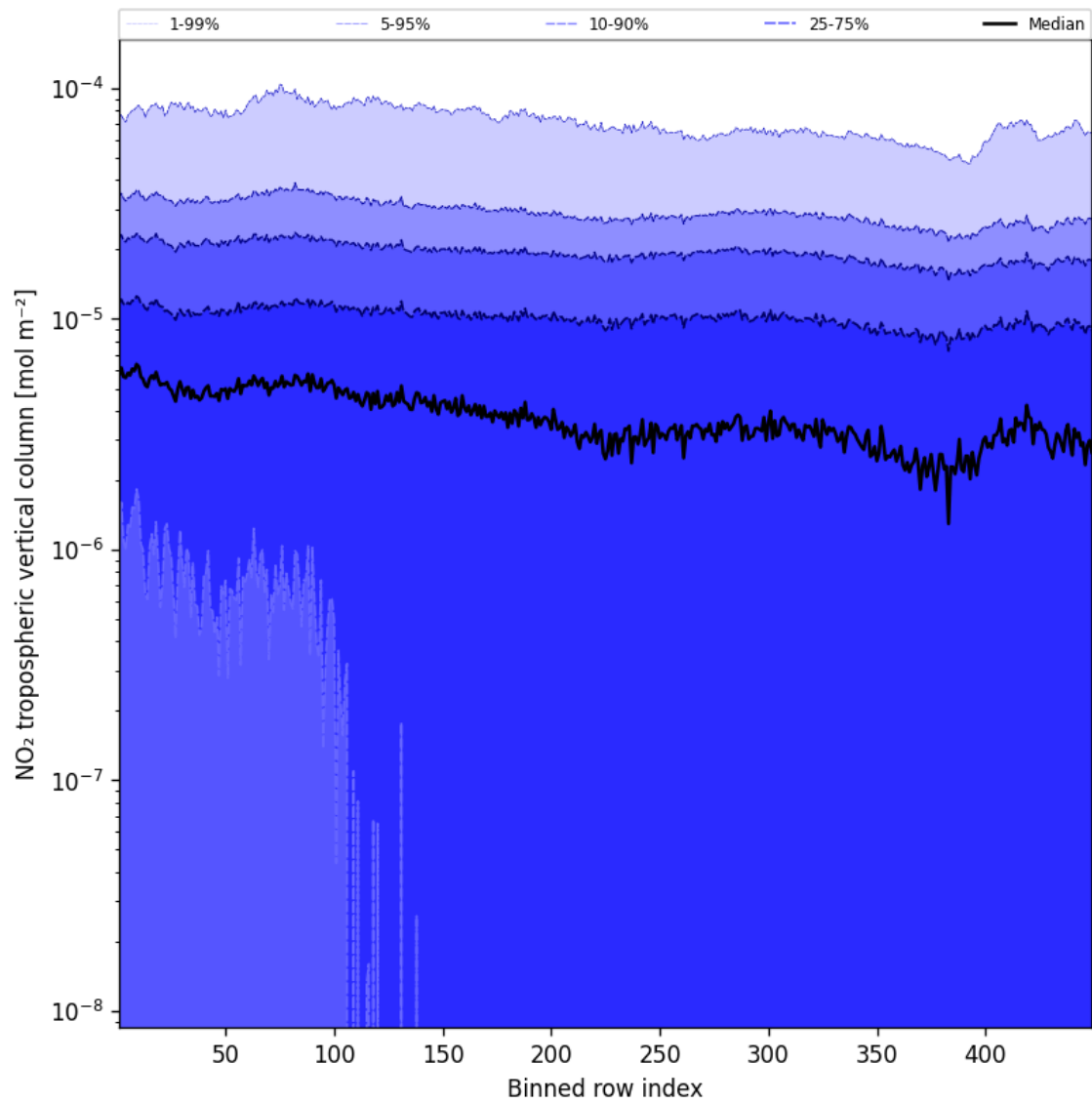
Figure 46: Along track statistics of “NO 2 tropospheric vertical column” for 2025-03-17 to 2025-03-18
