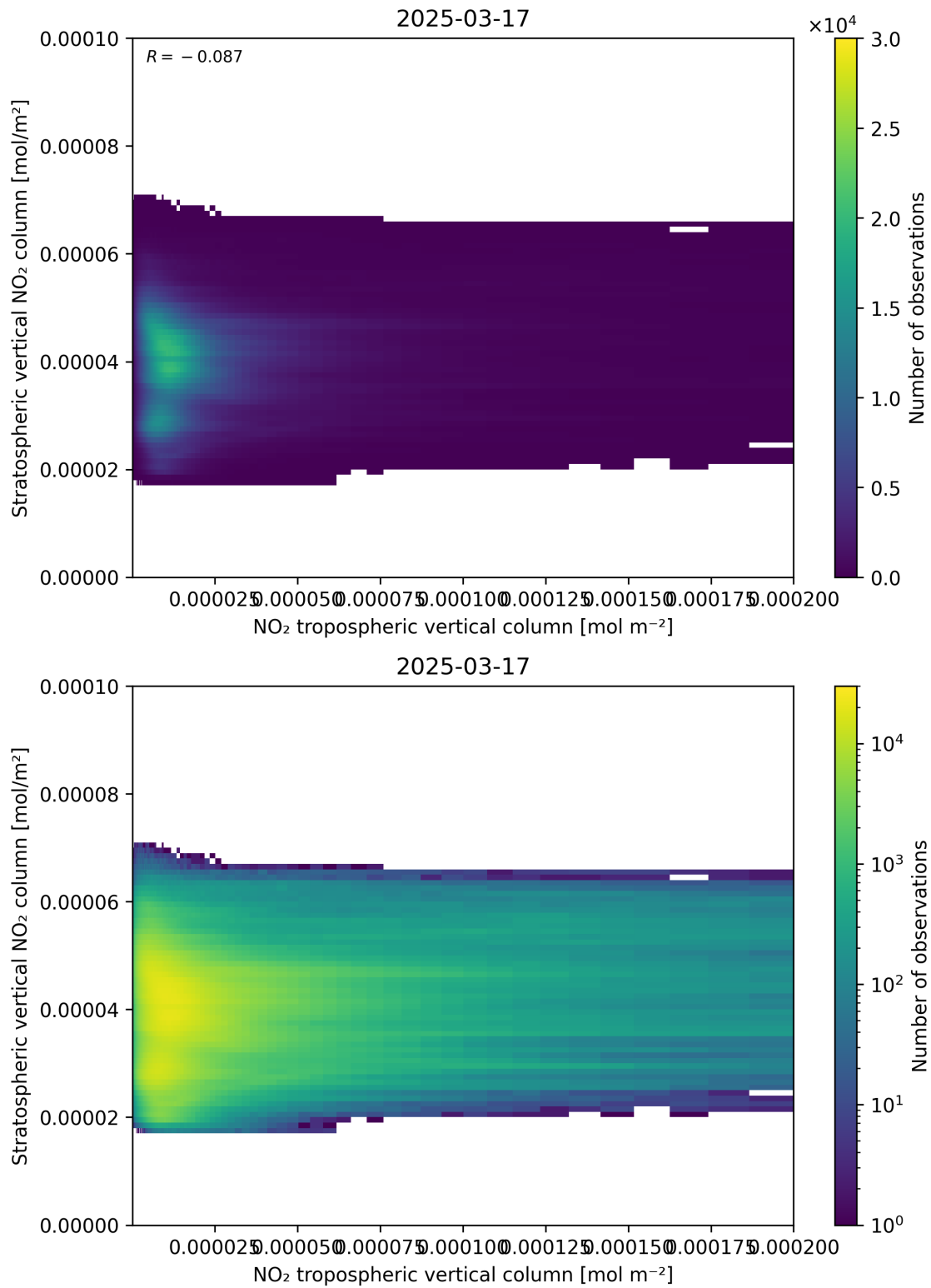
Figure 125: Scatter density plot of “NO 2 tropospheric vertical column” against “Stratospheric vertical NO 2 column” for 2025-03-17 to 2025-03-18.
