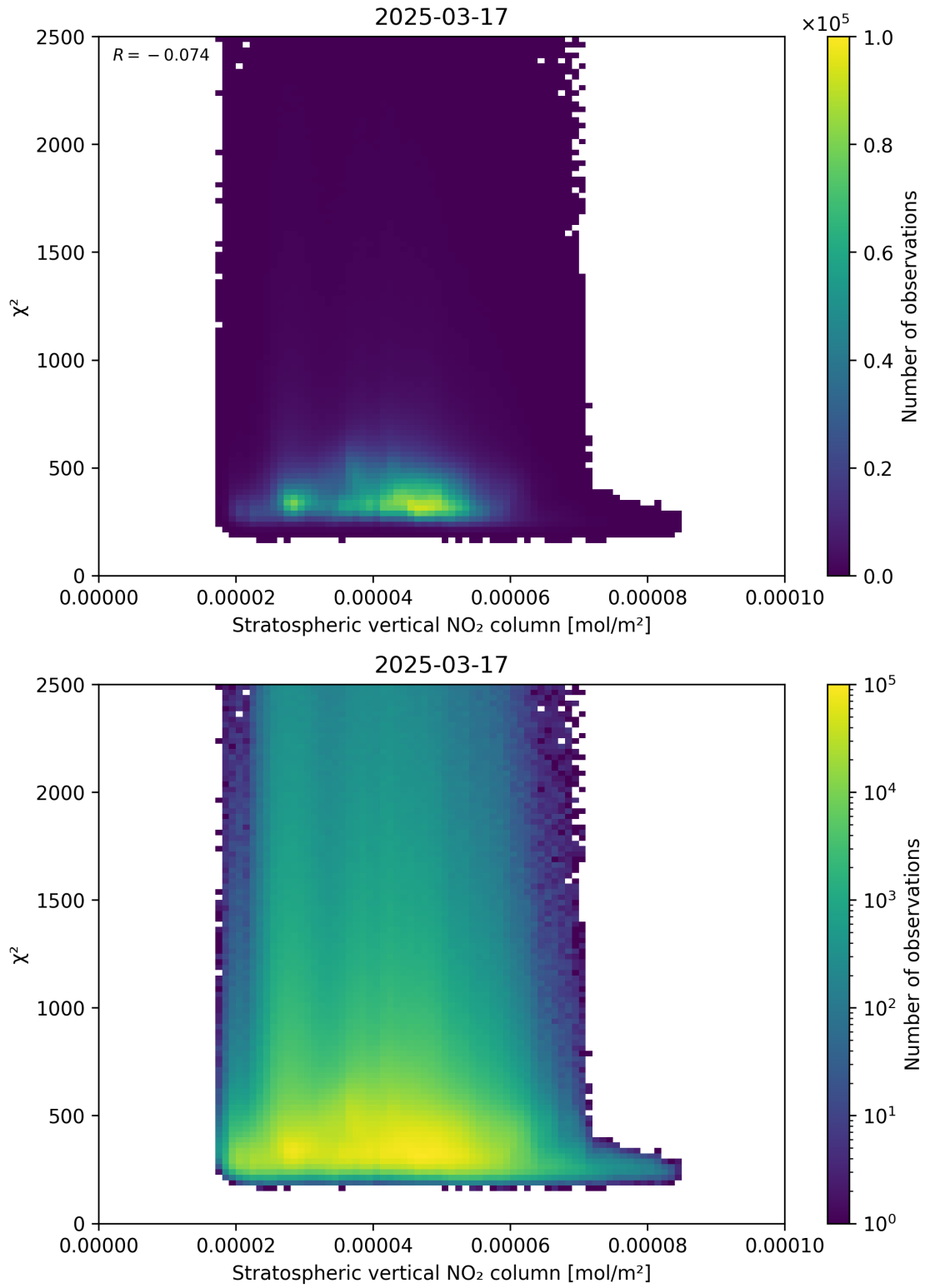
Figure 97: Scatter density plot of “Stratospheric vertical NO 2 column” against “ \chi^2 ” for 2025-03-17 to 2025-03-18.
