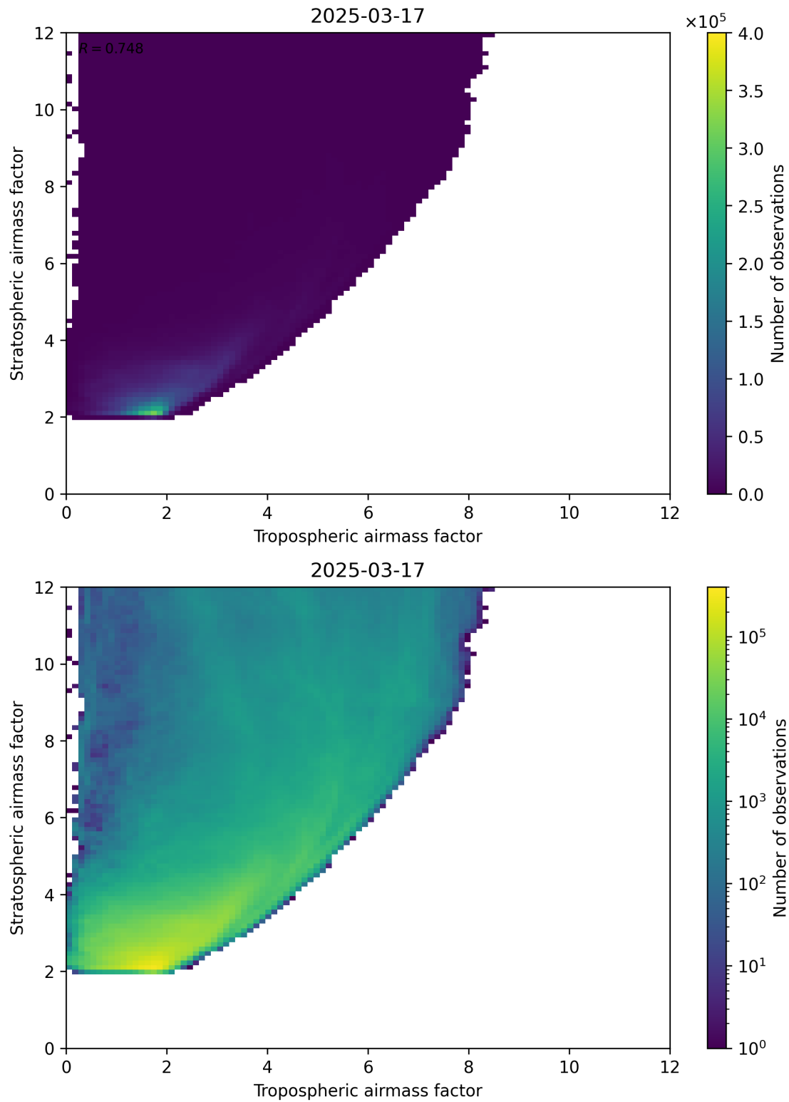
Figure 71: Scatter density plot of “Tropospheric airmass factor” against “Stratospheric airmass factor” for 2025-03-17 to 2025-03-18.
