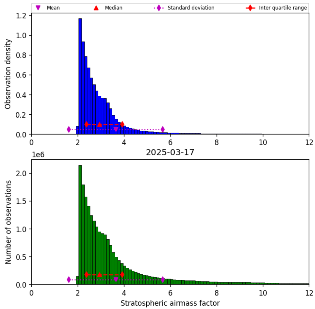
Figure 44: Histogram of “Stratospheric airmass factor” for 2025-03-17 to 2025-03-18
