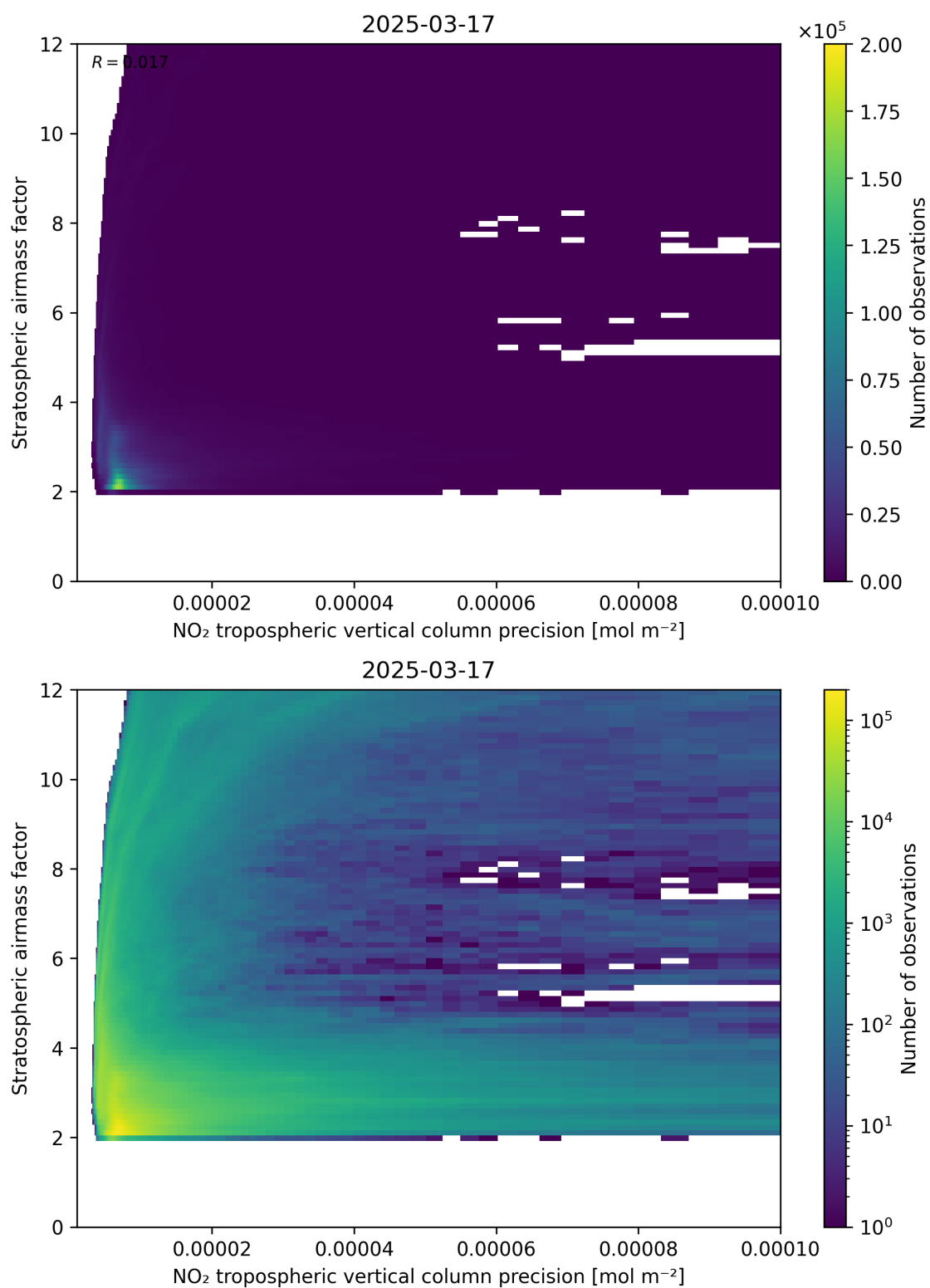
Figure 131: Scatter density plot of “NO 2 tropospheric vertical column precision” against “Stratospheric airmass factor” for 2025-03-17 to 2025-03-18.
