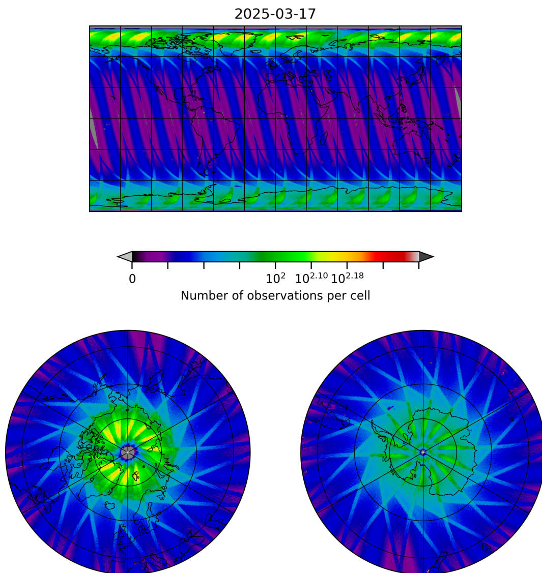
Figure 10: Map of the number of observations for 2025-03-17 to 2025-03-18
