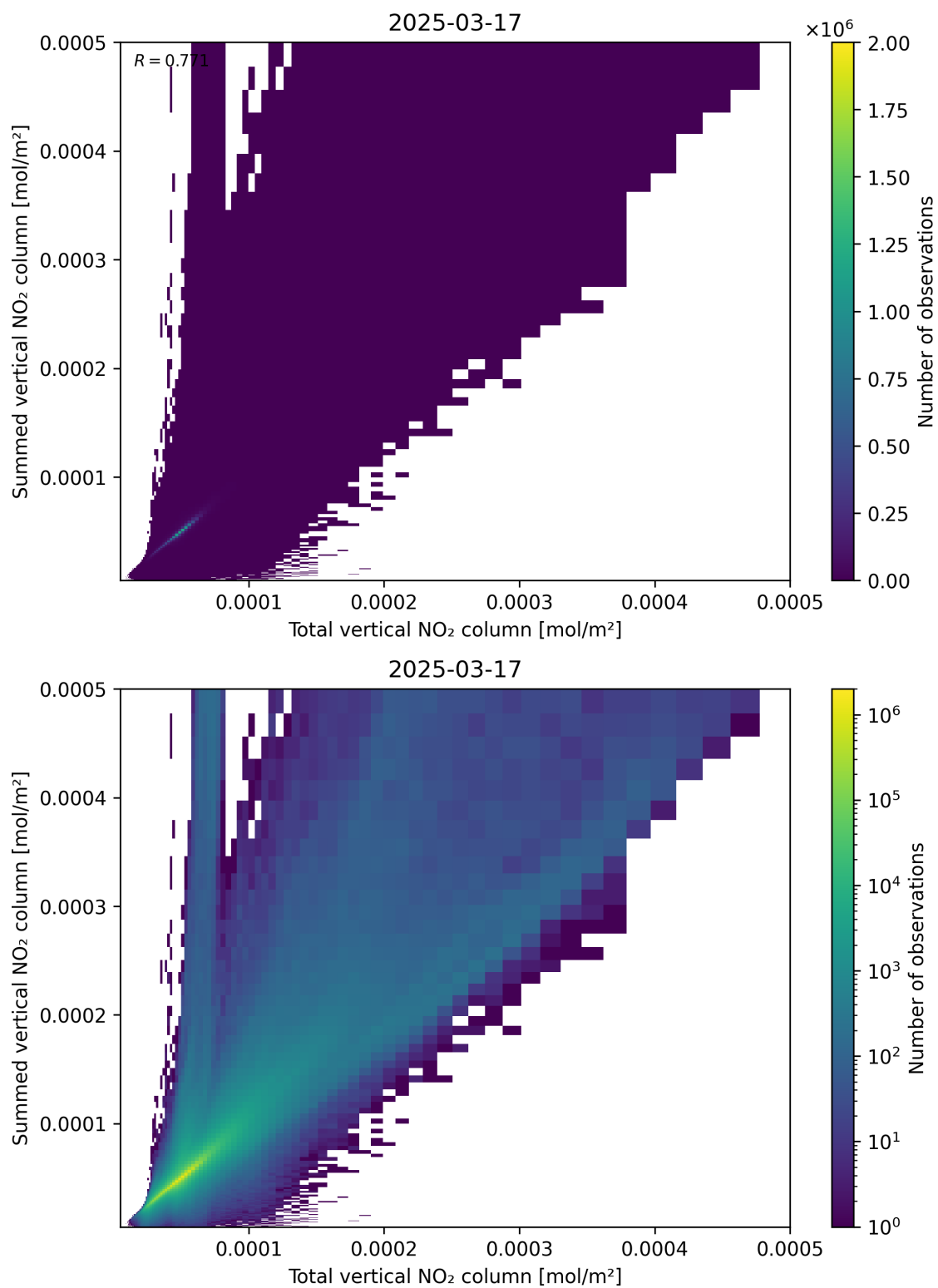
Figure 112: Scatter density plot of “Total vertical NO 2 column” against “Summed vertical NO 2 column” for 2025-03-17 to 2025-03-18.
