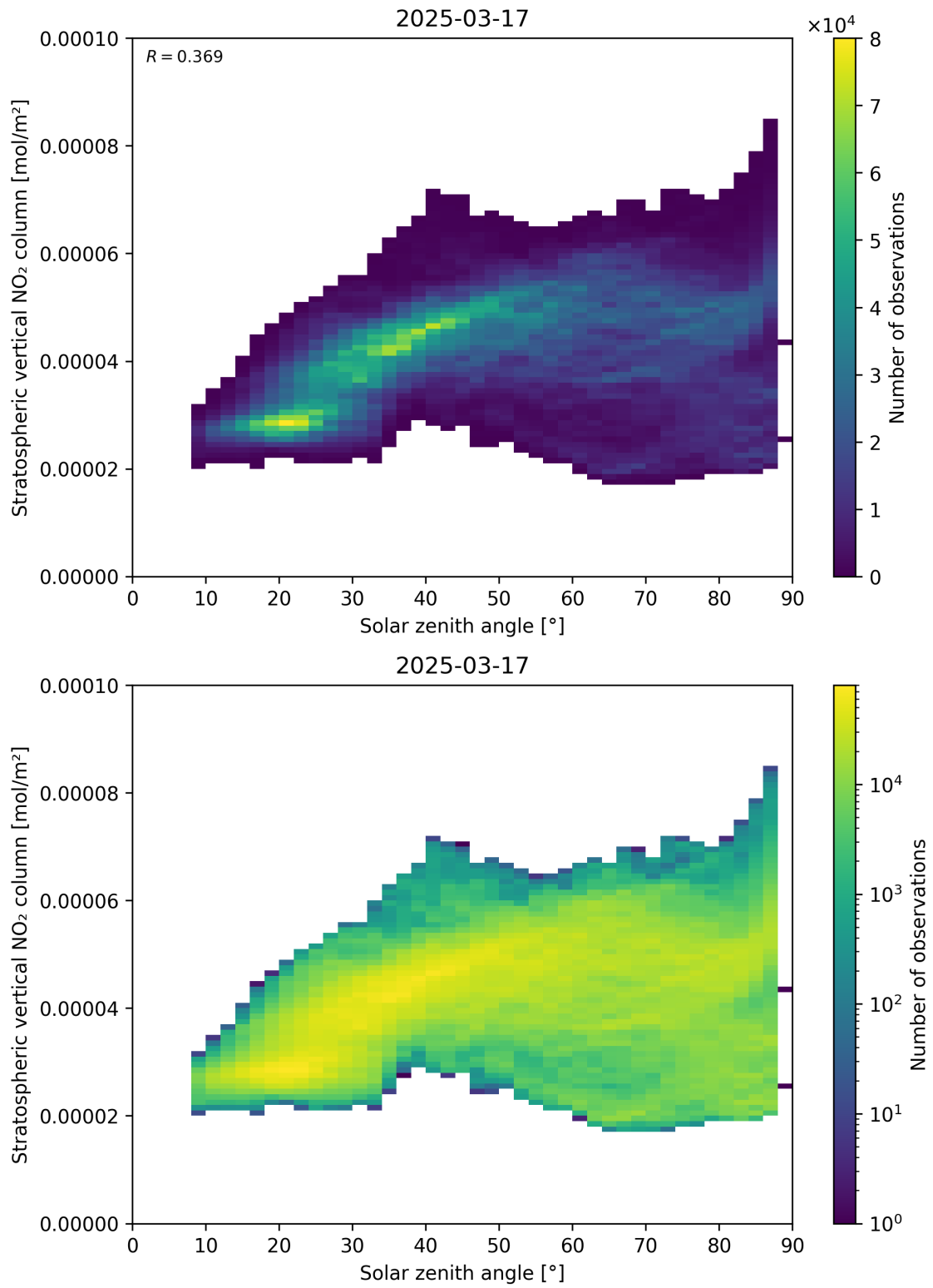
Figure 150: Scatter density plot of “Solar zenith angle” against “Stratospheric vertical \text{NO}_2 column” for 2025-03-17 to 2025-03-18.
