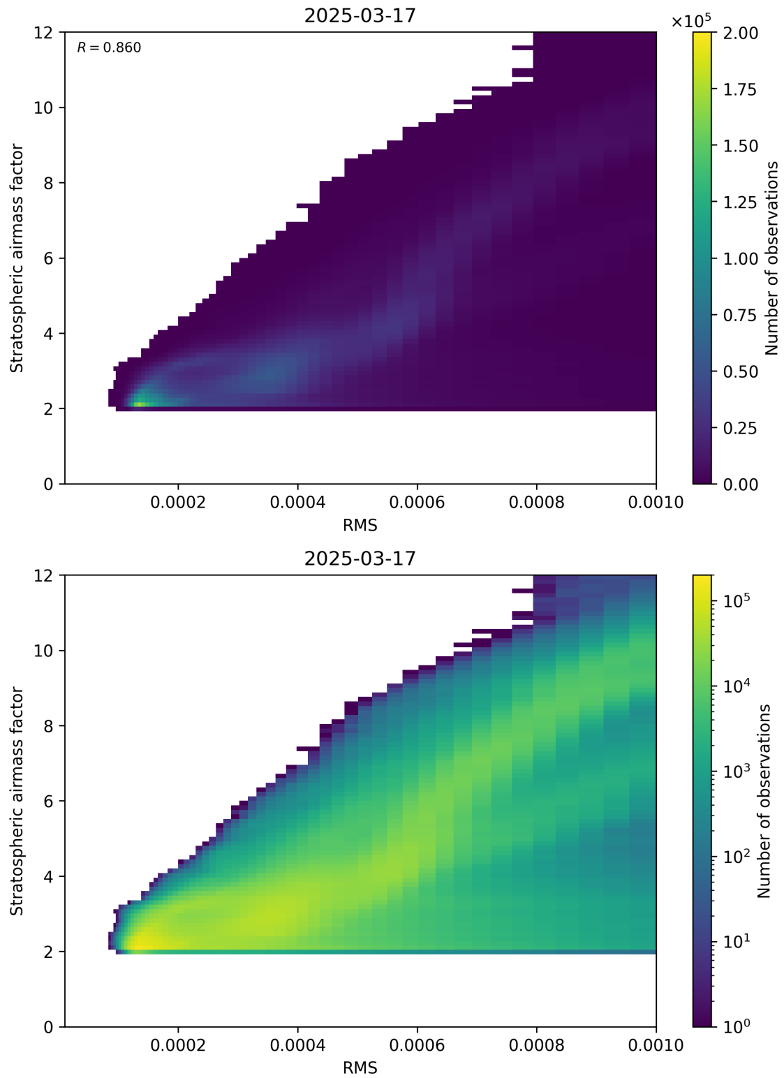
Figure 144: Scatter density plot of “RMS” against “Stratospheric airmass factor” for 2025-03-17 to 2025-03-18.
