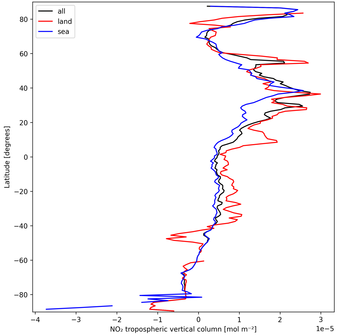
Figure 12: Zonal average of “NO 2 tropospheric vertical column” for 2025-03-17 to 2025-03-18.
