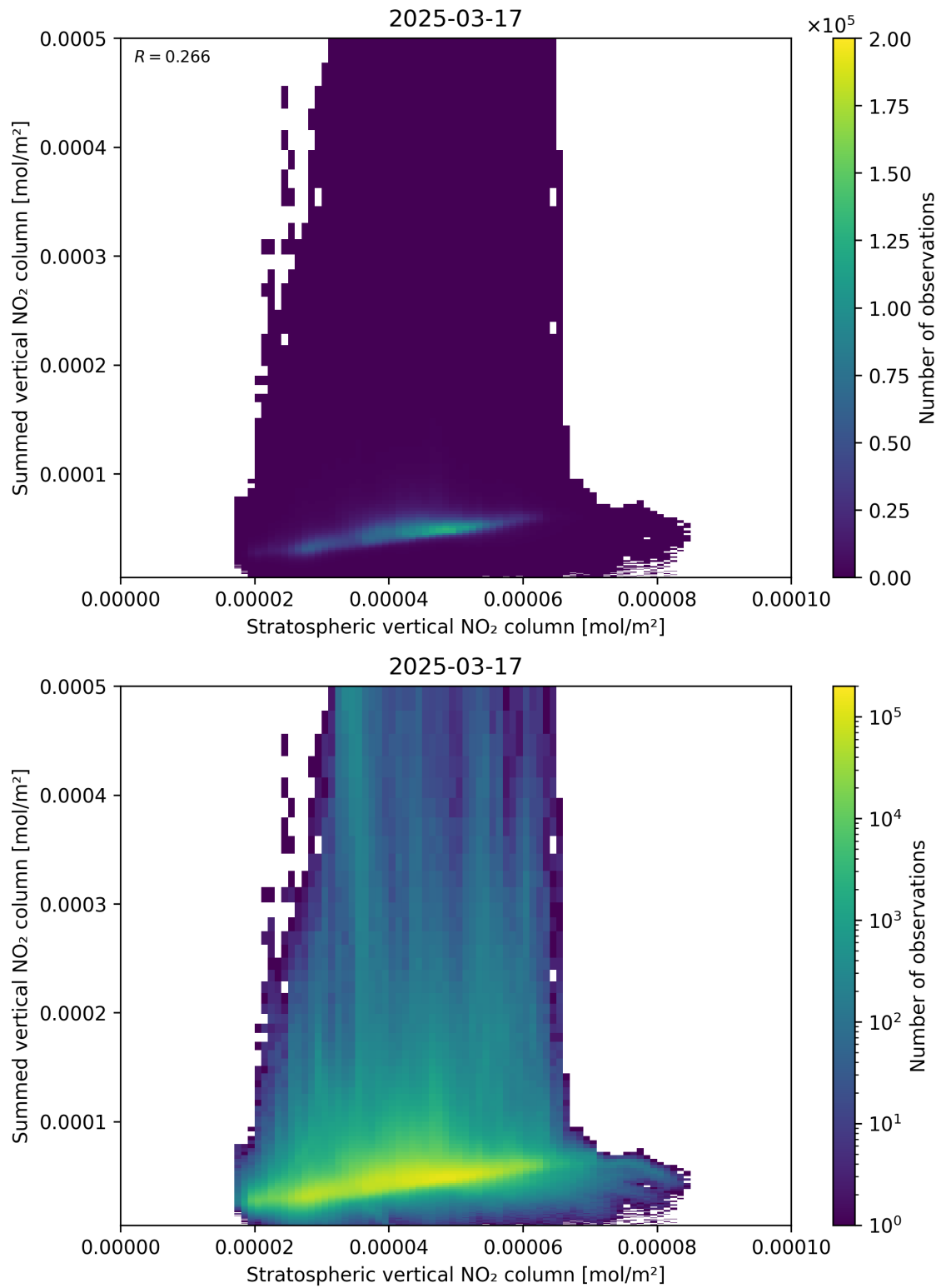
Figure 98: Scatter density plot of “Stratospheric vertical NO 2 column” against “Summed vertical NO 2 column” for 2025-03-17 to 2025-03-18.
