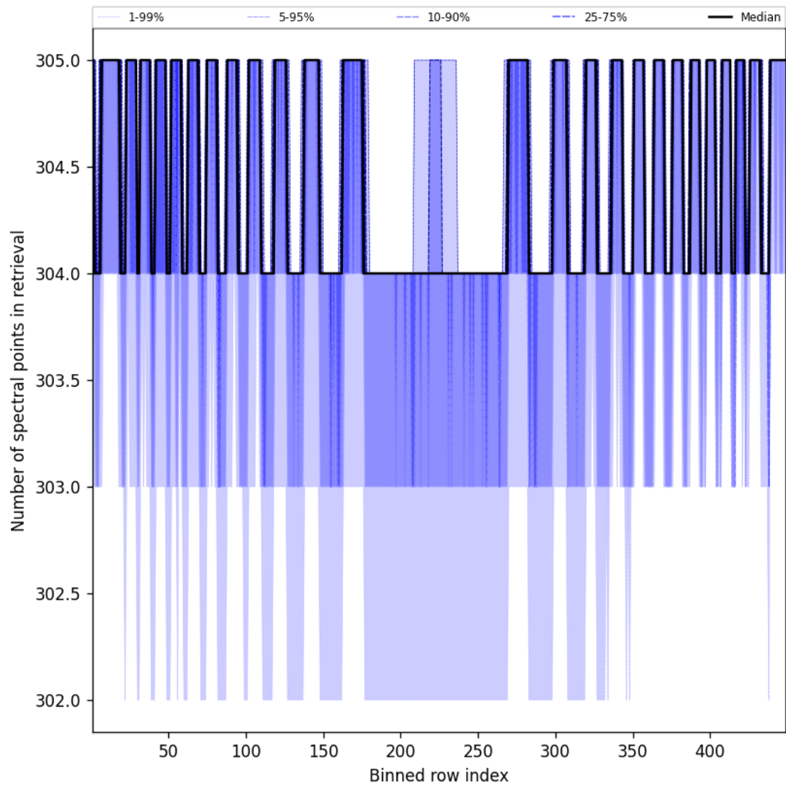
Figure 50: Along track statistics of “Number of spectral points in retrieval” for 2025-03-17 to 2025-03-18
