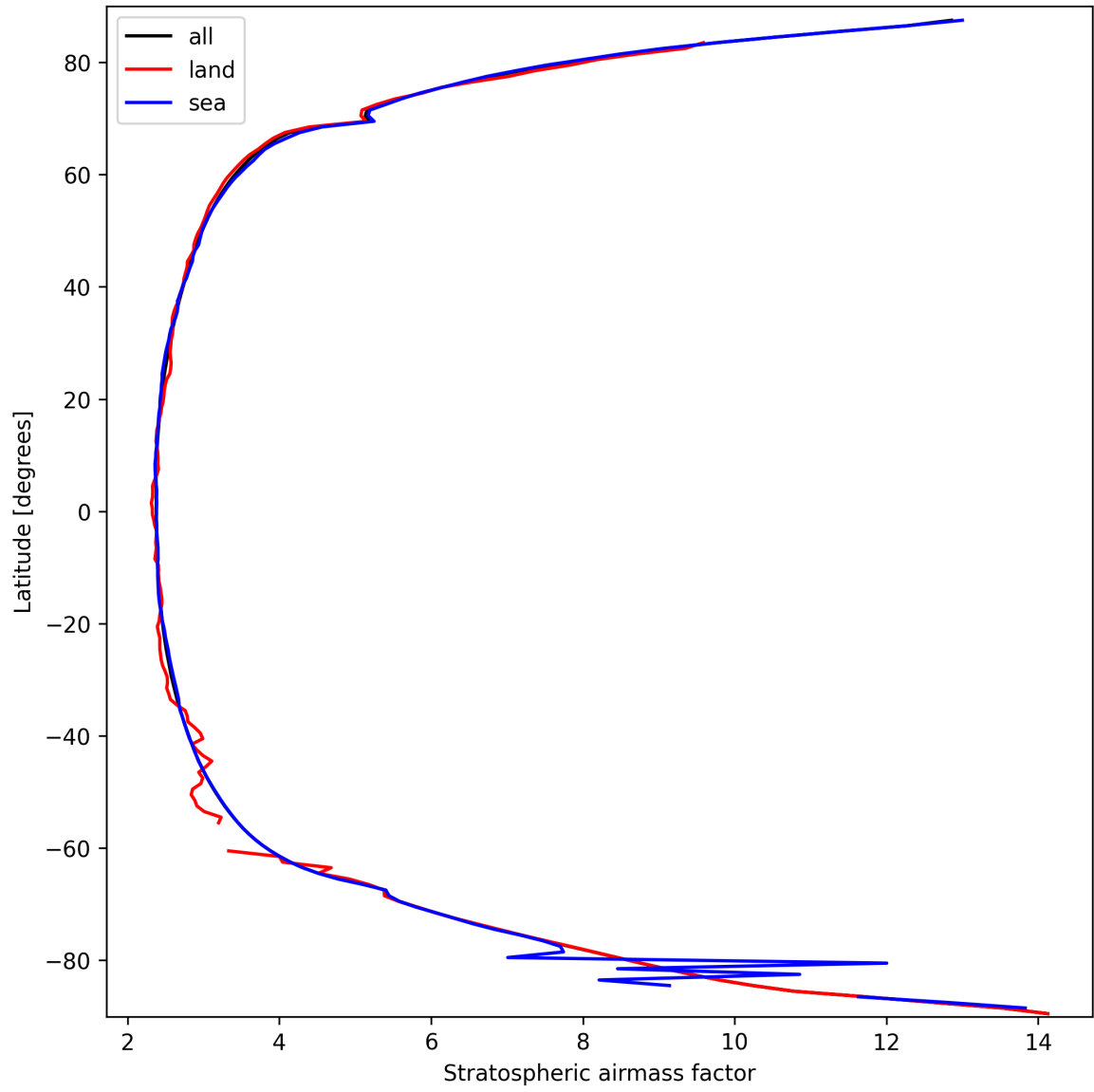
Figure 27: Zonal average of “Stratospheric air mass factor” for 2025-03-17 to 2025-03-18.
