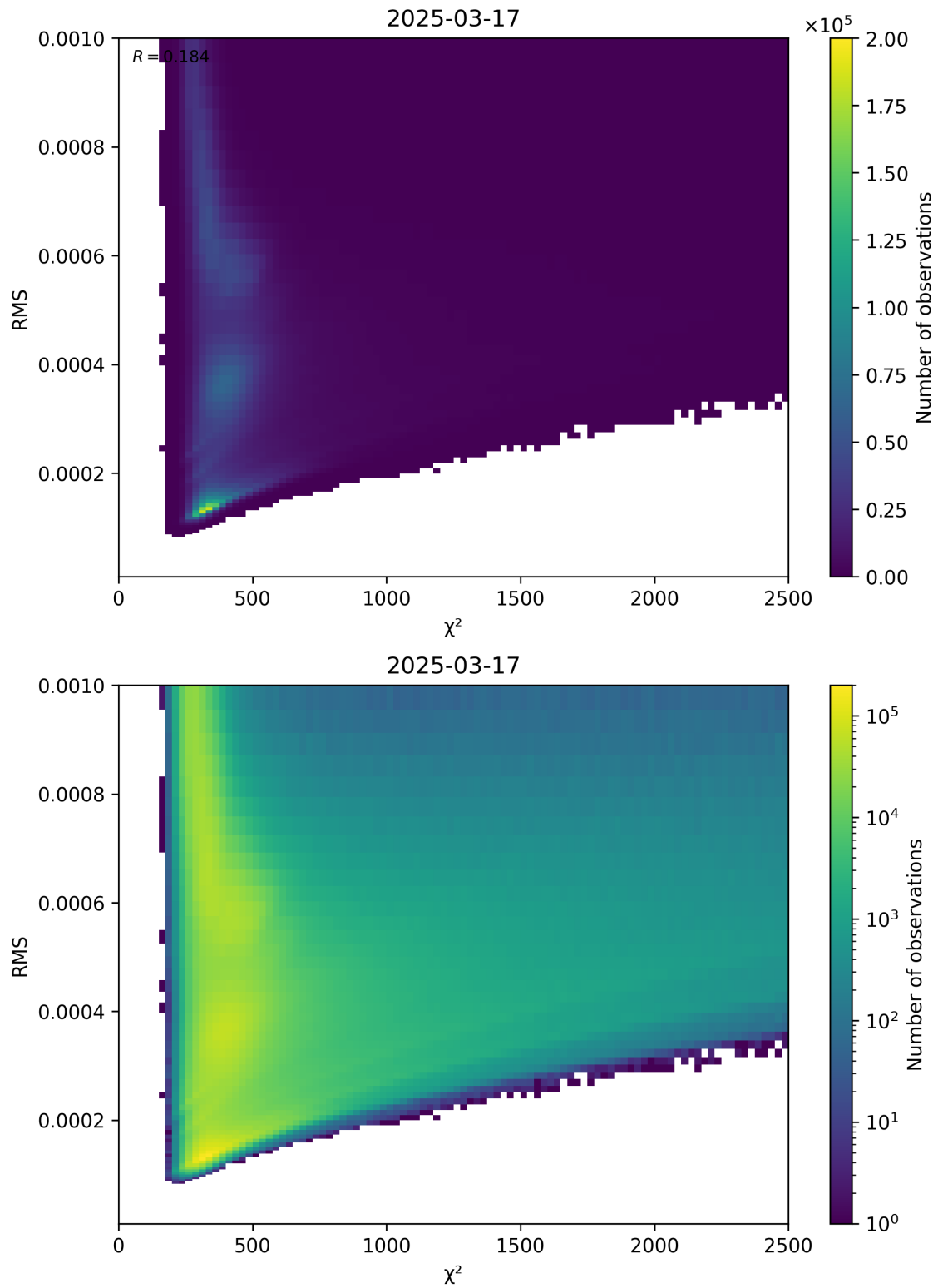
Figure 82: Scatter density plot of “ \chi^2 ” against “RMS” for 2025-03-17 to 2025-03-18.
