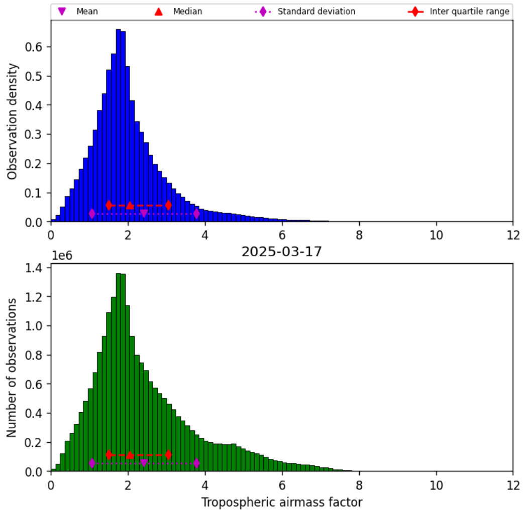
Figure 31: Histogram of “Tropospheric airmass factor” for 2025-03-17 to 2025-03-18
