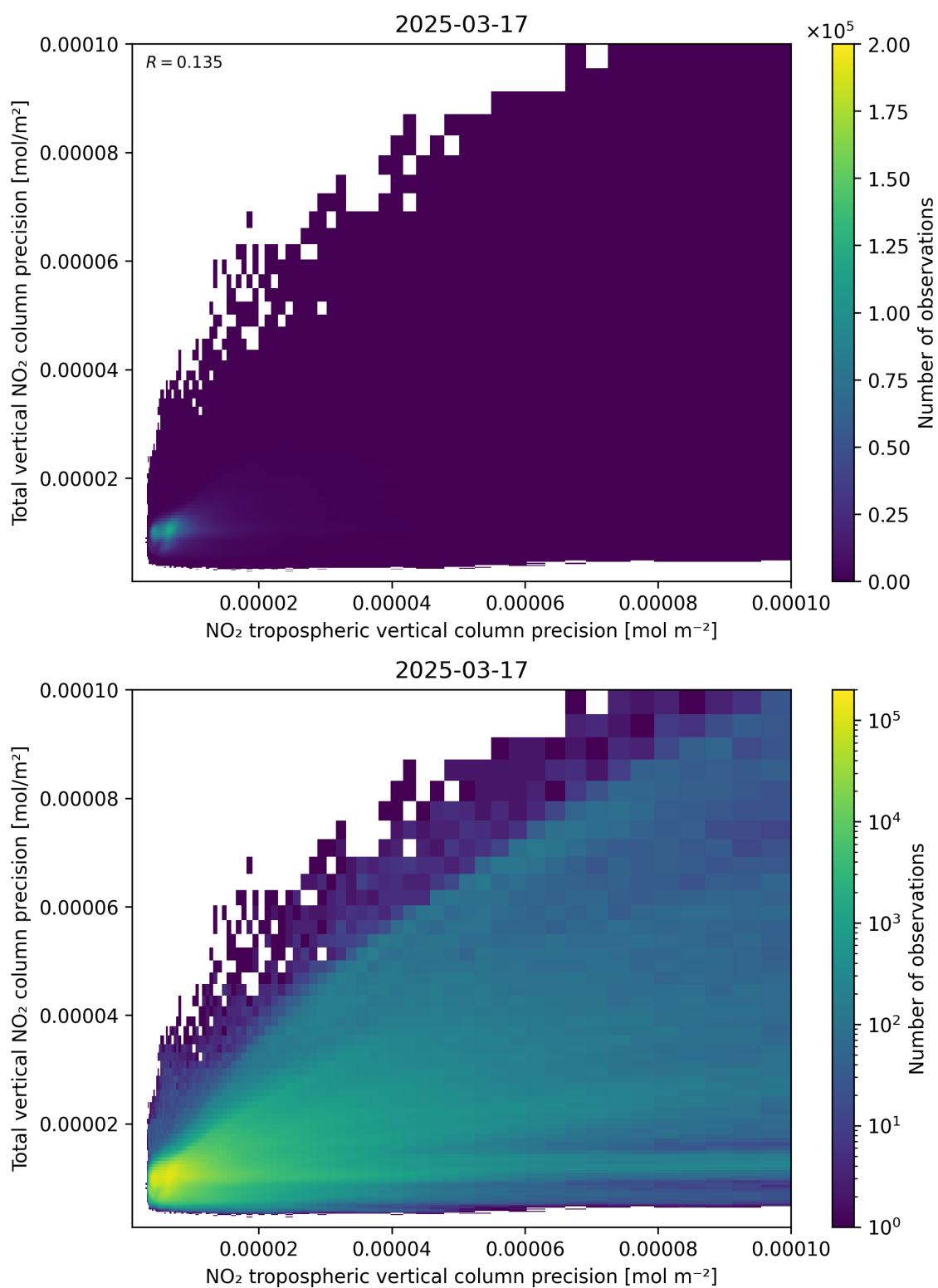
Figure 139: Scatter density plot of “NO 2 tropospheric vertical column precision” against “Total vertical NO 2 column precision” for 2025-03-17 to 2025-03-18.
