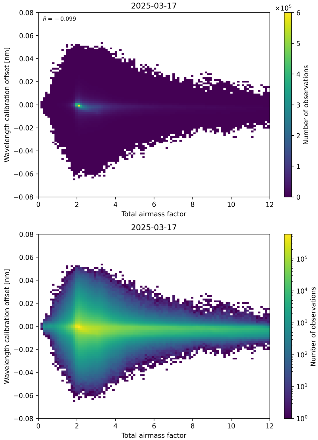
Figure 70: Scatter density plot of “Total airmass factor” against “Wavelength calibration offset” for 2025-03-17 to 2025-03-18.
