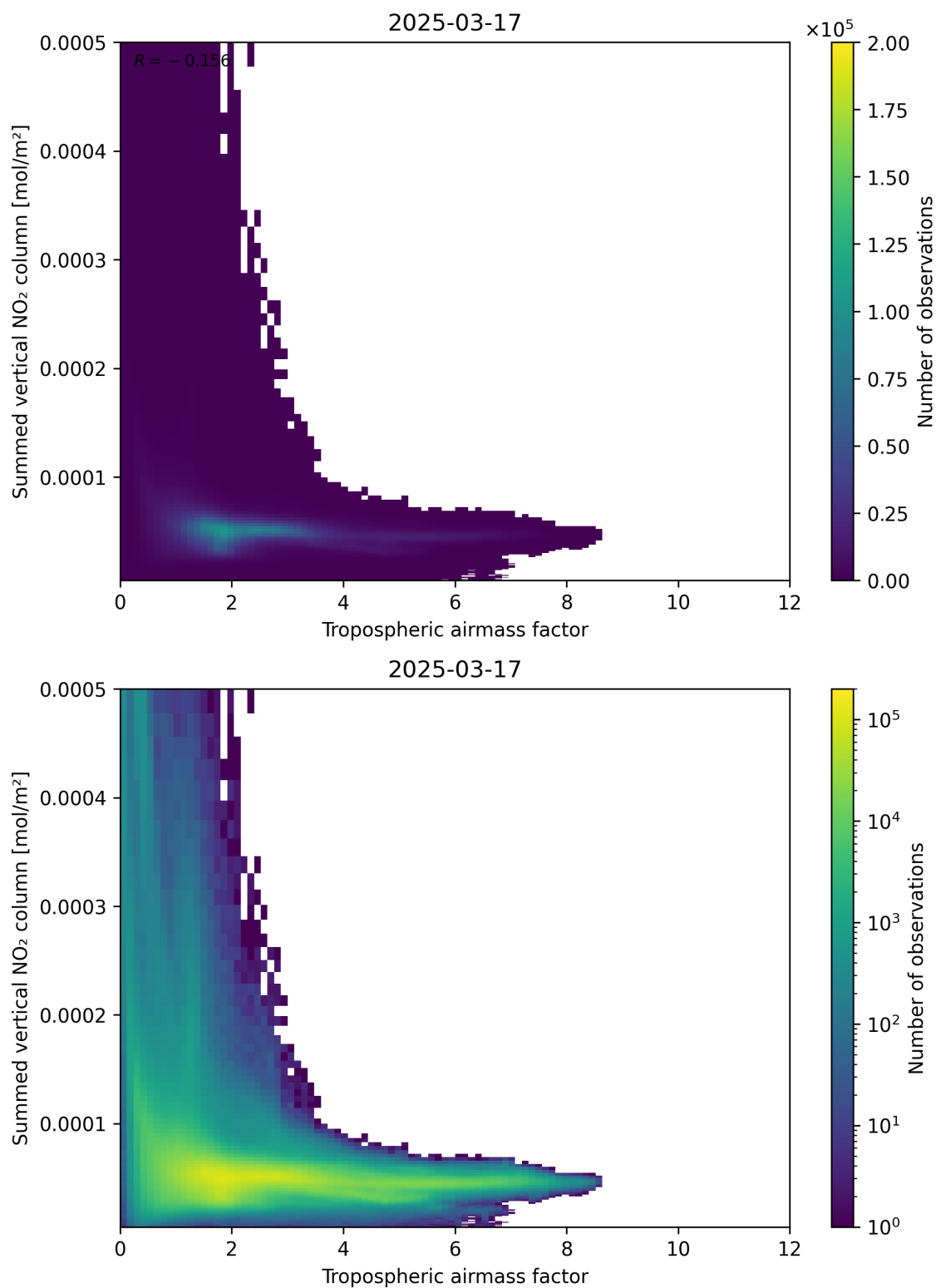
Figure 75: Scatter density plot of “Tropospheric airmass factor” against “Summed vertical NO 2 column” for 2025-03-17 to 2025-03-18.
