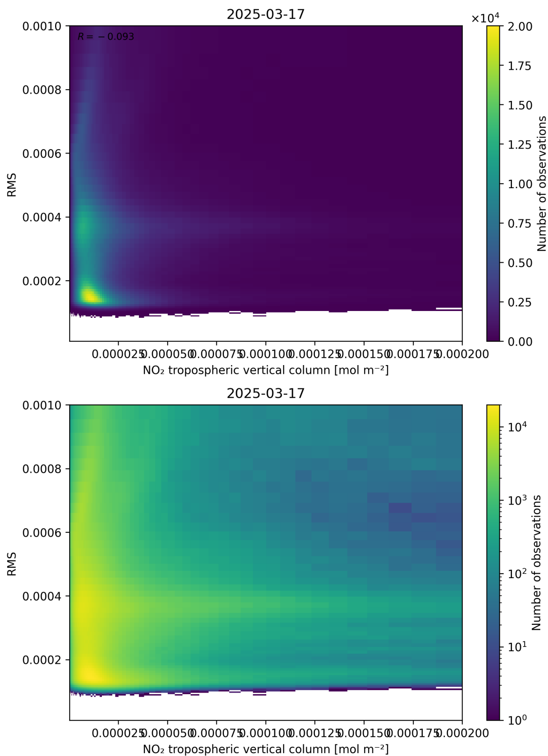
Figure 142: Scatter density plot of “NO 2 tropospheric vertical column” against “RMS” for 2025-03-17 to 2025-03-18.
