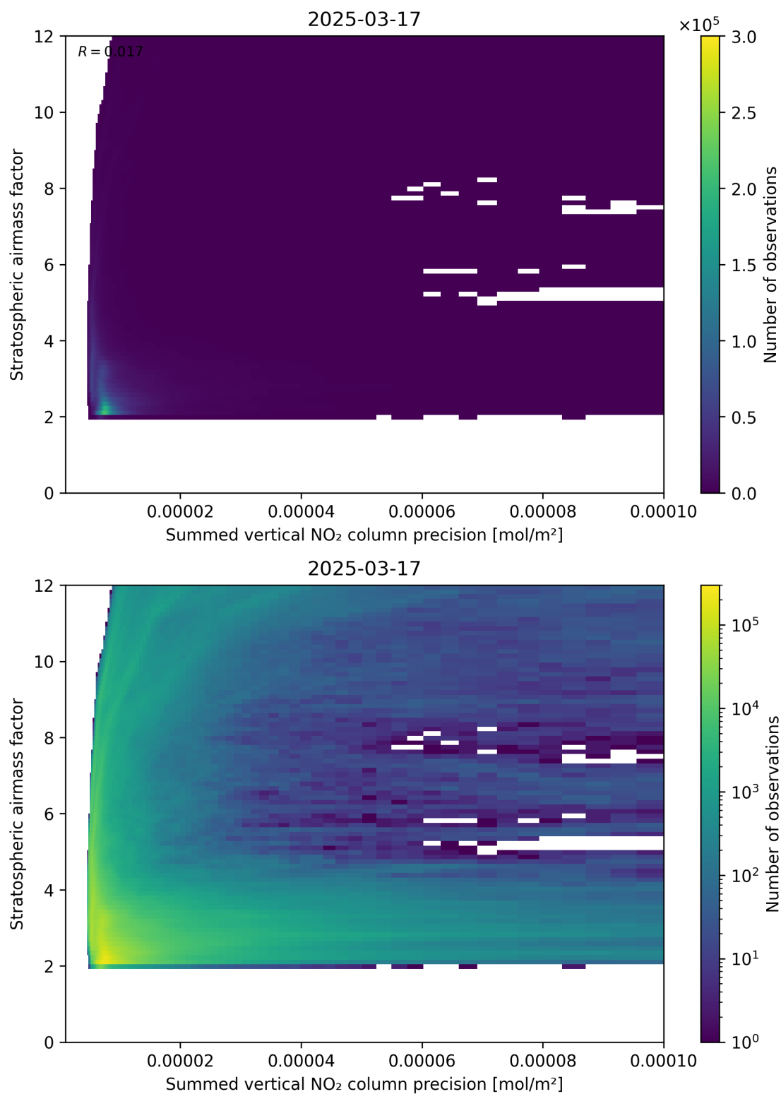
Figure 106: Scatter density plot of “Summed vertical NO 2 column precision” against “Stratospheric airmass factor” for 2025-03-17 to 2025-03-18.
