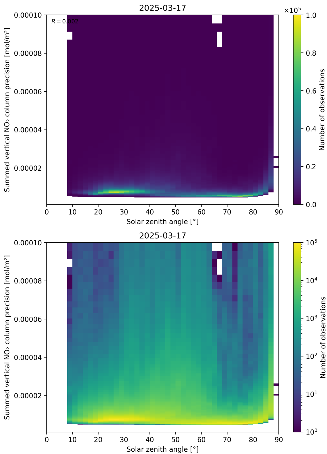
Figure 152: Scatter density plot of “Solar zenith angle” against “Summed vertical NO 2 column precision” for 2025-03-17 to 2025-03-18.
