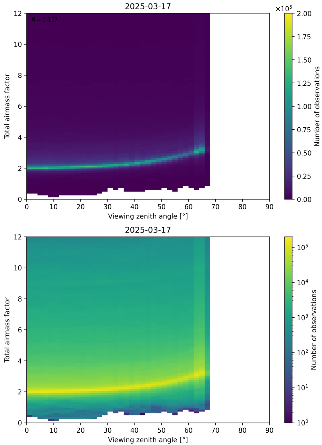
Figure 160: Scatter density plot of “Viewing zenith angle” against “Total airmass factor” for 2025-03-17 to 2025-03-18.
