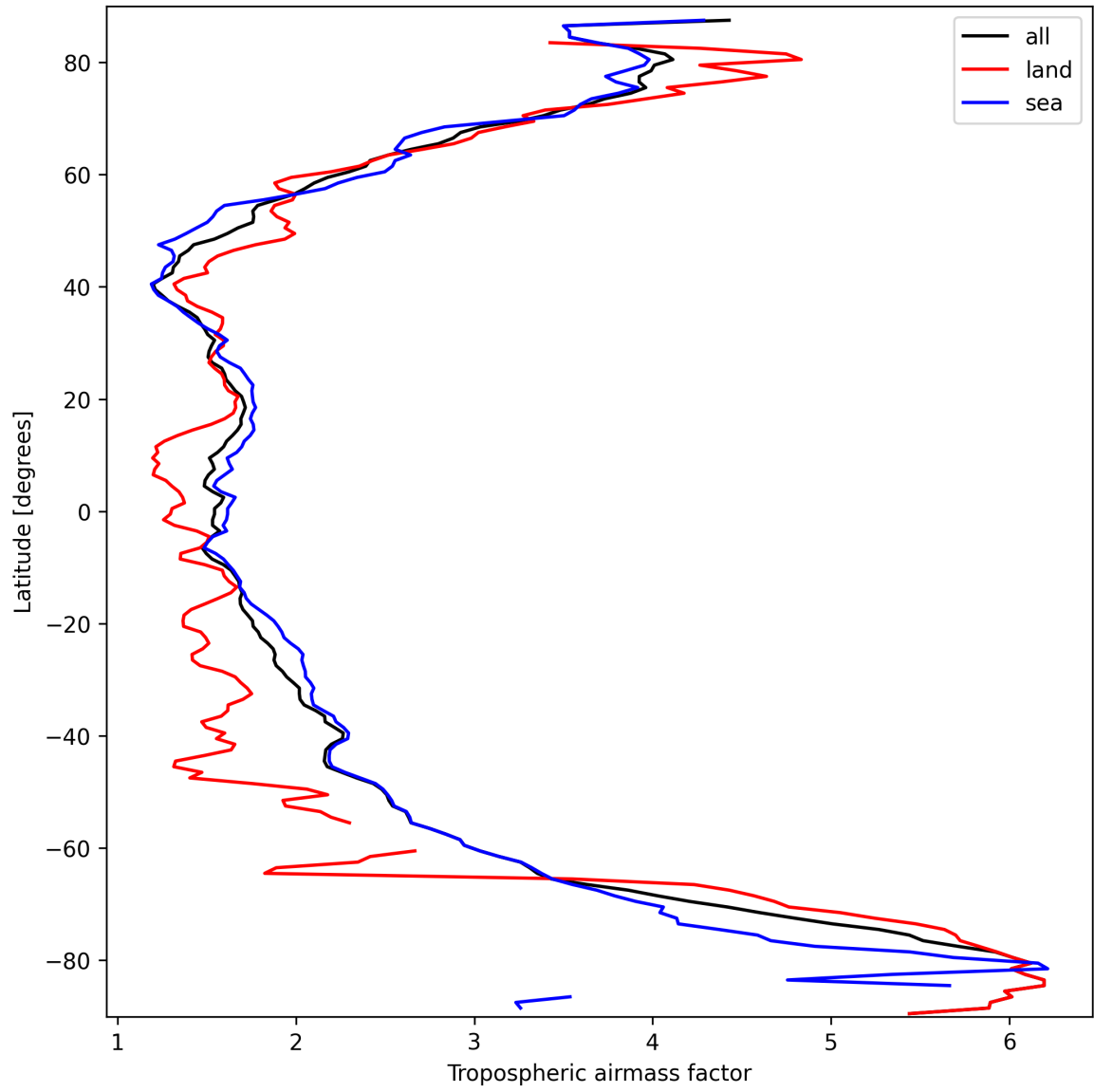
Figure 14: Zonal average of “Tropospheric airmass factor” for 2025-03-17 to 2025-03-18.
