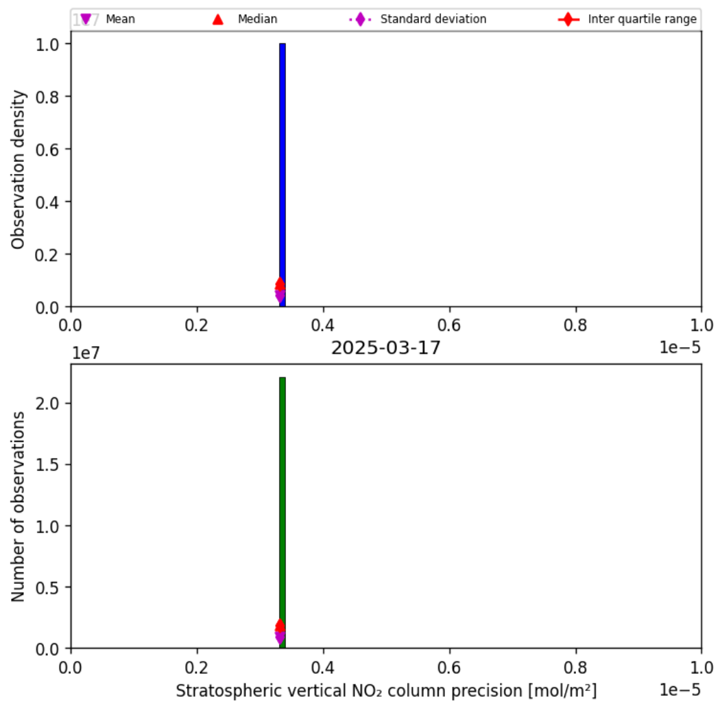
Figure 37: Histogram of “Stratospheric vertical NO 2 column precision” for 2025-03-17 to 2025-03-18
