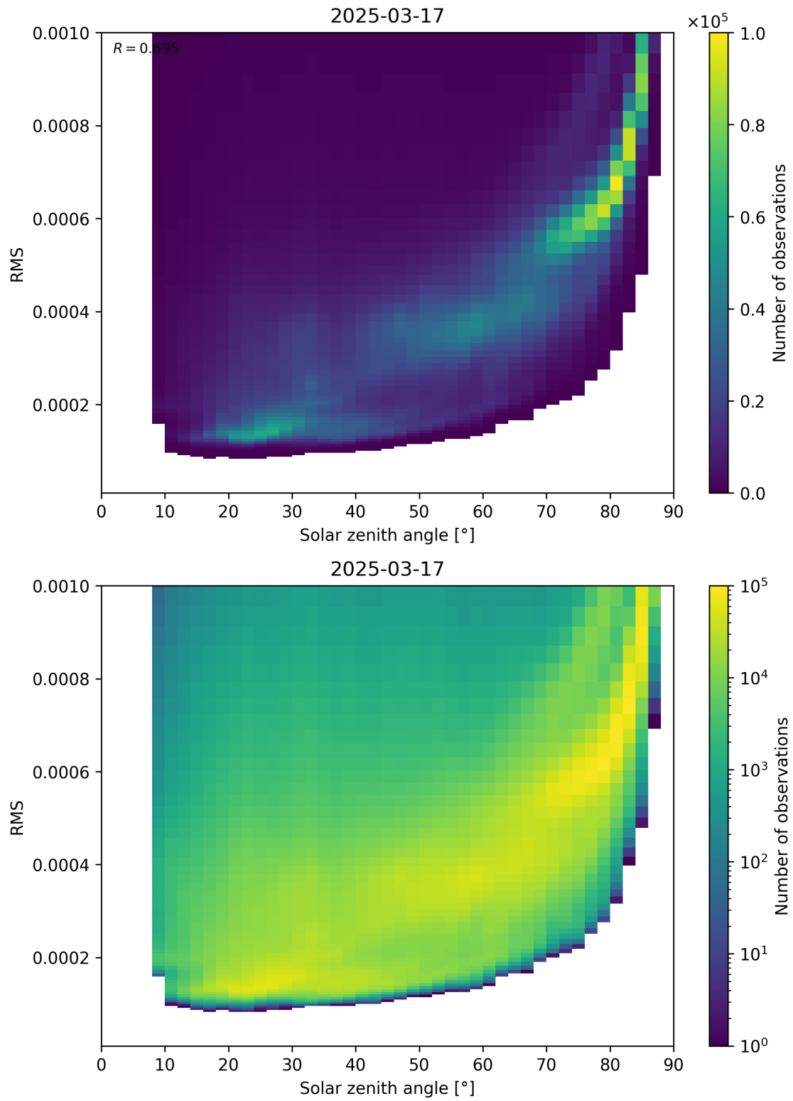
Figure 157: Scatter density plot of “Solar zenith angle” against “RMS” for 2025-03-17 to 2025-03-18.
