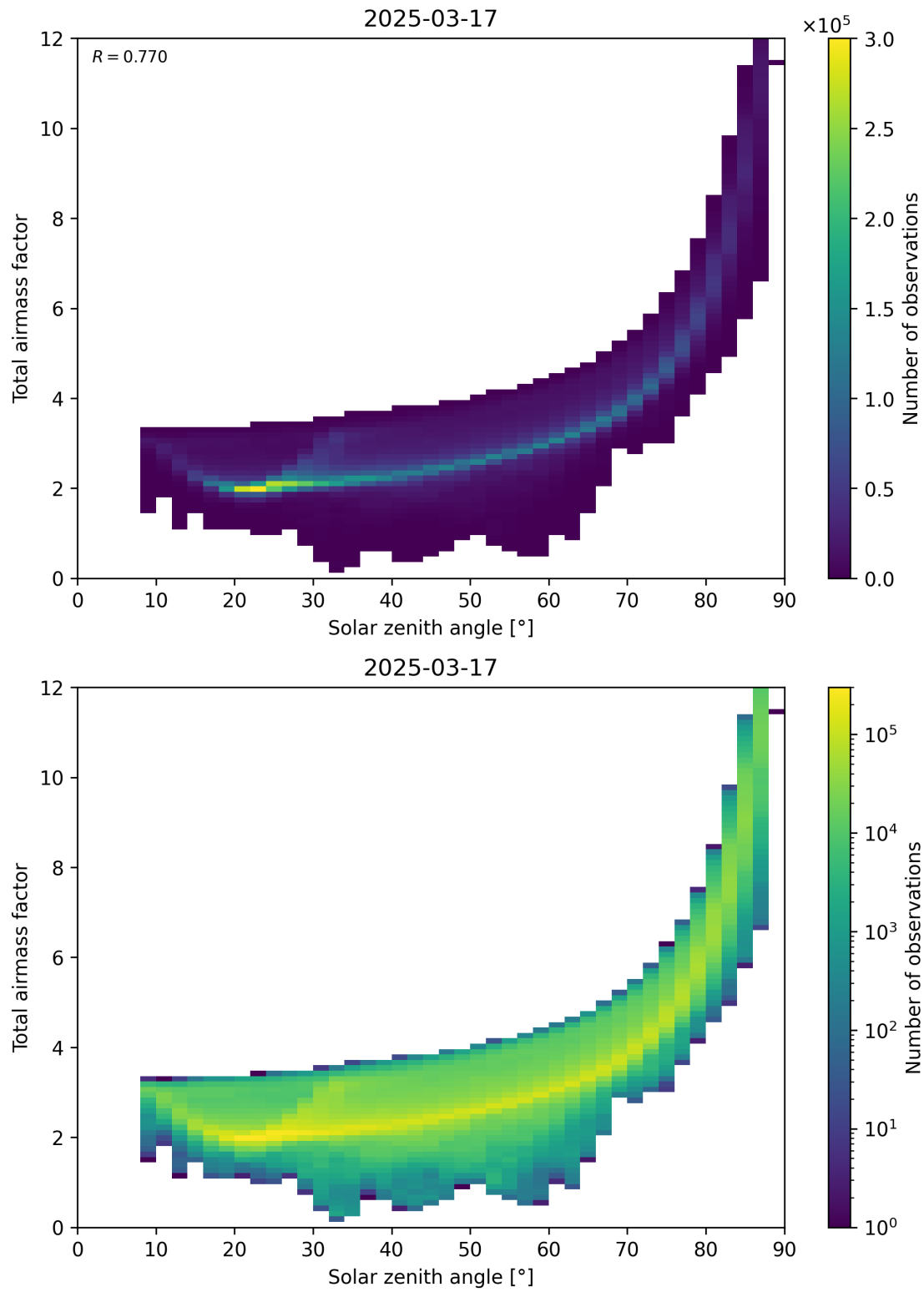
Figure 146: Scatter density plot of “Solar zenith angle” against “Total airmass factor” for 2025-03-17 to 2025-03-18.
