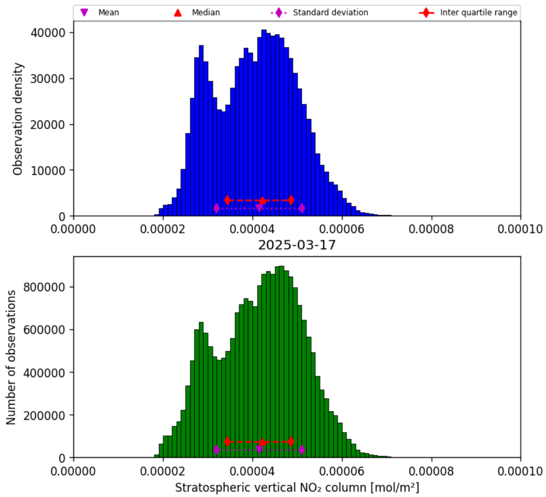
Figure 36: Histogram of “Stratospheric vertical NO 2 column” for 2025-03-17 to 2025-03-18
