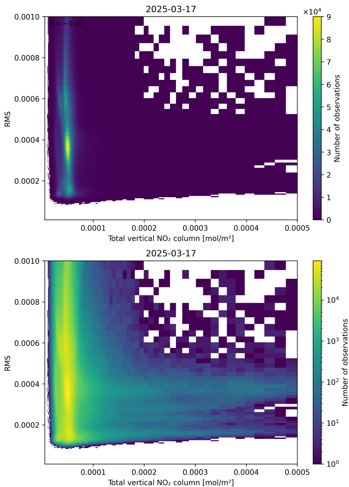
Figure 120: Scatter density plot of “Total vertical NO 2 column” against “RMS” for 2025-03-17 to 2025-03-18.
