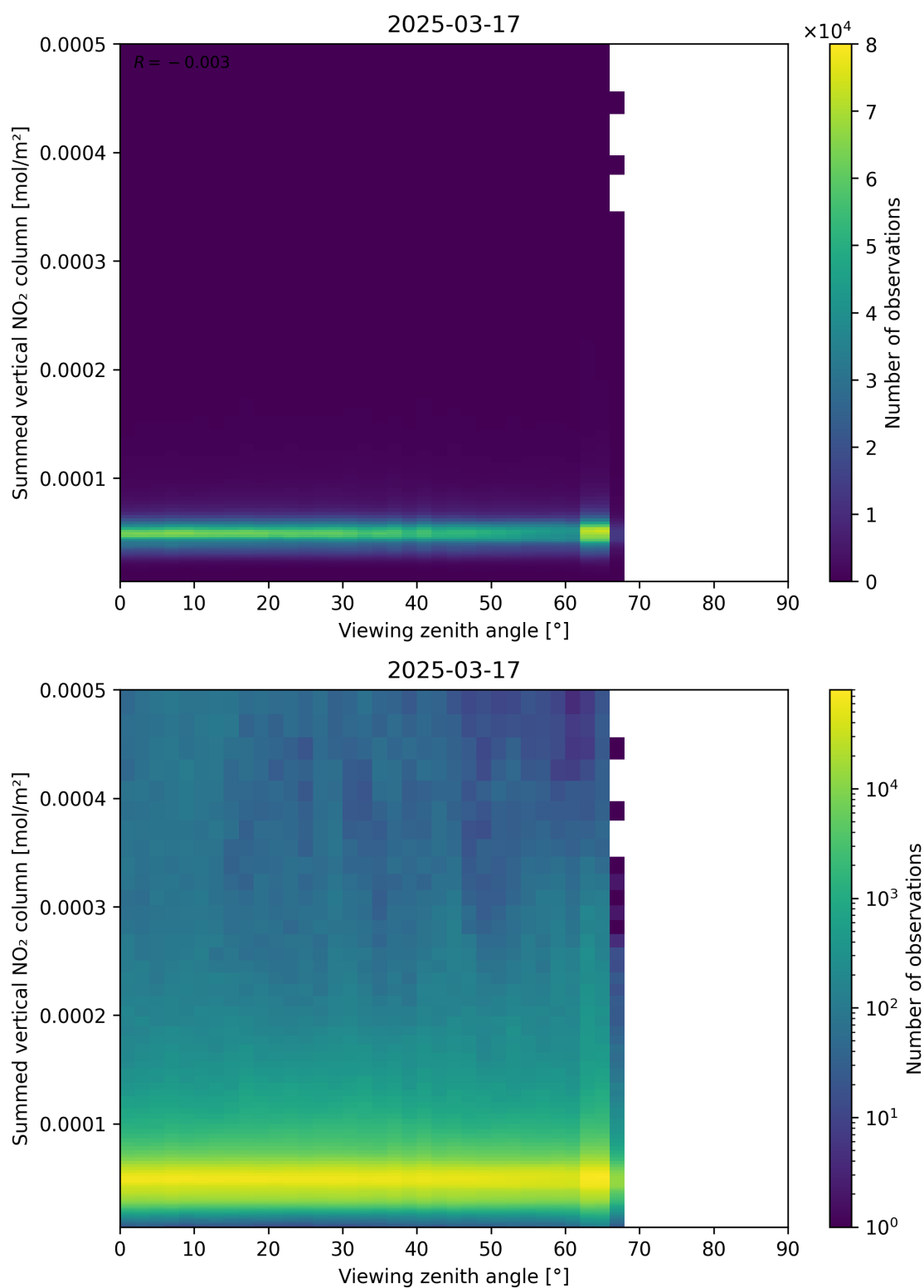
Figure 165: Scatter density plot of “Viewing zenith angle” against “Summed vertical NO 2 column” for 2025-03-17 to 2025-03-18.
