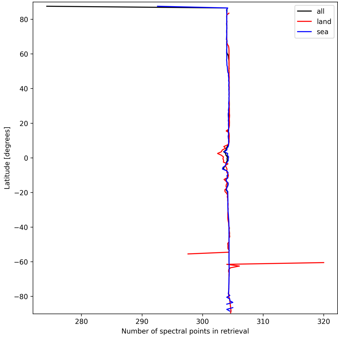
Figure 16: Zonal average of “Number of spectral points in retrieval” for 2025-03-17 to 2025-03-18.
