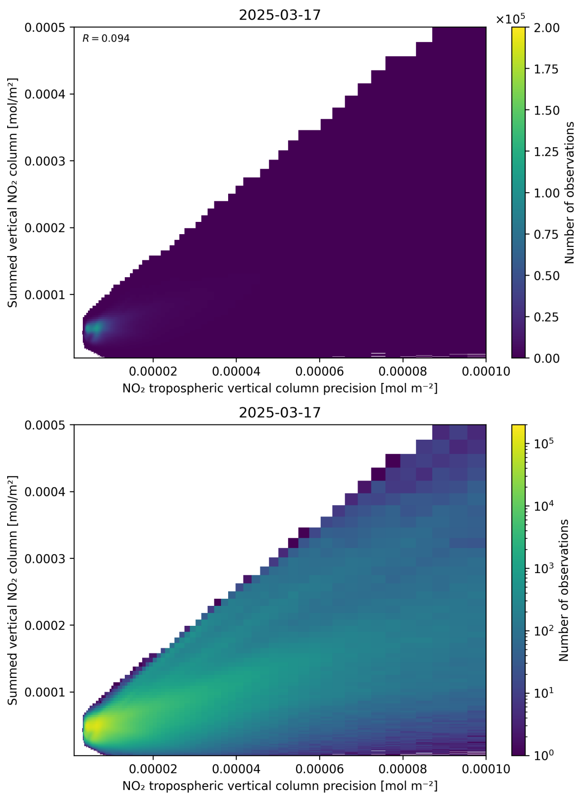
Figure 136: Scatter density plot of “NO 2 tropospheric vertical column precision” against “Summed vertical NO 2 column” for 2025-03-17 to 2025-03-18.
