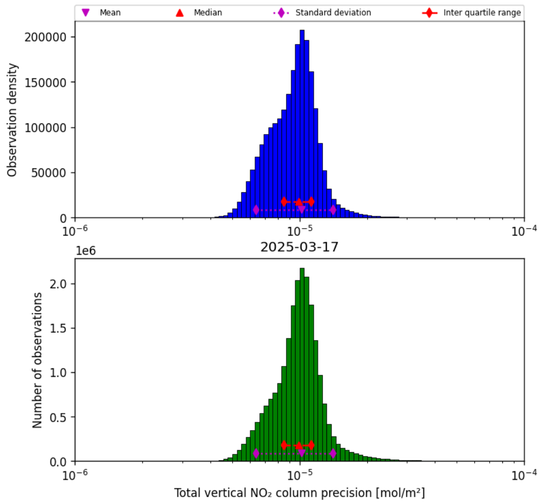
Figure 39: Histogram of “Total vertical NO 2 column precision” for 2025-03-17 to 2025-03-18
