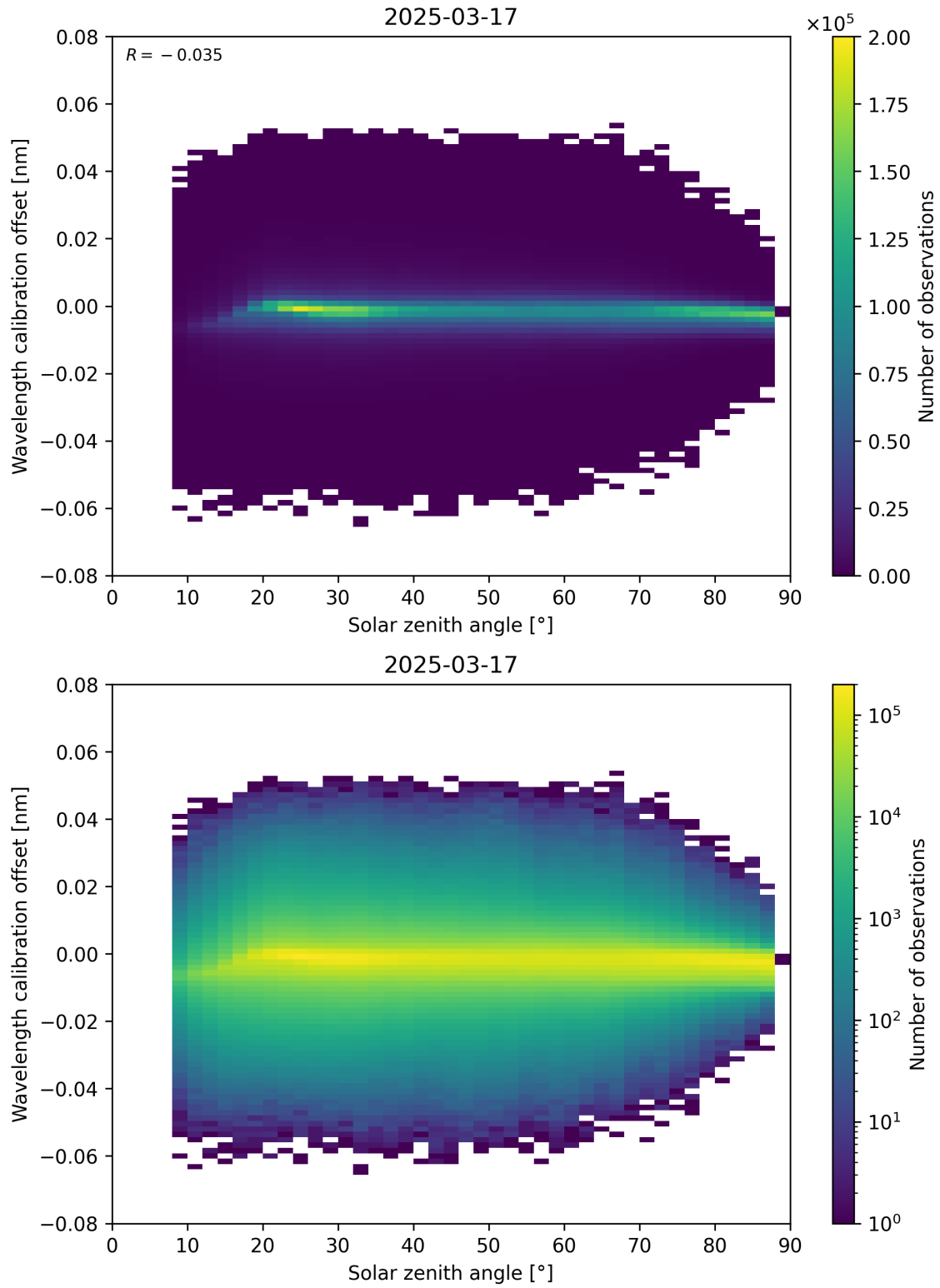
Figure 158: Scatter density plot of “Solar zenith angle” against “Wavelength calibration offset” for 2025-03-17 to 2025-03-18.
