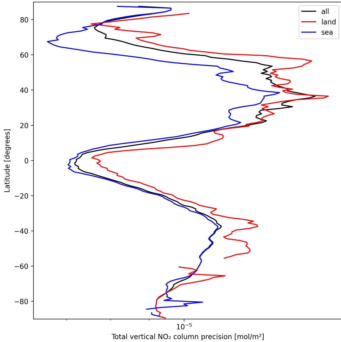
Figure 22: Zonal average of “Total vertical NO 2 column precision” for 2025-03-17 to 2025-03-18.
