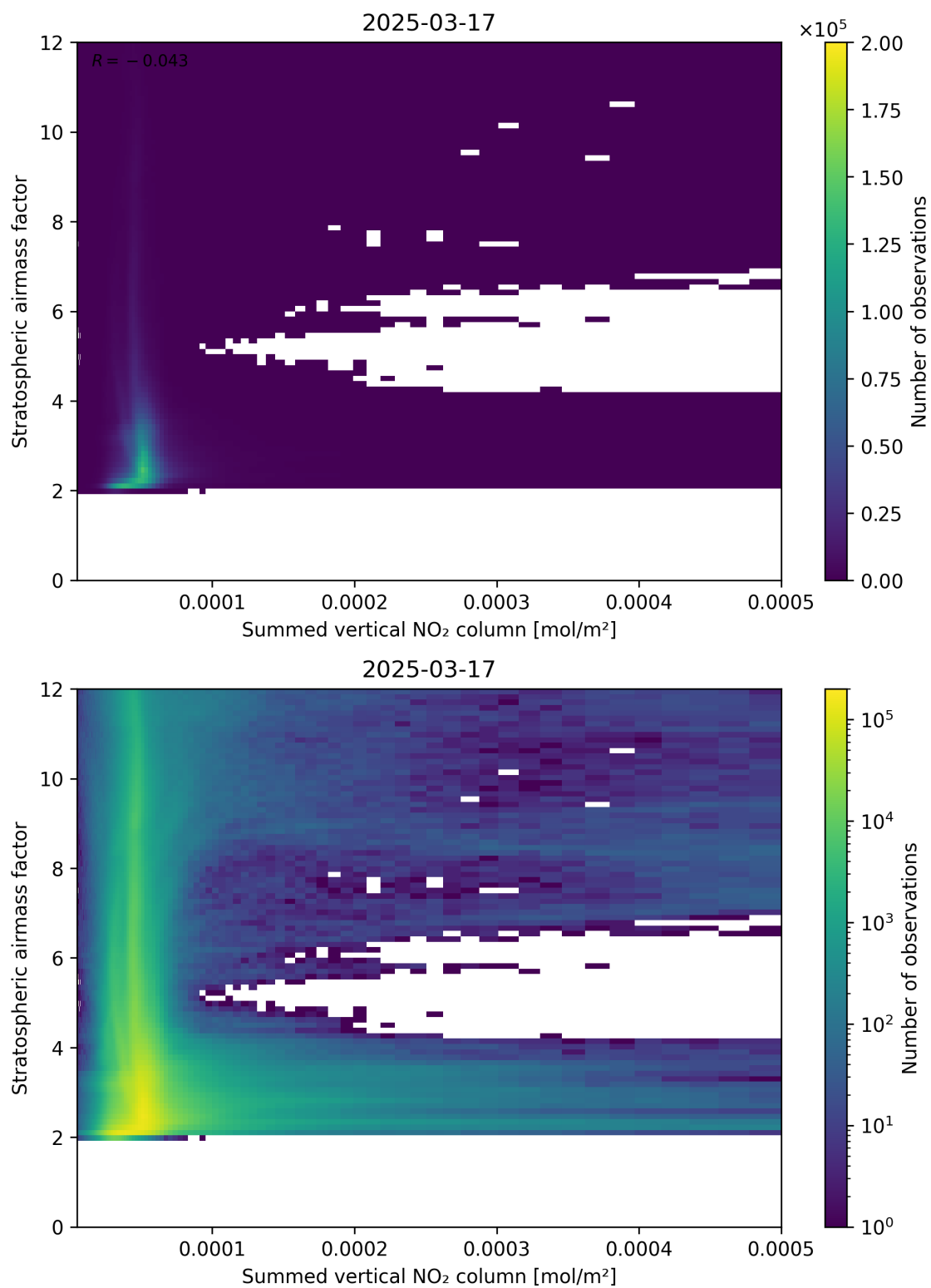
Figure 103: Scatter density plot of “Summed vertical NO 2 column” against “Stratospheric air mass factor” for 2025-03-17 to 2025-03-18.
