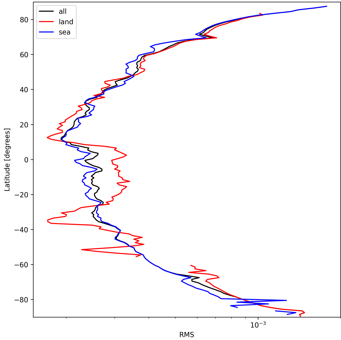
Figure 26: Zonal average of “RMS” for 2025-03-17 to 2025-03-18.
