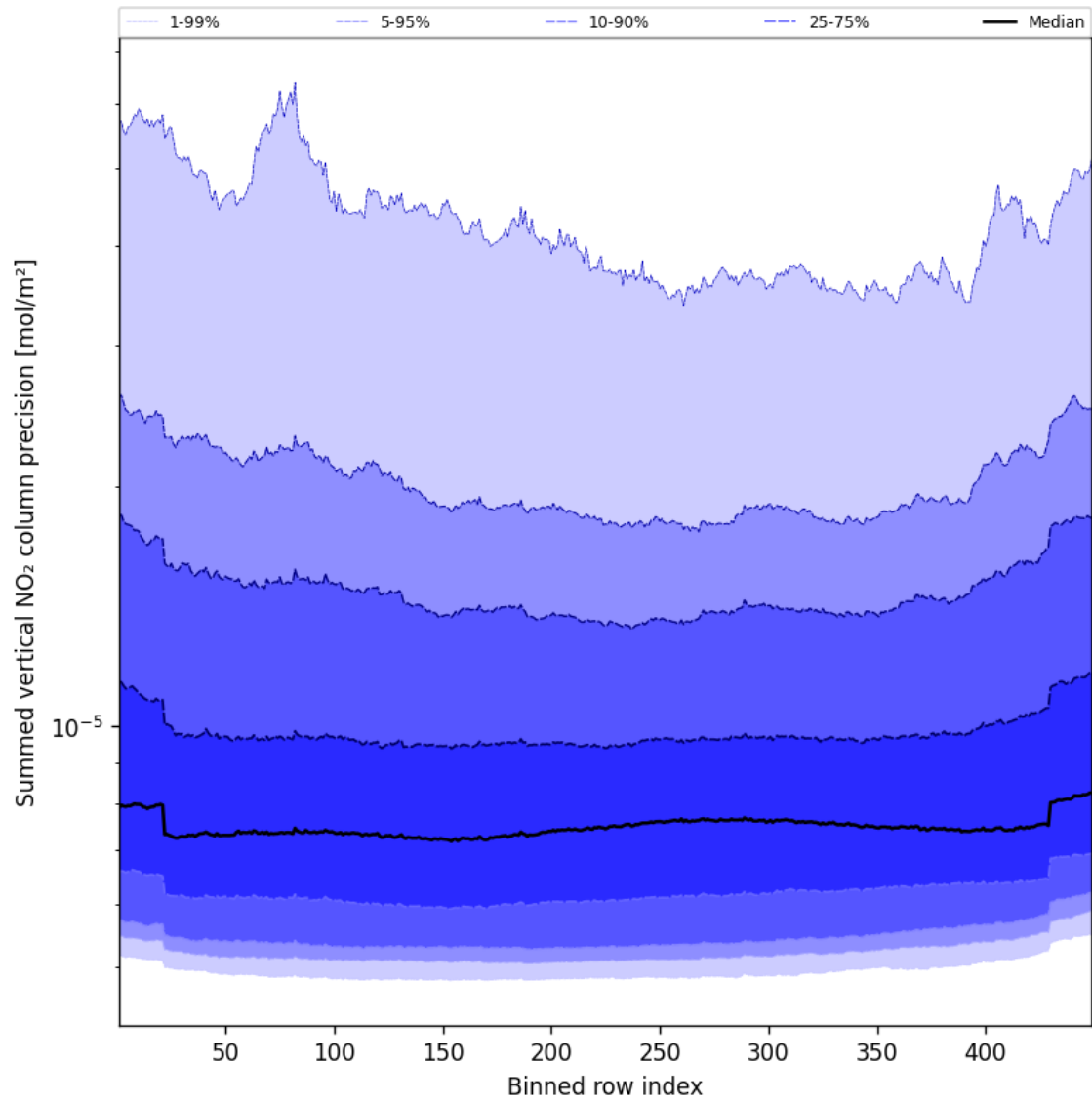
Figure 58: Along track statistics of “Summed vertical NO 2 column precision” for 2025-03-17 to 2025-03-18
