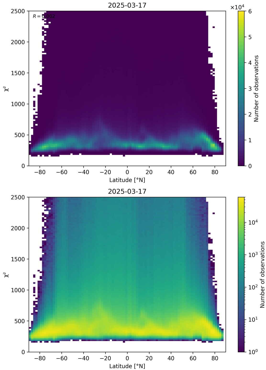
Figure 86: Scatter density plot of “Latitude” against “ \chi^2 ” for 2025-03-17 to 2025-03-18.
