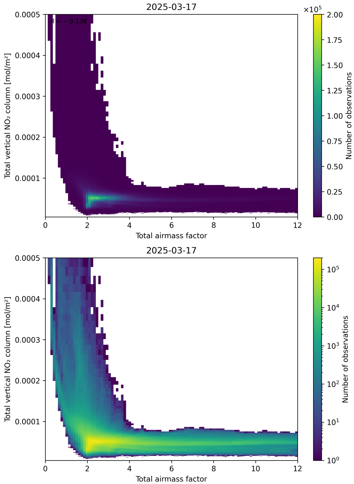
Figure 67: Scatter density plot of “Total airmass factor” against “Total vertical NO 2 column” for 2025-03-17 to 2025-03-18.
