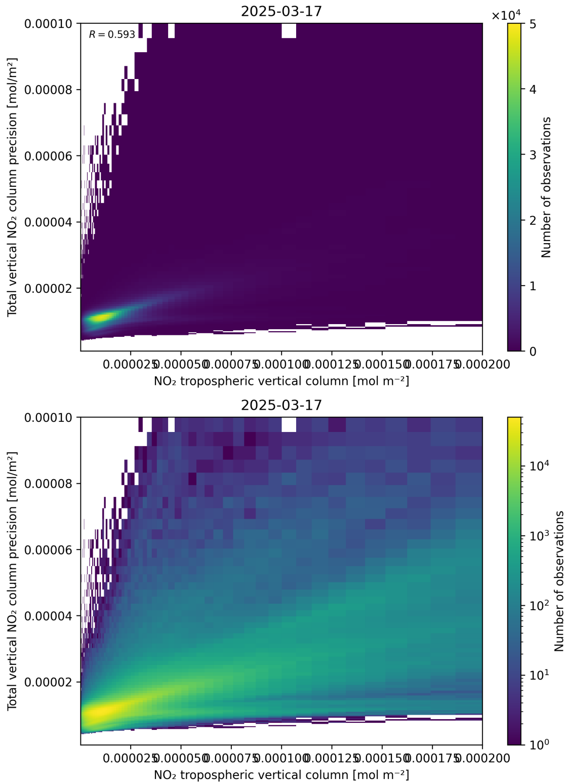
Figure 129: Scatter density plot of “NO 2 tropospheric vertical column” against “Total vertical NO 2 column precision” for 2025-03-17 to 2025-03-18.
