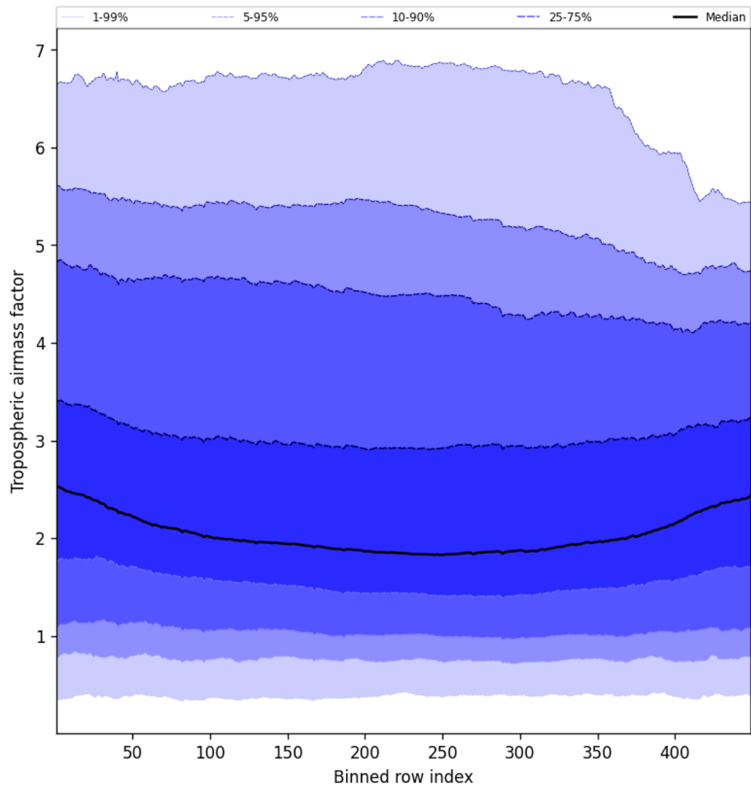
Figure 48: Along track statistics of “Tropospheric air mass factor” for 2025-03-17 to 2025-03-18
