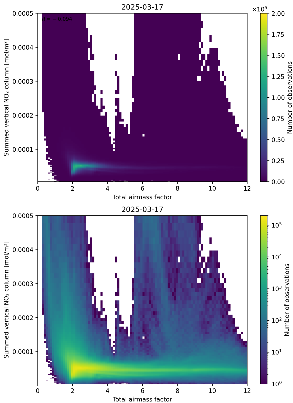
Figure 65: Scatter density plot of “Total airmass factor” against “Summed vertical NO 2 column” for 2025-03-17 to 2025-03-18.
