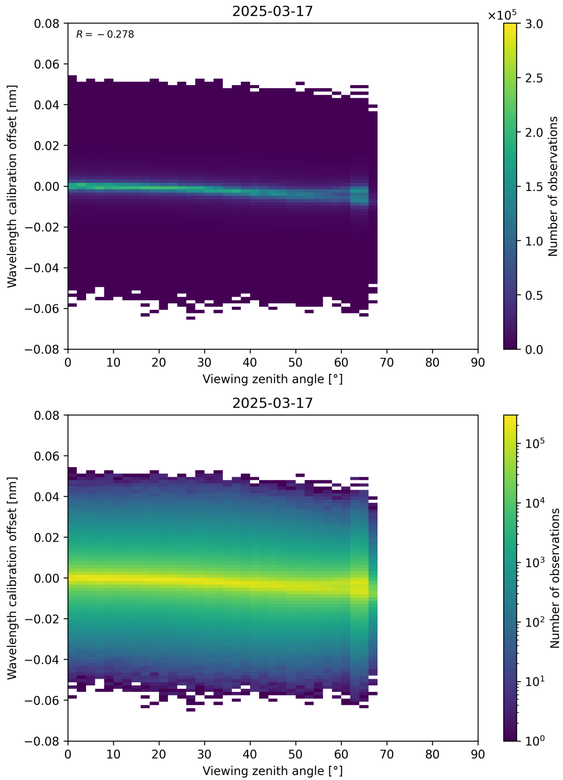
Figure 173: Scatter density plot of “Viewing zenith angle” against “Wavelength calibration offset” for 2025-03-17 to 2025-03-18.
