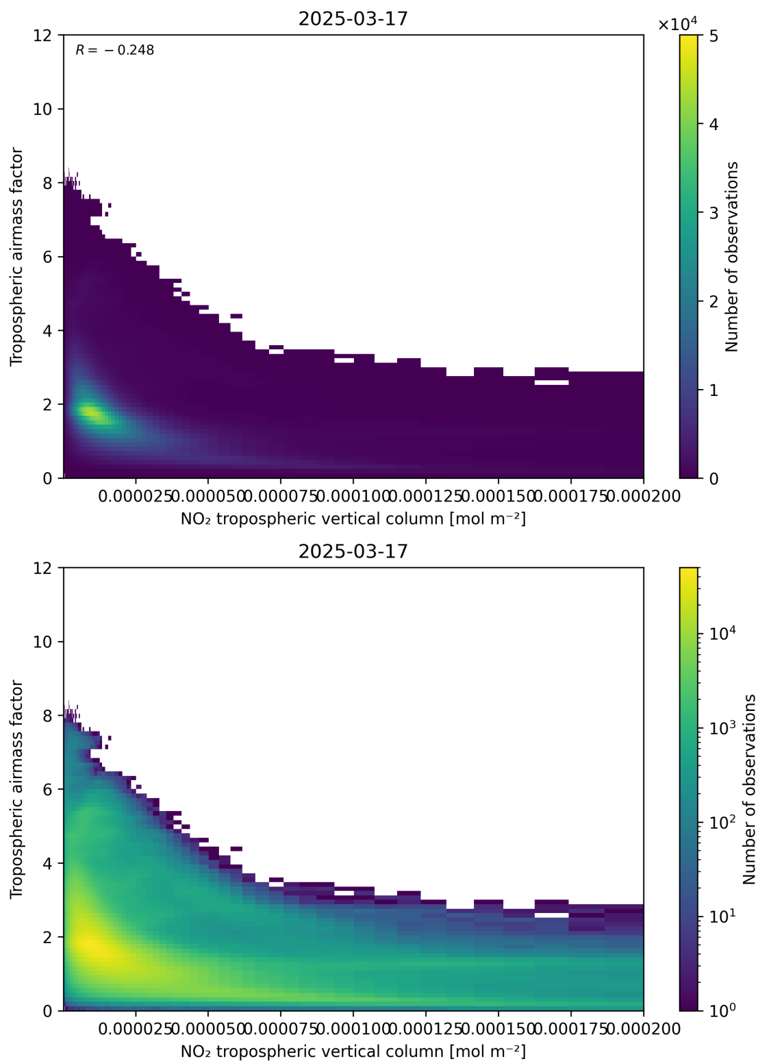
Figure 123: Scatter density plot of “NO 2 tropospheric vertical column” against “Tropospheric airmass factor” for 2025-03-17 to 2025-03-18.
