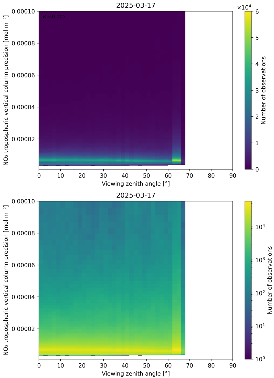
Figure 170: Scatter density plot of “Viewing zenith angle” against “NO 2 tropospheric vertical column precision” for 2025-03-17 to 2025-03-18.
