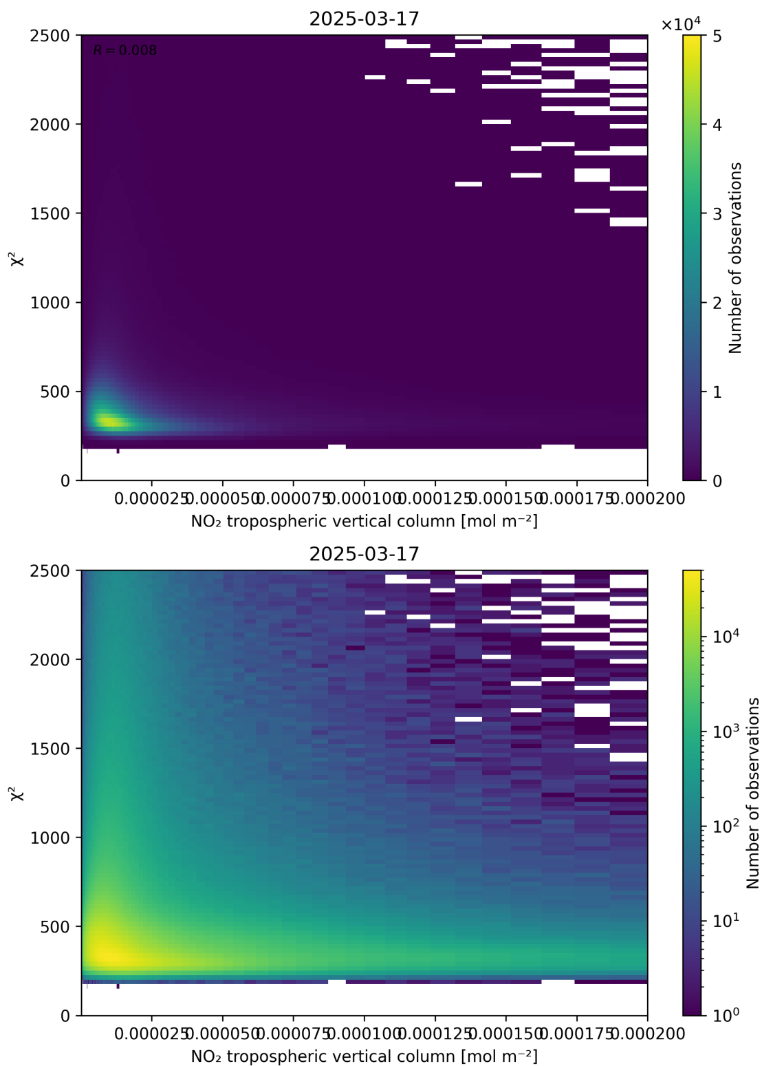
Figure 124: Scatter density plot of “NO 2 tropospheric vertical column” against “ \chi^2 ” for 2025-03-17 to 2025-03-18.
