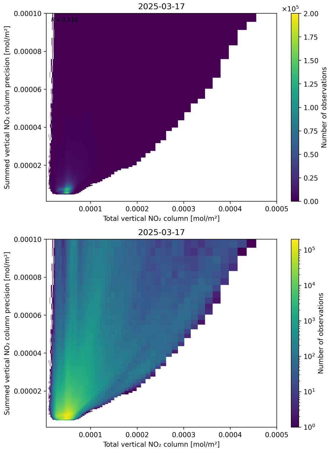
Figure 113: Scatter density plot of “Total vertical NO 2 column” against “Summed vertical NO 2 column precision” for 2025-03-17 to 2025-03-18.
