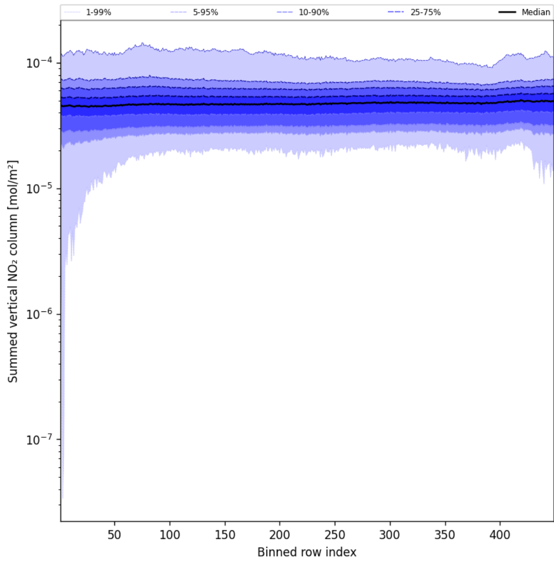
Figure 57: Along track statistics of “Summed vertical NO 2 column” for 2025-03-17 to 2025-03-18
