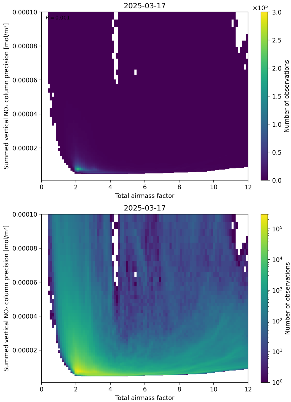
Figure 66: Scatter density plot of “Total airmass factor” against “Summed vertical NO 2 column precision” for 2025-03-17 to 2025-03-18.
