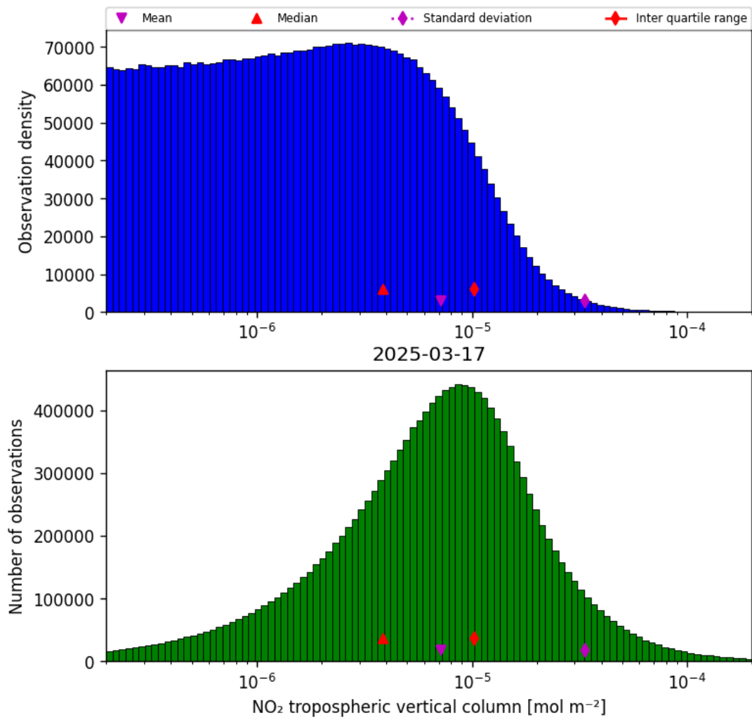
Figure 29: Histogram of “NO 2 tropospheric vertical column” for 2025-03-17 to 2025-03-18
