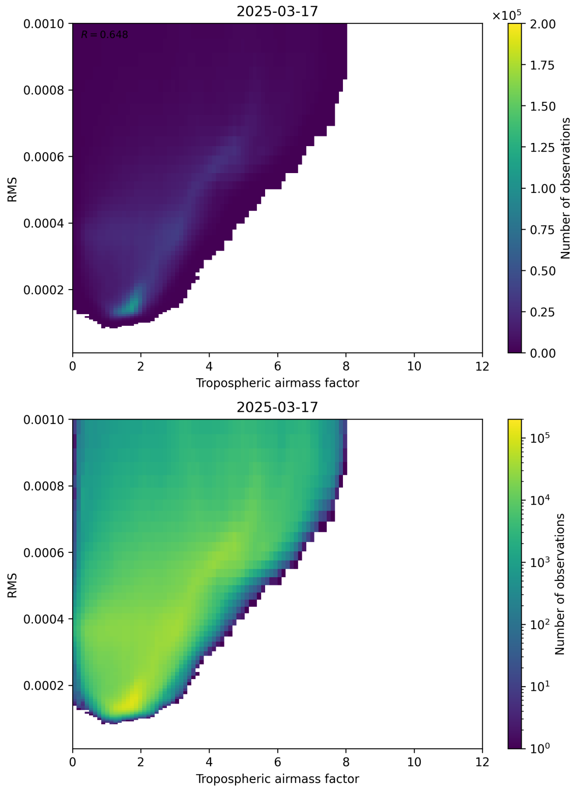
Figure 79: Scatter density plot of “Tropospheric airmass factor” against “RMS” for 2025-03-17 to 2025-03-18.
