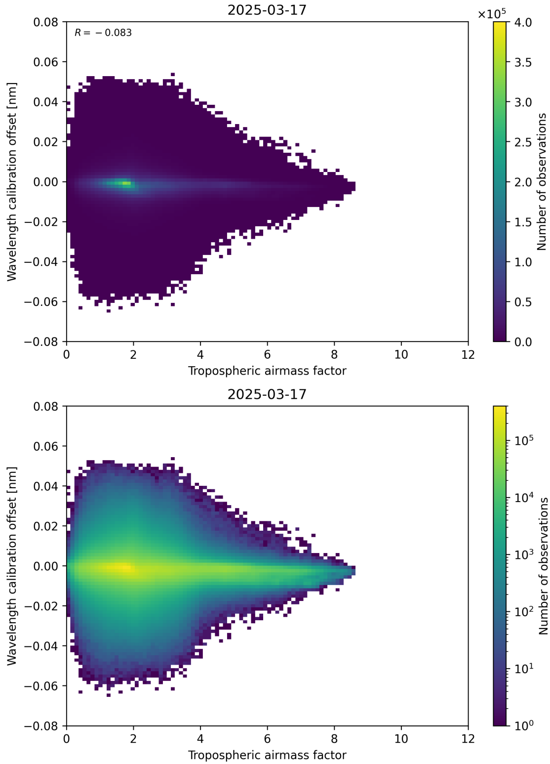
Figure 80: Scatter density plot of “Tropospheric airmass factor” against “Wavelength calibration offset” for 2025-03-17 to 2025-03-18.
