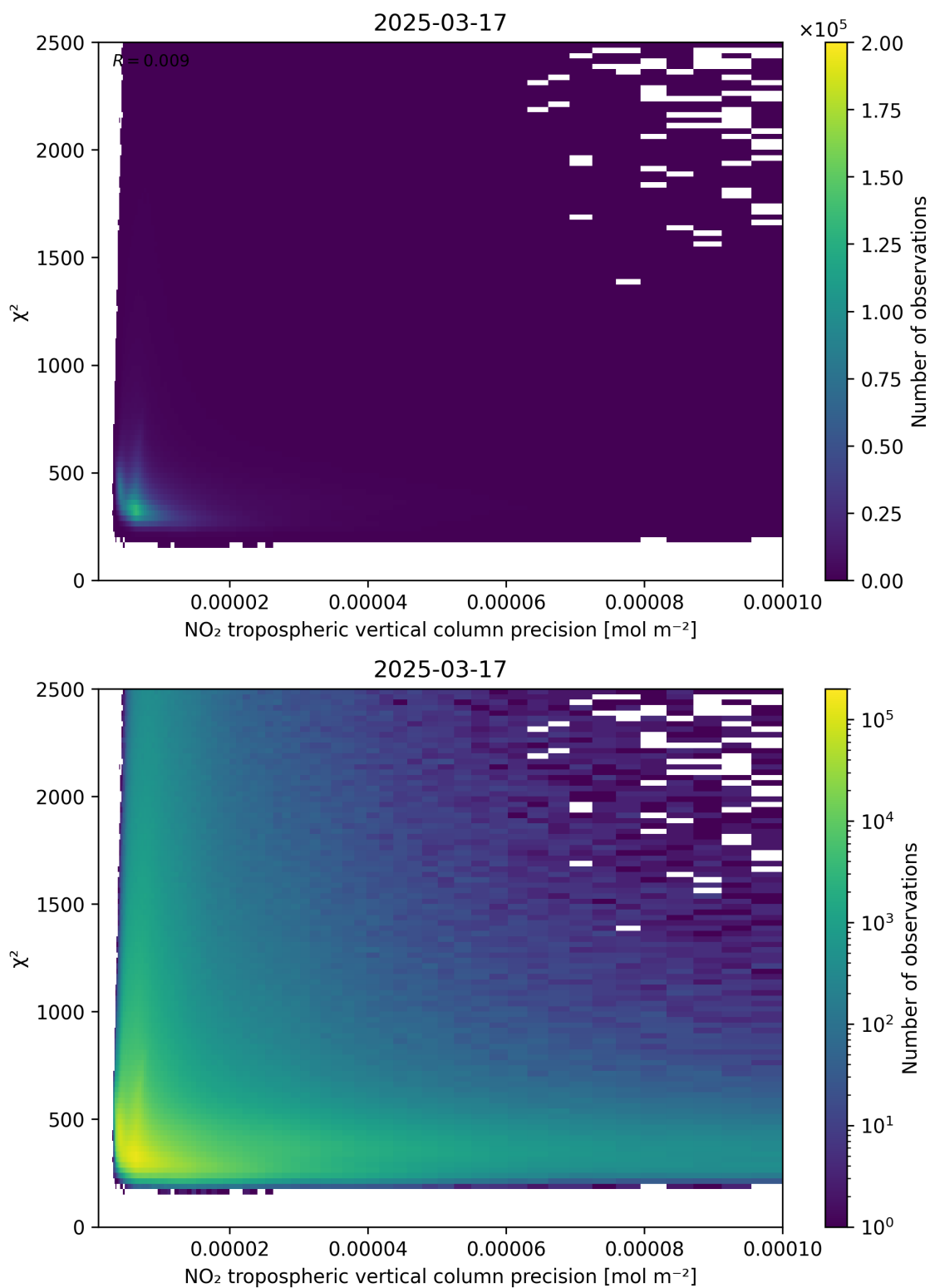
Figure 134: Scatter density plot of “NO 2 tropospheric vertical column precision” against “ \chi^2 ” for 2025-03-17 to 2025-03-18.
