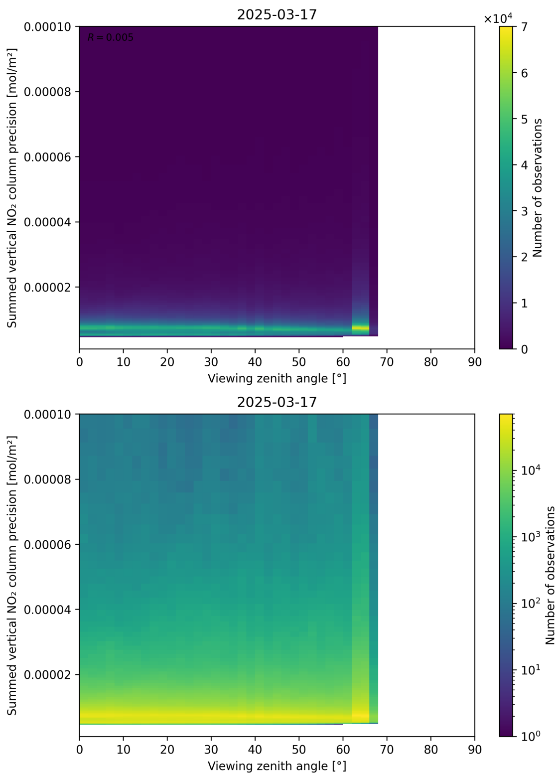
Figure 166: Scatter density plot of “Viewing zenith angle” against “Summed vertical NO 2 column precision” for 2025-03-17 to 2025-03-18.
