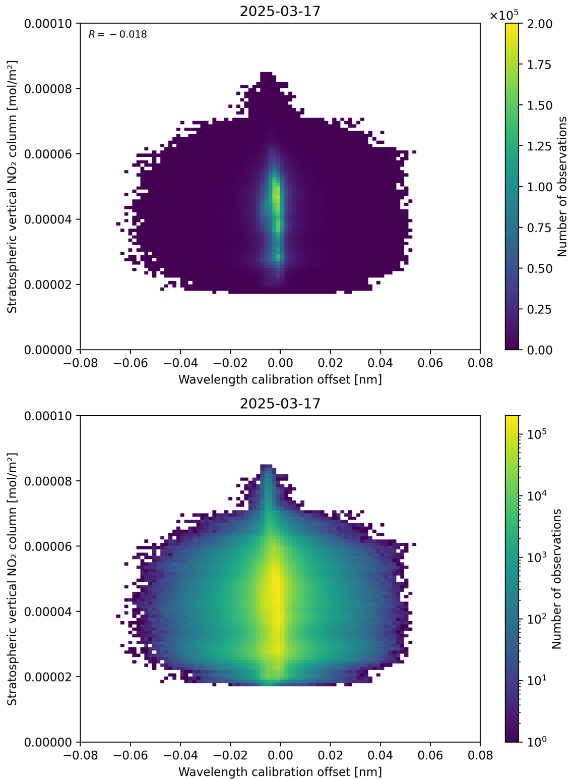
Figure 176: Scatter density plot of “Wavelength calibration offset” against “Stratospheric vertical NO 2 column” for 2025-03-17 to 2025-03-18.
