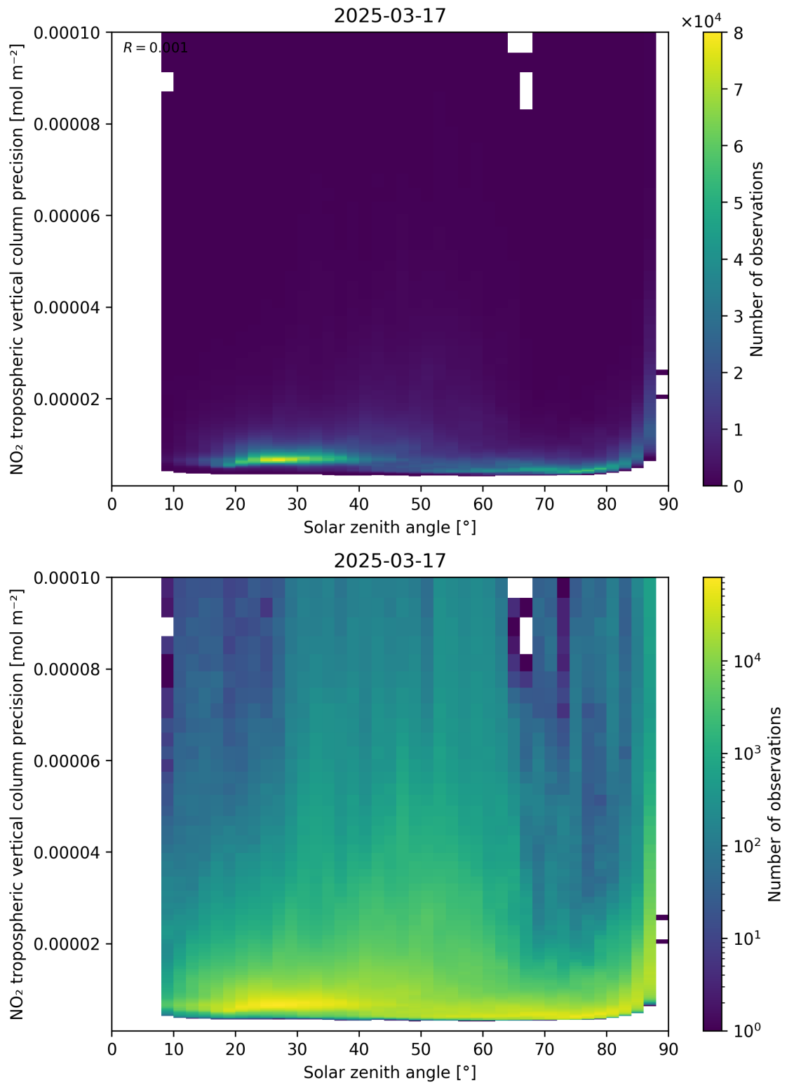
Figure 156: Scatter density plot of “Solar zenith angle” against “NO 2 tropospheric vertical column precision” for 2025-03-17 to 2025-03-18.
