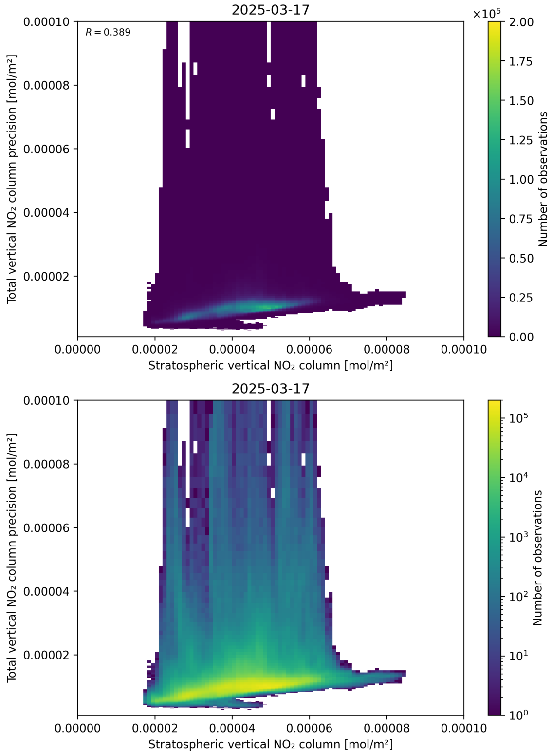
Figure 101: Scatter density plot of “Stratospheric vertical NO 2 column” against “Total vertical NO 2 column precision” for 2025-03-17 to 2025-03-18.
