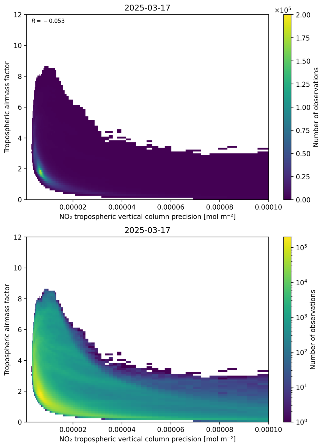
Figure 133: Scatter density plot of “NO 2 tropospheric vertical column precision” against “Tropospheric air mass factor” for 2025-03-17 to 2025-03-18.
