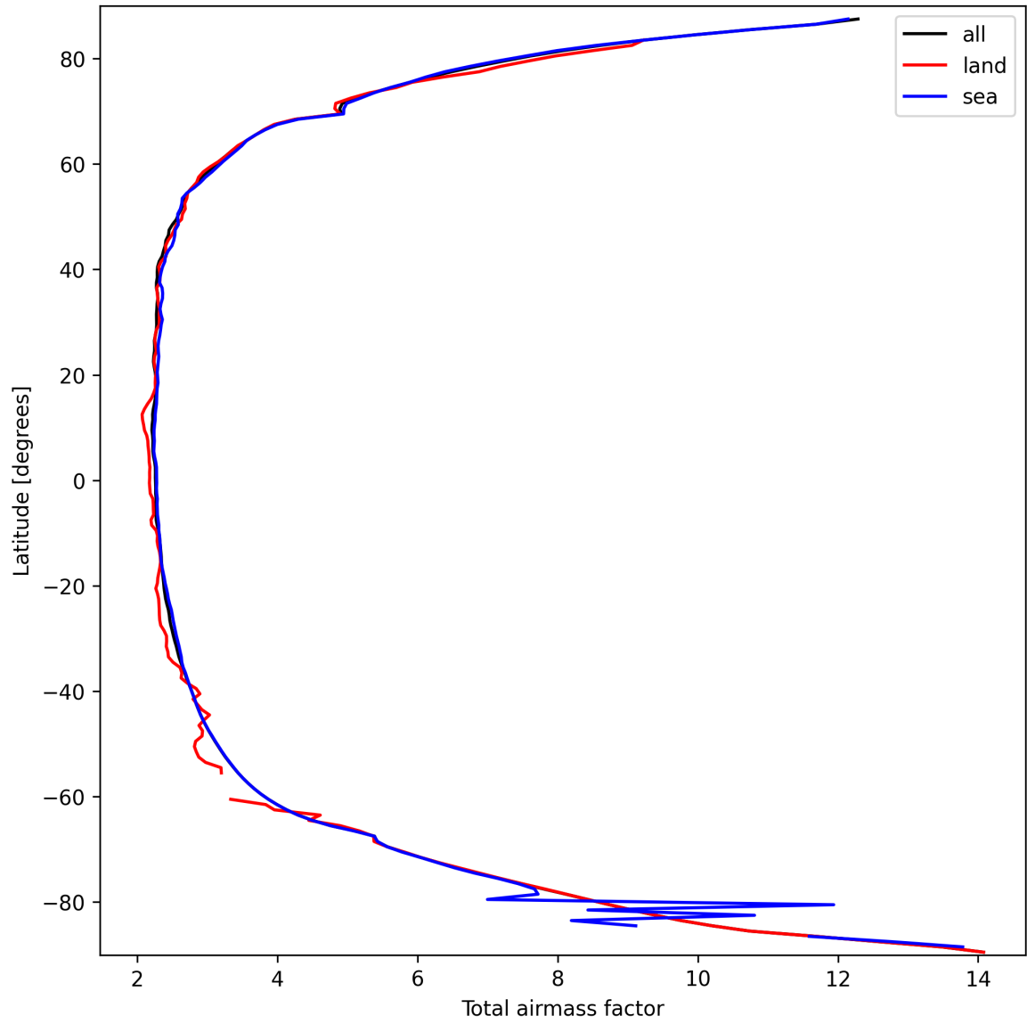
Figure 15: Zonal average of “Total airmass factor” for 2025-03-17 to 2025-03-18.
