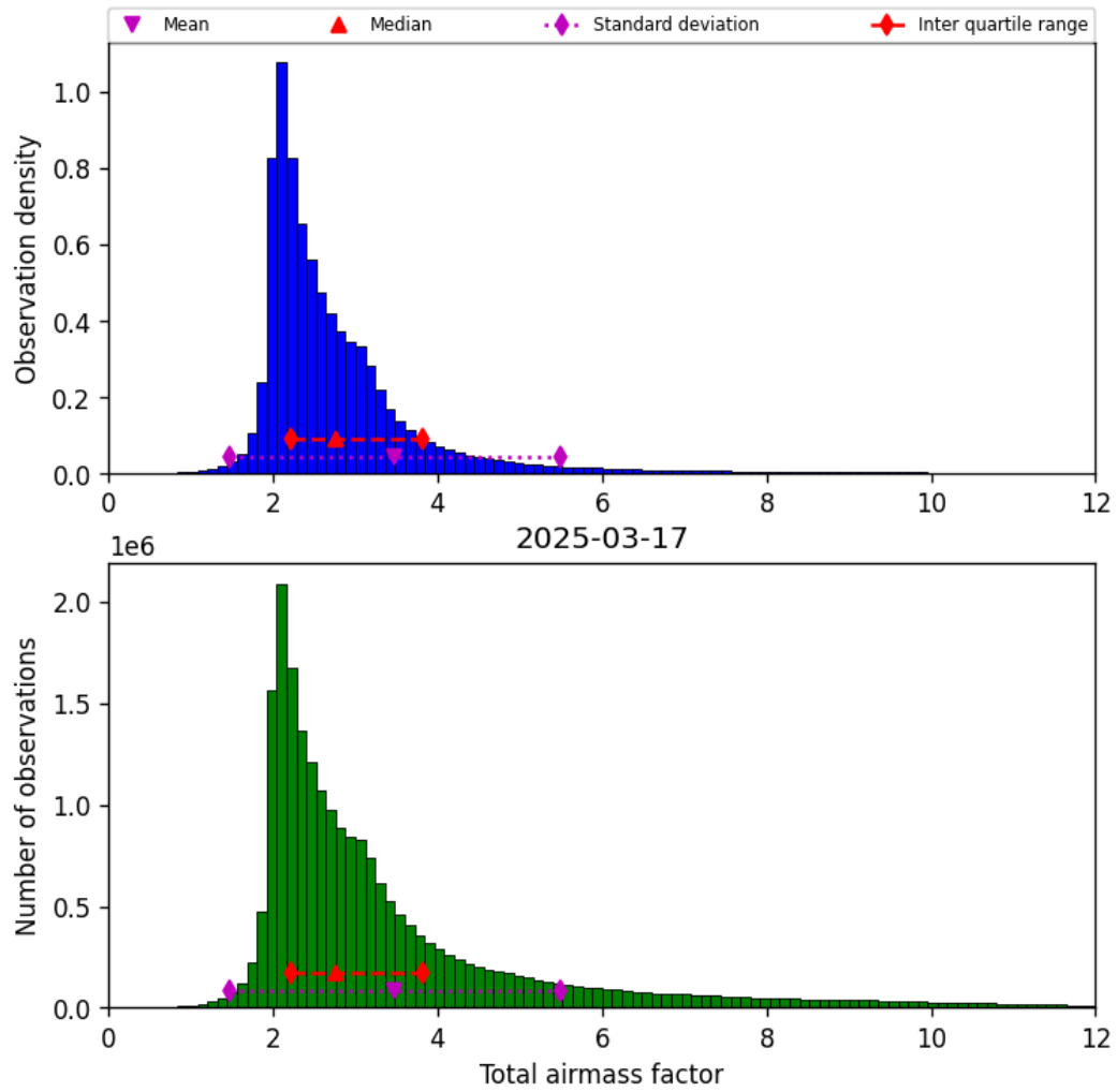
Figure 32: Histogram of “Total airmass factor” for 2025-03-17 to 2025-03-18
