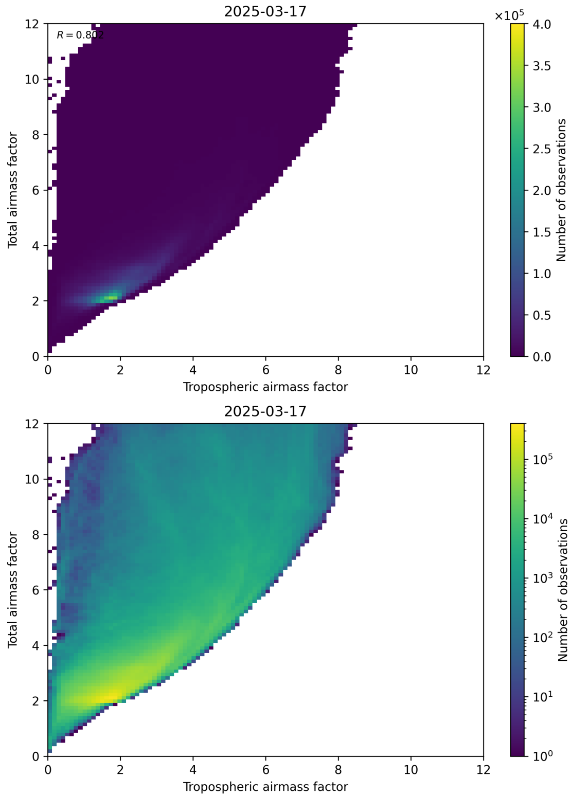
Figure 72: Scatter density plot of “Tropospheric airmass factor” against “Total airmass factor” for 2025-03-17 to 2025-03-18.
