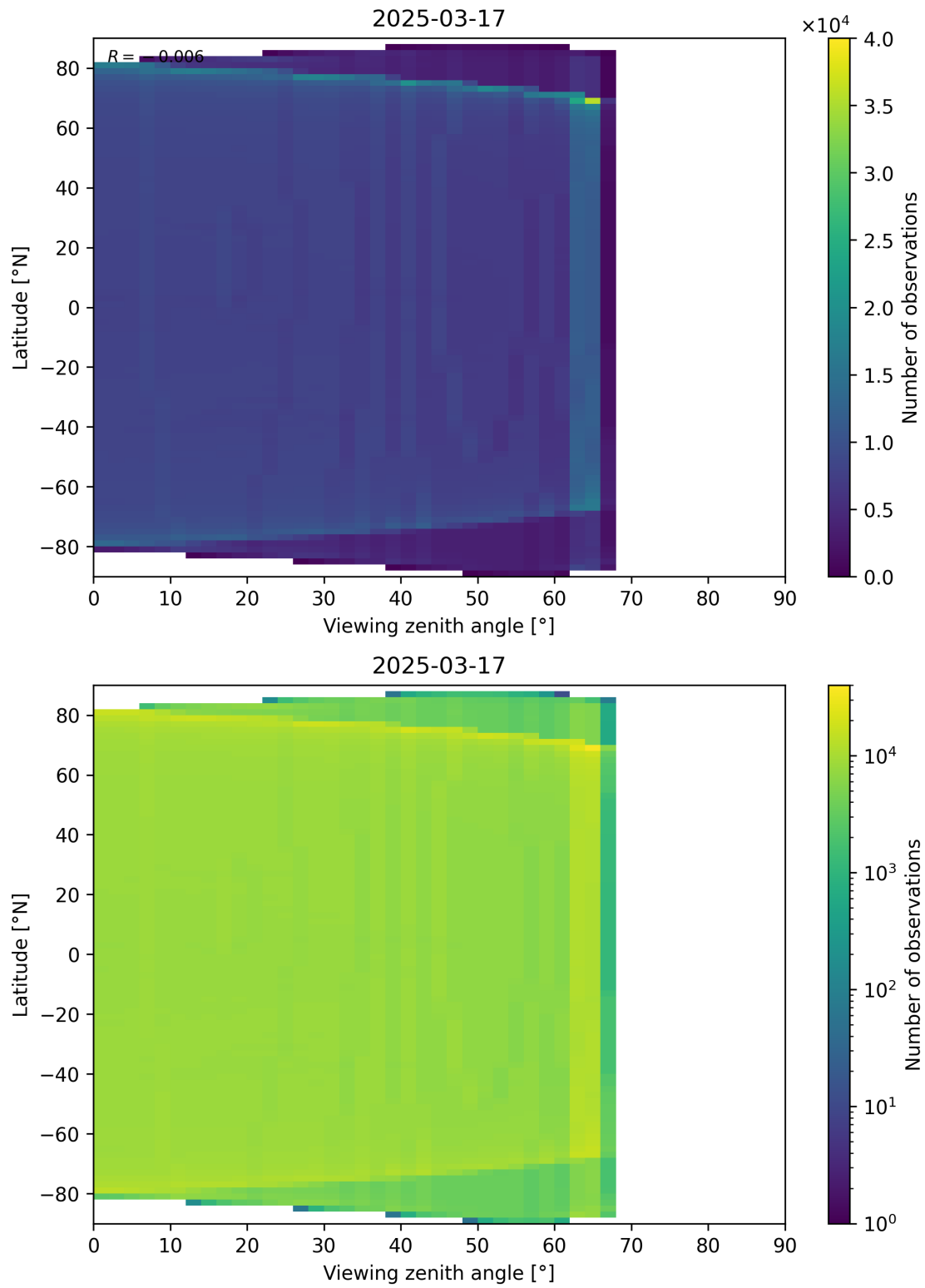
Figure 163: Scatter density plot of “Viewing zenith angle” against “Latitude” for 2025-03-17 to 2025-03-18.
