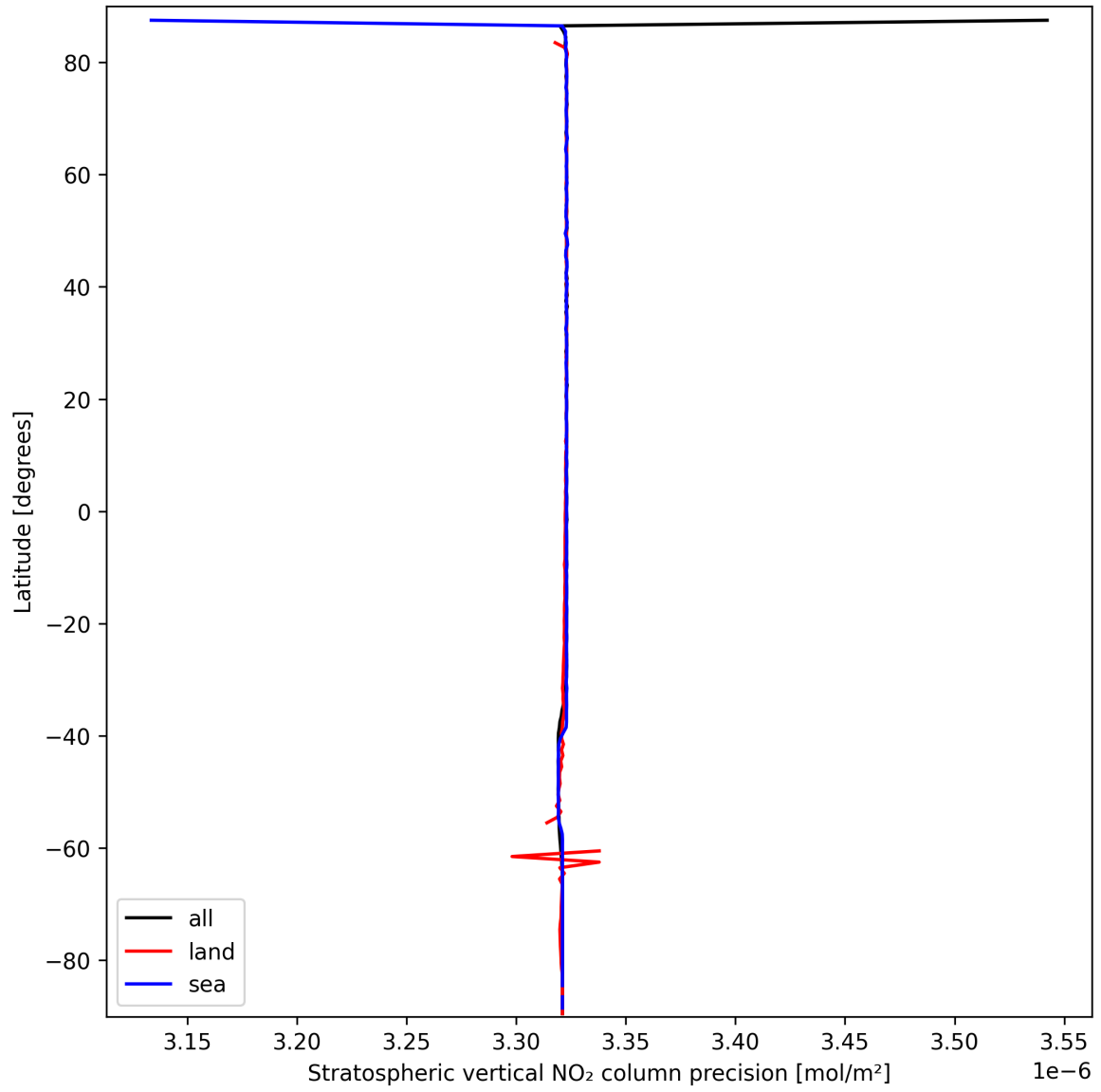
Figure 20: Zonal average of “Stratospheric vertical NO 2 column precision” for 2025-03-17 to 2025-03-18.
