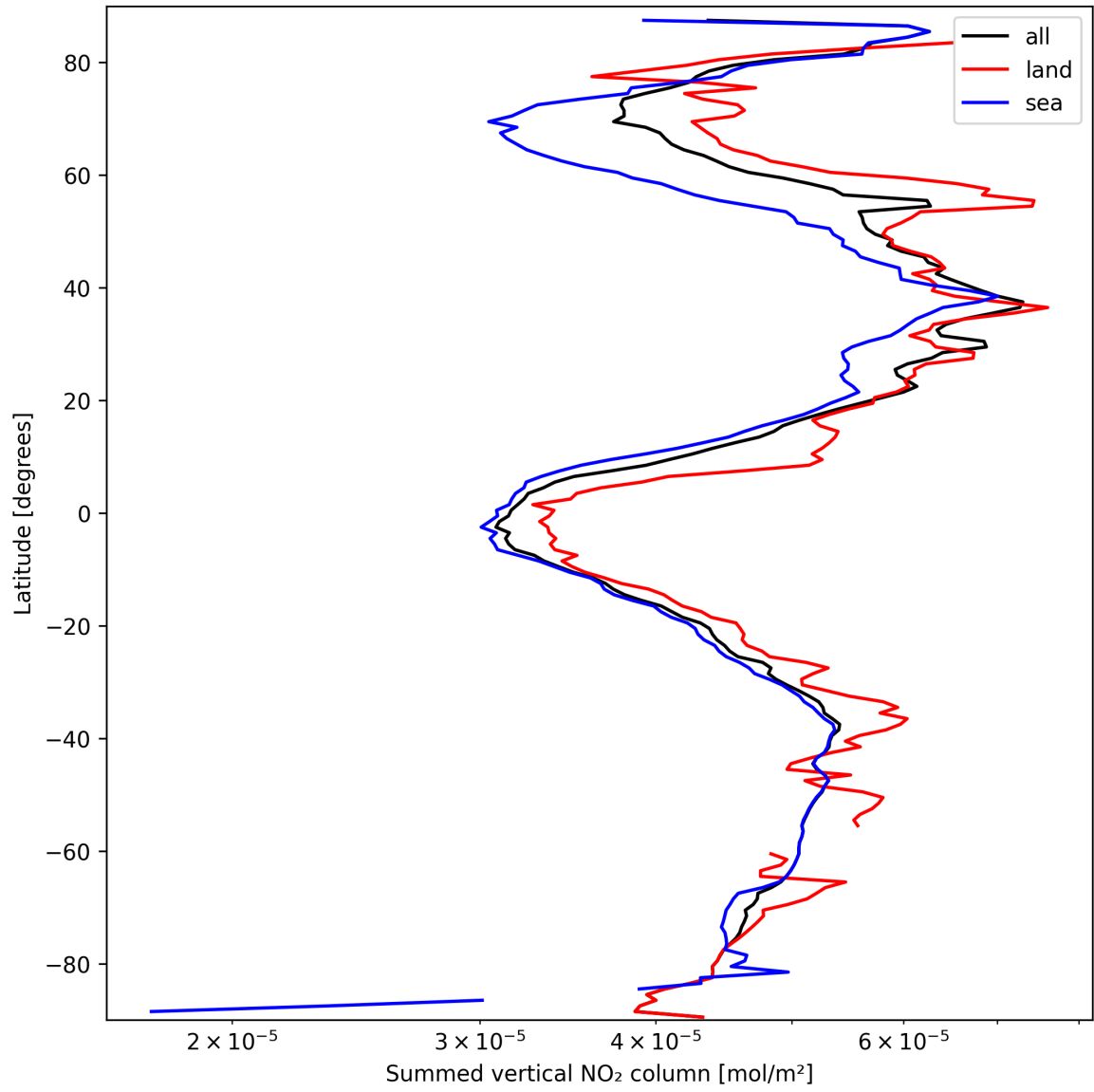
Figure 23: Zonal average of “Summed vertical NO 2 column” for 2025-03-17 to 2025-03-18.
