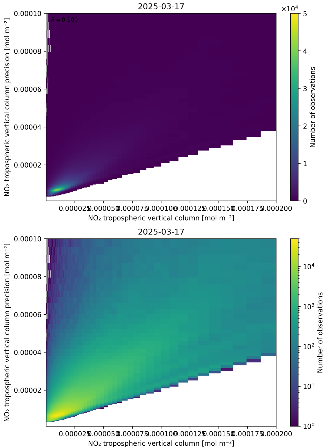
Figure 130: Scatter density plot of “NO 2 tropospheric vertical column” against “NO 2 tropospheric vertical column precision” for 2025-03-17 to 2025-03-18.
