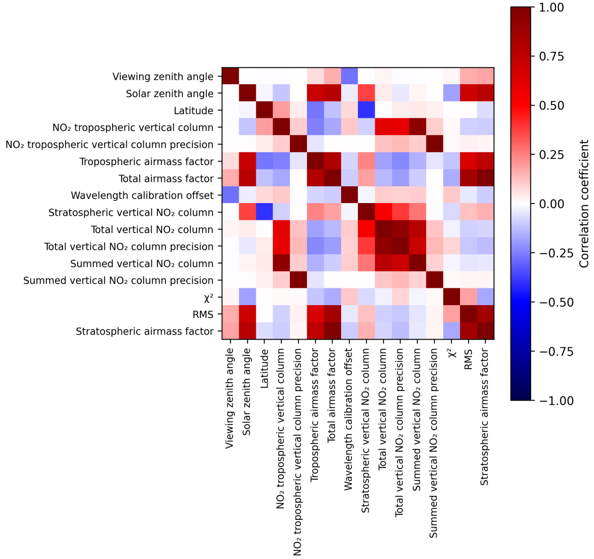
Figure 2: Map of correlation matrix for 2025-03-17 to 2025-03-18.
