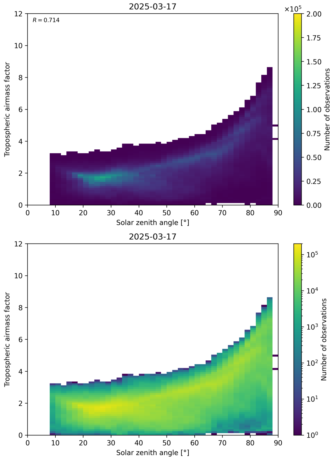
Figure 147: Scatter density plot of “Solar zenith angle” against “Tropospheric airmass factor” for 2025-03-17 to 2025-03-18.
