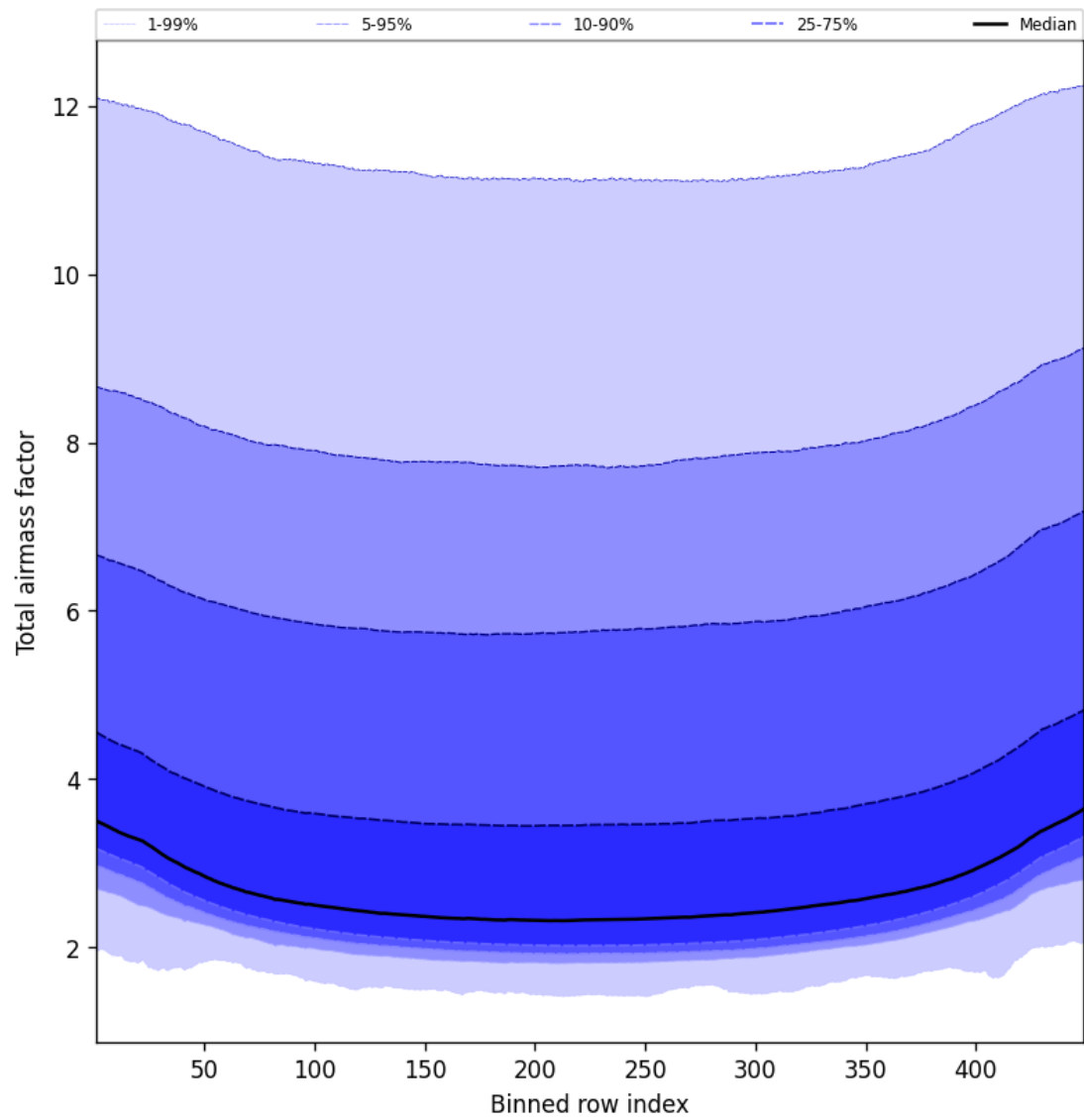
Figure 49: Along track statistics of “Total airmass factor” for 2025-03-17 to 2025-03-18
