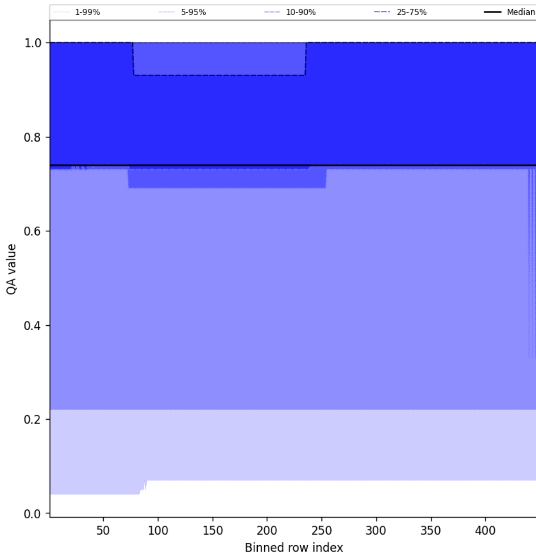
Figure 45: Along track statistics of “QA value” for 2025-03-17 to 2025-03-18
