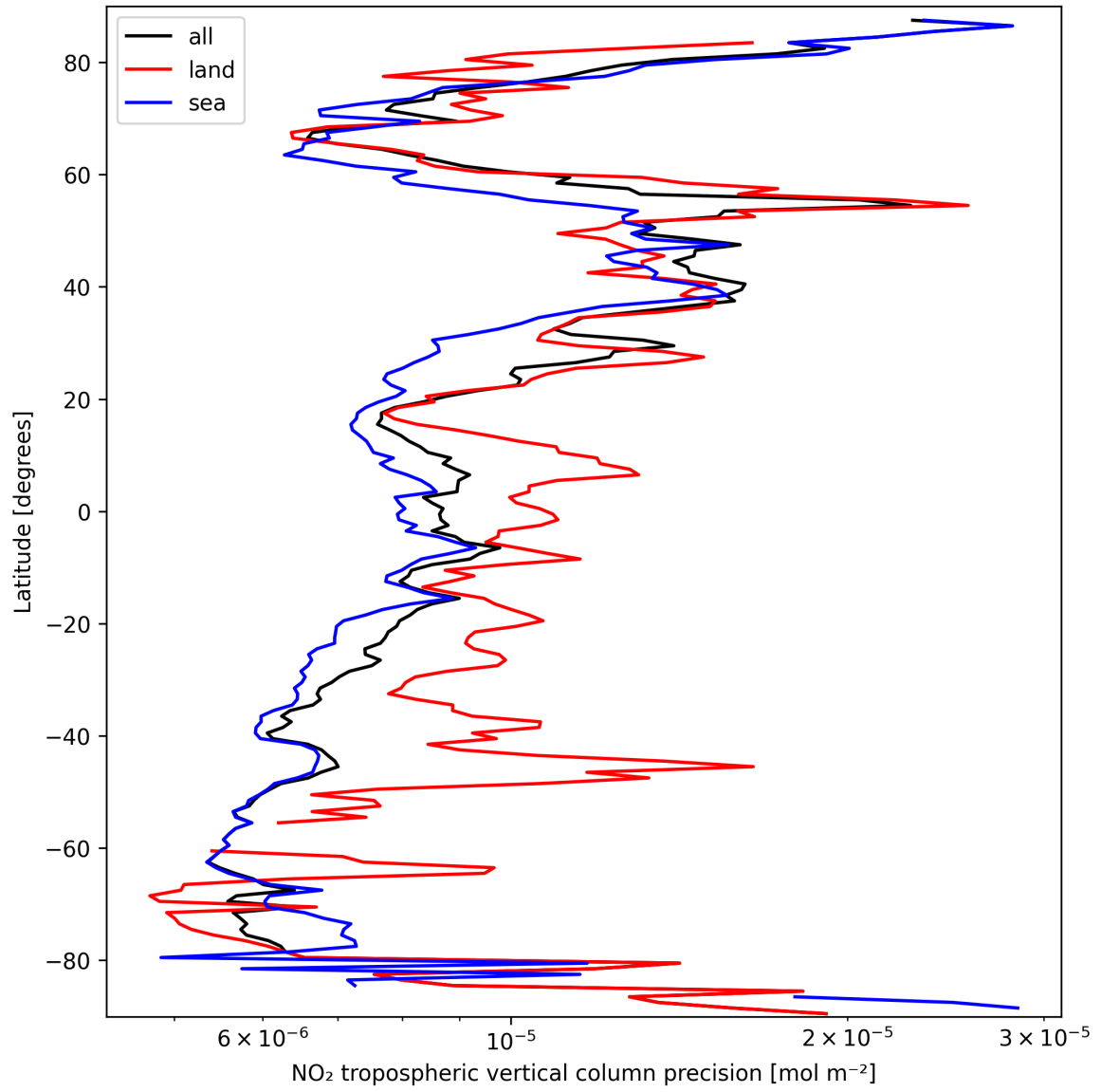
Figure 13: Zonal average of “NO 2 tropospheric vertical column precision” for 2025-03-17 to 2025-03-18.
