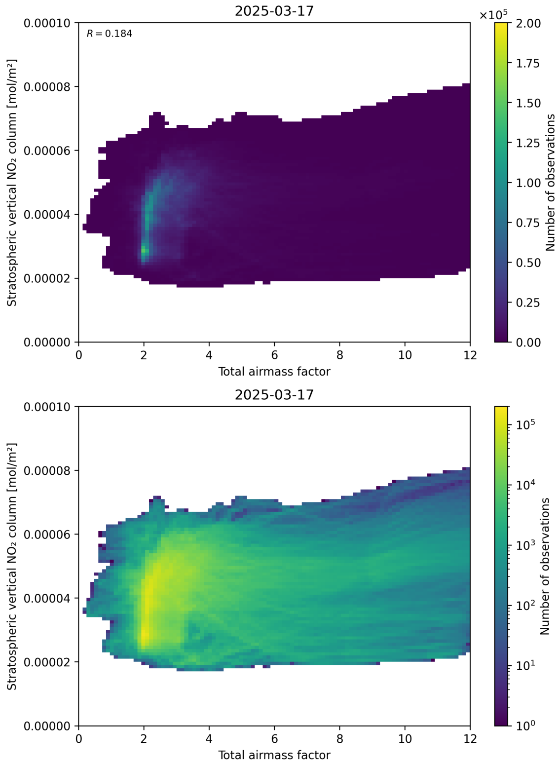
Figure 64: Scatter density plot of “Total airmass factor” against “Stratospheric vertical \text{NO}_2 column” for 2025-03-17 to 2025-03-18.
