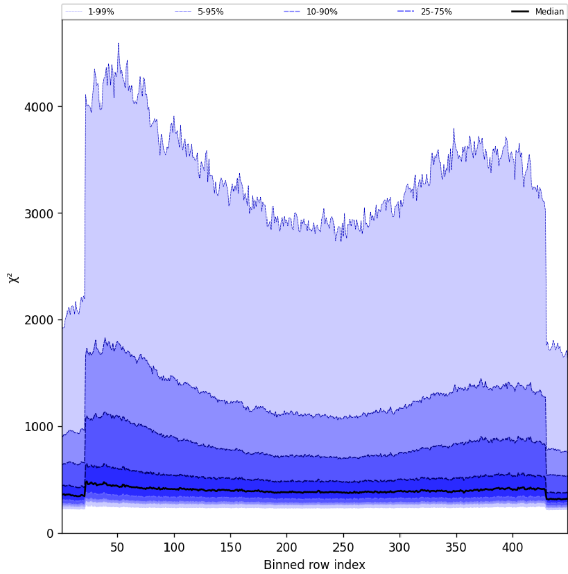
Figure 59: Along track statistics of “ \chi^2 ” for 2025-03-17 to 2025-03-18
