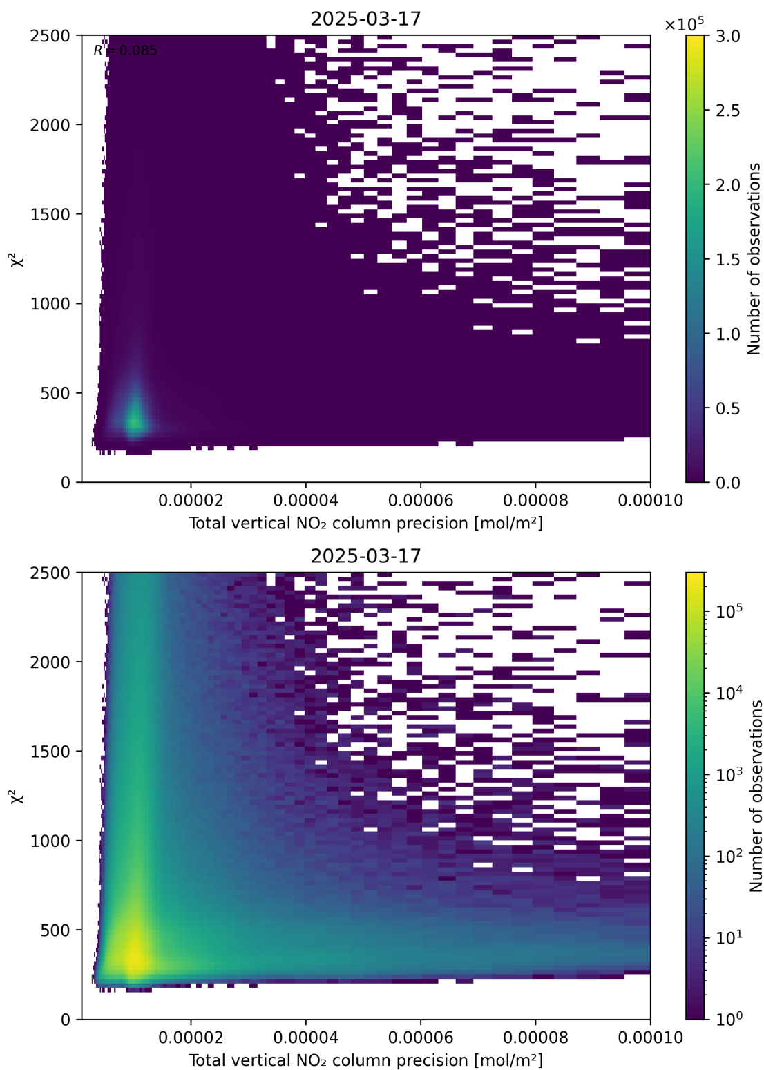
Figure 116: Scatter density plot of “Total vertical NO 2 column precision” against “ \chi^2 ” for 2025-03-17 to 2025-03-18.
