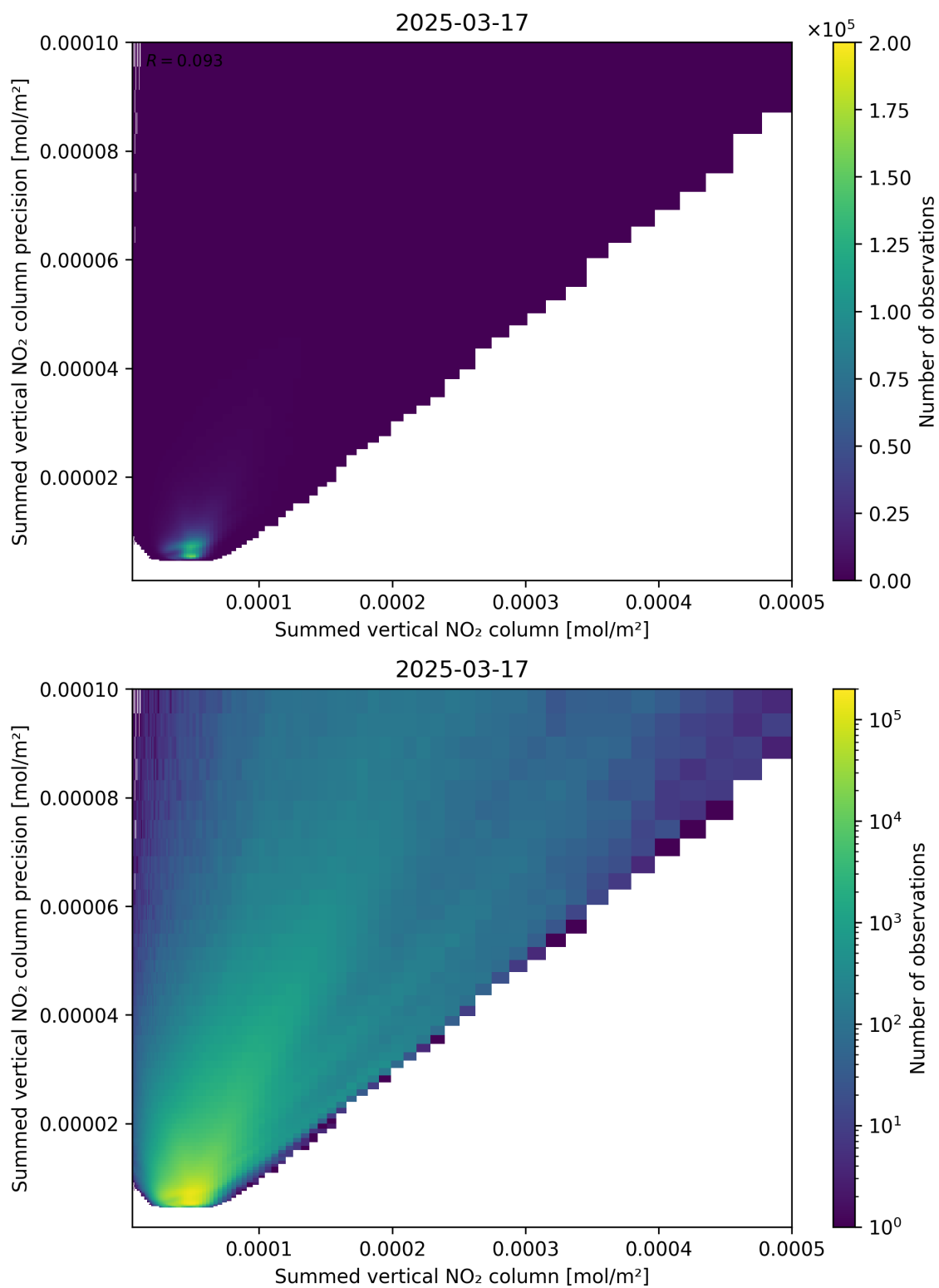
Figure 105: Scatter density plot of “Summed vertical NO 2 column” against “Summed vertical NO 2 column precision” for 2025-03-17 to 2025-03-18.
