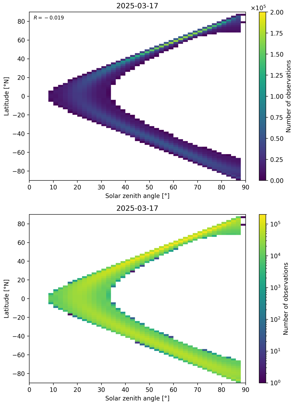
Figure 149: Scatter density plot of “Solar zenith angle” against “Latitude” for 2025-03-17 to 2025-03-18.
