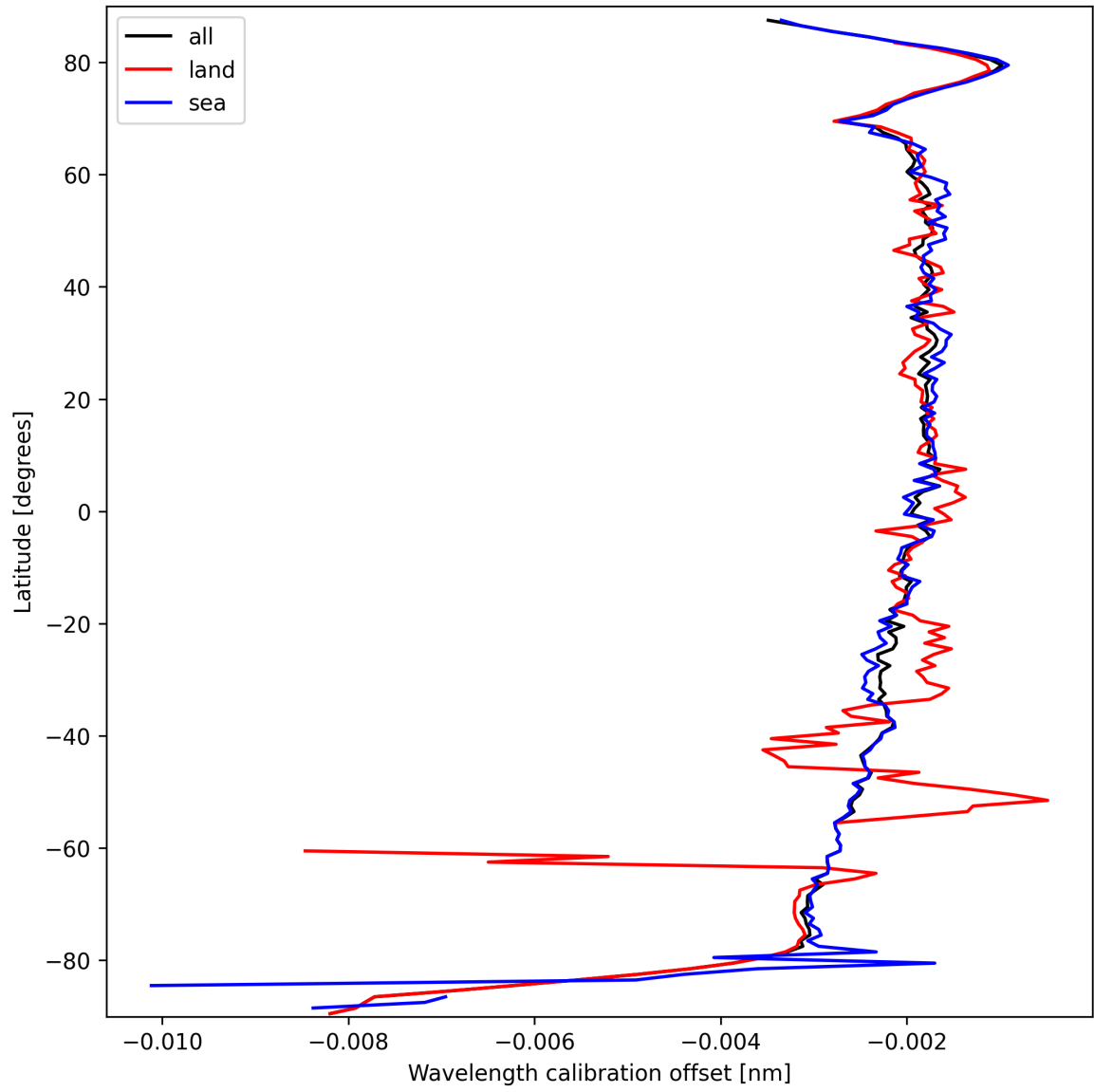
Figure 18: Zonal average of “Wavelength calibration offset” for 2025-03-17 to 2025-03-18.
