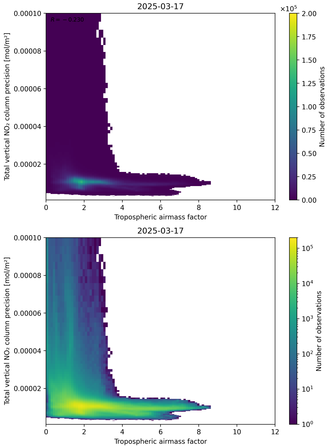
Figure 78: Scatter density plot of “Tropospheric airmass factor” against “Total vertical NO 2 column precision” for 2025-03-17 to 2025-03-18.
