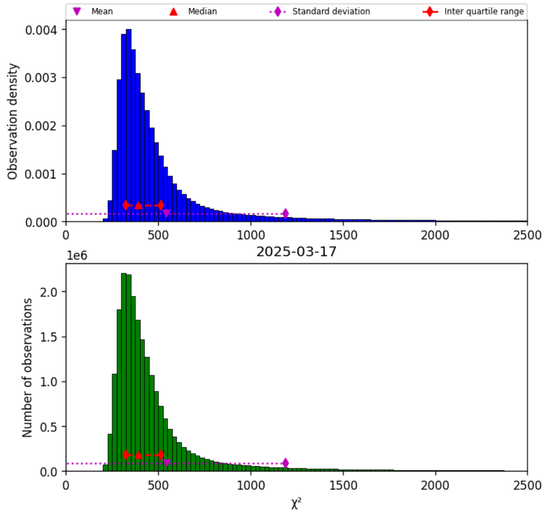
Figure 42: Histogram of “ \chi^2 ” for 2025-03-17 to 2025-03-18
