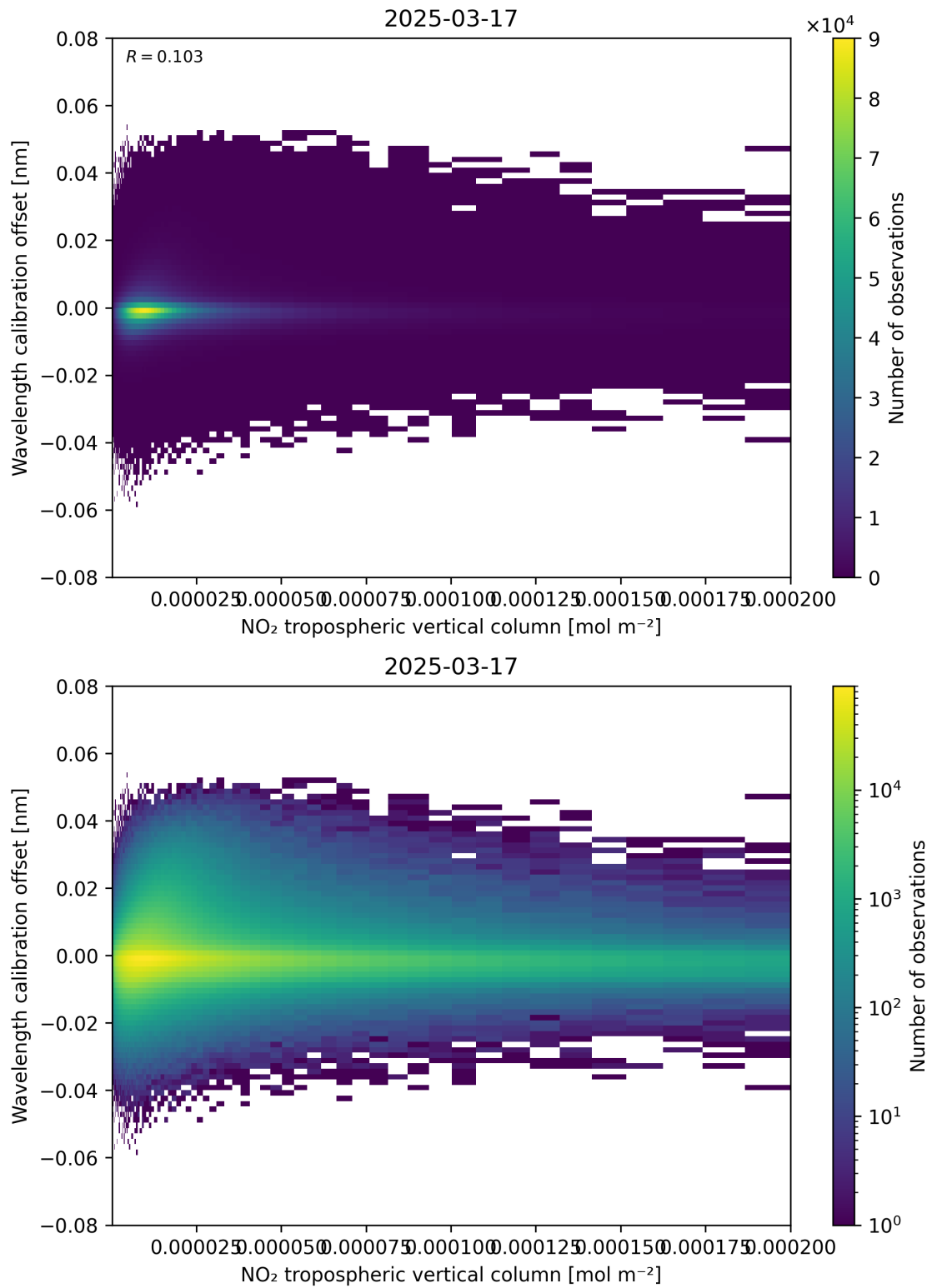
Figure 143: Scatter density plot of “NO 2 tropospheric vertical column” against “Wavelength calibration offset” for 2025-03-17 to 2025-03-18.
