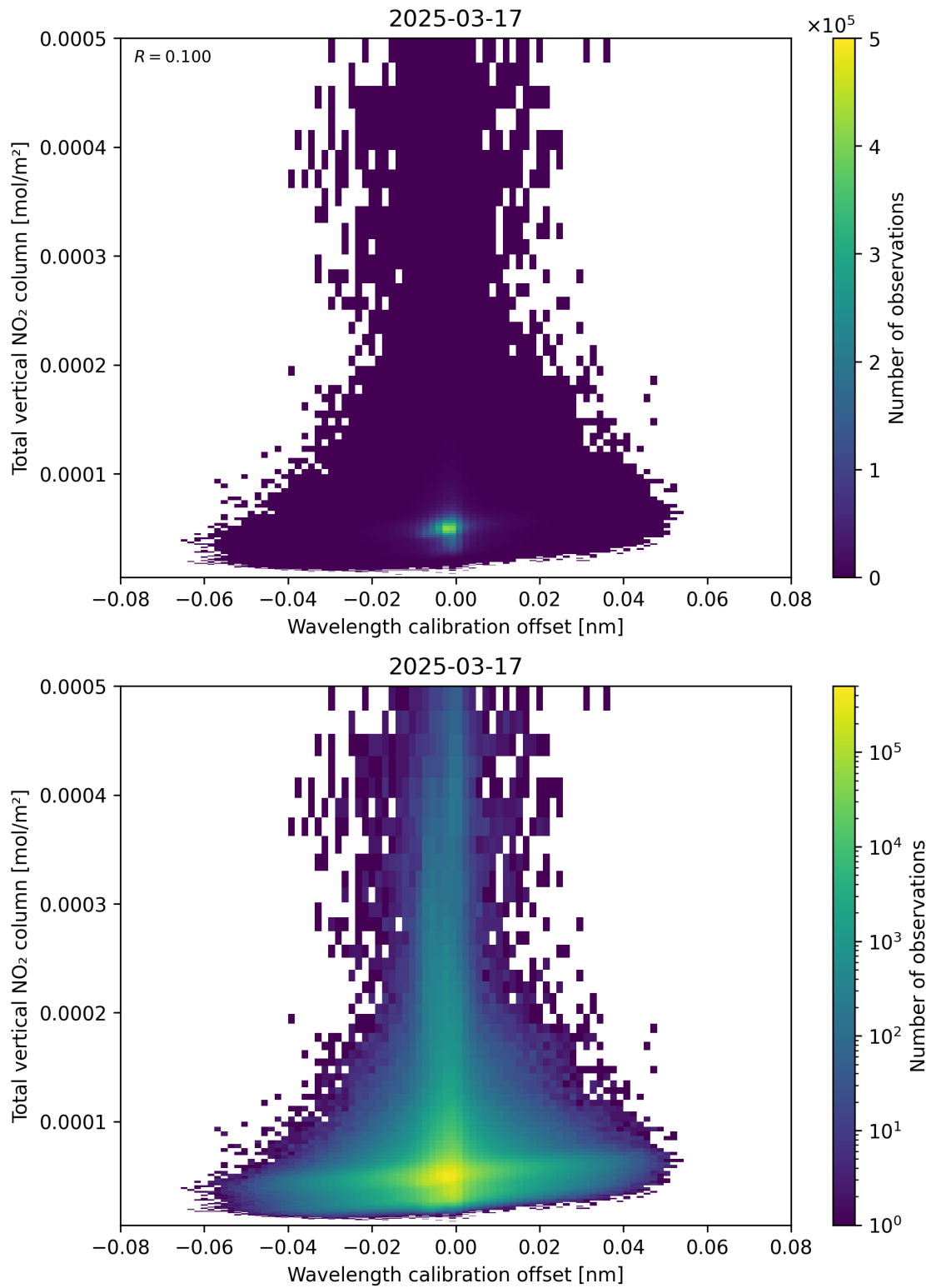
Figure 179: Scatter density plot of “Wavelength calibration offset” against “Total vertical NO 2 column” for 2025-03-17 to 2025-03-18.
