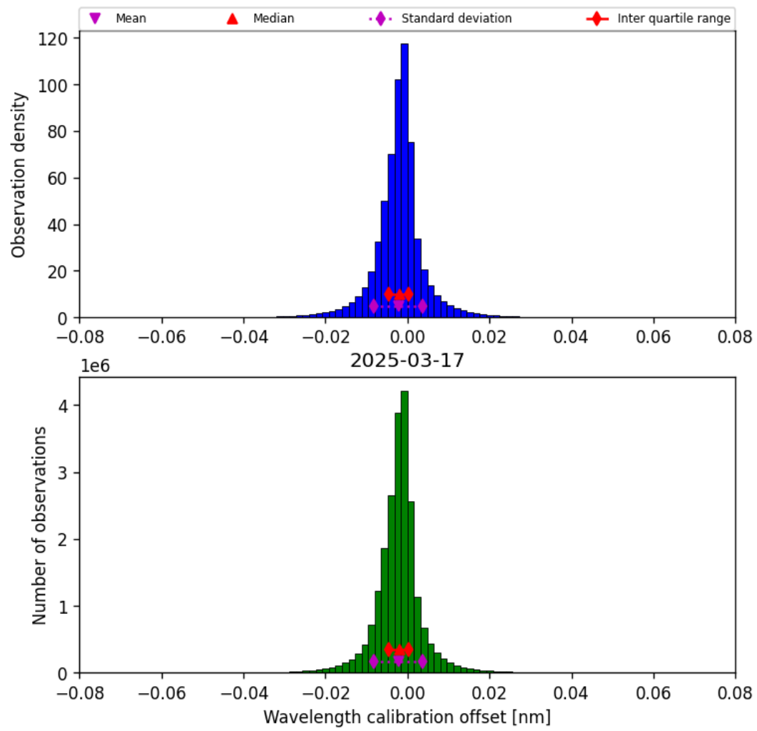
Figure 35: Histogram of “Wavelength calibration offset” for 2025-03-17 to 2025-03-18
