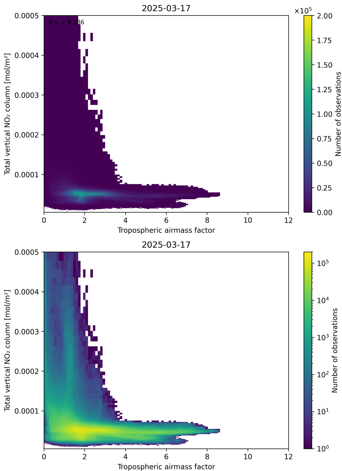
Figure 77: Scatter density plot of “Tropospheric airmass factor” against “Total vertical NO 2 column” for 2025-03-17 to 2025-03-18.
