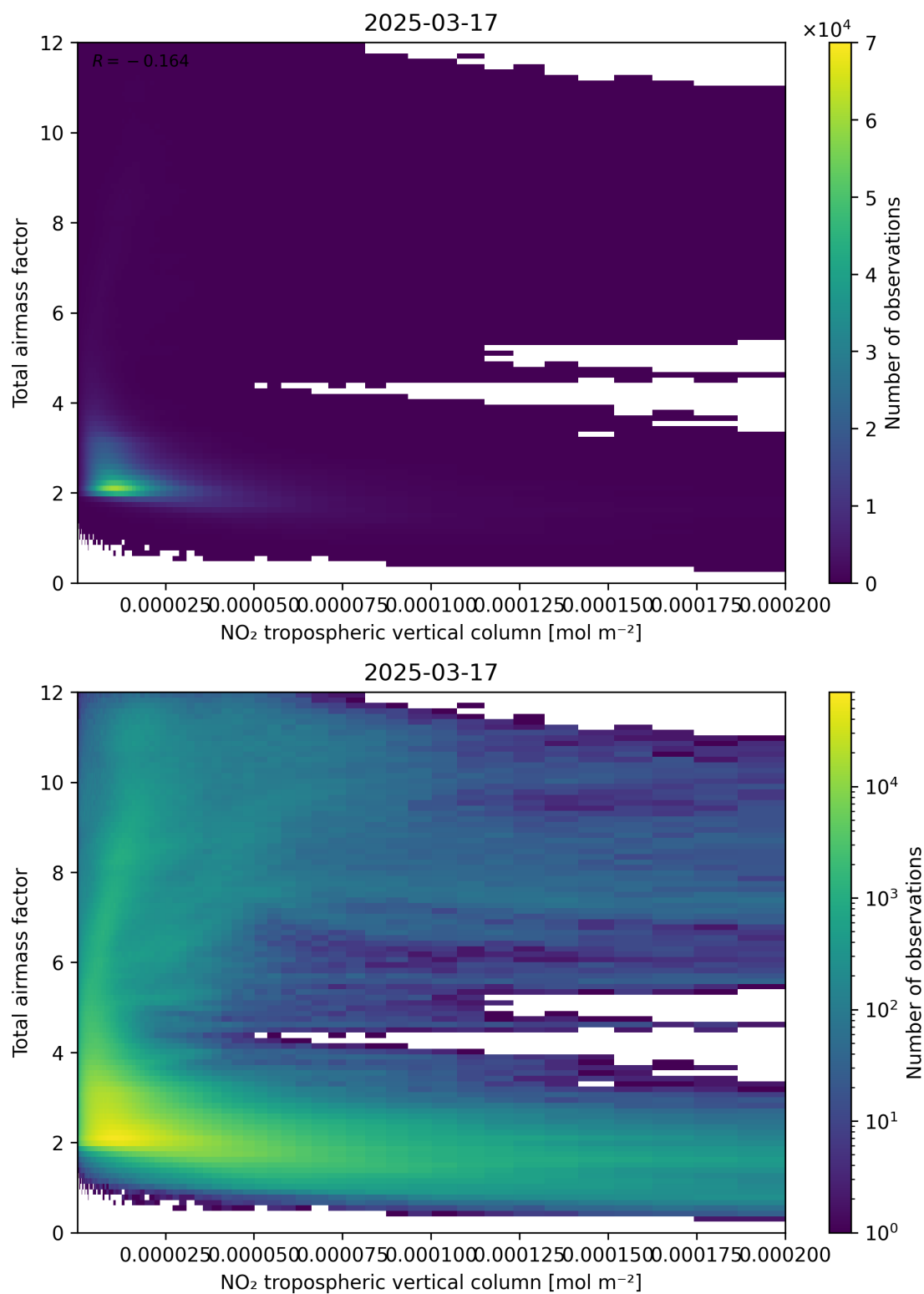
Figure 122: Scatter density plot of “NO 2 tropospheric vertical column” against “Total air mass factor” for 2025-03-17 to 2025-03-18.
