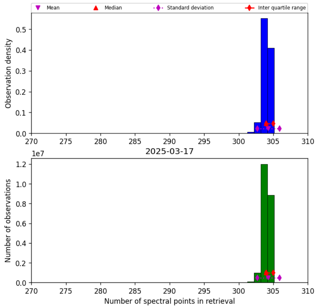
Figure 33: Histogram of “Number of spectral points in retrieval” for 2025-03-17 to 2025-03-18
