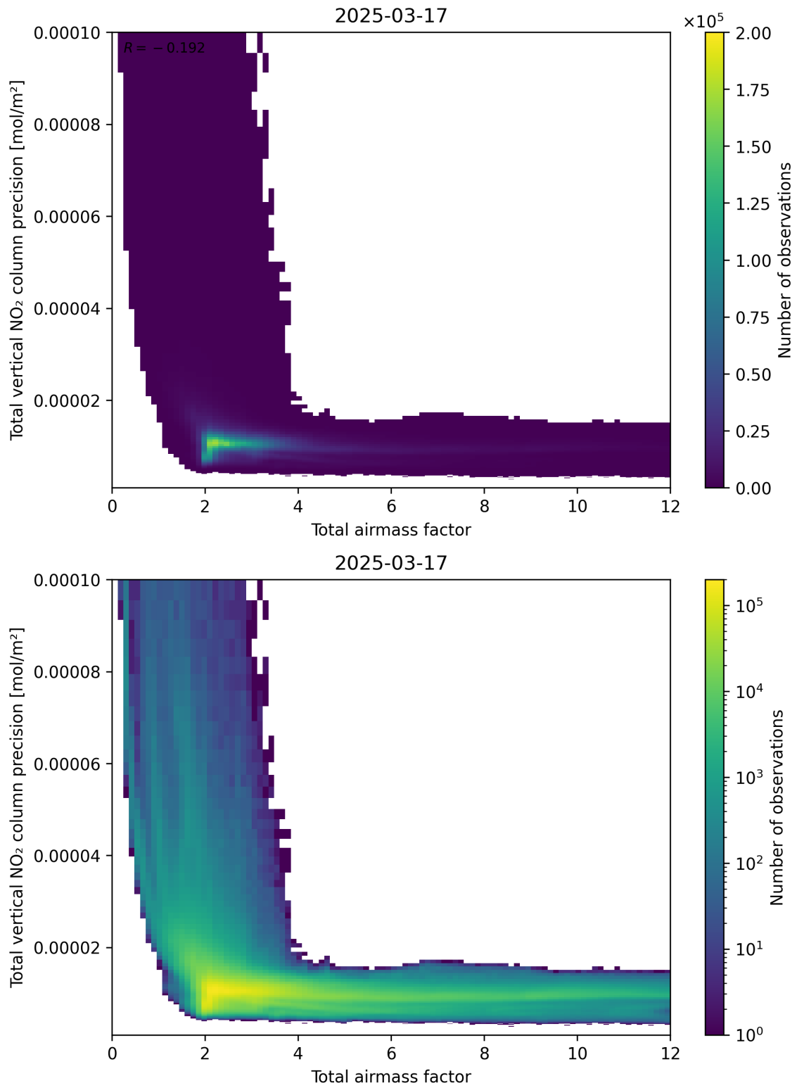
Figure 68: Scatter density plot of “Total airmass factor” against “Total vertical NO 2 column precision” for 2025-03-17 to 2025-03-18.
