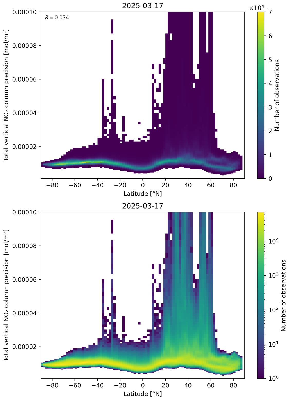
Figure 91: Scatter density plot of “Latitude” against “Total vertical NO 2 column precision” for 2025-03-17 to 2025-03-18.
