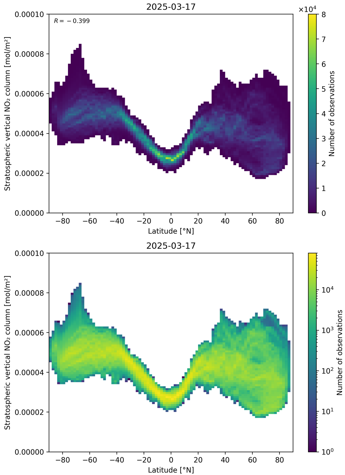
Figure 87: Scatter density plot of “Latitude” against “Stratospheric vertical \text{NO}_2 column” for 2025-03-17 to 2025-03-18.
