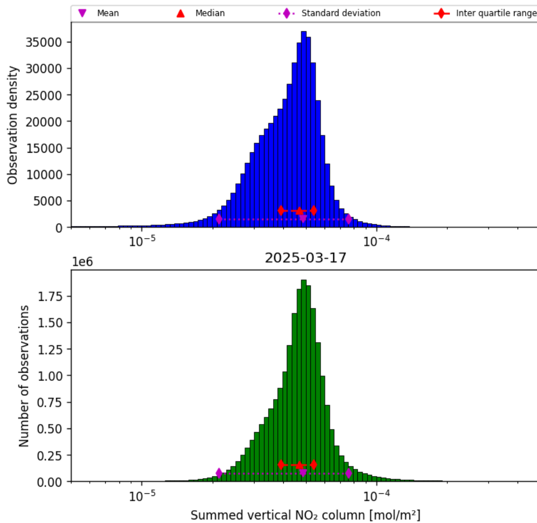
Figure 40: Histogram of “Summed vertical NO 2 column” for 2025-03-17 to 2025-03-18
