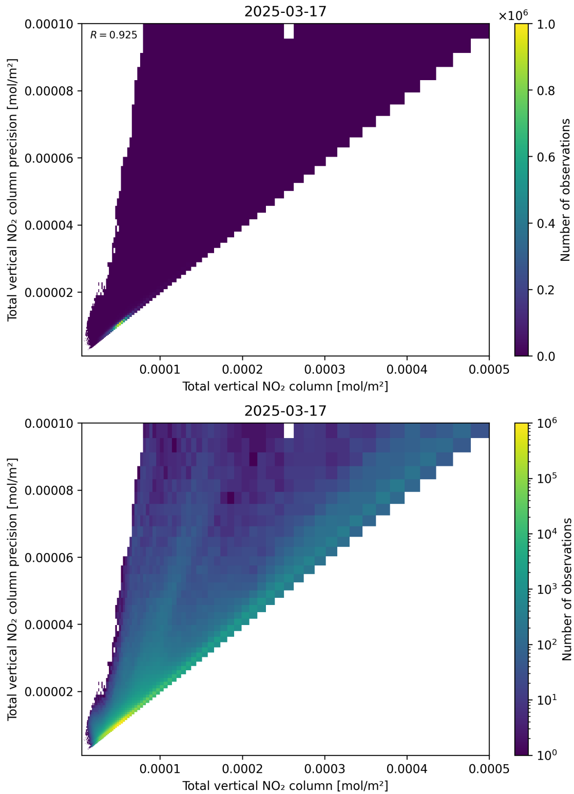
Figure 114: Scatter density plot of “Total vertical NO 2 column” against “Total vertical NO 2 column precision” for 2025-03-17 to 2025-03-18.
