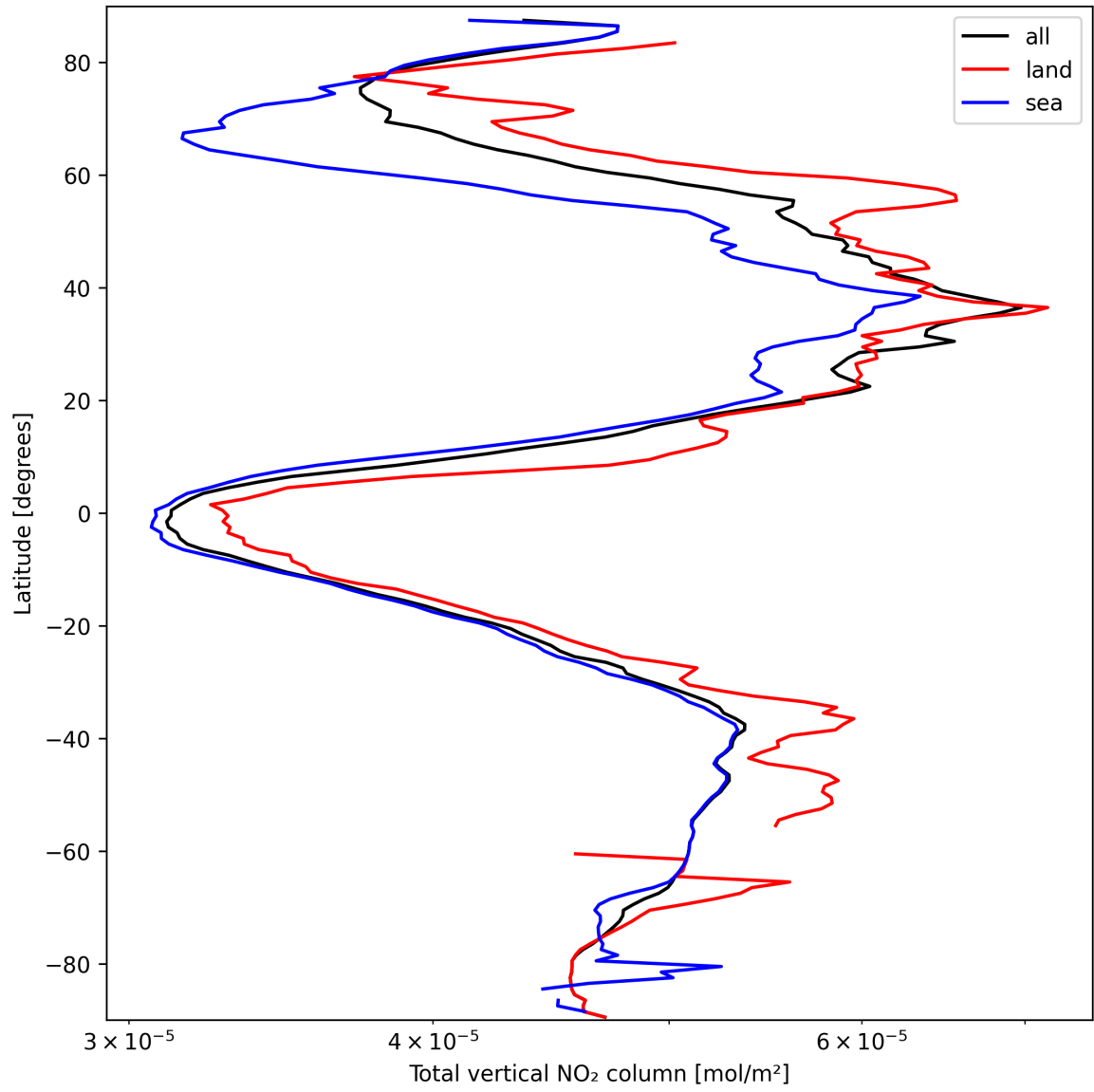
Figure 21: Zonal average of “Total vertical NO 2 column” for 2025-03-17 to 2025-03-18.
