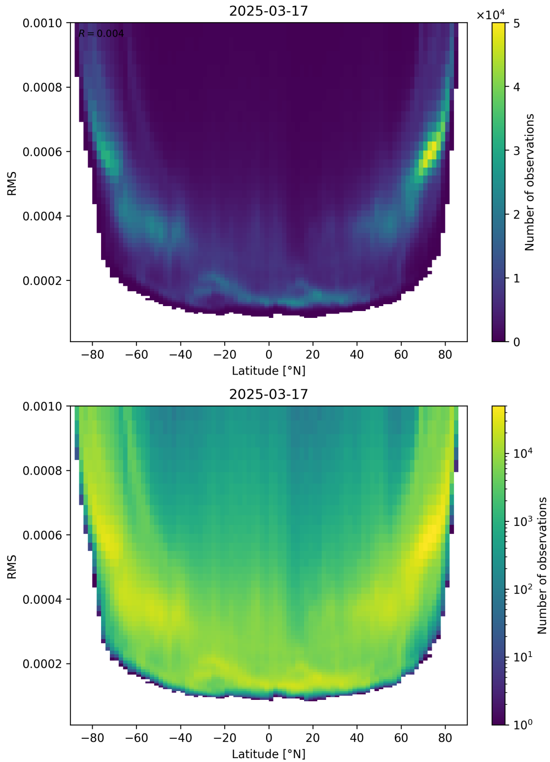
Figure 94: Scatter density plot of “Latitude” against “RMS” for 2025-03-17 to 2025-03-18.
