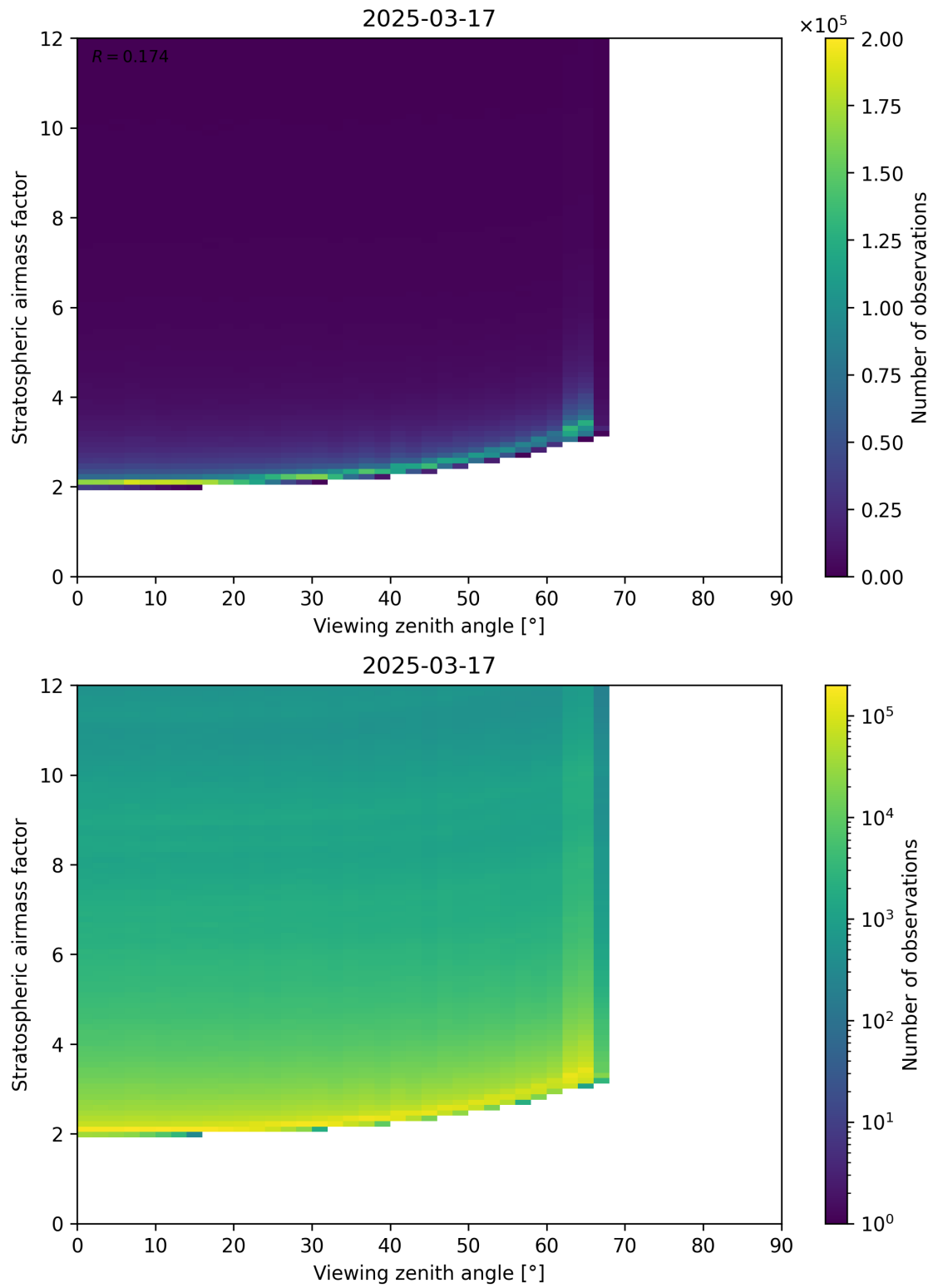
Figure 159: Scatter density plot of “Viewing zenith angle” against “Stratospheric airmass factor” for 2025-03-17 to 2025-03-18.
