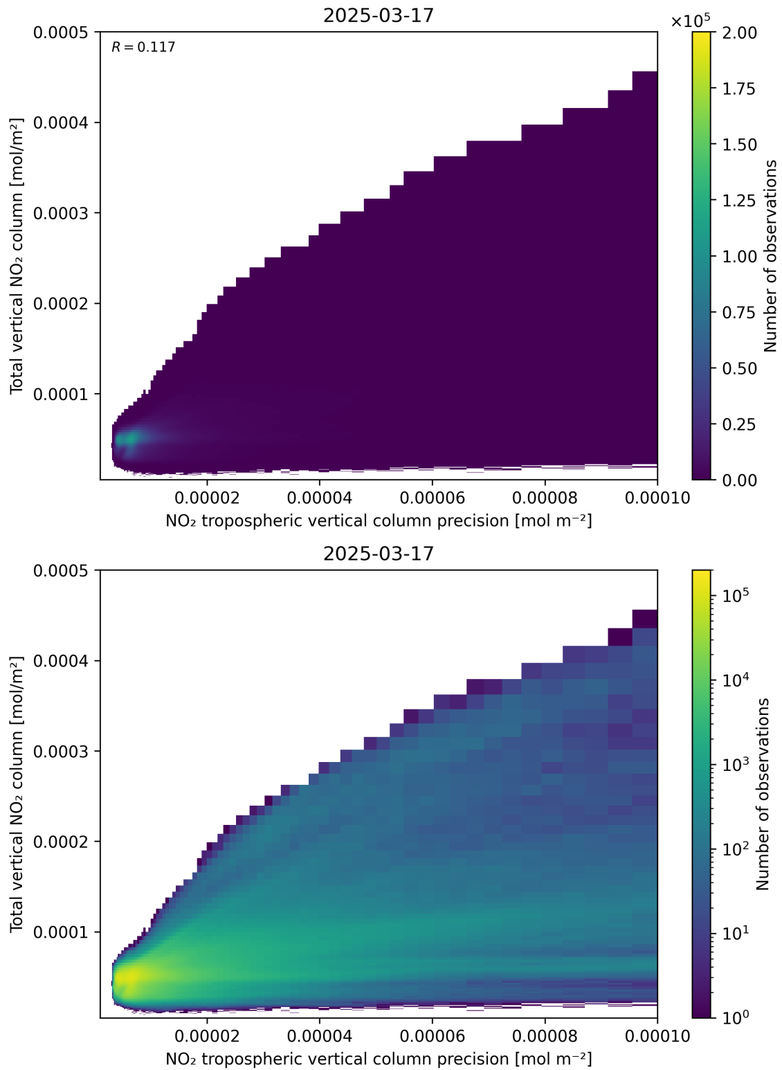
Figure 138: Scatter density plot of “NO 2 tropospheric vertical column precision” against “Total vertical NO 2 column” for 2025-03-17 to 2025-03-18.
