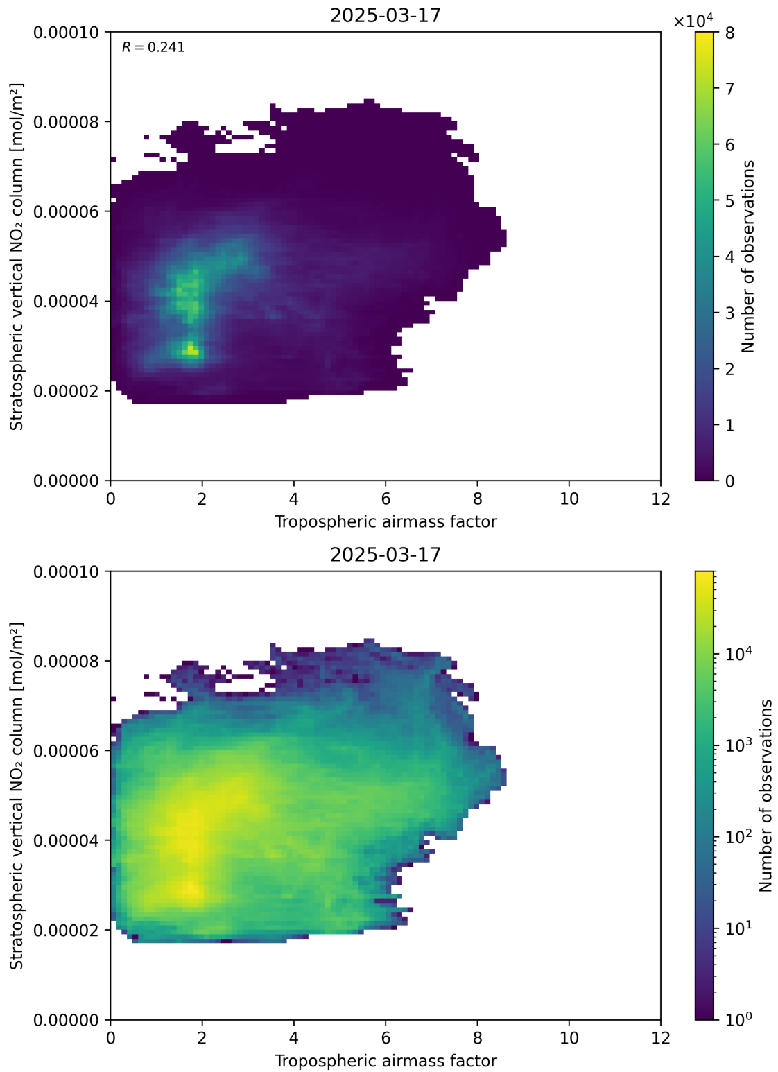
Figure 74: Scatter density plot of “Tropospheric airmass factor” against “Stratospheric vertical NO 2 column” for 2025-03-17 to 2025-03-18.
