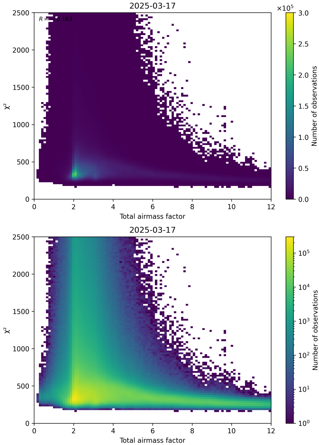
Figure 63: Scatter density plot of “Total airmass factor” against “ \chi^2 ” for 2025-03-17 to 2025-03-18.
