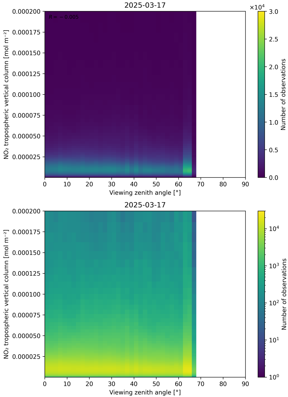
Figure 169: Scatter density plot of “Viewing zenith angle” against “NO 2 tropospheric vertical column” for 2025-03-17 to 2025-03-18.
