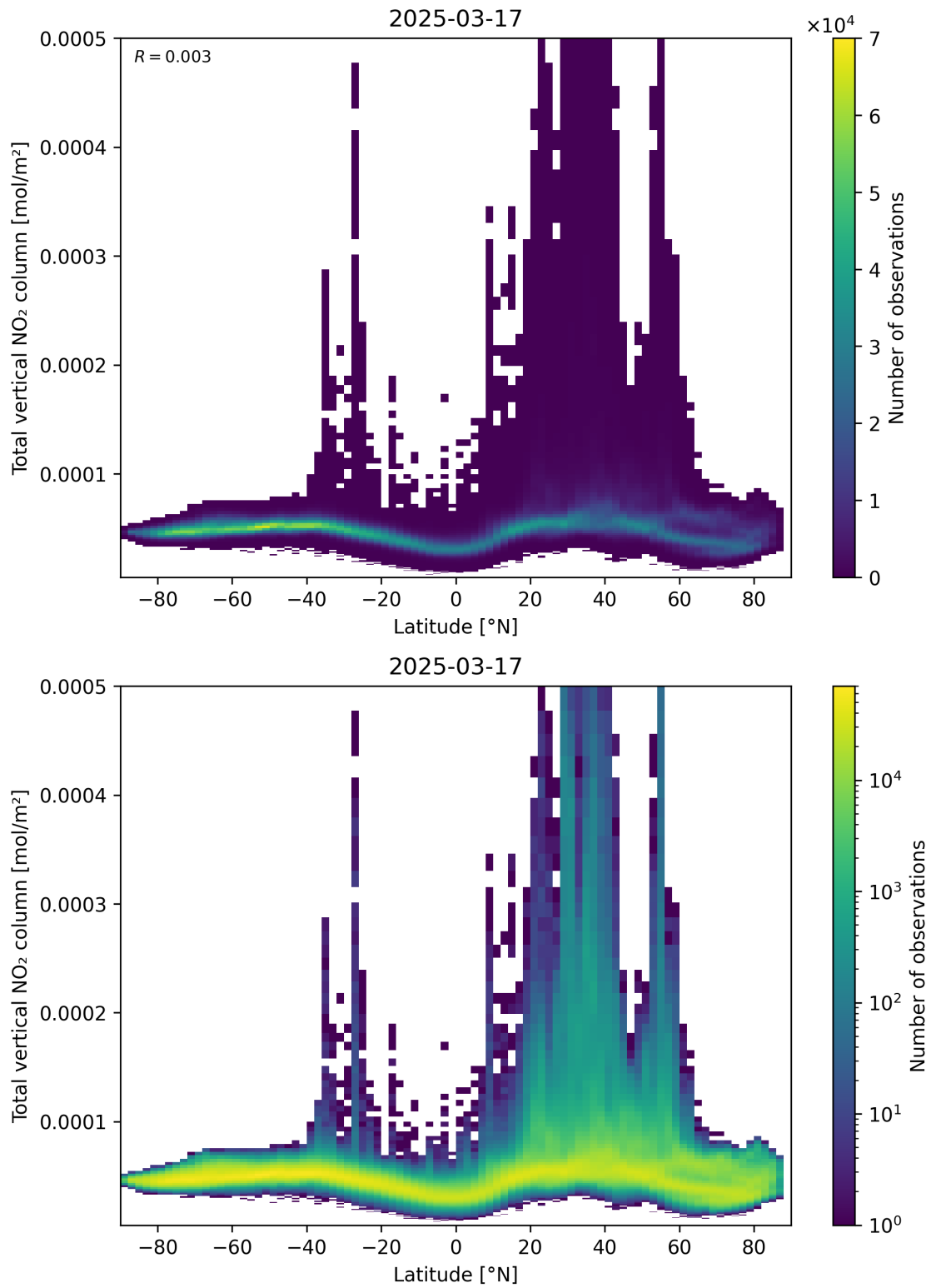
Figure 90: Scatter density plot of “Latitude” against “Total vertical NO 2 column” for 2025-03-17 to 2025-03-18.
