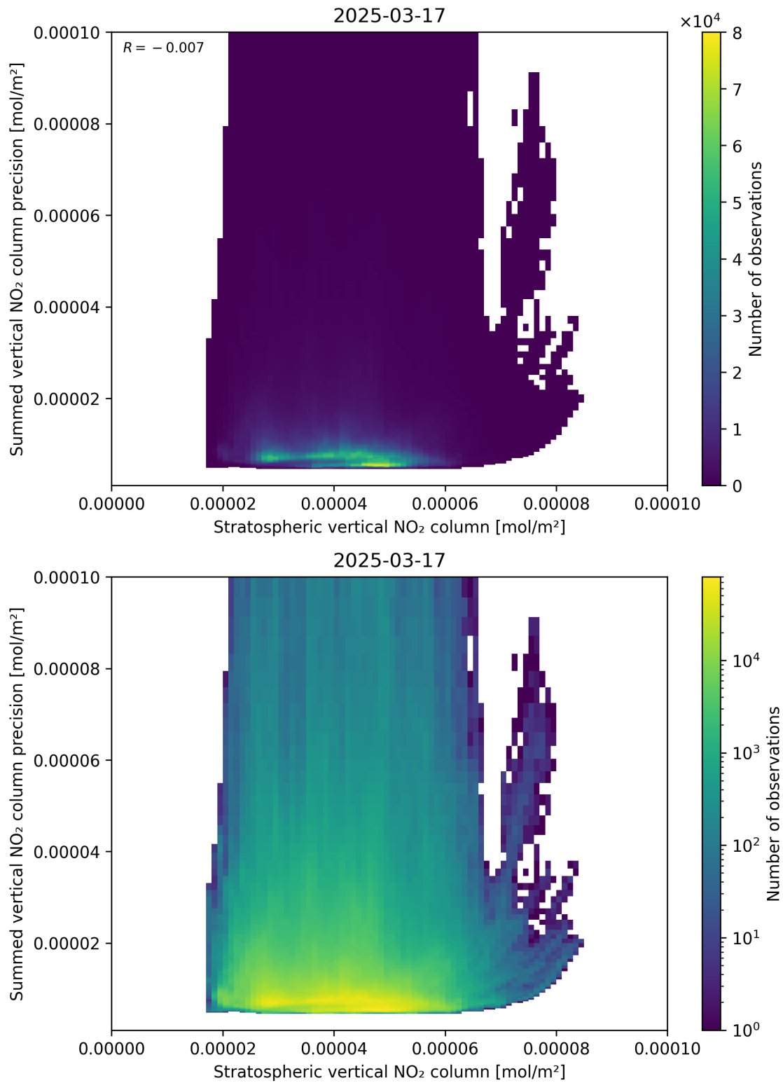
Figure 99: Scatter density plot of “Stratospheric vertical NO 2 column” against “Summed vertical NO 2 column precision” for 2025-03-17 to 2025-03-18.
