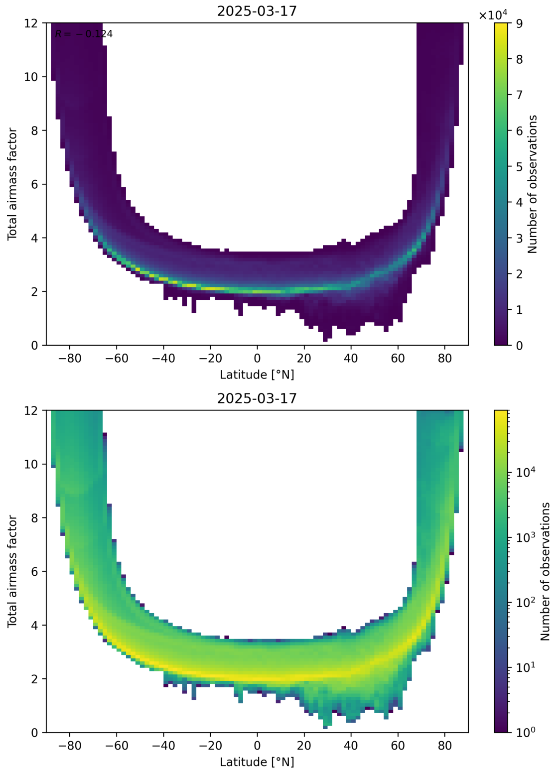
Figure 84: Scatter density plot of “Latitude” against “Total airmass factor” for 2025-03-17 to 2025-03-18.
