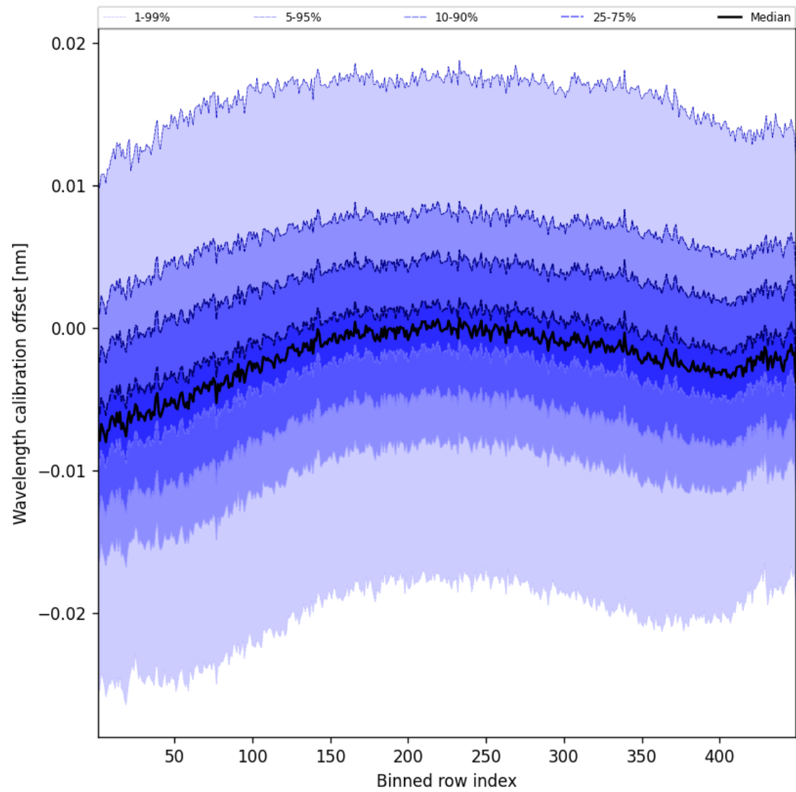
Figure 52: Along track statistics of “Wavelength calibration offset” for 2025-03-17 to 2025-03-18
