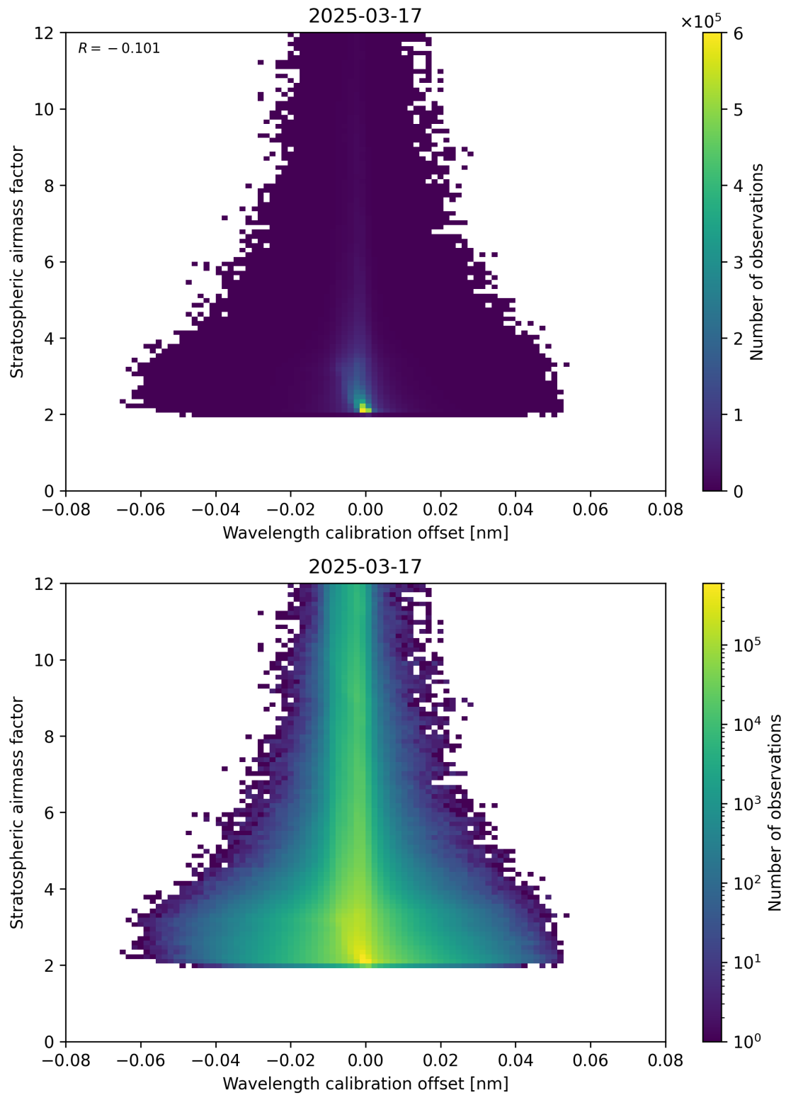
Figure 174: Scatter density plot of “Wavelength calibration offset” against “Stratospheric airmass factor” for 2025-03-17 to 2025-03-18.
