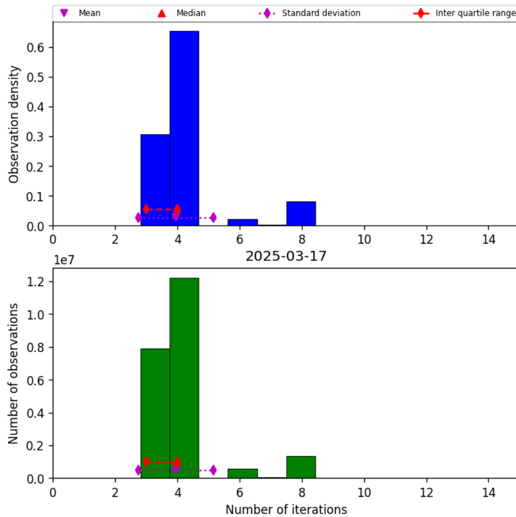
Figure 34: Histogram of “Number of iterations” for 2025-03-17 to 2025-03-18
