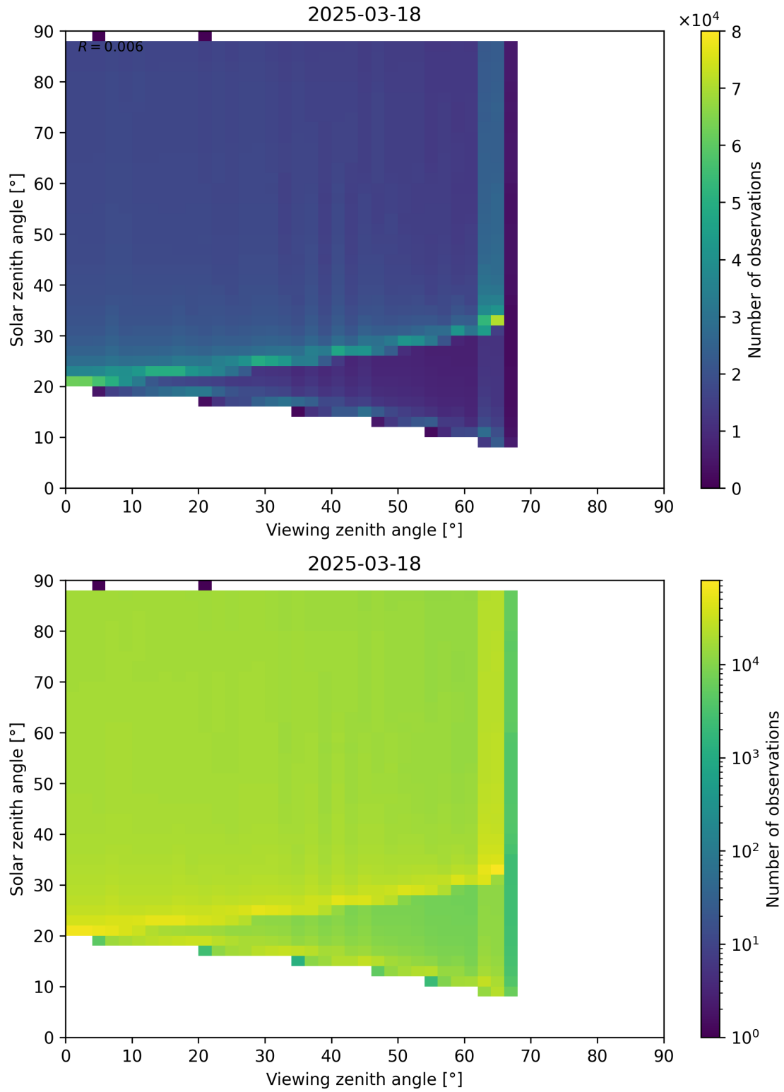
Figure 172: Scatter density plot of “Viewing zenith angle” against “Solar zenith angle” for 2025-03-18 to 2025-03-19.
