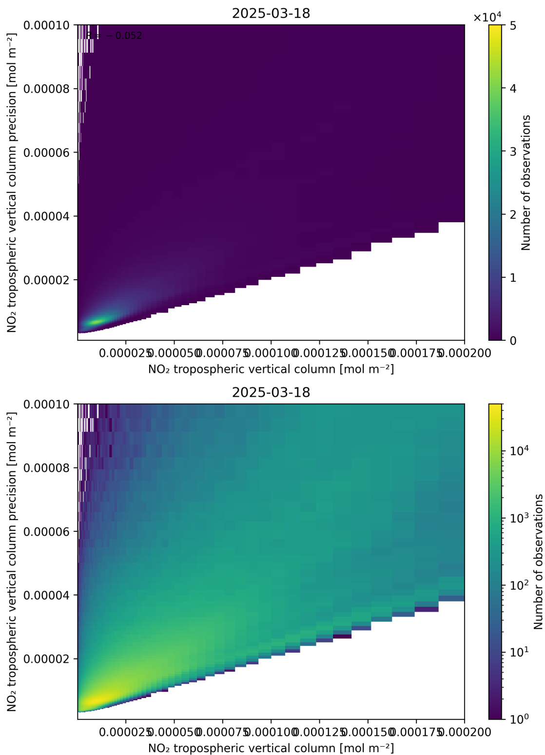
Figure 130: Scatter density plot of “NO 2 tropospheric vertical column” against “NO 2 tropospheric vertical column precision” for 2025-03-18 to 2025-03-19.
