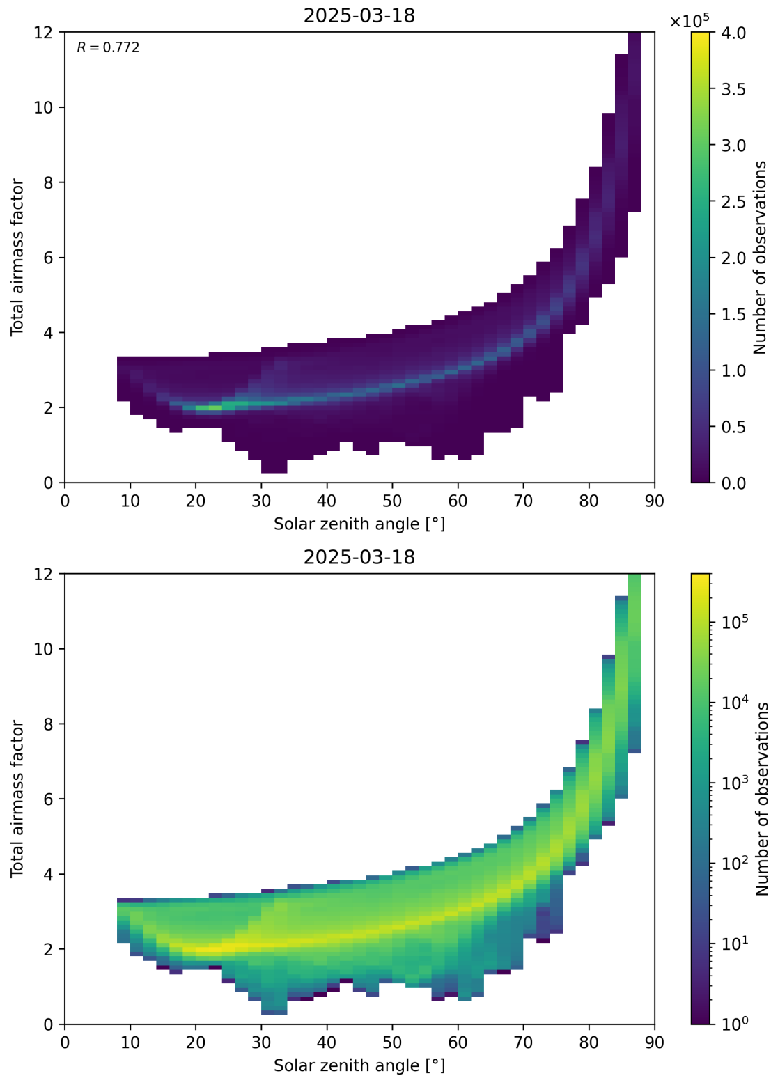
Figure 146: Scatter density plot of “Solar zenith angle” against “Total air mass factor” for 2025-03-18 to 2025-03-19.
