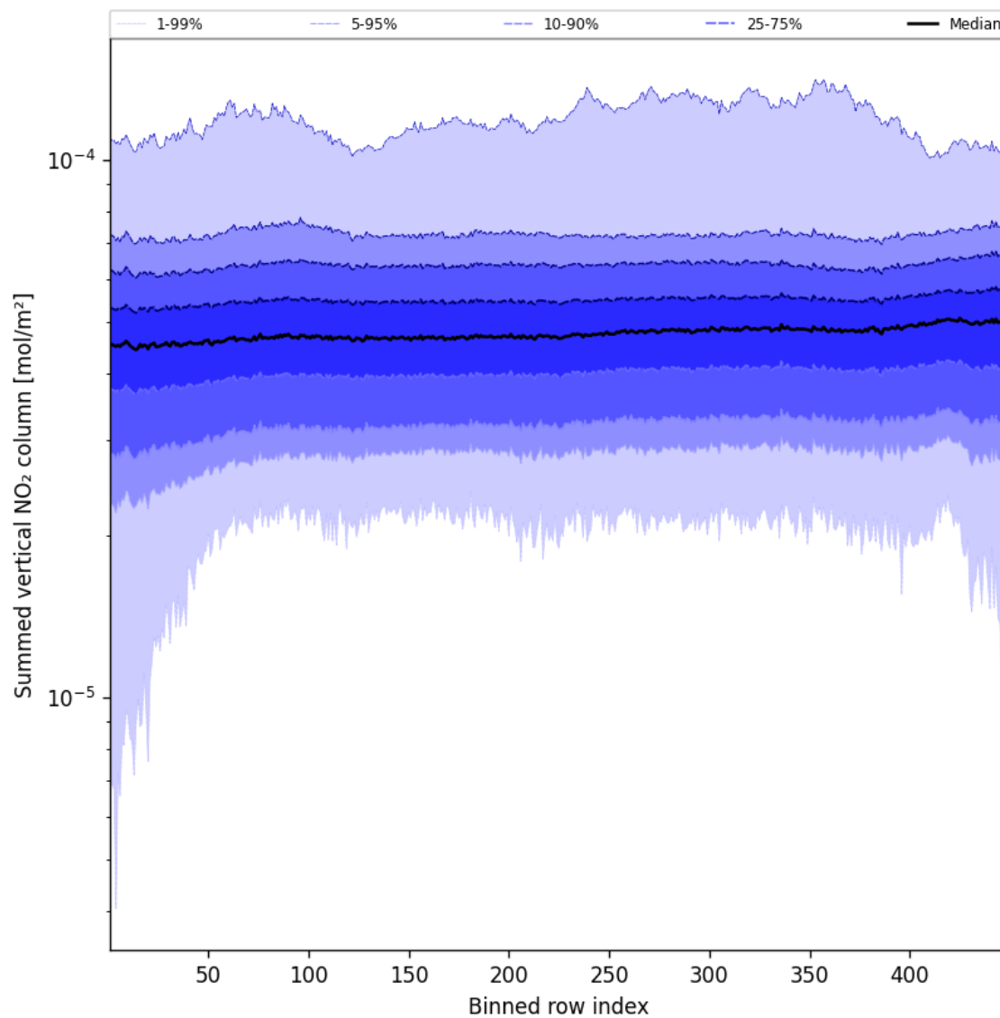
Figure 57: Along track statistics of “Summed vertical NO 2 column” for 2025-03-18 to 2025-03-19
