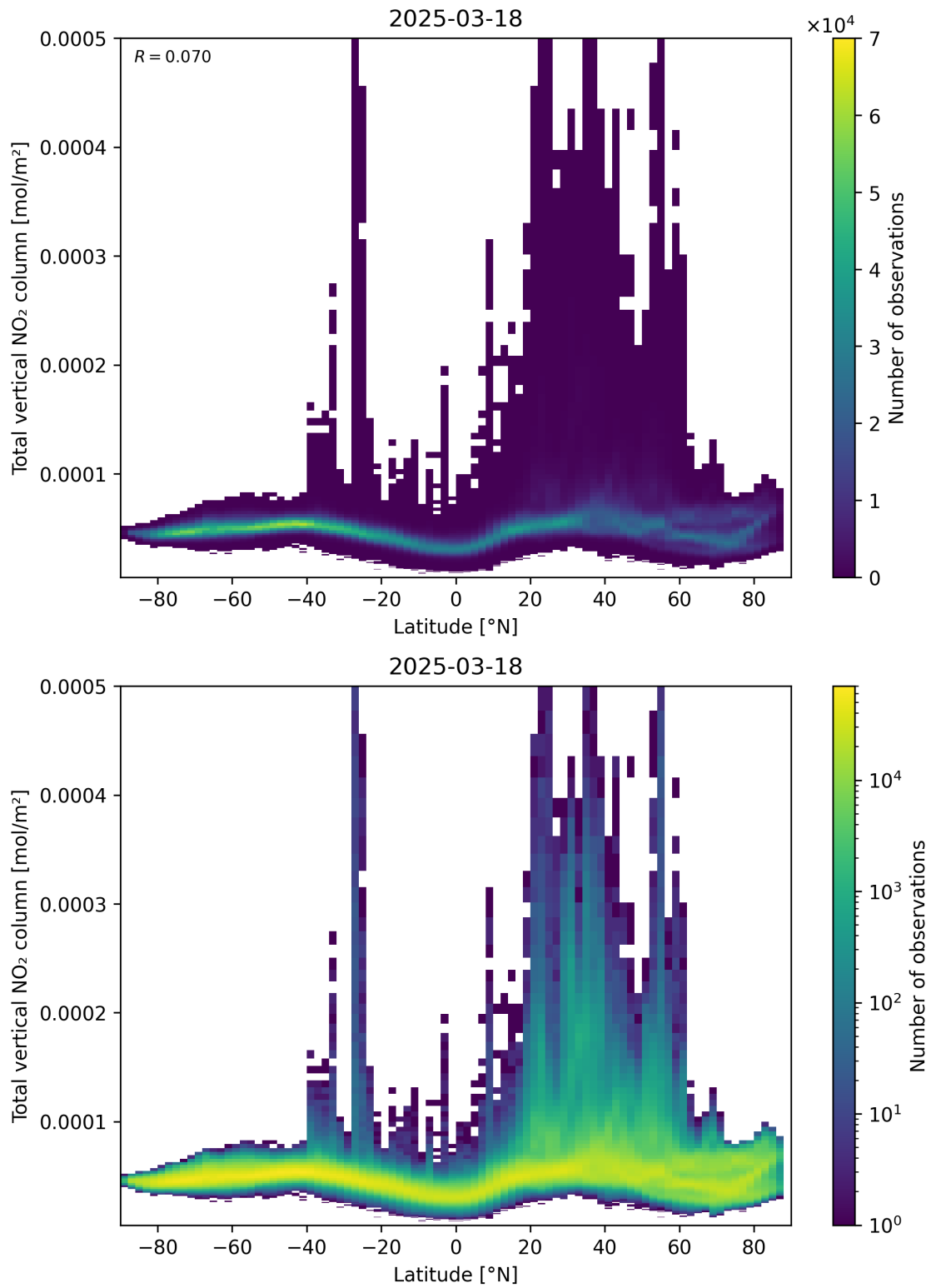
Figure 90: Scatter density plot of “Latitude” against “Total vertical NO 2 column” for 2025-03-18 to 2025-03-19.
