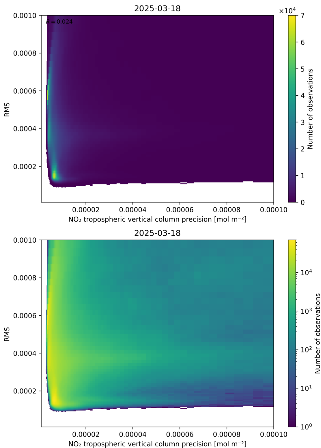
Figure 140: Scatter density plot of “NO 2 tropospheric vertical column precision” against “RMS” for 2025-03-18 to 2025-03-19.
