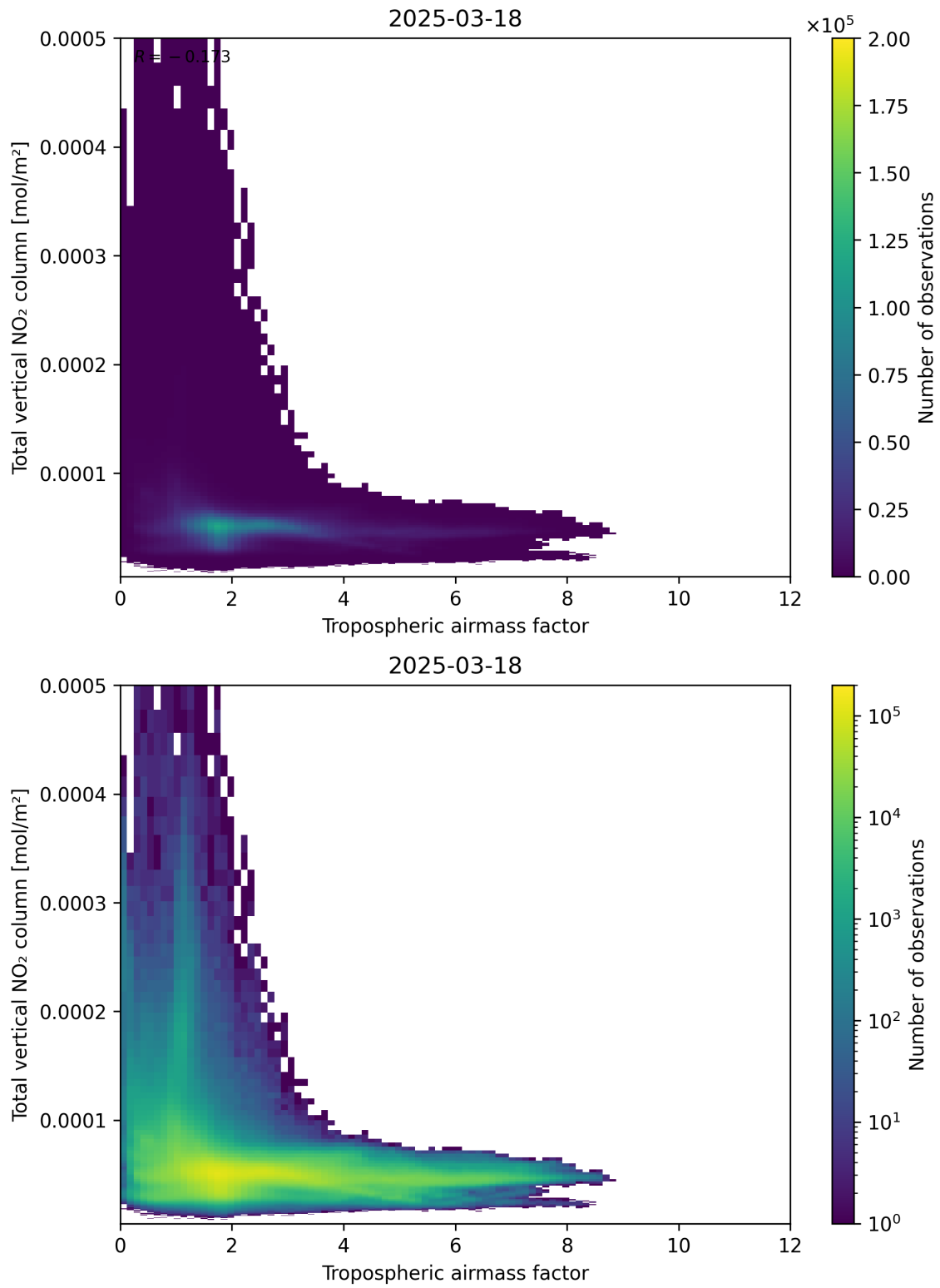
Figure 77: Scatter density plot of “Tropospheric airmass factor” against “Total vertical NO 2 column” for 2025-03-18 to 2025-03-19.
