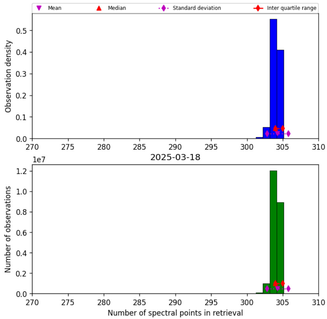
Figure 33: Histogram of “Number of spectral points in retrieval” for 2025-03-18 to 2025-03-19
