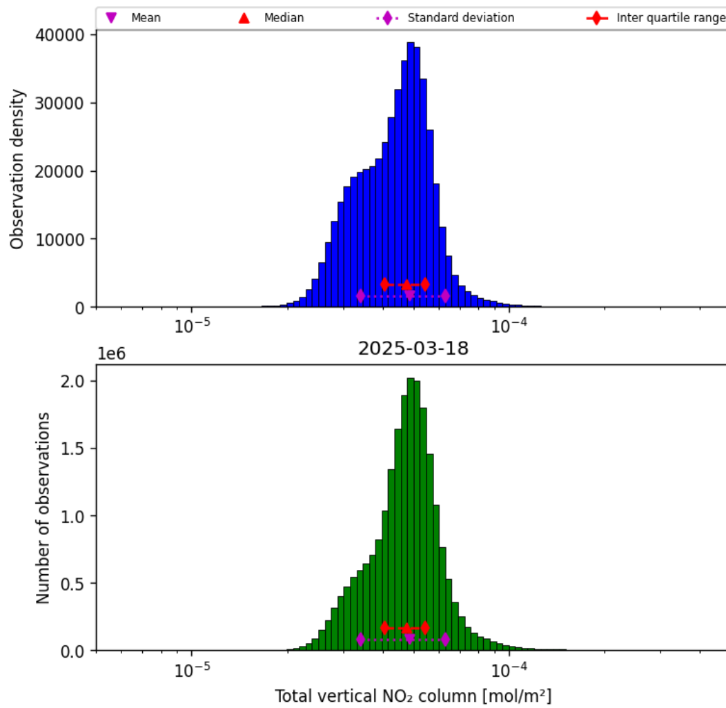
Figure 38: Histogram of “Total vertical NO 2 column” for 2025-03-18 to 2025-03-19
