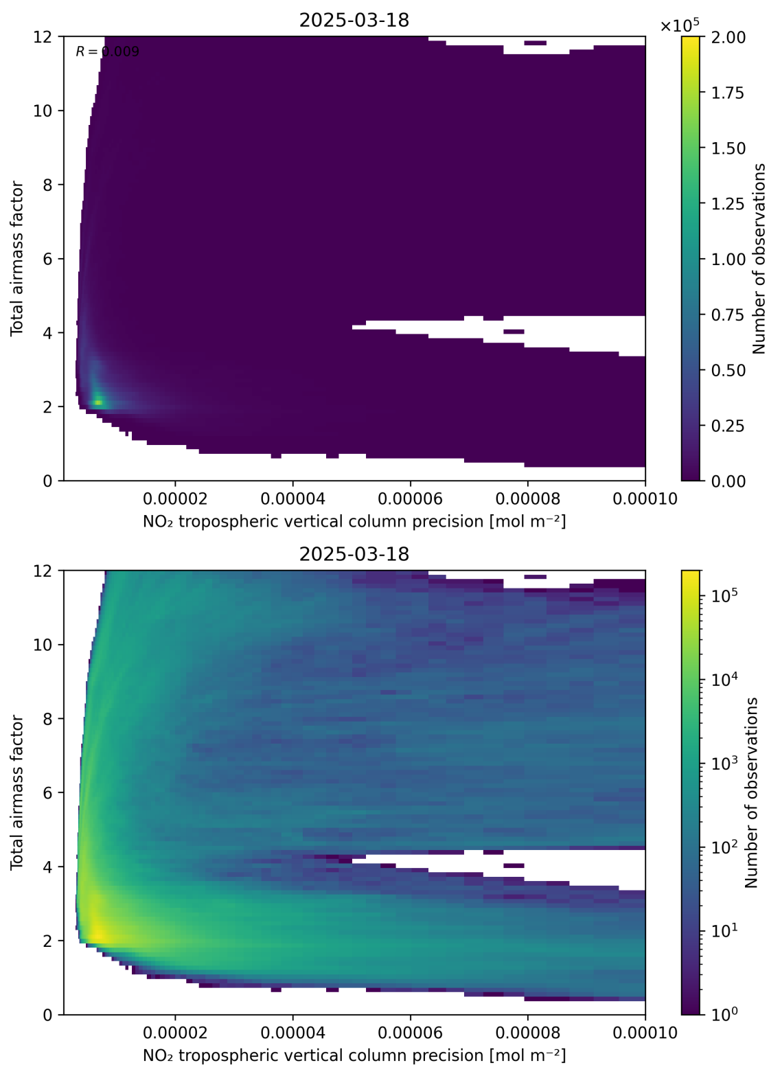
Figure 132: Scatter density plot of “NO 2 tropospheric vertical column precision” against “Total air mass factor” for 2025-03-18 to 2025-03-19.
