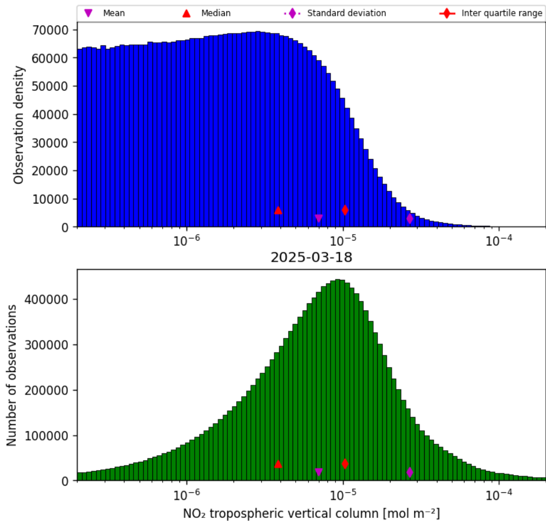
Figure 29: Histogram of “NO 2 tropospheric vertical column” for 2025-03-18 to 2025-03-19
