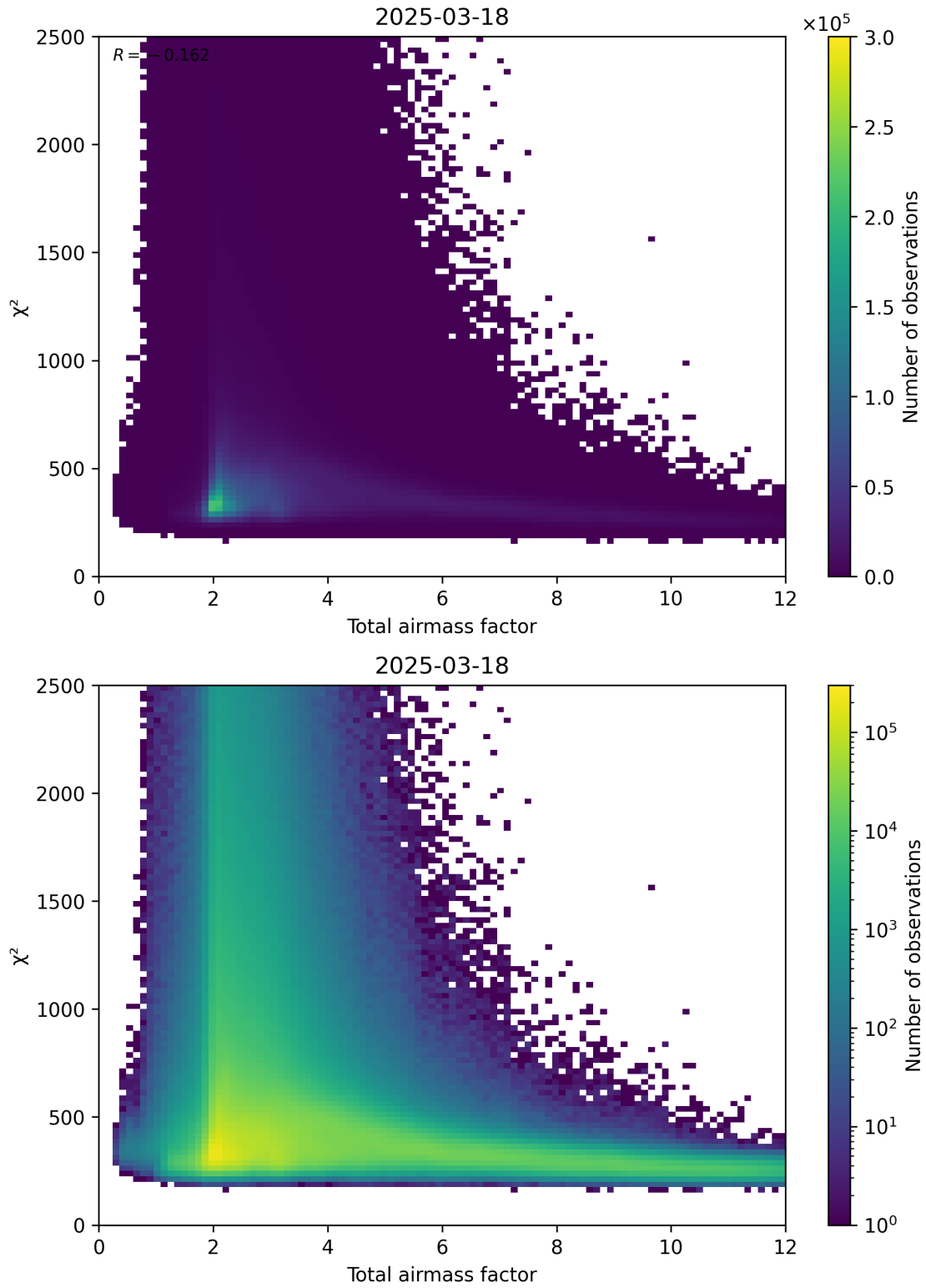
Figure 63: Scatter density plot of “Total airmass factor” against “ \chi^2 ” for 2025-03-18 to 2025-03-19.
