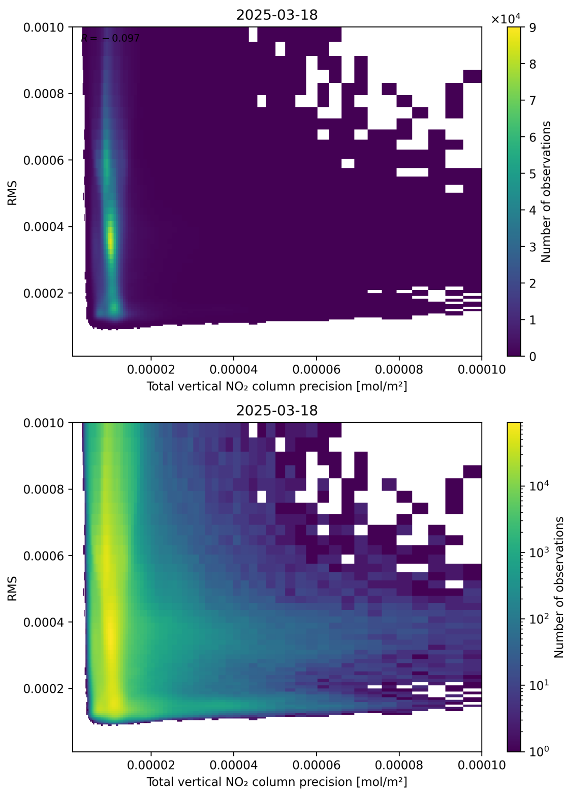
Figure 119: Scatter density plot of “Total vertical NO 2 column precision” against “RMS” for 2025-03-18 to 2025-03-19.
