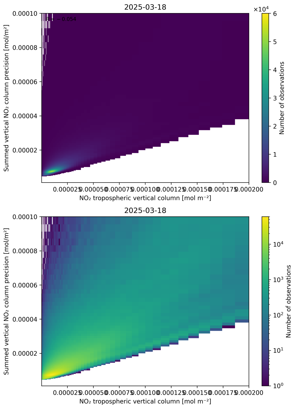
Figure 127: Scatter density plot of “NO 2 tropospheric vertical column” against “Summed vertical NO 2 column precision” for 2025-03-18 to 2025-03-19.
