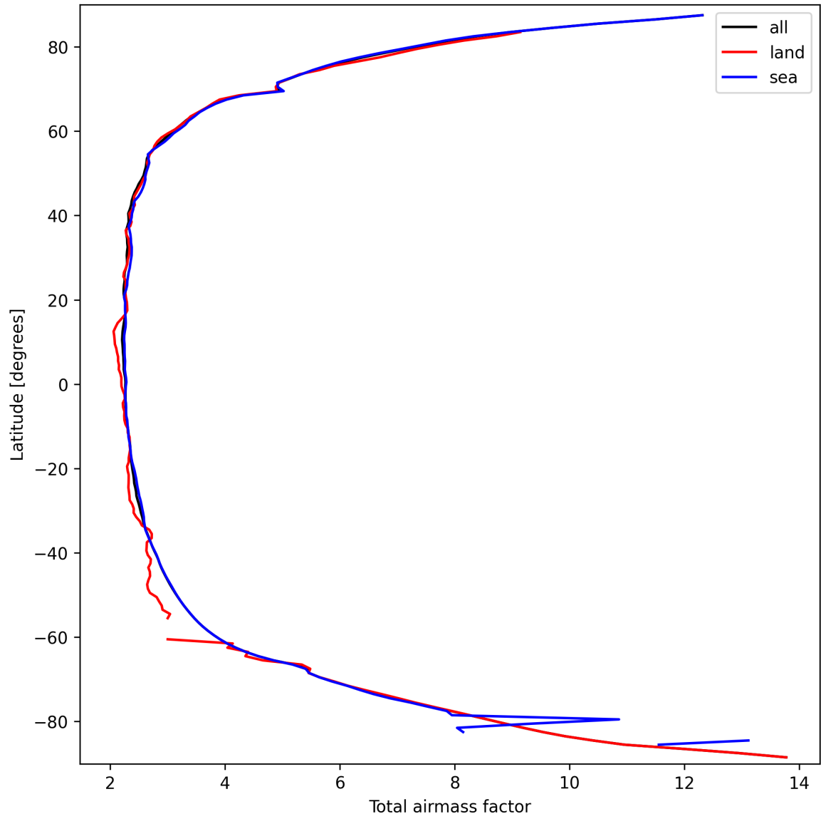
Figure 15: Zonal average of “Total airmass factor” for 2025-03-18 to 2025-03-19.
