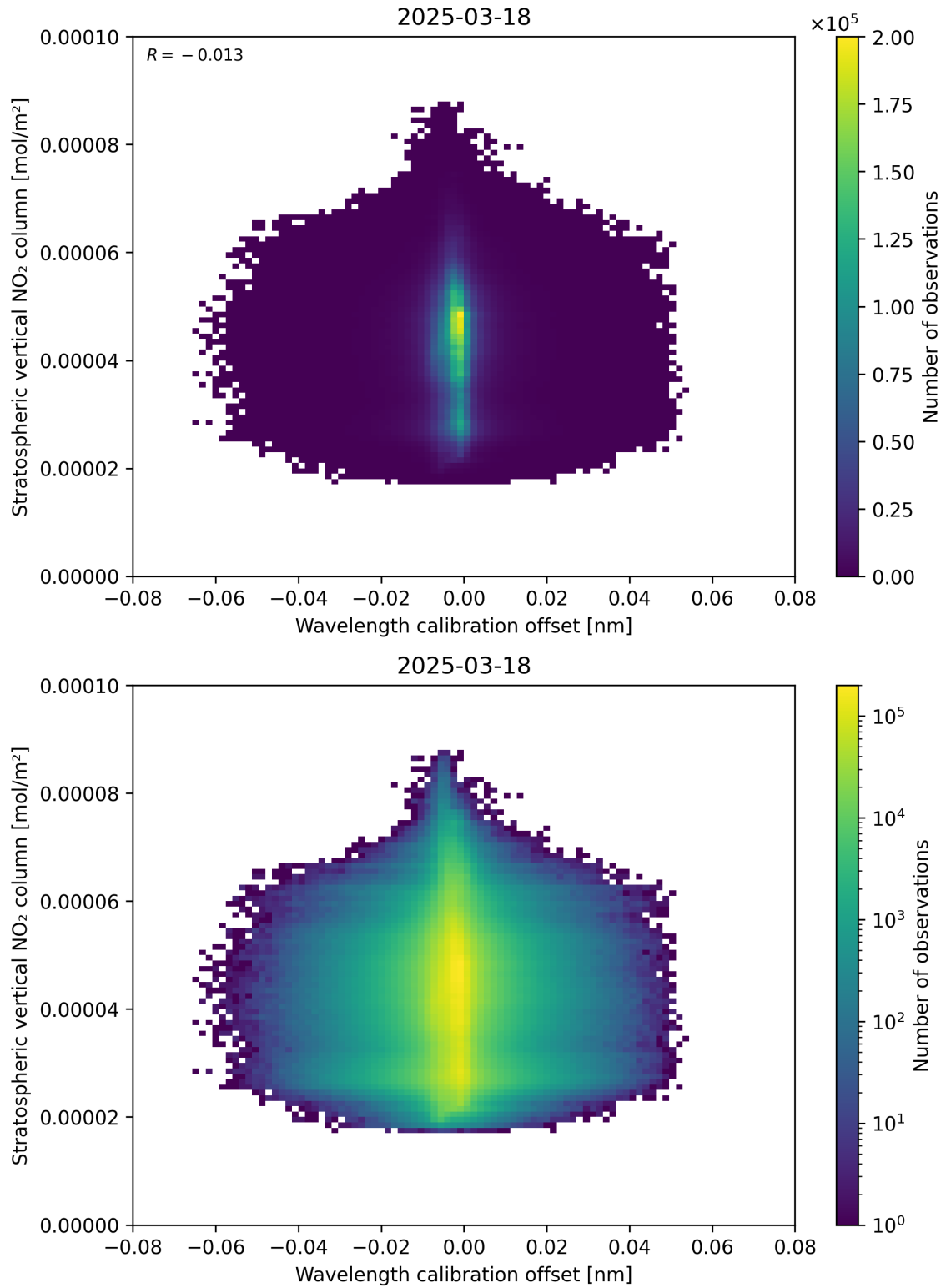
Figure 176: Scatter density plot of “Wavelength calibration offset” against “Stratospheric vertical NO 2 column” for 2025-03-18 to 2025-03-19.
