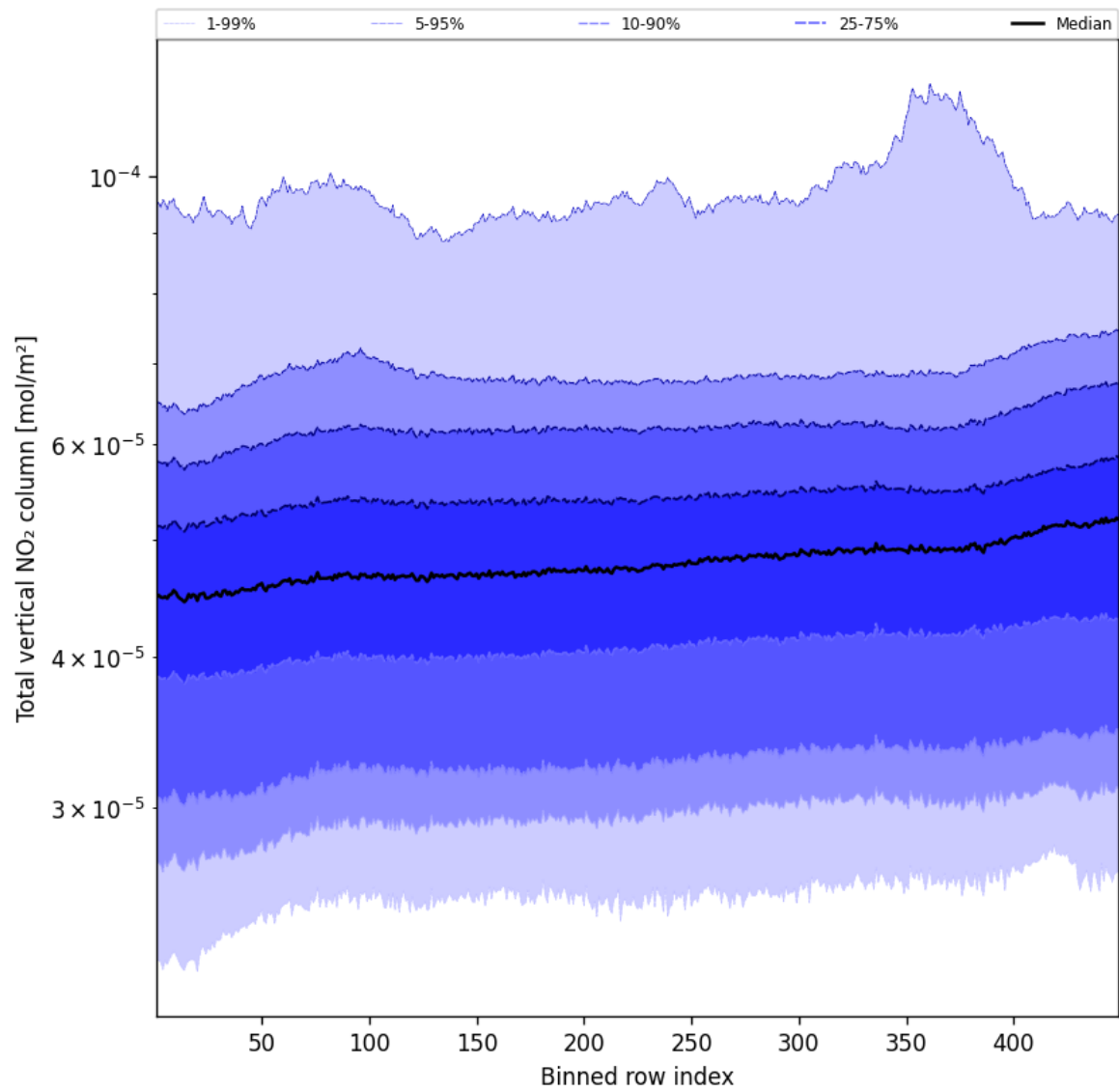
Figure 55: Along track statistics of “Total vertical NO 2 column” for 2025-03-18 to 2025-03-19
