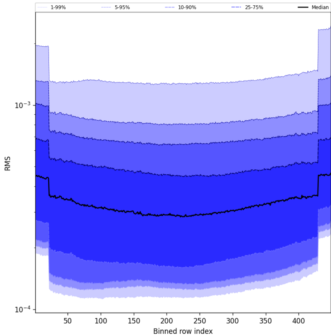
Figure 60: Along track statistics of “RMS” for 2025-03-18 to 2025-03-19
