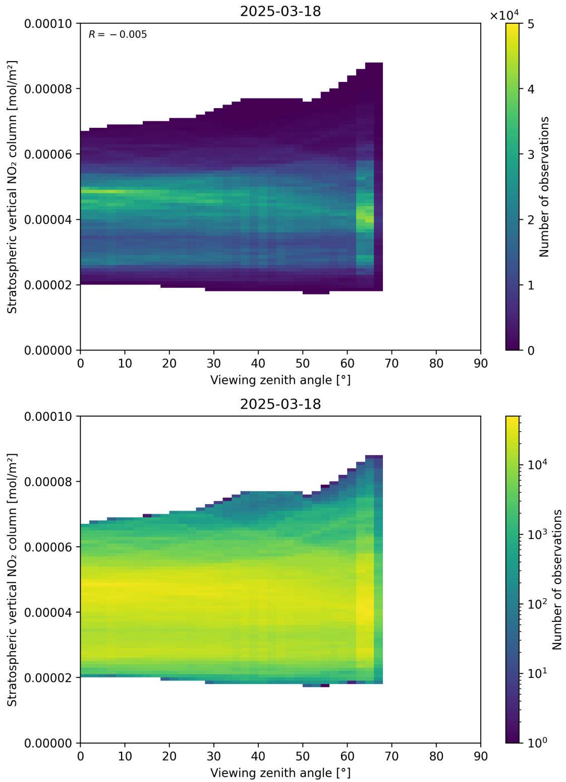
Figure 164: Scatter density plot of “Viewing zenith angle” against “Stratospheric vertical NO 2 column” for 2025-03-18 to 2025-03-19.
