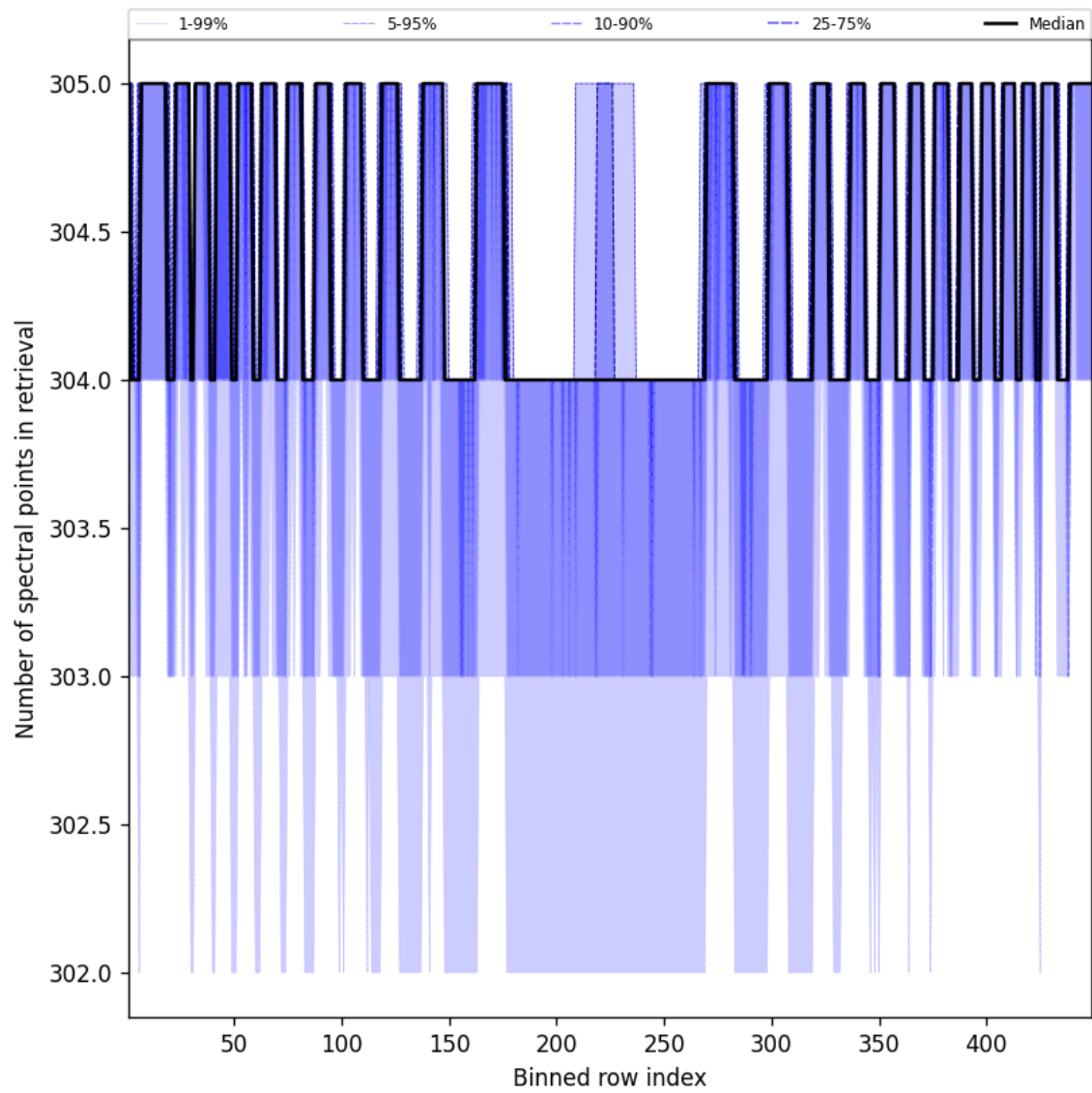
Figure 50: Along track statistics of “Number of spectral points in retrieval” for 2025-03-18 to 2025-03-19
