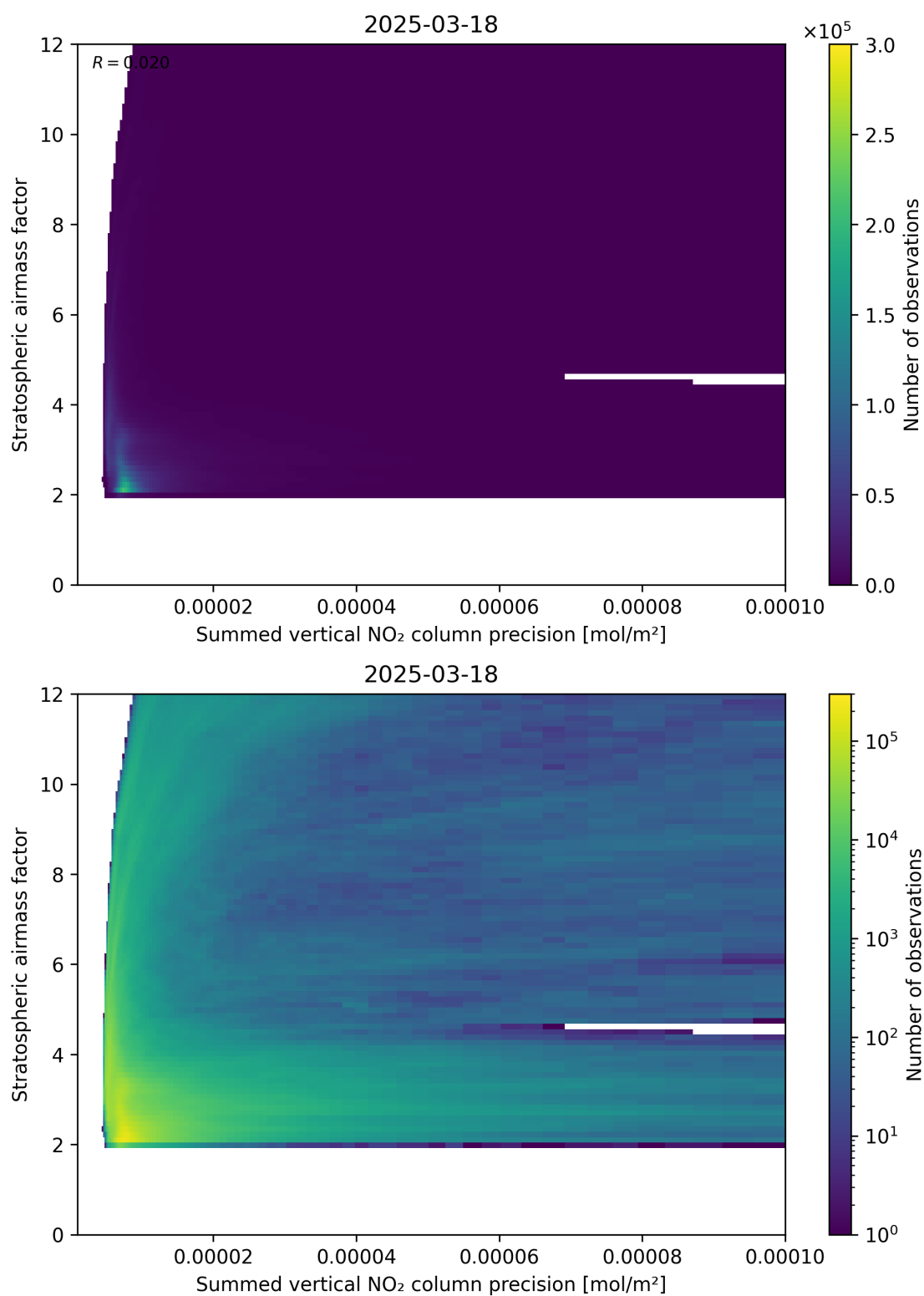
Figure 106: Scatter density plot of “Summed vertical NO 2 column precision” against “Stratospheric airmass factor” for 2025-03-18 to 2025-03-19.
