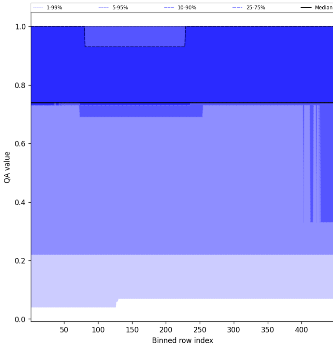
Figure 45: Along track statistics of "QA value" for 2025-03-18 to 2025-03-19
