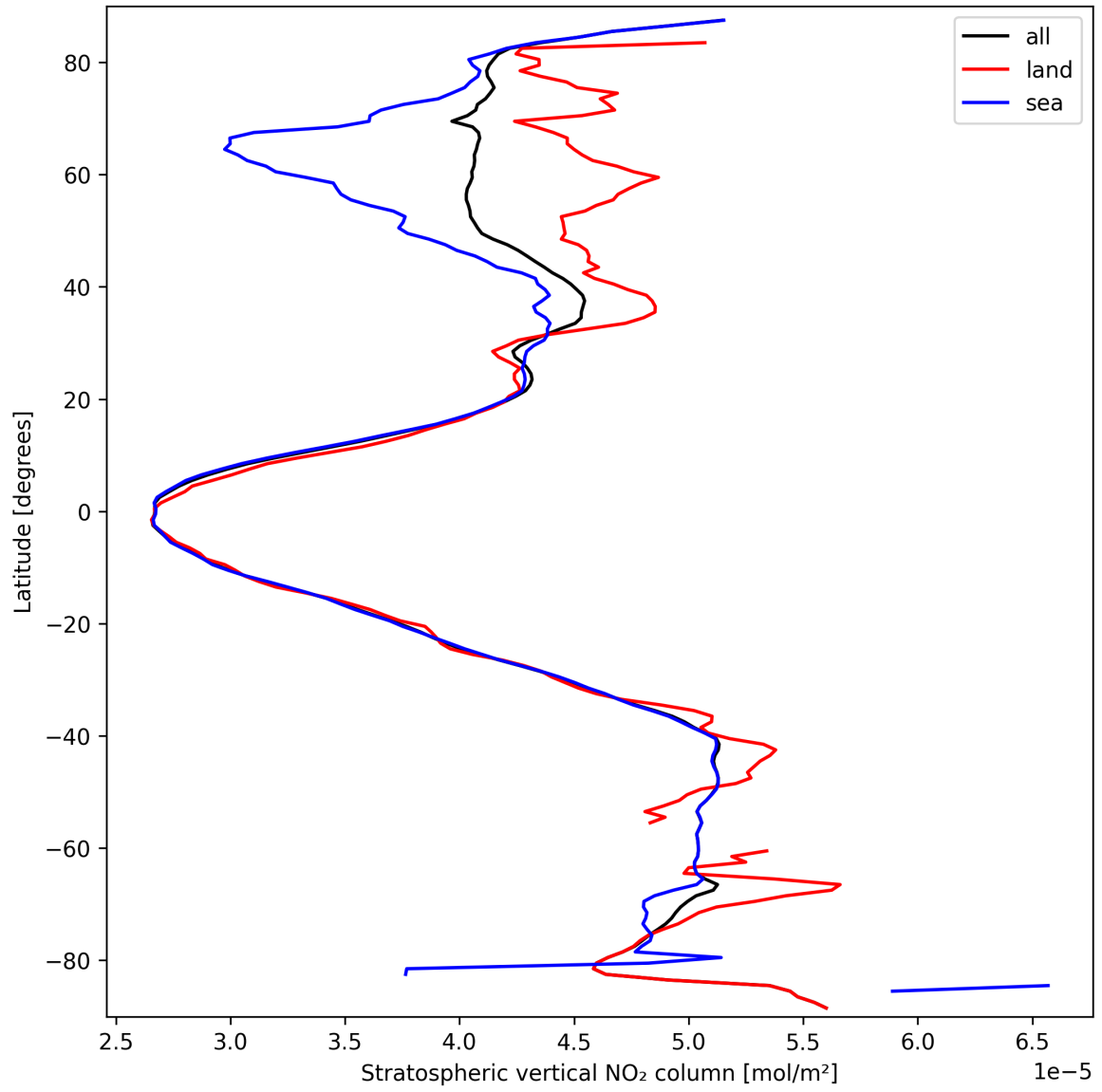
Figure 19: Zonal average of “Stratospheric vertical NO 2 column” for 2025-03-18 to 2025-03-19.
