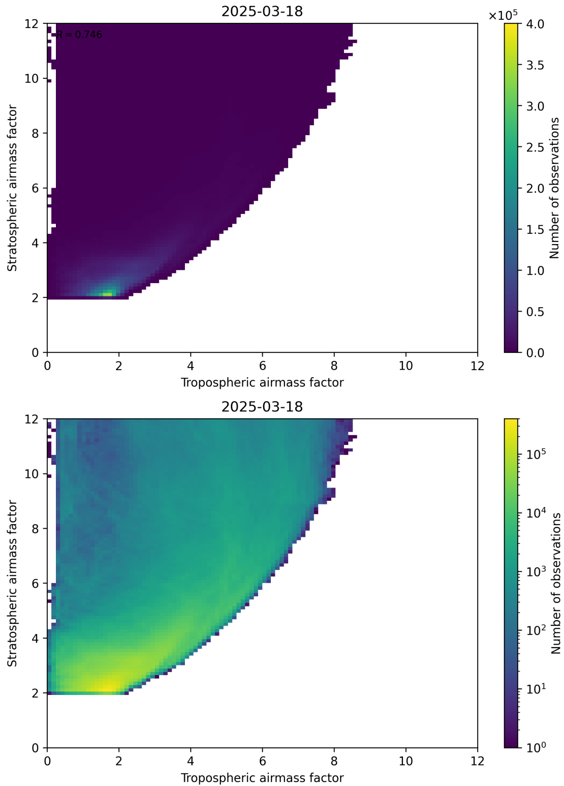
Figure 71: Scatter density plot of “Tropospheric airmass factor” against “Stratospheric airmass factor” for 2025-03-18 to 2025-03-19.
