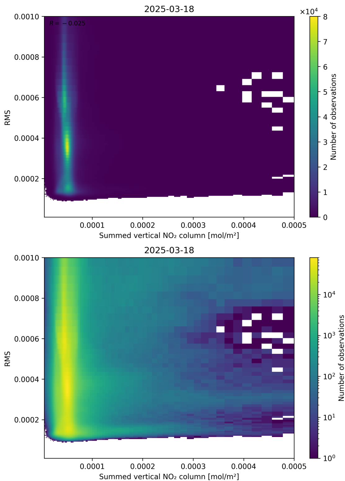
Figure 109: Scatter density plot of “Summed vertical NO 2 column” against “RMS” for 2025-03-18 to 2025-03-19.
