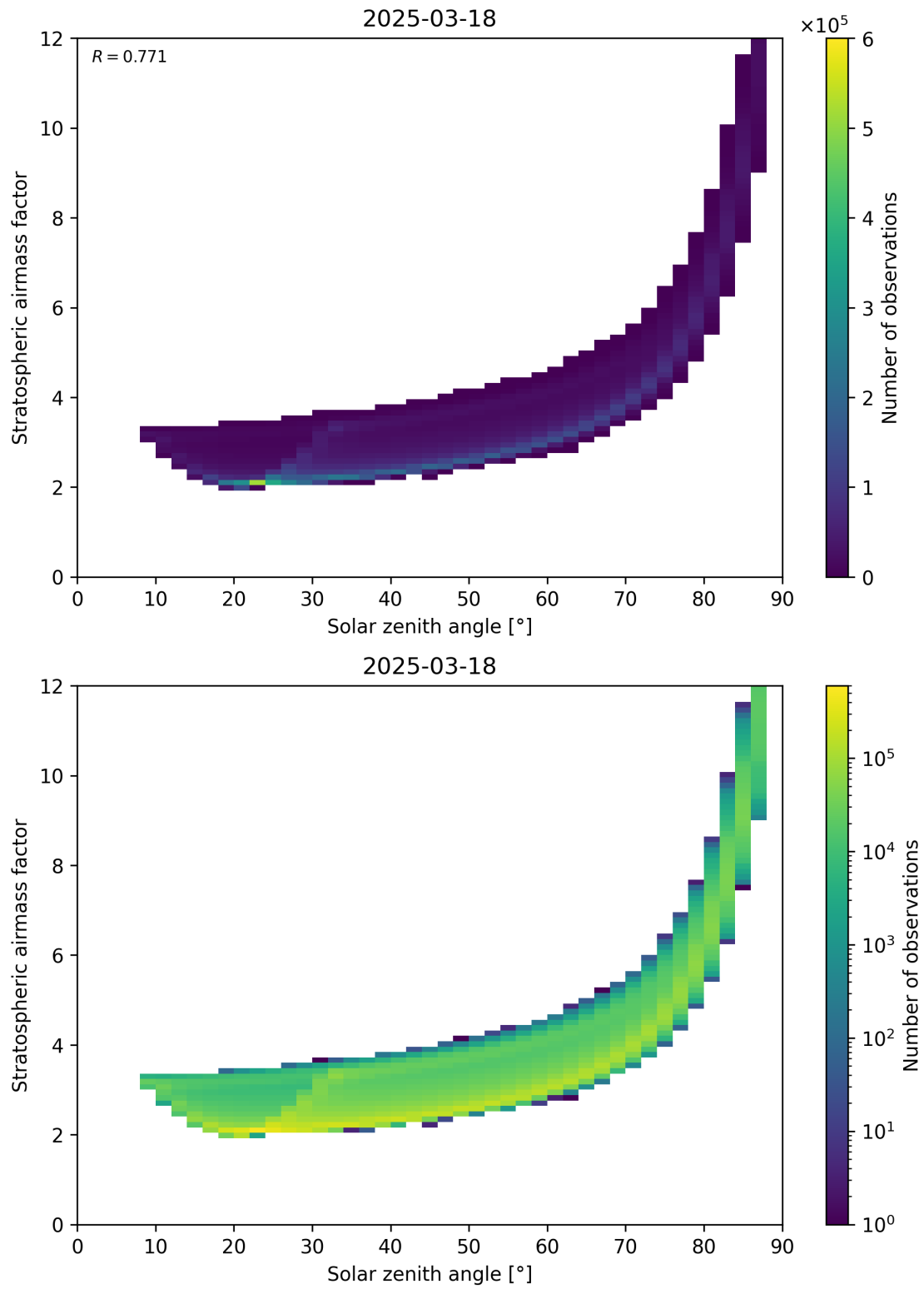
Figure 145: Scatter density plot of “Solar zenith angle” against “Stratospheric airmass factor” for 2025-03-18 to 2025-03-19.
