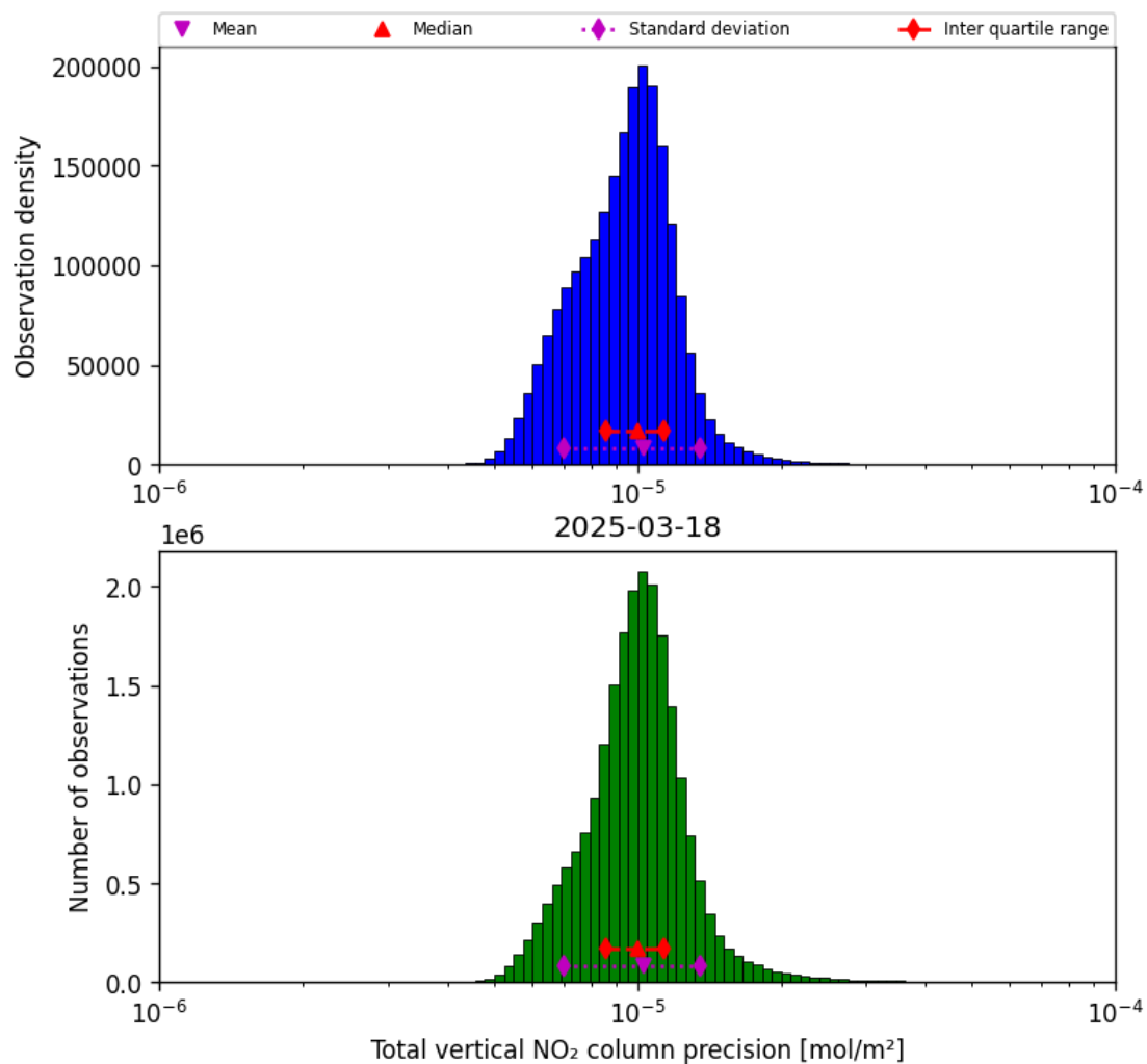
Figure 39: Histogram of “Total vertical NO 2 column precision” for 2025-03-18 to 2025-03-19
