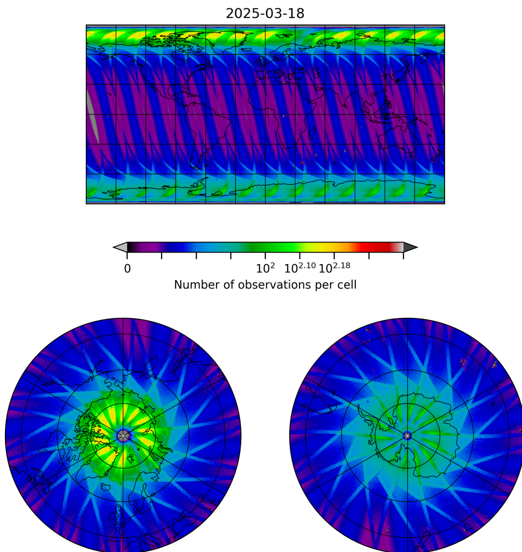
Figure 10: Map of the number of observations for 2025-03-18 to 2025-03-19
