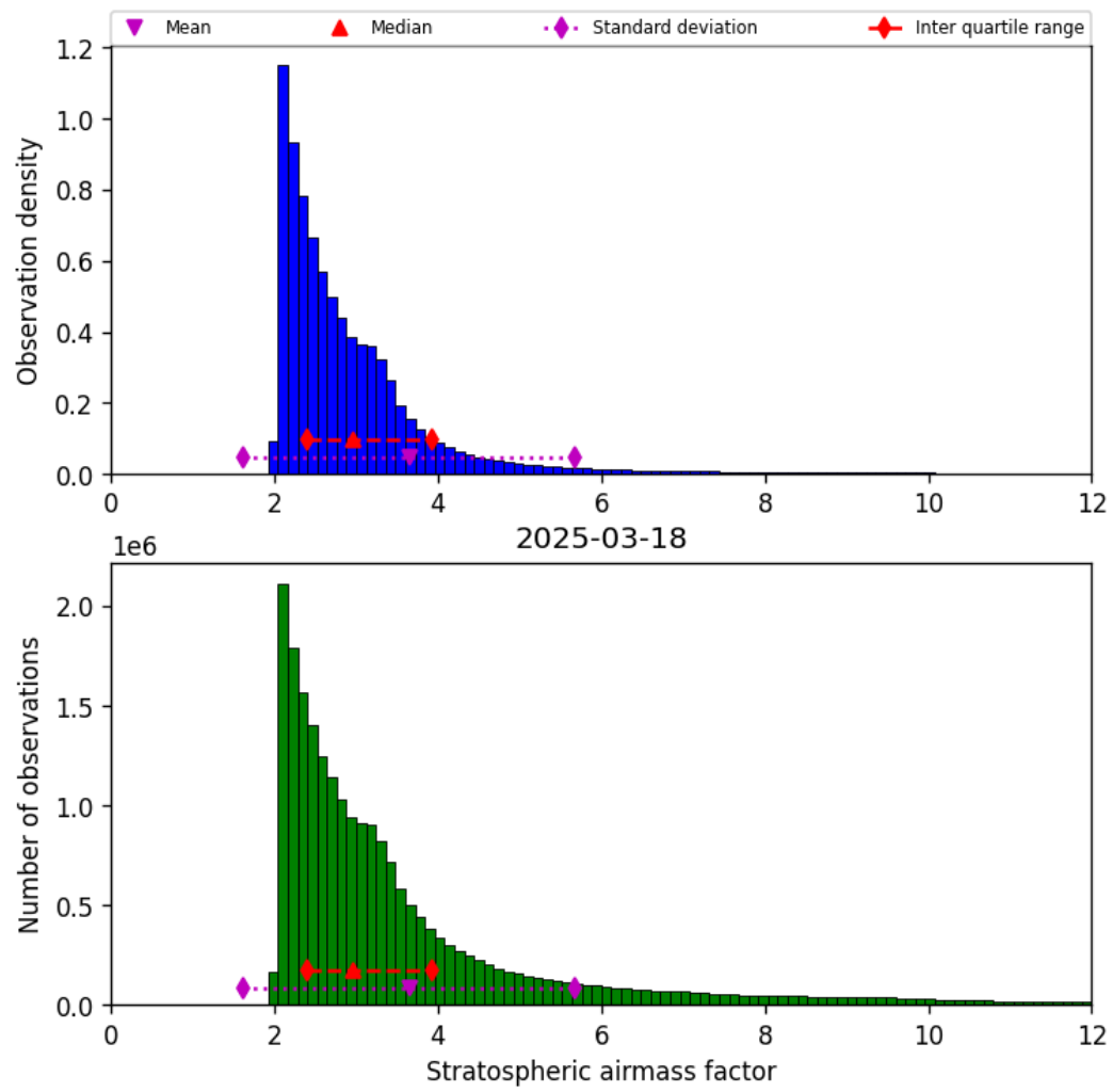
Figure 44: Histogram of “Stratospheric airmass factor” for 2025-03-18 to 2025-03-19
