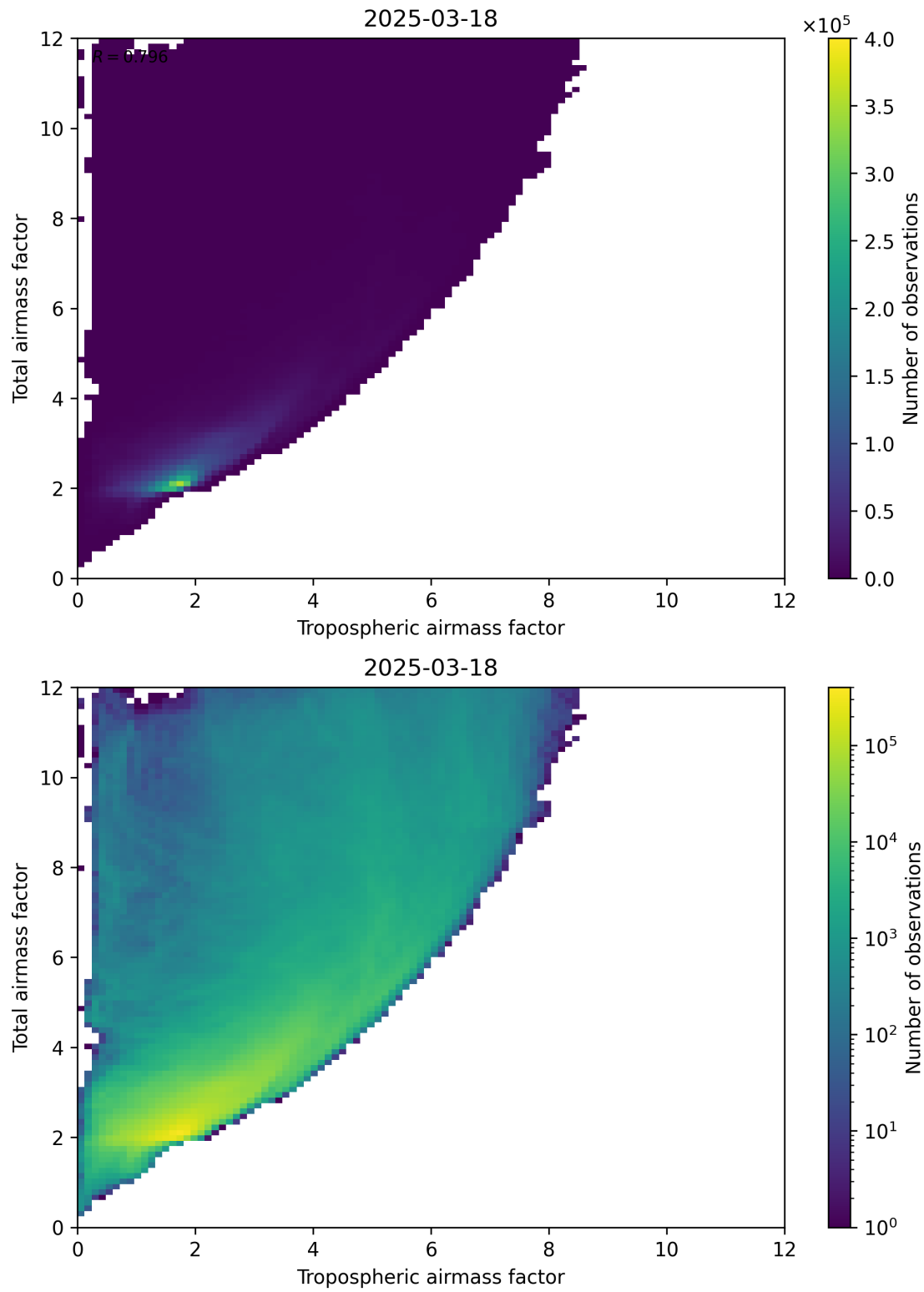
Figure 72: Scatter density plot of “Tropospheric airmass factor” against “Total airmass factor” for 2025-03-18 to 2025-03-19.
