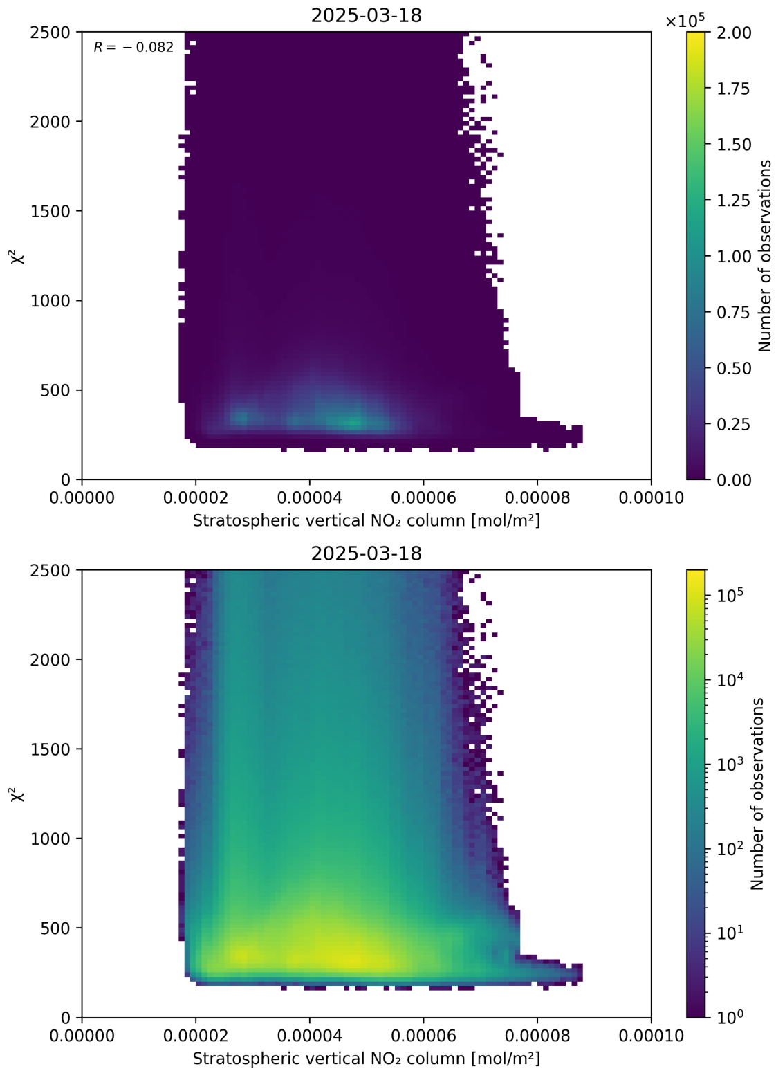
Figure 97: Scatter density plot of “Stratospheric vertical NO 2 column” against “ \chi^2 ” for 2025-03-18 to 2025-03-19.
