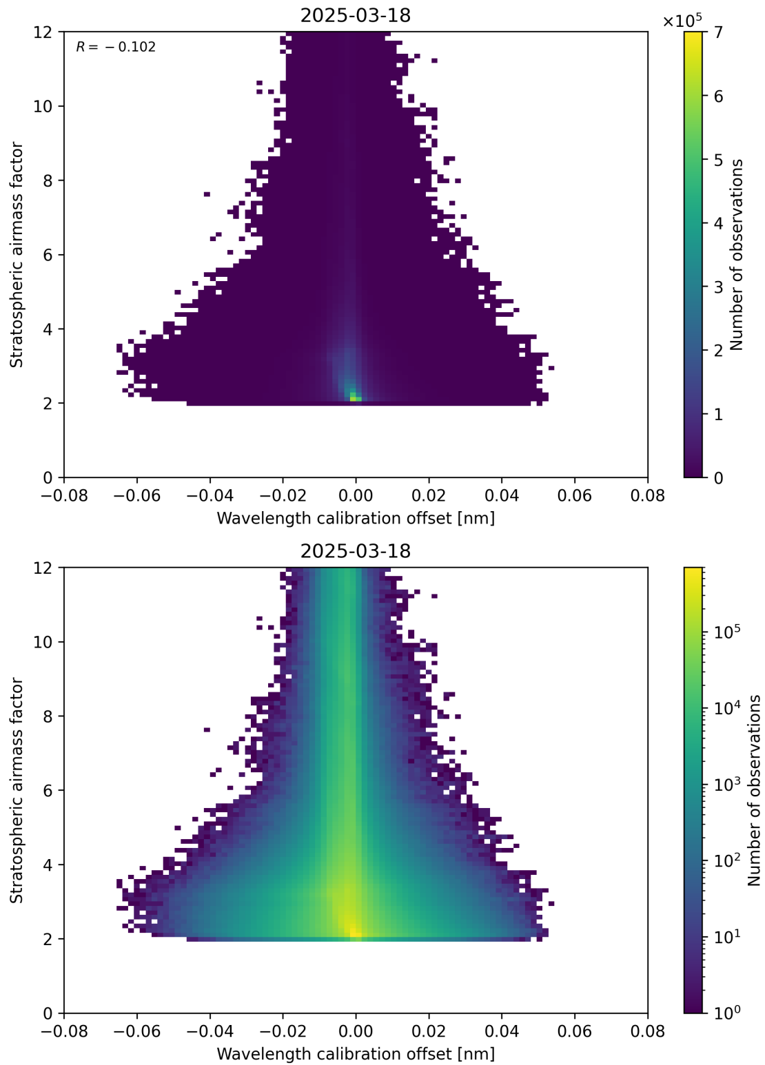
Figure 174: Scatter density plot of “Wavelength calibration offset” against “Stratospheric air mass factor” for 2025-03-18 to 2025-03-19.
