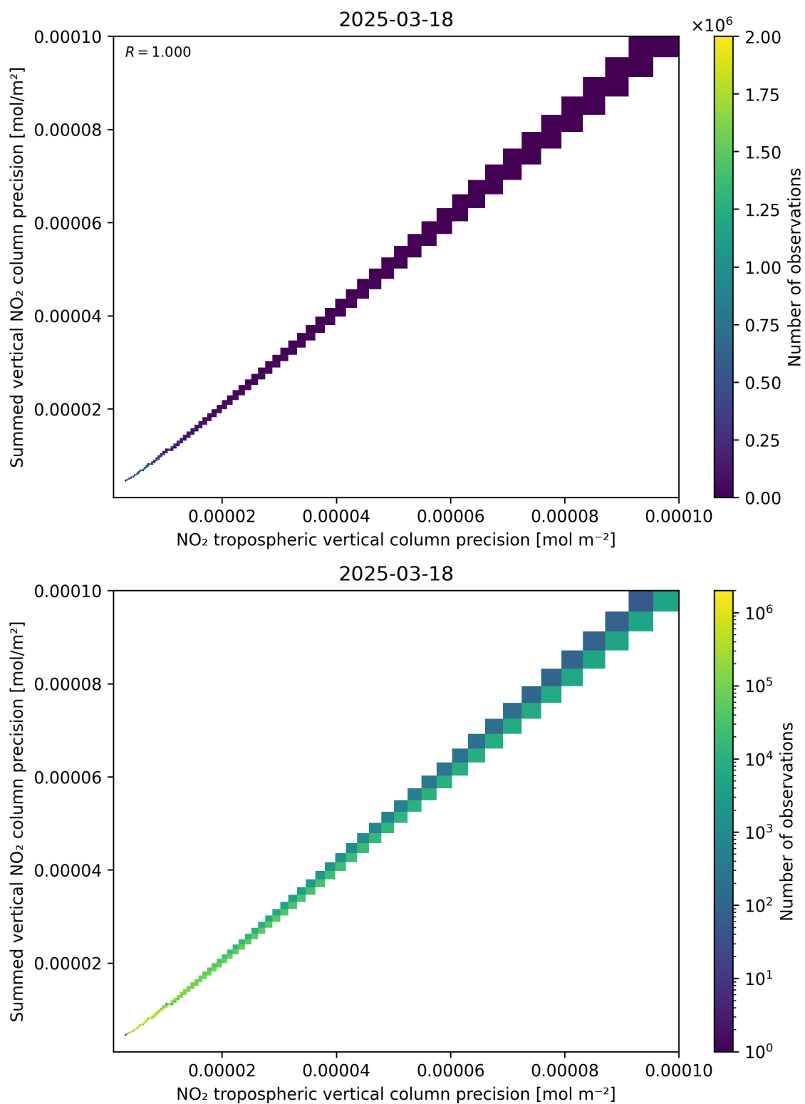
Figure 137: Scatter density plot of “NO 2 tropospheric vertical column precision” against “Summed vertical NO 2 column precision” for 2025-03-18 to 2025-03-19.
