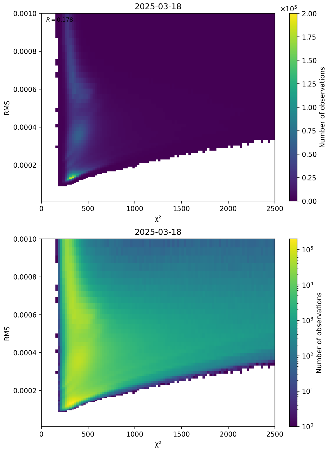
Figure 82: Scatter density plot of “ \chi^2 ” against “RMS” for 2025-03-18 to 2025-03-19.
