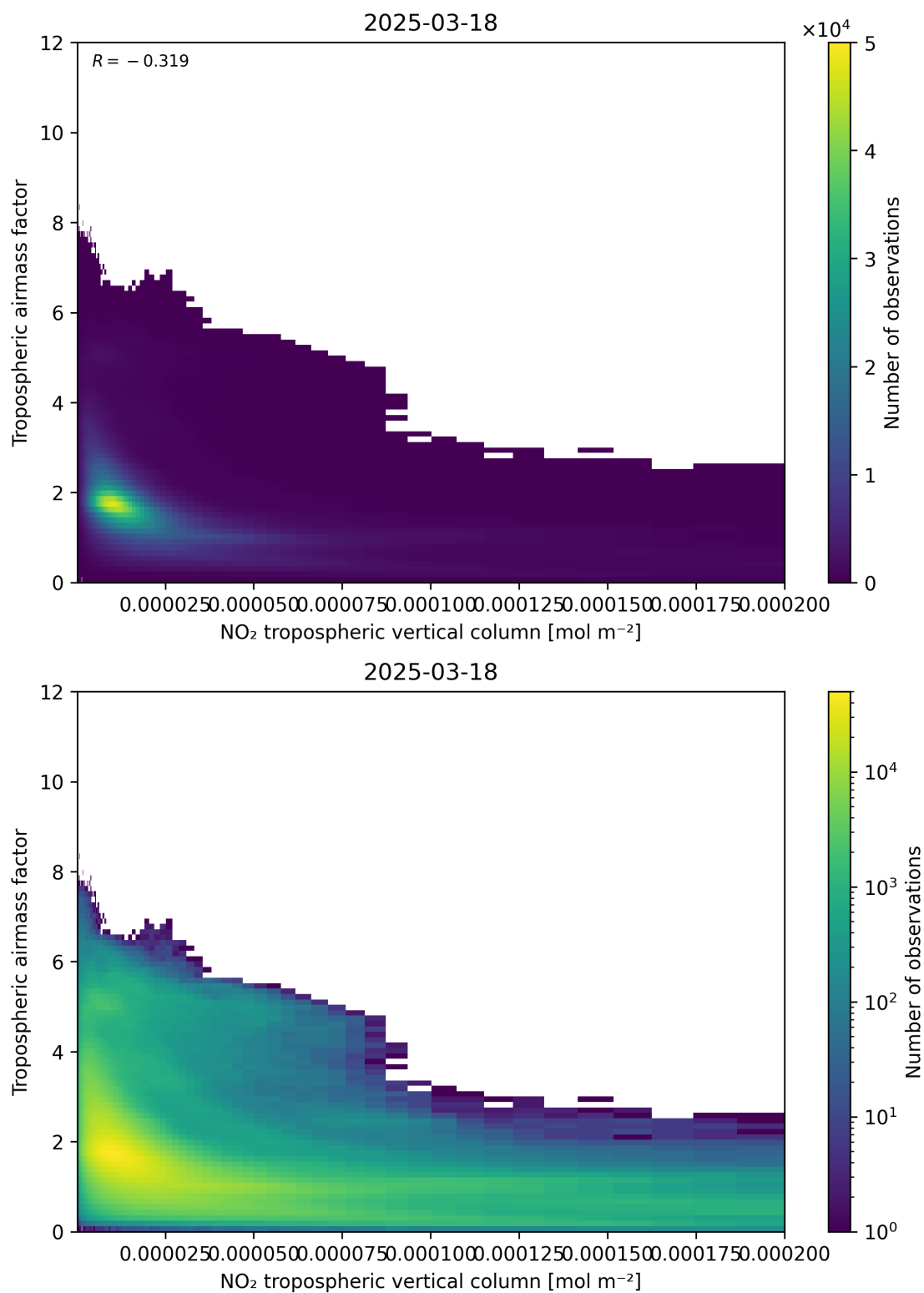
Figure 123: Scatter density plot of “NO 2 tropospheric vertical column” against “Tropospheric air mass factor” for 2025-03-18 to 2025-03-19.
