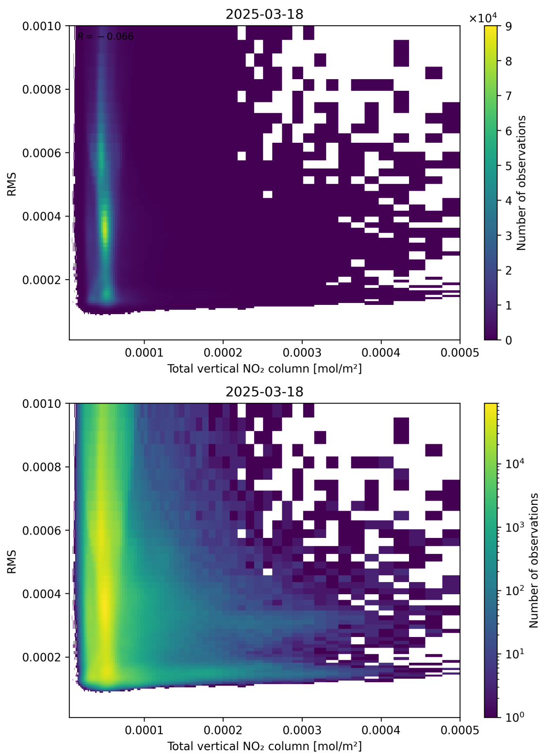
Figure 120: Scatter density plot of “Total vertical NO 2 column” against “RMS” for 2025-03-18 to 2025-03-19.
