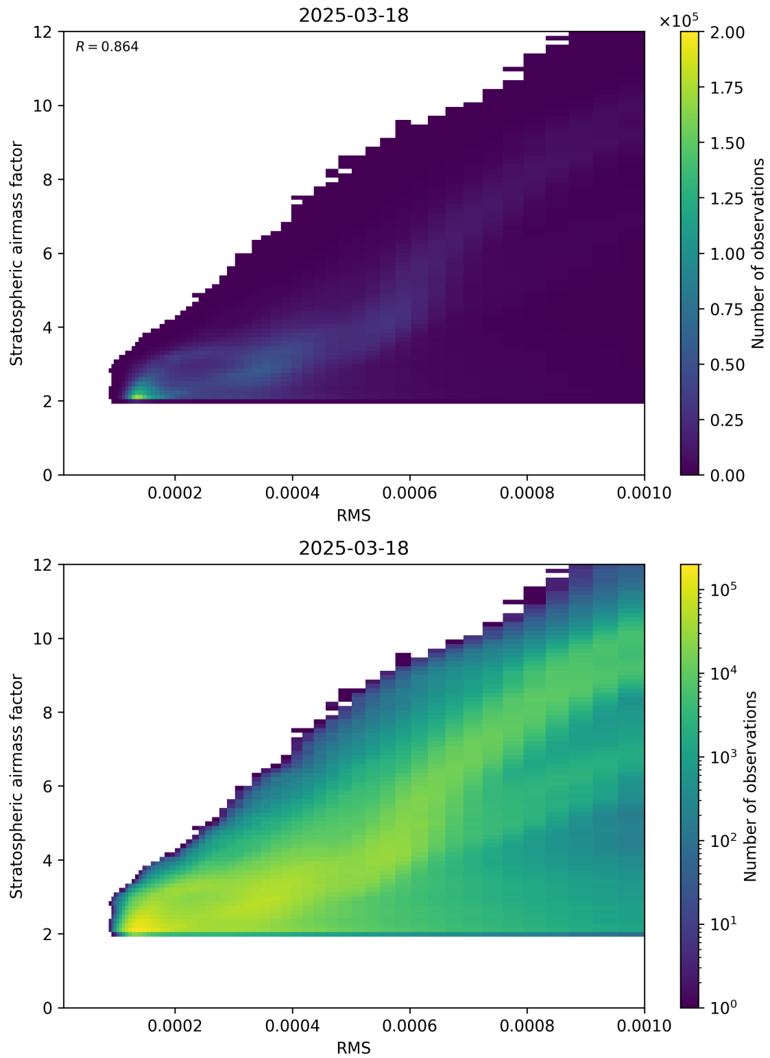
Figure 144: Scatter density plot of “RMS” against “Stratospheric air mass factor” for 2025-03-18 to 2025-03-19.
