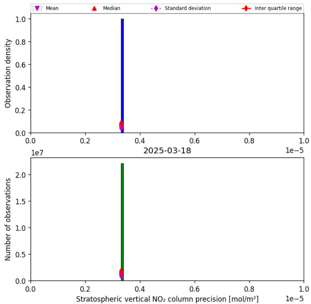
Figure 37: Histogram of “Stratospheric vertical NO 2 column precision” for 2025-03-18 to 2025-03-19
