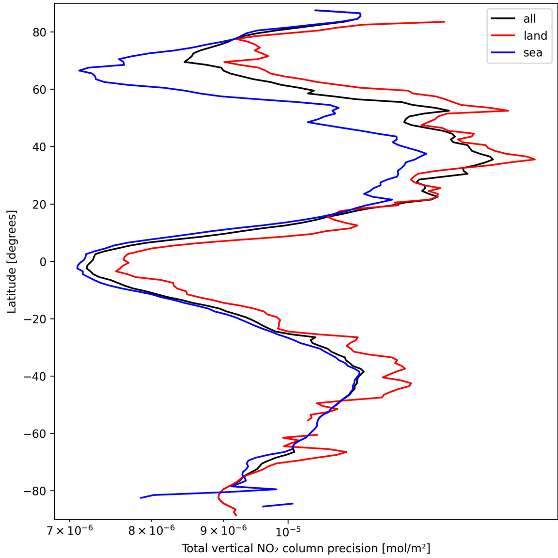
Figure 22: Zonal average of "Total vertical NO 2 column precision" for 2025-03-18 to 2025-03-19.
