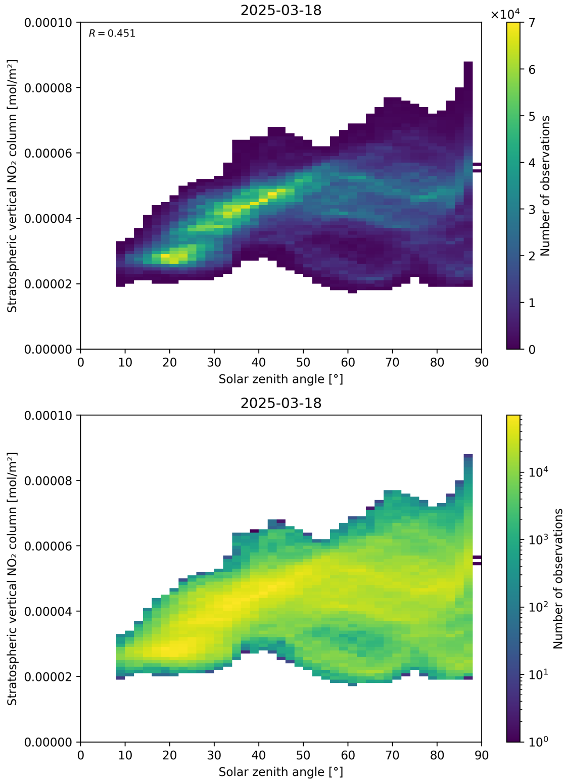
Figure 150: Scatter density plot of “Solar zenith angle” against “Stratospheric vertical NO 2 column” for 2025-03-18 to 2025-03-19.
