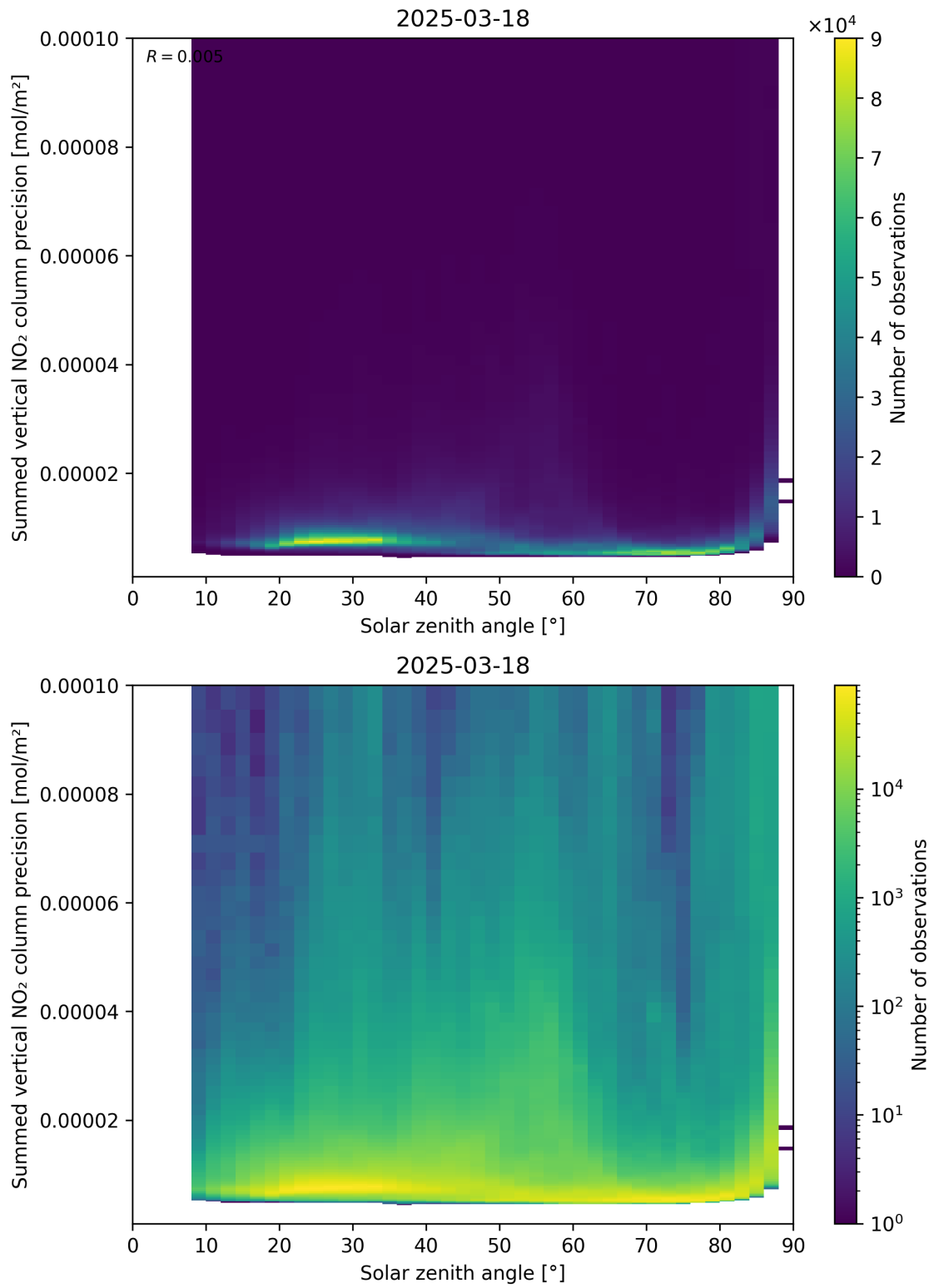
Figure 152: Scatter density plot of “Solar zenith angle” against “Summed vertical NO 2 column precision” for 2025-03-18 to 2025-03-19.
