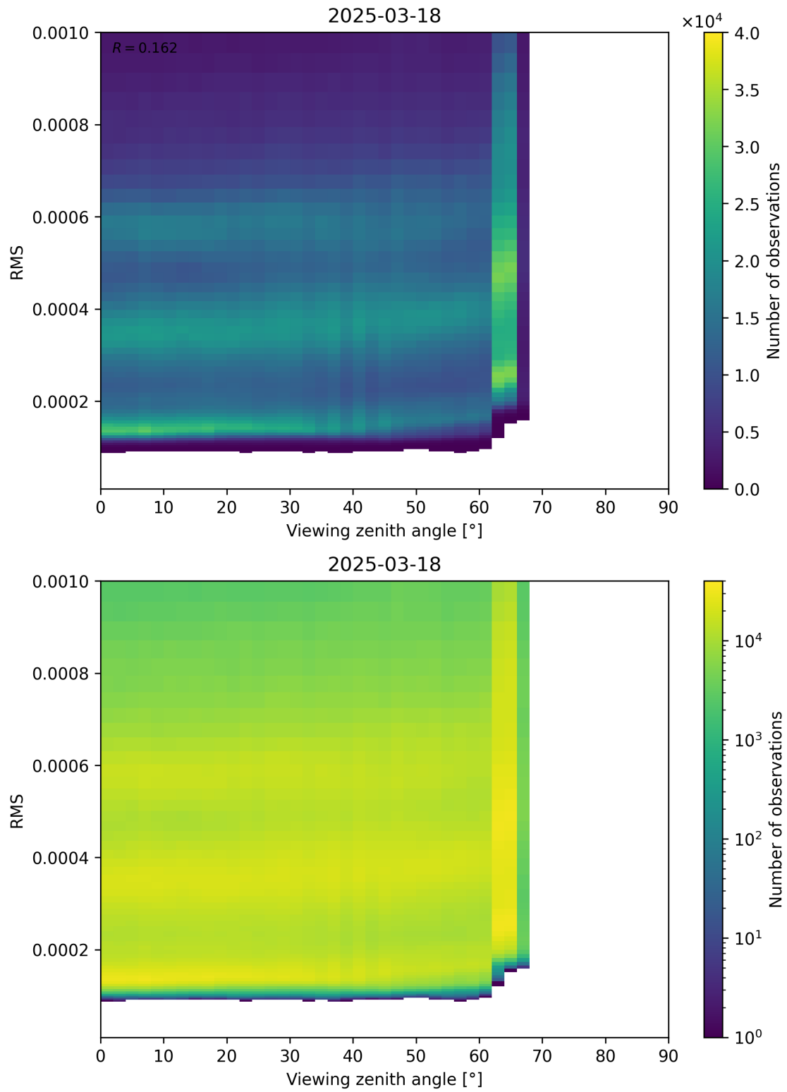
Figure 171: Scatter density plot of “Viewing zenith angle” against “RMS” for 2025-03-18 to 2025-03-19.
