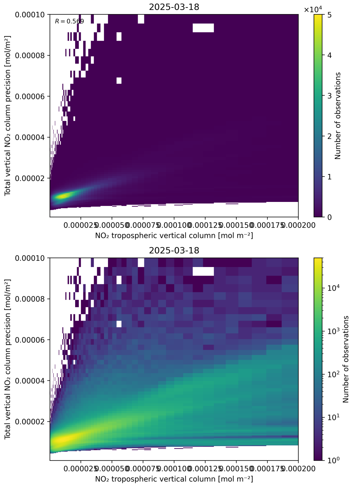
Figure 129: Scatter density plot of “NO 2 tropospheric vertical column” against “Total vertical NO 2 column precision” for 2025-03-18 to 2025-03-19.
