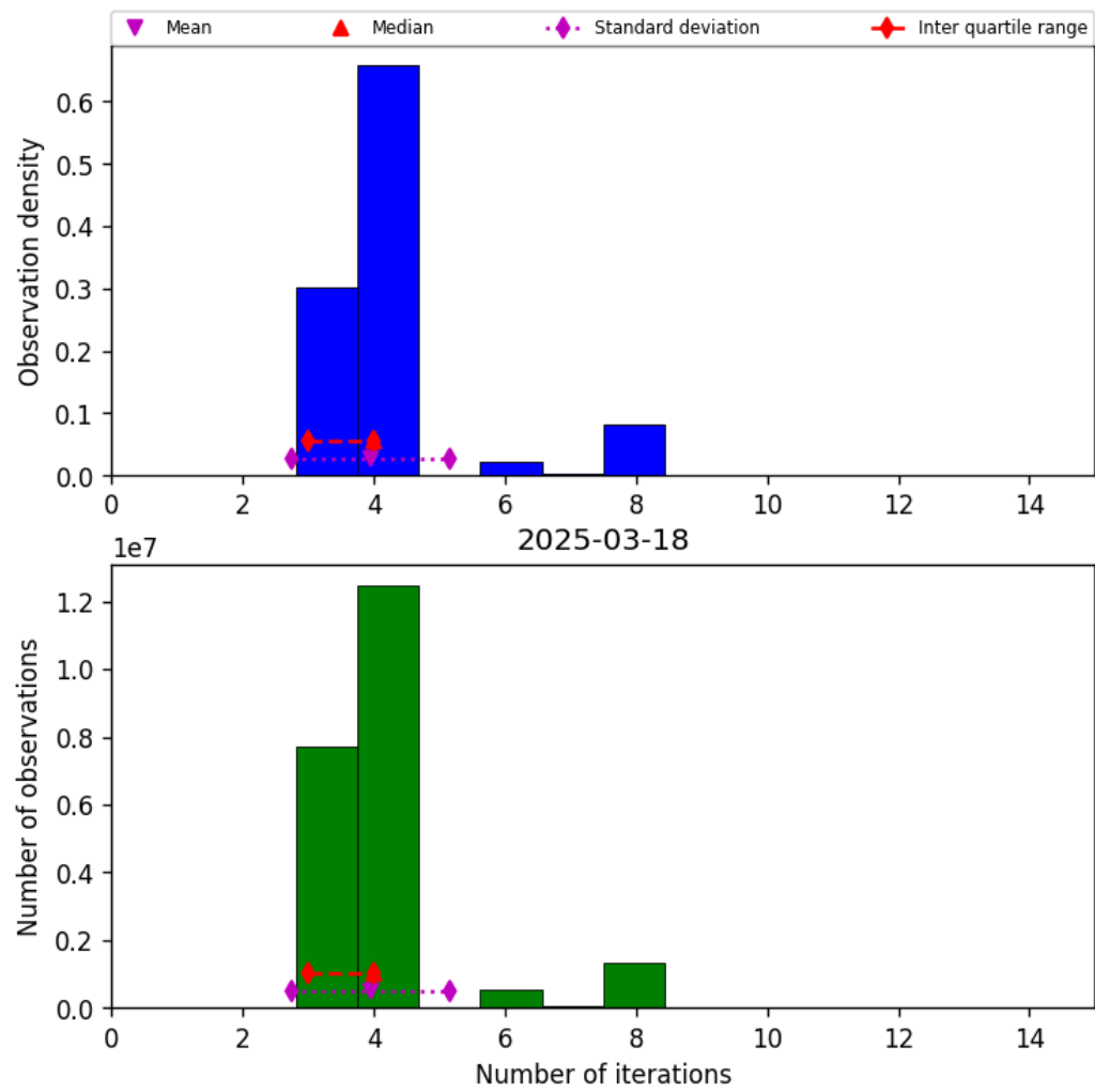
Figure 34: Histogram of “Number of iterations” for 2025-03-18 to 2025-03-19
