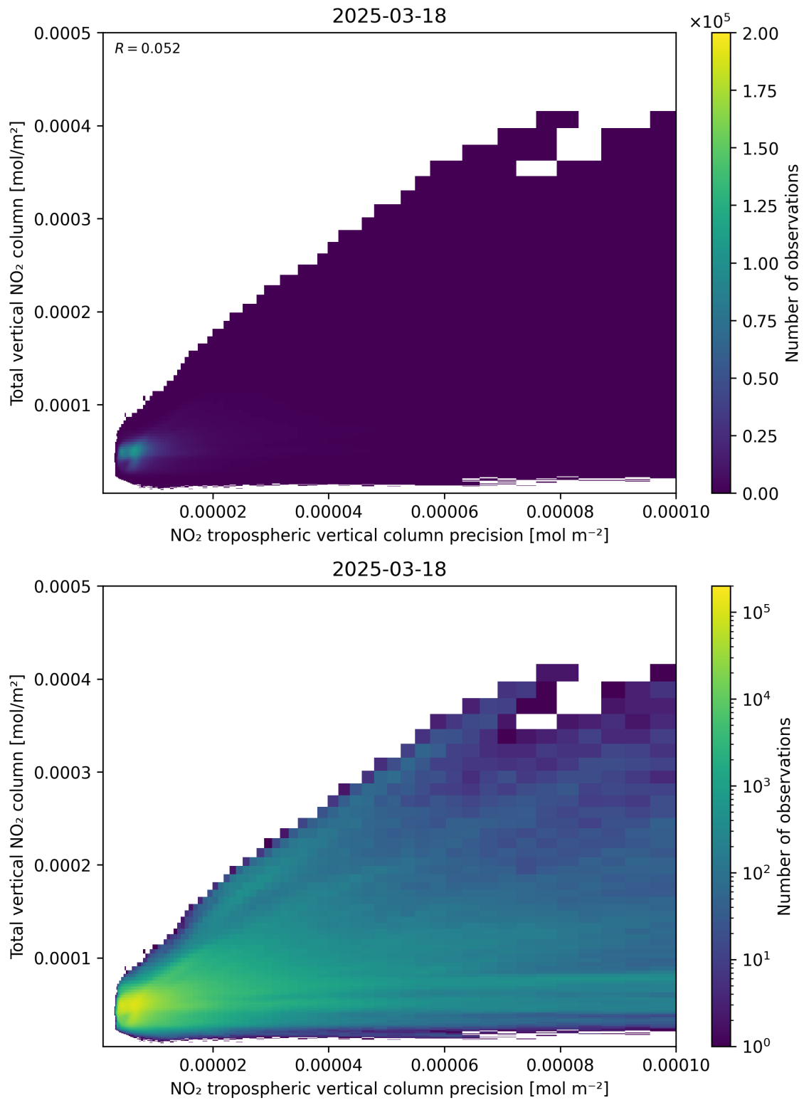
Figure 138: Scatter density plot of “NO 2 tropospheric vertical column precision” against “Total vertical NO 2 column” for 2025-03-18 to 2025-03-19.
