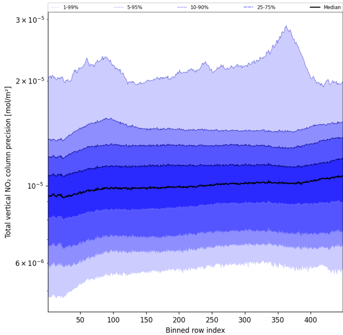
Figure 56: Along track statistics of “Total vertical NO 2 column precision” for 2025-03-18 to 2025-03-19
