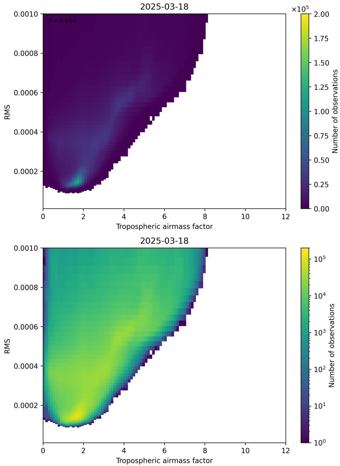
Figure 79: Scatter density plot of “Tropospheric airmass factor” against “RMS” for 2025-03-18 to 2025-03-19.
