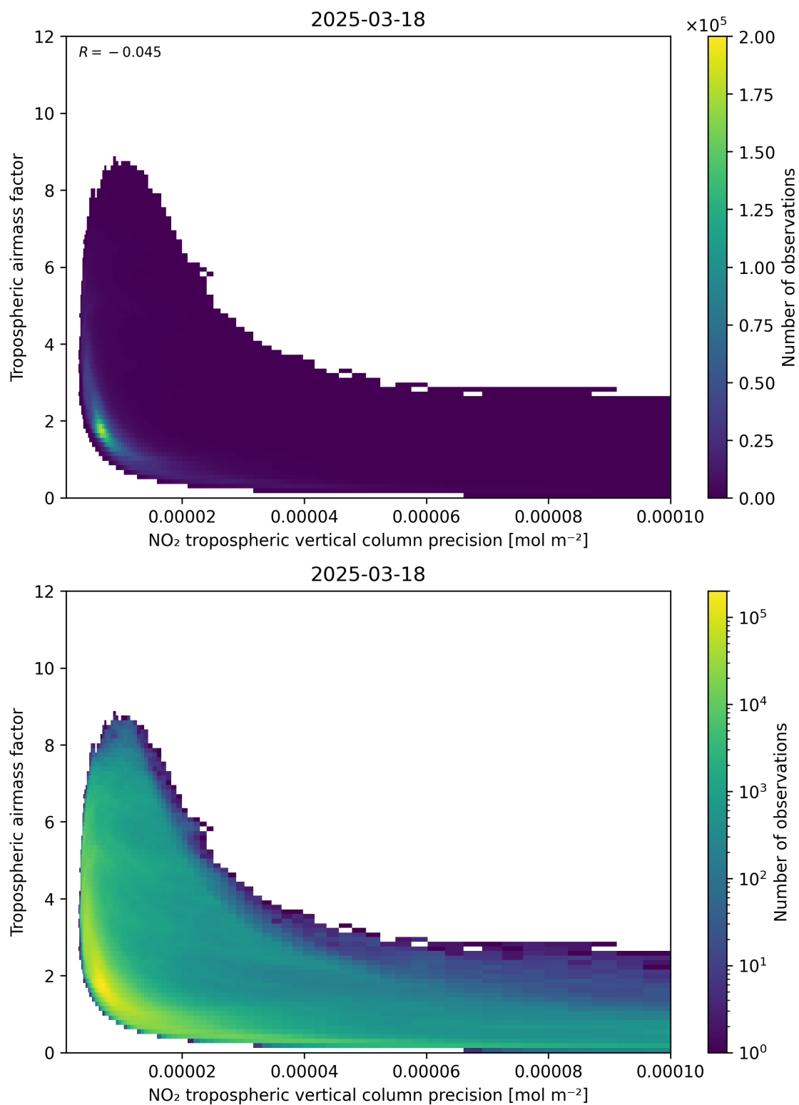
Figure 133: Scatter density plot of “NO 2 tropospheric vertical column precision” against “Tropospheric air mass factor” for 2025-03-18 to 2025-03-19.
