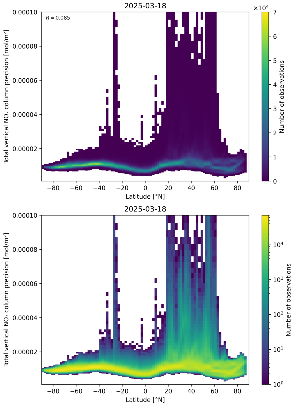
Figure 91: Scatter density plot of “Latitude” against “Total vertical NO 2 column precision” for 2025-03-18 to 2025-03-19.
