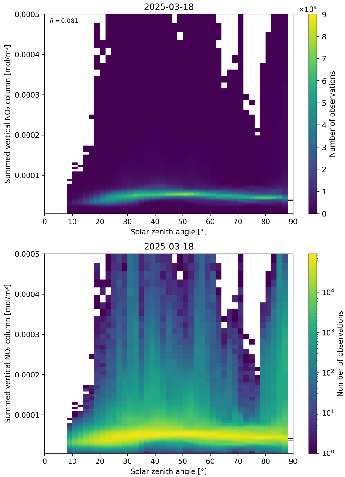
Figure 151: Scatter density plot of “Solar zenith angle” against “Summed vertical NO 2 column” for 2025-03-18 to 2025-03-19.
