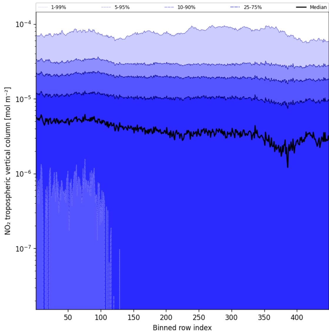
Figure 46: Along track statistics of “NO 2 tropospheric vertical column” for 2025-03-18 to 2025-03-19
