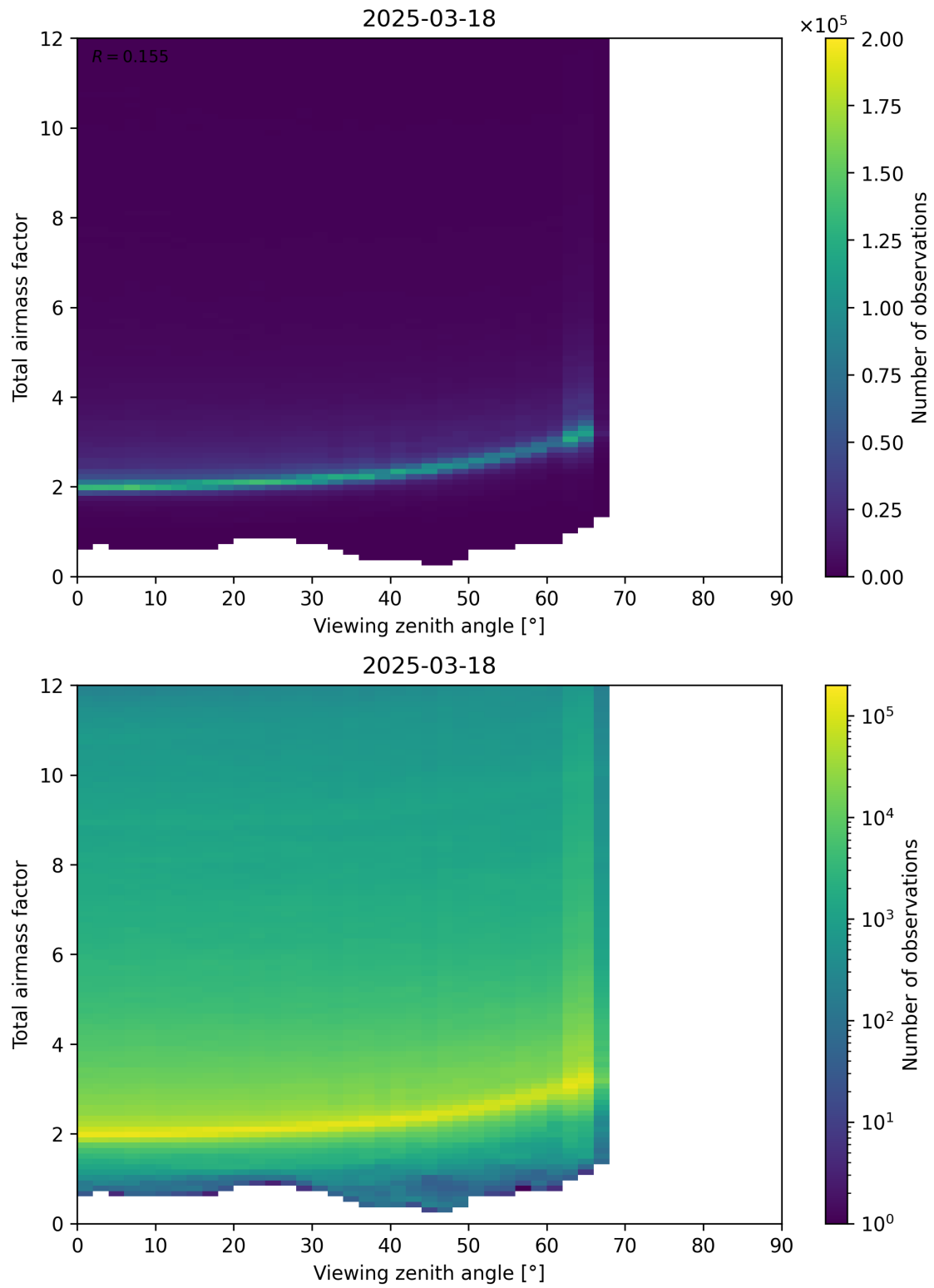
Figure 160: Scatter density plot of “Viewing zenith angle” against “Total airmass factor” for 2025-03-18 to 2025-03-19.
