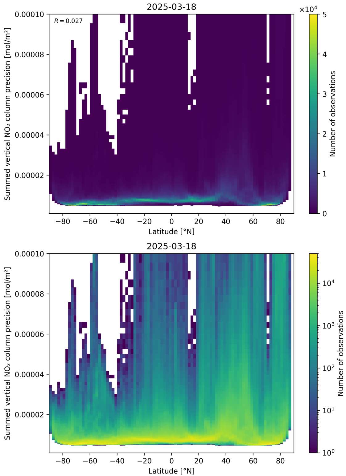
Figure 89: Scatter density plot of “Latitude” against “Summed vertical NO 2 column precision” for 2025-03-18 to 2025-03-19.
