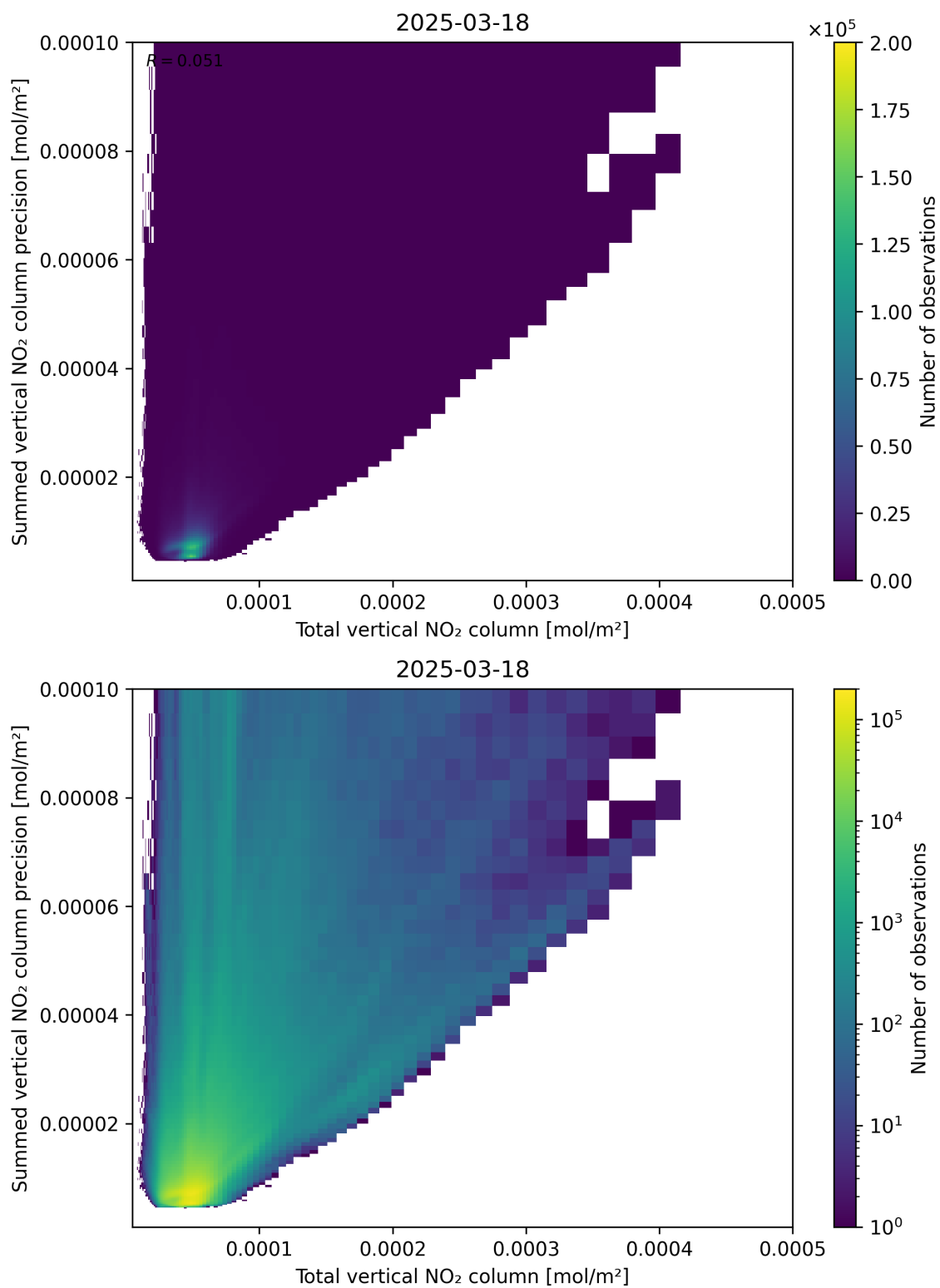
Figure 113: Scatter density plot of “Total vertical NO 2 column” against “Summed vertical NO 2 column precision” for 2025-03-18 to 2025-03-19.
