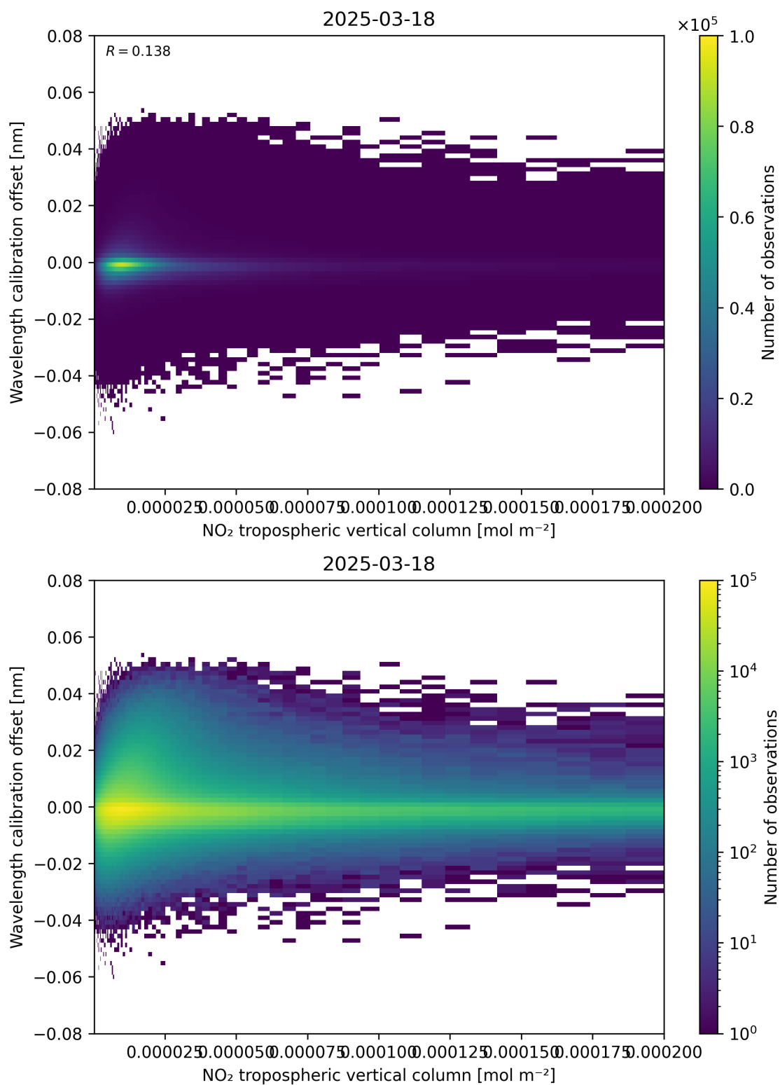
Figure 143: Scatter density plot of “NO 2 tropospheric vertical column” against “Wavelength calibration offset” for 2025-03-18 to 2025-03-19.
