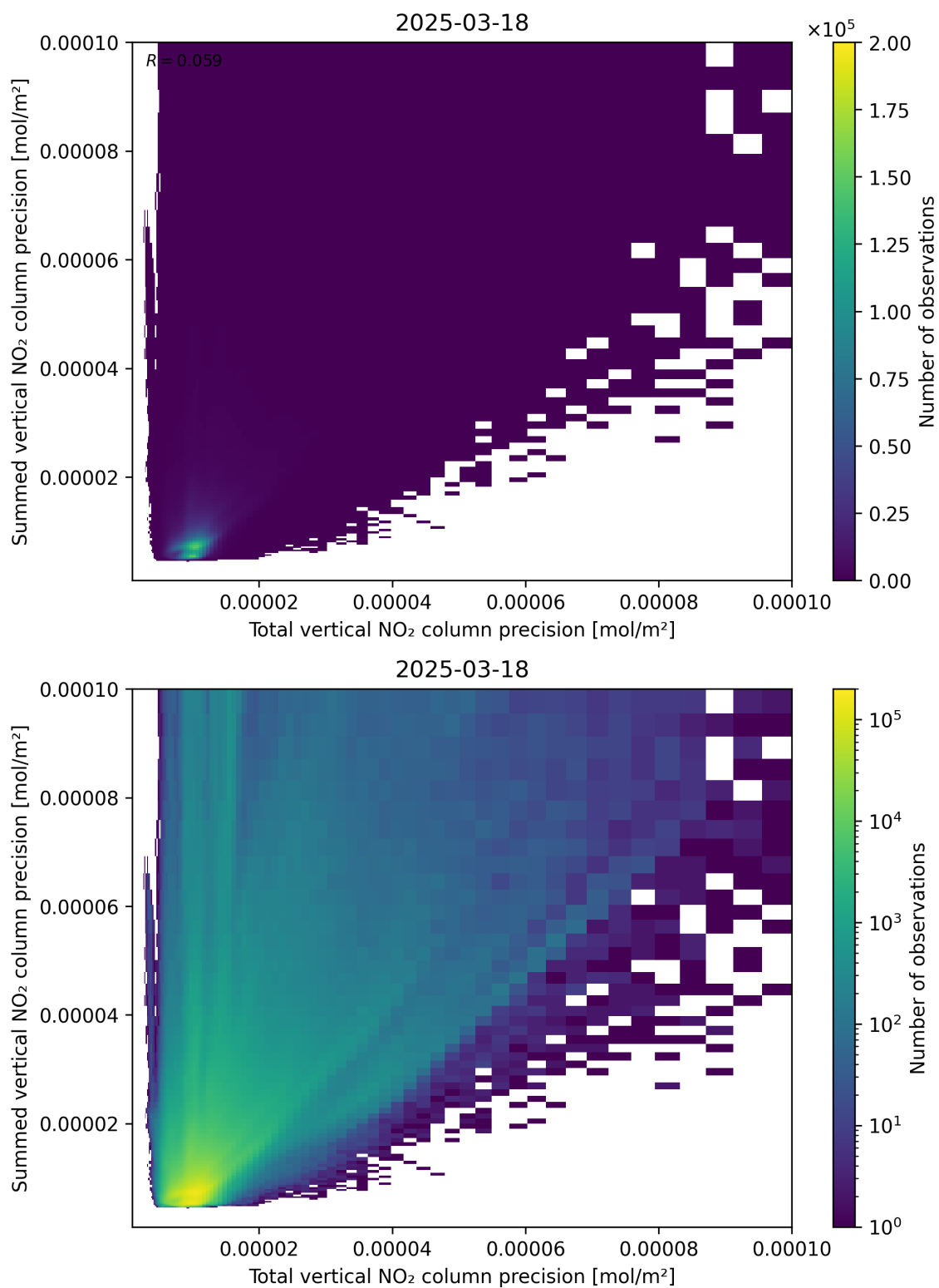
Figure 118: Scatter density plot of “Total vertical NO 2 column precision” against “Summed vertical NO 2 column precision” for 2025-03-18 to 2025-03-19.
