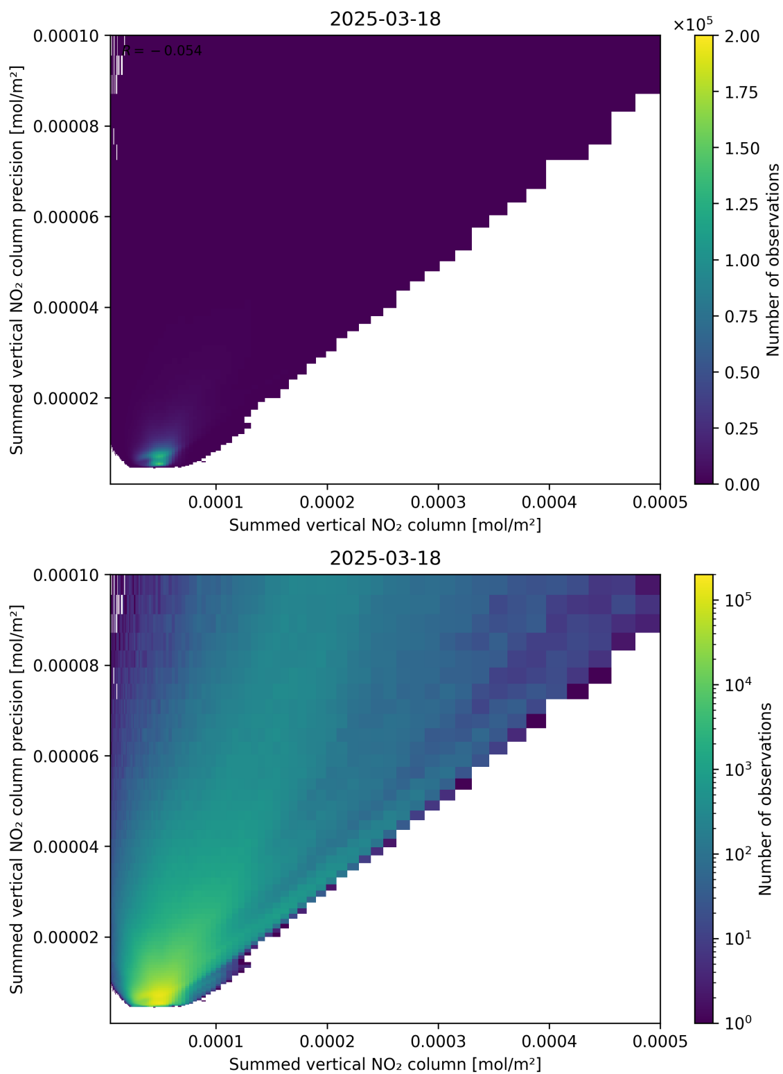
Figure 105: Scatter density plot of “Summed vertical NO 2 column” against “Summed vertical NO 2 column precision” for 2025-03-18 to 2025-03-19.
