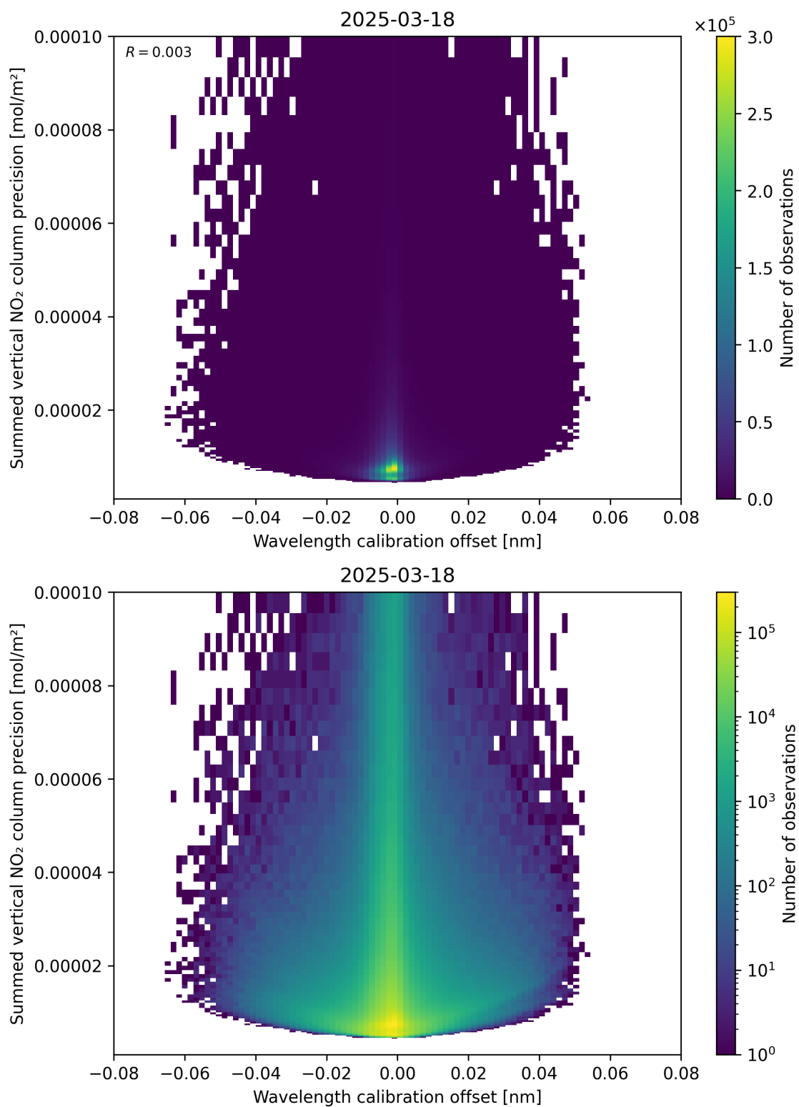
Figure 178: Scatter density plot of “Wavelength calibration offset” against “Summed vertical NO 2 column precision” for 2025-03-18 to 2025-03-19.
