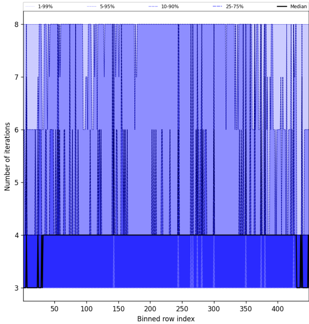
Figure 51: Along track statistics of “Number of iterations” for 2025-03-18 to 2025-03-19
