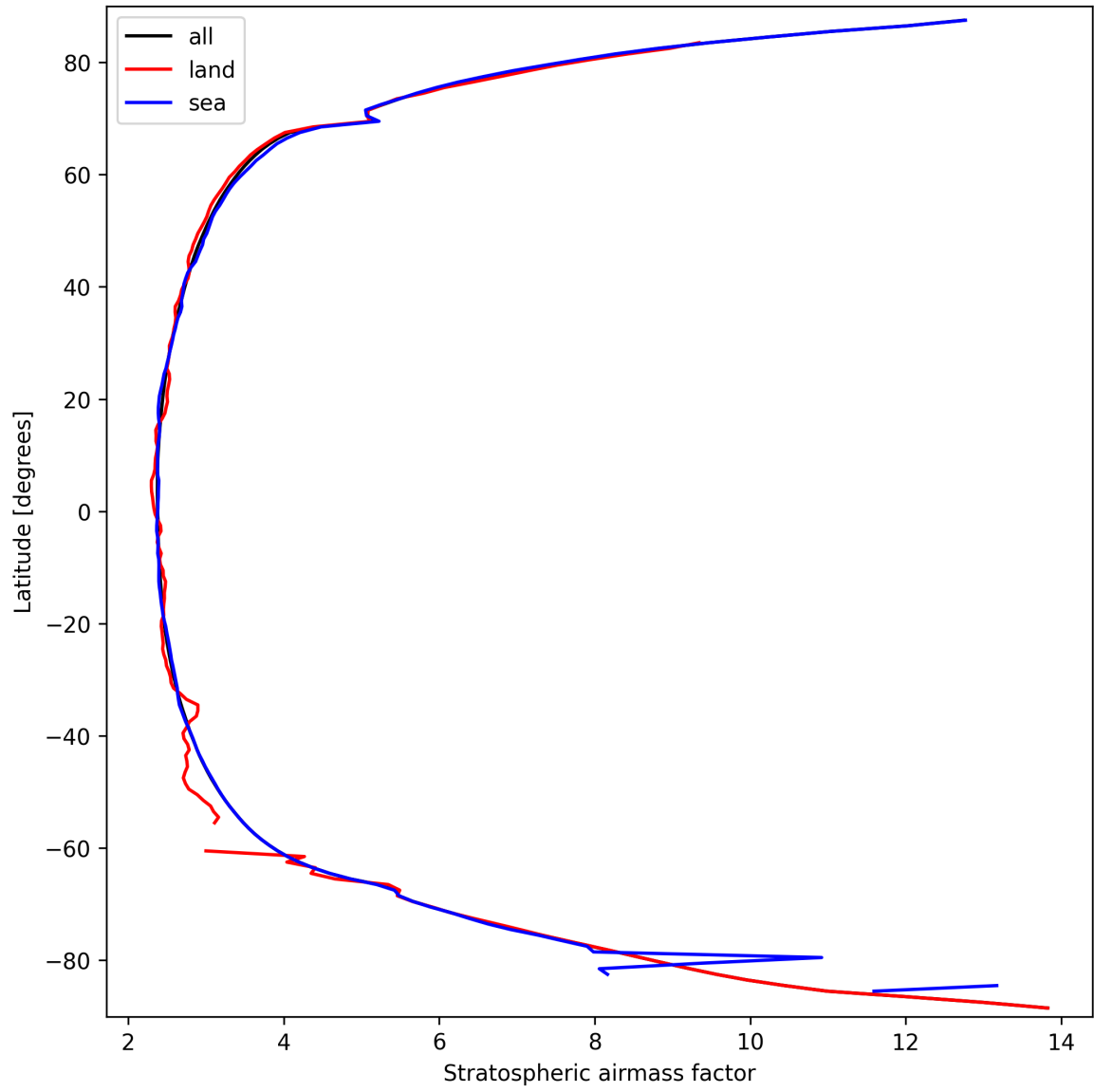
Figure 27: Zonal average of “Stratospheric airmass factor” for 2025-03-18 to 2025-03-19.
