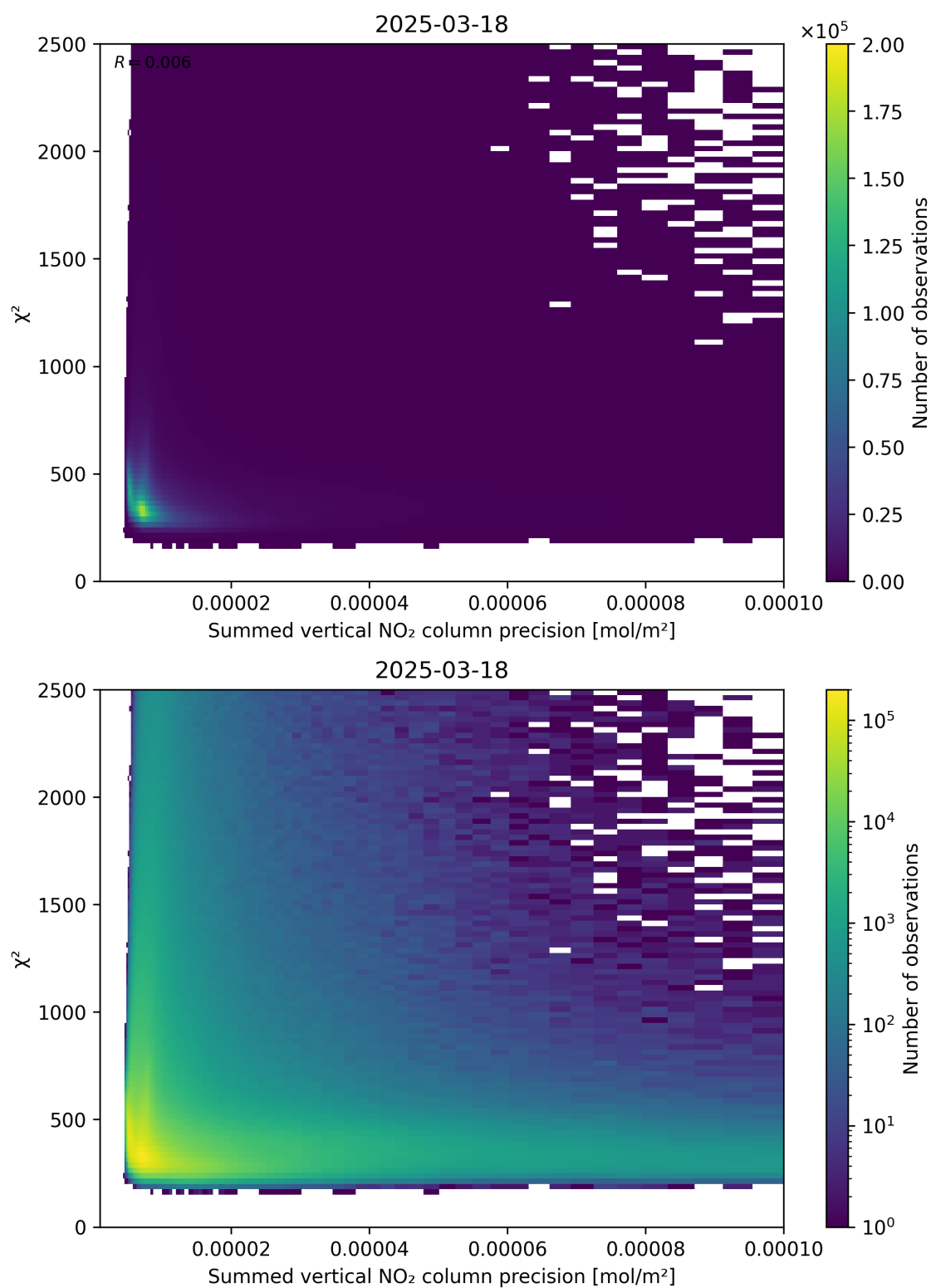
Figure 107: Scatter density plot of “Summed vertical NO 2 column precision” against “ \chi^2 ” for 2025-03-18 to 2025-03-19.
