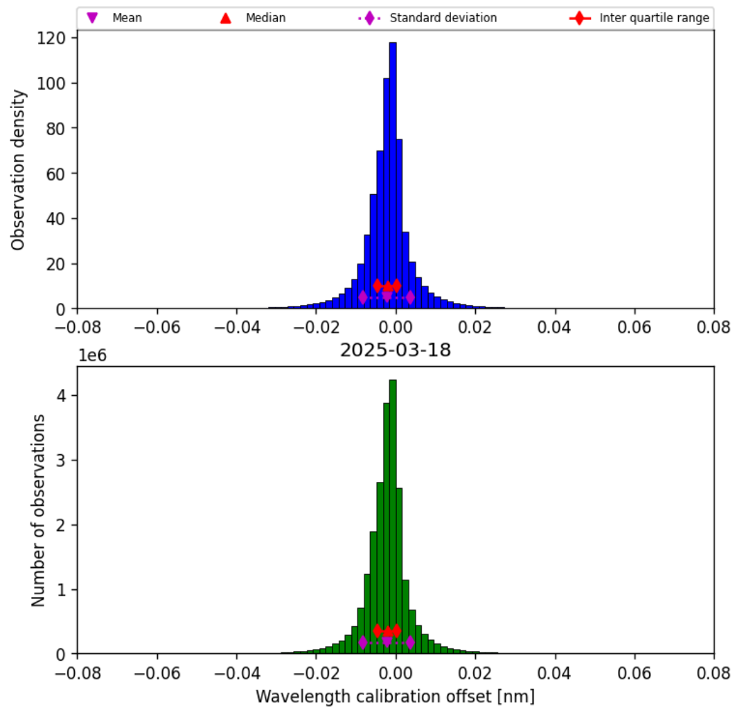
Figure 35: Histogram of “Wavelength calibration offset” for 2025-03-18 to 2025-03-19
