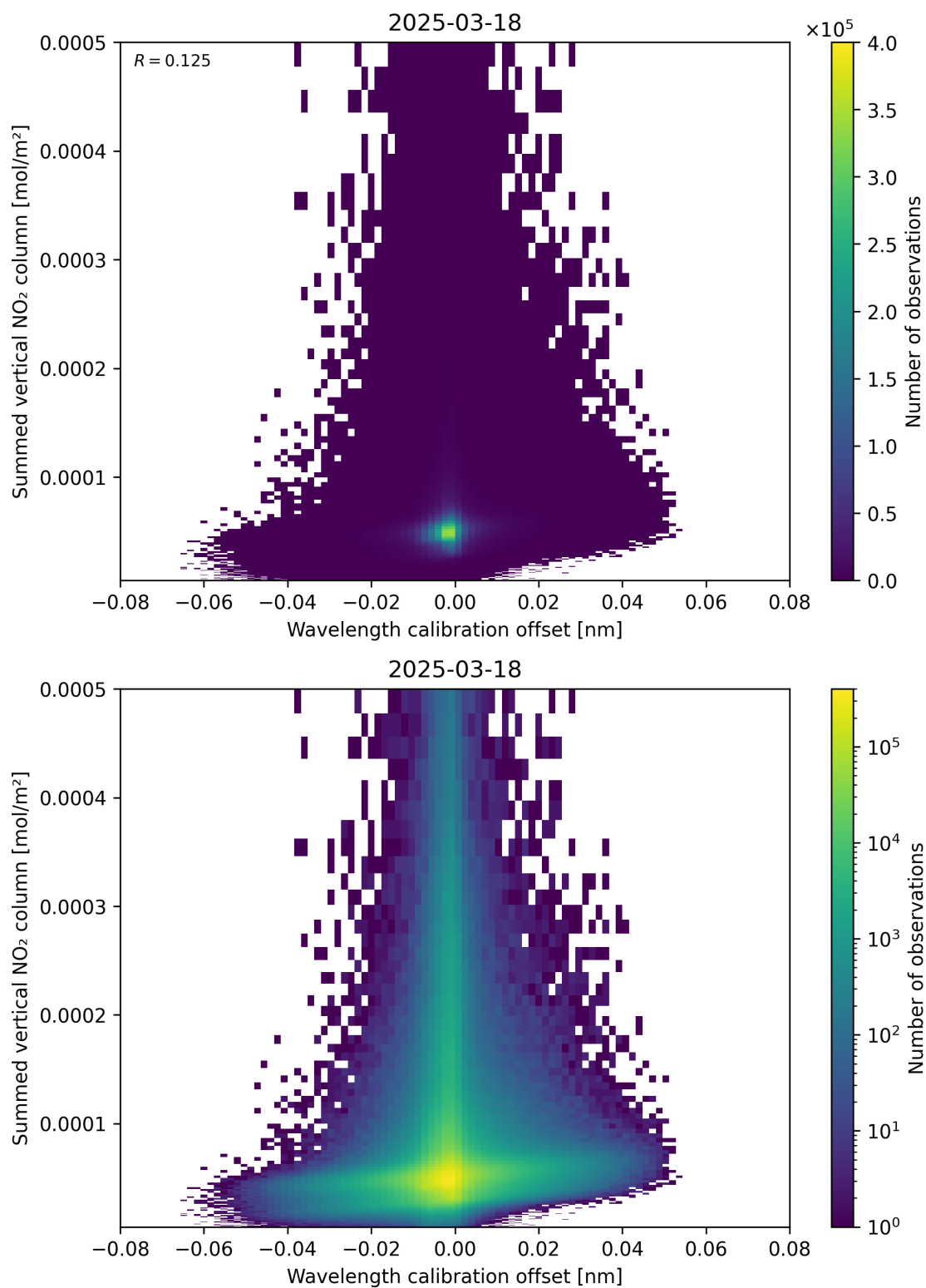
Figure 177: Scatter density plot of “Wavelength calibration offset” against “Summed vertical NO 2 column” for 2025-03-18 to 2025-03-19.
