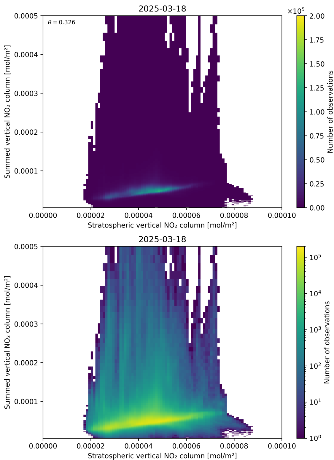
Figure 98: Scatter density plot of “Stratospheric vertical NO 2 column” against “Summed vertical NO 2 column” for 2025-03-18 to 2025-03-19.
