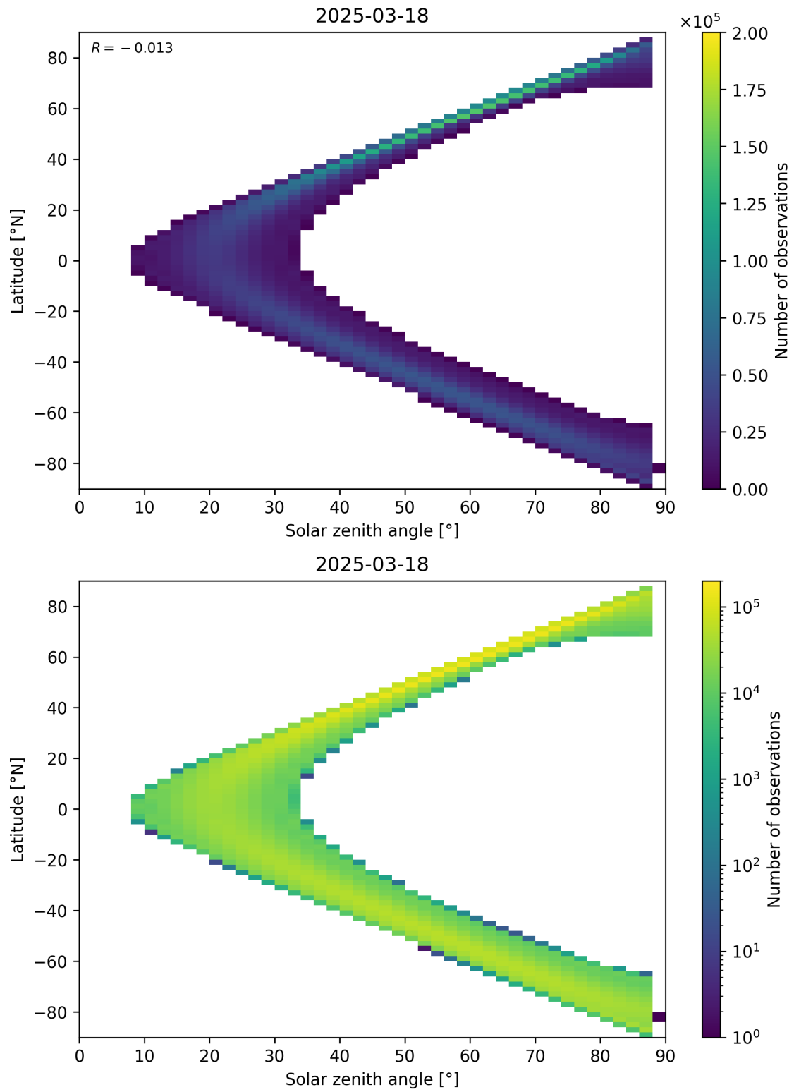
Figure 149: Scatter density plot of “Solar zenith angle” against “Latitude” for 2025-03-18 to 2025-03-19.
