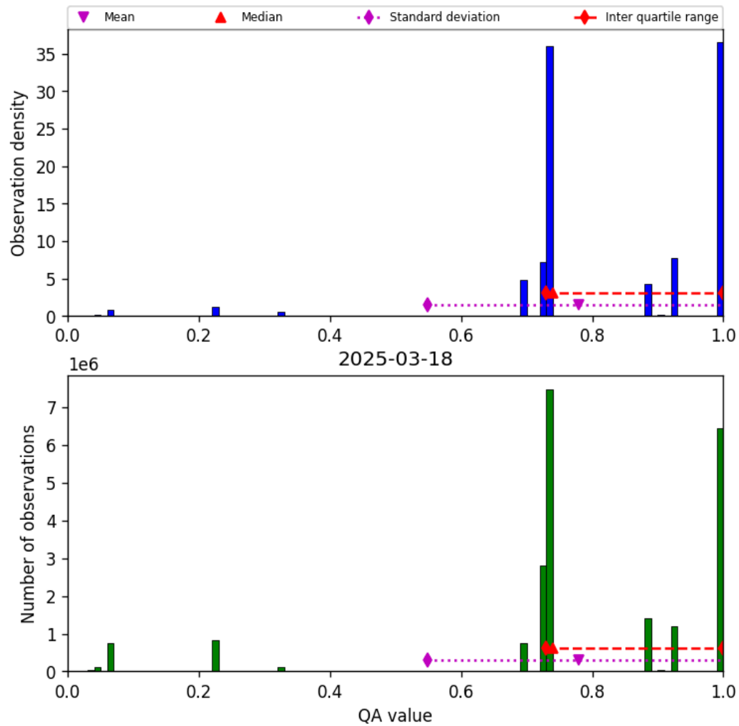
Figure 28: Histogram of “QA value” for 2025-03-18 to 2025-03-19
