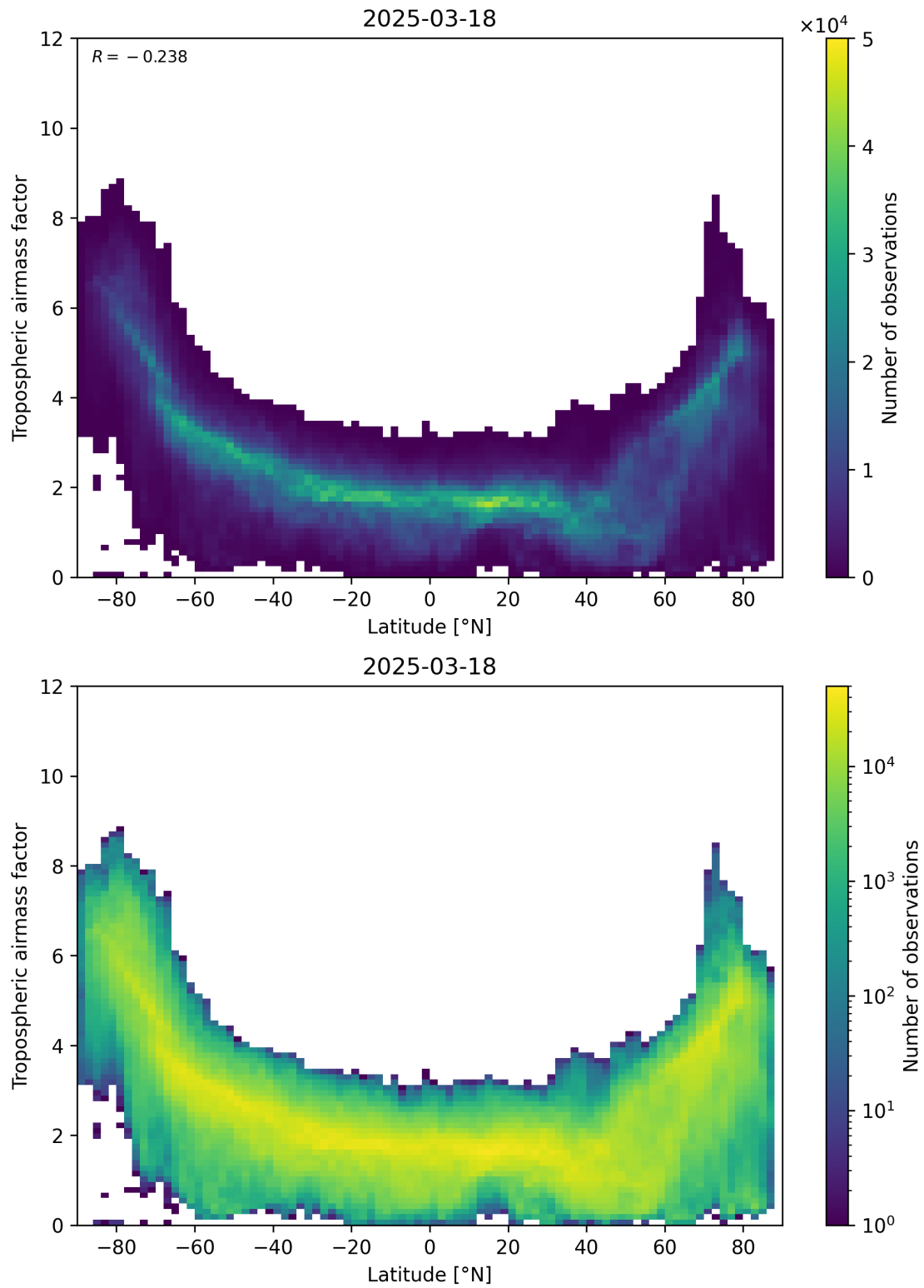
Figure 85: Scatter density plot of “Latitude” against “Tropospheric airmass factor” for 2025-03-18 to 2025-03-19.
