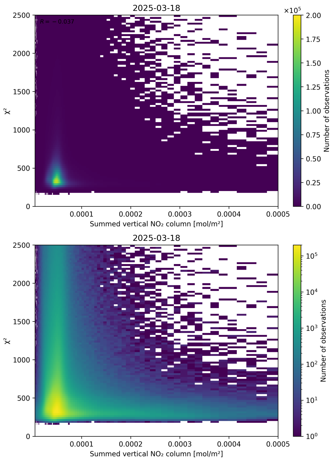
Figure 104: Scatter density plot of “Summed vertical NO 2 column” against “ \chi^2 ” for 2025-03-18 to 2025-03-19.
