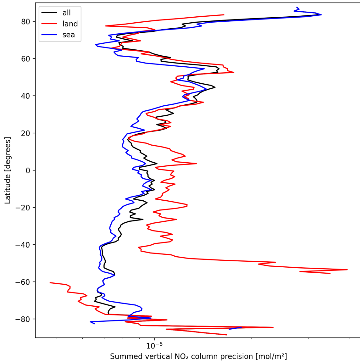
Figure 24: Zonal average of “Summed vertical NO 2 column precision” for 2025-03-18 to 2025-03-19.
