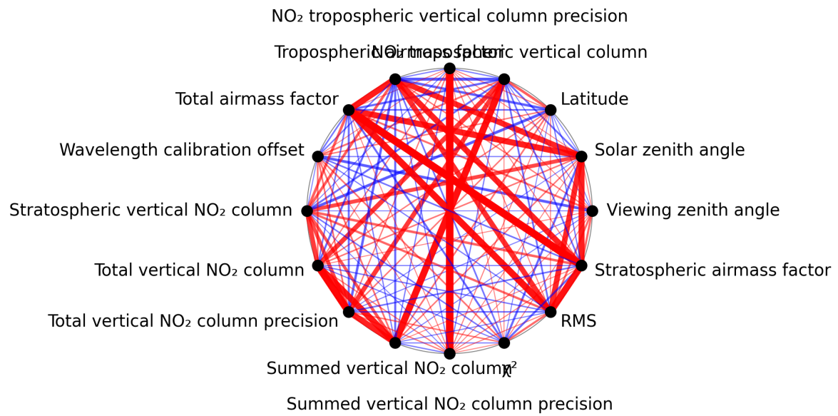
Figure 1: Map of correlation graph for 2025-03-18 to 2025-03-19.
