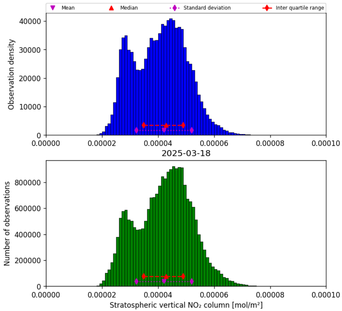
Figure 36: Histogram of “Stratospheric vertical NO 2 column” for 2025-03-18 to 2025-03-19
