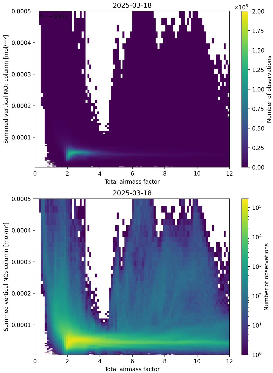
Figure 65: Scatter density plot of “Total airmass factor” against “Summed vertical NO 2 column” for 2025-03-18 to 2025-03-19.
