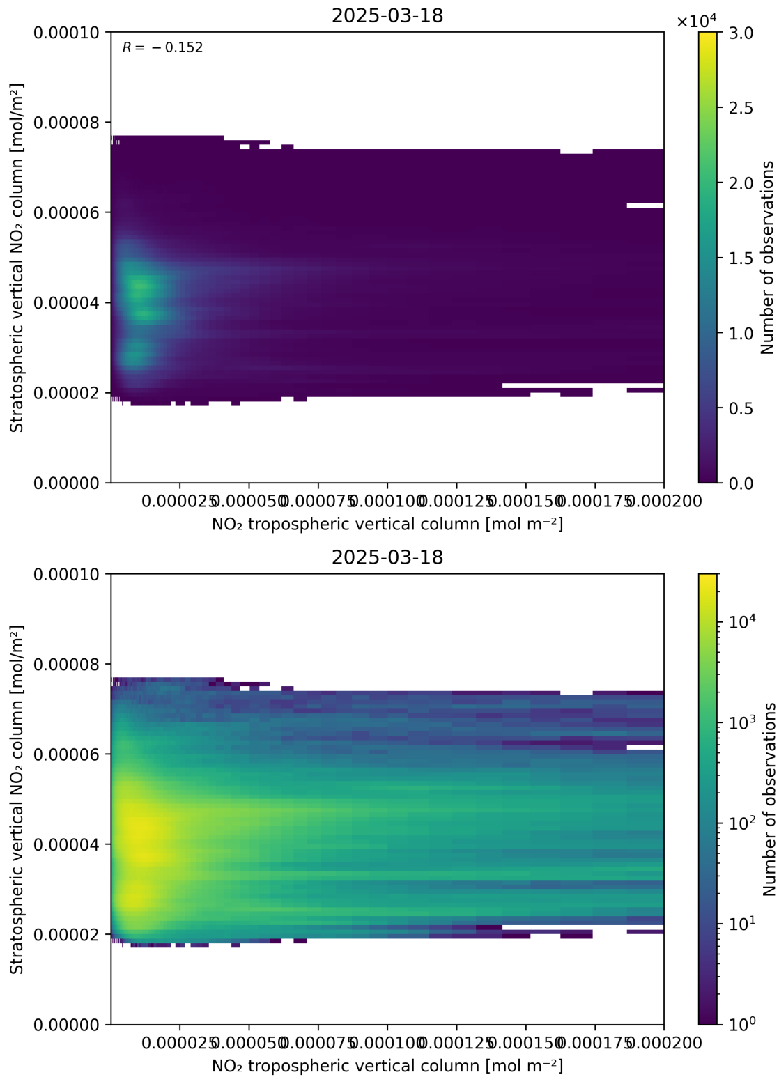
Figure 125: Scatter density plot of “NO 2 tropospheric vertical column” against “Stratospheric vertical NO 2 column” for 2025-03-18 to 2025-03-19.
