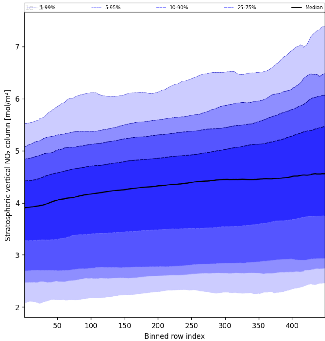
Figure 53: Along track statistics of “Stratospheric vertical NO 2 column” for 2025-03-18 to 2025-03-19
