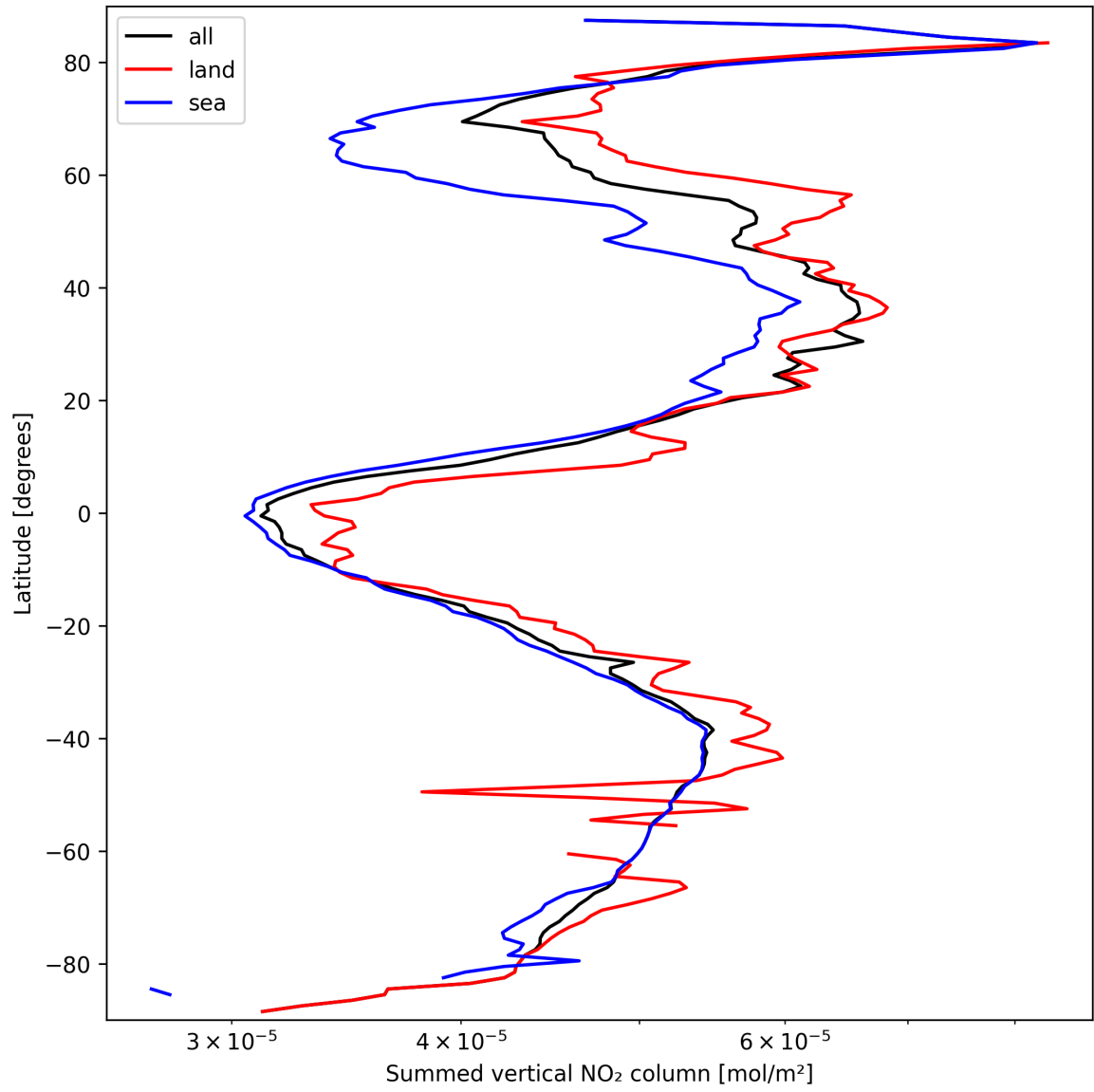
Figure 23: Zonal average of “Summed vertical NO 2 column” for 2025-03-18 to 2025-03-19.
