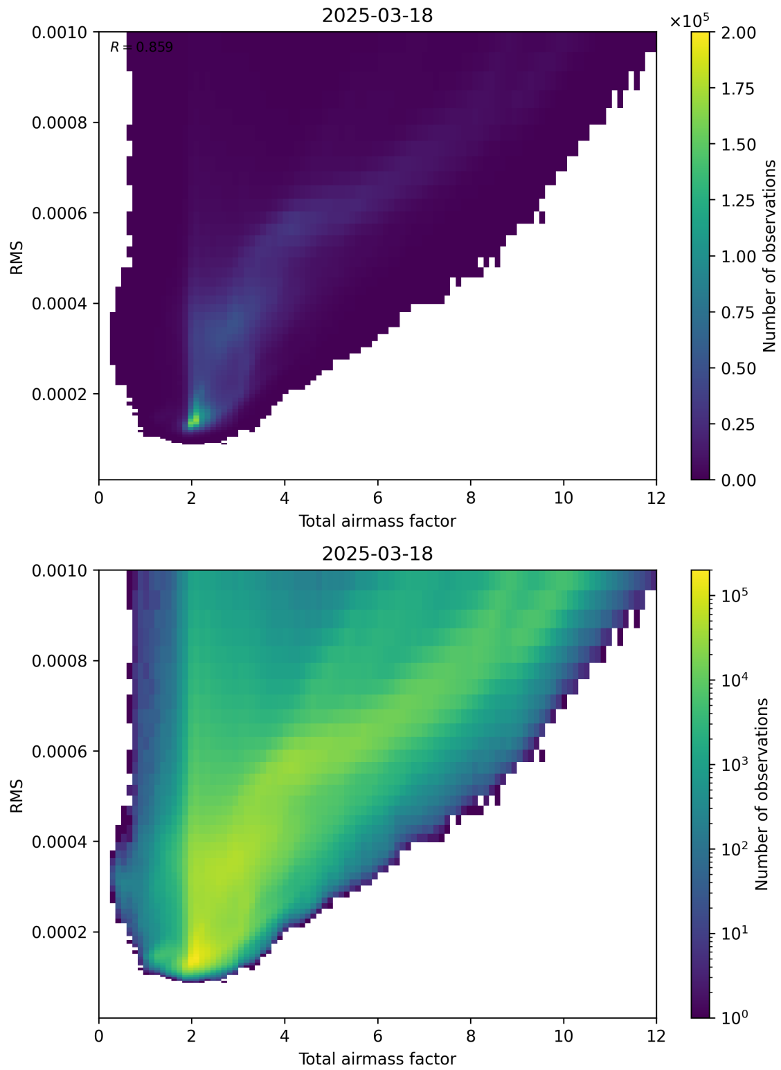
Figure 69: Scatter density plot of “Total airmass factor” against “RMS” for 2025-03-18 to 2025-03-19.
