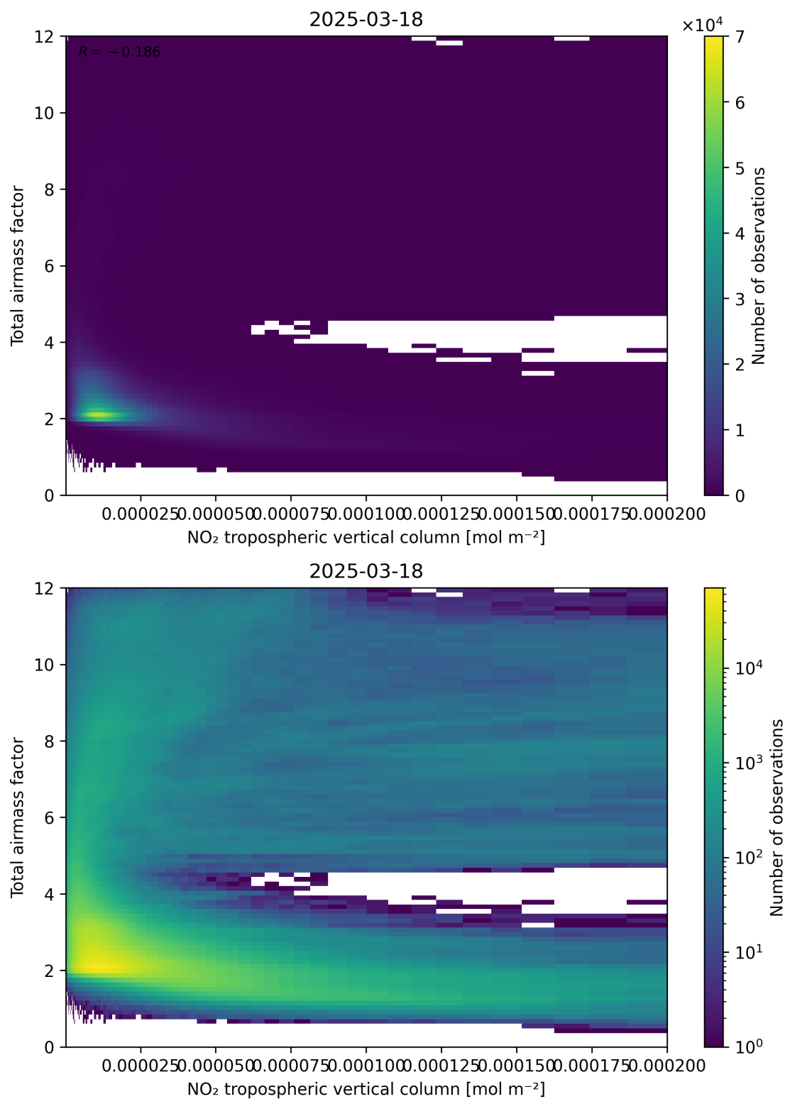
Figure 122: Scatter density plot of “NO 2 tropospheric vertical column” against “Total air mass factor” for 2025-03-18 to 2025-03-19.
