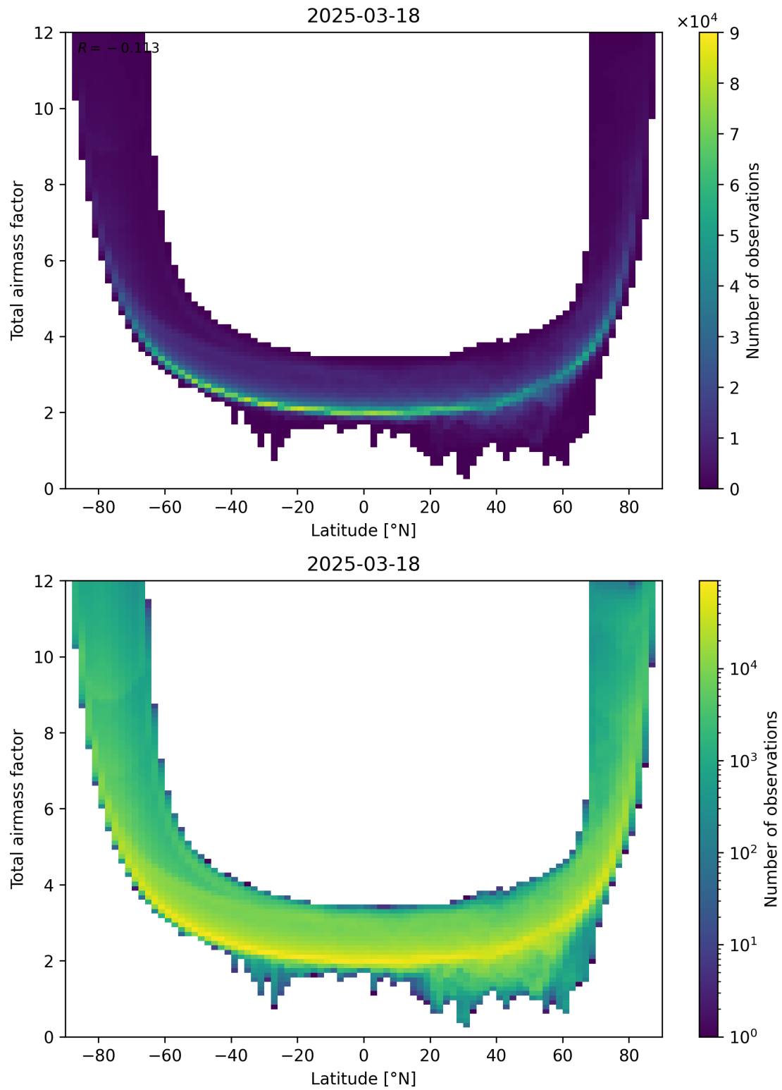
Figure 84: Scatter density plot of “Latitude” against “Total airmass factor” for 2025-03-18 to 2025-03-19.
