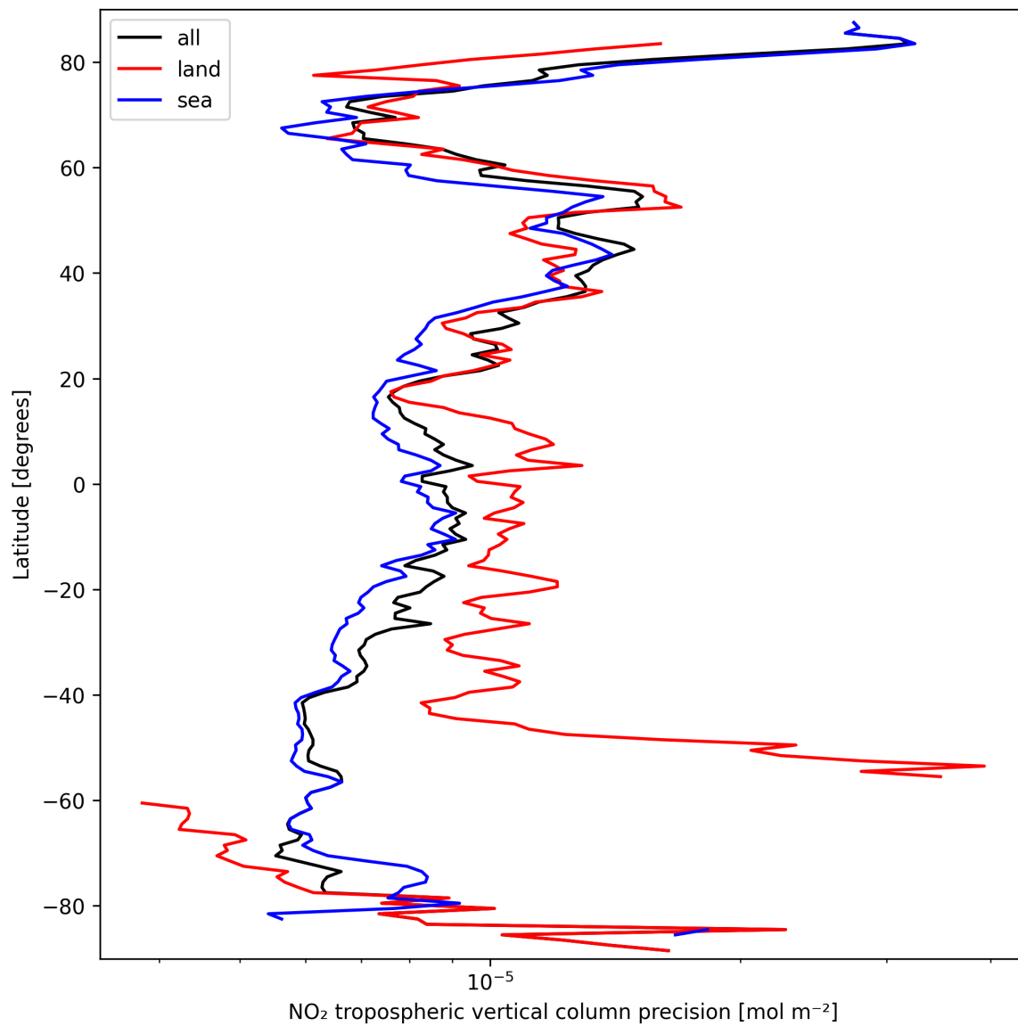
Figure 13: Zonal average of “NO 2 tropospheric vertical column precision” for 2025-03-18 to 2025-03-19.
