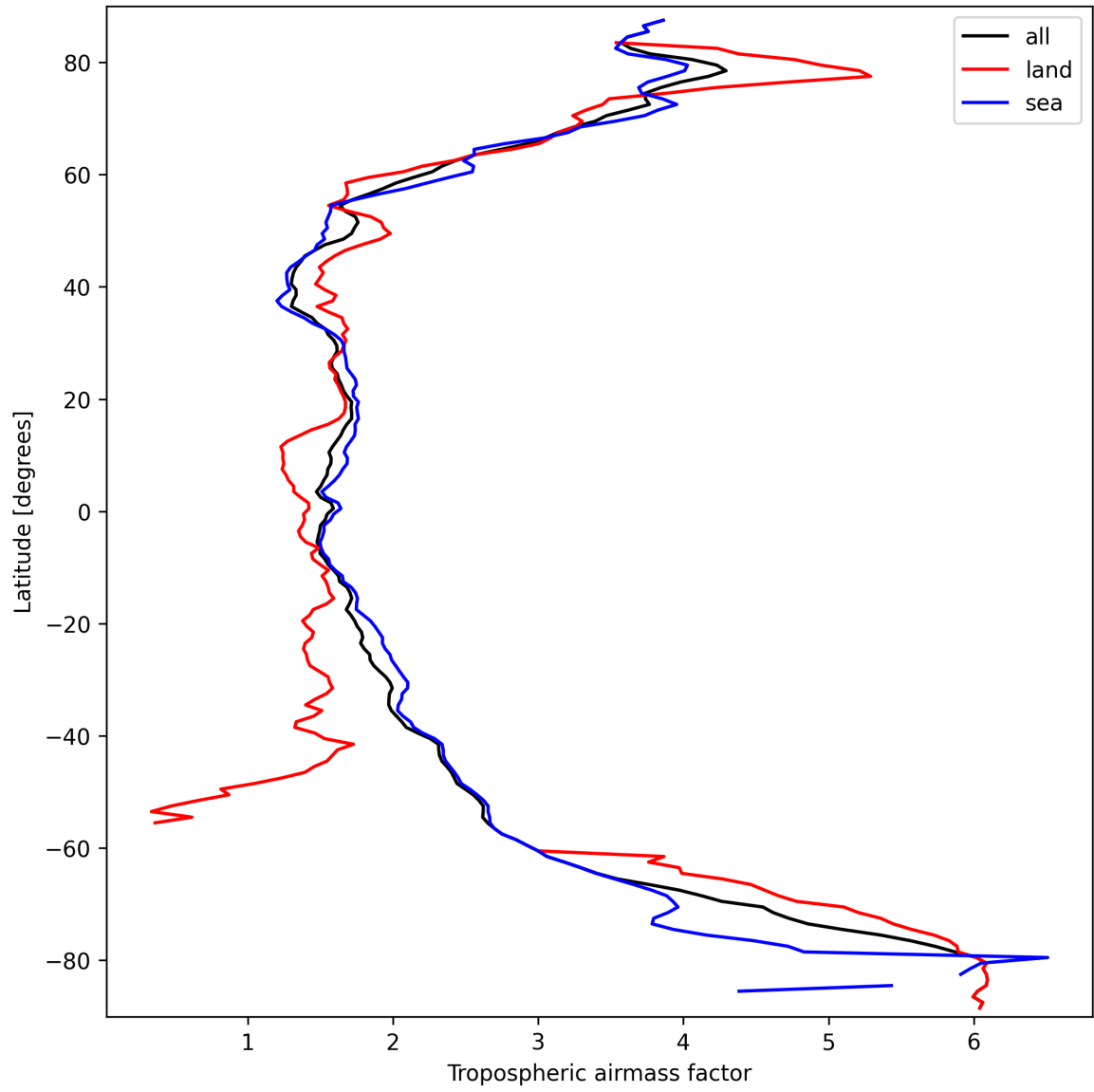
Figure 14: Zonal average of “Tropospheric airmass factor” for 2025-03-18 to 2025-03-19.
