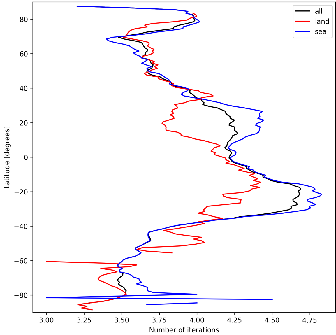
Figure 17: Zonal average of “Number of iterations” for 2025-03-18 to 2025-03-19.
