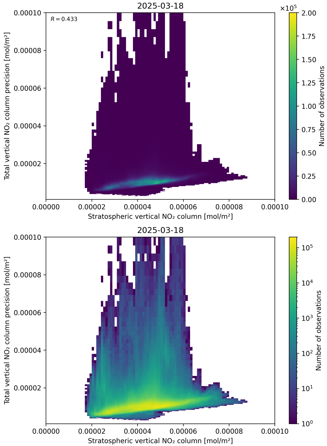
Figure 101: Scatter density plot of “Stratospheric vertical NO 2 column” against “Total vertical NO 2 column precision” for 2025-03-18 to 2025-03-19.
