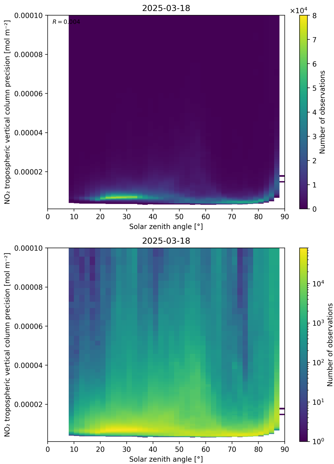
Figure 156: Scatter density plot of “Solar zenith angle” against “NO 2 tropospheric vertical column precision” for 2025-03-18 to 2025-03-19.
