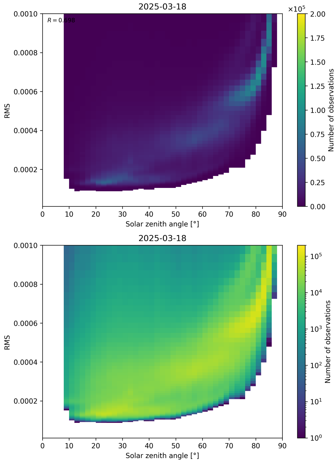
Figure 157: Scatter density plot of “Solar zenith angle” against “RMS” for 2025-03-18 to 2025-03-19.
