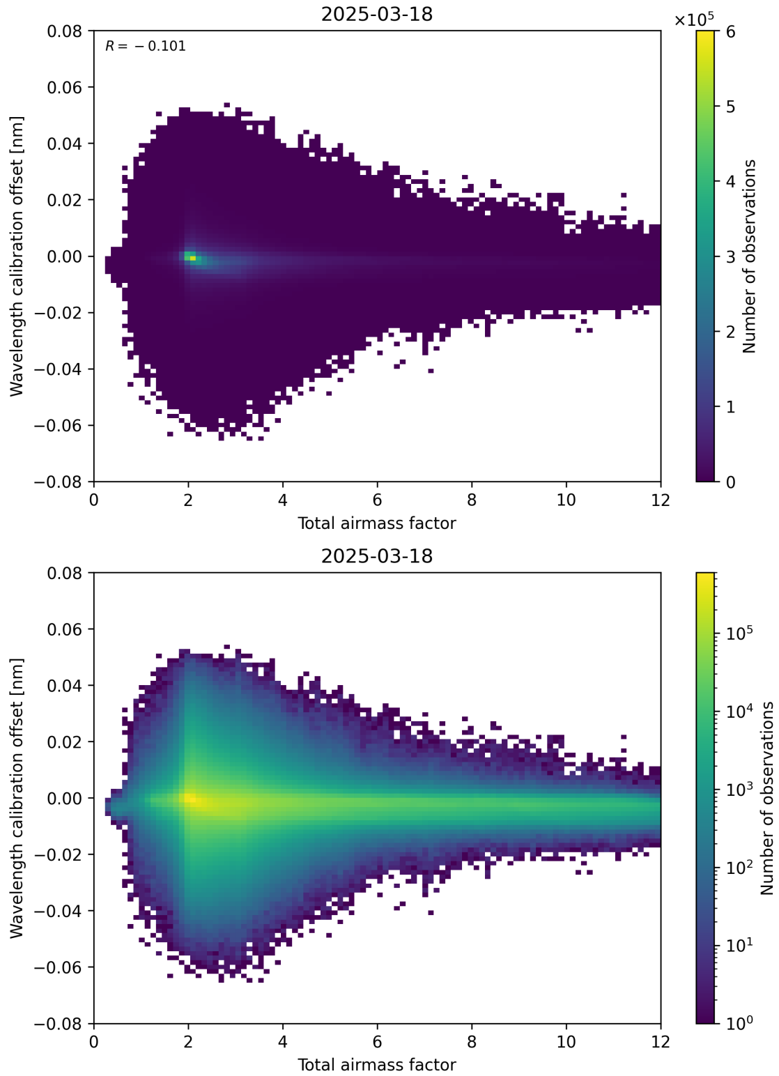
Figure 70: Scatter density plot of “Total airmass factor” against “Wavelength calibration offset” for 2025-03-18 to 2025-03-19.
