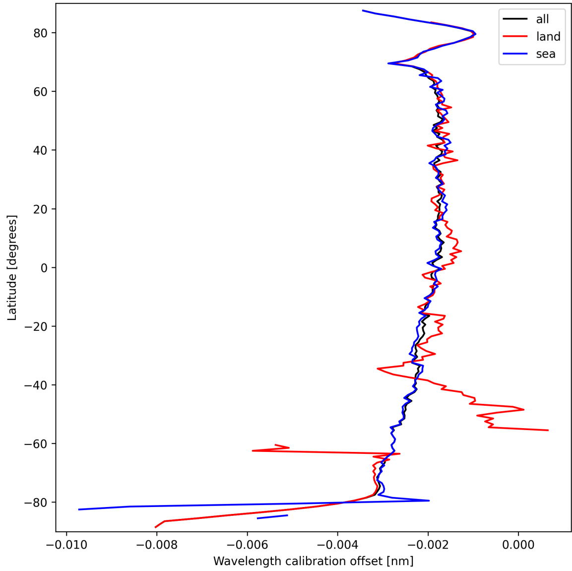
Figure 18: Zonal average of “Wavelength calibration offset” for 2025-03-18 to 2025-03-19.
