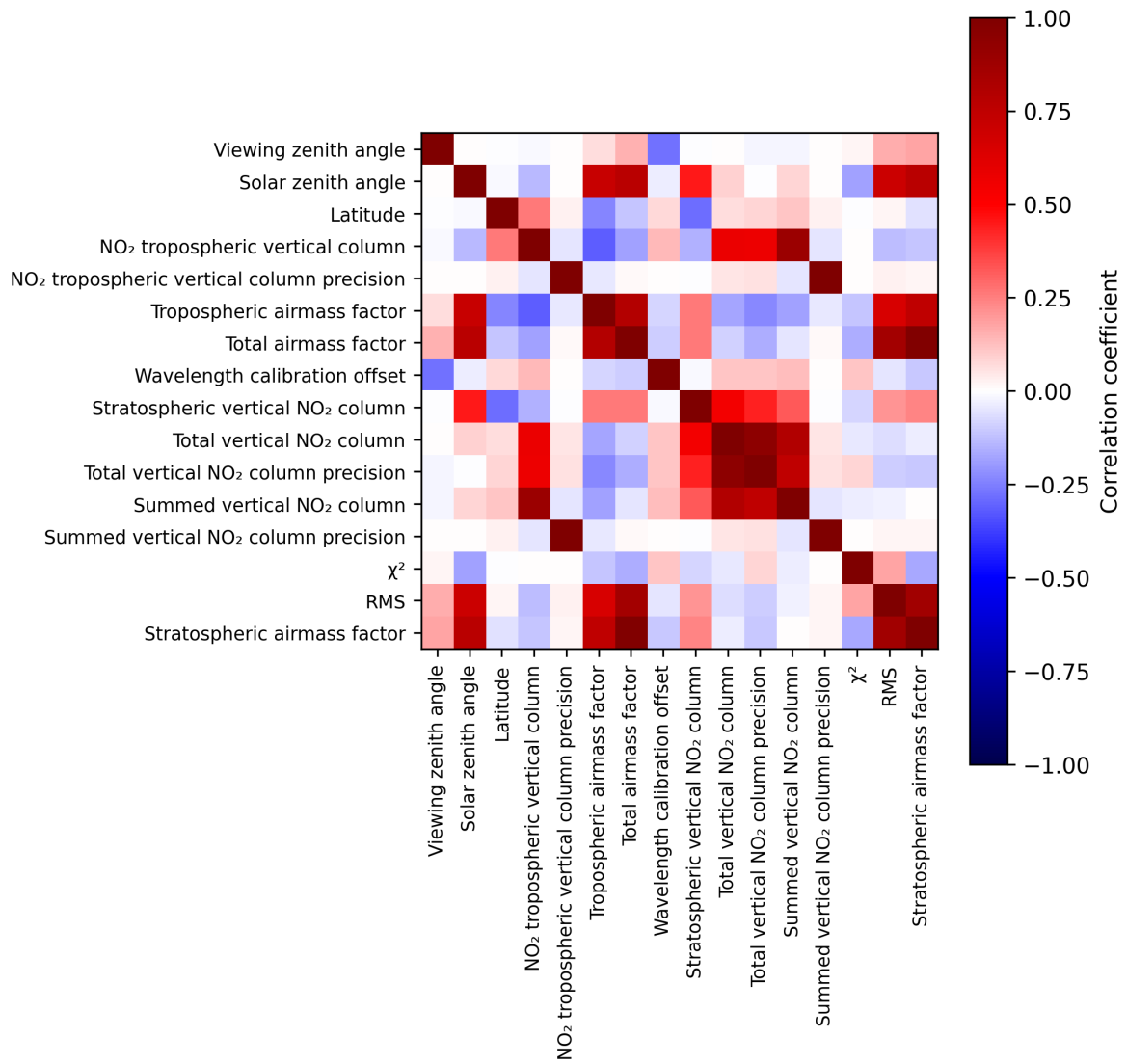
Figure 2: Map of correlation matrix for 2025-03-18 to 2025-03-19.
