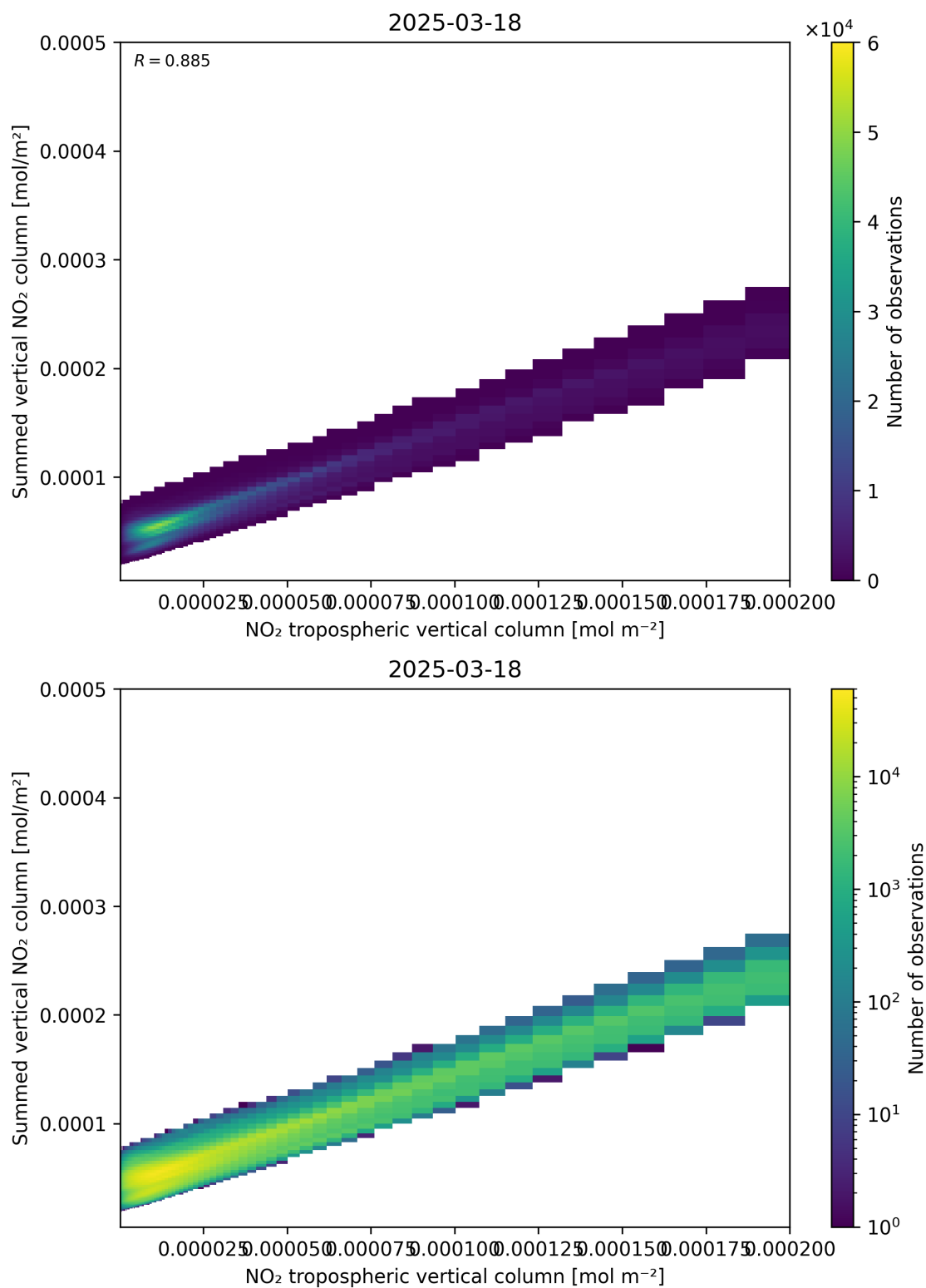
Figure 126: Scatter density plot of “NO 2 tropospheric vertical column” against “Summed vertical NO 2 column” for 2025-03-18 to 2025-03-19.
