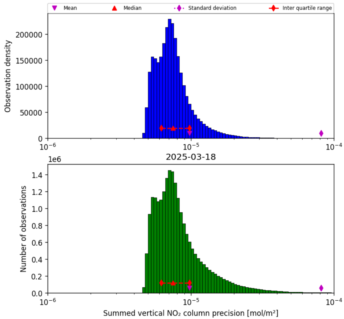
Figure 41: Histogram of "Summed vertical NO 2 column precision" for 2025-03-18 to 2025-03-19
