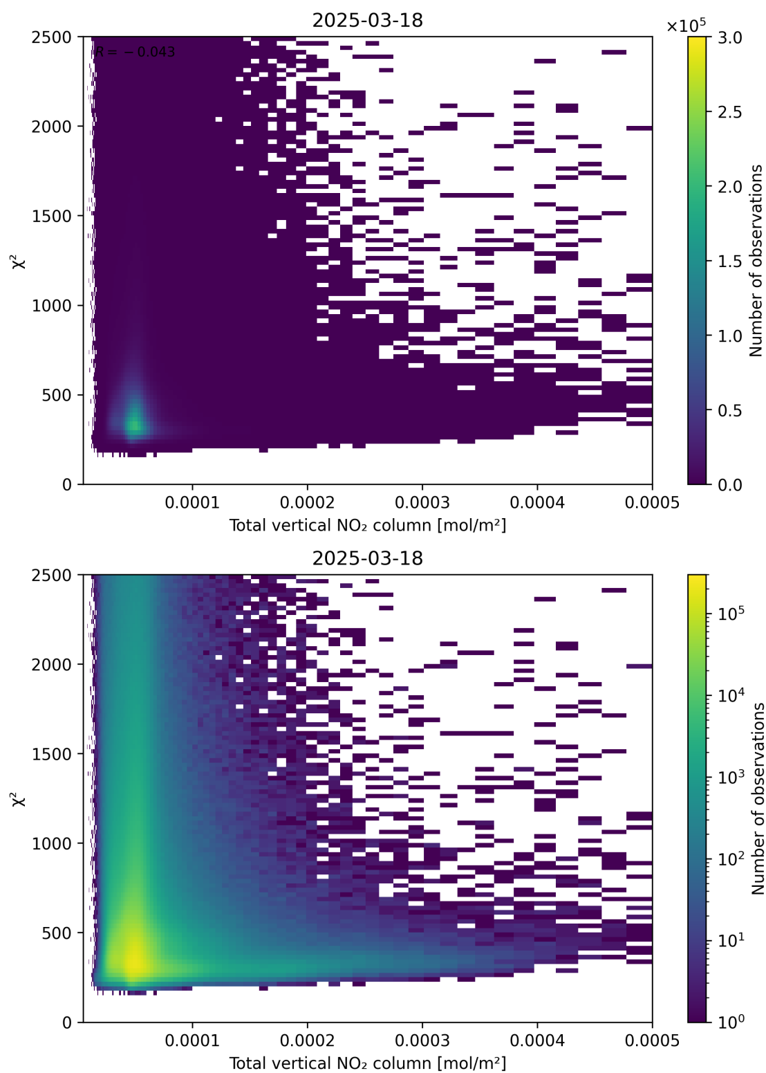
Figure 111: Scatter density plot of “Total vertical NO 2 column” against “ \chi^2 ” for 2025-03-18 to 2025-03-19.
