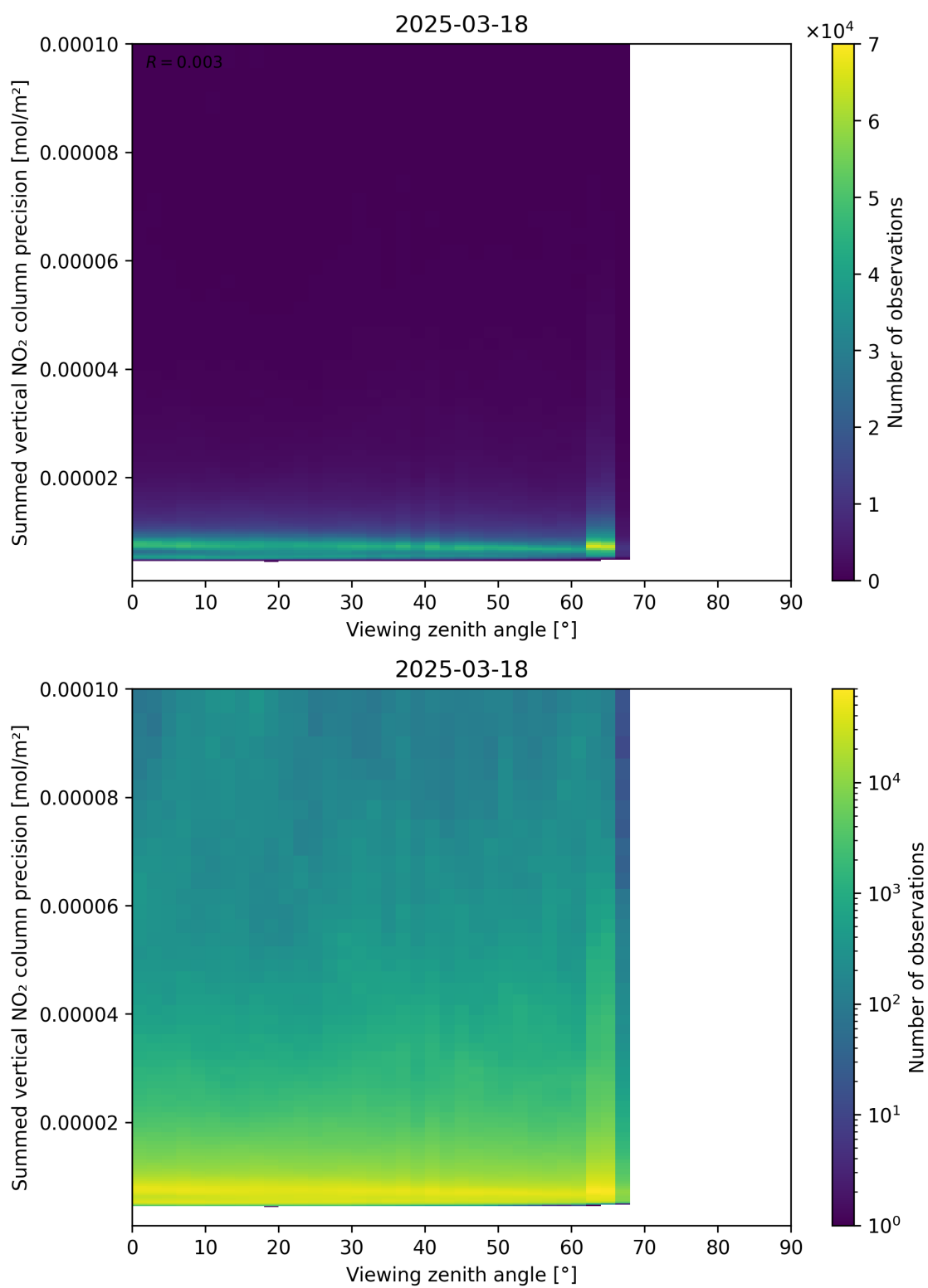
Figure 166: Scatter density plot of “Viewing zenith angle” against “Summed vertical NO 2 column precision” for 2025-03-18 to 2025-03-19.
