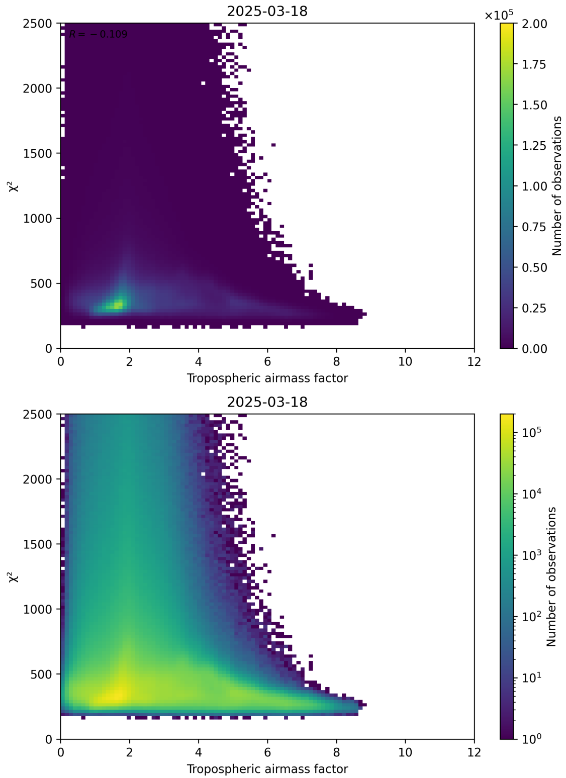
Figure 73: Scatter density plot of “Tropospheric airmass factor” against “ \chi^2 ” for 2025-03-18 to 2025-03-19.
