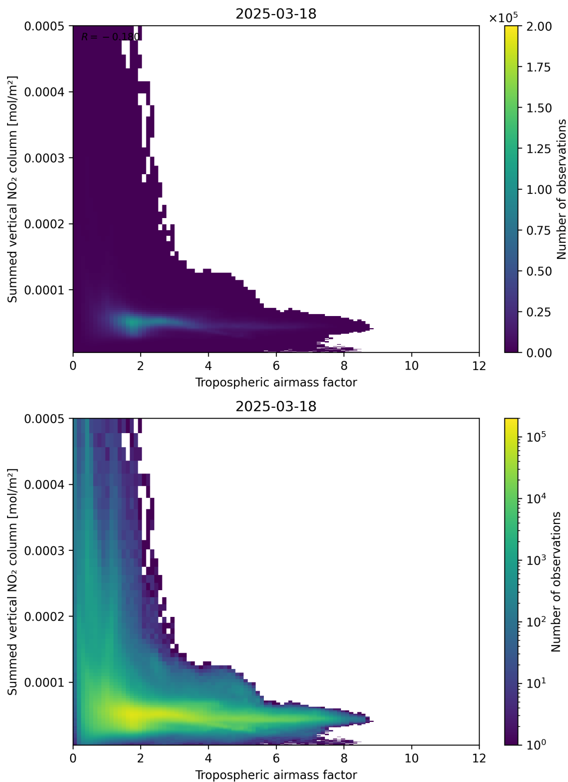
Figure 75: Scatter density plot of “Tropospheric air mass factor” against “Summed vertical NO 2 column” for 2025-03-18 to 2025-03-19.
