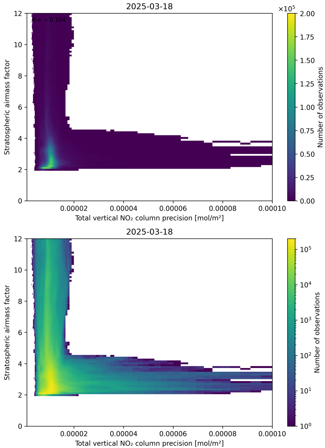
Figure 115: Scatter density plot of “Total vertical NO 2 column precision” against “Stratospheric air mass factor” for 2025-03-18 to 2025-03-19.
