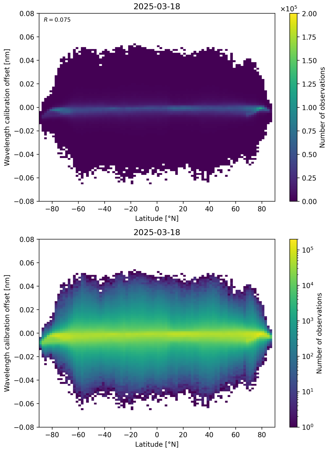
Figure 95: Scatter density plot of “Latitude” against “Wavelength calibration offset” for 2025-03-18 to 2025-03-19.
