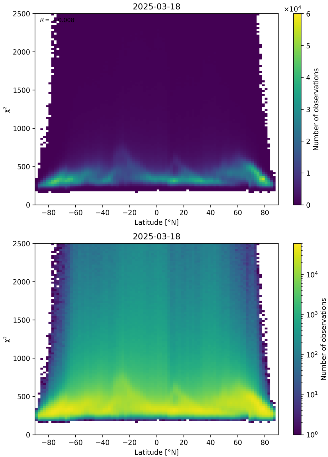
Figure 86: Scatter density plot of “Latitude” against “ \chi^2 ” for 2025-03-18 to 2025-03-19.
