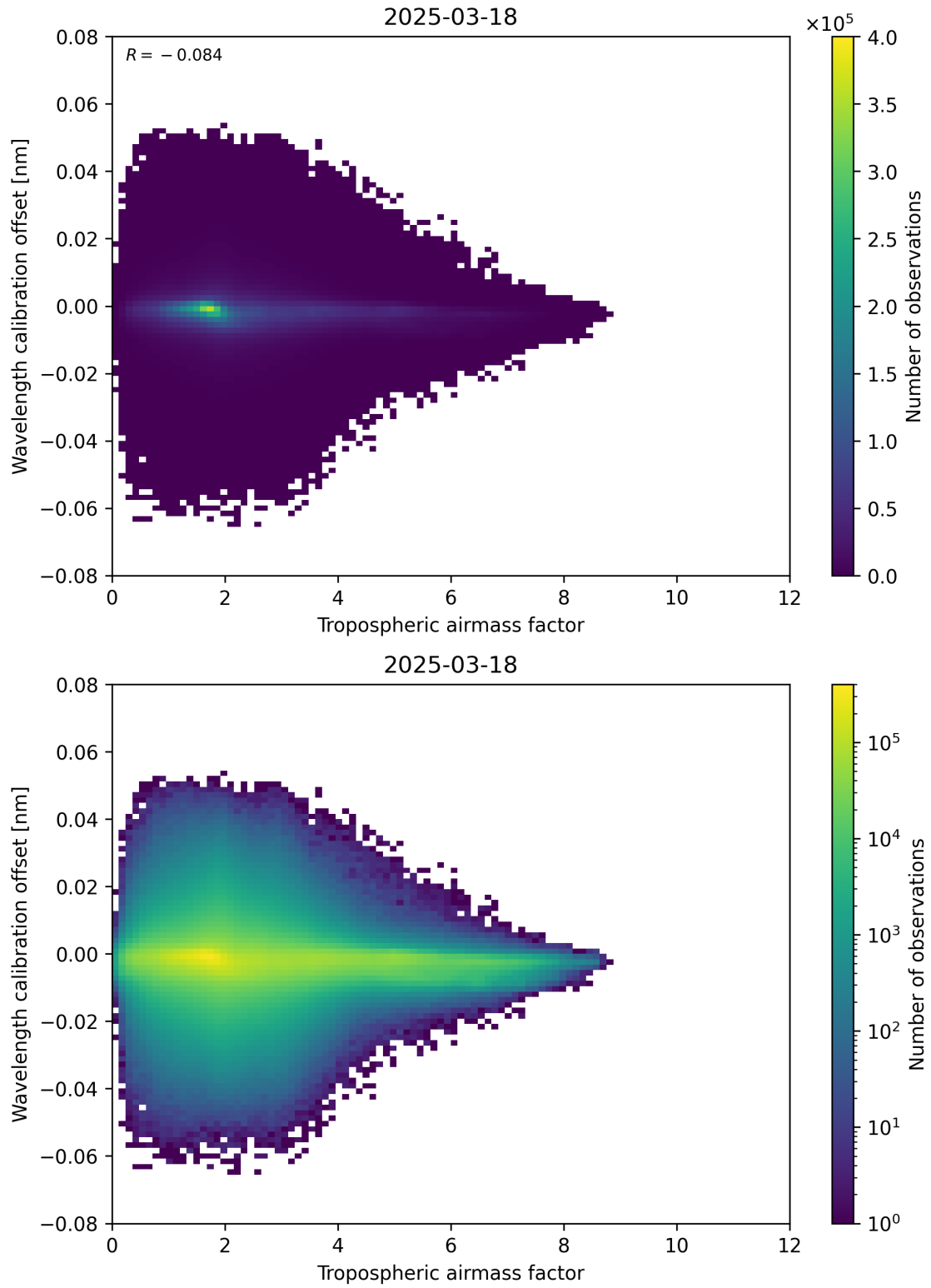
Figure 80: Scatter density plot of “Tropospheric airmass factor” against “Wavelength calibration offset” for 2025-03-18 to 2025-03-19.
