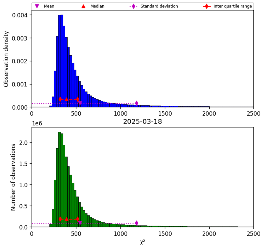
Figure 42: Histogram of “ \chi^2 ” for 2025-03-18 to 2025-03-19
