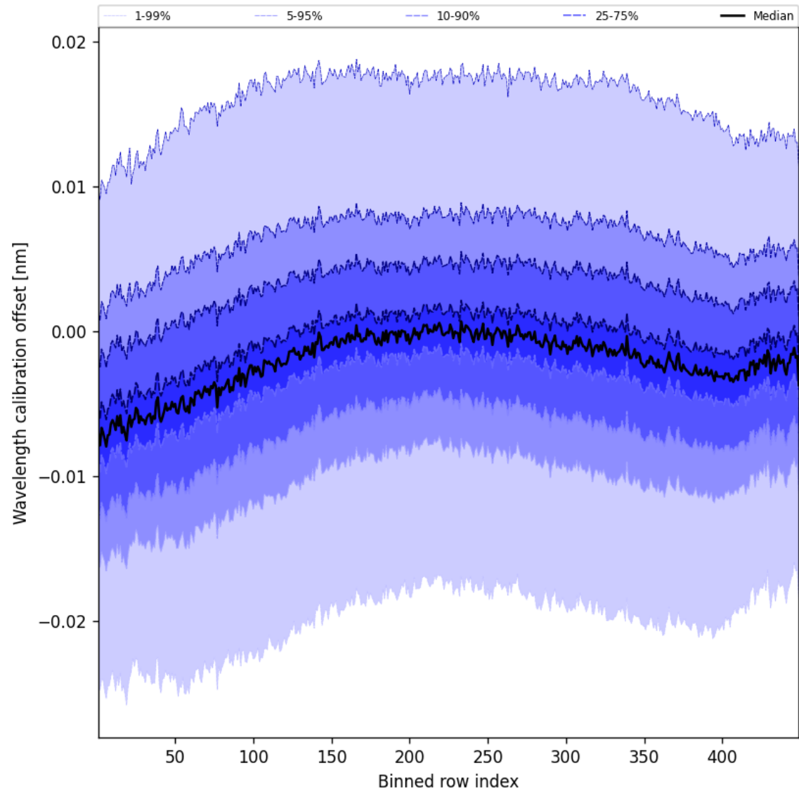
Figure 52: Along track statistics of “Wavelength calibration offset” for 2025-03-18 to 2025-03-19
