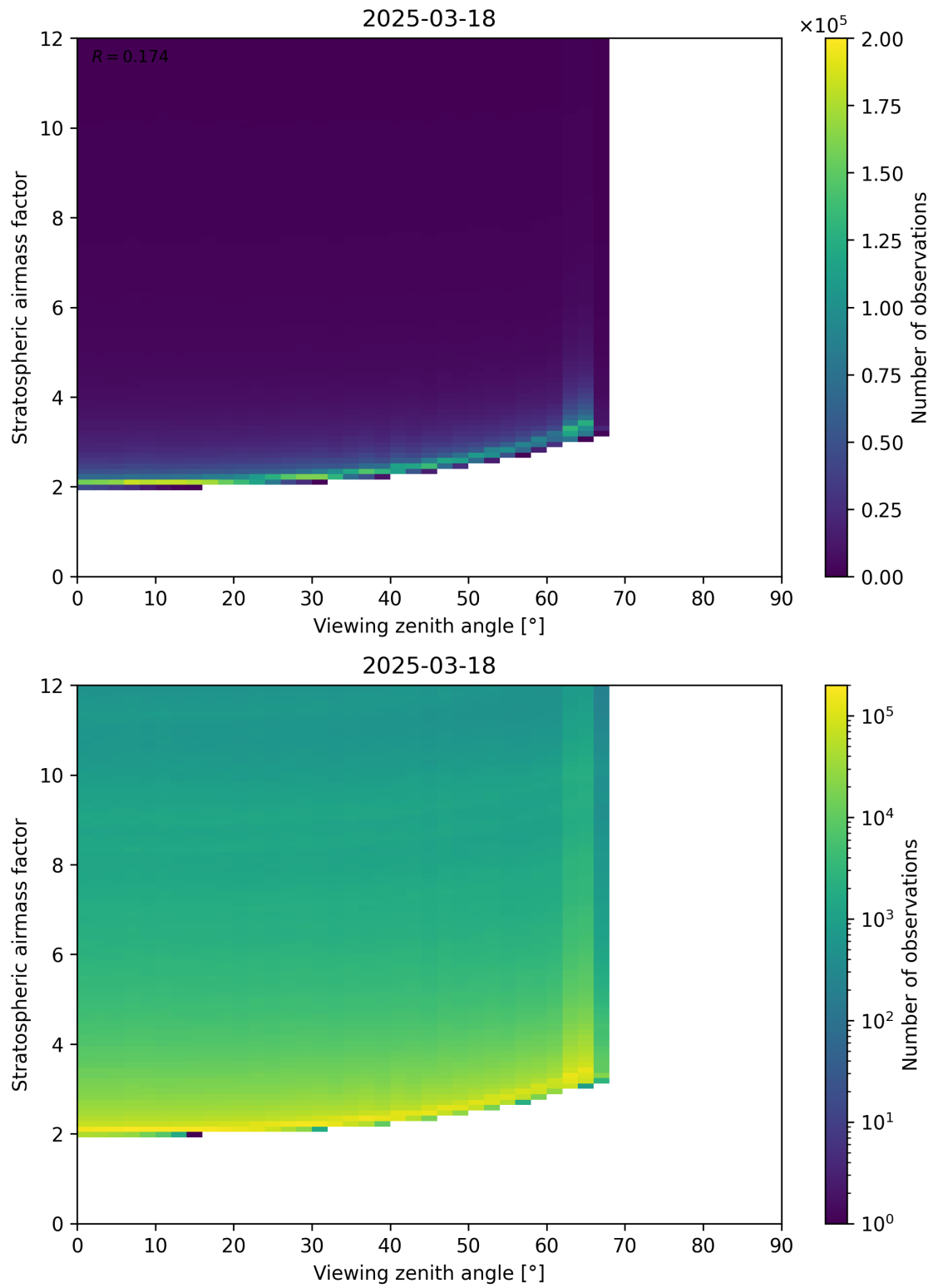
Figure 159: Scatter density plot of “Viewing zenith angle” against “Stratospheric airmass factor” for 2025-03-18 to 2025-03-19.
