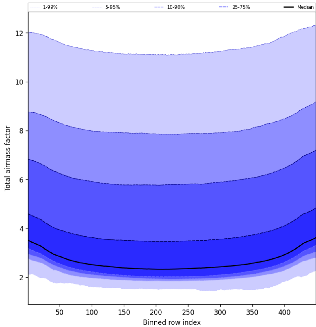
Figure 49: Along track statistics of “Total airmass factor” for 2025-03-18 to 2025-03-19
