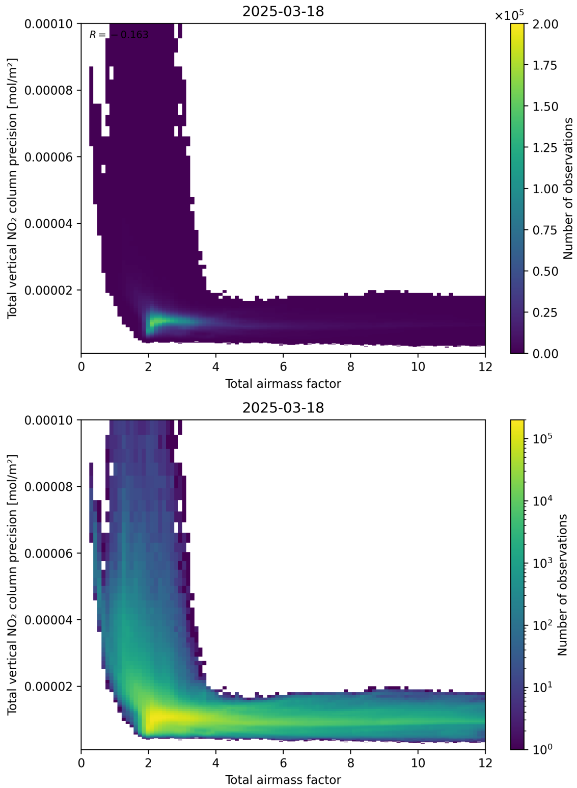
Figure 68: Scatter density plot of “Total airmass factor” against “Total vertical NO 2 column precision” for 2025-03-18 to 2025-03-19.
