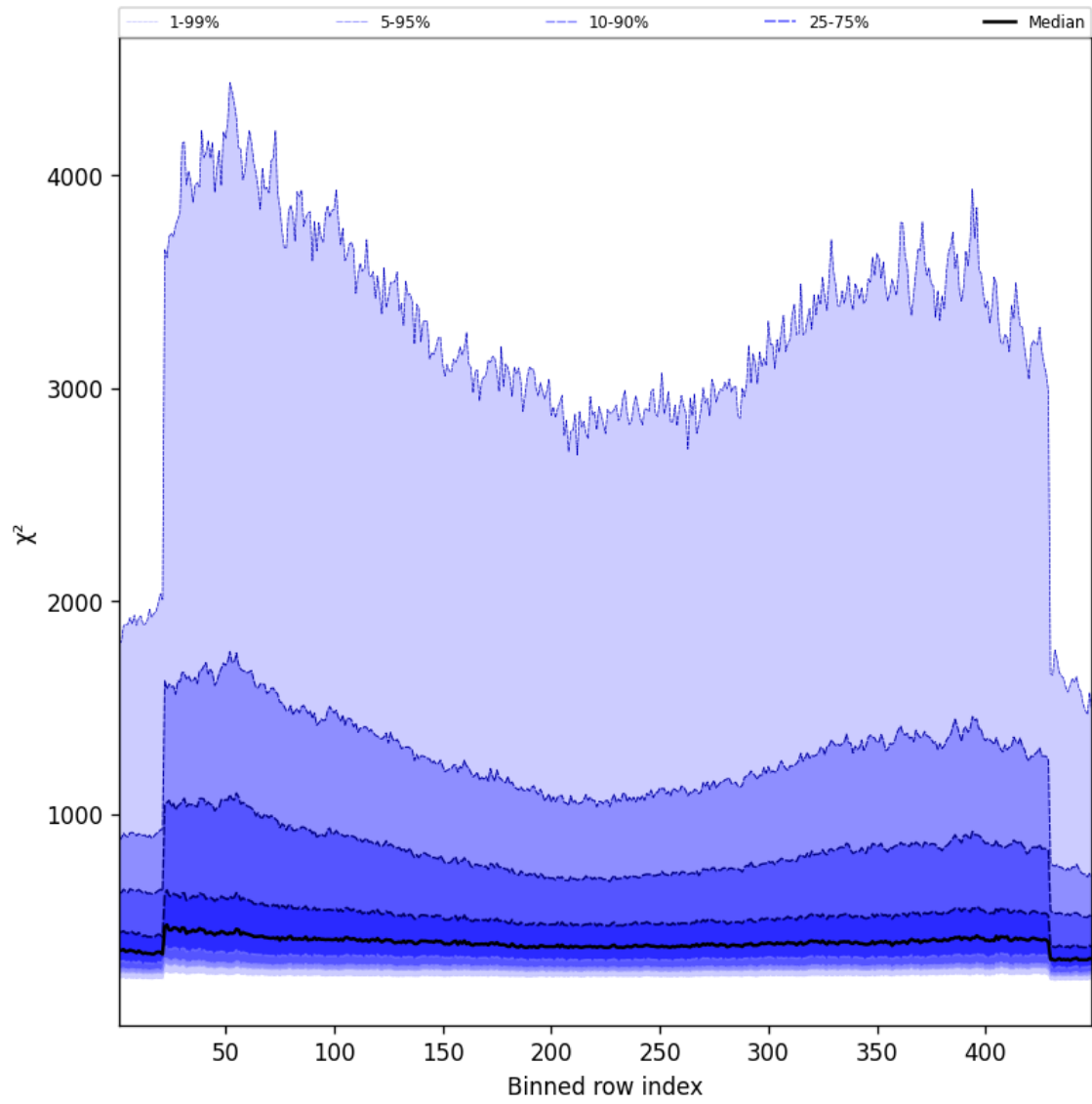
Figure 59: Along track statistics of “ \chi^2 ” for 2025-03-18 to 2025-03-19
