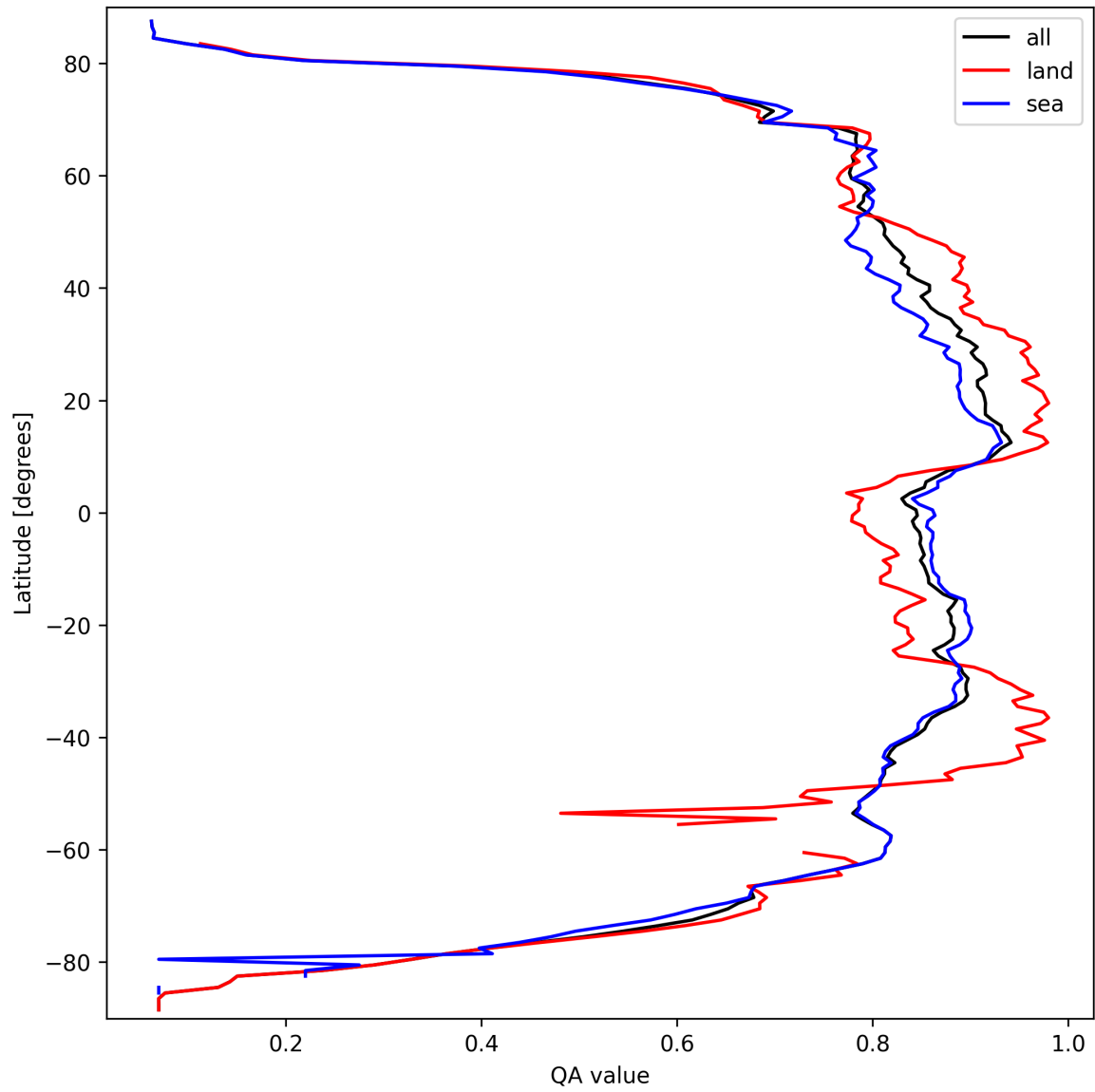
Figure 11: Zonal average of “QA value” for 2025-03-18 to 2025-03-19.
