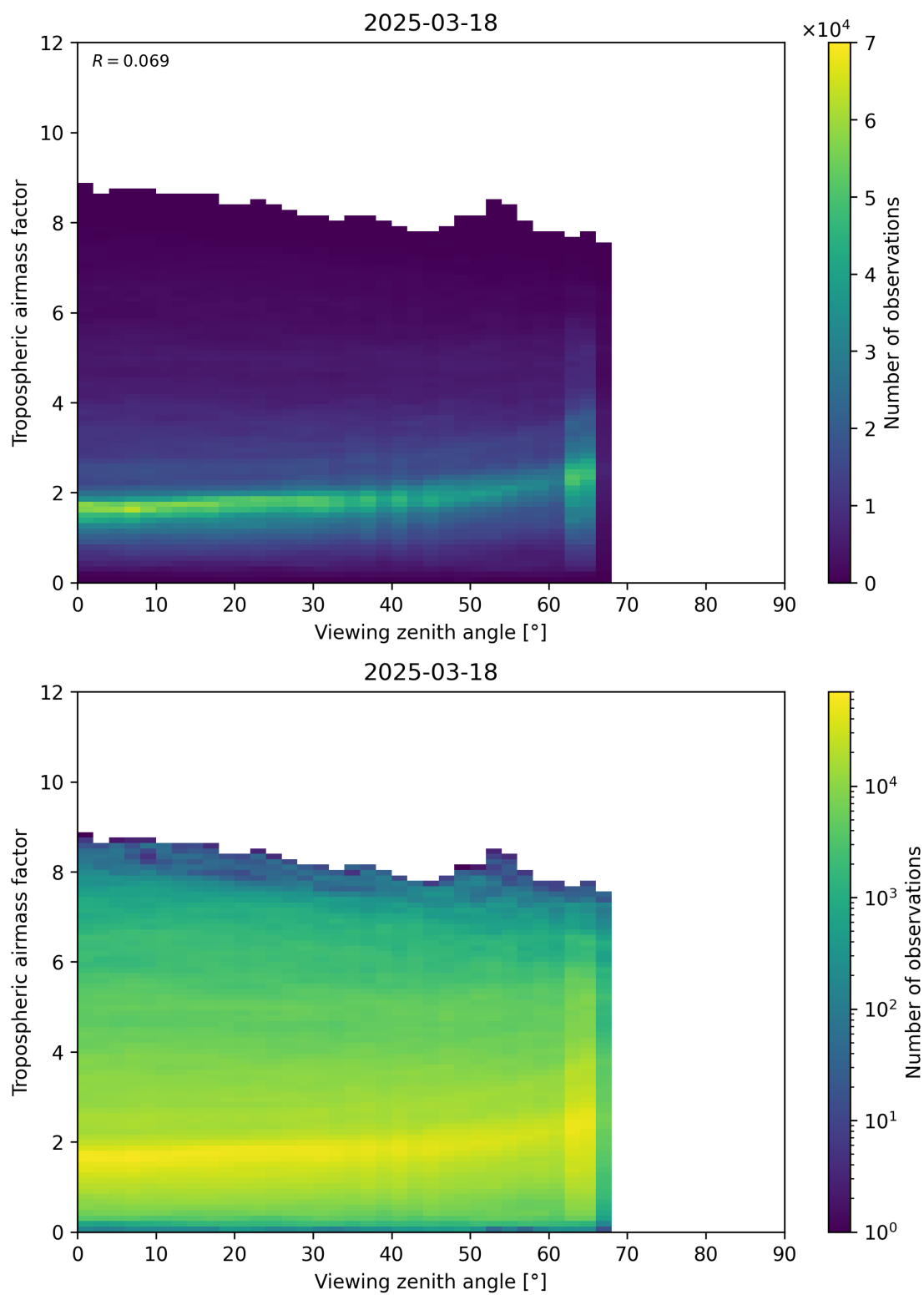
Figure 161: Scatter density plot of “Viewing zenith angle” against “Tropospheric airmass factor” for 2025-03-18 to 2025-03-19.
