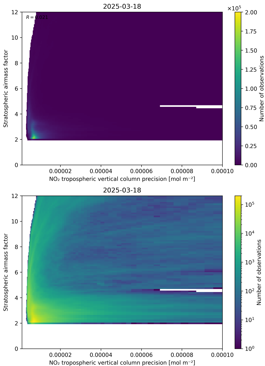
Figure 131: Scatter density plot of “NO 2 tropospheric vertical column precision” against “Stratospheric airmass factor” for 2025-03-18 to 2025-03-19.
