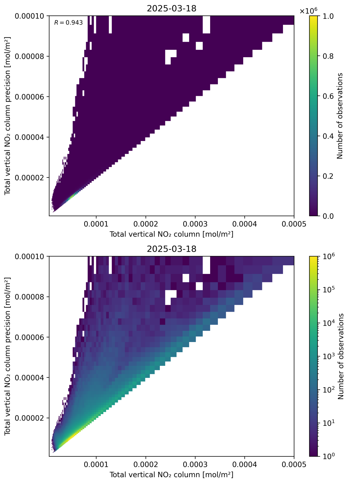
Figure 114: Scatter density plot of “Total vertical NO 2 column” against “Total vertical NO 2 column precision” for 2025-03-18 to 2025-03-19.
