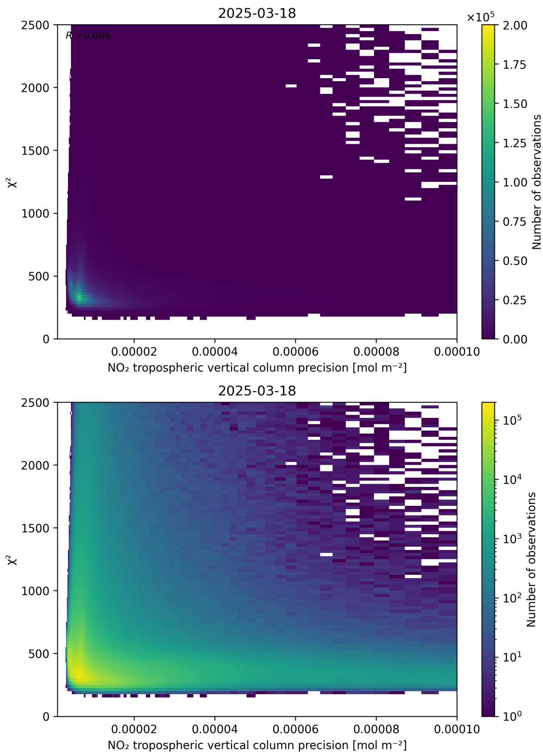
Figure 134: Scatter density plot of “NO 2 tropospheric vertical column precision” against “ \chi^2 ” for 2025-03-18 to 2025-03-19.
