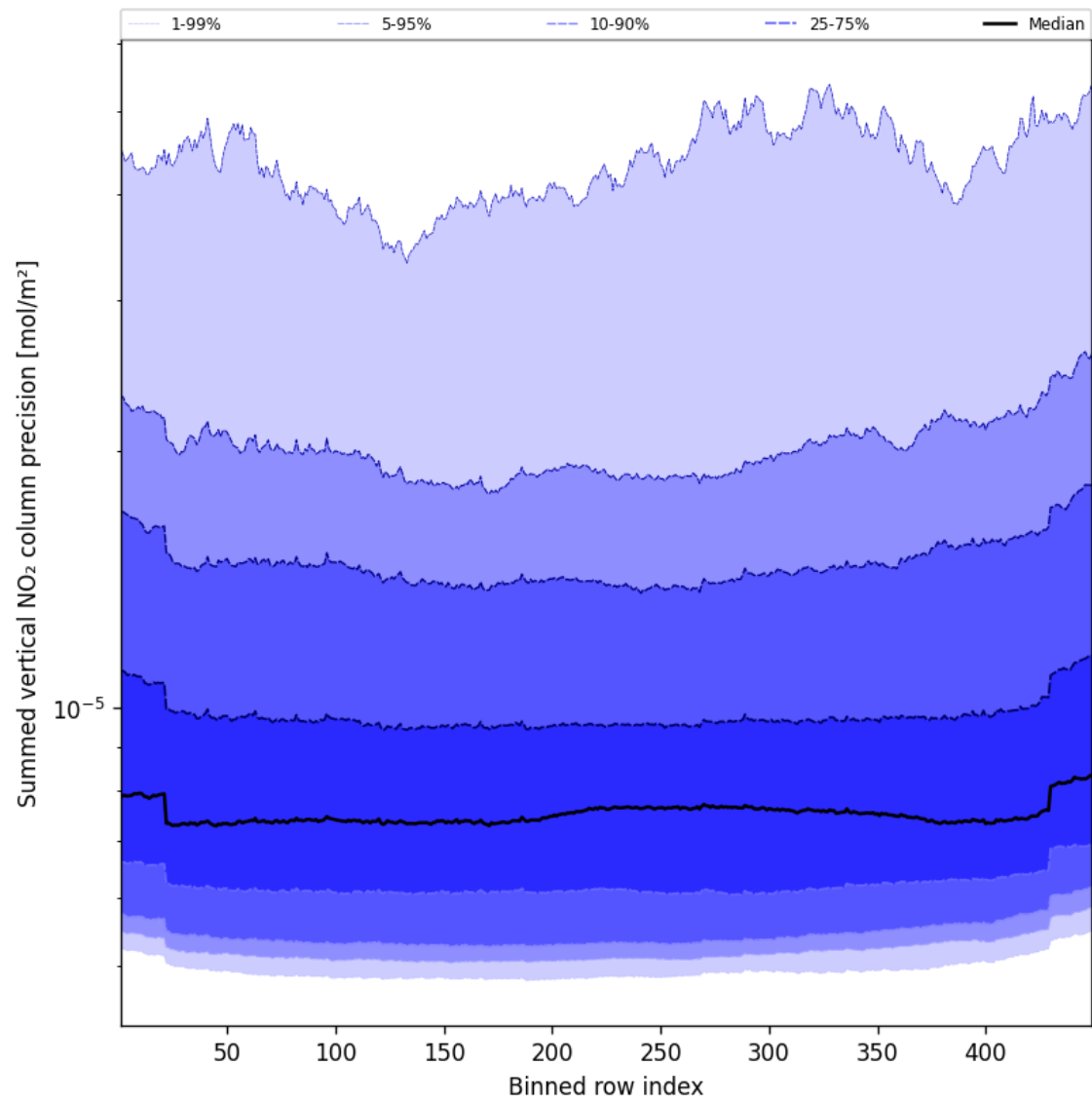
Figure 58: Along track statistics of “Summed vertical NO 2 column precision” for 2025-03-18 to 2025-03-19
