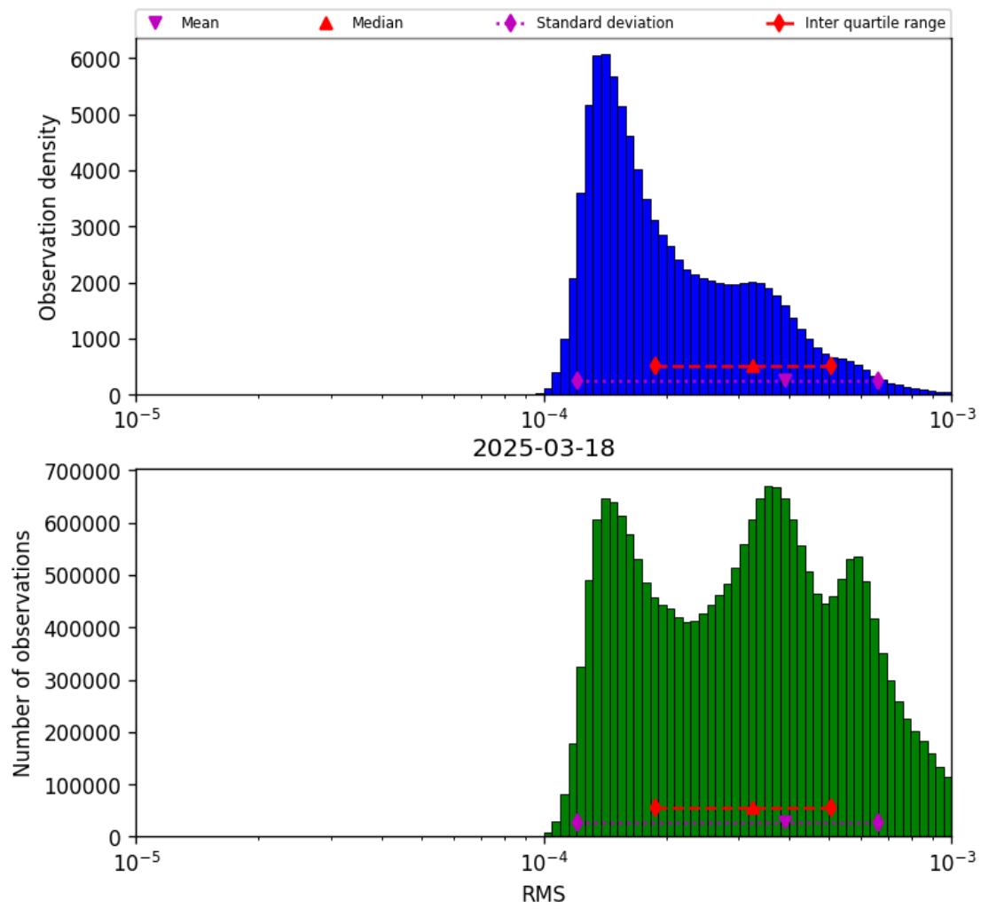
Figure 43: Histogram of “RMS” for 2025-03-18 to 2025-03-19
