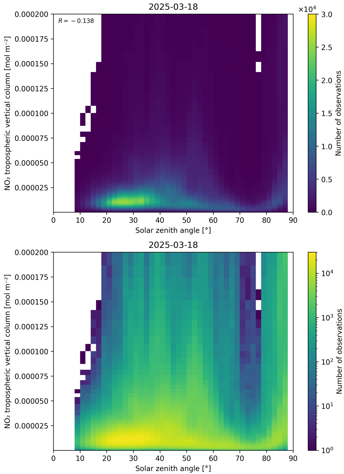
Figure 155: Scatter density plot of “Solar zenith angle” against “NO 2 tropospheric vertical column” for 2025-03-18 to 2025-03-19.
