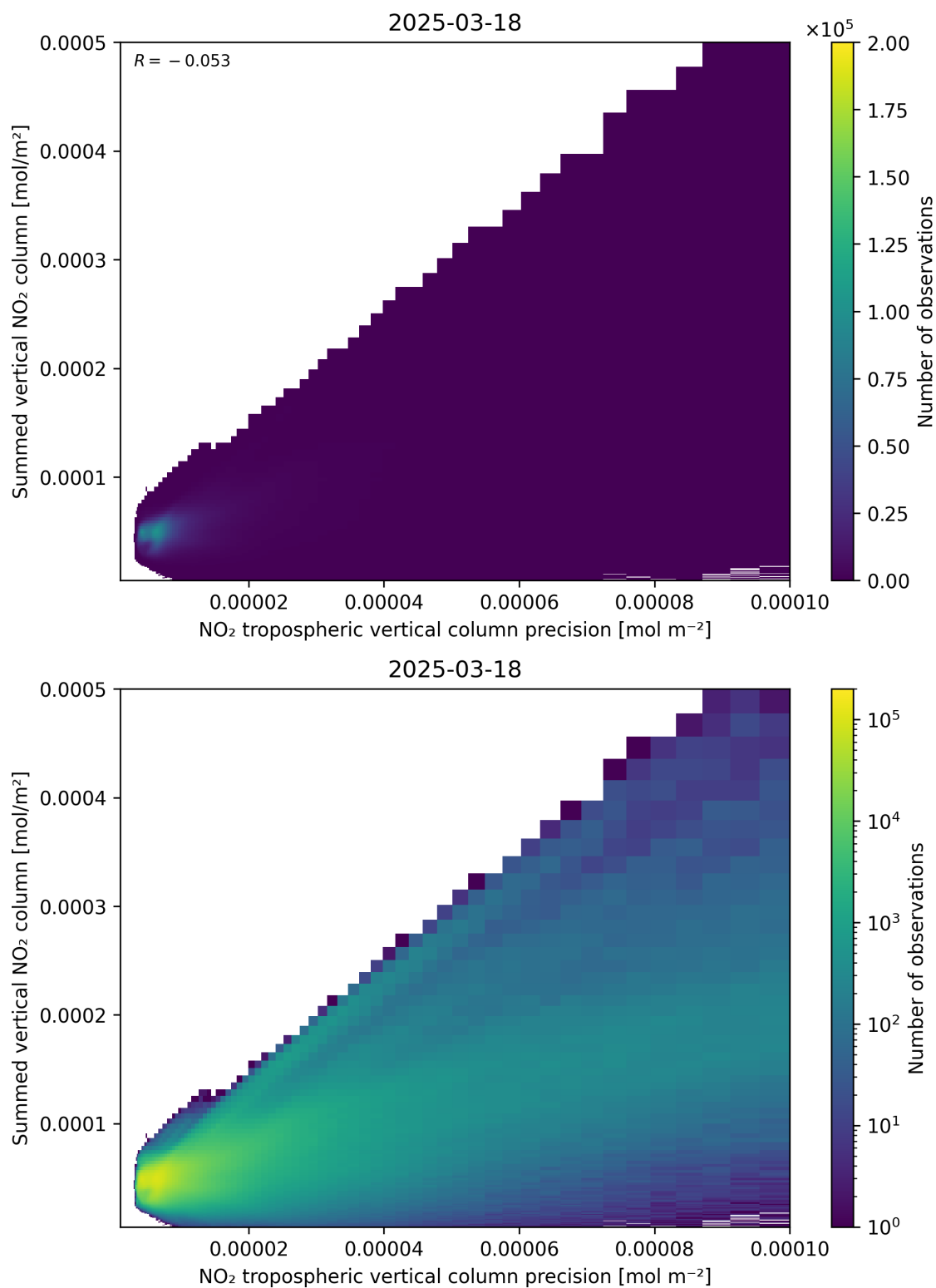
Figure 136: Scatter density plot of “NO 2 tropospheric vertical column precision” against “Summed vertical NO 2 column” for 2025-03-18 to 2025-03-19.
