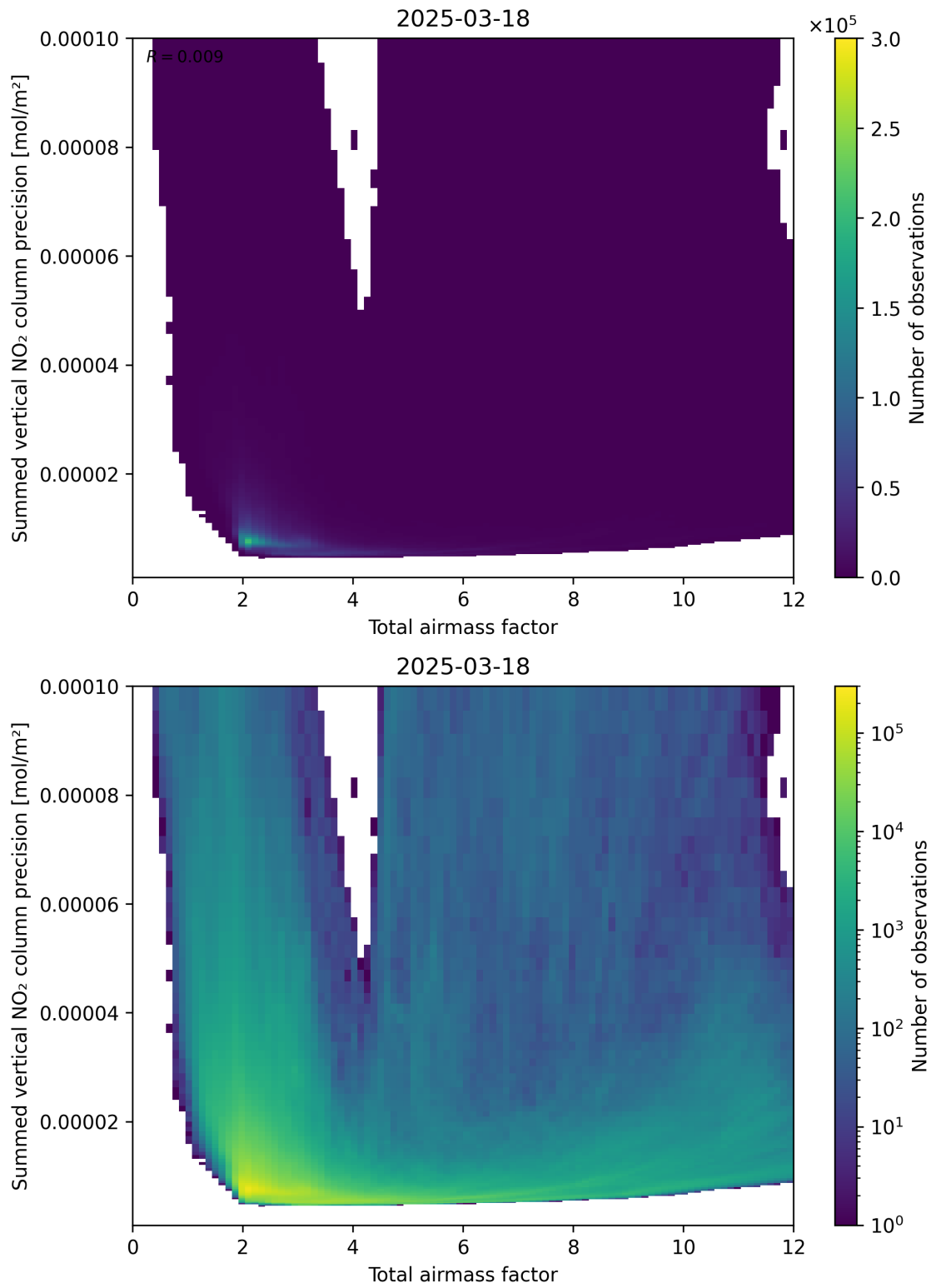
Figure 66: Scatter density plot of “Total airmass factor” against “Summed vertical NO 2 column precision” for 2025-03-18 to 2025-03-19.
