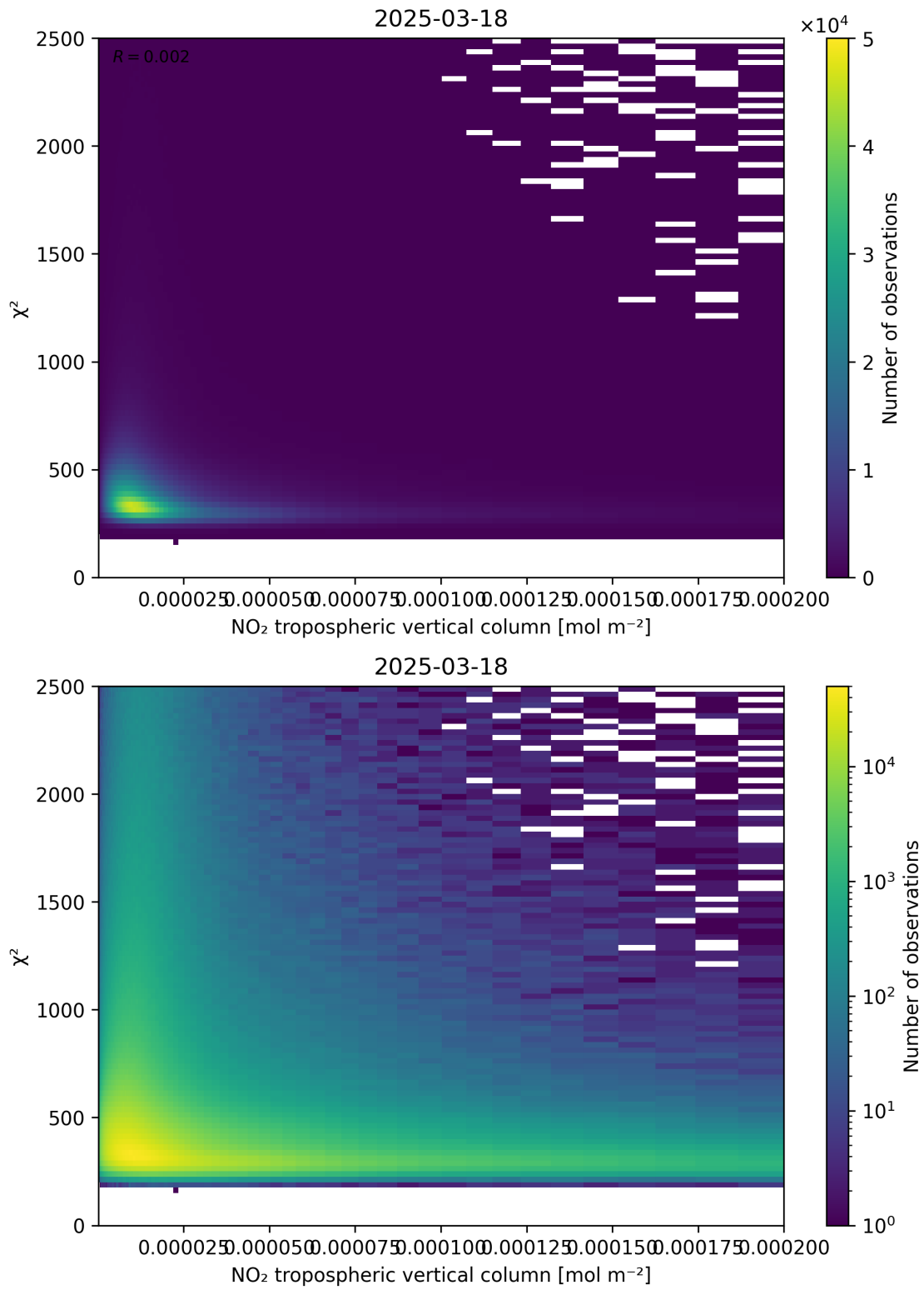
Figure 124: Scatter density plot of “NO 2 tropospheric vertical column” against “ \chi^2 ” for 2025-03-18 to 2025-03-19.
