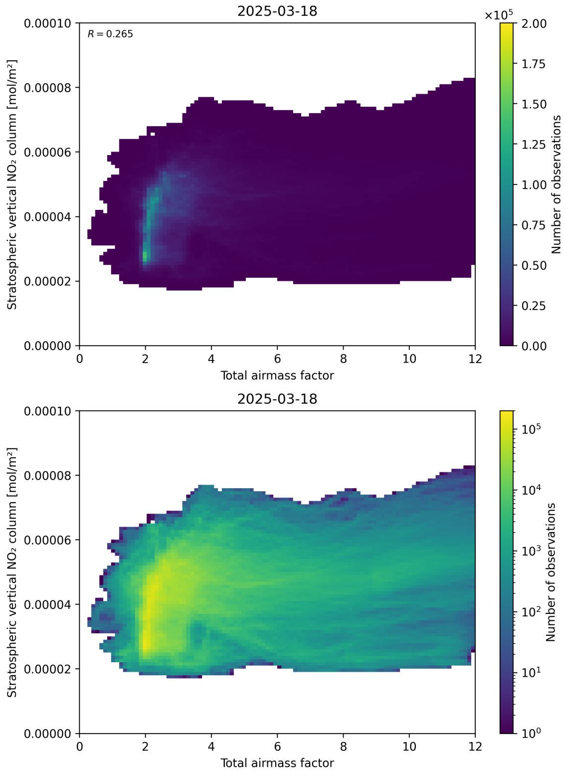
Figure 64: Scatter density plot of “Total airmass factor” against “Stratospheric vertical \text{NO}_2 column” for 2025-03-18 to 2025-03-19.
