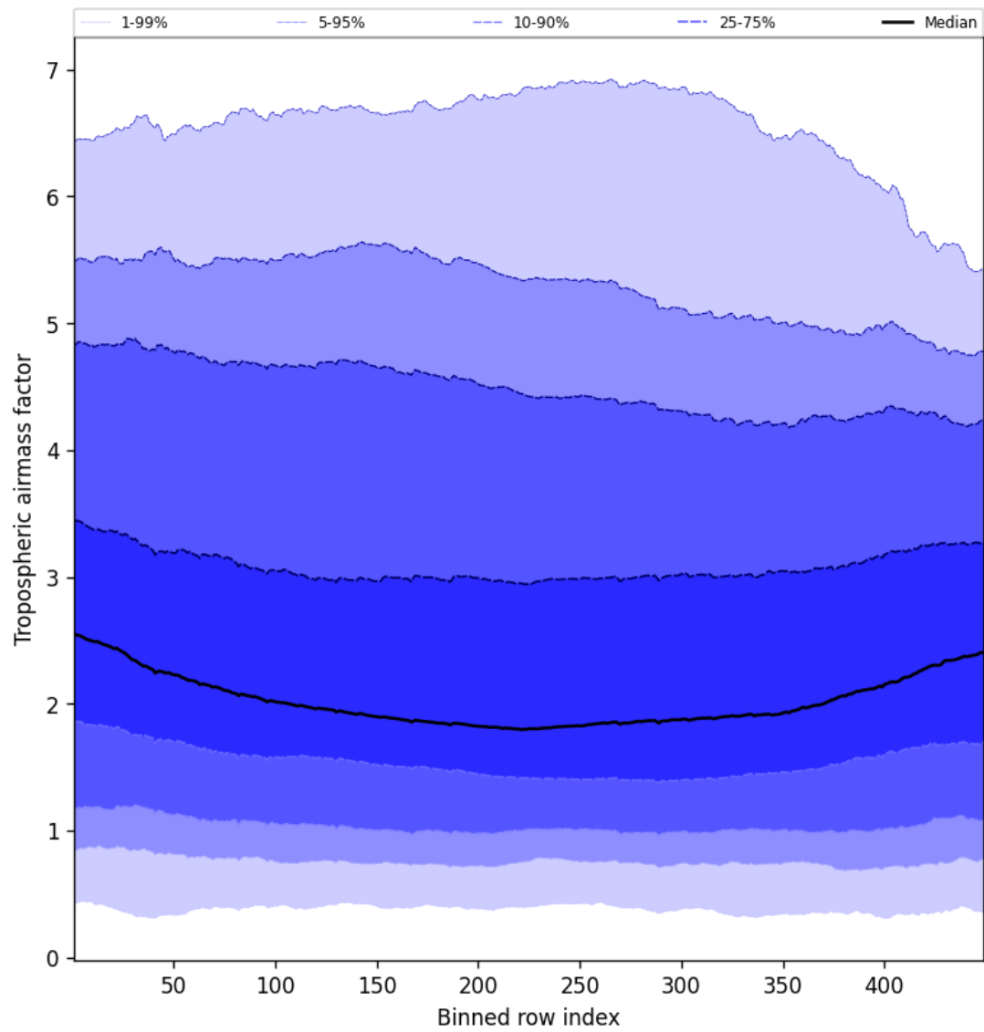
Figure 48: Along track statistics of “Tropospheric air mass factor” for 2025-03-18 to 2025-03-19
