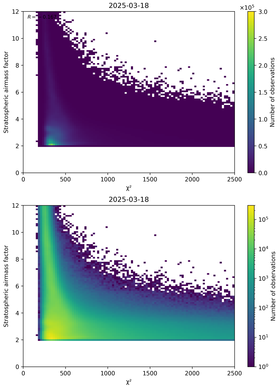
Figure 81: Scatter density plot of “ \chi^2 ” against “Stratospheric airmass factor” for 2025-03-18 to 2025-03-19.
