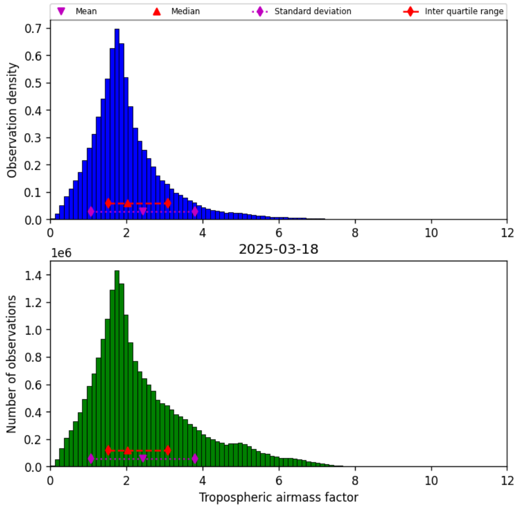
Figure 31: Histogram of “Tropospheric airmass factor” for 2025-03-18 to 2025-03-19
