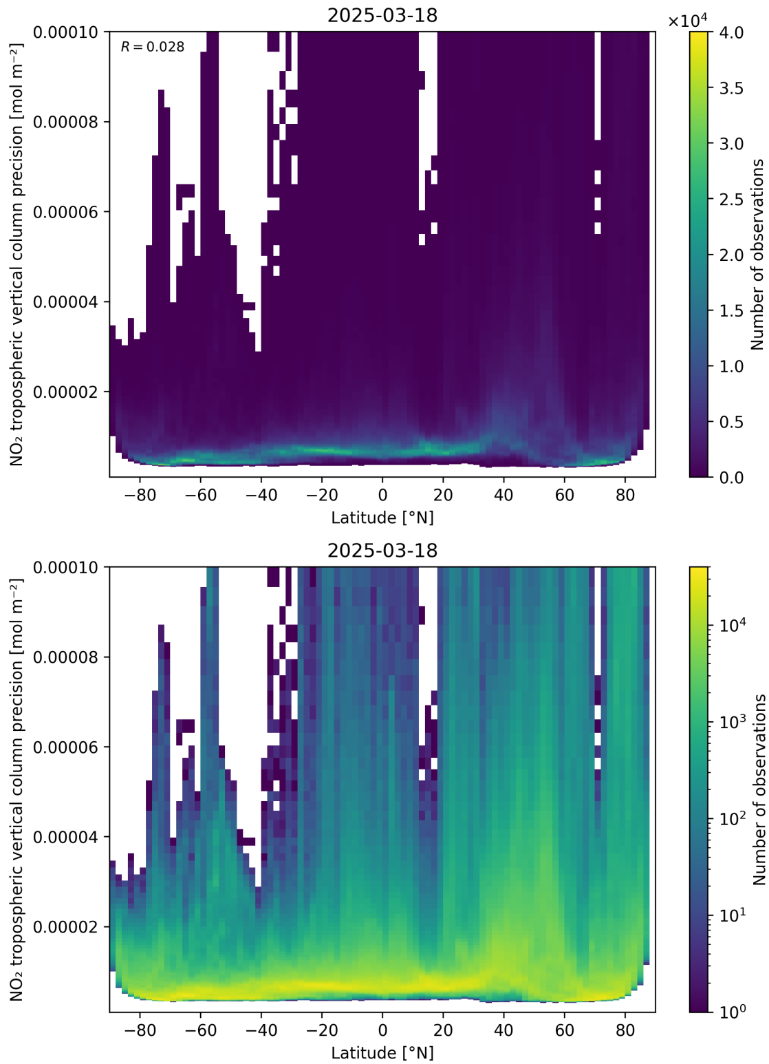
Figure 93: Scatter density plot of “Latitude” against “NO 2 tropospheric vertical column precision” for 2025-03-18 to 2025-03-19.
