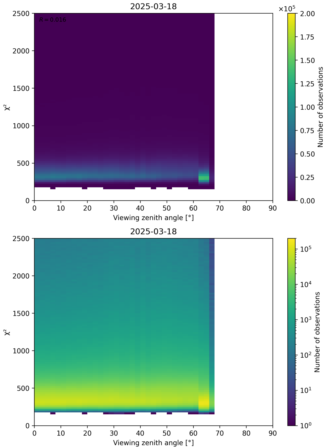
Figure 162: Scatter density plot of “Viewing zenith angle” against “ \chi^2 ” for 2025-03-18 to 2025-03-19.
