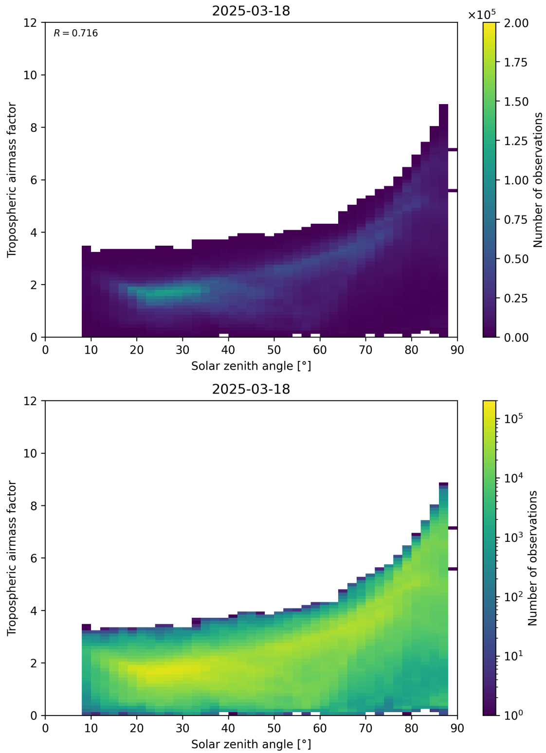
Figure 147: Scatter density plot of “Solar zenith angle” against “Tropospheric airmass factor” for 2025-03-18 to 2025-03-19.
