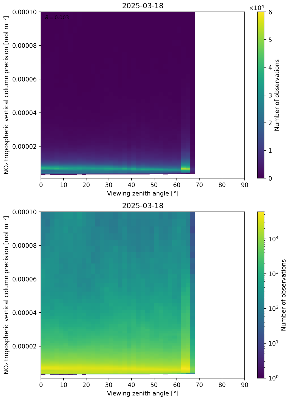
Figure 170: Scatter density plot of “Viewing zenith angle” against “NO 2 tropospheric vertical column precision” for 2025-03-18 to 2025-03-19.
