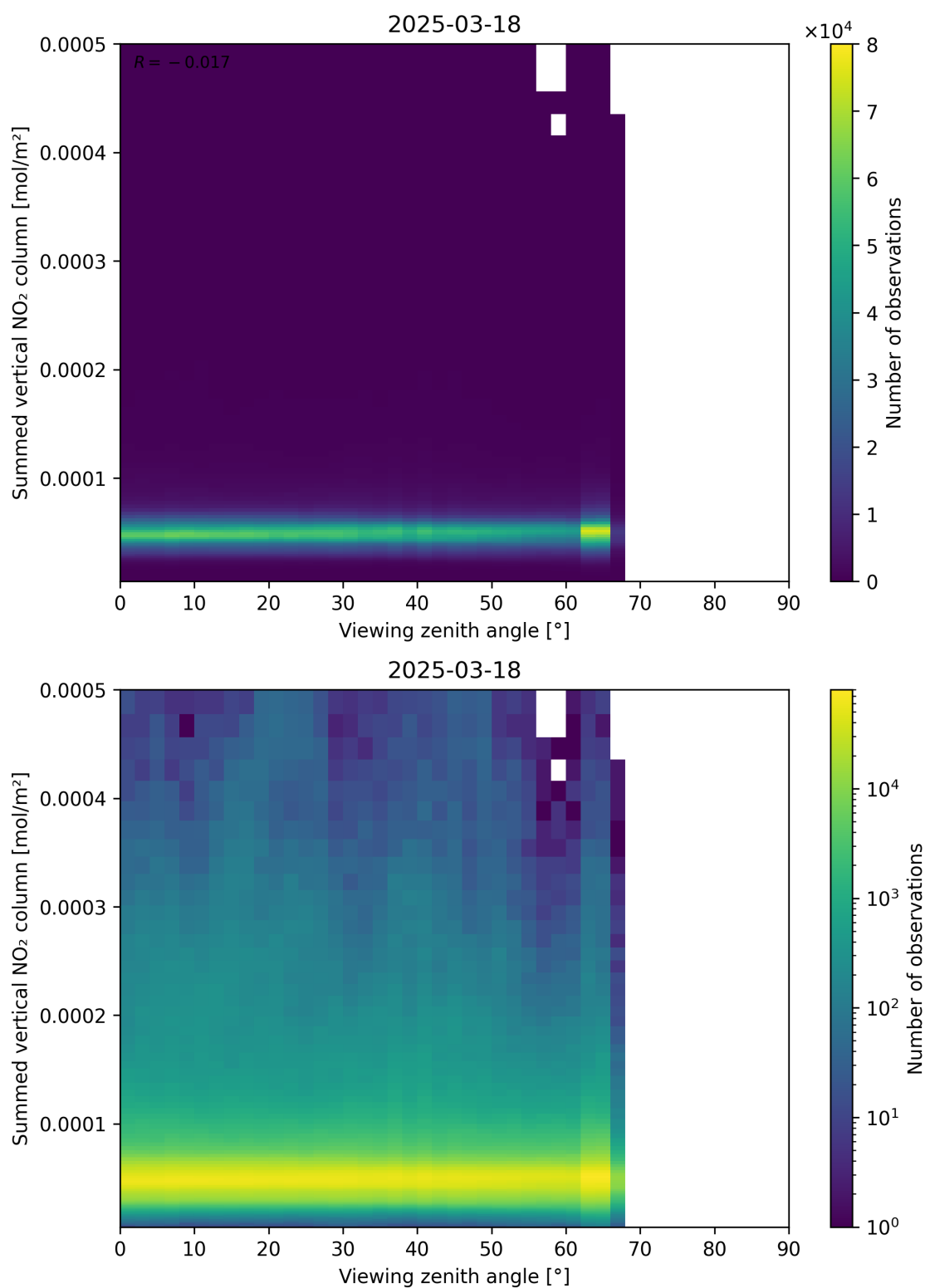
Figure 165: Scatter density plot of “Viewing zenith angle” against “Summed vertical NO 2 column” for 2025-03-18 to 2025-03-19.
