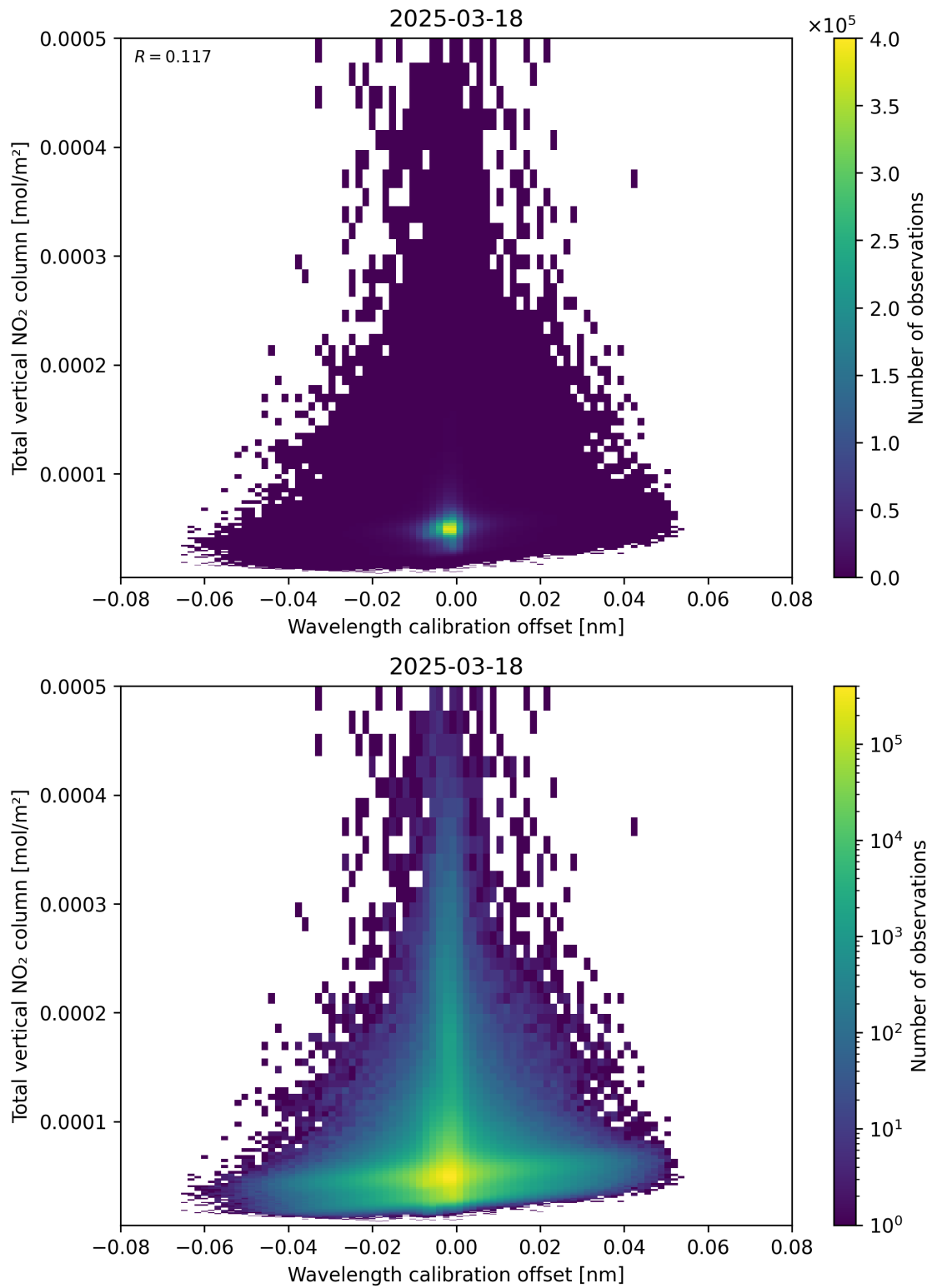
Figure 179: Scatter density plot of “Wavelength calibration offset” against “Total vertical NO 2 column” for 2025-03-18 to 2025-03-19.
