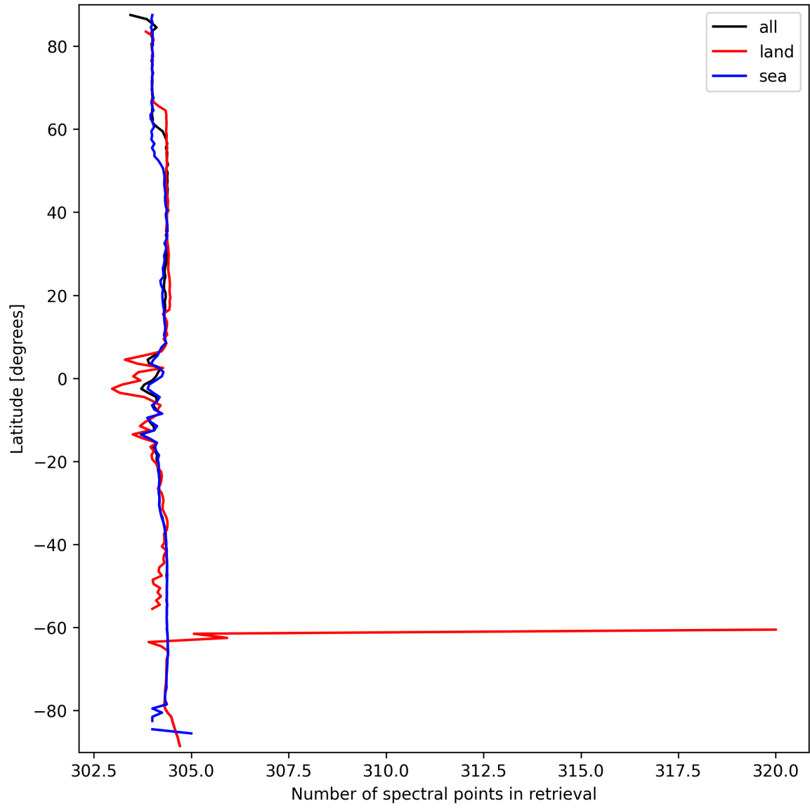
Figure 16: Zonal average of “Number of spectral points in retrieval” for 2025-03-18 to 2025-03-19.
