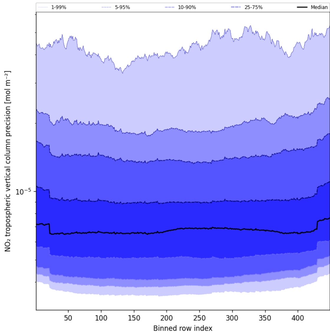
Figure 47: Along track statistics of “NO 2 tropospheric vertical column precision” for 2025-03-18 to 2025-03-19
