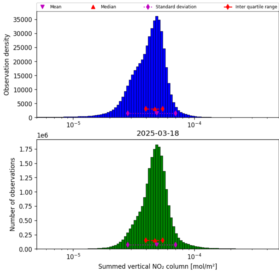
Figure 40: Histogram of “Summed vertical NO 2 column” for 2025-03-18 to 2025-03-19
