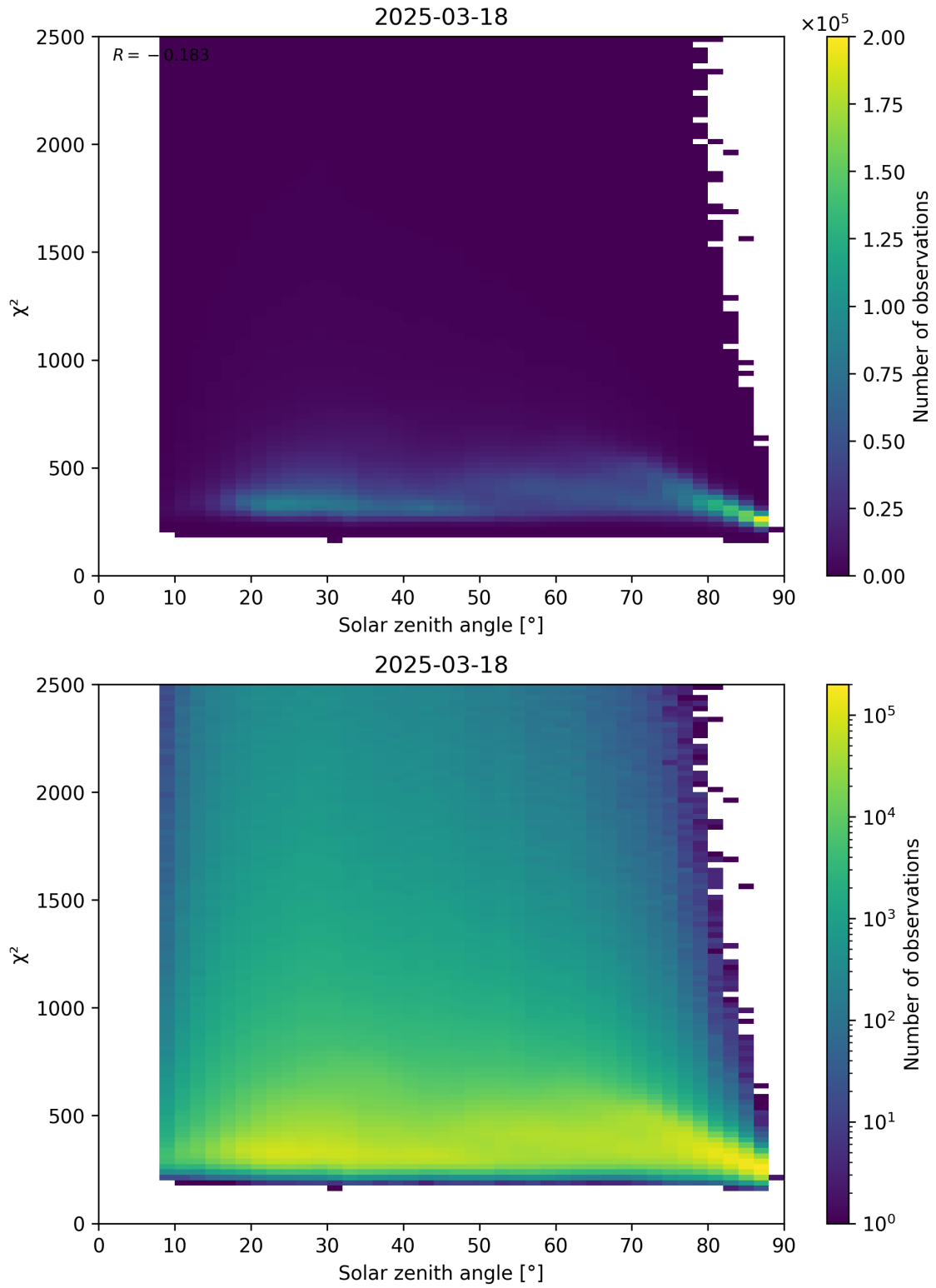
Figure 148: Scatter density plot of “Solar zenith angle” against “ \chi^2 ” for 2025-03-18 to 2025-03-19.
