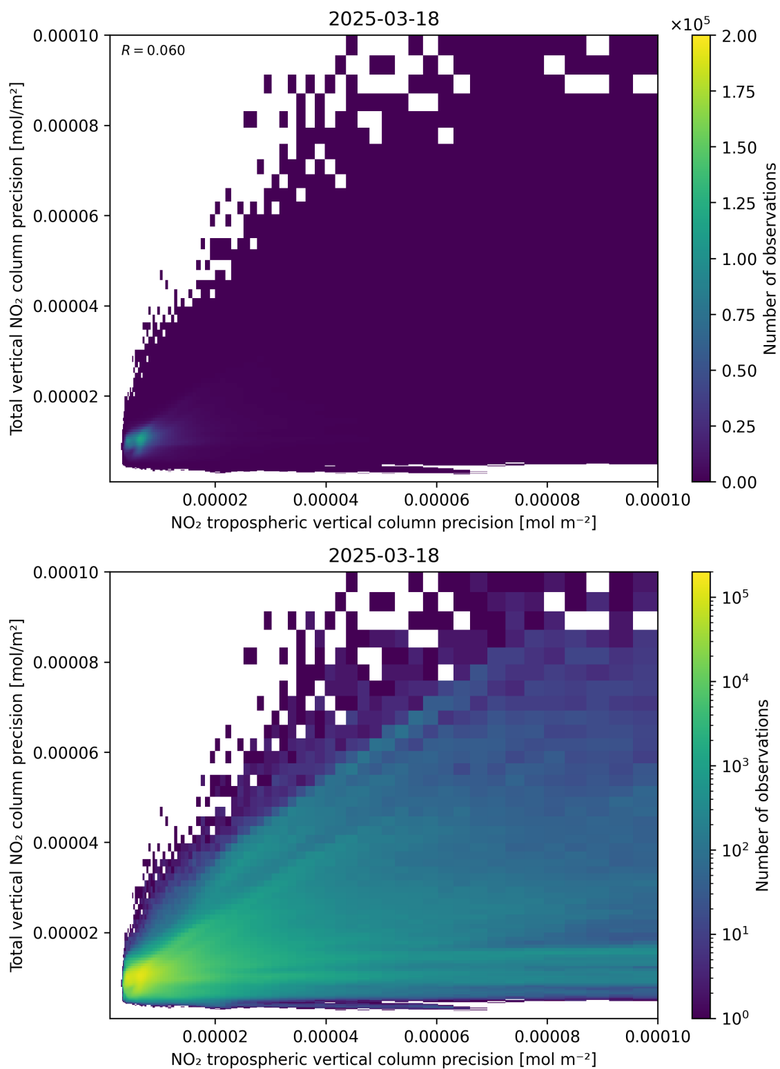
Figure 139: Scatter density plot of “NO 2 tropospheric vertical column precision” against “Total vertical NO 2 column precision” for 2025-03-18 to 2025-03-19.
