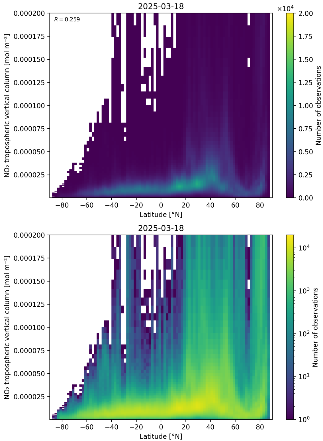
Figure 92: Scatter density plot of “Latitude” against “NO 2 tropospheric vertical column” for 2025-03-18 to 2025-03-19.
