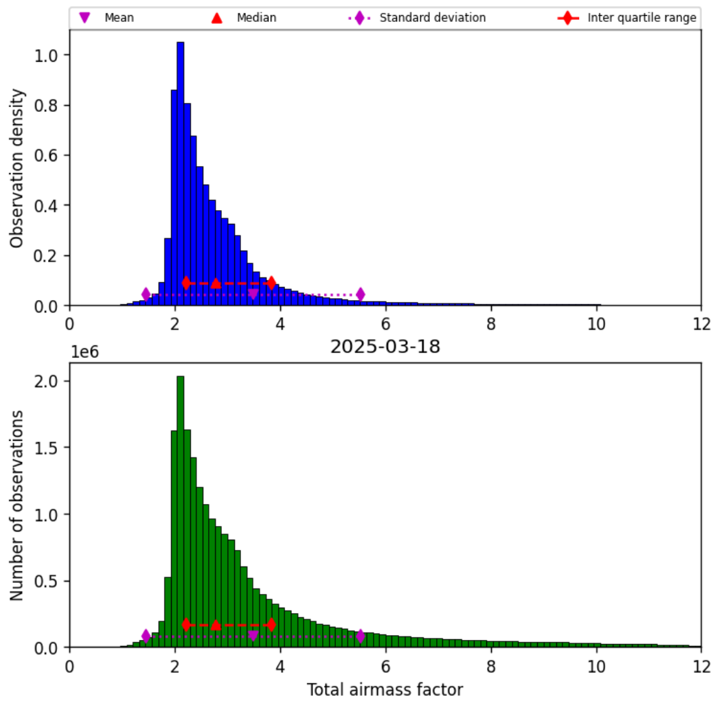
Figure 32: Histogram of “Total airmass factor” for 2025-03-18 to 2025-03-19
