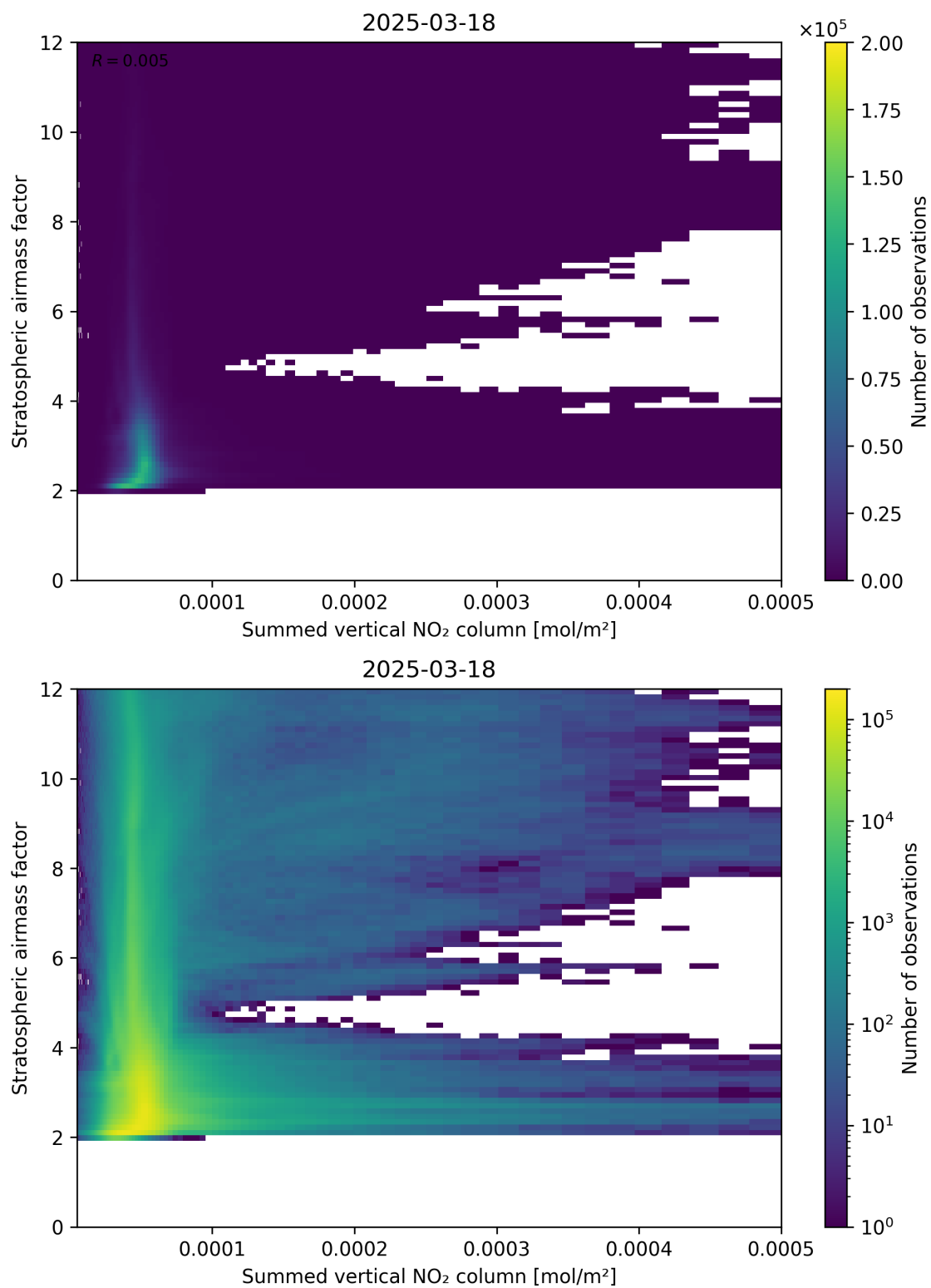
Figure 103: Scatter density plot of “Summed vertical NO 2 column” against “Stratospheric airmass factor” for 2025-03-18 to 2025-03-19.
