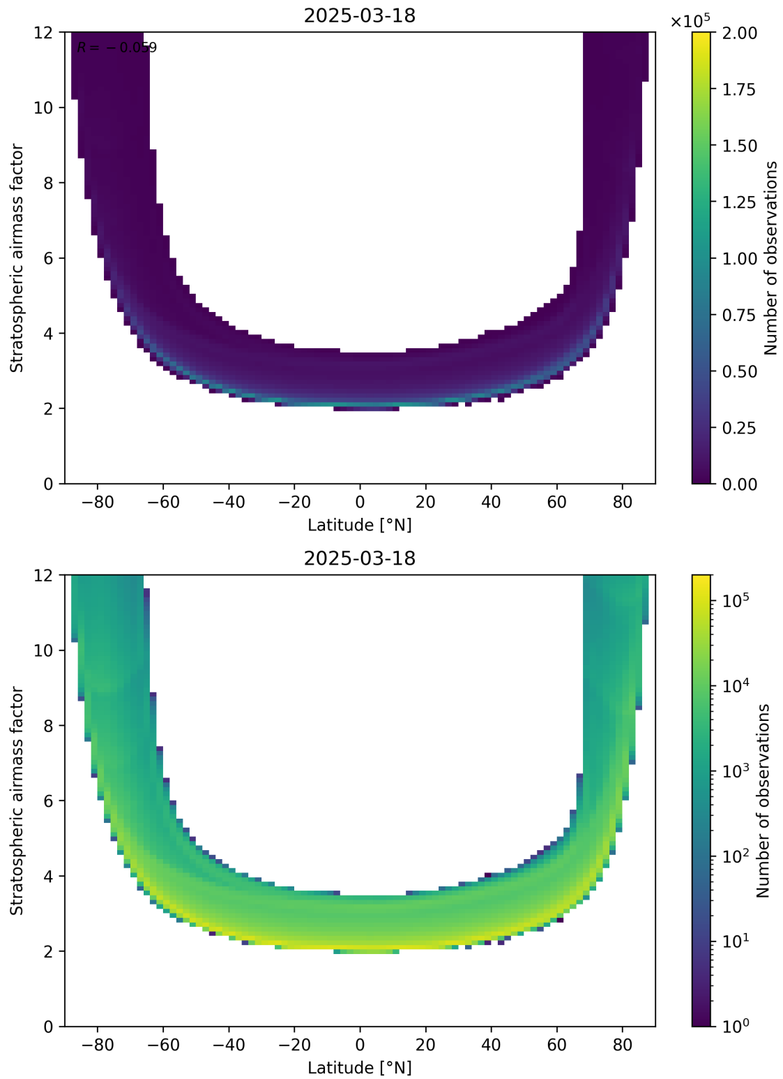
Figure 83: Scatter density plot of “Latitude” against “Stratospheric air mass factor” for 2025-03-18 to 2025-03-19.
