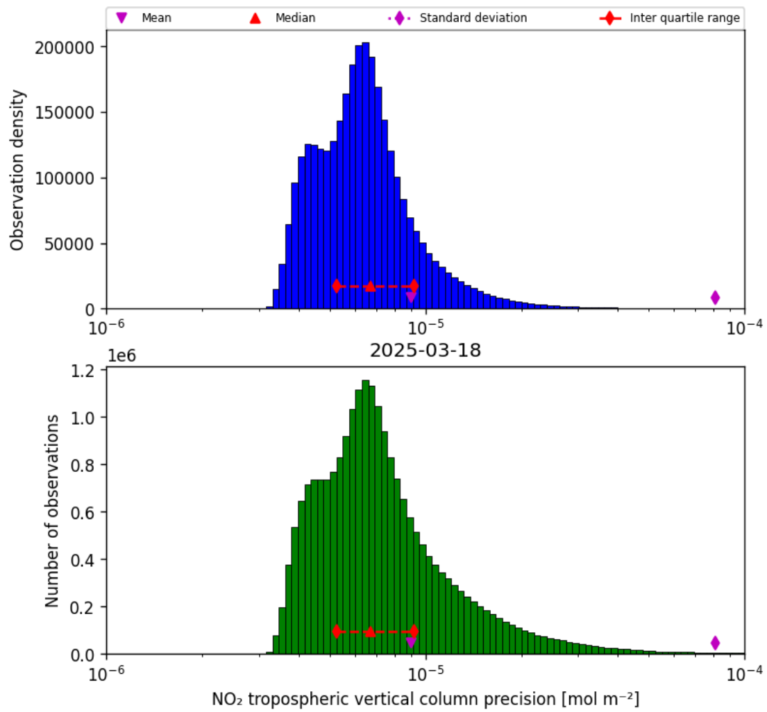
Figure 30: Histogram of “NO 2 tropospheric vertical column precision” for 2025-03-18 to 2025-03-19
