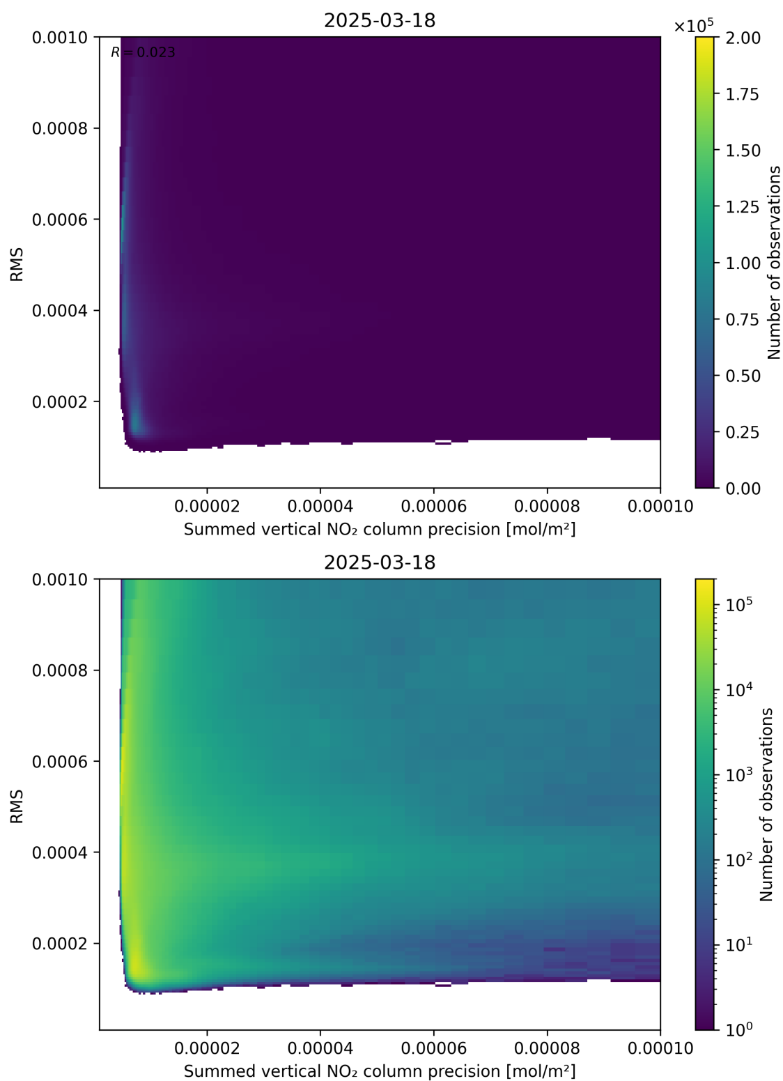
Figure 108: Scatter density plot of “Summed vertical NO 2 column precision” against “RMS” for 2025-03-18 to 2025-03-19.
