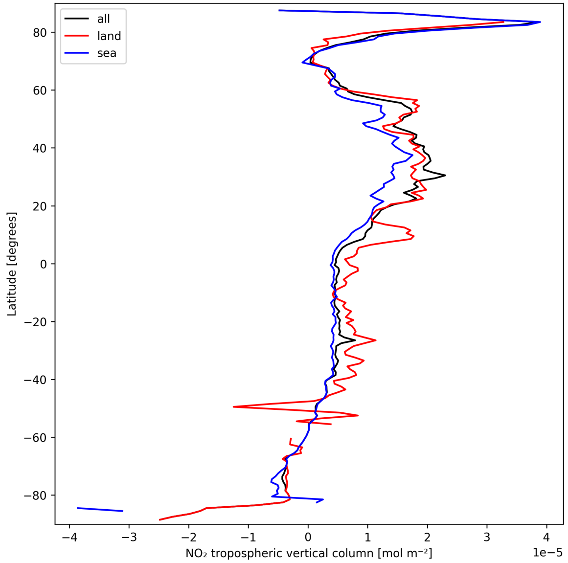
Figure 12: Zonal average of “NO 2 tropospheric vertical column” for 2025-03-18 to 2025-03-19.
