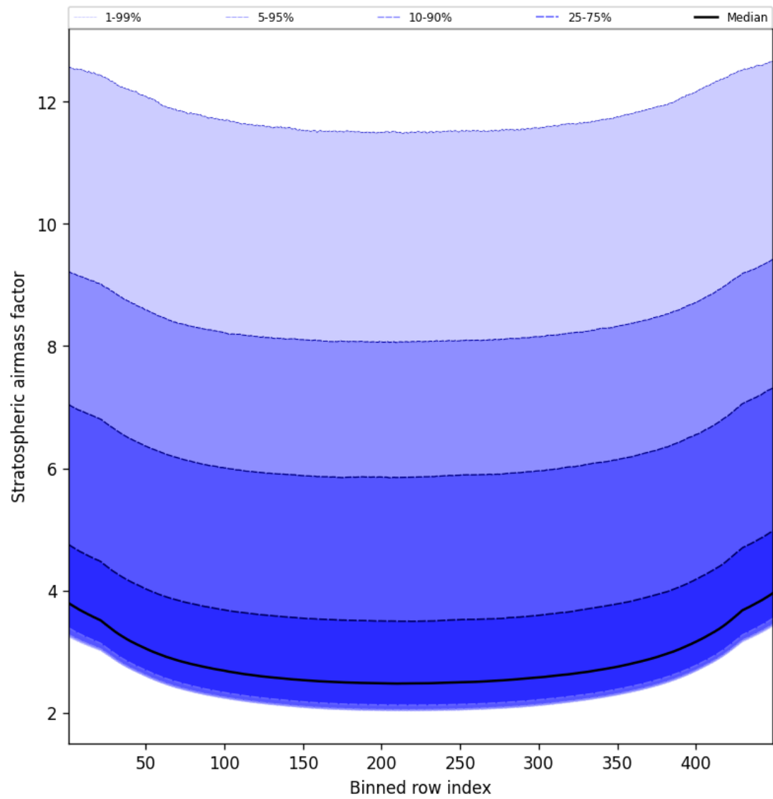
Figure 61: Along track statistics of “Stratospheric airmass factor” for 2025-03-18 to 2025-03-19
