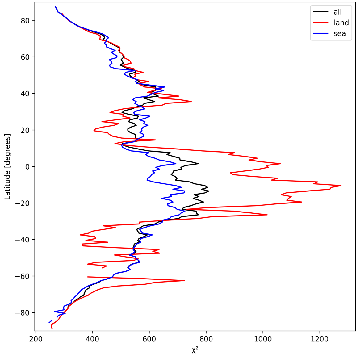
Figure 25: Zonal average of “ \chi^2 ” for 2025-03-18 to 2025-03-19.
