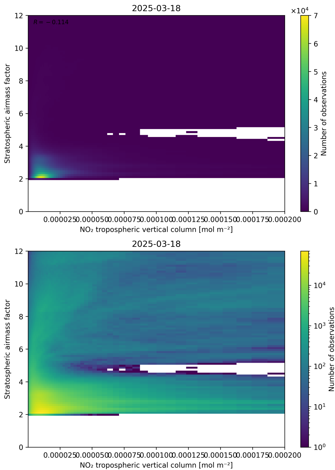
Figure 121: Scatter density plot of “NO 2 tropospheric vertical column” against “Stratospheric air mass factor” for 2025-03-18 to 2025-03-19.
