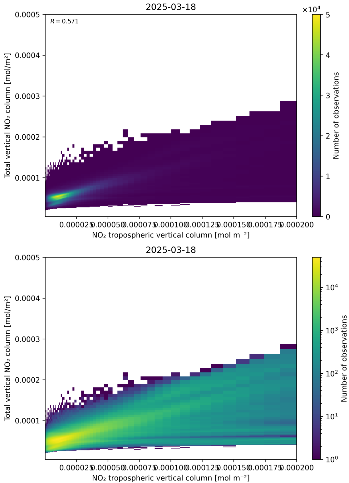
Figure 128: Scatter density plot of “NO 2 tropospheric vertical column” against “Total vertical NO 2 column” for 2025-03-18 to 2025-03-19.
