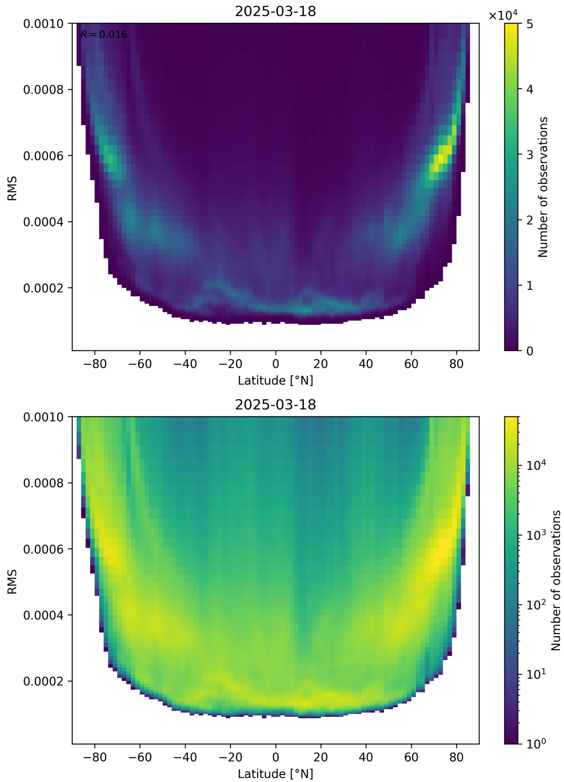
Figure 94: Scatter density plot of “Latitude” against “RMS” for 2025-03-18 to 2025-03-19.
