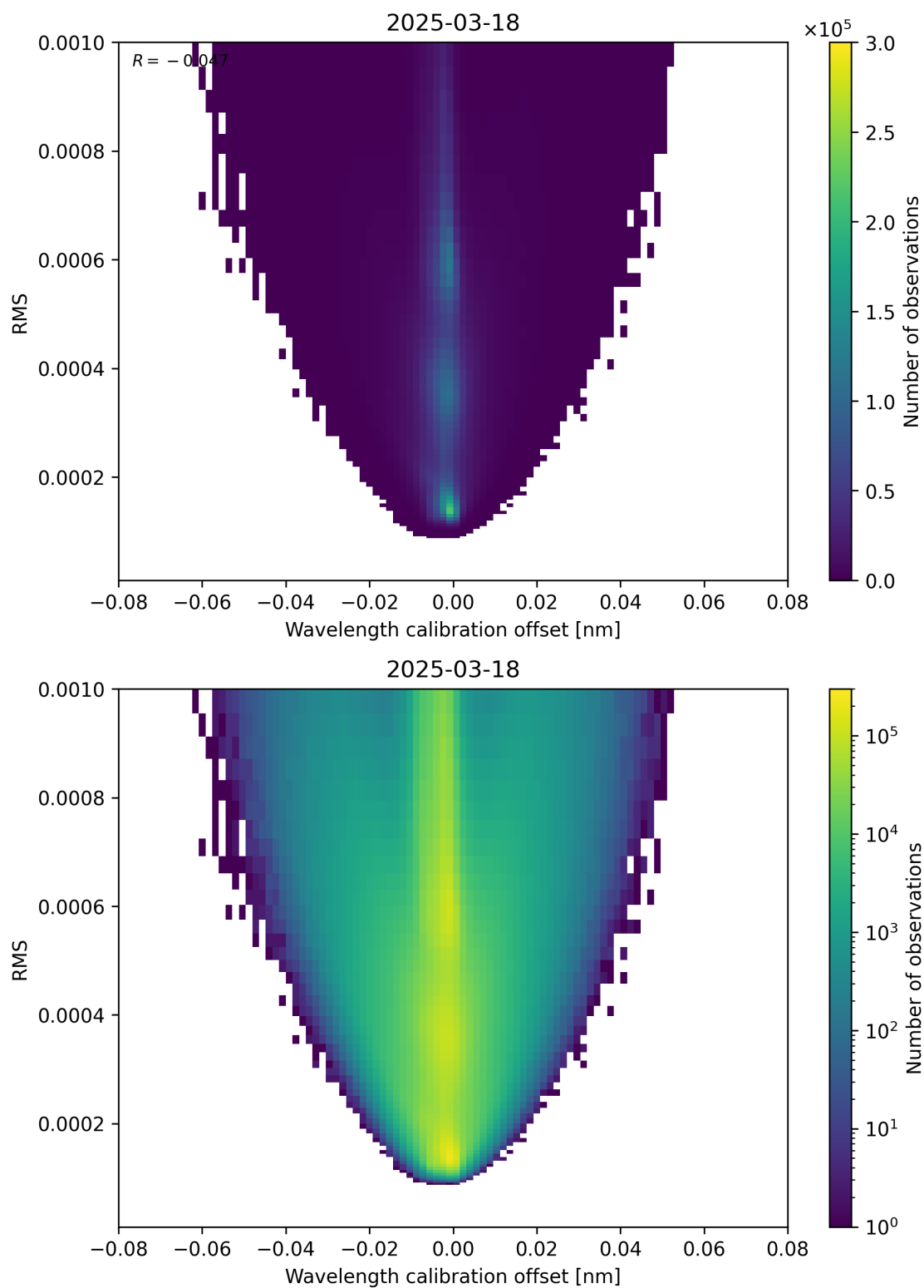
Figure 181: Scatter density plot of “Wavelength calibration offset” against “RMS” for 2025-03-18 to 2025-03-19.
