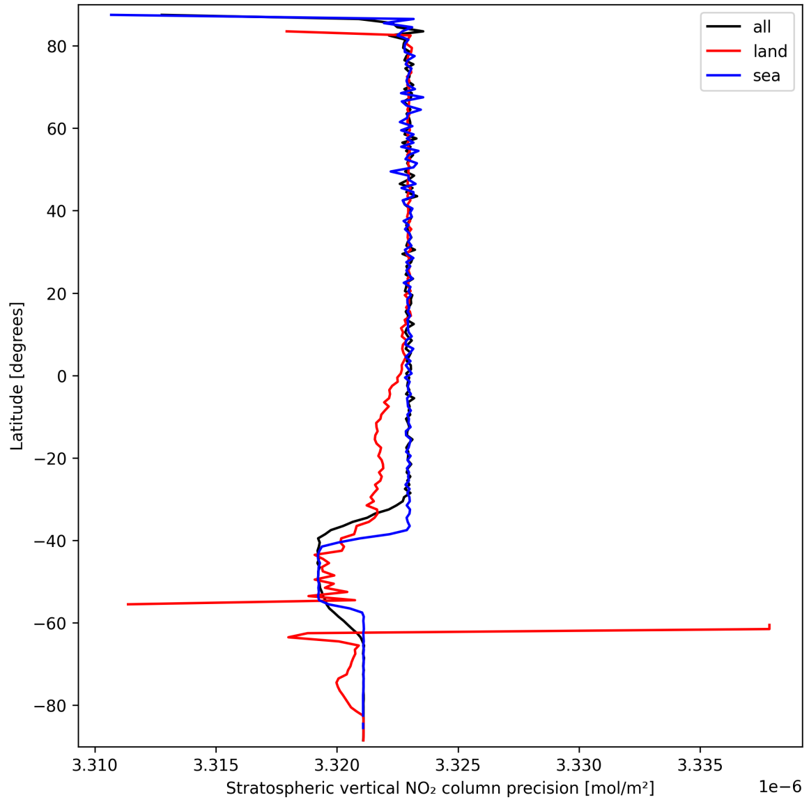
Figure 20: Zonal average of “Stratospheric vertical NO 2 column precision” for 2025-03-18 to 2025-03-19.
