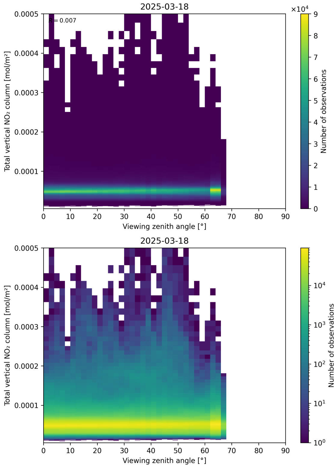
Figure 167: Scatter density plot of “Viewing zenith angle” against “Total vertical NO 2 column” for 2025-03-18 to 2025-03-19.
