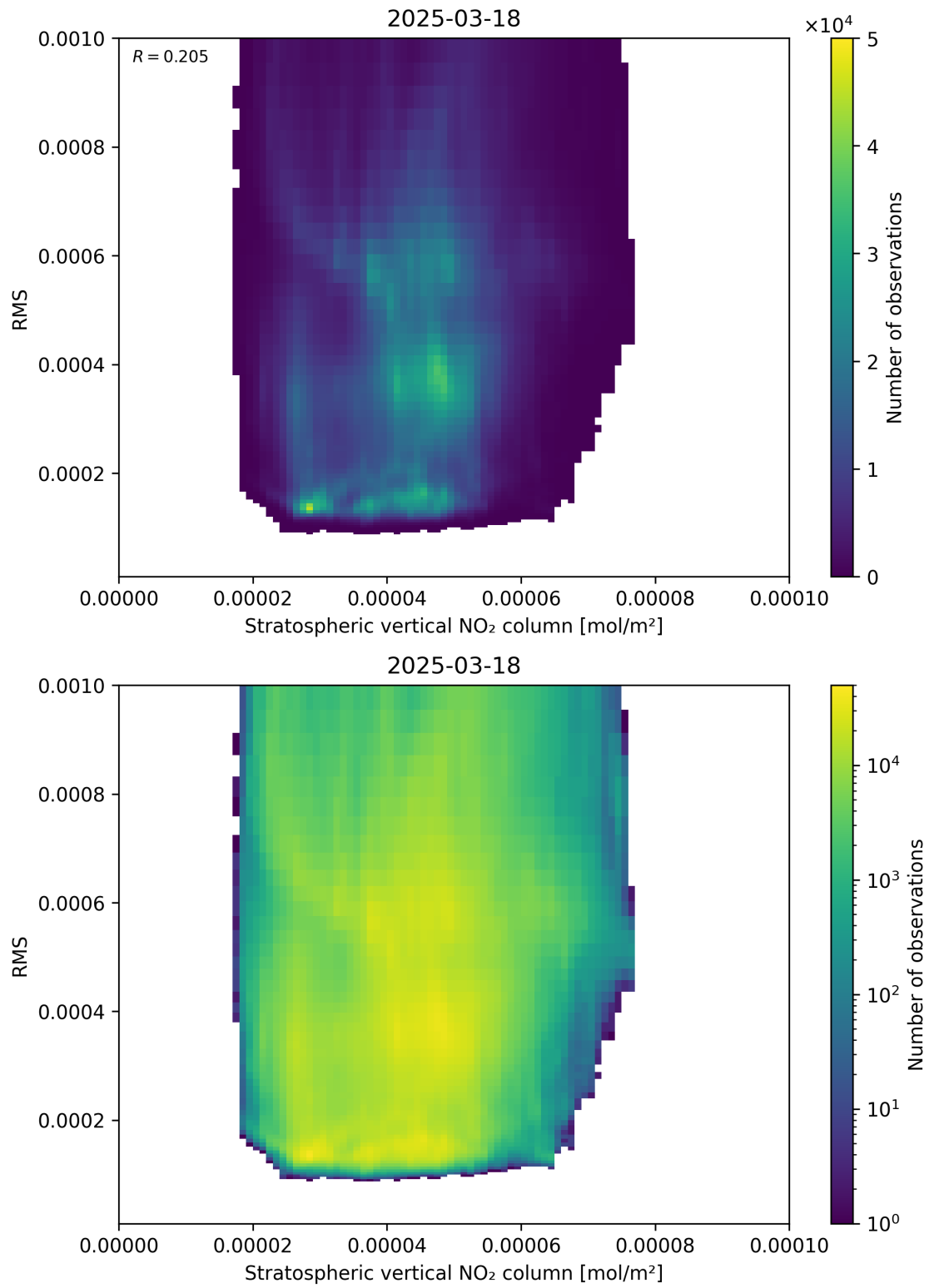
Figure 102: Scatter density plot of “Stratospheric vertical NO 2 column” against “RMS” for 2025-03-18 to 2025-03-19.
