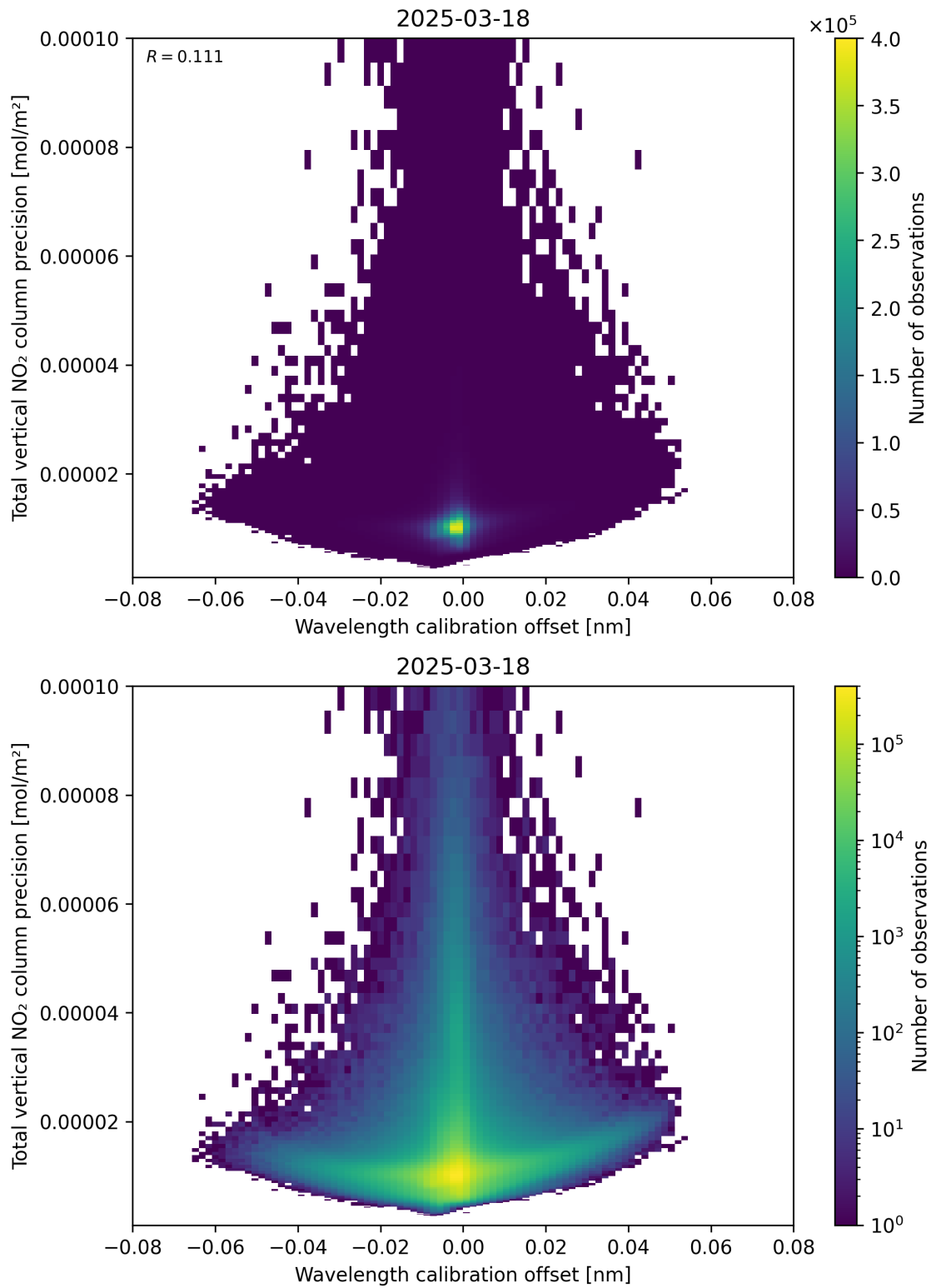
Figure 180: Scatter density plot of “Wavelength calibration offset” against “Total vertical NO 2 column precision” for 2025-03-18 to 2025-03-19.
