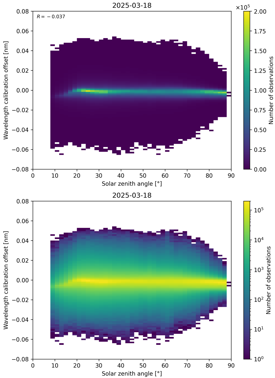
Figure 158: Scatter density plot of “Solar zenith angle” against “Wavelength calibration offset” for 2025-03-18 to 2025-03-19.
