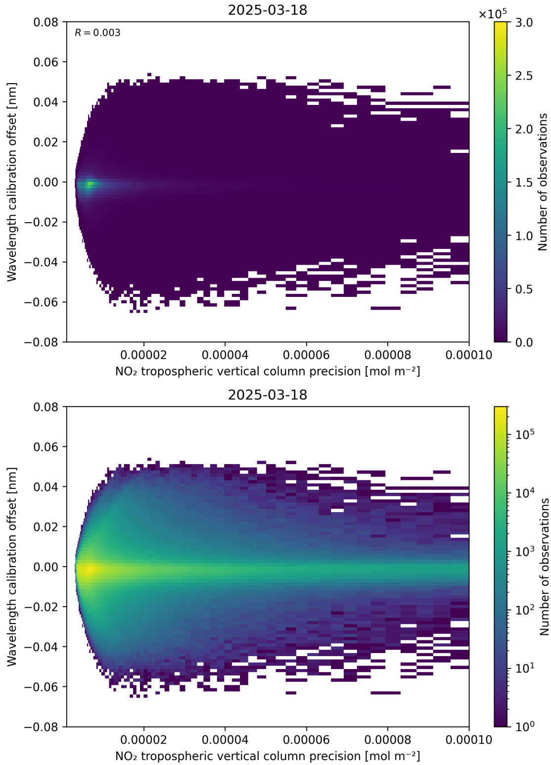
Figure 141: Scatter density plot of “NO 2 tropospheric vertical column precision” against “Wavelength calibration offset” for 2025-03-18 to 2025-03-19.
