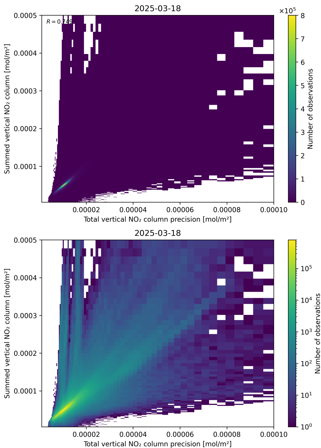
Figure 117: Scatter density plot of “Total vertical NO 2 column precision” against “Summed vertical NO 2 column” for 2025-03-18 to 2025-03-19.
