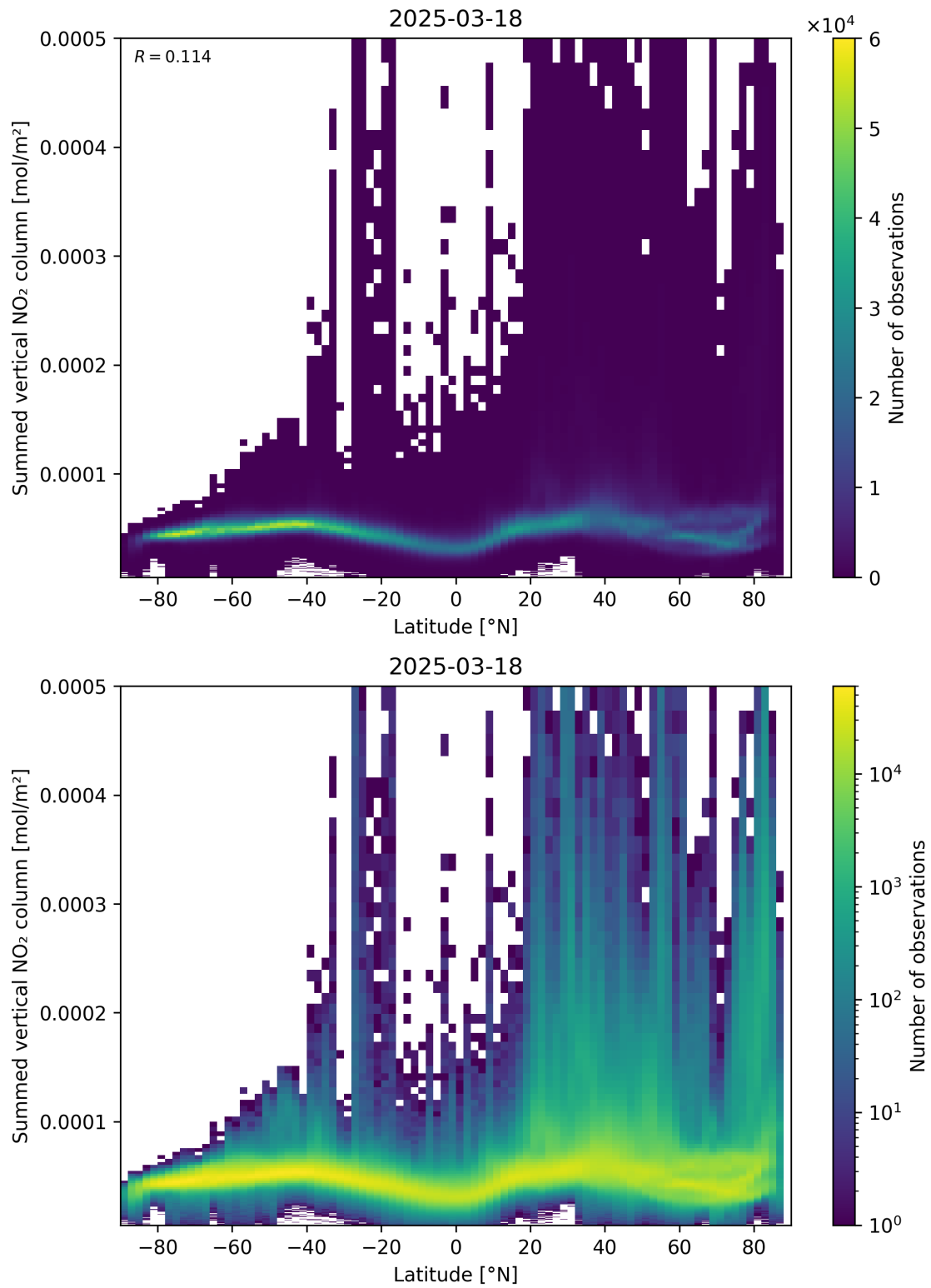
Figure 88: Scatter density plot of “Latitude” against “Summed vertical NO 2 column” for 2025-03-18 to 2025-03-19.
