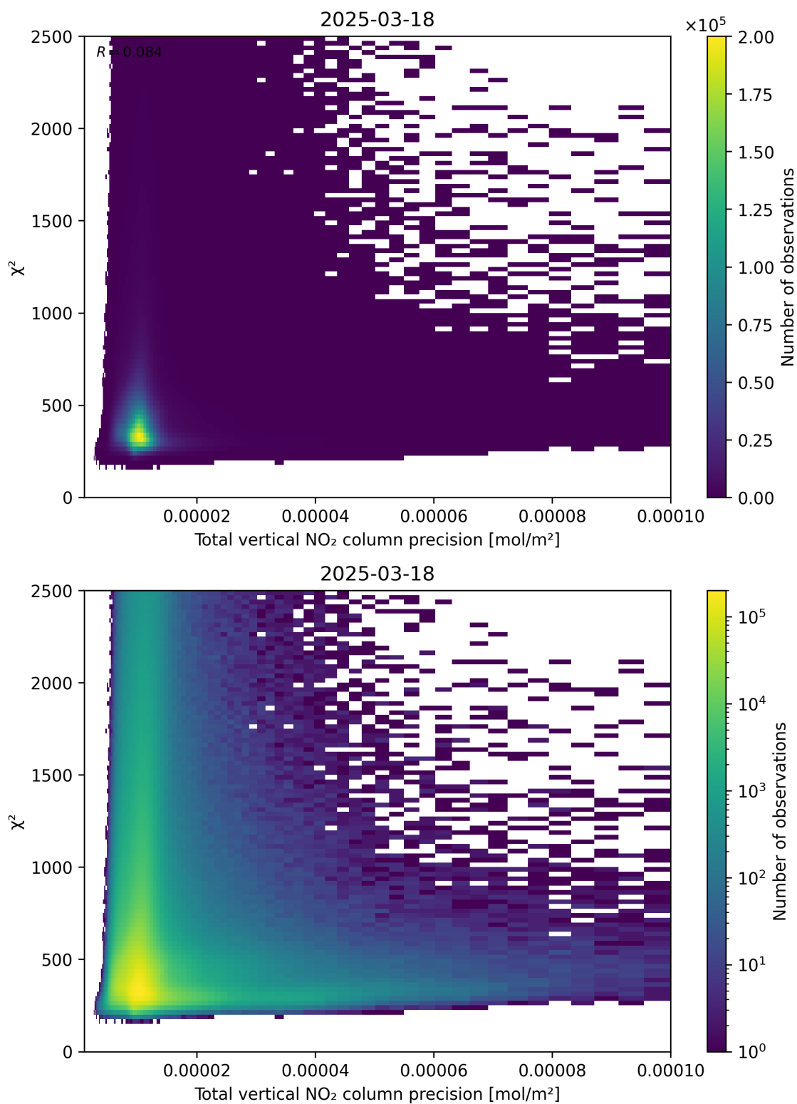
Figure 116: Scatter density plot of “Total vertical NO 2 column precision” against “ \chi^2 ” for 2025-03-18 to 2025-03-19.
