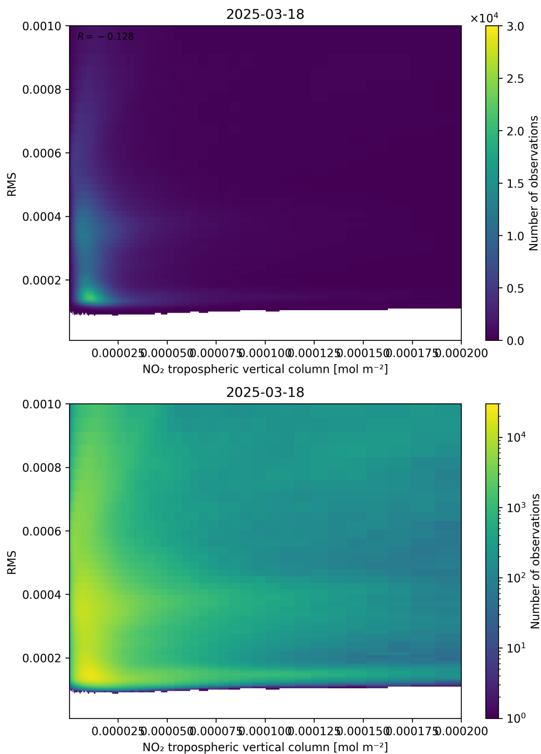
Figure 142: Scatter density plot of “NO 2 tropospheric vertical column” against “RMS” for 2025-03-18 to 2025-03-19.
