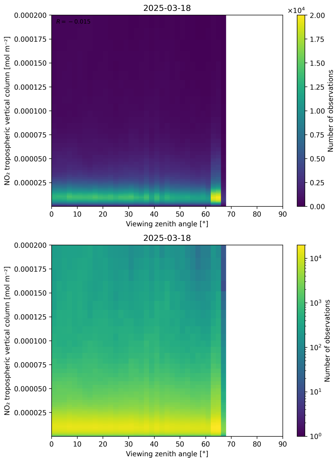
Figure 169: Scatter density plot of “Viewing zenith angle” against “NO 2 tropospheric vertical column” for 2025-03-18 to 2025-03-19.
