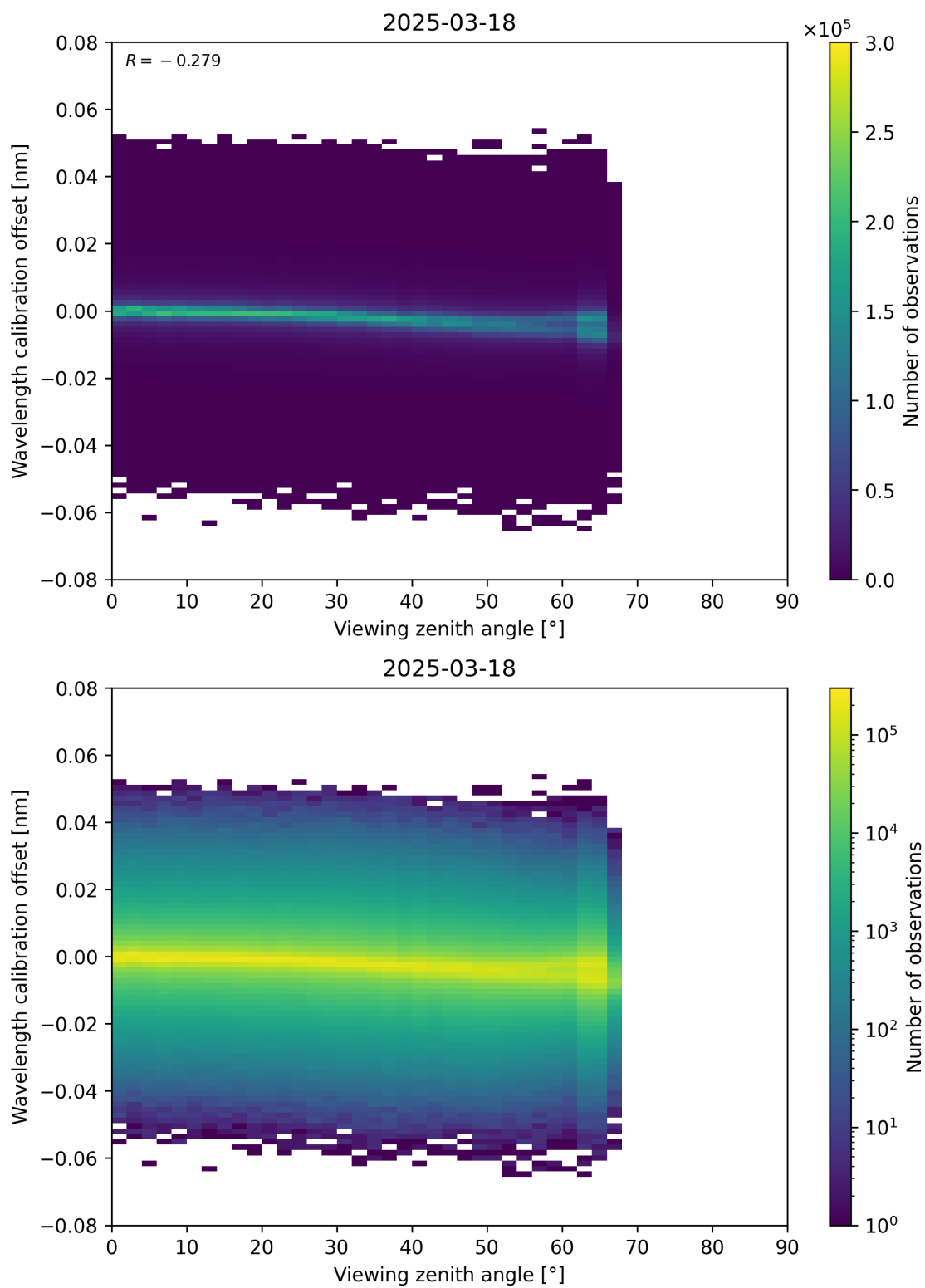
Figure 173: Scatter density plot of “Viewing zenith angle” against “Wavelength calibration offset” for 2025-03-18 to 2025-03-19.
