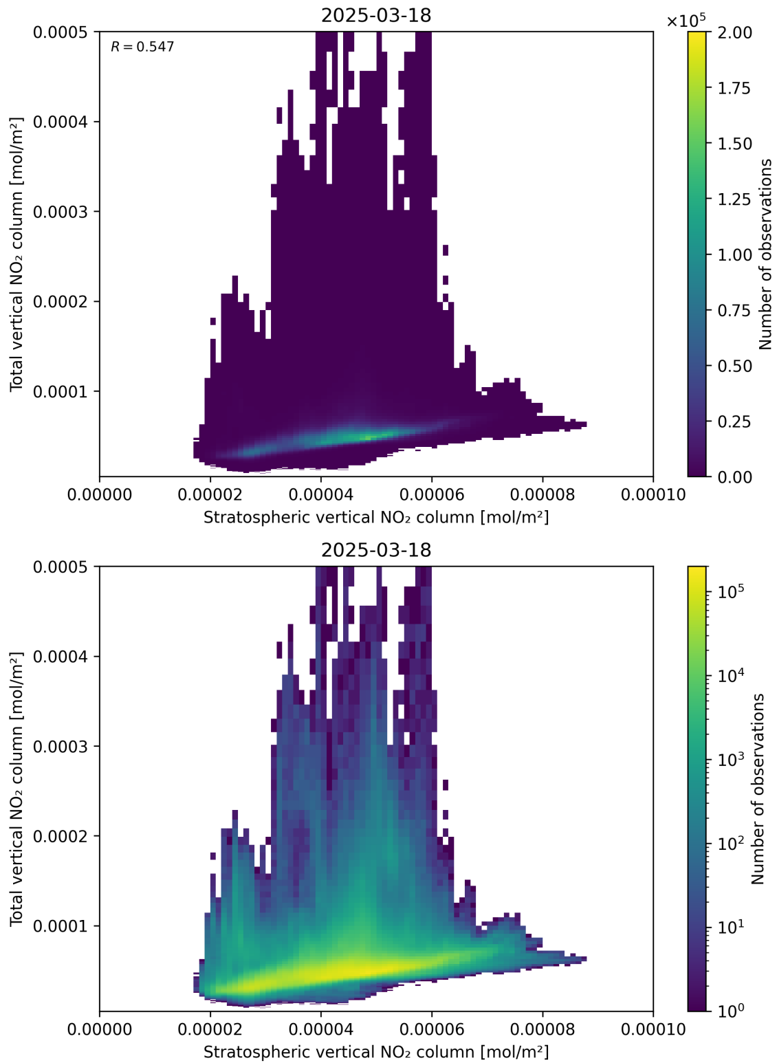
Figure 100: Scatter density plot of “Stratospheric vertical NO 2 column” against “Total vertical NO 2 column” for 2025-03-18 to 2025-03-19.
