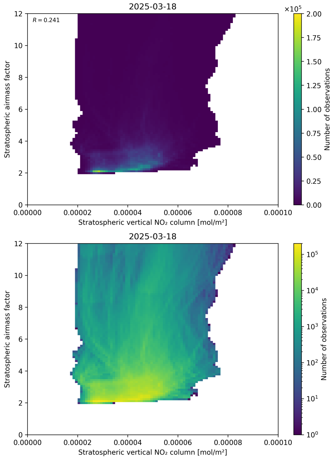
Figure 96: Scatter density plot of “Stratospheric vertical NO 2 column” against “Stratospheric airmass factor” for 2025-03-18 to 2025-03-19.
