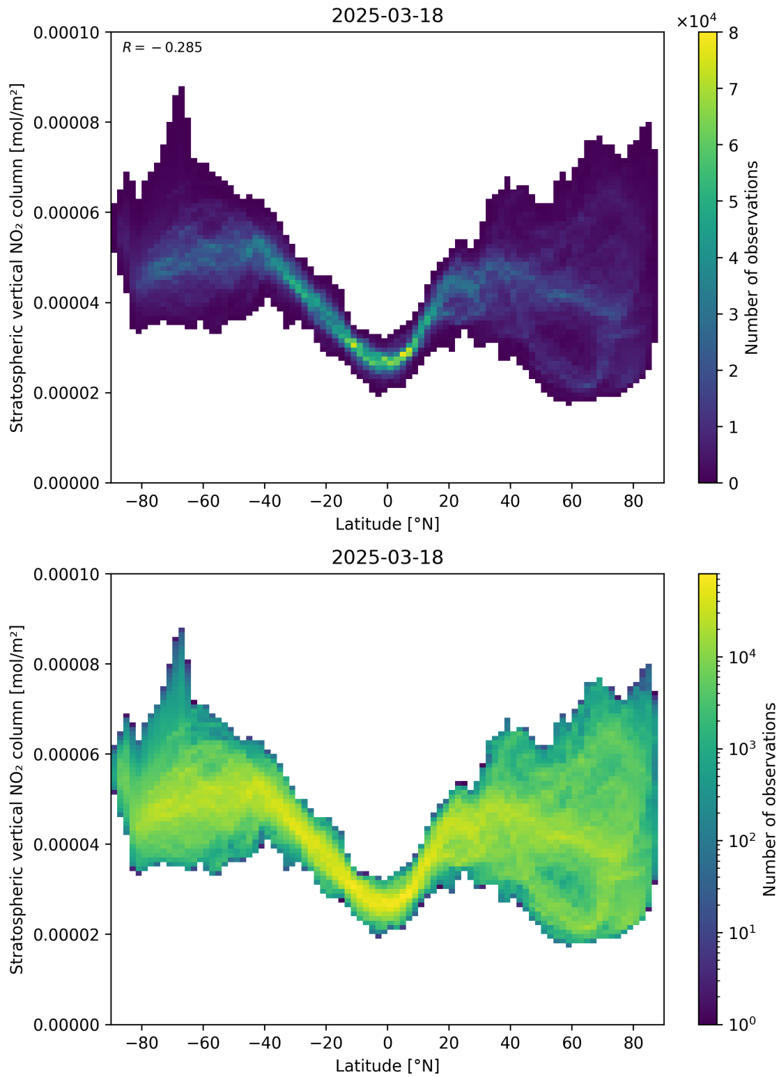
Figure 87: Scatter density plot of “Latitude” against “Stratospheric vertical NO 2 column” for 2025-03-18 to 2025-03-19.
