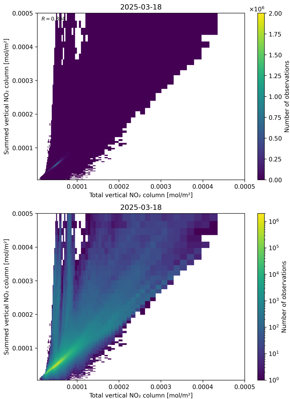
Figure 112: Scatter density plot of “Total vertical NO 2 column” against “Summed vertical NO 2 column” for 2025-03-18 to 2025-03-19.
