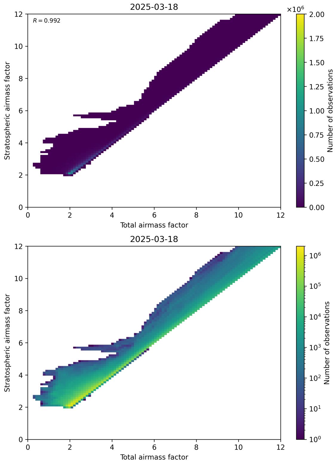
Figure 62: Scatter density plot of “Total airmass factor” against “Stratospheric airmass factor” for 2025-03-18 to 2025-03-19.
