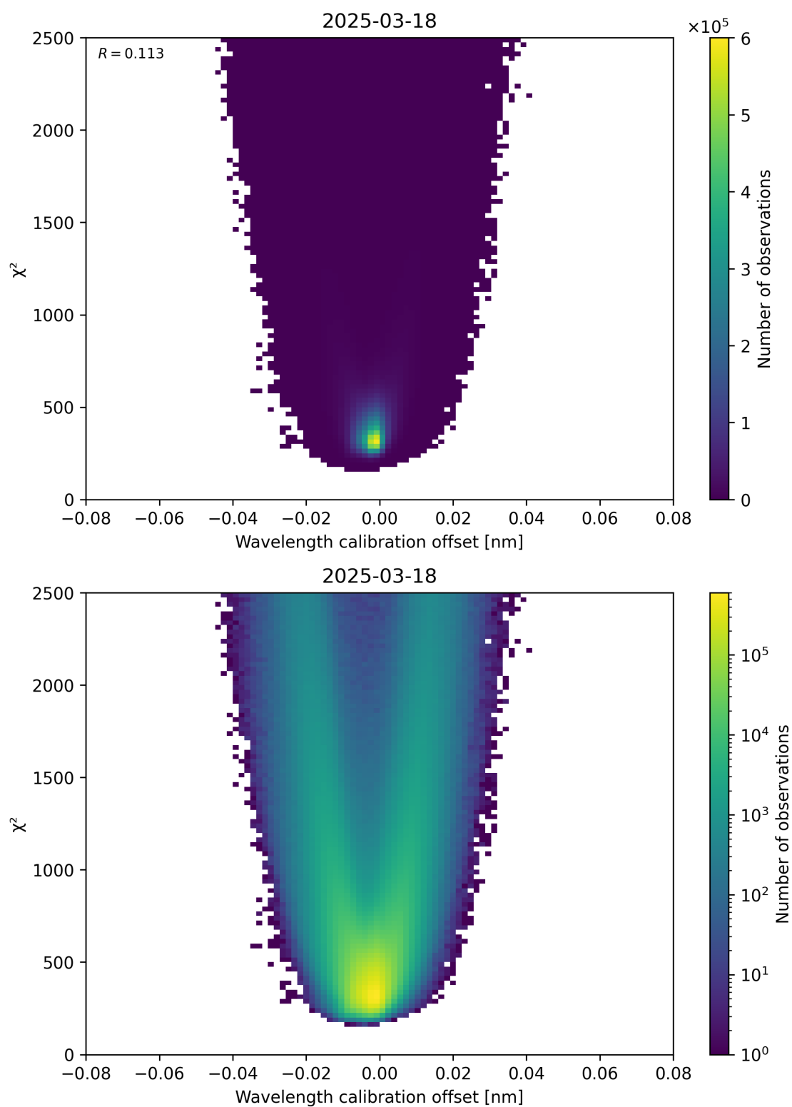
Figure 175: Scatter density plot of “Wavelength calibration offset” against “ \chi^2 ” for 2025-03-18 to 2025-03-19.
