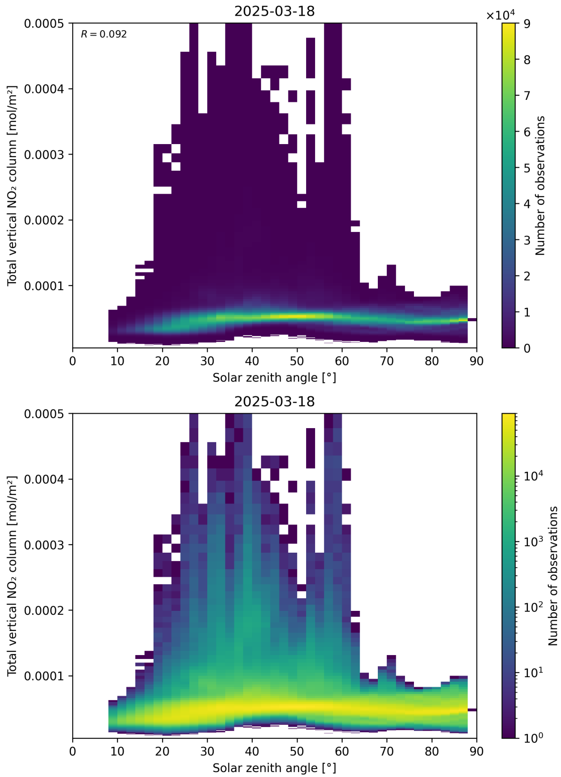
Figure 153: Scatter density plot of “Solar zenith angle” against “Total vertical NO 2 column” for 2025-03-18 to 2025-03-19.
