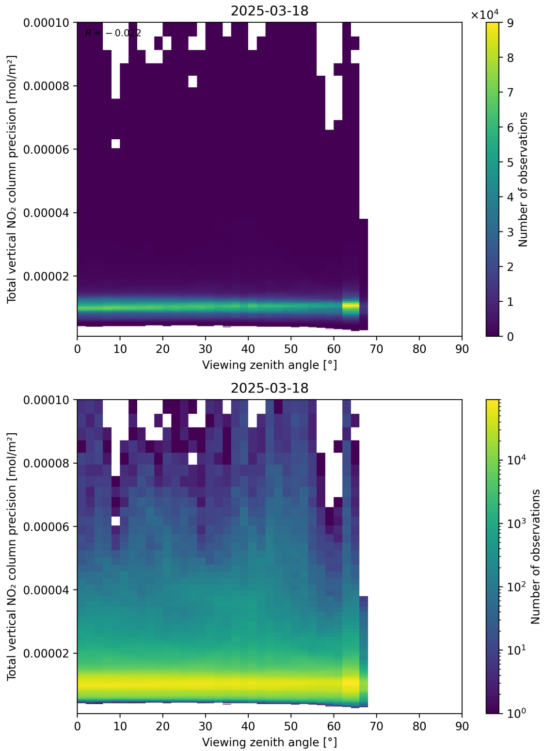
Figure 168: Scatter density plot of “Viewing zenith angle” against “Total vertical NO 2 column precision” for 2025-03-18 to 2025-03-19.
