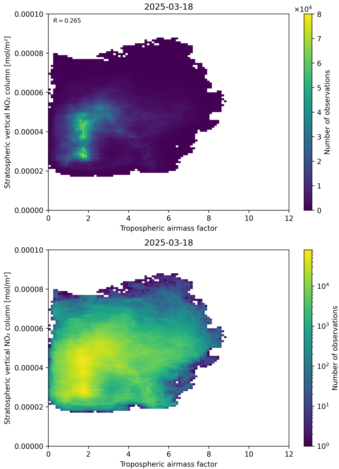
Figure 74: Scatter density plot of “Tropospheric air mass factor” against “Stratospheric vertical NO 2 column” for 2025-03-18 to 2025-03-19.
