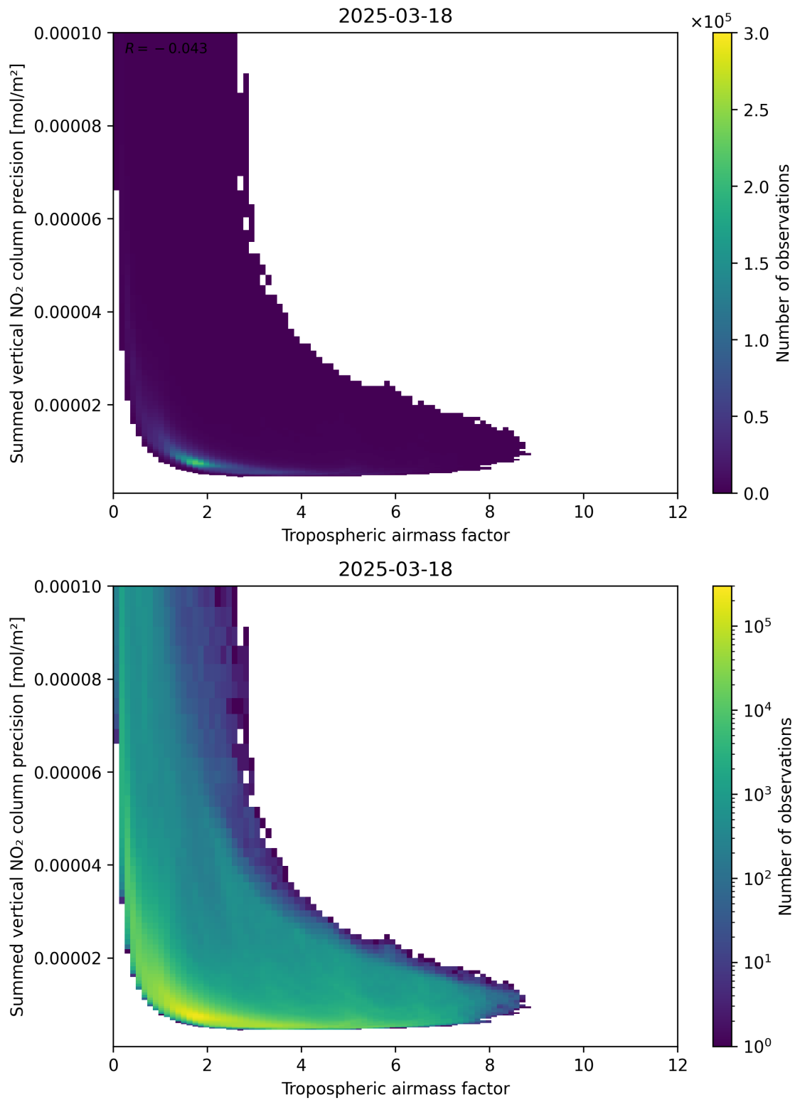
Figure 76: Scatter density plot of “Tropospheric air mass factor” against “Summed vertical NO 2 column precision” for 2025-03-18 to 2025-03-19.
