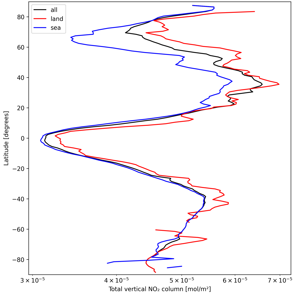
Figure 21: Zonal average of “Total vertical NO 2 column” for 2025-03-18 to 2025-03-19.
