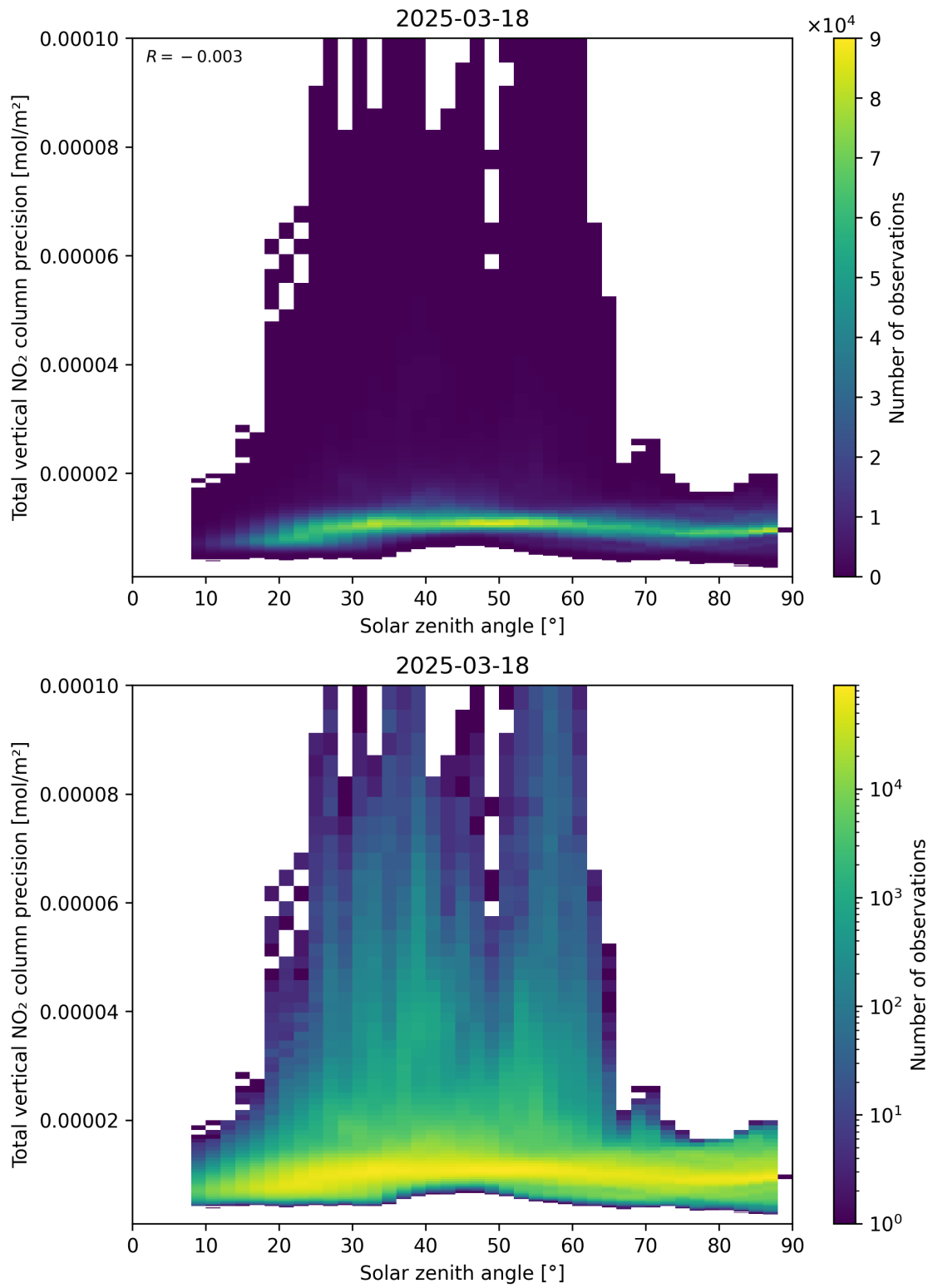
Figure 154: Scatter density plot of “Solar zenith angle” against “Total vertical NO 2 column precision” for 2025-03-18 to 2025-03-19.
