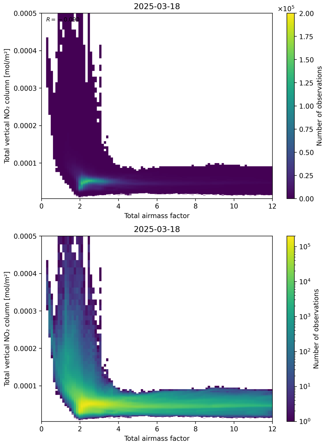
Figure 67: Scatter density plot of “Total airmass factor” against “Total vertical NO 2 column” for 2025-03-18 to 2025-03-19.
