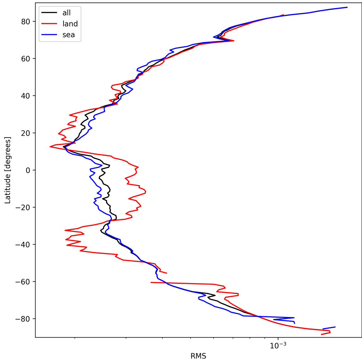
Figure 26: Zonal average of “RMS” for 2025-03-18 to 2025-03-19.
