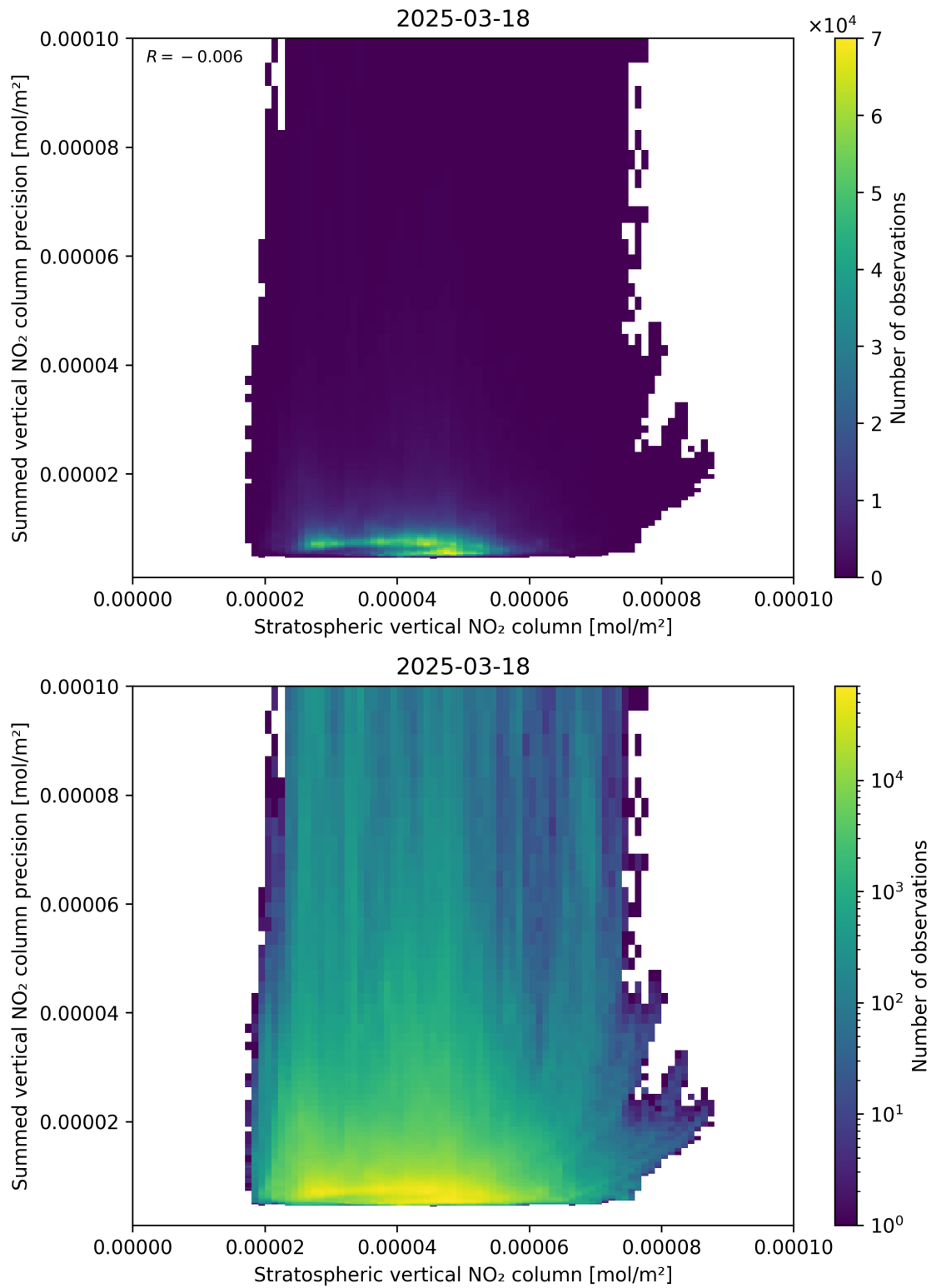
Figure 99: Scatter density plot of “Stratospheric vertical NO 2 column” against “Summed vertical NO 2 column precision” for 2025-03-18 to 2025-03-19.
