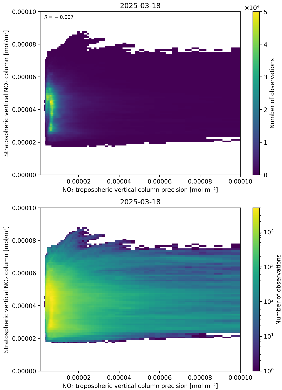
Figure 135: Scatter density plot of “NO 2 tropospheric vertical column precision” against “Stratospheric vertical NO 2 column” for 2025-03-18 to 2025-03-19.
