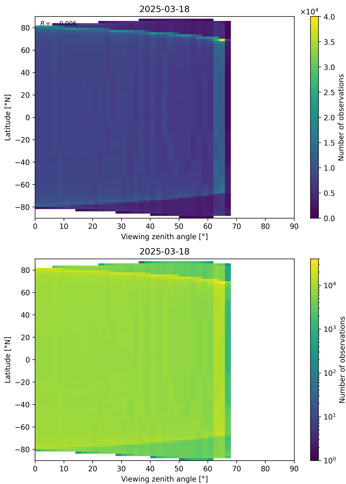
Figure 163: Scatter density plot of “Viewing zenith angle” against “Latitude” for 2025-03-18 to 2025-03-19.
