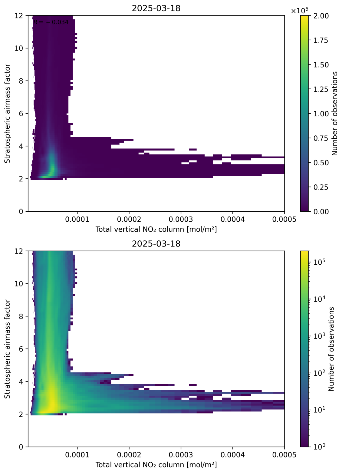
Figure 110: Scatter density plot of “Total vertical NO 2 column” against “Stratospheric airmass factor” for 2025-03-18 to 2025-03-19.
