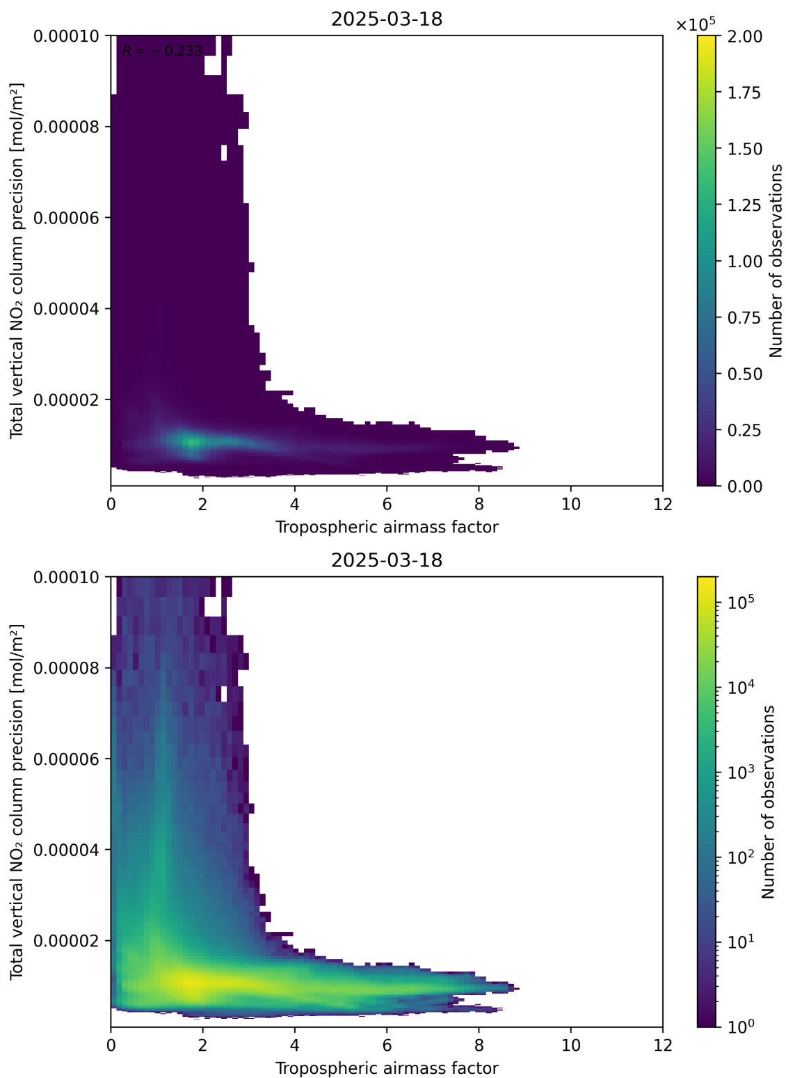
Figure 78: Scatter density plot of “Tropospheric airmass factor” against “Total vertical NO 2 column precision” for 2025-03-18 to 2025-03-19.
