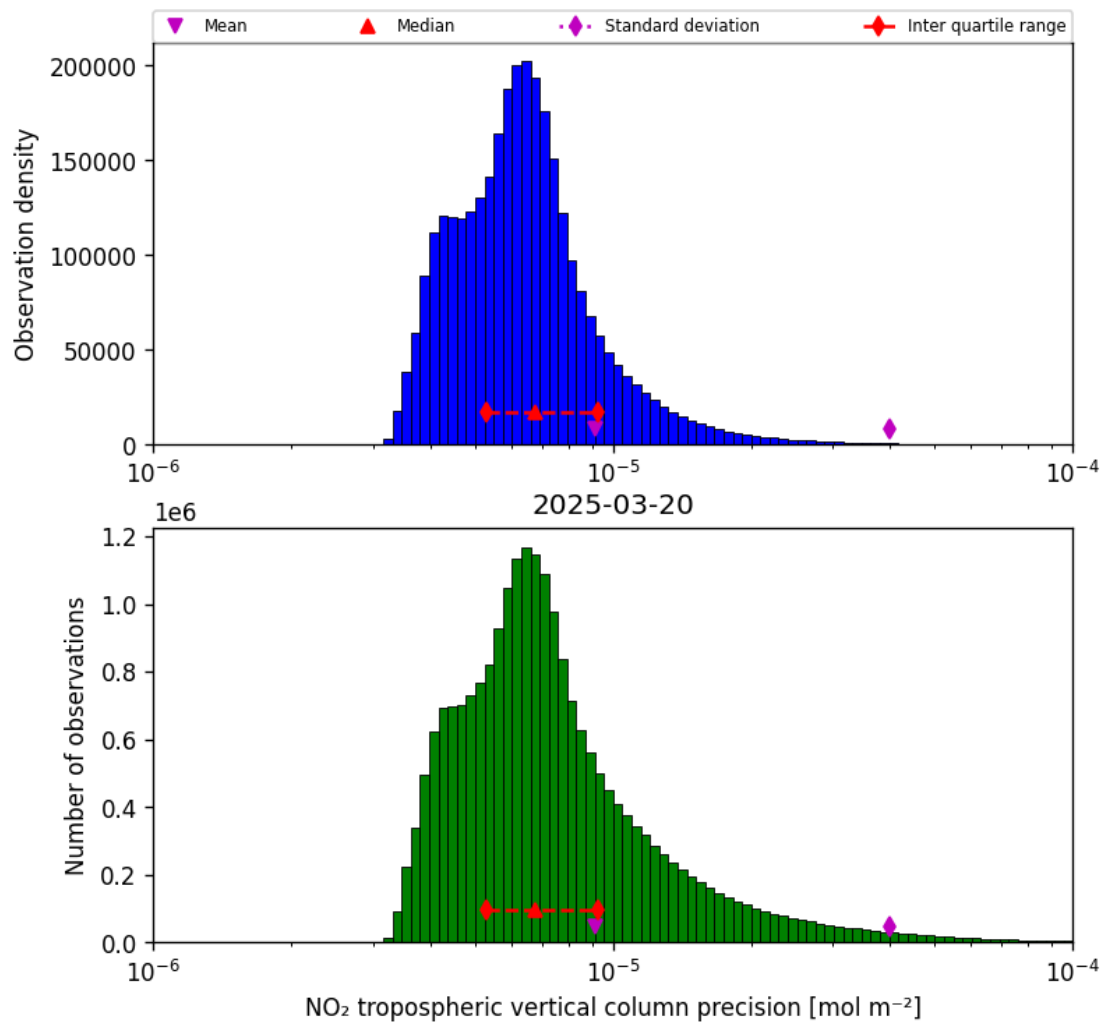
Figure 30: Histogram of “NO 2 tropospheric vertical column precision” for 2025-03-20 to 2025-03-21
