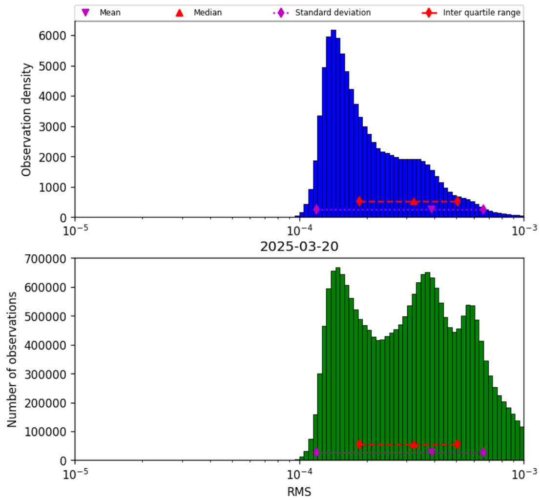
Figure 43: Histogram of “RMS” for 2025-03-20 to 2025-03-21
