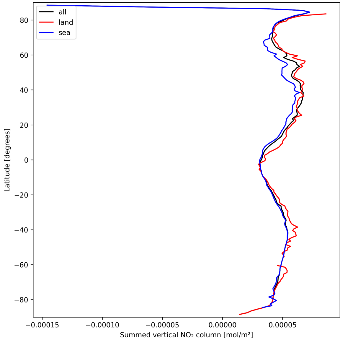
Figure 23: Zonal average of “Summed vertical NO 2 column” for 2025-03-20 to 2025-03-21.
