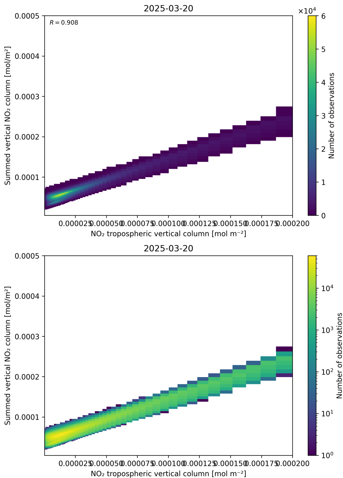
Figure 126: Scatter density plot of “NO 2 tropospheric vertical column” against “Summed vertical NO 2 column” for 2025-03-20 to 2025-03-21.
