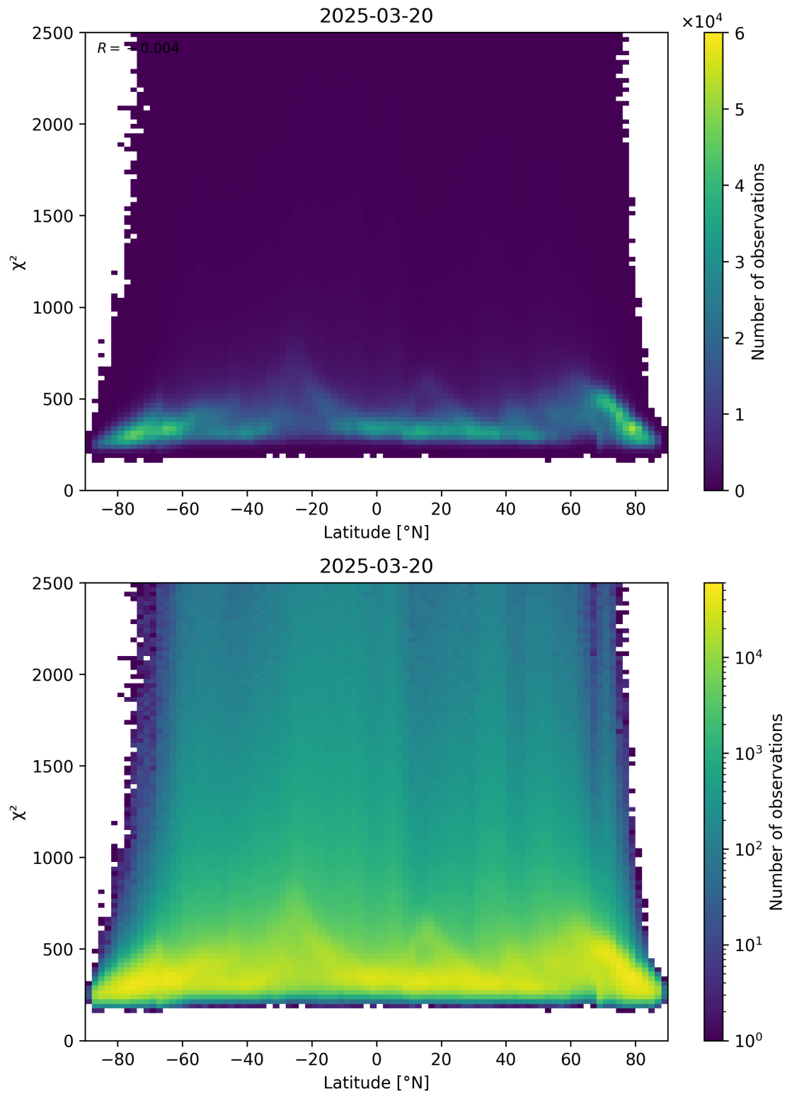
Figure 86: Scatter density plot of “Latitude” against “ \chi^2 ” for 2025-03-20 to 2025-03-21.
