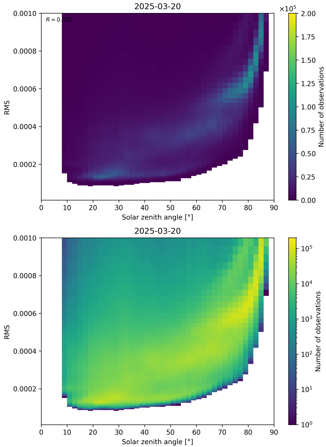
Figure 157: Scatter density plot of “Solar zenith angle” against “RMS” for 2025-03-20 to 2025-03-21.
