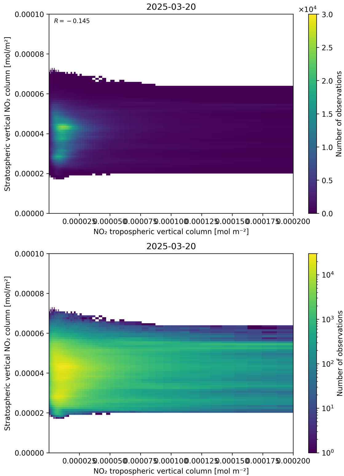
Figure 125: Scatter density plot of “NO 2 tropospheric vertical column” against “Stratospheric vertical NO 2 column” for 2025-03-20 to 2025-03-21.
