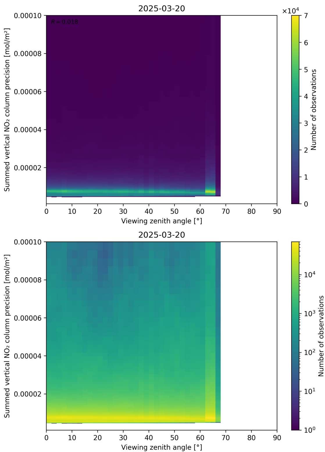
Figure 166: Scatter density plot of “Viewing zenith angle” against “Summed vertical NO 2 column precision” for 2025-03-20 to 2025-03-21.
