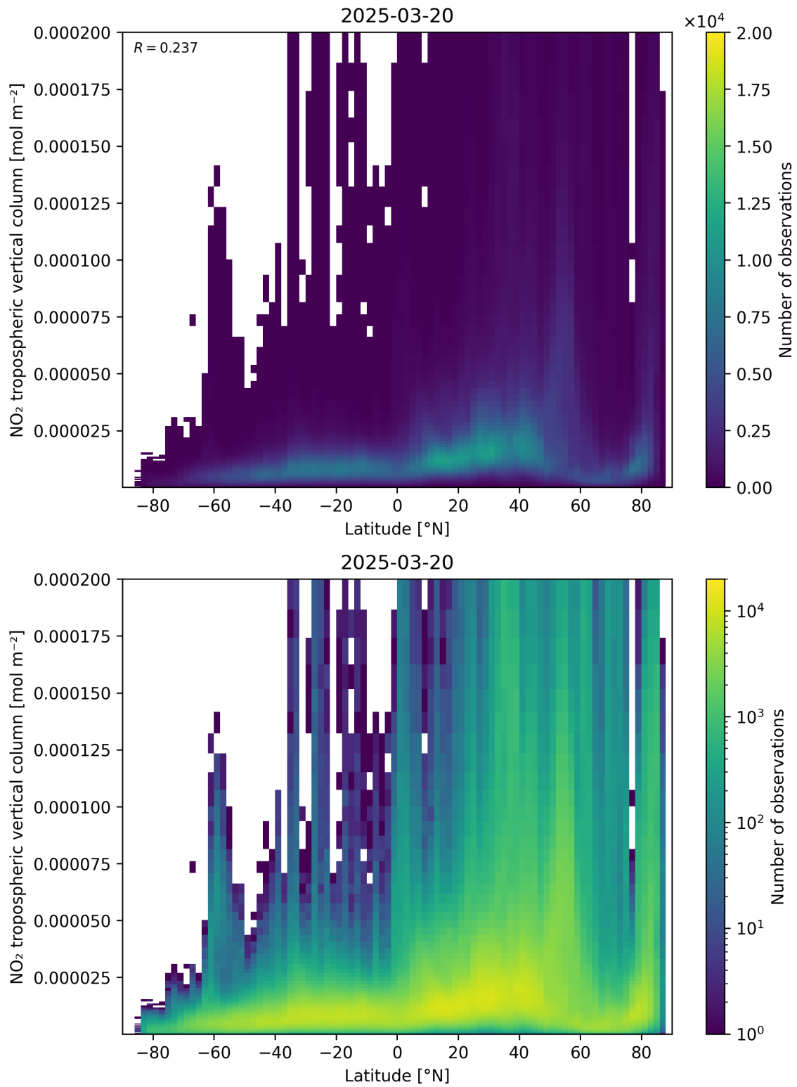
Figure 92: Scatter density plot of “Latitude” against “NO 2 tropospheric vertical column” for 2025-03-20 to 2025-03-21.
