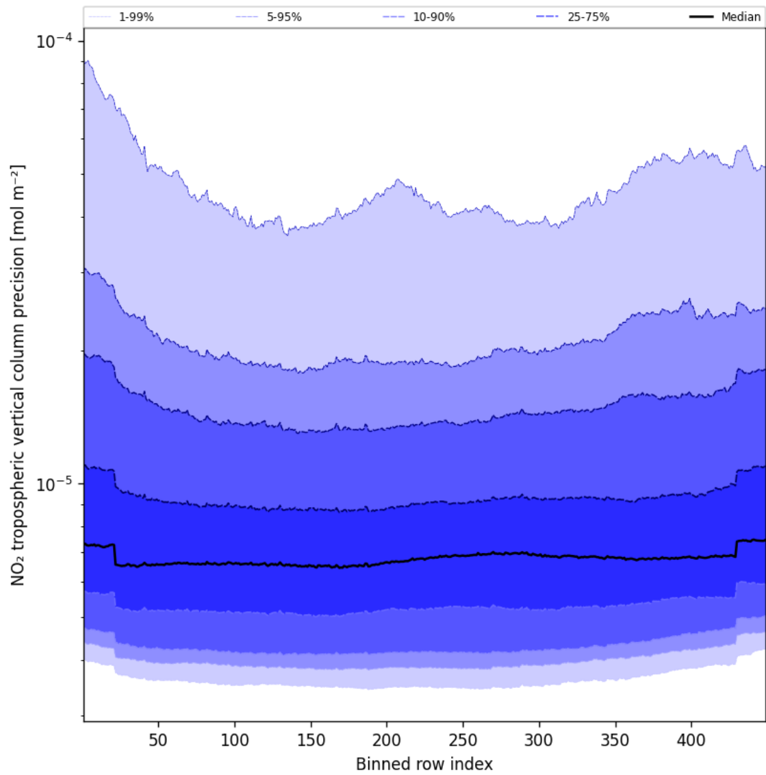
Figure 47: Along track statistics of “NO 2 tropospheric vertical column precision” for 2025-03-20 to 2025-03-21
