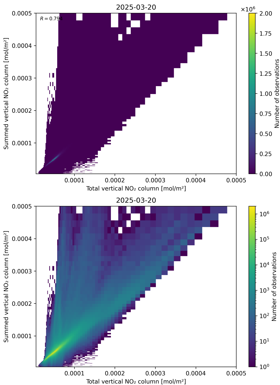
Figure 112: Scatter density plot of “Total vertical NO 2 column” against “Summed vertical NO 2 column” for 2025-03-20 to 2025-03-21.
