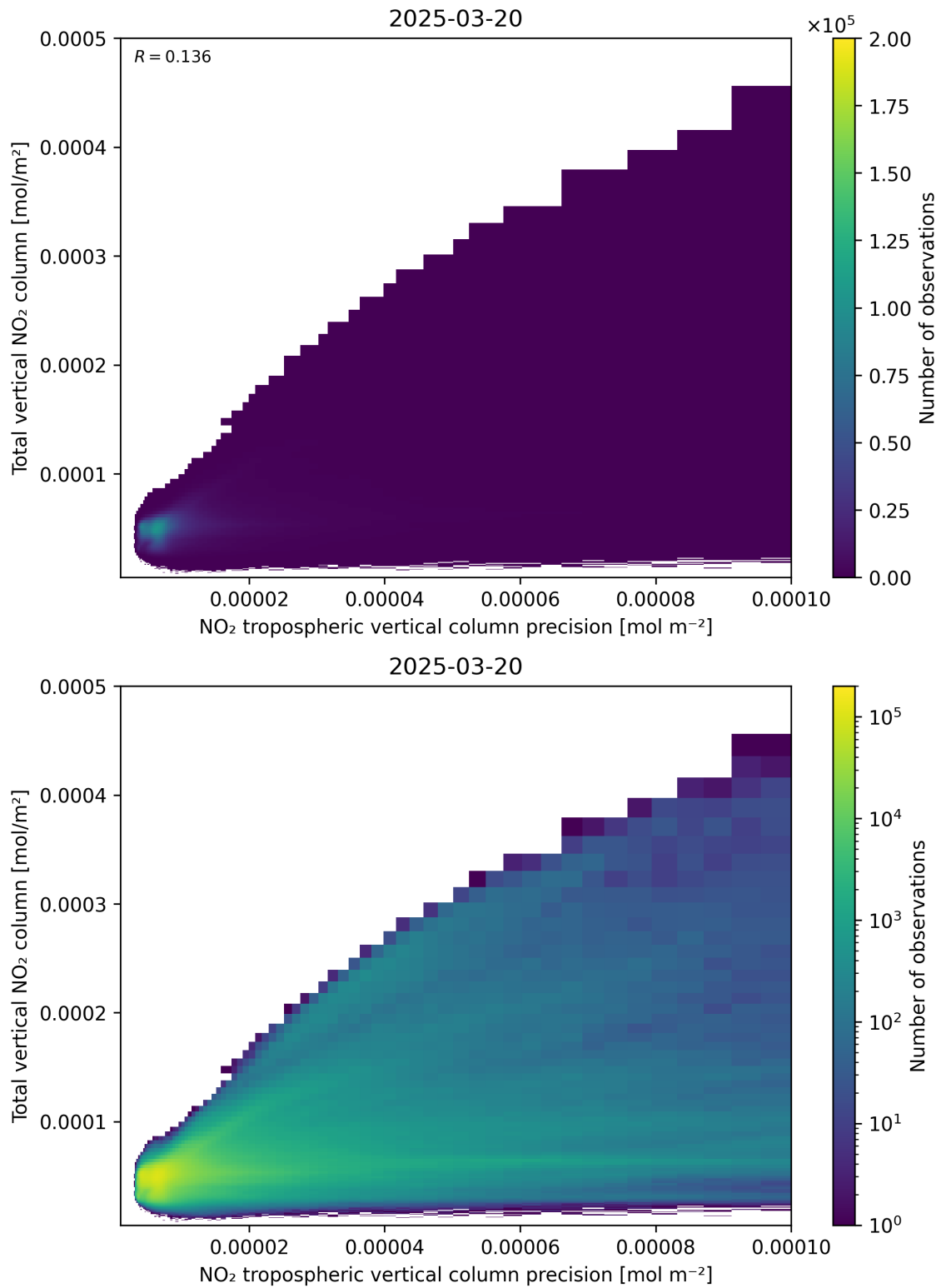
Figure 138: Scatter density plot of “NO 2 tropospheric vertical column precision” against “Total vertical NO 2 column” for 2025-03-20 to 2025-03-21.
