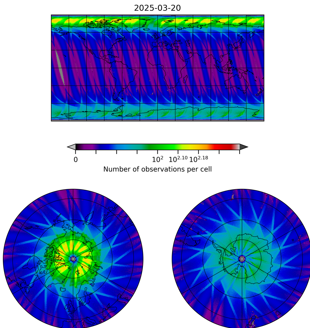
Figure 10: Map of the number of observations for 2025-03-20 to 2025-03-21
