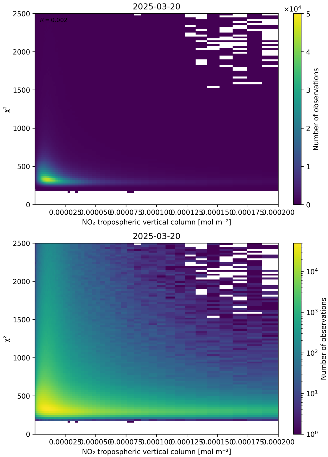
Figure 124: Scatter density plot of “NO 2 tropospheric vertical column” against “ \chi^2 ” for 2025-03-20 to 2025-03-21.
