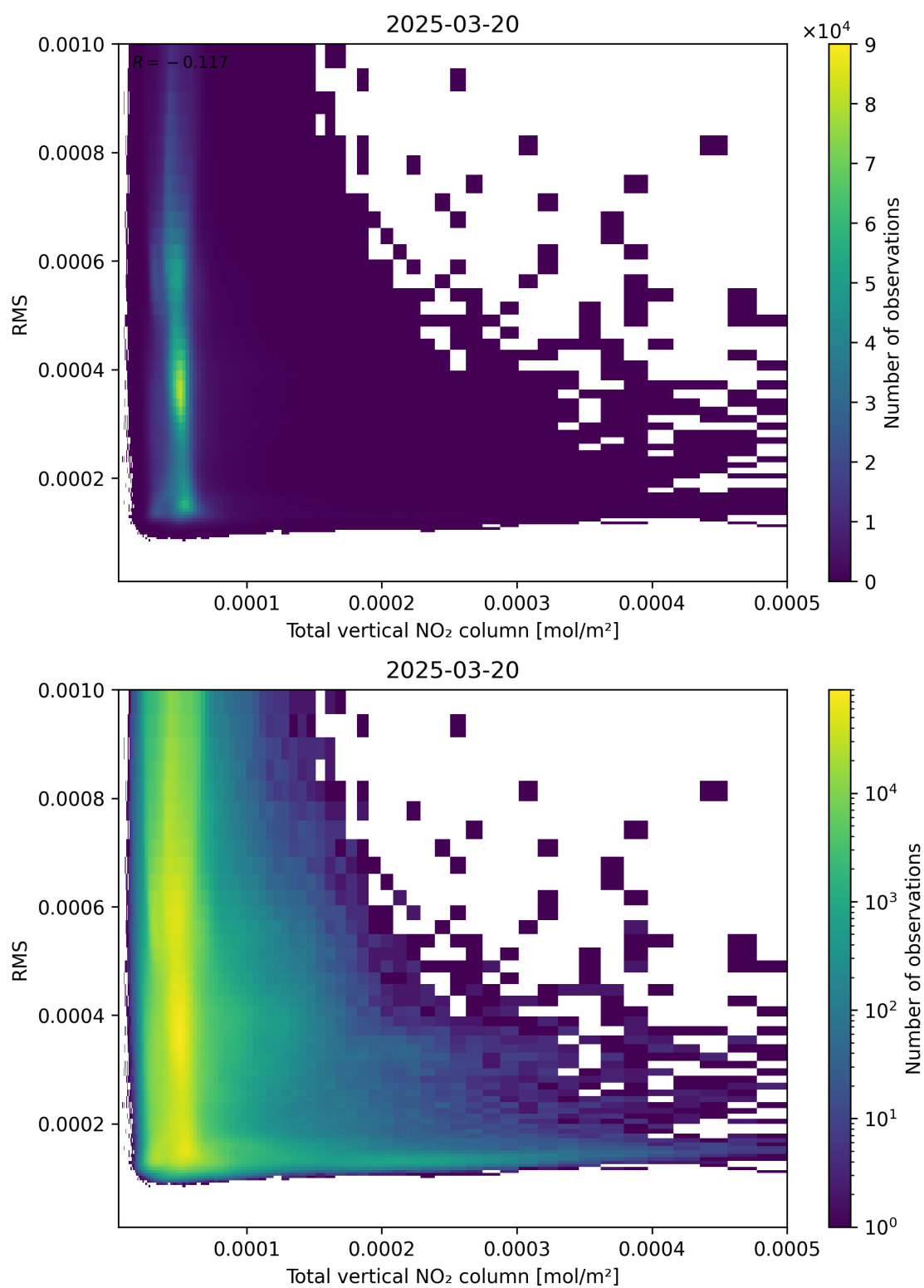
Figure 120: Scatter density plot of “Total vertical NO 2 column” against “RMS” for 2025-03-20 to 2025-03-21.
