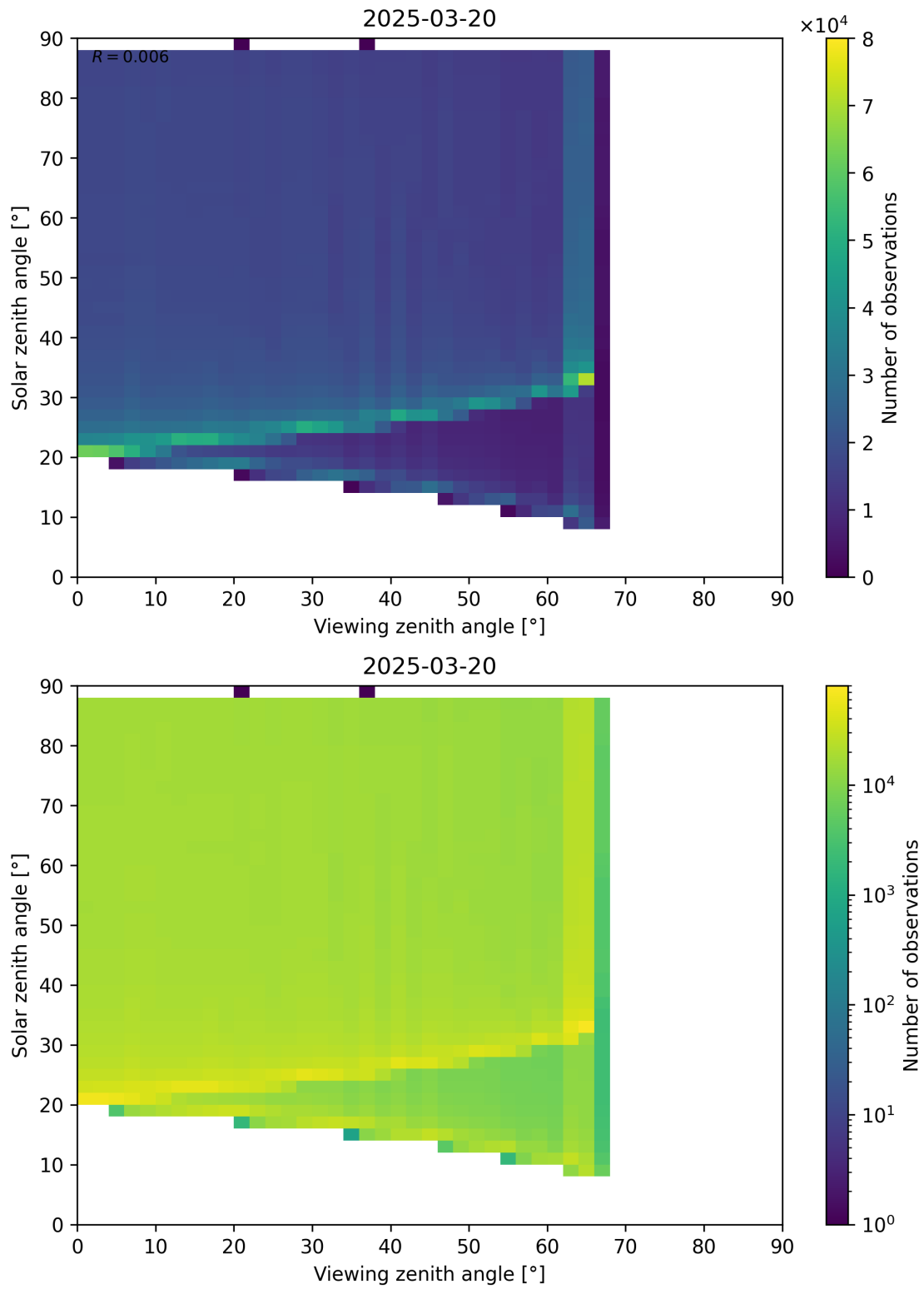
Figure 172: Scatter density plot of “Viewing zenith angle” against “Solar zenith angle” for 2025-03-20 to 2025-03-21.
