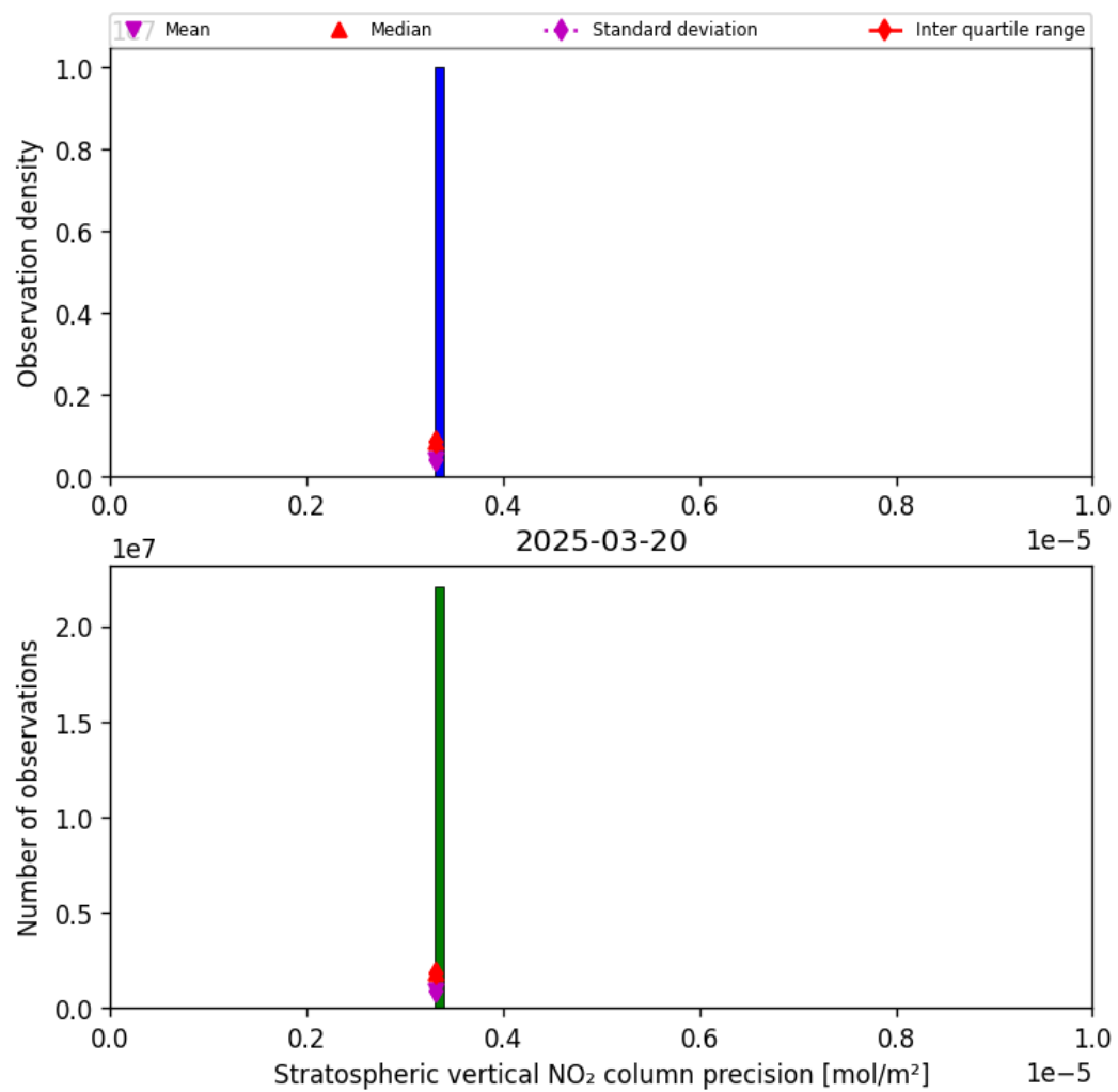
Figure 37: Histogram of “Stratospheric vertical NO 2 column precision” for 2025-03-20 to 2025-03-21
