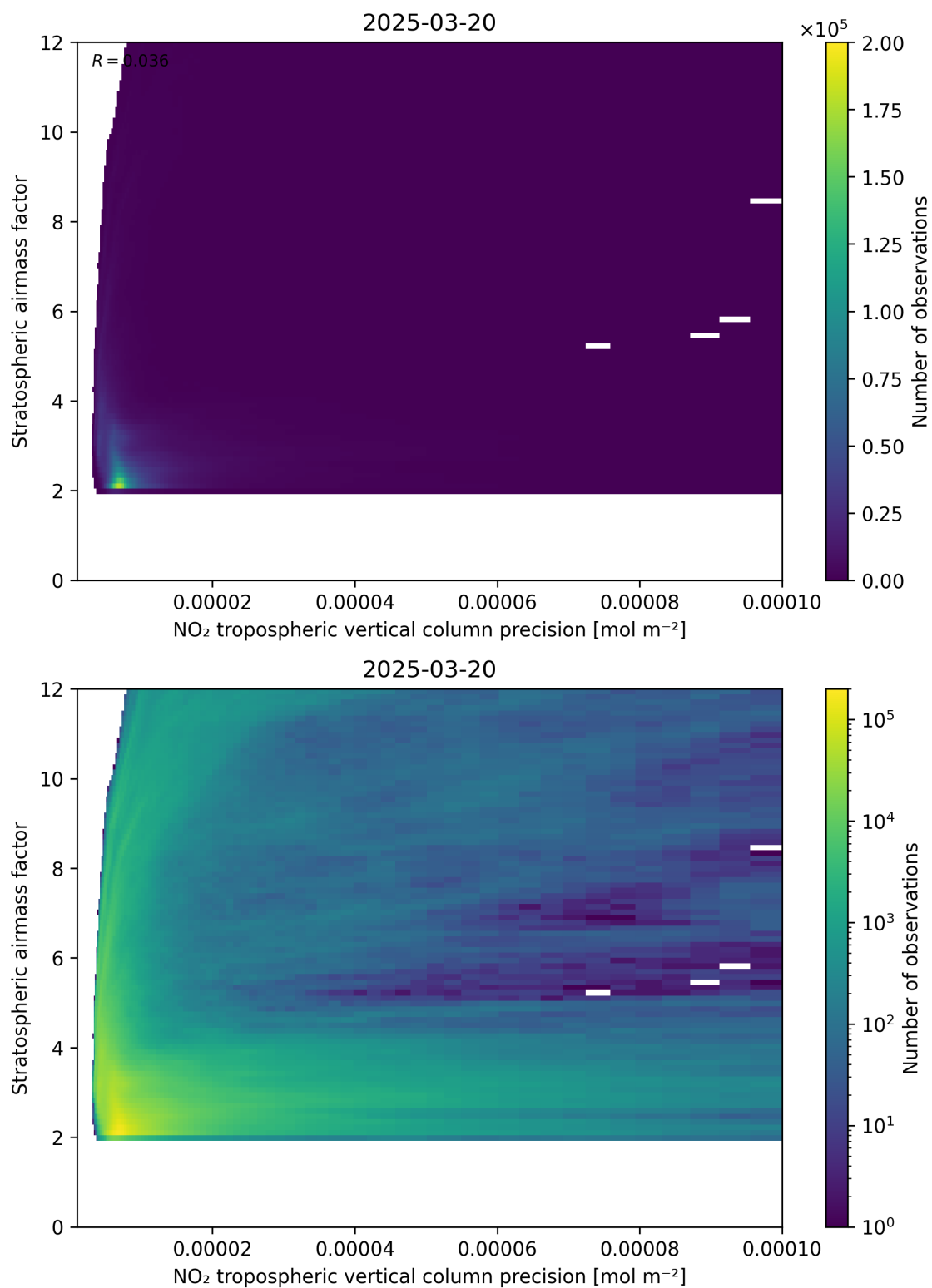
Figure 131: Scatter density plot of “NO 2 tropospheric vertical column precision” against “Stratospheric airmass factor” for 2025-03-20 to 2025-03-21.
