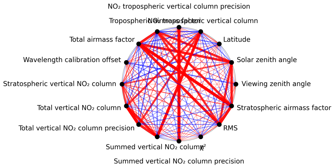
Figure 1: Map of correlation graph for 2025-03-20 to 2025-03-21.
