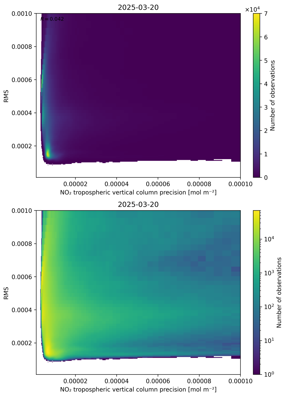
Figure 140: Scatter density plot of “NO 2 tropospheric vertical column precision” against “RMS” for 2025-03-20 to 2025-03-21.
