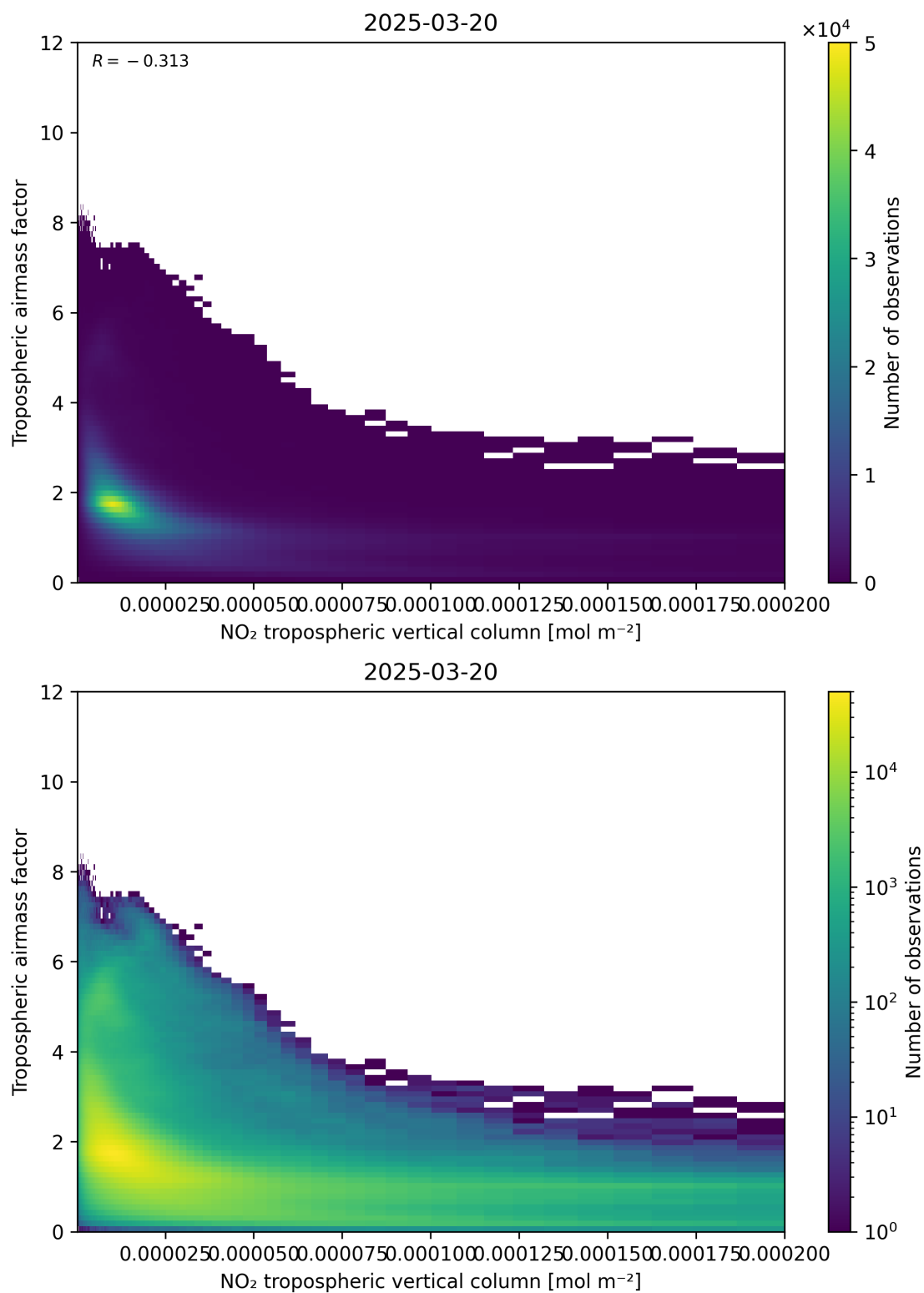
Figure 123: Scatter density plot of “NO 2 tropospheric vertical column” against “Tropospheric air mass factor” for 2025-03-20 to 2025-03-21.
