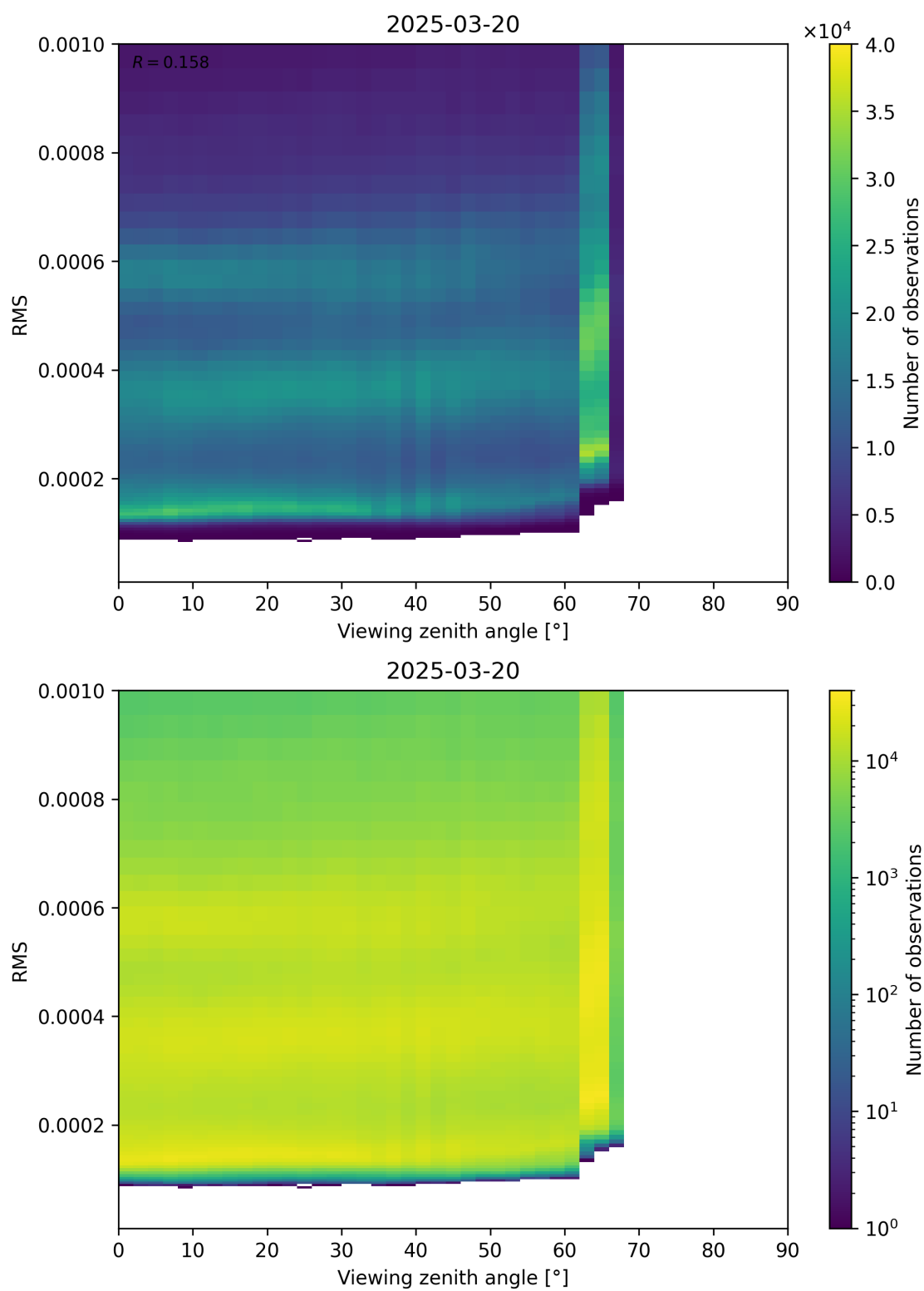
Figure 171: Scatter density plot of “Viewing zenith angle” against “RMS” for 2025-03-20 to 2025-03-21.
