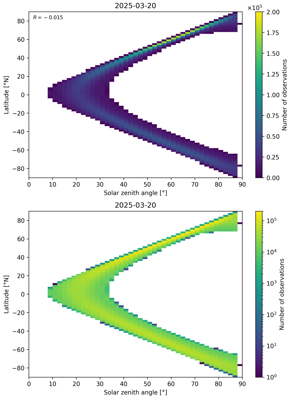
Figure 149: Scatter density plot of “Solar zenith angle” against “Latitude” for 2025-03-20 to 2025-03-21.
