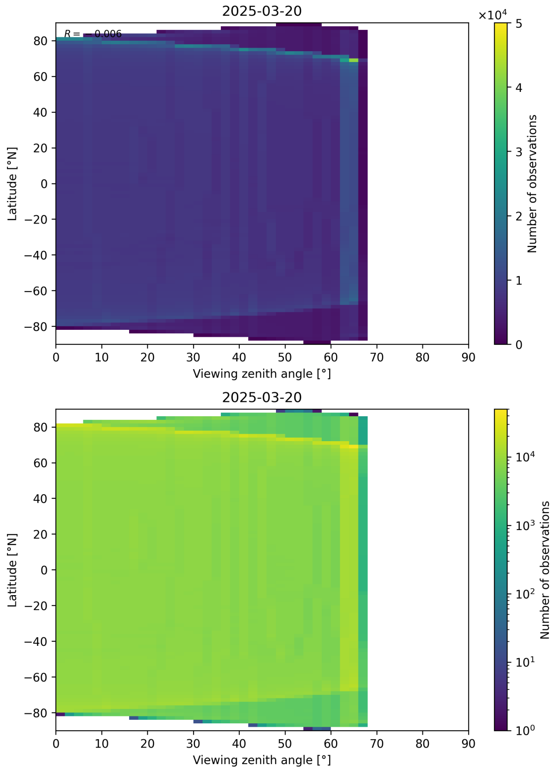
Figure 163: Scatter density plot of “Viewing zenith angle” against “Latitude” for 2025-03-20 to 2025-03-21.
