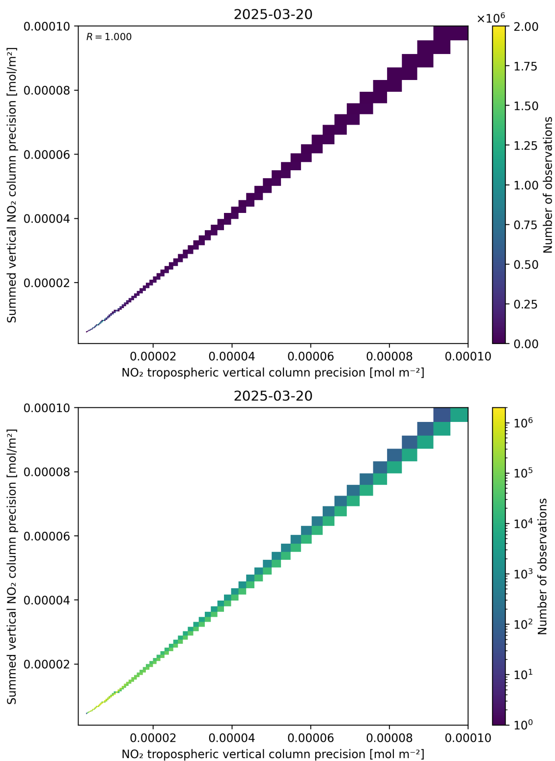
Figure 137: Scatter density plot of “NO 2 tropospheric vertical column precision” against “Summed vertical NO 2 column precision” for 2025-03-20 to 2025-03-21.
