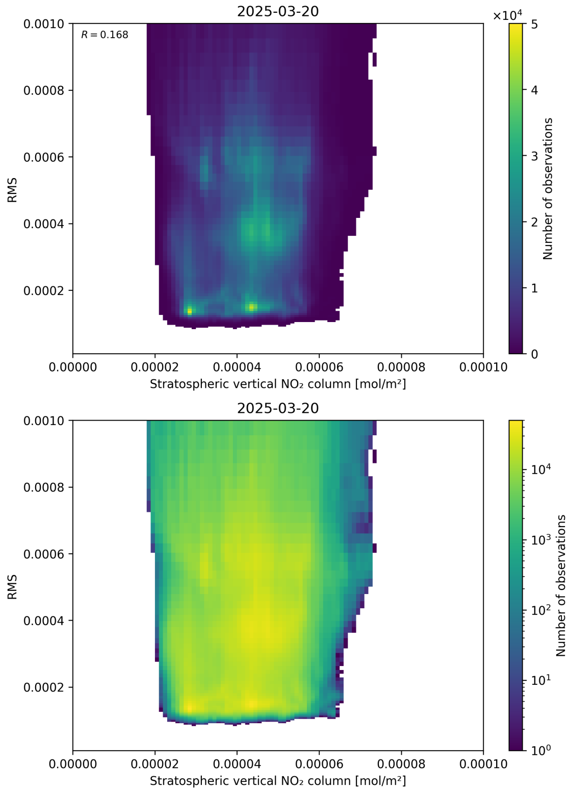
Figure 102: Scatter density plot of “Stratospheric vertical NO 2 column” against “RMS” for 2025-03-20 to 2025-03-21.
