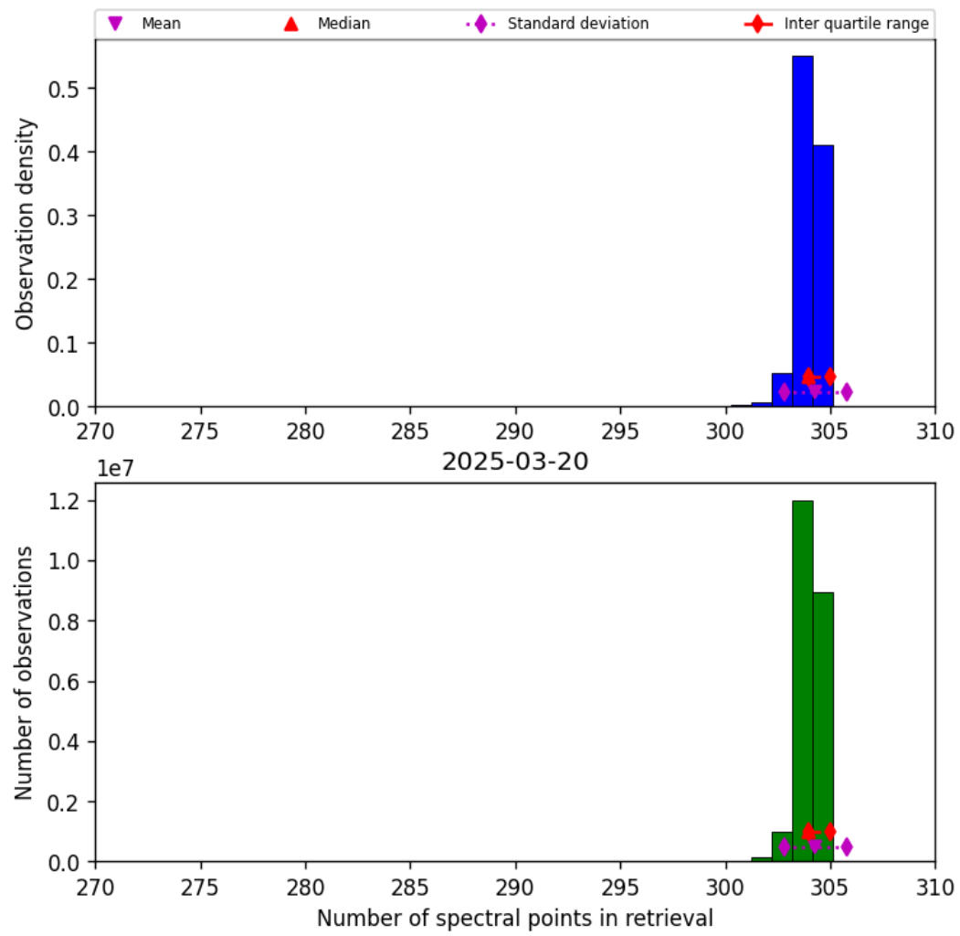
Figure 33: Histogram of “Number of spectral points in retrieval” for 2025-03-20 to 2025-03-21
