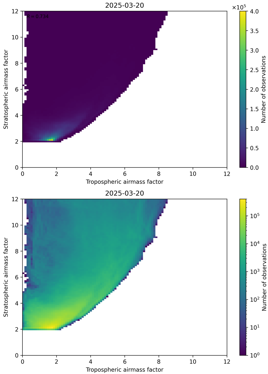
Figure 71: Scatter density plot of “Tropospheric airmass factor” against “Stratospheric airmass factor” for 2025-03-20 to 2025-03-21.
