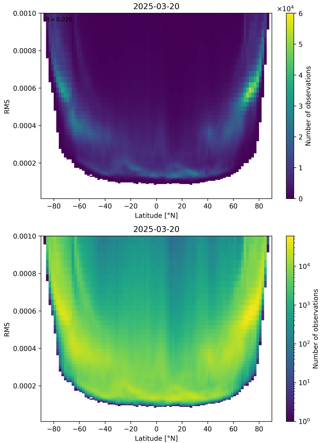
Figure 94: Scatter density plot of “Latitude” against “RMS” for 2025-03-20 to 2025-03-21.
