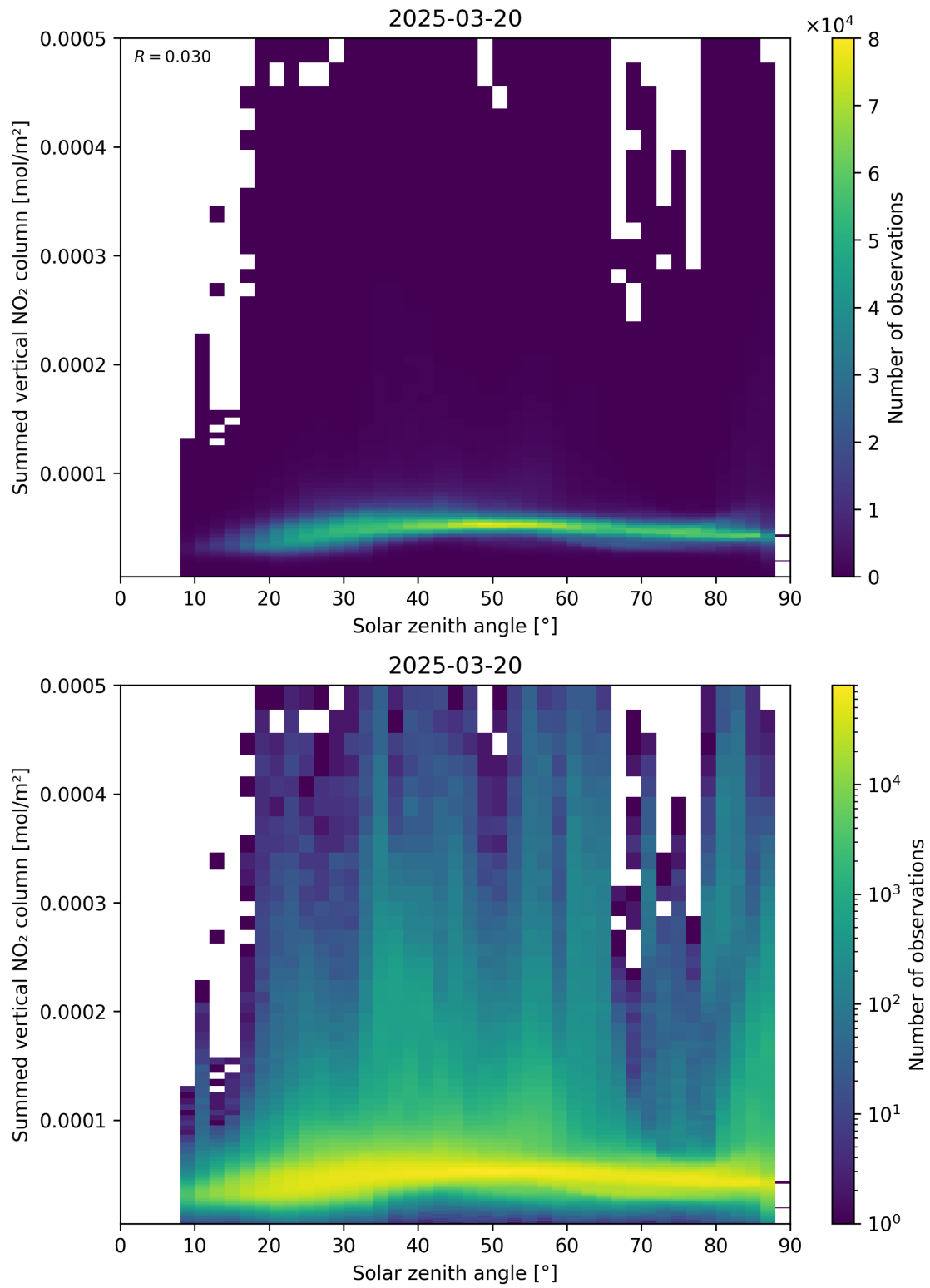
Figure 151: Scatter density plot of “Solar zenith angle” against “Summed vertical NO 2 column” for 2025-03-20 to 2025-03-21.
