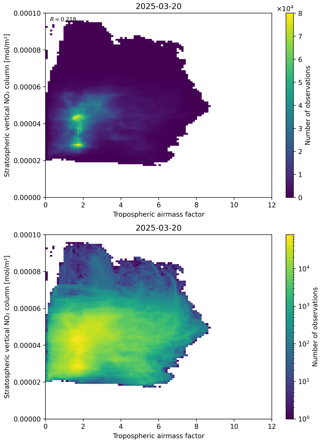
Figure 74: Scatter density plot of “Tropospheric air mass factor” against “Stratospheric vertical NO 2 column” for 2025-03-20 to 2025-03-21.
