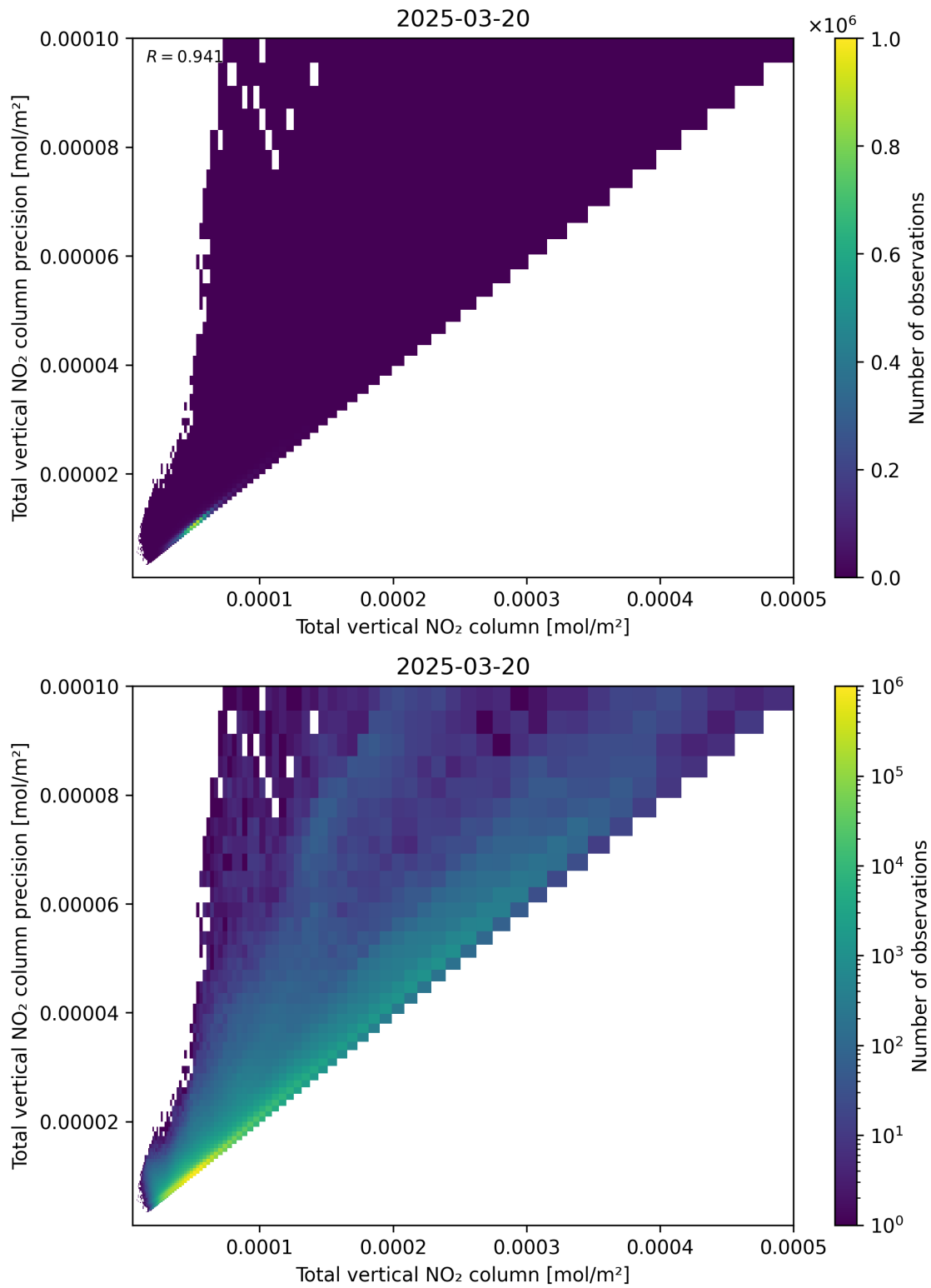
Figure 114: Scatter density plot of “Total vertical NO 2 column” against “Total vertical NO 2 column precision” for 2025-03-20 to 2025-03-21.
