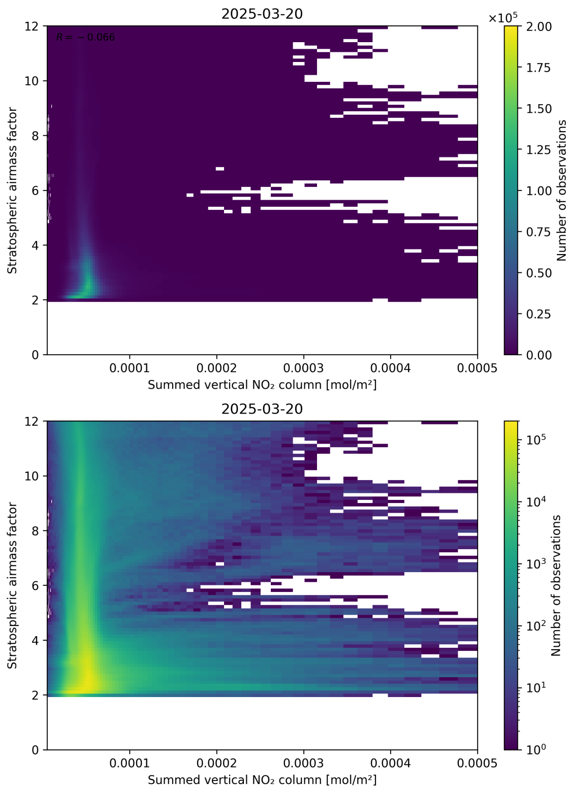
Figure 103: Scatter density plot of “Summed vertical NO 2 column” against “Stratospheric airmass factor” for 2025-03-20 to 2025-03-21.
