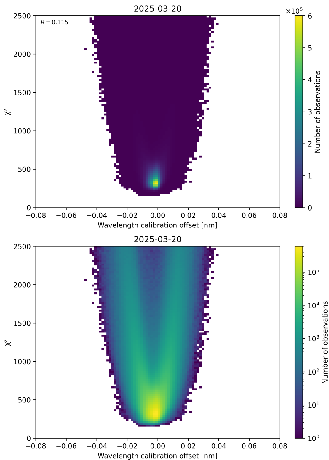
Figure 175: Scatter density plot of “Wavelength calibration offset” against “ \chi^2 ” for 2025-03-20 to 2025-03-21.
