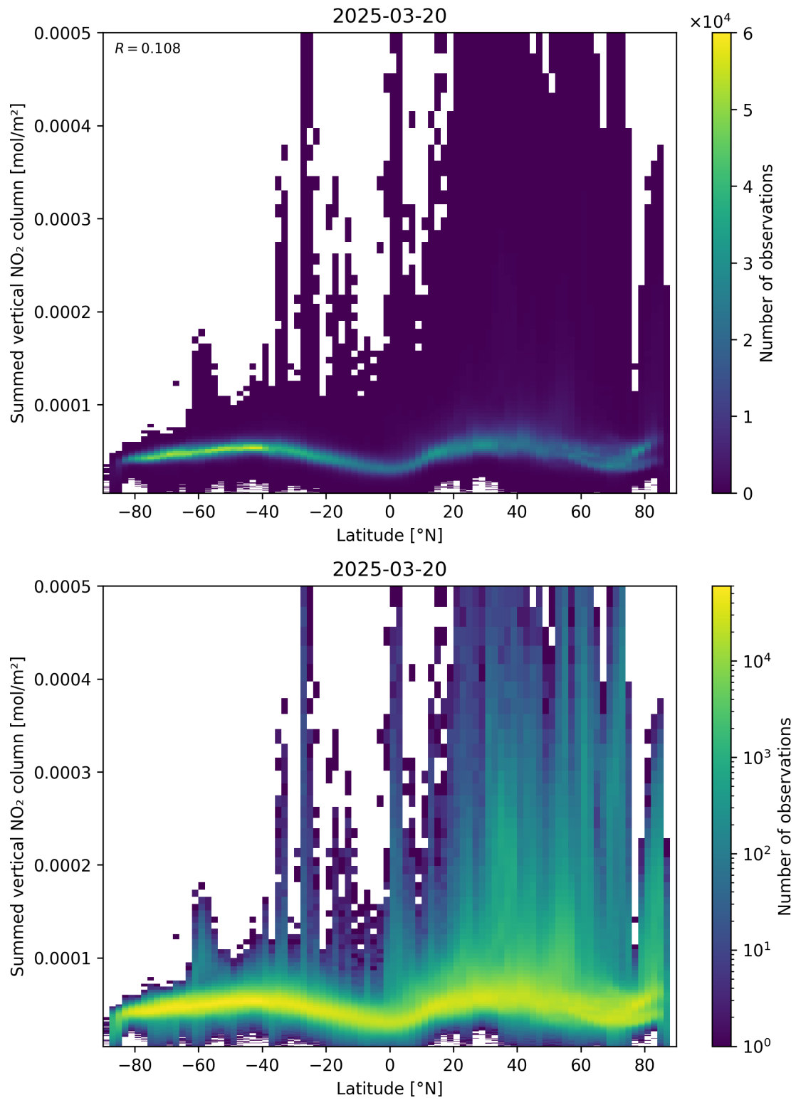
Figure 88: Scatter density plot of “Latitude” against “Summed vertical NO 2 column” for 2025-03-20 to 2025-03-21.
