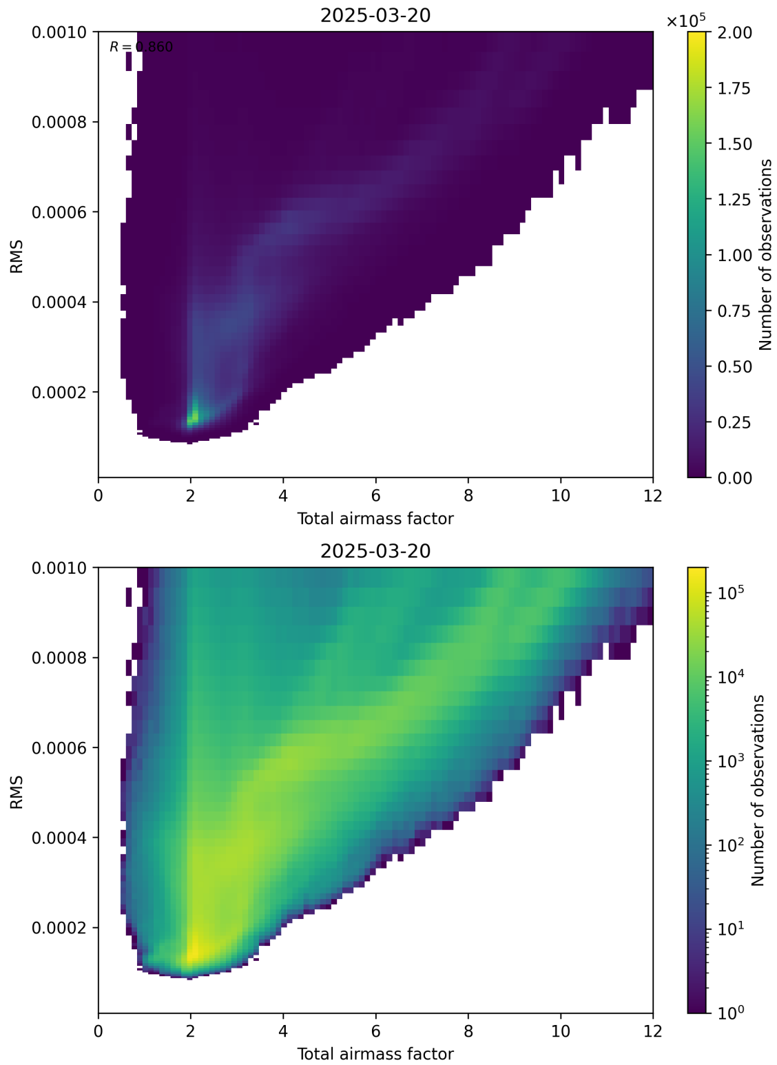
Figure 69: Scatter density plot of “Total airmass factor” against “RMS” for 2025-03-20 to 2025-03-21.
