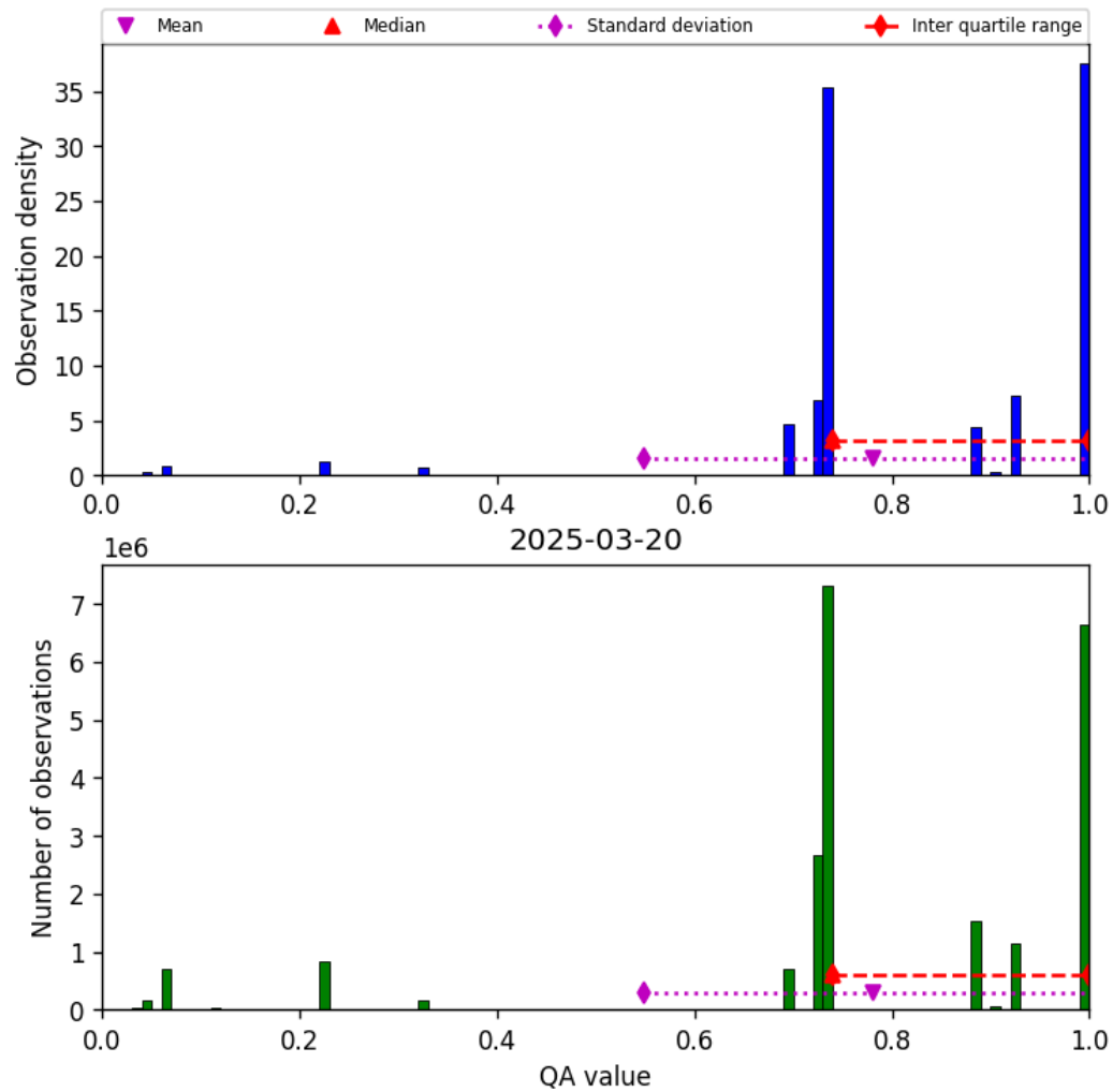
Figure 28: Histogram of “QA value” for 2025-03-20 to 2025-03-21
