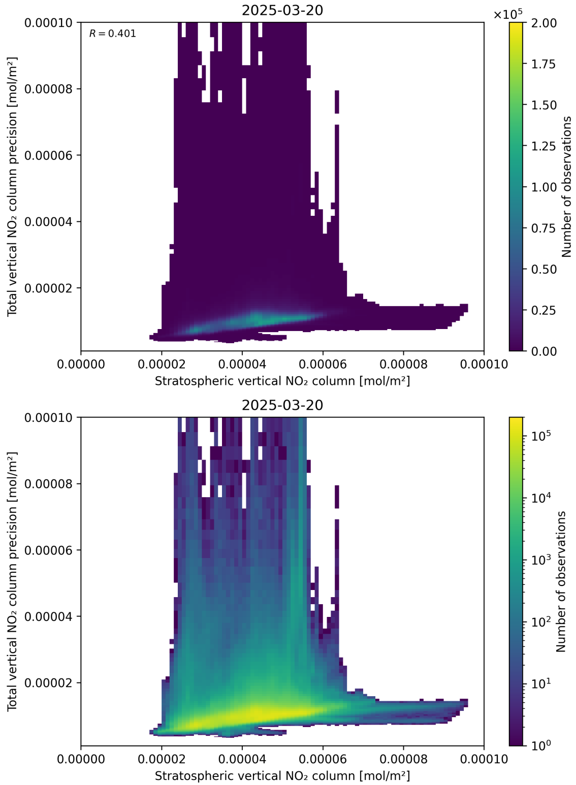
Figure 101: Scatter density plot of “Stratospheric vertical NO 2 column” against “Total vertical NO 2 column precision” for 2025-03-20 to 2025-03-21.
