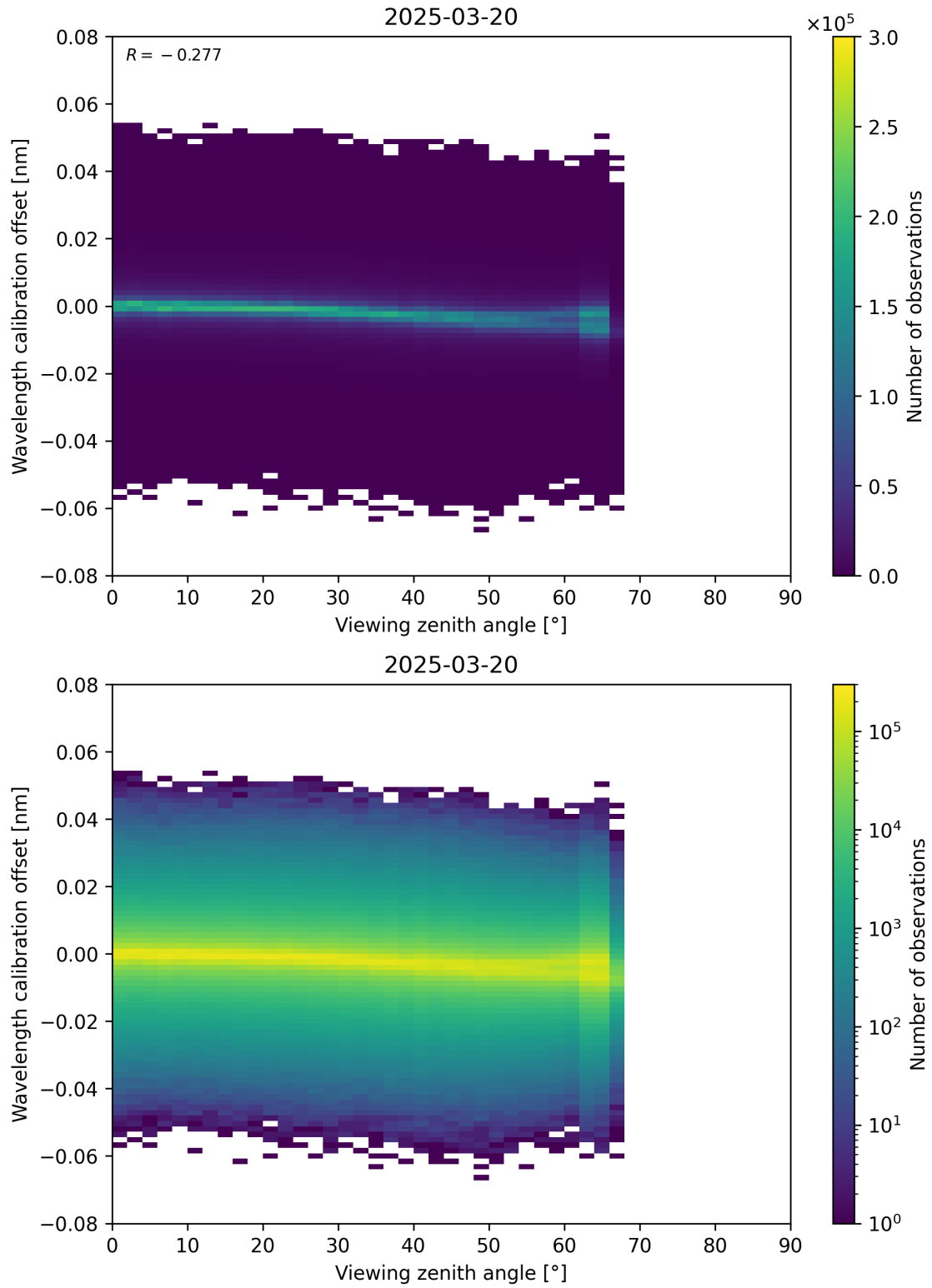
Figure 173: Scatter density plot of “Viewing zenith angle” against “Wavelength calibration offset” for 2025-03-20 to 2025-03-21.
