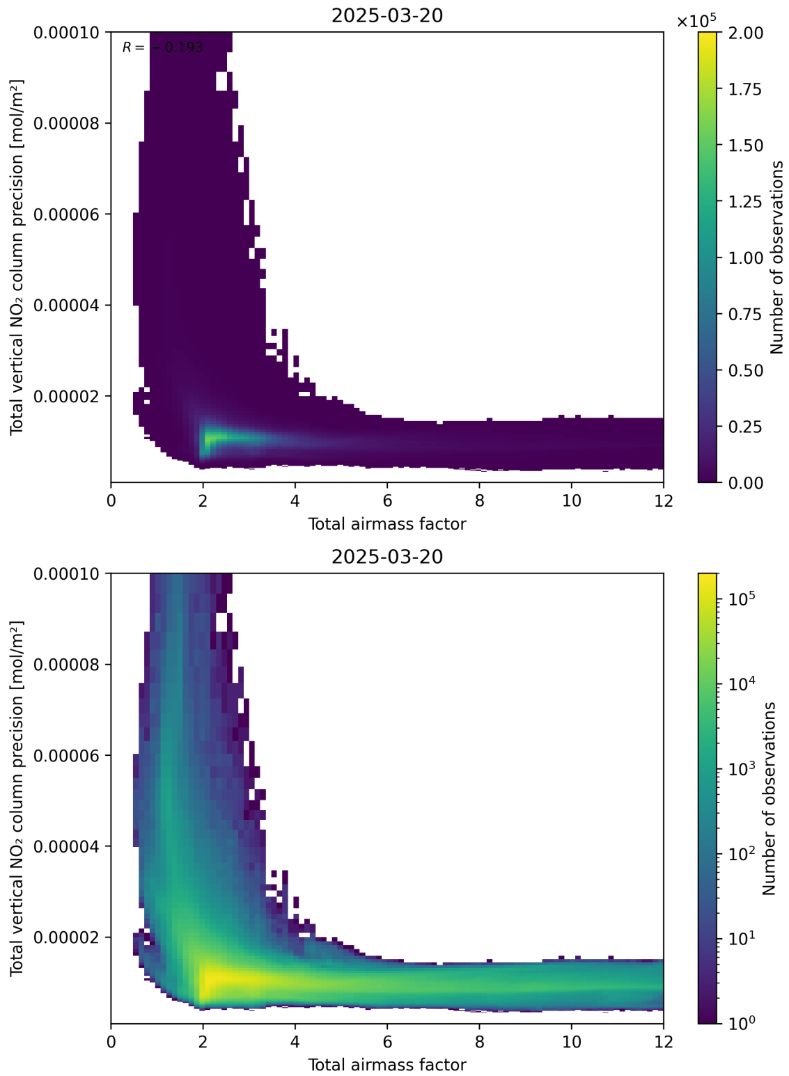
Figure 68: Scatter density plot of “Total airmass factor” against “Total vertical NO 2 column precision” for 2025-03-20 to 2025-03-21.
