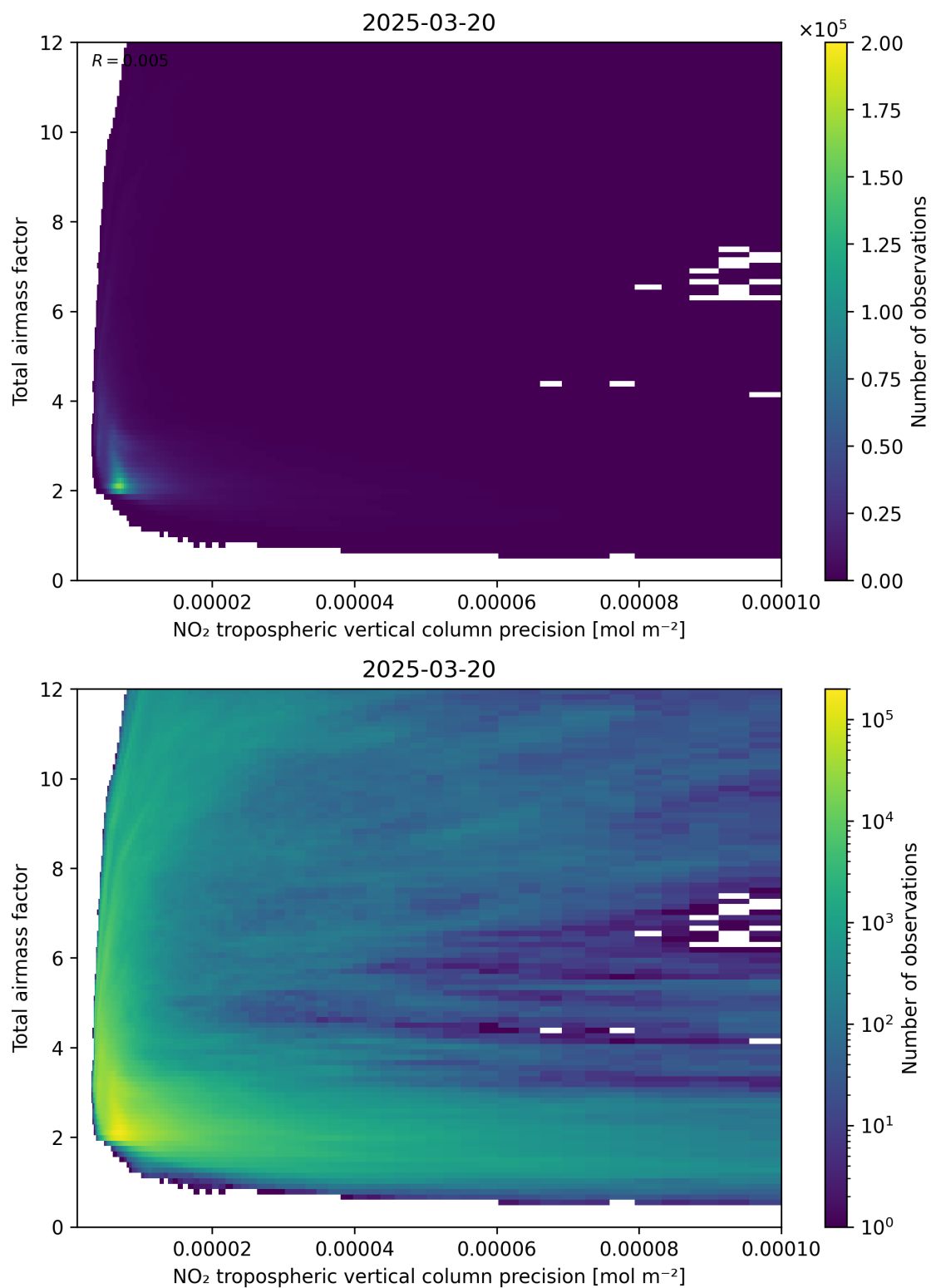
Figure 132: Scatter density plot of “NO 2 tropospheric vertical column precision” against “Total air mass factor” for 2025-03-20 to 2025-03-21.
