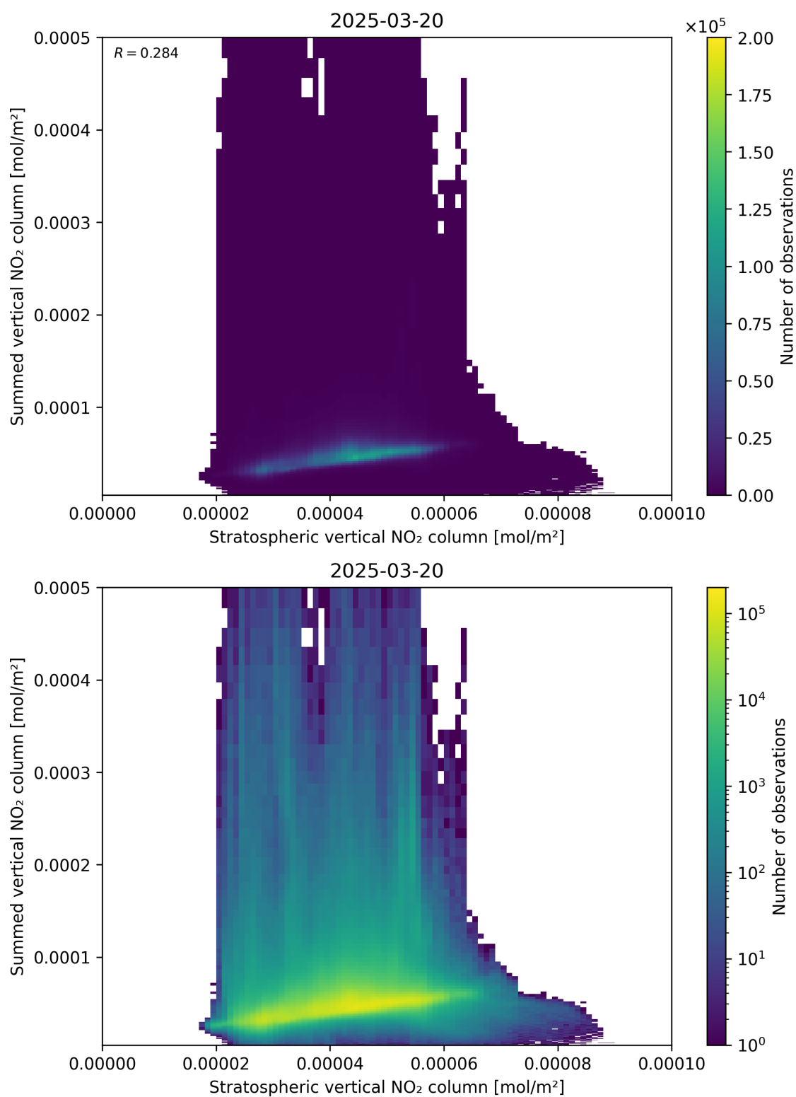
Figure 98: Scatter density plot of “Stratospheric vertical NO 2 column” against “Summed vertical NO 2 column” for 2025-03-20 to 2025-03-21.
