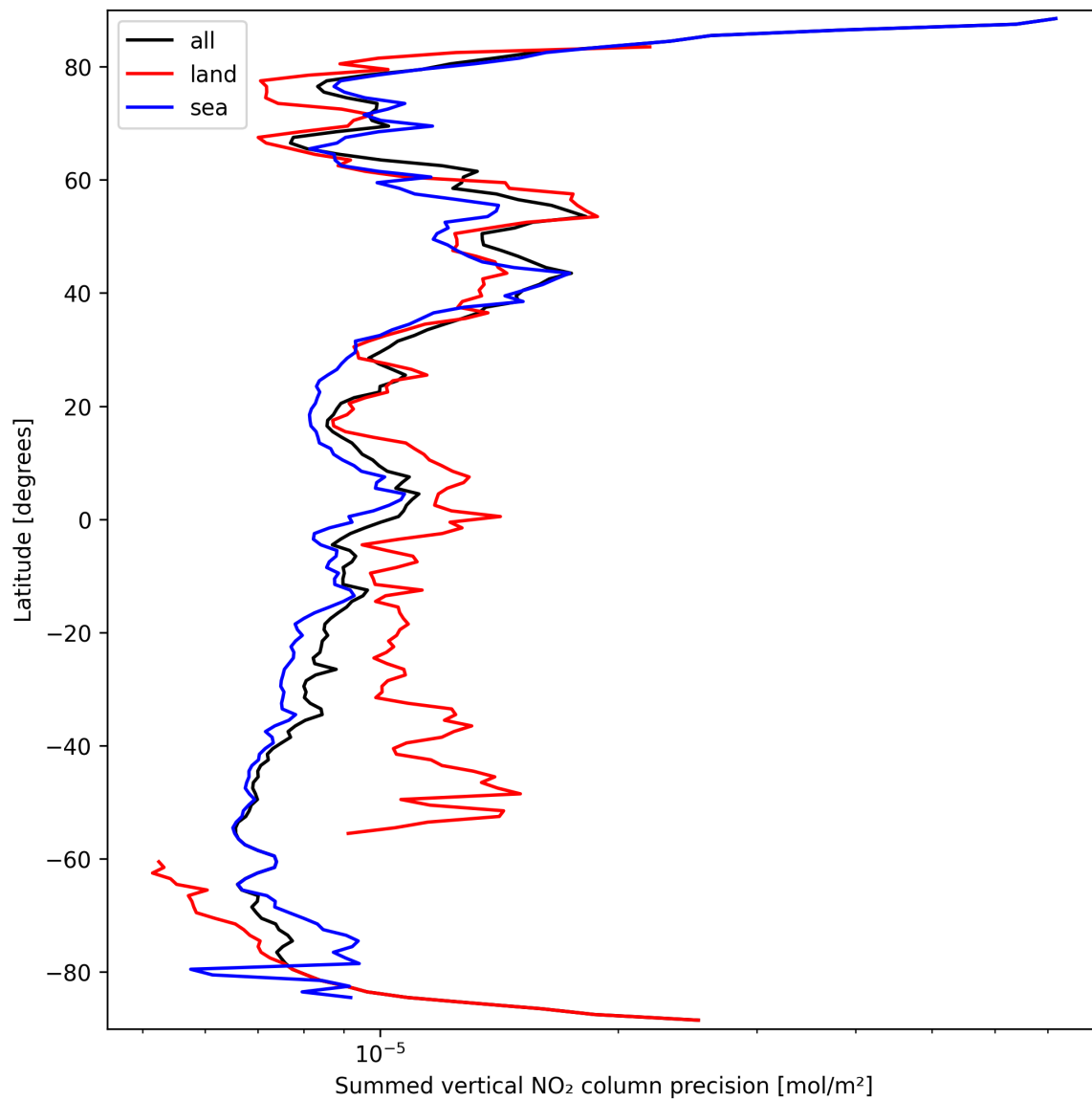
Figure 24: Zonal average of “Summed vertical NO 2 column precision” for 2025-03-20 to 2025-03-21.
