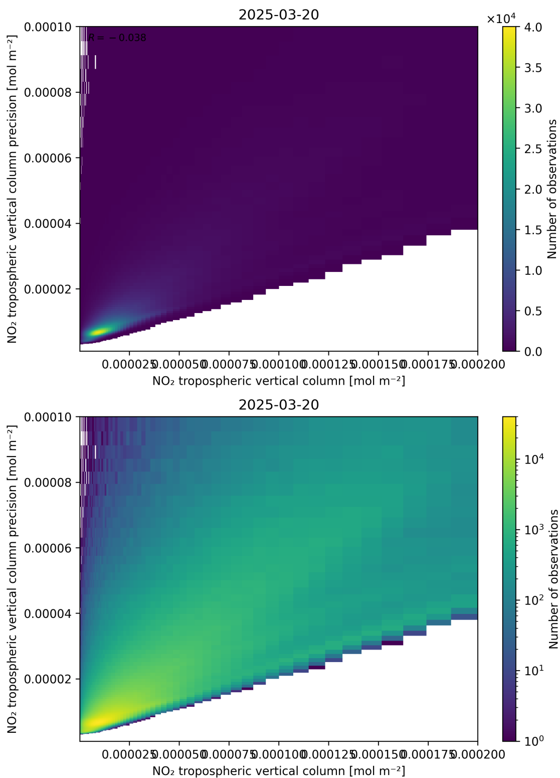
Figure 130: Scatter density plot of “NO 2 tropospheric vertical column” against “NO 2 tropospheric vertical column precision” for 2025-03-20 to 2025-03-21.
