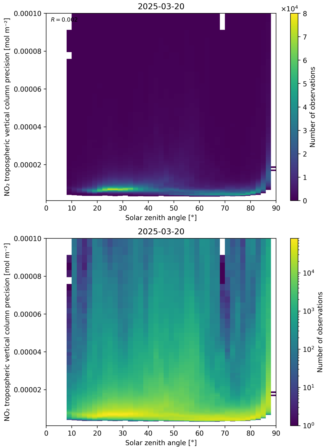
Figure 156: Scatter density plot of “Solar zenith angle” against “NO 2 tropospheric vertical column precision” for 2025-03-20 to 2025-03-21.
