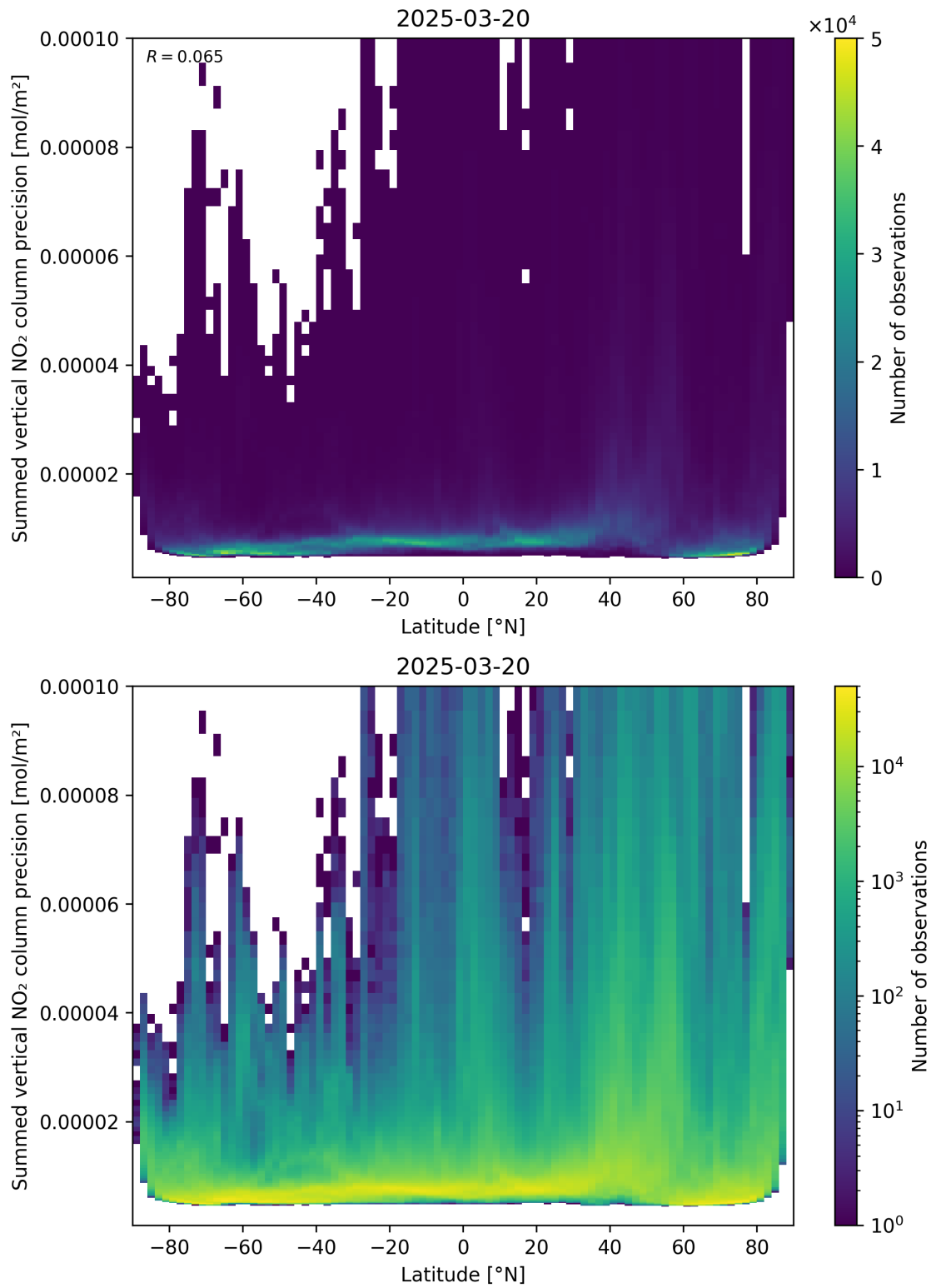
Figure 89: Scatter density plot of “Latitude” against “Summed vertical NO 2 column precision” for 2025-03-20 to 2025-03-21.
