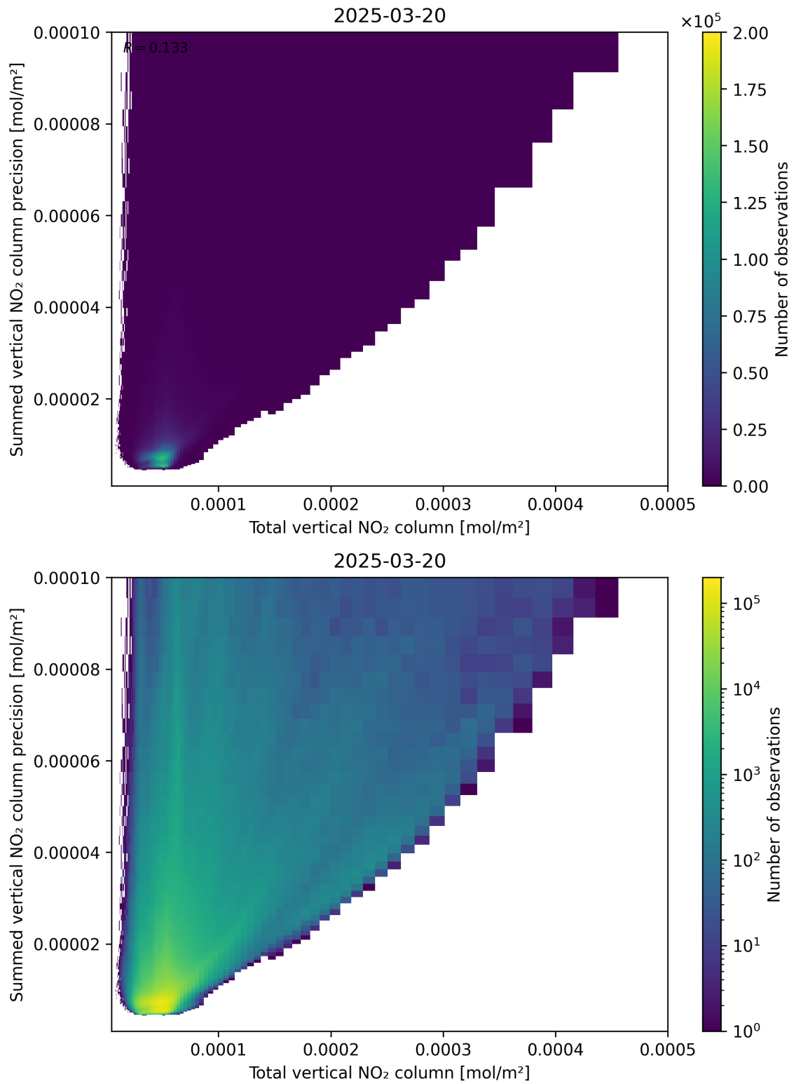
Figure 113: Scatter density plot of “Total vertical NO 2 column” against “Summed vertical NO 2 column precision” for 2025-03-20 to 2025-03-21.
