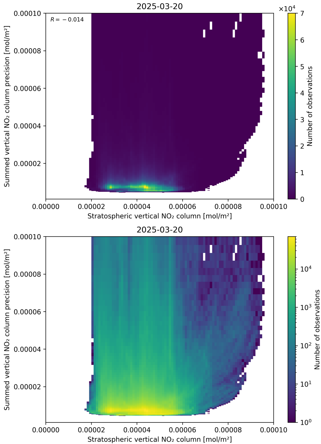
Figure 99: Scatter density plot of “Stratospheric vertical NO 2 column” against “Summed vertical NO 2 column precision” for 2025-03-20 to 2025-03-21.
