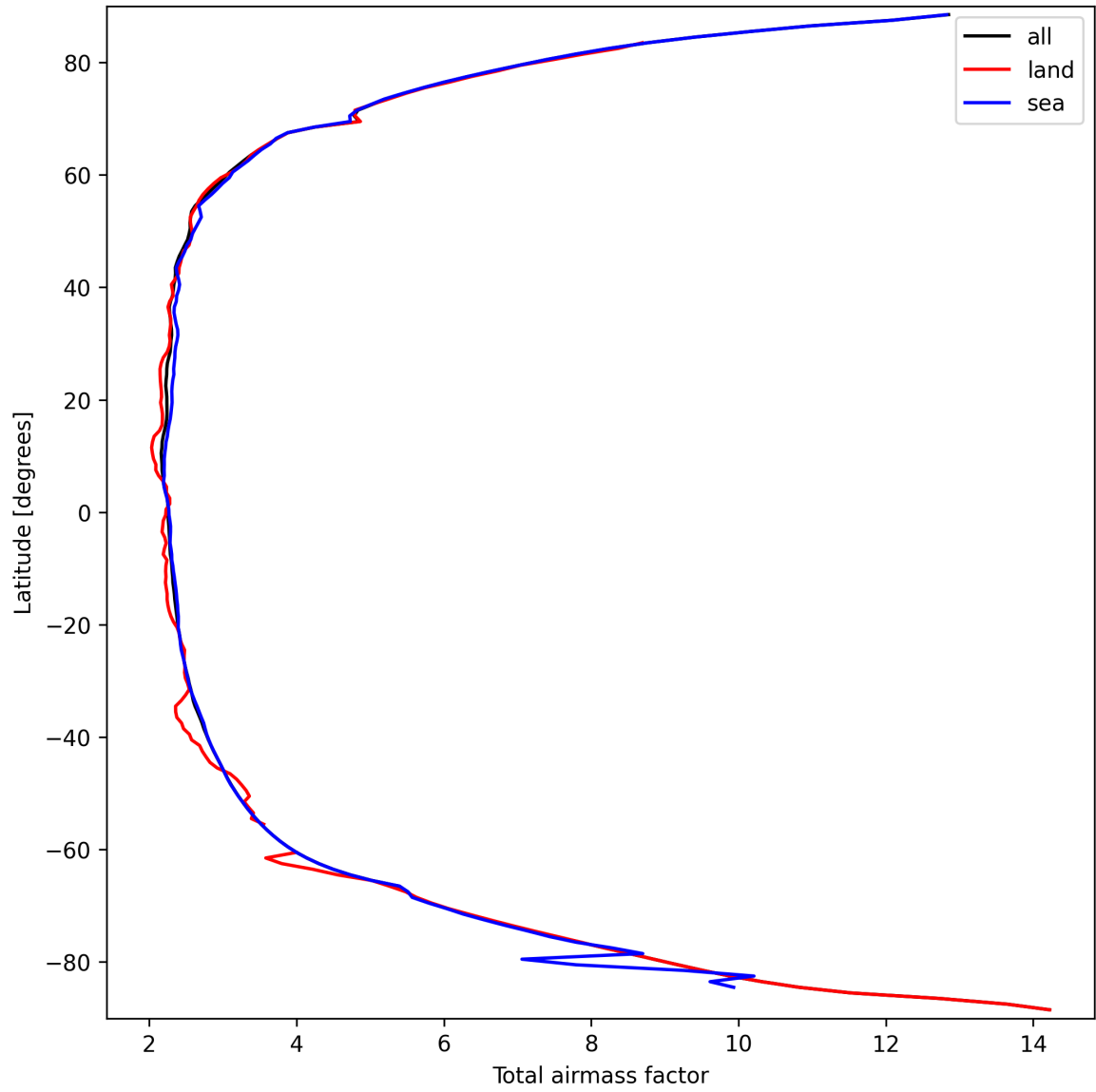
Figure 15: Zonal average of “Total airmass factor” for 2025-03-20 to 2025-03-21.
