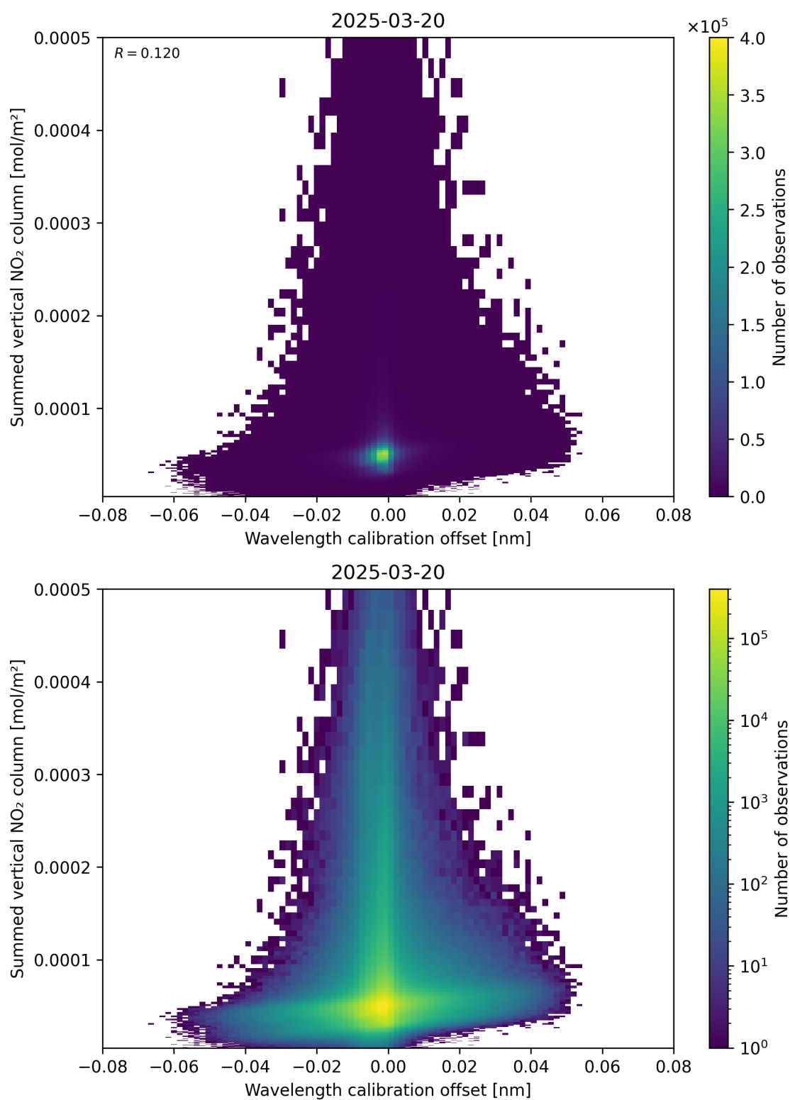
Figure 177: Scatter density plot of “Wavelength calibration offset” against “Summed vertical NO 2 column” for 2025-03-20 to 2025-03-21.
