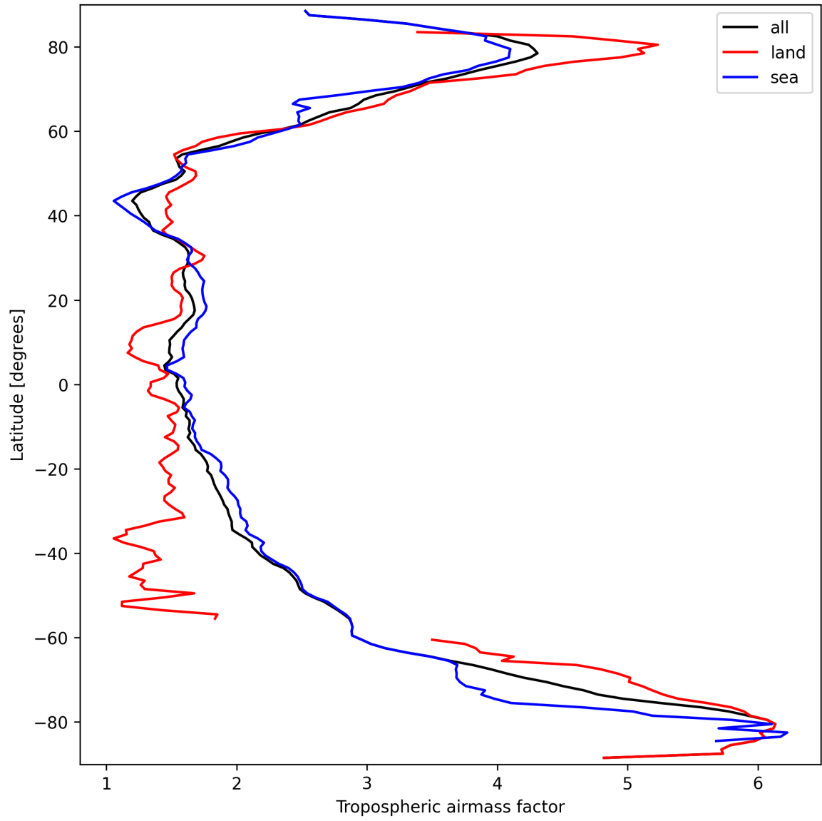
Figure 14: Zonal average of “Tropospheric airmass factor” for 2025-03-20 to 2025-03-21.
