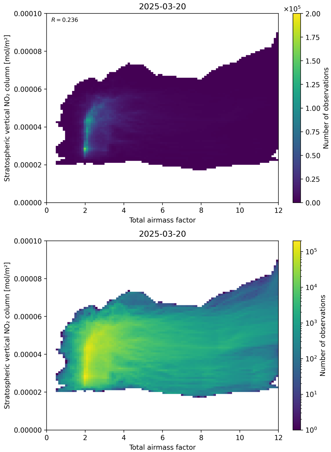
Figure 64: Scatter density plot of “Total airmass factor” against “Stratospheric vertical NO 2 column” for 2025-03-20 to 2025-03-21.
