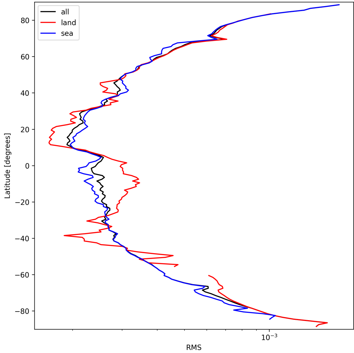
Figure 26: Zonal average of “RMS” for 2025-03-20 to 2025-03-21.
