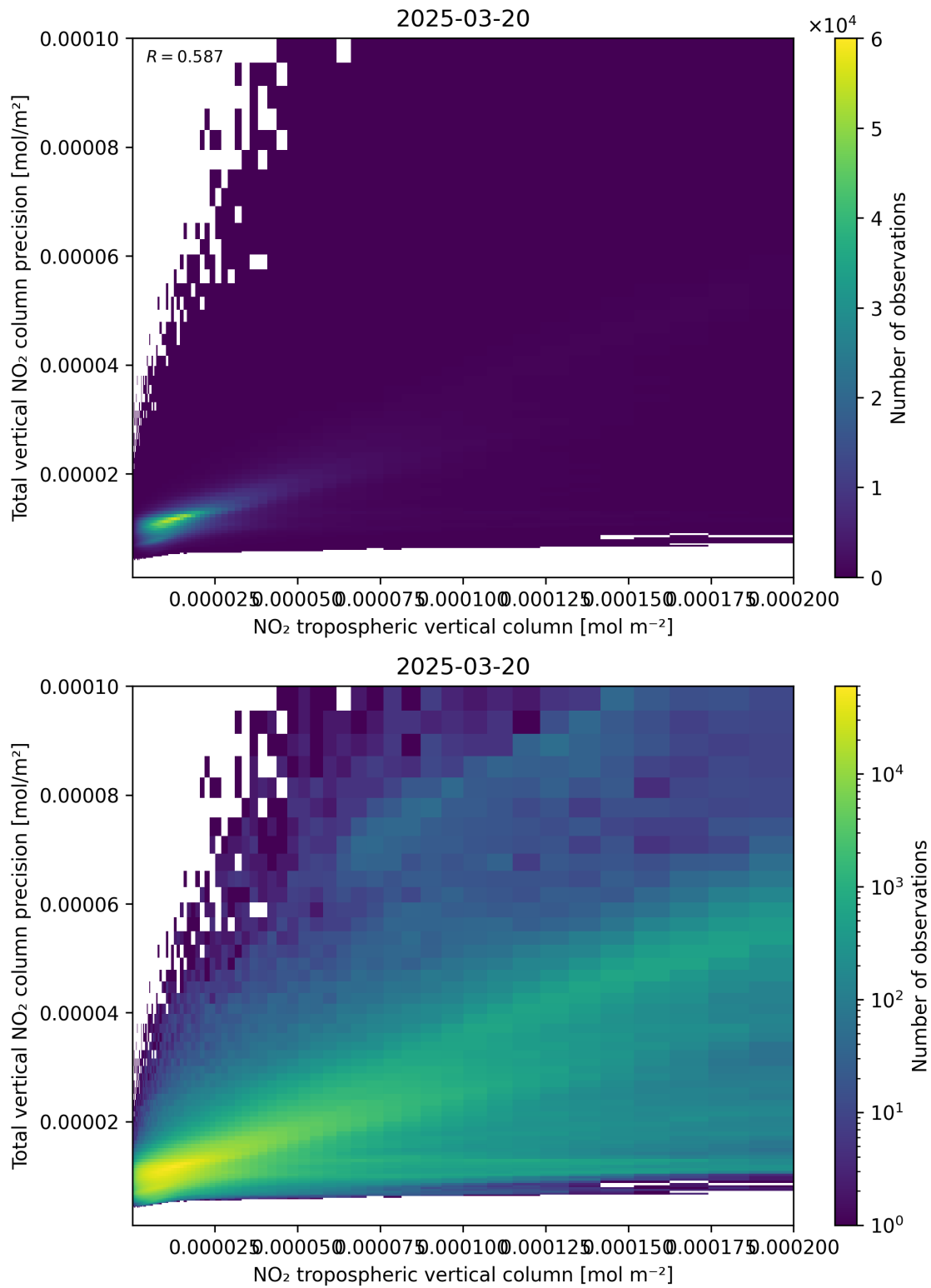
Figure 129: Scatter density plot of “NO 2 tropospheric vertical column” against “Total vertical NO 2 column precision” for 2025-03-20 to 2025-03-21.
