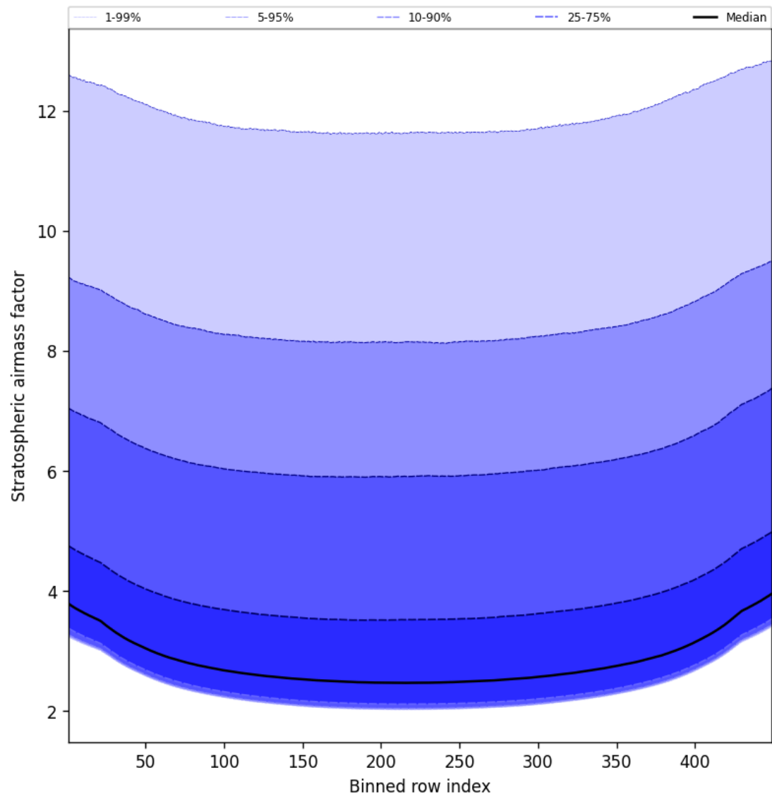
Figure 61: Along track statistics of “Stratospheric airmass factor” for 2025-03-20 to 2025-03-21
