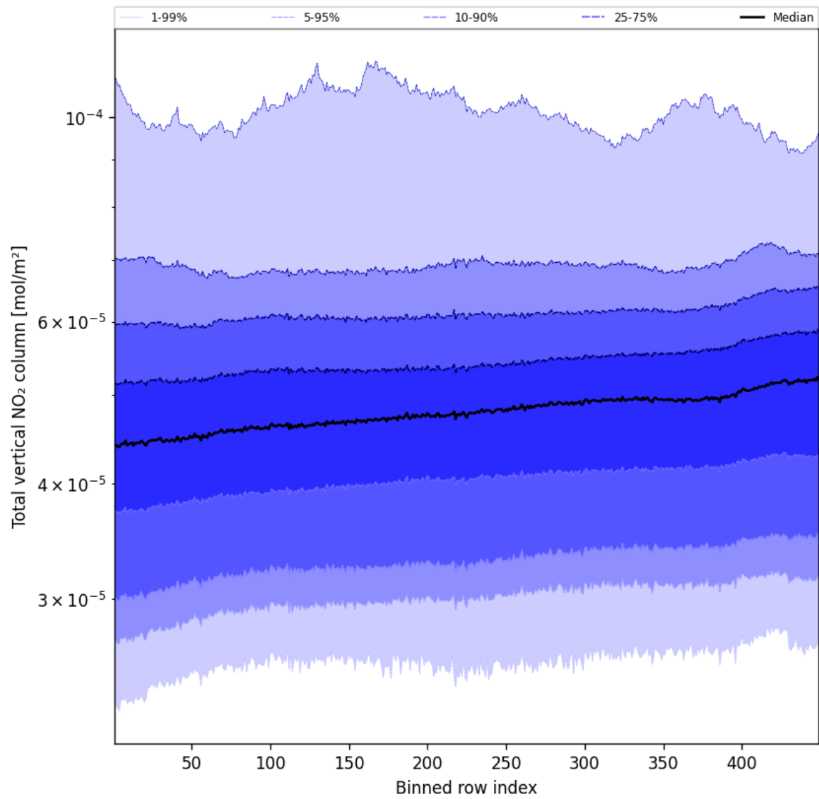
Figure 55: Along track statistics of “Total vertical NO 2 column” for 2025-03-20 to 2025-03-21
