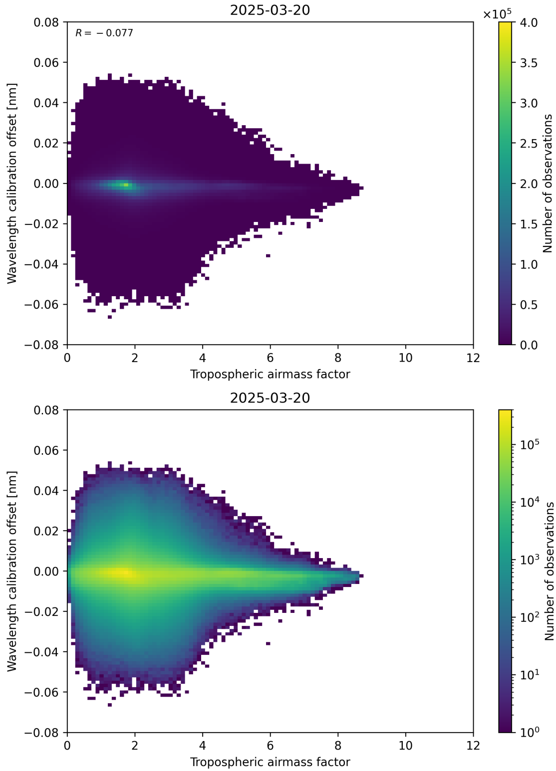
Figure 80: Scatter density plot of “Tropospheric airmass factor” against “Wavelength calibration offset” for 2025-03-20 to 2025-03-21.
