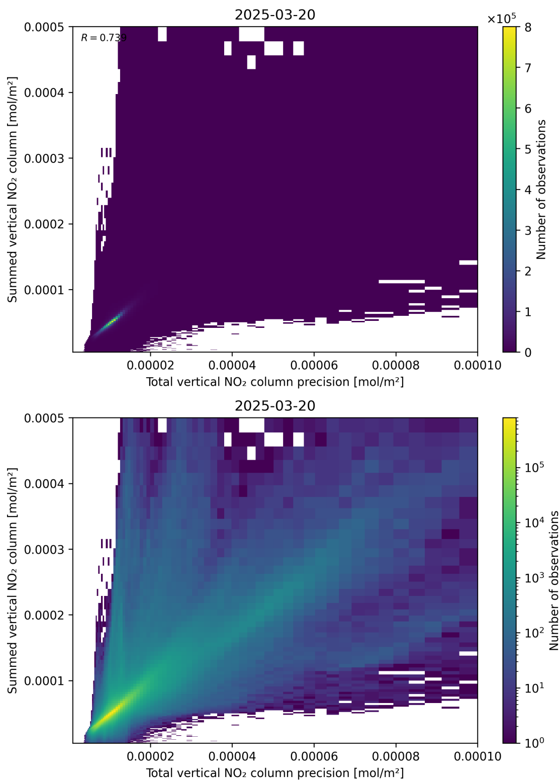
Figure 117: Scatter density plot of “Total vertical NO 2 column precision” against “Summed vertical NO 2 column” for 2025-03-20 to 2025-03-21.
