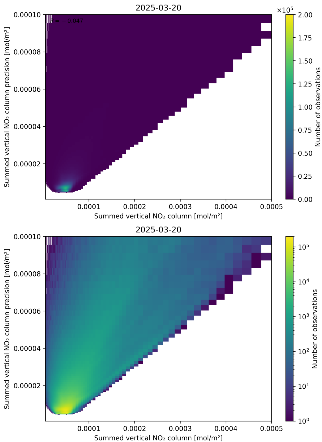
Figure 105: Scatter density plot of “Summed vertical NO 2 column” against “Summed vertical NO 2 column precision” for 2025-03-20 to 2025-03-21.
