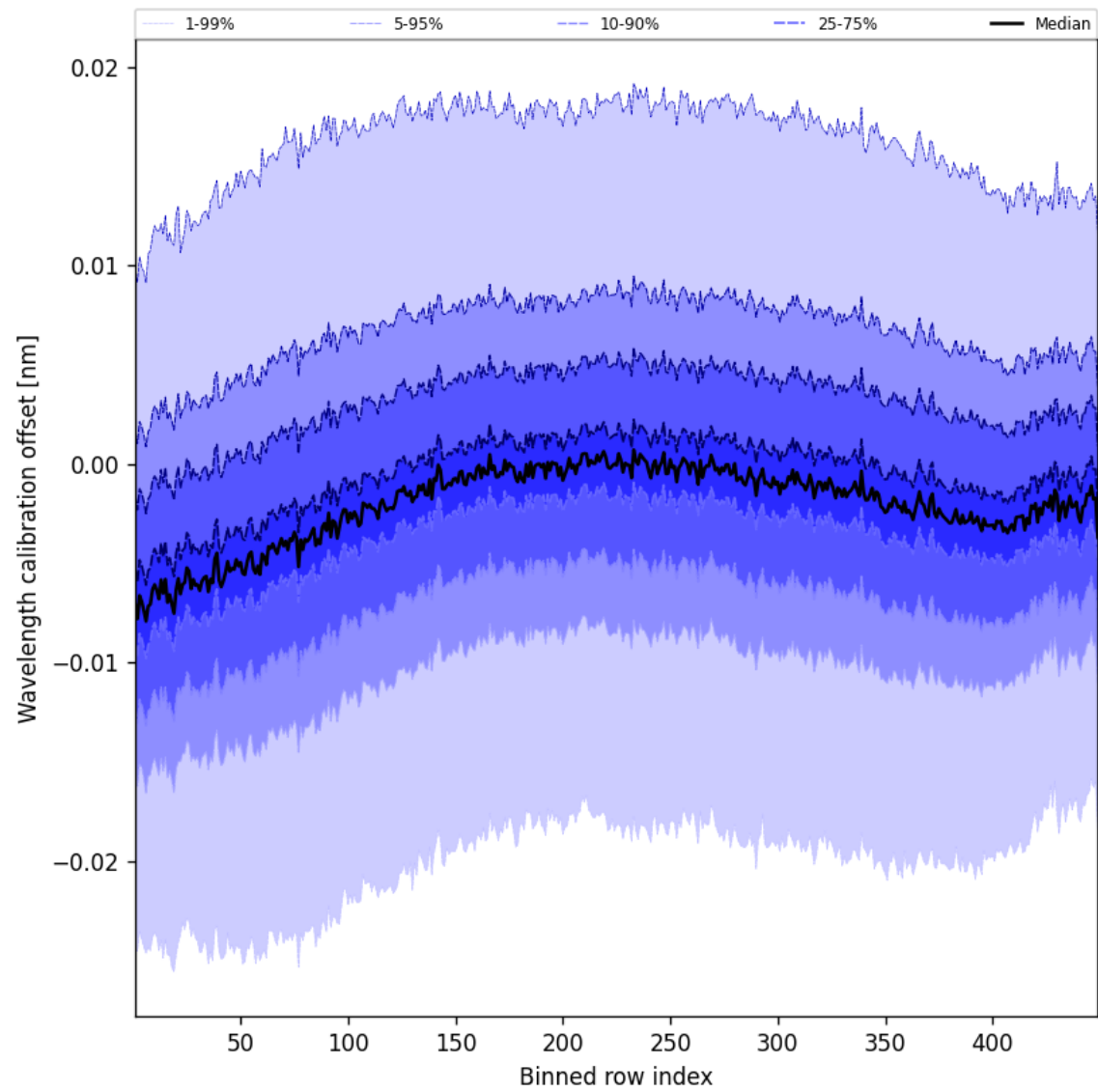
Figure 52: Along track statistics of “Wavelength calibration offset” for 2025-03-20 to 2025-03-21
