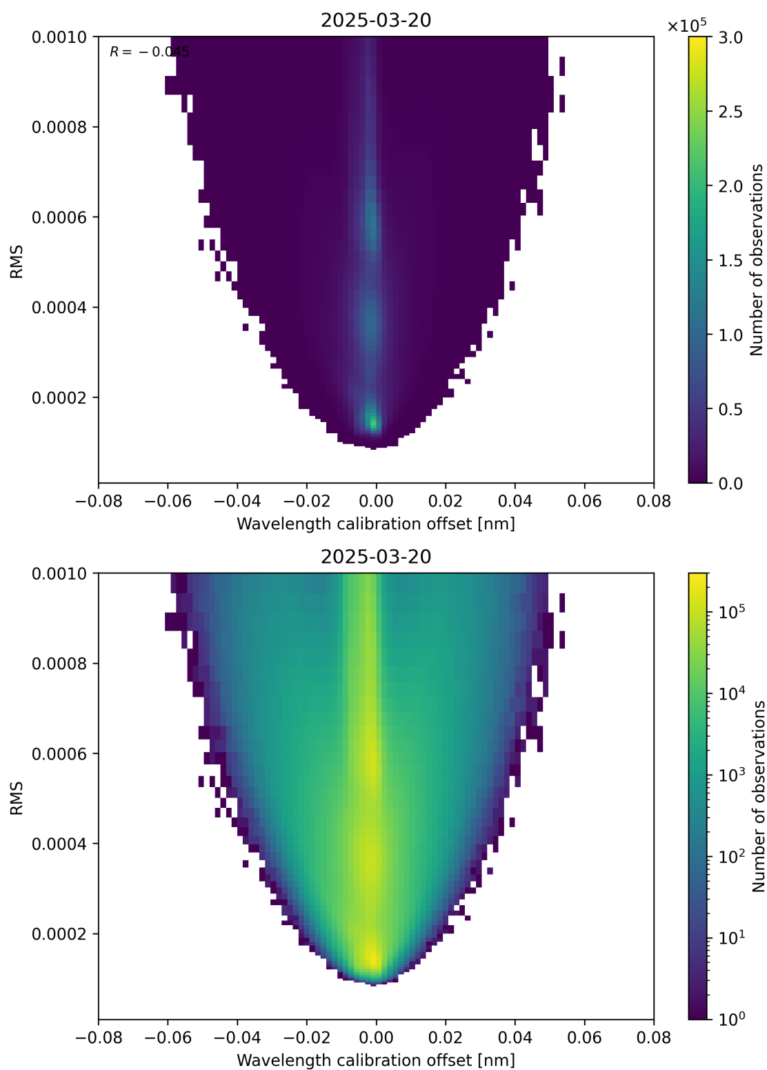
Figure 181: Scatter density plot of “Wavelength calibration offset” against “RMS” for 2025-03-20 to 2025-03-21.
