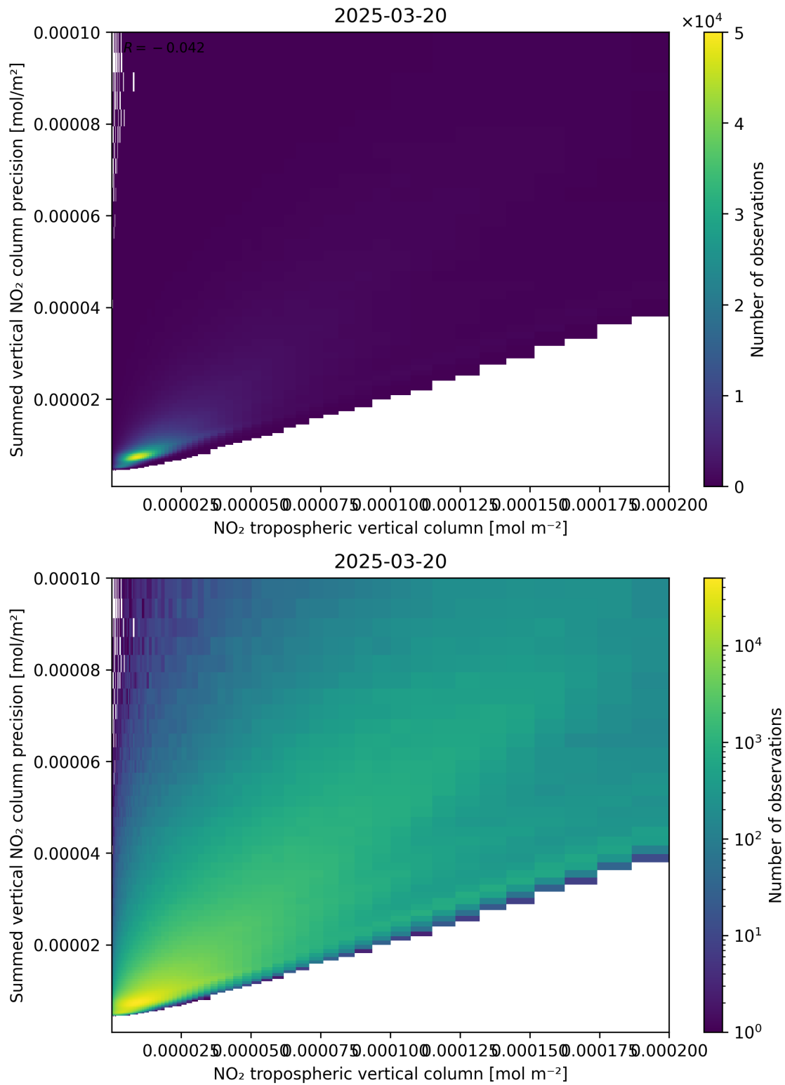
Figure 127: Scatter density plot of “NO 2 tropospheric vertical column” against “Summed vertical NO 2 column precision” for 2025-03-20 to 2025-03-21.
