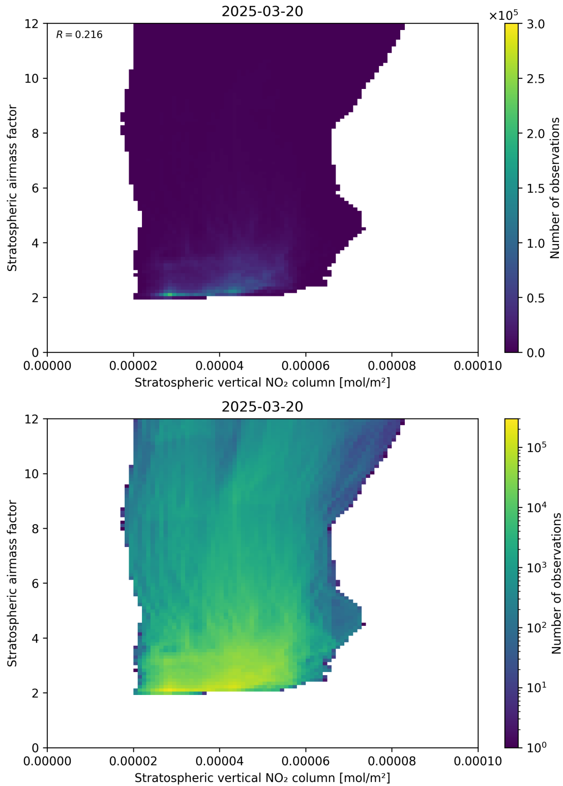
Figure 96: Scatter density plot of “Stratospheric vertical NO 2 column” against “Stratospheric airmass factor” for 2025-03-20 to 2025-03-21.
