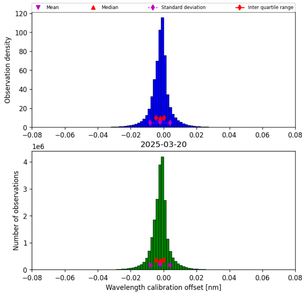
Figure 35: Histogram of “Wavelength calibration offset” for 2025-03-20 to 2025-03-21
