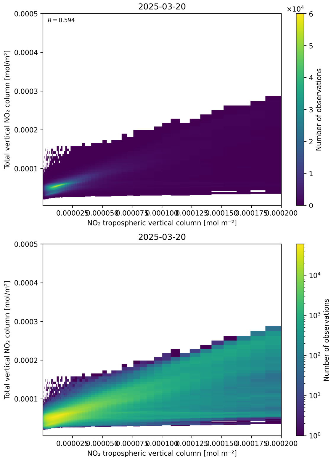
Figure 128: Scatter density plot of “NO 2 tropospheric vertical column” against “Total vertical NO 2 column” for 2025-03-20 to 2025-03-21.
