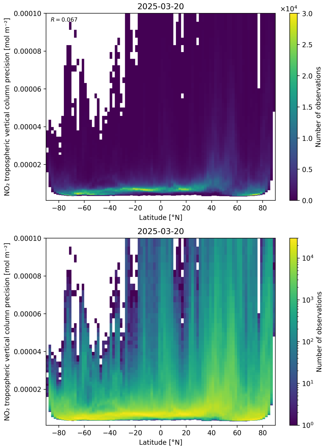
Figure 93: Scatter density plot of “Latitude” against “NO 2 tropospheric vertical column precision” for 2025-03-20 to 2025-03-21.
