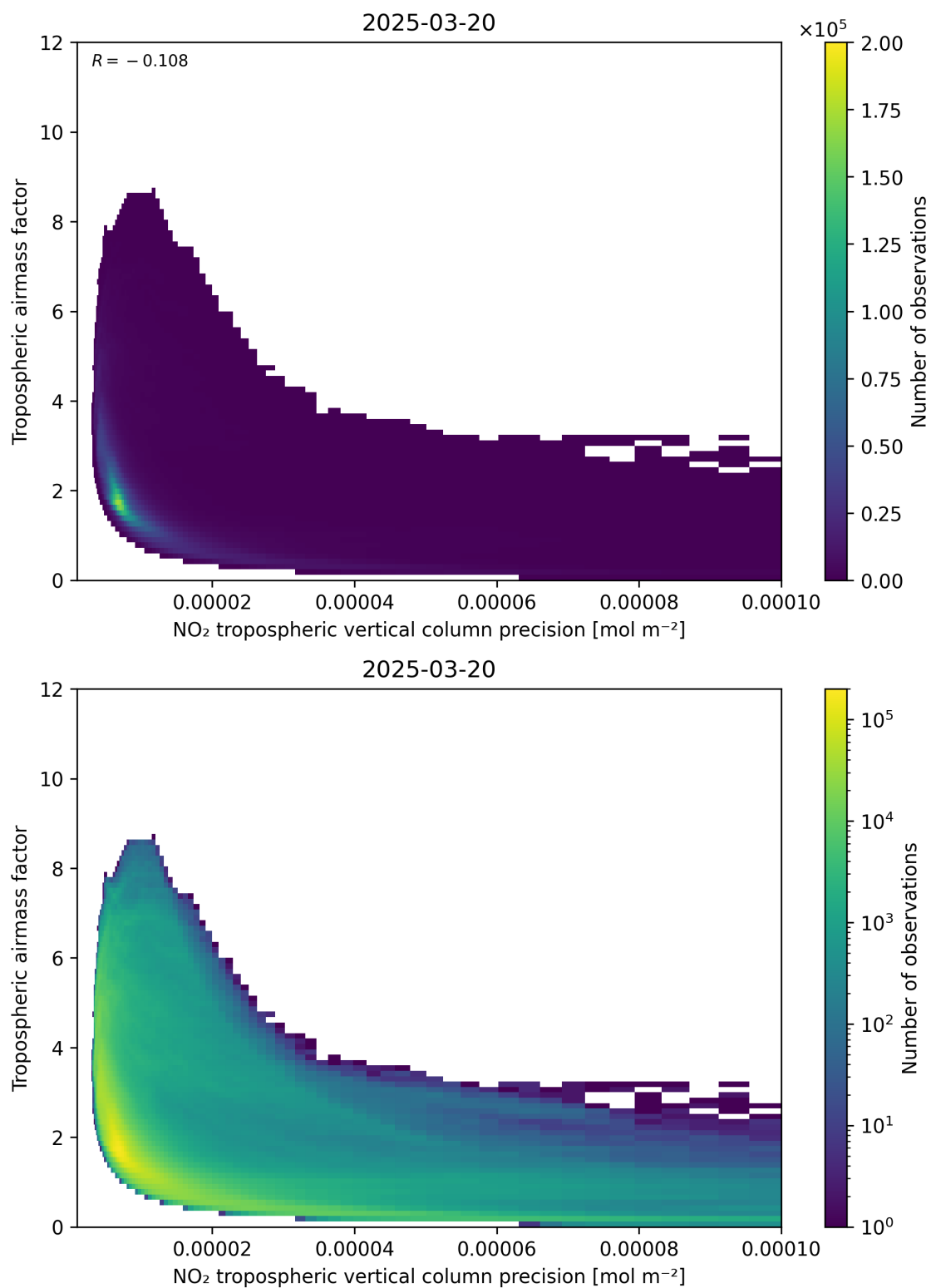
Figure 133: Scatter density plot of “NO 2 tropospheric vertical column precision” against “Tropospheric air mass factor” for 2025-03-20 to 2025-03-21.
