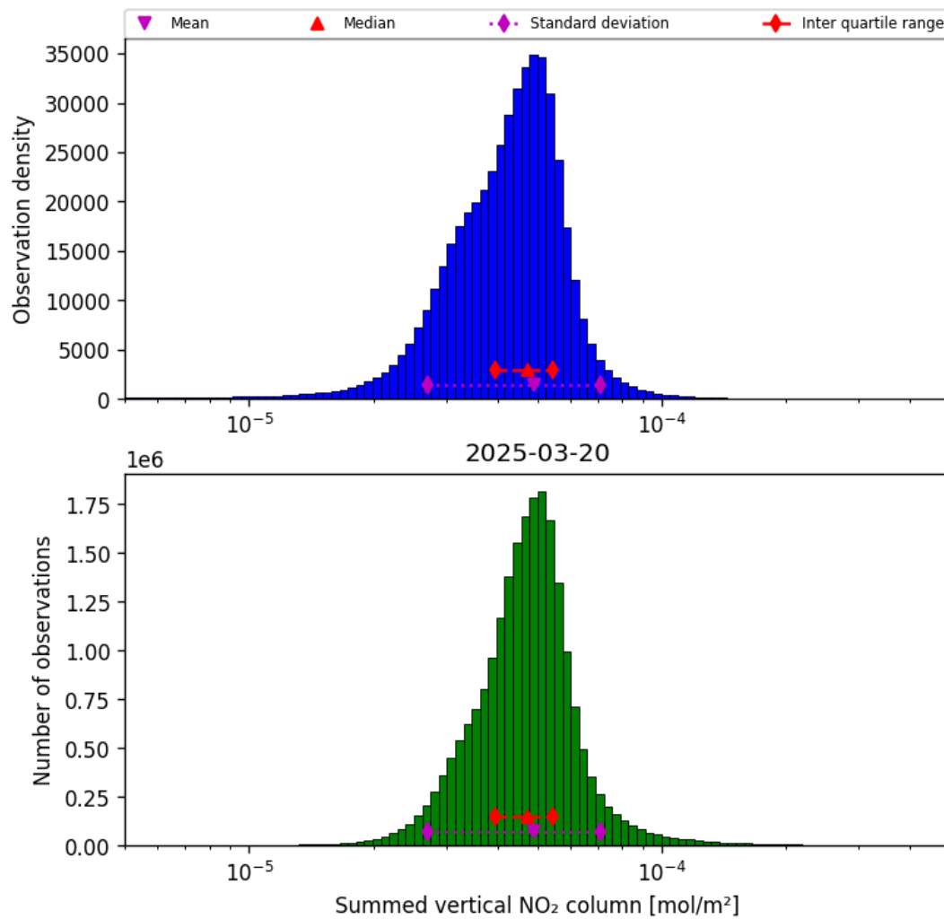
Figure 40: Histogram of “Summed vertical NO 2 column” for 2025-03-20 to 2025-03-21
