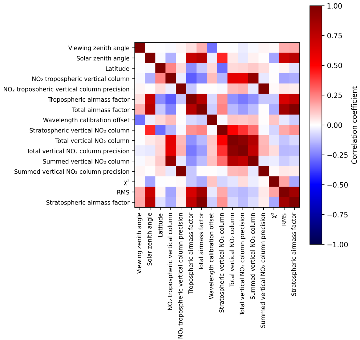
Figure 2: Map of correlation matrix for 2025-03-20 to 2025-03-21.
