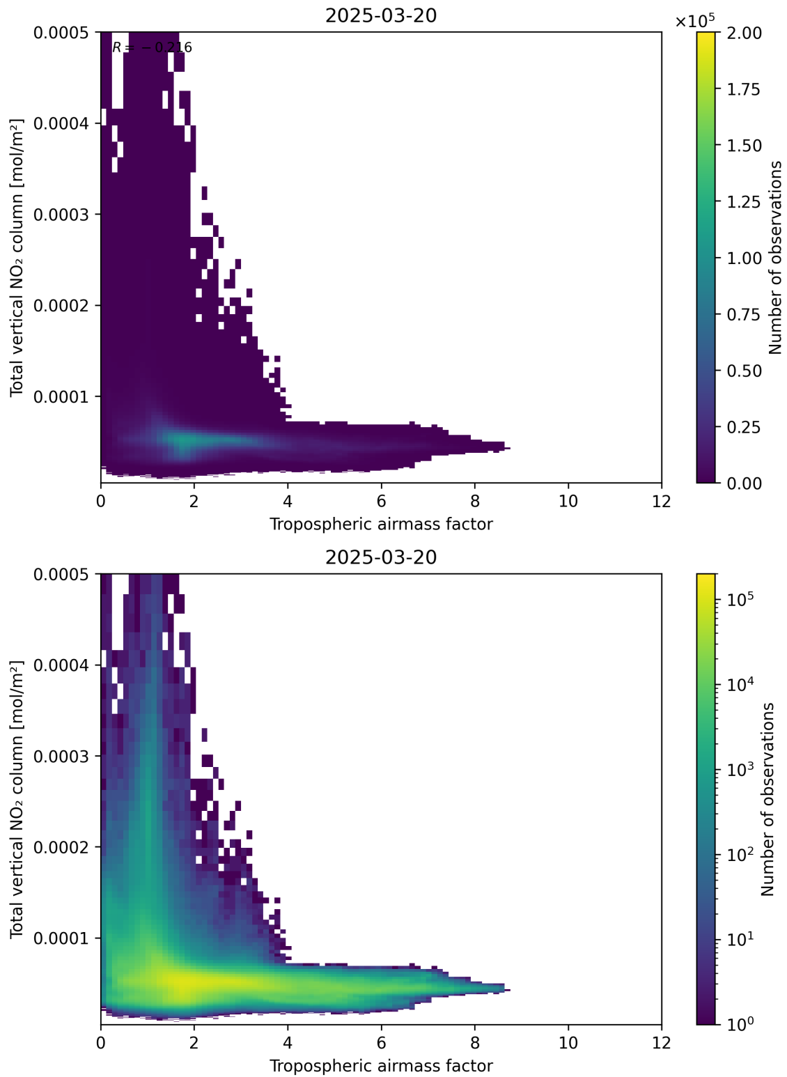
Figure 77: Scatter density plot of “Tropospheric air mass factor” against “Total vertical NO 2 column” for 2025-03-20 to 2025-03-21.
