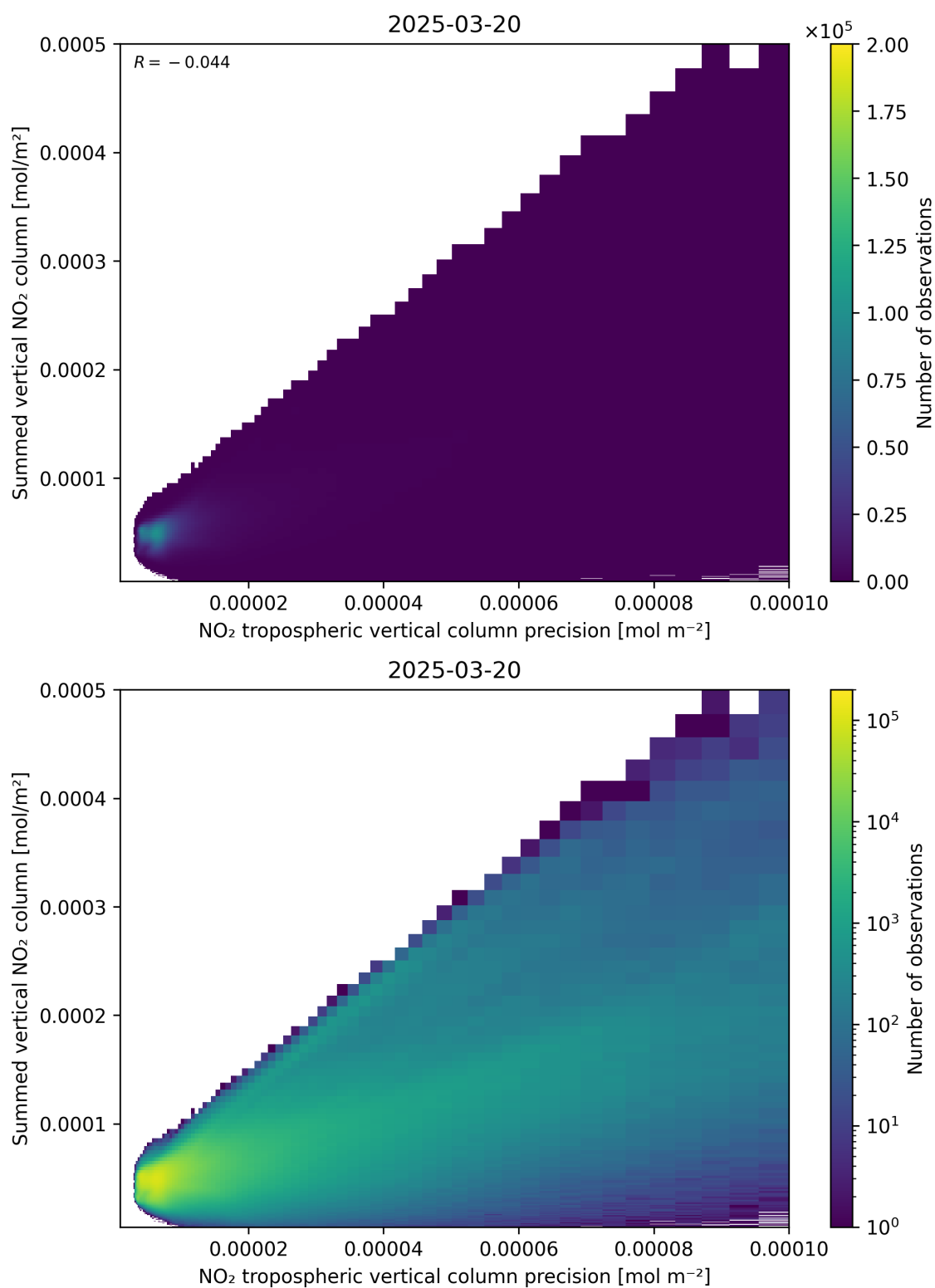
Figure 136: Scatter density plot of “NO 2 tropospheric vertical column precision” against “Summed vertical NO 2 column” for 2025-03-20 to 2025-03-21.
