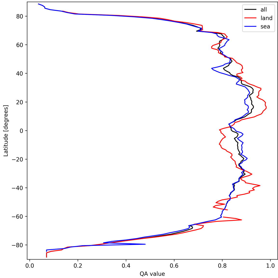
Figure 11: Zonal average of “QA value” for 2025-03-20 to 2025-03-21.
