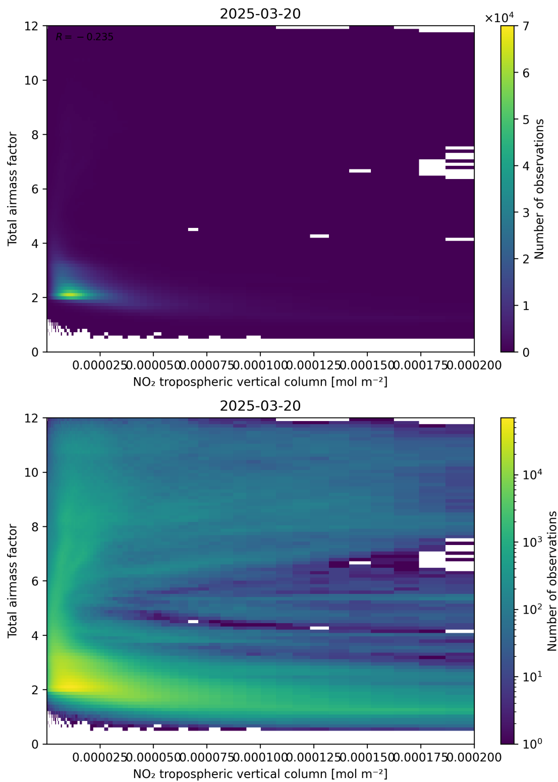
Figure 122: Scatter density plot of “NO 2 tropospheric vertical column” against “Total air mass factor” for 2025-03-20 to 2025-03-21.
