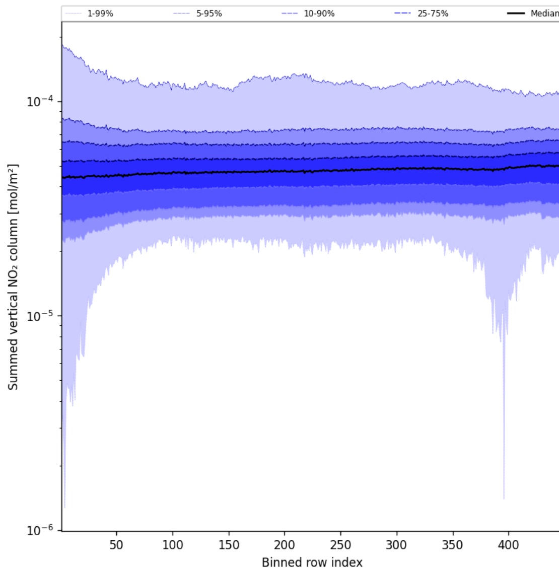
Figure 57: Along track statistics of “Summed vertical NO 2 column” for 2025-03-20 to 2025-03-21
