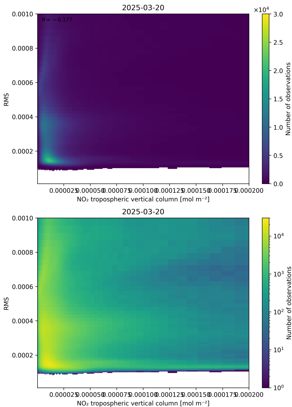
Figure 142: Scatter density plot of “NO 2 tropospheric vertical column” against “RMS” for 2025-03-20 to 2025-03-21.
