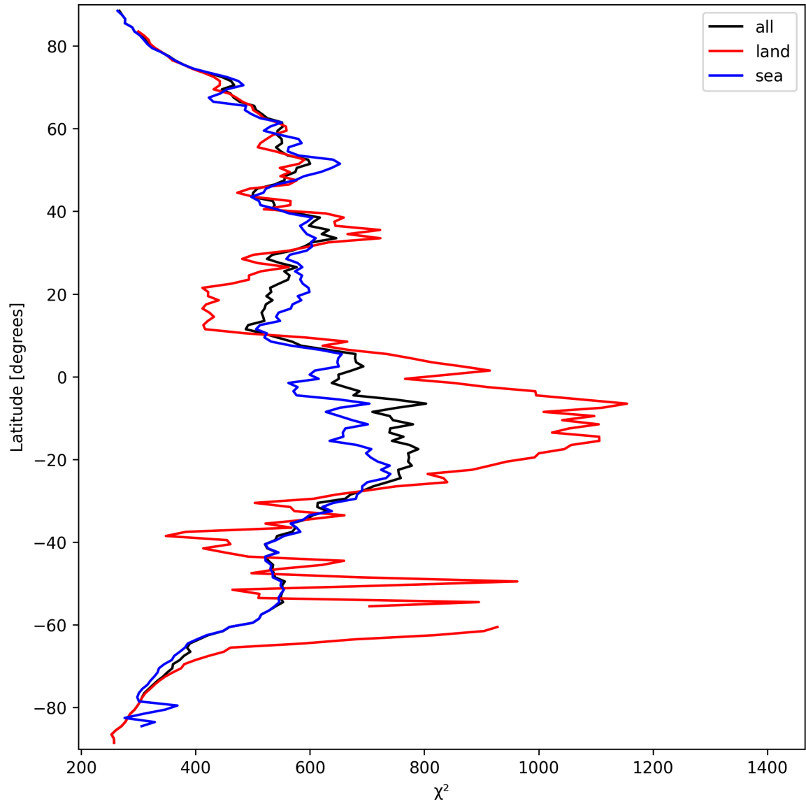
Figure 25: Zonal average of “ \chi^2 ” for 2025-03-20 to 2025-03-21.
