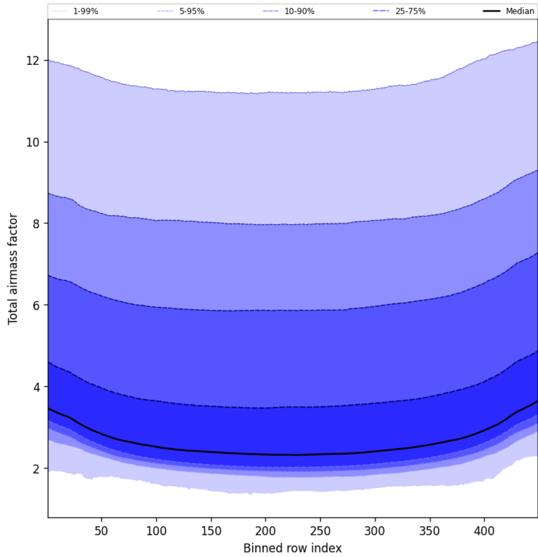
Figure 49: Along track statistics of “Total airmass factor” for 2025-03-20 to 2025-03-21
