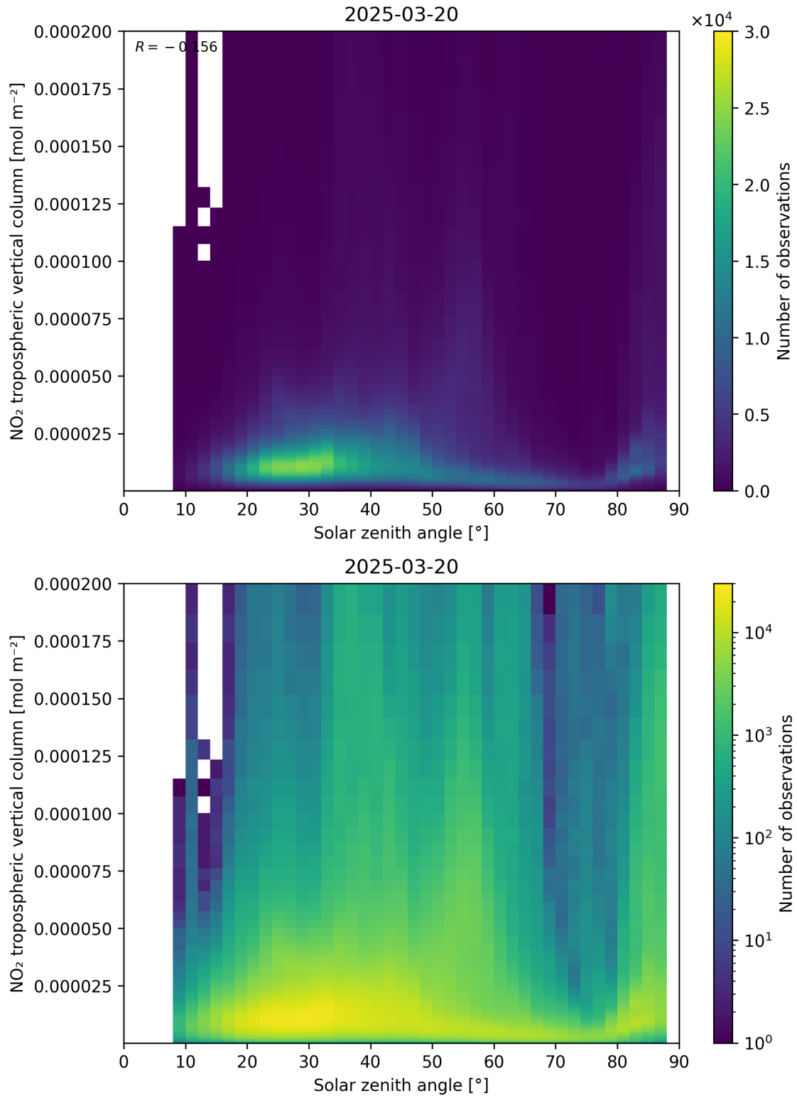
Figure 155: Scatter density plot of “Solar zenith angle” against “NO 2 tropospheric vertical column” for 2025-03-20 to 2025-03-21.
