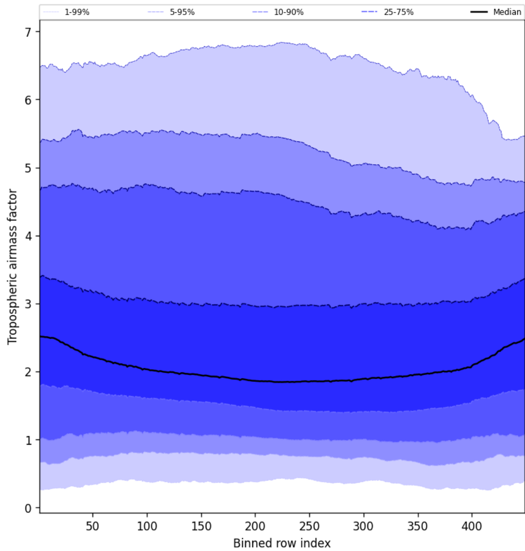
Figure 48: Along track statistics of “Tropospheric airmass factor” for 2025-03-20 to 2025-03-21
