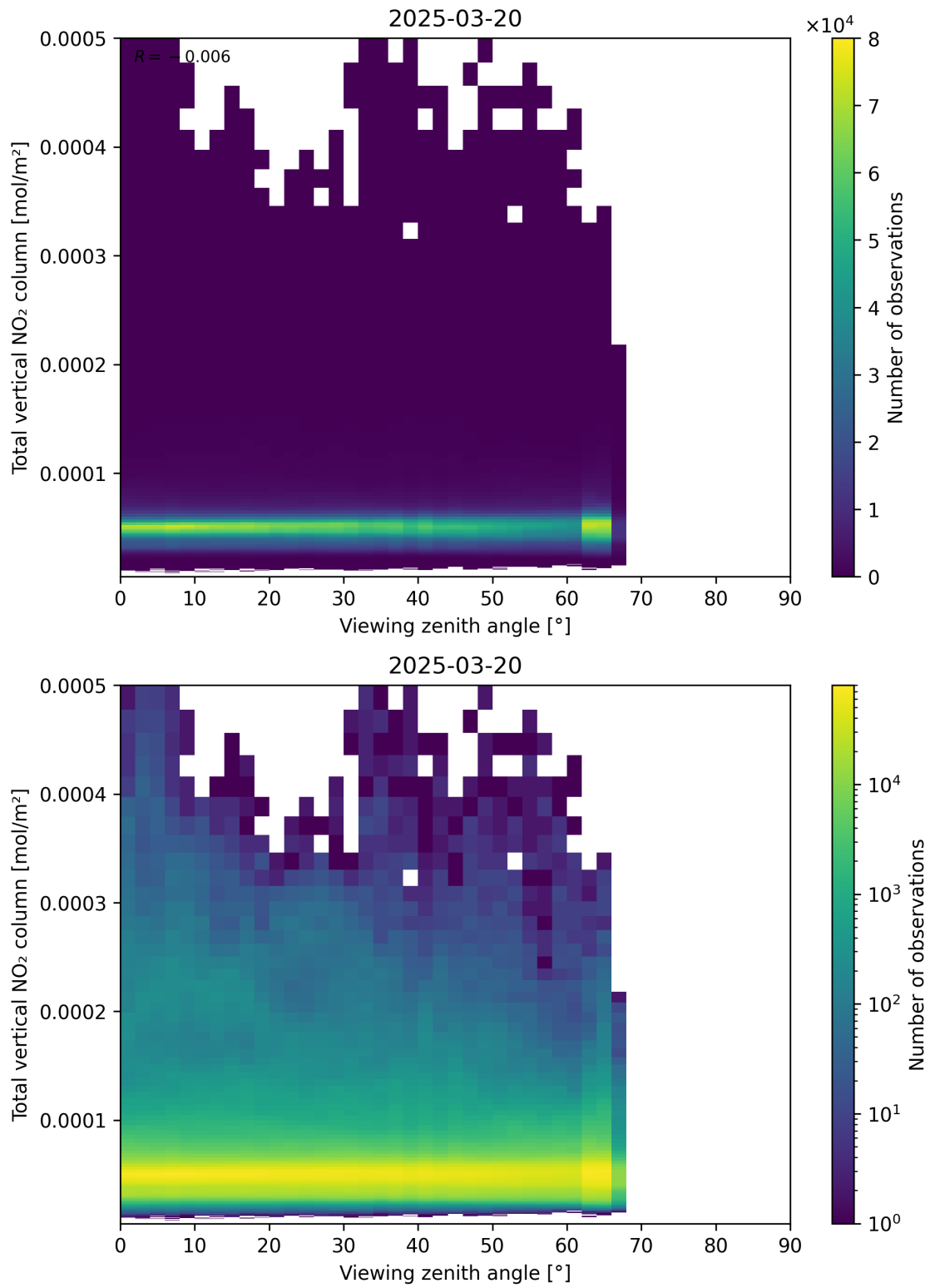
Figure 167: Scatter density plot of “Viewing zenith angle” against “Total vertical NO 2 column” for 2025-03-20 to 2025-03-21.
