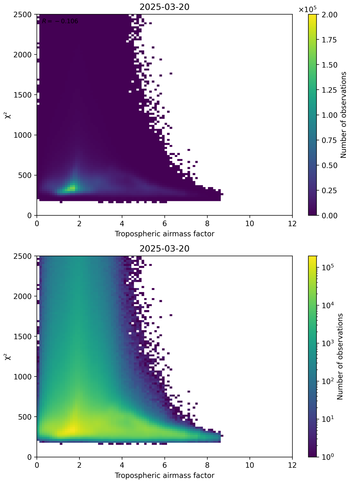
Figure 73: Scatter density plot of “Tropospheric airmass factor” against “ \chi^2 ” for 2025-03-20 to 2025-03-21.
