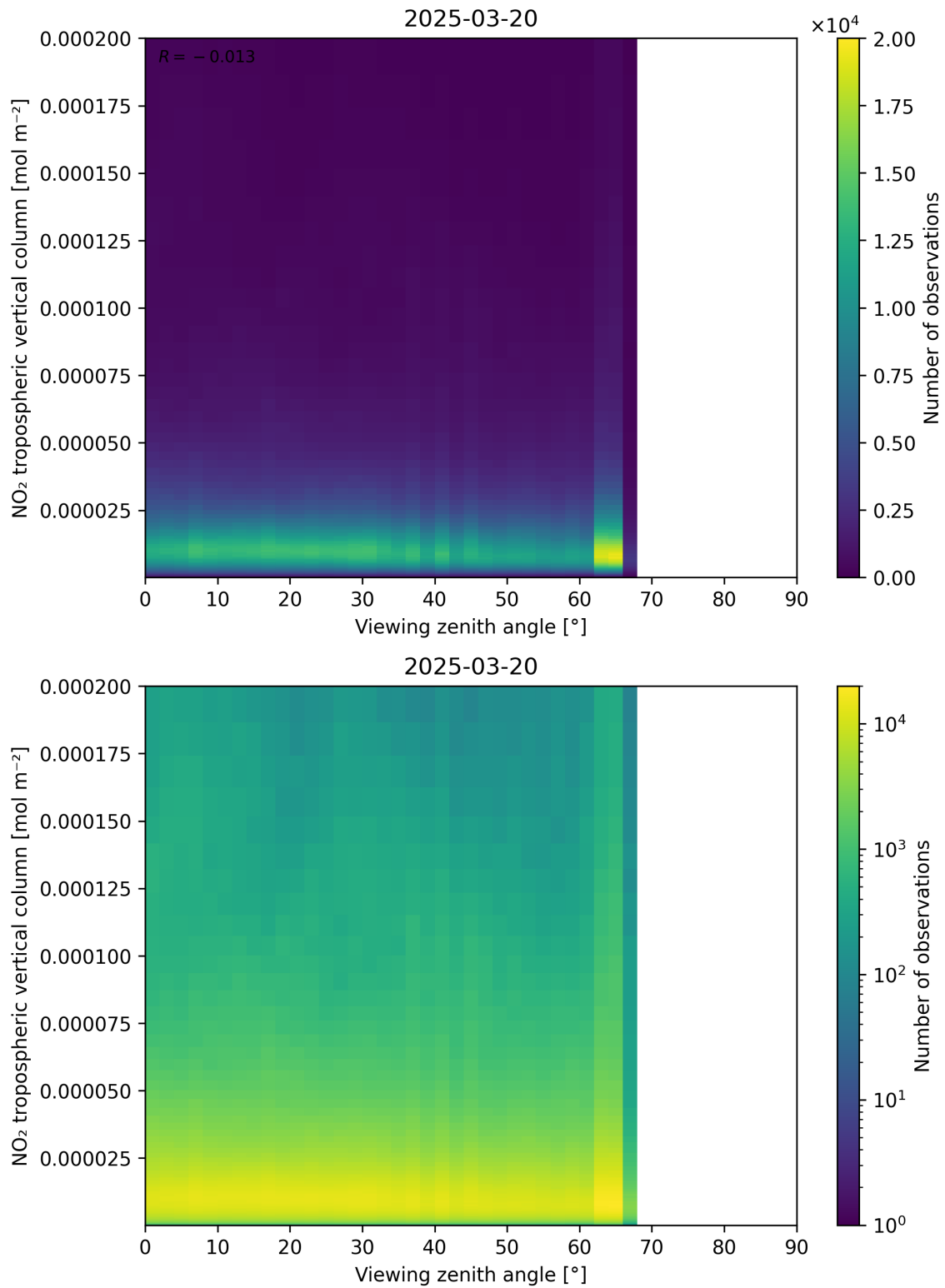
Figure 169: Scatter density plot of “Viewing zenith angle” against “NO 2 tropospheric vertical column” for 2025-03-20 to 2025-03-21.
