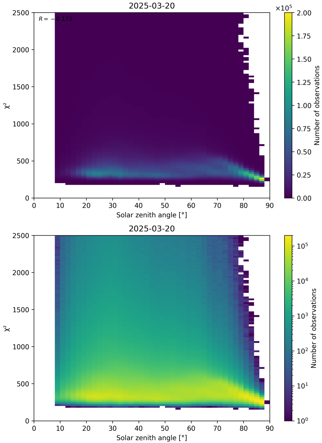
Figure 148: Scatter density plot of “Solar zenith angle” against “ \chi^2 ” for 2025-03-20 to 2025-03-21.
