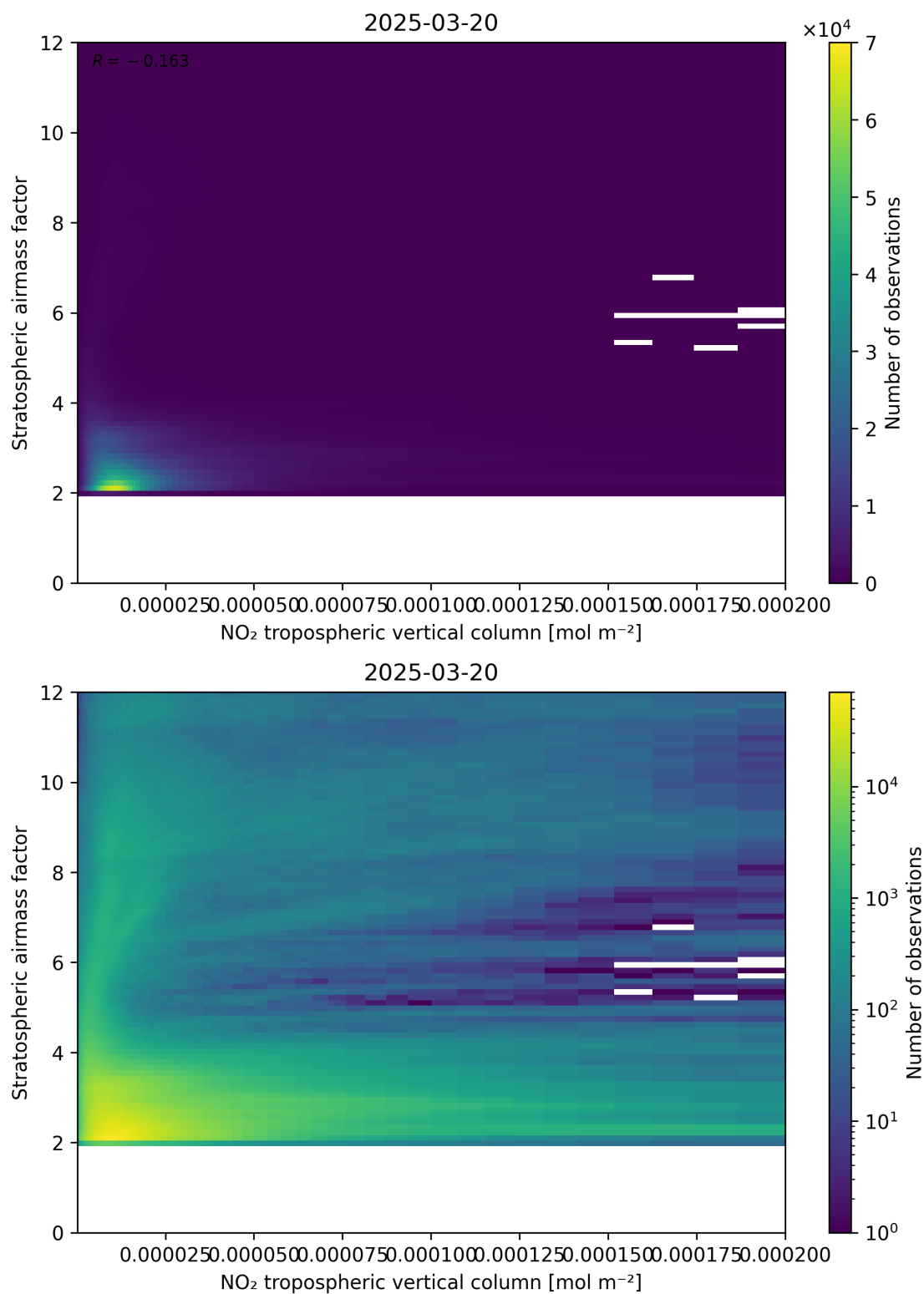
Figure 121: Scatter density plot of “NO 2 tropospheric vertical column” against “Stratospheric air mass factor” for 2025-03-20 to 2025-03-21.
