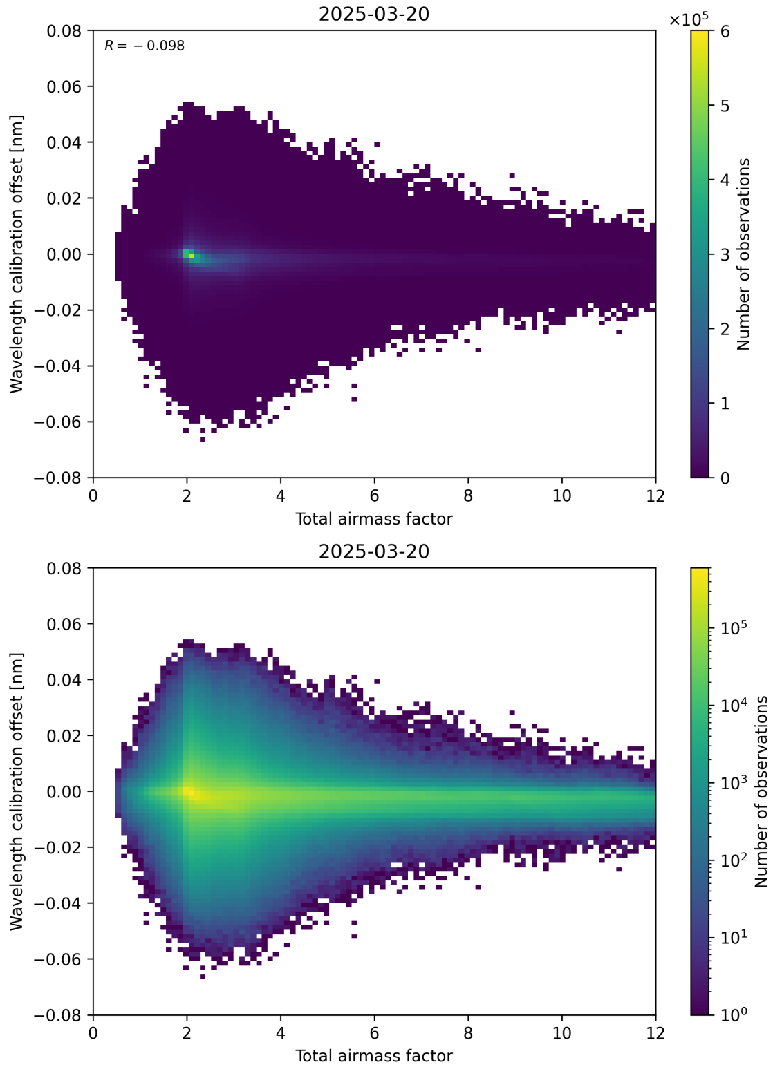
Figure 70: Scatter density plot of “Total airmass factor” against “Wavelength calibration offset” for 2025-03-20 to 2025-03-21.
