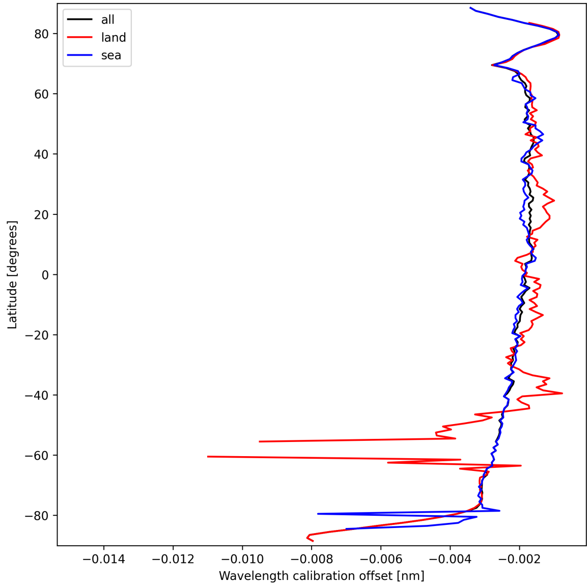
Figure 18: Zonal average of “Wavelength calibration offset” for 2025-03-20 to 2025-03-21.
