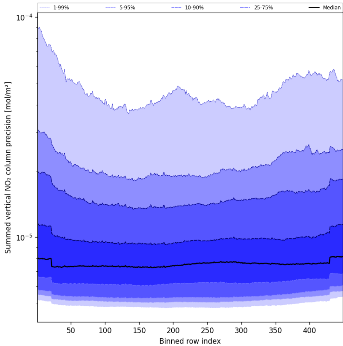
Figure 58: Along track statistics of “Summed vertical NO 2 column precision” for 2025-03-20 to 2025-03-21
