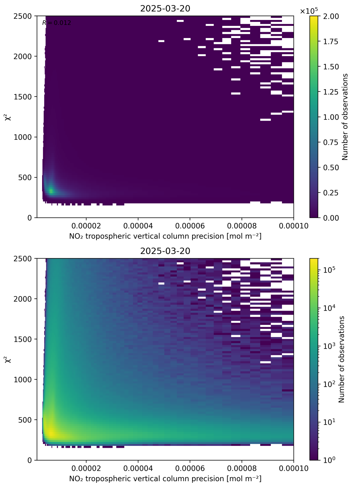
Figure 134: Scatter density plot of “NO 2 tropospheric vertical column precision” against “ \chi^2 ” for 2025-03-20 to 2025-03-21.
