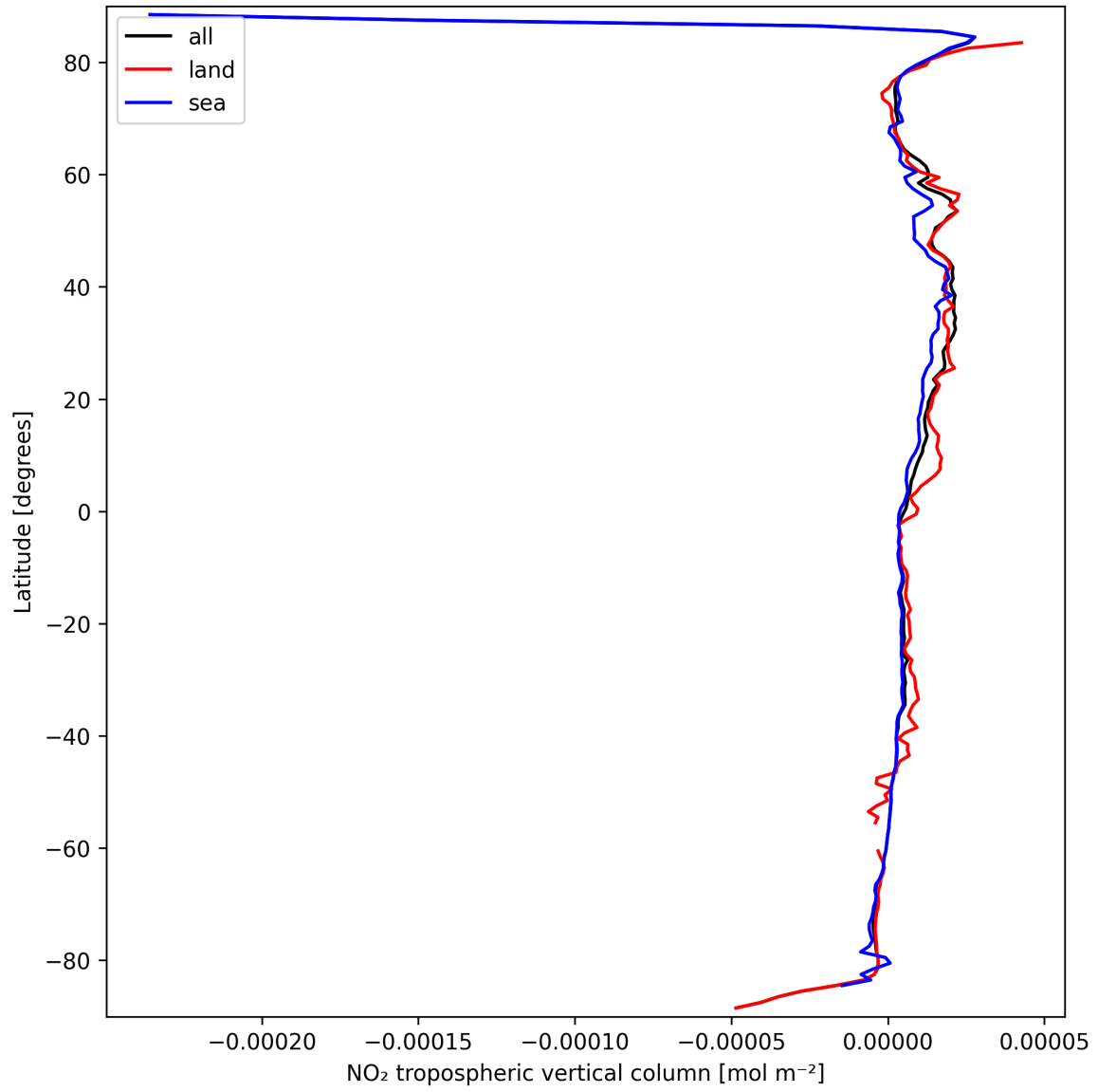
Figure 12: Zonal average of “NO 2 tropospheric vertical column” for 2025-03-20 to 2025-03-21.
