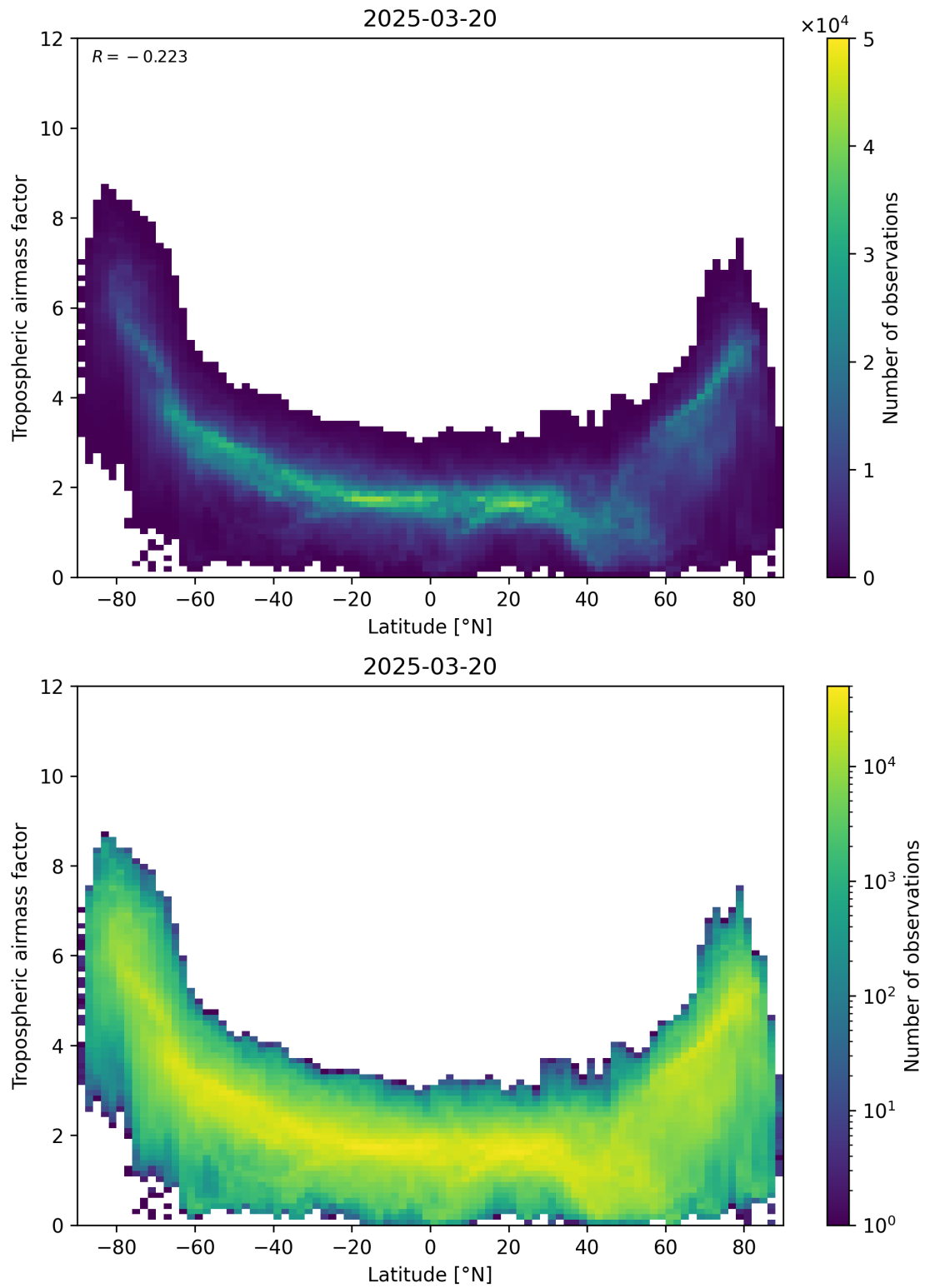
Figure 85: Scatter density plot of “Latitude” against “Tropospheric airmass factor” for 2025-03-20 to 2025-03-21.
