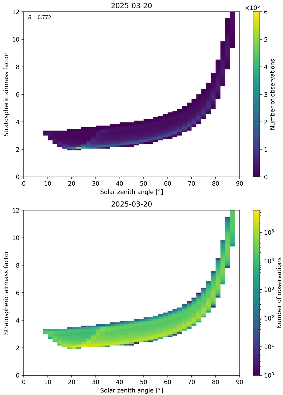
Figure 145: Scatter density plot of “Solar zenith angle” against “Stratospheric airmass factor” for 2025-03-20 to 2025-03-21.
