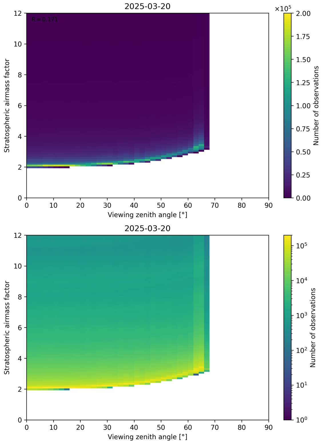
Figure 159: Scatter density plot of “Viewing zenith angle” against “Stratospheric airmass factor” for 2025-03-20 to 2025-03-21.
