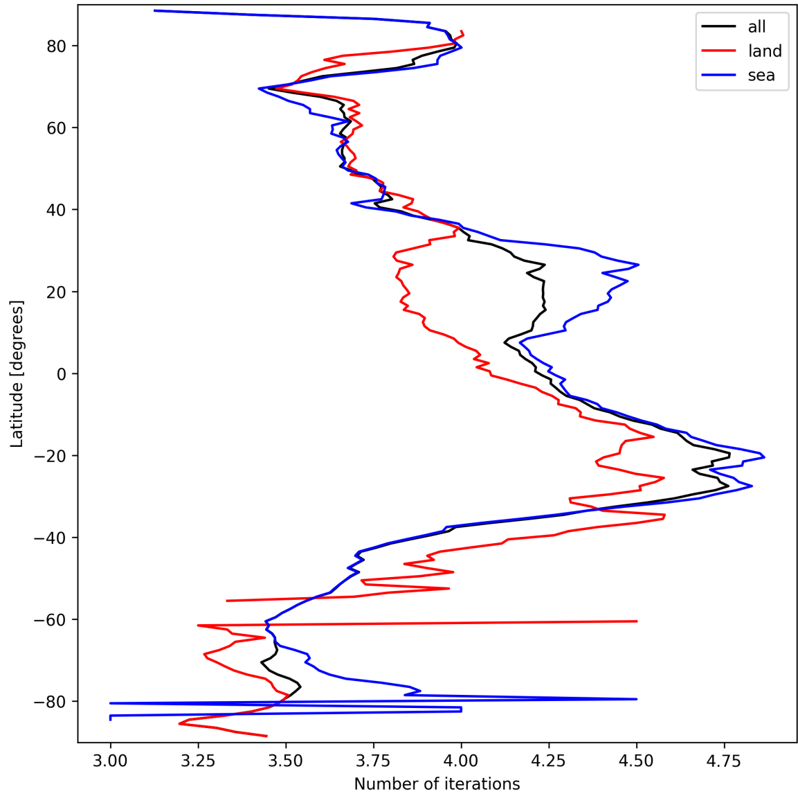
Figure 17: Zonal average of “Number of iterations” for 2025-03-20 to 2025-03-21.
