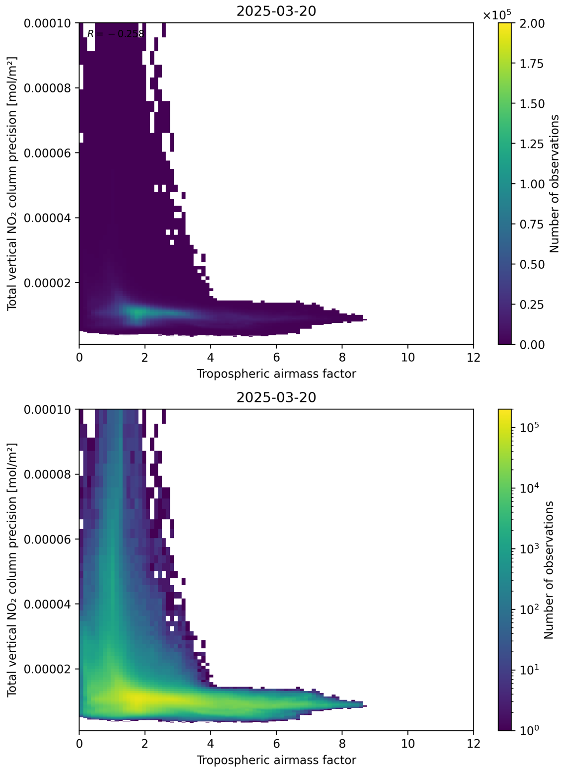
Figure 78: Scatter density plot of “Tropospheric air mass factor” against “Total vertical NO 2 column precision” for 2025-03-20 to 2025-03-21.
