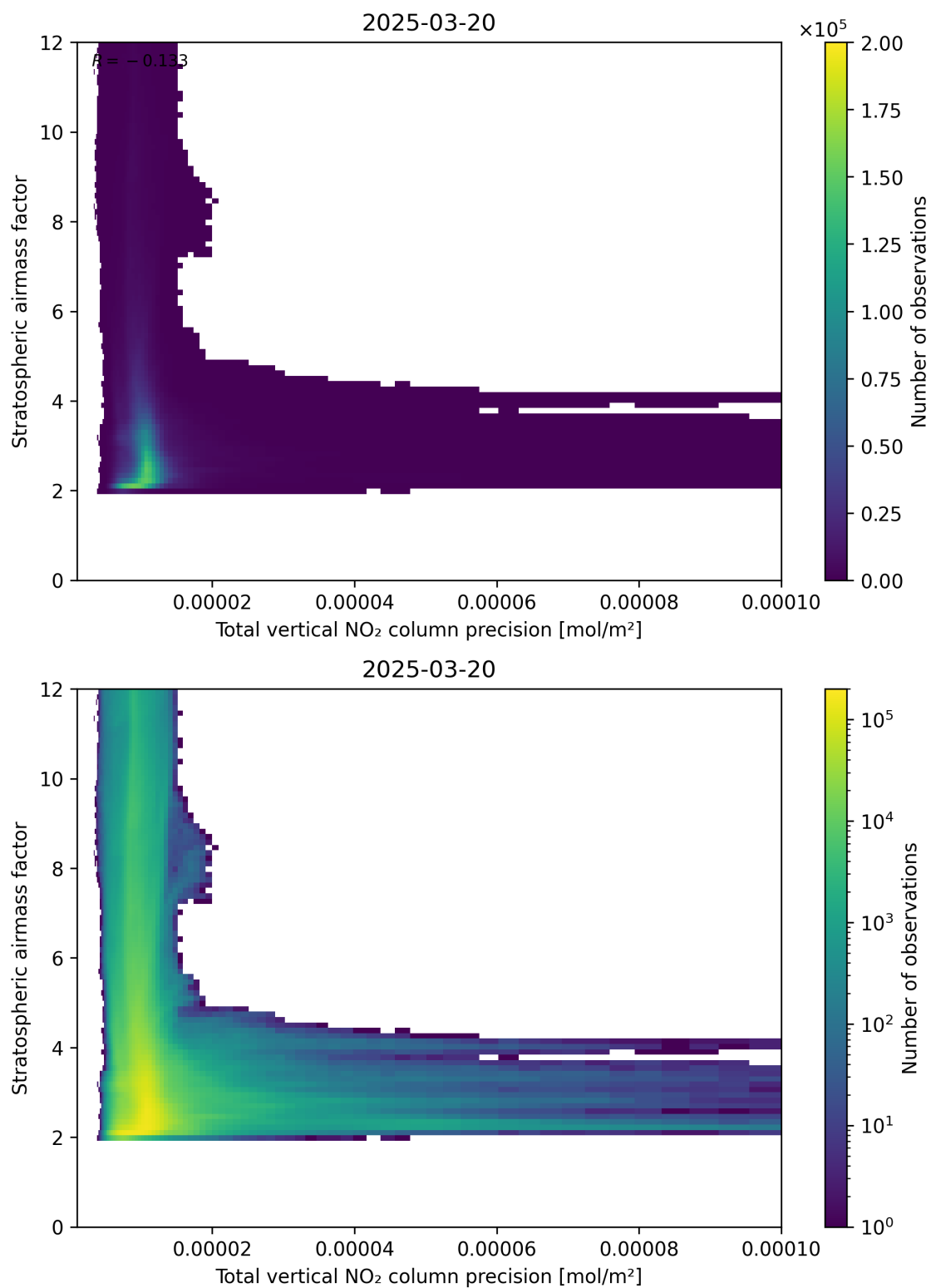
Figure 115: Scatter density plot of “Total vertical NO 2 column precision” against “Stratospheric air mass factor” for 2025-03-20 to 2025-03-21.
