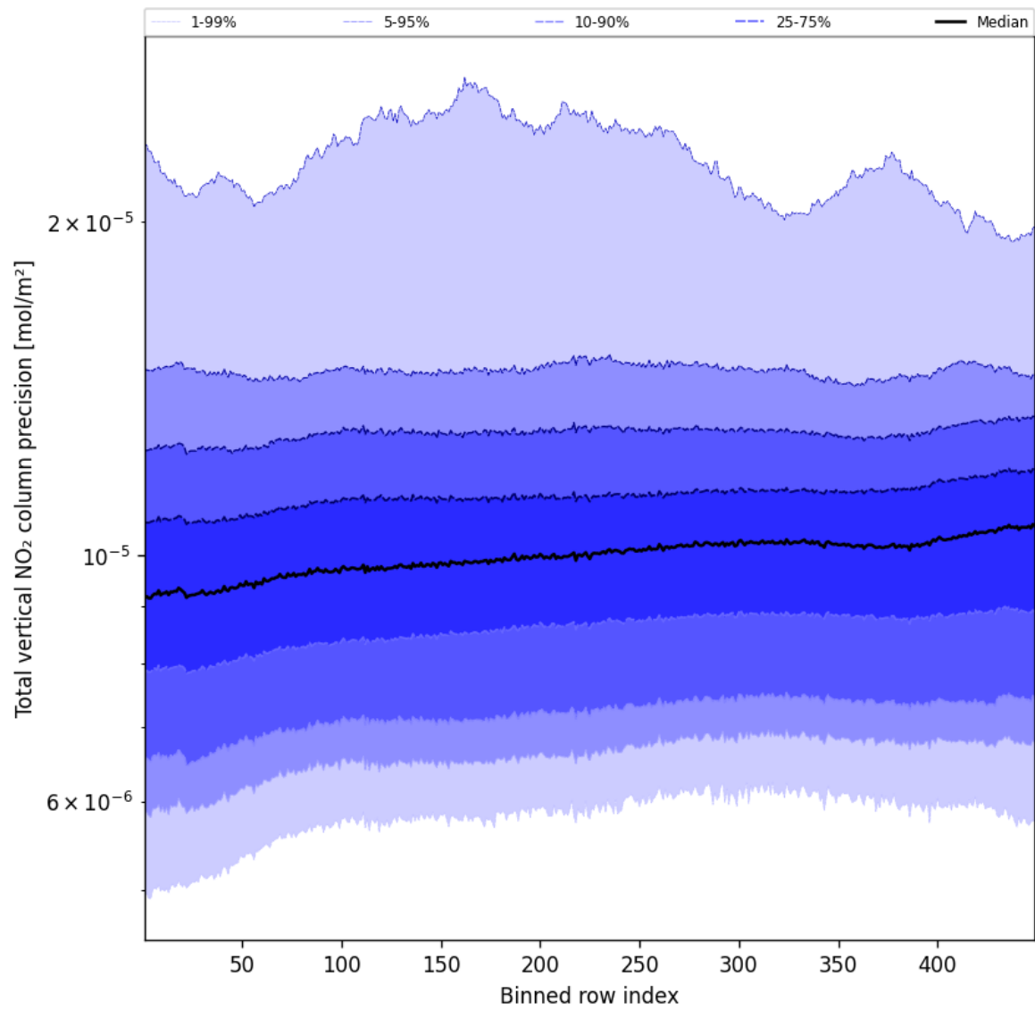
Figure 56: Along track statistics of “Total vertical NO 2 column precision” for 2025-03-20 to 2025-03-21
