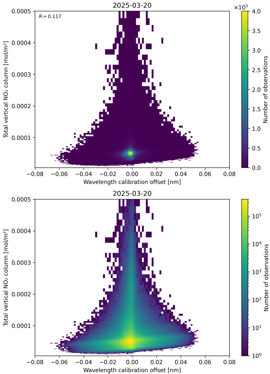
Figure 179: Scatter density plot of “Wavelength calibration offset” against “Total vertical NO 2 column” for 2025-03-20 to 2025-03-21.
