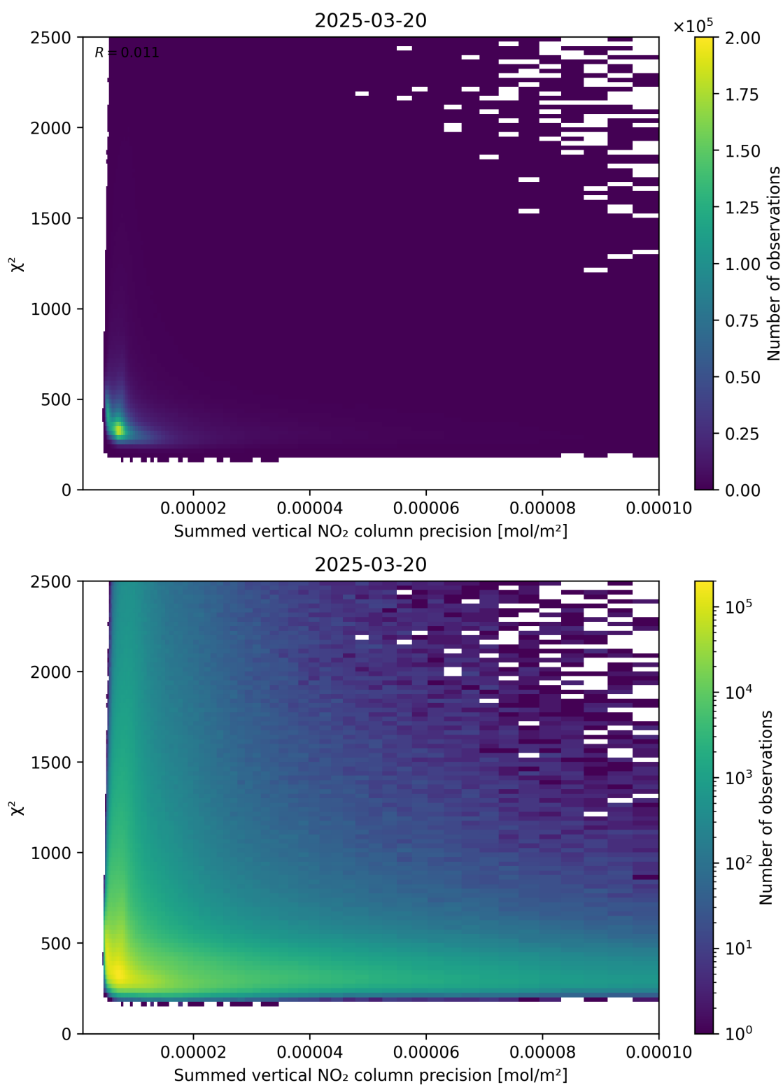
Figure 107: Scatter density plot of “Summed vertical NO 2 column precision” against “ \chi^2 ” for 2025-03-20 to 2025-03-21.
