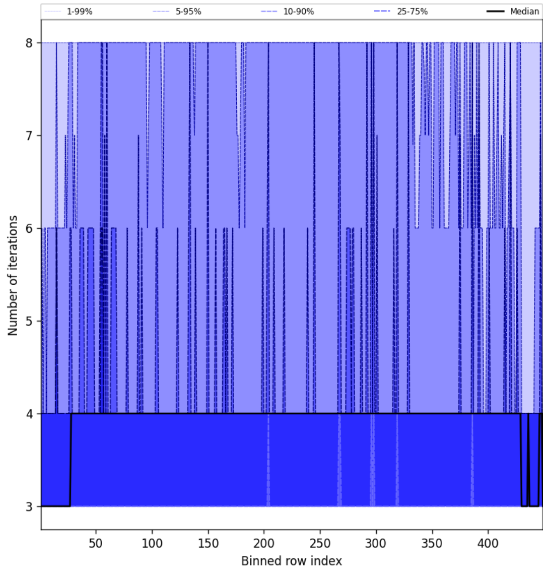
Figure 51: Along track statistics of “Number of iterations” for 2025-03-20 to 2025-03-21
