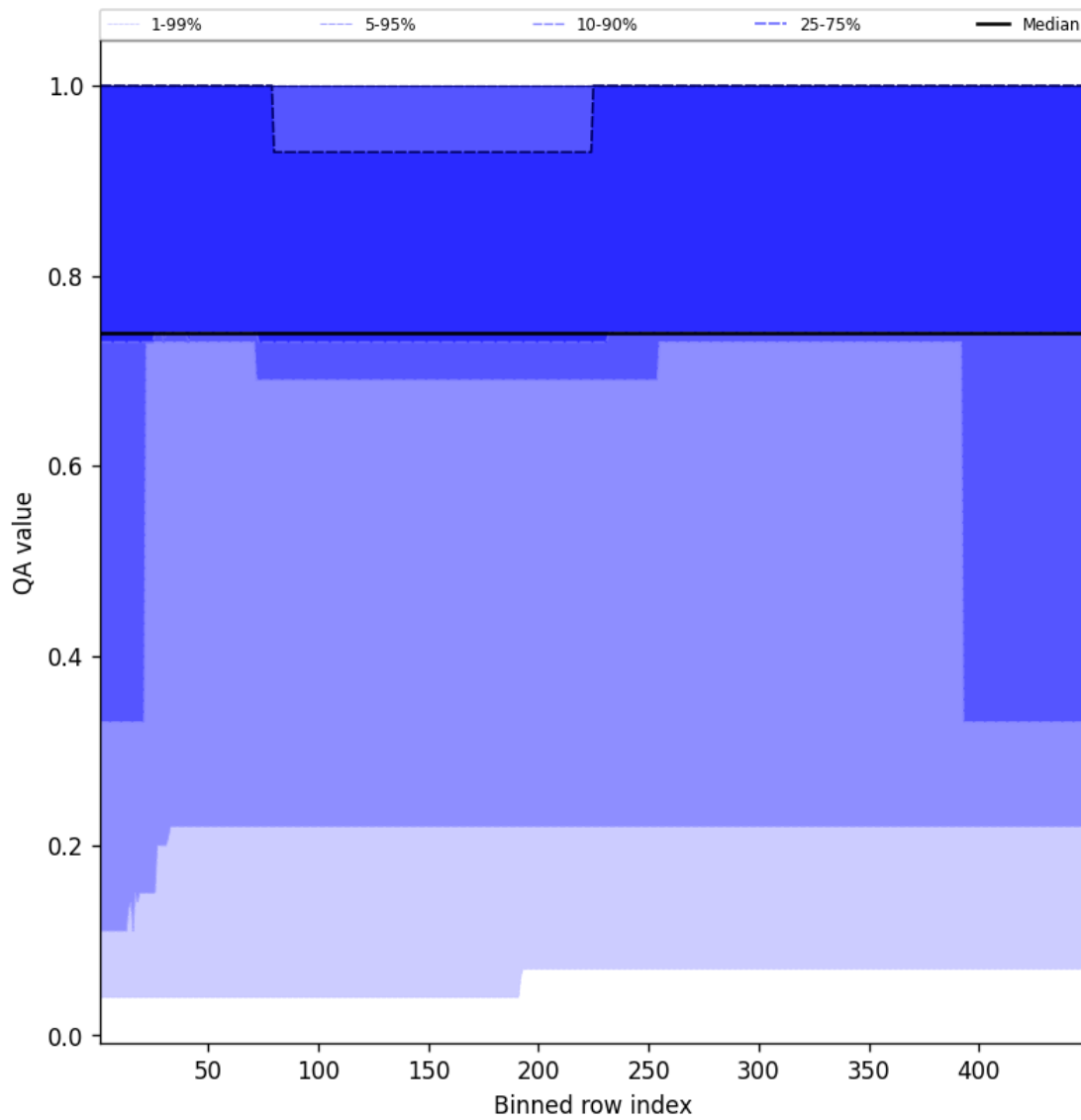
Figure 45: Along track statistics of “QA value” for 2025-03-20 to 2025-03-21
