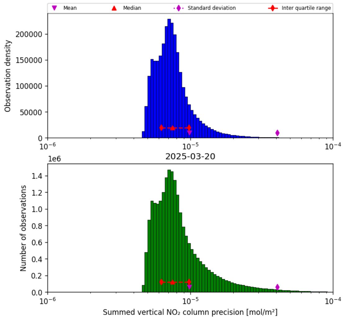
Figure 41: Histogram of “Summed vertical NO 2 column precision” for 2025-03-20 to 2025-03-21
