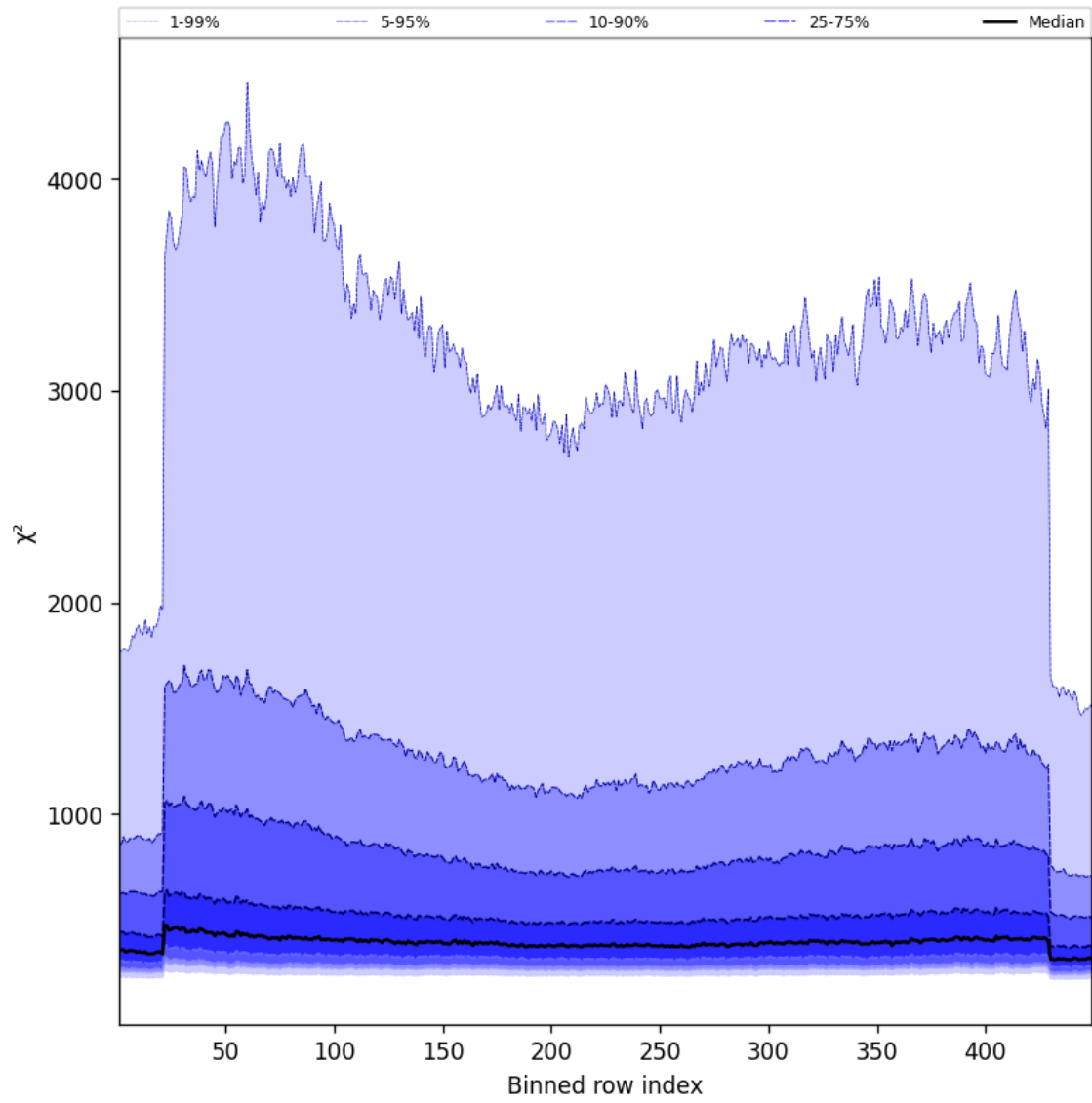
Figure 59: Along track statistics of “ \chi^2 ” for 2025-03-20 to 2025-03-21
