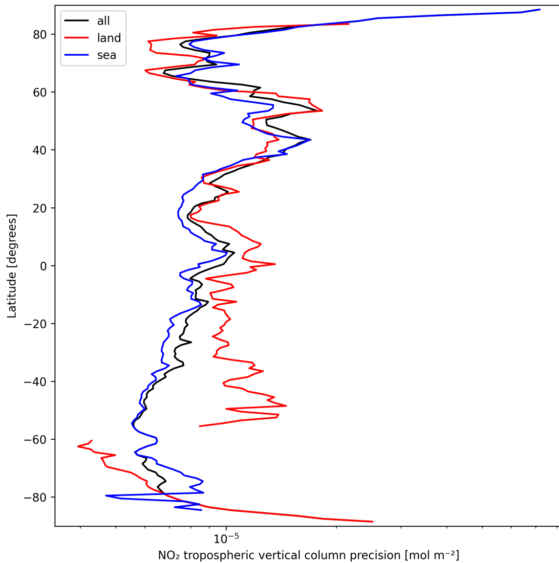
Figure 13: Zonal average of “NO 2 tropospheric vertical column precision” for 2025-03-20 to 2025-03-21.
