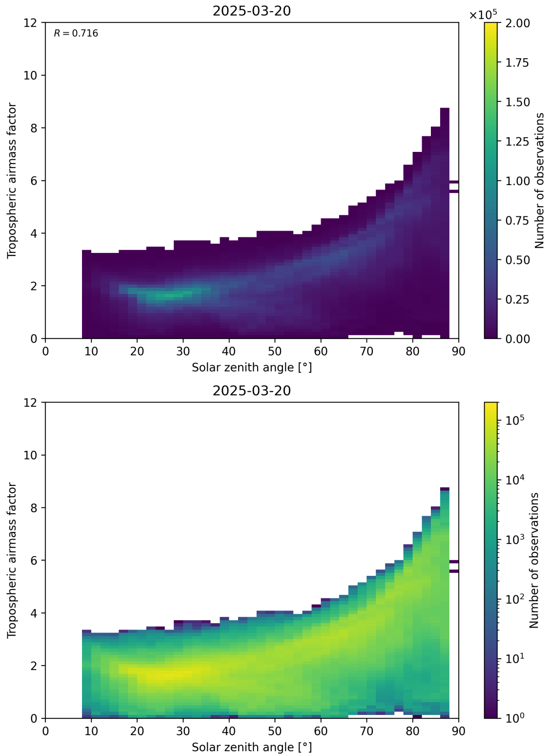
Figure 147: Scatter density plot of “Solar zenith angle” against “Tropospheric airmass factor” for 2025-03-20 to 2025-03-21.
