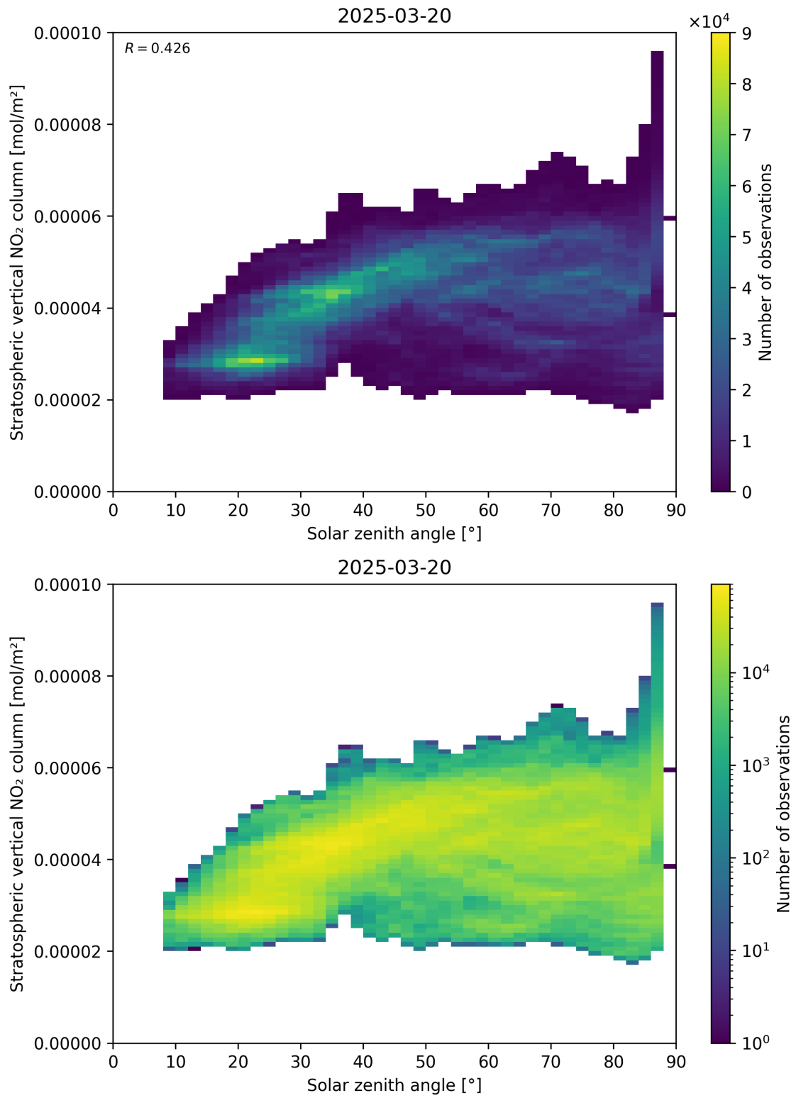
Figure 150: Scatter density plot of “Solar zenith angle” against “Stratospheric vertical NO 2 column” for 2025-03-20 to 2025-03-21.
