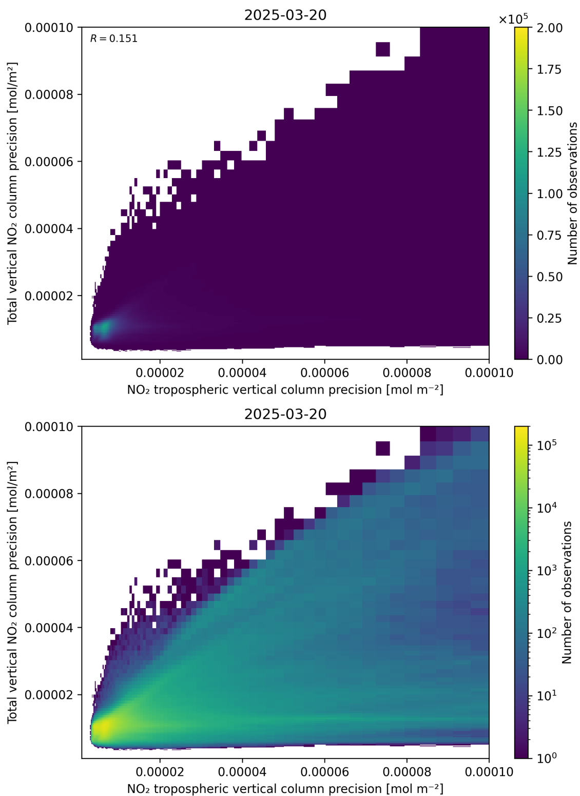
Figure 139: Scatter density plot of “NO 2 tropospheric vertical column precision” against “Total vertical NO 2 column precision” for 2025-03-20 to 2025-03-21.
