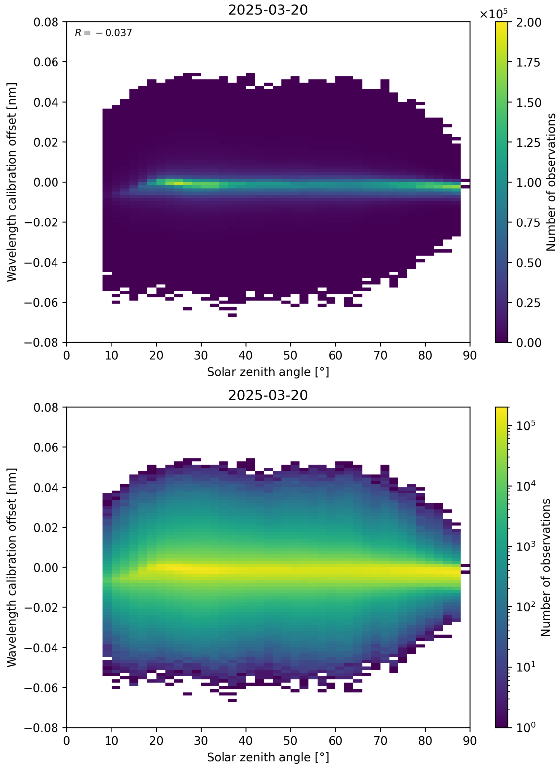
Figure 158: Scatter density plot of “Solar zenith angle” against “Wavelength calibration offset” for 2025-03-20 to 2025-03-21.
