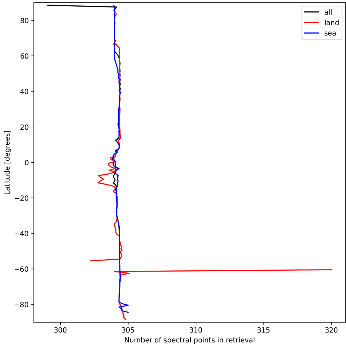
Figure 16: Zonal average of “Number of spectral points in retrieval” for 2025-03-20 to 2025-03-21.
