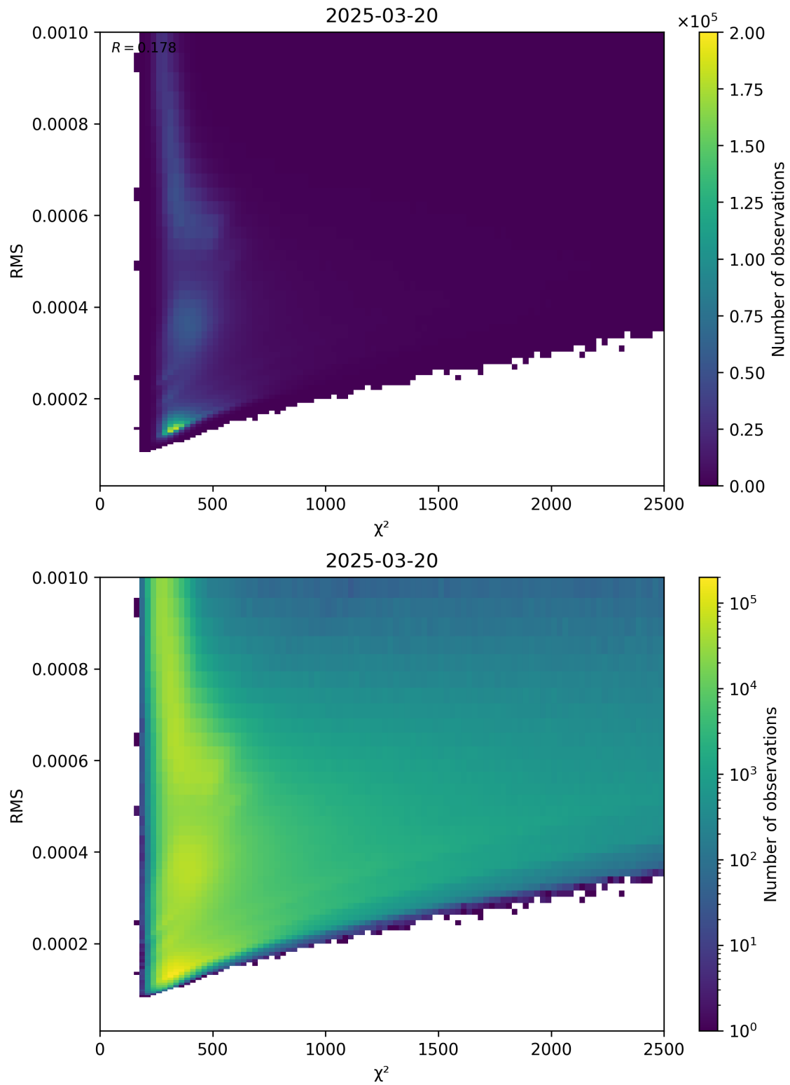
Figure 82: Scatter density plot of “ \chi^2 ” against “RMS” for 2025-03-20 to 2025-03-21.
