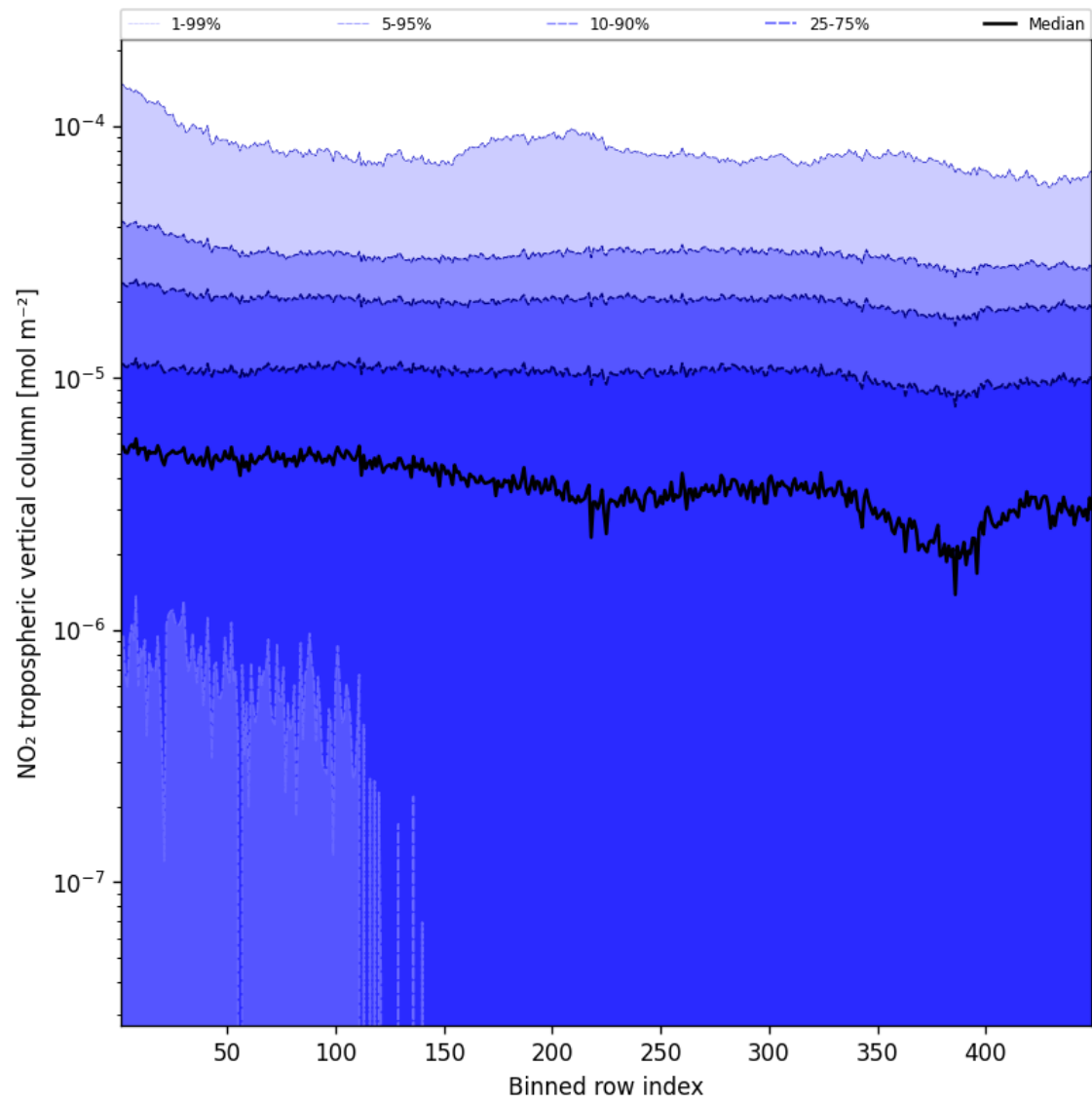
Figure 46: Along track statistics of “NO 2 tropospheric vertical column” for 2025-03-20 to 2025-03-21
