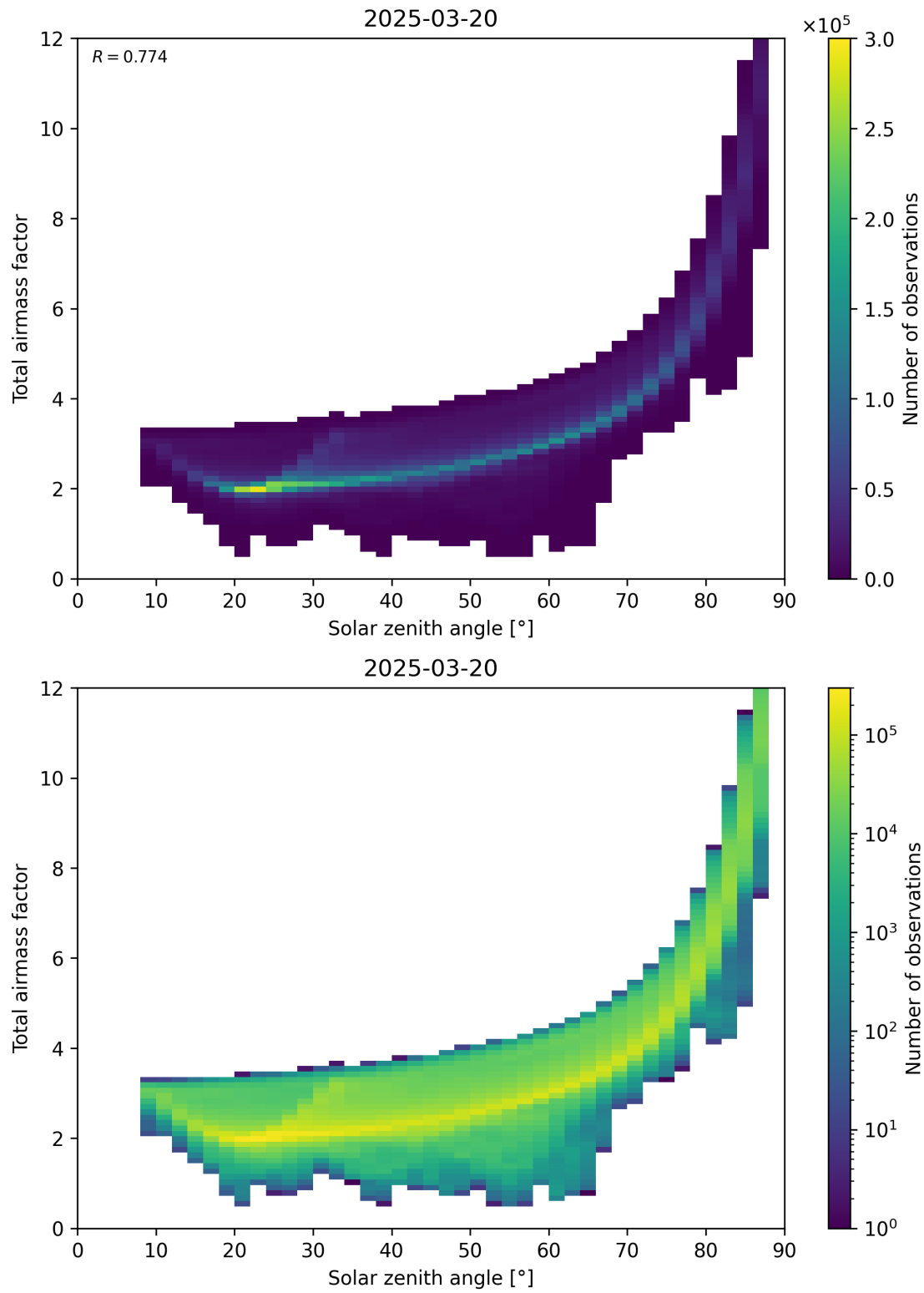
Figure 146: Scatter density plot of “Solar zenith angle” against “Total air mass factor” for 2025-03-20 to 2025-03-21.
