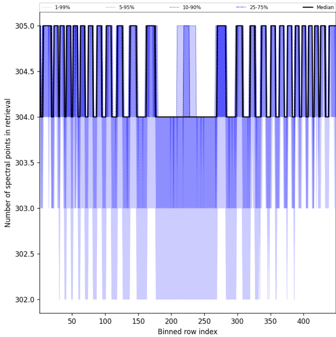
Figure 50: Along track statistics of “Number of spectral points in retrieval” for 2025-03-20 to 2025-03-21
