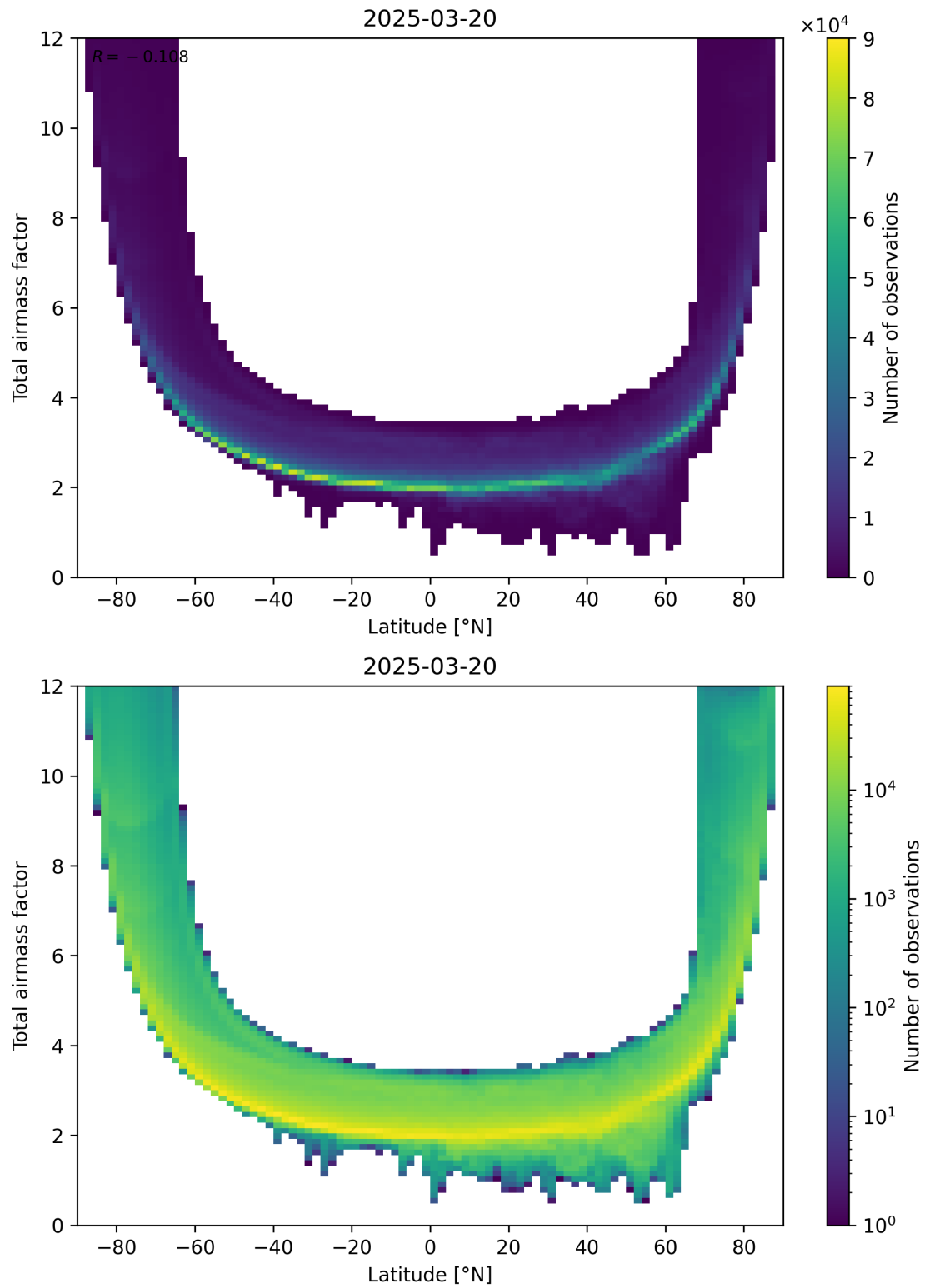
Figure 84: Scatter density plot of “Latitude” against “Total airmass factor” for 2025-03-20 to 2025-03-21.
