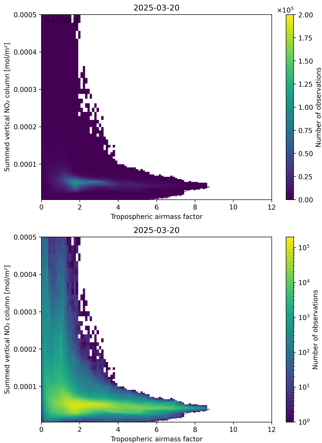
Figure 75: Scatter density plot of “Tropospheric air mass factor” against “Summed vertical NO 2 column” for 2025-03-20 to 2025-03-21.
