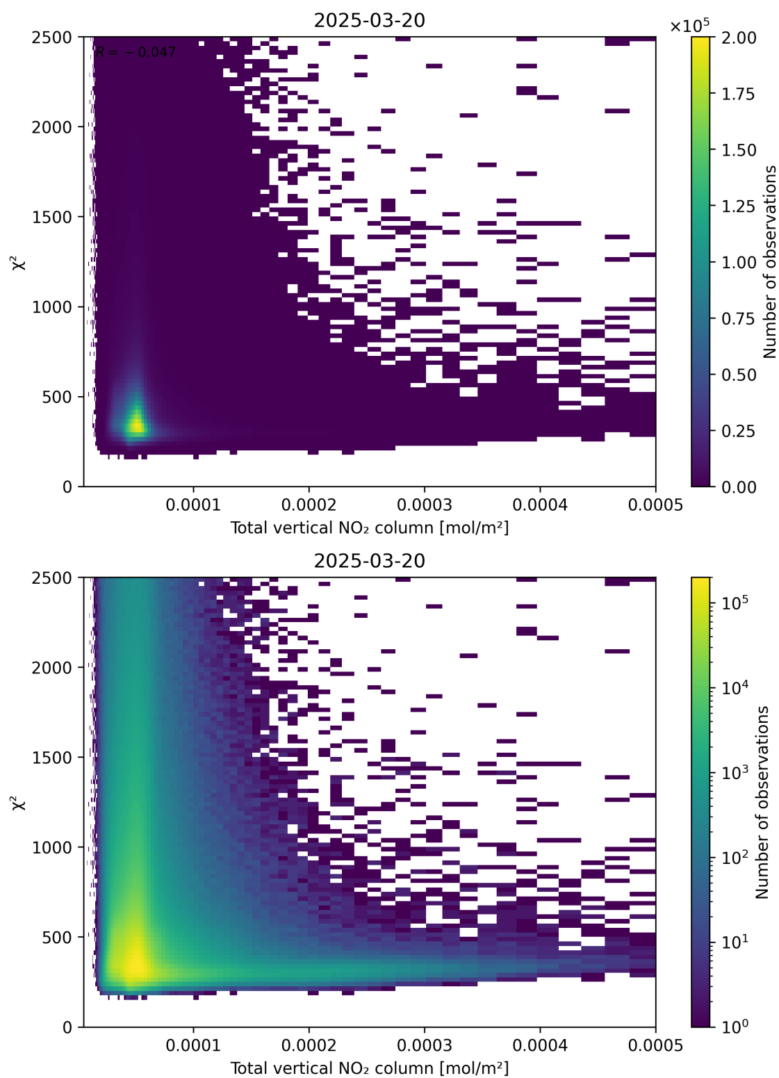
Figure 111: Scatter density plot of “Total vertical NO 2 column” against “ \chi^2 ” for 2025-03-20 to 2025-03-21.
