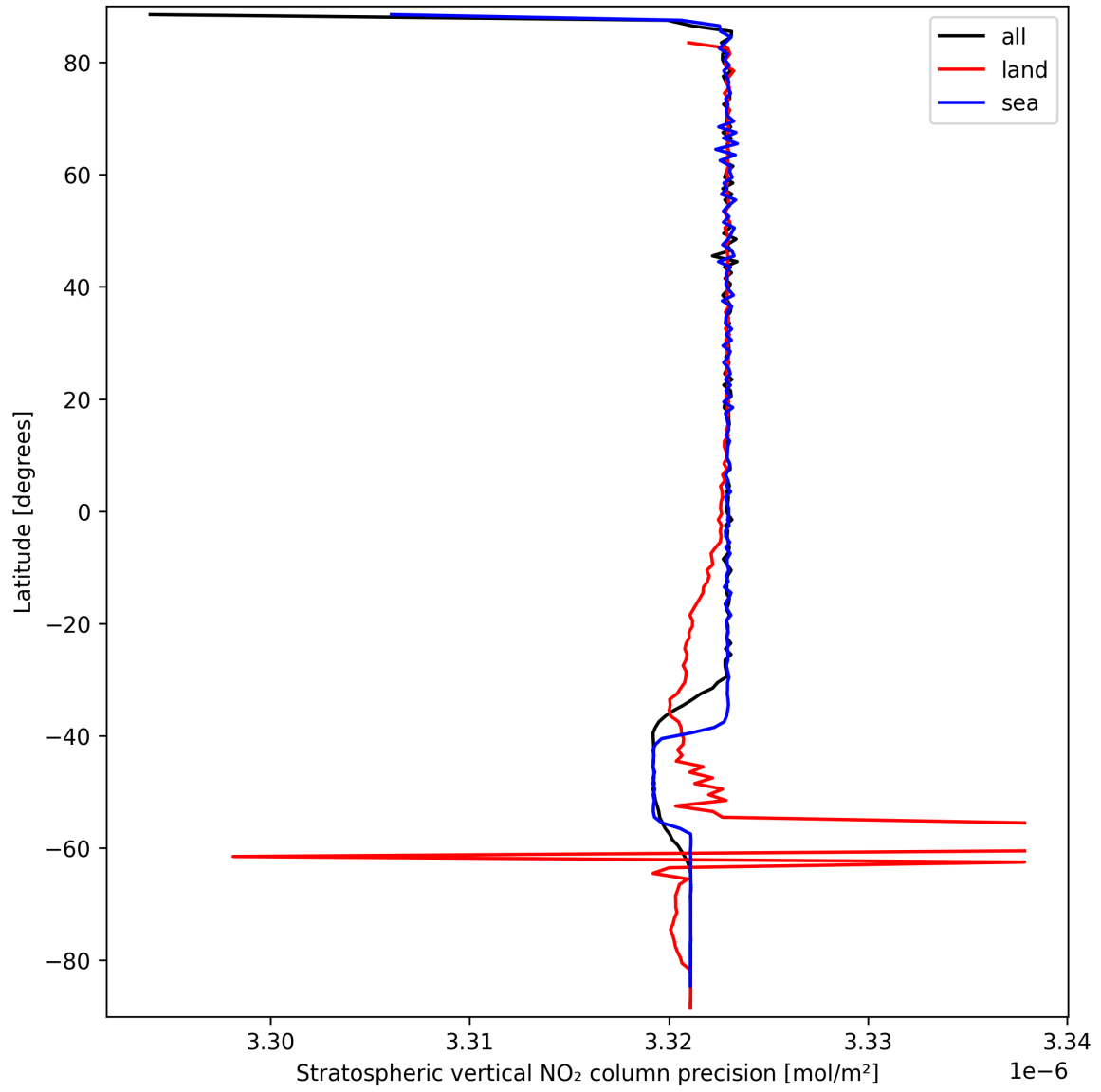
Figure 20: Zonal average of “Stratospheric vertical NO 2 column precision” for 2025-03-20 to 2025-03-21.
