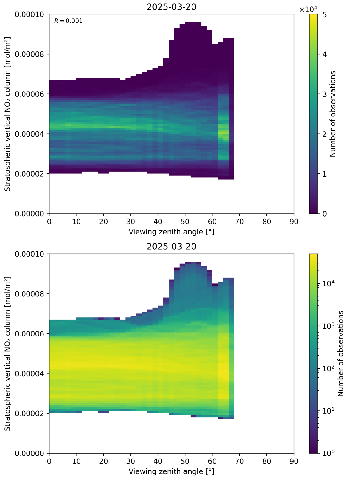
Figure 164: Scatter density plot of “Viewing zenith angle” against “Stratospheric vertical NO 2 column” for 2025-03-20 to 2025-03-21.
