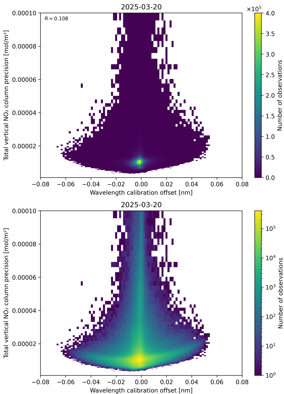
Figure 180: Scatter density plot of “Wavelength calibration offset” against “Total vertical NO 2 column precision” for 2025-03-20 to 2025-03-21.
