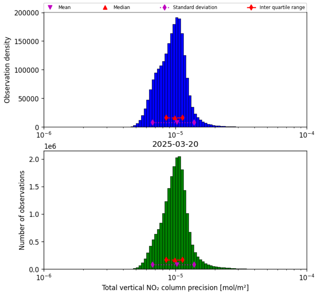
Figure 39: Histogram of "Total vertical NO 2 column precision" for 2025-03-20 to 2025-03-21
