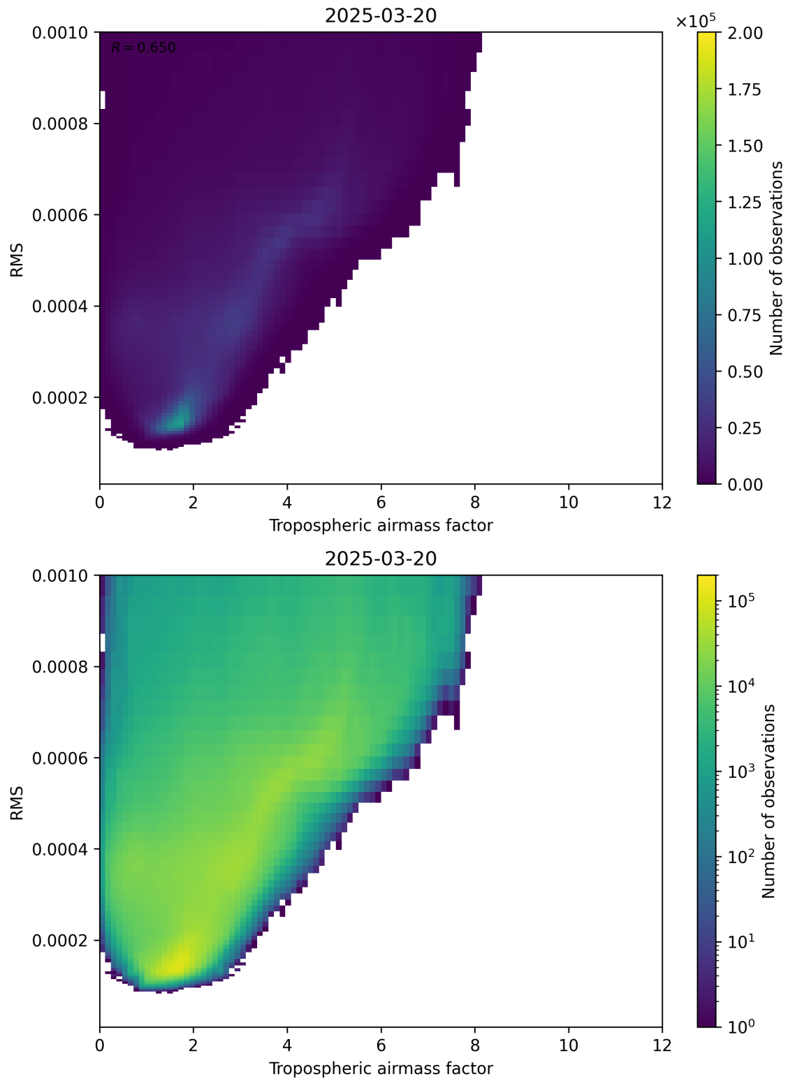
Figure 79: Scatter density plot of “Tropospheric airmass factor” against “RMS” for 2025-03-20 to 2025-03-21.
