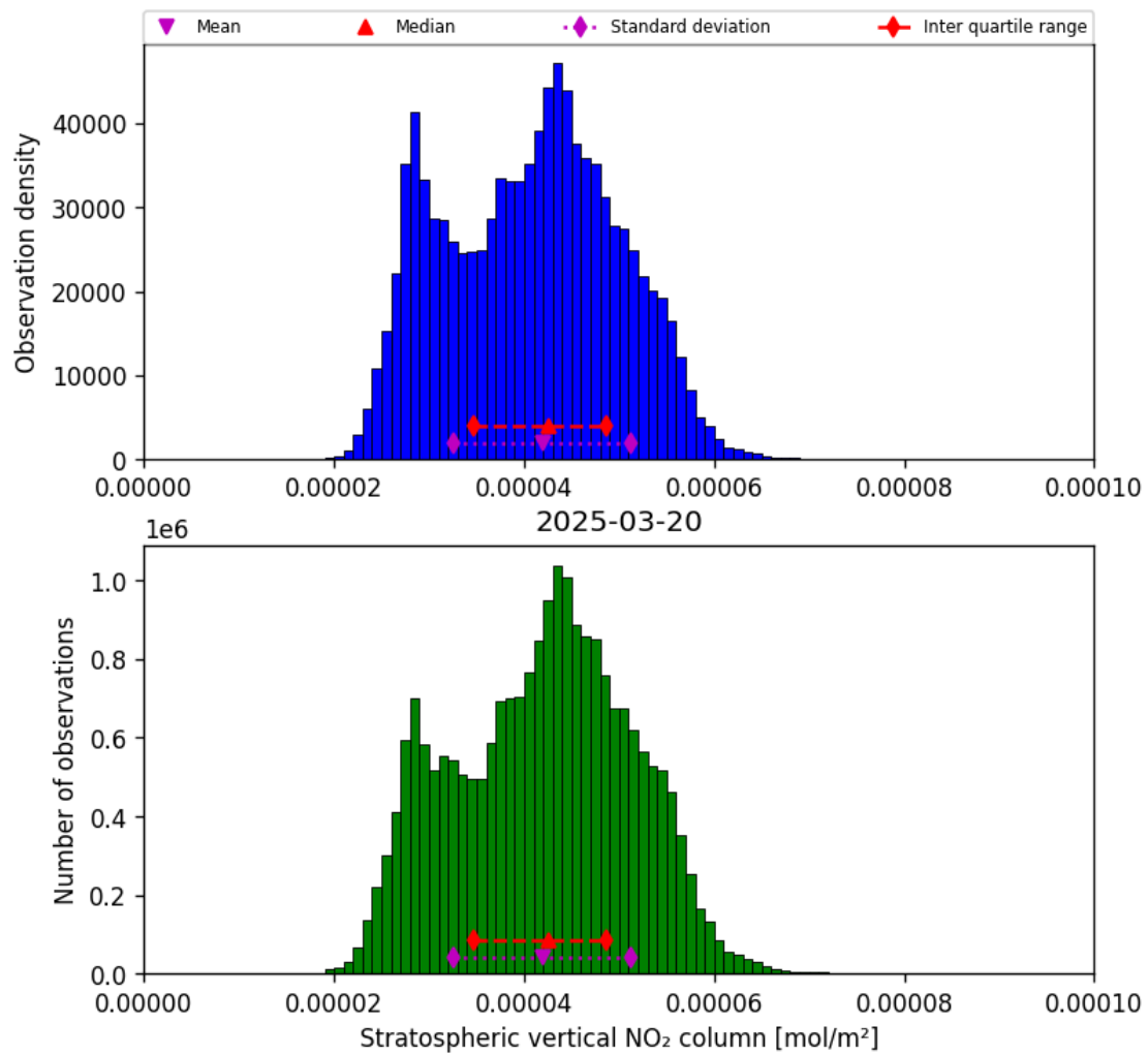
Figure 36: Histogram of “Stratospheric vertical NO 2 column” for 2025-03-20 to 2025-03-21
