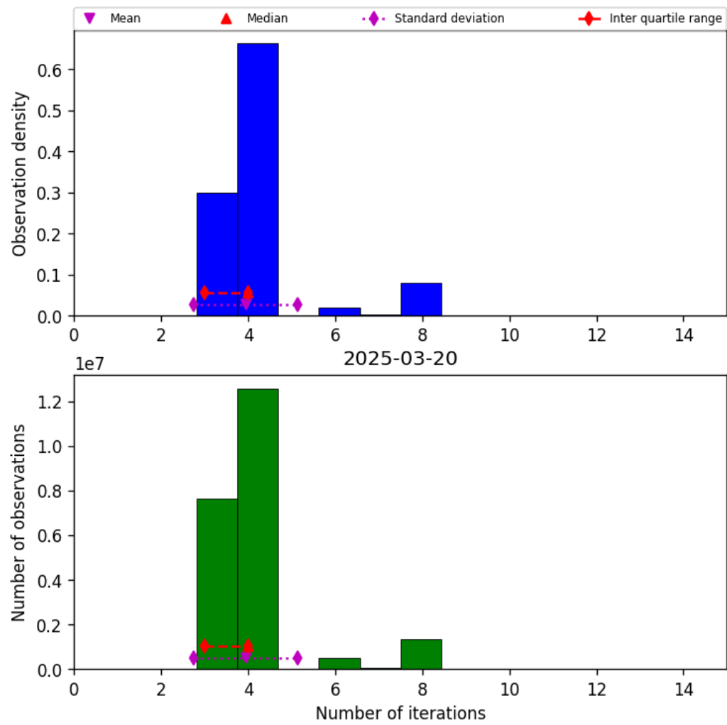
Figure 34: Histogram of “Number of iterations” for 2025-03-20 to 2025-03-21
