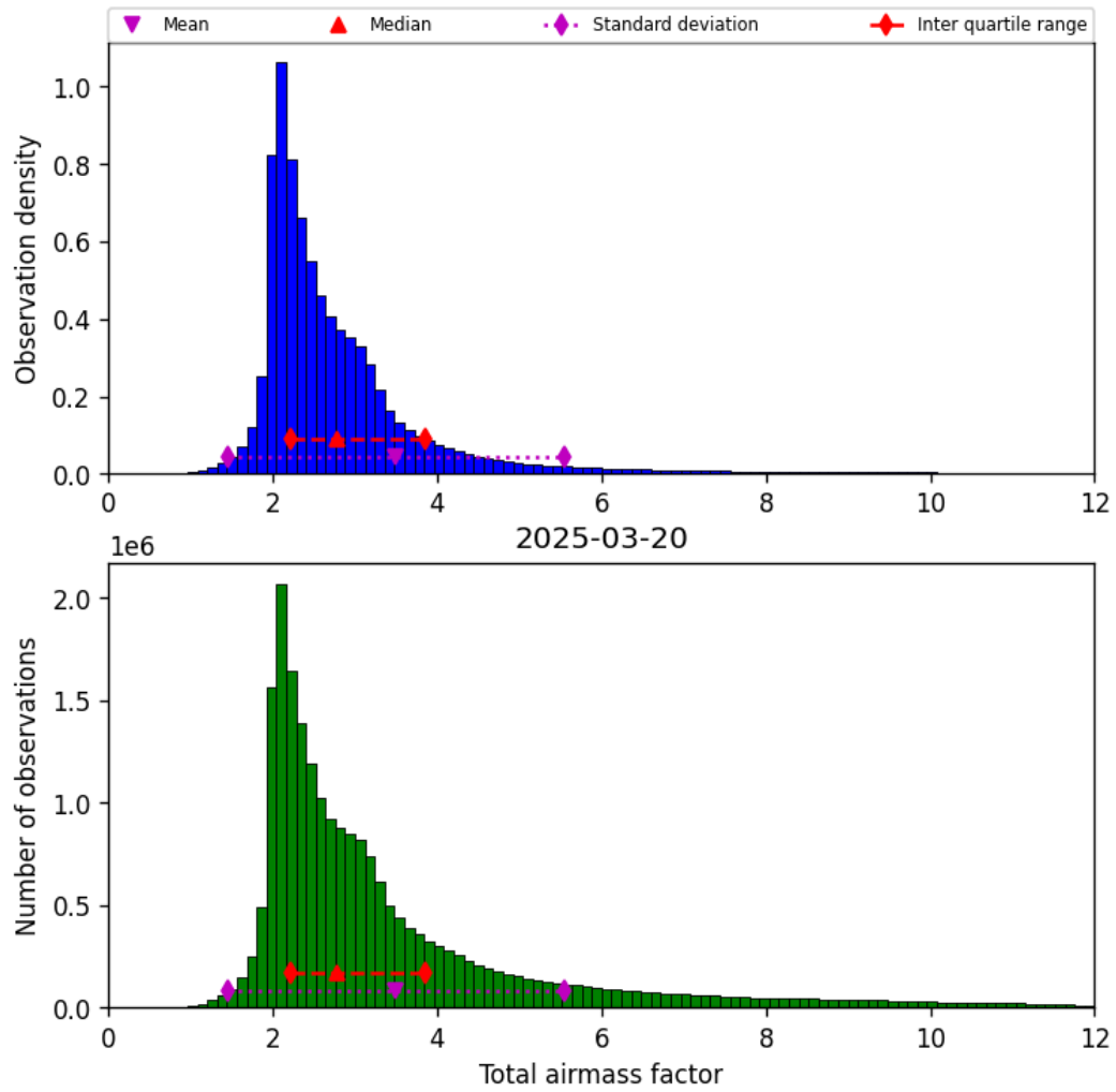
Figure 32: Histogram of “Total airmass factor” for 2025-03-20 to 2025-03-21
