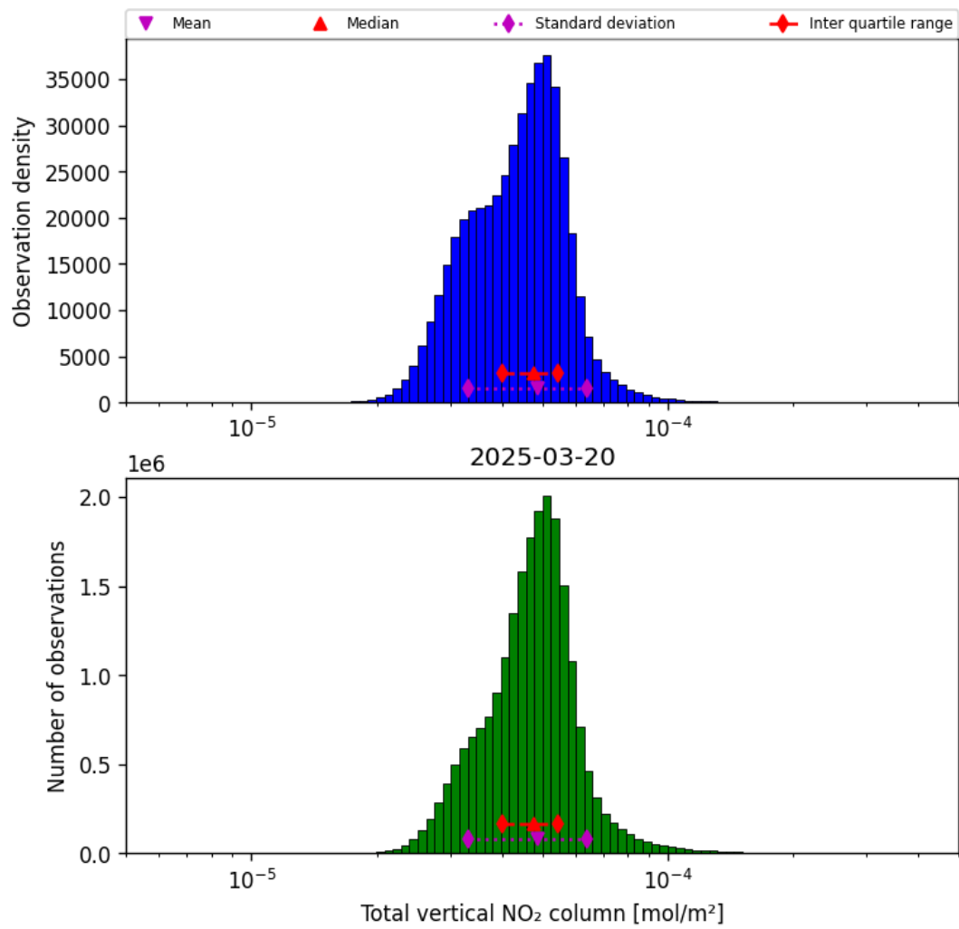
Figure 38: Histogram of “Total vertical NO 2 column” for 2025-03-20 to 2025-03-21
