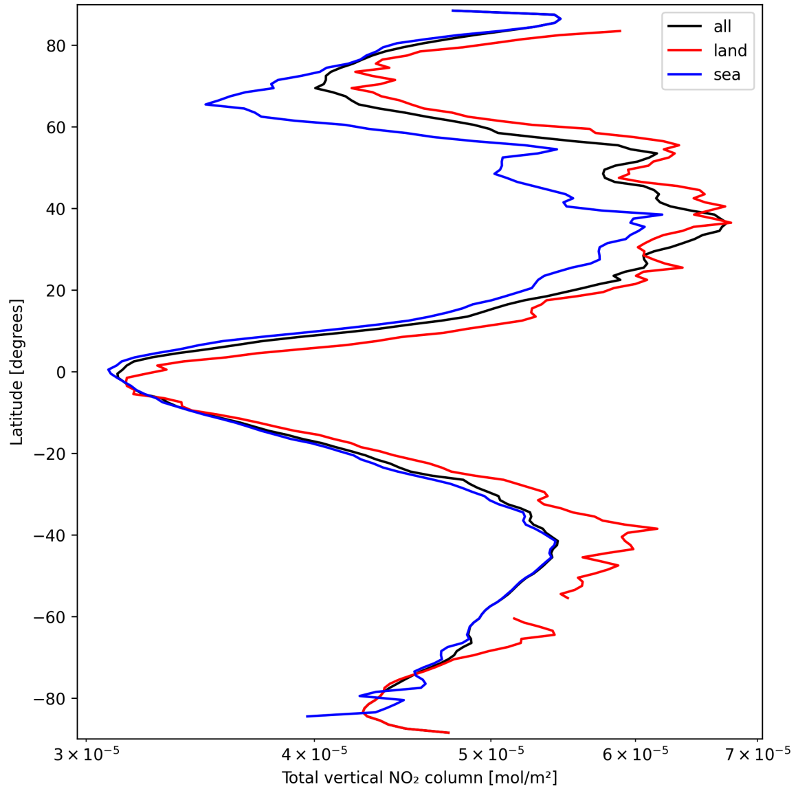
Figure 21: Zonal average of “Total vertical NO 2 column” for 2025-03-20 to 2025-03-21.
