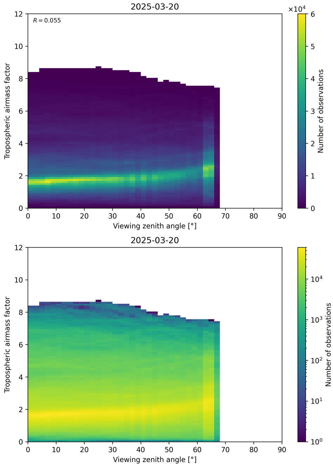
Figure 161: Scatter density plot of “Viewing zenith angle” against “Tropospheric airmass factor” for 2025-03-20 to 2025-03-21.
