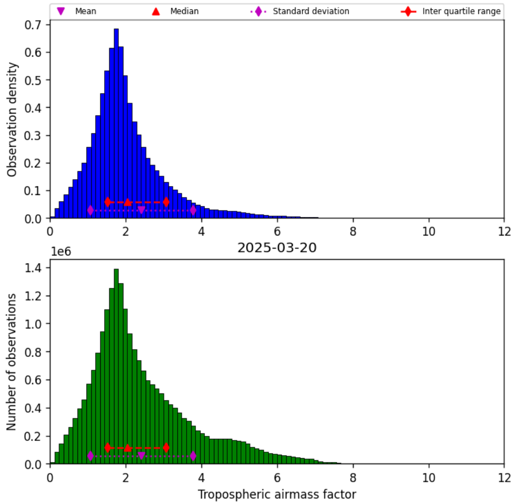
Figure 31: Histogram of “Tropospheric airmass factor” for 2025-03-20 to 2025-03-21
