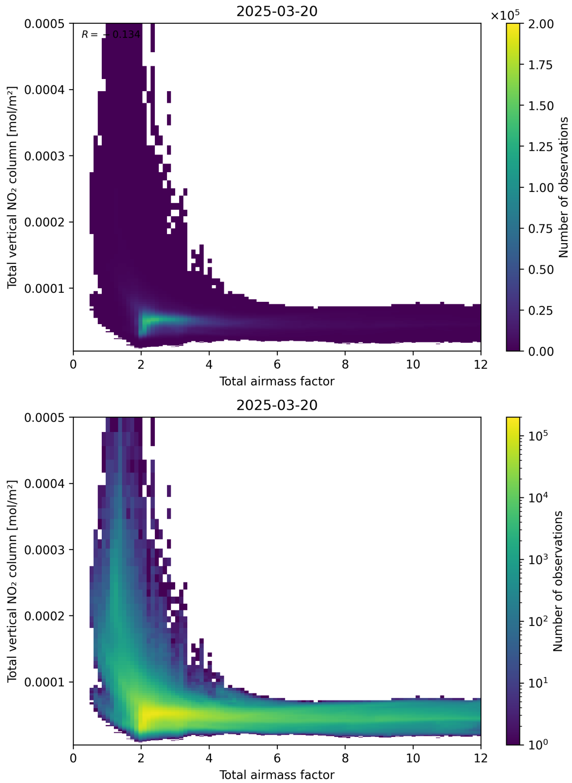
Figure 67: Scatter density plot of “Total airmass factor” against “Total vertical NO 2 column” for 2025-03-20 to 2025-03-21.
