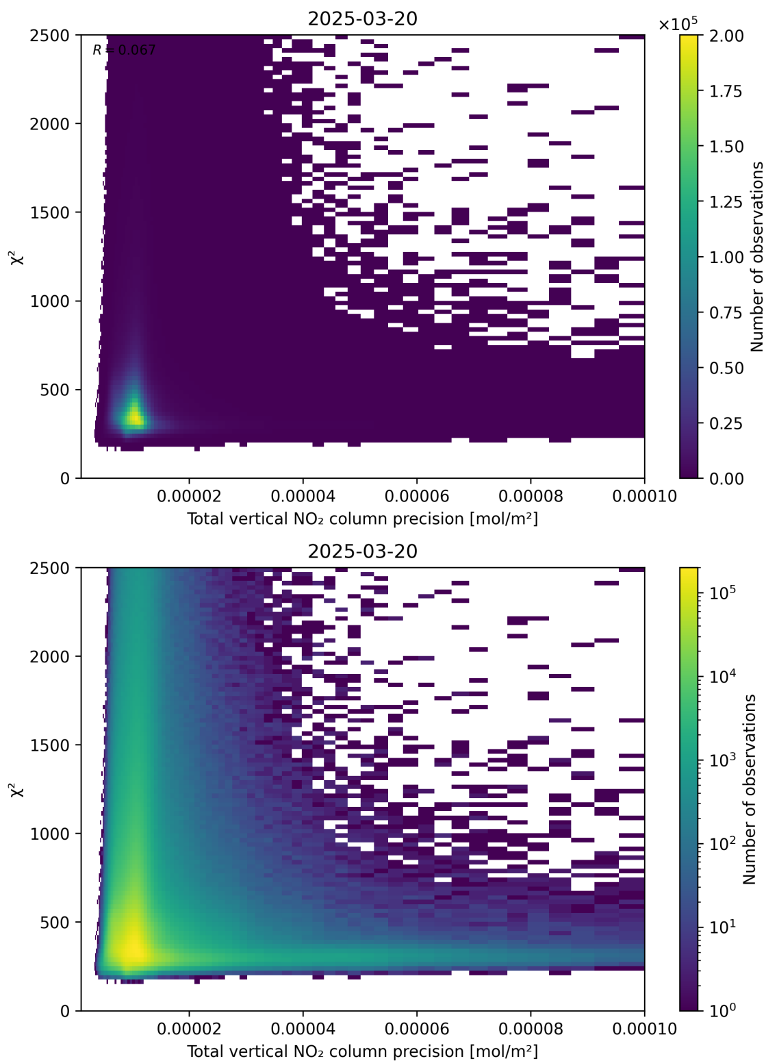
Figure 116: Scatter density plot of “Total vertical NO 2 column precision” against “ \chi^2 ” for 2025-03-20 to 2025-03-21.
