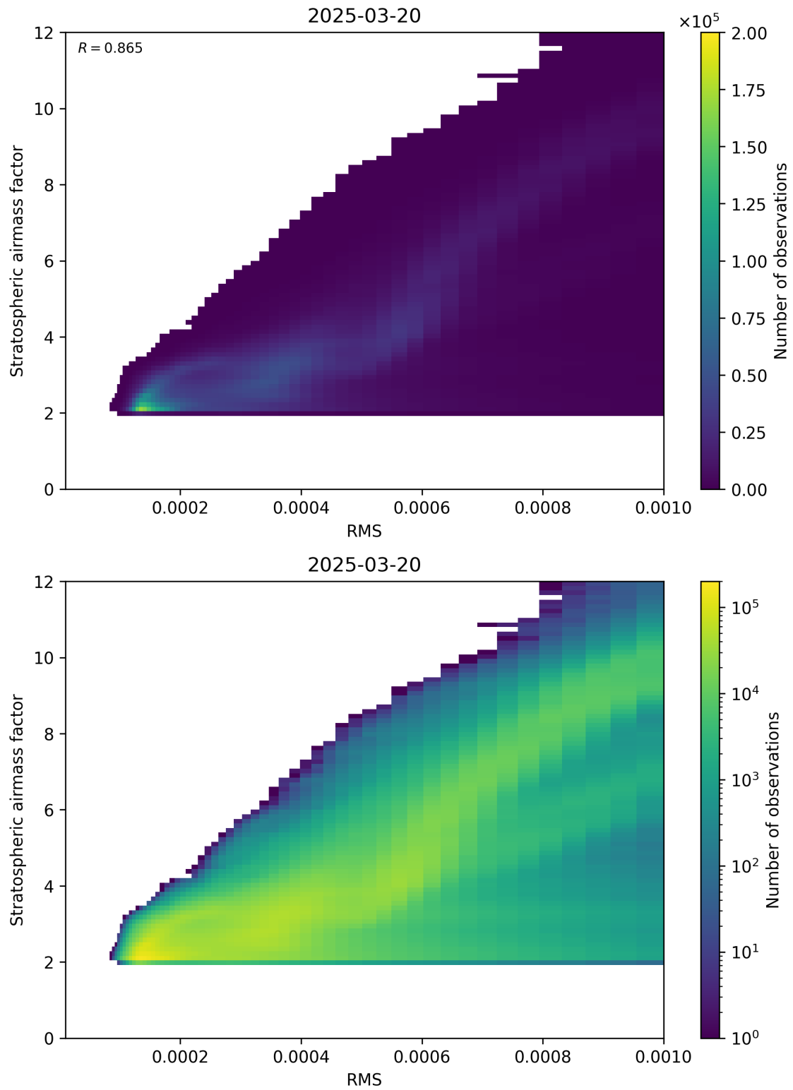
Figure 144: Scatter density plot of “RMS” against “Stratospheric airmass factor” for 2025-03-20 to 2025-03-21.
