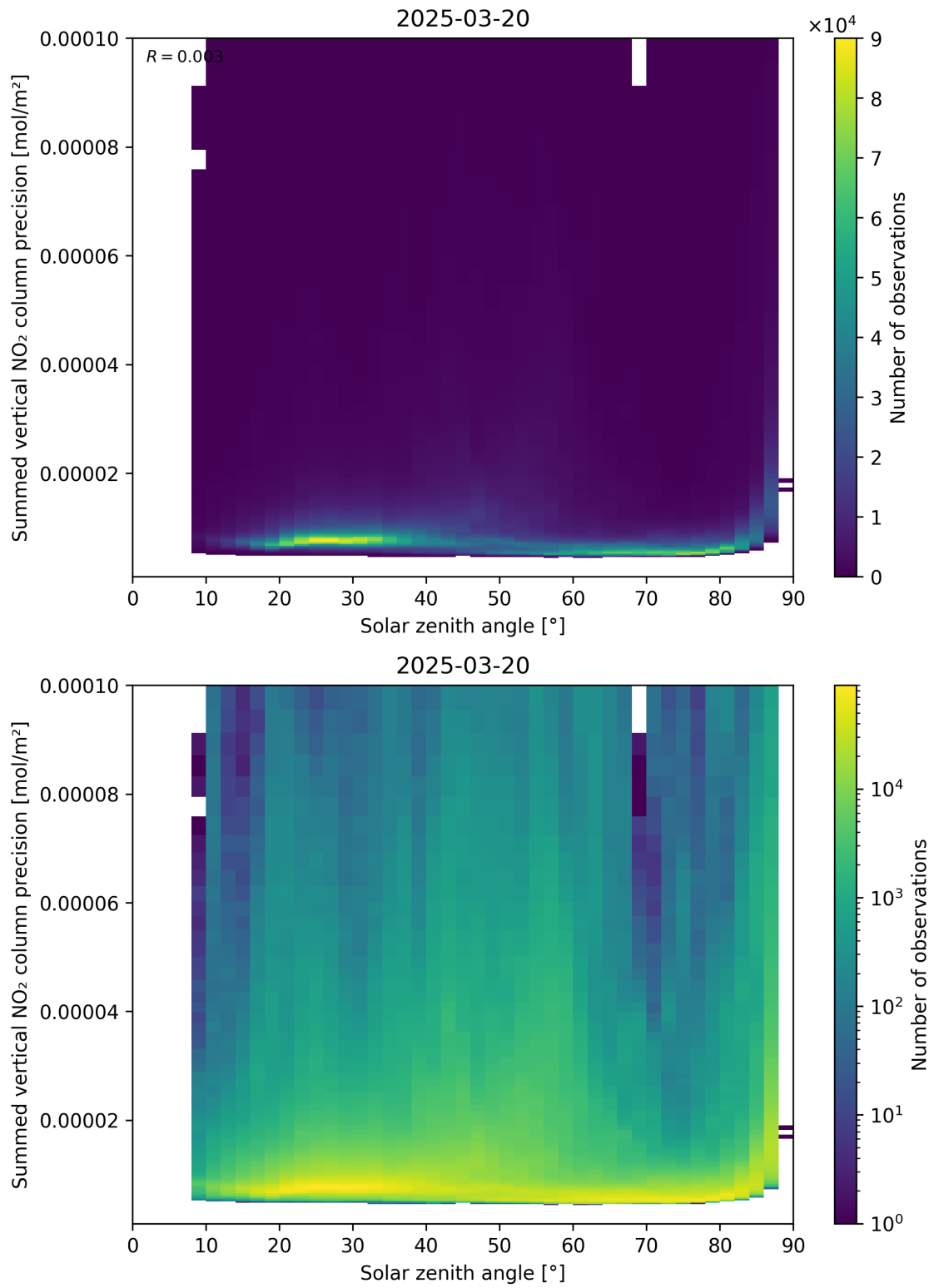
Figure 152: Scatter density plot of “Solar zenith angle” against “Summed vertical NO 2 column precision” for 2025-03-20 to 2025-03-21.
