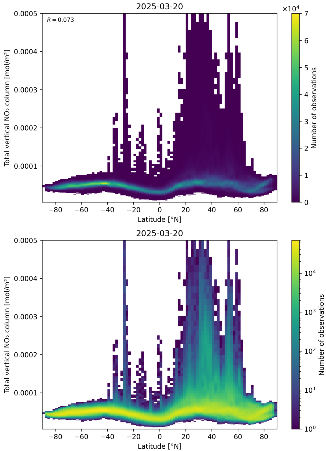
Figure 90: Scatter density plot of “Latitude” against “Total vertical NO 2 column” for 2025-03-20 to 2025-03-21.
