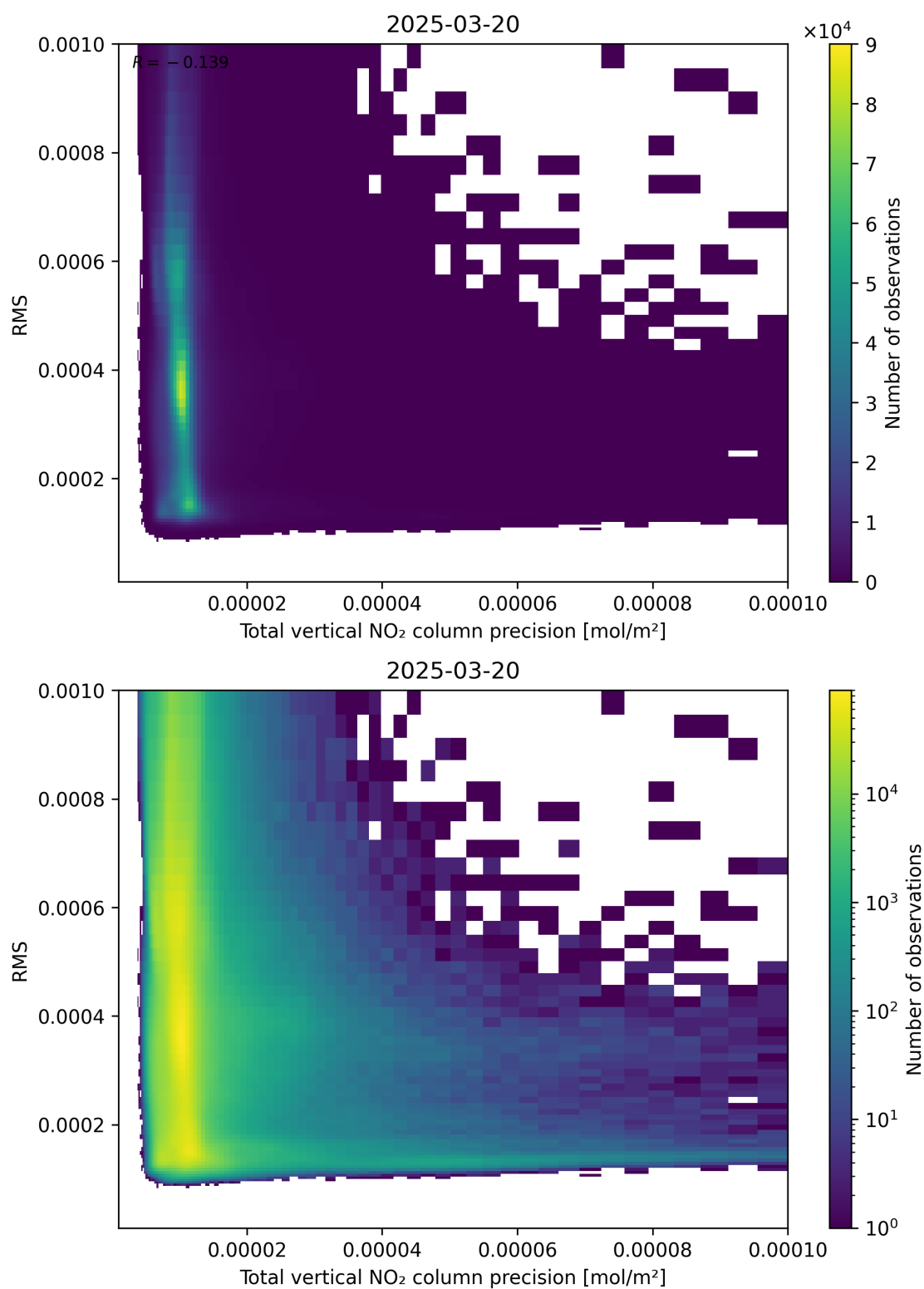
Figure 119: Scatter density plot of “Total vertical NO 2 column precision” against “RMS” for 2025-03-20 to 2025-03-21.
