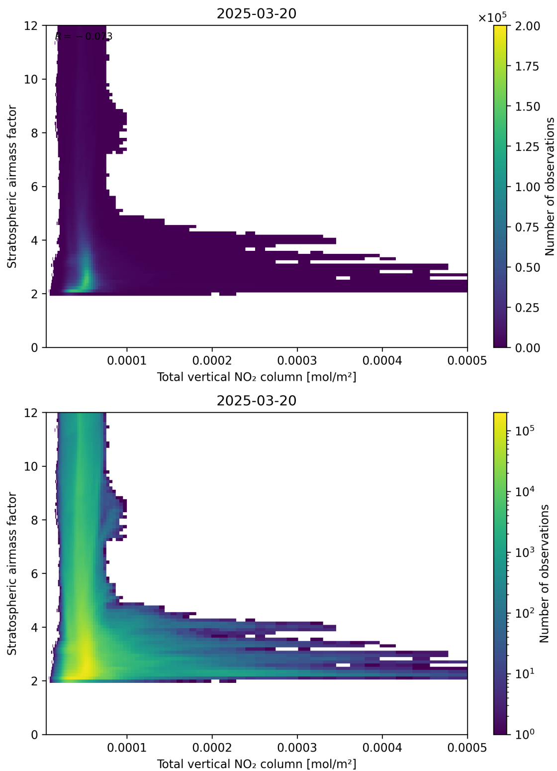
Figure 110: Scatter density plot of “Total vertical NO 2 column” against “Stratospheric airmass factor” for 2025-03-20 to 2025-03-21.
