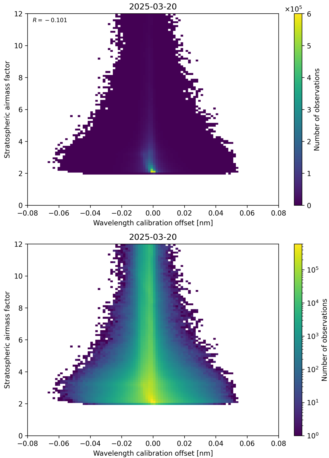
Figure 174: Scatter density plot of “Wavelength calibration offset” against “Stratospheric air mass factor” for 2025-03-20 to 2025-03-21.
