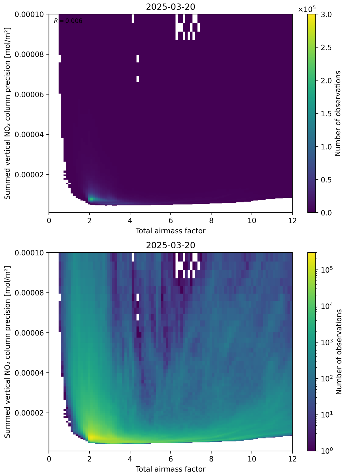
Figure 66: Scatter density plot of “Total airmass factor” against “Summed vertical NO 2 column precision” for 2025-03-20 to 2025-03-21.
