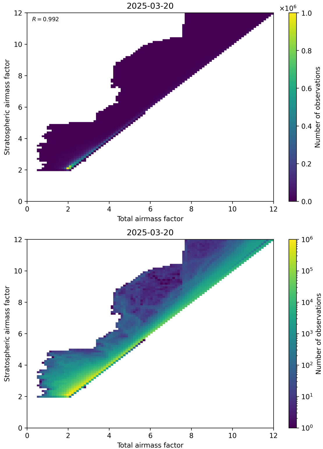
Figure 62: Scatter density plot of “Total airmass factor” against “Stratospheric airmass factor” for 2025-03-20 to 2025-03-21.
