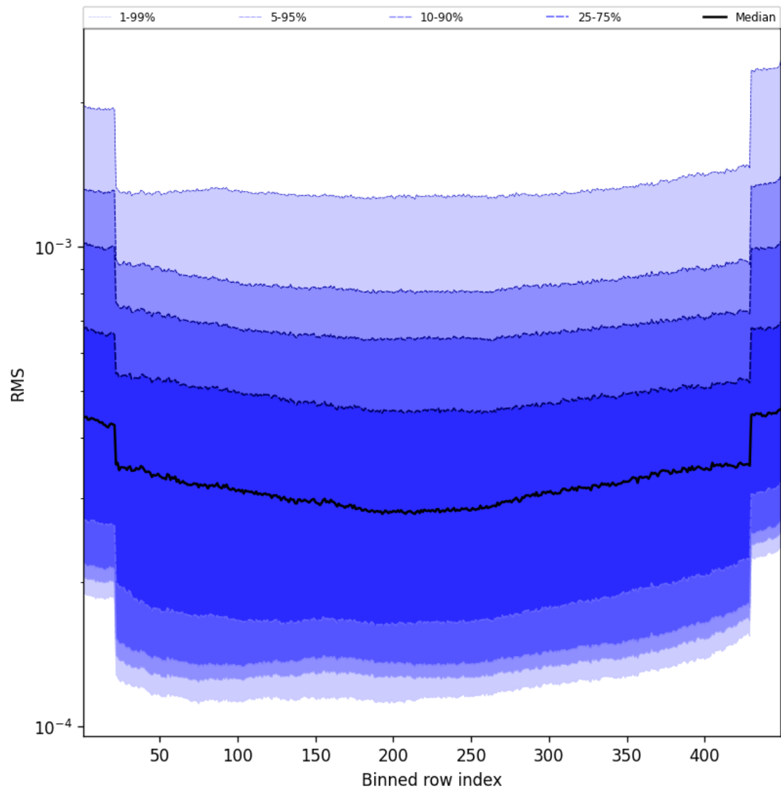
Figure 60: Along track statistics of "RMS" for 2025-03-20 to 2025-03-21
