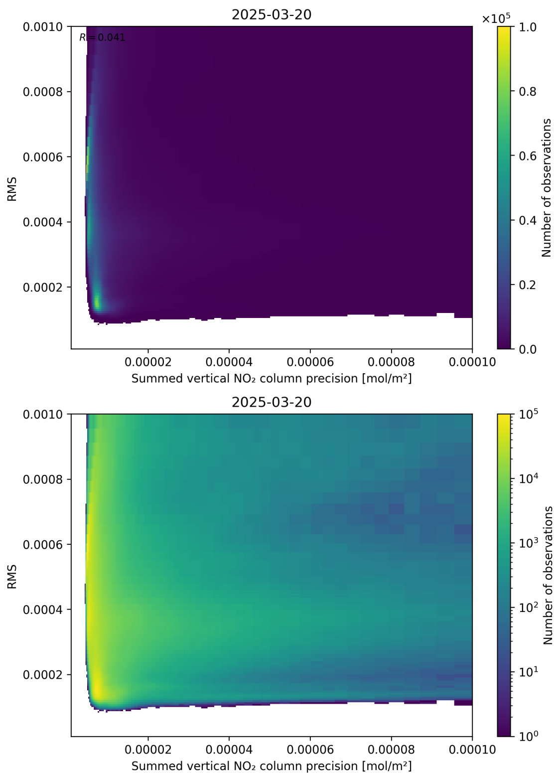
Figure 108: Scatter density plot of “Summed vertical NO 2 column precision” against “RMS” for 2025-03-20 to 2025-03-21.
