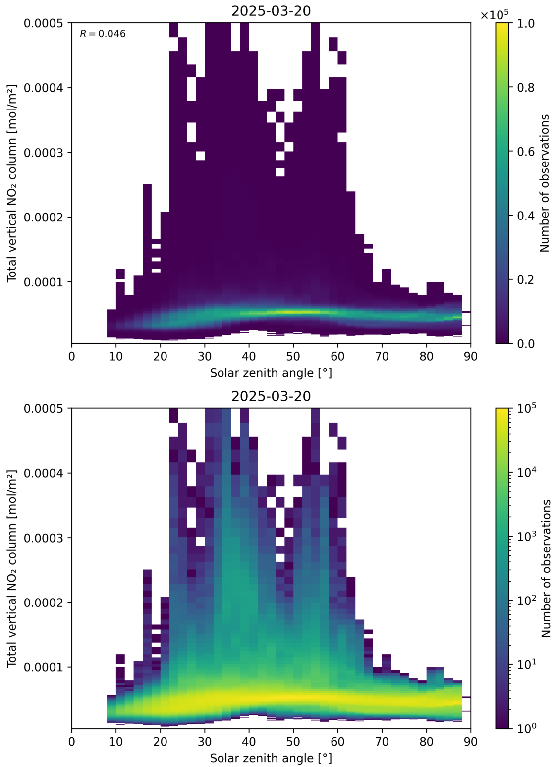
Figure 153: Scatter density plot of “Solar zenith angle” against “Total vertical NO 2 column” for 2025-03-20 to 2025-03-21.
