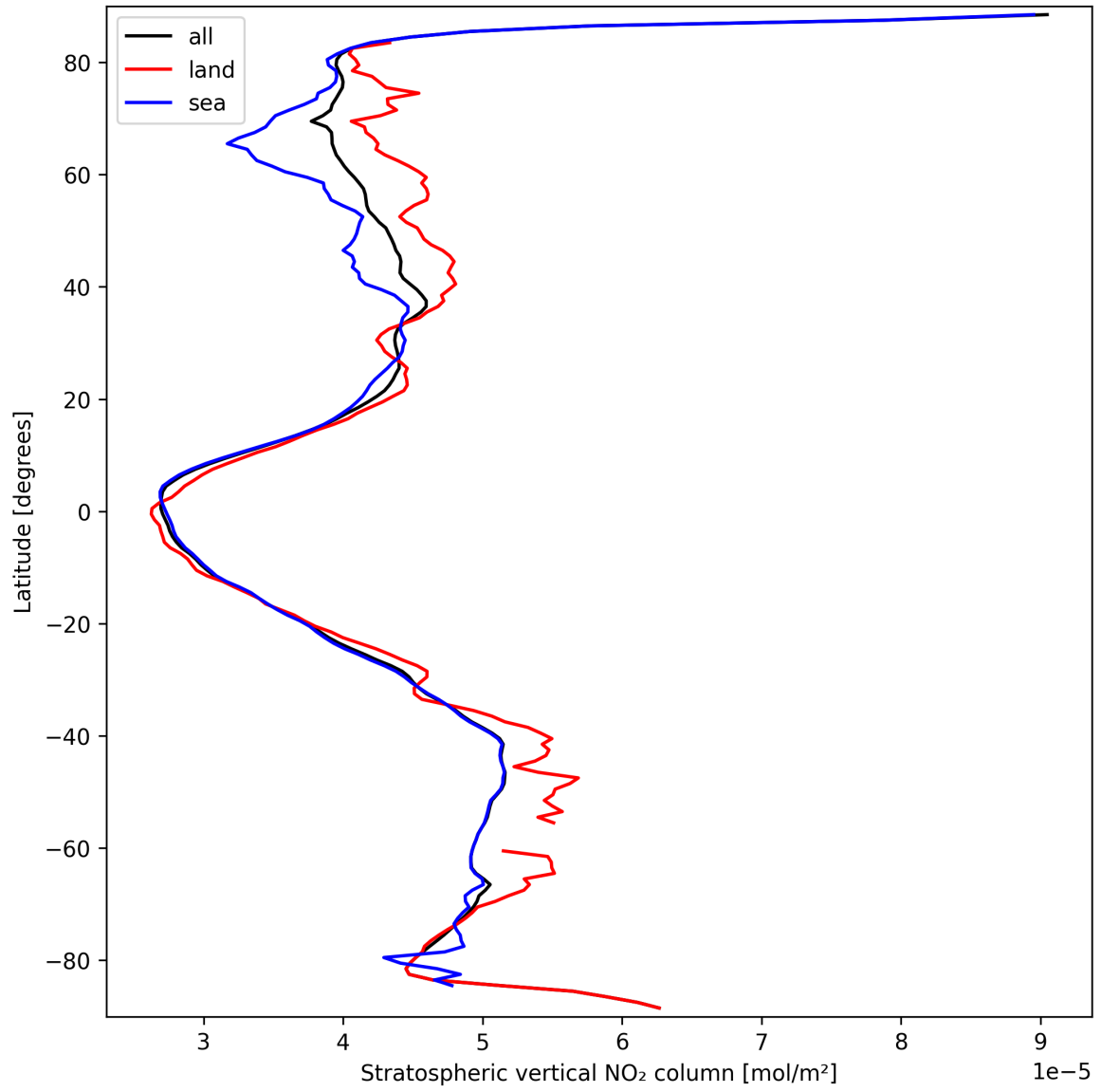
Figure 19: Zonal average of “Stratospheric vertical NO 2 column” for 2025-03-20 to 2025-03-21.
