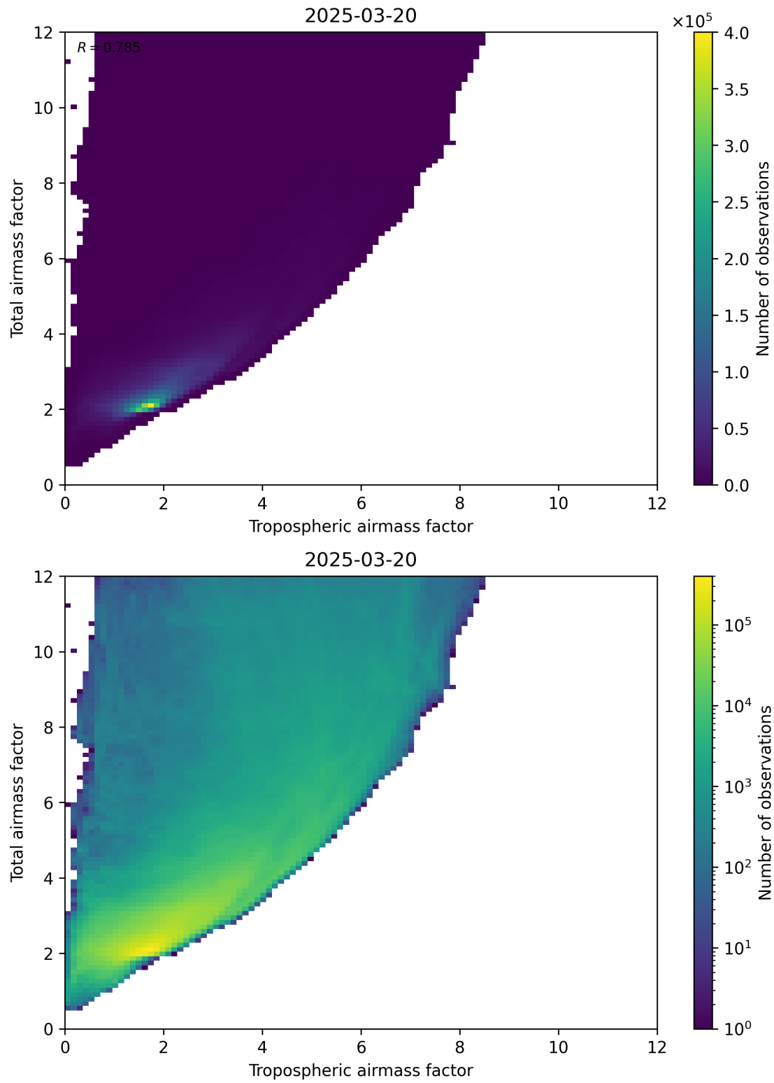
Figure 72: Scatter density plot of “Tropospheric airmass factor” against “Total airmass factor” for 2025-03-20 to 2025-03-21.
