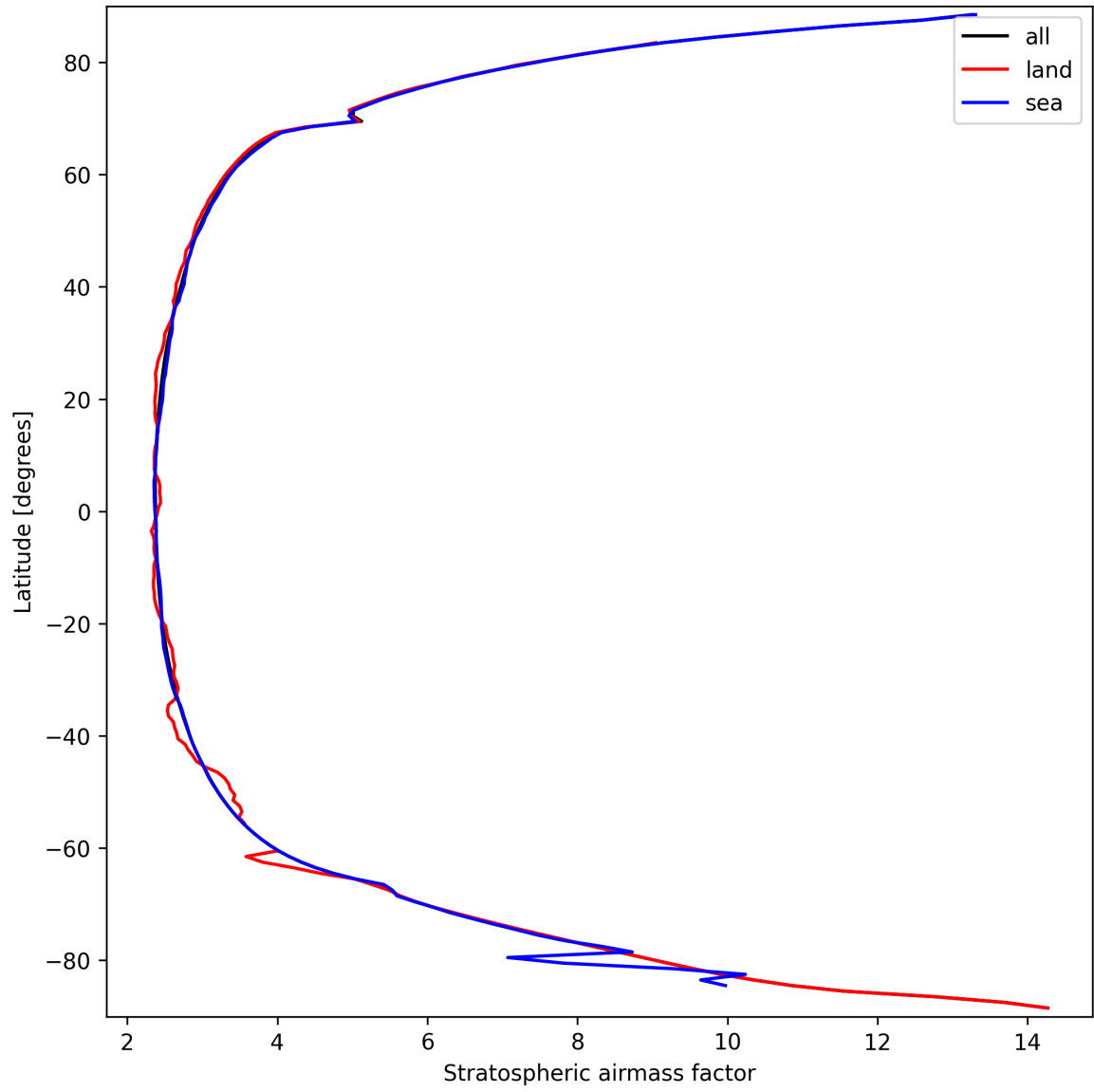
Figure 27: Zonal average of “Stratospheric airmass factor” for 2025-03-20 to 2025-03-21.
