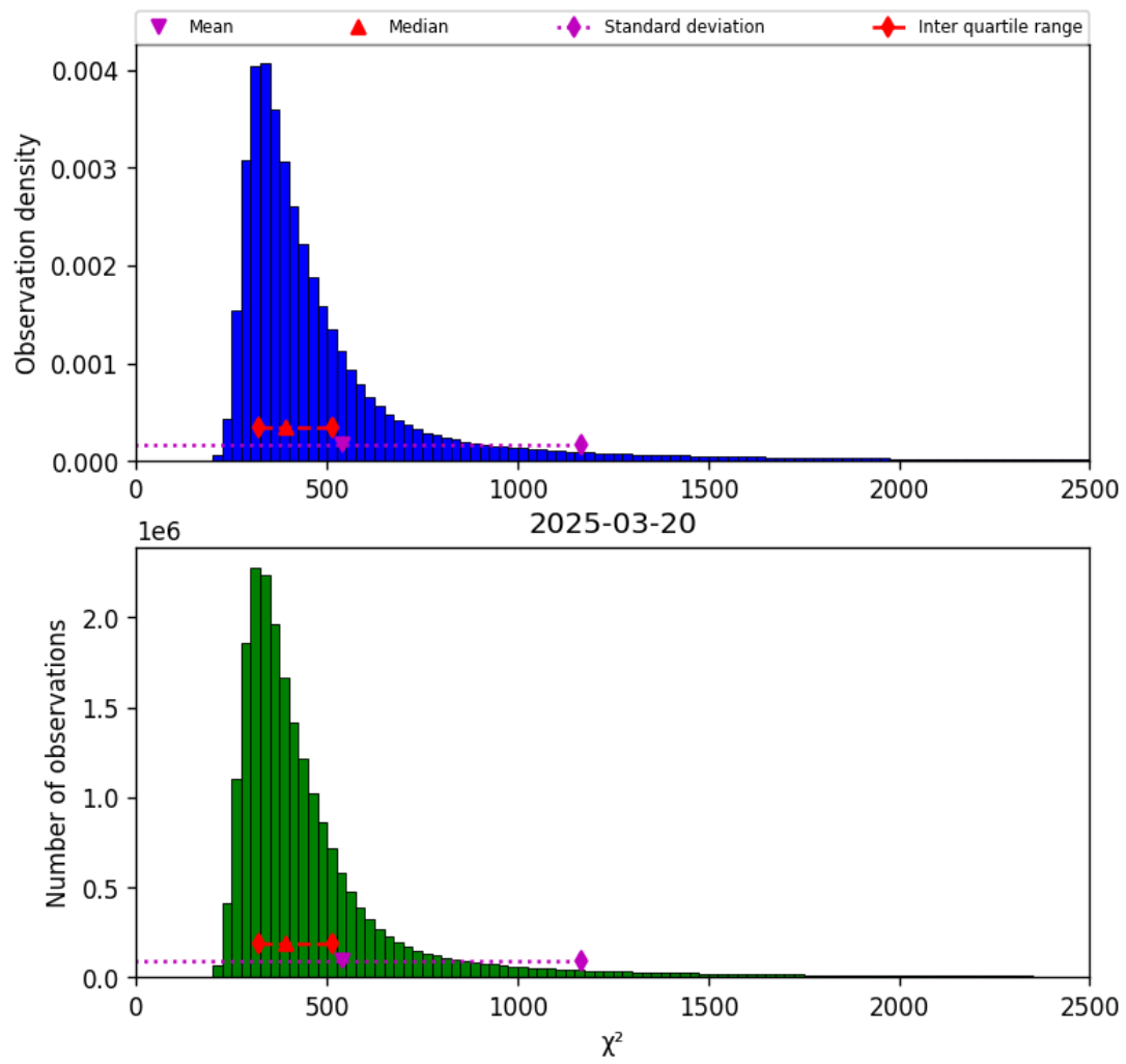
Figure 42: Histogram of “ \chi^2 ” for 2025-03-20 to 2025-03-21
