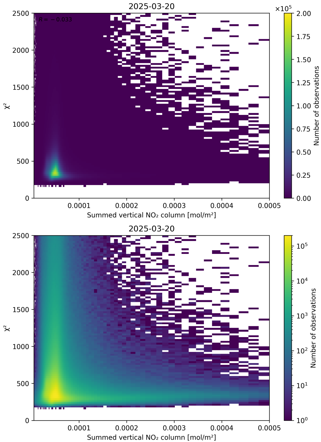
Figure 104: Scatter density plot of “Summed vertical NO 2 column” against “ \chi^2 ” for 2025-03-20 to 2025-03-21.
