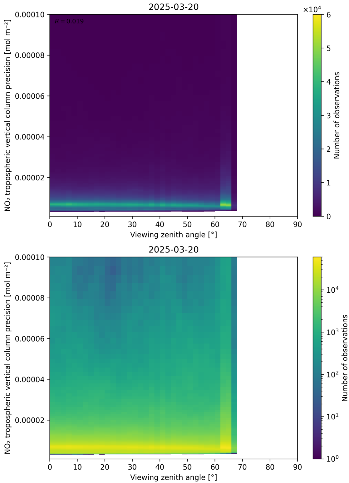
Figure 170: Scatter density plot of “Viewing zenith angle” against “NO 2 tropospheric vertical column precision” for 2025-03-20 to 2025-03-21.
