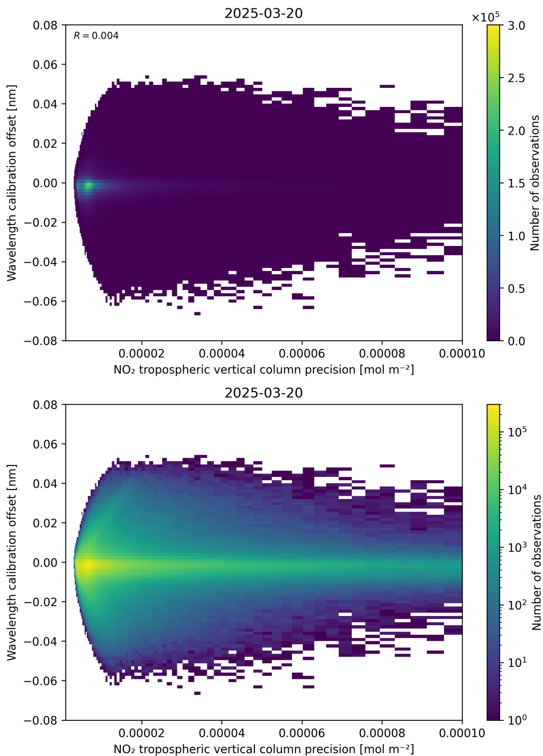
Figure 141: Scatter density plot of “NO 2 tropospheric vertical column precision” against “Wavelength calibration offset” for 2025-03-20 to 2025-03-21.
