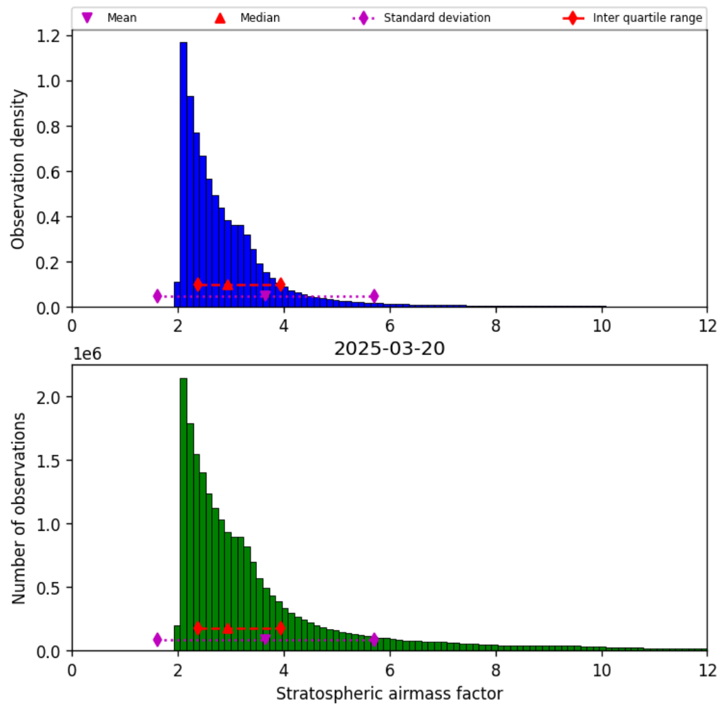
Figure 44: Histogram of “Stratospheric airmass factor” for 2025-03-20 to 2025-03-21
