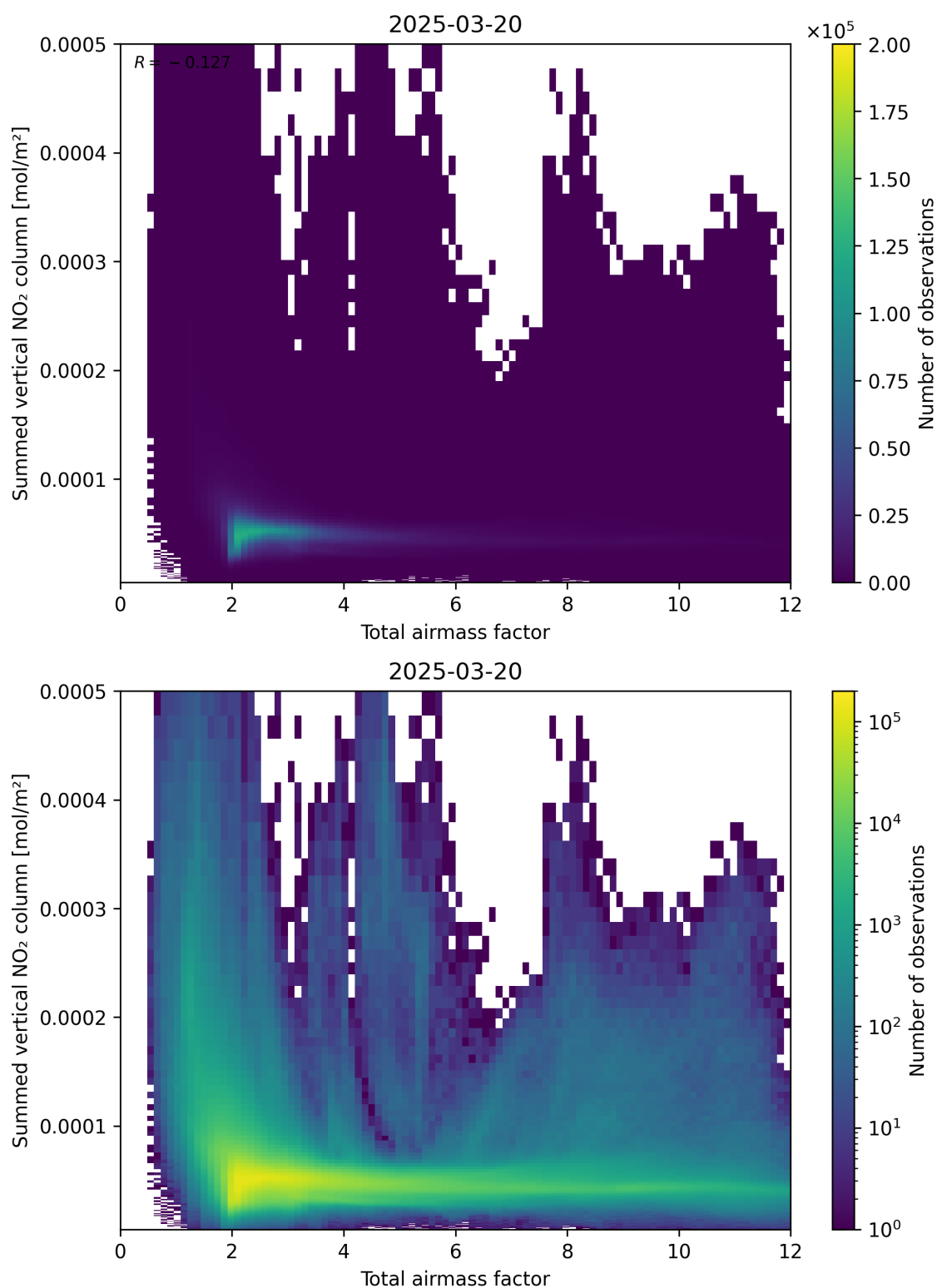
Figure 65: Scatter density plot of “Total airmass factor” against “Summed vertical NO 2 column” for 2025-03-20 to 2025-03-21.
