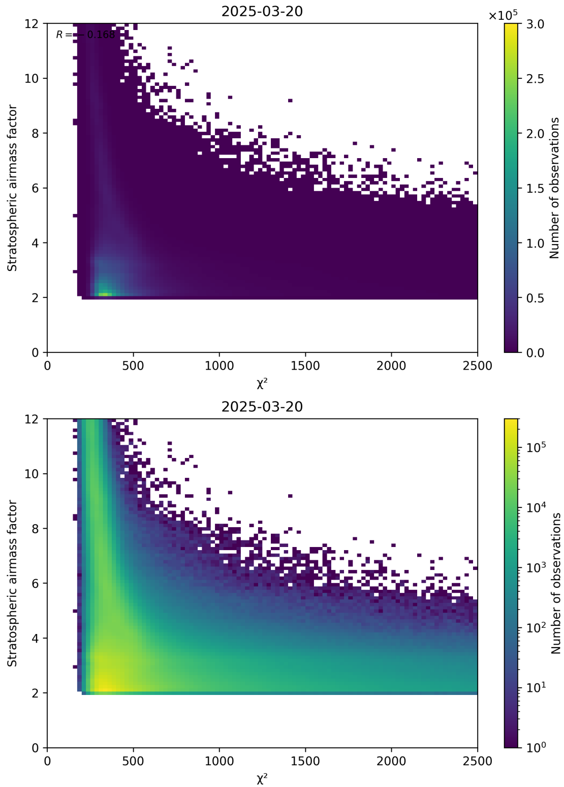
Figure 81: Scatter density plot of “ \chi^2 ” against “Stratospheric airmass factor” for 2025-03-20 to 2025-03-21.
