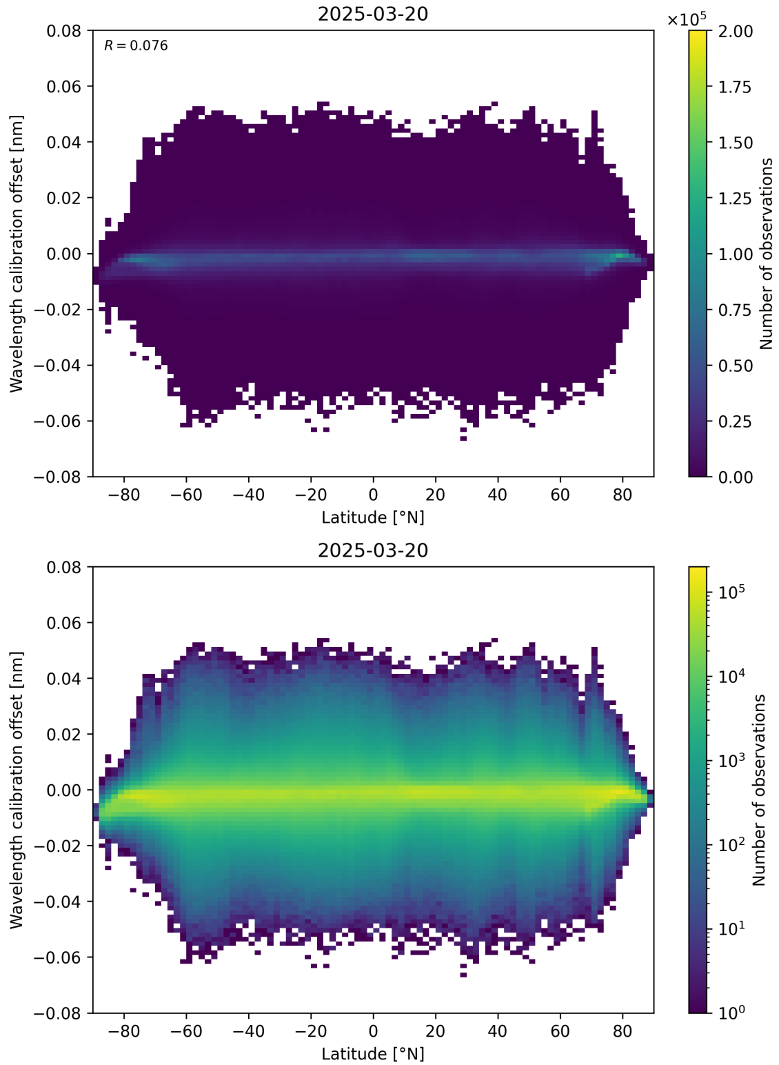
Figure 95: Scatter density plot of “Latitude” against “Wavelength calibration offset” for 2025-03-20 to 2025-03-21.
