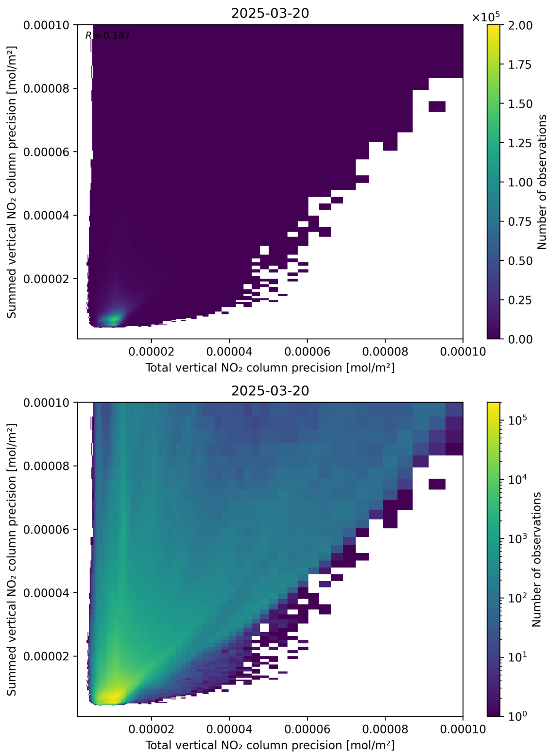
Figure 118: Scatter density plot of “Total vertical NO 2 column precision” against “Summed vertical NO 2 column precision” for 2025-03-20 to 2025-03-21.
