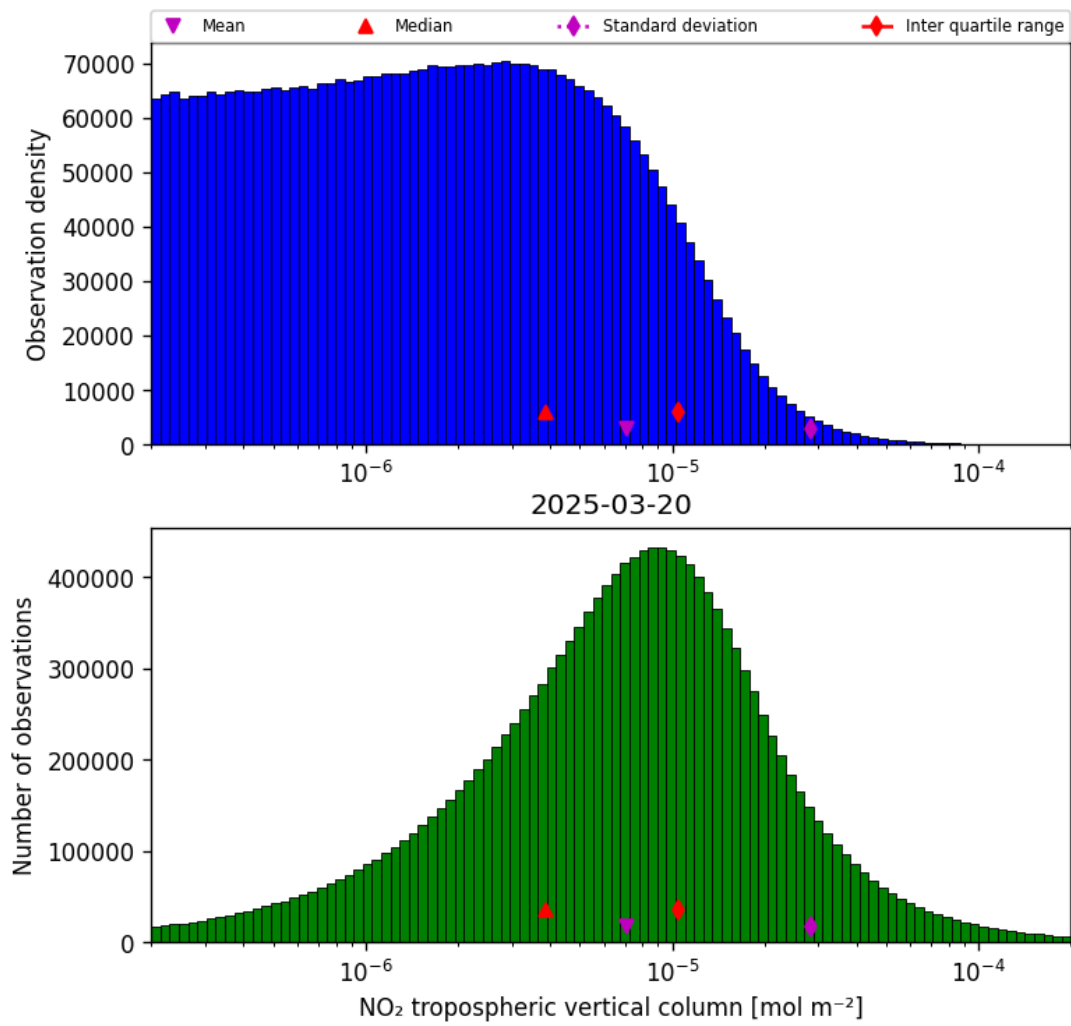
Figure 29: Histogram of “NO 2 tropospheric vertical column” for 2025-03-20 to 2025-03-21
