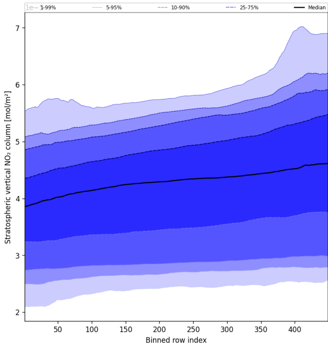
Figure 53: Along track statistics of “Stratospheric vertical NO 2 column” for 2025-03-20 to 2025-03-21
