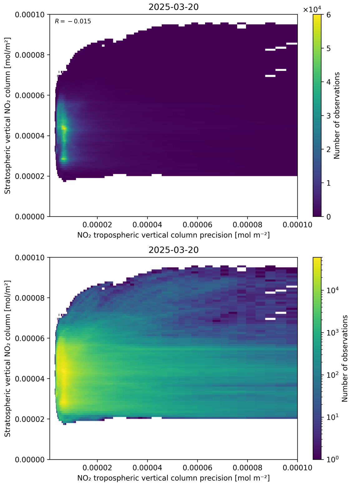
Figure 135: Scatter density plot of “NO 2 tropospheric vertical column precision” against “Stratospheric vertical NO 2 column” for 2025-03-20 to 2025-03-21.
