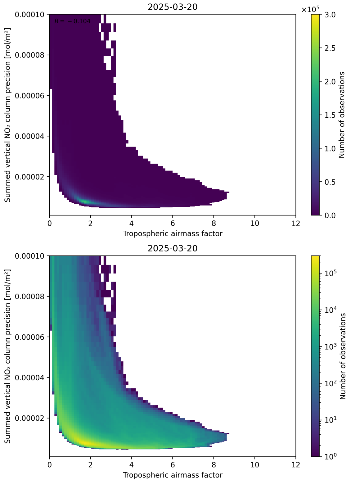
Figure 76: Scatter density plot of “Tropospheric air mass factor” against “Summed vertical NO 2 column precision” for 2025-03-20 to 2025-03-21.
