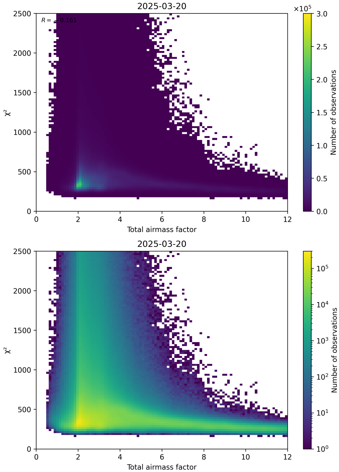
Figure 63: Scatter density plot of “Total airmass factor” against “ \chi^2 ” for 2025-03-20 to 2025-03-21.
