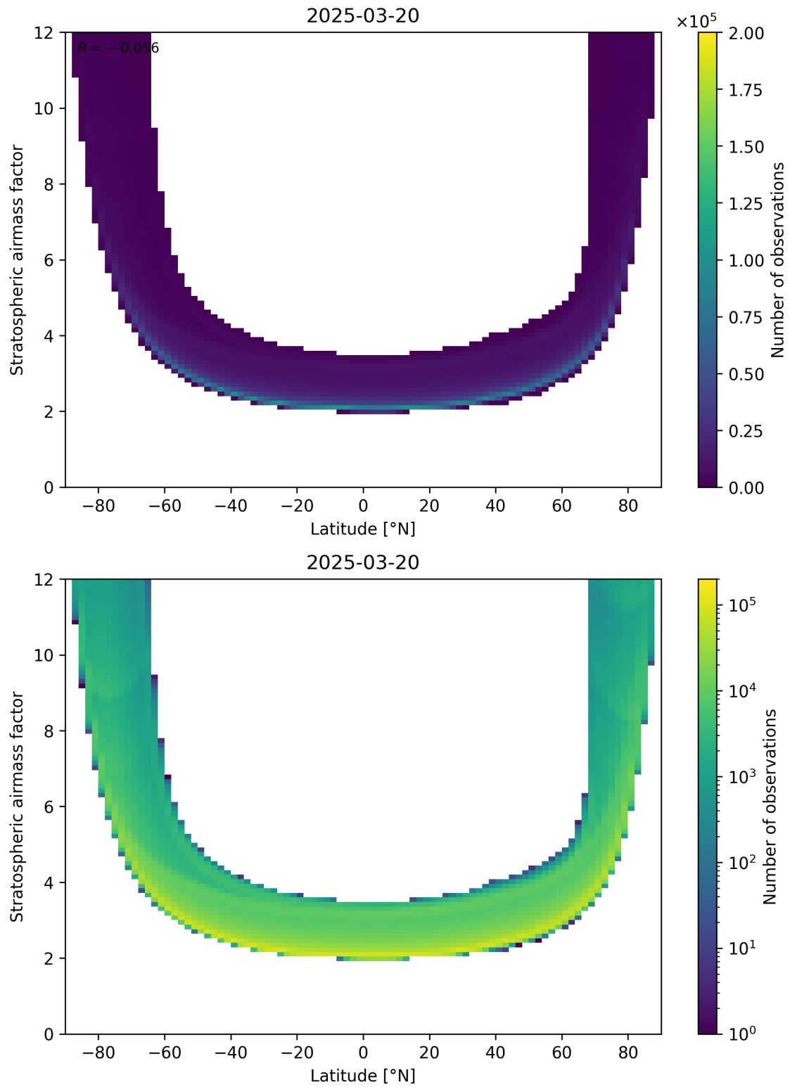
Figure 83: Scatter density plot of “Latitude” against “Stratospheric air mass factor” for 2025-03-20 to 2025-03-21.
