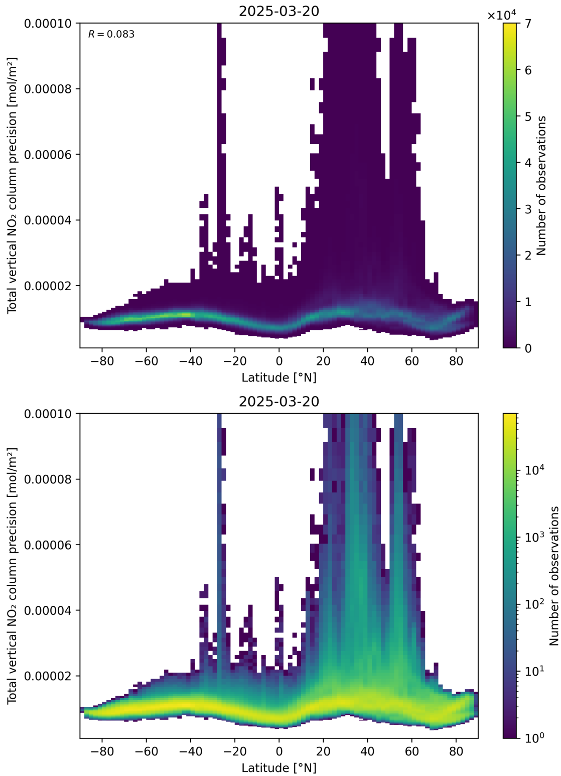
Figure 91: Scatter density plot of “Latitude” against “Total vertical NO 2 column precision” for 2025-03-20 to 2025-03-21.
