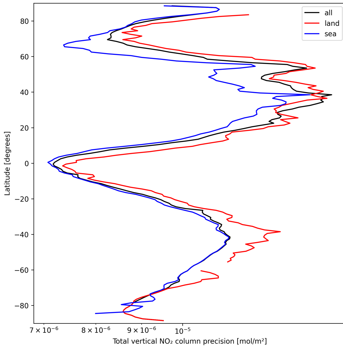
Figure 22: Zonal average of “Total vertical NO 2 column precision” for 2025-03-20 to 2025-03-21.
