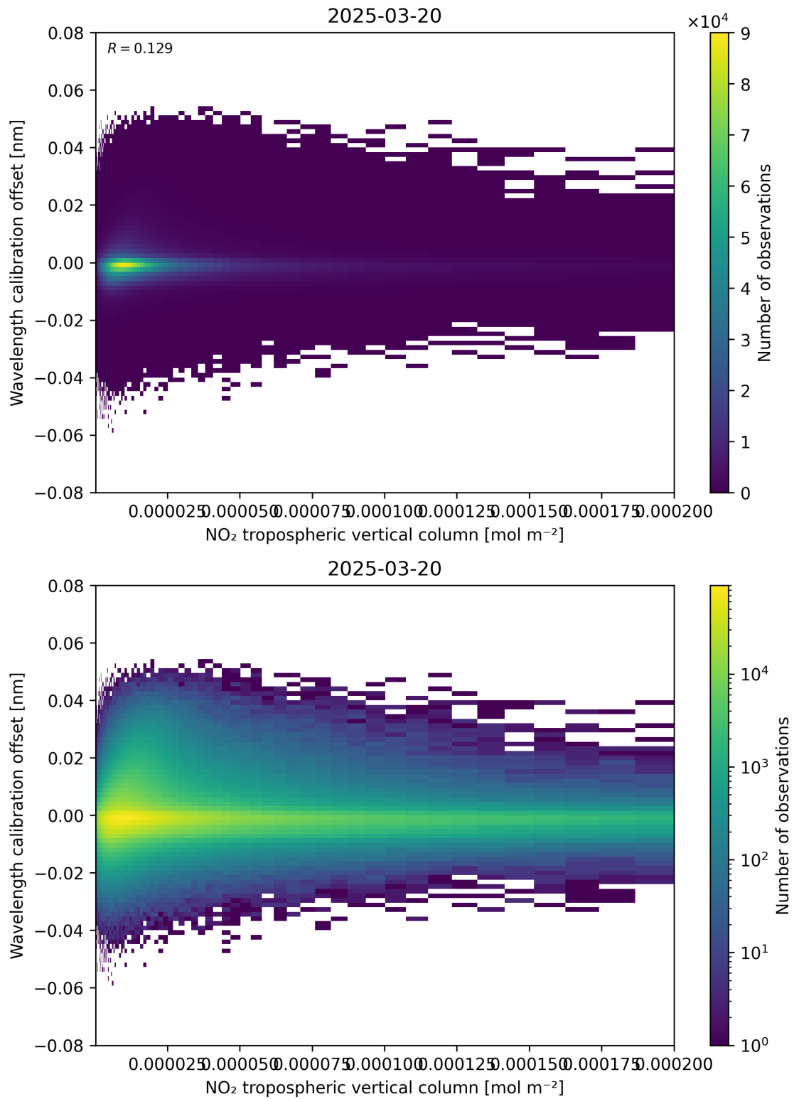
Figure 143: Scatter density plot of “NO 2 tropospheric vertical column” against “Wavelength calibration offset” for 2025-03-20 to 2025-03-21.
