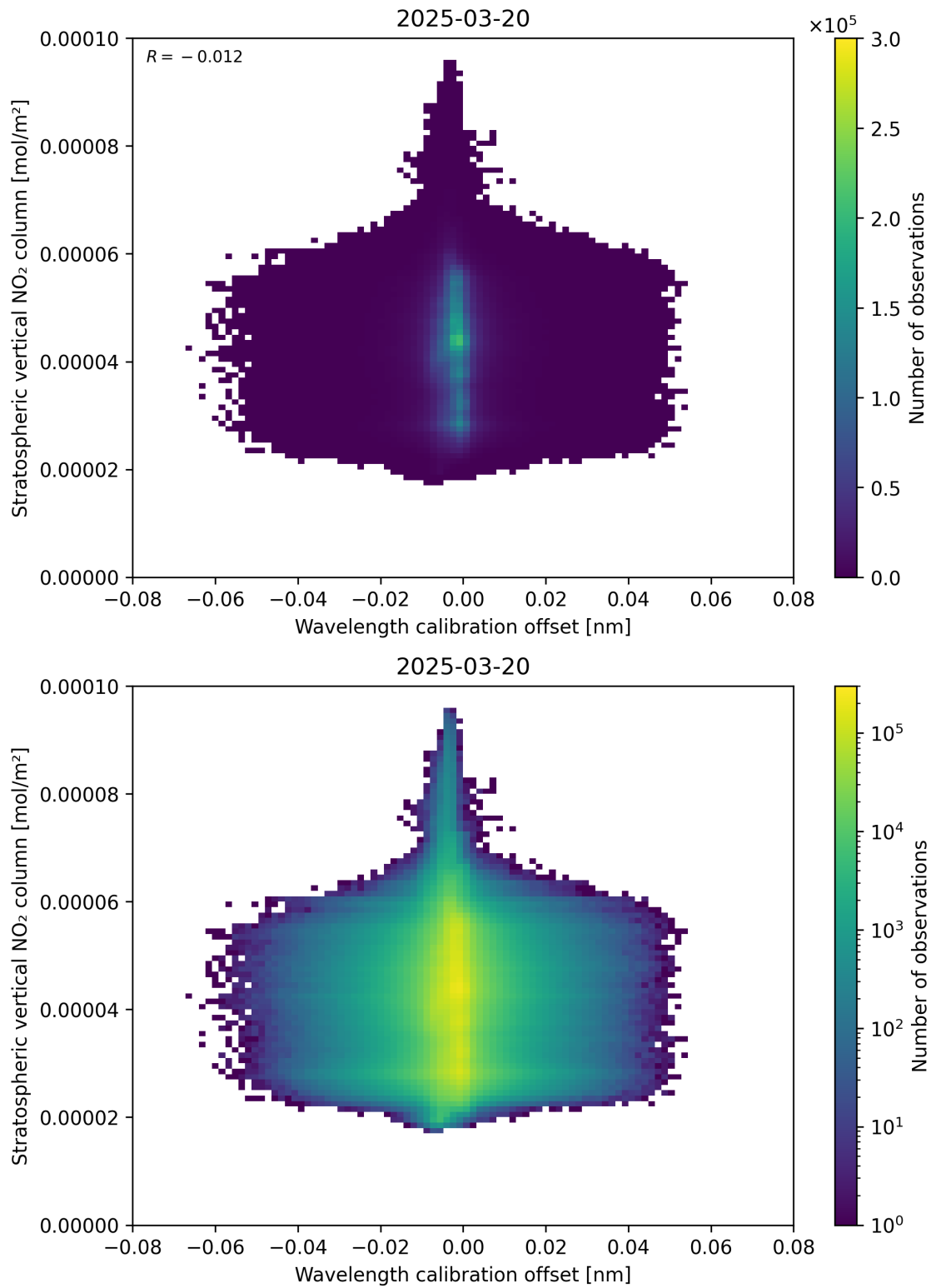
Figure 176: Scatter density plot of “Wavelength calibration offset” against “Stratospheric vertical NO 2 column” for 2025-03-20 to 2025-03-21.
