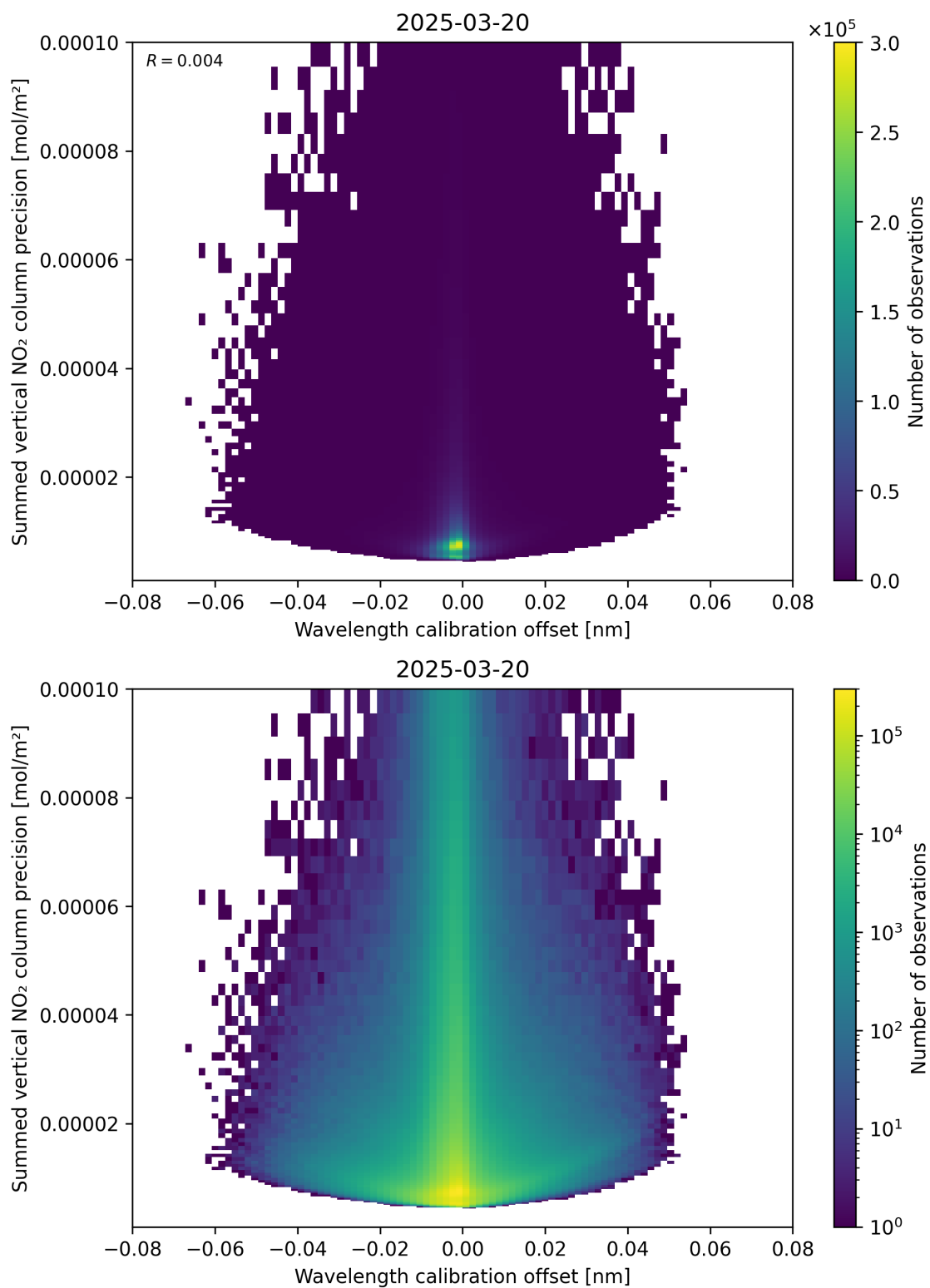
Figure 178: Scatter density plot of “Wavelength calibration offset” against “Summed vertical NO 2 column precision” for 2025-03-20 to 2025-03-21.
