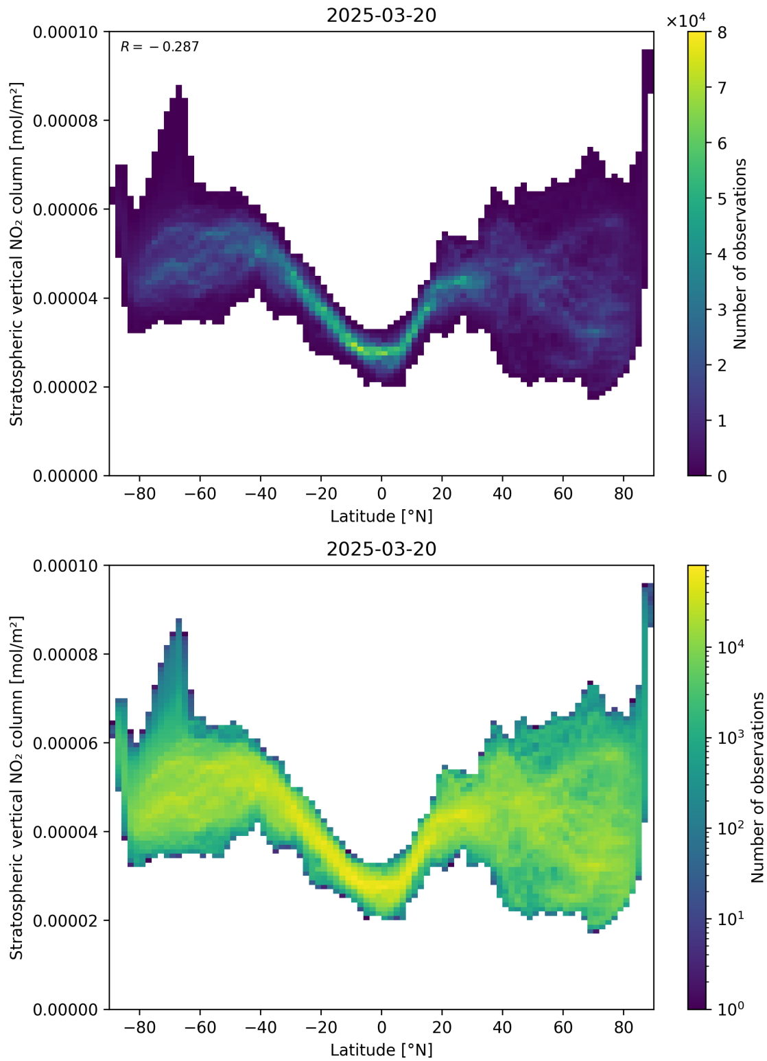
Figure 87: Scatter density plot of “Latitude” against “Stratospheric vertical NO 2 column” for 2025-03-20 to 2025-03-21.
