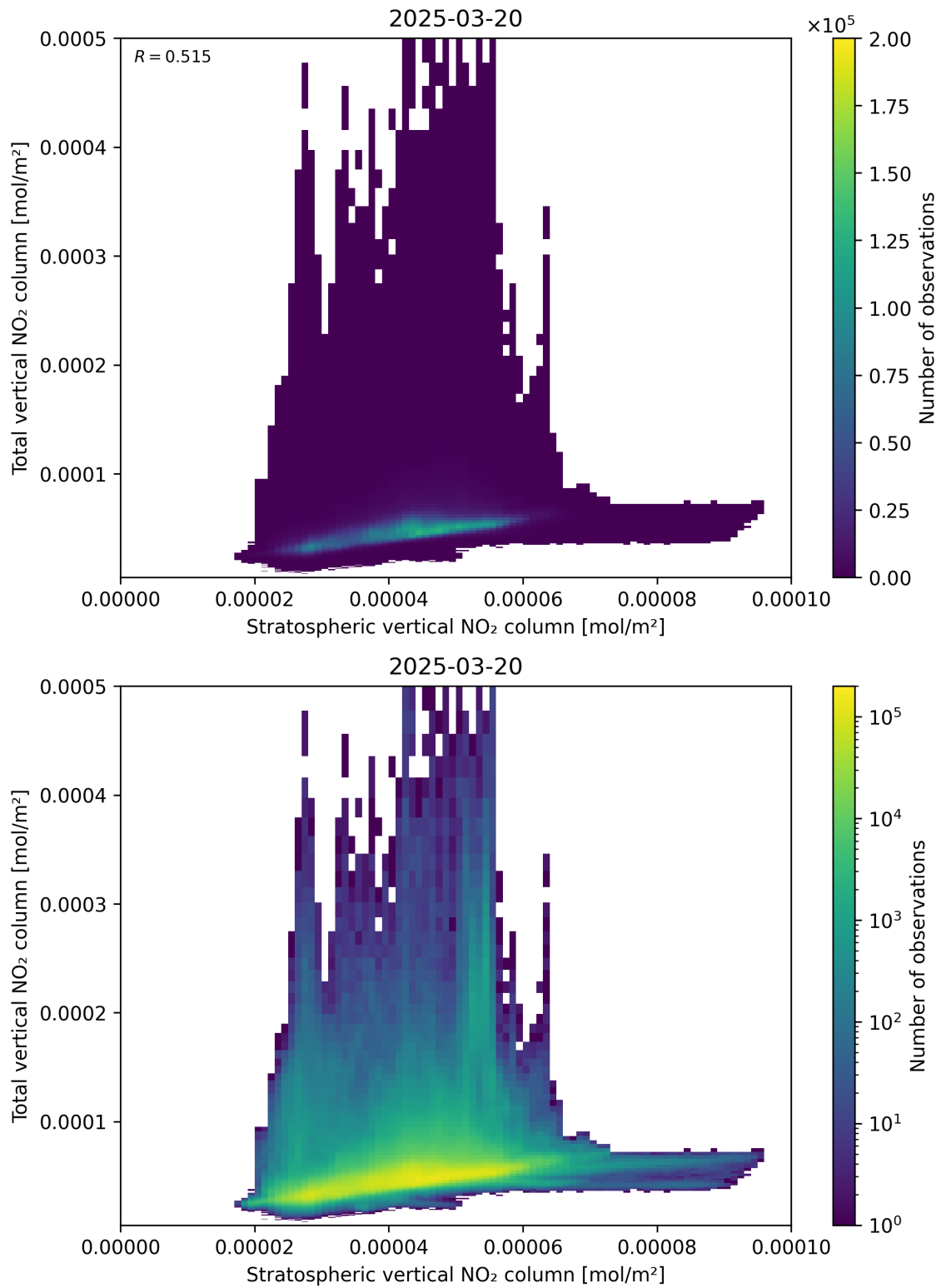
Figure 100: Scatter density plot of “Stratospheric vertical NO 2 column” against “Total vertical NO 2 column” for 2025-03-20 to 2025-03-21.
