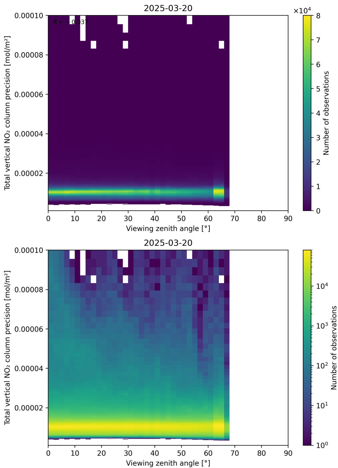
Figure 168: Scatter density plot of “Viewing zenith angle” against “Total vertical NO 2 column precision” for 2025-03-20 to 2025-03-21.
