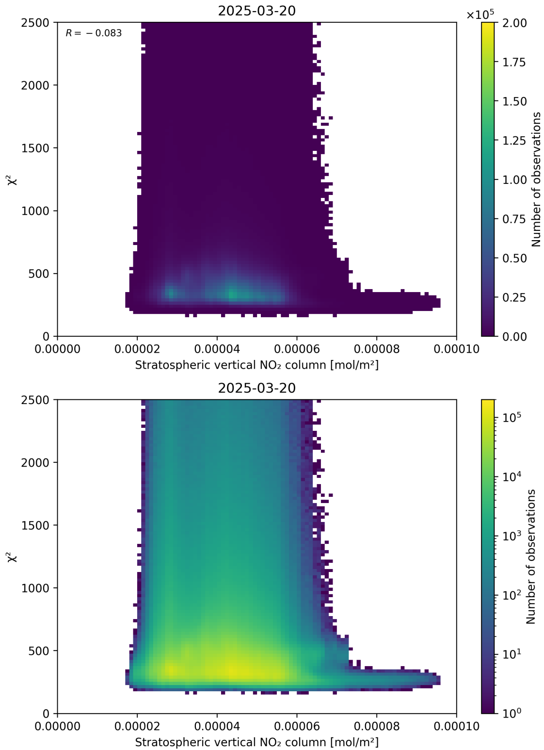
Figure 97: Scatter density plot of “Stratospheric vertical NO 2 column” against “ \chi^2 ” for 2025-03-20 to 2025-03-21.
