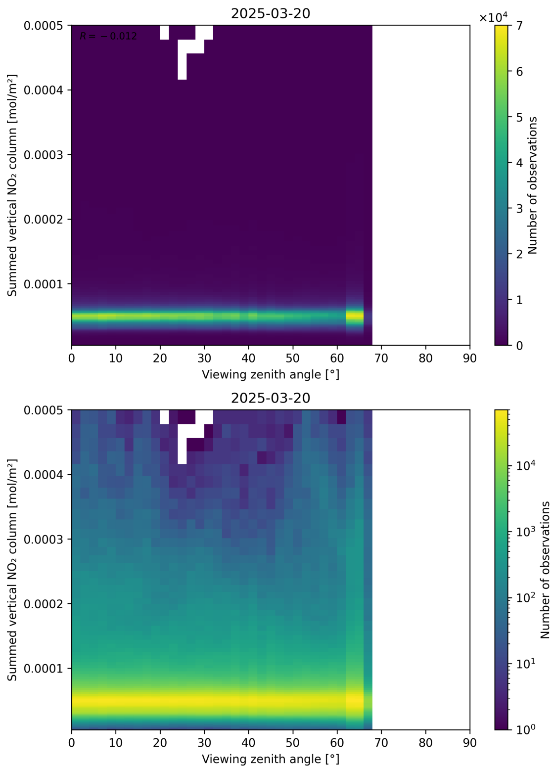
Figure 165: Scatter density plot of “Viewing zenith angle” against “Summed vertical NO 2 column” for 2025-03-20 to 2025-03-21.
