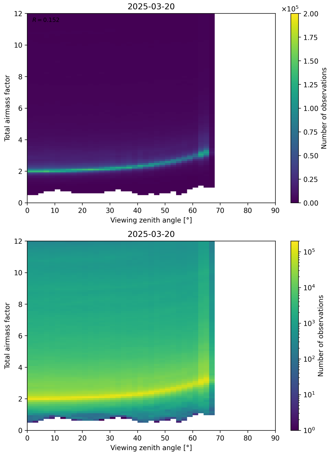
Figure 160: Scatter density plot of “Viewing zenith angle” against “Total airmass factor” for 2025-03-20 to 2025-03-21.
