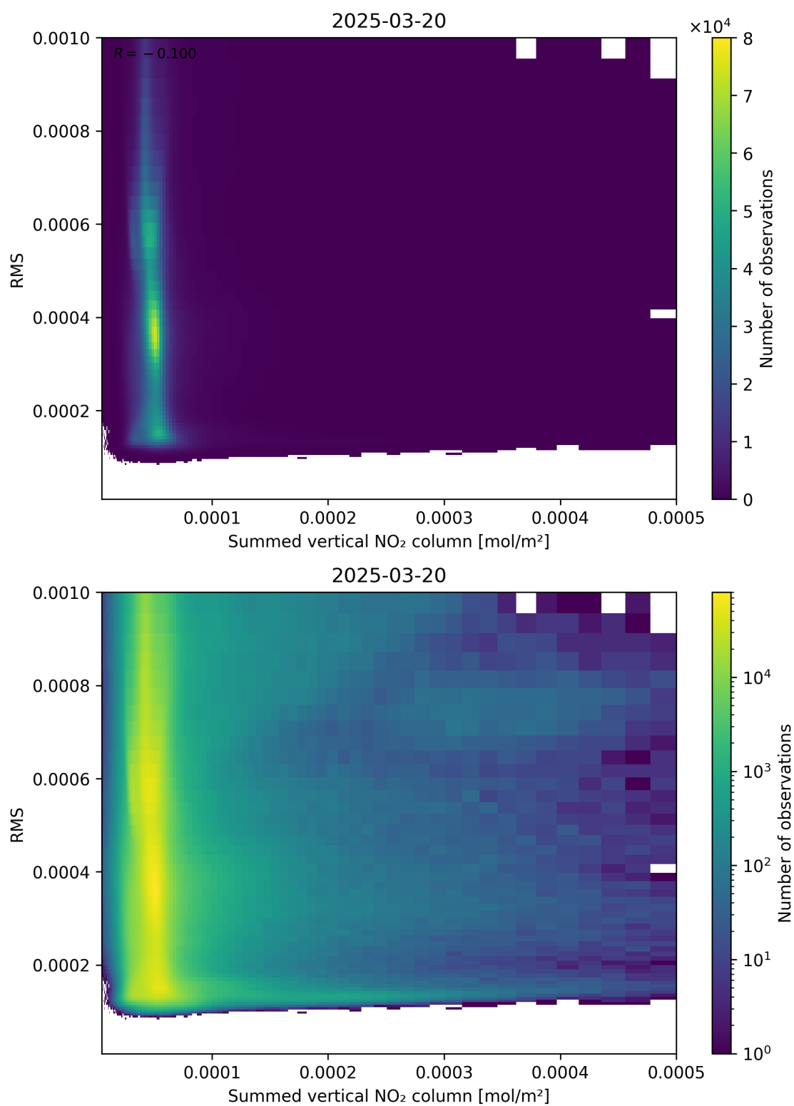
Figure 109: Scatter density plot of “Summed vertical NO 2 column” against “RMS” for 2025-03-20 to 2025-03-21.
