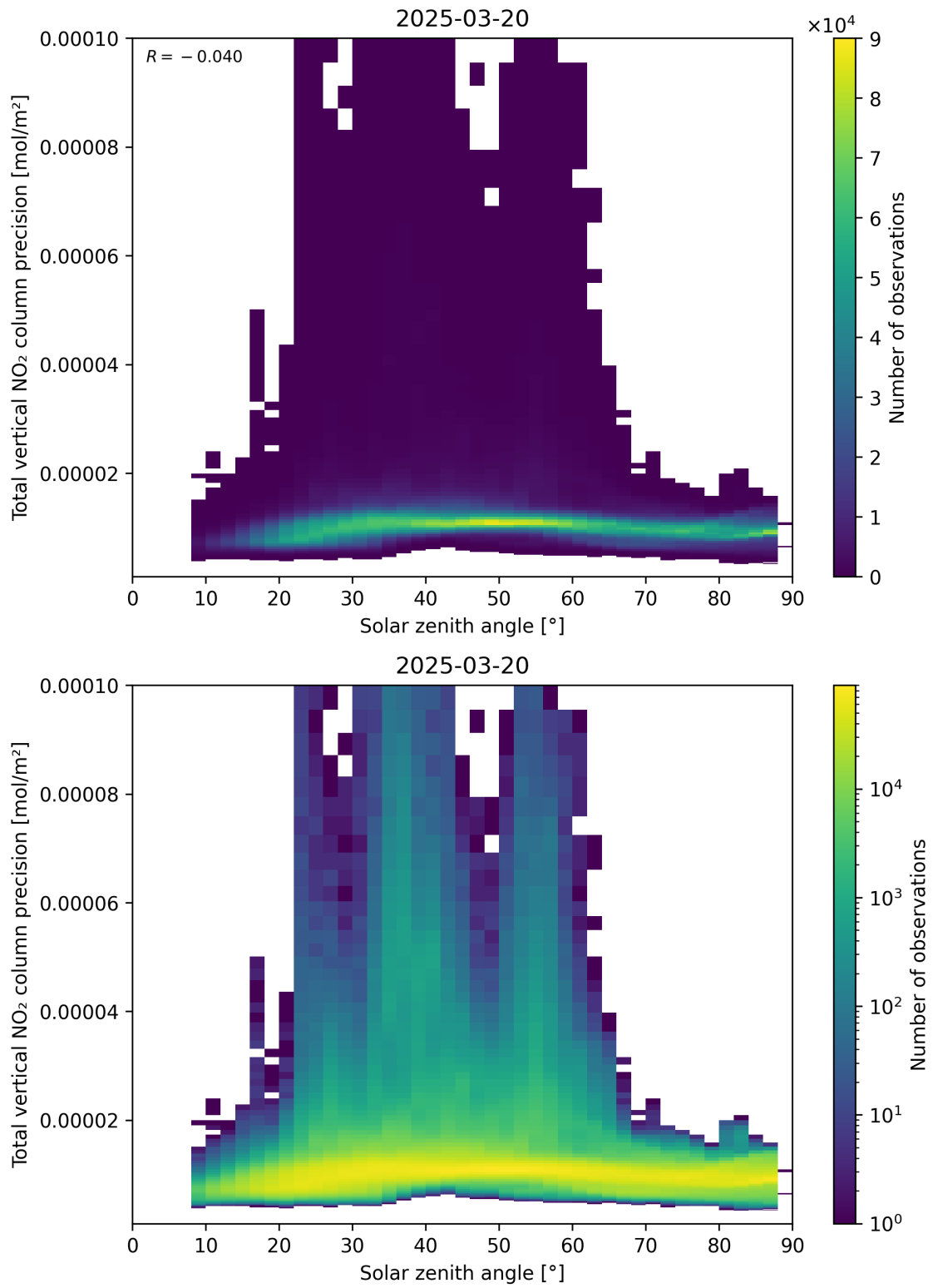
Figure 154: Scatter density plot of “Solar zenith angle” against “Total vertical NO 2 column precision” for 2025-03-20 to 2025-03-21.
