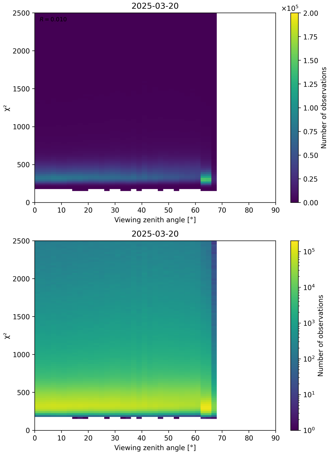
Figure 162: Scatter density plot of “Viewing zenith angle” against “ \chi^2 ” for 2025-03-20 to 2025-03-21.
