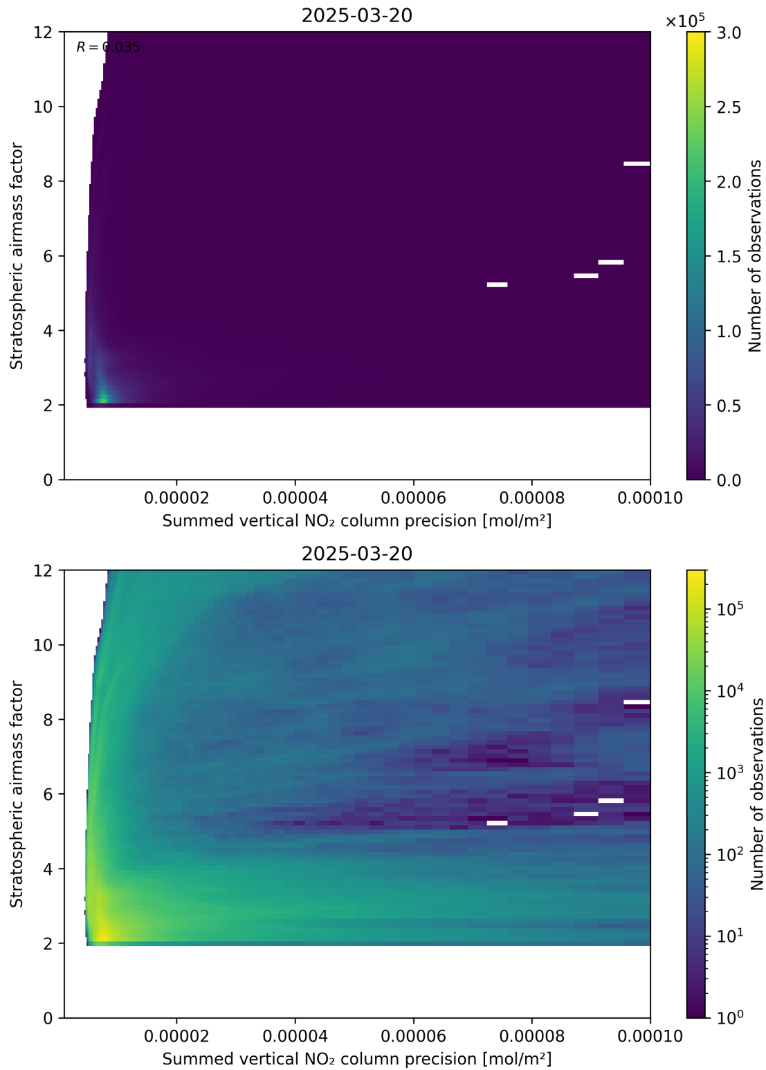
Figure 106: Scatter density plot of “Summed vertical NO 2 column precision” against “Stratospheric airmass factor” for 2025-03-20 to 2025-03-21.
