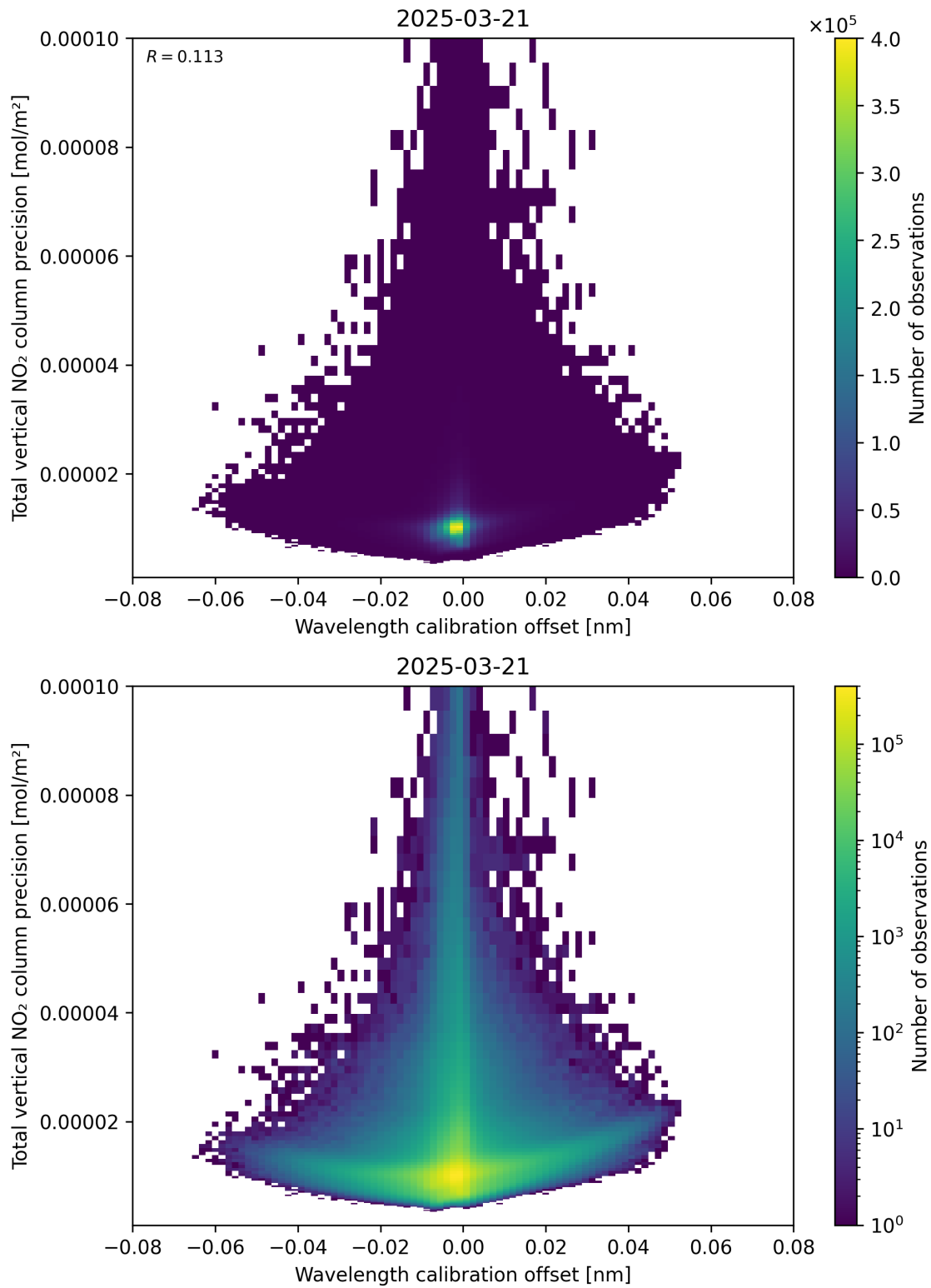
Figure 180: Scatter density plot of “Wavelength calibration offset” against “Total vertical NO 2 column precision” for 2025-03-21 to 2025-03-21.
