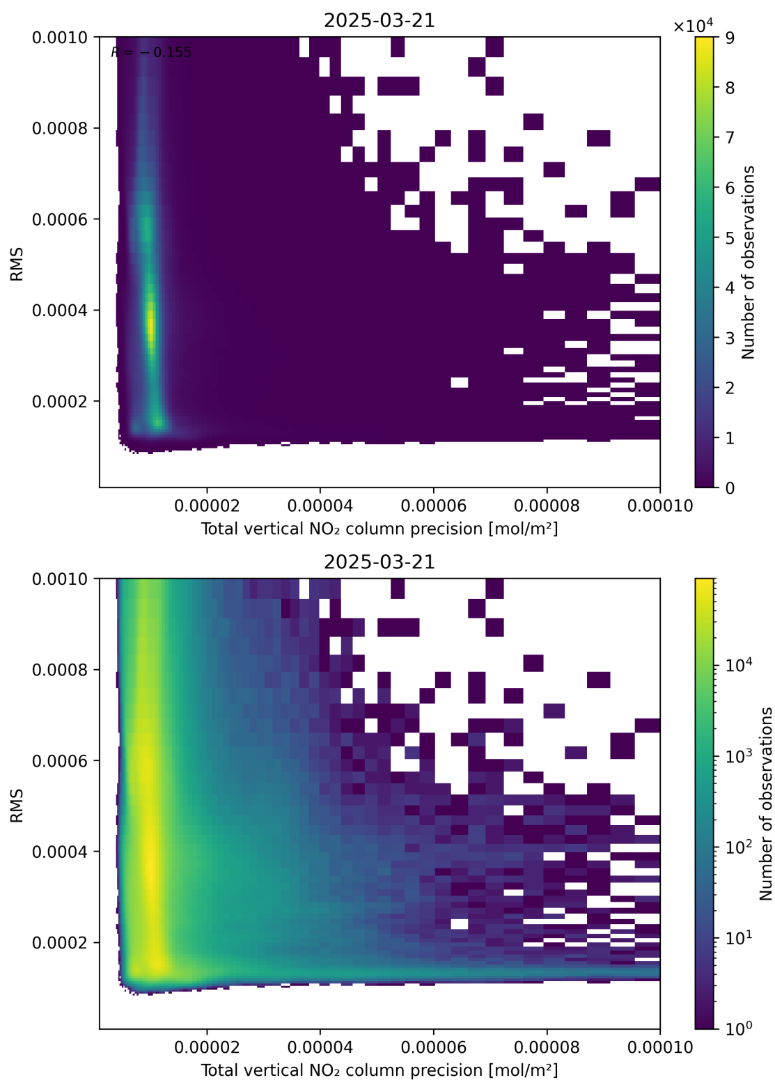
Figure 119: Scatter density plot of “Total vertical NO 2 column precision” against “RMS” for 2025-03-21 to 2025-03-21.
