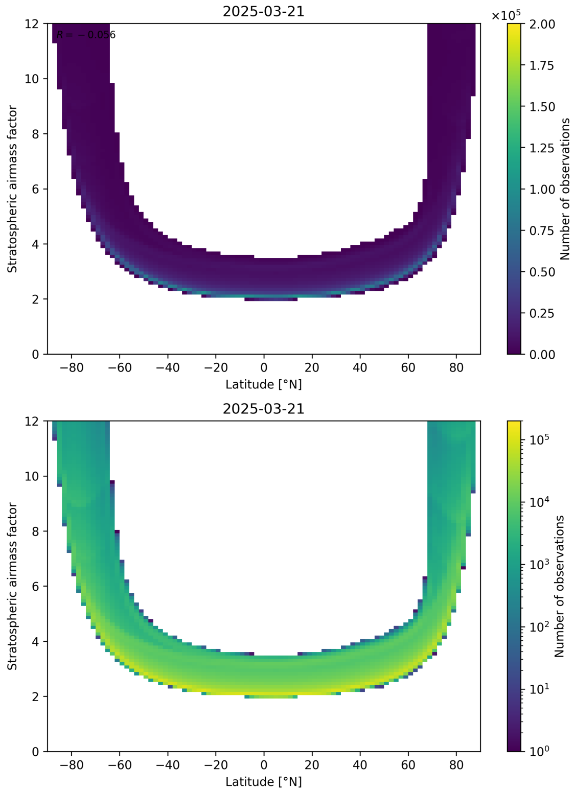
Figure 83: Scatter density plot of “Latitude” against “Stratospheric air mass factor” for 2025-03-21 to 2025-03-21.
