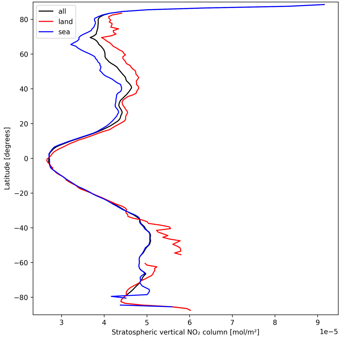
Figure 19: Zonal average of “Stratospheric vertical NO 2 column” for 2025-03-21 to 2025-03-21.
