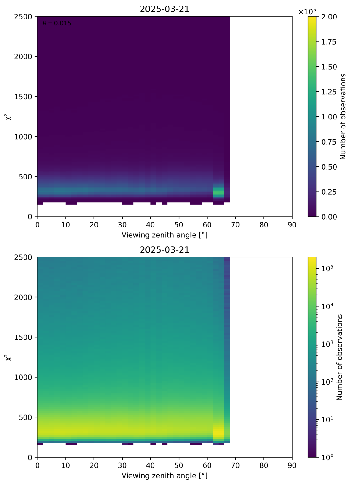
Figure 162: Scatter density plot of “Viewing zenith angle” against “ \chi^2 ” for 2025-03-21 to 2025-03-21.
