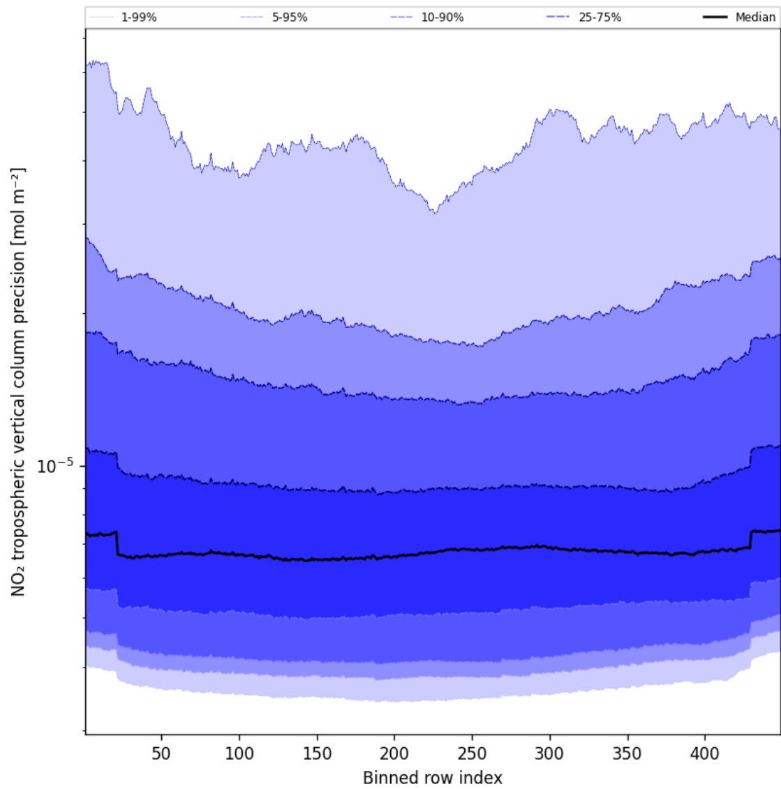
Figure 47: Along track statistics of “NO 2 tropospheric vertical column precision” for 2025-03-21 to 2025-03-21
