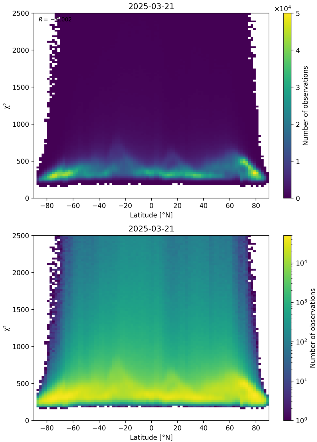
Figure 86: Scatter density plot of “Latitude” against “ \chi^2 ” for 2025-03-21 to 2025-03-21.
