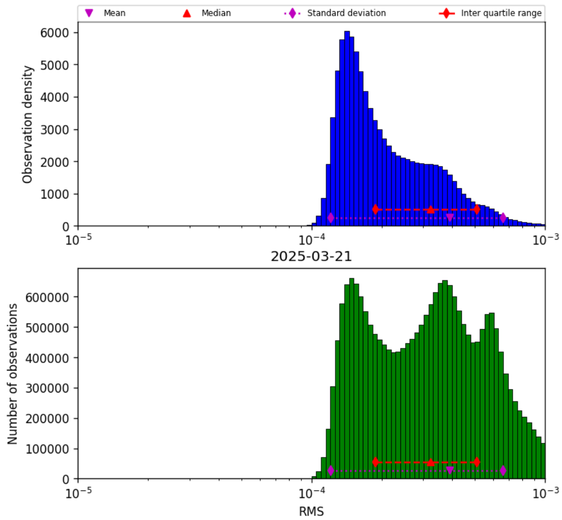
Figure 43: Histogram of “RMS” for 2025-03-21 to 2025-03-21
