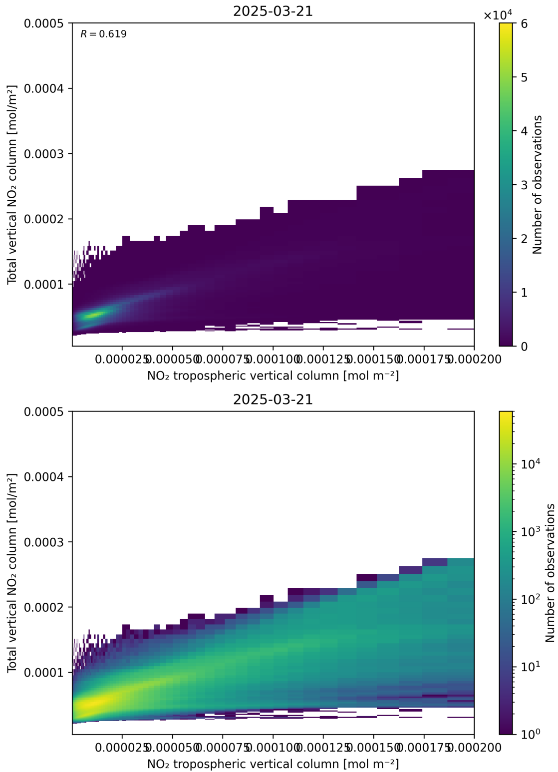
Figure 128: Scatter density plot of “NO 2 tropospheric vertical column” against “Total vertical NO 2 column” for 2025-03-21 to 2025-03-21.
