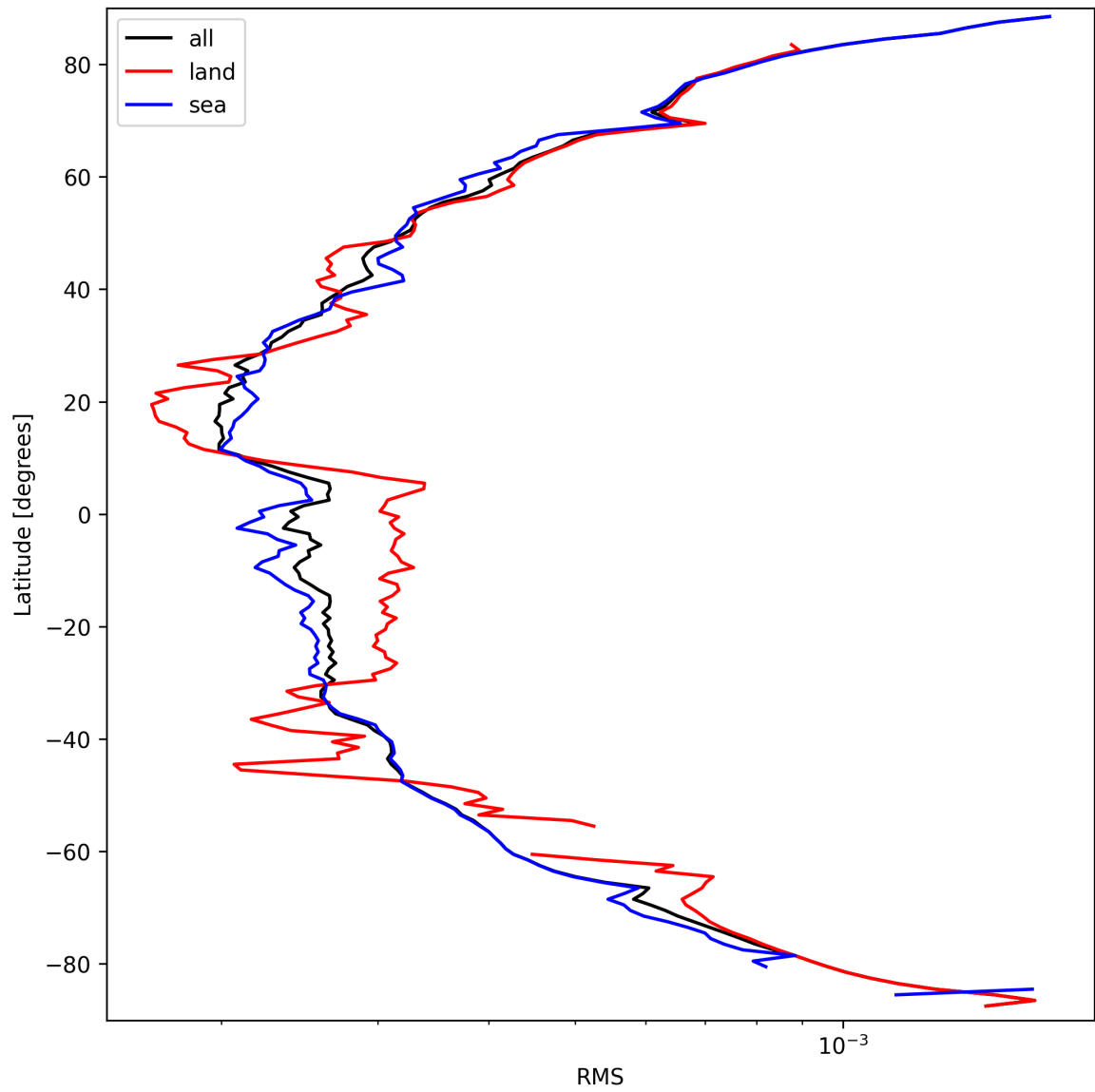
Figure 26: Zonal average of “RMS” for 2025-03-21 to 2025-03-21.
