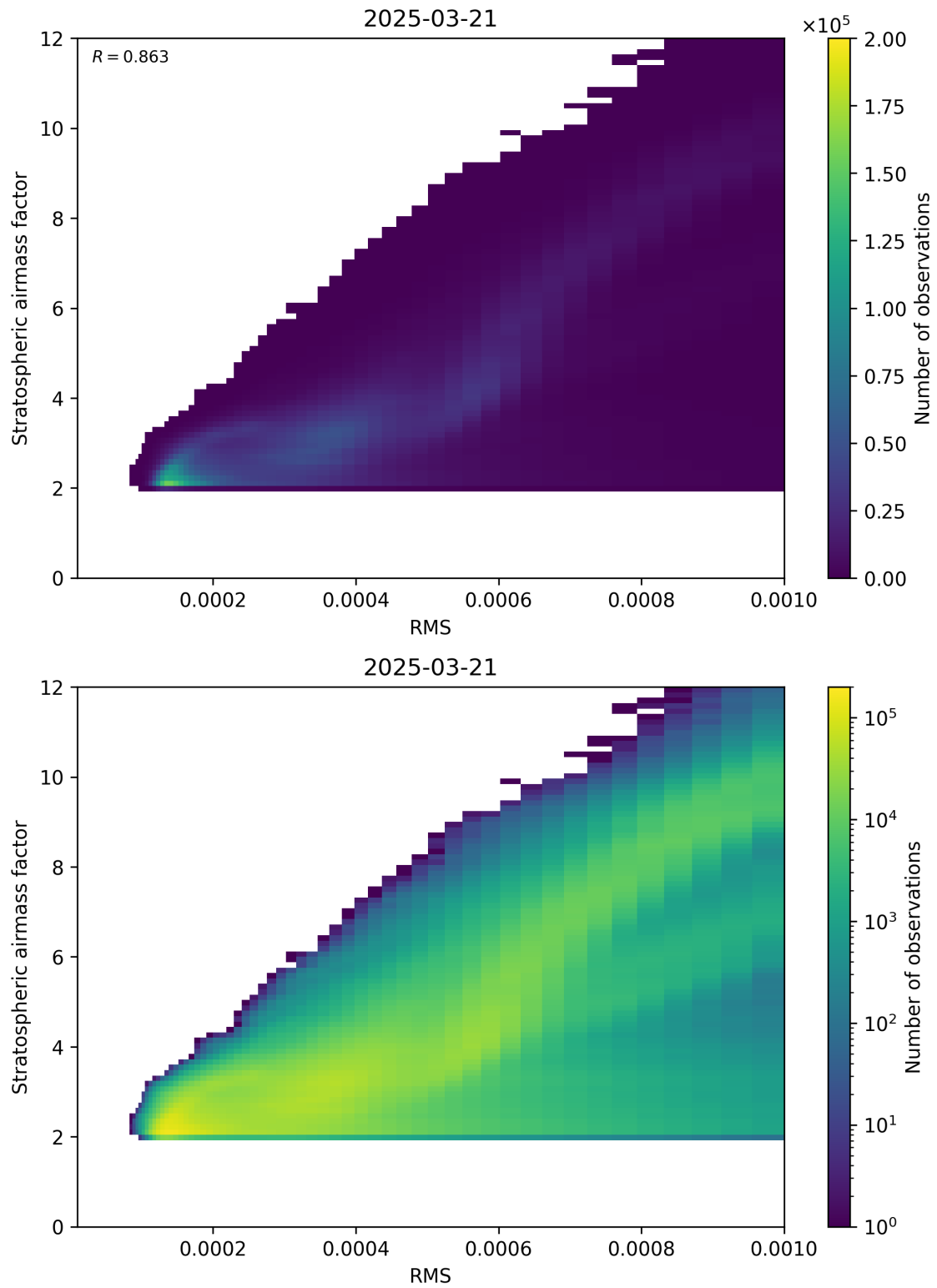
Figure 144: Scatter density plot of “RMS” against “Stratospheric airmass factor” for 2025-03-21 to 2025-03-21.
