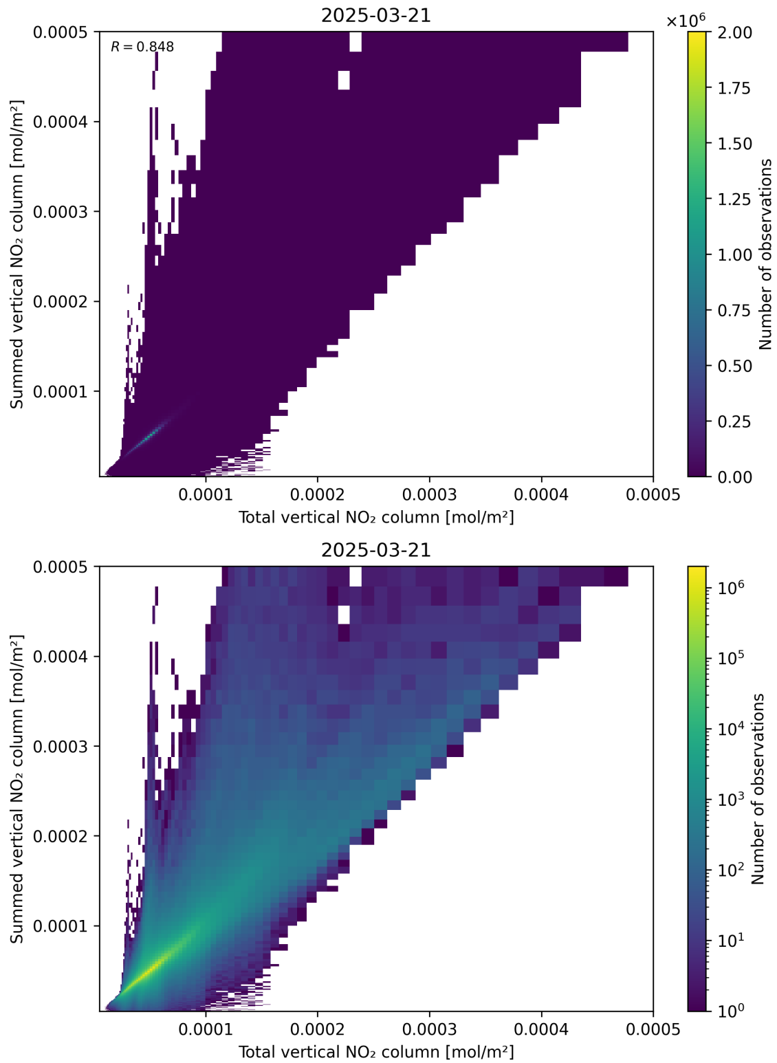
Figure 112: Scatter density plot of “Total vertical NO 2 column” against “Summed vertical NO 2 column” for 2025-03-21 to 2025-03-21.
