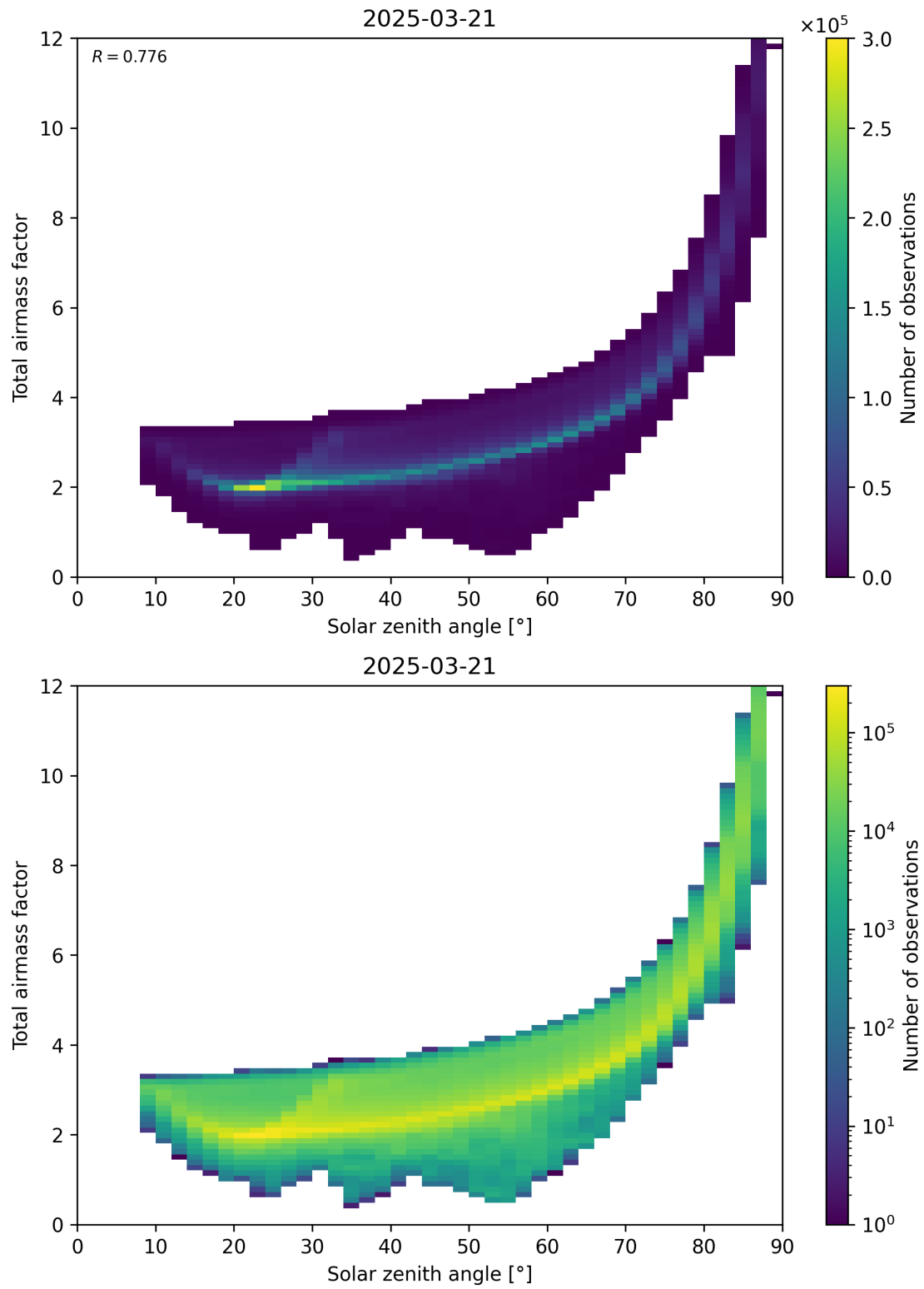
Figure 146: Scatter density plot of “Solar zenith angle” against “Total air mass factor” for 2025-03-21 to 2025-03-21.
