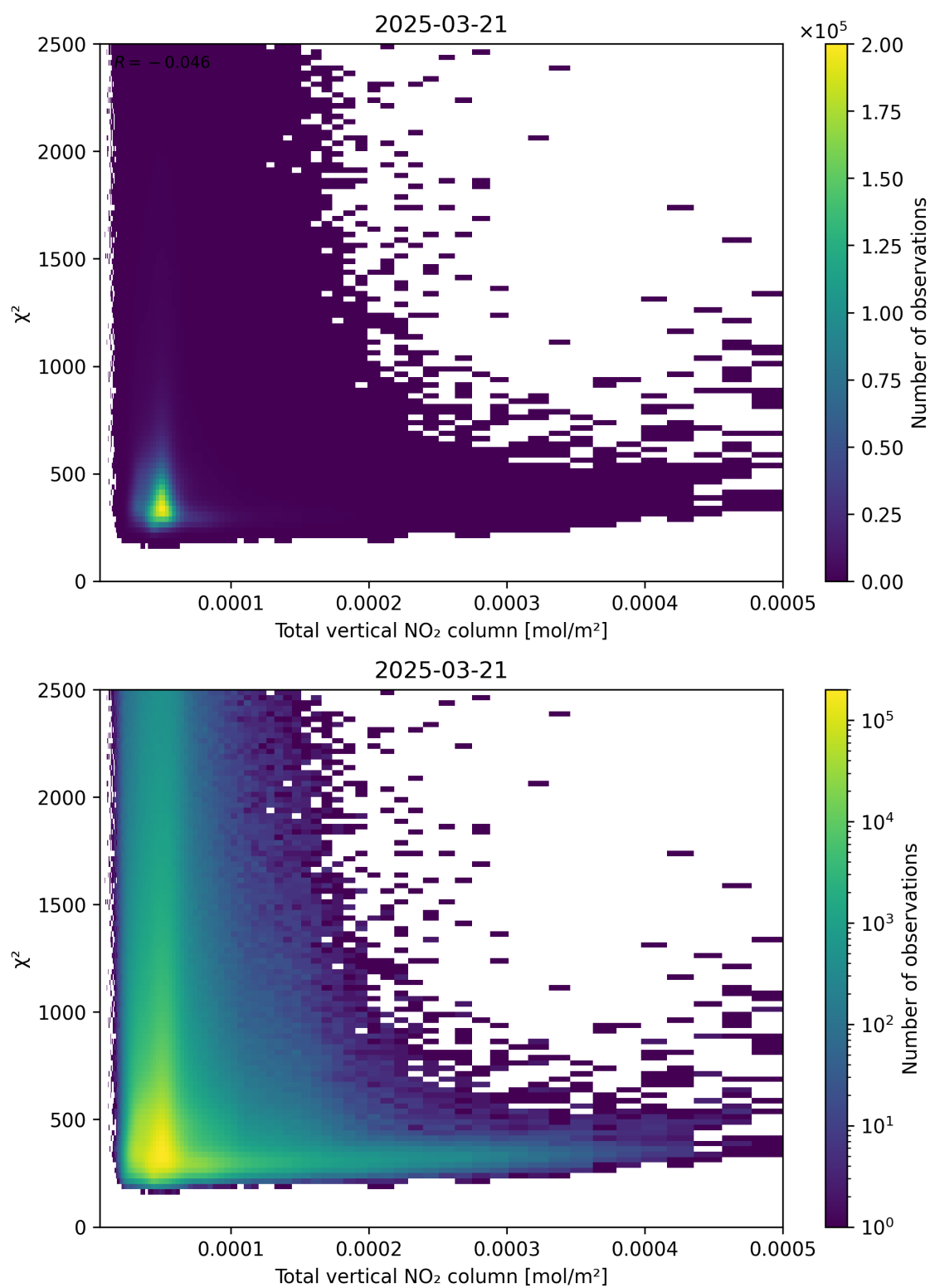
Figure 111: Scatter density plot of “Total vertical NO 2 column” against “ \chi^2 ” for 2025-03-21 to 2025-03-21.
