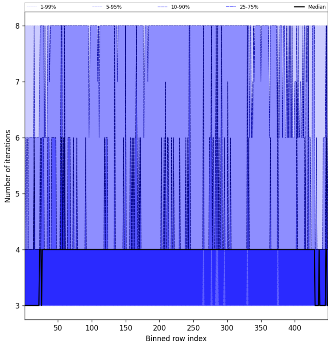
Figure 51: Along track statistics of “Number of iterations” for 2025-03-21 to 2025-03-21
