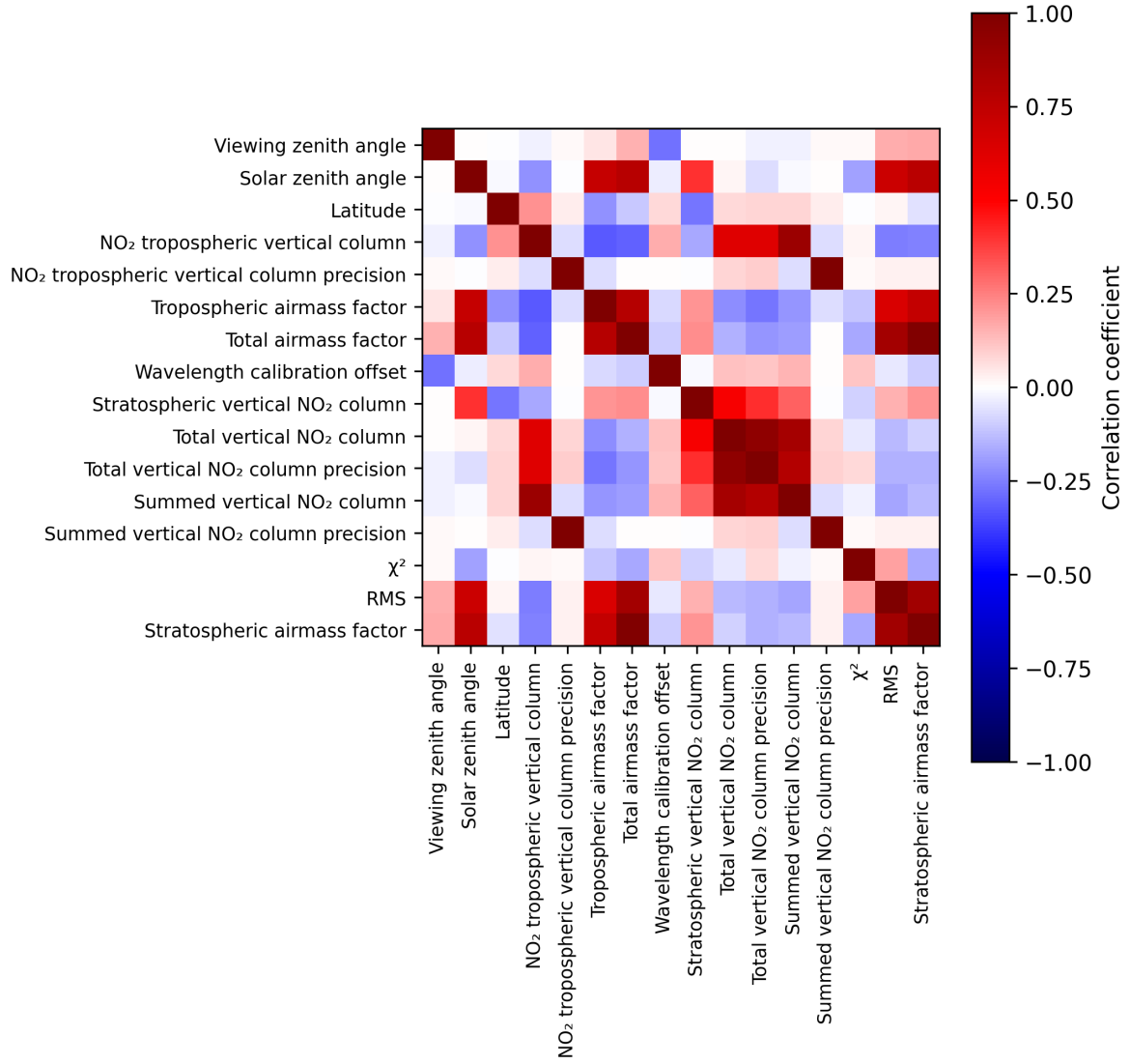
Figure 2: Map of correlation matrix for 2025-03-21 to 2025-03-21.
