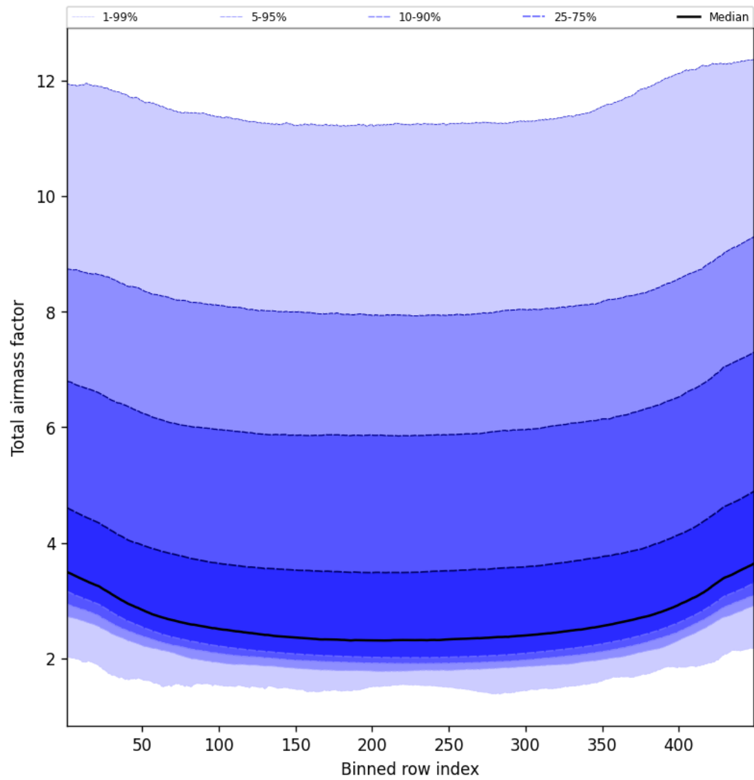
Figure 49: Along track statistics of “Total airmass factor” for 2025-03-21 to 2025-03-21
