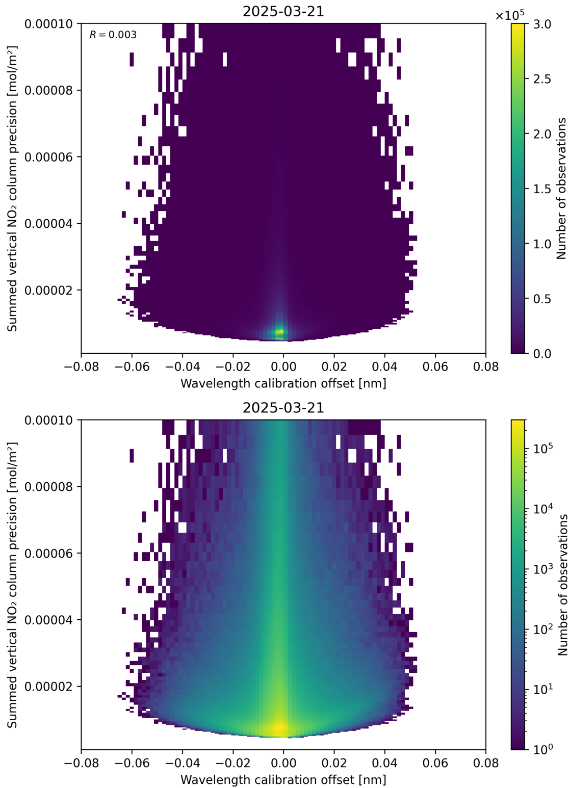
Figure 178: Scatter density plot of “Wavelength calibration offset” against “Summed vertical NO 2 column precision” for 2025-03-21 to 2025-03-21.
