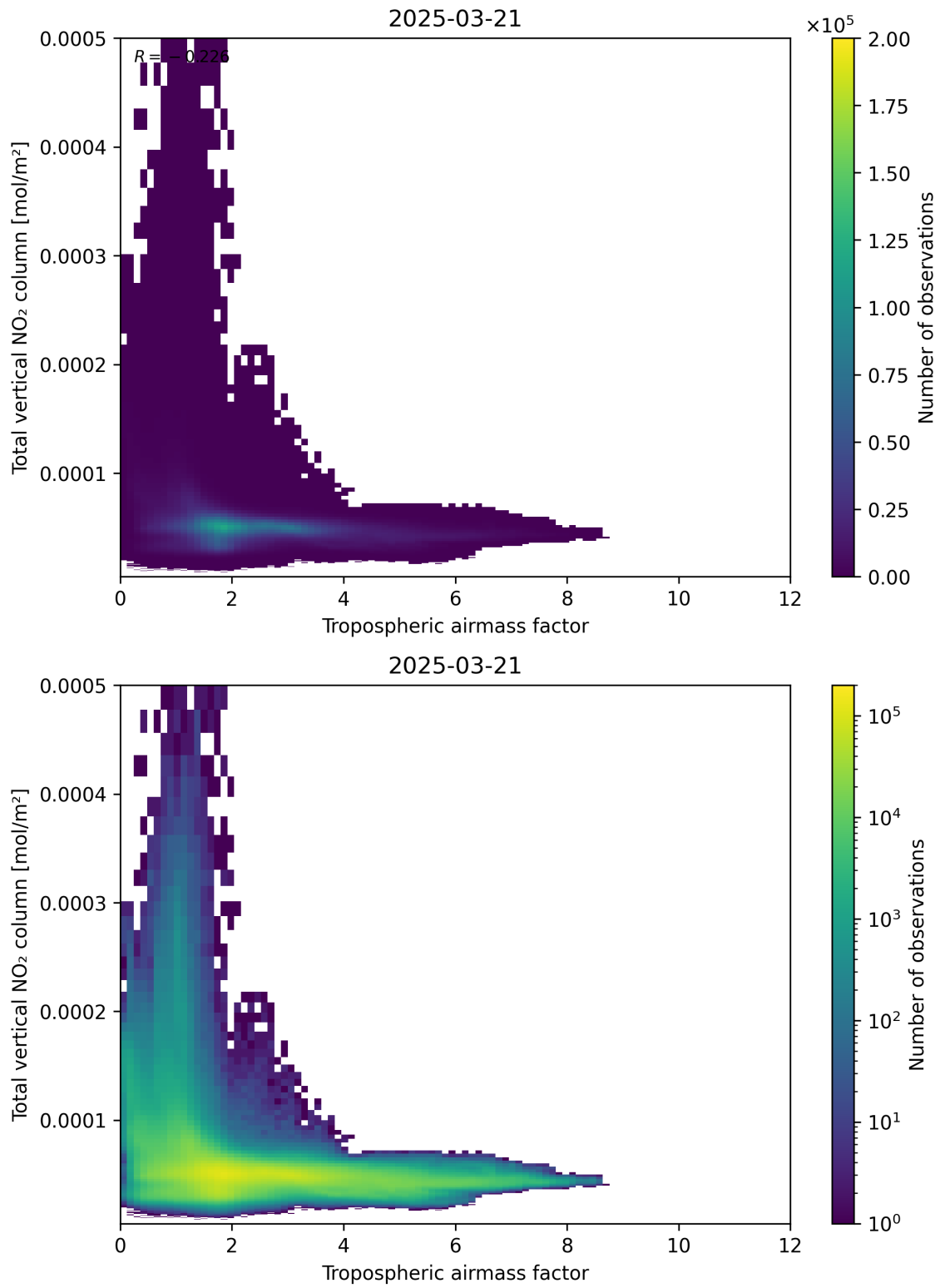
Figure 77: Scatter density plot of “Tropospheric airmass factor” against “Total vertical NO 2 column” for 2025-03-21 to 2025-03-21.
