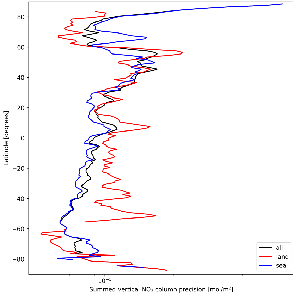
Figure 24: Zonal average of “Summed vertical NO 2 column precision” for 2025-03-21 to 2025-03-21.
