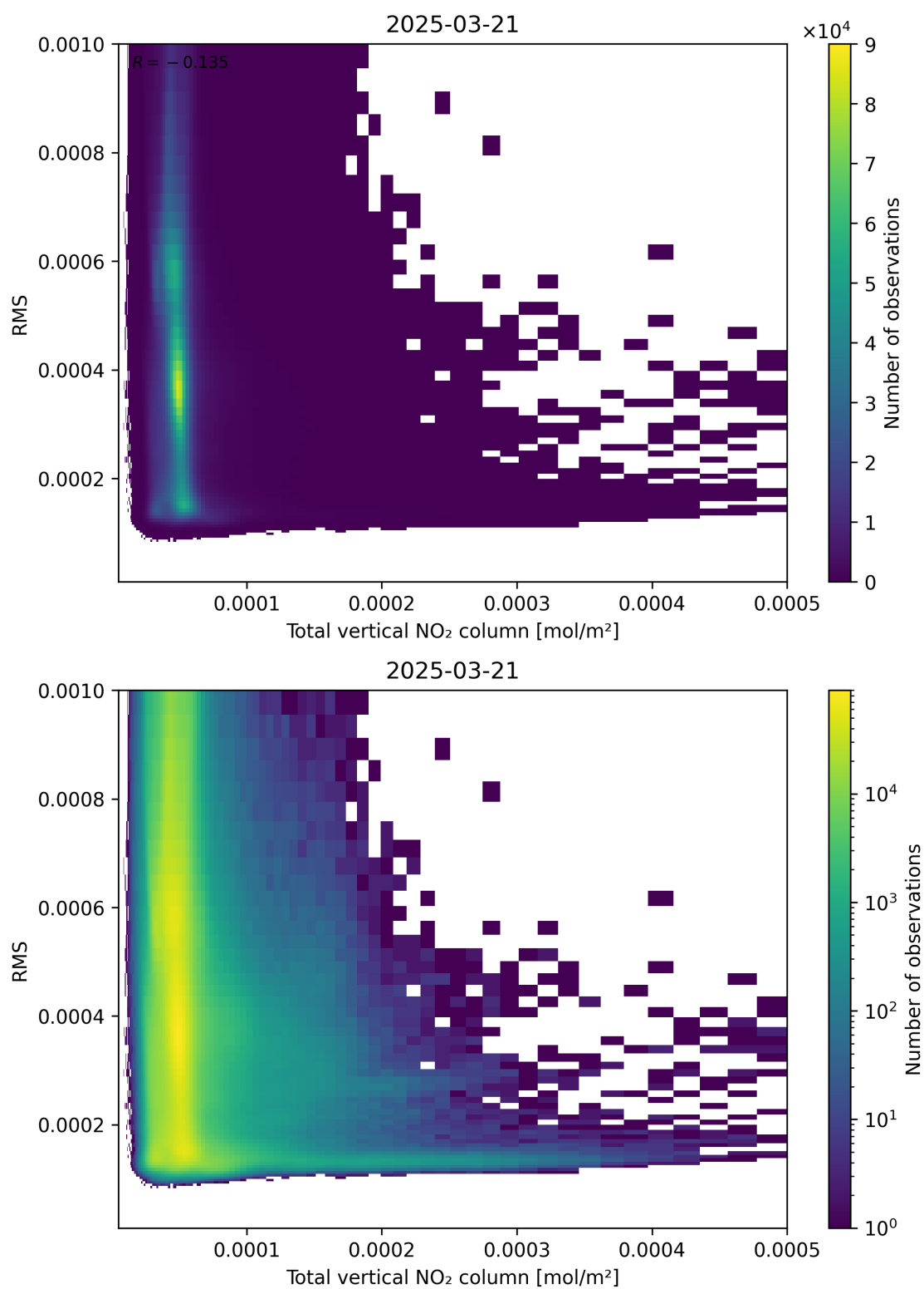
Figure 120: Scatter density plot of “Total vertical NO 2 column” against “RMS” for 2025-03-21 to 2025-03-21.
