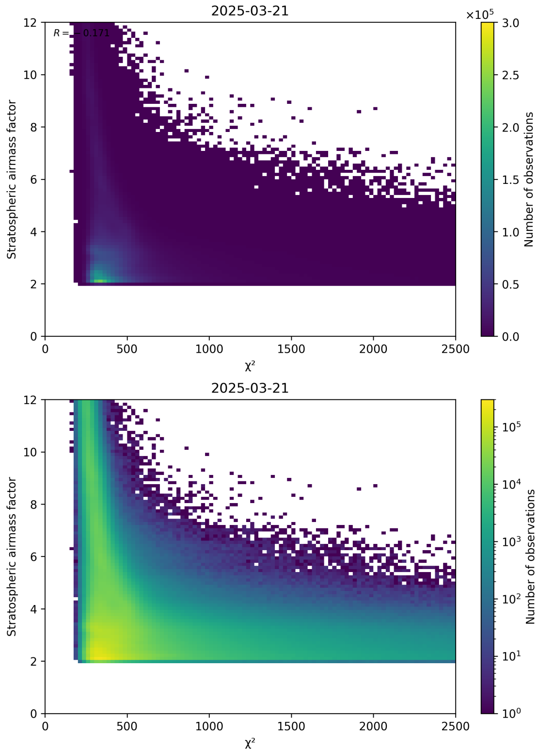
Figure 81: Scatter density plot of “ \chi^2 ” against “Stratospheric airmass factor” for 2025-03-21 to 2025-03-21.
