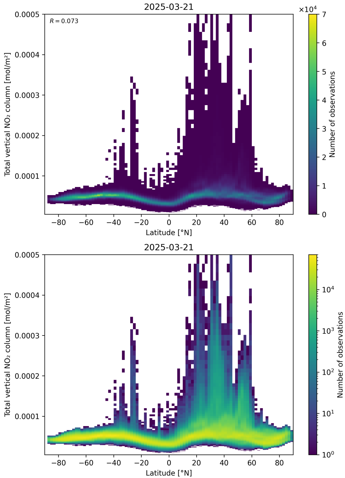
Figure 90: Scatter density plot of “Latitude” against “Total vertical NO 2 column” for 2025-03-21 to 2025-03-21.
