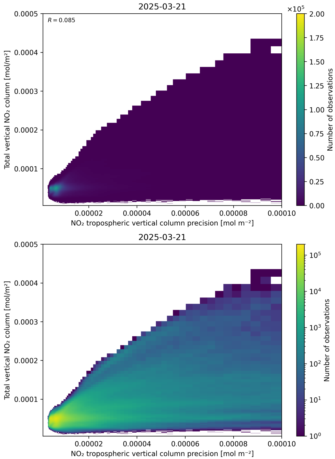
Figure 138: Scatter density plot of “NO 2 tropospheric vertical column precision” against “Total vertical NO 2 column” for 2025-03-21 to 2025-03-21.
