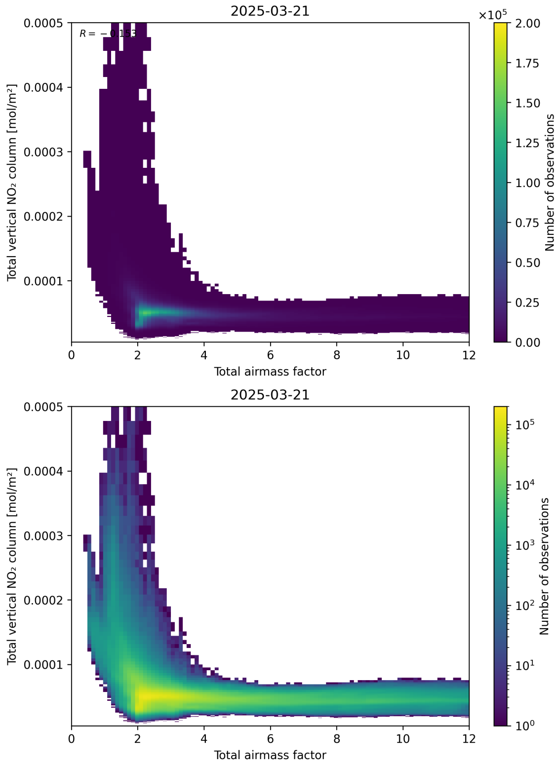
Figure 67: Scatter density plot of “Total airmass factor” against “Total vertical NO 2 column” for 2025-03-21 to 2025-03-21.
