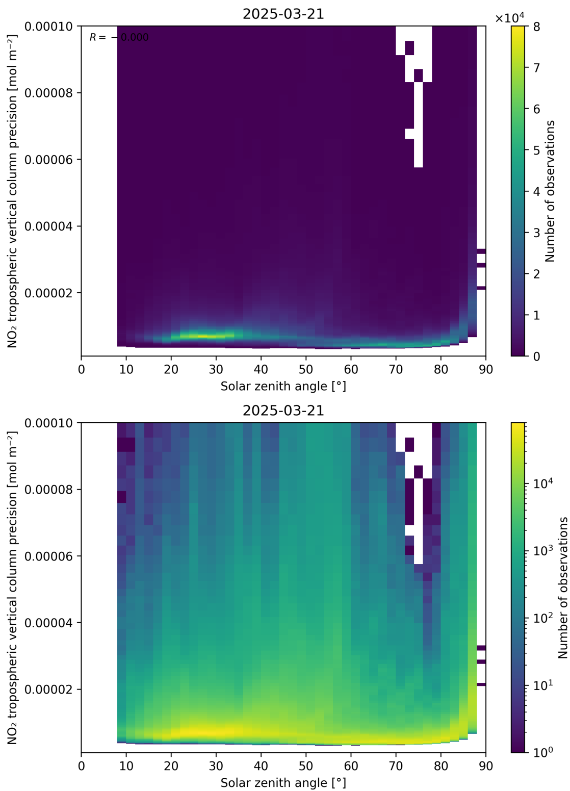
Figure 156: Scatter density plot of “Solar zenith angle” against “NO 2 tropospheric vertical column precision” for 2025-03-21 to 2025-03-21.
