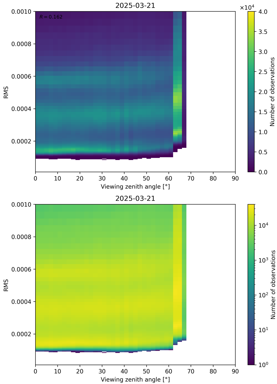
Figure 171: Scatter density plot of “Viewing zenith angle” against “RMS” for 2025-03-21 to 2025-03-21.
