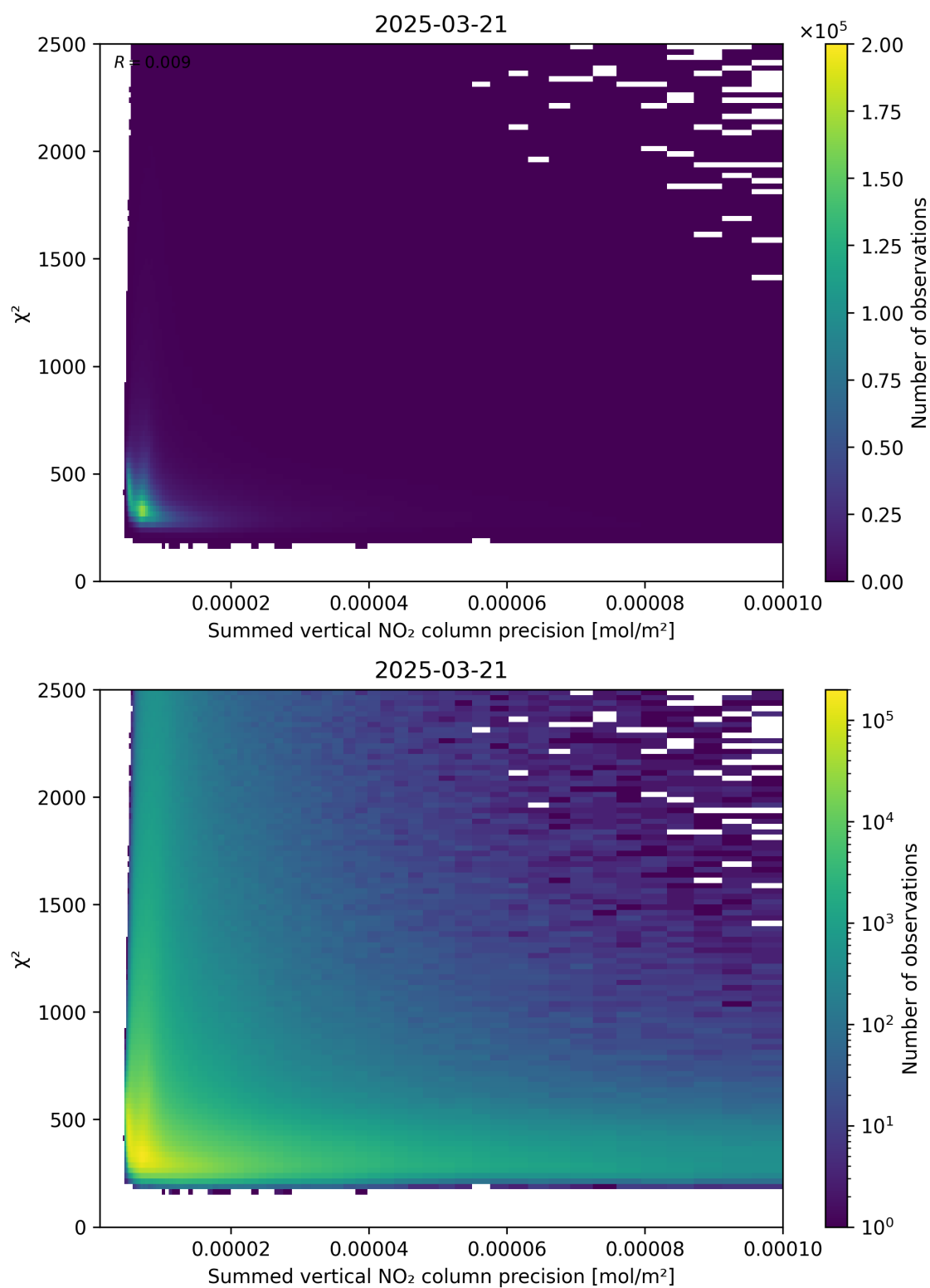
Figure 107: Scatter density plot of “Summed vertical NO 2 column precision” against “ \chi^2 ” for 2025-03-21 to 2025-03-21.
