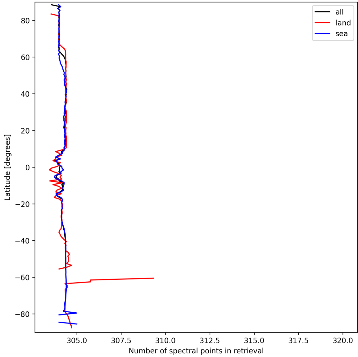
Figure 16: Zonal average of “Number of spectral points in retrieval” for 2025-03-21 to 2025-03-21.
