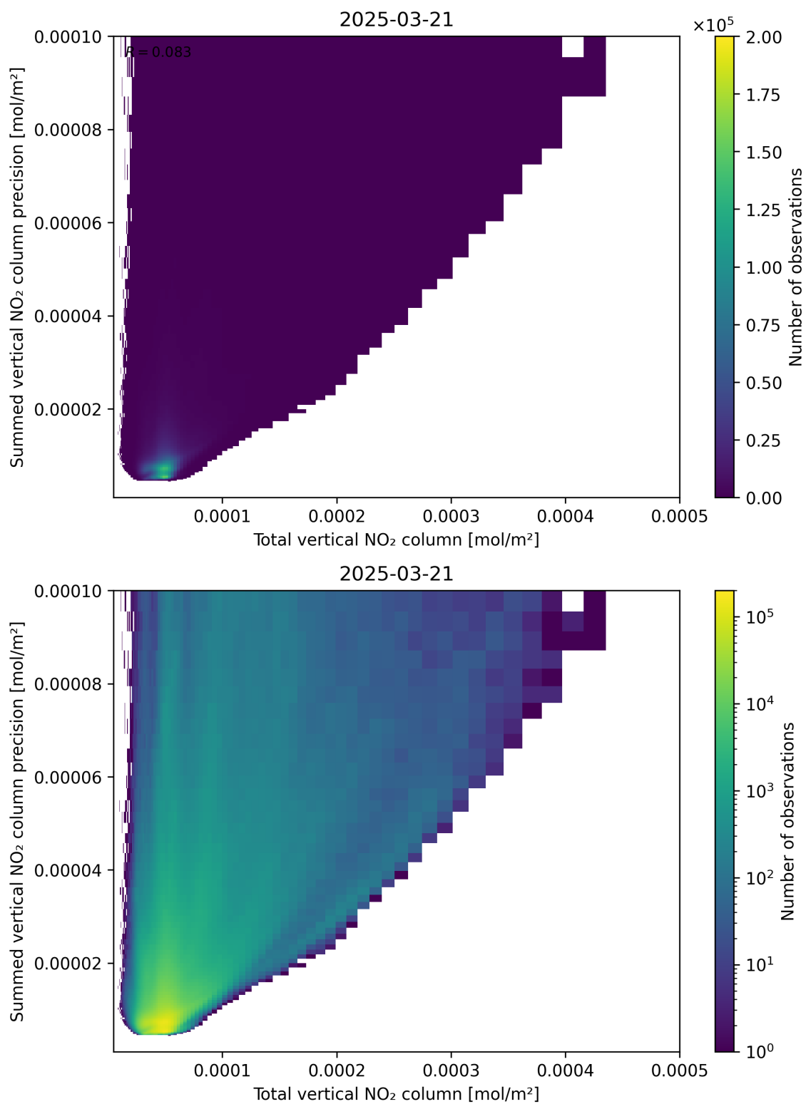
Figure 113: Scatter density plot of “Total vertical NO 2 column” against “Summed vertical NO 2 column precision” for 2025-03-21 to 2025-03-21.
