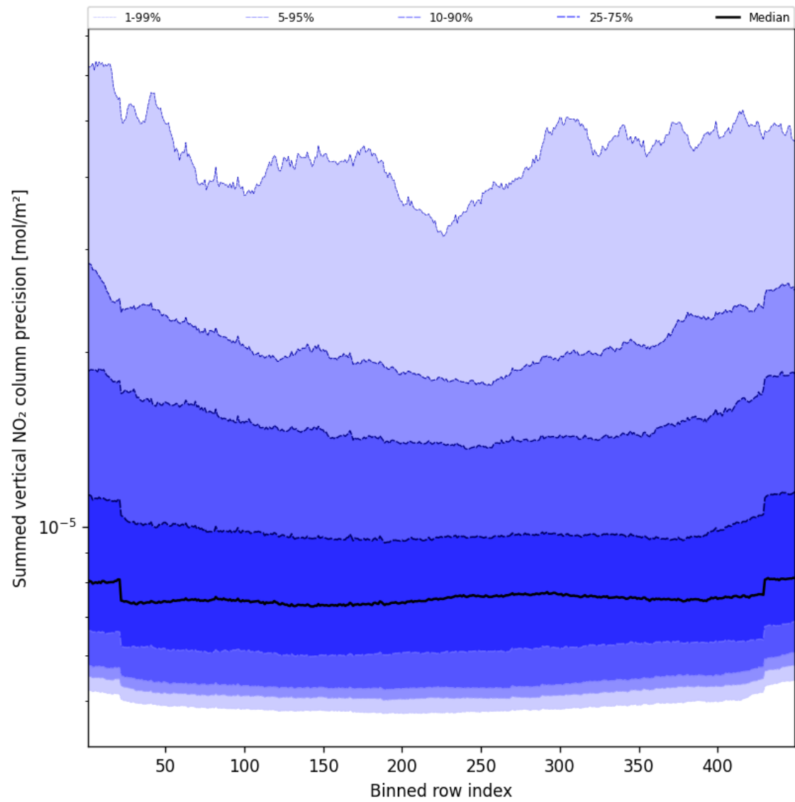
Figure 58: Along track statistics of “Summed vertical NO 2 column precision” for 2025-03-21 to 2025-03-21
