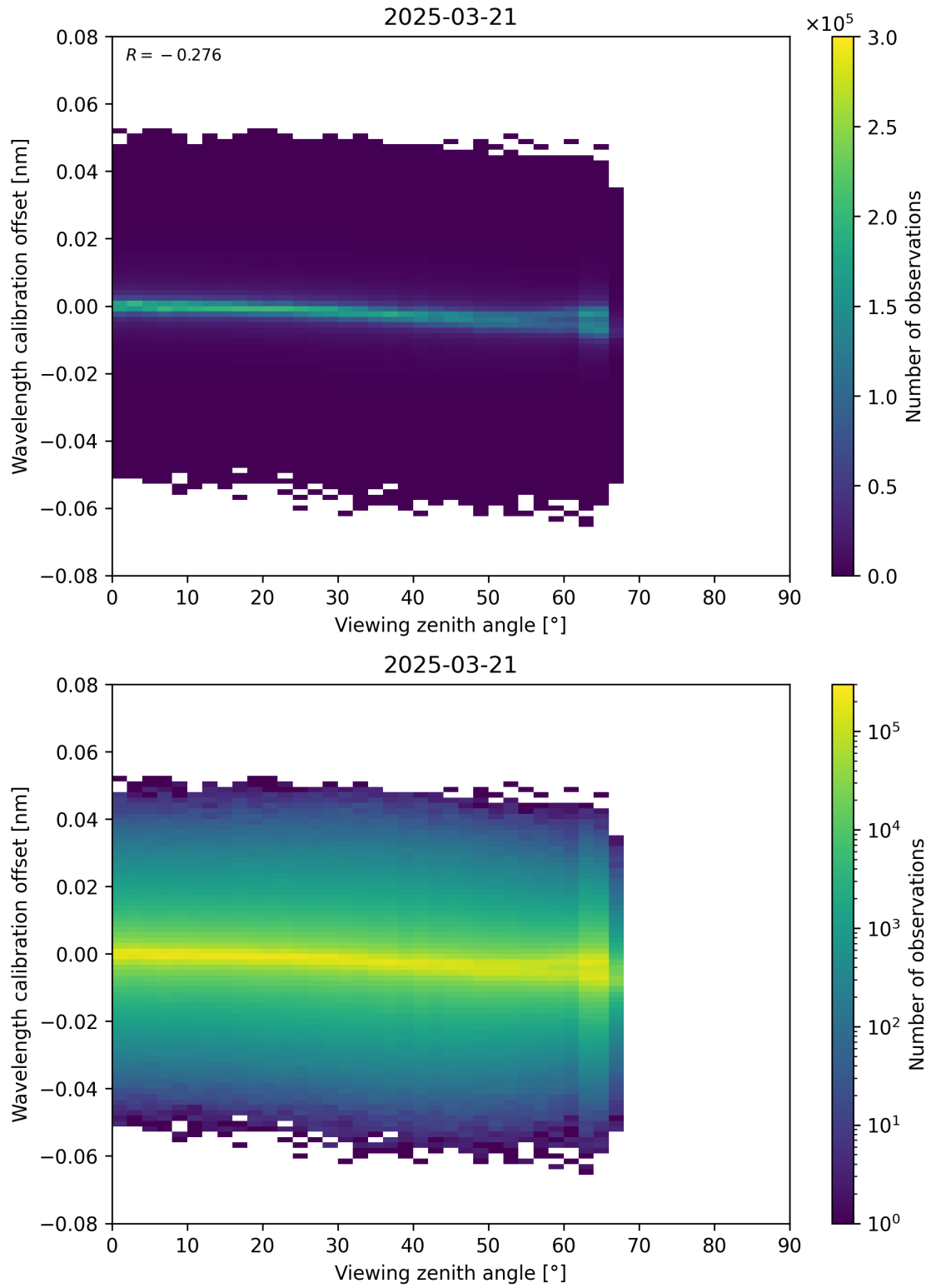
Figure 173: Scatter density plot of “Viewing zenith angle” against “Wavelength calibration offset” for 2025-03-21 to 2025-03-21.
