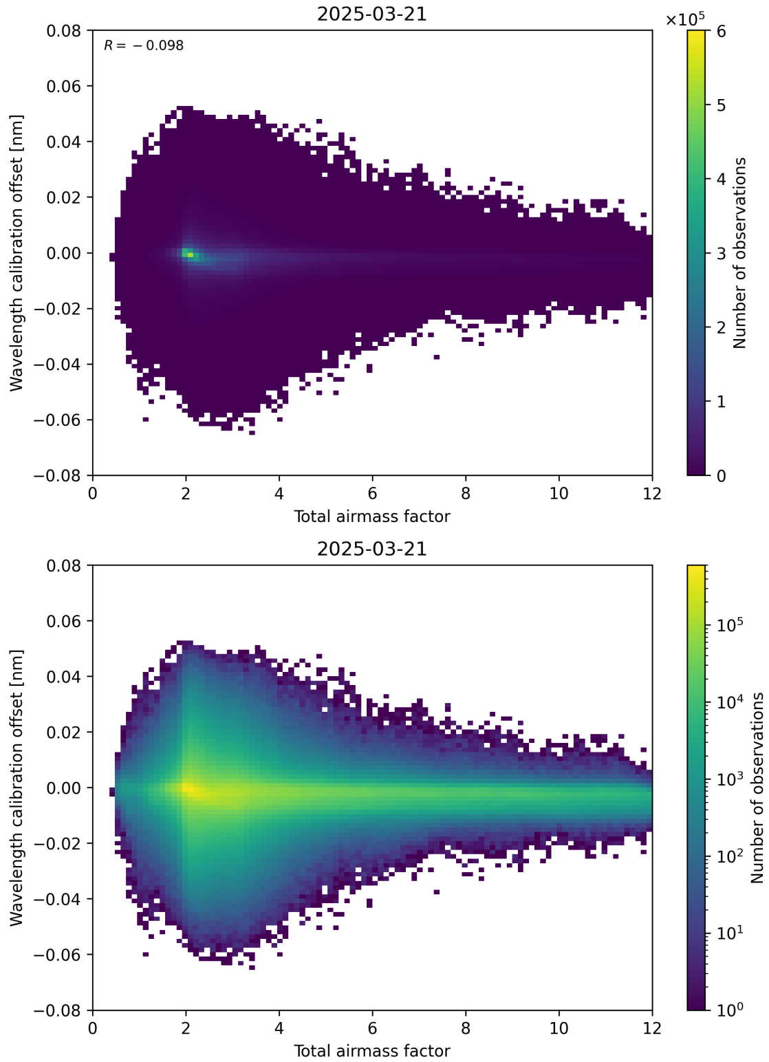
Figure 70: Scatter density plot of “Total airmass factor” against “Wavelength calibration offset” for 2025-03-21 to 2025-03-21.
