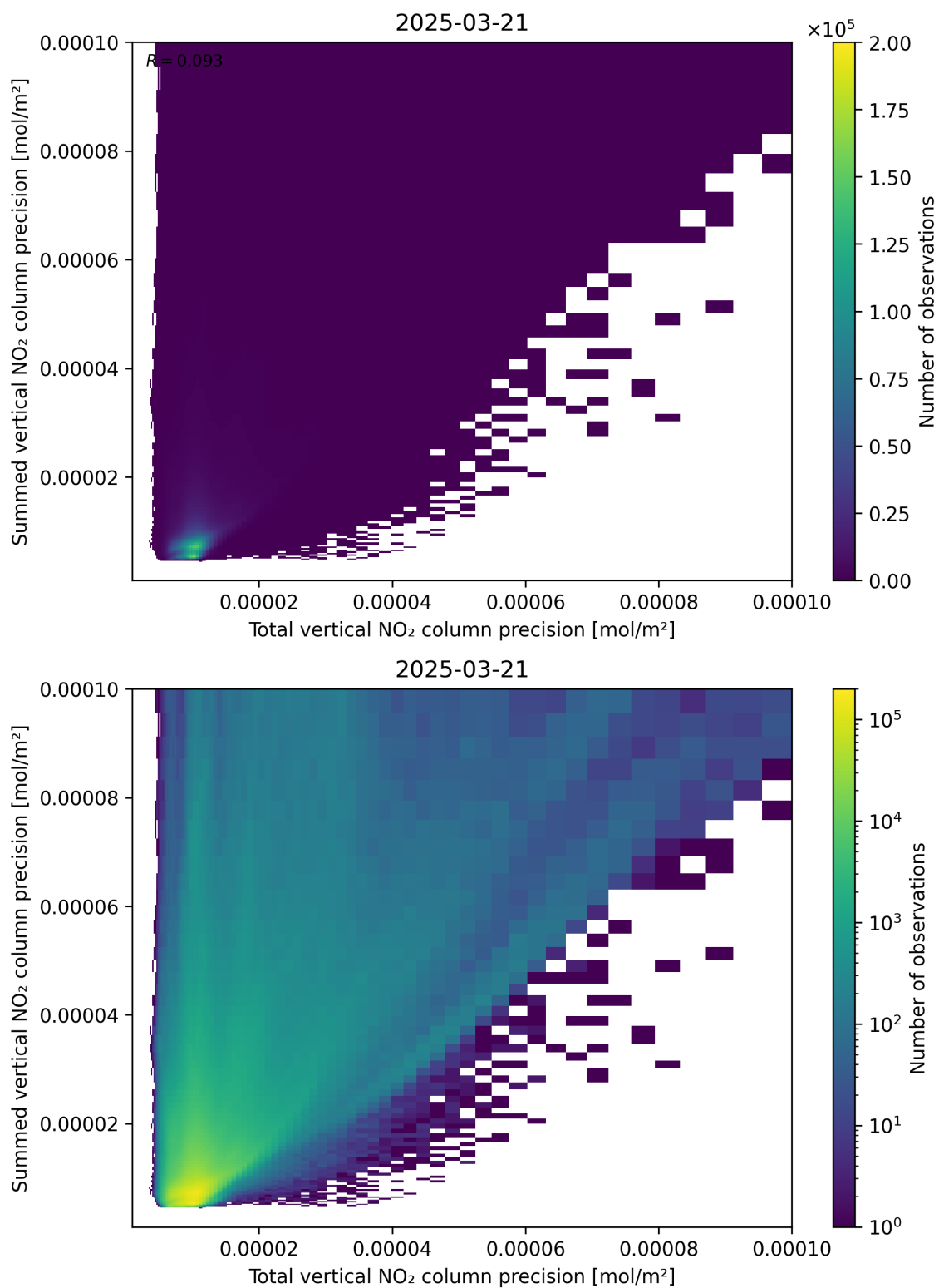
Figure 118: Scatter density plot of “Total vertical NO 2 column precision” against “Summed vertical NO 2 column precision” for 2025-03-21 to 2025-03-21.
