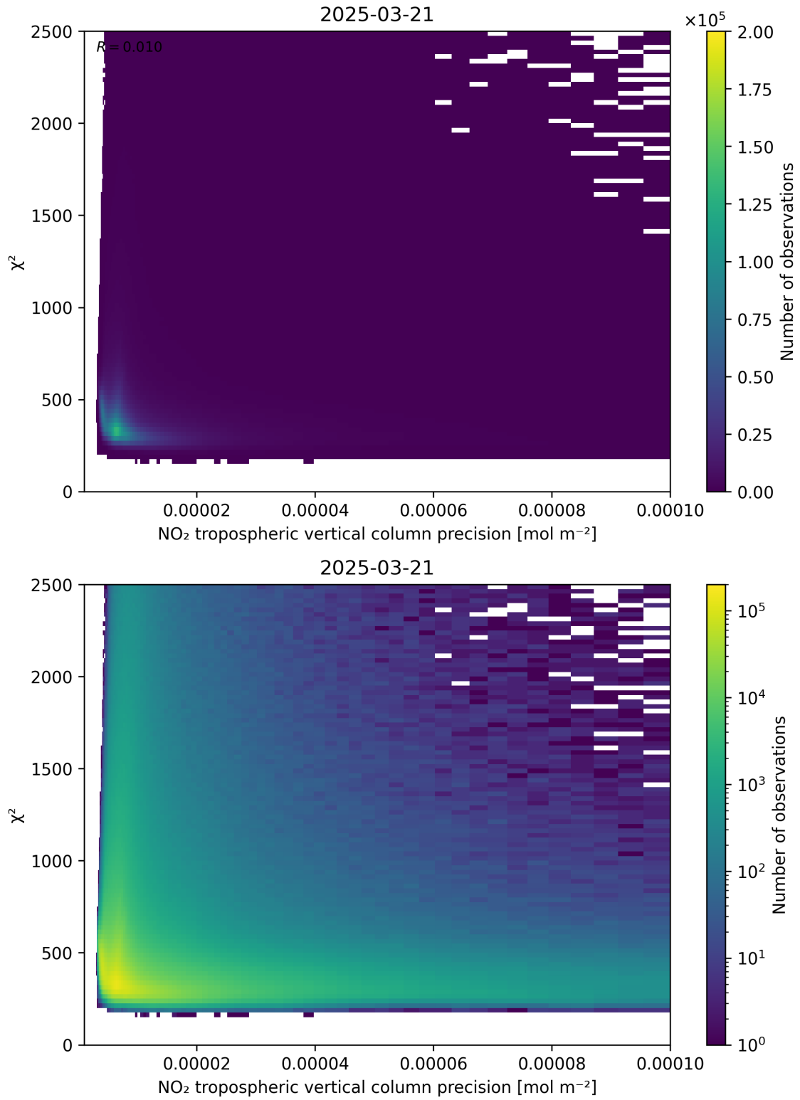
Figure 134: Scatter density plot of “NO 2 tropospheric vertical column precision” against “ \chi^2 ” for 2025-03-21 to 2025-03-21.
