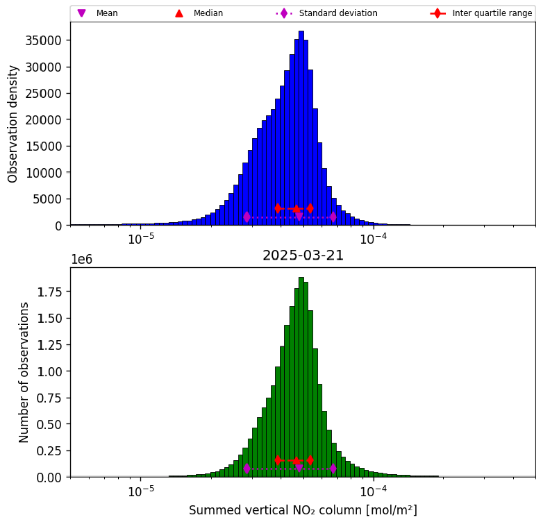
Figure 40: Histogram of “Summed vertical NO 2 column” for 2025-03-21 to 2025-03-21
