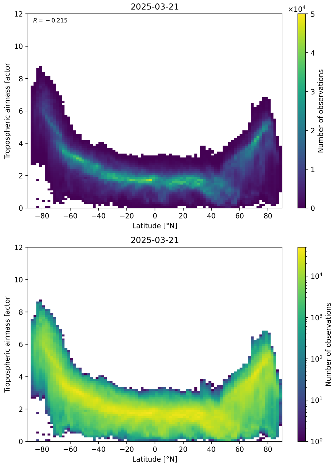
Figure 85: Scatter density plot of “Latitude” against “Tropospheric airmass factor” for 2025-03-21 to 2025-03-21.
