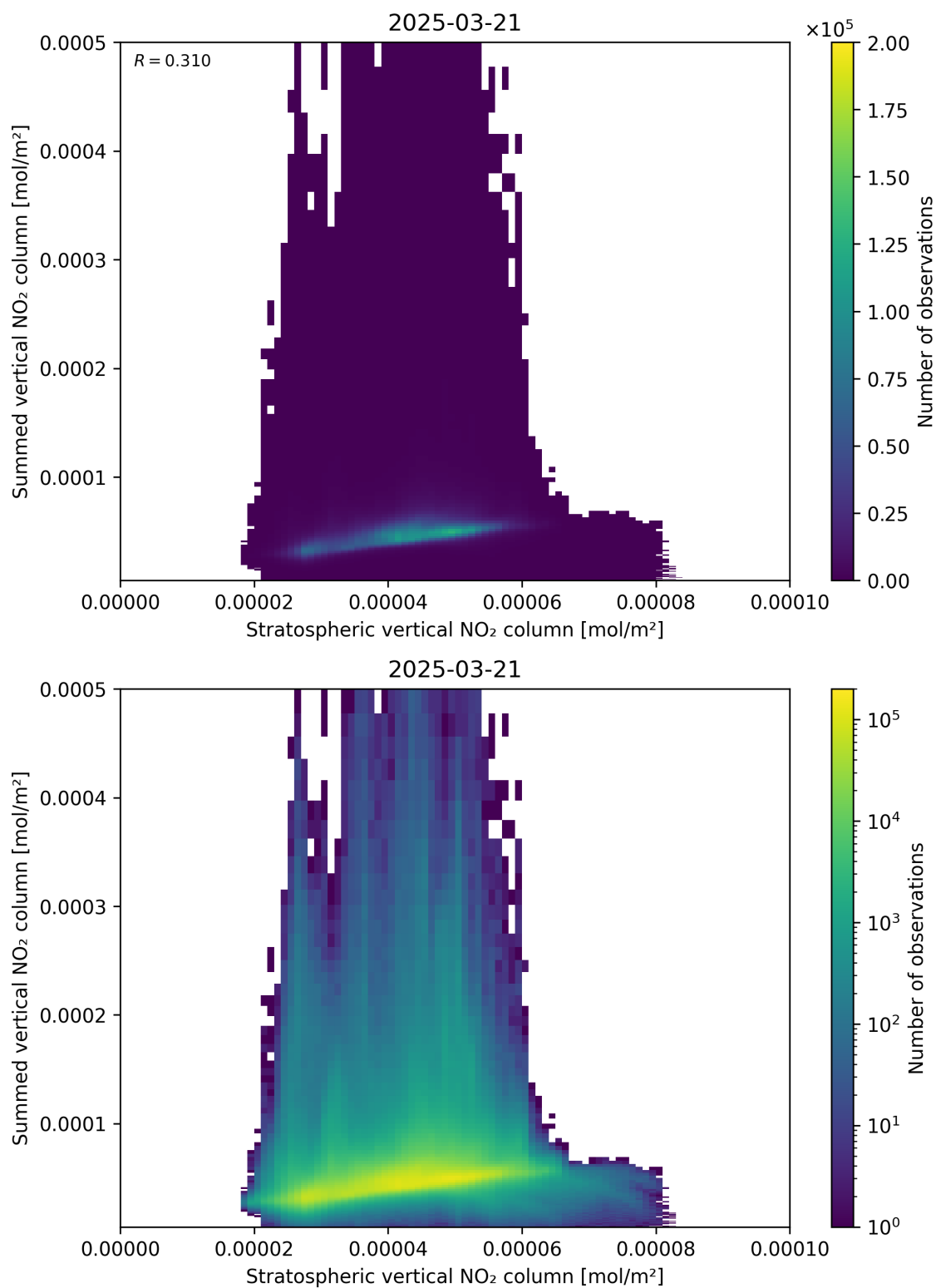
Figure 98: Scatter density plot of “Stratospheric vertical NO 2 column” against “Summed vertical NO 2 column” for 2025-03-21 to 2025-03-21.
