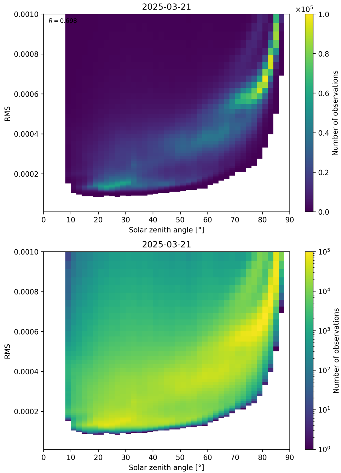
Figure 157: Scatter density plot of “Solar zenith angle” against “RMS” for 2025-03-21 to 2025-03-21.
