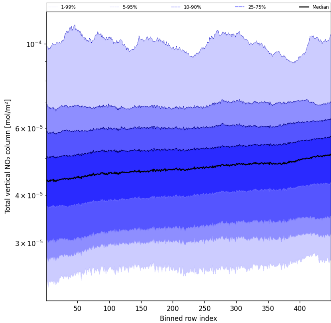
Figure 55: Along track statistics of “Total vertical NO 2 column” for 2025-03-21 to 2025-03-21
