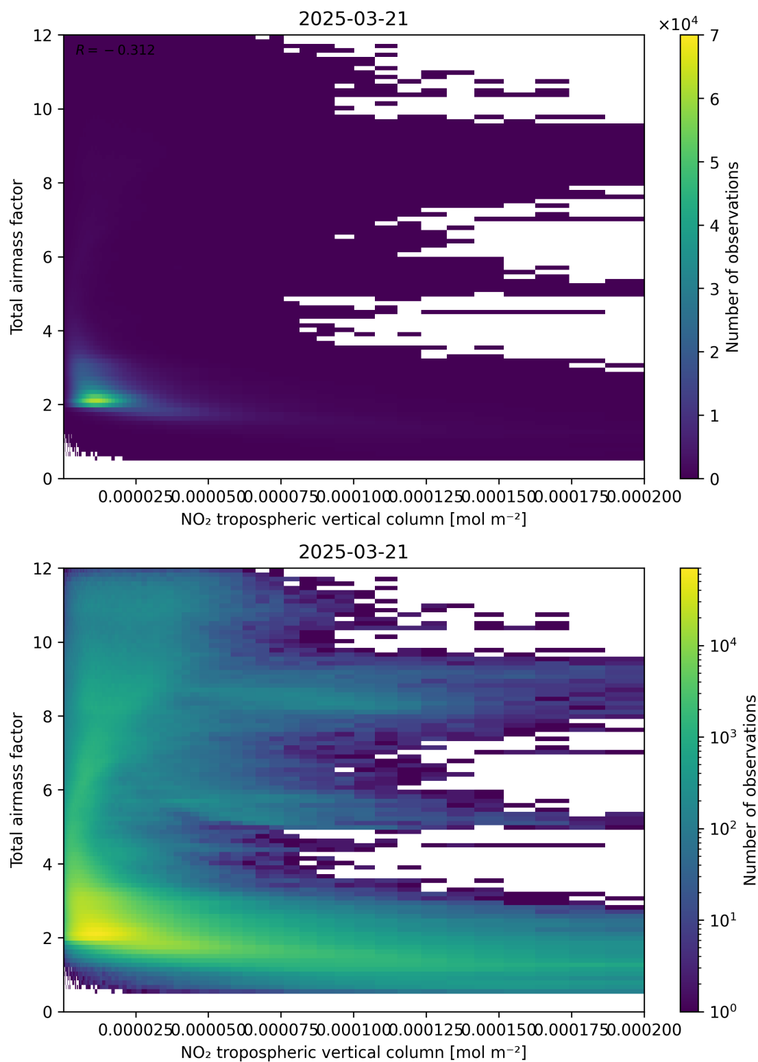
Figure 122: Scatter density plot of “NO 2 tropospheric vertical column” against “Total air mass factor” for 2025-03-21 to 2025-03-21.
