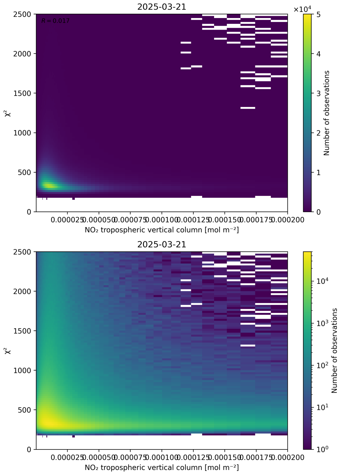
Figure 124: Scatter density plot of “NO 2 tropospheric vertical column” against “ \chi^2 ” for 2025-03-21 to 2025-03-21.
