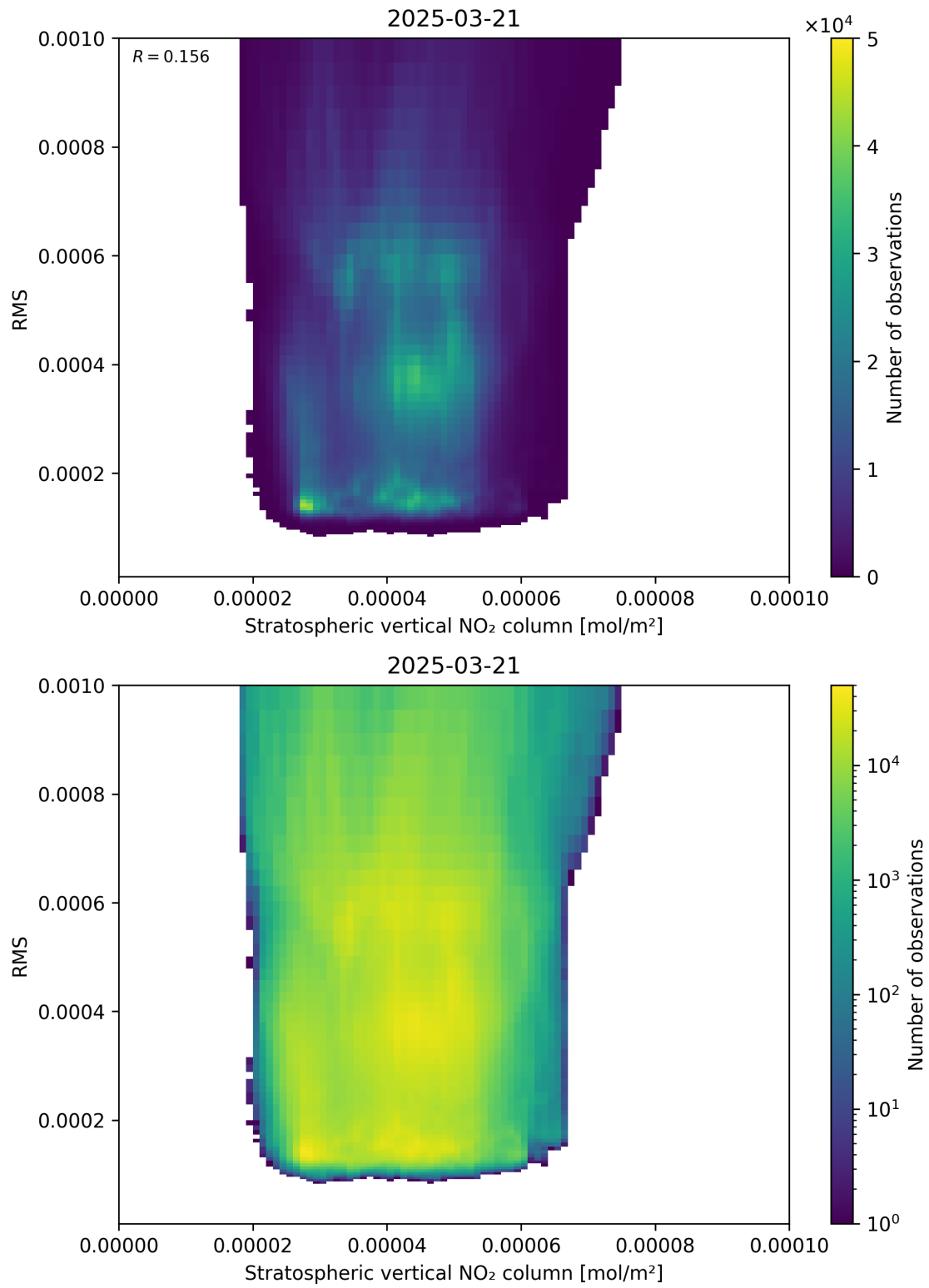
Figure 102: Scatter density plot of “Stratospheric vertical NO 2 column” against “RMS” for 2025-03-21 to 2025-03-21.
