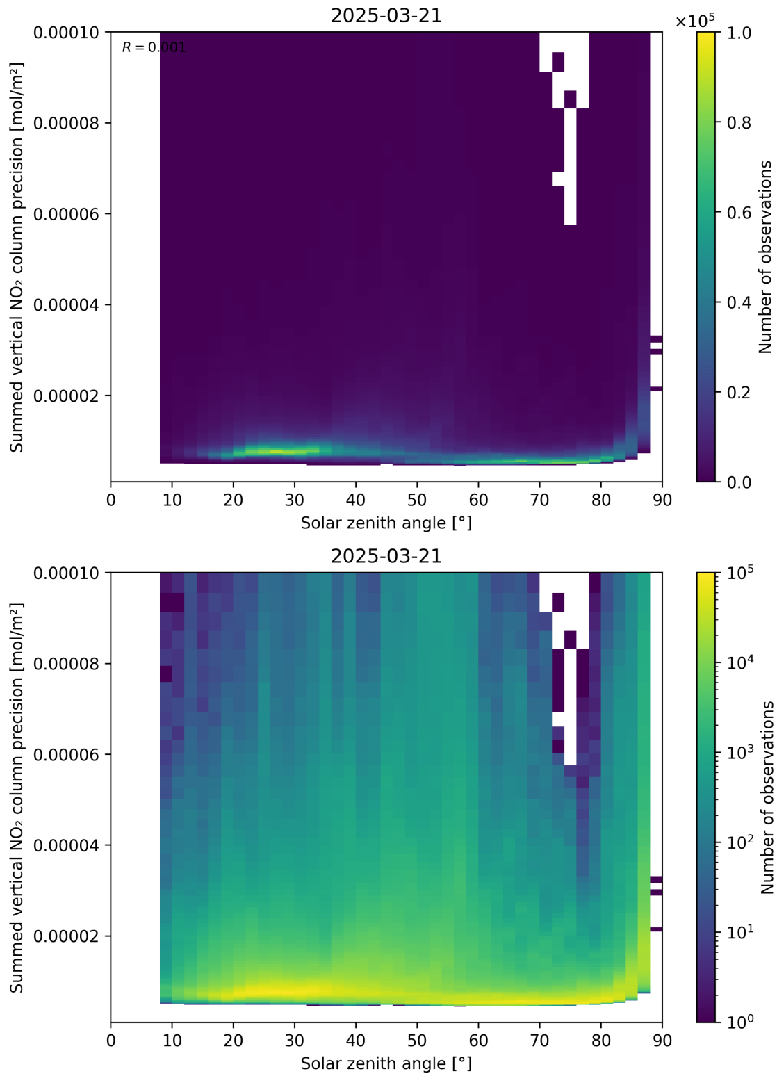
Figure 152: Scatter density plot of “Solar zenith angle” against “Summed vertical NO 2 column precision” for 2025-03-21 to 2025-03-21.
