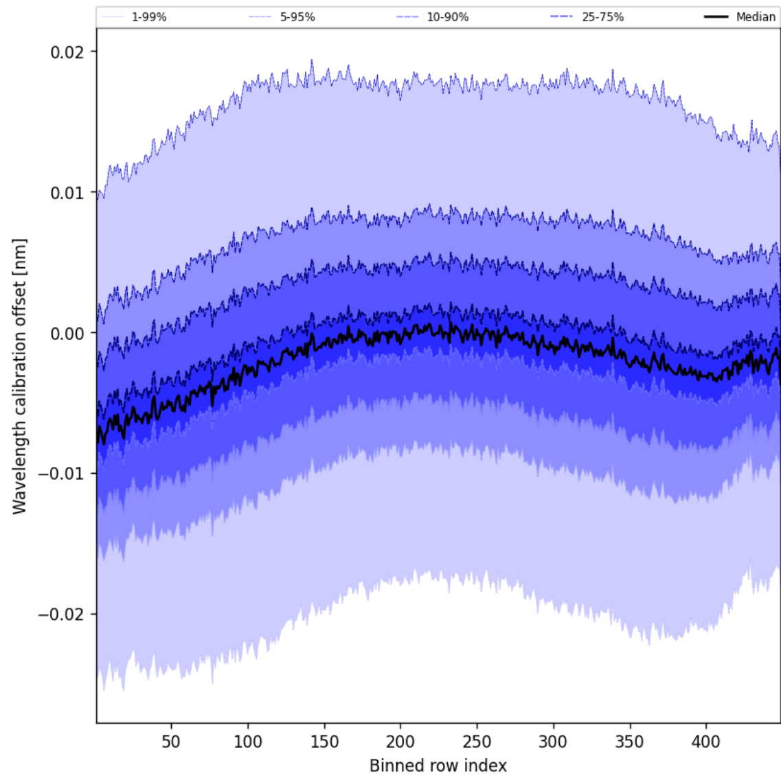
Figure 52: Along track statistics of “Wavelength calibration offset” for 2025-03-21 to 2025-03-21
