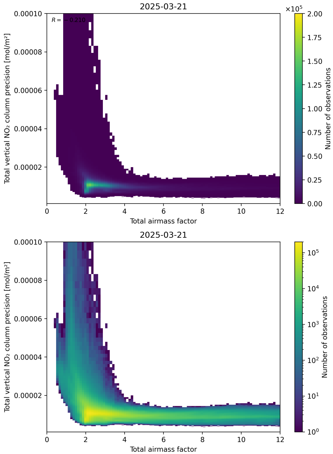
Figure 68: Scatter density plot of “Total airmass factor” against “Total vertical NO 2 column precision” for 2025-03-21 to 2025-03-21.
