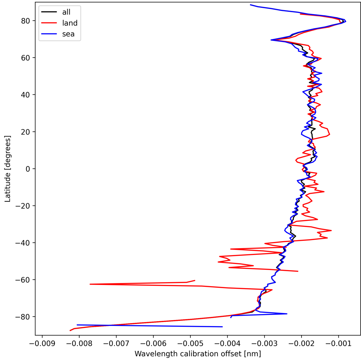
Figure 18: Zonal average of “Wavelength calibration offset” for 2025-03-21 to 2025-03-21.
