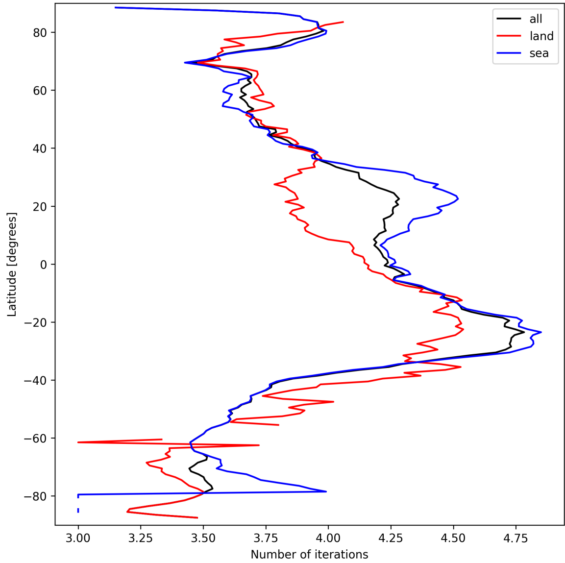
Figure 17: Zonal average of “Number of iterations” for 2025-03-21 to 2025-03-21.
