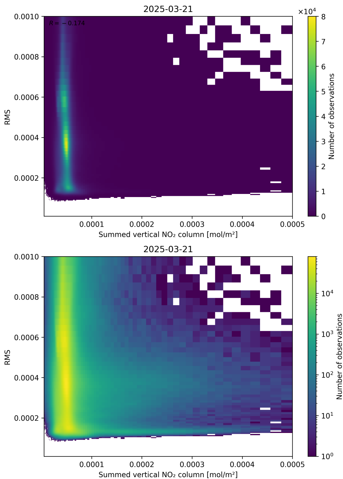
Figure 109: Scatter density plot of “Summed vertical NO 2 column” against “RMS” for 2025-03-21 to 2025-03-21.
