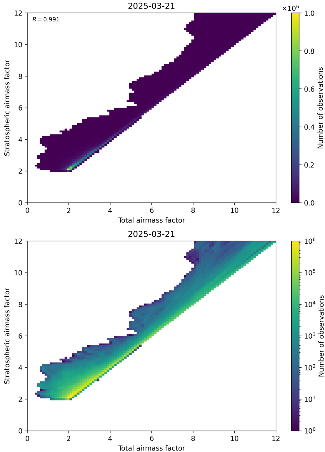
Figure 62: Scatter density plot of “Total airmass factor” against “Stratospheric airmass factor” for 2025-03-21 to 2025-03-21.
