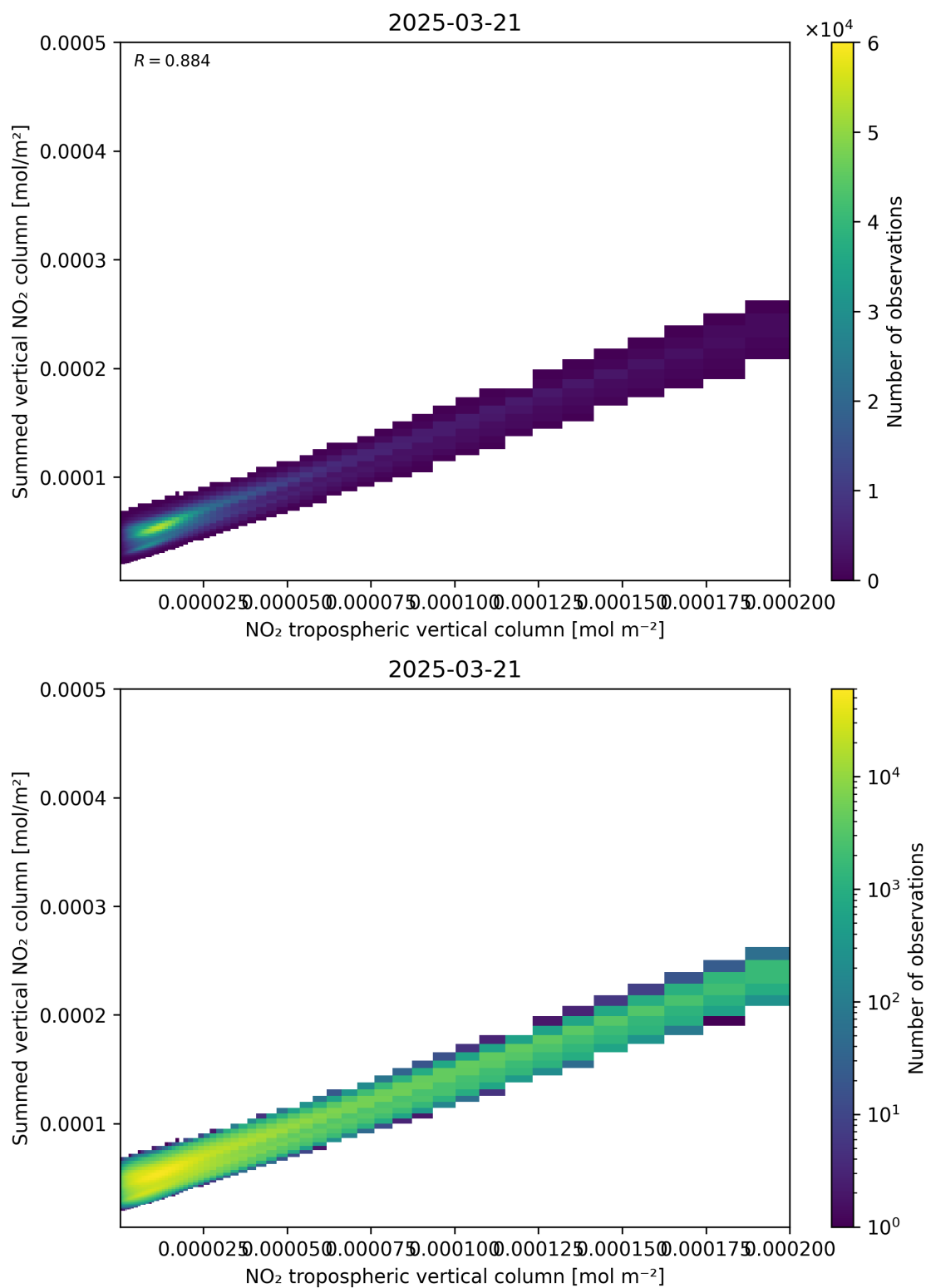
Figure 126: Scatter density plot of “NO 2 tropospheric vertical column” against “Summed vertical NO 2 column” for 2025-03-21 to 2025-03-21.
