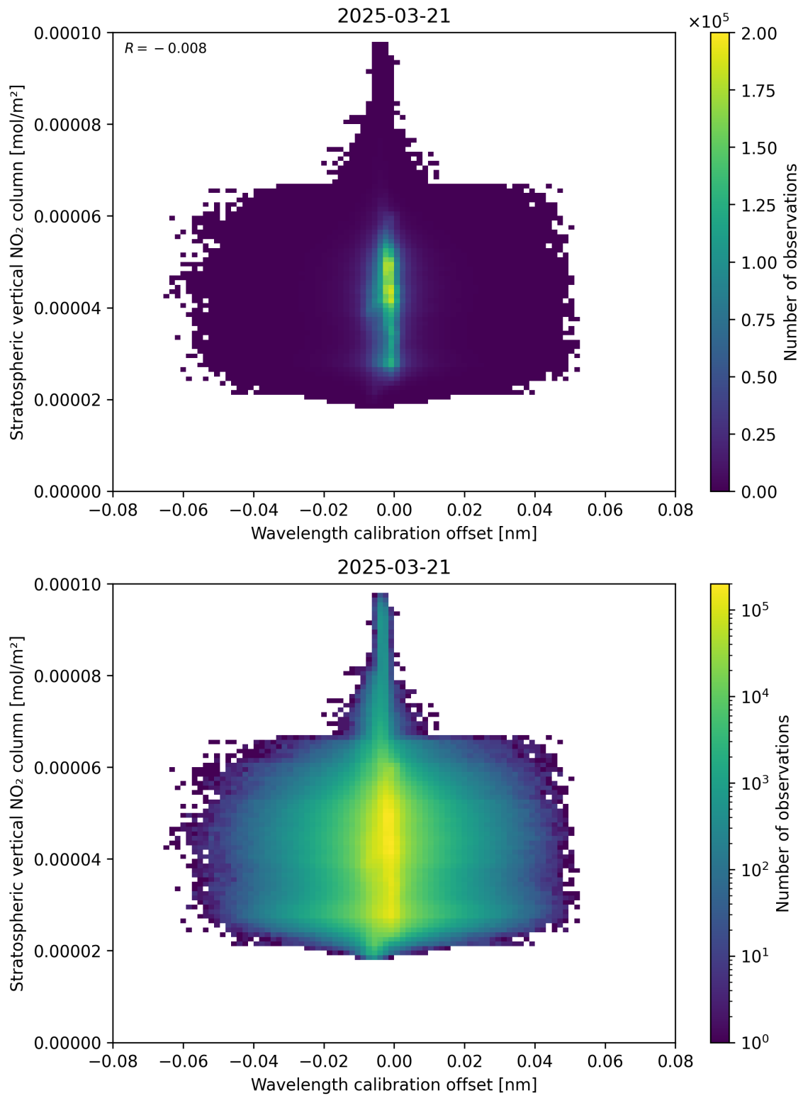
Figure 176: Scatter density plot of “Wavelength calibration offset” against “Stratospheric vertical NO 2 column” for 2025-03-21 to 2025-03-21.
