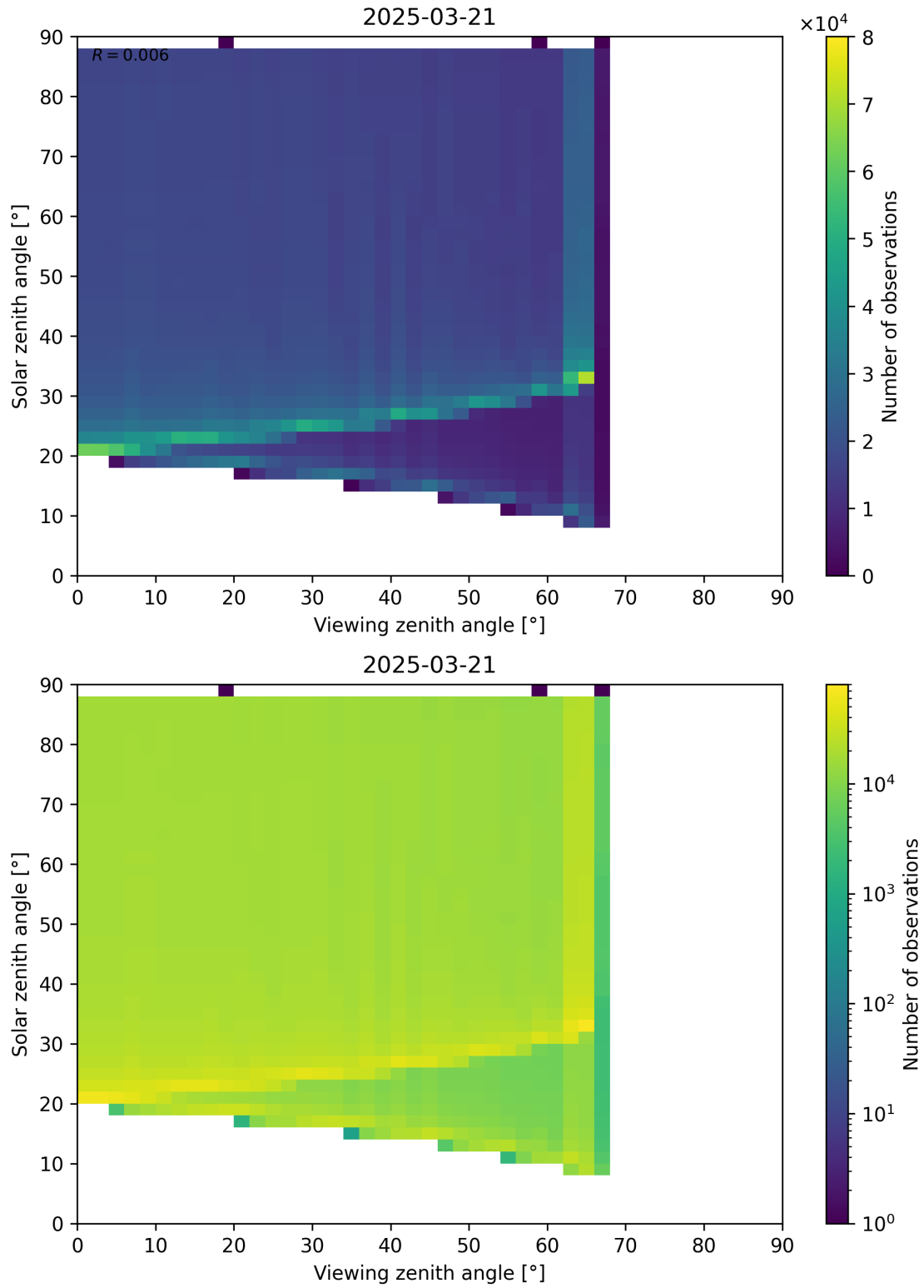
Figure 172: Scatter density plot of “Viewing zenith angle” against “Solar zenith angle” for 2025-03-21 to 2025-03-21.
