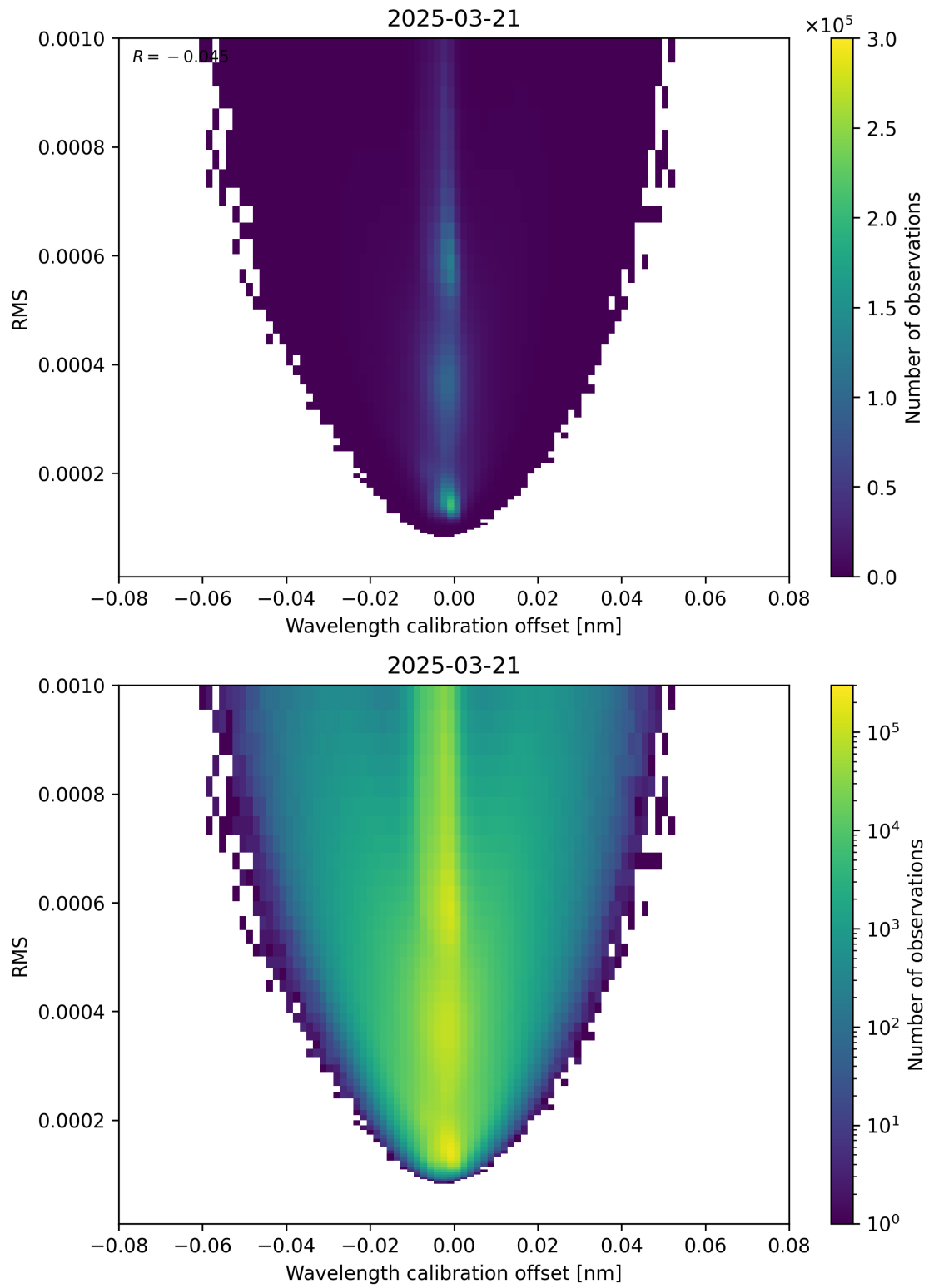
Figure 181: Scatter density plot of “Wavelength calibration offset” against “RMS” for 2025-03-21 to 2025-03-21.
