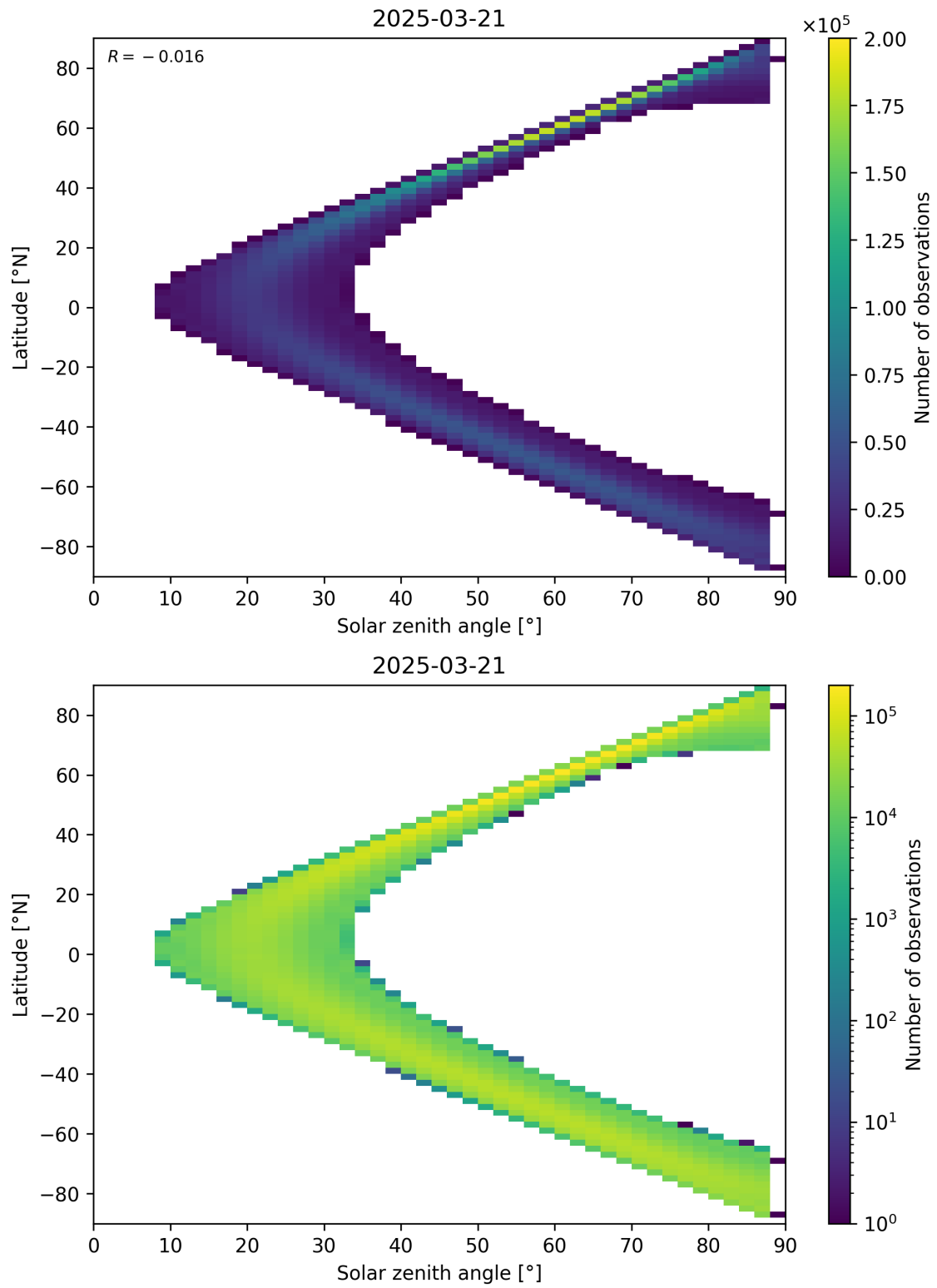
Figure 149: Scatter density plot of “Solar zenith angle” against “Latitude” for 2025-03-21 to 2025-03-21.
