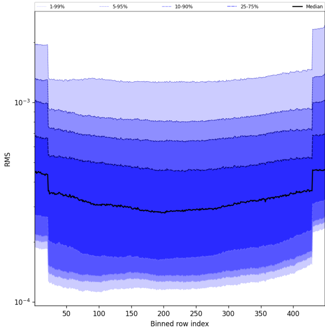
Figure 60: Along track statistics of “RMS” for 2025-03-21 to 2025-03-21
