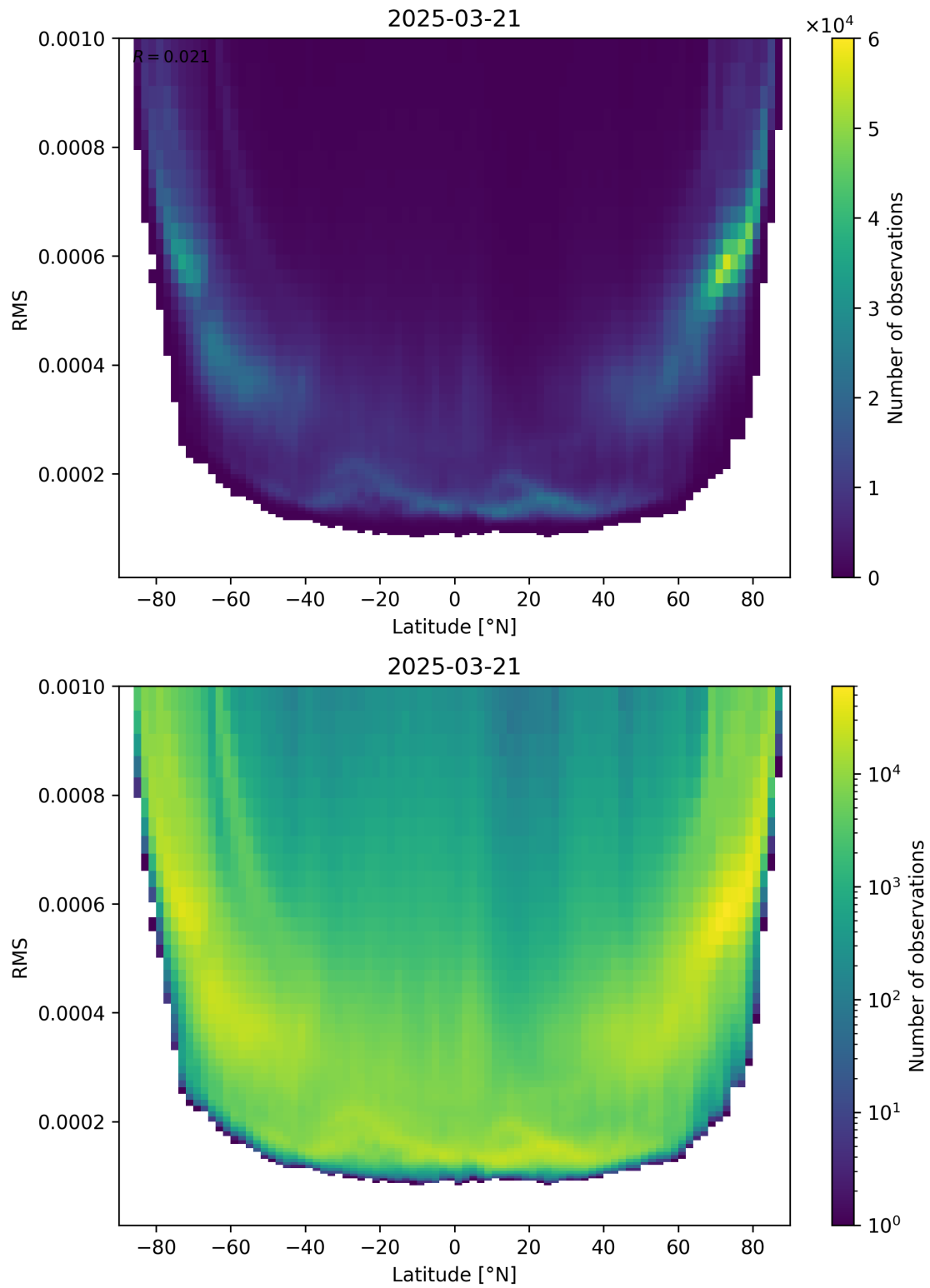
Figure 94: Scatter density plot of “Latitude” against “RMS” for 2025-03-21 to 2025-03-21.
