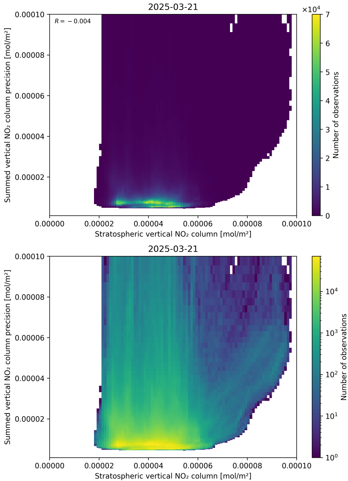
Figure 99: Scatter density plot of “Stratospheric vertical NO 2 column” against “Summed vertical NO 2 column precision” for 2025-03-21 to 2025-03-21.
