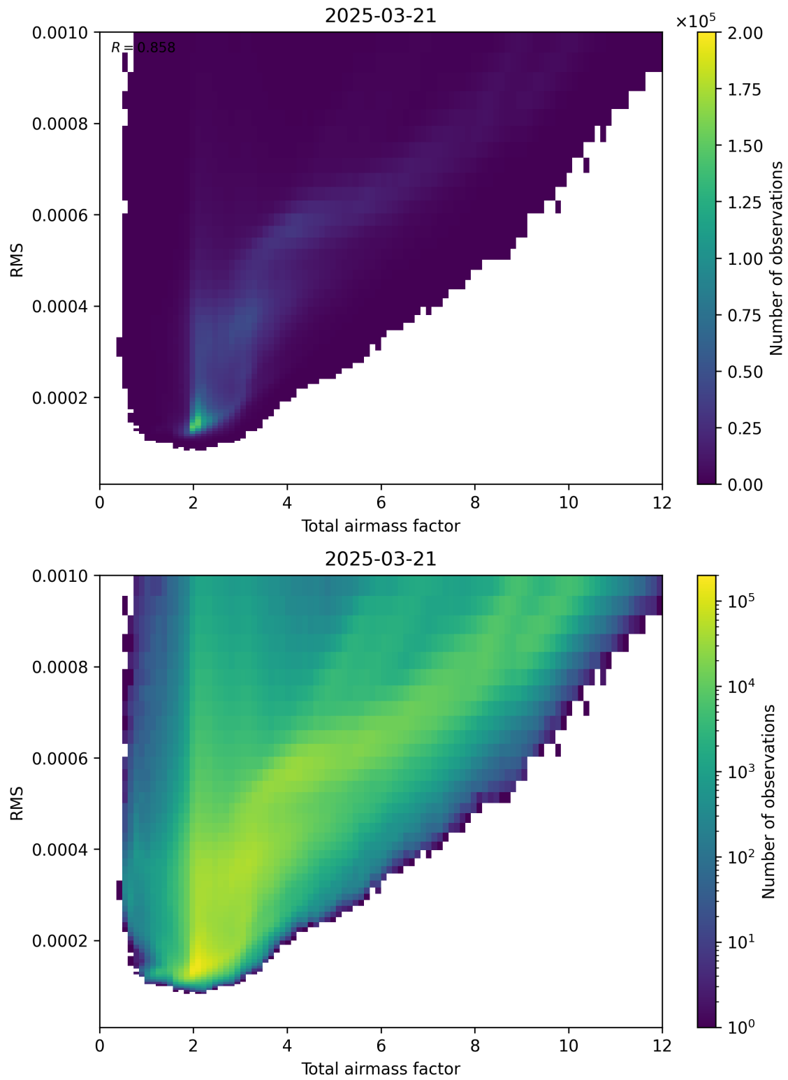
Figure 69: Scatter density plot of “Total airmass factor” against “RMS” for 2025-03-21 to 2025-03-21.
