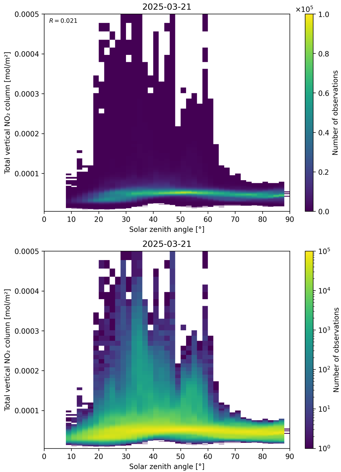
Figure 153: Scatter density plot of “Solar zenith angle” against “Total vertical NO 2 column” for 2025-03-21 to 2025-03-21.
