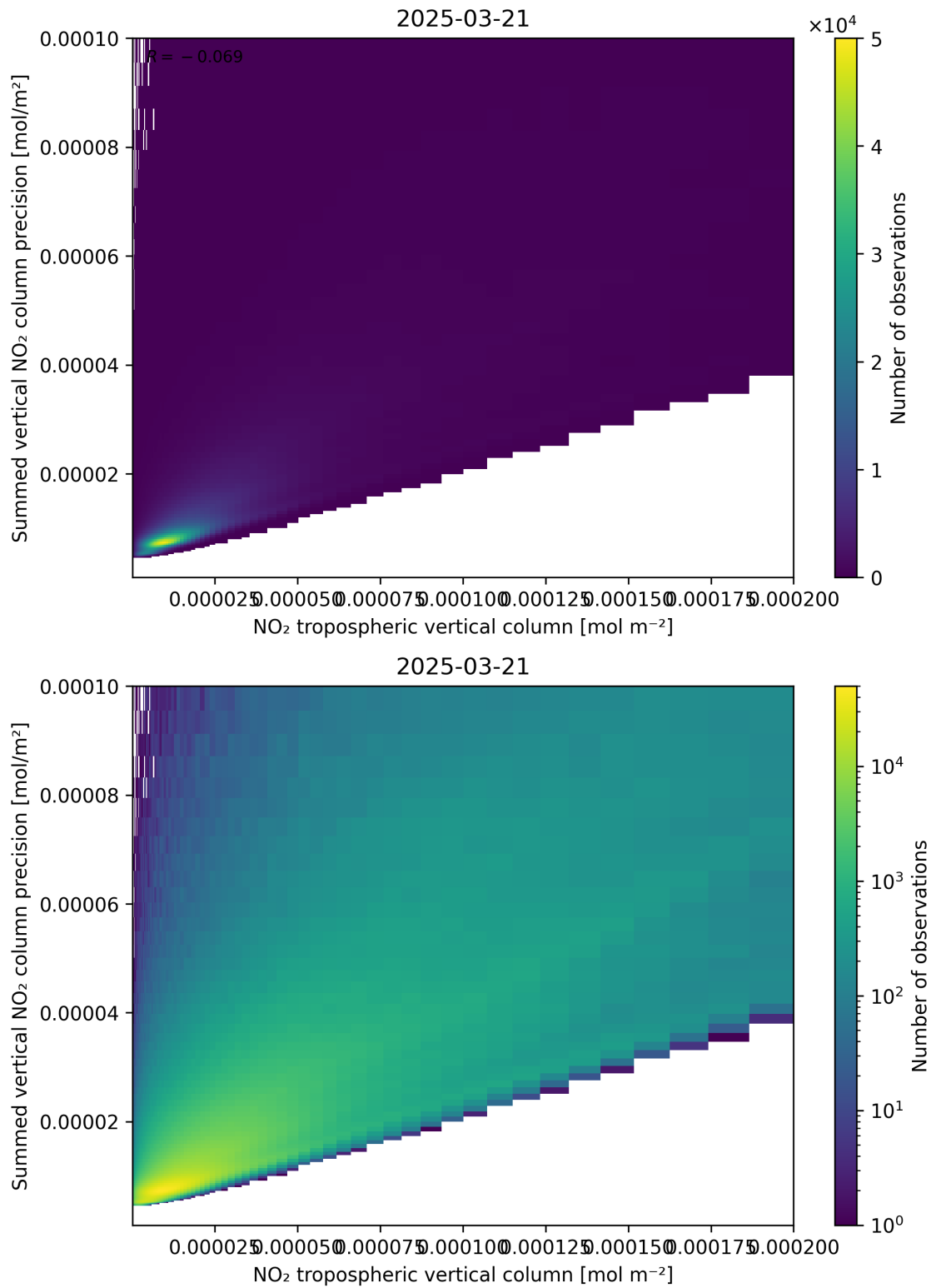
Figure 127: Scatter density plot of “NO 2 tropospheric vertical column” against “Summed vertical NO 2 column precision” for 2025-03-21 to 2025-03-21.
