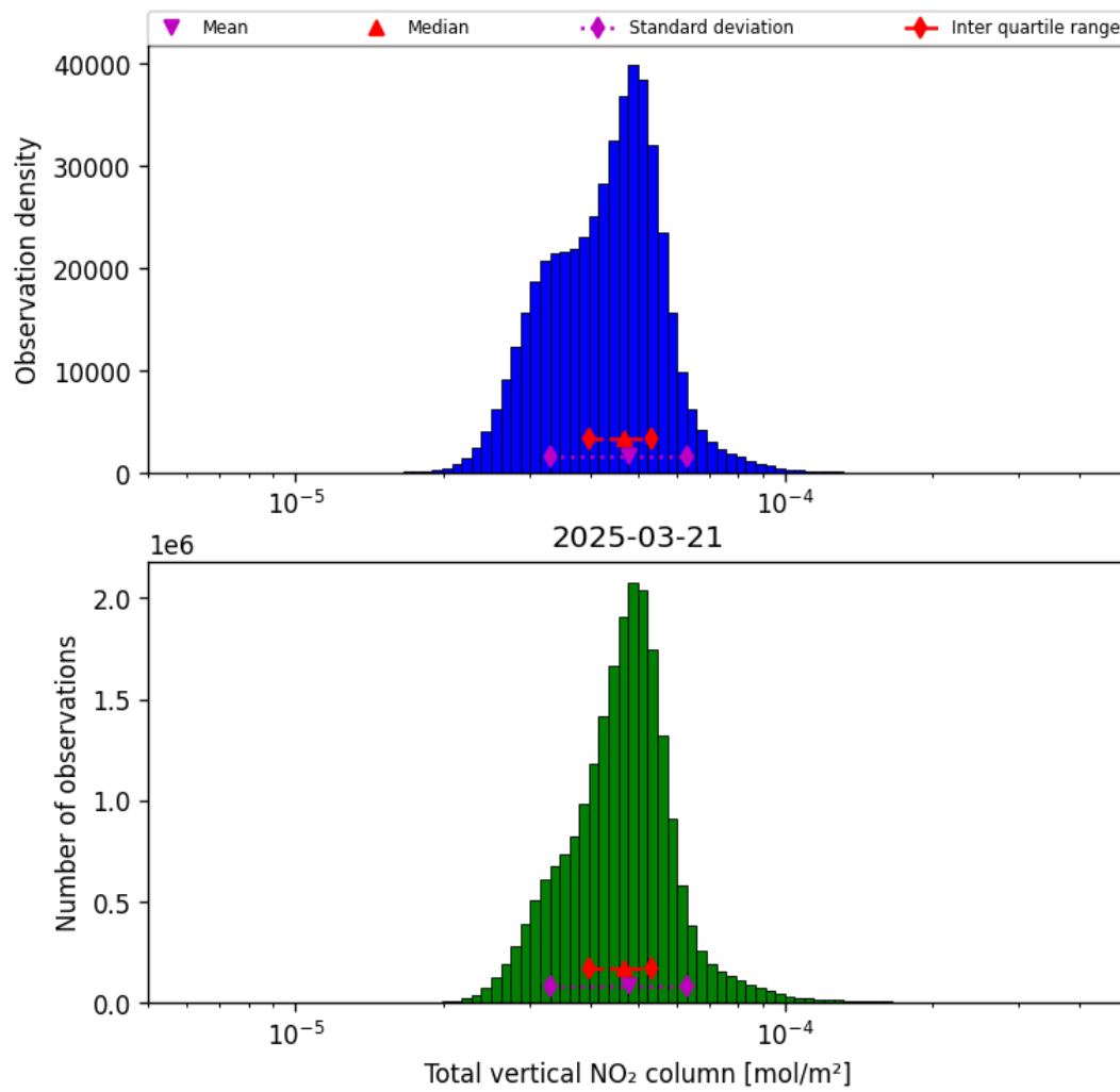
Figure 38: Histogram of “Total vertical NO 2 column” for 2025-03-21 to 2025-03-21
