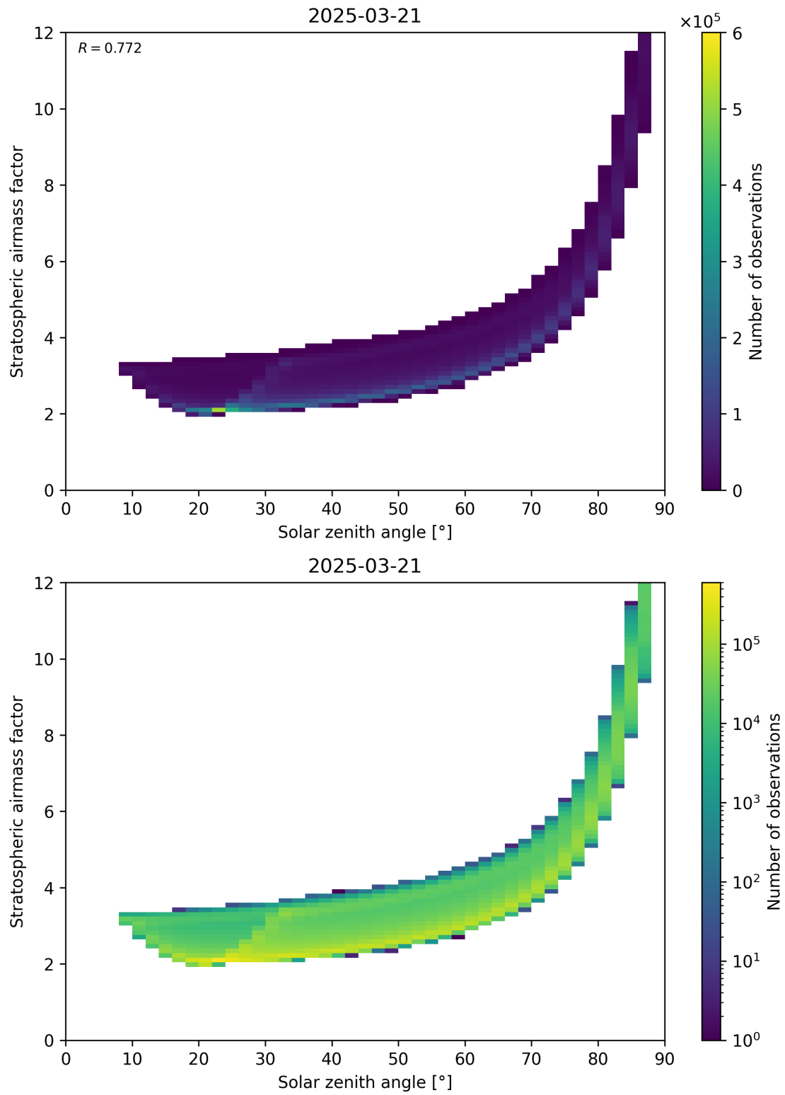
Figure 145: Scatter density plot of “Solar zenith angle” against “Stratospheric airmass factor” for 2025-03-21 to 2025-03-21.
