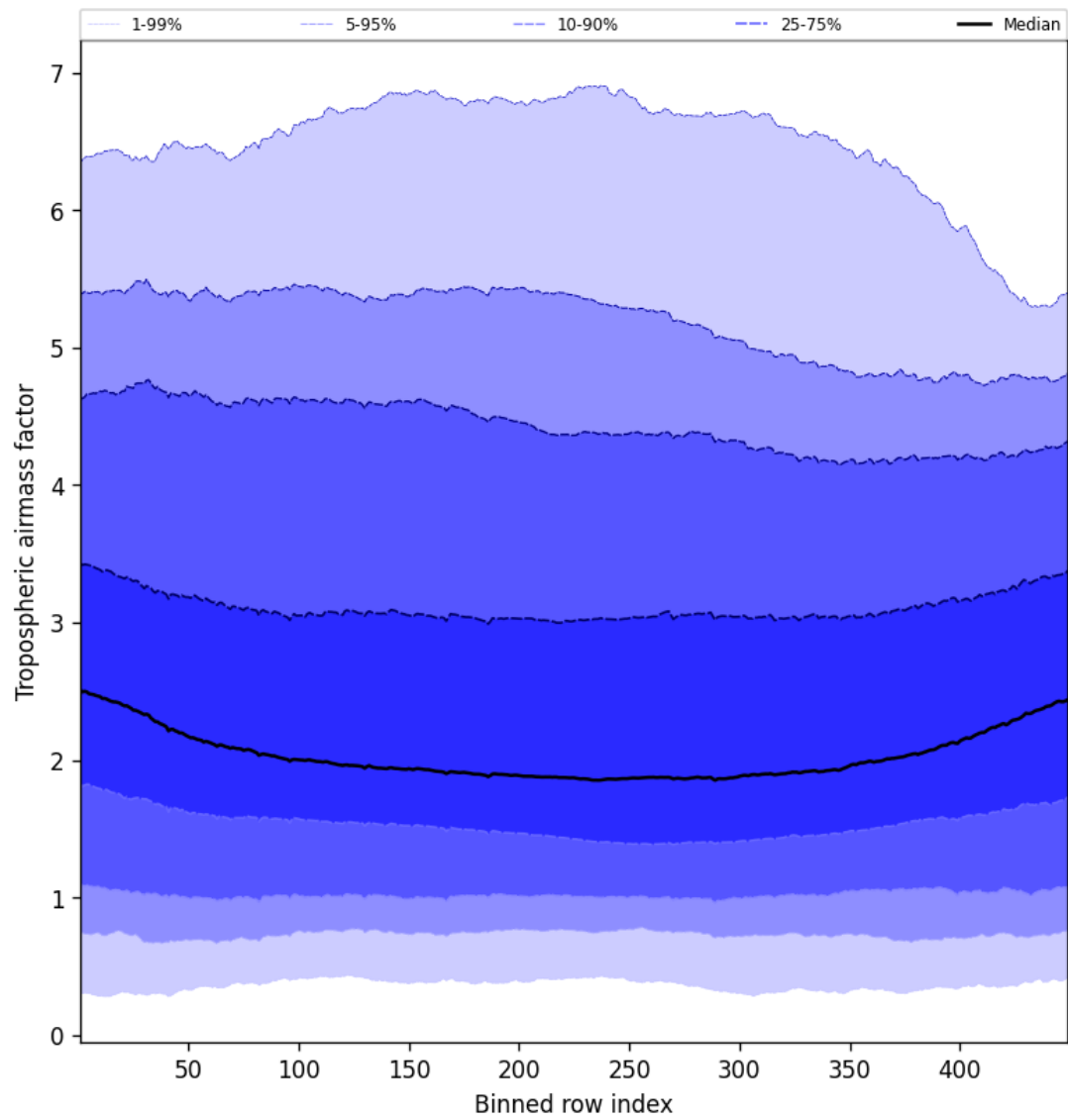
Figure 48: Along track statistics of “Tropospheric airmass factor” for 2025-03-21 to 2025-03-21
