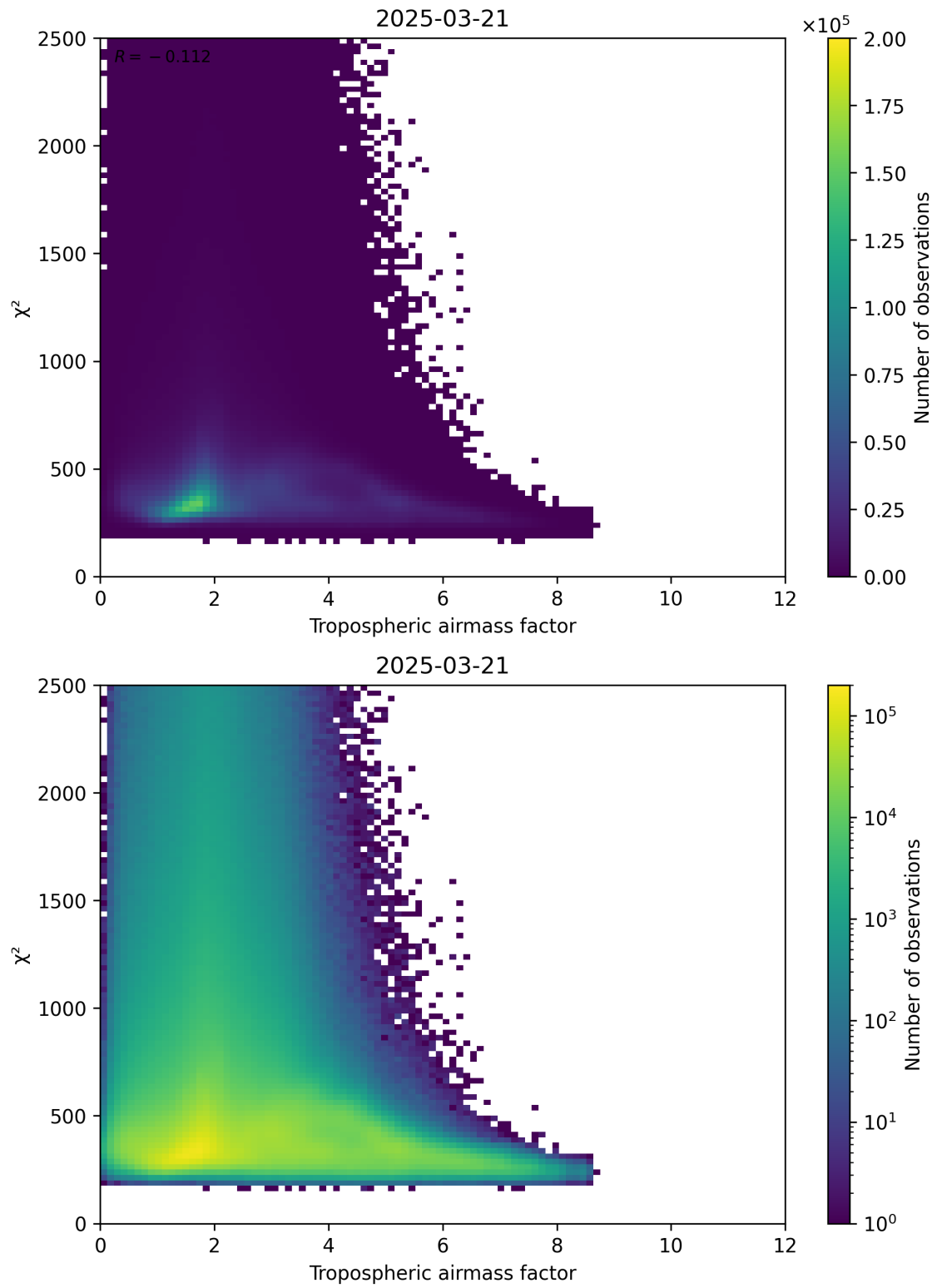
Figure 73: Scatter density plot of “Tropospheric airmass factor” against “ \chi^2 ” for 2025-03-21 to 2025-03-21.
