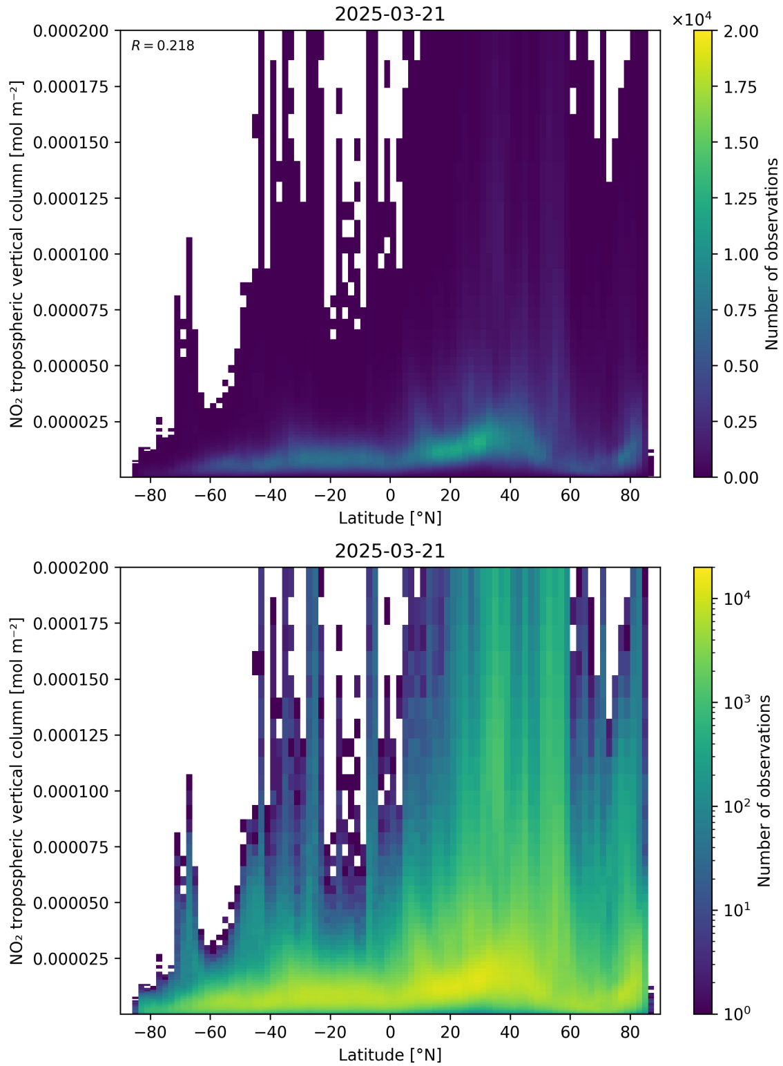
Figure 92: Scatter density plot of “Latitude” against “NO 2 tropospheric vertical column” for 2025-03-21 to 2025-03-21.
