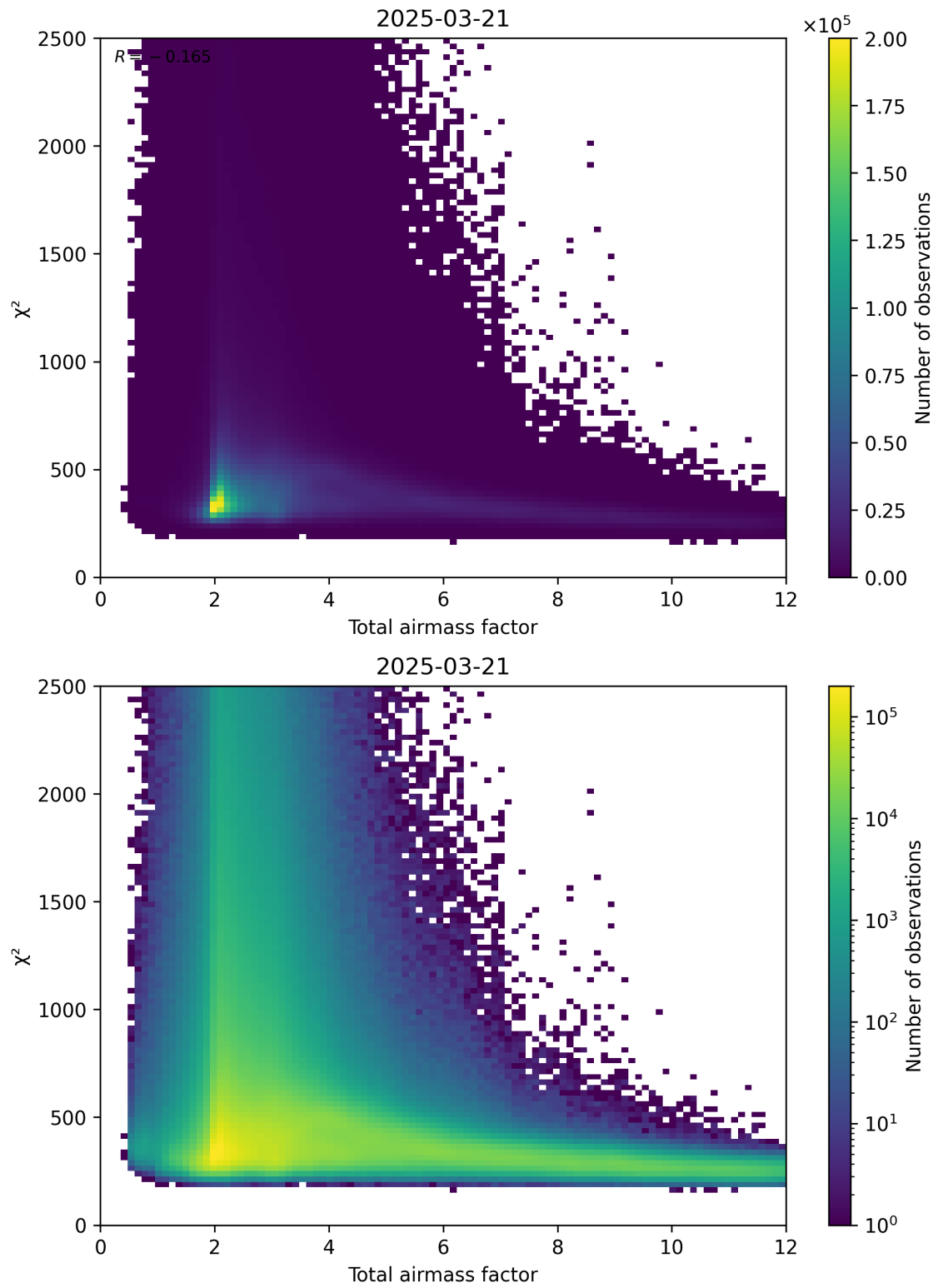
Figure 63: Scatter density plot of “Total airmass factor” against “ \chi^2 ” for 2025-03-21 to 2025-03-21.
