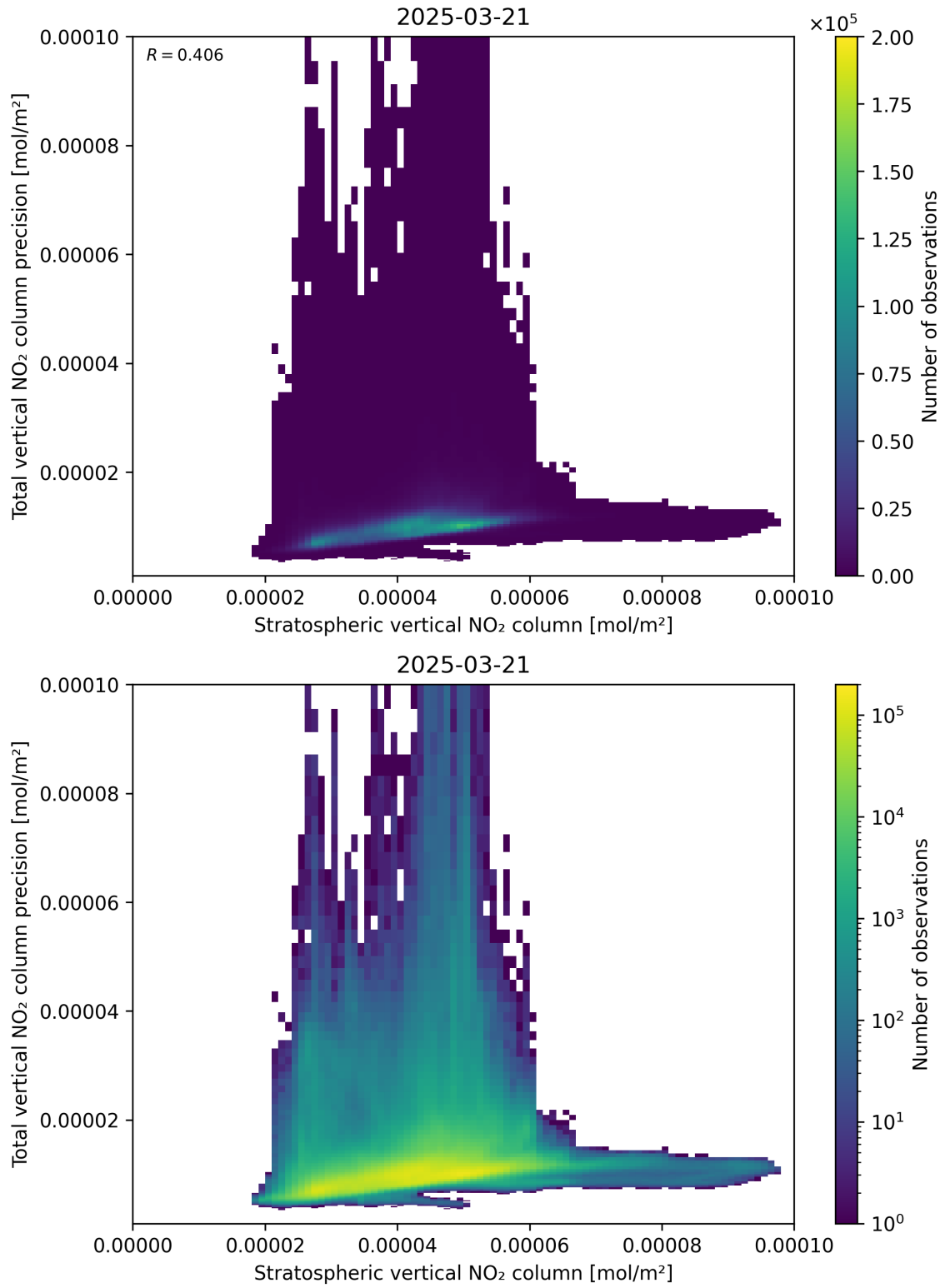
Figure 101: Scatter density plot of “Stratospheric vertical NO 2 column” against “Total vertical NO 2 column precision” for 2025-03-21 to 2025-03-21.
