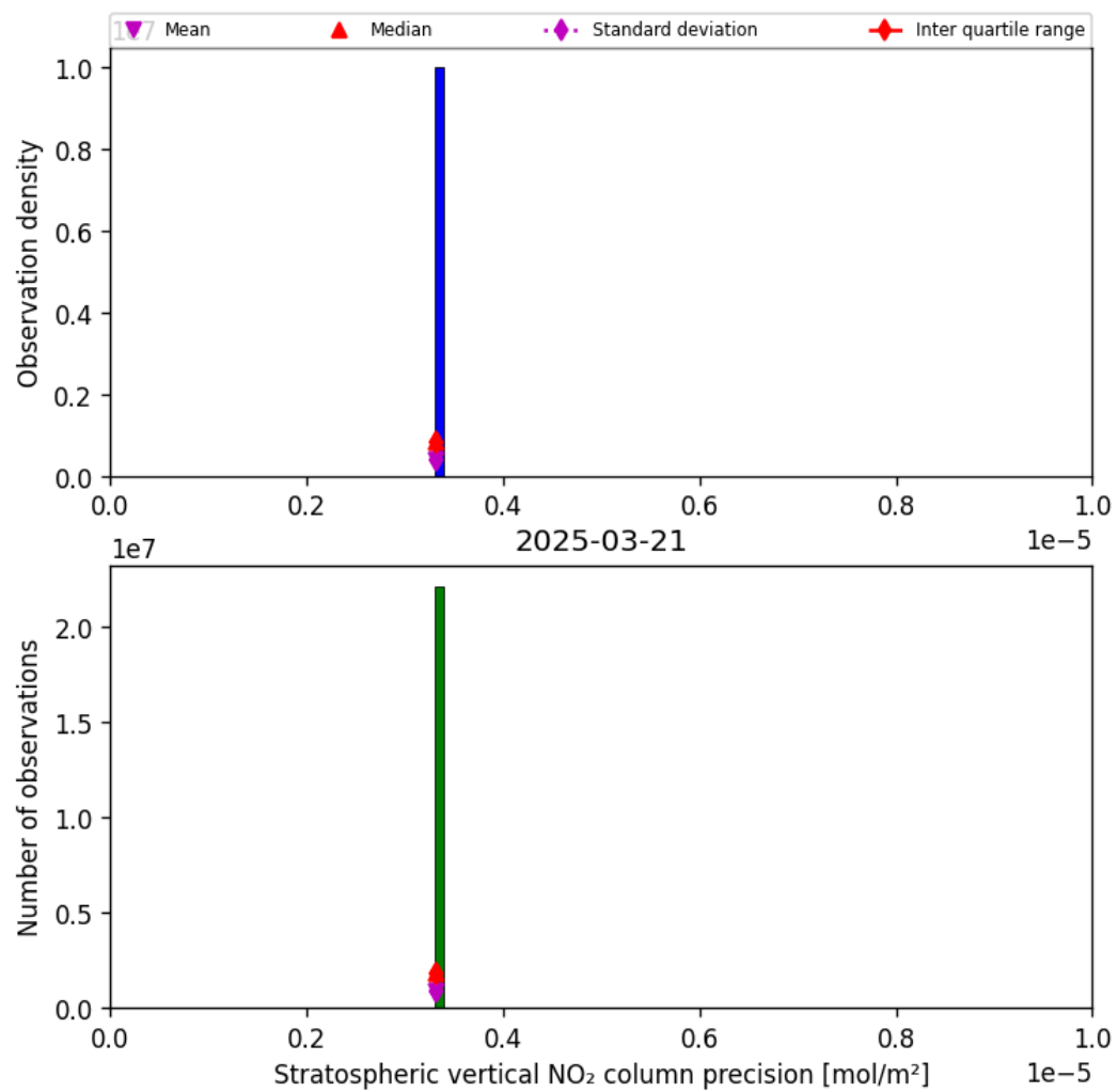
Figure 37: Histogram of “Stratospheric vertical NO 2 column precision” for 2025-03-21 to 2025-03-21
