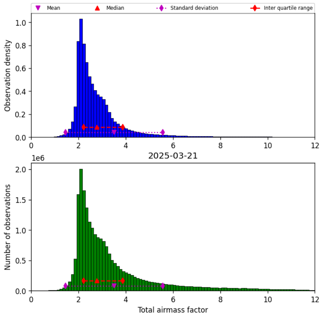
Figure 32: Histogram of “Total airmass factor” for 2025-03-21 to 2025-03-21
