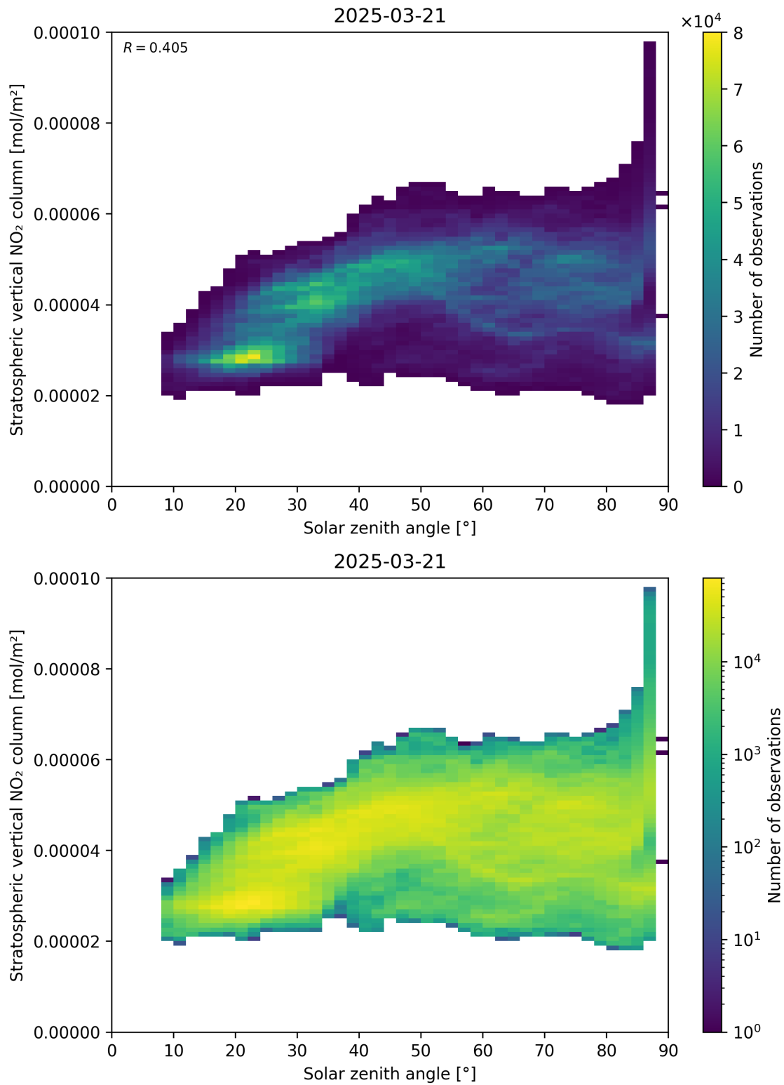
Figure 150: Scatter density plot of “Solar zenith angle” against “Stratospheric vertical NO 2 column” for 2025-03-21 to 2025-03-21.
