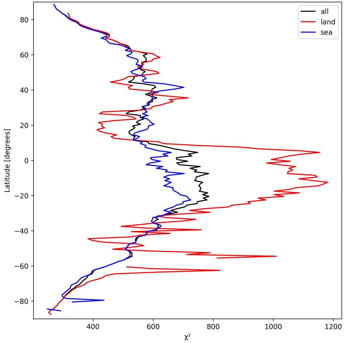
Figure 25: Zonal average of “ \chi^2 ” for 2025-03-21 to 2025-03-21.
