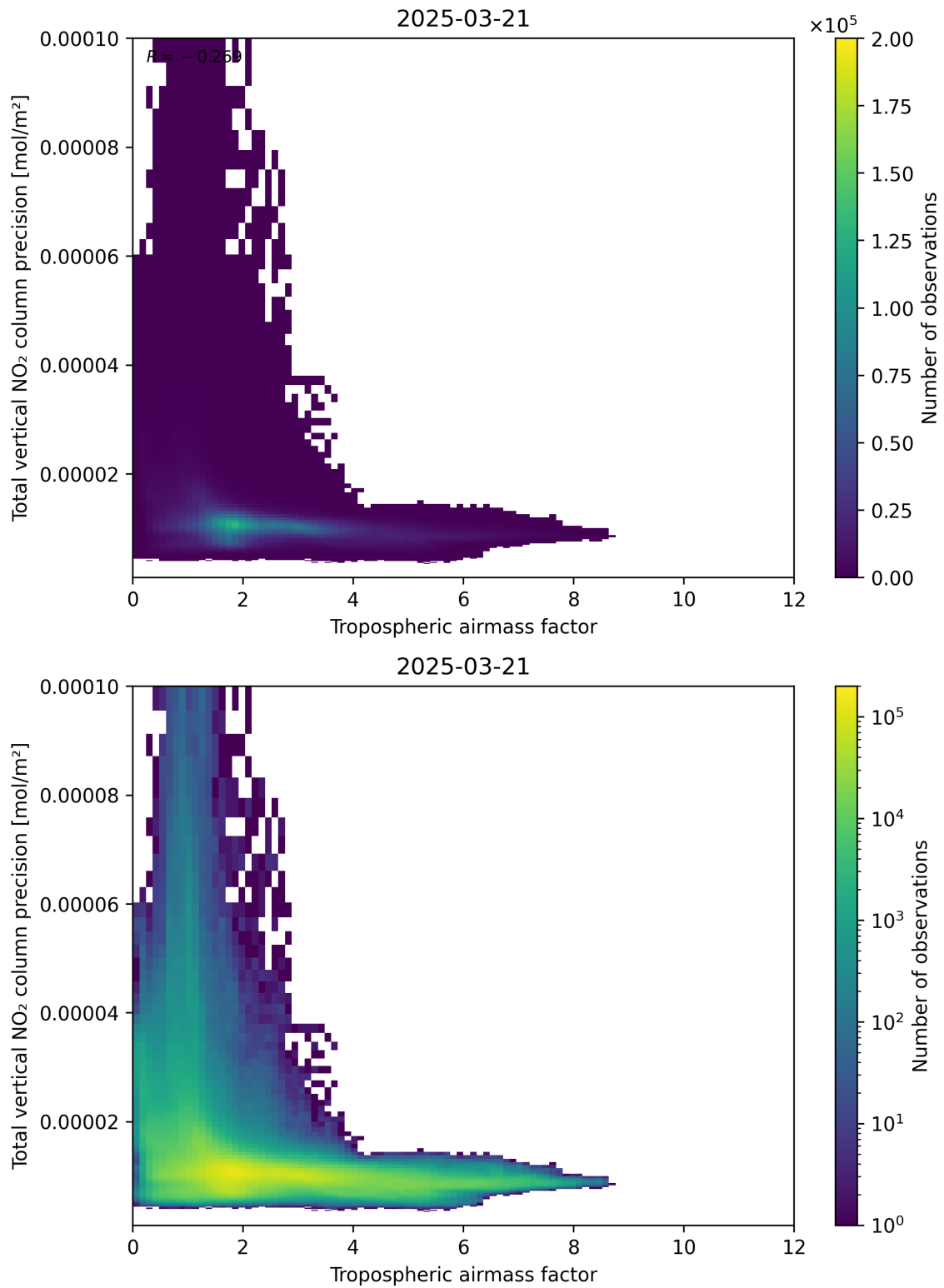
Figure 78: Scatter density plot of “Tropospheric airmass factor” against “Total vertical NO 2 column precision” for 2025-03-21 to 2025-03-21.
