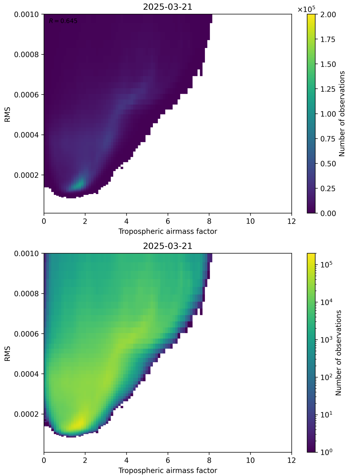
Figure 79: Scatter density plot of “Tropospheric airmass factor” against “RMS” for 2025-03-21 to 2025-03-21.
