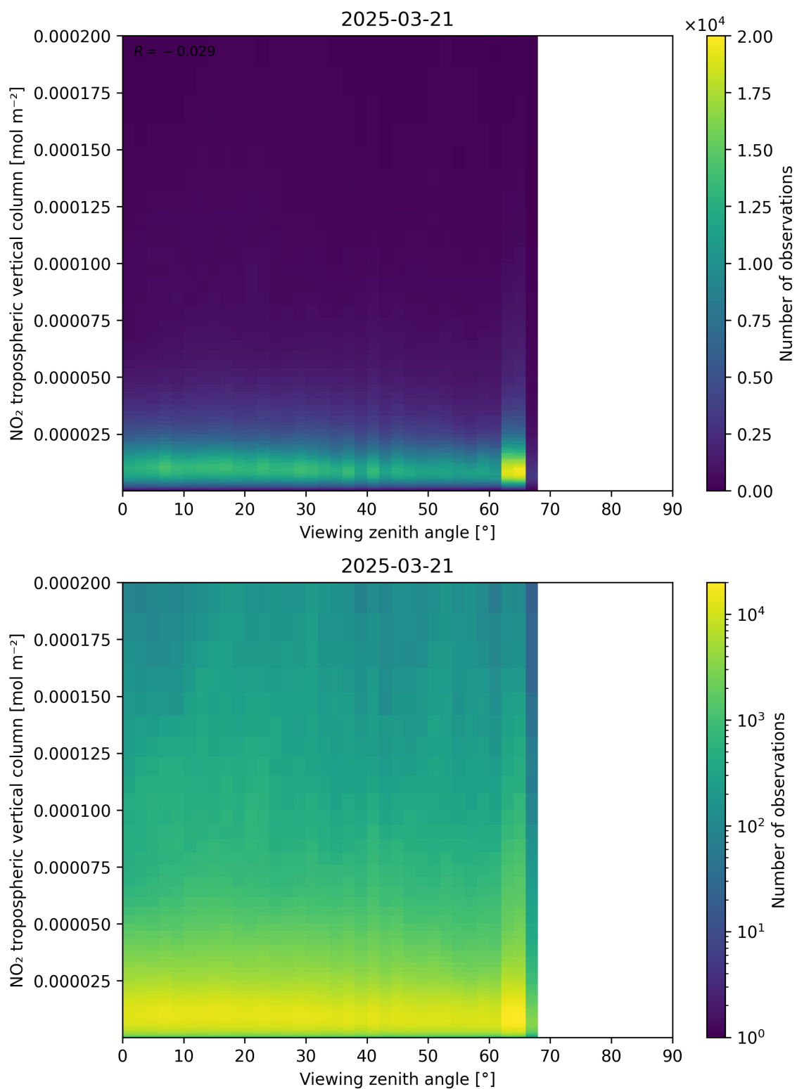
Figure 169: Scatter density plot of “Viewing zenith angle” against “NO 2 tropospheric vertical column” for 2025-03-21 to 2025-03-21.
