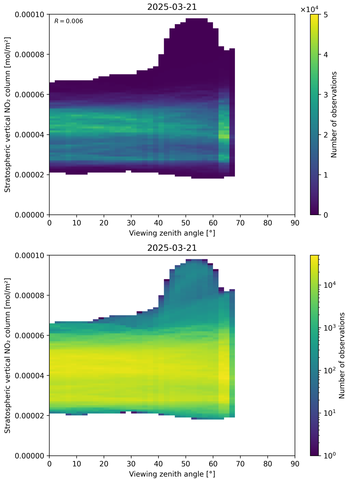
Figure 164: Scatter density plot of “Viewing zenith angle” against “Stratospheric vertical NO 2 column” for 2025-03-21 to 2025-03-21.
