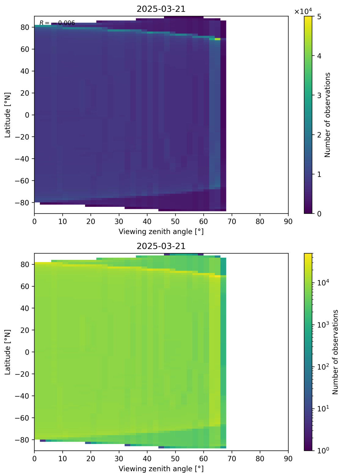
Figure 163: Scatter density plot of “Viewing zenith angle” against “Latitude” for 2025-03-21 to 2025-03-21.
