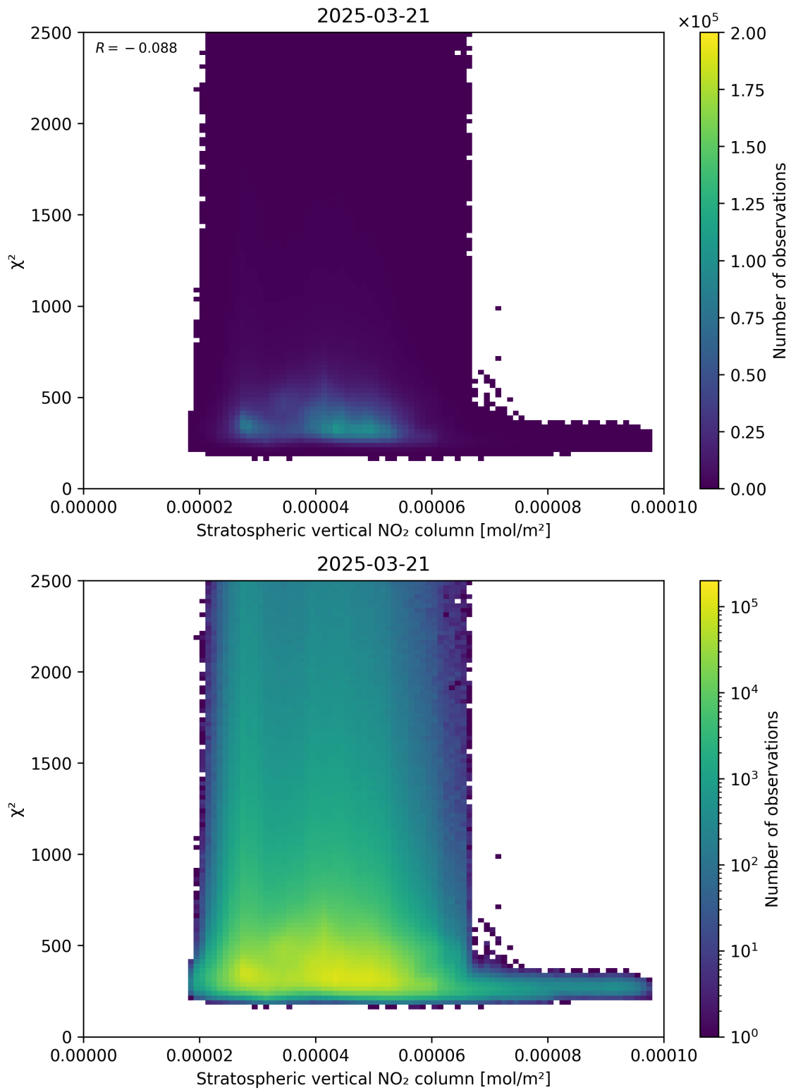
Figure 97: Scatter density plot of “Stratospheric vertical NO 2 column” against “ \chi^2 ” for 2025-03-21 to 2025-03-21.
