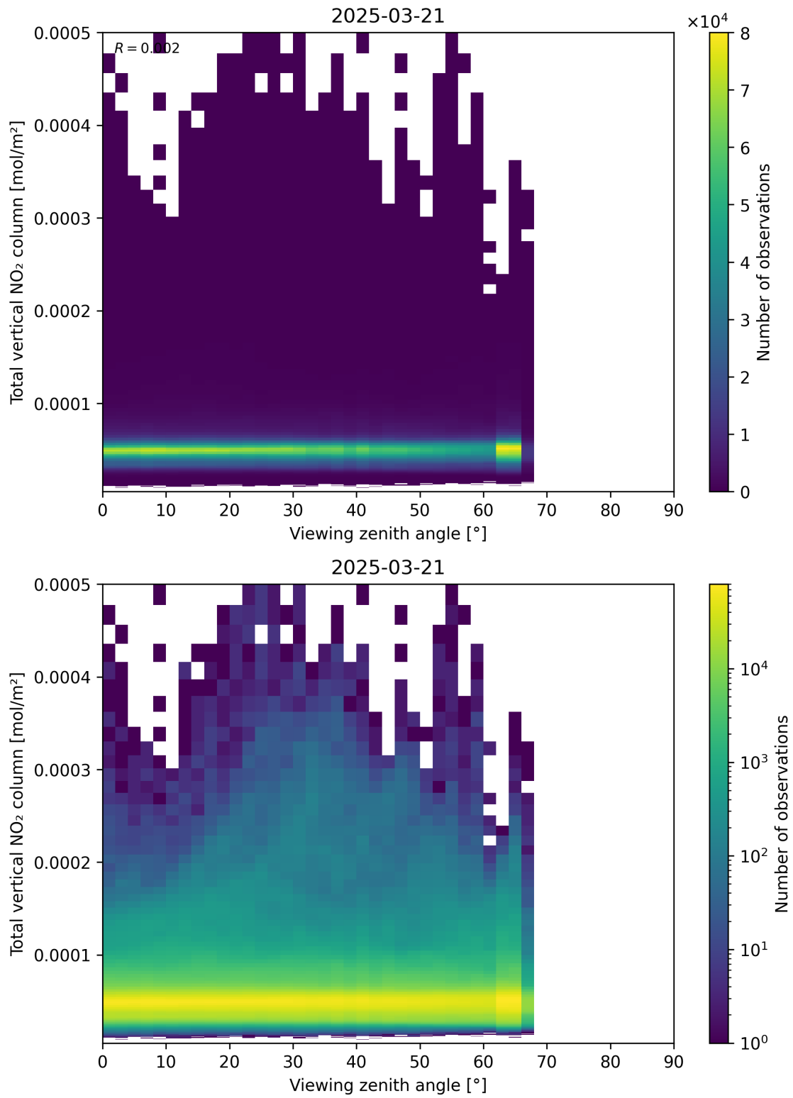
Figure 167: Scatter density plot of “Viewing zenith angle” against “Total vertical NO 2 column” for 2025-03-21 to 2025-03-21.
