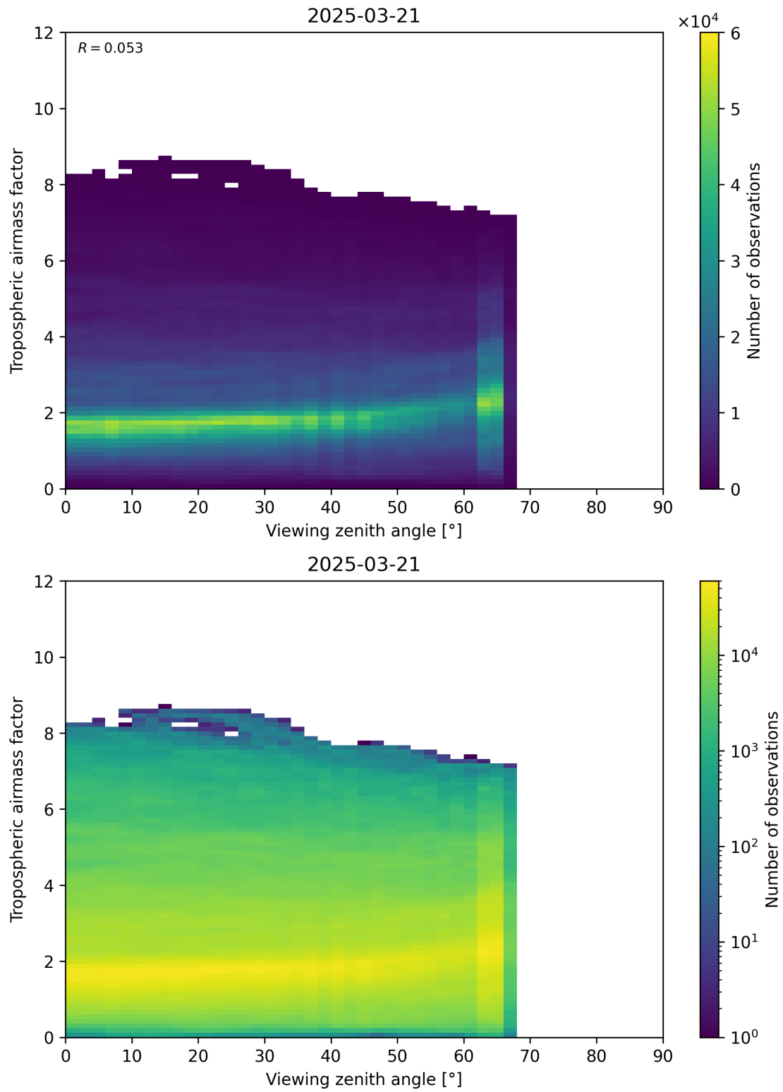
Figure 161: Scatter density plot of “Viewing zenith angle” against “Tropospheric airmass factor” for 2025-03-21 to 2025-03-21.
