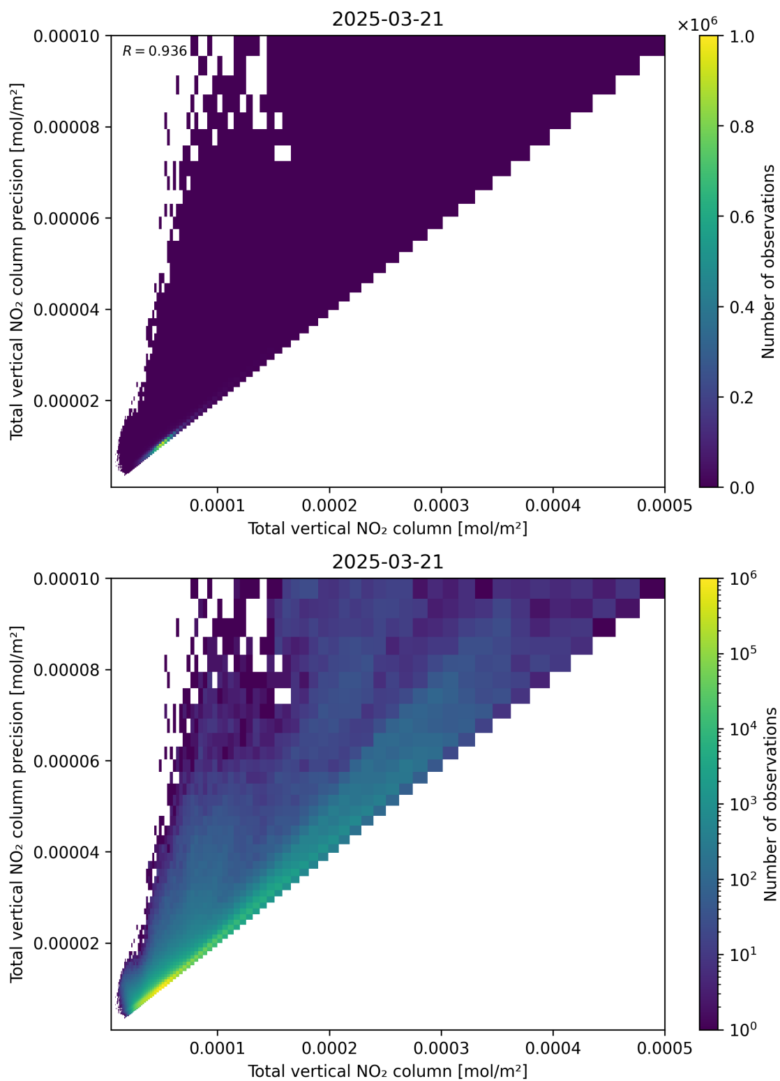
Figure 114: Scatter density plot of “Total vertical NO 2 column” against “Total vertical NO 2 column precision” for 2025-03-21 to 2025-03-21.
