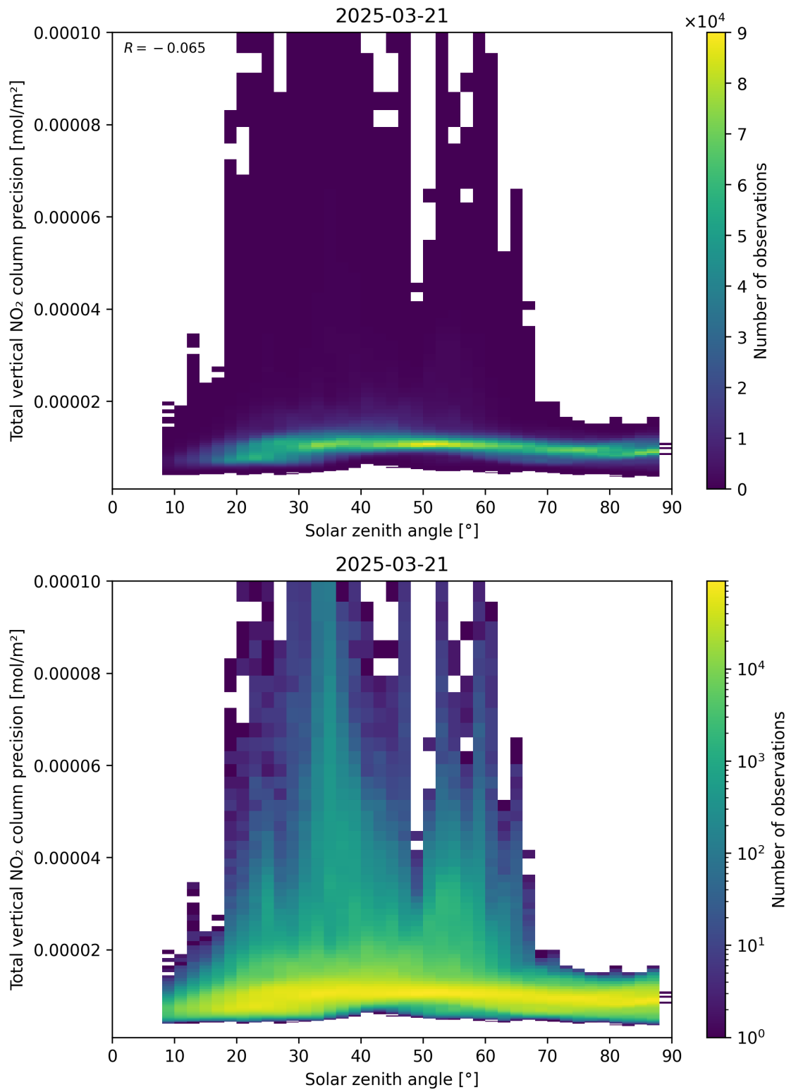
Figure 154: Scatter density plot of “Solar zenith angle” against “Total vertical NO 2 column precision” for 2025-03-21 to 2025-03-21.
