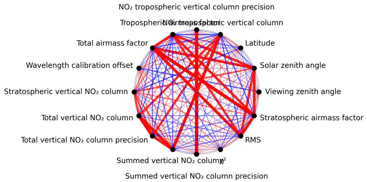
Figure 1: Map of correlation graph for 2025-03-21 to 2025-03-21.
