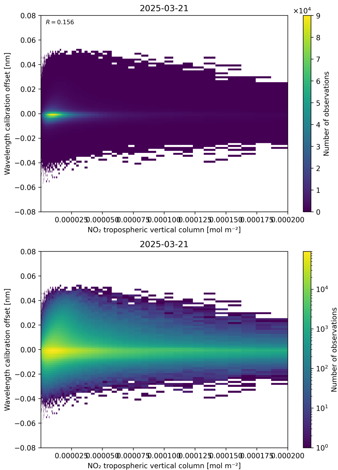
Figure 143: Scatter density plot of “NO 2 tropospheric vertical column” against “Wavelength calibration offset” for 2025-03-21 to 2025-03-21.
