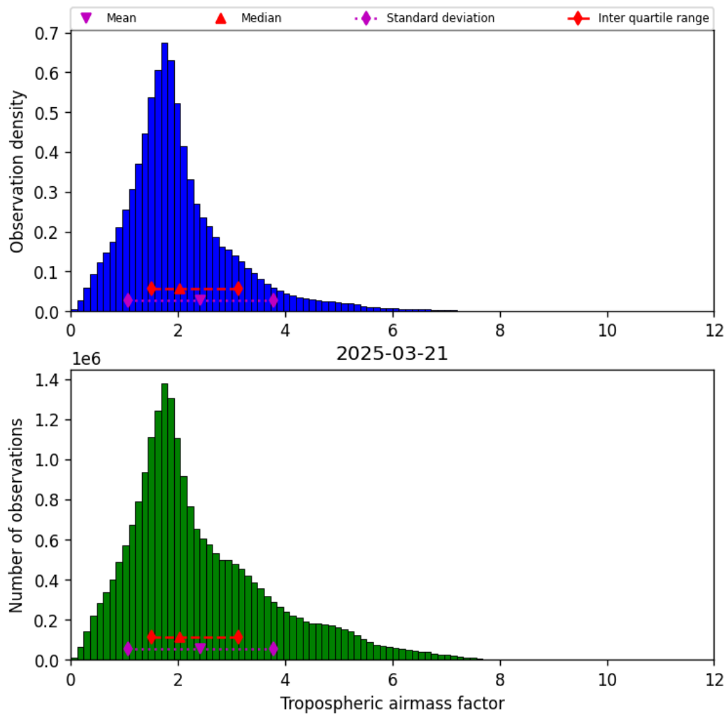
Figure 31: Histogram of “Tropospheric airmass factor” for 2025-03-21 to 2025-03-21
