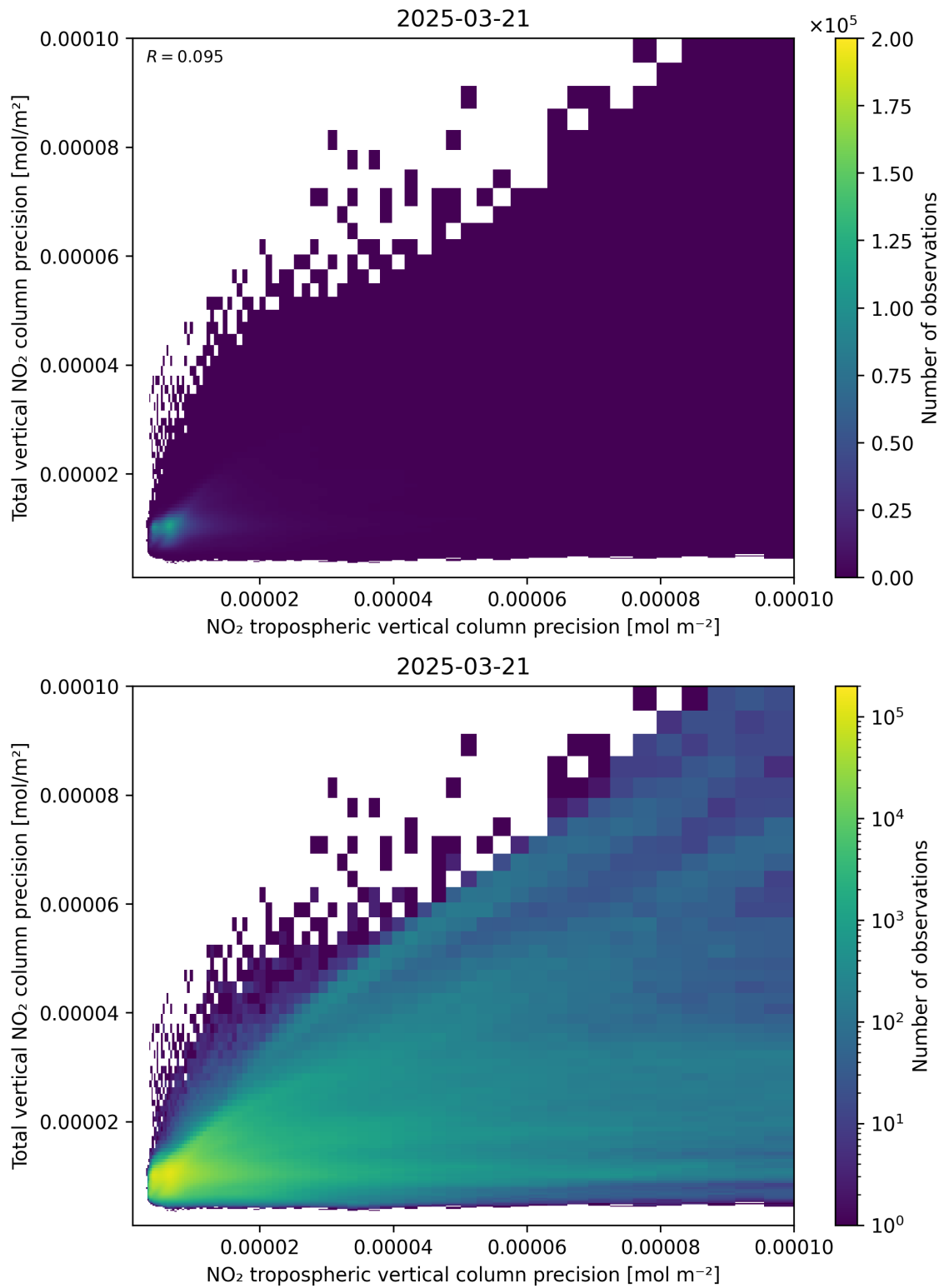
Figure 139: Scatter density plot of “NO 2 tropospheric vertical column precision” against “Total vertical NO 2 column precision” for 2025-03-21 to 2025-03-21.
