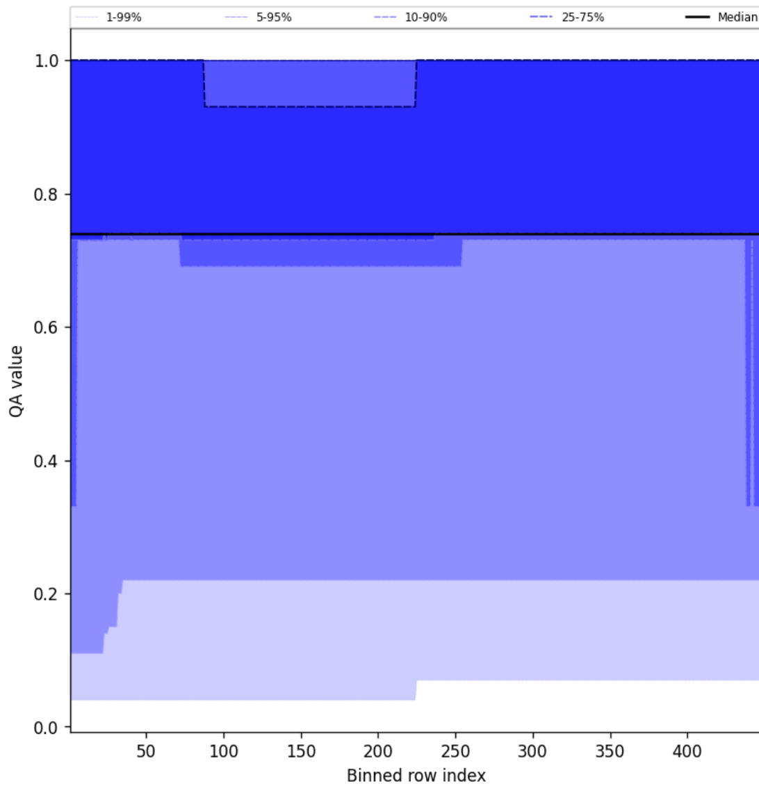
Figure 45: Along track statistics of “QA value” for 2025-03-21 to 2025-03-21
