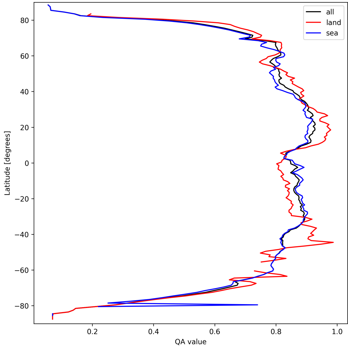
Figure 11: Zonal average of “QA value” for 2025-03-21 to 2025-03-21.
