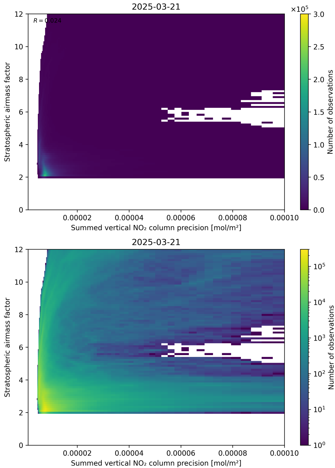
Figure 106: Scatter density plot of “Summed vertical NO 2 column precision” against “Stratospheric airmass factor” for 2025-03-21 to 2025-03-21.
