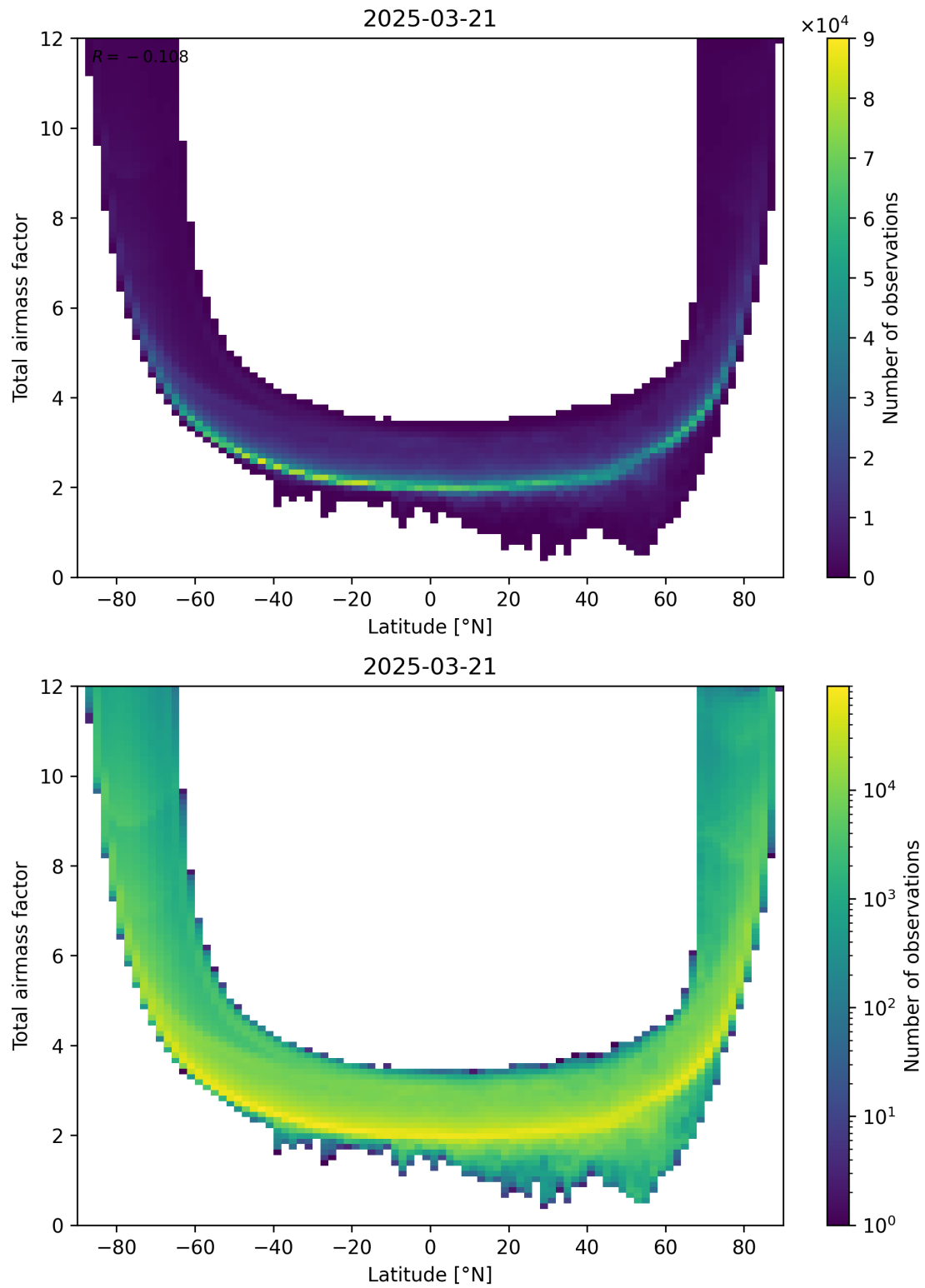
Figure 84: Scatter density plot of “Latitude” against “Total airmass factor” for 2025-03-21 to 2025-03-21.
