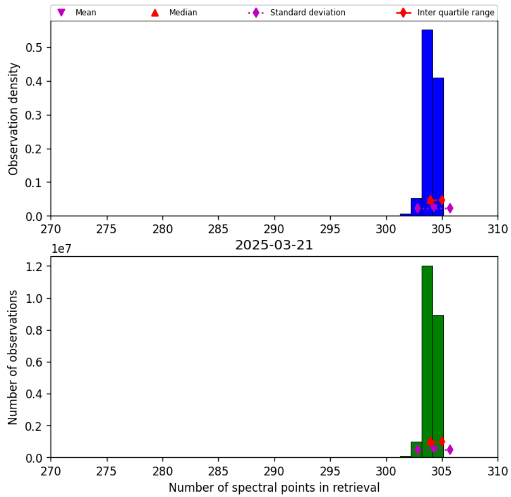
Figure 33: Histogram of “Number of spectral points in retrieval” for 2025-03-21 to 2025-03-21
