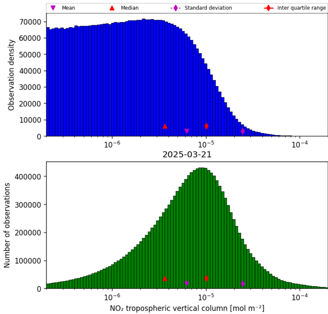
Figure 29: Histogram of “NO 2 tropospheric vertical column” for 2025-03-21 to 2025-03-21
