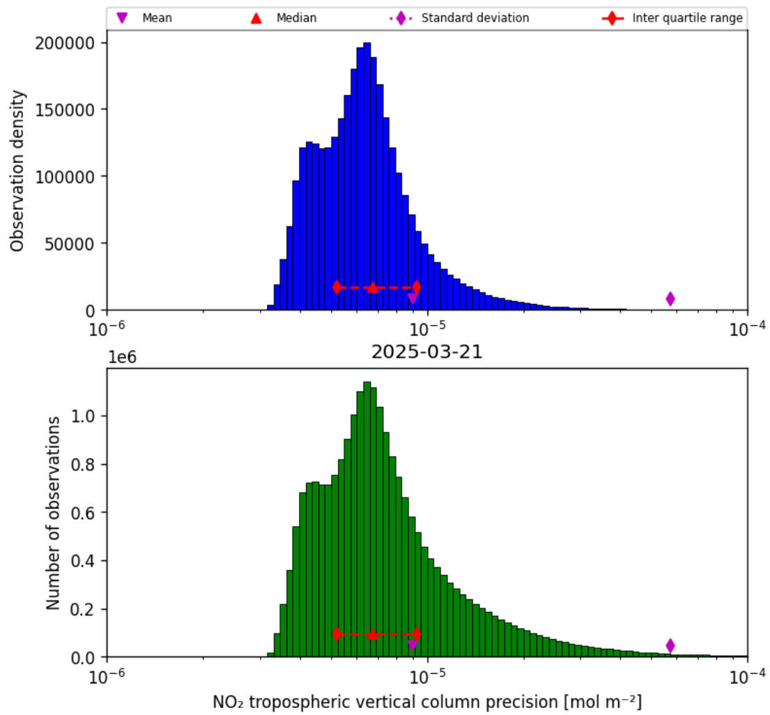
Figure 30: Histogram of “NO 2 tropospheric vertical column precision” for 2025-03-21 to 2025-03-21
