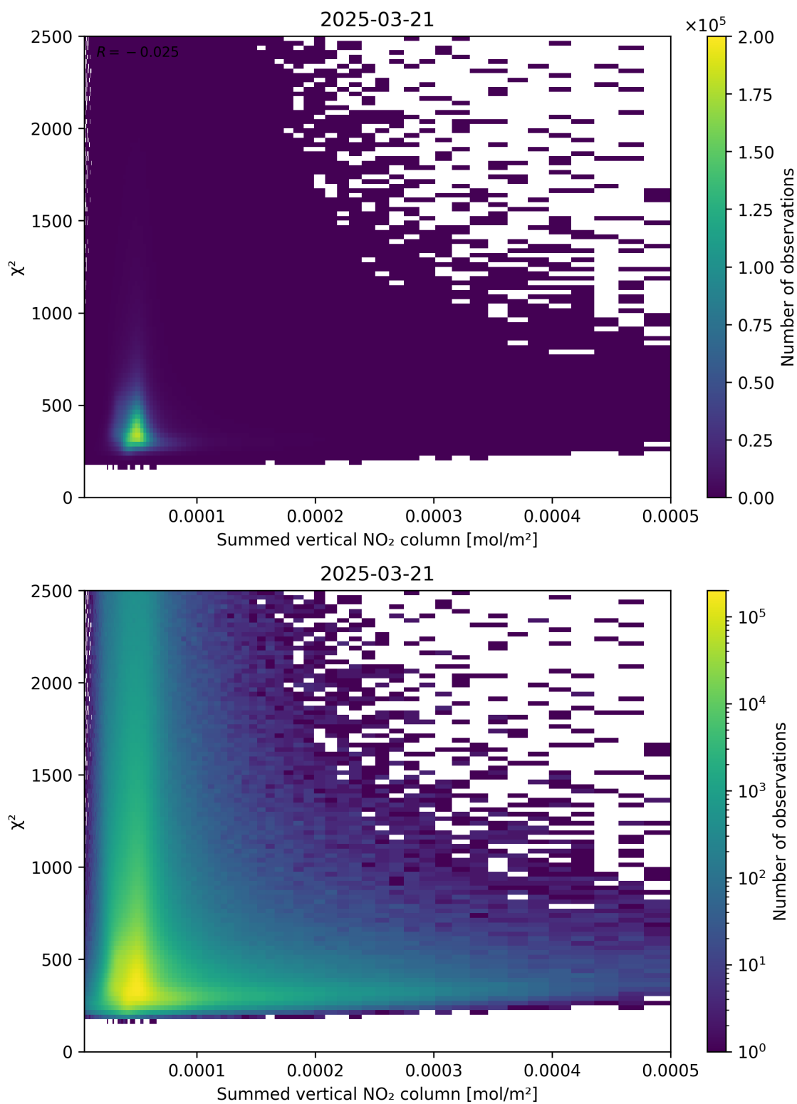
Figure 104: Scatter density plot of “Summed vertical NO 2 column” against “ \chi^2 ” for 2025-03-21 to 2025-03-21.
