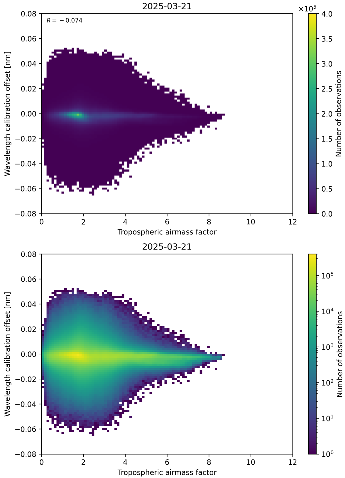
Figure 80: Scatter density plot of “Tropospheric airmass factor” against “Wavelength calibration offset” for 2025-03-21 to 2025-03-21.
