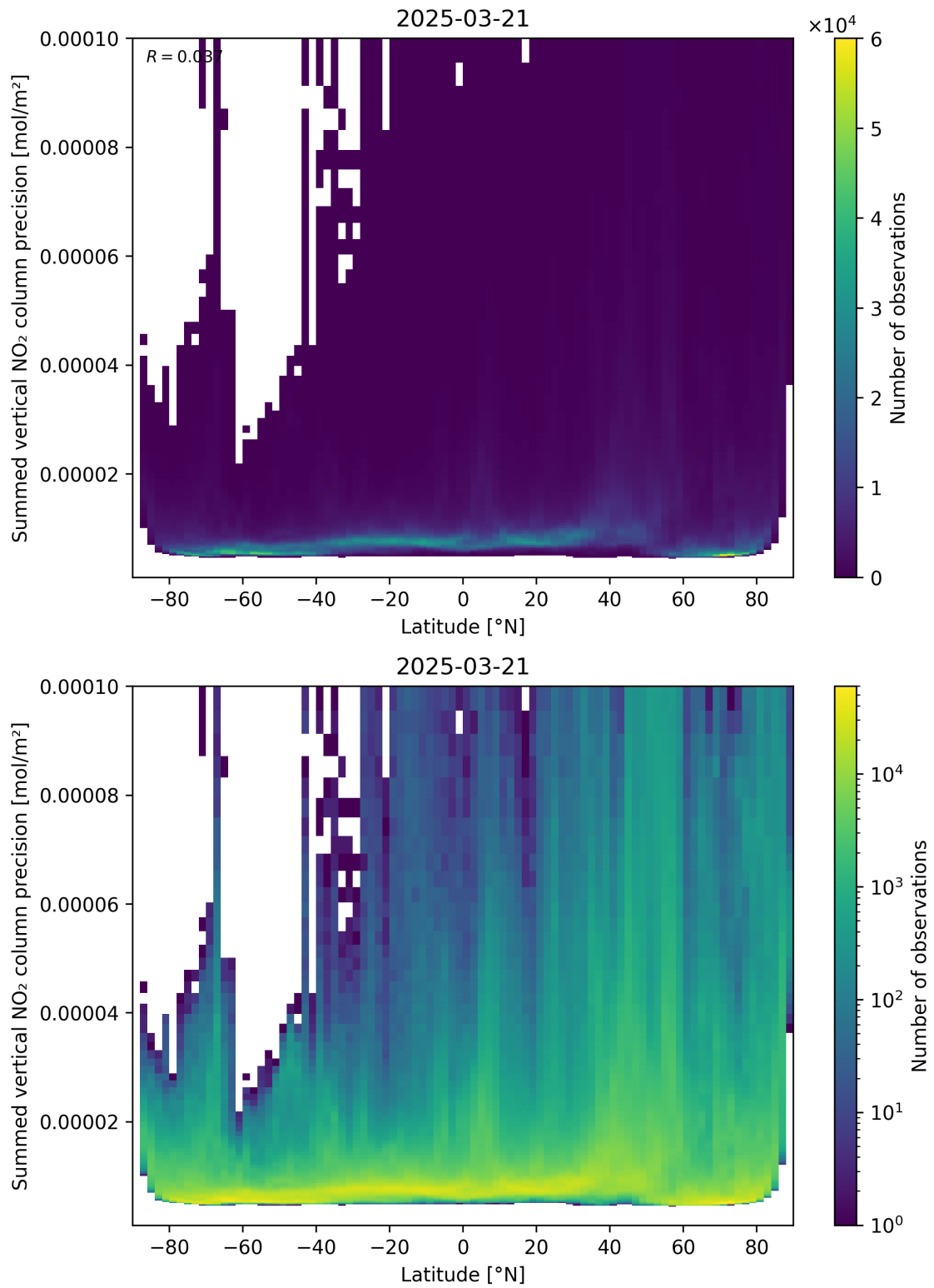
Figure 89: Scatter density plot of “Latitude” against “Summed vertical NO 2 column precision” for 2025-03-21 to 2025-03-21.
