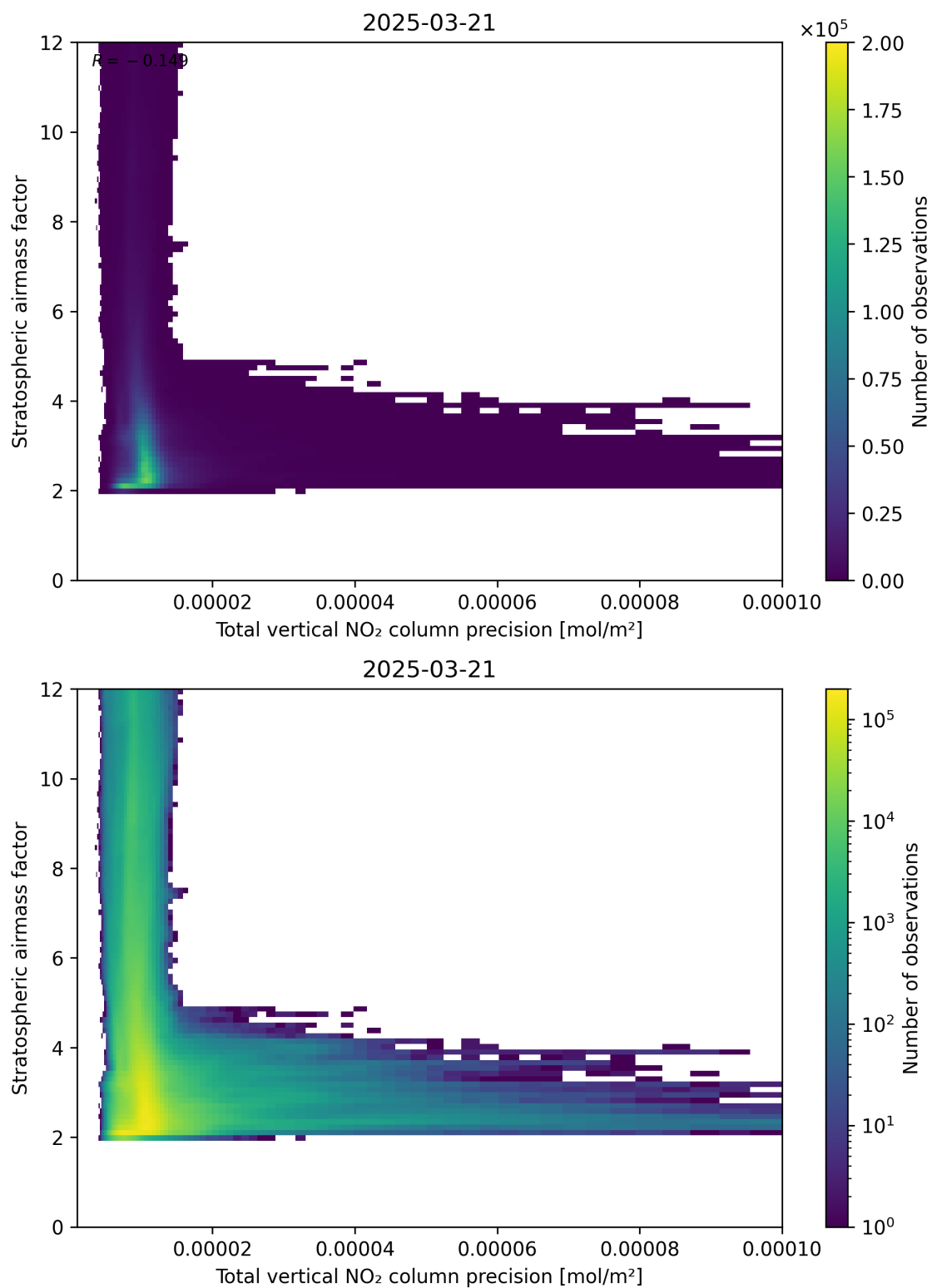
Figure 115: Scatter density plot of “Total vertical NO 2 column precision” against “Stratospheric air mass factor” for 2025-03-21 to 2025-03-21.
