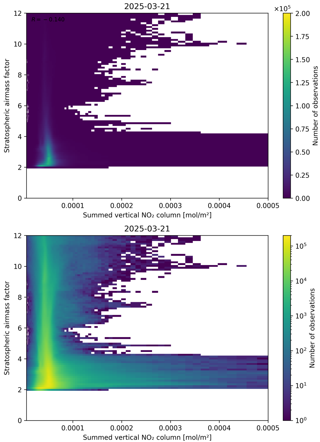
Figure 103: Scatter density plot of “Summed vertical NO 2 column” against “Stratospheric airmass factor” for 2025-03-21 to 2025-03-21.
