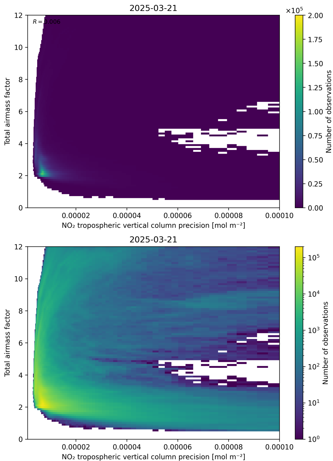
Figure 132: Scatter density plot of “NO 2 tropospheric vertical column precision” against “Total air mass factor” for 2025-03-21 to 2025-03-21.
