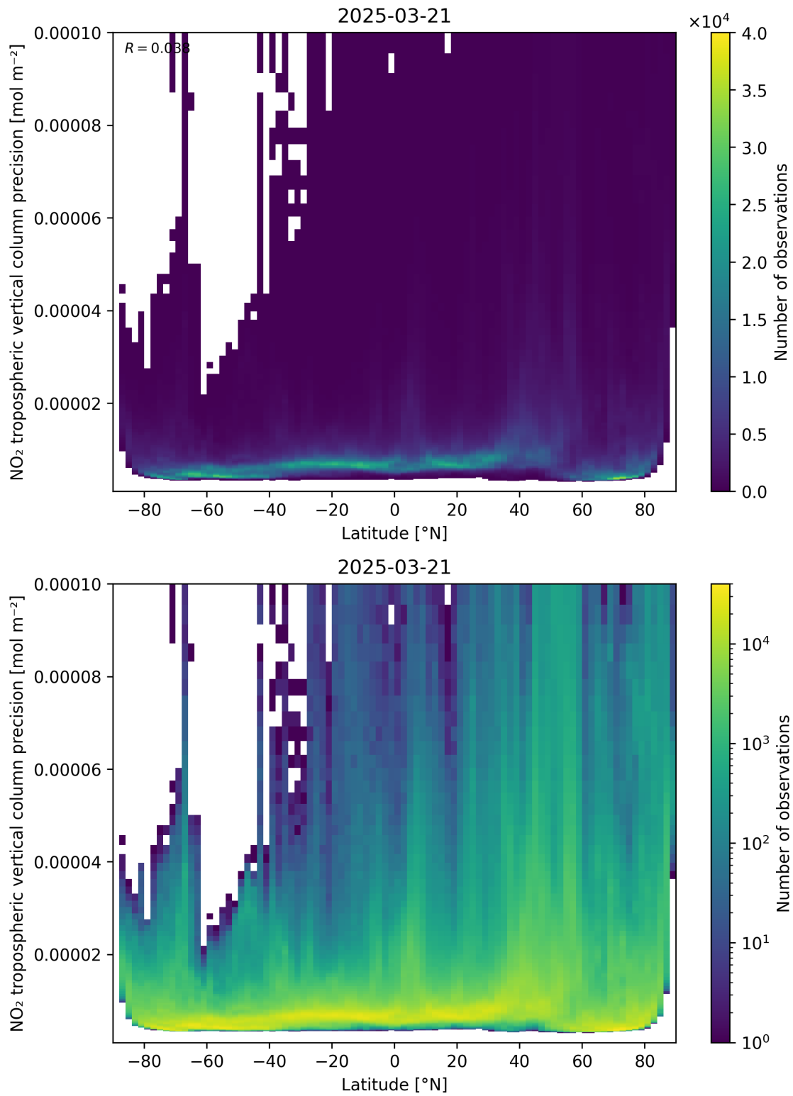
Figure 93: Scatter density plot of “Latitude” against “NO 2 tropospheric vertical column precision” for 2025-03-21 to 2025-03-21.
