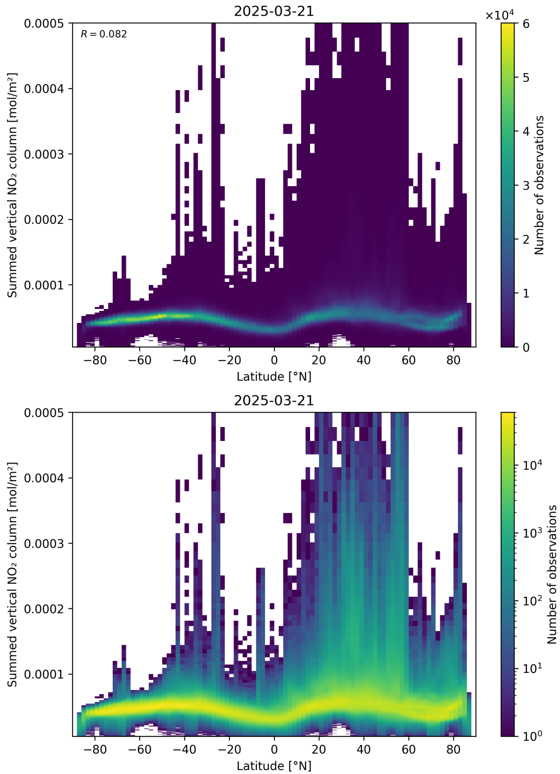
Figure 88: Scatter density plot of “Latitude” against “Summed vertical NO 2 column” for 2025-03-21 to 2025-03-21.
