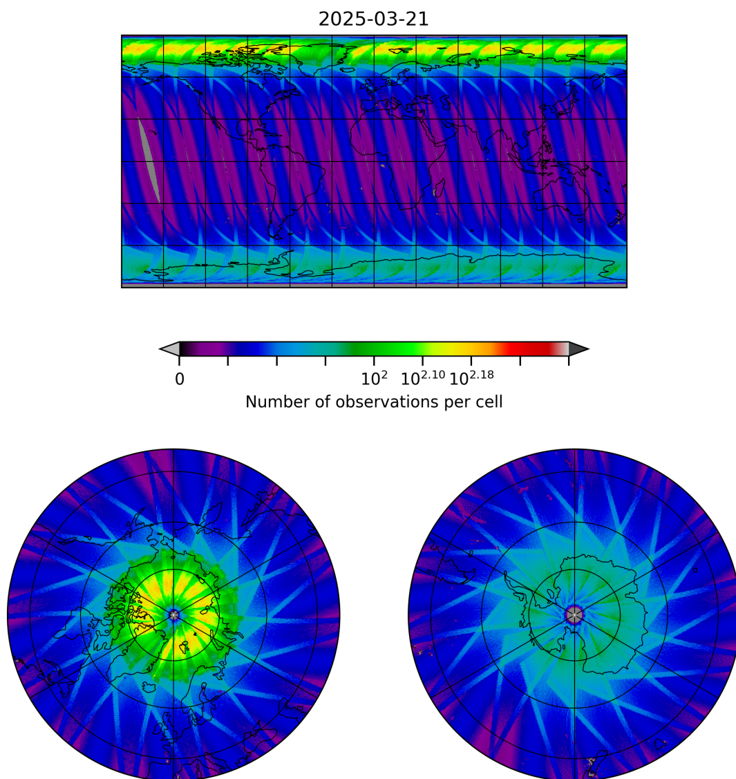
Figure 10: Map of the number of observations for 2025-03-21 to 2025-03-21
