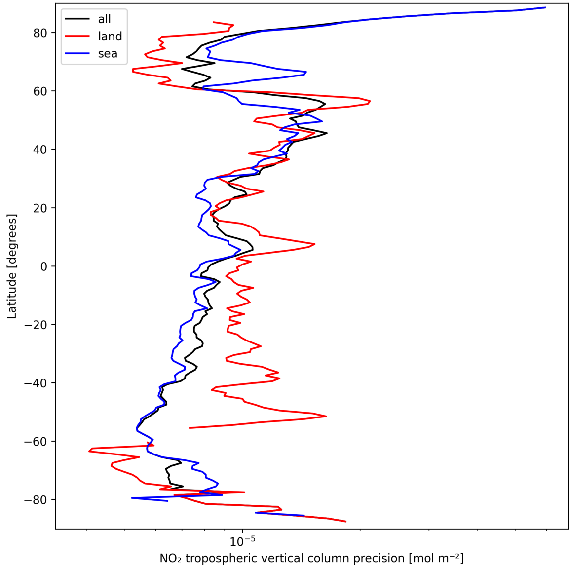
Figure 13: Zonal average of “NO 2 tropospheric vertical column precision” for 2025-03-21 to 2025-03-21.
