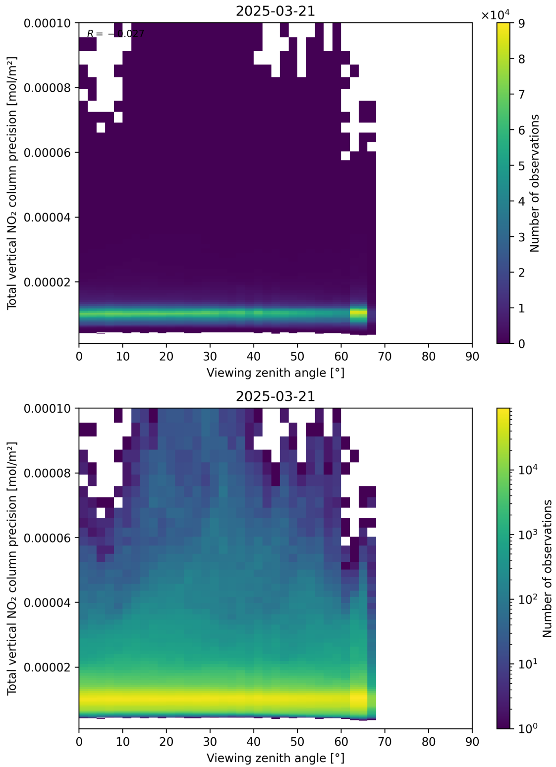
Figure 168: Scatter density plot of “Viewing zenith angle” against “Total vertical NO 2 column precision” for 2025-03-21 to 2025-03-21.
