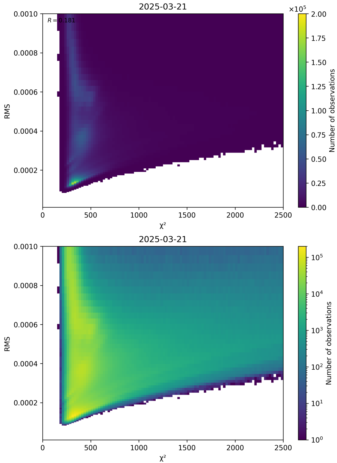
Figure 82: Scatter density plot of “ \chi^2 ” against “RMS” for 2025-03-21 to 2025-03-21.
