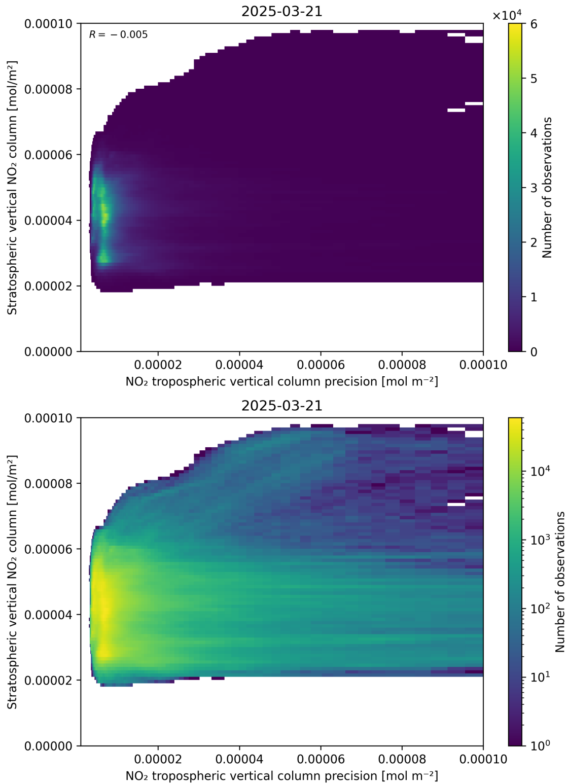
Figure 135: Scatter density plot of “NO 2 tropospheric vertical column precision” against “Stratospheric vertical NO 2 column” for 2025-03-21 to 2025-03-21.
