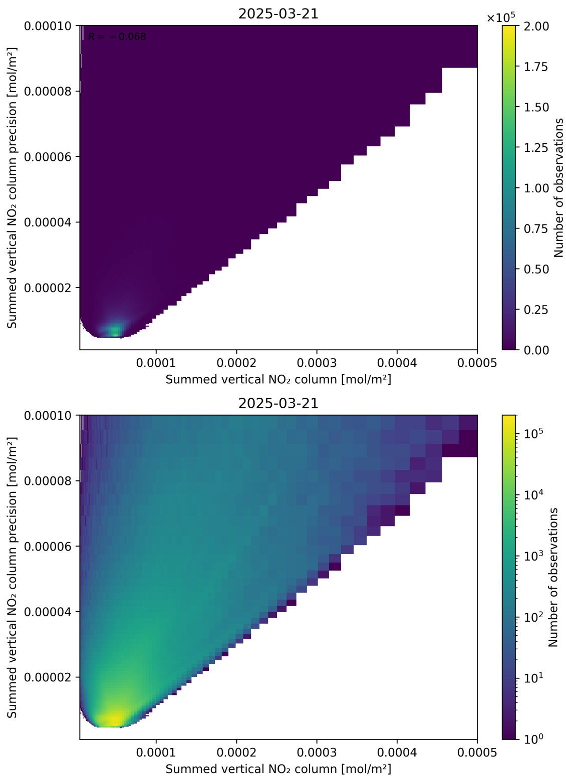
Figure 105: Scatter density plot of “Summed vertical NO 2 column” against “Summed vertical NO 2 column precision” for 2025-03-21 to 2025-03-21.
