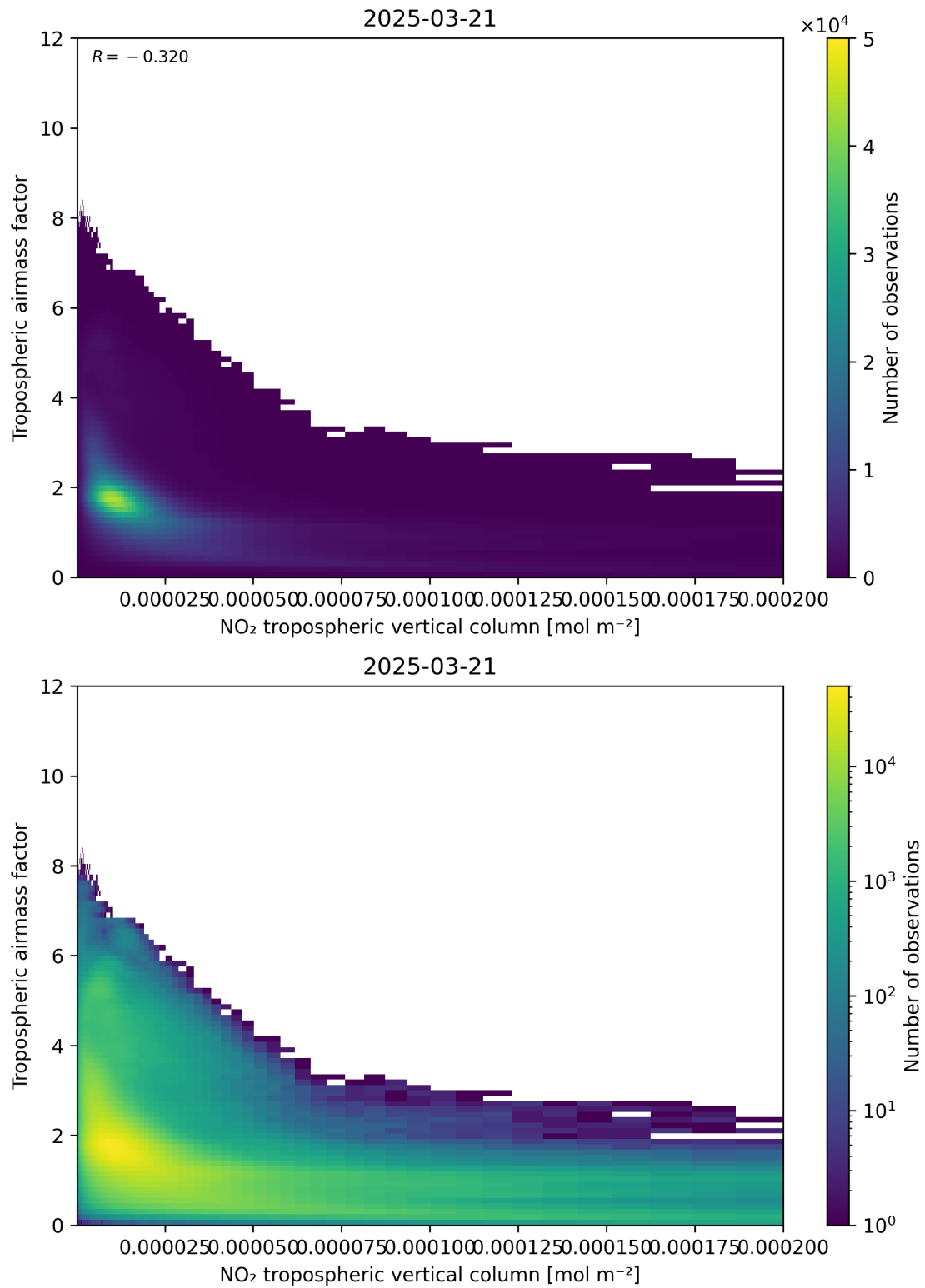
Figure 123: Scatter density plot of “NO 2 tropospheric vertical column” against “Tropospheric air mass factor” for 2025-03-21 to 2025-03-21.
