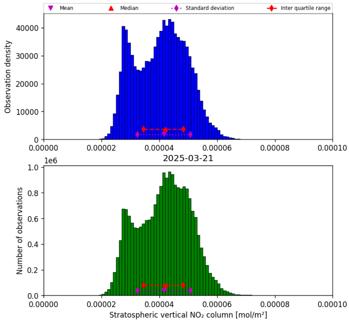
Figure 36: Histogram of “Stratospheric vertical NO 2 column” for 2025-03-21 to 2025-03-21
