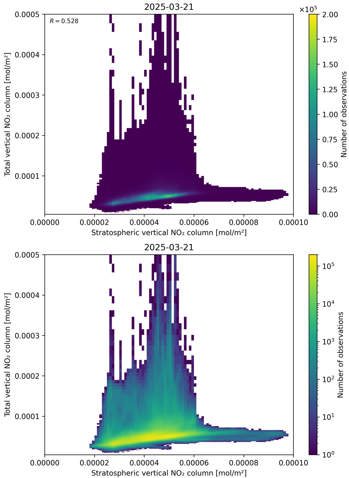
Figure 100: Scatter density plot of “Stratospheric vertical NO 2 column” against “Total vertical NO 2 column” for 2025-03-21 to 2025-03-21.
