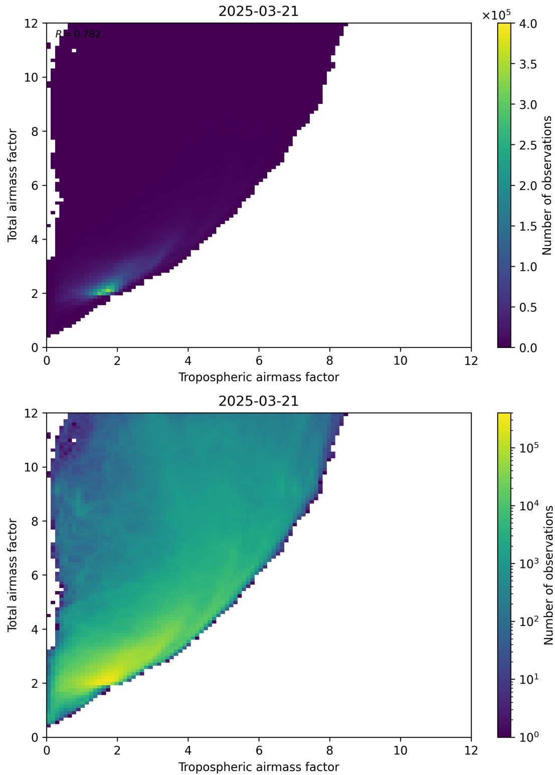
Figure 72: Scatter density plot of “Tropospheric airmass factor” against “Total airmass factor” for 2025-03-21 to 2025-03-21.
