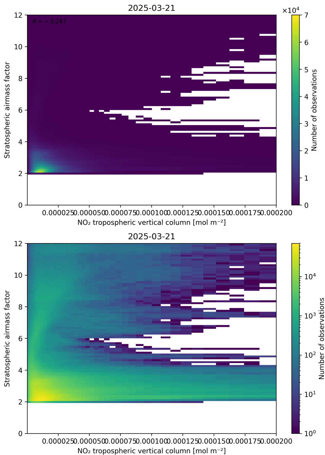
Figure 121: Scatter density plot of “NO 2 tropospheric vertical column” against “Stratospheric airmass factor” for 2025-03-21 to 2025-03-21.
