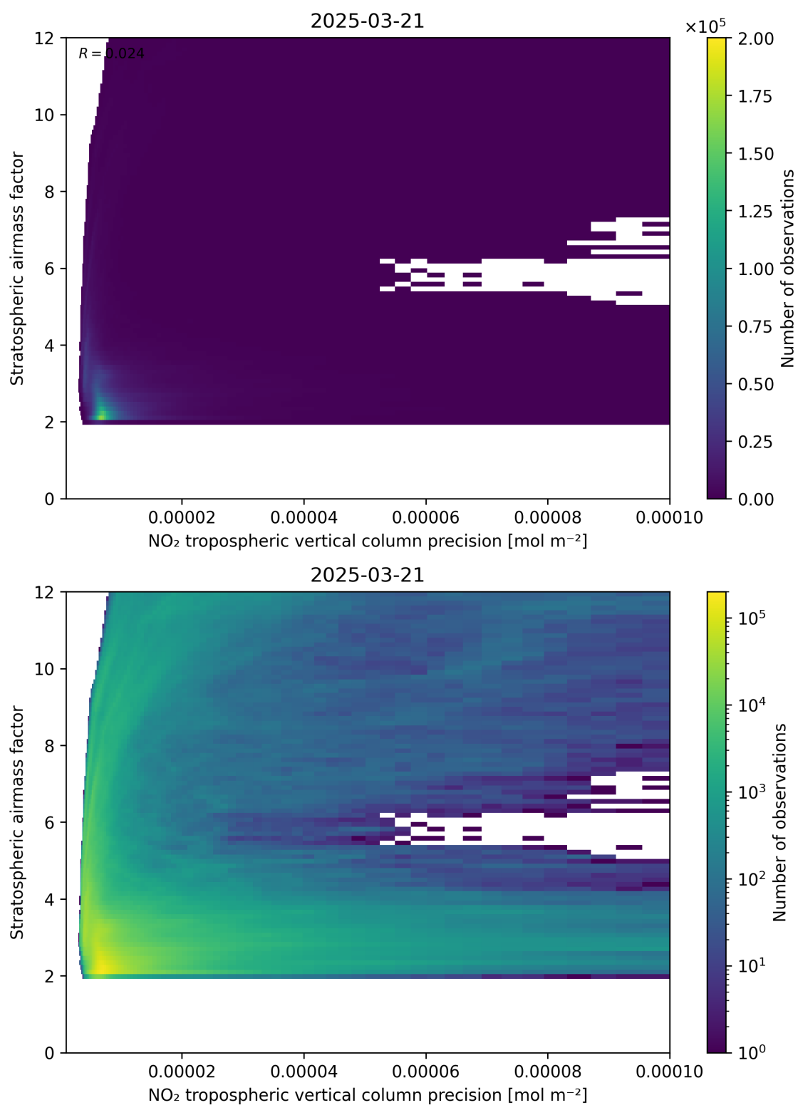
Figure 131: Scatter density plot of “NO 2 tropospheric vertical column precision” against “Stratospheric airmass factor” for 2025-03-21 to 2025-03-21.
