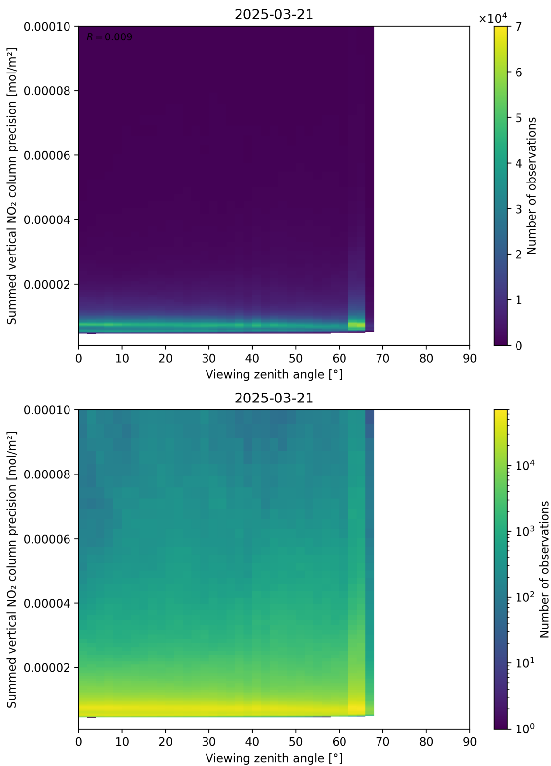
Figure 166: Scatter density plot of “Viewing zenith angle” against “Summed vertical NO 2 column precision” for 2025-03-21 to 2025-03-21.
