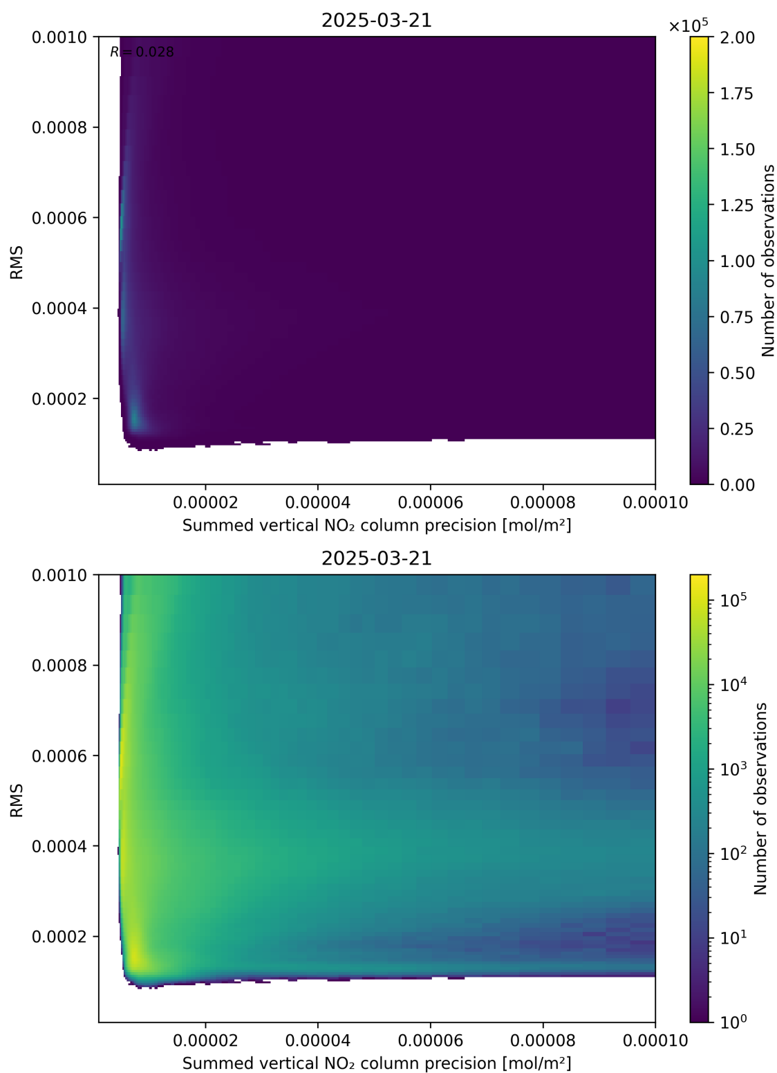
Figure 108: Scatter density plot of “Summed vertical NO 2 column precision” against “RMS” for 2025-03-21 to 2025-03-21.
