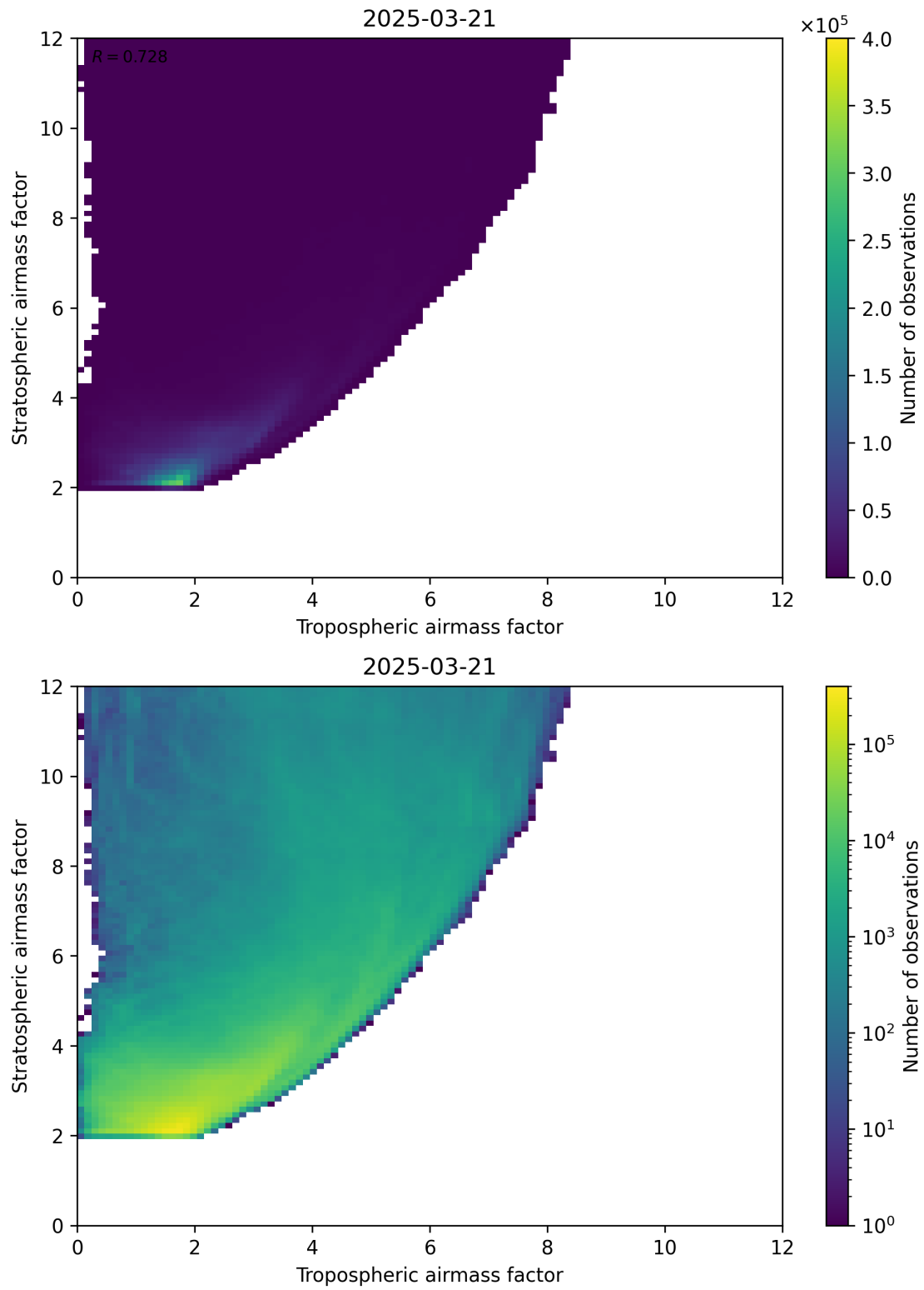
Figure 71: Scatter density plot of “Tropospheric airmass factor” against “Stratospheric airmass factor” for 2025-03-21 to 2025-03-21.
