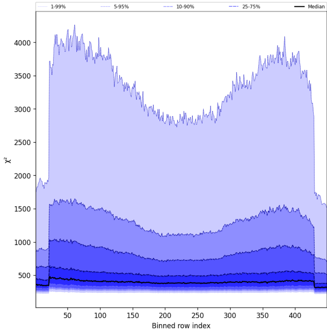
Figure 59: Along track statistics of “ \chi^2 ” for 2025-03-21 to 2025-03-21
