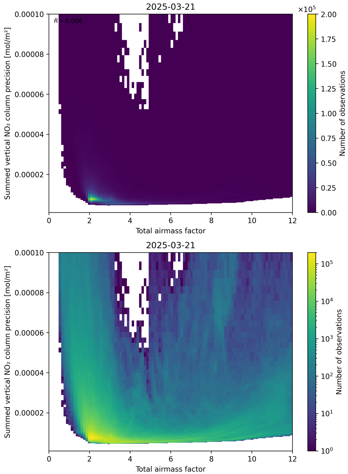
Figure 66: Scatter density plot of “Total airmass factor” against “Summed vertical NO 2 column precision” for 2025-03-21 to 2025-03-21.
