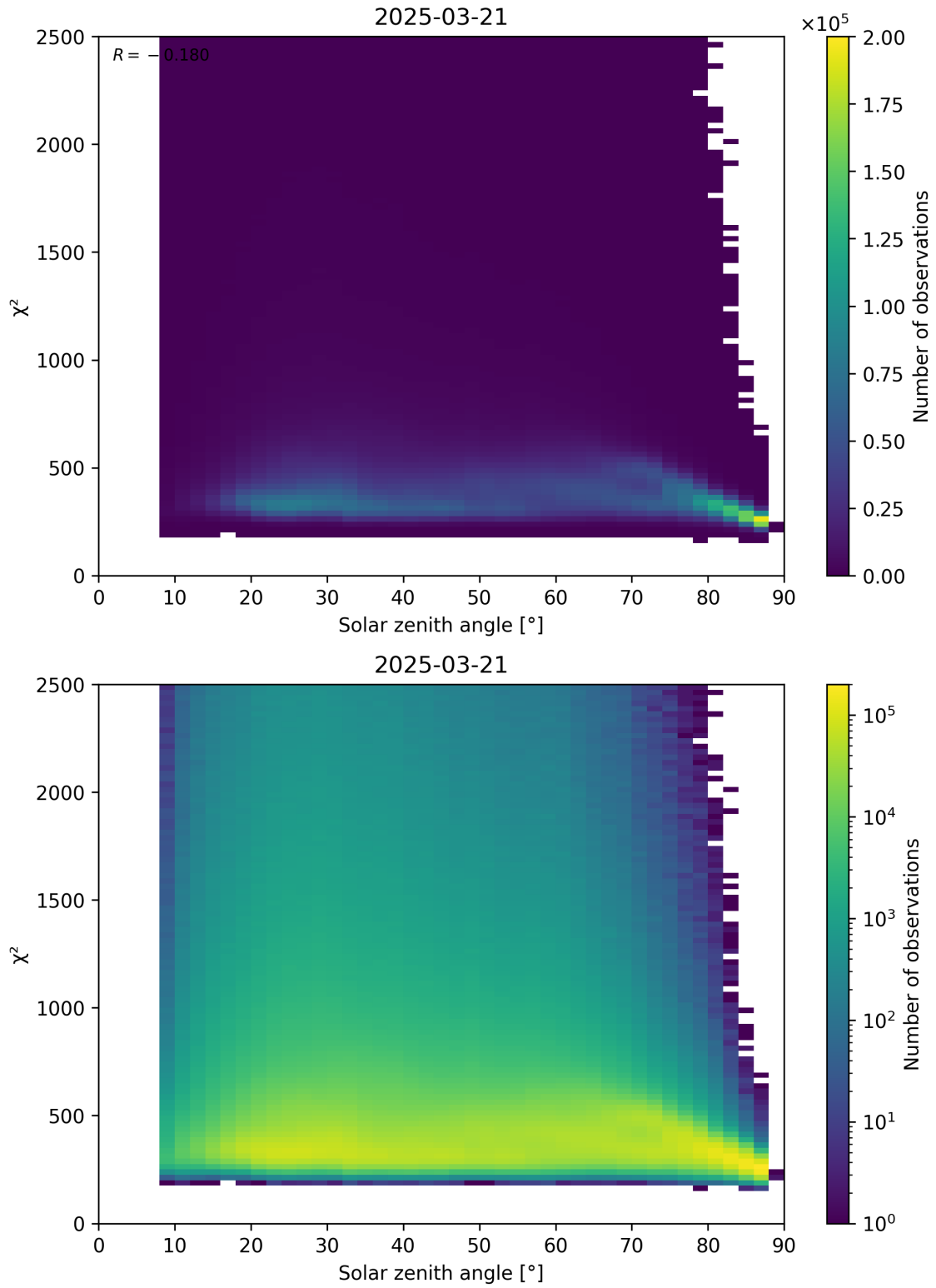
Figure 148: Scatter density plot of “Solar zenith angle” against “ \chi^2 ” for 2025-03-21 to 2025-03-21.
