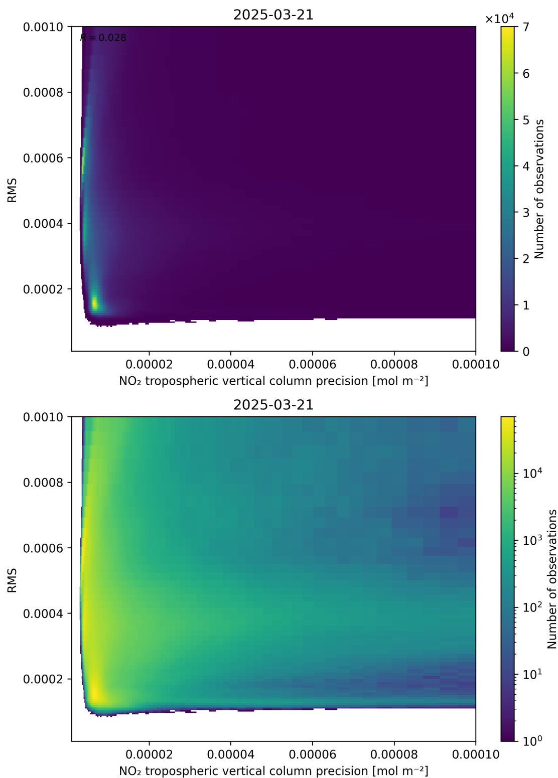
Figure 140: Scatter density plot of “NO 2 tropospheric vertical column precision” against “RMS” for 2025-03-21 to 2025-03-21.
