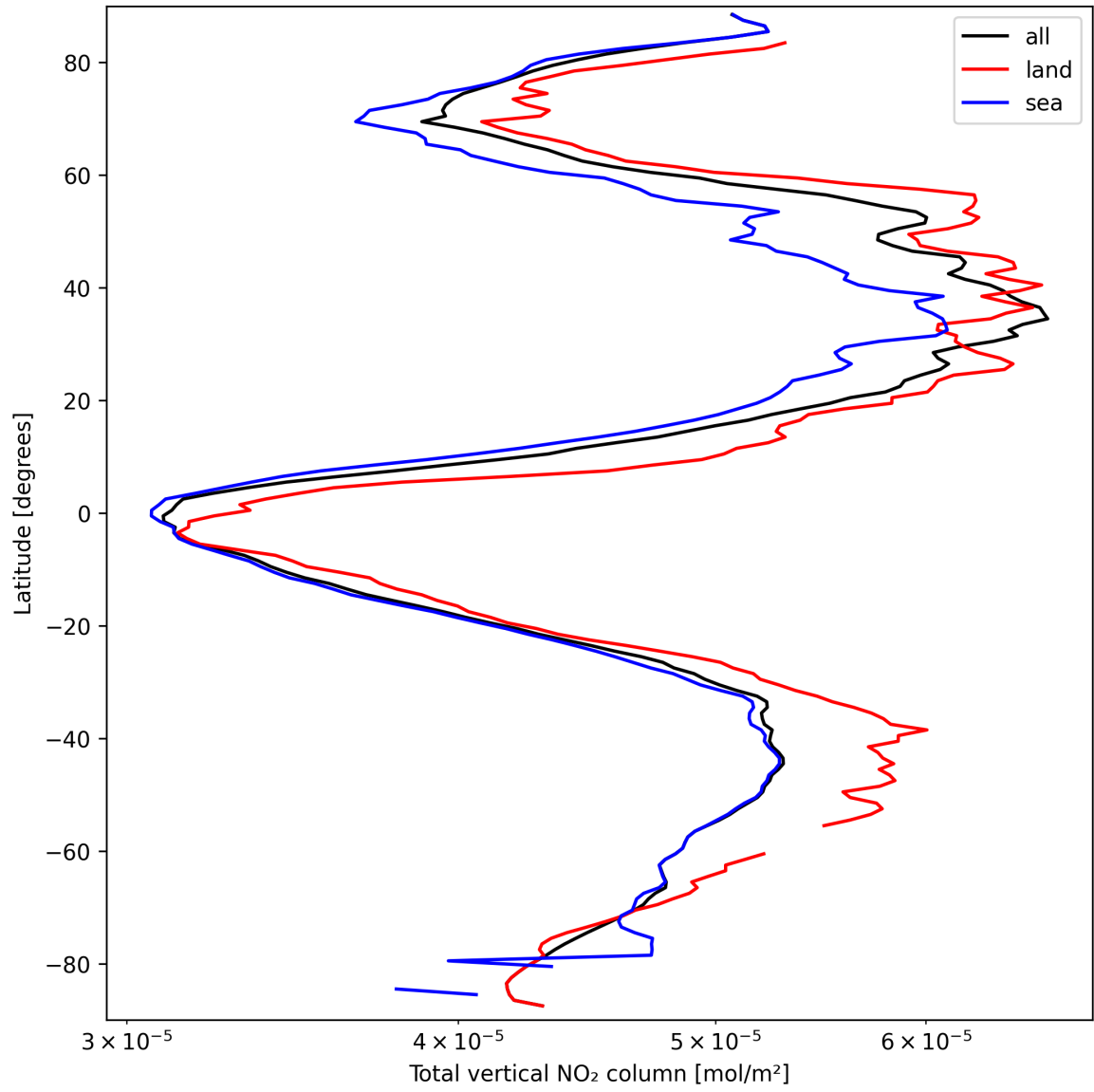
Figure 21: Zonal average of “Total vertical NO 2 column” for 2025-03-21 to 2025-03-21.
