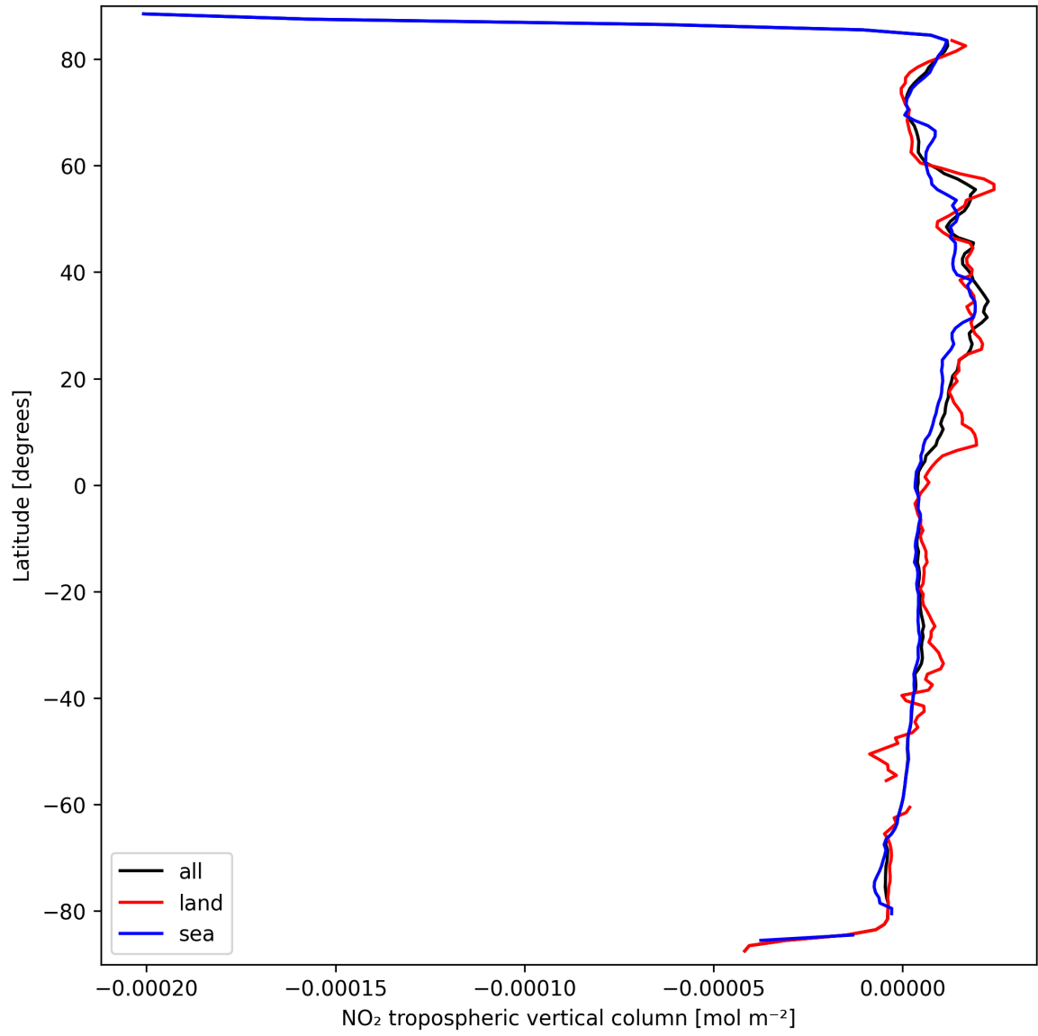
Figure 12: Zonal average of “NO 2 tropospheric vertical column” for 2025-03-21 to 2025-03-21.
