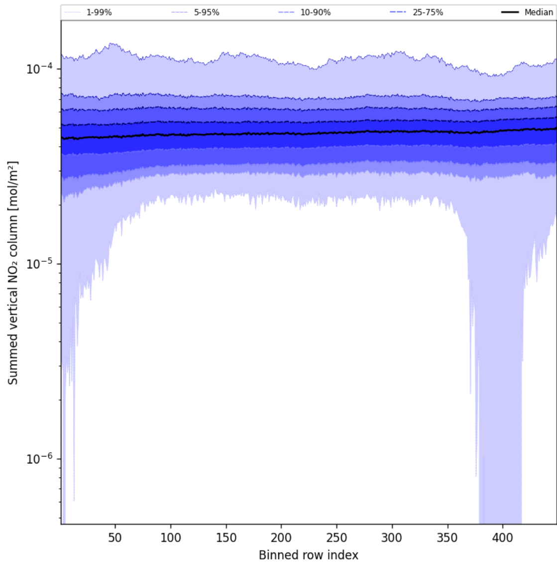
Figure 57: Along track statistics of “Summed vertical NO 2 column” for 2025-03-21 to 2025-03-21
