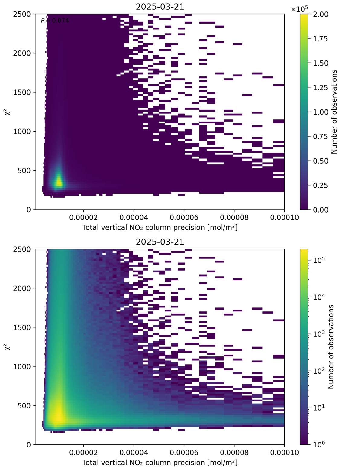
Figure 116: Scatter density plot of “Total vertical NO 2 column precision” against “ \chi^2 ” for 2025-03-21 to 2025-03-21.
