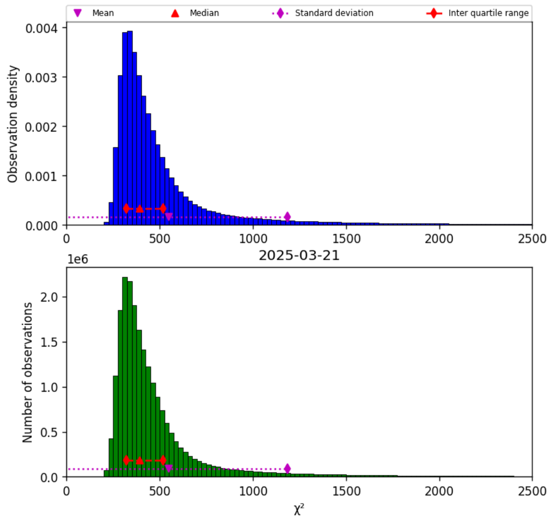
Figure 42: Histogram of “ \chi^2 ” for 2025-03-21 to 2025-03-21
