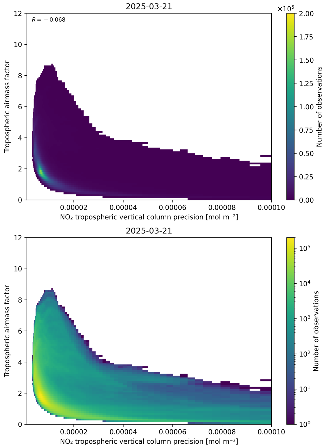
Figure 133: Scatter density plot of “NO 2 tropospheric vertical column precision” against “Tropospheric airmass factor” for 2025-03-21 to 2025-03-21.
