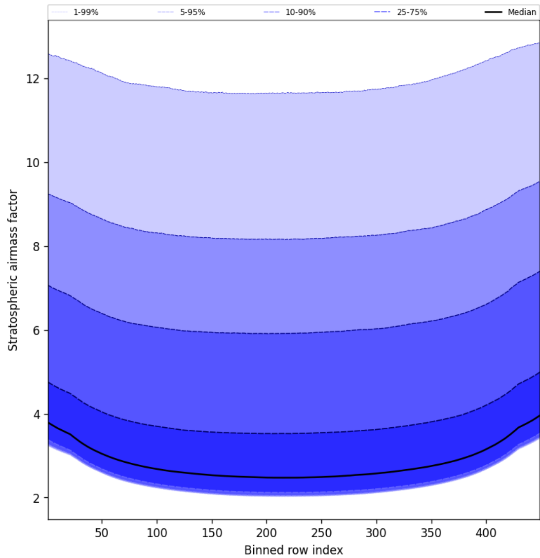
Figure 61: Along track statistics of “Stratospheric airmass factor” for 2025-03-21 to 2025-03-21
