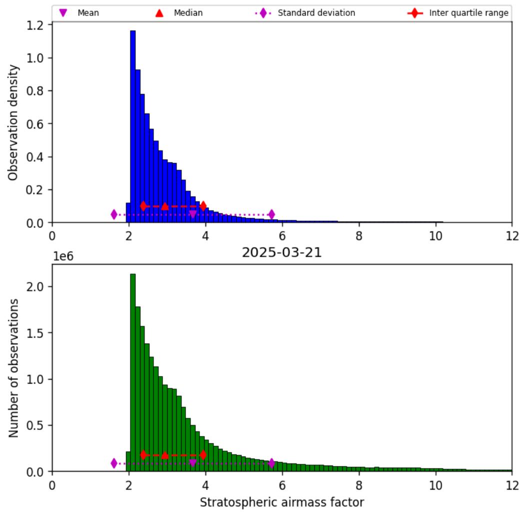
Figure 44: Histogram of “Stratospheric airmass factor” for 2025-03-21 to 2025-03-21
