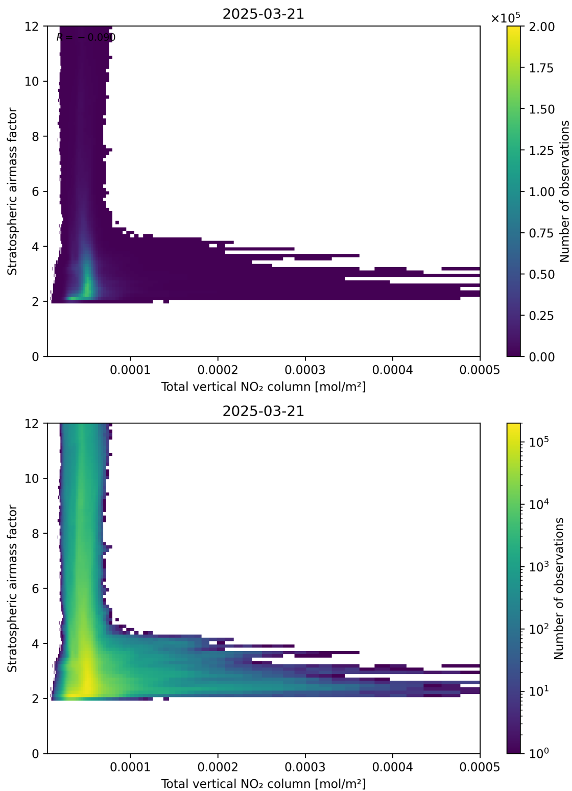
Figure 110: Scatter density plot of “Total vertical NO 2 column” against “Stratospheric airmass factor” for 2025-03-21 to 2025-03-21.
