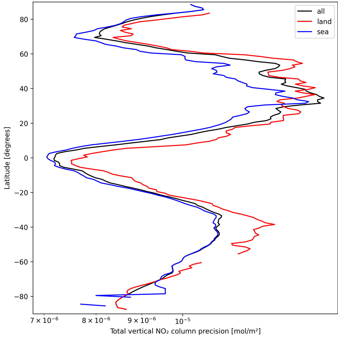
Figure 22: Zonal average of “Total vertical NO 2 column precision” for 2025-03-21 to 2025-03-21.
