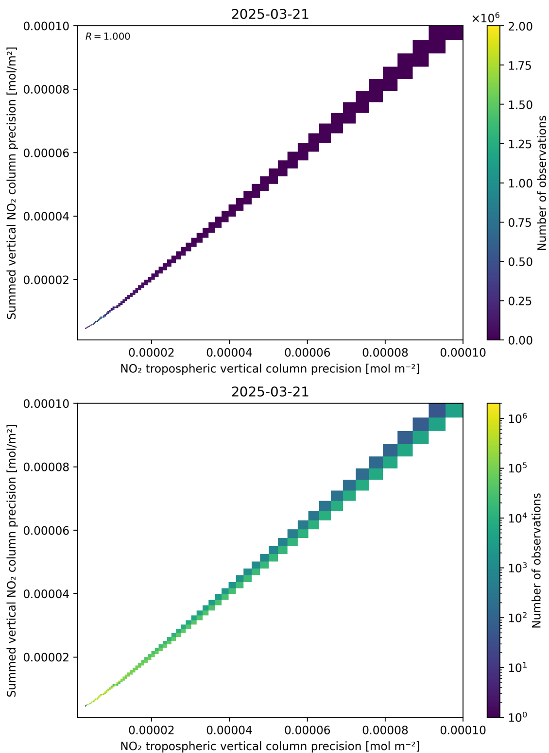
Figure 137: Scatter density plot of “NO 2 tropospheric vertical column precision” against “Summed vertical NO 2 column precision” for 2025-03-21 to 2025-03-21.
