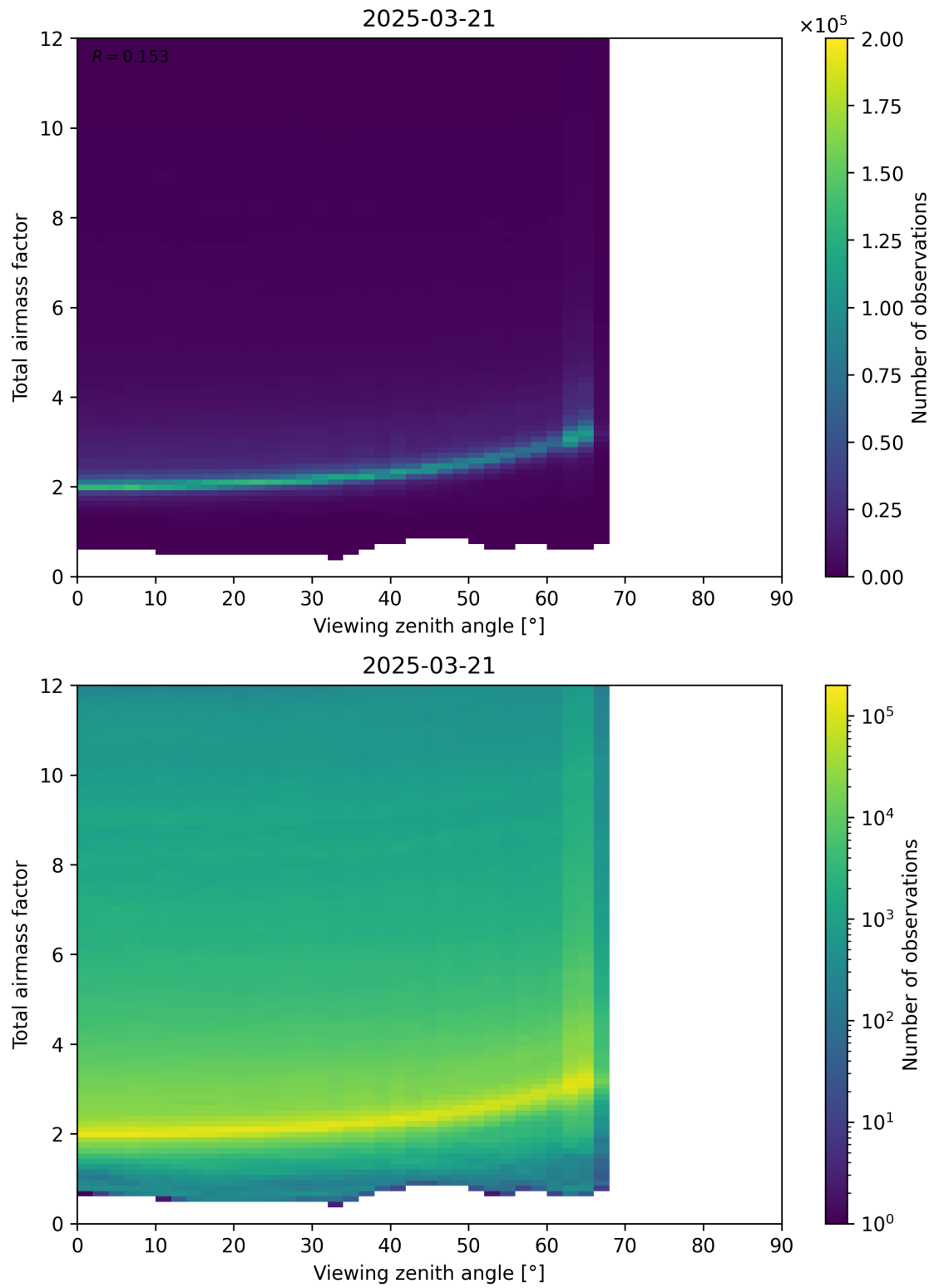
Figure 160: Scatter density plot of “Viewing zenith angle” against “Total airmass factor” for 2025-03-21 to 2025-03-21.
