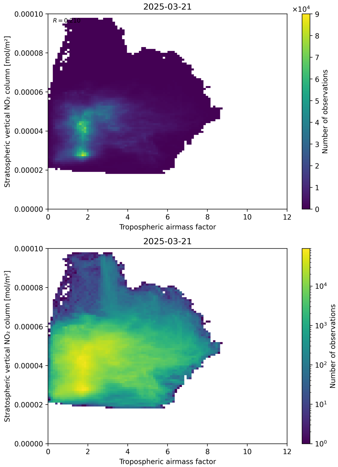
Figure 74: Scatter density plot of “Tropospheric air mass factor” against “Stratospheric vertical NO 2 column” for 2025-03-21 to 2025-03-21.
