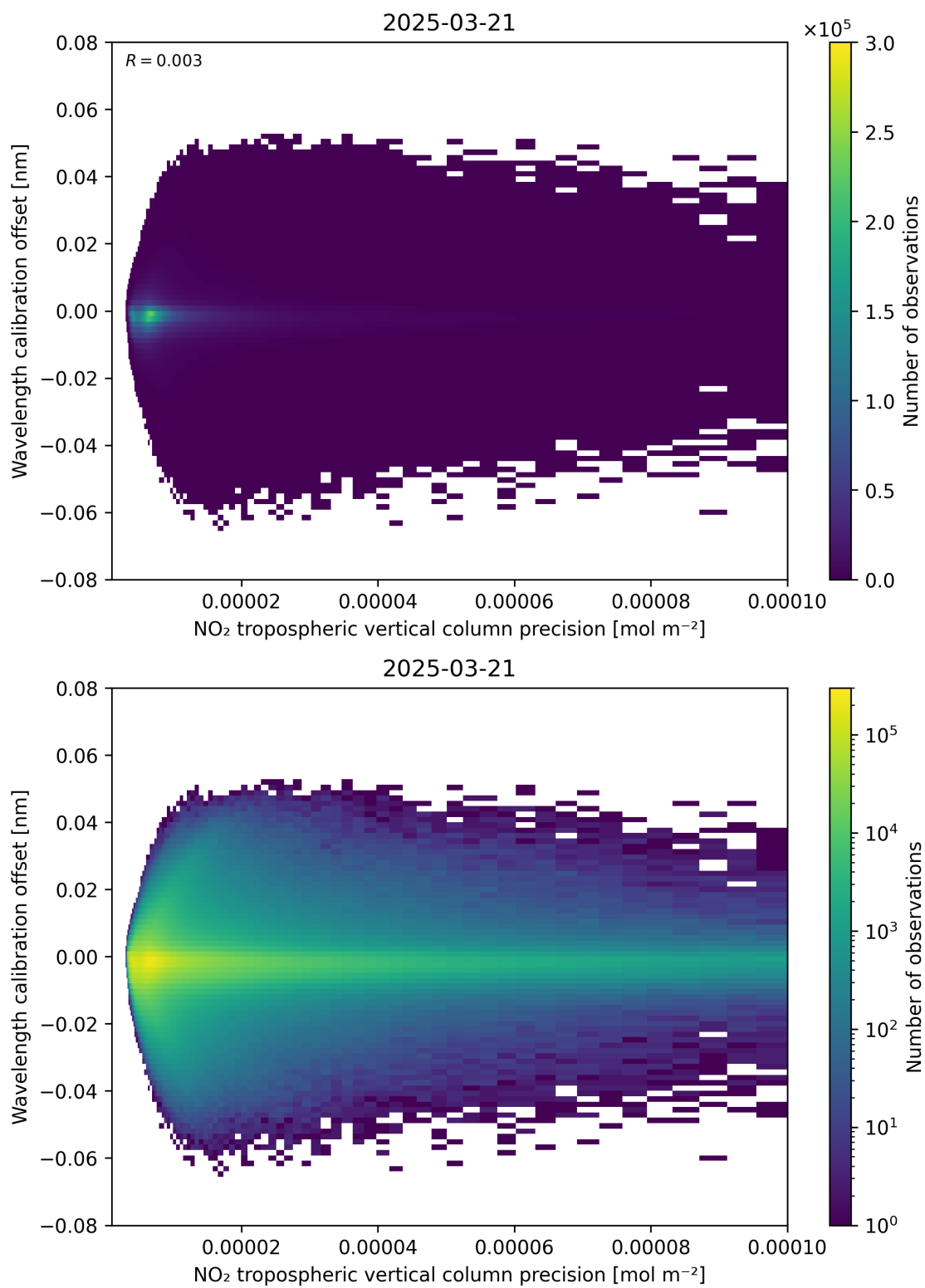
Figure 141: Scatter density plot of “NO 2 tropospheric vertical column precision” against “Wavelength calibration offset” for 2025-03-21 to 2025-03-21.
