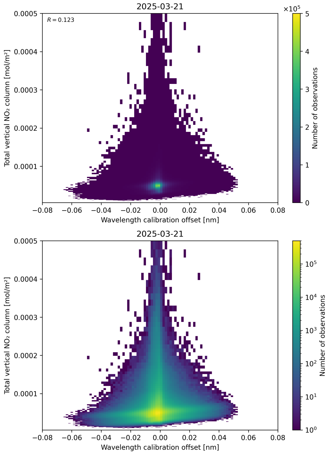
Figure 179: Scatter density plot of “Wavelength calibration offset” against “Total vertical NO 2 column” for 2025-03-21 to 2025-03-21.
