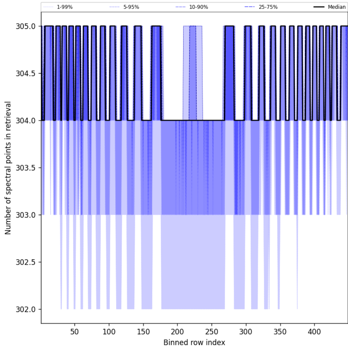
Figure 50: Along track statistics of “Number of spectral points in retrieval” for 2025-03-21 to 2025-03-21
