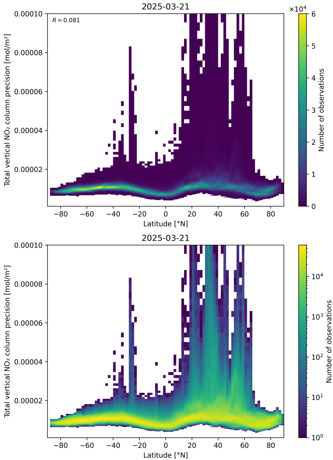
Figure 91: Scatter density plot of “Latitude” against “Total vertical NO 2 column precision” for 2025-03-21 to 2025-03-21.
