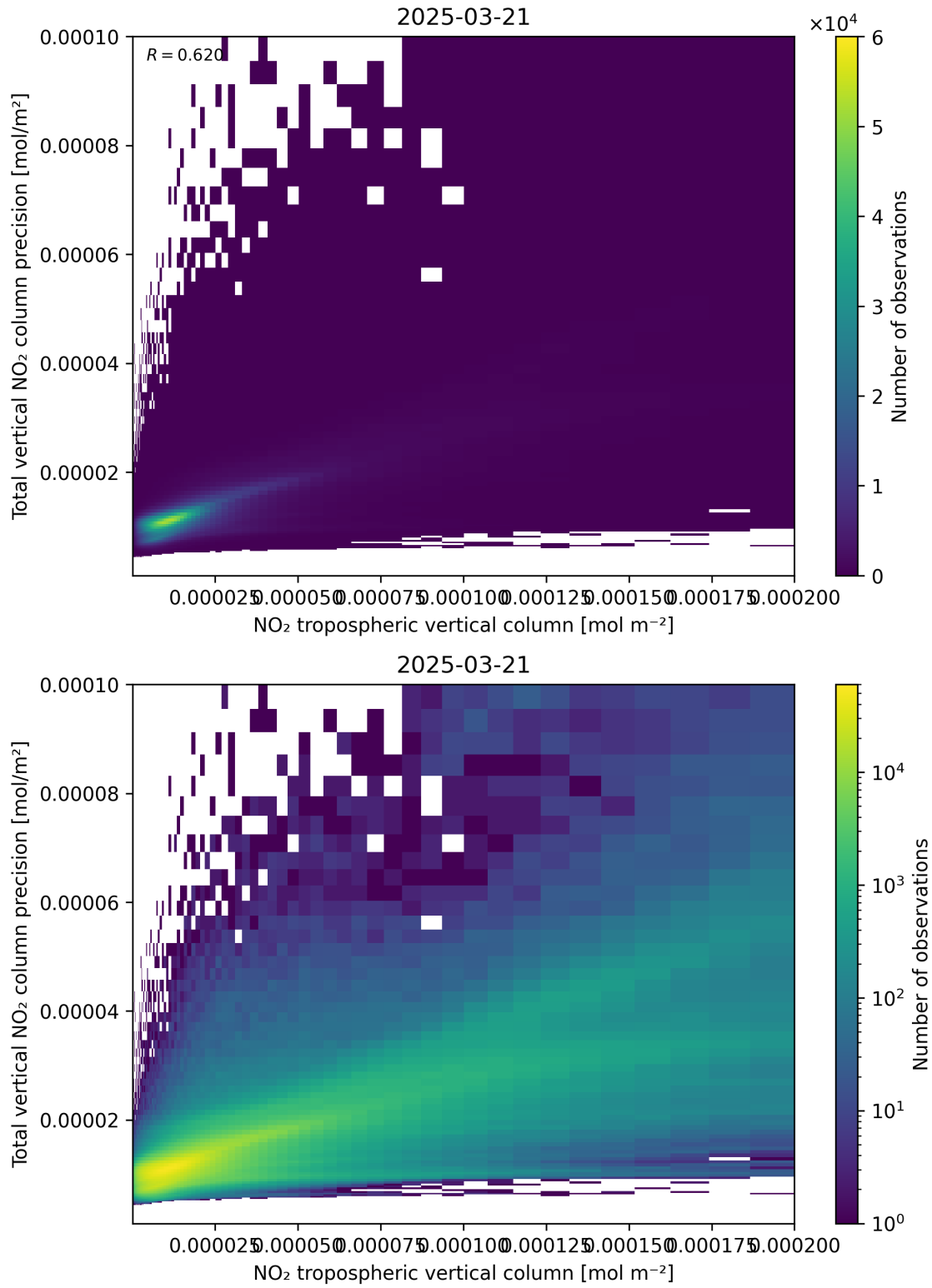
Figure 129: Scatter density plot of “NO 2 tropospheric vertical column” against “Total vertical NO 2 column precision” for 2025-03-21 to 2025-03-21.
