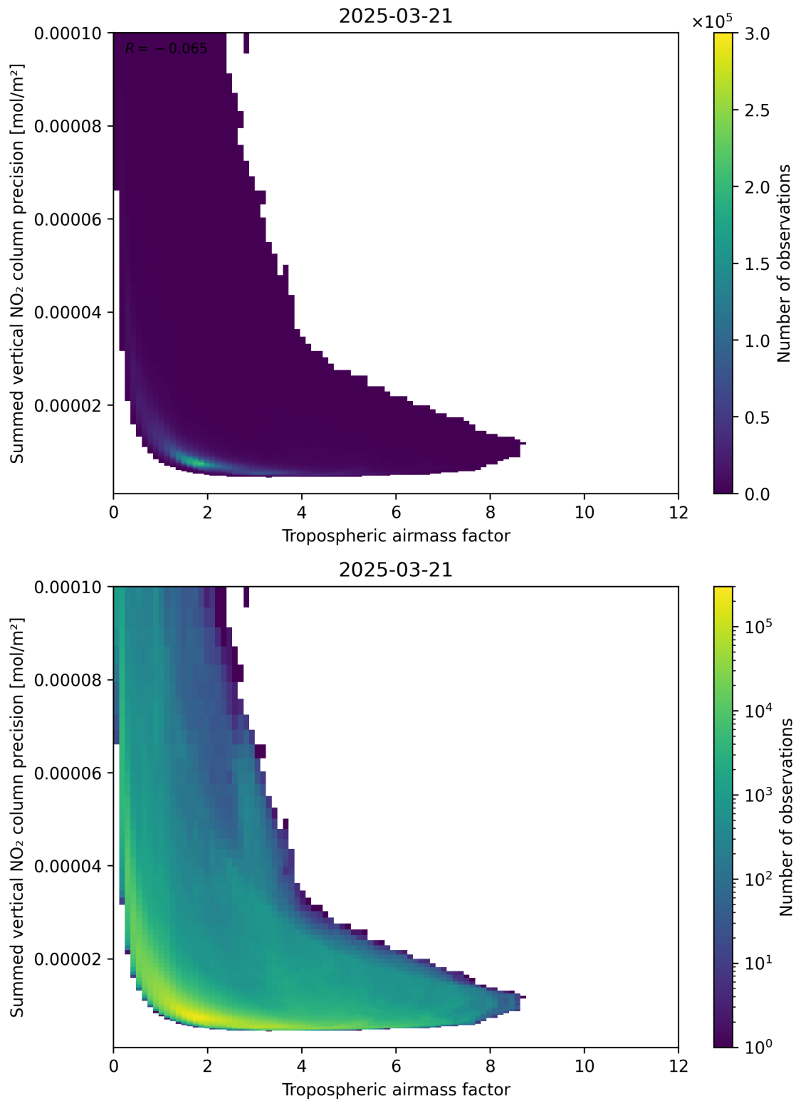
Figure 76: Scatter density plot of “Tropospheric air mass factor” against “Summed vertical NO 2 column precision” for 2025-03-21 to 2025-03-21.
