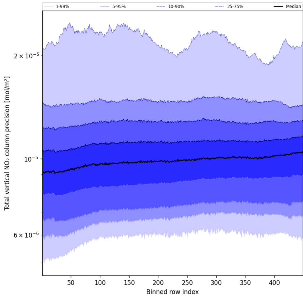
Figure 56: Along track statistics of “Total vertical NO 2 column precision” for 2025-03-21 to 2025-03-21
