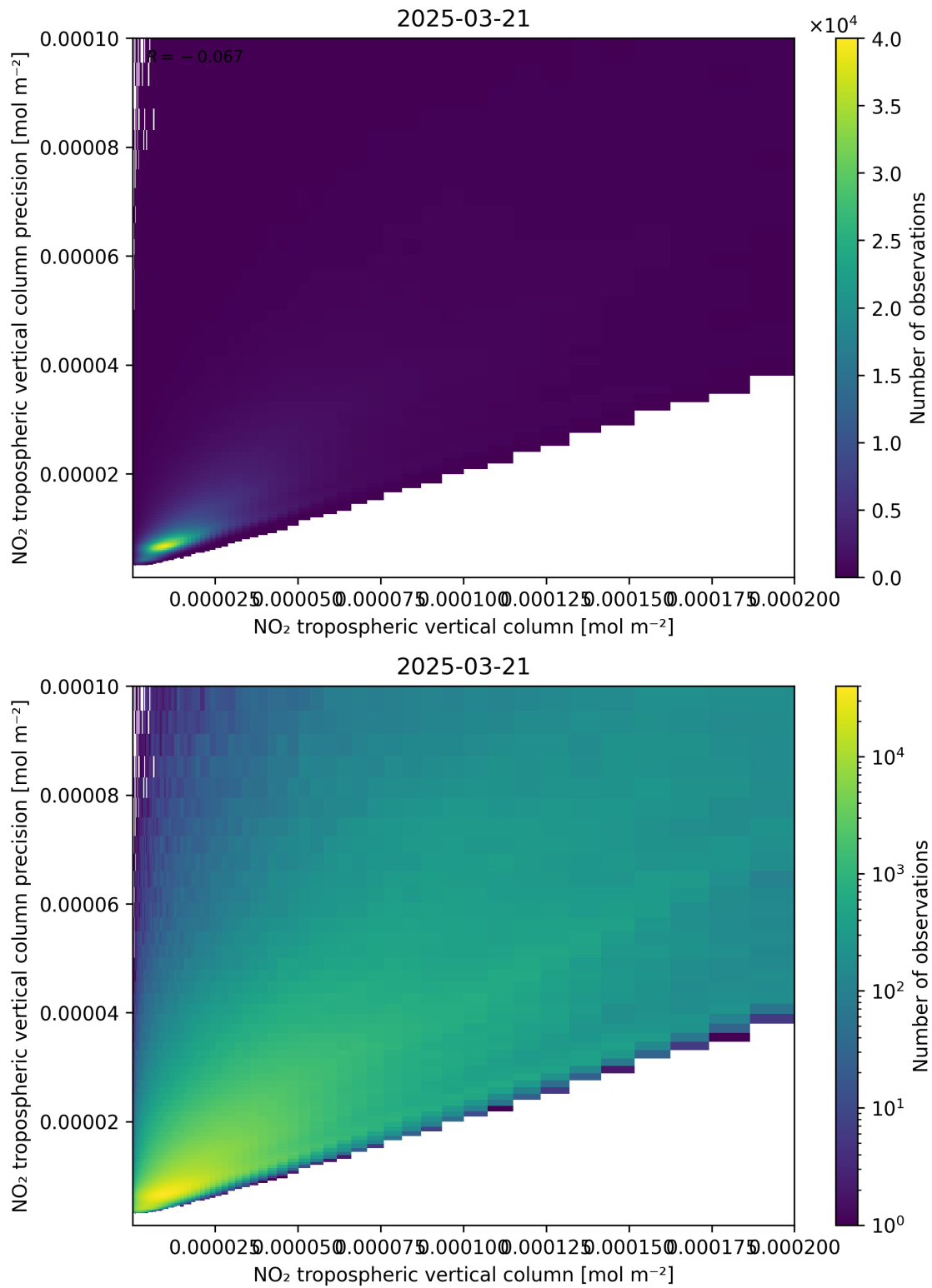
Figure 130: Scatter density plot of “NO 2 tropospheric vertical column” against “NO 2 tropospheric vertical column precision” for 2025-03-21 to 2025-03-21.
