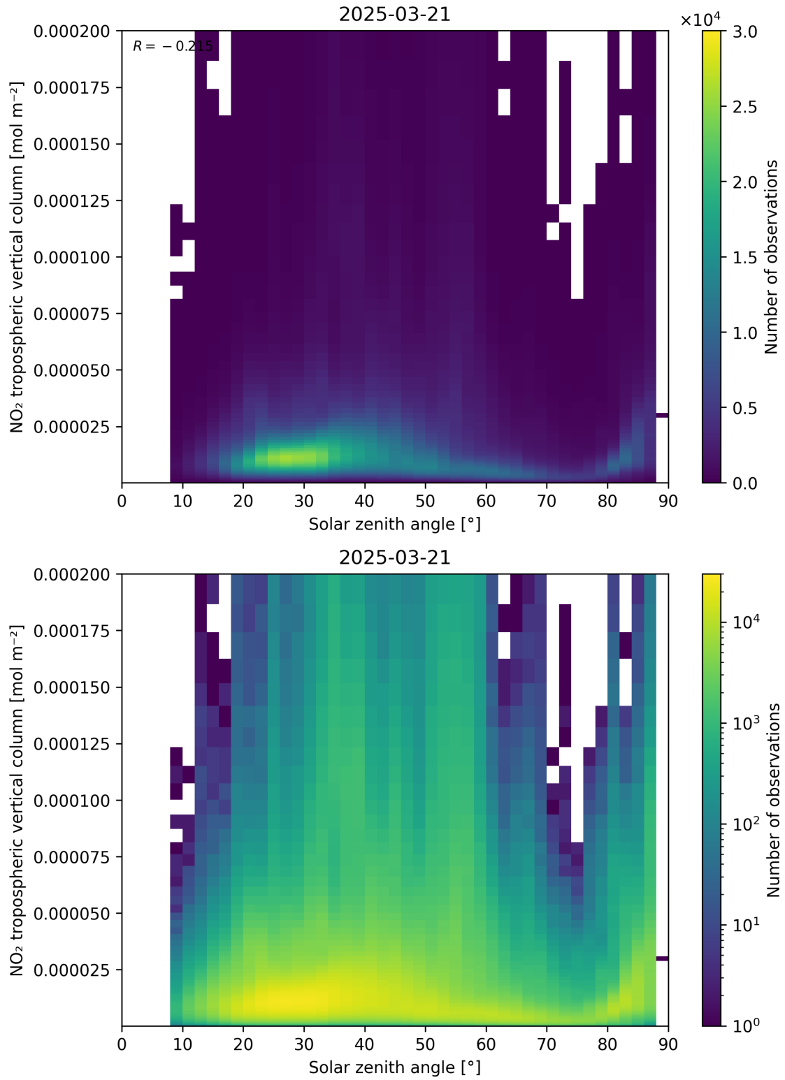
Figure 155: Scatter density plot of “Solar zenith angle” against “NO 2 tropospheric vertical column” for 2025-03-21 to 2025-03-21.
