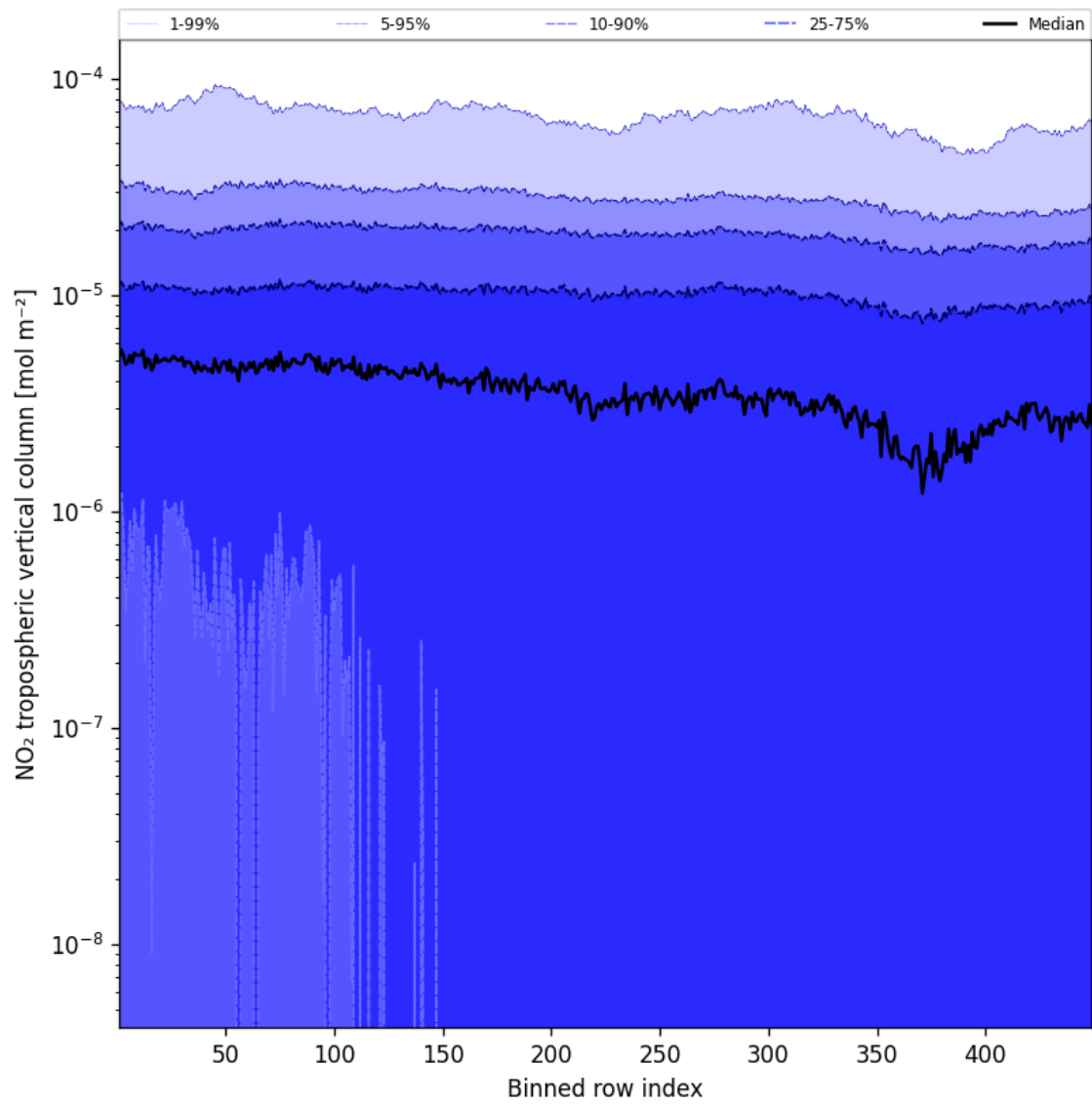
Figure 46: Along track statistics of “NO 2 tropospheric vertical column” for 2025-03-21 to 2025-03-21
