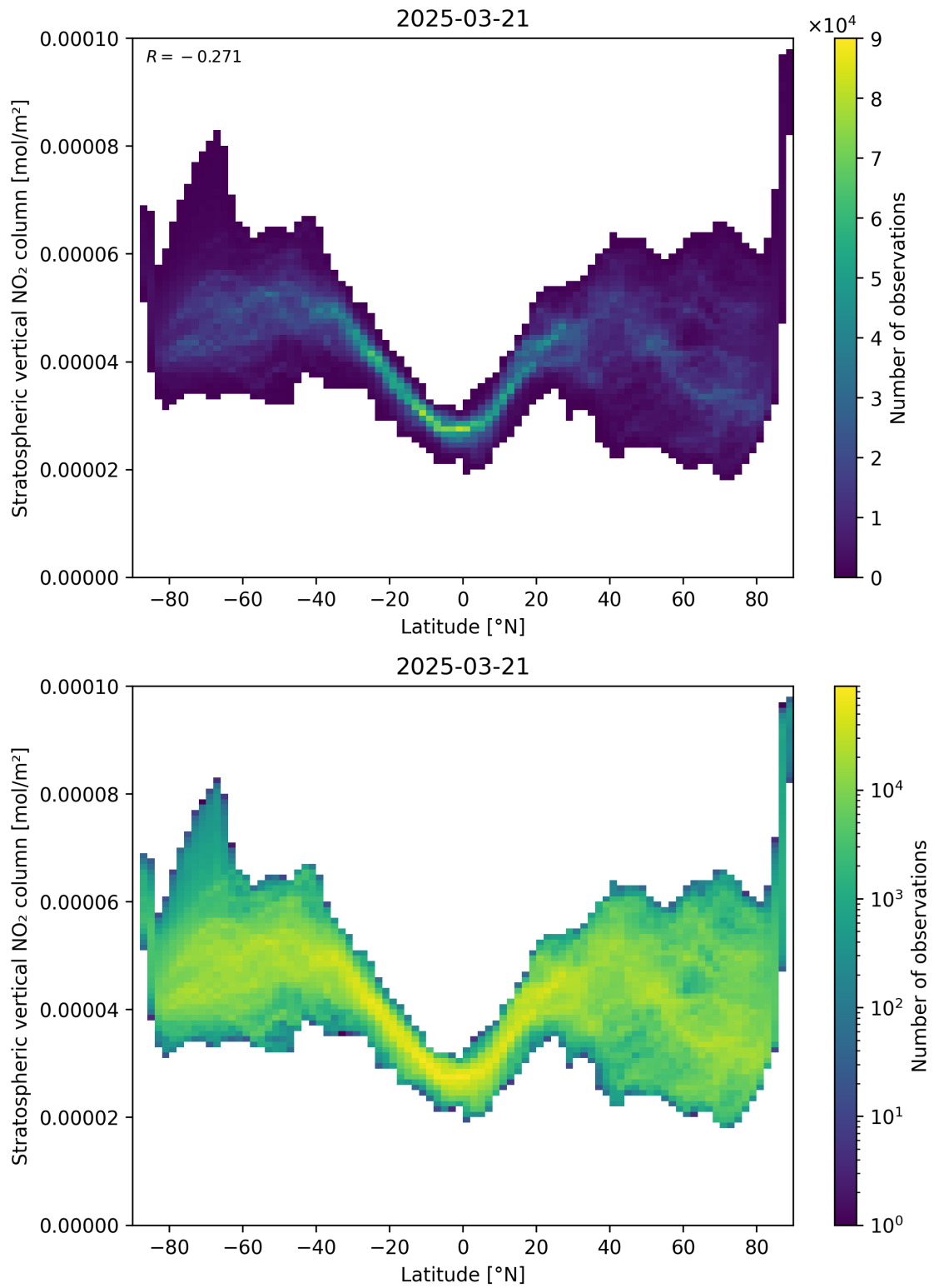
Figure 87: Scatter density plot of “Latitude” against “Stratospheric vertical NO 2 column” for 2025-03-21 to 2025-03-21.
