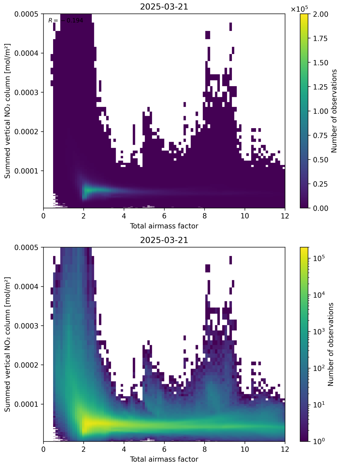
Figure 65: Scatter density plot of “Total airmass factor” against “Summed vertical NO 2 column” for 2025-03-21 to 2025-03-21.
