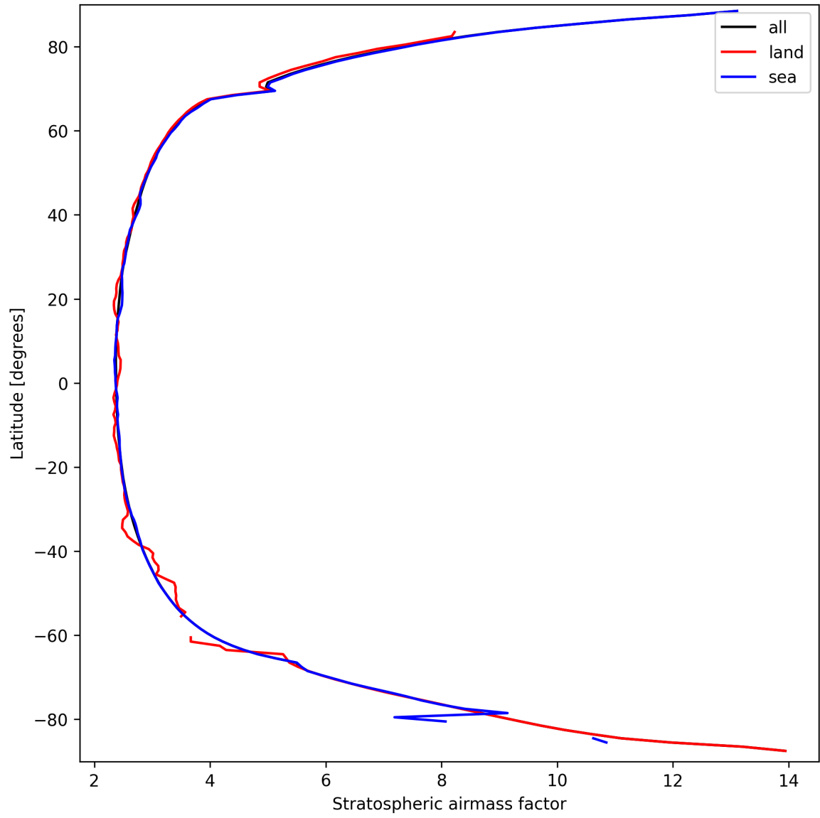
Figure 27: Zonal average of “Stratospheric airmass factor” for 2025-03-21 to 2025-03-21.
