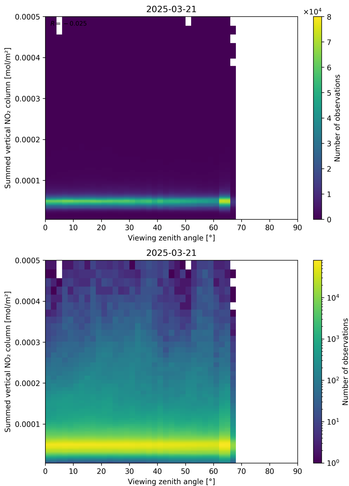
Figure 165: Scatter density plot of “Viewing zenith angle” against “Summed vertical NO 2 column” for 2025-03-21 to 2025-03-21.
