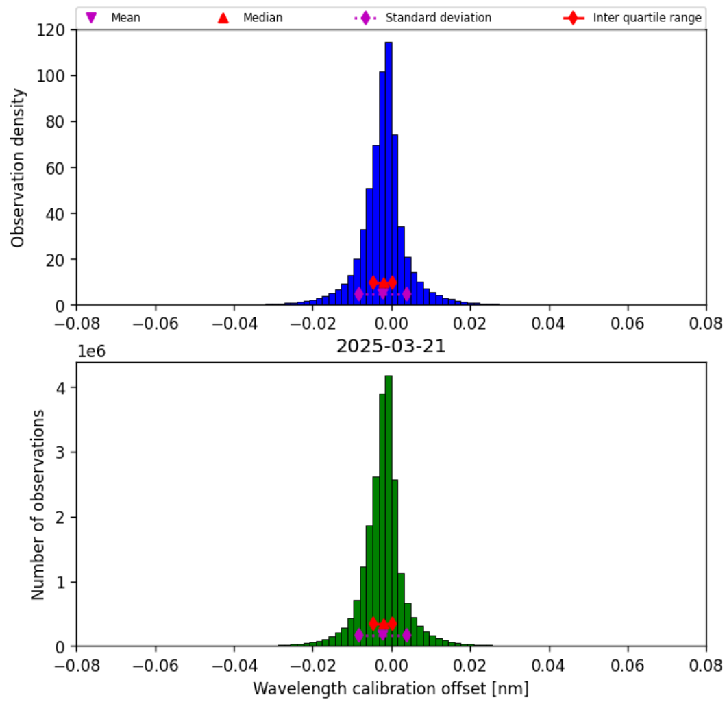
Figure 35: Histogram of “Wavelength calibration offset” for 2025-03-21 to 2025-03-21
