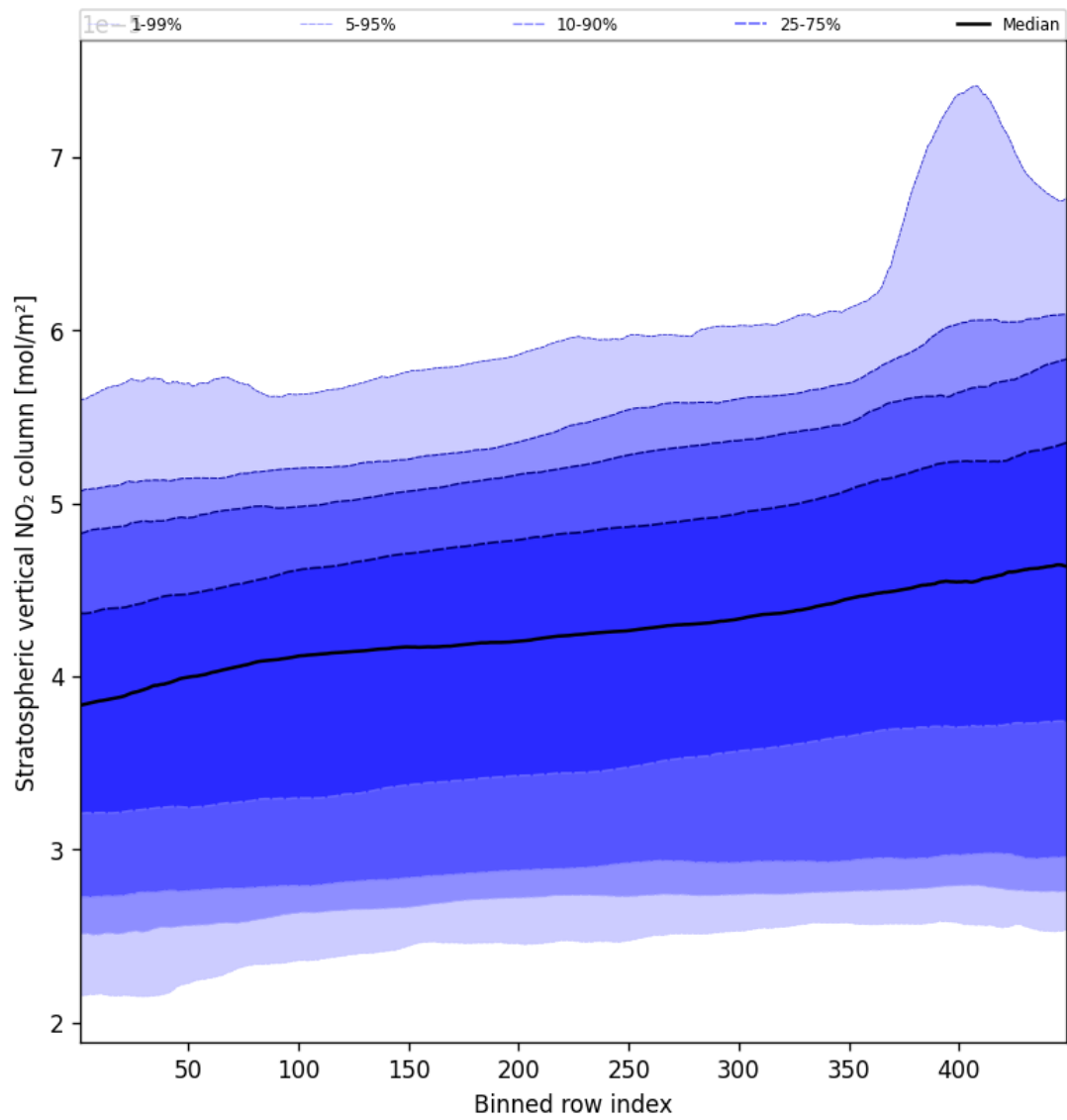
Figure 53: Along track statistics of “Stratospheric vertical NO 2 column” for 2025-03-21 to 2025-03-21
