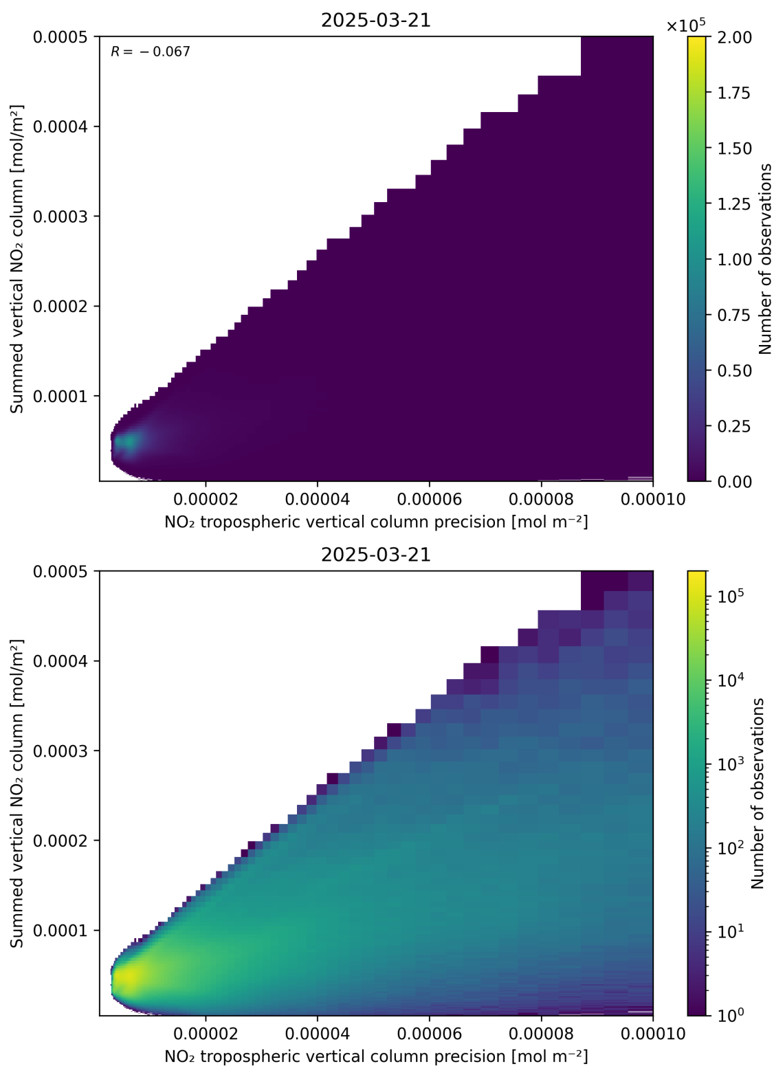
Figure 136: Scatter density plot of “NO 2 tropospheric vertical column precision” against “Summed vertical NO 2 column” for 2025-03-21 to 2025-03-21.
