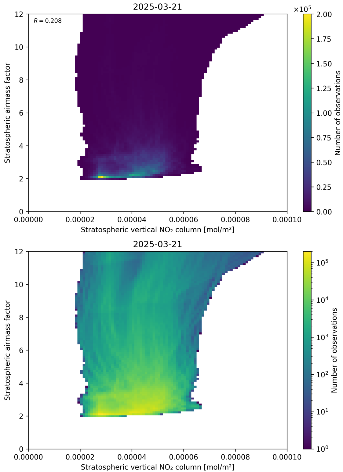
Figure 96: Scatter density plot of “Stratospheric vertical NO 2 column” against “Stratospheric airmass factor” for 2025-03-21 to 2025-03-21.
