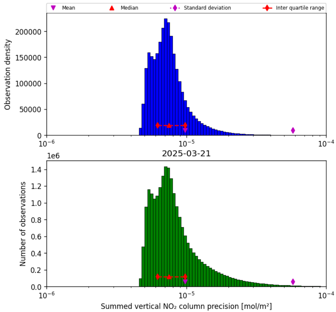
Figure 41: Histogram of "Summed vertical NO 2 column precision" for 2025-03-21 to 2025-03-21
