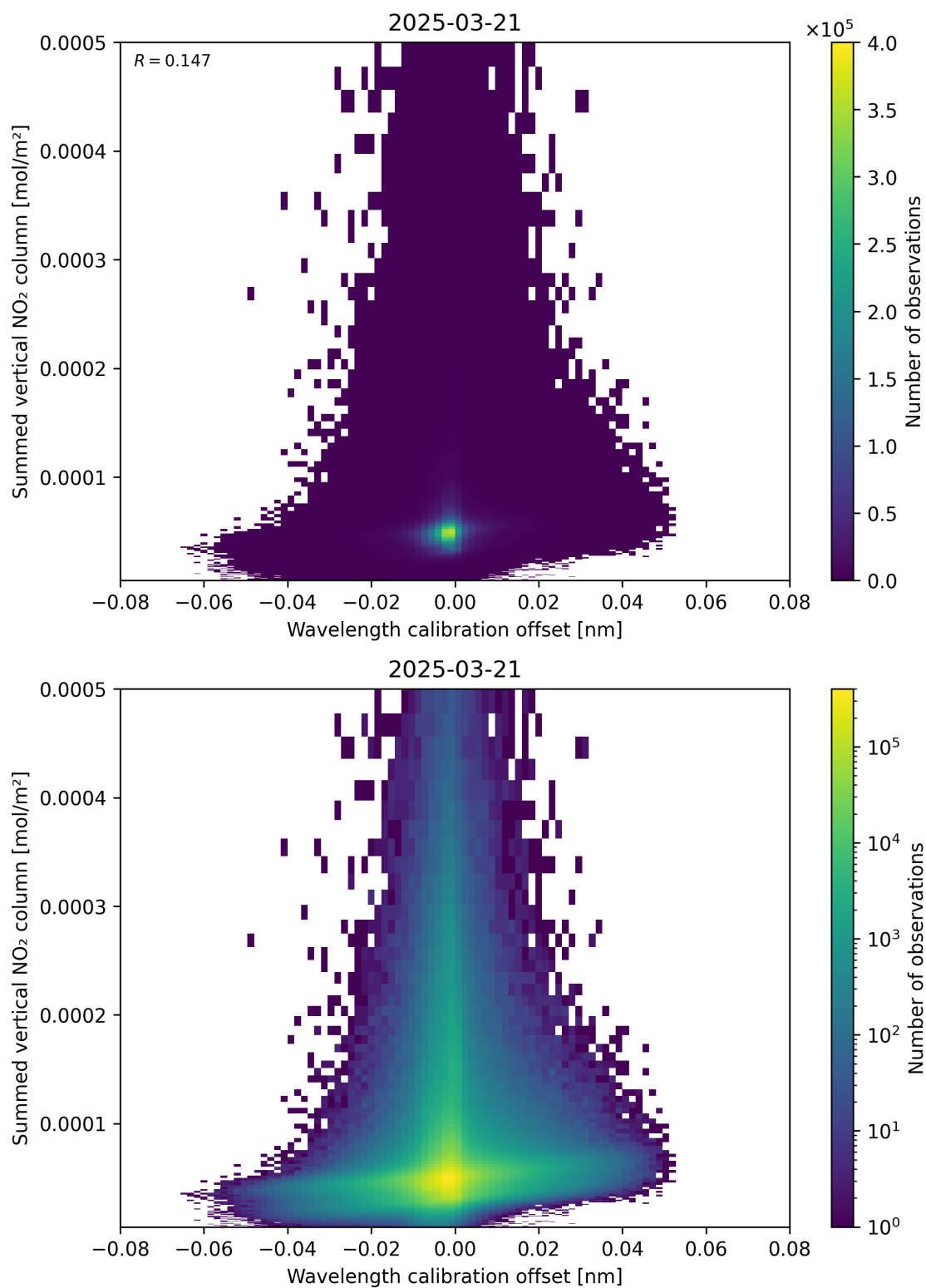
Figure 177: Scatter density plot of “Wavelength calibration offset” against “Summed vertical NO 2 column” for 2025-03-21 to 2025-03-21.
