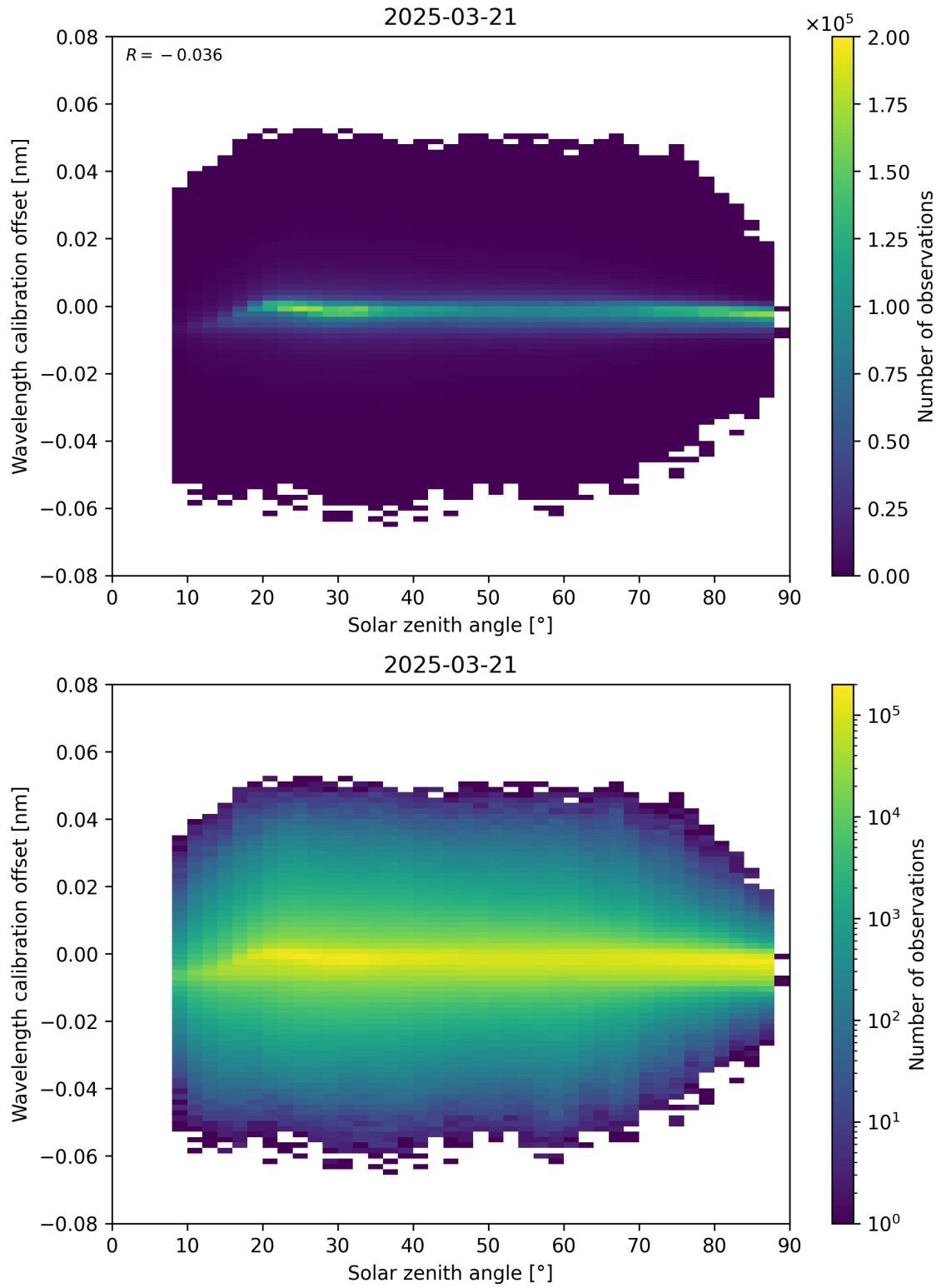
Figure 158: Scatter density plot of “Solar zenith angle” against “Wavelength calibration offset” for 2025-03-21 to 2025-03-21.
