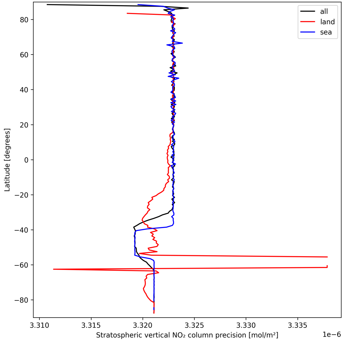
Figure 20: Zonal average of “Stratospheric vertical NO 2 column precision” for 2025-03-21 to 2025-03-21.
