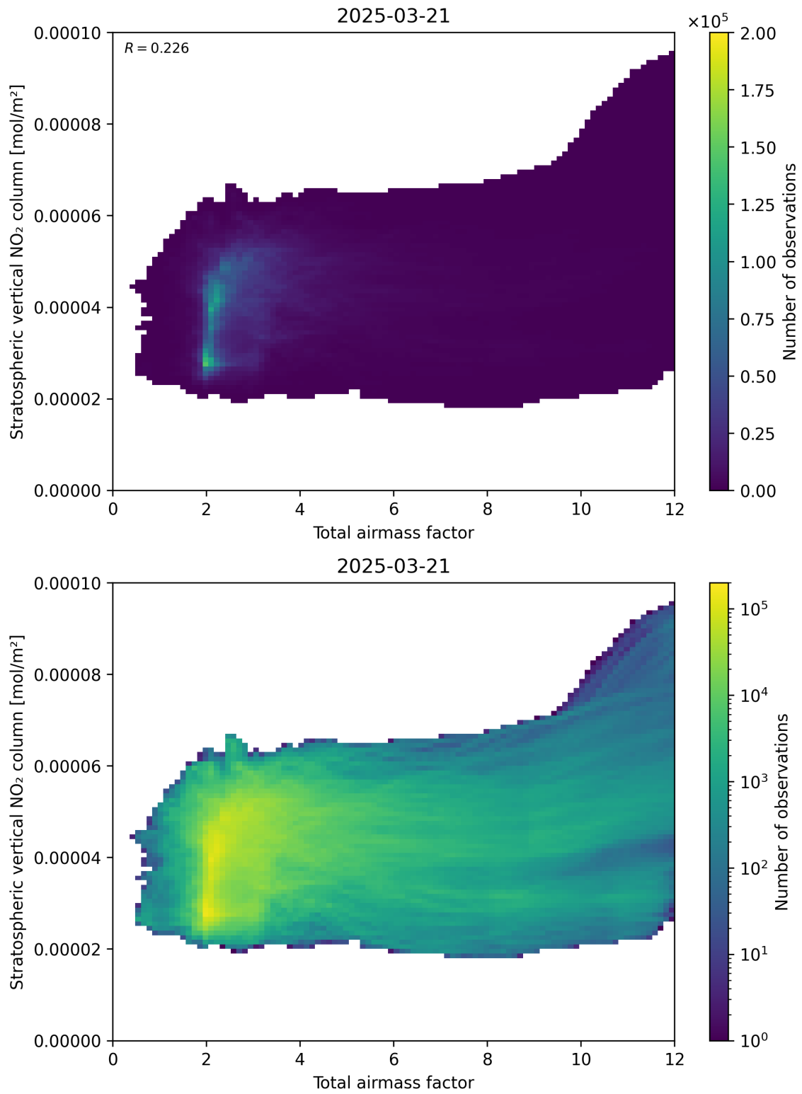
Figure 64: Scatter density plot of “Total airmass factor” against “Stratospheric vertical NO 2 column” for 2025-03-21 to 2025-03-21.
