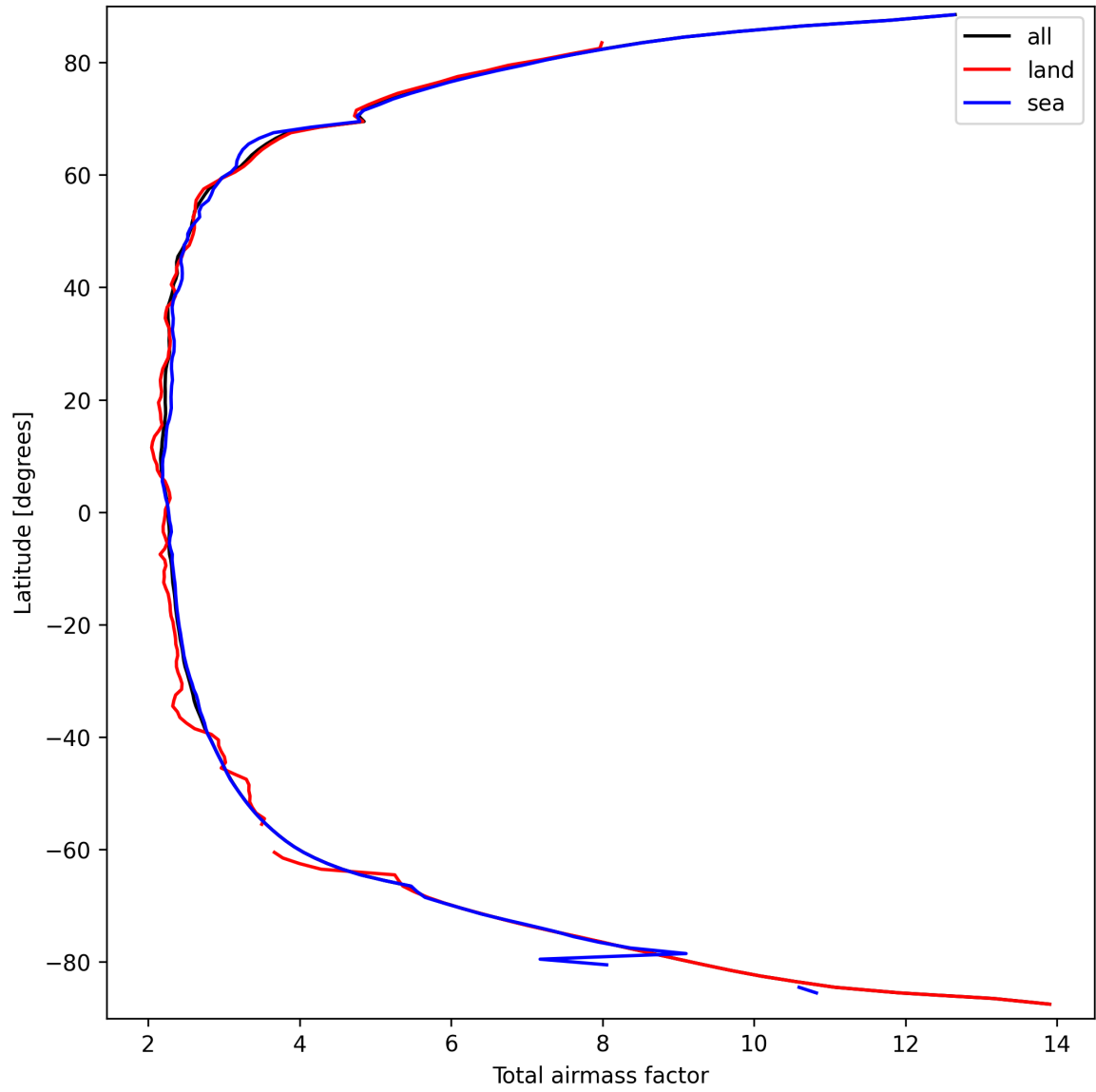
Figure 15: Zonal average of “Total airmass factor” for 2025-03-21 to 2025-03-21.
