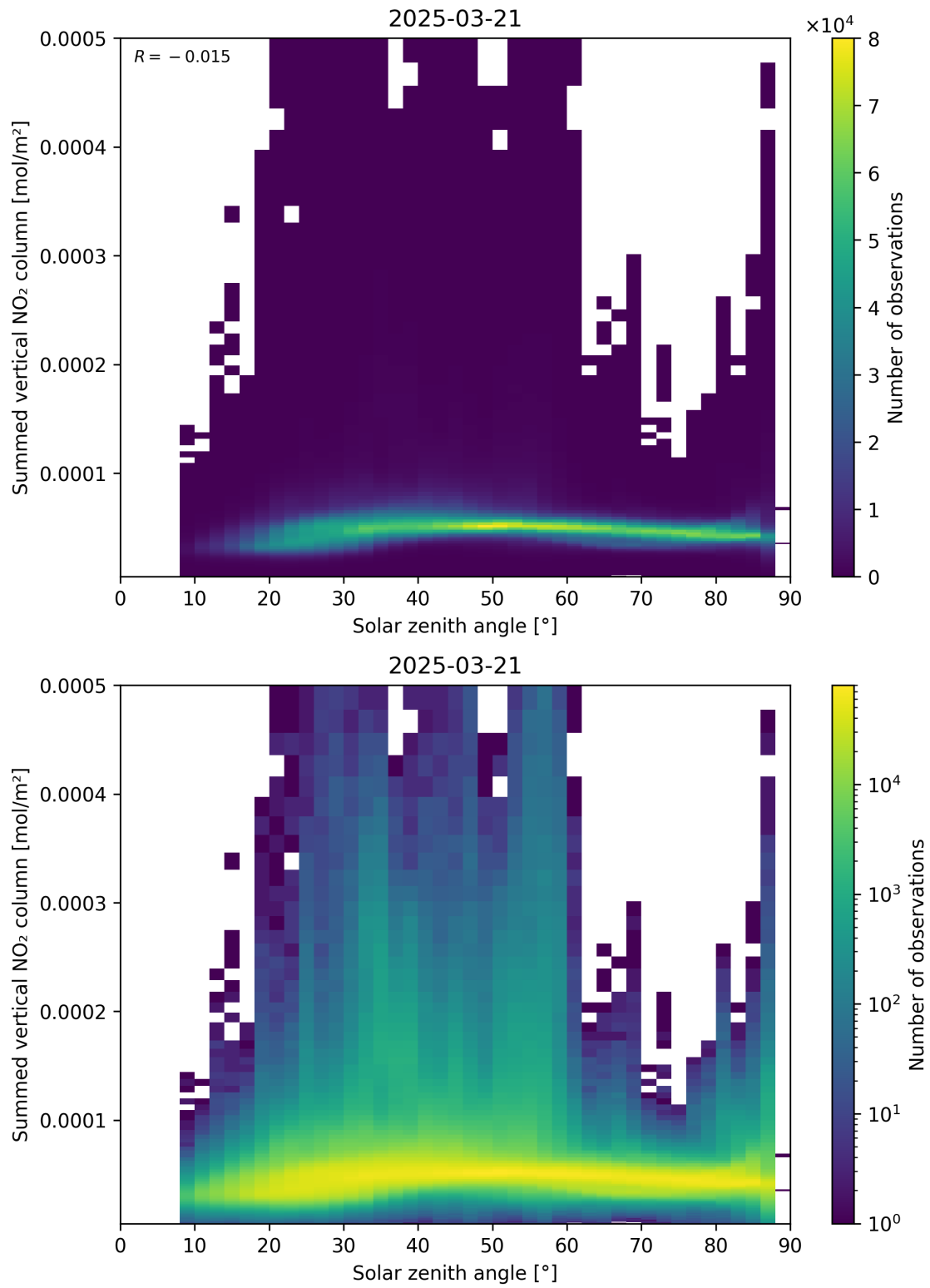
Figure 151: Scatter density plot of “Solar zenith angle” against “Summed vertical NO 2 column” for 2025-03-21 to 2025-03-21.
