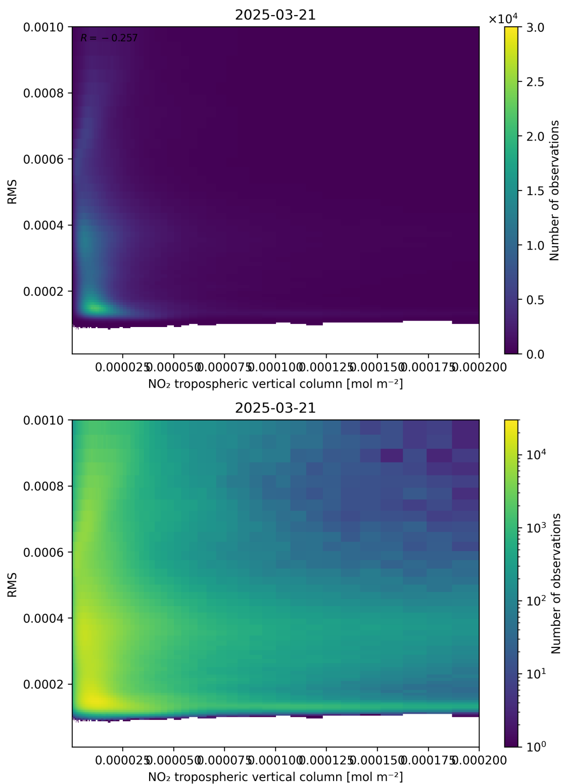
Figure 142: Scatter density plot of “NO 2 tropospheric vertical column” against “RMS” for 2025-03-21 to 2025-03-21.
