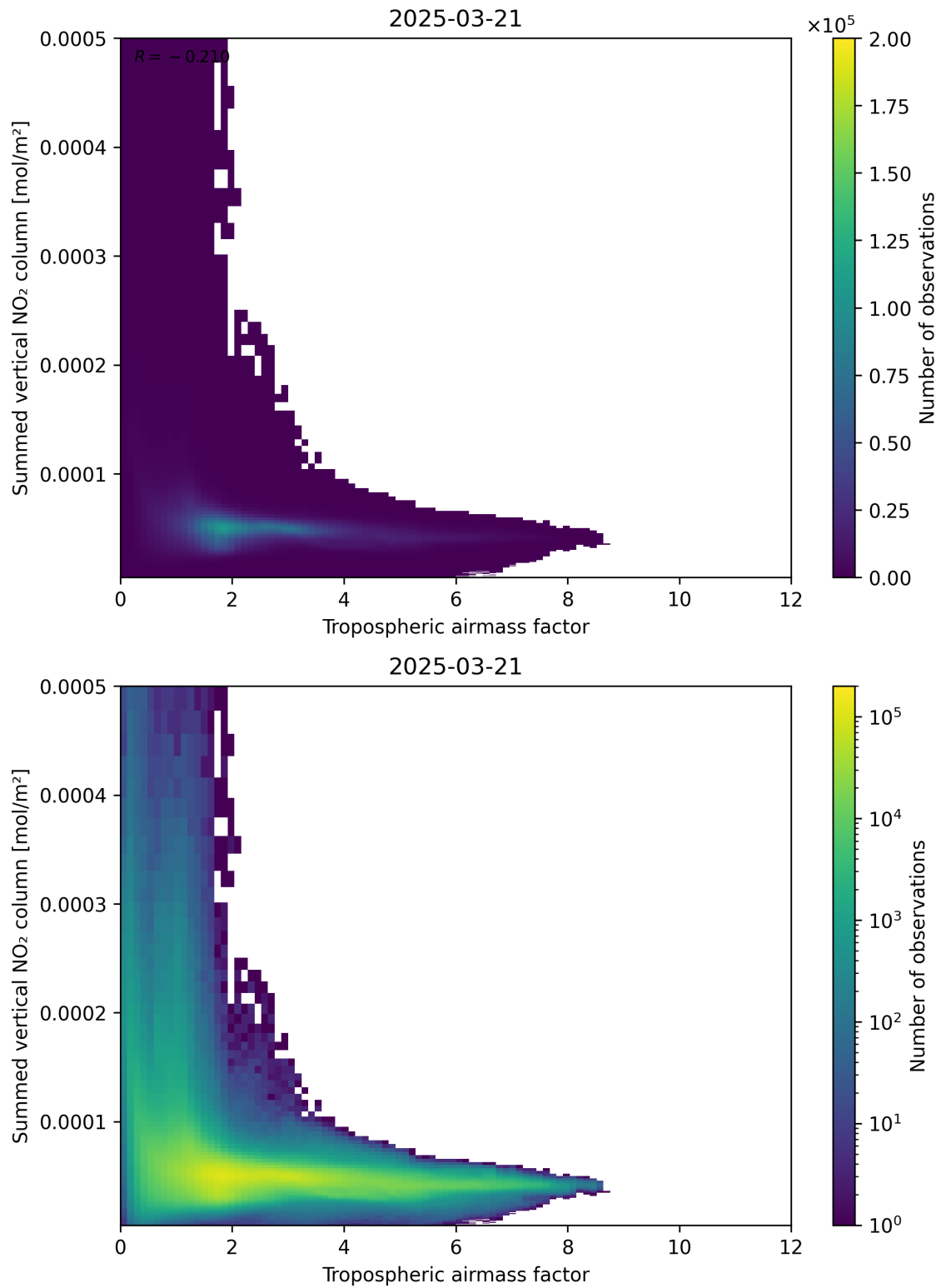
Figure 75: Scatter density plot of “Tropospheric airmass factor” against “Summed vertical NO 2 column” for 2025-03-21 to 2025-03-21.
