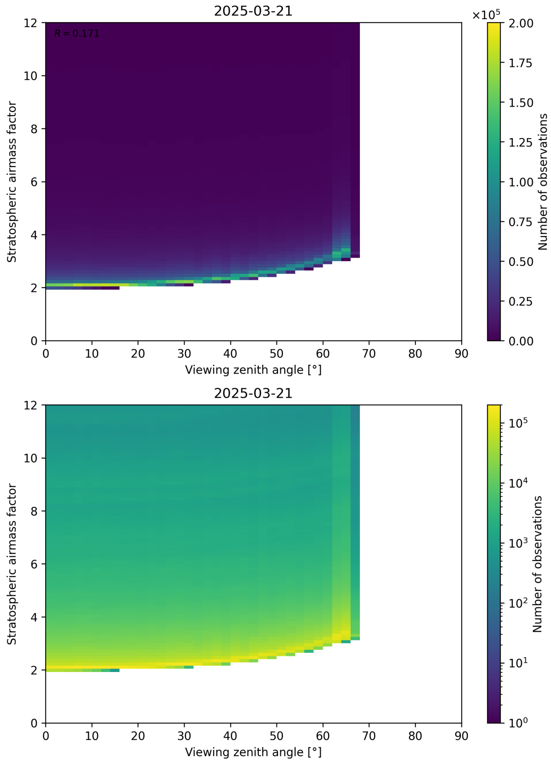
Figure 159: Scatter density plot of “Viewing zenith angle” against “Stratospheric airmass factor” for 2025-03-21 to 2025-03-21.
