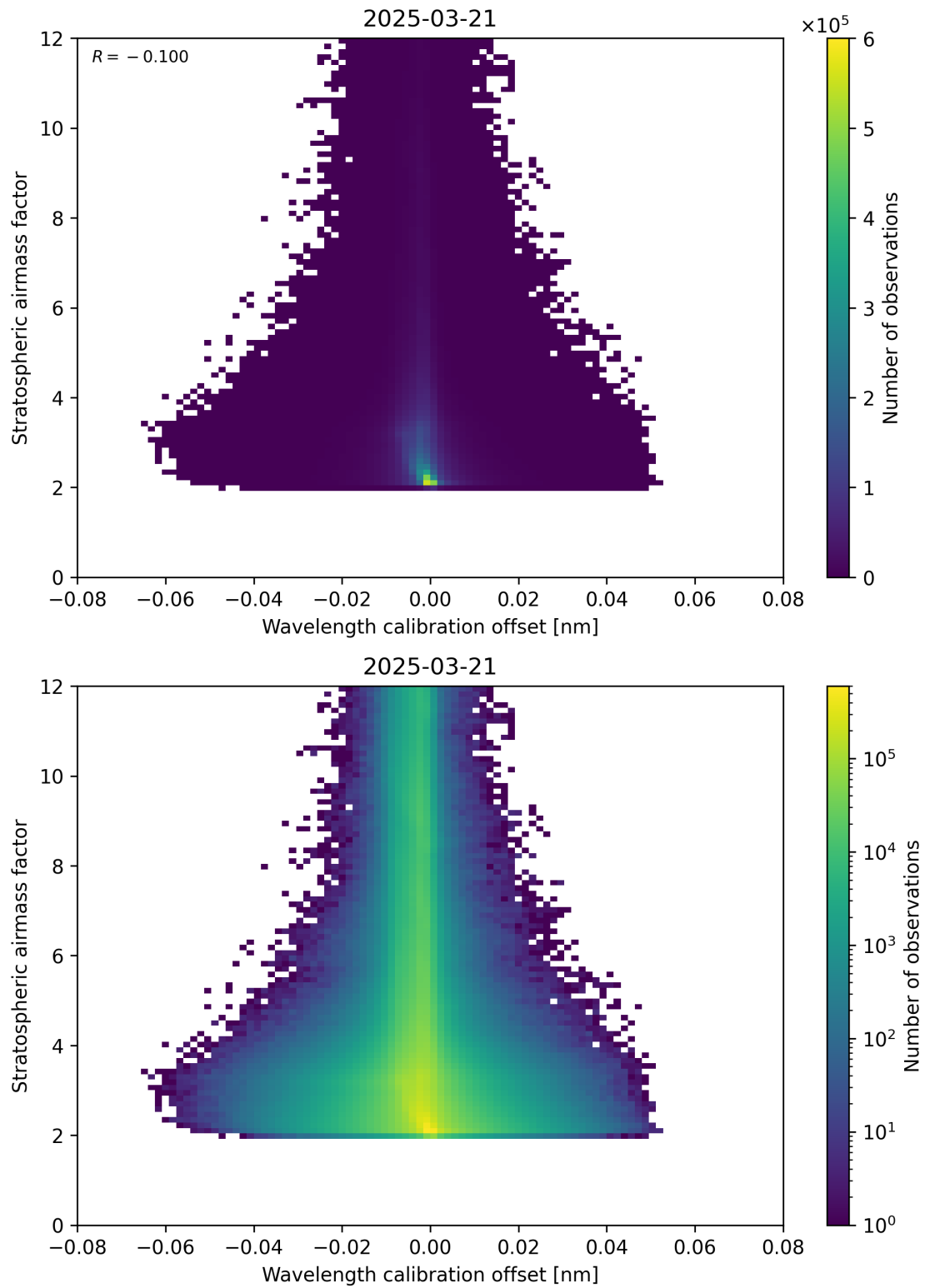
Figure 174: Scatter density plot of “Wavelength calibration offset” against “Stratospheric airmass factor” for 2025-03-21 to 2025-03-21.
