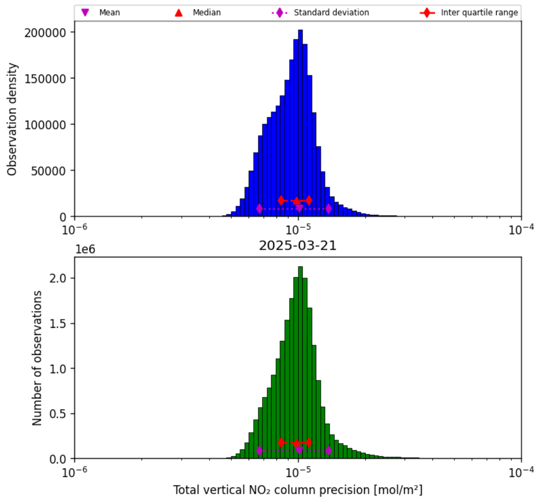
Figure 39: Histogram of "Total vertical NO 2 column precision" for 2025-03-21 to 2025-03-21
