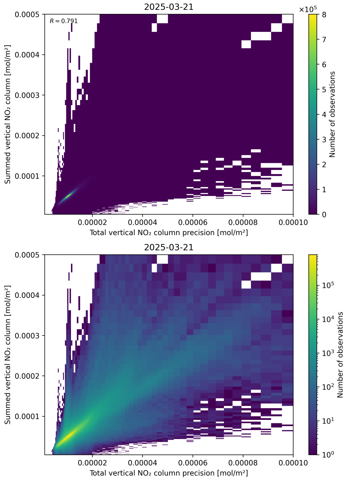
Figure 117: Scatter density plot of “Total vertical NO 2 column precision” against “Summed vertical NO 2 column” for 2025-03-21 to 2025-03-21.
