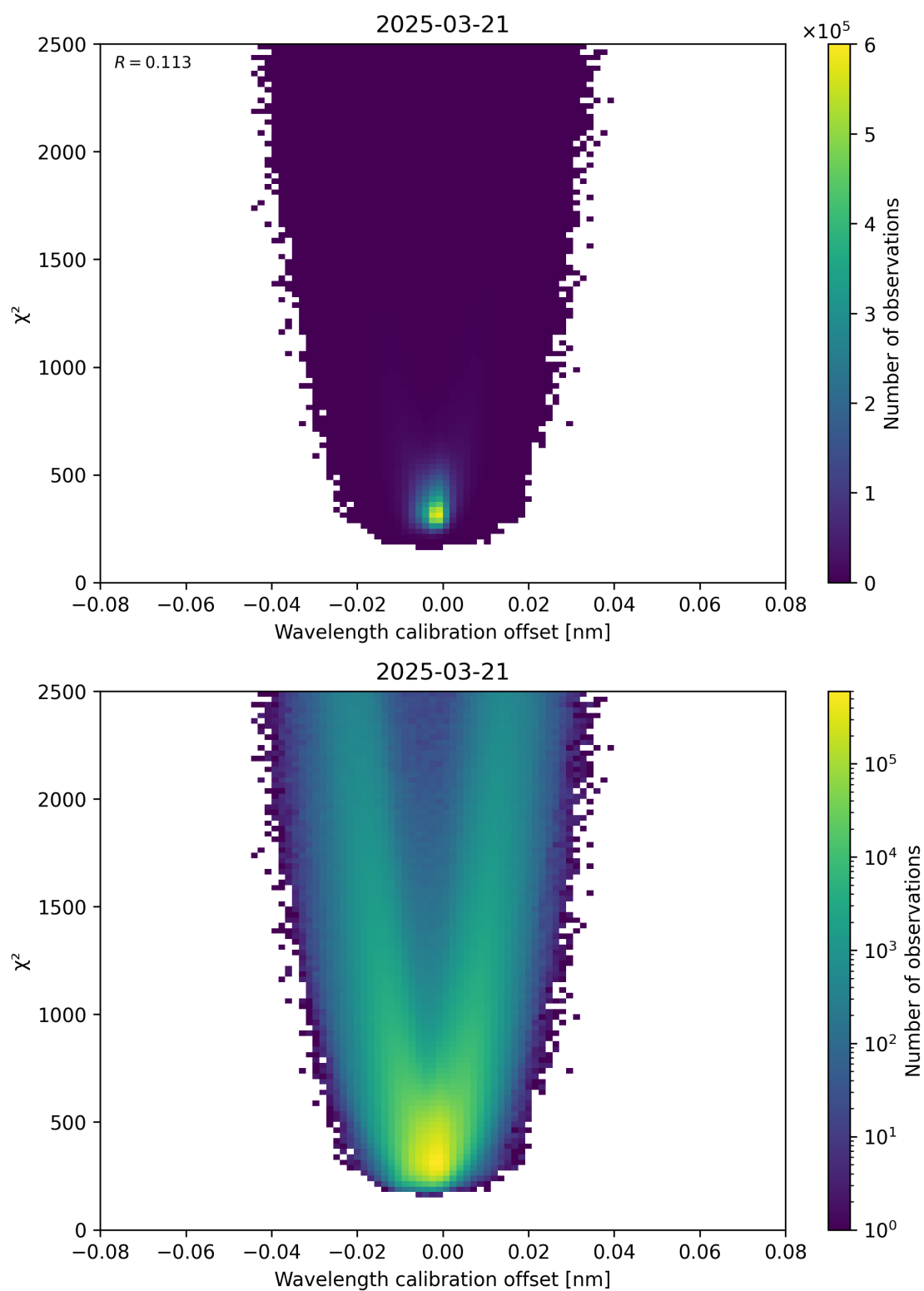
Figure 175: Scatter density plot of “Wavelength calibration offset” against “ \chi^2 ” for 2025-03-21 to 2025-03-21.
