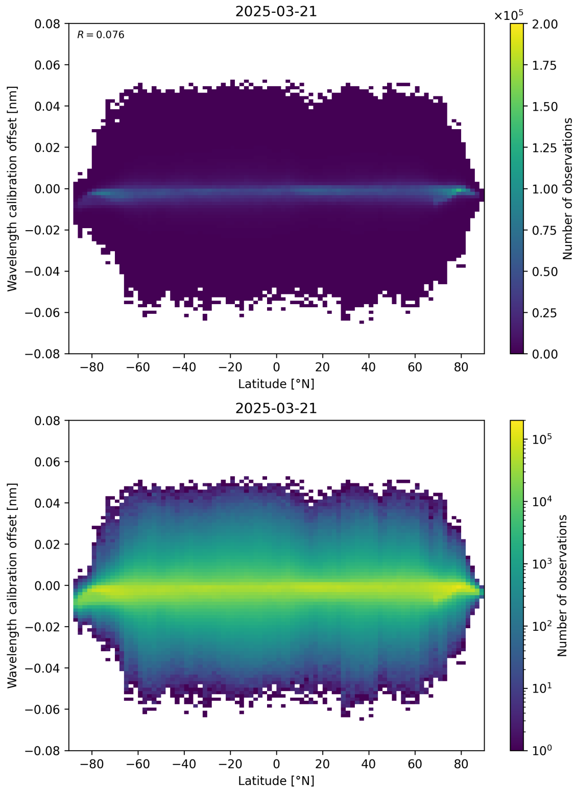
Figure 95: Scatter density plot of “Latitude” against “Wavelength calibration offset” for 2025-03-21 to 2025-03-21.
