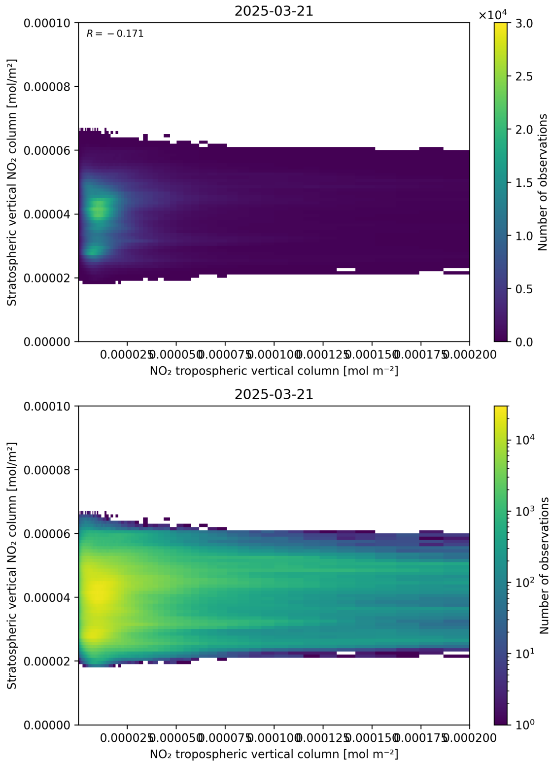
Figure 125: Scatter density plot of “NO 2 tropospheric vertical column” against “Stratospheric vertical NO 2 column” for 2025-03-21 to 2025-03-21.
