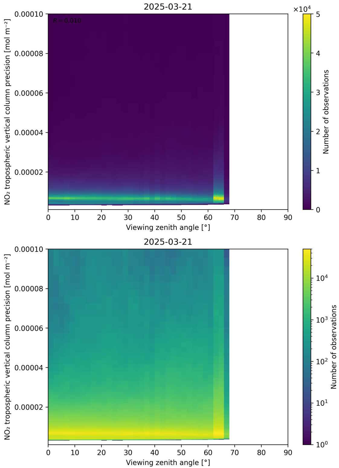
Figure 170: Scatter density plot of “Viewing zenith angle” against “NO 2 tropospheric vertical column precision” for 2025-03-21 to 2025-03-21.
