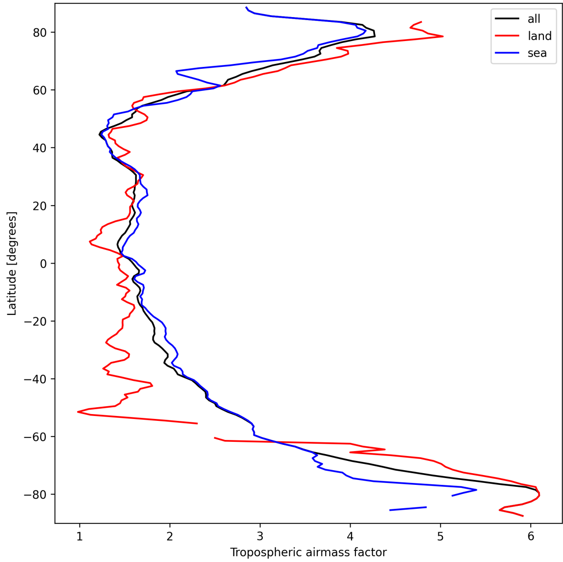
Figure 14: Zonal average of “Tropospheric airmass factor” for 2025-03-21 to 2025-03-21.
