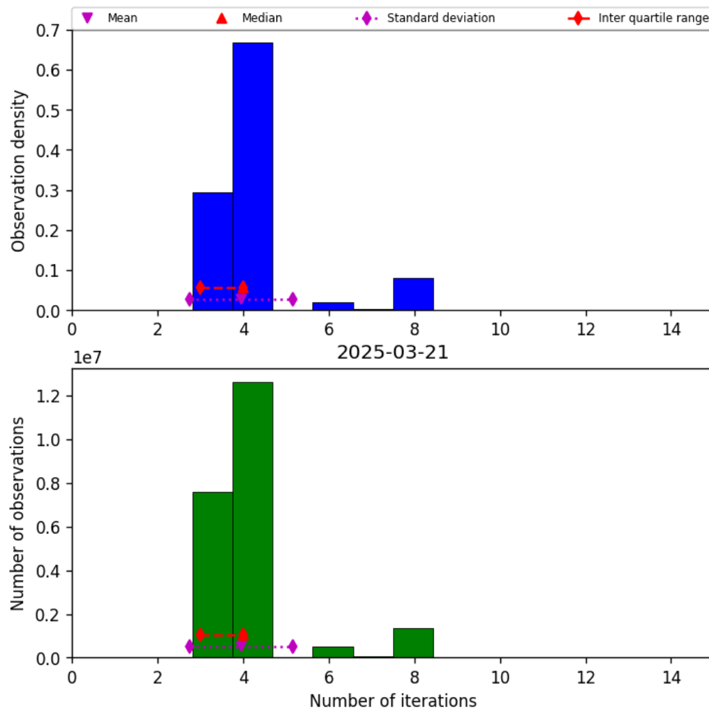
Figure 34: Histogram of “Number of iterations” for 2025-03-21 to 2025-03-21
