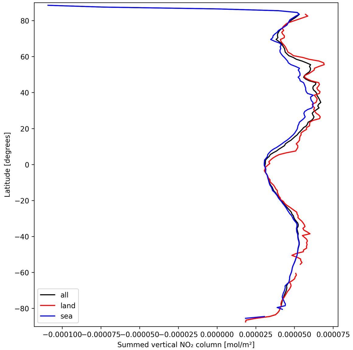
Figure 23: Zonal average of “Summed vertical NO 2 column” for 2025-03-21 to 2025-03-21.
