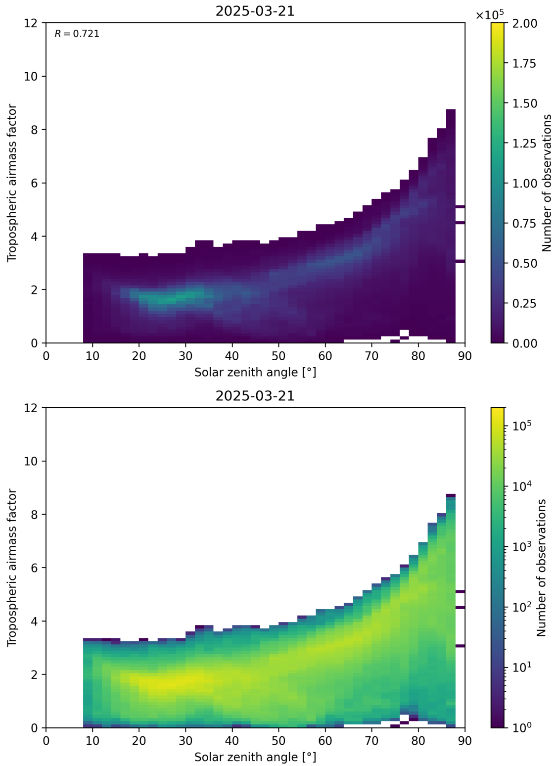
Figure 147: Scatter density plot of “Solar zenith angle” against “Tropospheric airmass factor” for 2025-03-21 to 2025-03-21.
