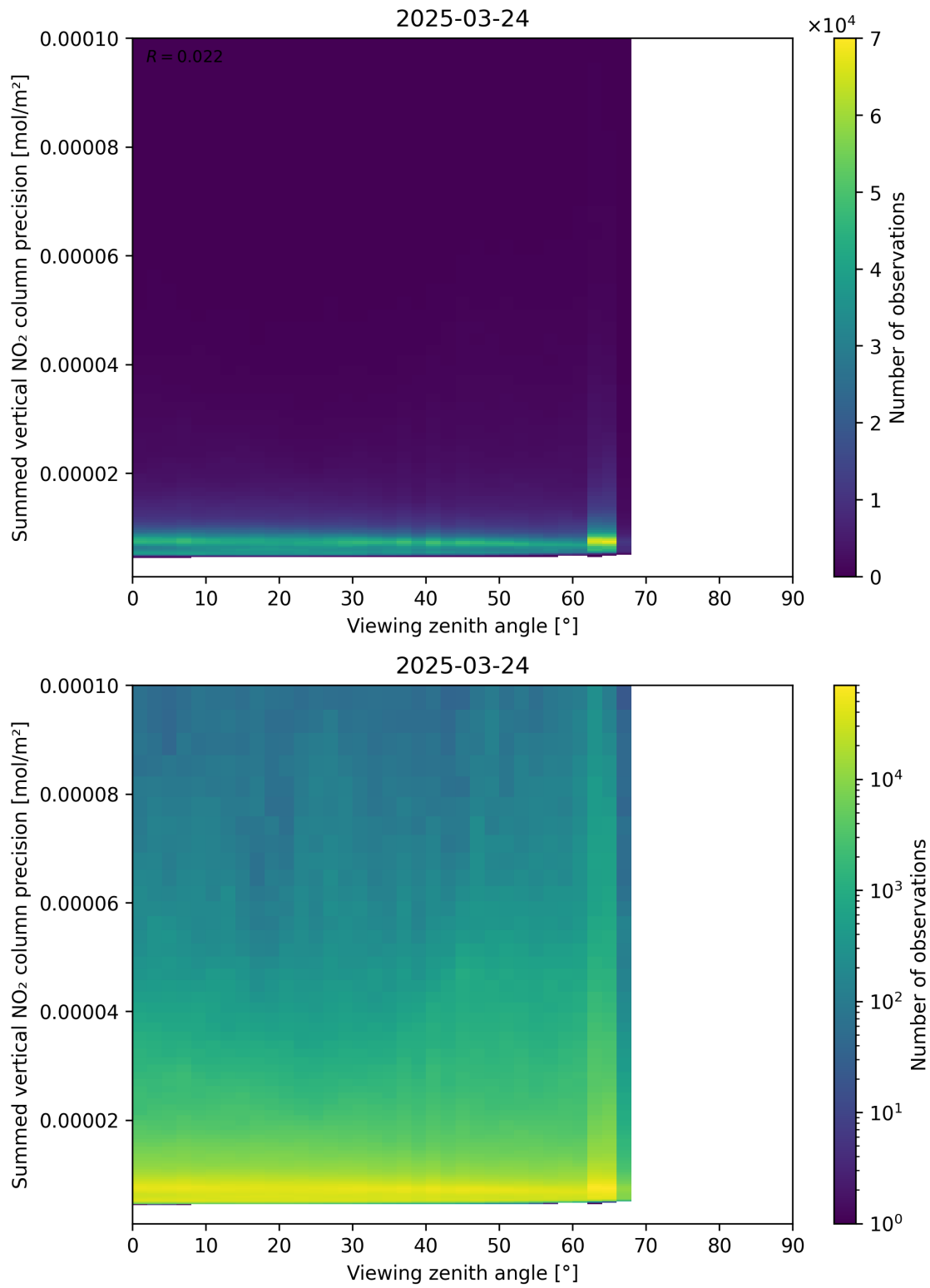
Figure 166: Scatter density plot of “Viewing zenith angle” against “Summed vertical NO 2 column precision” for 2025-03-24 to 2025-03-25.
