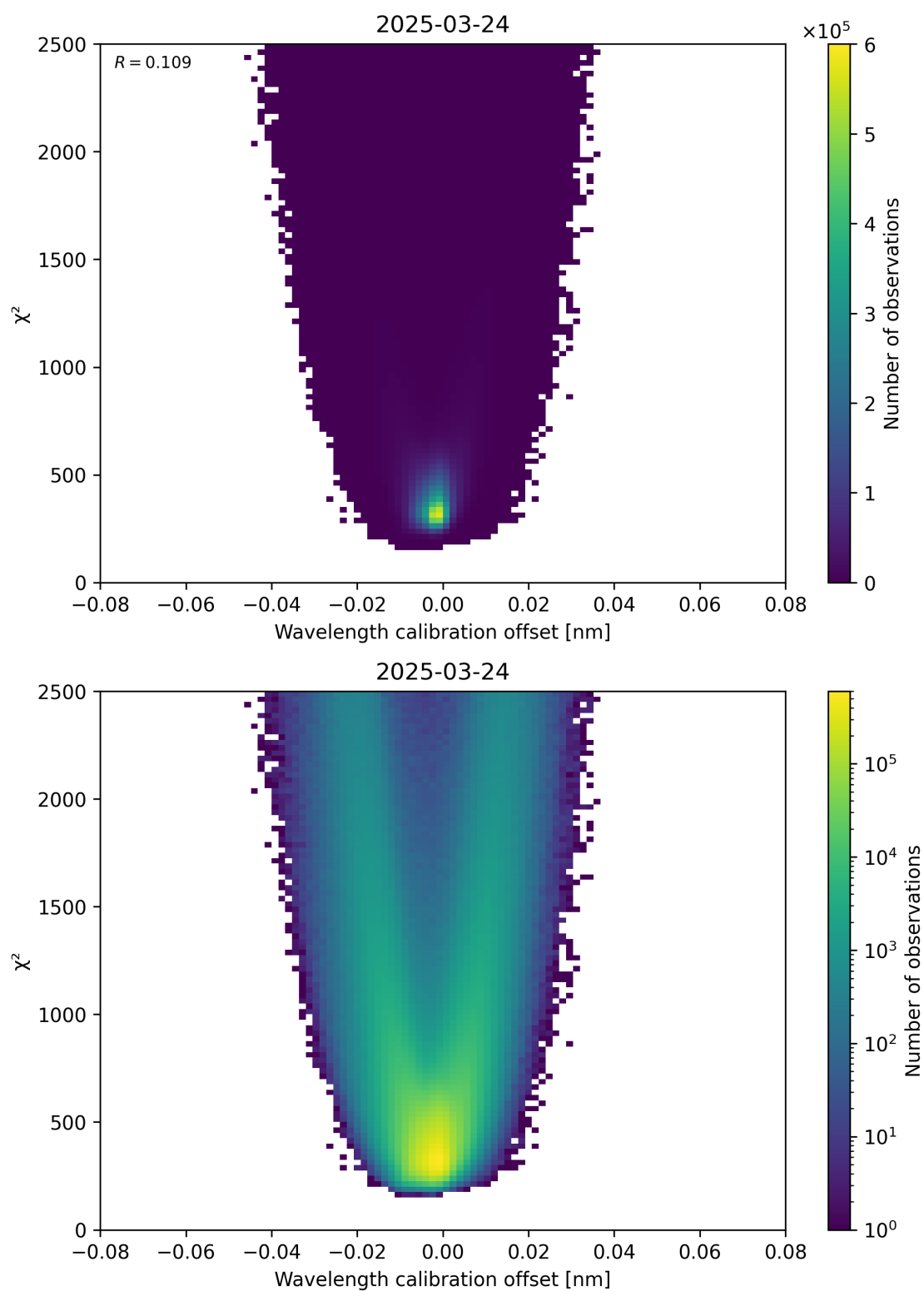
Figure 175: Scatter density plot of “Wavelength calibration offset” against “ \chi^2 ” for 2025-03-24 to 2025-03-25.
