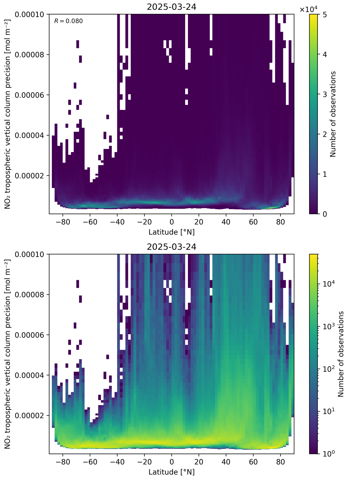
Figure 93: Scatter density plot of “Latitude” against “NO 2 tropospheric vertical column precision” for 2025-03-24 to 2025-03-25.
