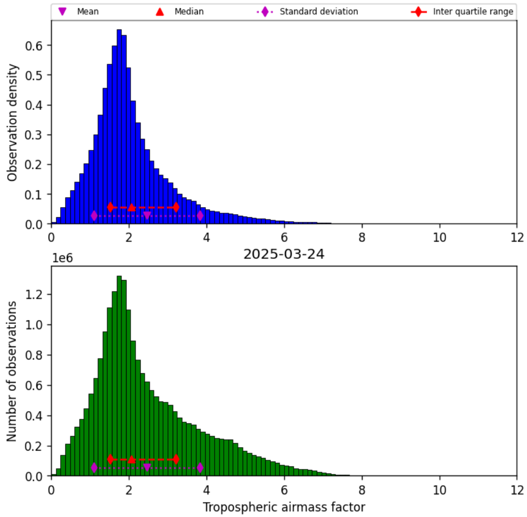
Figure 31: Histogram of “Tropospheric airmass factor” for 2025-03-24 to 2025-03-25
