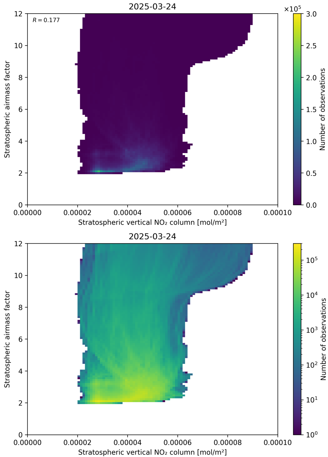
Figure 96: Scatter density plot of “Stratospheric vertical NO 2 column” against “Stratospheric airmass factor” for 2025-03-24 to 2025-03-25.
