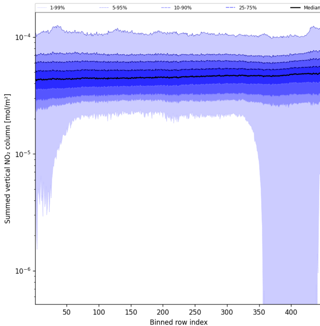
Figure 57: Along track statistics of “Summed vertical NO 2 column” for 2025-03-24 to 2025-03-25
