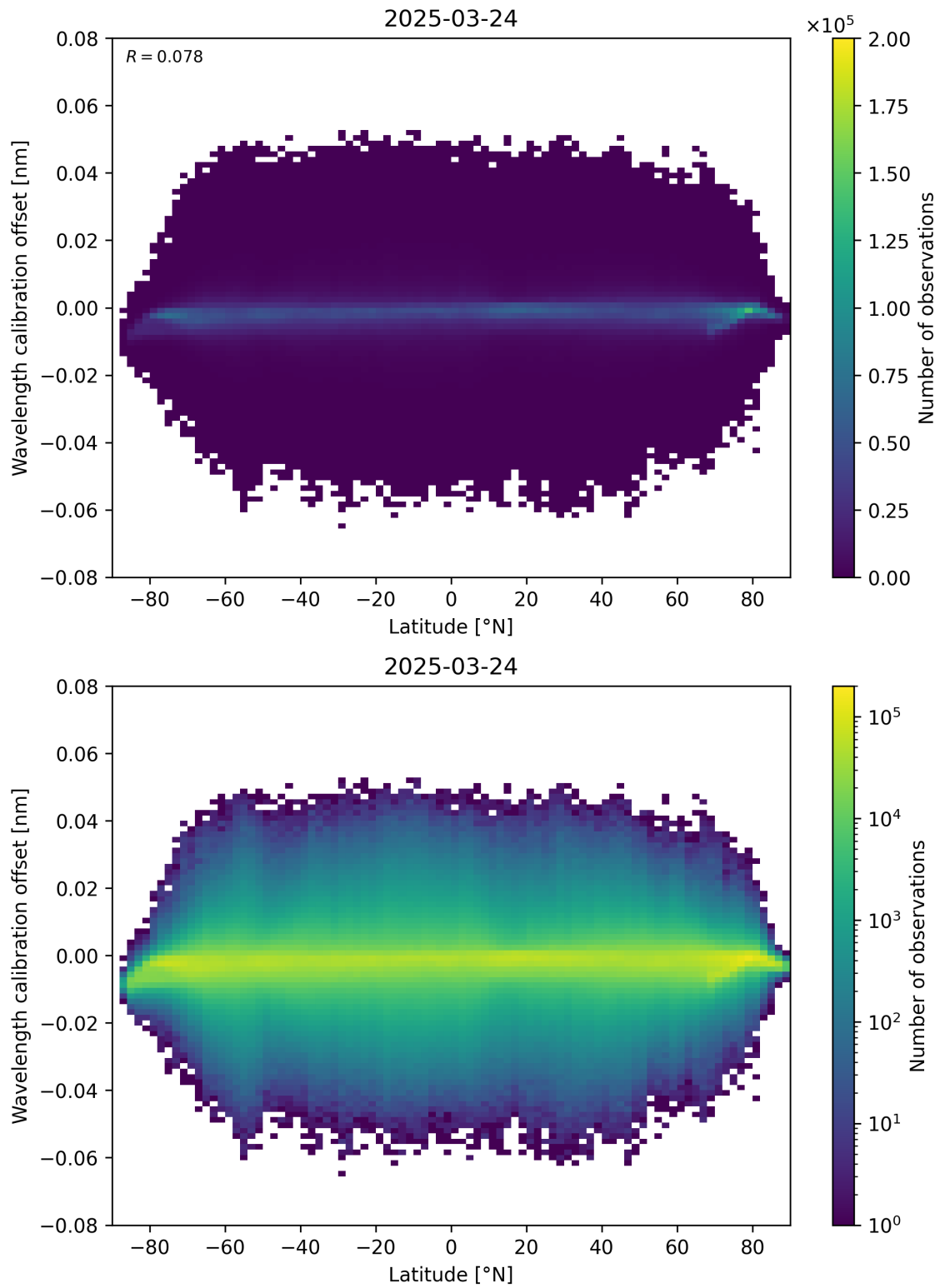
Figure 95: Scatter density plot of “Latitude” against “Wavelength calibration offset” for 2025-03-24 to 2025-03-25.
