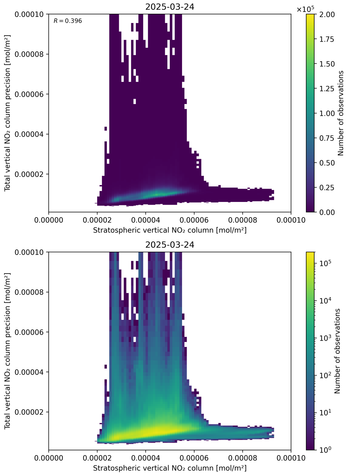
Figure 101: Scatter density plot of “Stratospheric vertical NO 2 column” against “Total vertical NO 2 column precision” for 2025-03-24 to 2025-03-25.
