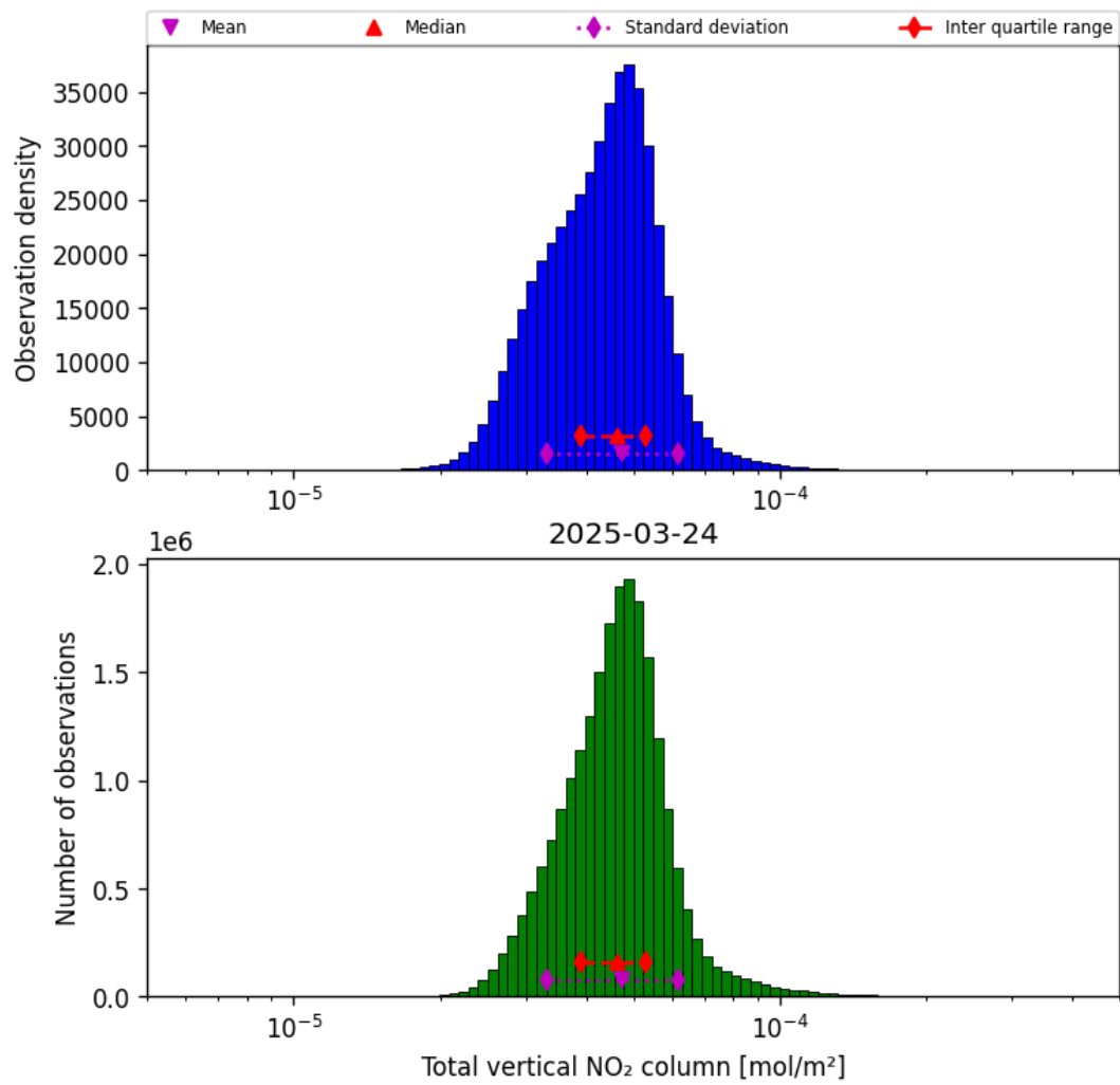
Figure 38: Histogram of “Total vertical NO 2 column” for 2025-03-24 to 2025-03-25
