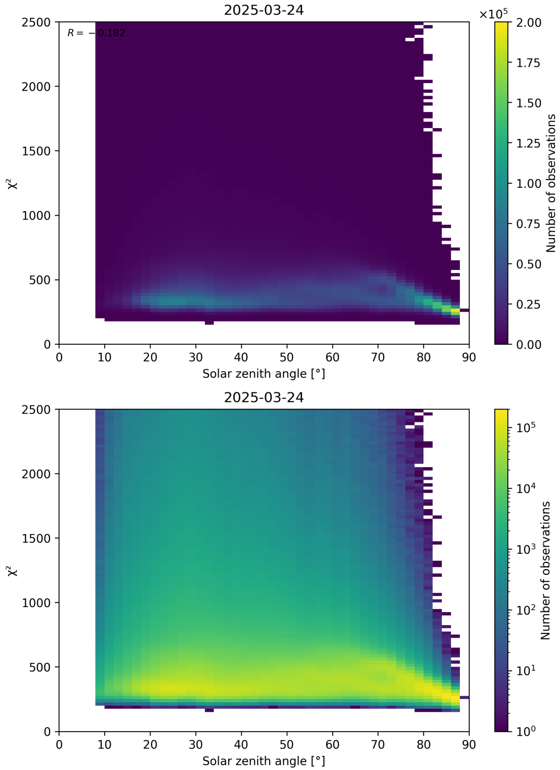
Figure 148: Scatter density plot of “Solar zenith angle” against “ \chi^2 ” for 2025-03-24 to 2025-03-25.
