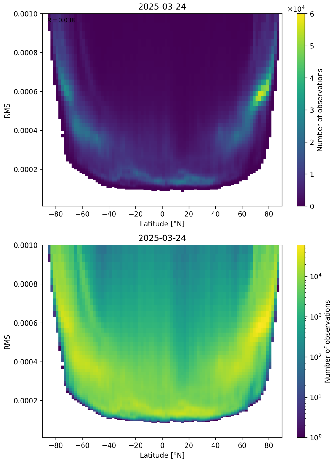
Figure 94: Scatter density plot of “Latitude” against “RMS” for 2025-03-24 to 2025-03-25.
