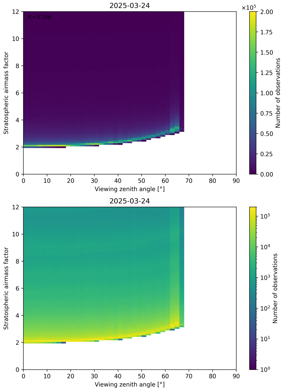
Figure 159: Scatter density plot of “Viewing zenith angle” against “Stratospheric airmass factor” for 2025-03-24 to 2025-03-25.
