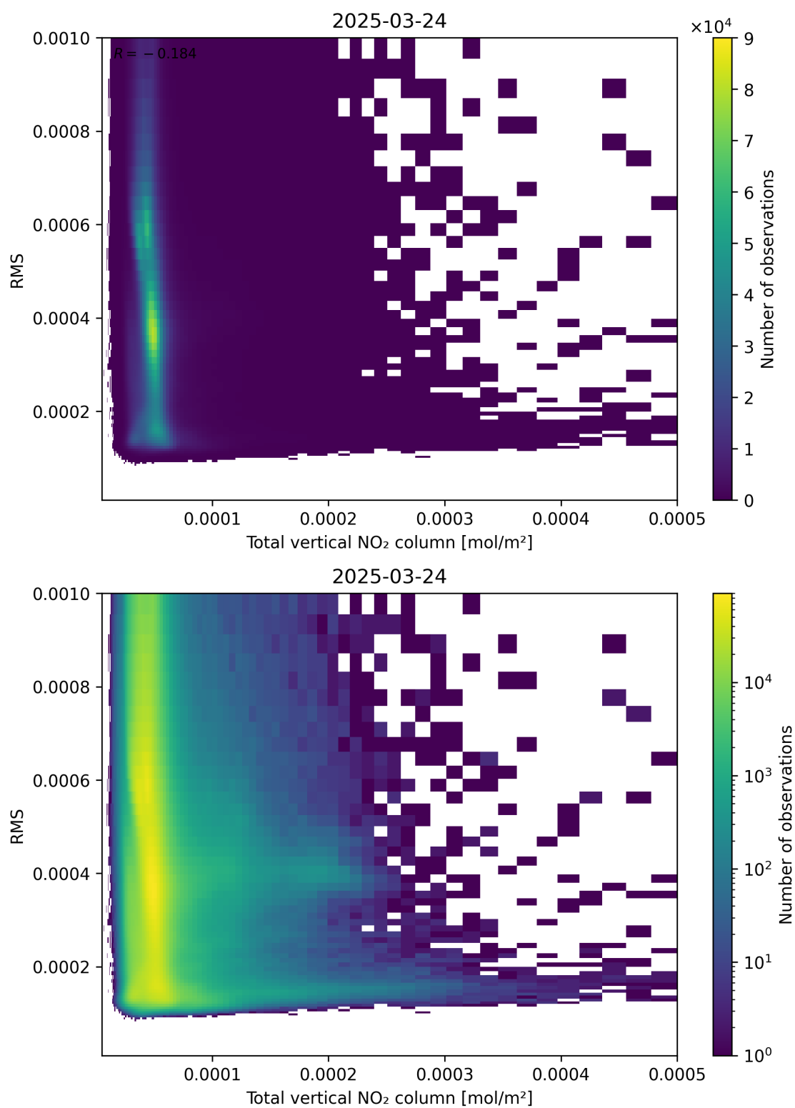
Figure 120: Scatter density plot of “Total vertical NO 2 column” against “RMS” for 2025-03-24 to 2025-03-25.
