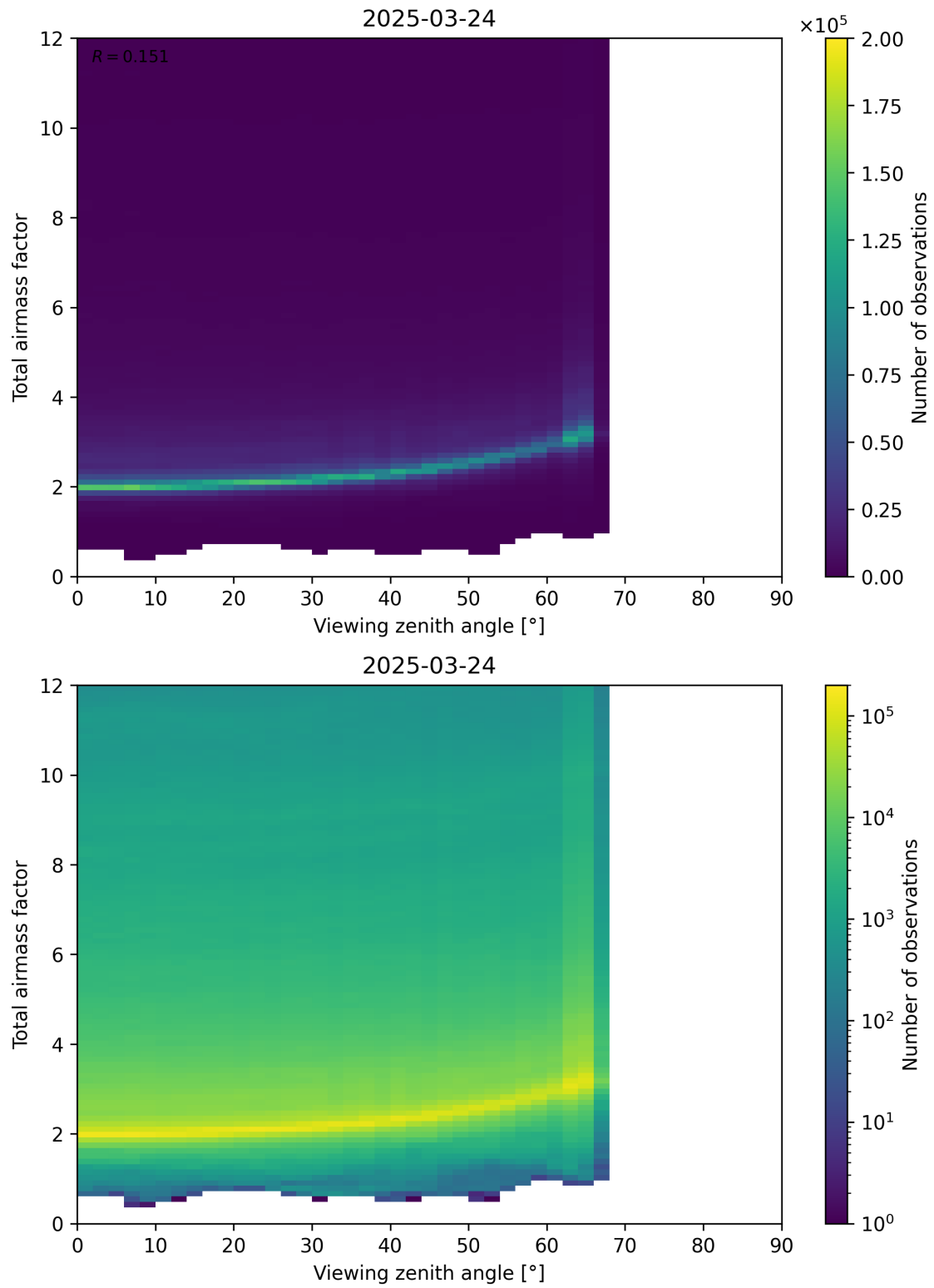
Figure 160: Scatter density plot of “Viewing zenith angle” against “Total airmass factor” for 2025-03-24 to 2025-03-25.
