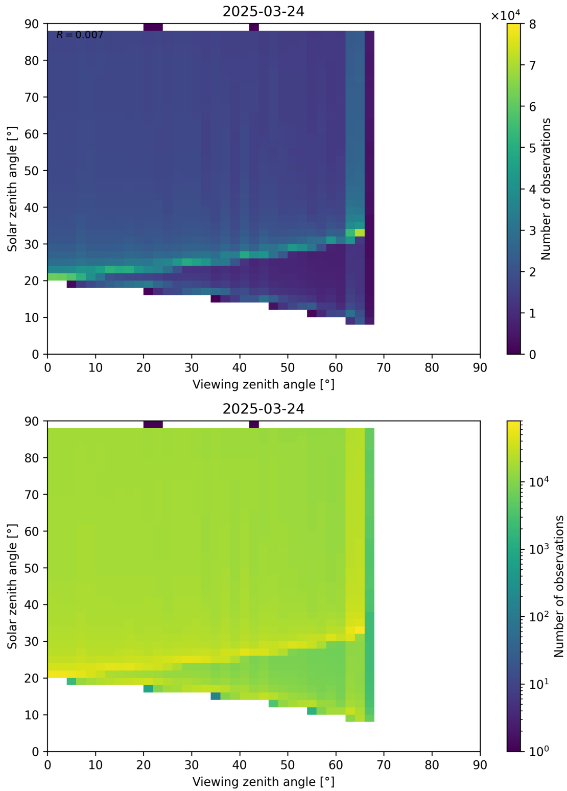
Figure 172: Scatter density plot of “Viewing zenith angle” against “Solar zenith angle” for 2025-03-24 to 2025-03-25.
