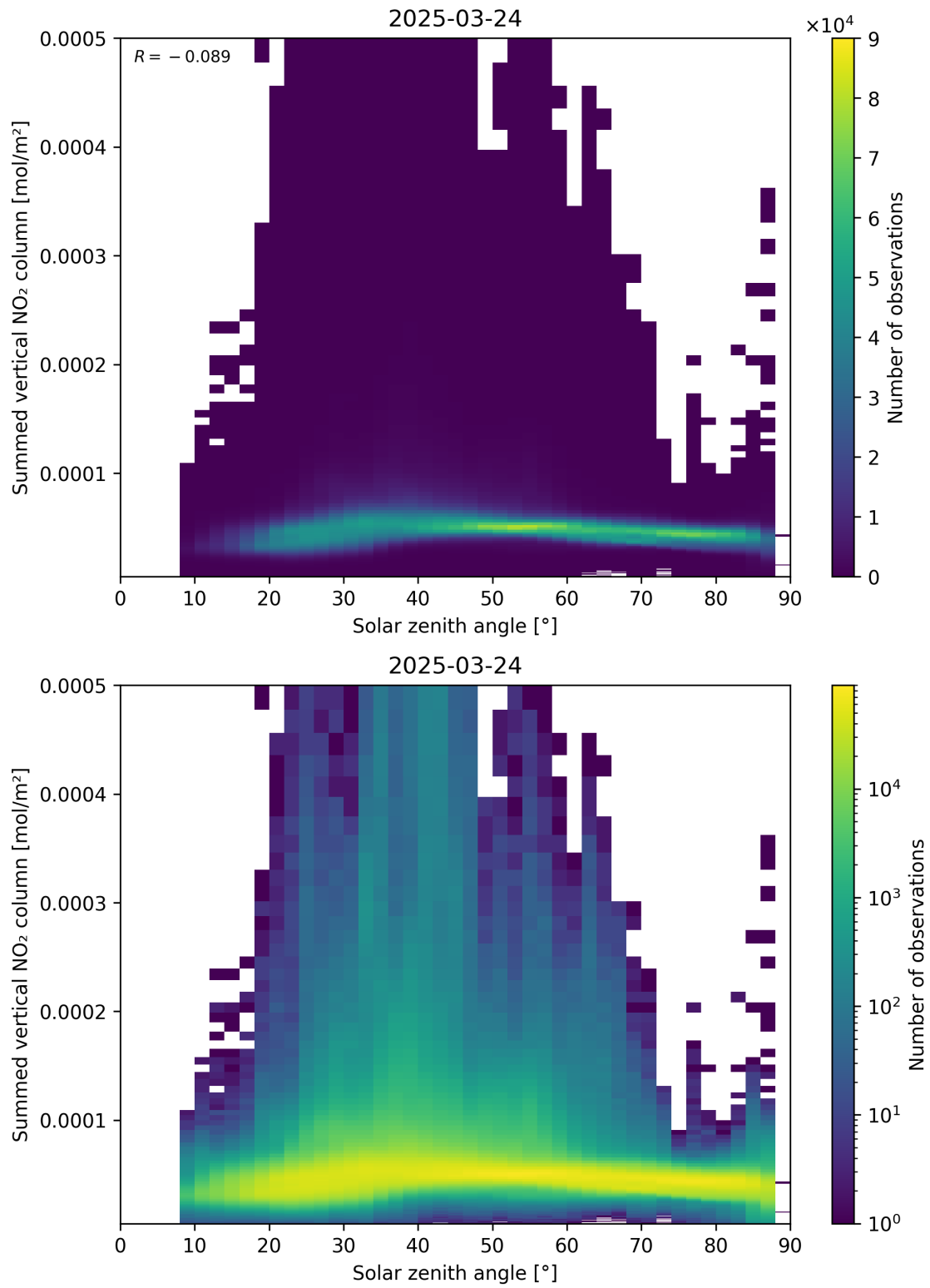
Figure 151: Scatter density plot of “Solar zenith angle” against “Summed vertical NO 2 column” for 2025-03-24 to 2025-03-25.
