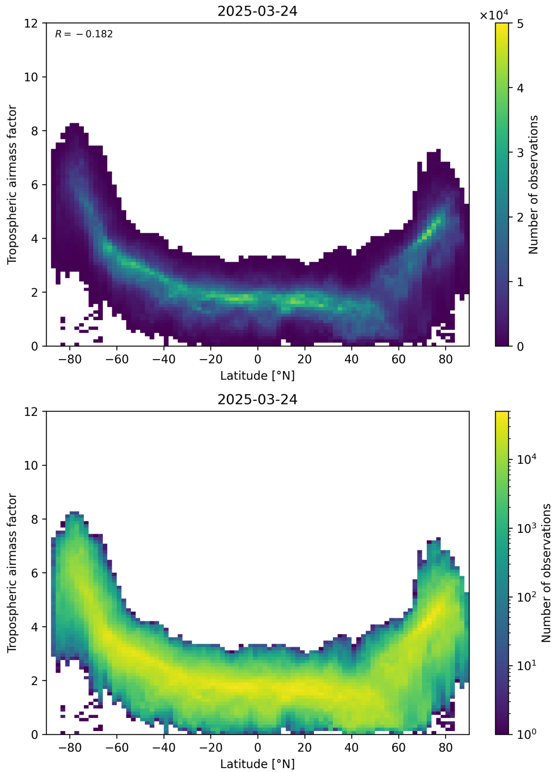
Figure 85: Scatter density plot of “Latitude” against “Tropospheric airmass factor” for 2025-03-24 to 2025-03-25.
