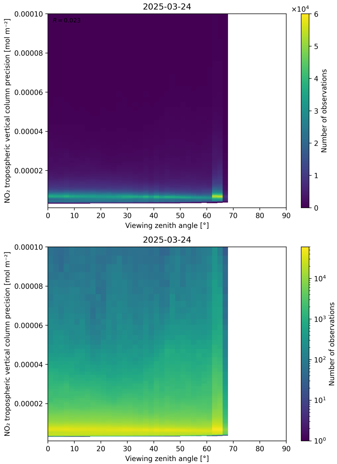
Figure 170: Scatter density plot of “Viewing zenith angle” against “NO 2 tropospheric vertical column precision” for 2025-03-24 to 2025-03-25.
