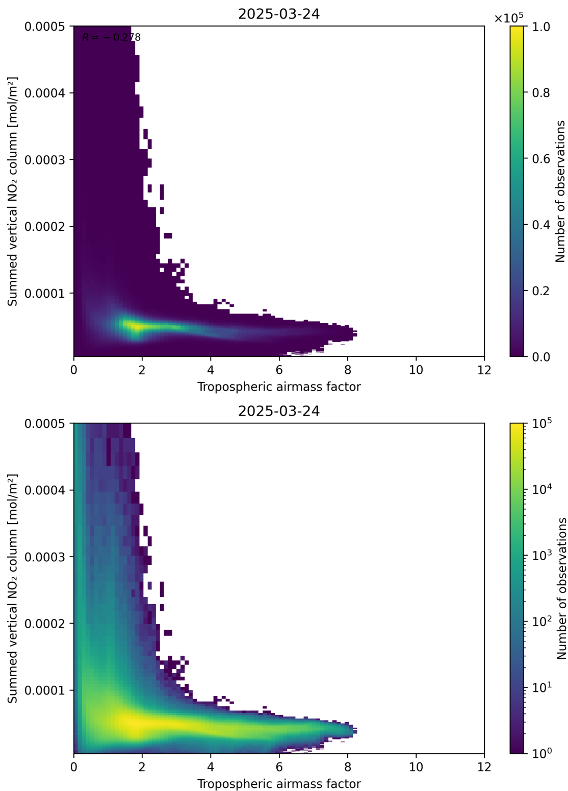
Figure 75: Scatter density plot of “Tropospheric air mass factor” against “Summed vertical NO 2 column” for 2025-03-24 to 2025-03-25.
