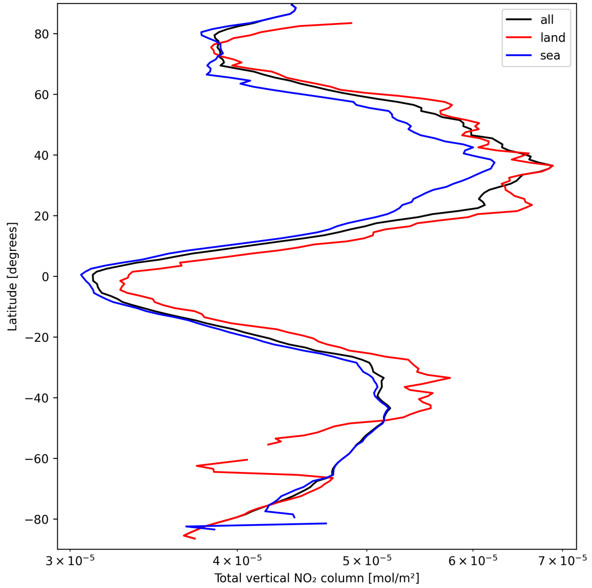
Figure 21: Zonal average of “Total vertical NO 2 column” for 2025-03-24 to 2025-03-25.
