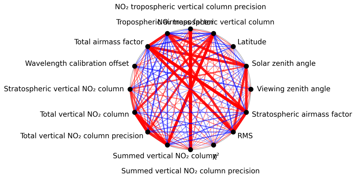
Figure 1: Map of correlation graph for 2025-03-24 to 2025-03-25.
