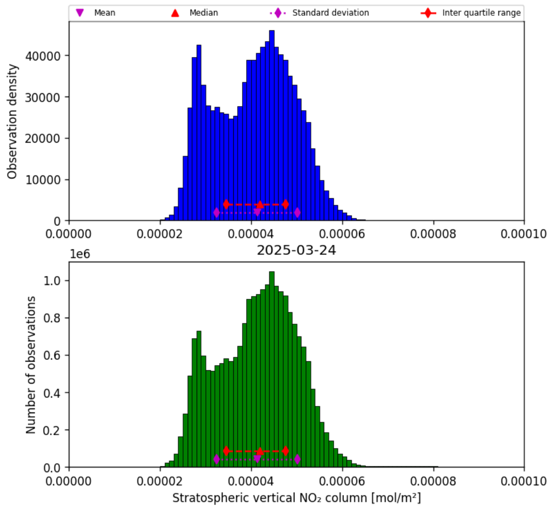
Figure 36: Histogram of “Stratospheric vertical NO 2 column” for 2025-03-24 to 2025-03-25
