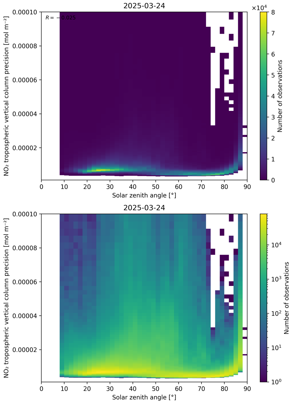
Figure 156: Scatter density plot of “Solar zenith angle” against “NO 2 tropospheric vertical column precision” for 2025-03-24 to 2025-03-25.
