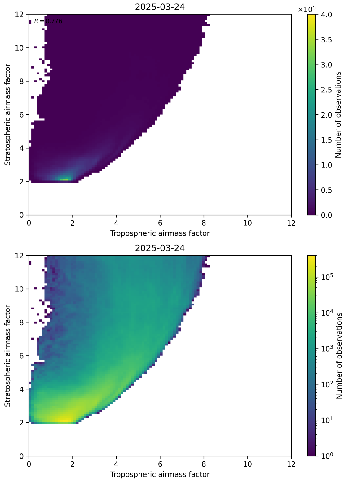
Figure 71: Scatter density plot of “Tropospheric airmass factor” against “Stratospheric airmass factor” for 2025-03-24 to 2025-03-25.
