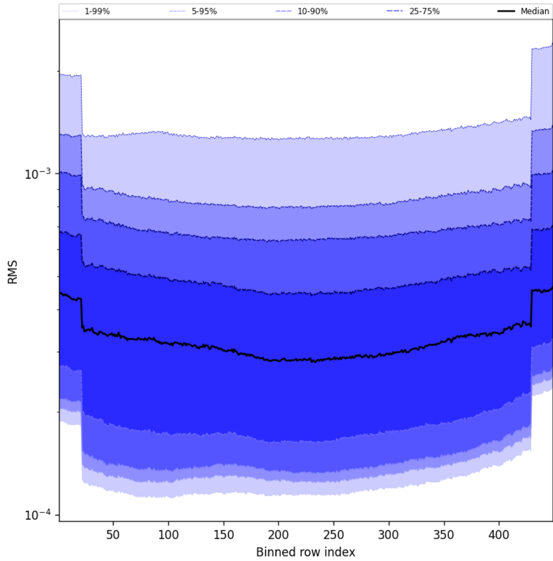
Figure 60: Along track statistics of “RMS” for 2025-03-24 to 2025-03-25
