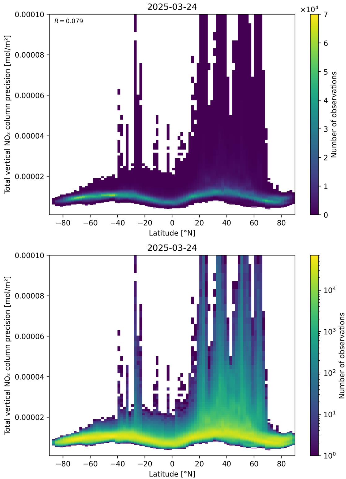
Figure 91: Scatter density plot of “Latitude” against “Total vertical NO 2 column precision” for 2025-03-24 to 2025-03-25.
