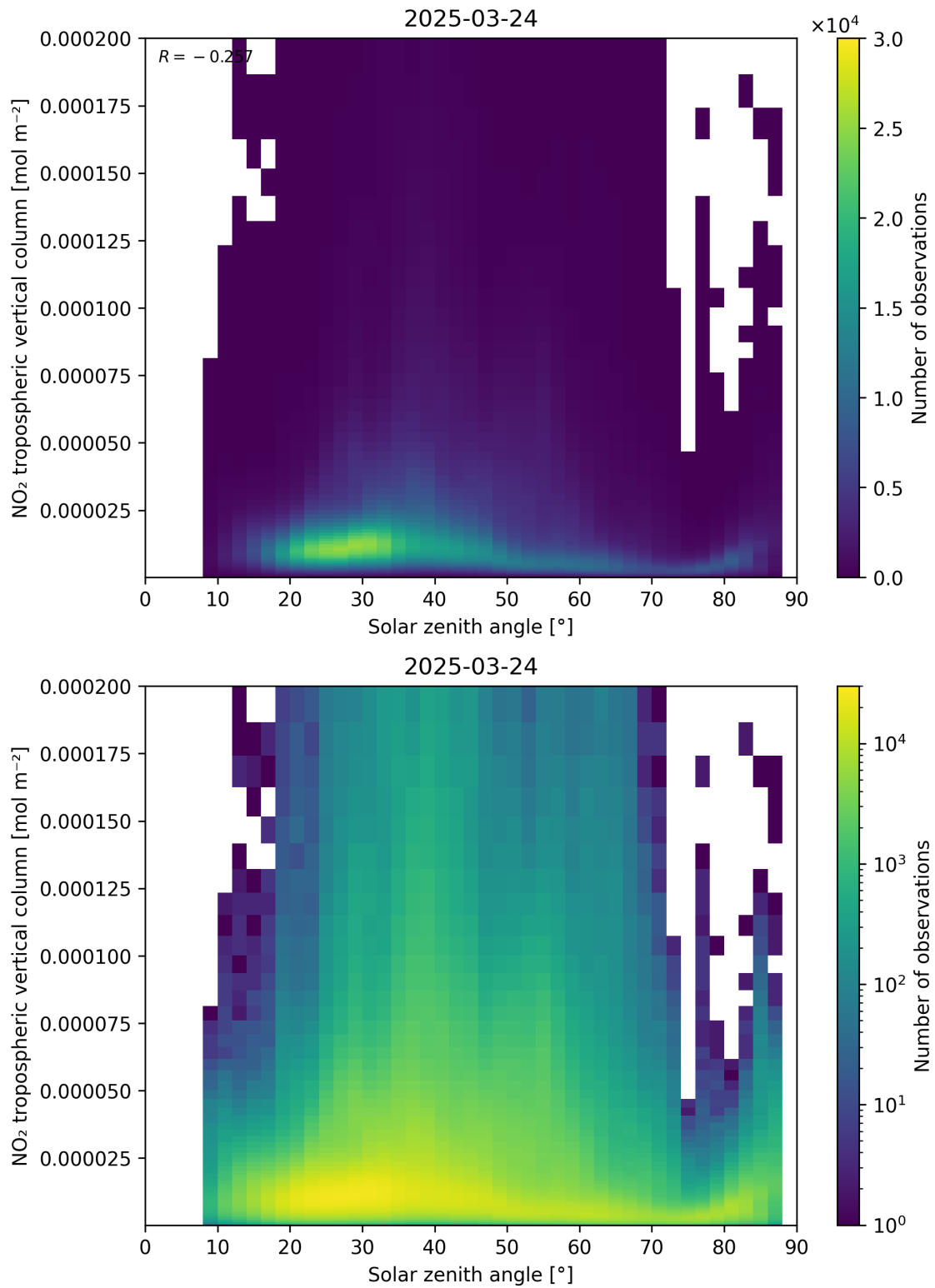
Figure 155: Scatter density plot of “Solar zenith angle” against “NO 2 tropospheric vertical column” for 2025-03-24 to 2025-03-25.
