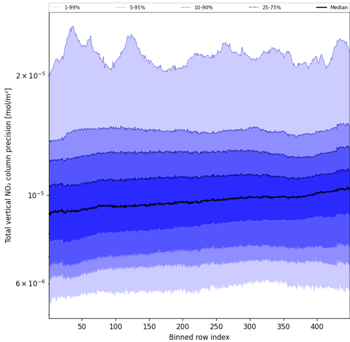
Figure 56: Along track statistics of "Total vertical NO 2 column precision" for 2025-03-24 to 2025-03-25
