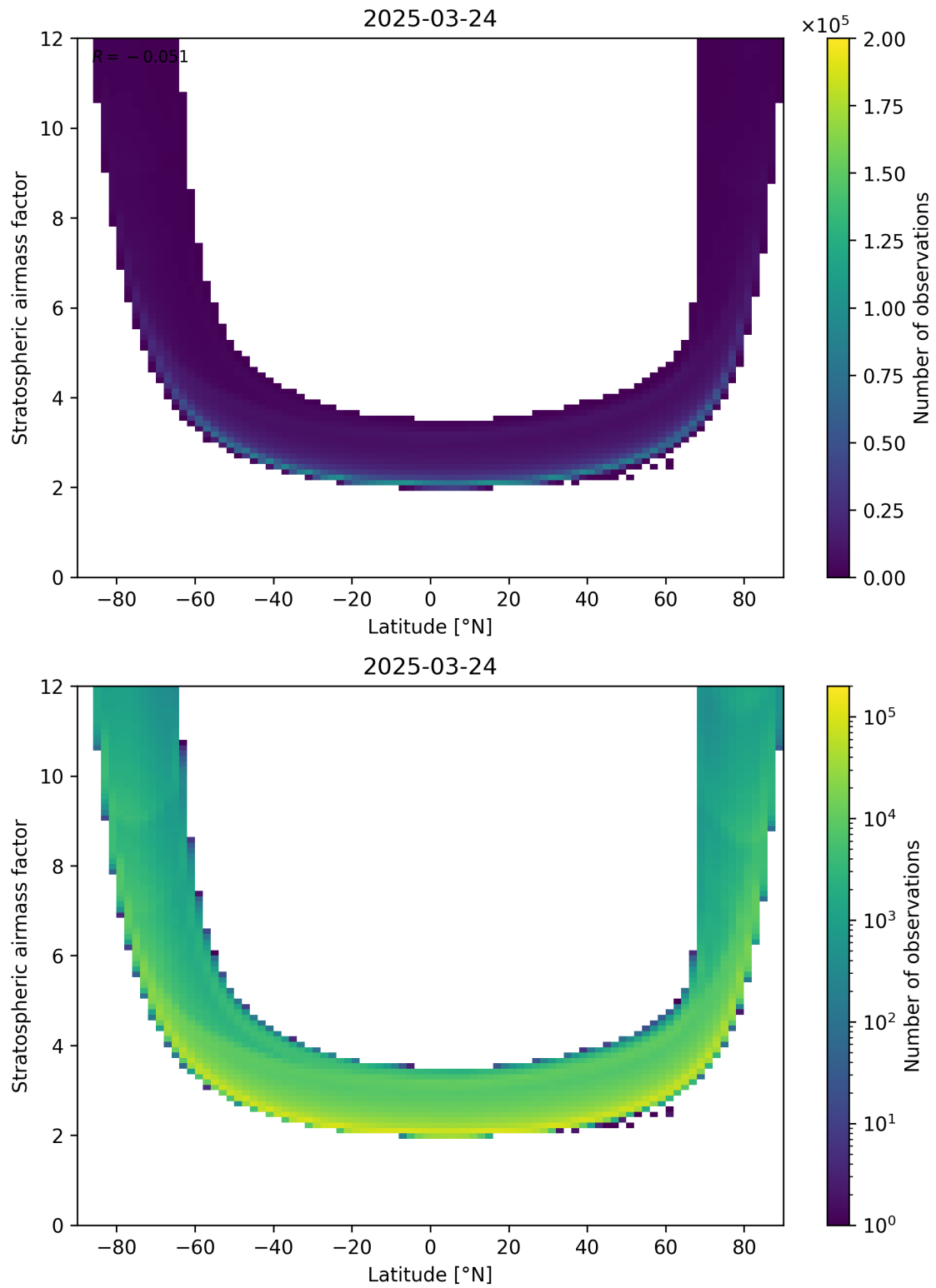
Figure 83: Scatter density plot of “Latitude” against “Stratospheric airmass factor” for 2025-03-24 to 2025-03-25.
