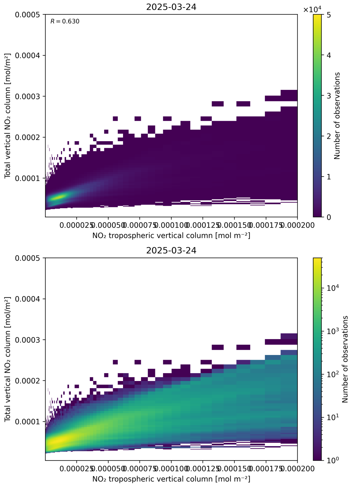
Figure 128: Scatter density plot of “NO 2 tropospheric vertical column” against “Total vertical NO 2 column” for 2025-03-24 to 2025-03-25.
