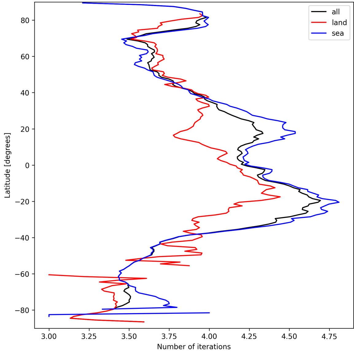
Figure 17: Zonal average of “Number of iterations” for 2025-03-24 to 2025-03-25.
