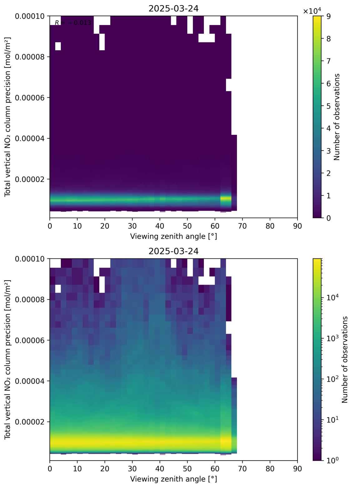
Figure 168: Scatter density plot of “Viewing zenith angle” against “Total vertical NO 2 column precision” for 2025-03-24 to 2025-03-25.
