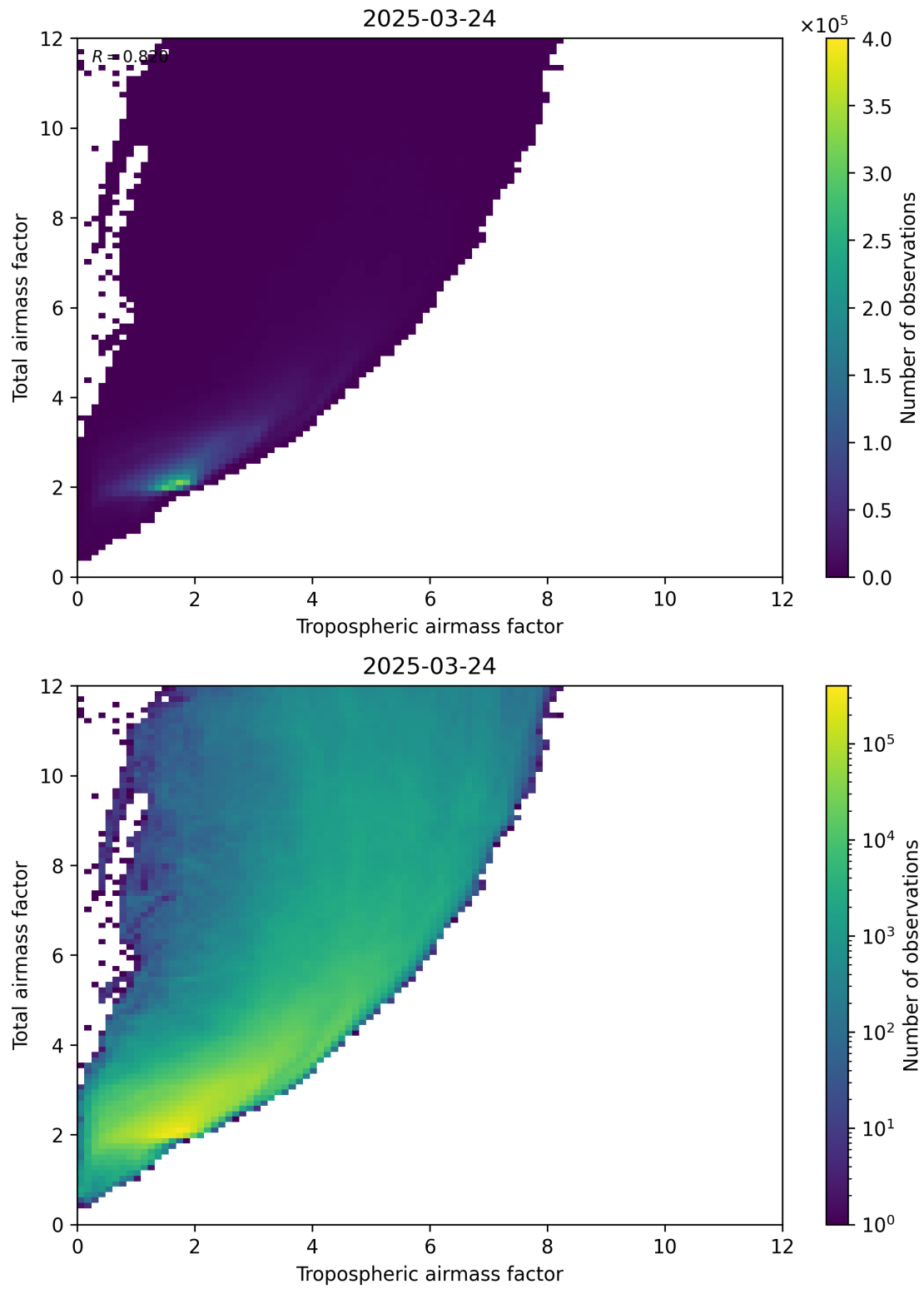
Figure 72: Scatter density plot of “Tropospheric airmass factor” against “Total airmass factor” for 2025-03-24 to 2025-03-25.
