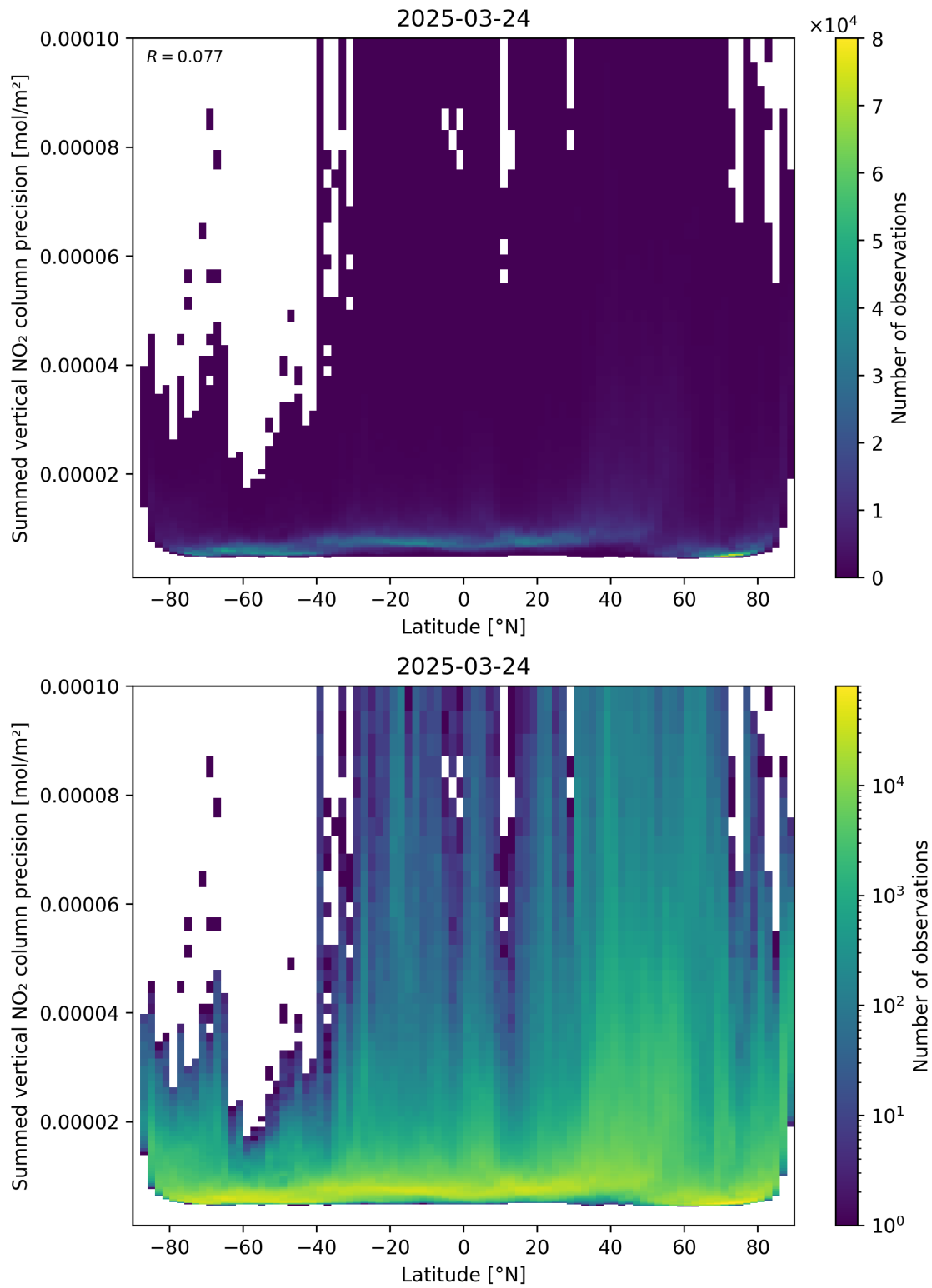
Figure 89: Scatter density plot of “Latitude” against “Summed vertical NO 2 column precision” for 2025-03-24 to 2025-03-25.
