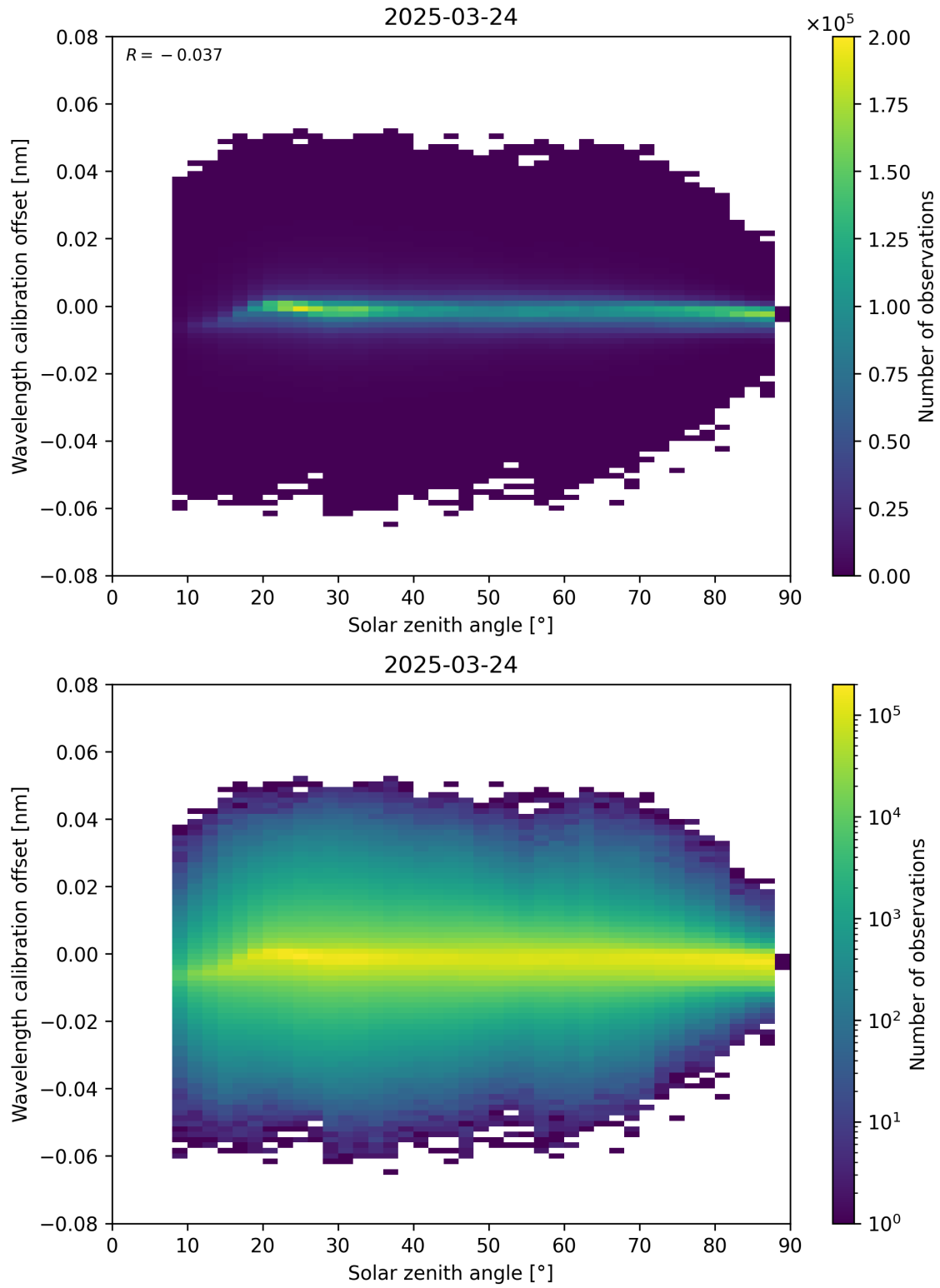
Figure 158: Scatter density plot of “Solar zenith angle” against “Wavelength calibration offset” for 2025-03-24 to 2025-03-25.
