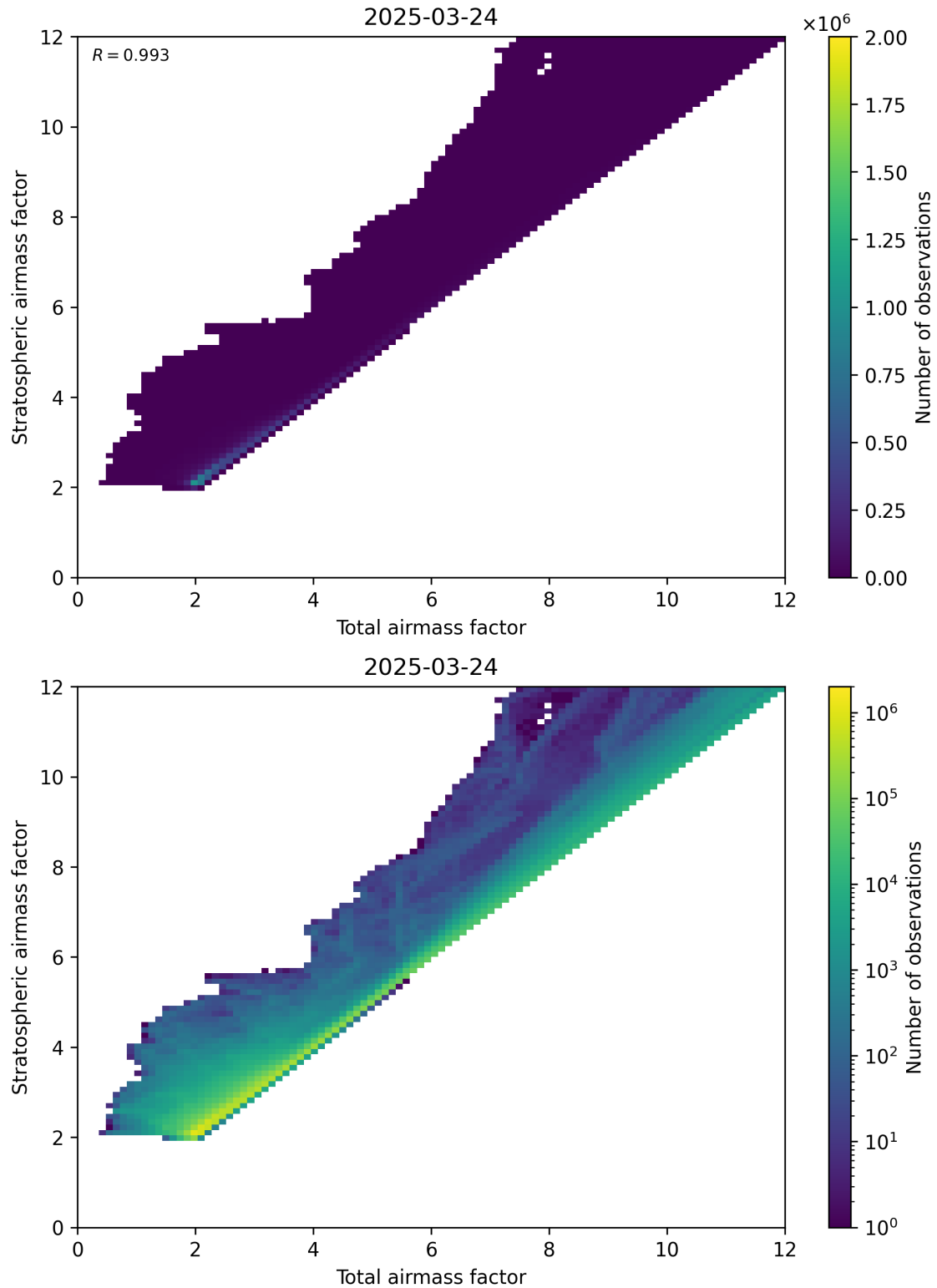
Figure 62: Scatter density plot of “Total airmass factor” against “Stratospheric airmass factor” for 2025-03-24 to 2025-03-25.
