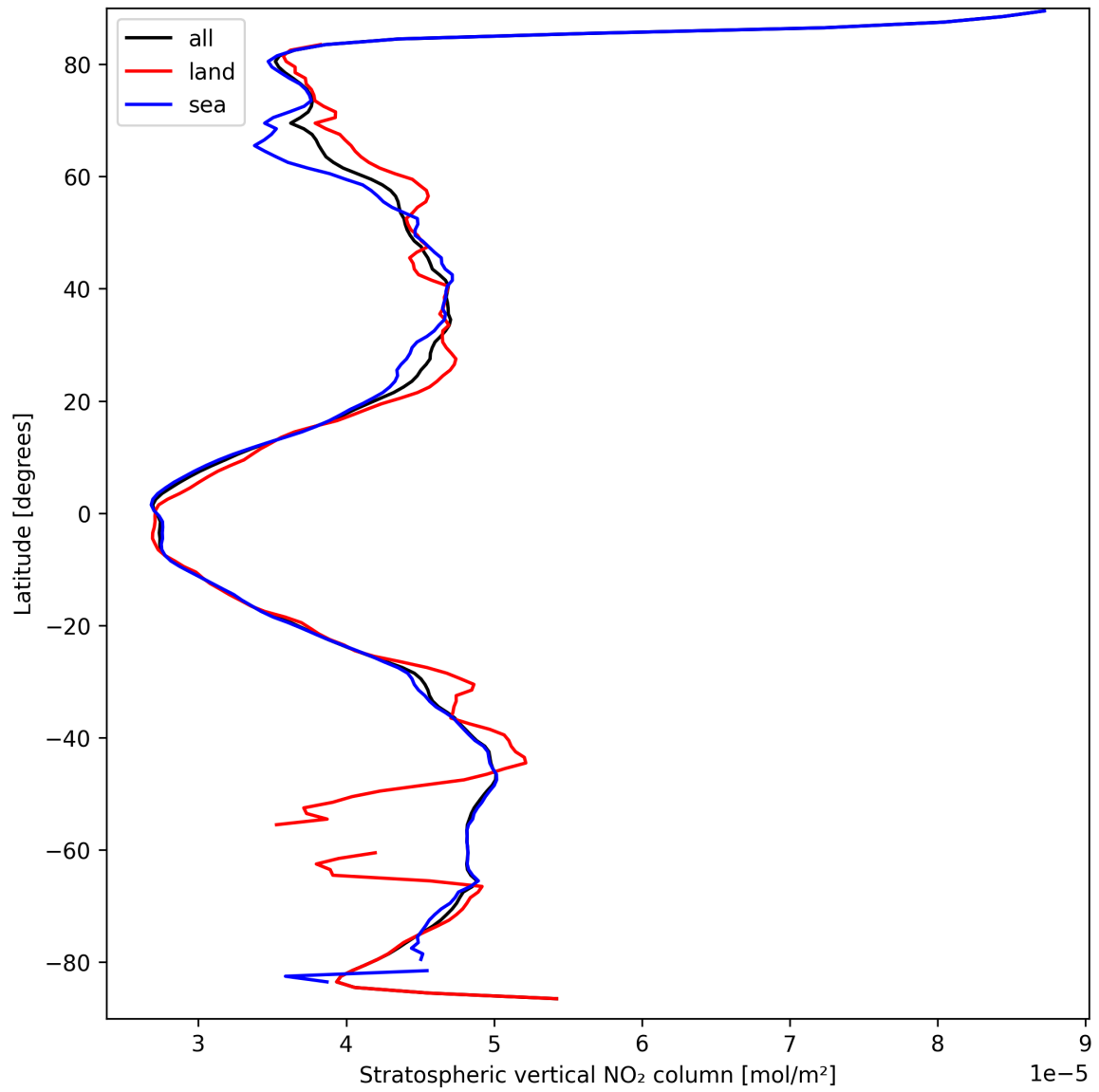
Figure 19: Zonal average of “Stratospheric vertical NO 2 column” for 2025-03-24 to 2025-03-25.
