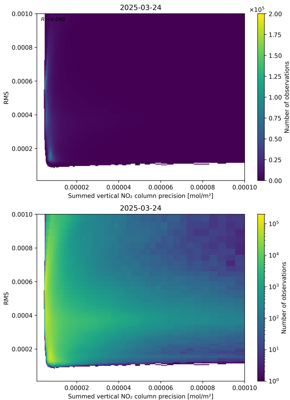
Figure 108: Scatter density plot of “Summed vertical NO 2 column precision” against “RMS” for 2025-03-24 to 2025-03-25.
