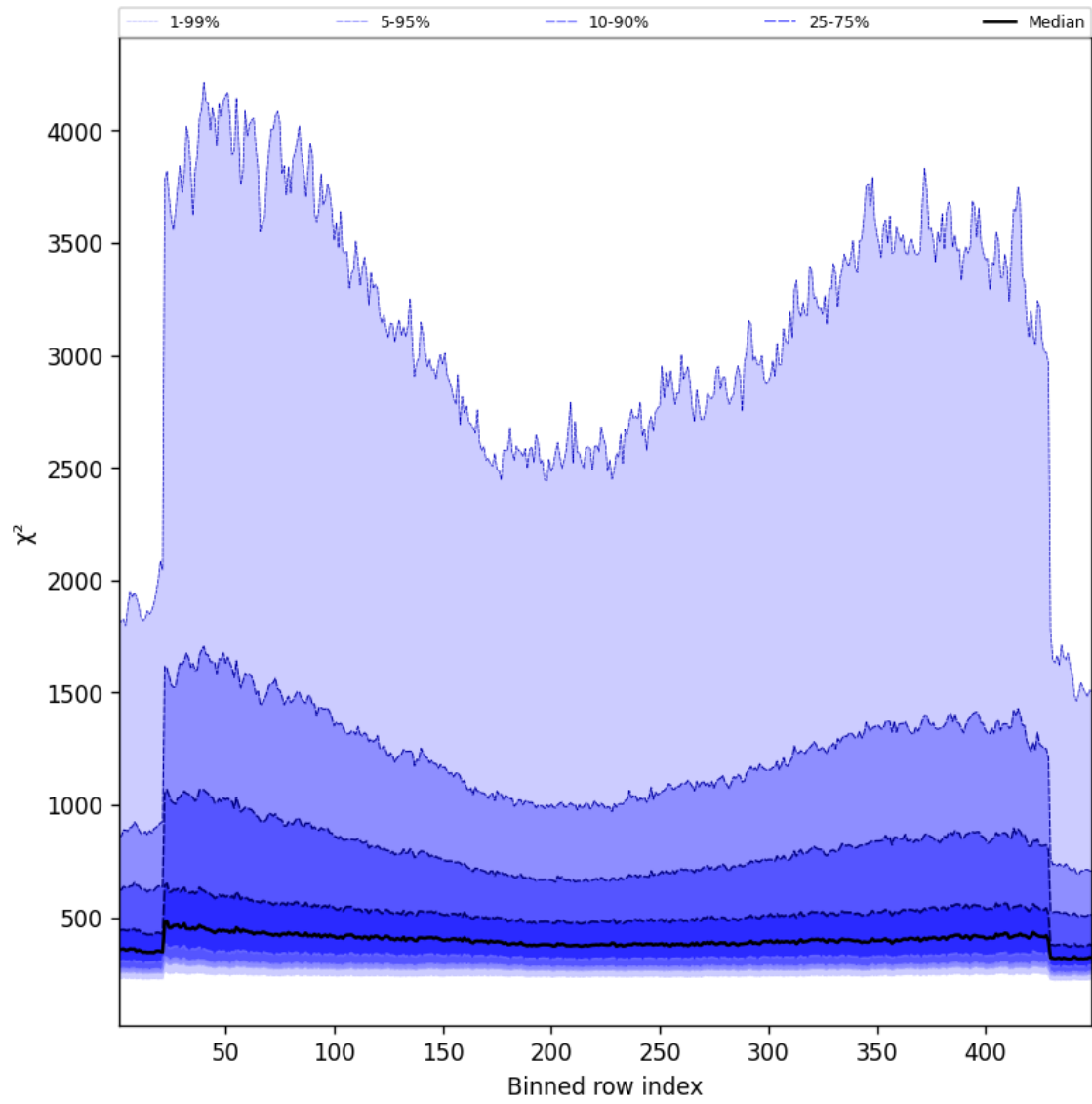
Figure 59: Along track statistics of “ \chi^2 ” for 2025-03-24 to 2025-03-25
