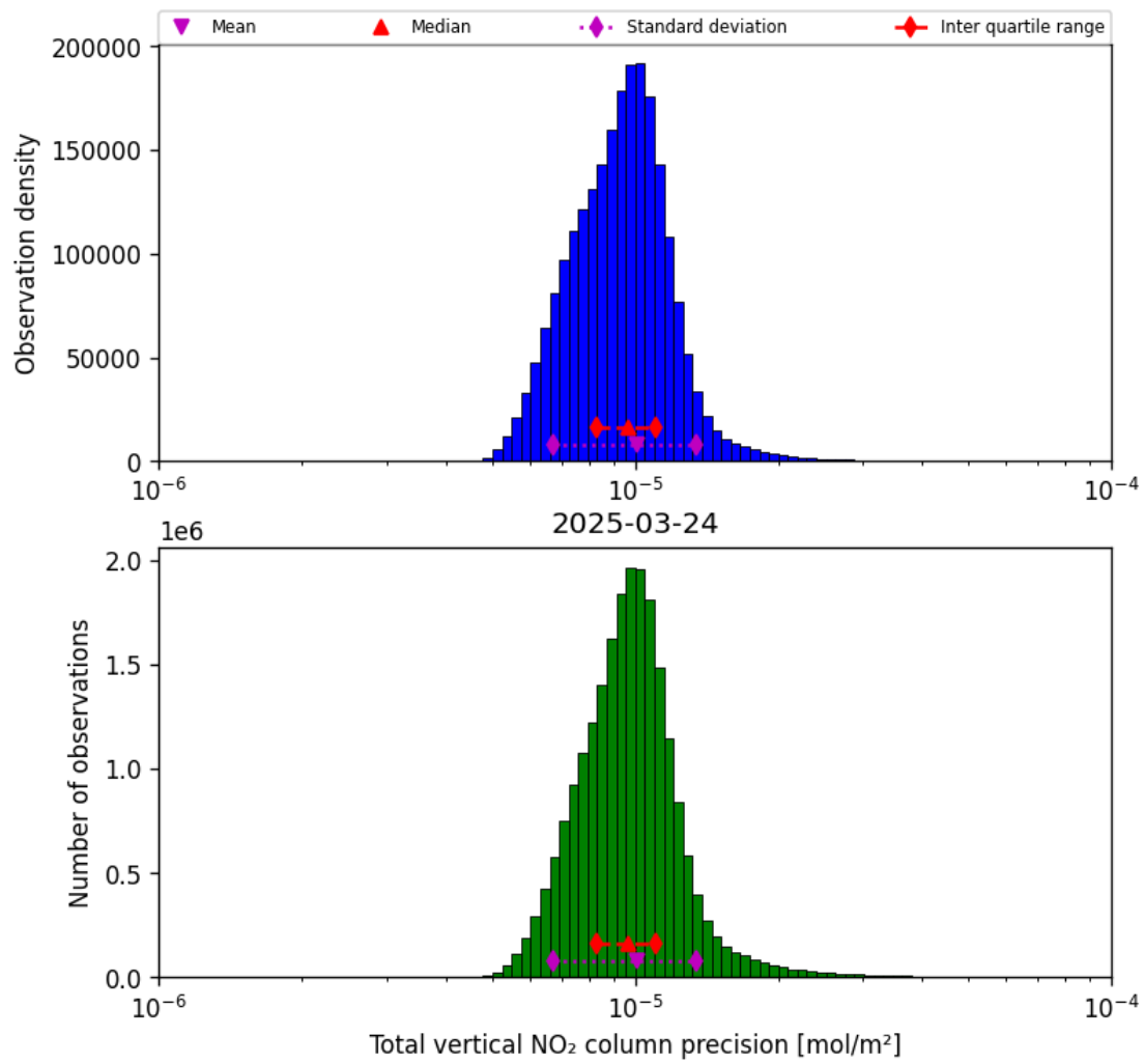
Figure 39: Histogram of “Total vertical NO 2 column precision” for 2025-03-24 to 2025-03-25
