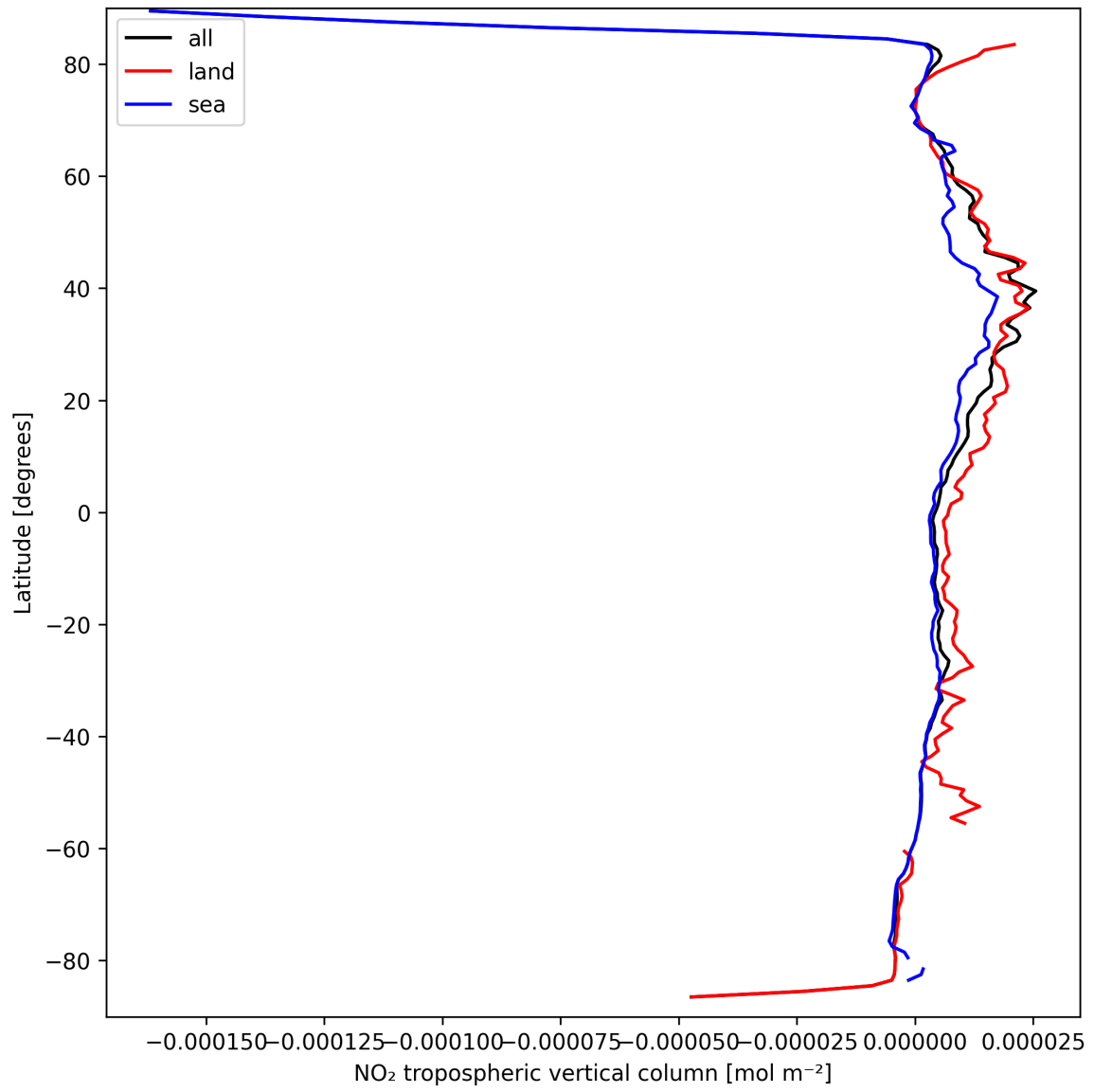
Figure 12: Zonal average of “NO 2 tropospheric vertical column” for 2025-03-24 to 2025-03-25.
