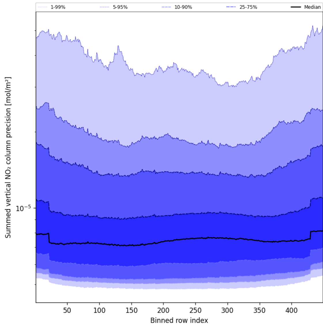
Figure 58: Along track statistics of “Summed vertical NO 2 column precision” for 2025-03-24 to 2025-03-25
