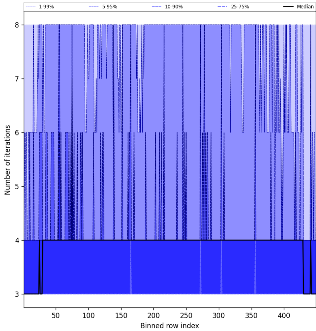
Figure 51: Along track statistics of “Number of iterations” for 2025-03-24 to 2025-03-25
