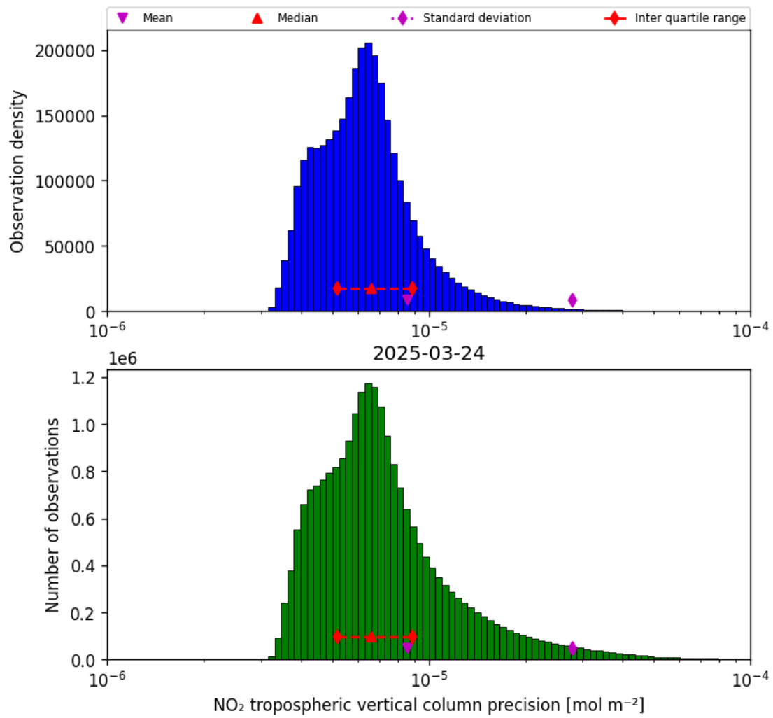
Figure 30: Histogram of “NO 2 tropospheric vertical column precision” for 2025-03-24 to 2025-03-25
