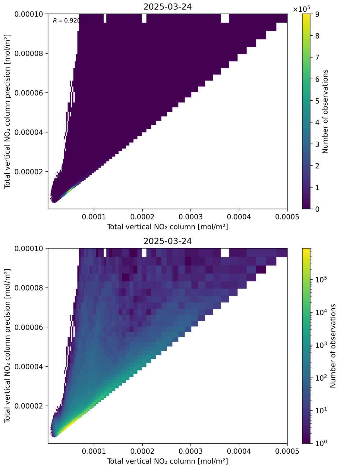
Figure 114: Scatter density plot of “Total vertical NO 2 column” against “Total vertical NO 2 column precision” for 2025-03-24 to 2025-03-25.
