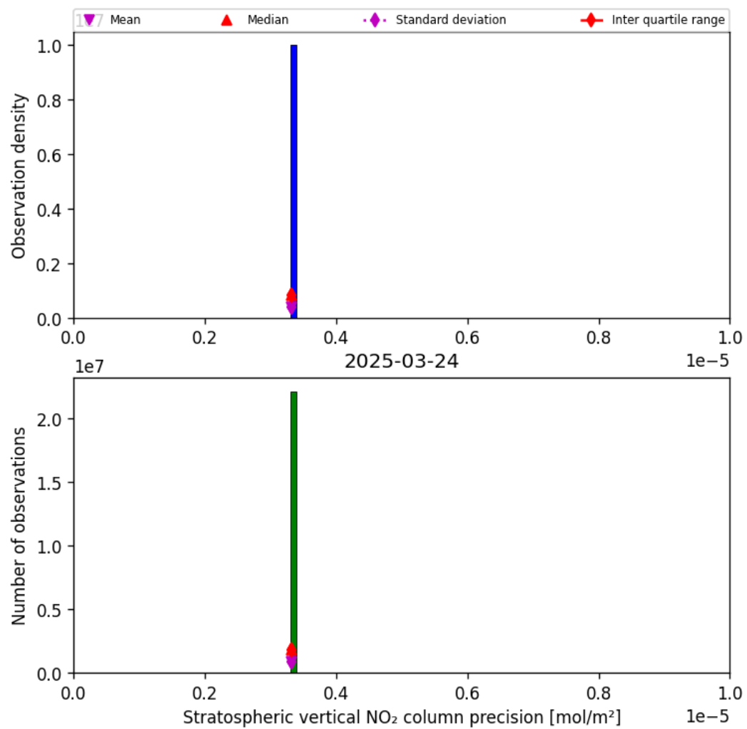
Figure 37: Histogram of “Stratospheric vertical NO 2 column precision” for 2025-03-24 to 2025-03-25
