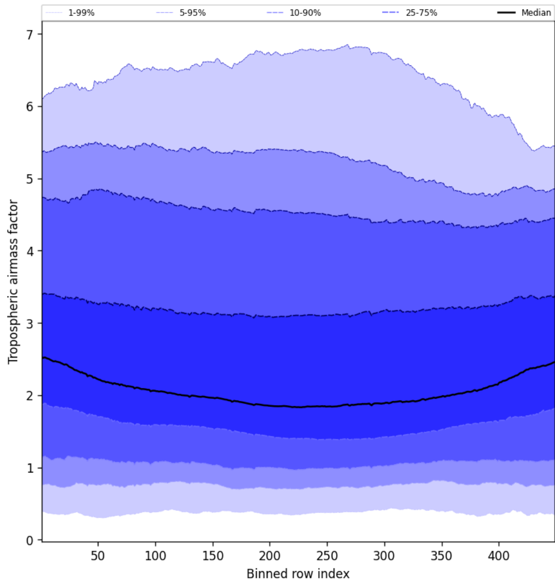
Figure 48: Along track statistics of “Tropospheric airmass factor” for 2025-03-24 to 2025-03-25
