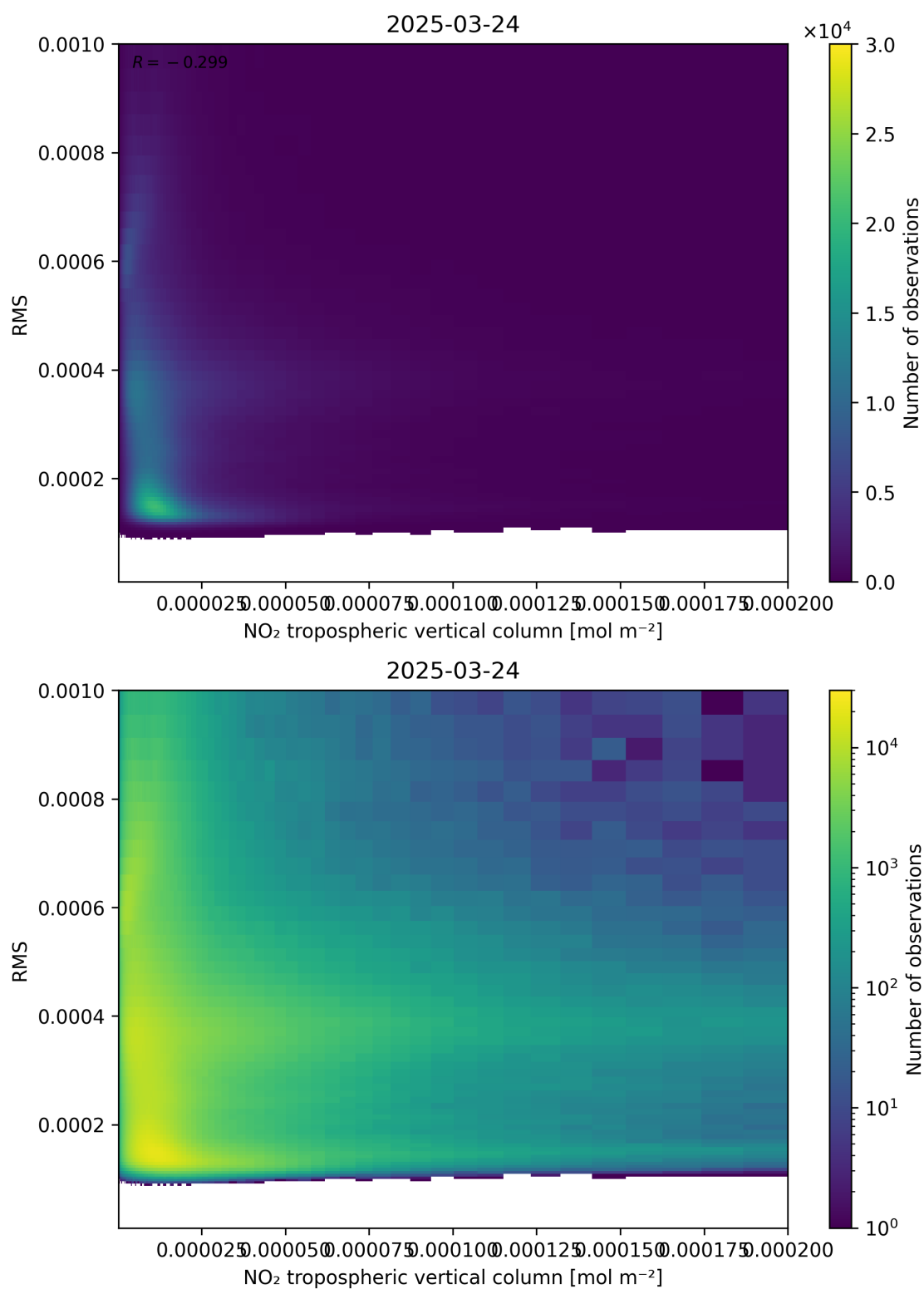
Figure 142: Scatter density plot of “NO 2 tropospheric vertical column” against “RMS” for 2025-03-24 to 2025-03-25.
