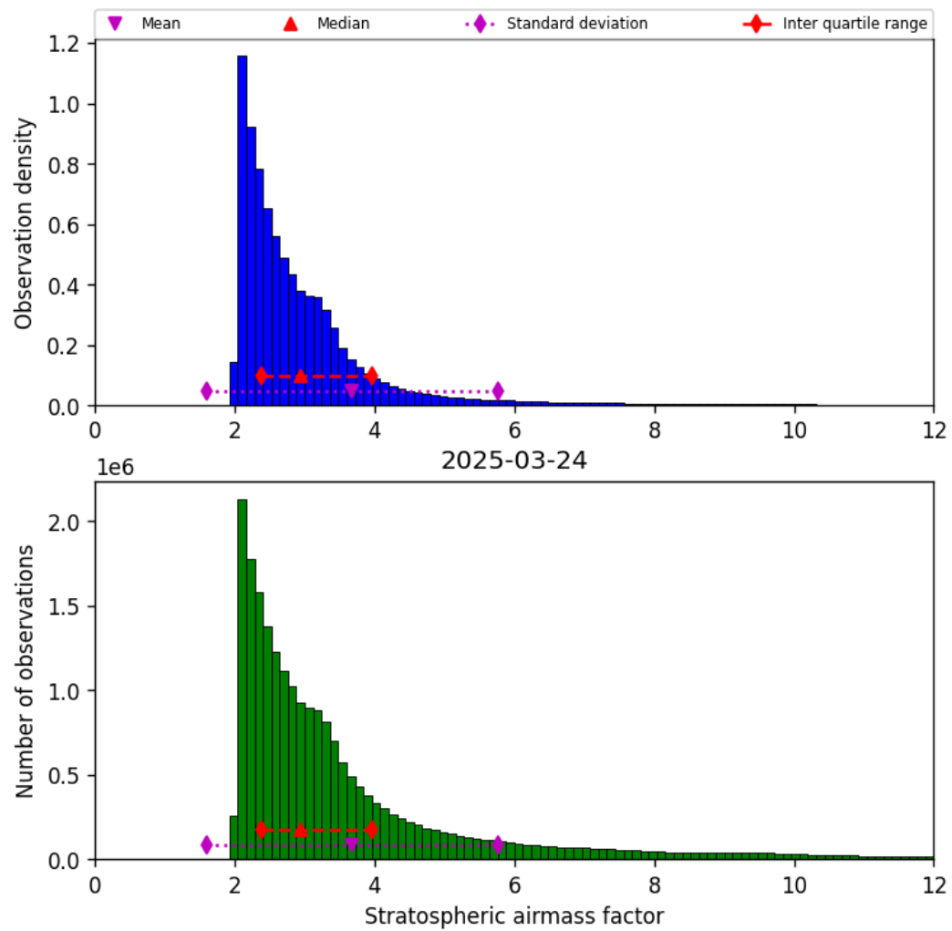
Figure 44: Histogram of “Stratospheric airmass factor” for 2025-03-24 to 2025-03-25
