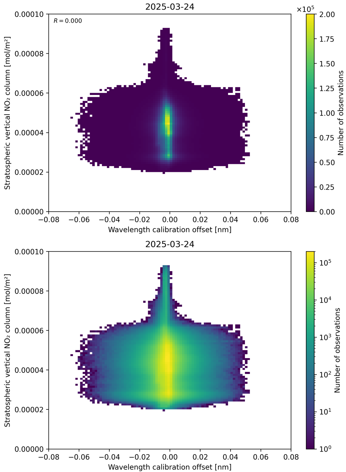
Figure 176: Scatter density plot of “Wavelength calibration offset” against “Stratospheric vertical NO 2 column” for 2025-03-24 to 2025-03-25.
