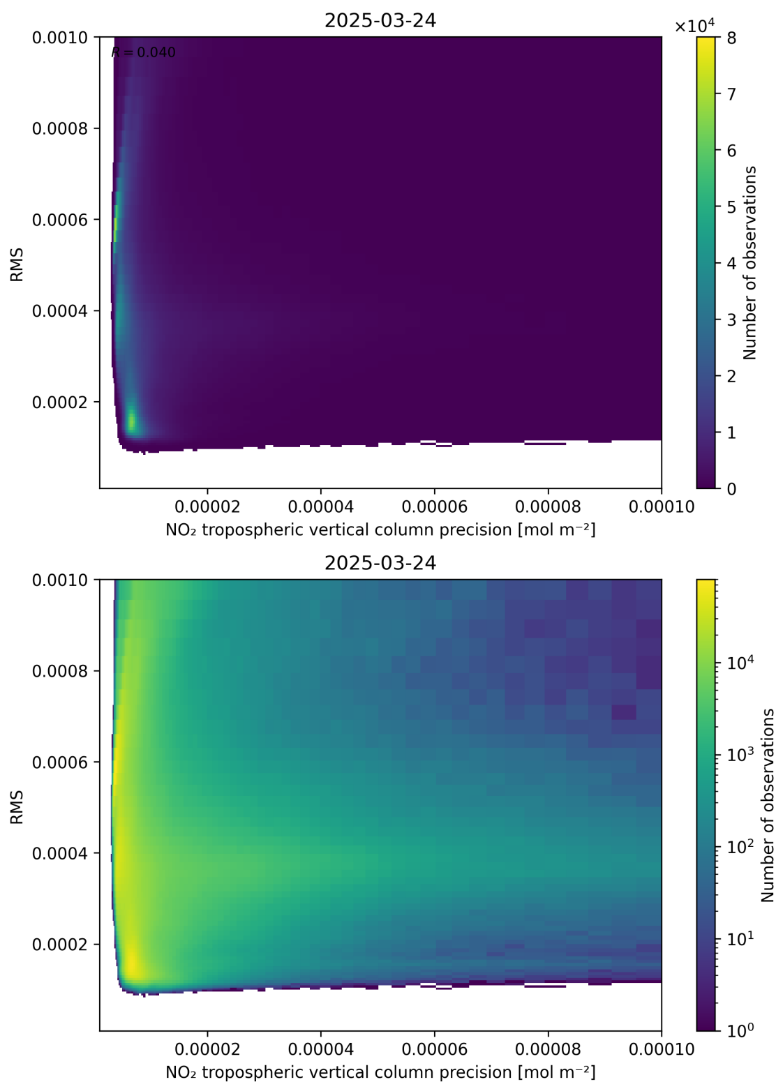
Figure 140: Scatter density plot of “NO 2 tropospheric vertical column precision” against “RMS” for 2025-03-24 to 2025-03-25.
