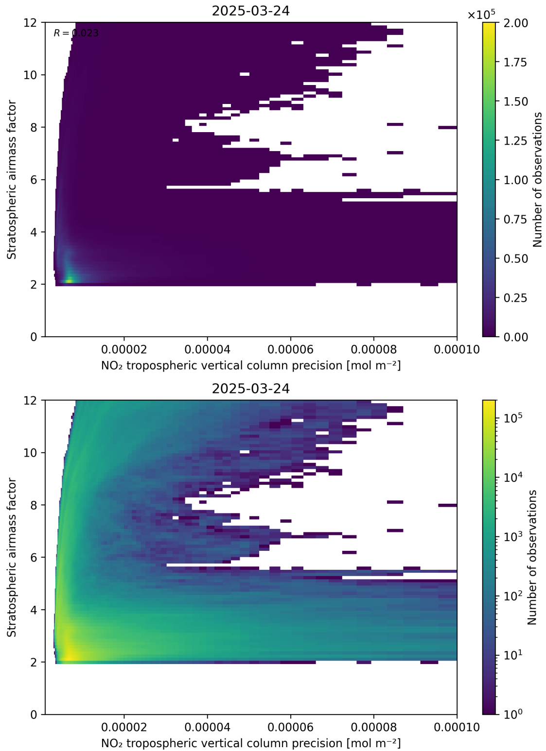
Figure 131: Scatter density plot of “NO 2 tropospheric vertical column precision” against “Stratospheric airmass factor” for 2025-03-24 to 2025-03-25.
