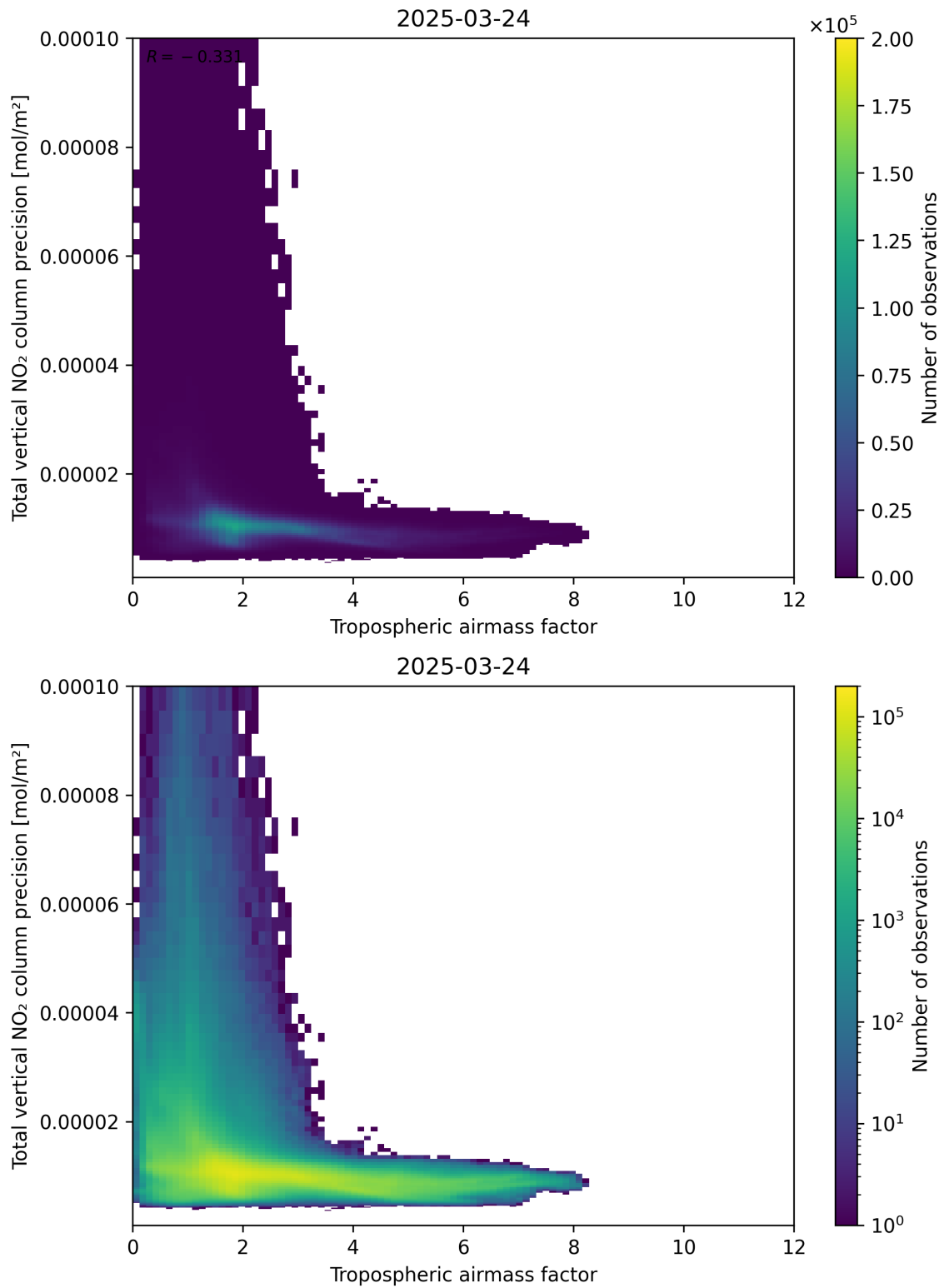
Figure 78: Scatter density plot of “Tropospheric air mass factor” against “Total vertical NO 2 column precision” for 2025-03-24 to 2025-03-25.
