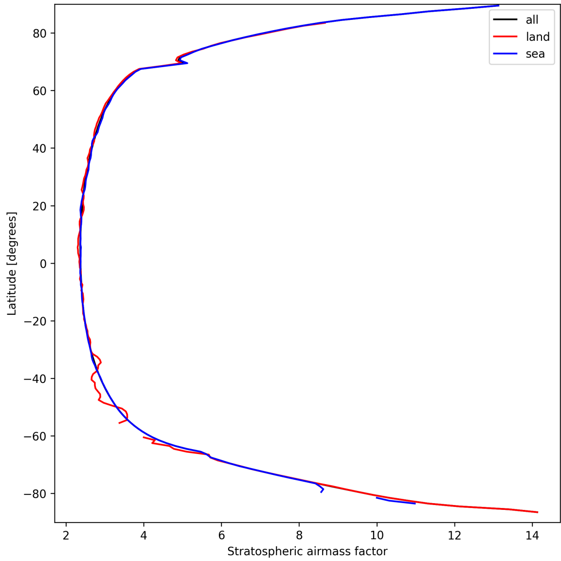
Figure 27: Zonal average of “Stratospheric airmass factor” for 2025-03-24 to 2025-03-25.
