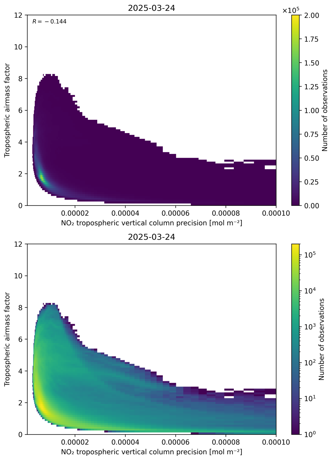
Figure 133: Scatter density plot of “NO 2 tropospheric vertical column precision” against “Tropospheric air mass factor” for 2025-03-24 to 2025-03-25.
