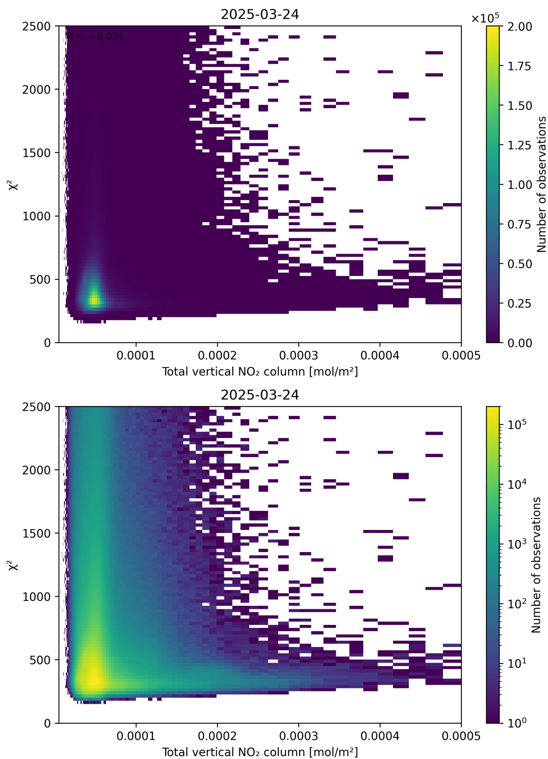
Figure 111: Scatter density plot of “Total vertical NO 2 column” against “ \chi^2 ” for 2025-03-24 to 2025-03-25.
