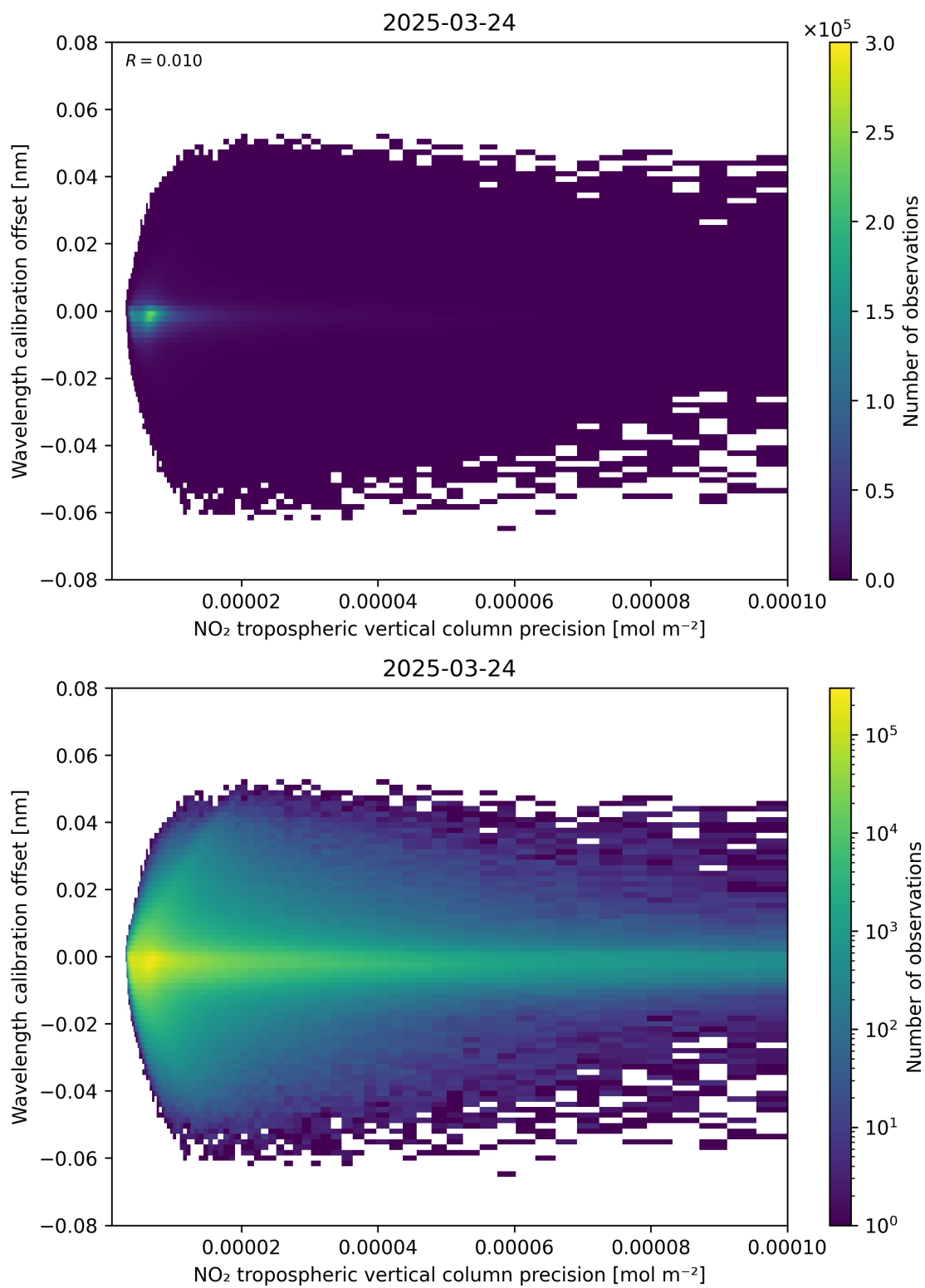
Figure 141: Scatter density plot of “NO 2 tropospheric vertical column precision” against “Wavelength calibration offset” for 2025-03-24 to 2025-03-25.
