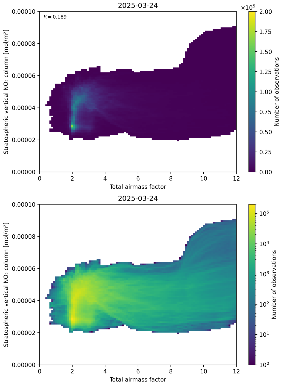
Figure 64: Scatter density plot of “Total airmass factor” against “Stratospheric vertical \text{NO}_2 column” for 2025-03-24 to 2025-03-25.
