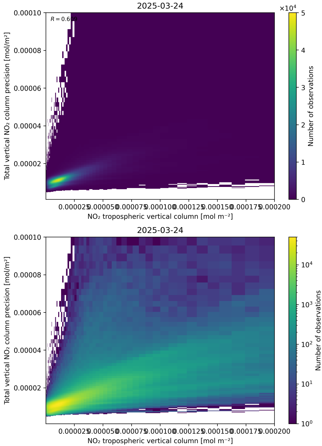
Figure 129: Scatter density plot of “NO 2 tropospheric vertical column” against “Total vertical NO 2 column precision” for 2025-03-24 to 2025-03-25.
