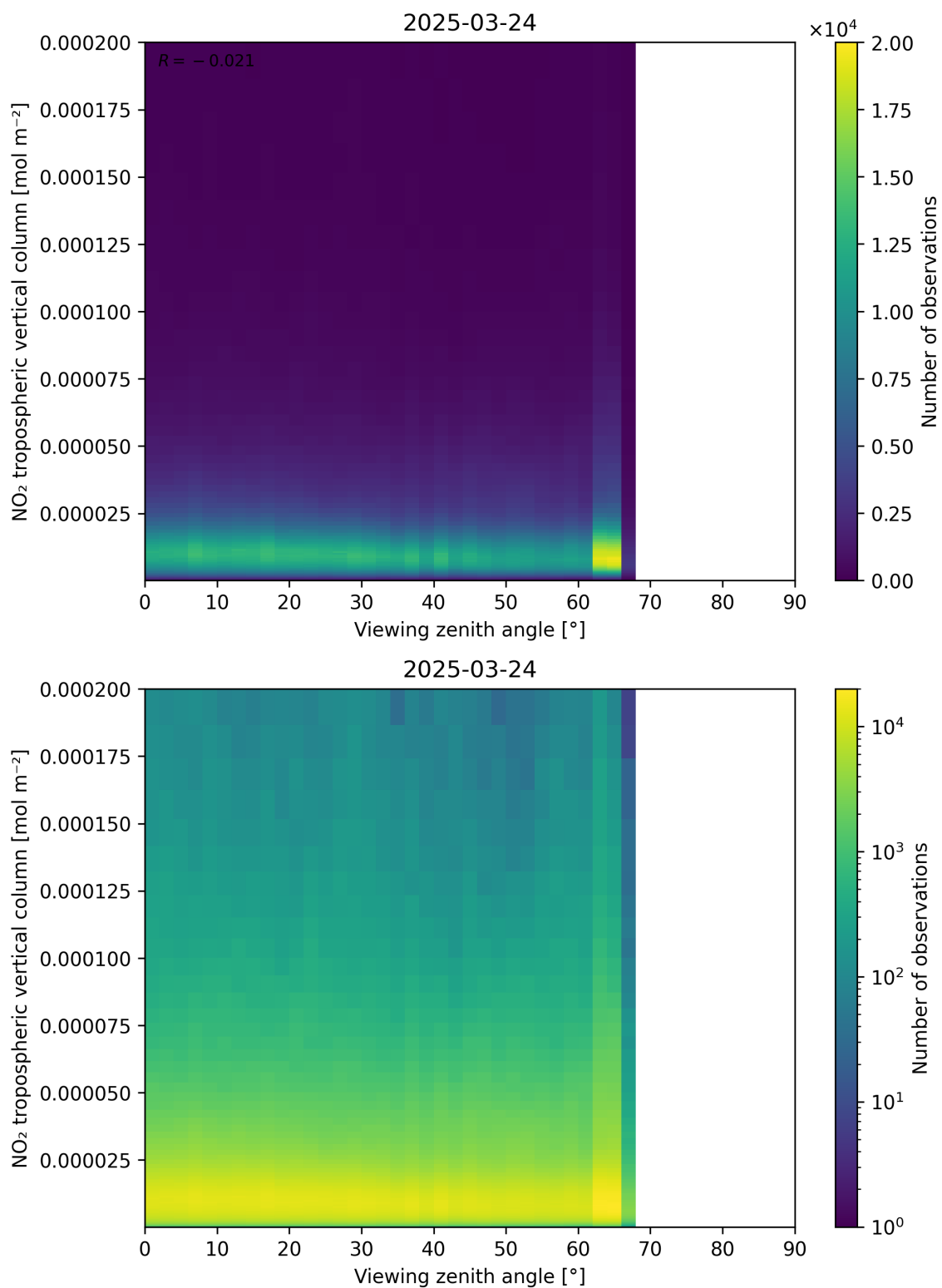
Figure 169: Scatter density plot of “Viewing zenith angle” against “NO 2 tropospheric vertical column” for 2025-03-24 to 2025-03-25.
