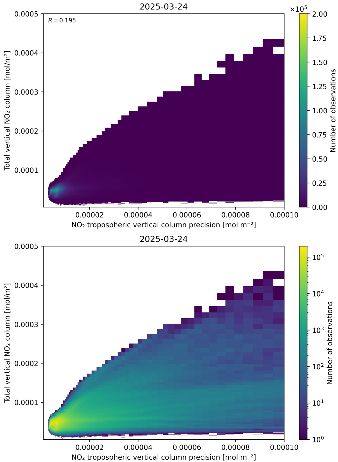
Figure 138: Scatter density plot of “NO 2 tropospheric vertical column precision” against “Total vertical NO 2 column” for 2025-03-24 to 2025-03-25.
