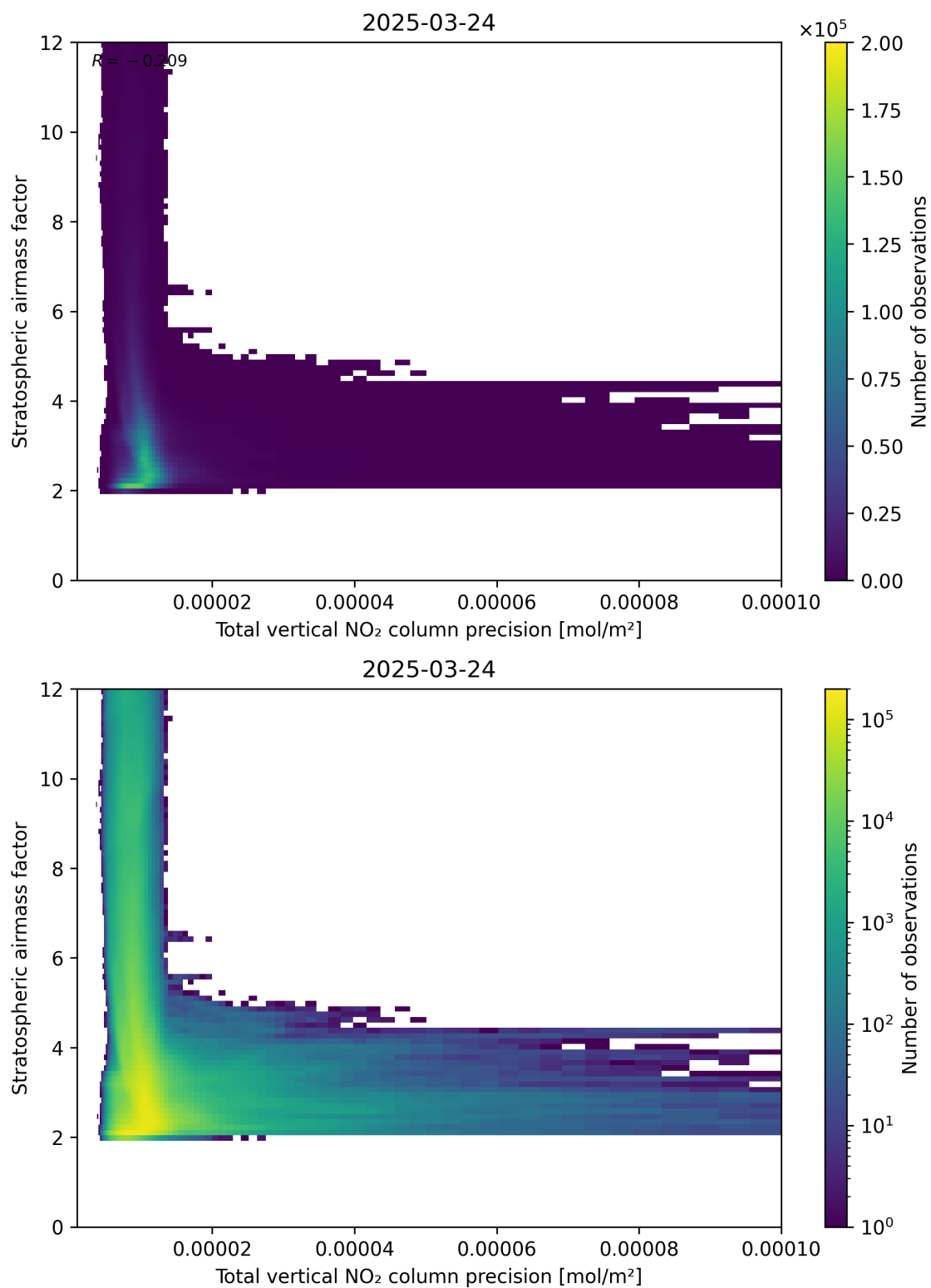
Figure 115: Scatter density plot of “Total vertical NO 2 column precision” against “Stratospheric air mass factor” for 2025-03-24 to 2025-03-25.
