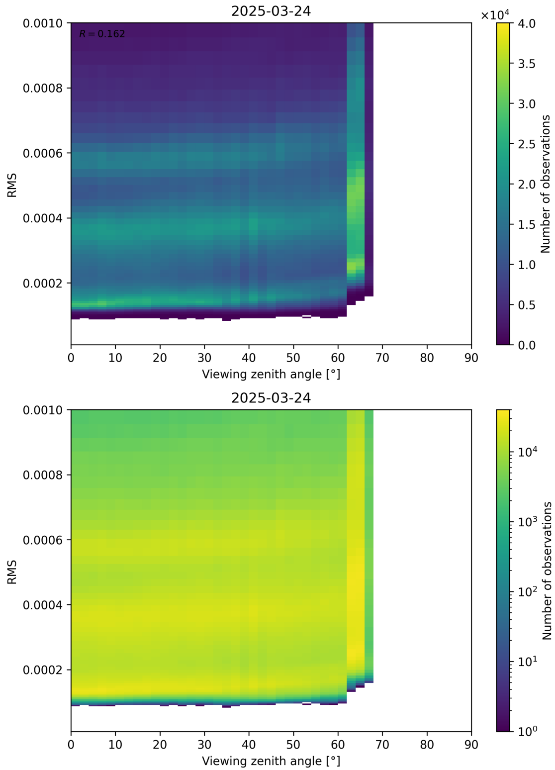
Figure 171: Scatter density plot of “Viewing zenith angle” against “RMS” for 2025-03-24 to 2025-03-25.
