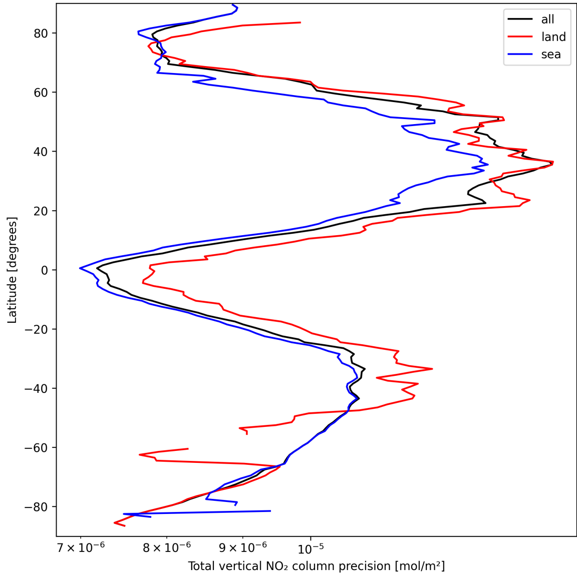
Figure 22: Zonal average of “Total vertical NO 2 column precision” for 2025-03-24 to 2025-03-25.
