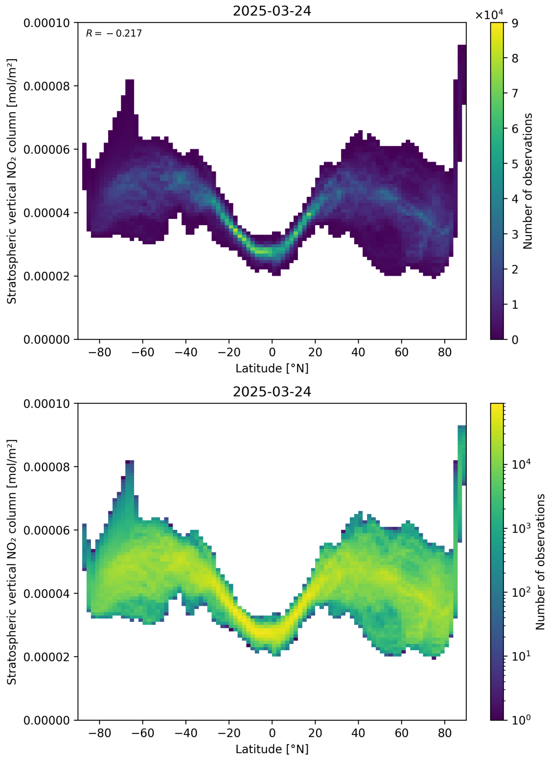
Figure 87: Scatter density plot of “Latitude” against “Stratospheric vertical NO 2 column” for 2025-03-24 to 2025-03-25.
