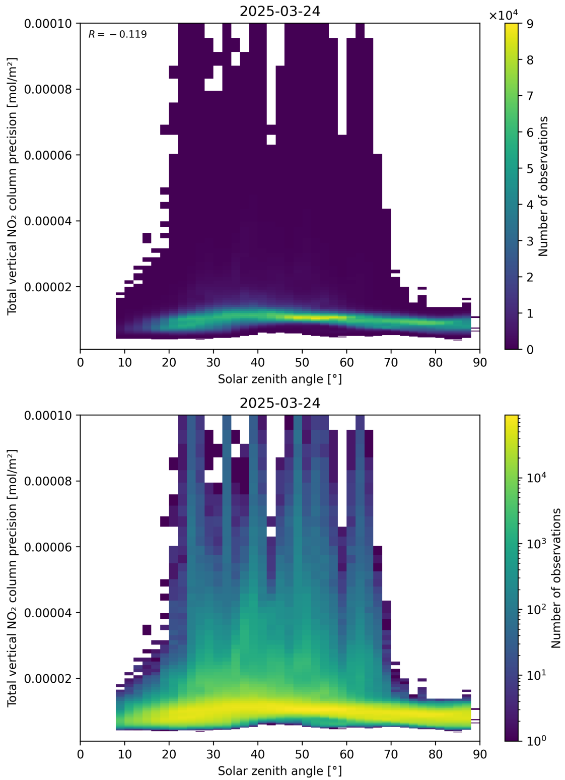
Figure 154: Scatter density plot of “Solar zenith angle” against “Total vertical NO 2 column precision” for 2025-03-24 to 2025-03-25.
