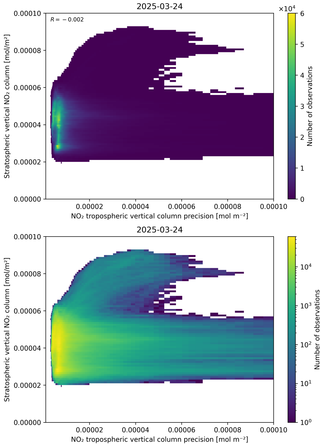
Figure 135: Scatter density plot of “NO 2 tropospheric vertical column precision” against “Stratospheric vertical NO 2 column” for 2025-03-24 to 2025-03-25.
