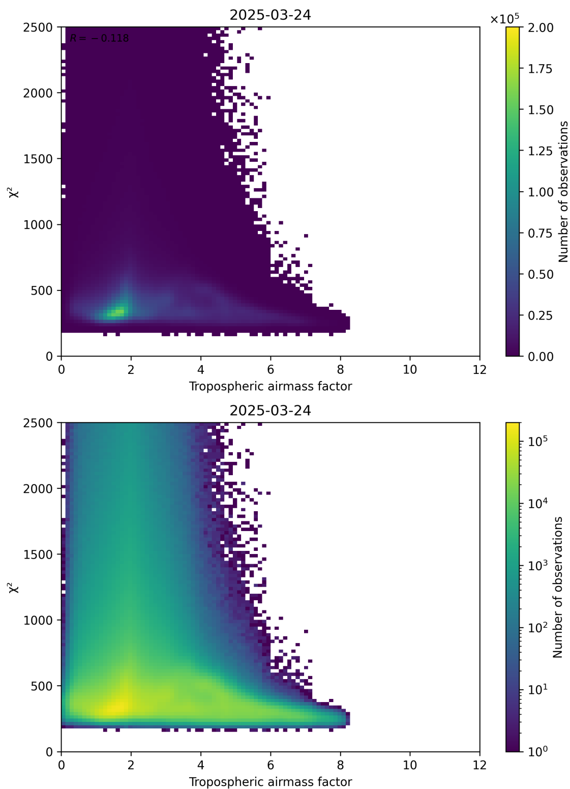
Figure 73: Scatter density plot of “Tropospheric airmass factor” against “ \chi^2 ” for 2025-03-24 to 2025-03-25.
