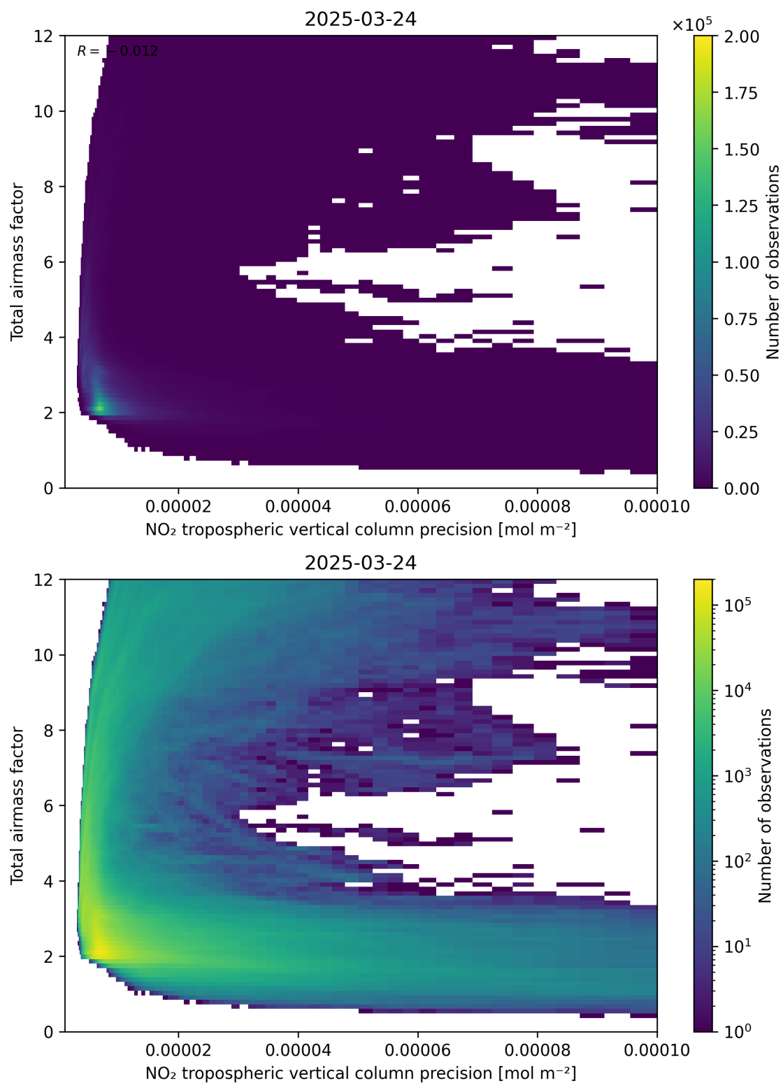
Figure 132: Scatter density plot of “NO 2 tropospheric vertical column precision” against “Total air mass factor” for 2025-03-24 to 2025-03-25.
