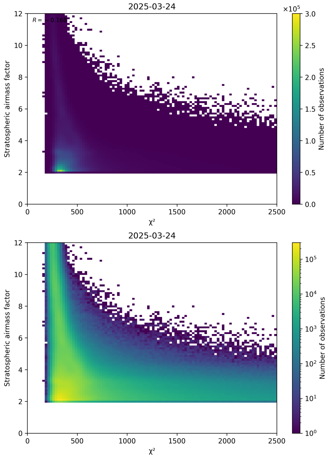
Figure 81: Scatter density plot of “ \chi^2 ” against “Stratospheric airmass factor” for 2025-03-24 to 2025-03-25.
