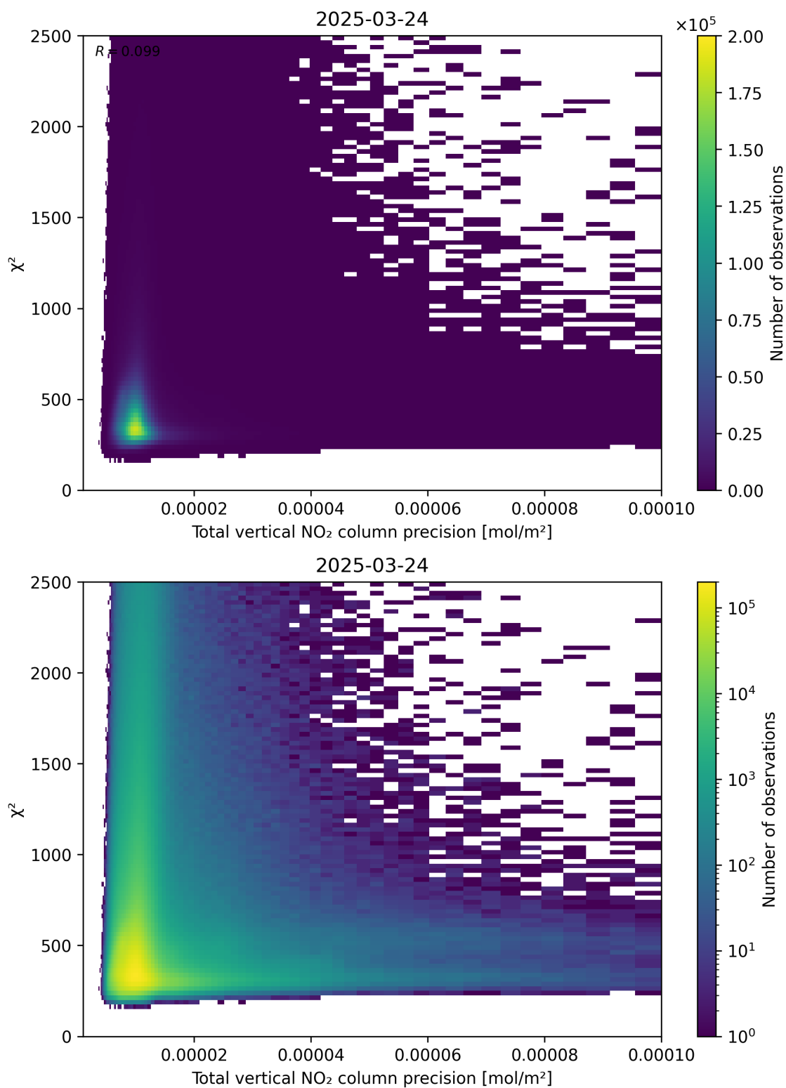
Figure 116: Scatter density plot of “Total vertical NO 2 column precision” against “ \chi^2 ” for 2025-03-24 to 2025-03-25.
