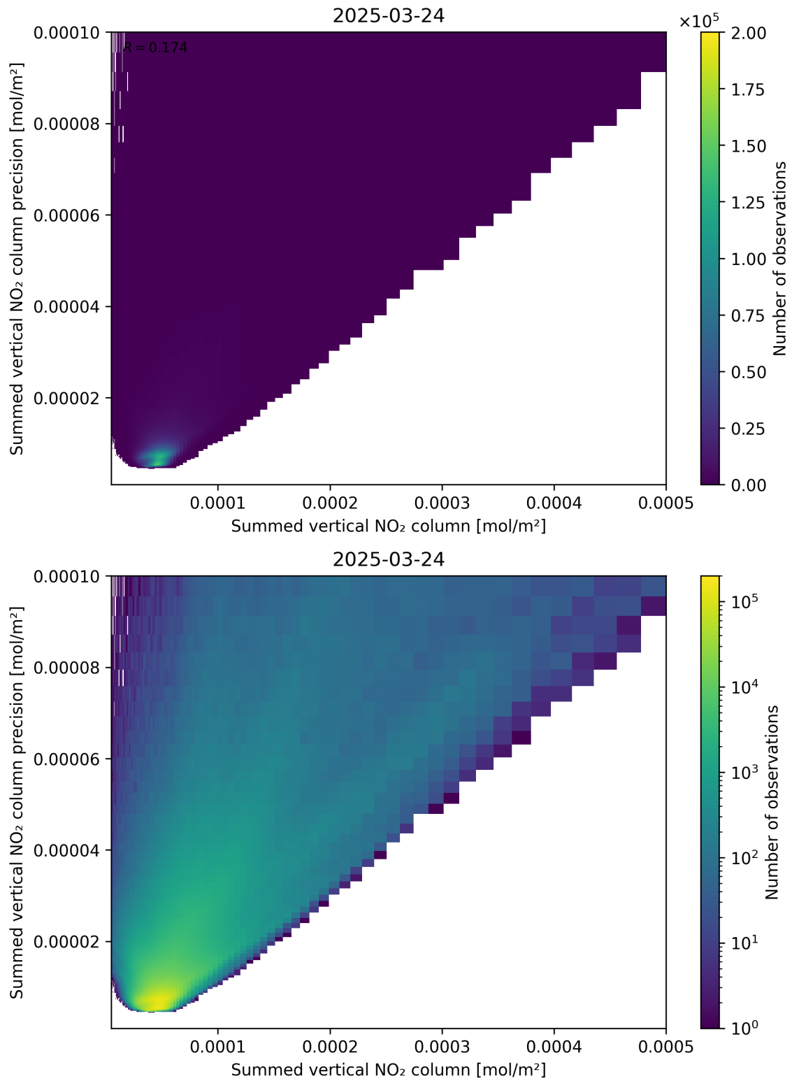
Figure 105: Scatter density plot of “Summed vertical NO 2 column” against “Summed vertical NO 2 column precision” for 2025-03-24 to 2025-03-25.
