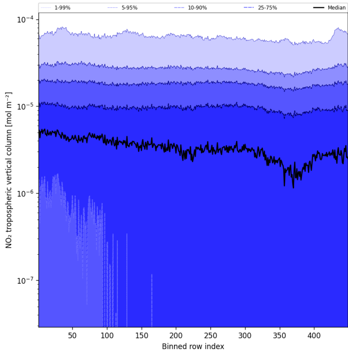
Figure 46: Along track statistics of “NO 2 tropospheric vertical column” for 2025-03-24 to 2025-03-25
