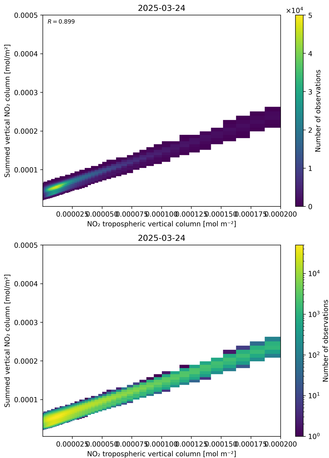
Figure 126: Scatter density plot of “NO 2 tropospheric vertical column” against “Summed vertical NO 2 column” for 2025-03-24 to 2025-03-25.
