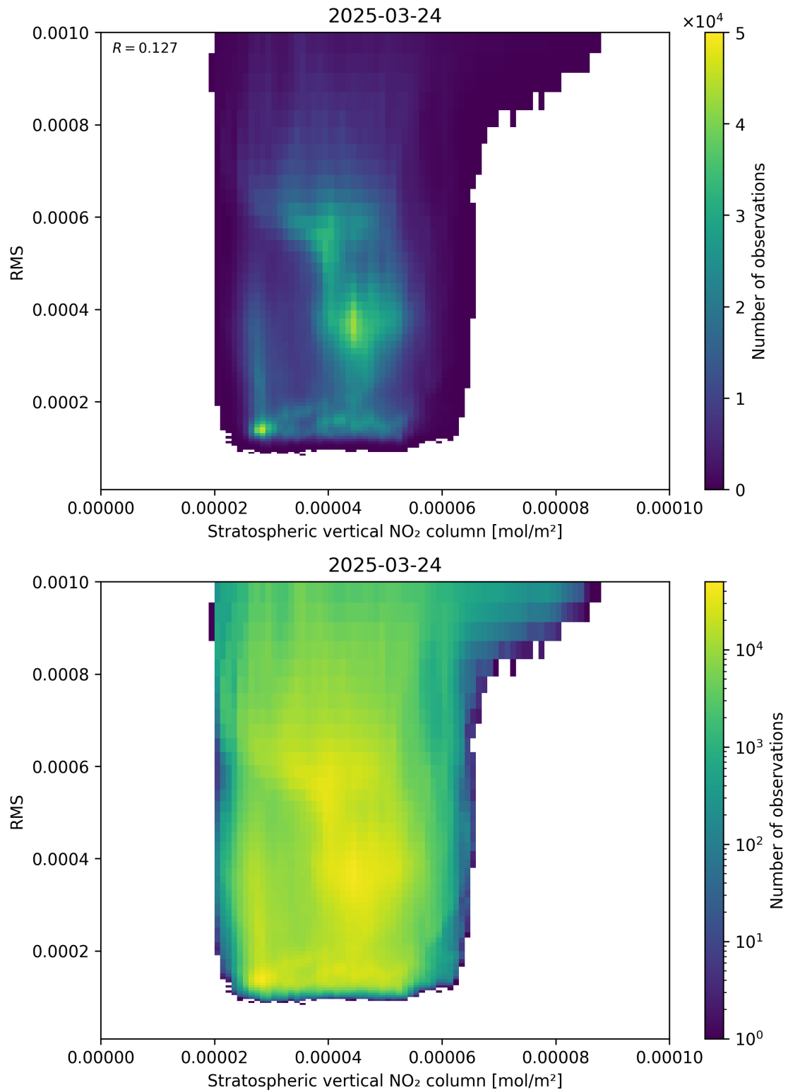
Figure 102: Scatter density plot of “Stratospheric vertical NO 2 column” against “RMS” for 2025-03-24 to 2025-03-25.
