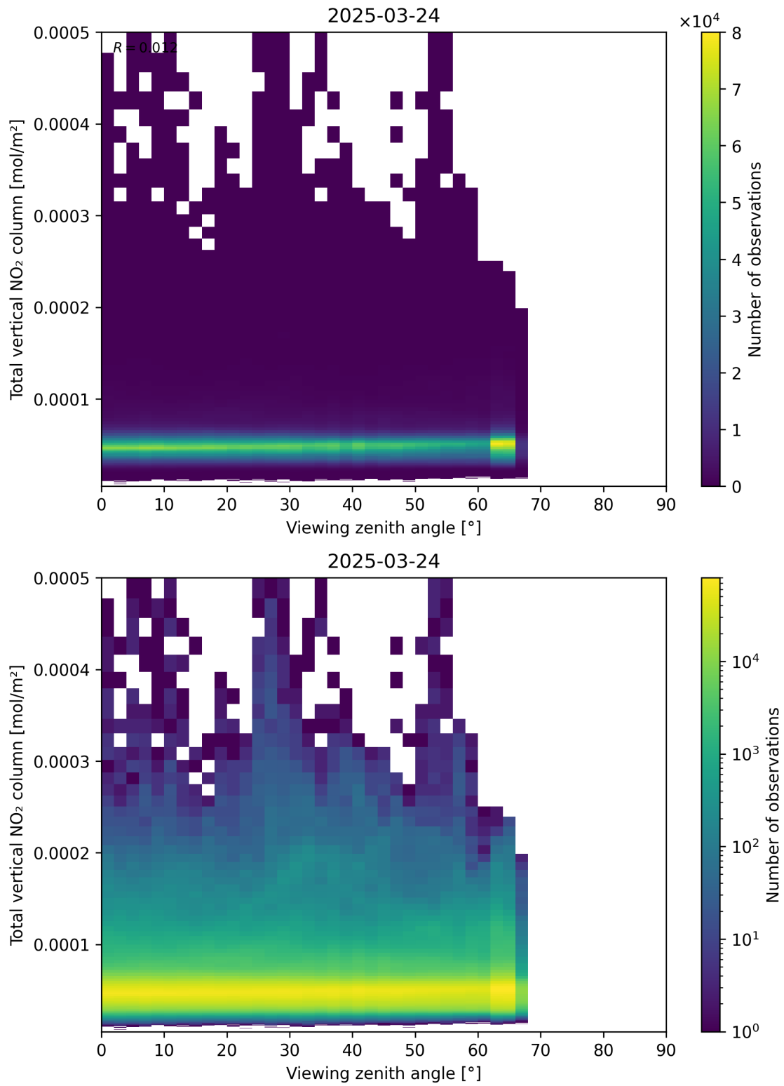
Figure 167: Scatter density plot of “Viewing zenith angle” against “Total vertical NO 2 column” for 2025-03-24 to 2025-03-25.
