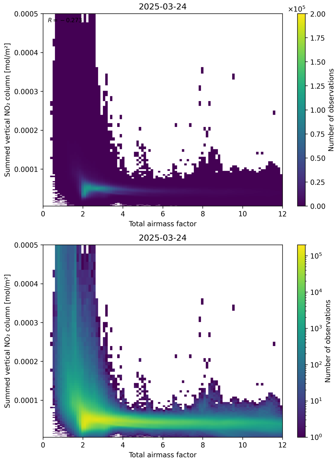
Figure 65: Scatter density plot of “Total airmass factor” against “Summed vertical NO 2 column” for 2025-03-24 to 2025-03-25.
