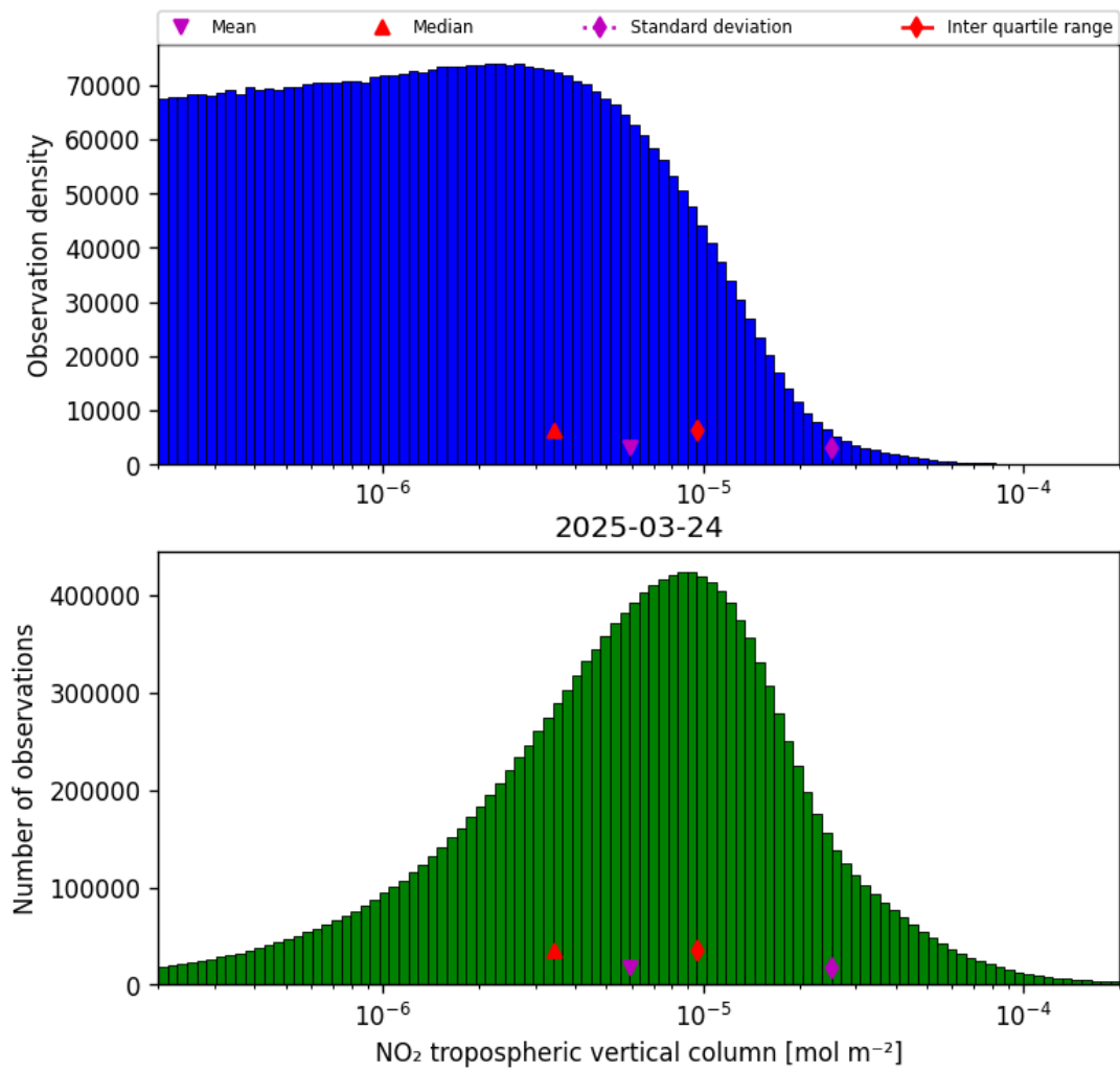
Figure 29: Histogram of “NO 2 tropospheric vertical column” for 2025-03-24 to 2025-03-25
