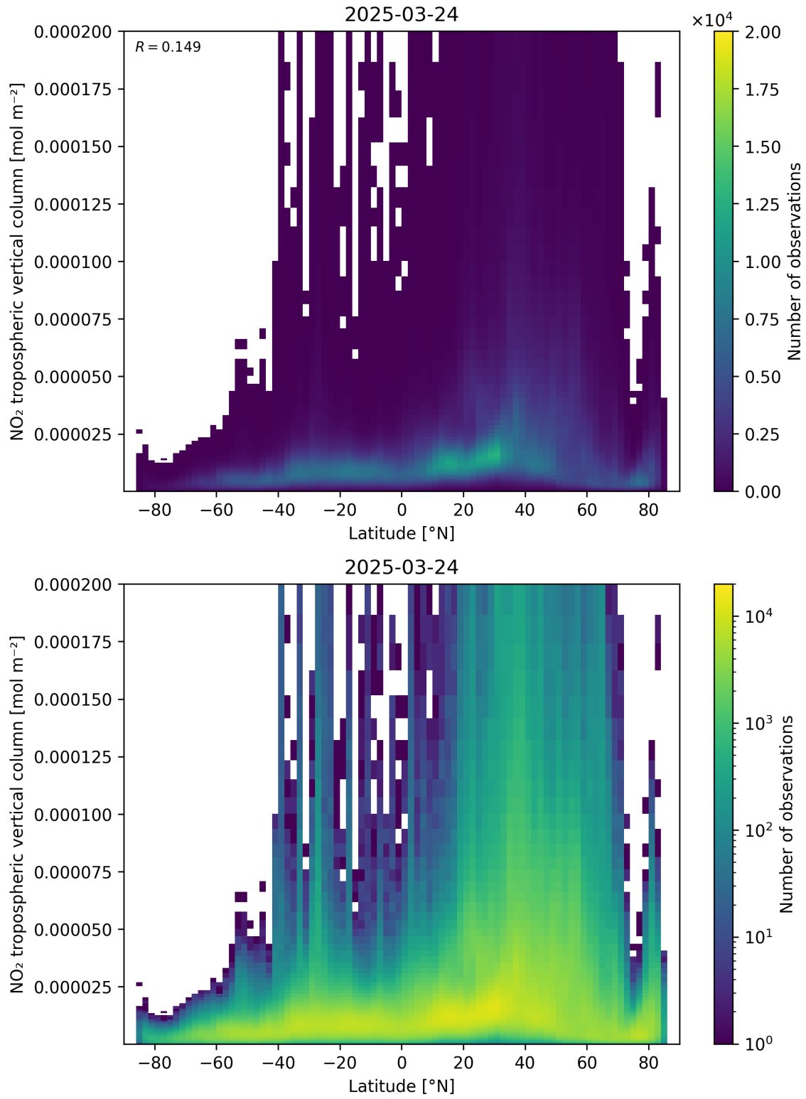
Figure 92: Scatter density plot of “Latitude” against “NO 2 tropospheric vertical column” for 2025-03-24 to 2025-03-25.
