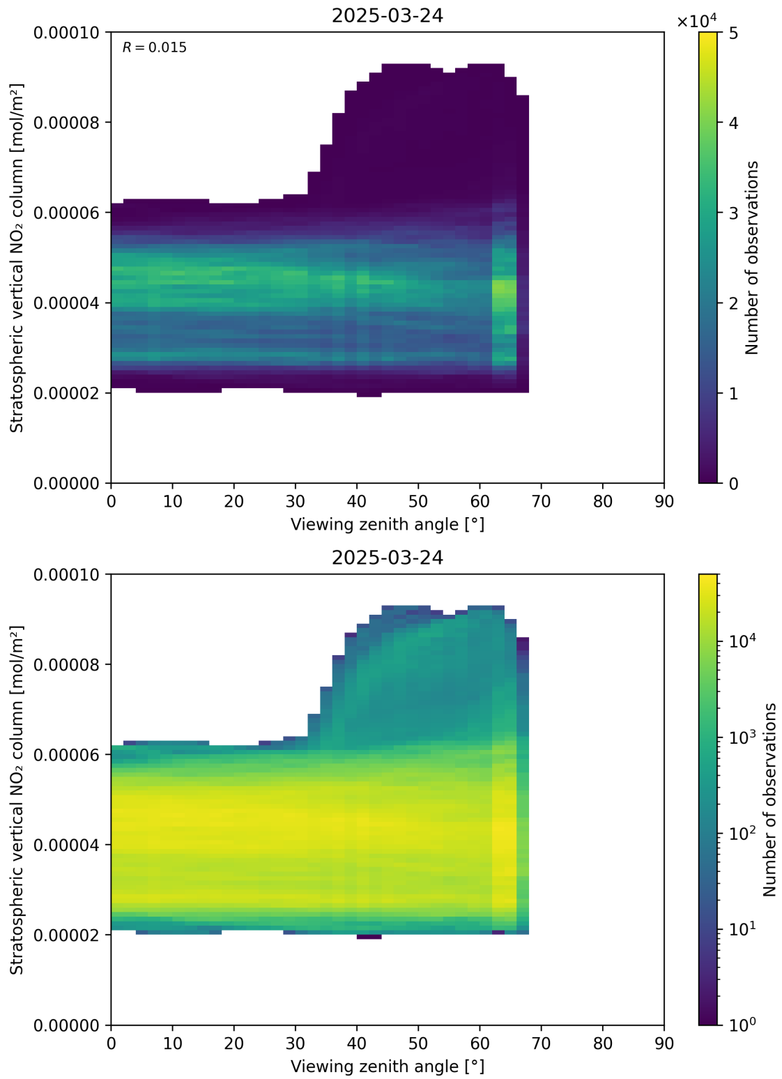
Figure 164: Scatter density plot of “Viewing zenith angle” against “Stratospheric vertical NO 2 column” for 2025-03-24 to 2025-03-25.
