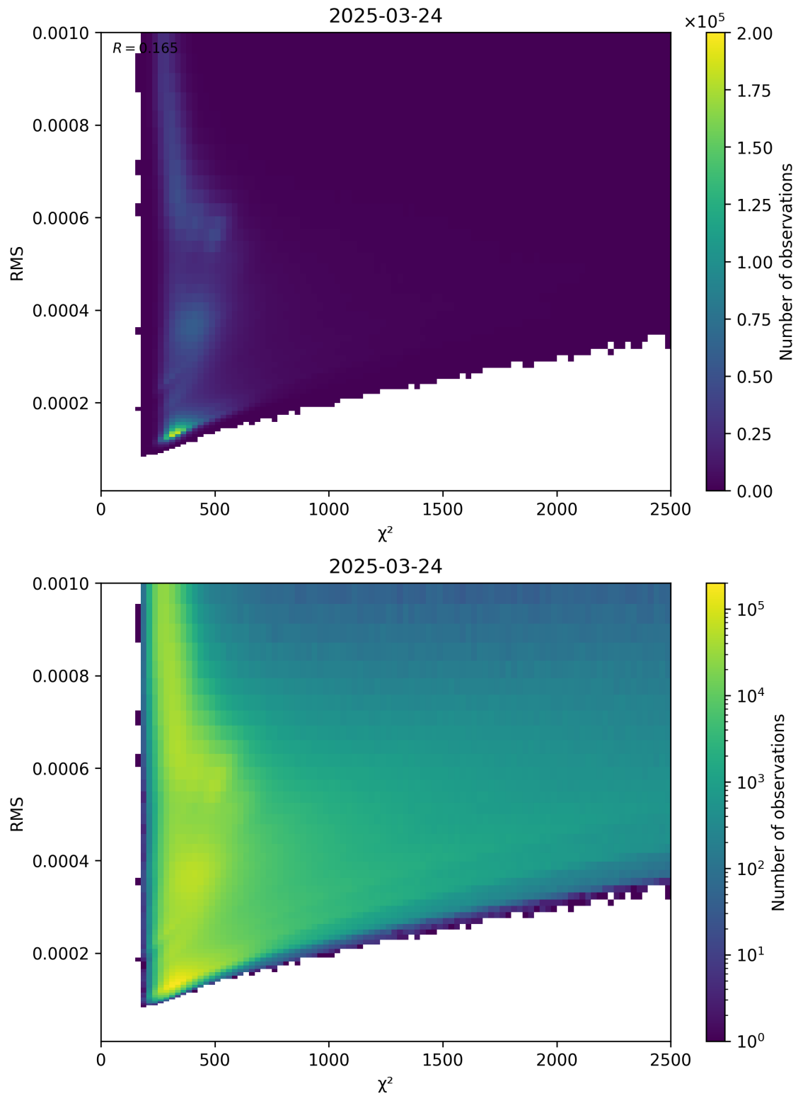
Figure 82: Scatter density plot of “ \chi^2 ” against “RMS” for 2025-03-24 to 2025-03-25.
