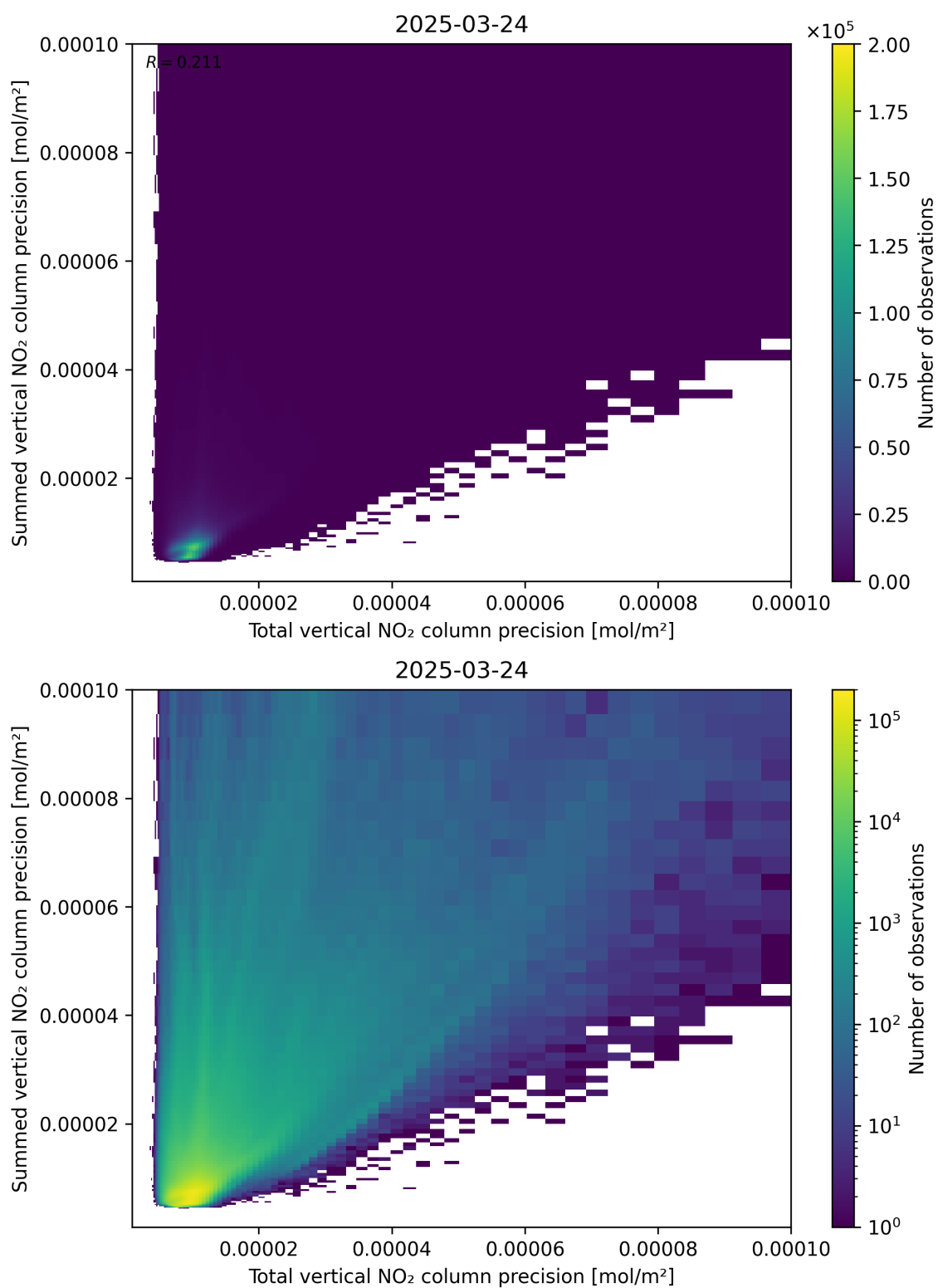
Figure 118: Scatter density plot of “Total vertical NO 2 column precision” against “Summed vertical NO 2 column precision” for 2025-03-24 to 2025-03-25.
