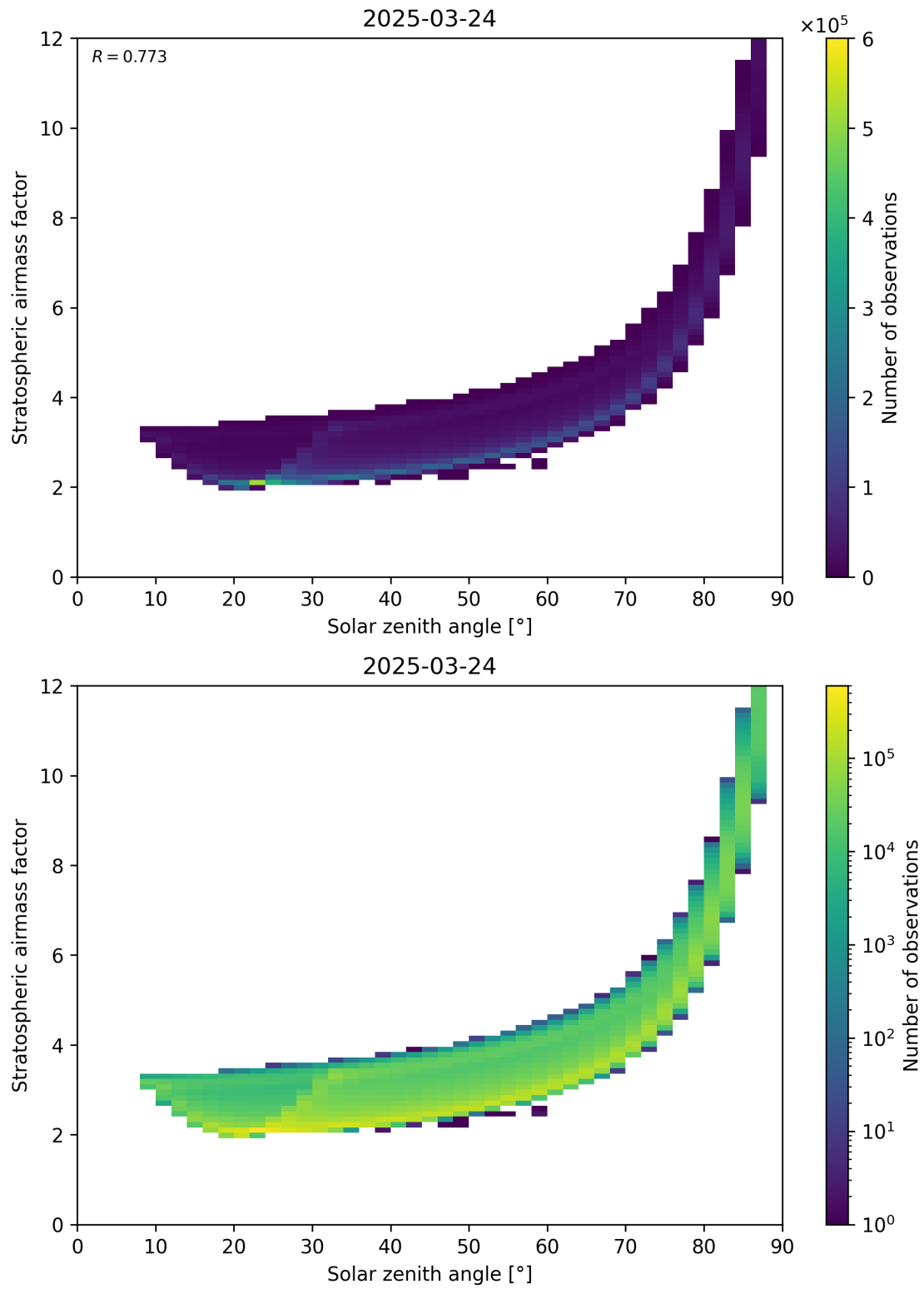
Figure 145: Scatter density plot of “Solar zenith angle” against “Stratospheric airmass factor” for 2025-03-24 to 2025-03-25.
