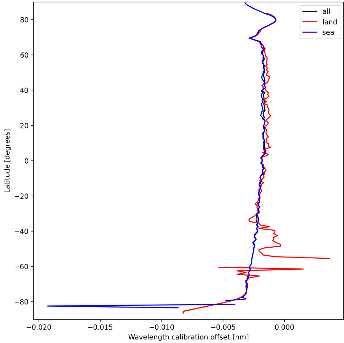
Figure 18: Zonal average of “Wavelength calibration offset” for 2025-03-24 to 2025-03-25.
