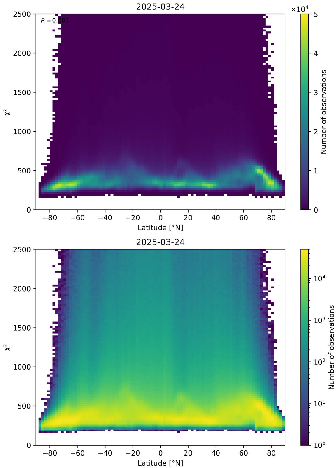
Figure 86: Scatter density plot of “Latitude” against “ \chi^2 ” for 2025-03-24 to 2025-03-25.
