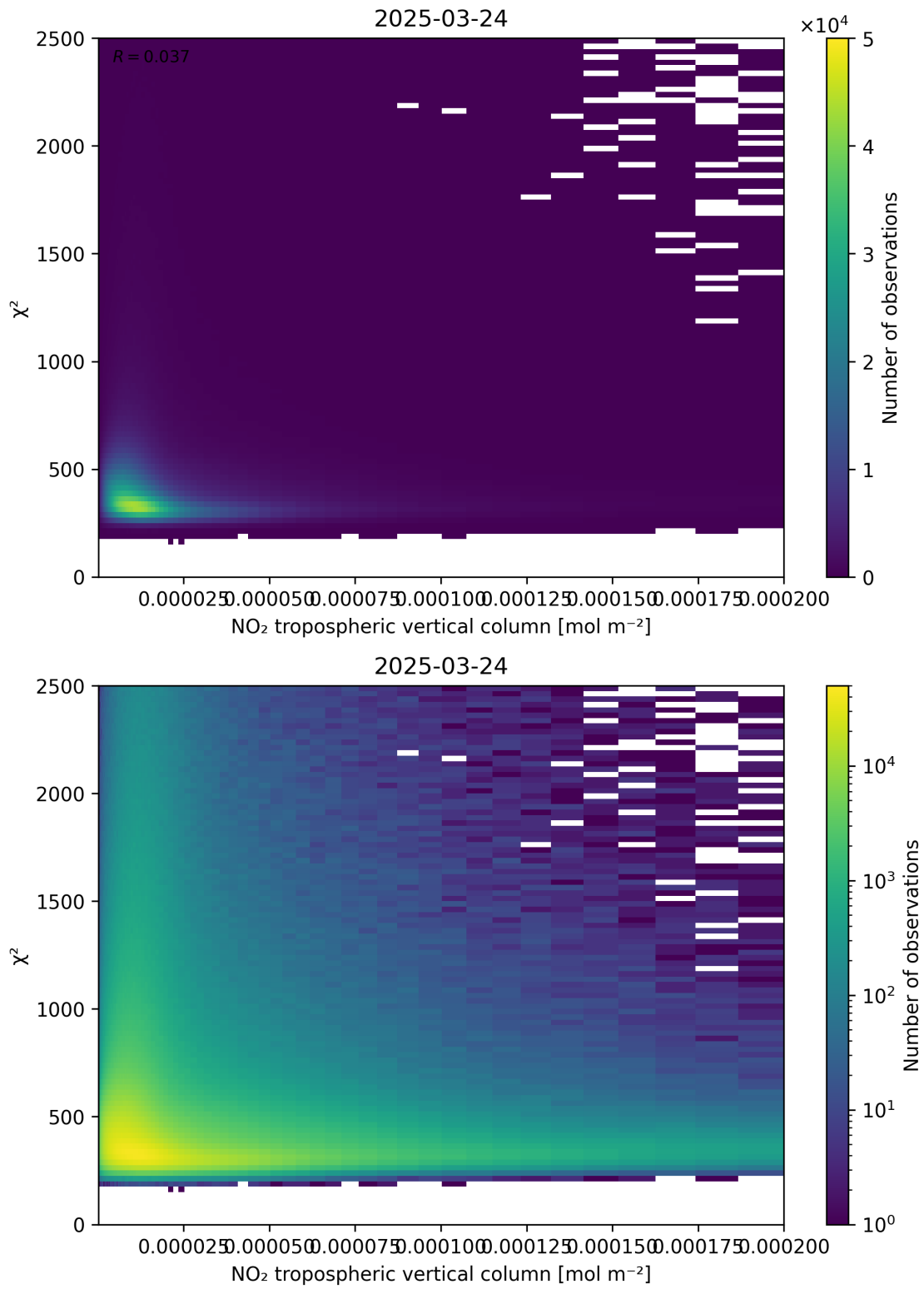
Figure 124: Scatter density plot of “NO 2 tropospheric vertical column” against “ \chi^2 ” for 2025-03-24 to 2025-03-25.
