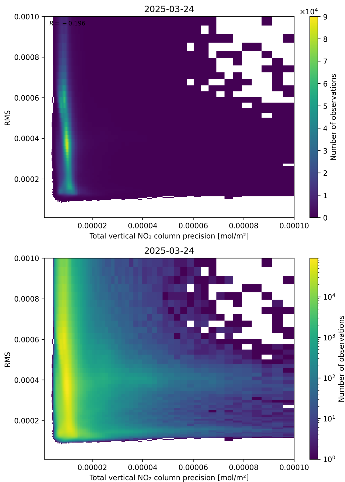
Figure 119: Scatter density plot of “Total vertical NO 2 column precision” against “RMS” for 2025-03-24 to 2025-03-25.
