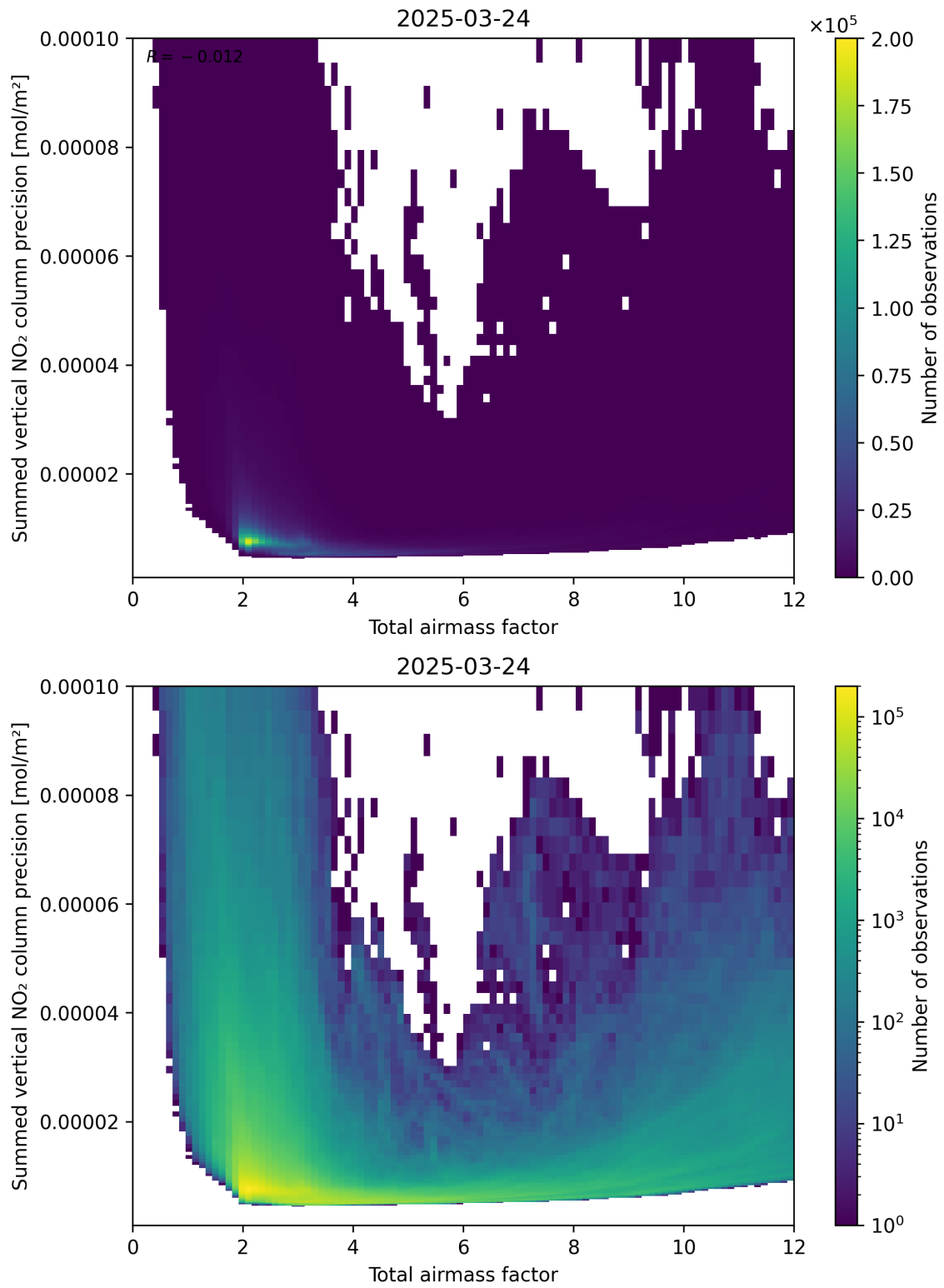
Figure 66: Scatter density plot of “Total airmass factor” against “Summed vertical NO 2 column precision” for 2025-03-24 to 2025-03-25.
