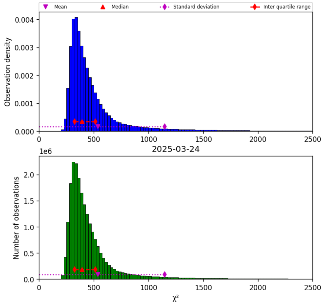
Figure 42: Histogram of “ \chi^2 ” for 2025-03-24 to 2025-03-25
