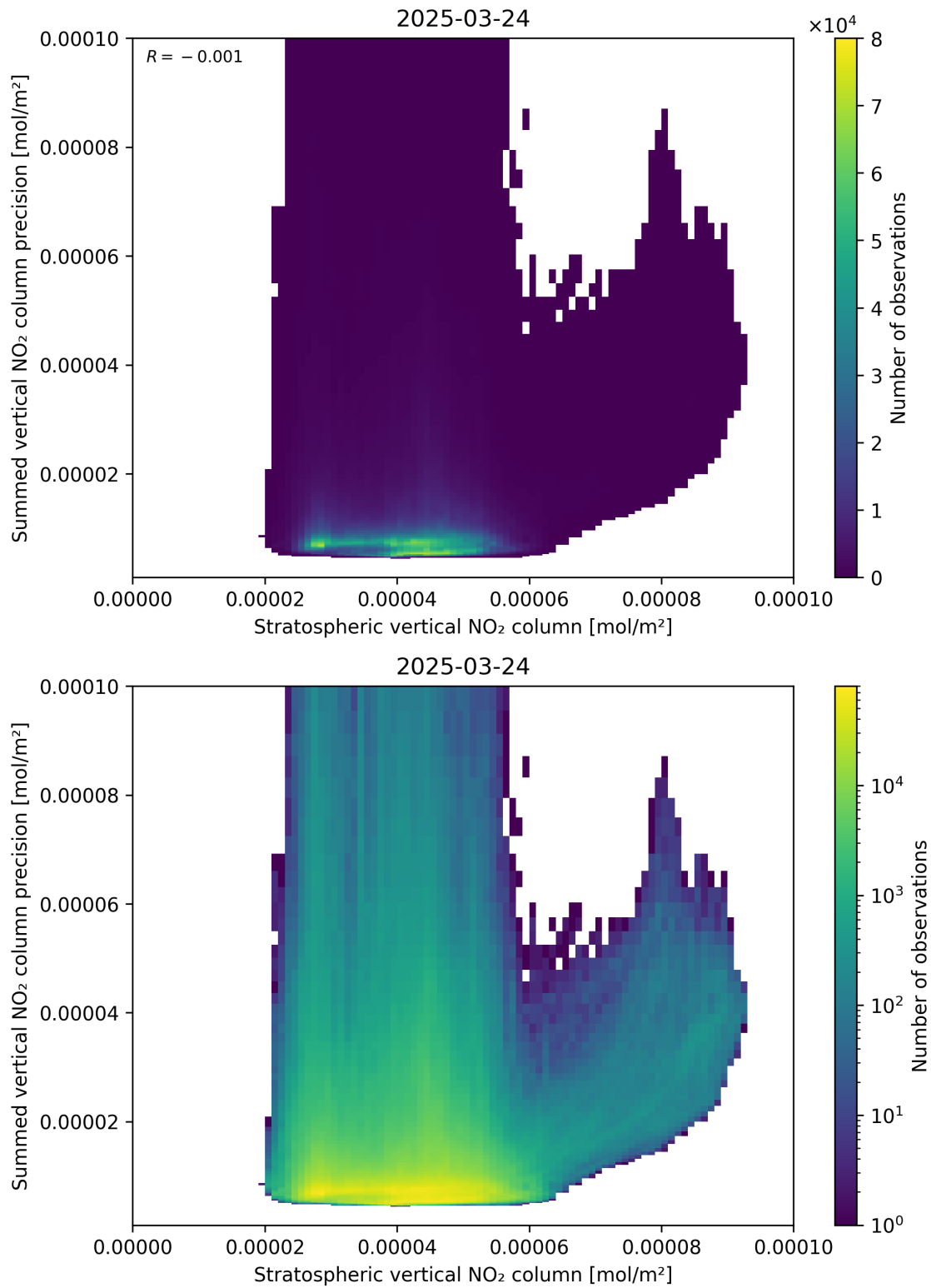
Figure 99: Scatter density plot of “Stratospheric vertical NO 2 column” against “Summed vertical NO 2 column precision” for 2025-03-24 to 2025-03-25.
