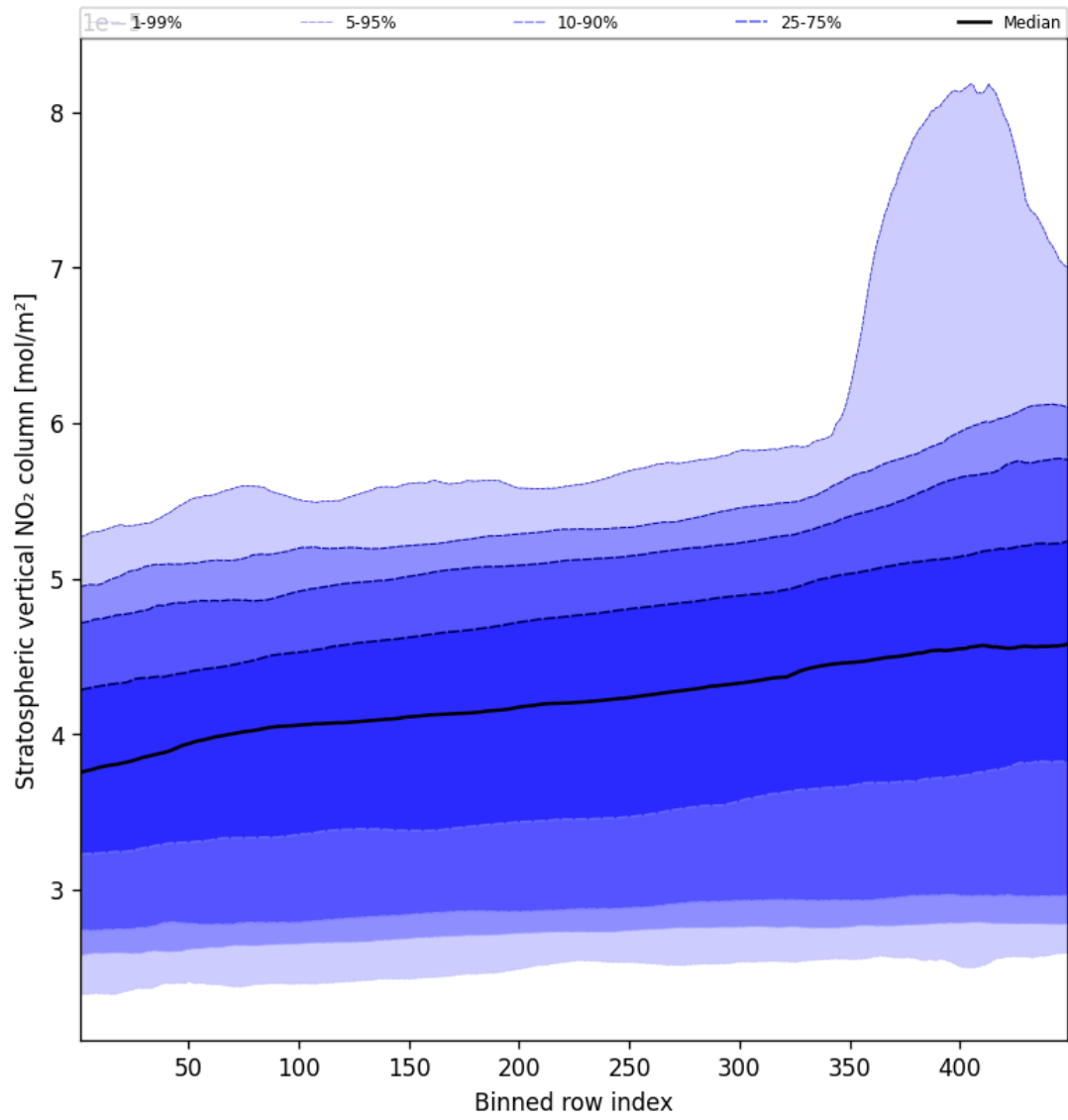
Figure 53: Along track statistics of “Stratospheric vertical NO 2 column” for 2025-03-24 to 2025-03-25
