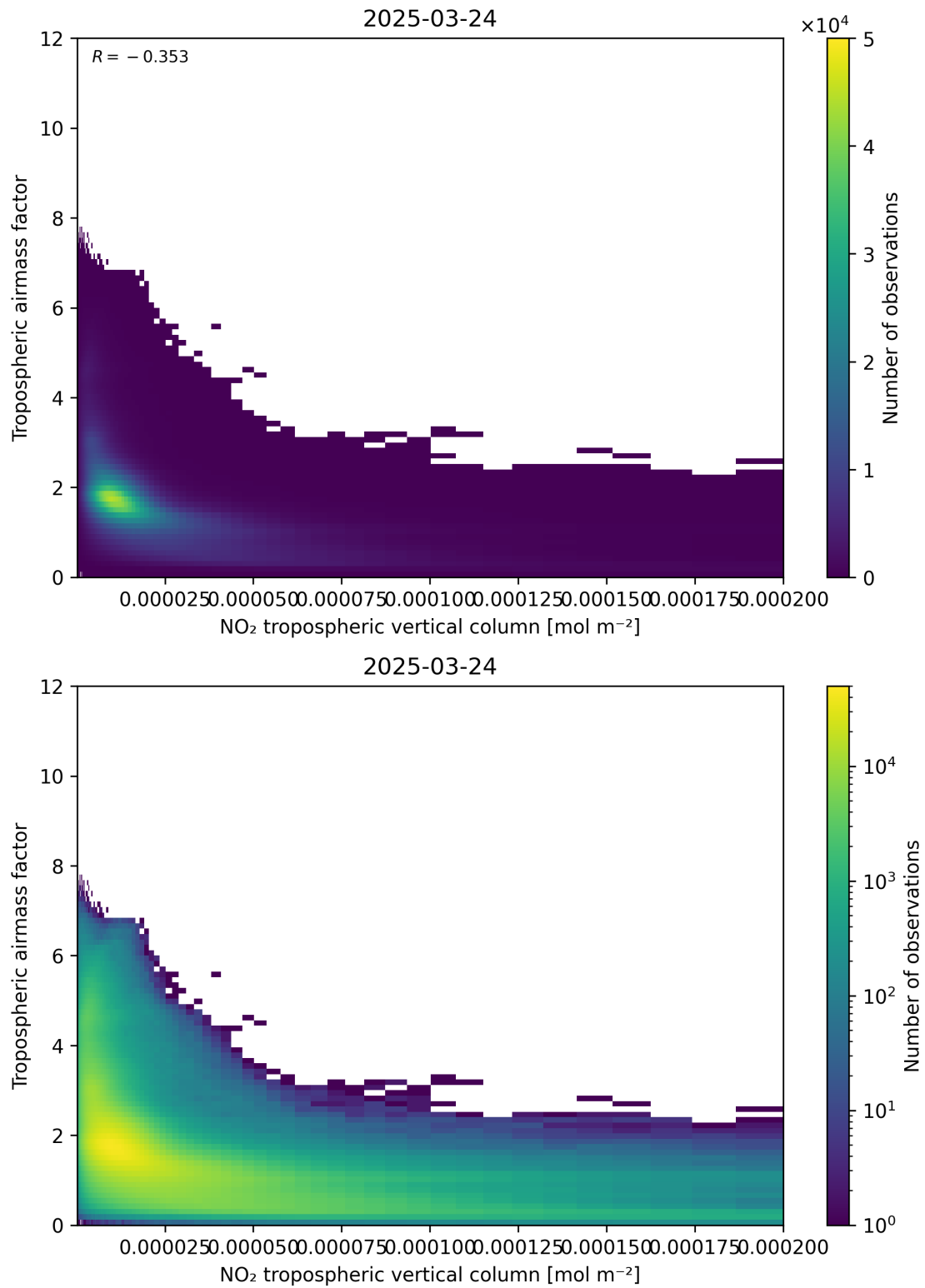
Figure 123: Scatter density plot of “NO 2 tropospheric vertical column” against “Tropospheric air mass factor” for 2025-03-24 to 2025-03-25.
