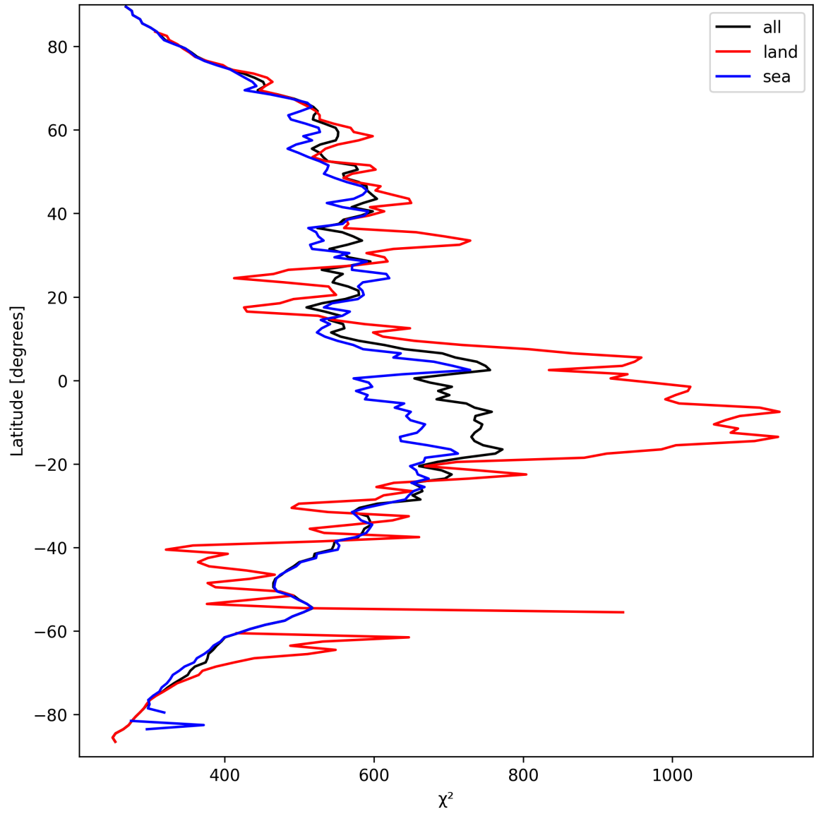
Figure 25: Zonal average of “ \chi^2 ” for 2025-03-24 to 2025-03-25.
