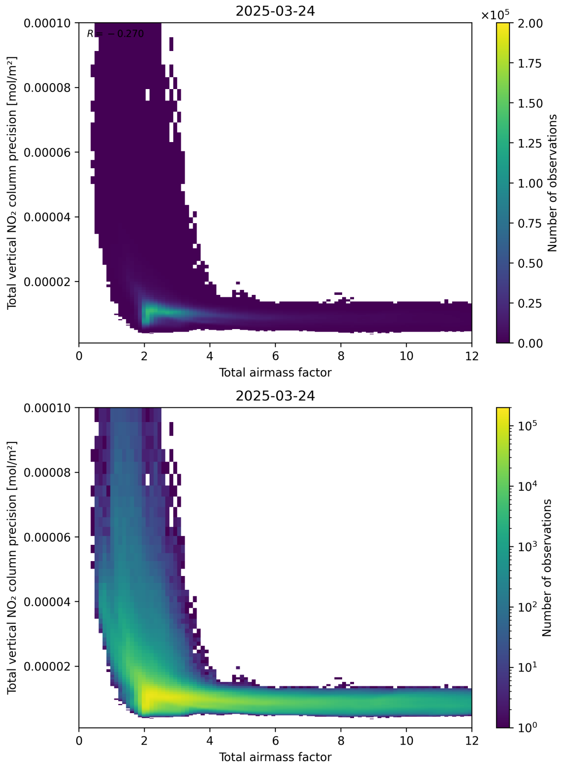
Figure 68: Scatter density plot of “Total airmass factor” against “Total vertical NO 2 column precision” for 2025-03-24 to 2025-03-25.
