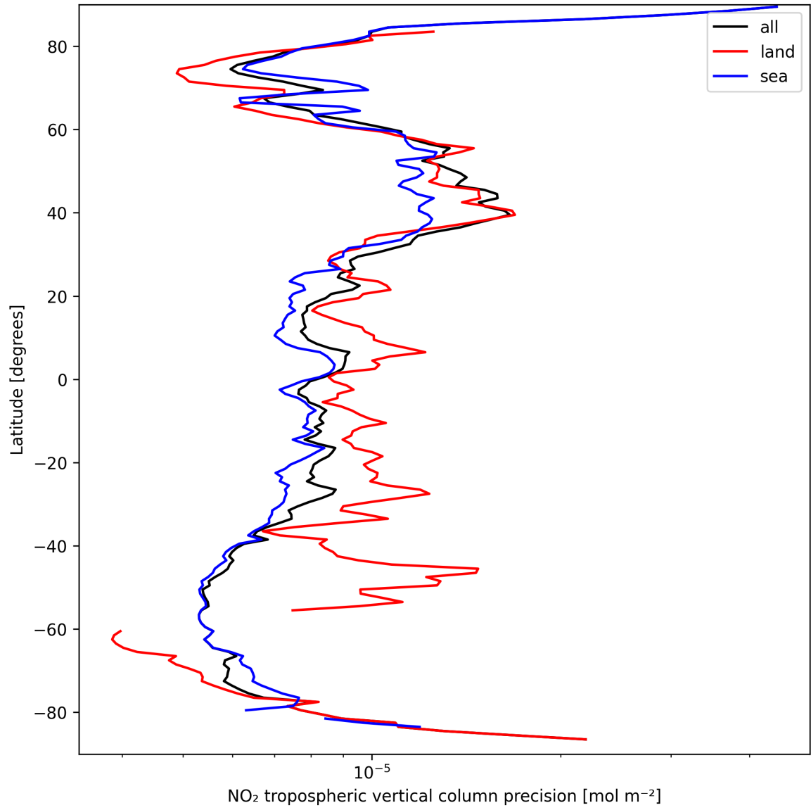
Figure 13: Zonal average of “NO 2 tropospheric vertical column precision” for 2025-03-24 to 2025-03-25.
