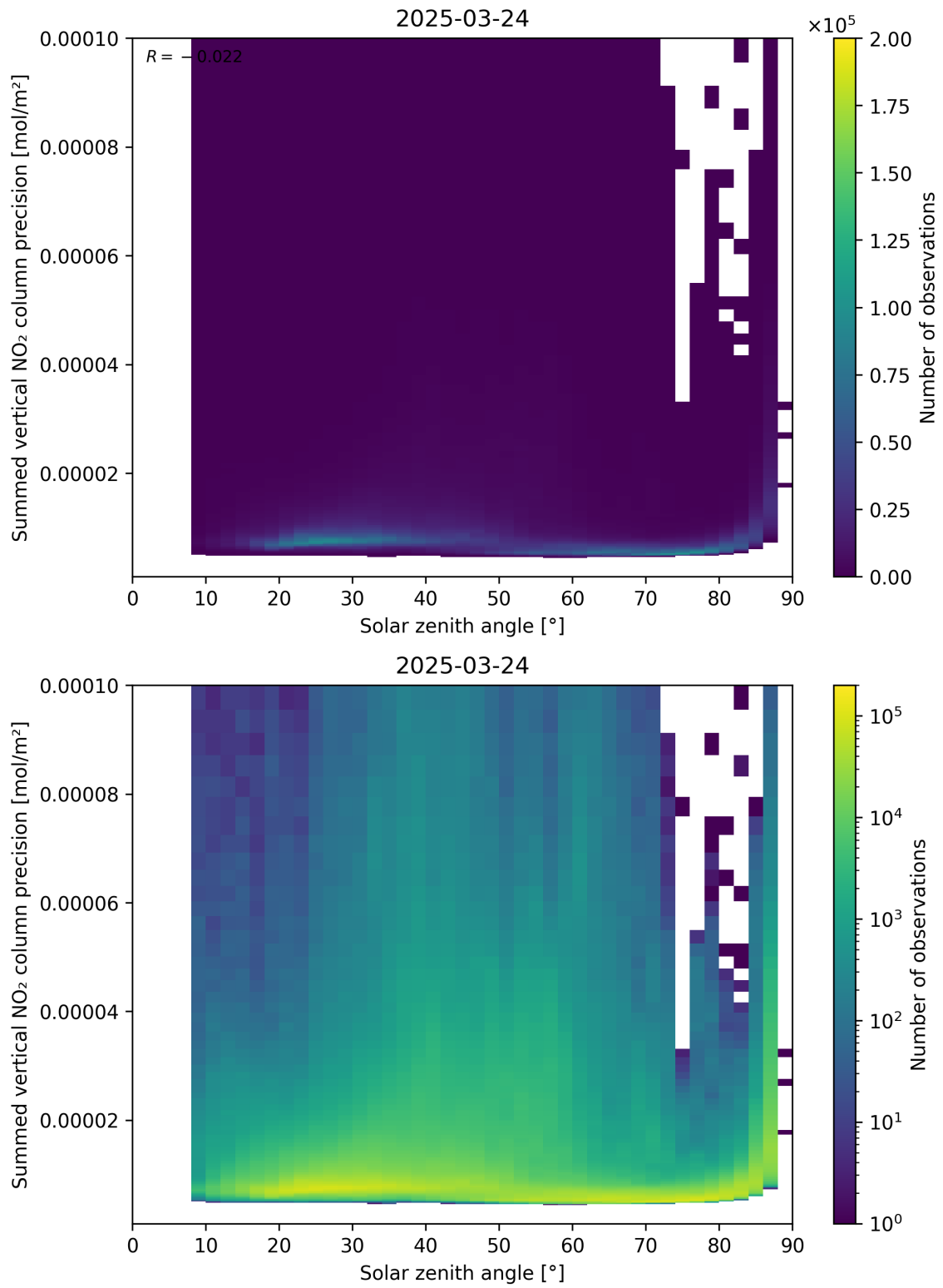
Figure 152: Scatter density plot of “Solar zenith angle” against “Summed vertical NO 2 column precision” for 2025-03-24 to 2025-03-25.
