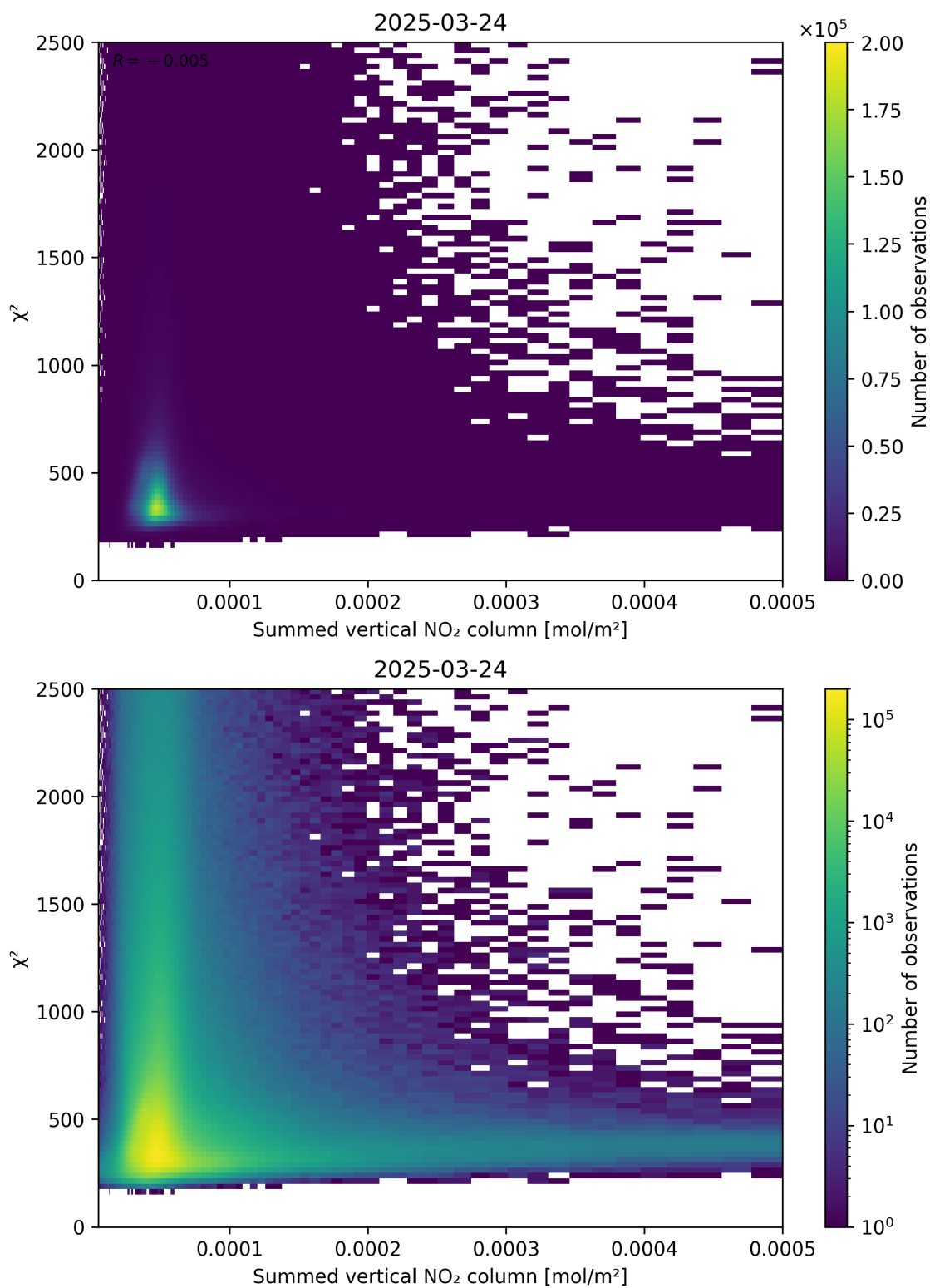
Figure 104: Scatter density plot of “Summed vertical NO 2 column” against “ \chi^2 ” for 2025-03-24 to 2025-03-25.
