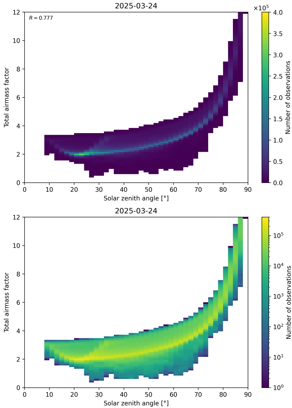
Figure 146: Scatter density plot of “Solar zenith angle” against “Total air mass factor” for 2025-03-24 to 2025-03-25.
