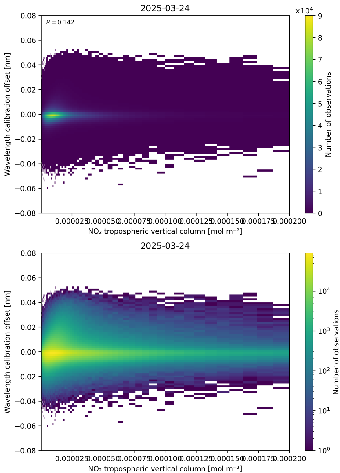
Figure 143: Scatter density plot of “NO 2 tropospheric vertical column” against “Wavelength calibration offset” for 2025-03-24 to 2025-03-25.
