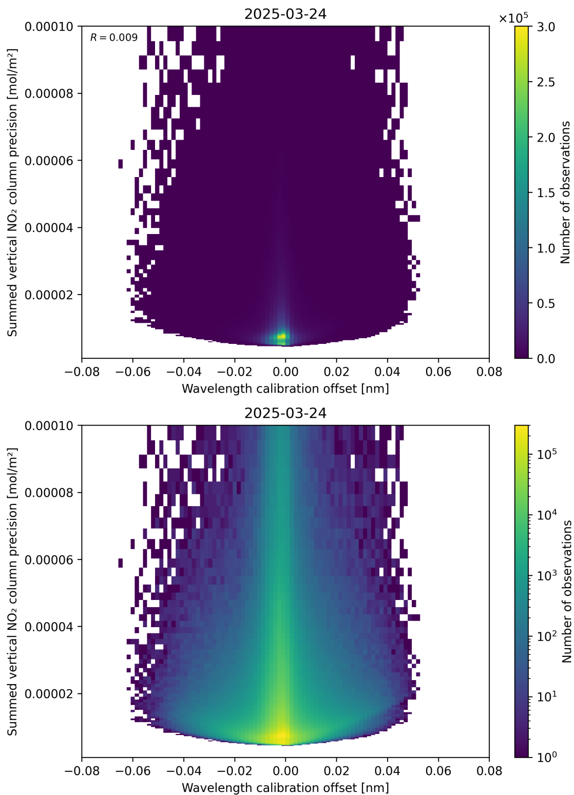
Figure 178: Scatter density plot of “Wavelength calibration offset” against “Summed vertical NO 2 column precision” for 2025-03-24 to 2025-03-25.
