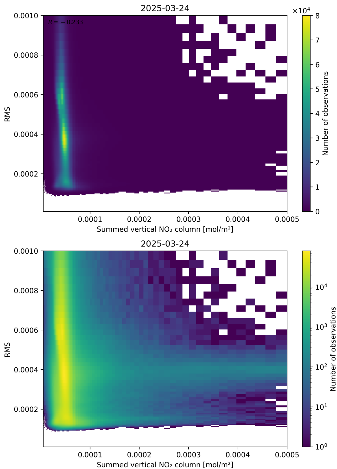
Figure 109: Scatter density plot of “Summed vertical NO 2 column” against “RMS” for 2025-03-24 to 2025-03-25.
