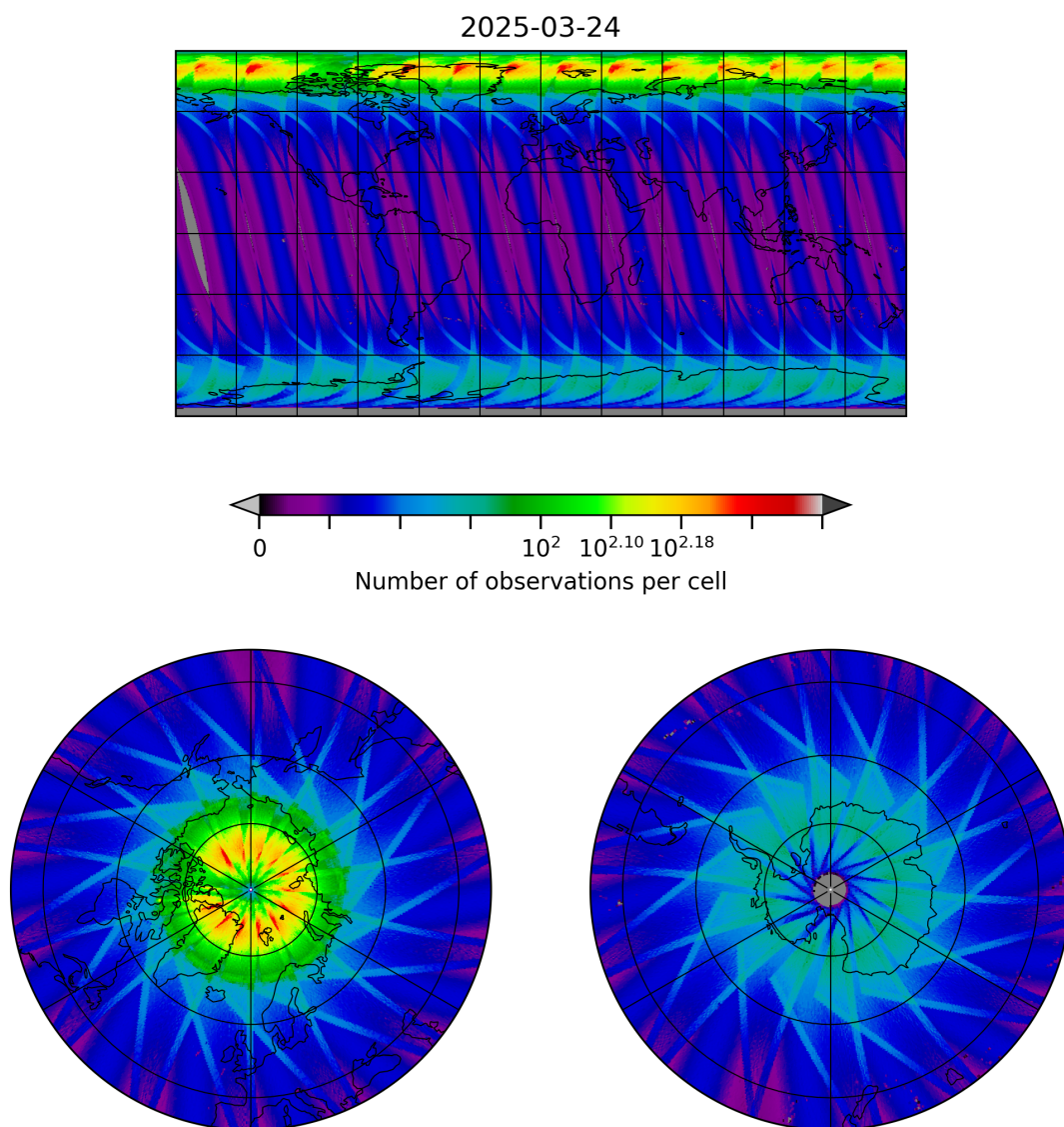
Figure 10: Map of the number of observations for 2025-03-24 to 2025-03-25
