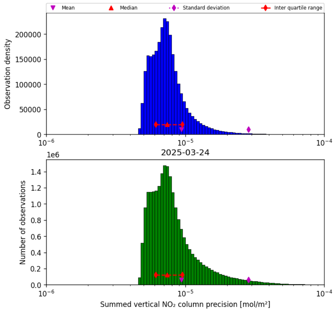
Figure 41: Histogram of “Summed vertical NO 2 column precision” for 2025-03-24 to 2025-03-25
