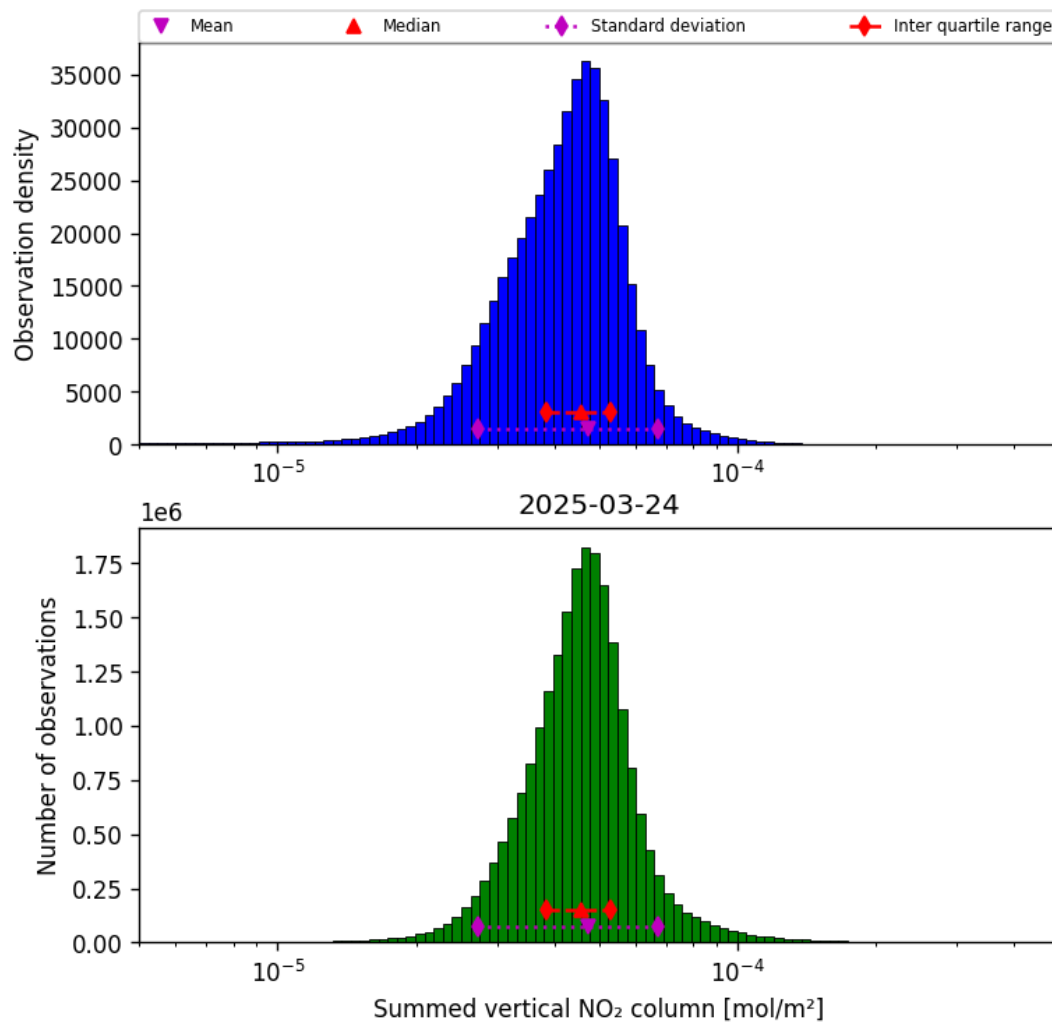
Figure 40: Histogram of “Summed vertical NO 2 column” for 2025-03-24 to 2025-03-25
