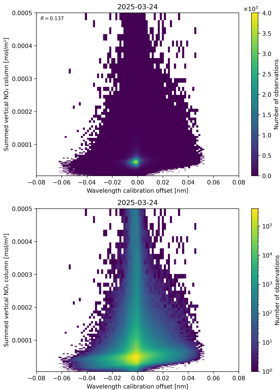
Figure 177: Scatter density plot of “Wavelength calibration offset” against “Summed vertical NO 2 column” for 2025-03-24 to 2025-03-25.
