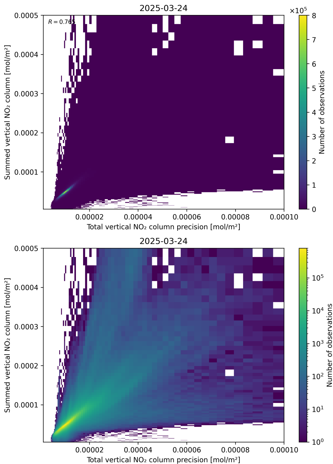
Figure 117: Scatter density plot of “Total vertical NO 2 column precision” against “Summed vertical NO 2 column” for 2025-03-24 to 2025-03-25.
