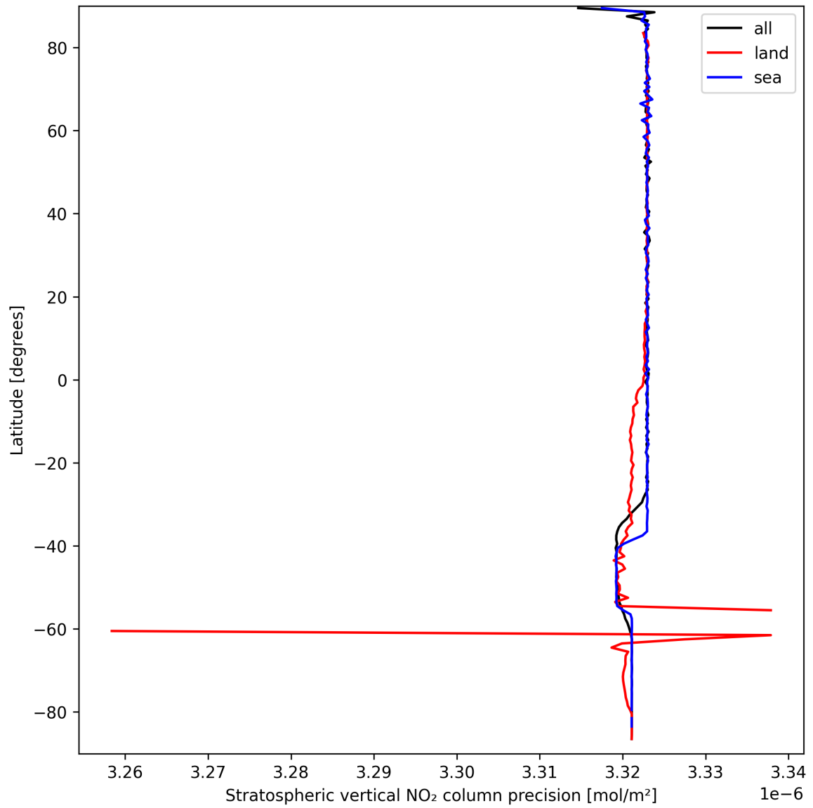
Figure 20: Zonal average of “Stratospheric vertical NO 2 column precision” for 2025-03-24 to 2025-03-25.
