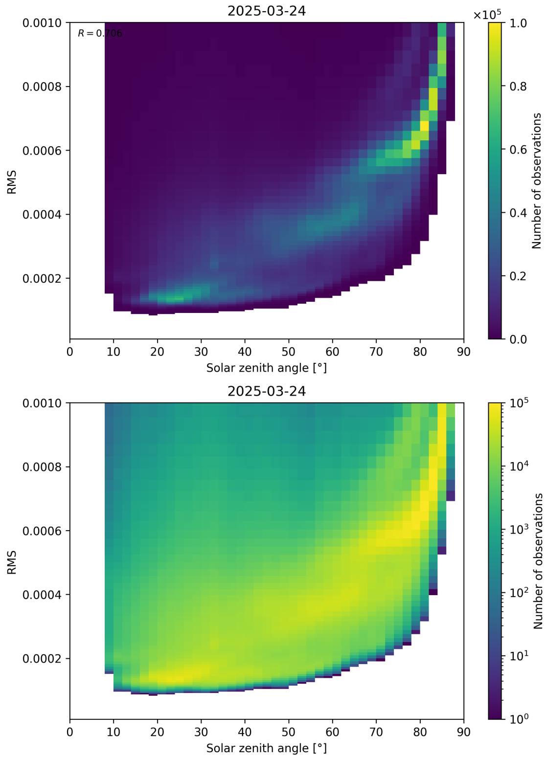
Figure 157: Scatter density plot of “Solar zenith angle” against “RMS” for 2025-03-24 to 2025-03-25.
