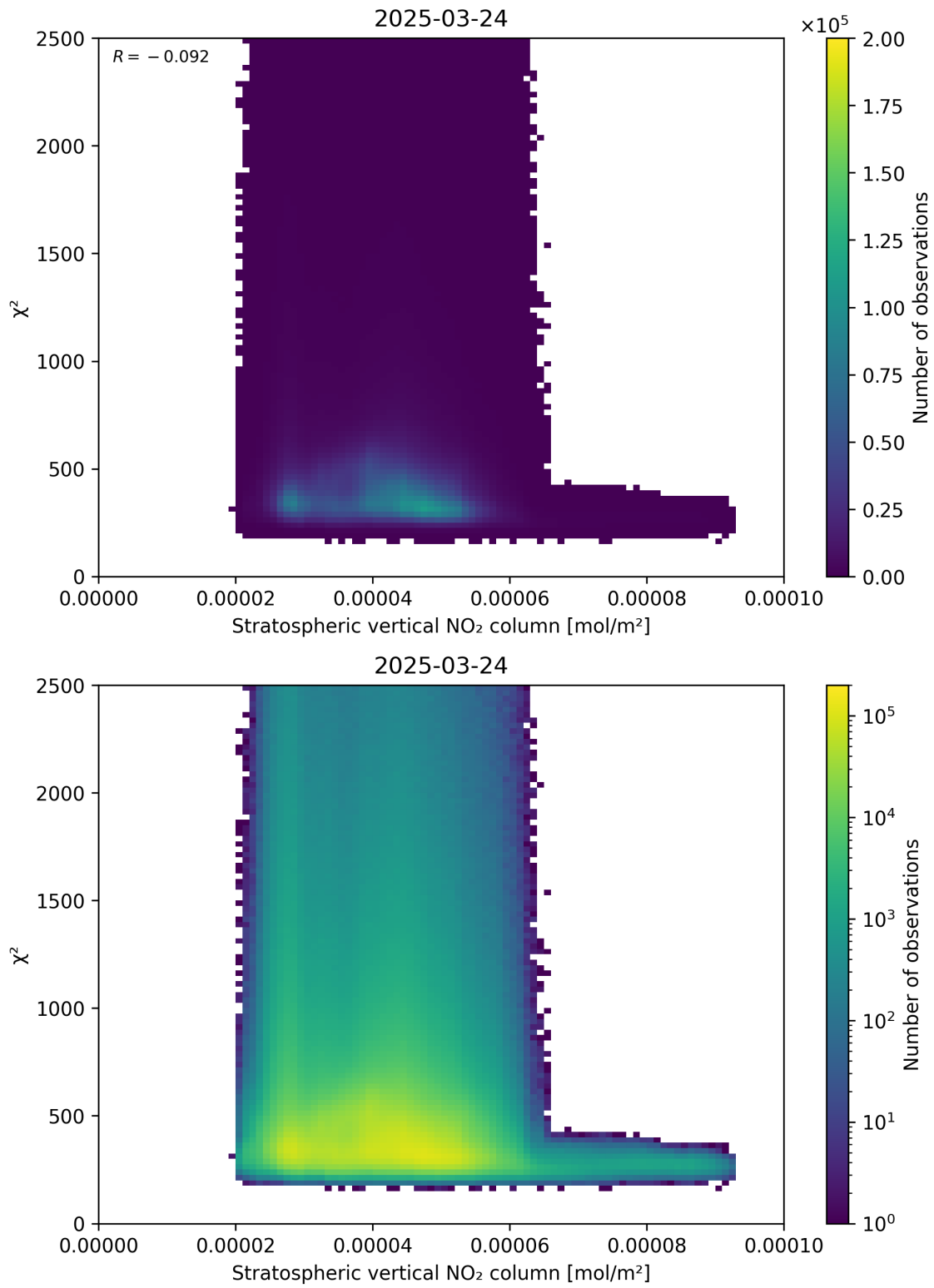
Figure 97: Scatter density plot of “Stratospheric vertical NO 2 column” against “ \chi^2 ” for 2025-03-24 to 2025-03-25.
