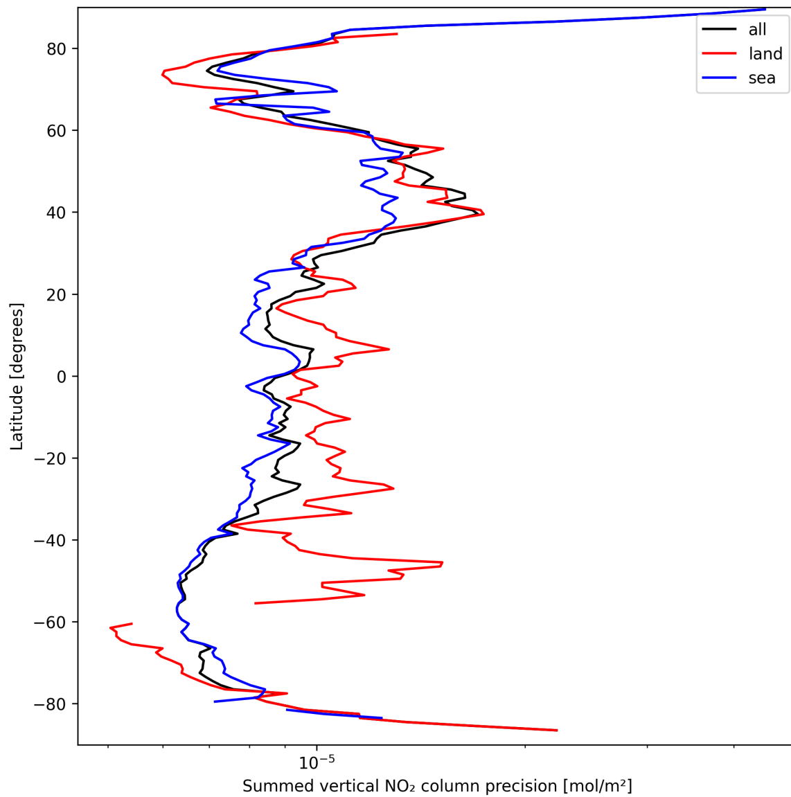
Figure 24: Zonal average of “Summed vertical NO 2 column precision” for 2025-03-24 to 2025-03-25.
