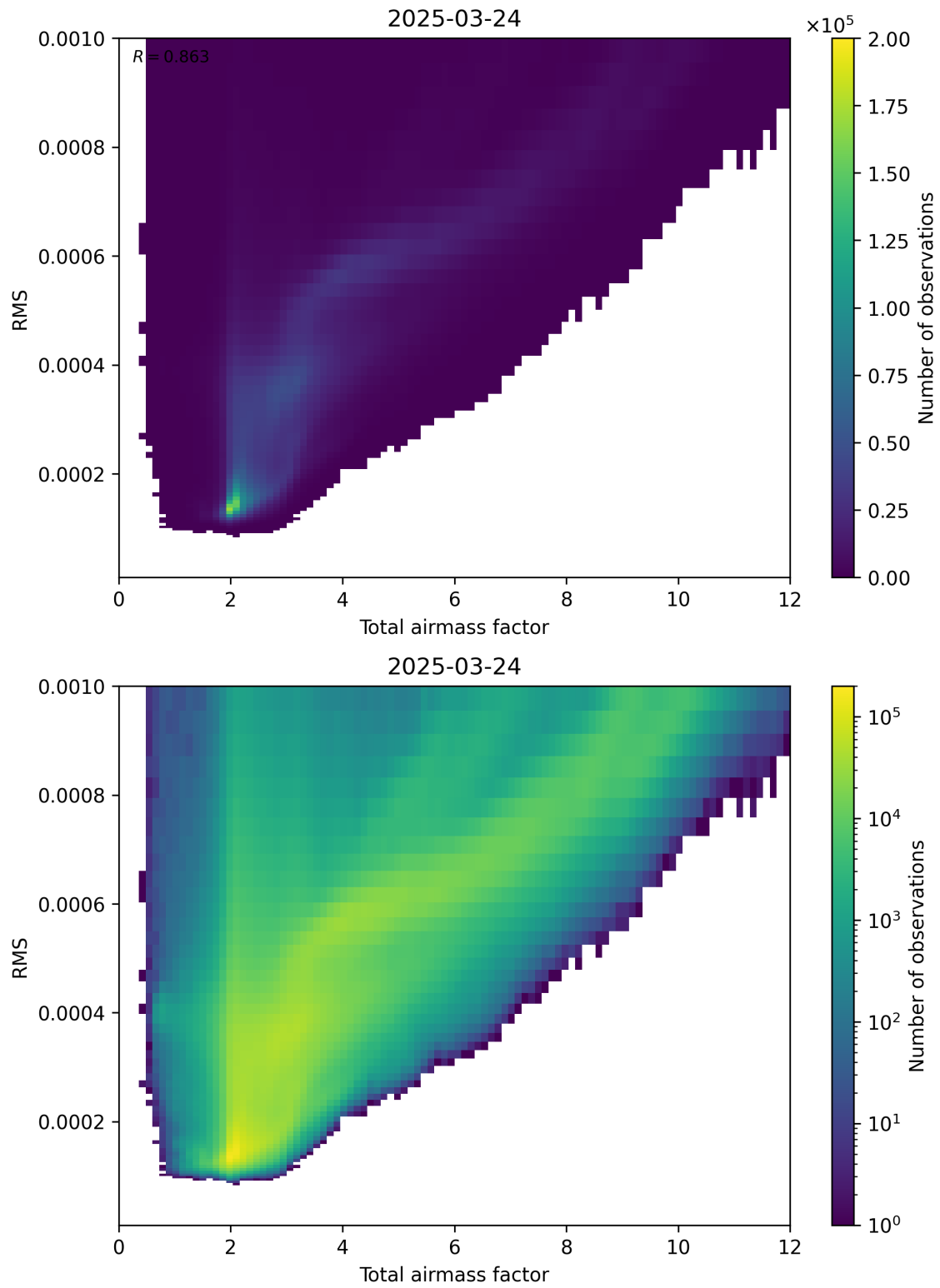
Figure 69: Scatter density plot of “Total airmass factor” against “RMS” for 2025-03-24 to 2025-03-25.
