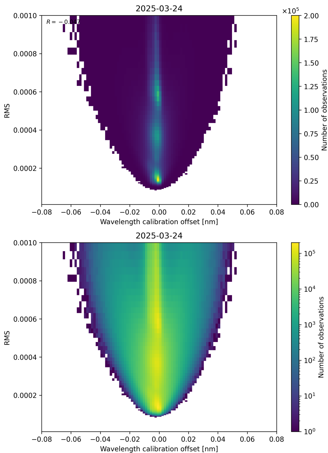
Figure 181: Scatter density plot of “Wavelength calibration offset” against “RMS” for 2025-03-24 to 2025-03-25.
