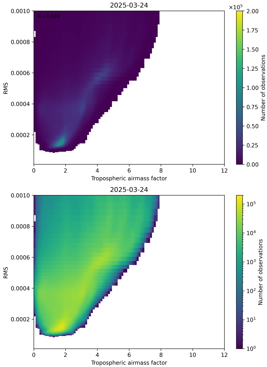
Figure 79: Scatter density plot of “Tropospheric airmass factor” against “RMS” for 2025-03-24 to 2025-03-25.
