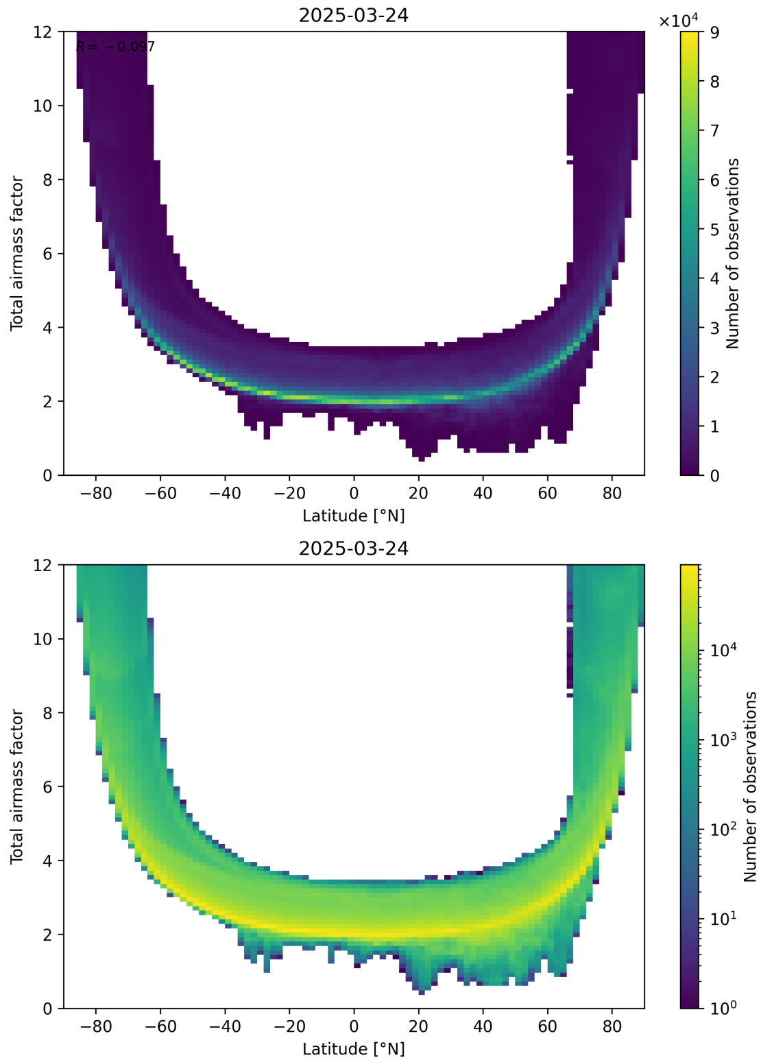
Figure 84: Scatter density plot of “Latitude” against “Total airmass factor” for 2025-03-24 to 2025-03-25.
