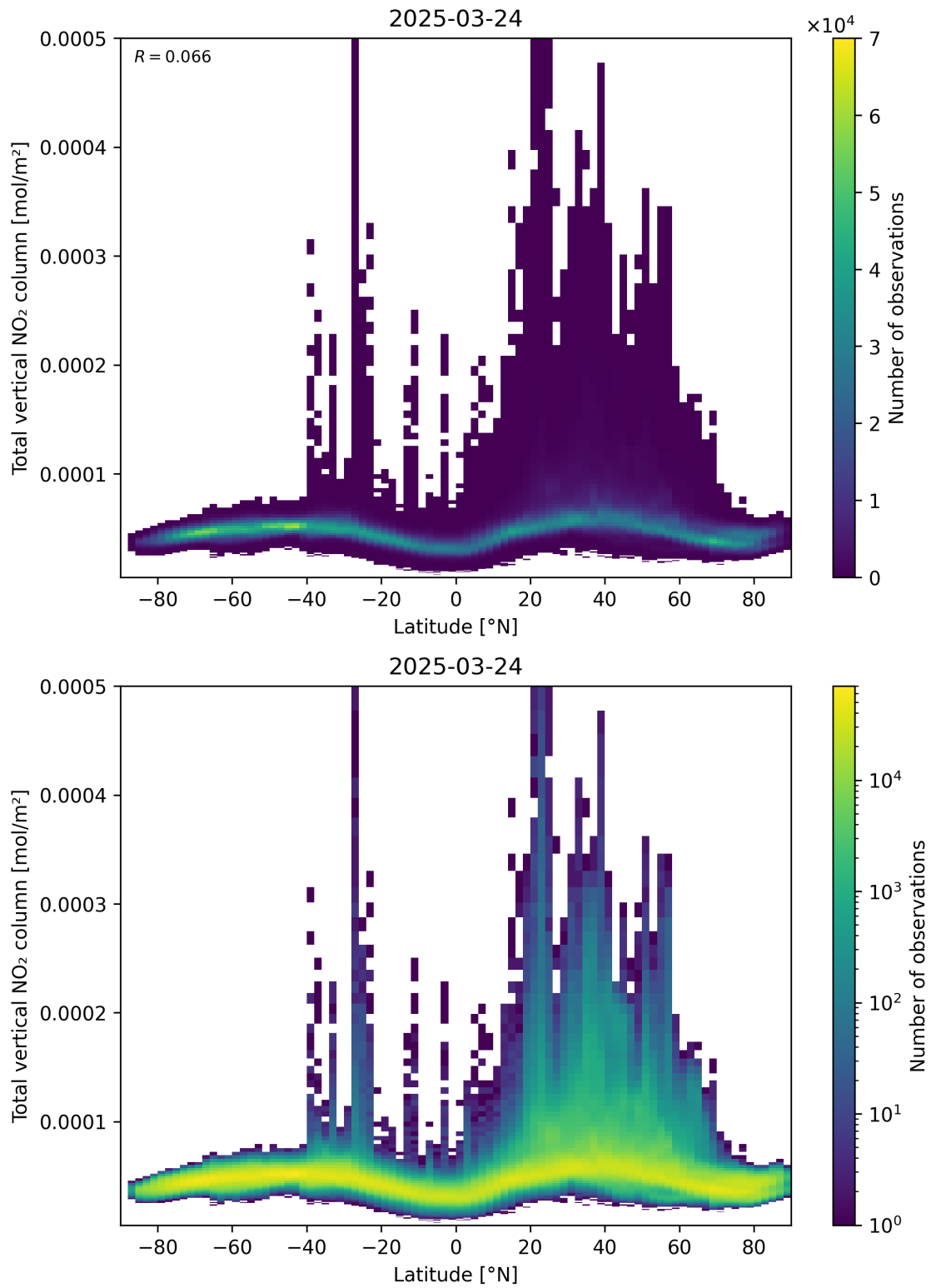
Figure 90: Scatter density plot of “Latitude” against “Total vertical NO 2 column” for 2025-03-24 to 2025-03-25.
