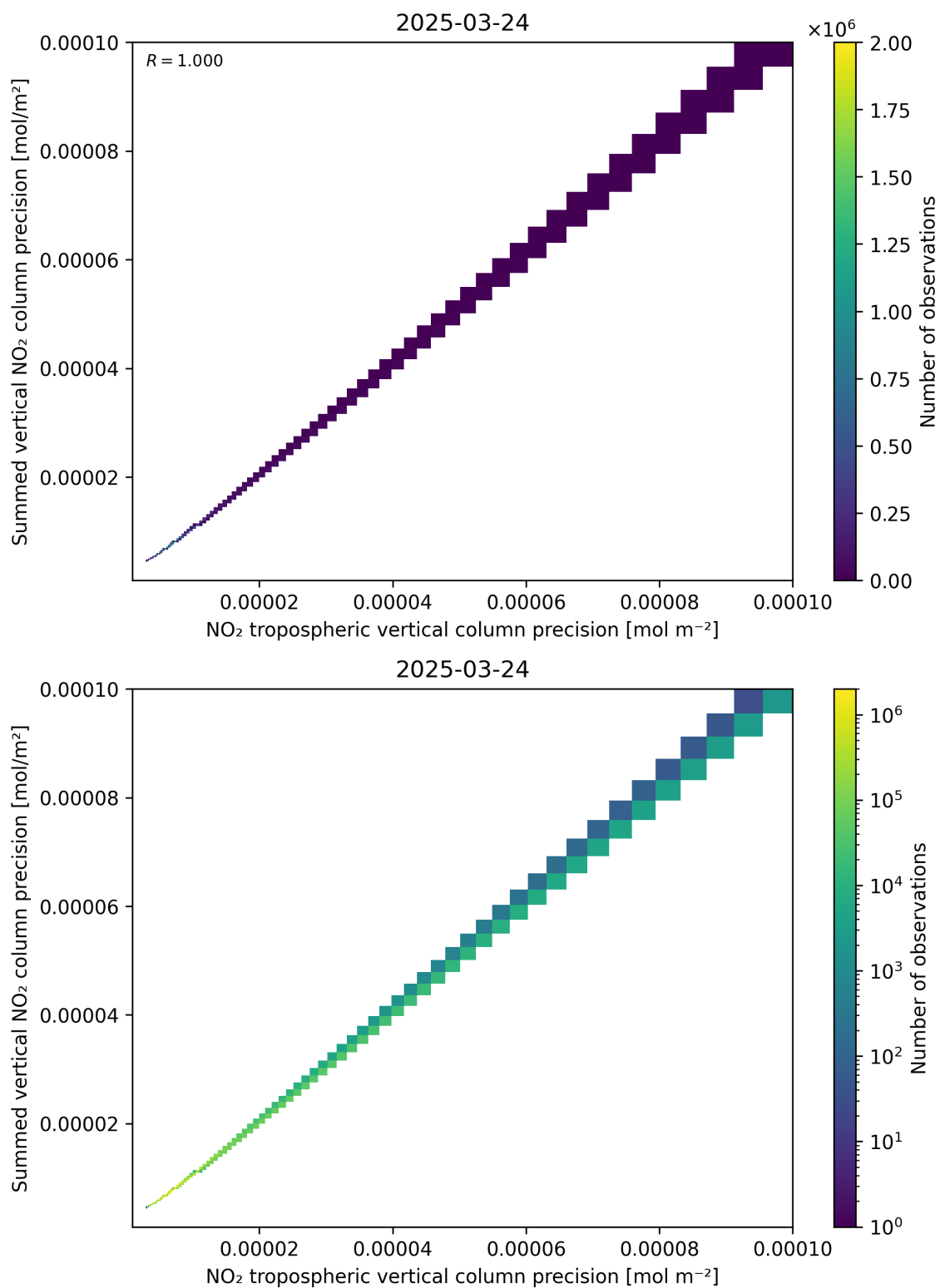
Figure 137: Scatter density plot of “NO 2 tropospheric vertical column precision” against “Summed vertical NO 2 column precision” for 2025-03-24 to 2025-03-25.
