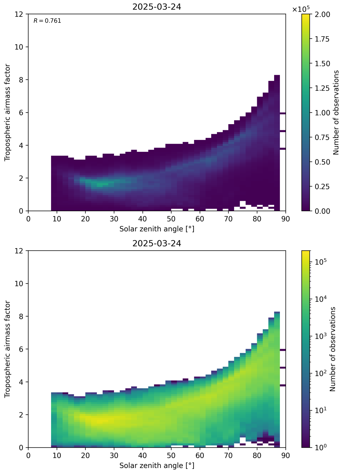
Figure 147: Scatter density plot of “Solar zenith angle” against “Tropospheric airmass factor” for 2025-03-24 to 2025-03-25.
