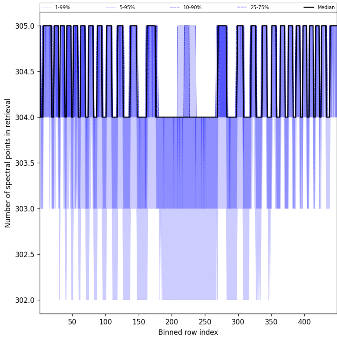
Figure 50: Along track statistics of “Number of spectral points in retrieval” for 2025-03-24 to 2025-03-25
