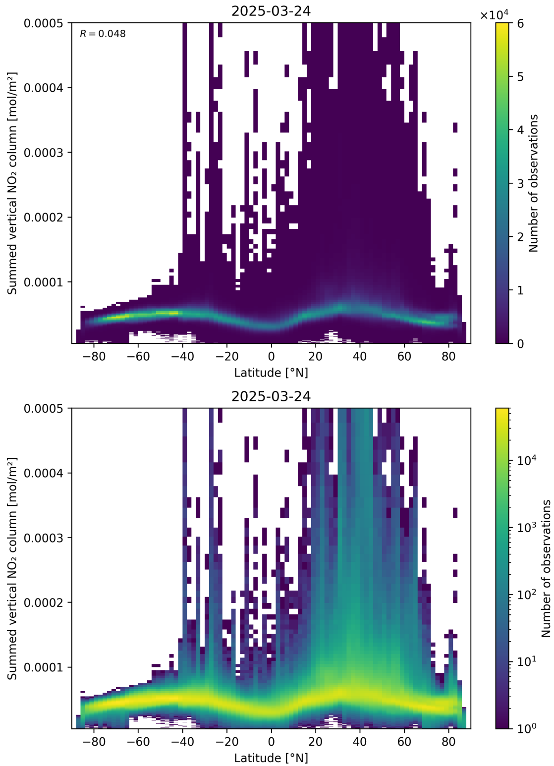
Figure 88: Scatter density plot of “Latitude” against “Summed vertical NO 2 column” for 2025-03-24 to 2025-03-25.
