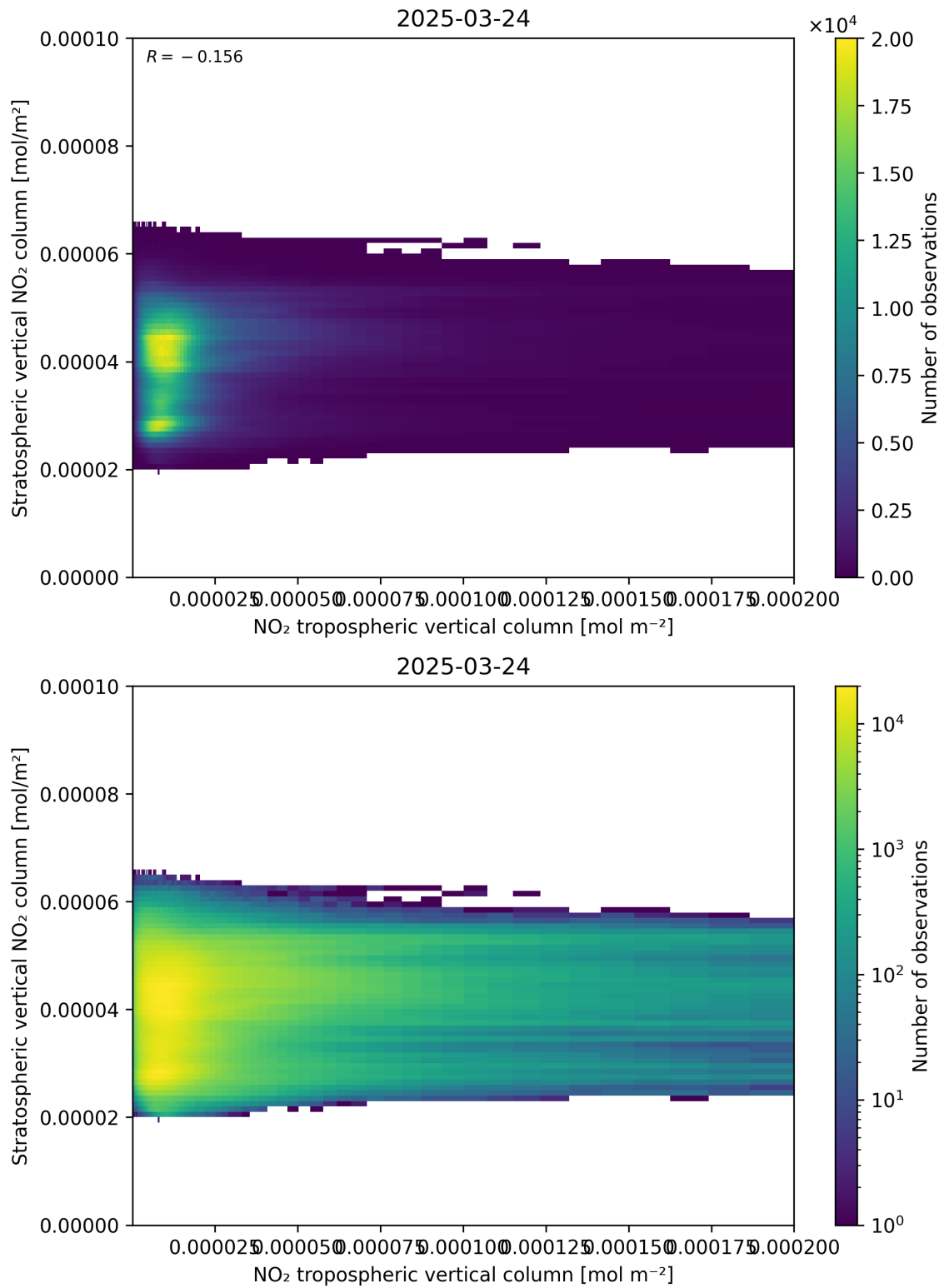
Figure 125: Scatter density plot of “NO 2 tropospheric vertical column” against “Stratospheric vertical NO 2 column” for 2025-03-24 to 2025-03-25.
