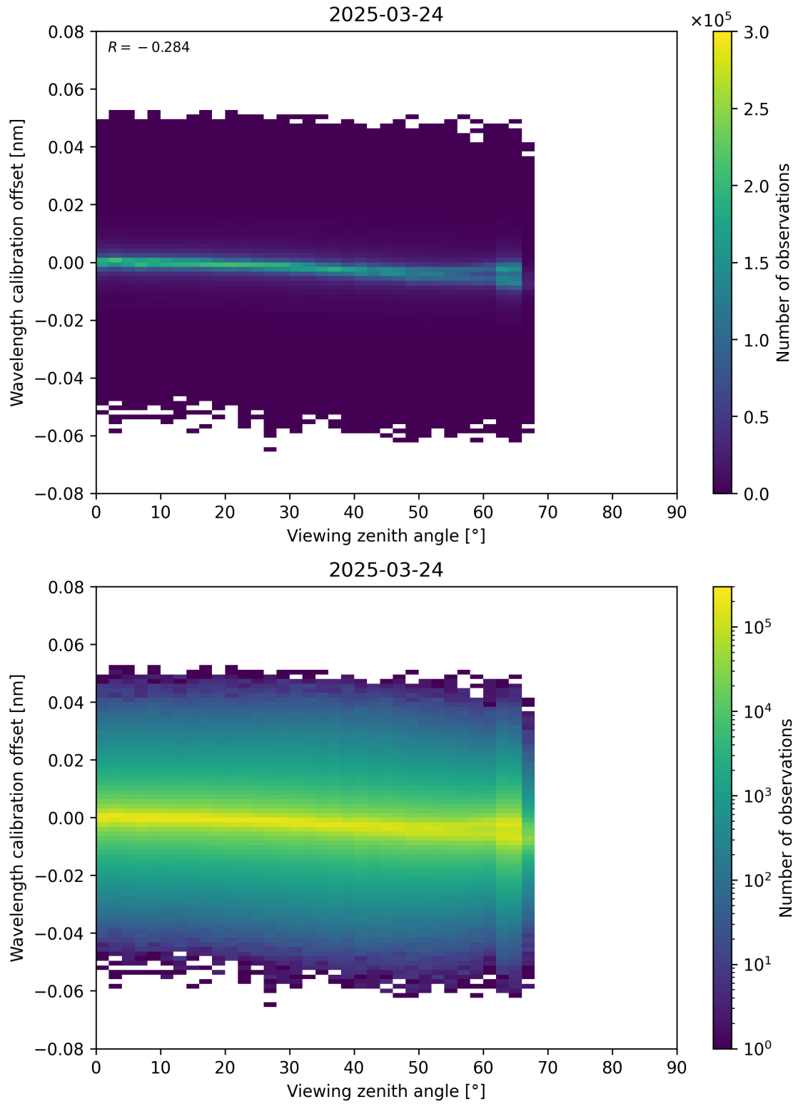
Figure 173: Scatter density plot of “Viewing zenith angle” against “Wavelength calibration offset” for 2025-03-24 to 2025-03-25.
