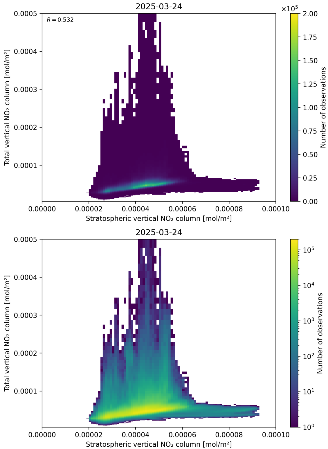
Figure 100: Scatter density plot of “Stratospheric vertical NO 2 column” against “Total vertical NO 2 column” for 2025-03-24 to 2025-03-25.
