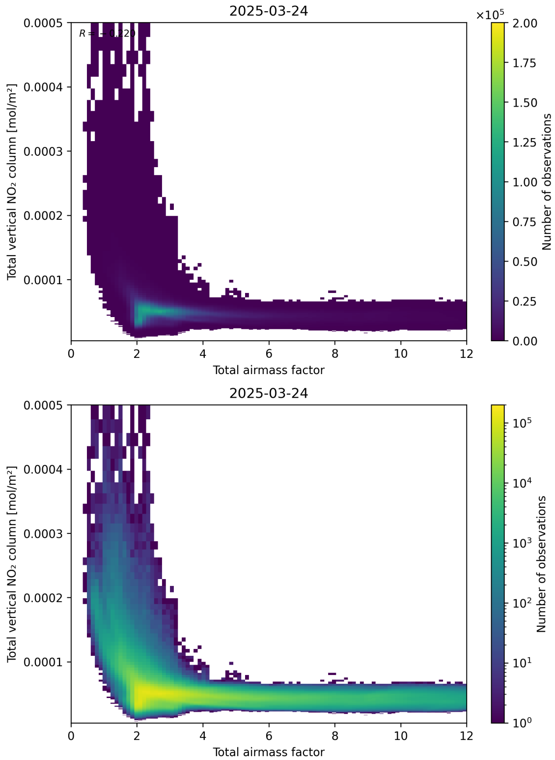
Figure 67: Scatter density plot of “Total airmass factor” against “Total vertical NO 2 column” for 2025-03-24 to 2025-03-25.
