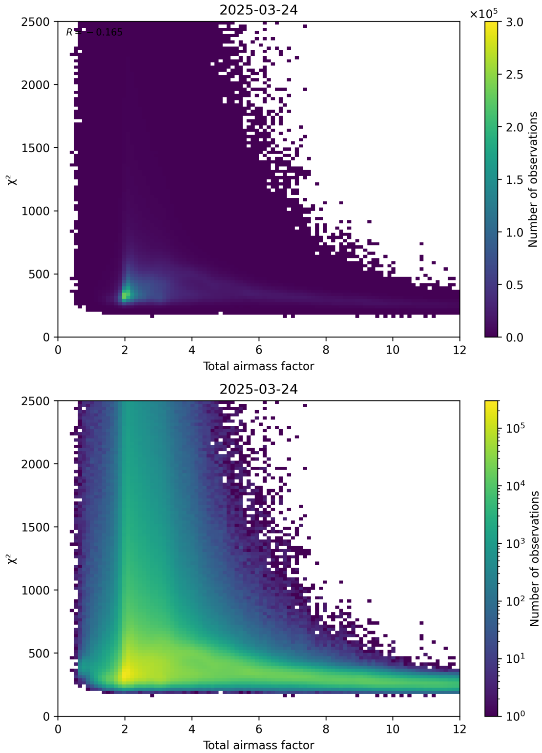
Figure 63: Scatter density plot of “Total airmass factor” against “ \chi^2 ” for 2025-03-24 to 2025-03-25.
