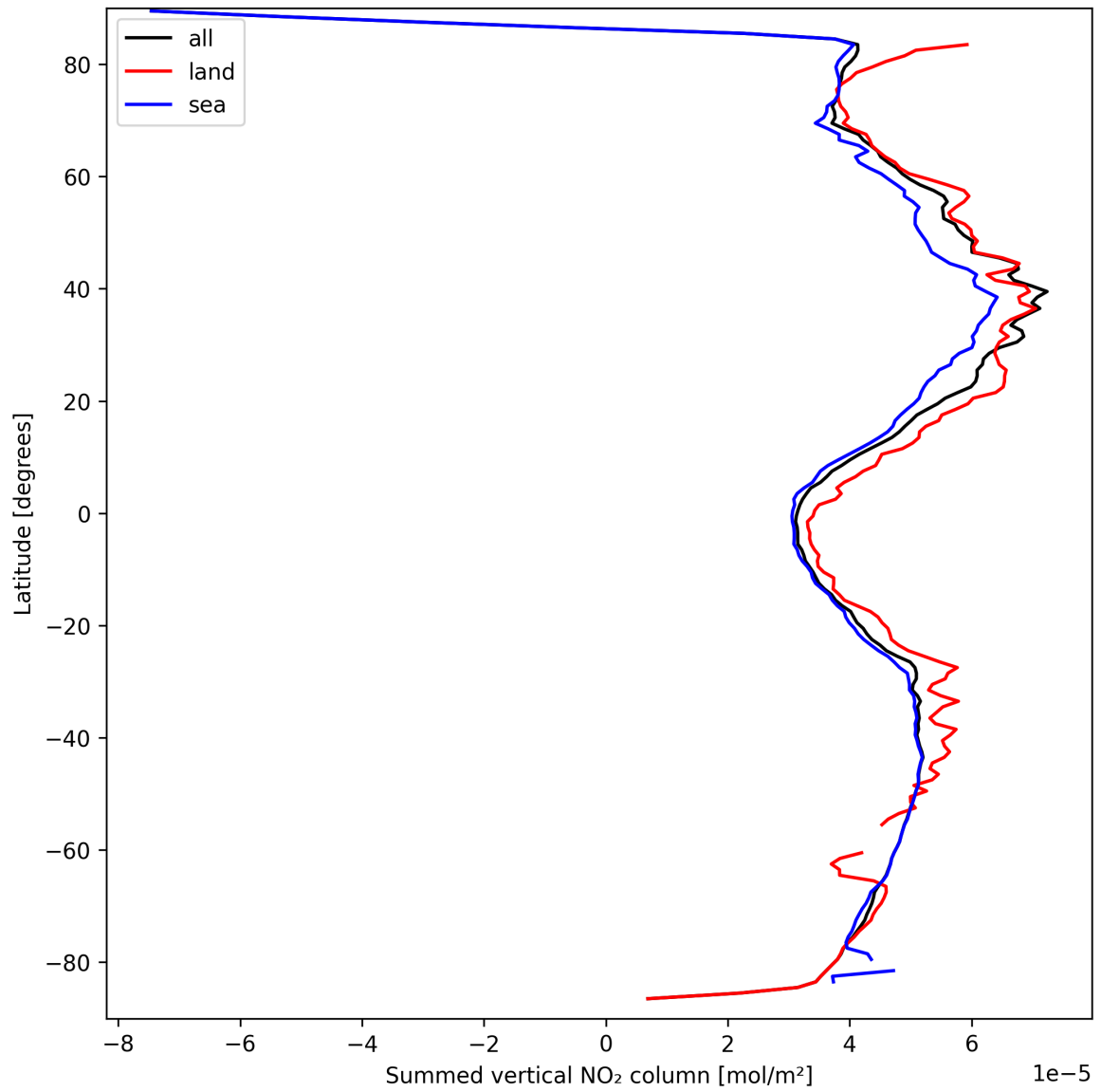
Figure 23: Zonal average of “Summed vertical NO 2 column” for 2025-03-24 to 2025-03-25.
