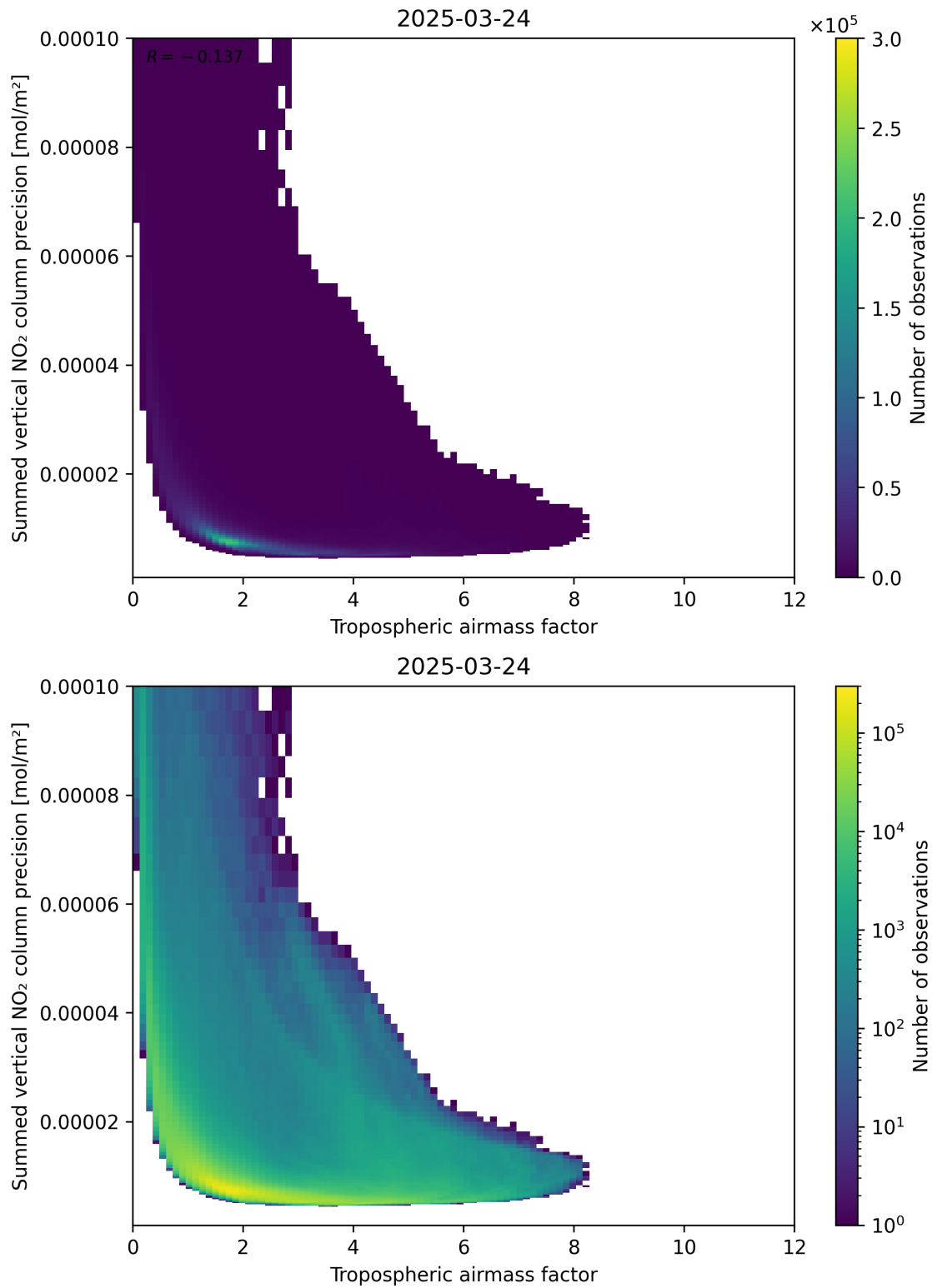
Figure 76: Scatter density plot of “Tropospheric air mass factor” against “Summed vertical NO 2 column precision” for 2025-03-24 to 2025-03-25.
