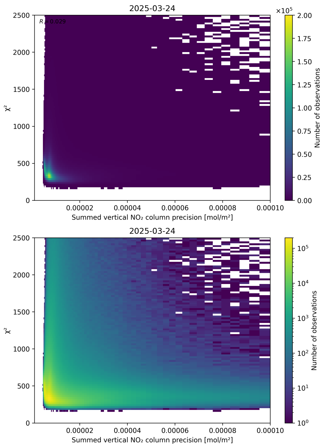
Figure 107: Scatter density plot of “Summed vertical NO 2 column precision” against “ \chi^2 ” for 2025-03-24 to 2025-03-25.
