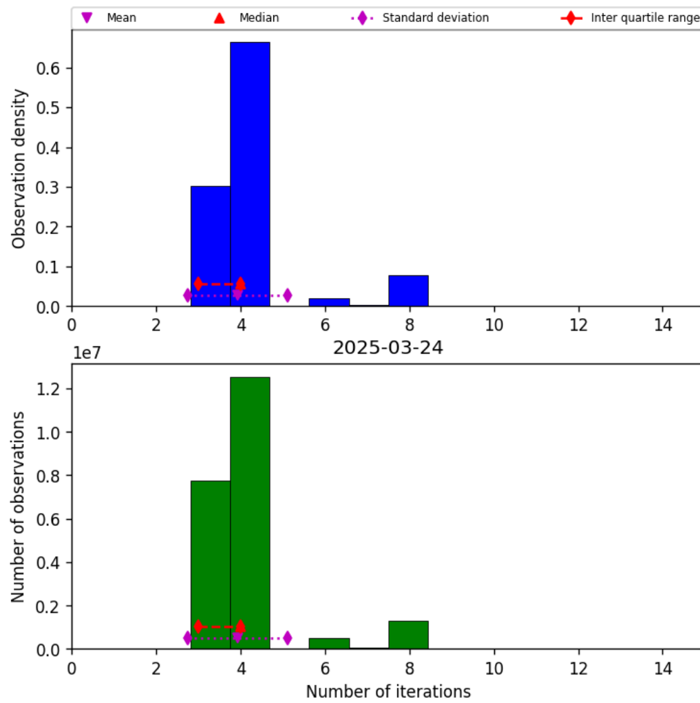
Figure 34: Histogram of “Number of iterations” for 2025-03-24 to 2025-03-25
