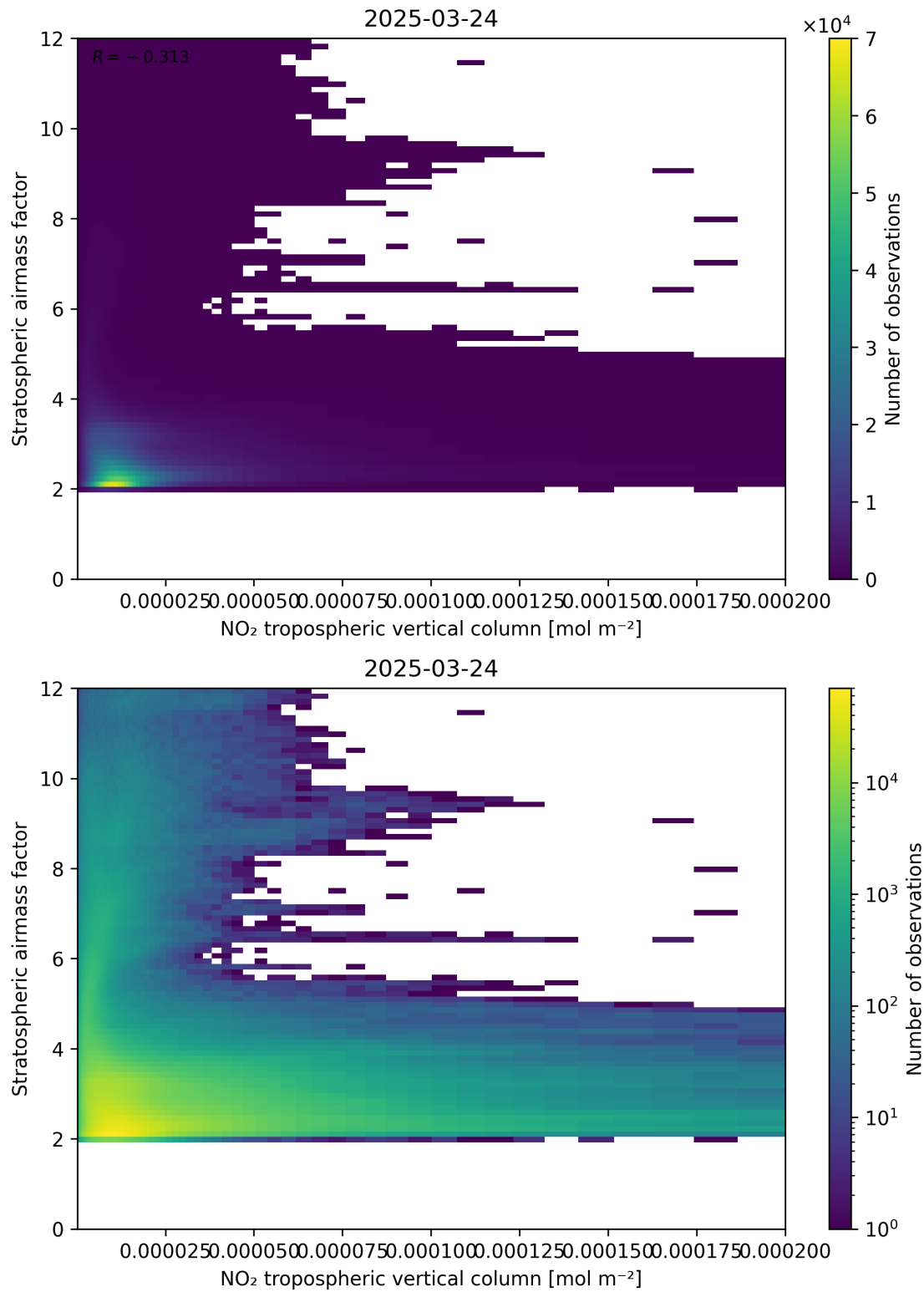
Figure 121: Scatter density plot of “NO 2 tropospheric vertical column” against “Stratospheric air mass factor” for 2025-03-24 to 2025-03-25.
