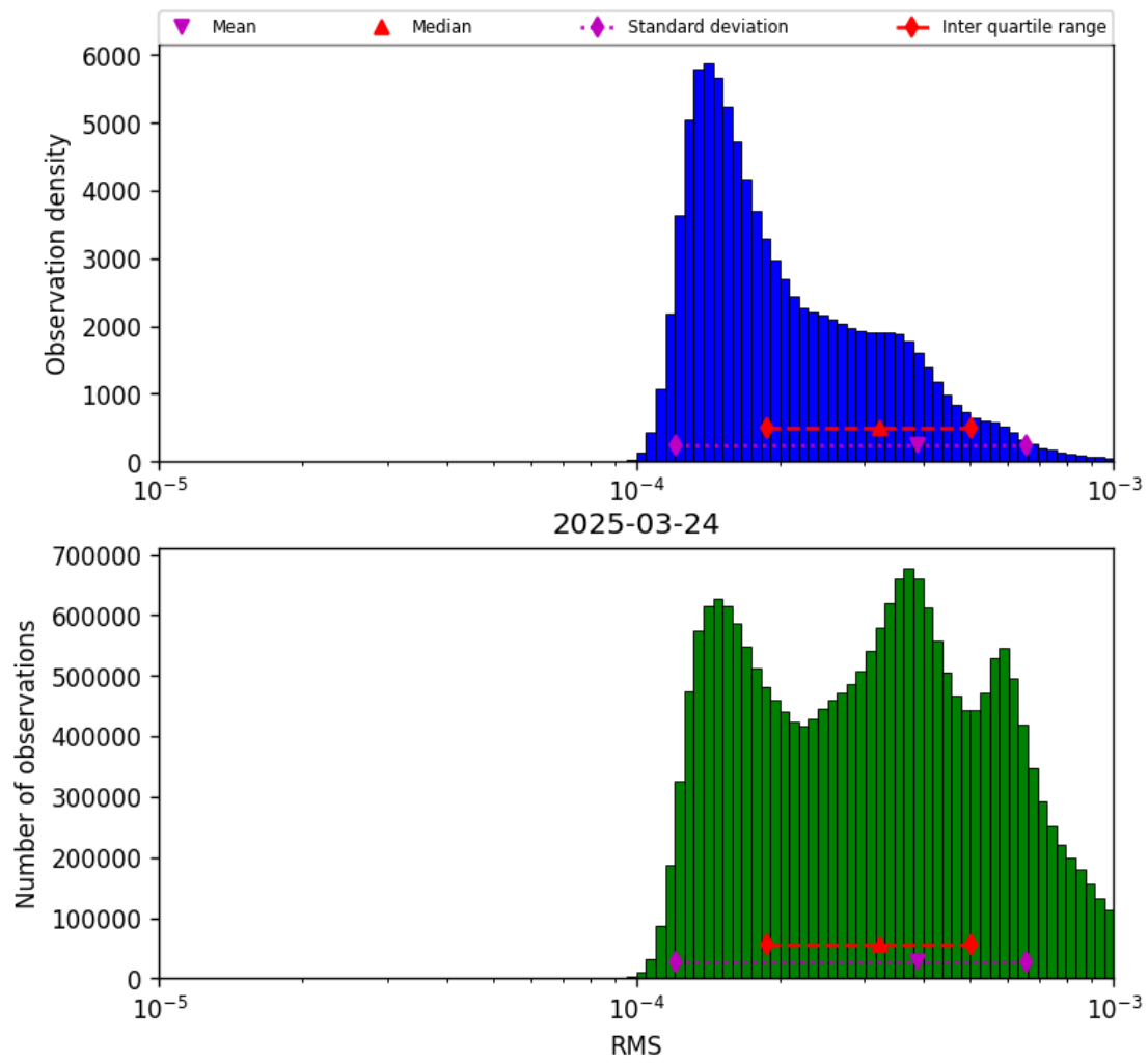
Figure 43: Histogram of “RMS” for 2025-03-24 to 2025-03-25
