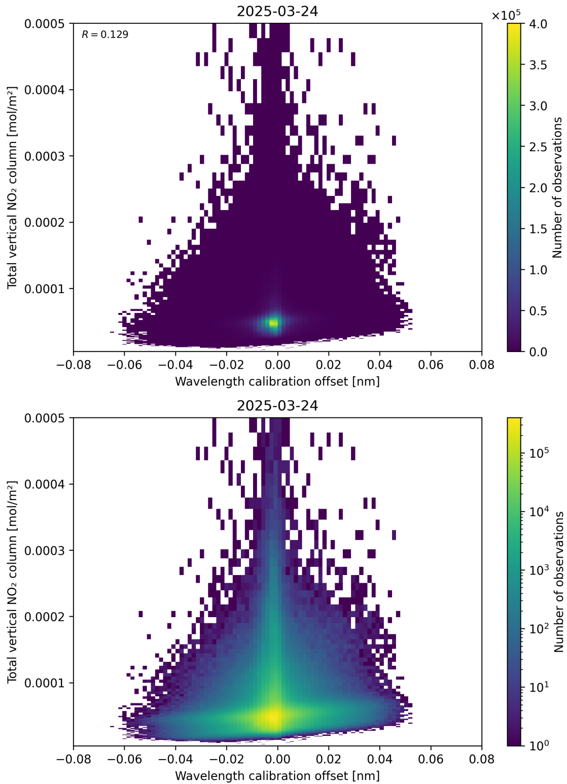
Figure 179: Scatter density plot of “Wavelength calibration offset” against “Total vertical NO 2 column” for 2025-03-24 to 2025-03-25.
