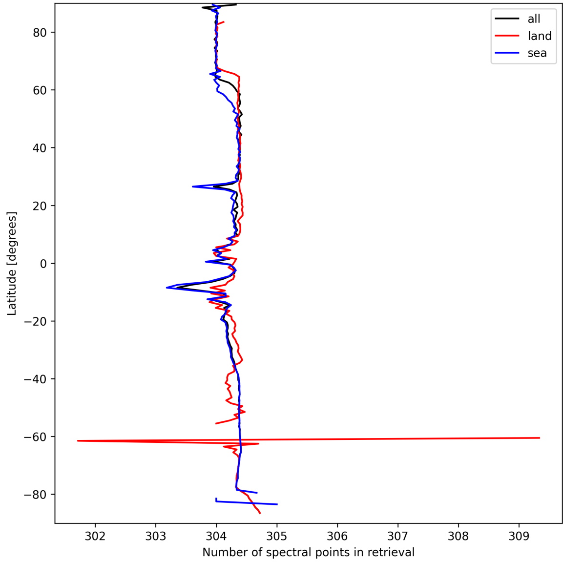
Figure 16: Zonal average of “Number of spectral points in retrieval” for 2025-03-24 to 2025-03-25.
