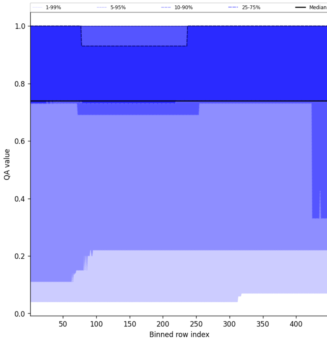
Figure 45: Along track statistics of “QA value” for 2025-03-24 to 2025-03-25
