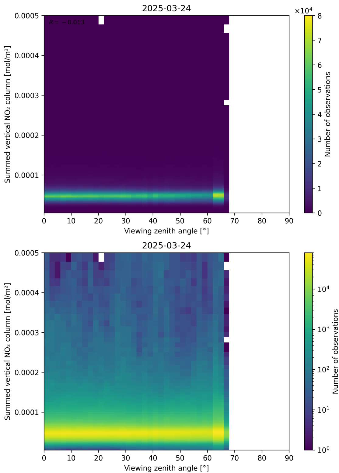
Figure 165: Scatter density plot of “Viewing zenith angle” against “Summed vertical NO 2 column” for 2025-03-24 to 2025-03-25.
