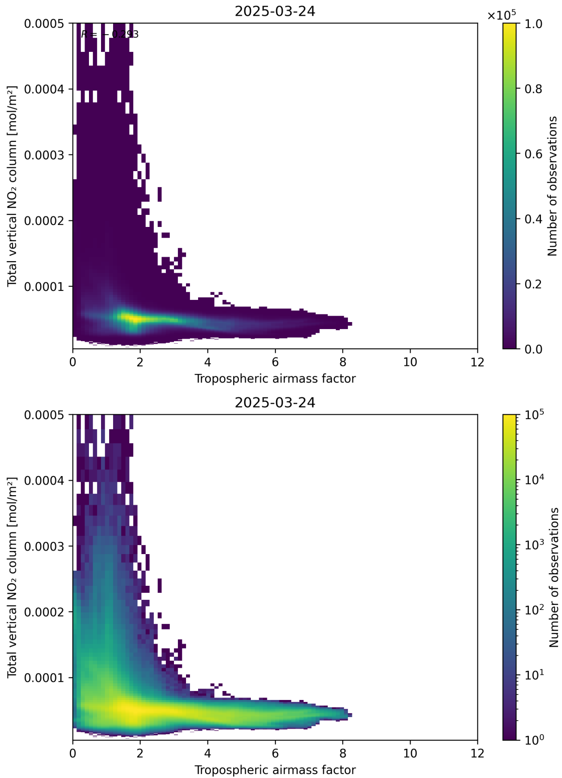
Figure 77: Scatter density plot of “Tropospheric airmass factor” against “Total vertical NO 2 column” for 2025-03-24 to 2025-03-25.
