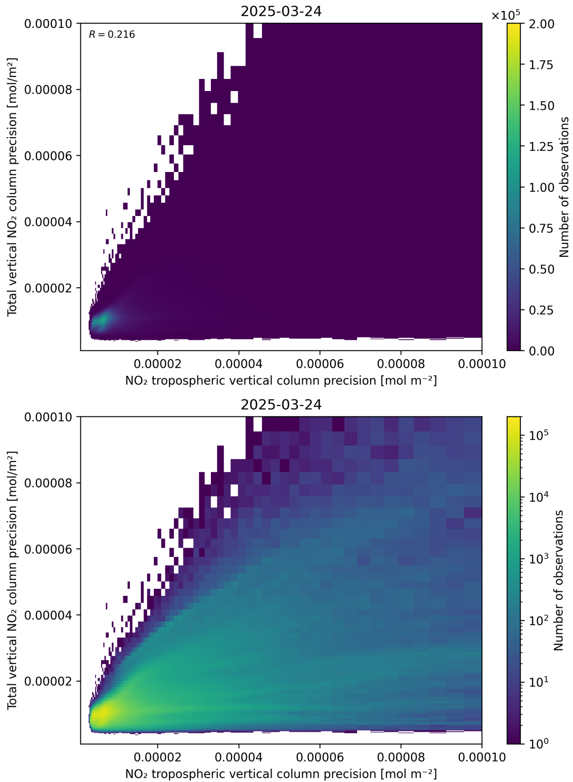
Figure 139: Scatter density plot of “NO 2 tropospheric vertical column precision” against “Total vertical NO 2 column precision” for 2025-03-24 to 2025-03-25.
