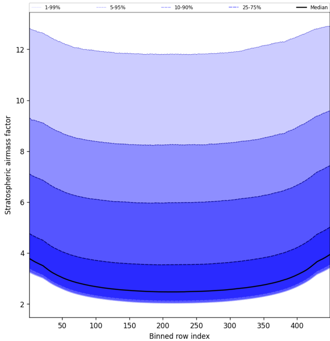
Figure 61: Along track statistics of “Stratospheric airmass factor” for 2025-03-24 to 2025-03-25
