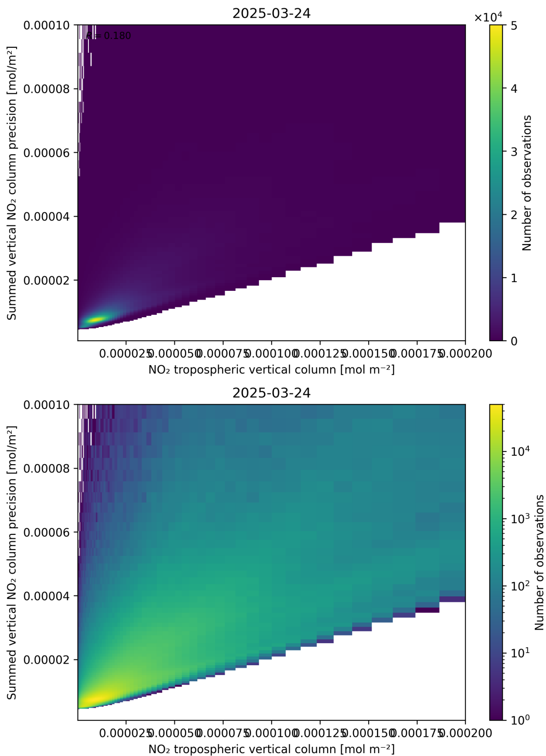
Figure 127: Scatter density plot of “NO 2 tropospheric vertical column” against “Summed vertical NO 2 column precision” for 2025-03-24 to 2025-03-25.
