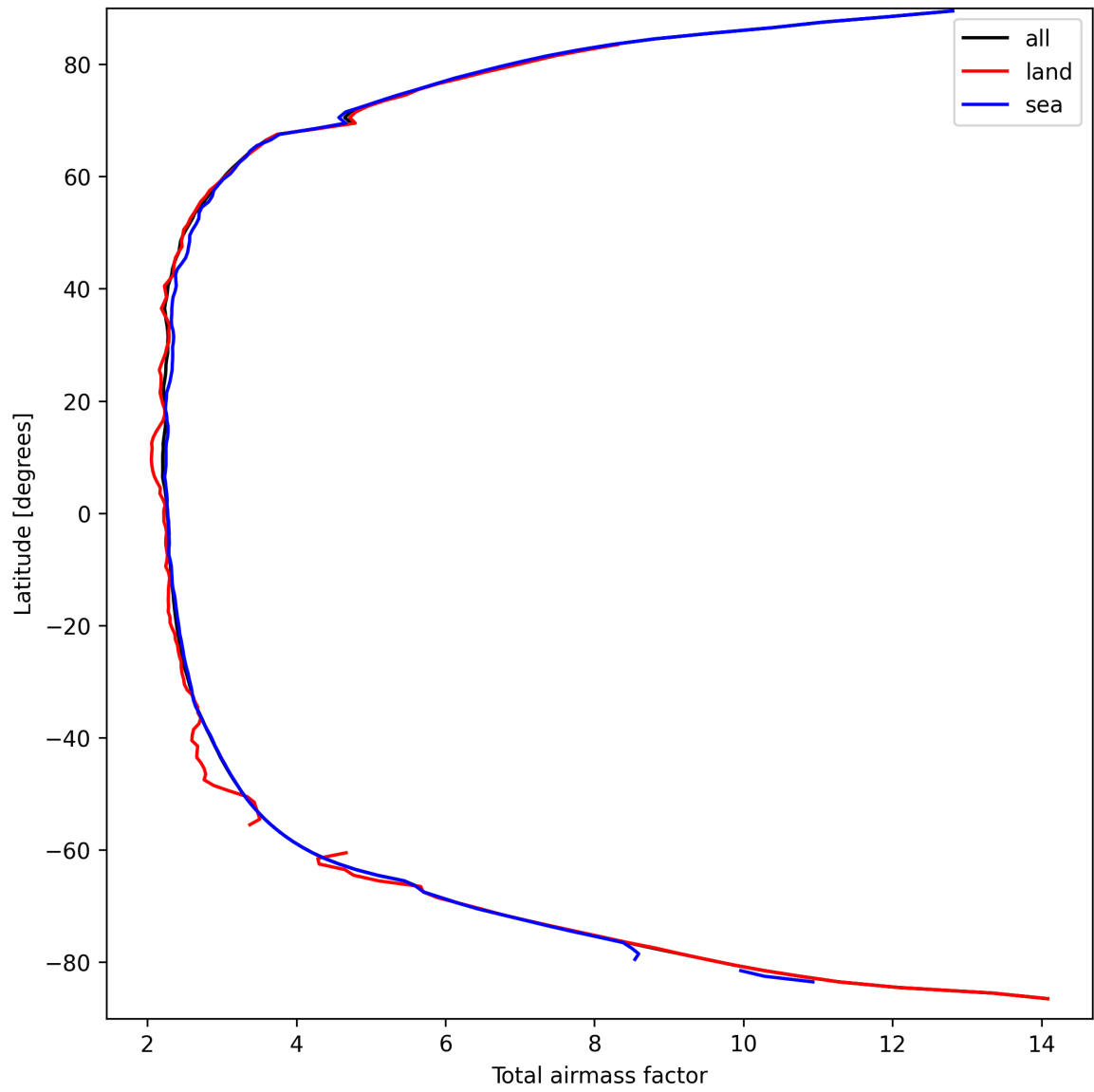
Figure 15: Zonal average of “Total airmass factor” for 2025-03-24 to 2025-03-25.
