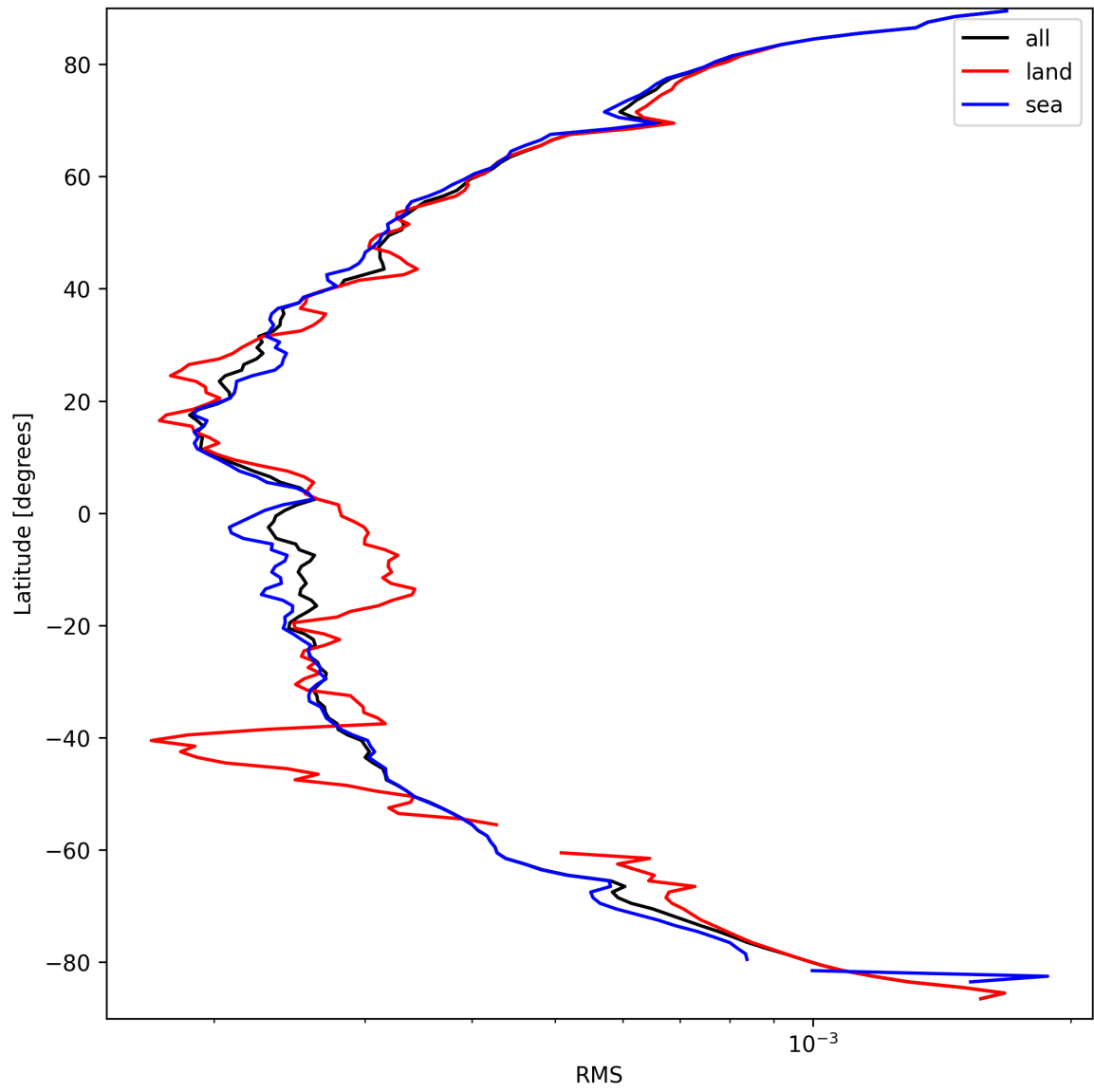
Figure 26: Zonal average of “RMS” for 2025-03-24 to 2025-03-25.
