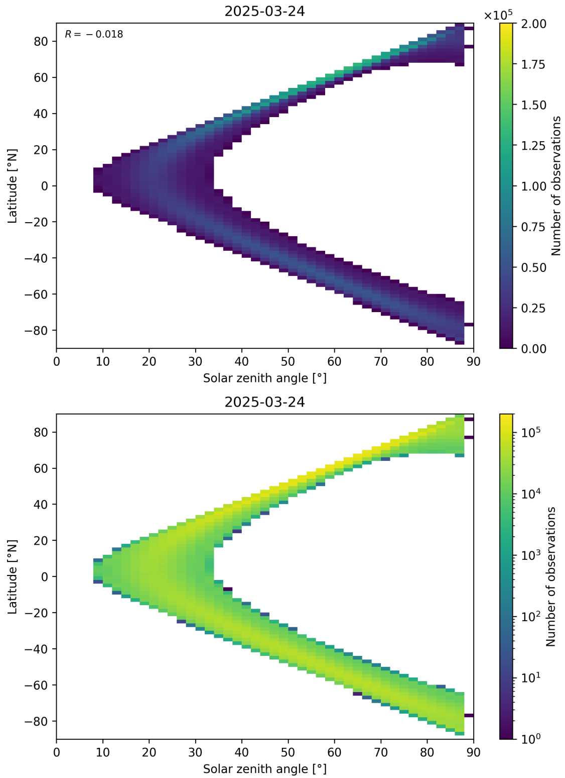
Figure 149: Scatter density plot of “Solar zenith angle” against “Latitude” for 2025-03-24 to 2025-03-25.
