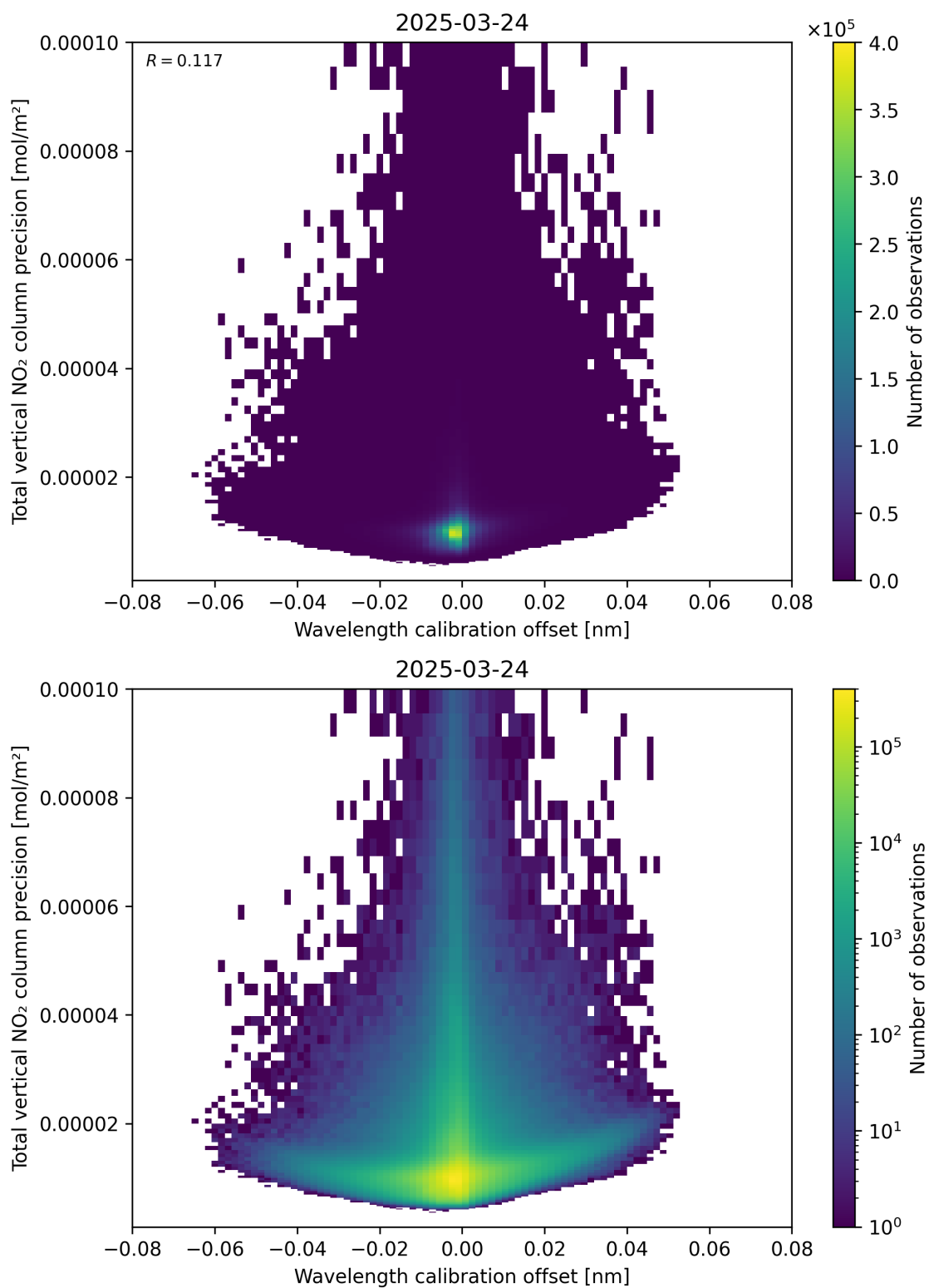
Figure 180: Scatter density plot of “Wavelength calibration offset” against “Total vertical NO 2 column precision” for 2025-03-24 to 2025-03-25.
