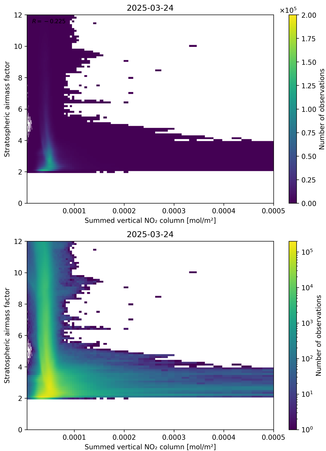
Figure 103: Scatter density plot of “Summed vertical NO 2 column” against “Stratospheric air mass factor” for 2025-03-24 to 2025-03-25.
