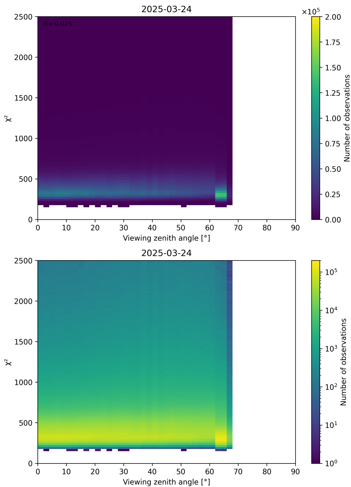
Figure 162: Scatter density plot of “Viewing zenith angle” against “ \chi^2 ” for 2025-03-24 to 2025-03-25.
