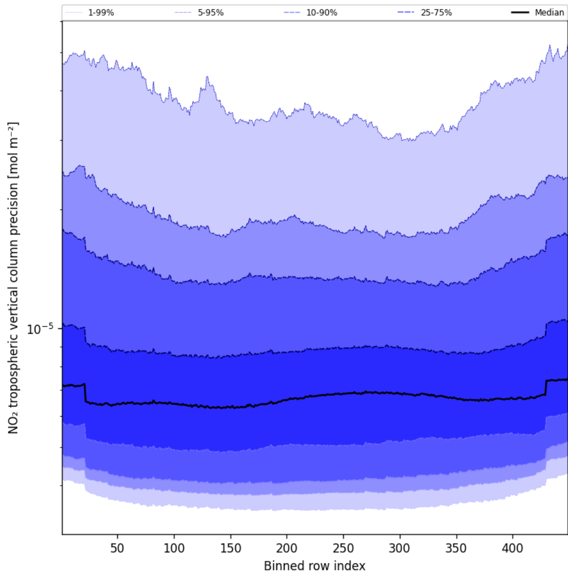
Figure 47: Along track statistics of “NO 2 tropospheric vertical column precision” for 2025-03-24 to 2025-03-25
