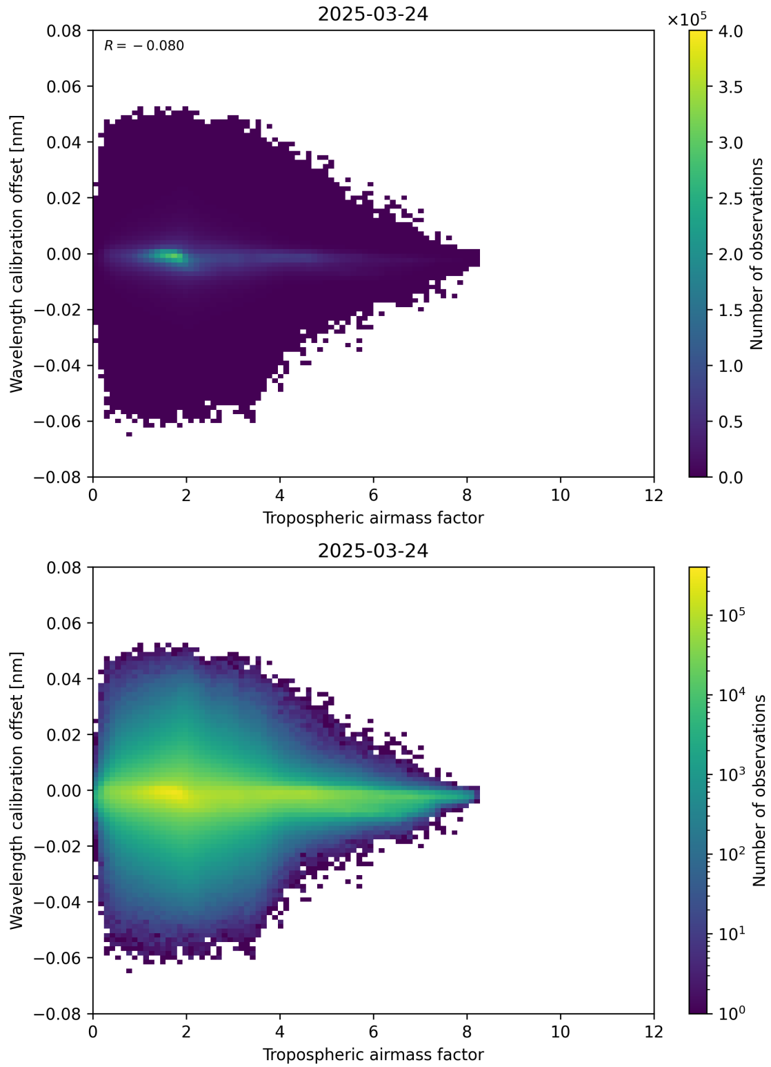
Figure 80: Scatter density plot of “Tropospheric airmass factor” against “Wavelength calibration offset” for 2025-03-24 to 2025-03-25.
