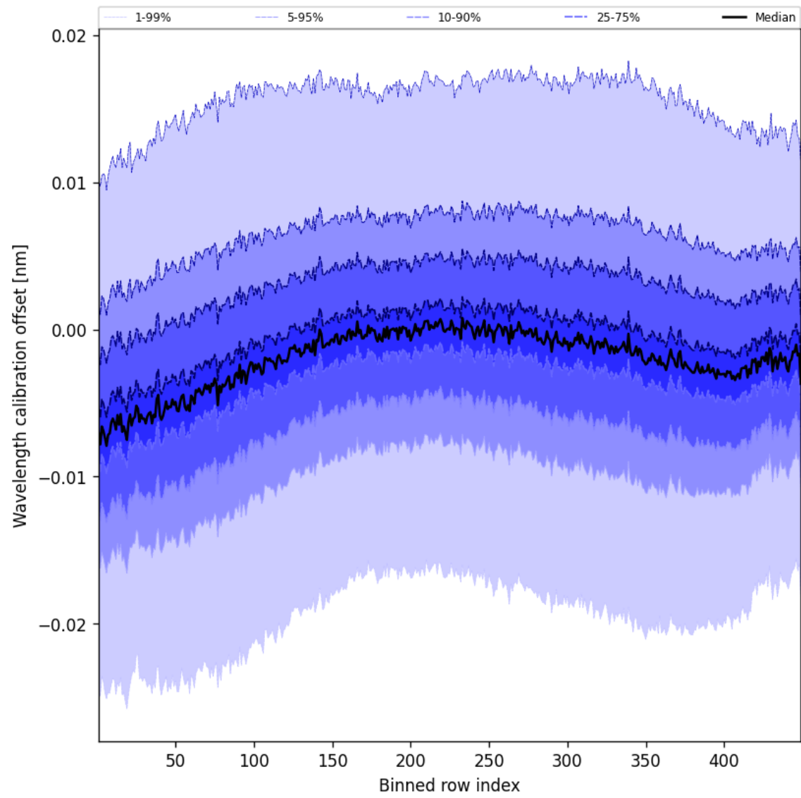
Figure 52: Along track statistics of “Wavelength calibration offset” for 2025-03-24 to 2025-03-25
