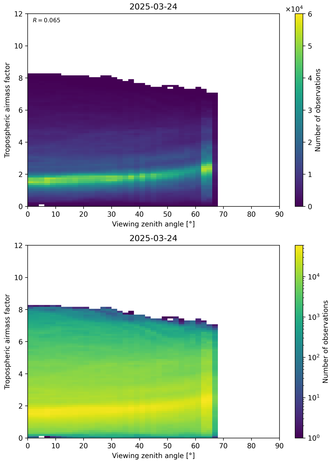
Figure 161: Scatter density plot of “Viewing zenith angle” against “Tropospheric airmass factor” for 2025-03-24 to 2025-03-25.
