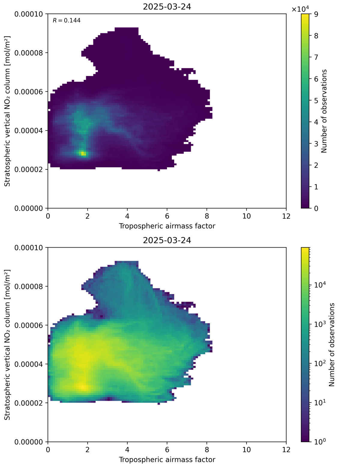
Figure 74: Scatter density plot of “Tropospheric airmass factor” against “Stratospheric vertical NO 2 column” for 2025-03-24 to 2025-03-25.
