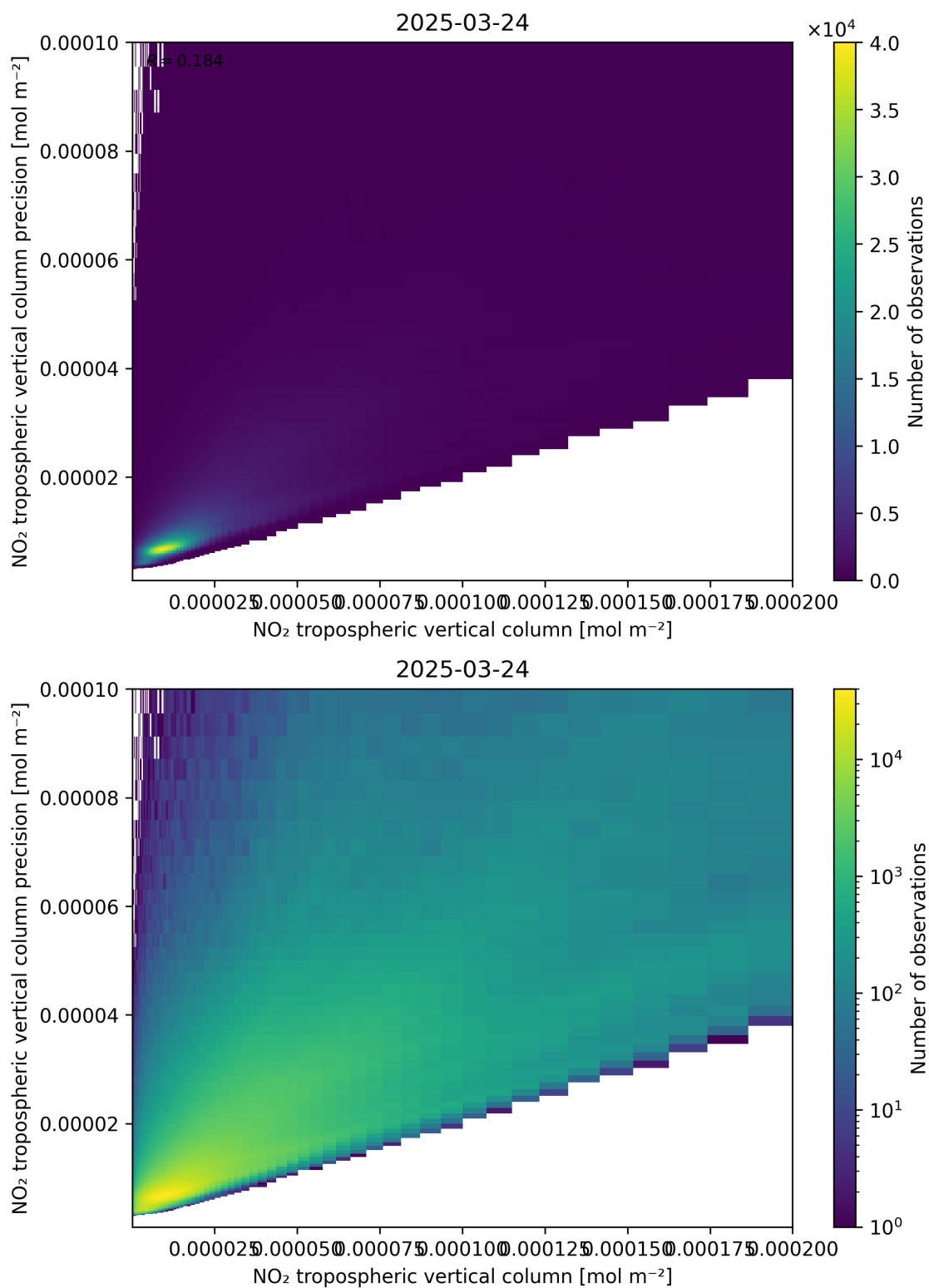
Figure 130: Scatter density plot of “NO 2 tropospheric vertical column” against “NO 2 tropospheric vertical column precision” for 2025-03-24 to 2025-03-25.
