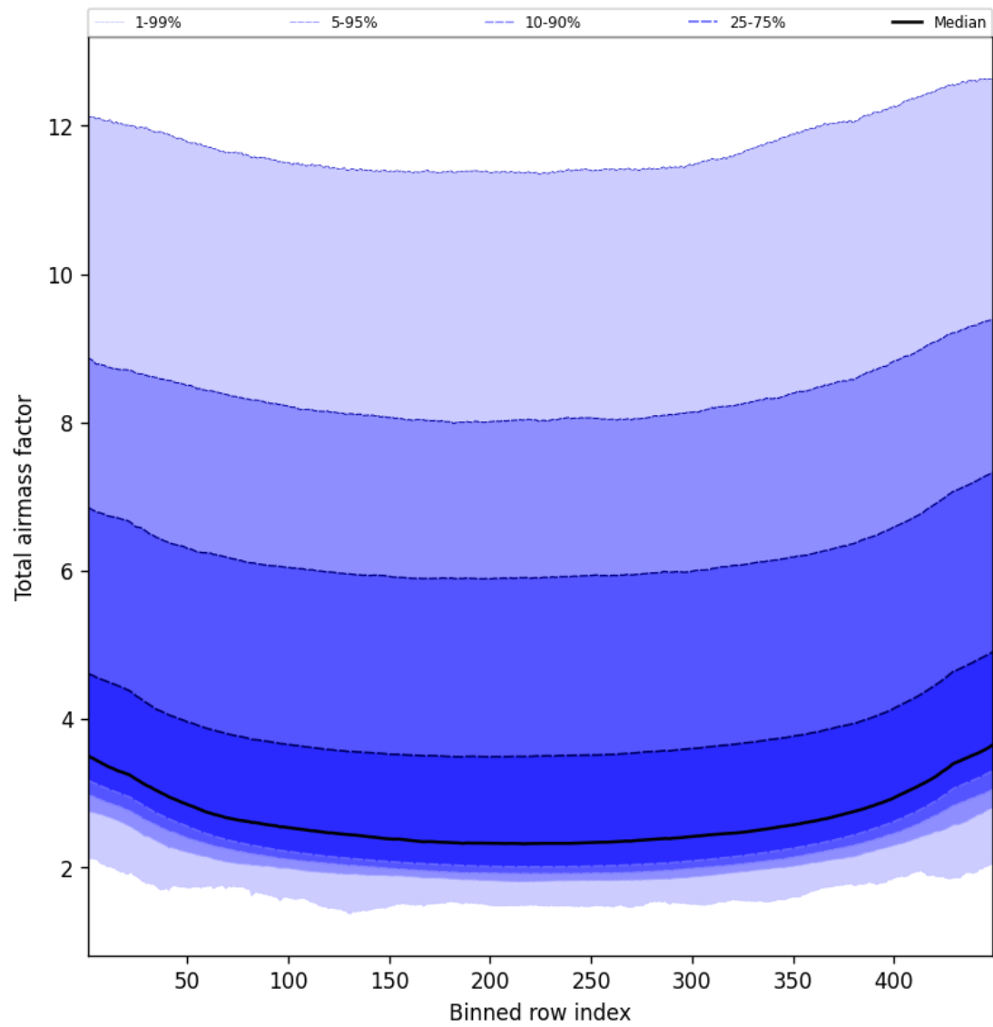
Figure 49: Along track statistics of “Total airmass factor” for 2025-03-24 to 2025-03-25
