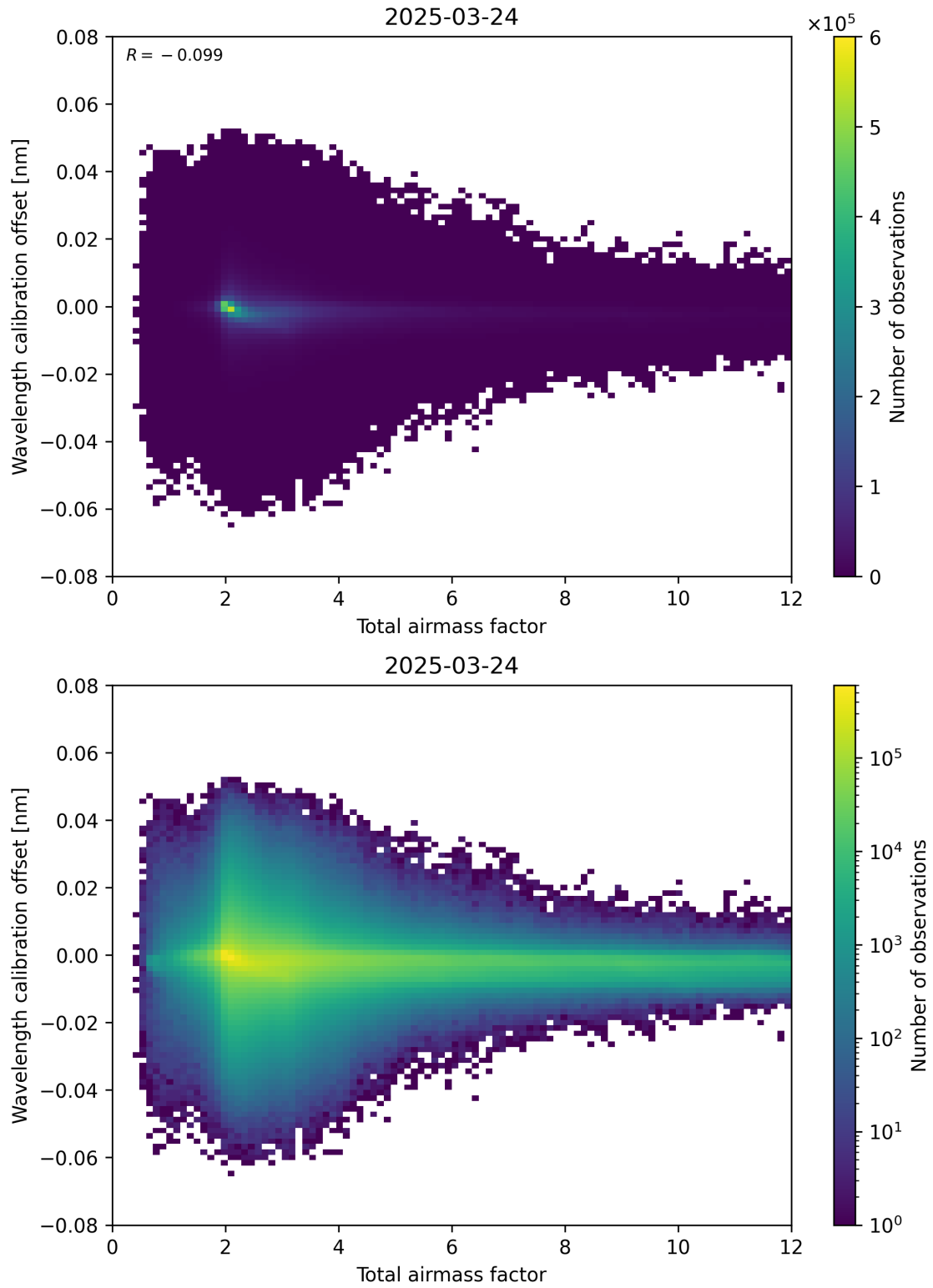
Figure 70: Scatter density plot of “Total airmass factor” against “Wavelength calibration offset” for 2025-03-24 to 2025-03-25.
