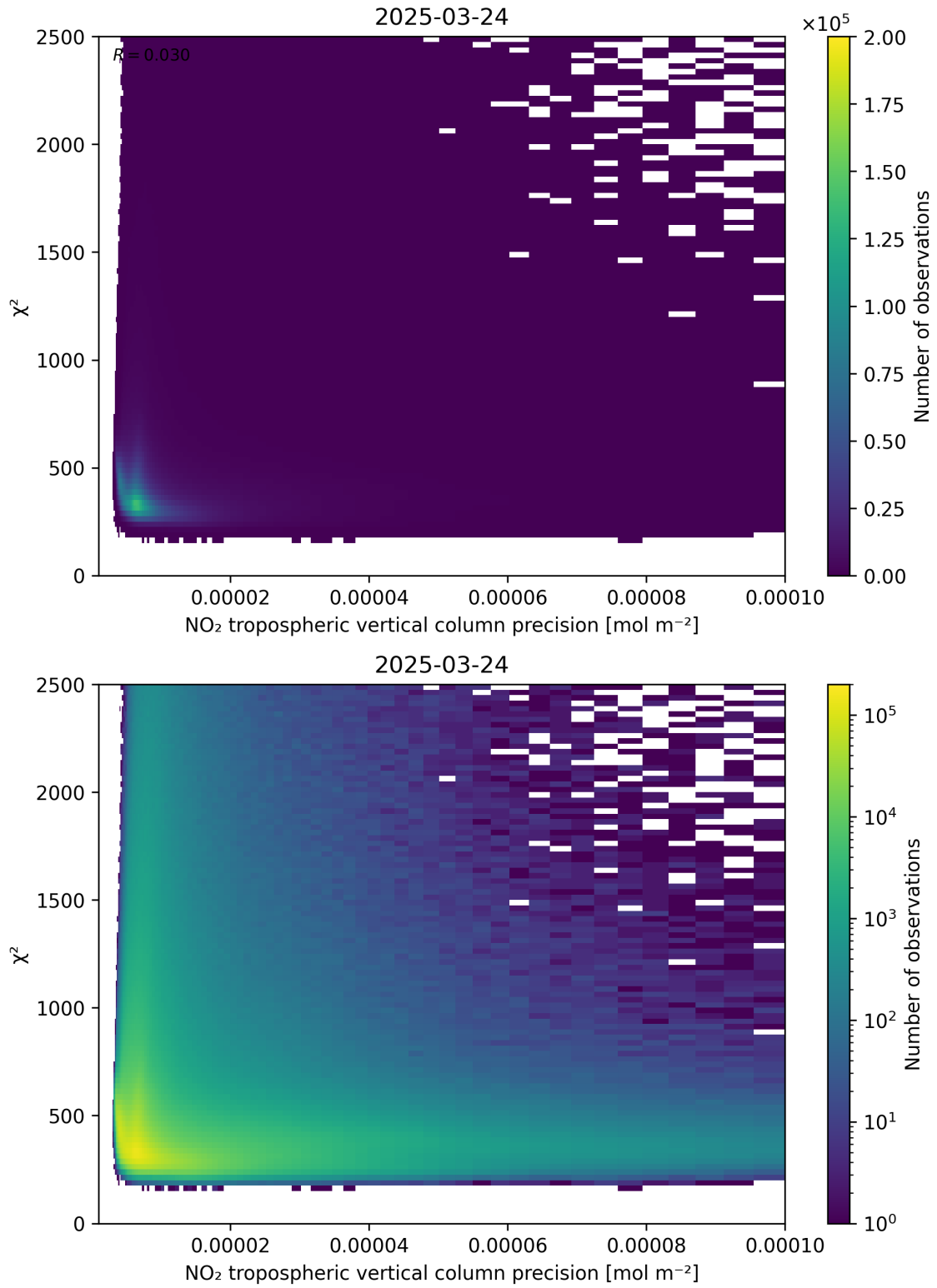
Figure 134: Scatter density plot of “NO 2 tropospheric vertical column precision” against “ \chi^2 ” for 2025-03-24 to 2025-03-25.
