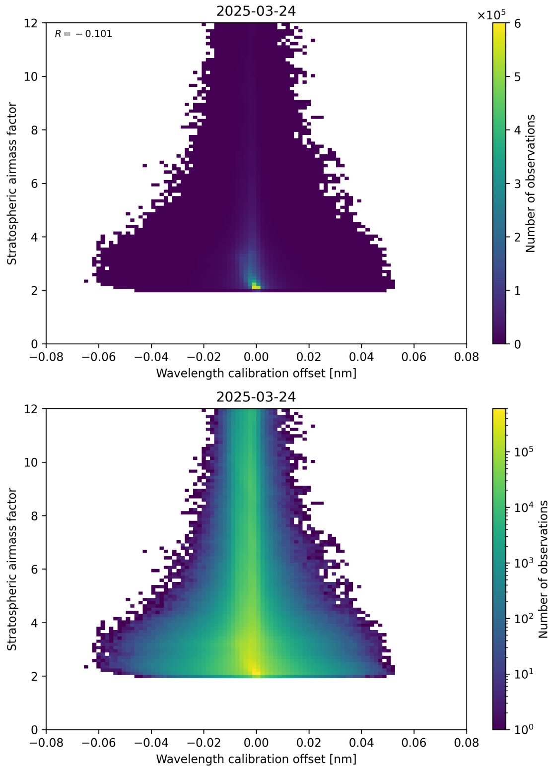
Figure 174: Scatter density plot of “Wavelength calibration offset” against “Stratospheric air mass factor” for 2025-03-24 to 2025-03-25.
