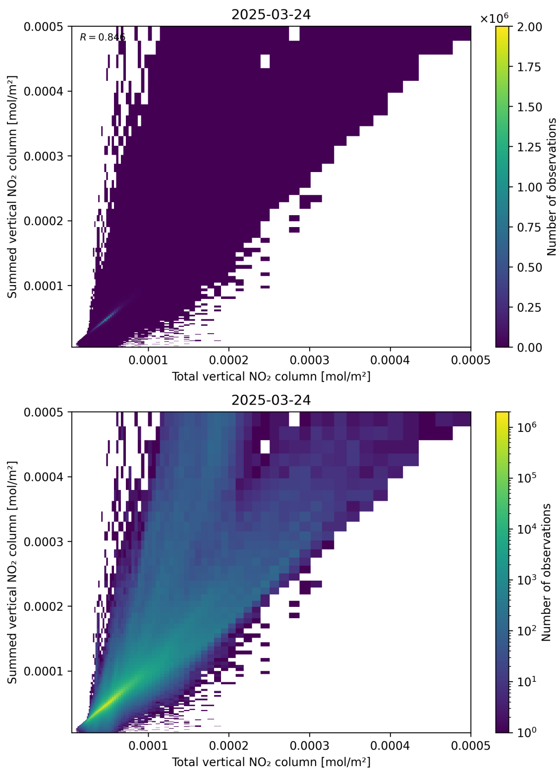
Figure 112: Scatter density plot of “Total vertical NO 2 column” against “Summed vertical NO 2 column” for 2025-03-24 to 2025-03-25.
