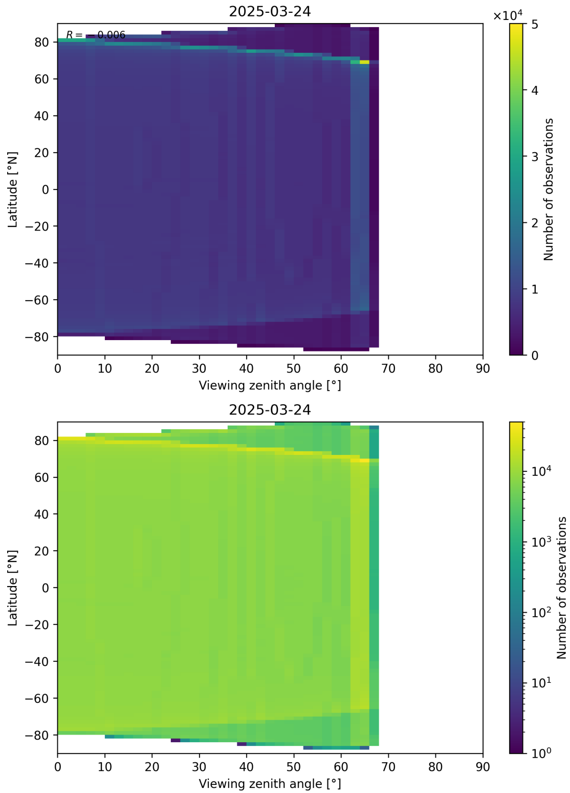
Figure 163: Scatter density plot of “Viewing zenith angle” against “Latitude” for 2025-03-24 to 2025-03-25.
