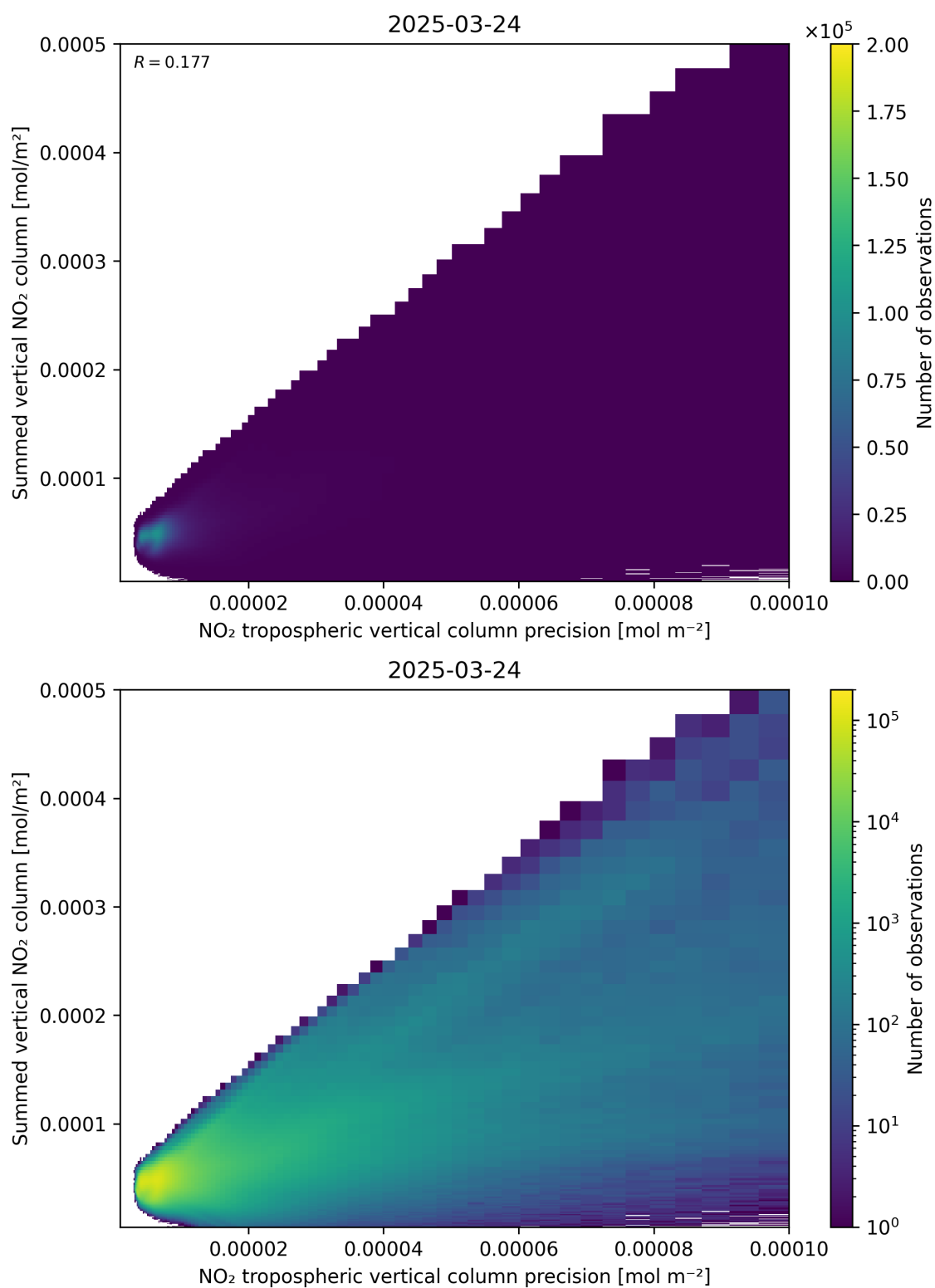
Figure 136: Scatter density plot of “NO 2 tropospheric vertical column precision” against “Summed vertical NO 2 column” for 2025-03-24 to 2025-03-25.
