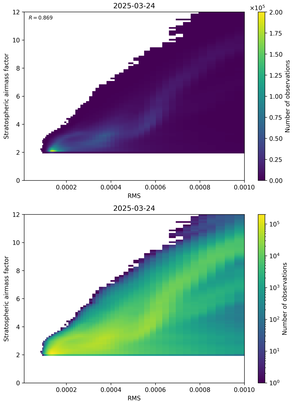
Figure 144: Scatter density plot of “RMS” against “Stratospheric airmass factor” for 2025-03-24 to 2025-03-25.
