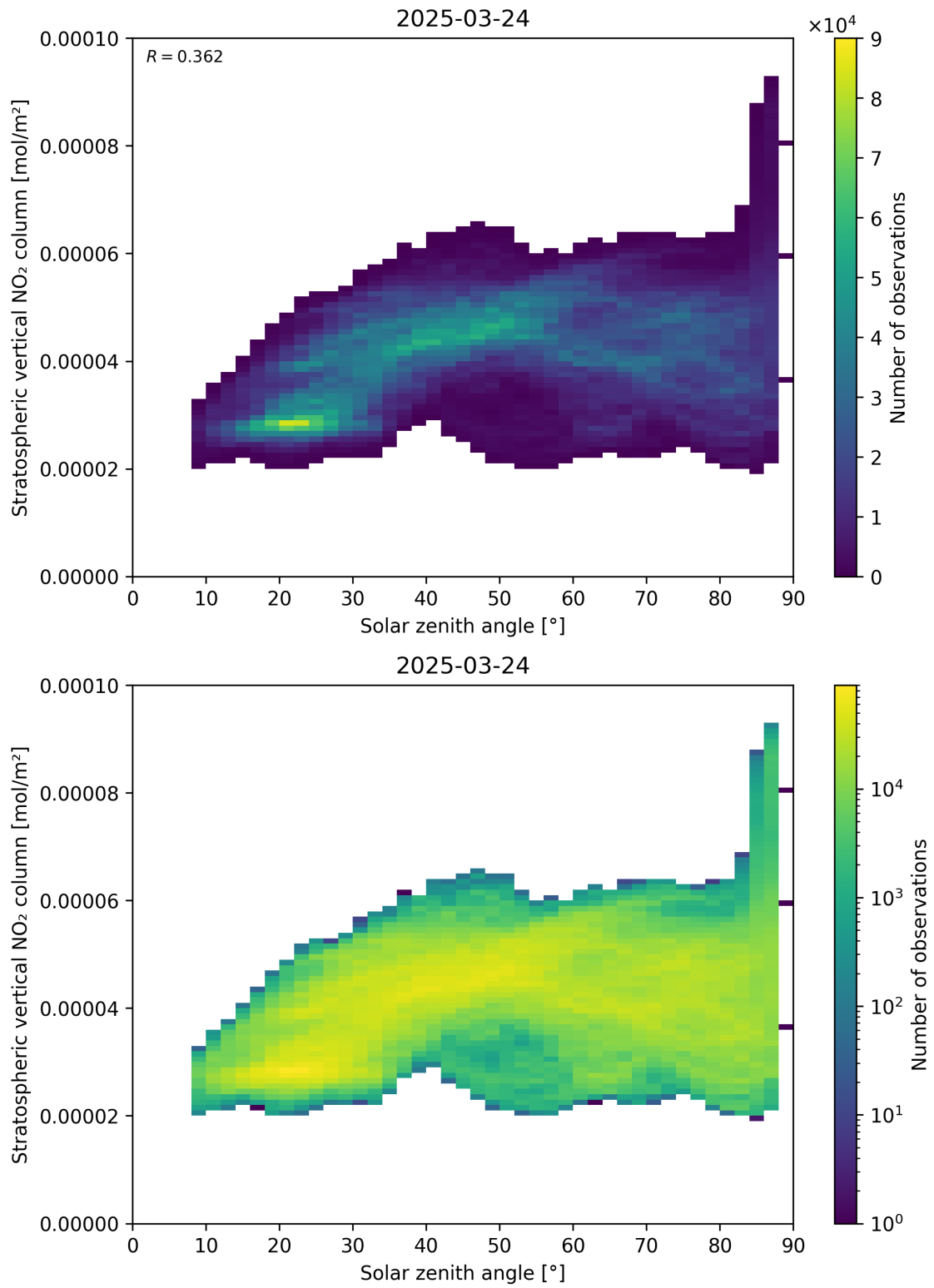
Figure 150: Scatter density plot of “Solar zenith angle” against “Stratospheric vertical NO 2 column” for 2025-03-24 to 2025-03-25.
