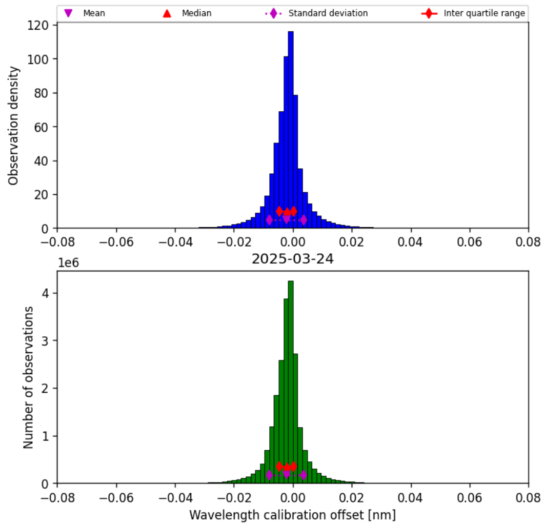
Figure 35: Histogram of “Wavelength calibration offset” for 2025-03-24 to 2025-03-25
