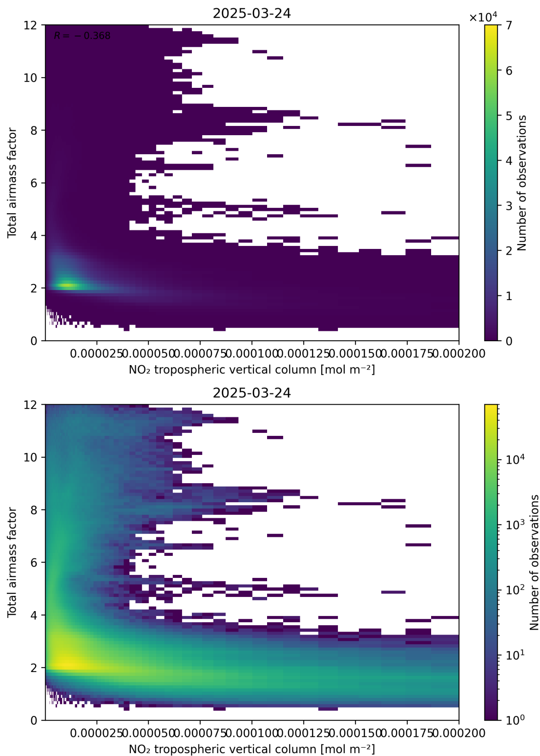
Figure 122: Scatter density plot of “NO 2 tropospheric vertical column” against “Total air mass factor” for 2025-03-24 to 2025-03-25.
