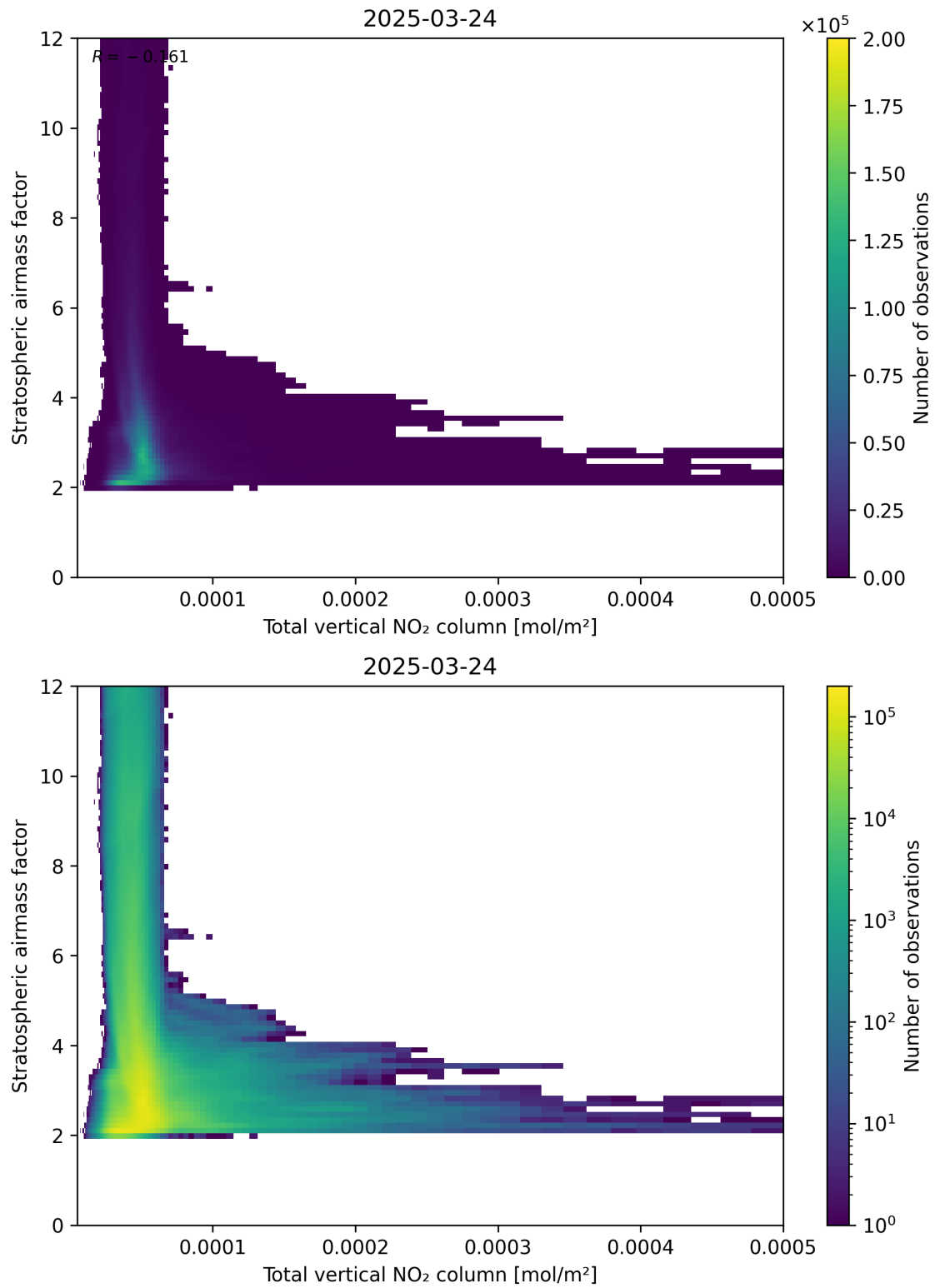
Figure 110: Scatter density plot of “Total vertical NO 2 column” against “Stratospheric airmass factor” for 2025-03-24 to 2025-03-25.
