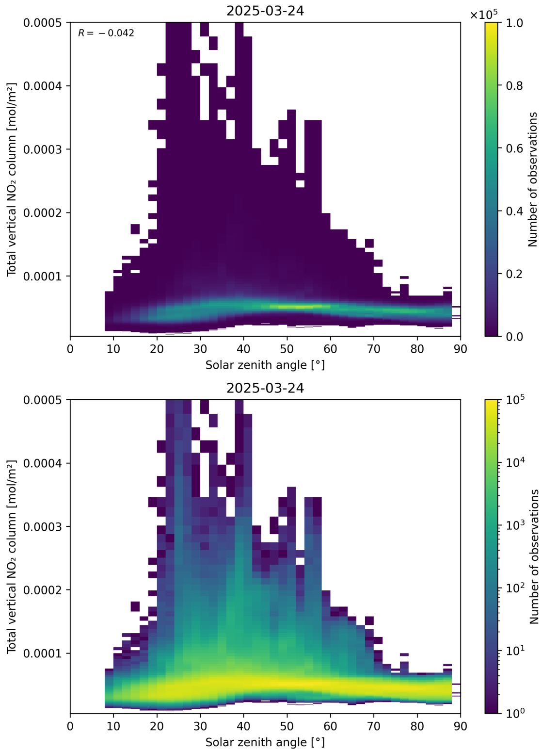
Figure 153: Scatter density plot of “Solar zenith angle” against “Total vertical NO 2 column” for 2025-03-24 to 2025-03-25.
