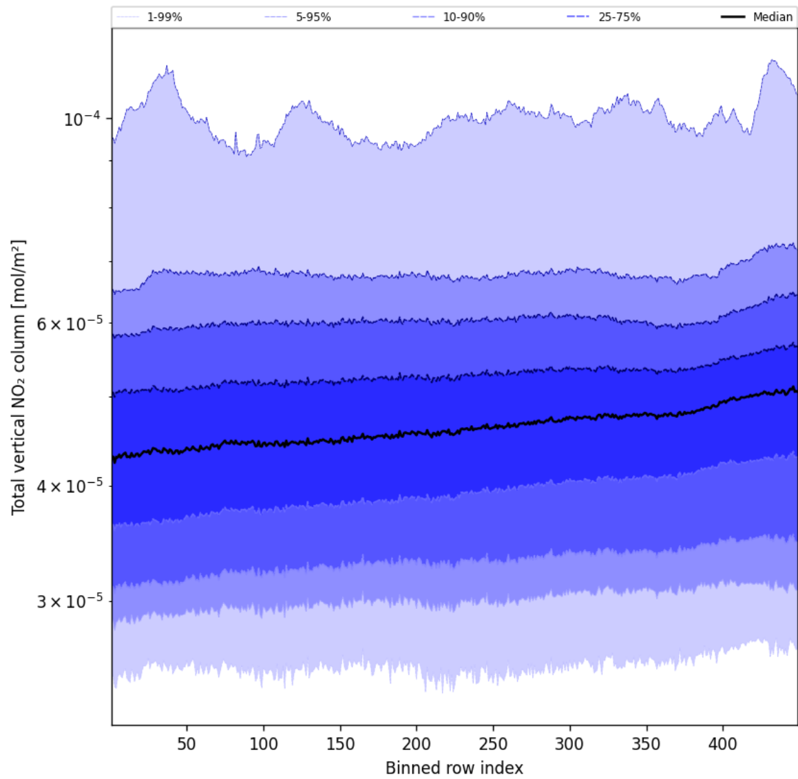
Figure 55: Along track statistics of “Total vertical NO 2 column” for 2025-03-24 to 2025-03-25
