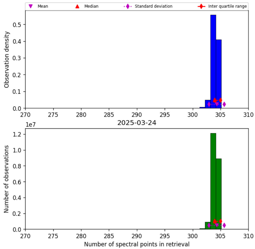
Figure 33: Histogram of “Number of spectral points in retrieval” for 2025-03-24 to 2025-03-25
