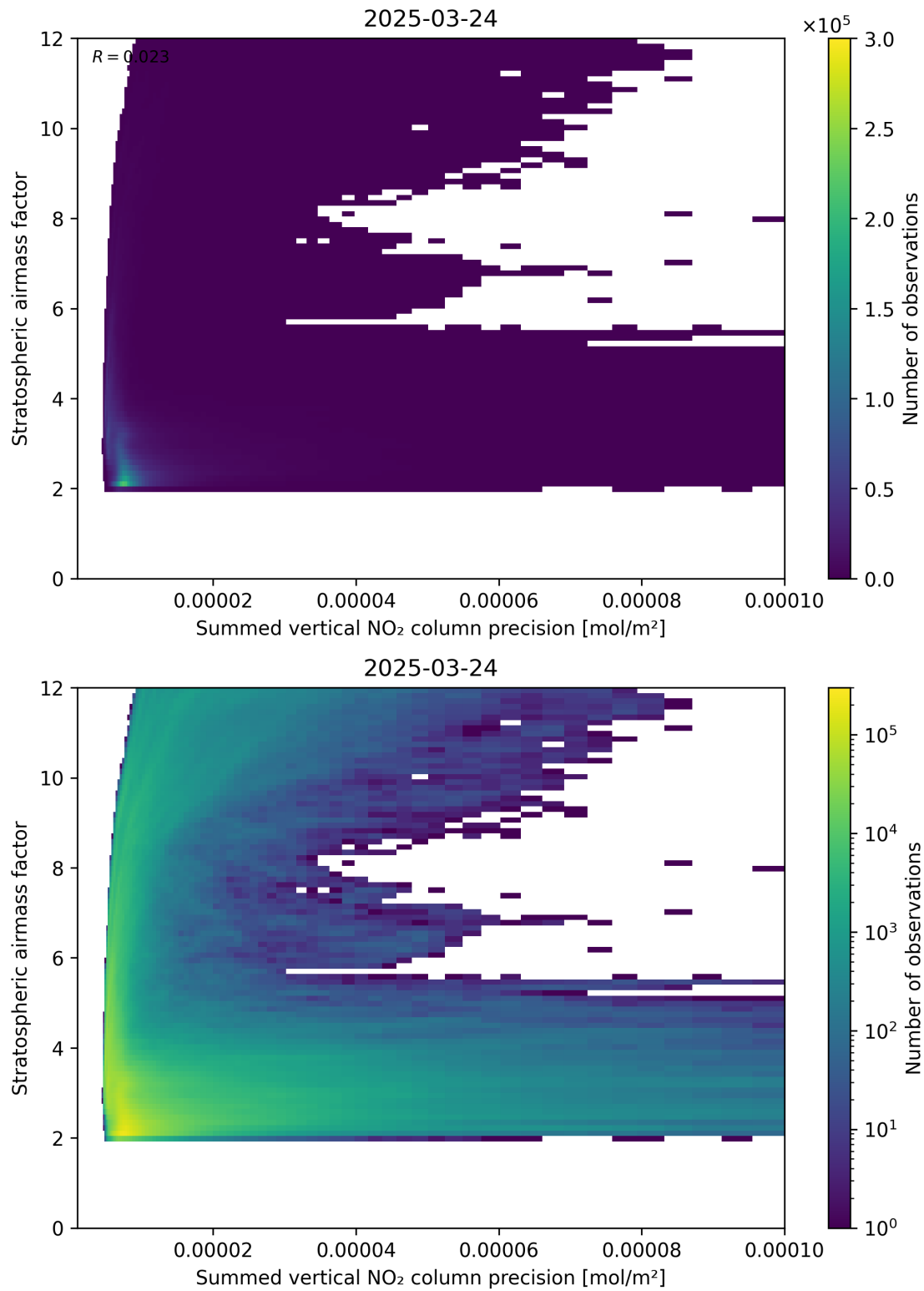
Figure 106: Scatter density plot of “Summed vertical NO 2 column precision” against “Stratospheric airmass factor” for 2025-03-24 to 2025-03-25.
