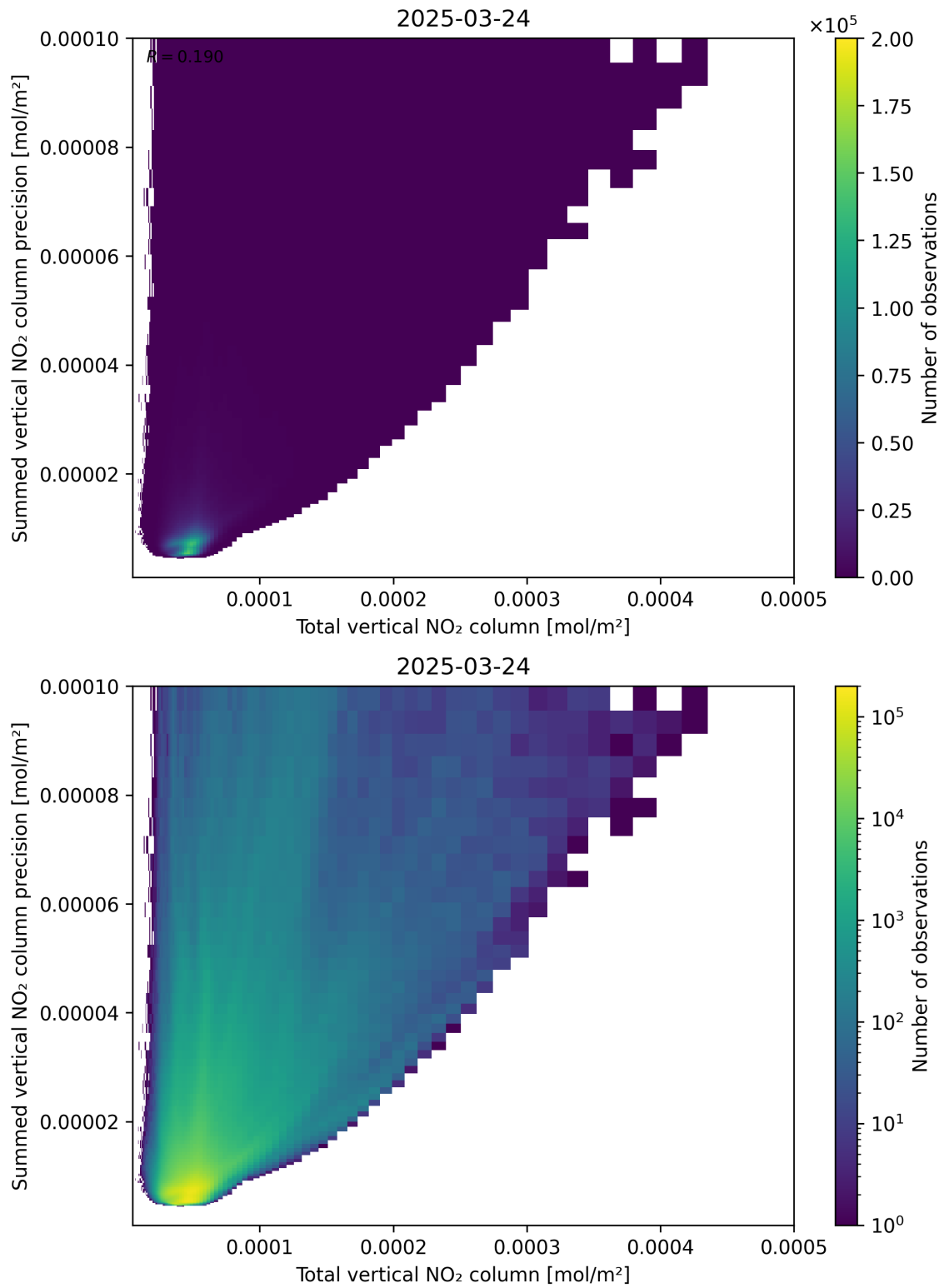
Figure 113: Scatter density plot of “Total vertical NO 2 column” against “Summed vertical NO 2 column precision” for 2025-03-24 to 2025-03-25.
