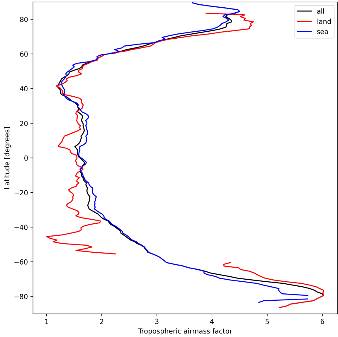
Figure 14: Zonal average of “Tropospheric airmass factor” for 2025-03-24 to 2025-03-25.
