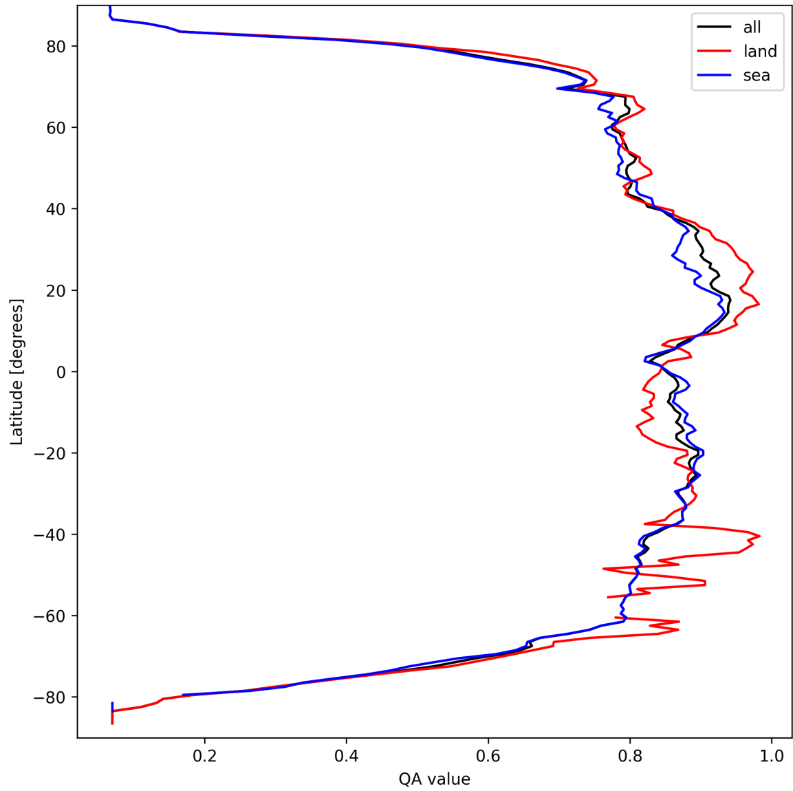
Figure 11: Zonal average of “QA value” for 2025-03-24 to 2025-03-25.
