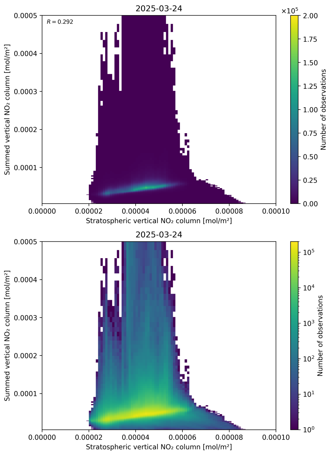
Figure 98: Scatter density plot of “Stratospheric vertical NO 2 column” against “Summed vertical NO 2 column” for 2025-03-24 to 2025-03-25.
