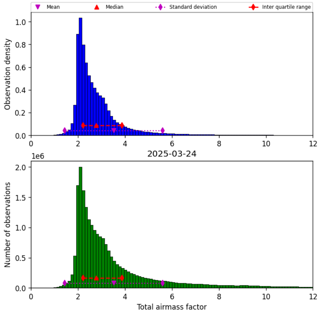
Figure 32: Histogram of “Total airmass factor” for 2025-03-24 to 2025-03-25
