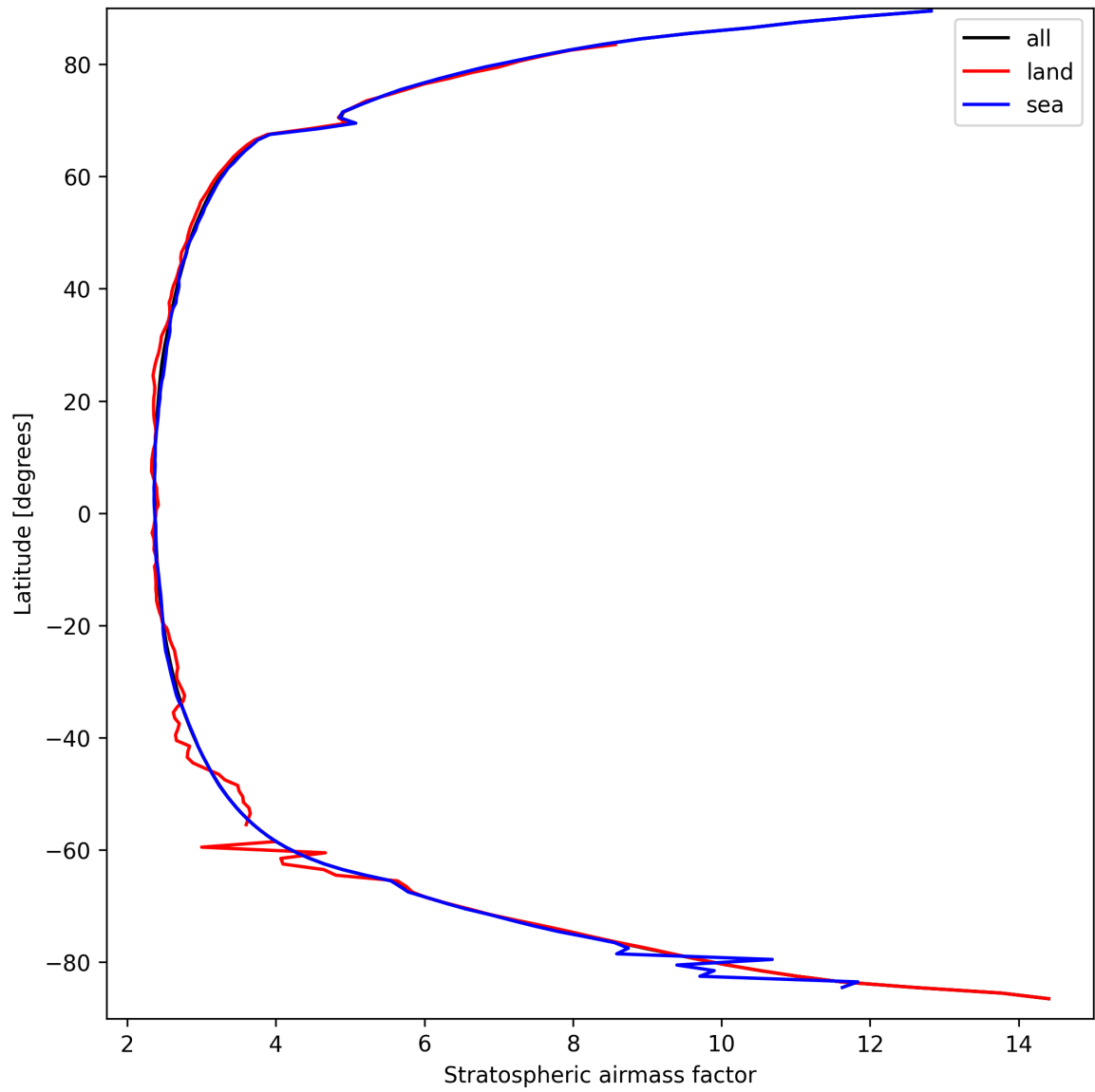
Figure 27: Zonal average of “Stratospheric airmass factor” for 2025-03-25 to 2025-03-26.
