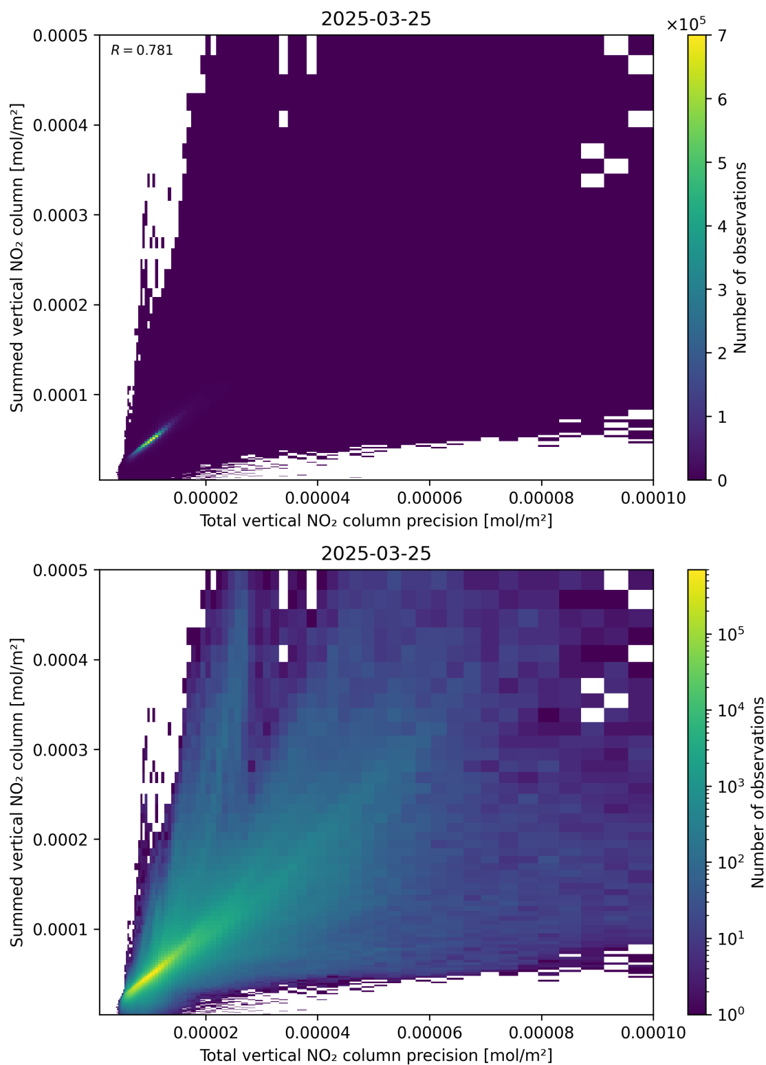
Figure 117: Scatter density plot of “Total vertical NO 2 column precision” against “Summed vertical NO 2 column” for 2025-03-25 to 2025-03-26.
