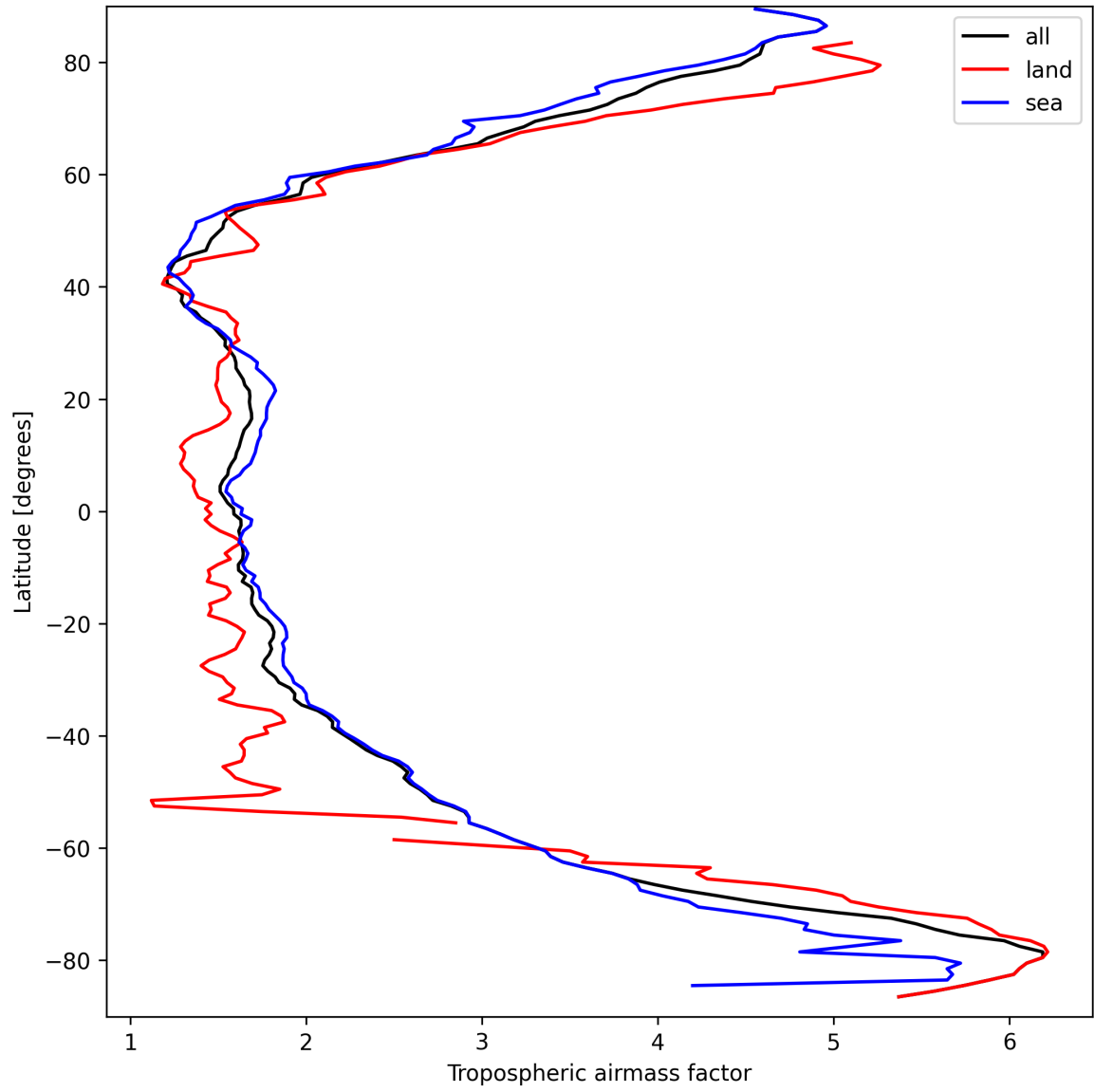
Figure 14: Zonal average of “Tropospheric airmass factor” for 2025-03-25 to 2025-03-26.
