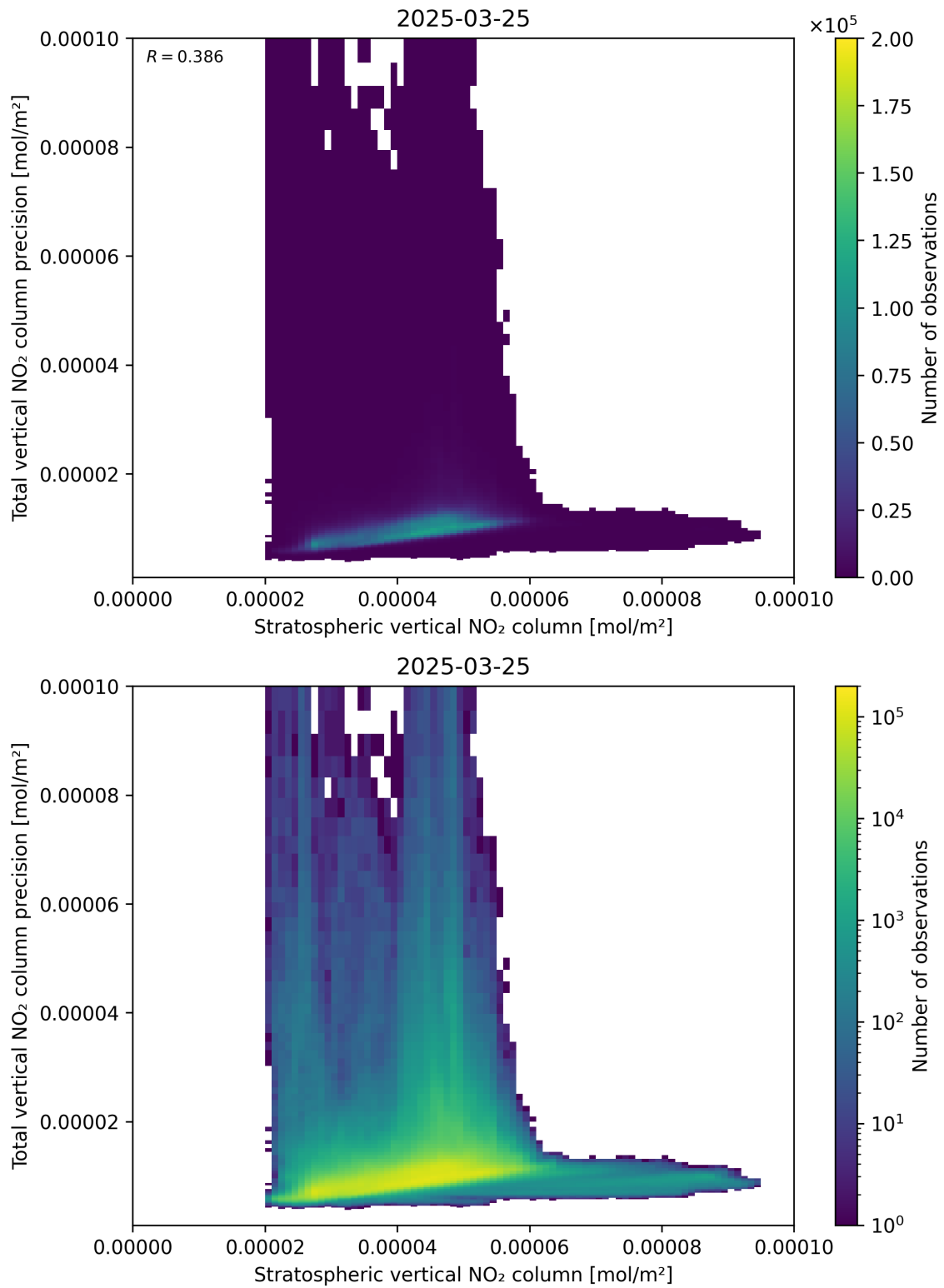
Figure 101: Scatter density plot of “Stratospheric vertical NO 2 column” against “Total vertical NO 2 column precision” for 2025-03-25 to 2025-03-26.
