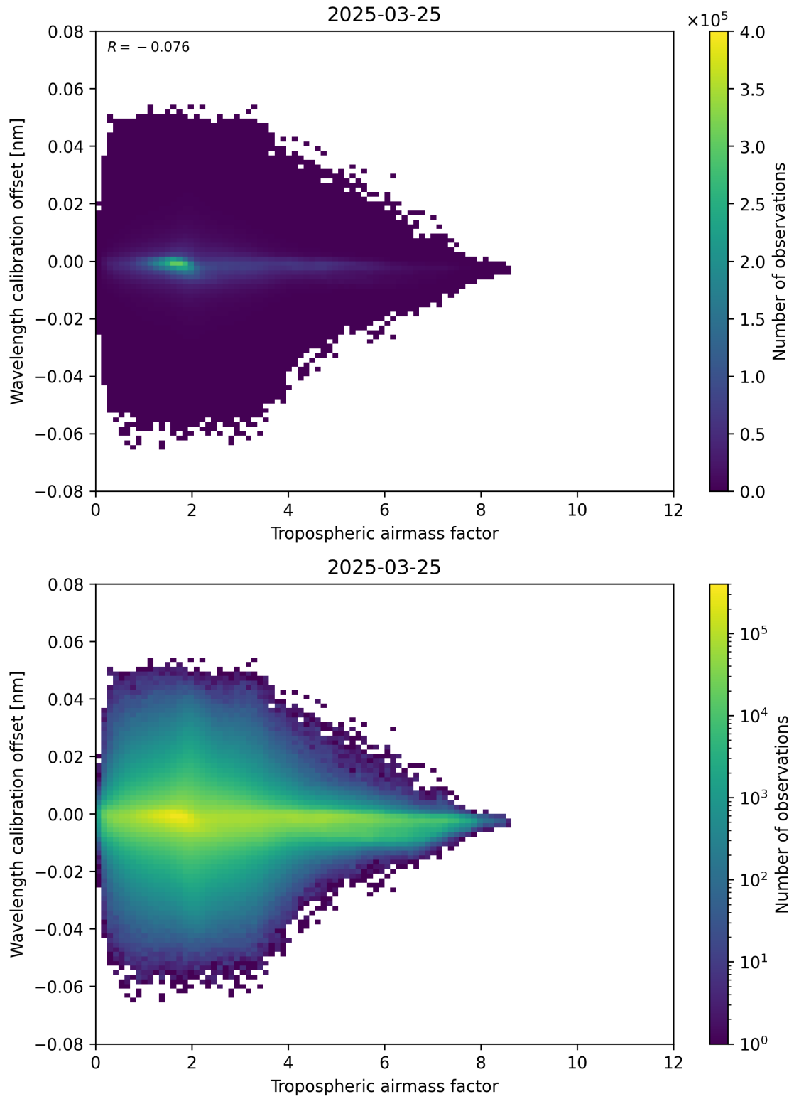
Figure 80: Scatter density plot of “Tropospheric airmass factor” against “Wavelength calibration offset” for 2025-03-25 to 2025-03-26.
