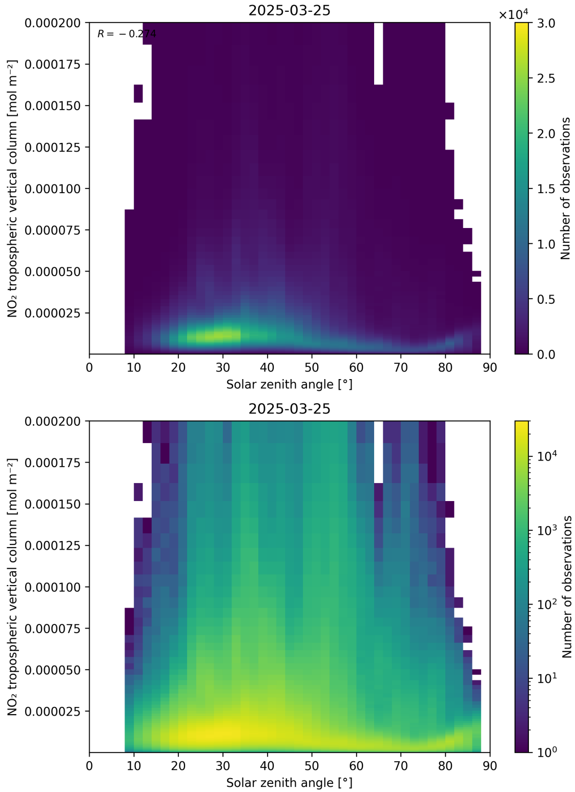
Figure 155: Scatter density plot of “Solar zenith angle” against “NO 2 tropospheric vertical column” for 2025-03-25 to 2025-03-26.
