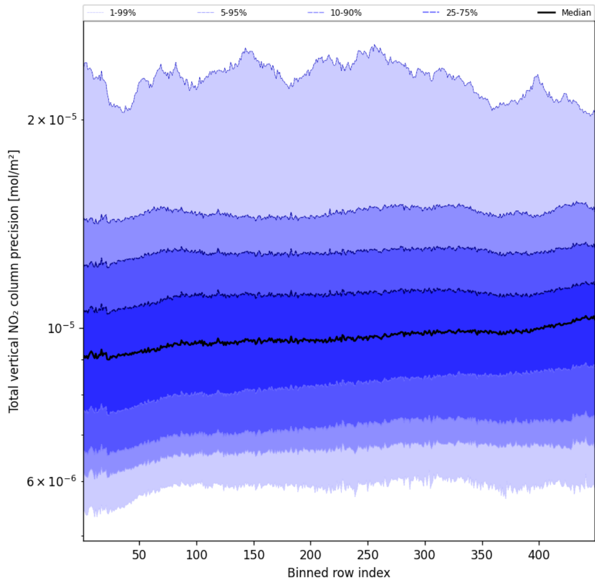
Figure 56: Along track statistics of “Total vertical NO 2 column precision” for 2025-03-25 to 2025-03-26
