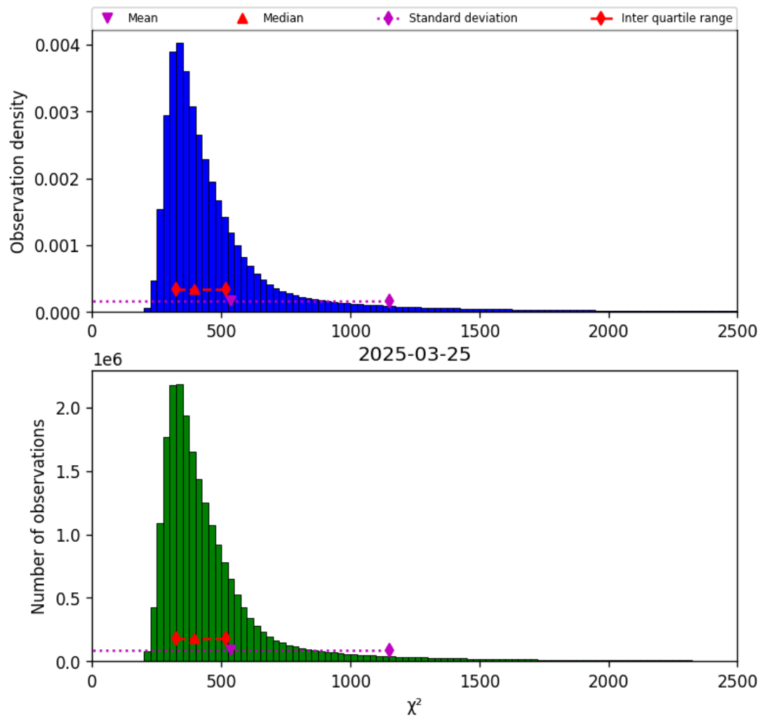
Figure 42: Histogram of “ \chi^2 ” for 2025-03-25 to 2025-03-26
