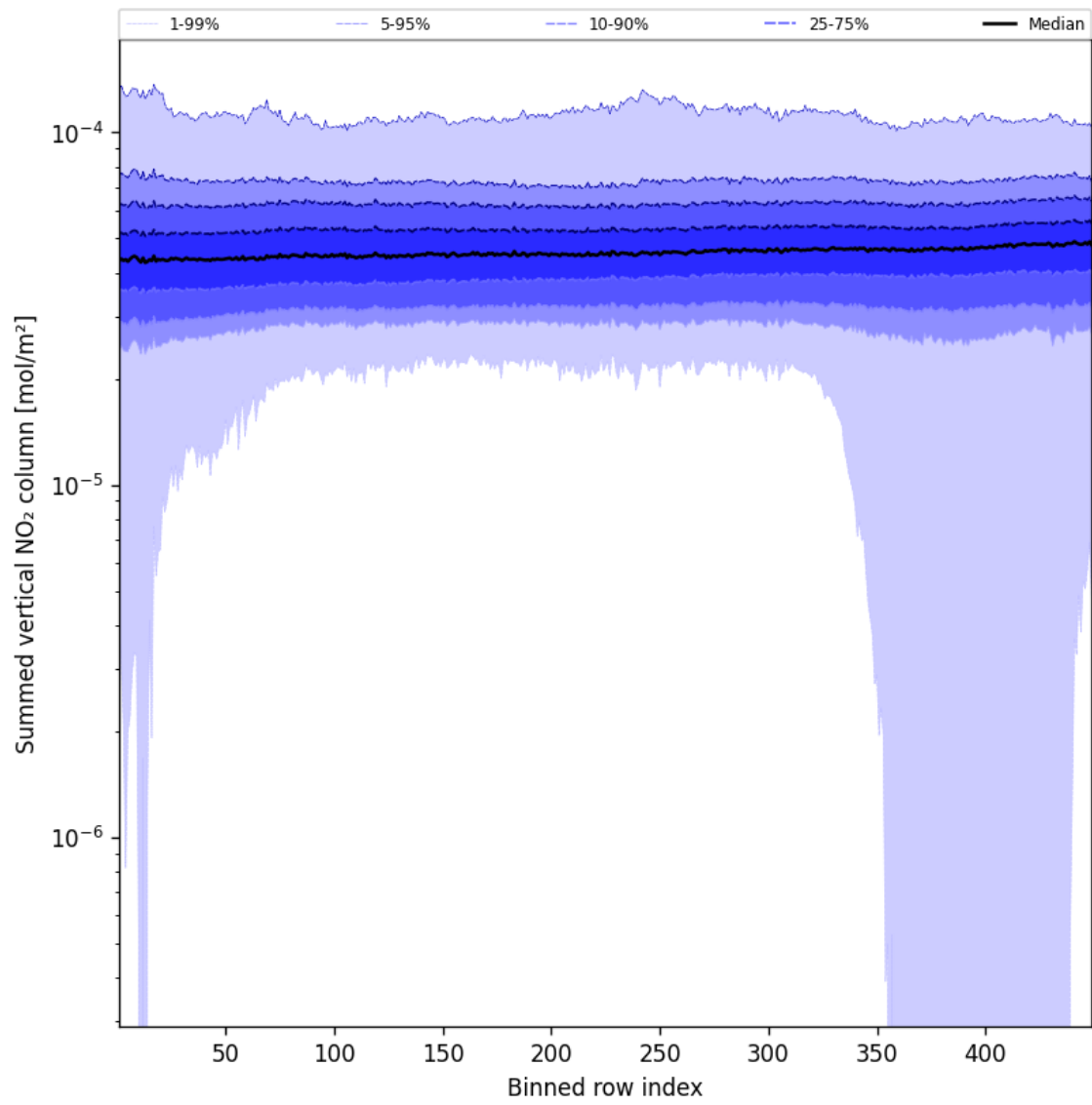
Figure 57: Along track statistics of “Summed vertical NO 2 column” for 2025-03-25 to 2025-03-26
