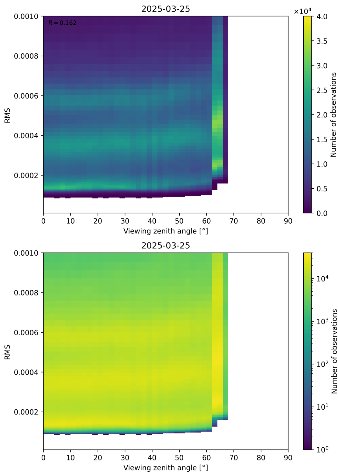
Figure 171: Scatter density plot of “Viewing zenith angle” against “RMS” for 2025-03-25 to 2025-03-26.
