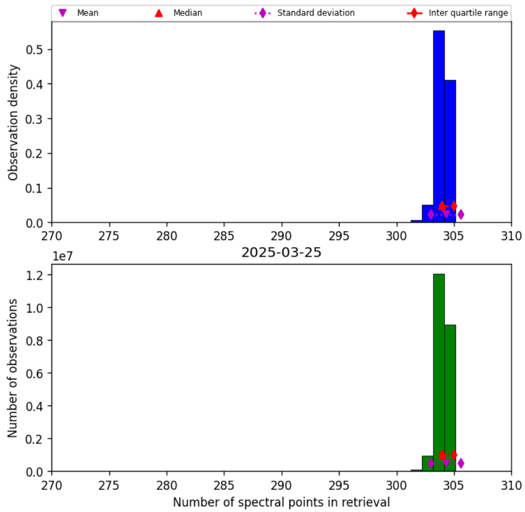
Figure 33: Histogram of “Number of spectral points in retrieval” for 2025-03-25 to 2025-03-26
