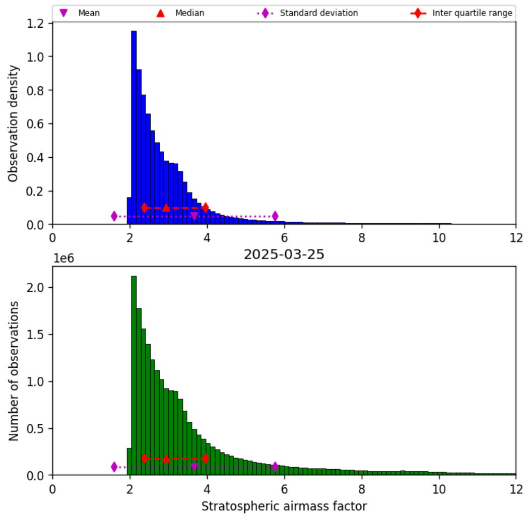
Figure 44: Histogram of “Stratospheric airmass factor” for 2025-03-25 to 2025-03-26
