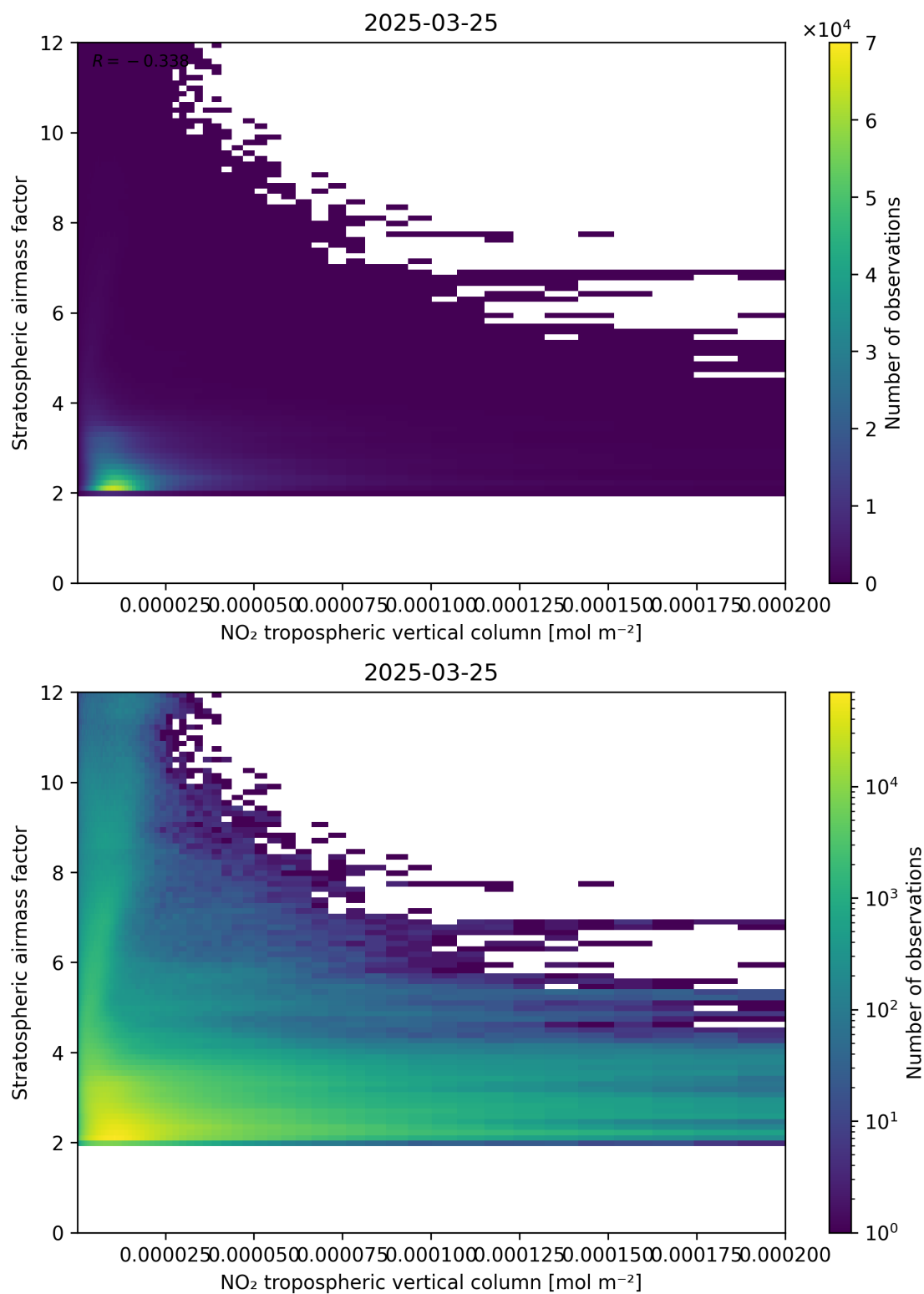
Figure 121: Scatter density plot of “NO 2 tropospheric vertical column” against “Stratospheric air mass factor” for 2025-03-25 to 2025-03-26.
