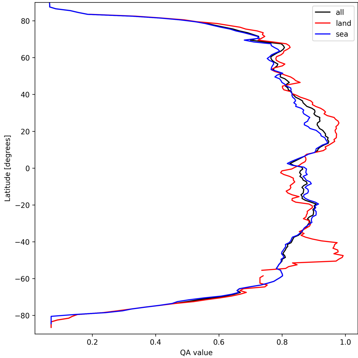
Figure 11: Zonal average of “QA value” for 2025-03-25 to 2025-03-26.
