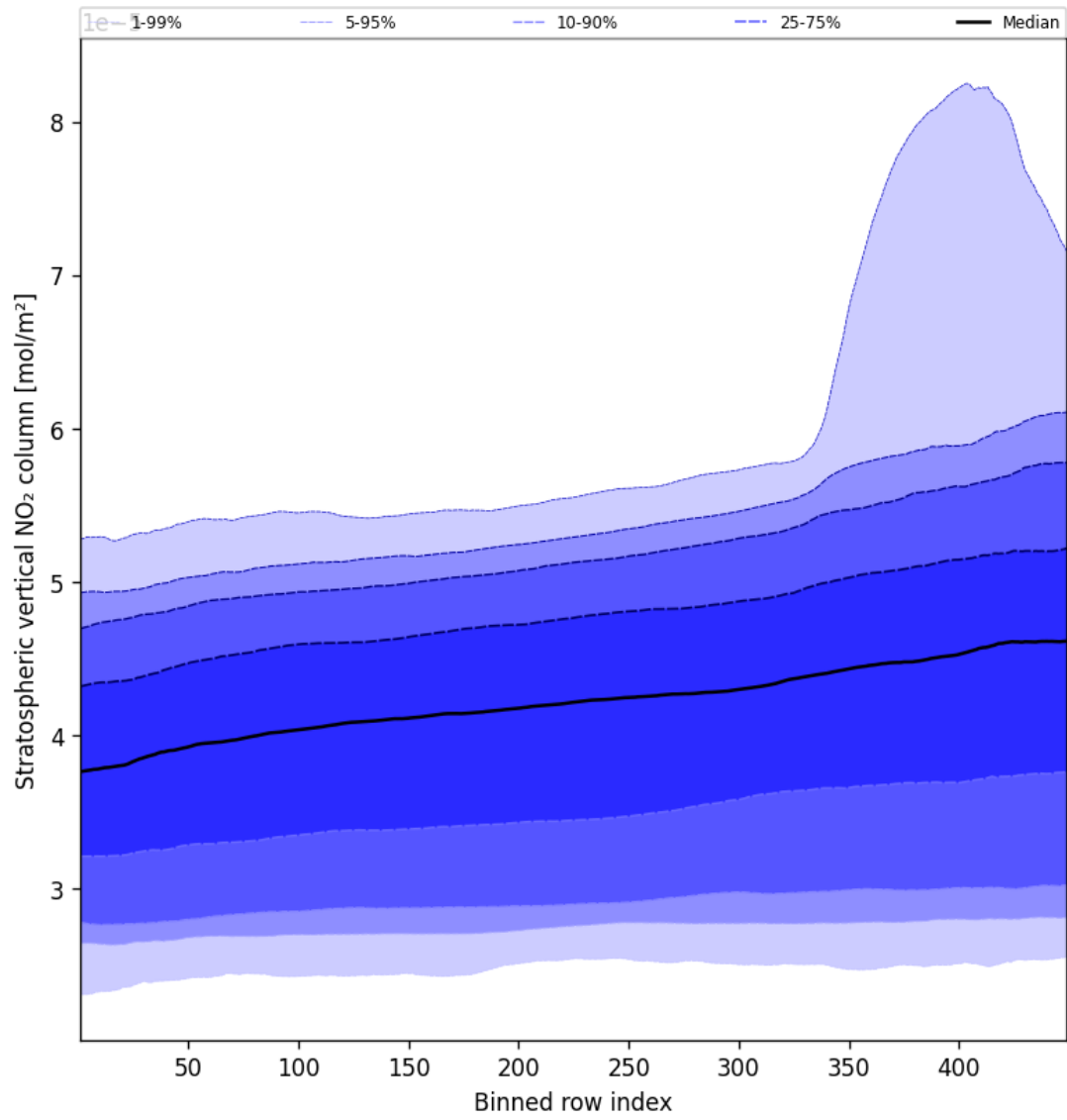
Figure 53: Along track statistics of “Stratospheric vertical NO 2 column” for 2025-03-25 to 2025-03-26
