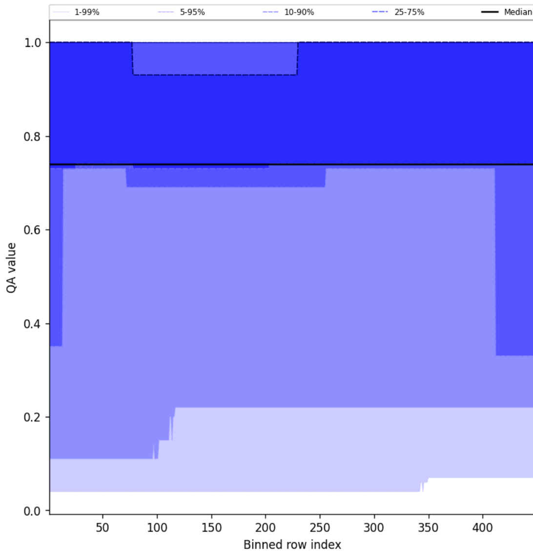
Figure 45: Along track statistics of “QA value” for 2025-03-25 to 2025-03-26
