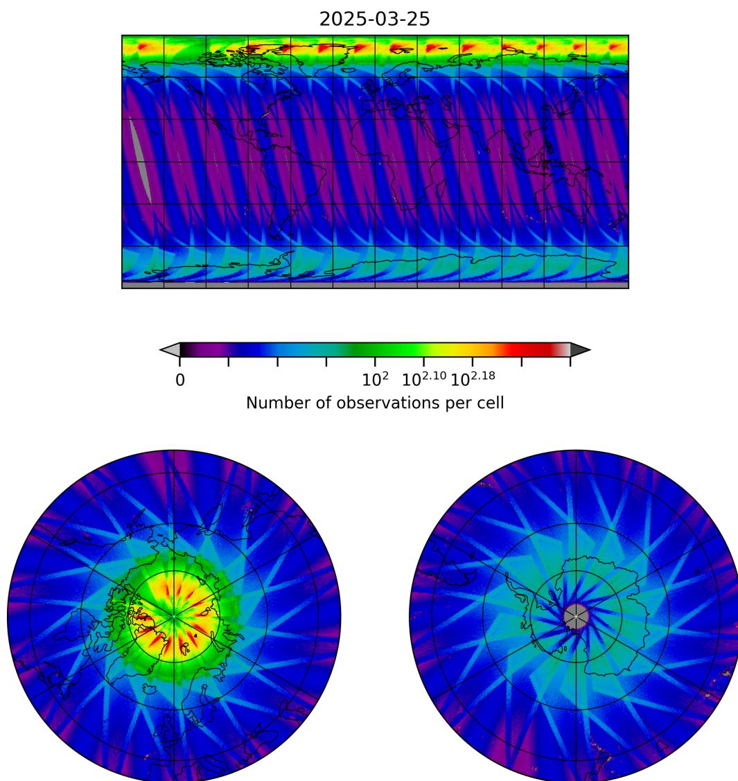
Figure 10: Map of the number of observations for 2025-03-25 to 2025-03-26
