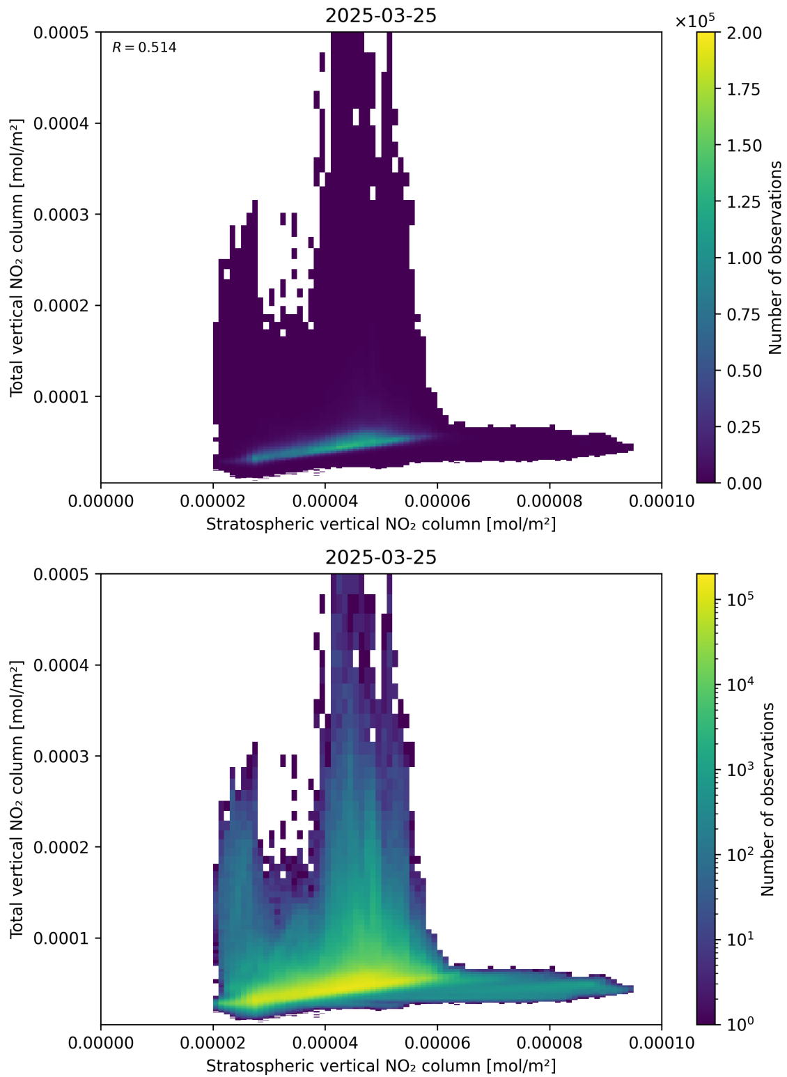
Figure 100: Scatter density plot of “Stratospheric vertical NO 2 column” against “Total vertical NO 2 column” for 2025-03-25 to 2025-03-26.
