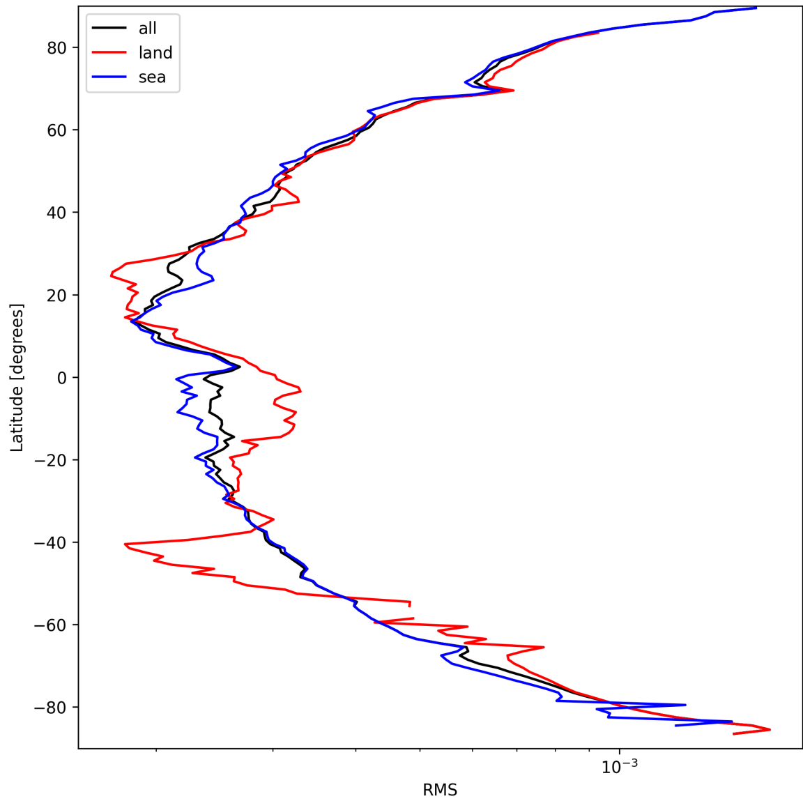
Figure 26: Zonal average of “RMS” for 2025-03-25 to 2025-03-26.
