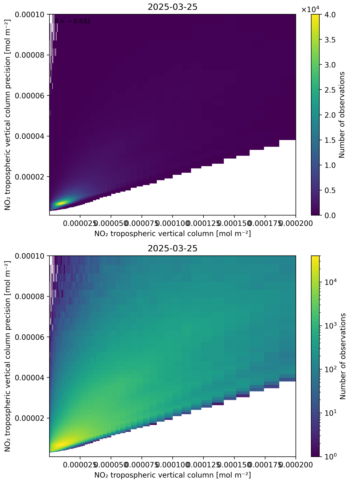
Figure 130: Scatter density plot of “NO 2 tropospheric vertical column” against “NO 2 tropospheric vertical column precision” for 2025-03-25 to 2025-03-26.
