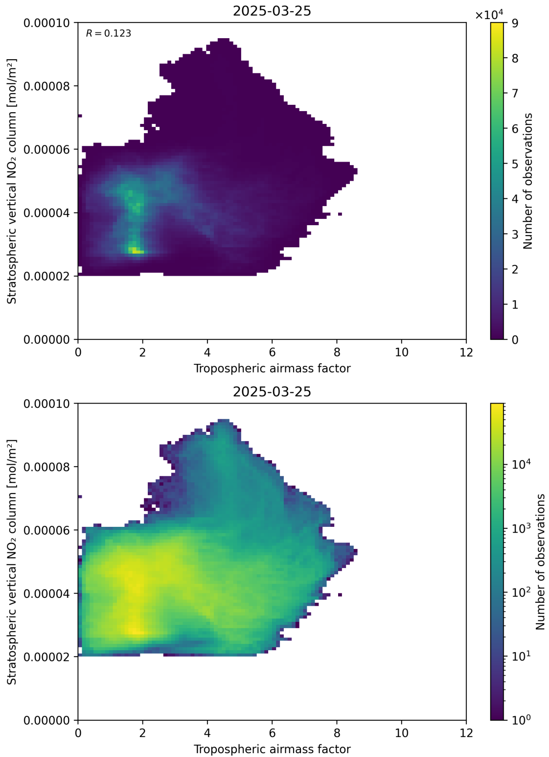
Figure 74: Scatter density plot of “Tropospheric air mass factor” against “Stratospheric vertical NO 2 column” for 2025-03-25 to 2025-03-26.
