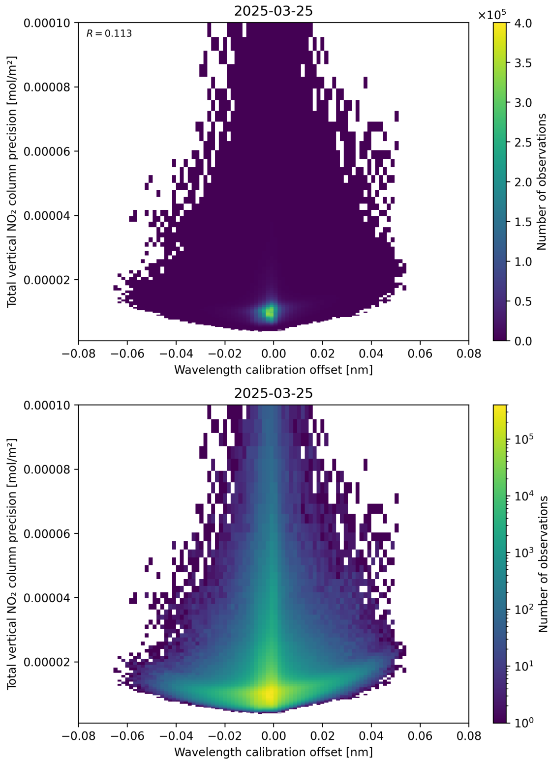
Figure 180: Scatter density plot of “Wavelength calibration offset” against “Total vertical NO 2 column precision” for 2025-03-25 to 2025-03-26.
