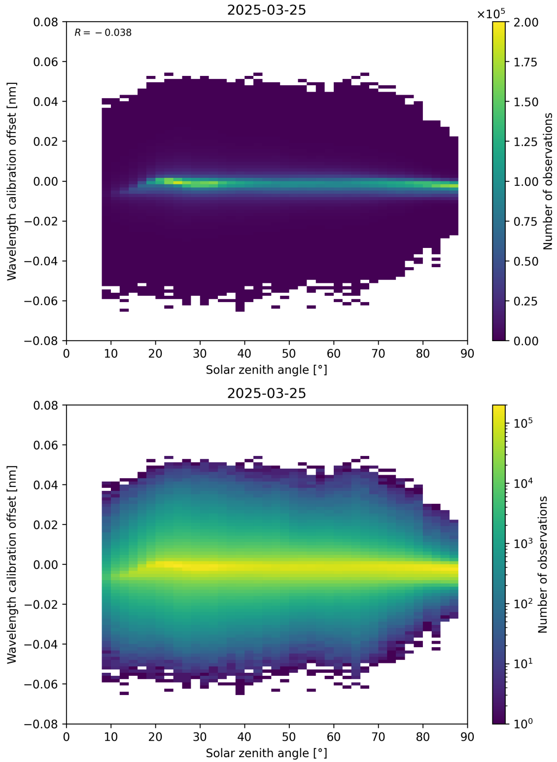
Figure 158: Scatter density plot of “Solar zenith angle” against “Wavelength calibration offset” for 2025-03-25 to 2025-03-26.
