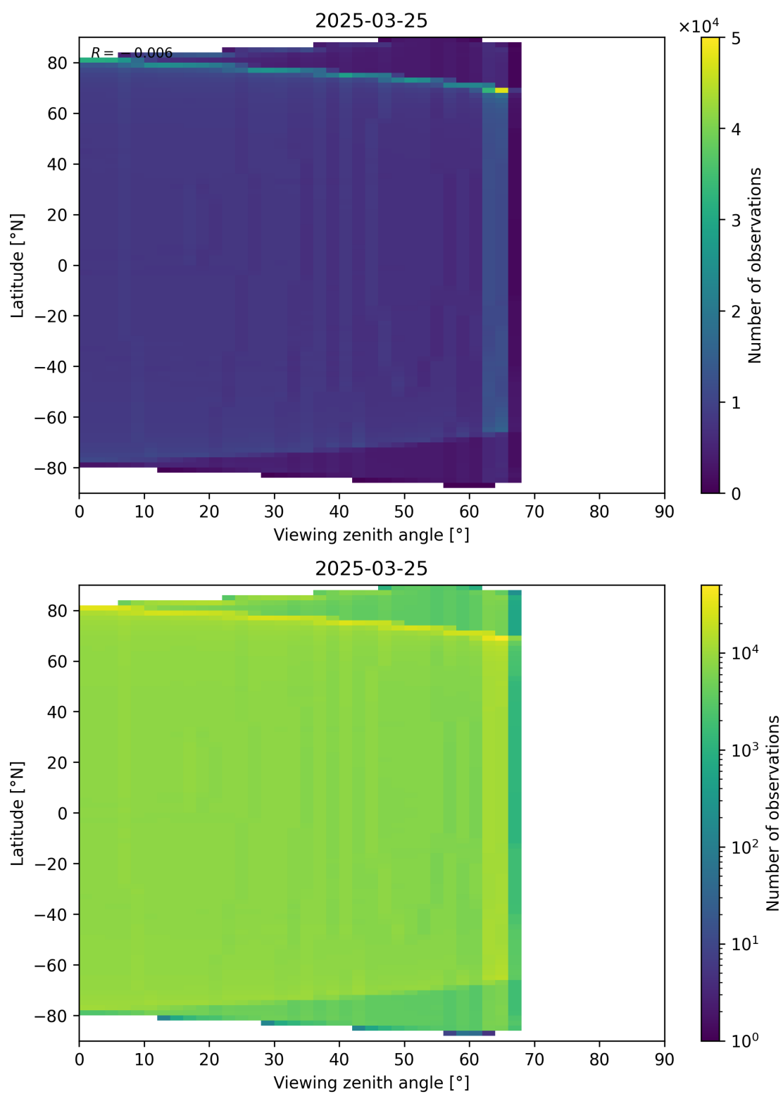
Figure 163: Scatter density plot of “Viewing zenith angle” against “Latitude” for 2025-03-25 to 2025-03-26.
