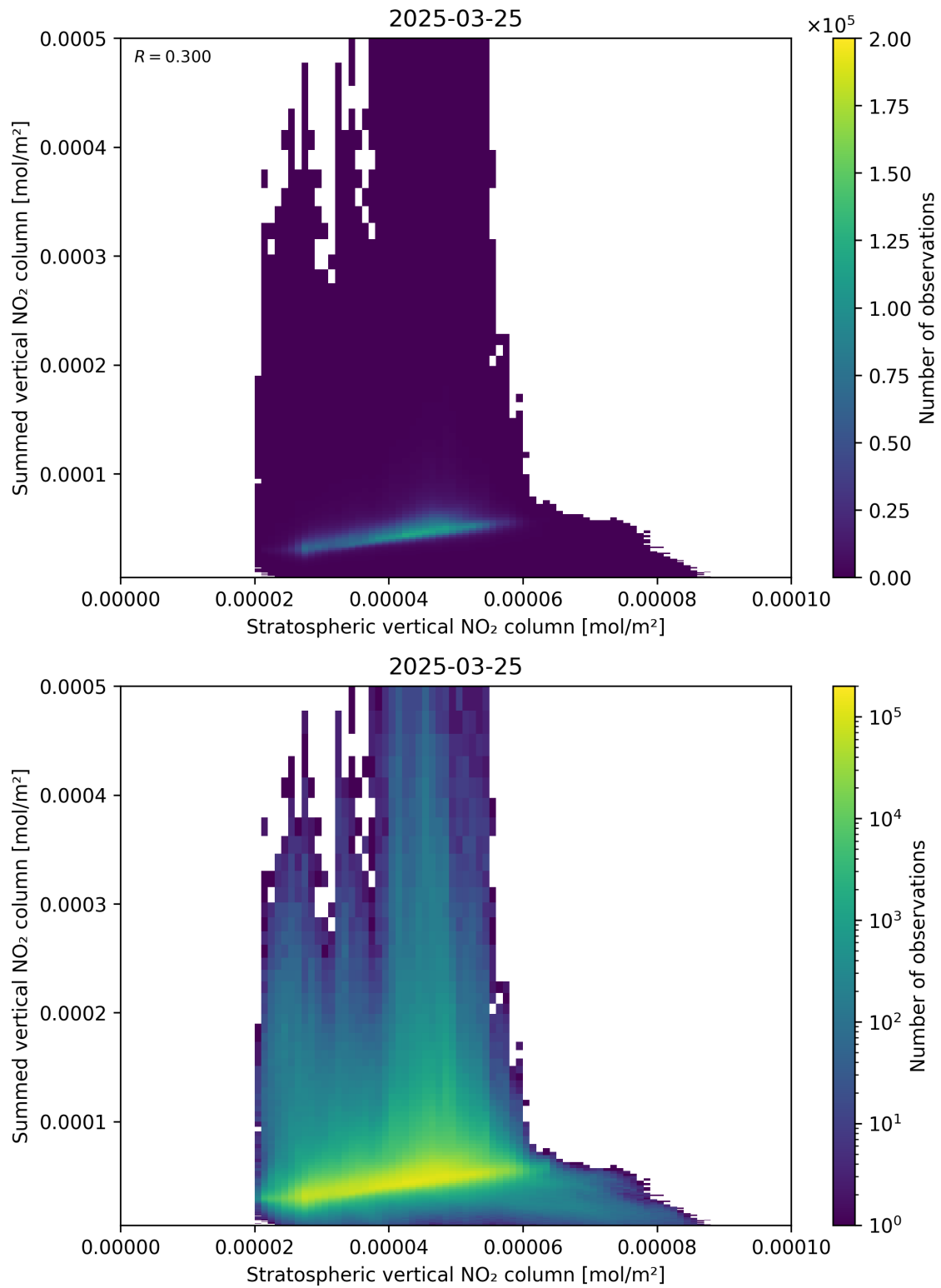
Figure 98: Scatter density plot of “Stratospheric vertical NO 2 column” against “Summed vertical NO 2 column” for 2025-03-25 to 2025-03-26.
