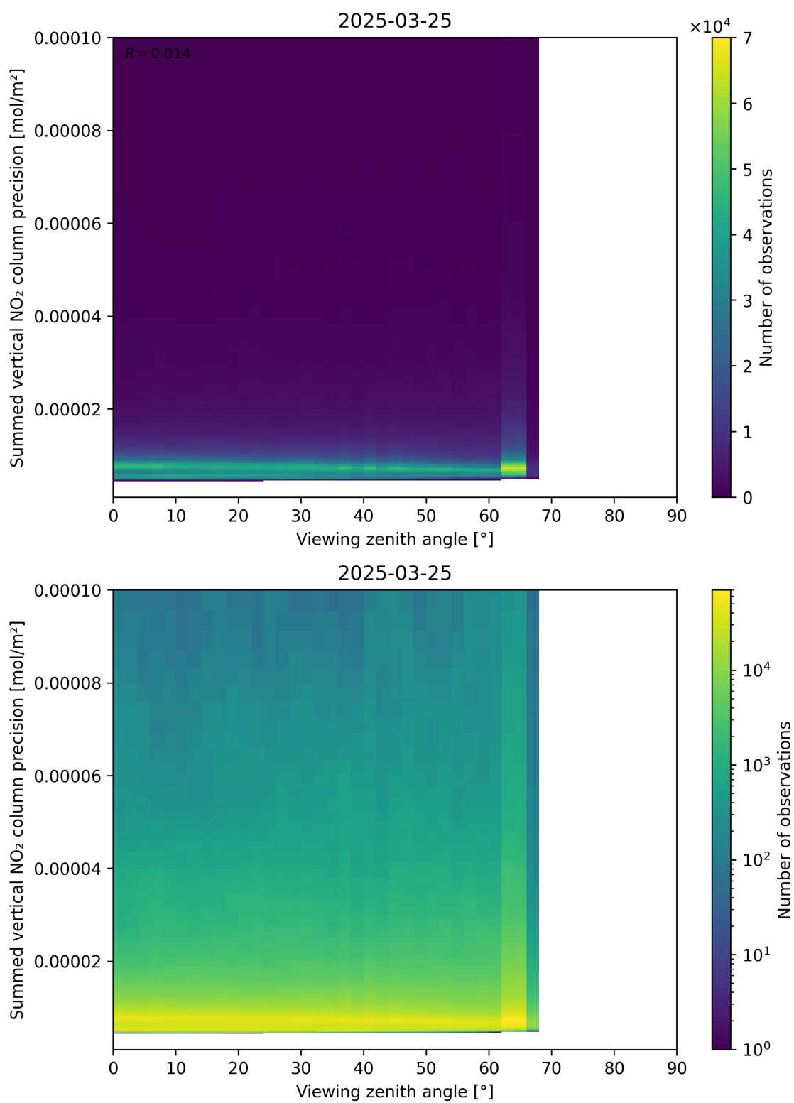
Figure 166: Scatter density plot of “Viewing zenith angle” against “Summed vertical NO 2 column precision” for 2025-03-25 to 2025-03-26.
