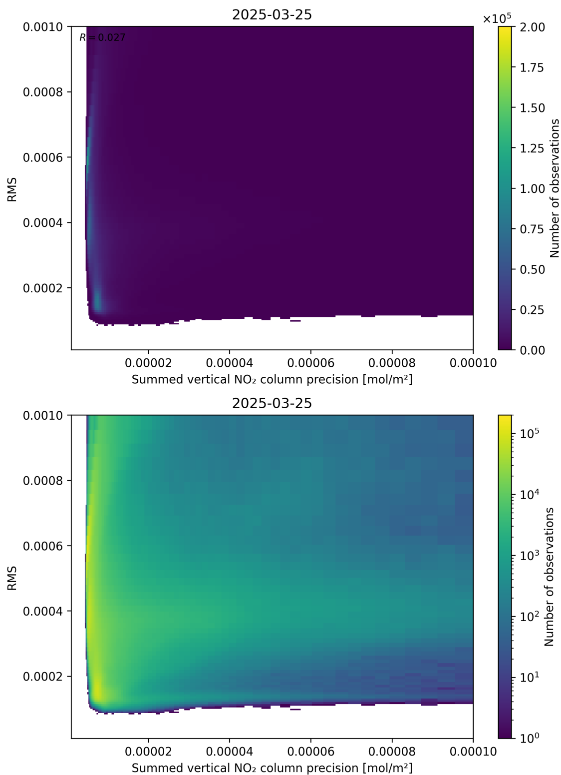
Figure 108: Scatter density plot of “Summed vertical NO 2 column precision” against “RMS” for 2025-03-25 to 2025-03-26.
