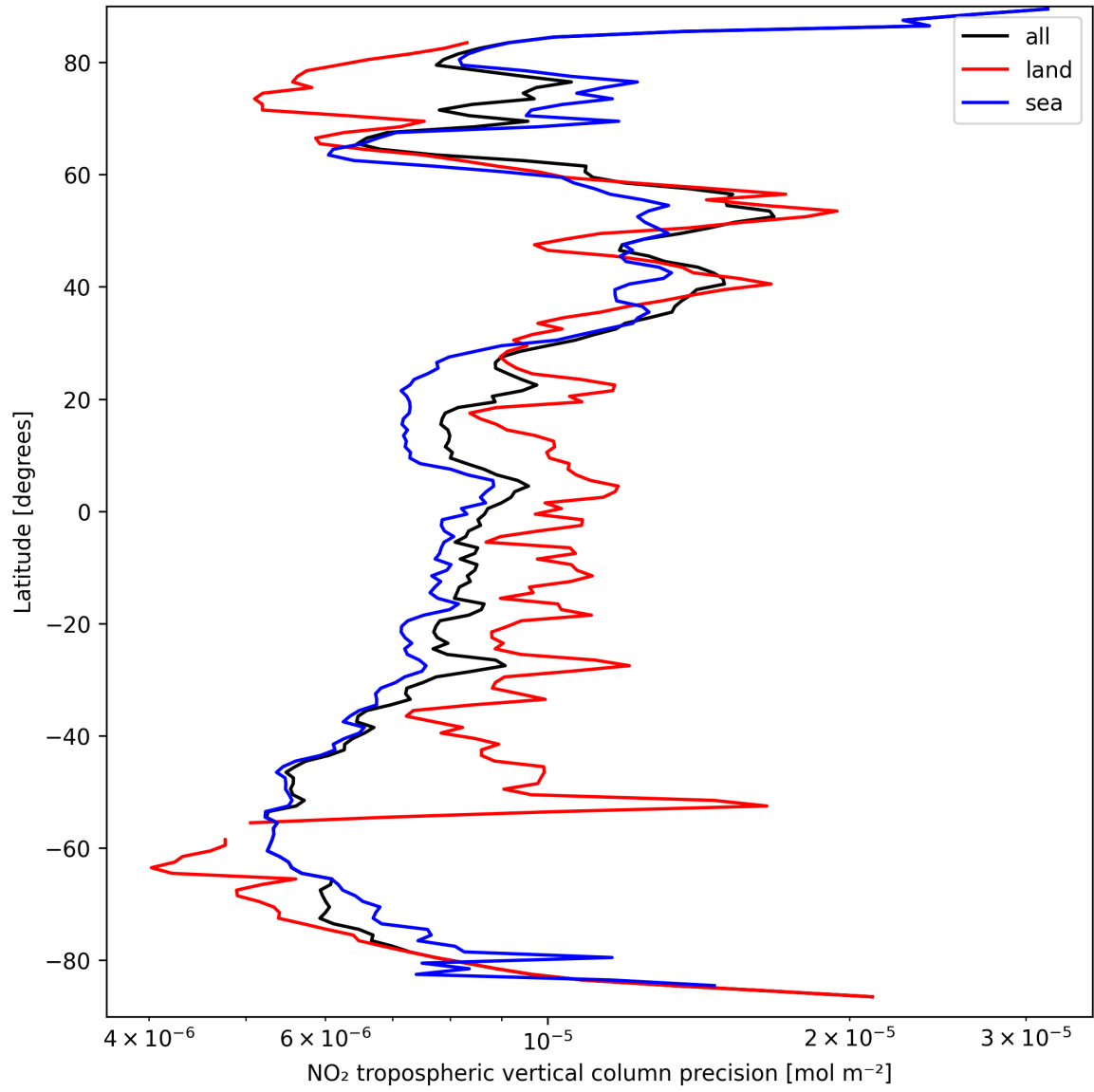
Figure 13: Zonal average of “NO 2 tropospheric vertical column precision” for 2025-03-25 to 2025-03-26.
