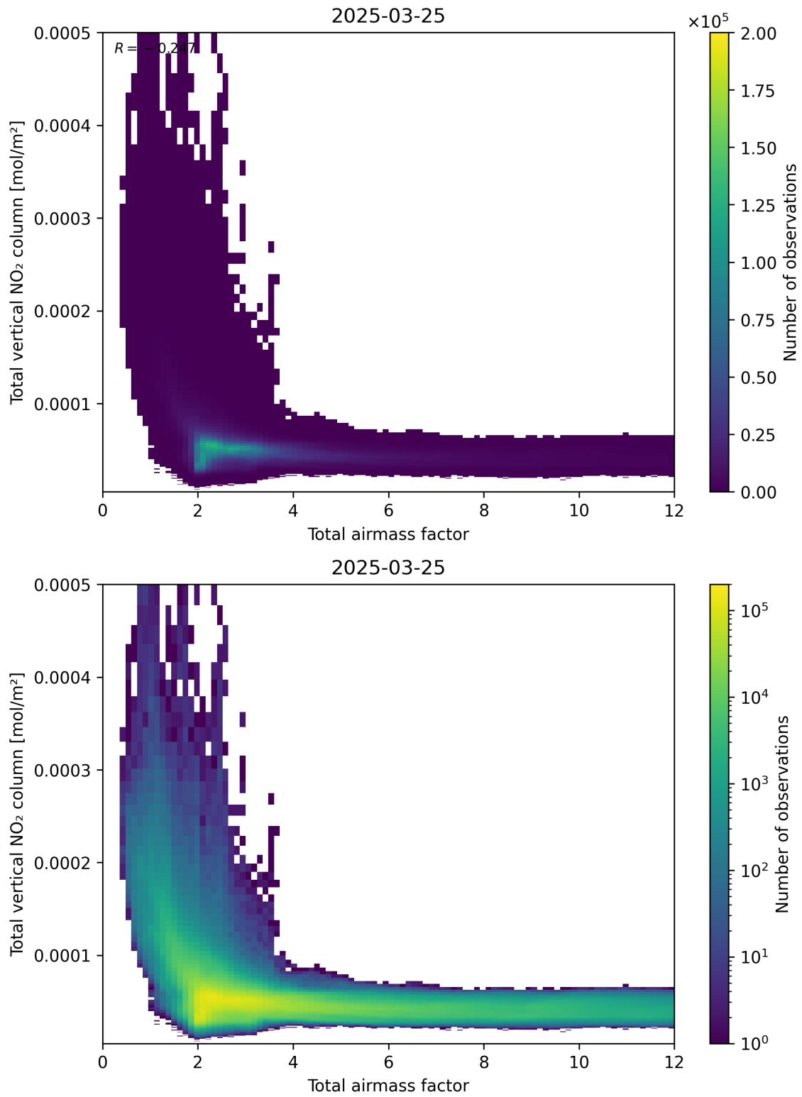
Figure 67: Scatter density plot of “Total airmass factor” against “Total vertical NO 2 column” for 2025-03-25 to 2025-03-26.
