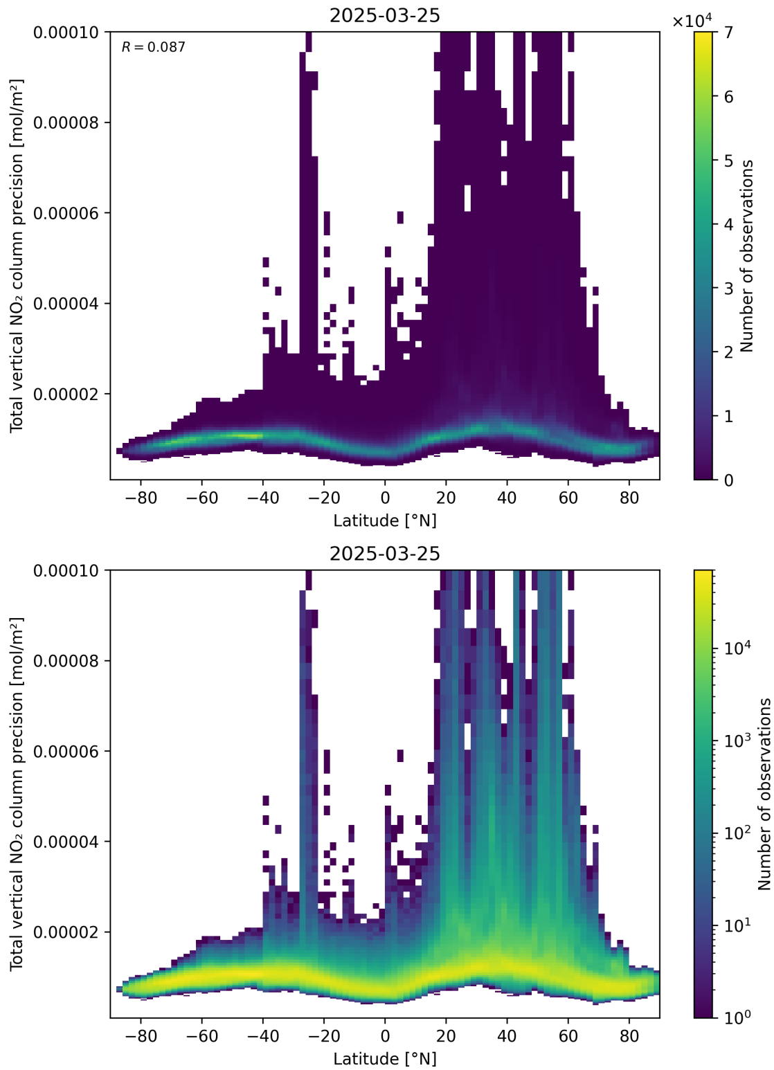
Figure 91: Scatter density plot of “Latitude” against “Total vertical NO 2 column precision” for 2025-03-25 to 2025-03-26.
