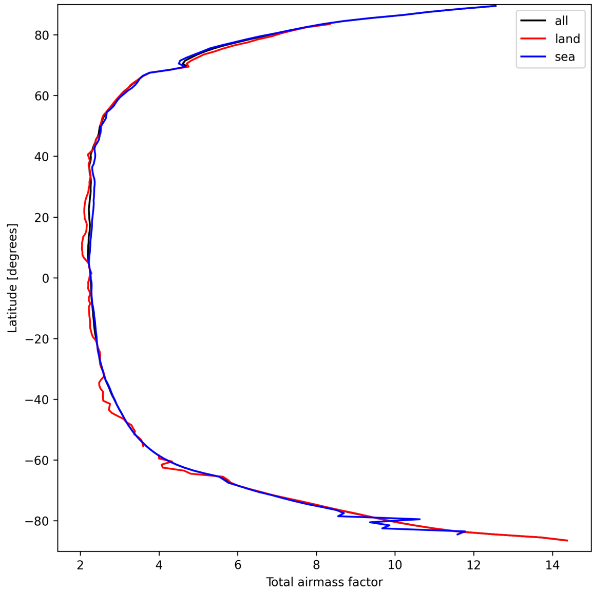
Figure 15: Zonal average of “Total airmass factor” for 2025-03-25 to 2025-03-26.
