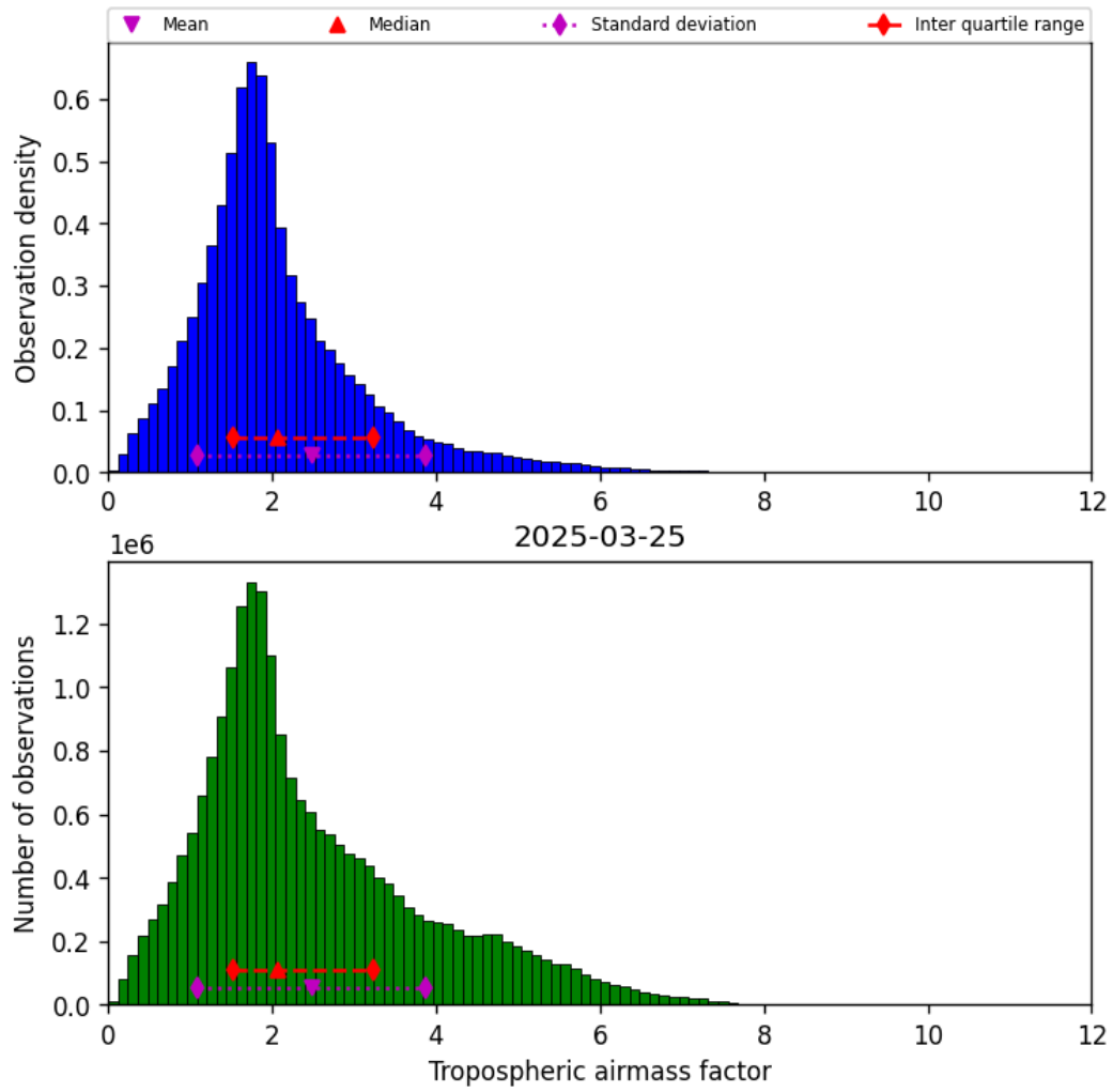
Figure 31: Histogram of “Tropospheric airmass factor” for 2025-03-25 to 2025-03-26
