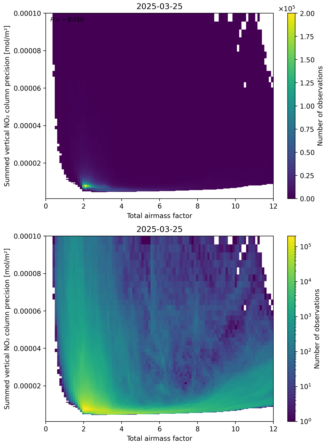
Figure 66: Scatter density plot of “Total airmass factor” against “Summed vertical NO 2 column precision” for 2025-03-25 to 2025-03-26.
