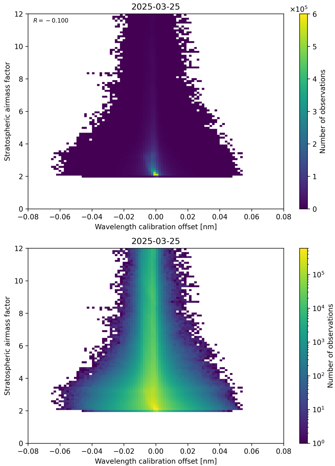
Figure 174: Scatter density plot of “Wavelength calibration offset” against “Stratospheric airmass factor” for 2025-03-25 to 2025-03-26.
