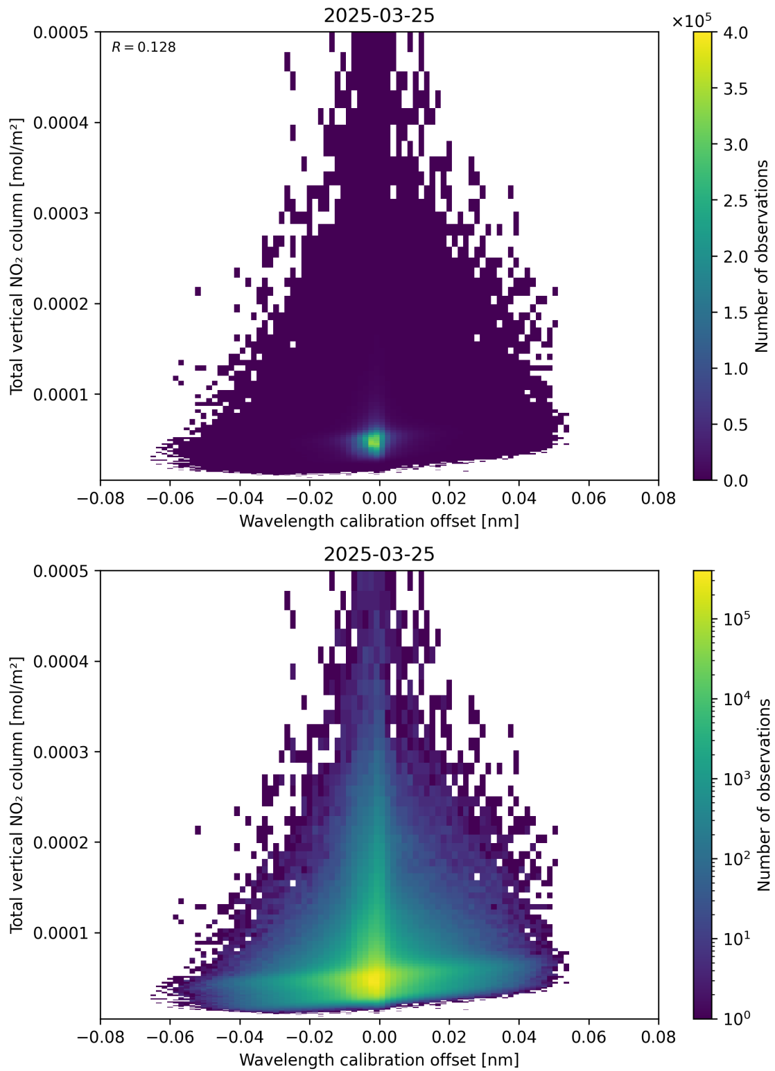
Figure 179: Scatter density plot of “Wavelength calibration offset” against “Total vertical NO 2 column” for 2025-03-25 to 2025-03-26.
