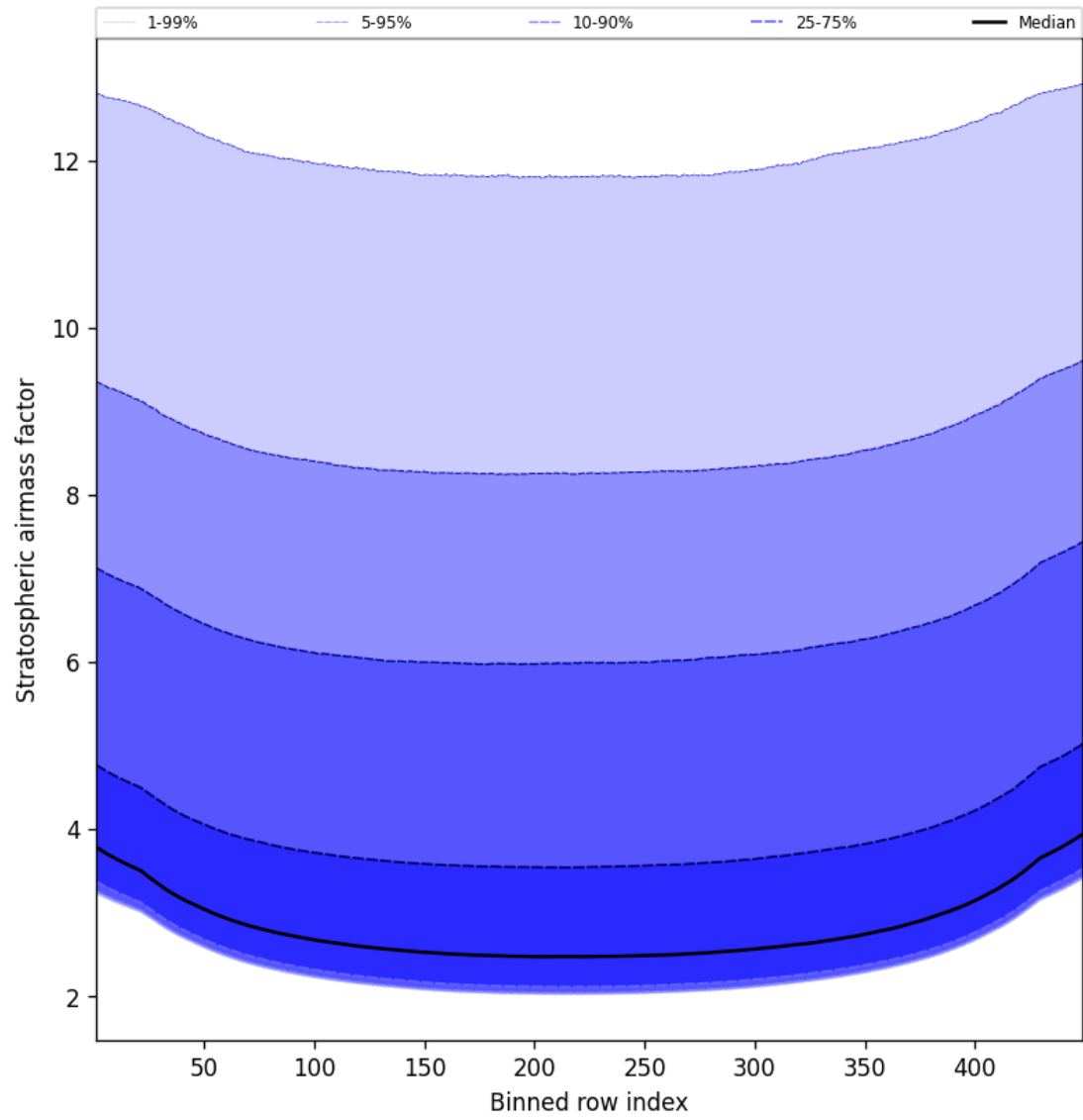
Figure 61: Along track statistics of “Stratospheric airmass factor” for 2025-03-25 to 2025-03-26
