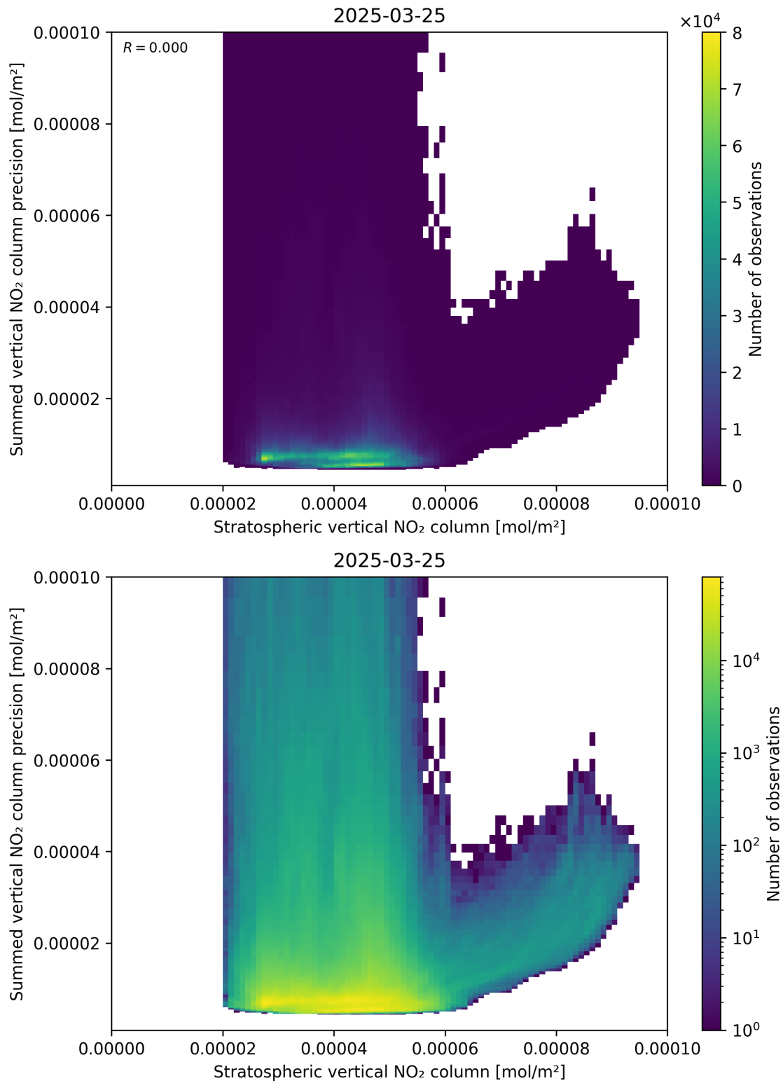
Figure 99: Scatter density plot of “Stratospheric vertical NO 2 column” against “Summed vertical NO 2 column precision” for 2025-03-25 to 2025-03-26.
