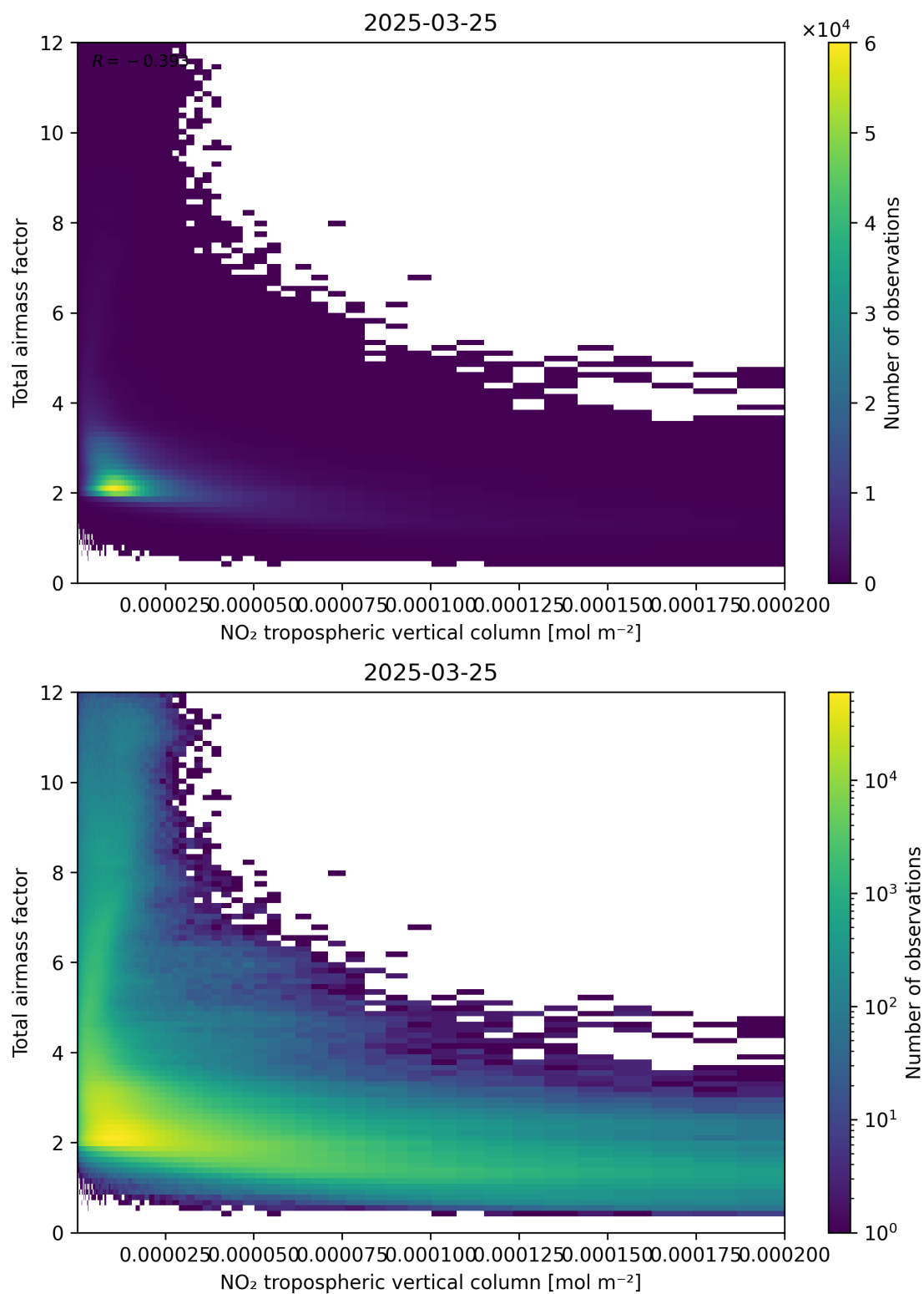
Figure 122: Scatter density plot of “NO 2 tropospheric vertical column” against “Total air mass factor” for 2025-03-25 to 2025-03-26.
