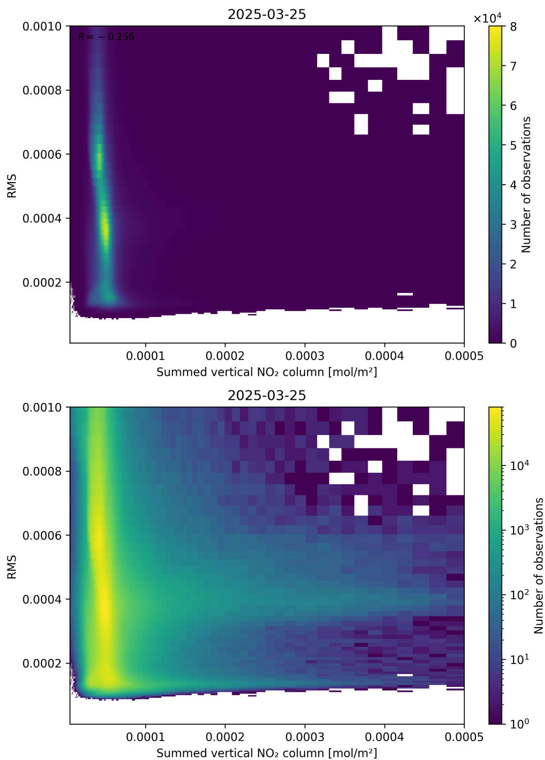
Figure 109: Scatter density plot of “Summed vertical NO 2 column” against “RMS” for 2025-03-25 to 2025-03-26.
