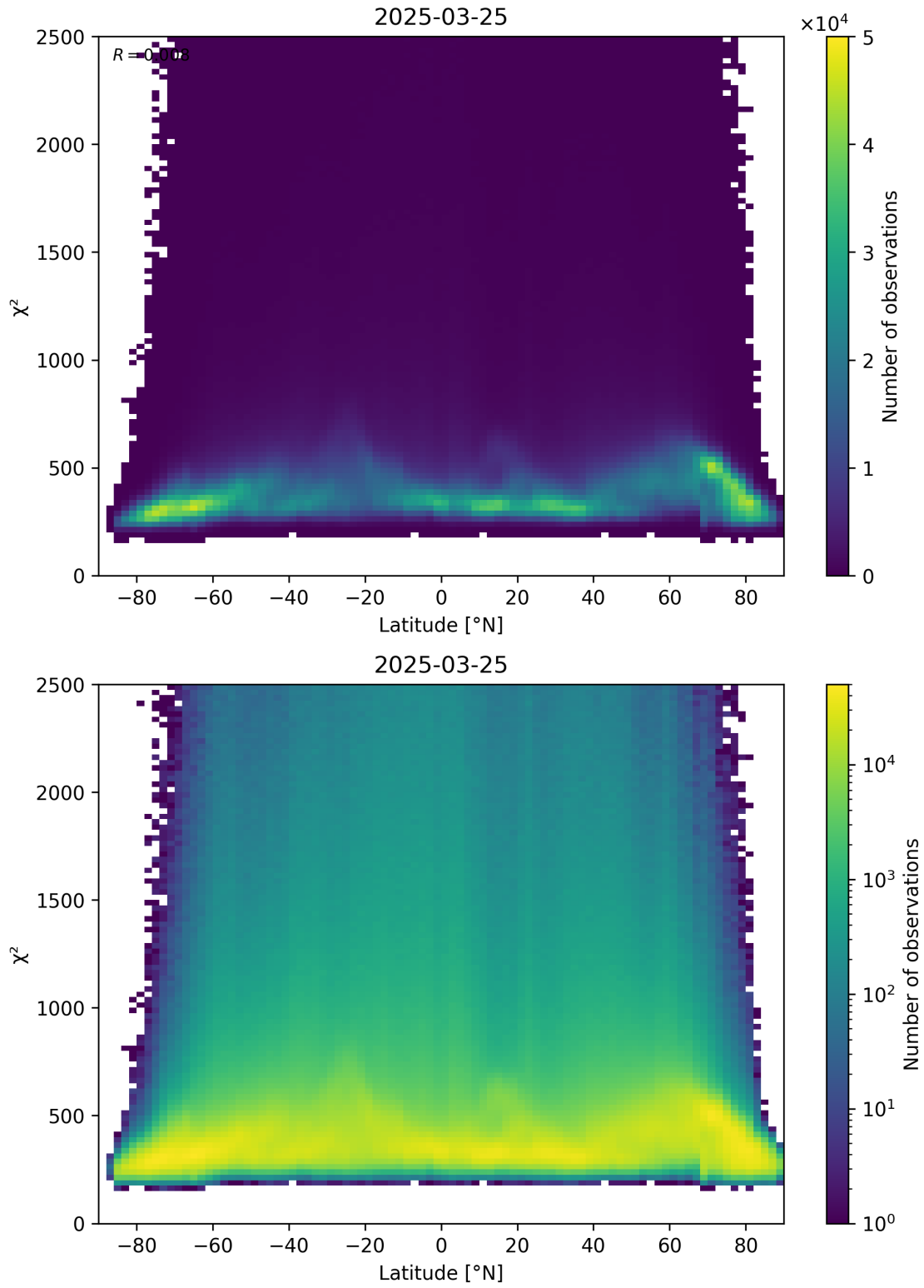
Figure 86: Scatter density plot of “Latitude” against “ \chi^2 ” for 2025-03-25 to 2025-03-26.
