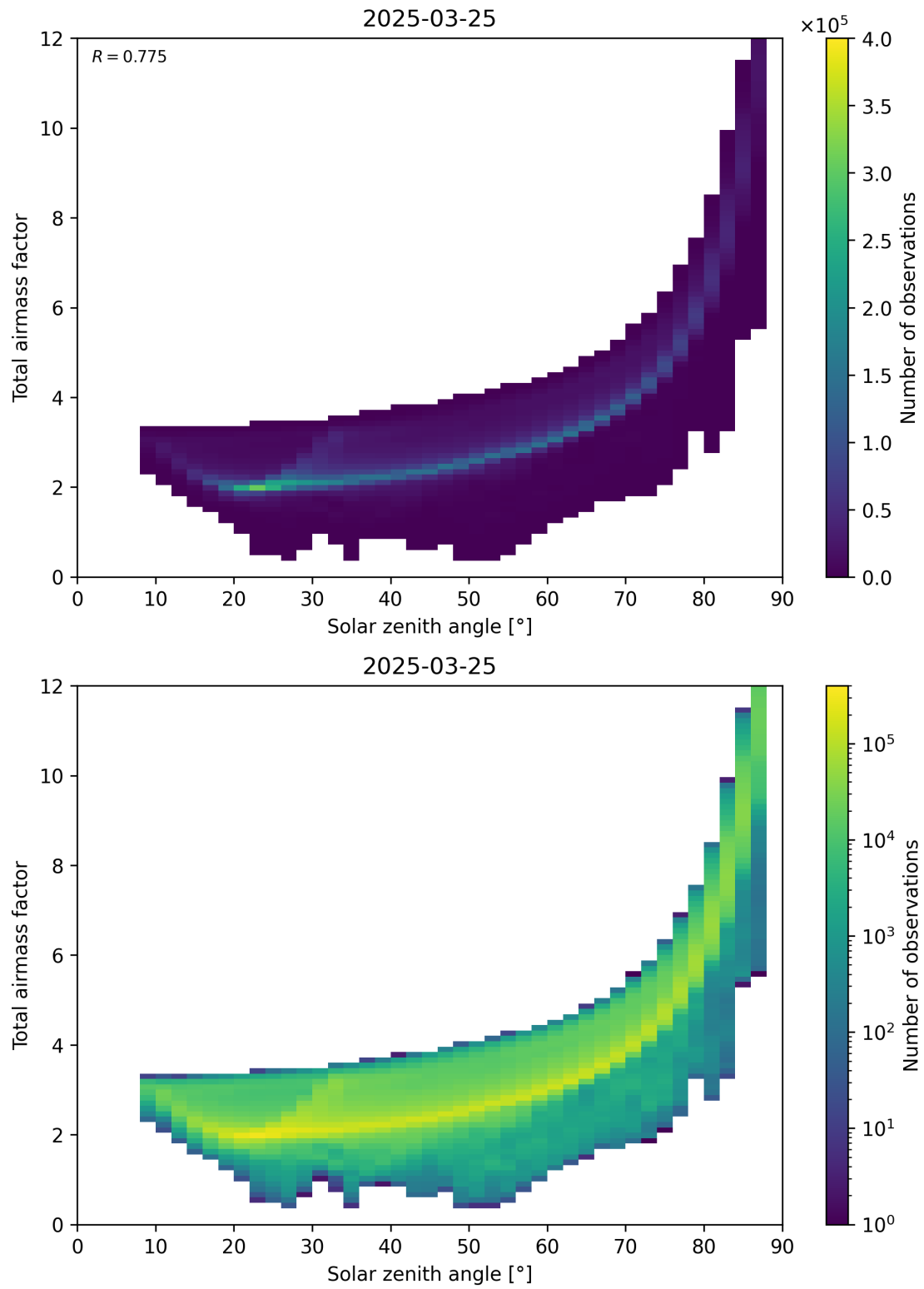
Figure 146: Scatter density plot of “Solar zenith angle” against “Total air mass factor” for 2025-03-25 to 2025-03-26.
