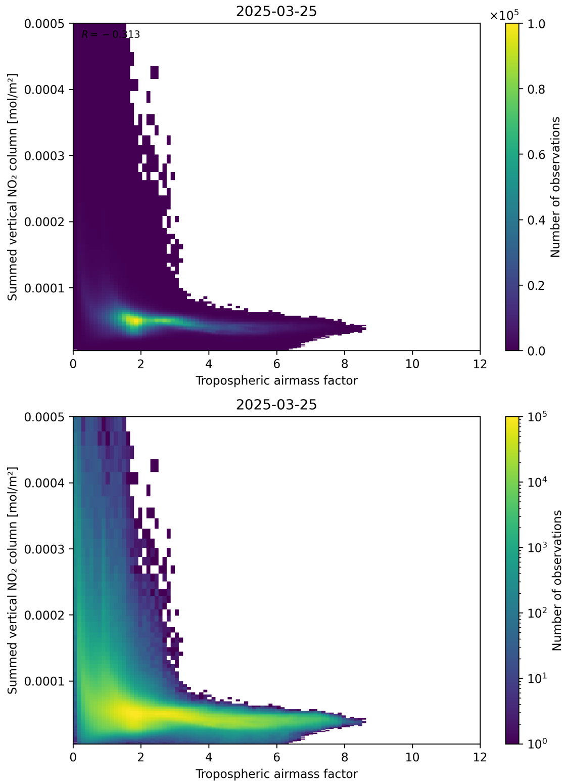
Figure 75: Scatter density plot of “Tropospheric air mass factor” against “Summed vertical NO 2 column” for 2025-03-25 to 2025-03-26.
