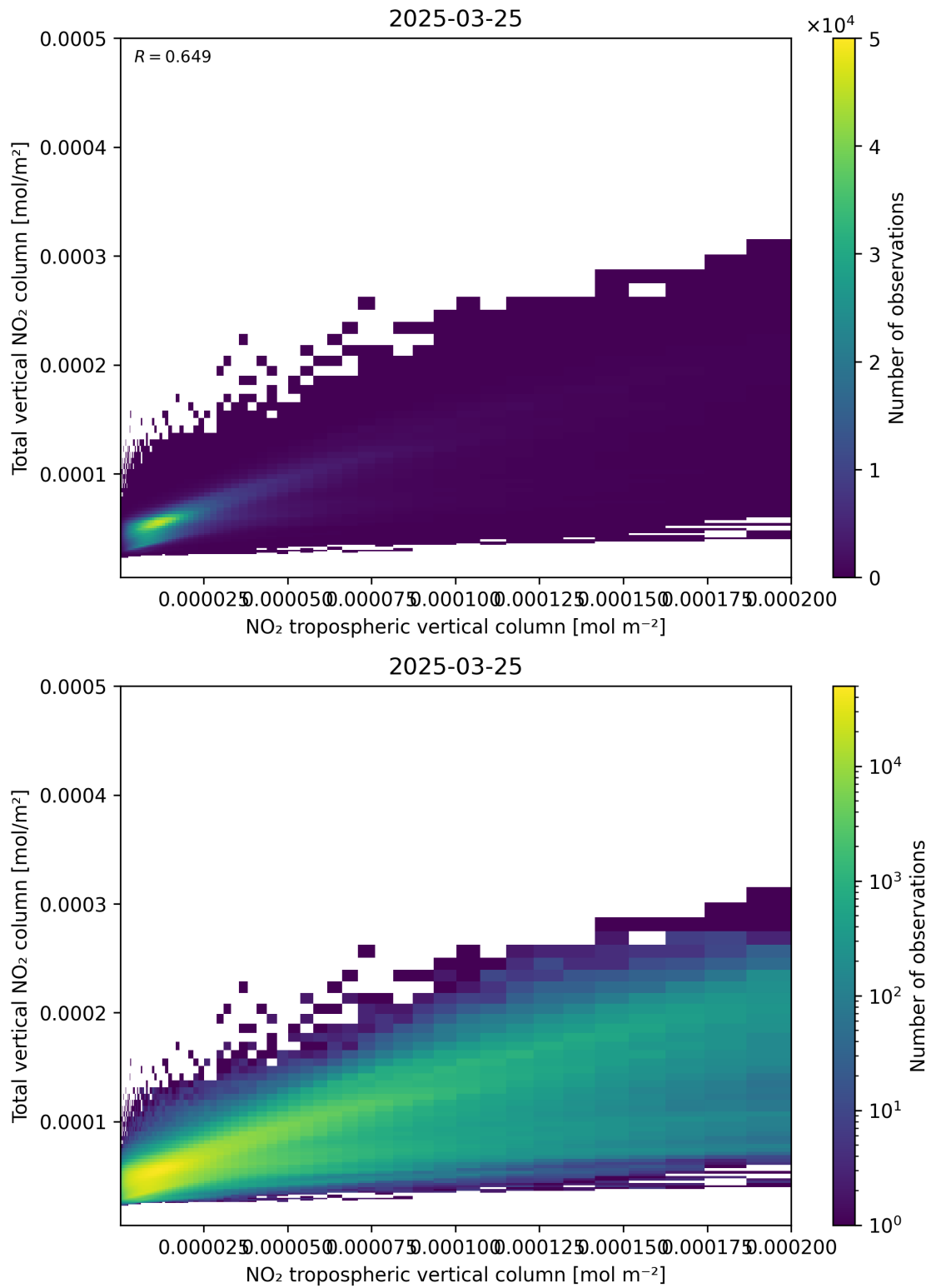
Figure 128: Scatter density plot of “NO 2 tropospheric vertical column” against “Total vertical NO 2 column” for 2025-03-25 to 2025-03-26.
