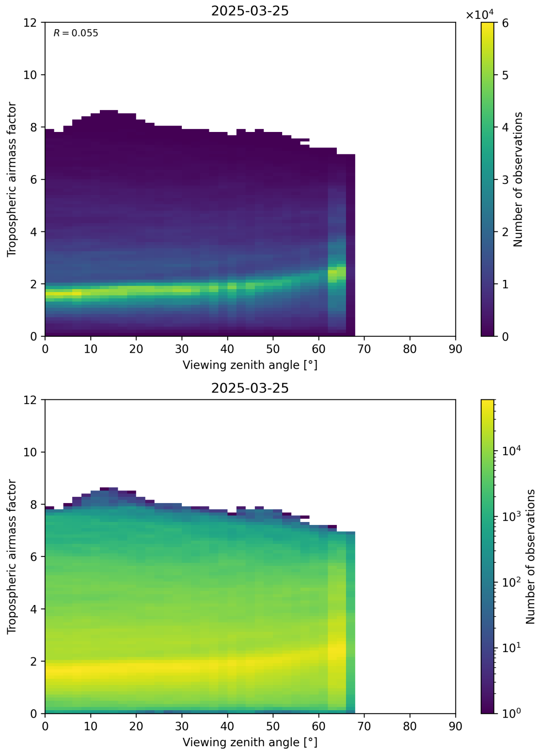
Figure 161: Scatter density plot of “Viewing zenith angle” against “Tropospheric airmass factor” for 2025-03-25 to 2025-03-26.
