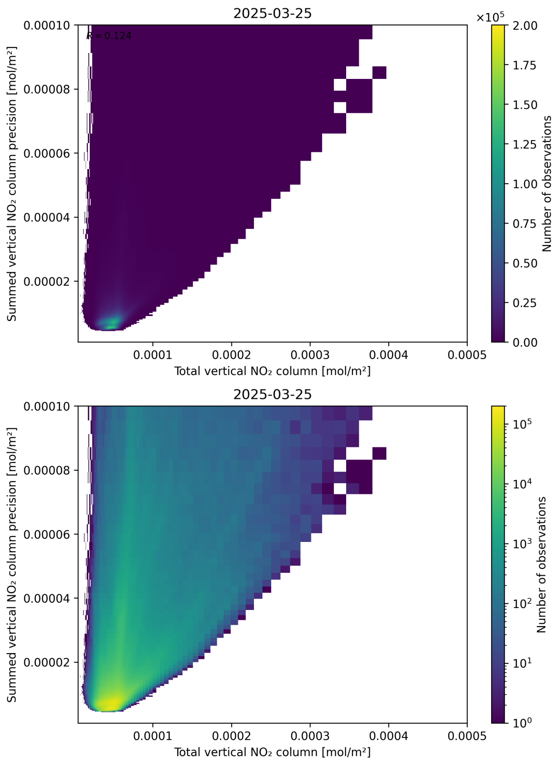
Figure 113: Scatter density plot of “Total vertical NO 2 column” against “Summed vertical NO 2 column precision” for 2025-03-25 to 2025-03-26.
