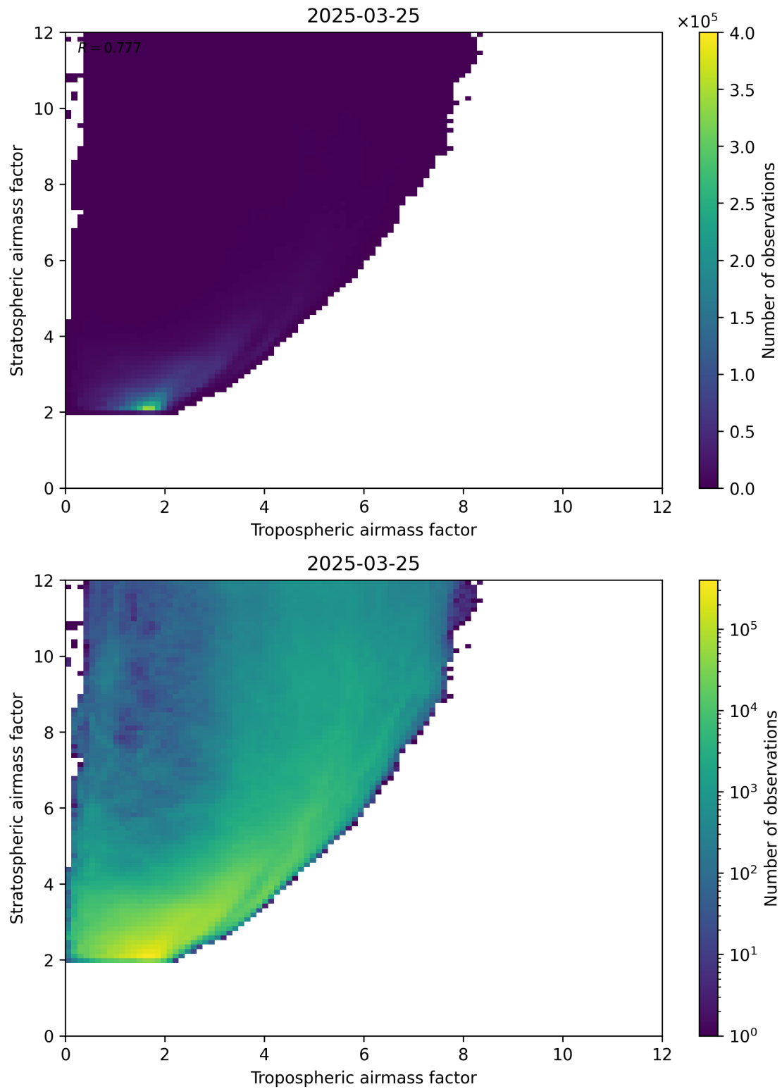
Figure 71: Scatter density plot of “Tropospheric airmass factor” against “Stratospheric airmass factor” for 2025-03-25 to 2025-03-26.
