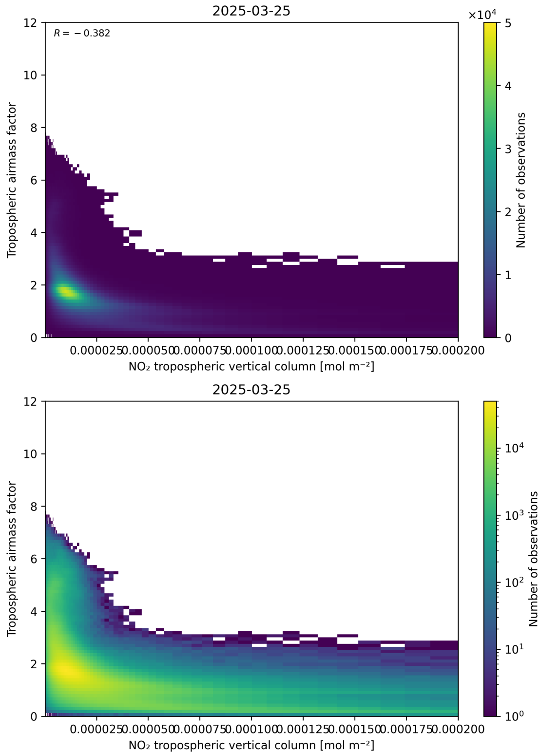
Figure 123: Scatter density plot of “NO 2 tropospheric vertical column” against “Tropospheric air mass factor” for 2025-03-25 to 2025-03-26.
