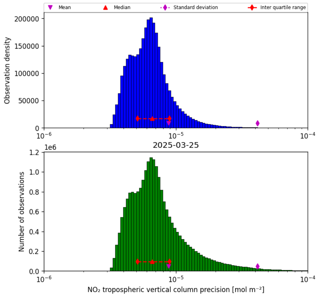
Figure 30: Histogram of “NO 2 tropospheric vertical column precision” for 2025-03-25 to 2025-03-26
