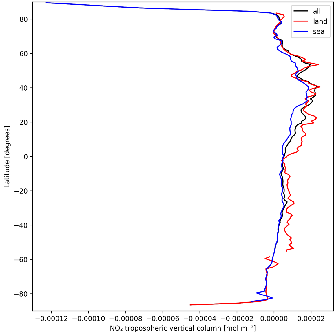
Figure 12: Zonal average of “NO 2 tropospheric vertical column” for 2025-03-25 to 2025-03-26.
