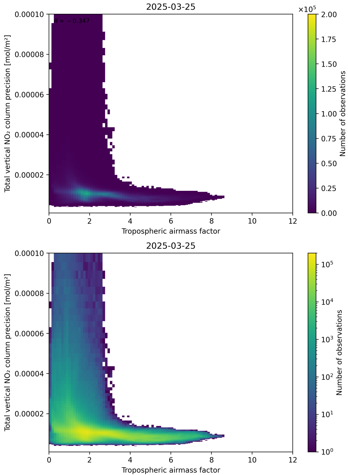
Figure 78: Scatter density plot of “Tropospheric air mass factor” against “Total vertical NO 2 column precision” for 2025-03-25 to 2025-03-26.
