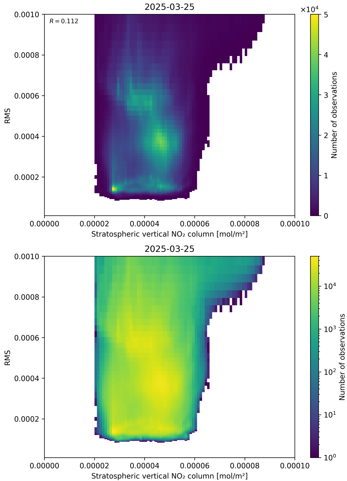
Figure 102: Scatter density plot of “Stratospheric vertical NO 2 column” against “RMS” for 2025-03-25 to 2025-03-26.
