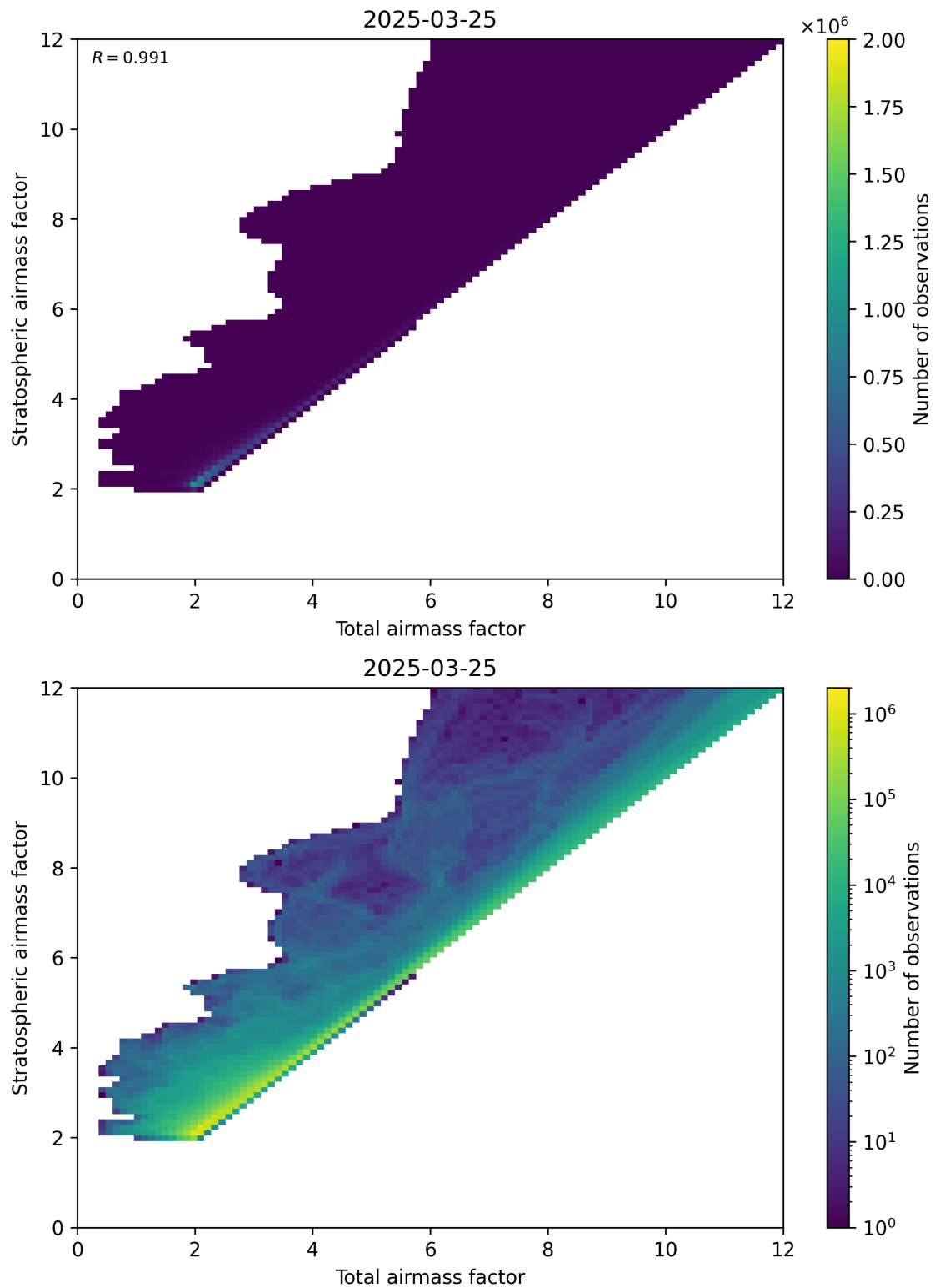
Figure 62: Scatter density plot of “Total airmass factor” against “Stratospheric airmass factor” for 2025-03-25 to 2025-03-26.
