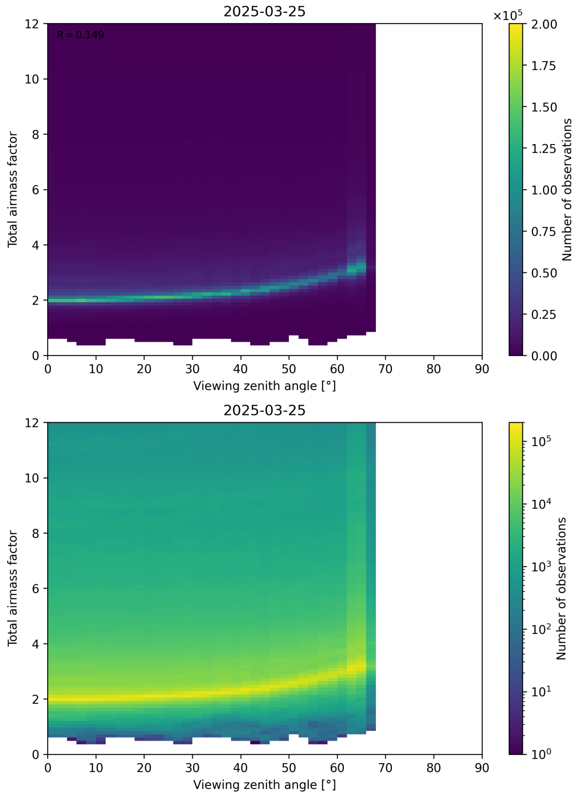
Figure 160: Scatter density plot of “Viewing zenith angle” against “Total airmass factor” for 2025-03-25 to 2025-03-26.
