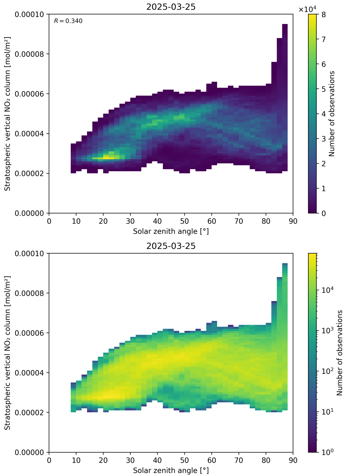
Figure 150: Scatter density plot of “Solar zenith angle” against “Stratospheric vertical NO 2 column” for 2025-03-25 to 2025-03-26.
