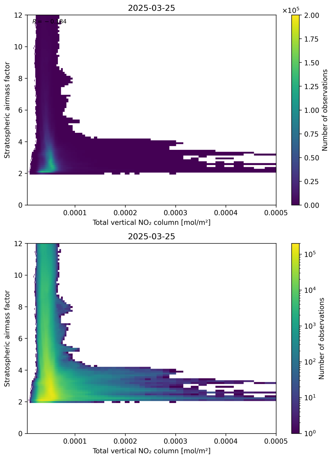
Figure 110: Scatter density plot of “Total vertical NO 2 column” against “Stratospheric airmass factor” for 2025-03-25 to 2025-03-26.
