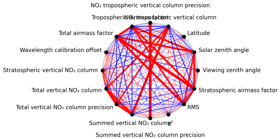
Figure 1: Map of correlation graph for 2025-03-25 to 2025-03-26.
