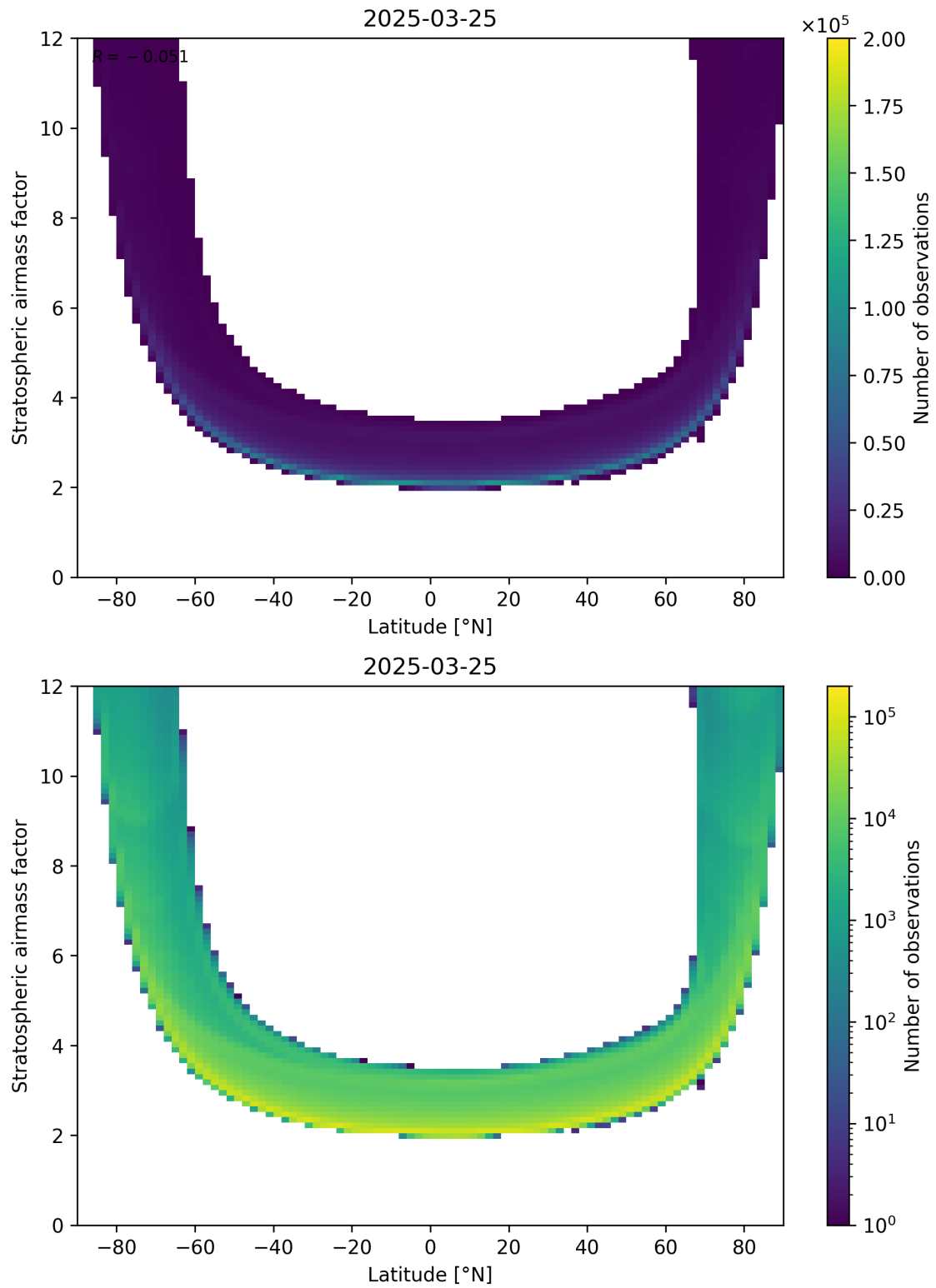
Figure 83: Scatter density plot of “Latitude” against “Stratospheric air mass factor” for 2025-03-25 to 2025-03-26.
