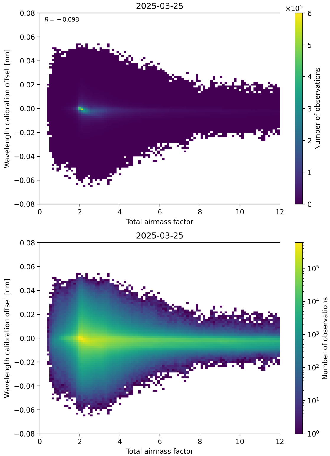
Figure 70: Scatter density plot of “Total airmass factor” against “Wavelength calibration offset” for 2025-03-25 to 2025-03-26.
