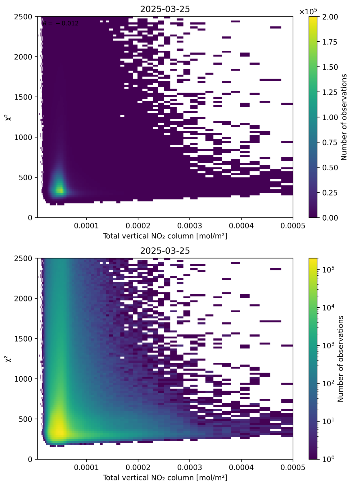
Figure 111: Scatter density plot of “Total vertical NO 2 column” against “ \chi^2 ” for 2025-03-25 to 2025-03-26.
