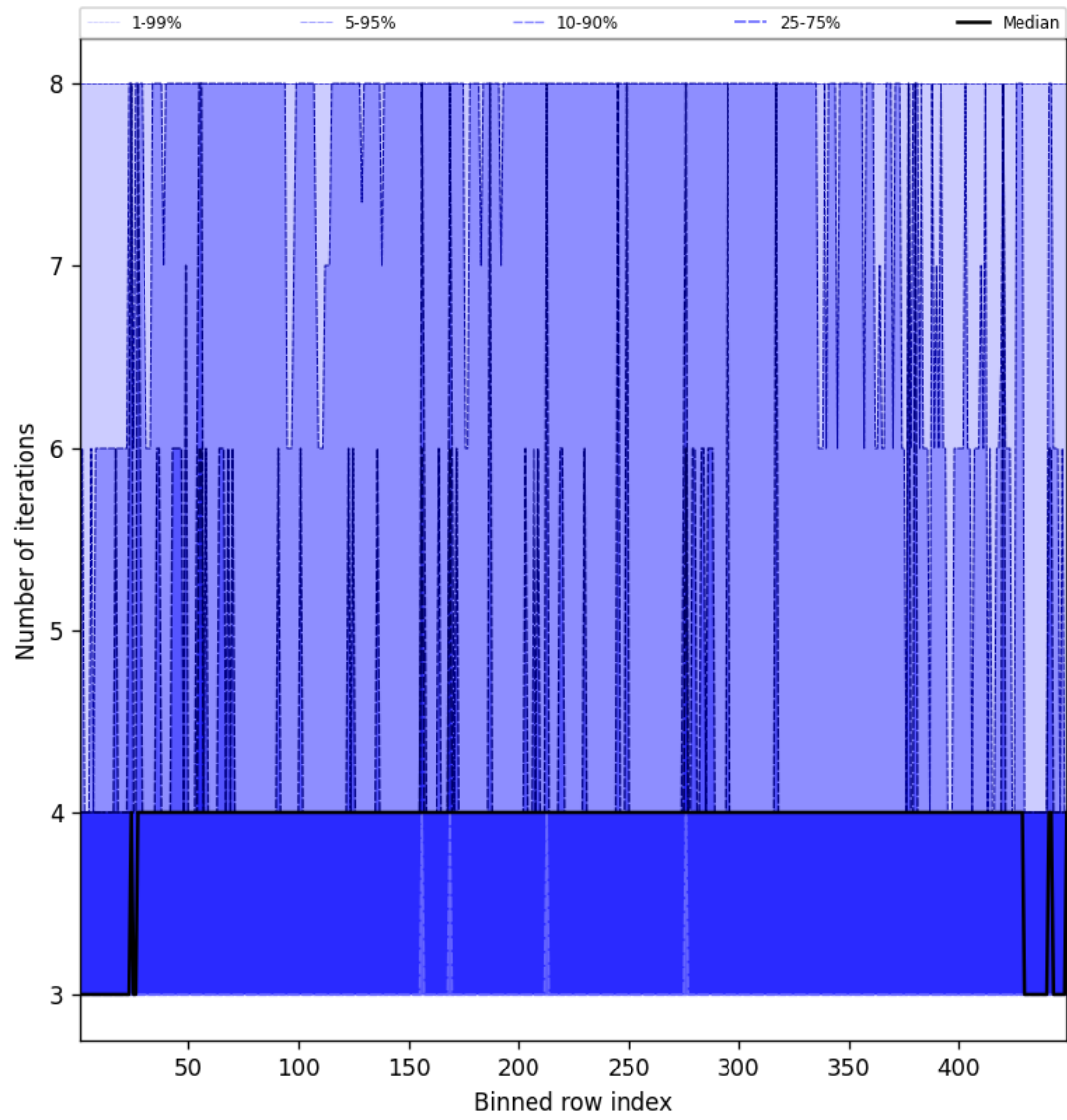
Figure 51: Along track statistics of “Number of iterations” for 2025-03-25 to 2025-03-26
