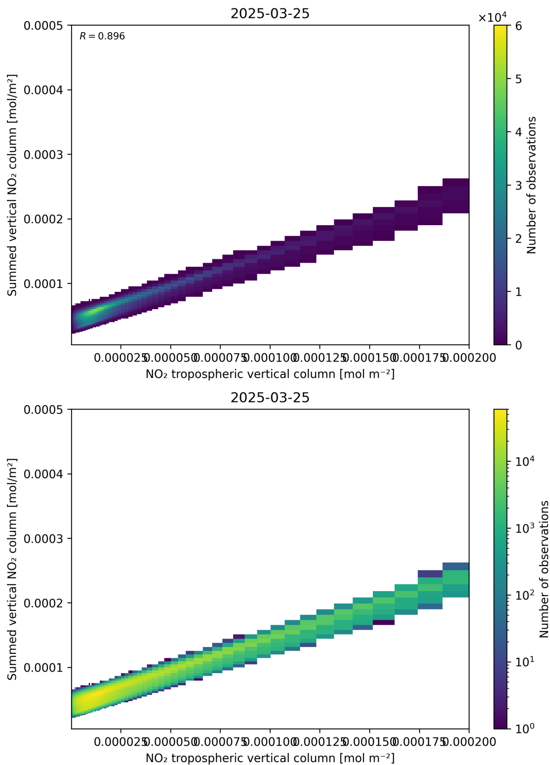
Figure 126: Scatter density plot of “NO 2 tropospheric vertical column” against “Summed vertical NO 2 column” for 2025-03-25 to 2025-03-26.
