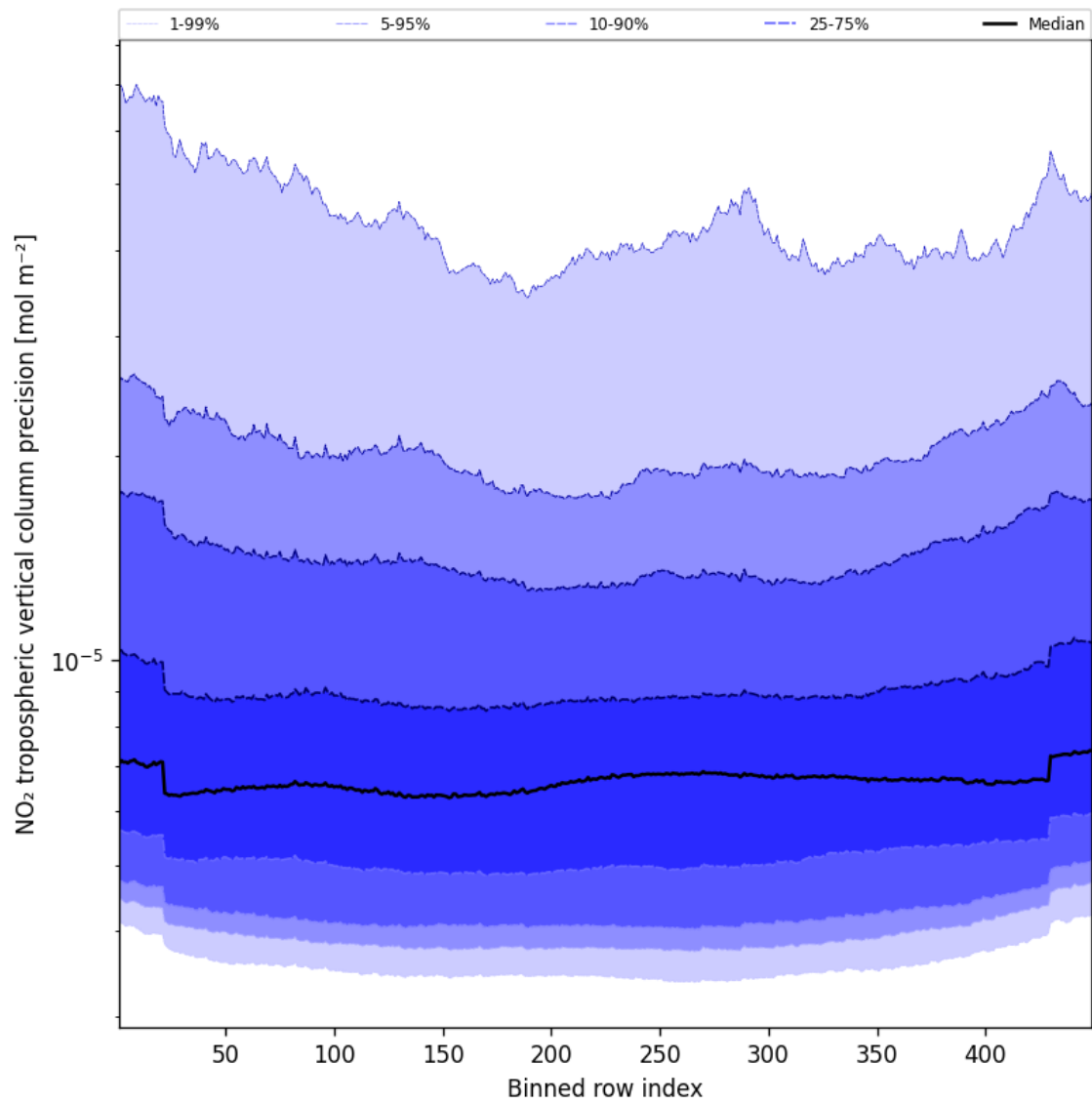
Figure 47: Along track statistics of “NO 2 tropospheric vertical column precision” for 2025-03-25 to 2025-03-26
