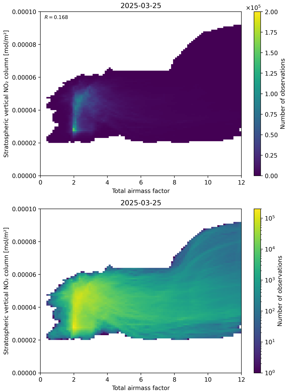
Figure 64: Scatter density plot of “Total airmass factor” against “Stratospheric vertical \text{NO}_2 column” for 2025-03-25 to 2025-03-26.
