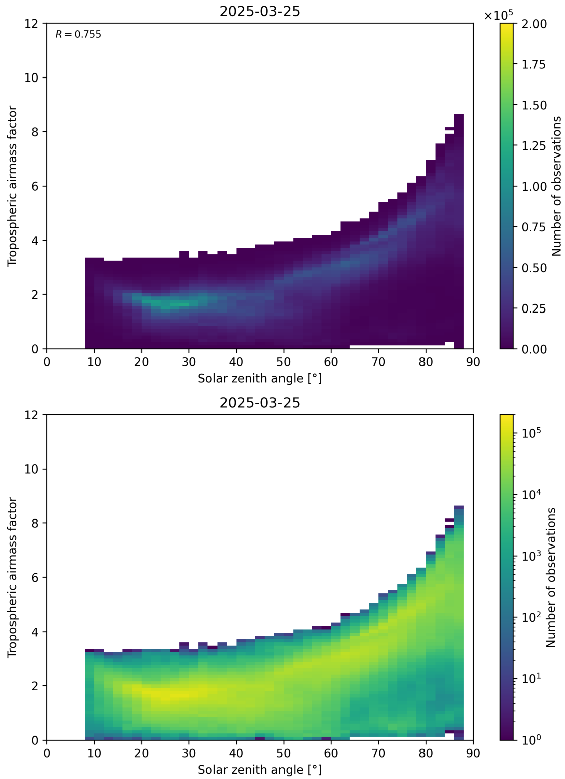
Figure 147: Scatter density plot of “Solar zenith angle” against “Tropospheric airmass factor” for 2025-03-25 to 2025-03-26.
