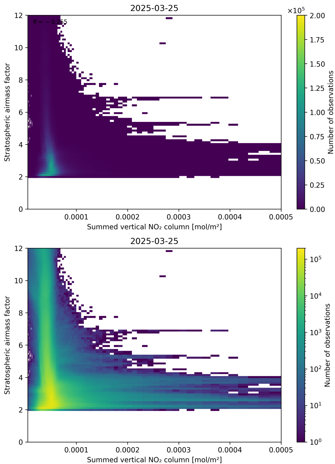
Figure 103: Scatter density plot of “Summed vertical NO 2 column” against “Stratospheric air mass factor” for 2025-03-25 to 2025-03-26.
