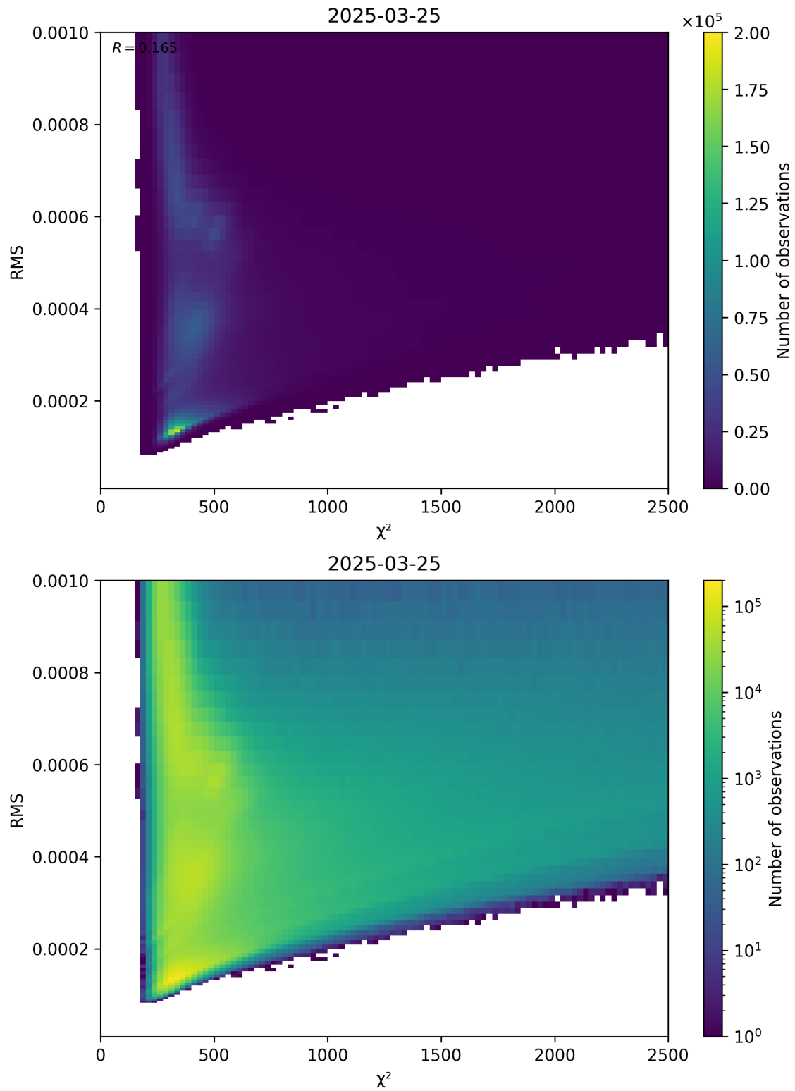
Figure 82: Scatter density plot of “ \chi^2 ” against “RMS” for 2025-03-25 to 2025-03-26.
