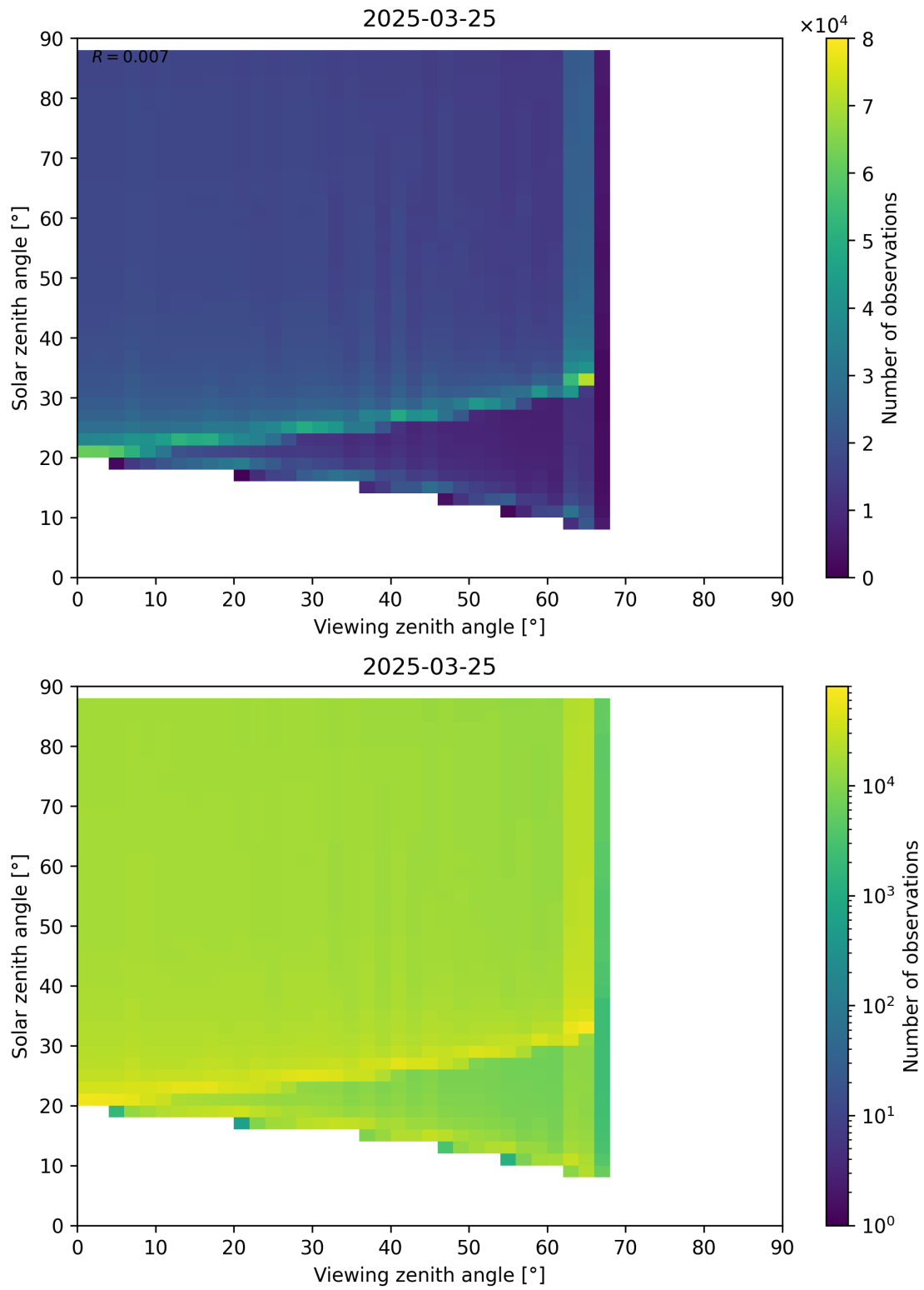
Figure 172: Scatter density plot of “Viewing zenith angle” against “Solar zenith angle” for 2025-03-25 to 2025-03-26.
