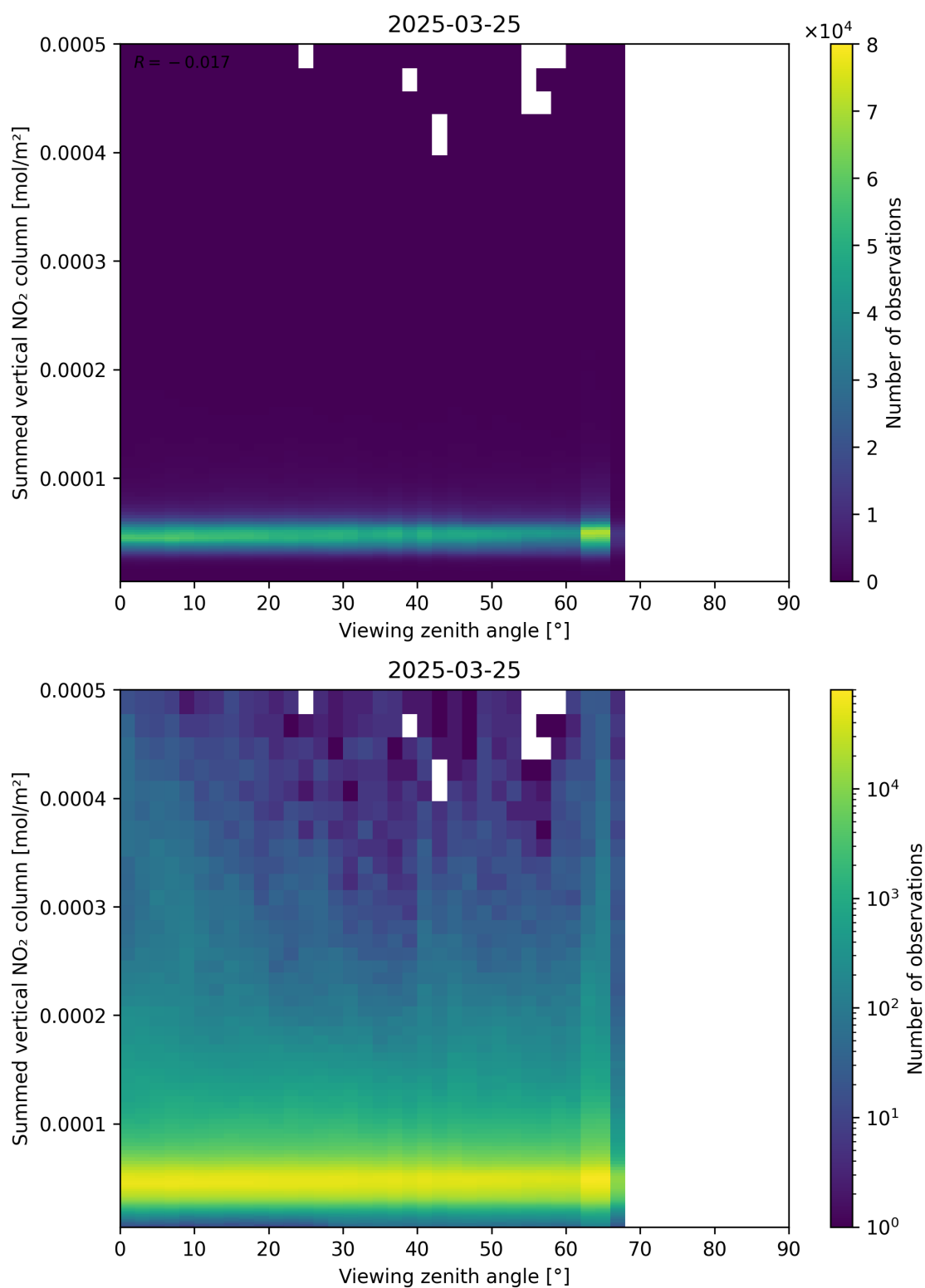
Figure 165: Scatter density plot of “Viewing zenith angle” against “Summed vertical NO 2 column” for 2025-03-25 to 2025-03-26.
