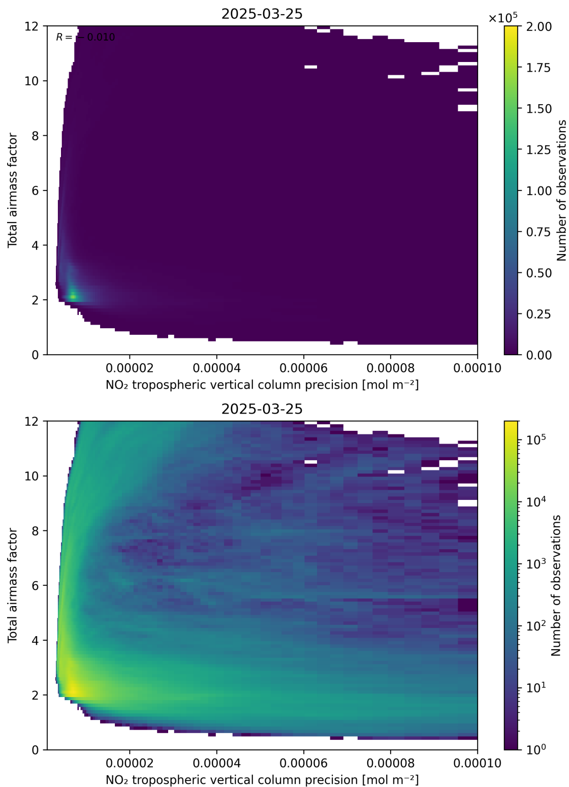
Figure 132: Scatter density plot of “NO 2 tropospheric vertical column precision” against “Total air mass factor” for 2025-03-25 to 2025-03-26.
