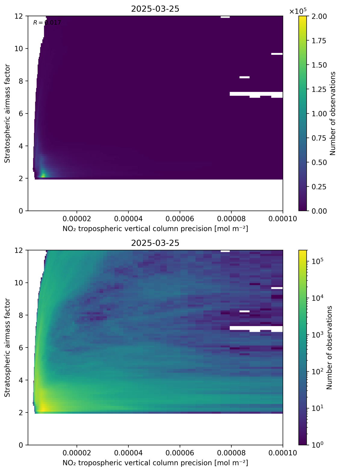
Figure 131: Scatter density plot of “NO 2 tropospheric vertical column precision” against “Stratospheric airmass factor” for 2025-03-25 to 2025-03-26.
