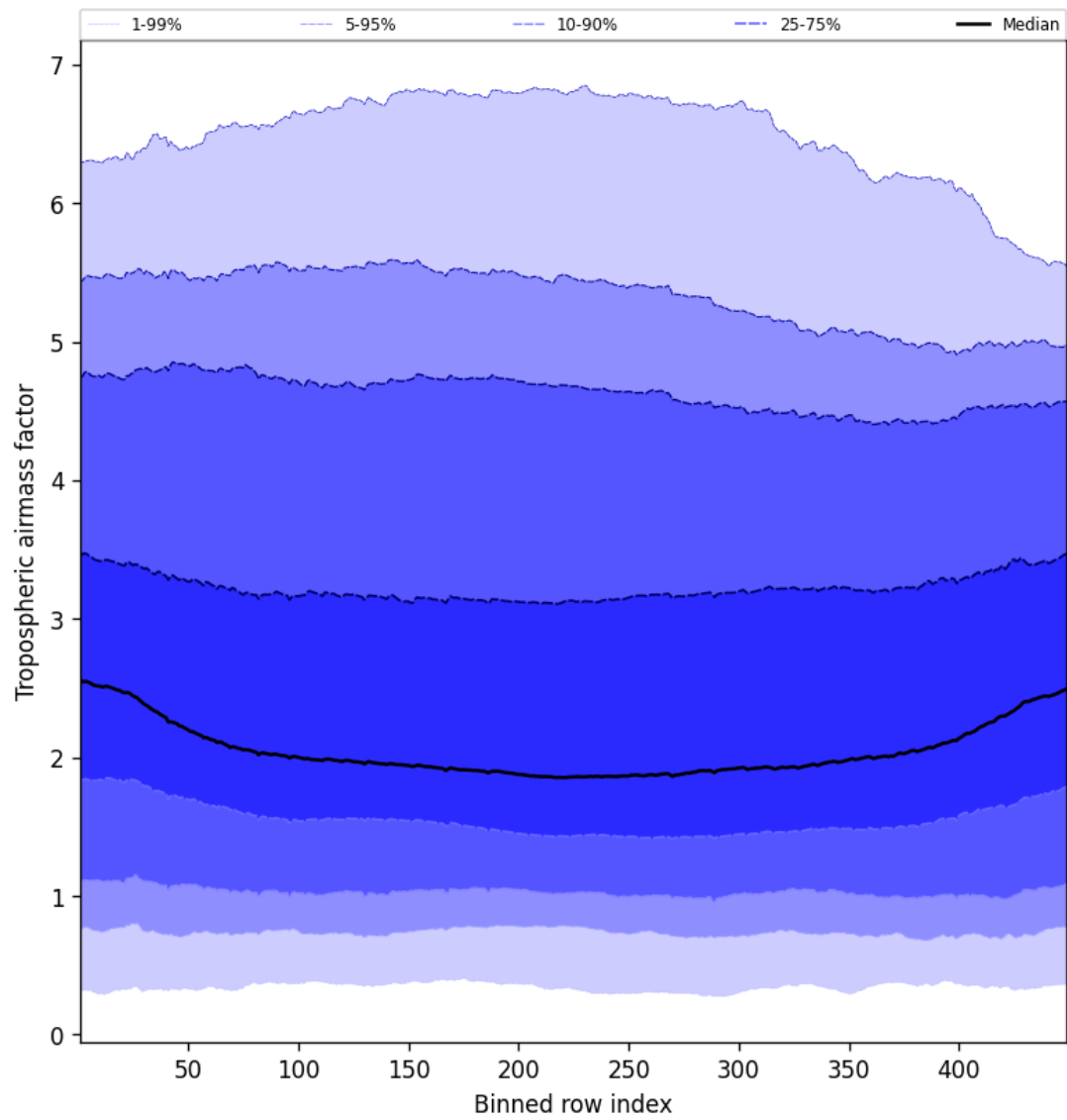
Figure 48: Along track statistics of “Tropospheric airmass factor” for 2025-03-25 to 2025-03-26
