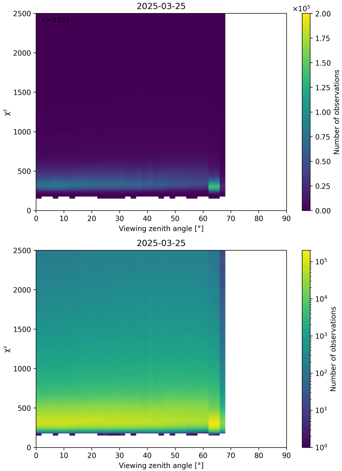
Figure 162: Scatter density plot of “Viewing zenith angle” against “ \chi^2 ” for 2025-03-25 to 2025-03-26.
