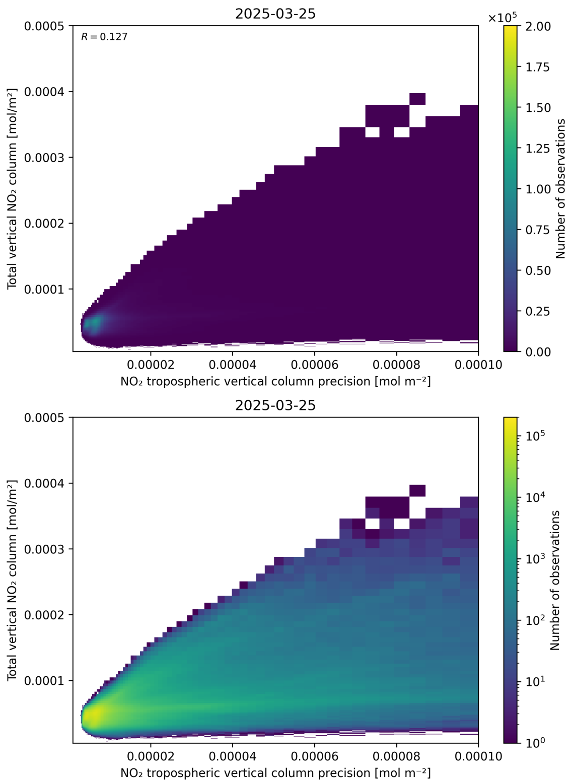
Figure 138: Scatter density plot of “NO 2 tropospheric vertical column precision” against “Total vertical NO 2 column” for 2025-03-25 to 2025-03-26.
