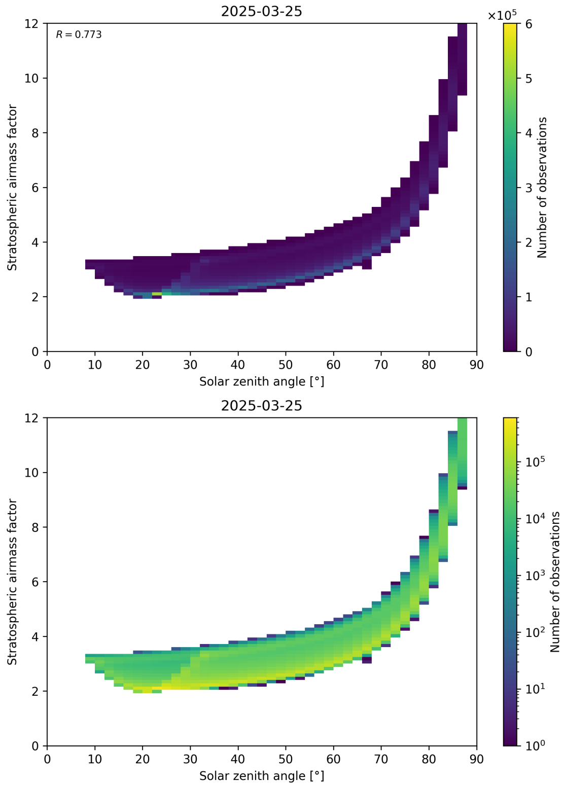
Figure 145: Scatter density plot of “Solar zenith angle” against “Stratospheric airmass factor” for 2025-03-25 to 2025-03-26.
