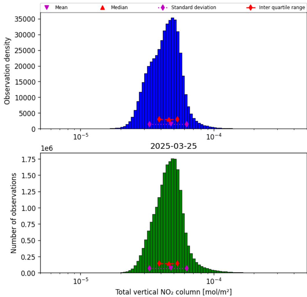
Figure 38: Histogram of "Total vertical NO 2 column" for 2025-03-25 to 2025-03-26
