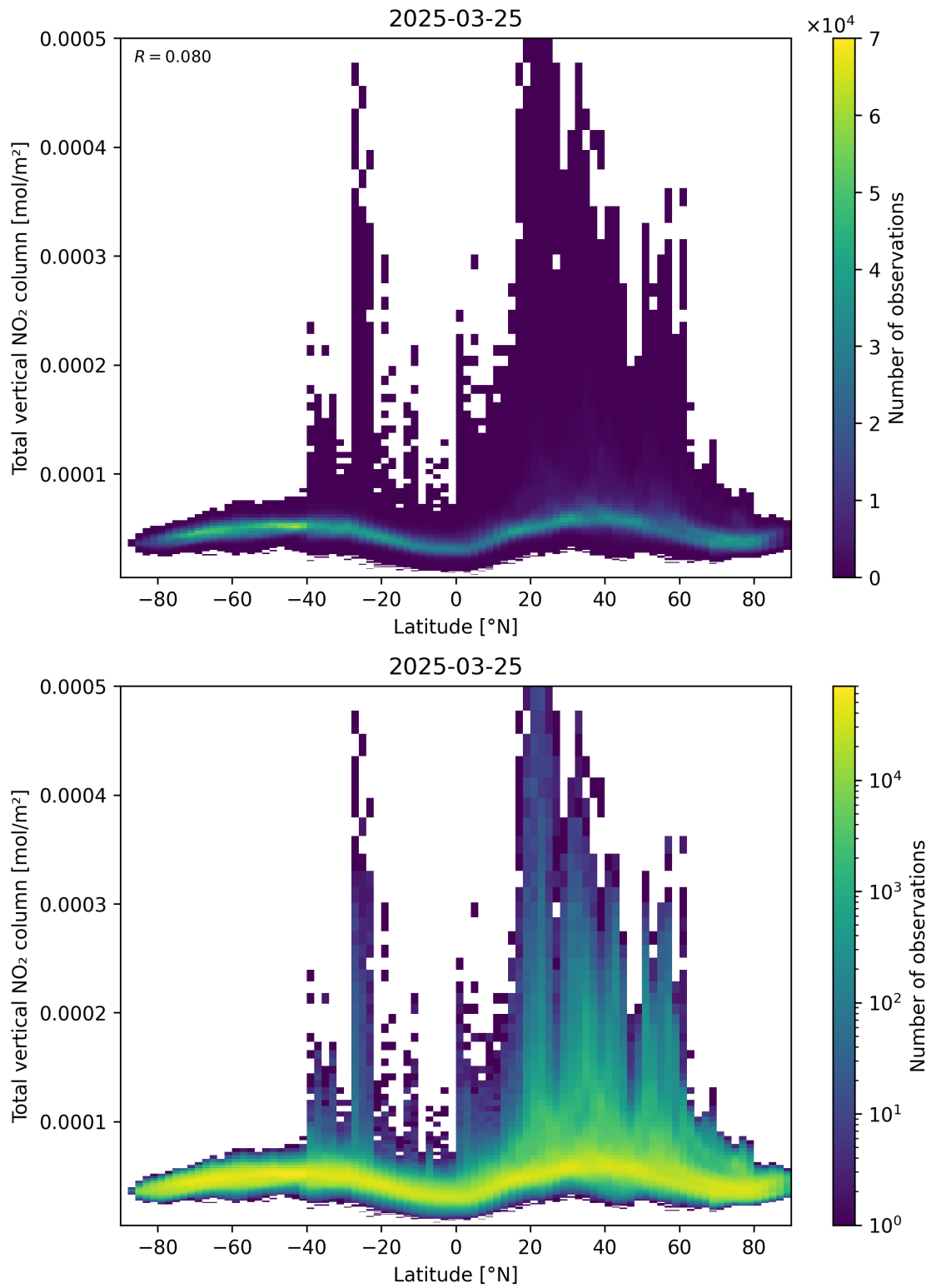
Figure 90: Scatter density plot of “Latitude” against “Total vertical NO 2 column” for 2025-03-25 to 2025-03-26.
