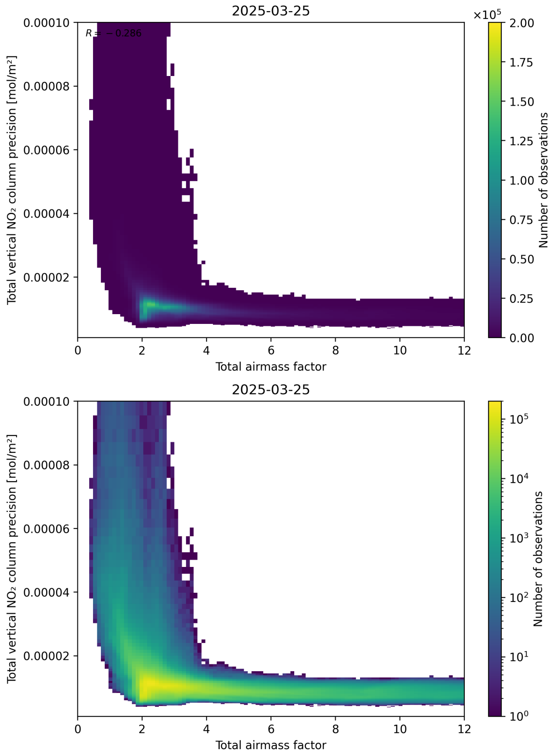
Figure 68: Scatter density plot of “Total airmass factor” against “Total vertical NO 2 column precision” for 2025-03-25 to 2025-03-26.
