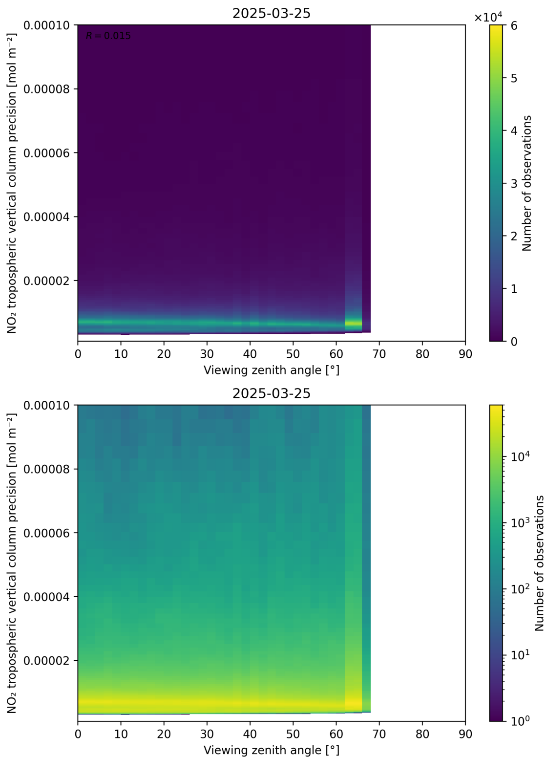
Figure 170: Scatter density plot of “Viewing zenith angle” against “NO 2 tropospheric vertical column precision” for 2025-03-25 to 2025-03-26.
