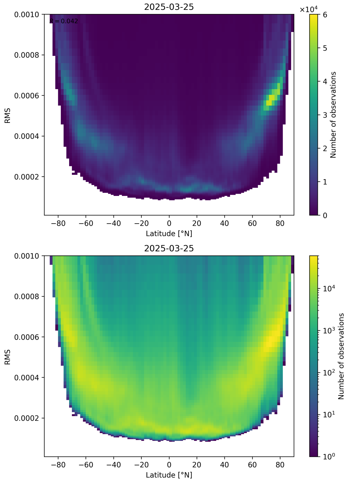
Figure 94: Scatter density plot of “Latitude” against “RMS” for 2025-03-25 to 2025-03-26.
