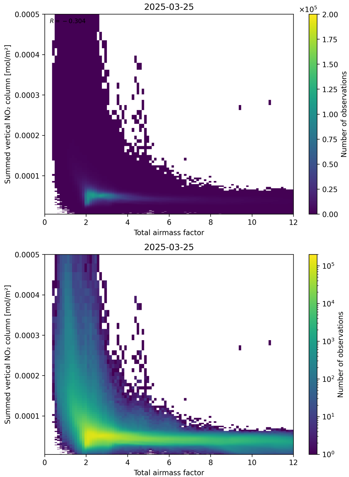
Figure 65: Scatter density plot of “Total airmass factor” against “Summed vertical NO 2 column” for 2025-03-25 to 2025-03-26.
