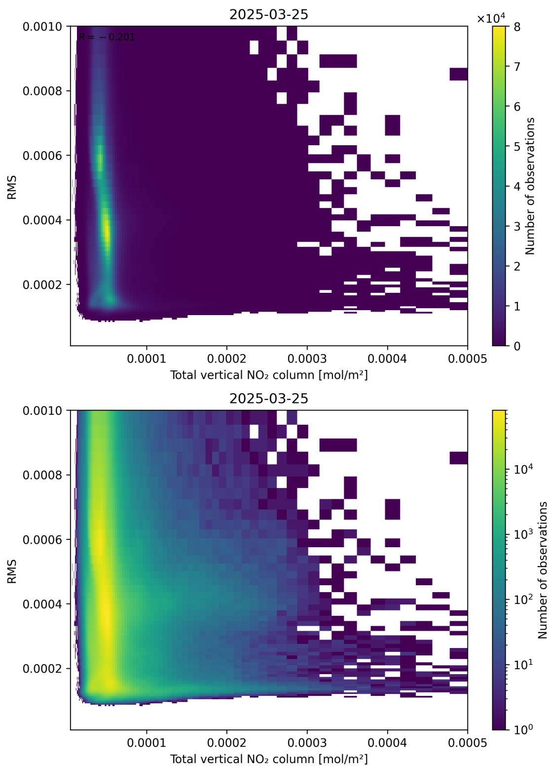
Figure 120: Scatter density plot of “Total vertical NO 2 column” against “RMS” for 2025-03-25 to 2025-03-26.
