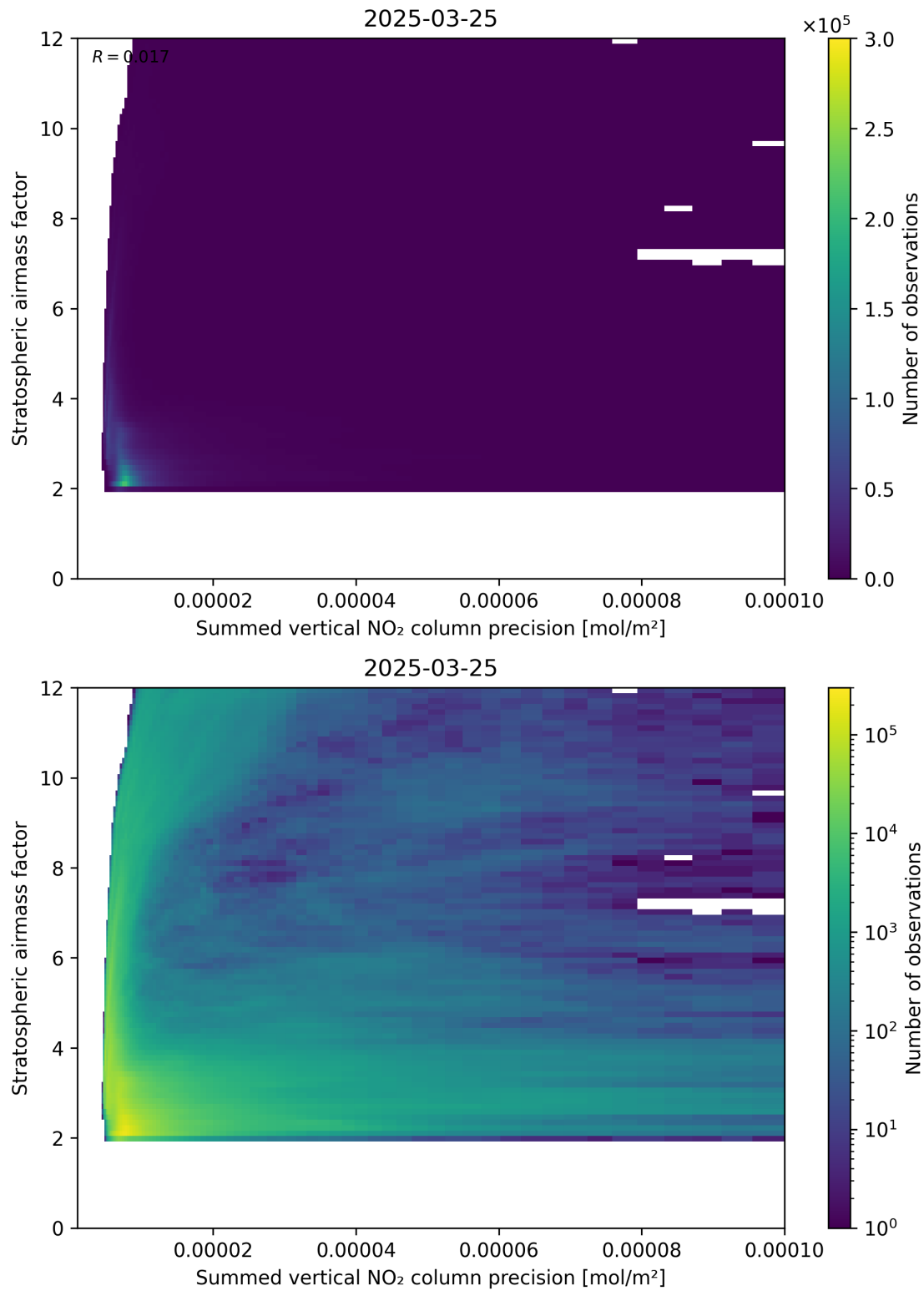
Figure 106: Scatter density plot of “Summed vertical NO 2 column precision” against “Stratospheric airmass factor” for 2025-03-25 to 2025-03-26.
