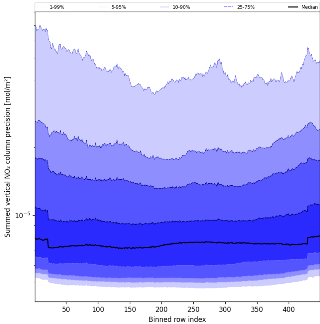
Figure 58: Along track statistics of “Summed vertical NO 2 column precision” for 2025-03-25 to 2025-03-26
