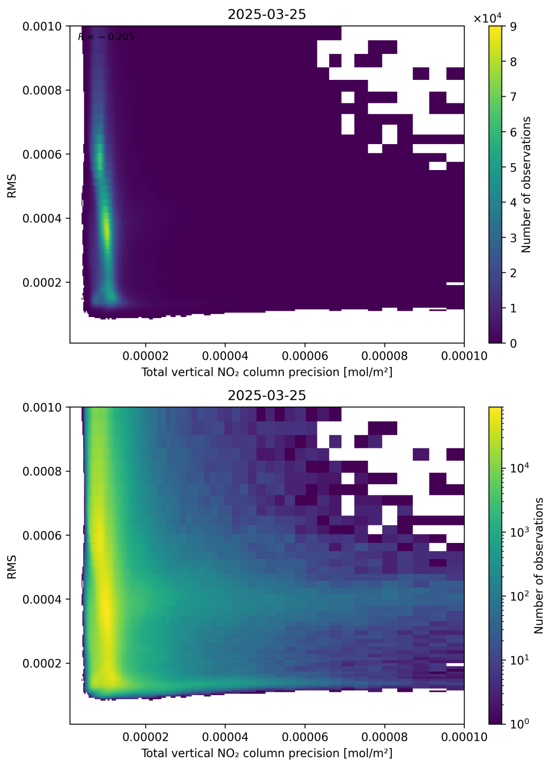
Figure 119: Scatter density plot of “Total vertical NO 2 column precision” against “RMS” for 2025-03-25 to 2025-03-26.
