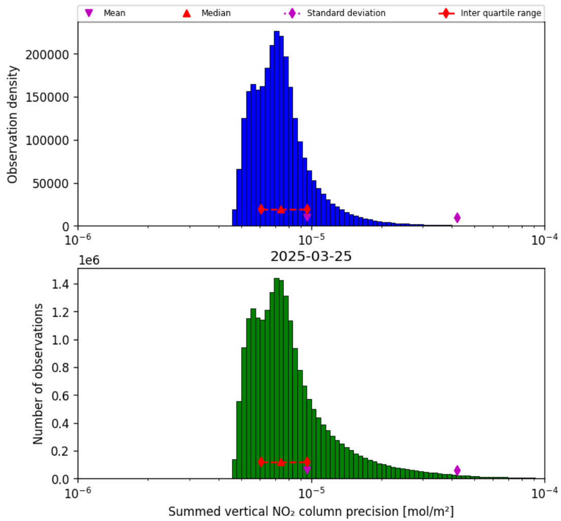
Figure 41: Histogram of "Summed vertical NO 2 column precision" for 2025-03-25 to 2025-03-26
