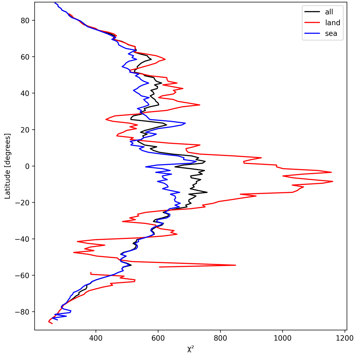
Figure 25: Zonal average of “ \chi^2 ” for 2025-03-25 to 2025-03-26.
