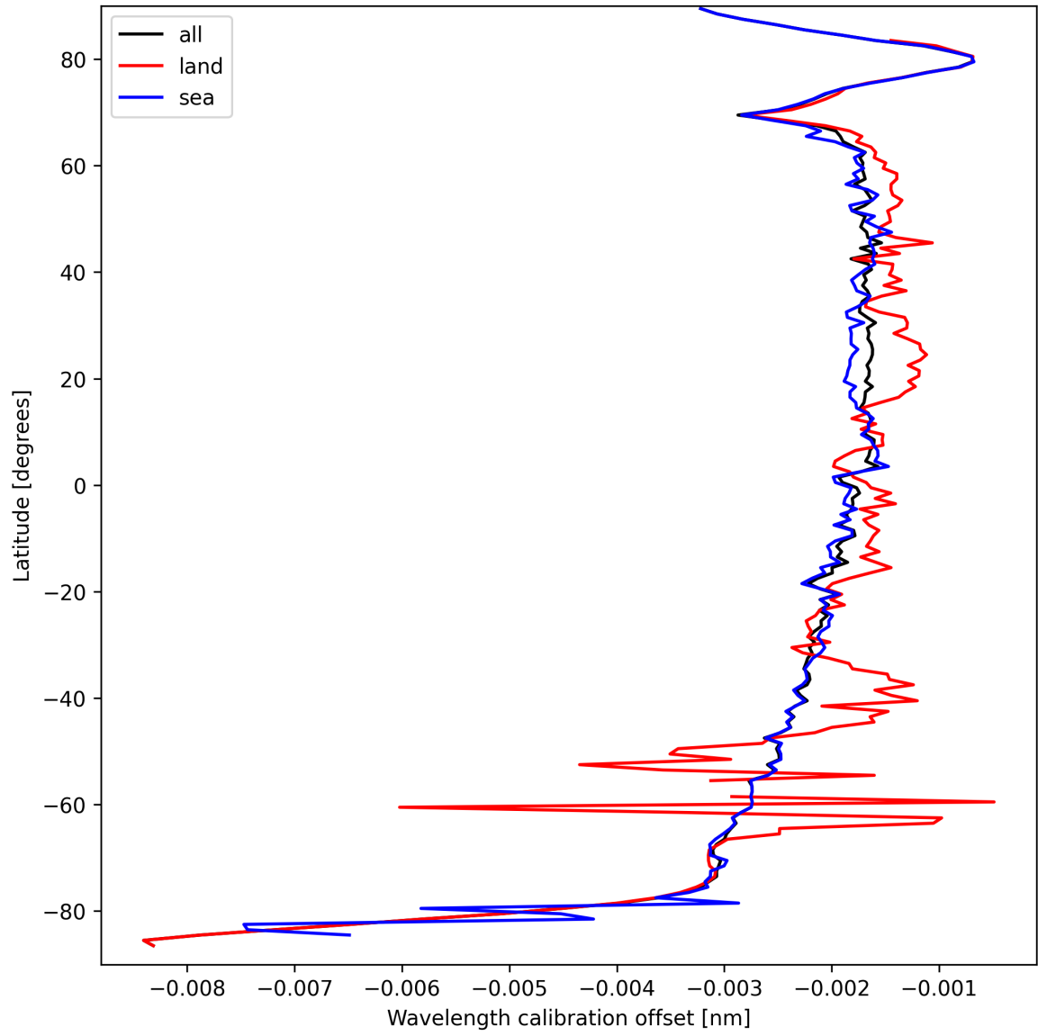
Figure 18: Zonal average of “Wavelength calibration offset” for 2025-03-25 to 2025-03-26.
