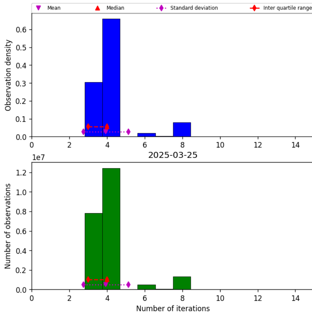
Figure 34: Histogram of “Number of iterations” for 2025-03-25 to 2025-03-26
