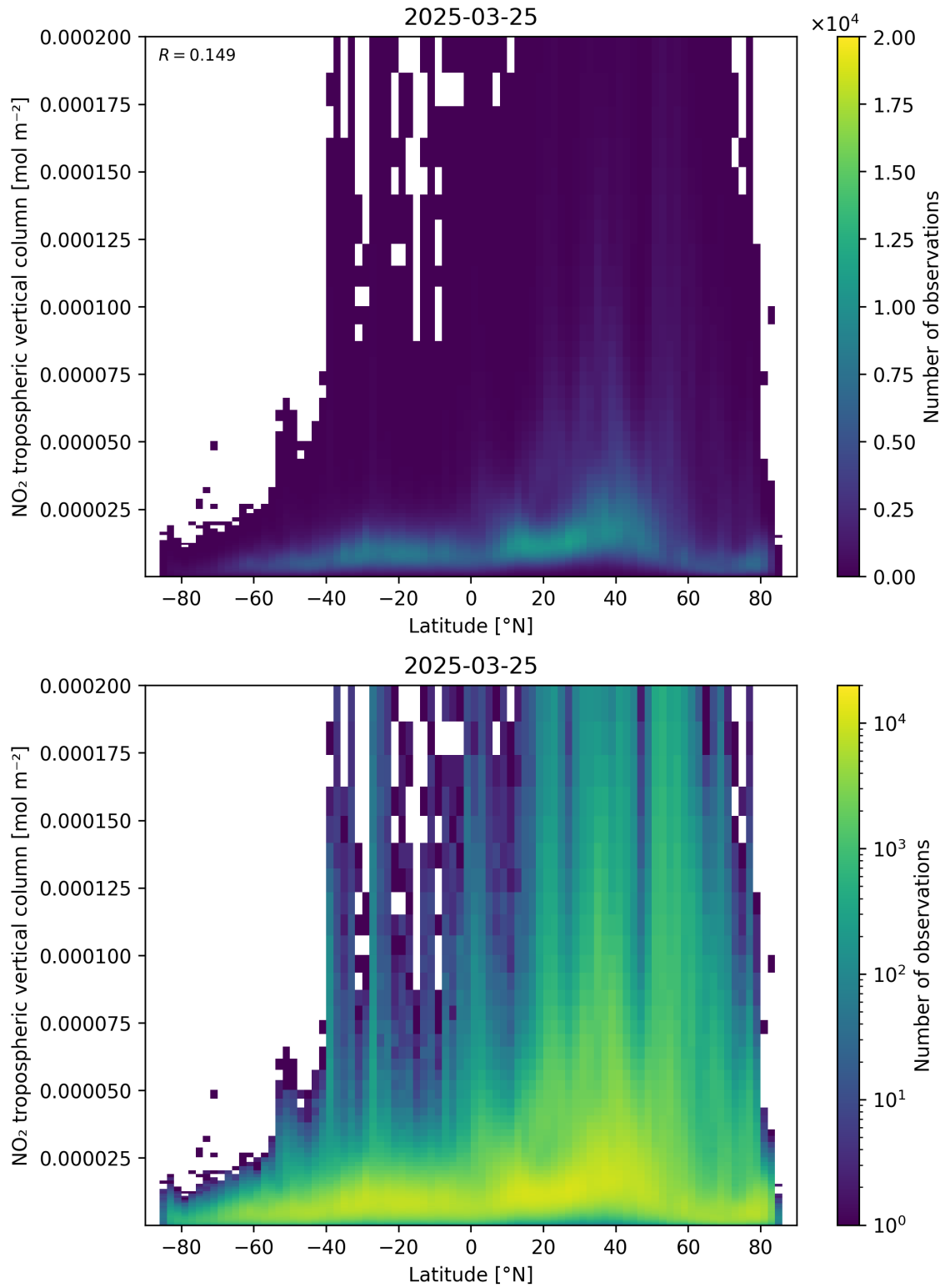
Figure 92: Scatter density plot of “Latitude” against “NO 2 tropospheric vertical column” for 2025-03-25 to 2025-03-26.
