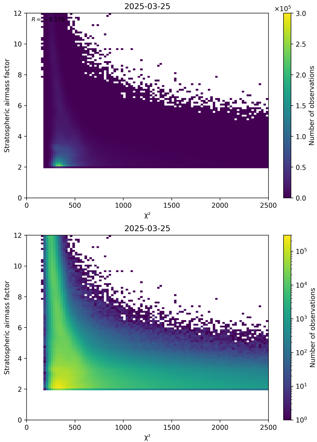
Figure 81: Scatter density plot of “ \chi^2 ” against “Stratospheric airmass factor” for 2025-03-25 to 2025-03-26.
