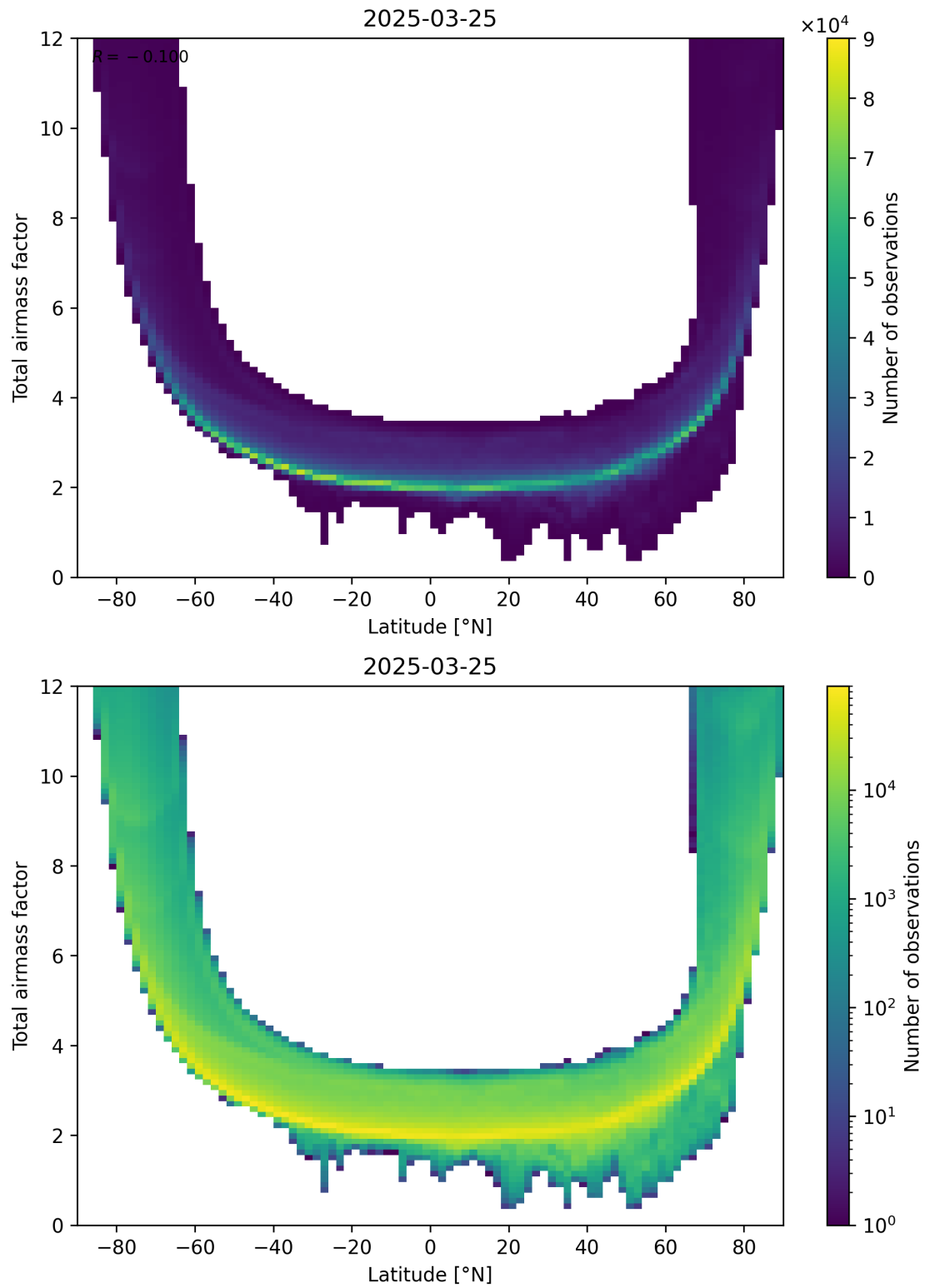
Figure 84: Scatter density plot of “Latitude” against “Total airmass factor” for 2025-03-25 to 2025-03-26.
