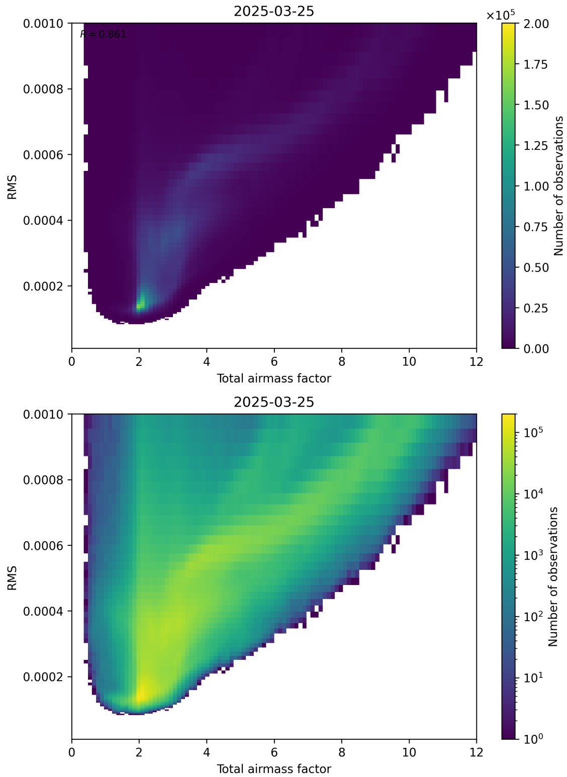
Figure 69: Scatter density plot of “Total airmass factor” against “RMS” for 2025-03-25 to 2025-03-26.
