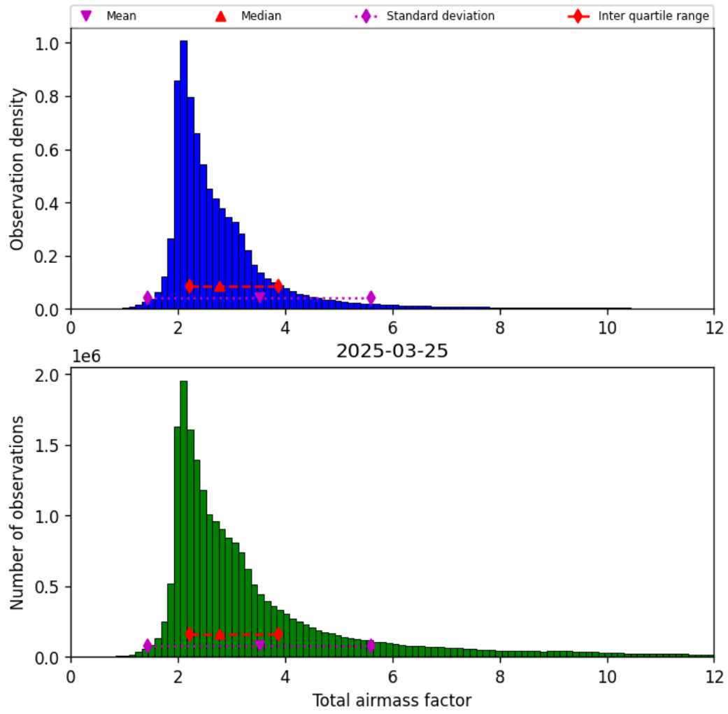
Figure 32: Histogram of “Total airmass factor” for 2025-03-25 to 2025-03-26
