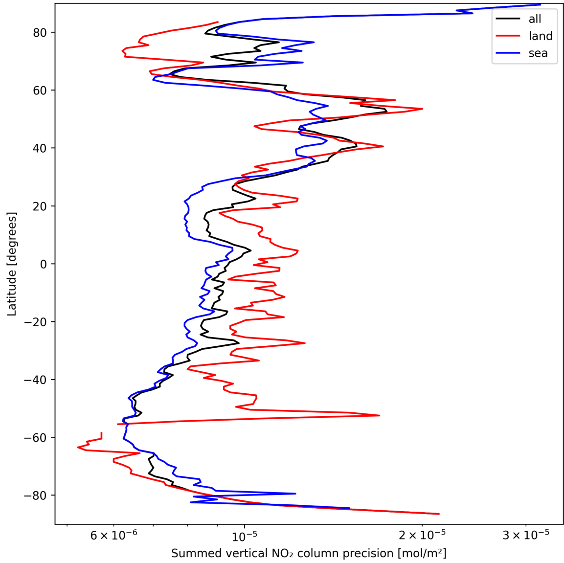
Figure 24: Zonal average of “Summed vertical NO 2 column precision” for 2025-03-25 to 2025-03-26.
