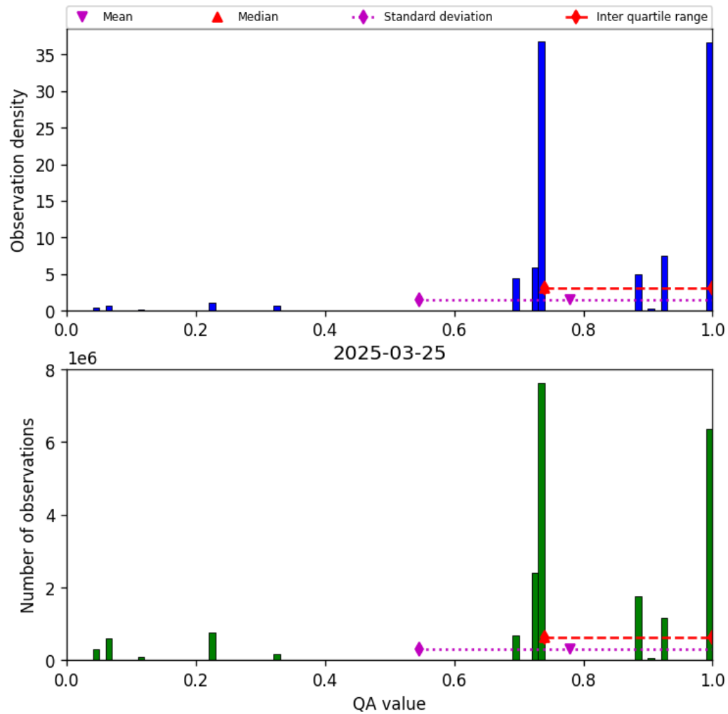
Figure 28: Histogram of “QA value” for 2025-03-25 to 2025-03-26
