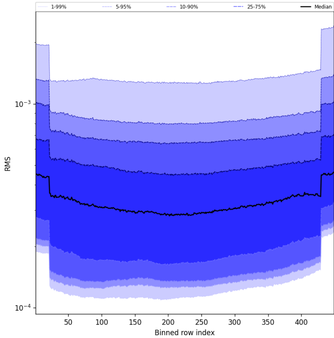
Figure 60: Along track statistics of “RMS” for 2025-03-25 to 2025-03-26
