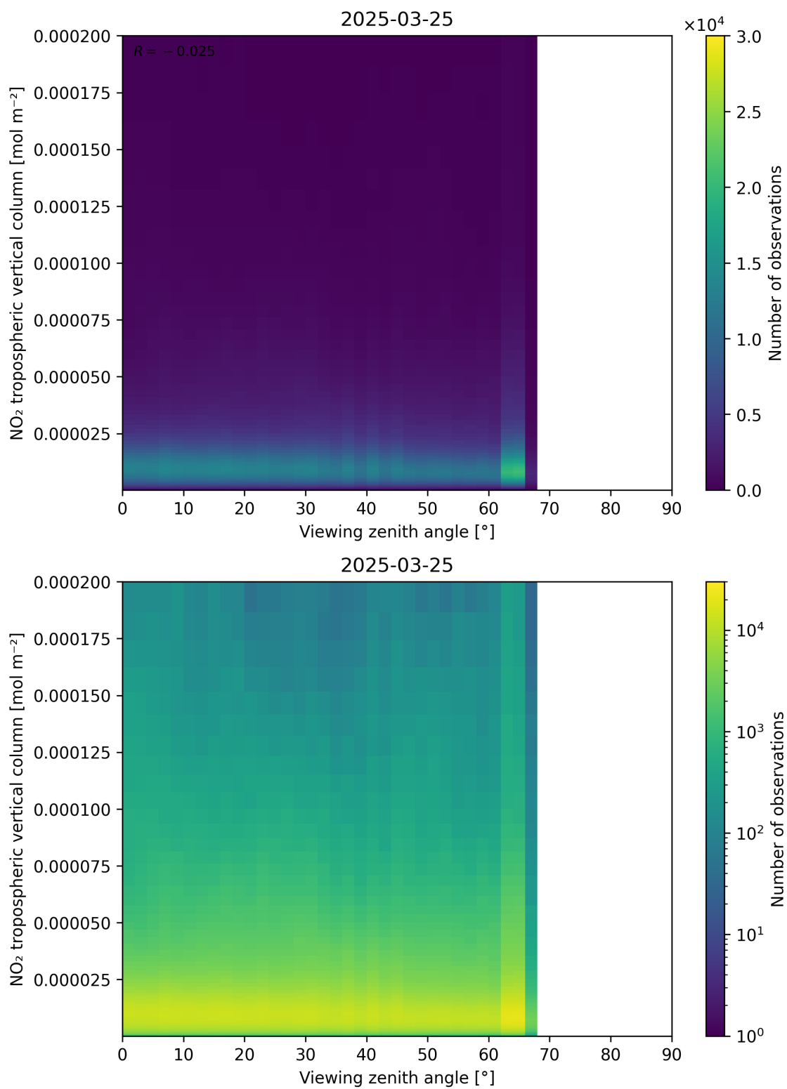
Figure 169: Scatter density plot of “Viewing zenith angle” against “NO 2 tropospheric vertical column” for 2025-03-25 to 2025-03-26.
