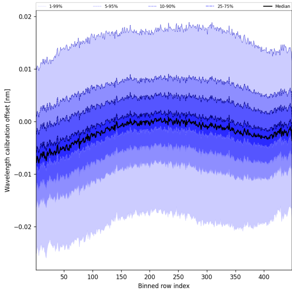
Figure 52: Along track statistics of “Wavelength calibration offset” for 2025-03-25 to 2025-03-26
