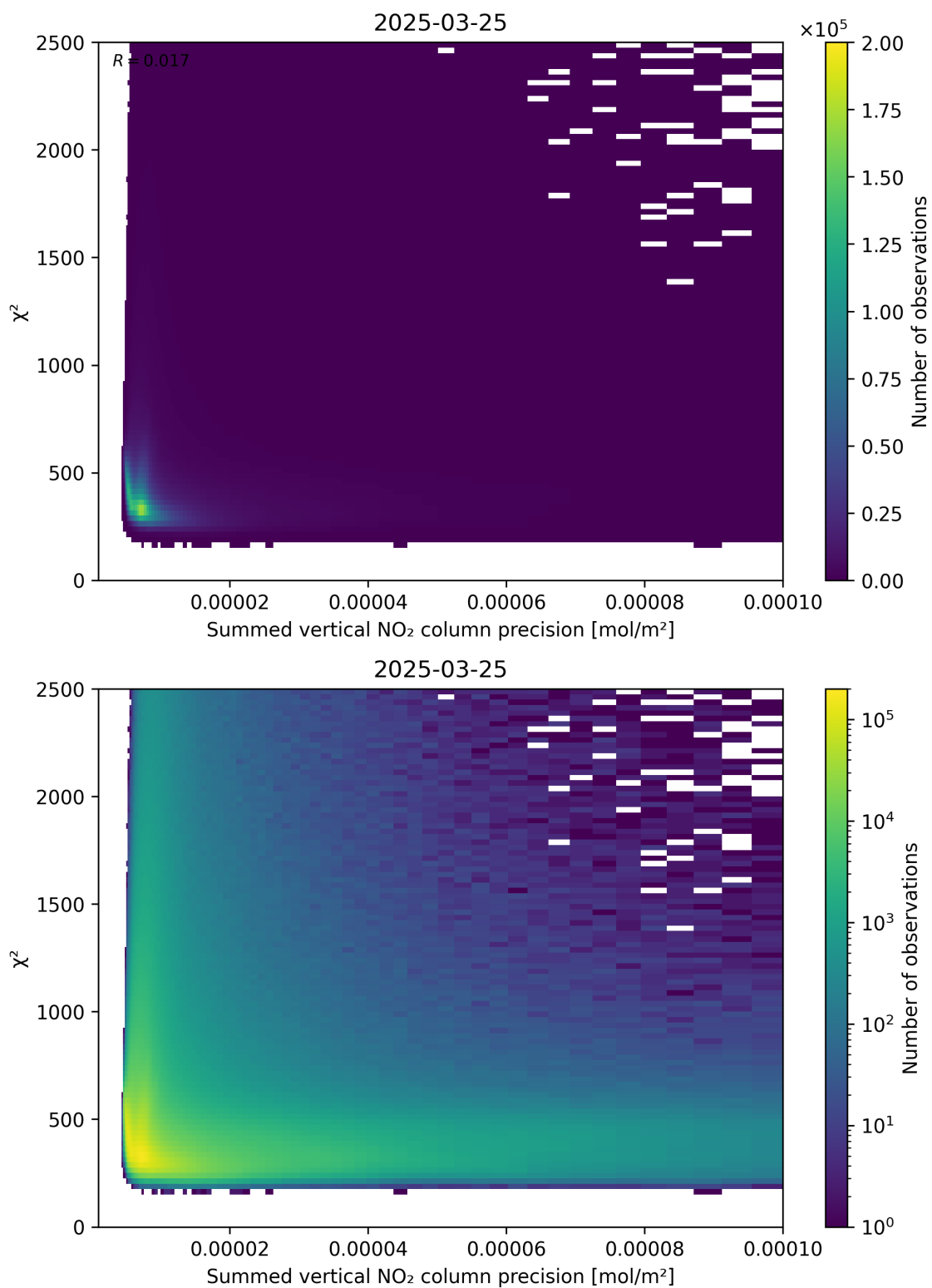
Figure 107: Scatter density plot of “Summed vertical NO 2 column precision” against “ \chi^2 ” for 2025-03-25 to 2025-03-26.
