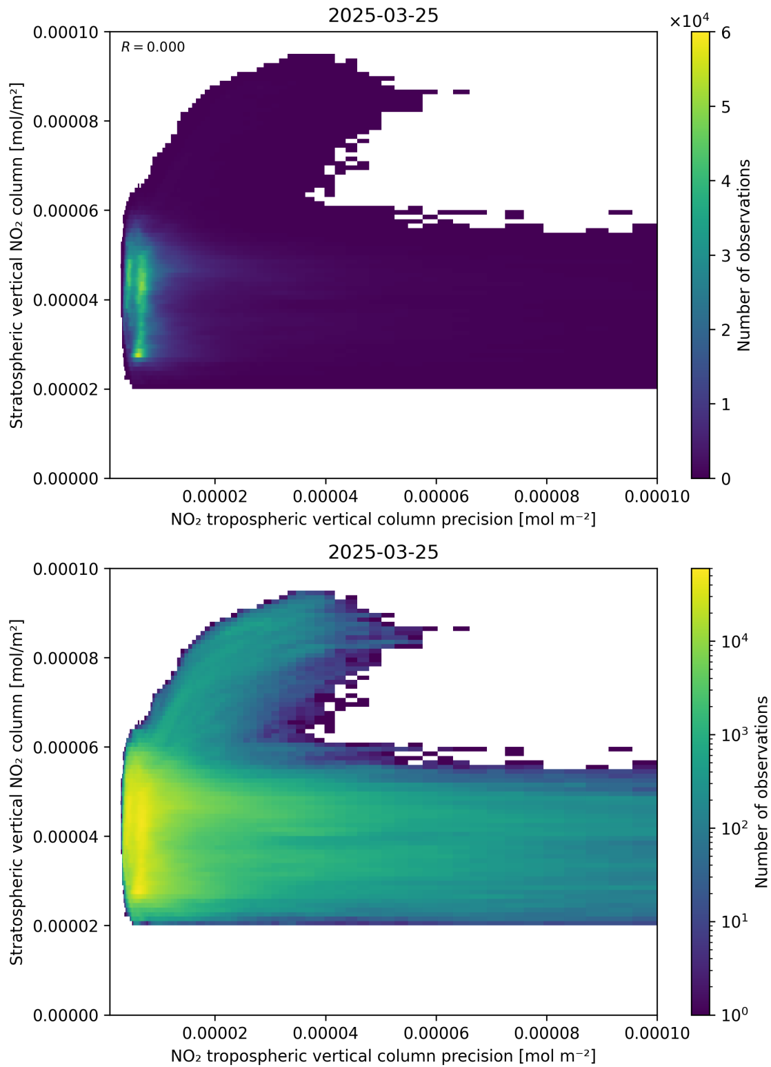
Figure 135: Scatter density plot of “NO 2 tropospheric vertical column precision” against “Stratospheric vertical NO 2 column” for 2025-03-25 to 2025-03-26.
