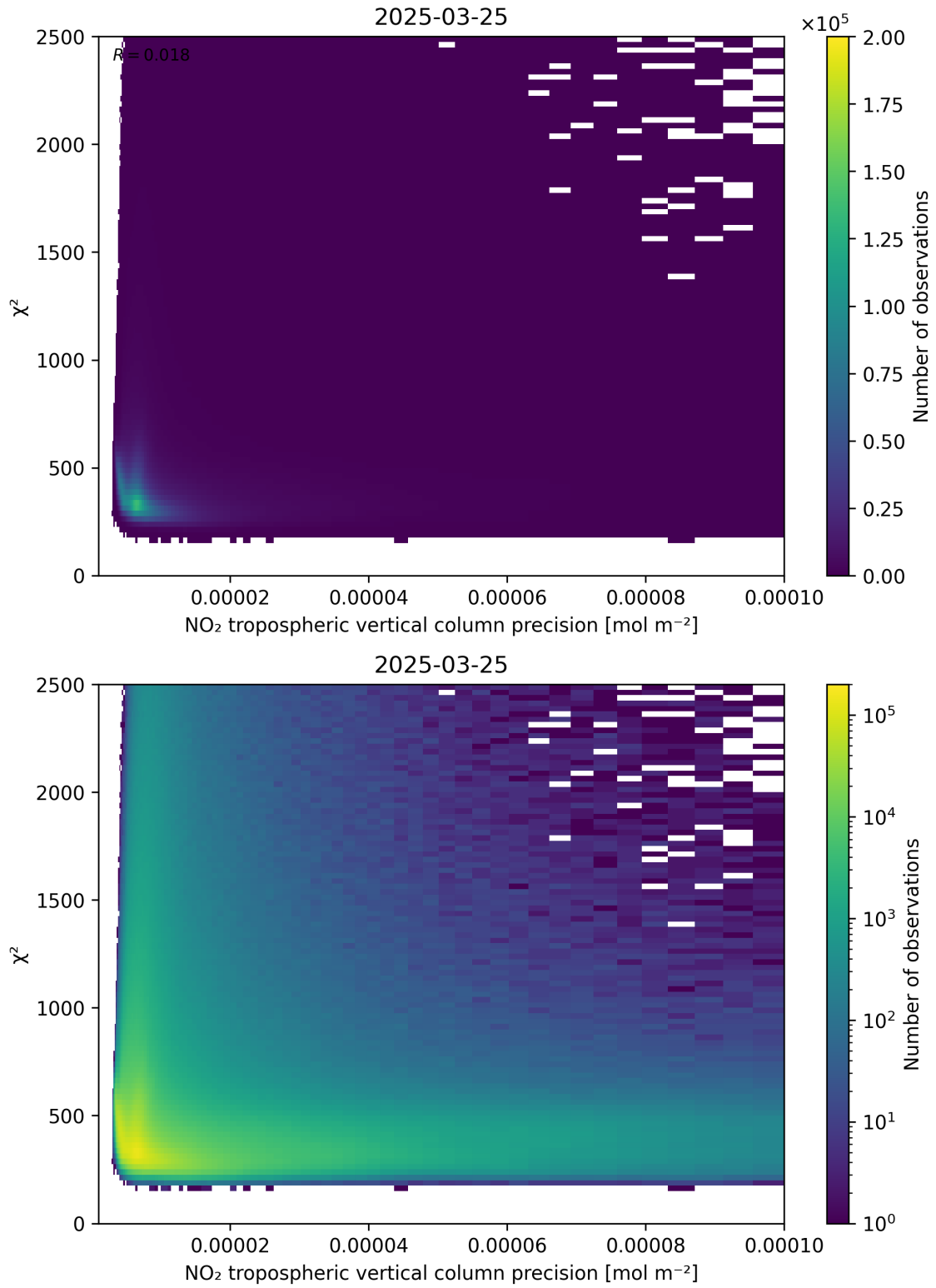
Figure 134: Scatter density plot of “NO 2 tropospheric vertical column precision” against “ \chi^2 ” for 2025-03-25 to 2025-03-26.
