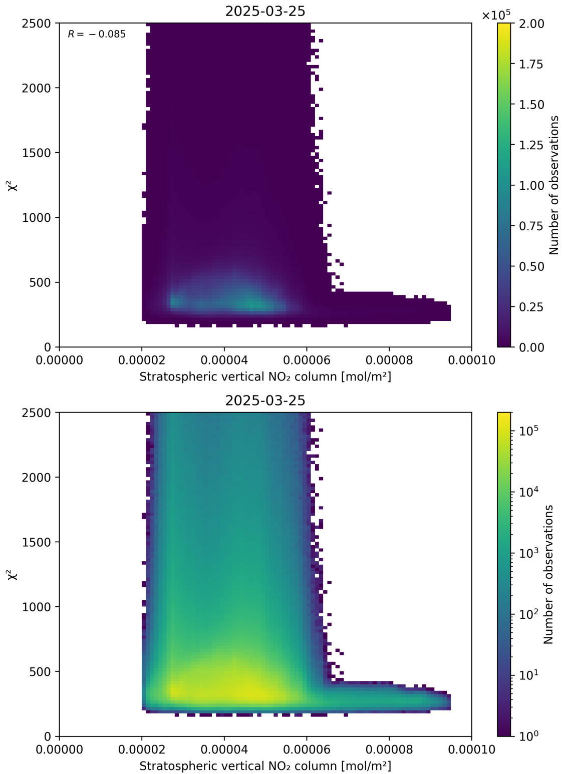
Figure 97: Scatter density plot of “Stratospheric vertical NO 2 column” against “ \chi^2 ” for 2025-03-25 to 2025-03-26.
