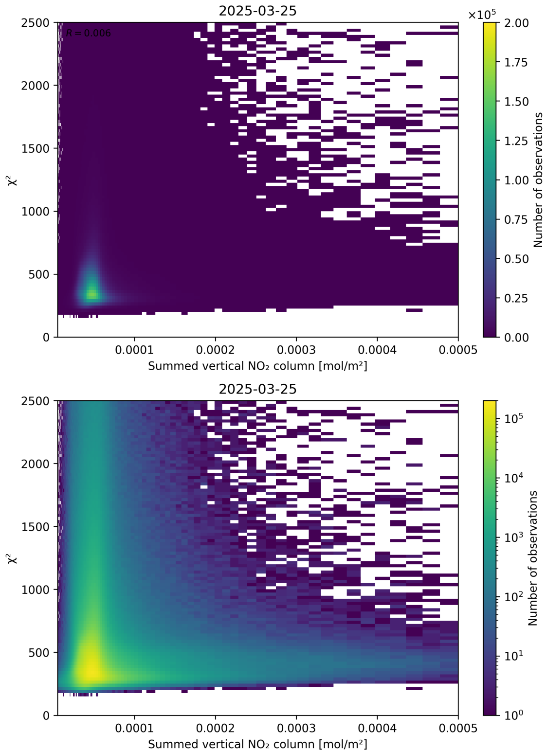
Figure 104: Scatter density plot of “Summed vertical NO 2 column” against “ \chi^2 ” for 2025-03-25 to 2025-03-26.
