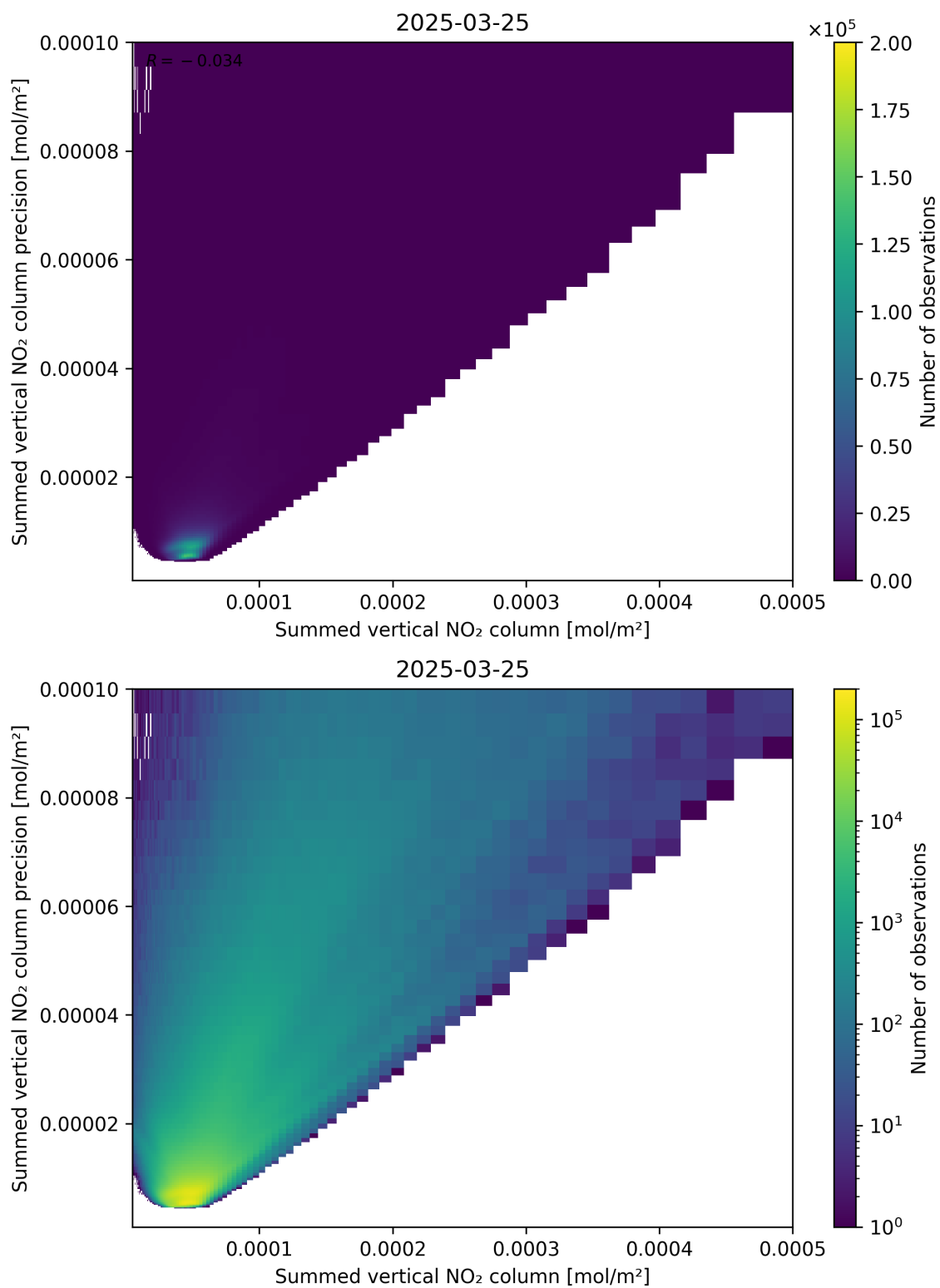
Figure 105: Scatter density plot of “Summed vertical NO 2 column” against “Summed vertical NO 2 column precision” for 2025-03-25 to 2025-03-26.
