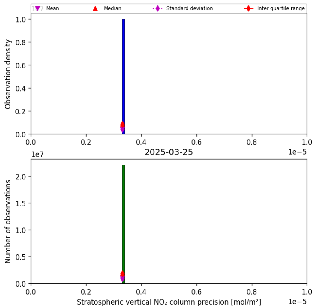
Figure 37: Histogram of “Stratospheric vertical NO 2 column precision” for 2025-03-25 to 2025-03-26
