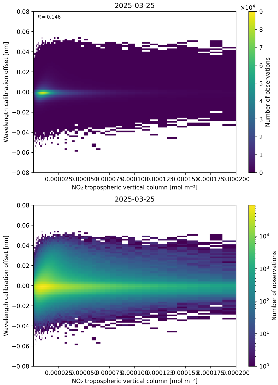
Figure 143: Scatter density plot of “NO 2 tropospheric vertical column” against “Wavelength calibration offset” for 2025-03-25 to 2025-03-26.
