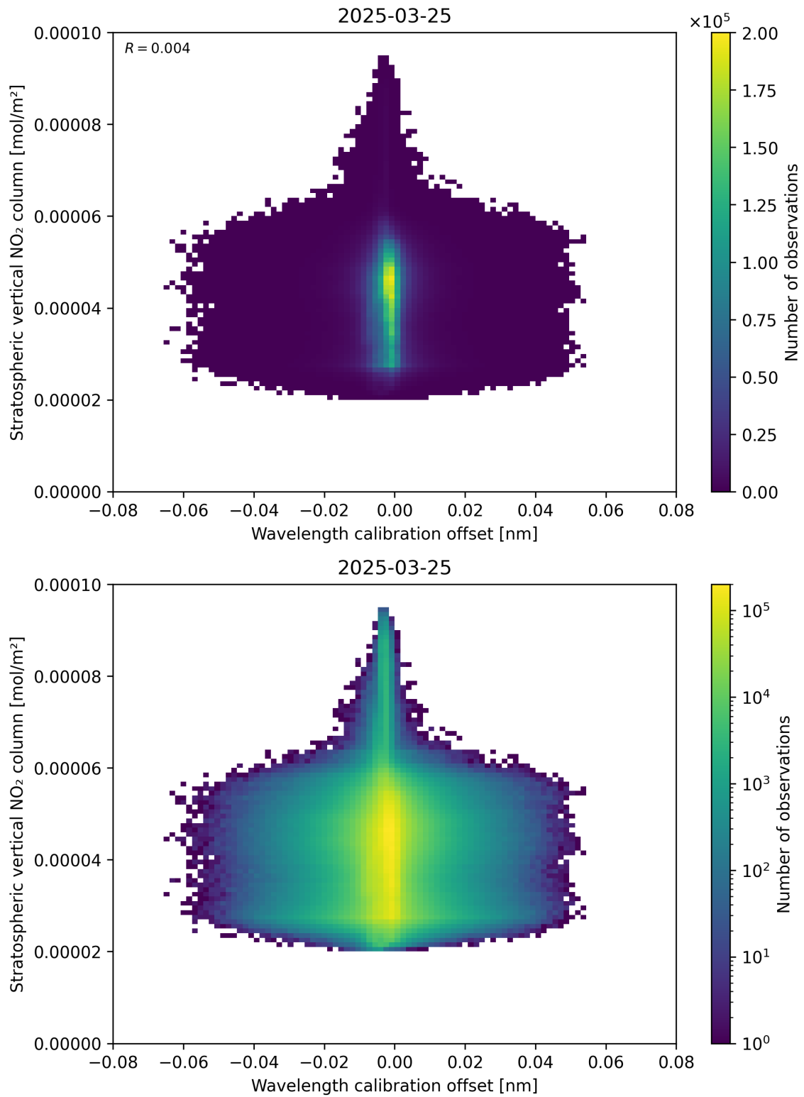
Figure 176: Scatter density plot of “Wavelength calibration offset” against “Stratospheric vertical NO 2 column” for 2025-03-25 to 2025-03-26.
