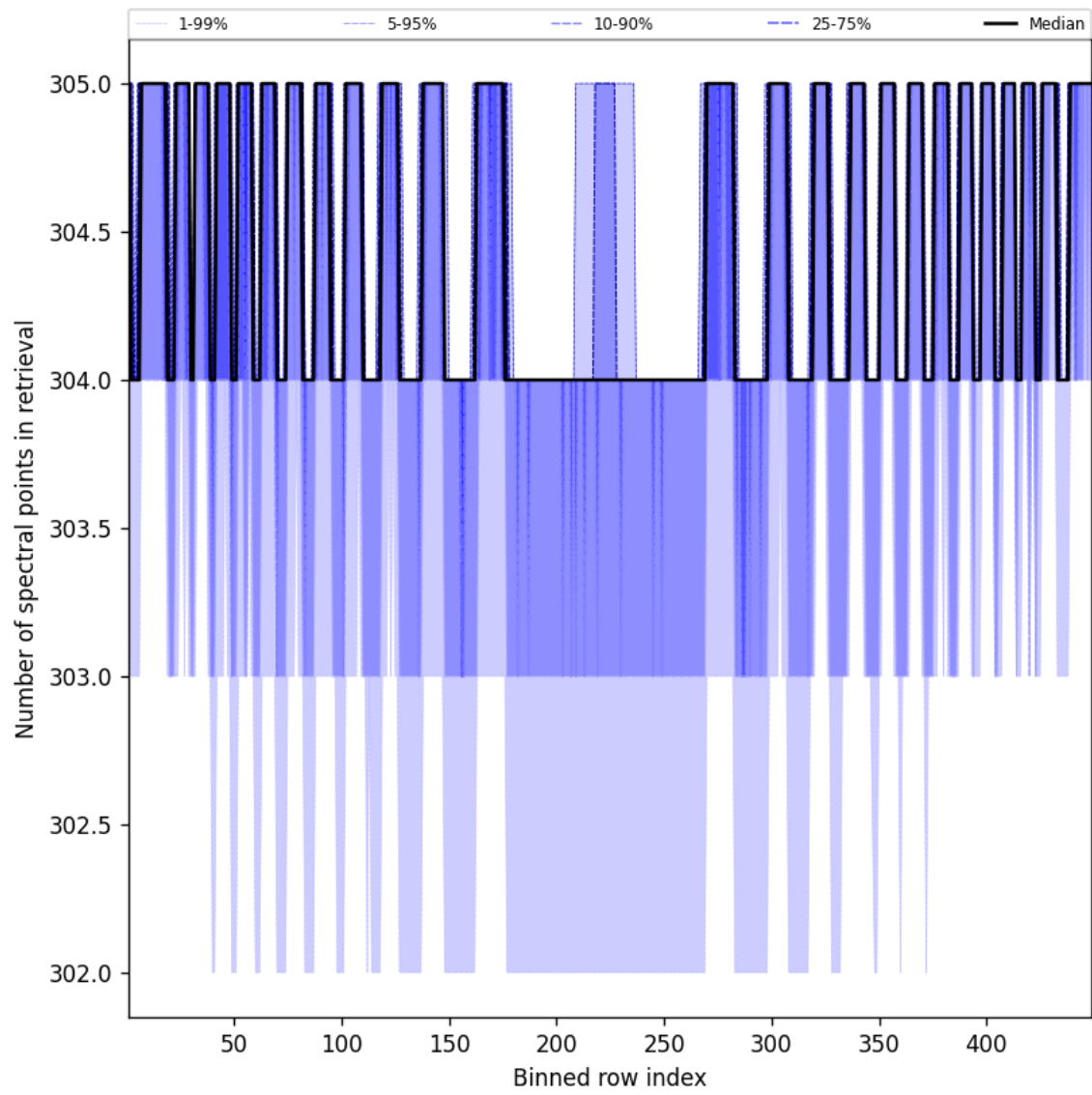
Figure 50: Along track statistics of “Number of spectral points in retrieval” for 2025-03-25 to 2025-03-26
