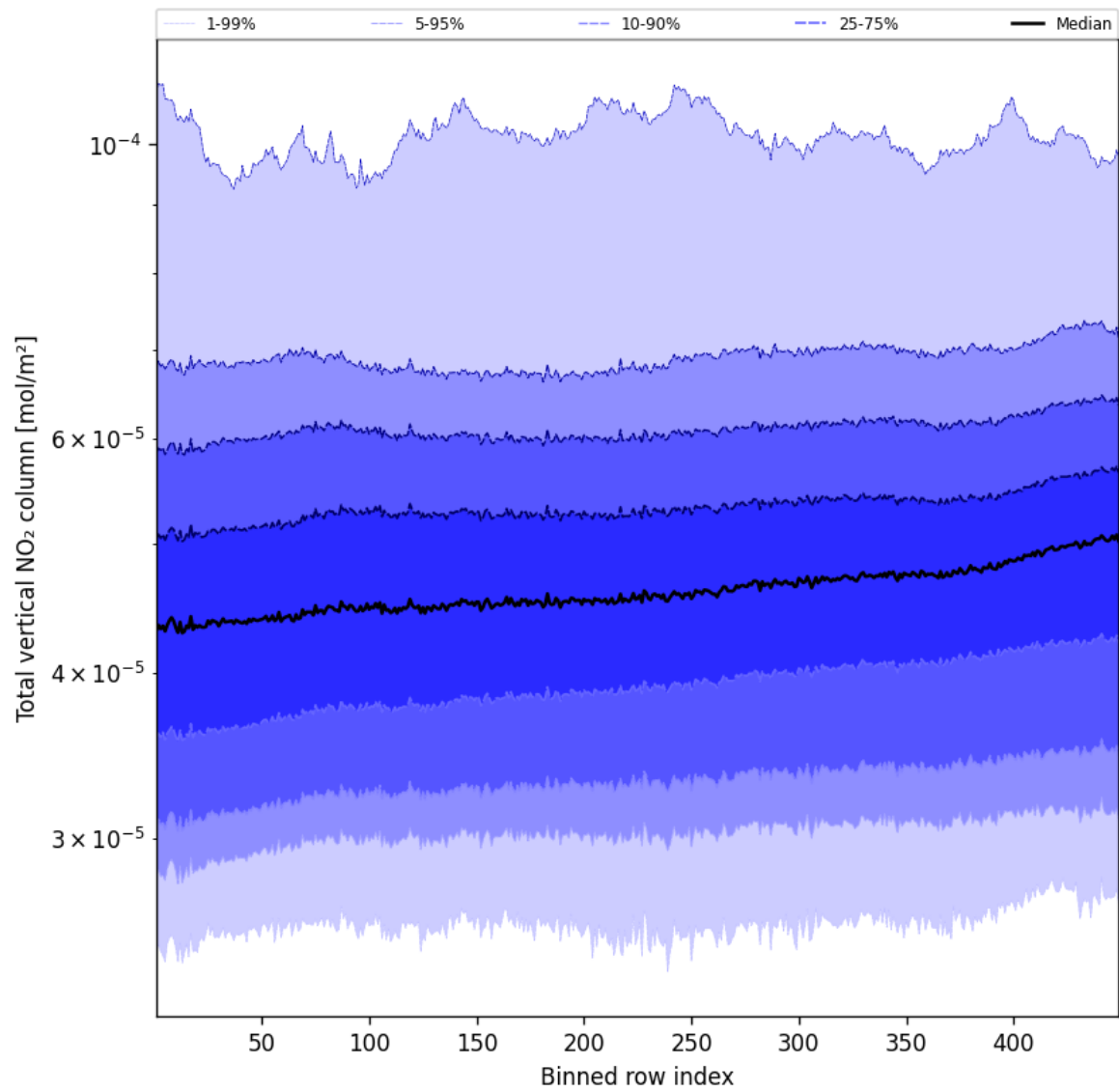
Figure 55: Along track statistics of “Total vertical NO 2 column” for 2025-03-25 to 2025-03-26
