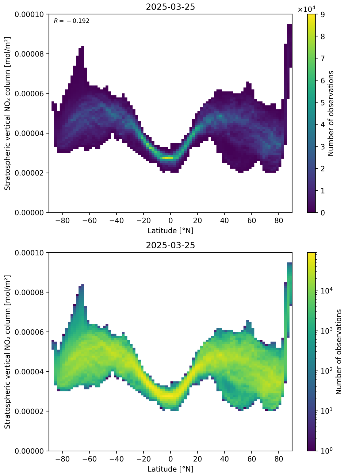
Figure 87: Scatter density plot of “Latitude” against “Stratospheric vertical NO 2 column” for 2025-03-25 to 2025-03-26.
