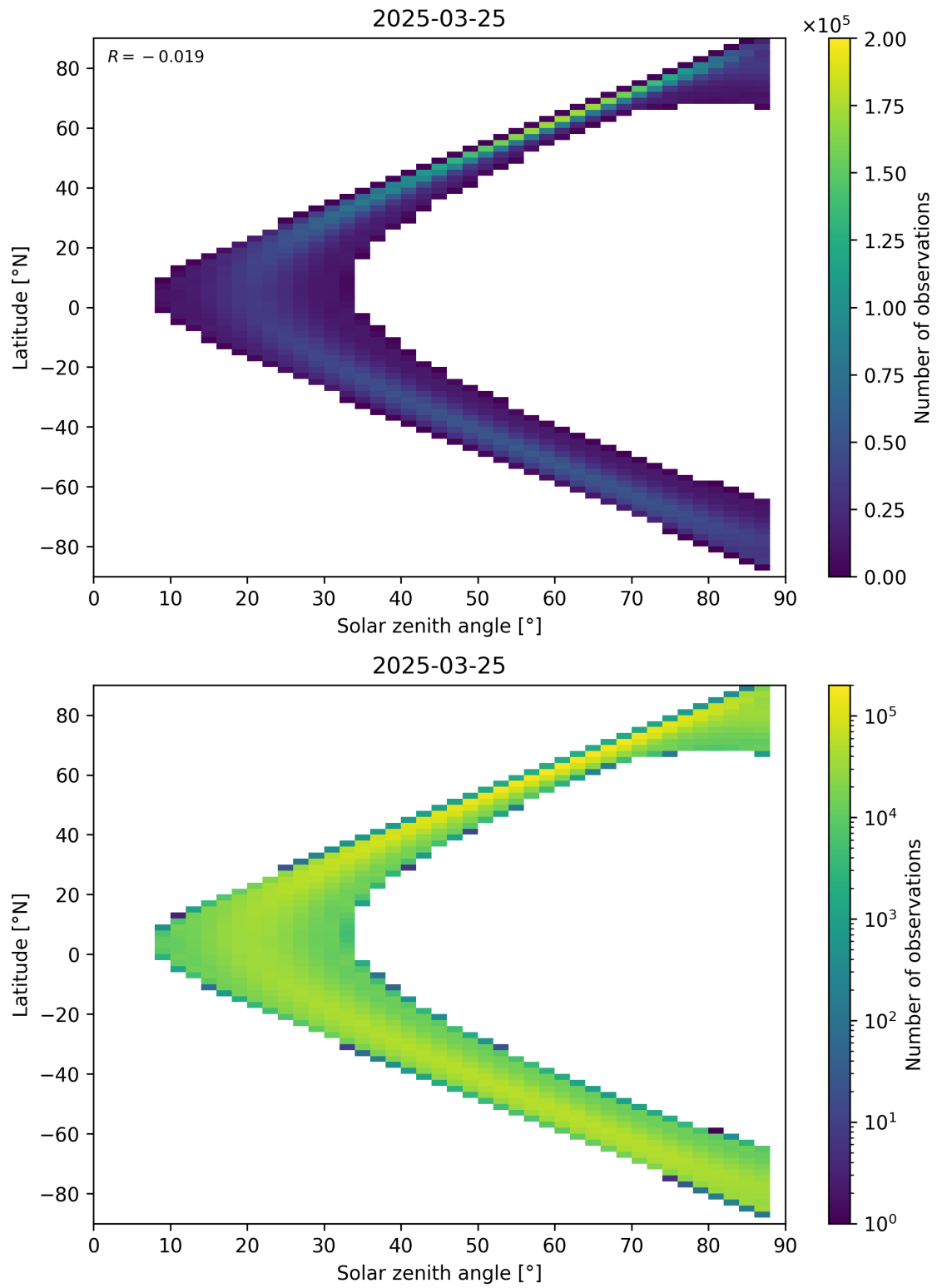
Figure 149: Scatter density plot of “Solar zenith angle” against “Latitude” for 2025-03-25 to 2025-03-26.
