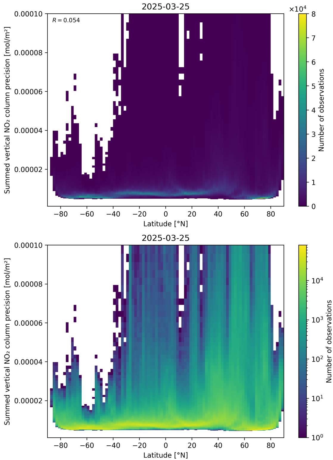
Figure 89: Scatter density plot of “Latitude” against “Summed vertical NO 2 column precision” for 2025-03-25 to 2025-03-26.
