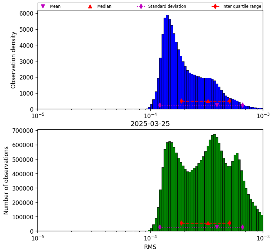
Figure 43: Histogram of “RMS” for 2025-03-25 to 2025-03-26
