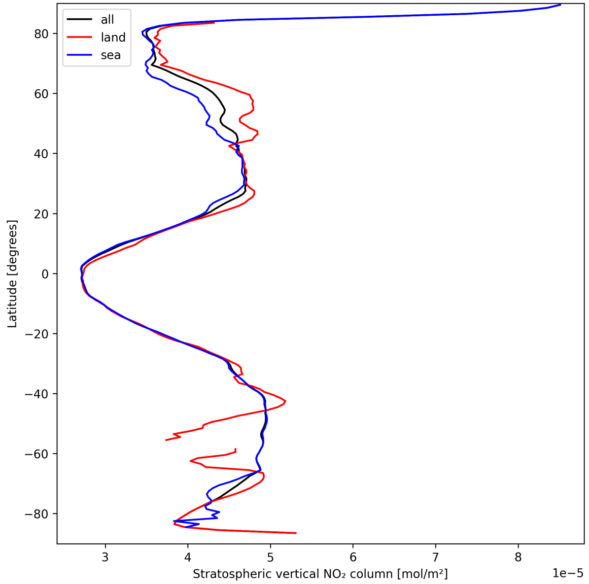
Figure 19: Zonal average of “Stratospheric vertical NO 2 column” for 2025-03-25 to 2025-03-26.
