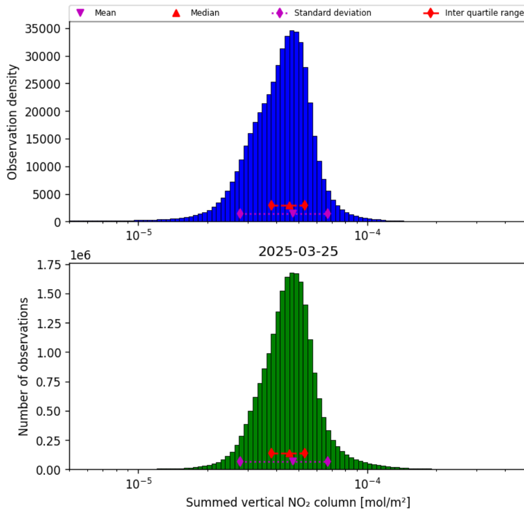
Figure 40: Histogram of “Summed vertical NO 2 column” for 2025-03-25 to 2025-03-26
