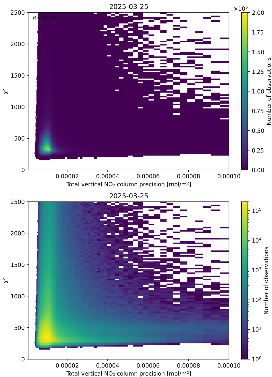
Figure 116: Scatter density plot of “Total vertical NO 2 column precision” against “ \chi^2 ” for 2025-03-25 to 2025-03-26.
