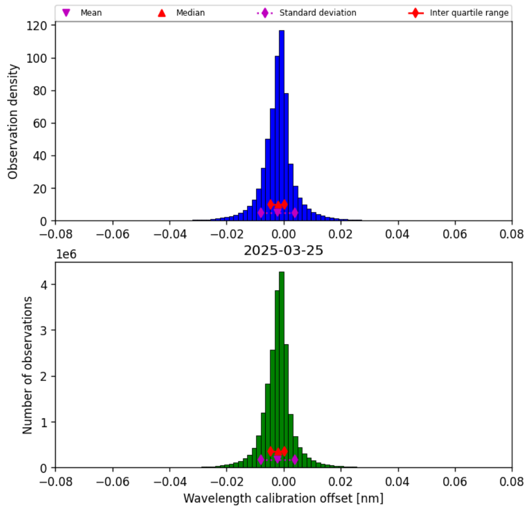
Figure 35: Histogram of “Wavelength calibration offset” for 2025-03-25 to 2025-03-26
