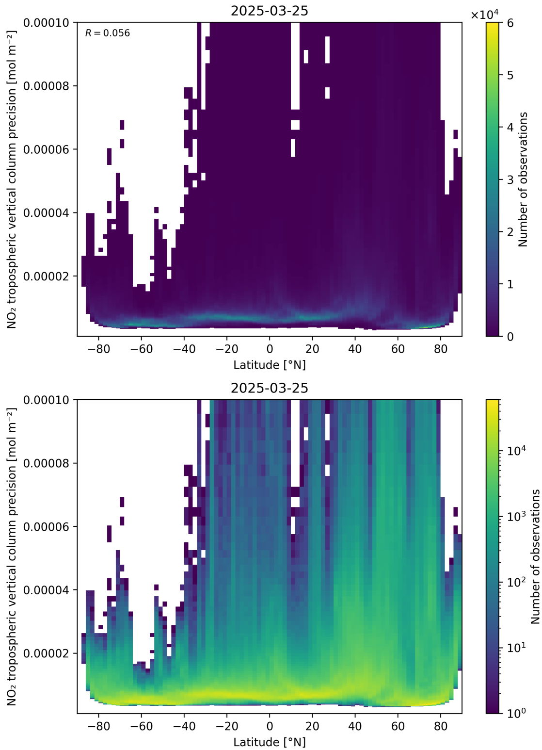
Figure 93: Scatter density plot of “Latitude” against “NO 2 tropospheric vertical column precision” for 2025-03-25 to 2025-03-26.
