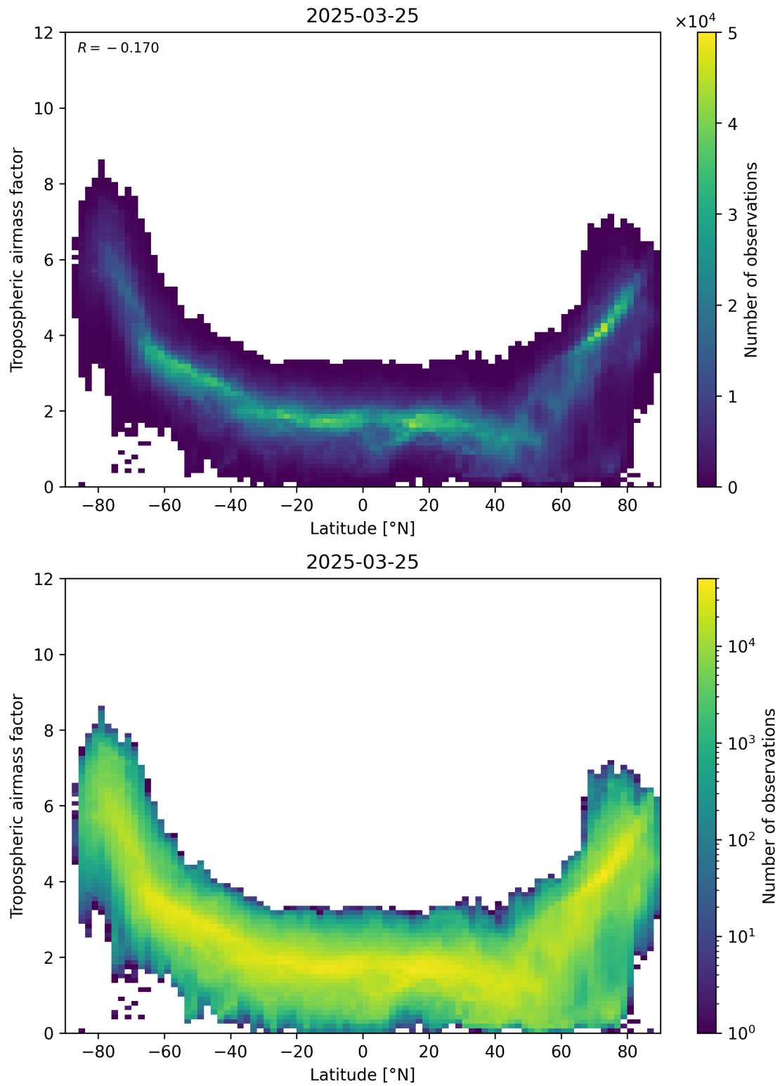
Figure 85: Scatter density plot of “Latitude” against “Tropospheric airmass factor” for 2025-03-25 to 2025-03-26.
