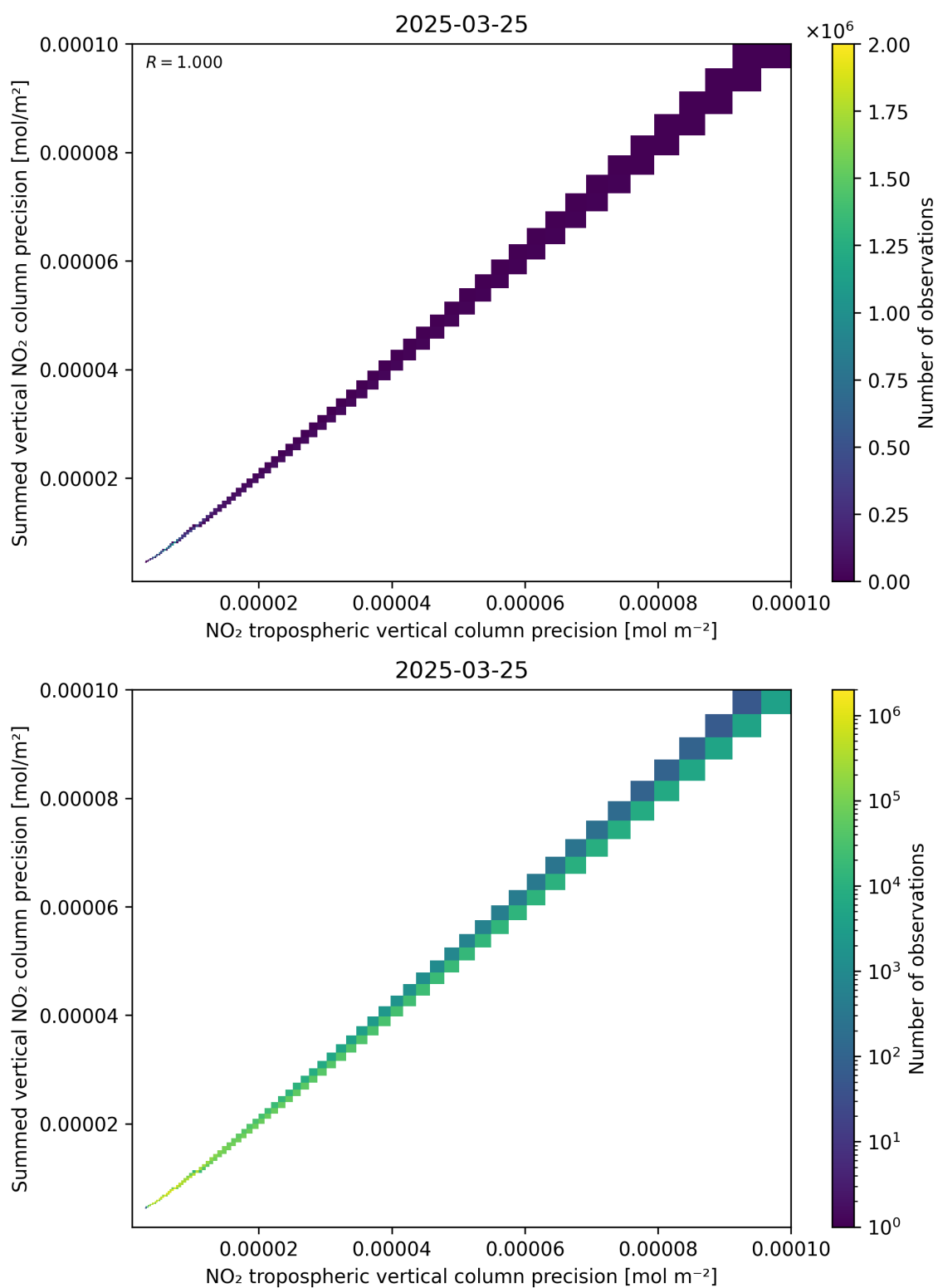
Figure 137: Scatter density plot of “NO 2 tropospheric vertical column precision” against “Summed vertical NO 2 column precision” for 2025-03-25 to 2025-03-26.
