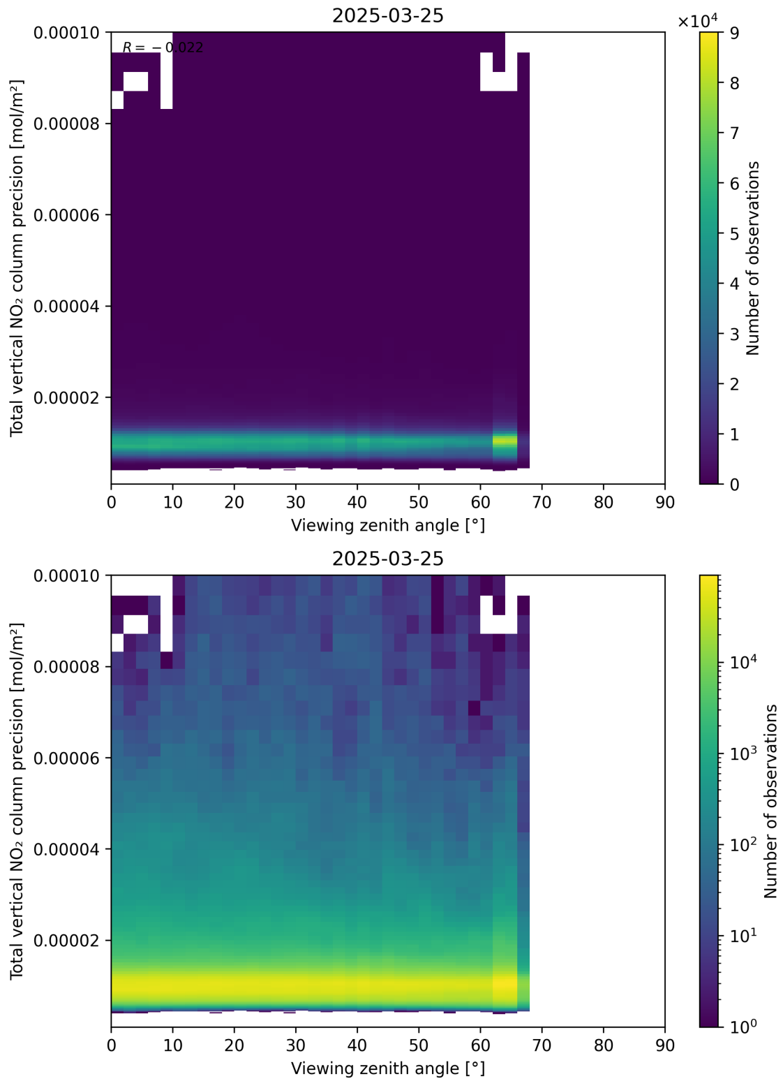
Figure 168: Scatter density plot of “Viewing zenith angle” against “Total vertical NO 2 column precision” for 2025-03-25 to 2025-03-26.
