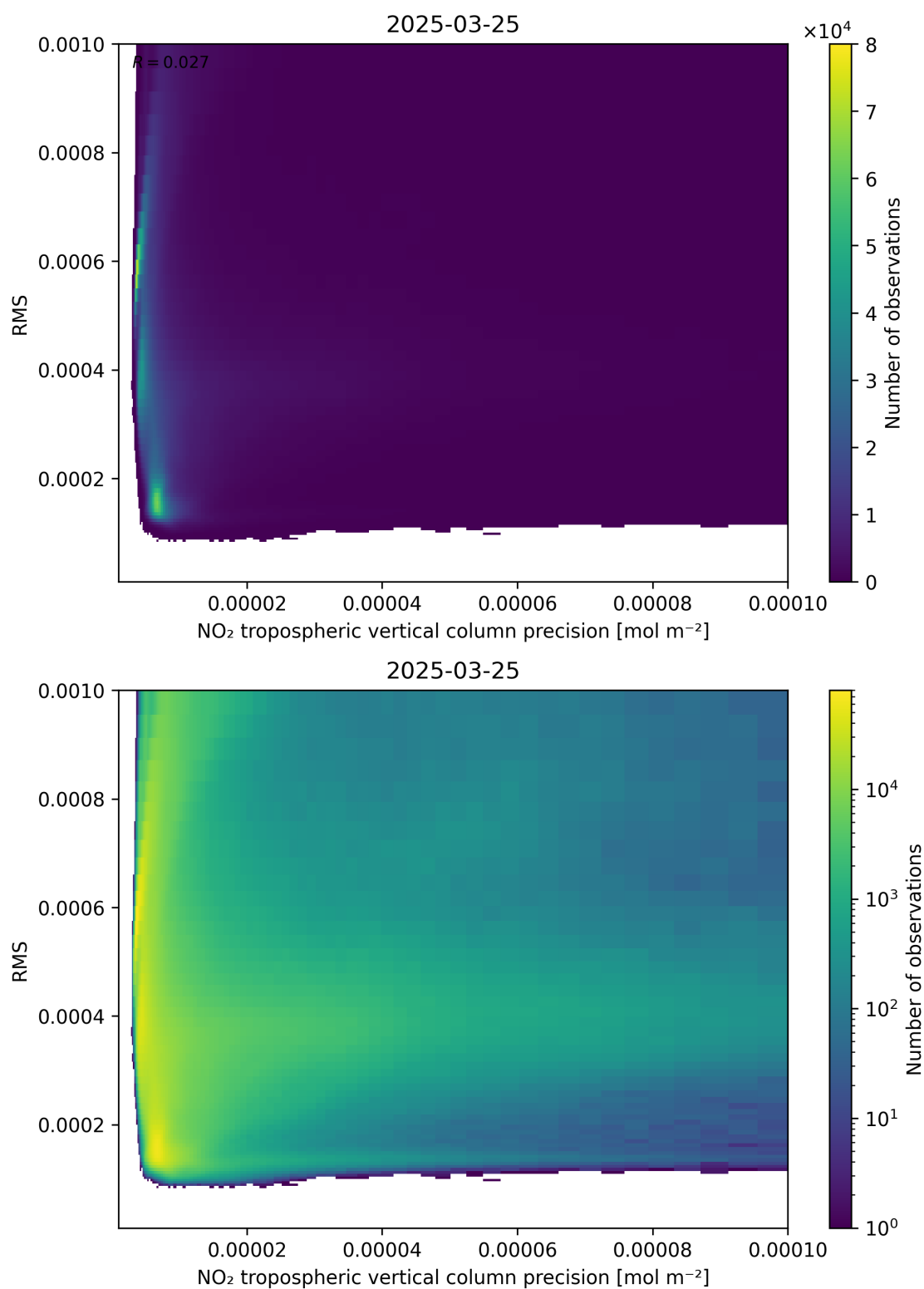
Figure 140: Scatter density plot of “NO 2 tropospheric vertical column precision” against “RMS” for 2025-03-25 to 2025-03-26.
