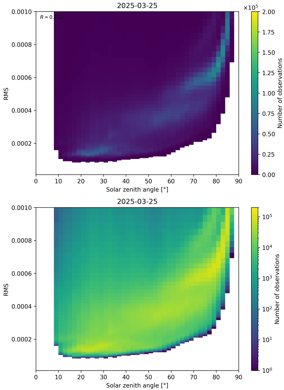
Figure 157: Scatter density plot of “Solar zenith angle” against “RMS” for 2025-03-25 to 2025-03-26.
