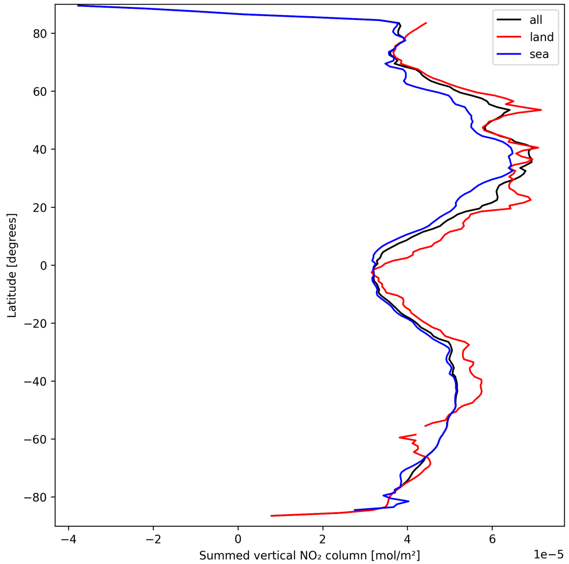
Figure 23: Zonal average of “Summed vertical NO 2 column” for 2025-03-25 to 2025-03-26.
