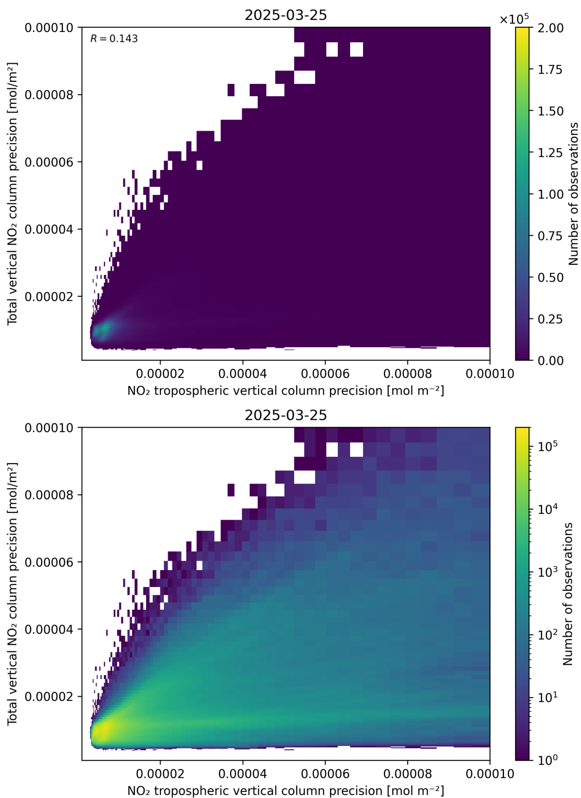
Figure 139: Scatter density plot of “NO 2 tropospheric vertical column precision” against “Total vertical NO 2 column precision” for 2025-03-25 to 2025-03-26.
