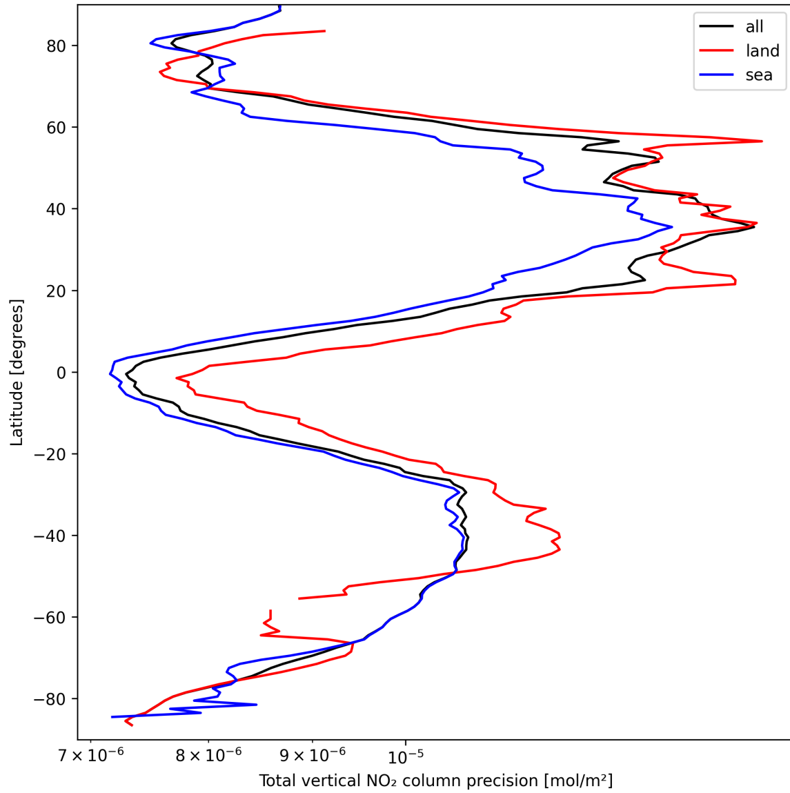
Figure 22: Zonal average of “Total vertical NO 2 column precision” for 2025-03-25 to 2025-03-26.
