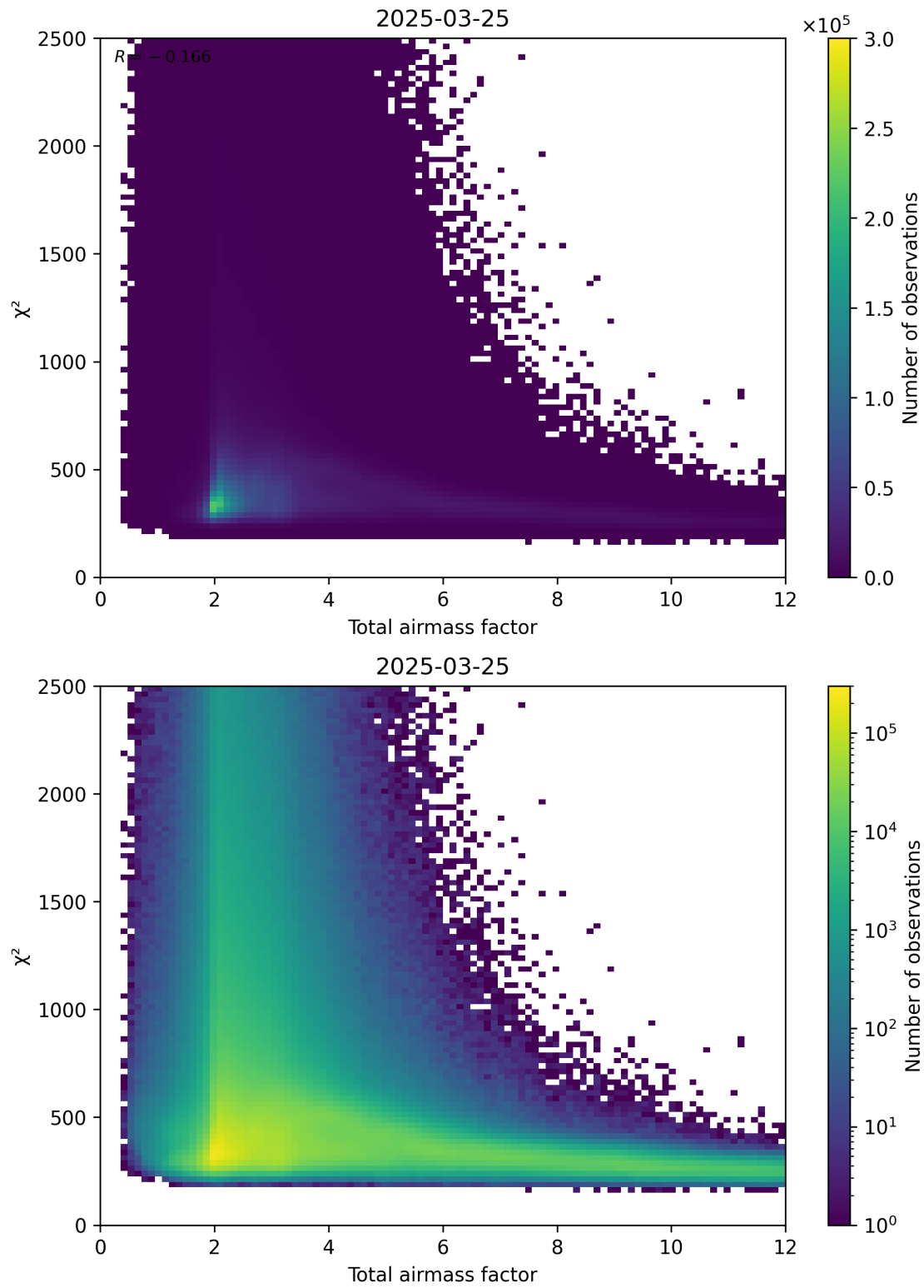
Figure 63: Scatter density plot of “Total airmass factor” against “ \chi^2 ” for 2025-03-25 to 2025-03-26.
