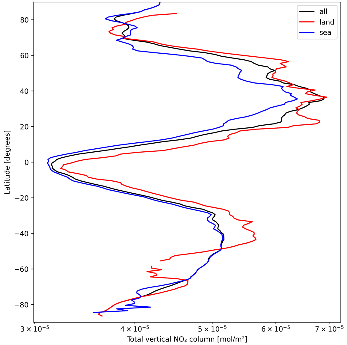
Figure 21: Zonal average of “Total vertical NO 2 column” for 2025-03-25 to 2025-03-26.
