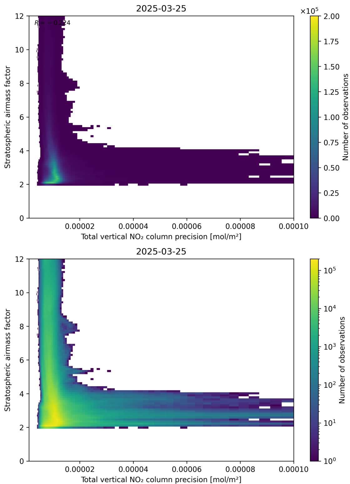
Figure 115: Scatter density plot of “Total vertical NO 2 column precision” against “Stratospheric air mass factor” for 2025-03-25 to 2025-03-26.
