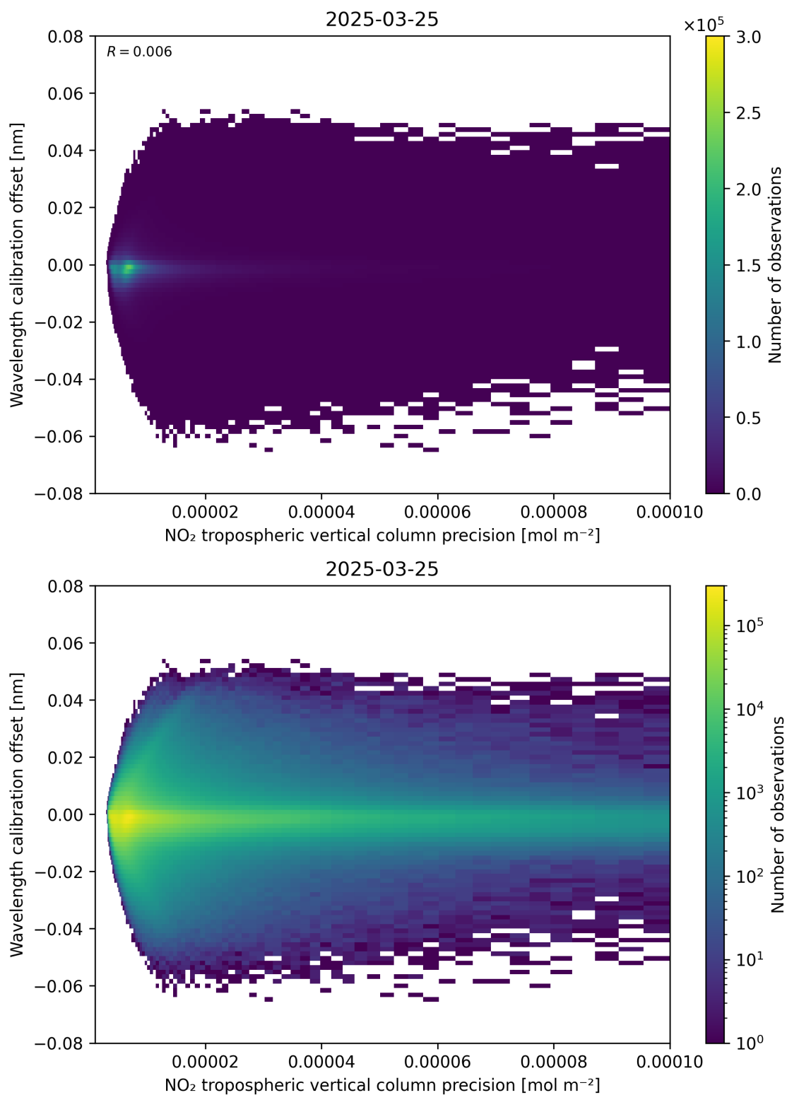
Figure 141: Scatter density plot of “NO 2 tropospheric vertical column precision” against “Wavelength calibration offset” for 2025-03-25 to 2025-03-26.
