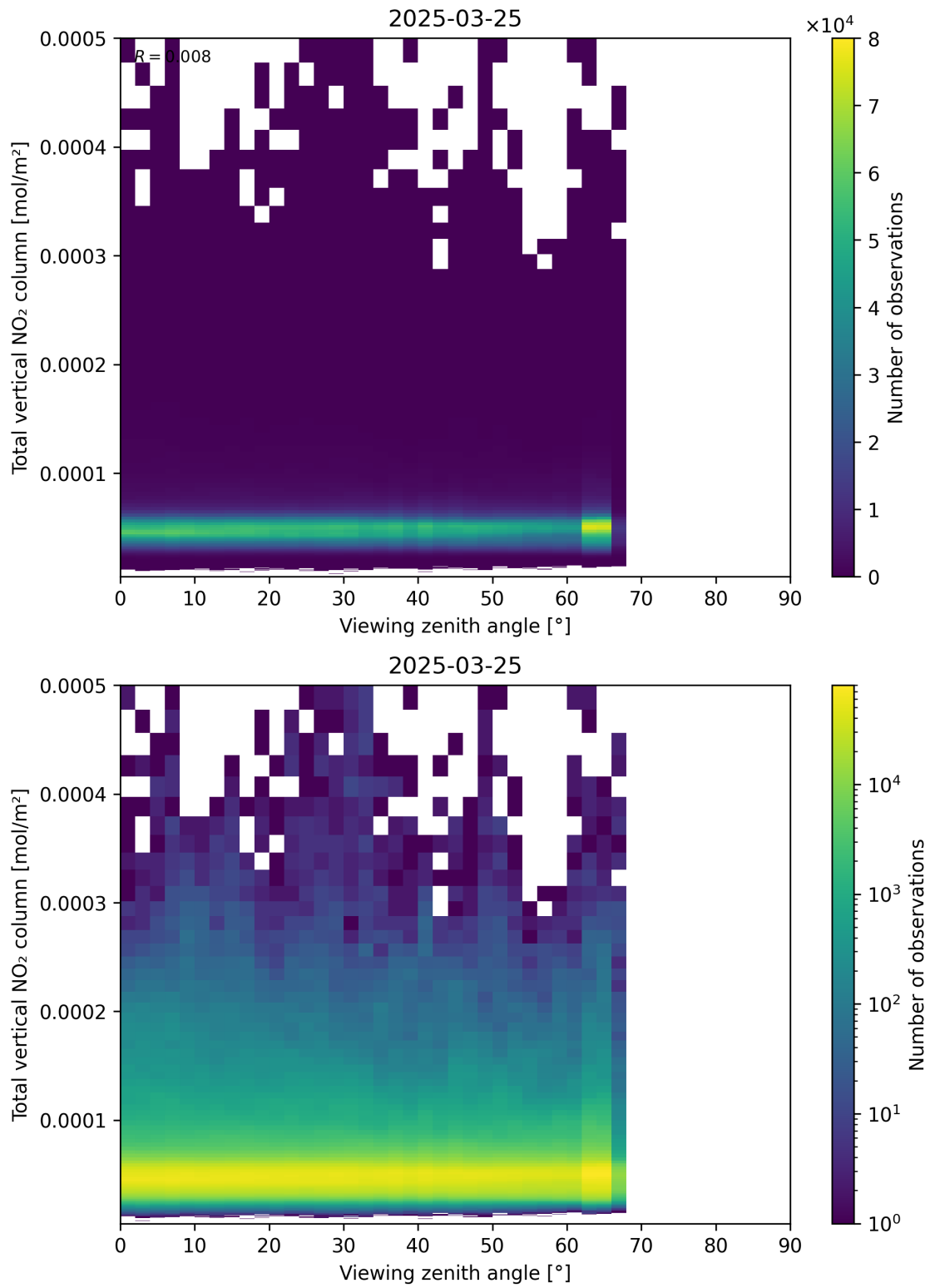
Figure 167: Scatter density plot of “Viewing zenith angle” against “Total vertical NO 2 column” for 2025-03-25 to 2025-03-26.
