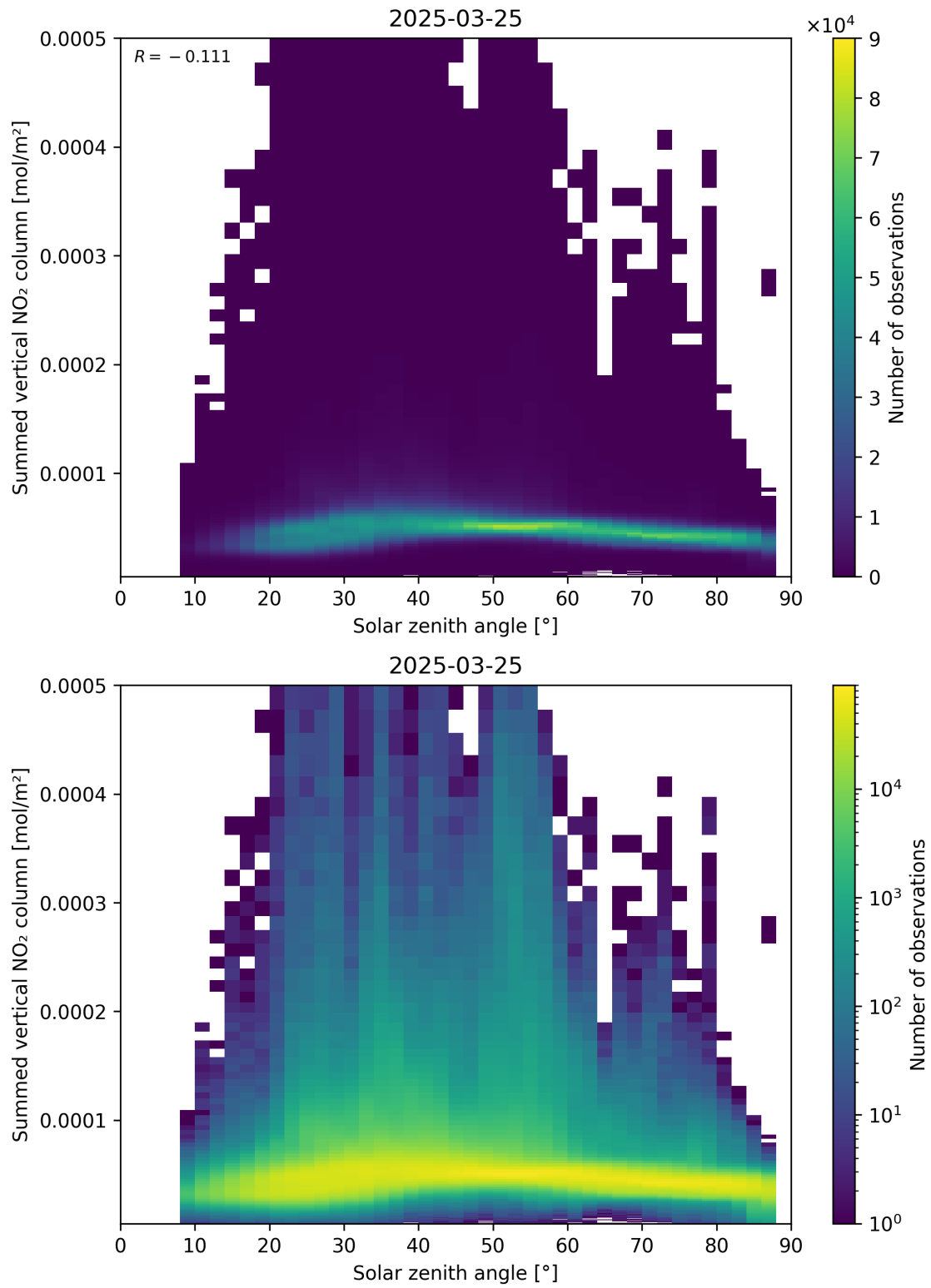
Figure 151: Scatter density plot of “Solar zenith angle” against “Summed vertical NO 2 column” for 2025-03-25 to 2025-03-26.
