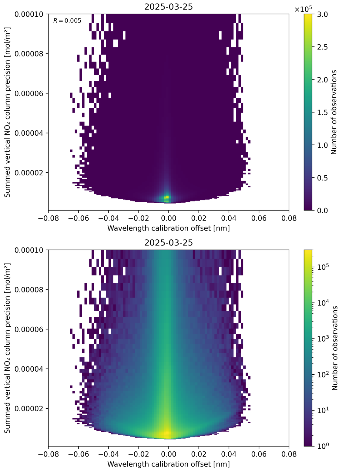
Figure 178: Scatter density plot of “Wavelength calibration offset” against “Summed vertical NO 2 column precision” for 2025-03-25 to 2025-03-26.
