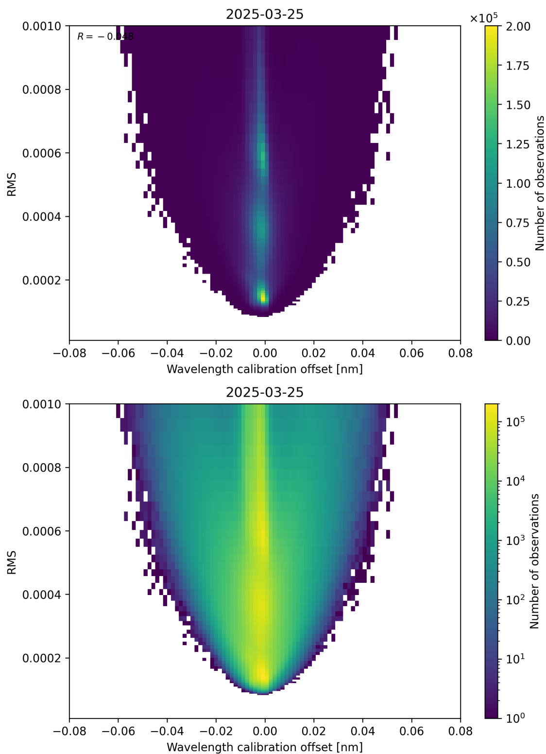
Figure 181: Scatter density plot of “Wavelength calibration offset” against “RMS” for 2025-03-25 to 2025-03-26.
