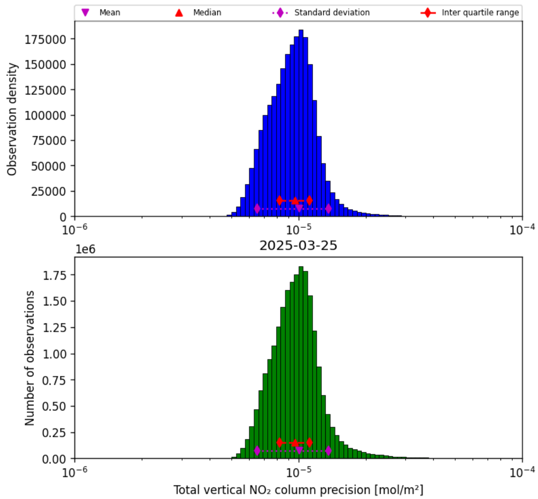
Figure 39: Histogram of “Total vertical NO 2 column precision” for 2025-03-25 to 2025-03-26
