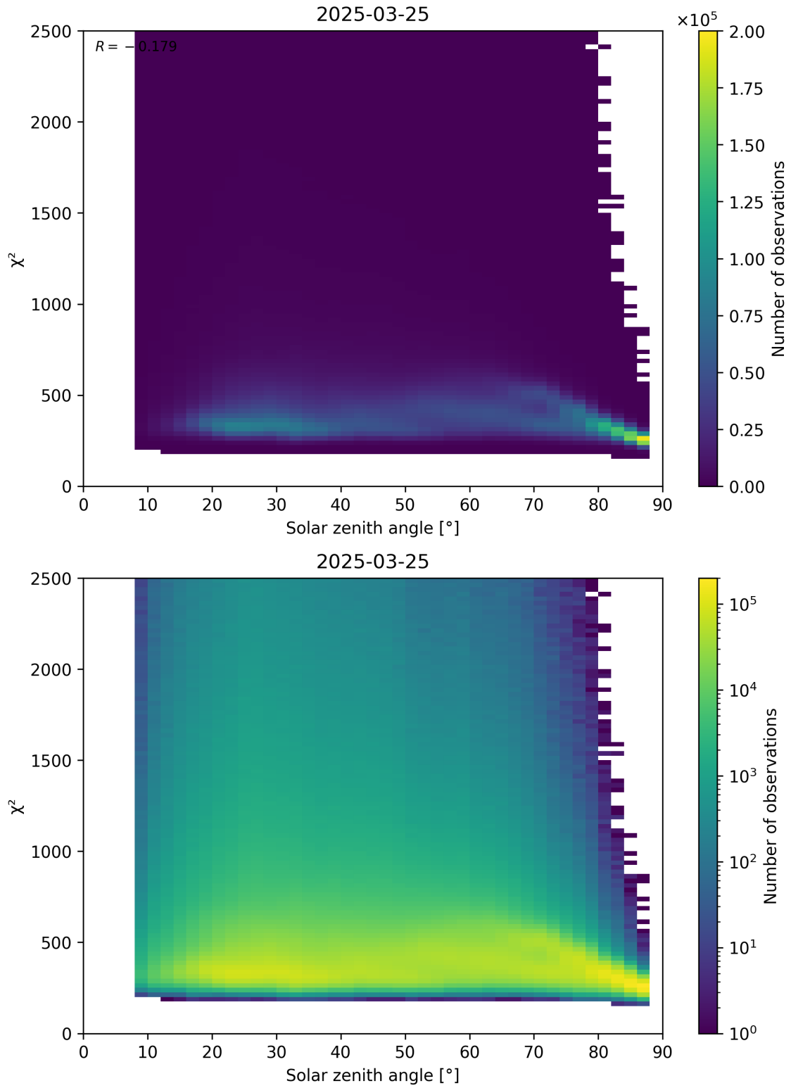
Figure 148: Scatter density plot of “Solar zenith angle” against “ \chi^2 ” for 2025-03-25 to 2025-03-26.
