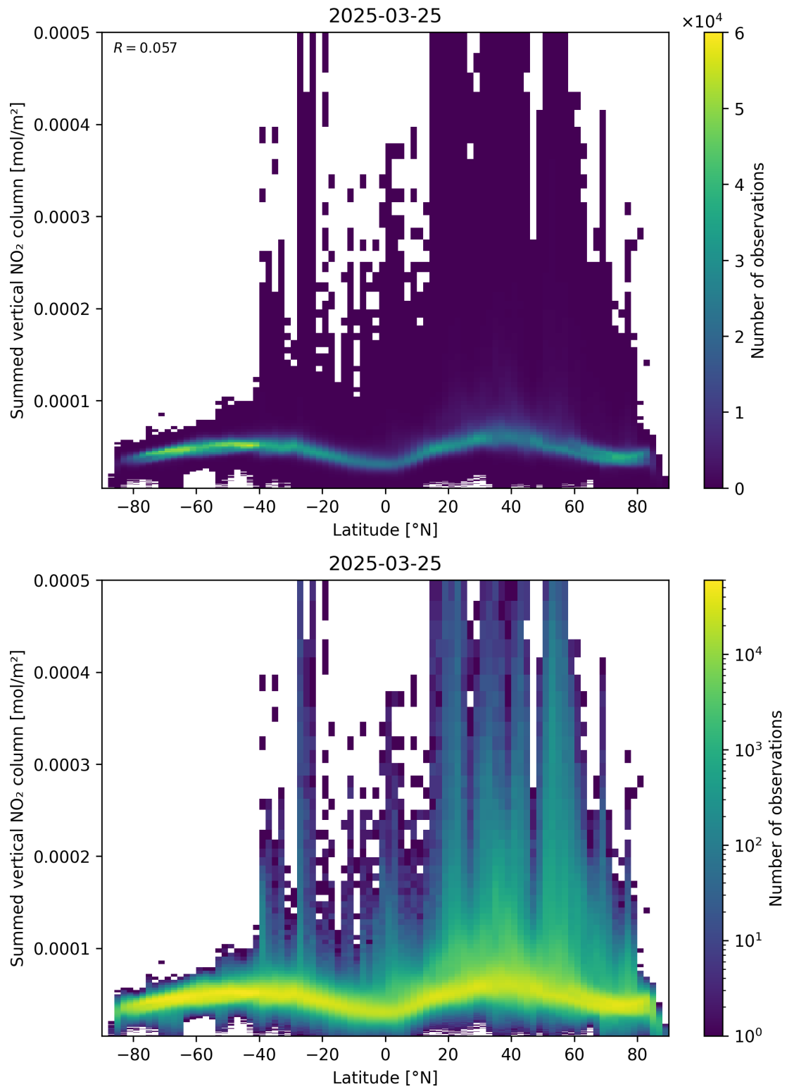
Figure 88: Scatter density plot of “Latitude” against “Summed vertical NO 2 column” for 2025-03-25 to 2025-03-26.
