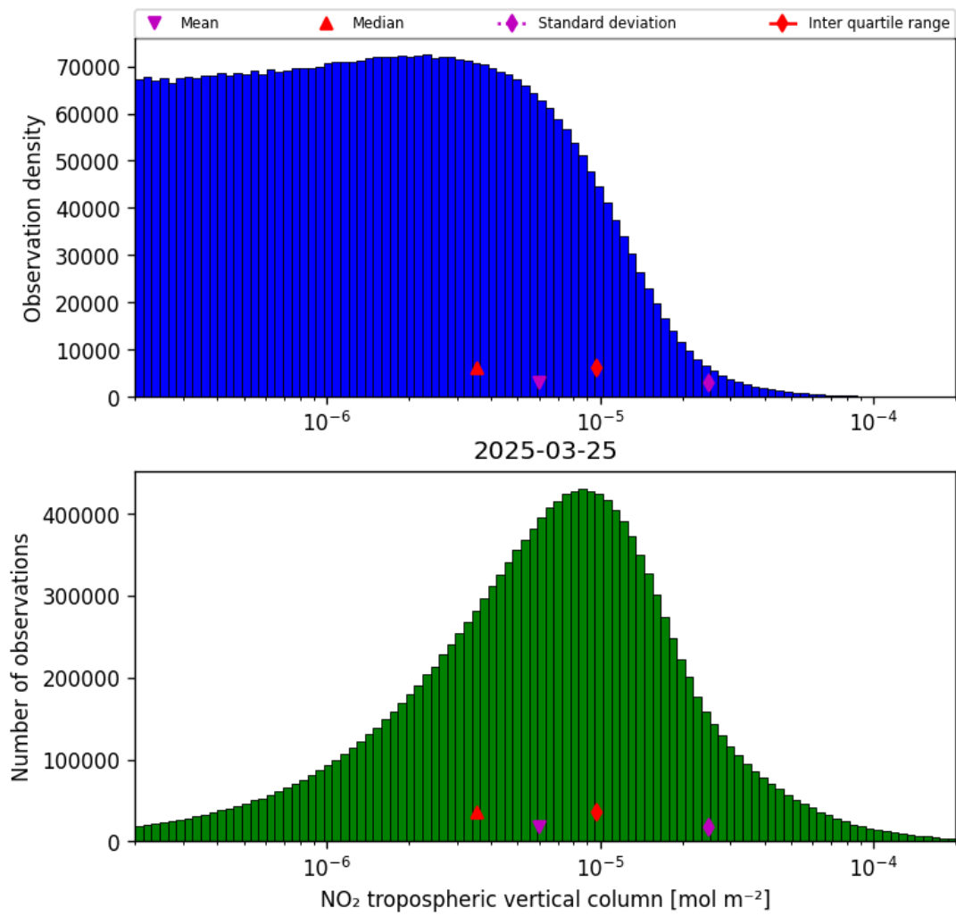
Figure 29: Histogram of “NO 2 tropospheric vertical column” for 2025-03-25 to 2025-03-26
