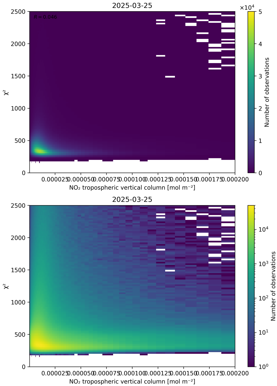
Figure 124: Scatter density plot of “NO 2 tropospheric vertical column” against “ \chi^2 ” for 2025-03-25 to 2025-03-26.
