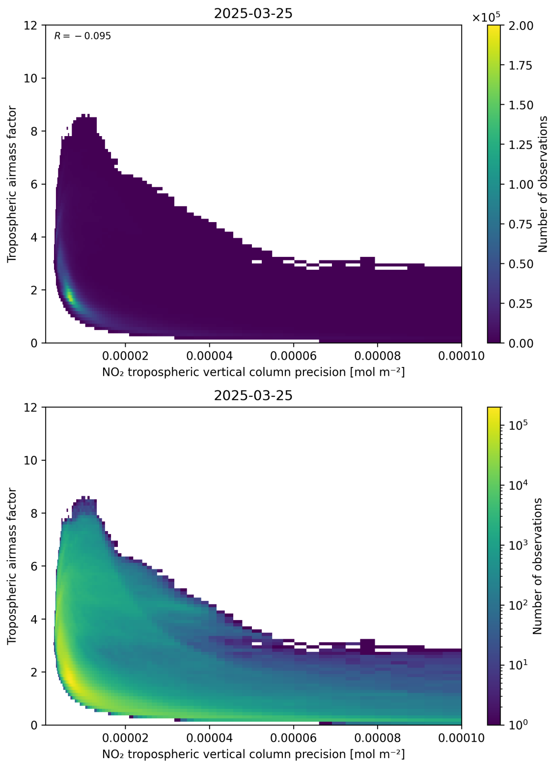
Figure 133: Scatter density plot of “NO 2 tropospheric vertical column precision” against “Tropospheric air mass factor” for 2025-03-25 to 2025-03-26.
