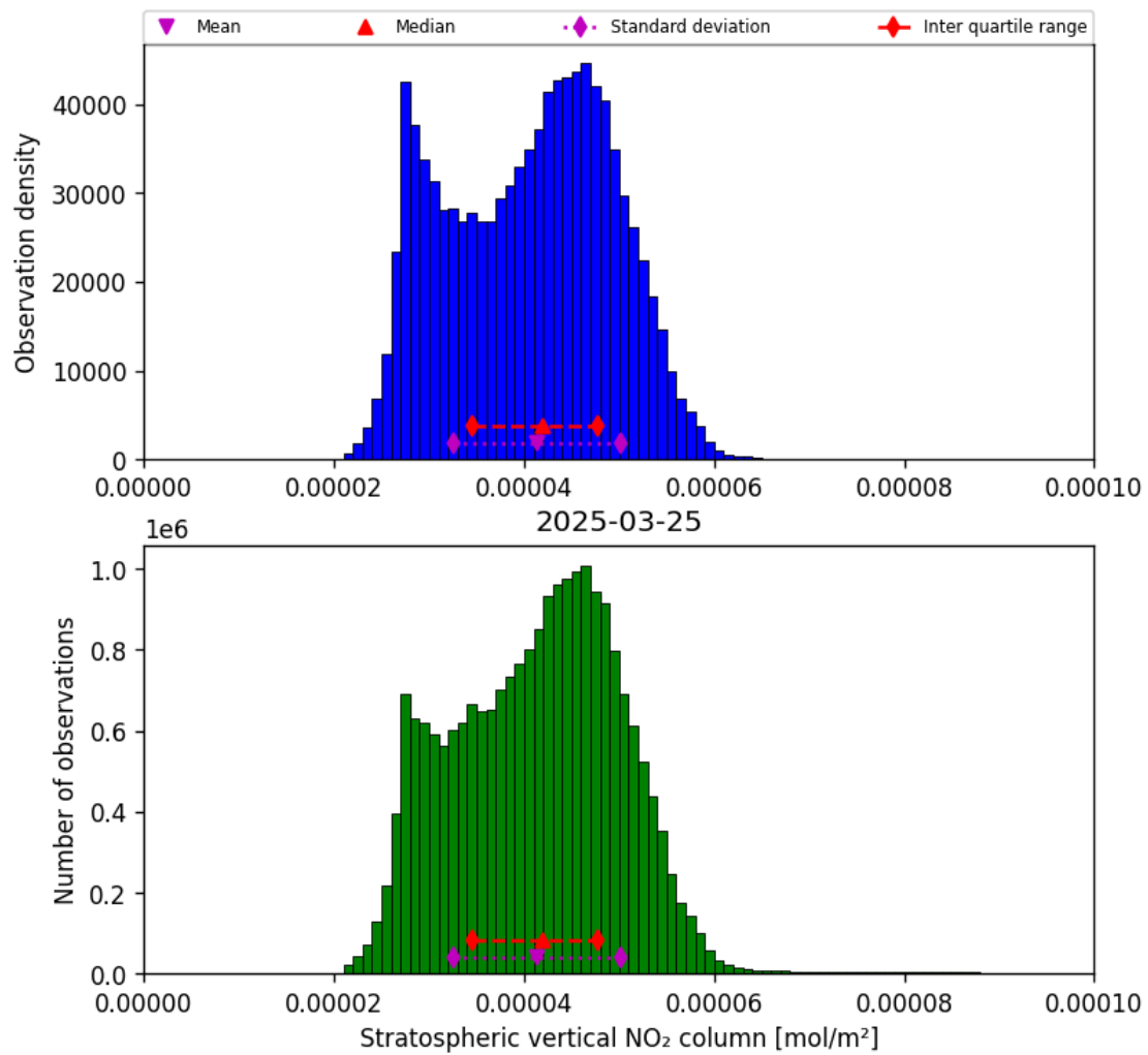
Figure 36: Histogram of “Stratospheric vertical NO 2 column” for 2025-03-25 to 2025-03-26
