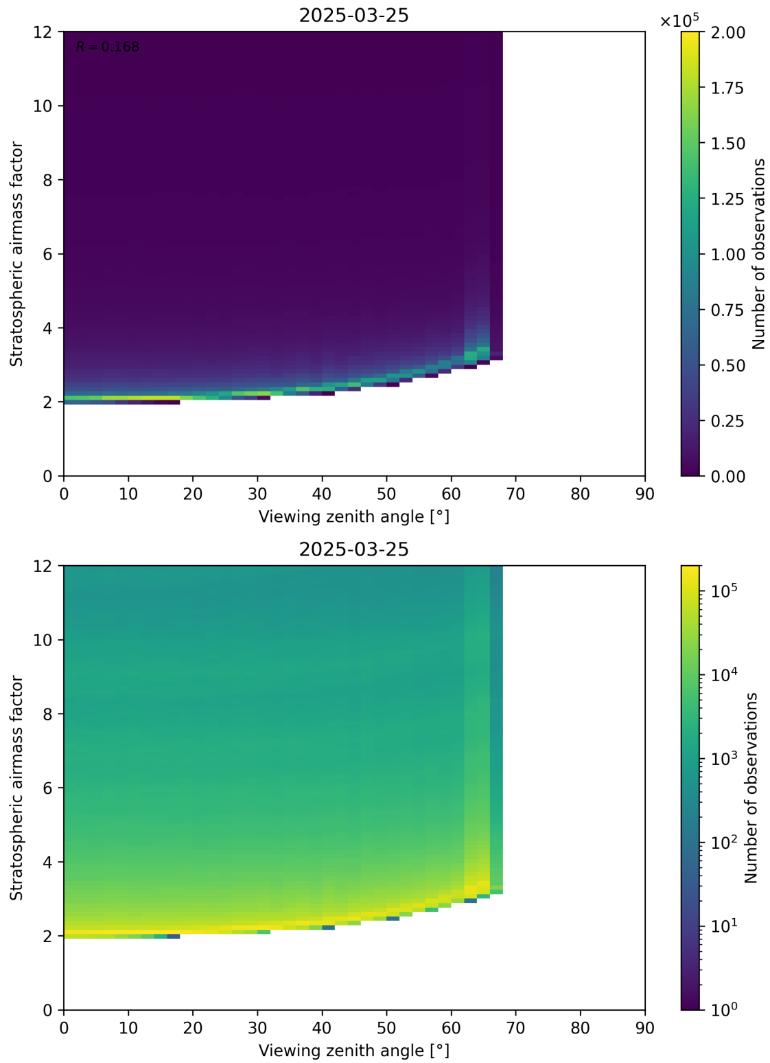
Figure 159: Scatter density plot of “Viewing zenith angle” against “Stratospheric airmass factor” for 2025-03-25 to 2025-03-26.
