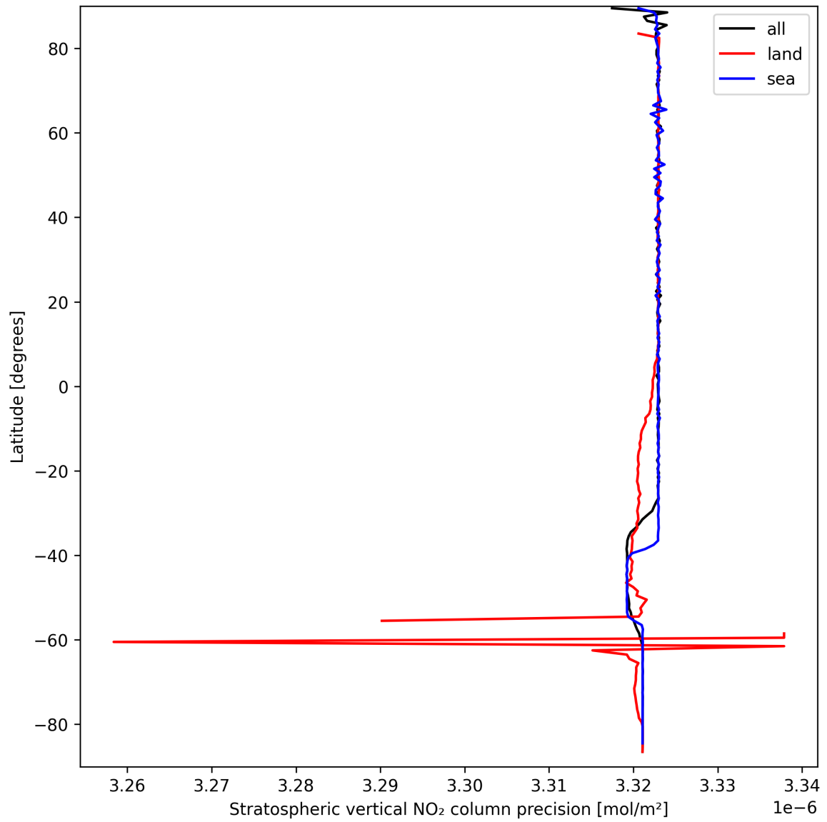
Figure 20: Zonal average of “Stratospheric vertical NO 2 column precision” for 2025-03-25 to 2025-03-26.
