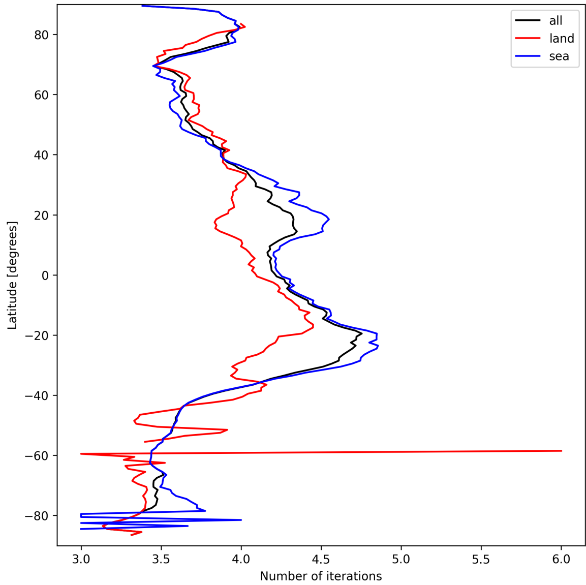
Figure 17: Zonal average of “Number of iterations” for 2025-03-25 to 2025-03-26.
