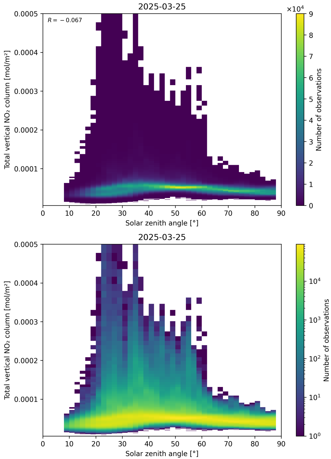
Figure 153: Scatter density plot of “Solar zenith angle” against “Total vertical NO 2 column” for 2025-03-25 to 2025-03-26.
