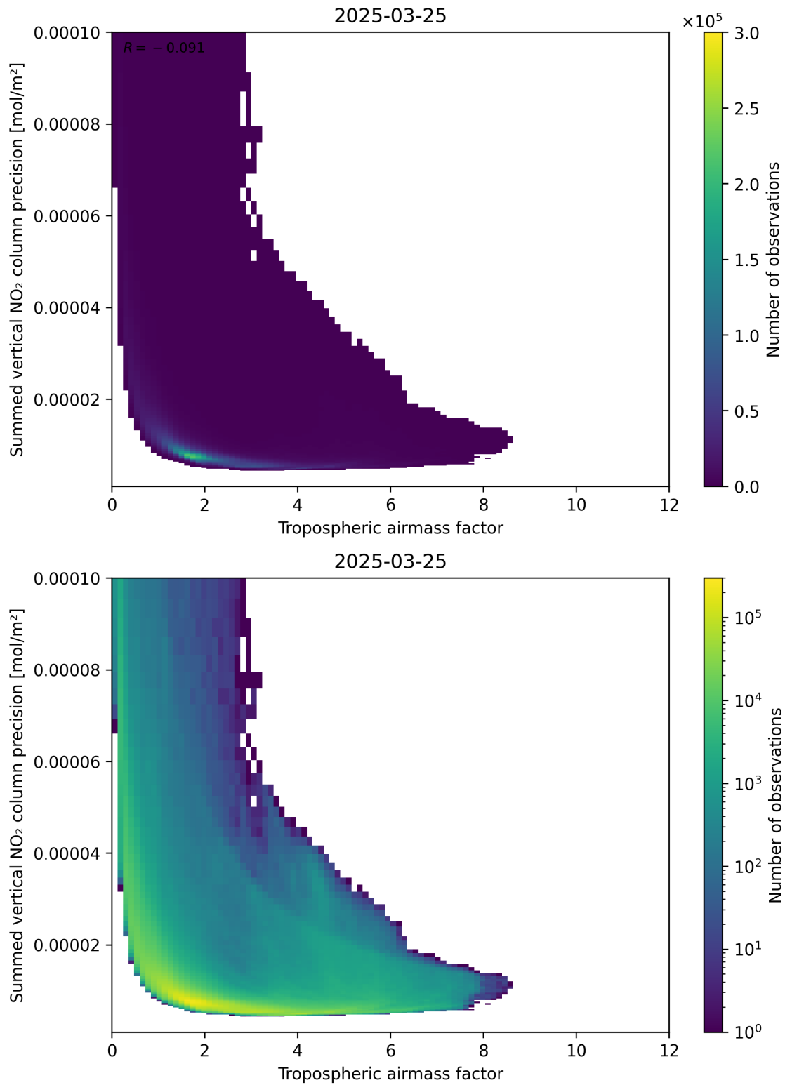
Figure 76: Scatter density plot of “Tropospheric airmass factor” against “Summed vertical NO 2 column precision” for 2025-03-25 to 2025-03-26.
