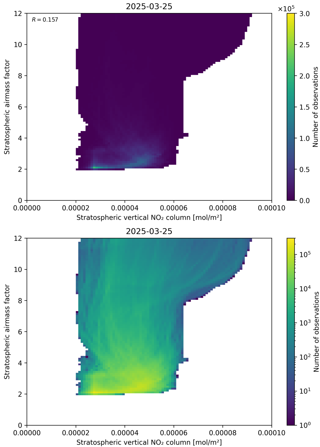
Figure 96: Scatter density plot of “Stratospheric vertical NO 2 column” against “Stratospheric airmass factor” for 2025-03-25 to 2025-03-26.
