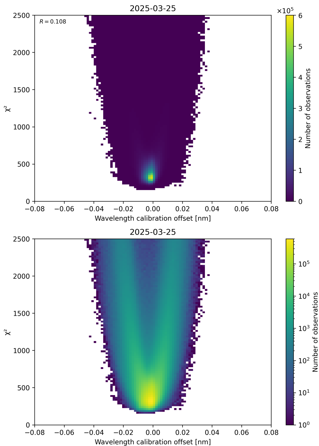
Figure 175: Scatter density plot of “Wavelength calibration offset” against “ \chi^2 ” for 2025-03-25 to 2025-03-26.
