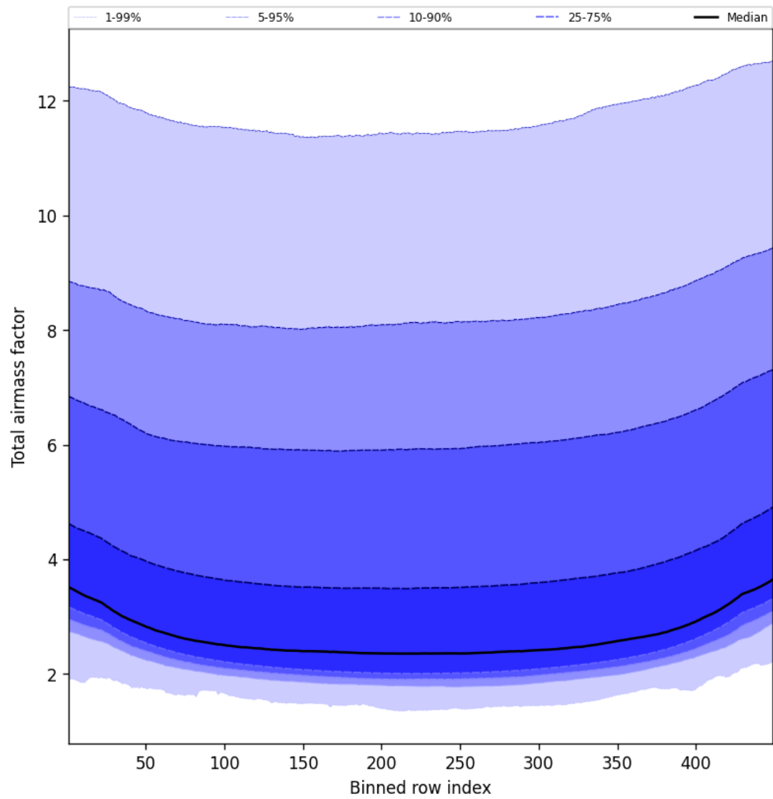
Figure 49: Along track statistics of “Total airmass factor” for 2025-03-25 to 2025-03-26
