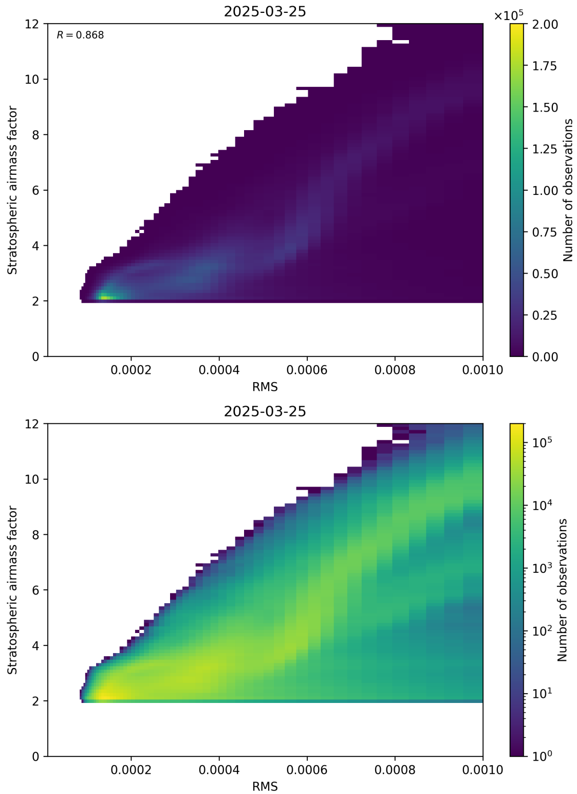
Figure 144: Scatter density plot of “RMS” against “Stratospheric airmass factor” for 2025-03-25 to 2025-03-26.
