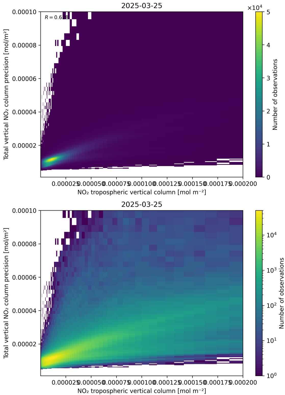
Figure 129: Scatter density plot of “NO 2 tropospheric vertical column” against “Total vertical NO 2 column precision” for 2025-03-25 to 2025-03-26.
