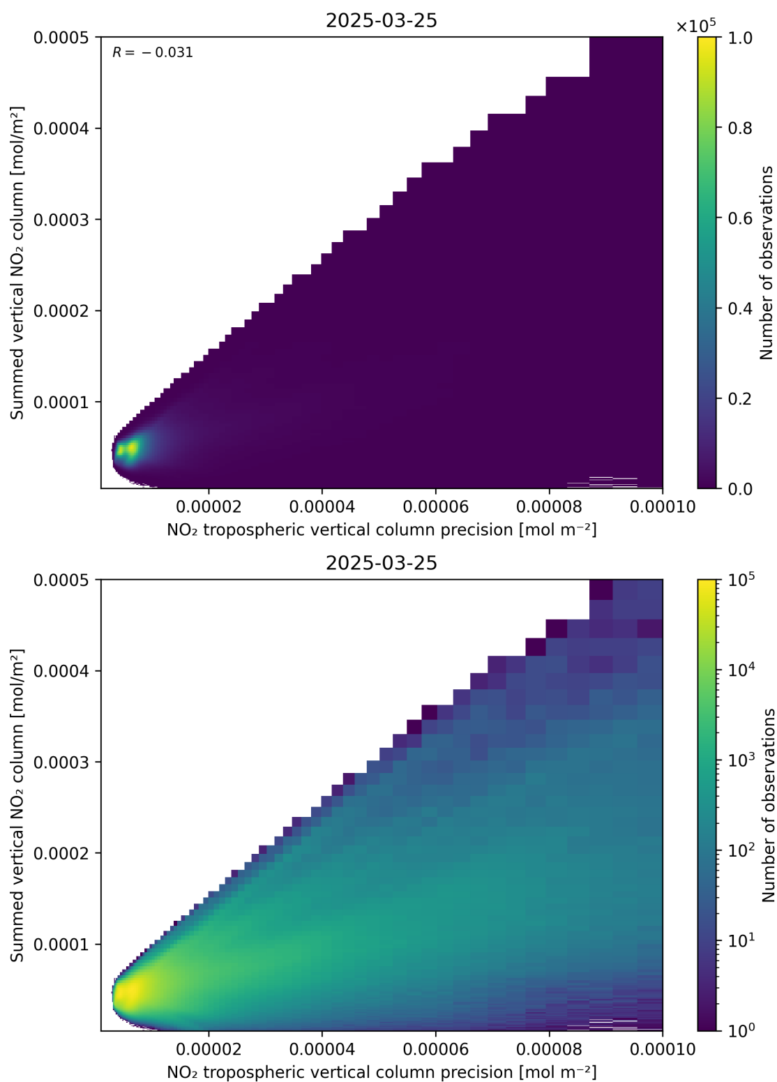
Figure 136: Scatter density plot of “NO 2 tropospheric vertical column precision” against “Summed vertical NO 2 column” for 2025-03-25 to 2025-03-26.
