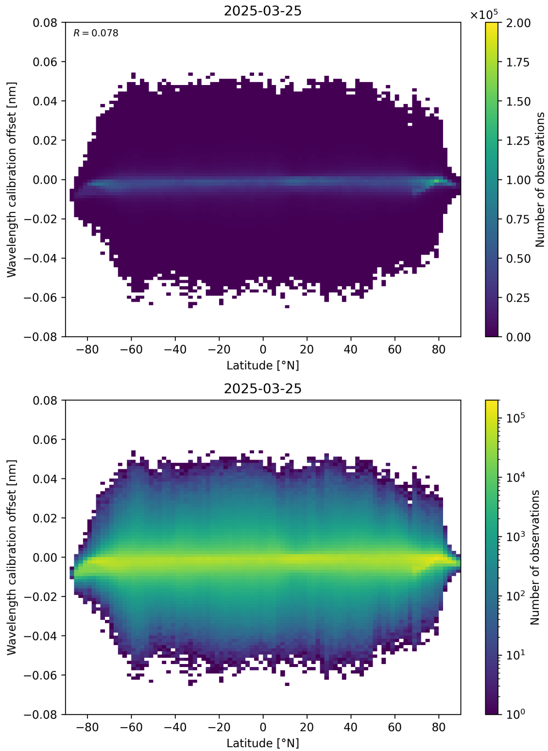
Figure 95: Scatter density plot of “Latitude” against “Wavelength calibration offset” for 2025-03-25 to 2025-03-26.
