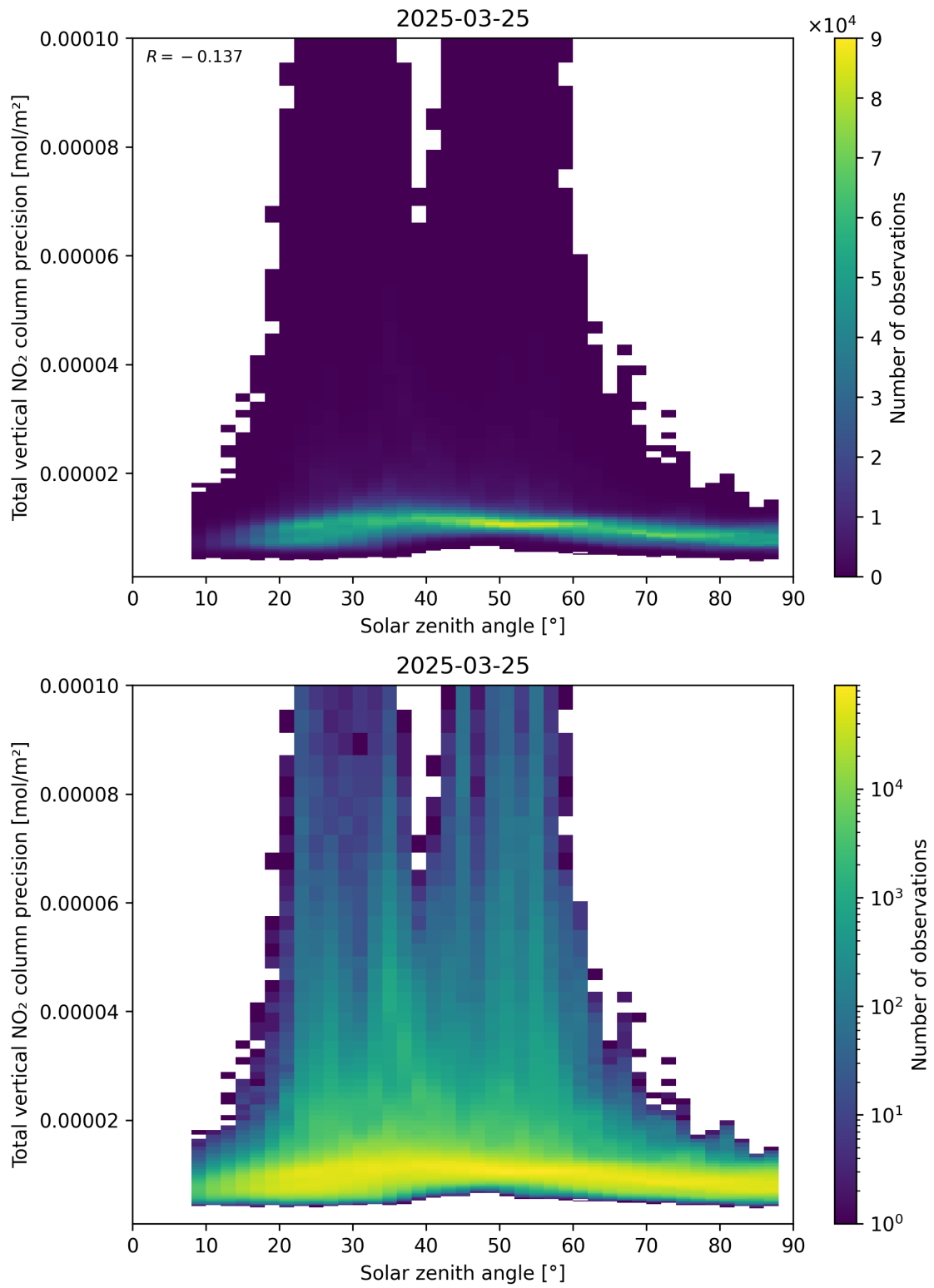
Figure 154: Scatter density plot of “Solar zenith angle” against “Total vertical NO 2 column precision” for 2025-03-25 to 2025-03-26.
