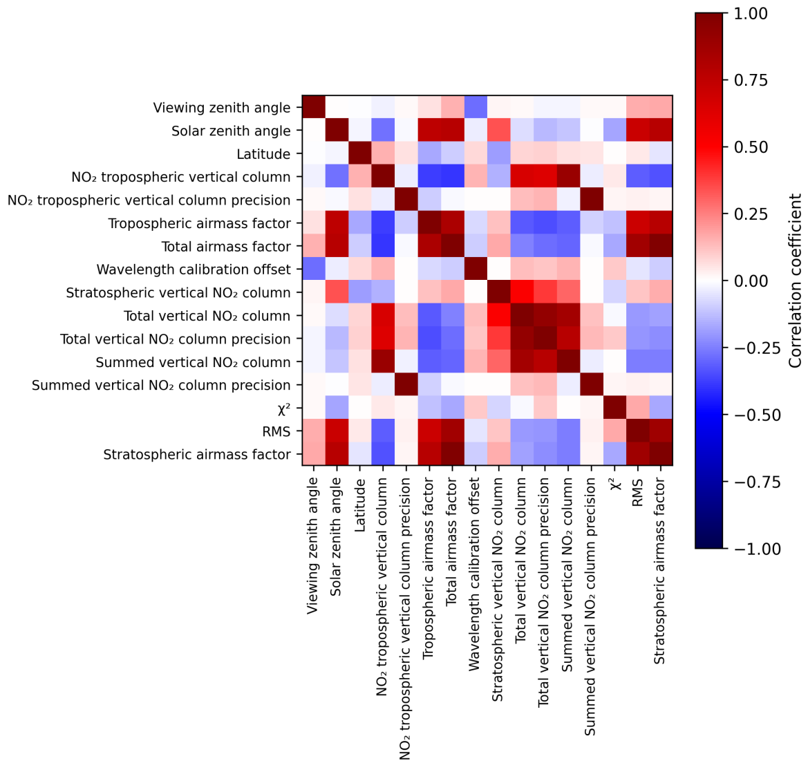
Figure 2: Map of correlation matrix for 2025-03-25 to 2025-03-26.
