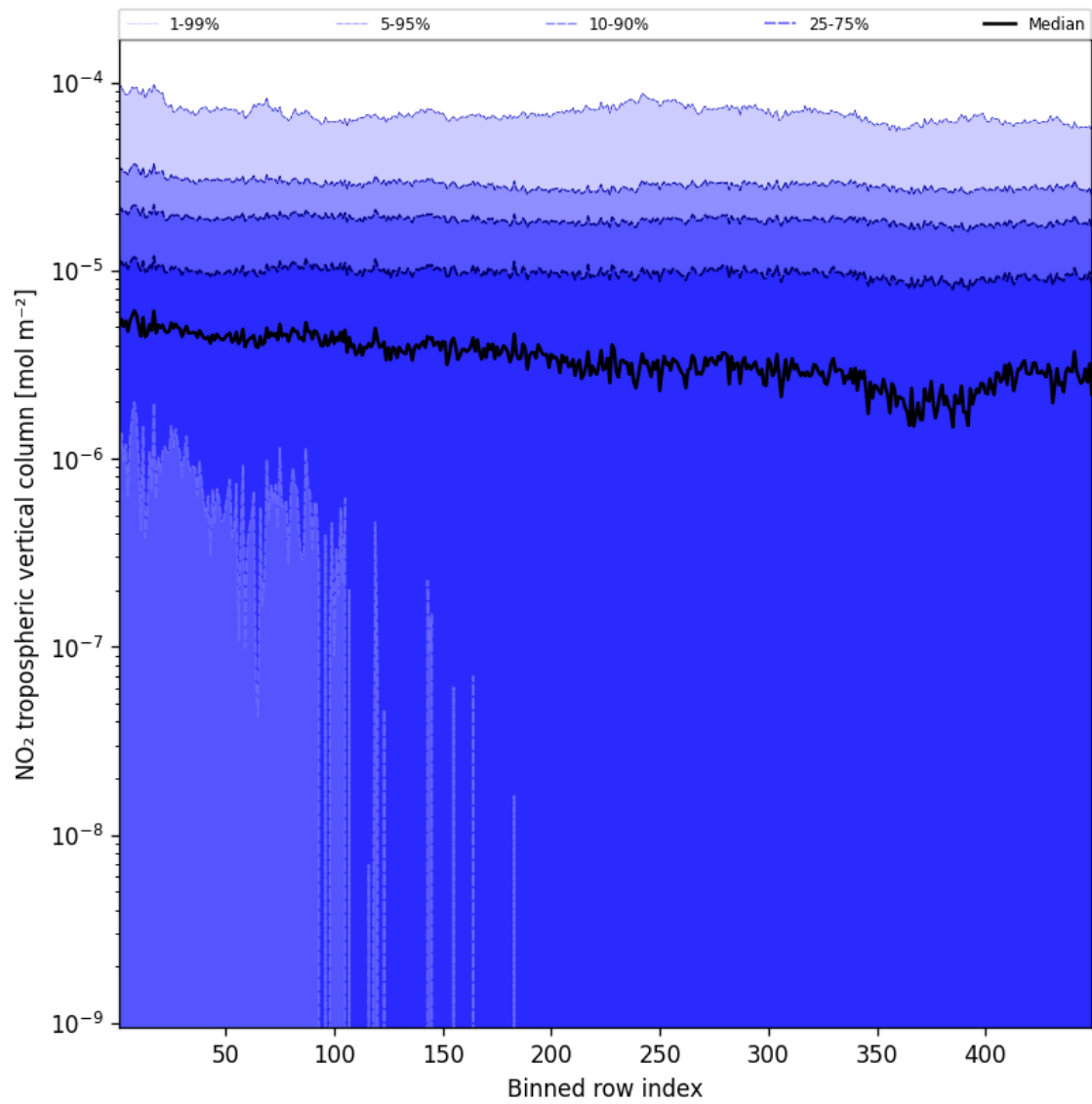
Figure 46: Along track statistics of “NO 2 tropospheric vertical column” for 2025-03-25 to 2025-03-26
