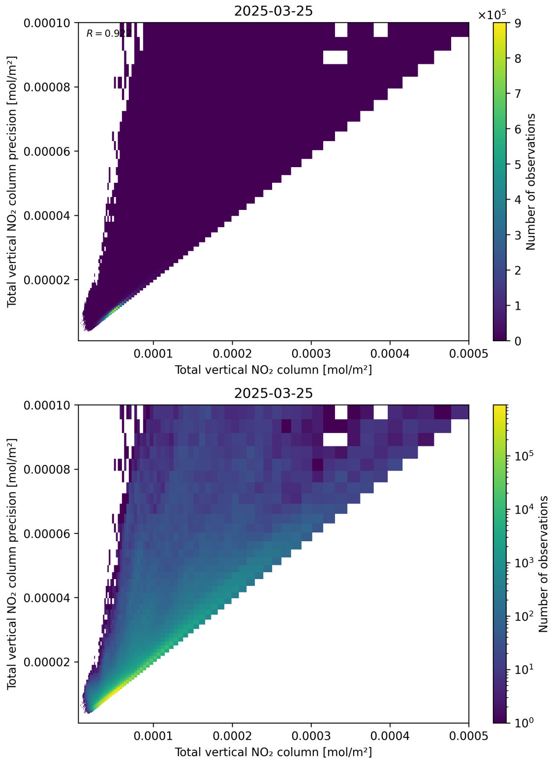
Figure 114: Scatter density plot of “Total vertical NO 2 column” against “Total vertical NO 2 column precision” for 2025-03-25 to 2025-03-26.
