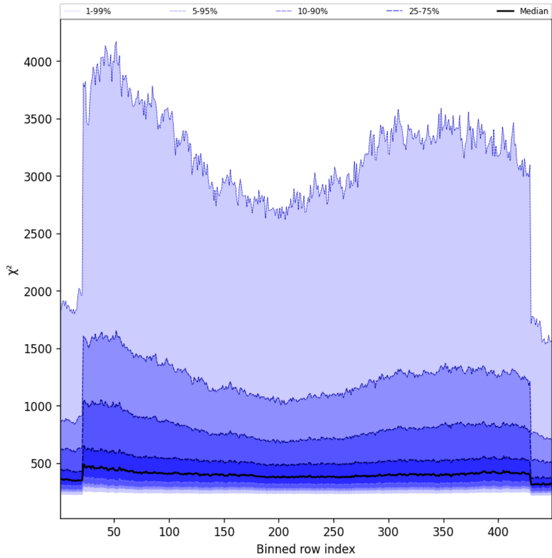
Figure 59: Along track statistics of “ \chi^2 ” for 2025-03-25 to 2025-03-26
