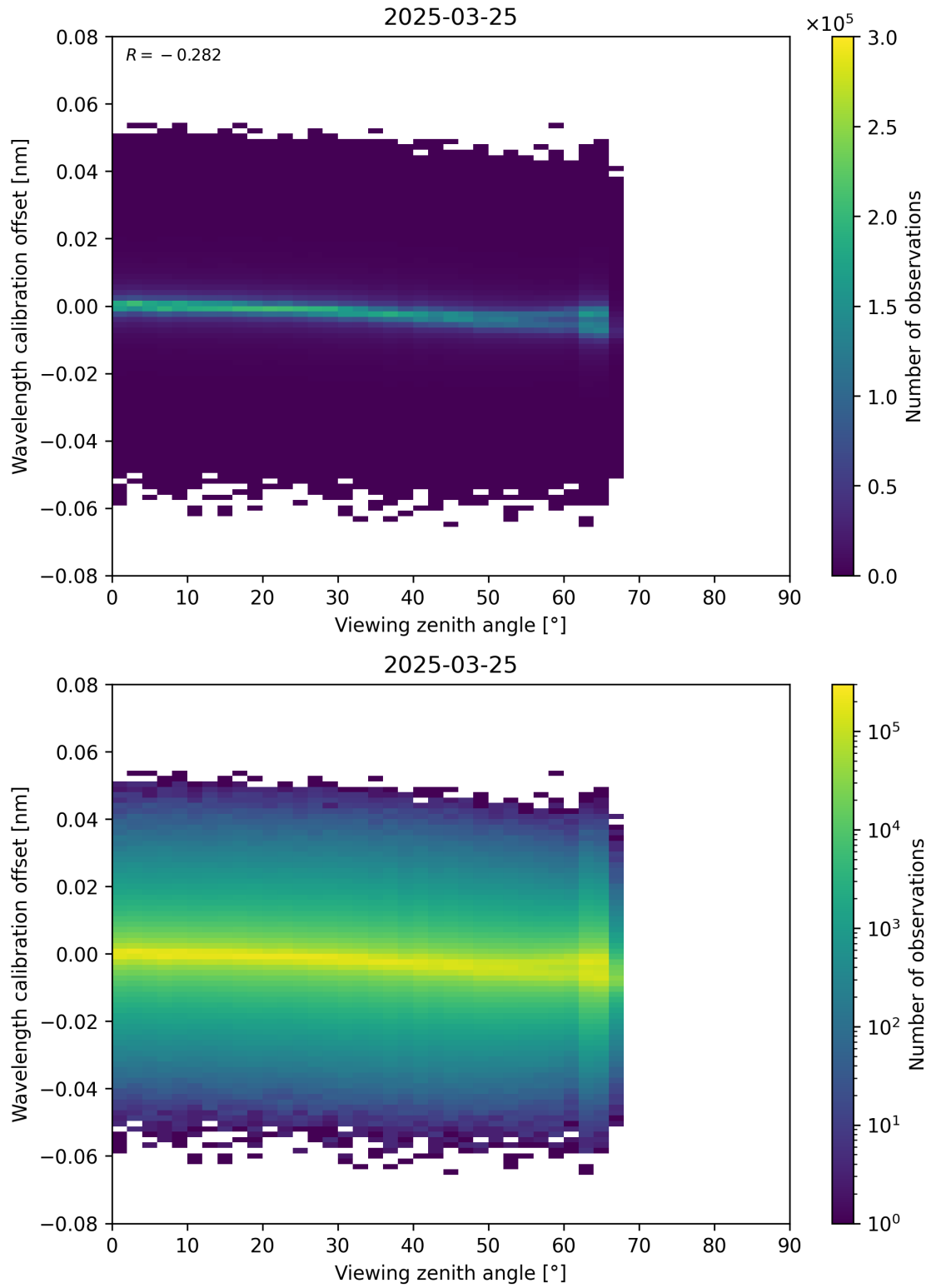
Figure 173: Scatter density plot of “Viewing zenith angle” against “Wavelength calibration offset” for 2025-03-25 to 2025-03-26.
