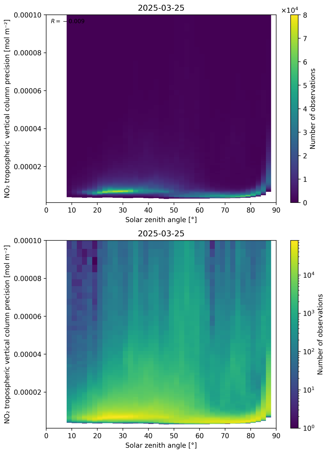
Figure 156: Scatter density plot of “Solar zenith angle” against “NO 2 tropospheric vertical column precision” for 2025-03-25 to 2025-03-26.
