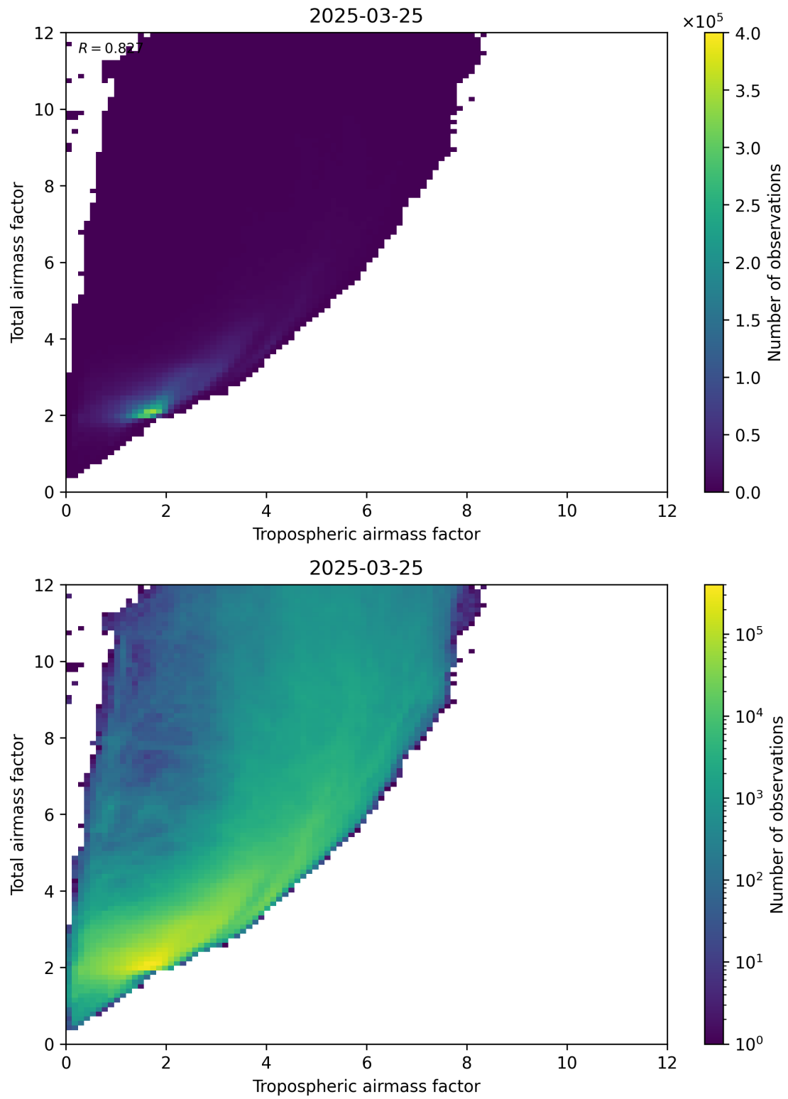
Figure 72: Scatter density plot of “Tropospheric airmass factor” against “Total airmass factor” for 2025-03-25 to 2025-03-26.
