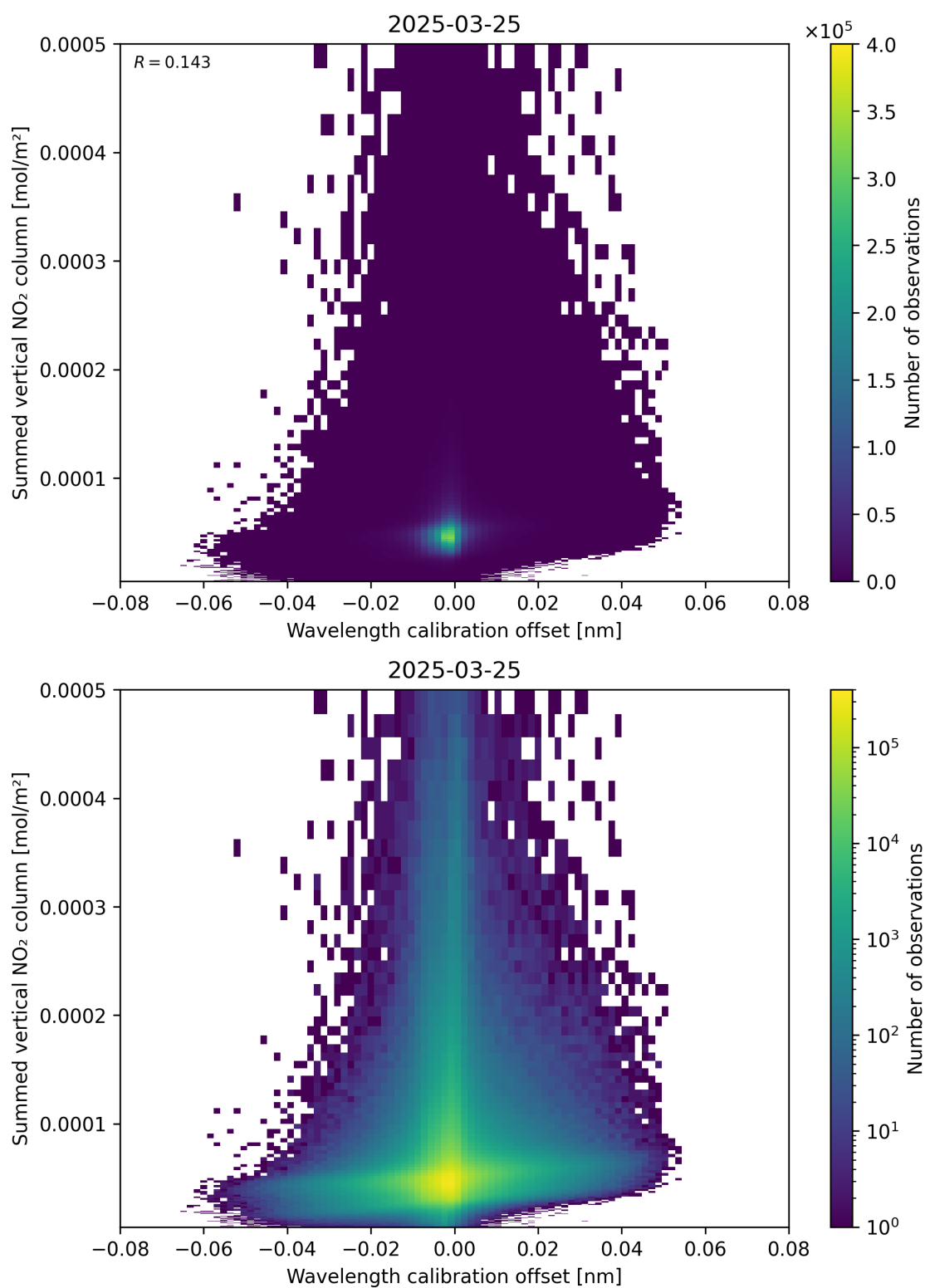
Figure 177: Scatter density plot of “Wavelength calibration offset” against “Summed vertical NO 2 column” for 2025-03-25 to 2025-03-26.
