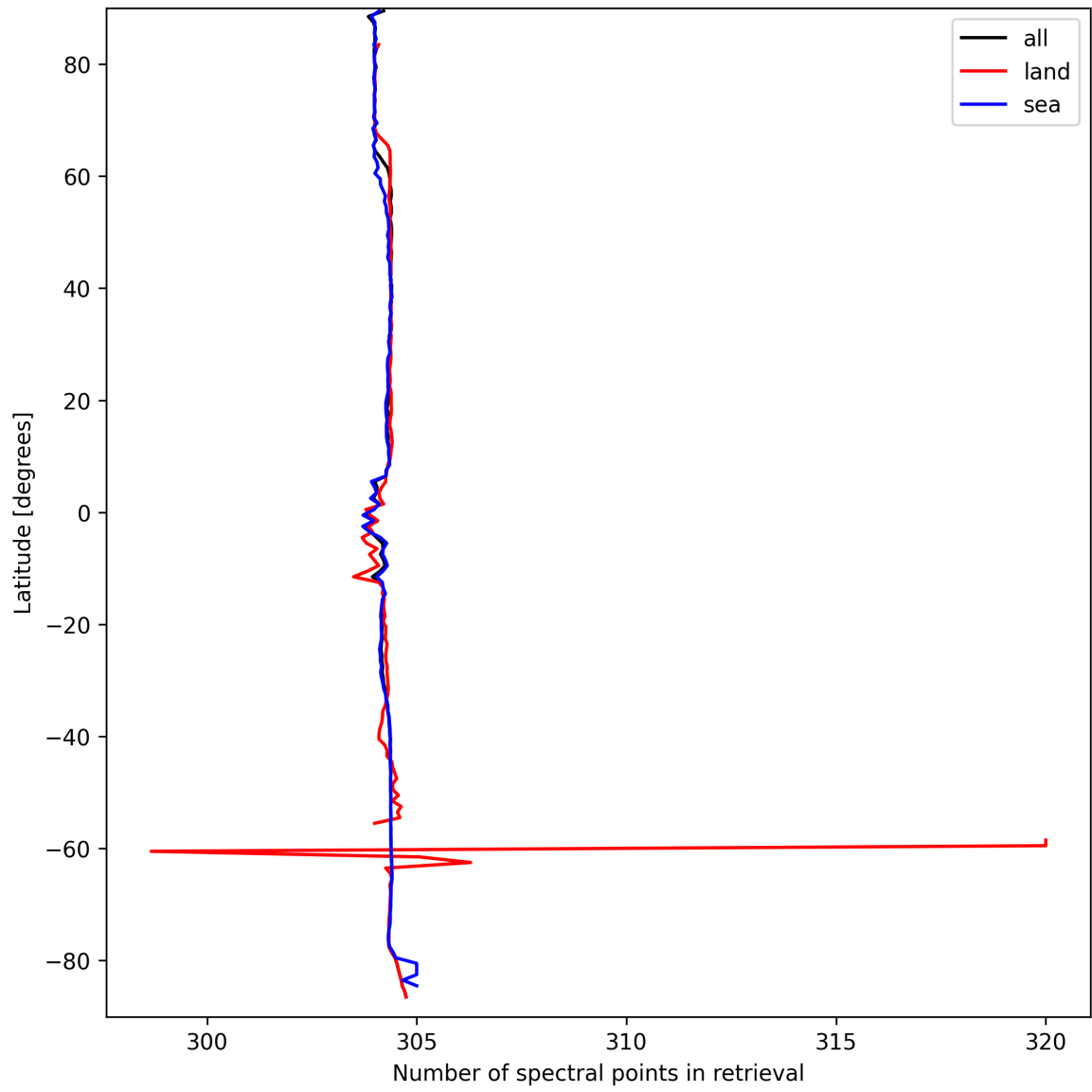
Figure 16: Zonal average of “Number of spectral points in retrieval” for 2025-03-25 to 2025-03-26.
