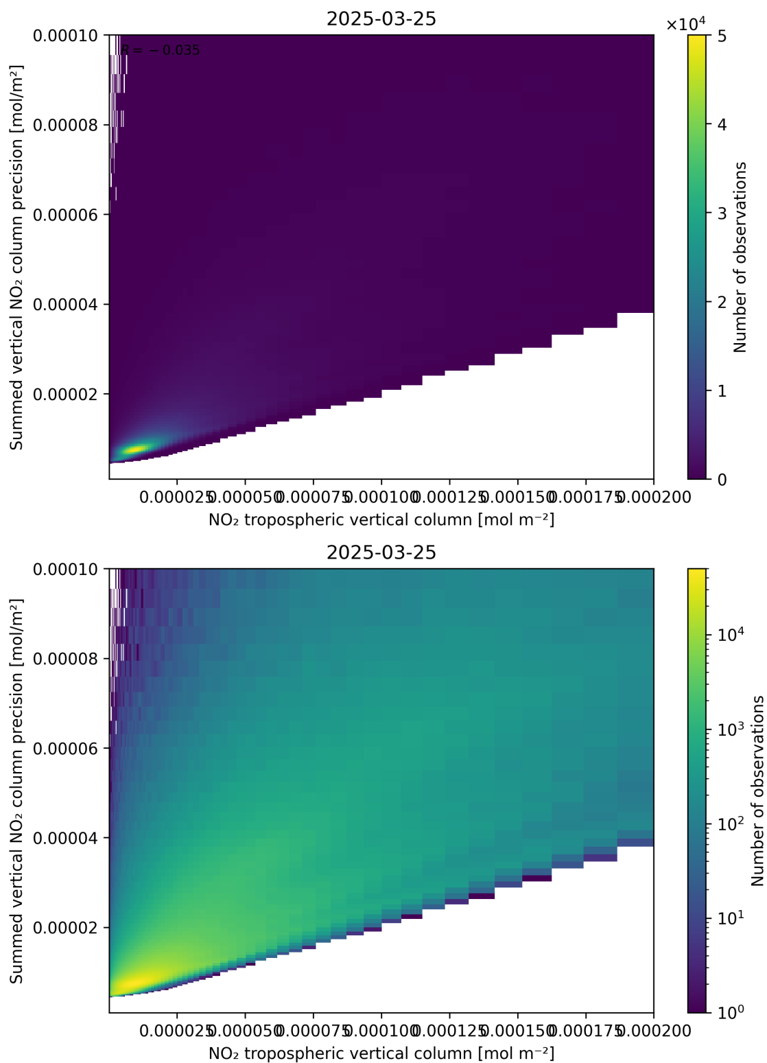
Figure 127: Scatter density plot of “NO 2 tropospheric vertical column” against “Summed vertical NO 2 column precision” for 2025-03-25 to 2025-03-26.
