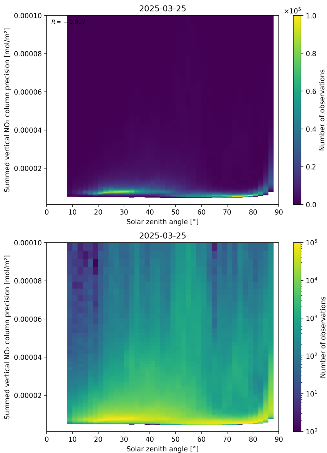
Figure 152: Scatter density plot of “Solar zenith angle” against “Summed vertical NO 2 column precision” for 2025-03-25 to 2025-03-26.
