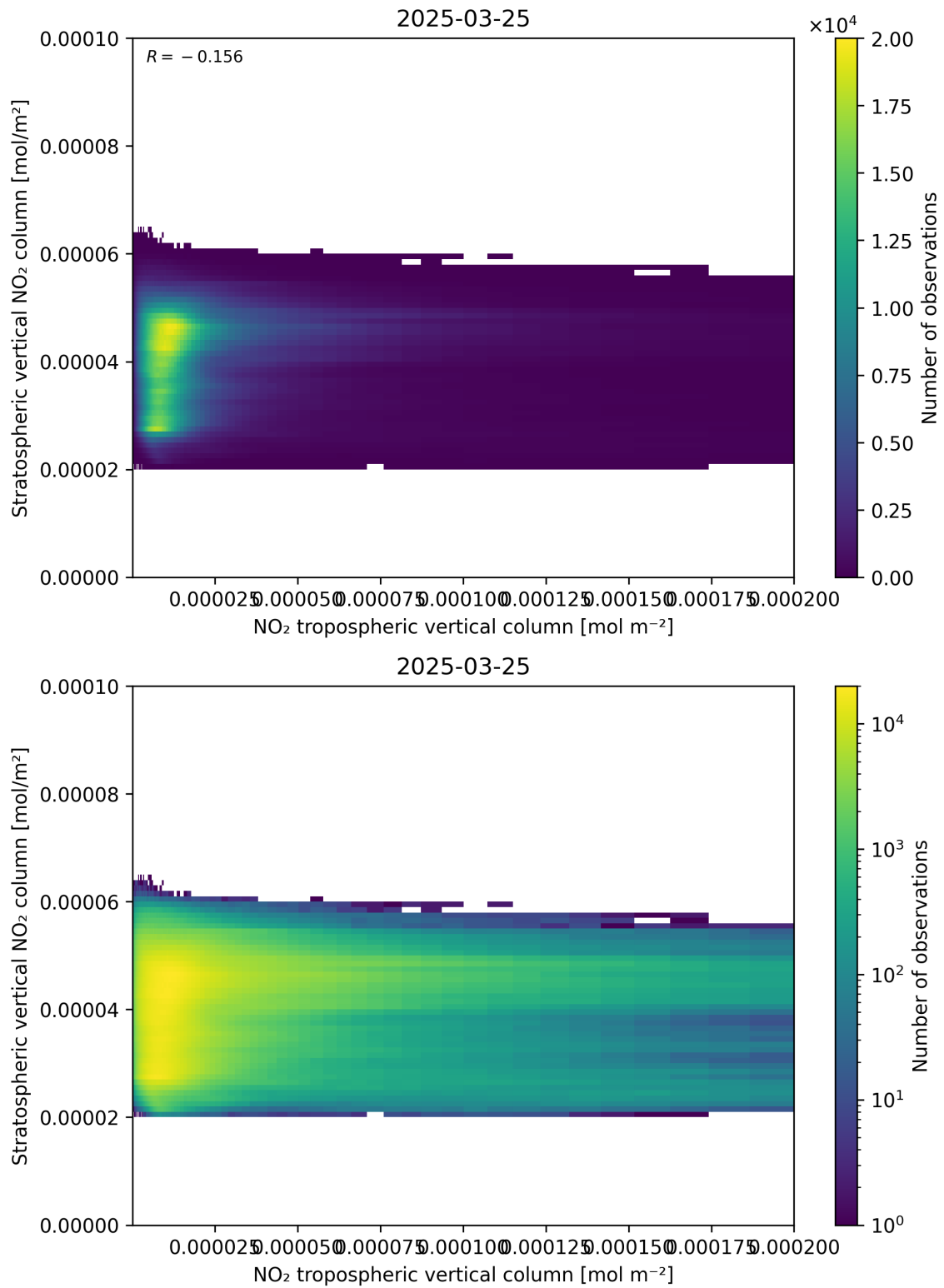
Figure 125: Scatter density plot of “NO 2 tropospheric vertical column” against “Stratospheric vertical NO 2 column” for 2025-03-25 to 2025-03-26.
