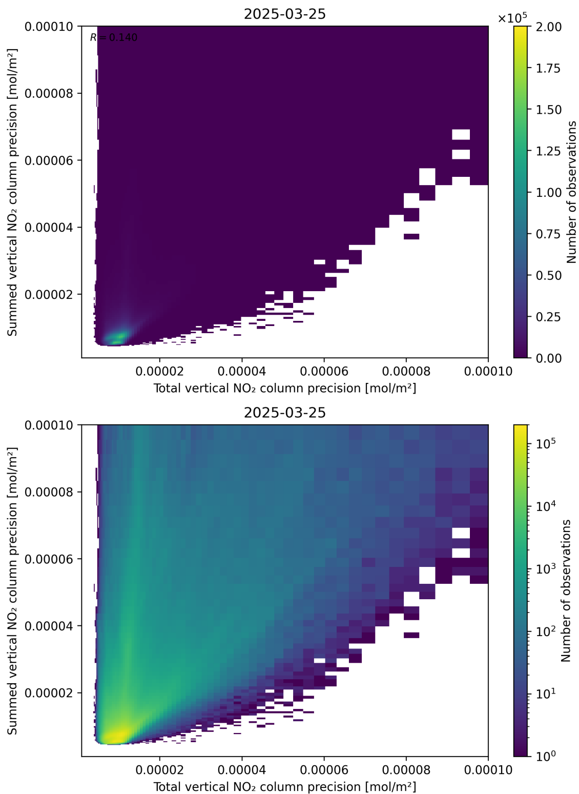
Figure 118: Scatter density plot of “Total vertical NO 2 column precision” against “Summed vertical NO 2 column precision” for 2025-03-25 to 2025-03-26.
