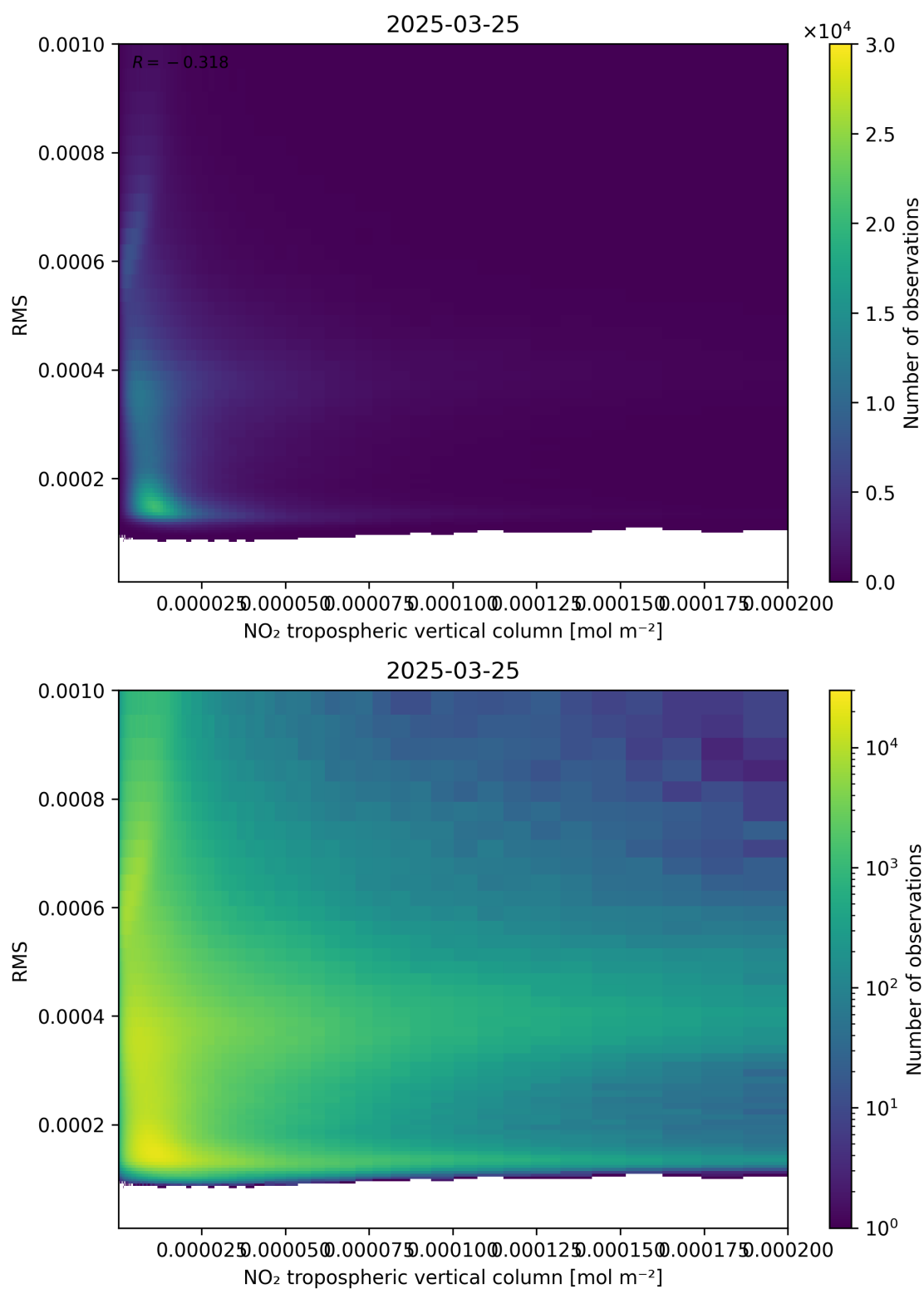
Figure 142: Scatter density plot of “NO 2 tropospheric vertical column” against “RMS” for 2025-03-25 to 2025-03-26.
