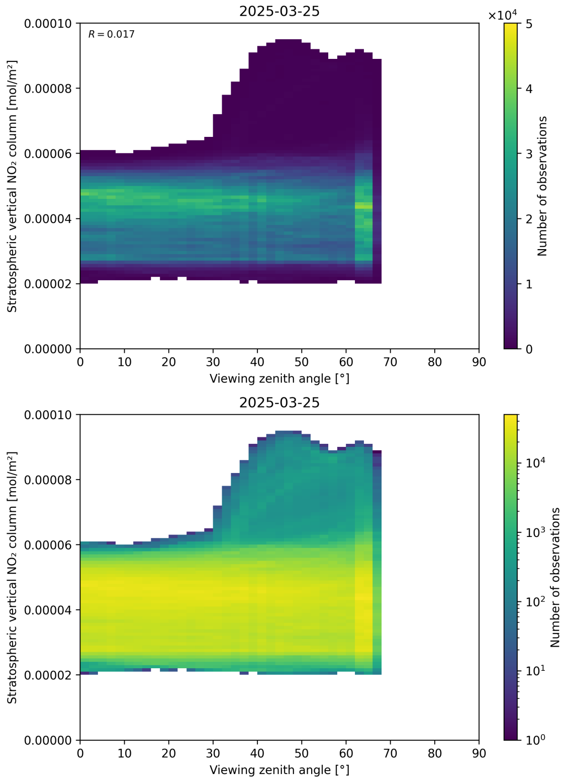
Figure 164: Scatter density plot of “Viewing zenith angle” against “Stratospheric vertical NO 2 column” for 2025-03-25 to 2025-03-26.
