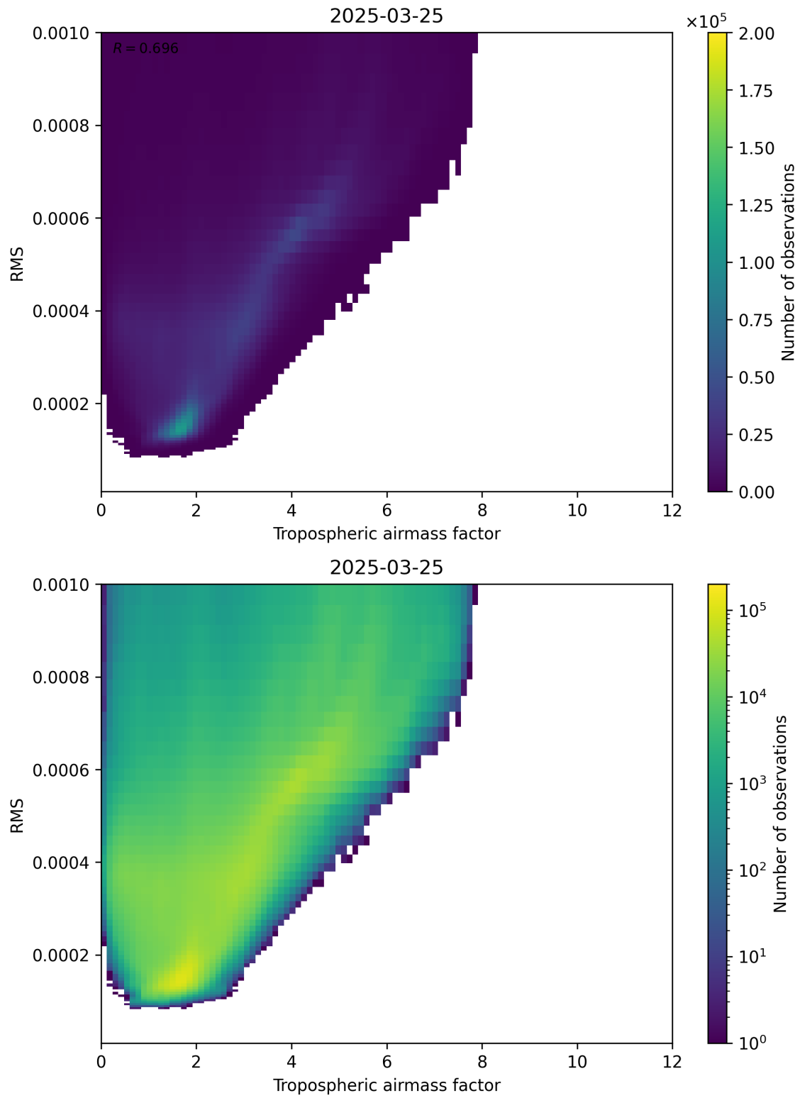
Figure 79: Scatter density plot of “Tropospheric airmass factor” against “RMS” for 2025-03-25 to 2025-03-26.
