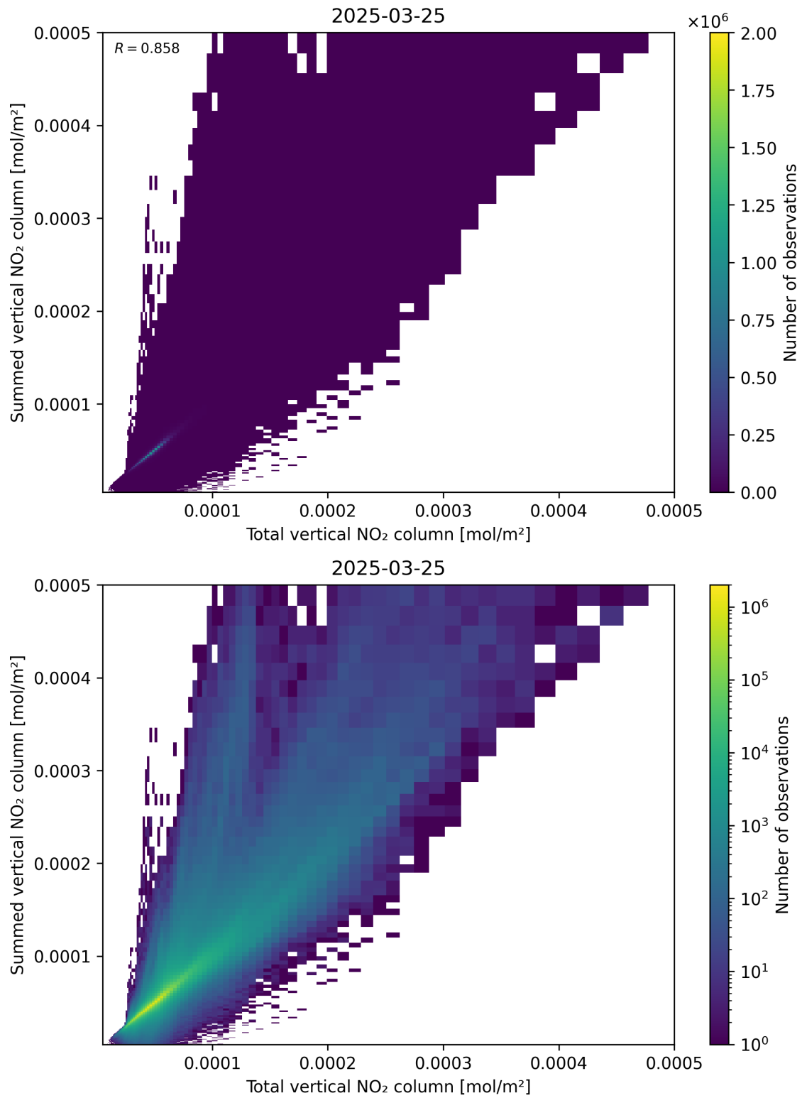
Figure 112: Scatter density plot of “Total vertical NO 2 column” against “Summed vertical NO 2 column” for 2025-03-25 to 2025-03-26.
