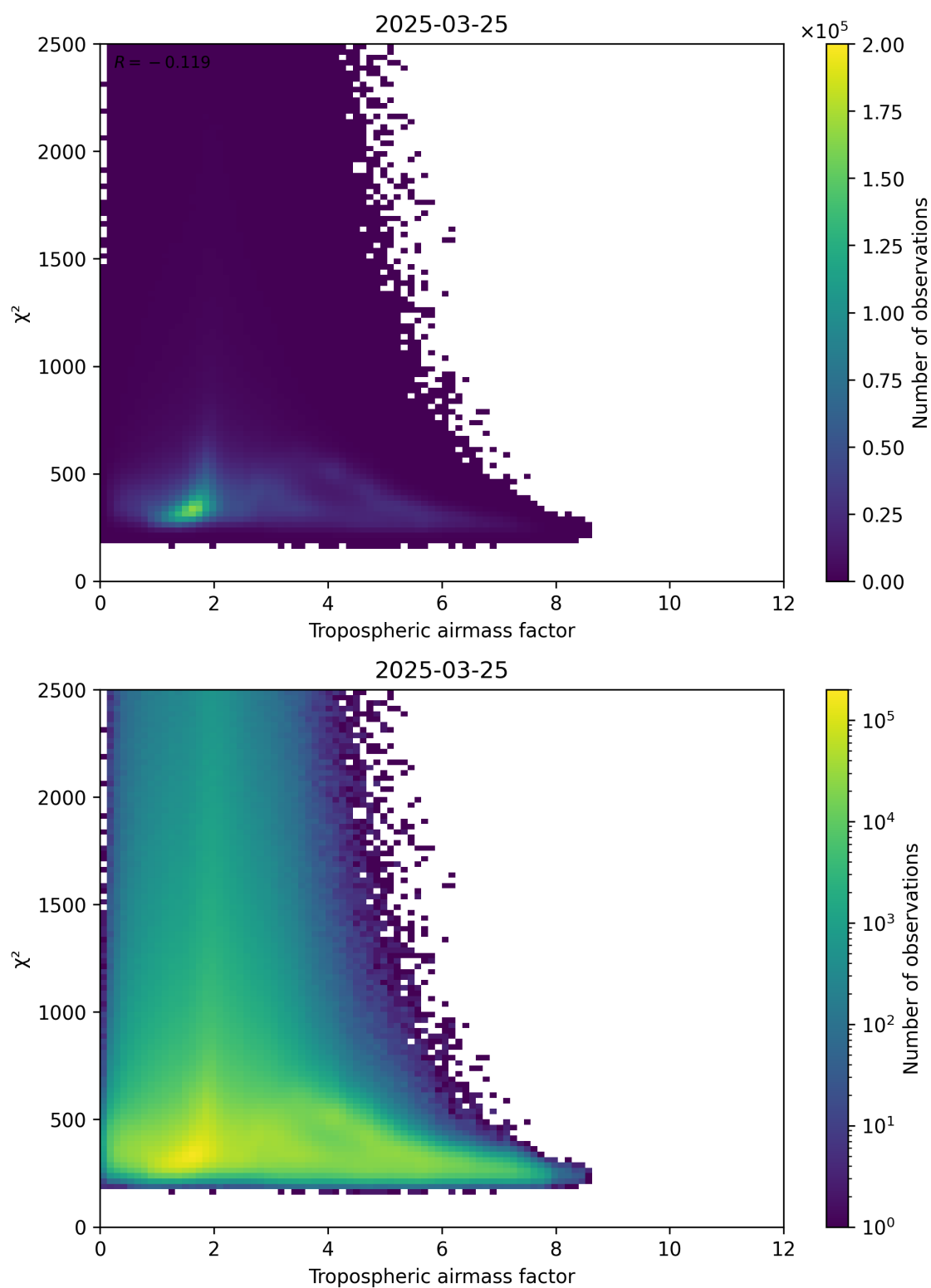
Figure 73: Scatter density plot of “Tropospheric airmass factor” against “ \chi^2 ” for 2025-03-25 to 2025-03-26.
