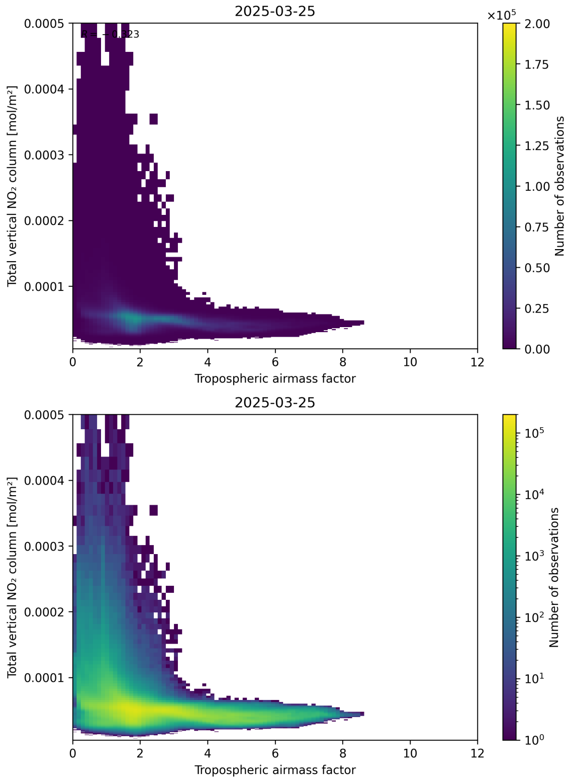
Figure 77: Scatter density plot of “Tropospheric airmass factor” against “Total vertical NO 2 column” for 2025-03-25 to 2025-03-26.
