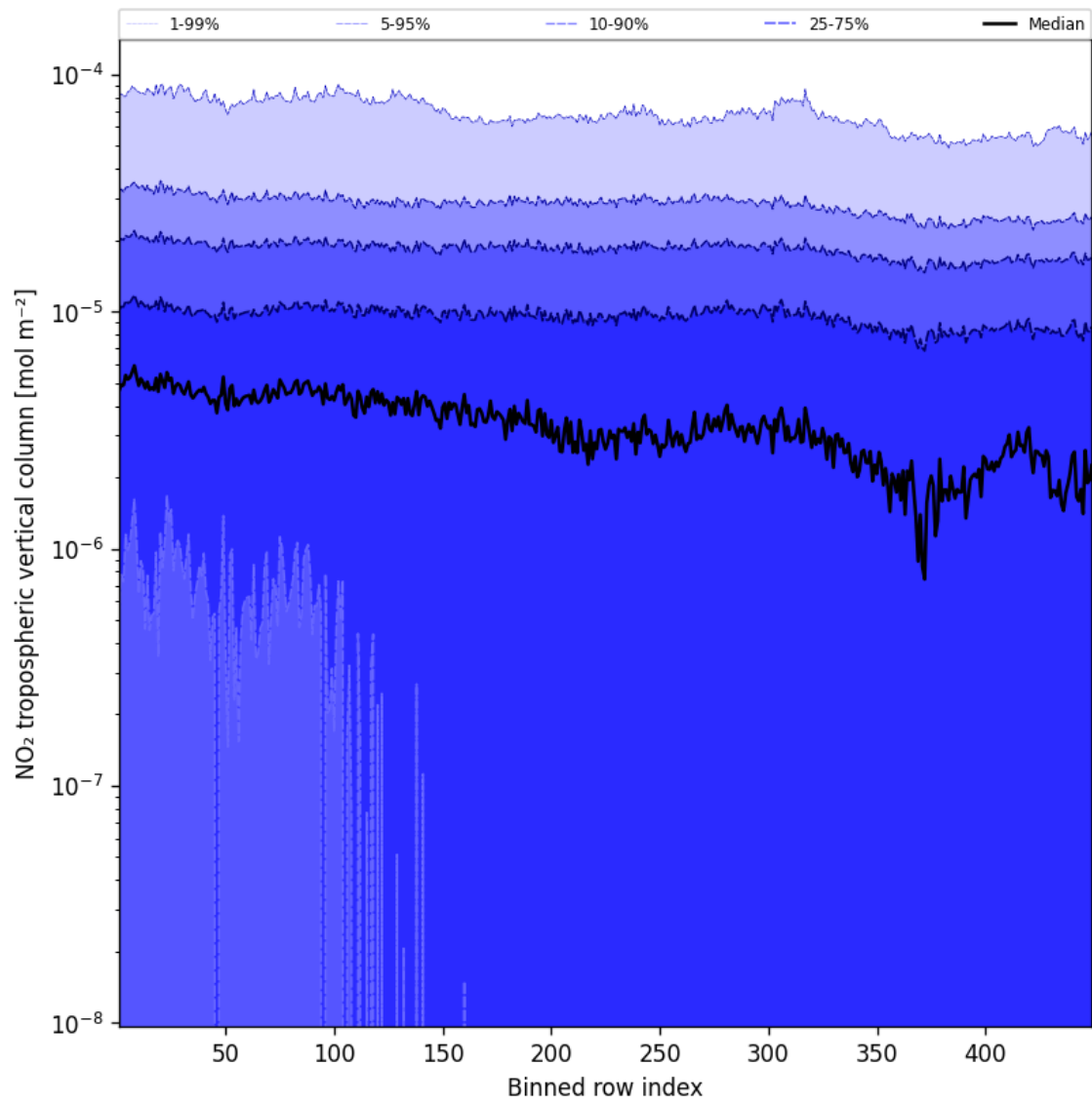
Figure 46: Along track statistics of “NO 2 tropospheric vertical column” for 2025-03-26 to 2025-03-26
