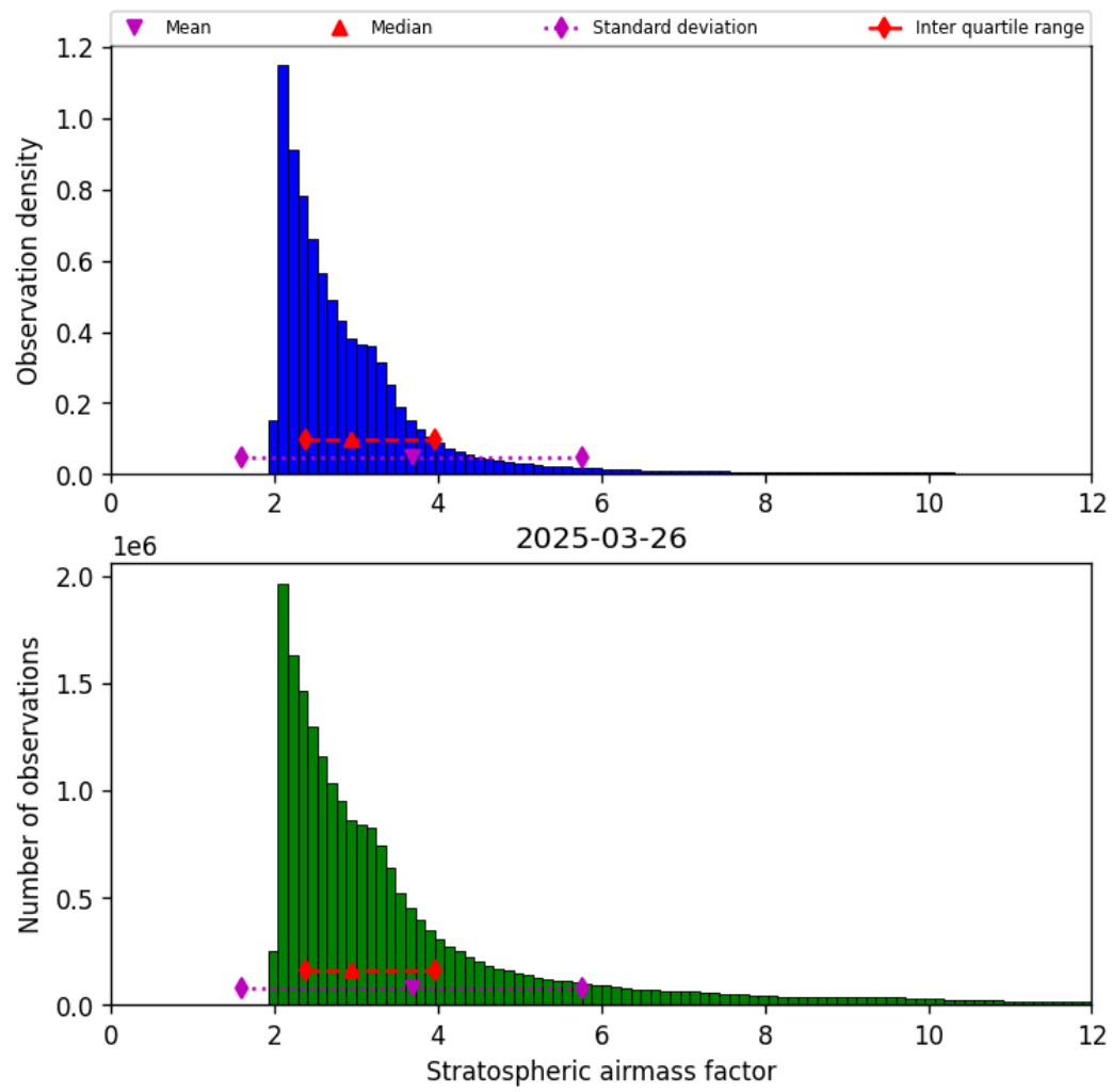
Figure 44: Histogram of “Stratospheric airmass factor” for 2025-03-26 to 2025-03-26
