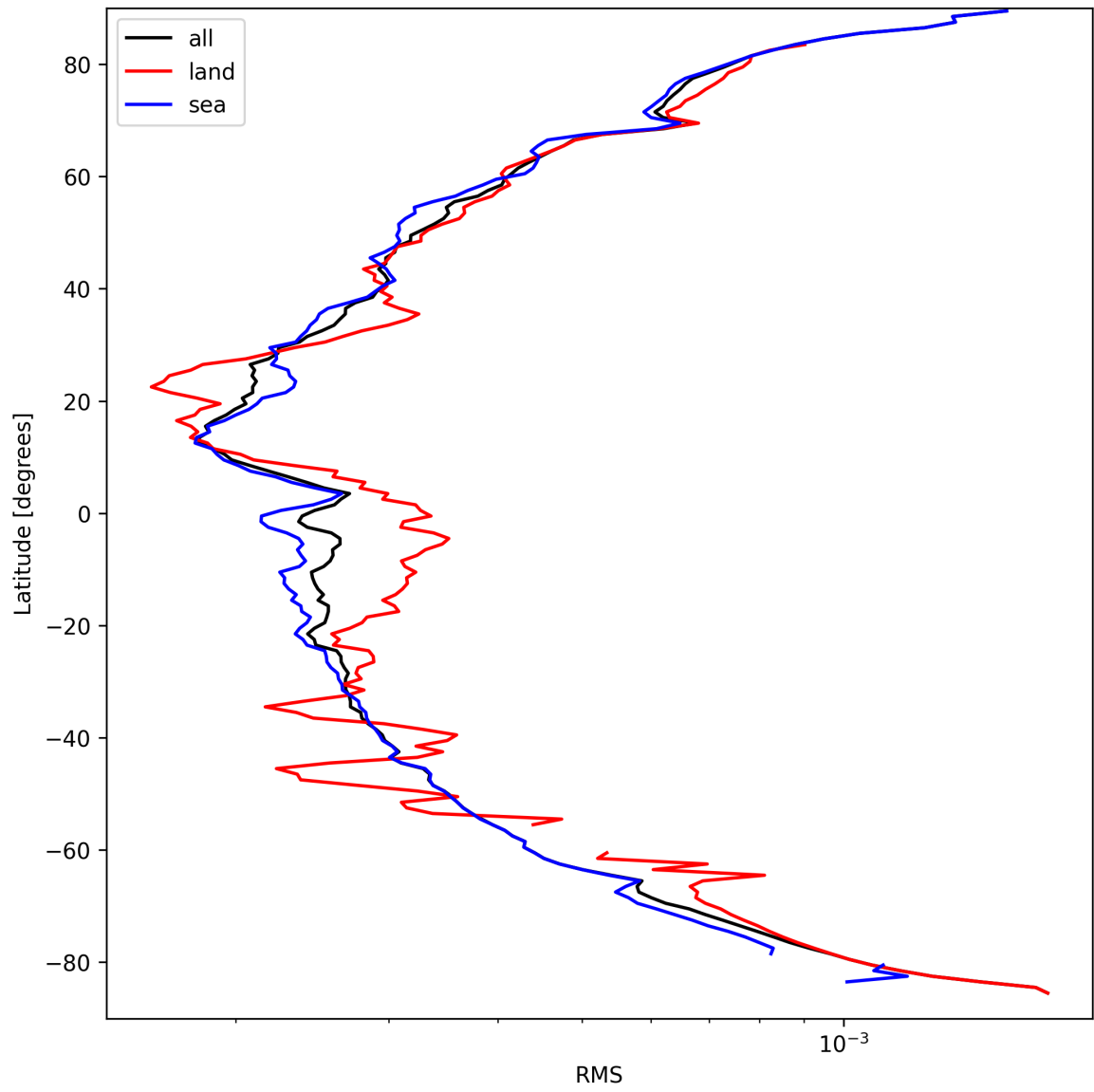
Figure 26: Zonal average of “RMS” for 2025-03-26 to 2025-03-26.
