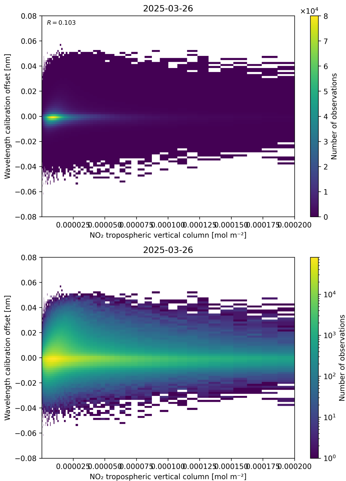
Figure 143: Scatter density plot of “NO 2 tropospheric vertical column” against “Wavelength calibration offset” for 2025-03-26 to 2025-03-26.
