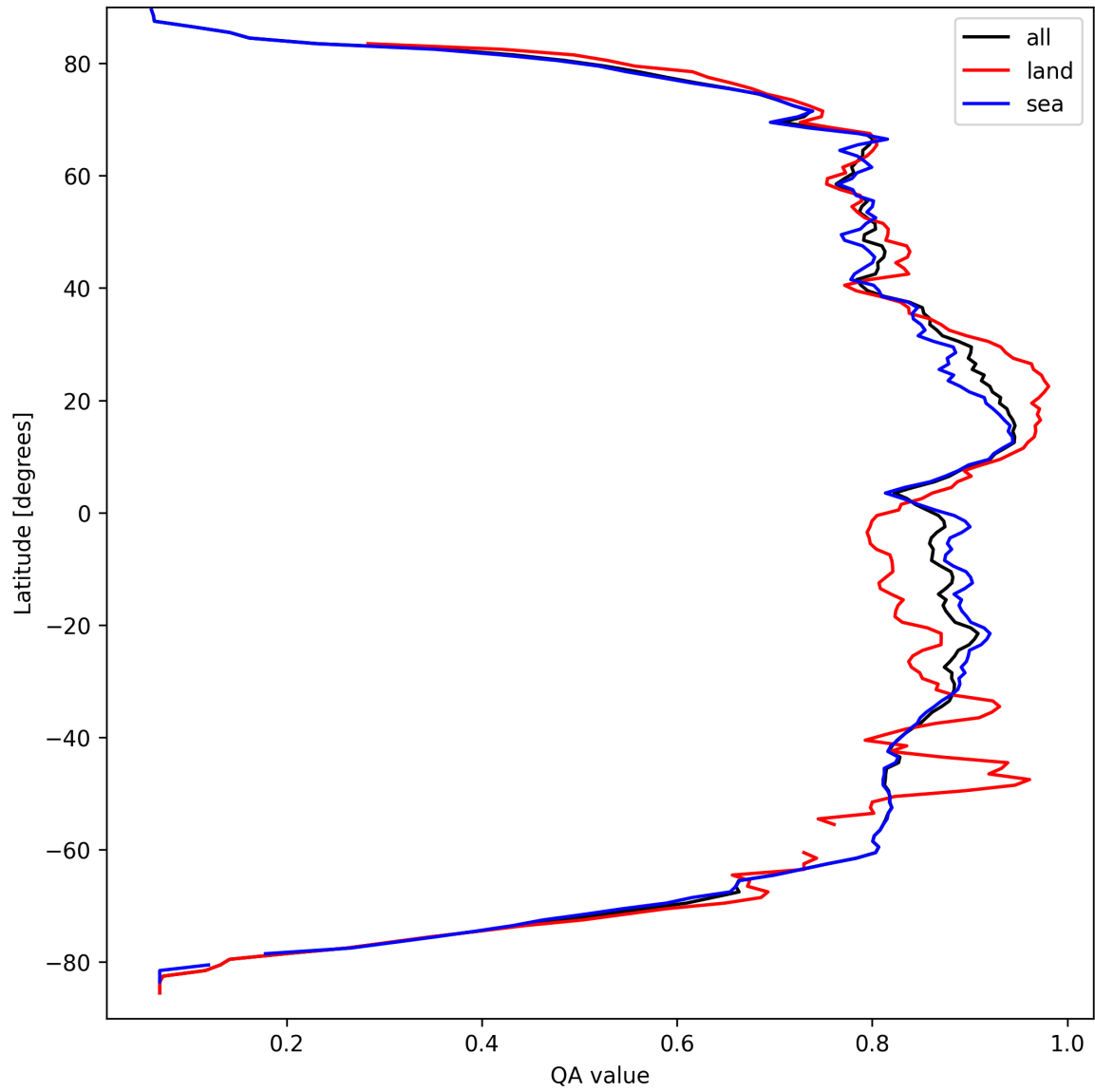
Figure 11: Zonal average of “QA value” for 2025-03-26 to 2025-03-26.
