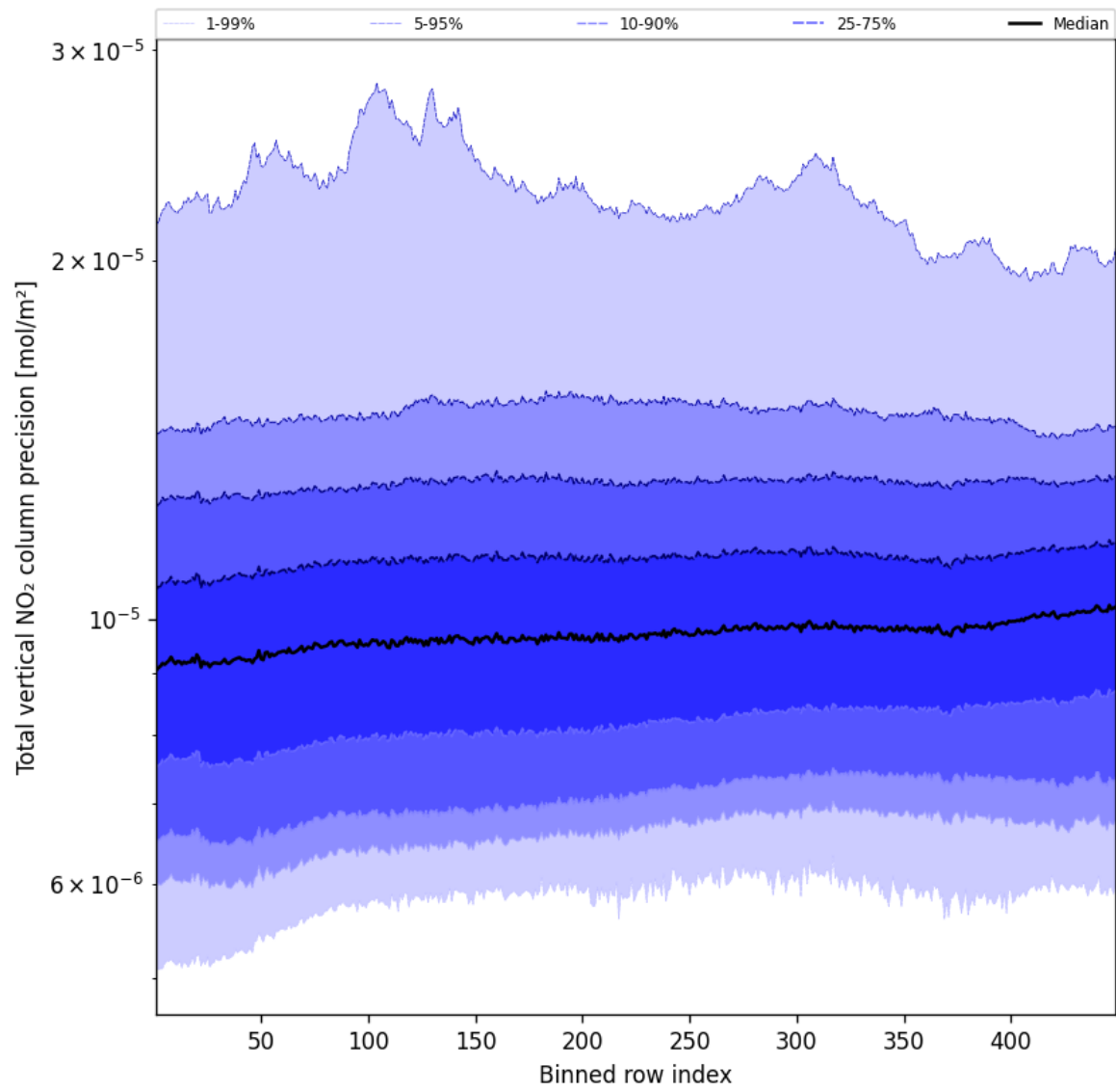
Figure 56: Along track statistics of “Total vertical NO 2 column precision” for 2025-03-26 to 2025-03-26
