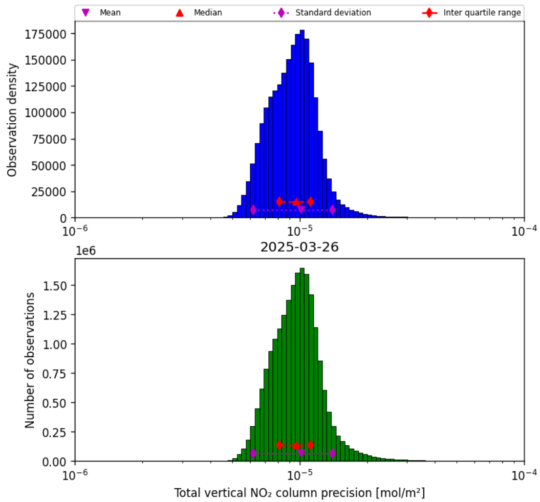
Figure 39: Histogram of "Total vertical NO 2 column precision" for 2025-03-26 to 2025-03-26
