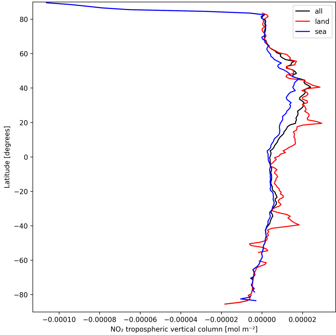
Figure 12: Zonal average of “NO 2 tropospheric vertical column” for 2025-03-26 to 2025-03-26.
