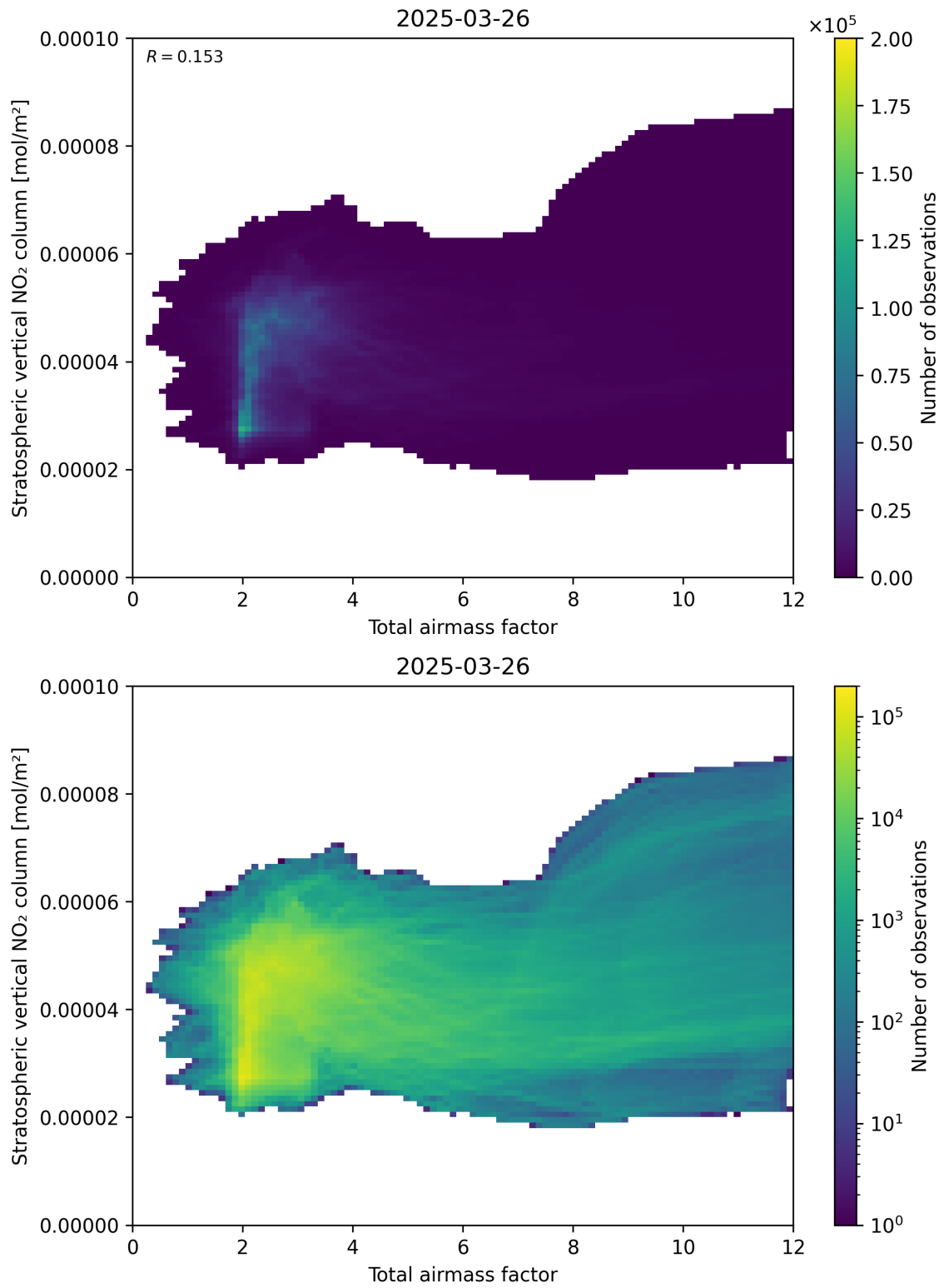
Figure 64: Scatter density plot of “Total airmass factor” against “Stratospheric vertical NO 2 column” for 2025-03-26 to 2025-03-26.
