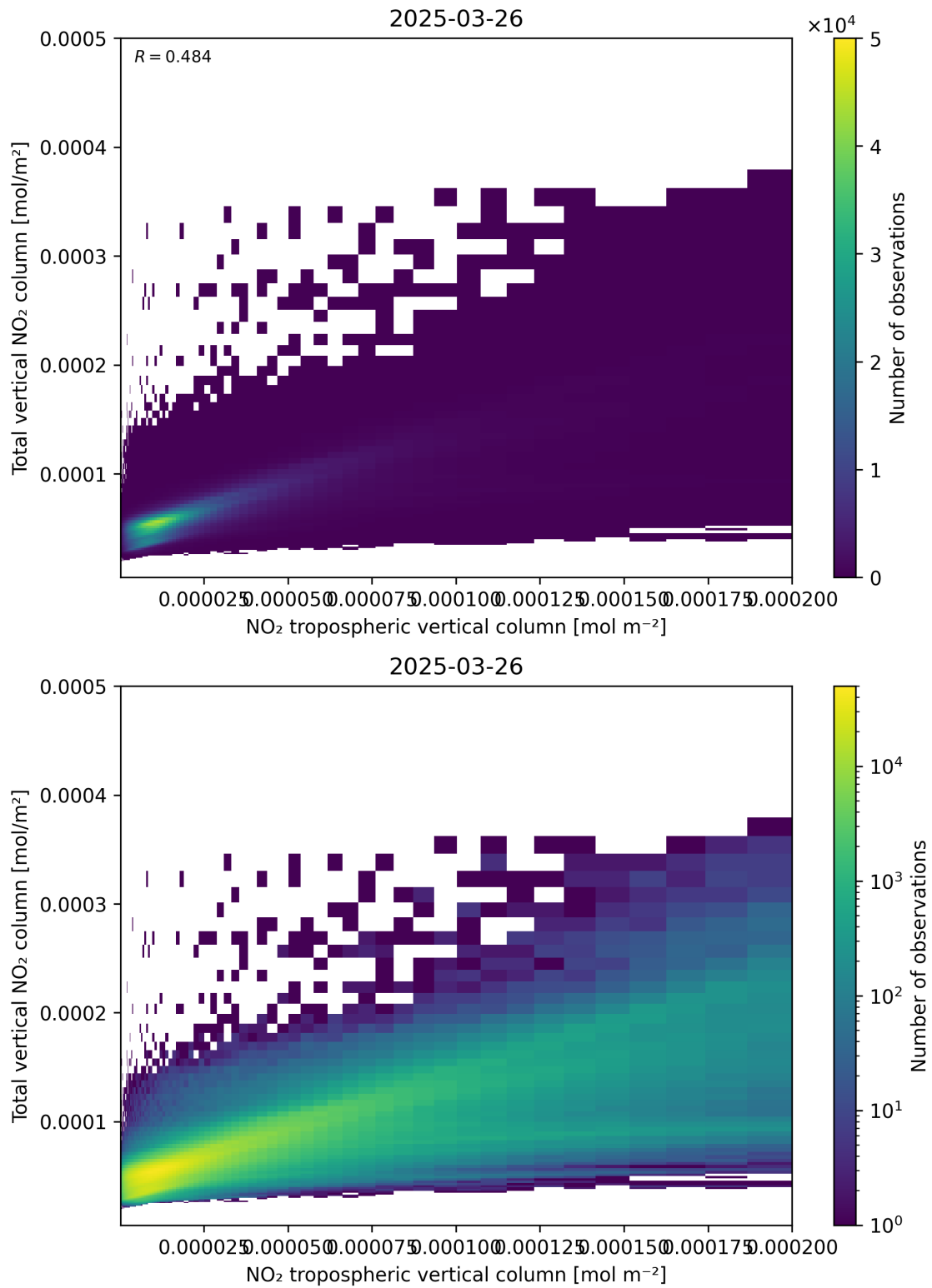
Figure 128: Scatter density plot of “NO 2 tropospheric vertical column” against “Total vertical NO 2 column” for 2025-03-26 to 2025-03-26.
