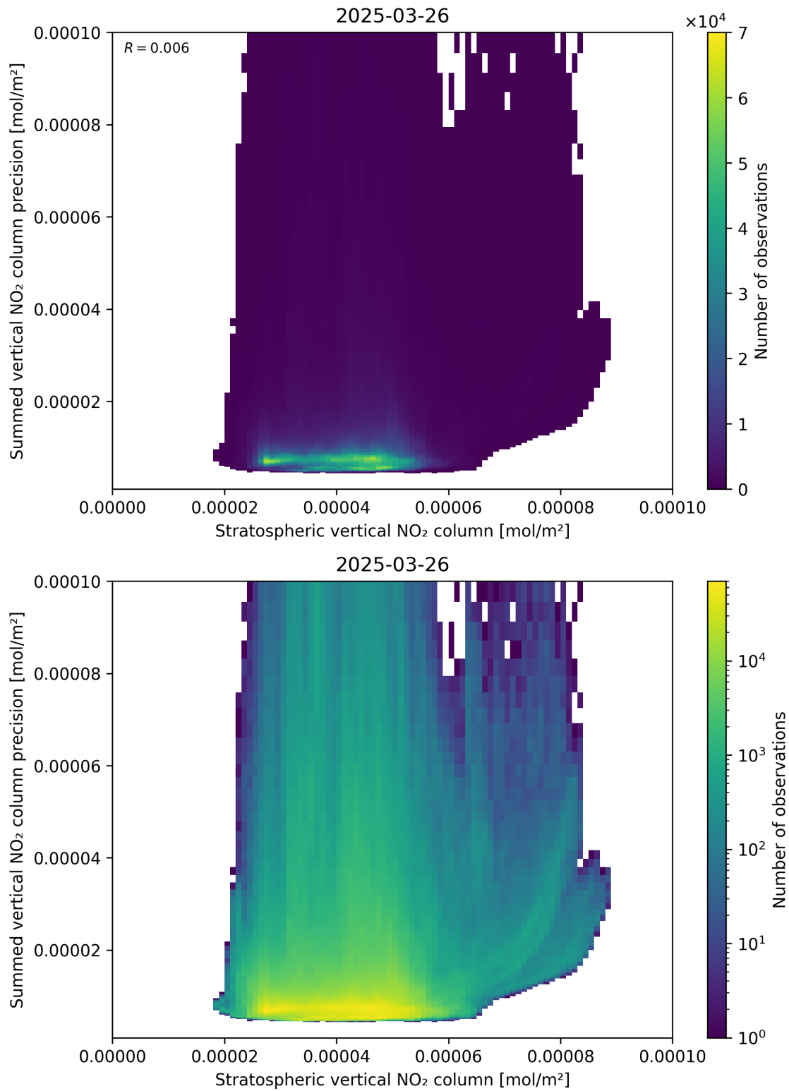
Figure 99: Scatter density plot of “Stratospheric vertical NO 2 column” against “Summed vertical NO 2 column precision” for 2025-03-26 to 2025-03-26.
