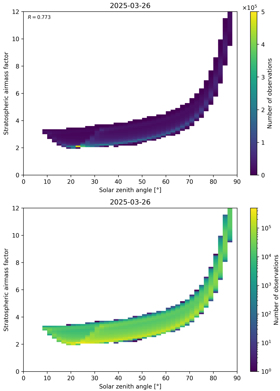
Figure 145: Scatter density plot of “Solar zenith angle” against “Stratospheric airmass factor” for 2025-03-26 to 2025-03-26.
