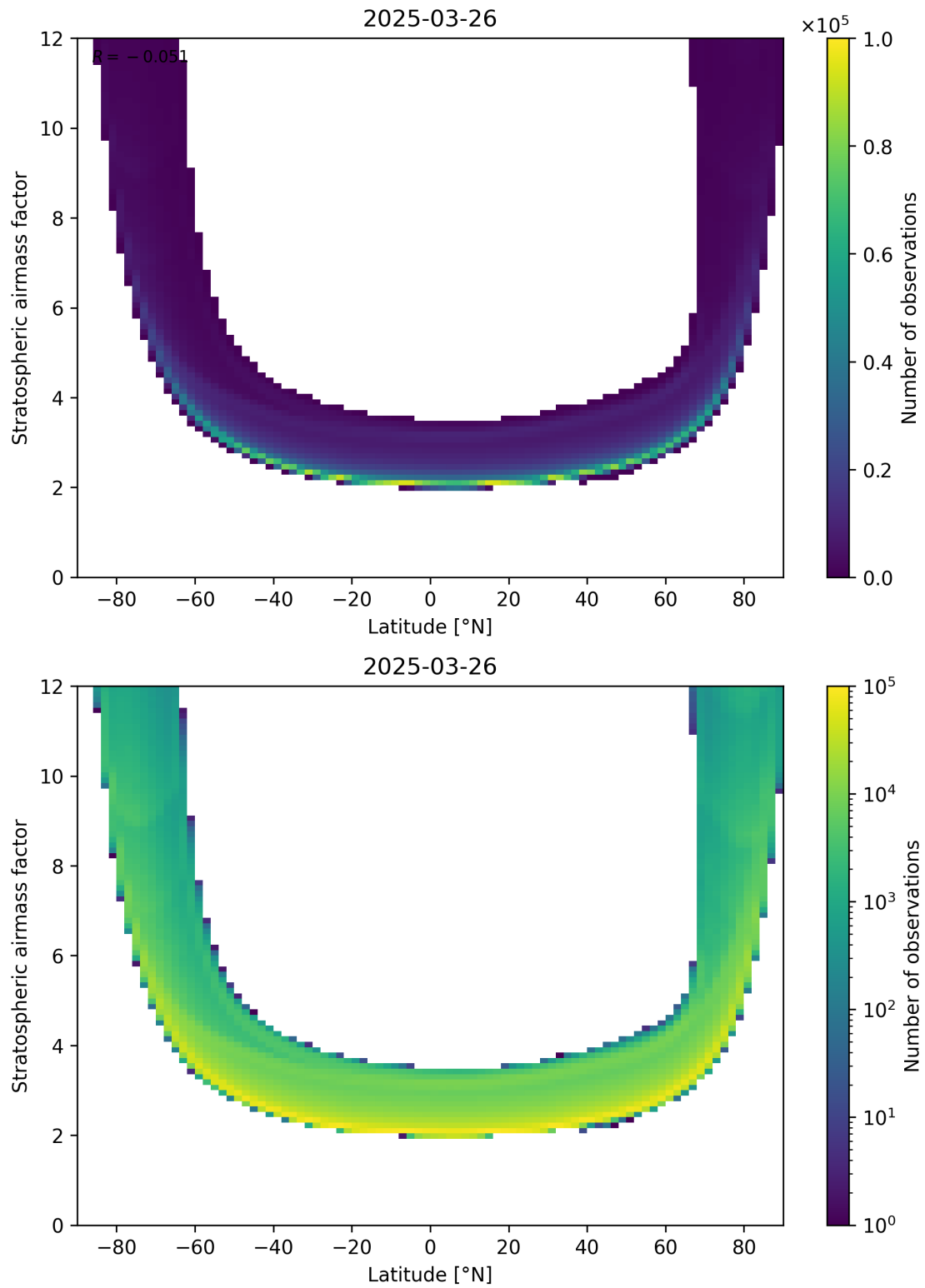
Figure 83: Scatter density plot of “Latitude” against “Stratospheric air mass factor” for 2025-03-26 to 2025-03-26.
