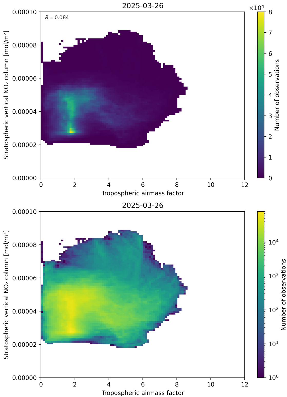
Figure 74: Scatter density plot of “Tropospheric airmass factor” against “Stratospheric vertical NO 2 column” for 2025-03-26 to 2025-03-26.
