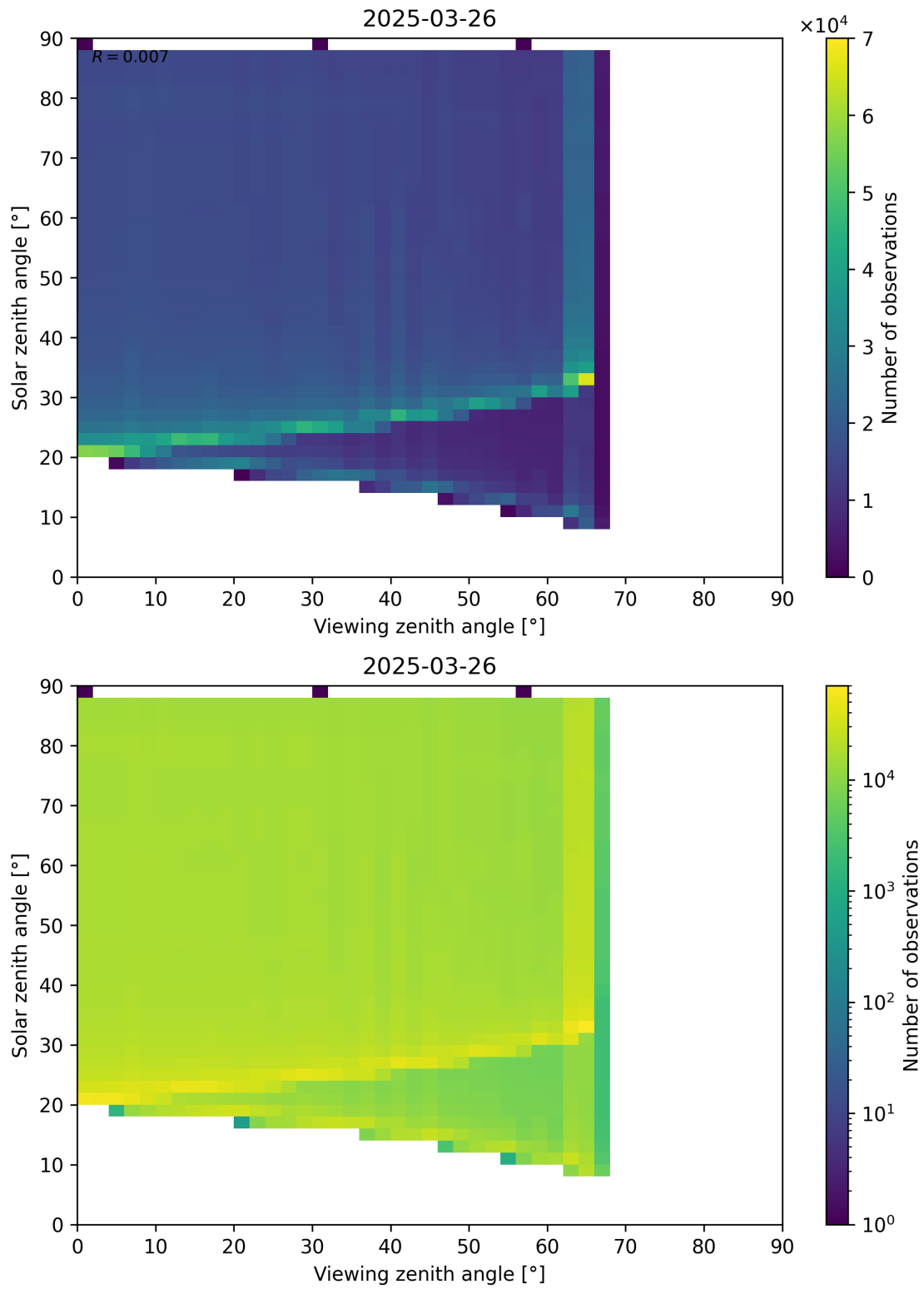
Figure 172: Scatter density plot of “Viewing zenith angle” against “Solar zenith angle” for 2025-03-26 to 2025-03-26.
