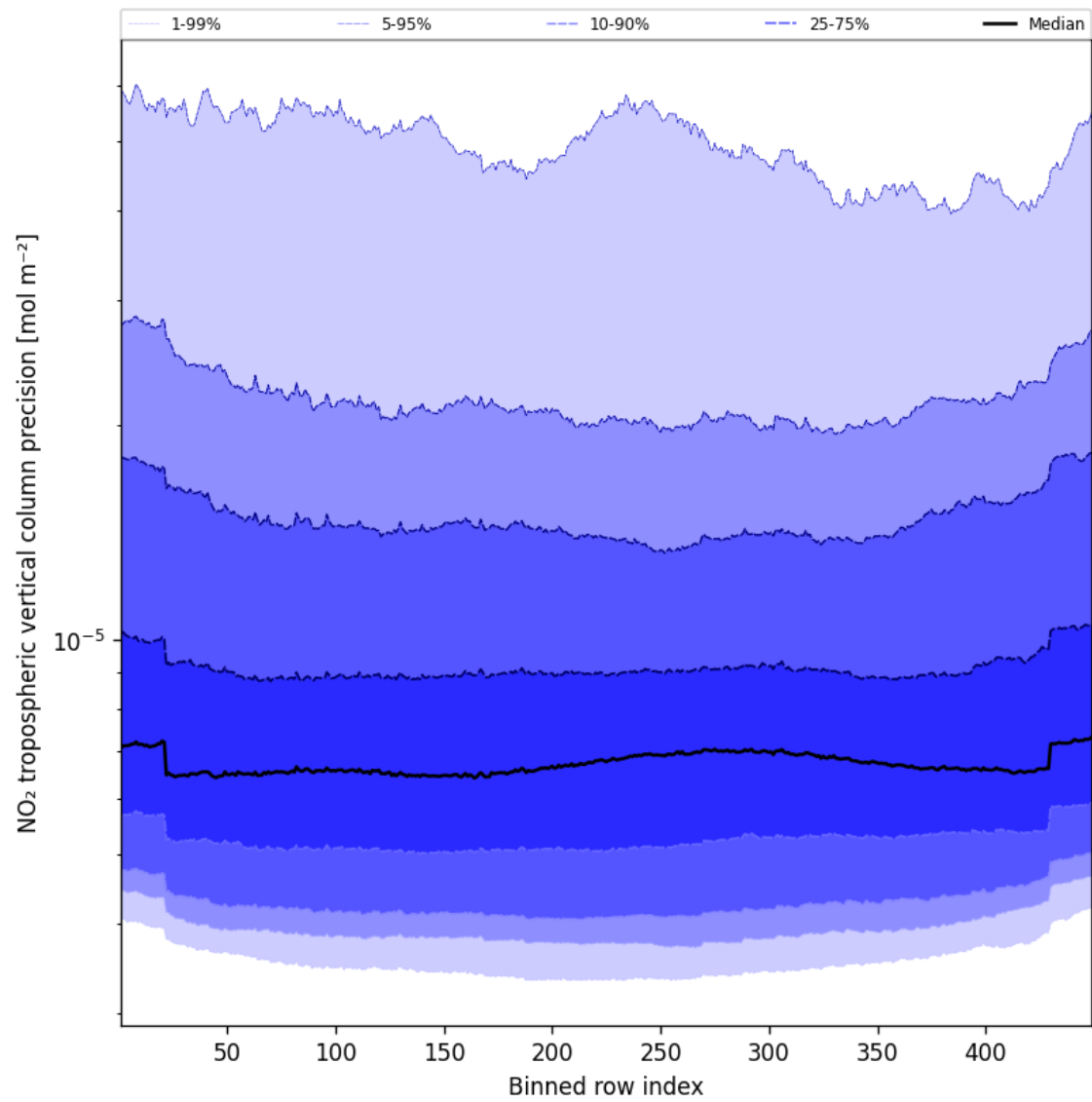
Figure 47: Along track statistics of “NO 2 tropospheric vertical column precision” for 2025-03-26 to 2025-03-26
