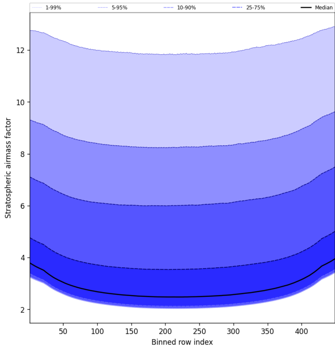
Figure 61: Along track statistics of “Stratospheric air mass factor” for 2025-03-26 to 2025-03-26
