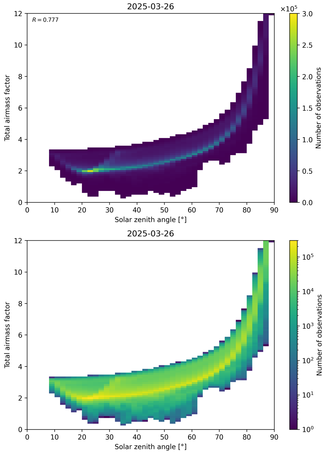
Figure 146: Scatter density plot of “Solar zenith angle” against “Total airmass factor” for 2025-03-26 to 2025-03-26.
