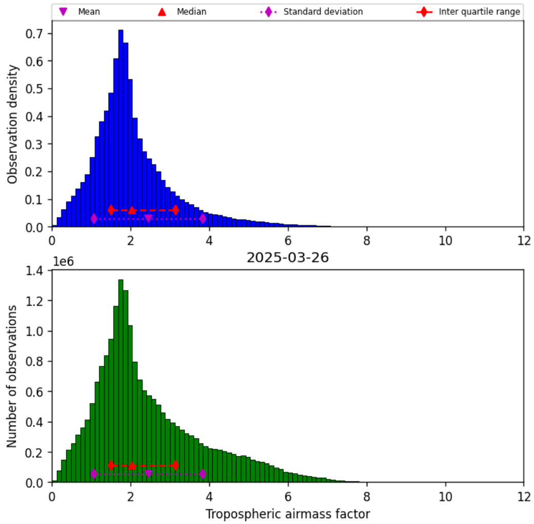
Figure 31: Histogram of “Tropospheric airmass factor” for 2025-03-26 to 2025-03-26
