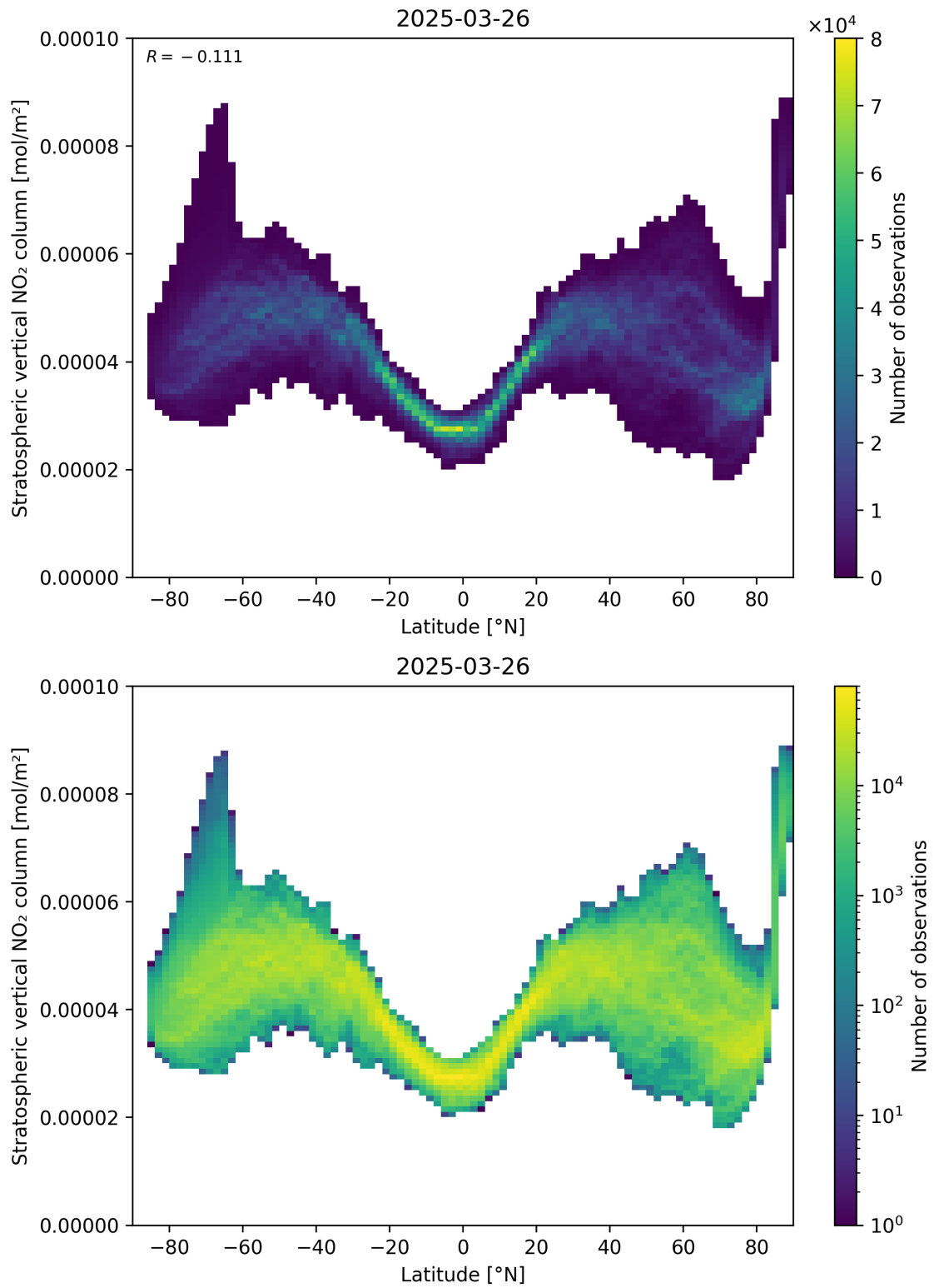
Figure 87: Scatter density plot of “Latitude” against “Stratospheric vertical NO 2 column” for 2025-03-26 to 2025-03-26.
