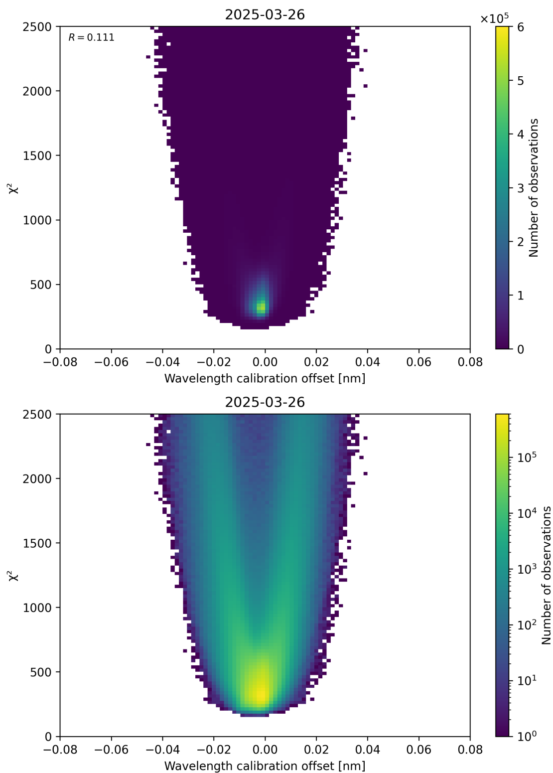
Figure 175: Scatter density plot of “Wavelength calibration offset” against “ \chi^2 ” for 2025-03-26 to 2025-03-26.
