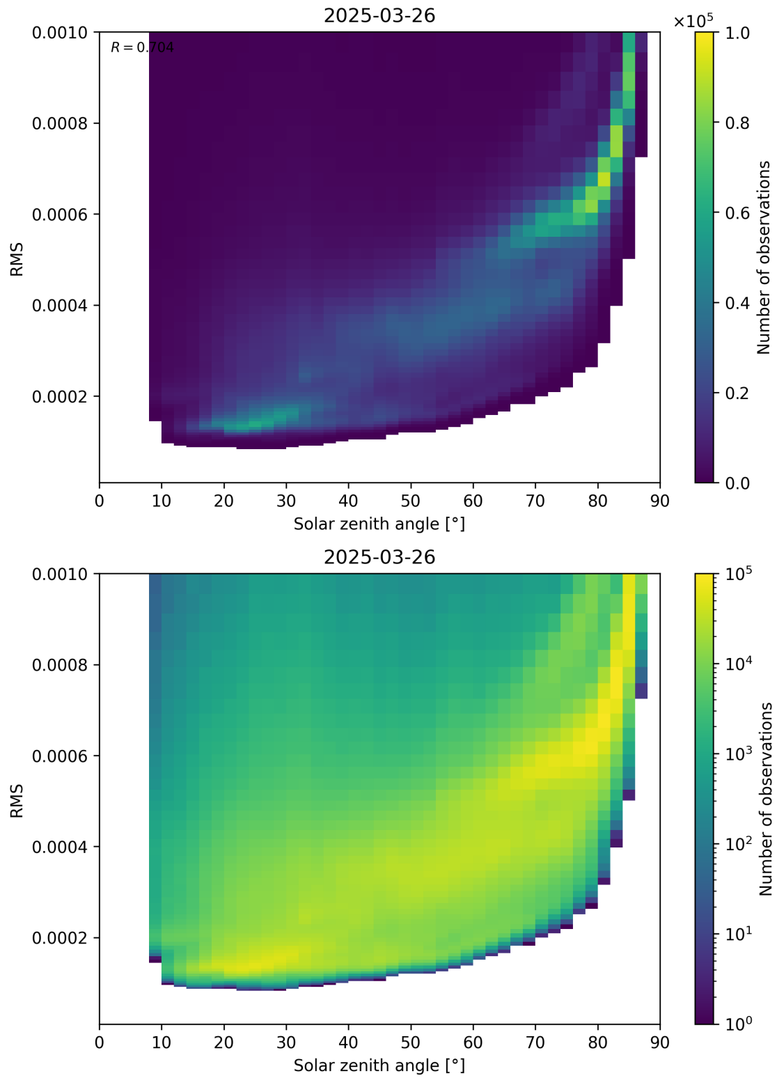
Figure 157: Scatter density plot of “Solar zenith angle” against “RMS” for 2025-03-26 to 2025-03-26.
