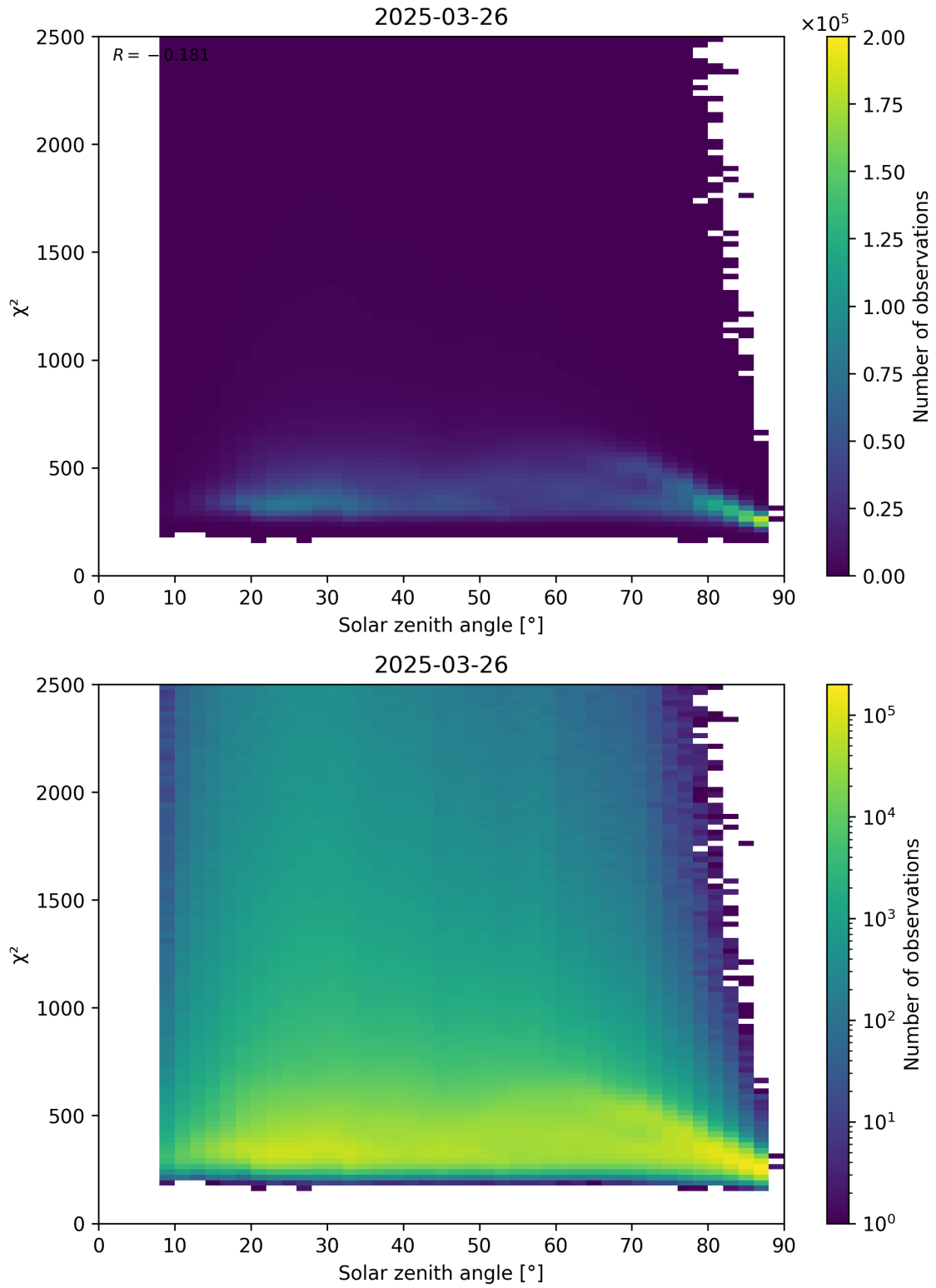
Figure 148: Scatter density plot of “Solar zenith angle” against “ \chi^2 ” for 2025-03-26 to 2025-03-26.
