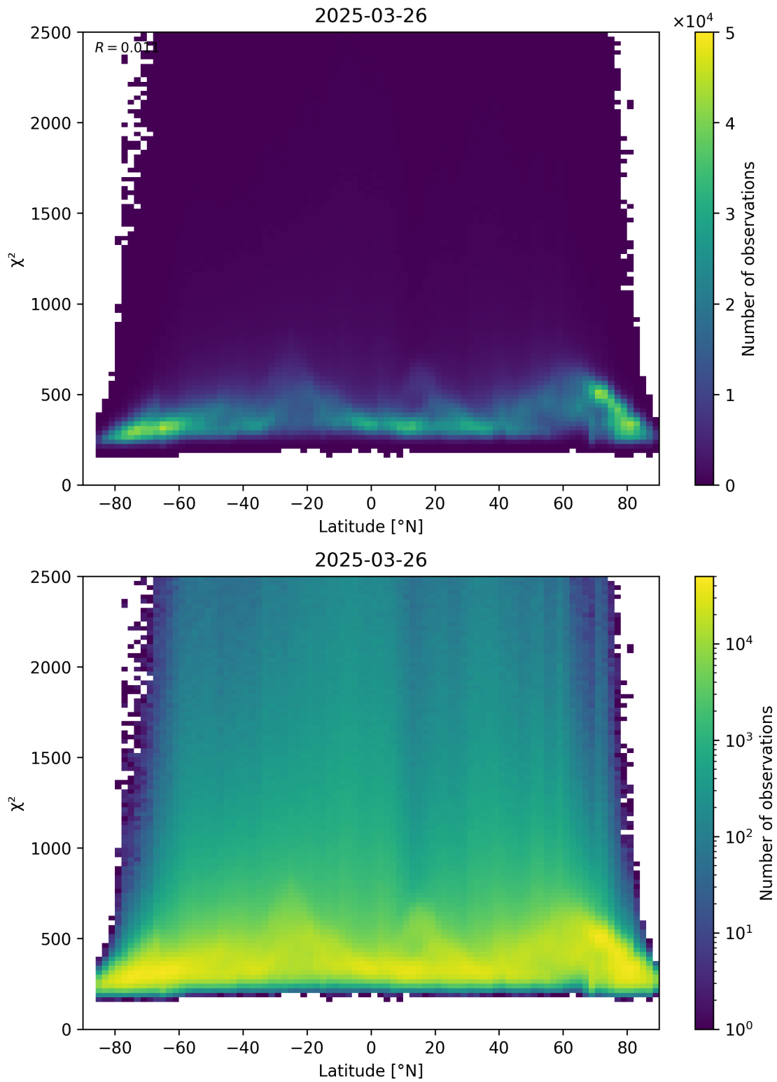
Figure 86: Scatter density plot of “Latitude” against “ \chi^2 ” for 2025-03-26 to 2025-03-26.
