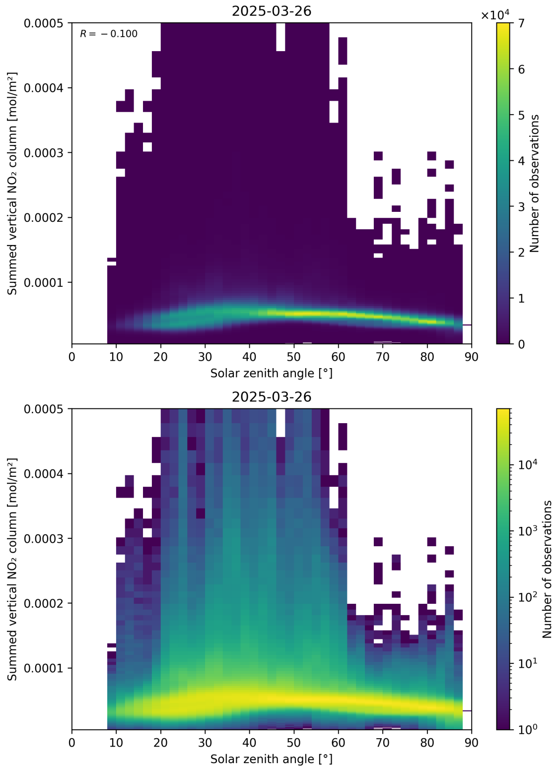
Figure 151: Scatter density plot of “Solar zenith angle” against “Summed vertical NO 2 column” for 2025-03-26 to 2025-03-26.
