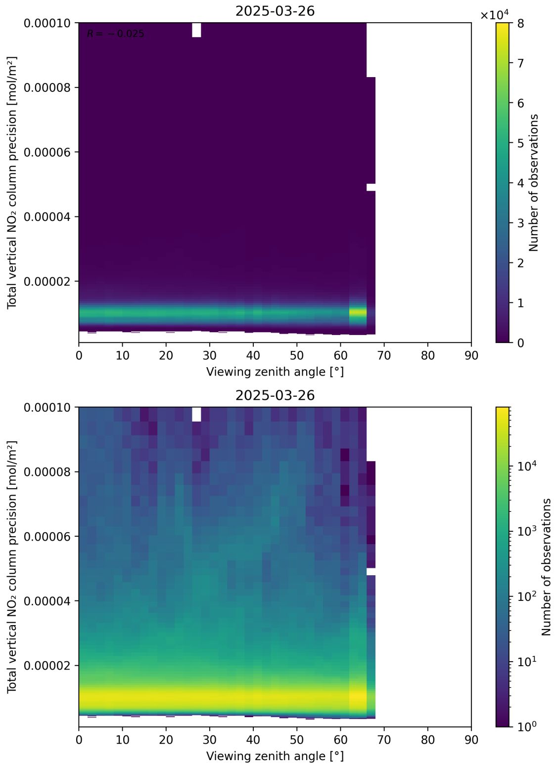
Figure 168: Scatter density plot of “Viewing zenith angle” against “Total vertical NO 2 column precision” for 2025-03-26 to 2025-03-26.
