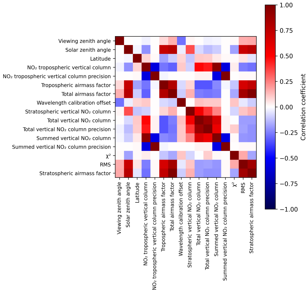
Figure 2: Map of correlation matrix for 2025-03-26 to 2025-03-26.
