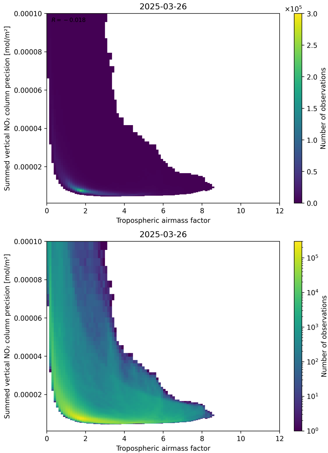
Figure 76: Scatter density plot of “Tropospheric air mass factor” against “Summed vertical NO 2 column precision” for 2025-03-26 to 2025-03-26.
