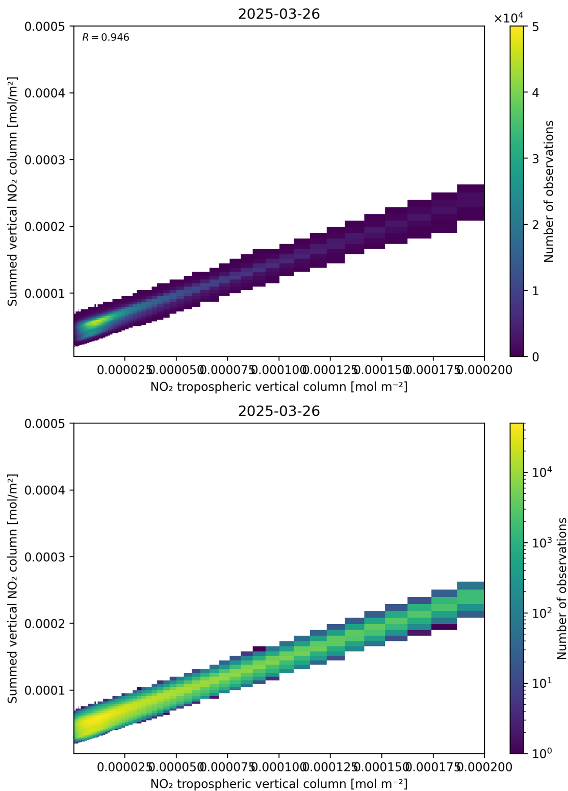
Figure 126: Scatter density plot of “NO 2 tropospheric vertical column” against “Summed vertical NO 2 column” for 2025-03-26 to 2025-03-26.
