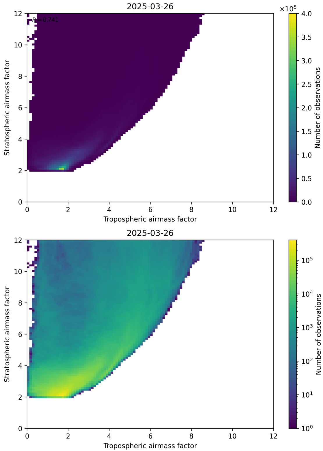
Figure 71: Scatter density plot of “Tropospheric airmass factor” against “Stratospheric airmass factor” for 2025-03-26 to 2025-03-26.
