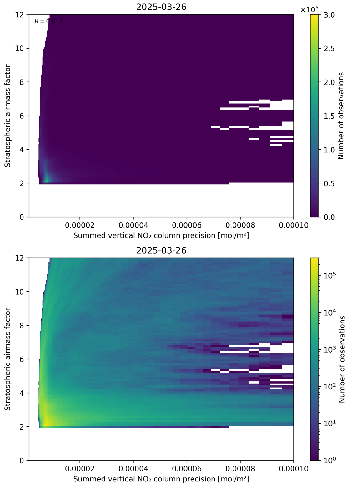
Figure 106: Scatter density plot of “Summed vertical NO 2 column precision” against “Stratospheric airmass factor” for 2025-03-26 to 2025-03-26.
