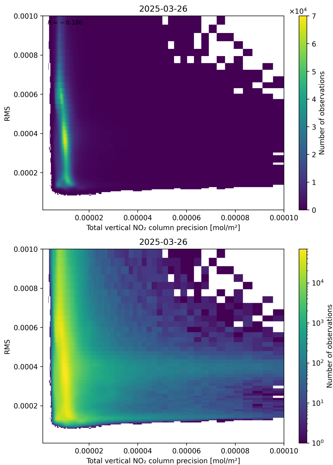
Figure 119: Scatter density plot of “Total vertical NO 2 column precision” against “RMS” for 2025-03-26 to 2025-03-26.
