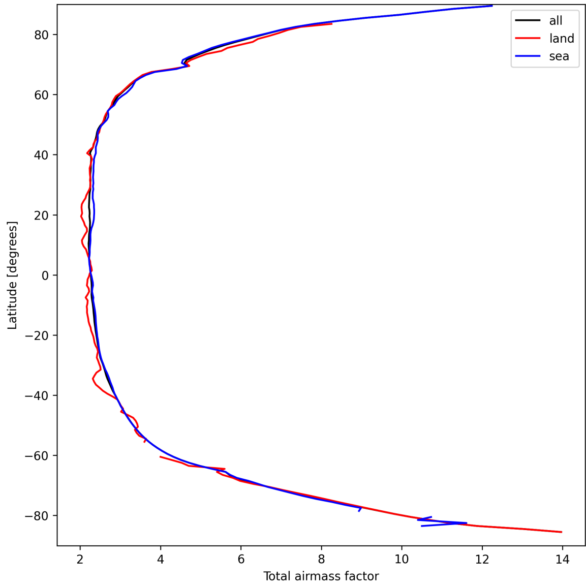
Figure 15: Zonal average of “Total airmass factor” for 2025-03-26 to 2025-03-26.
