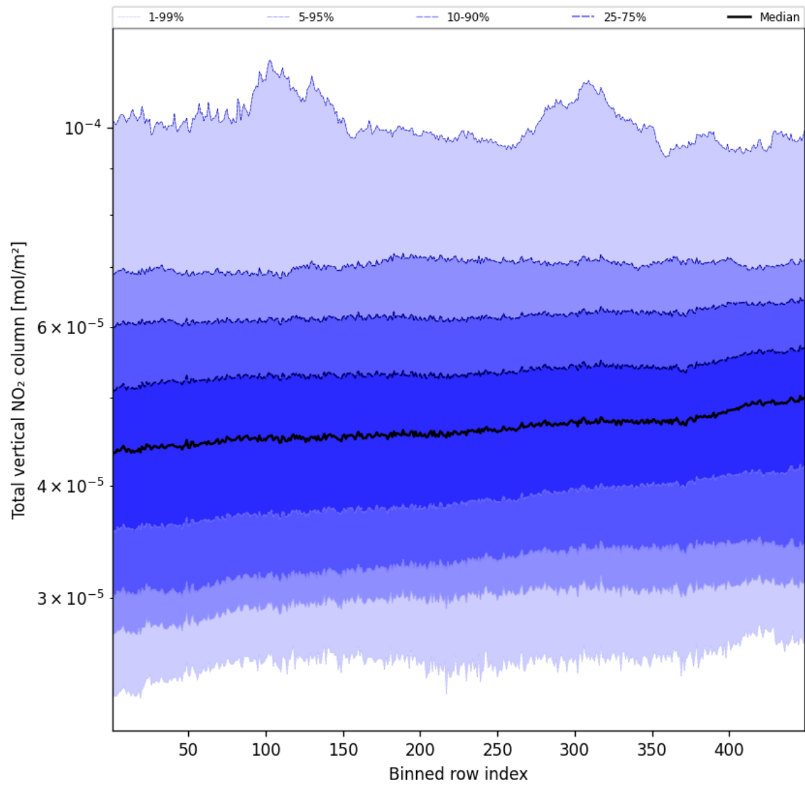
Figure 55: Along track statistics of “Total vertical NO 2 column” for 2025-03-26 to 2025-03-26
