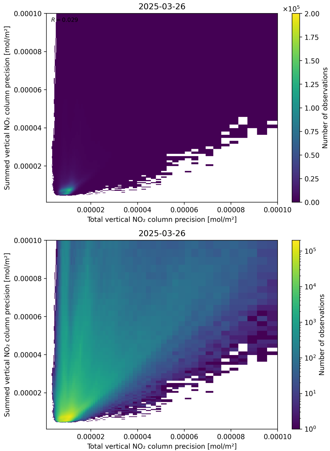
Figure 118: Scatter density plot of “Total vertical NO 2 column precision” against “Summed vertical NO 2 column precision” for 2025-03-26 to 2025-03-26.
