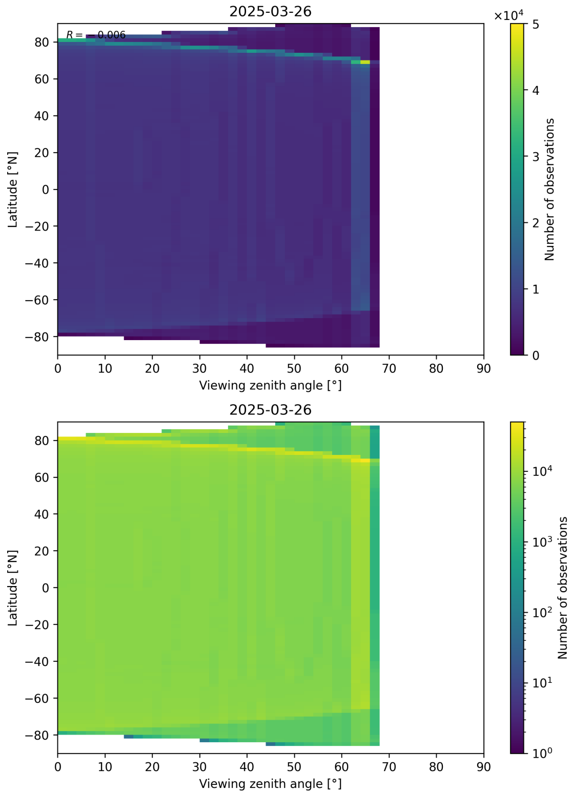
Figure 163: Scatter density plot of “Viewing zenith angle” against “Latitude” for 2025-03-26 to 2025-03-26.
