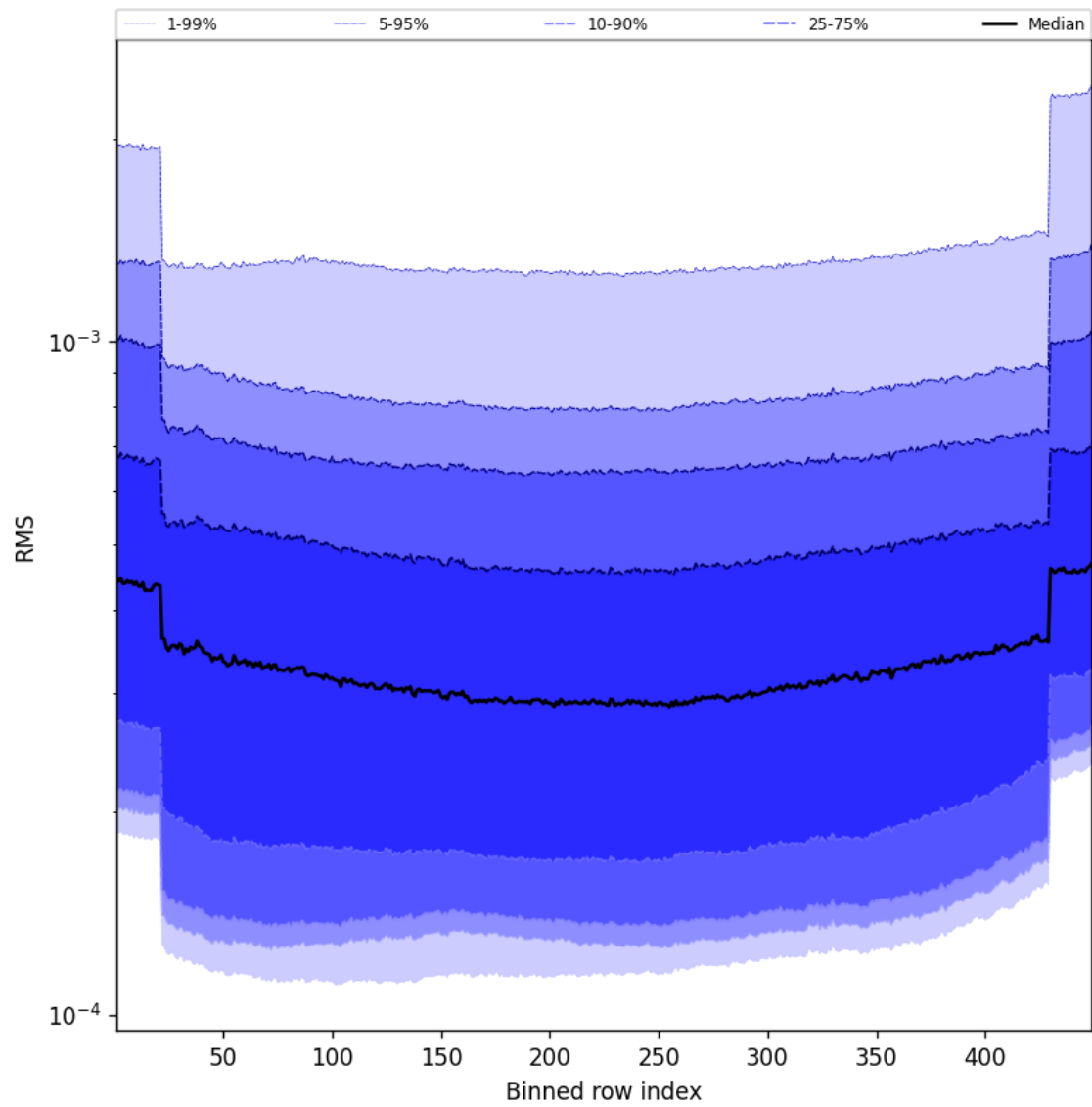
Figure 60: Along track statistics of “RMS” for 2025-03-26 to 2025-03-26
