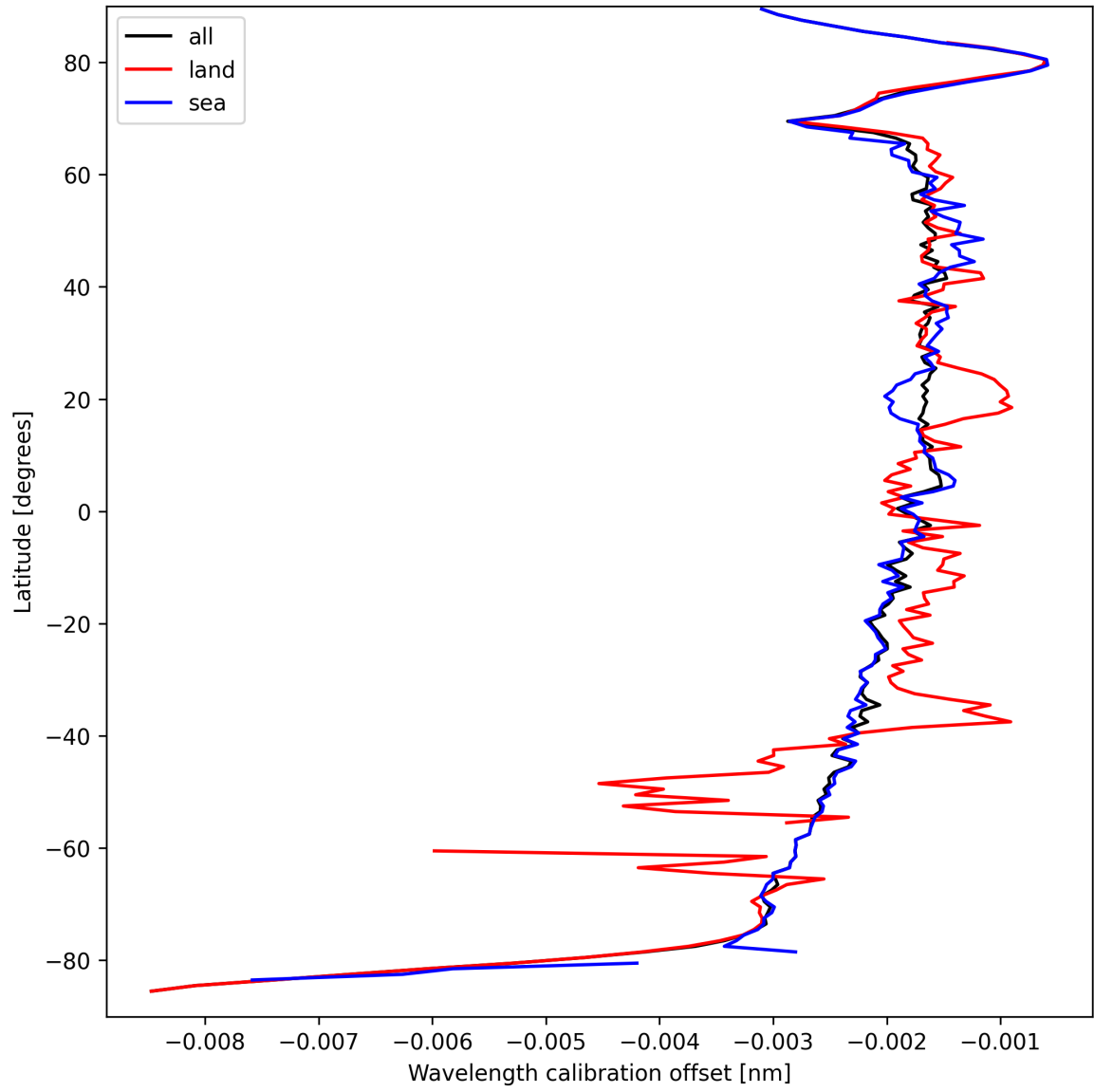
Figure 18: Zonal average of “Wavelength calibration offset” for 2025-03-26 to 2025-03-26.
