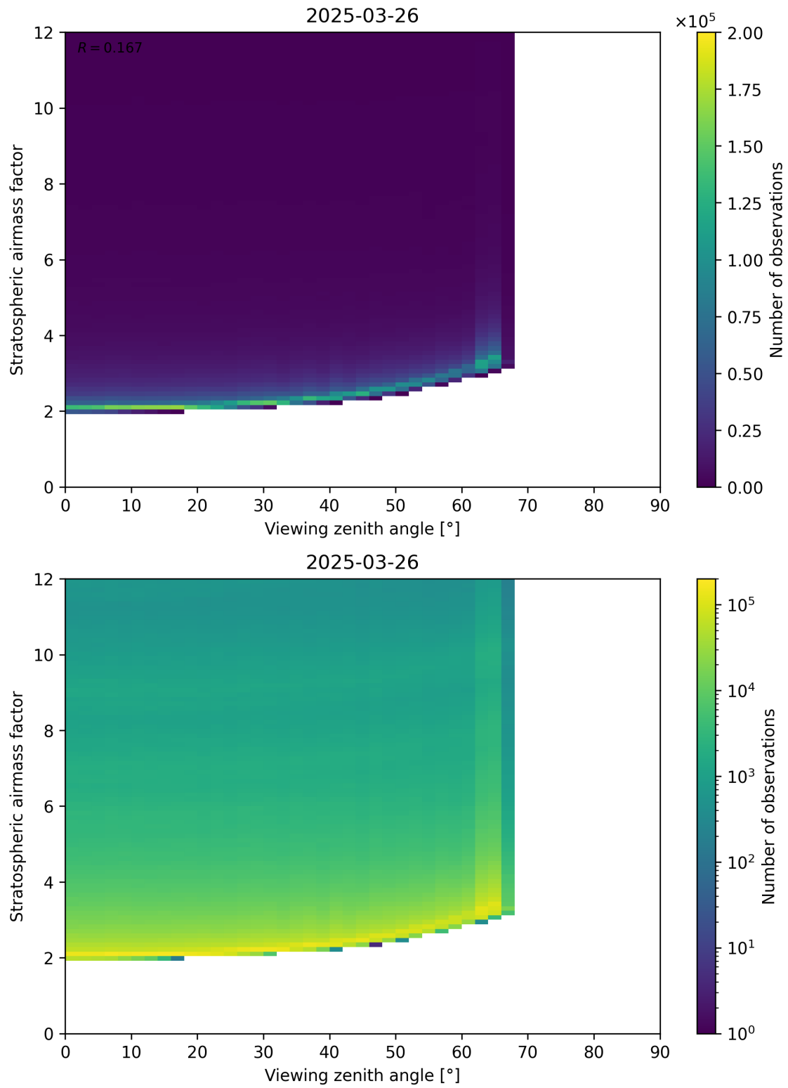
Figure 159: Scatter density plot of “Viewing zenith angle” against “Stratospheric airmass factor” for 2025-03-26 to 2025-03-26.
