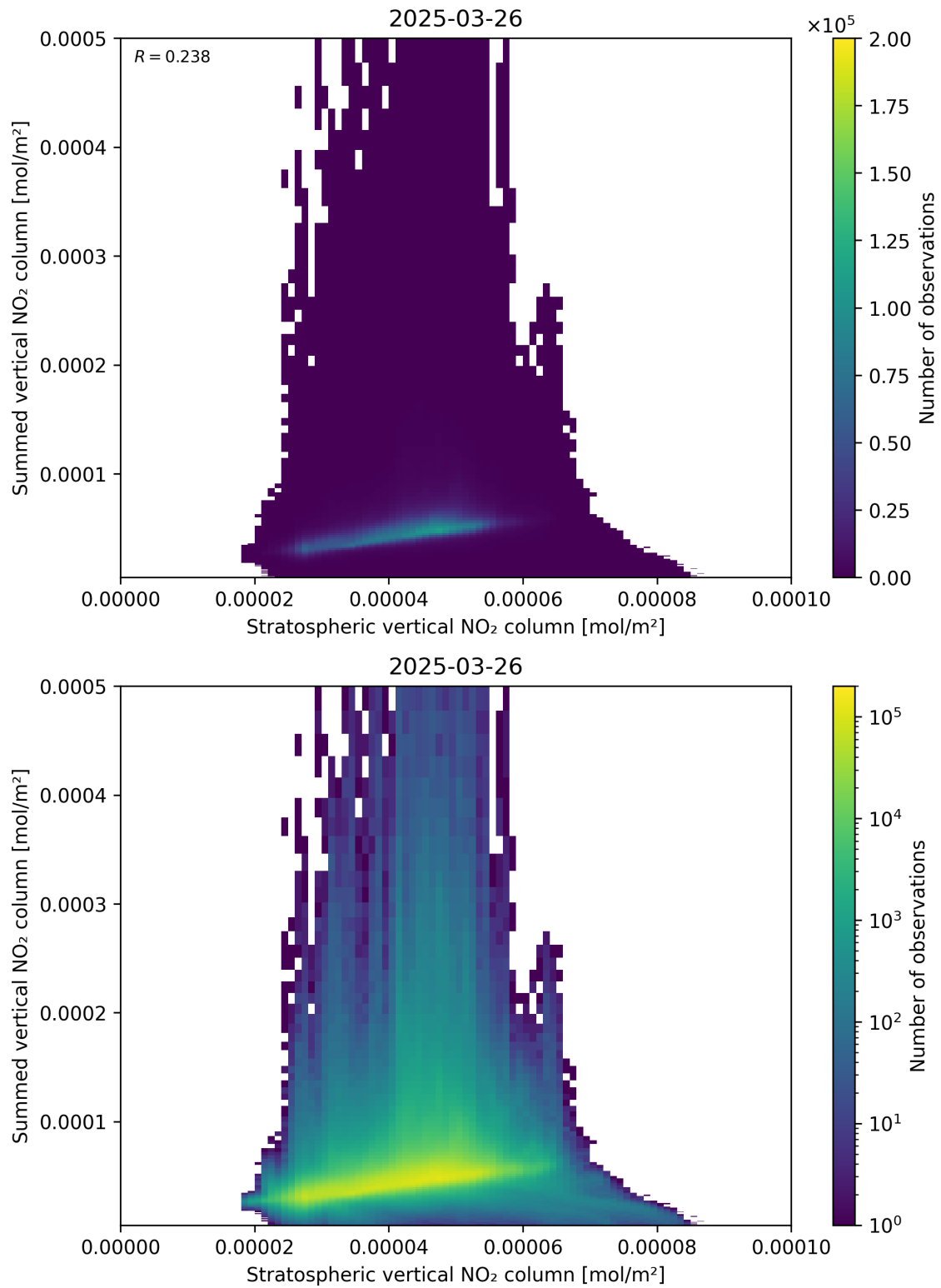
Figure 98: Scatter density plot of “Stratospheric vertical NO 2 column” against “Summed vertical NO 2 column” for 2025-03-26 to 2025-03-26.
