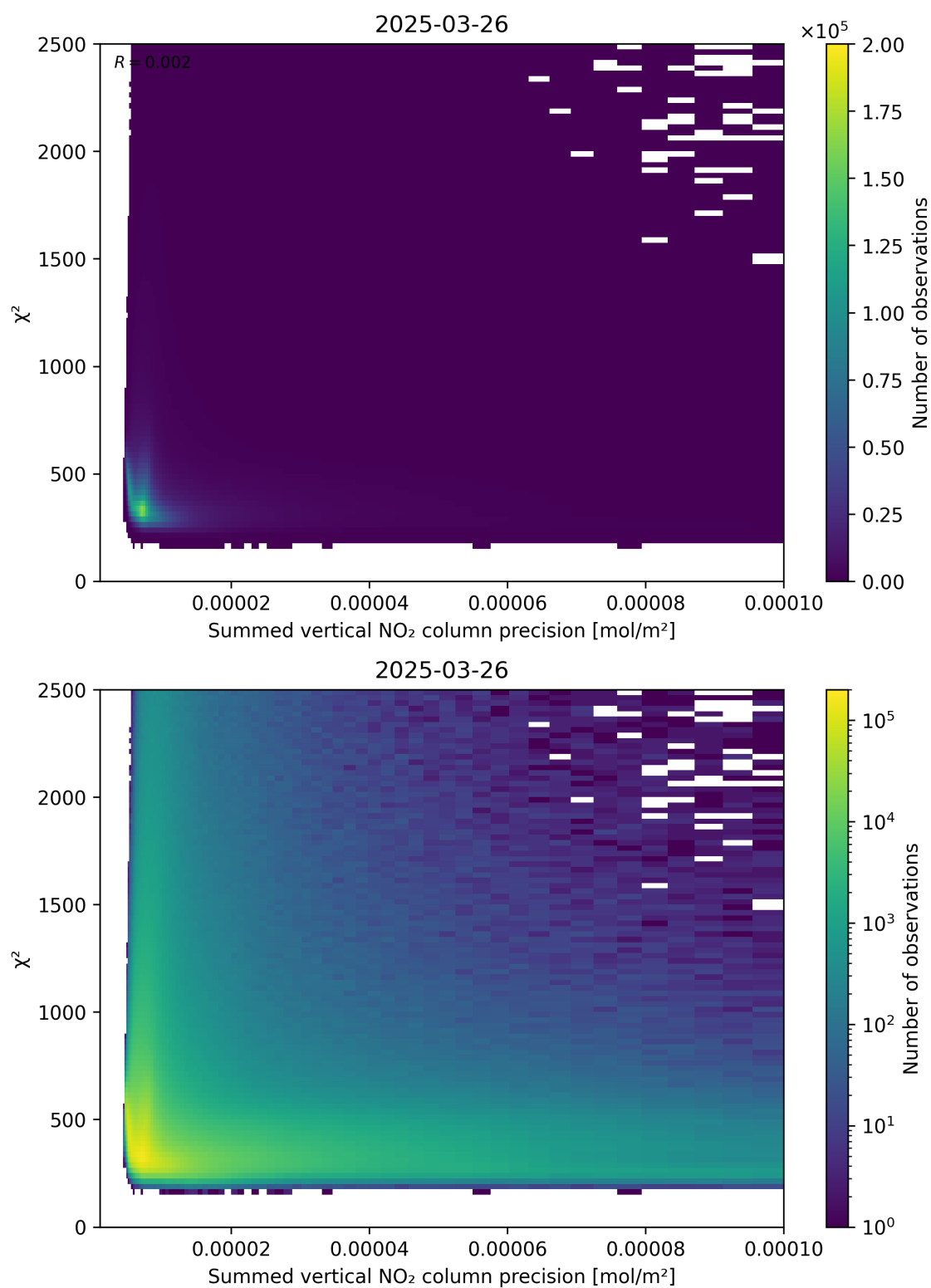
Figure 107: Scatter density plot of “Summed vertical NO 2 column precision” against “ \chi^2 ” for 2025-03-26 to 2025-03-26.
