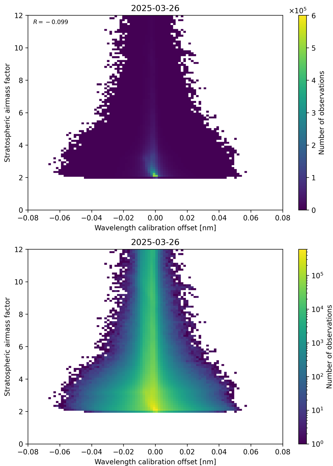
Figure 174: Scatter density plot of “Wavelength calibration offset” against “Stratospheric airmass factor” for 2025-03-26 to 2025-03-26.
