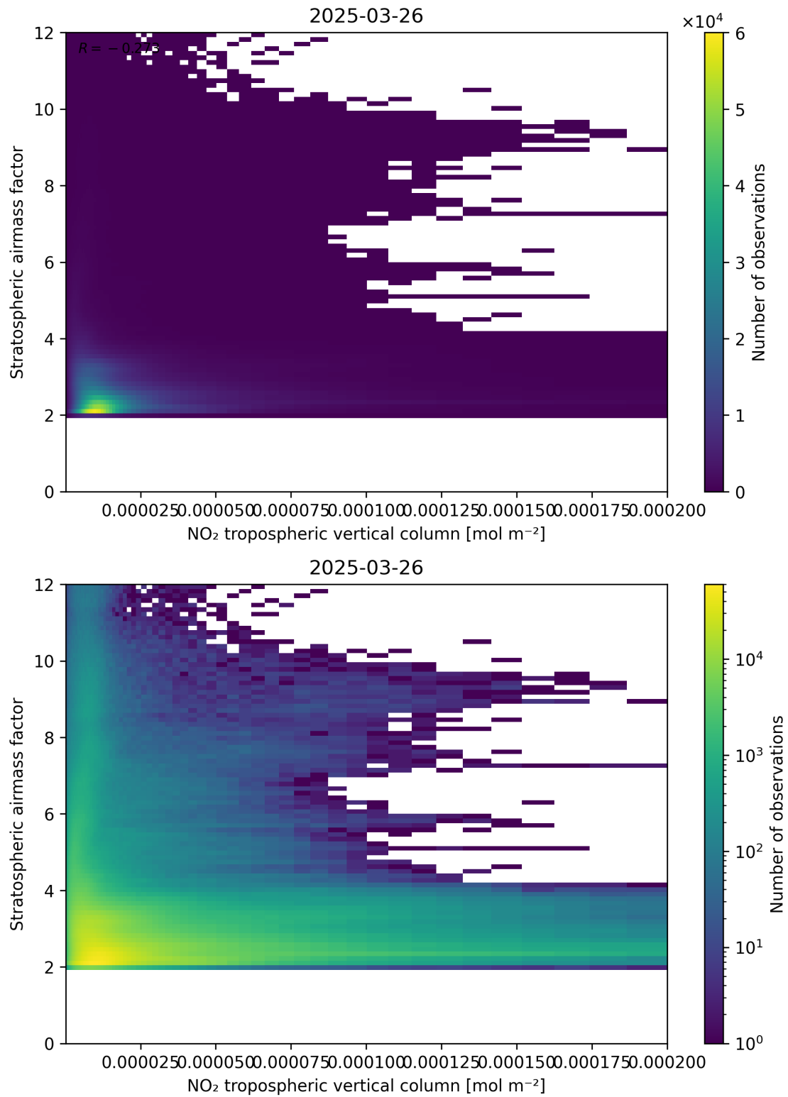
Figure 121: Scatter density plot of “NO 2 tropospheric vertical column” against “Stratospheric airmass factor” for 2025-03-26 to 2025-03-26.
