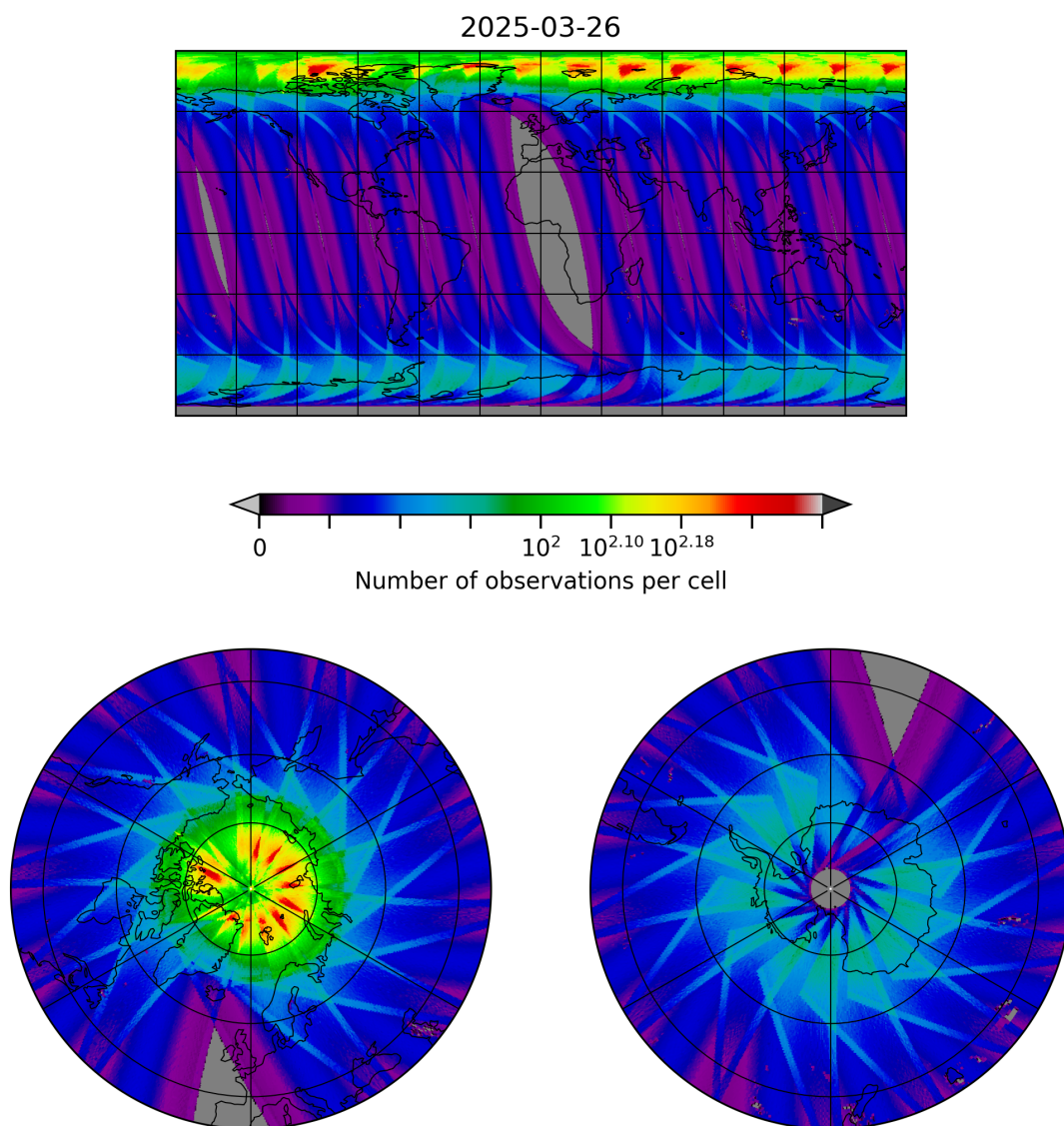
Figure 10: Map of the number of observations for 2025-03-26 to 2025-03-26
