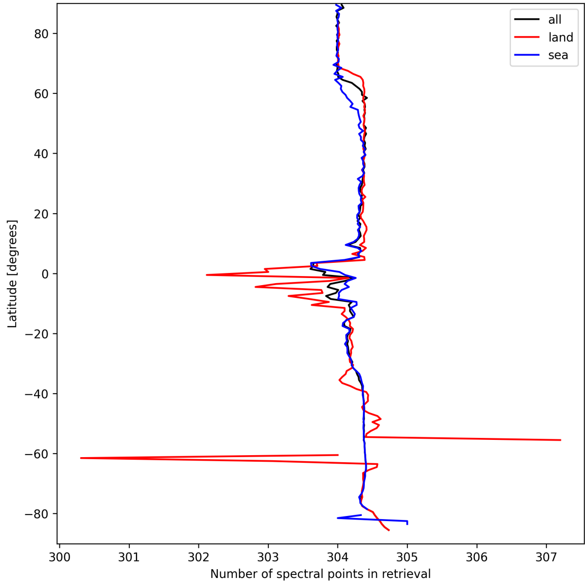
Figure 16: Zonal average of “Number of spectral points in retrieval” for 2025-03-26 to 2025-03-26.
