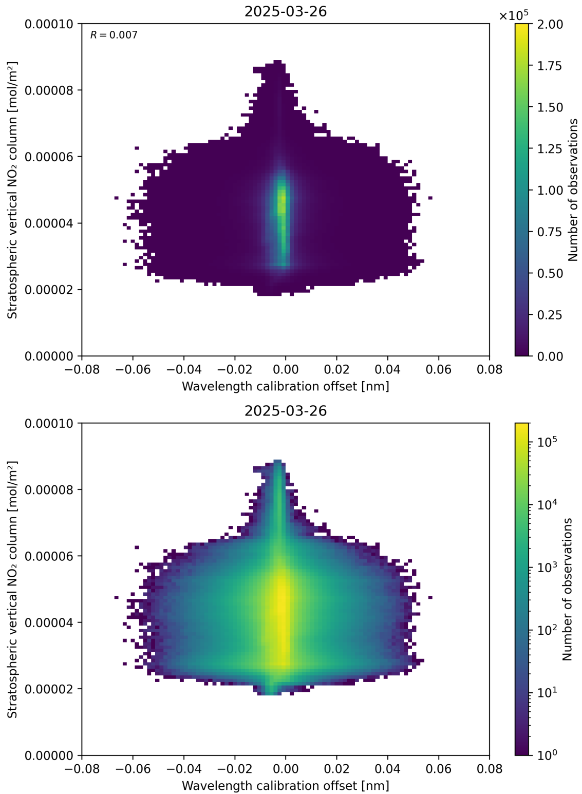
Figure 176: Scatter density plot of “Wavelength calibration offset” against “Stratospheric vertical NO 2 column” for 2025-03-26 to 2025-03-26.
