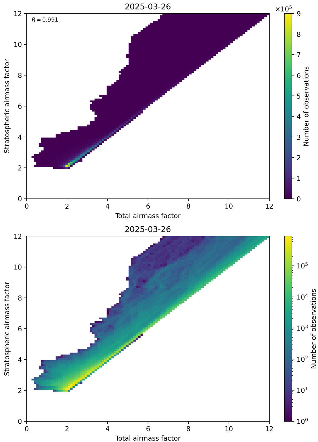
Figure 62: Scatter density plot of “Total airmass factor” against “Stratospheric airmass factor” for 2025-03-26 to 2025-03-26.
