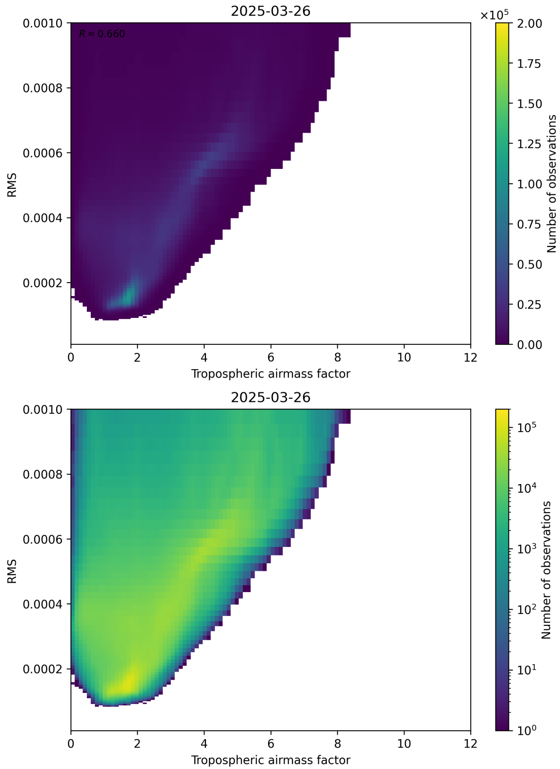
Figure 79: Scatter density plot of “Tropospheric airmass factor” against “RMS” for 2025-03-26 to 2025-03-26.
