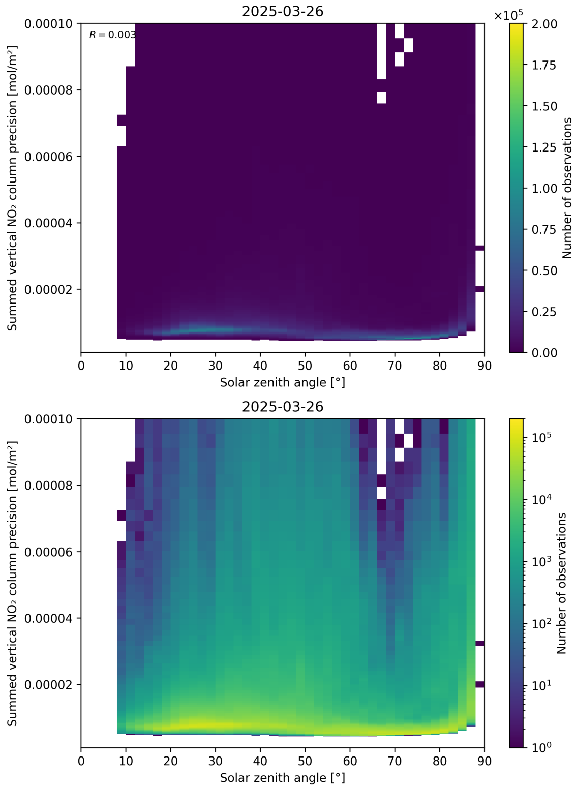
Figure 152: Scatter density plot of “Solar zenith angle” against “Summed vertical NO 2 column precision” for 2025-03-26 to 2025-03-26.
