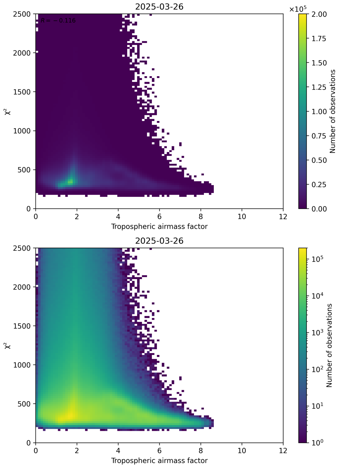
Figure 73: Scatter density plot of “Tropospheric airmass factor” against “ \chi^2 ” for 2025-03-26 to 2025-03-26.
