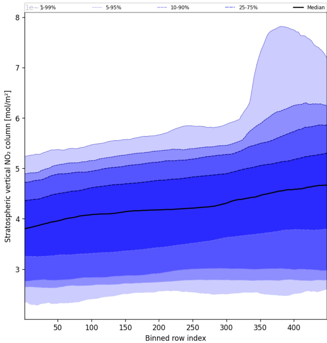
Figure 53: Along track statistics of “Stratospheric vertical NO 2 column” for 2025-03-26 to 2025-03-26
