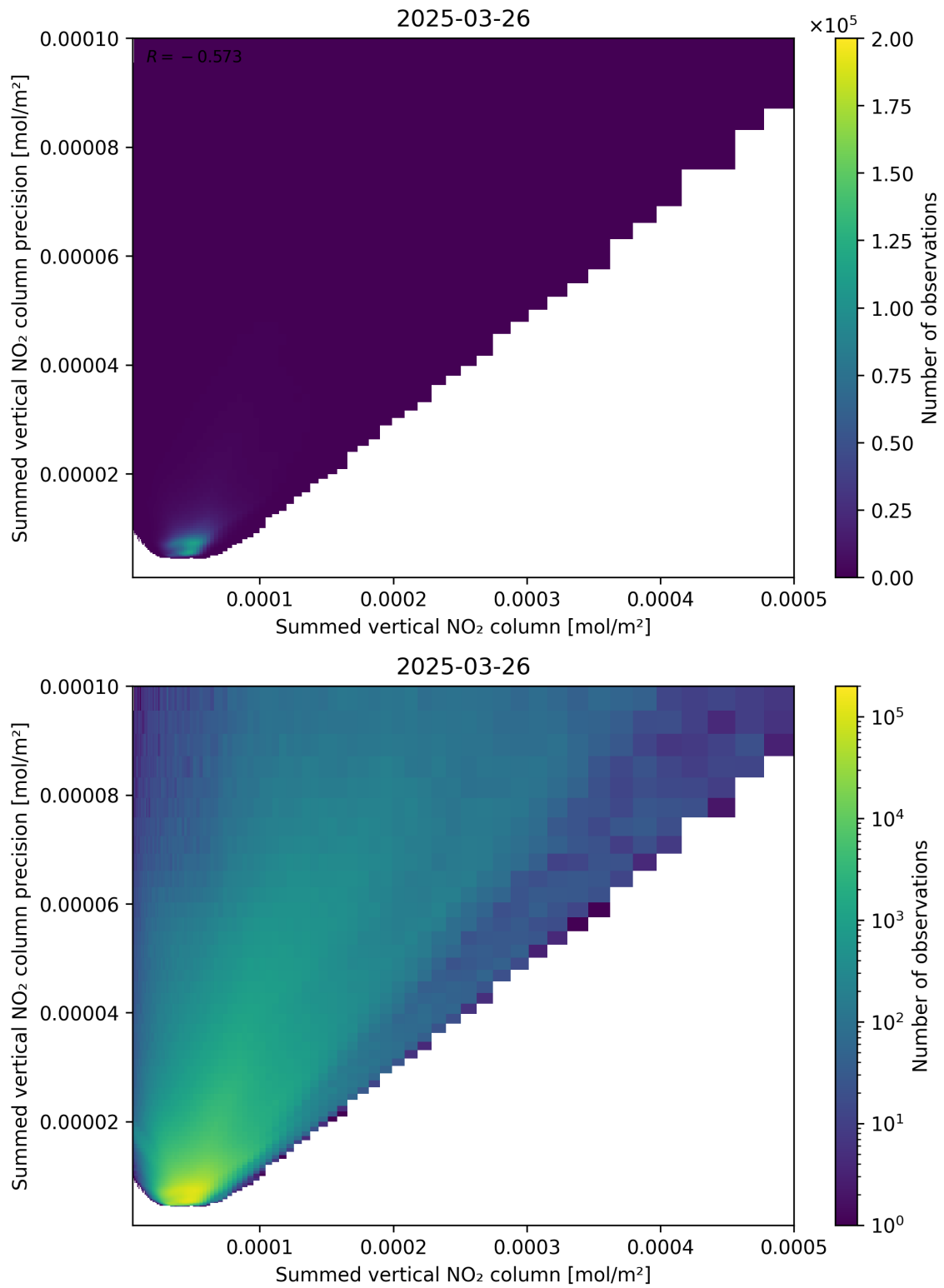
Figure 105: Scatter density plot of “Summed vertical NO 2 column” against “Summed vertical NO 2 column precision” for 2025-03-26 to 2025-03-26.
