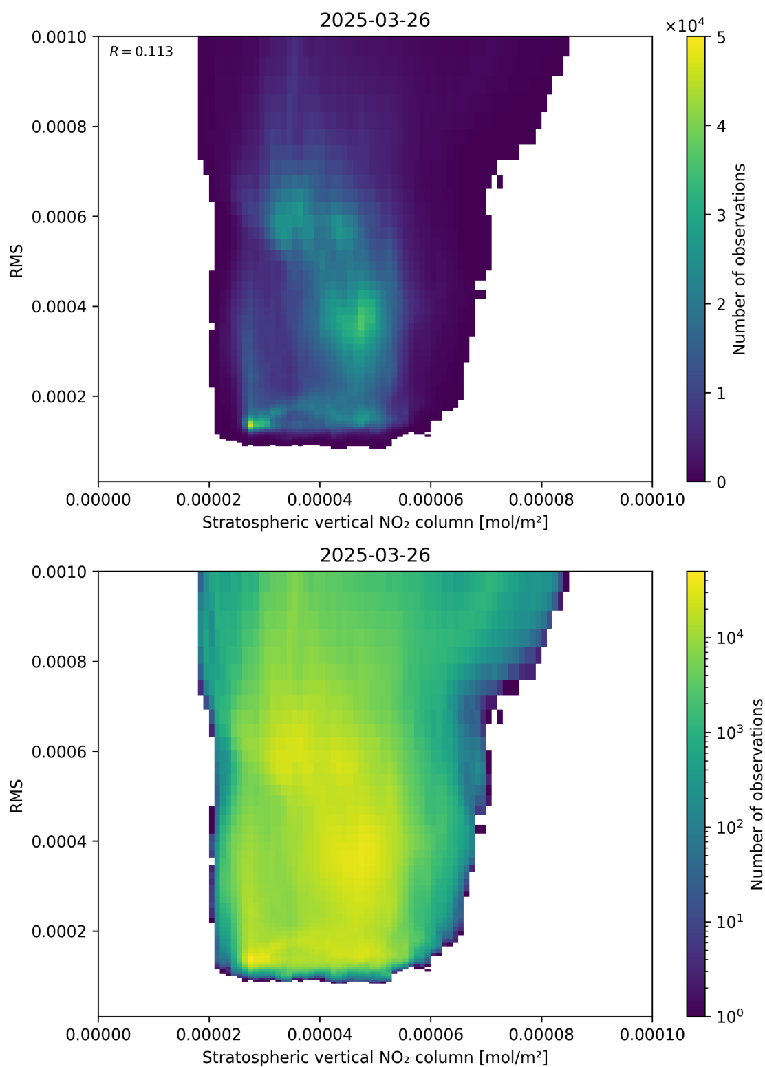
Figure 102: Scatter density plot of “Stratospheric vertical NO 2 column” against “RMS” for 2025-03-26 to 2025-03-26.
