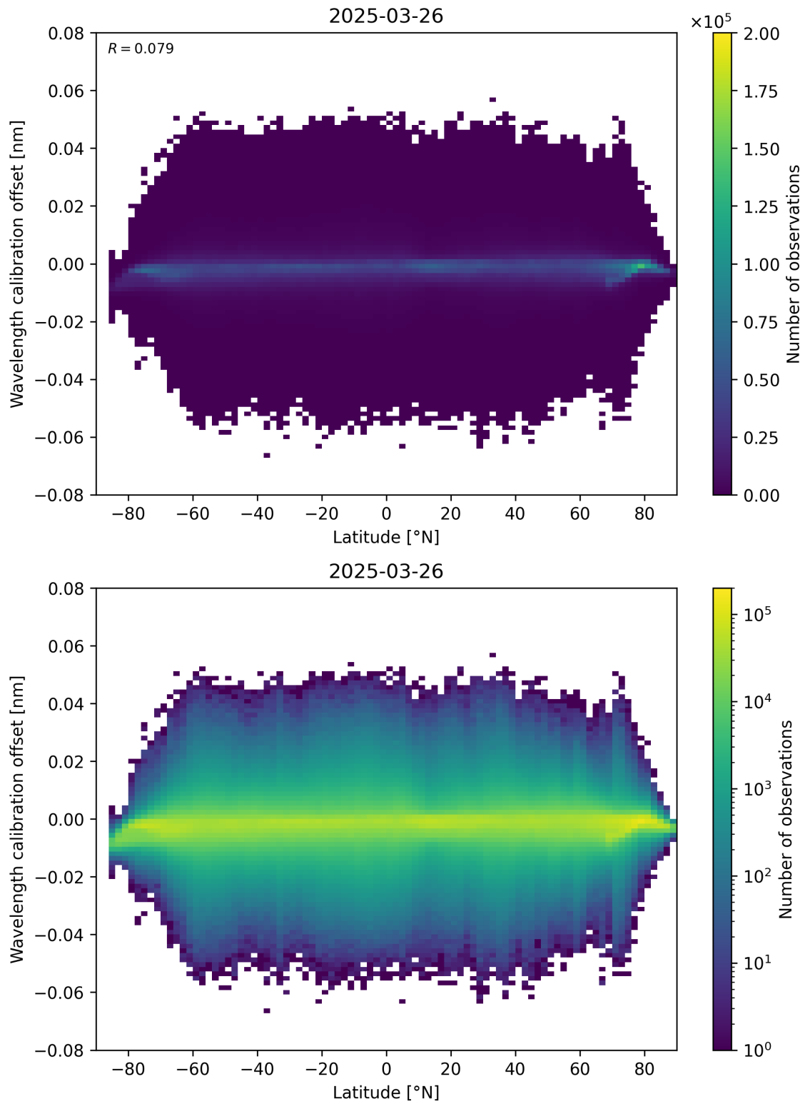
Figure 95: Scatter density plot of “Latitude” against “Wavelength calibration offset” for 2025-03-26 to 2025-03-26.
