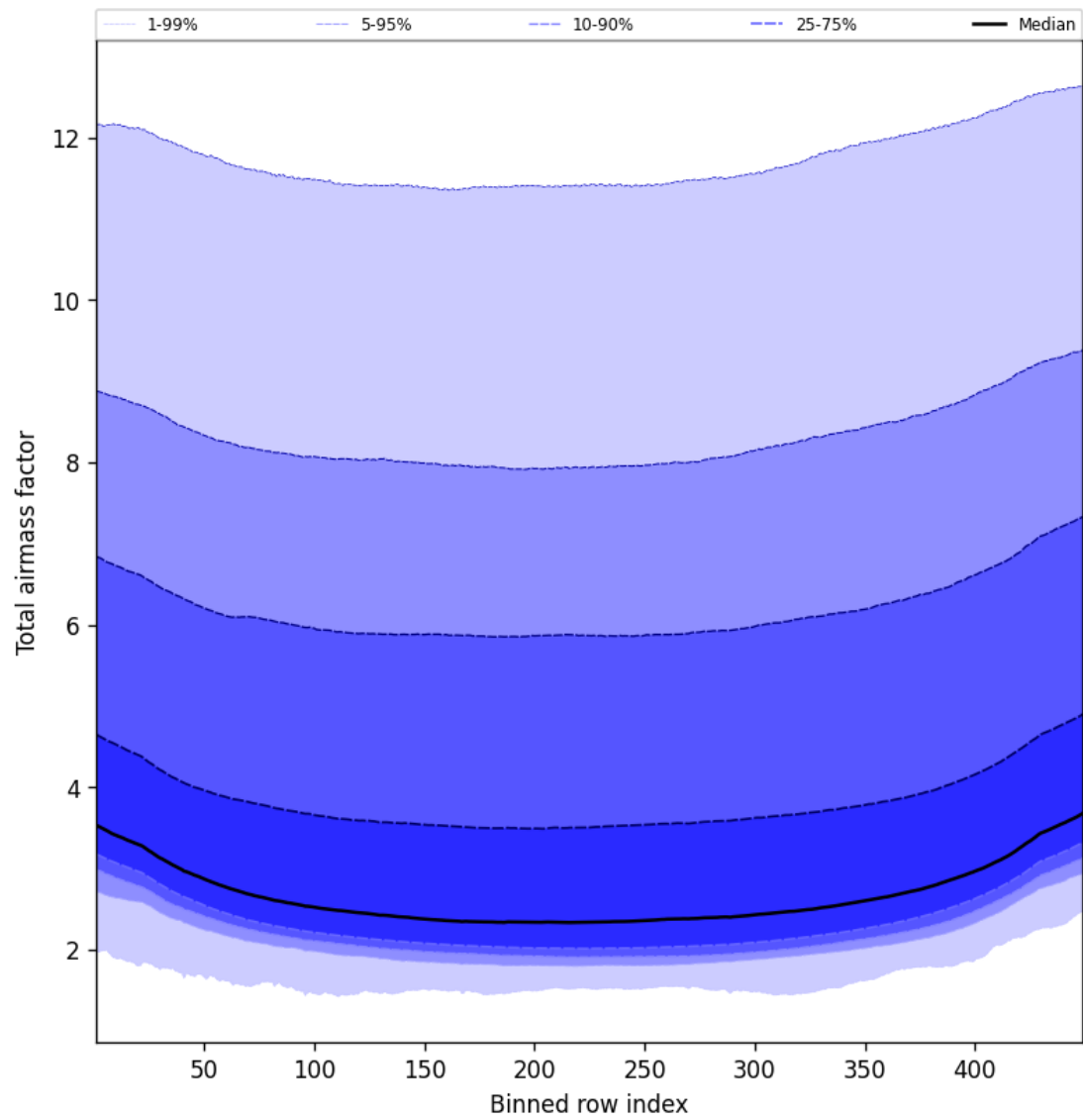
Figure 49: Along track statistics of “Total airmass factor” for 2025-03-26 to 2025-03-26
