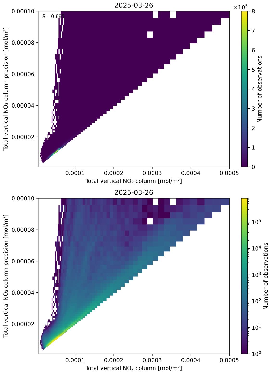
Figure 114: Scatter density plot of “Total vertical NO 2 column” against “Total vertical NO 2 column precision” for 2025-03-26 to 2025-03-26.
