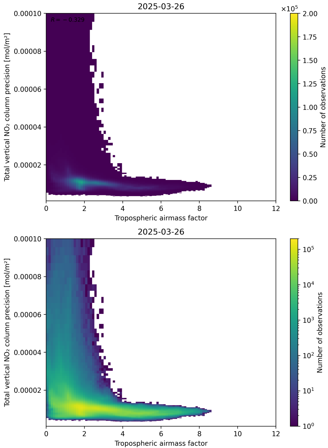
Figure 78: Scatter density plot of “Tropospheric air mass factor” against “Total vertical NO 2 column precision” for 2025-03-26 to 2025-03-26.
