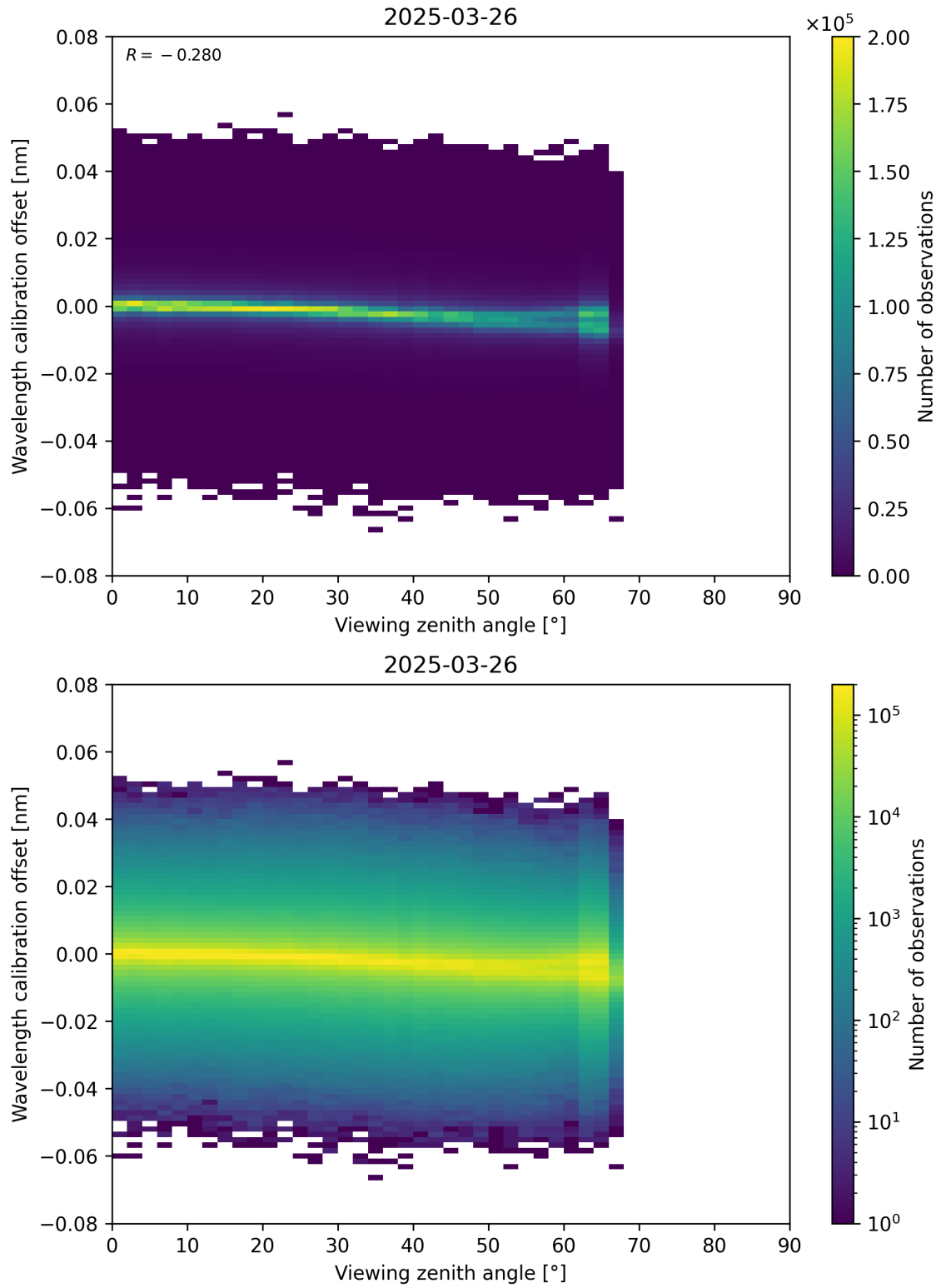
Figure 173: Scatter density plot of “Viewing zenith angle” against “Wavelength calibration offset” for 2025-03-26 to 2025-03-26.
