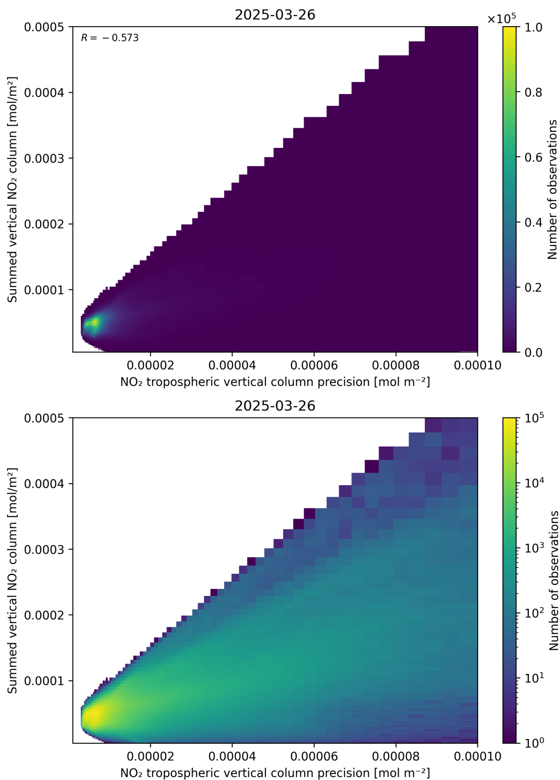
Figure 136: Scatter density plot of “NO 2 tropospheric vertical column precision” against “Summed vertical NO 2 column” for 2025-03-26 to 2025-03-26.
