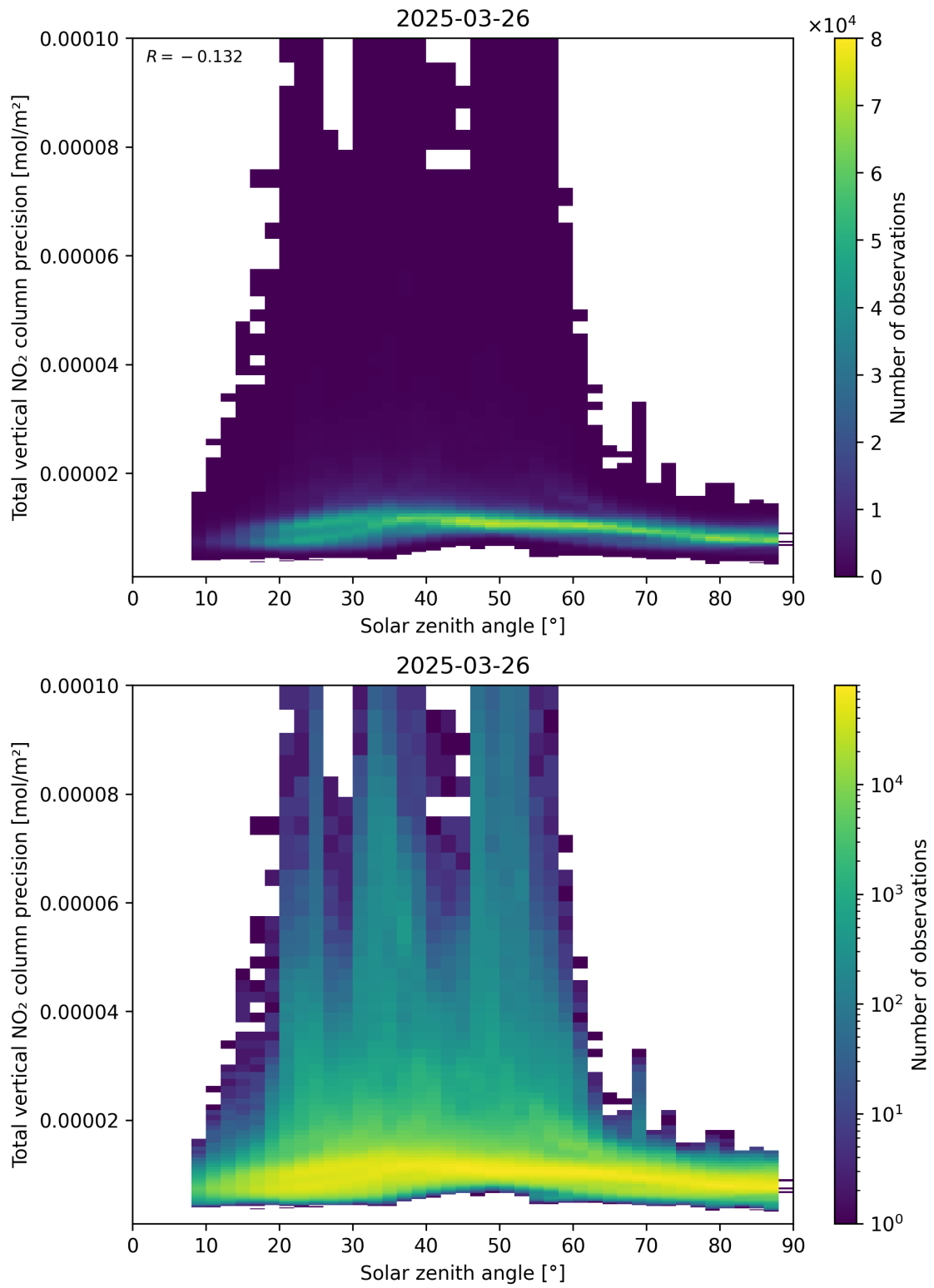
Figure 154: Scatter density plot of “Solar zenith angle” against “Total vertical NO 2 column precision” for 2025-03-26 to 2025-03-26.
