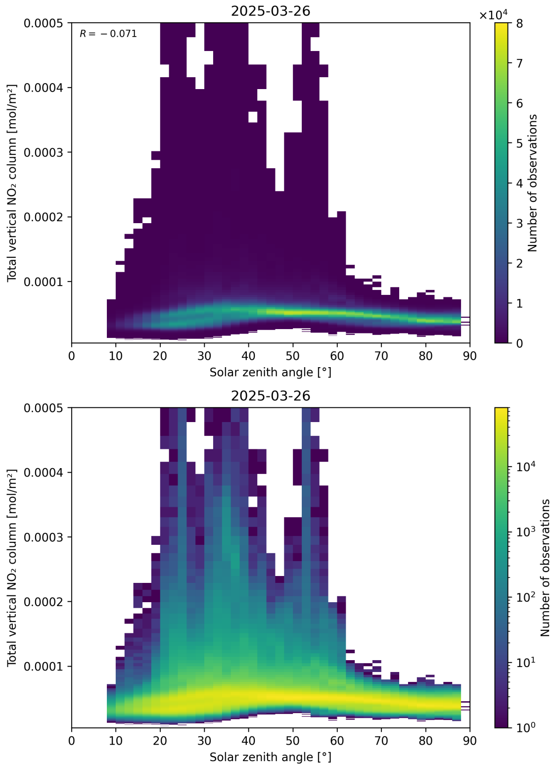
Figure 153: Scatter density plot of “Solar zenith angle” against “Total vertical NO 2 column” for 2025-03-26 to 2025-03-26.
