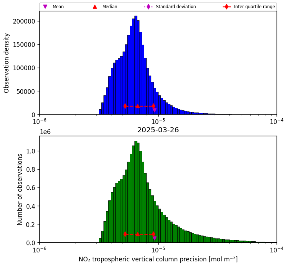
Figure 30: Histogram of “NO 2 tropospheric vertical column precision” for 2025-03-26 to 2025-03-26
