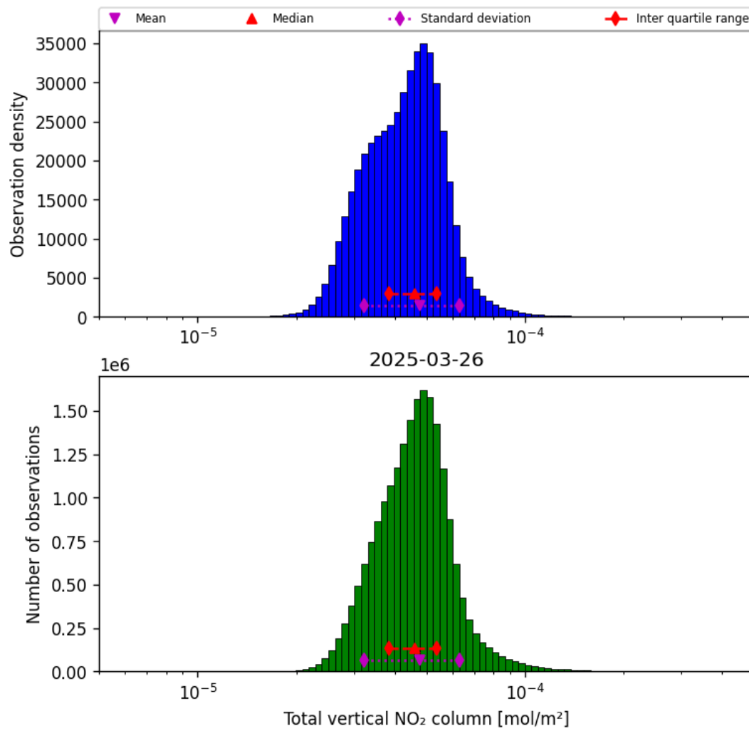
Figure 38: Histogram of "Total vertical NO 2 column" for 2025-03-26 to 2025-03-26
