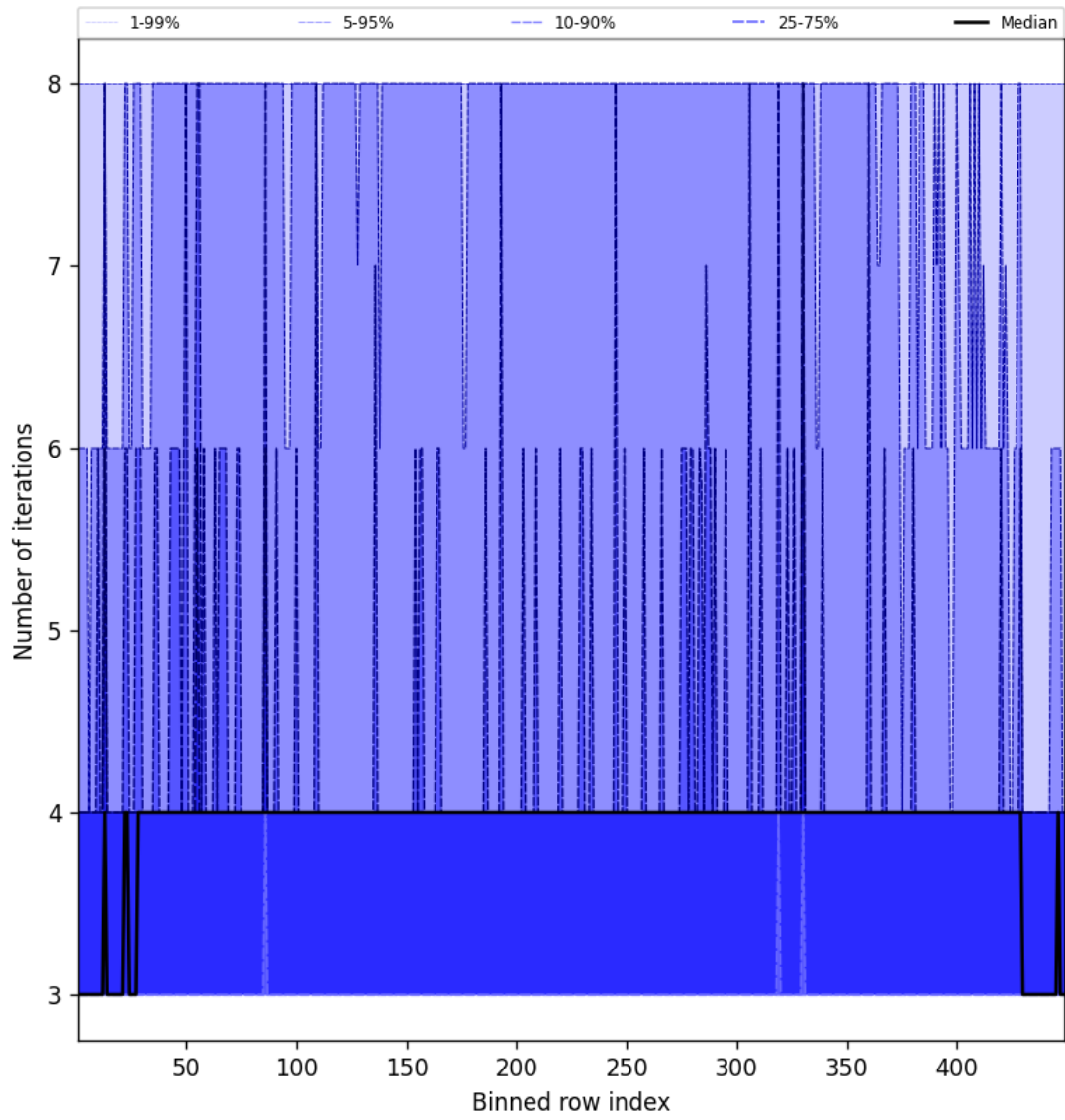
Figure 51: Along track statistics of “Number of iterations” for 2025-03-26 to 2025-03-26
