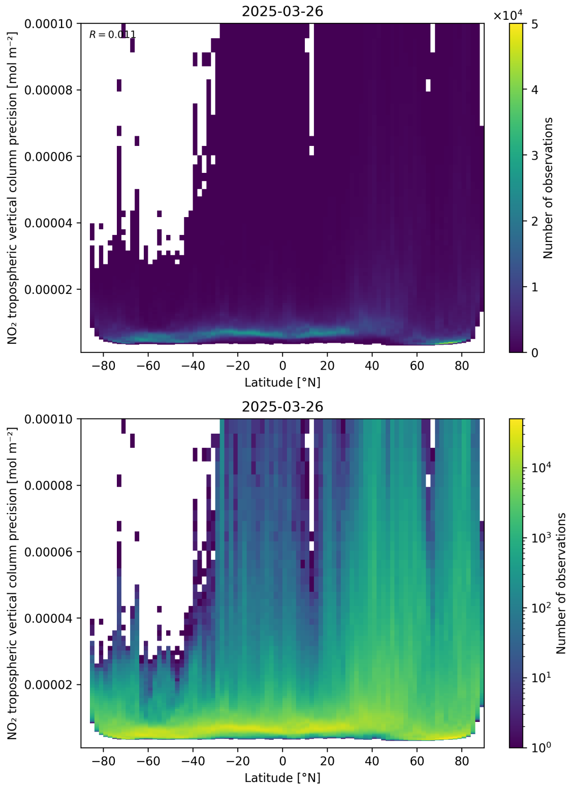
Figure 93: Scatter density plot of “Latitude” against “NO 2 tropospheric vertical column precision” for 2025-03-26 to 2025-03-26.
