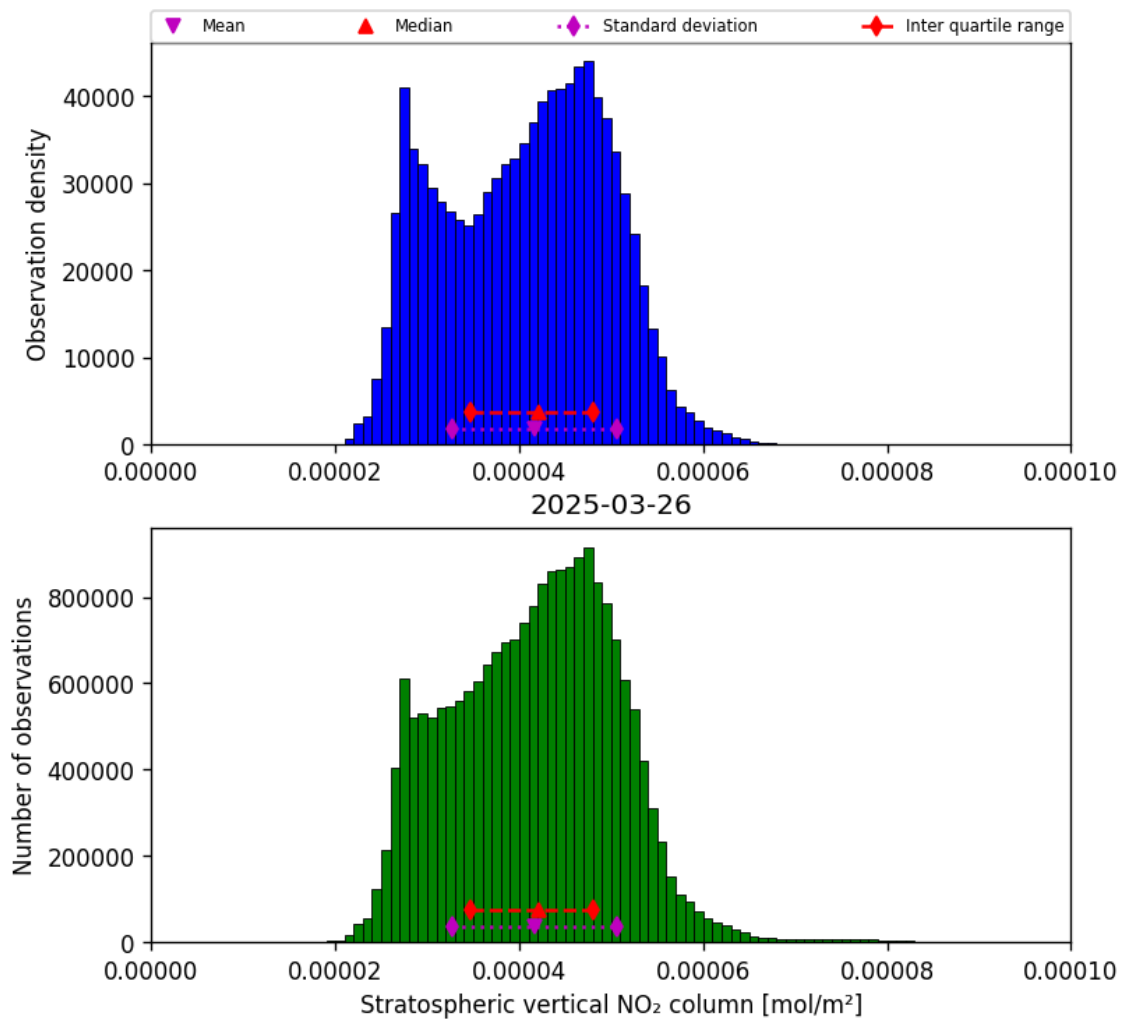
Figure 36: Histogram of “Stratospheric vertical NO 2 column” for 2025-03-26 to 2025-03-26
