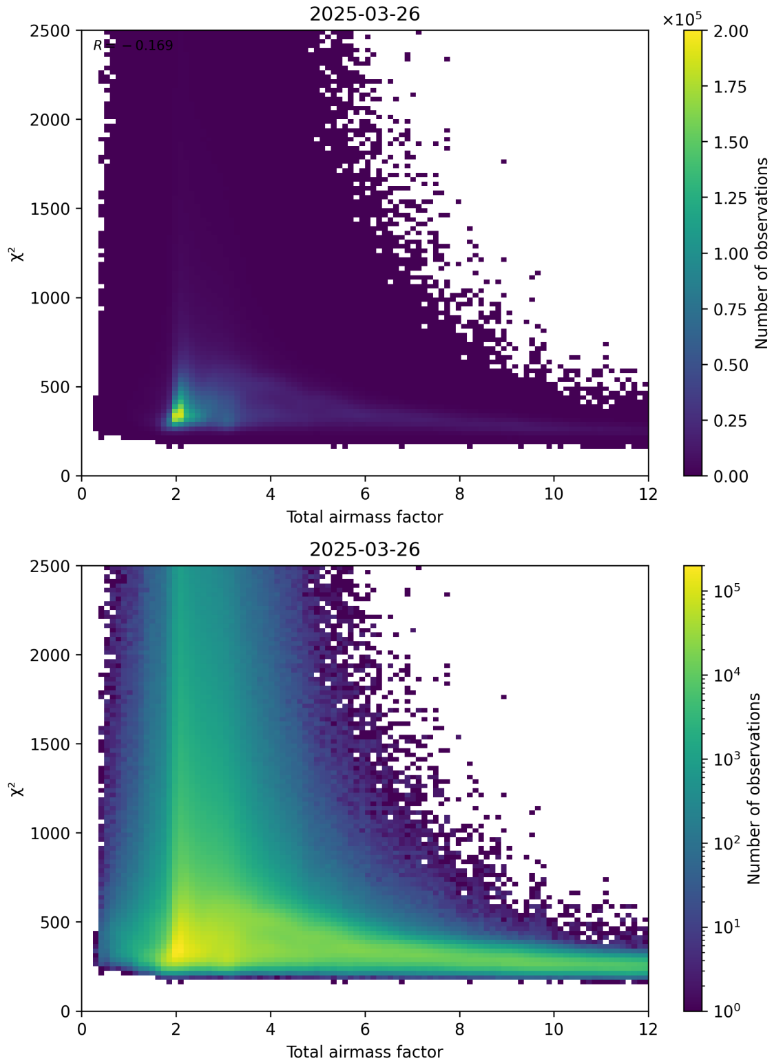
Figure 63: Scatter density plot of “Total airmass factor” against “ \chi^2 ” for 2025-03-26 to 2025-03-26.
