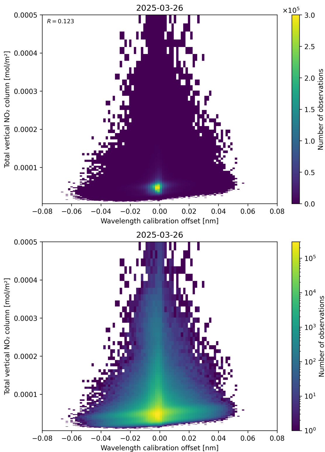
Figure 179: Scatter density plot of “Wavelength calibration offset” against “Total vertical NO 2 column” for 2025-03-26 to 2025-03-26.
