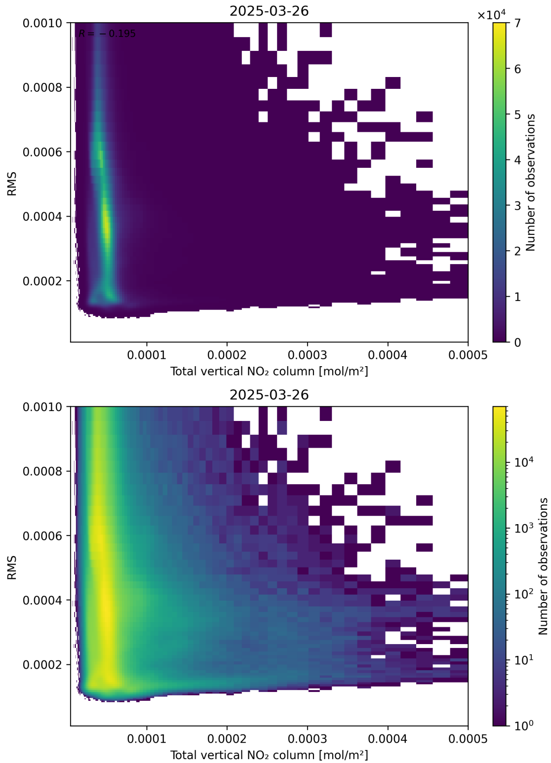
Figure 120: Scatter density plot of “Total vertical NO 2 column” against “RMS” for 2025-03-26 to 2025-03-26.
