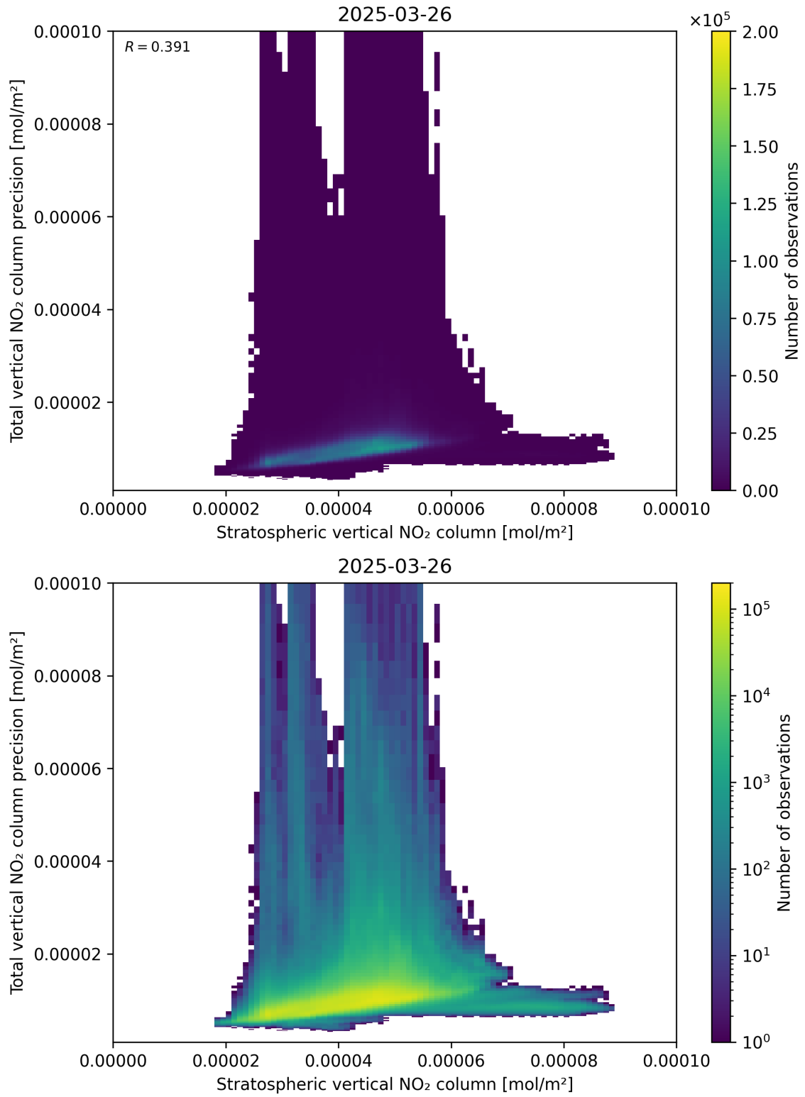
Figure 101: Scatter density plot of “Stratospheric vertical NO 2 column” against “Total vertical NO 2 column precision” for 2025-03-26 to 2025-03-26.
