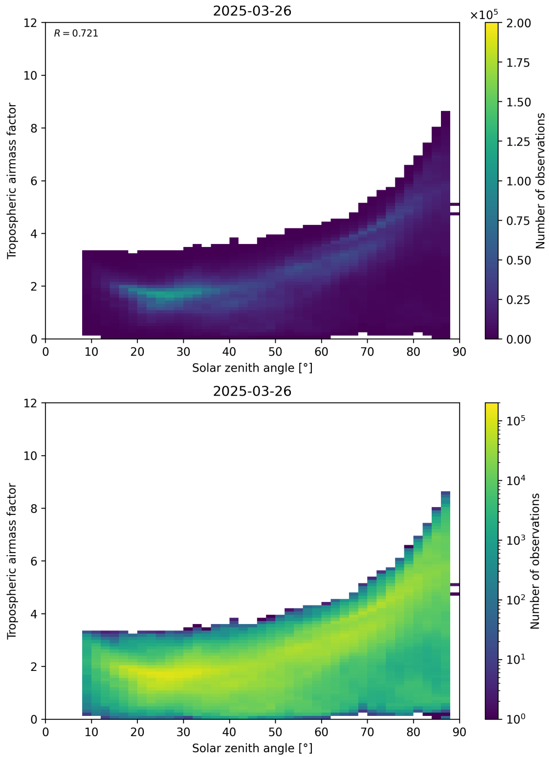
Figure 147: Scatter density plot of “Solar zenith angle” against “Tropospheric airmass factor” for 2025-03-26 to 2025-03-26.
