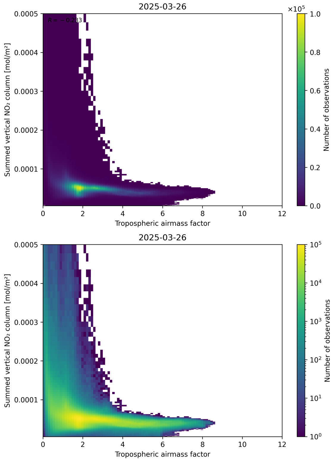
Figure 75: Scatter density plot of “Tropospheric air mass factor” against “Summed vertical NO 2 column” for 2025-03-26 to 2025-03-26.
