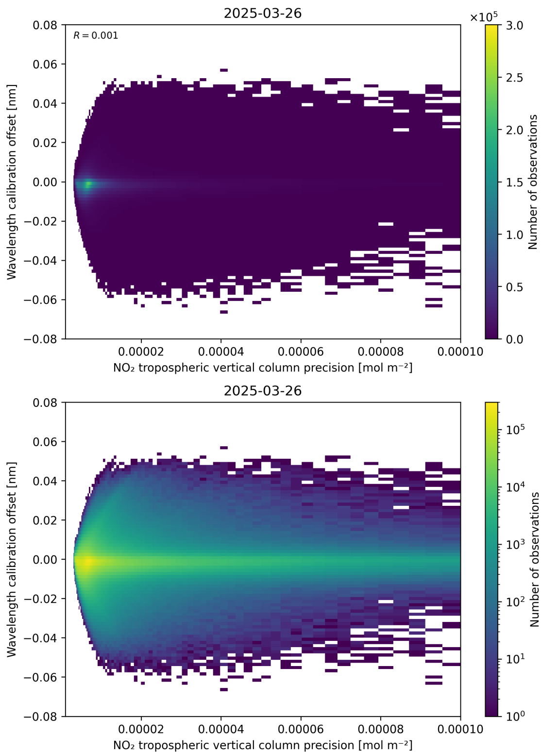
Figure 141: Scatter density plot of “NO 2 tropospheric vertical column precision” against “Wavelength calibration offset” for 2025-03-26 to 2025-03-26.
