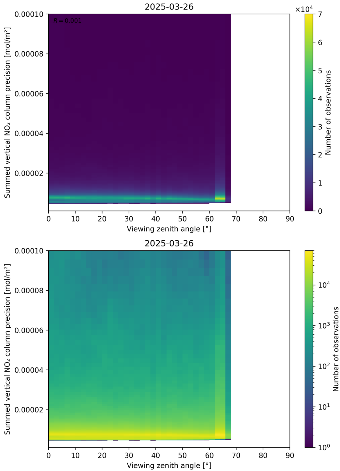
Figure 166: Scatter density plot of “Viewing zenith angle” against “Summed vertical NO 2 column precision” for 2025-03-26 to 2025-03-26.
