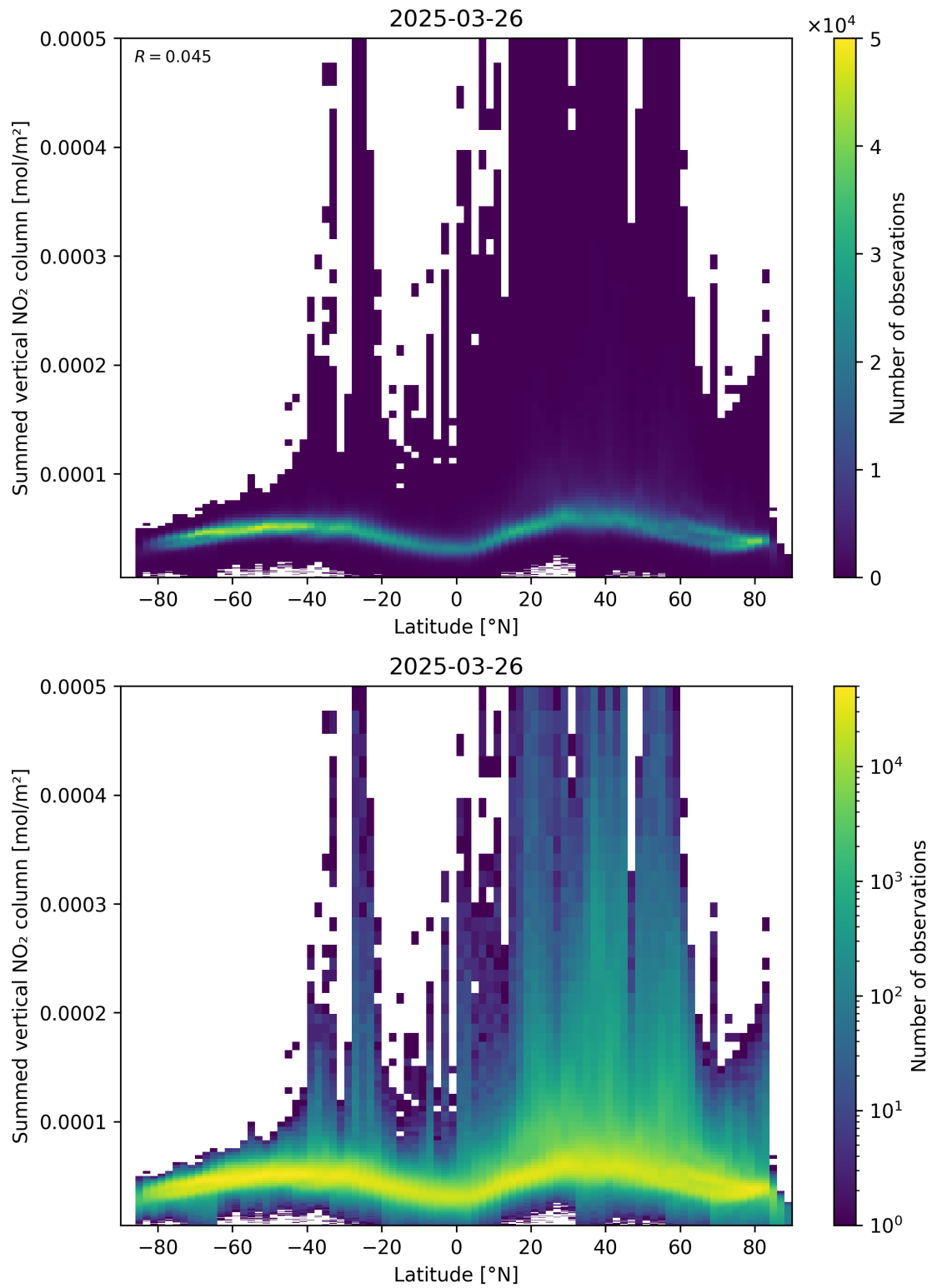
Figure 88: Scatter density plot of “Latitude” against “Summed vertical NO 2 column” for 2025-03-26 to 2025-03-26.
