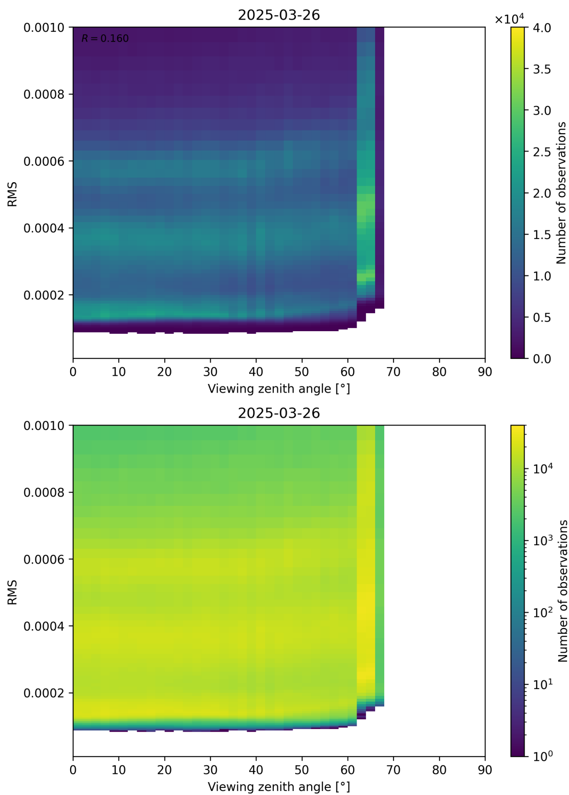
Figure 171: Scatter density plot of “Viewing zenith angle” against “RMS” for 2025-03-26 to 2025-03-26.
