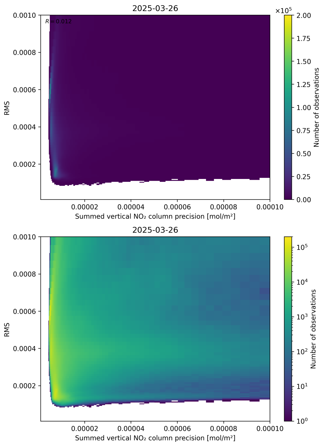
Figure 108: Scatter density plot of “Summed vertical NO 2 column precision” against “RMS” for 2025-03-26 to 2025-03-26.
