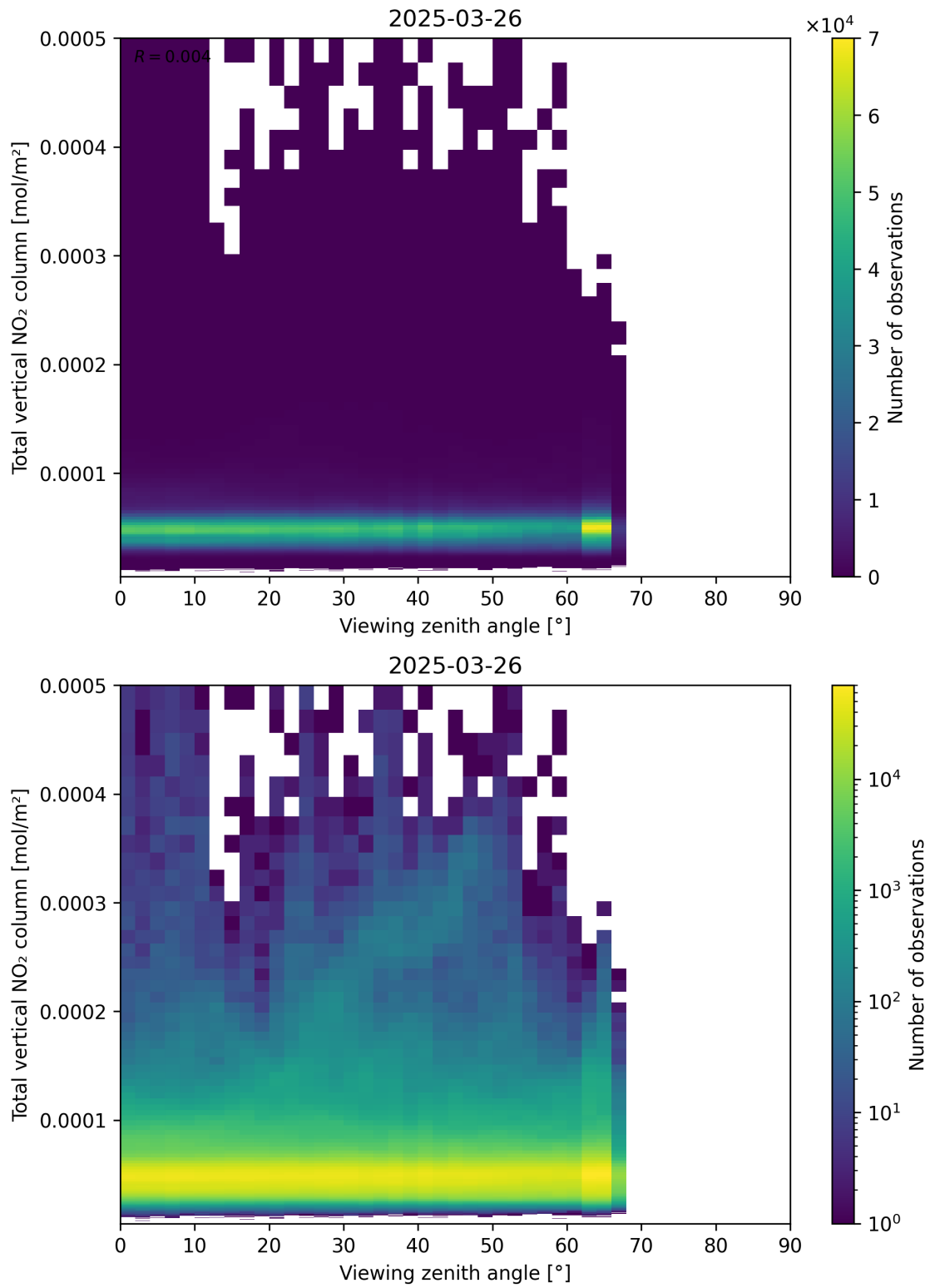
Figure 167: Scatter density plot of “Viewing zenith angle” against “Total vertical NO 2 column” for 2025-03-26 to 2025-03-26.
