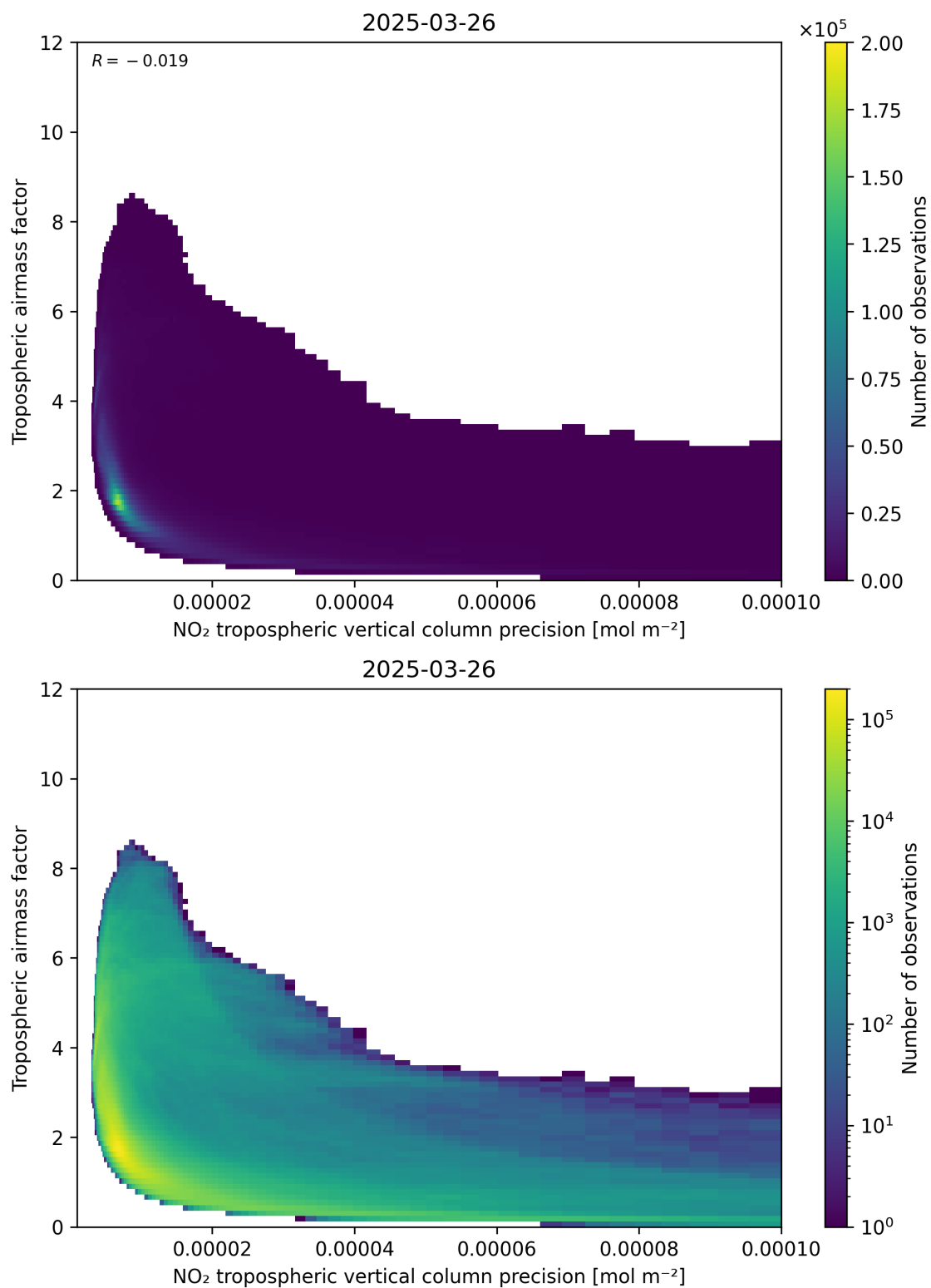
Figure 133: Scatter density plot of “NO 2 tropospheric vertical column precision” against “Tropospheric air mass factor” for 2025-03-26 to 2025-03-26.
