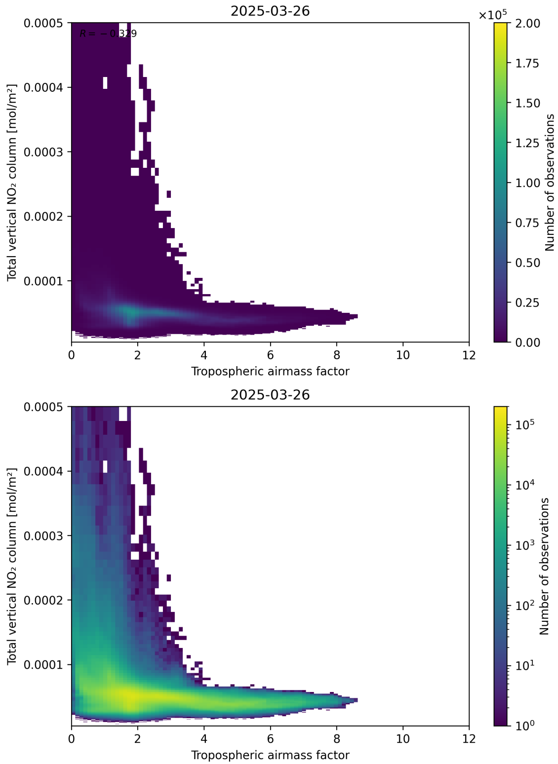
Figure 77: Scatter density plot of “Tropospheric airmass factor” against “Total vertical NO 2 column” for 2025-03-26 to 2025-03-26.
