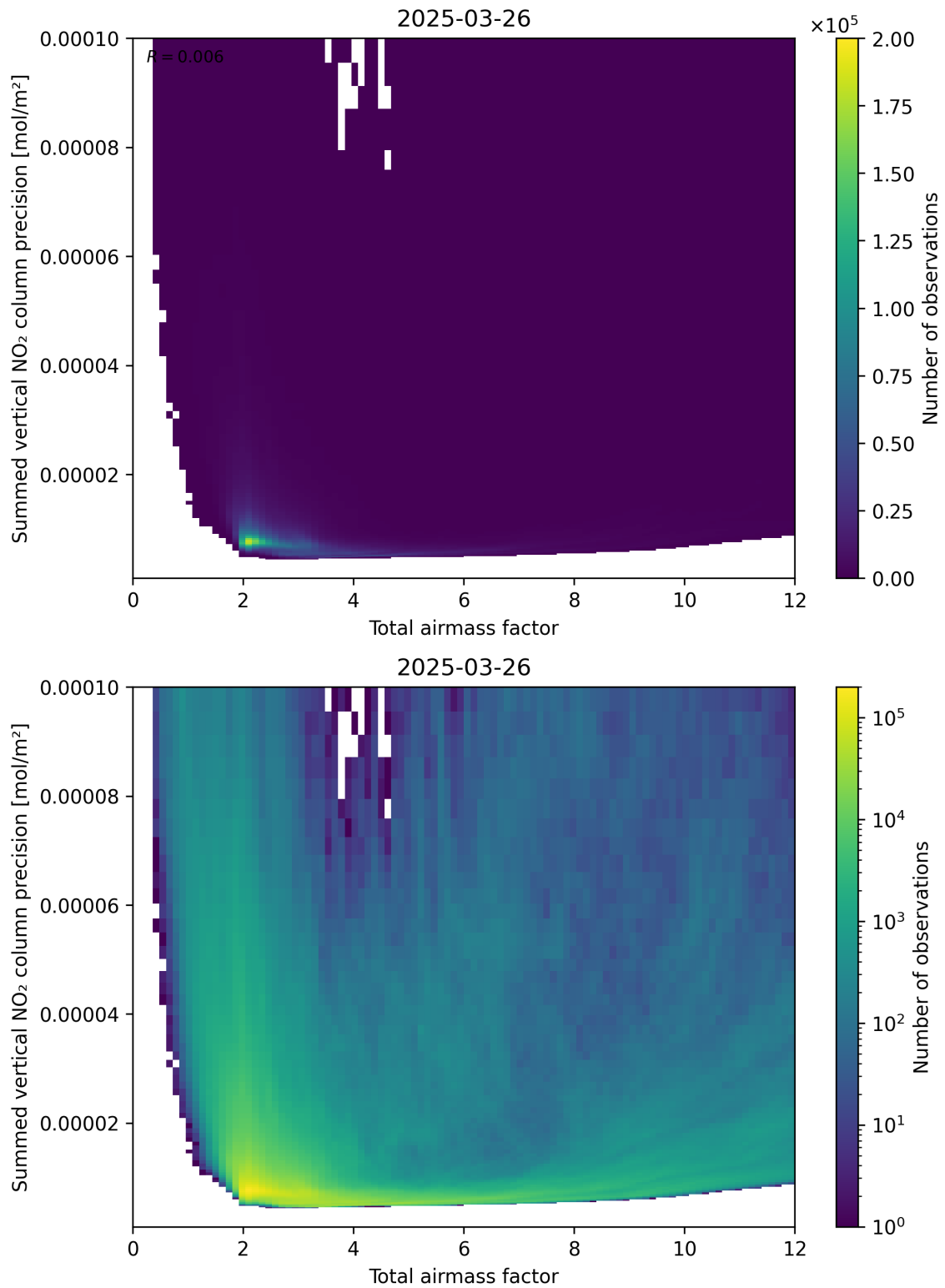
Figure 66: Scatter density plot of “Total airmass factor” against “Summed vertical NO 2 column precision” for 2025-03-26 to 2025-03-26.
