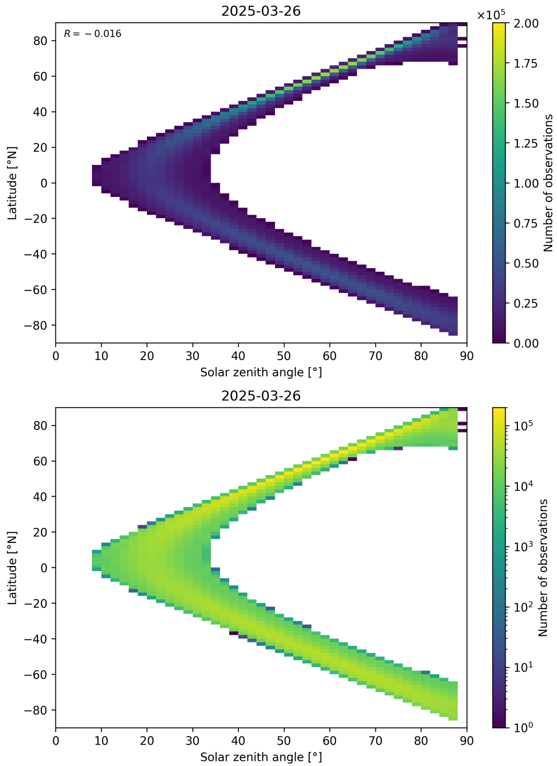
Figure 149: Scatter density plot of “Solar zenith angle” against “Latitude” for 2025-03-26 to 2025-03-26.
