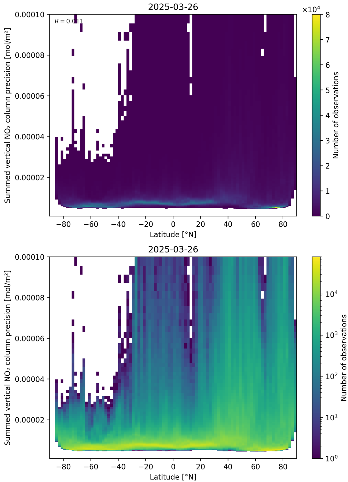
Figure 89: Scatter density plot of “Latitude” against “Summed vertical NO 2 column precision” for 2025-03-26 to 2025-03-26.
