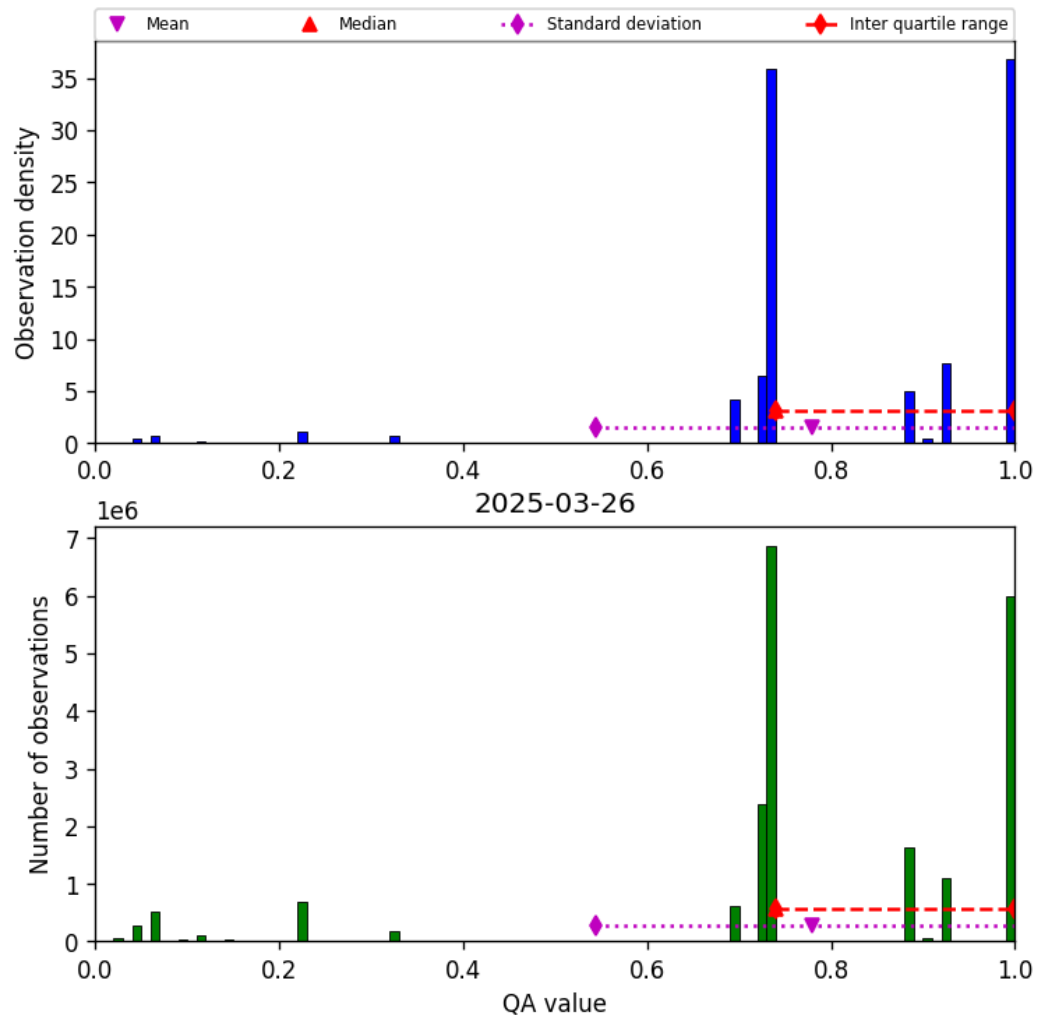
Figure 28: Histogram of “QA value” for 2025-03-26 to 2025-03-26
