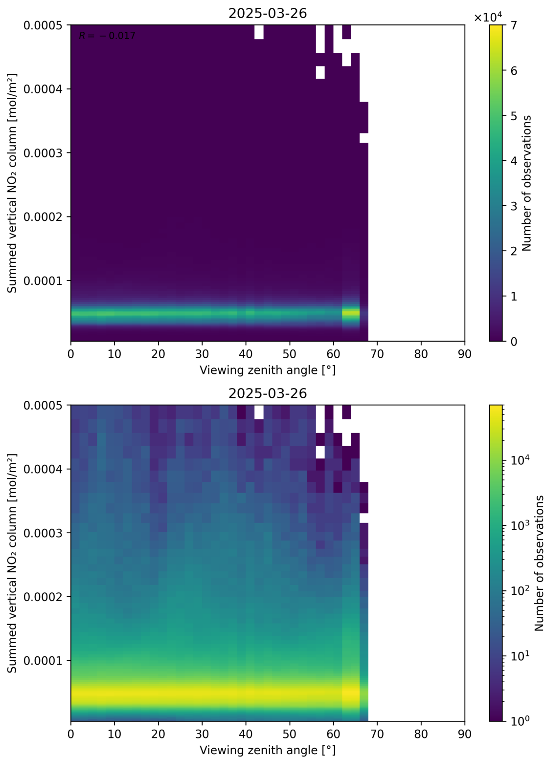
Figure 165: Scatter density plot of “Viewing zenith angle” against “Summed vertical NO 2 column” for 2025-03-26 to 2025-03-26.
