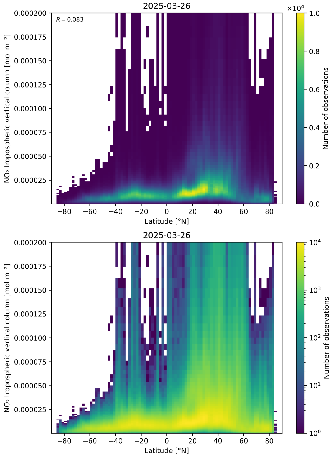
Figure 92: Scatter density plot of “Latitude” against “NO 2 tropospheric vertical column” for 2025-03-26 to 2025-03-26.
