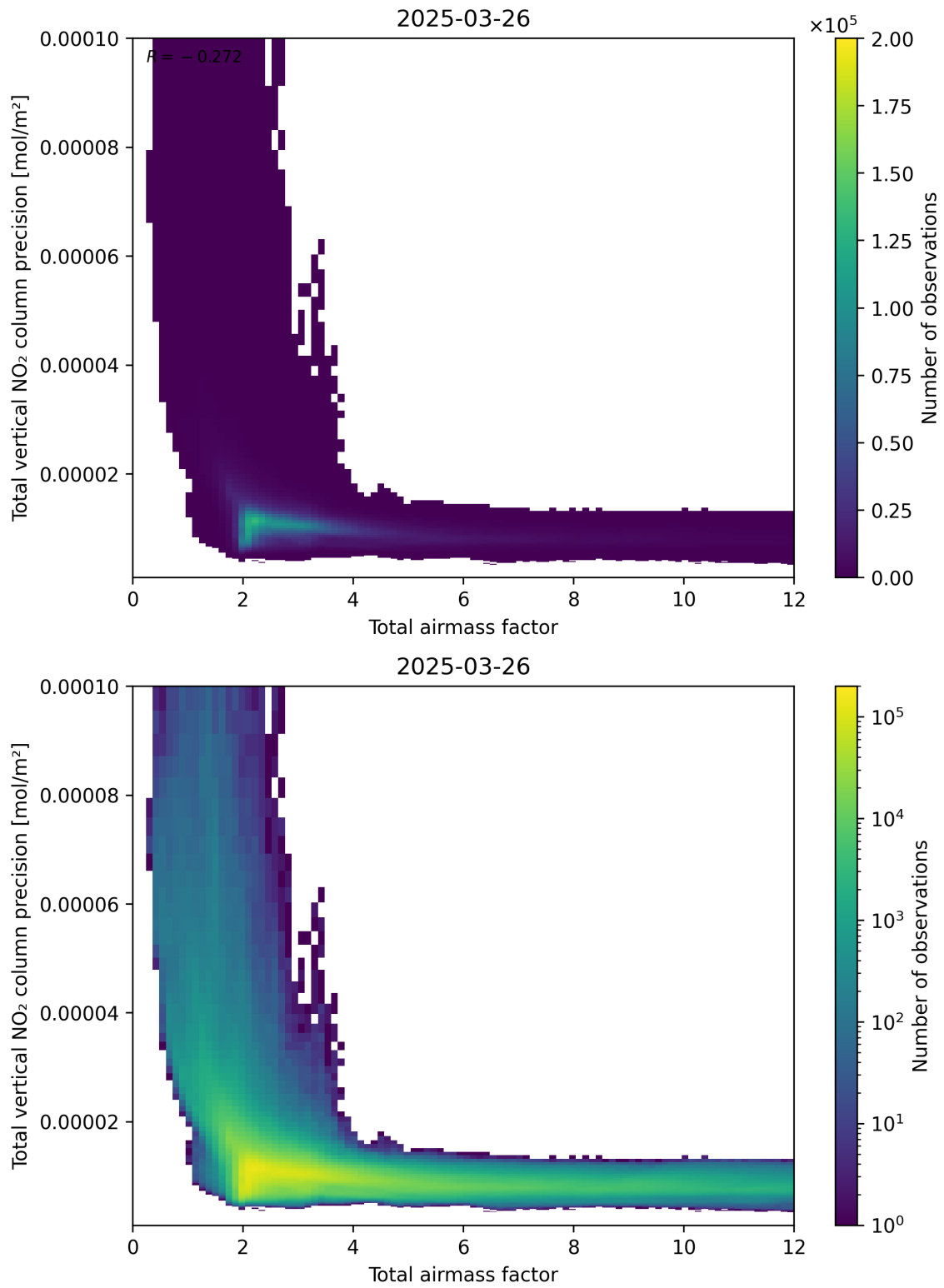
Figure 68: Scatter density plot of “Total airmass factor” against “Total vertical NO 2 column precision” for 2025-03-26 to 2025-03-26.
