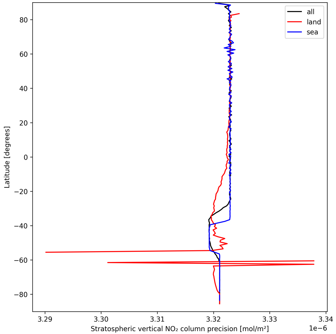
Figure 20: Zonal average of “Stratospheric vertical NO 2 column precision” for 2025-03-26 to 2025-03-26.
