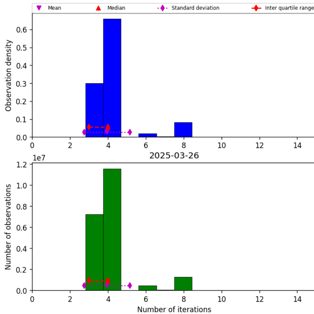
Figure 34: Histogram of “Number of iterations” for 2025-03-26 to 2025-03-26
