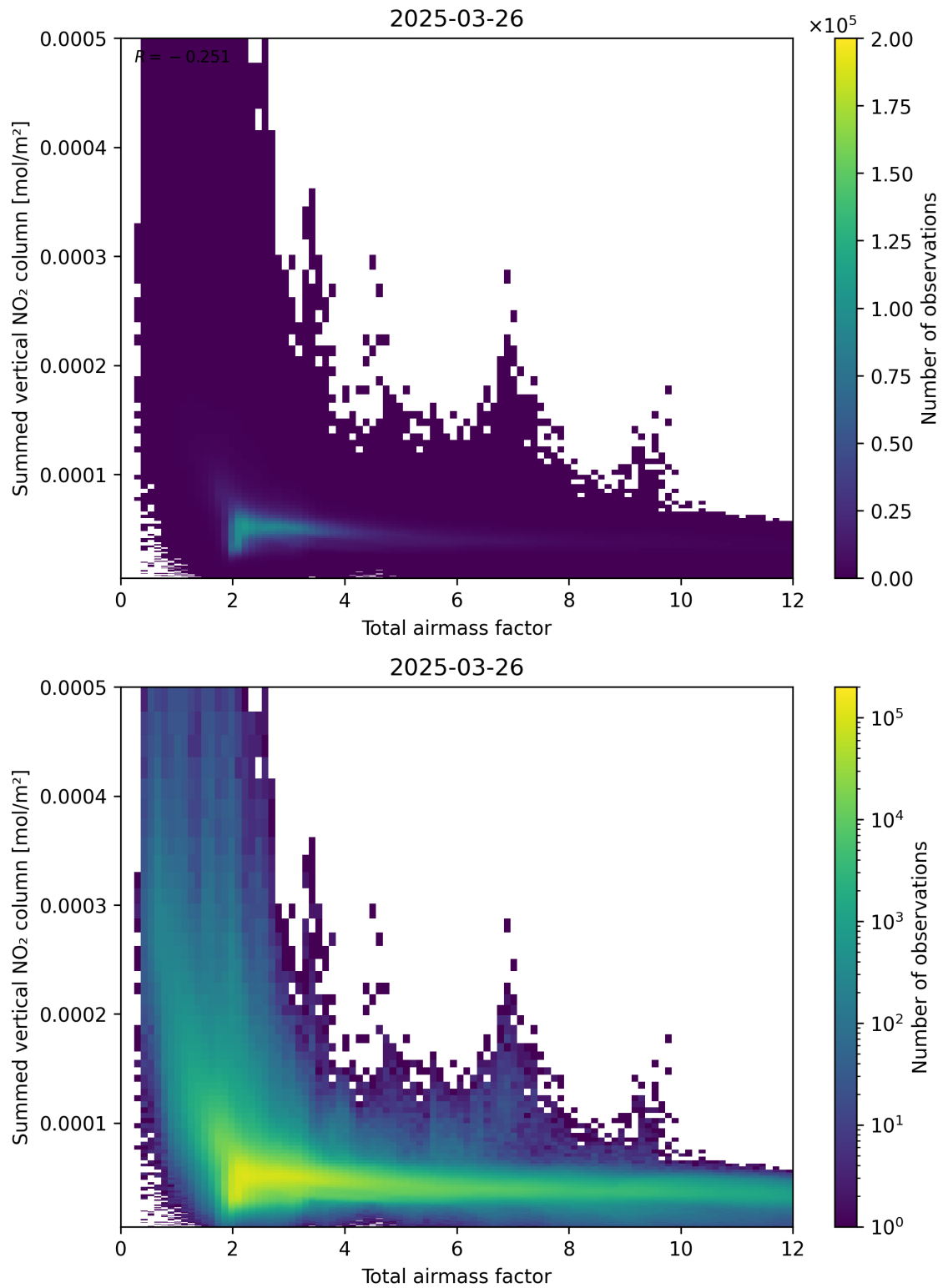
Figure 65: Scatter density plot of “Total airmass factor” against “Summed vertical NO 2 column” for 2025-03-26 to 2025-03-26.
