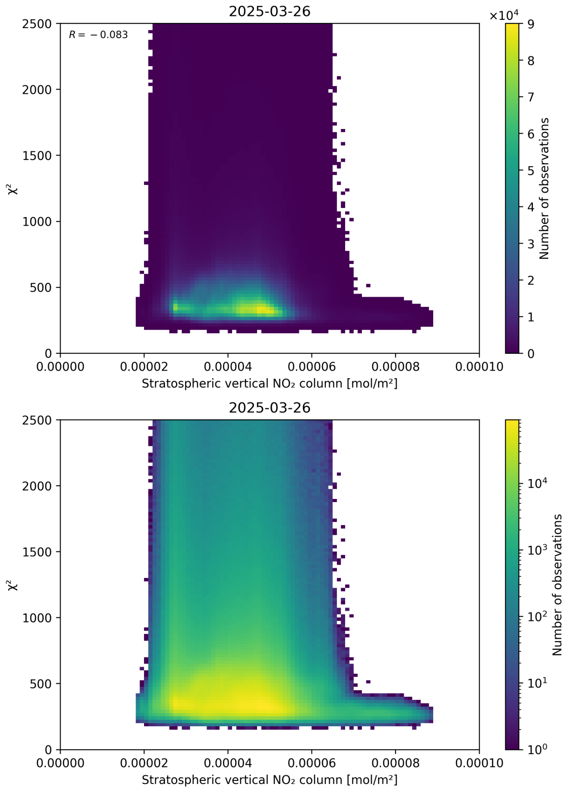
Figure 97: Scatter density plot of “Stratospheric vertical NO 2 column” against “ \chi^2 ” for 2025-03-26 to 2025-03-26.
