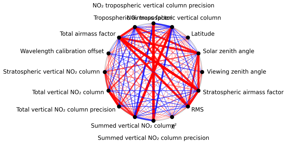
Figure 1: Map of correlation graph for 2025-03-26 to 2025-03-26.
