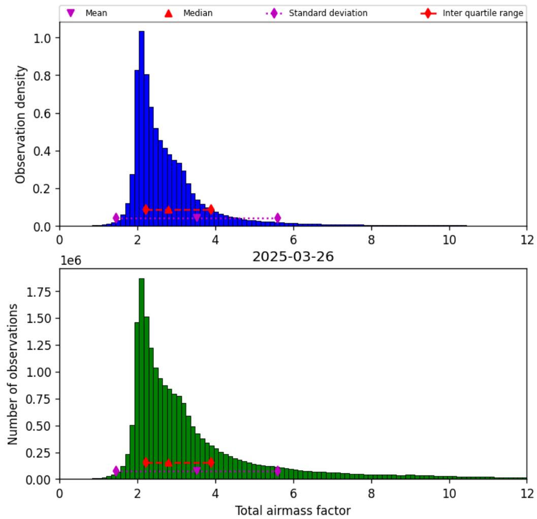
Figure 32: Histogram of “Total airmass factor” for 2025-03-26 to 2025-03-26
