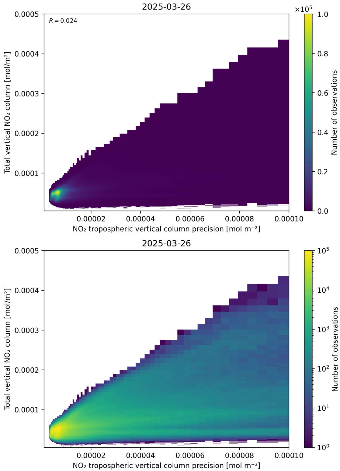
Figure 138: Scatter density plot of “NO 2 tropospheric vertical column precision” against “Total vertical NO 2 column” for 2025-03-26 to 2025-03-26.
