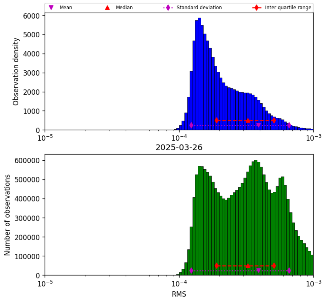
Figure 43: Histogram of “RMS” for 2025-03-26 to 2025-03-26
