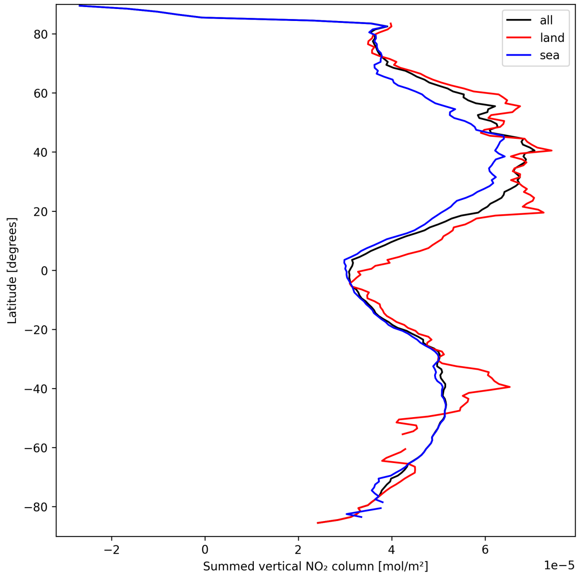
Figure 23: Zonal average of “Summed vertical NO 2 column” for 2025-03-26 to 2025-03-26.
