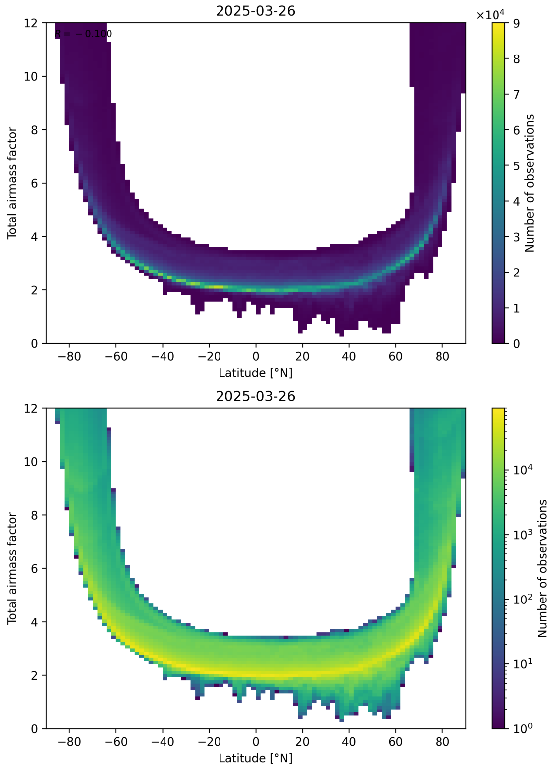
Figure 84: Scatter density plot of “Latitude” against “Total air mass factor” for 2025-03-26 to 2025-03-26.
