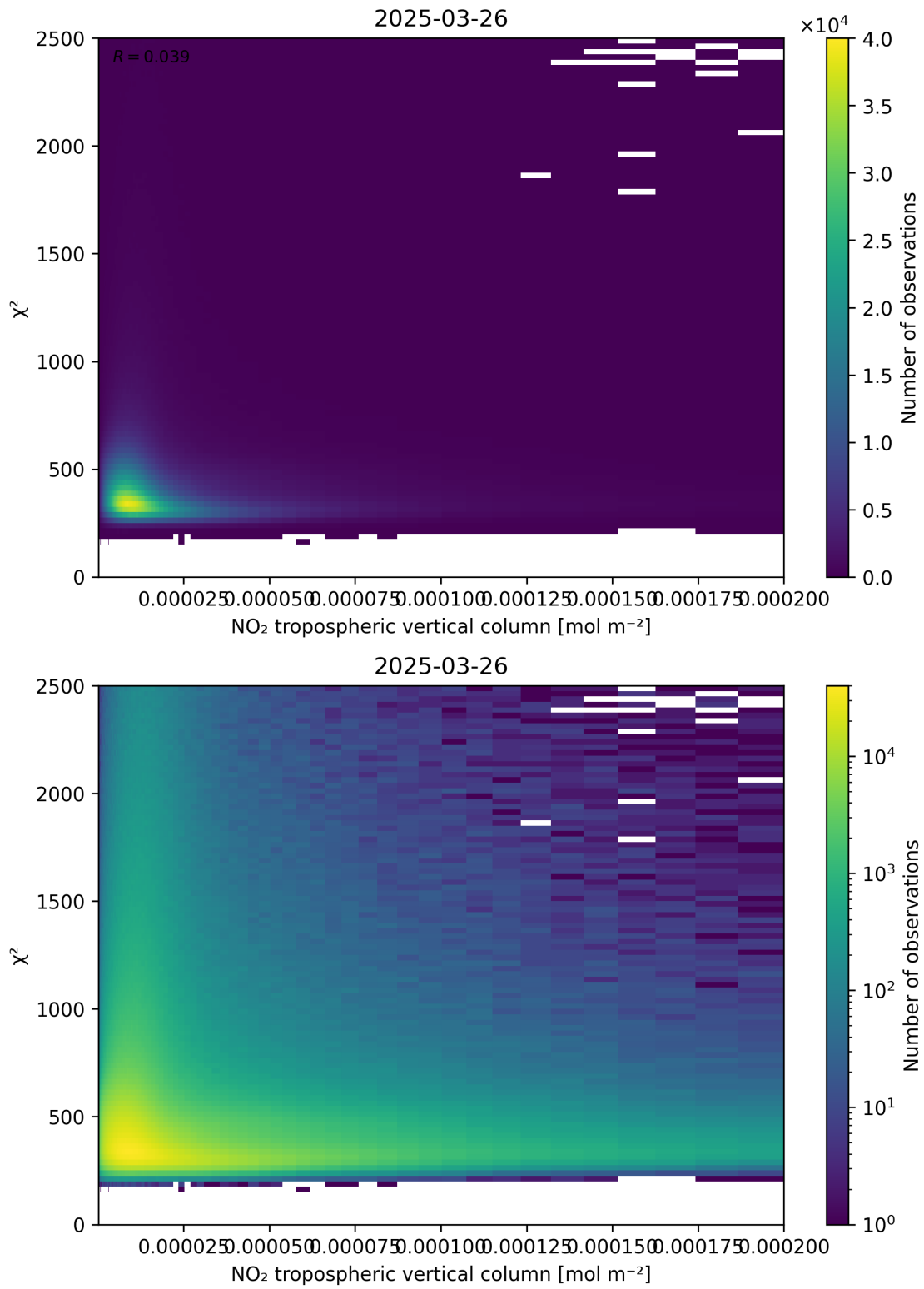
Figure 124: Scatter density plot of “NO 2 tropospheric vertical column” against “ \chi^2 ” for 2025-03-26 to 2025-03-26.
