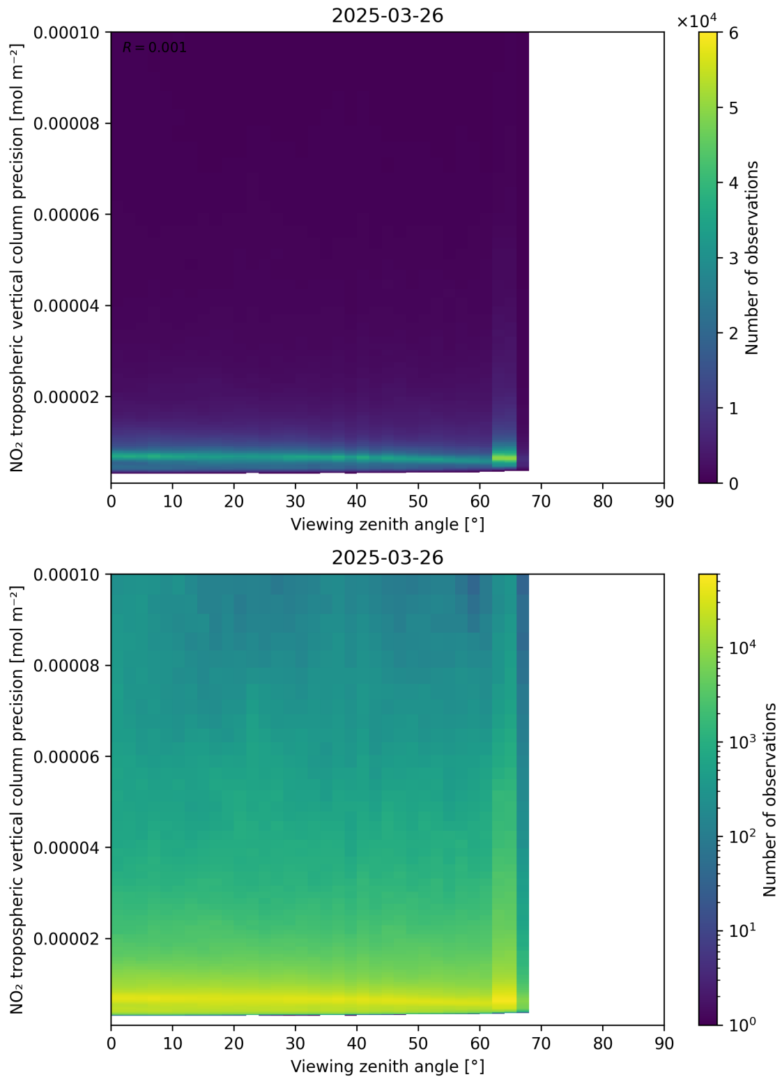
Figure 170: Scatter density plot of “Viewing zenith angle” against “NO 2 tropospheric vertical column precision” for 2025-03-26 to 2025-03-26.
