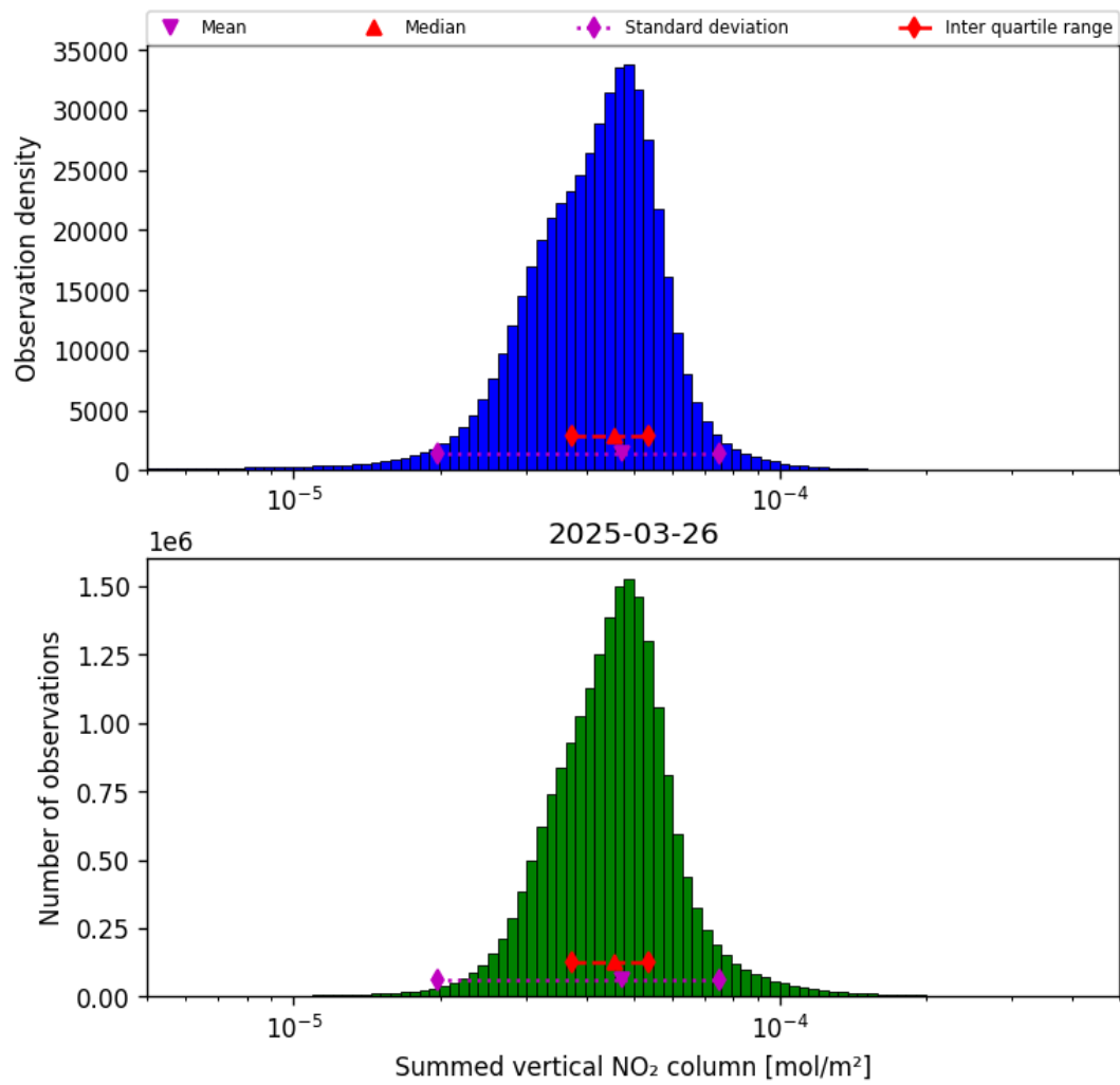
Figure 40: Histogram of “Summed vertical NO 2 column” for 2025-03-26 to 2025-03-26
