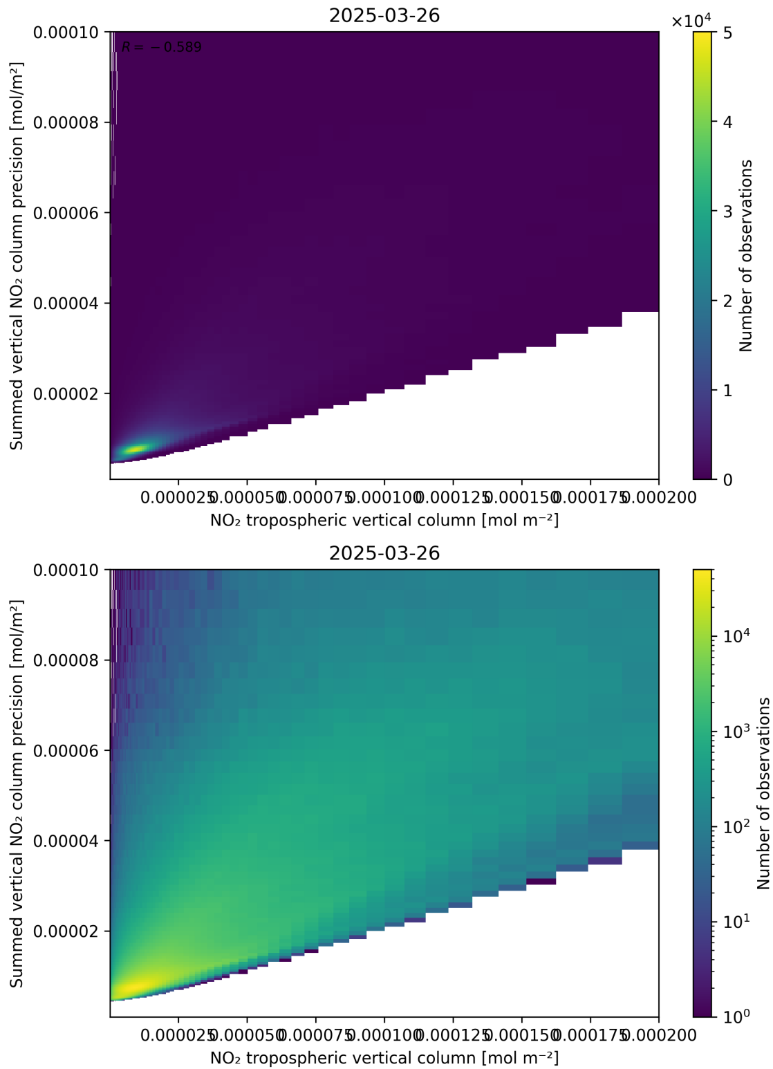
Figure 127: Scatter density plot of “NO 2 tropospheric vertical column” against “Summed vertical NO 2 column precision” for 2025-03-26 to 2025-03-26.
