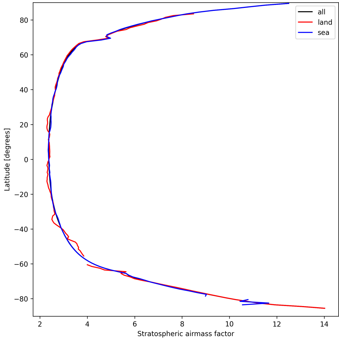
Figure 27: Zonal average of “Stratospheric airmass factor” for 2025-03-26 to 2025-03-26.
