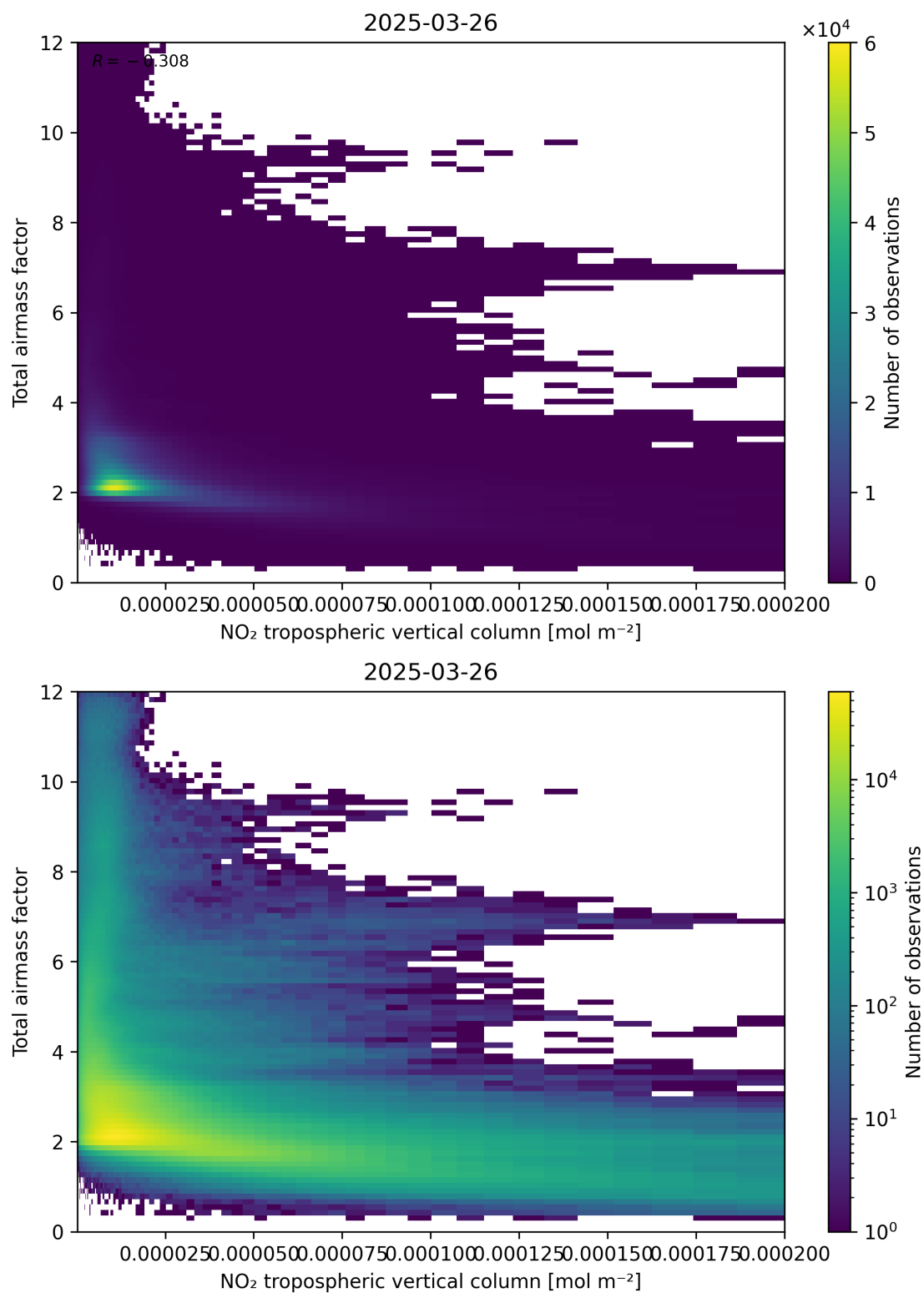
Figure 122: Scatter density plot of “NO 2 tropospheric vertical column” against “Total air mass factor” for 2025-03-26 to 2025-03-26.
