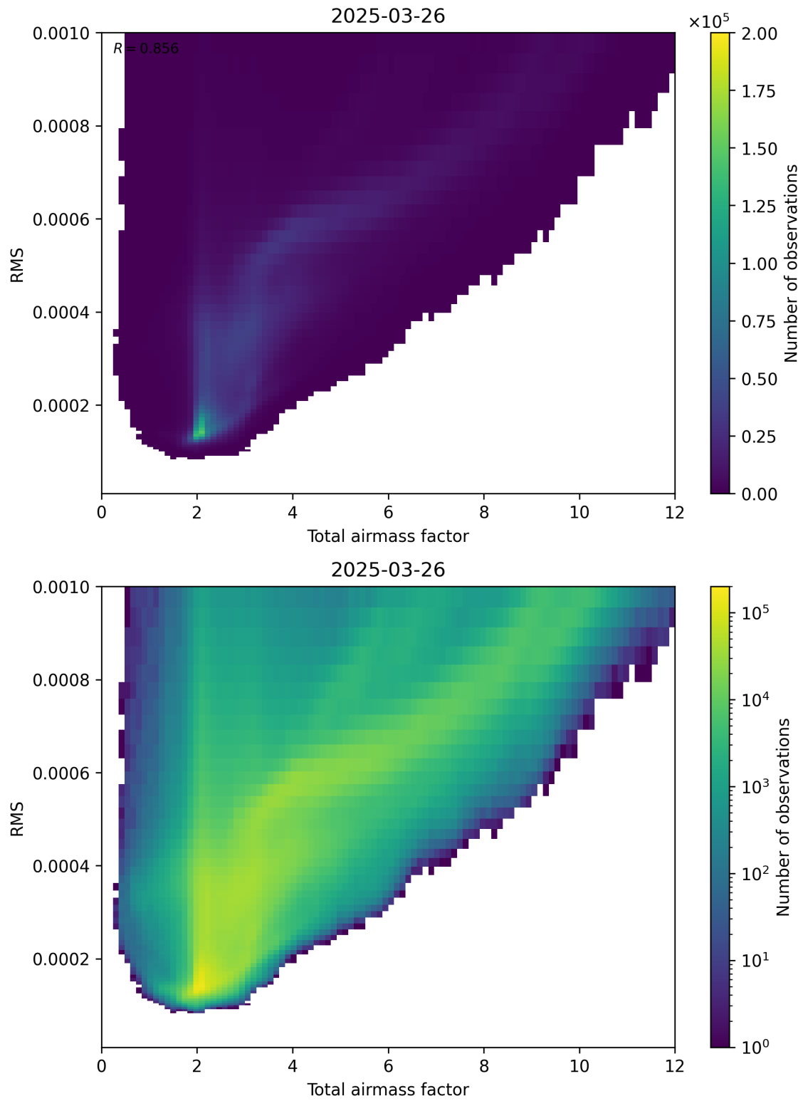
Figure 69: Scatter density plot of “Total airmass factor” against “RMS” for 2025-03-26 to 2025-03-26.
