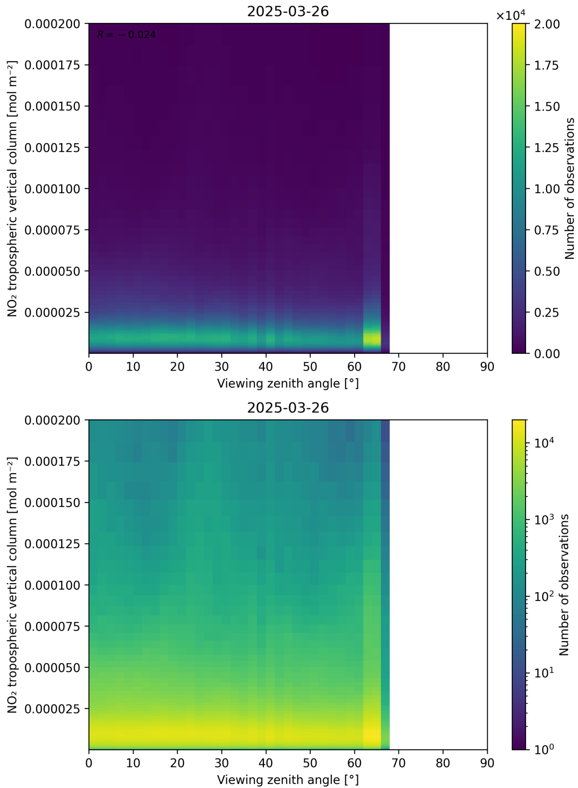
Figure 169: Scatter density plot of “Viewing zenith angle” against “NO 2 tropospheric vertical column” for 2025-03-26 to 2025-03-26.
