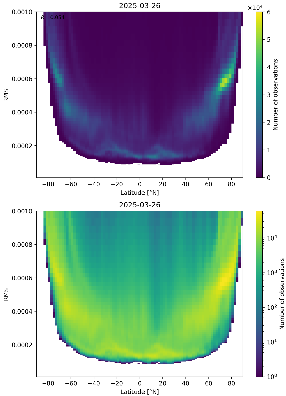
Figure 94: Scatter density plot of “Latitude” against “RMS” for 2025-03-26 to 2025-03-26.
