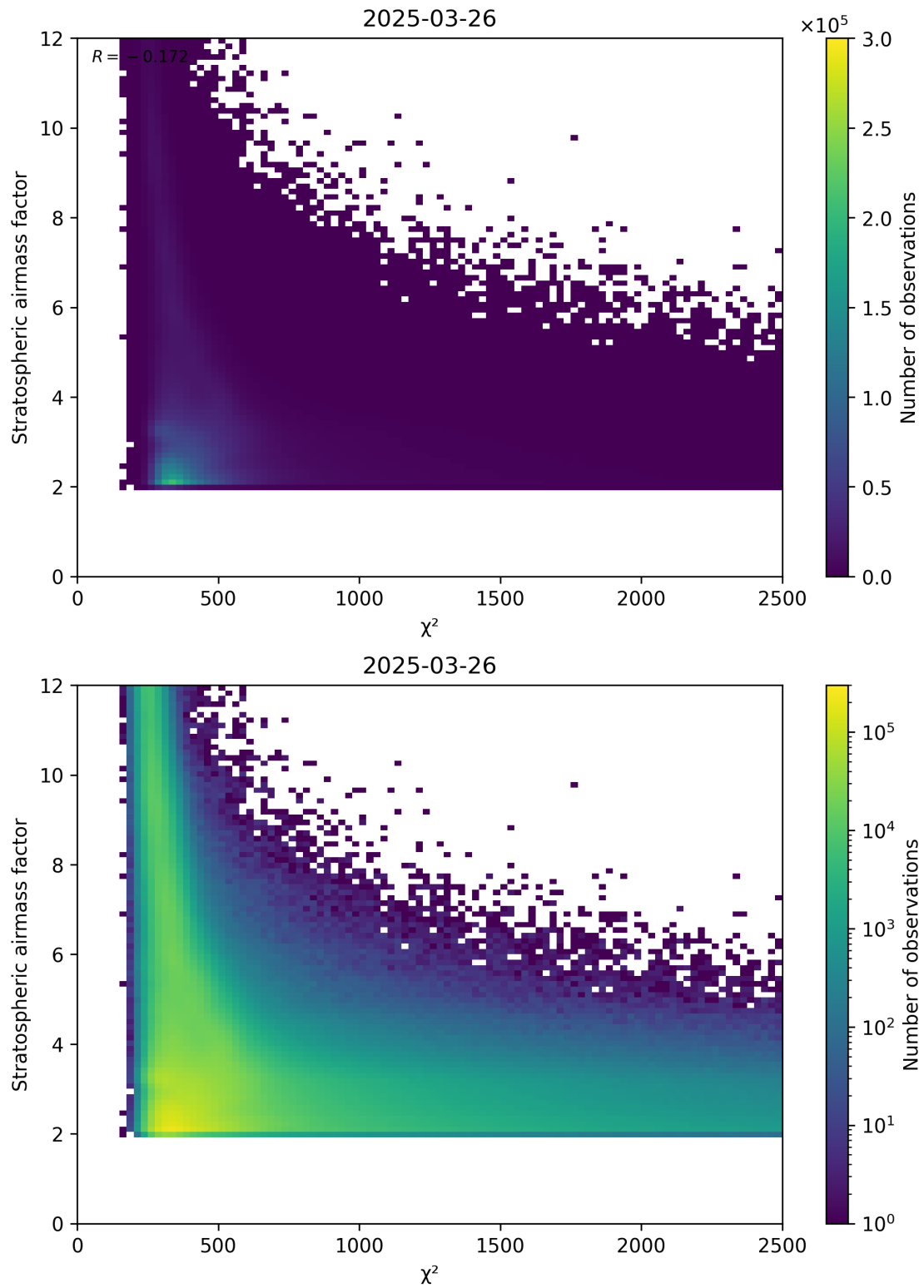
Figure 81: Scatter density plot of “ \chi^2 ” against “Stratospheric airmass factor” for 2025-03-26 to 2025-03-26.
