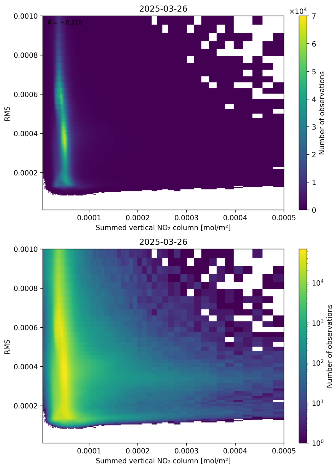
Figure 109: Scatter density plot of “Summed vertical NO 2 column” against “RMS” for 2025-03-26 to 2025-03-26.
