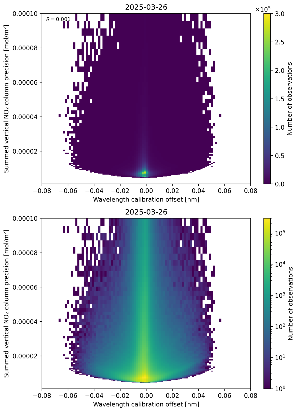
Figure 178: Scatter density plot of “Wavelength calibration offset” against “Summed vertical NO 2 column precision” for 2025-03-26 to 2025-03-26.
