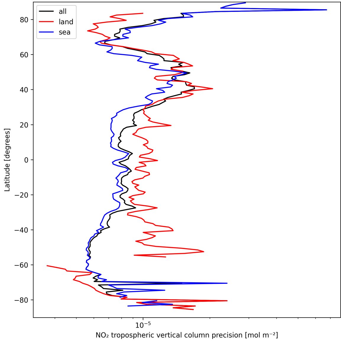
Figure 13: Zonal average of “NO 2 tropospheric vertical column precision” for 2025-03-26 to 2025-03-26.
