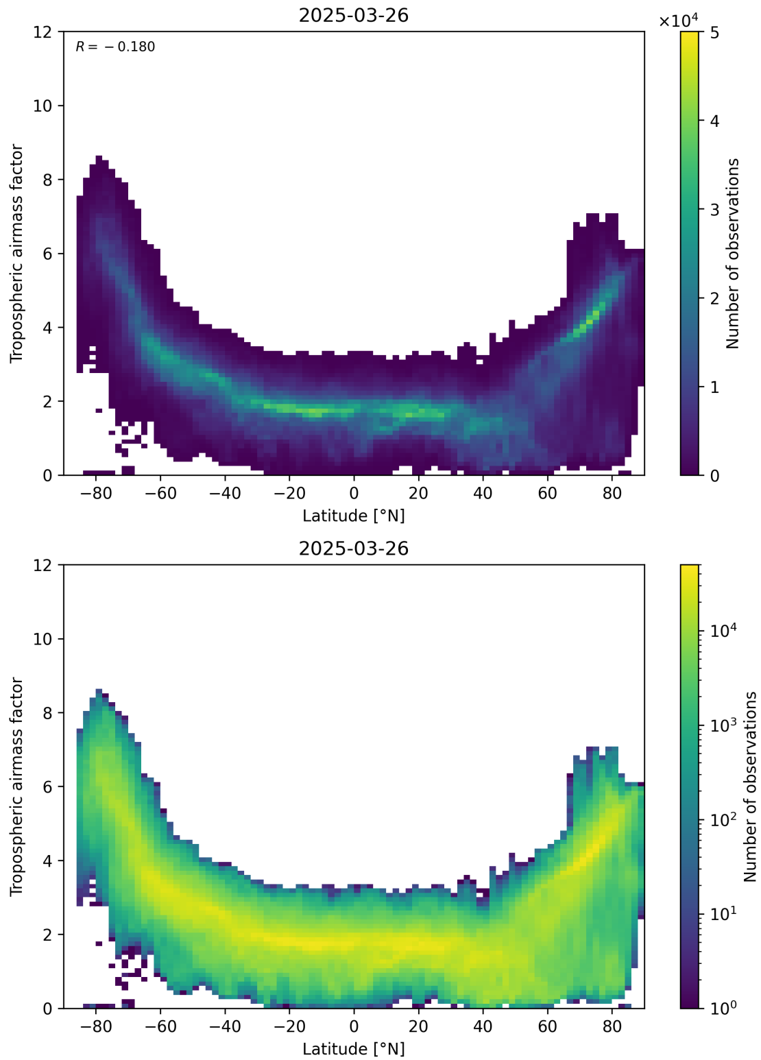
Figure 85: Scatter density plot of “Latitude” against “Tropospheric airmass factor” for 2025-03-26 to 2025-03-26.
