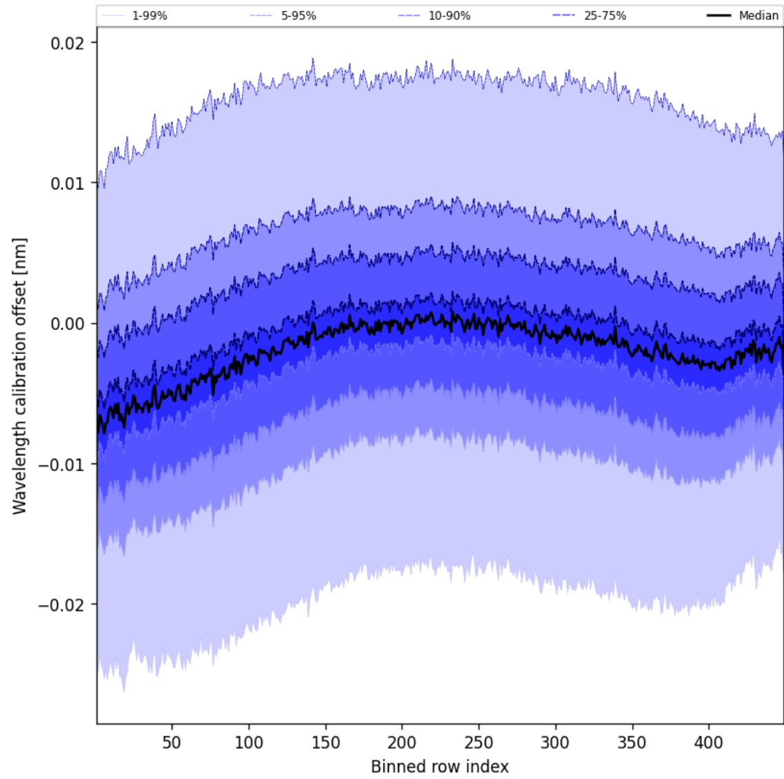
Figure 52: Along track statistics of “Wavelength calibration offset” for 2025-03-26 to 2025-03-26
