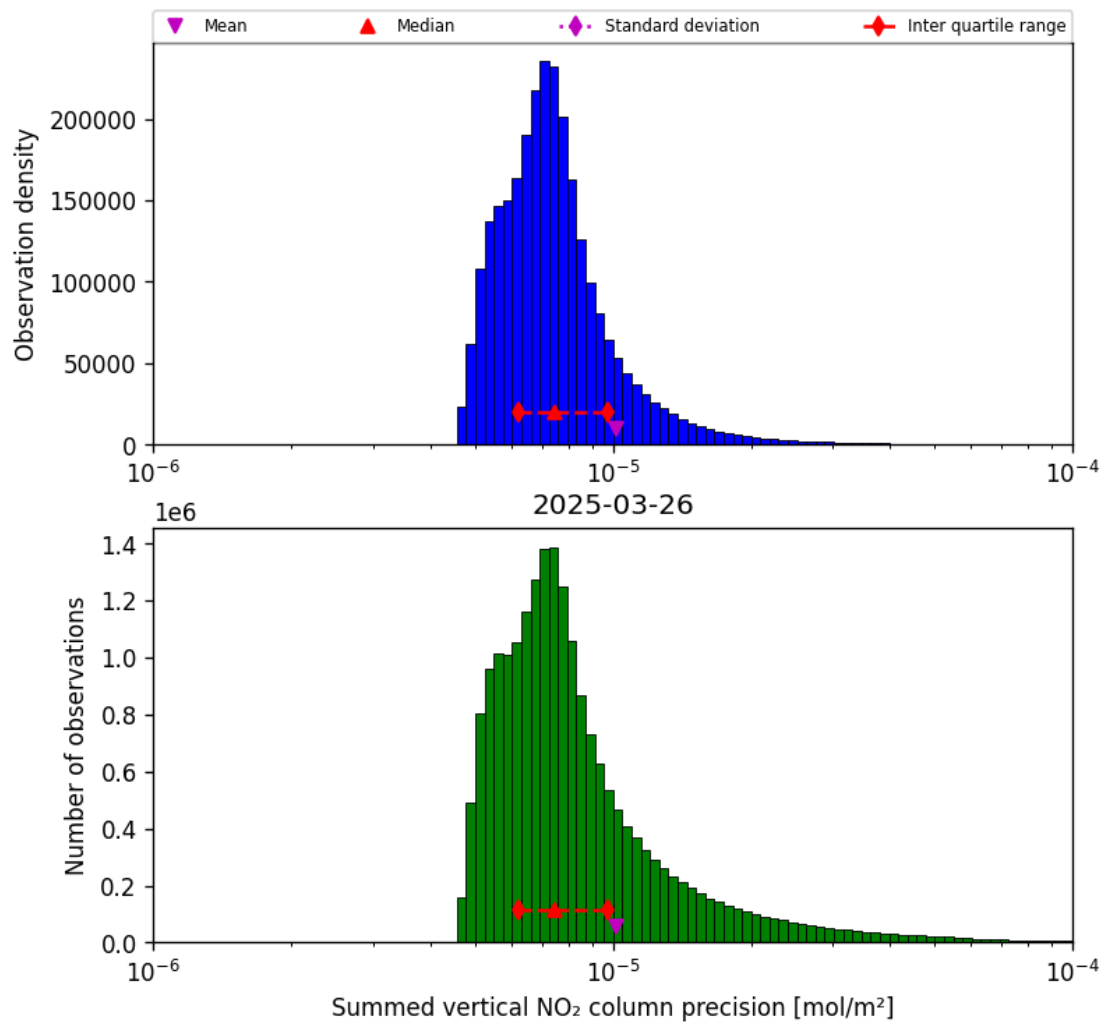
Figure 41: Histogram of "Summed vertical NO 2 column precision" for 2025-03-26 to 2025-03-26
