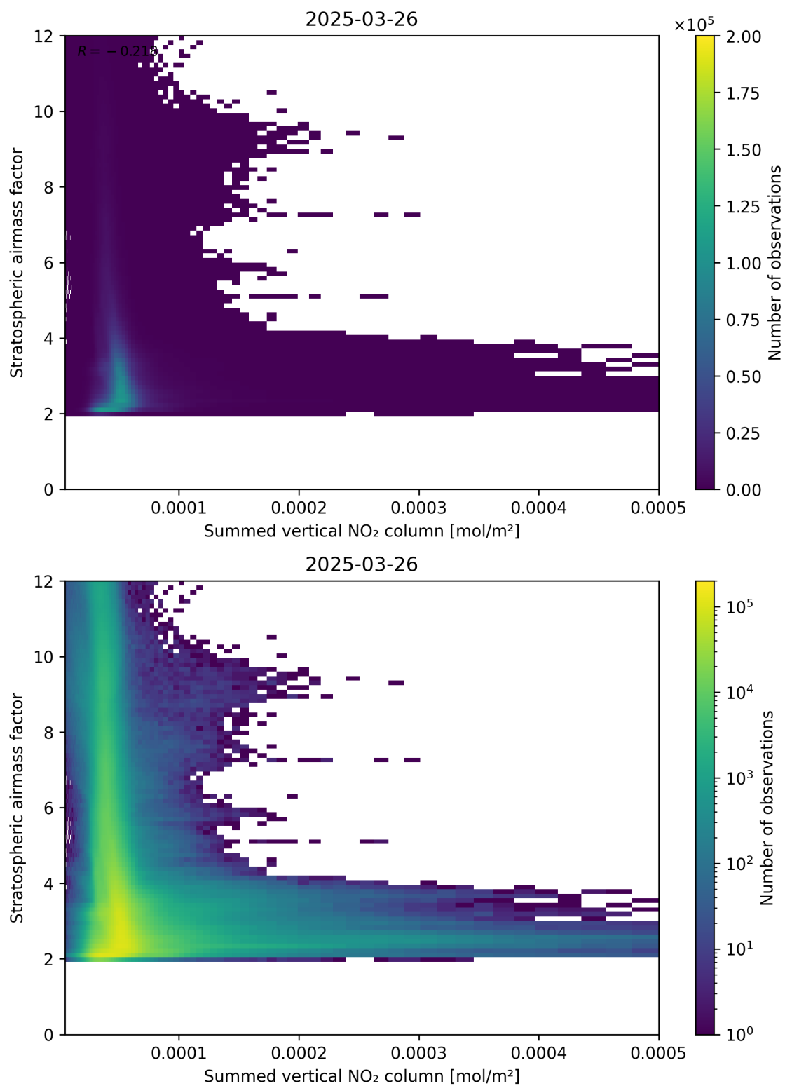
Figure 103: Scatter density plot of “Summed vertical NO 2 column” against “Stratospheric airmass factor” for 2025-03-26 to 2025-03-26.
