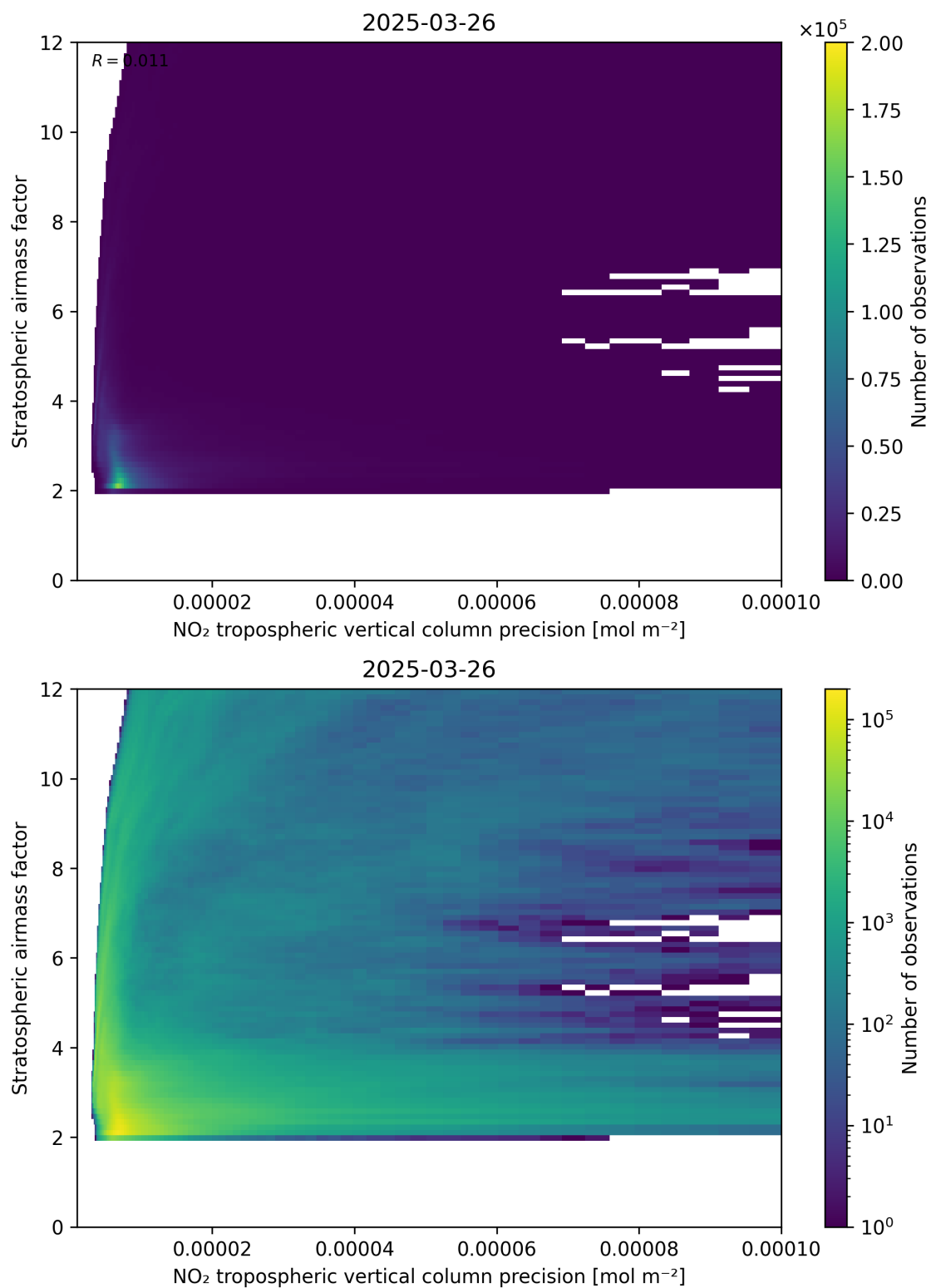
Figure 131: Scatter density plot of “NO 2 tropospheric vertical column precision” against “Stratospheric airmass factor” for 2025-03-26 to 2025-03-26.
