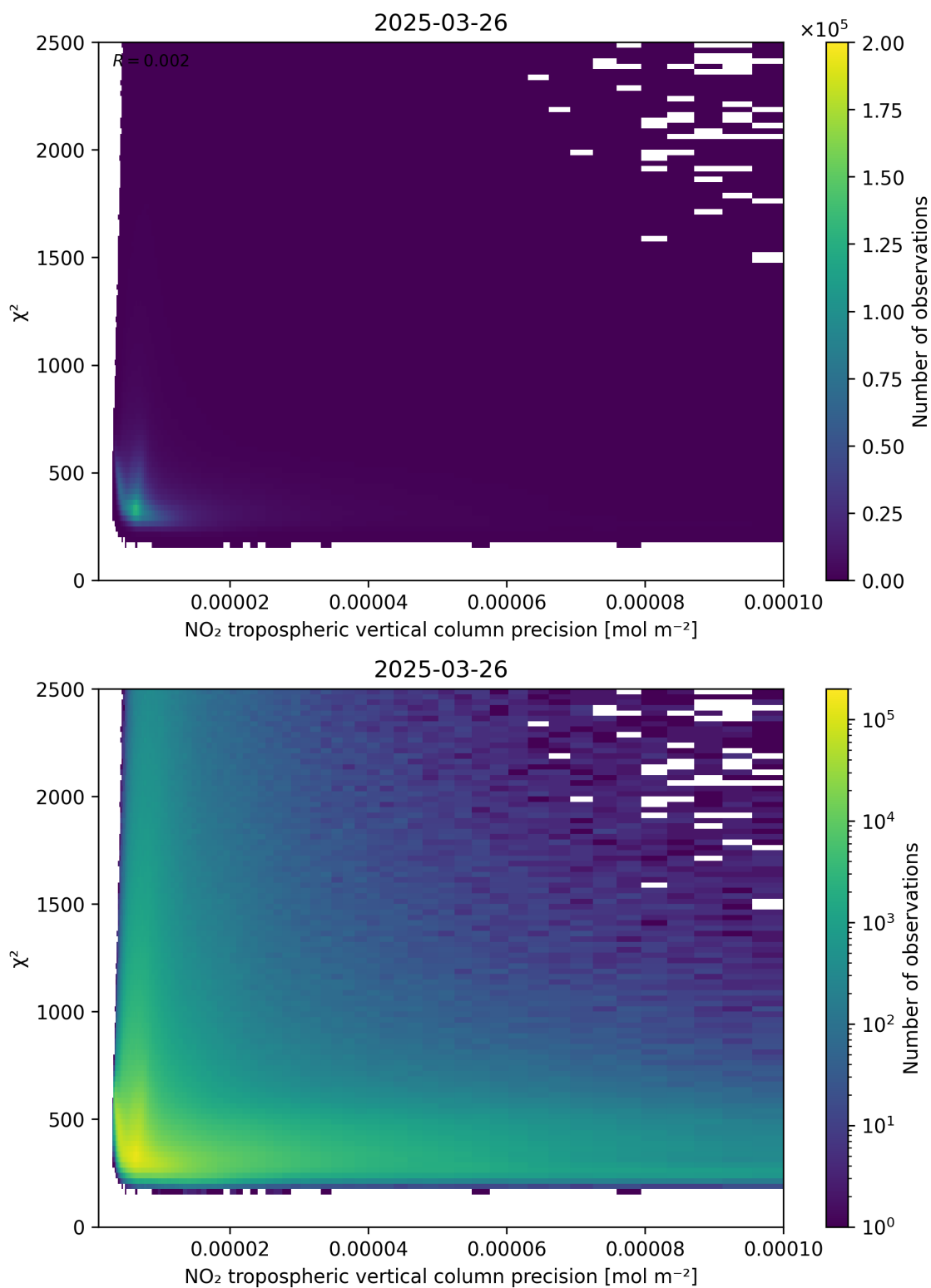
Figure 134: Scatter density plot of “NO 2 tropospheric vertical column precision” against “ \chi^2 ” for 2025-03-26 to 2025-03-26.
