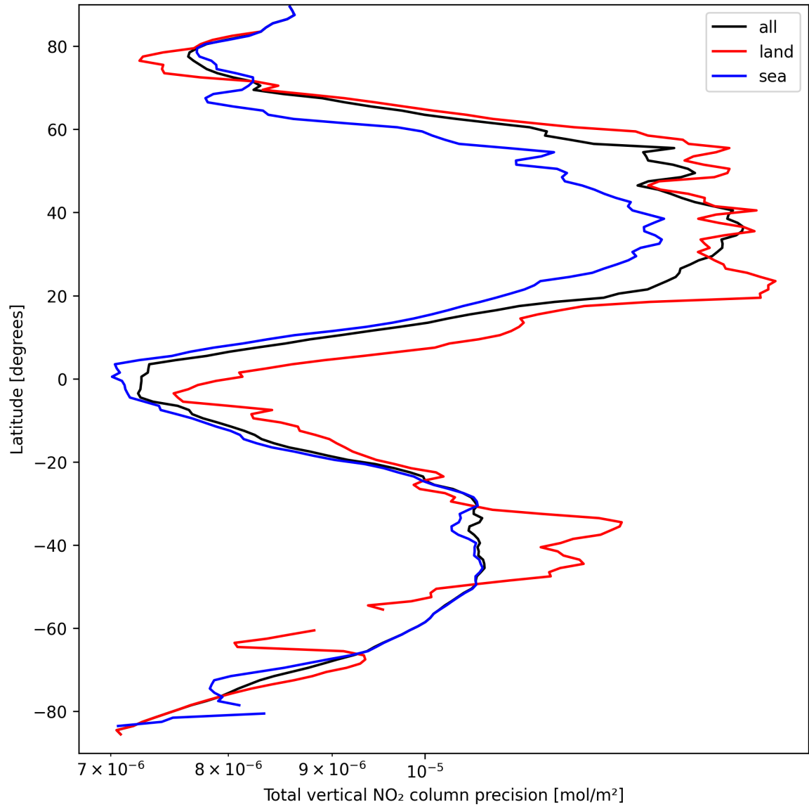
Figure 22: Zonal average of “Total vertical NO 2 column precision” for 2025-03-26 to 2025-03-26.
