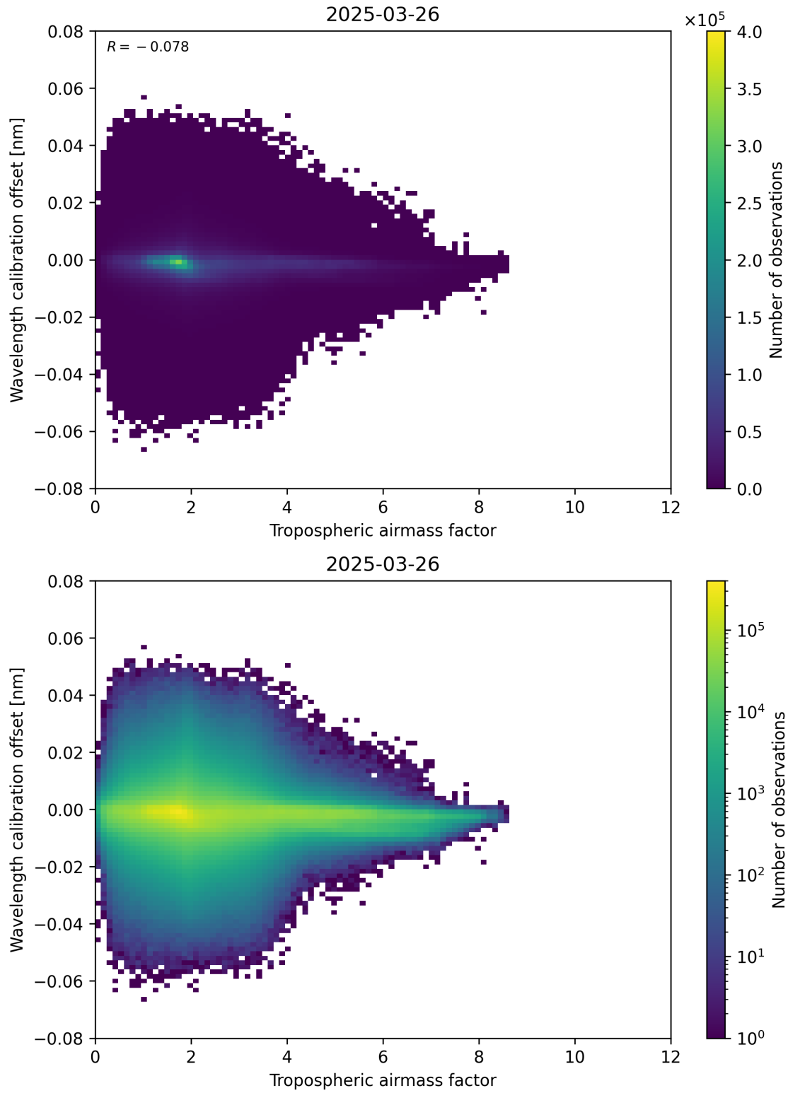
Figure 80: Scatter density plot of “Tropospheric airmass factor” against “Wavelength calibration offset” for 2025-03-26 to 2025-03-26.
