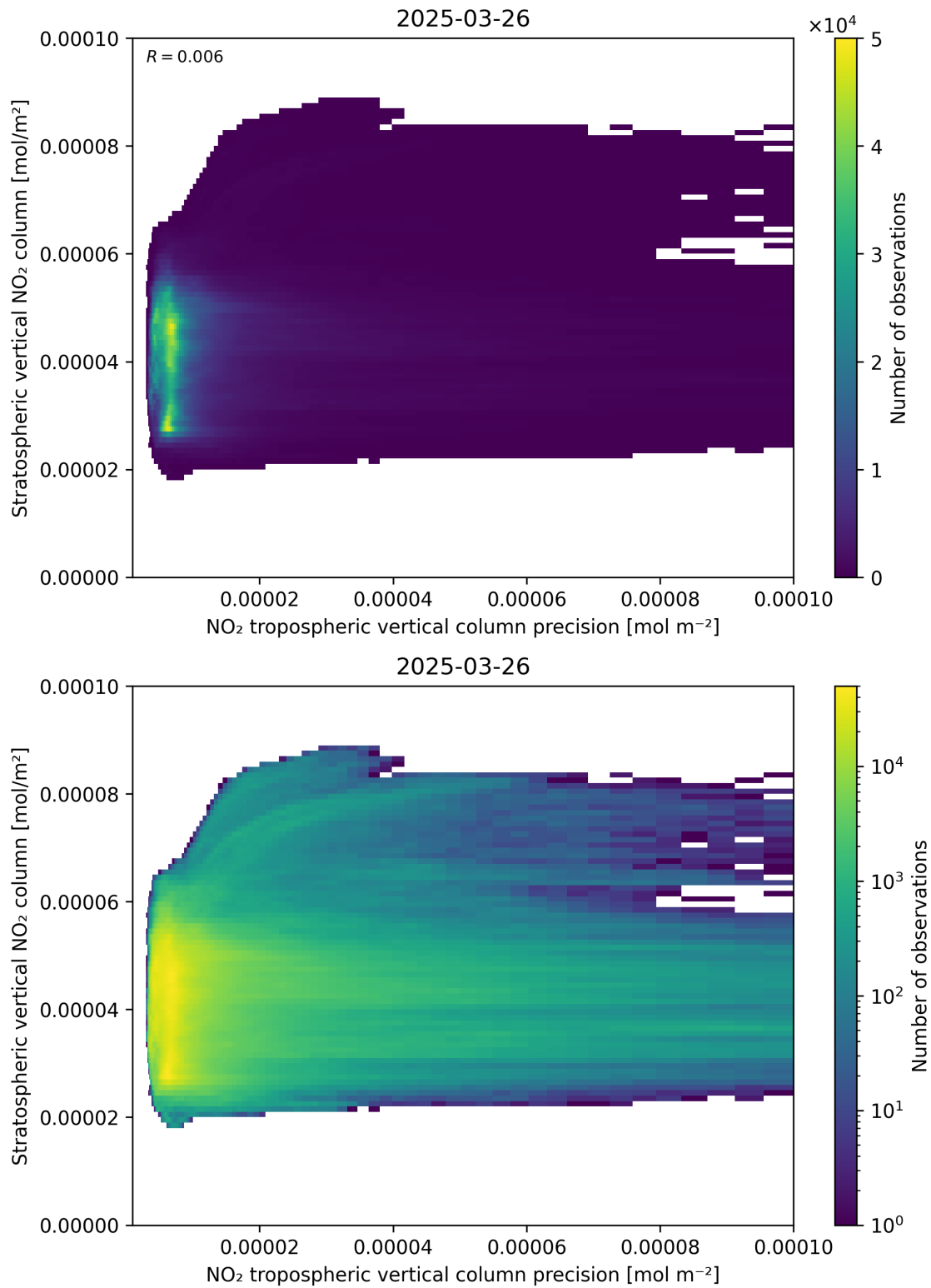
Figure 135: Scatter density plot of “NO 2 tropospheric vertical column precision” against “Stratospheric vertical NO 2 column” for 2025-03-26 to 2025-03-26.
