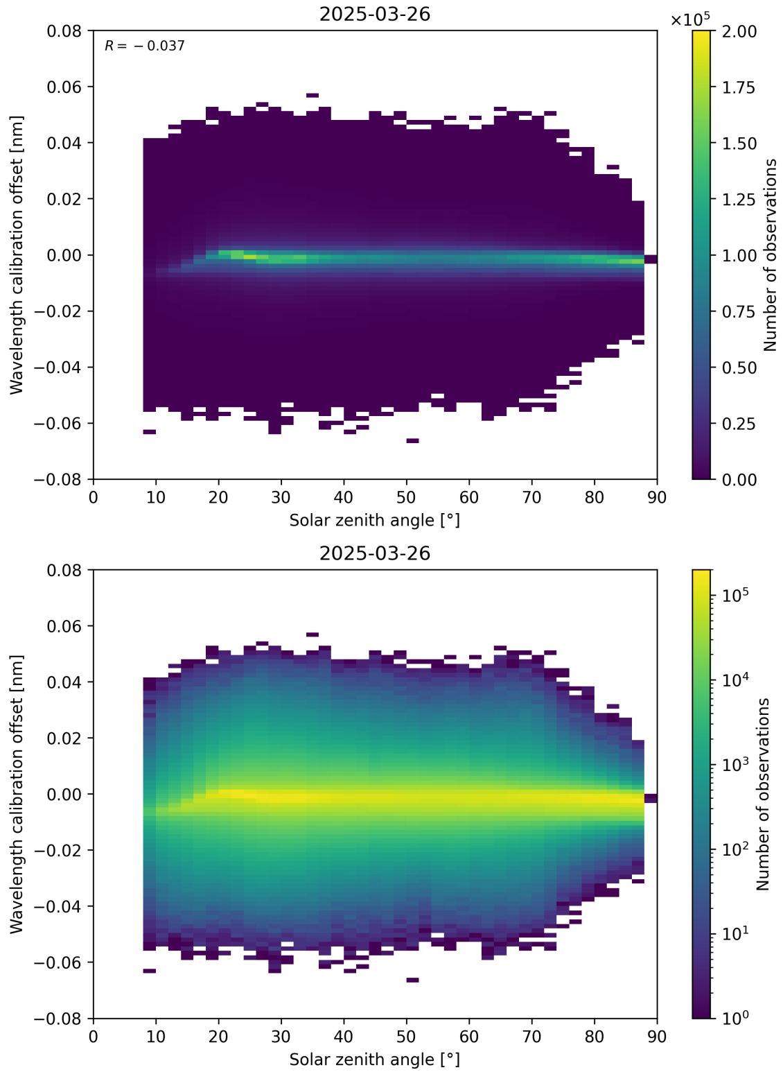
Figure 158: Scatter density plot of “Solar zenith angle” against “Wavelength calibration offset” for 2025-03-26 to 2025-03-26.
