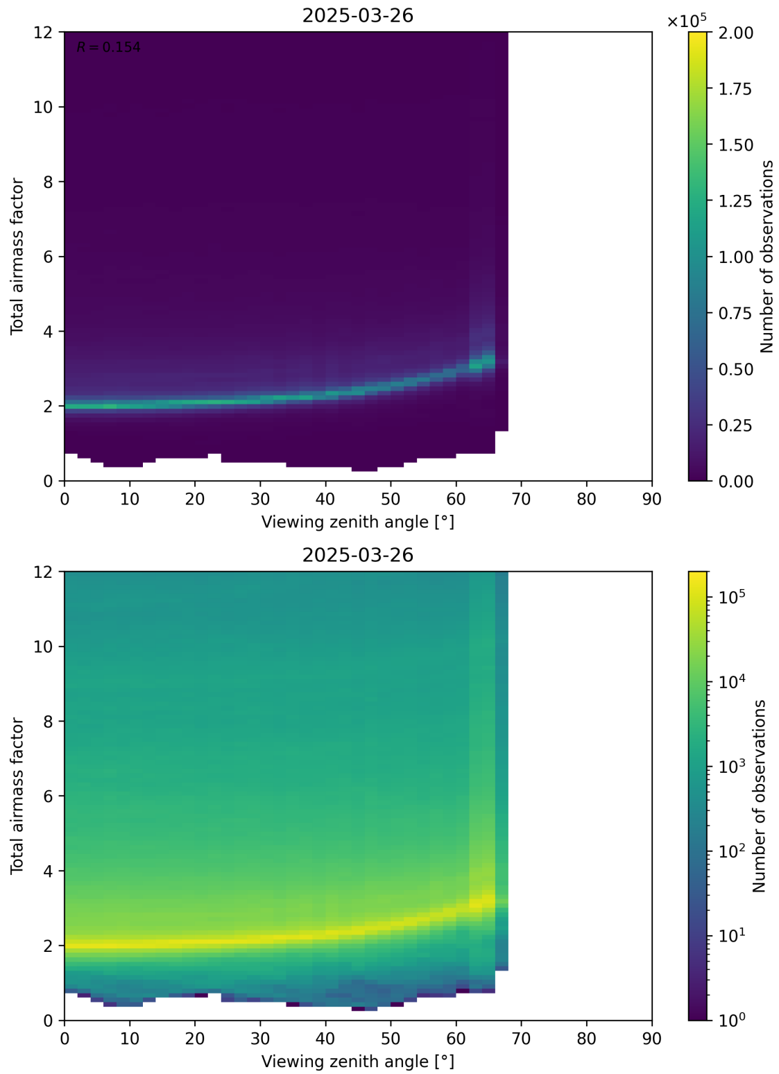
Figure 160: Scatter density plot of “Viewing zenith angle” against “Total airmass factor” for 2025-03-26 to 2025-03-26.
