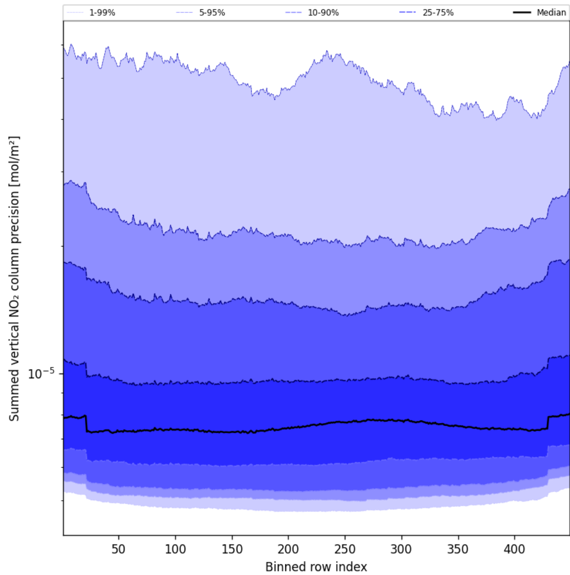
Figure 58: Along track statistics of “Summed vertical NO 2 column precision” for 2025-03-26 to 2025-03-26
