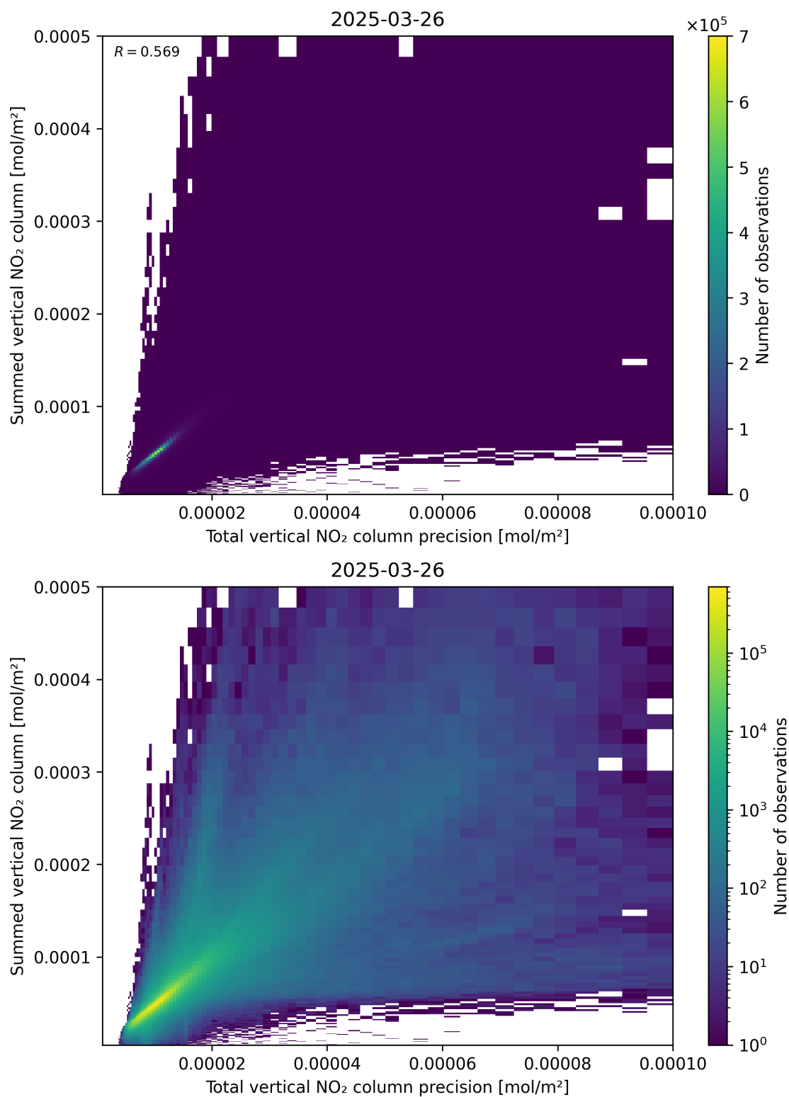
Figure 117: Scatter density plot of “Total vertical NO 2 column precision” against “Summed vertical NO 2 column” for 2025-03-26 to 2025-03-26.
