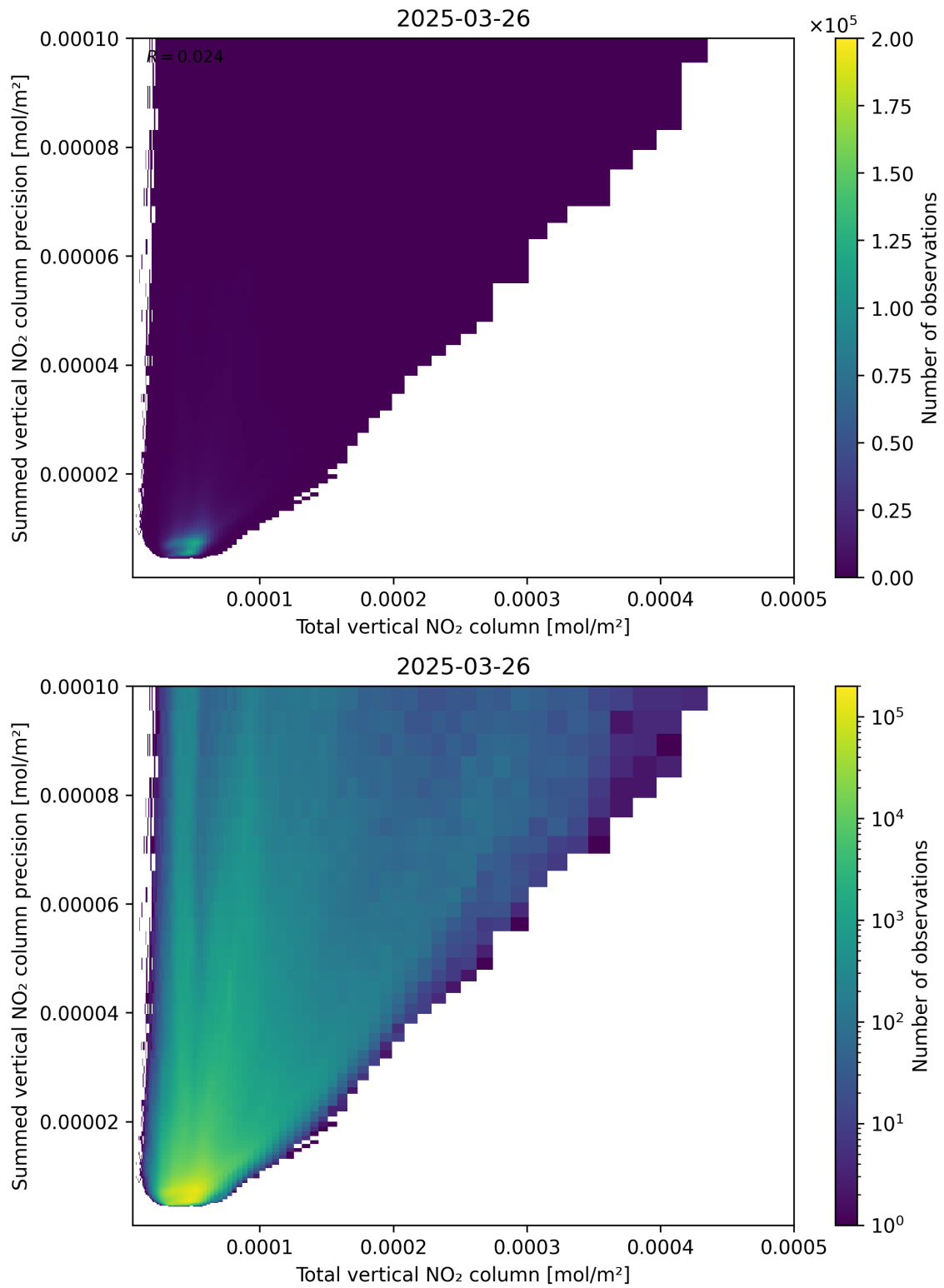
Figure 113: Scatter density plot of “Total vertical NO 2 column” against “Summed vertical NO 2 column precision” for 2025-03-26 to 2025-03-26.
