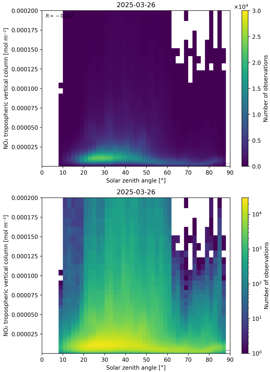
Figure 155: Scatter density plot of “Solar zenith angle” against “NO 2 tropospheric vertical column” for 2025-03-26 to 2025-03-26.
