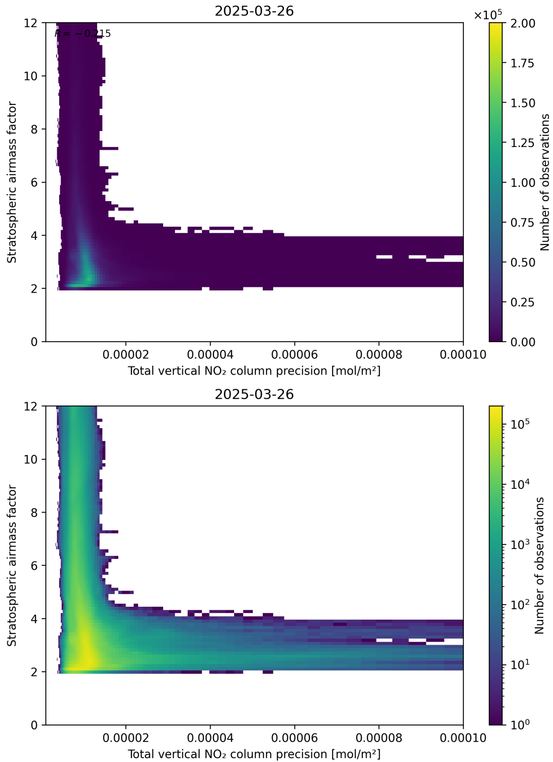
Figure 115: Scatter density plot of “Total vertical NO 2 column precision” against “Stratospheric air mass factor” for 2025-03-26 to 2025-03-26.
