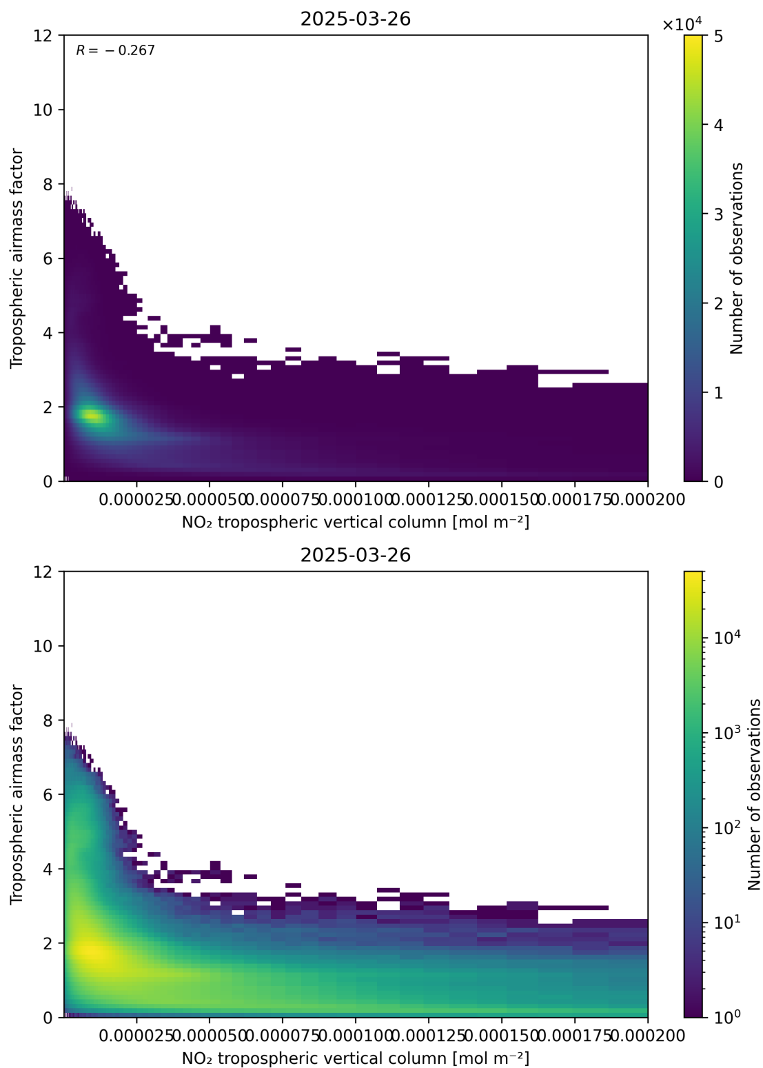
Figure 123: Scatter density plot of “NO 2 tropospheric vertical column” against “Tropospheric air mass factor” for 2025-03-26 to 2025-03-26.
