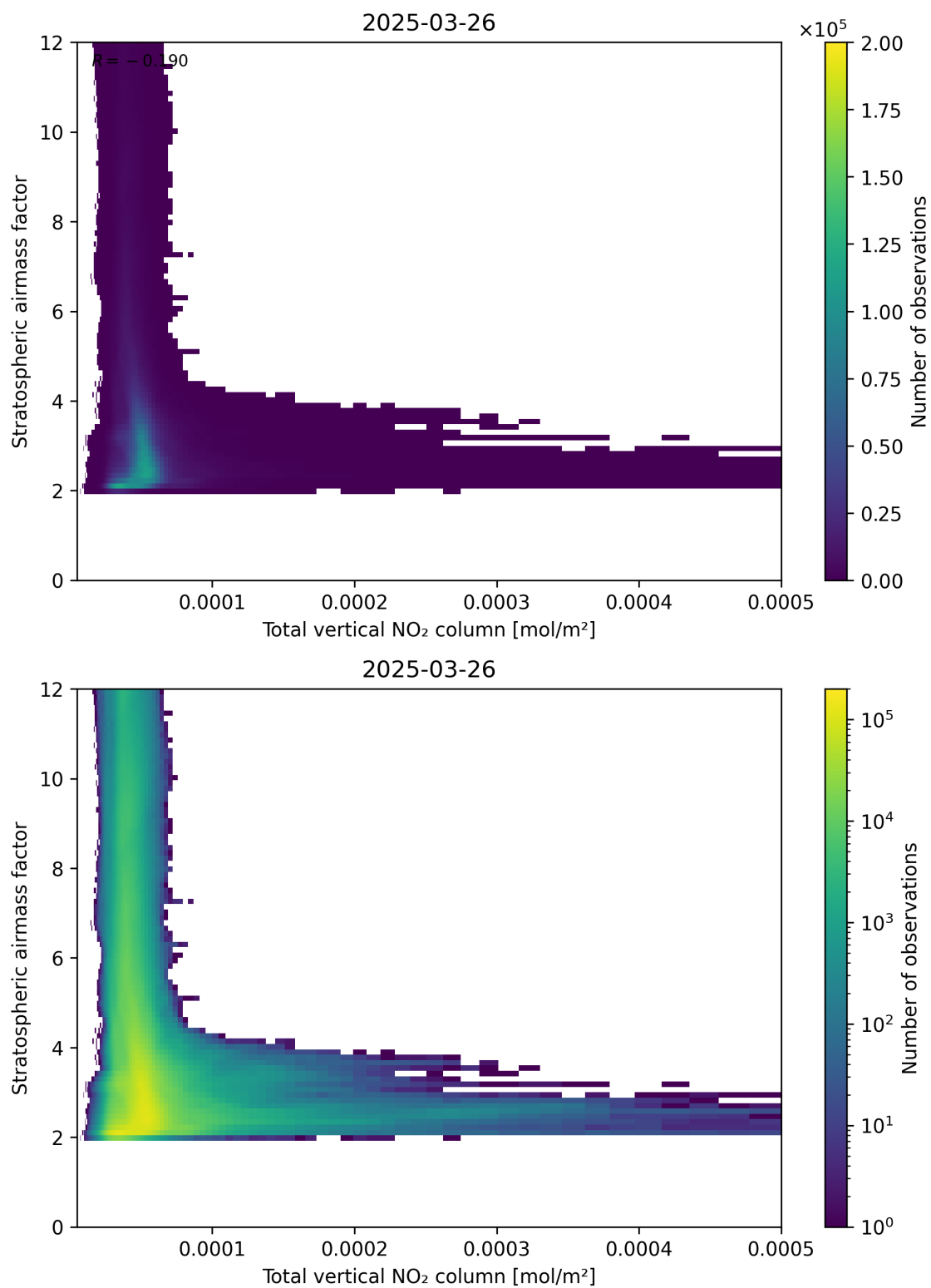
Figure 110: Scatter density plot of “Total vertical NO 2 column” against “Stratospheric airmass factor” for 2025-03-26 to 2025-03-26.
