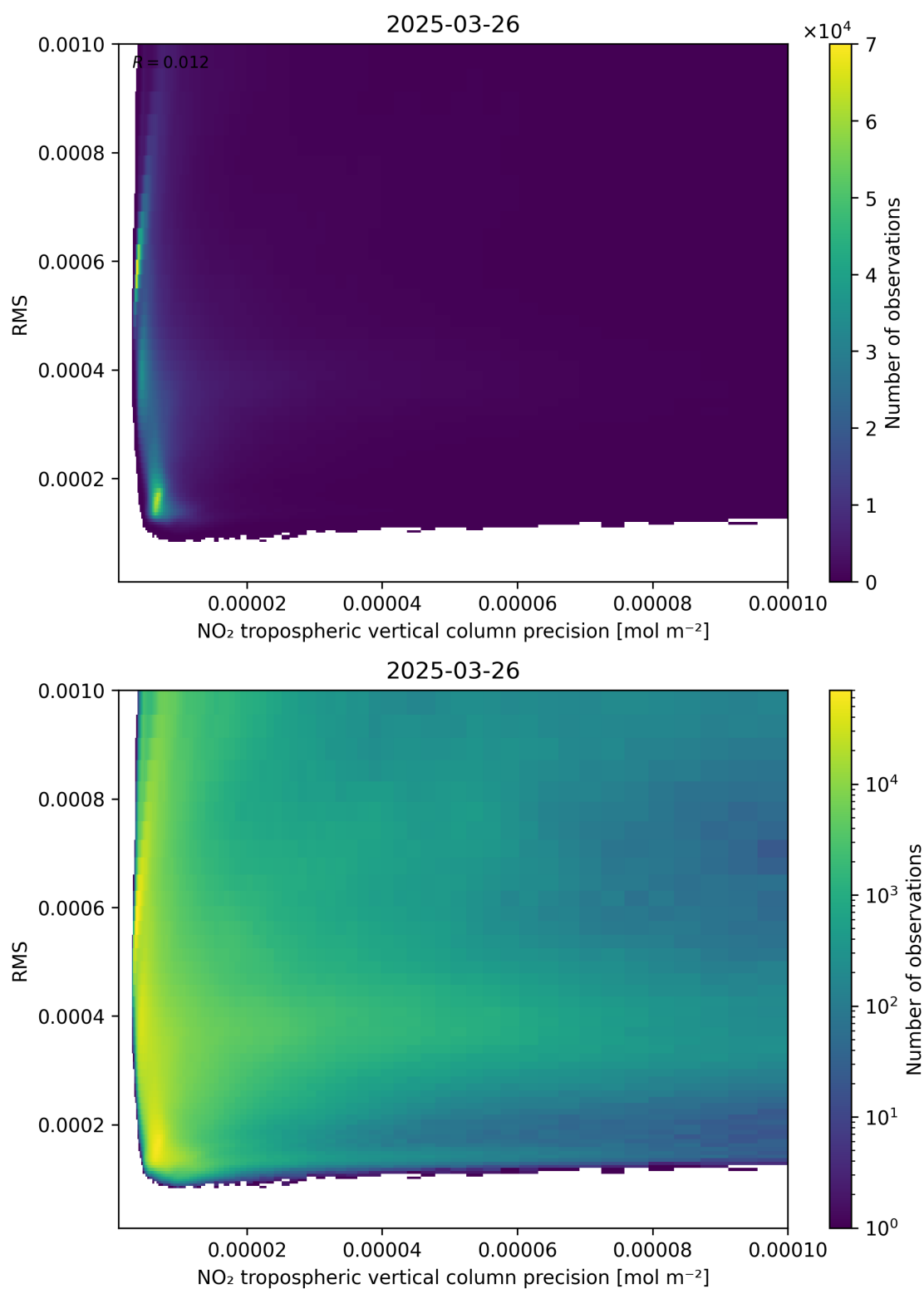
Figure 140: Scatter density plot of “NO 2 tropospheric vertical column precision” against “RMS” for 2025-03-26 to 2025-03-26.
