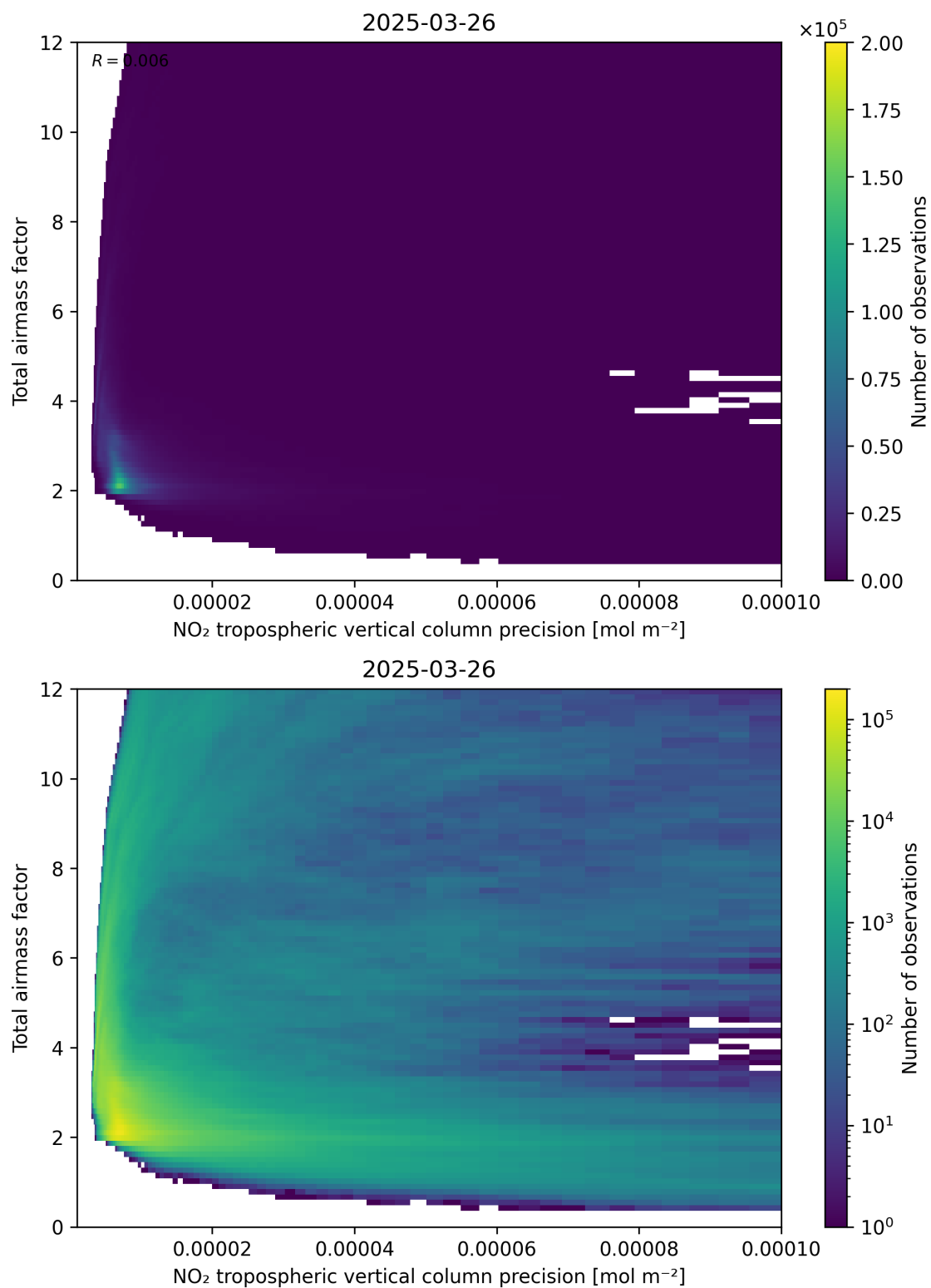
Figure 132: Scatter density plot of “NO 2 tropospheric vertical column precision” against “Total air mass factor” for 2025-03-26 to 2025-03-26.
