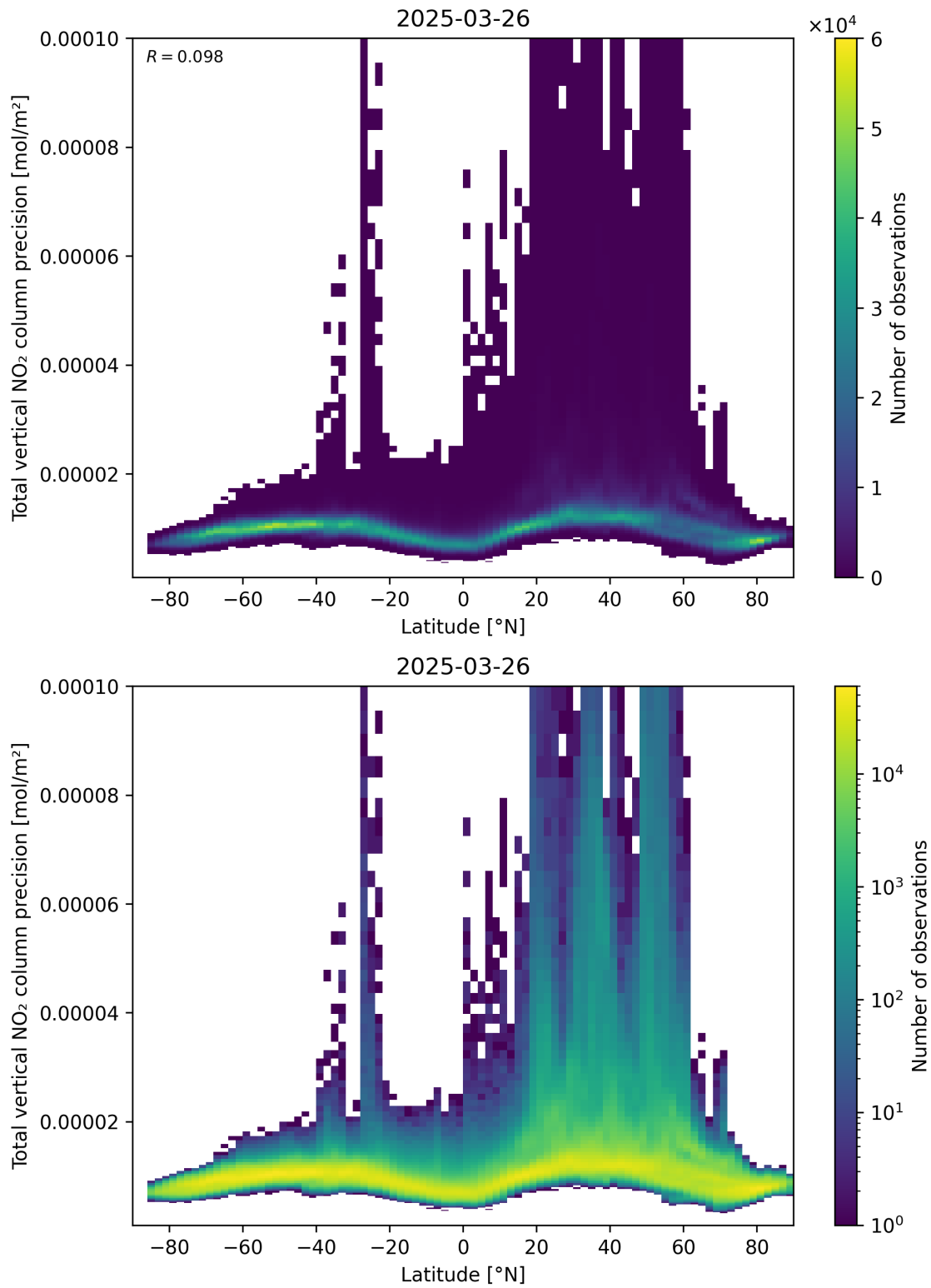
Figure 91: Scatter density plot of “Latitude” against “Total vertical NO 2 column precision” for 2025-03-26 to 2025-03-26.
