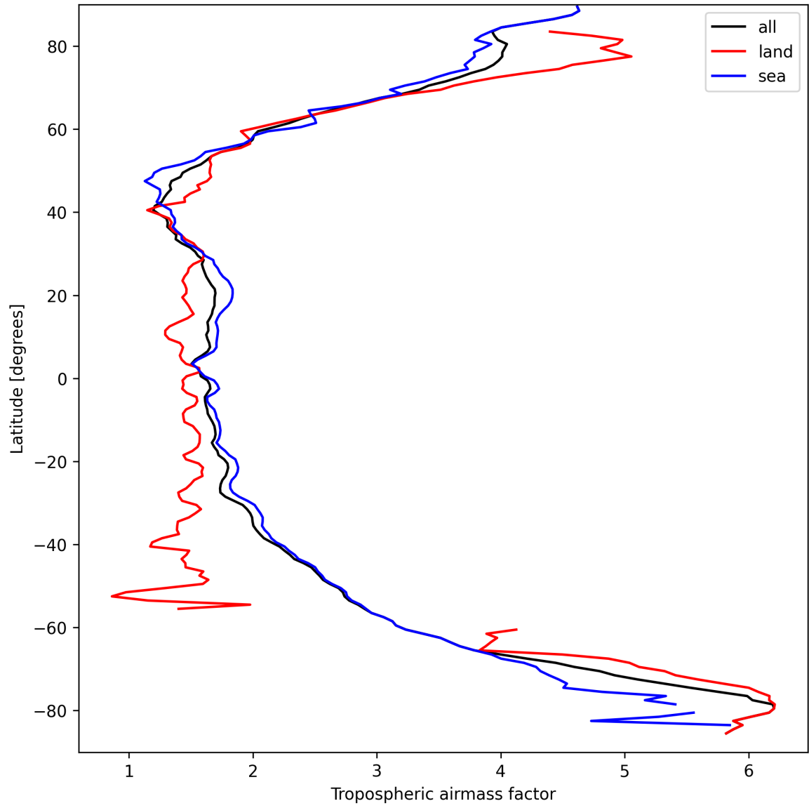
Figure 14: Zonal average of “Tropospheric airmass factor” for 2025-03-26 to 2025-03-26.
