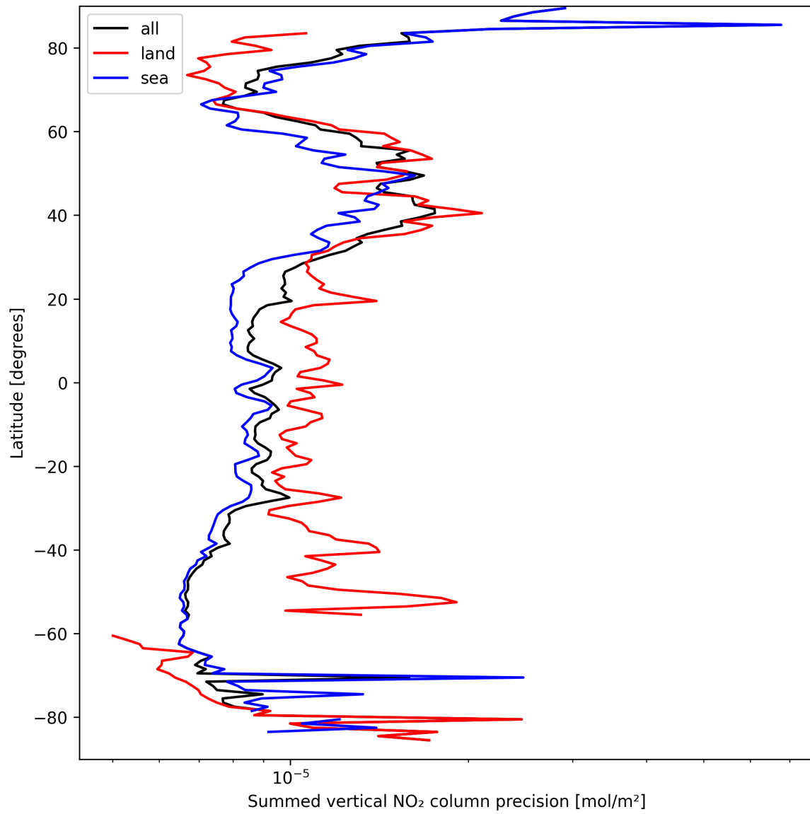
Figure 24: Zonal average of “Summed vertical NO 2 column precision” for 2025-03-26 to 2025-03-26.
