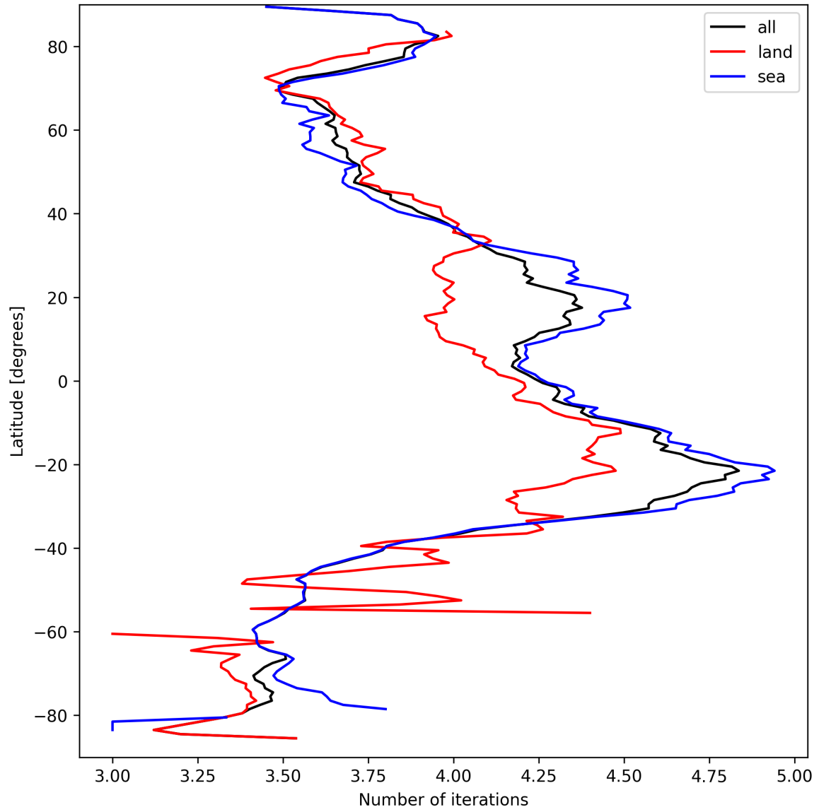
Figure 17: Zonal average of “Number of iterations” for 2025-03-26 to 2025-03-26.
