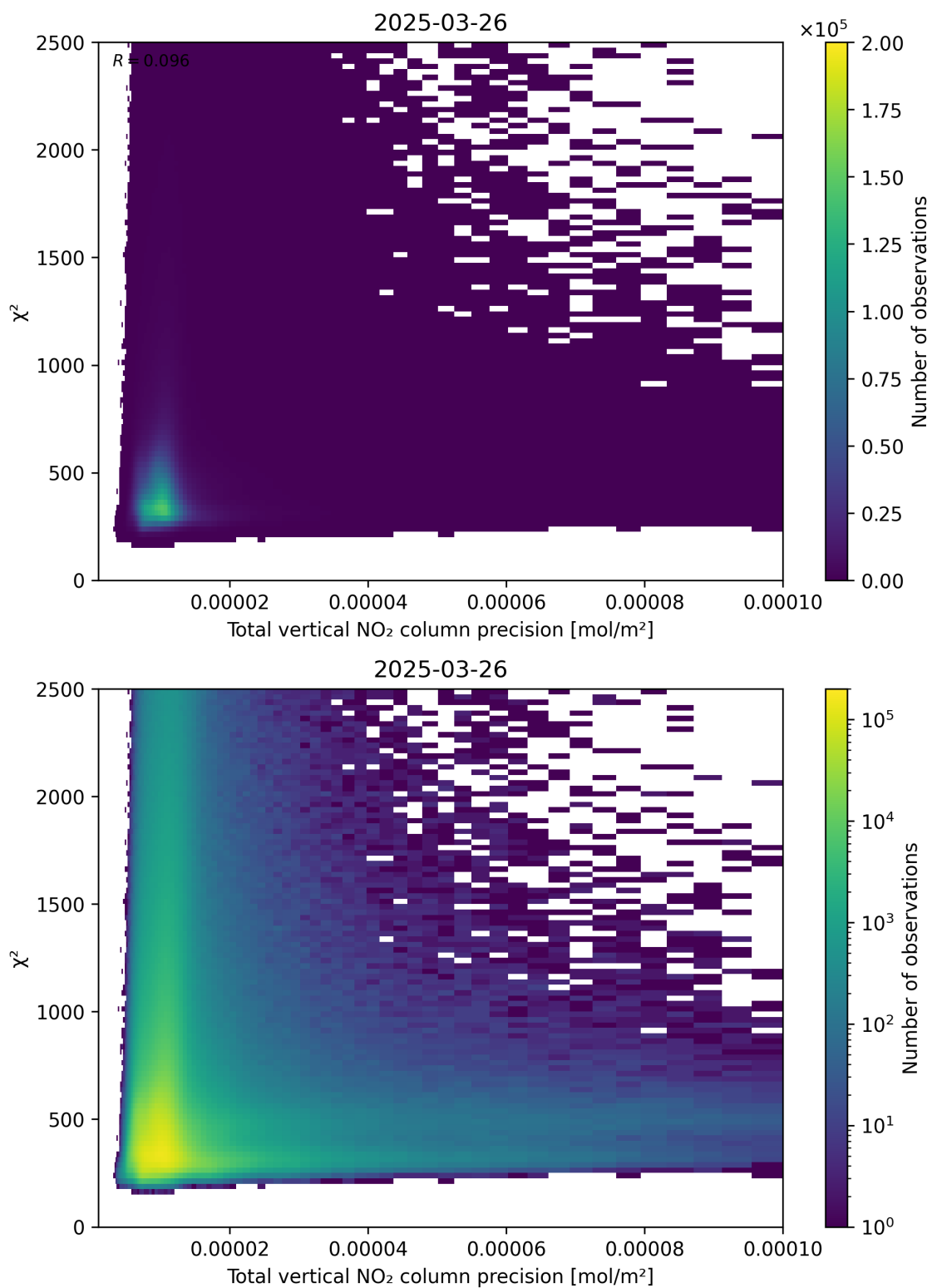
Figure 116: Scatter density plot of “Total vertical NO 2 column precision” against “ \chi^2 ” for 2025-03-26 to 2025-03-26.
