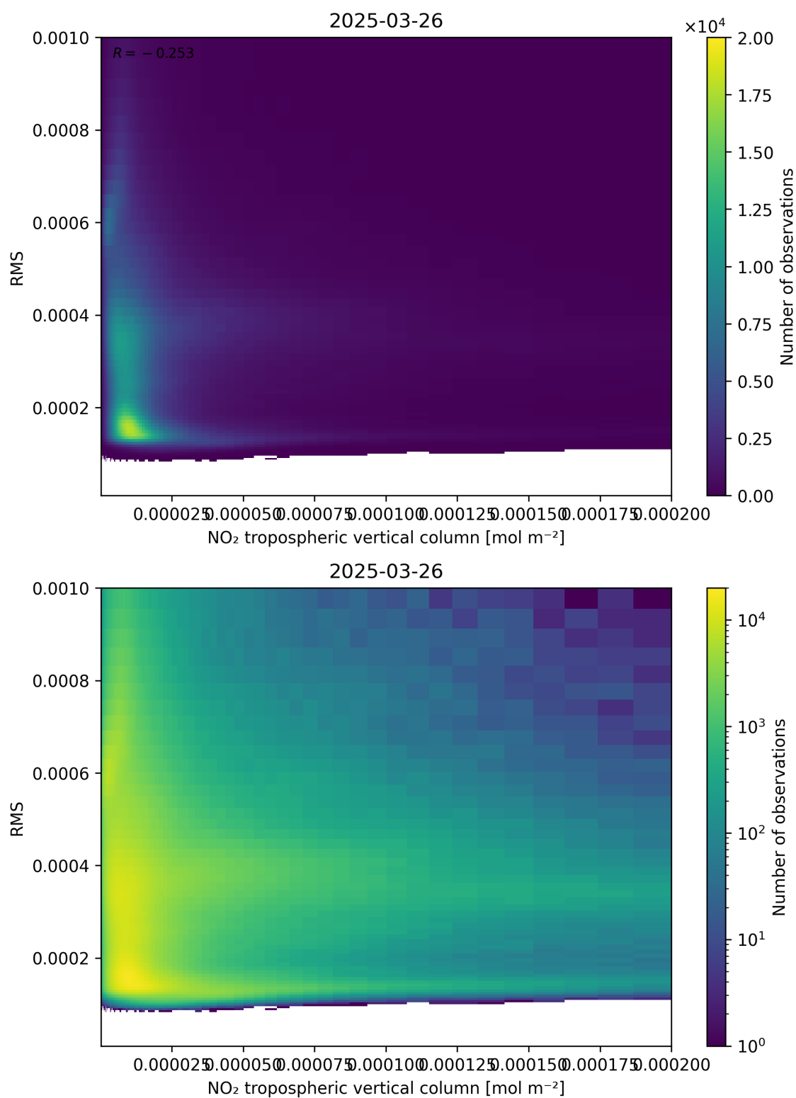
Figure 142: Scatter density plot of “NO 2 tropospheric vertical column” against “RMS” for 2025-03-26 to 2025-03-26.
