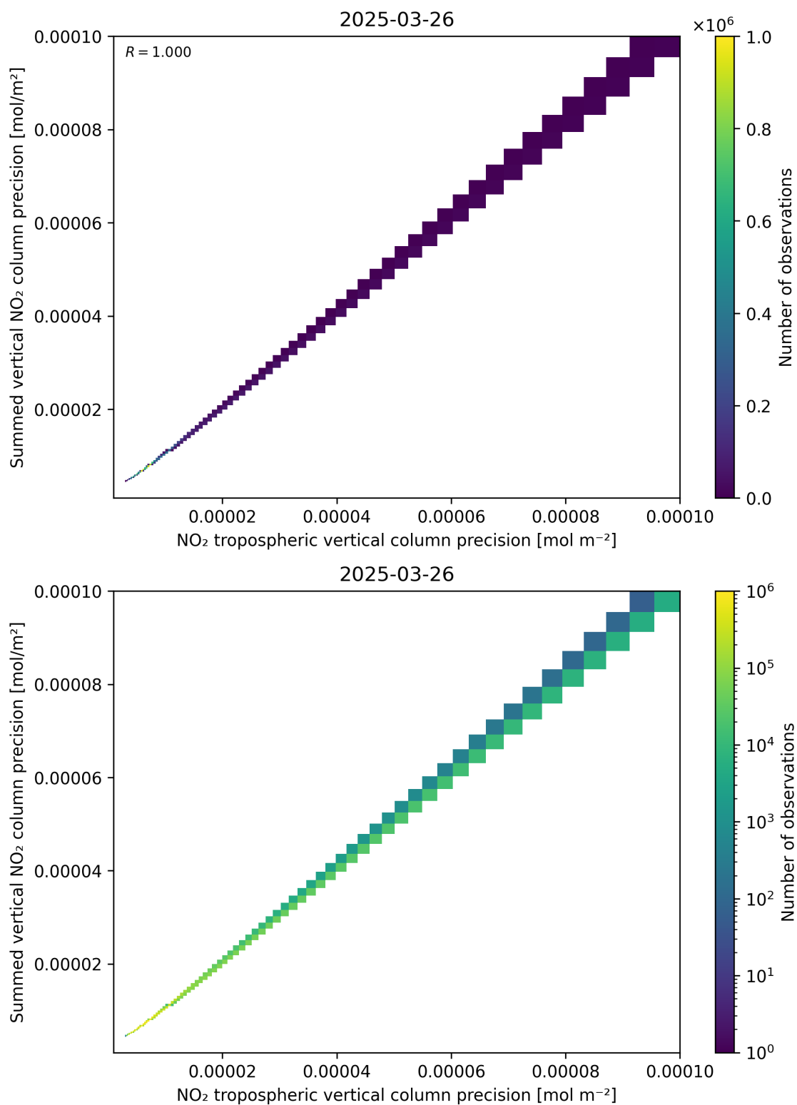
Figure 137: Scatter density plot of “NO 2 tropospheric vertical column precision” against “Summed vertical NO 2 column precision” for 2025-03-26 to 2025-03-26.
