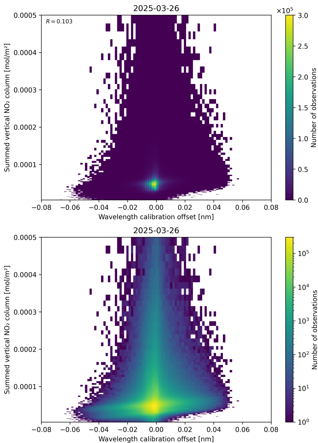
Figure 177: Scatter density plot of “Wavelength calibration offset” against “Summed vertical NO 2 column” for 2025-03-26 to 2025-03-26.
