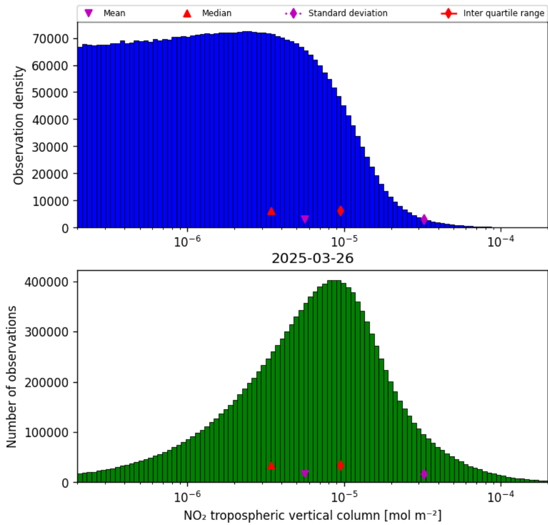
Figure 29: Histogram of “NO 2 tropospheric vertical column” for 2025-03-26 to 2025-03-26
