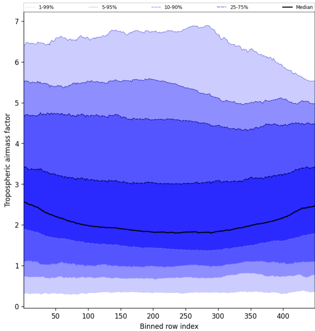
Figure 48: Along track statistics of “Tropospheric airmass factor” for 2025-03-26 to 2025-03-26
