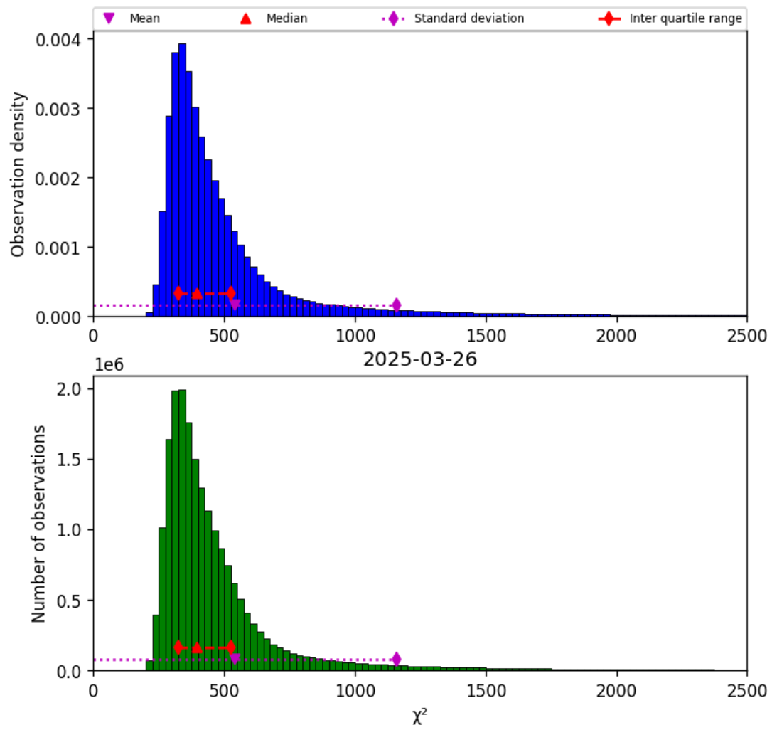
Figure 42: Histogram of “ \chi^2 ” for 2025-03-26 to 2025-03-26
