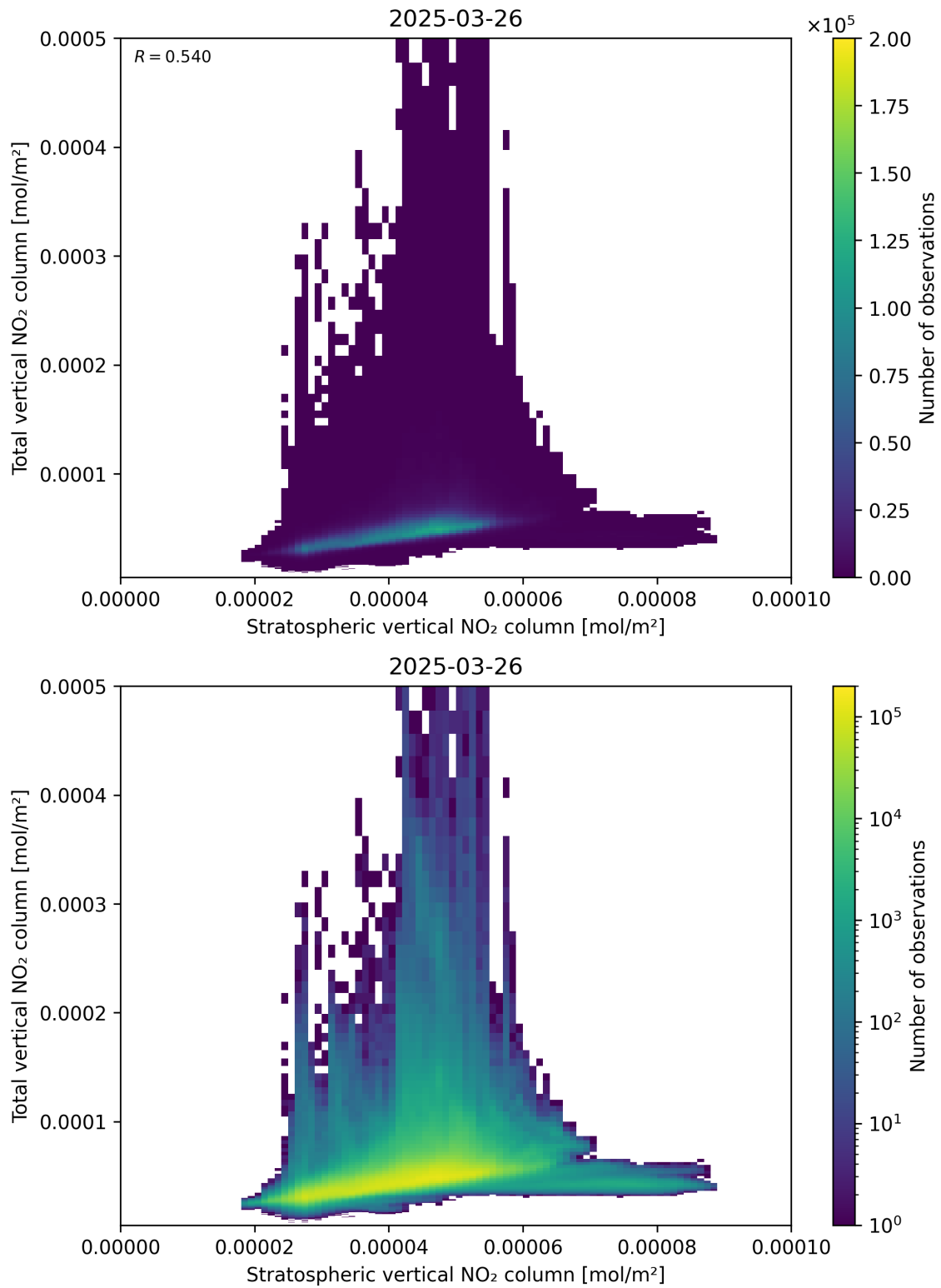
Figure 100: Scatter density plot of “Stratospheric vertical NO 2 column” against “Total vertical NO 2 column” for 2025-03-26 to 2025-03-26.
