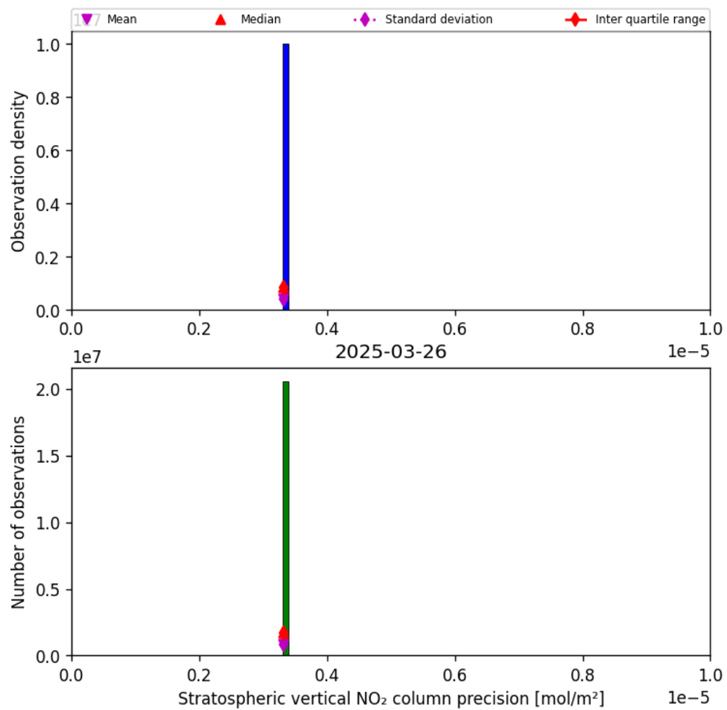
Figure 37: Histogram of “Stratospheric vertical NO 2 column precision” for 2025-03-26 to 2025-03-26
