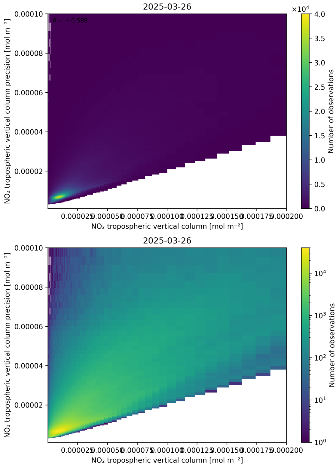
Figure 130: Scatter density plot of “NO 2 tropospheric vertical column” against “NO 2 tropospheric vertical column precision” for 2025-03-26 to 2025-03-26.
