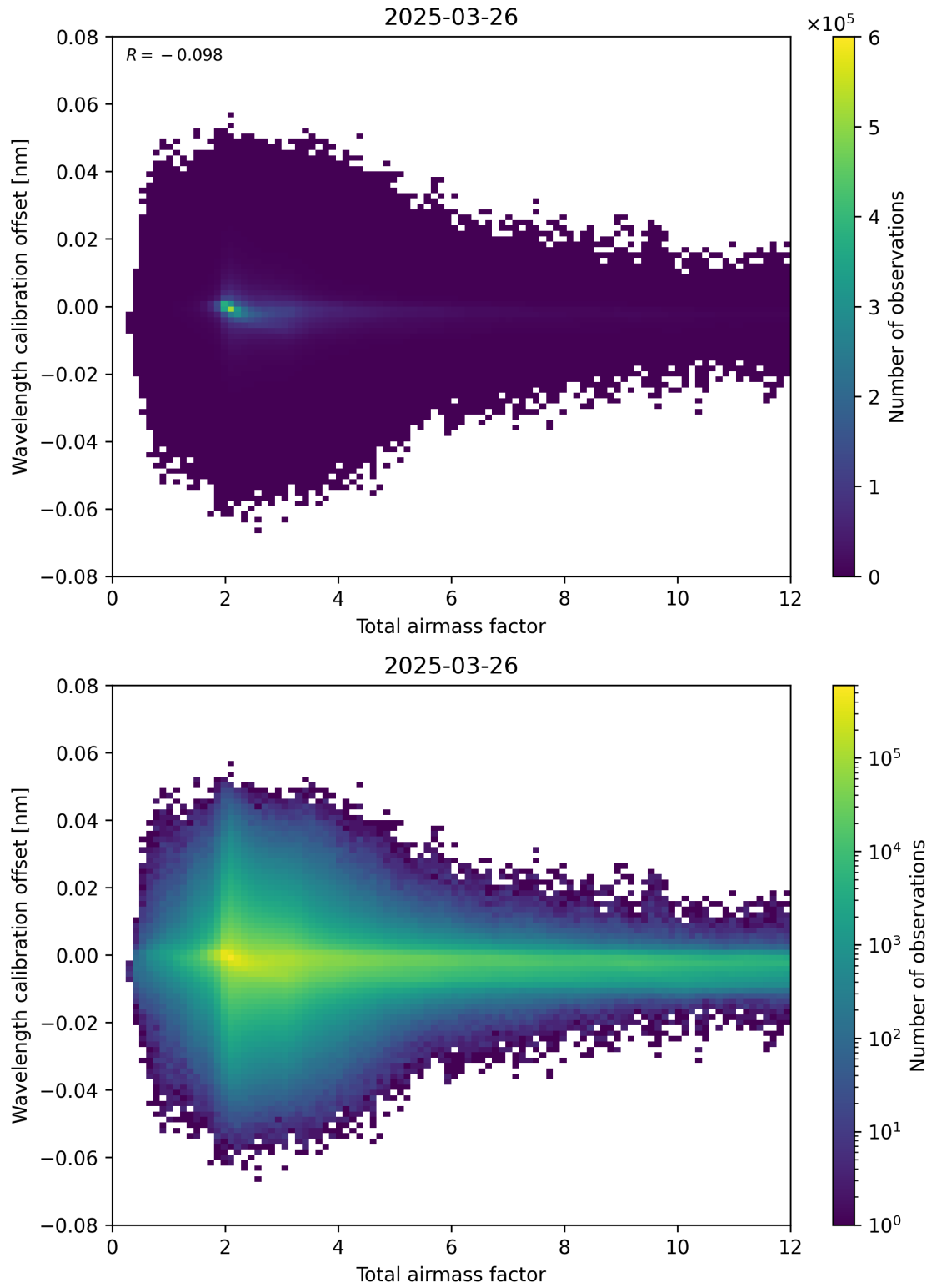
Figure 70: Scatter density plot of “Total airmass factor” against “Wavelength calibration offset” for 2025-03-26 to 2025-03-26.
