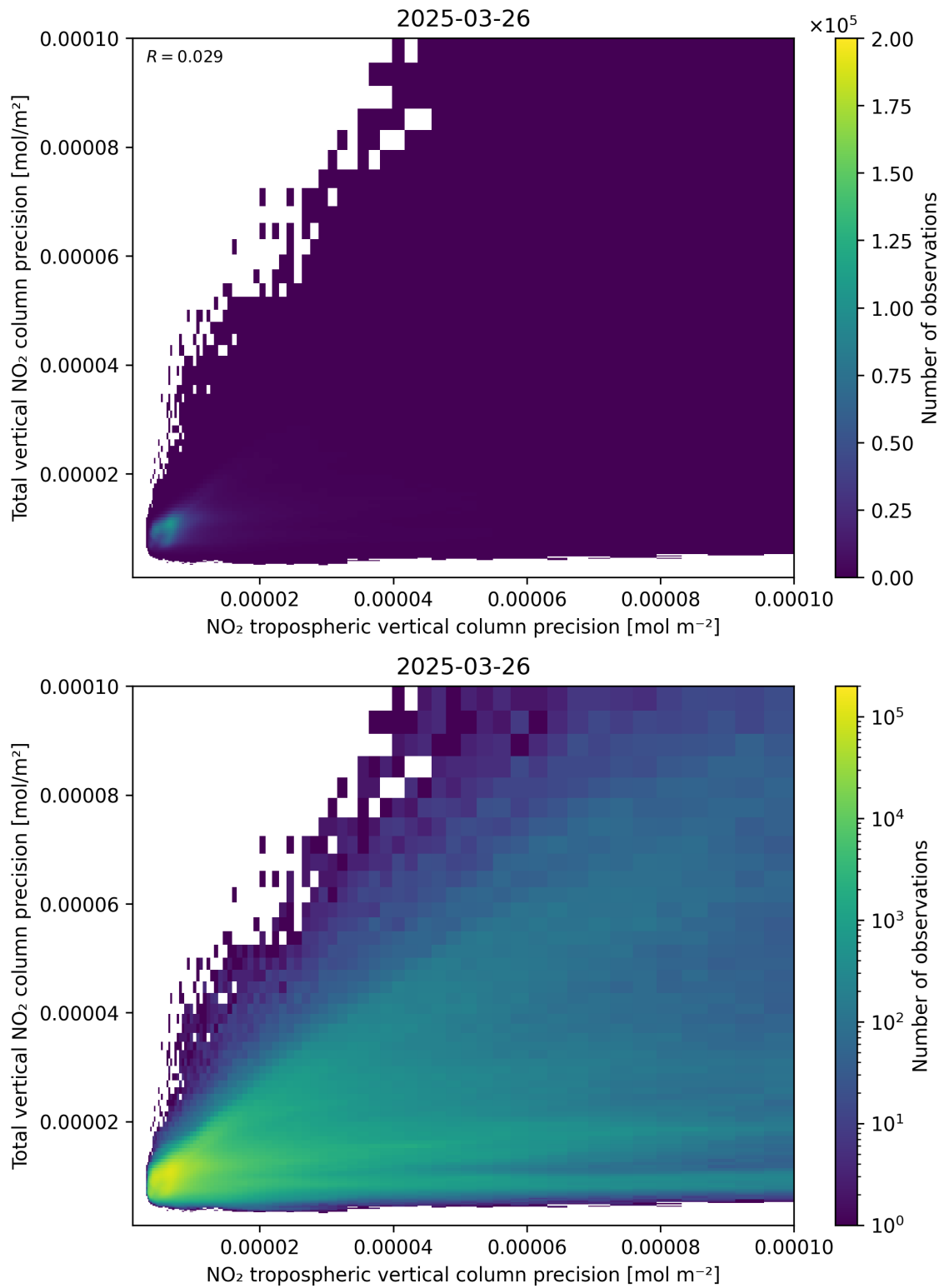
Figure 139: Scatter density plot of “NO 2 tropospheric vertical column precision” against “Total vertical NO 2 column precision” for 2025-03-26 to 2025-03-26.
