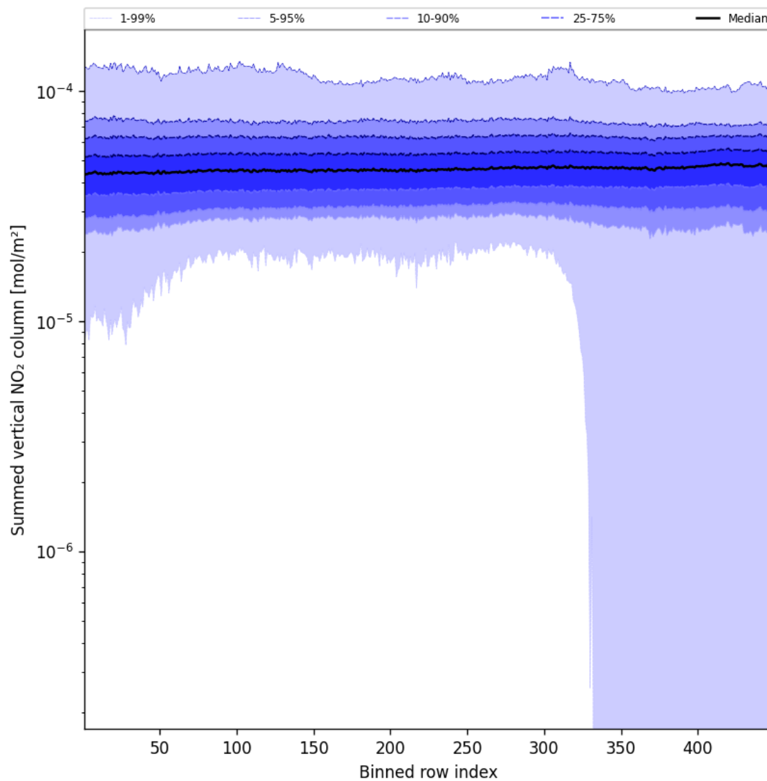
Figure 57: Along track statistics of “Summed vertical NO 2 column” for 2025-03-26 to 2025-03-26
