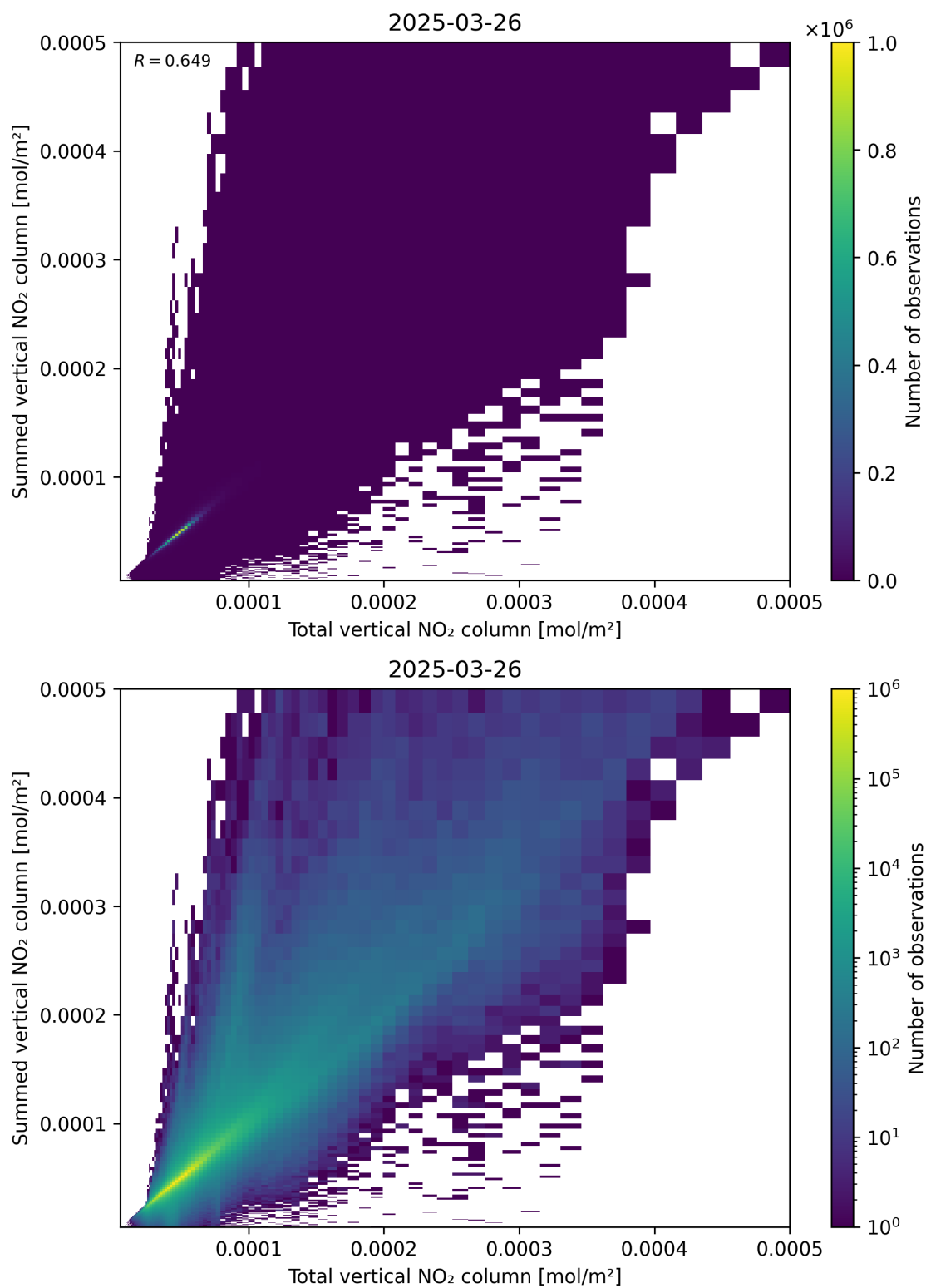
Figure 112: Scatter density plot of “Total vertical NO 2 column” against “Summed vertical NO 2 column” for 2025-03-26 to 2025-03-26.
