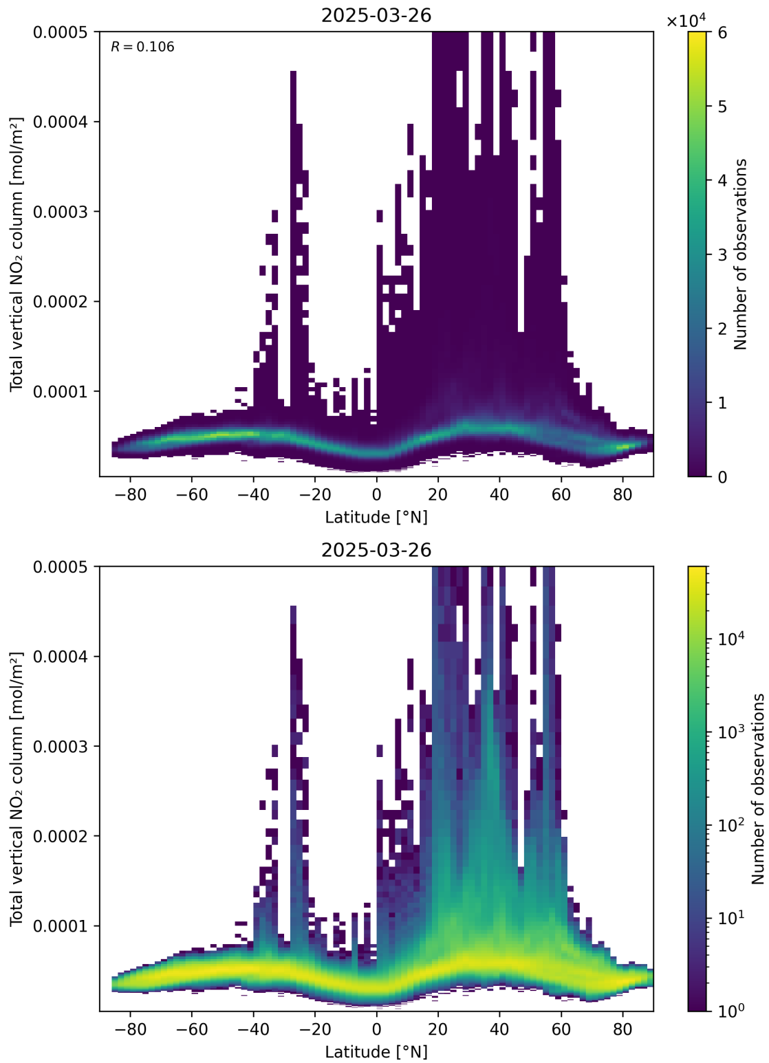
Figure 90: Scatter density plot of “Latitude” against “Total vertical NO 2 column” for 2025-03-26 to 2025-03-26.
