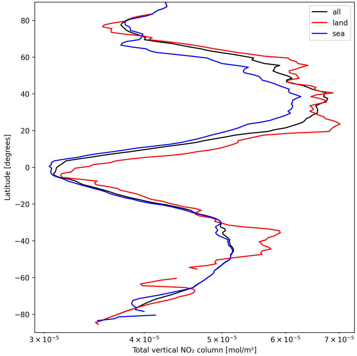
Figure 21: Zonal average of “Total vertical NO 2 column” for 2025-03-26 to 2025-03-26.
