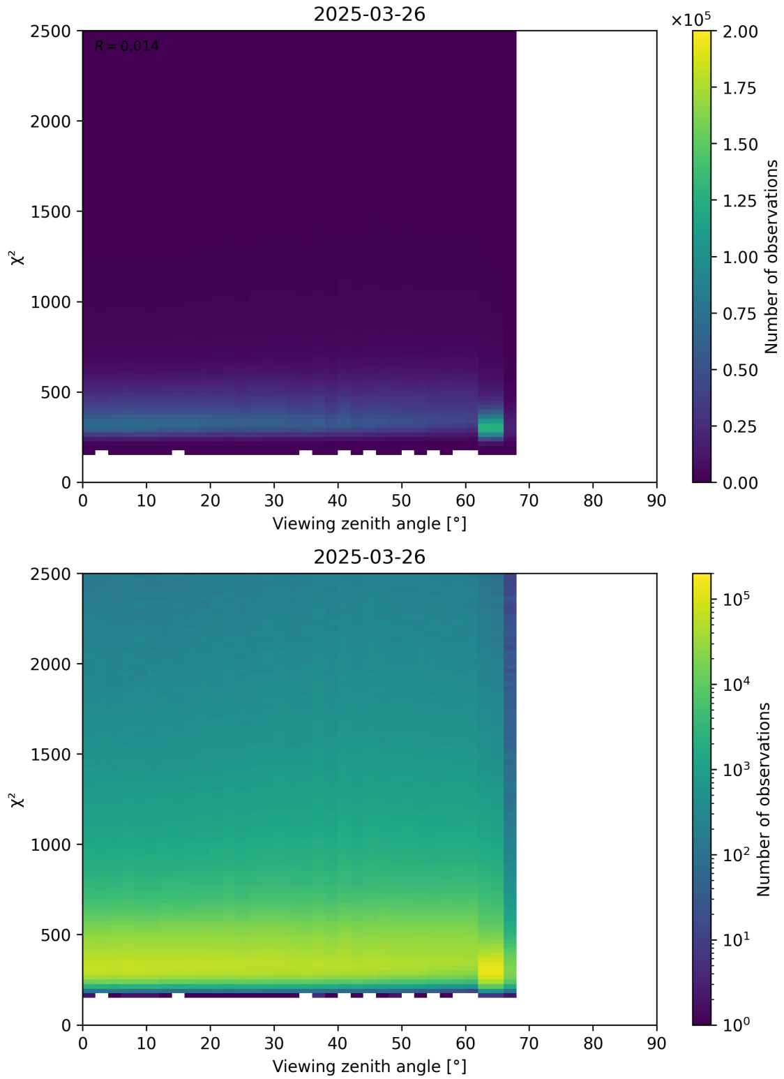
Figure 162: Scatter density plot of “Viewing zenith angle” against “ \chi^2 ” for 2025-03-26 to 2025-03-26.
