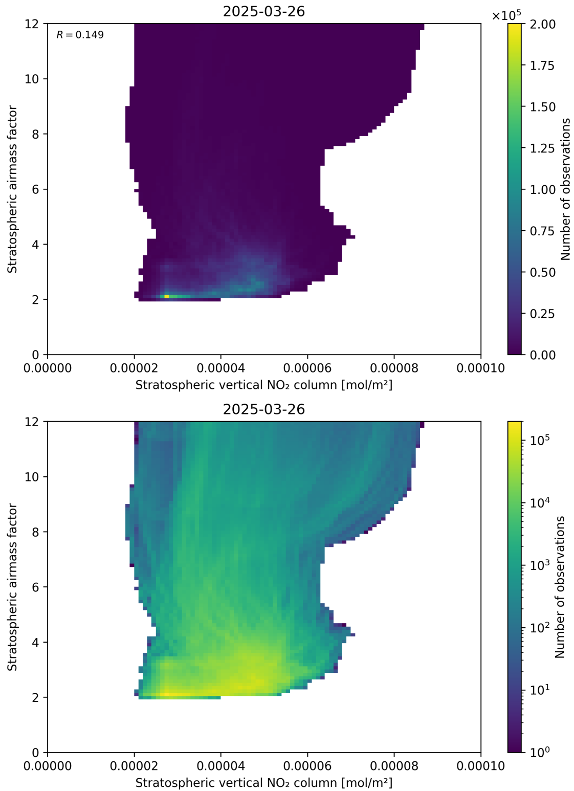
Figure 96: Scatter density plot of “Stratospheric vertical NO 2 column” against “Stratospheric airmass factor” for 2025-03-26 to 2025-03-26.
