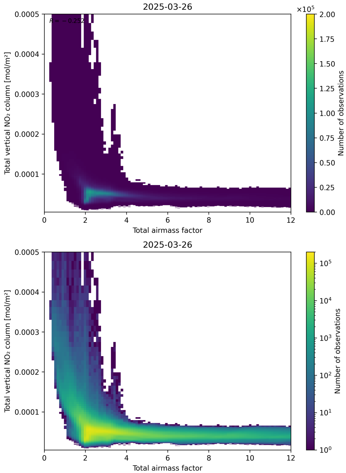
Figure 67: Scatter density plot of “Total airmass factor” against “Total vertical NO 2 column” for 2025-03-26 to 2025-03-26.
