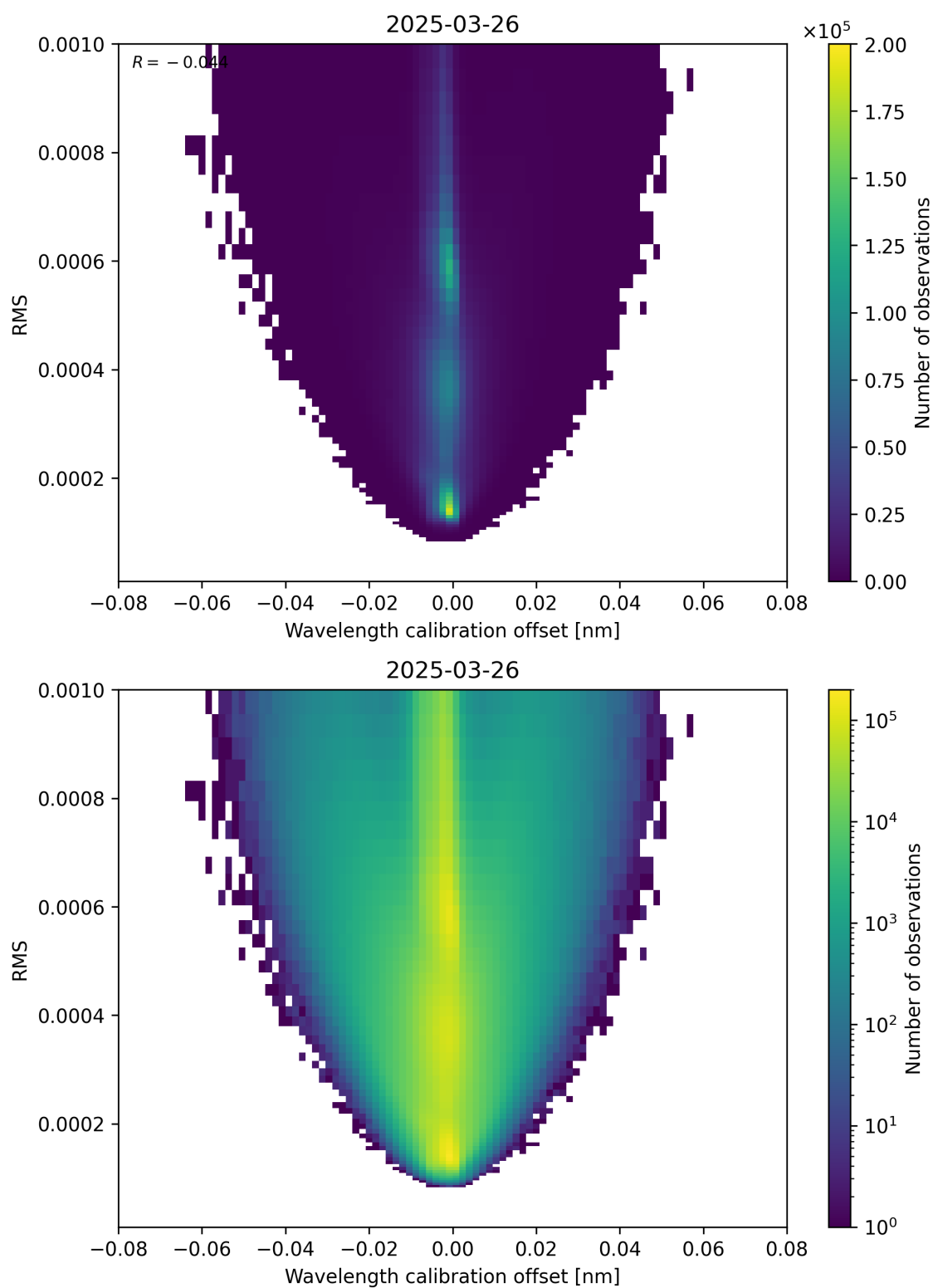
Figure 181: Scatter density plot of “Wavelength calibration offset” against “RMS” for 2025-03-26 to 2025-03-26.
