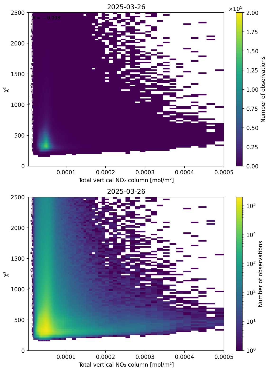
Figure 111: Scatter density plot of “Total vertical NO 2 column” against “ \chi^2 ” for 2025-03-26 to 2025-03-26.
