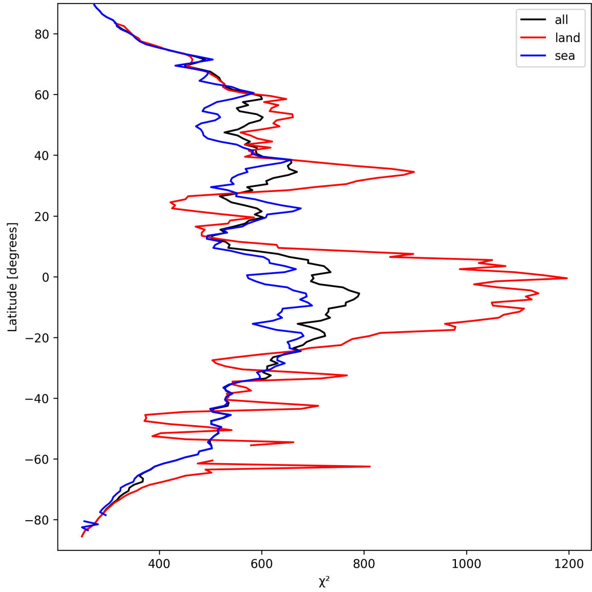
Figure 25: Zonal average of “ \chi^2 ” for 2025-03-26 to 2025-03-26.
