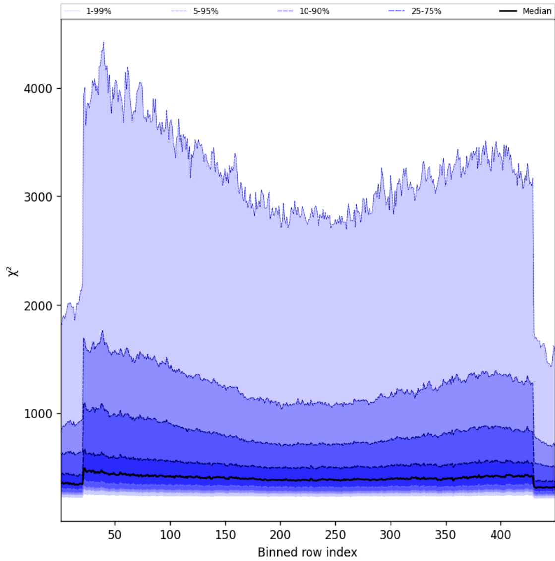
Figure 59: Along track statistics of “ \chi^2 ” for 2025-03-26 to 2025-03-26
