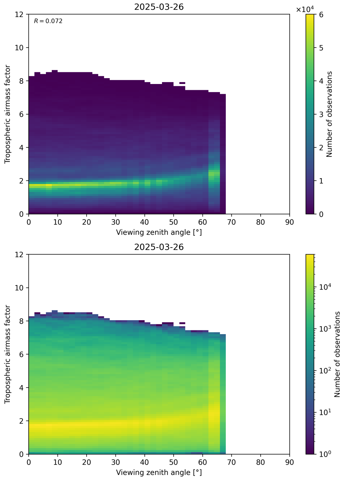
Figure 161: Scatter density plot of “Viewing zenith angle” against “Tropospheric airmass factor” for 2025-03-26 to 2025-03-26.
