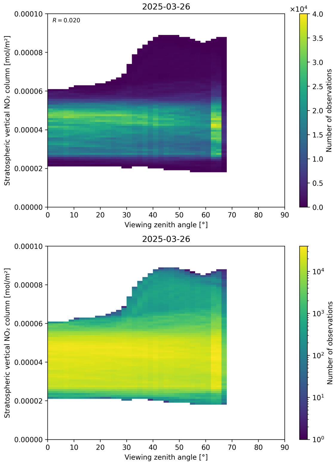
Figure 164: Scatter density plot of “Viewing zenith angle” against “Stratospheric vertical NO 2 column” for 2025-03-26 to 2025-03-26.
