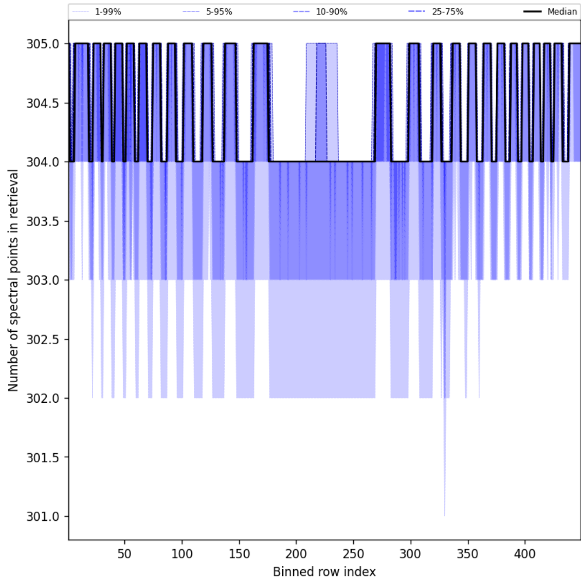
Figure 50: Along track statistics of “Number of spectral points in retrieval” for 2025-03-26 to 2025-03-26
