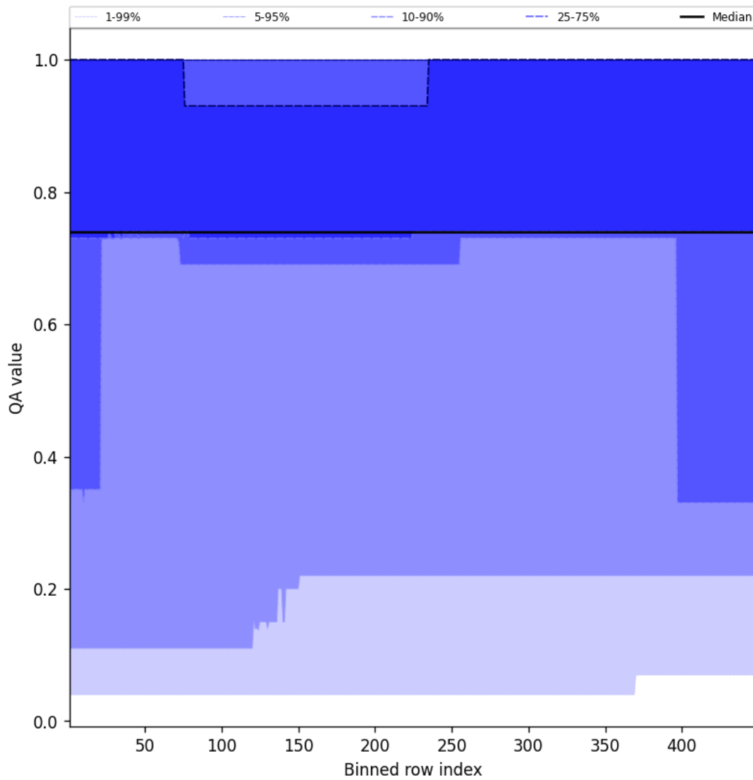
Figure 45: Along track statistics of “QA value” for 2025-03-26 to 2025-03-26
