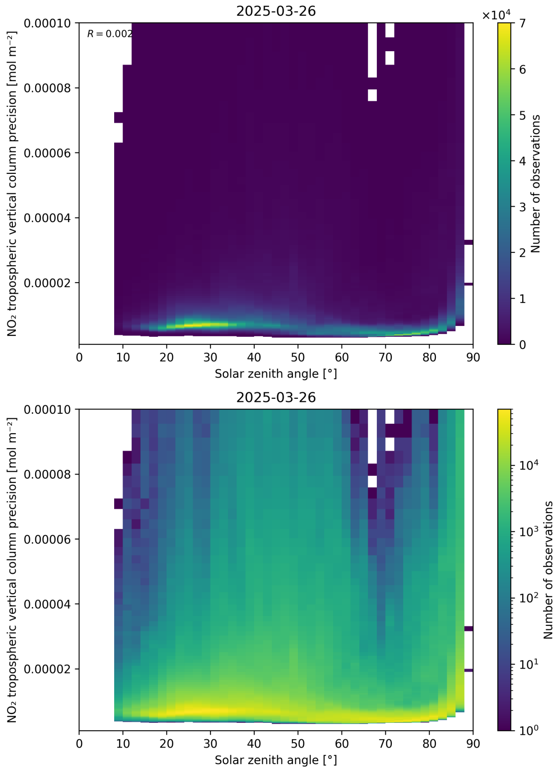
Figure 156: Scatter density plot of “Solar zenith angle” against “NO 2 tropospheric vertical column precision” for 2025-03-26 to 2025-03-26.
