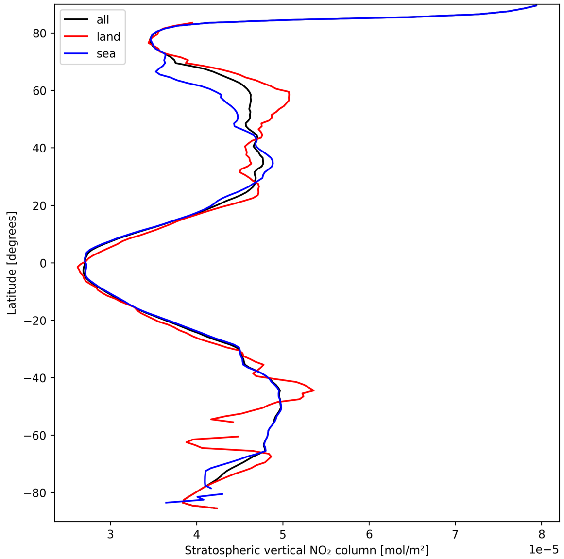
Figure 19: Zonal average of “Stratospheric vertical NO 2 column” for 2025-03-26 to 2025-03-26.
