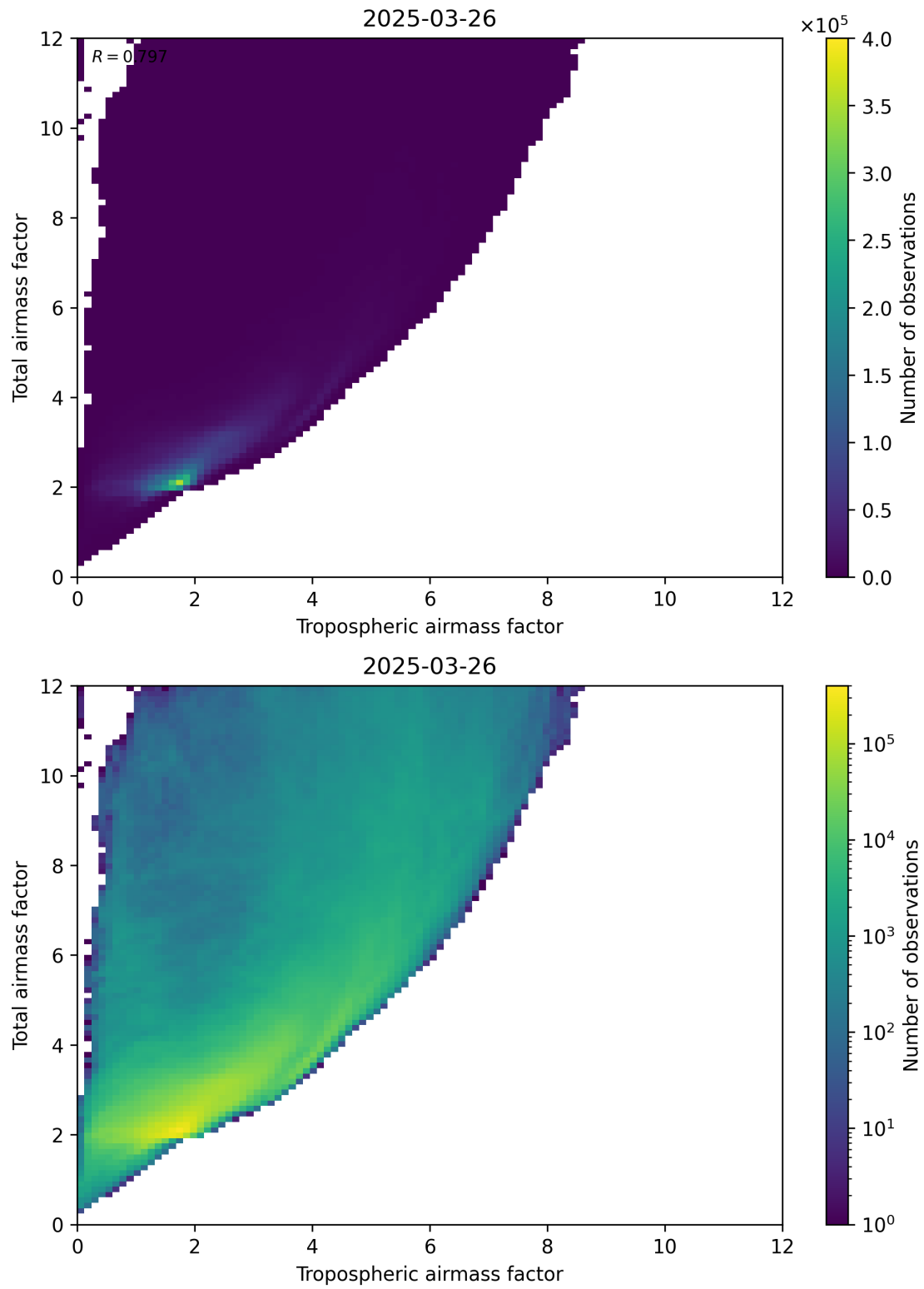
Figure 72: Scatter density plot of “Tropospheric airmass factor” against “Total airmass factor” for 2025-03-26 to 2025-03-26.
