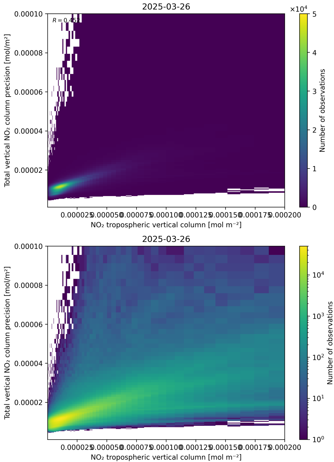
Figure 129: Scatter density plot of “NO 2 tropospheric vertical column” against “Total vertical NO 2 column precision” for 2025-03-26 to 2025-03-26.
