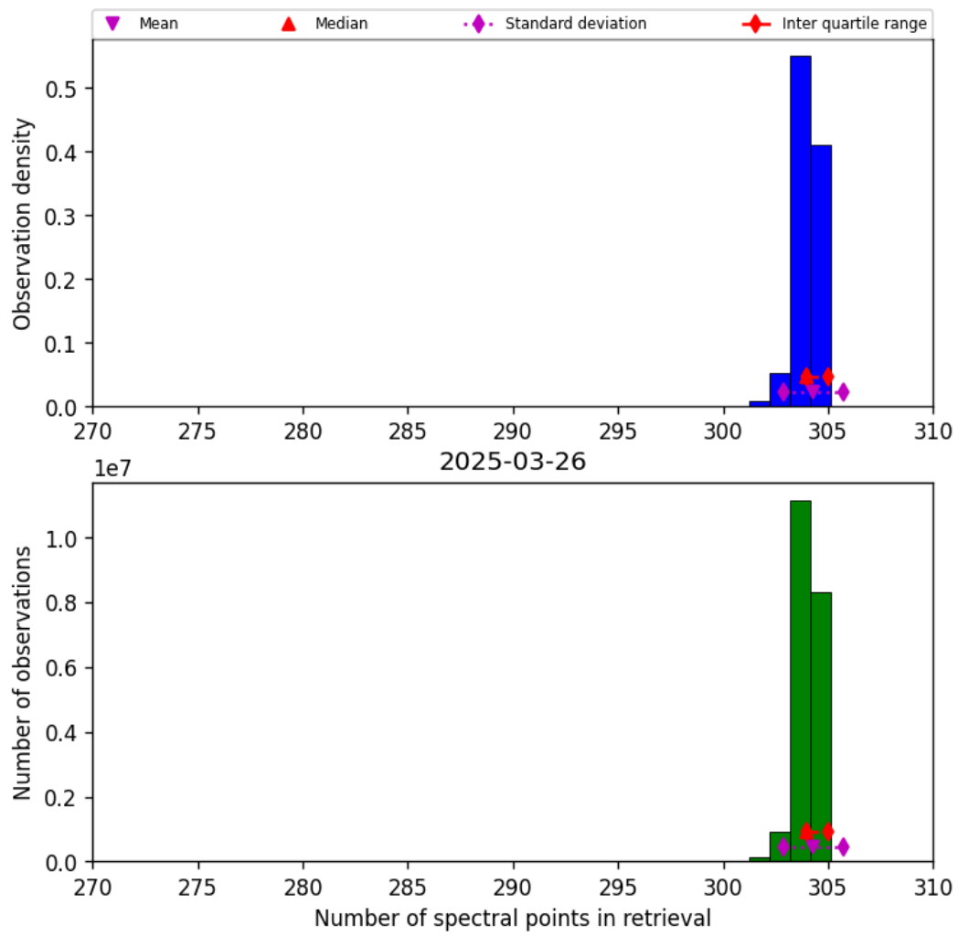
Figure 33: Histogram of “Number of spectral points in retrieval” for 2025-03-26 to 2025-03-26
