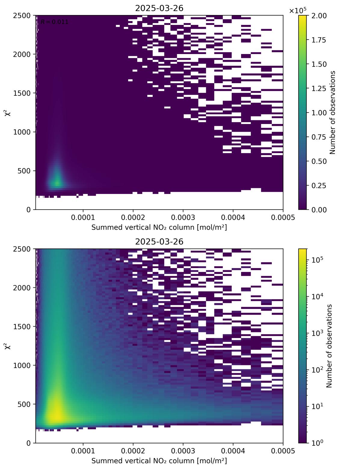
Figure 104: Scatter density plot of “Summed vertical NO 2 column” against “ \chi^2 ” for 2025-03-26 to 2025-03-26.
