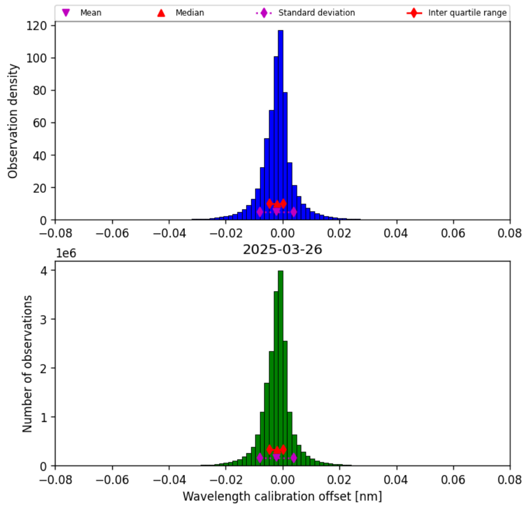
Figure 35: Histogram of “Wavelength calibration offset” for 2025-03-26 to 2025-03-26
