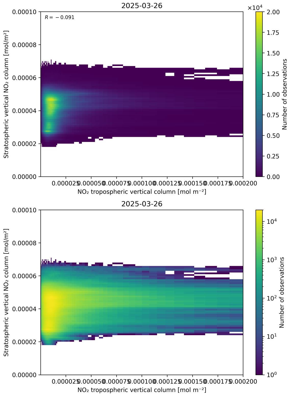
Figure 125: Scatter density plot of “NO 2 tropospheric vertical column” against “Stratospheric vertical NO 2 column” for 2025-03-26 to 2025-03-26.
