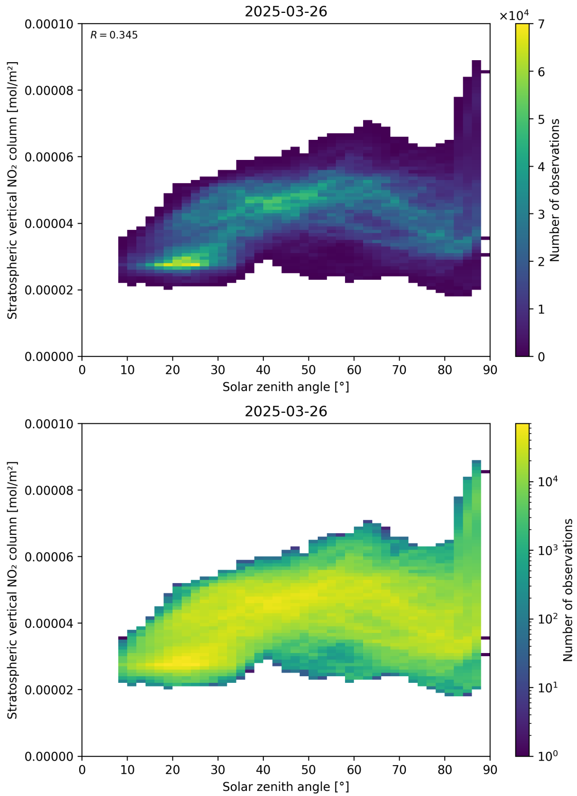
Figure 150: Scatter density plot of “Solar zenith angle” against “Stratospheric vertical NO 2 column” for 2025-03-26 to 2025-03-26.
