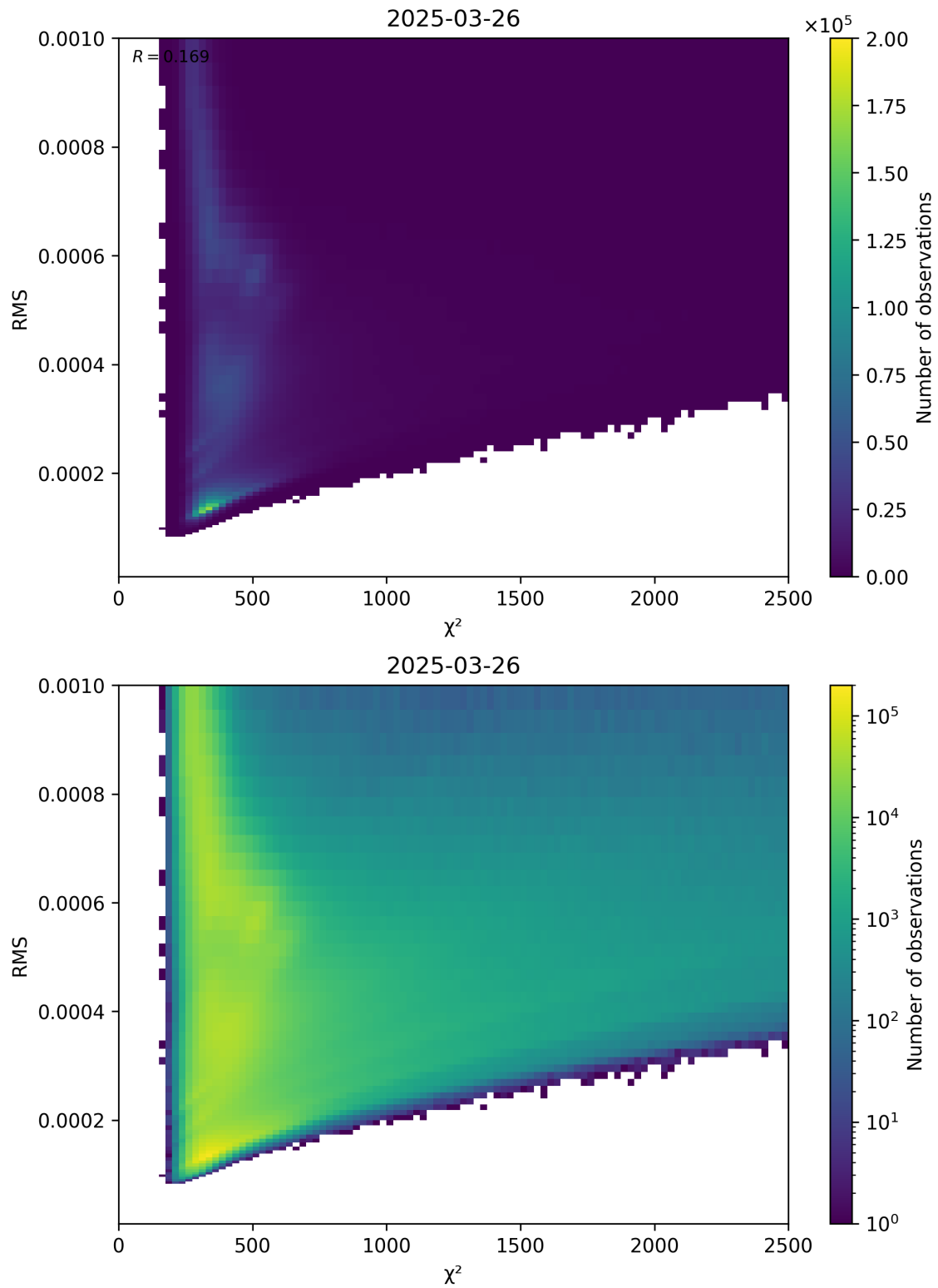
Figure 82: Scatter density plot of “ \chi^2 ” against “RMS” for 2025-03-26 to 2025-03-26.
