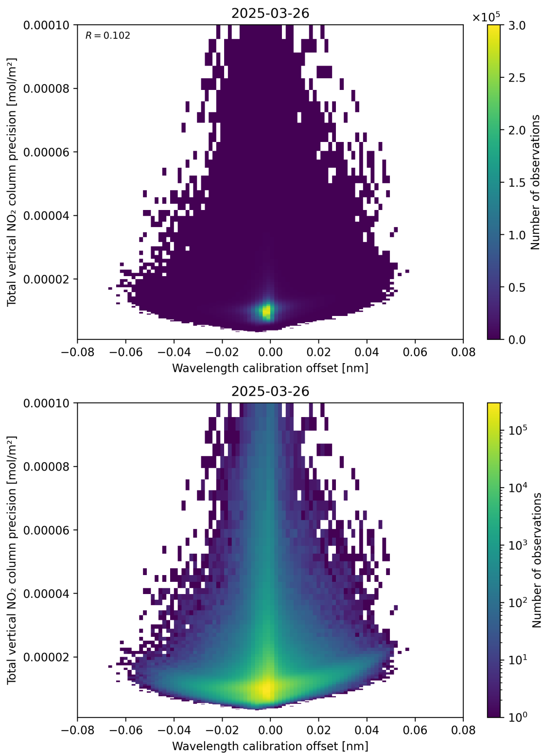
Figure 180: Scatter density plot of “Wavelength calibration offset” against “Total vertical NO 2 column precision” for 2025-03-26 to 2025-03-26.
