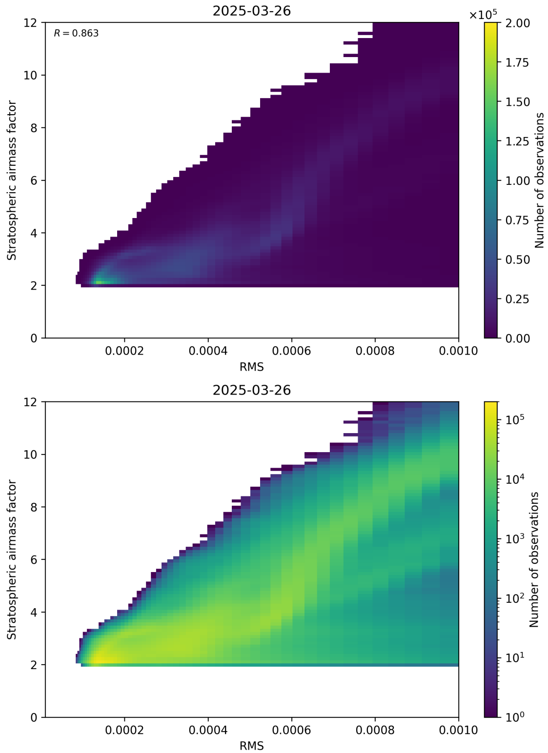
Figure 144: Scatter density plot of “RMS” against “Stratospheric airmass factor” for 2025-03-26 to 2025-03-26.
