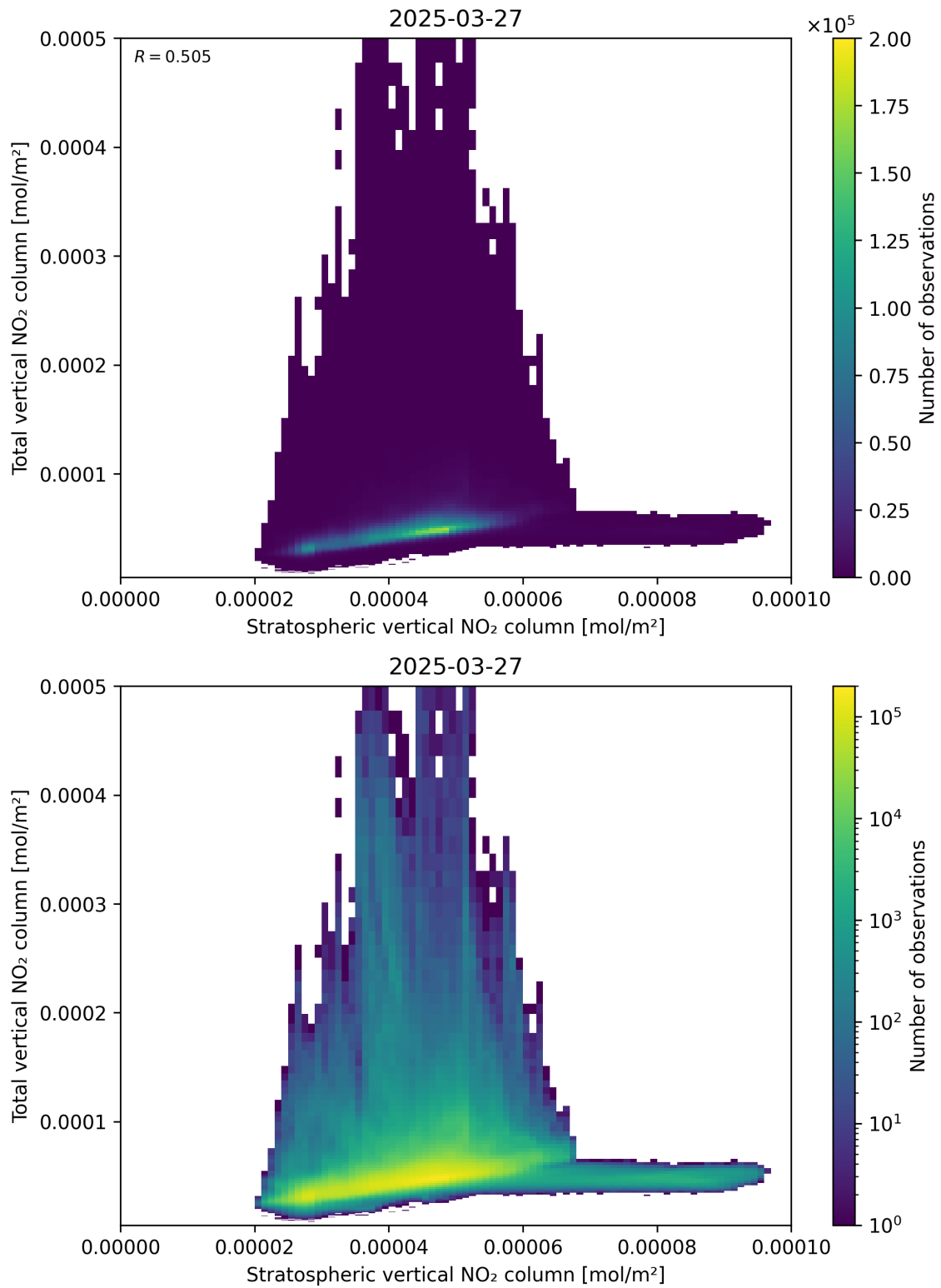
Figure 100: Scatter density plot of “Stratospheric vertical NO 2 column” against “Total vertical NO 2 column” for 2025-03-27 to 2025-03-28.
