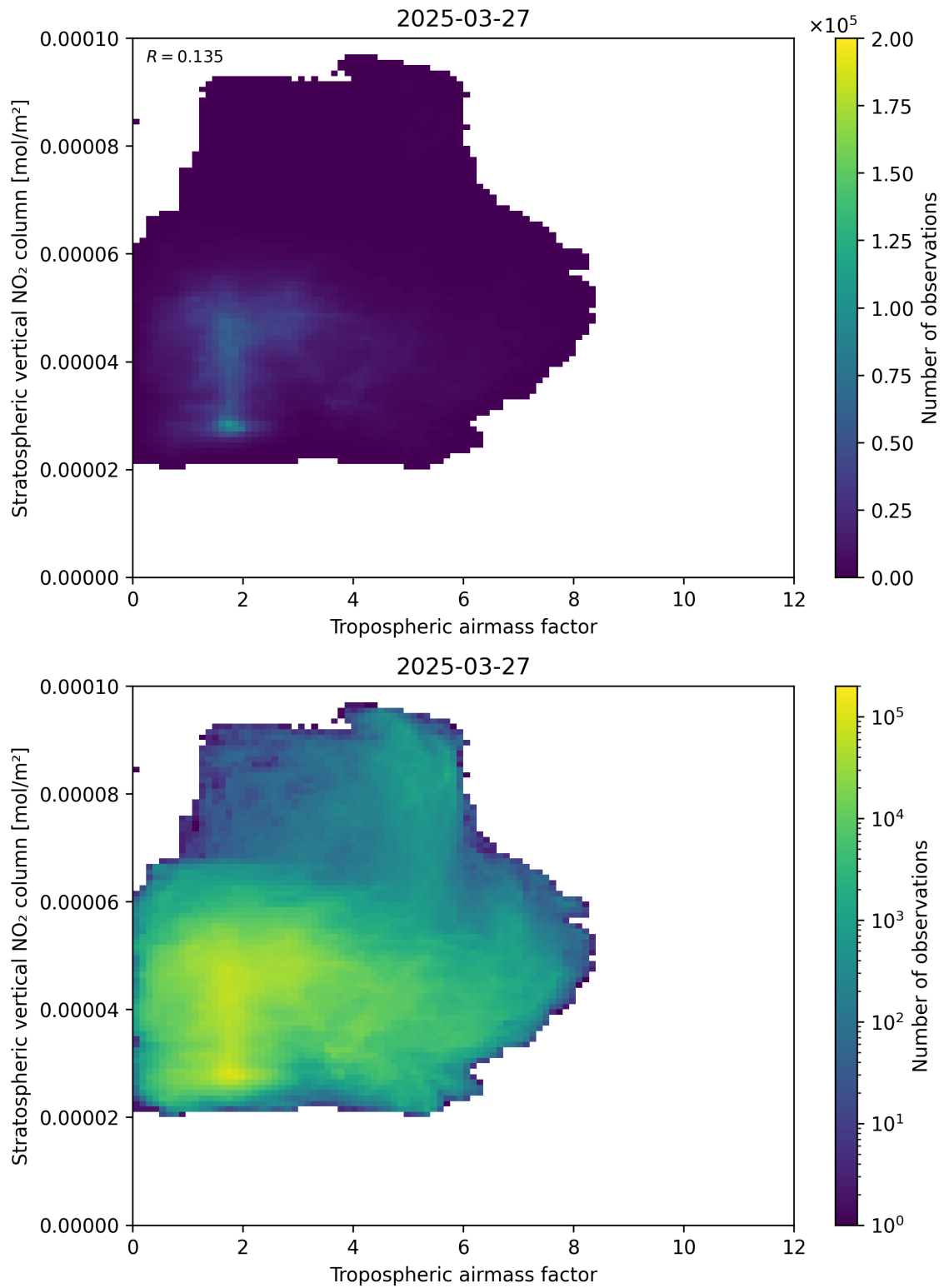
Figure 74: Scatter density plot of “Tropospheric airmass factor” against “Stratospheric vertical NO 2 column” for 2025-03-27 to 2025-03-28.
