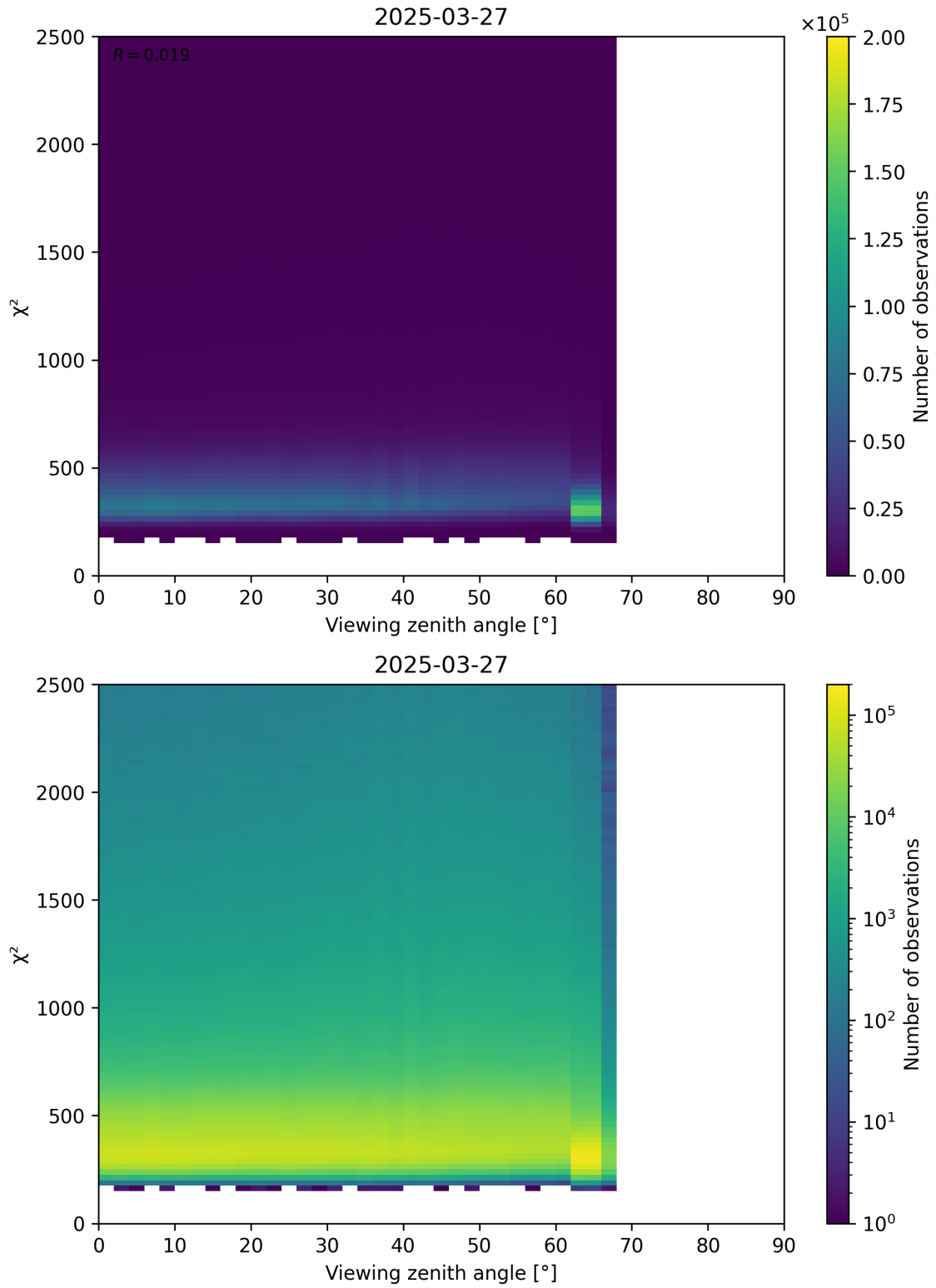
Figure 162: Scatter density plot of “Viewing zenith angle” against “ \chi^2 ” for 2025-03-27 to 2025-03-28.
