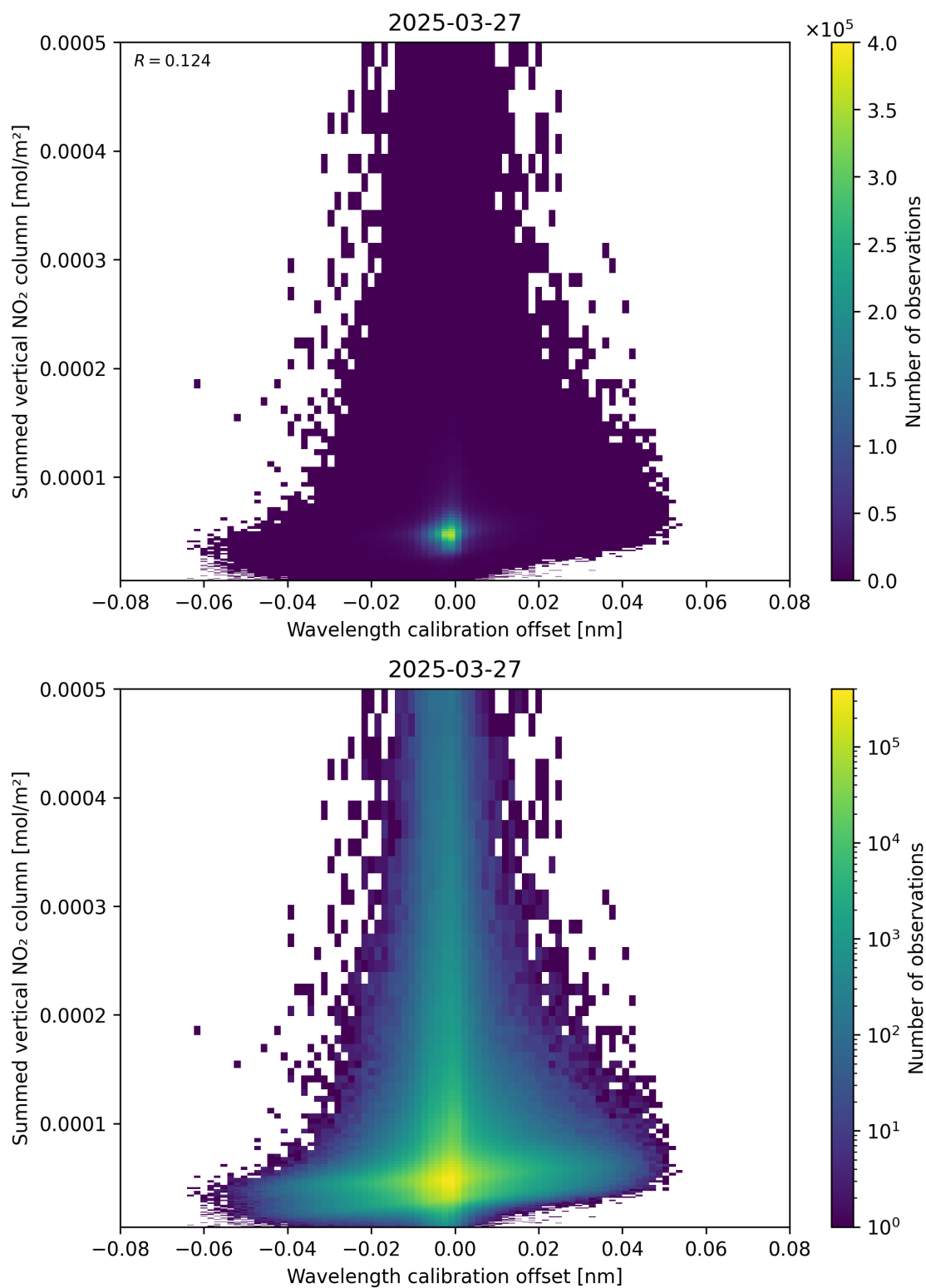
Figure 177: Scatter density plot of “Wavelength calibration offset” against “Summed vertical NO 2 column” for 2025-03-27 to 2025-03-28.
