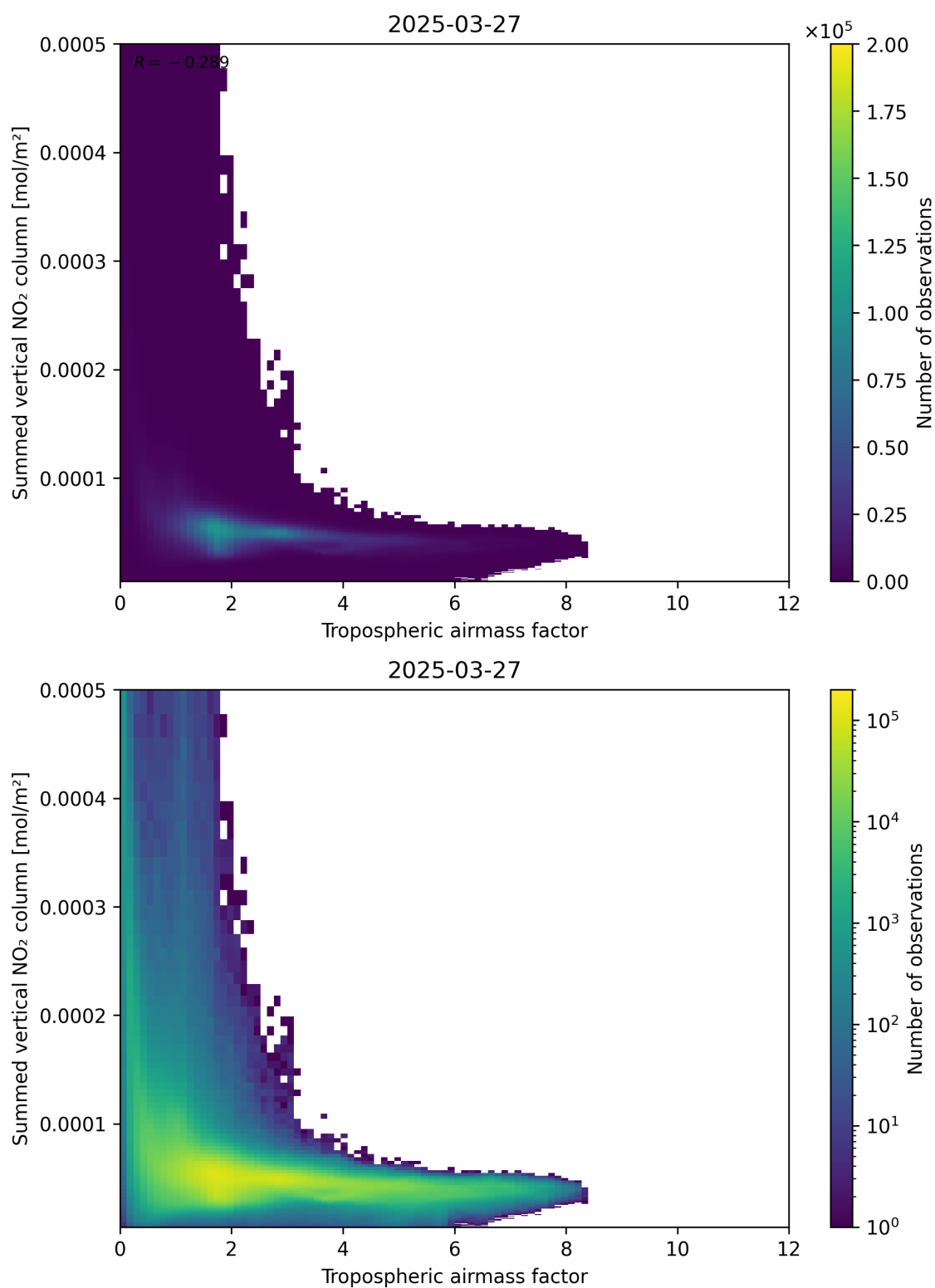
Figure 75: Scatter density plot of “Tropospheric air mass factor” against “Summed vertical NO 2 column” for 2025-03-27 to 2025-03-28.
