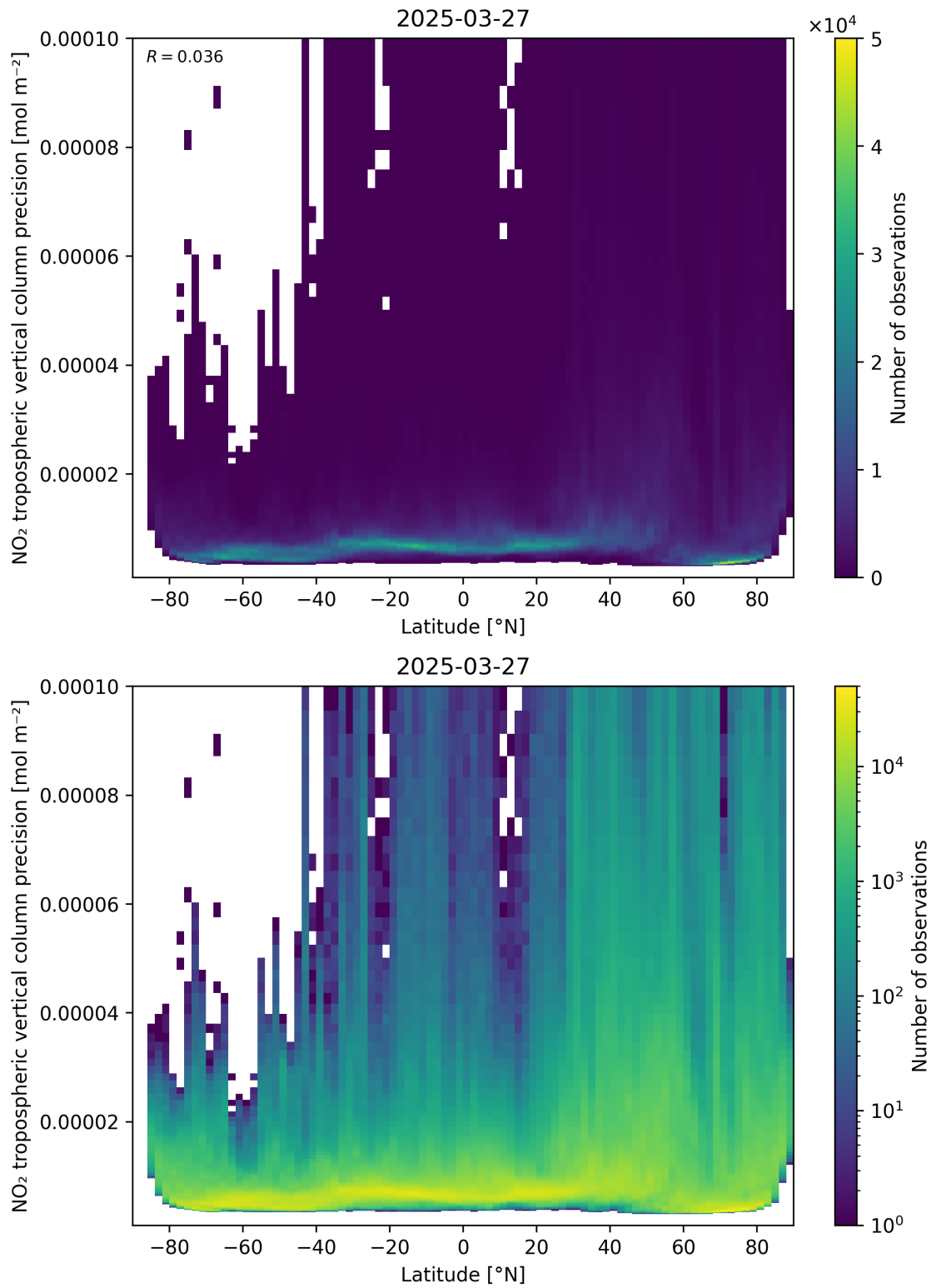
Figure 93: Scatter density plot of “Latitude” against “NO 2 tropospheric vertical column precision” for 2025-03-27 to 2025-03-28.
