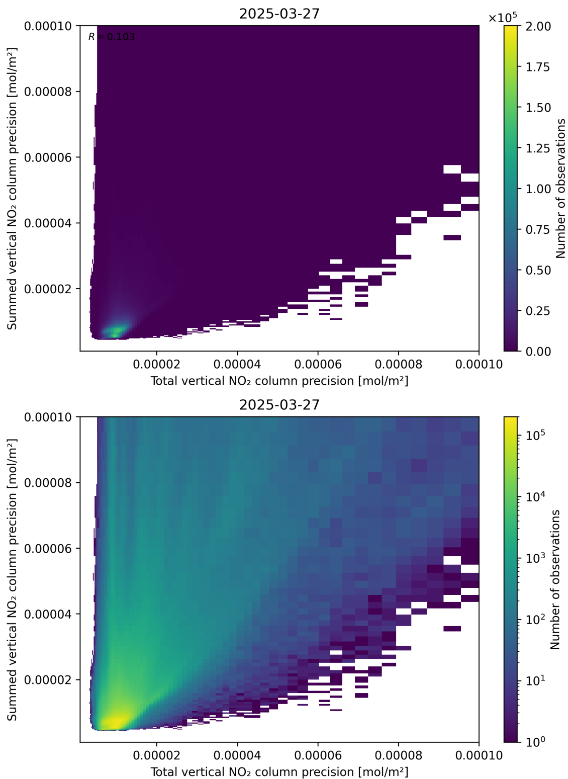
Figure 118: Scatter density plot of “Total vertical NO 2 column precision” against “Summed vertical NO 2 column precision” for 2025-03-27 to 2025-03-28.
