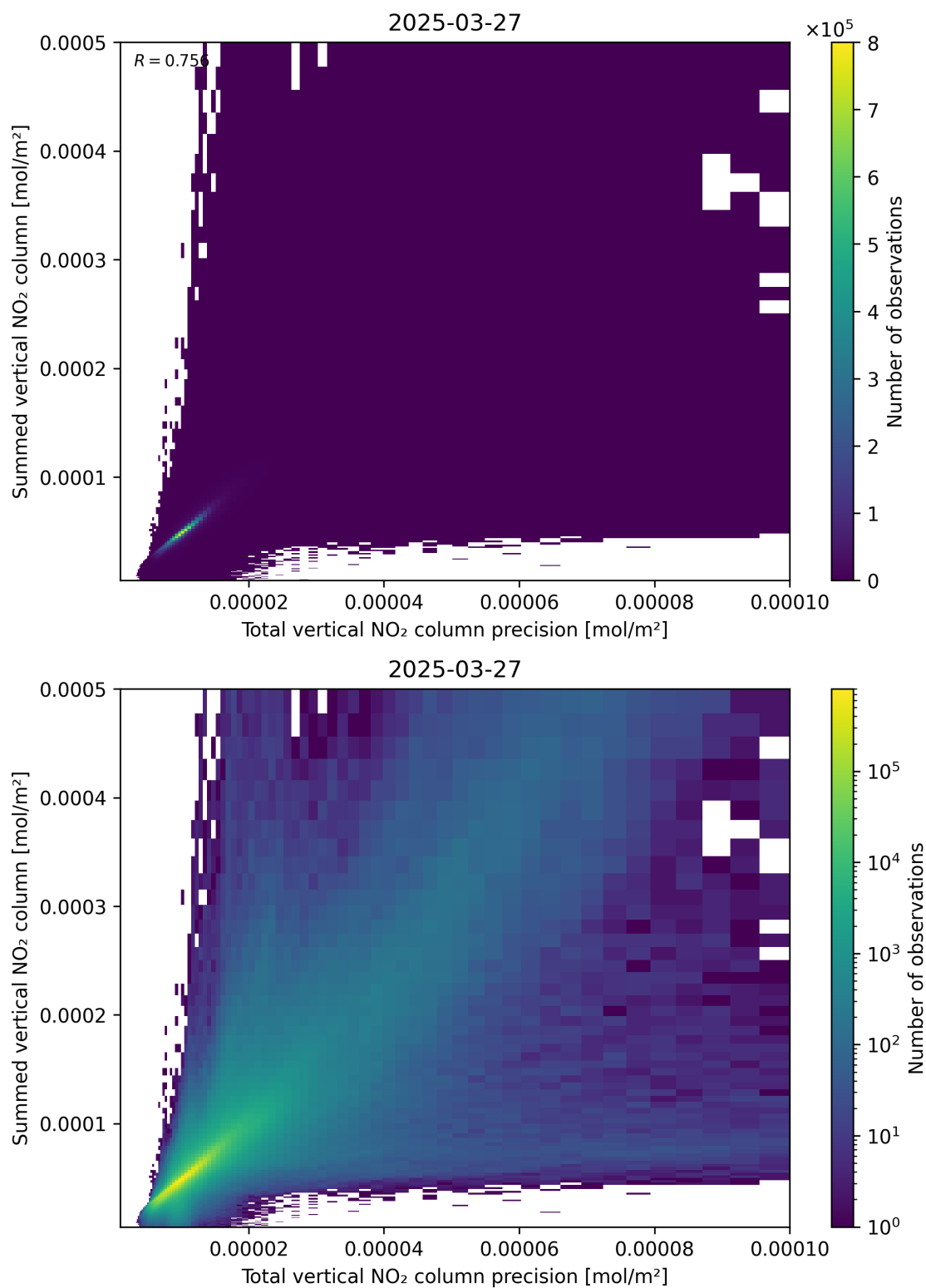
Figure 117: Scatter density plot of “Total vertical NO 2 column precision” against “Summed vertical NO 2 column” for 2025-03-27 to 2025-03-28.
