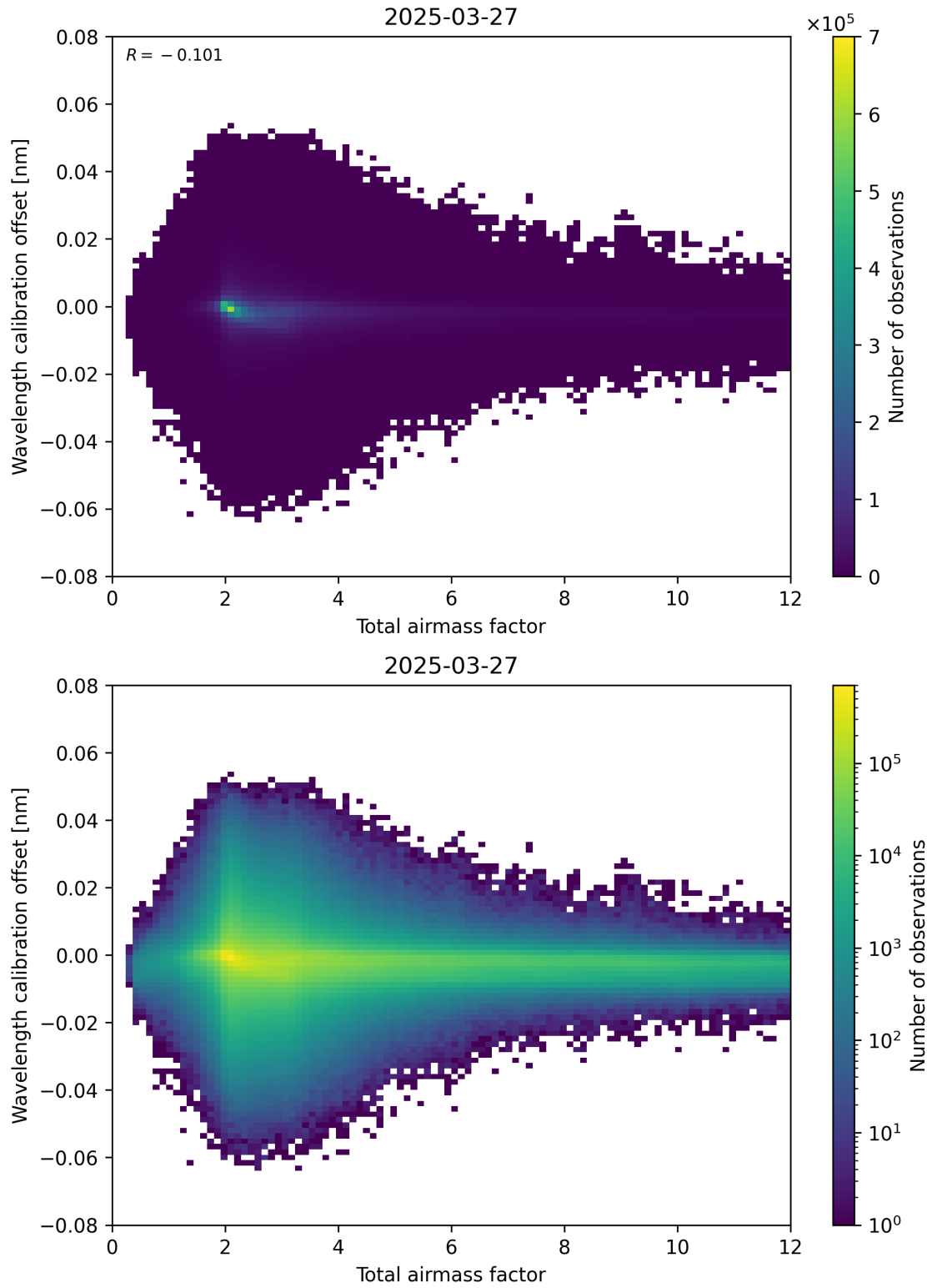
Figure 70: Scatter density plot of “Total airmass factor” against “Wavelength calibration offset” for 2025-03-27 to 2025-03-28.
