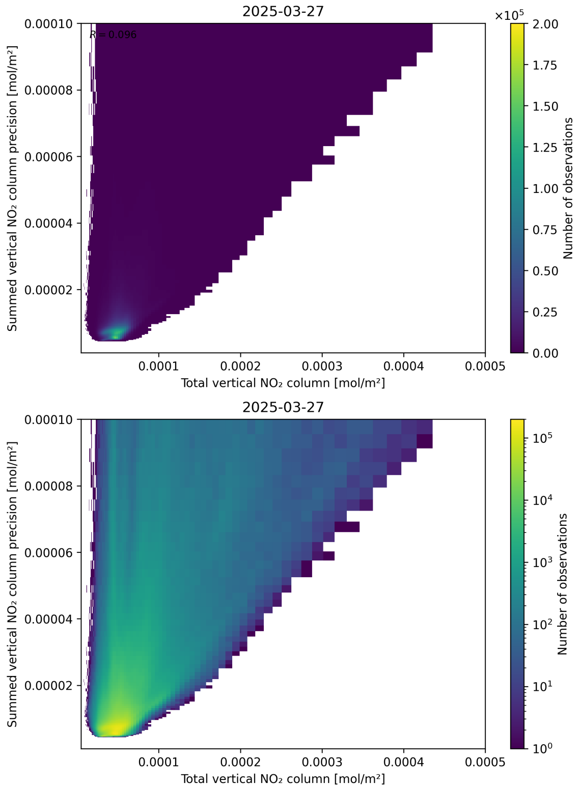
Figure 113: Scatter density plot of “Total vertical NO 2 column” against “Summed vertical NO 2 column precision” for 2025-03-27 to 2025-03-28.
