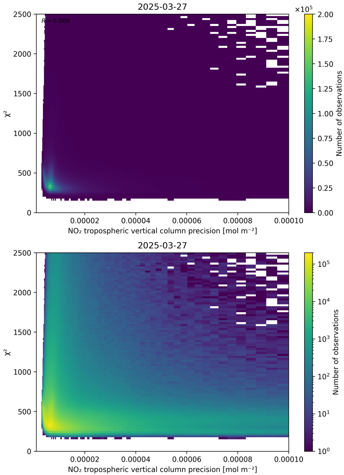
Figure 134: Scatter density plot of “NO 2 tropospheric vertical column precision” against “ \chi^2 ” for 2025-03-27 to 2025-03-28.
