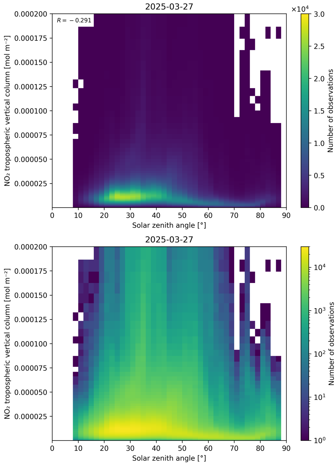
Figure 155: Scatter density plot of “Solar zenith angle” against “NO 2 tropospheric vertical column” for 2025-03-27 to 2025-03-28.
