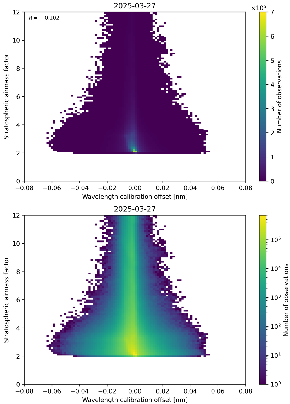
Figure 174: Scatter density plot of “Wavelength calibration offset” against “Stratospheric airmass factor” for 2025-03-27 to 2025-03-28.
