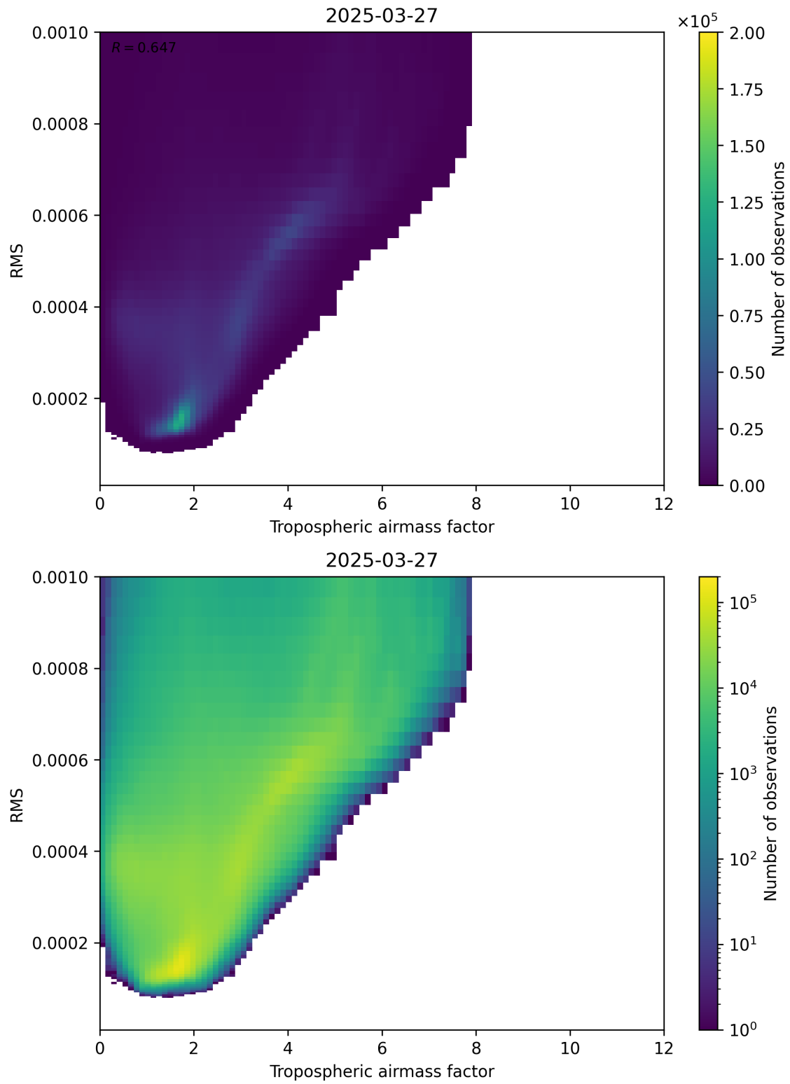
Figure 79: Scatter density plot of “Tropospheric airmass factor” against “RMS” for 2025-03-27 to 2025-03-28.
