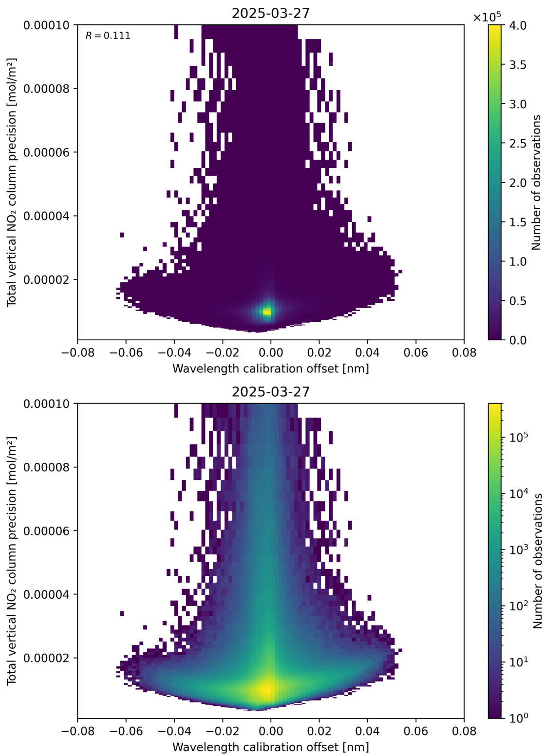
Figure 180: Scatter density plot of “Wavelength calibration offset” against “Total vertical NO 2 column precision” for 2025-03-27 to 2025-03-28.
