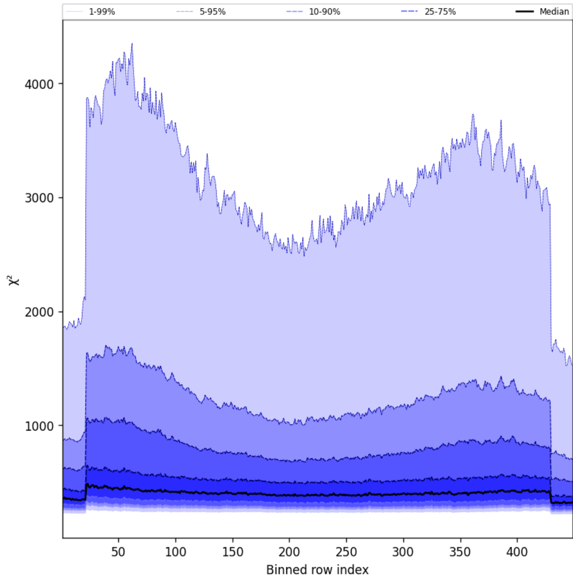
Figure 59: Along track statistics of “ \chi^2 ” for 2025-03-27 to 2025-03-28
