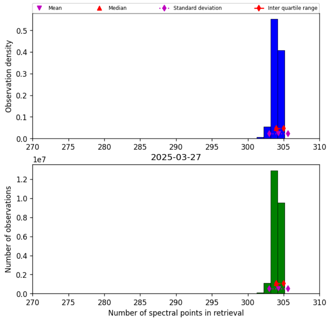
Figure 33: Histogram of “Number of spectral points in retrieval” for 2025-03-27 to 2025-03-28
