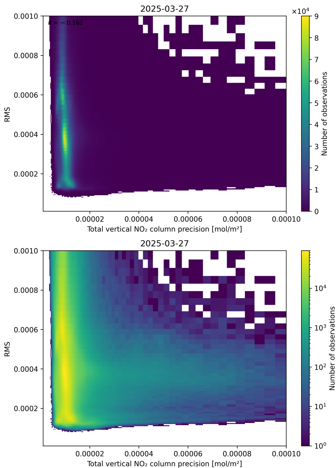
Figure 119: Scatter density plot of “Total vertical NO 2 column precision” against “RMS” for 2025-03-27 to 2025-03-28.
