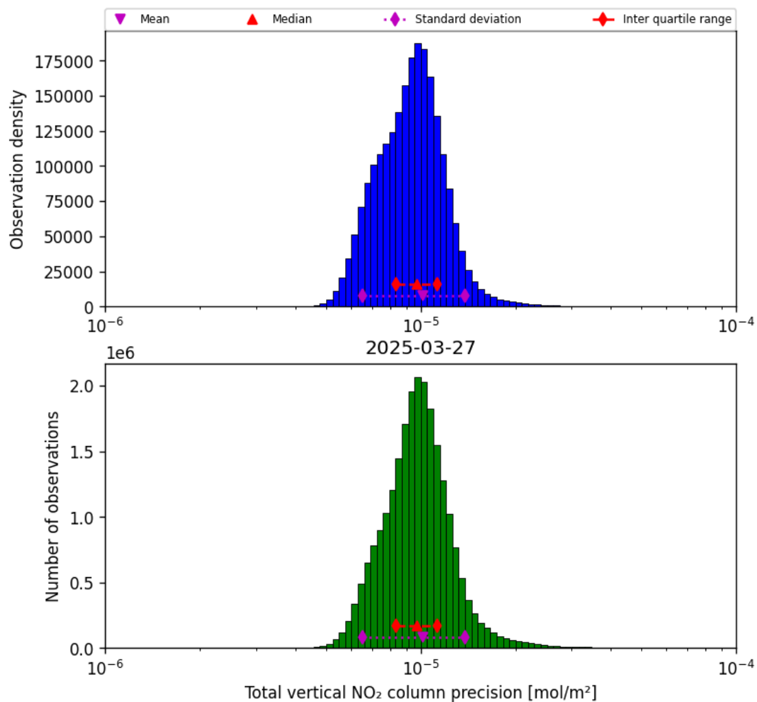
Figure 39: Histogram of “Total vertical NO 2 column precision” for 2025-03-27 to 2025-03-28
