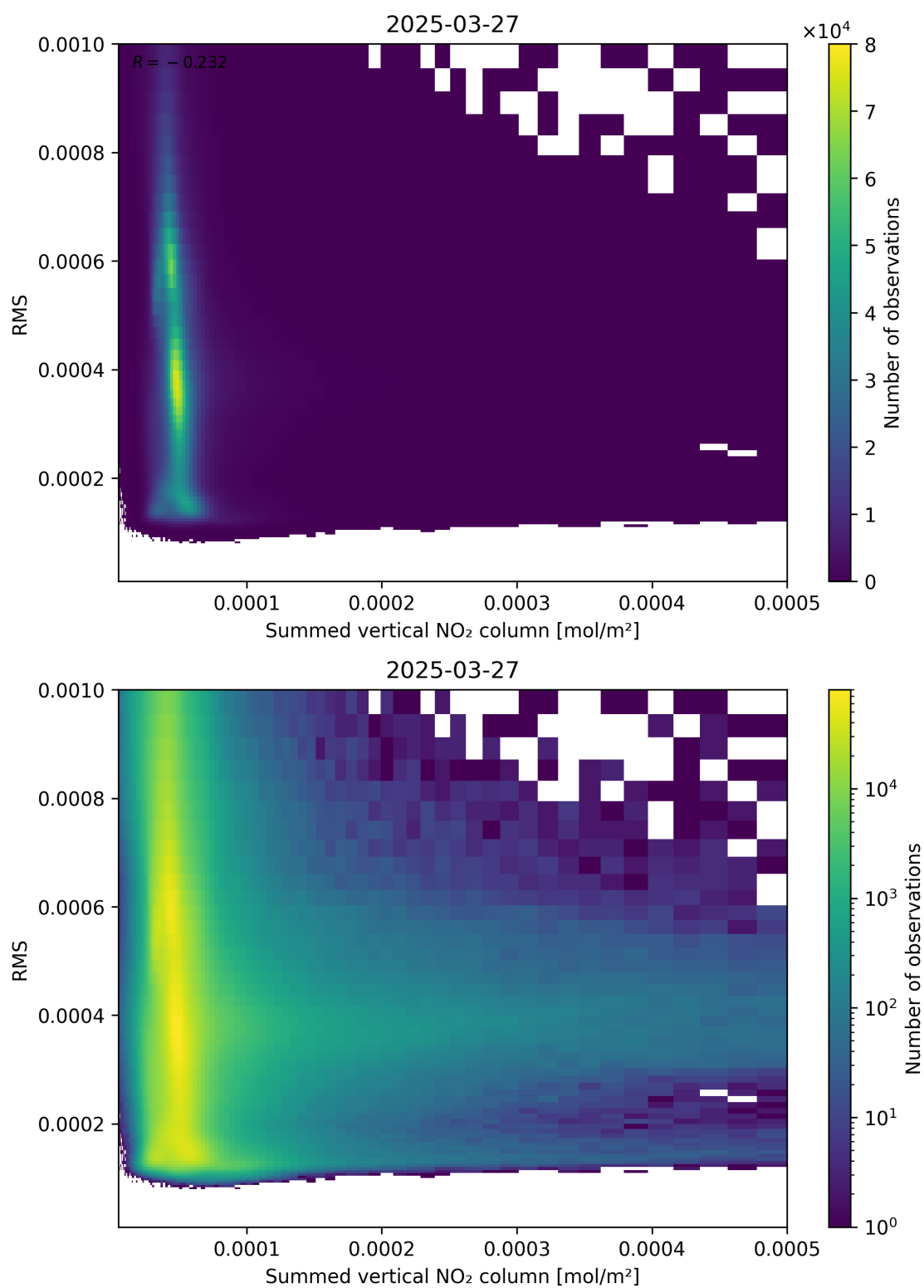
Figure 109: Scatter density plot of “Summed vertical NO 2 column” against “RMS” for 2025-03-27 to 2025-03-28.
