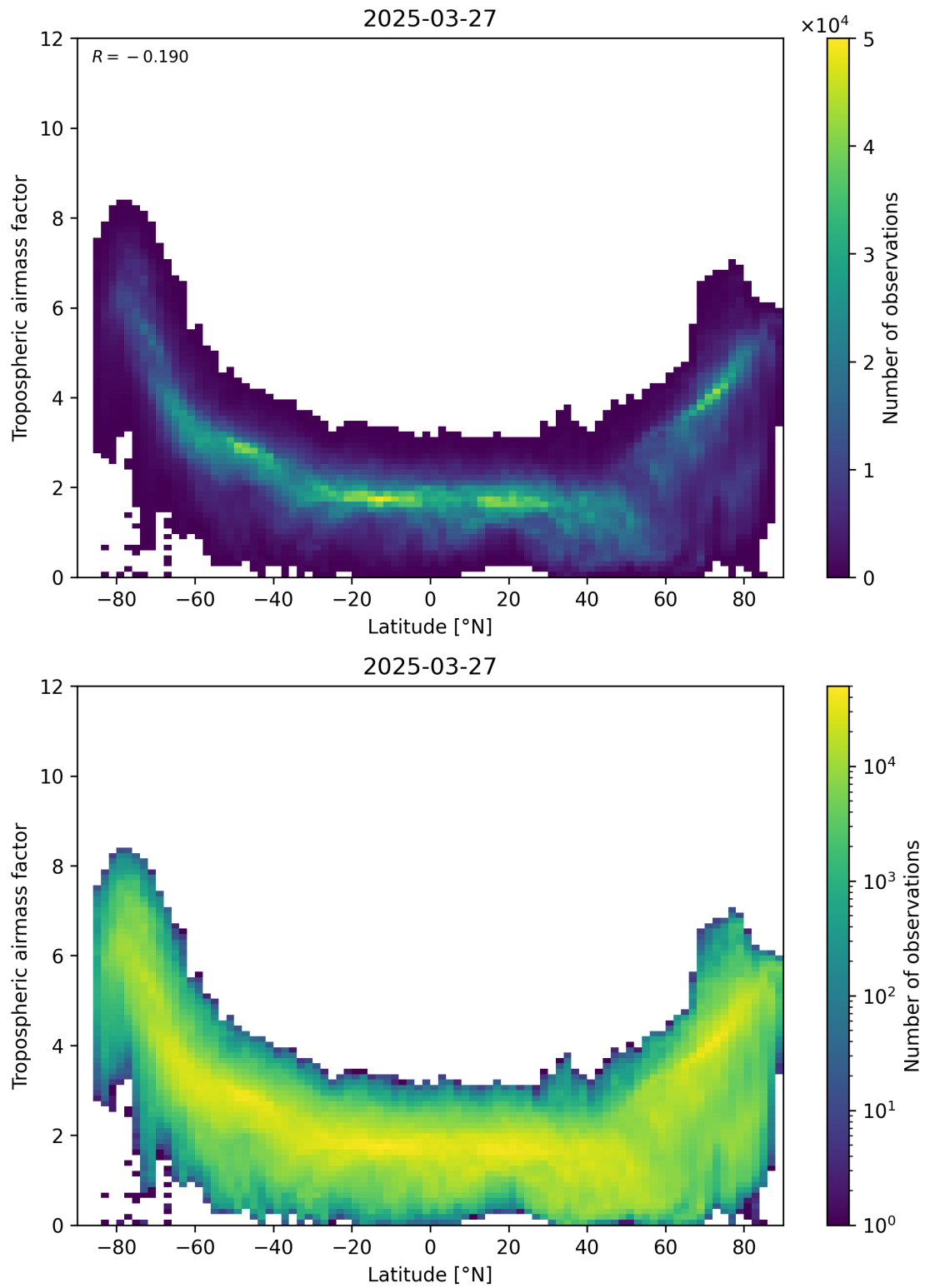
Figure 85: Scatter density plot of “Latitude” against “Tropospheric airmass factor” for 2025-03-27 to 2025-03-28.
