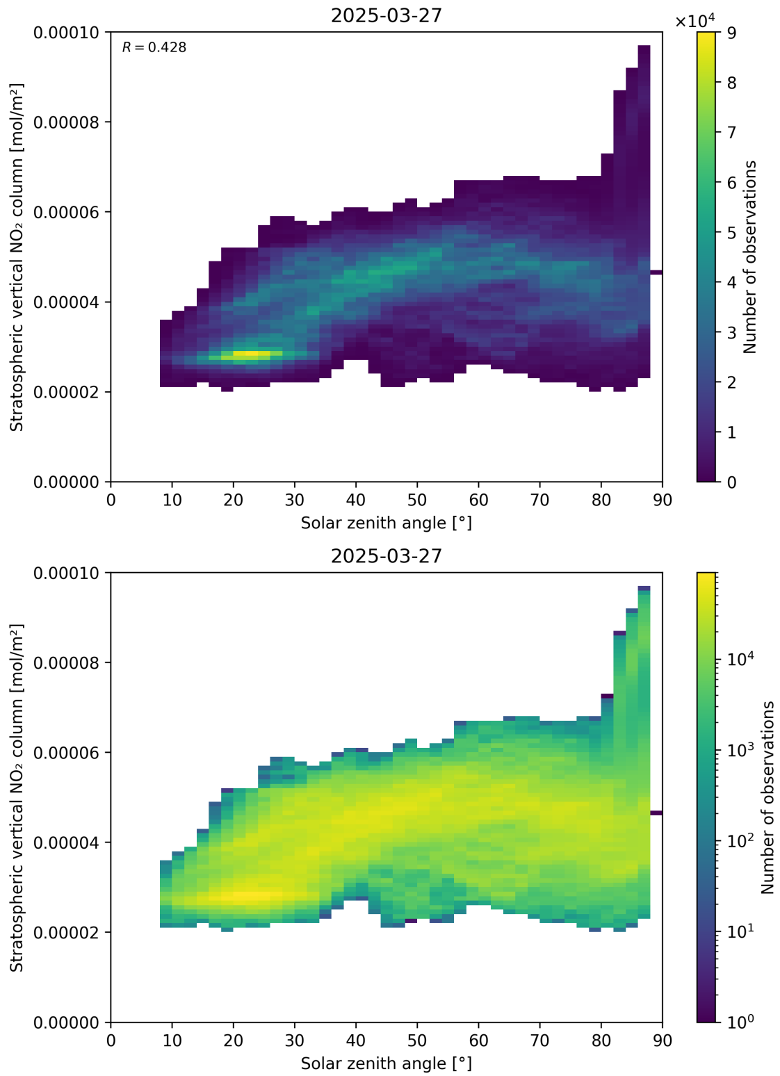
Figure 150: Scatter density plot of “Solar zenith angle” against “Stratospheric vertical \text{NO}_2 column” for 2025-03-27 to 2025-03-28.
