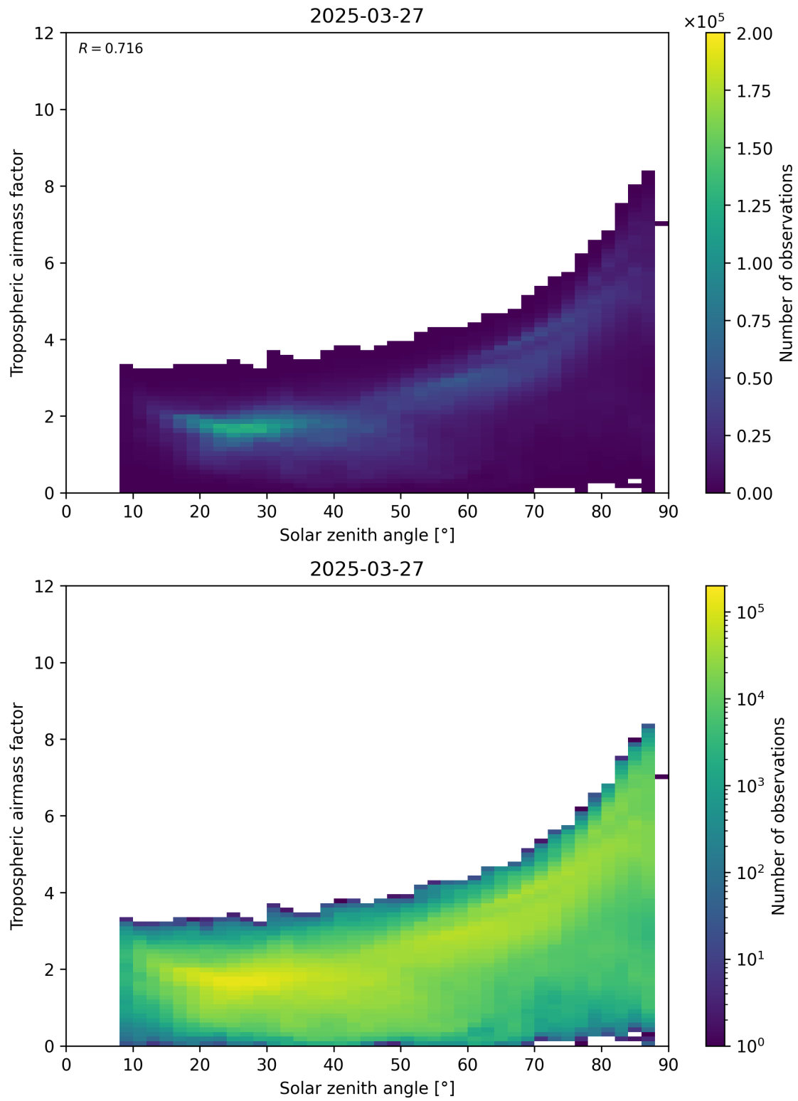
Figure 147: Scatter density plot of “Solar zenith angle” against “Tropospheric airmass factor” for 2025-03-27 to 2025-03-28.
