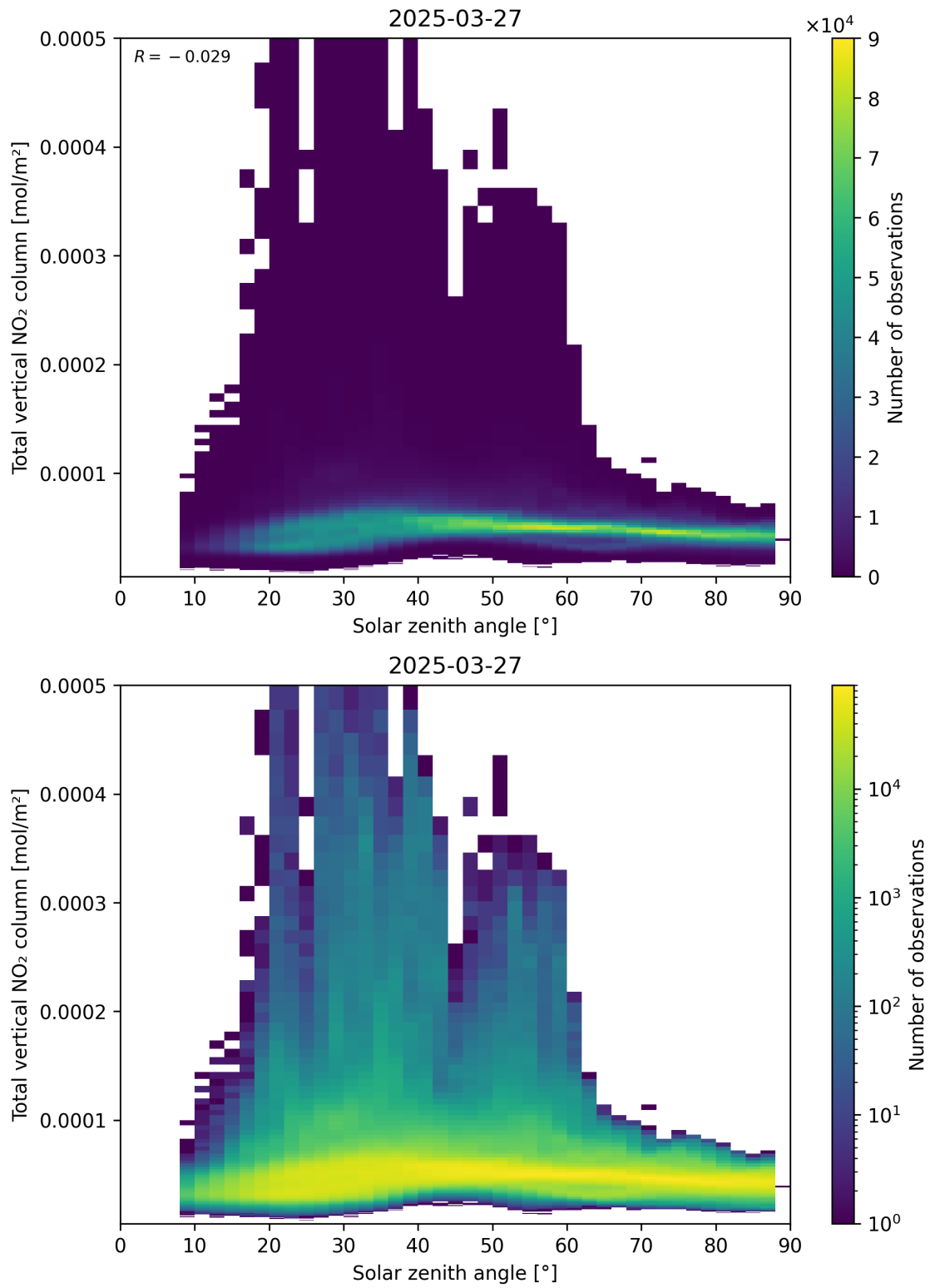
Figure 153: Scatter density plot of “Solar zenith angle” against “Total vertical NO 2 column” for 2025-03-27 to 2025-03-28.
