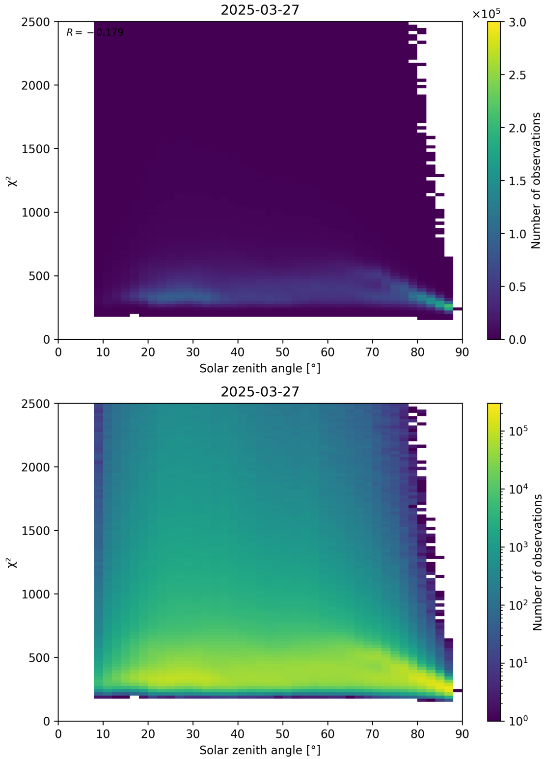
Figure 148: Scatter density plot of “Solar zenith angle” against “ \chi^2 ” for 2025-03-27 to 2025-03-28.
