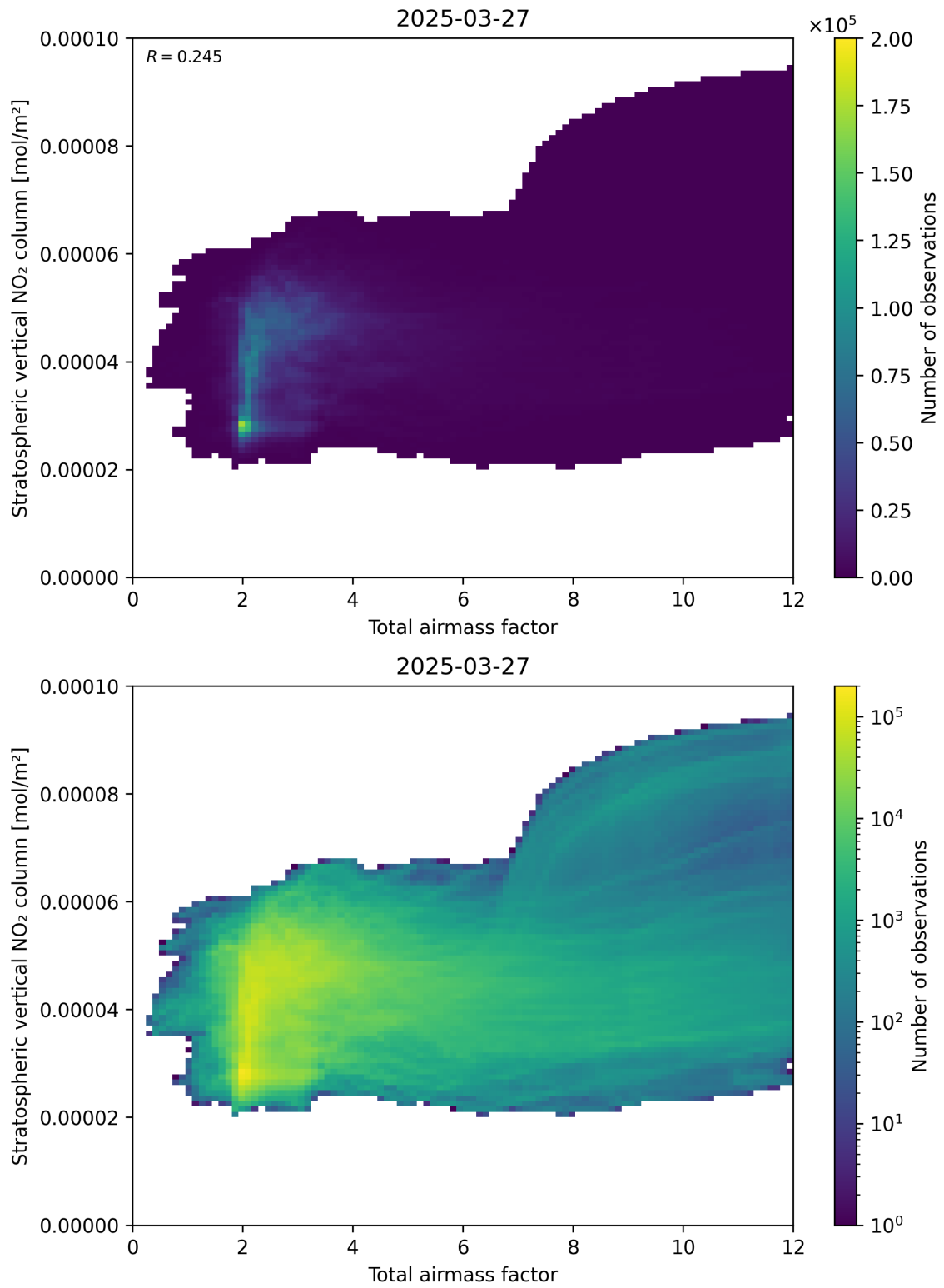
Figure 64: Scatter density plot of “Total airmass factor” against “Stratospheric vertical \text{NO}_2 column” for 2025-03-27 to 2025-03-28.
