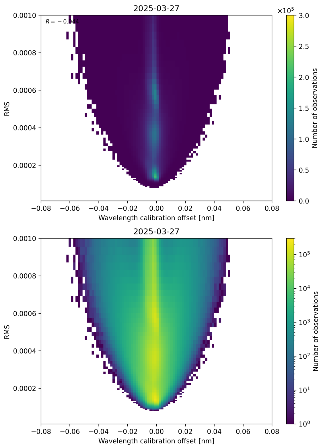
Figure 181: Scatter density plot of “Wavelength calibration offset” against “RMS” for 2025-03-27 to 2025-03-28.
