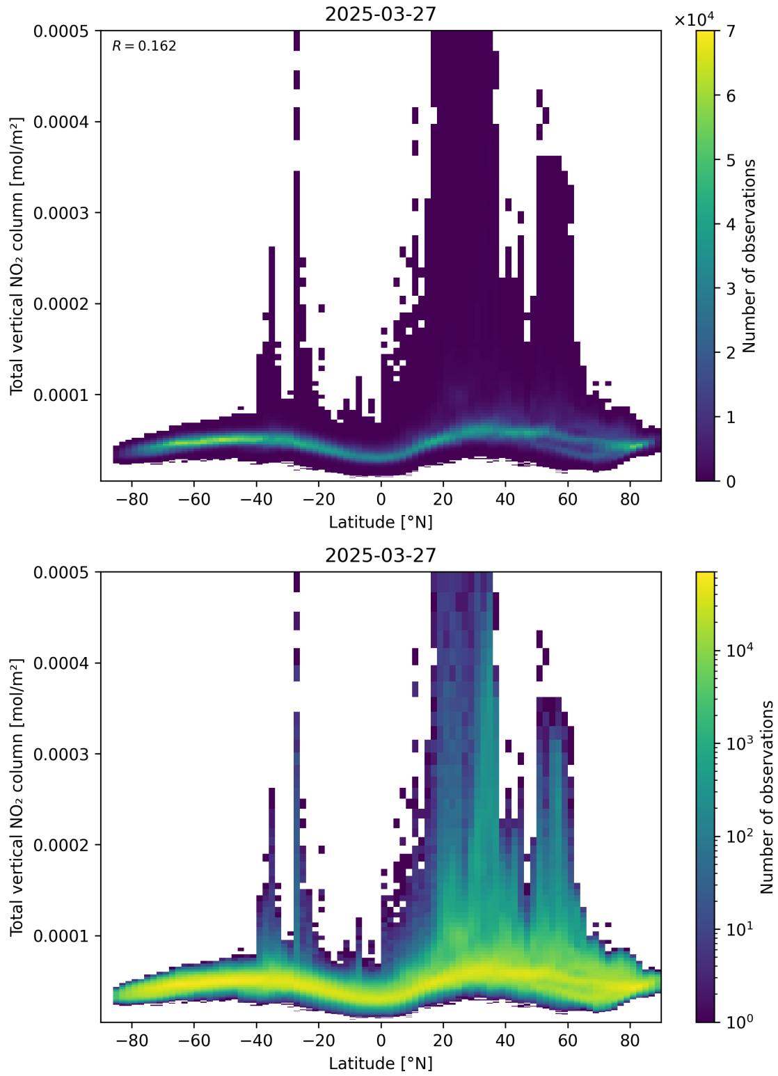
Figure 90: Scatter density plot of “Latitude” against “Total vertical NO 2 column” for 2025-03-27 to 2025-03-28.
