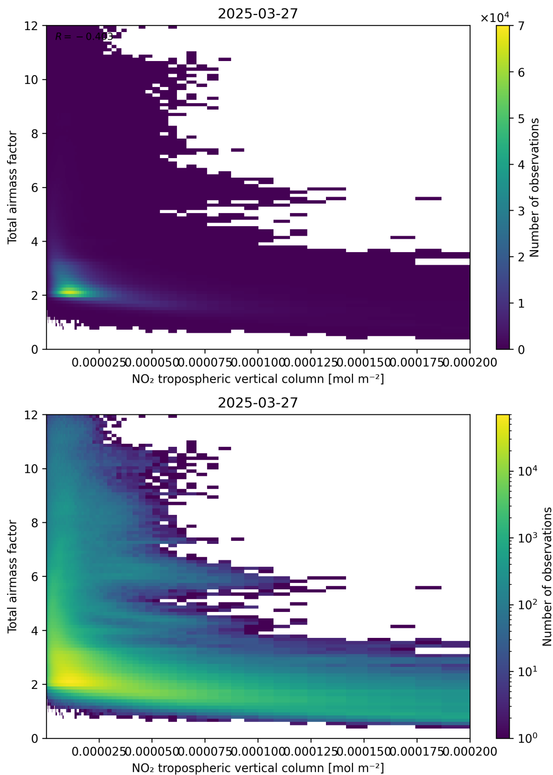
Figure 122: Scatter density plot of “NO 2 tropospheric vertical column” against “Total air mass factor” for 2025-03-27 to 2025-03-28.
