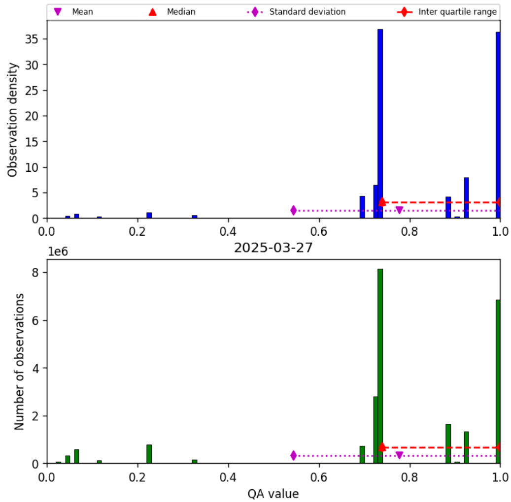
Figure 28: Histogram of “QA value” for 2025-03-27 to 2025-03-28
