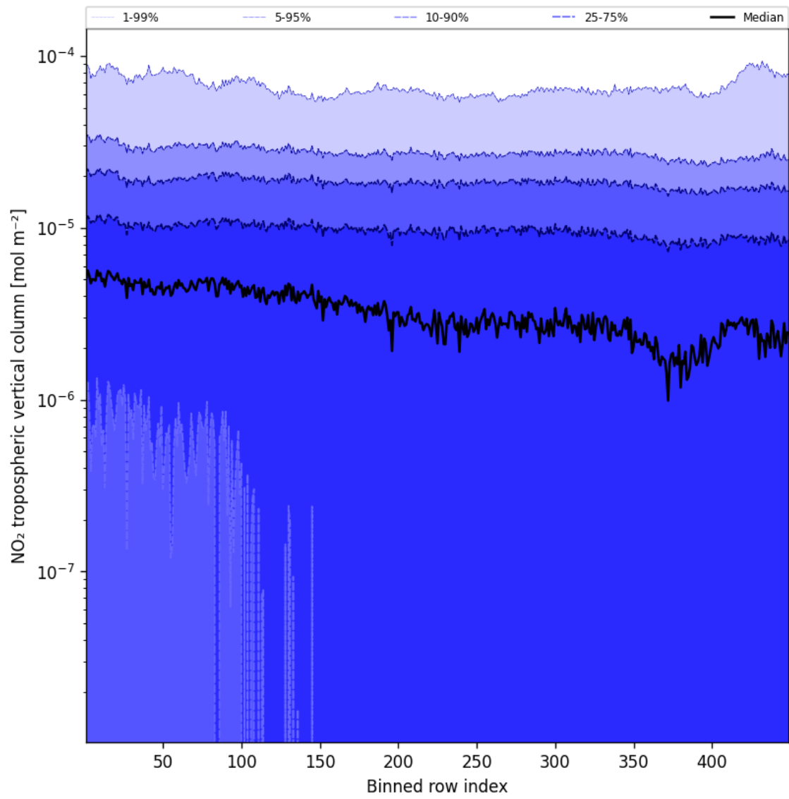
Figure 46: Along track statistics of “NO 2 tropospheric vertical column” for 2025-03-27 to 2025-03-28
