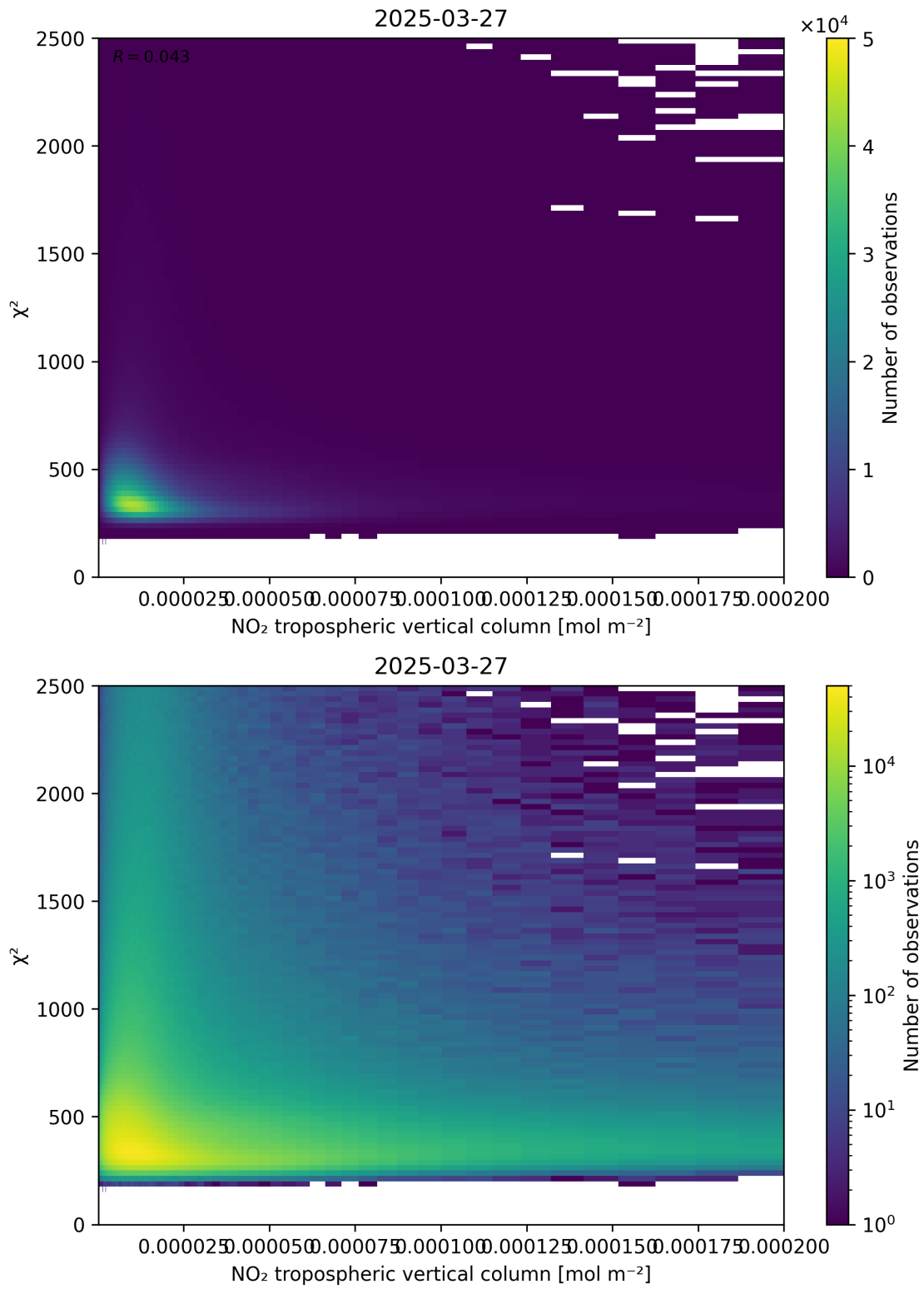
Figure 124: Scatter density plot of “NO 2 tropospheric vertical column” against “ \chi^2 ” for 2025-03-27 to 2025-03-28.
