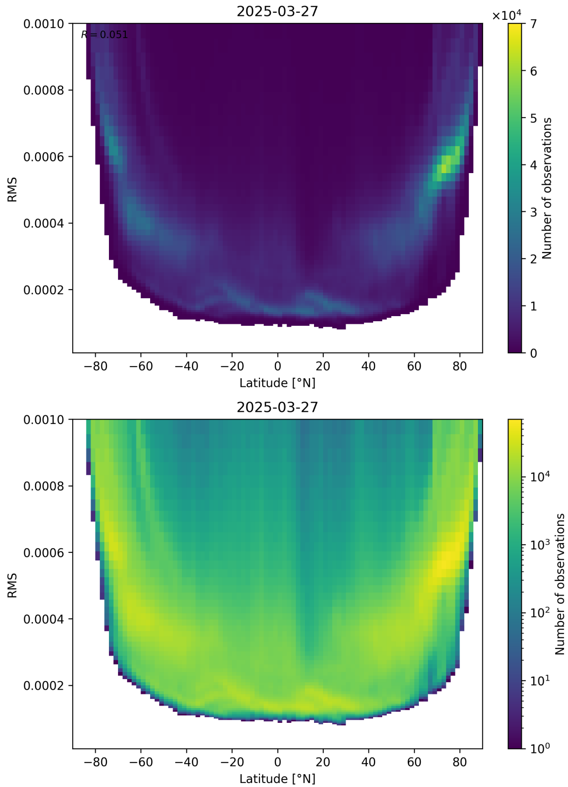
Figure 94: Scatter density plot of “Latitude” against “RMS” for 2025-03-27 to 2025-03-28.
