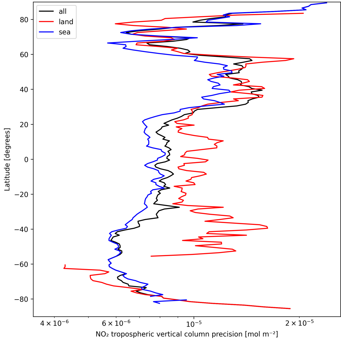
Figure 13: Zonal average of “NO 2 tropospheric vertical column precision” for 2025-03-27 to 2025-03-28.
