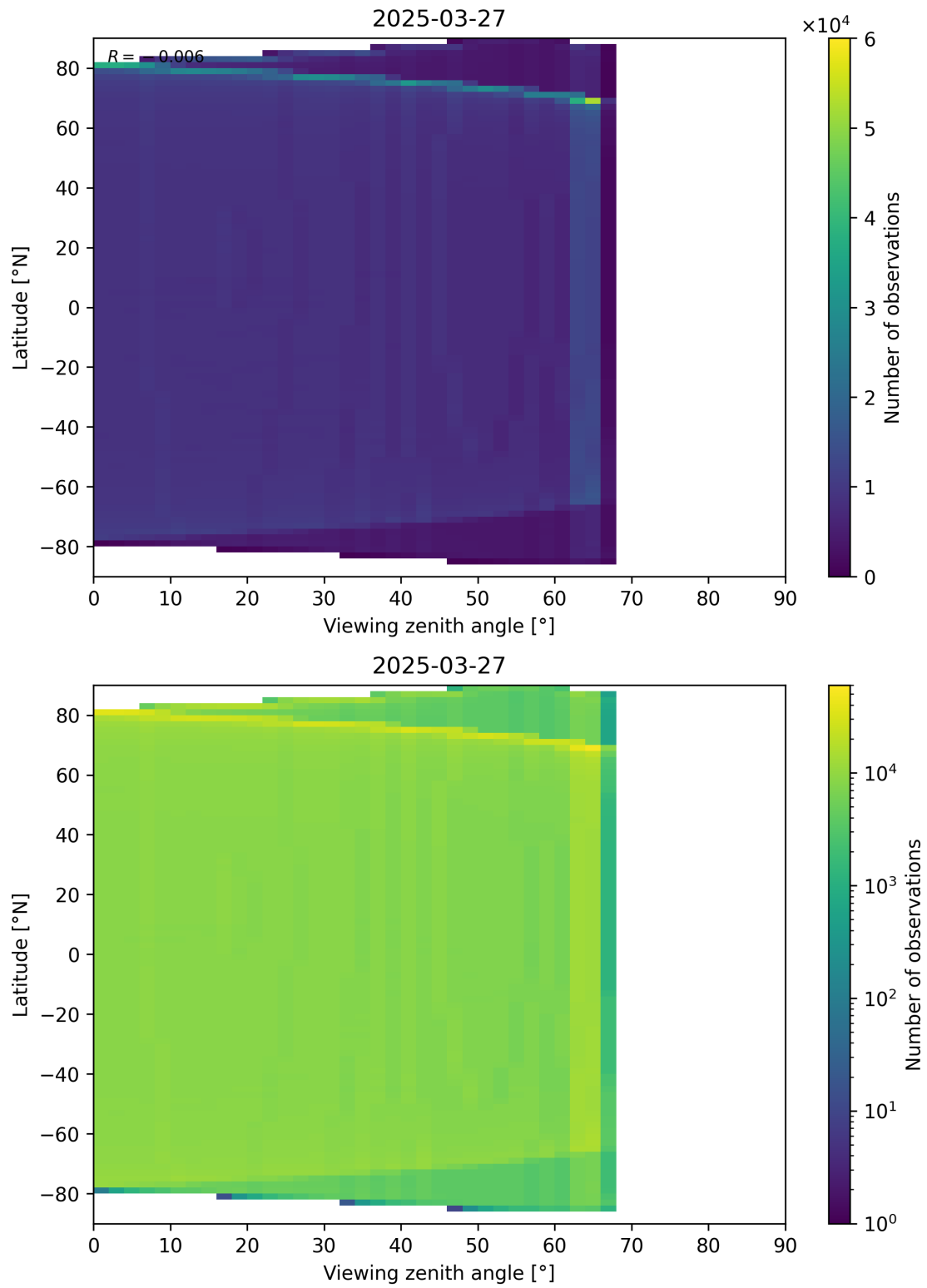
Figure 163: Scatter density plot of “Viewing zenith angle” against “Latitude” for 2025-03-27 to 2025-03-28.
