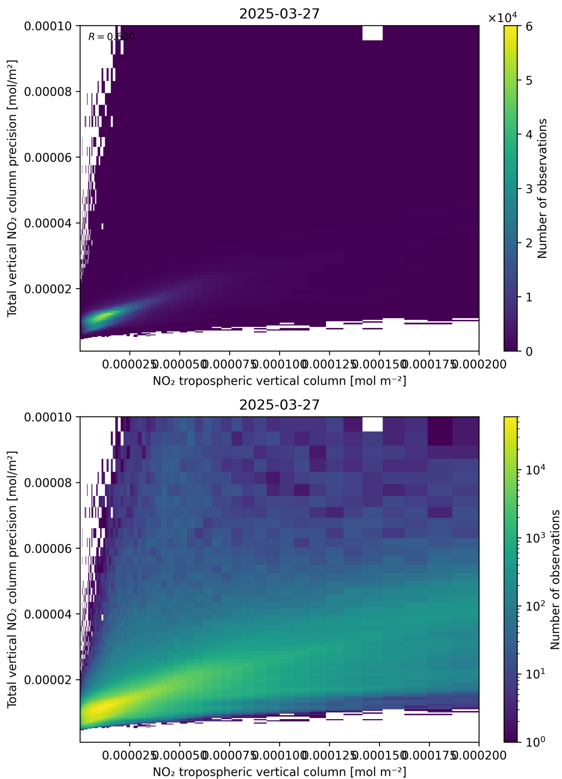
Figure 129: Scatter density plot of “NO 2 tropospheric vertical column” against “Total vertical NO 2 column precision” for 2025-03-27 to 2025-03-28.
