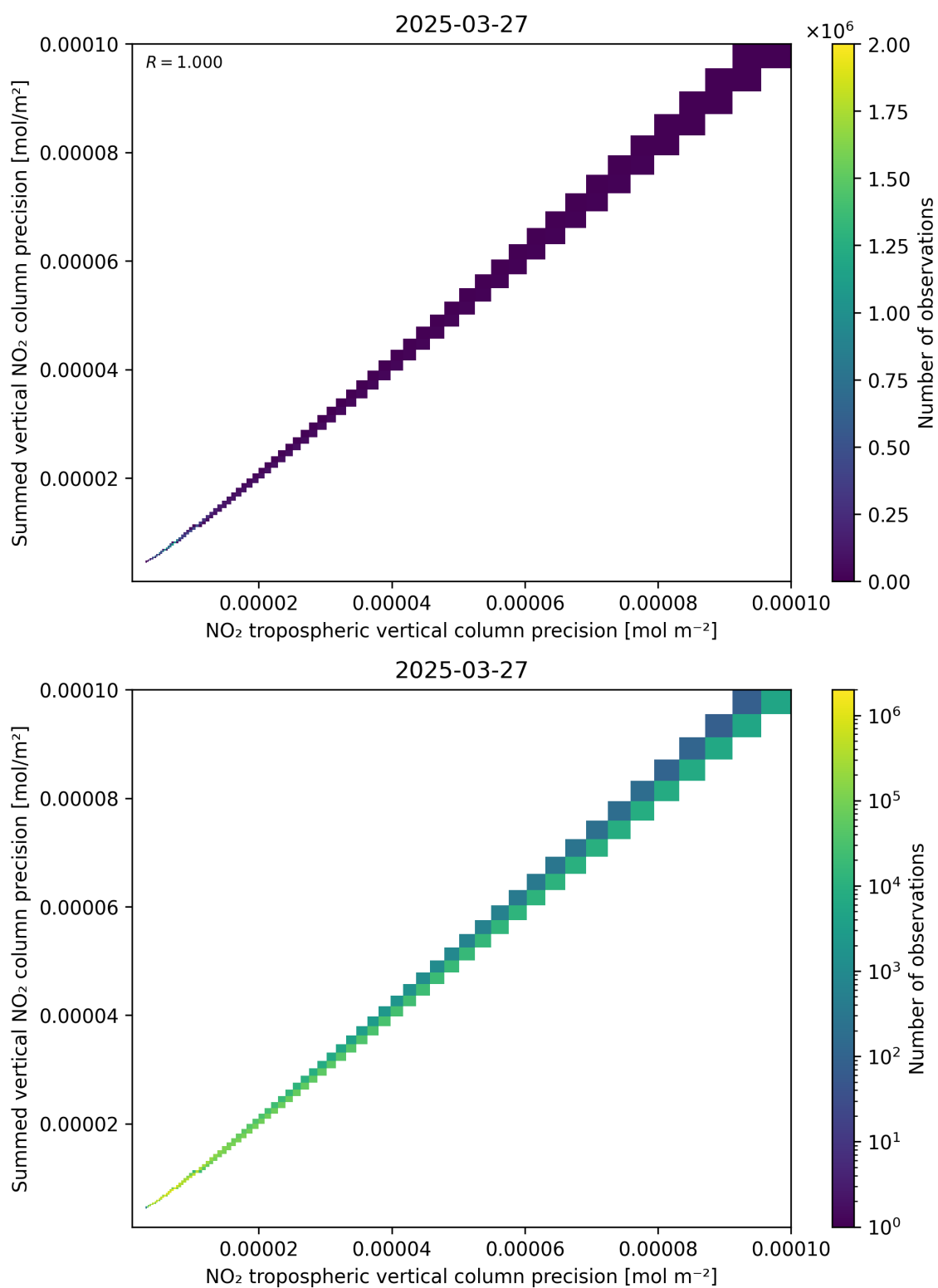
Figure 137: Scatter density plot of “NO 2 tropospheric vertical column precision” against “Summed vertical NO 2 column precision” for 2025-03-27 to 2025-03-28.
