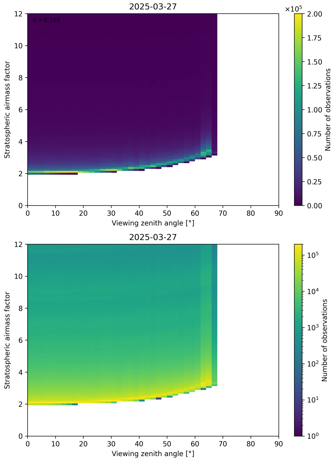
Figure 159: Scatter density plot of “Viewing zenith angle” against “Stratospheric airmass factor” for 2025-03-27 to 2025-03-28.
