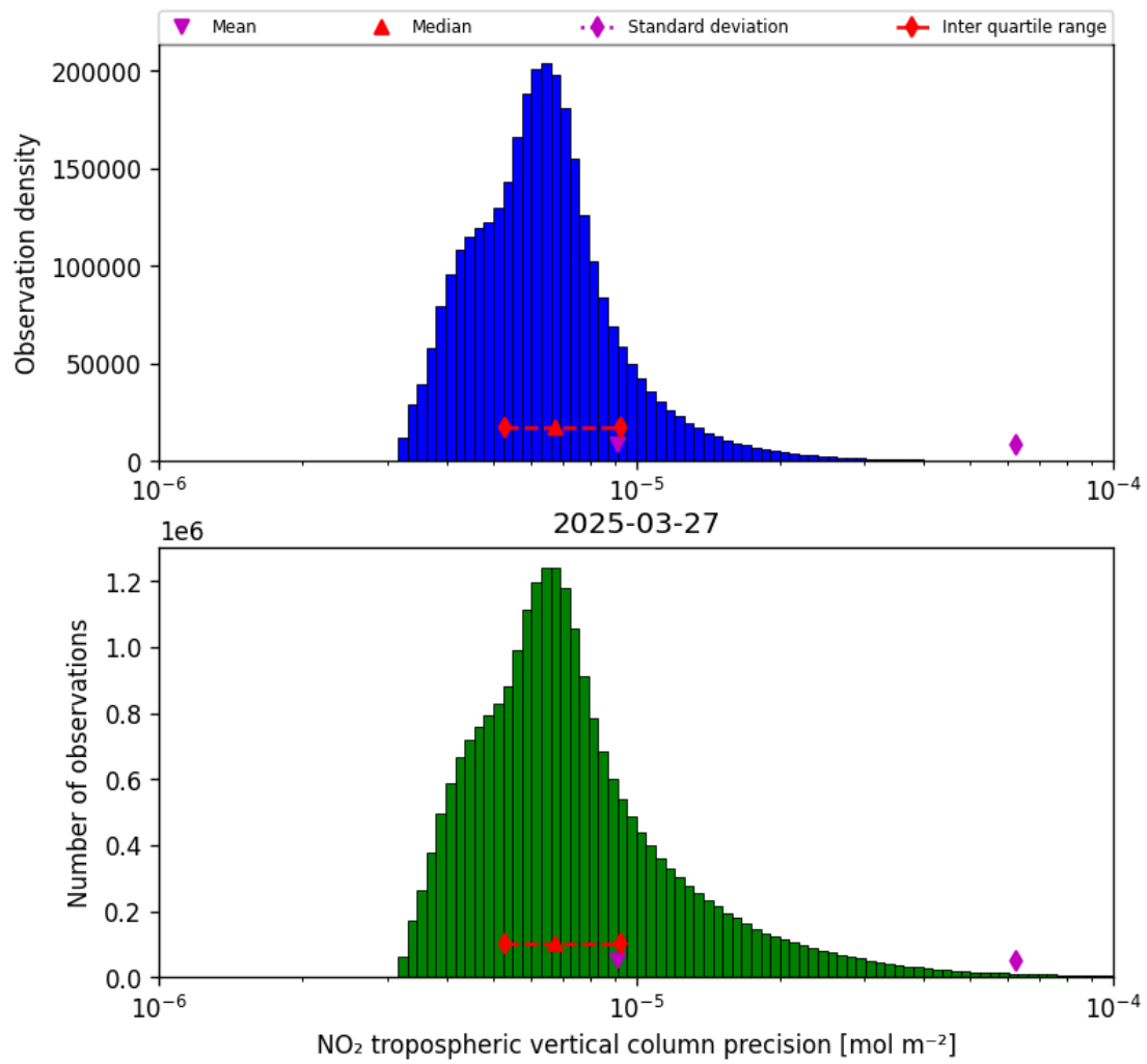
Figure 30: Histogram of “NO 2 tropospheric vertical column precision” for 2025-03-27 to 2025-03-28
