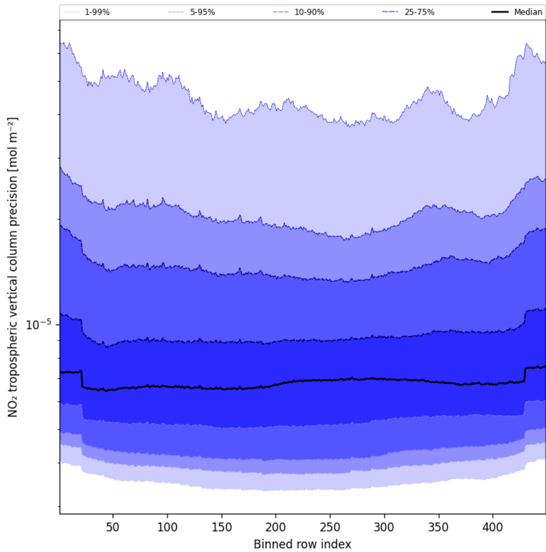
Figure 47: Along track statistics of “NO 2 tropospheric vertical column precision” for 2025-03-27 to 2025-03-28
