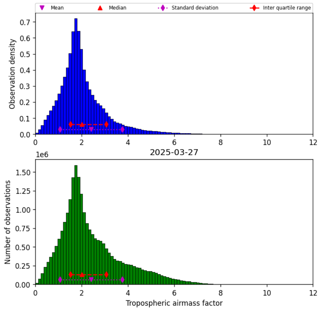
Figure 31: Histogram of “Tropospheric airmass factor” for 2025-03-27 to 2025-03-28
