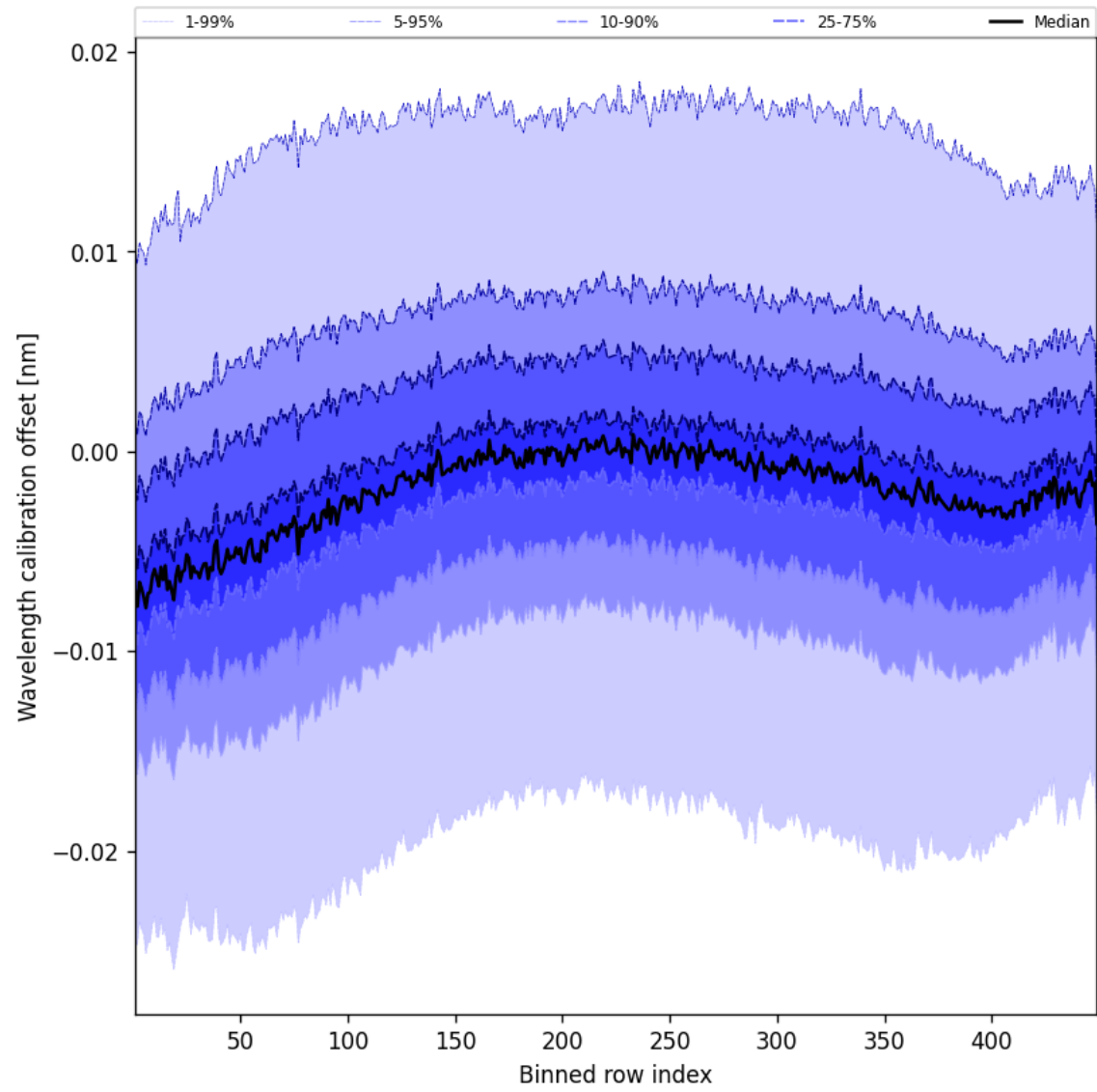
Figure 52: Along track statistics of “Wavelength calibration offset” for 2025-03-27 to 2025-03-28
