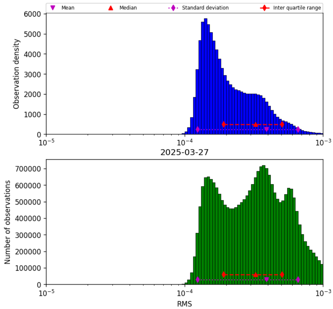
Figure 43: Histogram of “RMS” for 2025-03-27 to 2025-03-28
