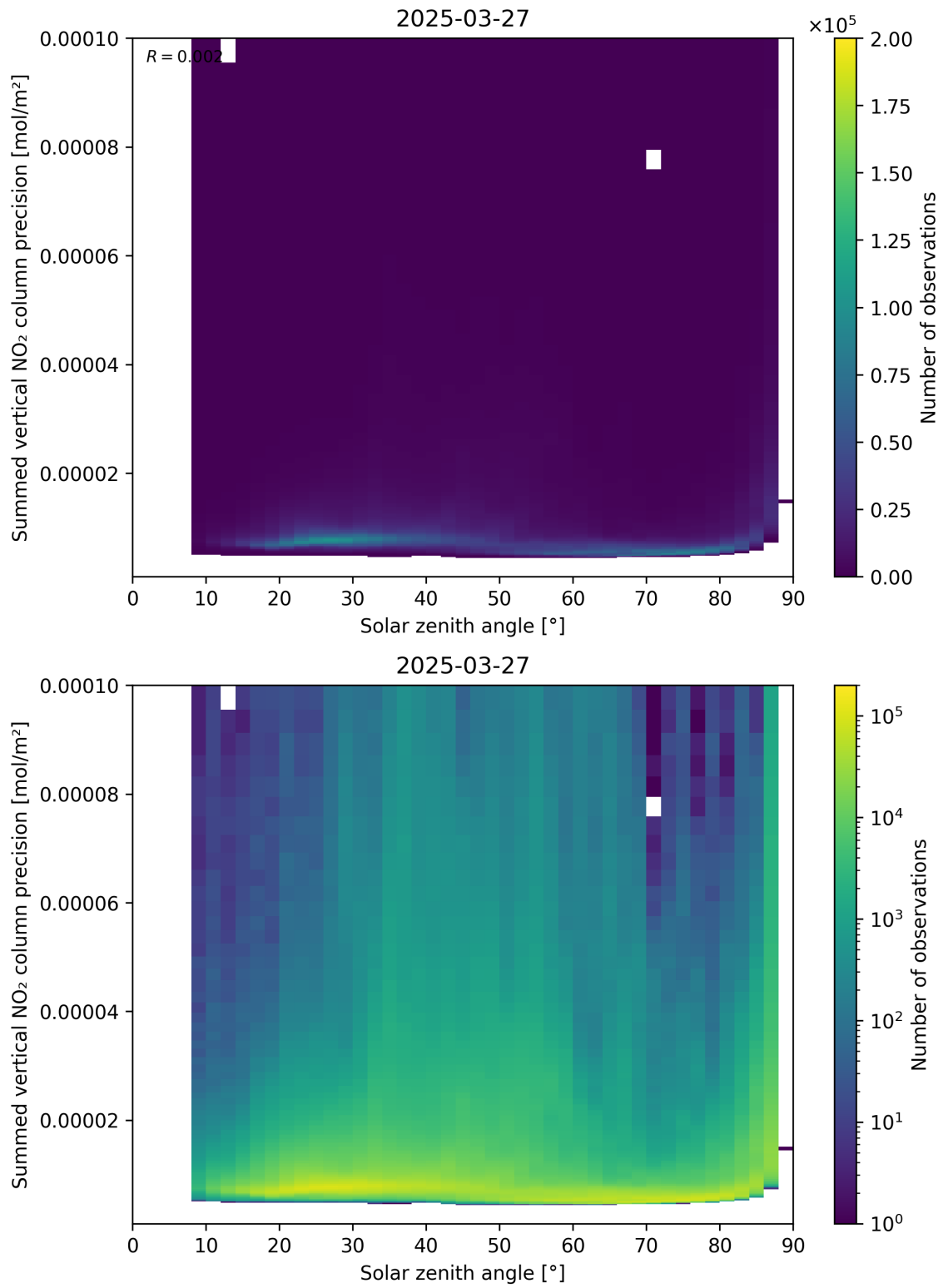
Figure 152: Scatter density plot of “Solar zenith angle” against “Summed vertical NO 2 column precision” for 2025-03-27 to 2025-03-28.
