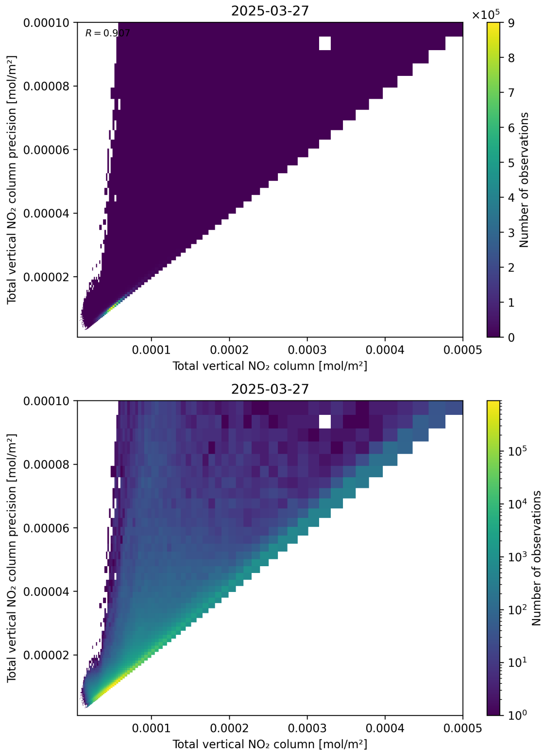
Figure 114: Scatter density plot of “Total vertical NO 2 column” against “Total vertical NO 2 column precision” for 2025-03-27 to 2025-03-28.
