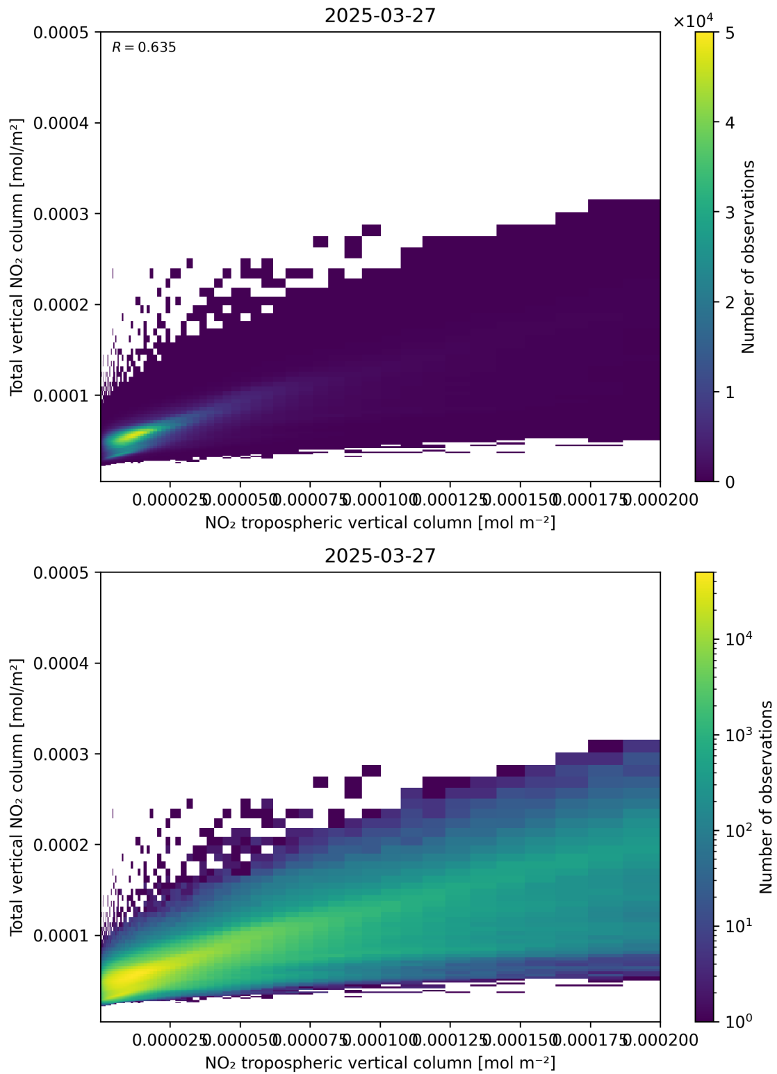
Figure 128: Scatter density plot of “NO 2 tropospheric vertical column” against “Total vertical NO 2 column” for 2025-03-27 to 2025-03-28.
