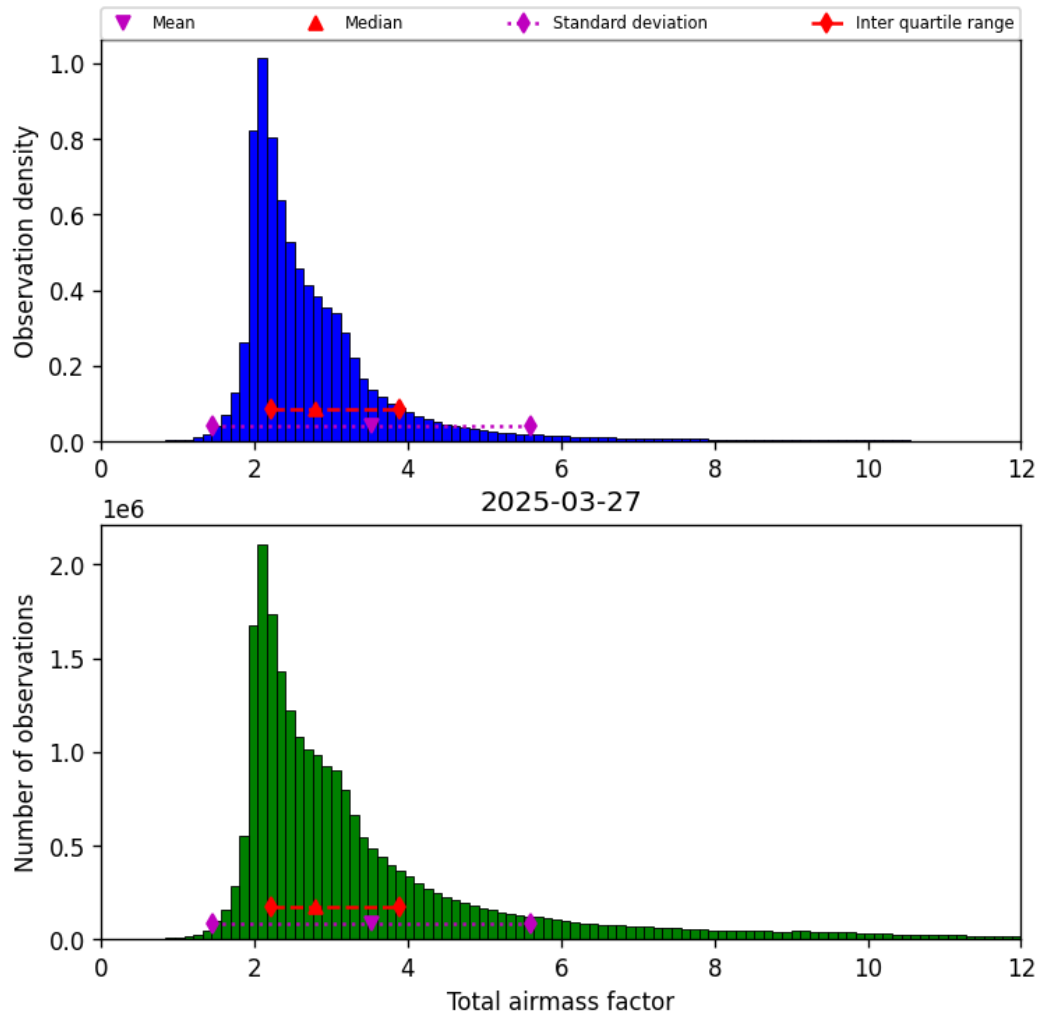
Figure 32: Histogram of “Total airmass factor” for 2025-03-27 to 2025-03-28
