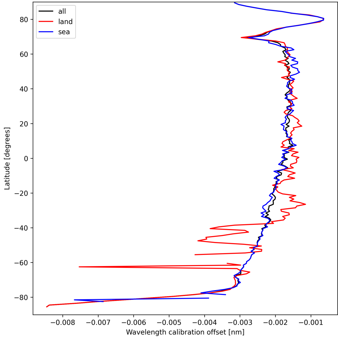
Figure 18: Zonal average of “Wavelength calibration offset” for 2025-03-27 to 2025-03-28.
