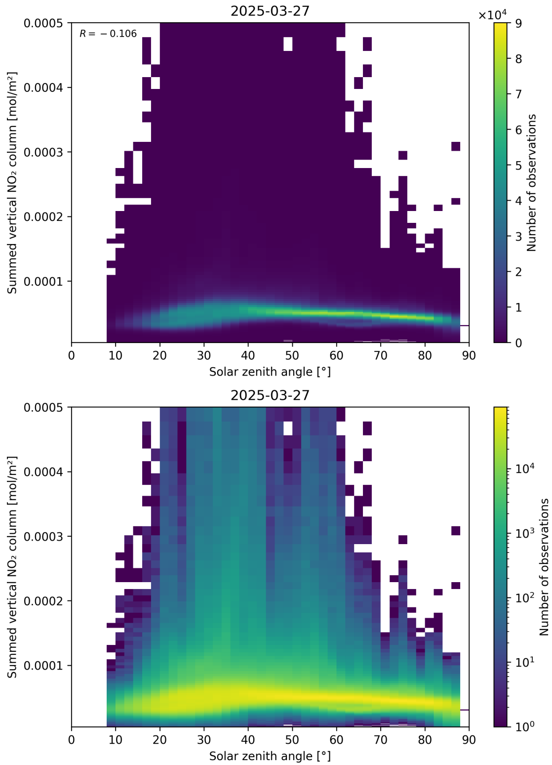
Figure 151: Scatter density plot of “Solar zenith angle” against “Summed vertical NO 2 column” for 2025-03-27 to 2025-03-28.
