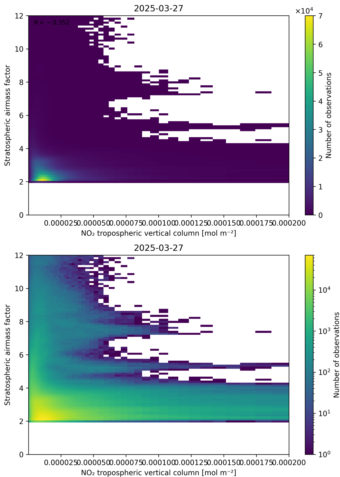
Figure 121: Scatter density plot of “NO 2 tropospheric vertical column” against “Stratospheric air mass factor” for 2025-03-27 to 2025-03-28.
