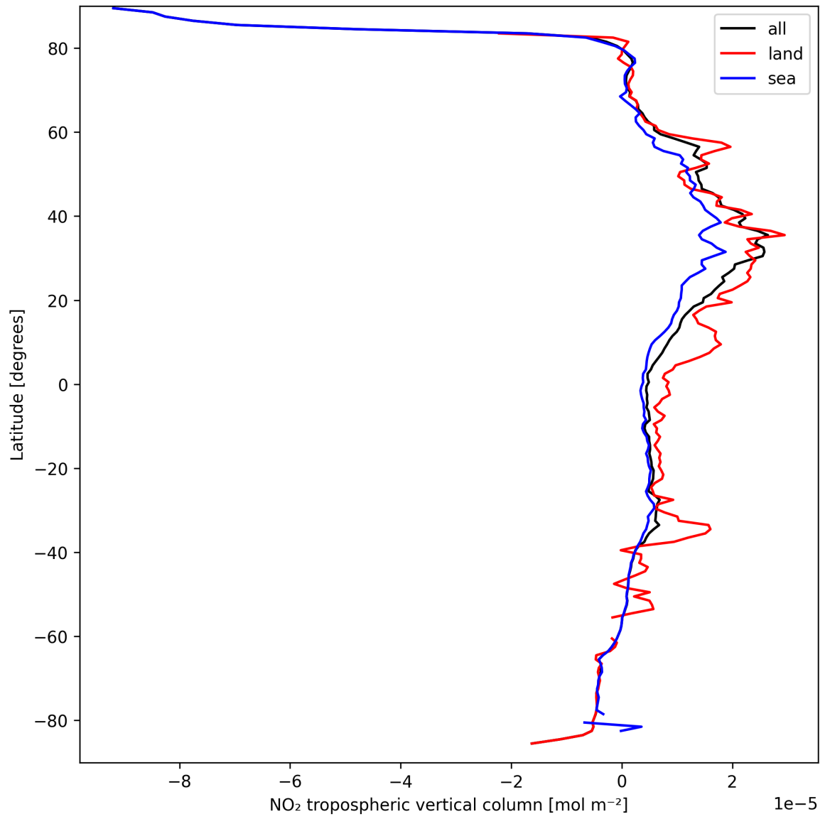
Figure 12: Zonal average of “NO 2 tropospheric vertical column” for 2025-03-27 to 2025-03-28.
