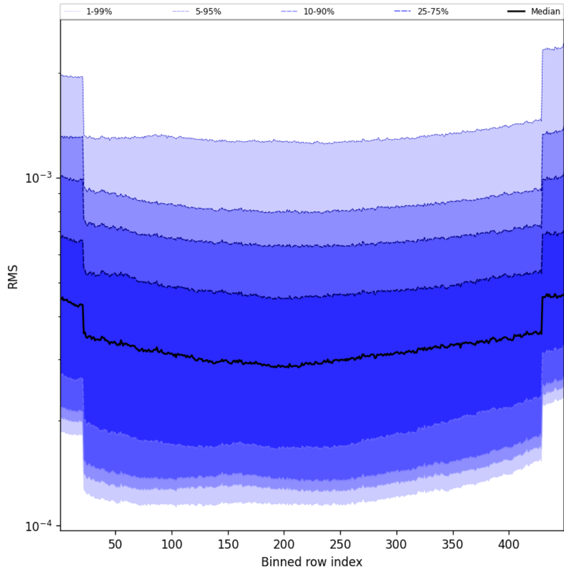
Figure 60: Along track statistics of “RMS” for 2025-03-27 to 2025-03-28
