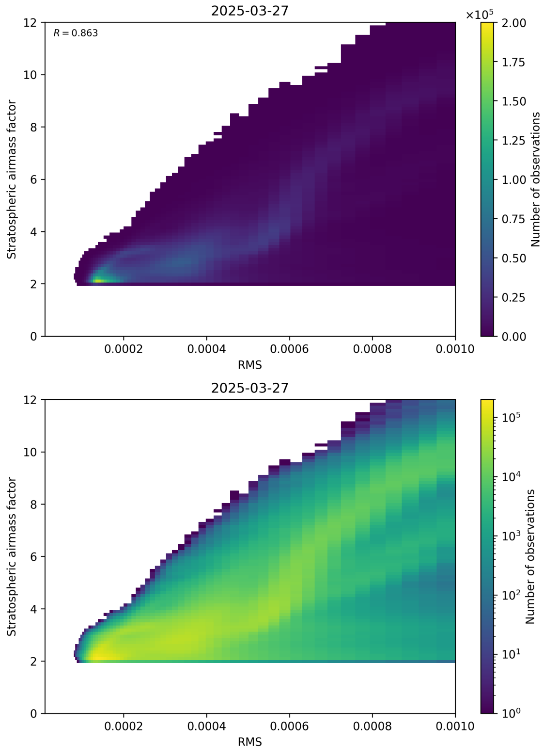
Figure 144: Scatter density plot of “RMS” against “Stratospheric airmass factor” for 2025-03-27 to 2025-03-28.
