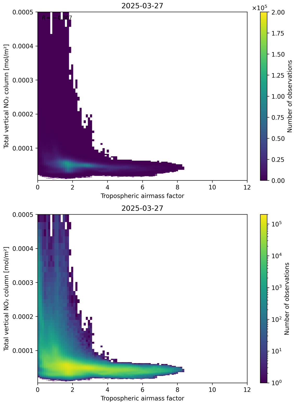
Figure 77: Scatter density plot of “Tropospheric airmass factor” against “Total vertical NO 2 column” for 2025-03-27 to 2025-03-28.
