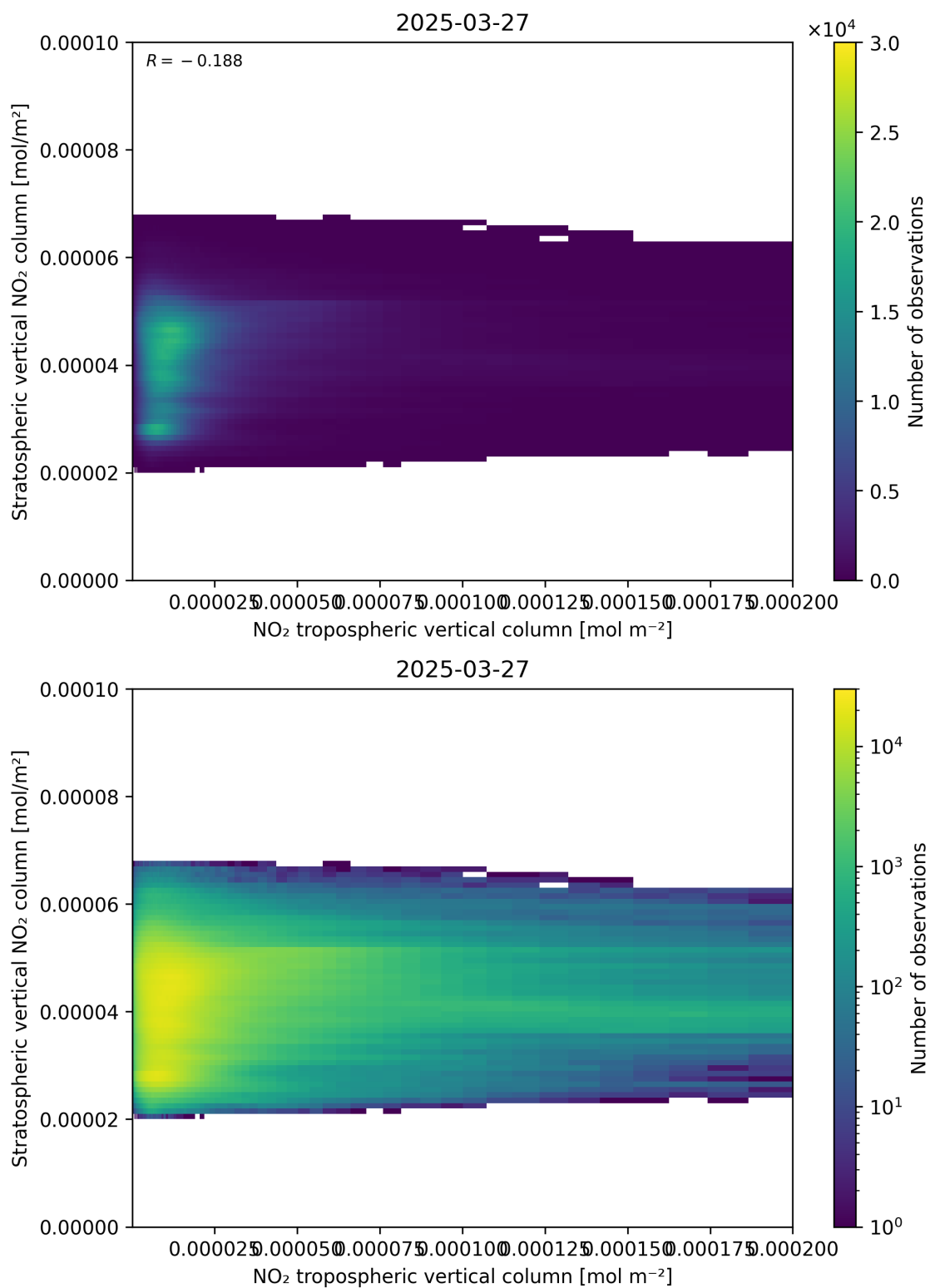
Figure 125: Scatter density plot of “NO 2 tropospheric vertical column” against “Stratospheric vertical NO 2 column” for 2025-03-27 to 2025-03-28.
