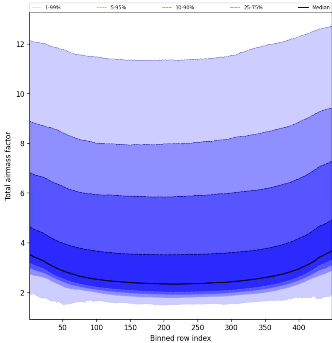
Figure 49: Along track statistics of “Total airmass factor” for 2025-03-27 to 2025-03-28
