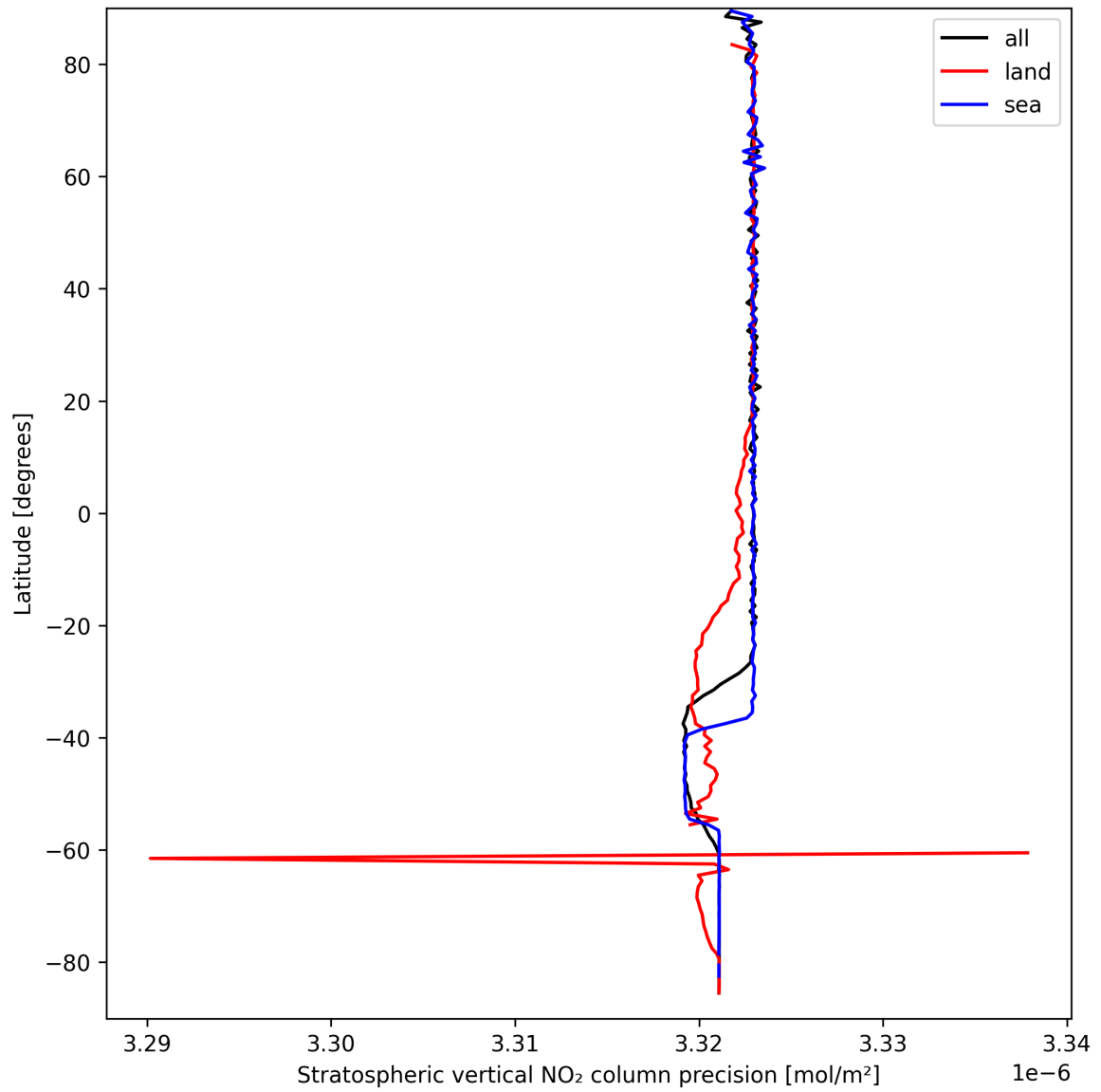
Figure 20: Zonal average of “Stratospheric vertical NO 2 column precision” for 2025-03-27 to 2025-03-28.
