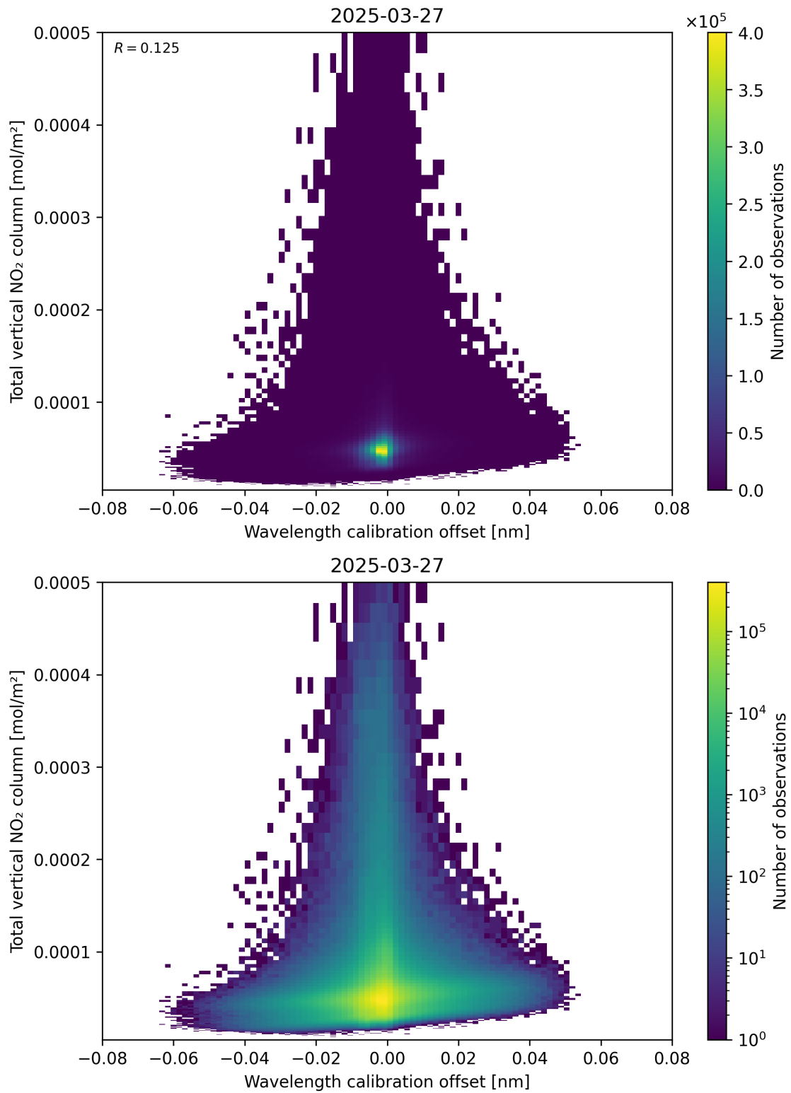
Figure 179: Scatter density plot of “Wavelength calibration offset” against “Total vertical NO 2 column” for 2025-03-27 to 2025-03-28.
