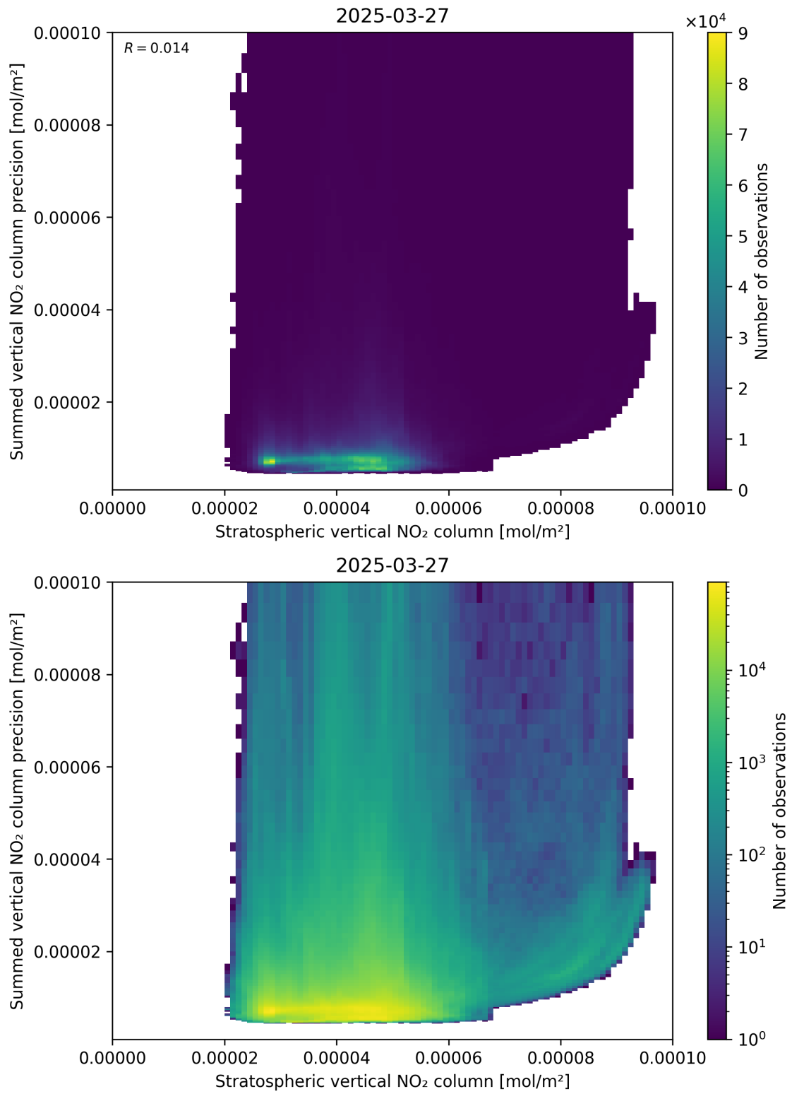
Figure 99: Scatter density plot of “Stratospheric vertical NO 2 column” against “Summed vertical NO 2 column precision” for 2025-03-27 to 2025-03-28.
