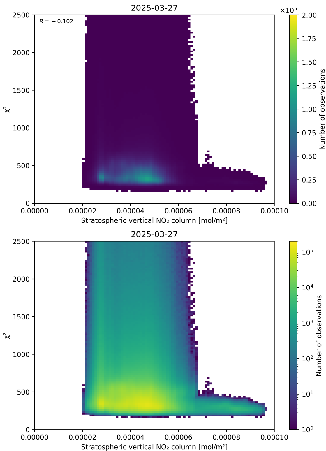
Figure 97: Scatter density plot of “Stratospheric vertical NO 2 column” against “ \chi^2 ” for 2025-03-27 to 2025-03-28.
