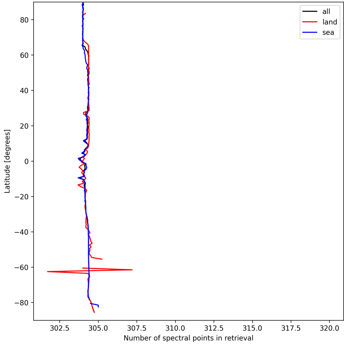
Figure 16: Zonal average of “Number of spectral points in retrieval” for 2025-03-27 to 2025-03-28.
