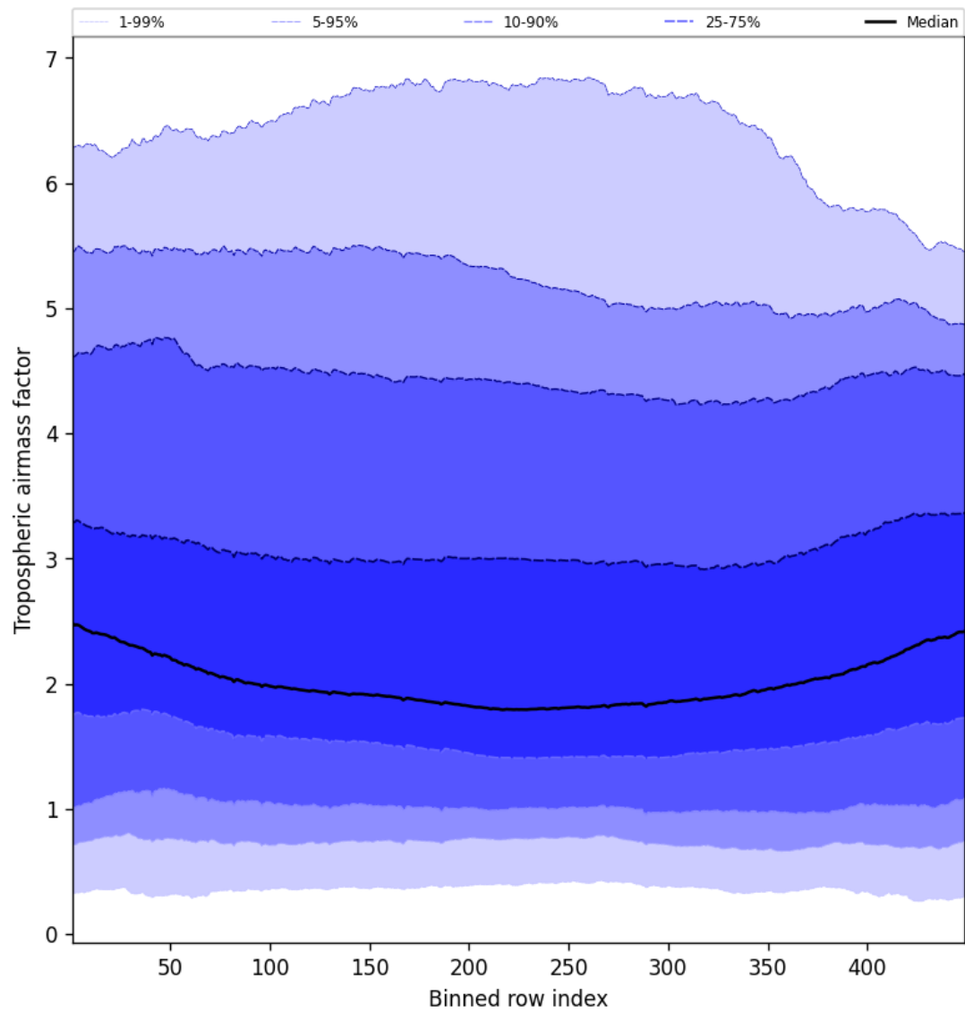
Figure 48: Along track statistics of “Tropospheric airmass factor” for 2025-03-27 to 2025-03-28
