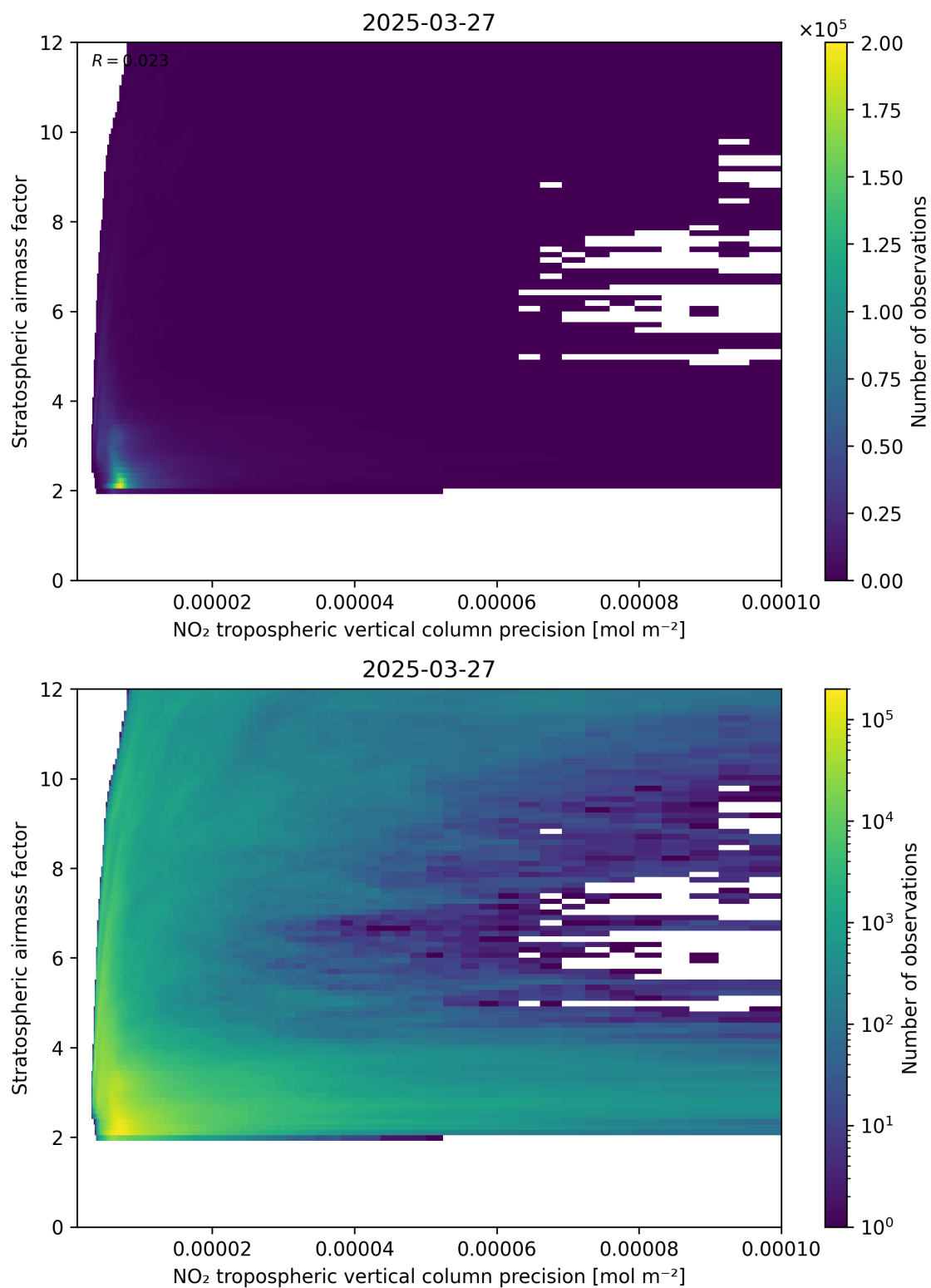
Figure 131: Scatter density plot of “NO 2 tropospheric vertical column precision” against “Stratospheric airmass factor” for 2025-03-27 to 2025-03-28.
