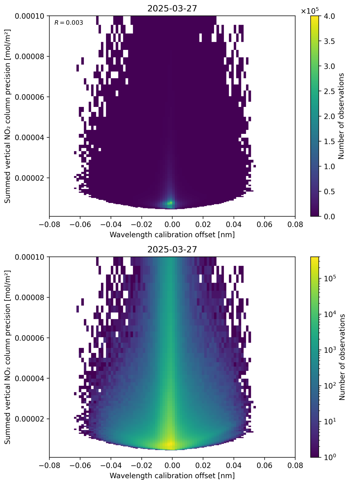
Figure 178: Scatter density plot of “Wavelength calibration offset” against “Summed vertical NO 2 column precision” for 2025-03-27 to 2025-03-28.
