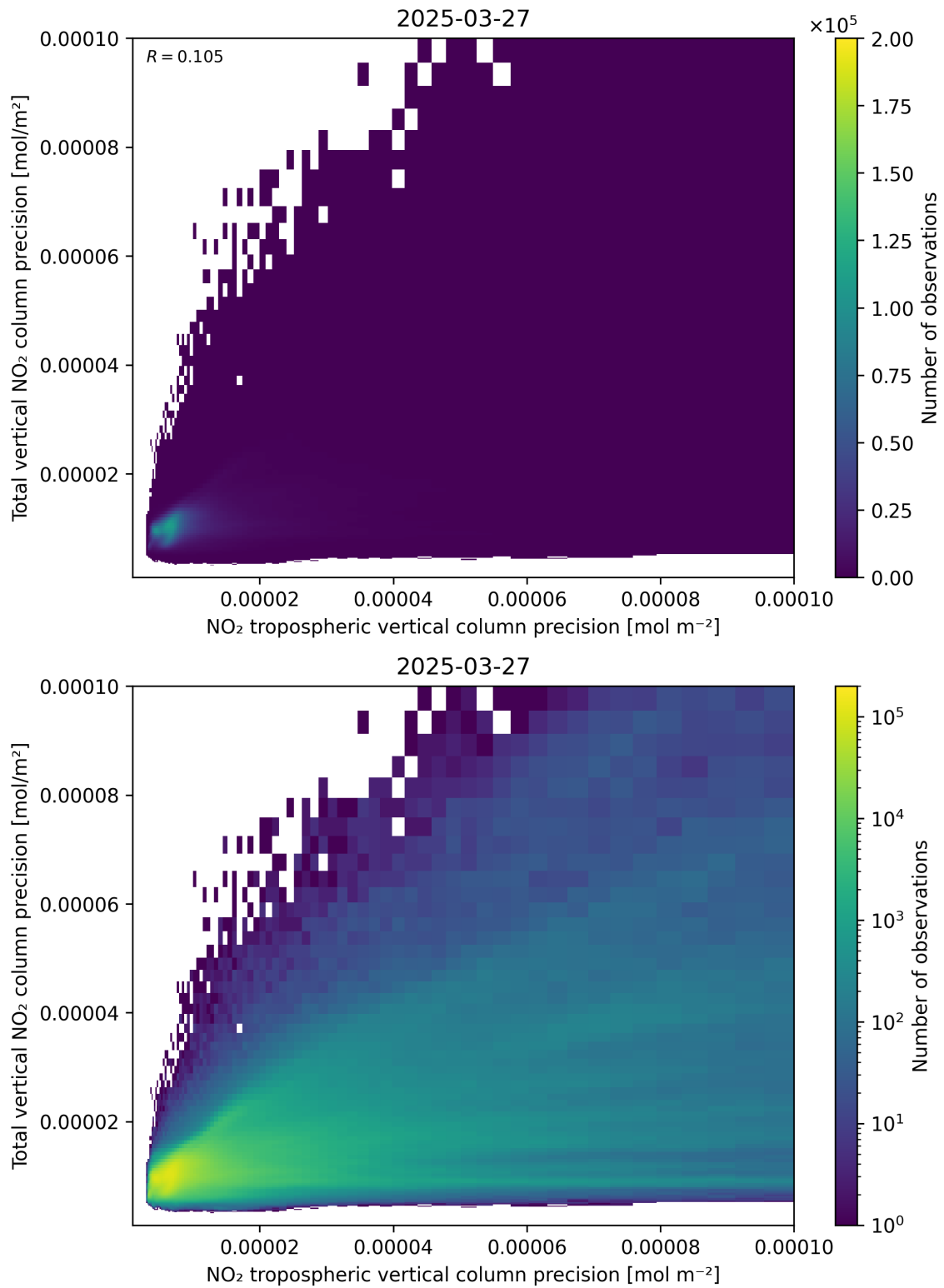
Figure 139: Scatter density plot of “NO 2 tropospheric vertical column precision” against “Total vertical NO 2 column precision” for 2025-03-27 to 2025-03-28.
