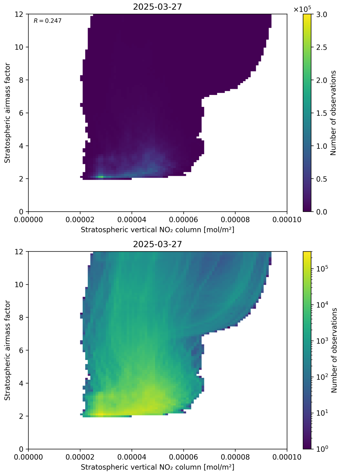
Figure 96: Scatter density plot of “Stratospheric vertical NO 2 column” against “Stratospheric airmass factor” for 2025-03-27 to 2025-03-28.
