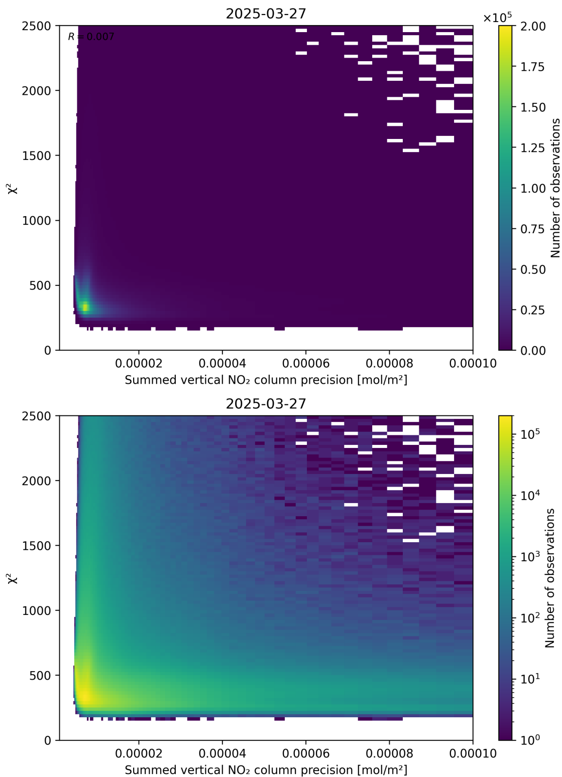
Figure 107: Scatter density plot of “Summed vertical NO 2 column precision” against “ \chi^2 ” for 2025-03-27 to 2025-03-28.
