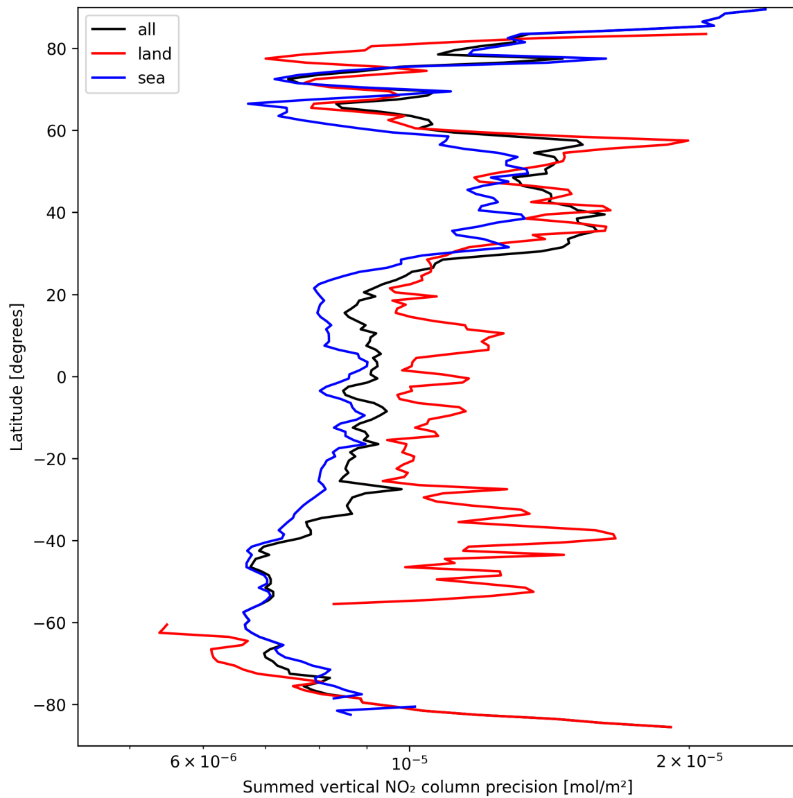
Figure 24: Zonal average of “Summed vertical NO 2 column precision” for 2025-03-27 to 2025-03-28.
