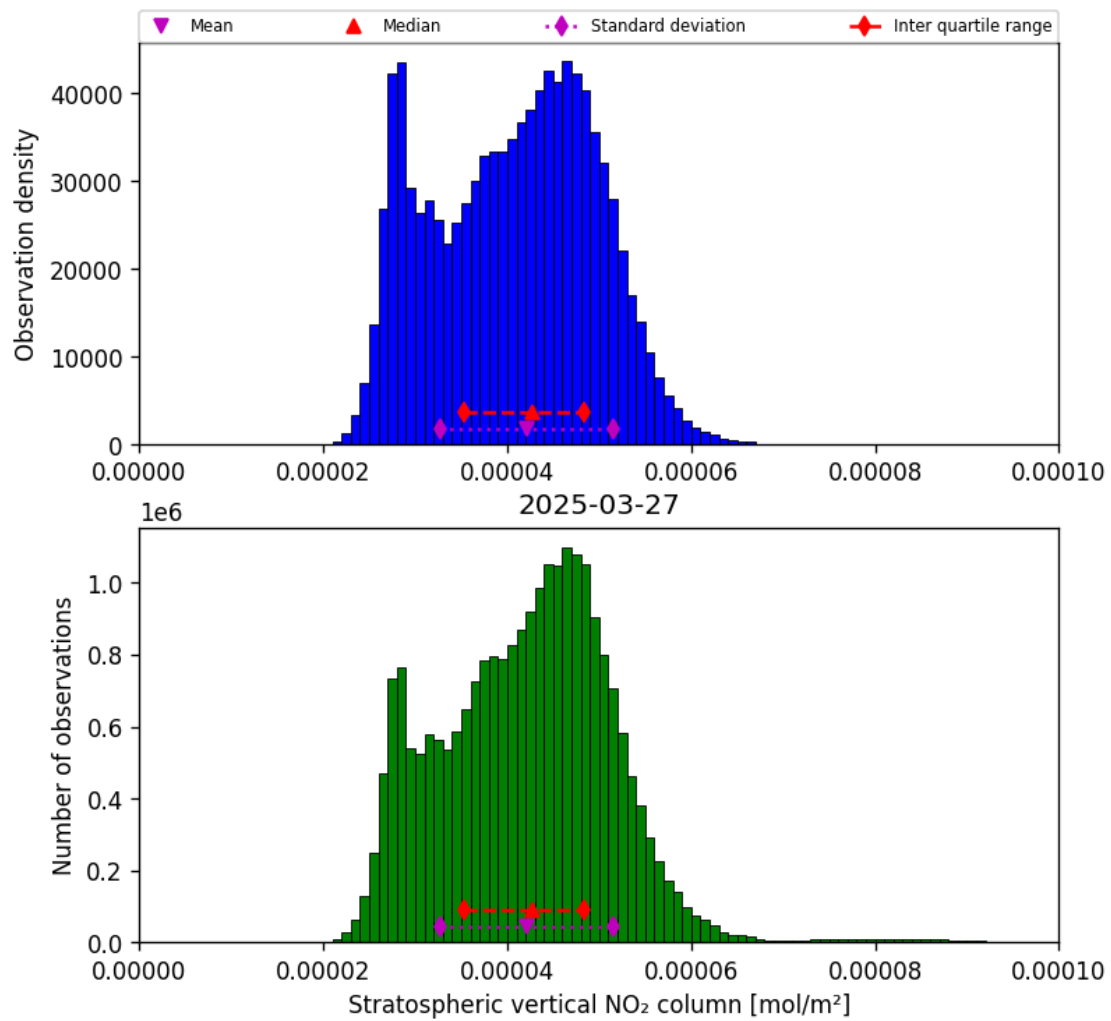
Figure 36: Histogram of “Stratospheric vertical NO 2 column” for 2025-03-27 to 2025-03-28
