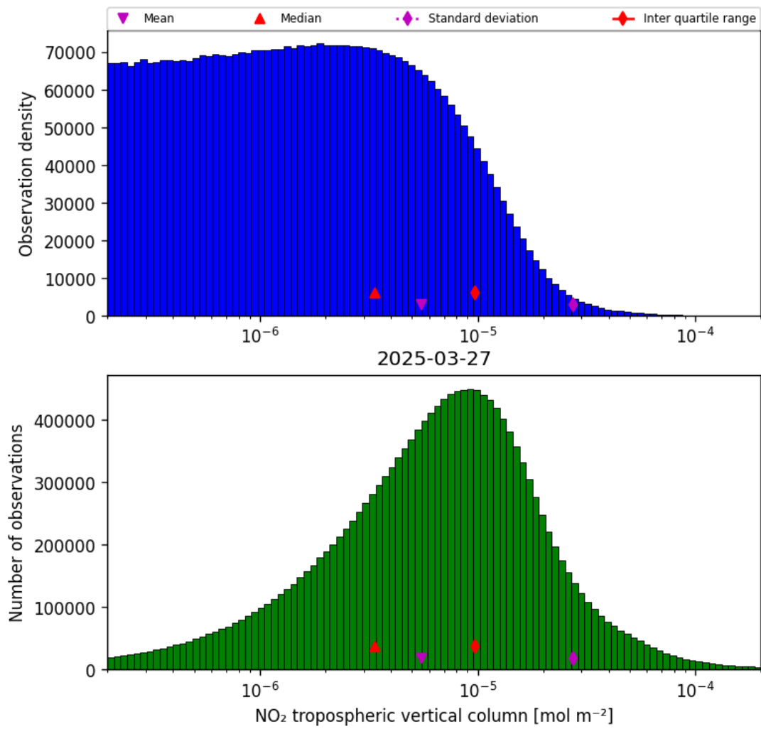
Figure 29: Histogram of “NO 2 tropospheric vertical column” for 2025-03-27 to 2025-03-28
