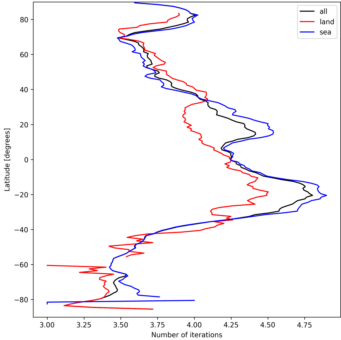
Figure 17: Zonal average of “Number of iterations” for 2025-03-27 to 2025-03-28.
