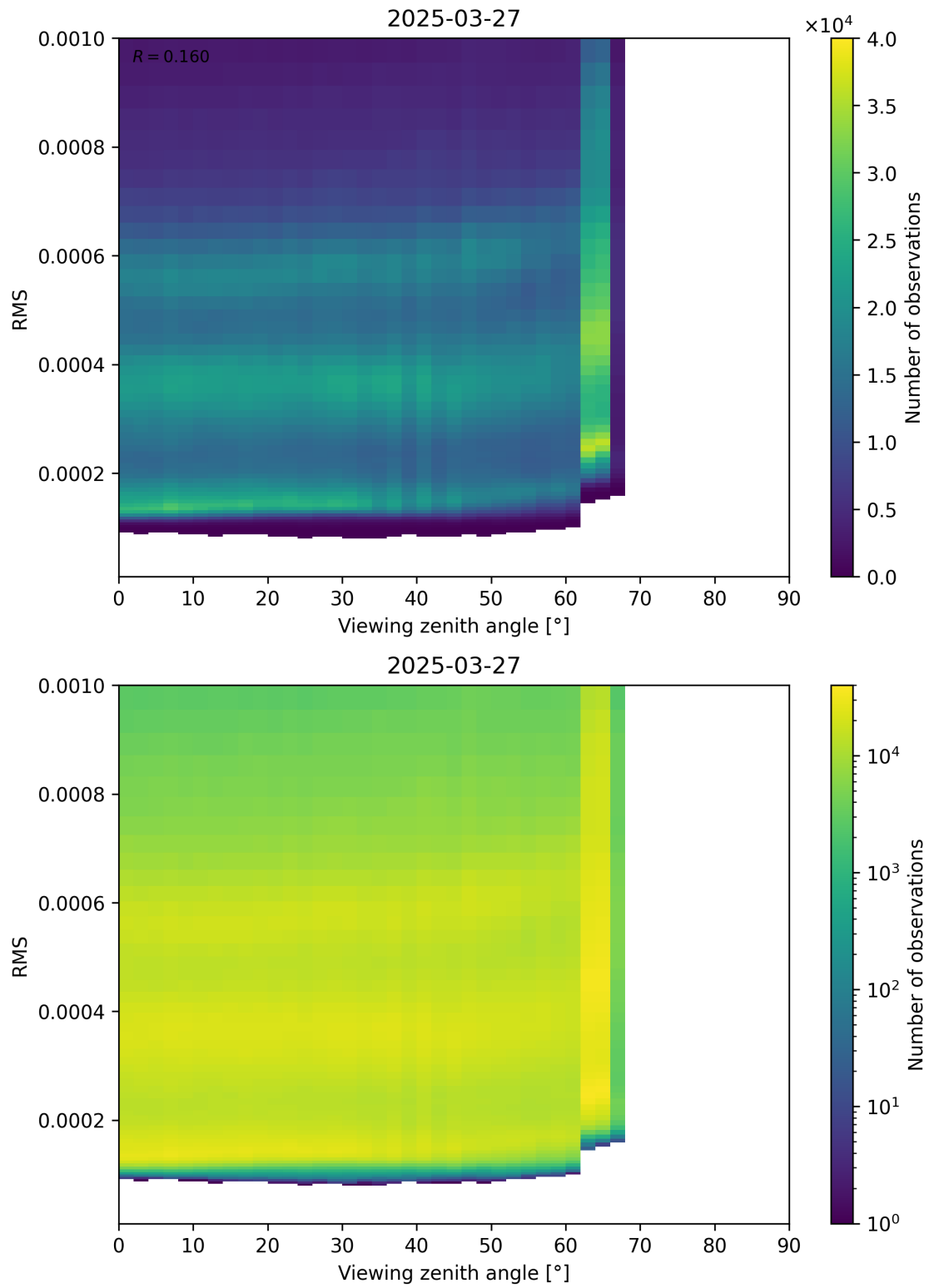
Figure 171: Scatter density plot of “Viewing zenith angle” against “RMS” for 2025-03-27 to 2025-03-28.
