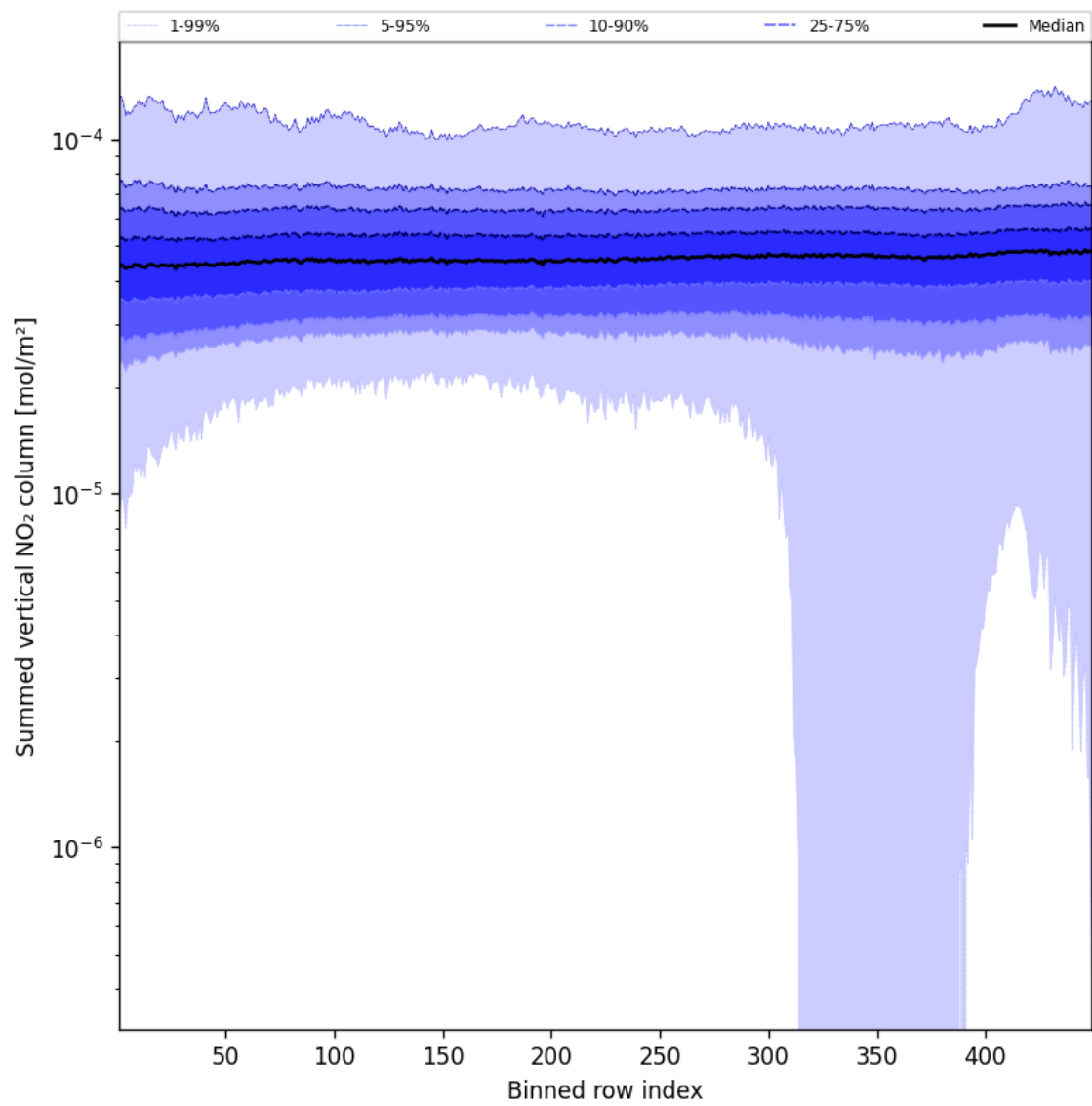
Figure 57: Along track statistics of “Summed vertical NO 2 column” for 2025-03-27 to 2025-03-28
