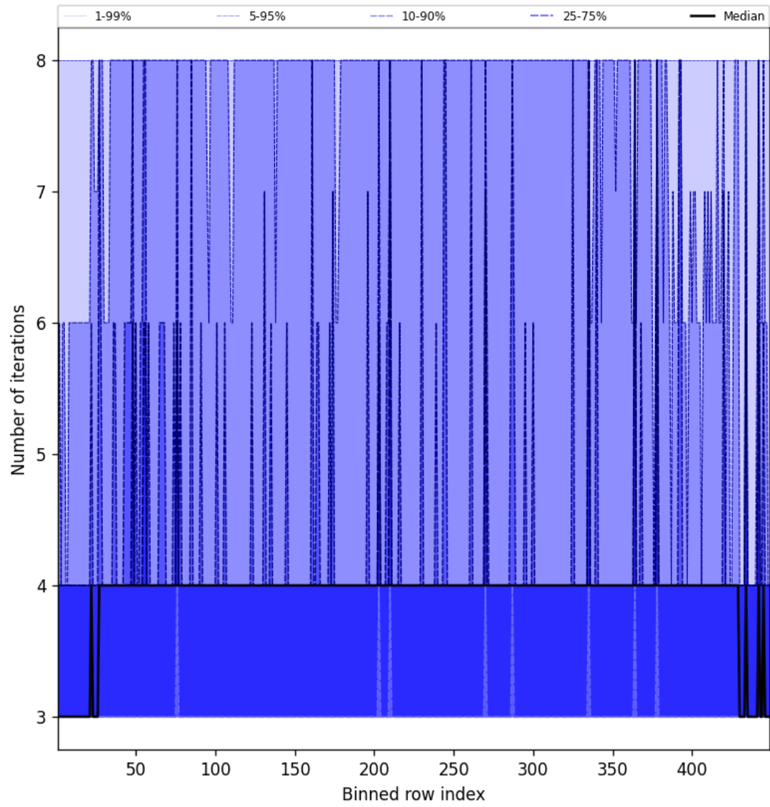
Figure 51: Along track statistics of “Number of iterations” for 2025-03-27 to 2025-03-28
