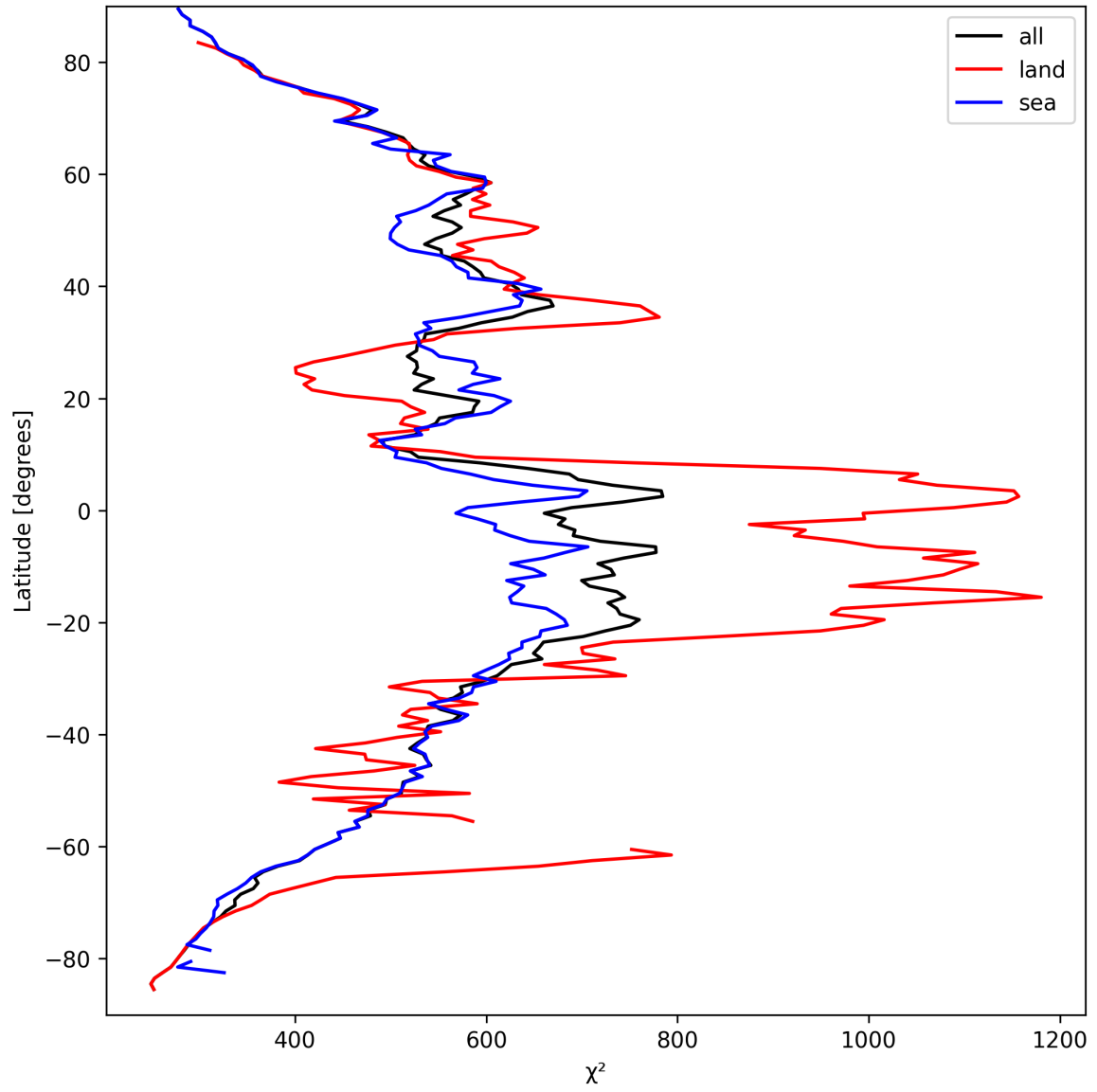
Figure 25: Zonal average of “ \chi^2 ” for 2025-03-27 to 2025-03-28.
