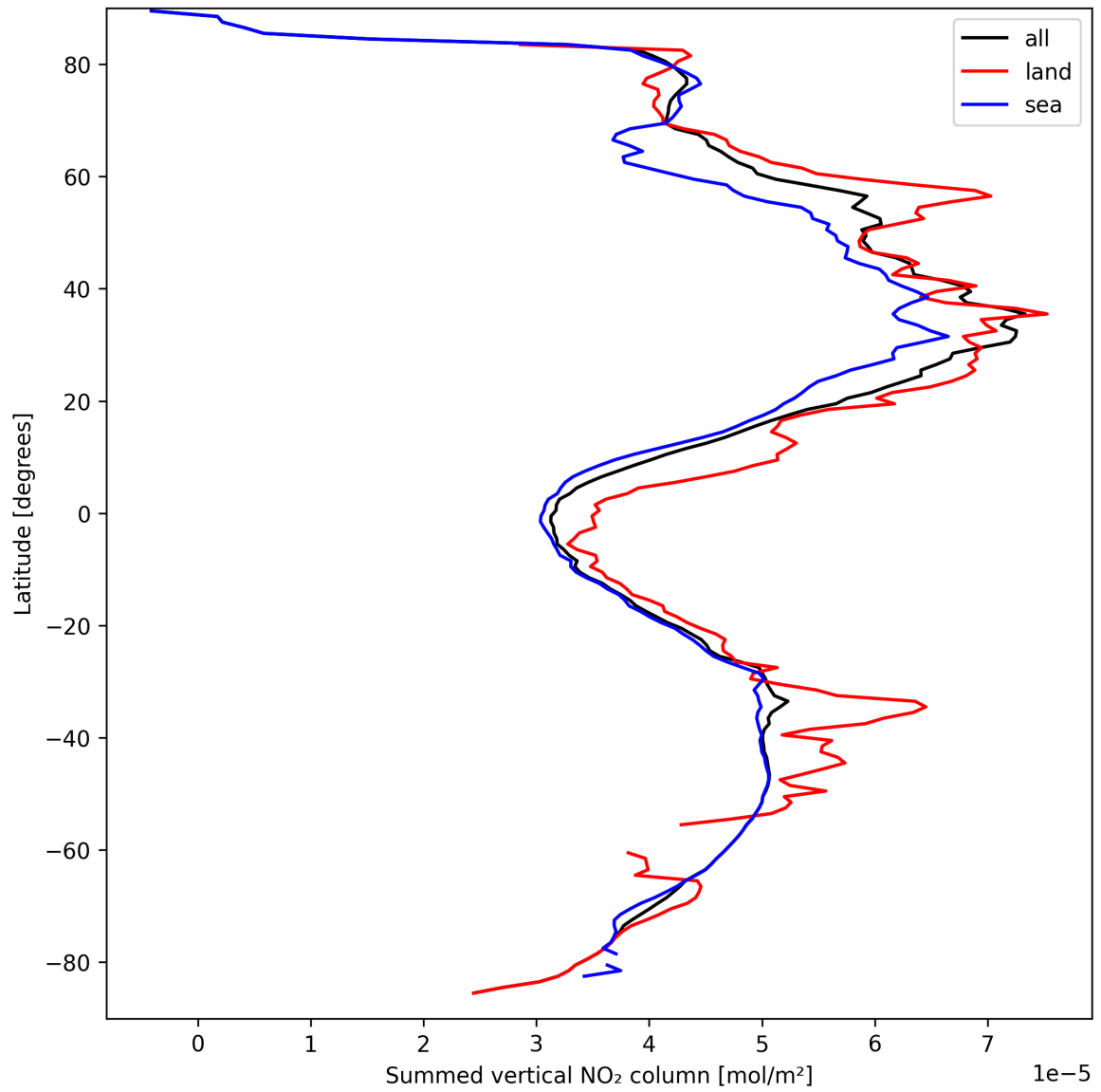
Figure 23: Zonal average of “Summed vertical NO 2 column” for 2025-03-27 to 2025-03-28.
