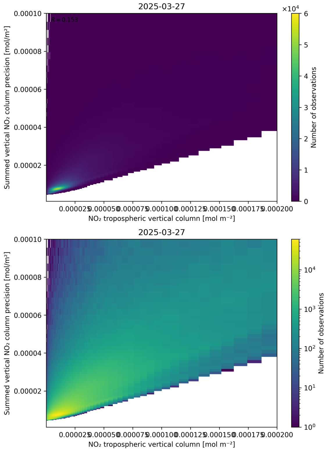
Figure 127: Scatter density plot of “NO 2 tropospheric vertical column” against “Summed vertical NO 2 column precision” for 2025-03-27 to 2025-03-28.
