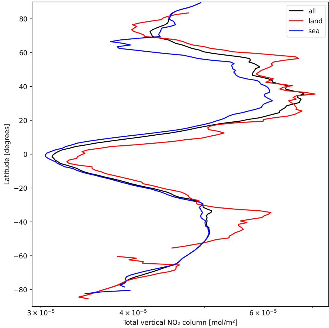
Figure 21: Zonal average of “Total vertical NO 2 column” for 2025-03-27 to 2025-03-28.
