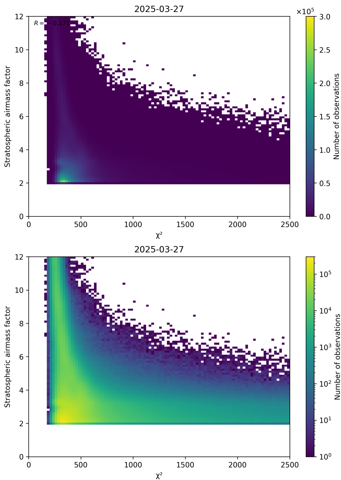
Figure 81: Scatter density plot of “ \chi^2 ” against “Stratospheric airmass factor” for 2025-03-27 to 2025-03-28.
