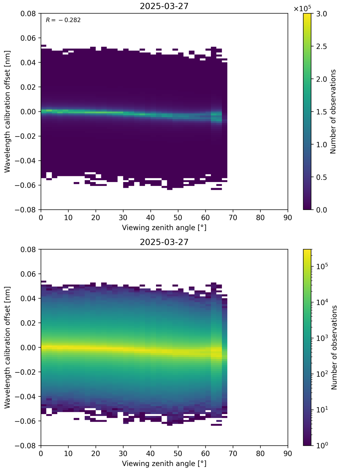
Figure 173: Scatter density plot of “Viewing zenith angle” against “Wavelength calibration offset” for 2025-03-27 to 2025-03-28.
