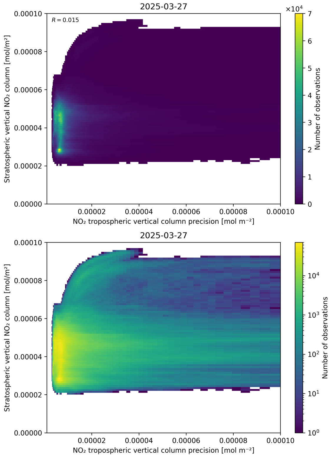
Figure 135: Scatter density plot of “NO 2 tropospheric vertical column precision” against “Stratospheric vertical NO 2 column” for 2025-03-27 to 2025-03-28.
