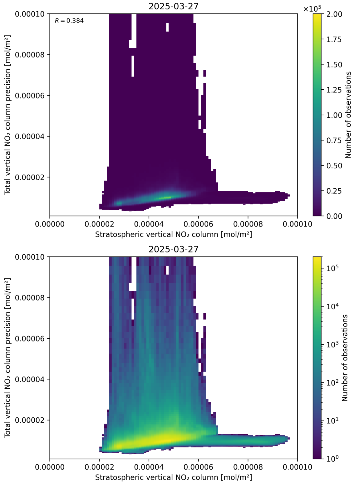
Figure 101: Scatter density plot of “Stratospheric vertical NO 2 column” against “Total vertical NO 2 column precision” for 2025-03-27 to 2025-03-28.
