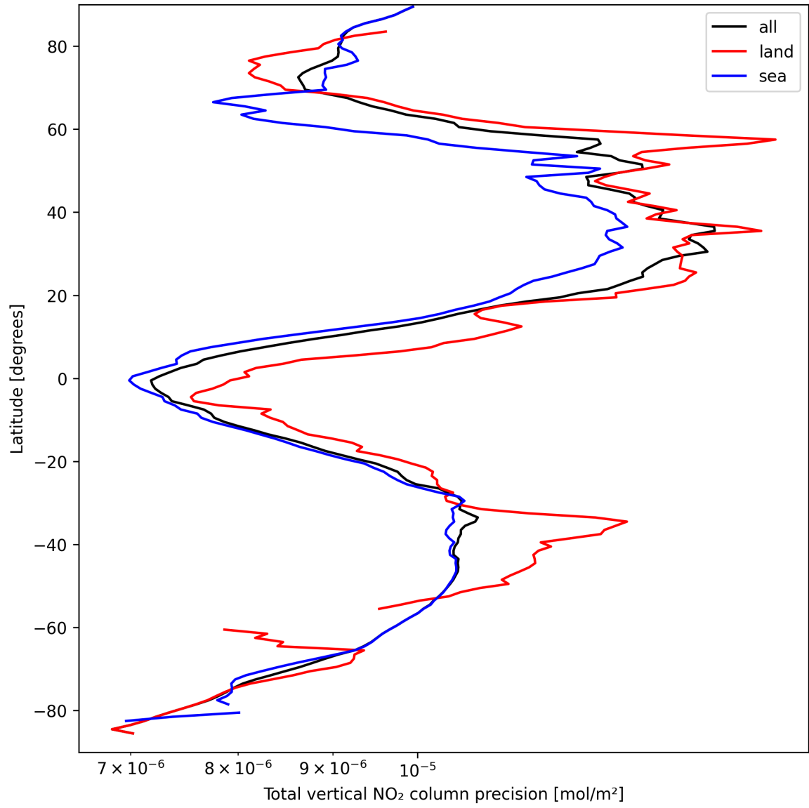
Figure 22: Zonal average of “Total vertical NO 2 column precision” for 2025-03-27 to 2025-03-28.
