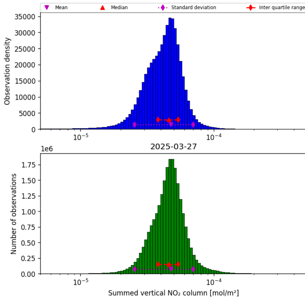
Figure 40: Histogram of “Summed vertical NO 2 column” for 2025-03-27 to 2025-03-28
