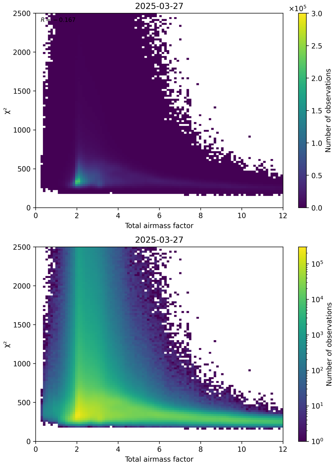
Figure 63: Scatter density plot of “Total airmass factor” against “ \chi^2 ” for 2025-03-27 to 2025-03-28.
