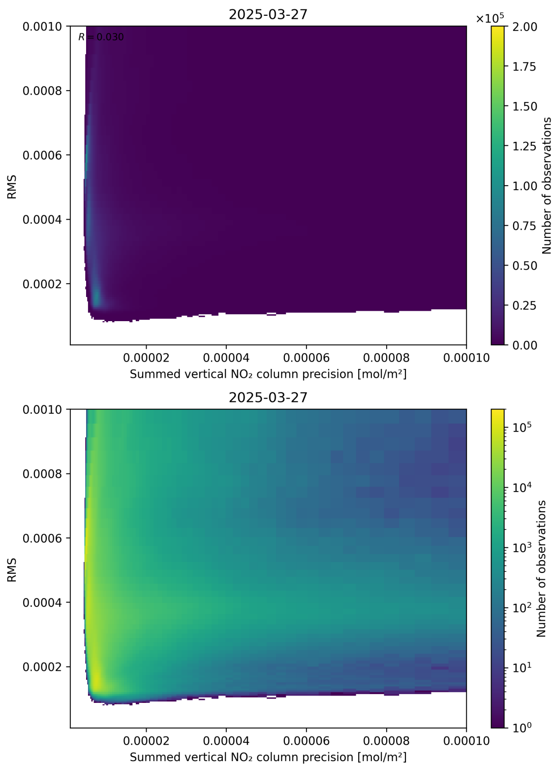
Figure 108: Scatter density plot of “Summed vertical NO 2 column precision” against “RMS” for 2025-03-27 to 2025-03-28.
