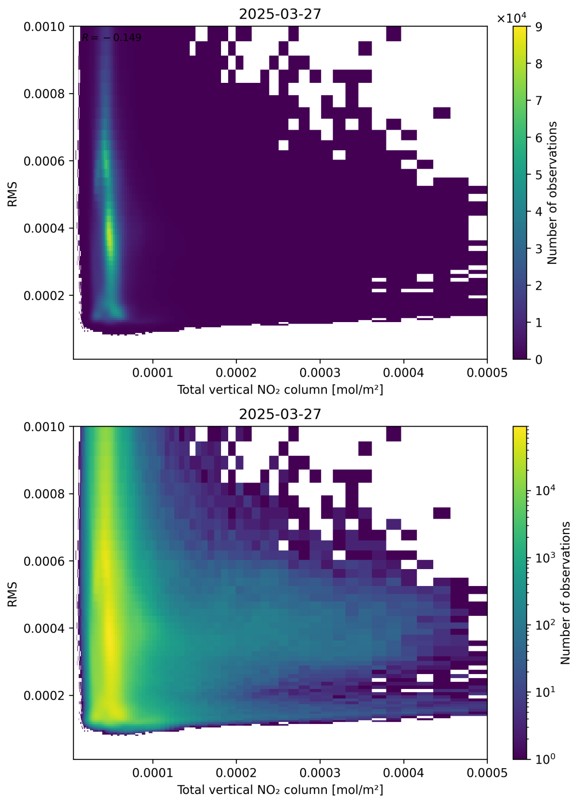
Figure 120: Scatter density plot of “Total vertical NO 2 column” against “RMS” for 2025-03-27 to 2025-03-28.
