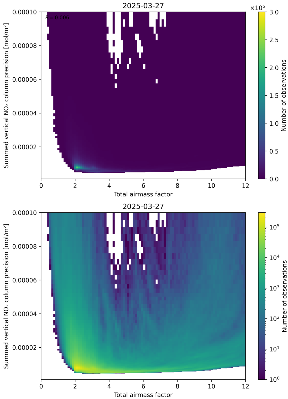
Figure 66: Scatter density plot of “Total airmass factor” against “Summed vertical NO 2 column precision” for 2025-03-27 to 2025-03-28.
