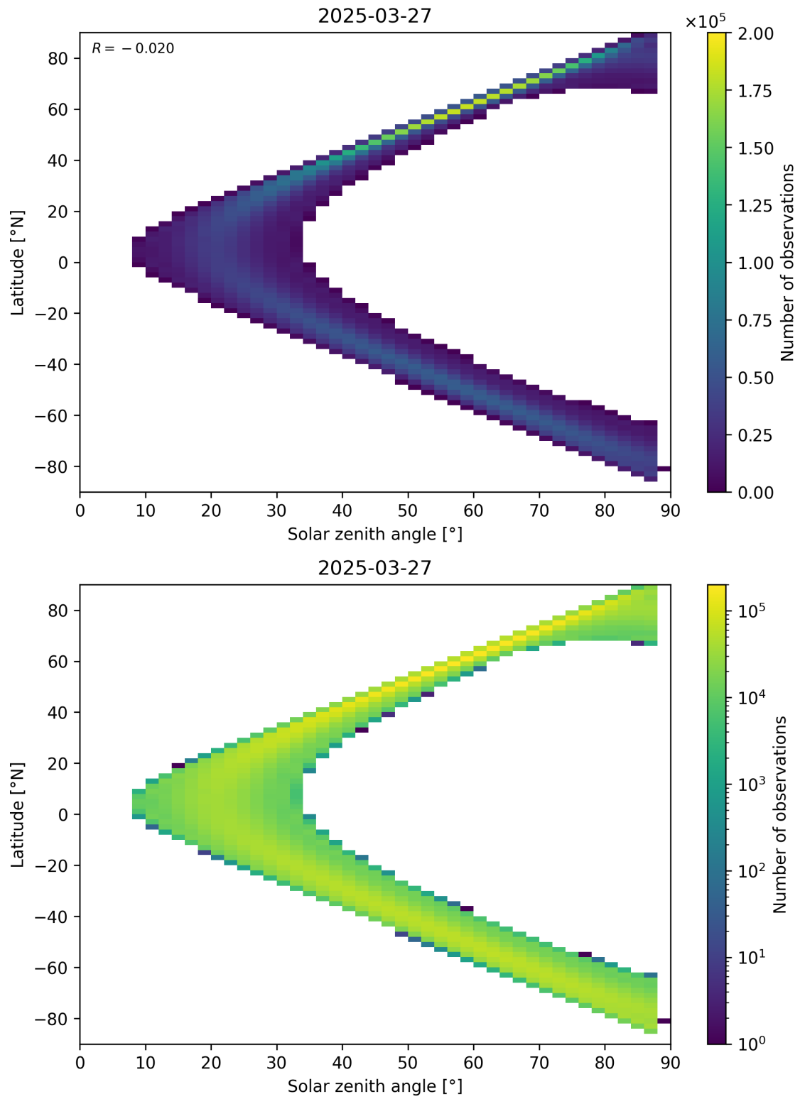
Figure 149: Scatter density plot of “Solar zenith angle” against “Latitude” for 2025-03-27 to 2025-03-28.
