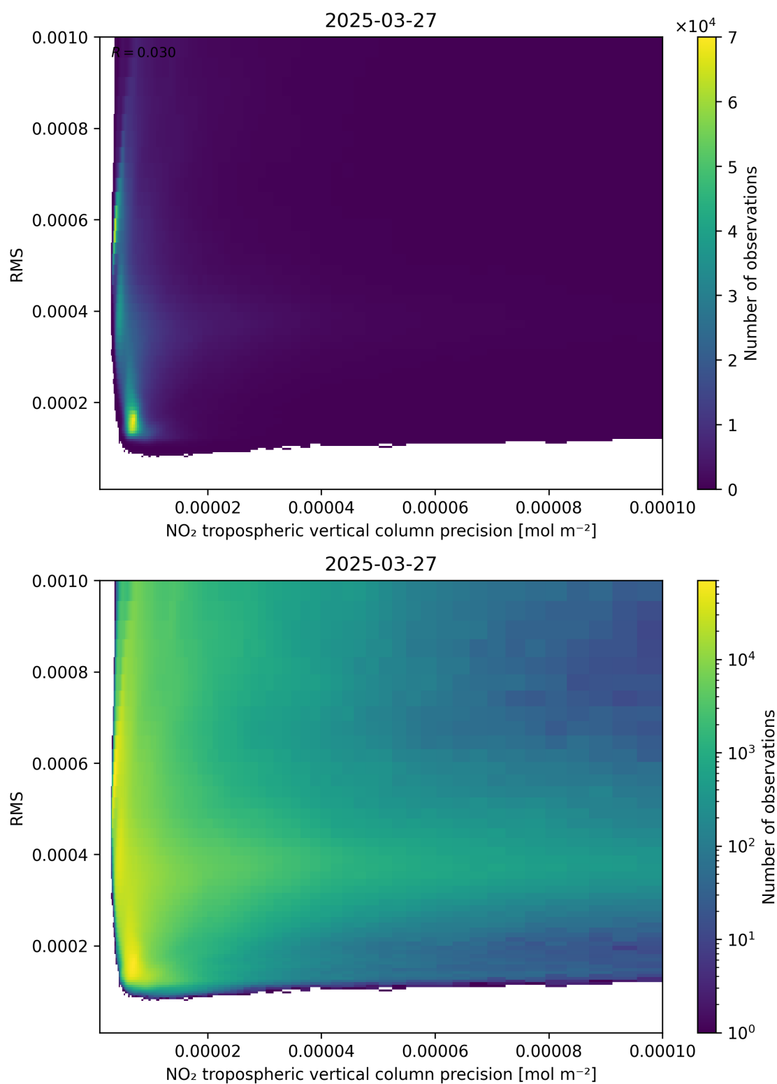
Figure 140: Scatter density plot of “NO 2 tropospheric vertical column precision” against “RMS” for 2025-03-27 to 2025-03-28.
