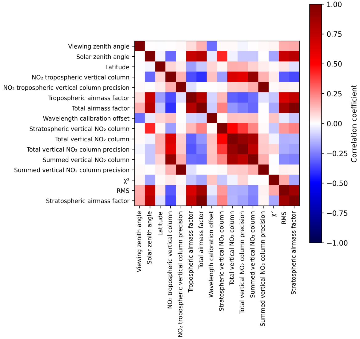
Figure 2: Map of correlation matrix for 2025-03-27 to 2025-03-28.
