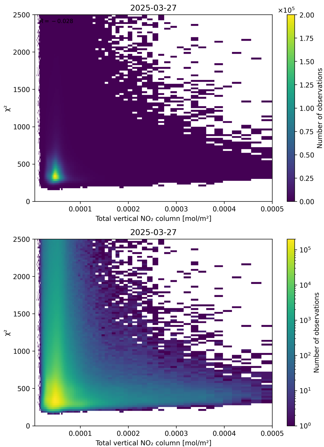
Figure 111: Scatter density plot of “Total vertical NO 2 column” against “ \chi^2 ” for 2025-03-27 to 2025-03-28.
