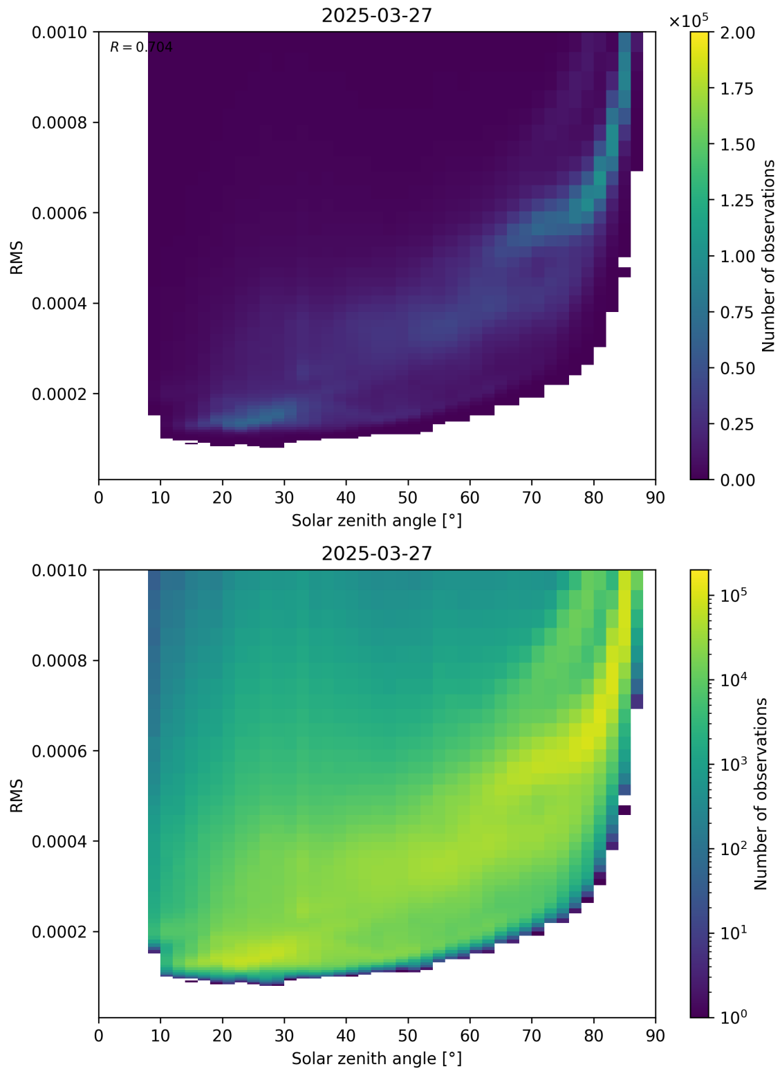
Figure 157: Scatter density plot of “Solar zenith angle” against “RMS” for 2025-03-27 to 2025-03-28.
