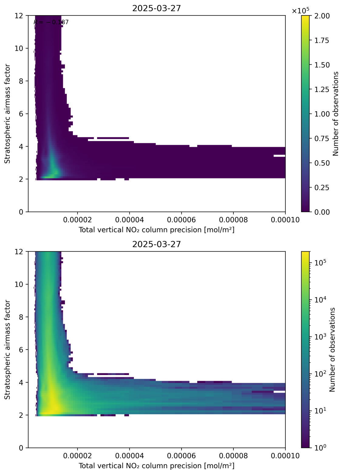
Figure 115: Scatter density plot of “Total vertical NO 2 column precision” against “Stratospheric air mass factor” for 2025-03-27 to 2025-03-28.
