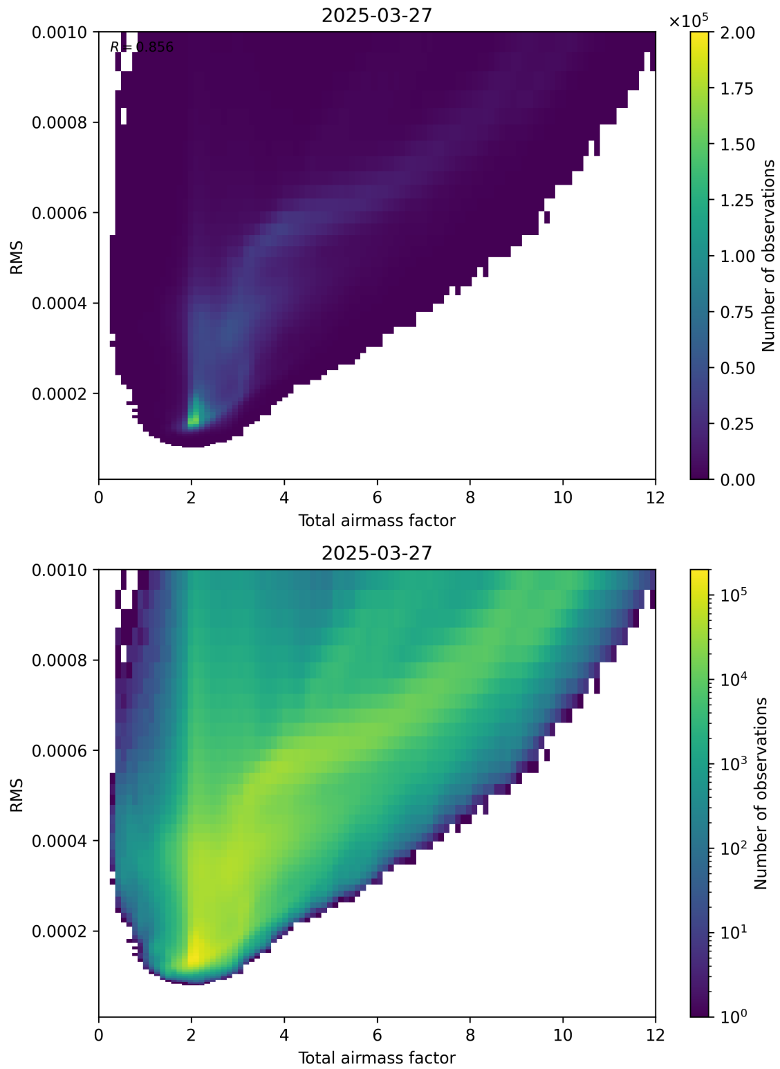
Figure 69: Scatter density plot of “Total airmass factor” against “RMS” for 2025-03-27 to 2025-03-28.
