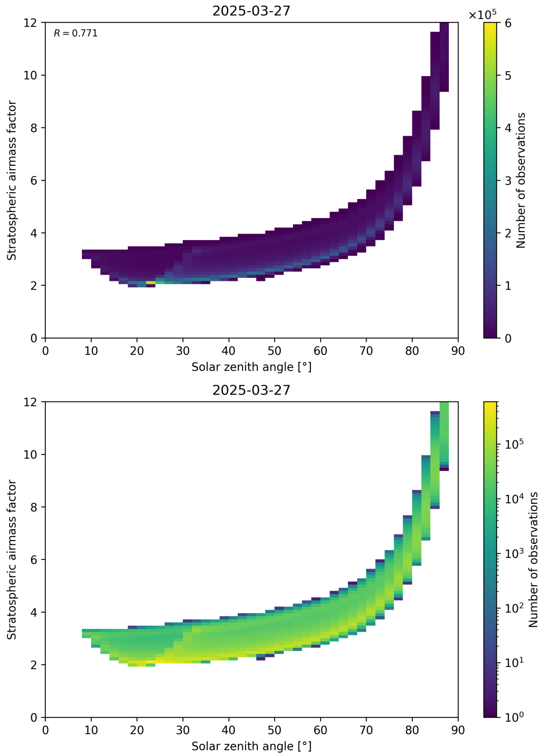
Figure 145: Scatter density plot of “Solar zenith angle” against “Stratospheric airmass factor” for 2025-03-27 to 2025-03-28.
