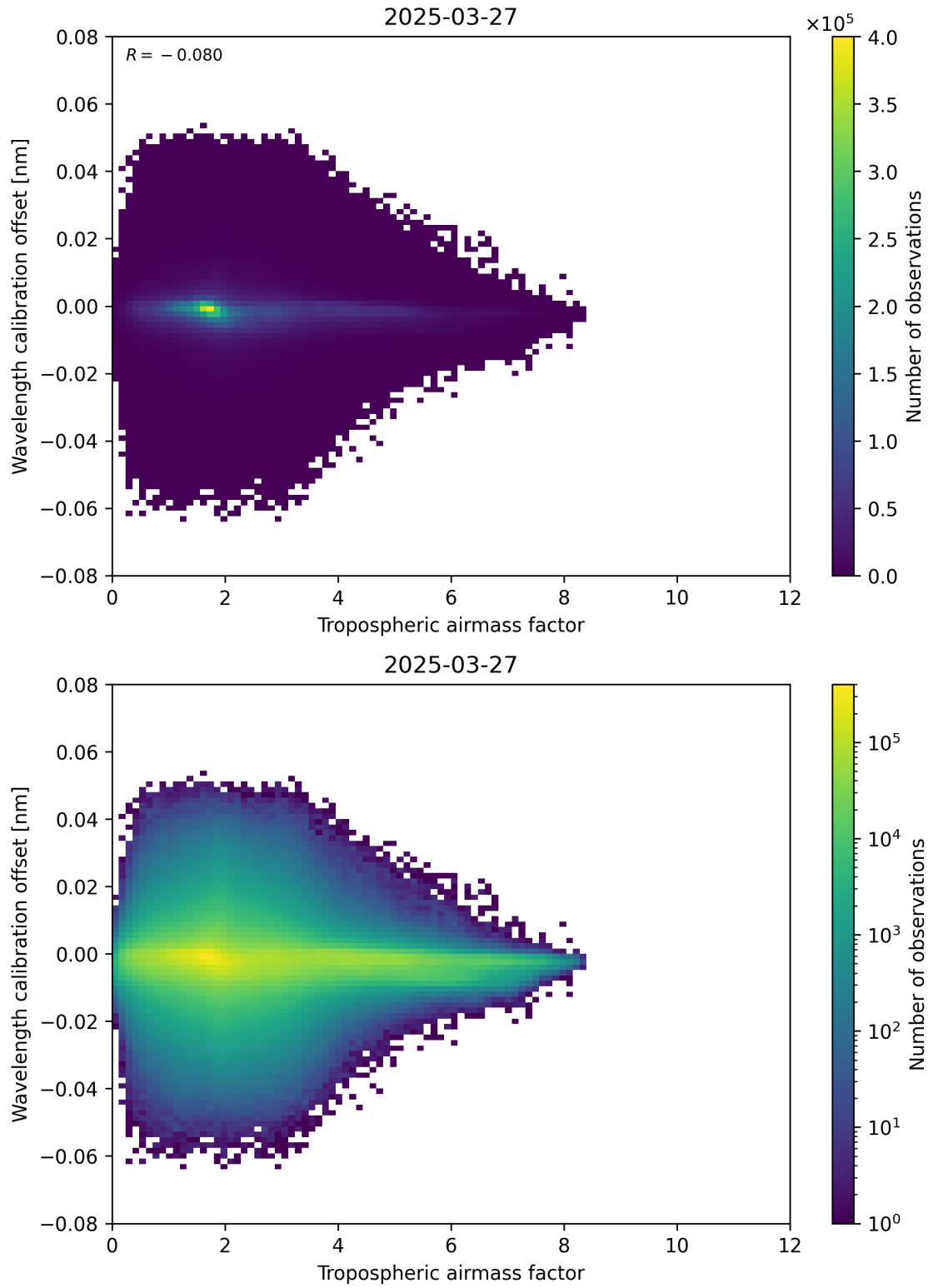
Figure 80: Scatter density plot of “Tropospheric airmass factor” against “Wavelength calibration offset” for 2025-03-27 to 2025-03-28.
