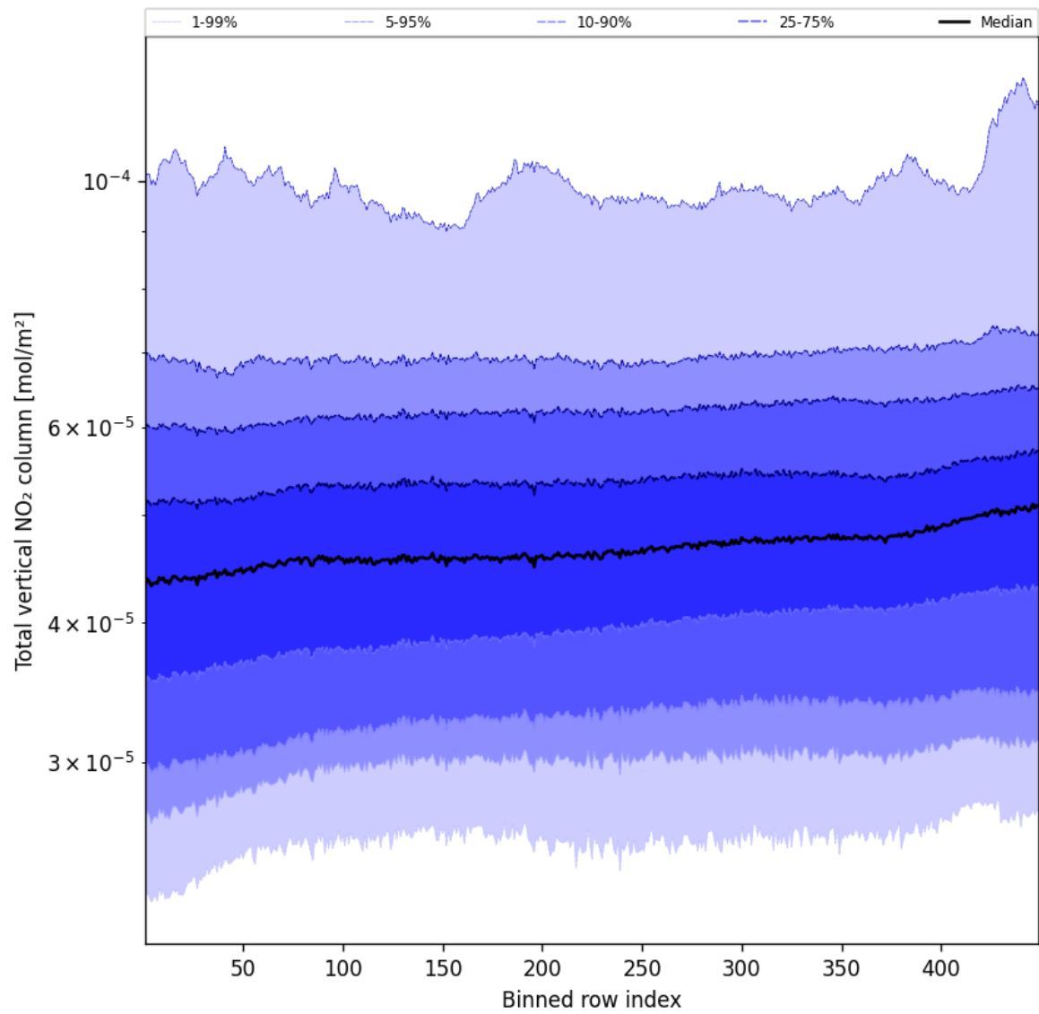
Figure 55: Along track statistics of “Total vertical NO 2 column” for 2025-03-27 to 2025-03-28
