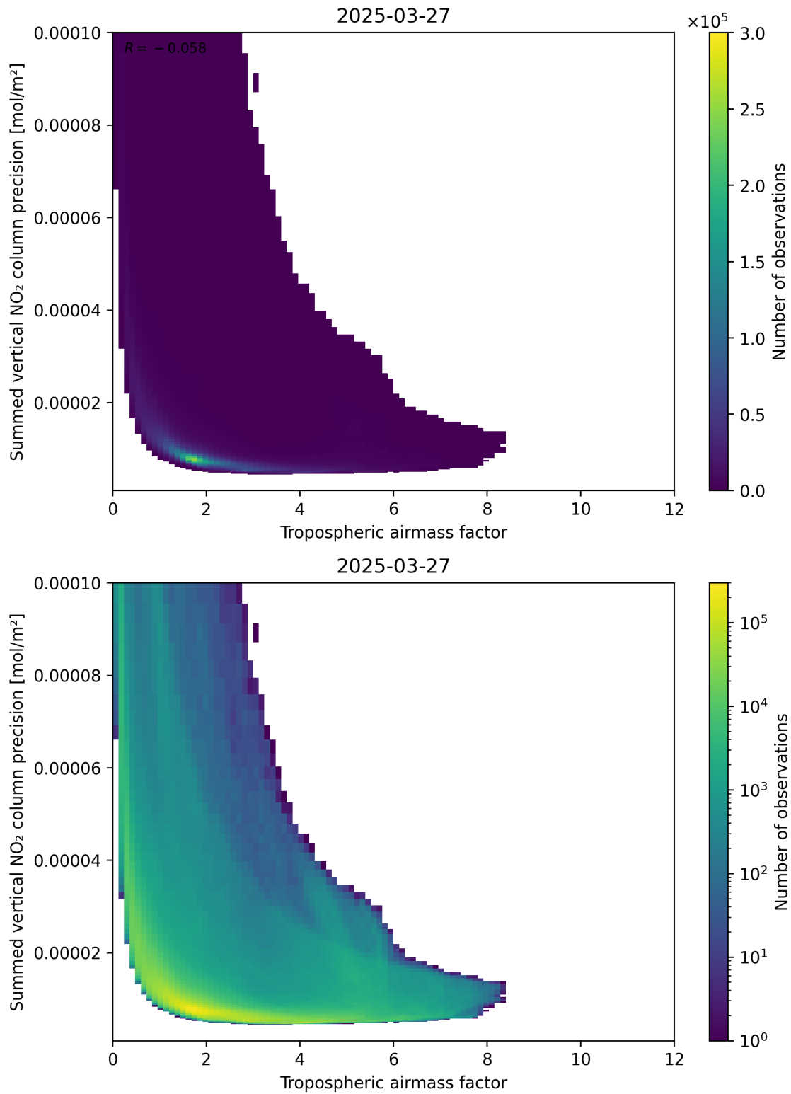
Figure 76: Scatter density plot of “Tropospheric air mass factor” against “Summed vertical NO 2 column precision” for 2025-03-27 to 2025-03-28.
