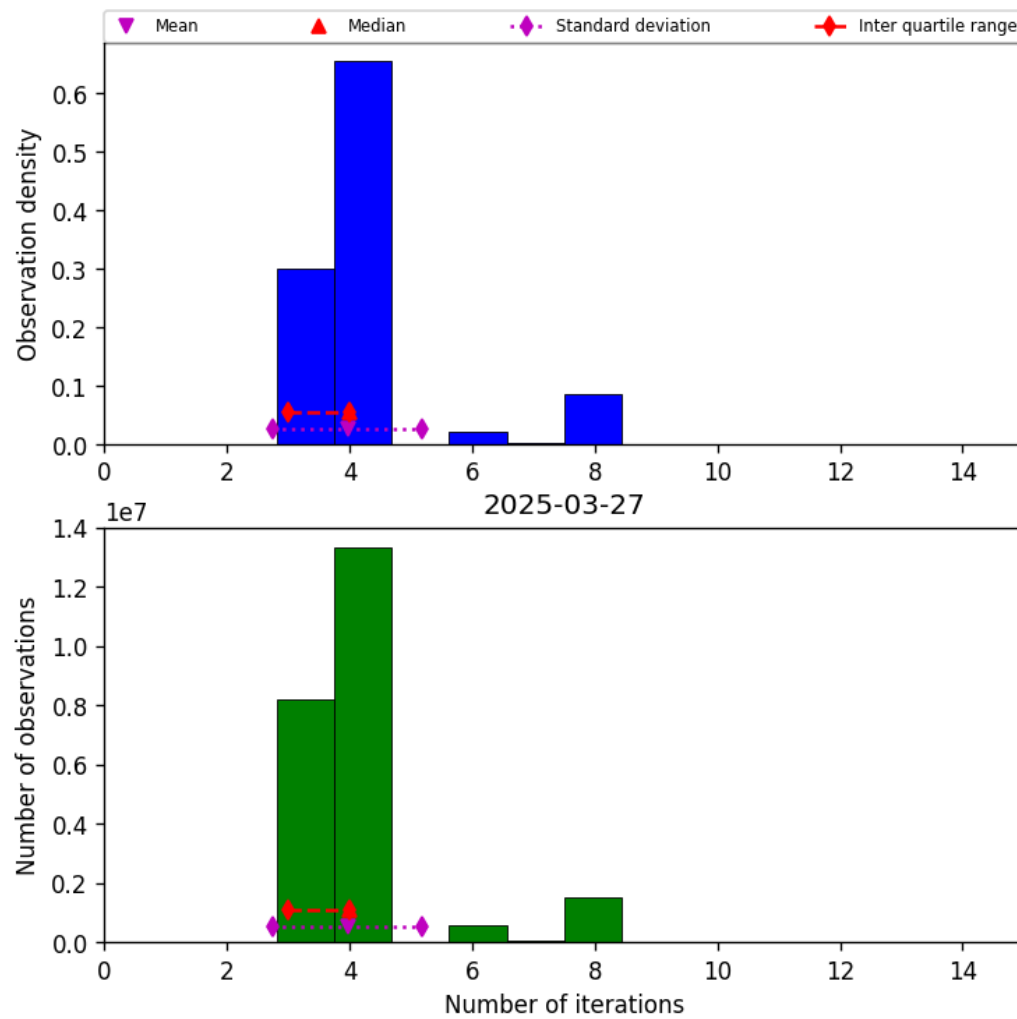
Figure 34: Histogram of “Number of iterations” for 2025-03-27 to 2025-03-28
