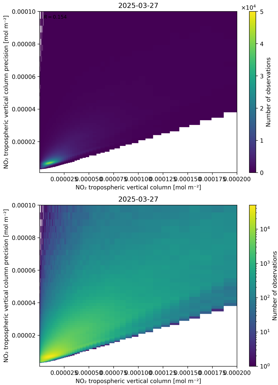
Figure 130: Scatter density plot of “NO 2 tropospheric vertical column” against “NO 2 tropospheric vertical column precision” for 2025-03-27 to 2025-03-28.
