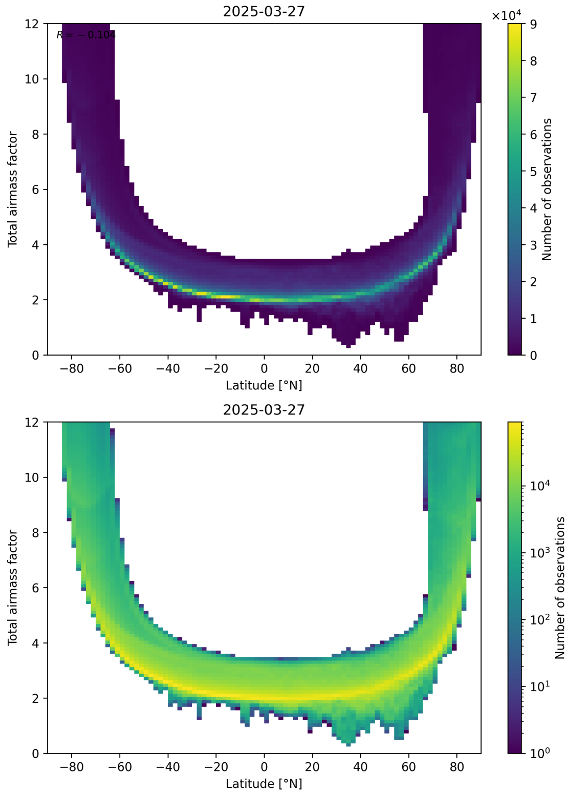
Figure 84: Scatter density plot of “Latitude” against “Total airmass factor” for 2025-03-27 to 2025-03-28.
