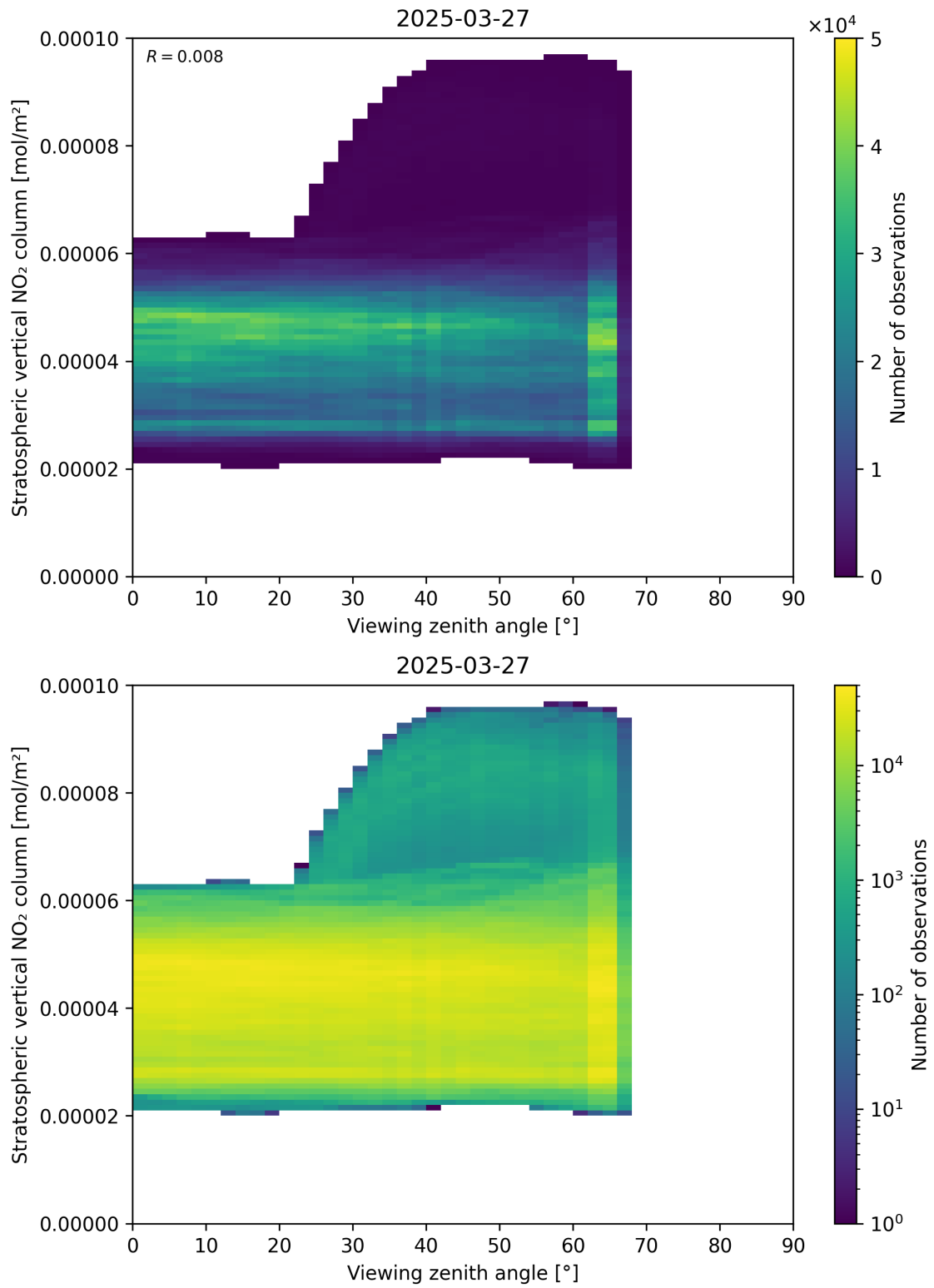
Figure 164: Scatter density plot of “Viewing zenith angle” against “Stratospheric vertical NO 2 column” for 2025-03-27 to 2025-03-28.
