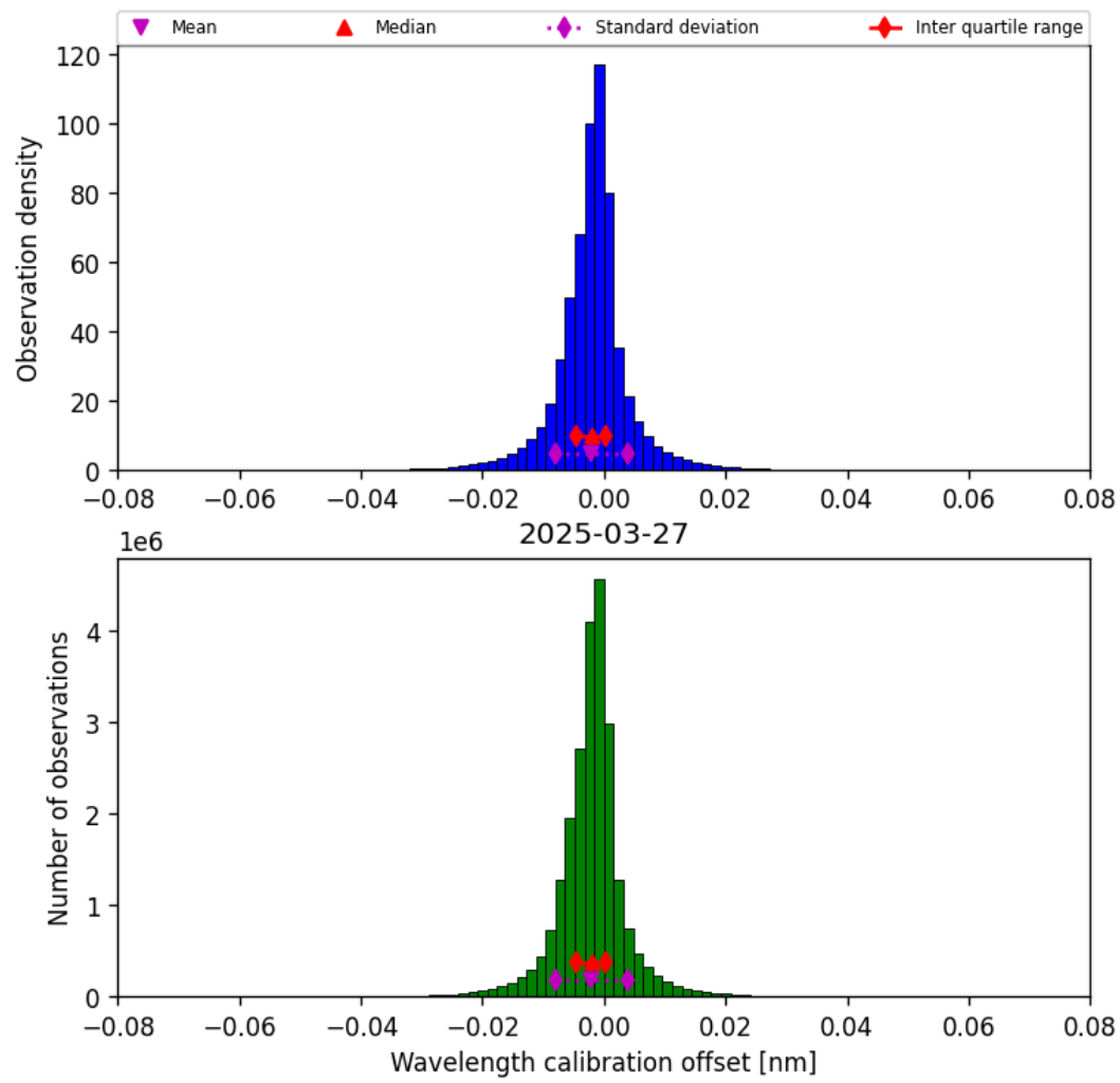
Figure 35: Histogram of “Wavelength calibration offset” for 2025-03-27 to 2025-03-28
