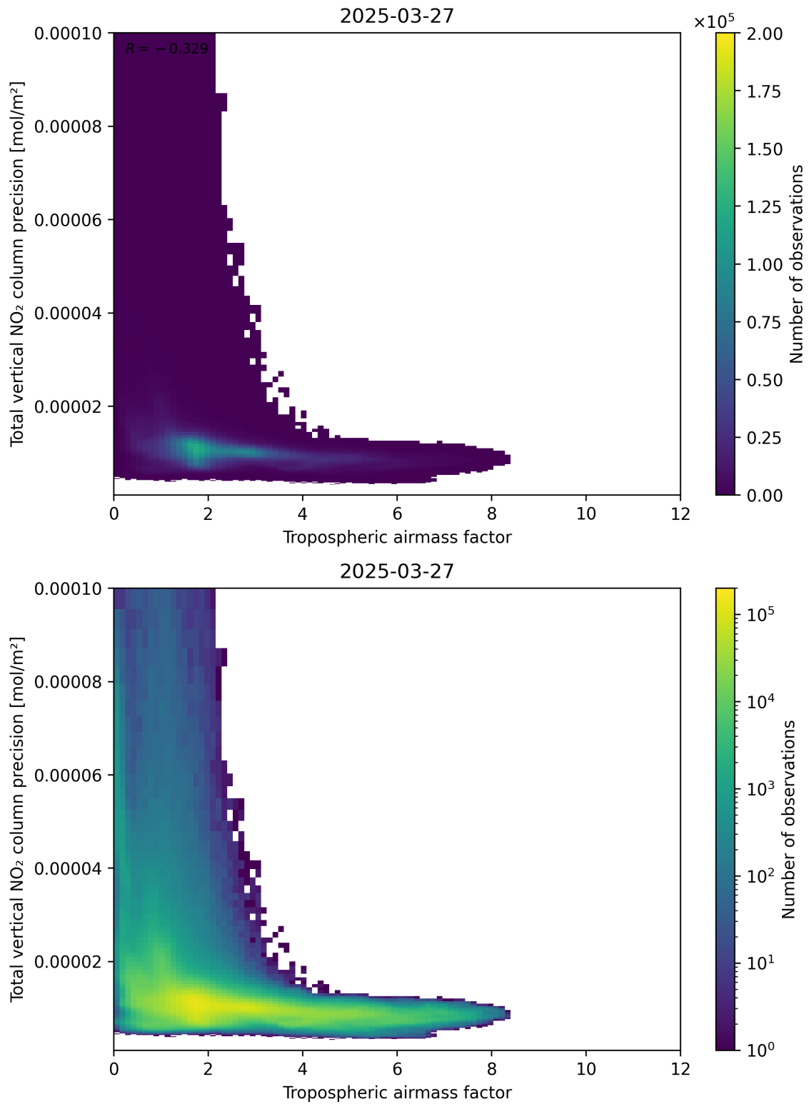
Figure 78: Scatter density plot of “Tropospheric air mass factor” against “Total vertical NO 2 column precision” for 2025-03-27 to 2025-03-28.
