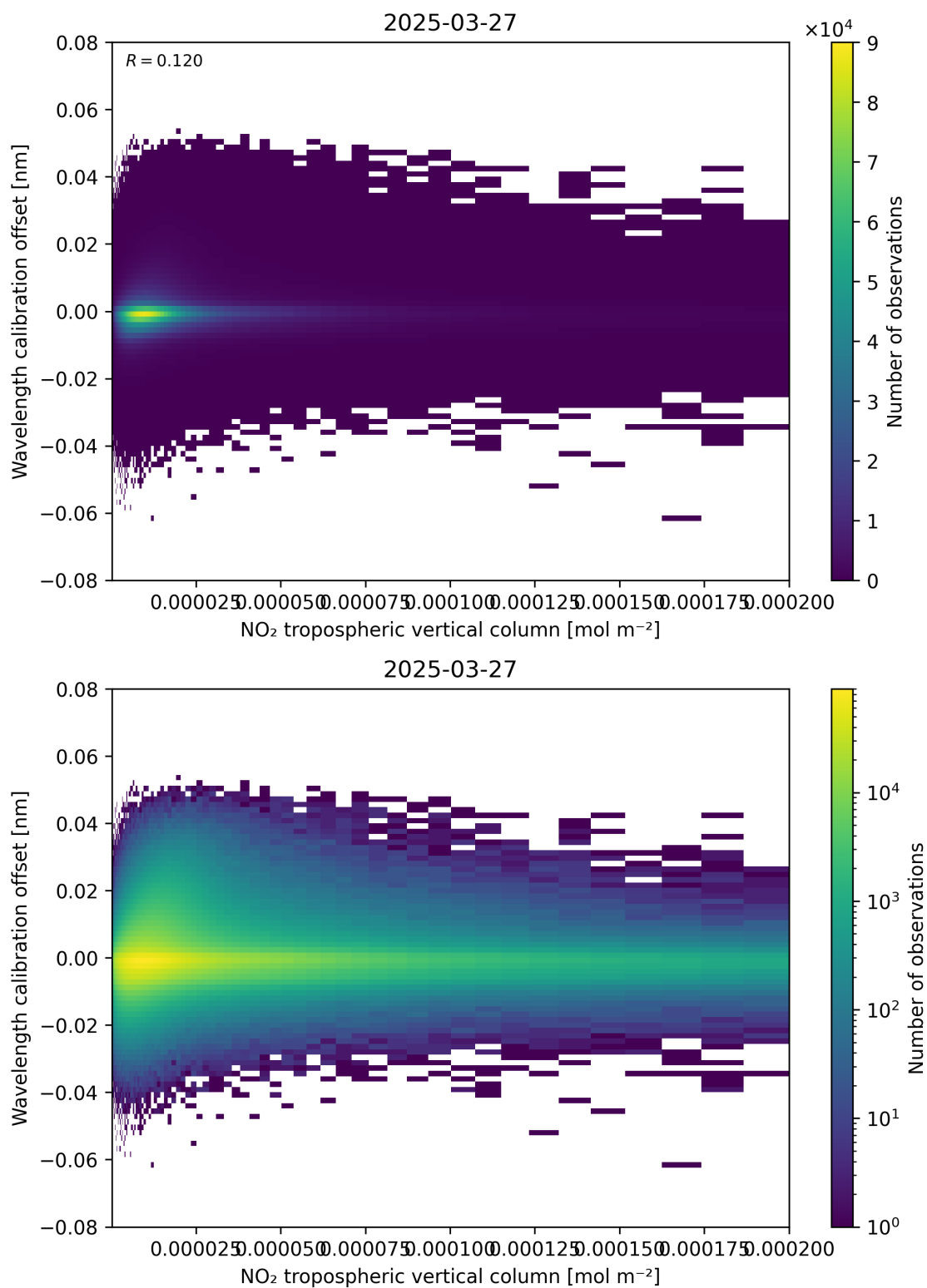
Figure 143: Scatter density plot of “NO 2 tropospheric vertical column” against “Wavelength calibration offset” for 2025-03-27 to 2025-03-28.
