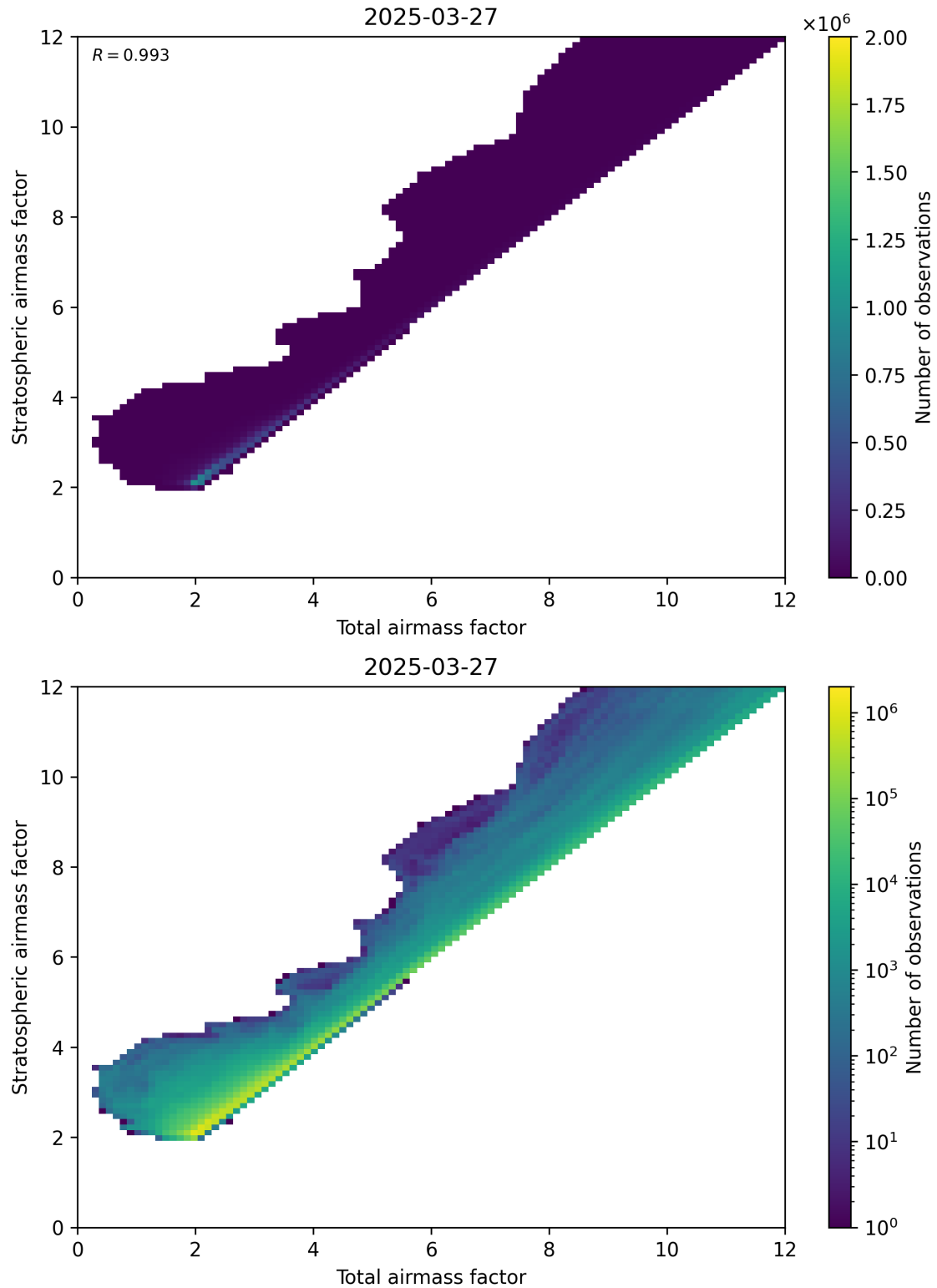
Figure 62: Scatter density plot of “Total airmass factor” against “Stratospheric airmass factor” for 2025-03-27 to 2025-03-28.
