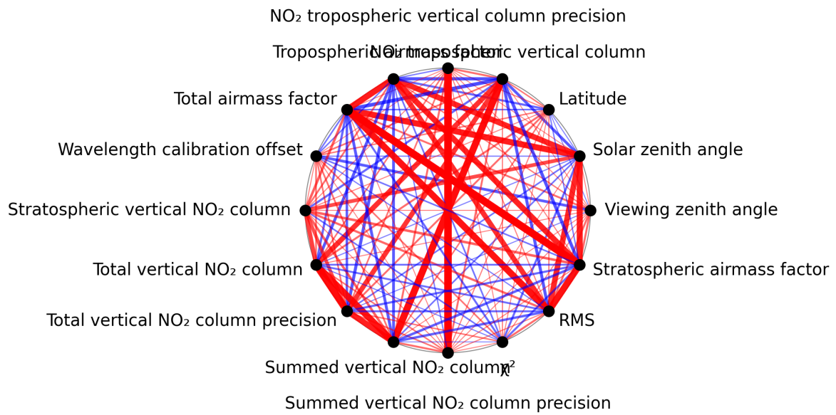
Figure 1: Map of correlation graph for 2025-03-27 to 2025-03-28.
