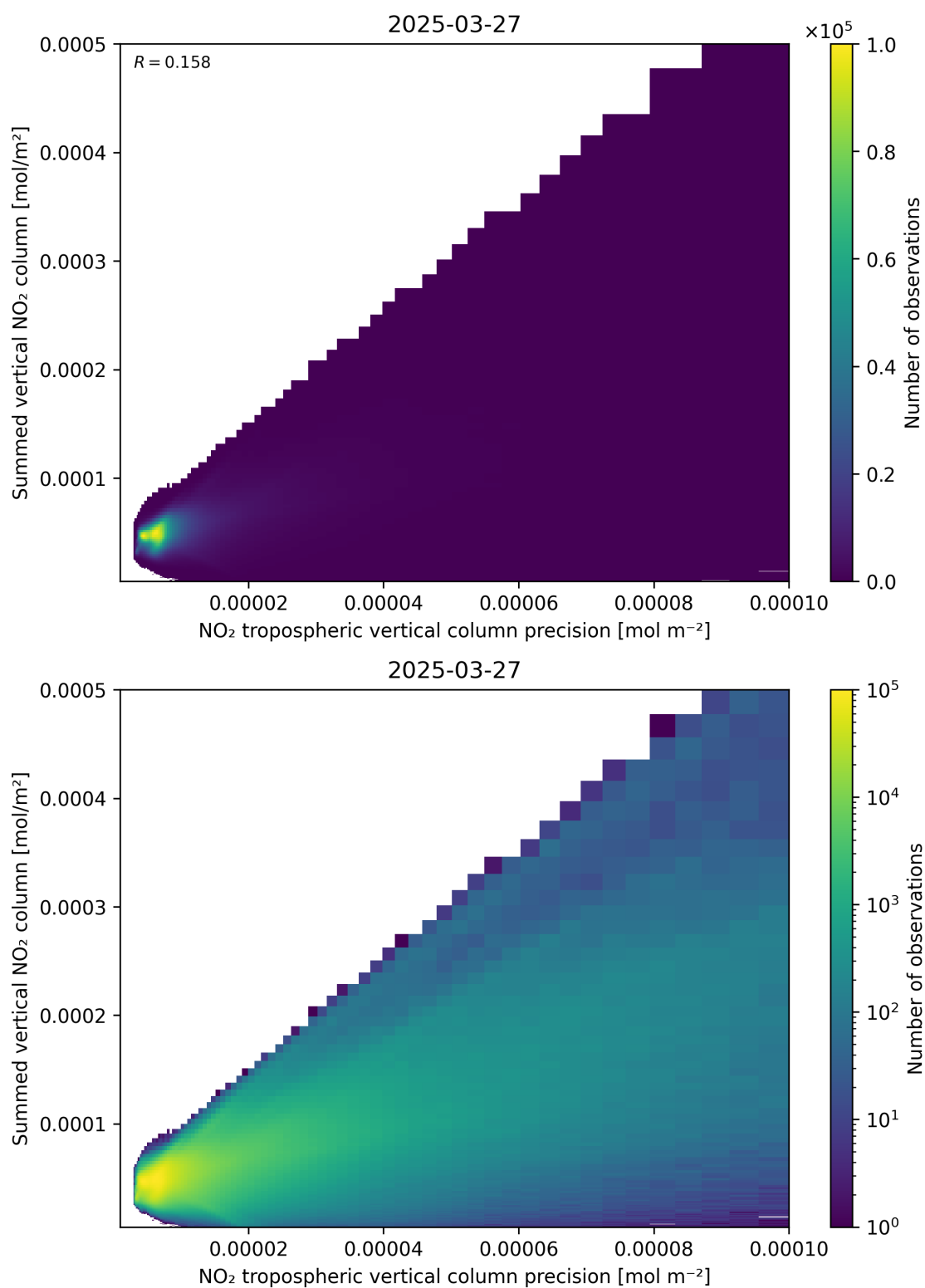
Figure 136: Scatter density plot of “NO 2 tropospheric vertical column precision” against “Summed vertical NO 2 column” for 2025-03-27 to 2025-03-28.
