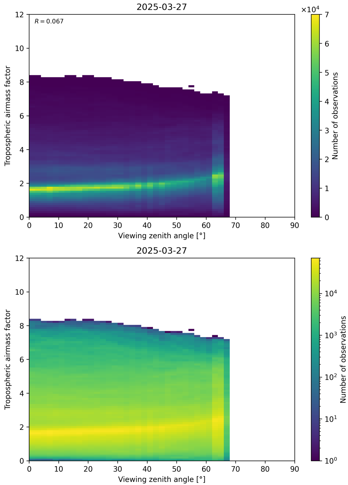
Figure 161: Scatter density plot of “Viewing zenith angle” against “Tropospheric airmass factor” for 2025-03-27 to 2025-03-28.
