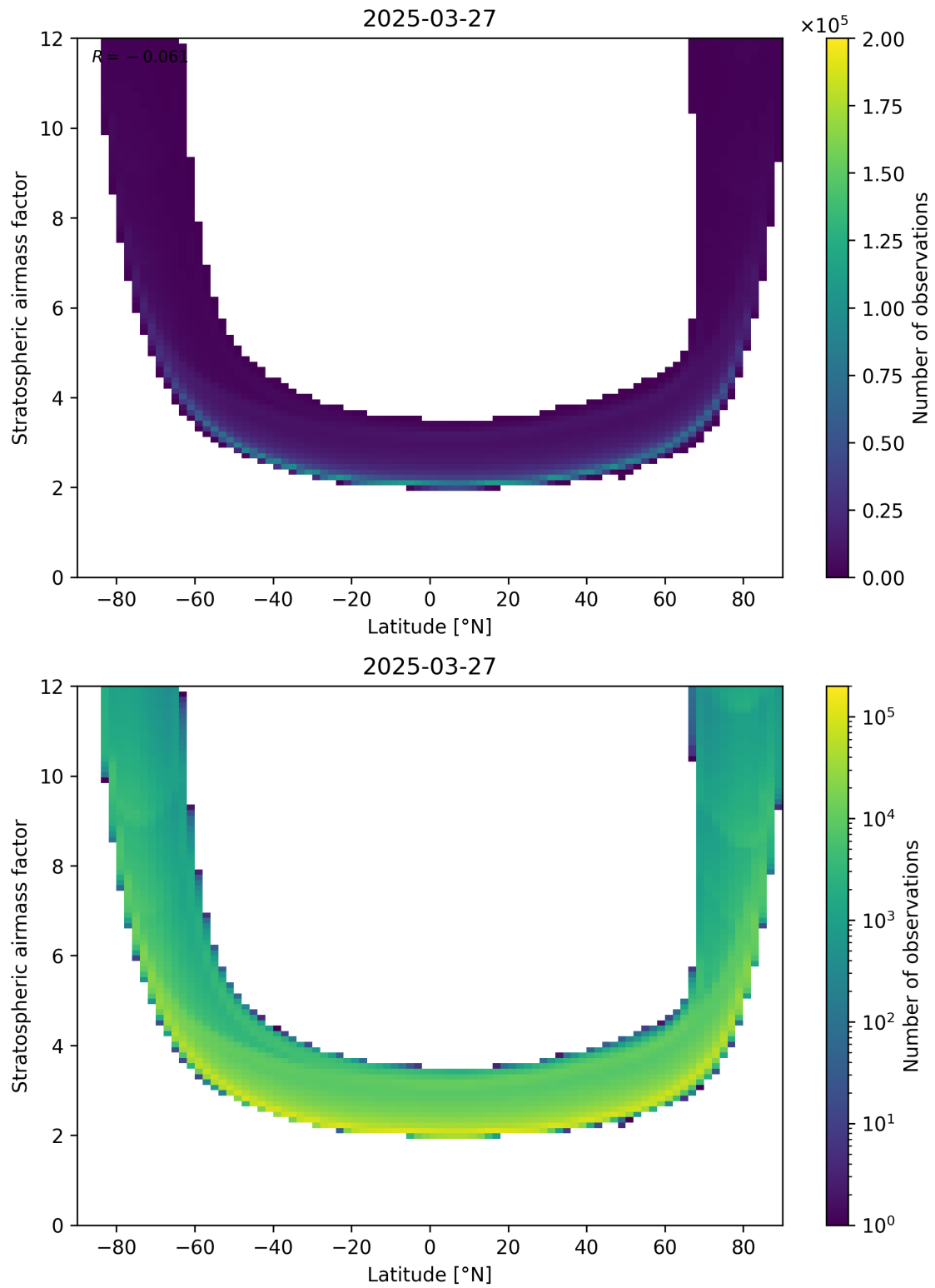
Figure 83: Scatter density plot of “Latitude” against “Stratospheric air mass factor” for 2025-03-27 to 2025-03-28.
