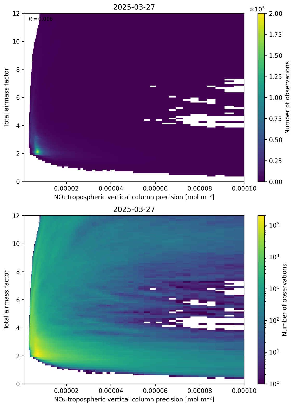
Figure 132: Scatter density plot of “NO 2 tropospheric vertical column precision” against “Total air mass factor” for 2025-03-27 to 2025-03-28.
