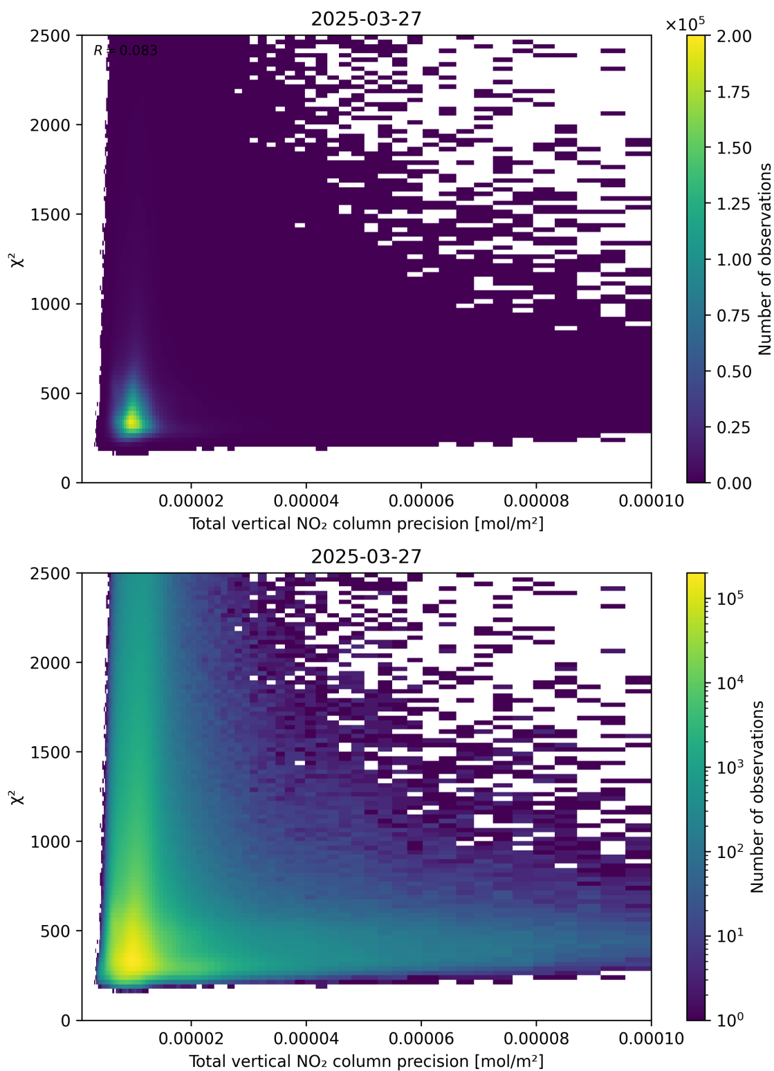
Figure 116: Scatter density plot of “Total vertical NO 2 column precision” against “ \chi^2 ” for 2025-03-27 to 2025-03-28.
