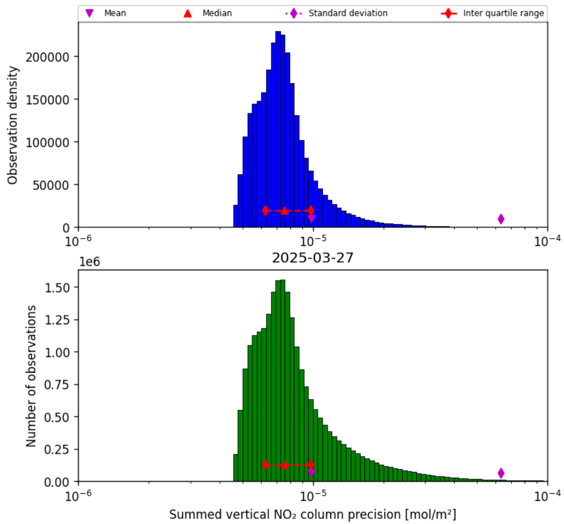
Figure 41: Histogram of “Summed vertical NO 2 column precision” for 2025-03-27 to 2025-03-28
