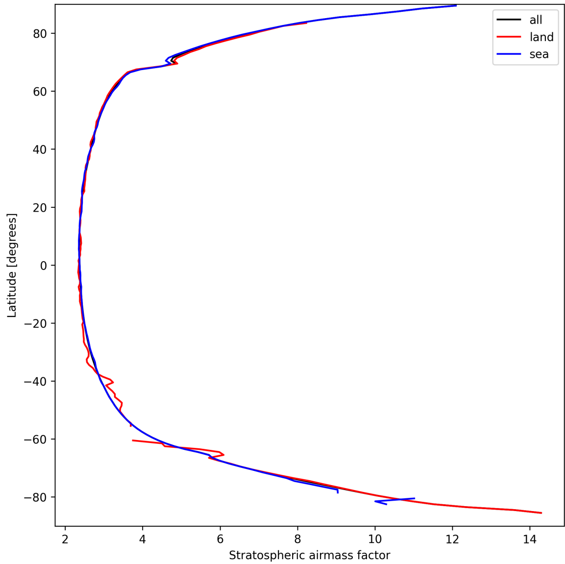
Figure 27: Zonal average of “Stratospheric airmass factor” for 2025-03-27 to 2025-03-28.
