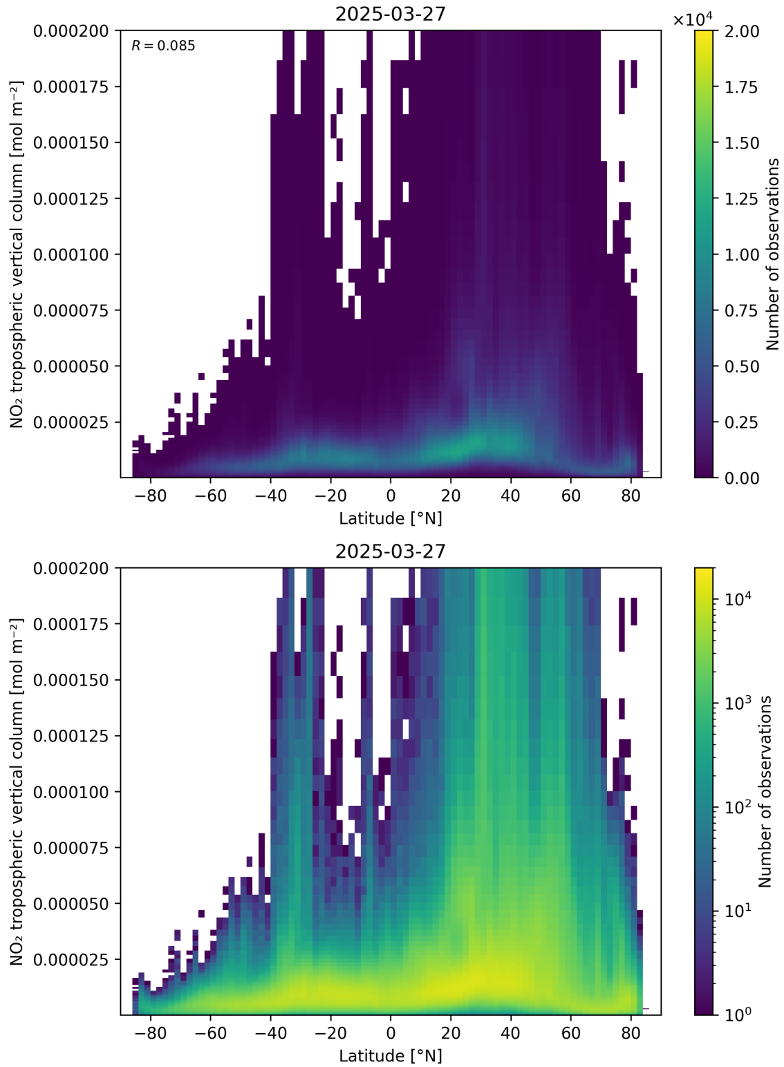
Figure 92: Scatter density plot of “Latitude” against “NO 2 tropospheric vertical column” for 2025-03-27 to 2025-03-28.
