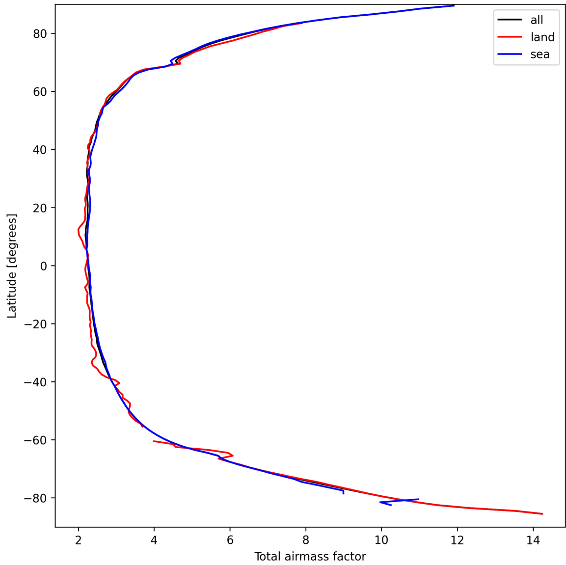
Figure 15: Zonal average of “Total airmass factor” for 2025-03-27 to 2025-03-28.
