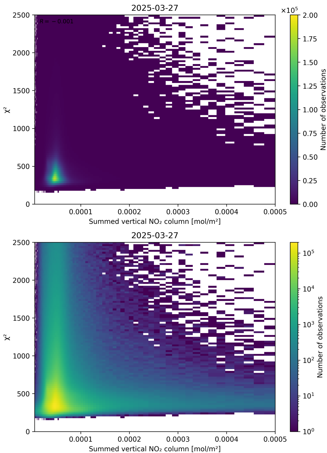
Figure 104: Scatter density plot of “Summed vertical NO 2 column” against “ \chi^2 ” for 2025-03-27 to 2025-03-28.
