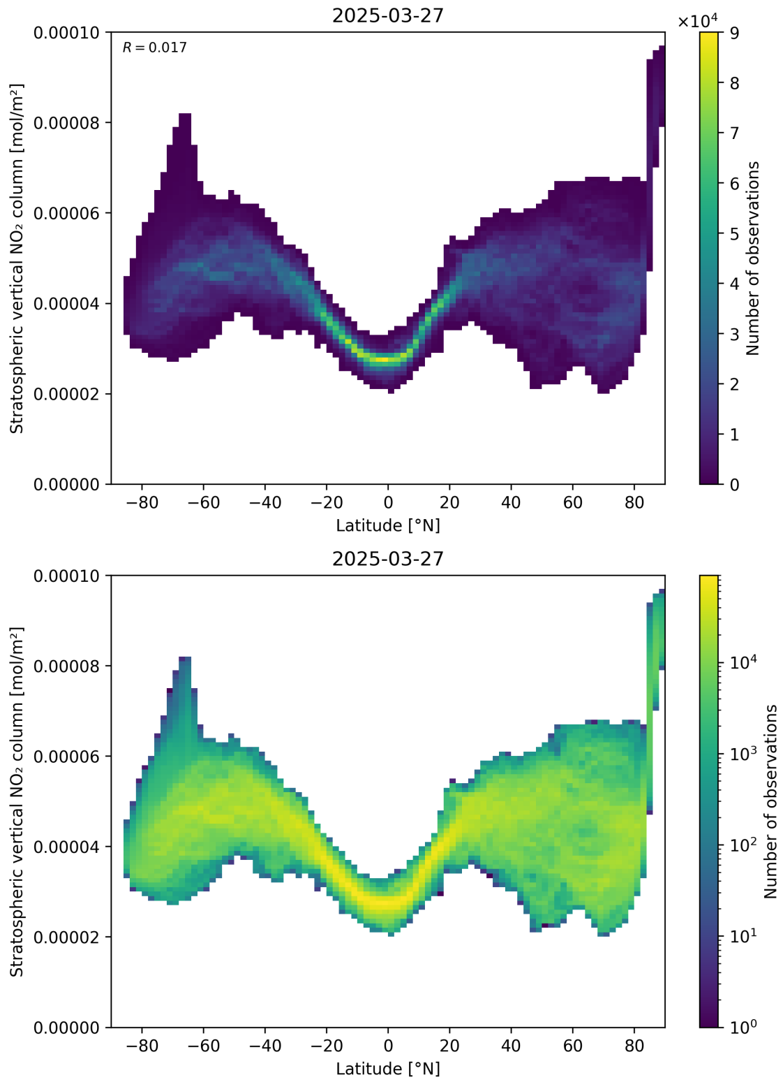
Figure 87: Scatter density plot of “Latitude” against “Stratospheric vertical NO 2 column” for 2025-03-27 to 2025-03-28.
