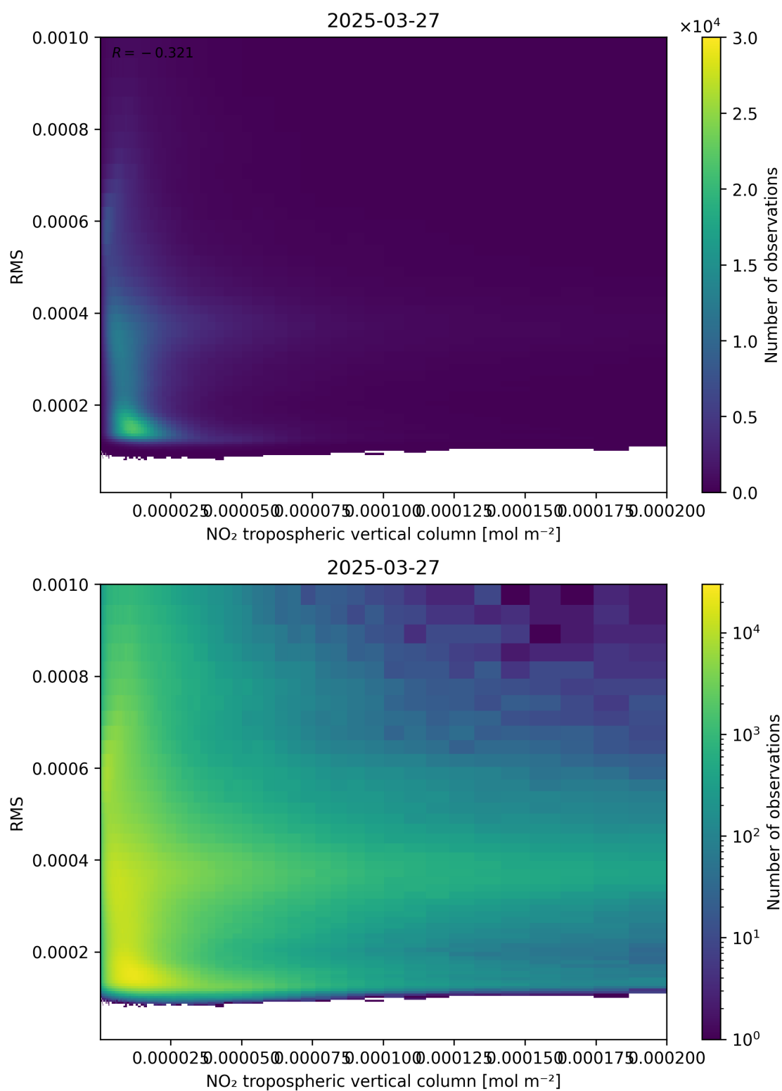
Figure 142: Scatter density plot of “NO 2 tropospheric vertical column” against “RMS” for 2025-03-27 to 2025-03-28.
