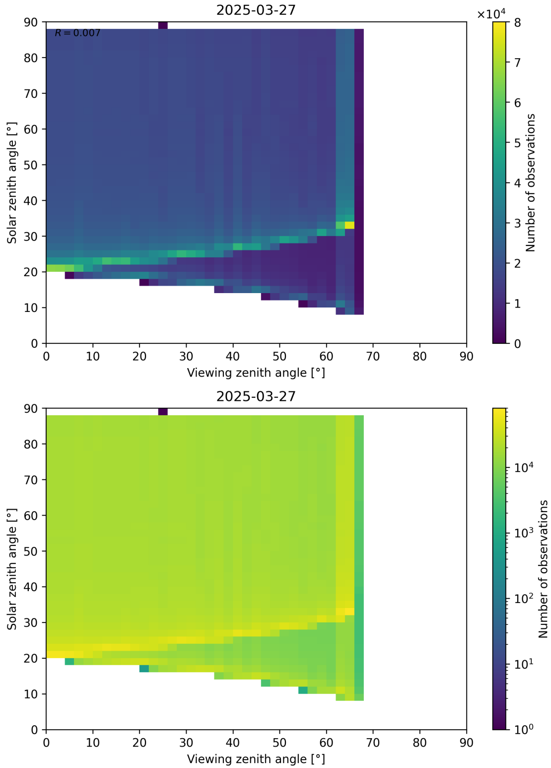
Figure 172: Scatter density plot of “Viewing zenith angle” against “Solar zenith angle” for 2025-03-27 to 2025-03-28.
