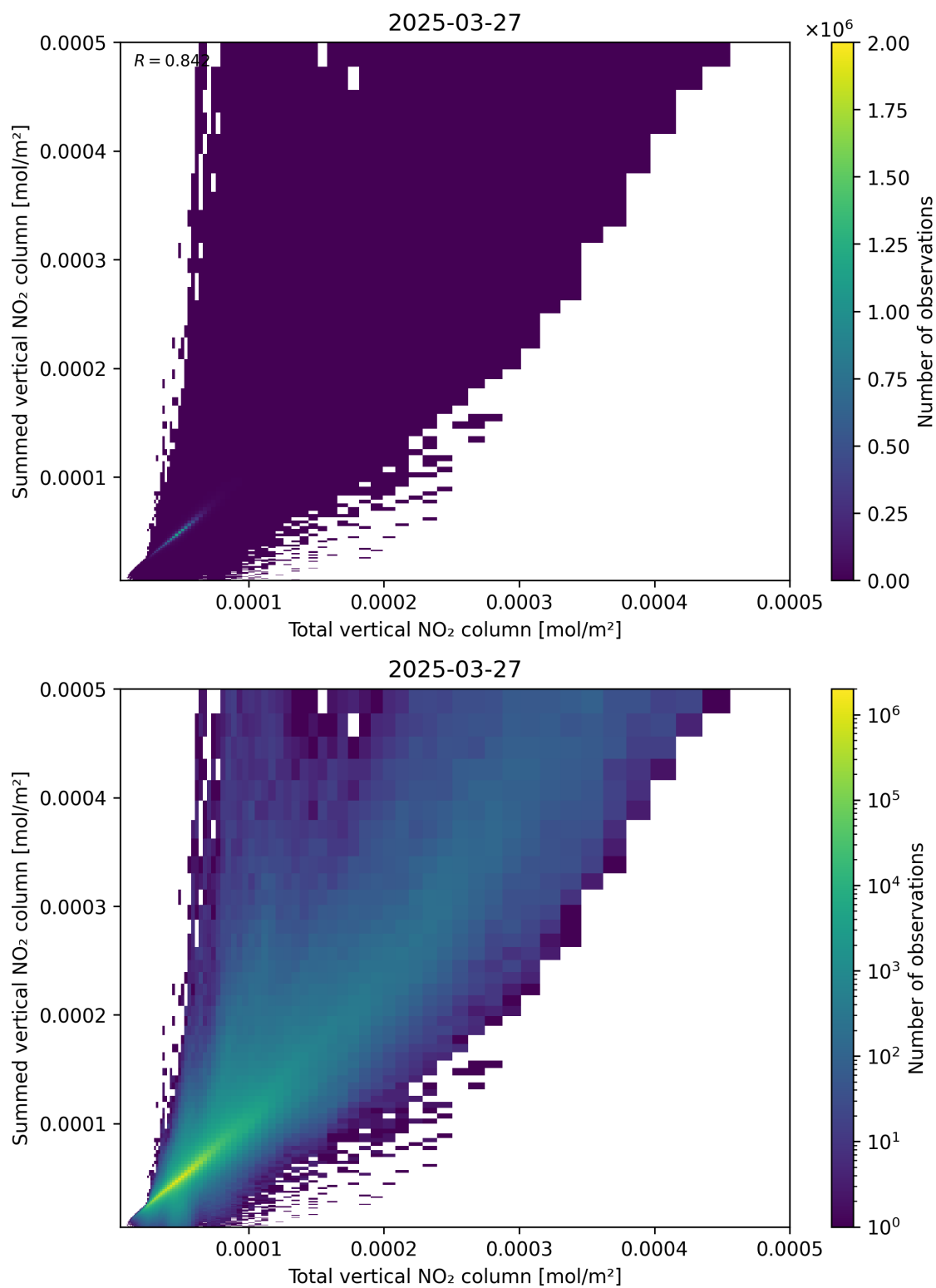
Figure 112: Scatter density plot of “Total vertical NO 2 column” against “Summed vertical NO 2 column” for 2025-03-27 to 2025-03-28.
