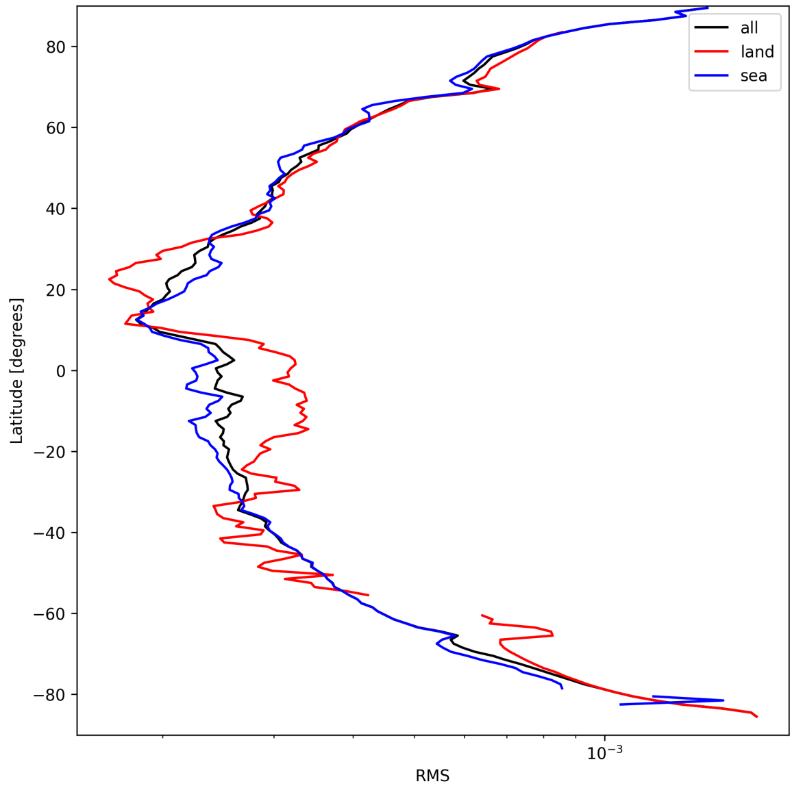
Figure 26: Zonal average of “RMS” for 2025-03-27 to 2025-03-28.
