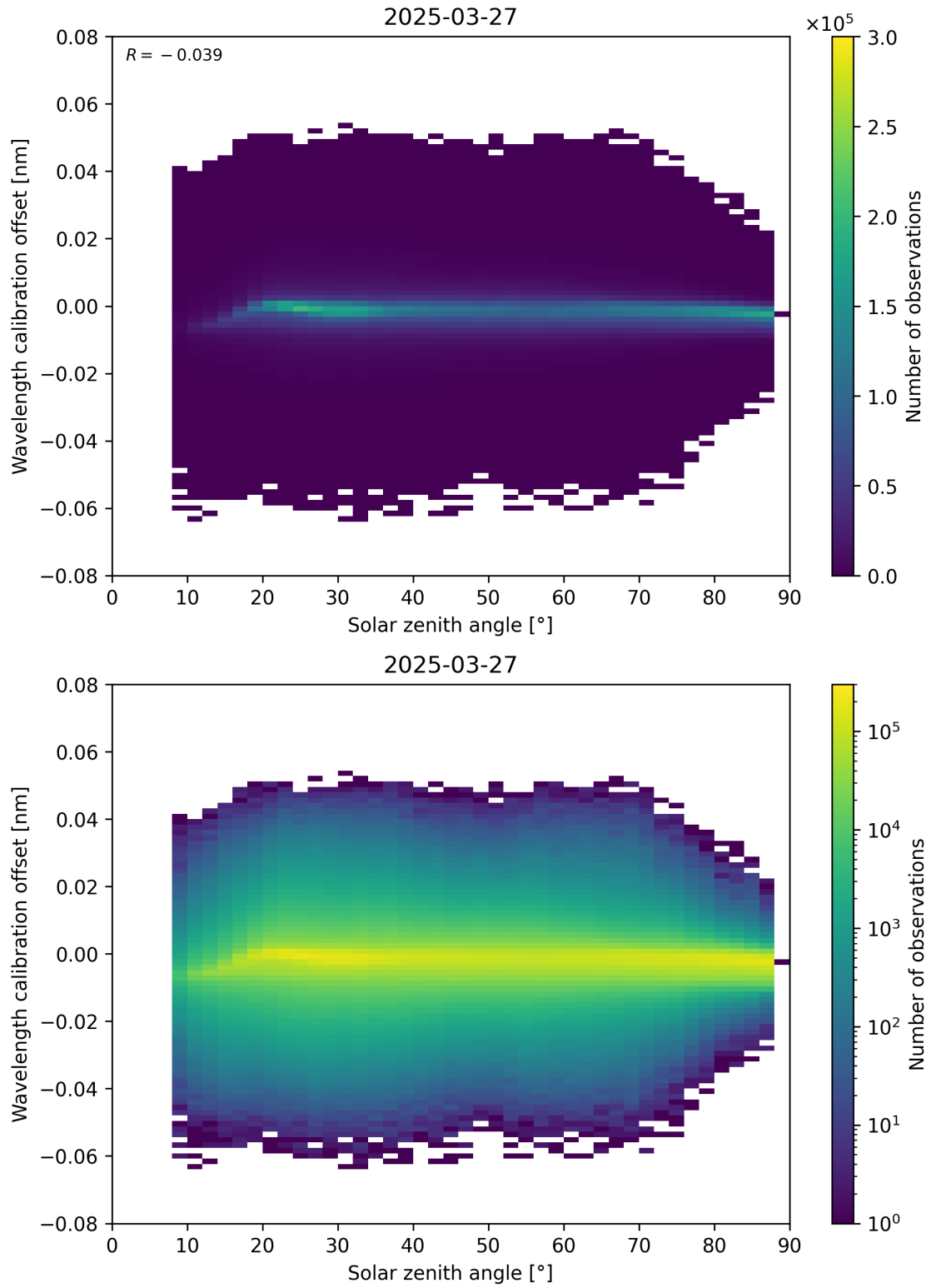
Figure 158: Scatter density plot of “Solar zenith angle” against “Wavelength calibration offset” for 2025-03-27 to 2025-03-28.
