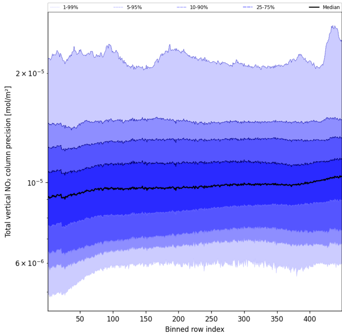
Figure 56: Along track statistics of "Total vertical NO 2 column precision" for 2025-03-27 to 2025-03-28
