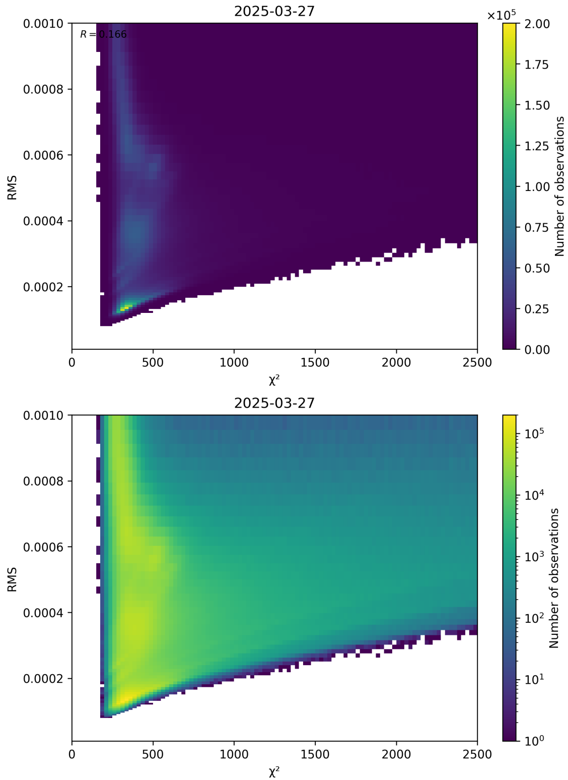
Figure 82: Scatter density plot of “ \chi^2 ” against “RMS” for 2025-03-27 to 2025-03-28.
