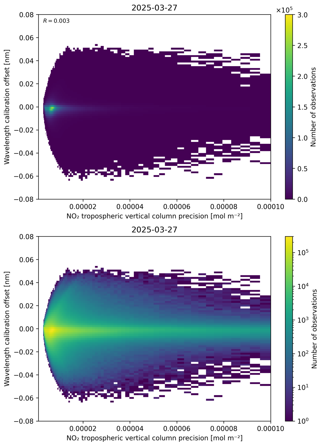
Figure 141: Scatter density plot of “NO 2 tropospheric vertical column precision” against “Wavelength calibration offset” for 2025-03-27 to 2025-03-28.
