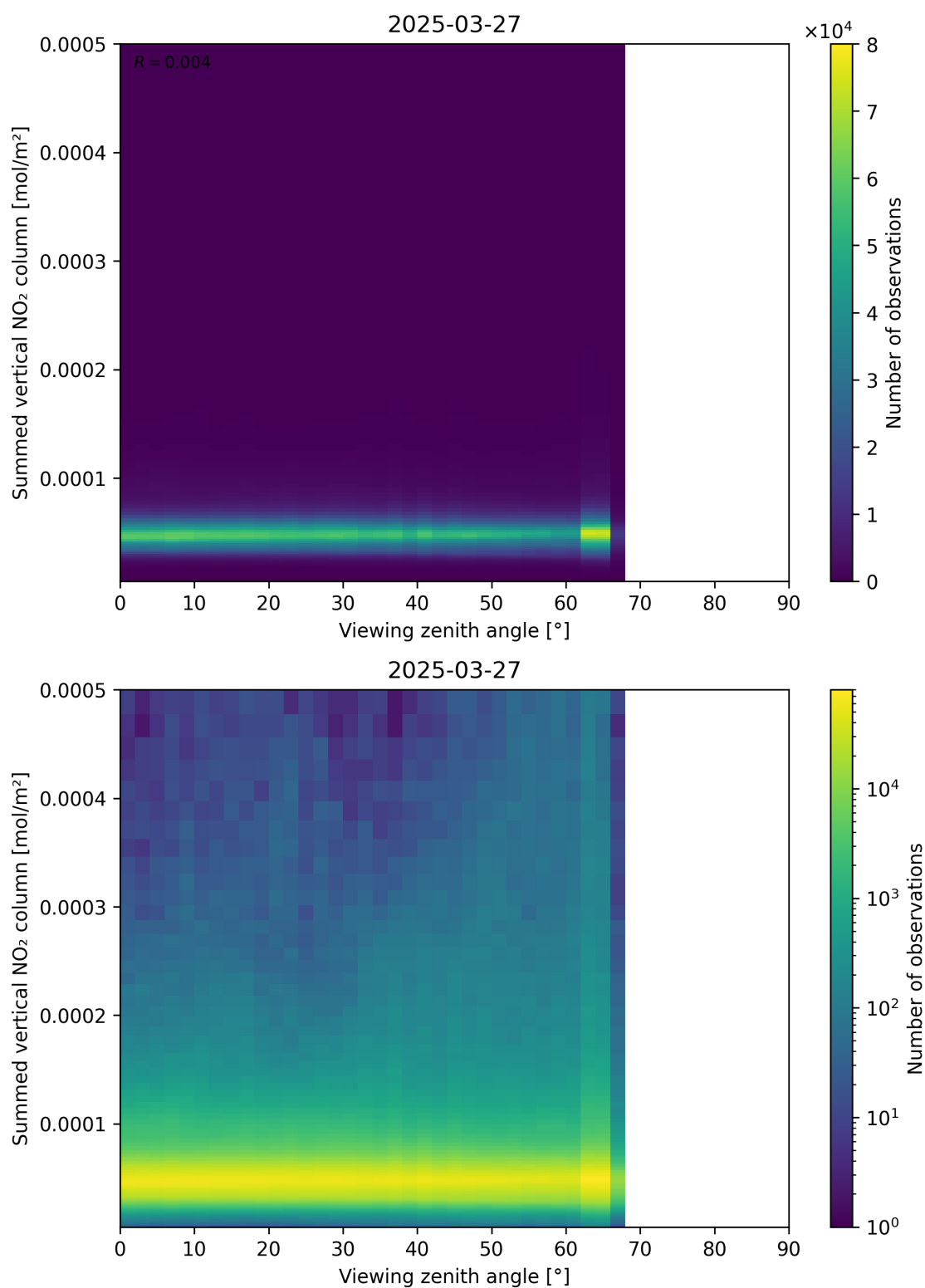
Figure 165: Scatter density plot of “Viewing zenith angle” against “Summed vertical NO 2 column” for 2025-03-27 to 2025-03-28.
