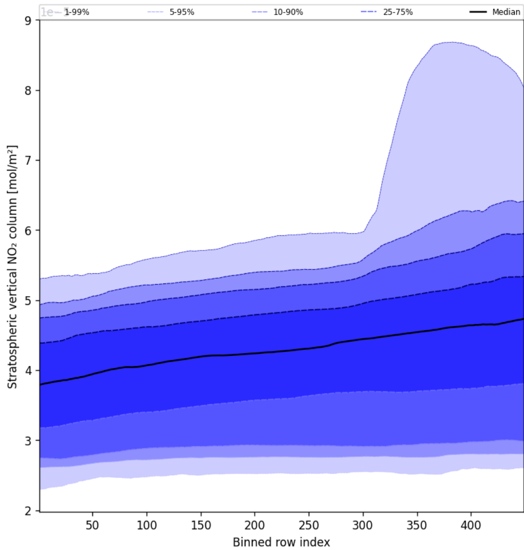
Figure 53: Along track statistics of “Stratospheric vertical NO 2 column” for 2025-03-27 to 2025-03-28
