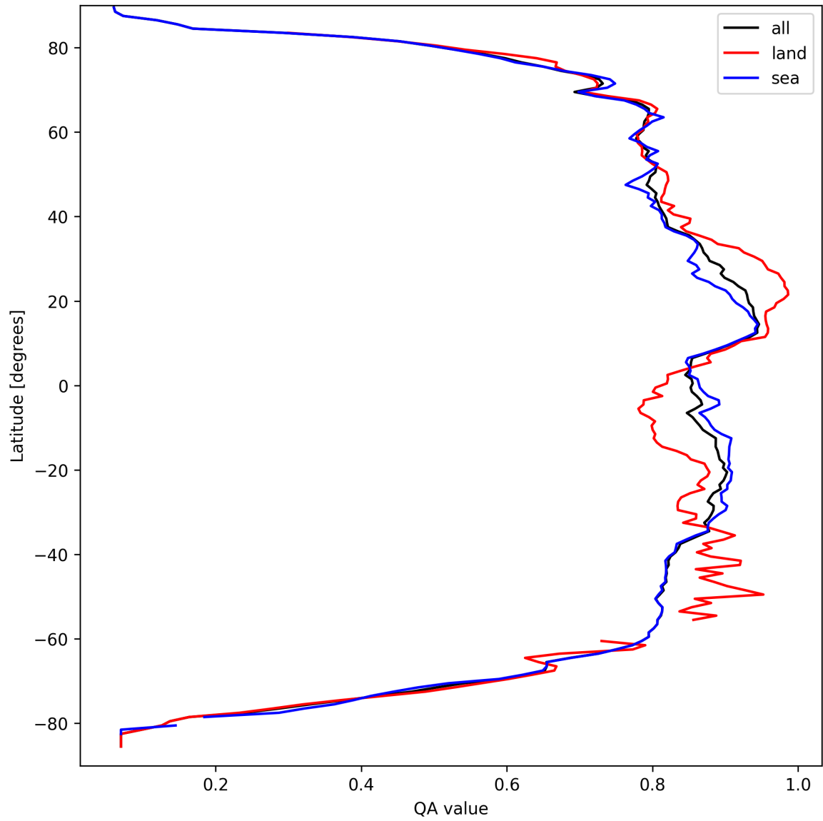
Figure 11: Zonal average of “QA value” for 2025-03-27 to 2025-03-28.
