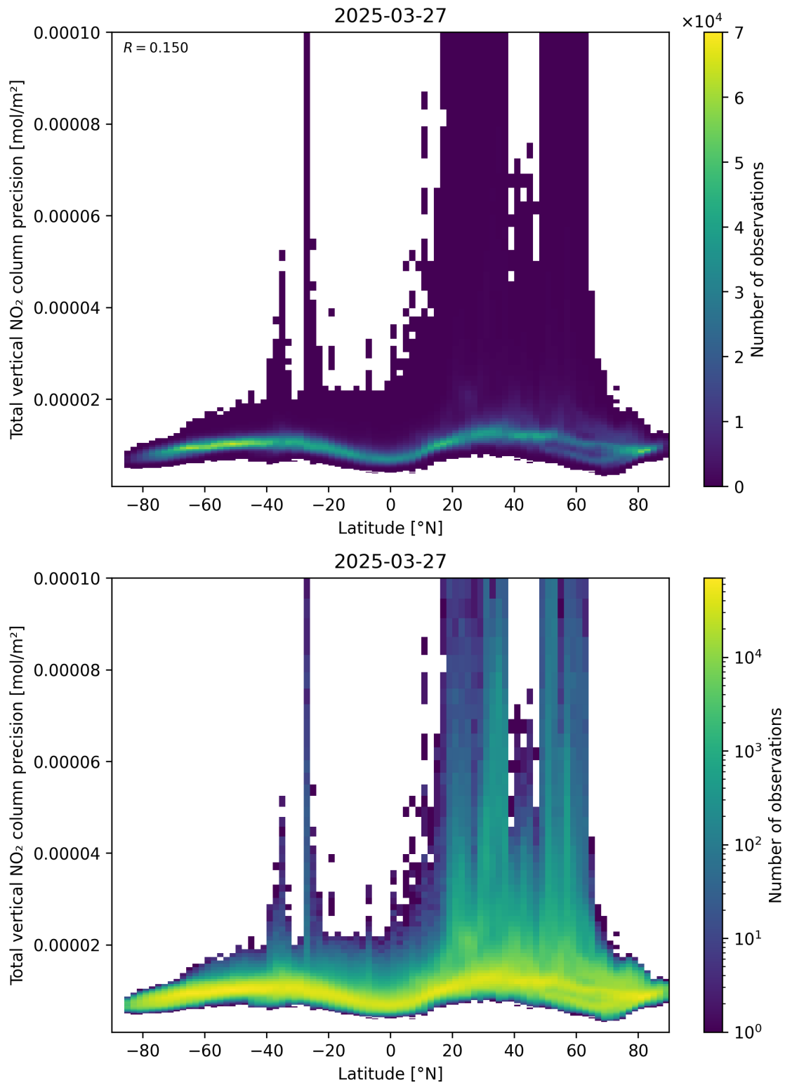
Figure 91: Scatter density plot of “Latitude” against “Total vertical NO 2 column precision” for 2025-03-27 to 2025-03-28.
