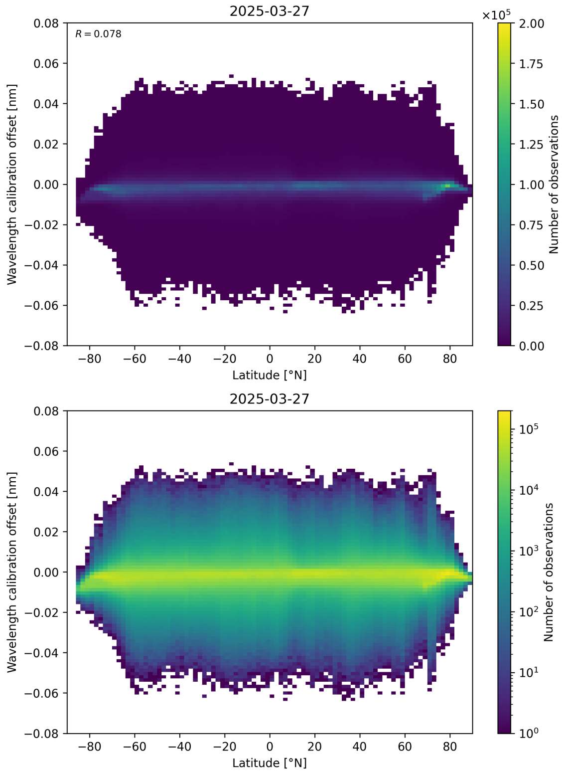
Figure 95: Scatter density plot of “Latitude” against “Wavelength calibration offset” for 2025-03-27 to 2025-03-28.
