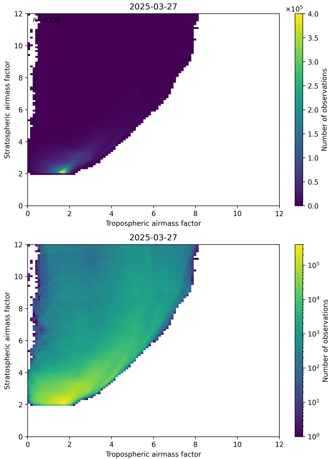
Figure 71: Scatter density plot of “Tropospheric airmass factor” against “Stratospheric airmass factor” for 2025-03-27 to 2025-03-28.
