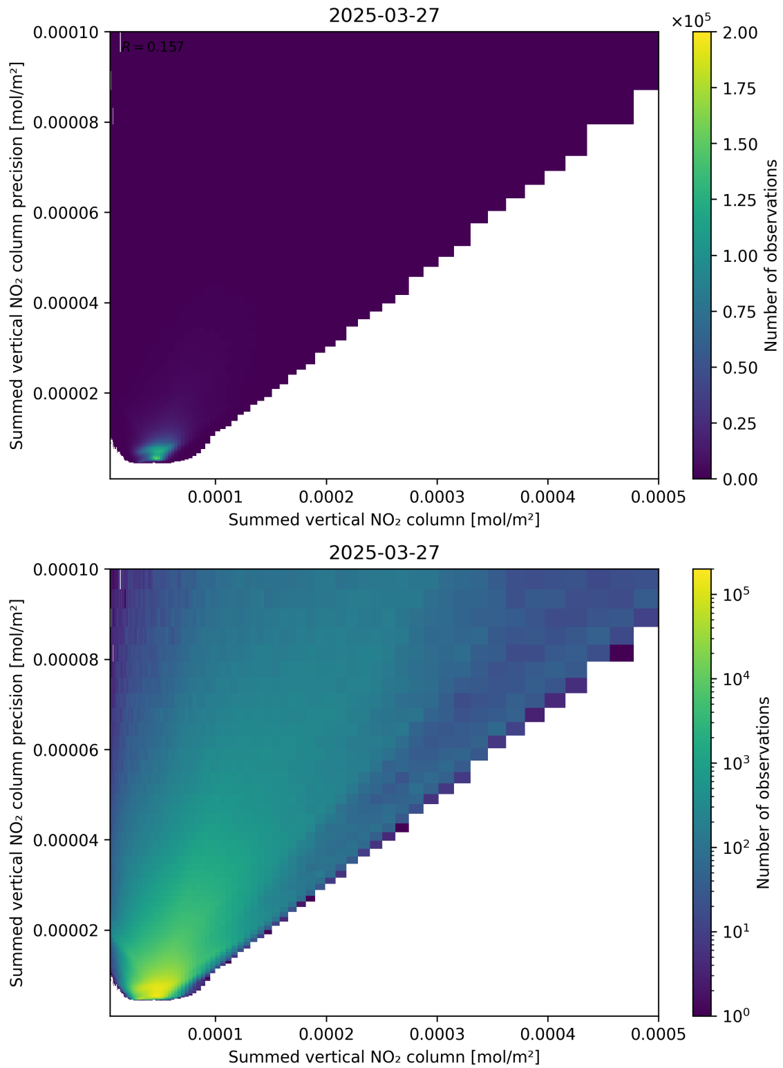
Figure 105: Scatter density plot of “Summed vertical NO 2 column” against “Summed vertical NO 2 column precision” for 2025-03-27 to 2025-03-28.
