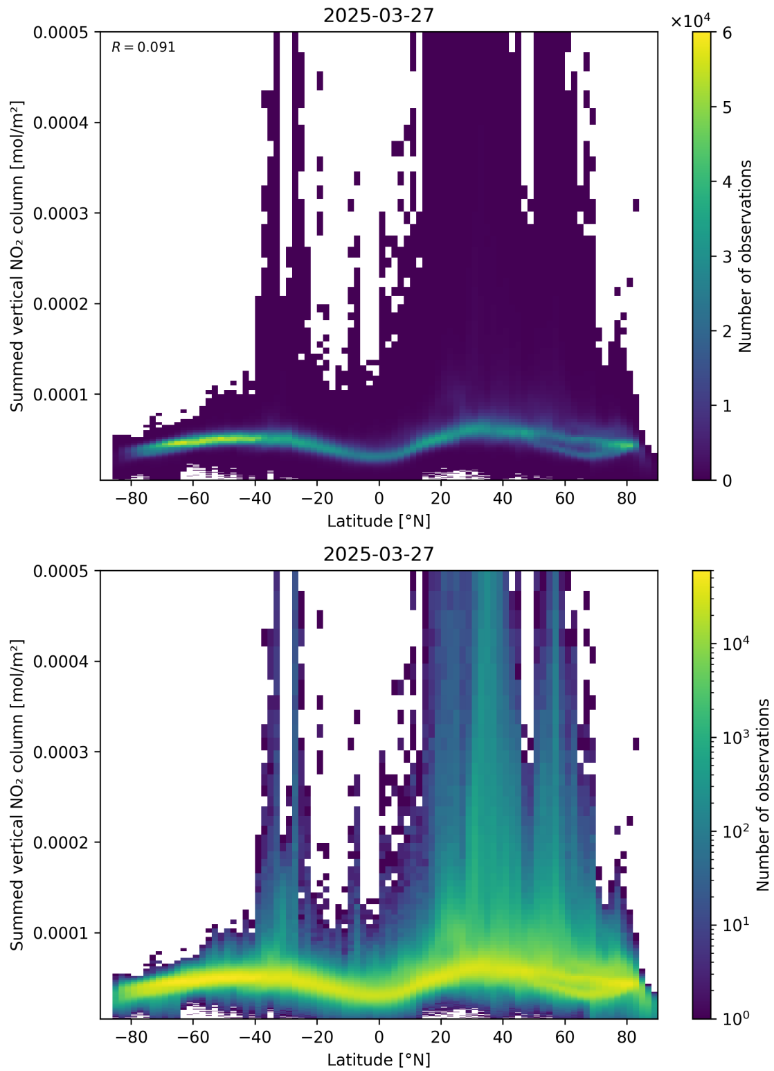
Figure 88: Scatter density plot of “Latitude” against “Summed vertical NO 2 column” for 2025-03-27 to 2025-03-28.
