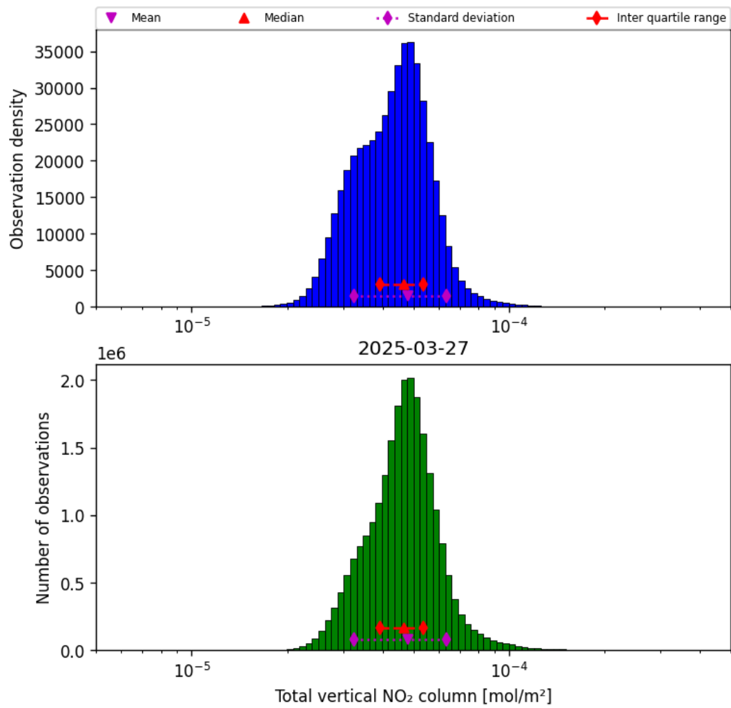
Figure 38: Histogram of “Total vertical NO 2 column” for 2025-03-27 to 2025-03-28
