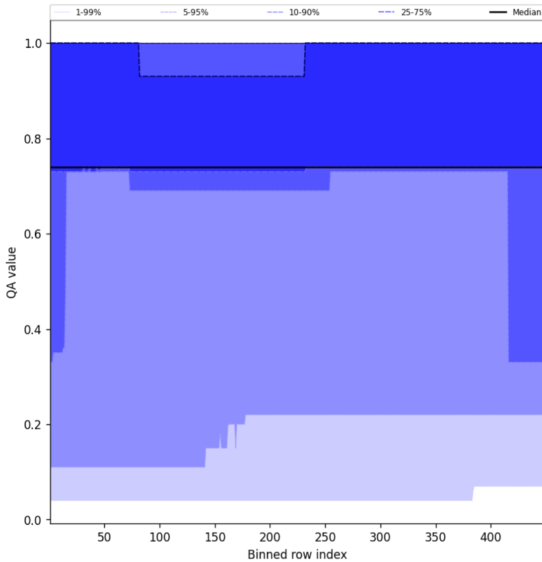
Figure 45: Along track statistics of “QA value” for 2025-03-27 to 2025-03-28
