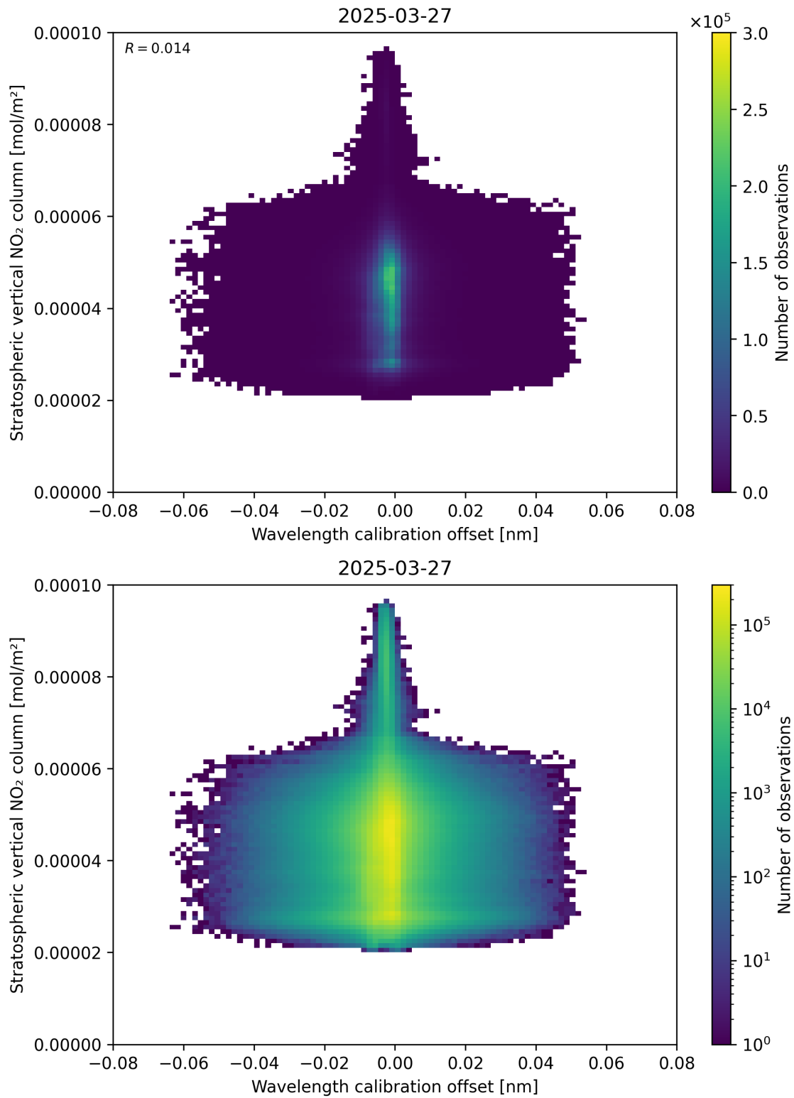
Figure 176: Scatter density plot of “Wavelength calibration offset” against “Stratospheric vertical NO 2 column” for 2025-03-27 to 2025-03-28.
