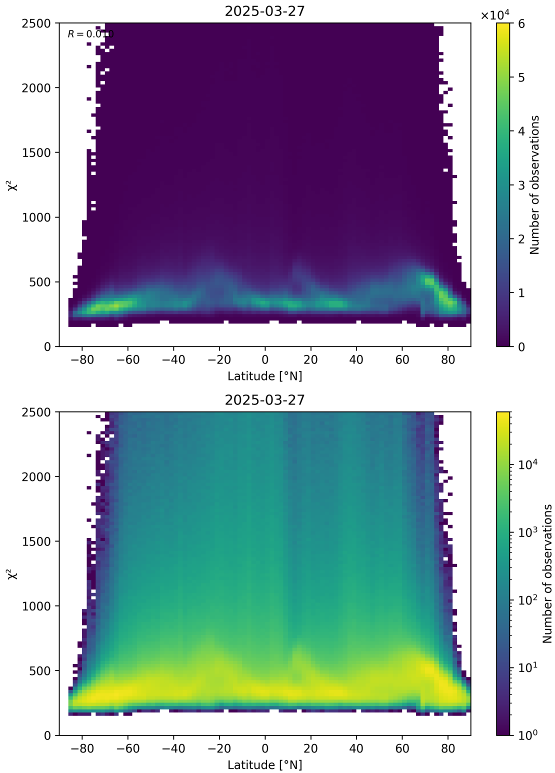
Figure 86: Scatter density plot of “Latitude” against “ \chi^2 ” for 2025-03-27 to 2025-03-28.
