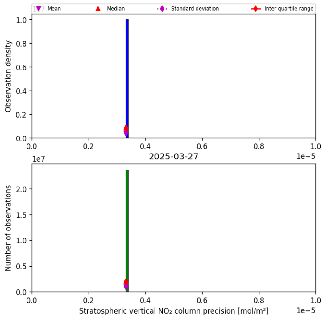
Figure 37: Histogram of “Stratospheric vertical NO 2 column precision” for 2025-03-27 to 2025-03-28
