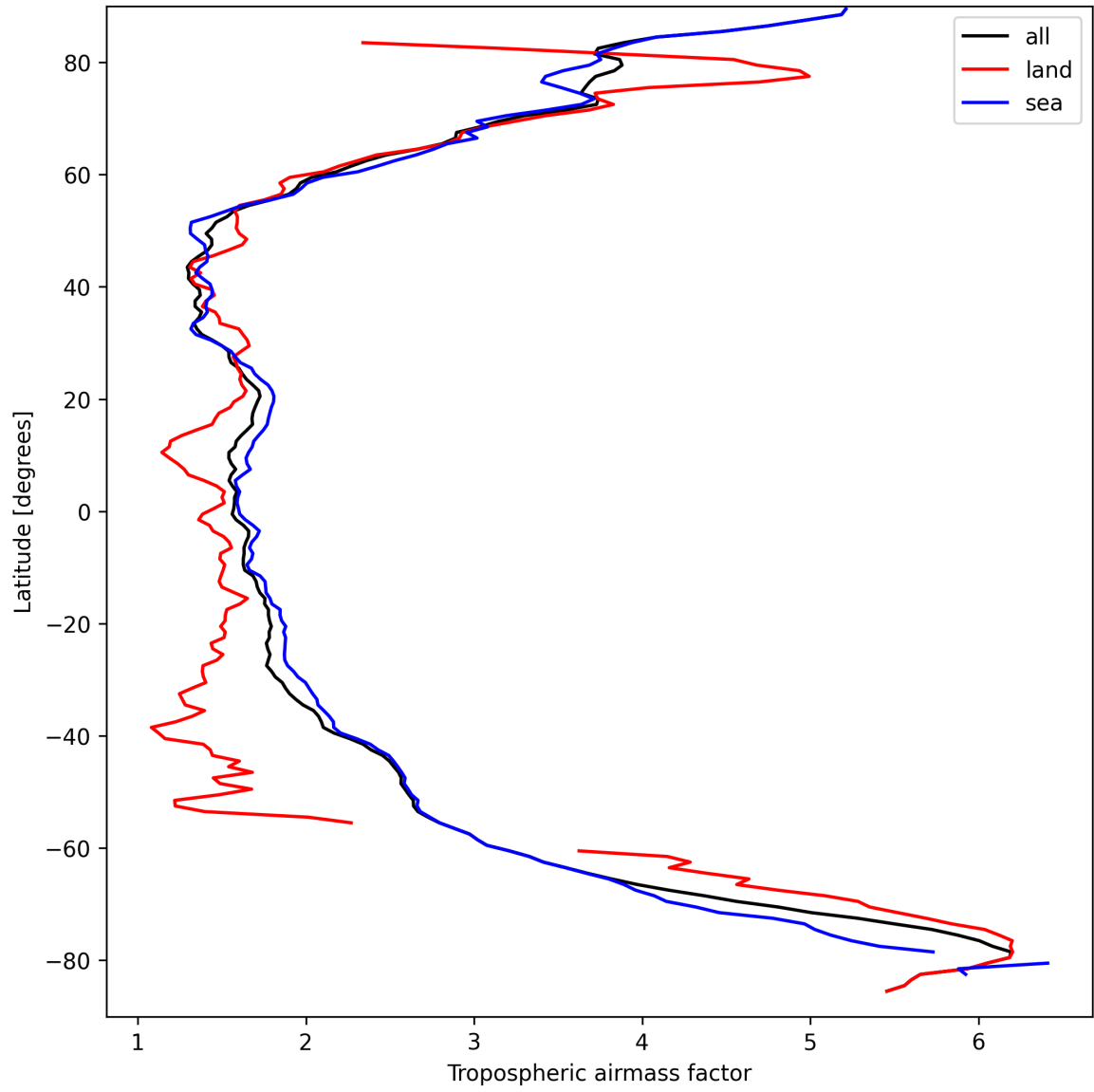
Figure 14: Zonal average of “Tropospheric airmass factor” for 2025-03-27 to 2025-03-28.
