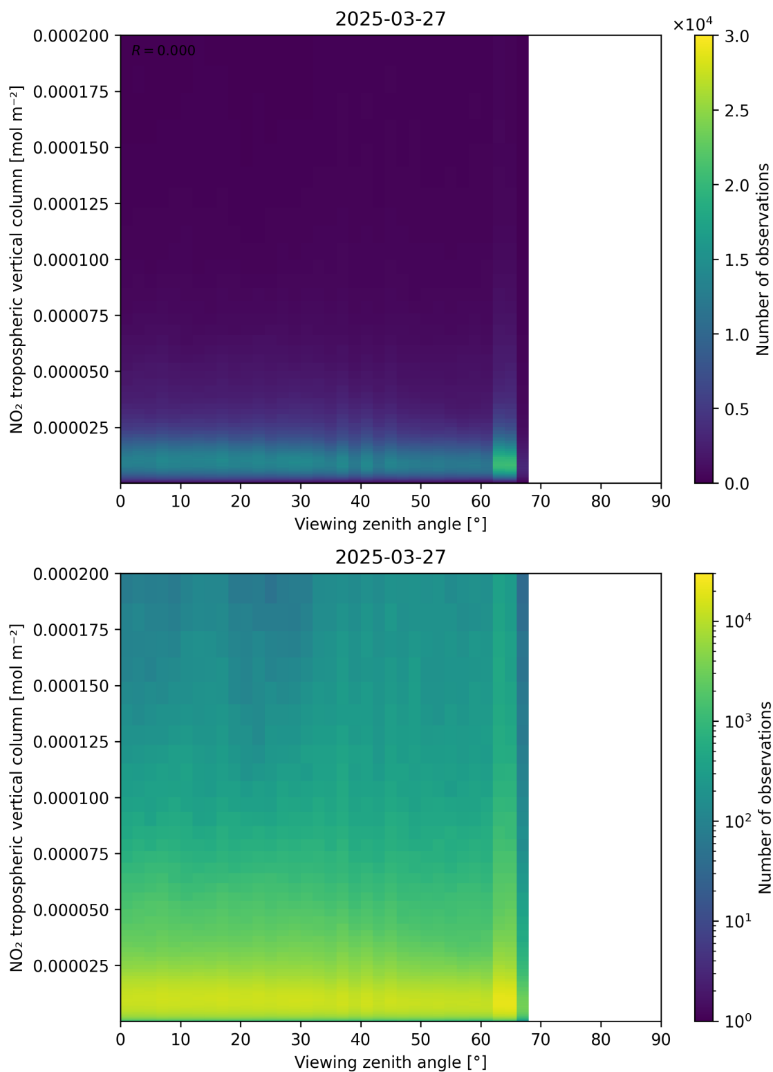
Figure 169: Scatter density plot of “Viewing zenith angle” against “NO 2 tropospheric vertical column” for 2025-03-27 to 2025-03-28.
