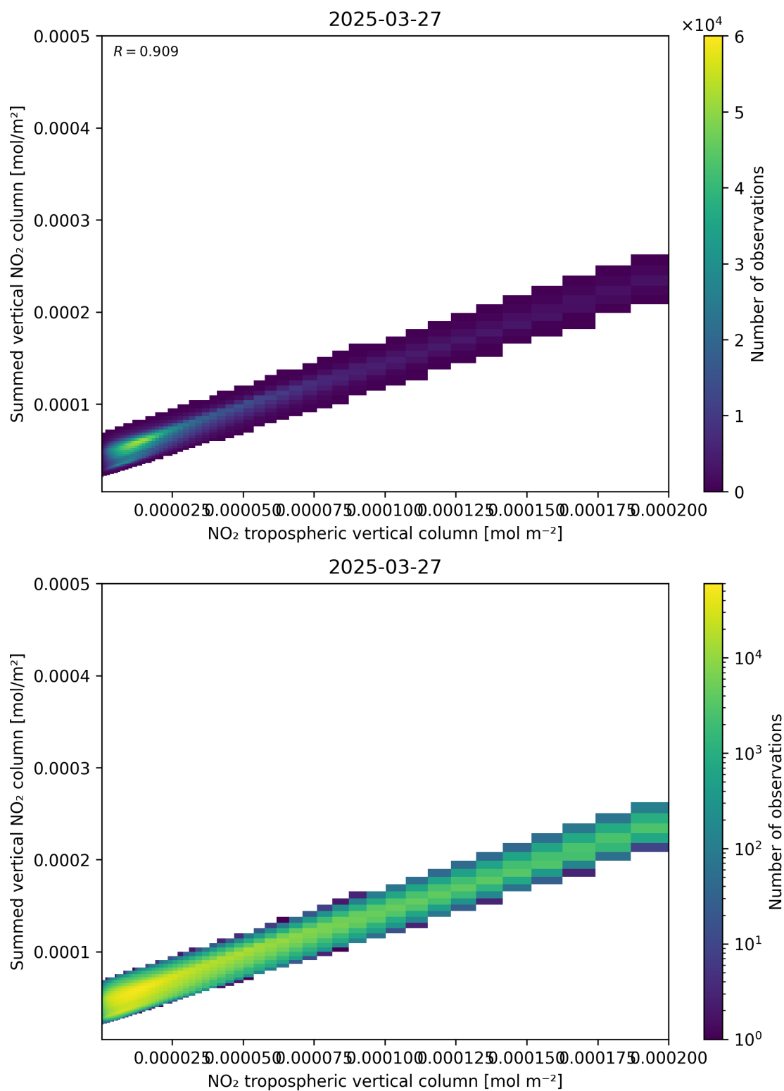
Figure 126: Scatter density plot of “NO 2 tropospheric vertical column” against “Summed vertical NO 2 column” for 2025-03-27 to 2025-03-28.
