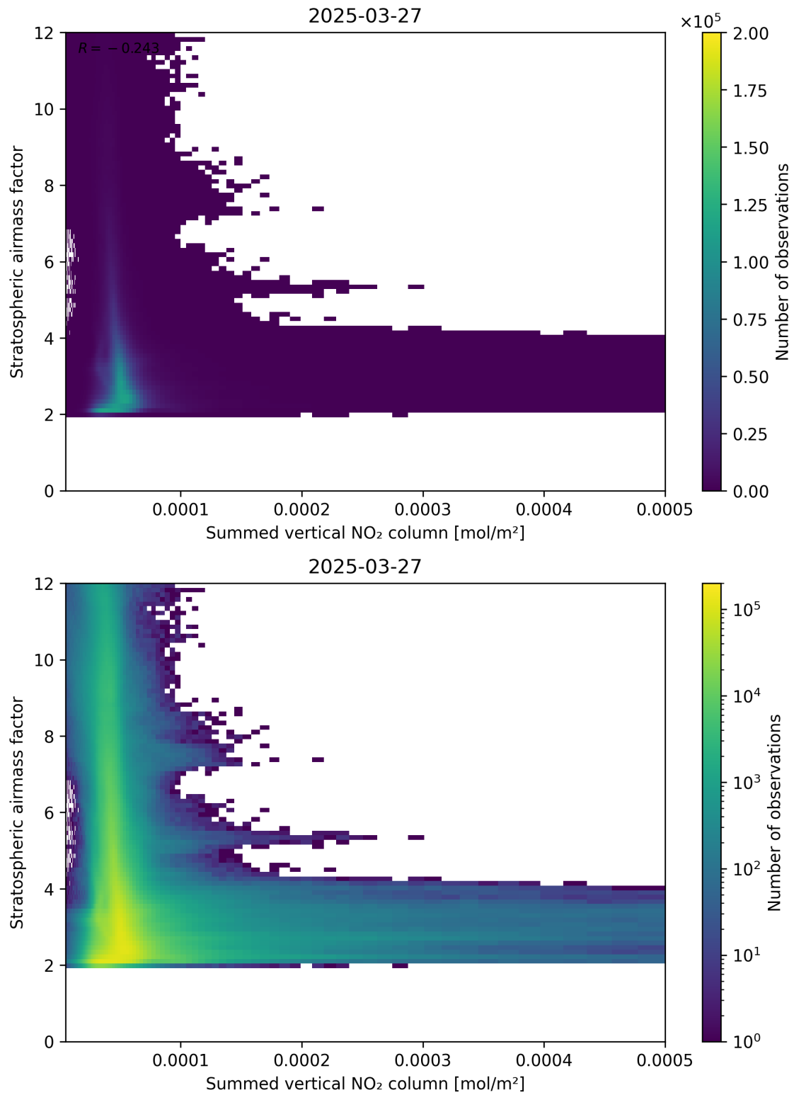
Figure 103: Scatter density plot of “Summed vertical NO 2 column” against “Stratospheric air mass factor” for 2025-03-27 to 2025-03-28.
