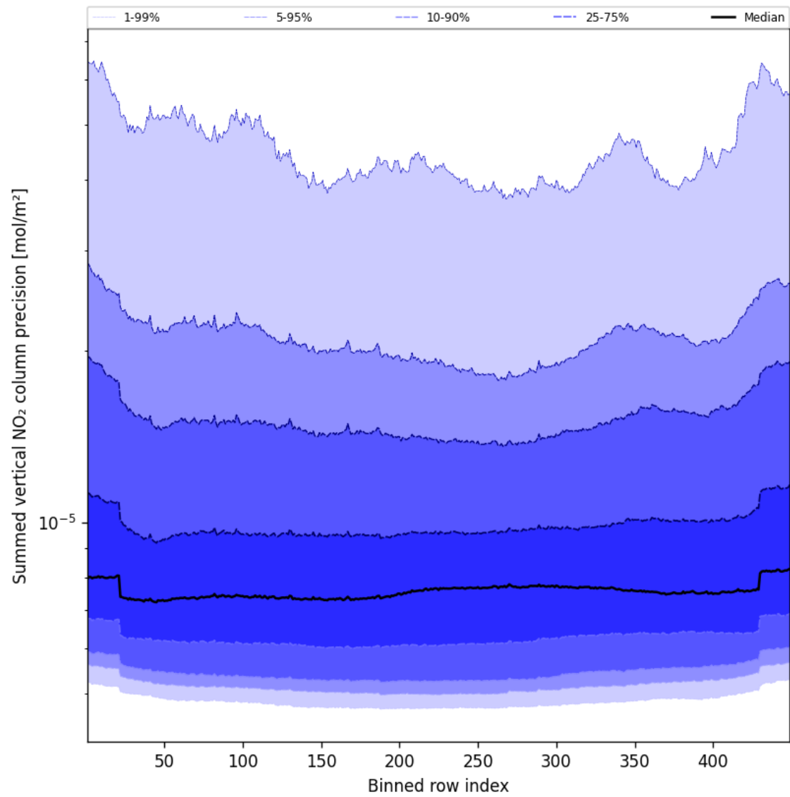
Figure 58: Along track statistics of “Summed vertical NO 2 column precision” for 2025-03-27 to 2025-03-28
