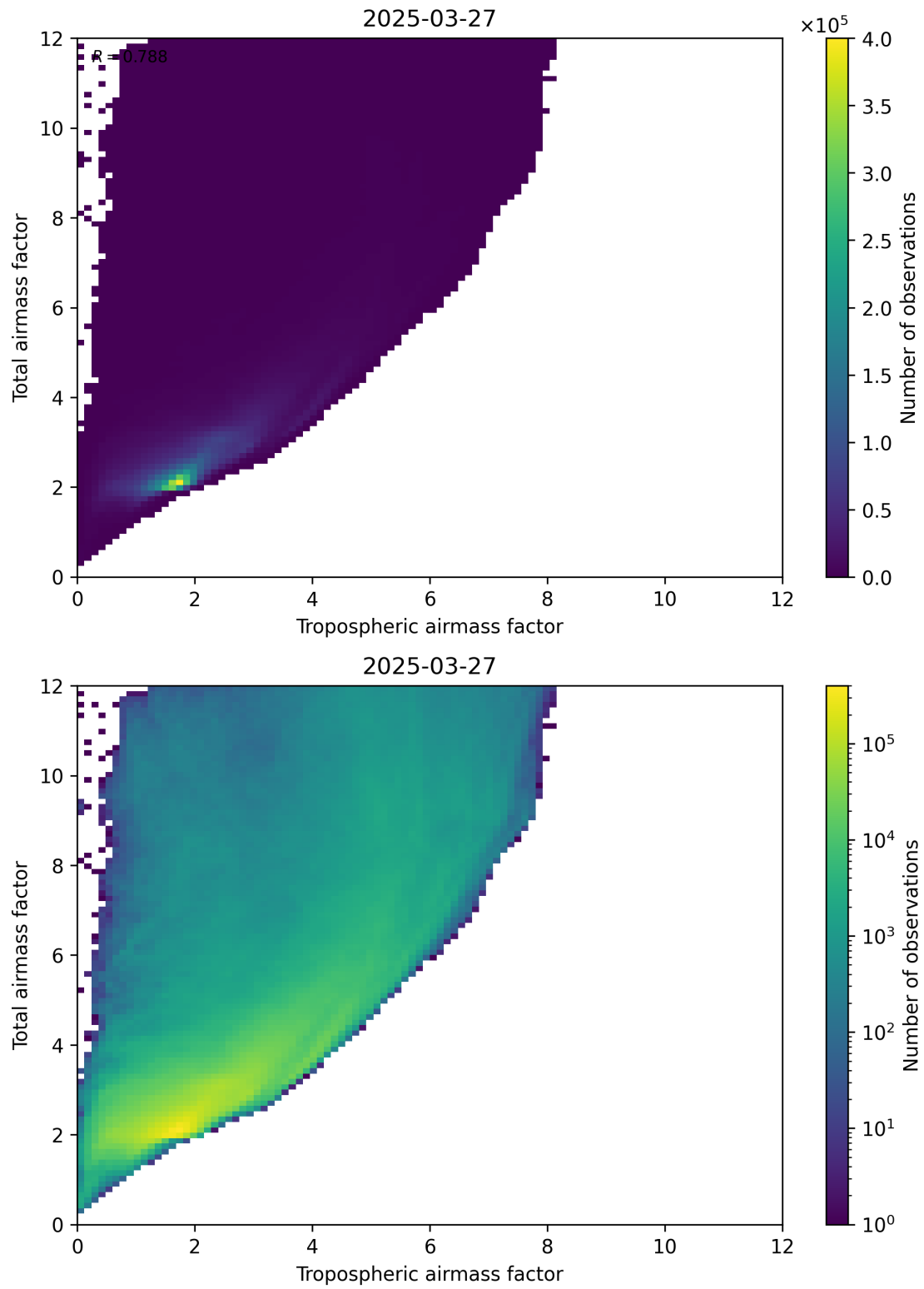
Figure 72: Scatter density plot of “Tropospheric airmass factor” against “Total airmass factor” for 2025-03-27 to 2025-03-28.
