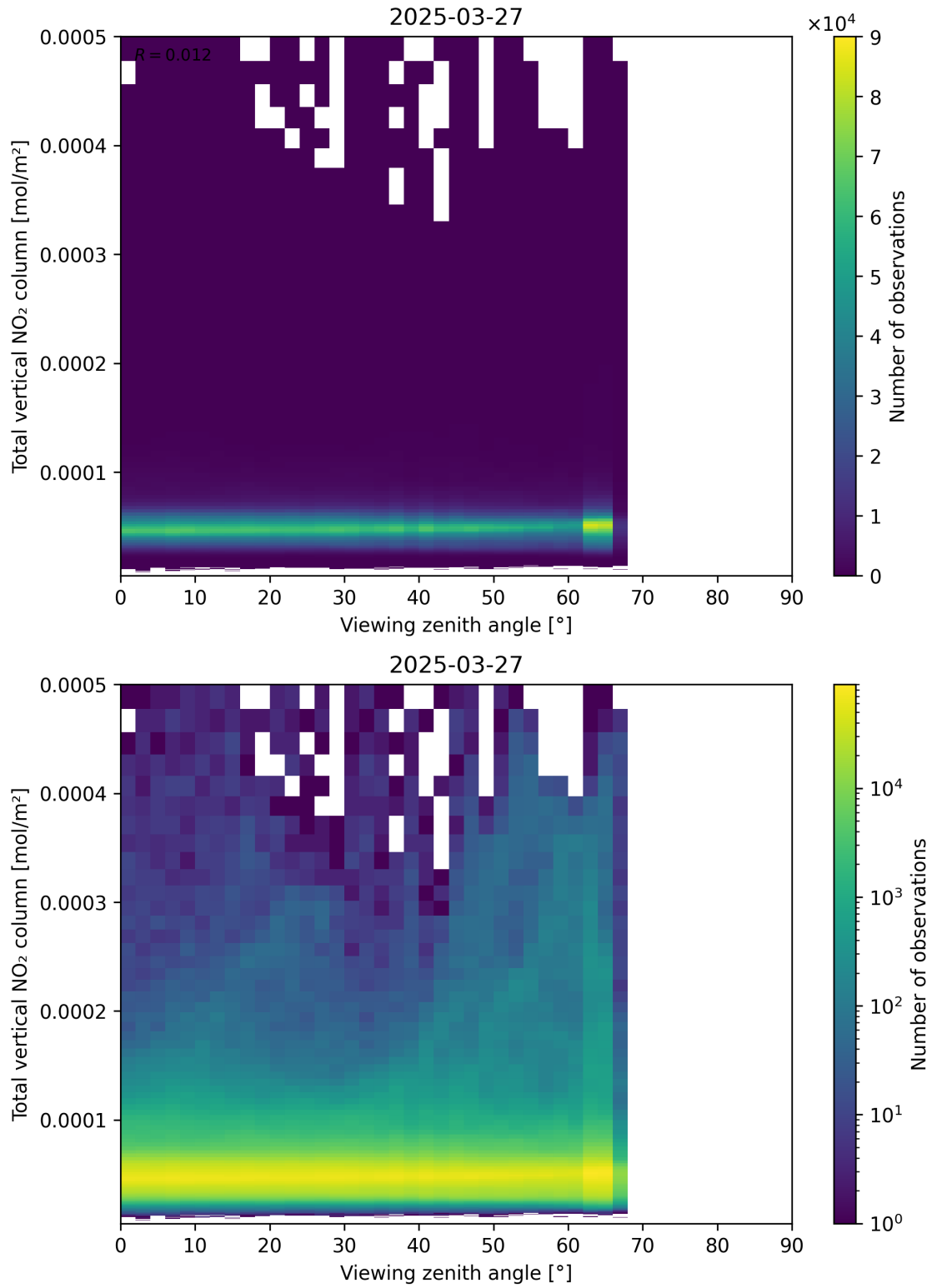
Figure 167: Scatter density plot of “Viewing zenith angle” against “Total vertical NO 2 column” for 2025-03-27 to 2025-03-28.
