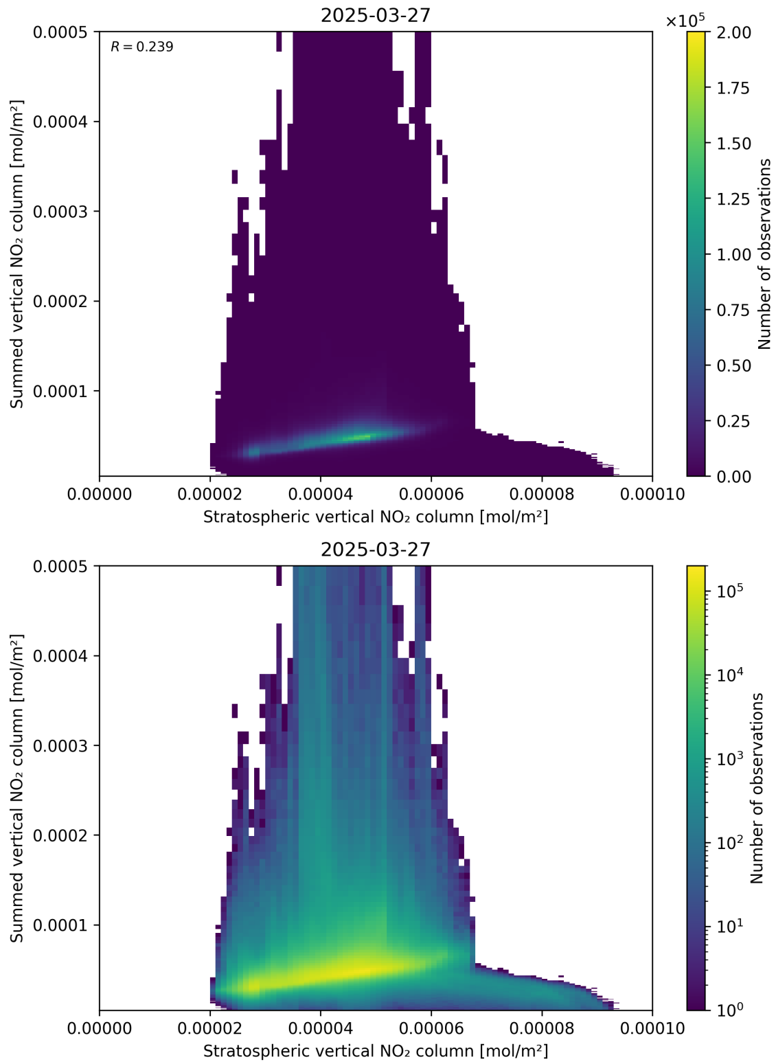
Figure 98: Scatter density plot of “Stratospheric vertical NO 2 column” against “Summed vertical NO 2 column” for 2025-03-27 to 2025-03-28.
