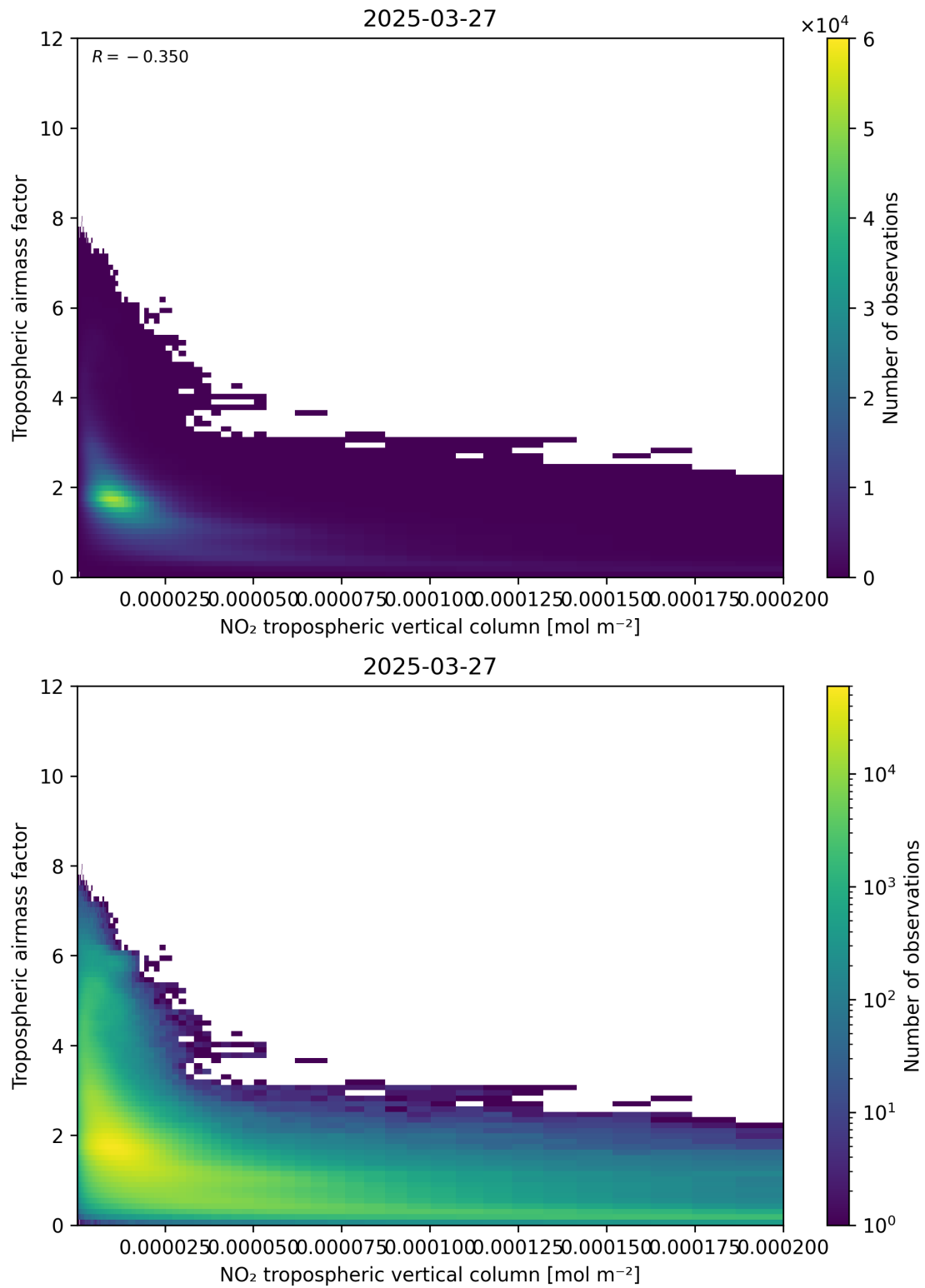
Figure 123: Scatter density plot of “NO 2 tropospheric vertical column” against “Tropospheric air mass factor” for 2025-03-27 to 2025-03-28.
