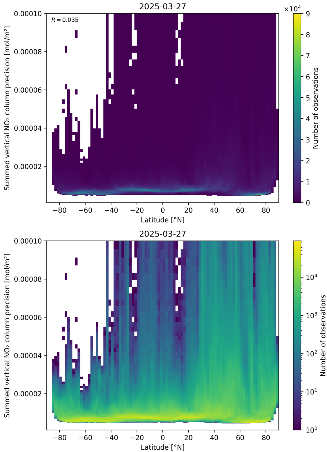
Figure 89: Scatter density plot of “Latitude” against “Summed vertical NO 2 column precision” for 2025-03-27 to 2025-03-28.
