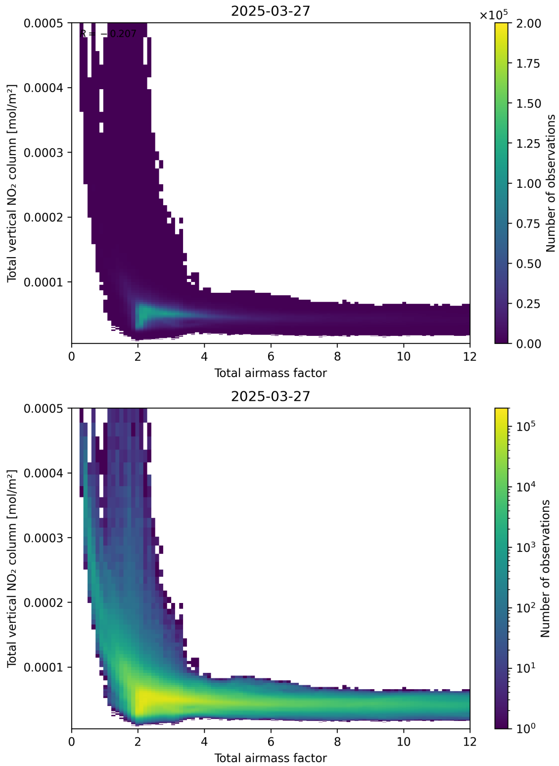
Figure 67: Scatter density plot of “Total airmass factor” against “Total vertical NO 2 column” for 2025-03-27 to 2025-03-28.
