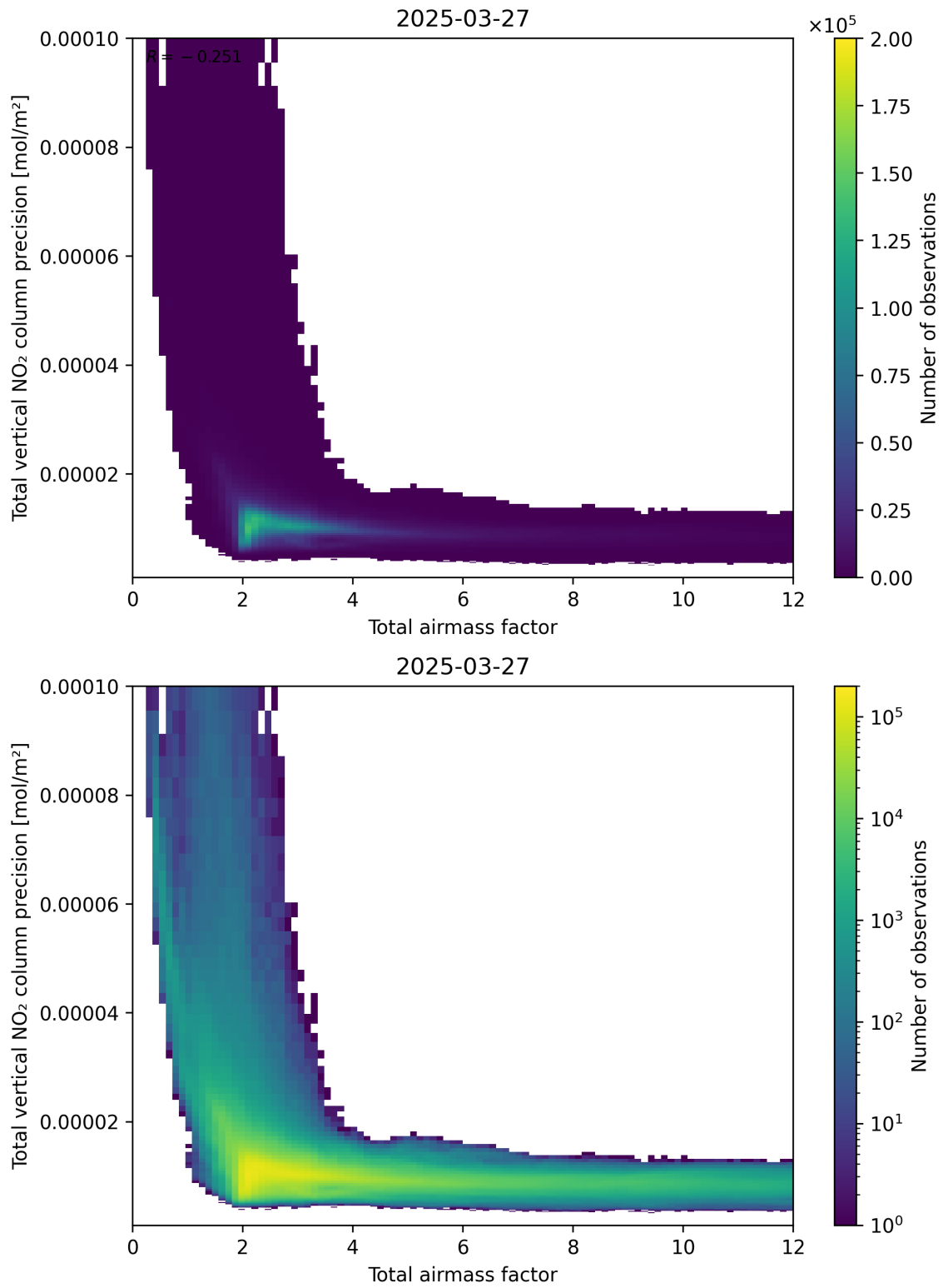
Figure 68: Scatter density plot of “Total airmass factor” against “Total vertical NO 2 column precision” for 2025-03-27 to 2025-03-28.
