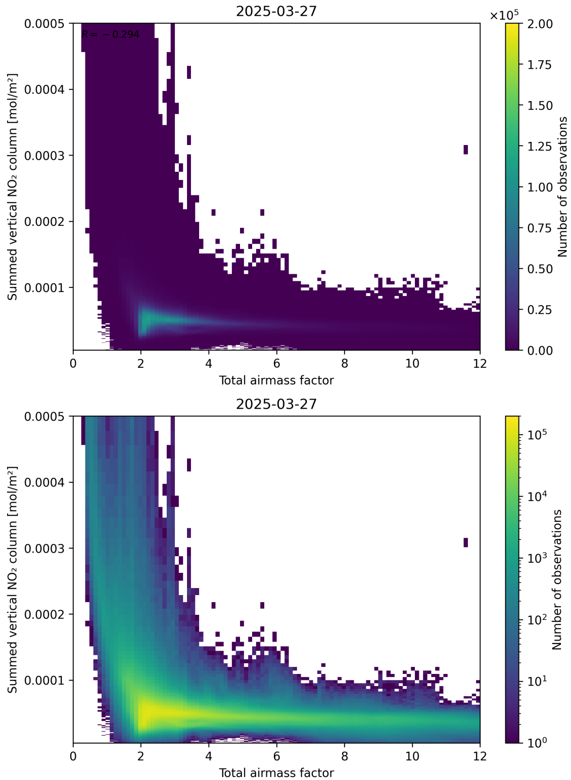
Figure 65: Scatter density plot of “Total airmass factor” against “Summed vertical NO 2 column” for 2025-03-27 to 2025-03-28.
