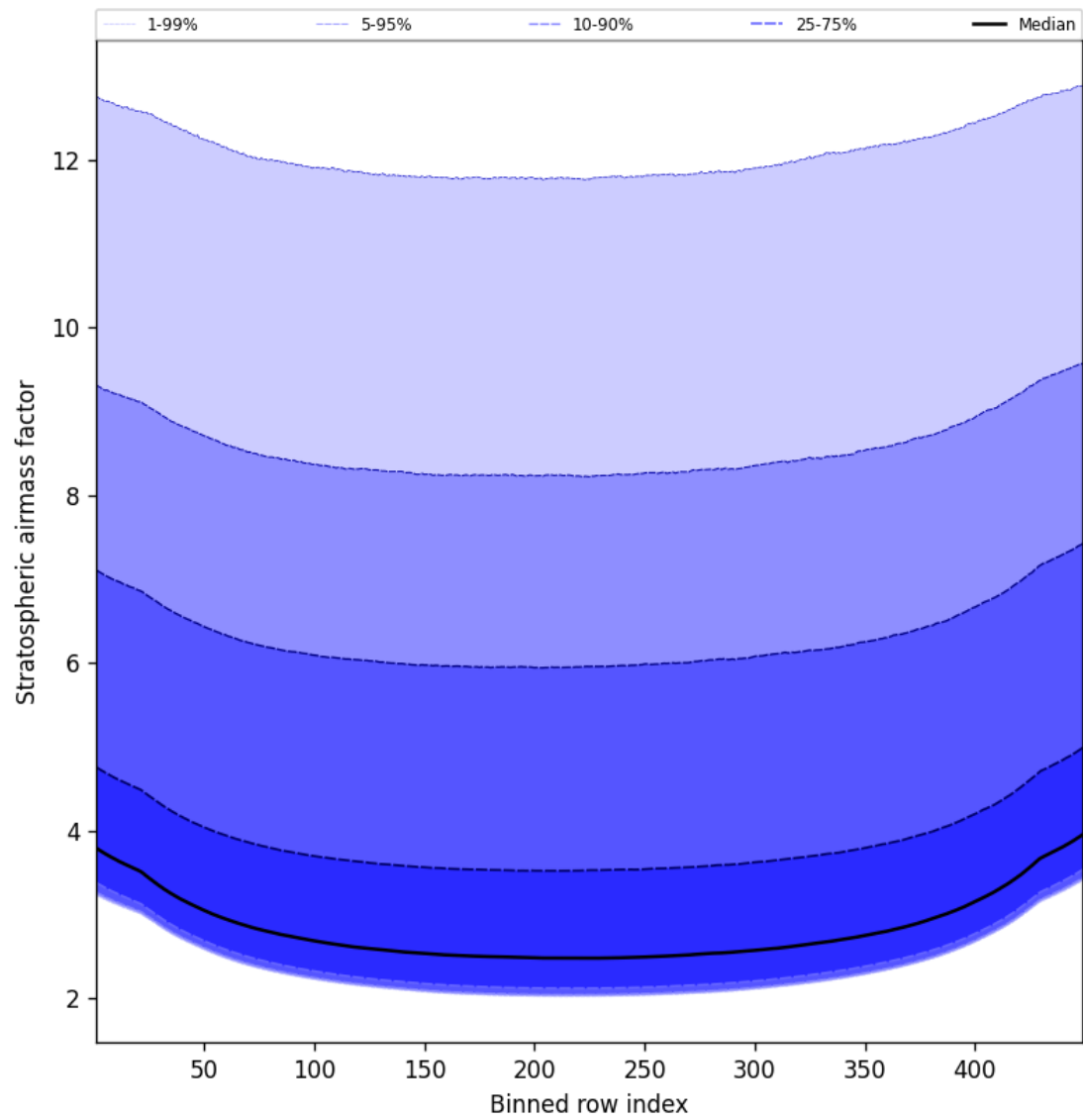
Figure 61: Along track statistics of “Stratospheric airmass factor” for 2025-03-27 to 2025-03-28
