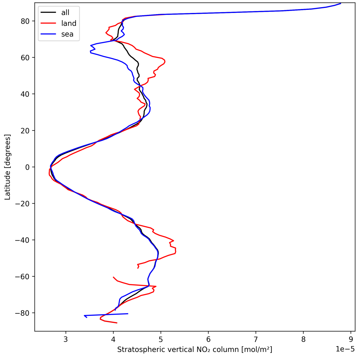
Figure 19: Zonal average of “Stratospheric vertical NO 2 column” for 2025-03-27 to 2025-03-28.
