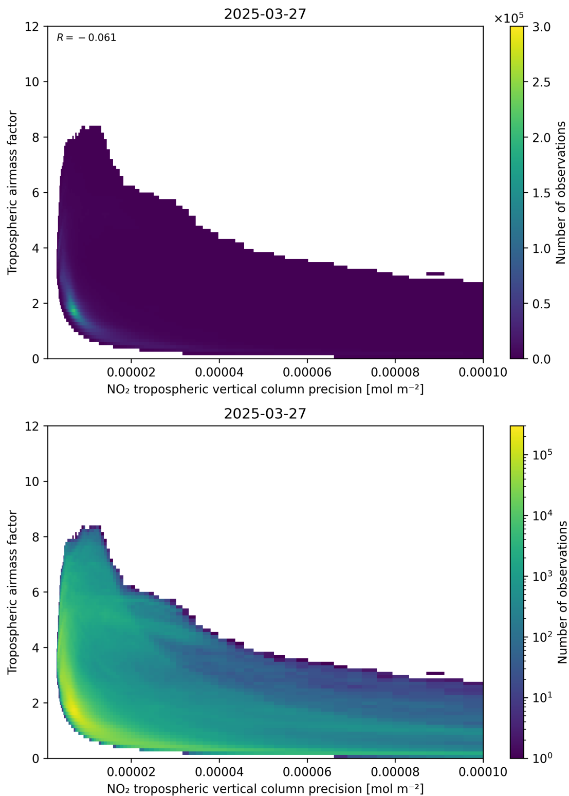
Figure 133: Scatter density plot of “NO 2 tropospheric vertical column precision” against “Tropospheric air mass factor” for 2025-03-27 to 2025-03-28.
