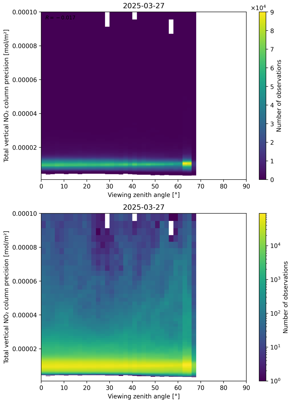
Figure 168: Scatter density plot of “Viewing zenith angle” against “Total vertical NO 2 column precision” for 2025-03-27 to 2025-03-28.
