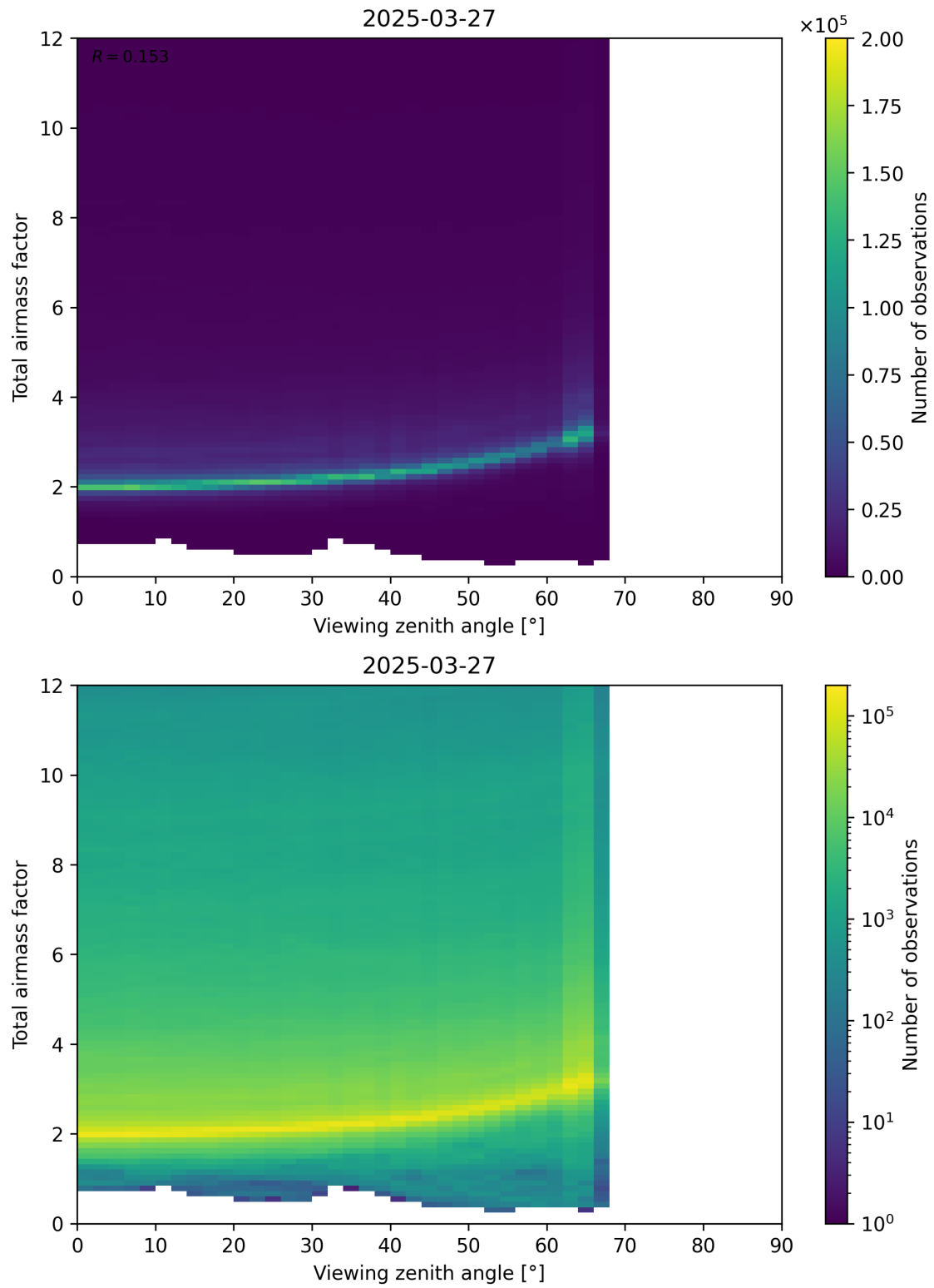
Figure 160: Scatter density plot of “Viewing zenith angle” against “Total airmass factor” for 2025-03-27 to 2025-03-28.
