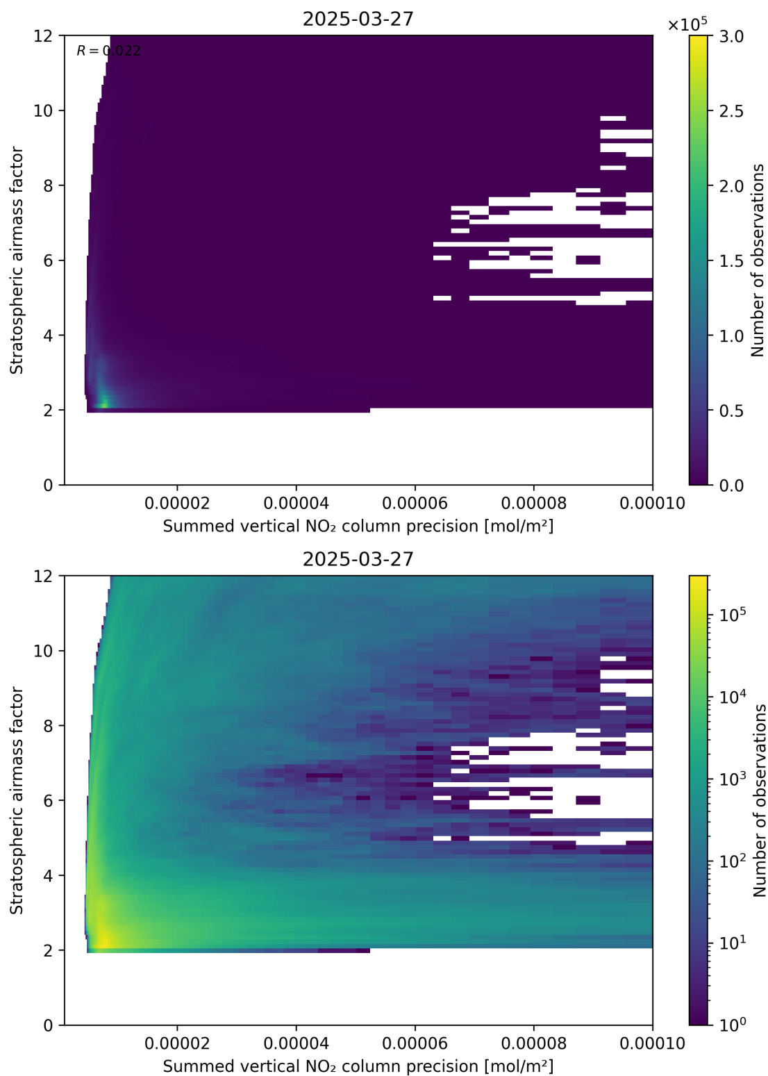
Figure 106: Scatter density plot of “Summed vertical NO 2 column precision” against “Stratospheric airmass factor” for 2025-03-27 to 2025-03-28.
