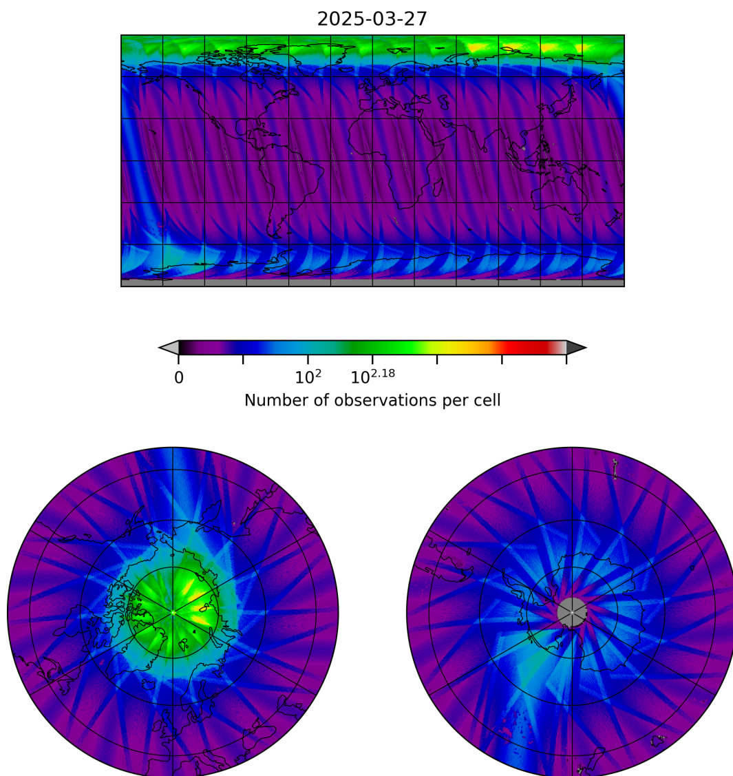
Figure 10: Map of the number of observations for 2025-03-27 to 2025-03-28
