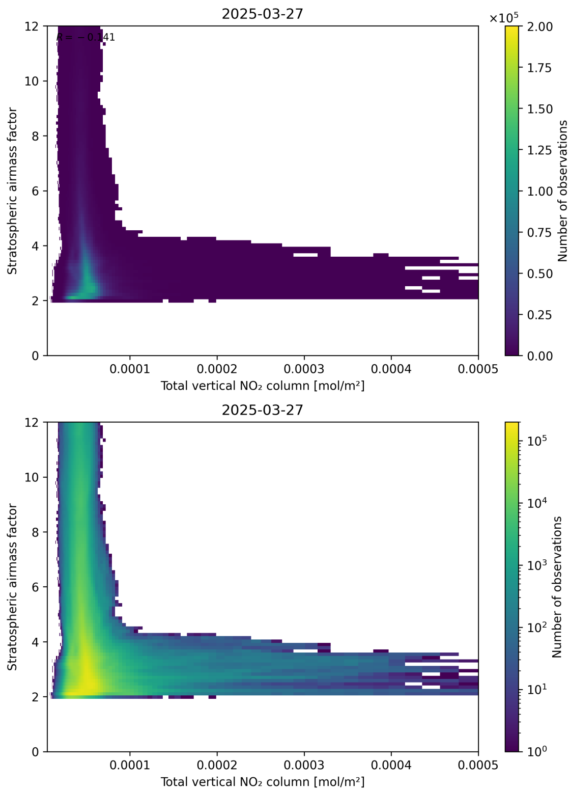
Figure 110: Scatter density plot of “Total vertical NO 2 column” against “Stratospheric air mass factor” for 2025-03-27 to 2025-03-28.
