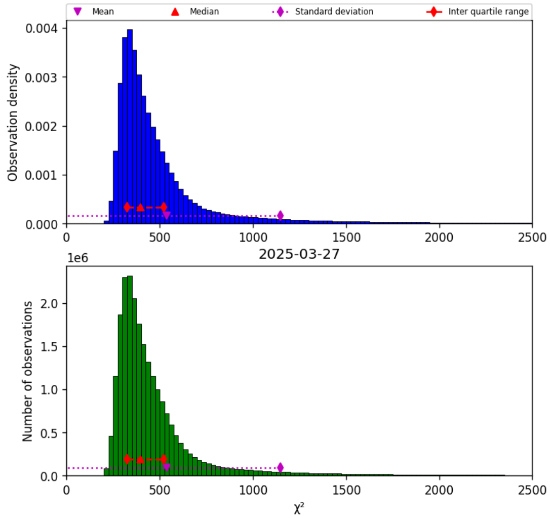
Figure 42: Histogram of “ \chi^2 ” for 2025-03-27 to 2025-03-28
