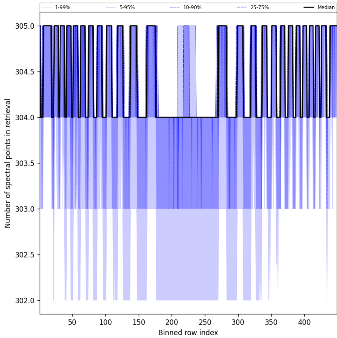
Figure 50: Along track statistics of “Number of spectral points in retrieval” for 2025-03-27 to 2025-03-28
