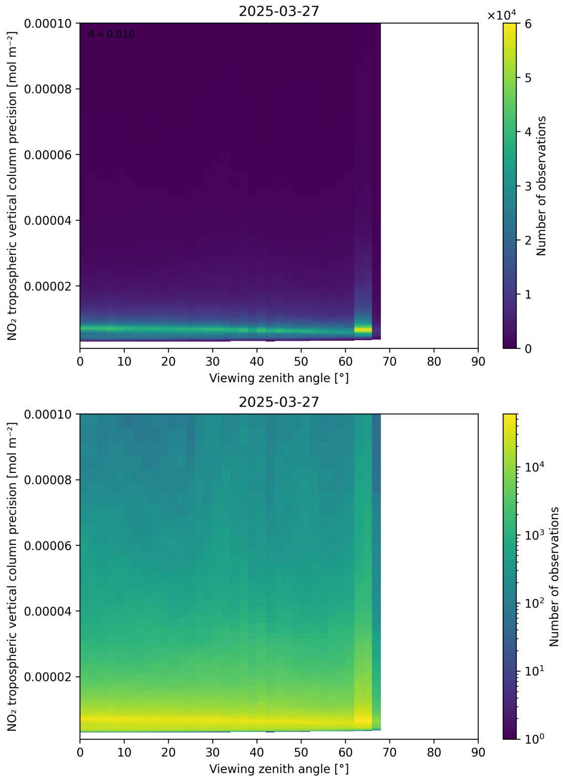
Figure 170: Scatter density plot of “Viewing zenith angle” against “NO 2 tropospheric vertical column precision” for 2025-03-27 to 2025-03-28.
