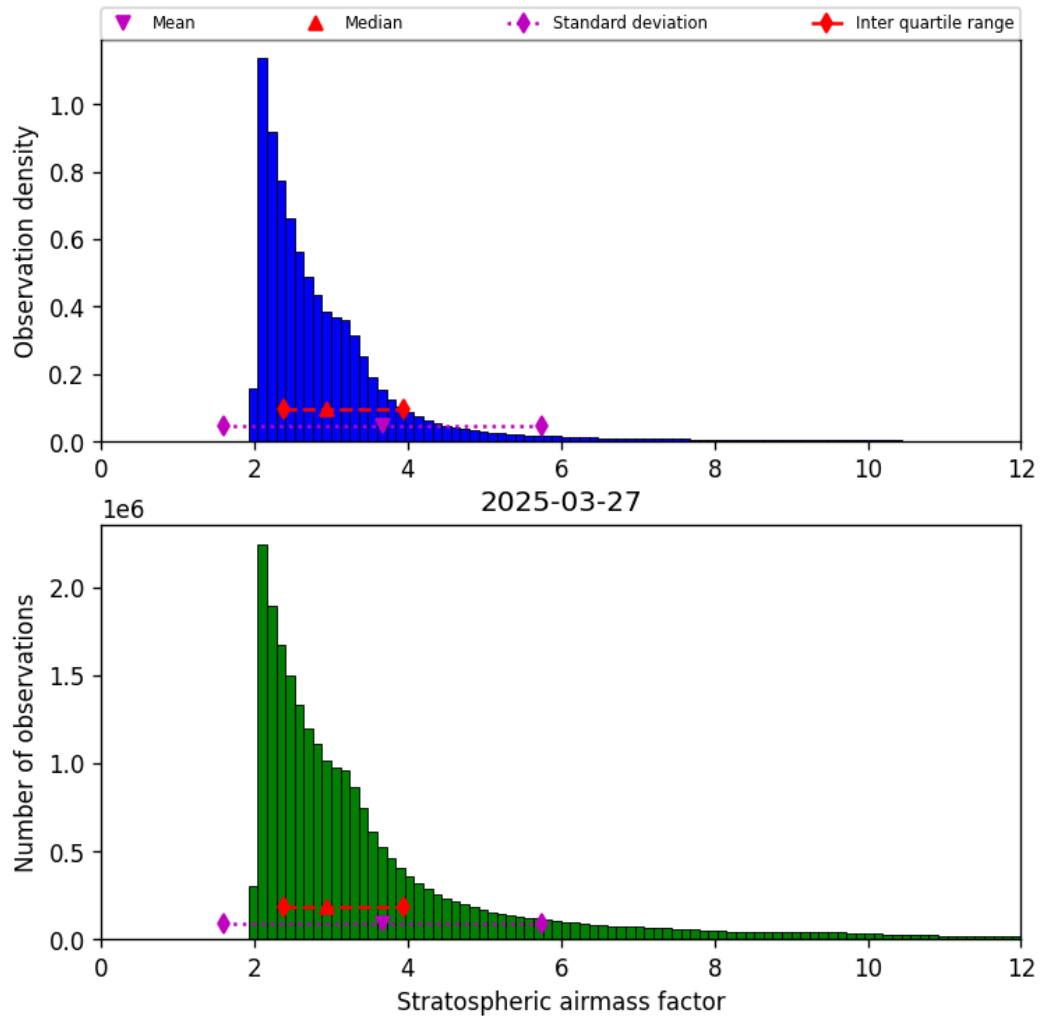
Figure 44: Histogram of “Stratospheric airmass factor” for 2025-03-27 to 2025-03-28
