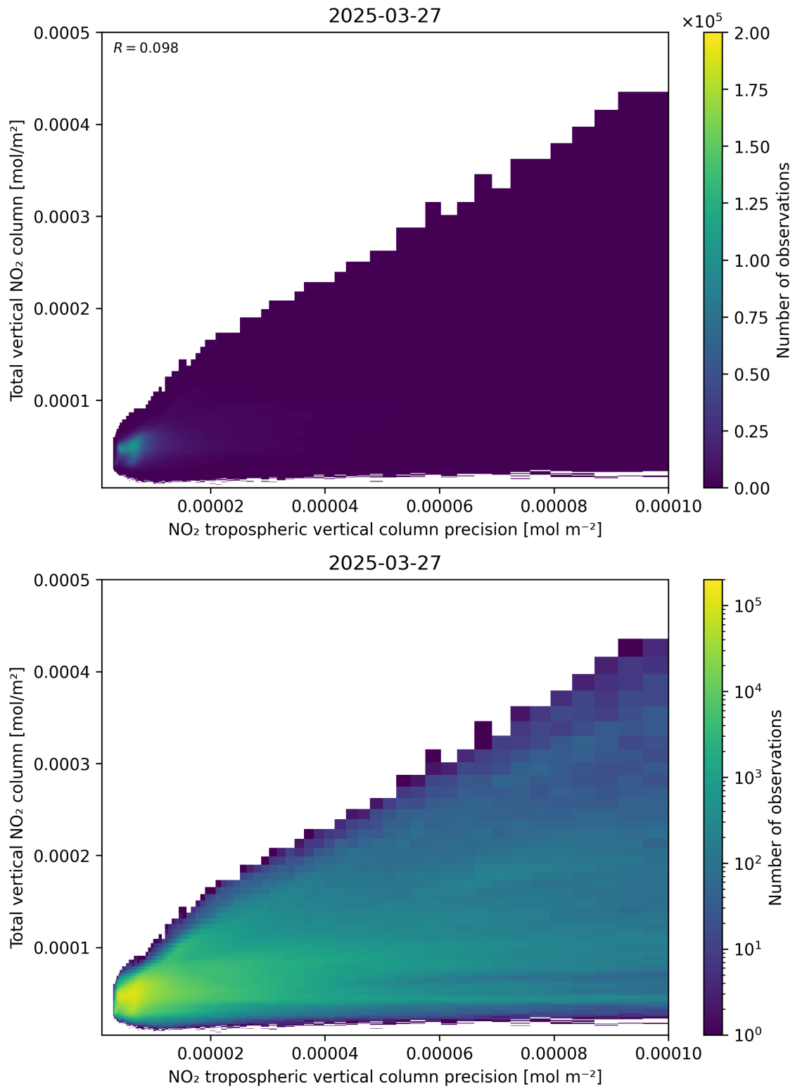
Figure 138: Scatter density plot of “NO 2 tropospheric vertical column precision” against “Total vertical NO 2 column” for 2025-03-27 to 2025-03-28.
