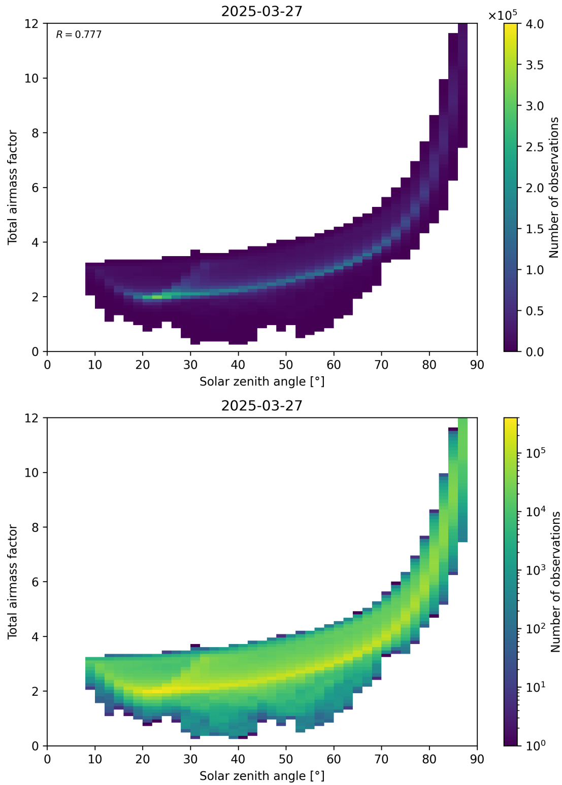
Figure 146: Scatter density plot of “Solar zenith angle” against “Total air mass factor” for 2025-03-27 to 2025-03-28.
