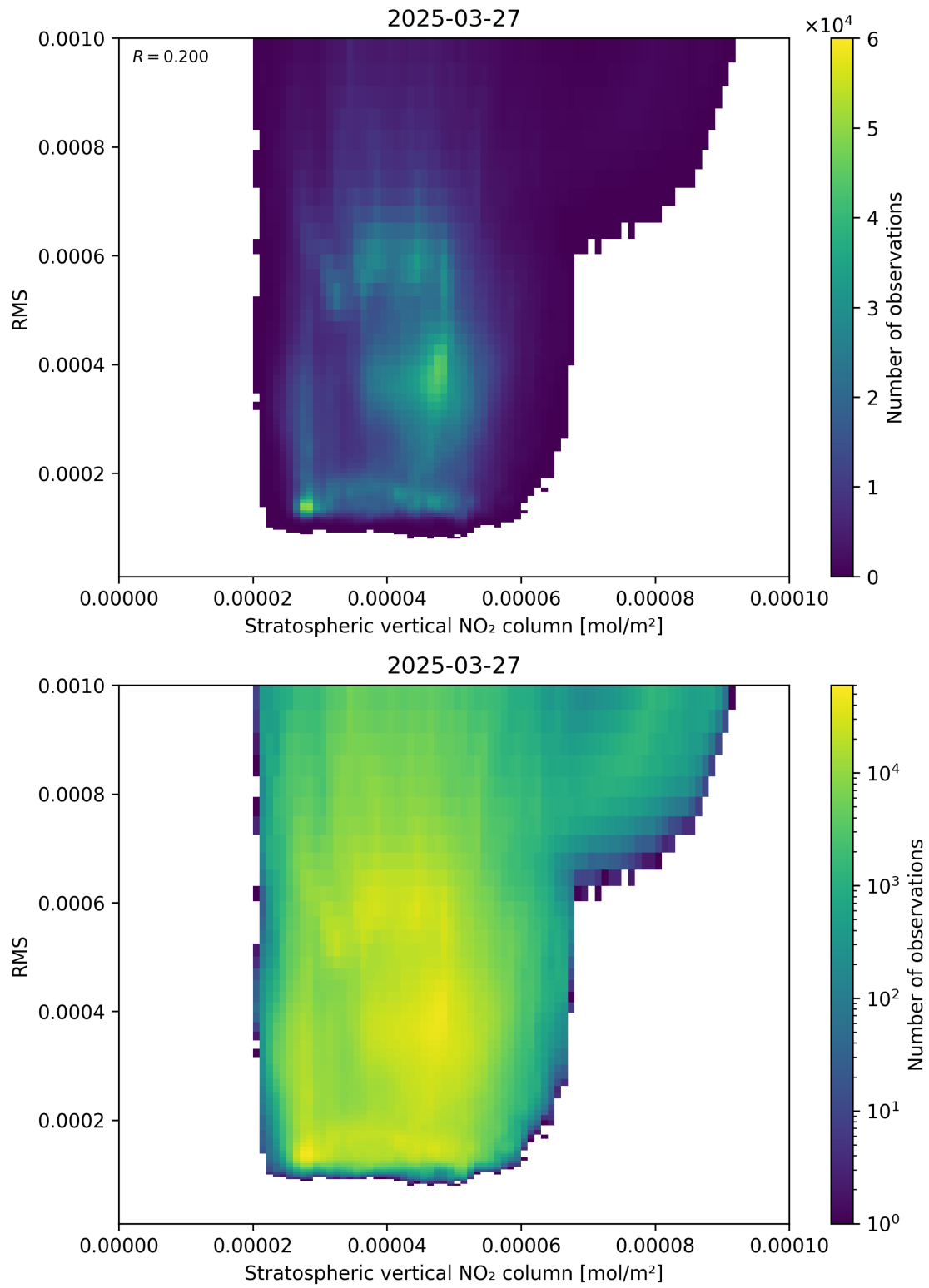
Figure 102: Scatter density plot of “Stratospheric vertical NO 2 column” against “RMS” for 2025-03-27 to 2025-03-28.
