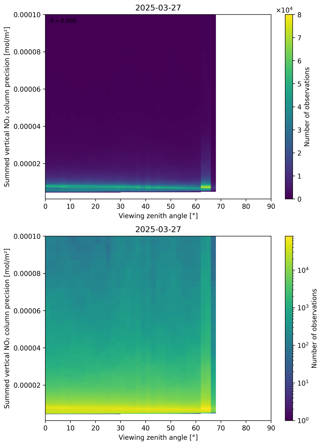
Figure 166: Scatter density plot of “Viewing zenith angle” against “Summed vertical NO 2 column precision” for 2025-03-27 to 2025-03-28.
