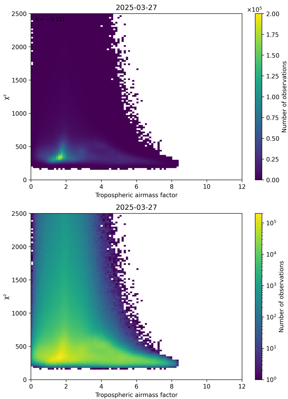
Figure 73: Scatter density plot of “Tropospheric airmass factor” against “ \chi^2 ” for 2025-03-27 to 2025-03-28.
