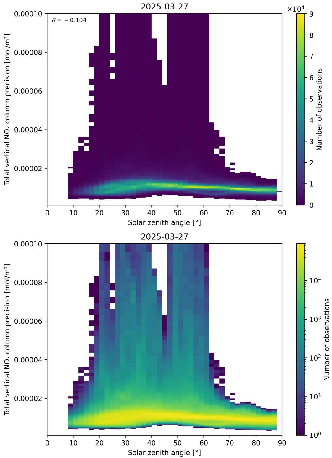
Figure 154: Scatter density plot of “Solar zenith angle” against “Total vertical NO 2 column precision” for 2025-03-27 to 2025-03-28.
