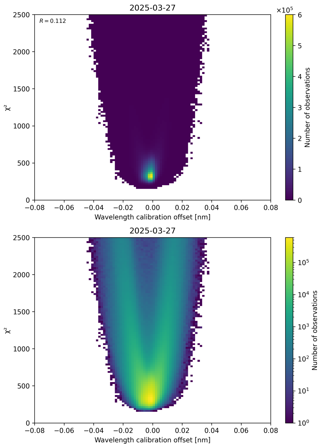
Figure 175: Scatter density plot of “Wavelength calibration offset” against “ \chi^2 ” for 2025-03-27 to 2025-03-28.
