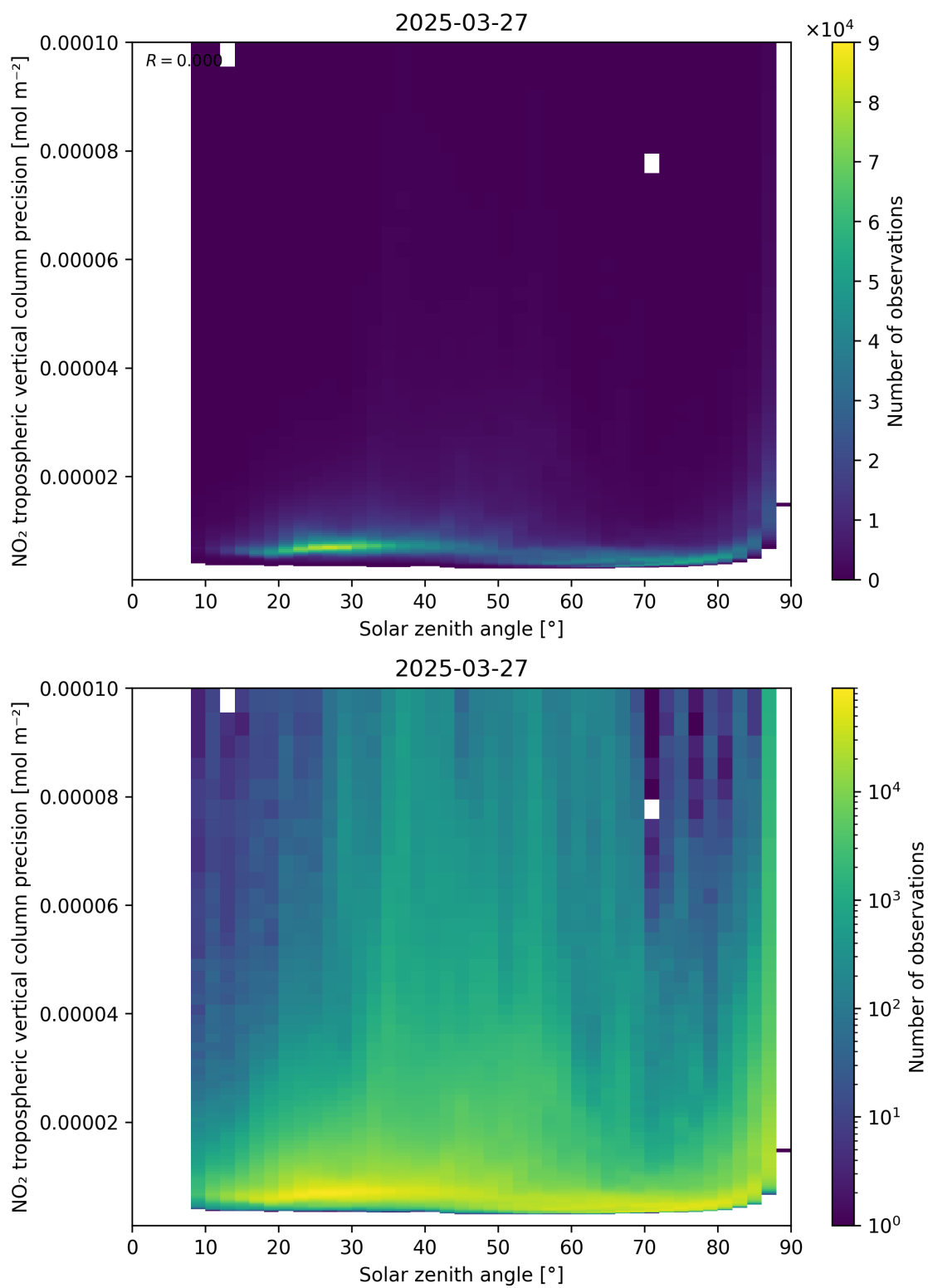
Figure 156: Scatter density plot of “Solar zenith angle” against “NO 2 tropospheric vertical column precision” for 2025-03-27 to 2025-03-28.
