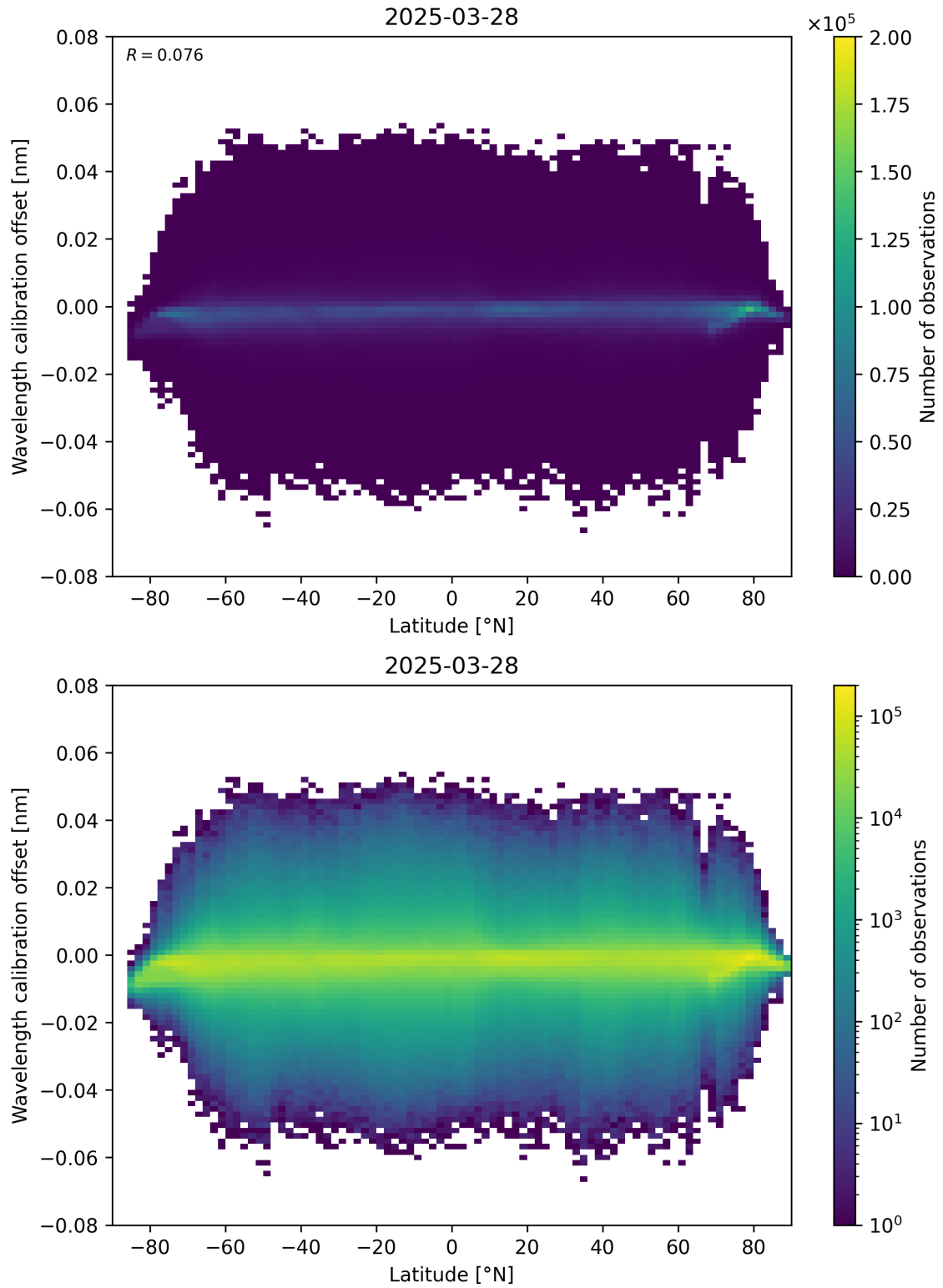
Figure 95: Scatter density plot of “Latitude” against “Wavelength calibration offset” for 2025-03-28 to 2025-03-29.
