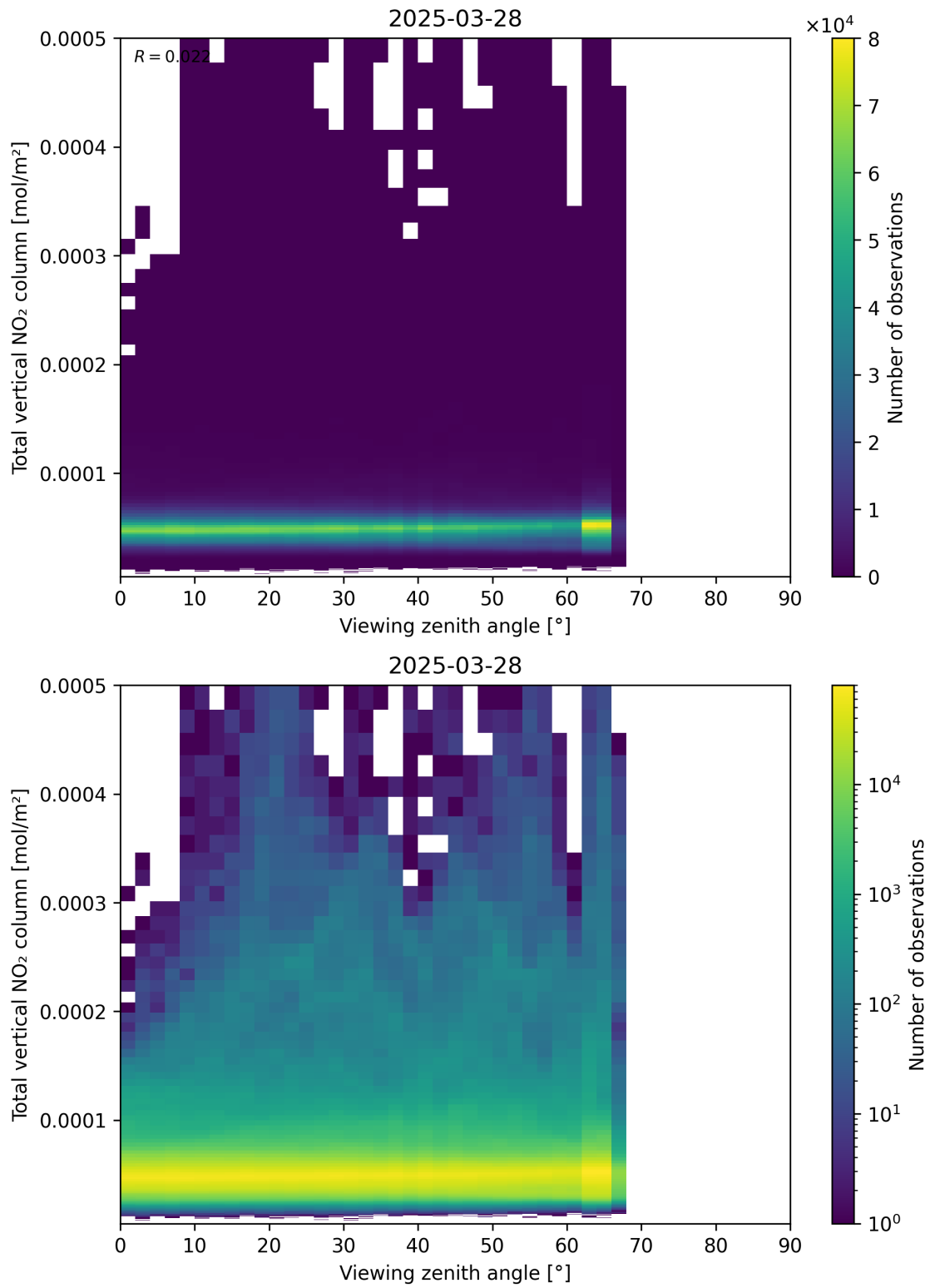
Figure 167: Scatter density plot of “Viewing zenith angle” against “Total vertical NO 2 column” for 2025-03-28 to 2025-03-29.
