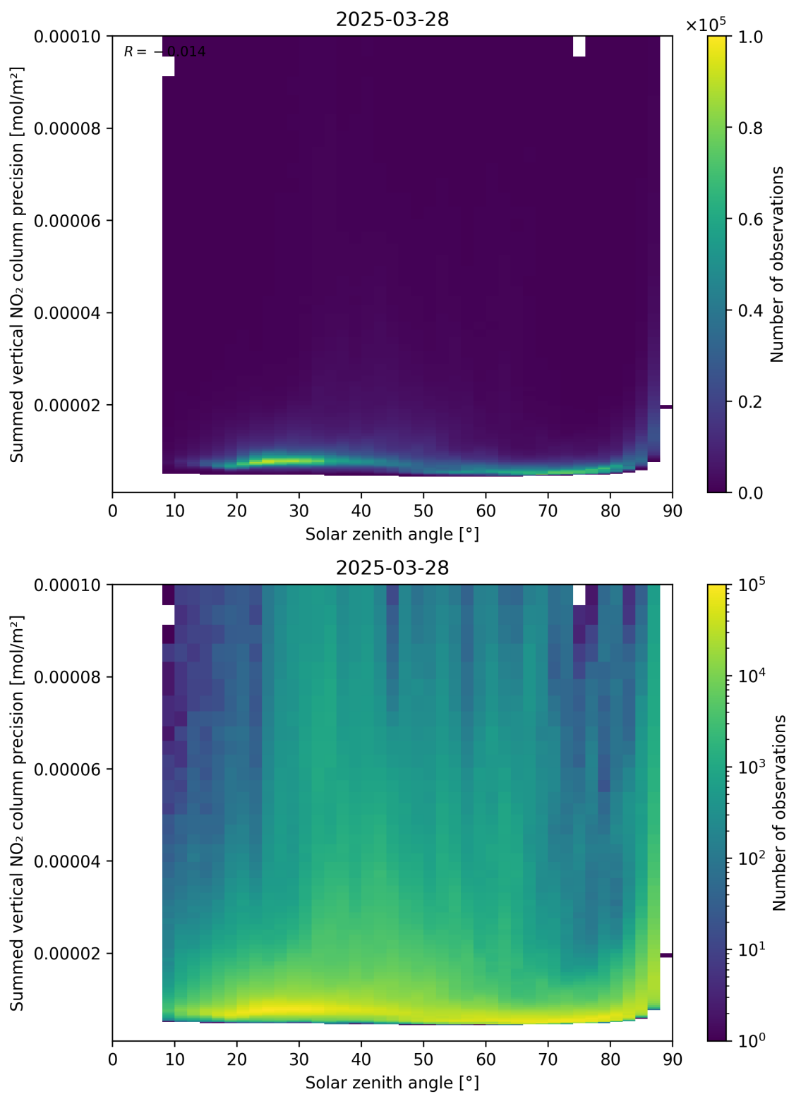
Figure 152: Scatter density plot of “Solar zenith angle” against “Summed vertical NO 2 column precision” for 2025-03-28 to 2025-03-29.
