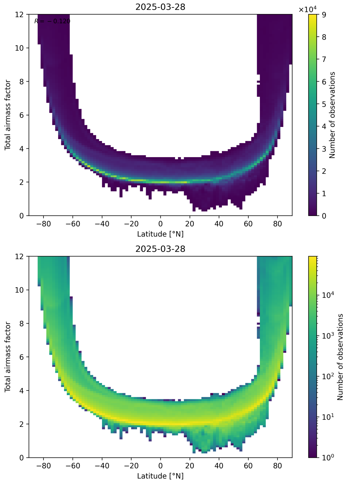
Figure 84: Scatter density plot of “Latitude” against “Total airmass factor” for 2025-03-28 to 2025-03-29.
