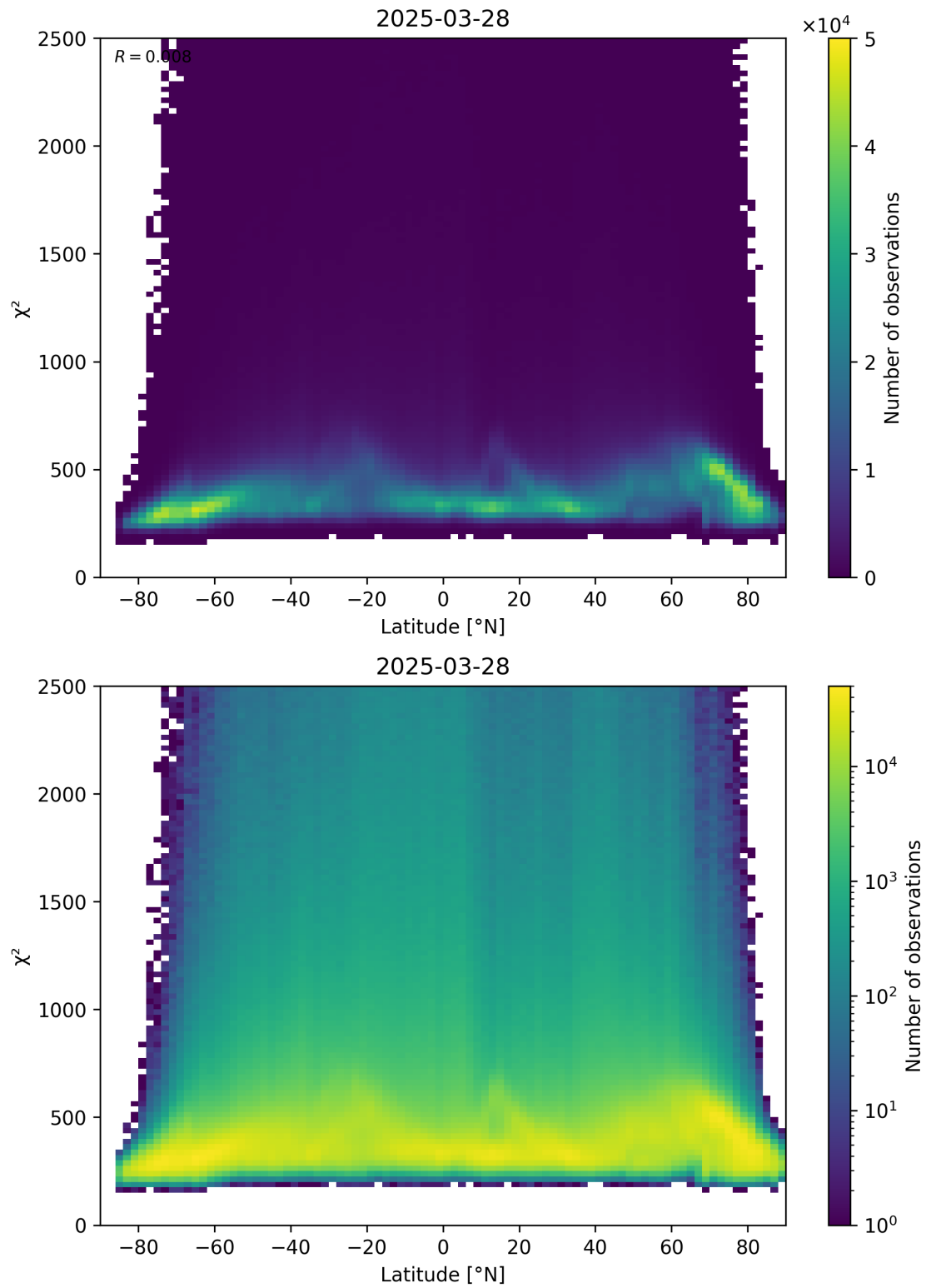
Figure 86: Scatter density plot of “Latitude” against “ \chi^2 ” for 2025-03-28 to 2025-03-29.
