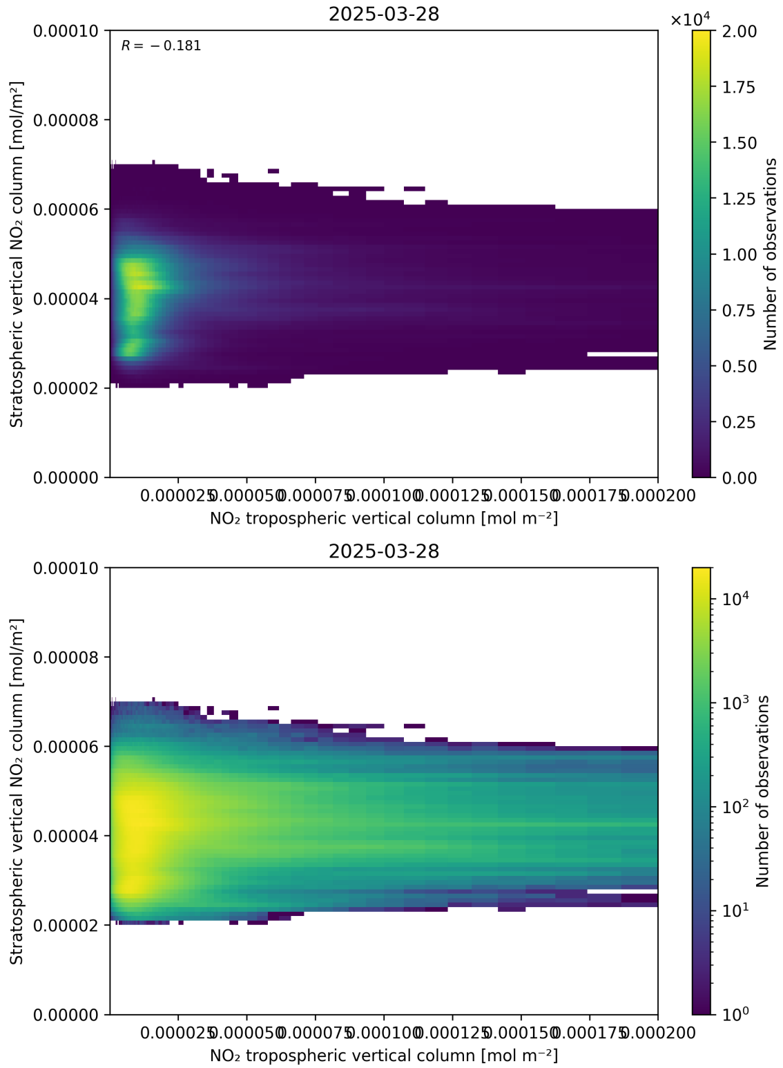
Figure 125: Scatter density plot of “NO 2 tropospheric vertical column” against “Stratospheric vertical NO 2 column” for 2025-03-28 to 2025-03-29.
