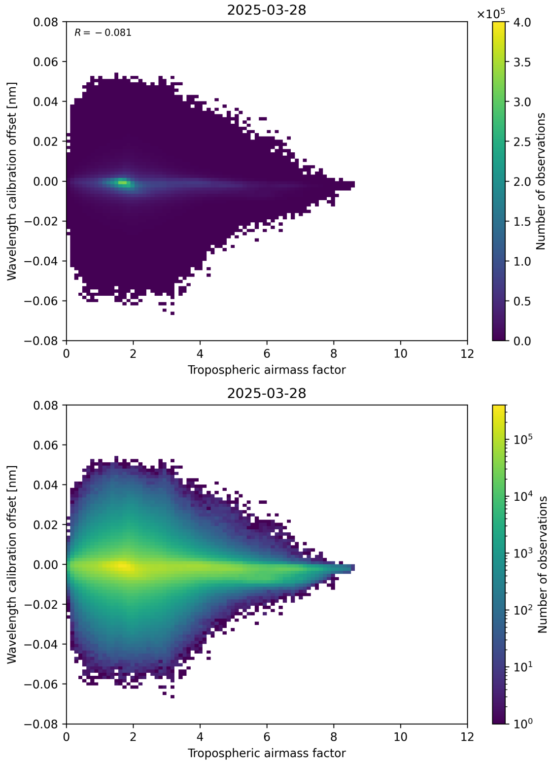
Figure 80: Scatter density plot of “Tropospheric airmass factor” against “Wavelength calibration offset” for 2025-03-28 to 2025-03-29.
