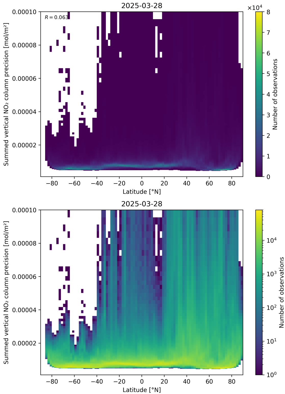
Figure 89: Scatter density plot of “Latitude” against “Summed vertical NO 2 column precision” for 2025-03-28 to 2025-03-29.
