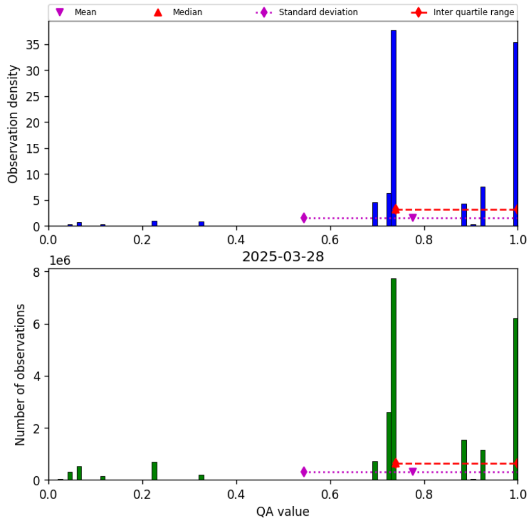
Figure 28: Histogram of “QA value” for 2025-03-28 to 2025-03-29
