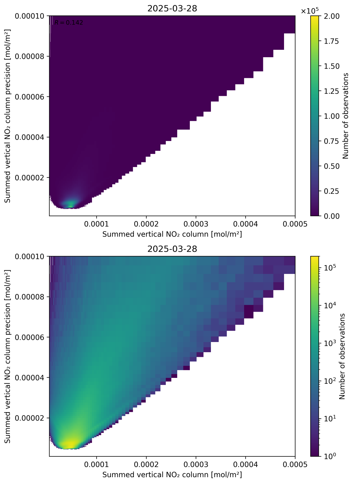
Figure 105: Scatter density plot of “Summed vertical NO 2 column” against “Summed vertical NO 2 column precision” for 2025-03-28 to 2025-03-29.
