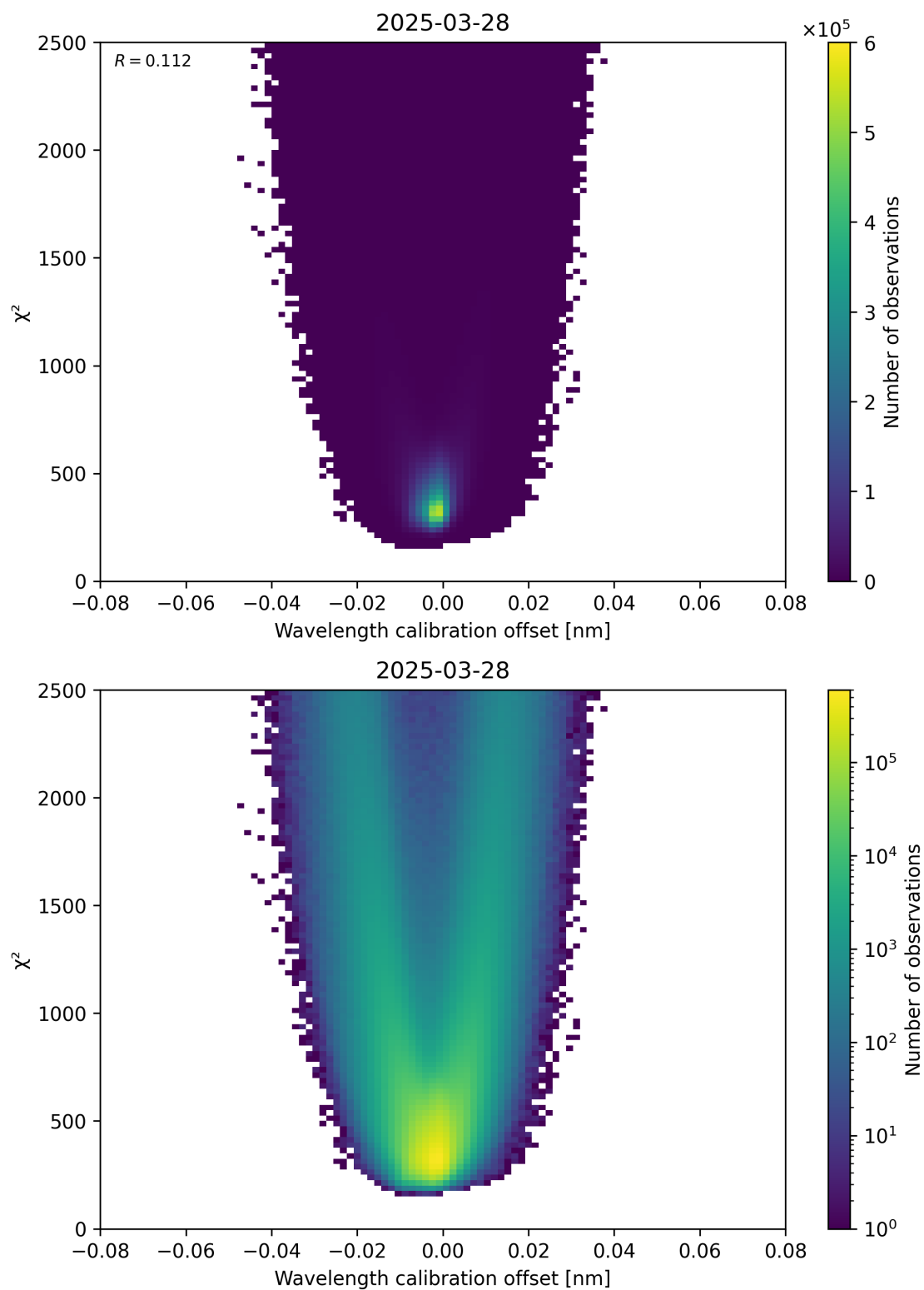
Figure 175: Scatter density plot of “Wavelength calibration offset” against “ \chi^2 ” for 2025-03-28 to 2025-03-29.
