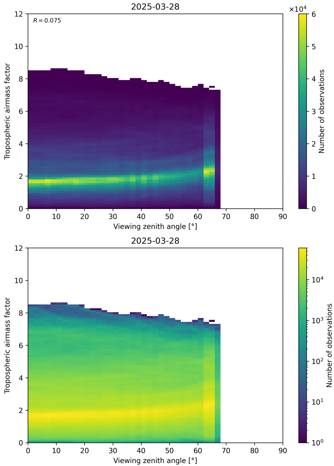
Figure 161: Scatter density plot of “Viewing zenith angle” against “Tropospheric airmass factor” for 2025-03-28 to 2025-03-29.
