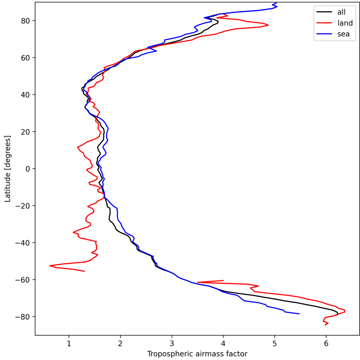
Figure 14: Zonal average of “Tropospheric airmass factor” for 2025-03-28 to 2025-03-29.
