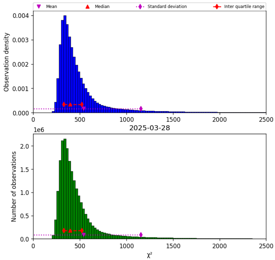
Figure 42: Histogram of “ \chi^2 ” for 2025-03-28 to 2025-03-29
