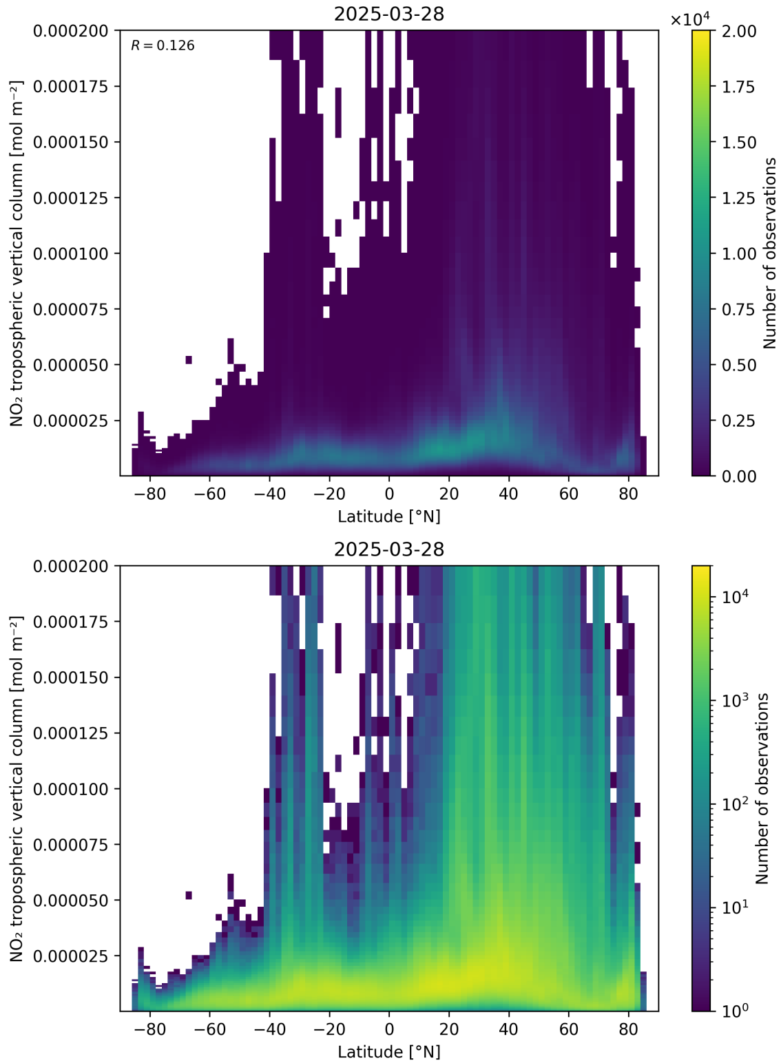
Figure 92: Scatter density plot of “Latitude” against “NO 2 tropospheric vertical column” for 2025-03-28 to 2025-03-29.
