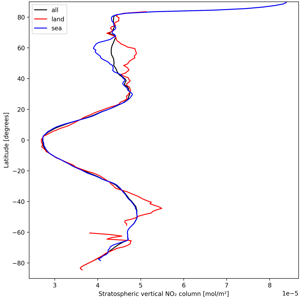
Figure 19: Zonal average of “Stratospheric vertical NO 2 column” for 2025-03-28 to 2025-03-29.
