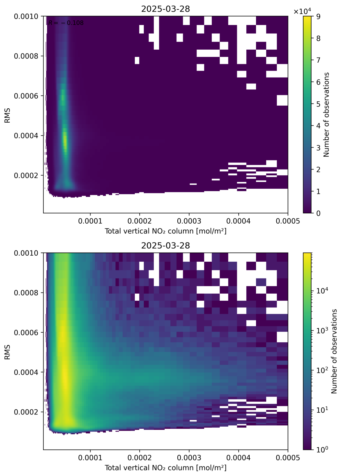
Figure 120: Scatter density plot of “Total vertical NO 2 column” against “RMS” for 2025-03-28 to 2025-03-29.
