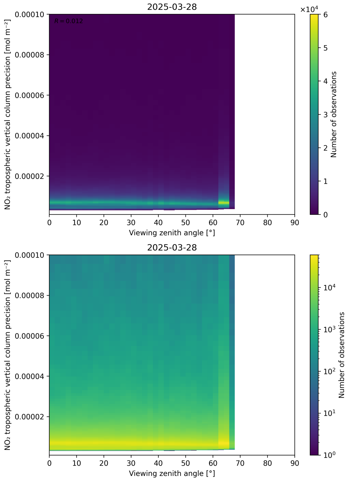
Figure 170: Scatter density plot of “Viewing zenith angle” against “NO 2 tropospheric vertical column precision” for 2025-03-28 to 2025-03-29.
