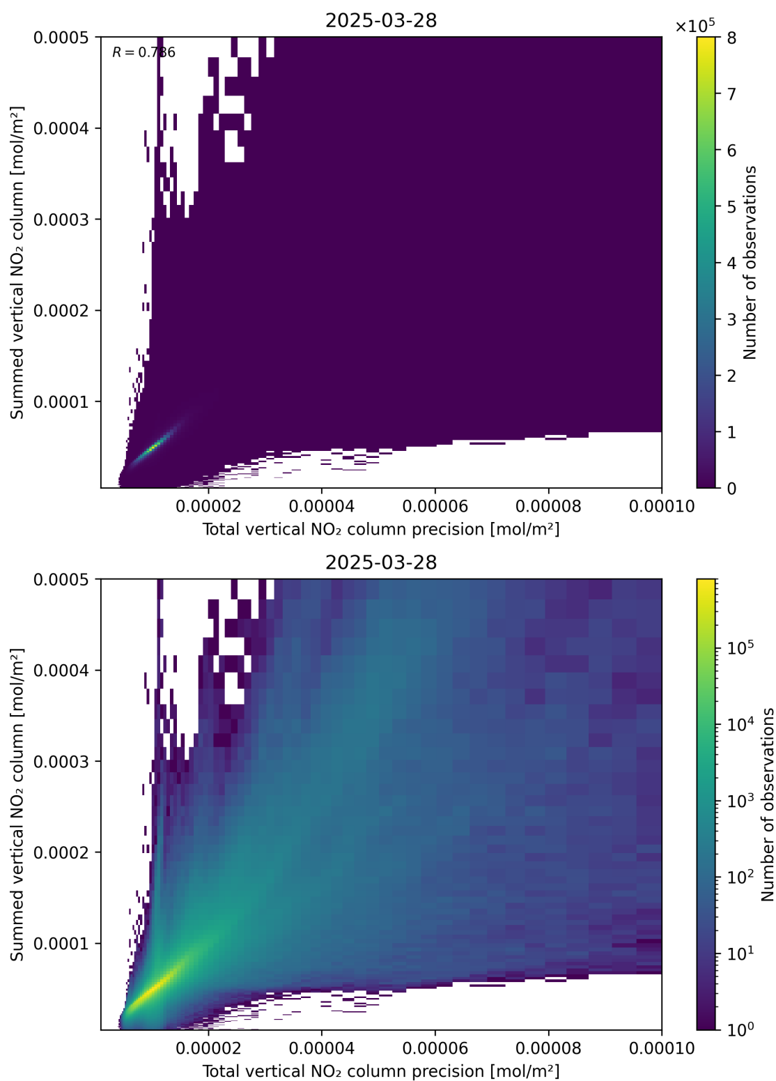
Figure 117: Scatter density plot of “Total vertical NO 2 column precision” against “Summed vertical NO 2 column” for 2025-03-28 to 2025-03-29.
