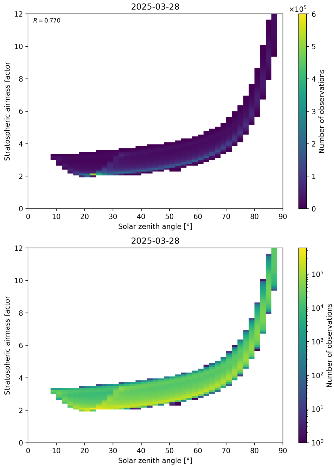
Figure 145: Scatter density plot of “Solar zenith angle” against “Stratospheric airmass factor” for 2025-03-28 to 2025-03-29.
