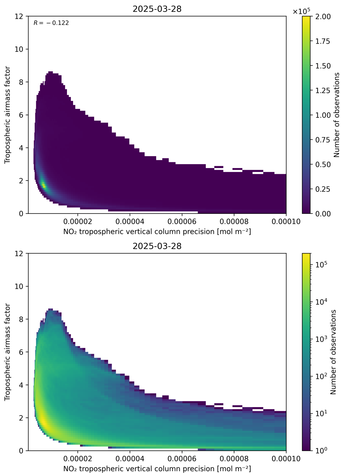
Figure 133: Scatter density plot of “NO 2 tropospheric vertical column precision” against “Tropospheric air mass factor” for 2025-03-28 to 2025-03-29.
