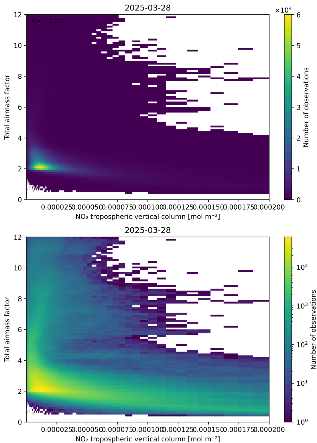
Figure 122: Scatter density plot of “NO 2 tropospheric vertical column” against “Total air mass factor” for 2025-03-28 to 2025-03-29.
