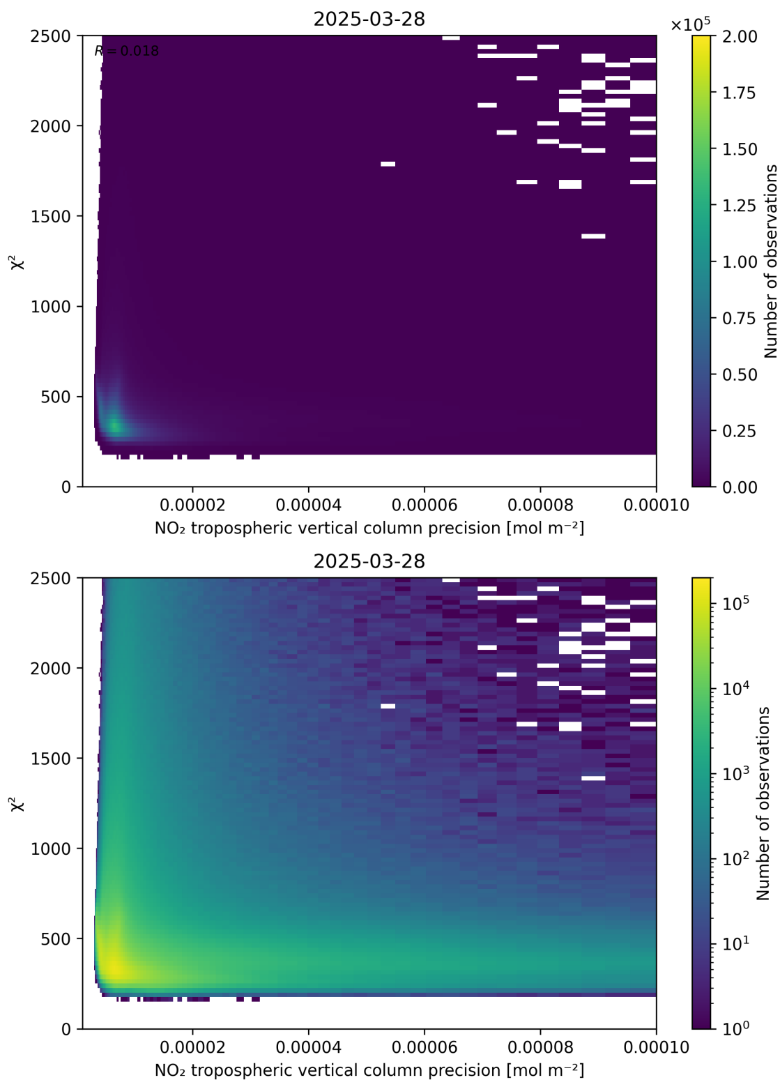
Figure 134: Scatter density plot of “NO 2 tropospheric vertical column precision” against “ \chi^2 ” for 2025-03-28 to 2025-03-29.
