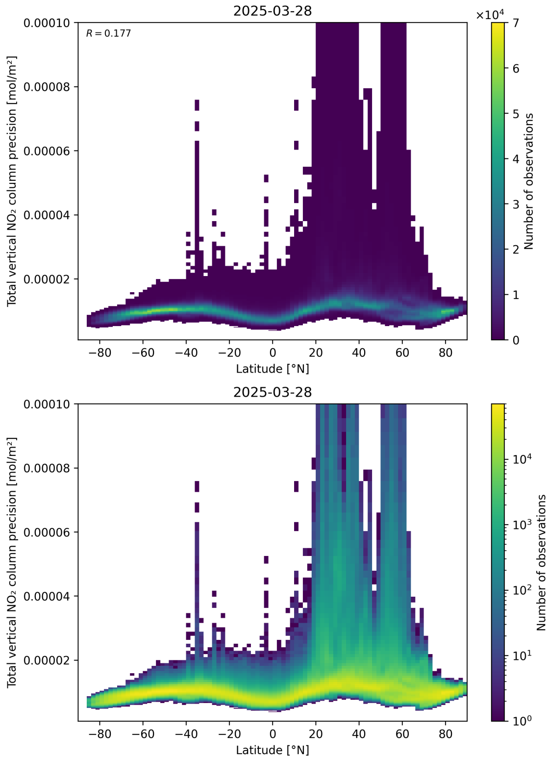
Figure 91: Scatter density plot of “Latitude” against “Total vertical NO 2 column precision” for 2025-03-28 to 2025-03-29.
