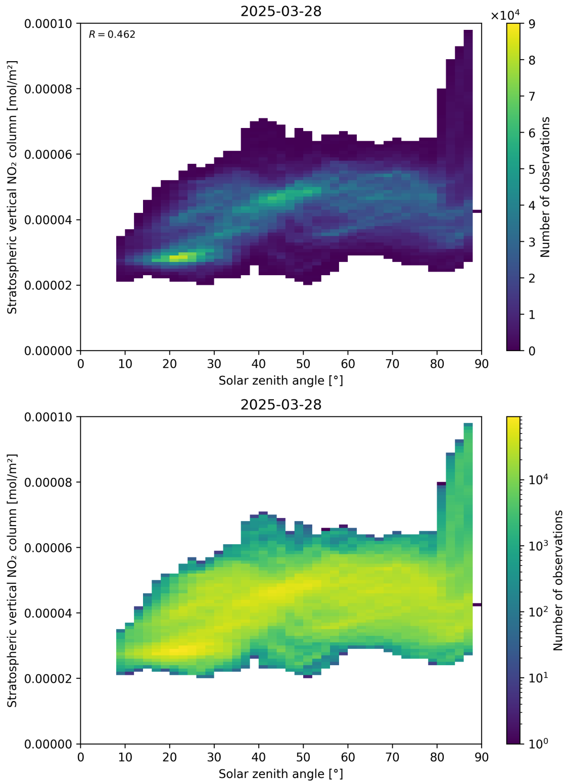
Figure 150: Scatter density plot of “Solar zenith angle” against “Stratospheric vertical NO 2 column” for 2025-03-28 to 2025-03-29.
