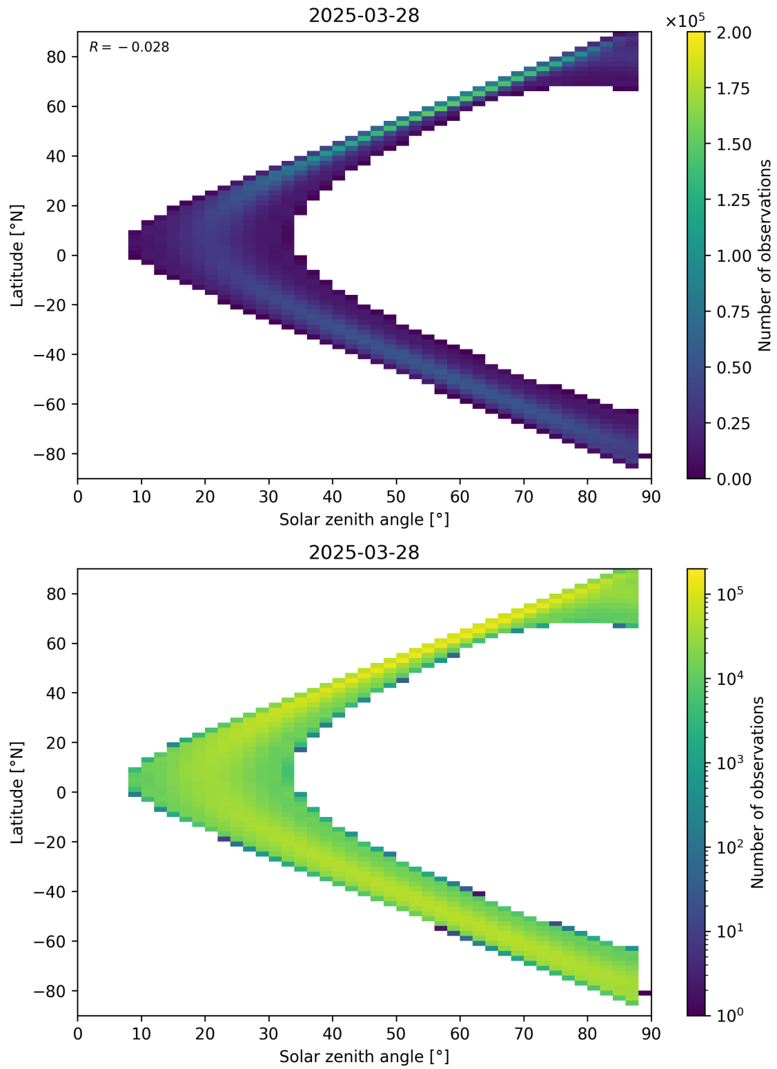
Figure 149: Scatter density plot of “Solar zenith angle” against “Latitude” for 2025-03-28 to 2025-03-29.
