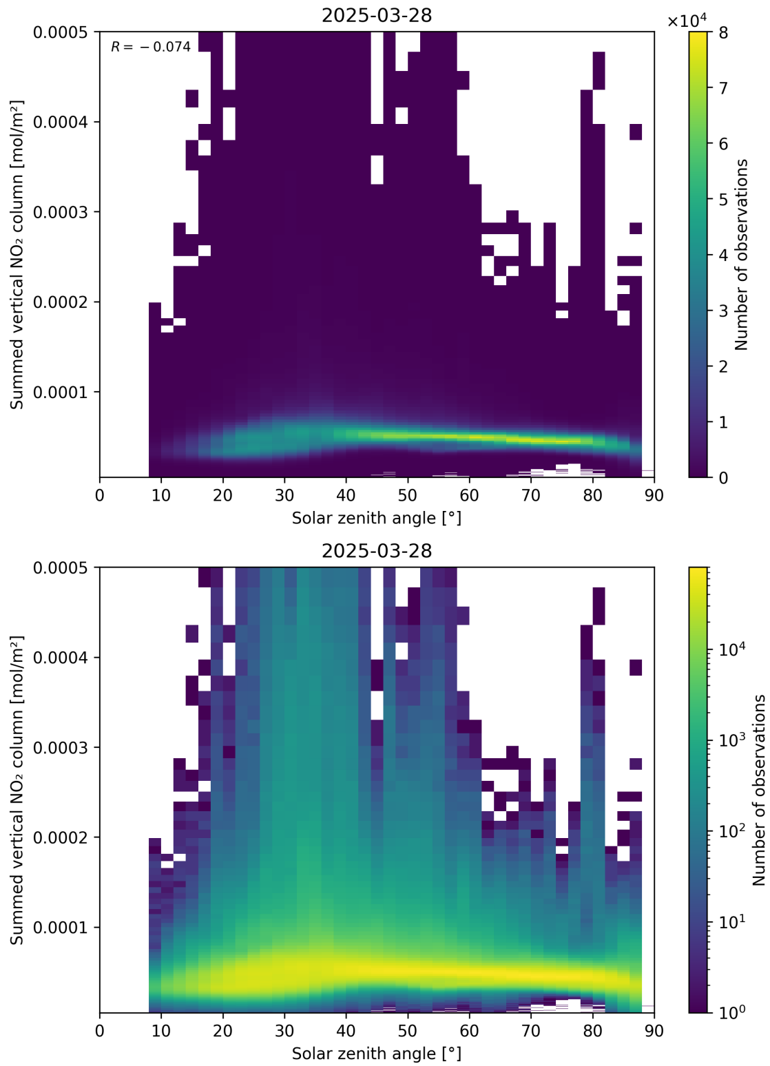
Figure 151: Scatter density plot of “Solar zenith angle” against “Summed vertical NO 2 column” for 2025-03-28 to 2025-03-29.
