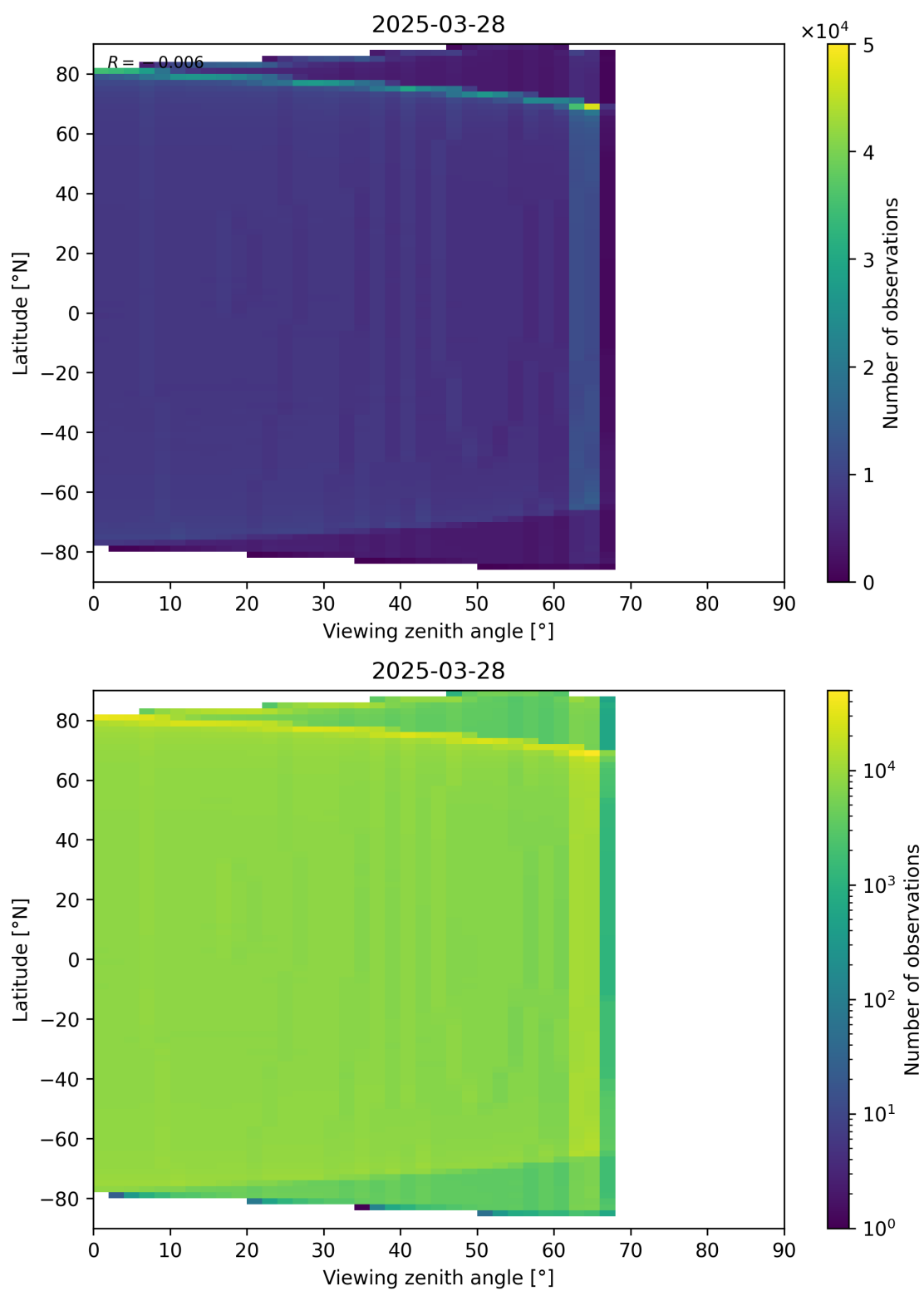
Figure 163: Scatter density plot of “Viewing zenith angle” against “Latitude” for 2025-03-28 to 2025-03-29.
