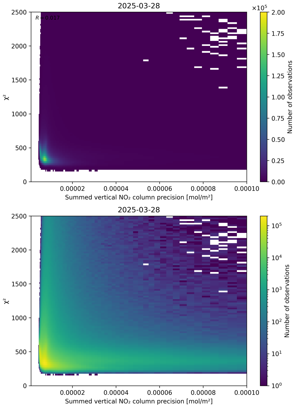
Figure 107: Scatter density plot of “Summed vertical NO 2 column precision” against “ \chi^2 ” for 2025-03-28 to 2025-03-29.
