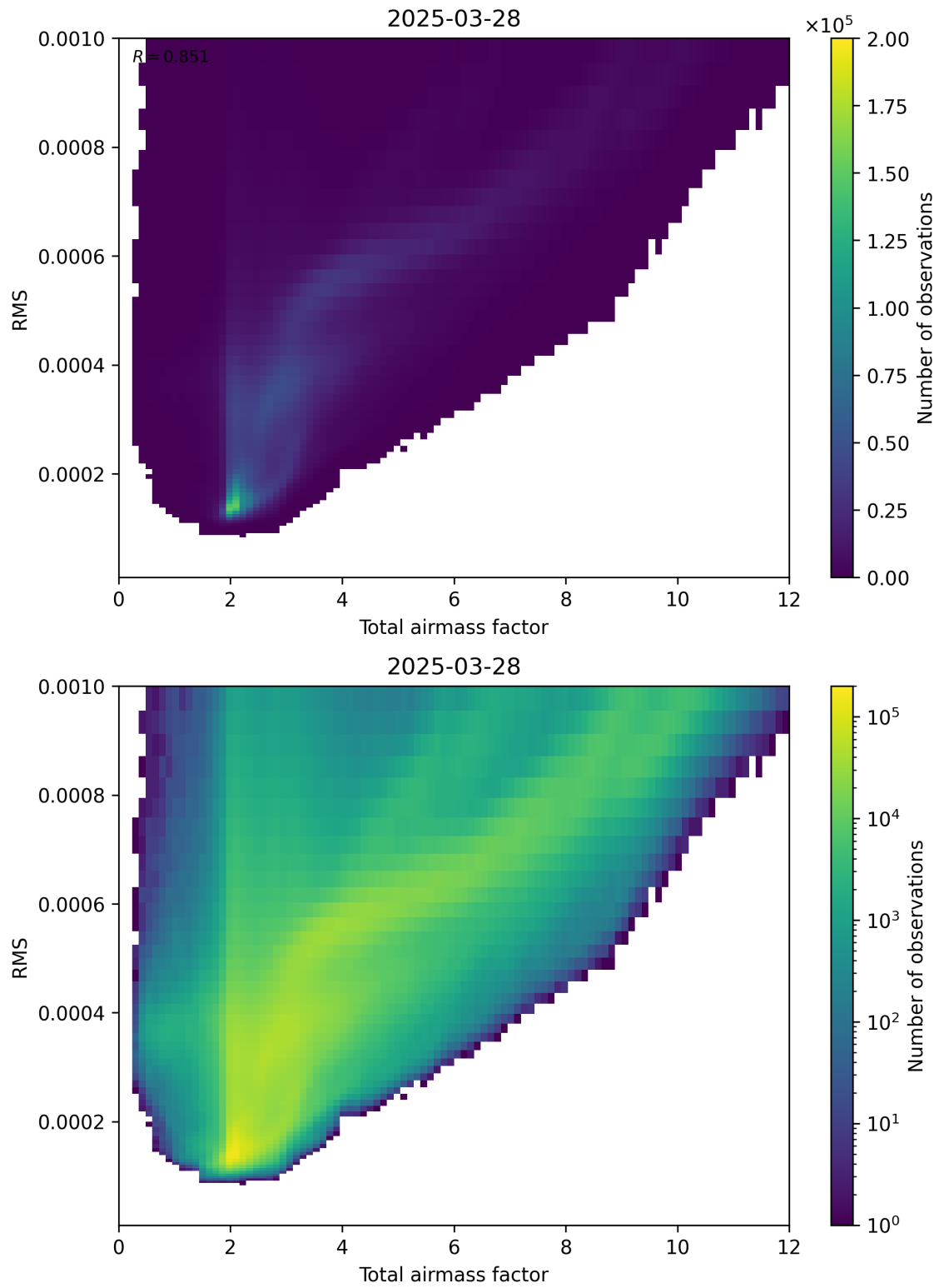
Figure 69: Scatter density plot of “Total airmass factor” against “RMS” for 2025-03-28 to 2025-03-29.
