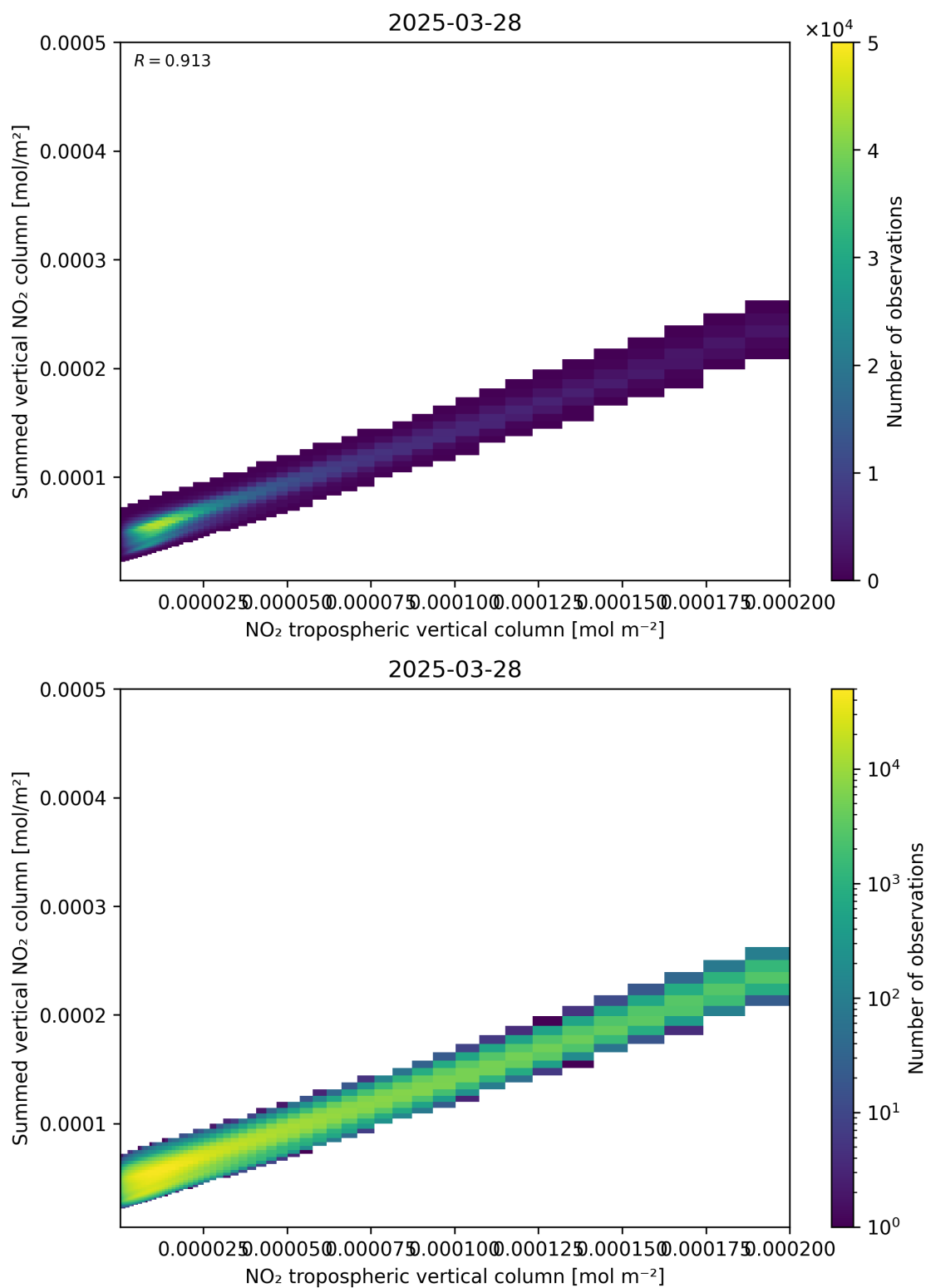
Figure 126: Scatter density plot of “NO 2 tropospheric vertical column” against “Summed vertical NO 2 column” for 2025-03-28 to 2025-03-29.
