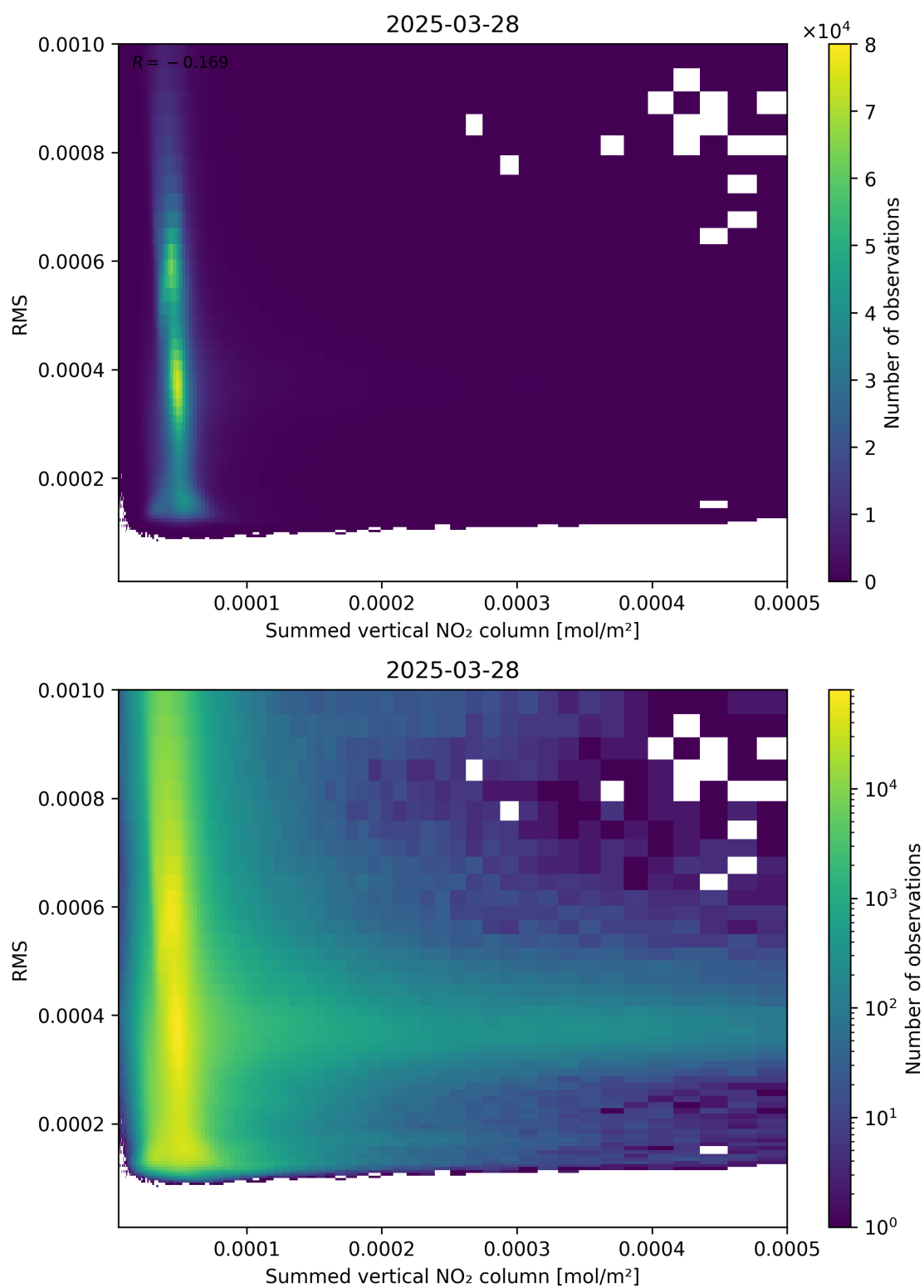
Figure 109: Scatter density plot of “Summed vertical NO 2 column” against “RMS” for 2025-03-28 to 2025-03-29.
