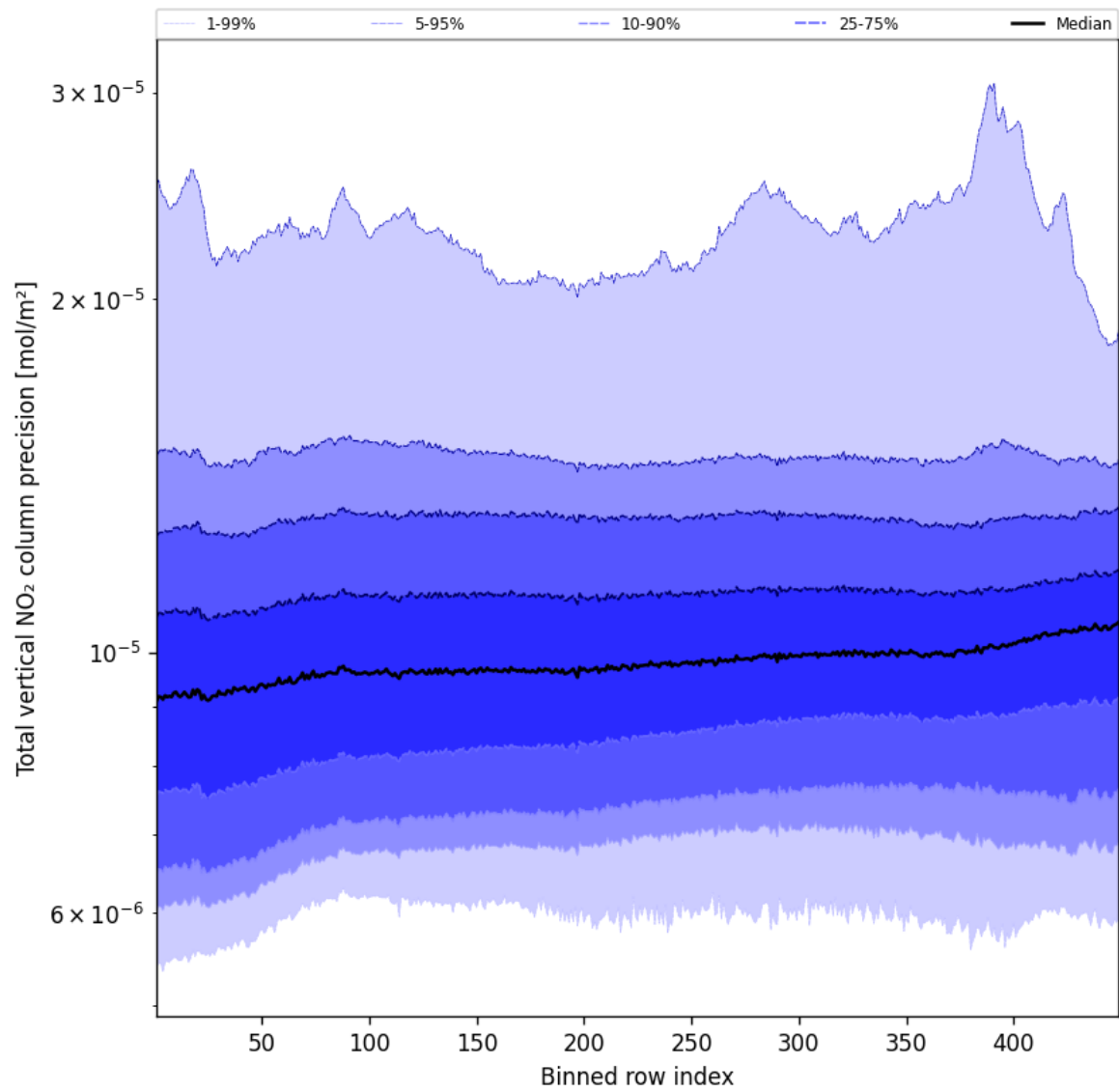
Figure 56: Along track statistics of “Total vertical NO 2 column precision” for 2025-03-28 to 2025-03-29
