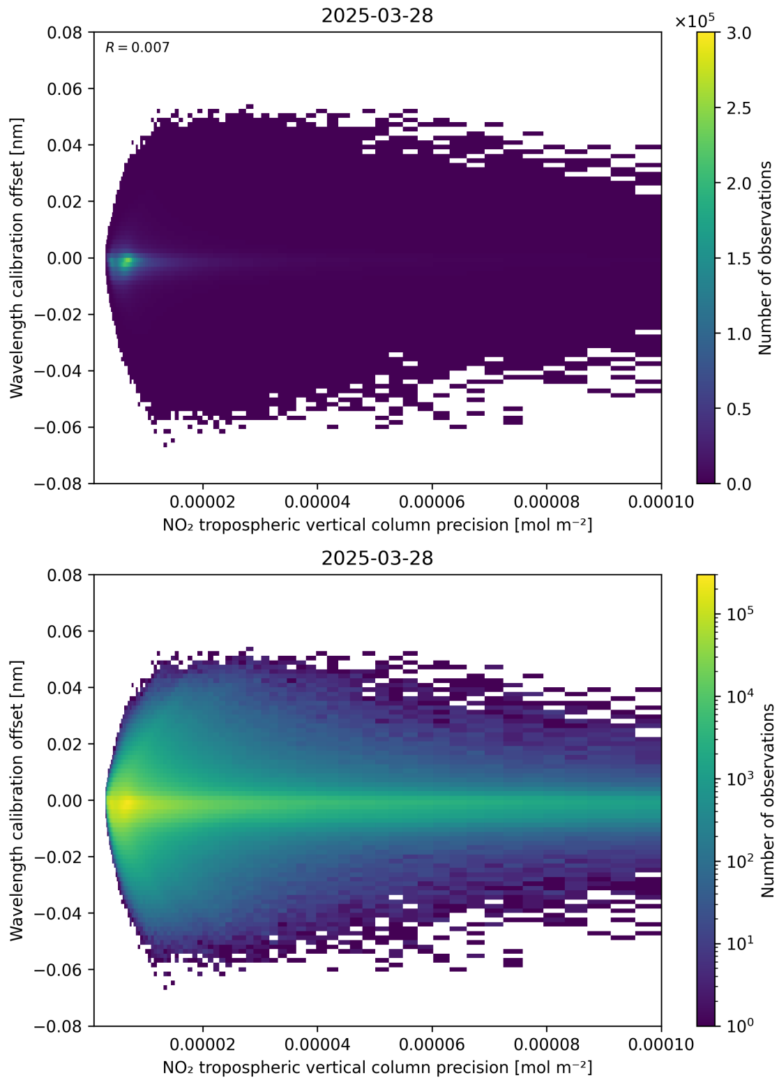
Figure 141: Scatter density plot of “NO 2 tropospheric vertical column precision” against “Wavelength calibration offset” for 2025-03-28 to 2025-03-29.
