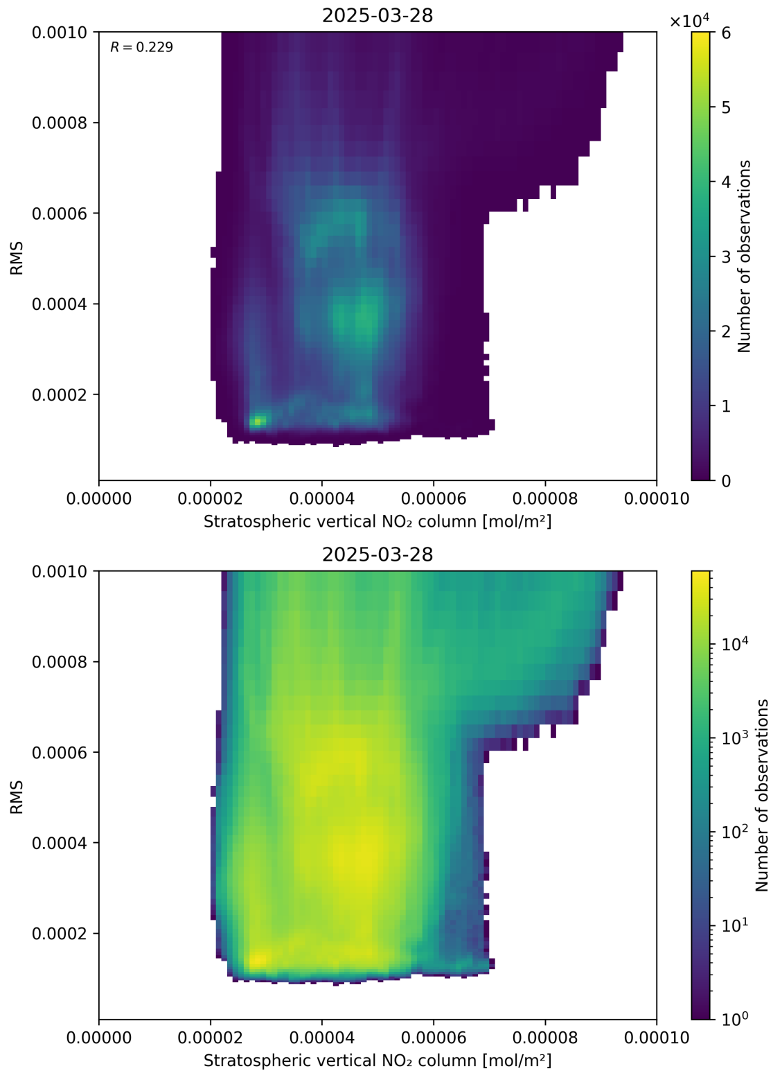
Figure 102: Scatter density plot of “Stratospheric vertical NO 2 column” against “RMS” for 2025-03-28 to 2025-03-29.
