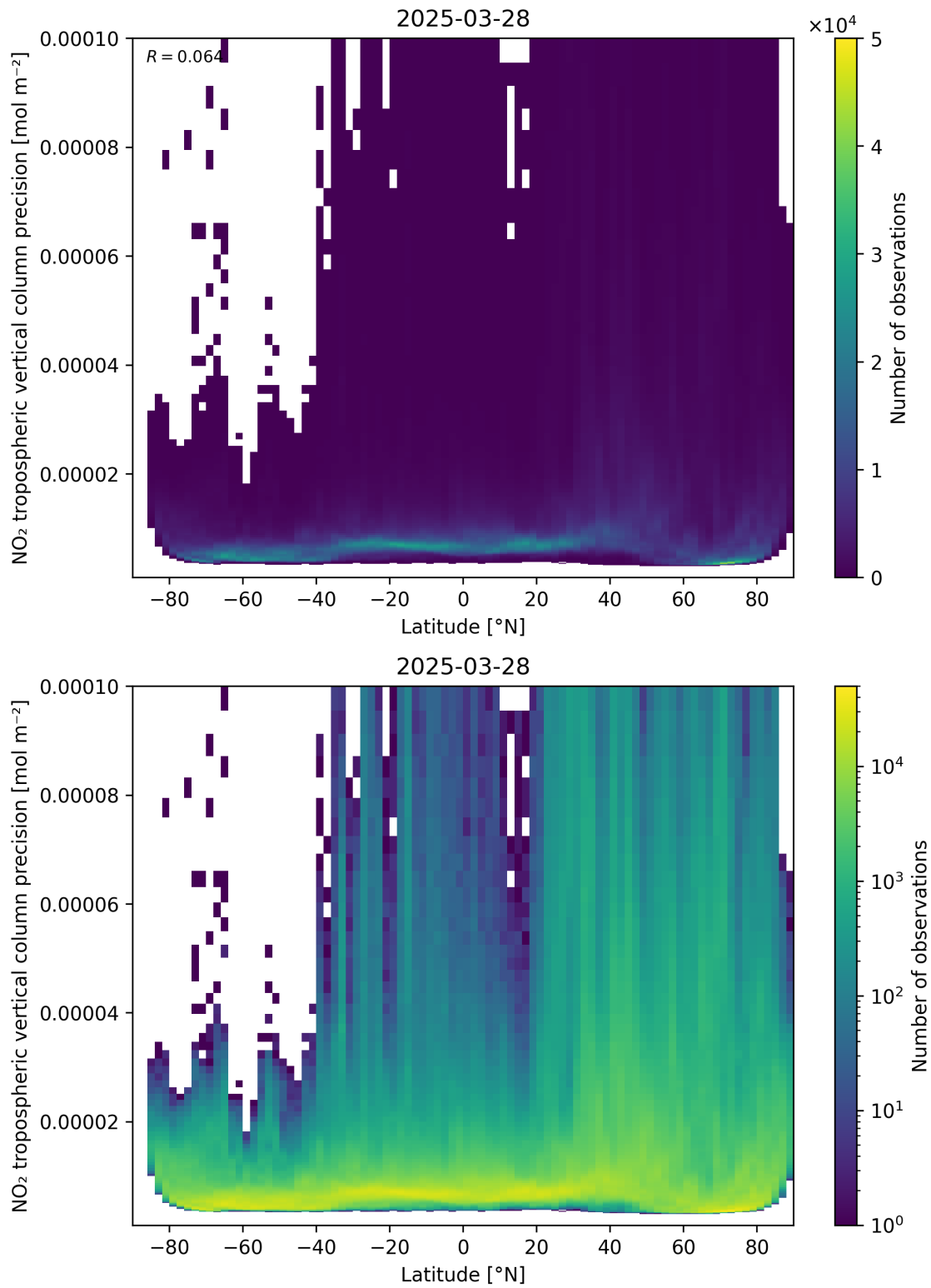
Figure 93: Scatter density plot of “Latitude” against “NO 2 tropospheric vertical column precision” for 2025-03-28 to 2025-03-29.
