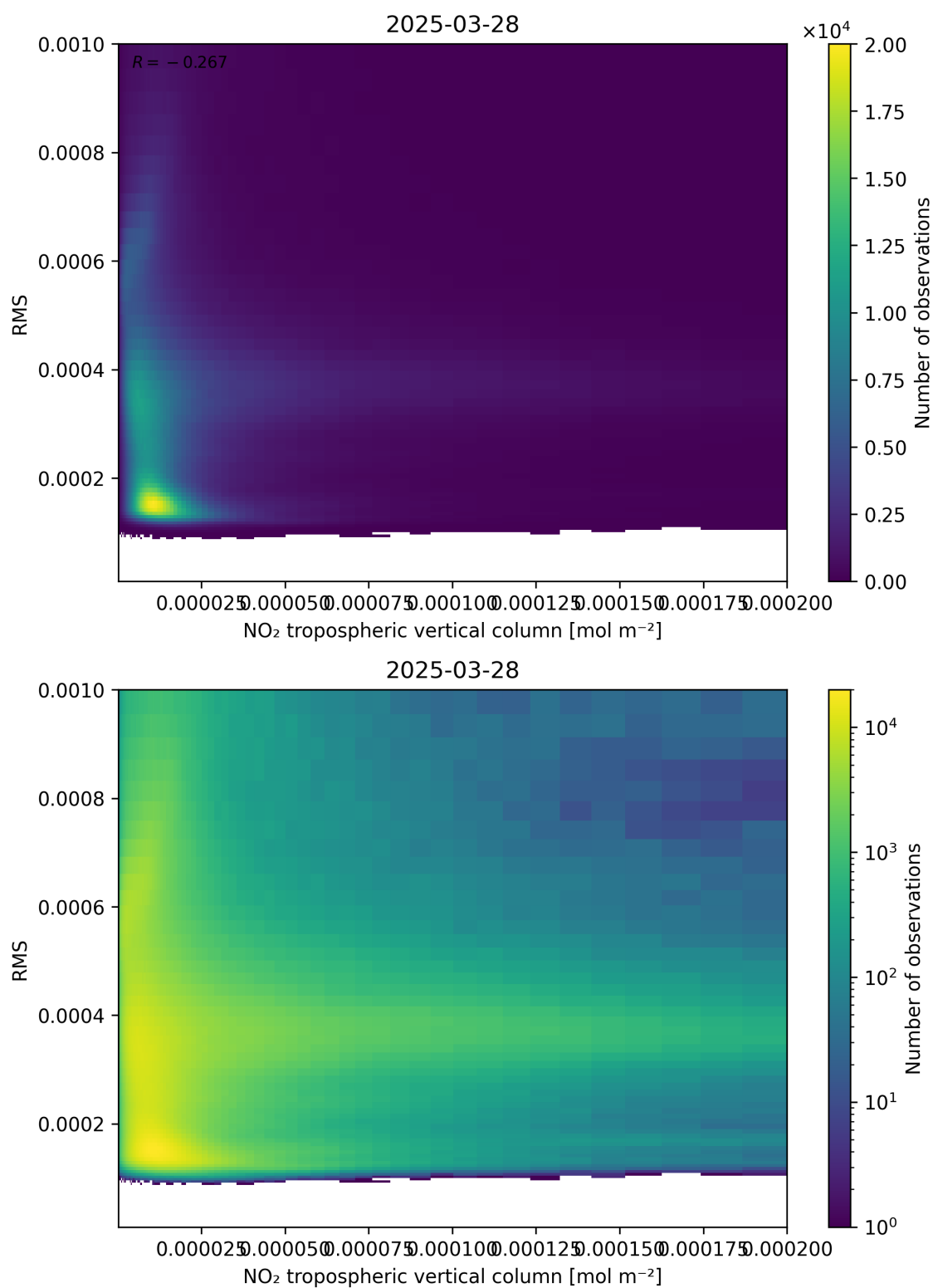
Figure 142: Scatter density plot of “NO 2 tropospheric vertical column” against “RMS” for 2025-03-28 to 2025-03-29.
