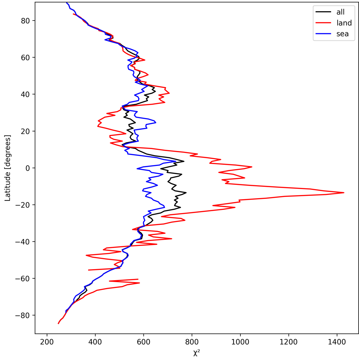
Figure 25: Zonal average of “ \chi^2 ” for 2025-03-28 to 2025-03-29.
