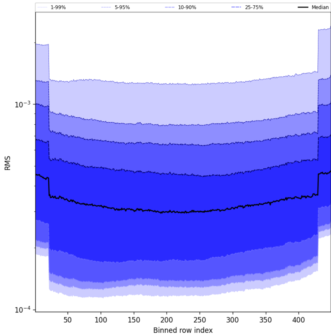
Figure 60: Along track statistics of “RMS” for 2025-03-28 to 2025-03-29
