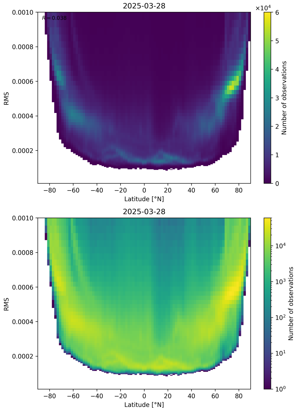
Figure 94: Scatter density plot of “Latitude” against “RMS” for 2025-03-28 to 2025-03-29.
