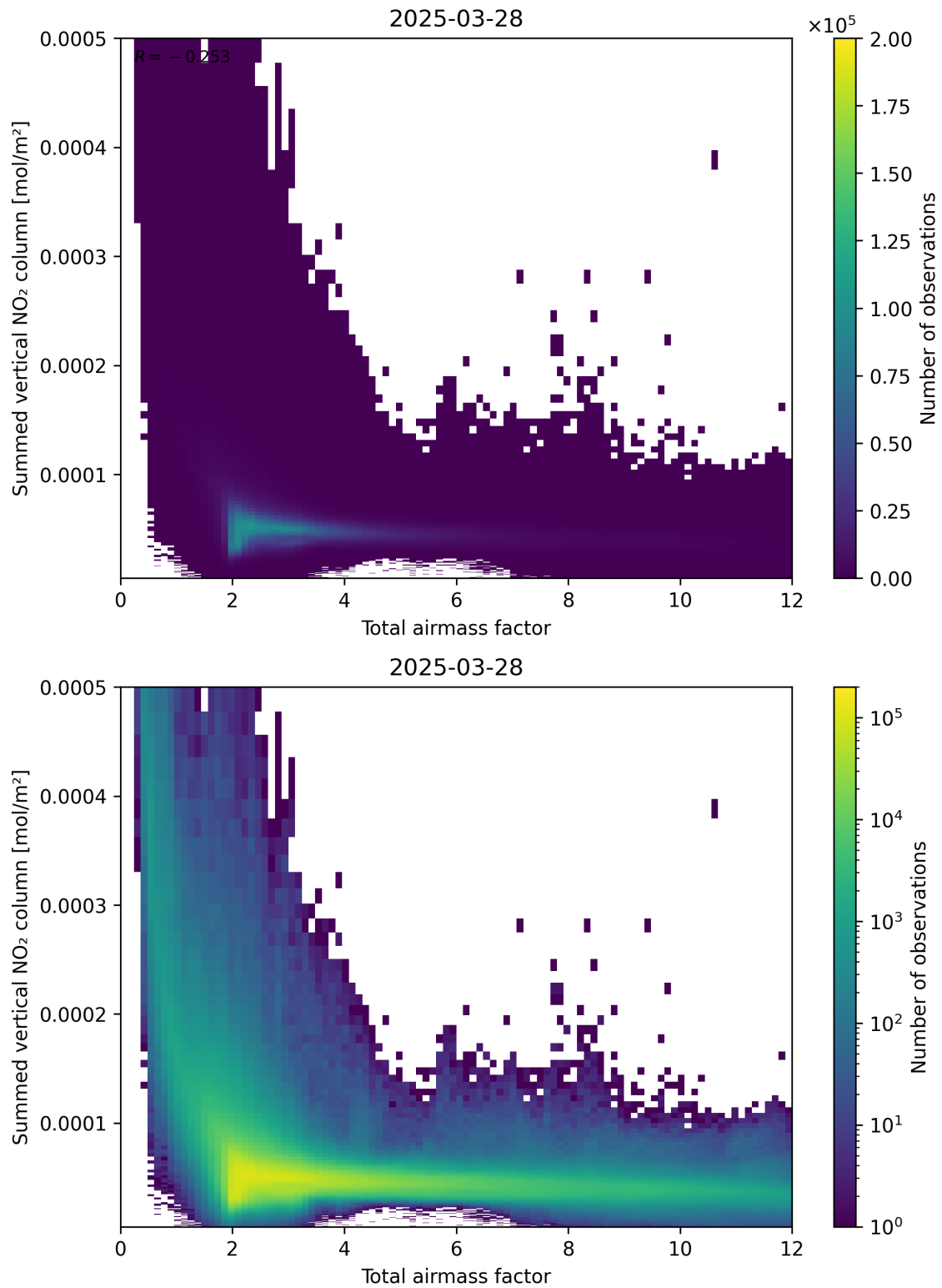
Figure 65: Scatter density plot of “Total airmass factor” against “Summed vertical NO 2 column” for 2025-03-28 to 2025-03-29.
