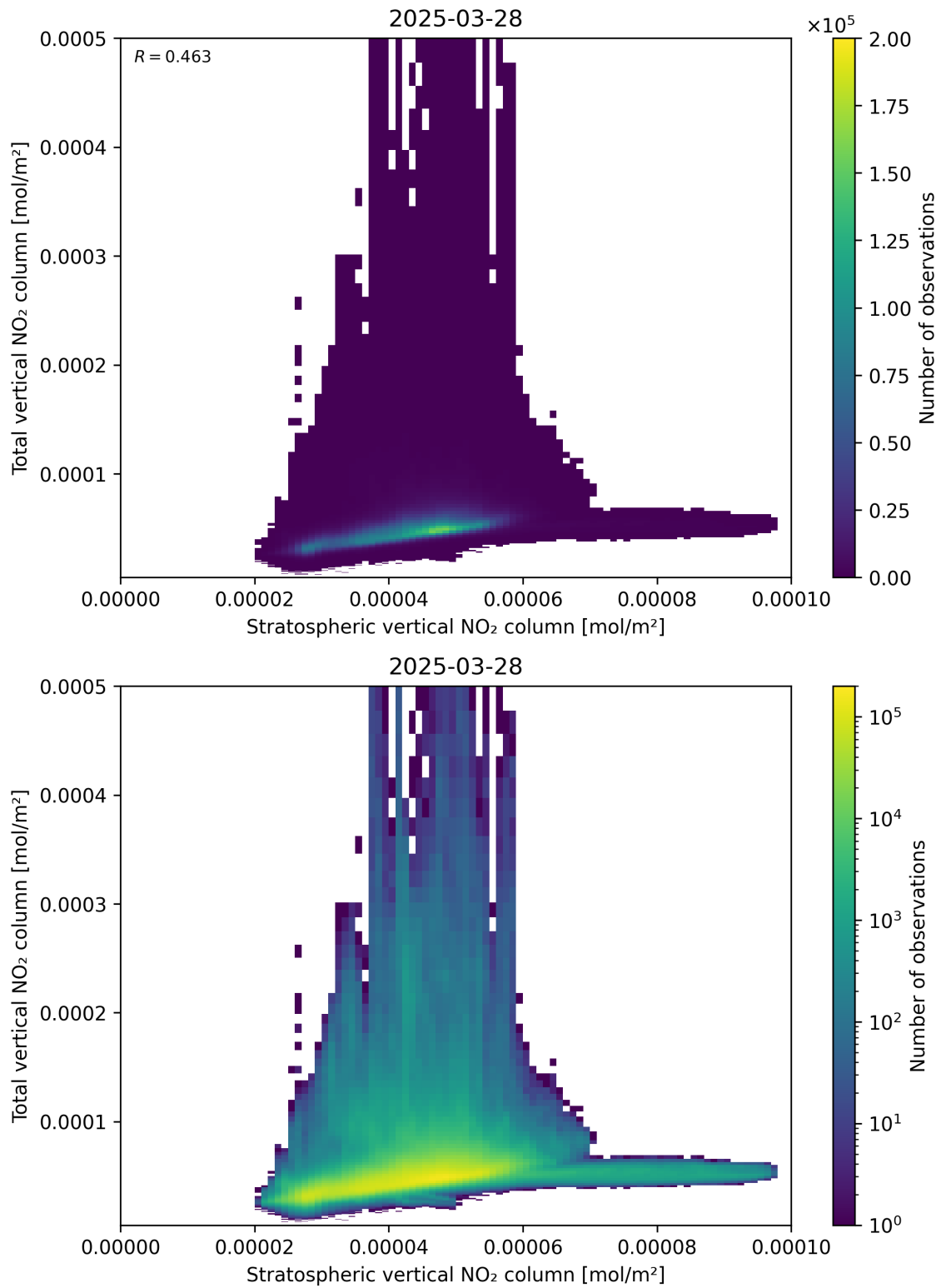
Figure 100: Scatter density plot of “Stratospheric vertical NO 2 column” against “Total vertical NO 2 column” for 2025-03-28 to 2025-03-29.
