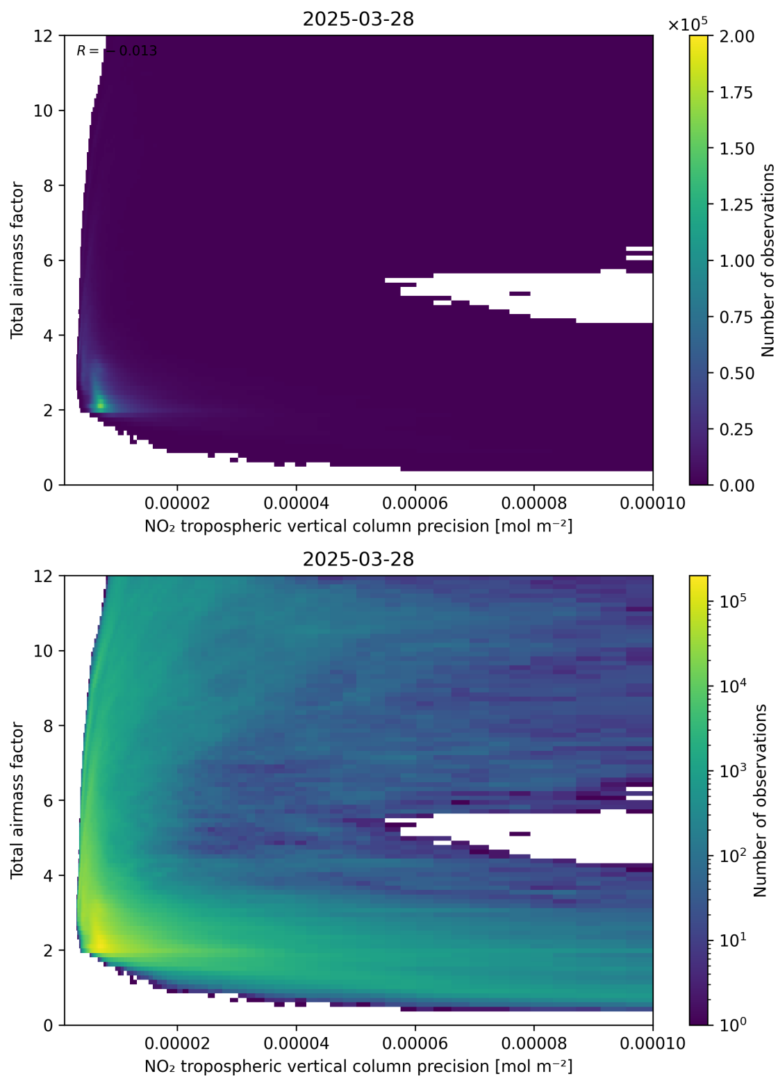
Figure 132: Scatter density plot of “NO 2 tropospheric vertical column precision” against “Total air mass factor” for 2025-03-28 to 2025-03-29.
