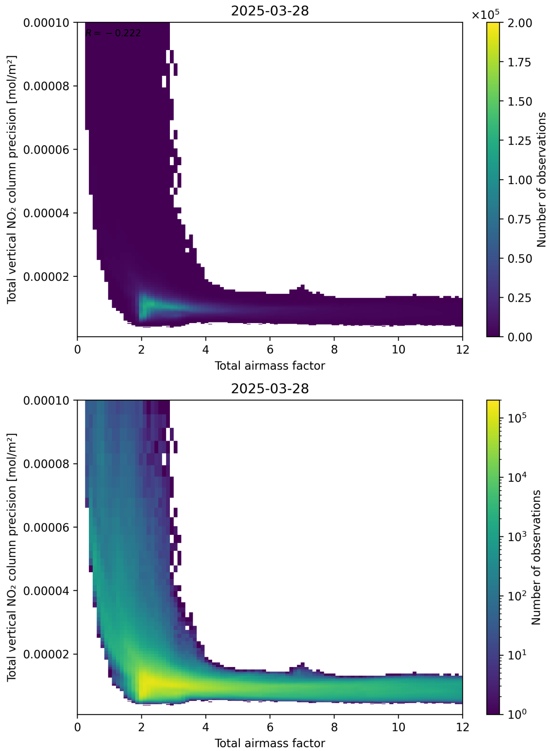
Figure 68: Scatter density plot of “Total airmass factor” against “Total vertical NO 2 column precision” for 2025-03-28 to 2025-03-29.
