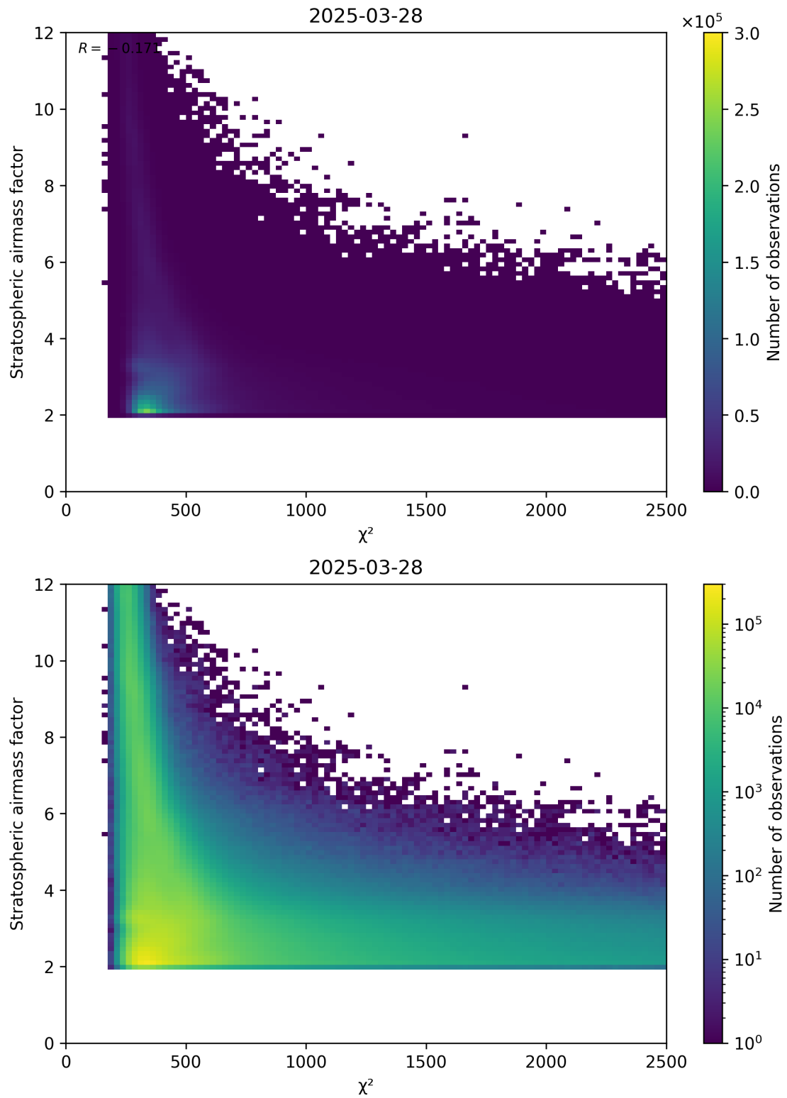
Figure 81: Scatter density plot of “ \chi^2 ” against “Stratospheric airmass factor” for 2025-03-28 to 2025-03-29.
