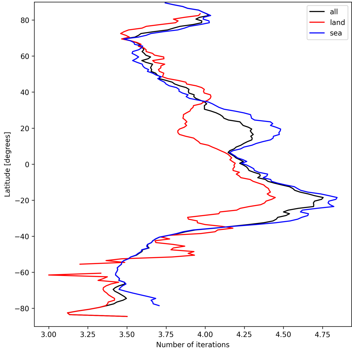
Figure 17: Zonal average of “Number of iterations” for 2025-03-28 to 2025-03-29.
