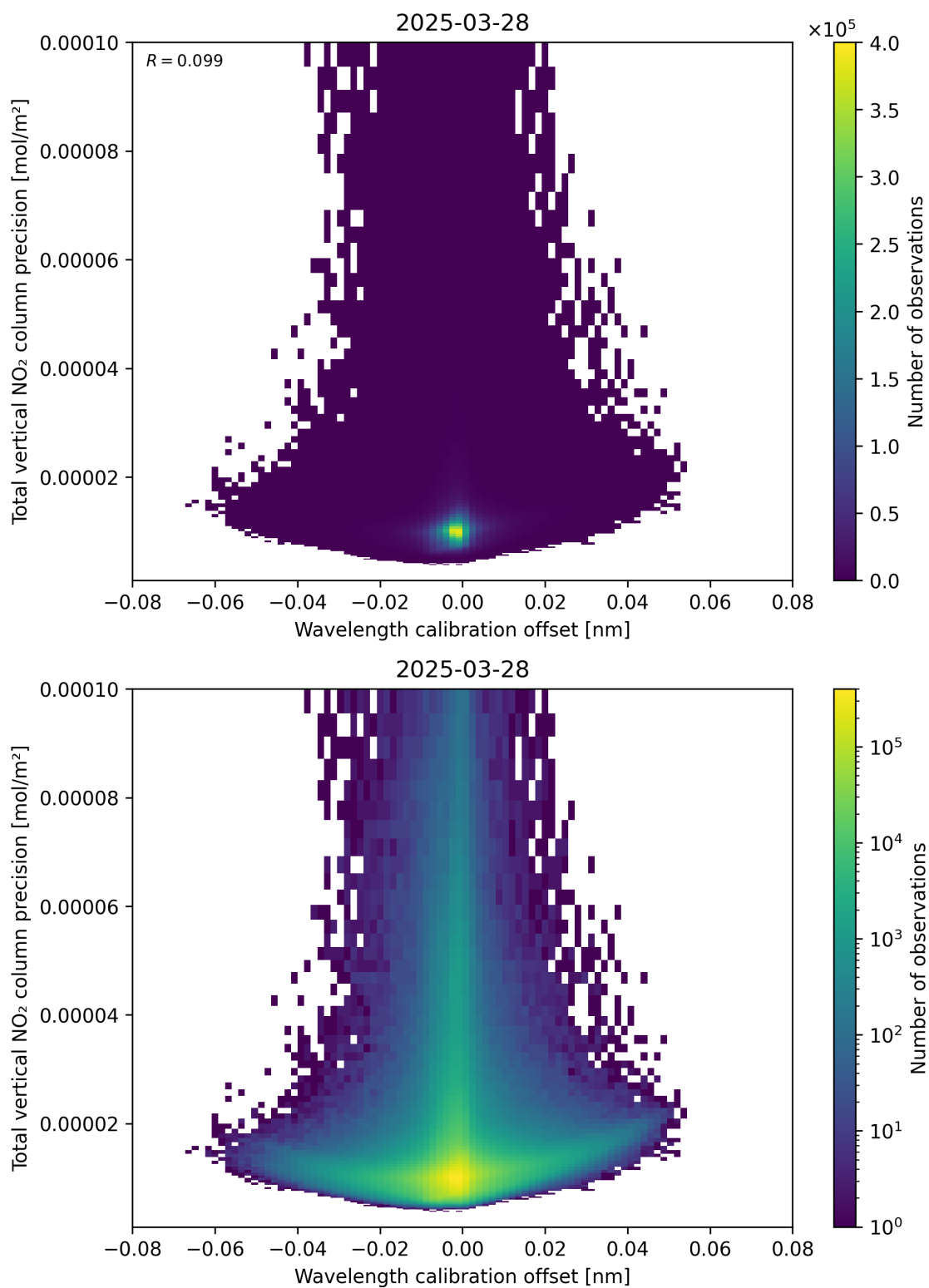
Figure 180: Scatter density plot of “Wavelength calibration offset” against “Total vertical NO 2 column precision” for 2025-03-28 to 2025-03-29.
