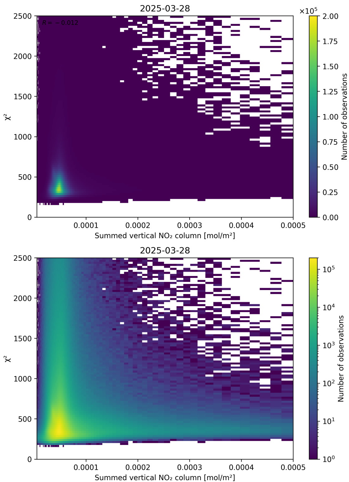
Figure 104: Scatter density plot of “Summed vertical NO 2 column” against “ \chi^2 ” for 2025-03-28 to 2025-03-29.
