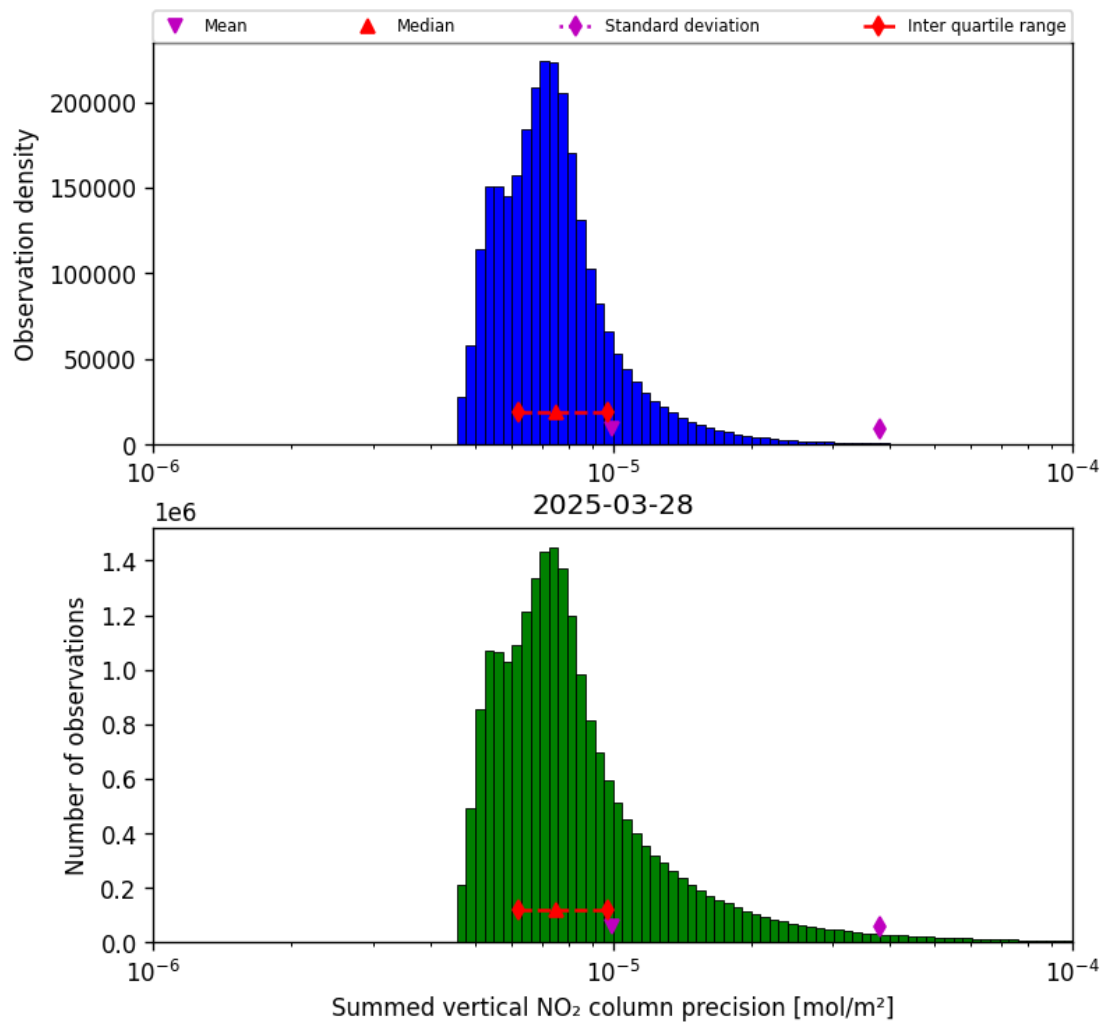
Figure 41: Histogram of “Summed vertical NO 2 column precision” for 2025-03-28 to 2025-03-29
