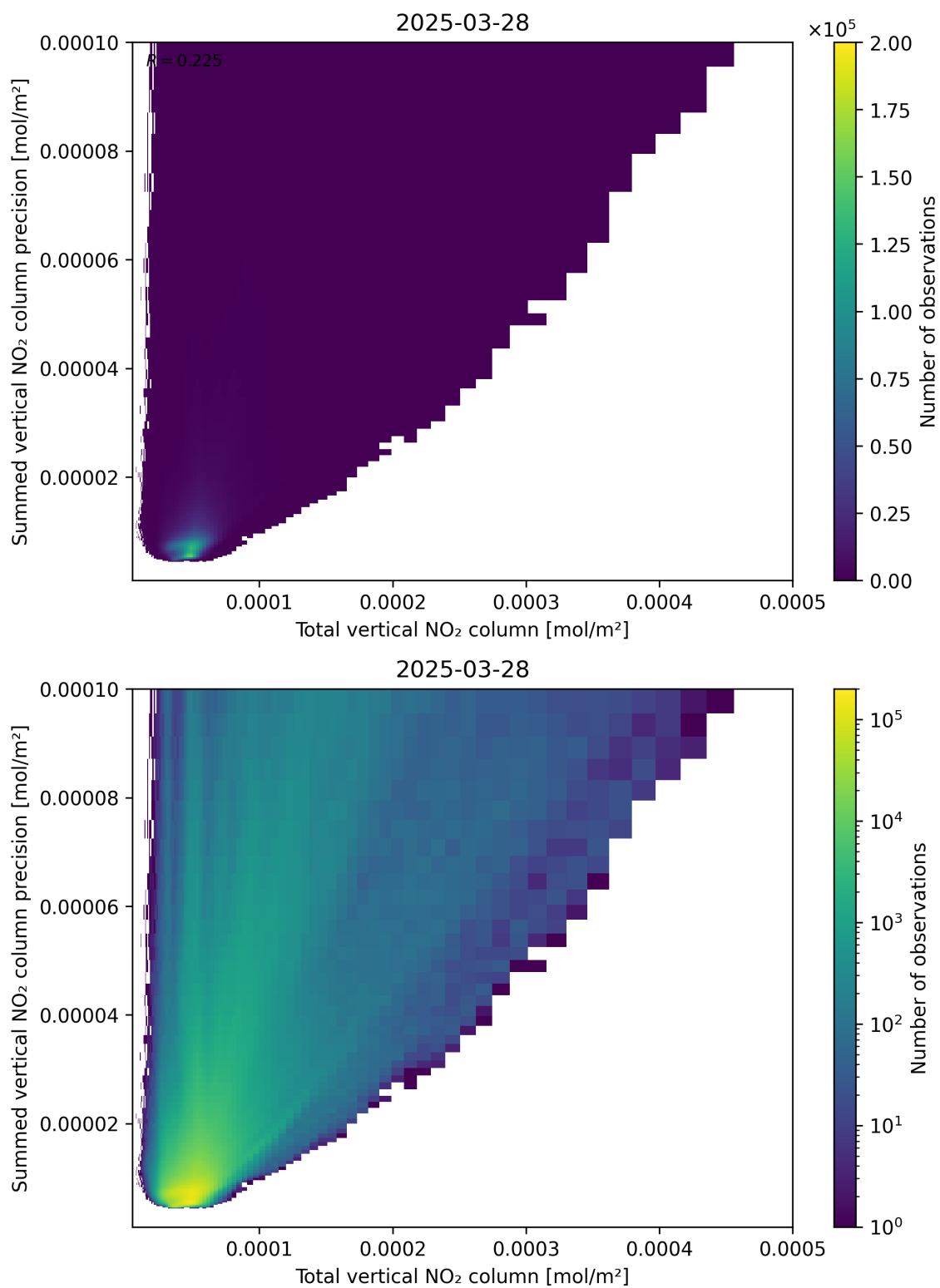
Figure 113: Scatter density plot of “Total vertical NO 2 column” against “Summed vertical NO 2 column precision” for 2025-03-28 to 2025-03-29.
