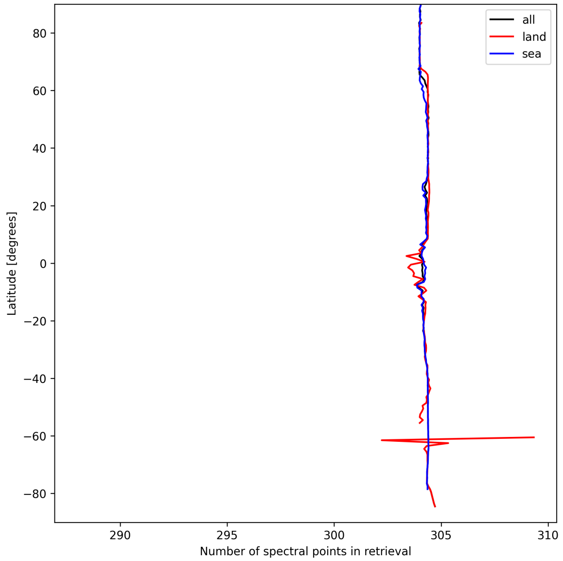
Figure 16: Zonal average of “Number of spectral points in retrieval” for 2025-03-28 to 2025-03-29.
