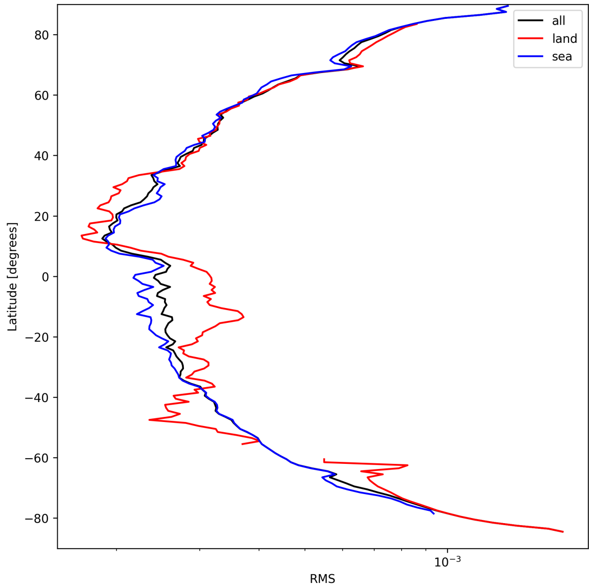
Figure 26: Zonal average of “RMS” for 2025-03-28 to 2025-03-29.
