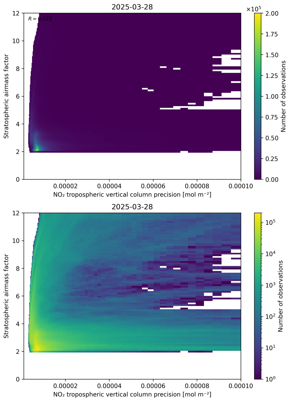
Figure 131: Scatter density plot of “NO 2 tropospheric vertical column precision” against “Stratospheric airmass factor” for 2025-03-28 to 2025-03-29.
