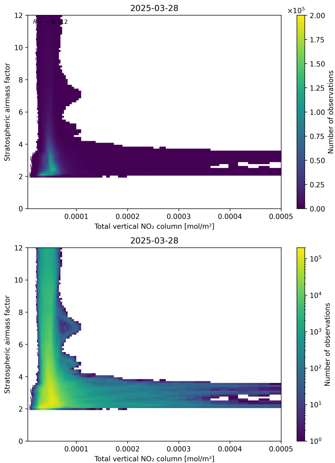
Figure 110: Scatter density plot of “Total vertical NO 2 column” against “Stratospheric airmass factor” for 2025-03-28 to 2025-03-29.
