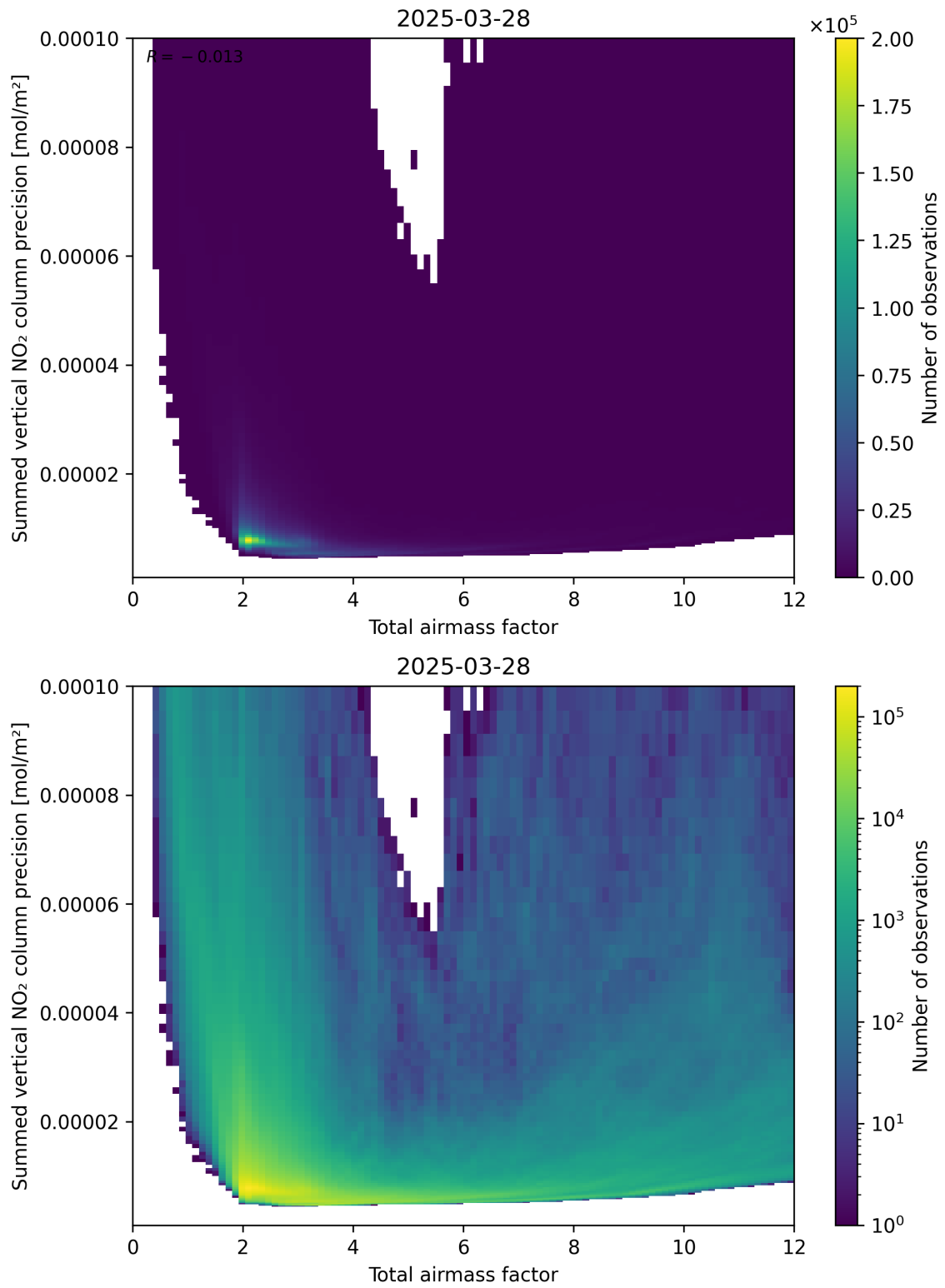
Figure 66: Scatter density plot of “Total airmass factor” against “Summed vertical NO 2 column precision” for 2025-03-28 to 2025-03-29.
