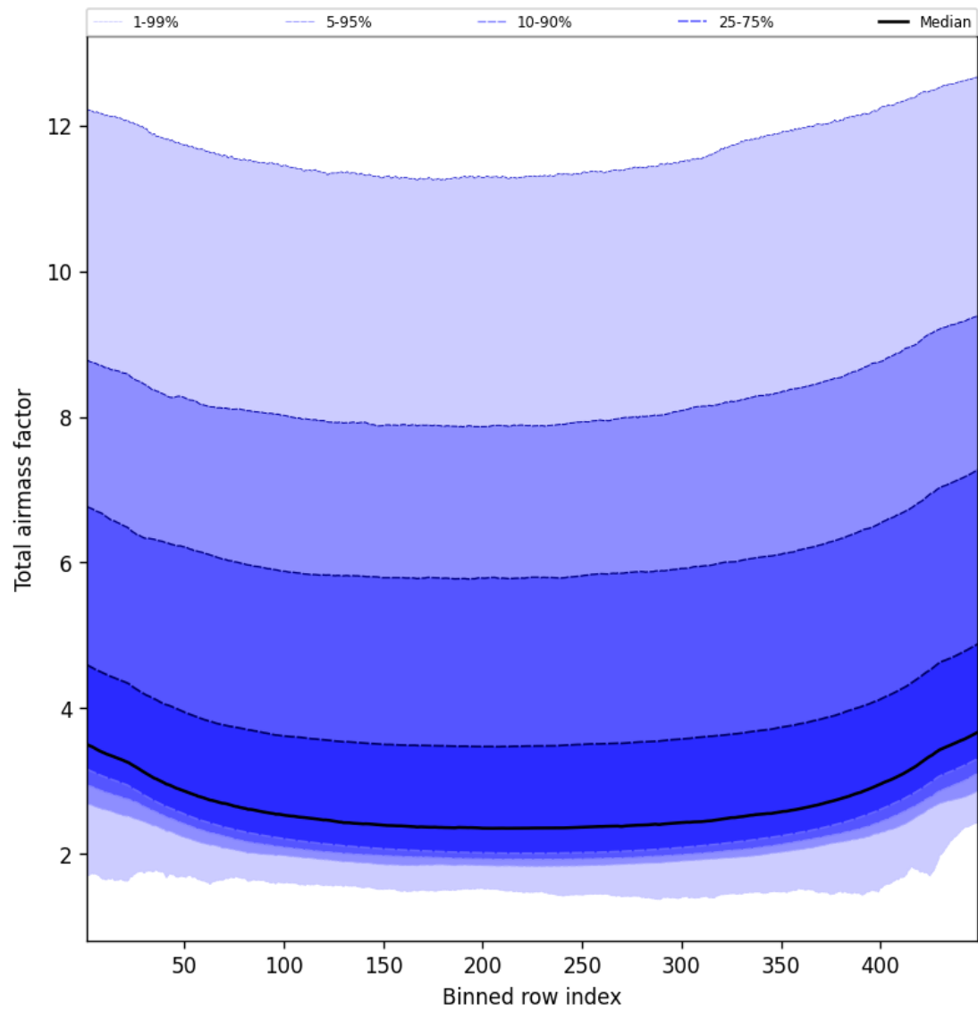
Figure 49: Along track statistics of “Total airmass factor” for 2025-03-28 to 2025-03-29
