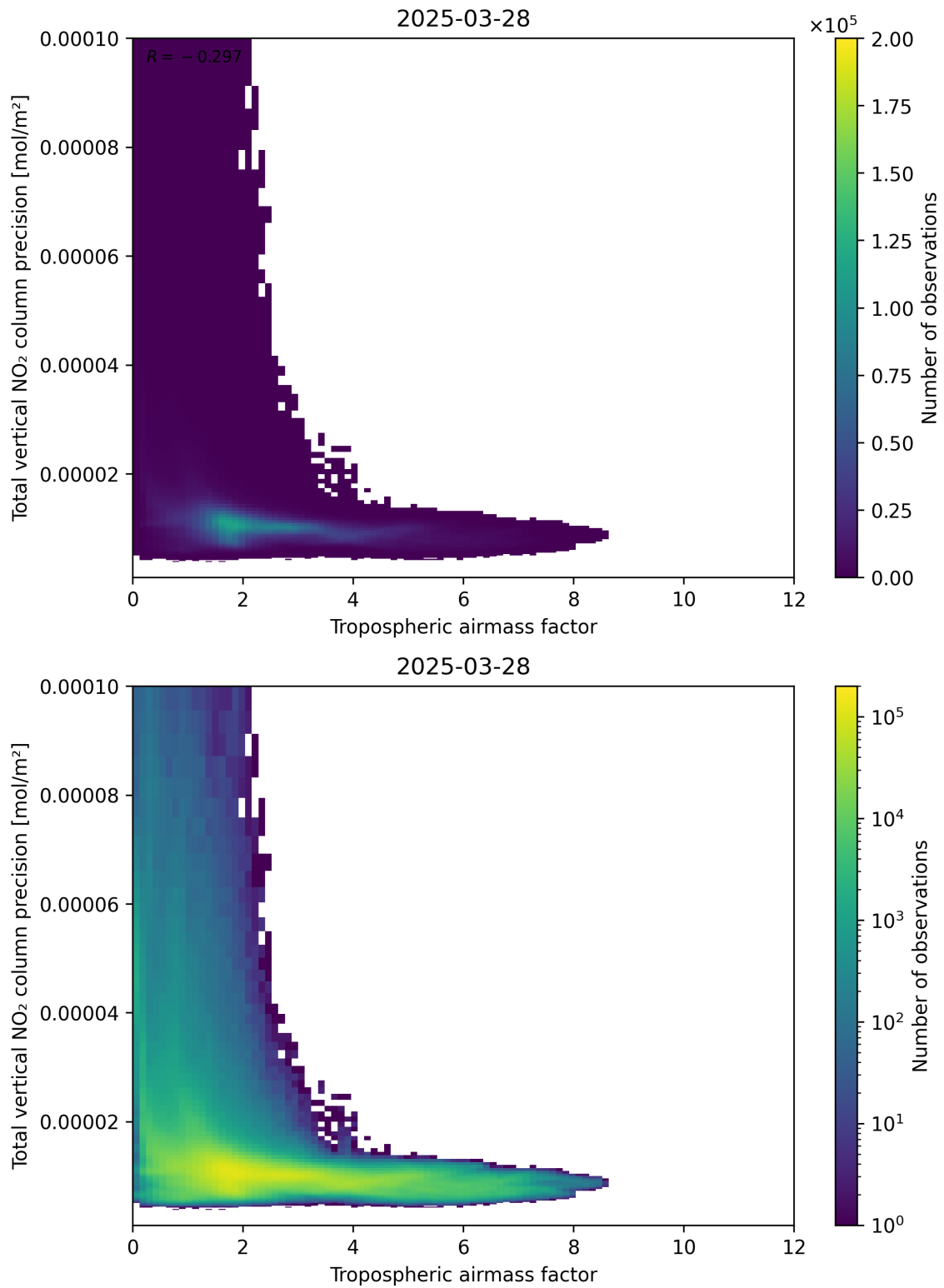
Figure 78: Scatter density plot of “Tropospheric airmass factor” against “Total vertical NO 2 column precision” for 2025-03-28 to 2025-03-29.
