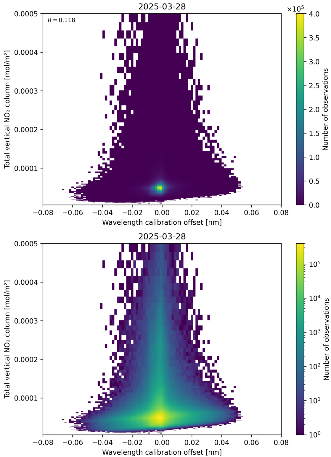
Figure 179: Scatter density plot of “Wavelength calibration offset” against “Total vertical NO 2 column” for 2025-03-28 to 2025-03-29.
