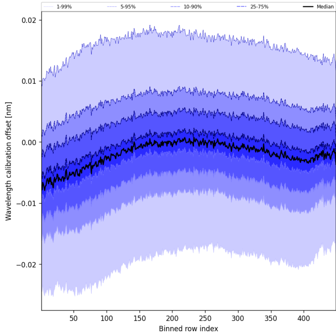
Figure 52: Along track statistics of “Wavelength calibration offset” for 2025-03-28 to 2025-03-29
