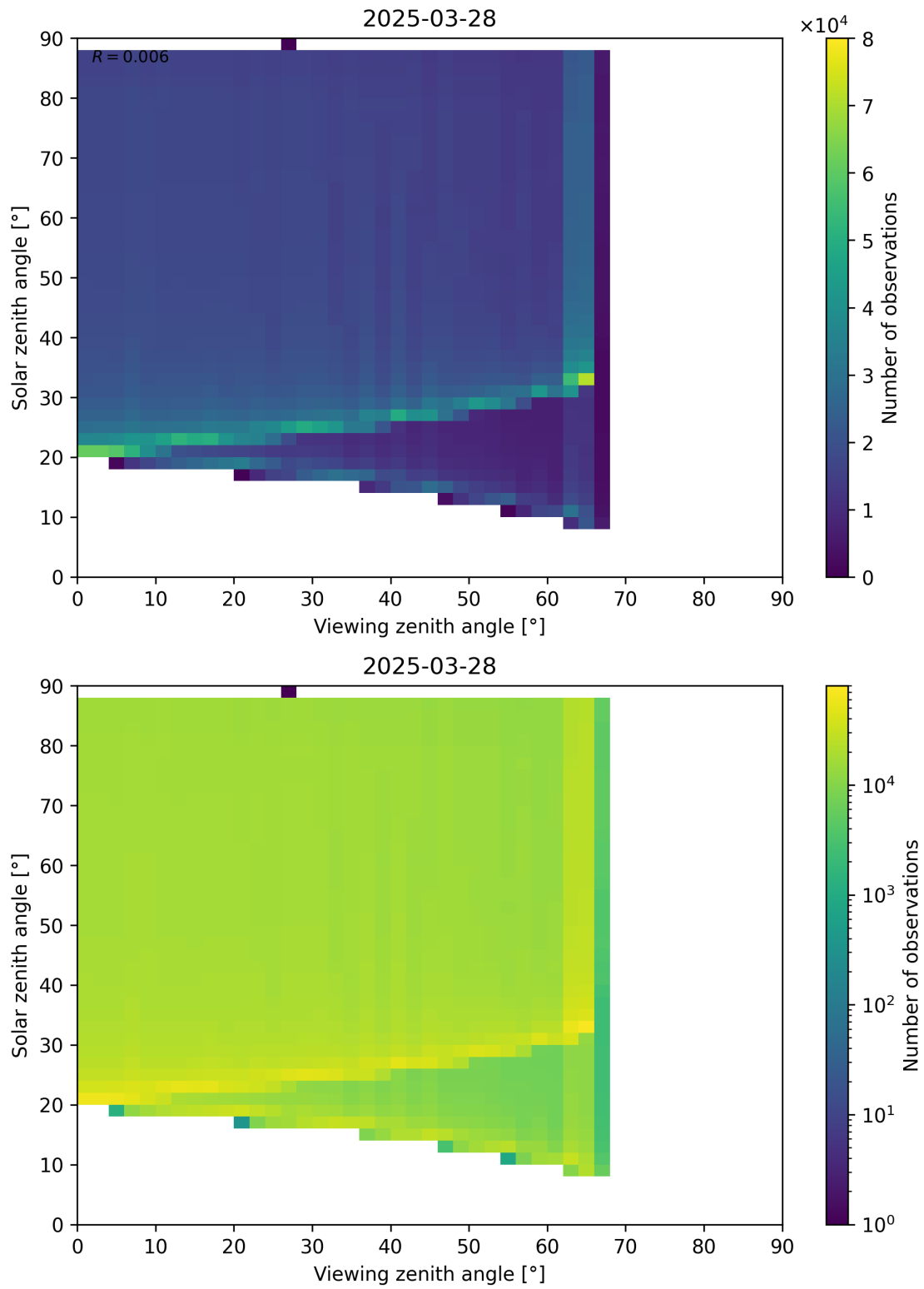
Figure 172: Scatter density plot of “Viewing zenith angle” against “Solar zenith angle” for 2025-03-28 to 2025-03-29.
