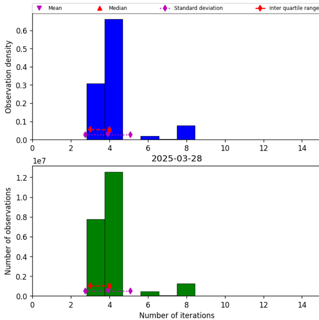
Figure 34: Histogram of “Number of iterations” for 2025-03-28 to 2025-03-29
