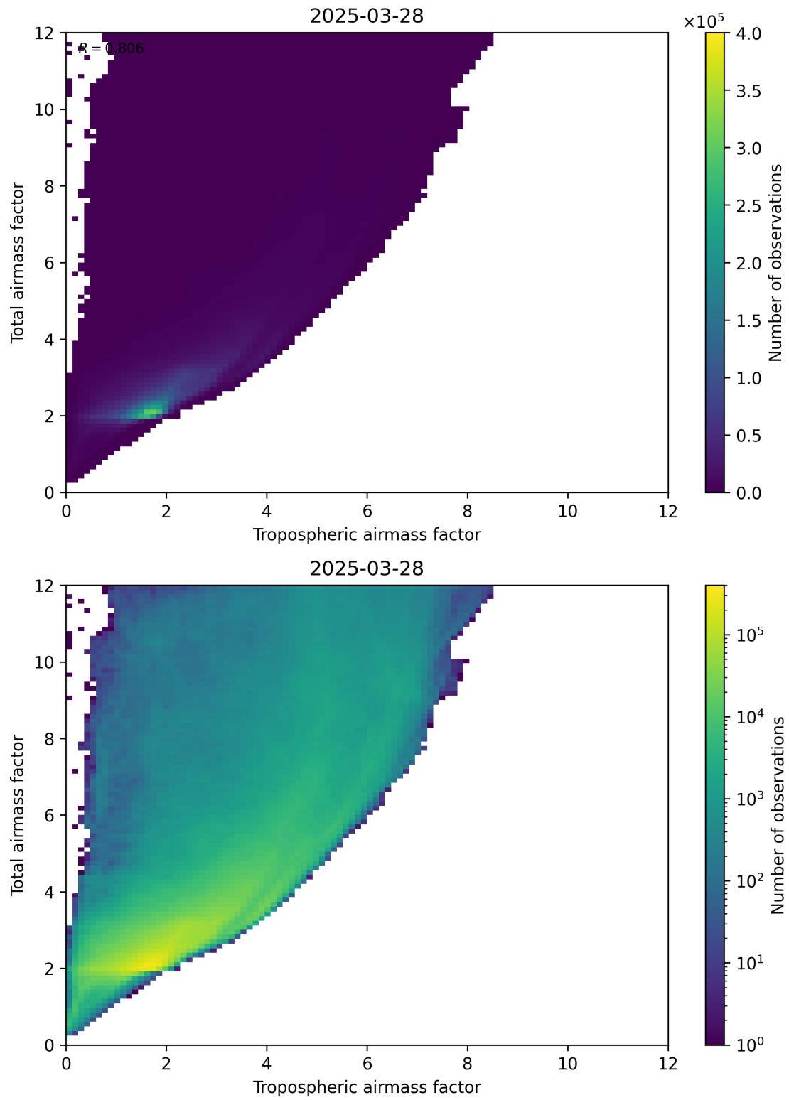
Figure 72: Scatter density plot of “Tropospheric airmass factor” against “Total airmass factor” for 2025-03-28 to 2025-03-29.
