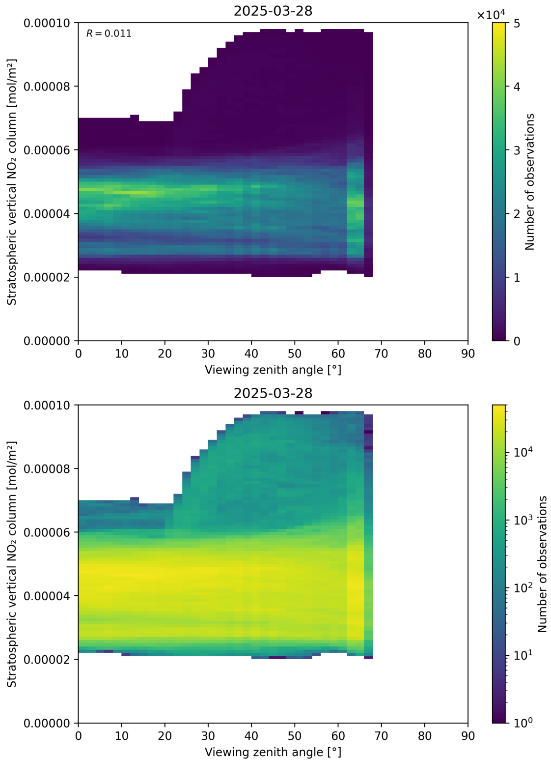
Figure 164: Scatter density plot of “Viewing zenith angle” against “Stratospheric vertical NO 2 column” for 2025-03-28 to 2025-03-29.
