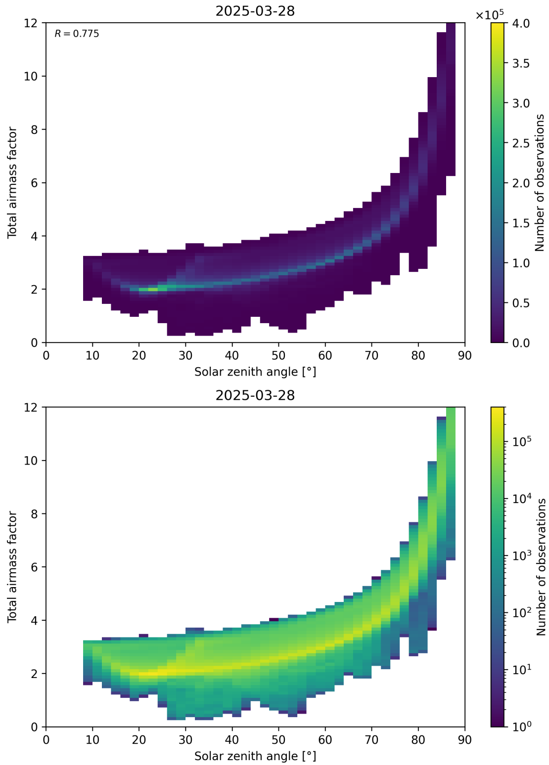
Figure 146: Scatter density plot of “Solar zenith angle” against “Total air mass factor” for 2025-03-28 to 2025-03-29.
