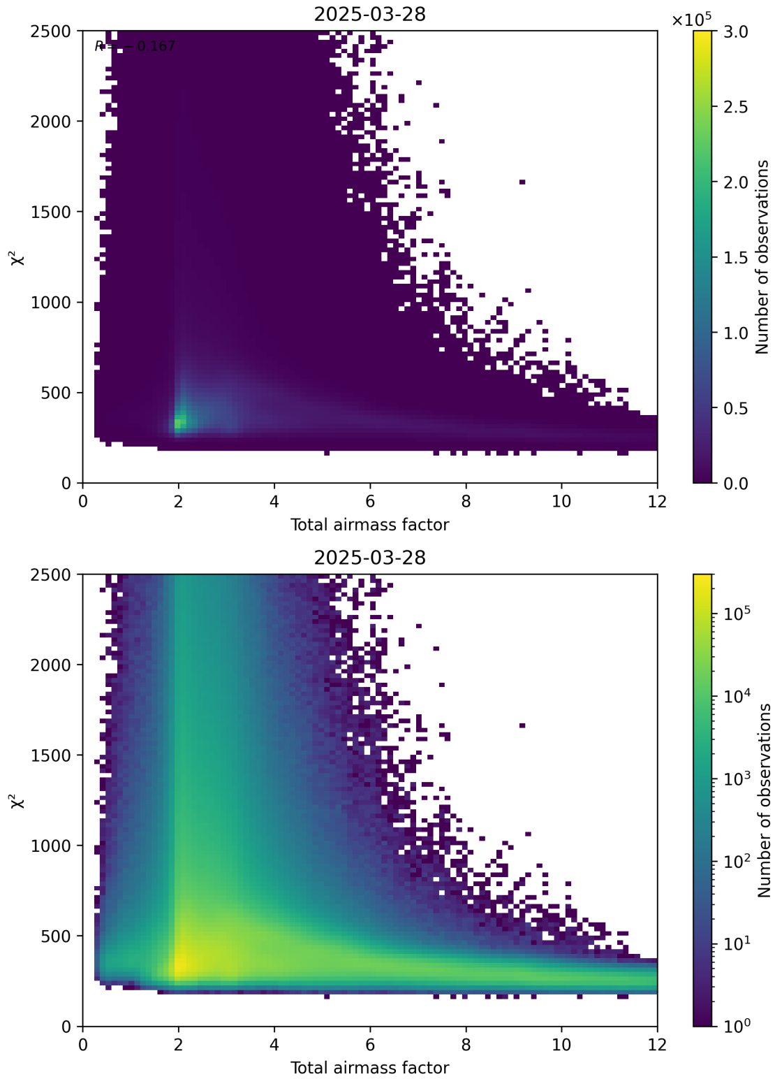
Figure 63: Scatter density plot of “Total airmass factor” against “ \chi^2 ” for 2025-03-28 to 2025-03-29.
