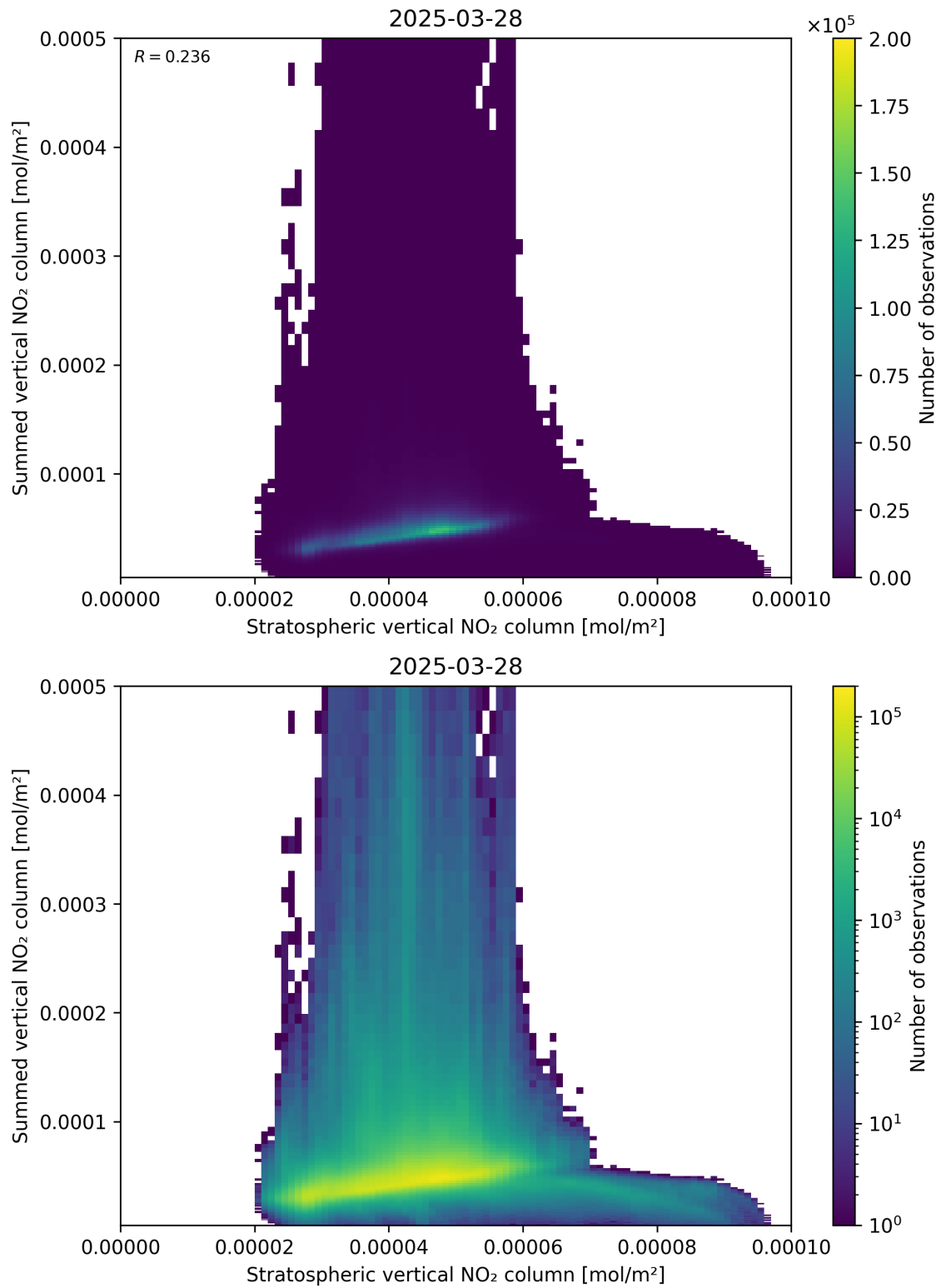
Figure 98: Scatter density plot of “Stratospheric vertical NO 2 column” against “Summed vertical NO 2 column” for 2025-03-28 to 2025-03-29.
