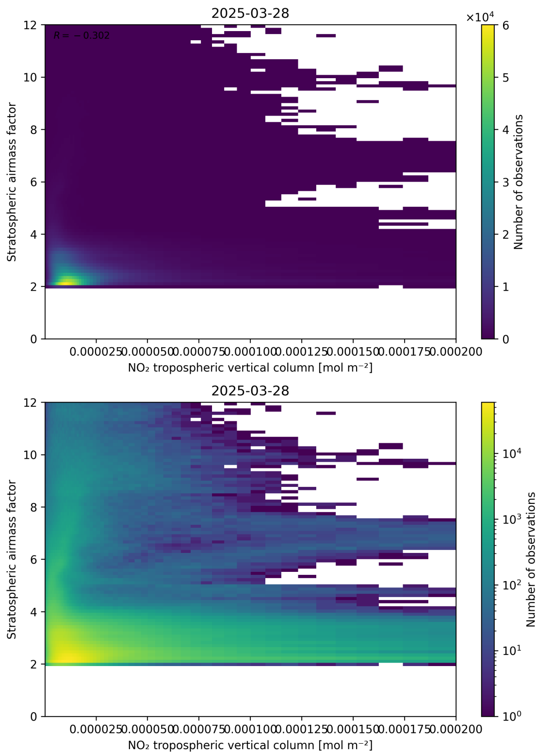
Figure 121: Scatter density plot of “NO 2 tropospheric vertical column” against “Stratospheric air mass factor” for 2025-03-28 to 2025-03-29.
