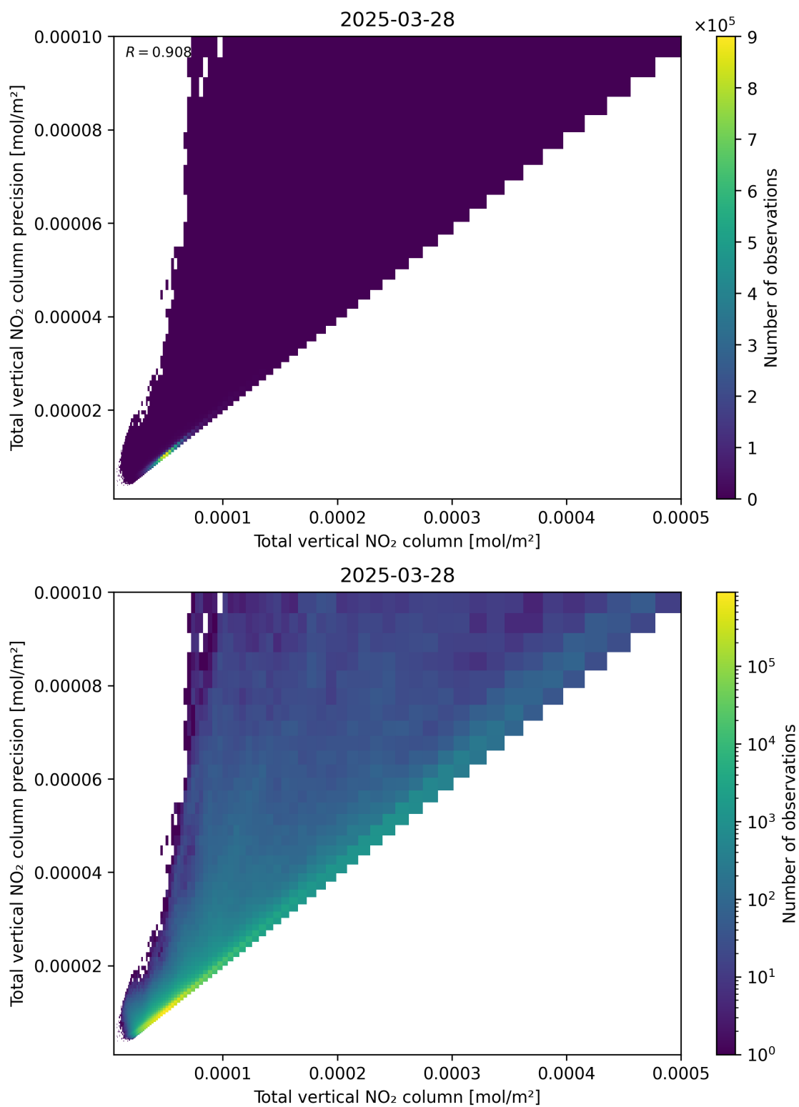
Figure 114: Scatter density plot of “Total vertical NO 2 column” against “Total vertical NO 2 column precision” for 2025-03-28 to 2025-03-29.
