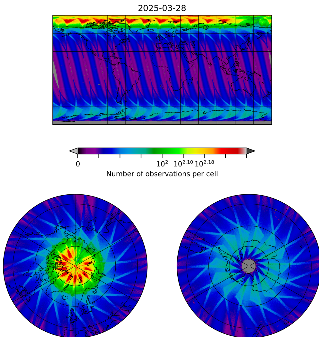
Figure 10: Map of the number of observations for 2025-03-28 to 2025-03-29
