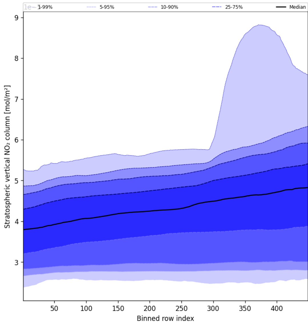
Figure 53: Along track statistics of “Stratospheric vertical NO 2 column” for 2025-03-28 to 2025-03-29
