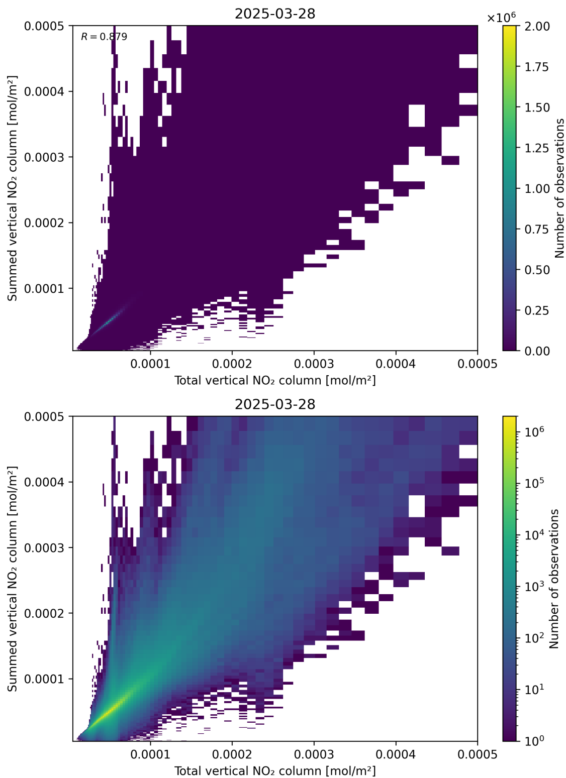
Figure 112: Scatter density plot of “Total vertical NO 2 column” against “Summed vertical NO 2 column” for 2025-03-28 to 2025-03-29.
