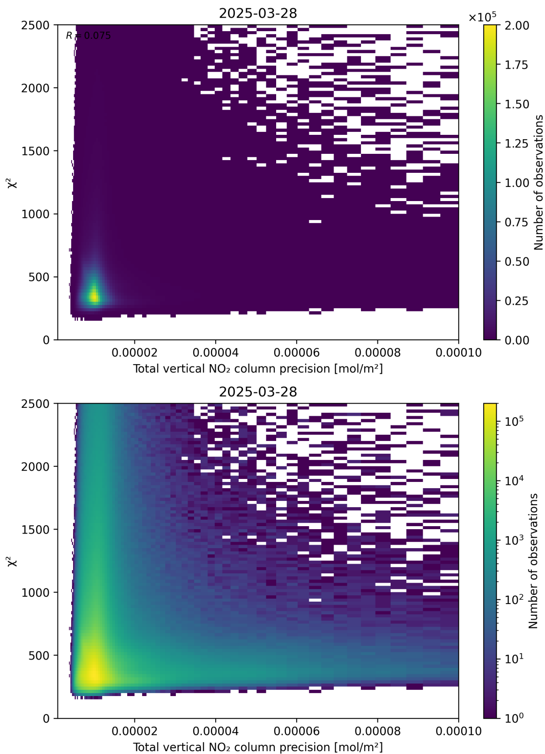
Figure 116: Scatter density plot of “Total vertical NO 2 column precision” against “ \chi^2 ” for 2025-03-28 to 2025-03-29.
