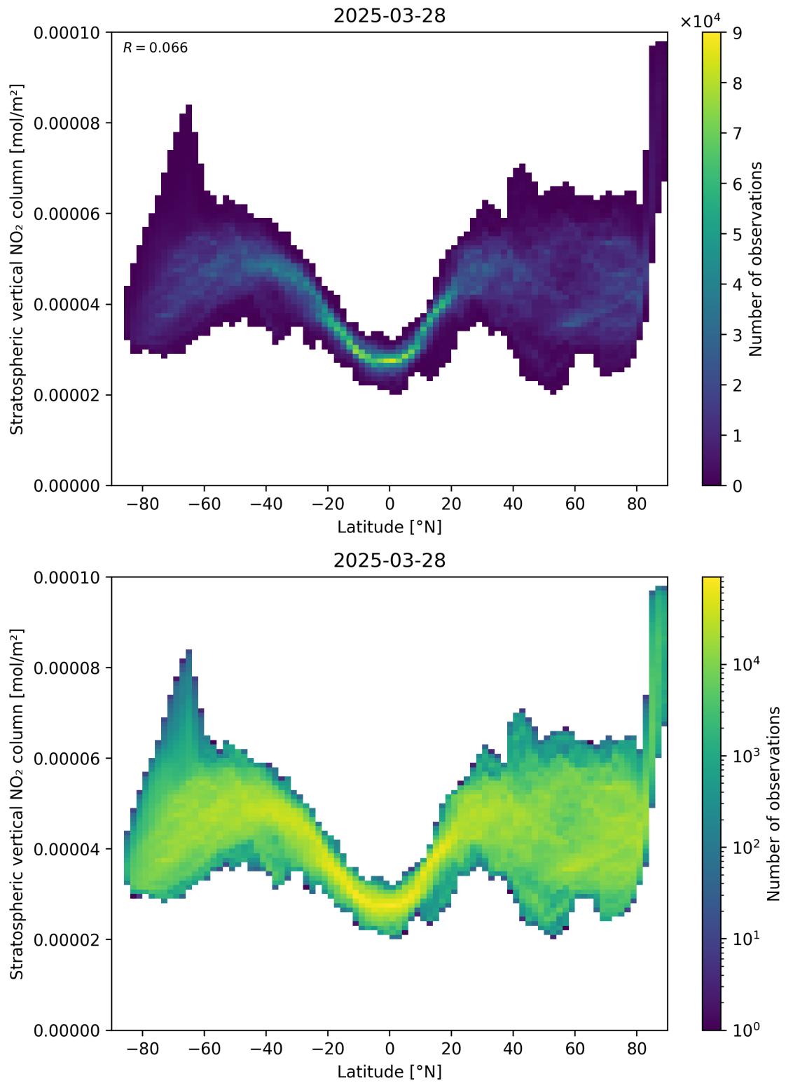
Figure 87: Scatter density plot of “Latitude” against “Stratospheric vertical NO 2 column” for 2025-03-28 to 2025-03-29.
