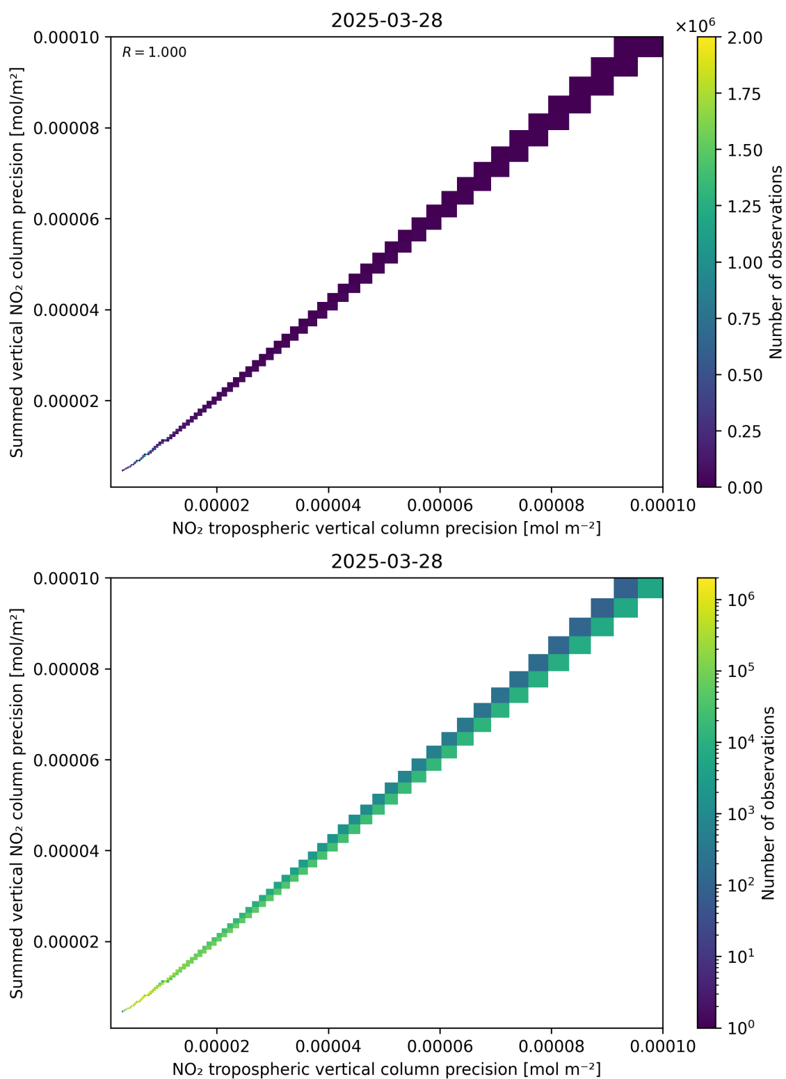
Figure 137: Scatter density plot of “NO 2 tropospheric vertical column precision” against “Summed vertical NO 2 column precision” for 2025-03-28 to 2025-03-29.
