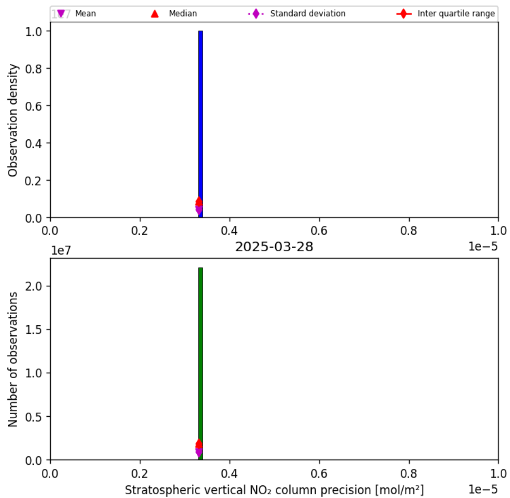
Figure 37: Histogram of “Stratospheric vertical NO 2 column precision” for 2025-03-28 to 2025-03-29
