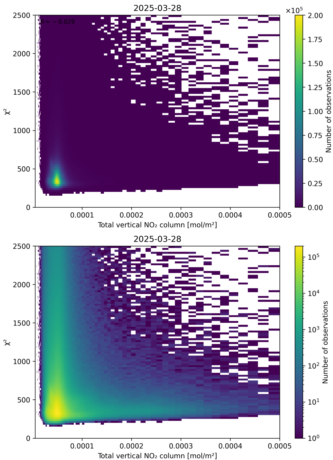
Figure 111: Scatter density plot of “Total vertical NO 2 column” against “ \chi^2 ” for 2025-03-28 to 2025-03-29.
