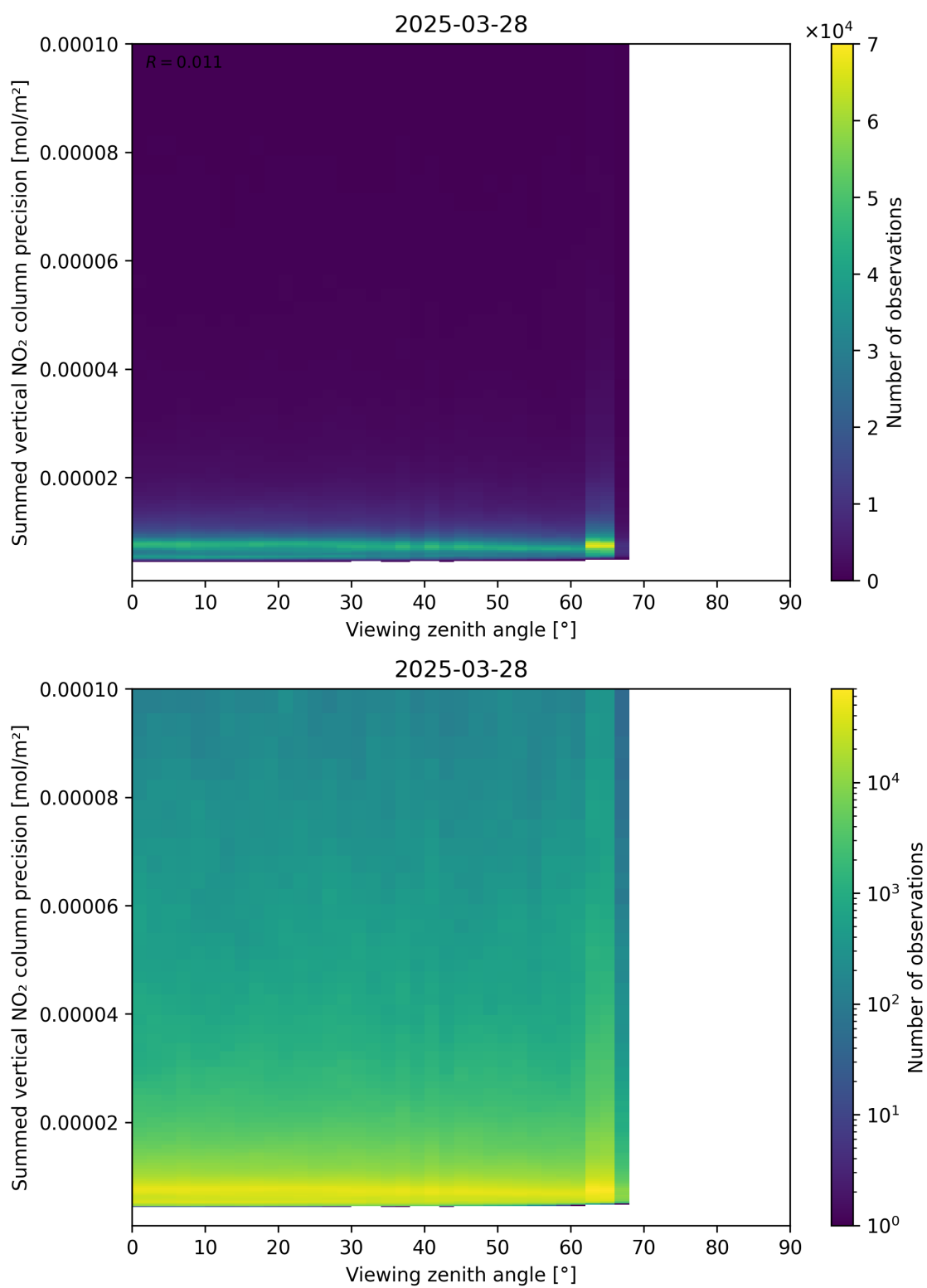
Figure 166: Scatter density plot of “Viewing zenith angle” against “Summed vertical NO 2 column precision” for 2025-03-28 to 2025-03-29.
