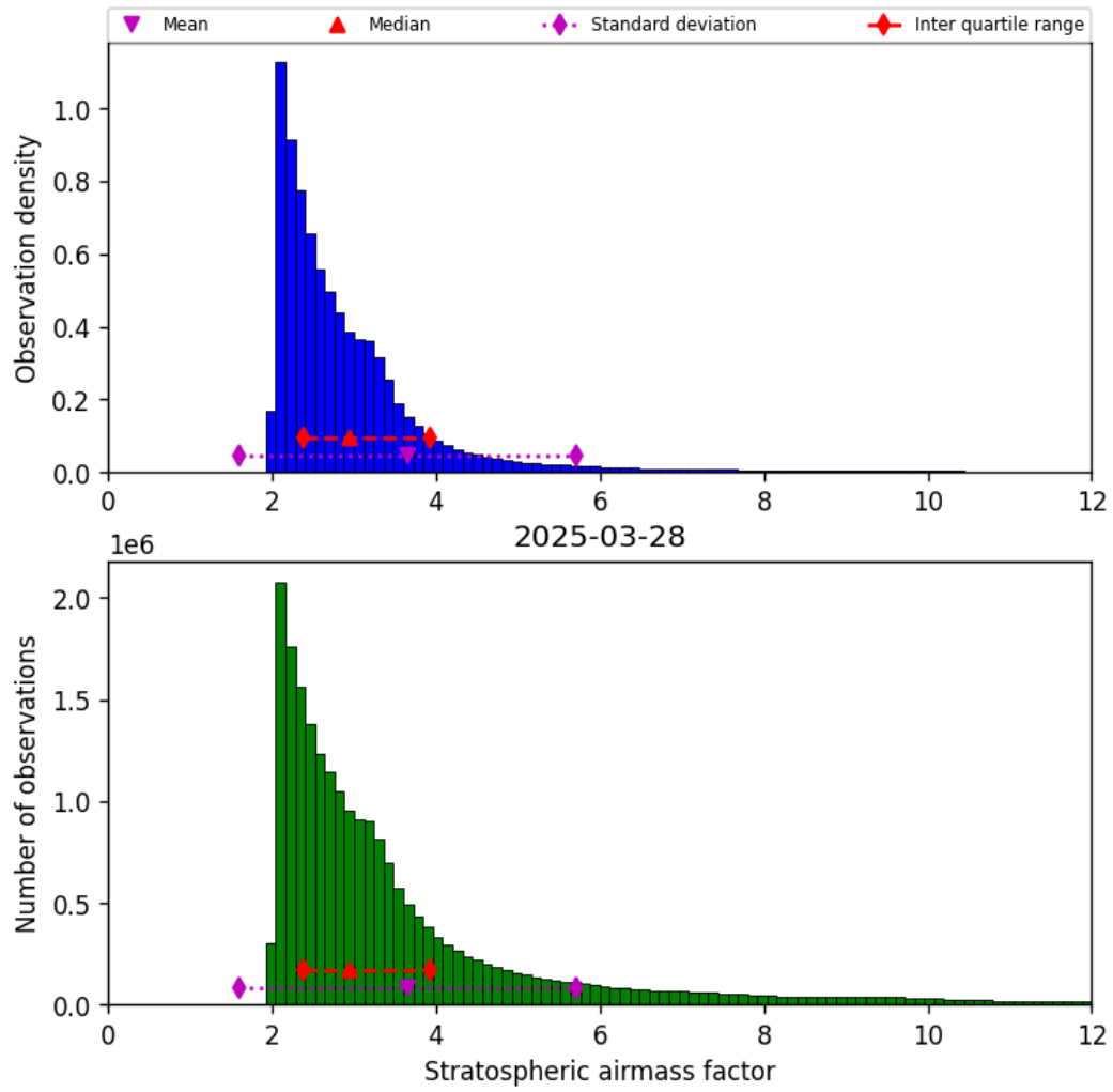
Figure 44: Histogram of “Stratospheric airmass factor” for 2025-03-28 to 2025-03-29
