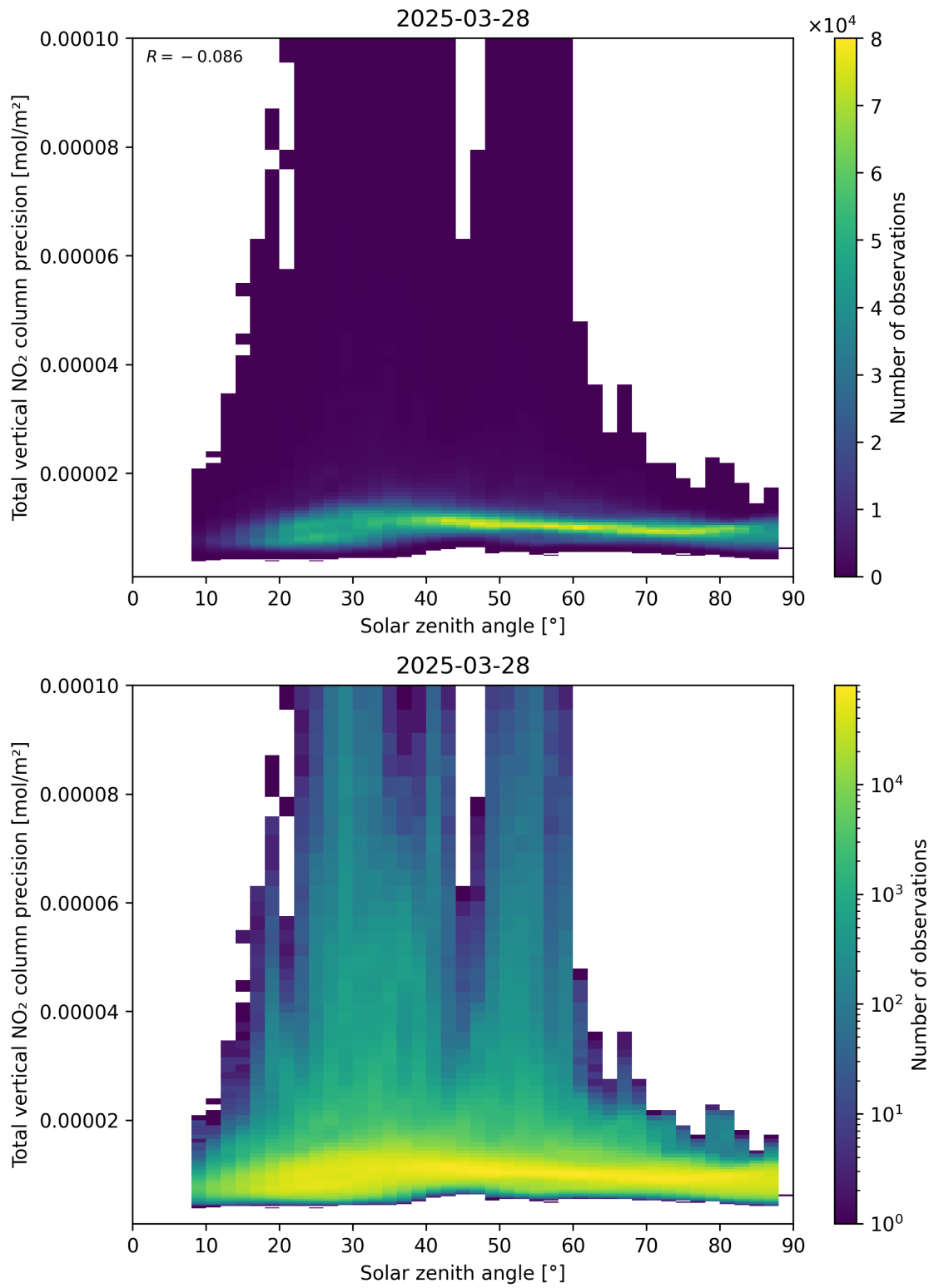
Figure 154: Scatter density plot of “Solar zenith angle” against “Total vertical NO 2 column precision” for 2025-03-28 to 2025-03-29.
