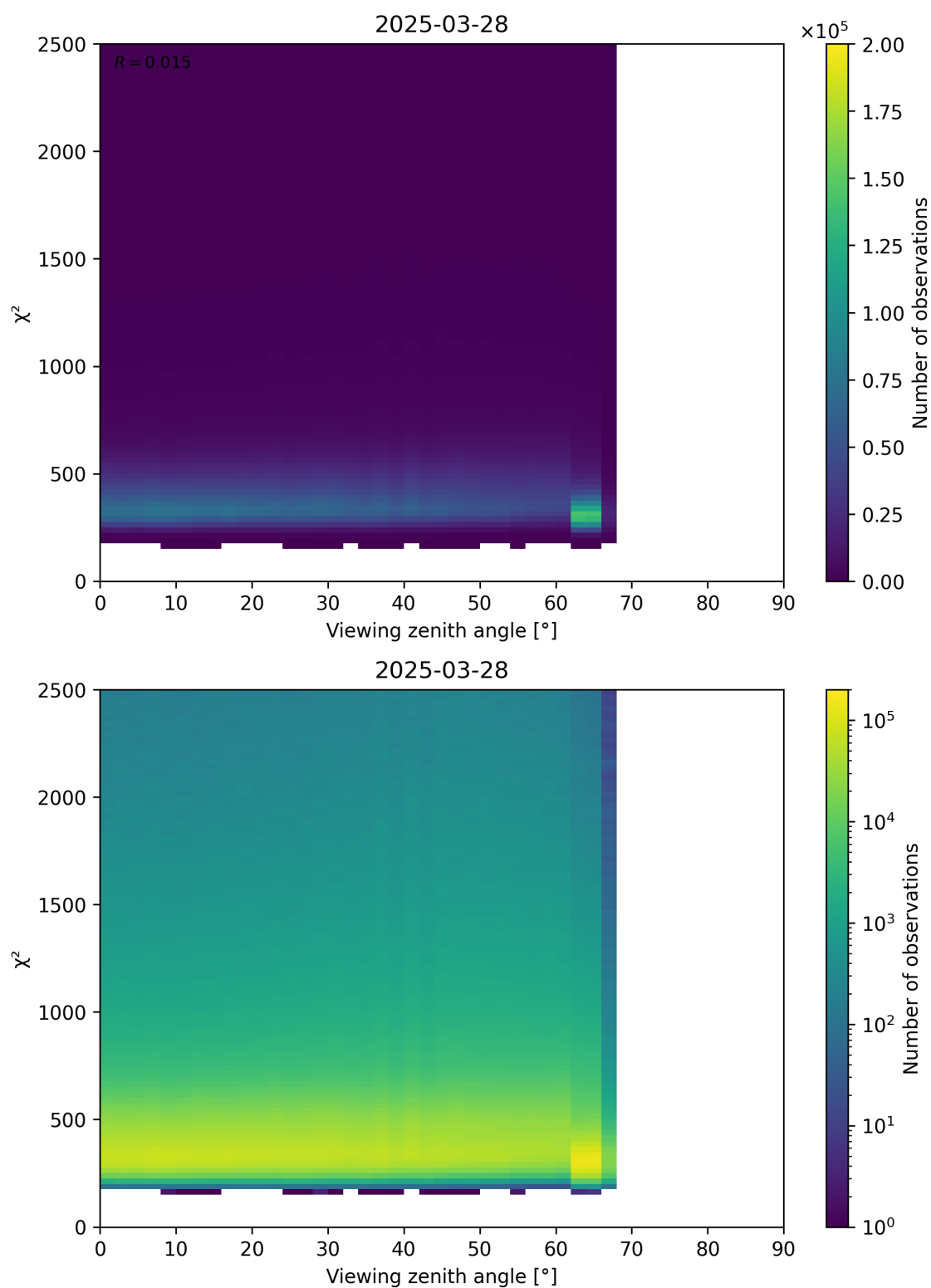
Figure 162: Scatter density plot of “Viewing zenith angle” against “ \chi^2 ” for 2025-03-28 to 2025-03-29.
