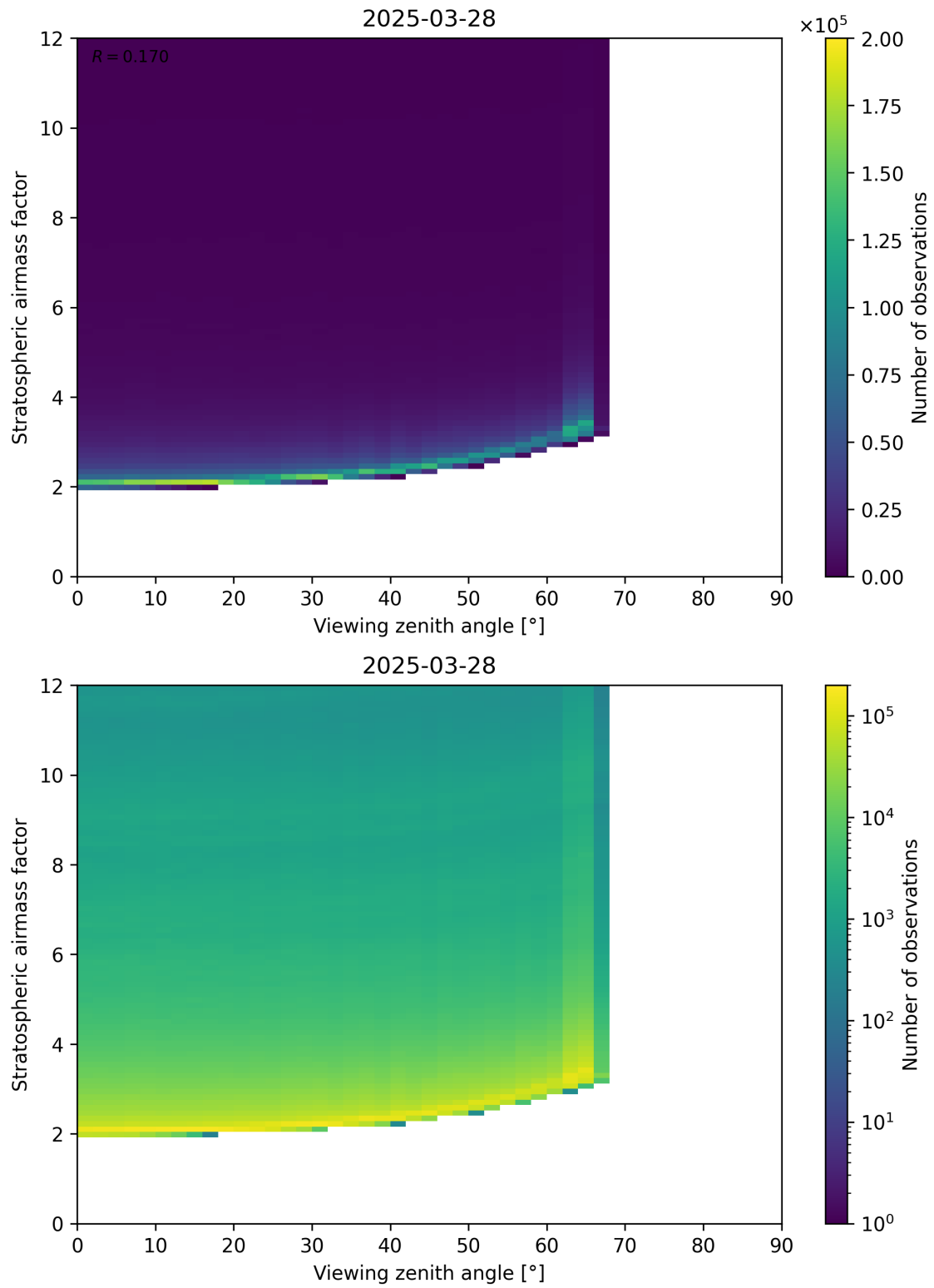
Figure 159: Scatter density plot of “Viewing zenith angle” against “Stratospheric airmass factor” for 2025-03-28 to 2025-03-29.
