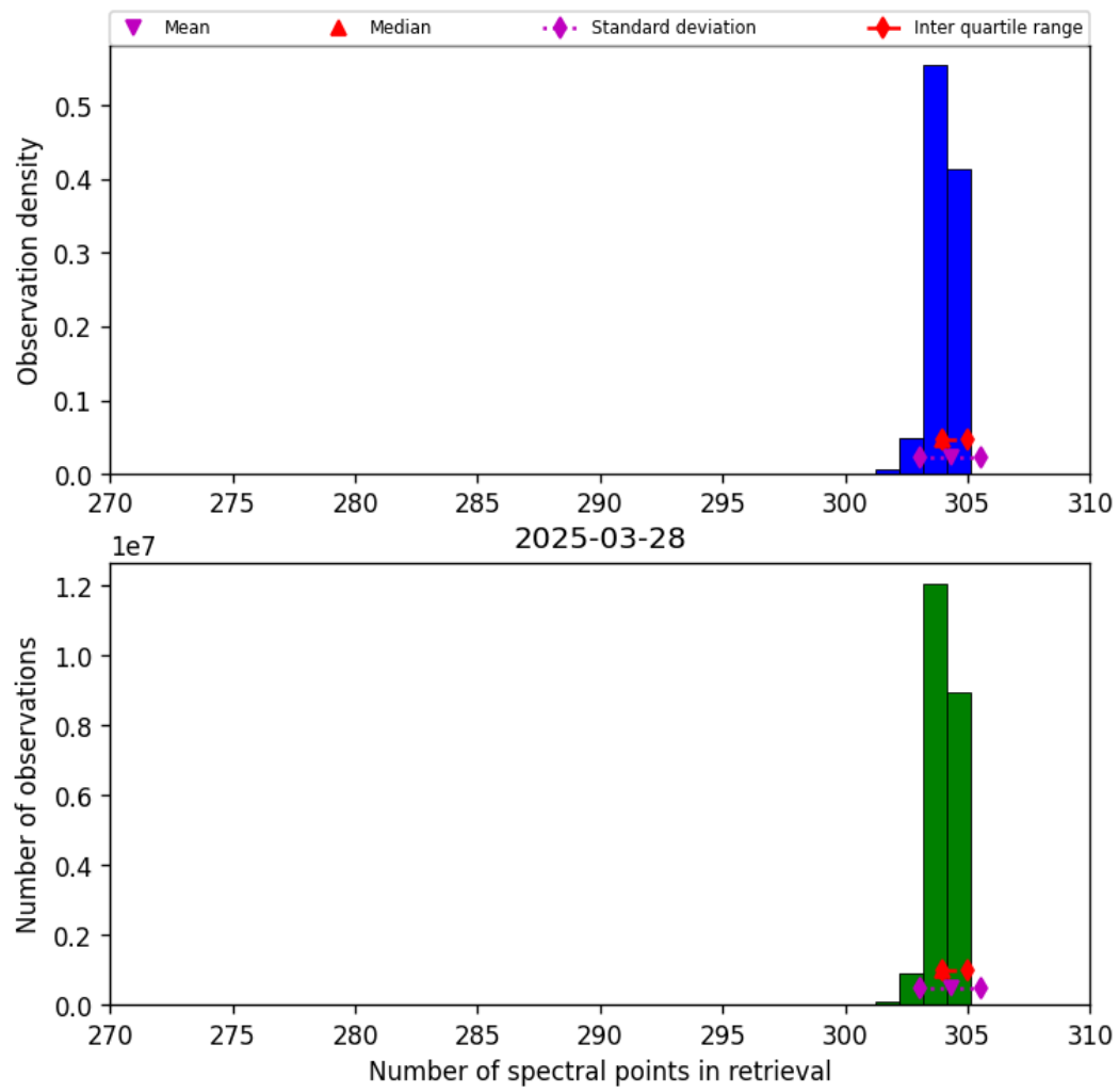
Figure 33: Histogram of “Number of spectral points in retrieval” for 2025-03-28 to 2025-03-29
