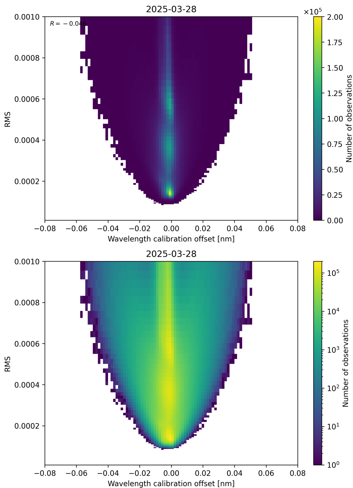
Figure 181: Scatter density plot of “Wavelength calibration offset” against “RMS” for 2025-03-28 to 2025-03-29.
