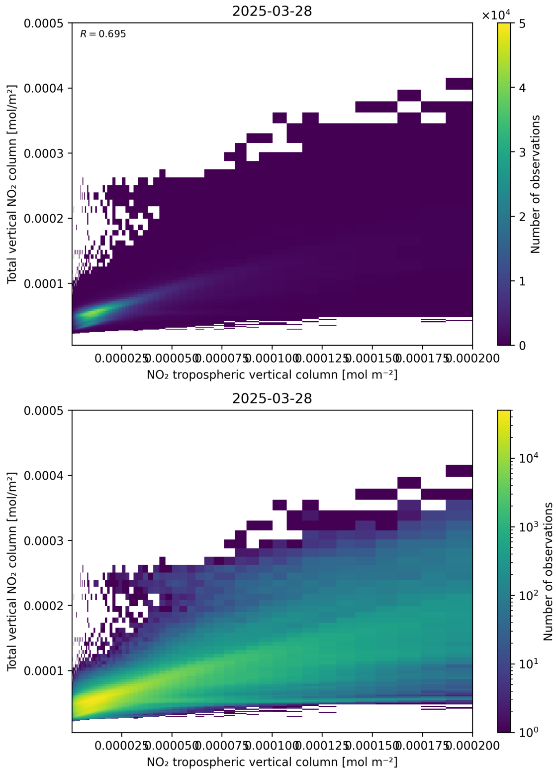
Figure 128: Scatter density plot of “NO 2 tropospheric vertical column” against “Total vertical NO 2 column” for 2025-03-28 to 2025-03-29.
