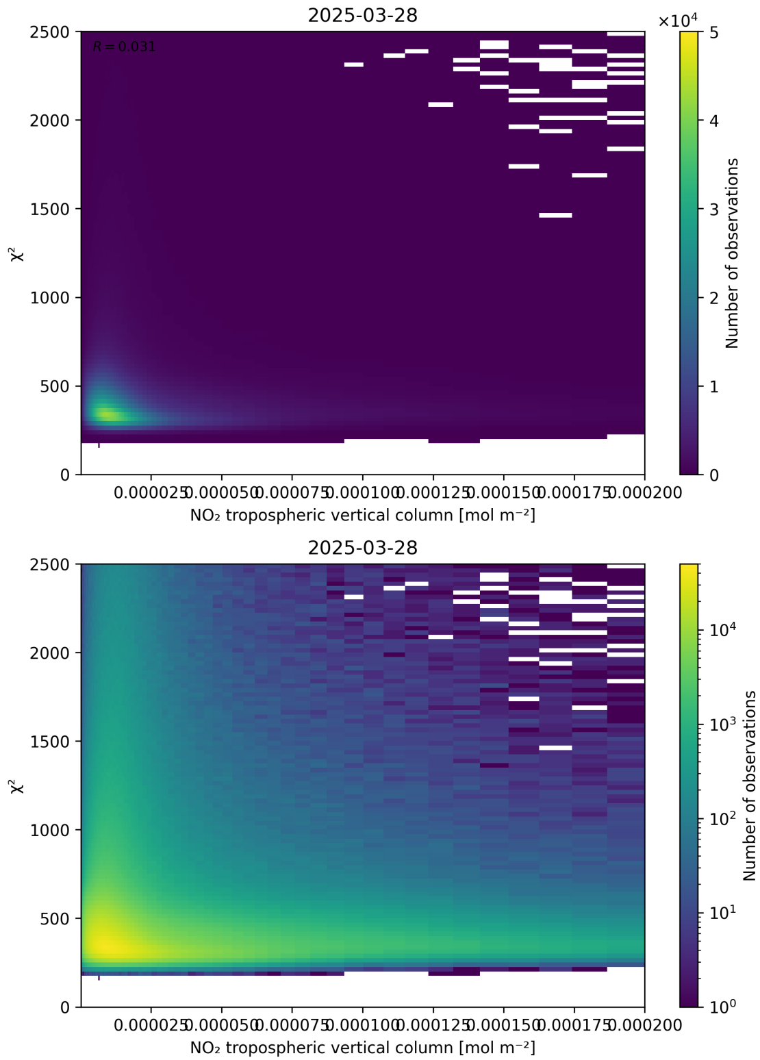
Figure 124: Scatter density plot of “NO 2 tropospheric vertical column” against “ \chi^2 ” for 2025-03-28 to 2025-03-29.
