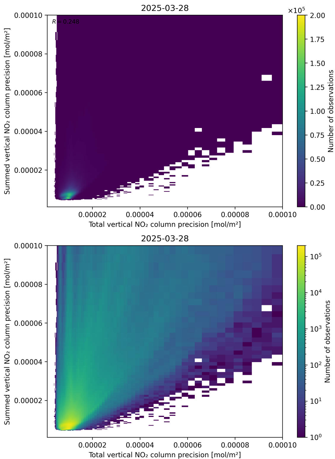
Figure 118: Scatter density plot of “Total vertical NO 2 column precision” against “Summed vertical NO 2 column precision” for 2025-03-28 to 2025-03-29.
