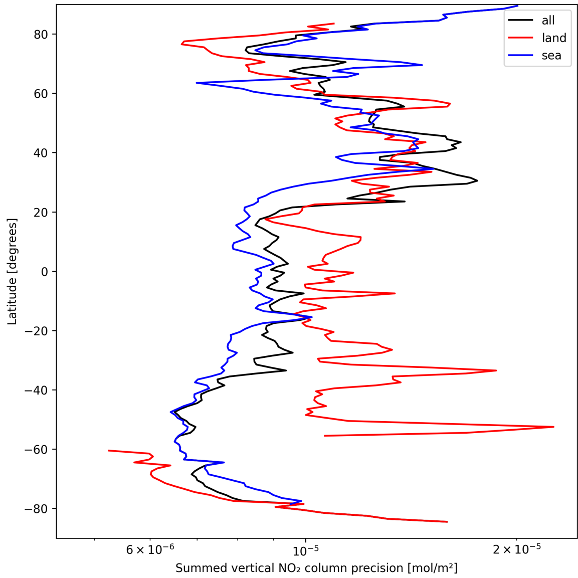
Figure 24: Zonal average of “Summed vertical NO 2 column precision” for 2025-03-28 to 2025-03-29.
