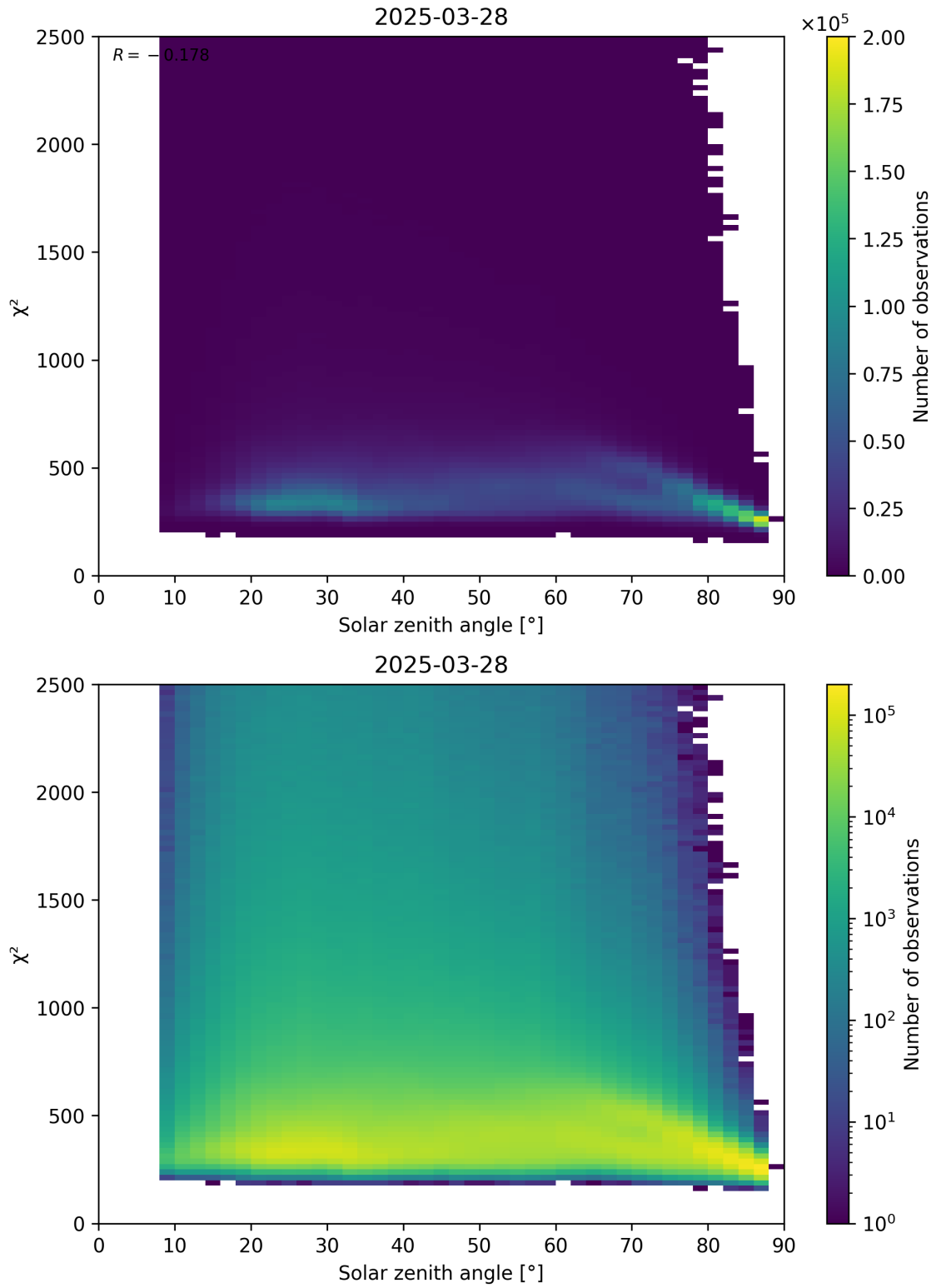
Figure 148: Scatter density plot of “Solar zenith angle” against “ \chi^2 ” for 2025-03-28 to 2025-03-29.
