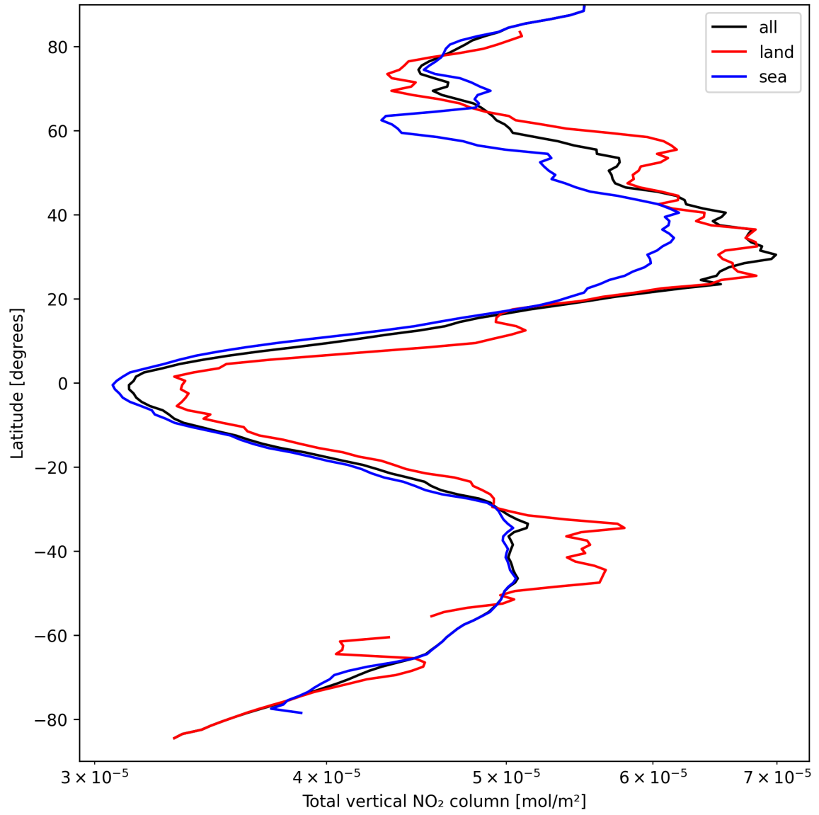
Figure 21: Zonal average of “Total vertical NO 2 column” for 2025-03-28 to 2025-03-29.
