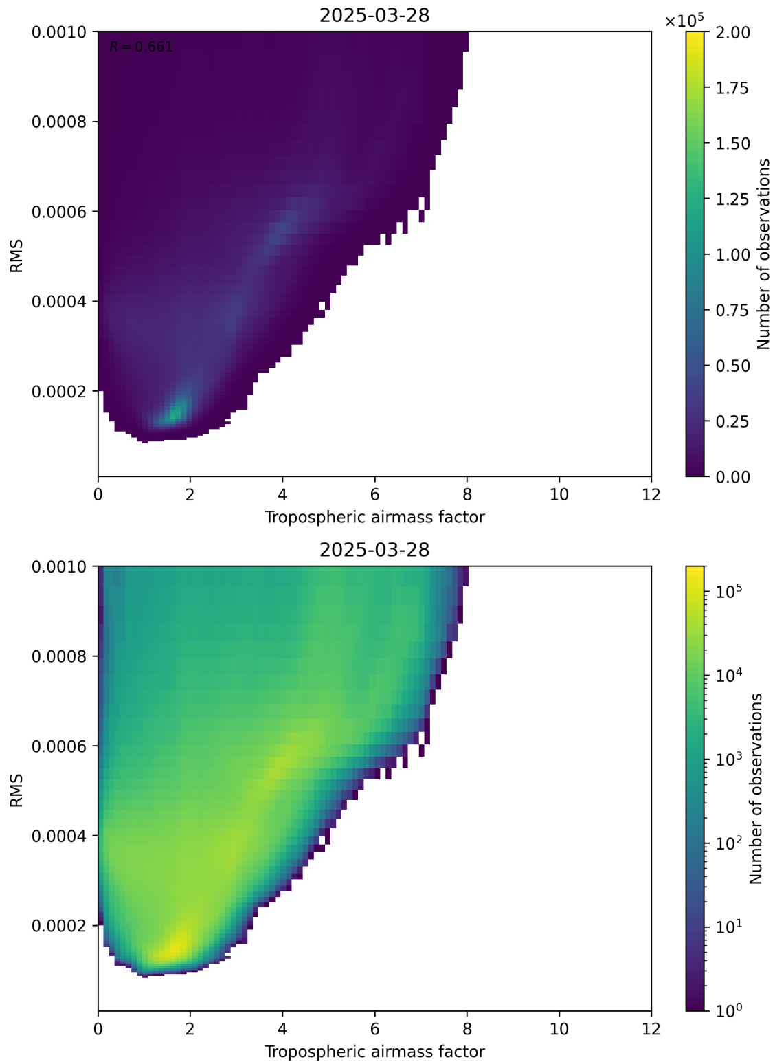
Figure 79: Scatter density plot of “Tropospheric airmass factor” against “RMS” for 2025-03-28 to 2025-03-29.
