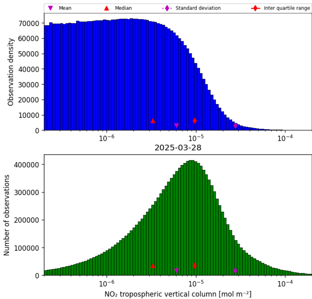
Figure 29: Histogram of “NO 2 tropospheric vertical column” for 2025-03-28 to 2025-03-29
