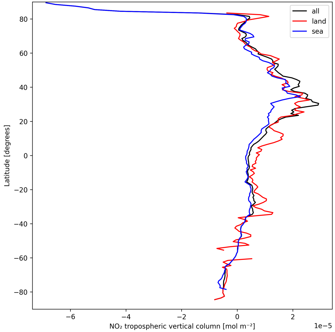
Figure 12: Zonal average of “NO 2 tropospheric vertical column” for 2025-03-28 to 2025-03-29.
