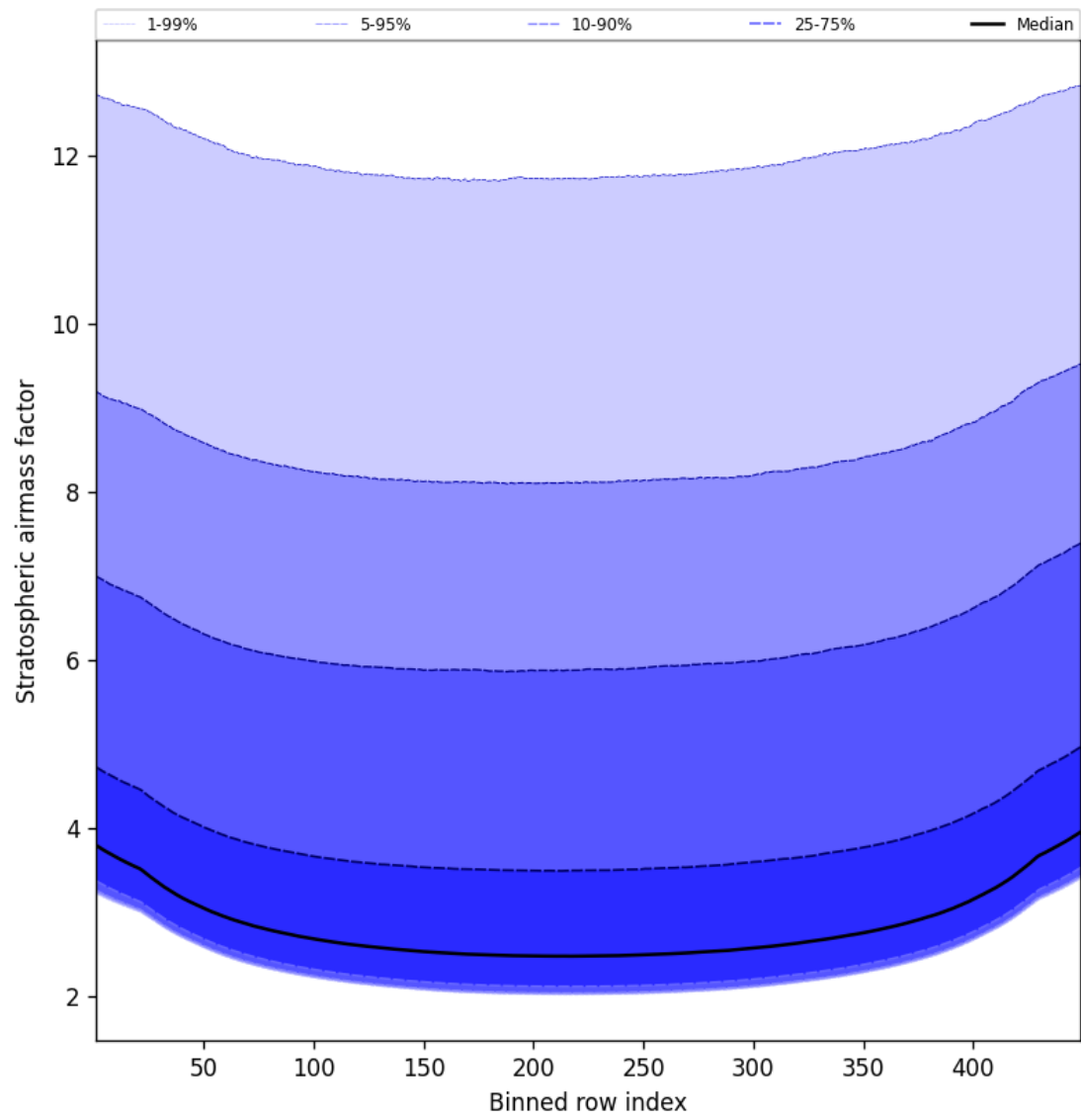
Figure 61: Along track statistics of “Stratospheric air mass factor” for 2025-03-28 to 2025-03-29
