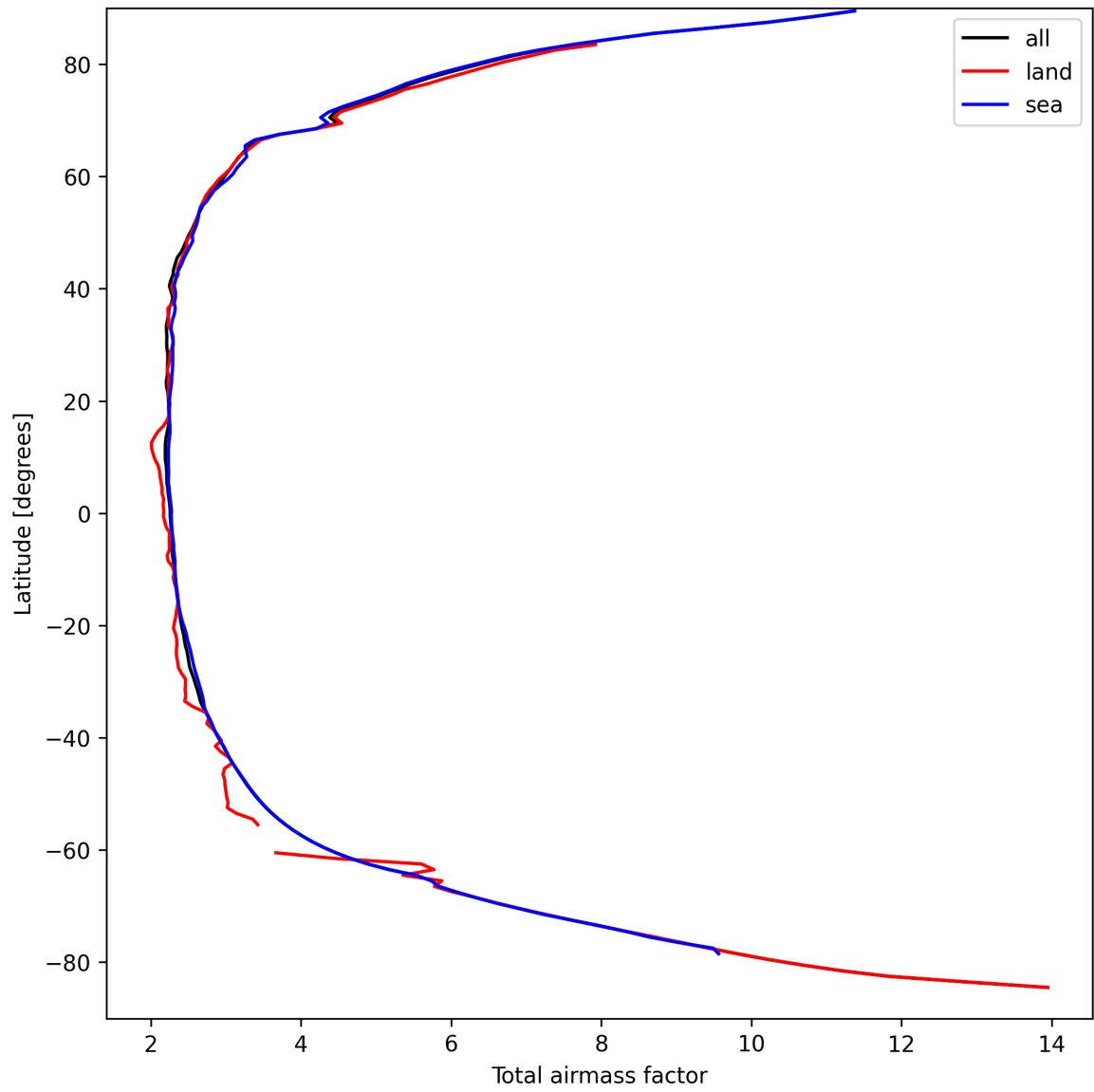
Figure 15: Zonal average of “Total airmass factor” for 2025-03-28 to 2025-03-29.
