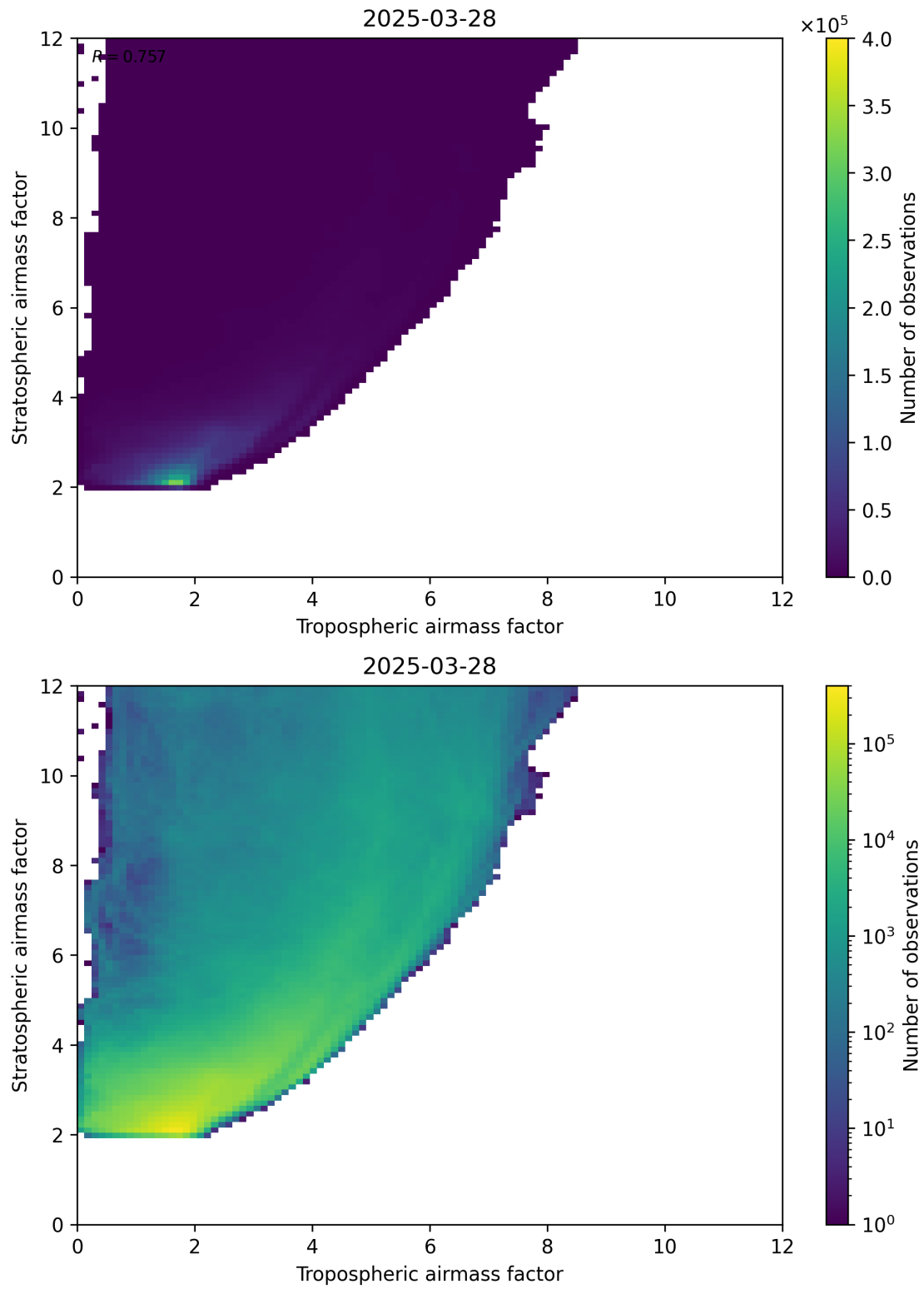
Figure 71: Scatter density plot of “Tropospheric airmass factor” against “Stratospheric airmass factor” for 2025-03-28 to 2025-03-29.
