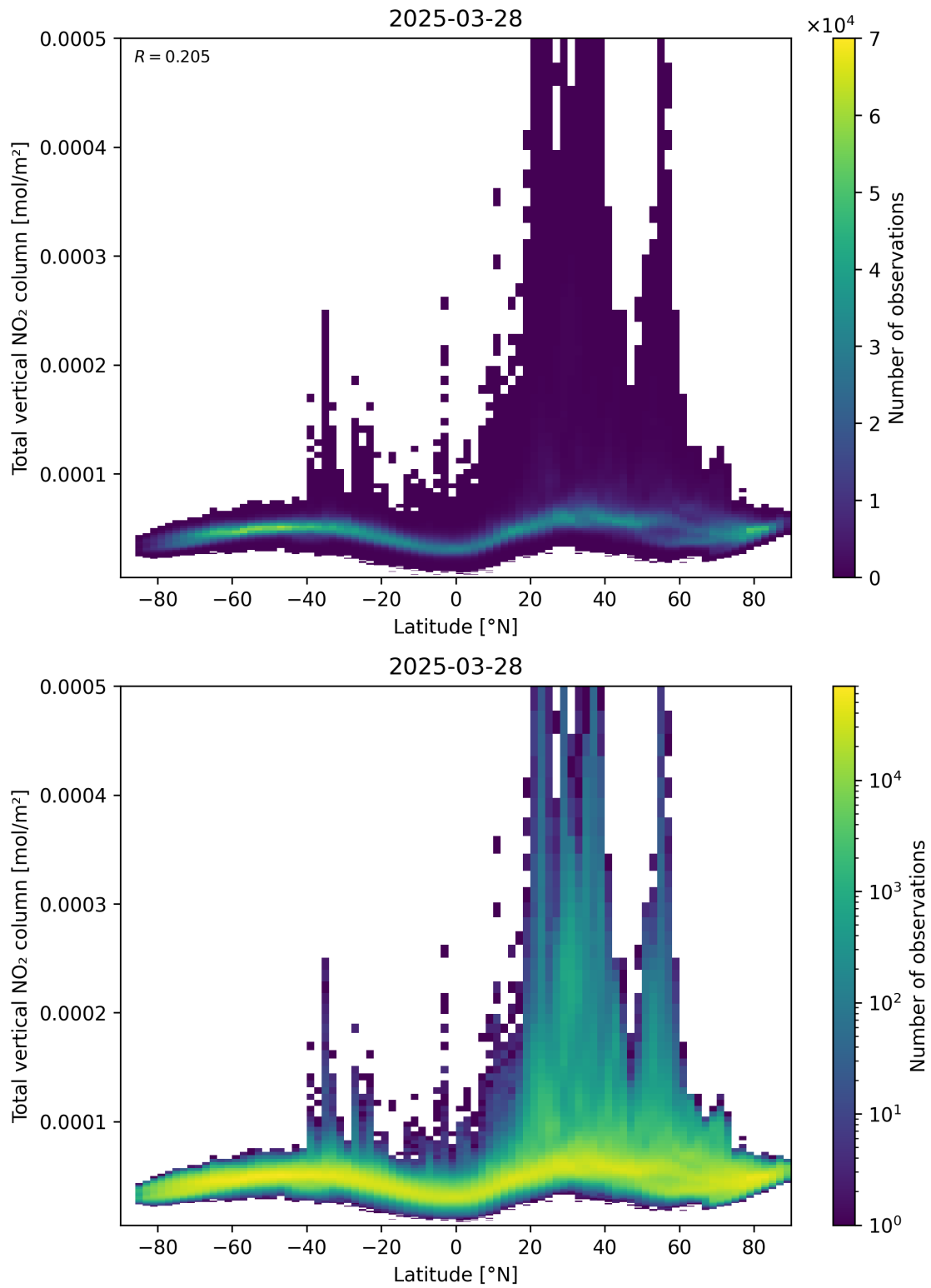
Figure 90: Scatter density plot of “Latitude” against “Total vertical NO 2 column” for 2025-03-28 to 2025-03-29.
