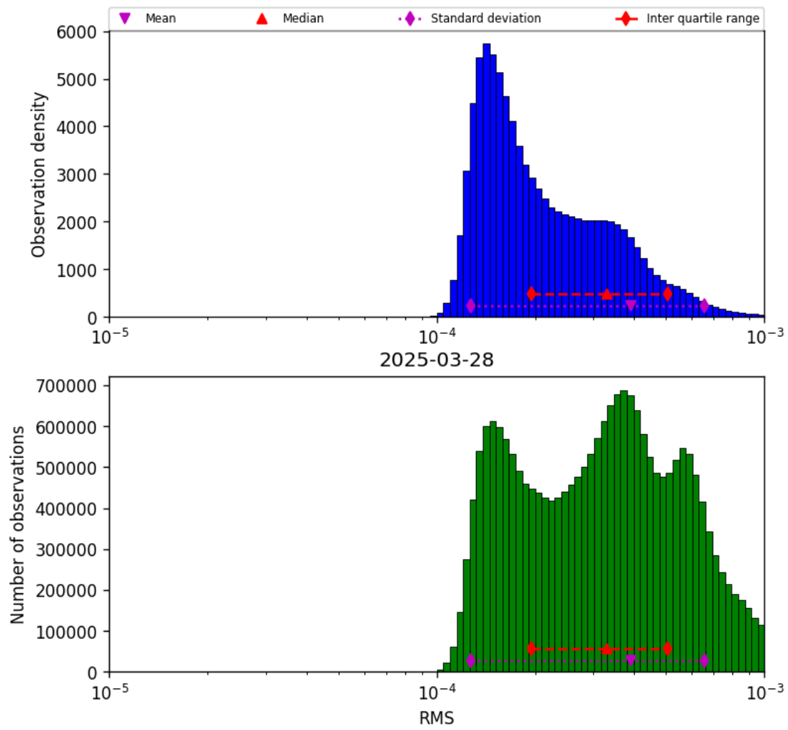
Figure 43: Histogram of “RMS” for 2025-03-28 to 2025-03-29
