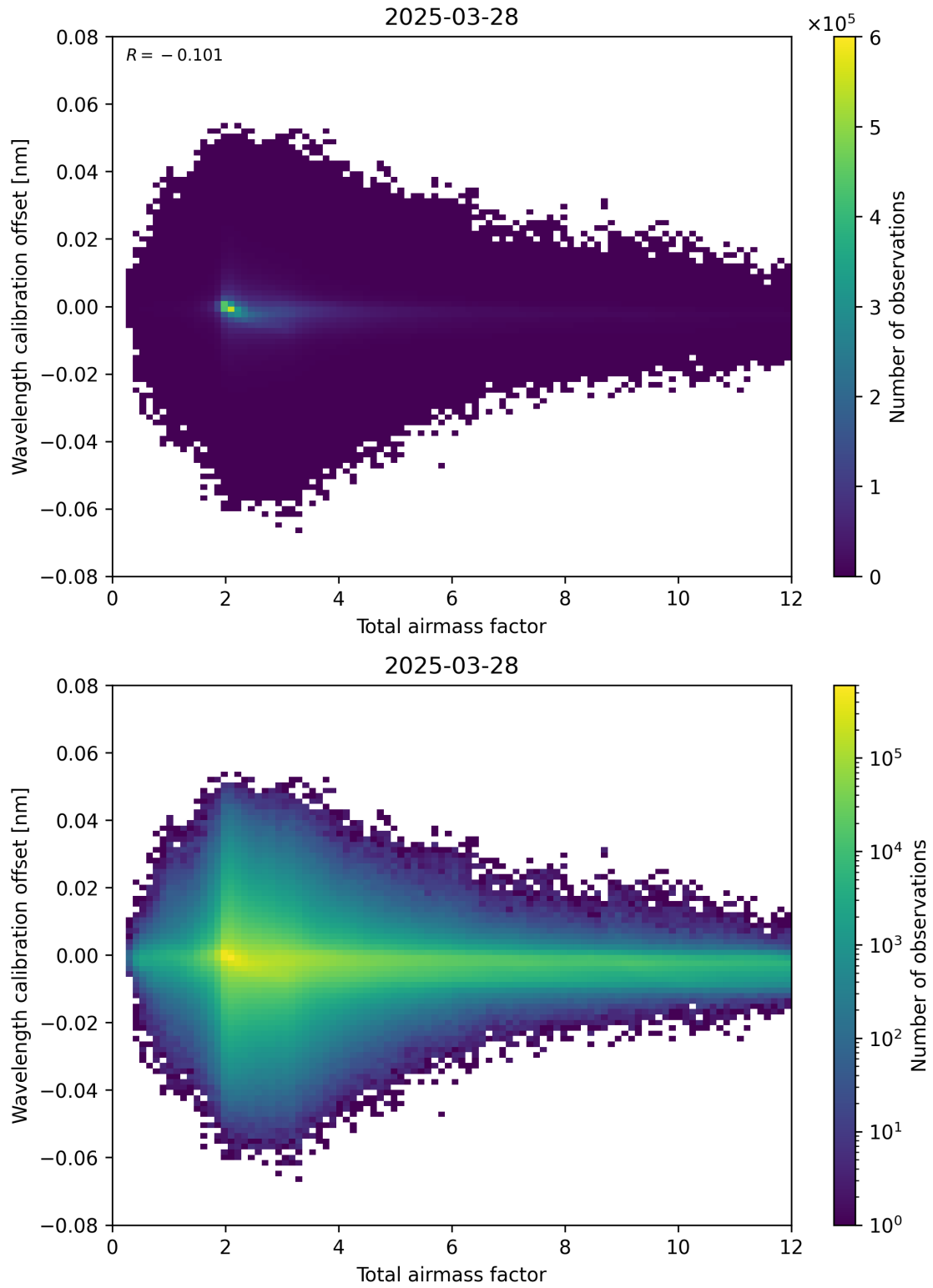
Figure 70: Scatter density plot of “Total airmass factor” against “Wavelength calibration offset” for 2025-03-28 to 2025-03-29.
