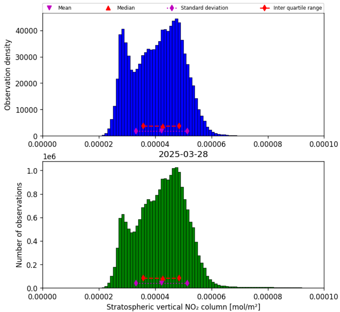
Figure 36: Histogram of “Stratospheric vertical NO 2 column” for 2025-03-28 to 2025-03-29
