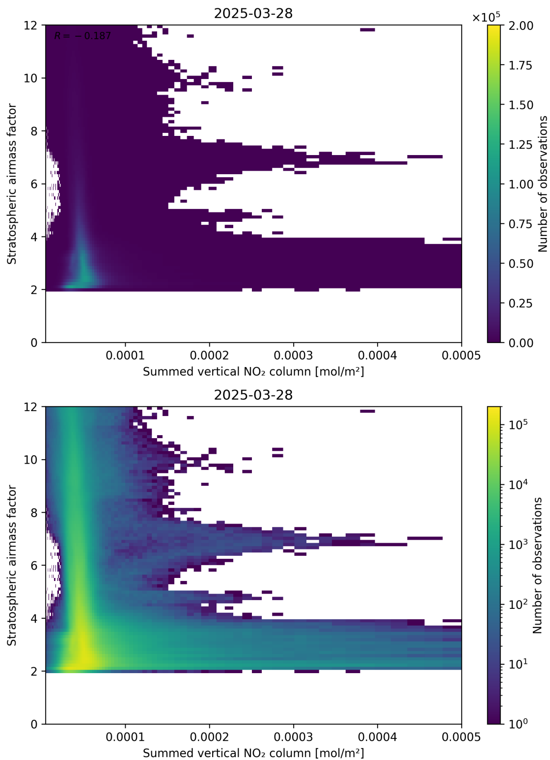
Figure 103: Scatter density plot of “Summed vertical NO 2 column” against “Stratospheric air mass factor” for 2025-03-28 to 2025-03-29.
