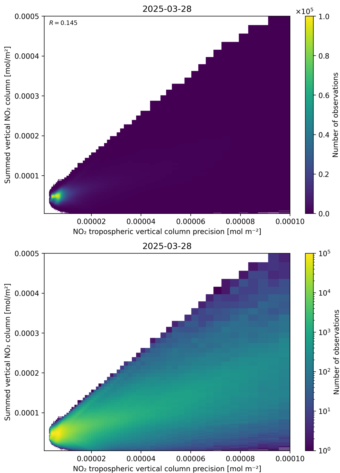
Figure 136: Scatter density plot of “NO 2 tropospheric vertical column precision” against “Summed vertical NO 2 column” for 2025-03-28 to 2025-03-29.
