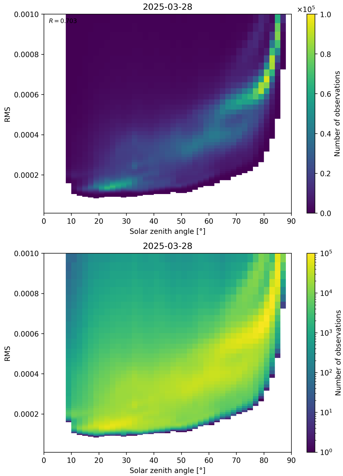
Figure 157: Scatter density plot of “Solar zenith angle” against “RMS” for 2025-03-28 to 2025-03-29.
