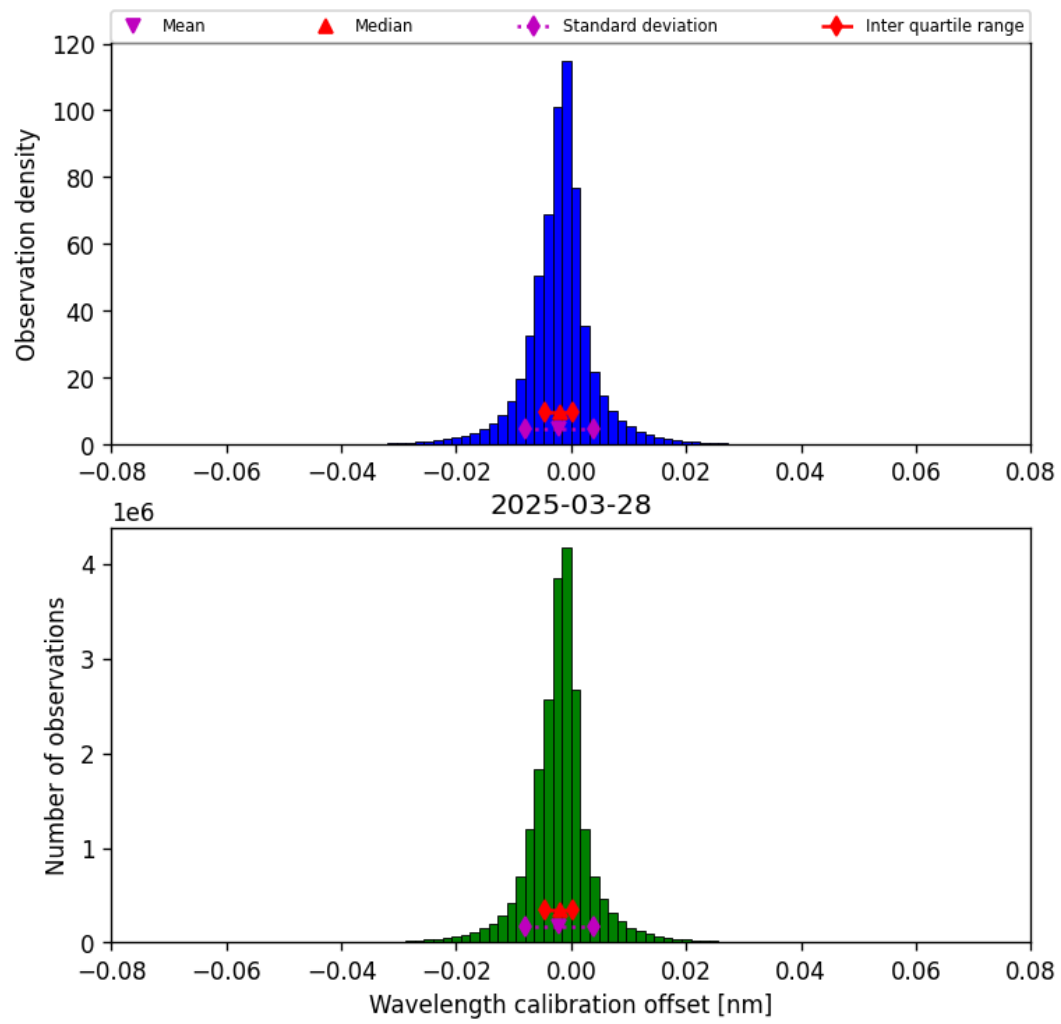
Figure 35: Histogram of “Wavelength calibration offset” for 2025-03-28 to 2025-03-29
