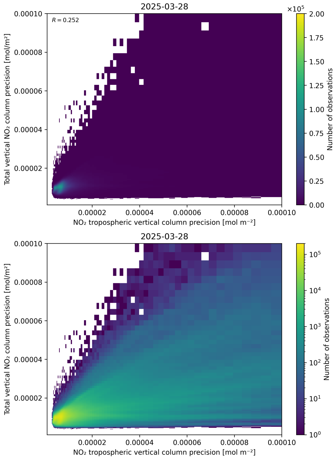
Figure 139: Scatter density plot of “NO 2 tropospheric vertical column precision” against “Total vertical NO 2 column precision” for 2025-03-28 to 2025-03-29.
