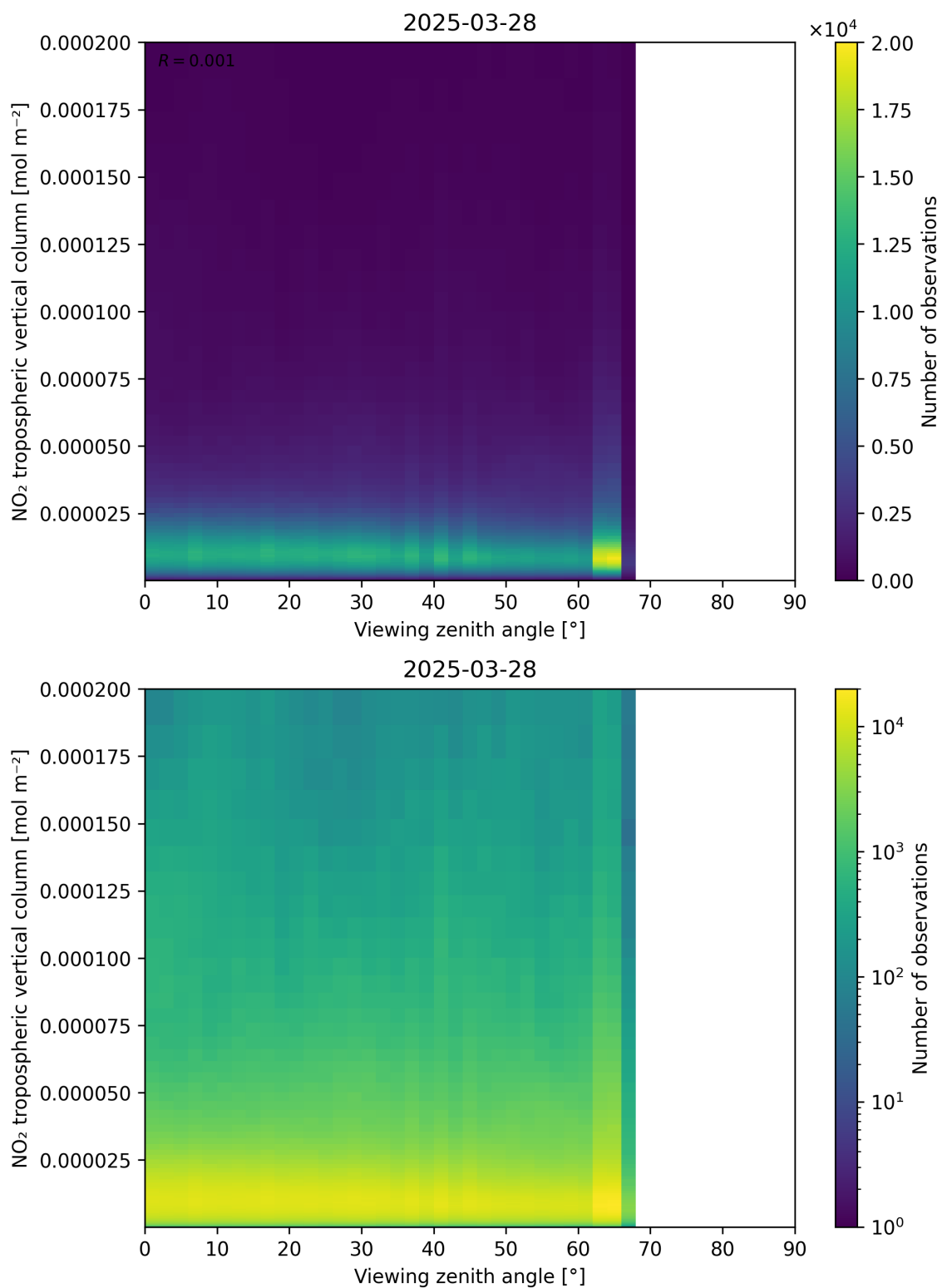
Figure 169: Scatter density plot of “Viewing zenith angle” against “NO 2 tropospheric vertical column” for 2025-03-28 to 2025-03-29.
