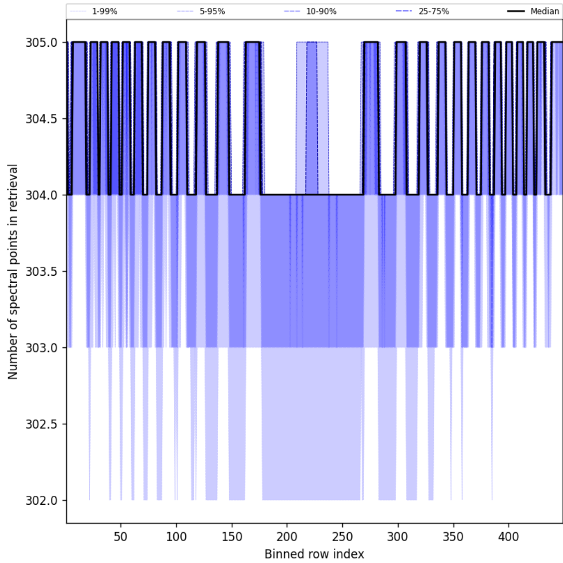
Figure 50: Along track statistics of “Number of spectral points in retrieval” for 2025-03-28 to 2025-03-29
