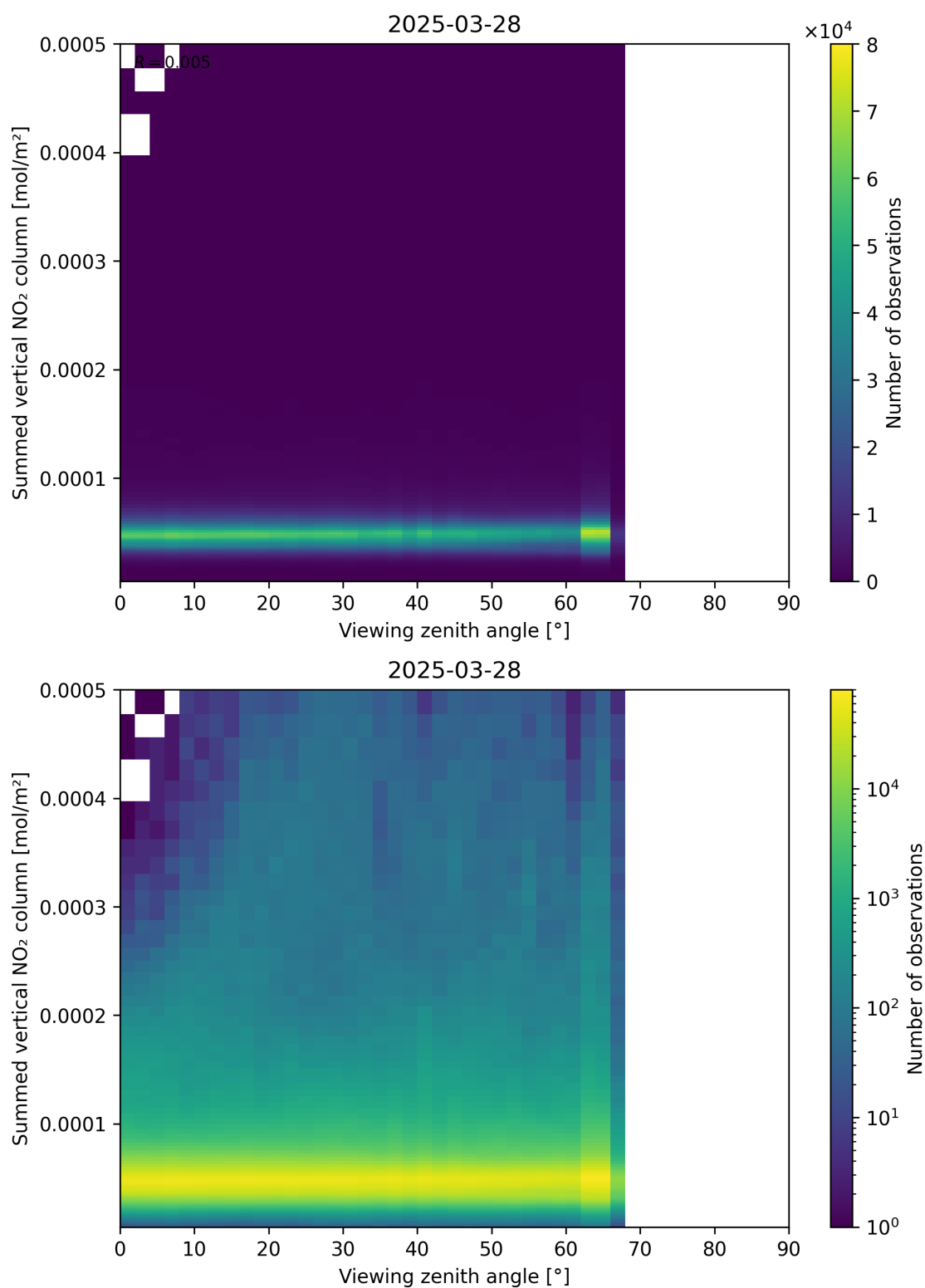
Figure 165: Scatter density plot of “Viewing zenith angle” against “Summed vertical NO 2 column” for 2025-03-28 to 2025-03-29.
