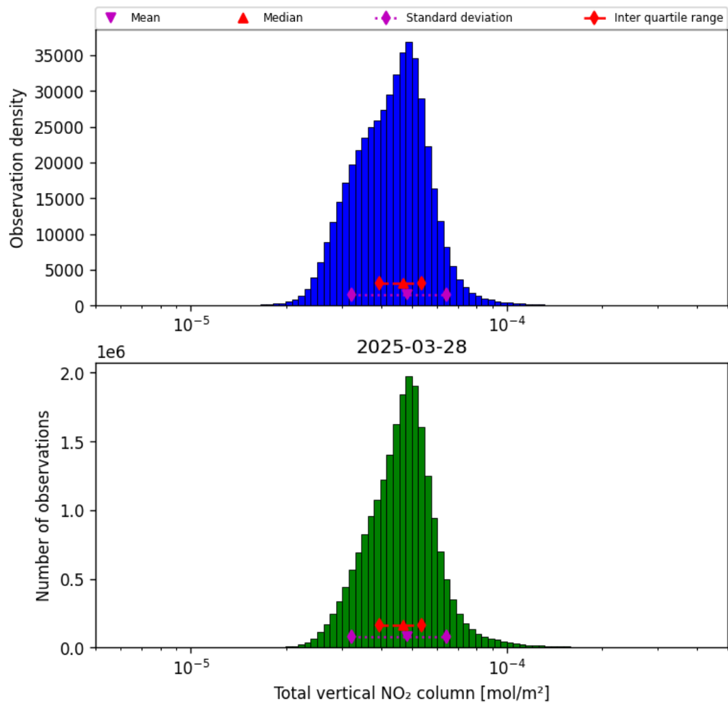
Figure 38: Histogram of "Total vertical NO 2 column" for 2025-03-28 to 2025-03-29
