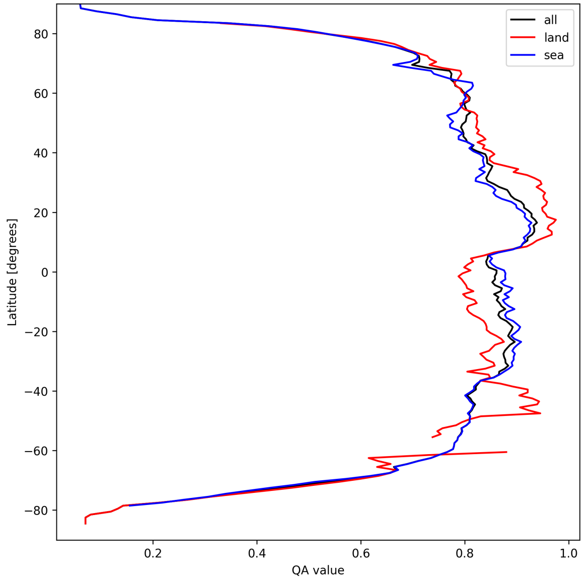
Figure 11: Zonal average of “QA value” for 2025-03-28 to 2025-03-29.
