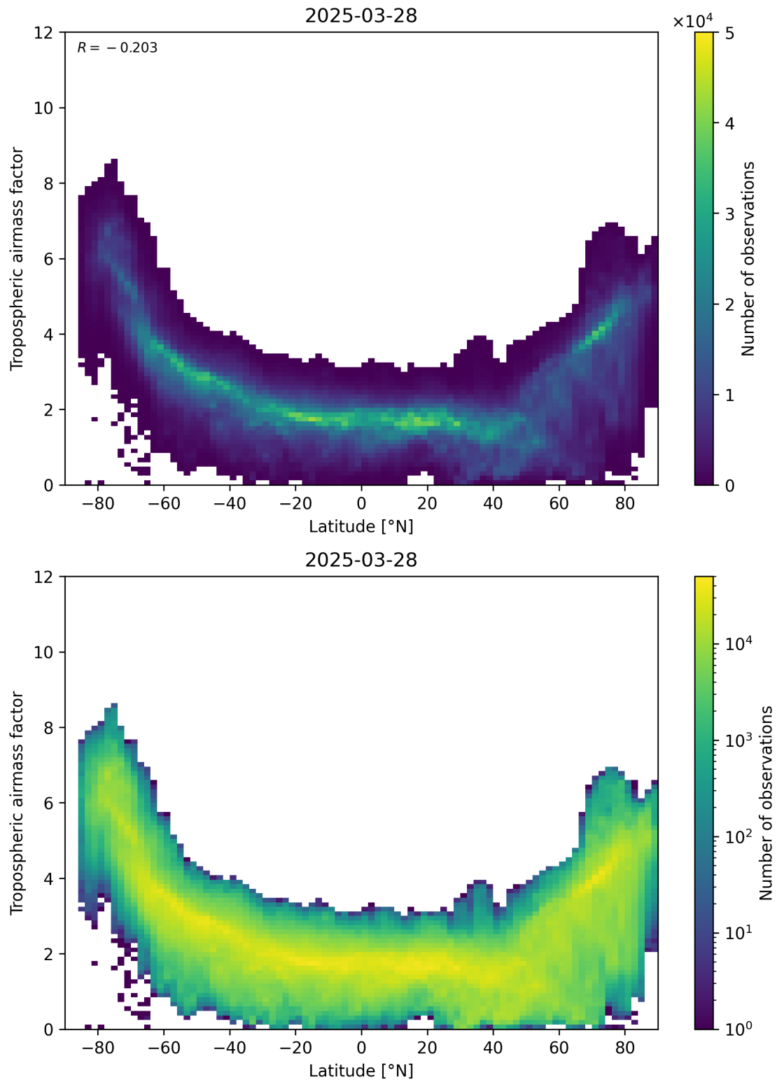
Figure 85: Scatter density plot of “Latitude” against “Tropospheric airmass factor” for 2025-03-28 to 2025-03-29.
