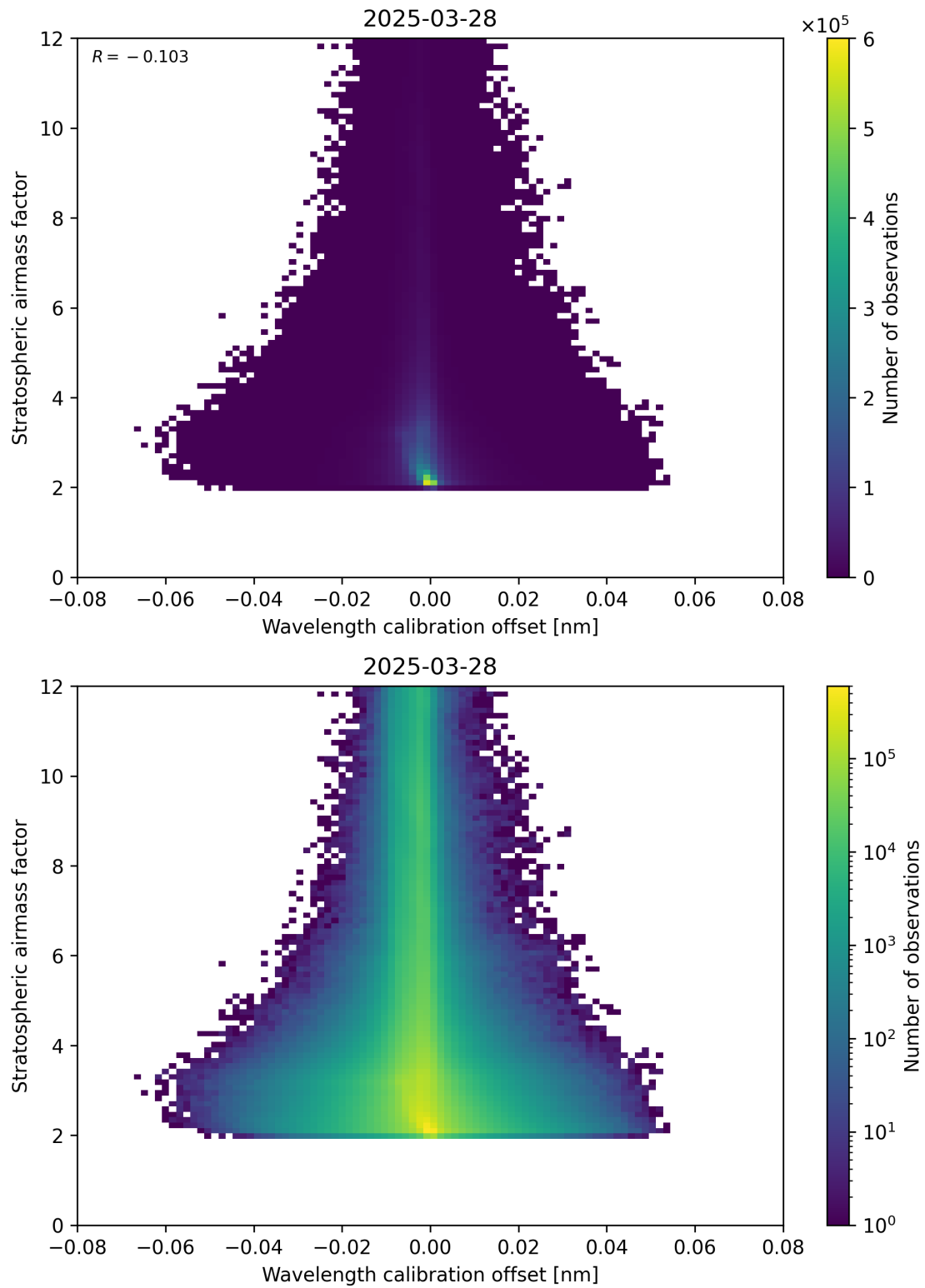
Figure 174: Scatter density plot of “Wavelength calibration offset” against “Stratospheric airmass factor” for 2025-03-28 to 2025-03-29.
