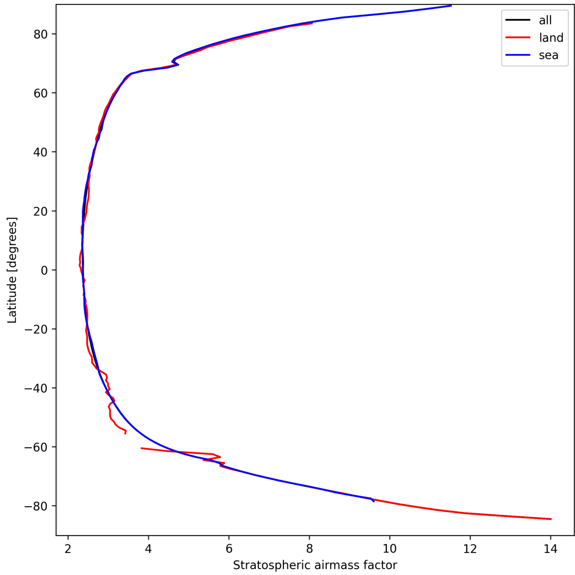
Figure 27: Zonal average of “Stratospheric airmass factor” for 2025-03-28 to 2025-03-29.
