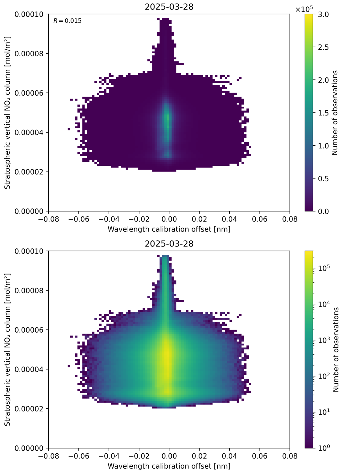
Figure 176: Scatter density plot of “Wavelength calibration offset” against “Stratospheric vertical NO 2 column” for 2025-03-28 to 2025-03-29.
