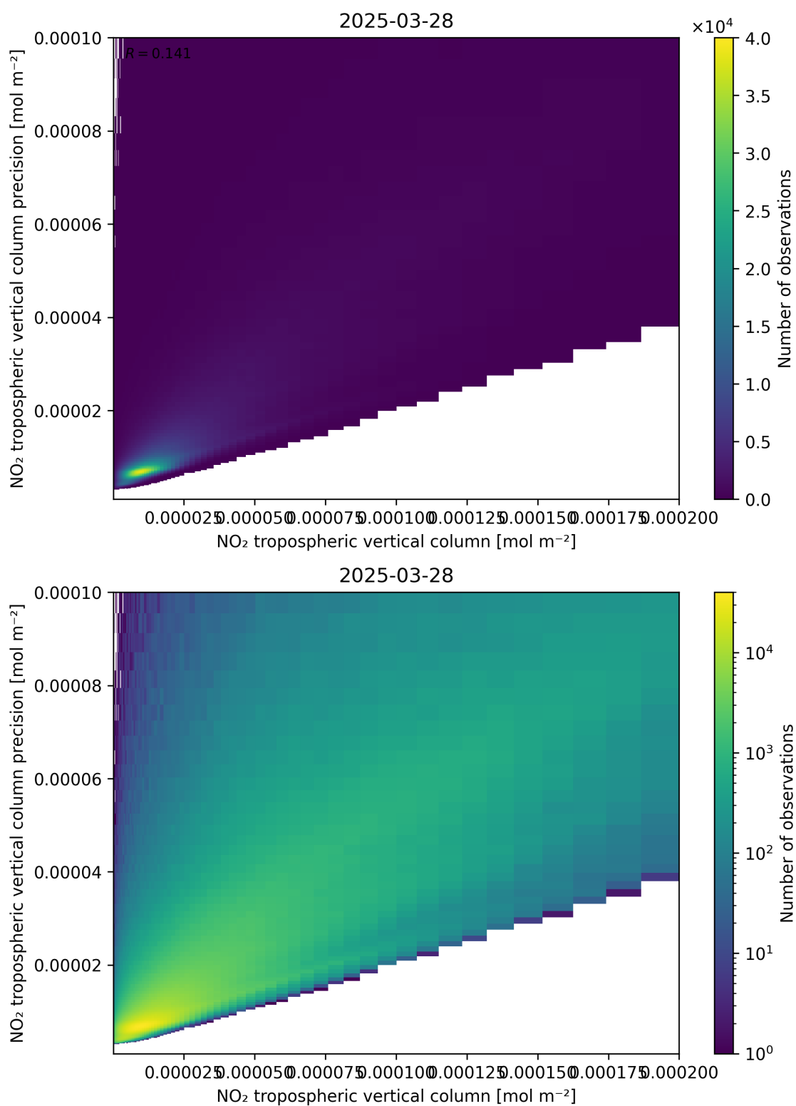
Figure 130: Scatter density plot of “NO 2 tropospheric vertical column” against “NO 2 tropospheric vertical column precision” for 2025-03-28 to 2025-03-29.
