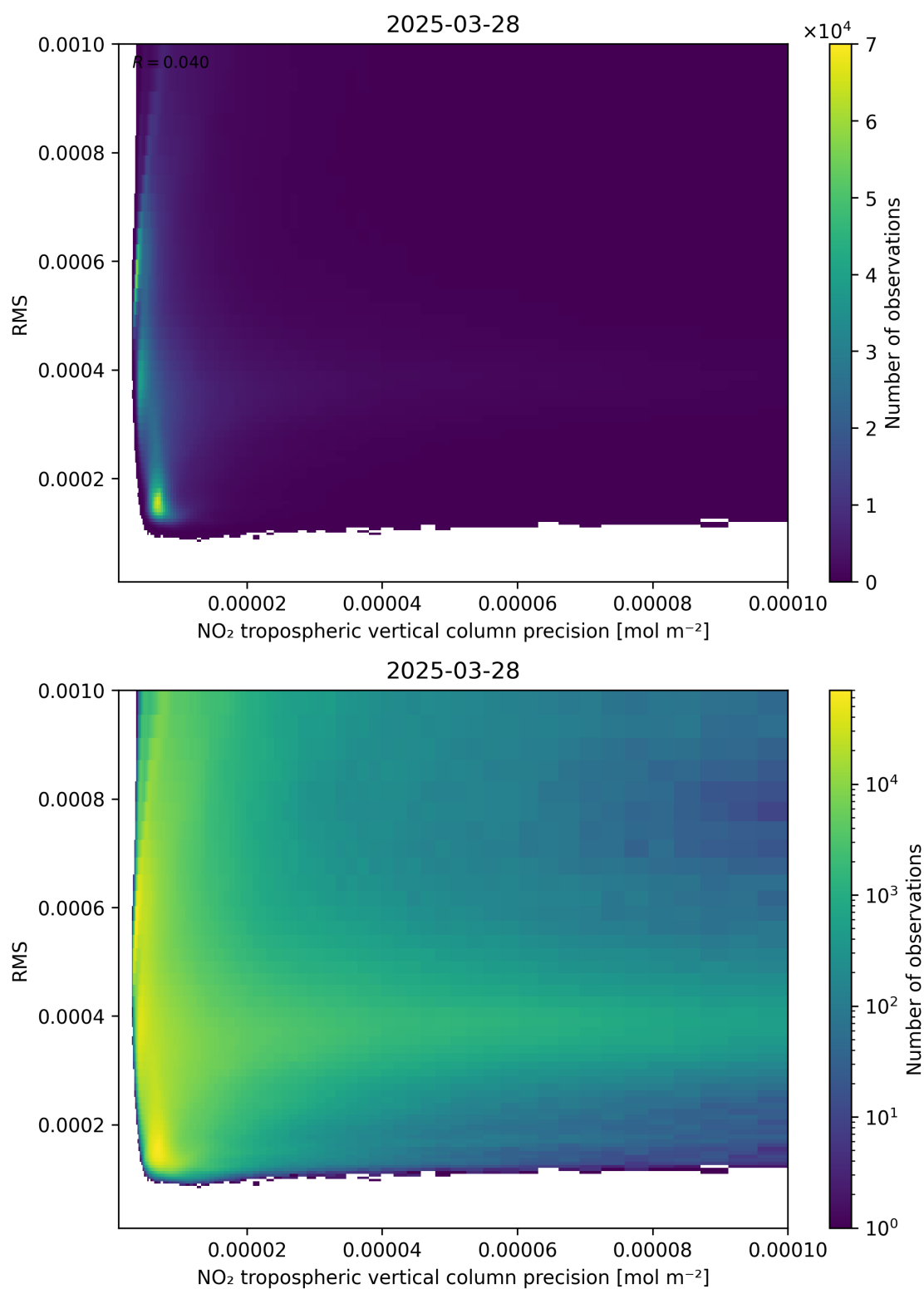
Figure 140: Scatter density plot of “NO 2 tropospheric vertical column precision” against “RMS” for 2025-03-28 to 2025-03-29.
