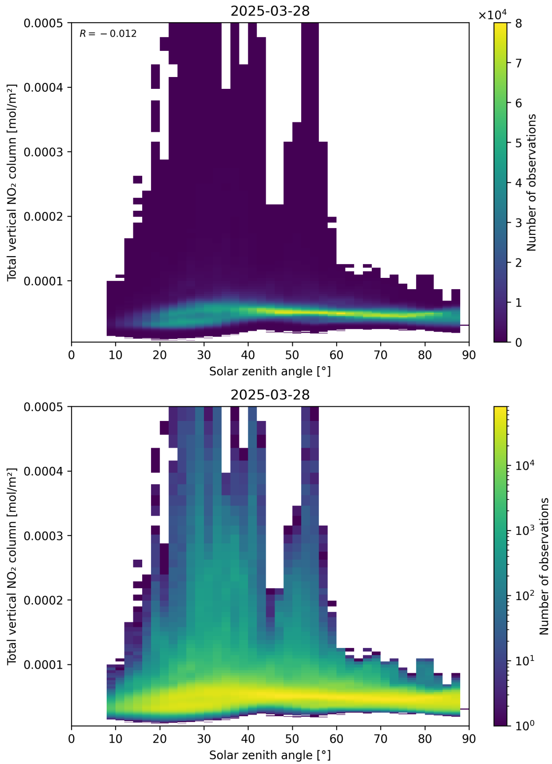
Figure 153: Scatter density plot of “Solar zenith angle” against “Total vertical NO 2 column” for 2025-03-28 to 2025-03-29.
