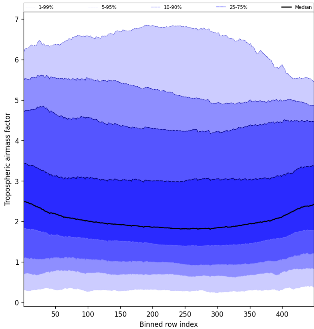
Figure 48: Along track statistics of “Tropospheric air mass factor” for 2025-03-28 to 2025-03-29
