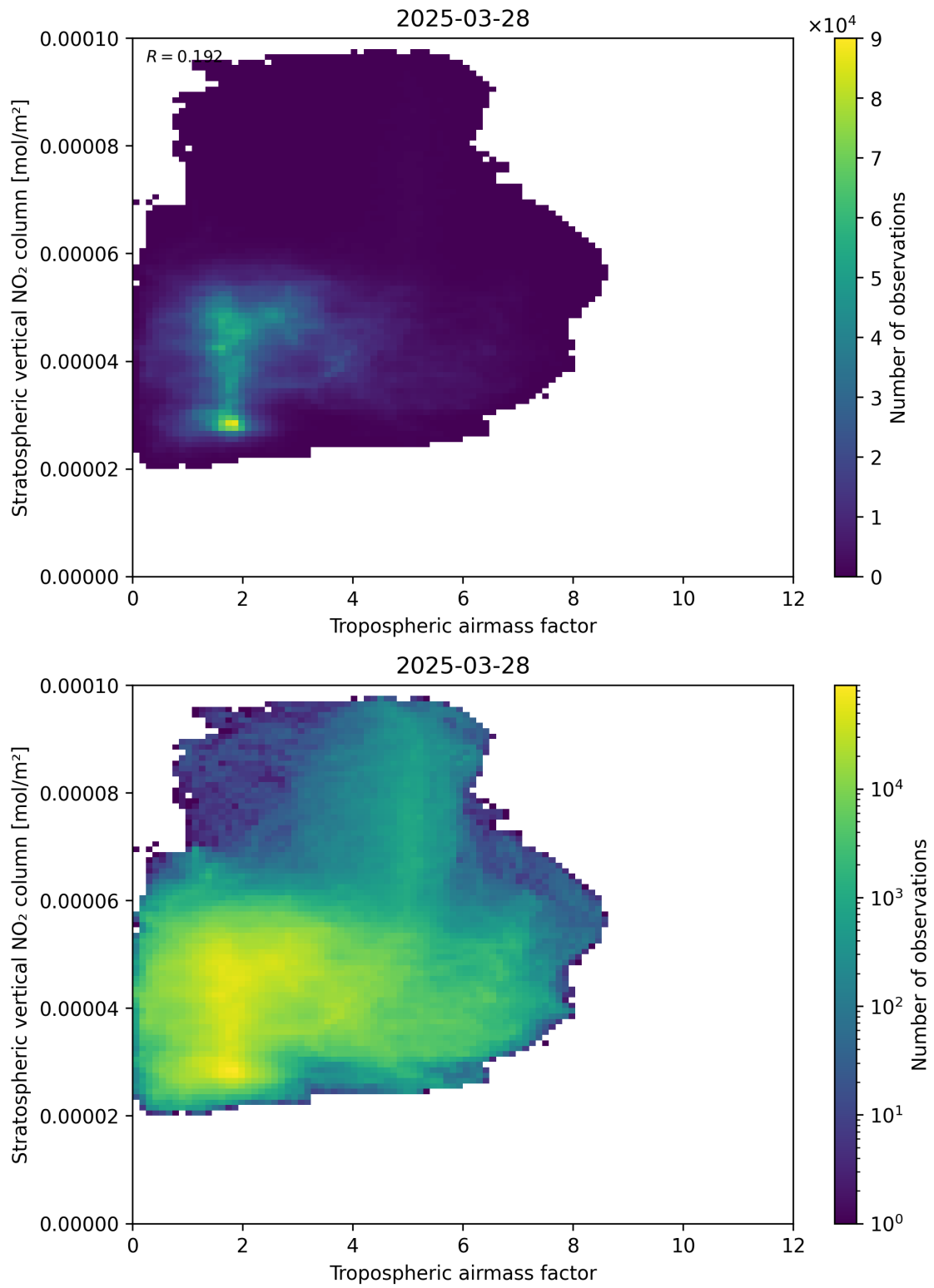
Figure 74: Scatter density plot of “Tropospheric air mass factor” against “Stratospheric vertical NO 2 column” for 2025-03-28 to 2025-03-29.
