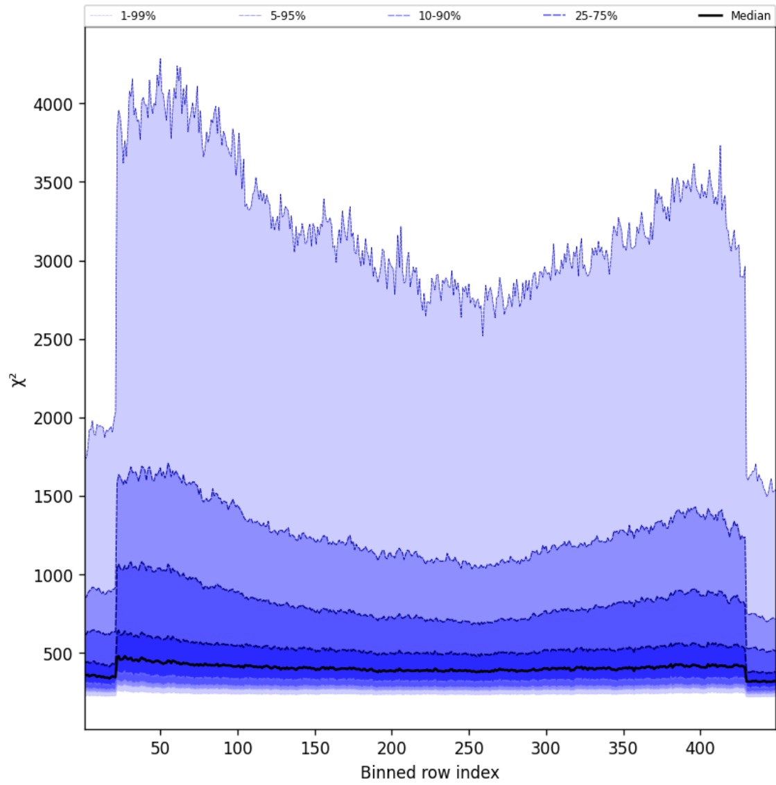
Figure 59: Along track statistics of “ \chi^2 ” for 2025-03-28 to 2025-03-29
