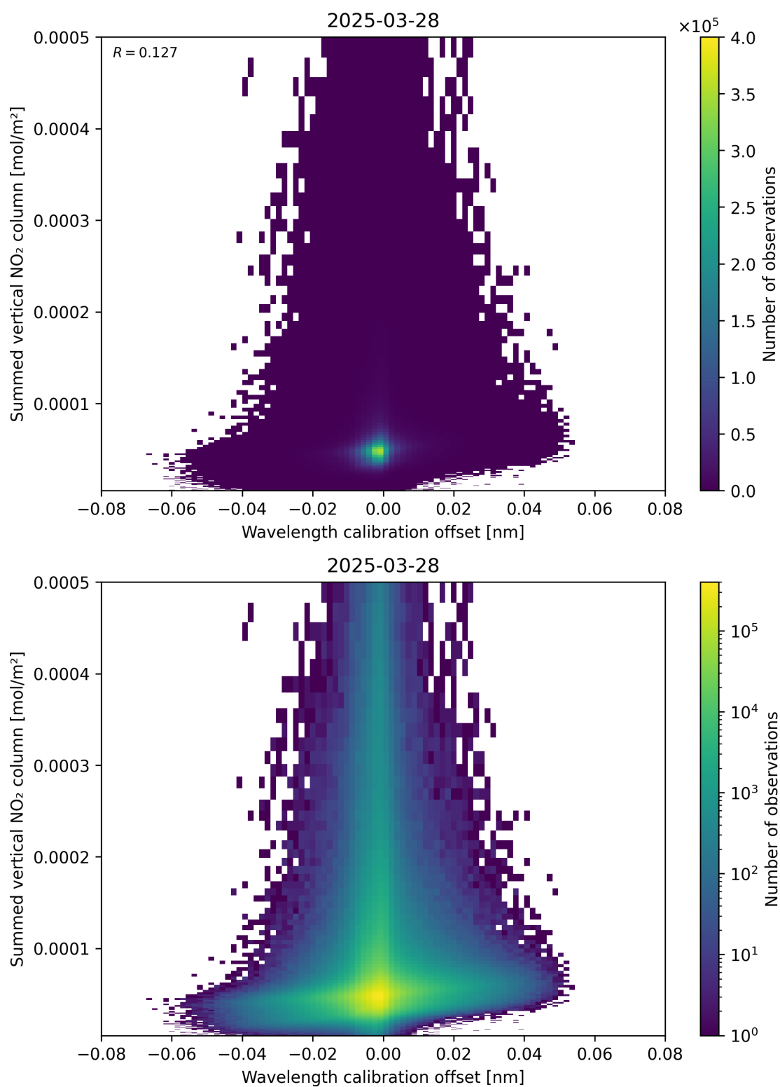
Figure 177: Scatter density plot of “Wavelength calibration offset” against “Summed vertical NO 2 column” for 2025-03-28 to 2025-03-29.
