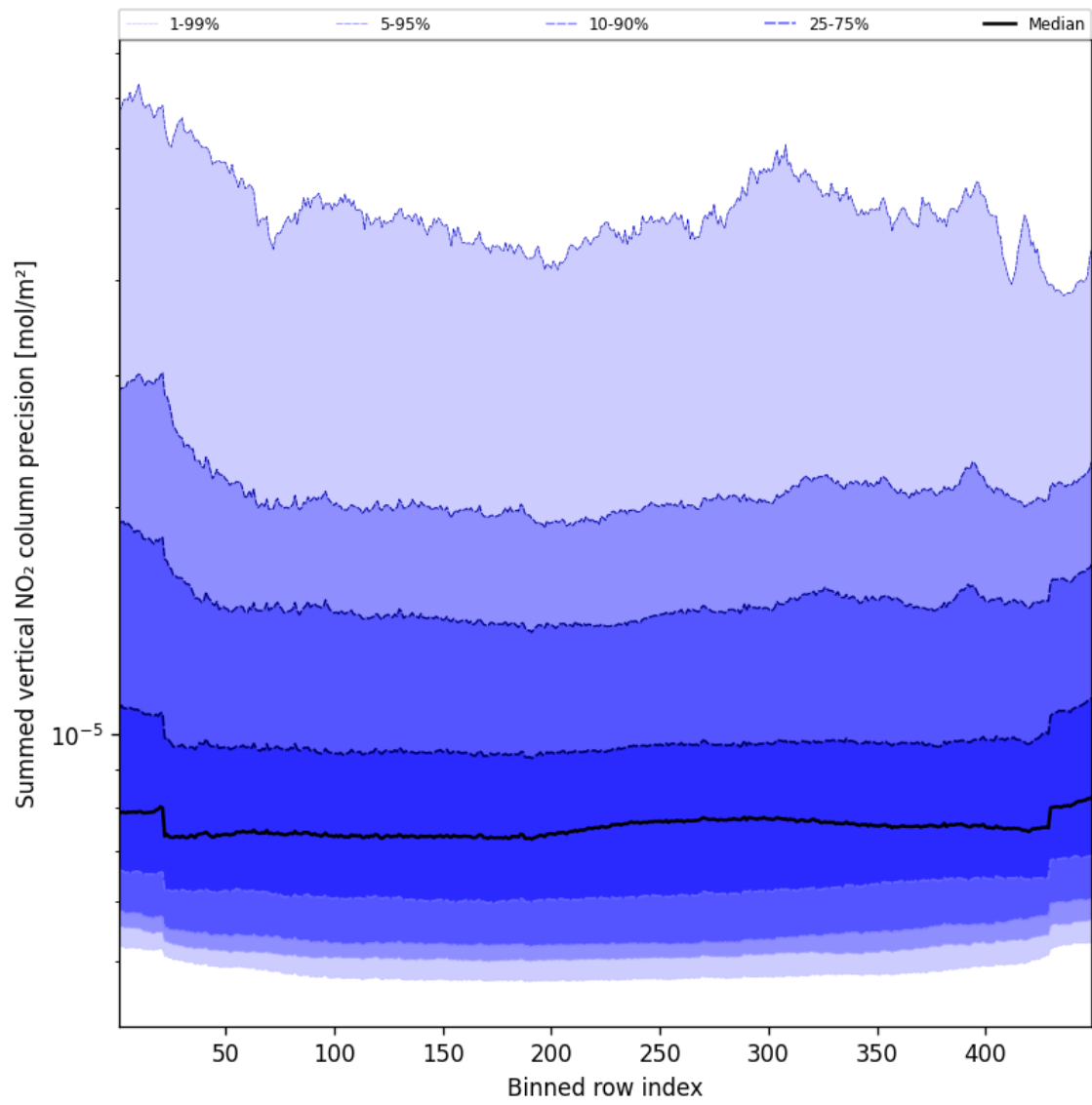
Figure 58: Along track statistics of “Summed vertical NO 2 column precision” for 2025-03-28 to 2025-03-29
