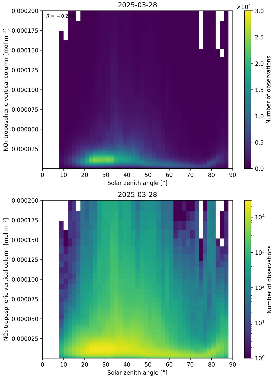
Figure 155: Scatter density plot of “Solar zenith angle” against “NO 2 tropospheric vertical column” for 2025-03-28 to 2025-03-29.
