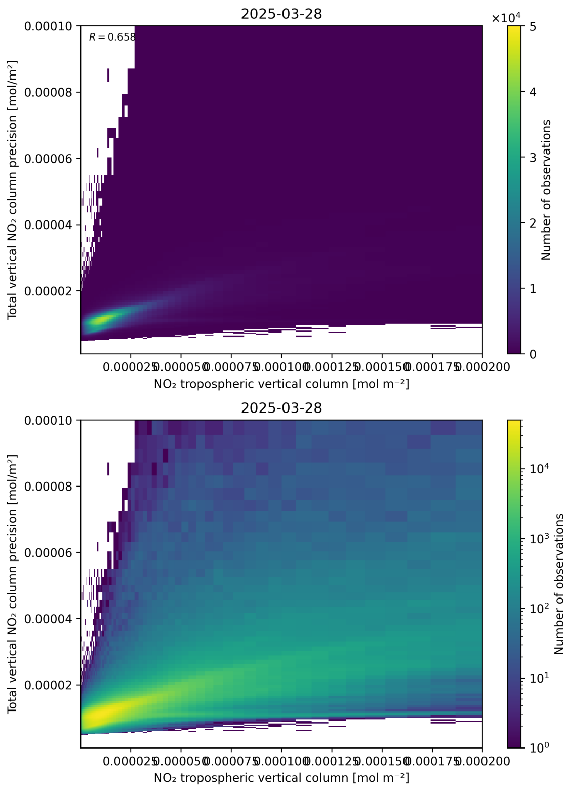
Figure 129: Scatter density plot of “NO 2 tropospheric vertical column” against “Total vertical NO 2 column precision” for 2025-03-28 to 2025-03-29.
