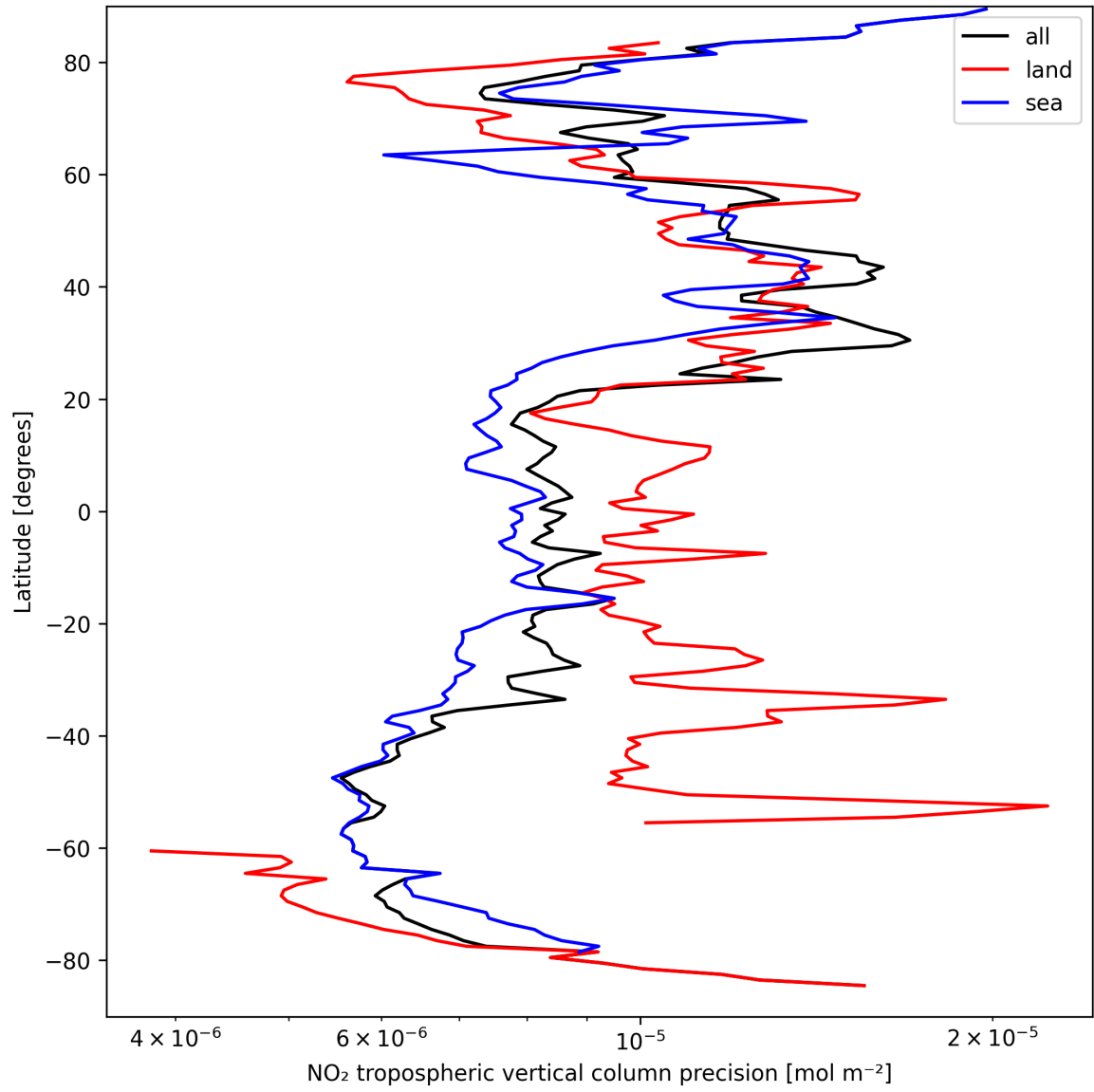
Figure 13: Zonal average of “NO 2 tropospheric vertical column precision” for 2025-03-28 to 2025-03-29.
