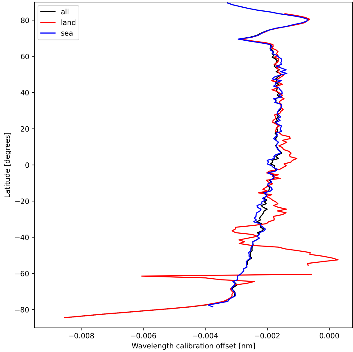
Figure 18: Zonal average of “Wavelength calibration offset” for 2025-03-28 to 2025-03-29.
