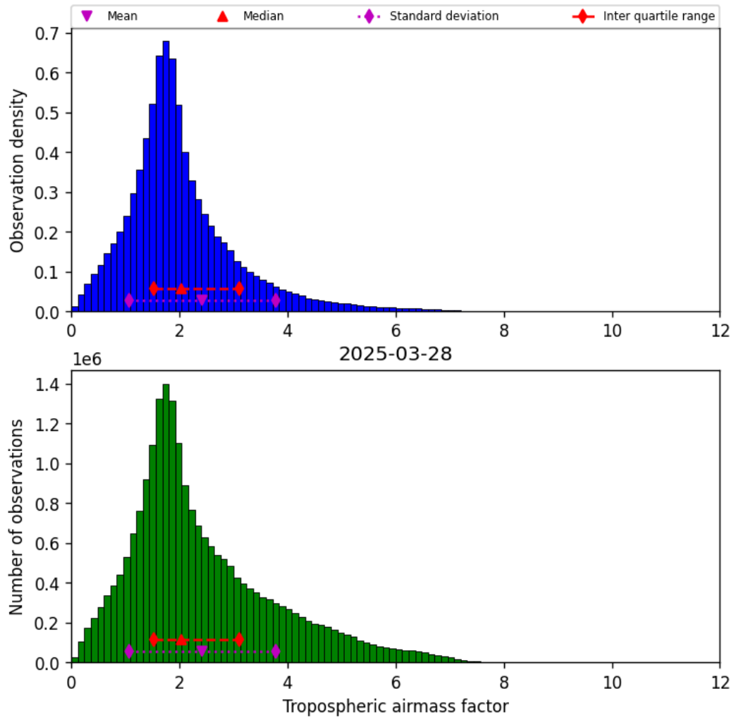
Figure 31: Histogram of “Tropospheric airmass factor” for 2025-03-28 to 2025-03-29
