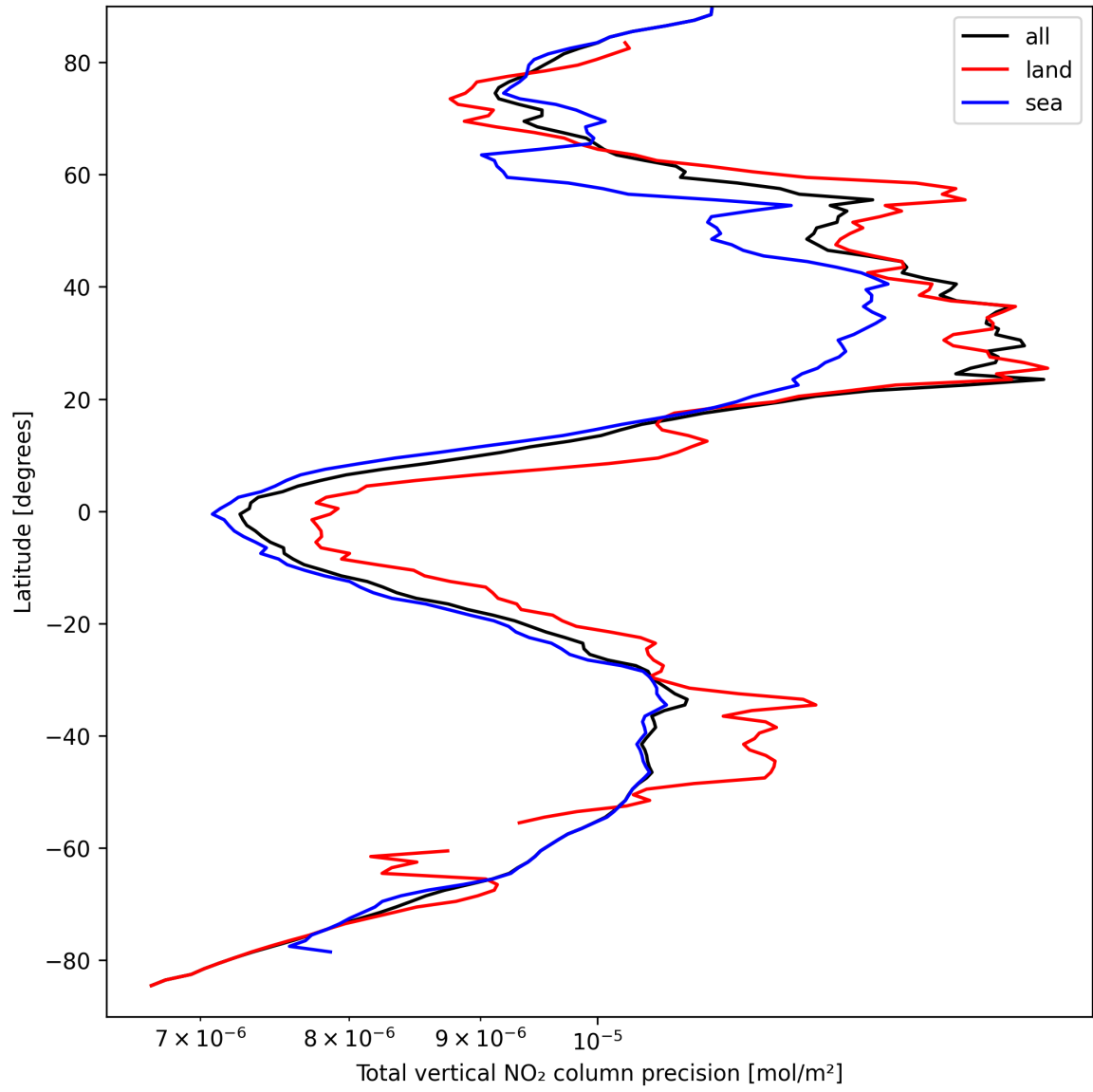
Figure 22: Zonal average of “Total vertical NO 2 column precision” for 2025-03-28 to 2025-03-29.
