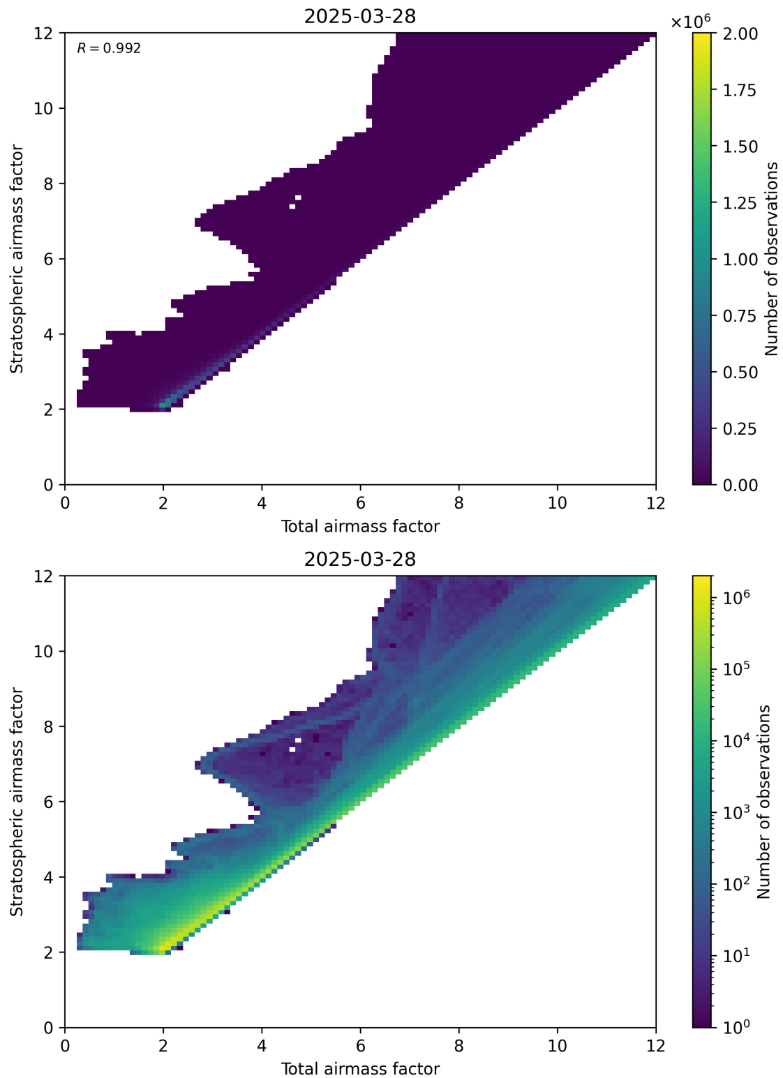
Figure 62: Scatter density plot of “Total airmass factor” against “Stratospheric airmass factor” for 2025-03-28 to 2025-03-29.
