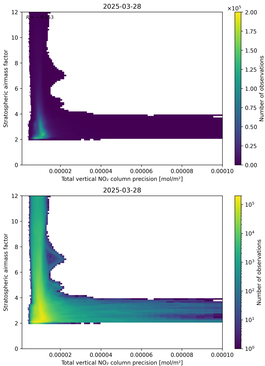
Figure 115: Scatter density plot of “Total vertical NO 2 column precision” against “Stratospheric air mass factor” for 2025-03-28 to 2025-03-29.
