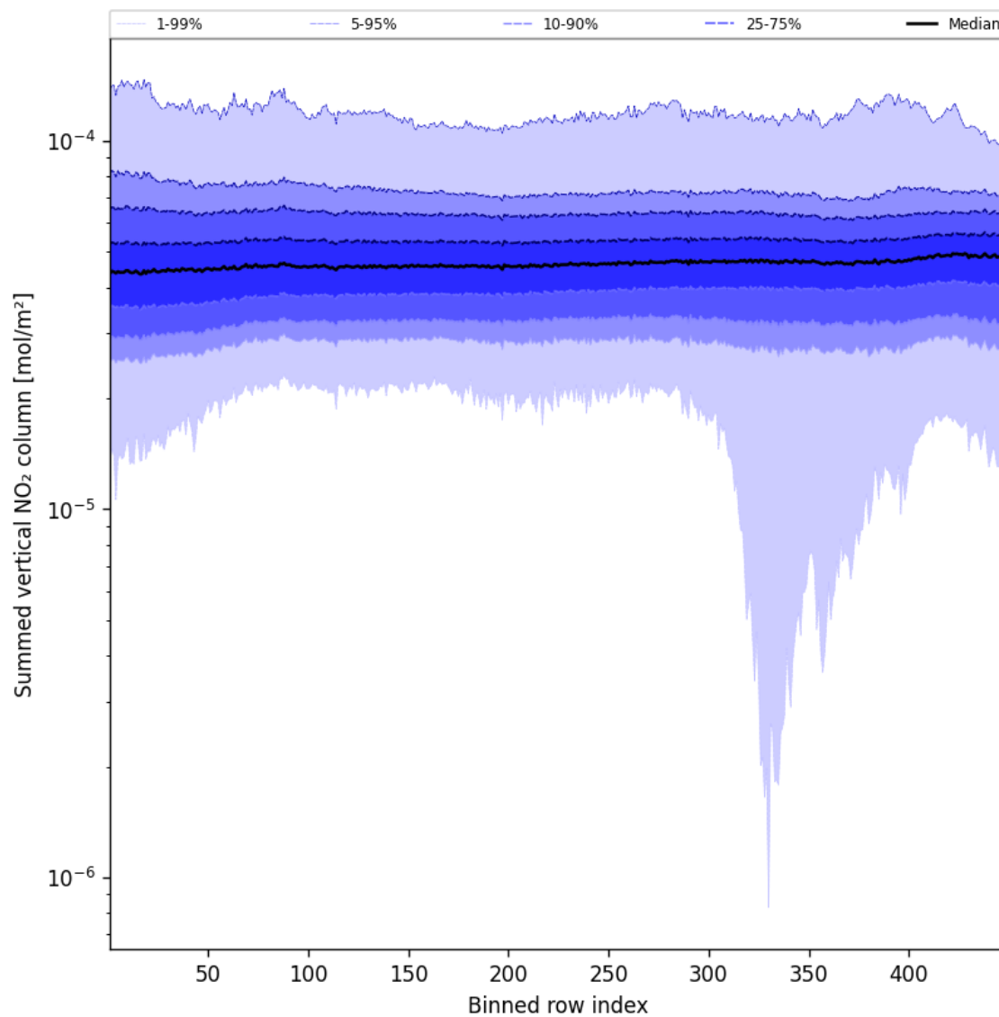
Figure 57: Along track statistics of “Summed vertical NO 2 column” for 2025-03-28 to 2025-03-29
