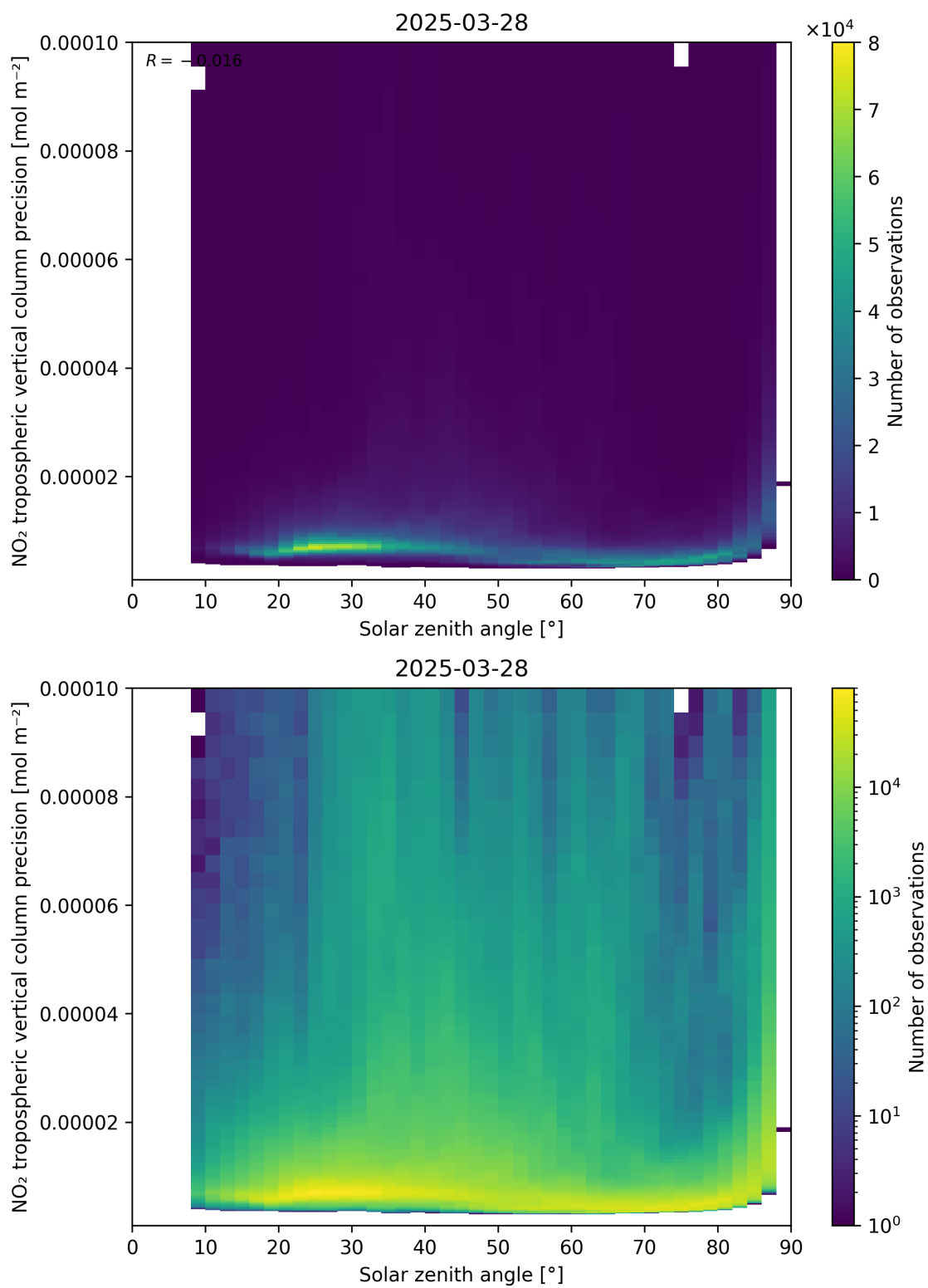
Figure 156: Scatter density plot of “Solar zenith angle” against “NO 2 tropospheric vertical column precision” for 2025-03-28 to 2025-03-29.
