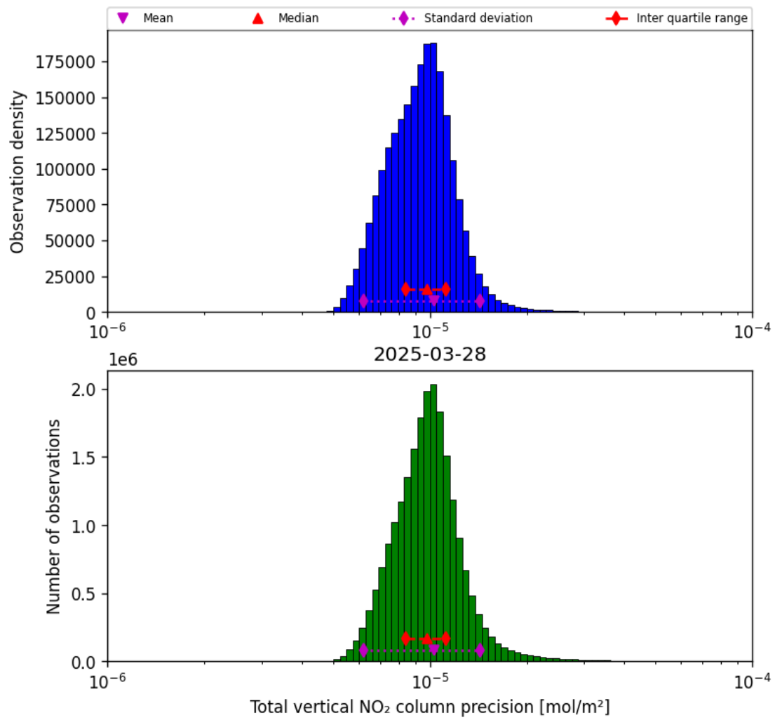
Figure 39: Histogram of “Total vertical NO 2 column precision” for 2025-03-28 to 2025-03-29
