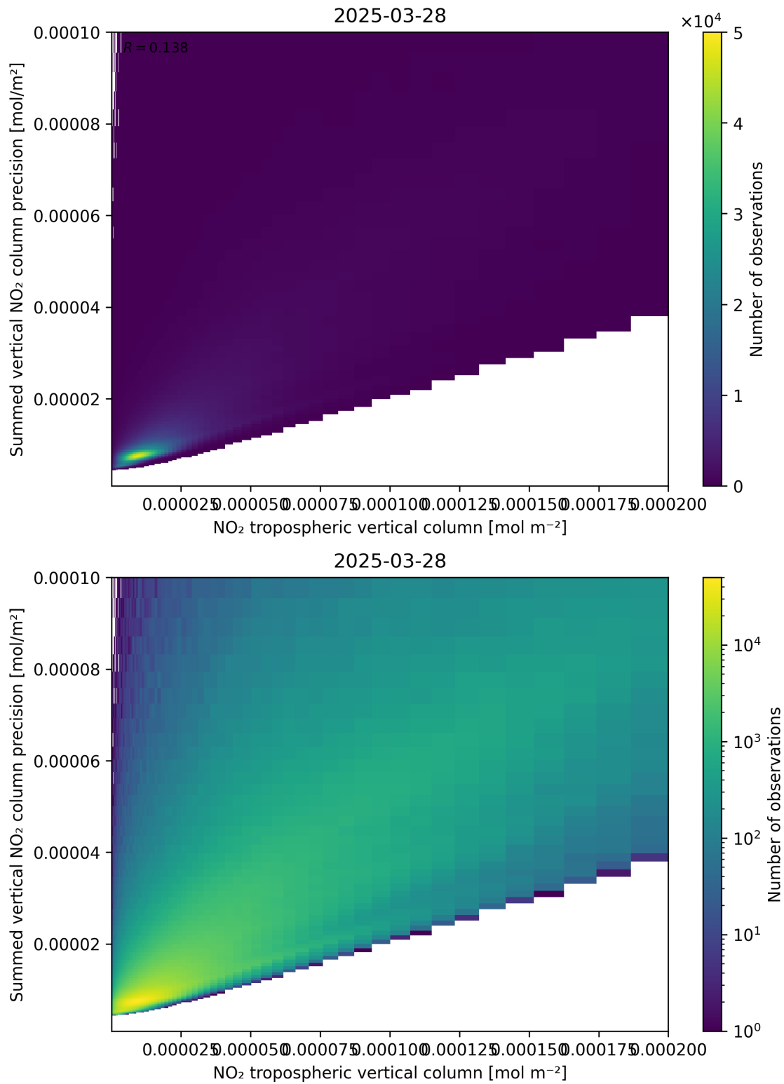
Figure 127: Scatter density plot of “NO 2 tropospheric vertical column” against “Summed vertical NO 2 column precision” for 2025-03-28 to 2025-03-29.
