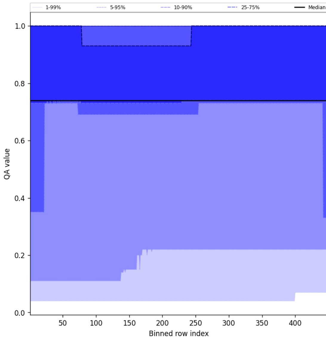
Figure 45: Along track statistics of “QA value” for 2025-03-28 to 2025-03-29
