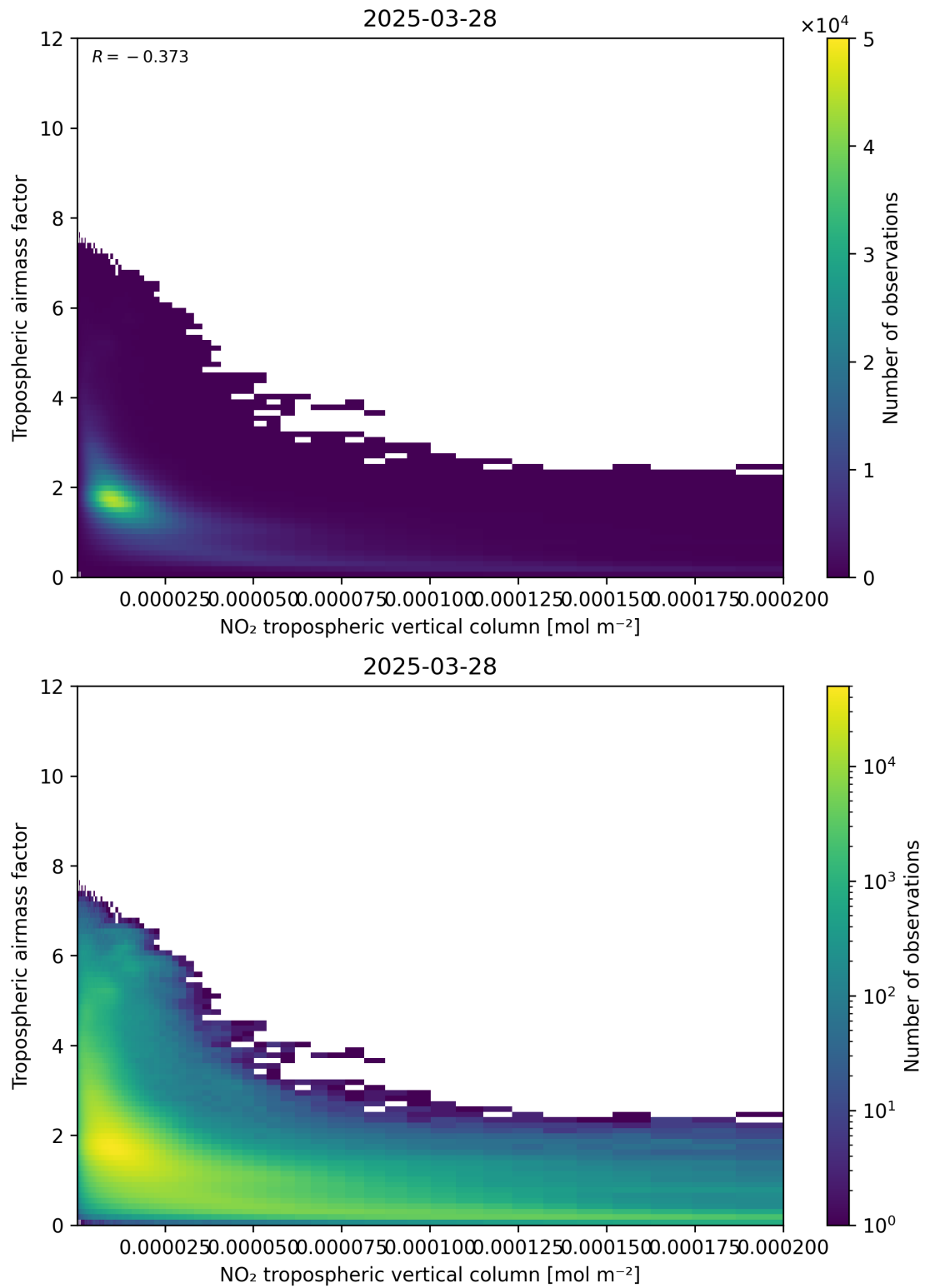
Figure 123: Scatter density plot of “NO 2 tropospheric vertical column” against “Tropospheric air mass factor” for 2025-03-28 to 2025-03-29.
