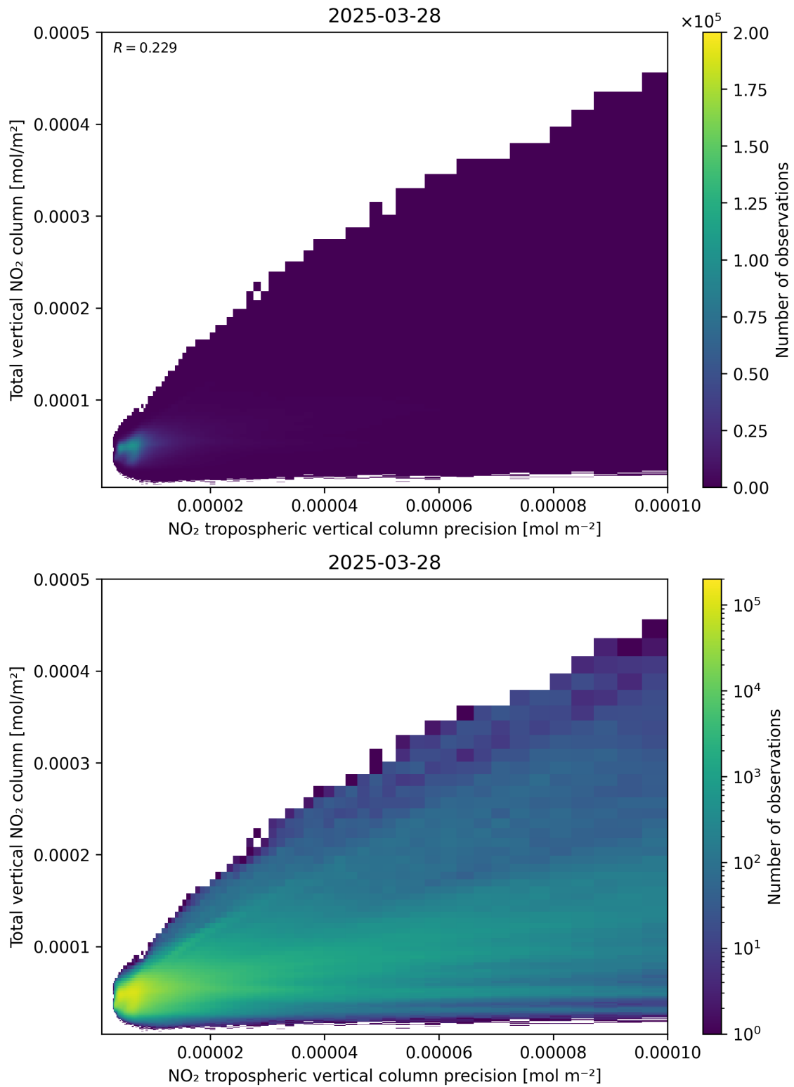
Figure 138: Scatter density plot of “NO 2 tropospheric vertical column precision” against “Total vertical NO 2 column” for 2025-03-28 to 2025-03-29.
