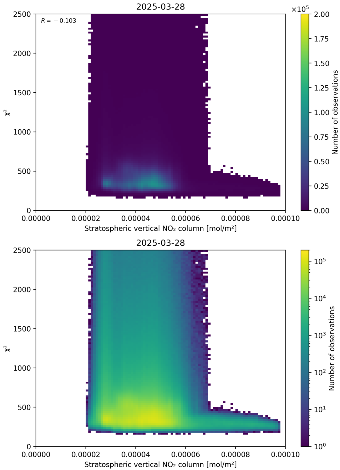
Figure 97: Scatter density plot of “Stratospheric vertical NO 2 column” against “ \chi^2 ” for 2025-03-28 to 2025-03-29.
