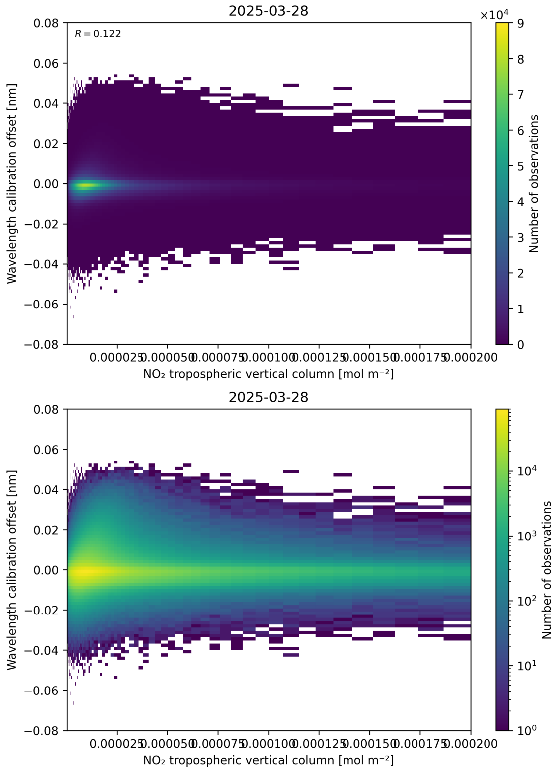
Figure 143: Scatter density plot of “NO 2 tropospheric vertical column” against “Wavelength calibration offset” for 2025-03-28 to 2025-03-29.
