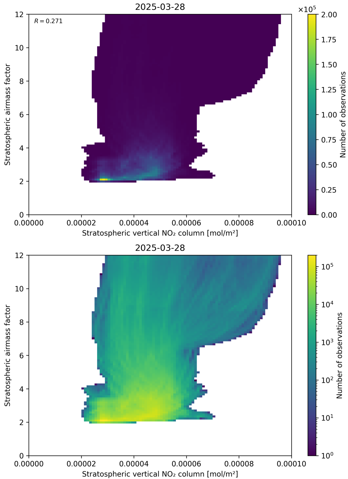
Figure 96: Scatter density plot of “Stratospheric vertical NO 2 column” against “Stratospheric airmass factor” for 2025-03-28 to 2025-03-29.
