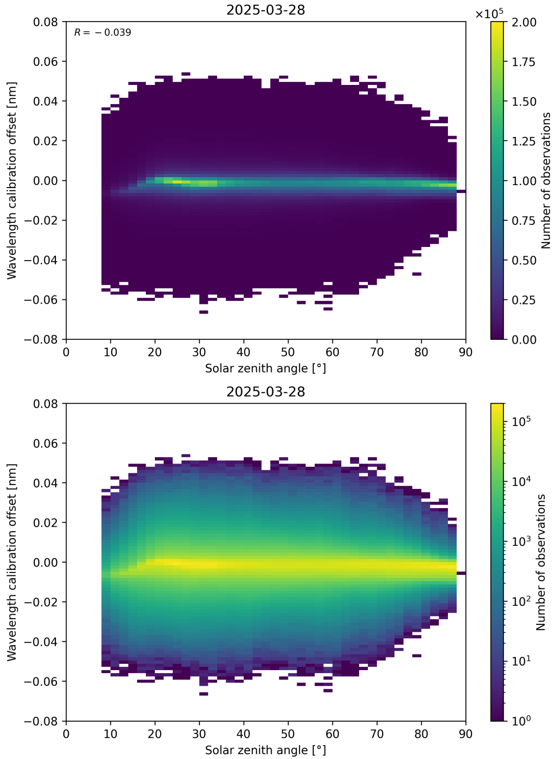
Figure 158: Scatter density plot of “Solar zenith angle” against “Wavelength calibration offset” for 2025-03-28 to 2025-03-29.
