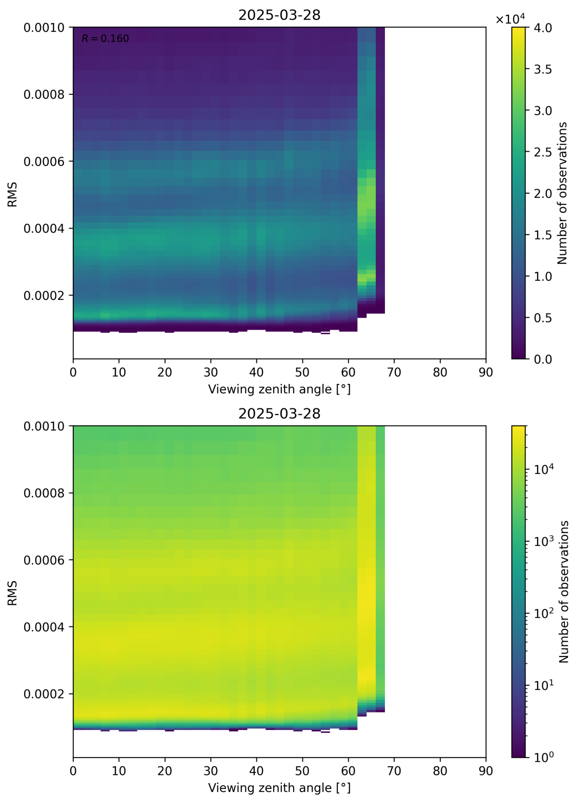
Figure 171: Scatter density plot of “Viewing zenith angle” against “RMS” for 2025-03-28 to 2025-03-29.
