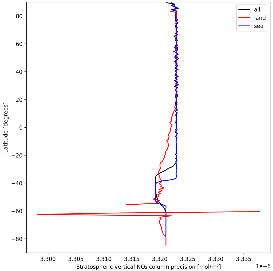
Figure 20: Zonal average of “Stratospheric vertical NO 2 column precision” for 2025-03-28 to 2025-03-29.
