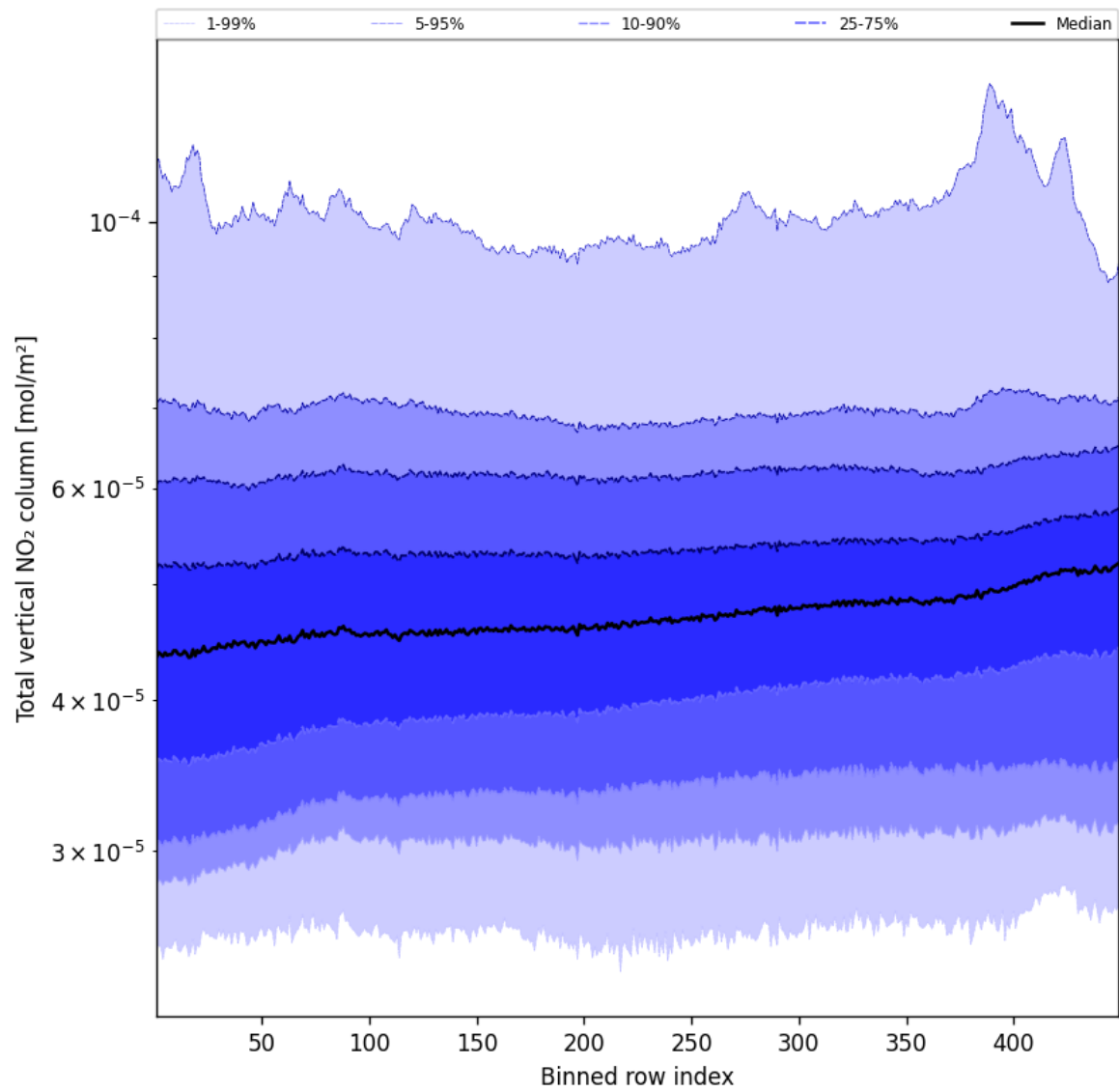
Figure 55: Along track statistics of “Total vertical NO 2 column” for 2025-03-28 to 2025-03-29
