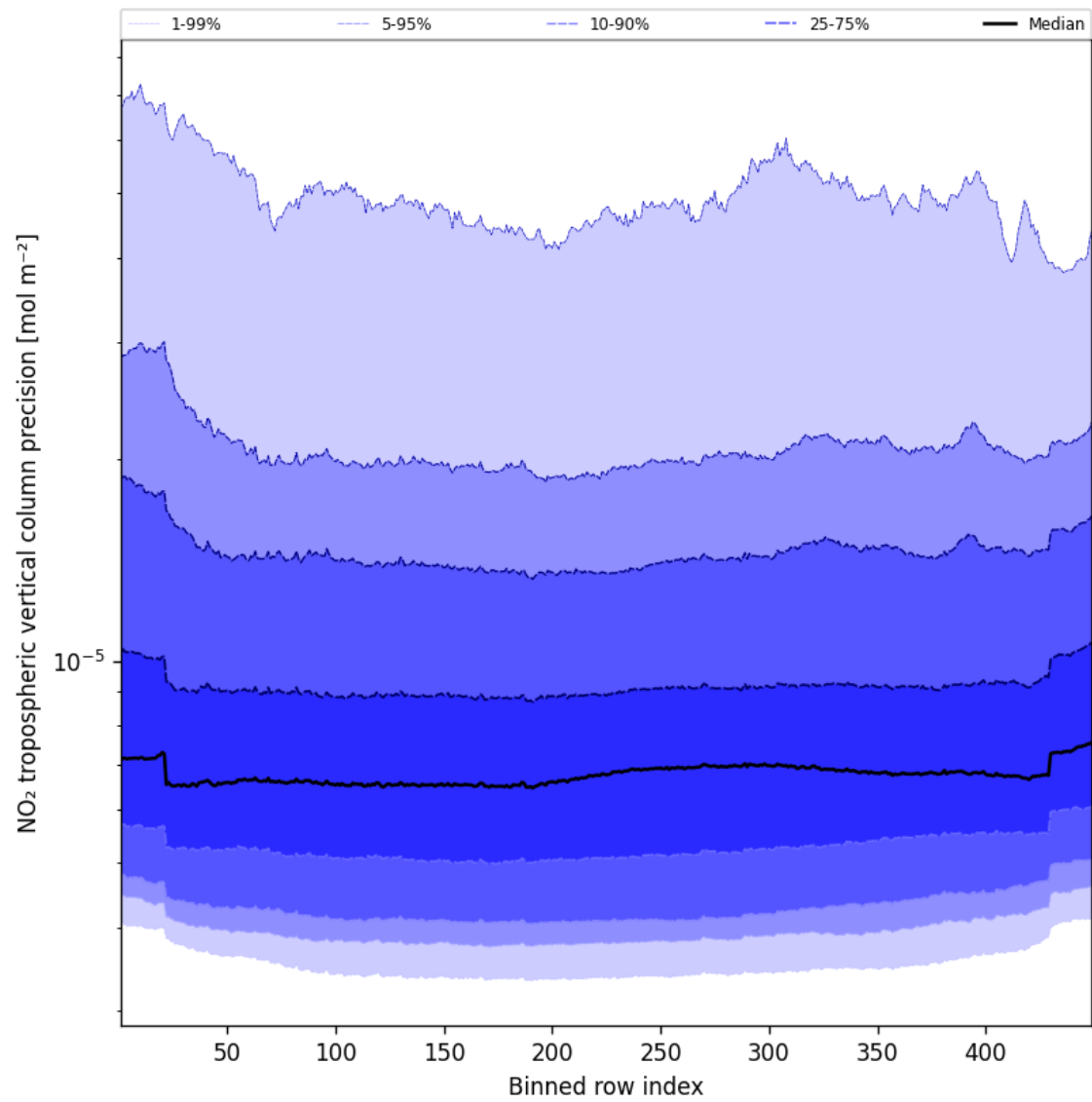
Figure 47: Along track statistics of “NO 2 tropospheric vertical column precision” for 2025-03-28 to 2025-03-29
