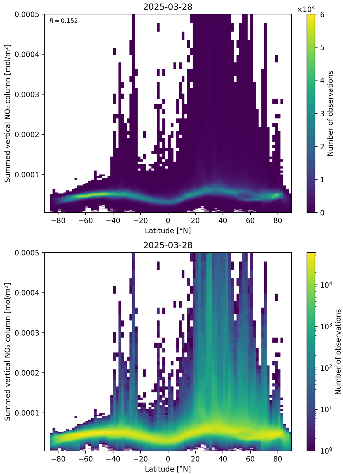
Figure 88: Scatter density plot of “Latitude” against “Summed vertical NO 2 column” for 2025-03-28 to 2025-03-29.
