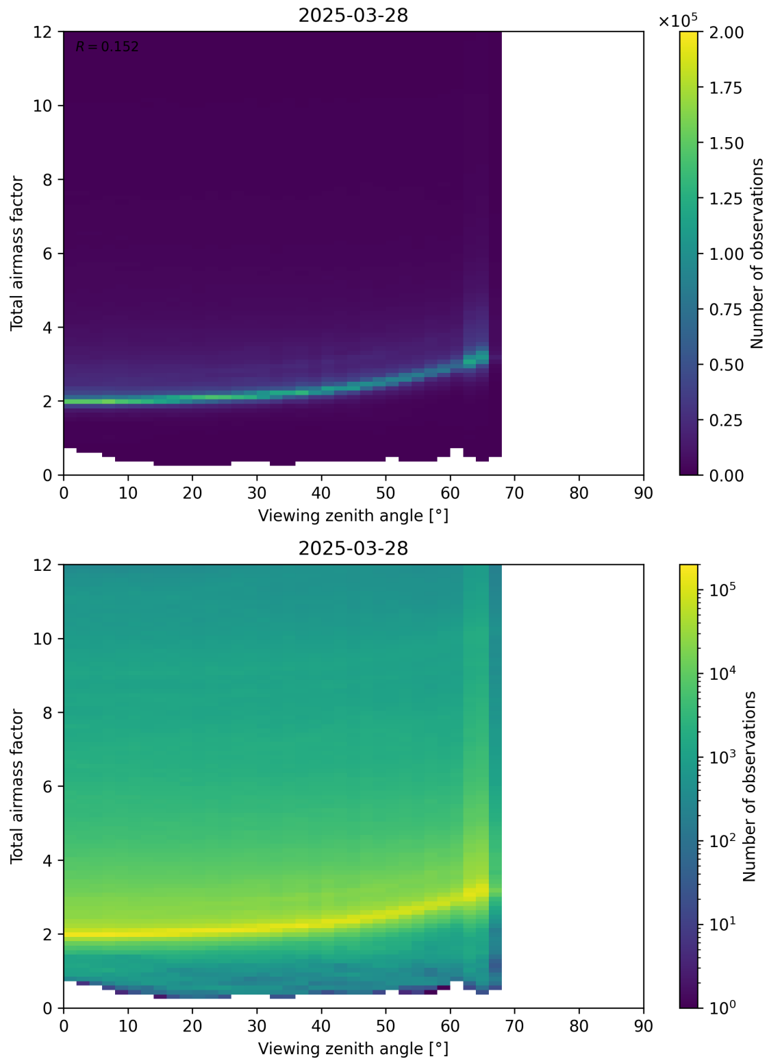
Figure 160: Scatter density plot of “Viewing zenith angle” against “Total airmass factor” for 2025-03-28 to 2025-03-29.
