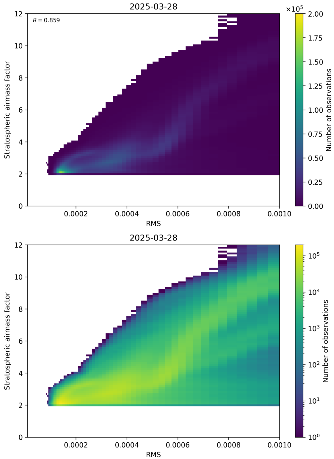
Figure 144: Scatter density plot of “RMS” against “Stratospheric airmass factor” for 2025-03-28 to 2025-03-29.
