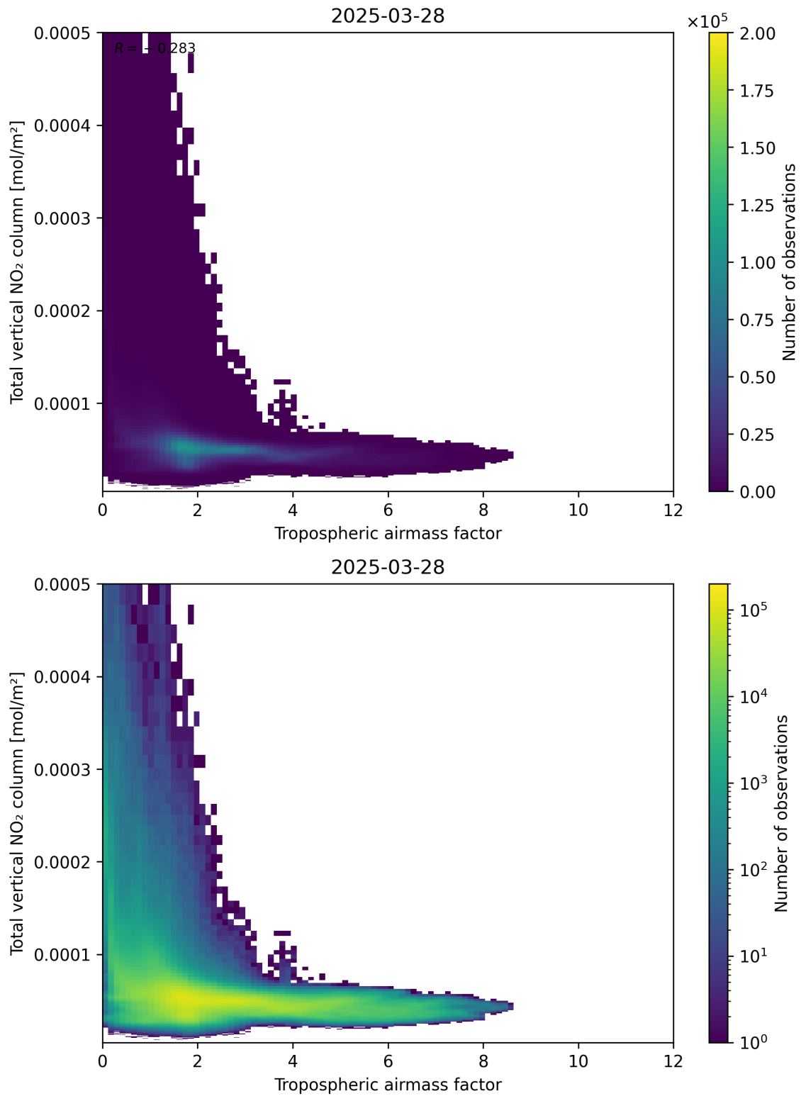
Figure 77: Scatter density plot of “Tropospheric airmass factor” against “Total vertical NO 2 column” for 2025-03-28 to 2025-03-29.
