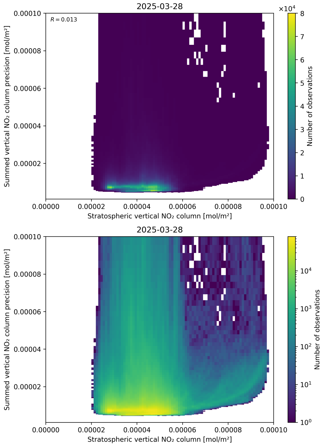
Figure 99: Scatter density plot of “Stratospheric vertical NO 2 column” against “Summed vertical NO 2 column precision” for 2025-03-28 to 2025-03-29.
