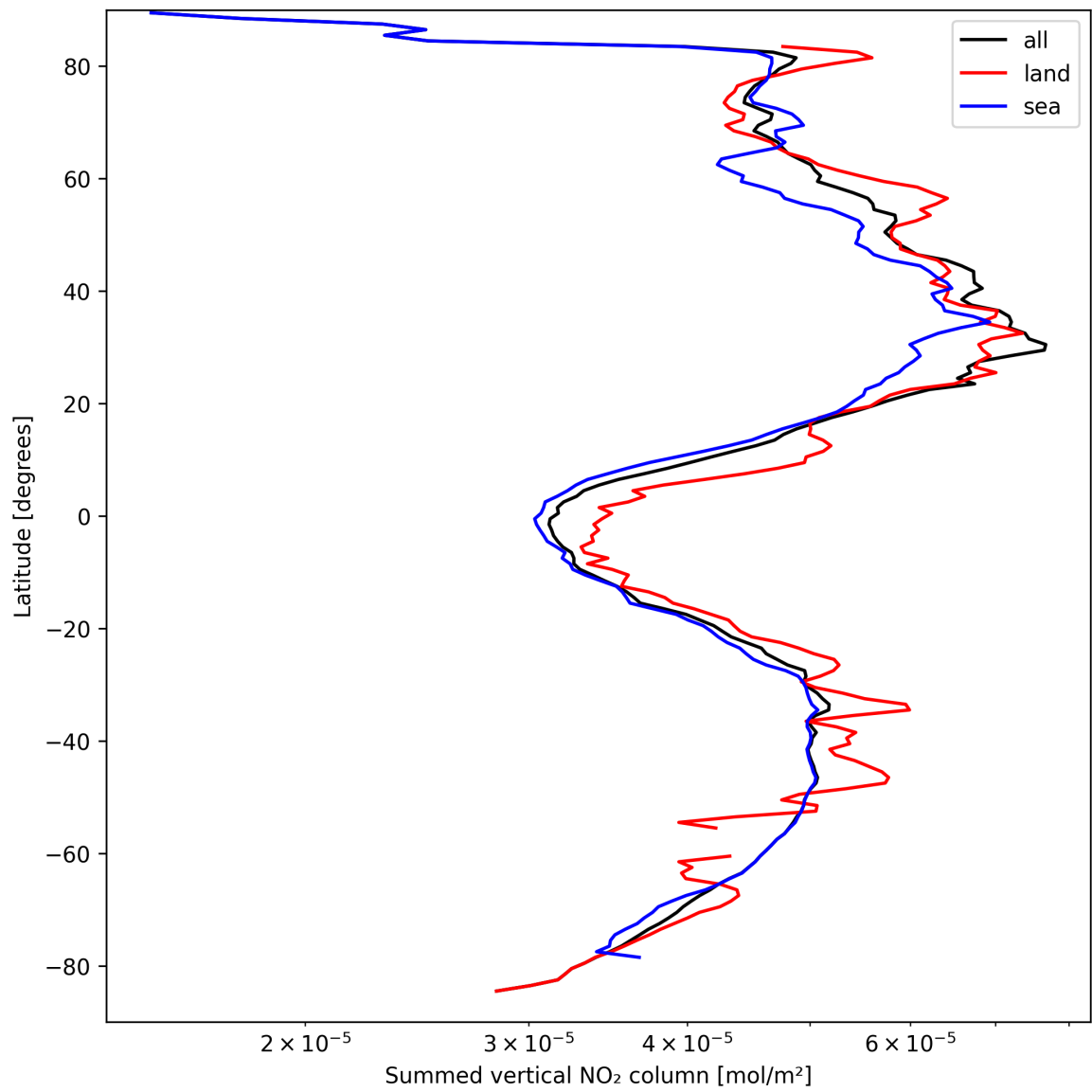
Figure 23: Zonal average of “Summed vertical NO 2 column” for 2025-03-28 to 2025-03-29.
