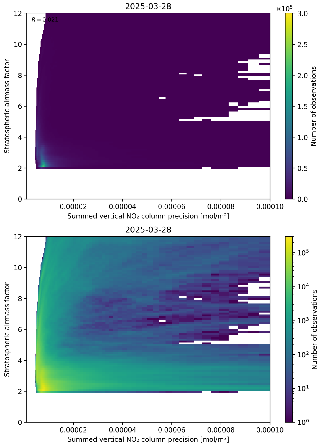
Figure 106: Scatter density plot of “Summed vertical NO 2 column precision” against “Stratospheric airmass factor” for 2025-03-28 to 2025-03-29.
