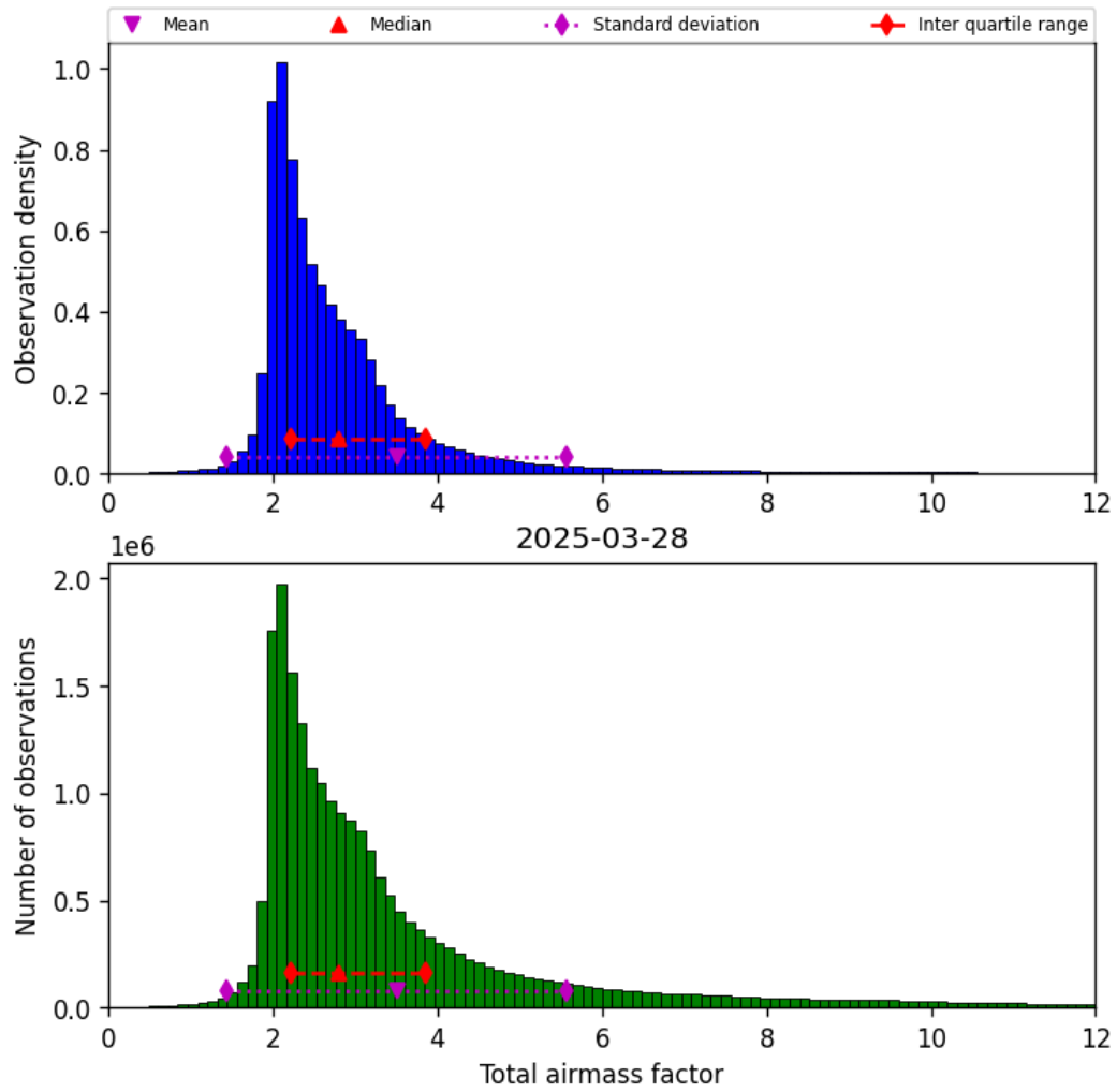
Figure 32: Histogram of “Total airmass factor” for 2025-03-28 to 2025-03-29
