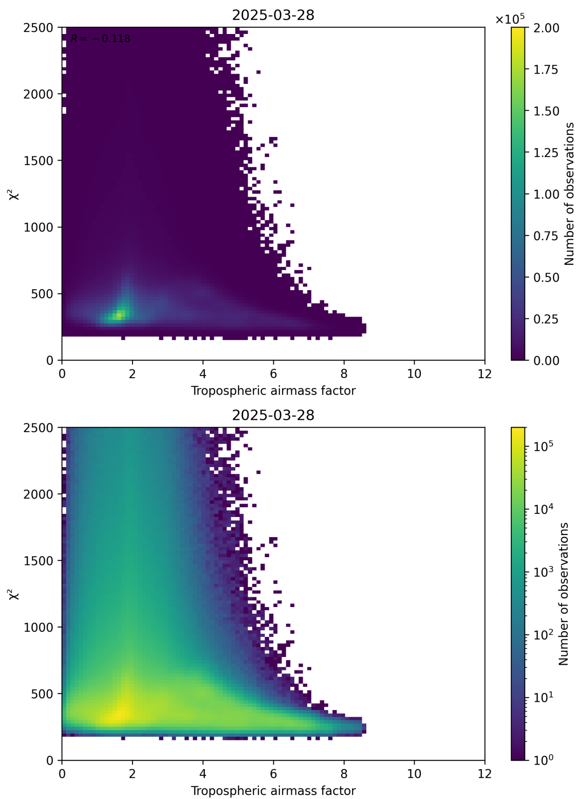
Figure 73: Scatter density plot of “Tropospheric airmass factor” against “ \chi^2 ” for 2025-03-28 to 2025-03-29.
