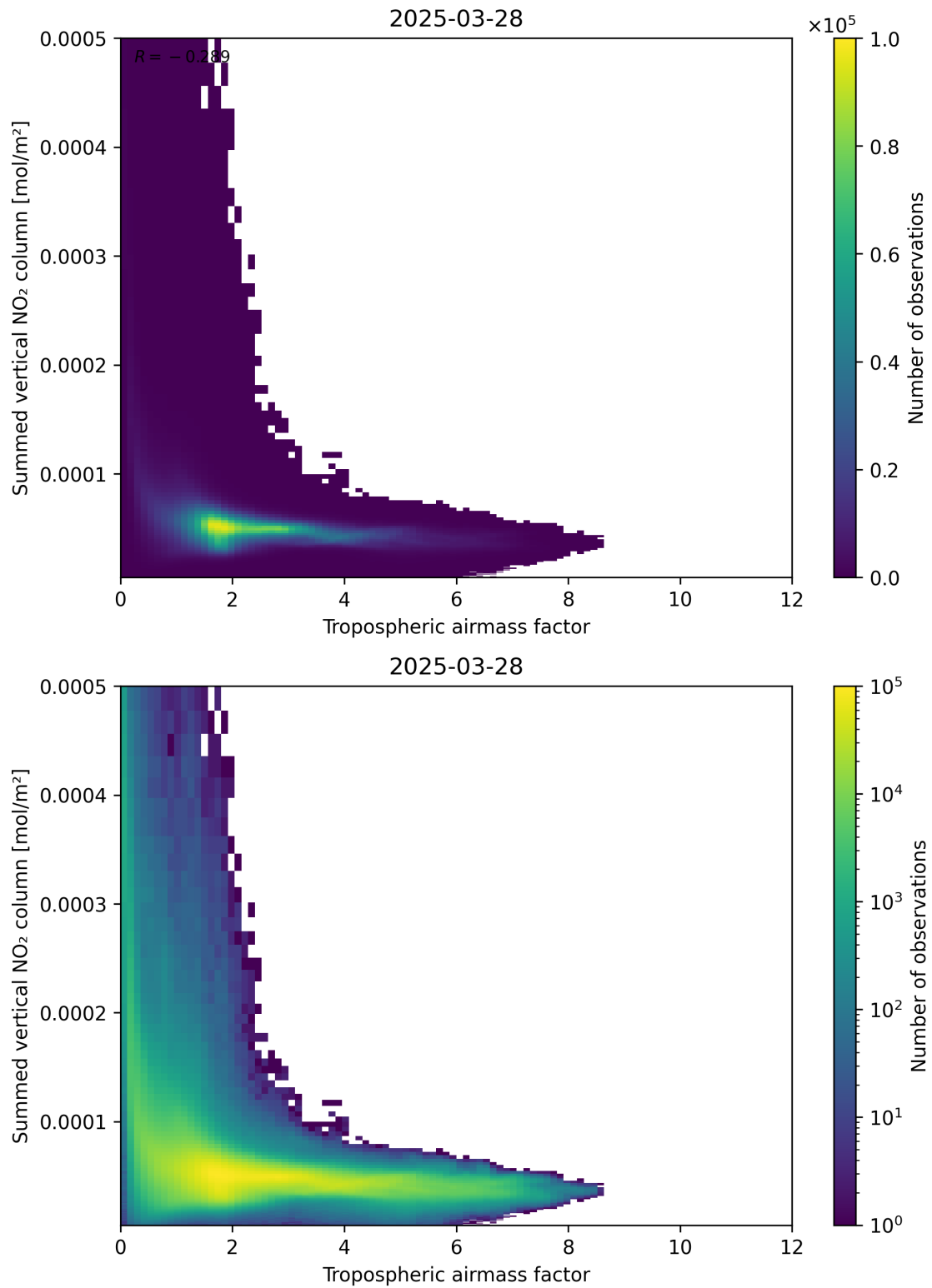
Figure 75: Scatter density plot of “Tropospheric air mass factor” against “Summed vertical NO 2 column” for 2025-03-28 to 2025-03-29.
