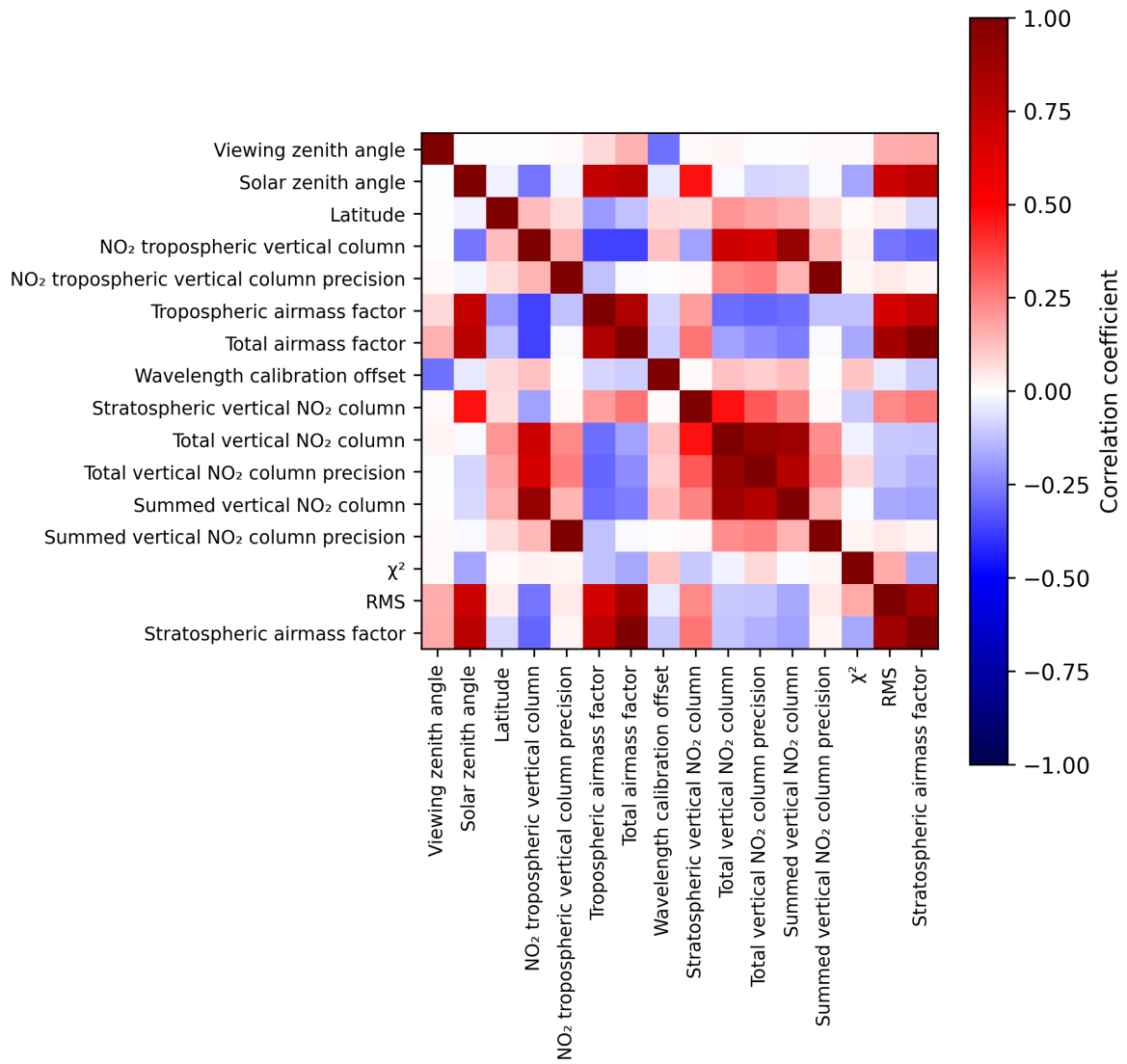
Figure 2: Map of correlation matrix for 2025-03-28 to 2025-03-29.
