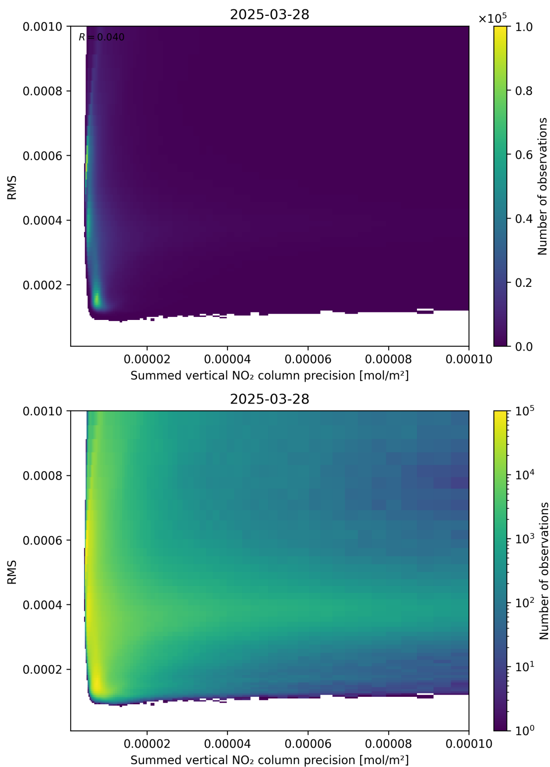
Figure 108: Scatter density plot of “Summed vertical NO 2 column precision” against “RMS” for 2025-03-28 to 2025-03-29.
