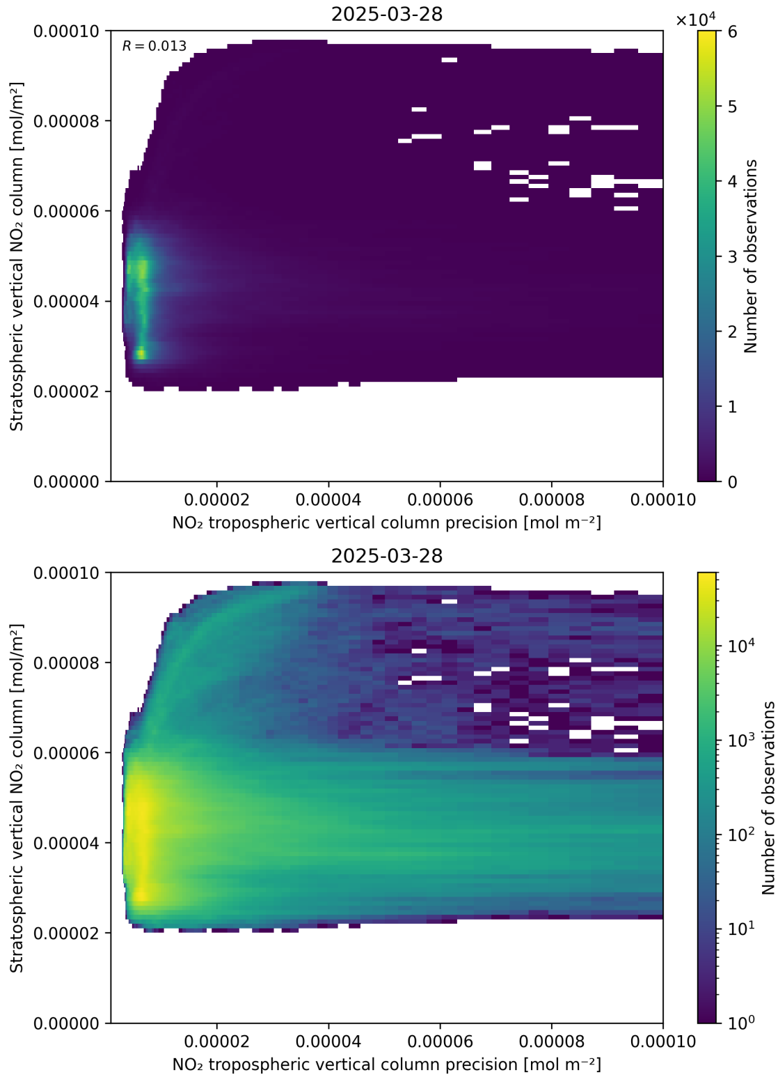
Figure 135: Scatter density plot of “NO 2 tropospheric vertical column precision” against “Stratospheric vertical NO 2 column” for 2025-03-28 to 2025-03-29.
