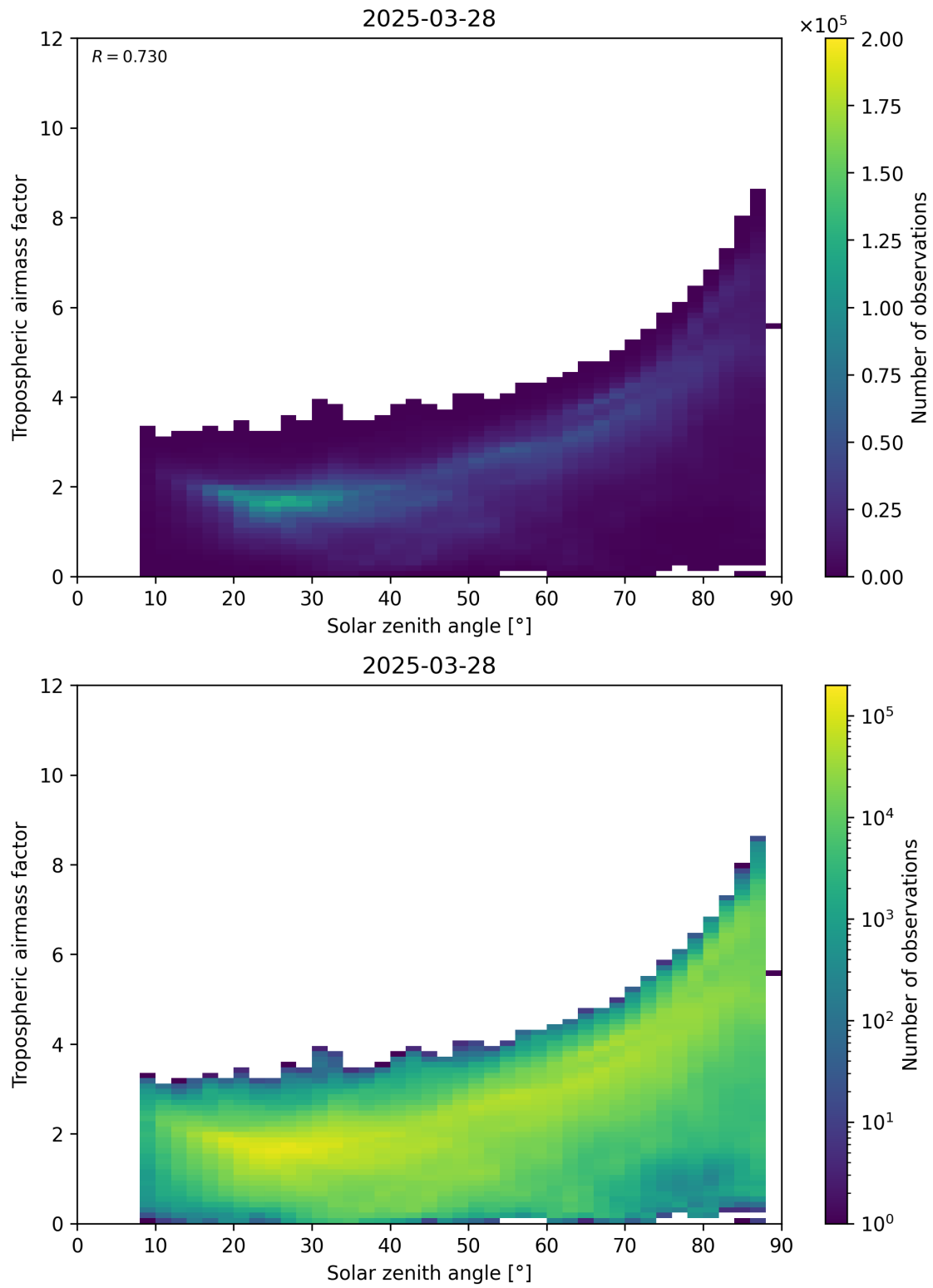
Figure 147: Scatter density plot of “Solar zenith angle” against “Tropospheric airmass factor” for 2025-03-28 to 2025-03-29.
