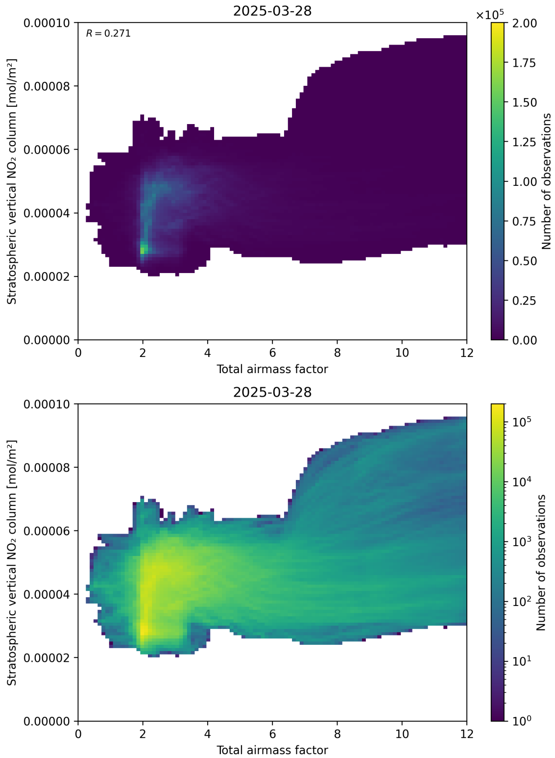
Figure 64: Scatter density plot of “Total airmass factor” against “Stratospheric vertical NO 2 column” for 2025-03-28 to 2025-03-29.
