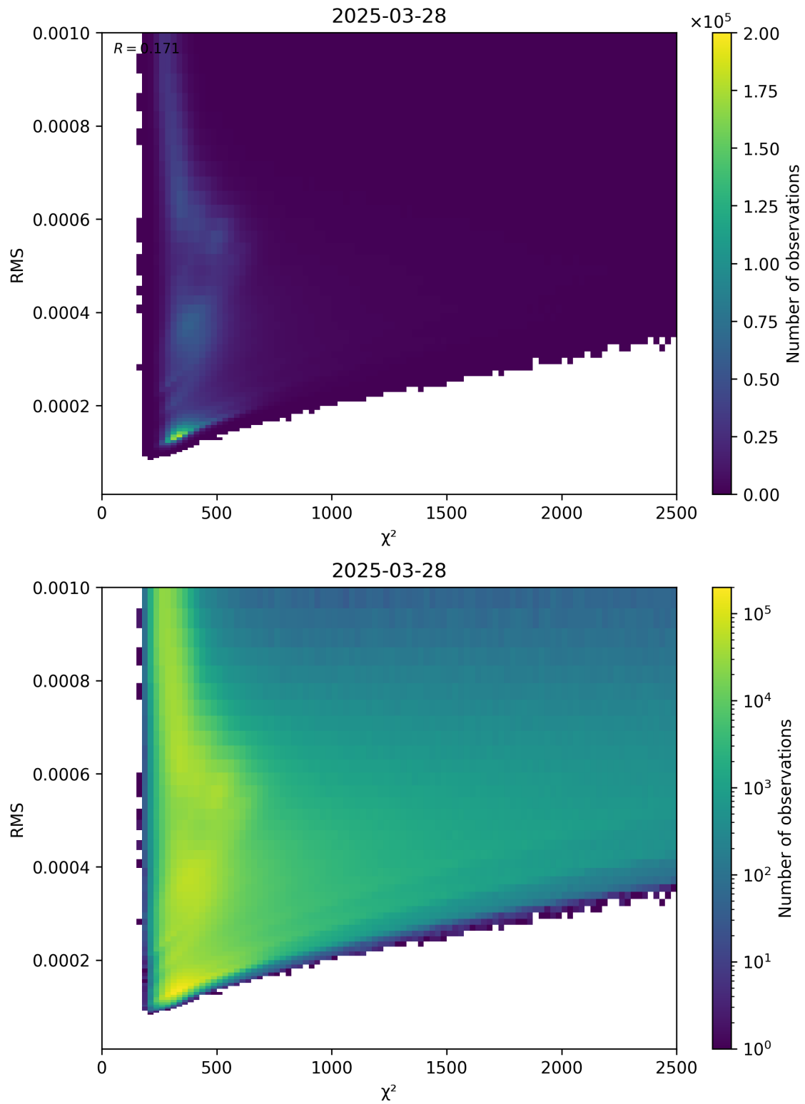
Figure 82: Scatter density plot of “ \chi^2 ” against “RMS” for 2025-03-28 to 2025-03-29.
