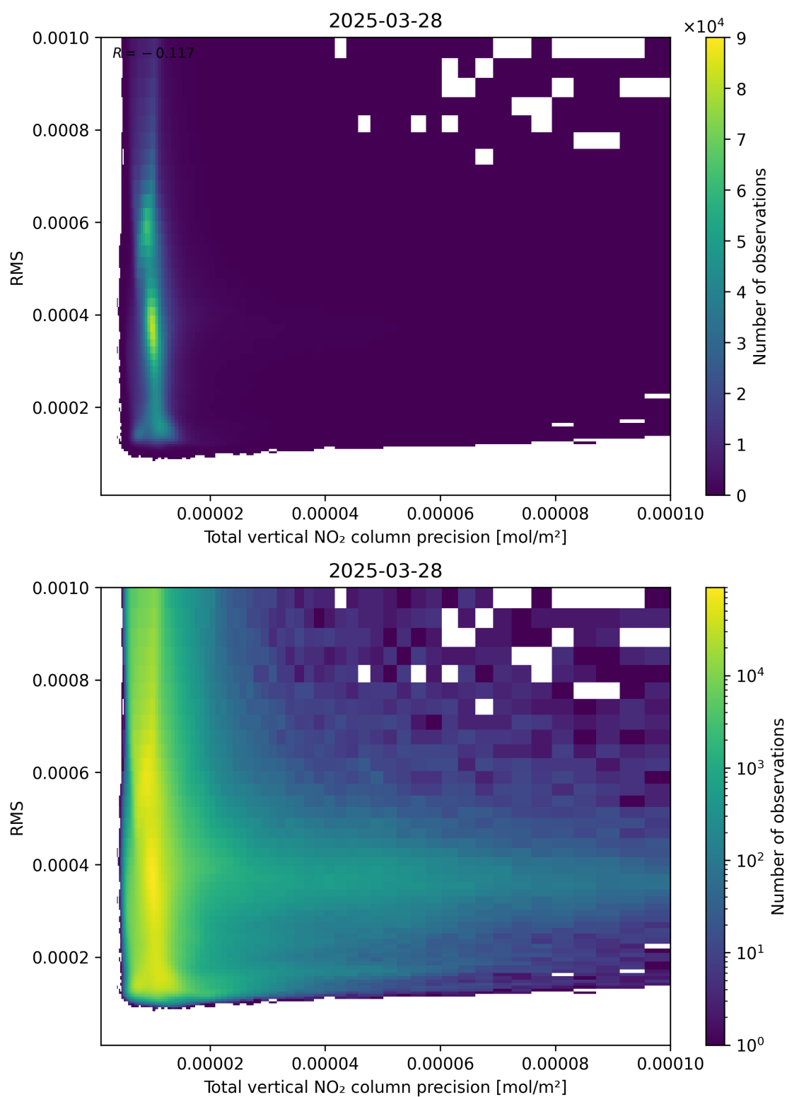
Figure 119: Scatter density plot of “Total vertical NO 2 column precision” against “RMS” for 2025-03-28 to 2025-03-29.
