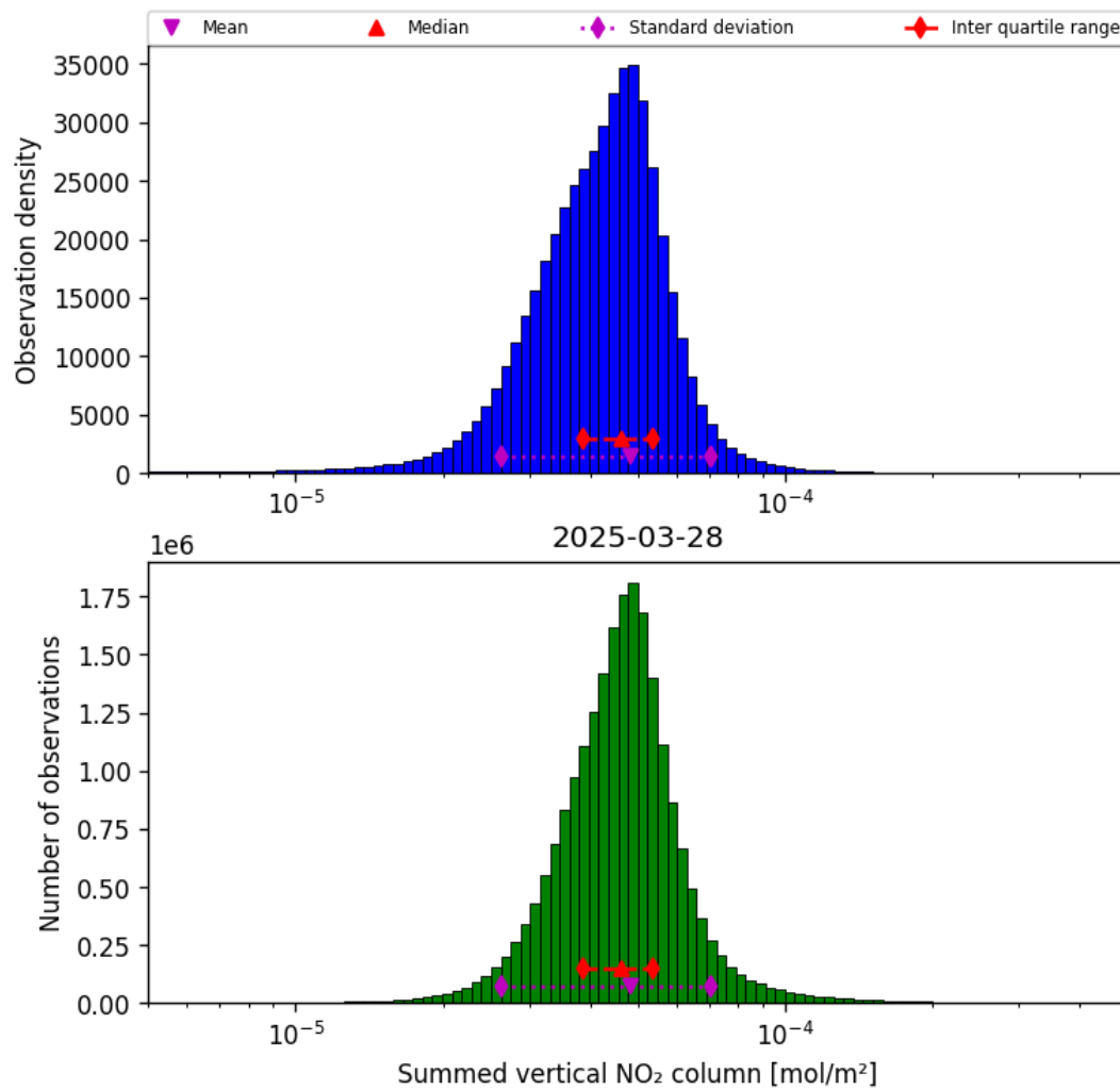
Figure 40: Histogram of “Summed vertical NO 2 column” for 2025-03-28 to 2025-03-29
