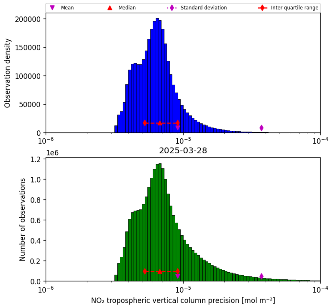
Figure 30: Histogram of “NO 2 tropospheric vertical column precision” for 2025-03-28 to 2025-03-29
