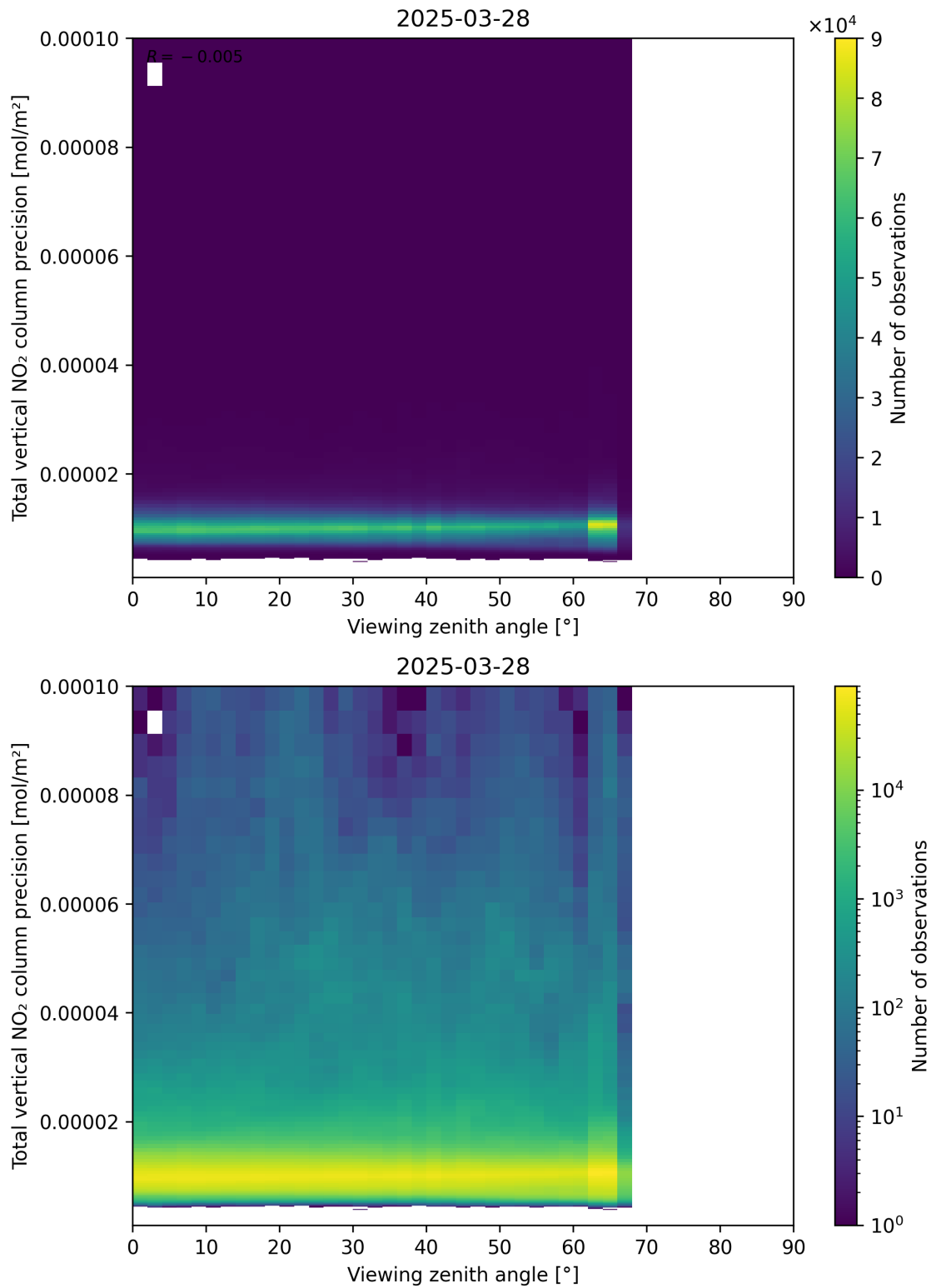
Figure 168: Scatter density plot of “Viewing zenith angle” against “Total vertical NO 2 column precision” for 2025-03-28 to 2025-03-29.
