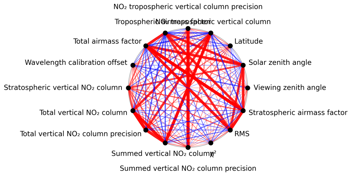
Figure 1: Map of correlation graph for 2025-03-28 to 2025-03-29.
