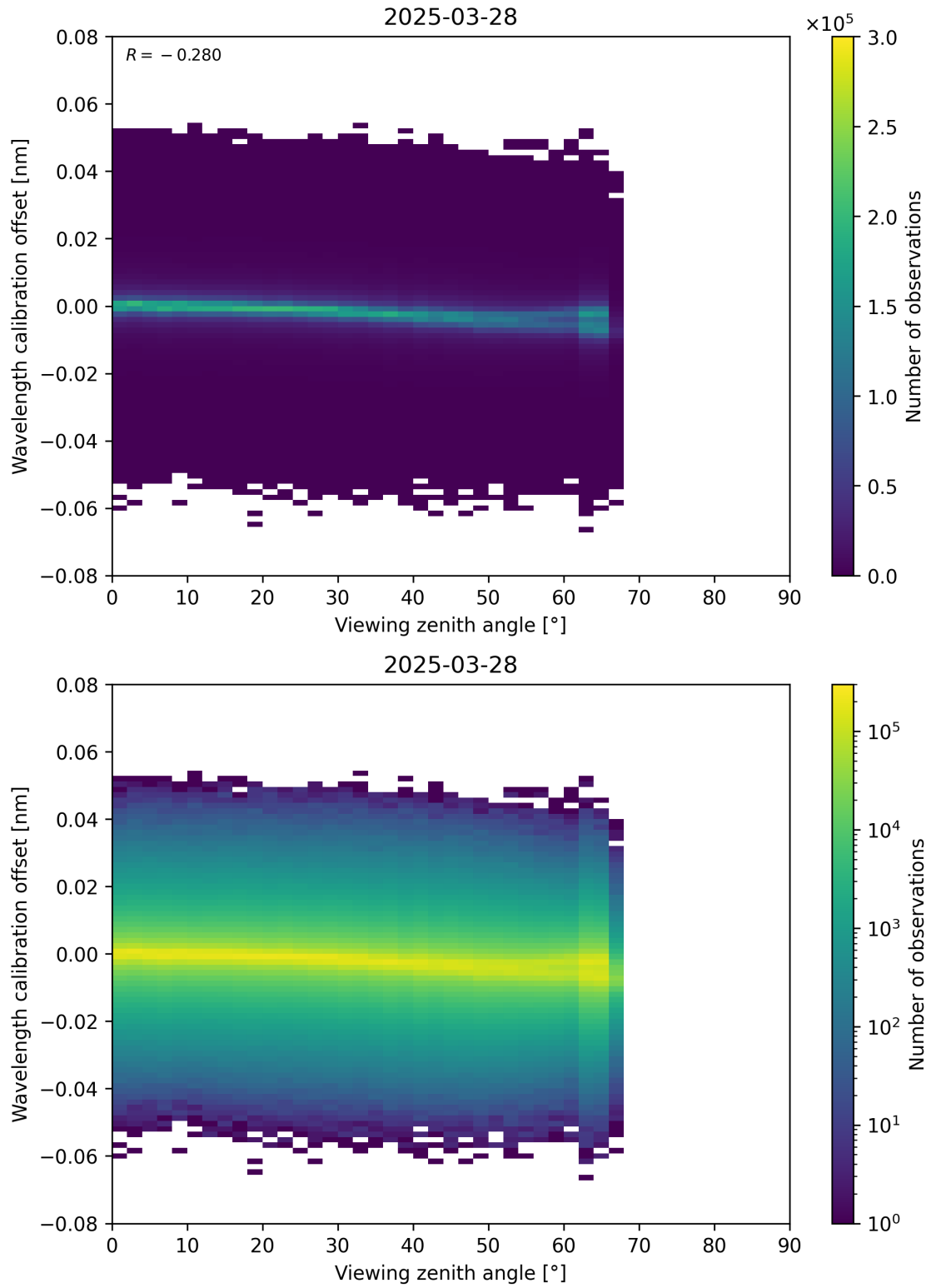
Figure 173: Scatter density plot of “Viewing zenith angle” against “Wavelength calibration offset” for 2025-03-28 to 2025-03-29.
