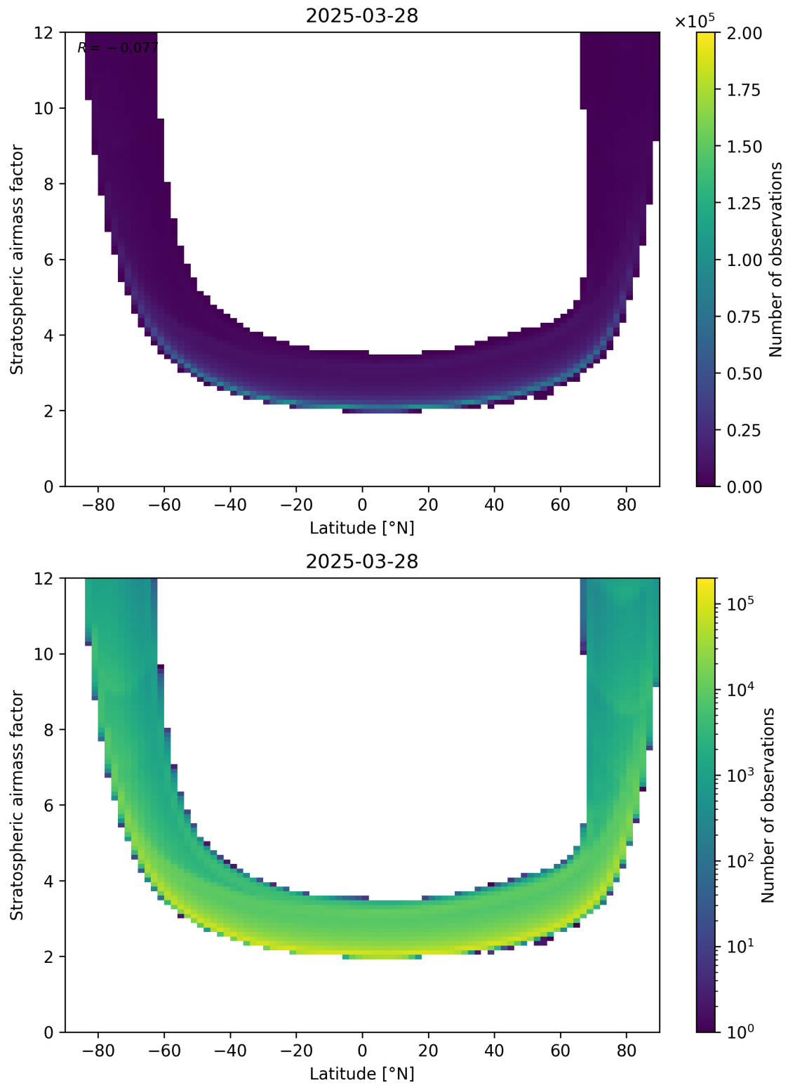
Figure 83: Scatter density plot of “Latitude” against “Stratospheric airmass factor” for 2025-03-28 to 2025-03-29.
