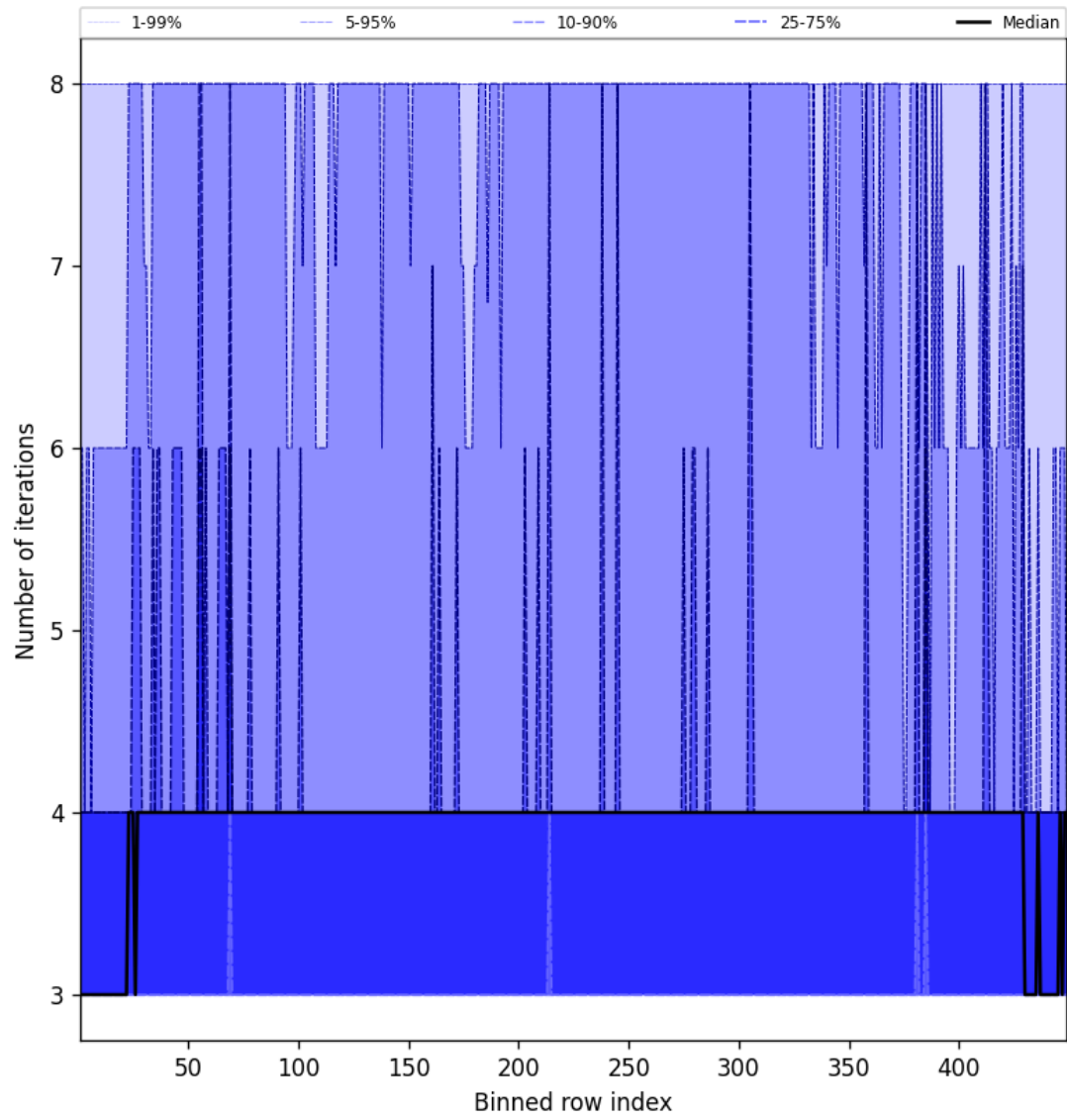
Figure 51: Along track statistics of “Number of iterations” for 2025-03-28 to 2025-03-29
