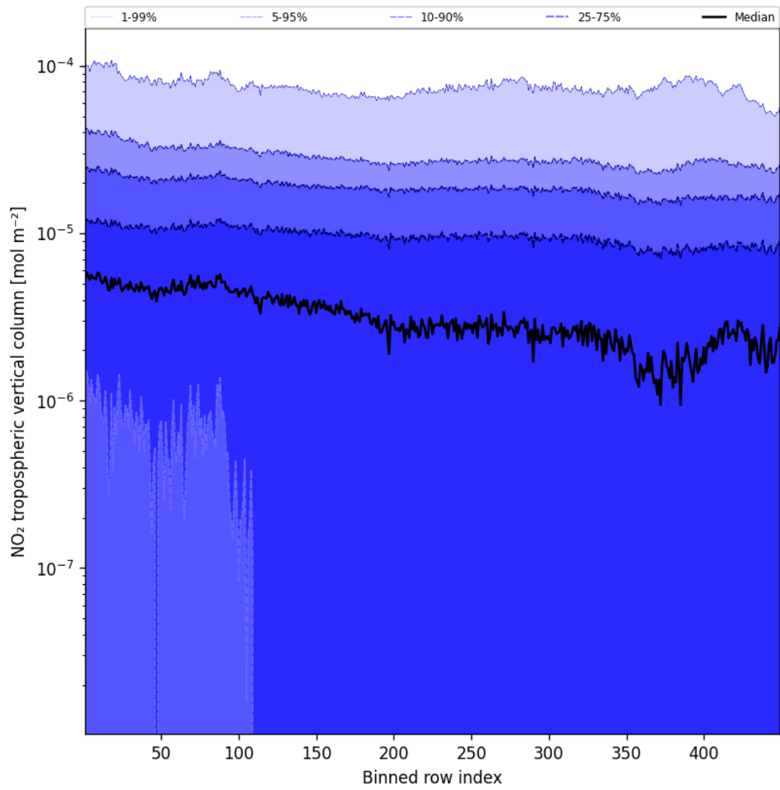
Figure 46: Along track statistics of “NO 2 tropospheric vertical column” for 2025-03-28 to 2025-03-29
