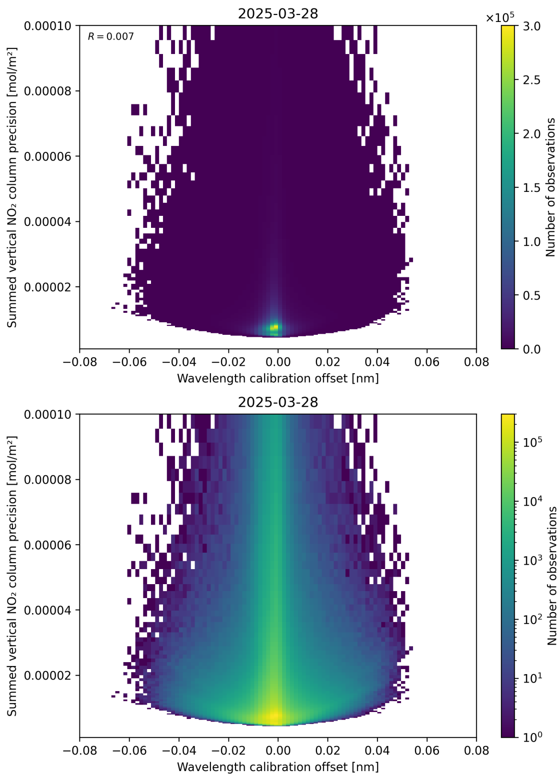
Figure 178: Scatter density plot of “Wavelength calibration offset” against “Summed vertical NO 2 column precision” for 2025-03-28 to 2025-03-29.
