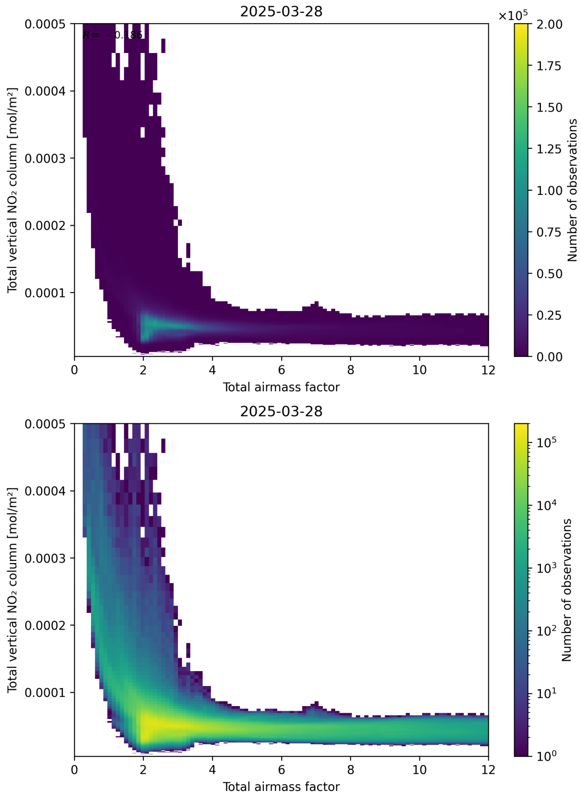
Figure 67: Scatter density plot of “Total airmass factor” against “Total vertical NO 2 column” for 2025-03-28 to 2025-03-29.
