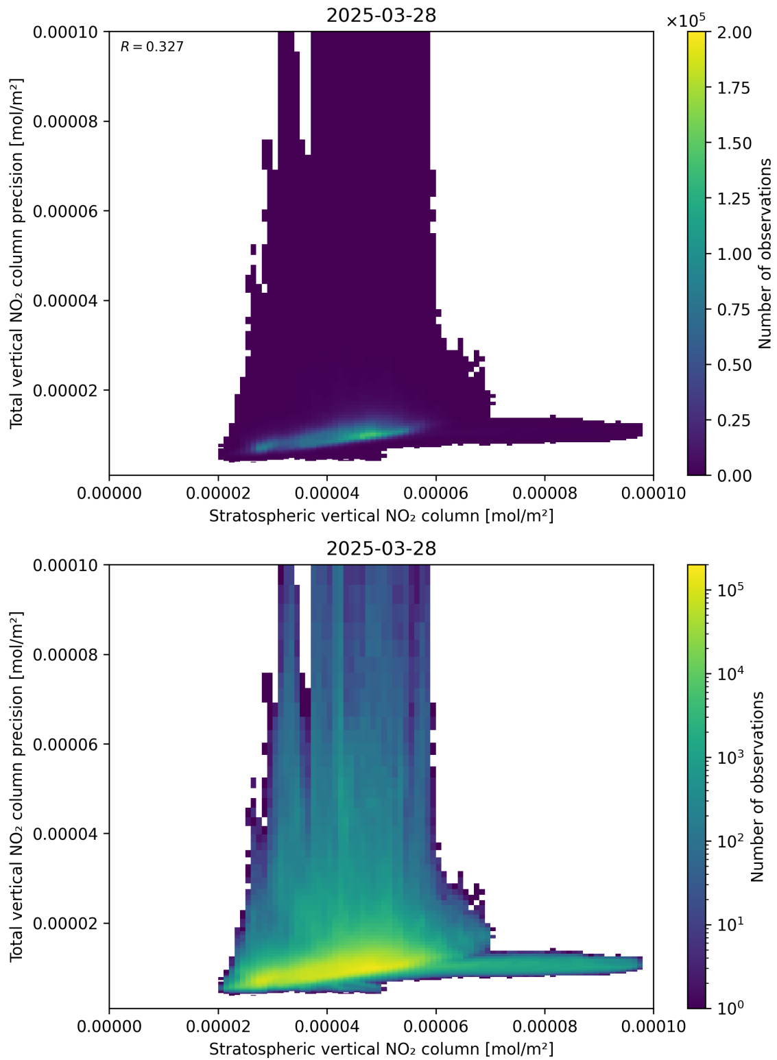
Figure 101: Scatter density plot of “Stratospheric vertical NO 2 column” against “Total vertical NO 2 column precision” for 2025-03-28 to 2025-03-29.
