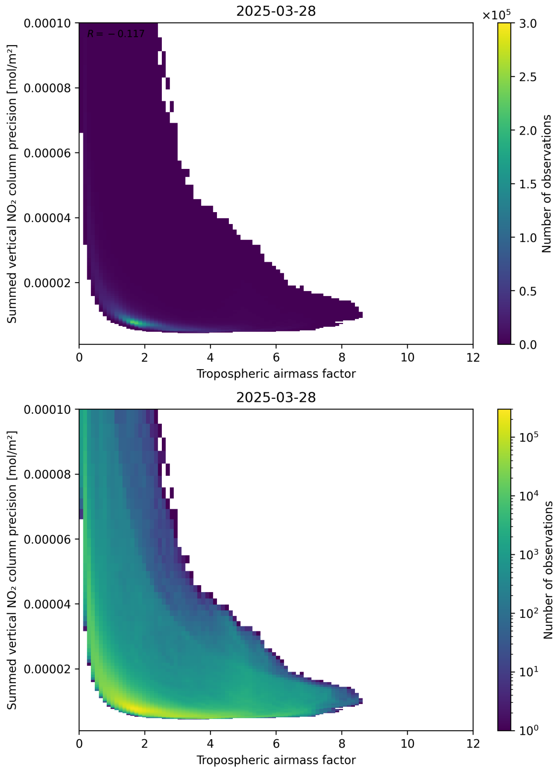
Figure 76: Scatter density plot of “Tropospheric air mass factor” against “Summed vertical NO 2 column precision” for 2025-03-28 to 2025-03-29.
