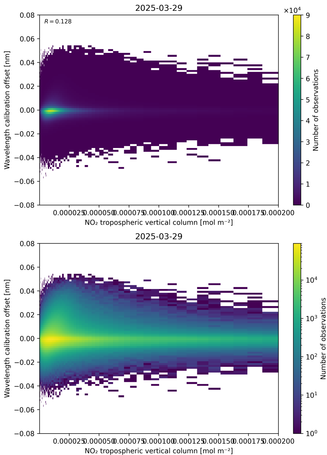
Figure 143: Scatter density plot of “NO 2 tropospheric vertical column” against “Wavelength calibration offset” for 2025-03-29 to 2025-03-30.
