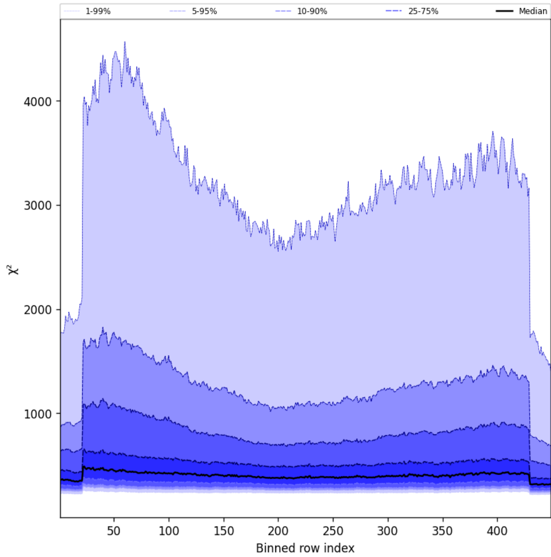
Figure 59: Along track statistics of “ \chi^2 ” for 2025-03-29 to 2025-03-30
