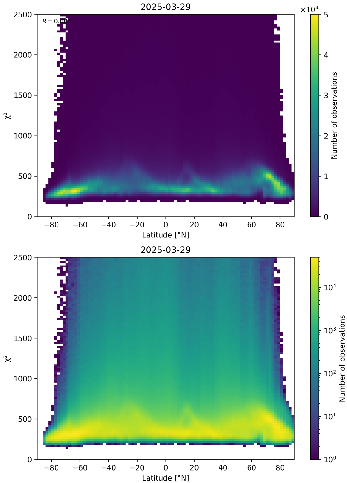
Figure 86: Scatter density plot of “Latitude” against “ \chi^2 ” for 2025-03-29 to 2025-03-30.
