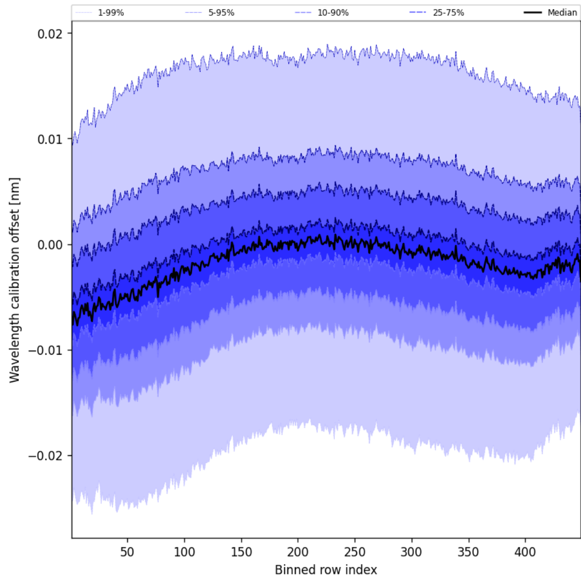
Figure 52: Along track statistics of “Wavelength calibration offset” for 2025-03-29 to 2025-03-30
