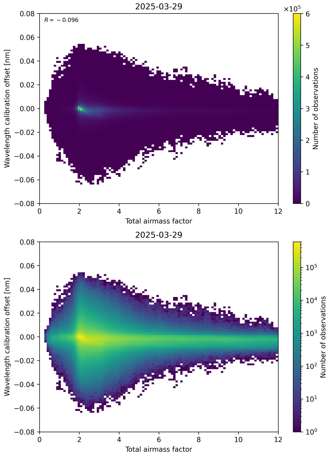
Figure 70: Scatter density plot of “Total airmass factor” against “Wavelength calibration offset” for 2025-03-29 to 2025-03-30.
