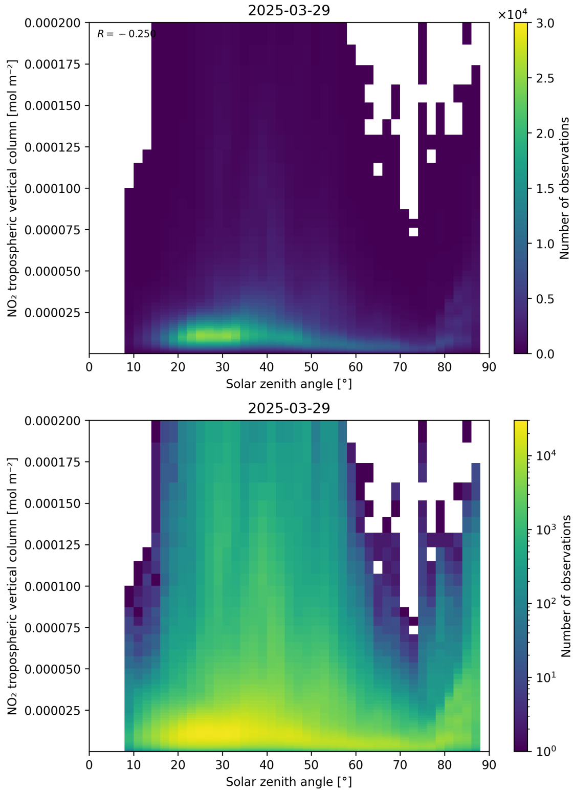
Figure 155: Scatter density plot of “Solar zenith angle” against “NO 2 tropospheric vertical column” for 2025-03-29 to 2025-03-30.
