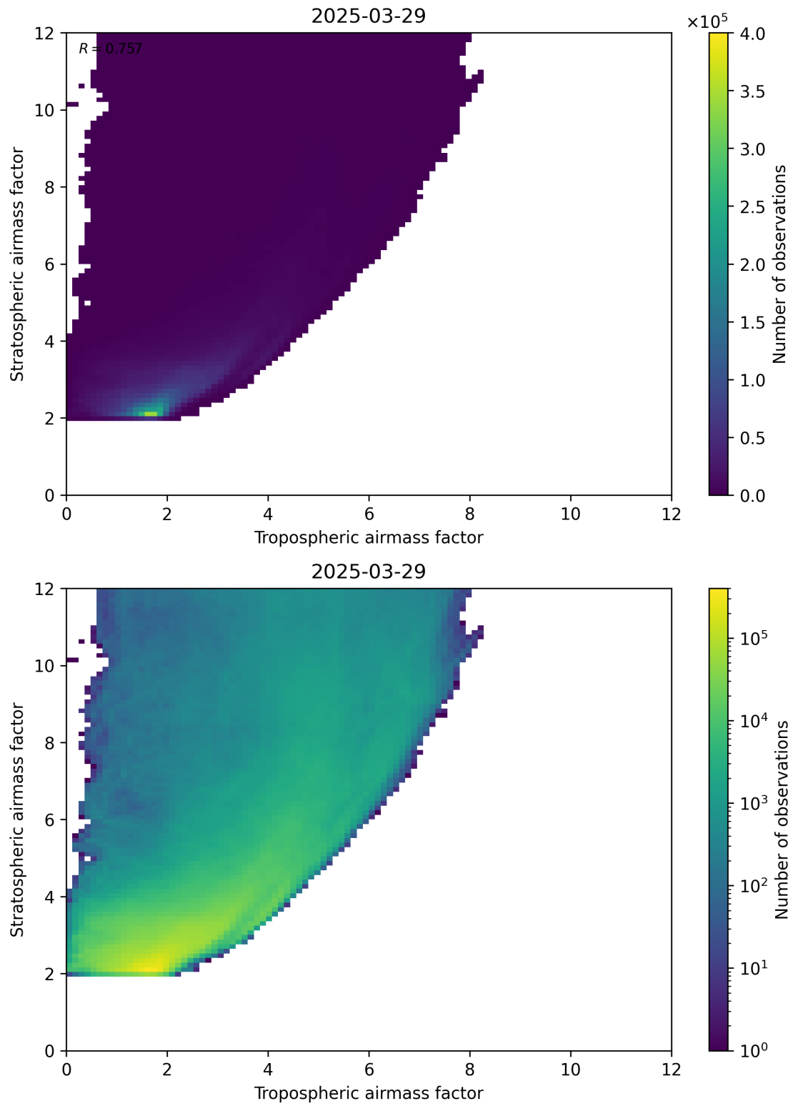
Figure 71: Scatter density plot of “Tropospheric airmass factor” against “Stratospheric airmass factor” for 2025-03-29 to 2025-03-30.
