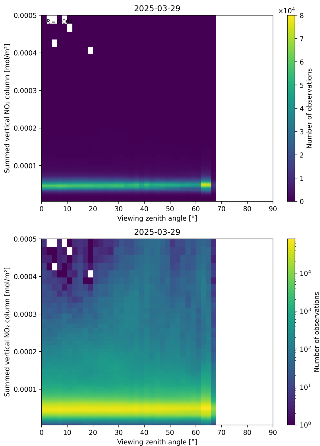
Figure 165: Scatter density plot of “Viewing zenith angle” against “Summed vertical NO 2 column” for 2025-03-29 to 2025-03-30.
