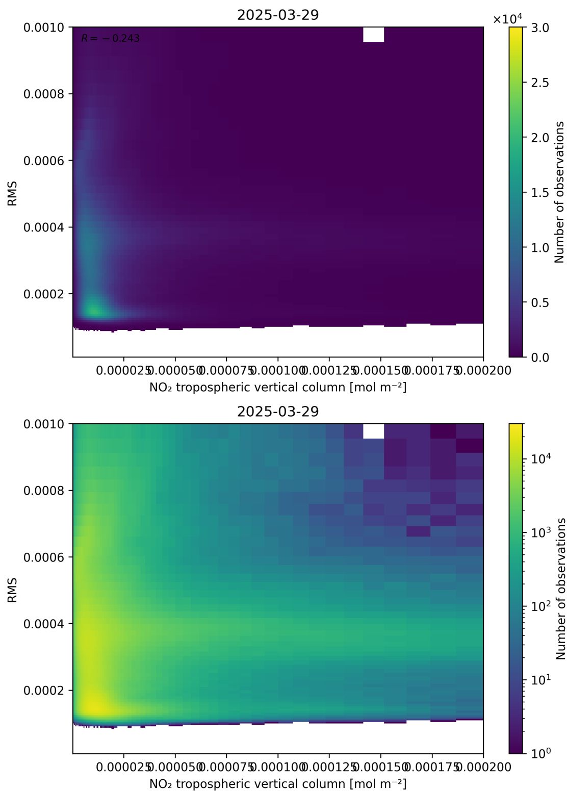
Figure 142: Scatter density plot of “NO 2 tropospheric vertical column” against “RMS” for 2025-03-29 to 2025-03-30.
