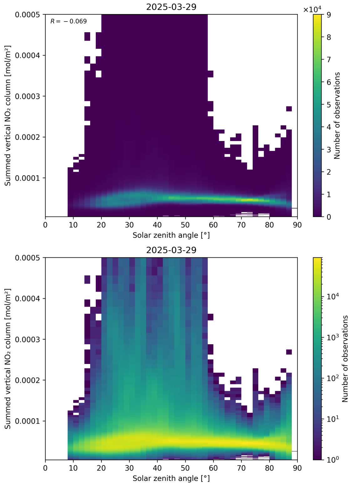
Figure 151: Scatter density plot of “Solar zenith angle” against “Summed vertical NO 2 column” for 2025-03-29 to 2025-03-30.
