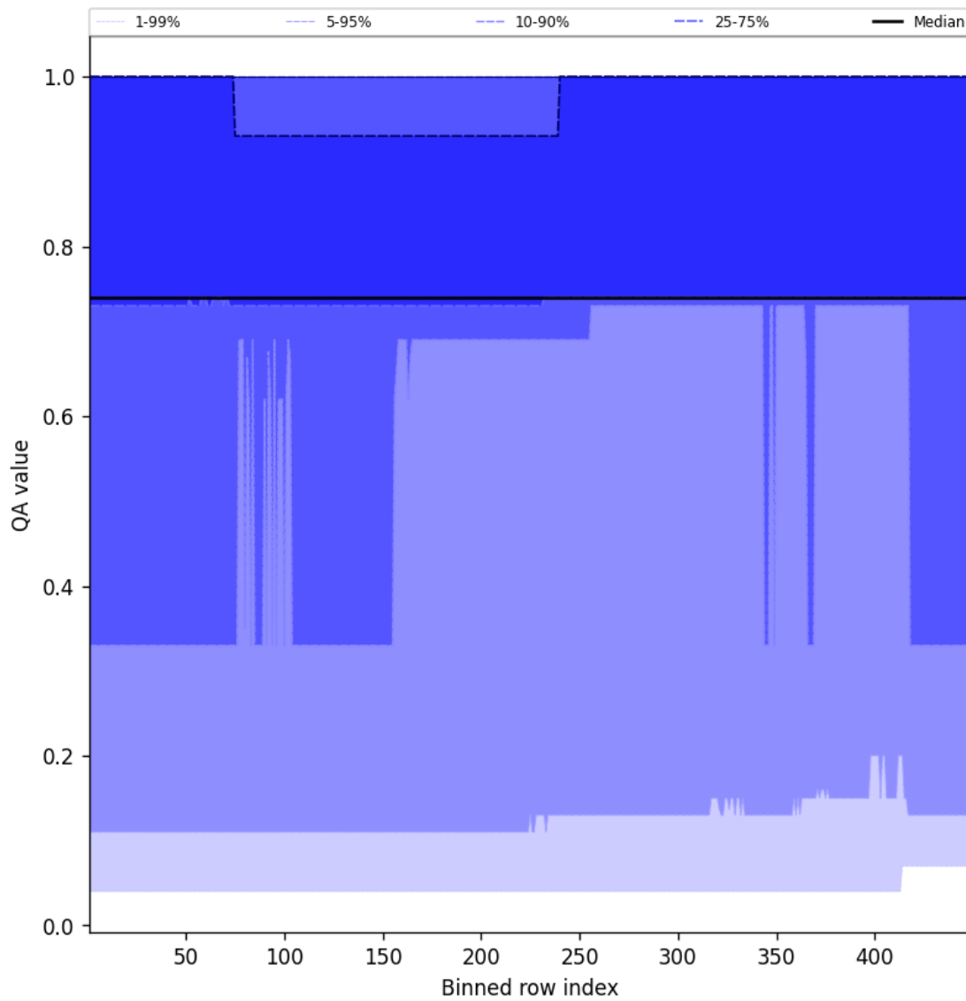
Figure 45: Along track statistics of “QA value” for 2025-03-29 to 2025-03-30
