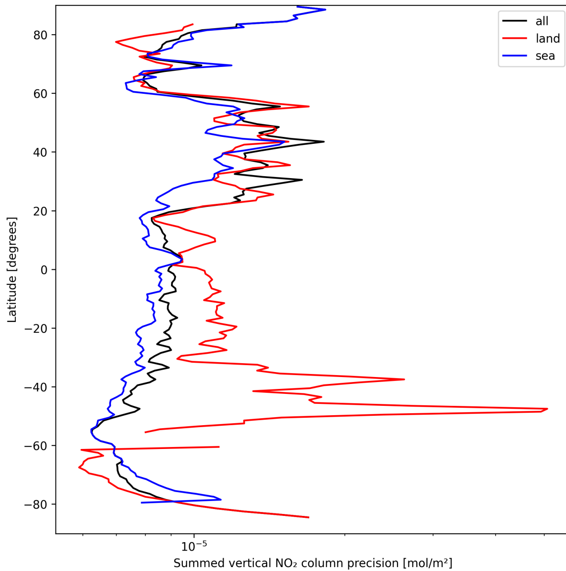
Figure 24: Zonal average of “Summed vertical NO 2 column precision” for 2025-03-29 to 2025-03-30.
