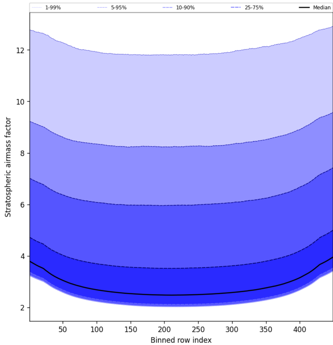
Figure 61: Along track statistics of “Stratospheric airmass factor” for 2025-03-29 to 2025-03-30
