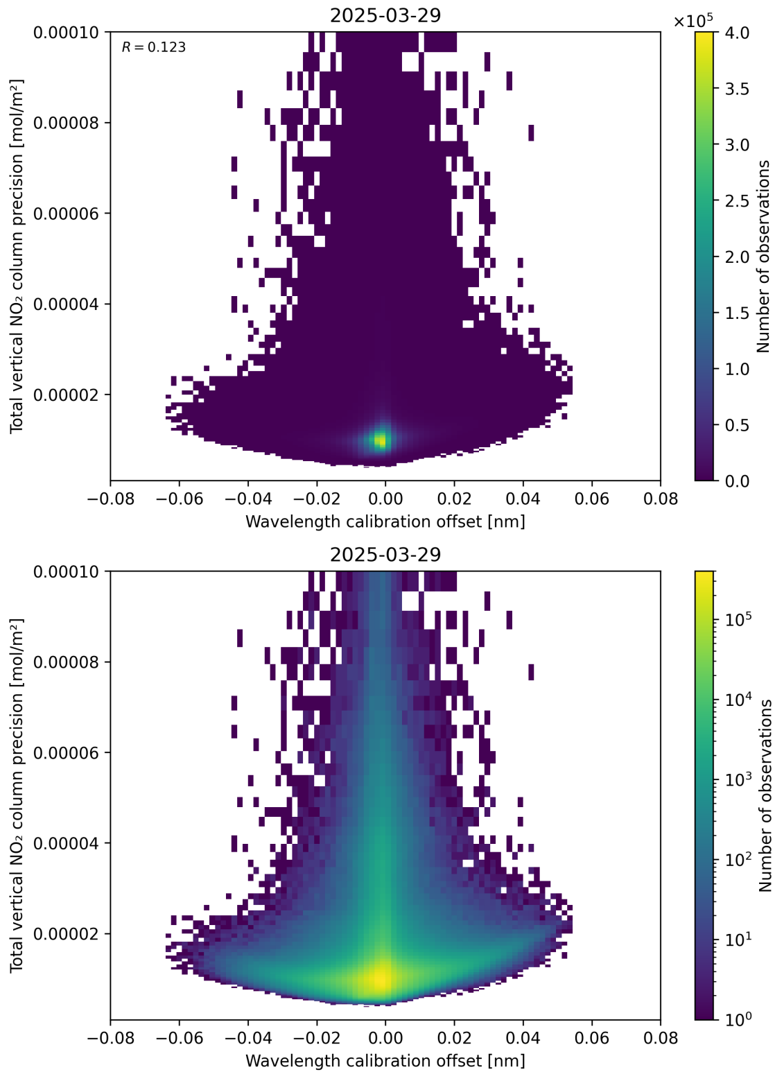
Figure 180: Scatter density plot of “Wavelength calibration offset” against “Total vertical NO 2 column precision” for 2025-03-29 to 2025-03-30.
