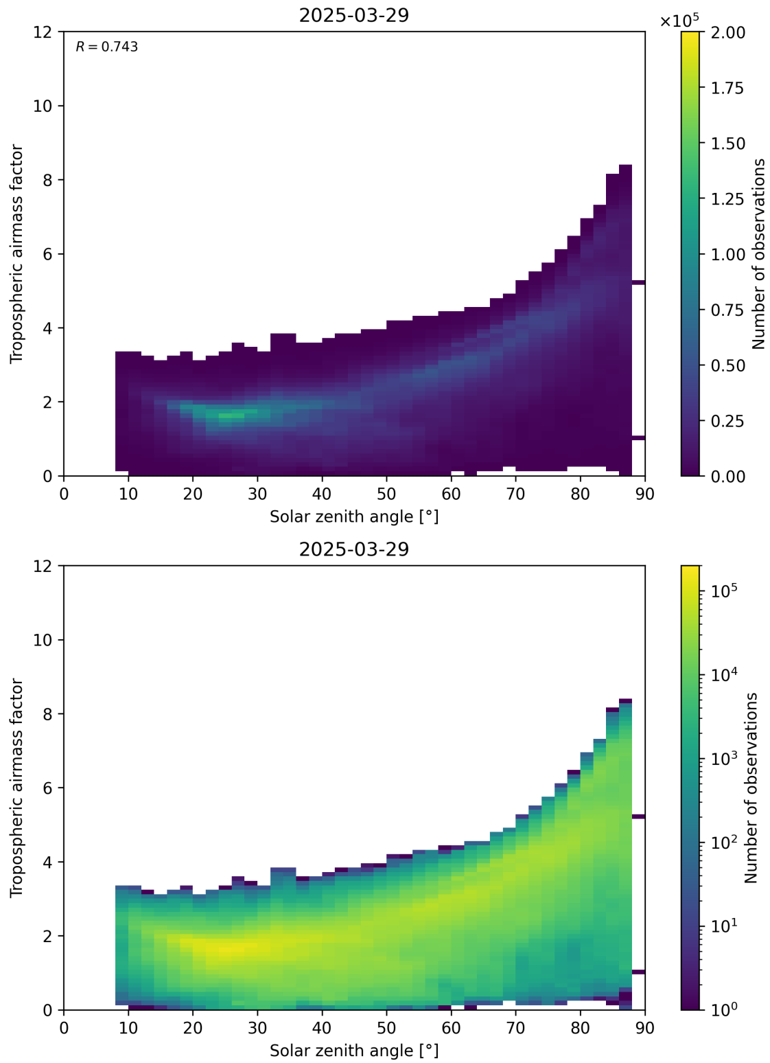
Figure 147: Scatter density plot of “Solar zenith angle” against “Tropospheric airmass factor” for 2025-03-29 to 2025-03-30.
