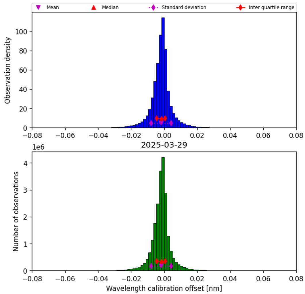
Figure 35: Histogram of “Wavelength calibration offset” for 2025-03-29 to 2025-03-30
