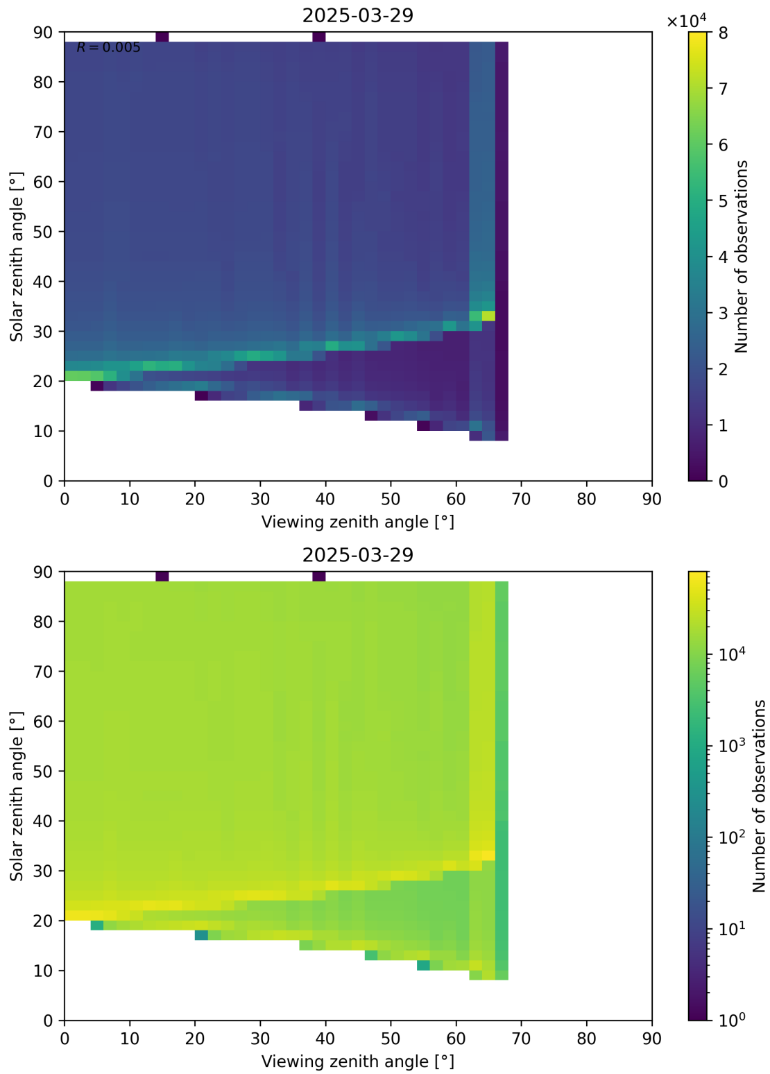
Figure 172: Scatter density plot of “Viewing zenith angle” against “Solar zenith angle” for 2025-03-29 to 2025-03-30.
