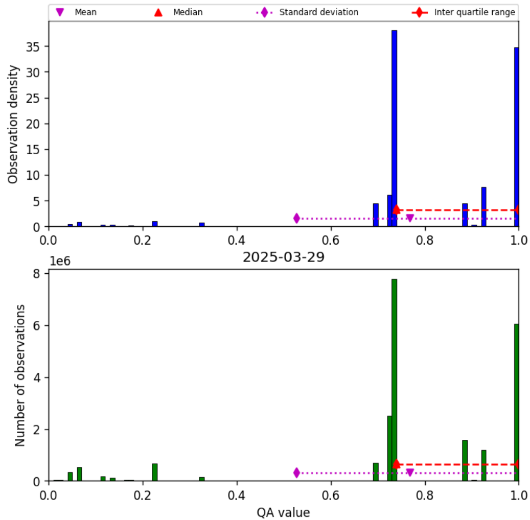
Figure 28: Histogram of “QA value” for 2025-03-29 to 2025-03-30
