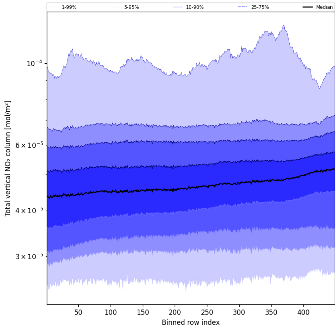
Figure 55: Along track statistics of “Total vertical NO 2 column” for 2025-03-29 to 2025-03-30
