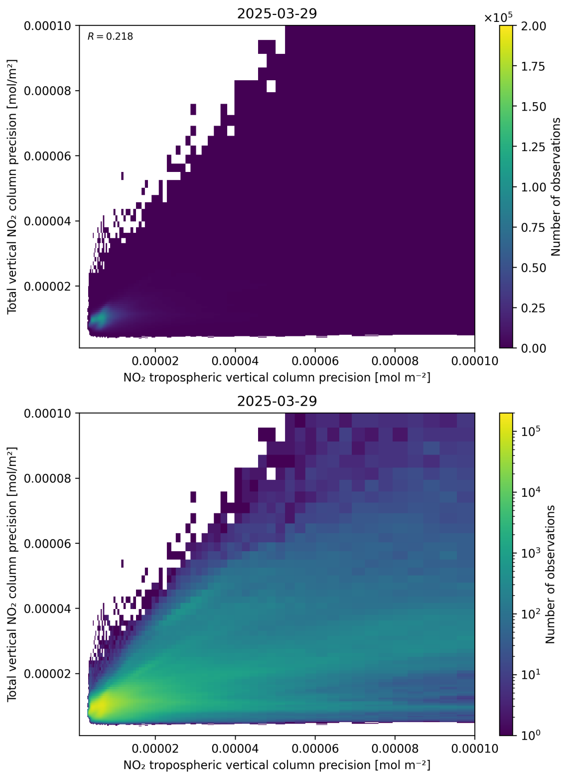
Figure 139: Scatter density plot of “NO 2 tropospheric vertical column precision” against “Total vertical NO 2 column precision” for 2025-03-29 to 2025-03-30.
