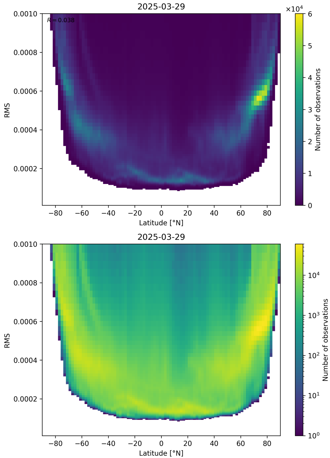
Figure 94: Scatter density plot of “Latitude” against “RMS” for 2025-03-29 to 2025-03-30.
