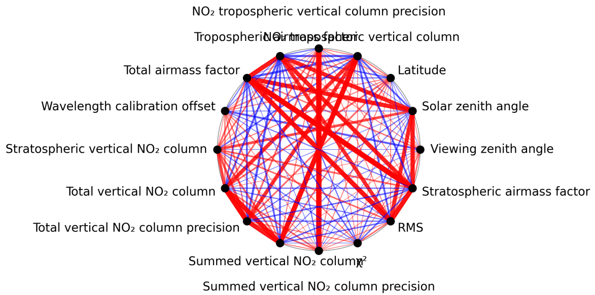
Figure 1: Map of correlation graph for 2025-03-29 to 2025-03-30.
