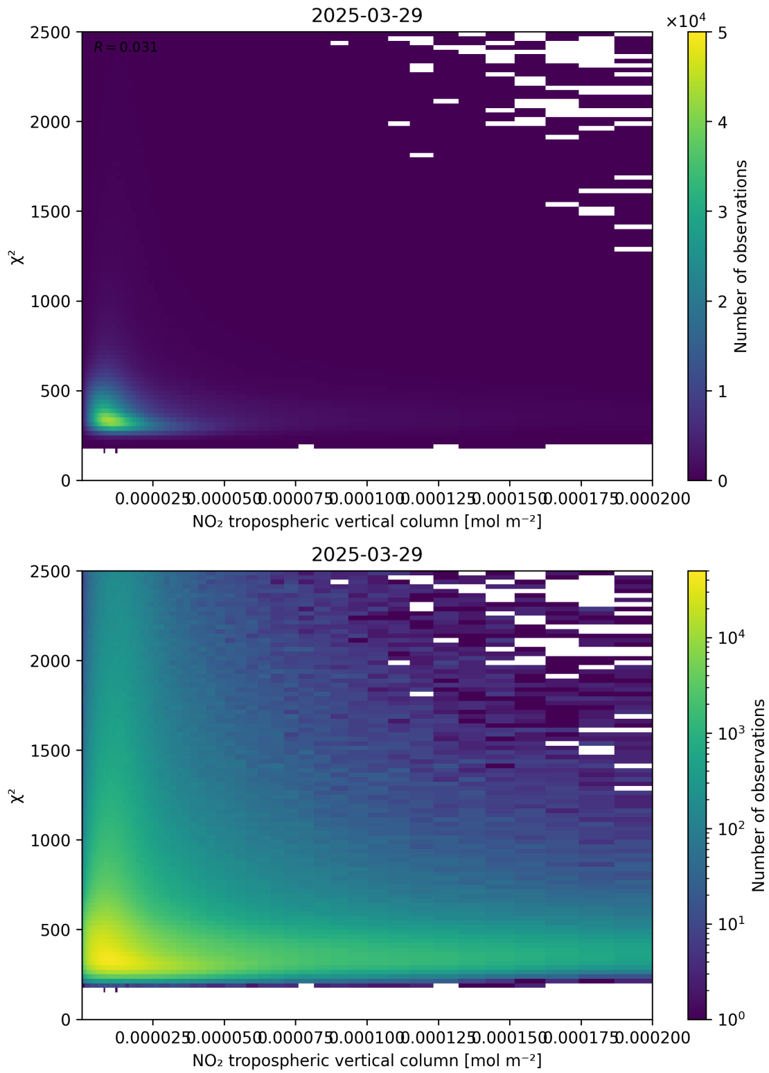
Figure 124: Scatter density plot of “NO 2 tropospheric vertical column” against “ \chi^2 ” for 2025-03-29 to 2025-03-30.
