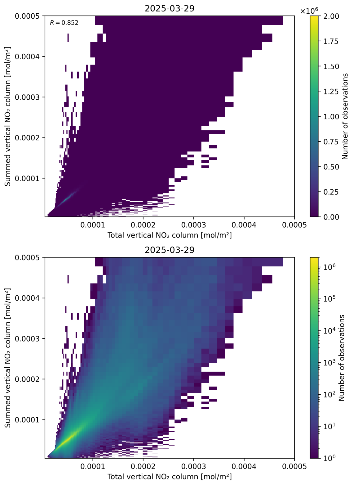
Figure 112: Scatter density plot of “Total vertical NO 2 column” against “Summed vertical NO 2 column” for 2025-03-29 to 2025-03-30.
