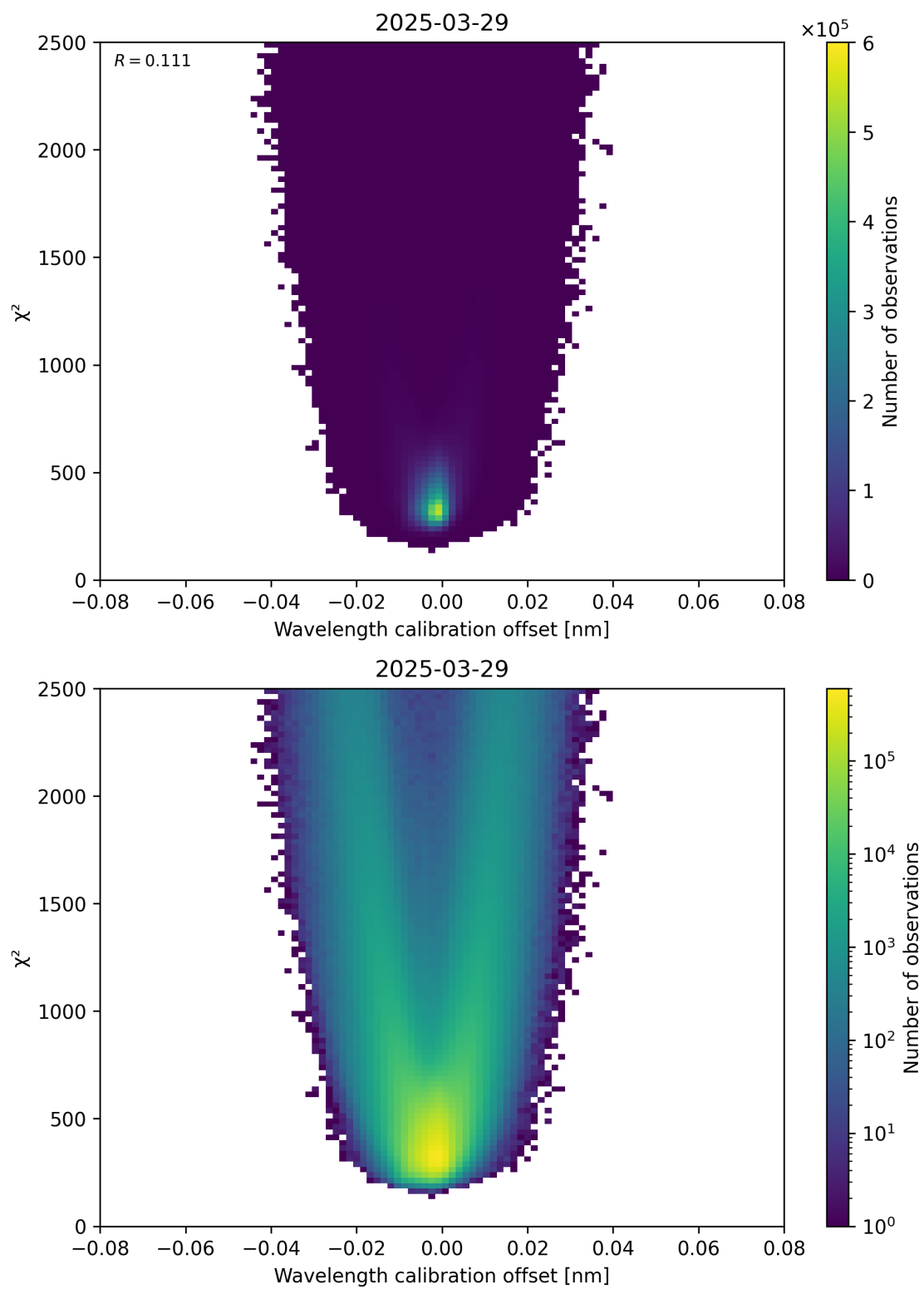
Figure 175: Scatter density plot of “Wavelength calibration offset” against “ \chi^2 ” for 2025-03-29 to 2025-03-30.
