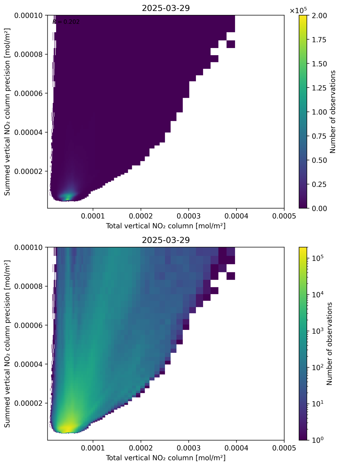
Figure 113: Scatter density plot of “Total vertical NO 2 column” against “Summed vertical NO 2 column precision” for 2025-03-29 to 2025-03-30.
