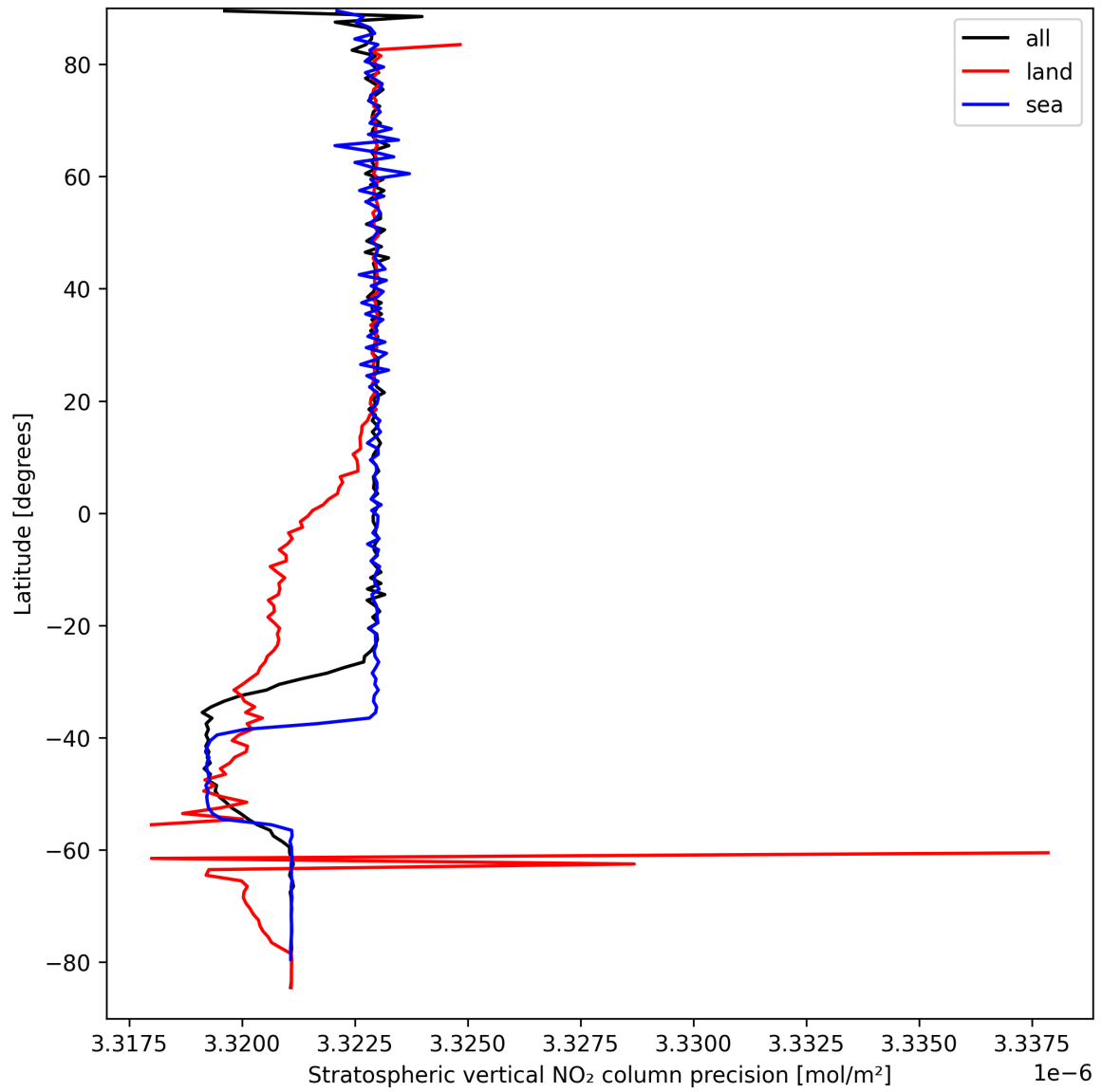
Figure 20: Zonal average of “Stratospheric vertical NO 2 column precision” for 2025-03-29 to 2025-03-30.
