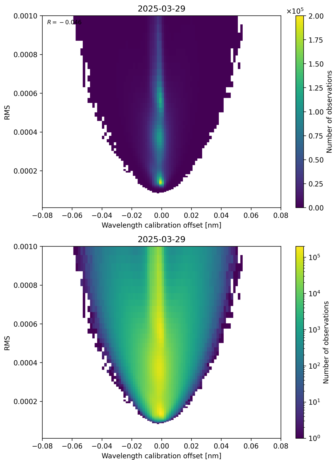
Figure 181: Scatter density plot of “Wavelength calibration offset” against “RMS” for 2025-03-29 to 2025-03-30.
