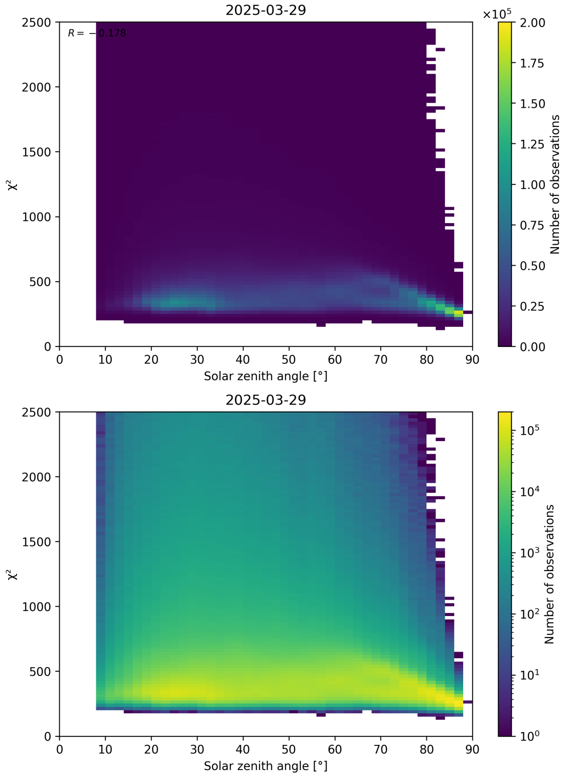
Figure 148: Scatter density plot of “Solar zenith angle” against “ \chi^2 ” for 2025-03-29 to 2025-03-30.
