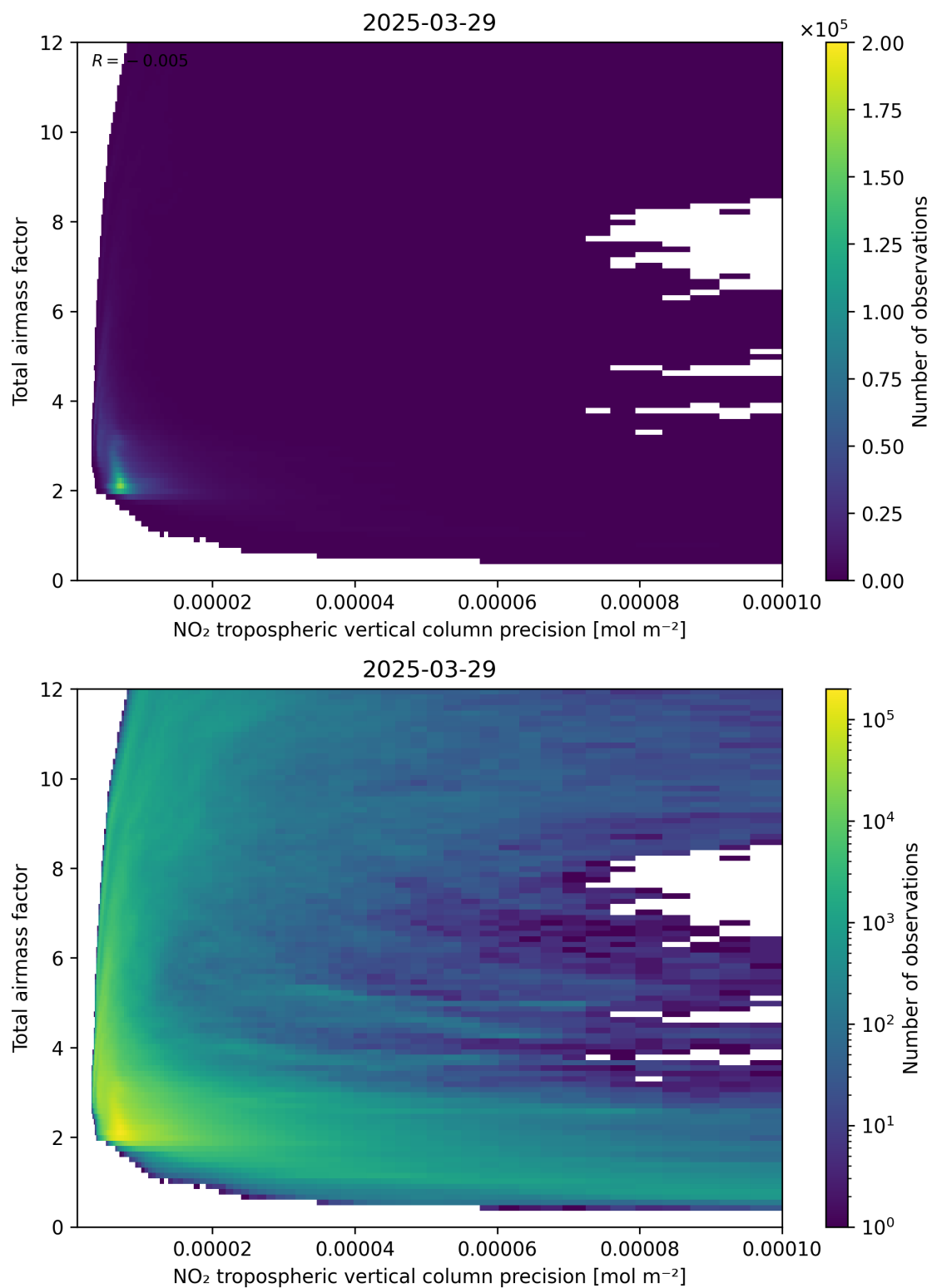
Figure 132: Scatter density plot of “NO 2 tropospheric vertical column precision” against “Total air mass factor” for 2025-03-29 to 2025-03-30.
