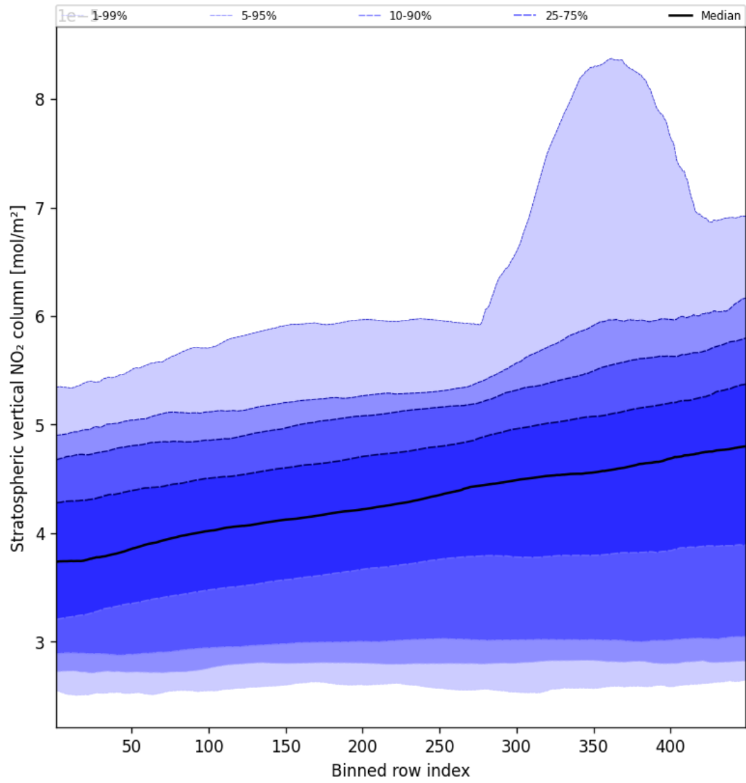
Figure 53: Along track statistics of “Stratospheric vertical NO 2 column” for 2025-03-29 to 2025-03-30
