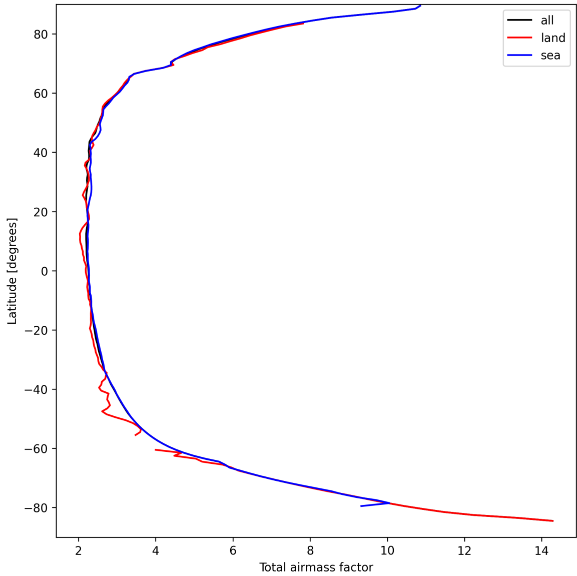
Figure 15: Zonal average of “Total airmass factor” for 2025-03-29 to 2025-03-30.
