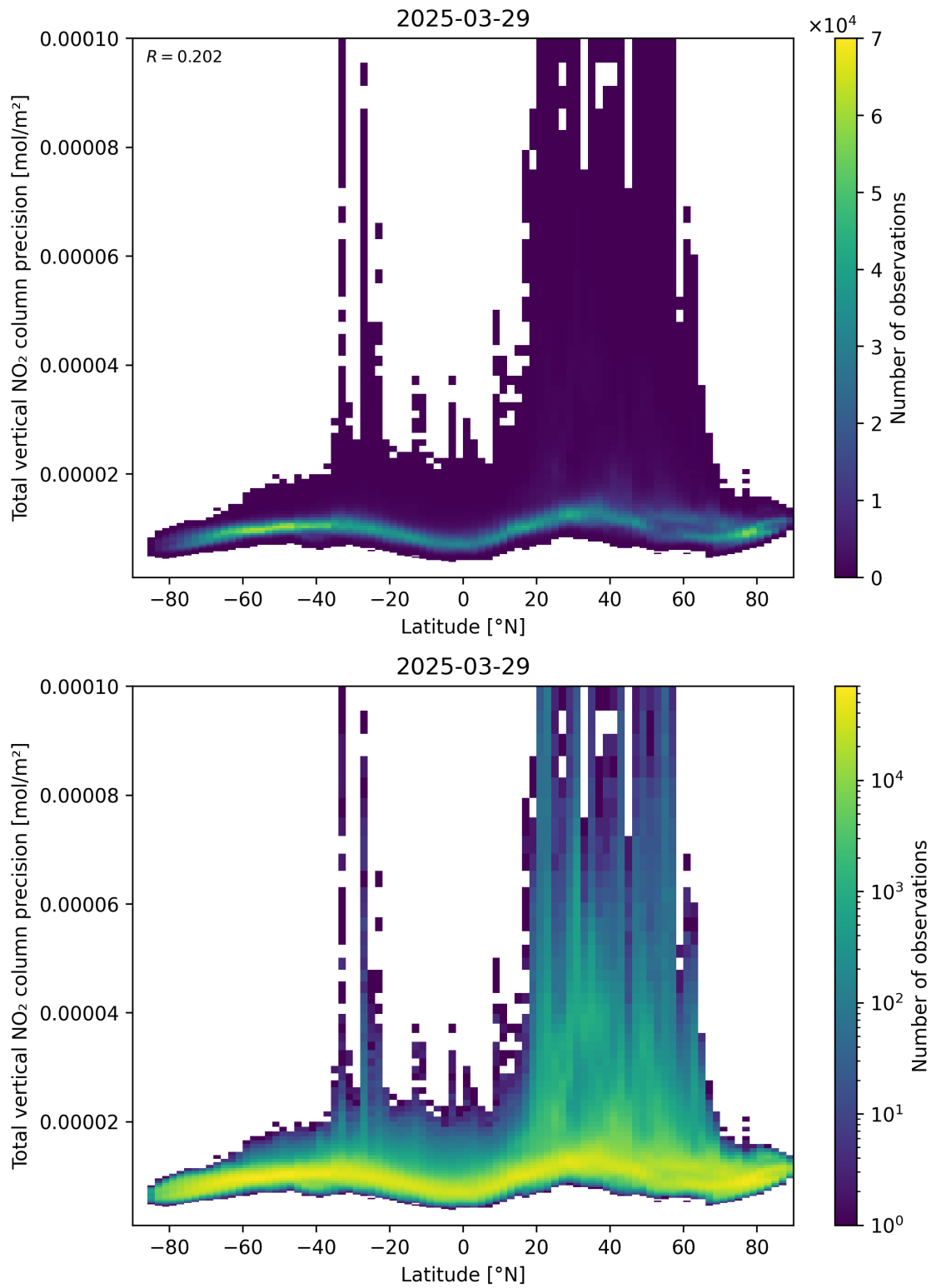
Figure 91: Scatter density plot of “Latitude” against “Total vertical NO 2 column precision” for 2025-03-29 to 2025-03-30.
