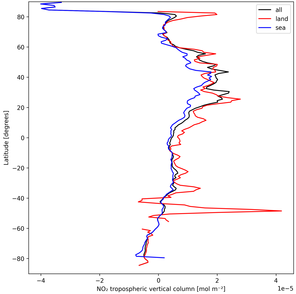
Figure 12: Zonal average of “NO 2 tropospheric vertical column” for 2025-03-29 to 2025-03-30.
