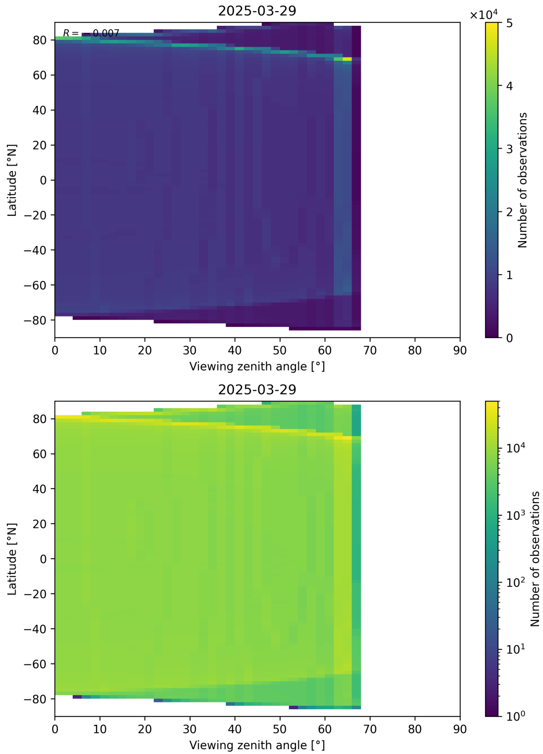
Figure 163: Scatter density plot of “Viewing zenith angle” against “Latitude” for 2025-03-29 to 2025-03-30.
