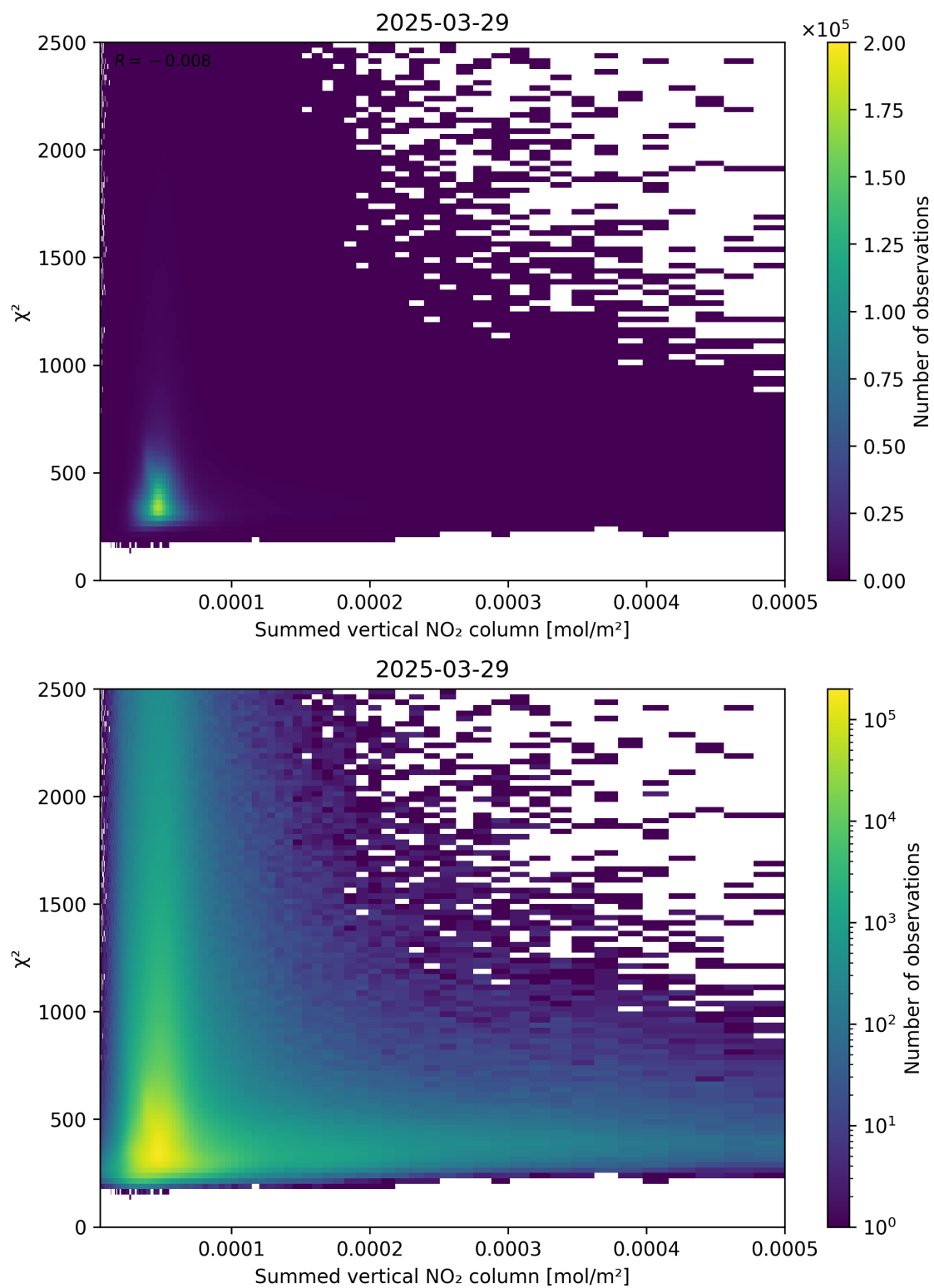
Figure 104: Scatter density plot of “Summed vertical NO 2 column” against “ \chi^2 ” for 2025-03-29 to 2025-03-30.
