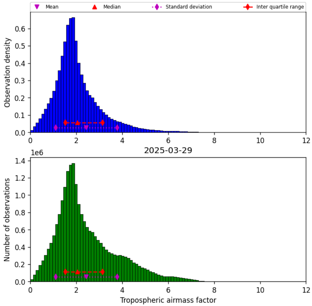
Figure 31: Histogram of “Tropospheric airmass factor” for 2025-03-29 to 2025-03-30
