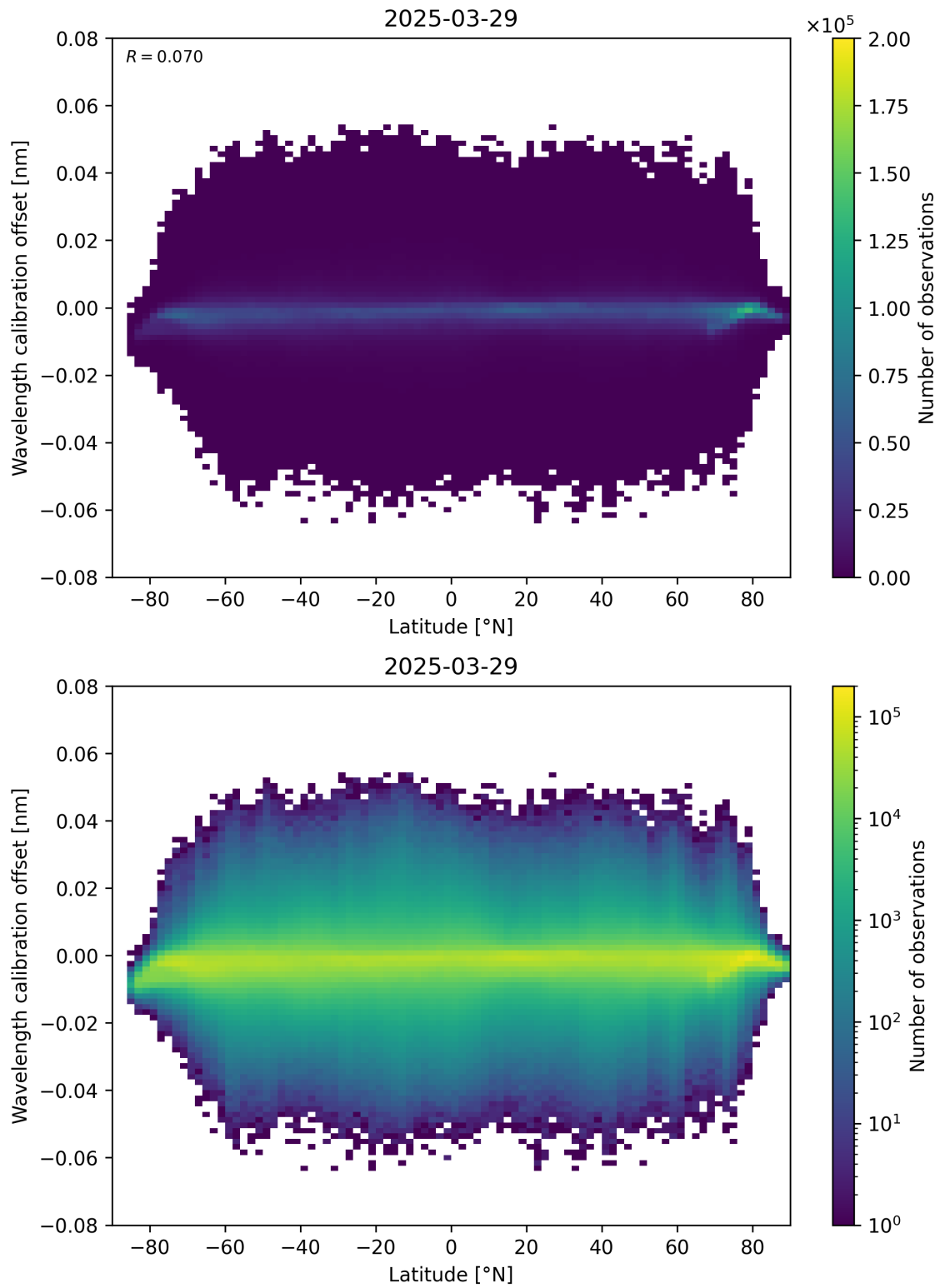
Figure 95: Scatter density plot of “Latitude” against “Wavelength calibration offset” for 2025-03-29 to 2025-03-30.
