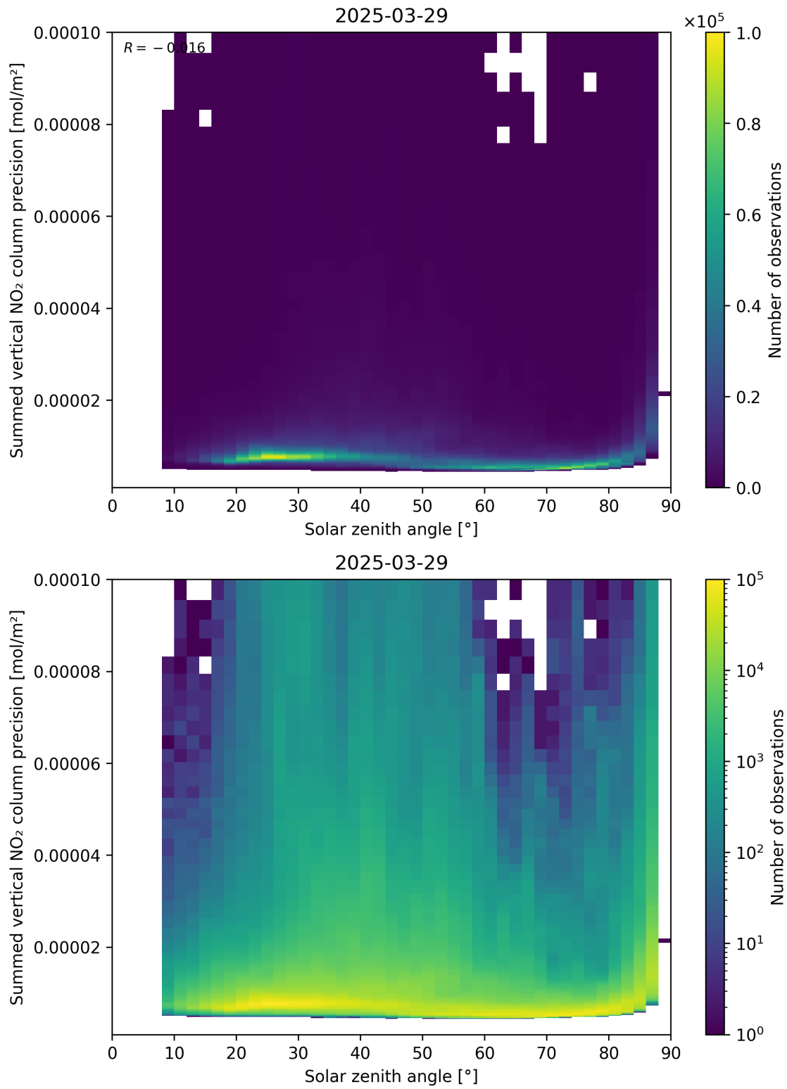
Figure 152: Scatter density plot of “Solar zenith angle” against “Summed vertical NO 2 column precision” for 2025-03-29 to 2025-03-30.
