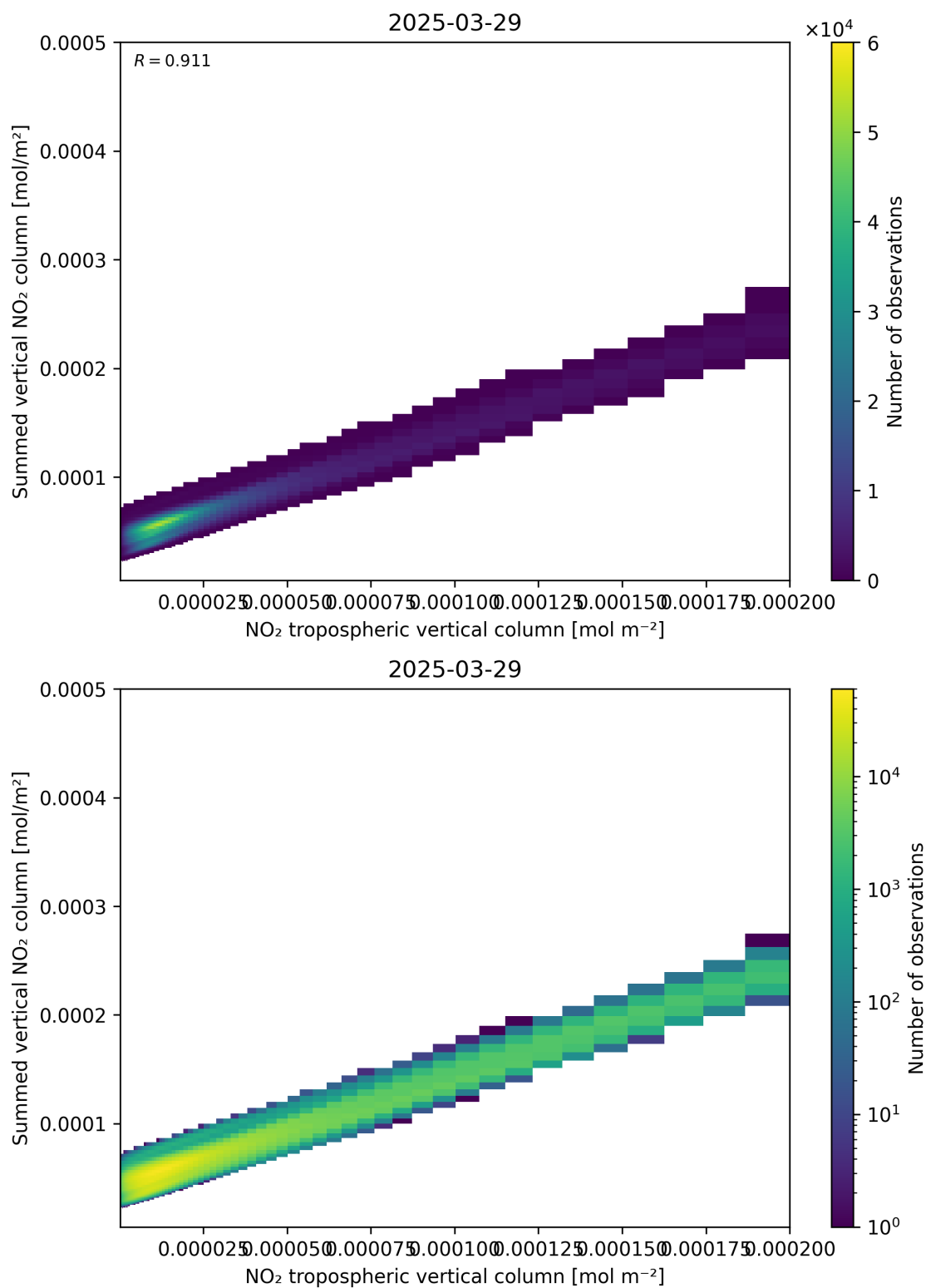
Figure 126: Scatter density plot of “NO 2 tropospheric vertical column” against “Summed vertical NO 2 column” for 2025-03-29 to 2025-03-30.
