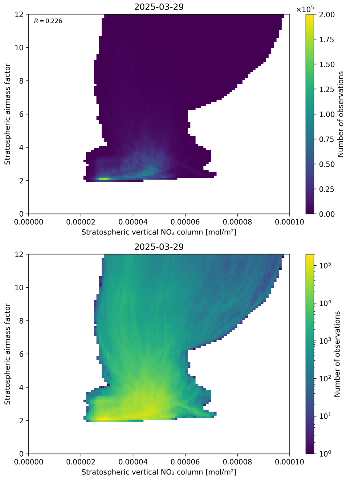
Figure 96: Scatter density plot of “Stratospheric vertical NO 2 column” against “Stratospheric airmass factor” for 2025-03-29 to 2025-03-30.
