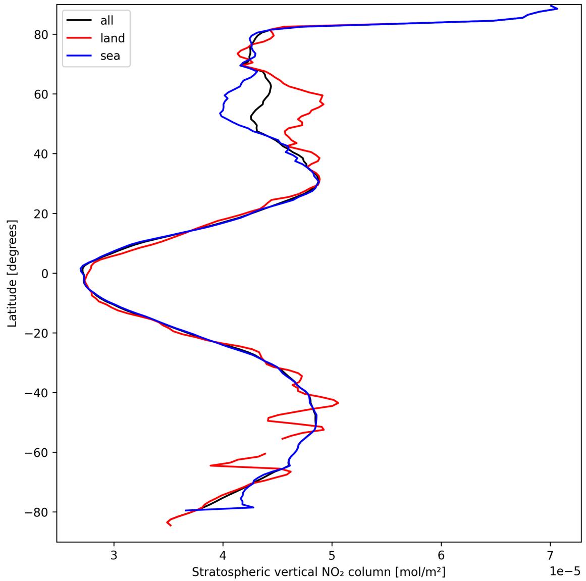
Figure 19: Zonal average of “Stratospheric vertical NO 2 column” for 2025-03-29 to 2025-03-30.
