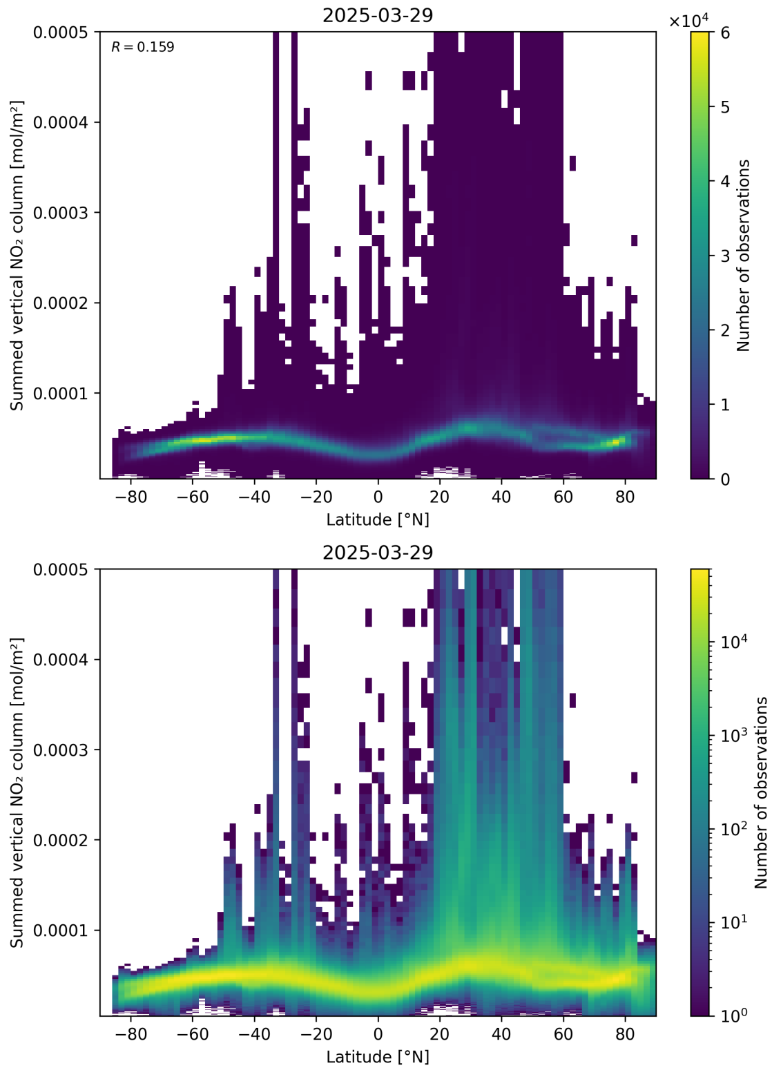
Figure 88: Scatter density plot of “Latitude” against “Summed vertical NO 2 column” for 2025-03-29 to 2025-03-30.
