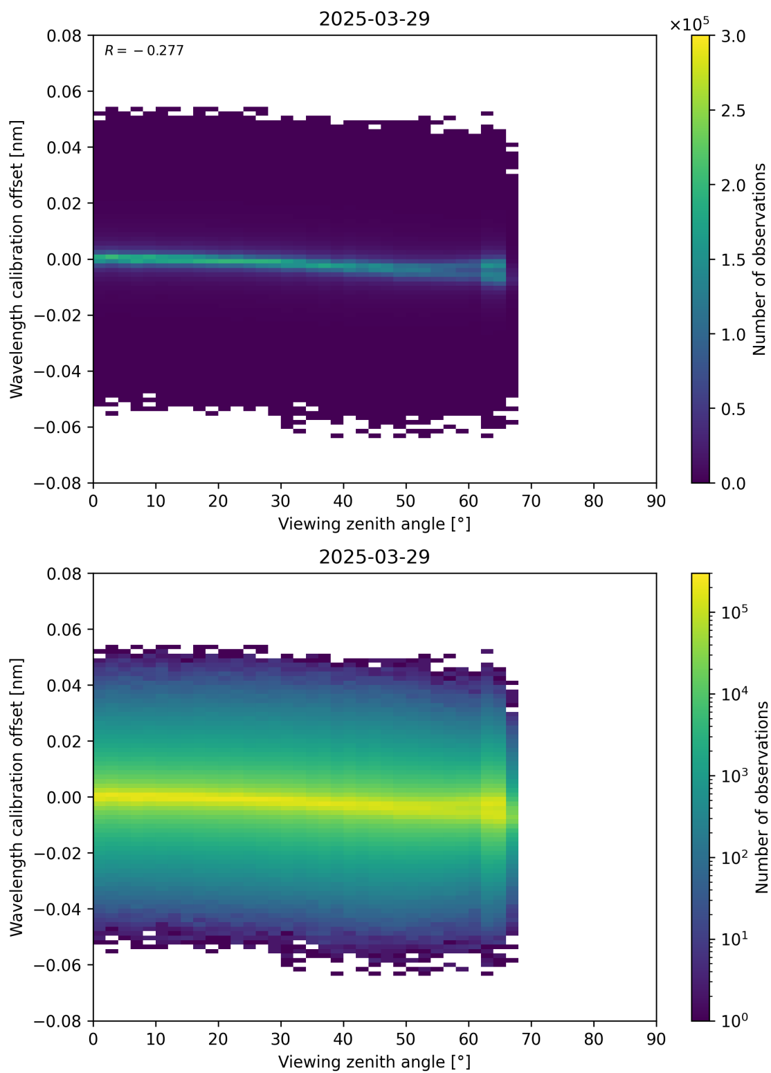
Figure 173: Scatter density plot of “Viewing zenith angle” against “Wavelength calibration offset” for 2025-03-29 to 2025-03-30.
