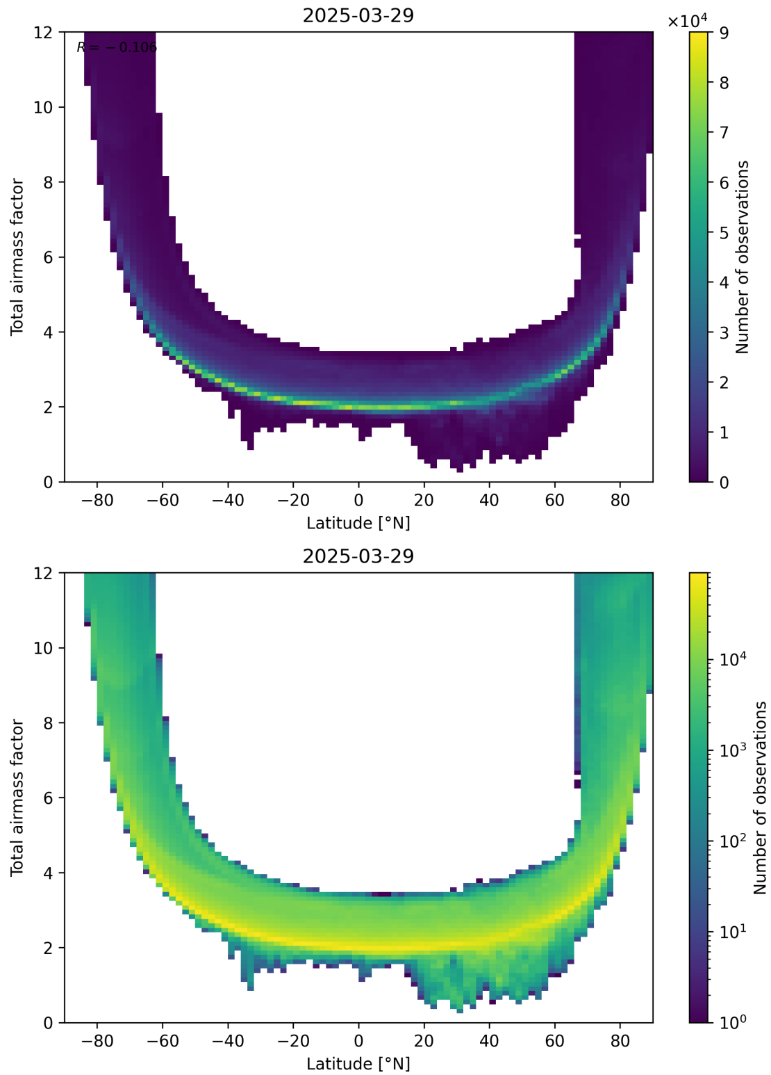
Figure 84: Scatter density plot of “Latitude” against “Total airmass factor” for 2025-03-29 to 2025-03-30.
