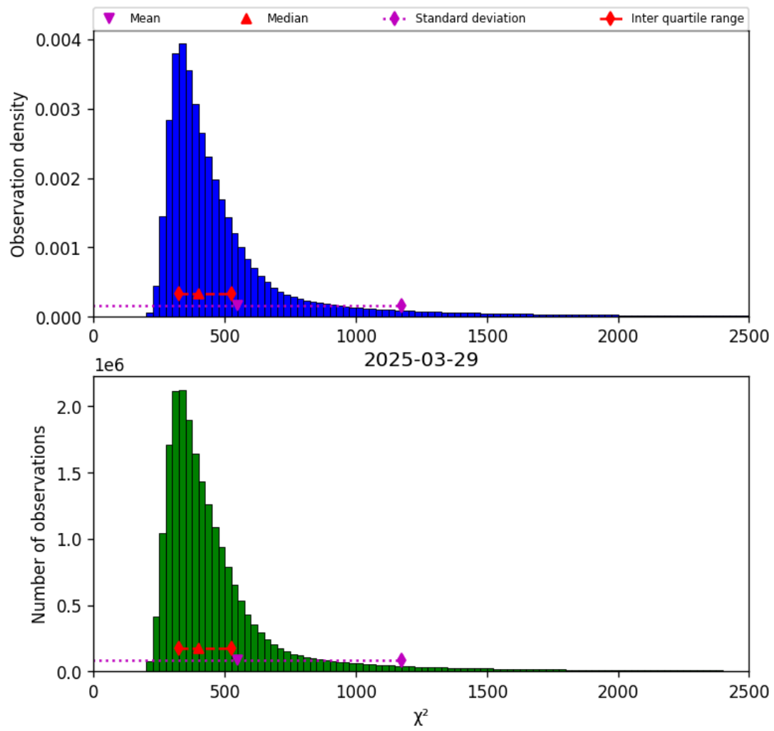
Figure 42: Histogram of “ \chi^2 ” for 2025-03-29 to 2025-03-30
