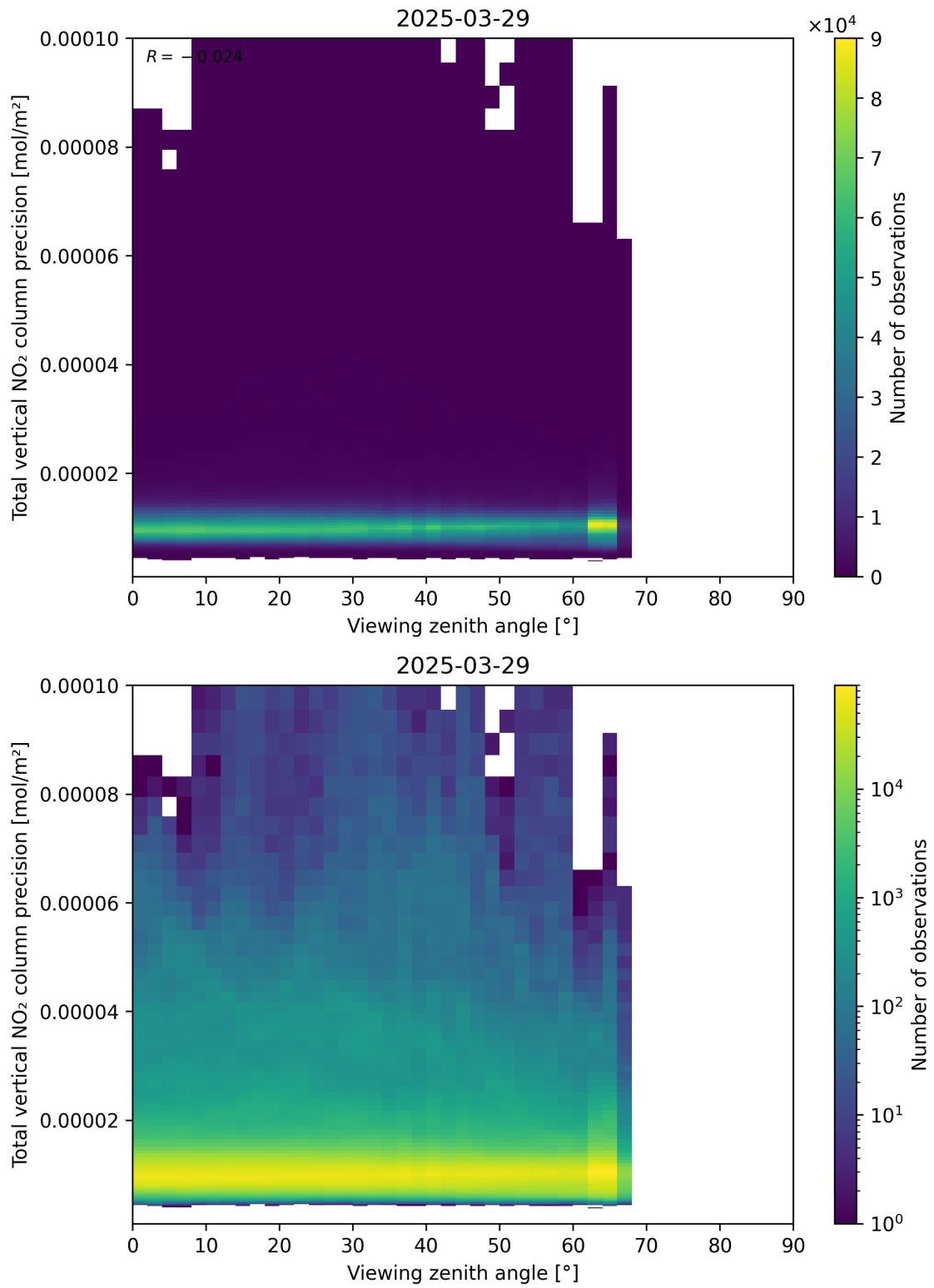
Figure 168: Scatter density plot of “Viewing zenith angle” against “Total vertical NO 2 column precision” for 2025-03-29 to 2025-03-30.
