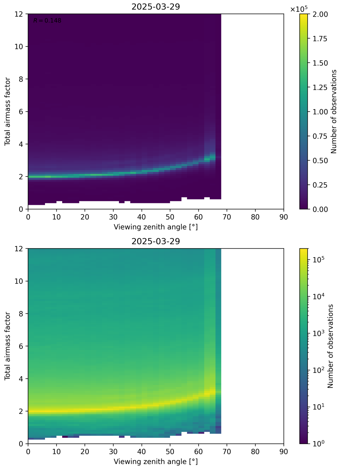
Figure 160: Scatter density plot of “Viewing zenith angle” against “Total airmass factor” for 2025-03-29 to 2025-03-30.
