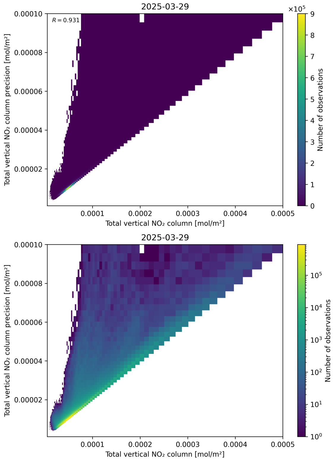
Figure 114: Scatter density plot of “Total vertical NO 2 column” against “Total vertical NO 2 column precision” for 2025-03-29 to 2025-03-30.
