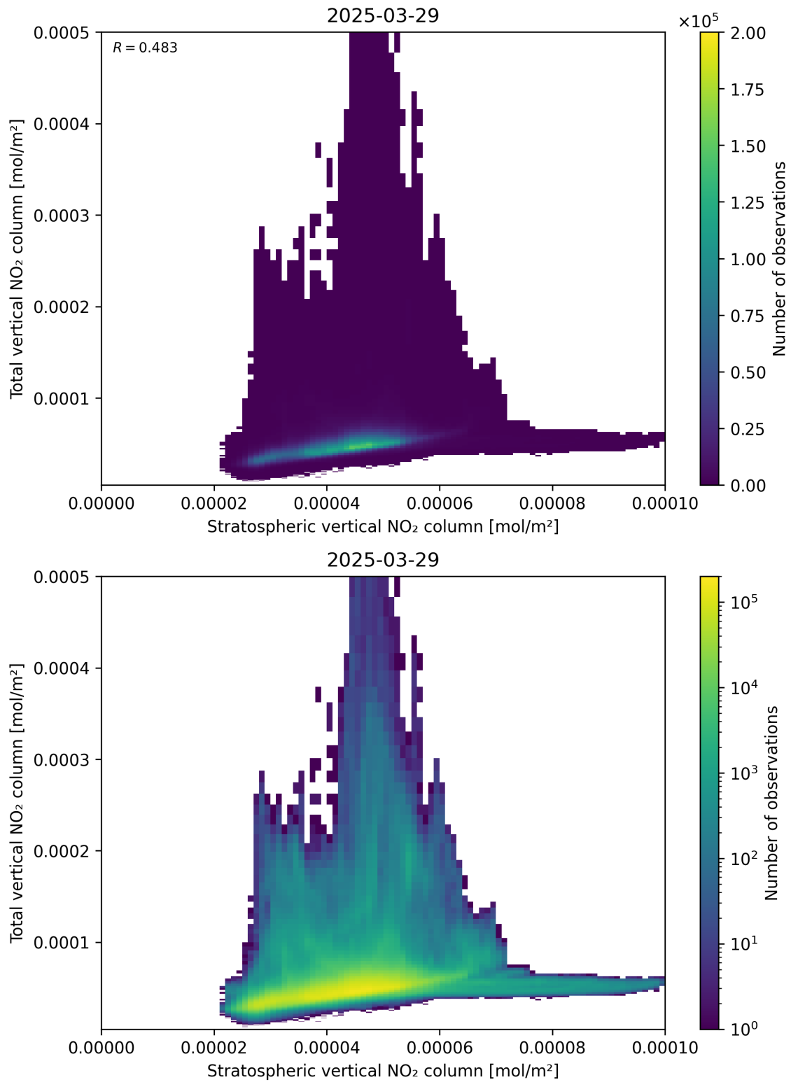
Figure 100: Scatter density plot of “Stratospheric vertical NO 2 column” against “Total vertical NO 2 column” for 2025-03-29 to 2025-03-30.
