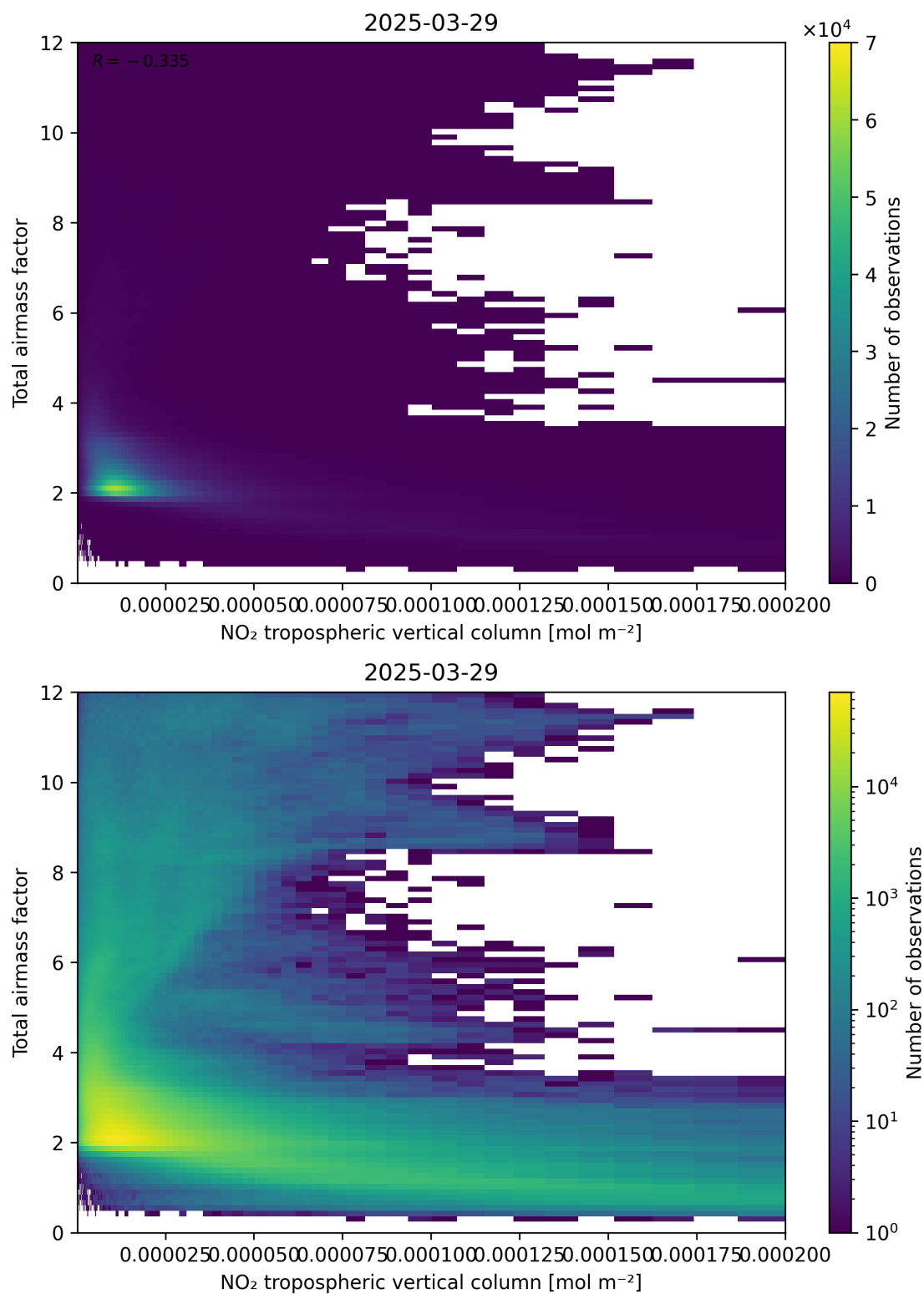
Figure 122: Scatter density plot of “NO 2 tropospheric vertical column” against “Total air mass factor” for 2025-03-29 to 2025-03-30.
