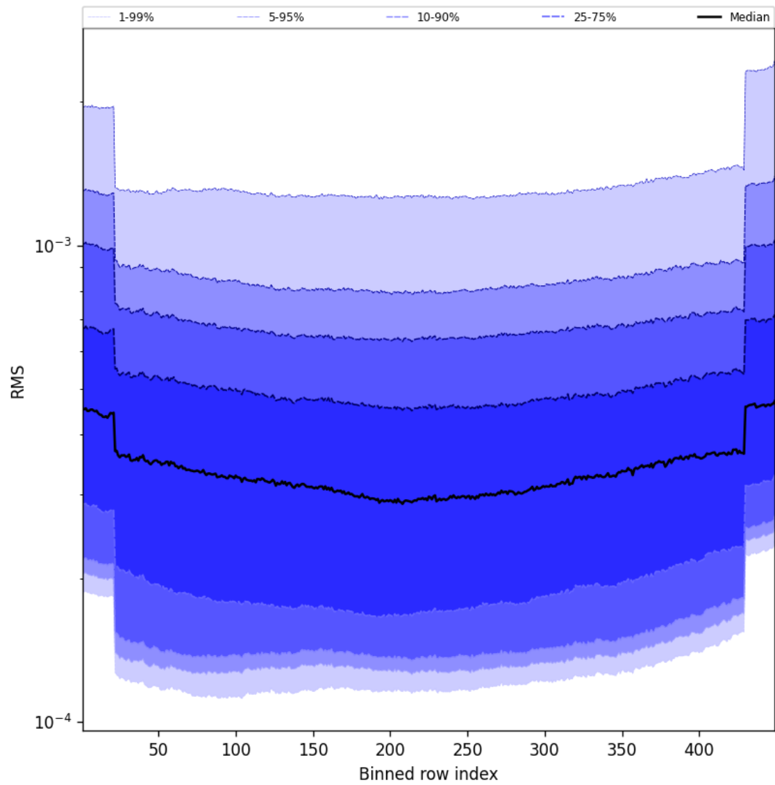
Figure 60: Along track statistics of “RMS” for 2025-03-29 to 2025-03-30
