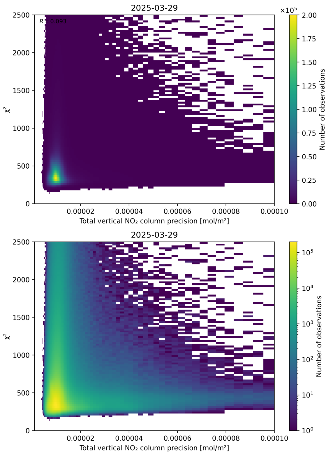
Figure 116: Scatter density plot of “Total vertical NO 2 column precision” against “ \chi^2 ” for 2025-03-29 to 2025-03-30.
