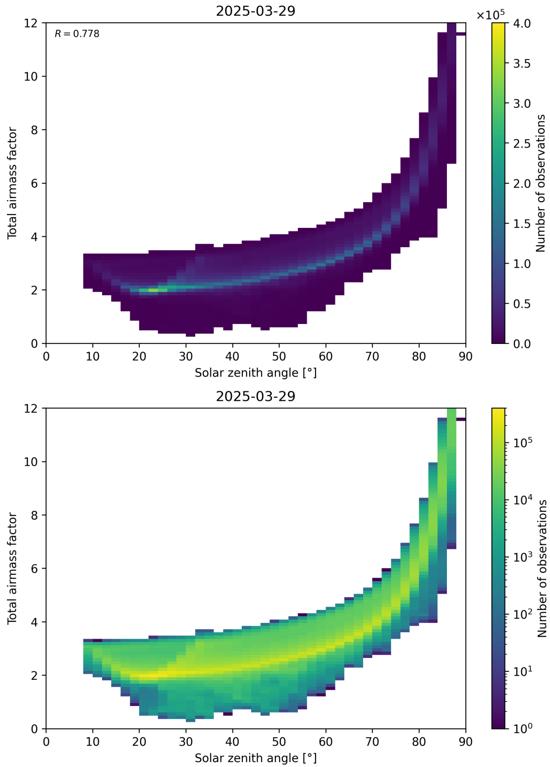
Figure 146: Scatter density plot of “Solar zenith angle” against “Total air mass factor” for 2025-03-29 to 2025-03-30.
