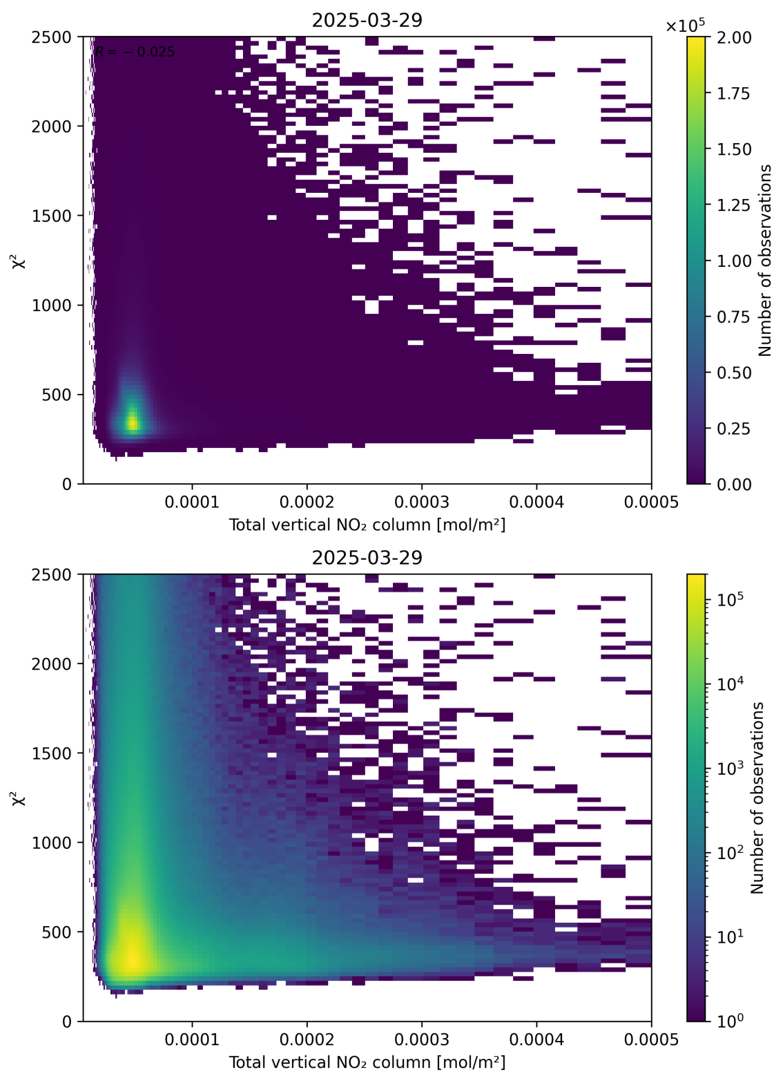
Figure 111: Scatter density plot of “Total vertical NO 2 column” against “ \chi^2 ” for 2025-03-29 to 2025-03-30.
