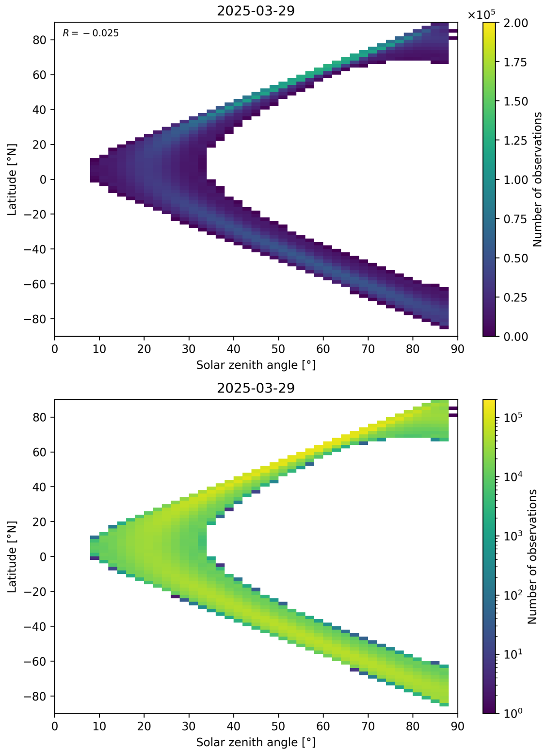
Figure 149: Scatter density plot of “Solar zenith angle” against “Latitude” for 2025-03-29 to 2025-03-30.
