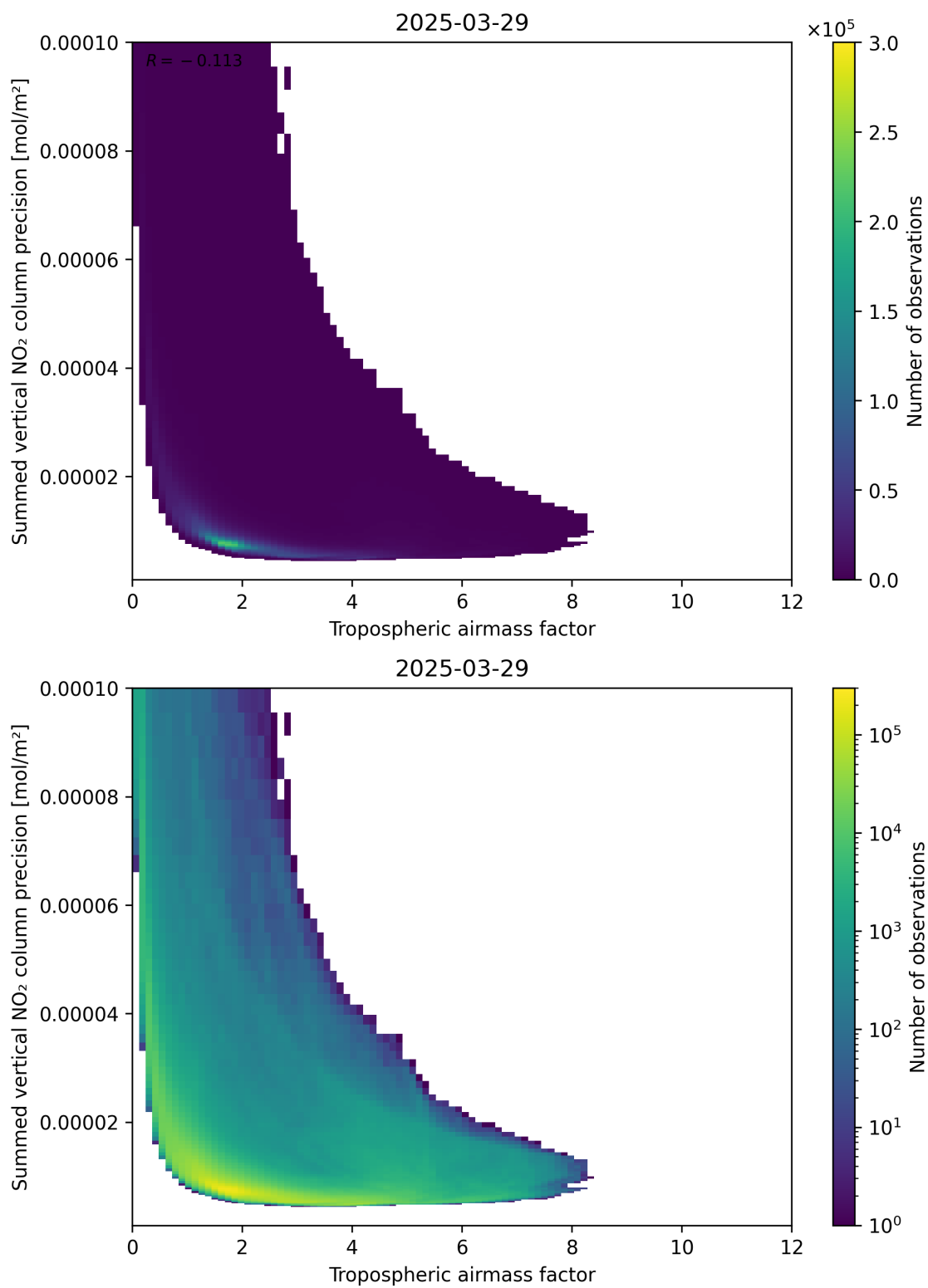
Figure 76: Scatter density plot of “Tropospheric air mass factor” against “Summed vertical NO 2 column precision” for 2025-03-29 to 2025-03-30.
