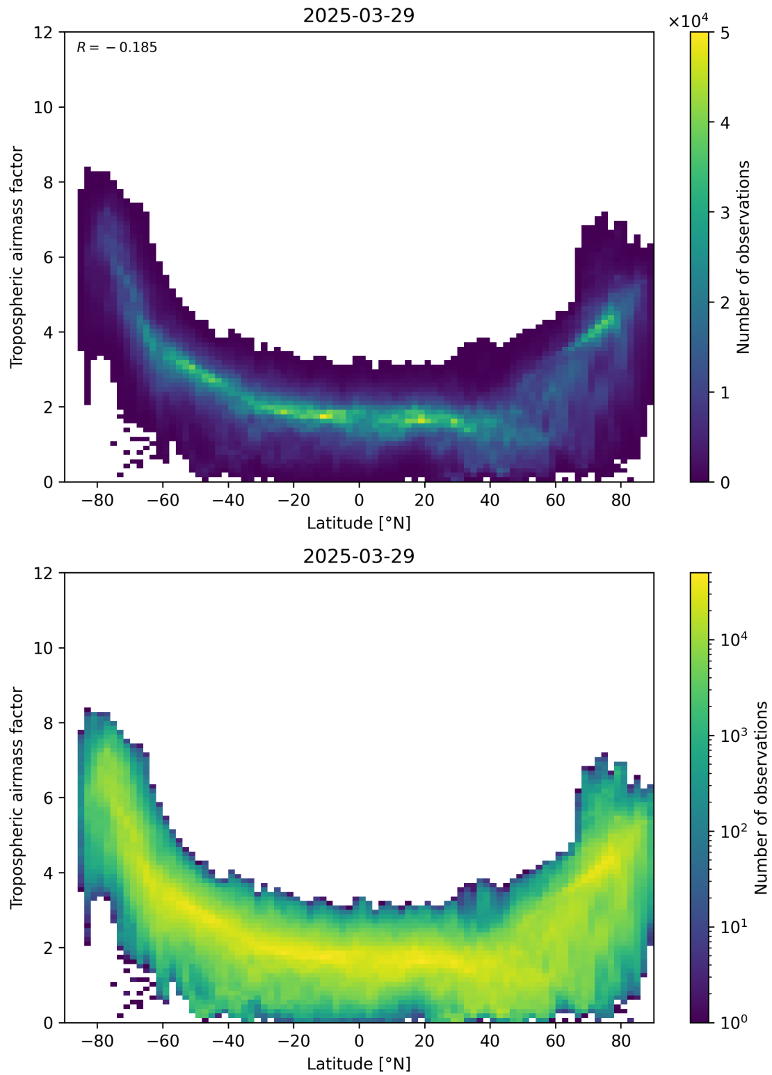
Figure 85: Scatter density plot of “Latitude” against “Tropospheric airmass factor” for 2025-03-29 to 2025-03-30.
