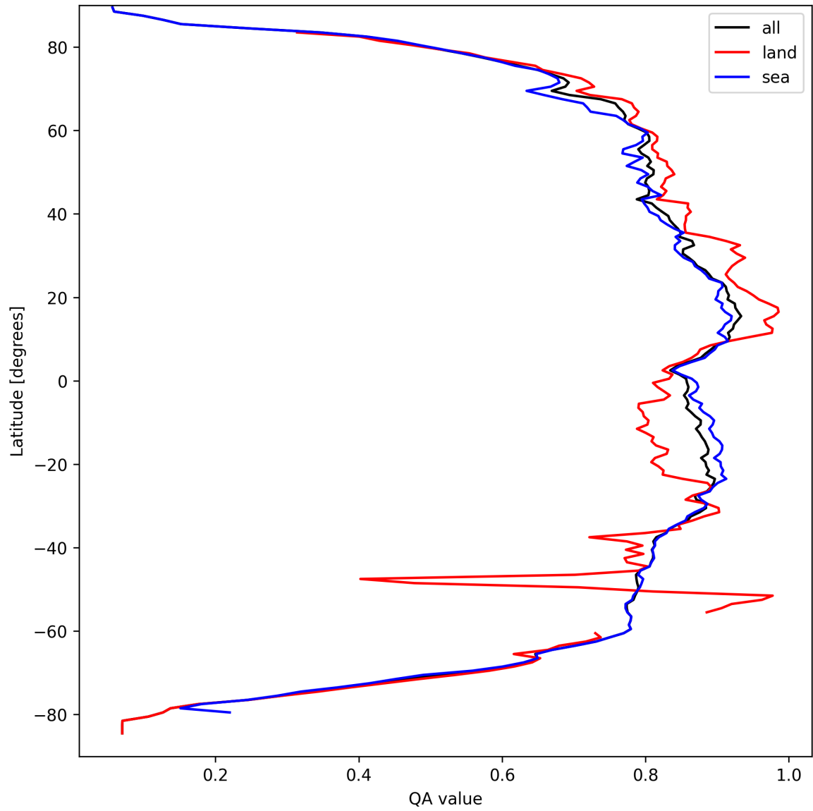
Figure 11: Zonal average of “QA value” for 2025-03-29 to 2025-03-30.
