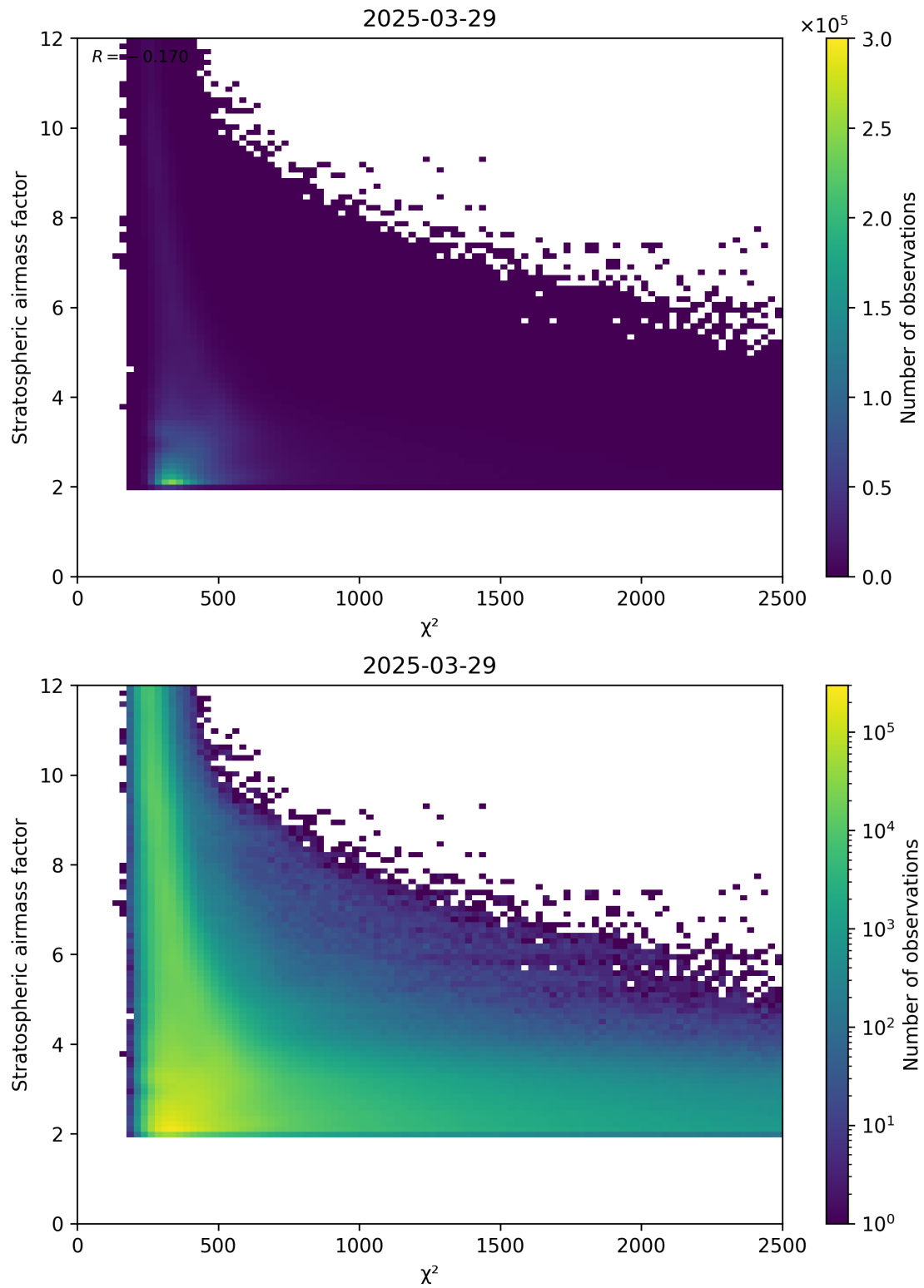
Figure 81: Scatter density plot of “ \chi^2 ” against “Stratospheric airmass factor” for 2025-03-29 to 2025-03-30.
