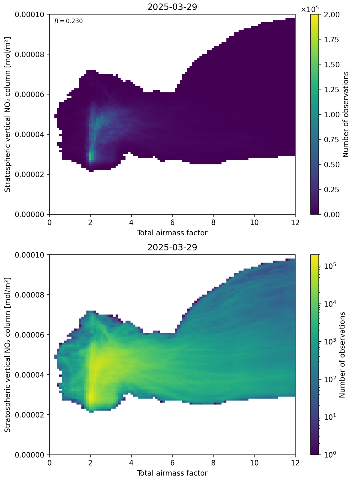
Figure 64: Scatter density plot of “Total airmass factor” against “Stratospheric vertical \text{NO}_2 column” for 2025-03-29 to 2025-03-30.
