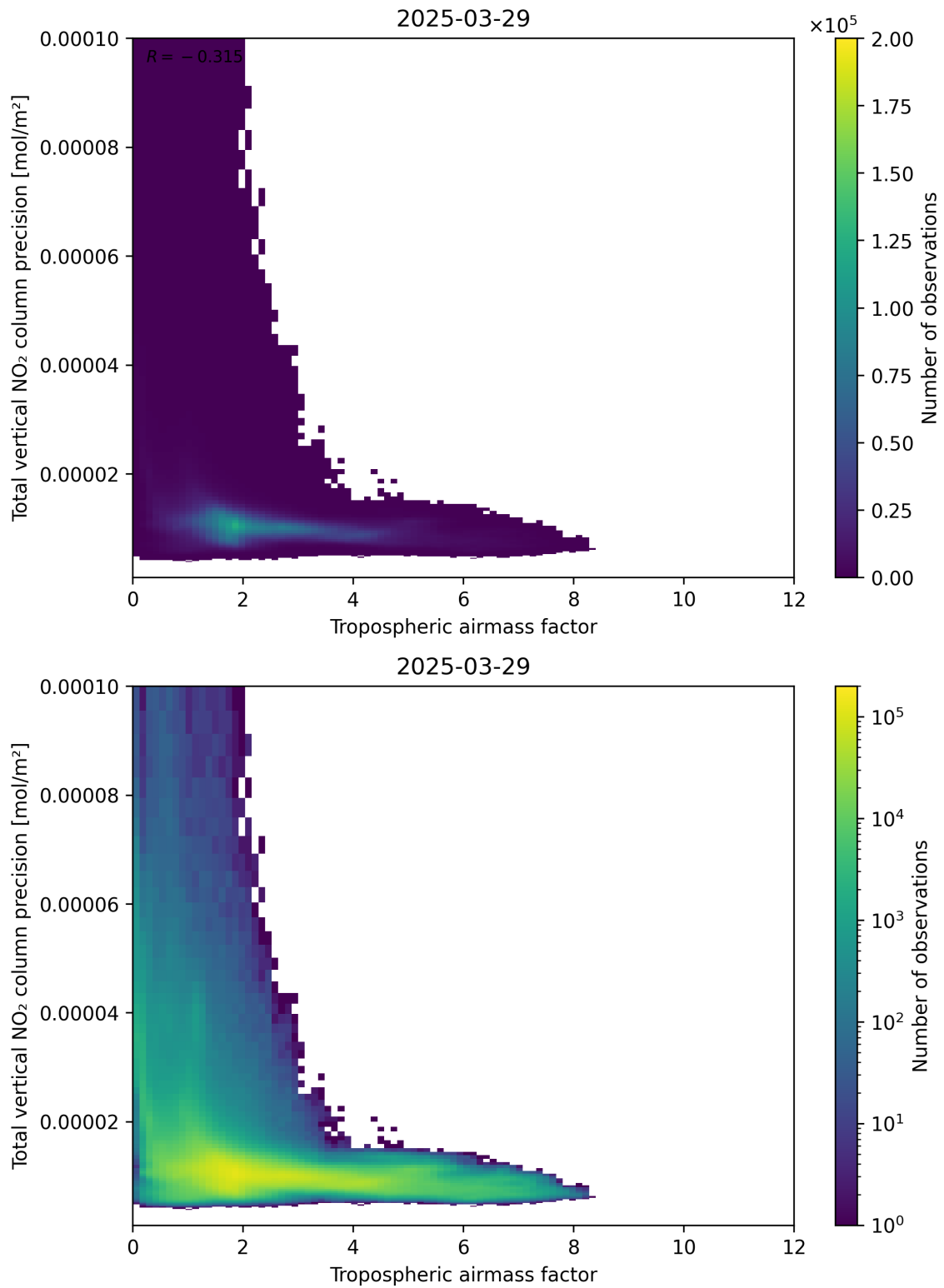
Figure 78: Scatter density plot of “Tropospheric air mass factor” against “Total vertical NO 2 column precision” for 2025-03-29 to 2025-03-30.
