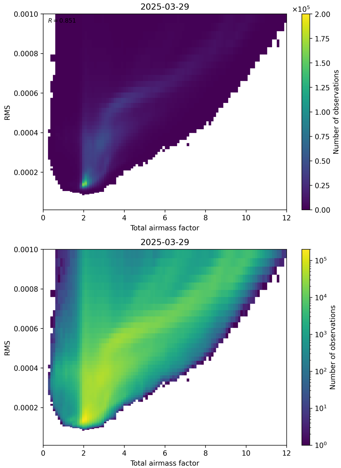
Figure 69: Scatter density plot of “Total airmass factor” against “RMS” for 2025-03-29 to 2025-03-30.
