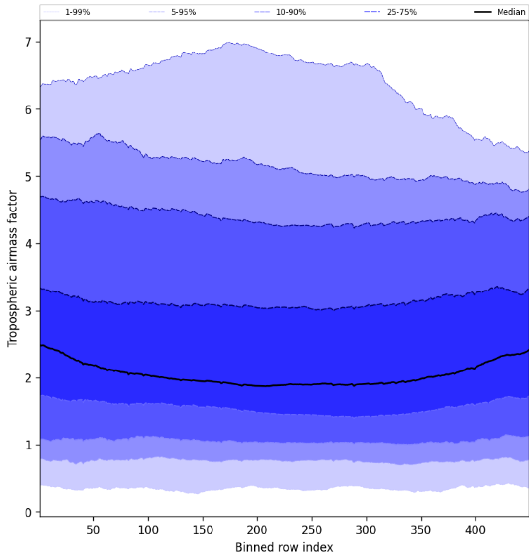
Figure 48: Along track statistics of “Tropospheric airmass factor” for 2025-03-29 to 2025-03-30
