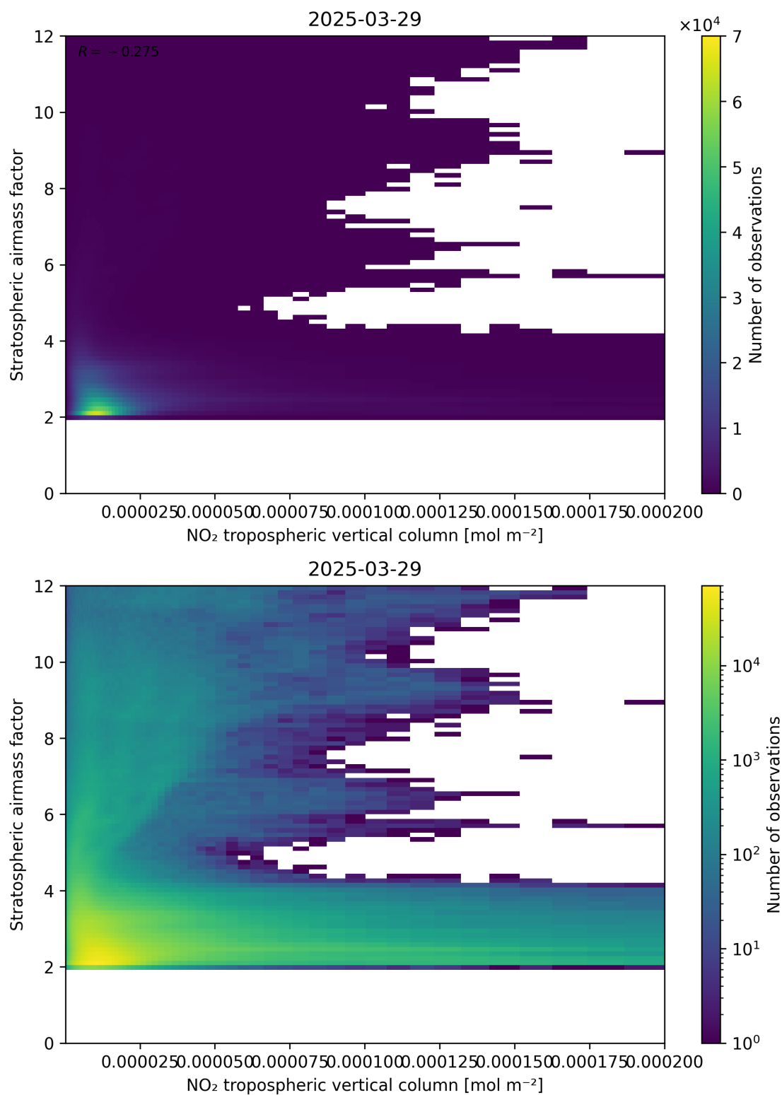
Figure 121: Scatter density plot of “NO 2 tropospheric vertical column” against “Stratospheric air mass factor” for 2025-03-29 to 2025-03-30.
