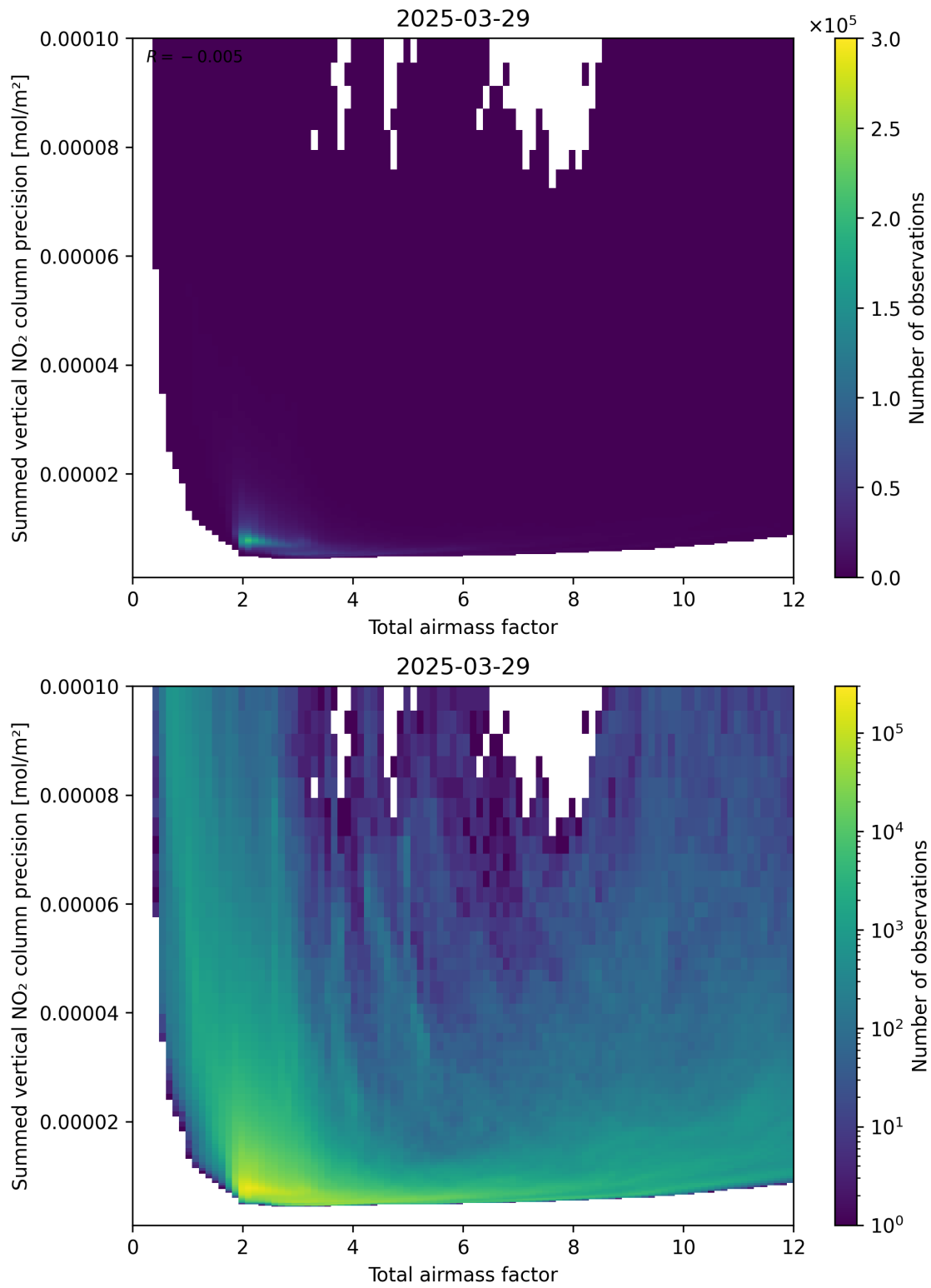
Figure 66: Scatter density plot of “Total airmass factor” against “Summed vertical NO 2 column precision” for 2025-03-29 to 2025-03-30.
