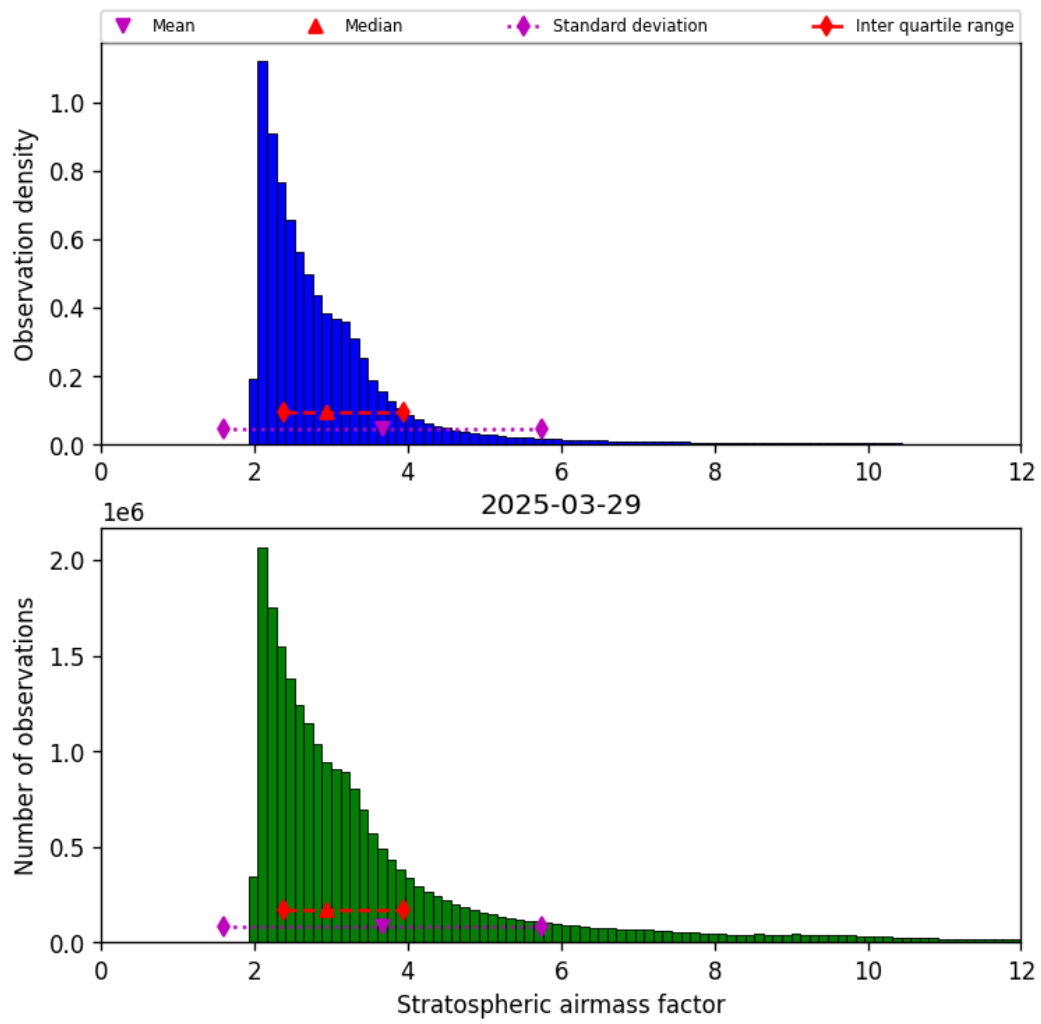
Figure 44: Histogram of “Stratospheric airmass factor” for 2025-03-29 to 2025-03-30
