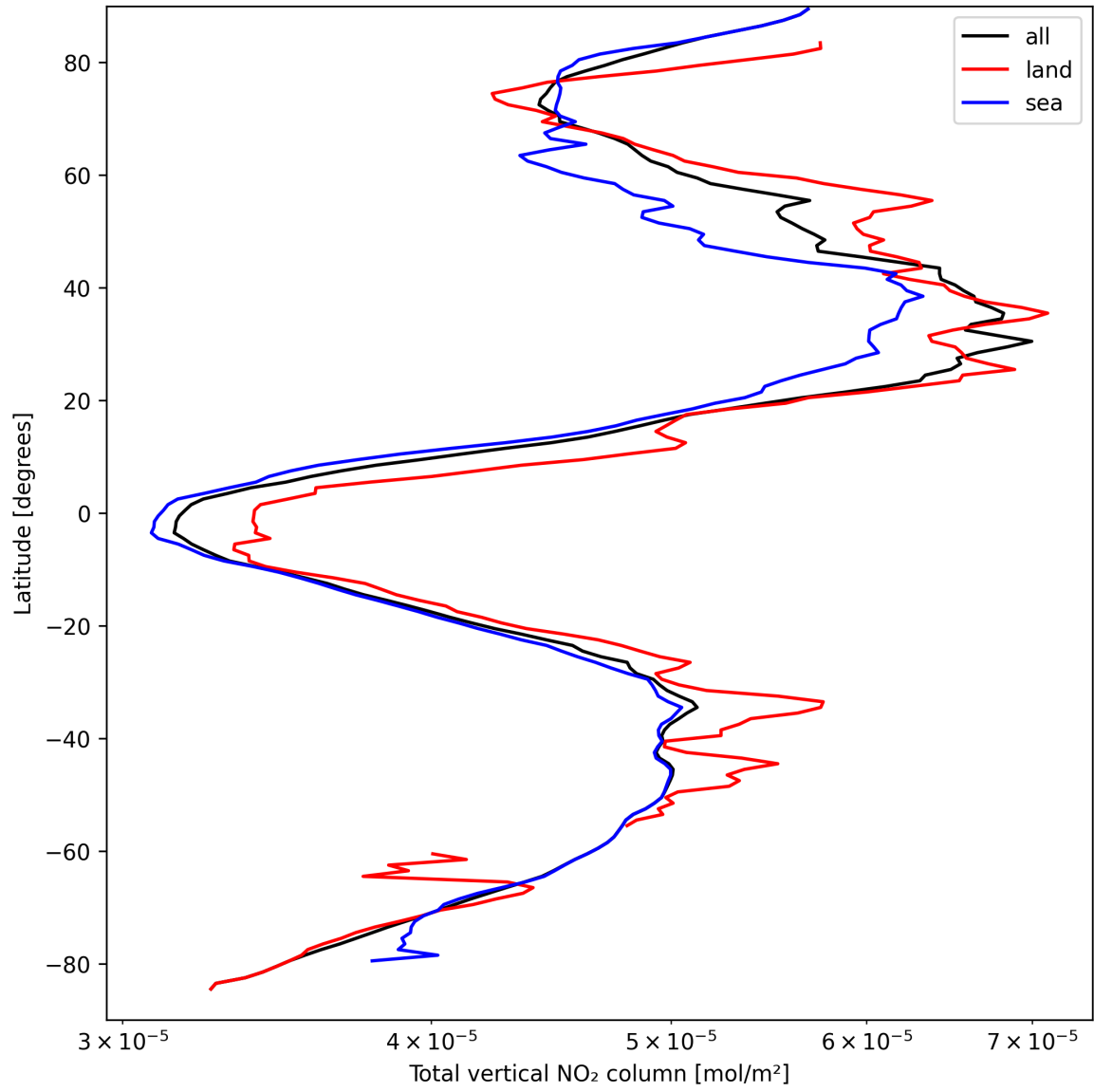
Figure 21: Zonal average of “Total vertical NO 2 column” for 2025-03-29 to 2025-03-30.
