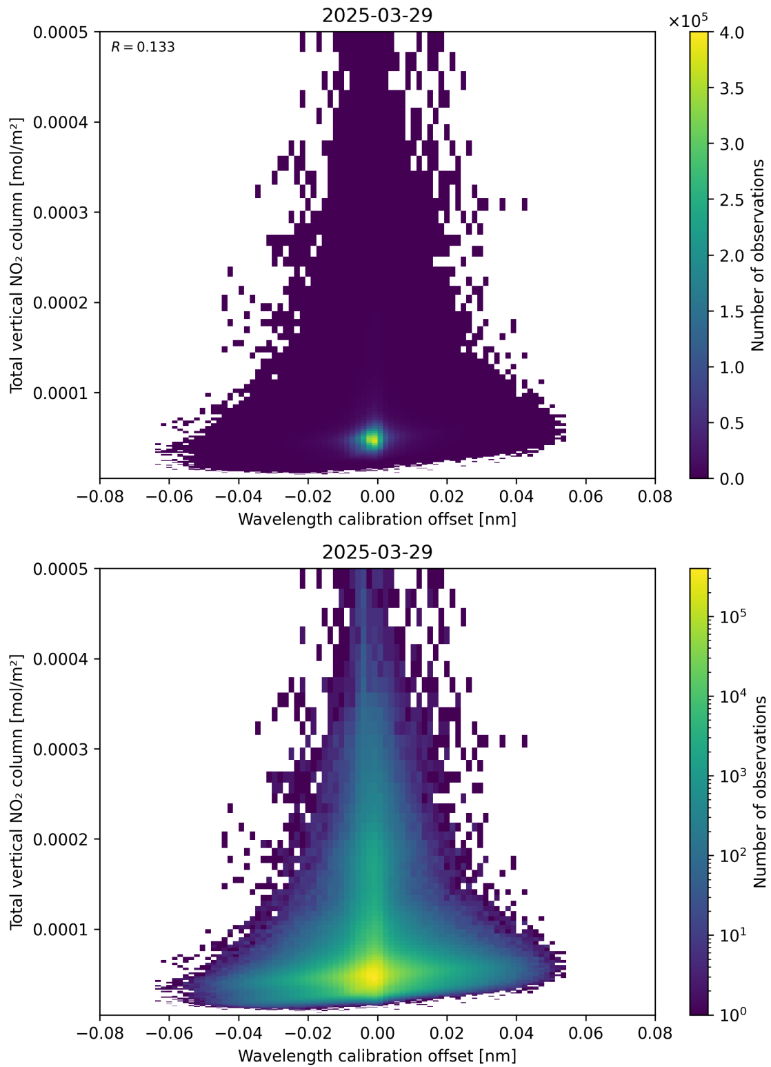
Figure 179: Scatter density plot of “Wavelength calibration offset” against “Total vertical NO 2 column” for 2025-03-29 to 2025-03-30.
