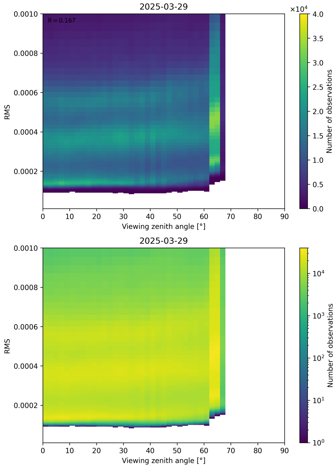
Figure 171: Scatter density plot of “Viewing zenith angle” against “RMS” for 2025-03-29 to 2025-03-30.
