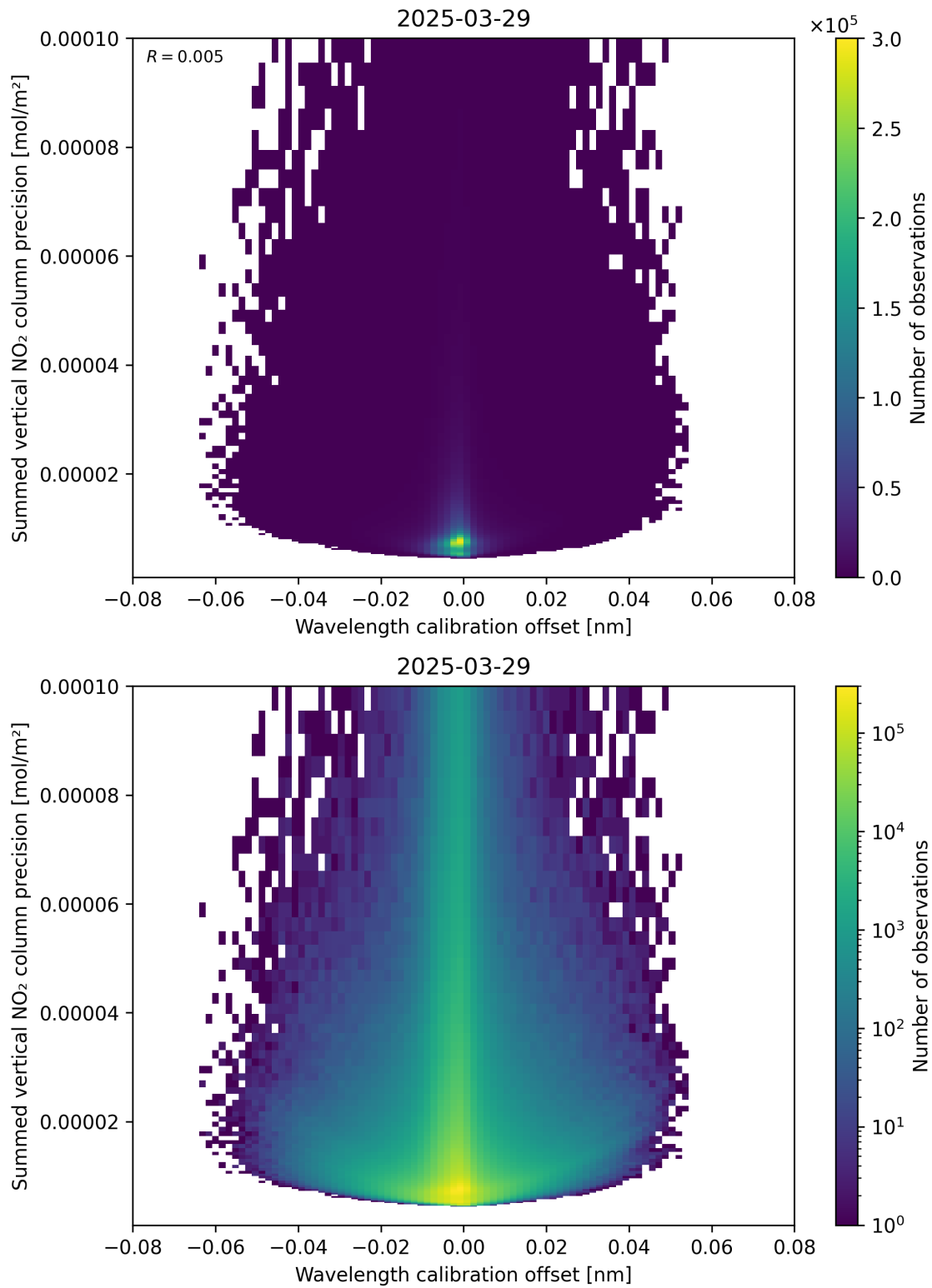
Figure 178: Scatter density plot of “Wavelength calibration offset” against “Summed vertical NO 2 column precision” for 2025-03-29 to 2025-03-30.
