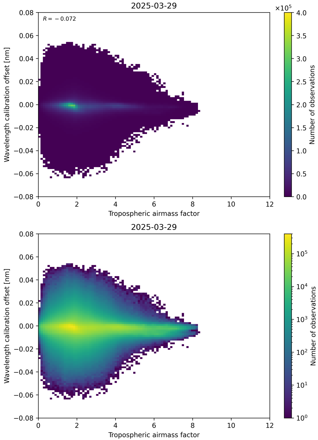
Figure 80: Scatter density plot of “Tropospheric airmass factor” against “Wavelength calibration offset” for 2025-03-29 to 2025-03-30.
