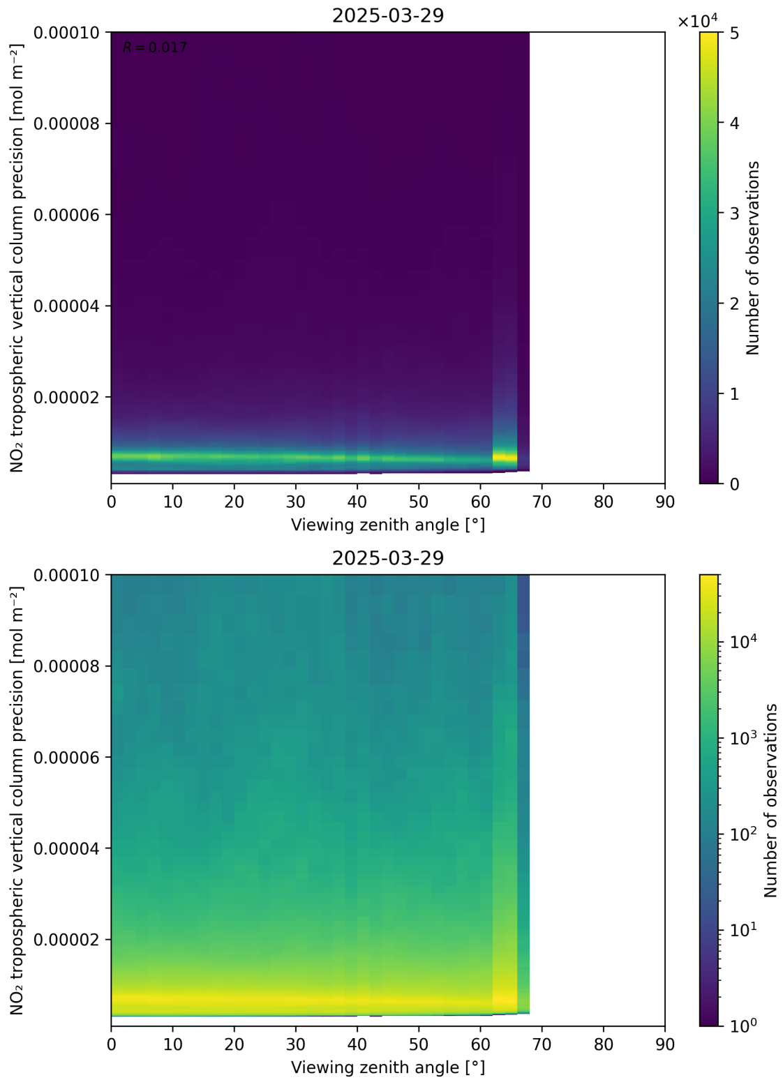
Figure 170: Scatter density plot of “Viewing zenith angle” against “NO 2 tropospheric vertical column precision” for 2025-03-29 to 2025-03-30.
