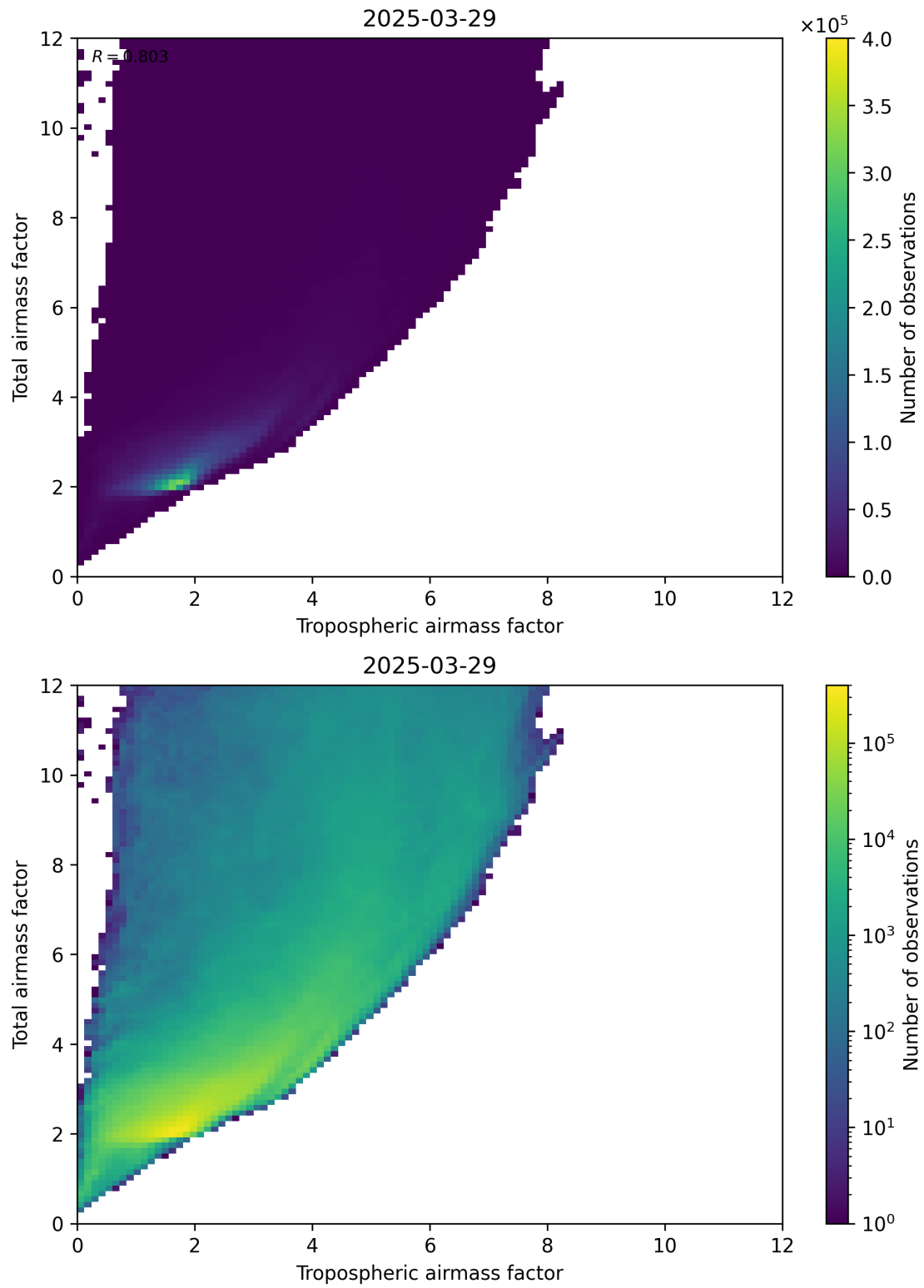
Figure 72: Scatter density plot of “Tropospheric airmass factor” against “Total airmass factor” for 2025-03-29 to 2025-03-30.
