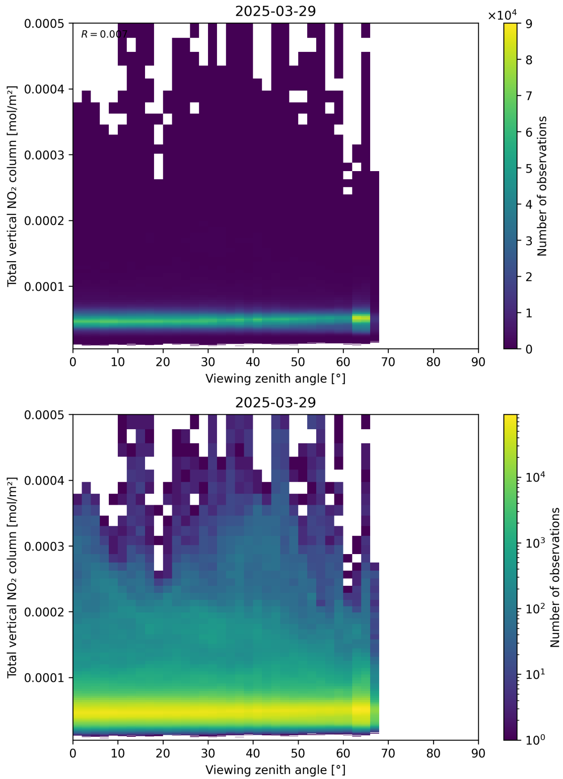
Figure 167: Scatter density plot of “Viewing zenith angle” against “Total vertical NO 2 column” for 2025-03-29 to 2025-03-30.
