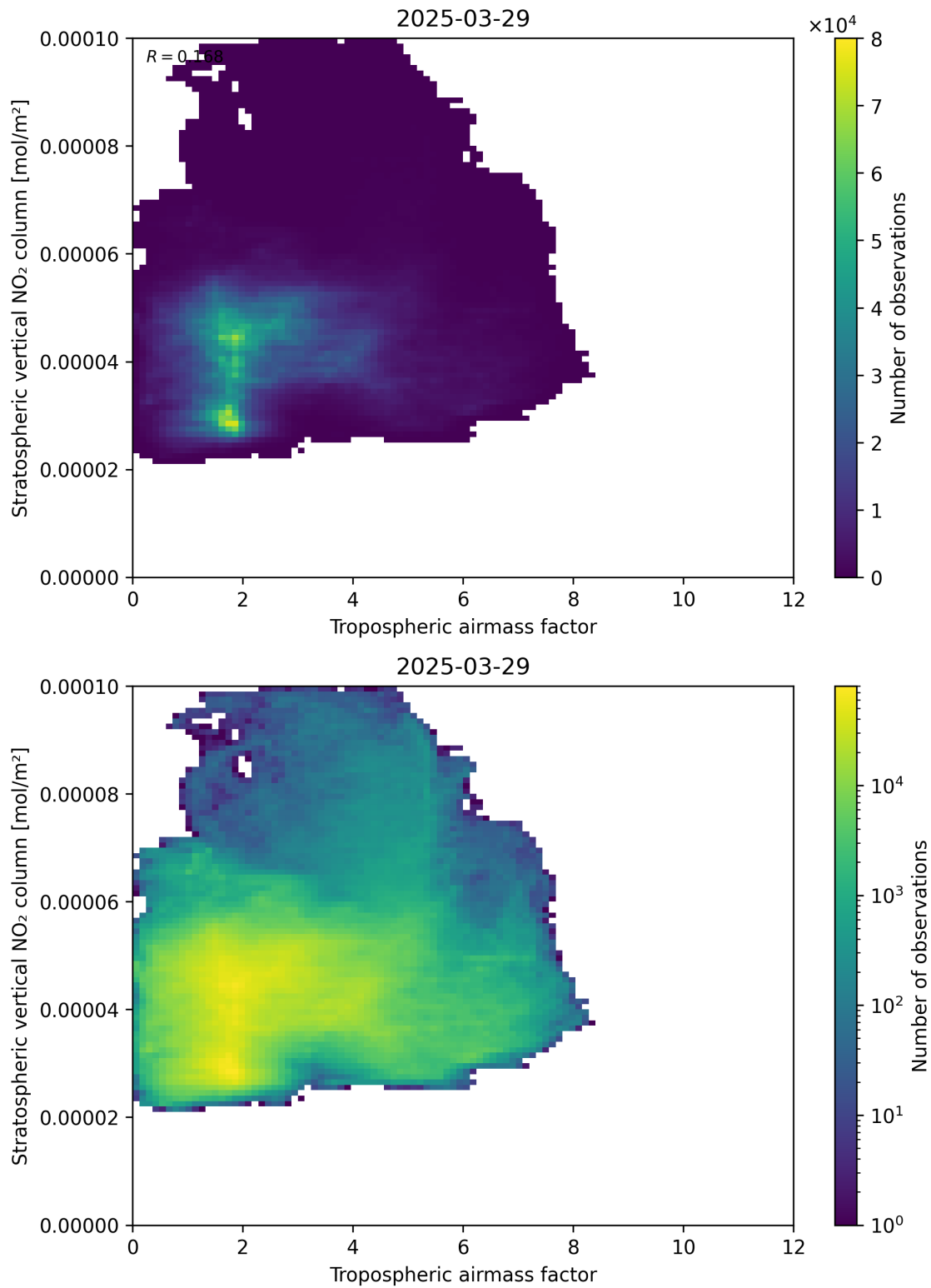
Figure 74: Scatter density plot of “Tropospheric air mass factor” against “Stratospheric vertical NO 2 column” for 2025-03-29 to 2025-03-30.
