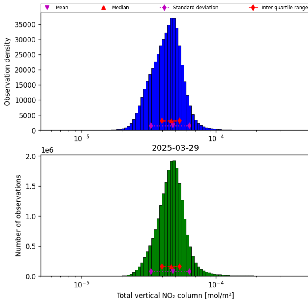
Figure 38: Histogram of “Total vertical NO 2 column” for 2025-03-29 to 2025-03-30
