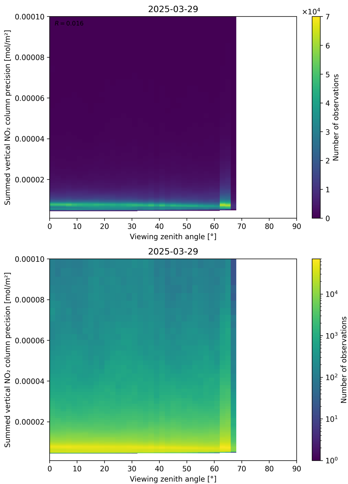
Figure 166: Scatter density plot of “Viewing zenith angle” against “Summed vertical NO 2 column precision” for 2025-03-29 to 2025-03-30.
