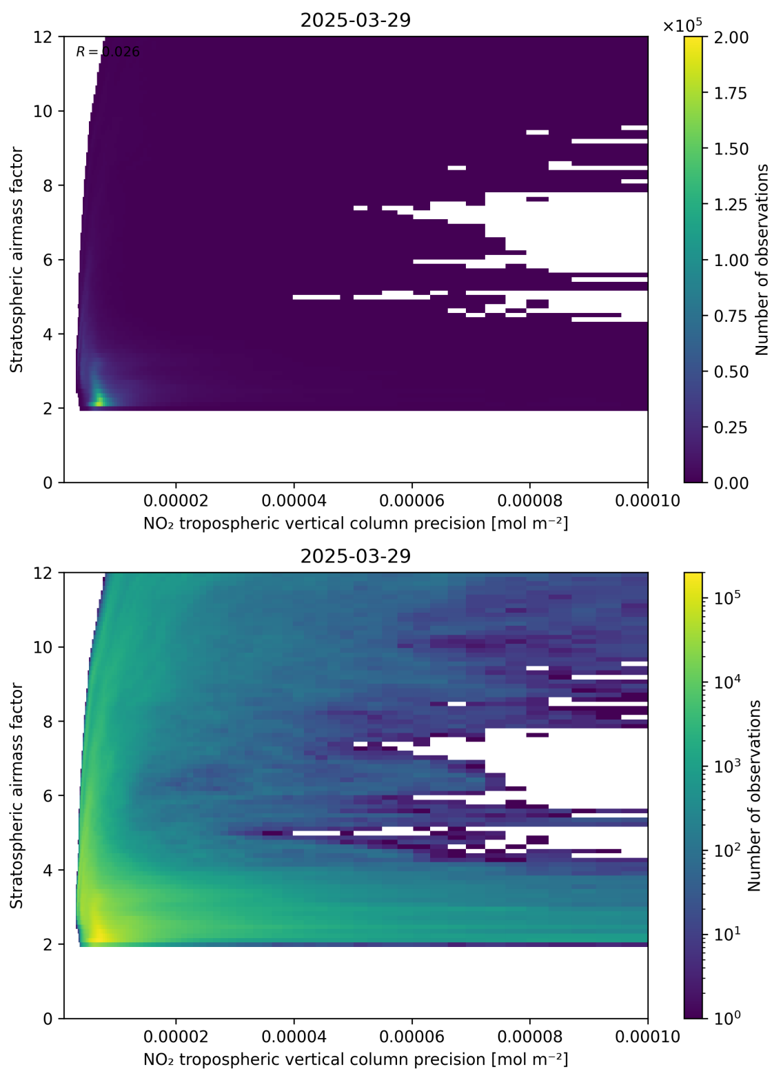
Figure 131: Scatter density plot of “NO 2 tropospheric vertical column precision” against “Stratospheric airmass factor” for 2025-03-29 to 2025-03-30.
