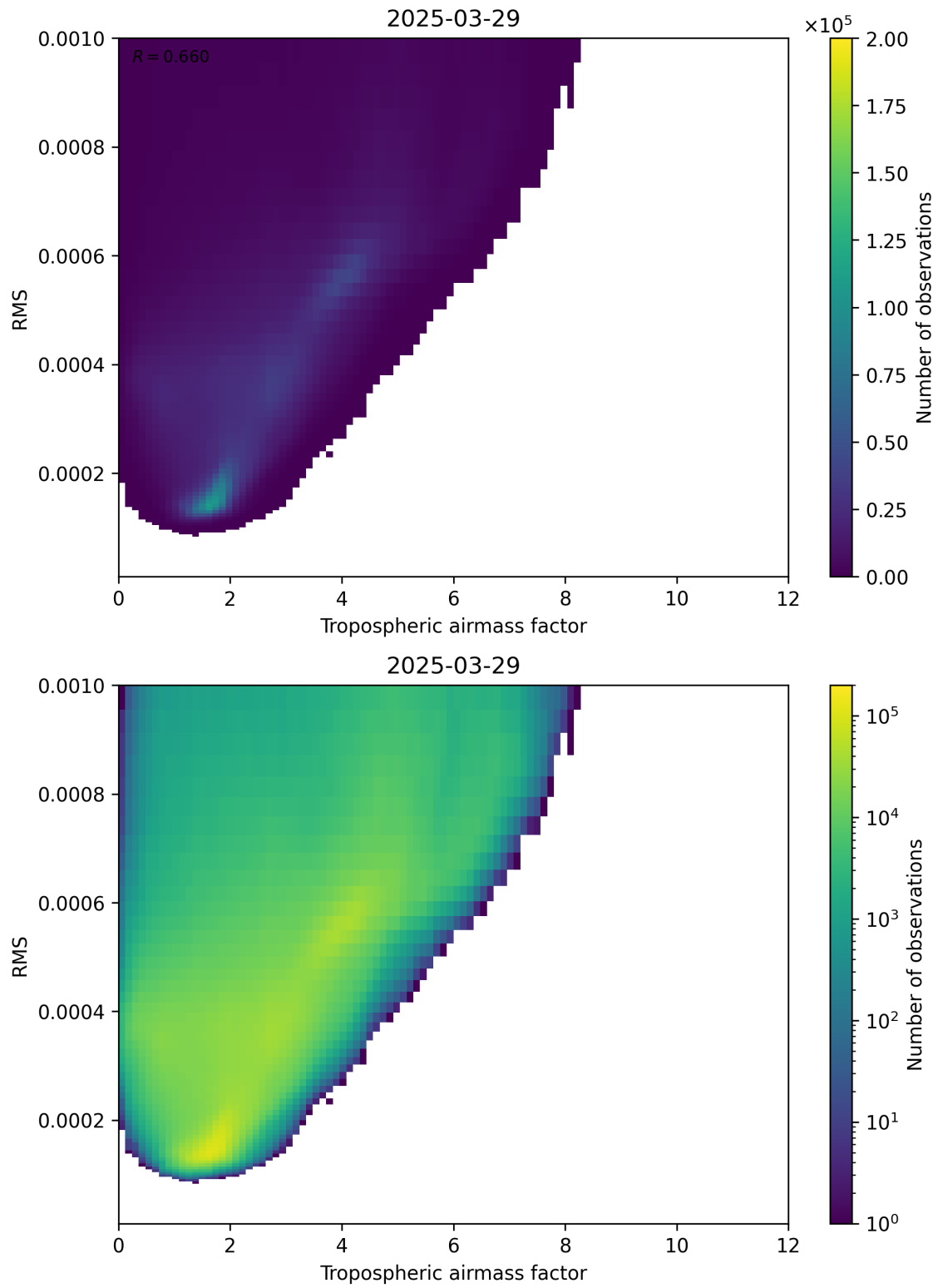
Figure 79: Scatter density plot of “Tropospheric airmass factor” against “RMS” for 2025-03-29 to 2025-03-30.
