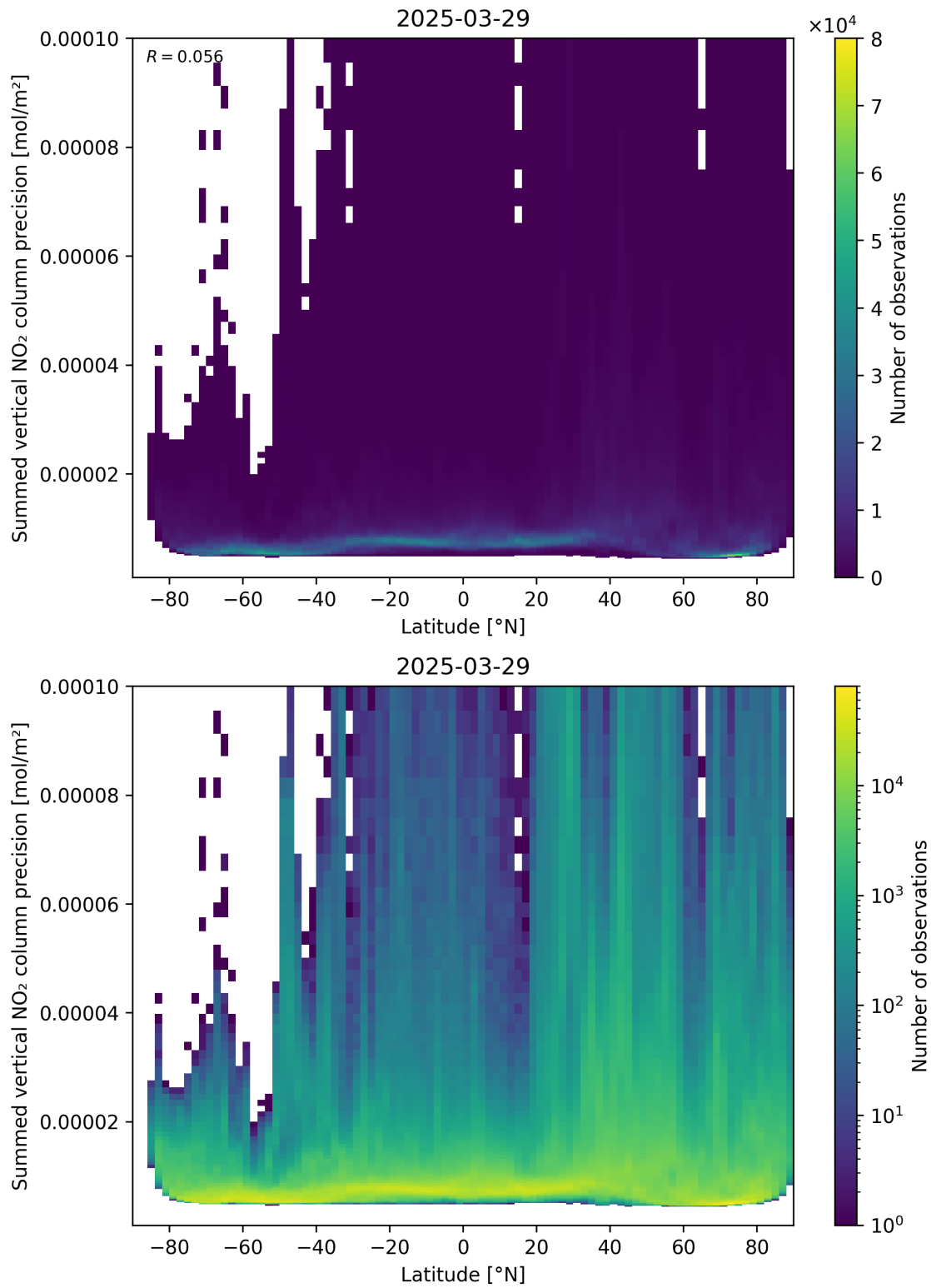
Figure 89: Scatter density plot of “Latitude” against “Summed vertical NO 2 column precision” for 2025-03-29 to 2025-03-30.
