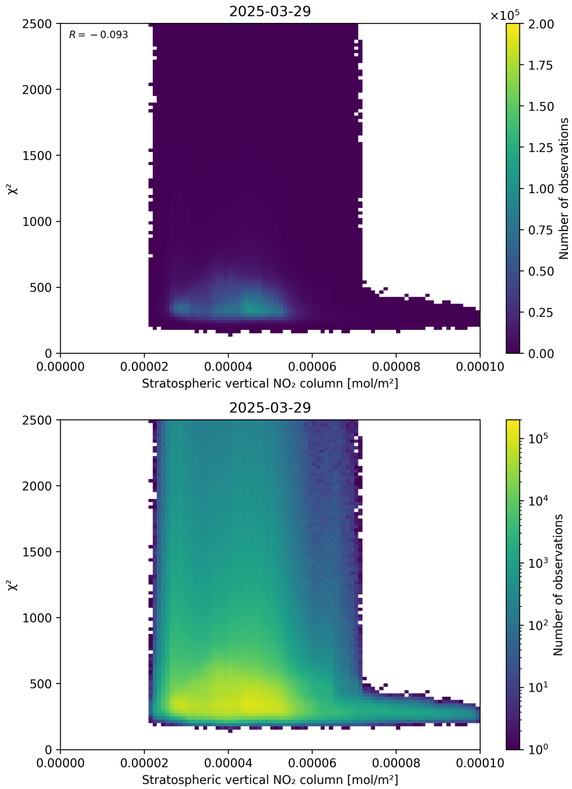
Figure 97: Scatter density plot of “Stratospheric vertical NO 2 column” against “ \chi^2 ” for 2025-03-29 to 2025-03-30.
