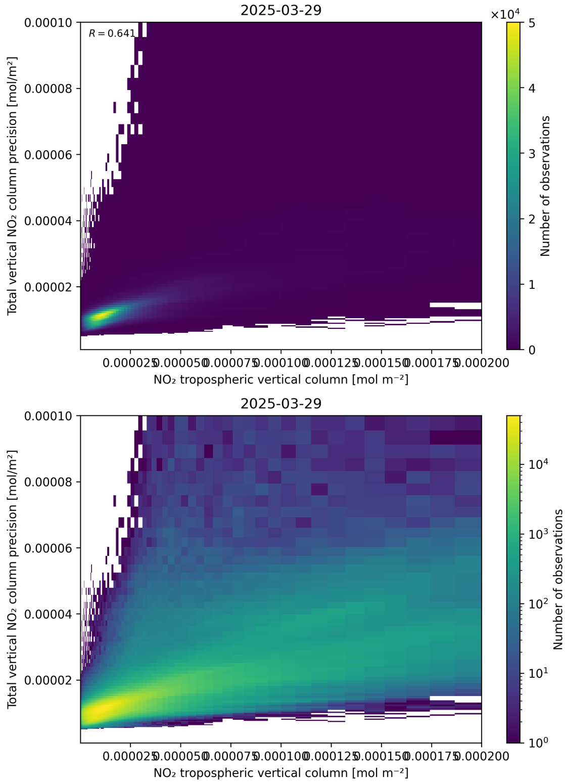
Figure 129: Scatter density plot of “NO 2 tropospheric vertical column” against “Total vertical NO 2 column precision” for 2025-03-29 to 2025-03-30.
