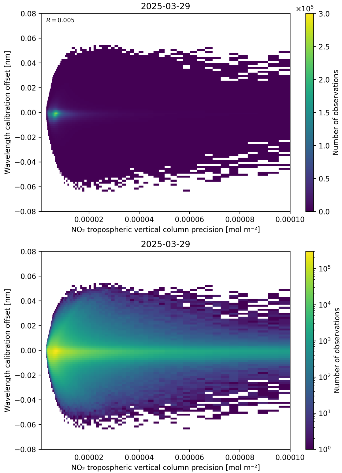
Figure 141: Scatter density plot of “NO 2 tropospheric vertical column precision” against “Wavelength calibration offset” for 2025-03-29 to 2025-03-30.
