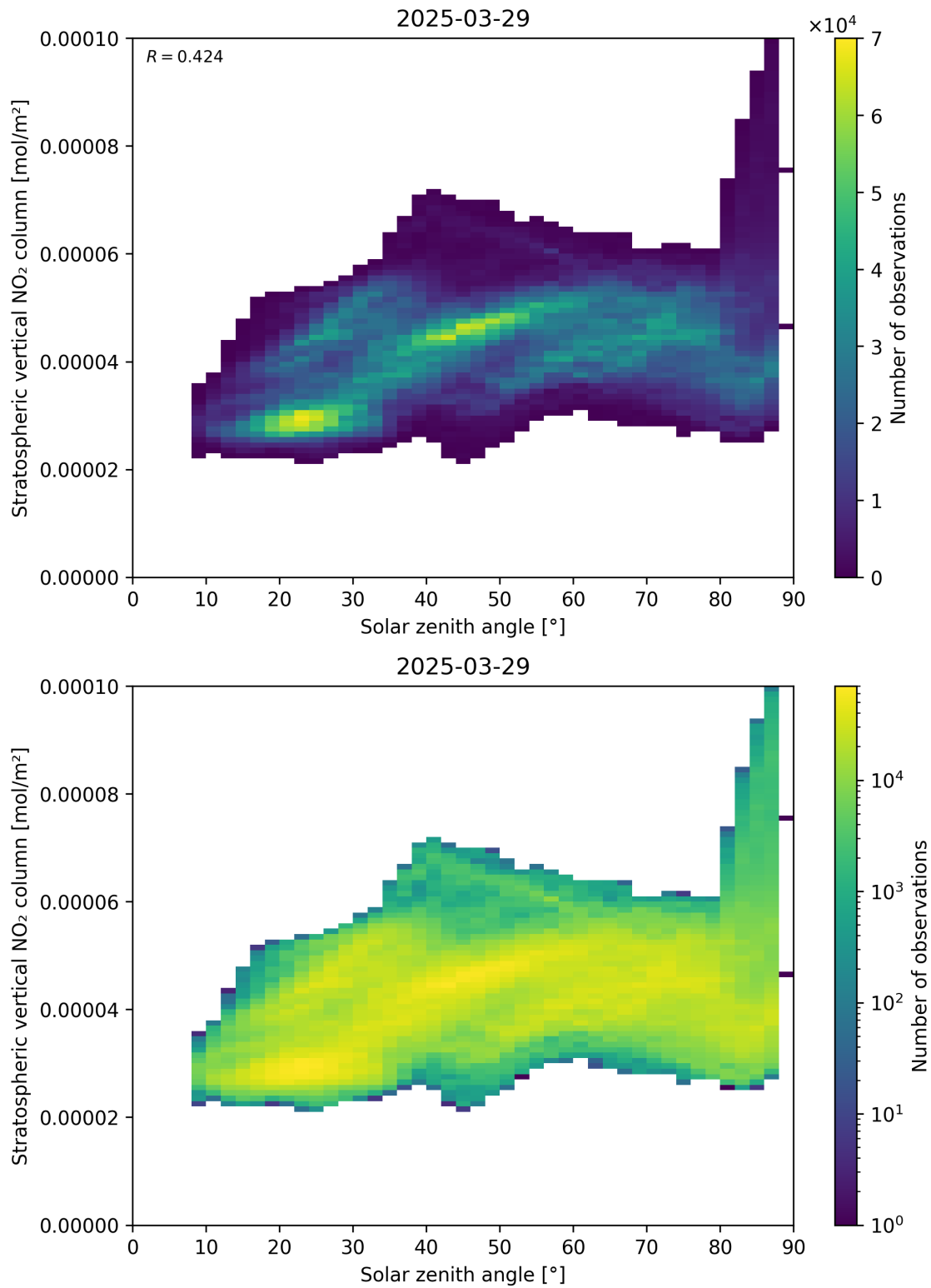
Figure 150: Scatter density plot of “Solar zenith angle” against “Stratospheric vertical NO 2 column” for 2025-03-29 to 2025-03-30.
