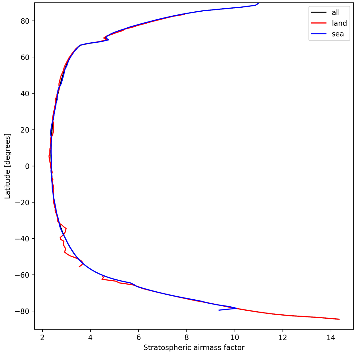
Figure 27: Zonal average of “Stratospheric air mass factor” for 2025-03-29 to 2025-03-30.
