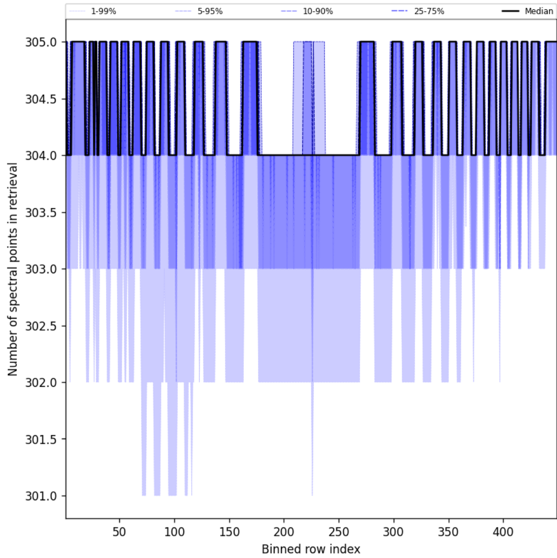
Figure 50: Along track statistics of “Number of spectral points in retrieval” for 2025-03-29 to 2025-03-30
