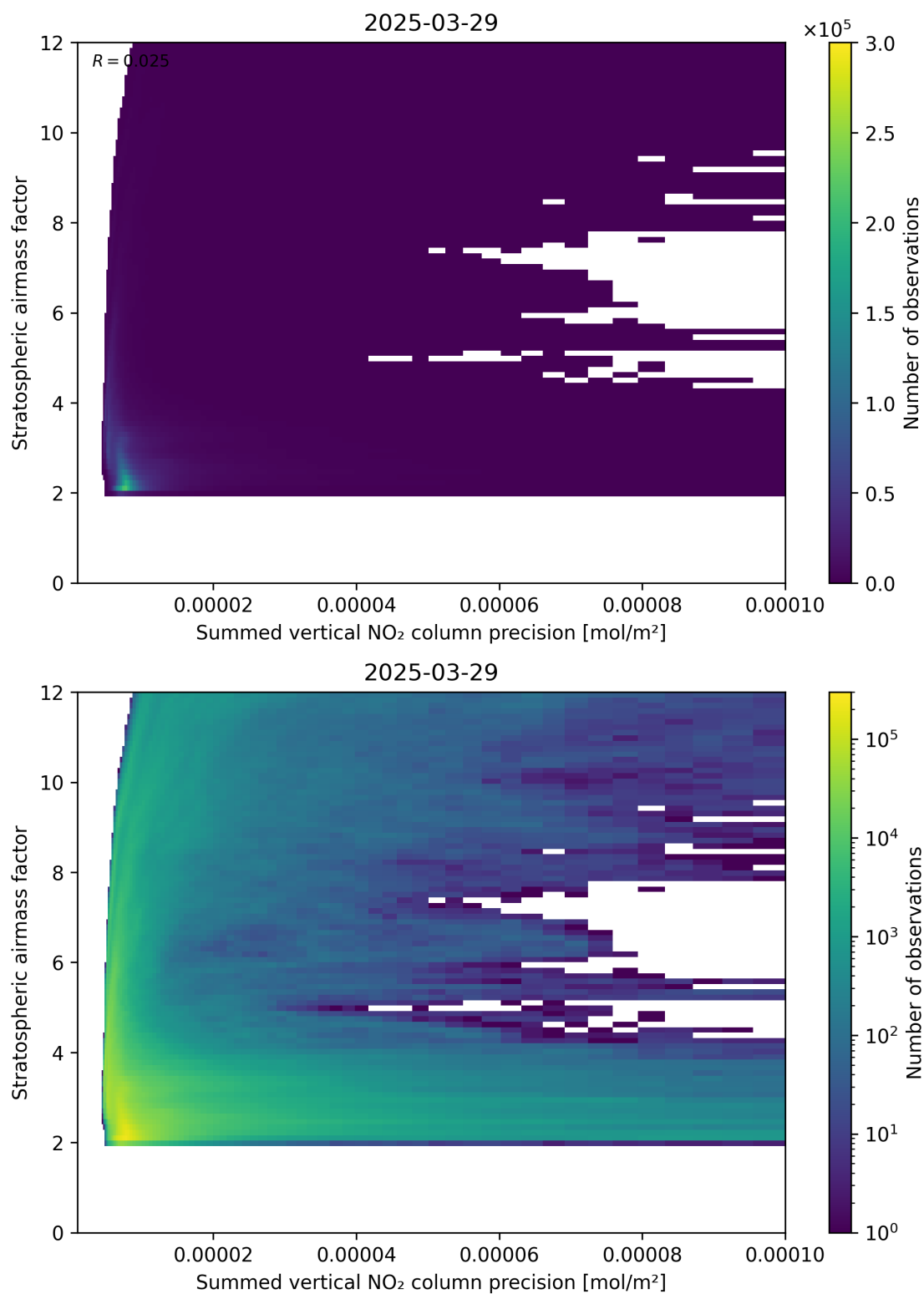
Figure 106: Scatter density plot of “Summed vertical NO 2 column precision” against “Stratospheric airmass factor” for 2025-03-29 to 2025-03-30.
