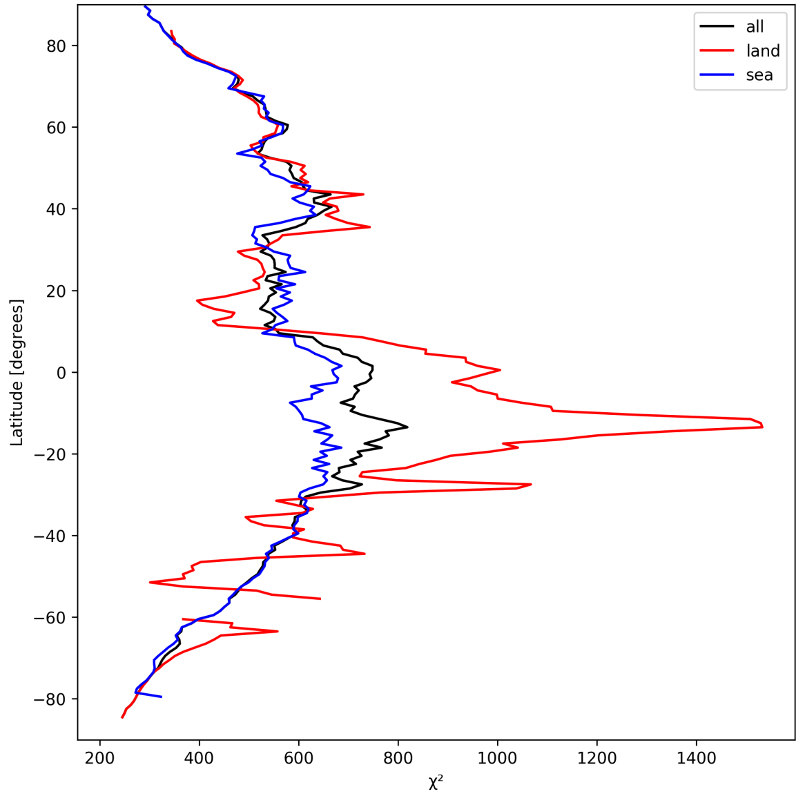
Figure 25: Zonal average of “ \chi^2 ” for 2025-03-29 to 2025-03-30.
