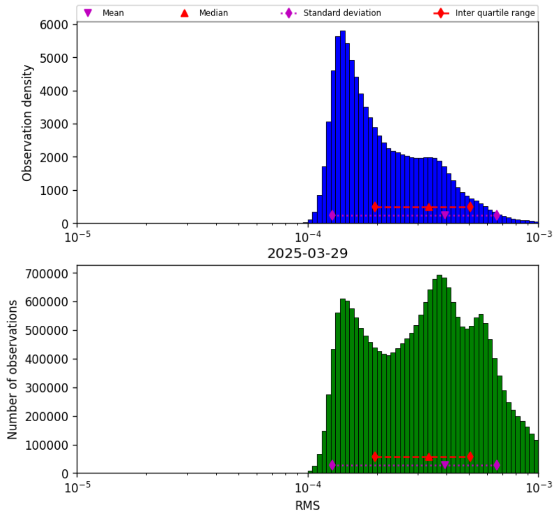
Figure 43: Histogram of “RMS” for 2025-03-29 to 2025-03-30
