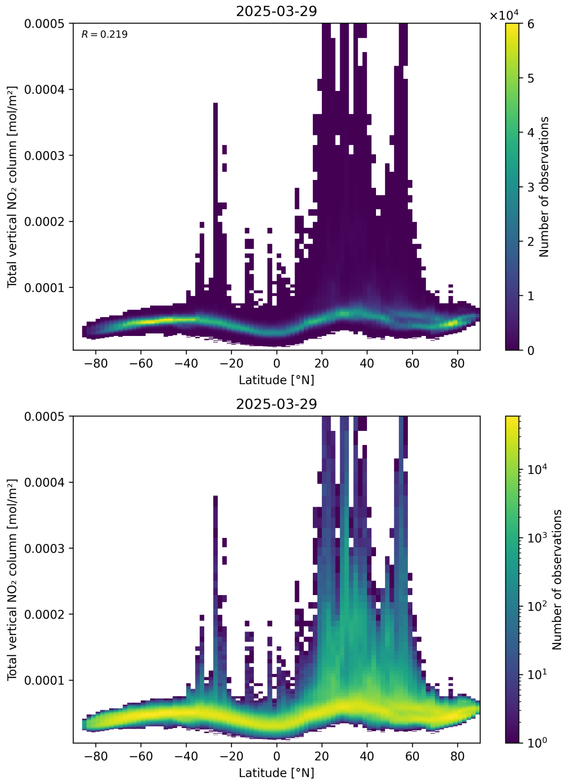
Figure 90: Scatter density plot of “Latitude” against “Total vertical NO 2 column” for 2025-03-29 to 2025-03-30.
