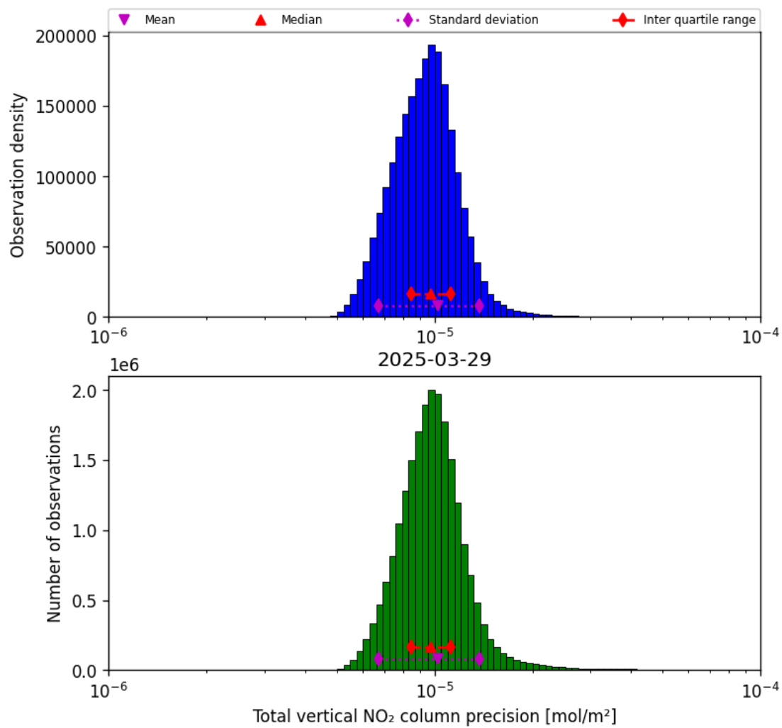
Figure 39: Histogram of "Total vertical NO 2 column precision" for 2025-03-29 to 2025-03-30
