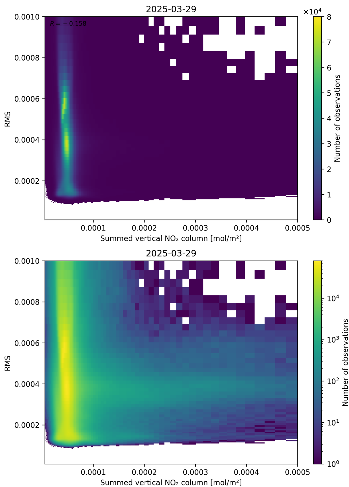
Figure 109: Scatter density plot of “Summed vertical NO 2 column” against “RMS” for 2025-03-29 to 2025-03-30.
