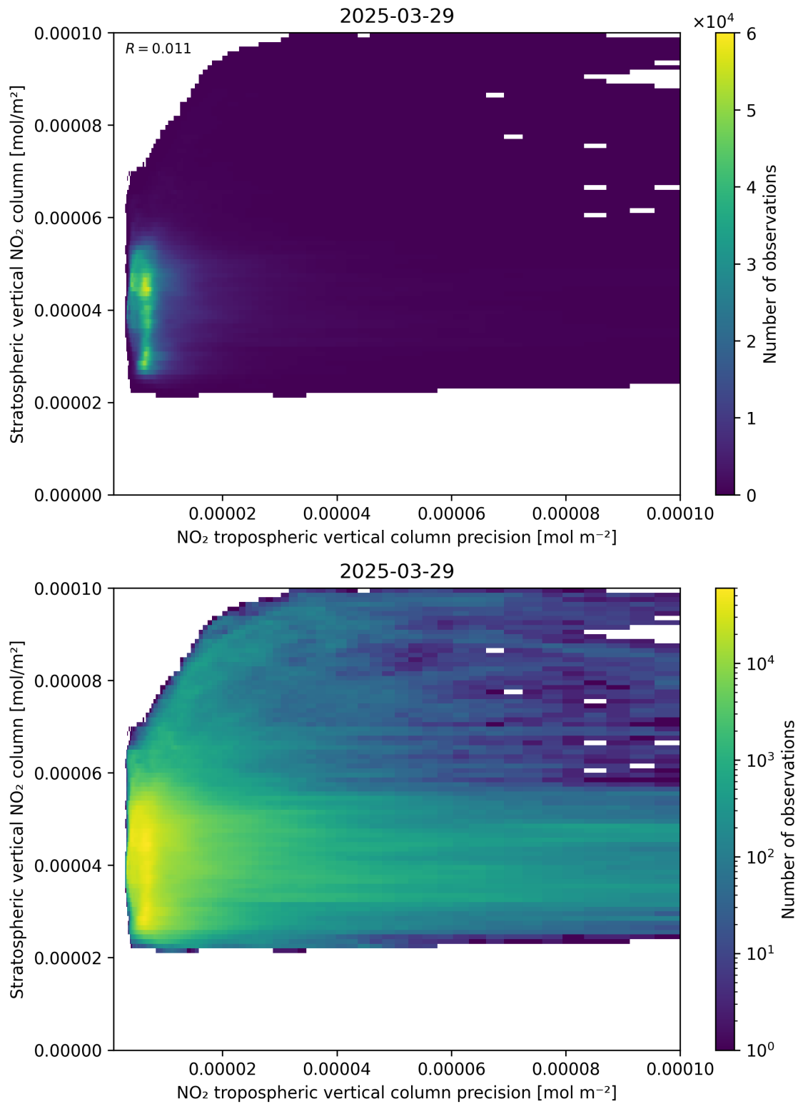
Figure 135: Scatter density plot of “NO 2 tropospheric vertical column precision” against “Stratospheric vertical NO 2 column” for 2025-03-29 to 2025-03-30.
