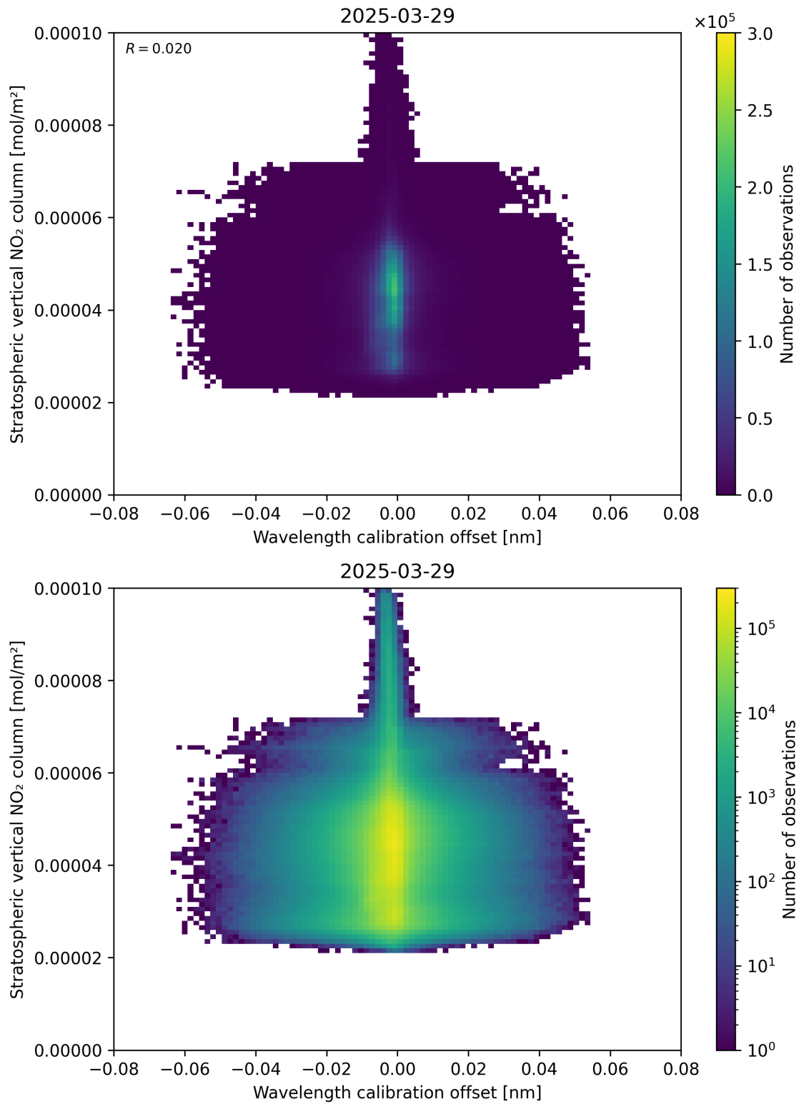
Figure 176: Scatter density plot of “Wavelength calibration offset” against “Stratospheric vertical NO 2 column” for 2025-03-29 to 2025-03-30.
