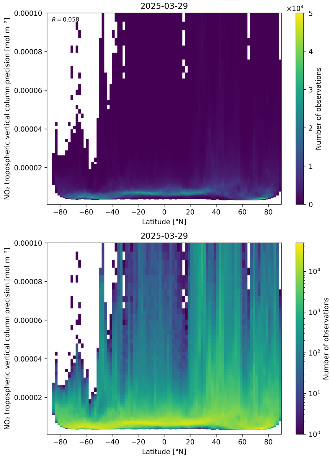
Figure 93: Scatter density plot of “Latitude” against “NO 2 tropospheric vertical column precision” for 2025-03-29 to 2025-03-30.
