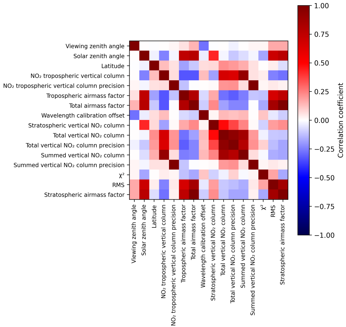
Figure 2: Map of correlation matrix for 2025-03-29 to 2025-03-30.
