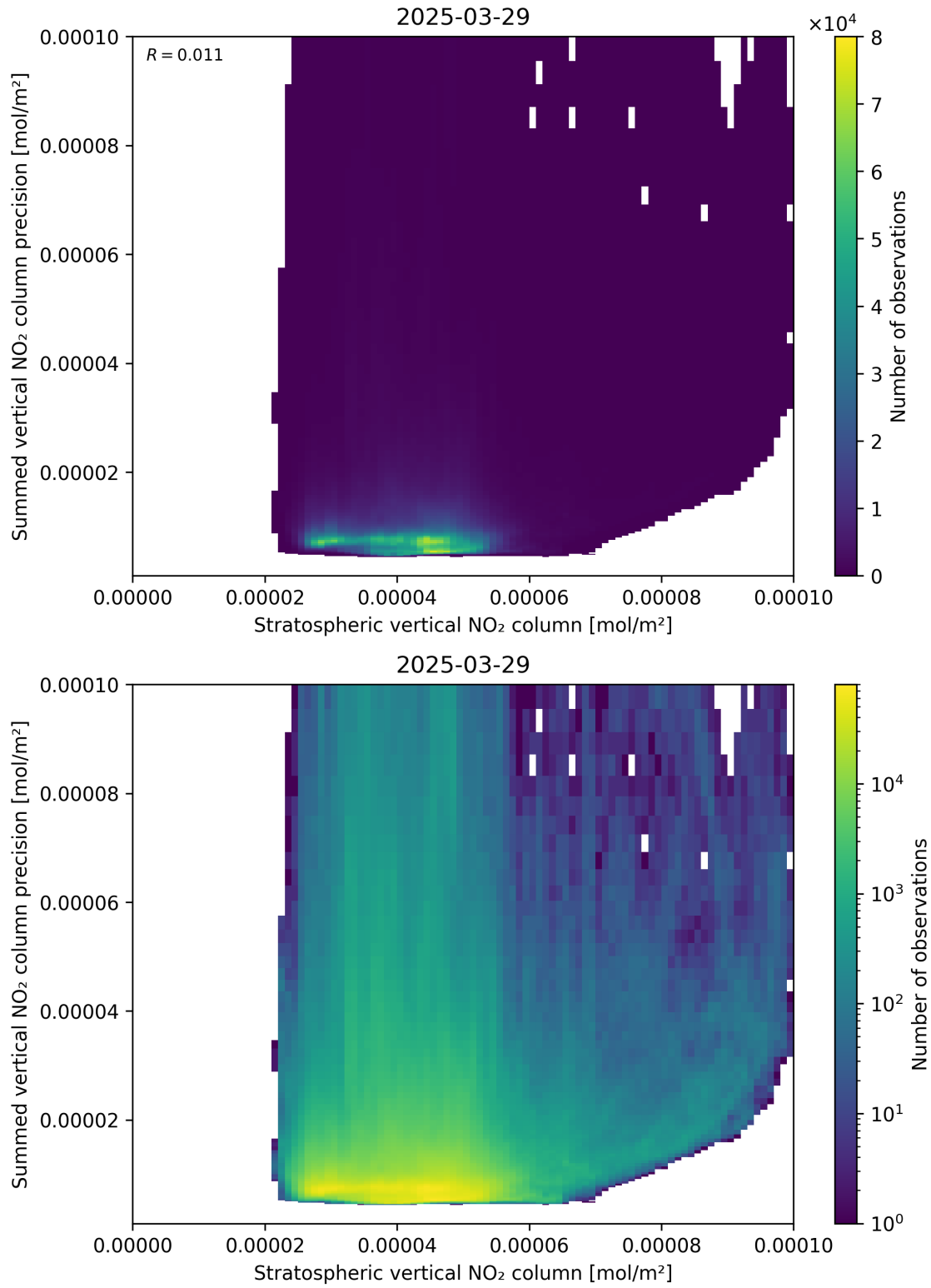
Figure 99: Scatter density plot of “Stratospheric vertical NO 2 column” against “Summed vertical NO 2 column precision” for 2025-03-29 to 2025-03-30.
