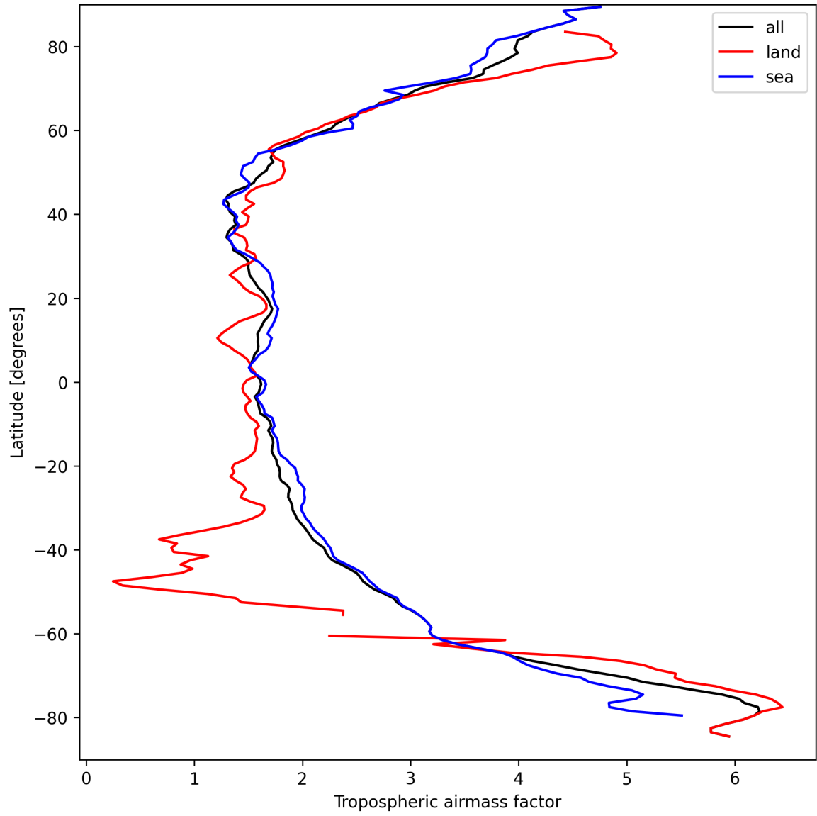
Figure 14: Zonal average of “Tropospheric air mass factor” for 2025-03-29 to 2025-03-30.
