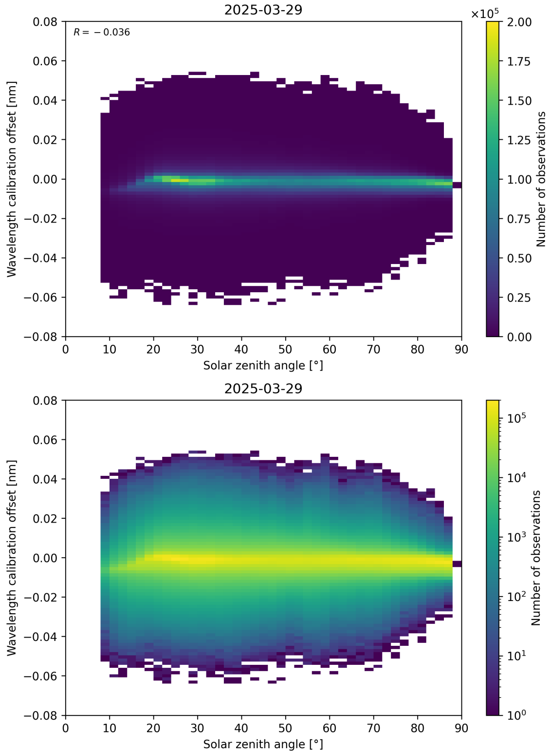
Figure 158: Scatter density plot of “Solar zenith angle” against “Wavelength calibration offset” for 2025-03-29 to 2025-03-30.
