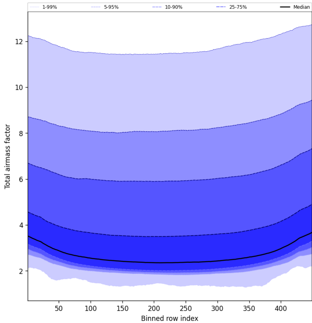
Figure 49: Along track statistics of “Total airmass factor” for 2025-03-29 to 2025-03-30
