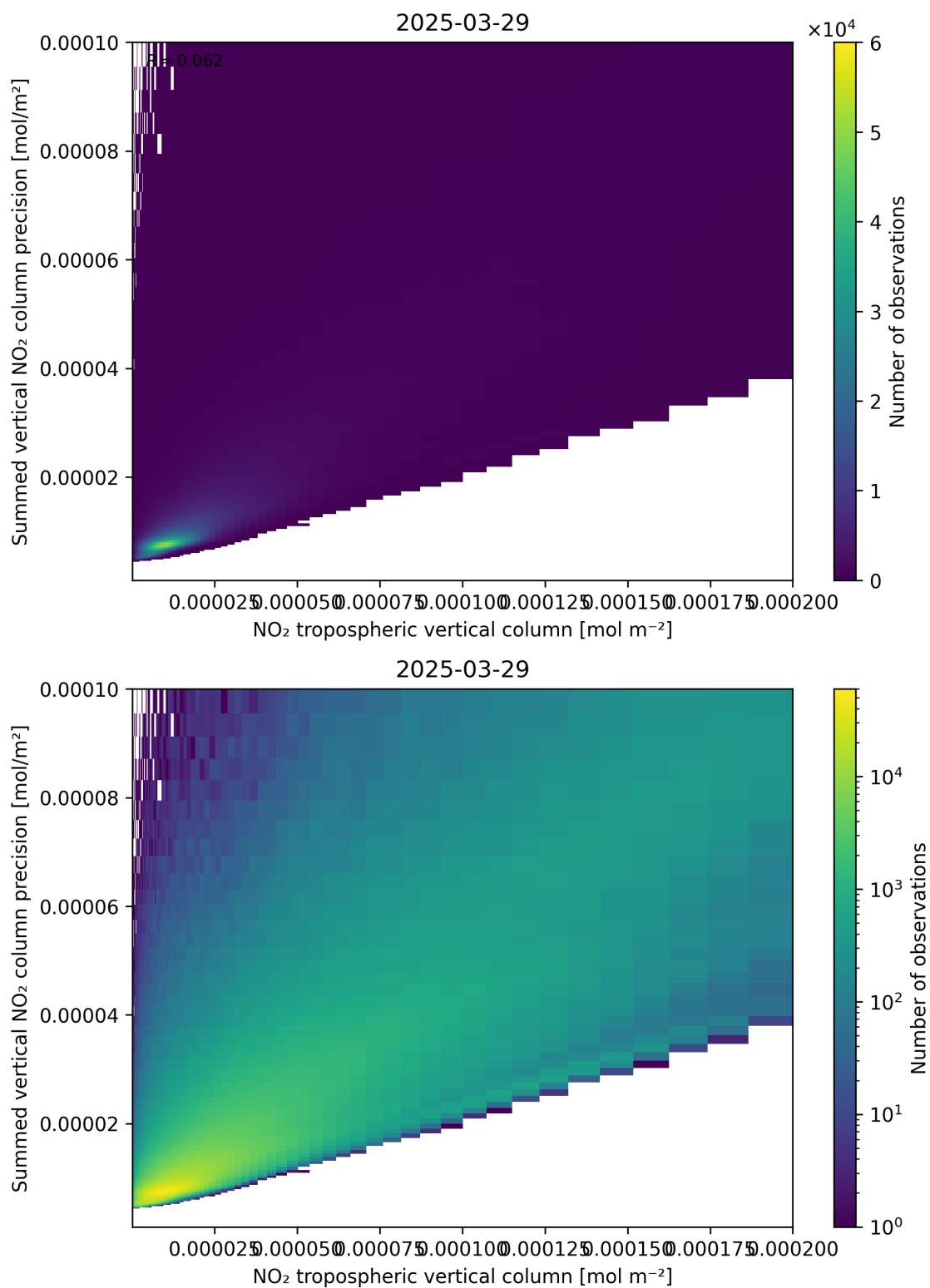
Figure 127: Scatter density plot of “NO 2 tropospheric vertical column” against “Summed vertical NO 2 column precision” for 2025-03-29 to 2025-03-30.
