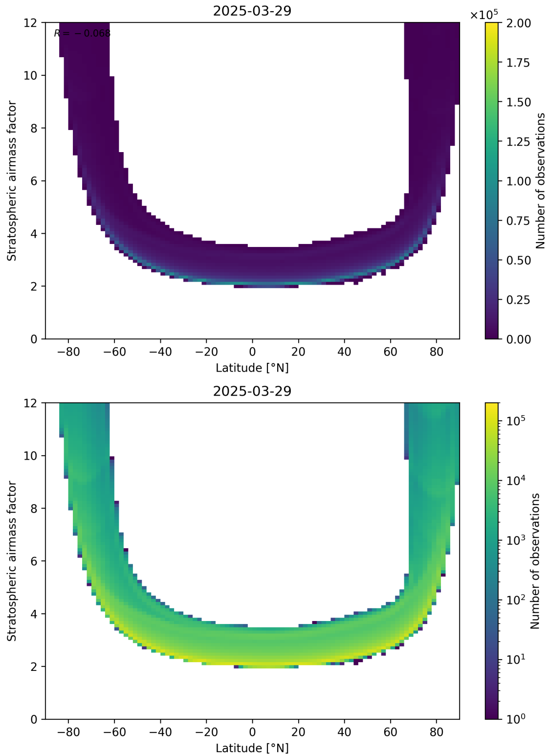
Figure 83: Scatter density plot of “Latitude” against “Stratospheric air mass factor” for 2025-03-29 to 2025-03-30.
