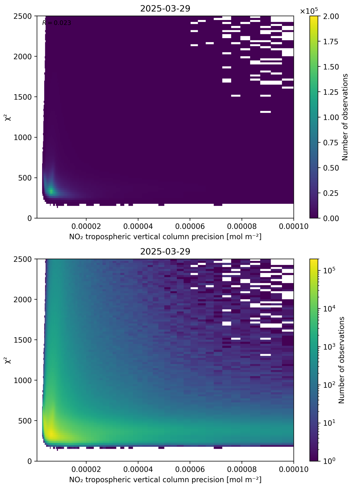
Figure 134: Scatter density plot of “NO 2 tropospheric vertical column precision” against “ \chi^2 ” for 2025-03-29 to 2025-03-30.
