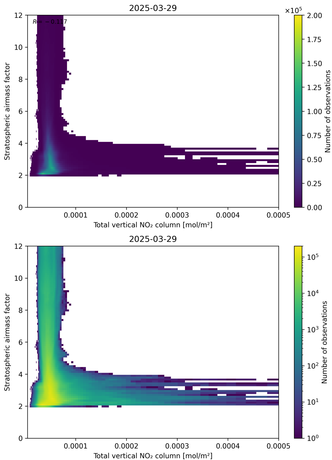
Figure 110: Scatter density plot of “Total vertical NO 2 column” against “Stratospheric airmass factor” for 2025-03-29 to 2025-03-30.
