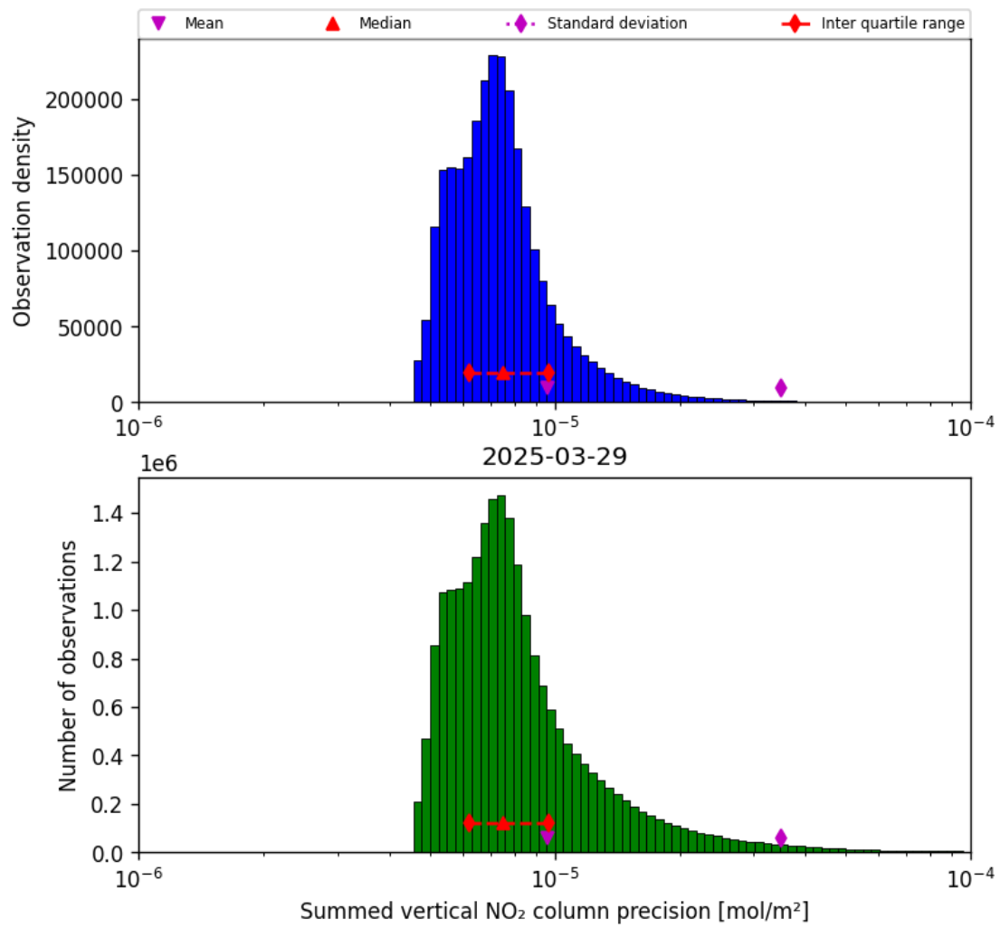
Figure 41: Histogram of "Summed vertical NO 2 column precision" for 2025-03-29 to 2025-03-30
