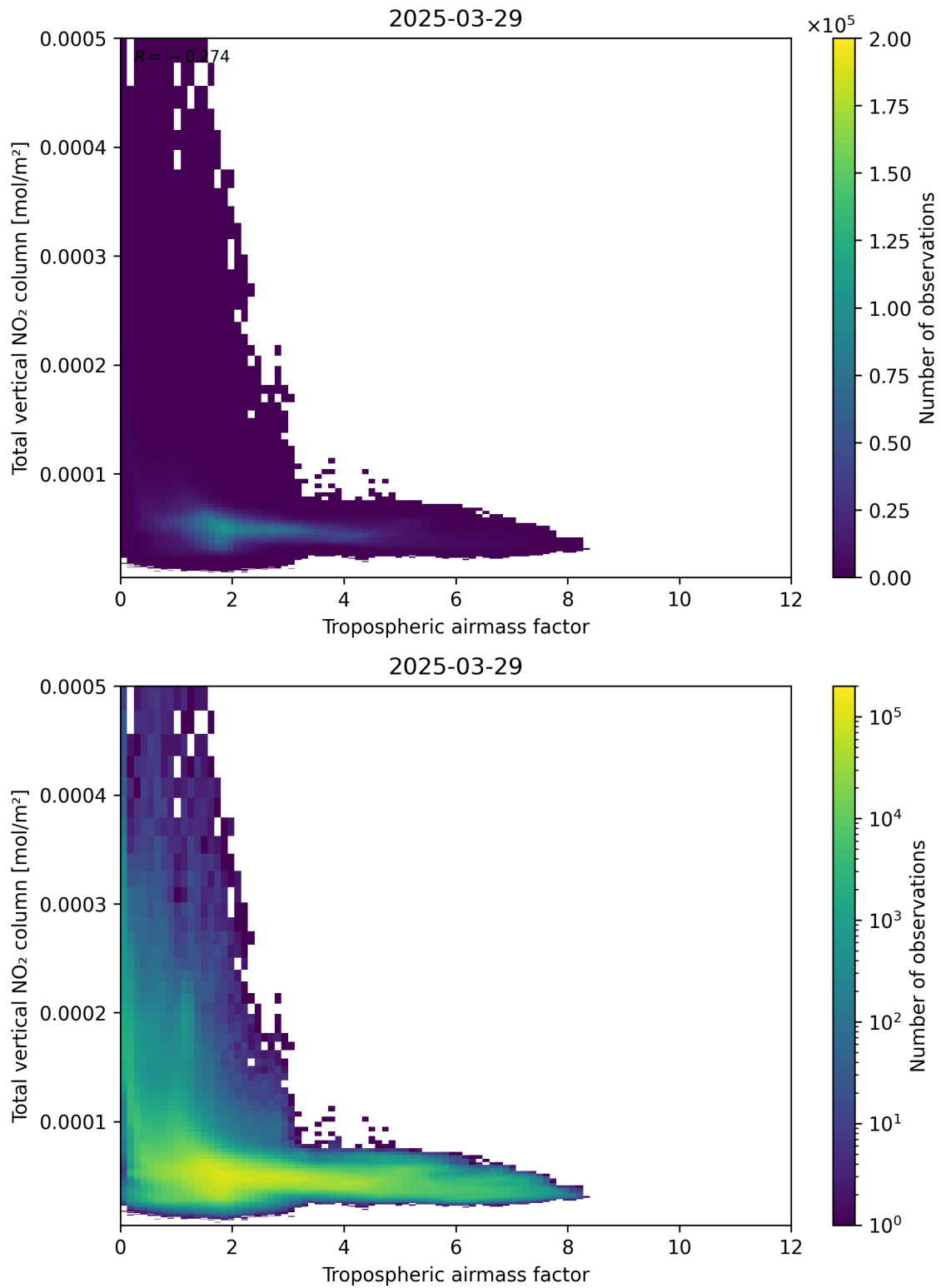
Figure 77: Scatter density plot of “Tropospheric airmass factor” against “Total vertical NO 2 column” for 2025-03-29 to 2025-03-30.
