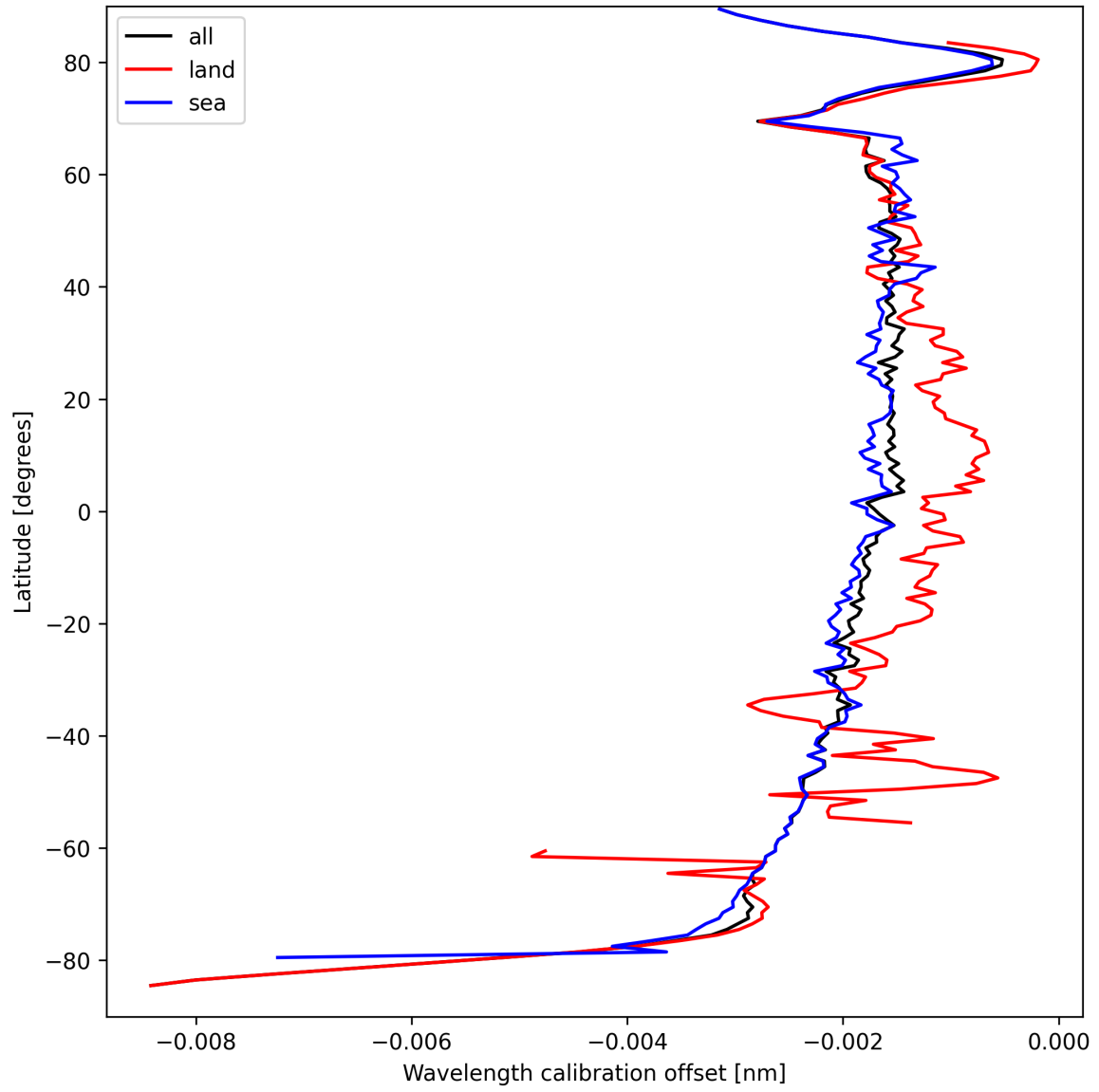
Figure 18: Zonal average of “Wavelength calibration offset” for 2025-03-29 to 2025-03-30.
