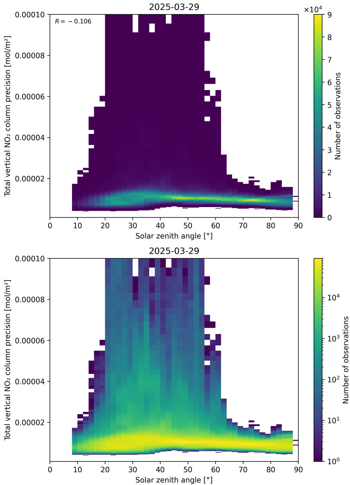
Figure 154: Scatter density plot of “Solar zenith angle” against “Total vertical NO 2 column precision” for 2025-03-29 to 2025-03-30.
