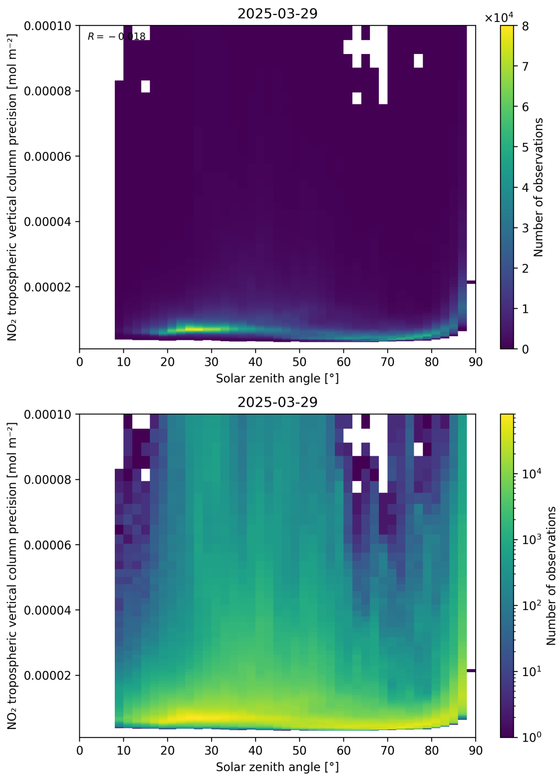
Figure 156: Scatter density plot of “Solar zenith angle” against “NO 2 tropospheric vertical column precision” for 2025-03-29 to 2025-03-30.
