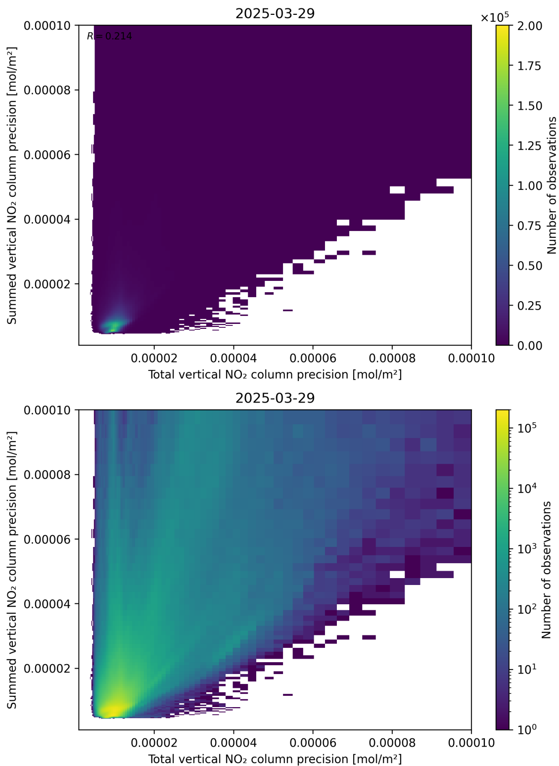
Figure 118: Scatter density plot of “Total vertical NO 2 column precision” against “Summed vertical NO 2 column precision” for 2025-03-29 to 2025-03-30.
