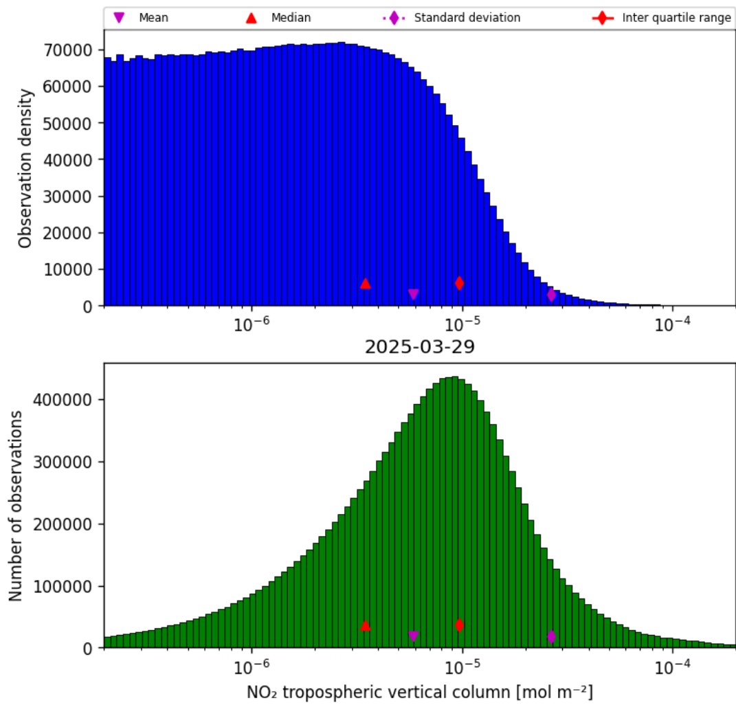
Figure 29: Histogram of “NO 2 tropospheric vertical column” for 2025-03-29 to 2025-03-30
