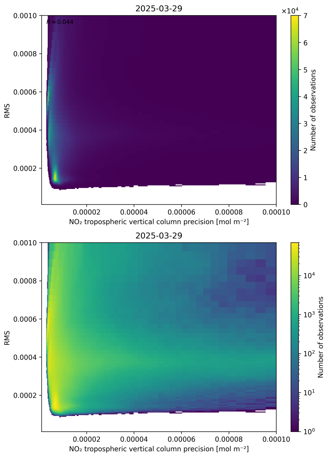
Figure 140: Scatter density plot of “NO 2 tropospheric vertical column precision” against “RMS” for 2025-03-29 to 2025-03-30.
