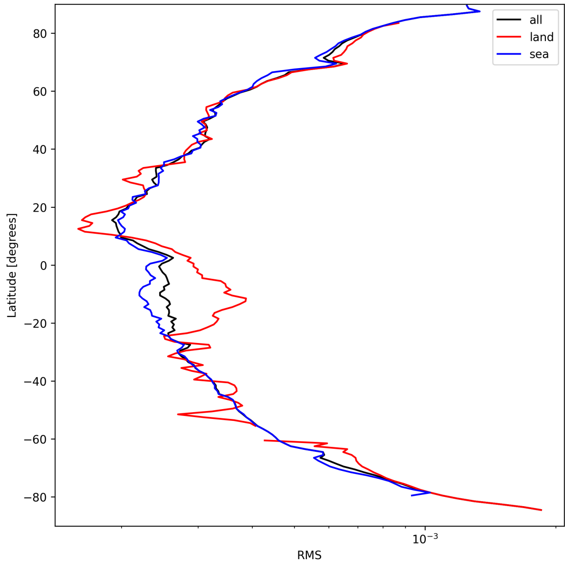
Figure 26: Zonal average of “RMS” for 2025-03-29 to 2025-03-30.
