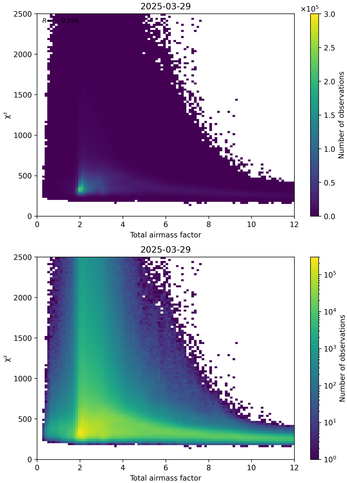
Figure 63: Scatter density plot of “Total airmass factor” against “ \chi^2 ” for 2025-03-29 to 2025-03-30.
