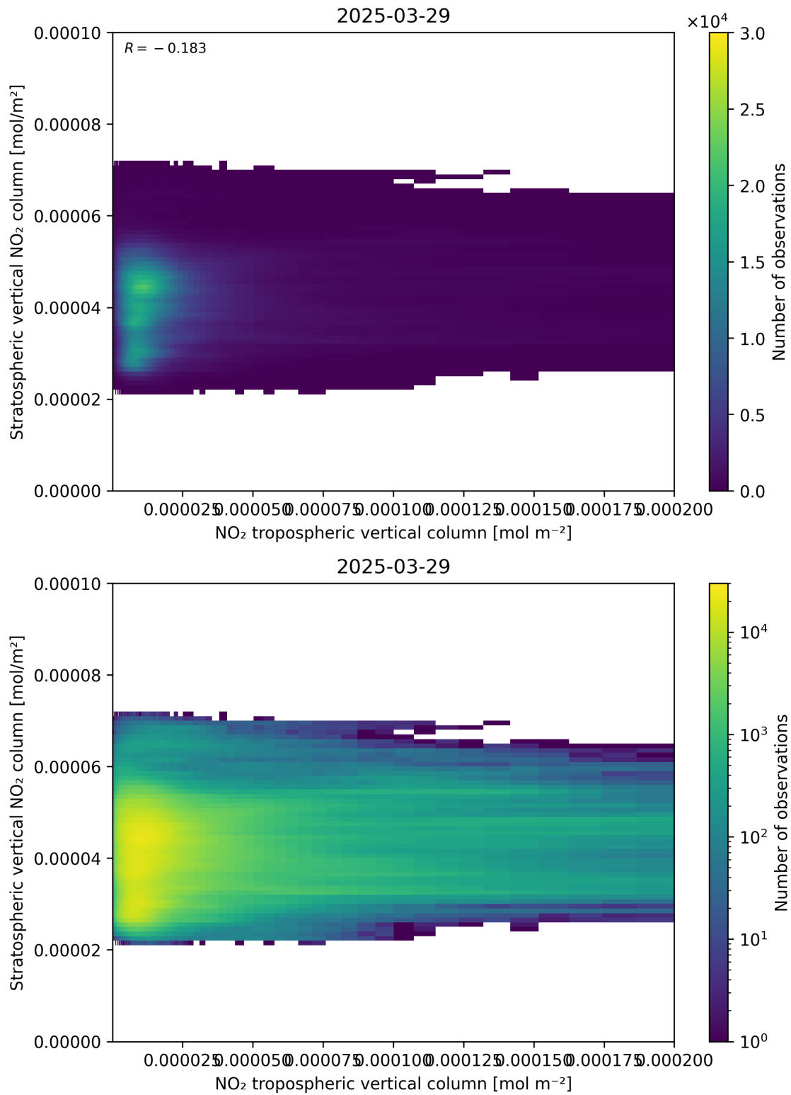
Figure 125: Scatter density plot of “NO 2 tropospheric vertical column” against “Stratospheric vertical NO 2 column” for 2025-03-29 to 2025-03-30.
