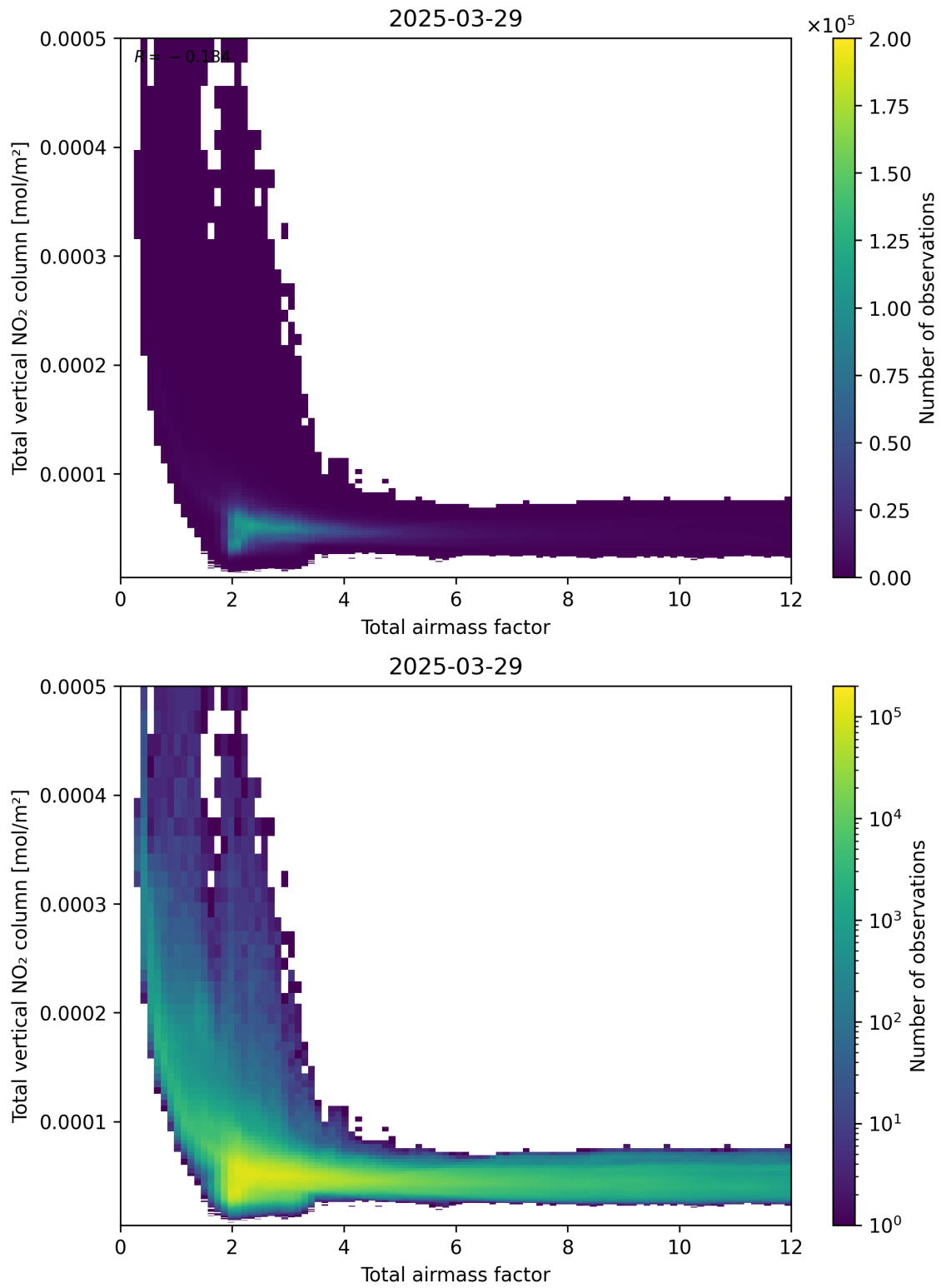
Figure 67: Scatter density plot of “Total airmass factor” against “Total vertical NO 2 column” for 2025-03-29 to 2025-03-30.
