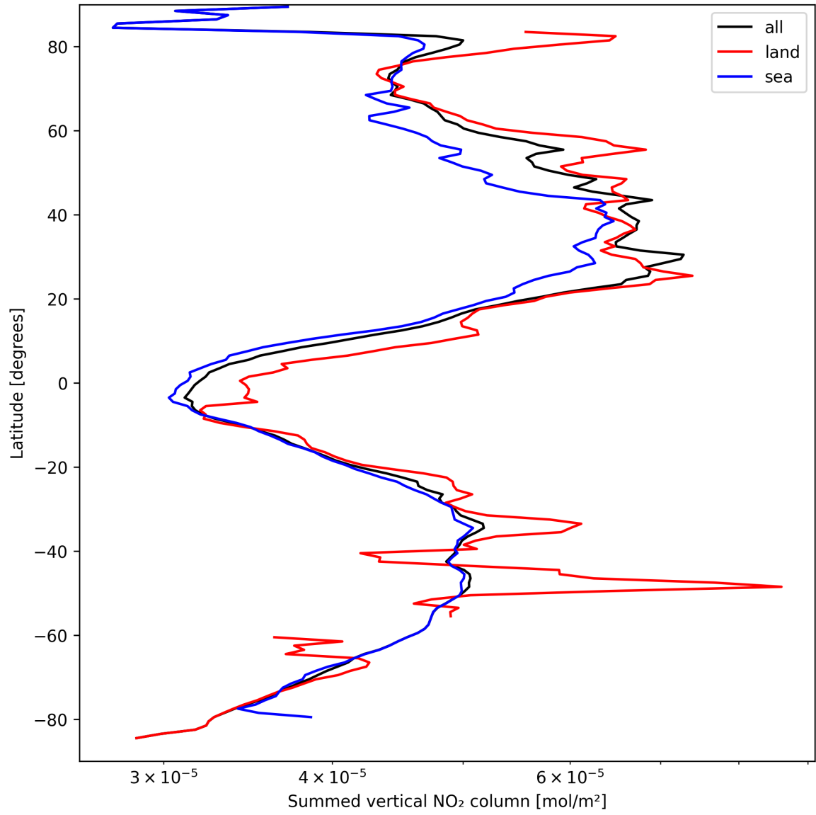
Figure 23: Zonal average of “Summed vertical NO 2 column” for 2025-03-29 to 2025-03-30.
