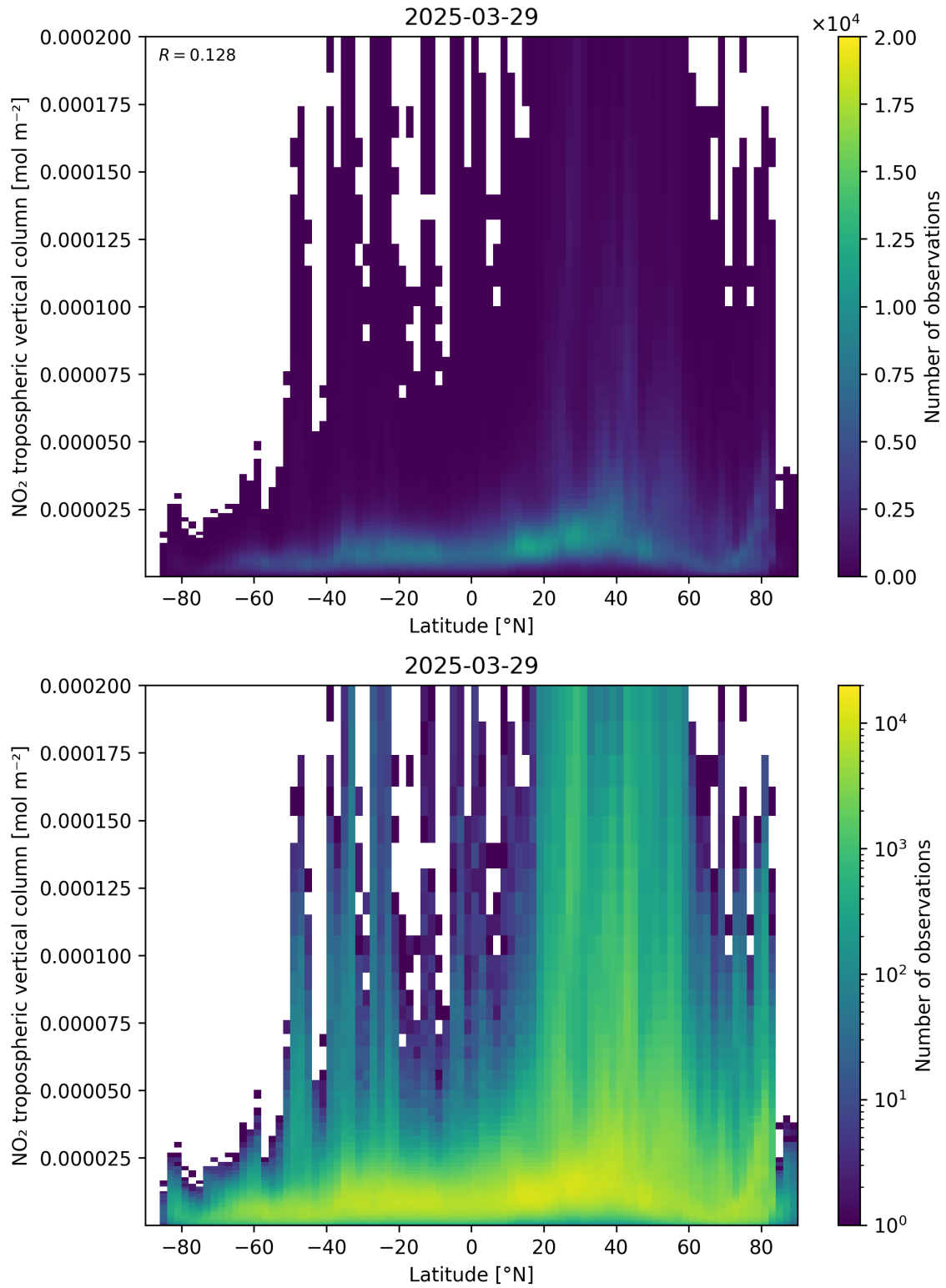
Figure 92: Scatter density plot of “Latitude” against “NO 2 tropospheric vertical column” for 2025-03-29 to 2025-03-30.
