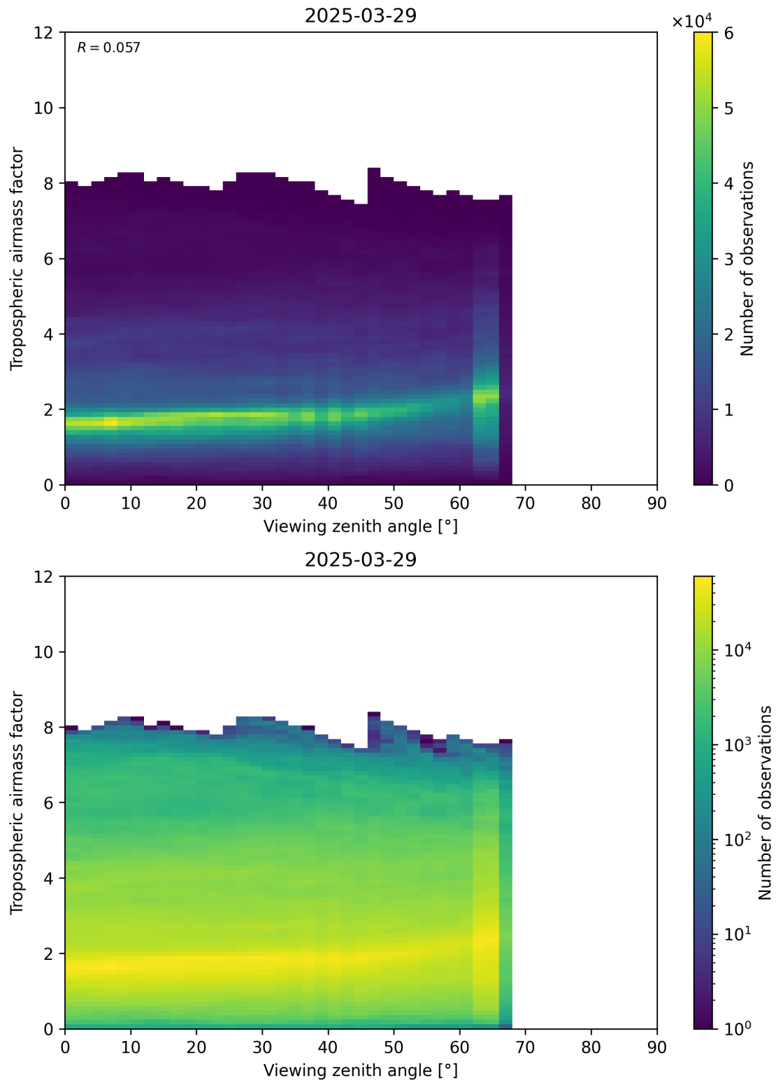
Figure 161: Scatter density plot of “Viewing zenith angle” against “Tropospheric airmass factor” for 2025-03-29 to 2025-03-30.
