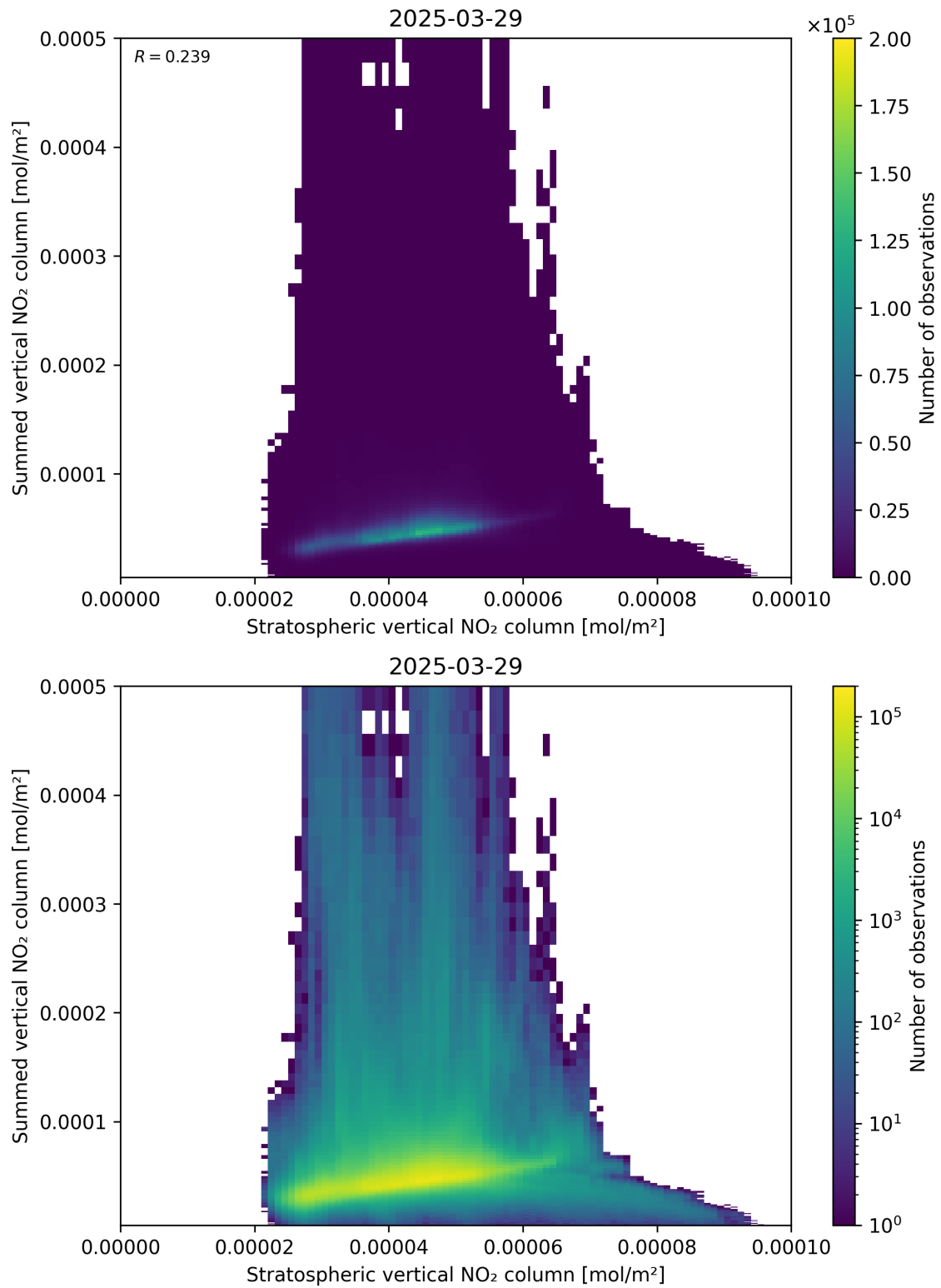
Figure 98: Scatter density plot of “Stratospheric vertical NO 2 column” against “Summed vertical NO 2 column” for 2025-03-29 to 2025-03-30.
