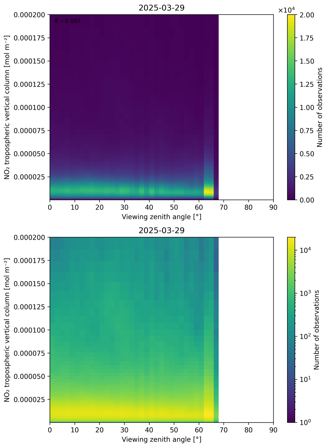
Figure 169: Scatter density plot of “Viewing zenith angle” against “NO 2 tropospheric vertical column” for 2025-03-29 to 2025-03-30.
