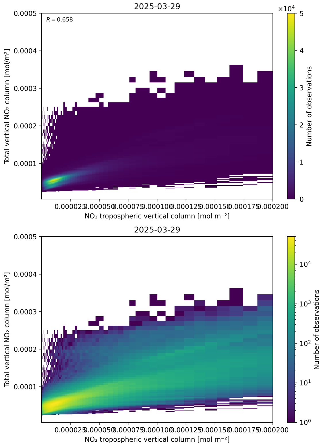
Figure 128: Scatter density plot of “NO 2 tropospheric vertical column” against “Total vertical NO 2 column” for 2025-03-29 to 2025-03-30.
