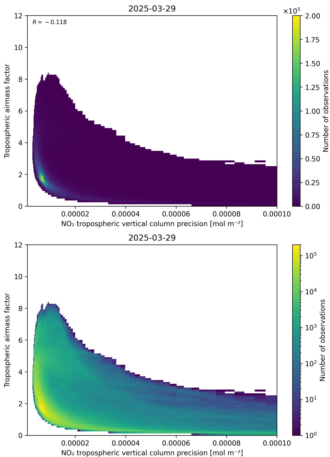
Figure 133: Scatter density plot of “NO 2 tropospheric vertical column precision” against “Tropospheric air mass factor” for 2025-03-29 to 2025-03-30.
