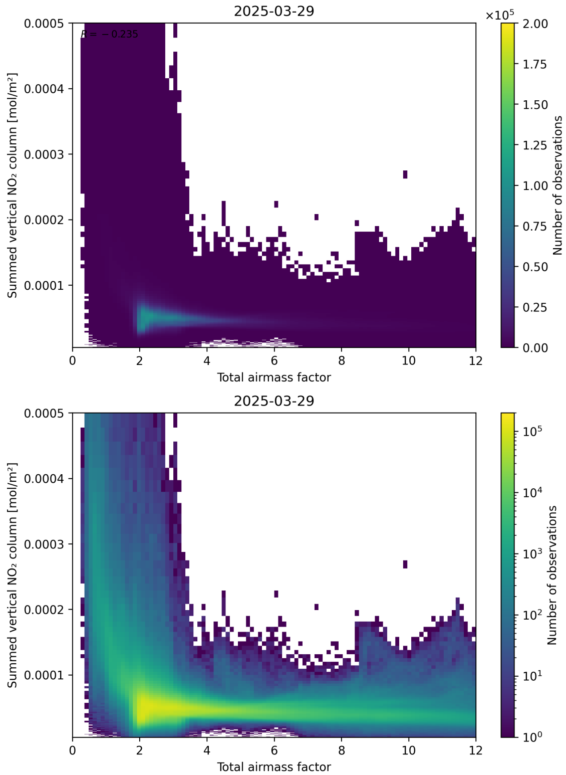
Figure 65: Scatter density plot of “Total airmass factor” against “Summed vertical NO 2 column” for 2025-03-29 to 2025-03-30.
