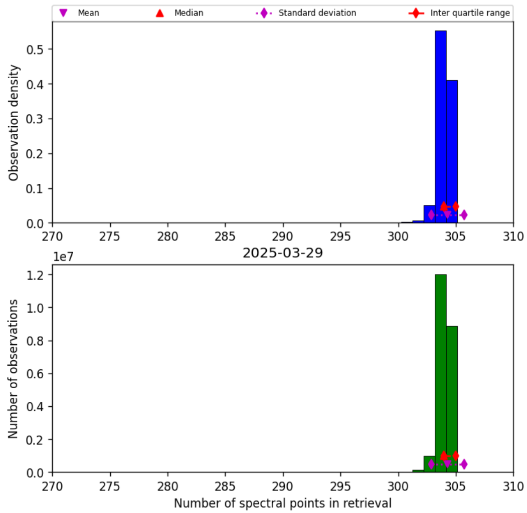
Figure 33: Histogram of “Number of spectral points in retrieval” for 2025-03-29 to 2025-03-30
