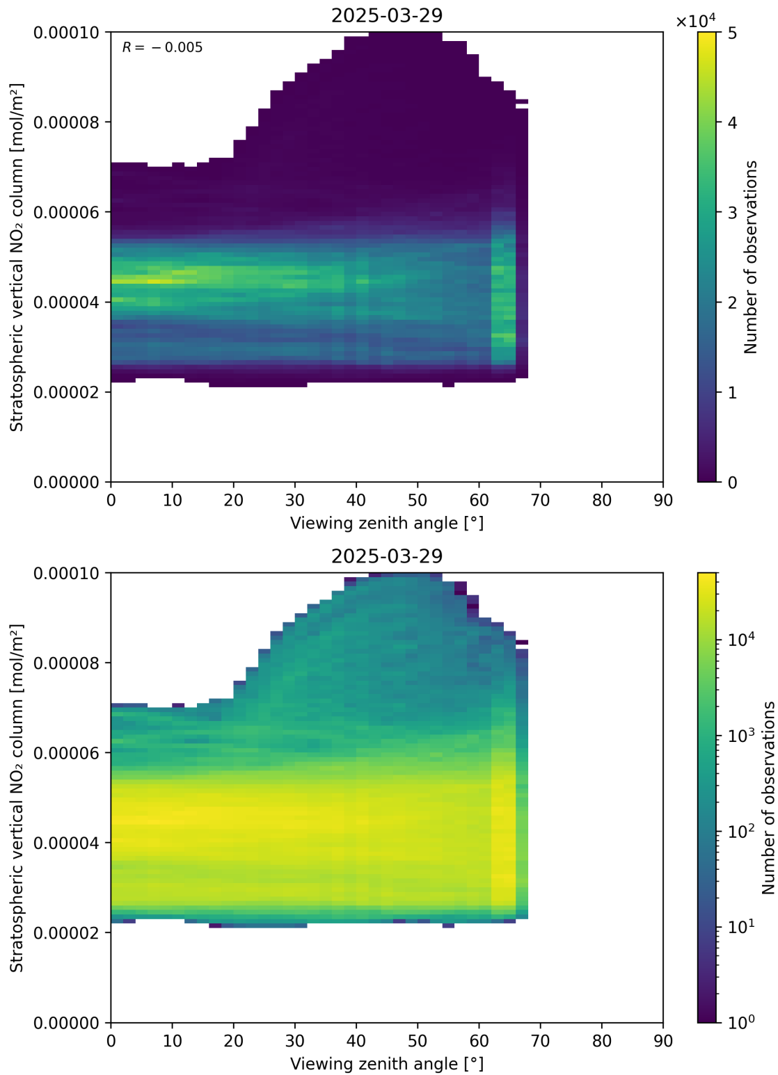
Figure 164: Scatter density plot of “Viewing zenith angle” against “Stratospheric vertical NO 2 column” for 2025-03-29 to 2025-03-30.
