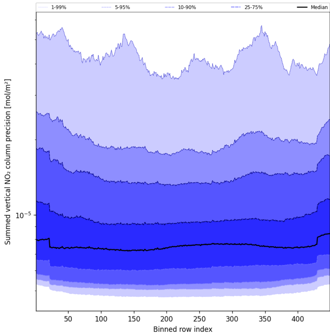
Figure 58: Along track statistics of “Summed vertical NO 2 column precision” for 2025-03-29 to 2025-03-30
