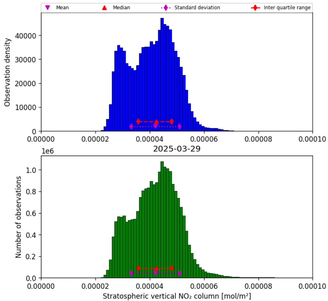
Figure 36: Histogram of “Stratospheric vertical NO 2 column” for 2025-03-29 to 2025-03-30
