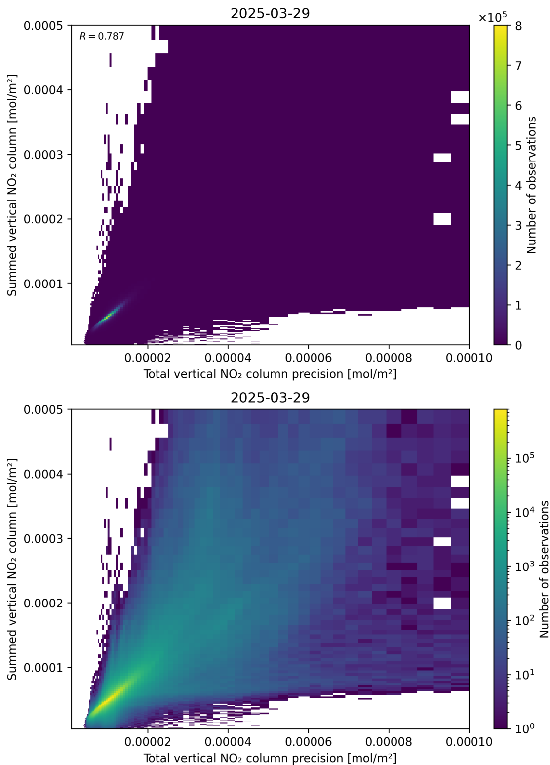
Figure 117: Scatter density plot of “Total vertical NO 2 column precision” against “Summed vertical NO 2 column” for 2025-03-29 to 2025-03-30.
