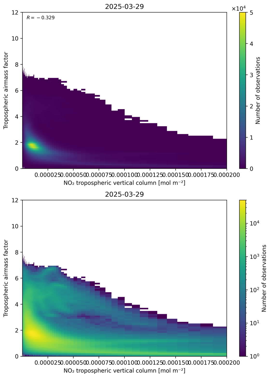
Figure 123: Scatter density plot of “NO 2 tropospheric vertical column” against “Tropospheric air mass factor” for 2025-03-29 to 2025-03-30.
