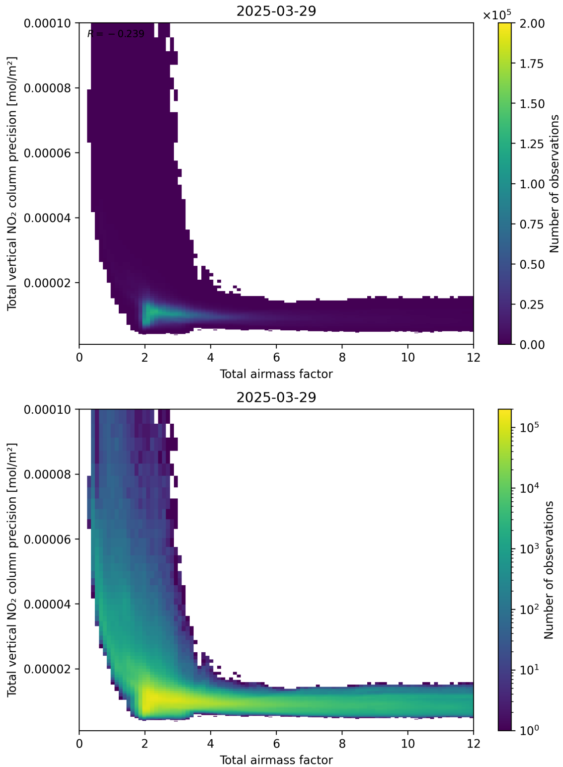
Figure 68: Scatter density plot of “Total airmass factor” against “Total vertical NO 2 column precision” for 2025-03-29 to 2025-03-30.
