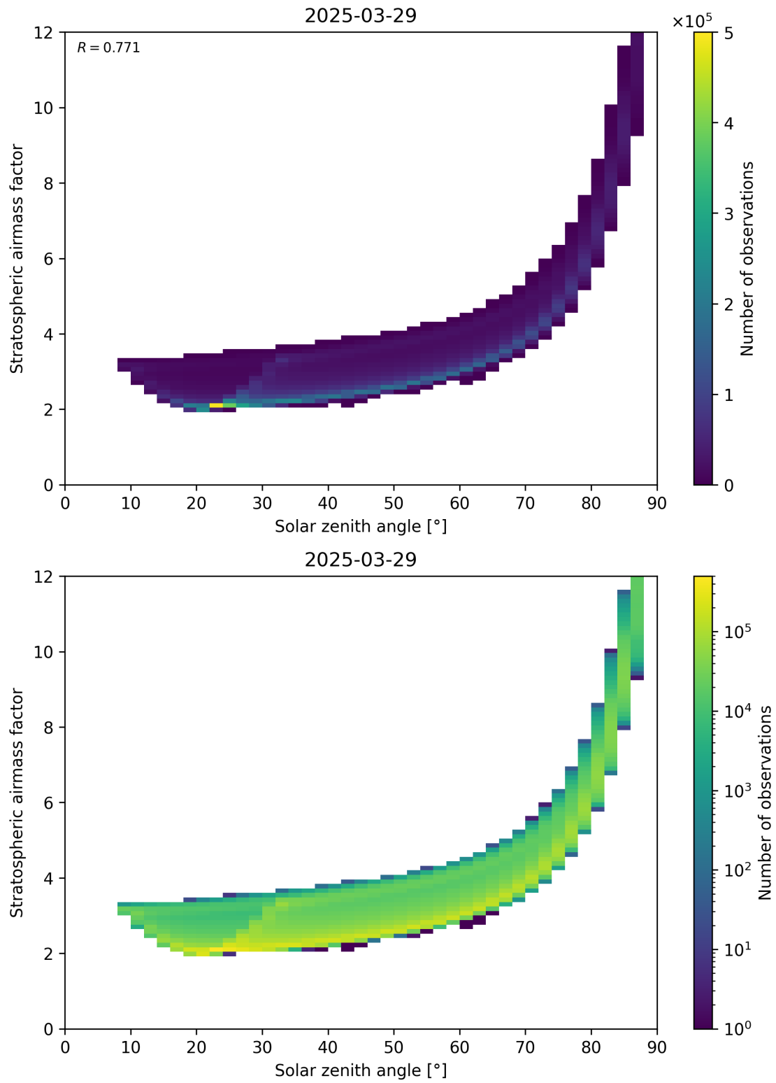
Figure 145: Scatter density plot of “Solar zenith angle” against “Stratospheric airmass factor” for 2025-03-29 to 2025-03-30.
