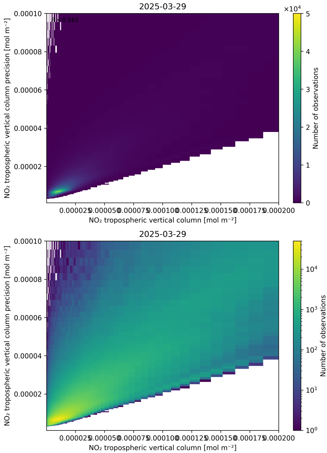
Figure 130: Scatter density plot of “NO 2 tropospheric vertical column” against “NO 2 tropospheric vertical column precision” for 2025-03-29 to 2025-03-30.
