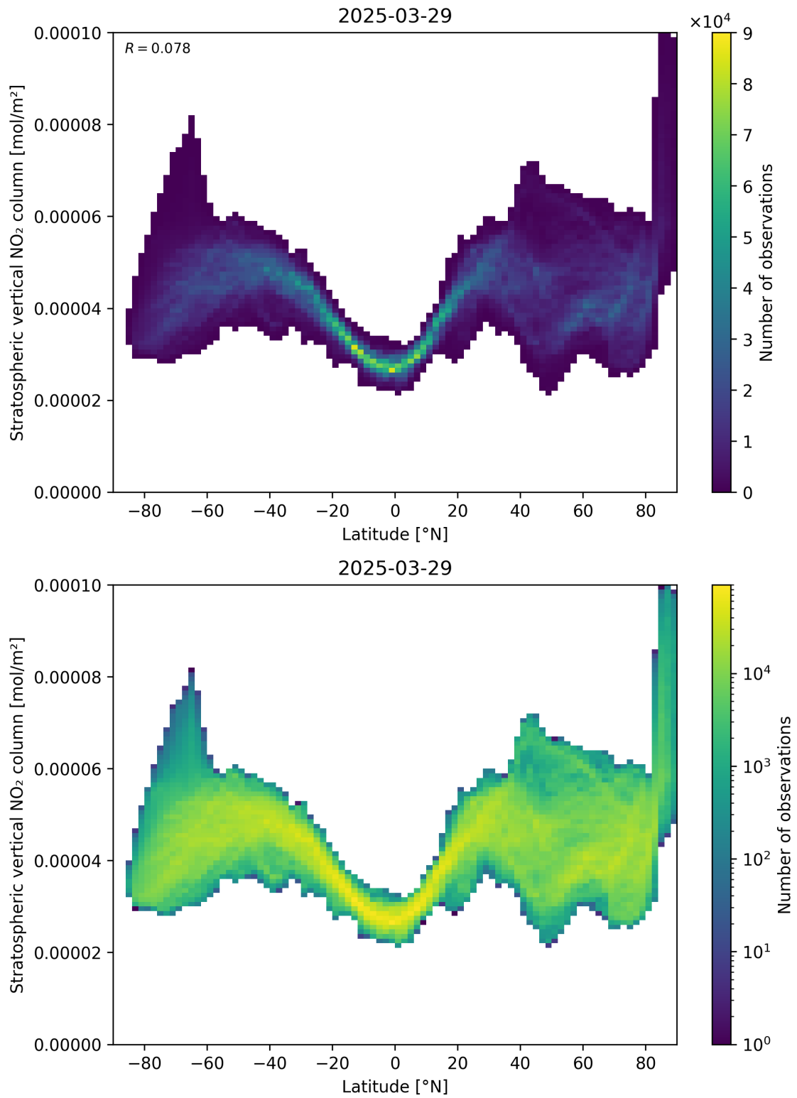
Figure 87: Scatter density plot of “Latitude” against “Stratospheric vertical NO 2 column” for 2025-03-29 to 2025-03-30.
