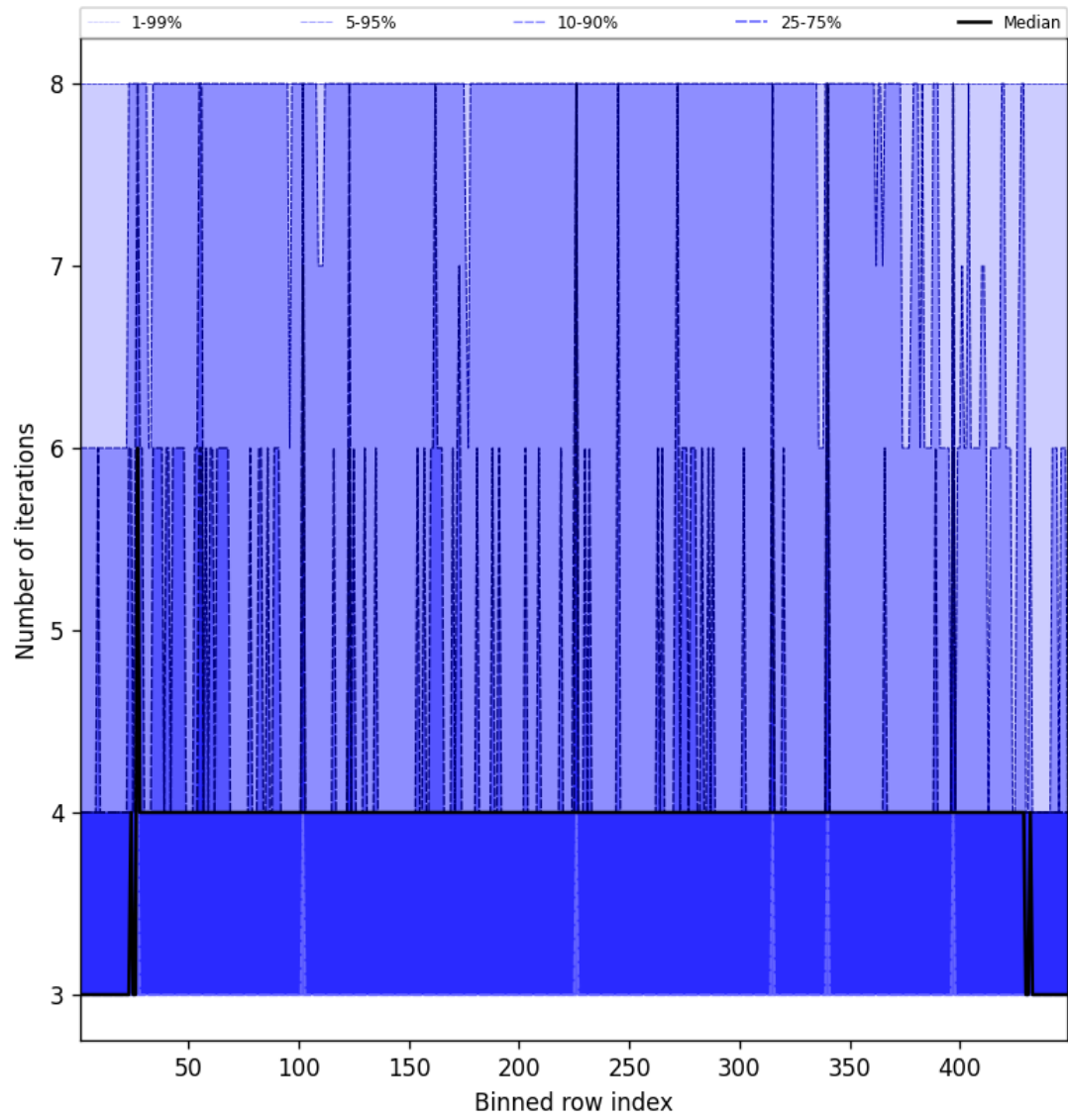
Figure 51: Along track statistics of “Number of iterations” for 2025-03-29 to 2025-03-30
