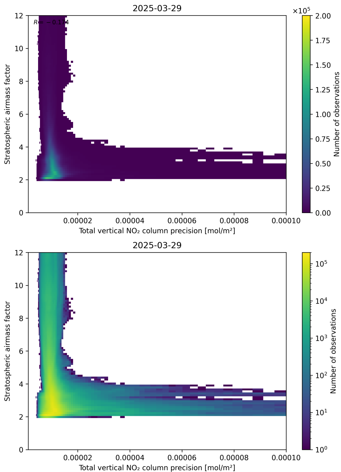
Figure 115: Scatter density plot of “Total vertical NO 2 column precision” against “Stratospheric air mass factor” for 2025-03-29 to 2025-03-30.
