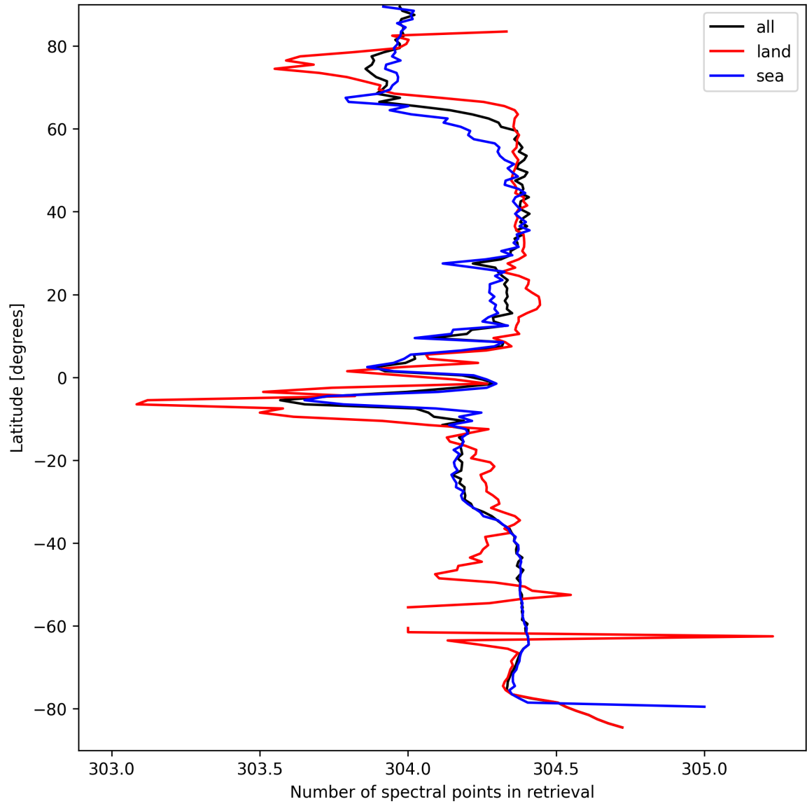
Figure 16: Zonal average of “Number of spectral points in retrieval” for 2025-03-29 to 2025-03-30.
