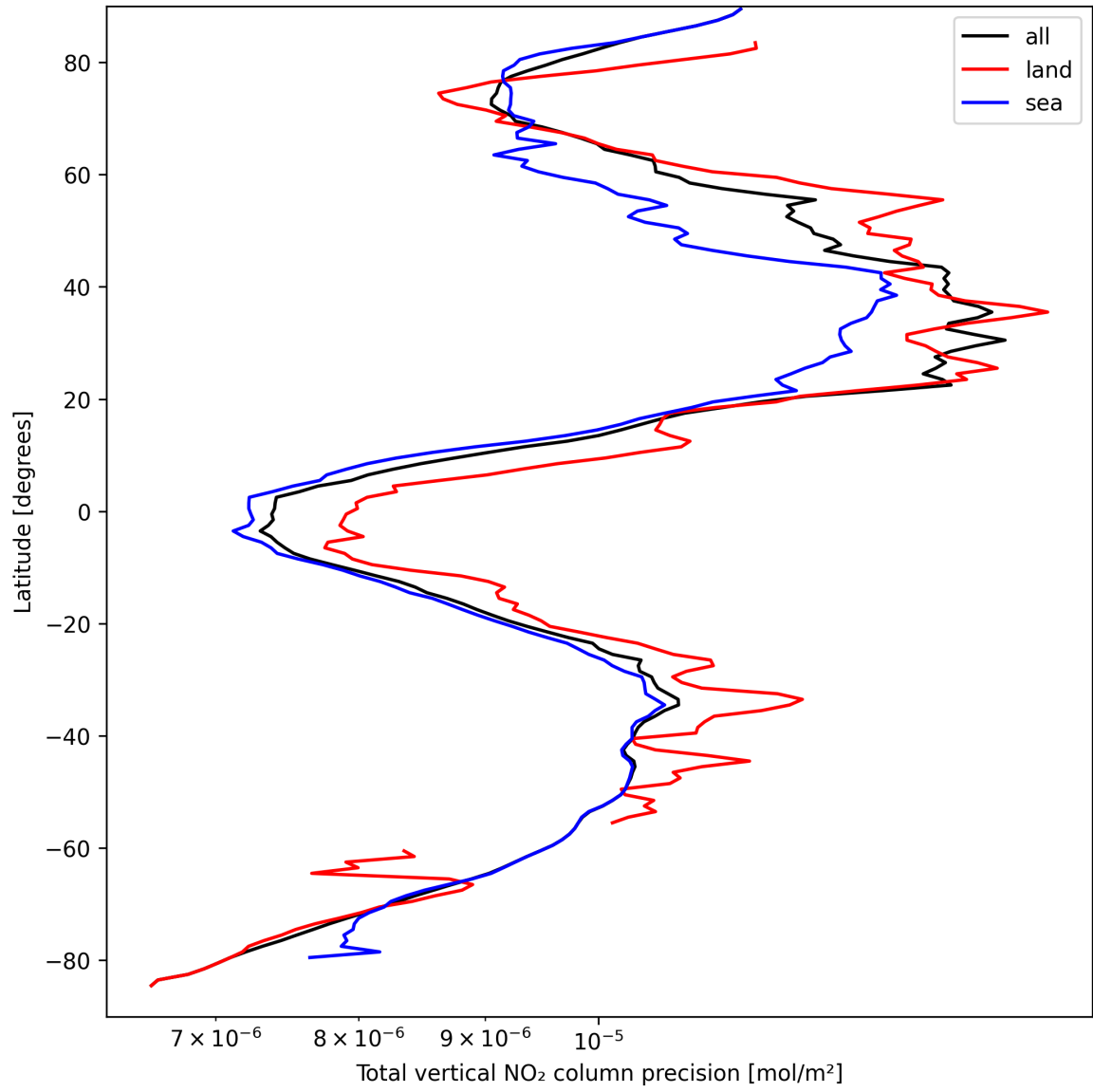
Figure 22: Zonal average of "Total vertical NO 2 column precision" for 2025-03-29 to 2025-03-30.
