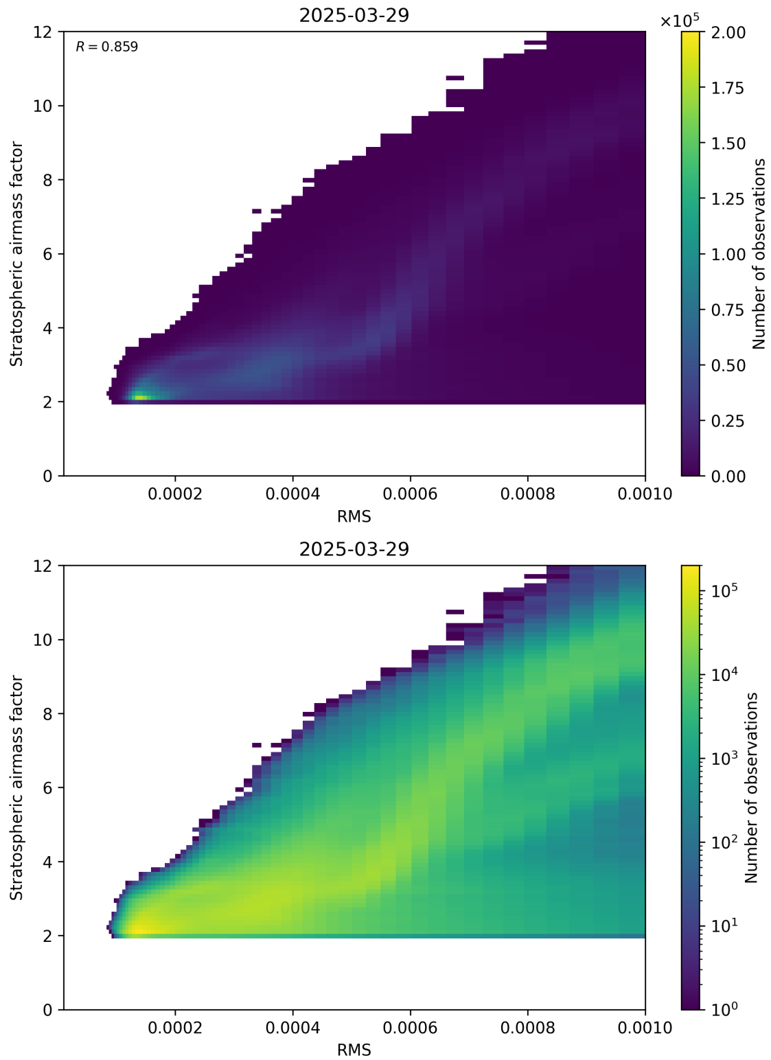
Figure 144: Scatter density plot of “RMS” against “Stratospheric airmass factor” for 2025-03-29 to 2025-03-30.
