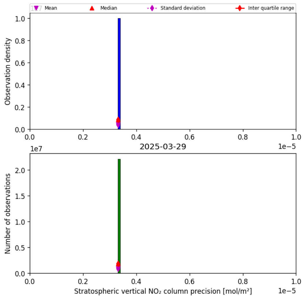
Figure 37: Histogram of “Stratospheric vertical NO 2 column precision” for 2025-03-29 to 2025-03-30
