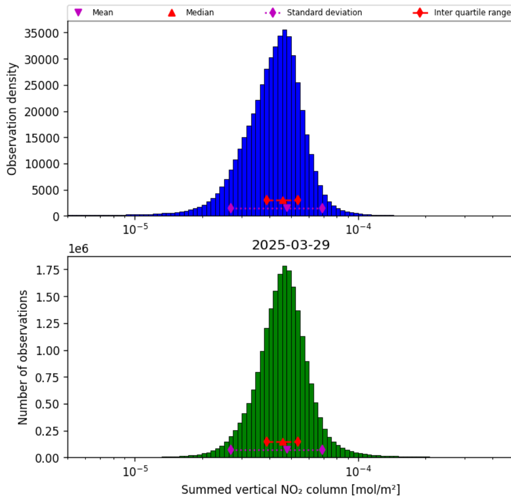
Figure 40: Histogram of “Summed vertical NO 2 column” for 2025-03-29 to 2025-03-30
