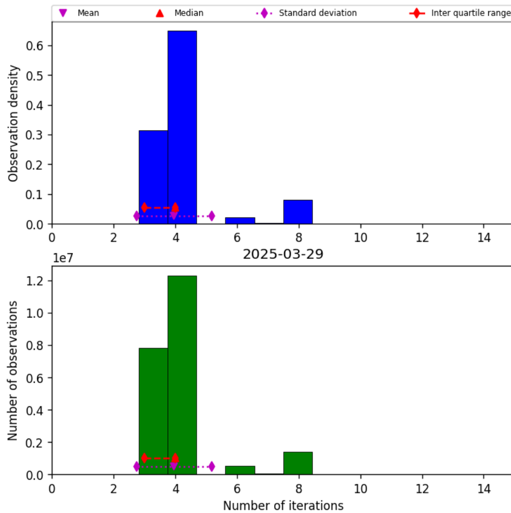
Figure 34: Histogram of “Number of iterations” for 2025-03-29 to 2025-03-30
