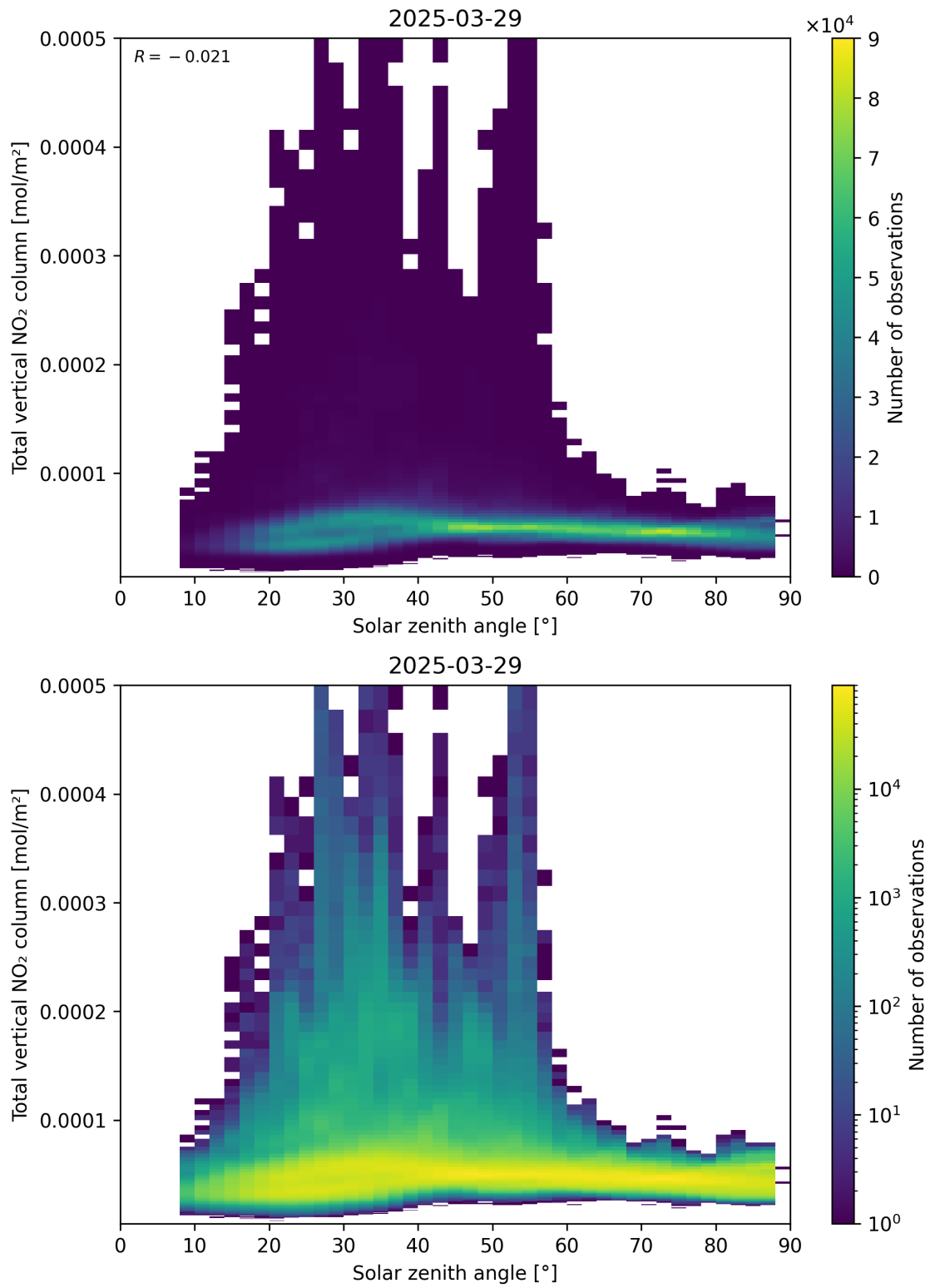
Figure 153: Scatter density plot of “Solar zenith angle” against “Total vertical NO 2 column” for 2025-03-29 to 2025-03-30.
