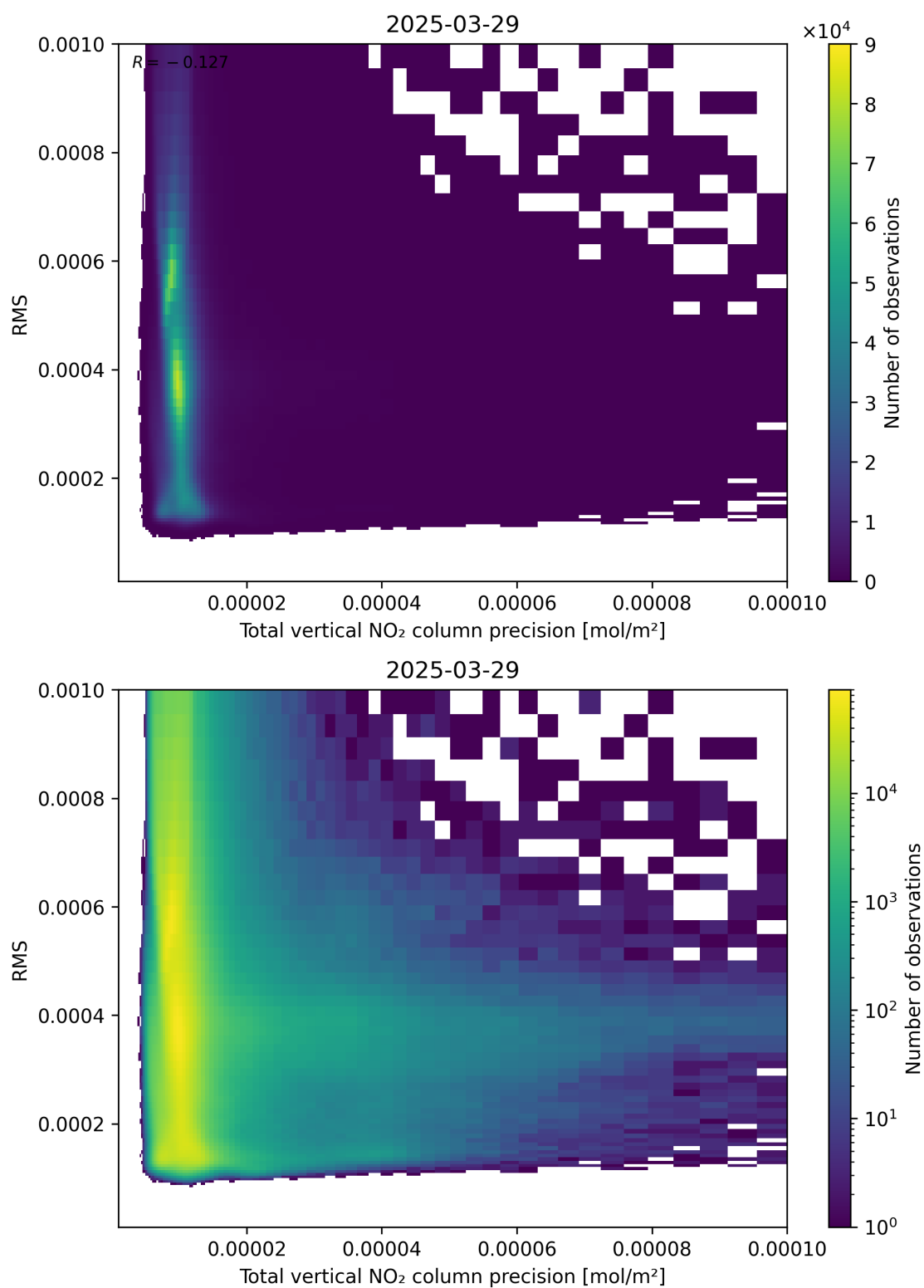
Figure 119: Scatter density plot of “Total vertical NO 2 column precision” against “RMS” for 2025-03-29 to 2025-03-30.
