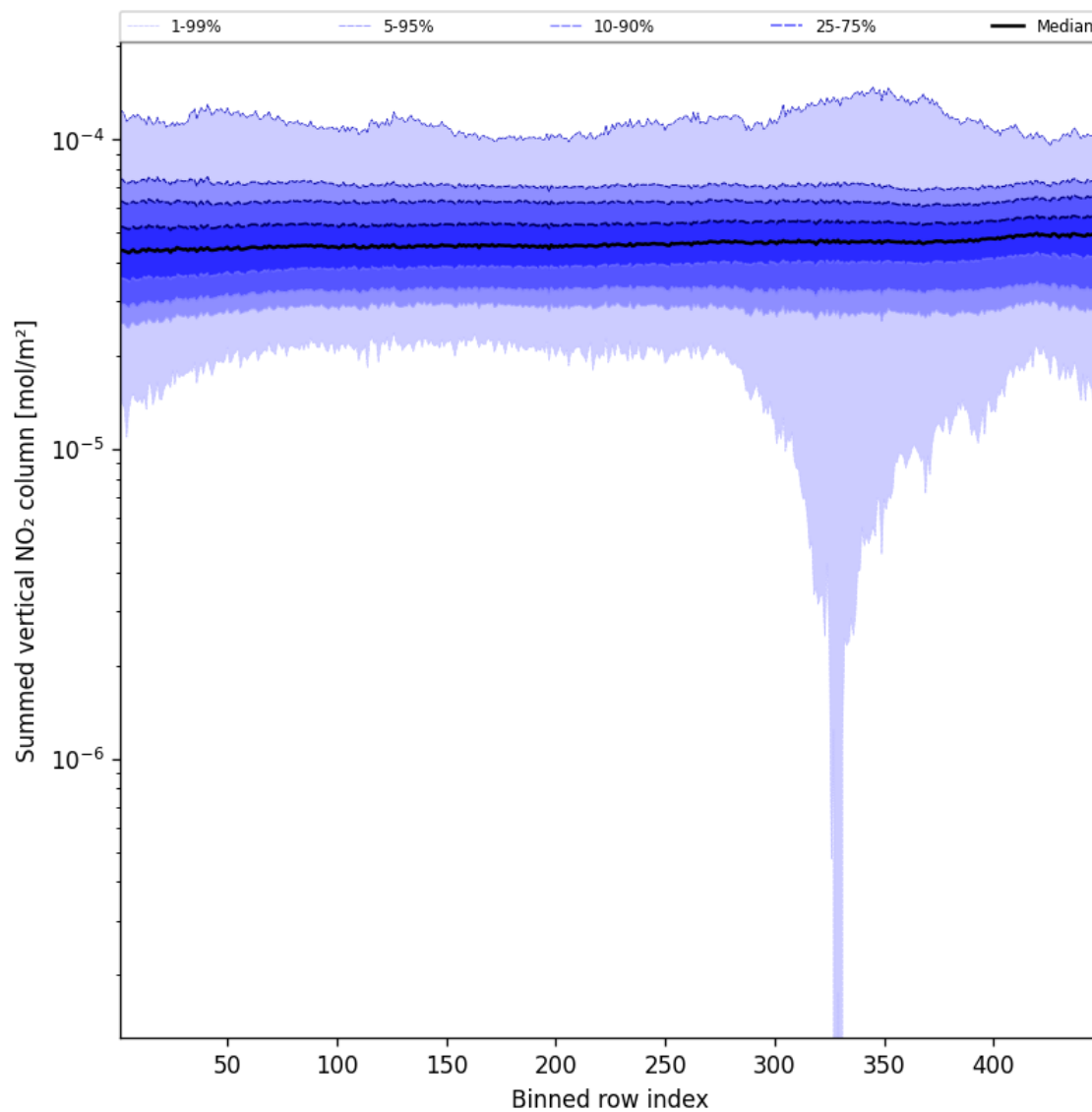
Figure 57: Along track statistics of “Summed vertical NO 2 column” for 2025-03-29 to 2025-03-30
