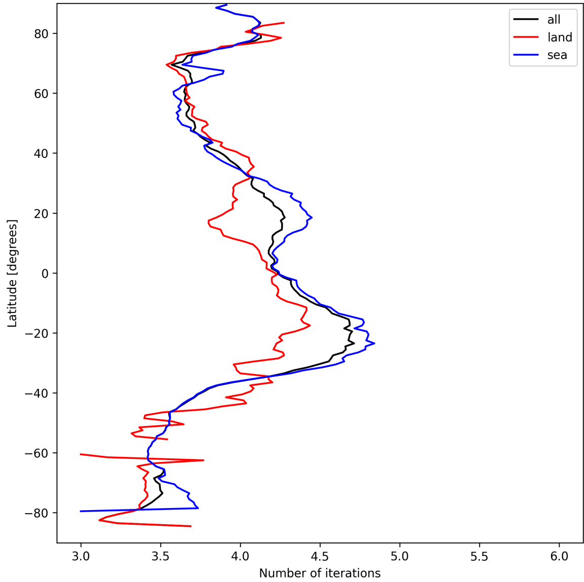
Figure 17: Zonal average of “Number of iterations” for 2025-03-29 to 2025-03-30.
