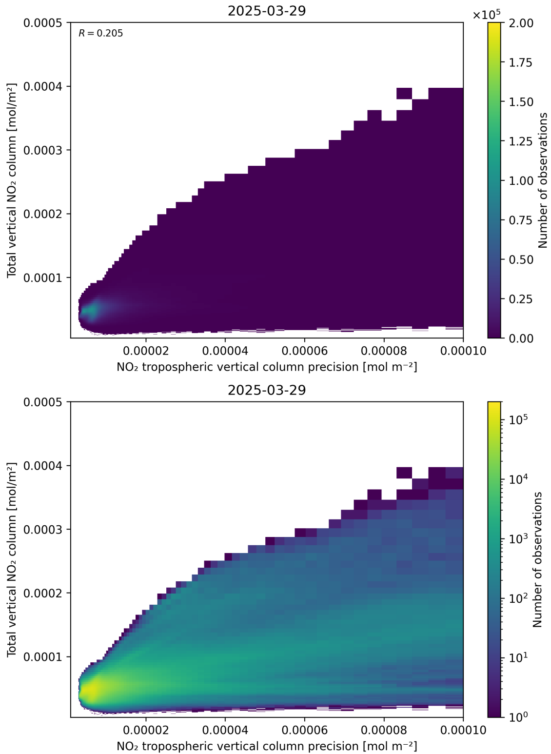
Figure 138: Scatter density plot of “NO 2 tropospheric vertical column precision” against “Total vertical NO 2 column” for 2025-03-29 to 2025-03-30.
