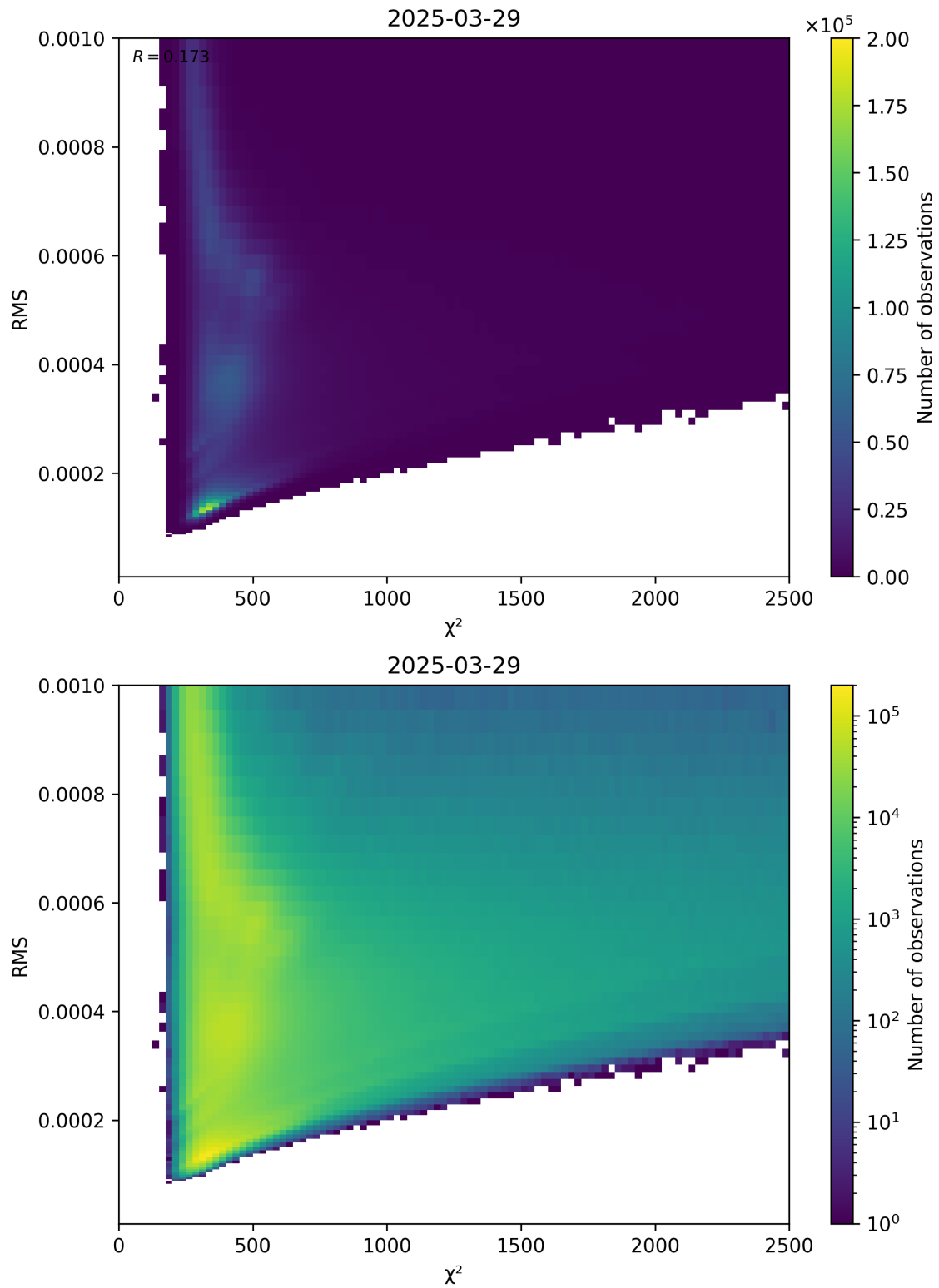
Figure 82: Scatter density plot of “ \chi^2 ” against “RMS” for 2025-03-29 to 2025-03-30.
