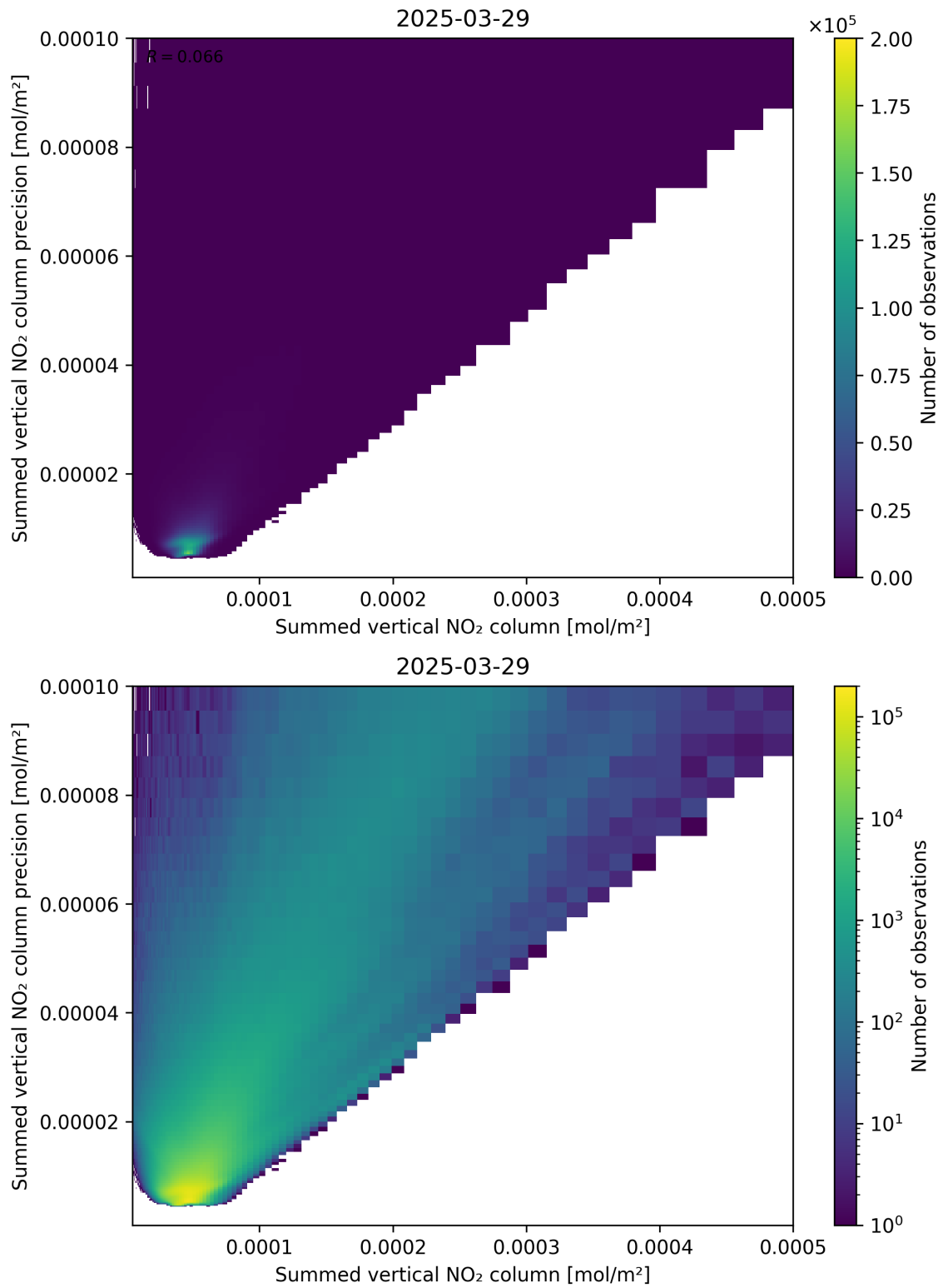
Figure 105: Scatter density plot of “Summed vertical NO 2 column” against “Summed vertical NO 2 column precision” for 2025-03-29 to 2025-03-30.
