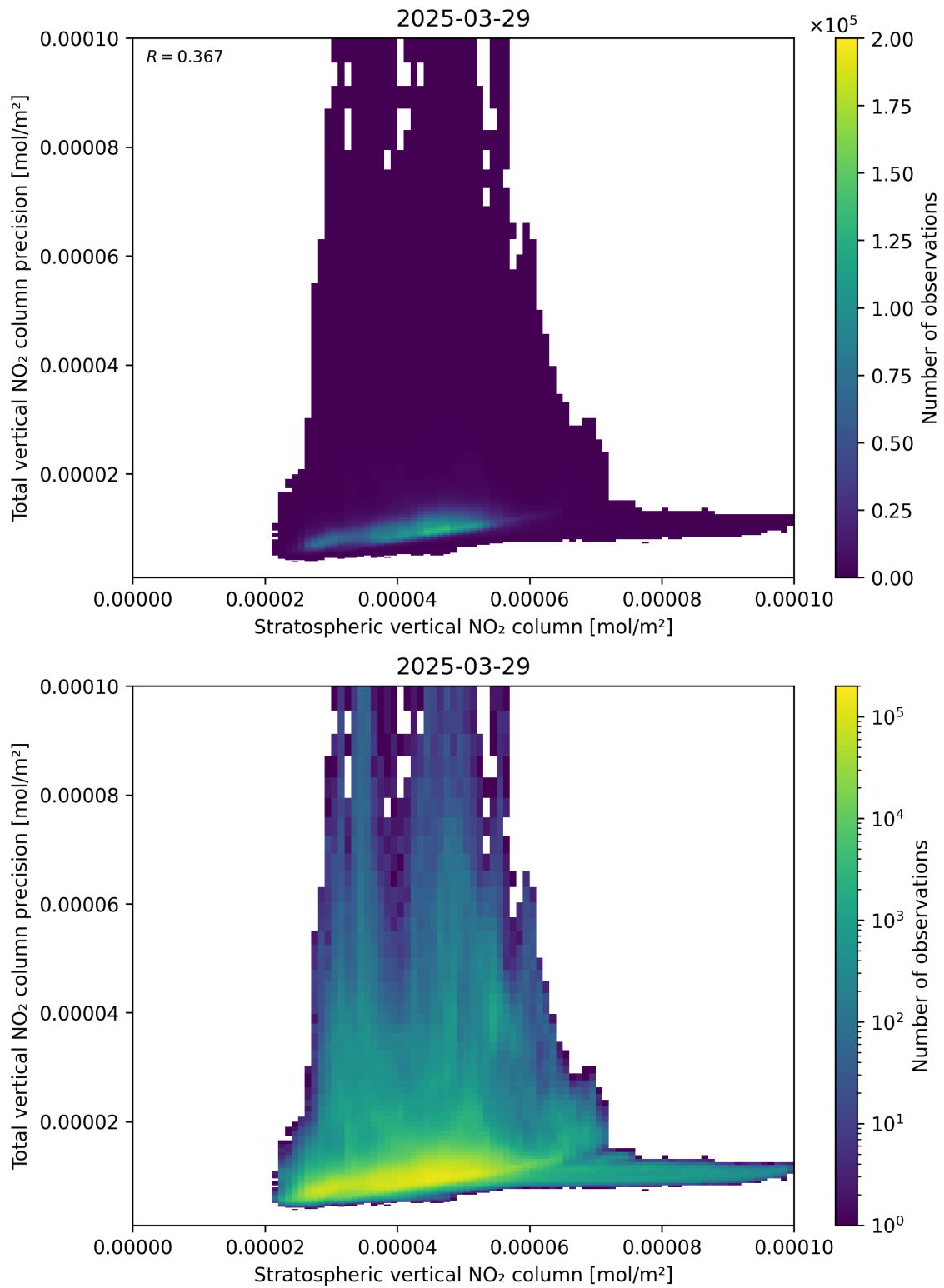
Figure 101: Scatter density plot of “Stratospheric vertical NO 2 column” against “Total vertical NO 2 column precision” for 2025-03-29 to 2025-03-30.
