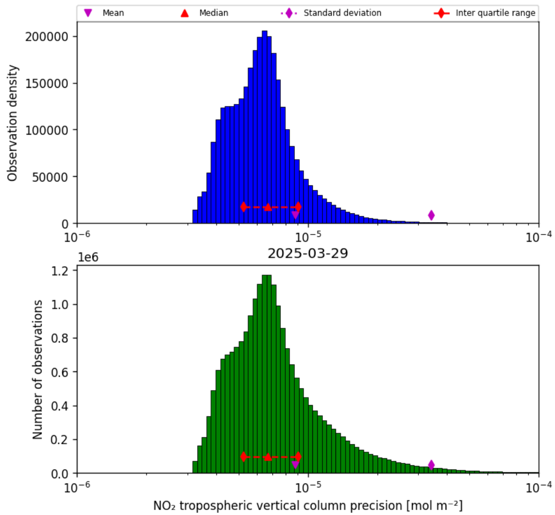
Figure 30: Histogram of “NO 2 tropospheric vertical column precision” for 2025-03-29 to 2025-03-30
