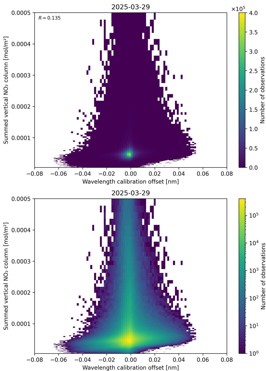
Figure 177: Scatter density plot of “Wavelength calibration offset” against “Summed vertical NO 2 column” for 2025-03-29 to 2025-03-30.
