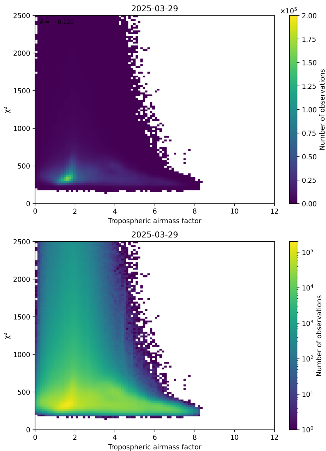
Figure 73: Scatter density plot of “Tropospheric airmass factor” against “ \chi^2 ” for 2025-03-29 to 2025-03-30.
