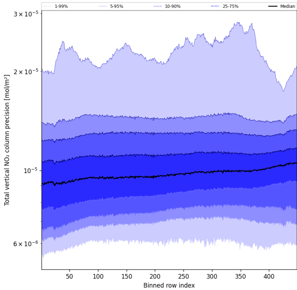
Figure 56: Along track statistics of “Total vertical NO 2 column precision” for 2025-03-29 to 2025-03-30
