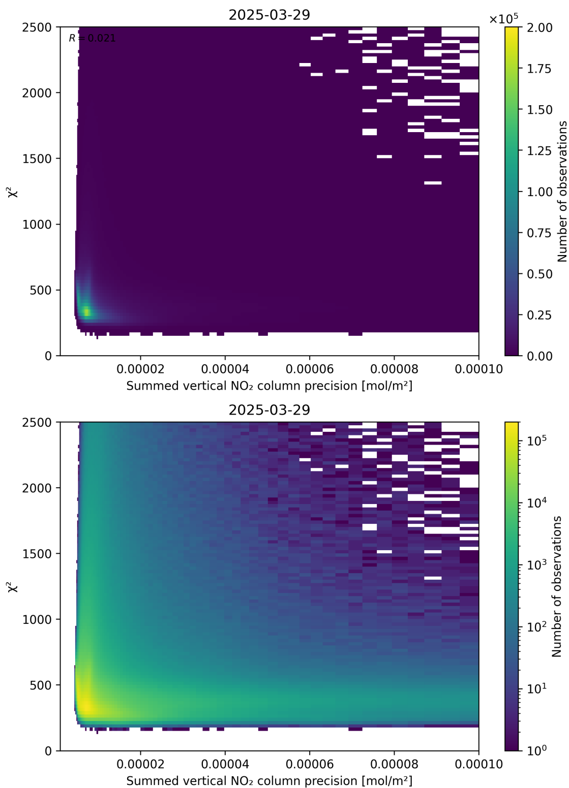
Figure 107: Scatter density plot of “Summed vertical NO 2 column precision” against “ \chi^2 ” for 2025-03-29 to 2025-03-30.
