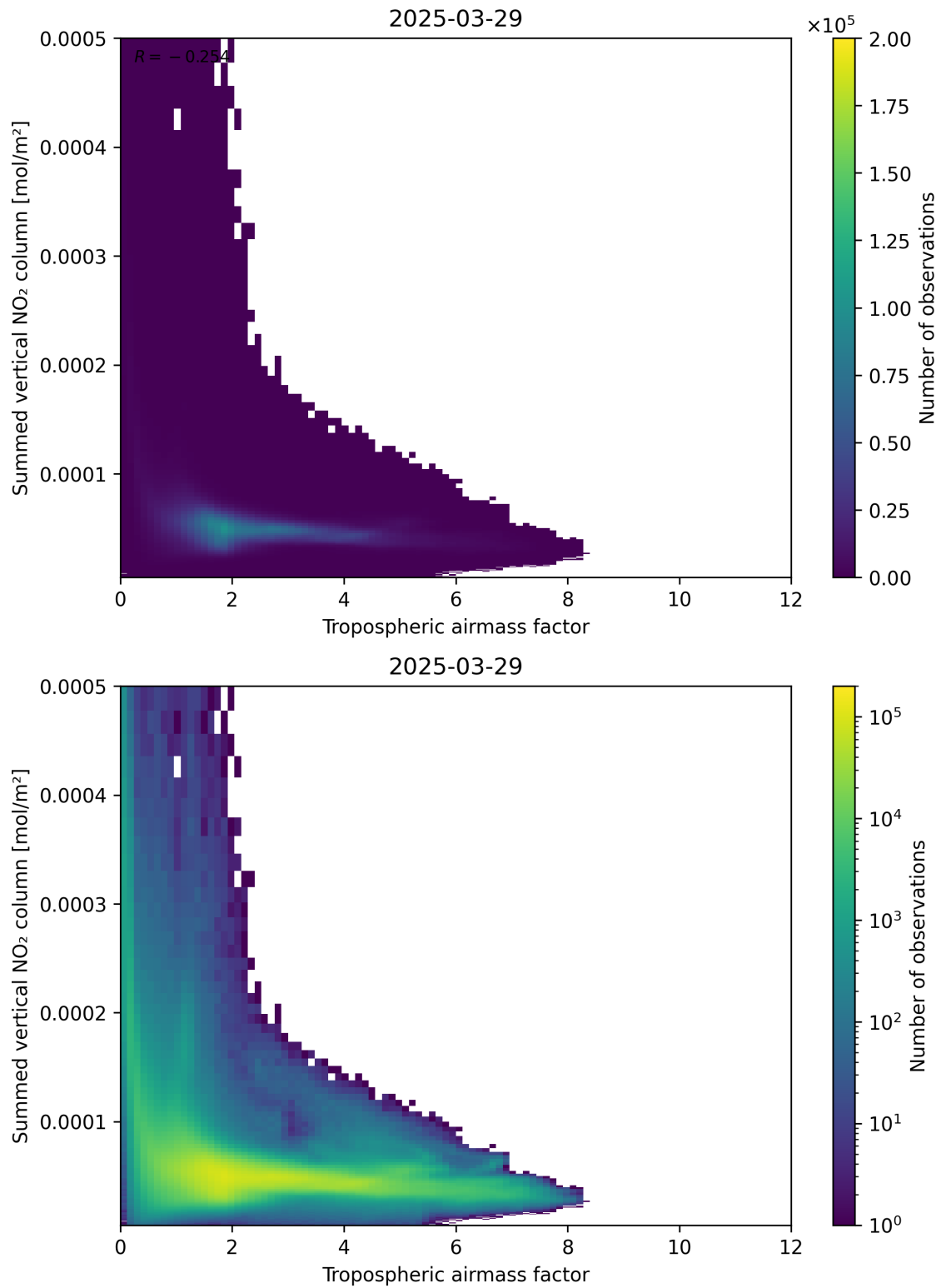
Figure 75: Scatter density plot of “Tropospheric air mass factor” against “Summed vertical NO 2 column” for 2025-03-29 to 2025-03-30.
