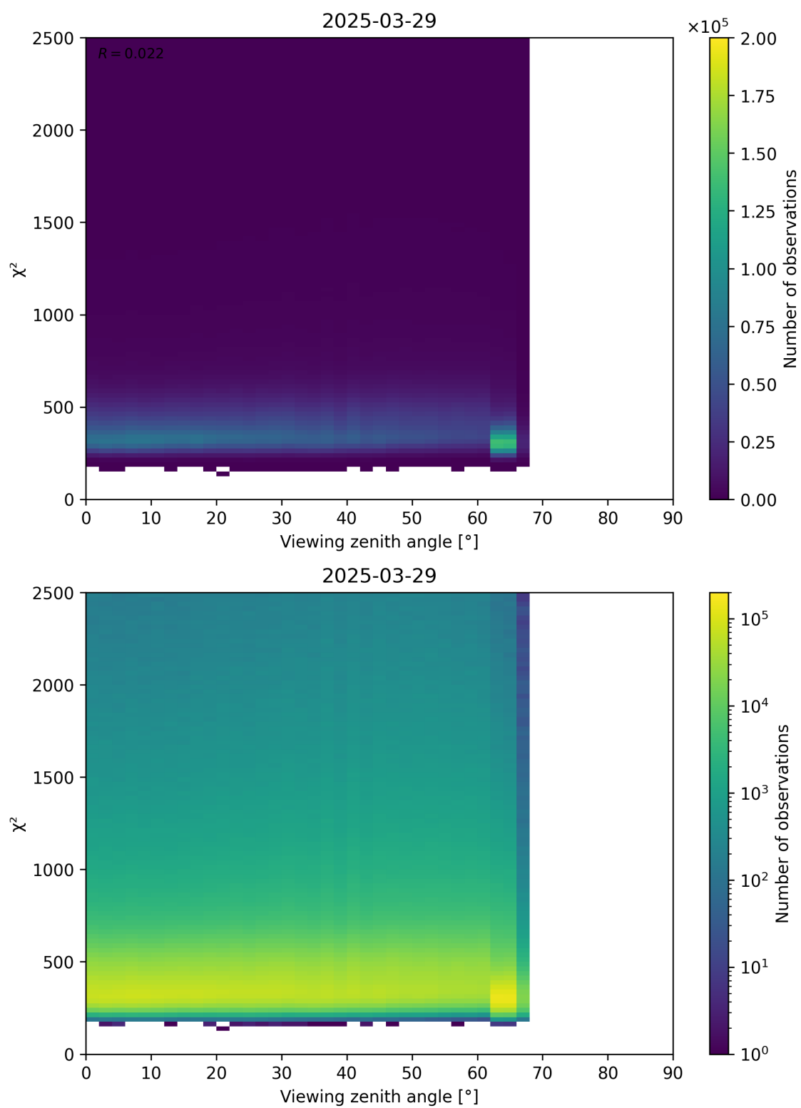
Figure 162: Scatter density plot of “Viewing zenith angle” against “ \chi^2 ” for 2025-03-29 to 2025-03-30.
