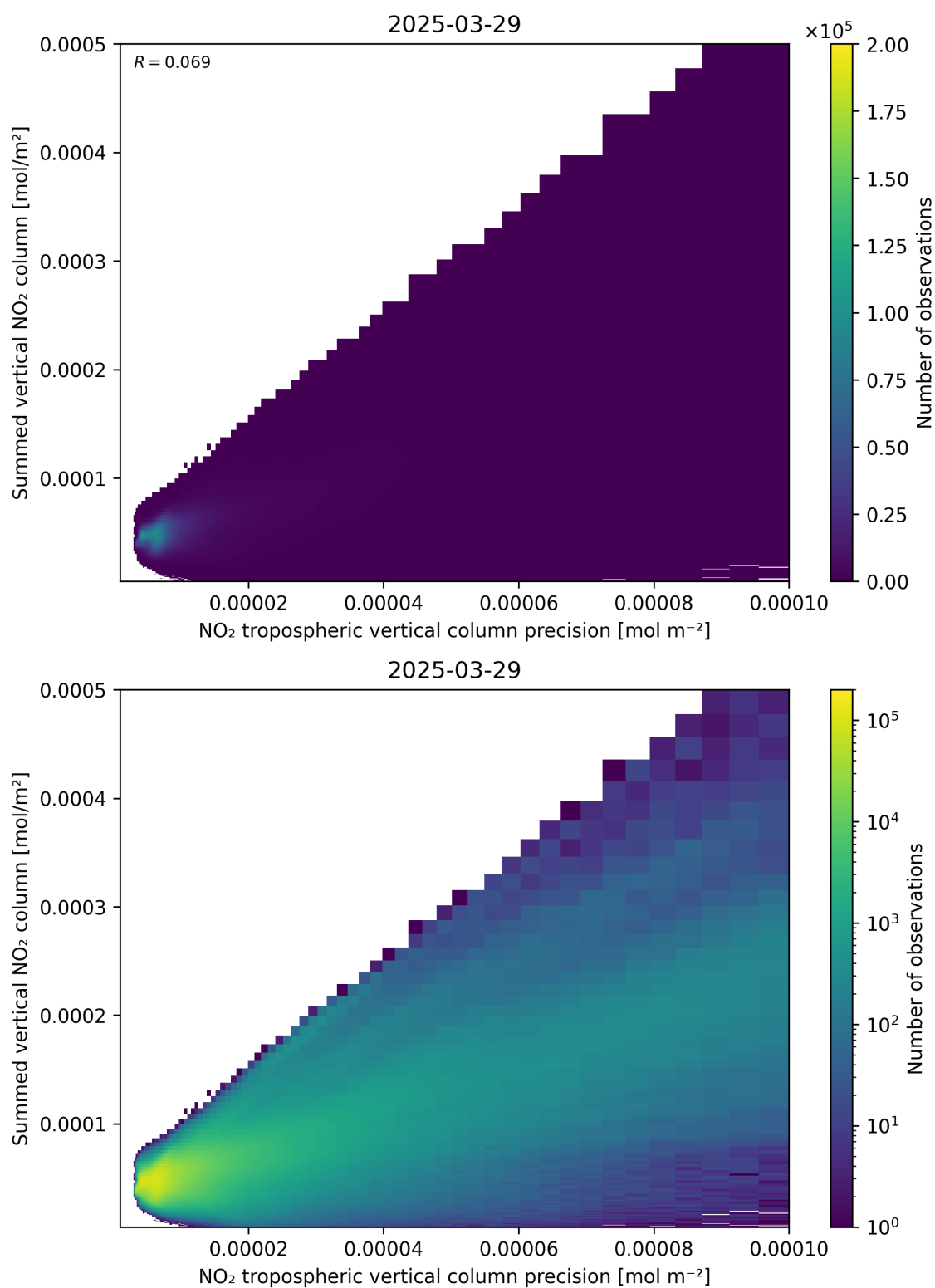
Figure 136: Scatter density plot of “NO 2 tropospheric vertical column precision” against “Summed vertical NO 2 column” for 2025-03-29 to 2025-03-30.
