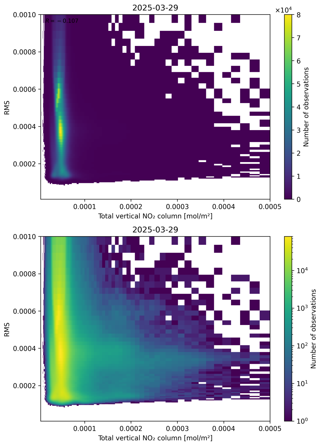
Figure 120: Scatter density plot of “Total vertical NO 2 column” against “RMS” for 2025-03-29 to 2025-03-30.
