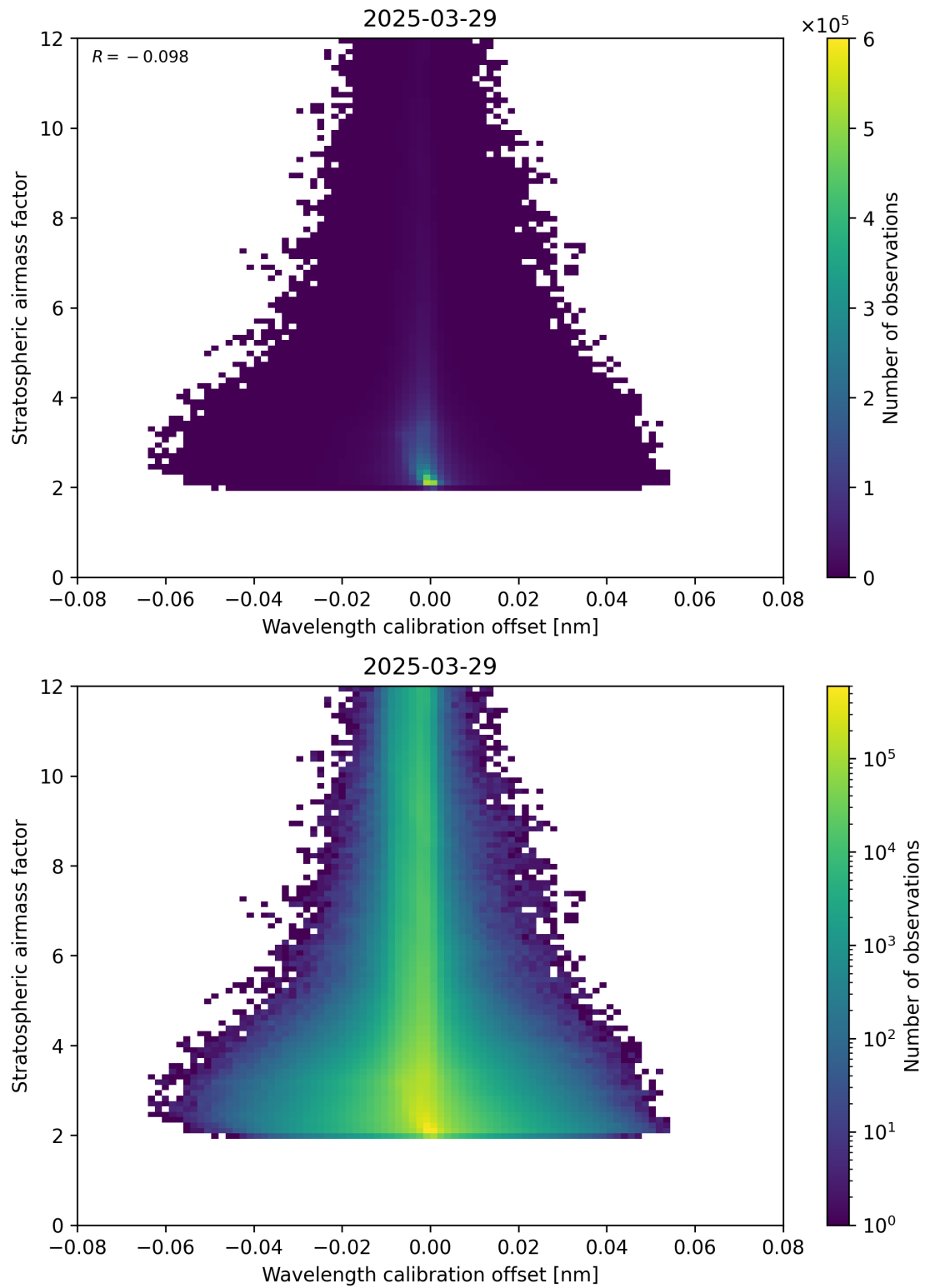
Figure 174: Scatter density plot of “Wavelength calibration offset” against “Stratospheric air mass factor” for 2025-03-29 to 2025-03-30.
