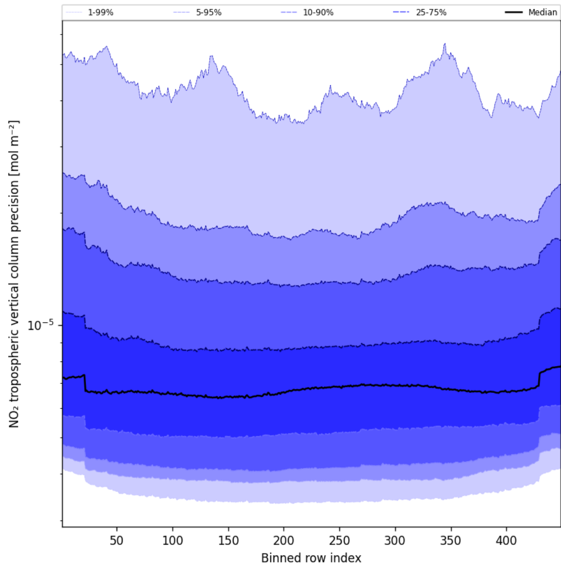
Figure 47: Along track statistics of “NO 2 tropospheric vertical column precision” for 2025-03-29 to 2025-03-30
