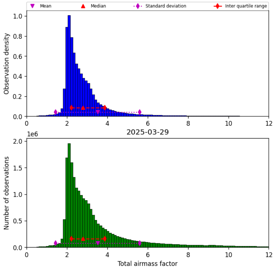
Figure 32: Histogram of “Total airmass factor” for 2025-03-29 to 2025-03-30
