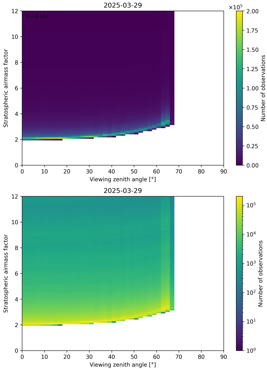
Figure 159: Scatter density plot of “Viewing zenith angle” against “Stratospheric airmass factor” for 2025-03-29 to 2025-03-30.
