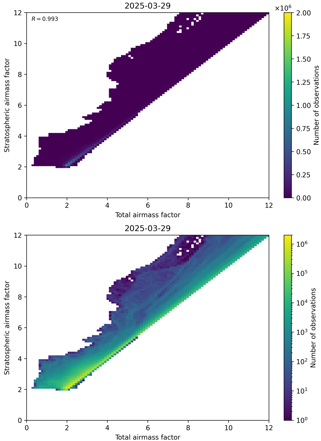
Figure 62: Scatter density plot of “Total airmass factor” against “Stratospheric airmass factor” for 2025-03-29 to 2025-03-30.
