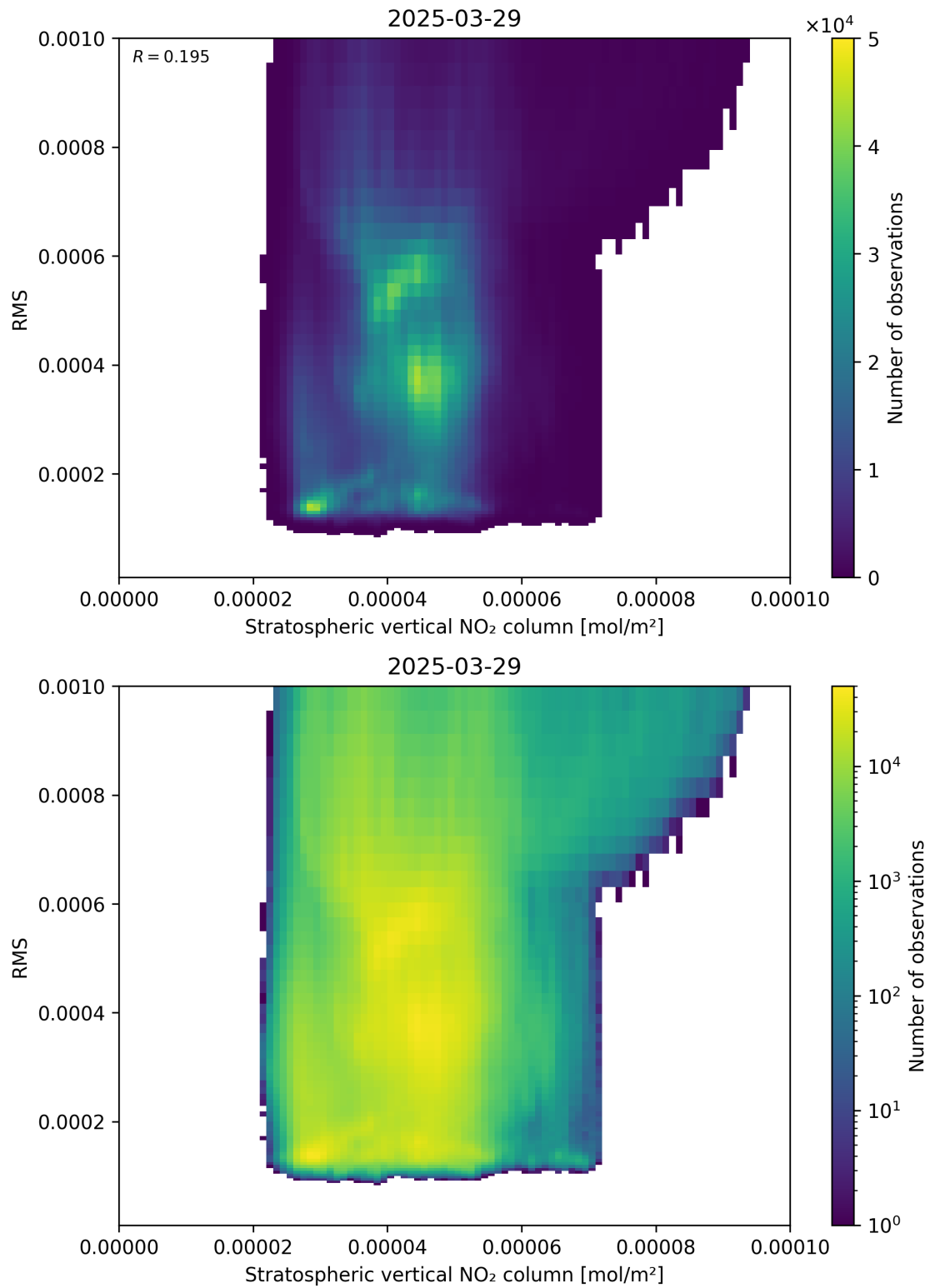
Figure 102: Scatter density plot of “Stratospheric vertical NO 2 column” against “RMS” for 2025-03-29 to 2025-03-30.
