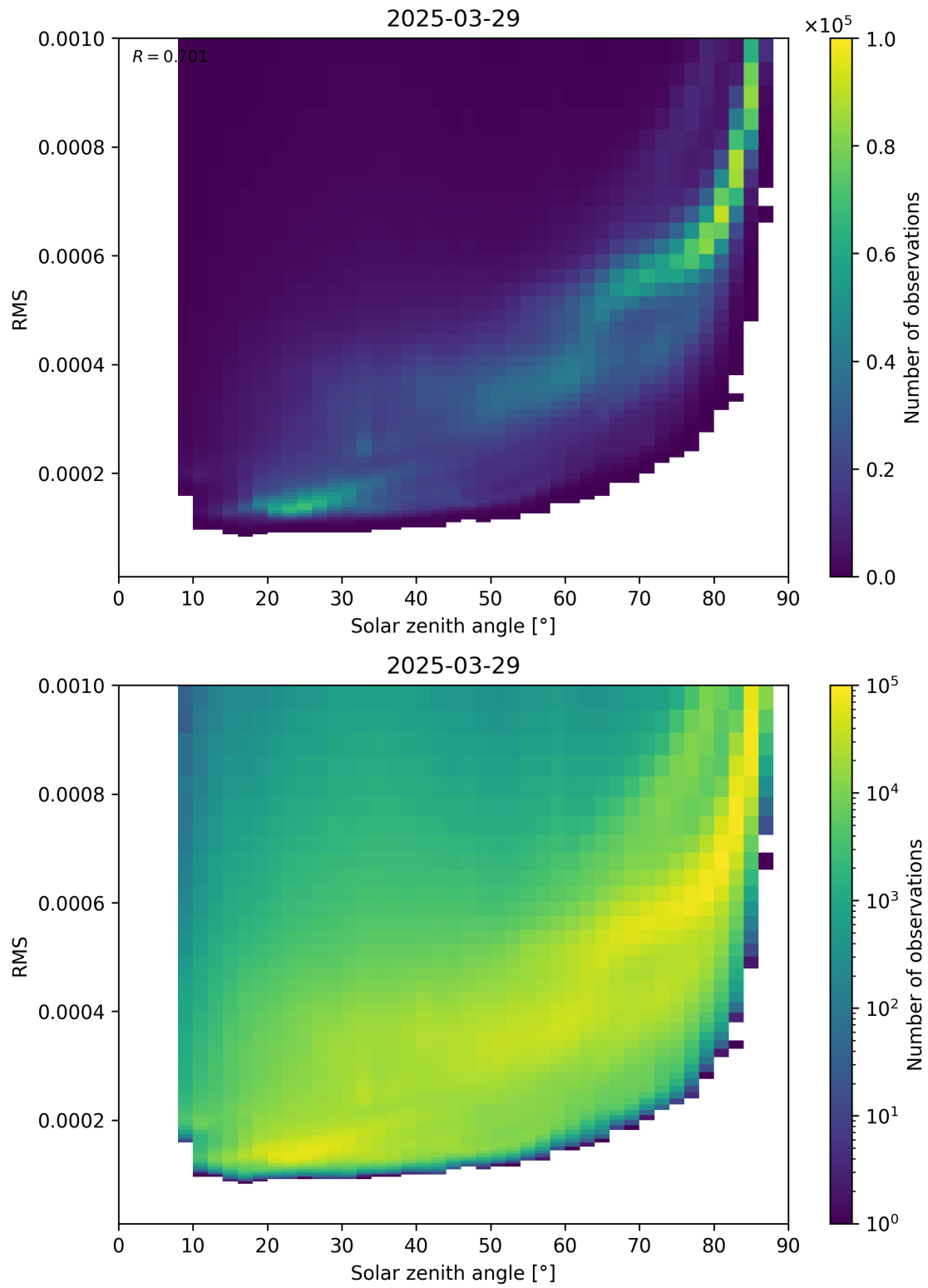
Figure 157: Scatter density plot of “Solar zenith angle” against “RMS” for 2025-03-29 to 2025-03-30.
