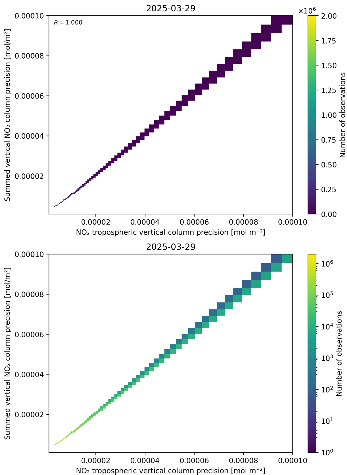
Figure 137: Scatter density plot of “NO 2 tropospheric vertical column precision” against “Summed vertical NO 2 column precision” for 2025-03-29 to 2025-03-30.
