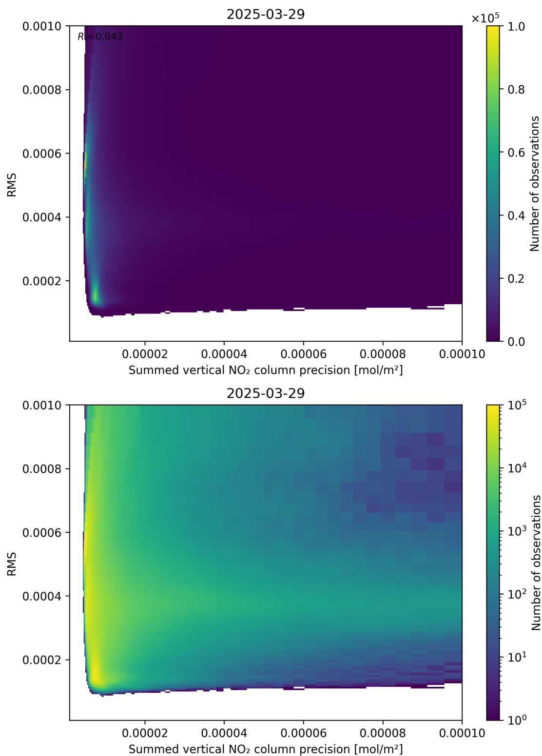
Figure 108: Scatter density plot of “Summed vertical NO 2 column precision” against “RMS” for 2025-03-29 to 2025-03-30.
