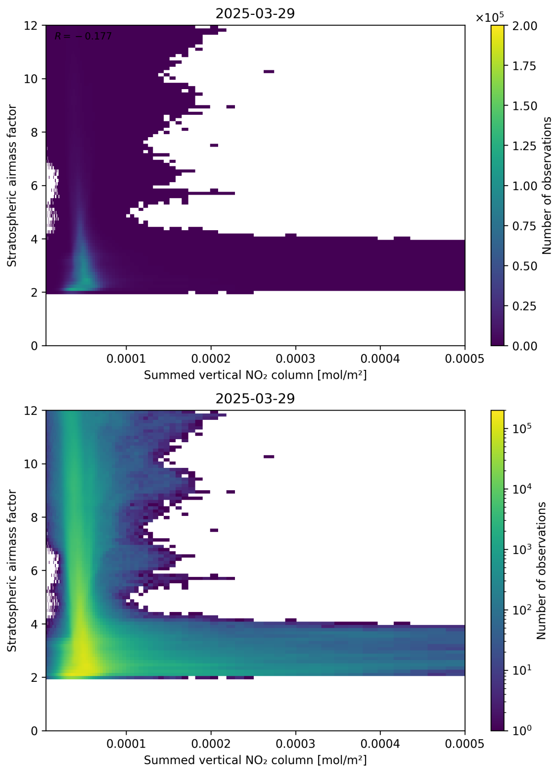
Figure 103: Scatter density plot of “Summed vertical NO 2 column” against “Stratospheric airmass factor” for 2025-03-29 to 2025-03-30.
