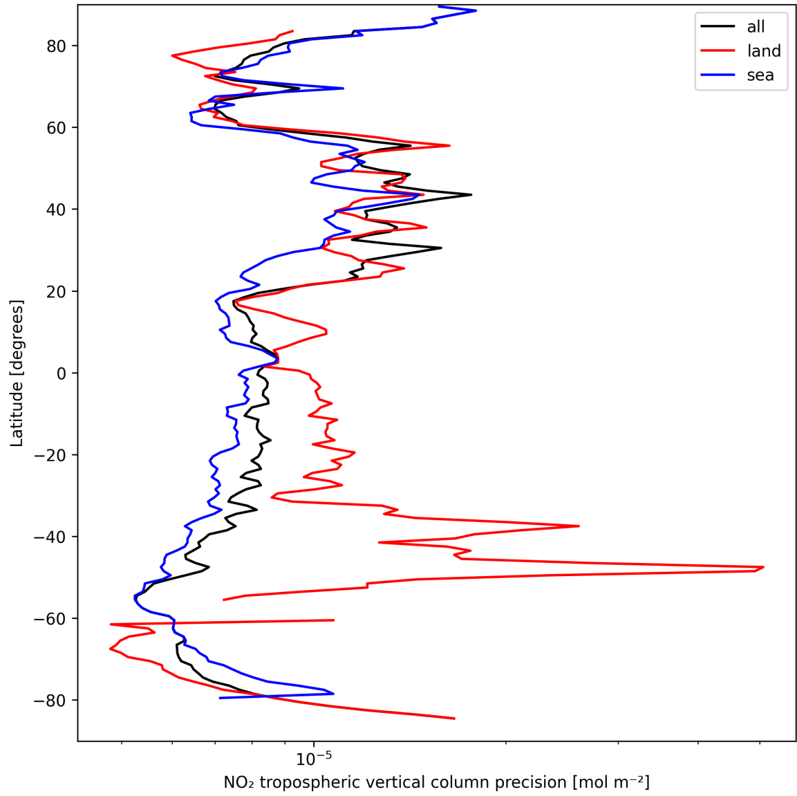
Figure 13: Zonal average of “NO 2 tropospheric vertical column precision” for 2025-03-29 to 2025-03-30.
