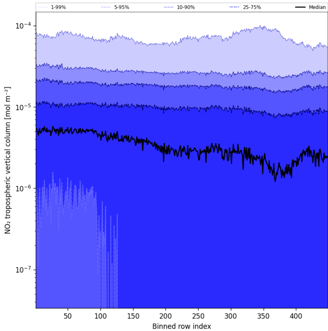
Figure 46: Along track statistics of “NO 2 tropospheric vertical column” for 2025-03-29 to 2025-03-30
