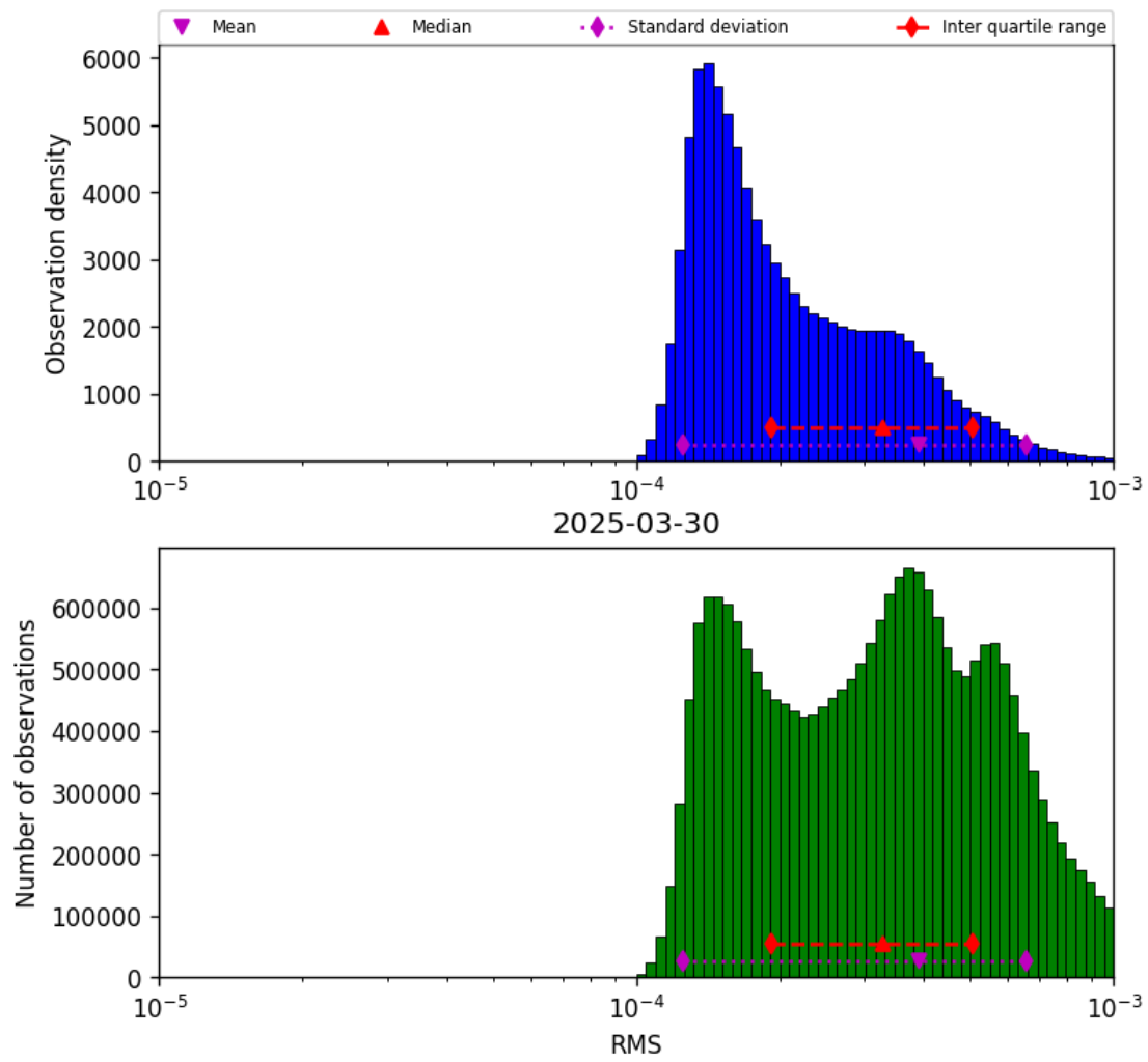
Figure 43: Histogram of “RMS” for 2025-03-30 to 2025-03-31
