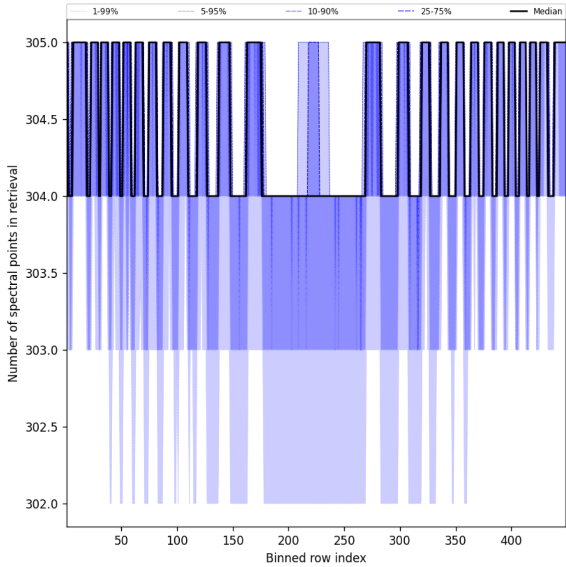
Figure 50: Along track statistics of “Number of spectral points in retrieval” for 2025-03-30 to 2025-03-31
