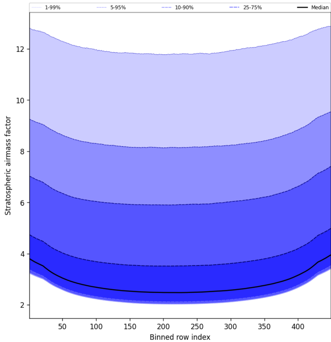
Figure 61: Along track statistics of “Stratospheric airmass factor” for 2025-03-30 to 2025-03-31
