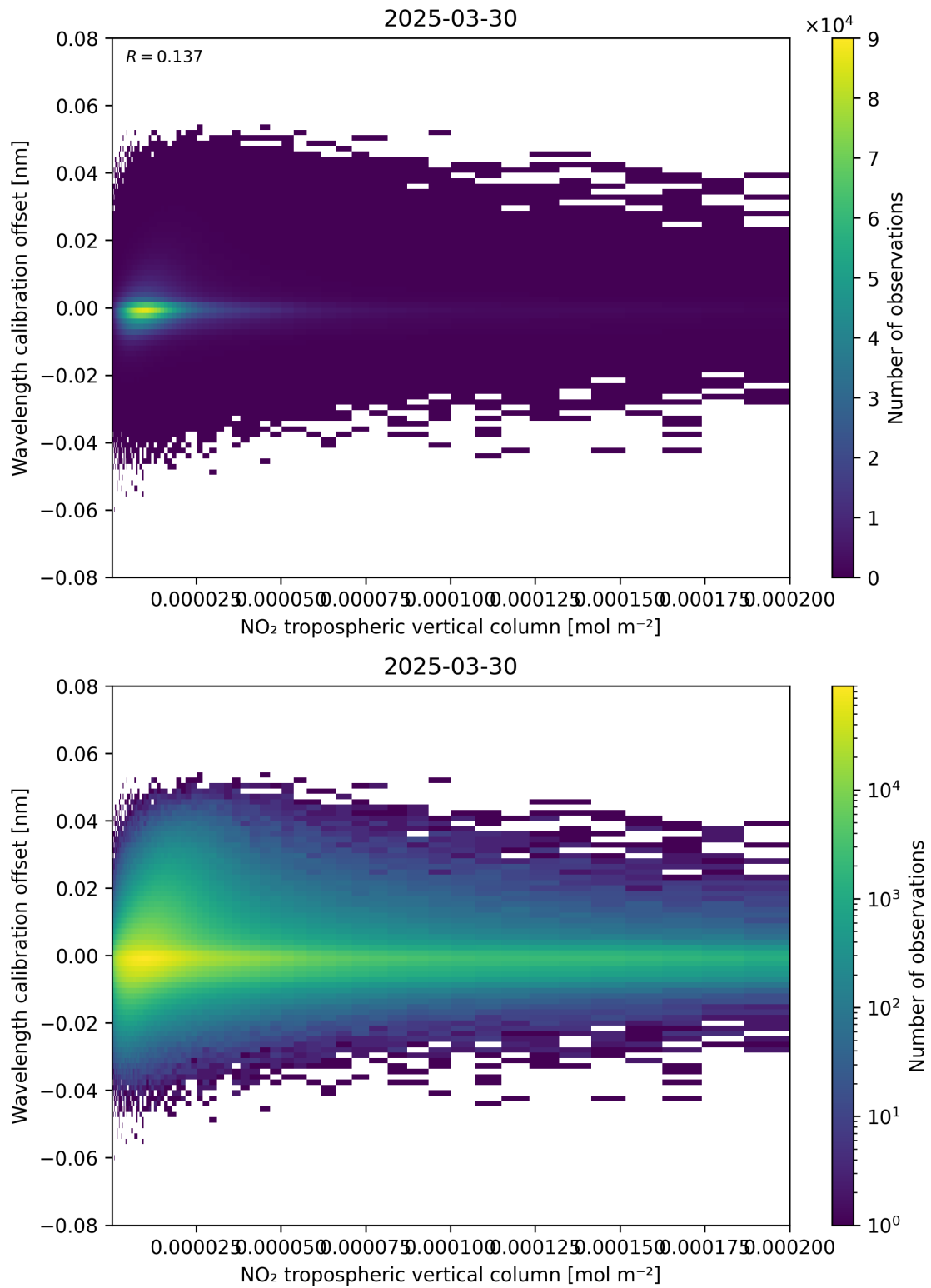
Figure 143: Scatter density plot of “NO 2 tropospheric vertical column” against “Wavelength calibration offset” for 2025-03-30 to 2025-03-31.
