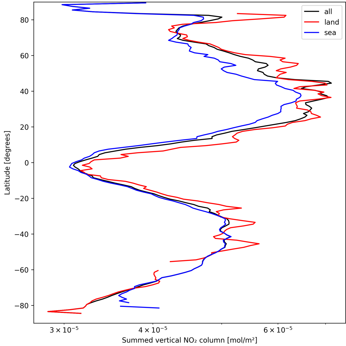
Figure 23: Zonal average of “Summed vertical NO 2 column” for 2025-03-30 to 2025-03-31.
