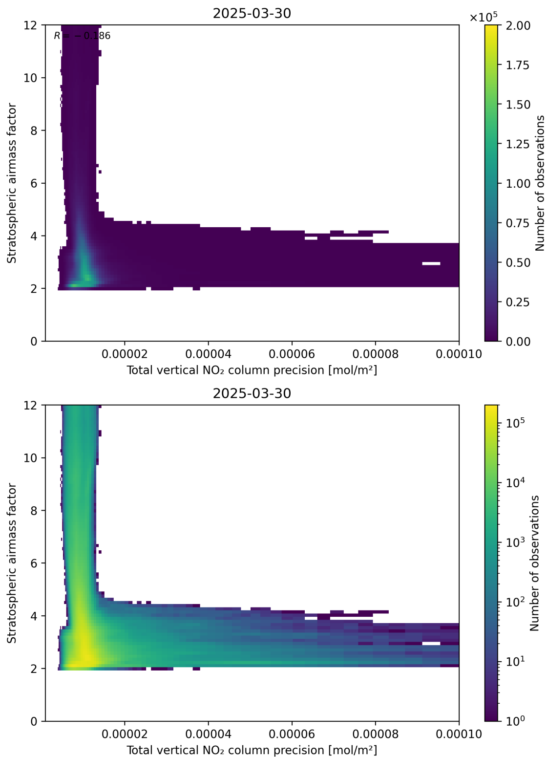
Figure 115: Scatter density plot of “Total vertical NO 2 column precision” against “Stratospheric air mass factor” for 2025-03-30 to 2025-03-31.
