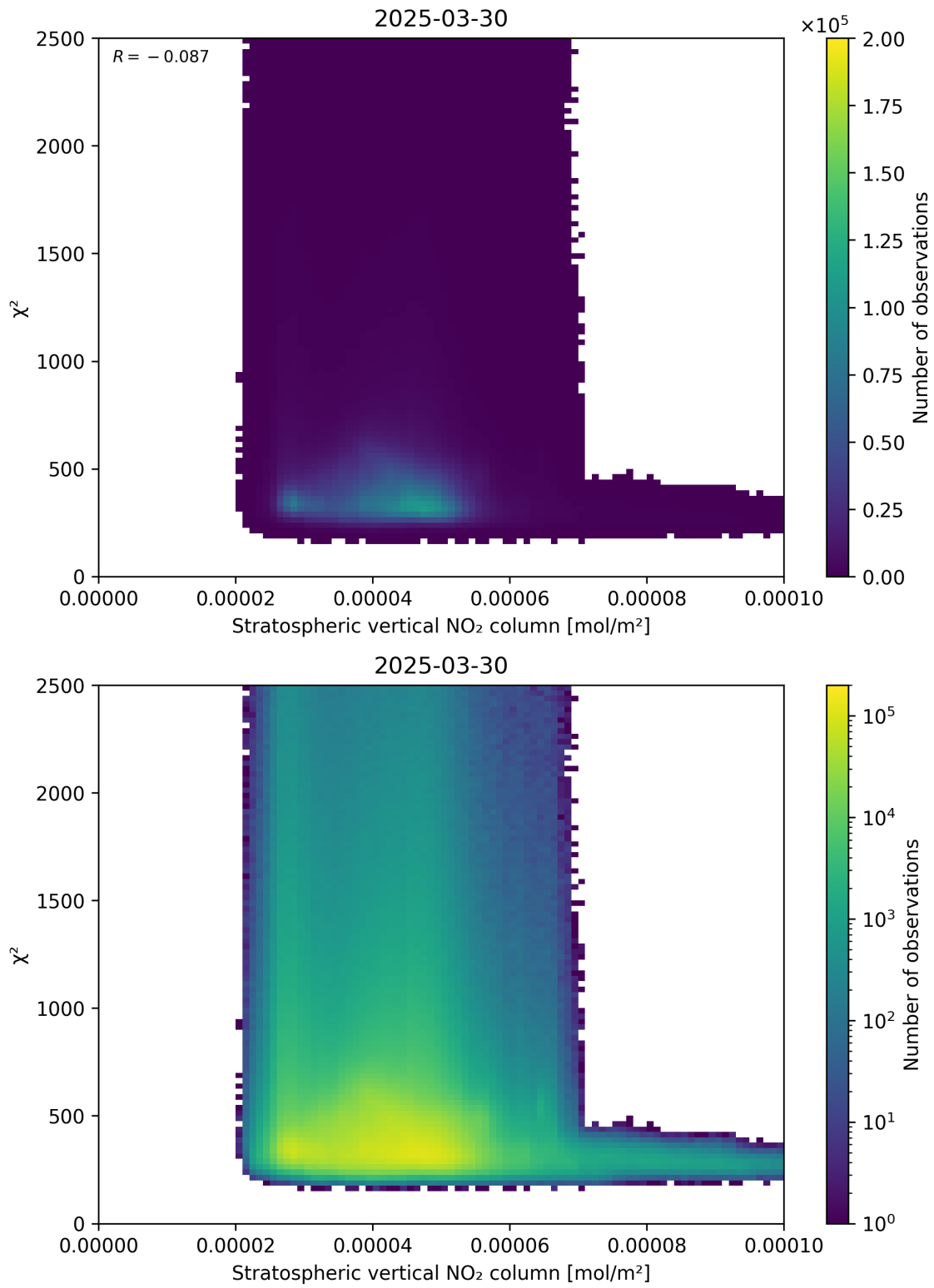
Figure 97: Scatter density plot of “Stratospheric vertical NO 2 column” against “ \chi^2 ” for 2025-03-30 to 2025-03-31.
