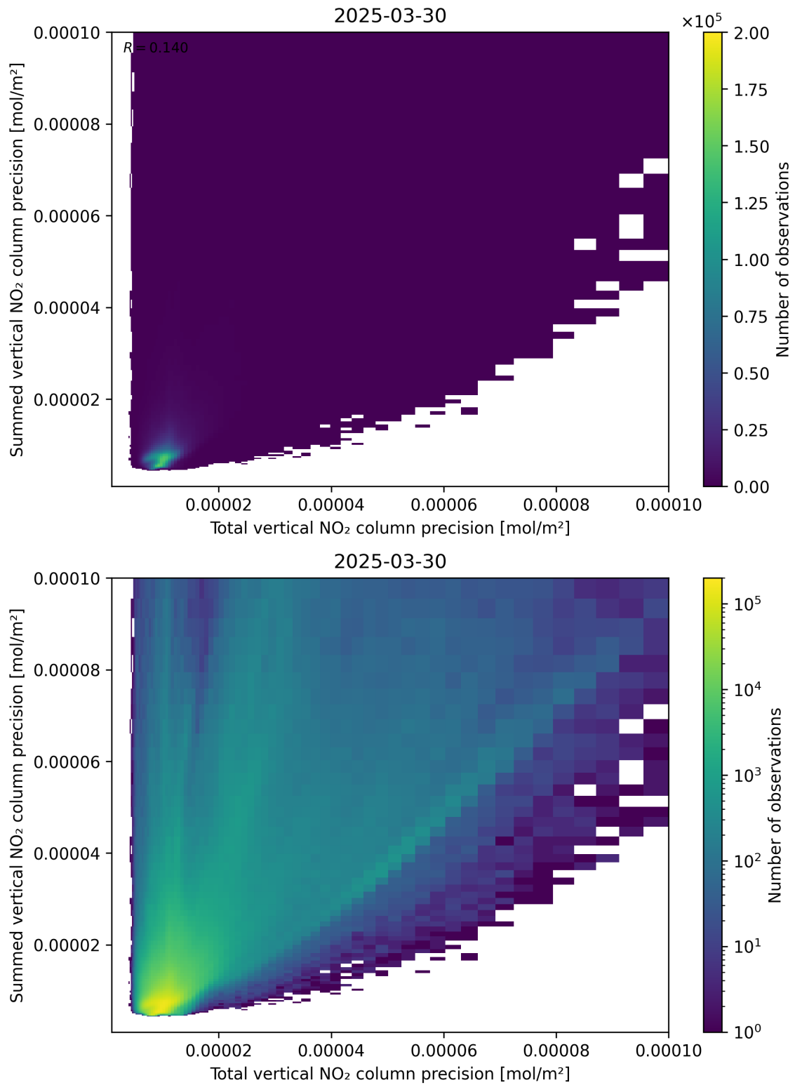
Figure 118: Scatter density plot of “Total vertical NO 2 column precision” against “Summed vertical NO 2 column precision” for 2025-03-30 to 2025-03-31.
