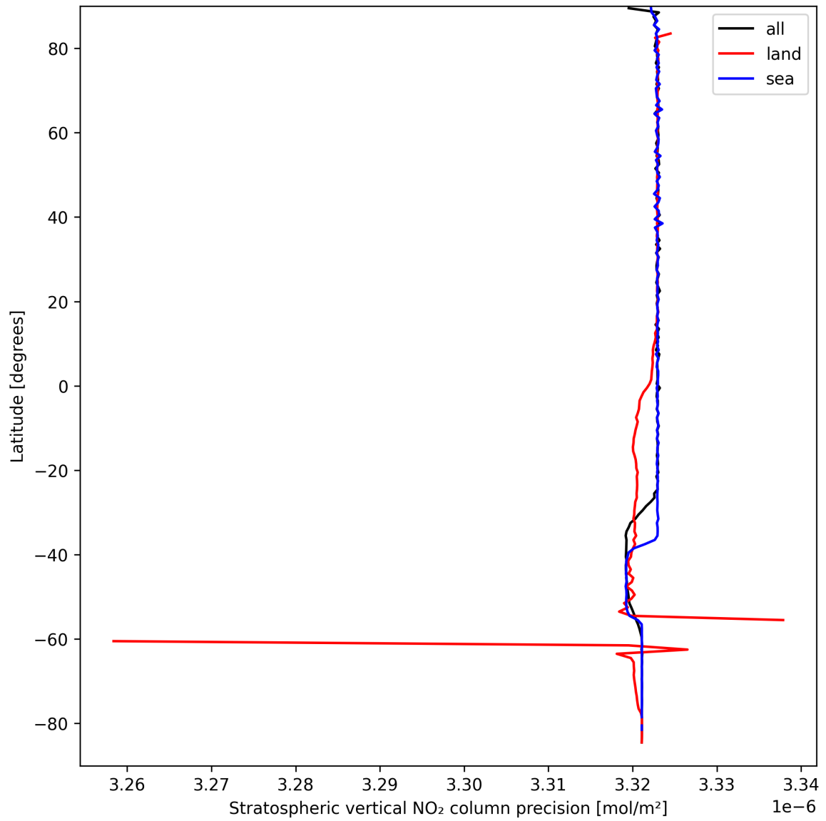
Figure 20: Zonal average of “Stratospheric vertical NO 2 column precision” for 2025-03-30 to 2025-03-31.
