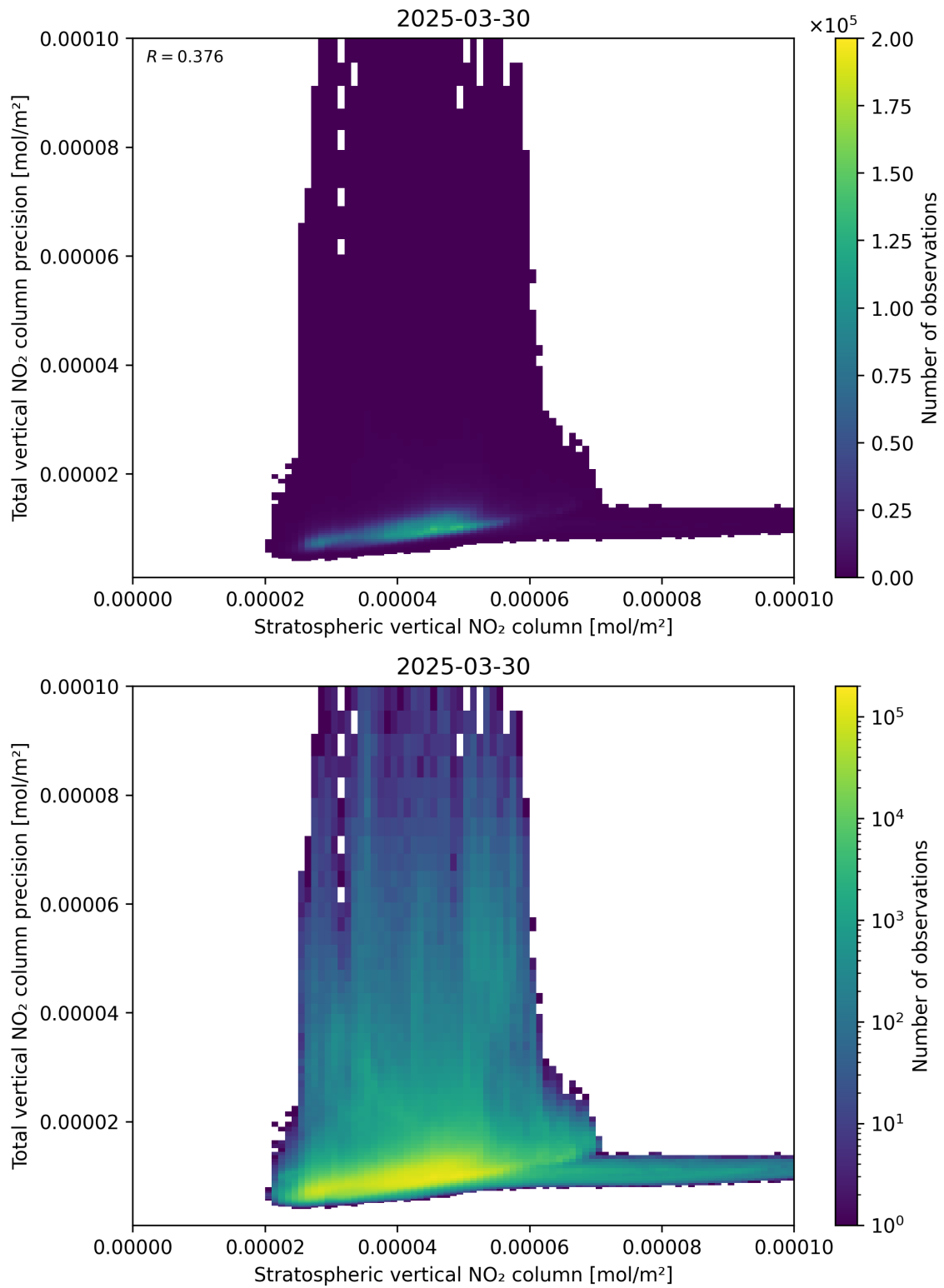
Figure 101: Scatter density plot of “Stratospheric vertical NO 2 column” against “Total vertical NO 2 column precision” for 2025-03-30 to 2025-03-31.
