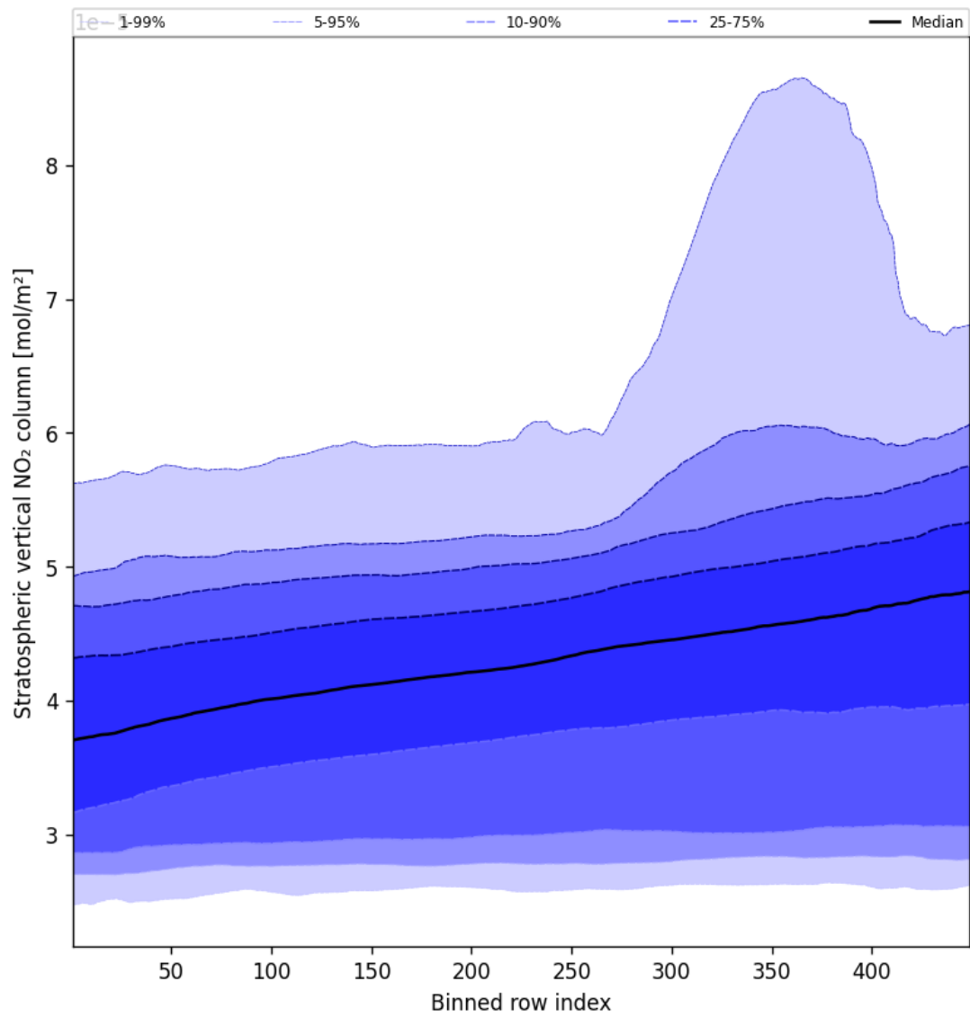
Figure 53: Along track statistics of “Stratospheric vertical NO 2 column” for 2025-03-30 to 2025-03-31
