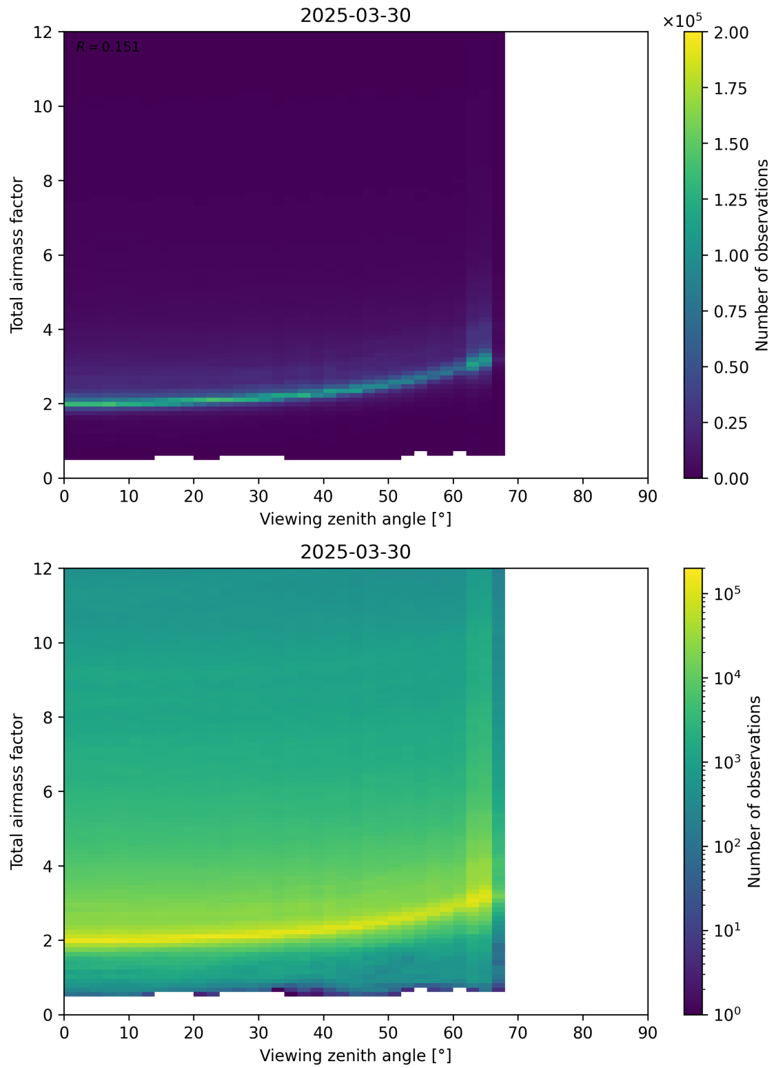
Figure 160: Scatter density plot of “Viewing zenith angle” against “Total airmass factor” for 2025-03-30 to 2025-03-31.
