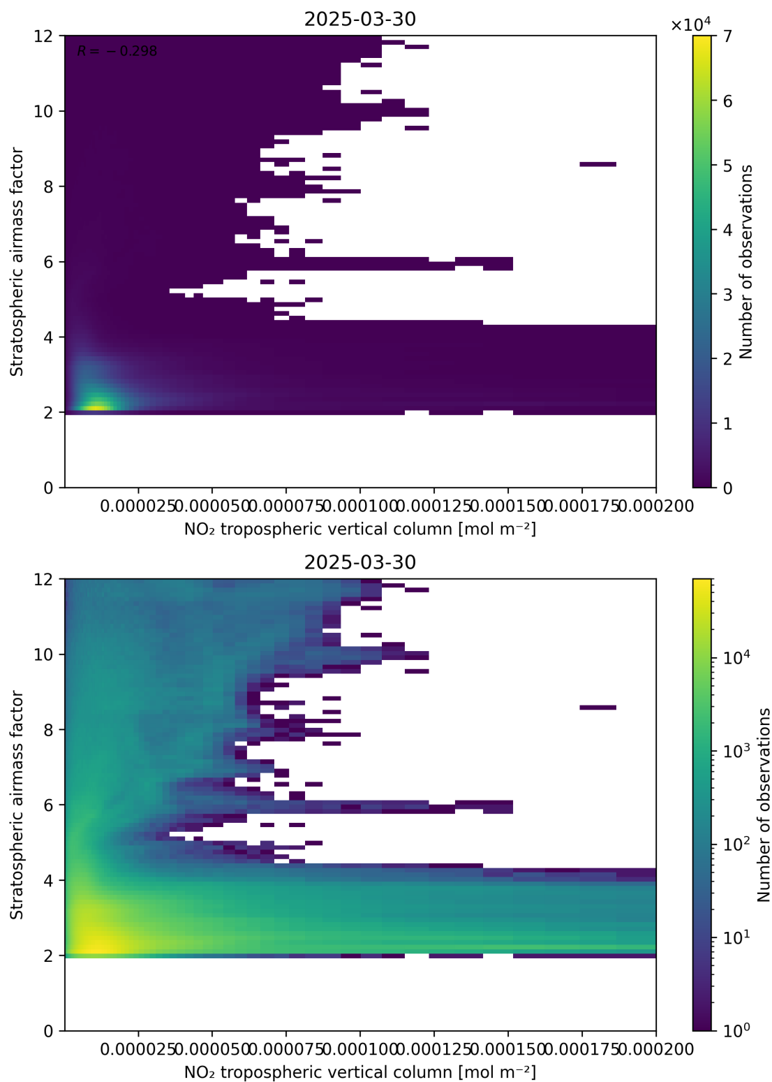
Figure 121: Scatter density plot of “NO 2 tropospheric vertical column” against “Stratospheric air mass factor” for 2025-03-30 to 2025-03-31.
