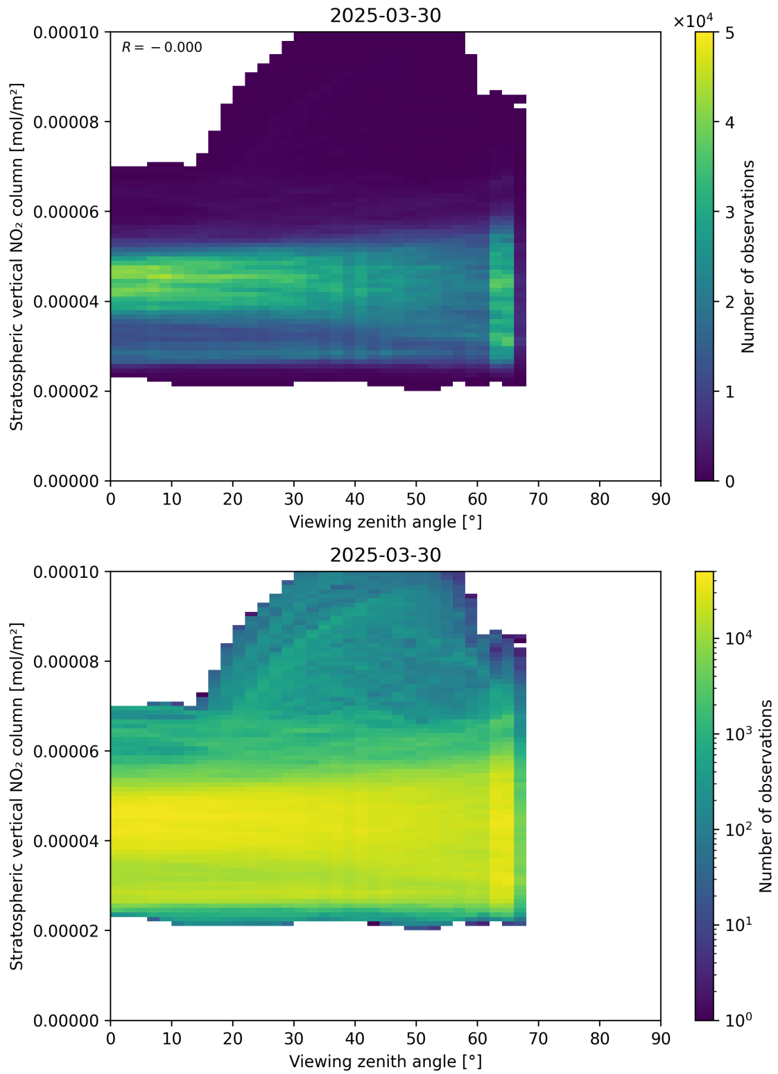
Figure 164: Scatter density plot of “Viewing zenith angle” against “Stratospheric vertical NO 2 column” for 2025-03-30 to 2025-03-31.
