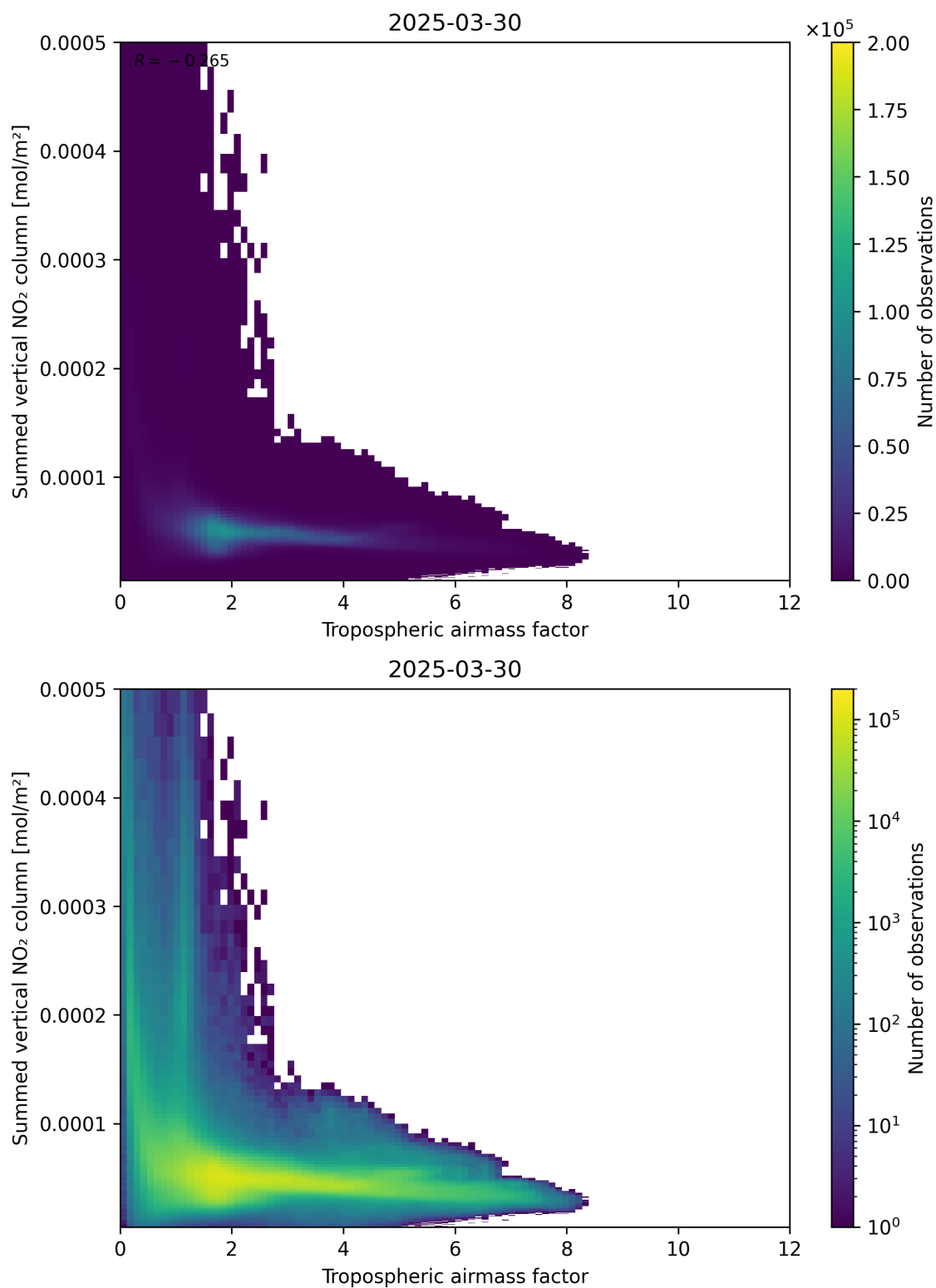
Figure 75: Scatter density plot of “Tropospheric air mass factor” against “Summed vertical NO 2 column” for 2025-03-30 to 2025-03-31.
