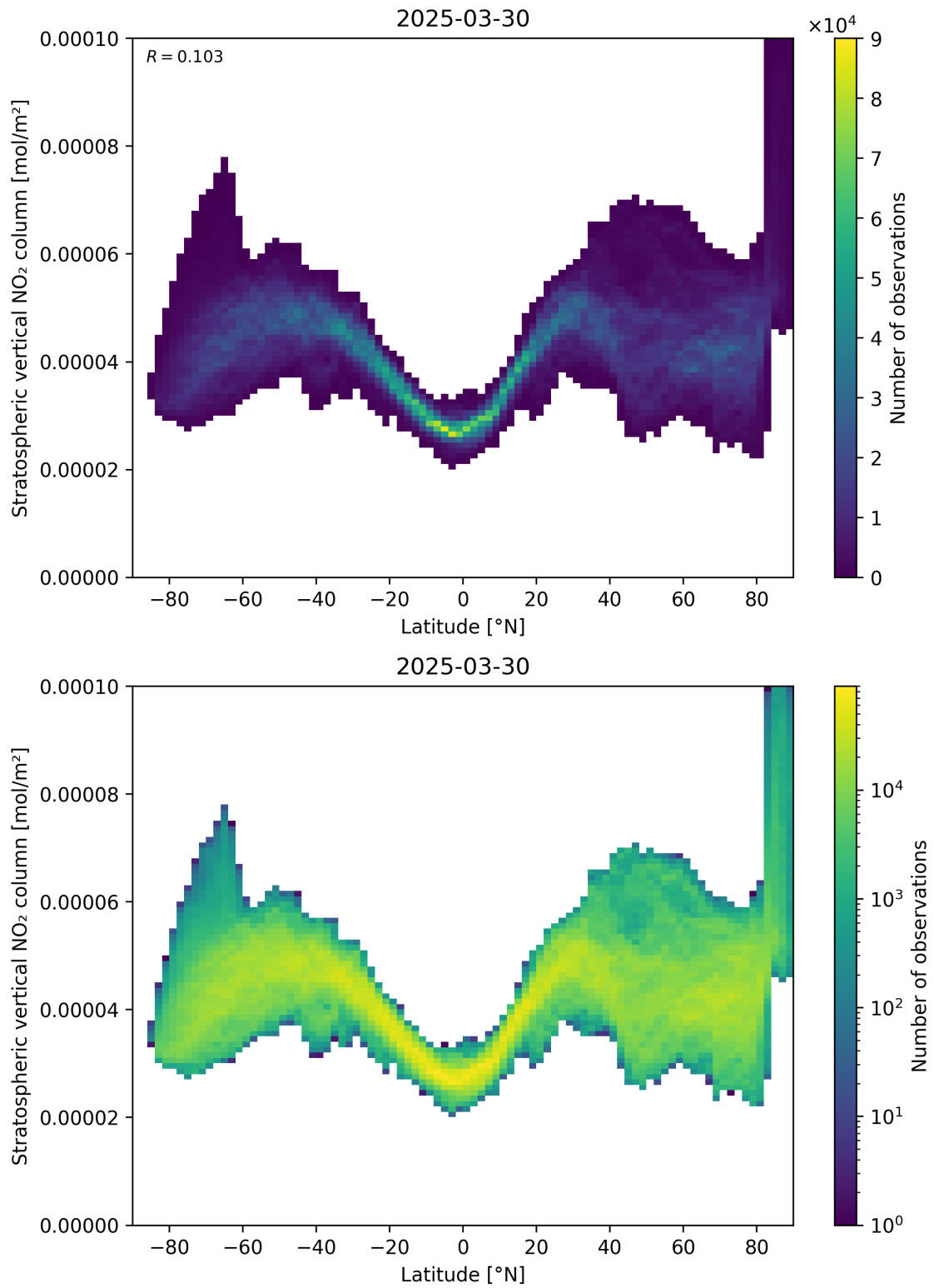
Figure 87: Scatter density plot of “Latitude” against “Stratospheric vertical NO 2 column” for 2025-03-30 to 2025-03-31.
