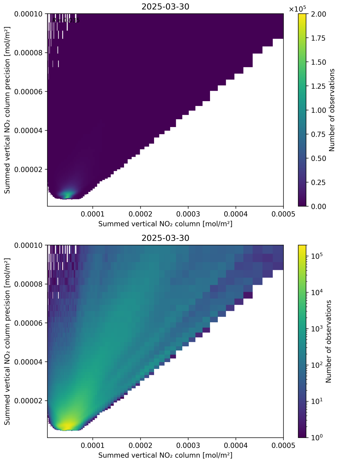
Figure 105: Scatter density plot of “Summed vertical NO 2 column” against “Summed vertical NO 2 column precision” for 2025-03-30 to 2025-03-31.
