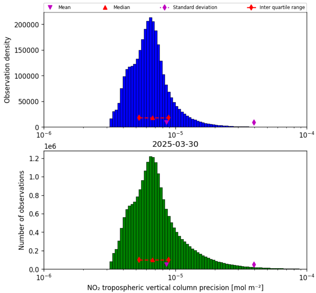
Figure 30: Histogram of “NO 2 tropospheric vertical column precision” for 2025-03-30 to 2025-03-31
