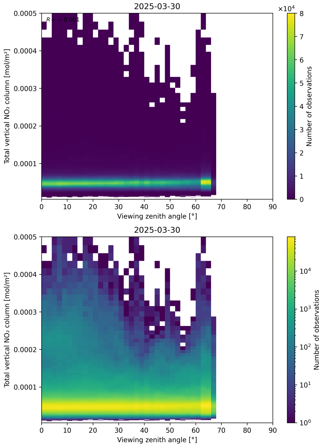
Figure 167: Scatter density plot of “Viewing zenith angle” against “Total vertical NO 2 column” for 2025-03-30 to 2025-03-31.
