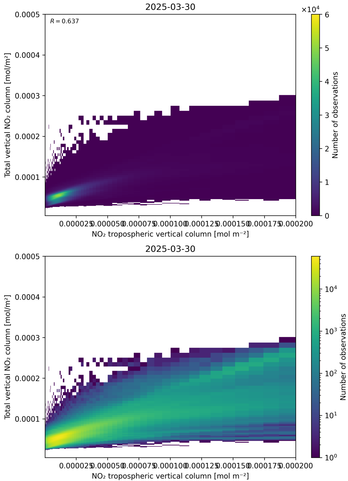
Figure 128: Scatter density plot of “NO 2 tropospheric vertical column” against “Total vertical NO 2 column” for 2025-03-30 to 2025-03-31.
