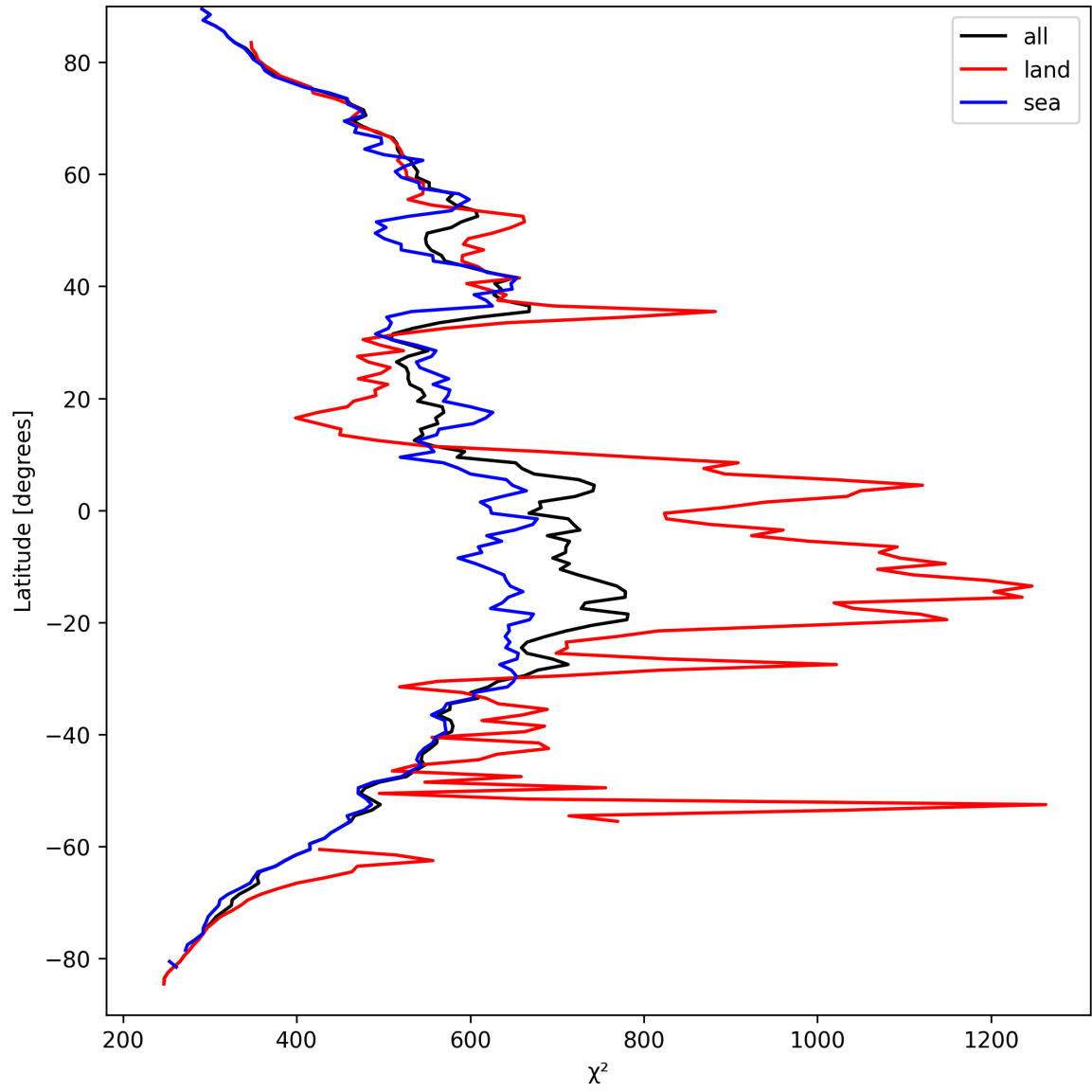
Figure 25: Zonal average of “ \chi^2 ” for 2025-03-30 to 2025-03-31.
