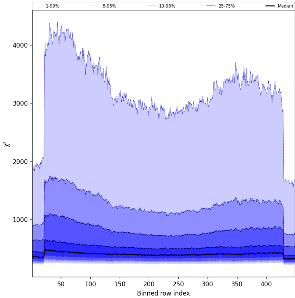
Figure 59: Along track statistics of “ \chi^2 ” for 2025-03-30 to 2025-03-31
