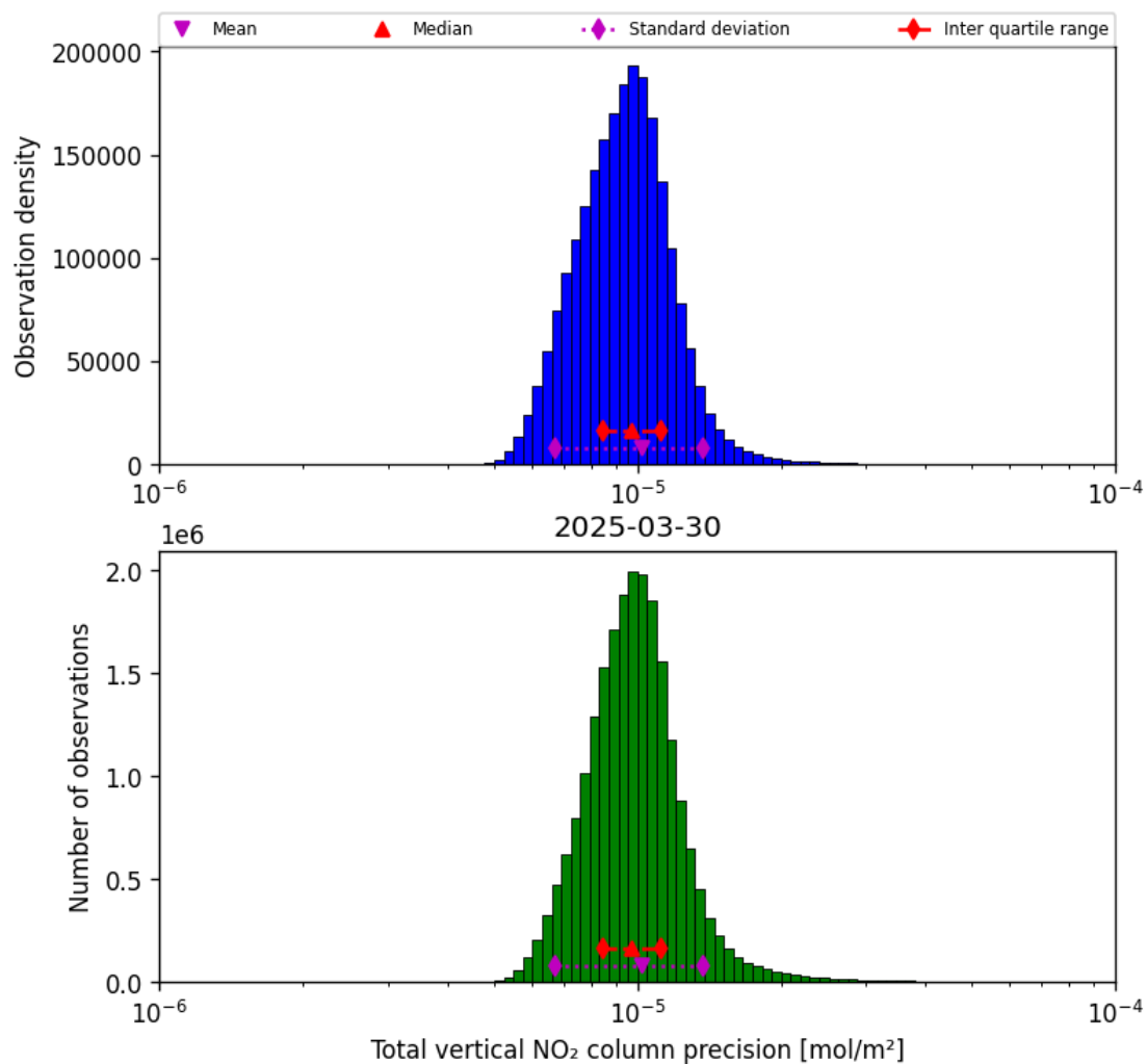
Figure 39: Histogram of "Total vertical NO 2 column precision" for 2025-03-30 to 2025-03-31
