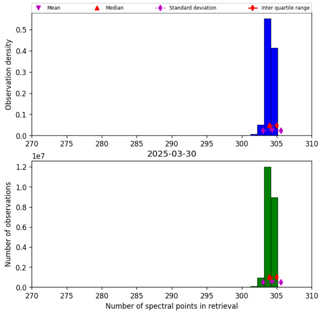
Figure 33: Histogram of “Number of spectral points in retrieval” for 2025-03-30 to 2025-03-31
