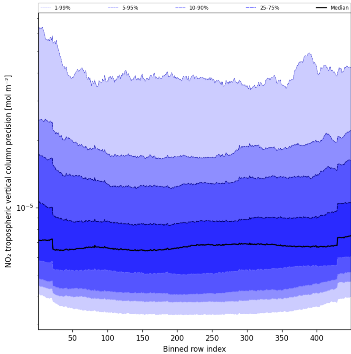
Figure 47: Along track statistics of “NO 2 tropospheric vertical column precision” for 2025-03-30 to 2025-03-31
