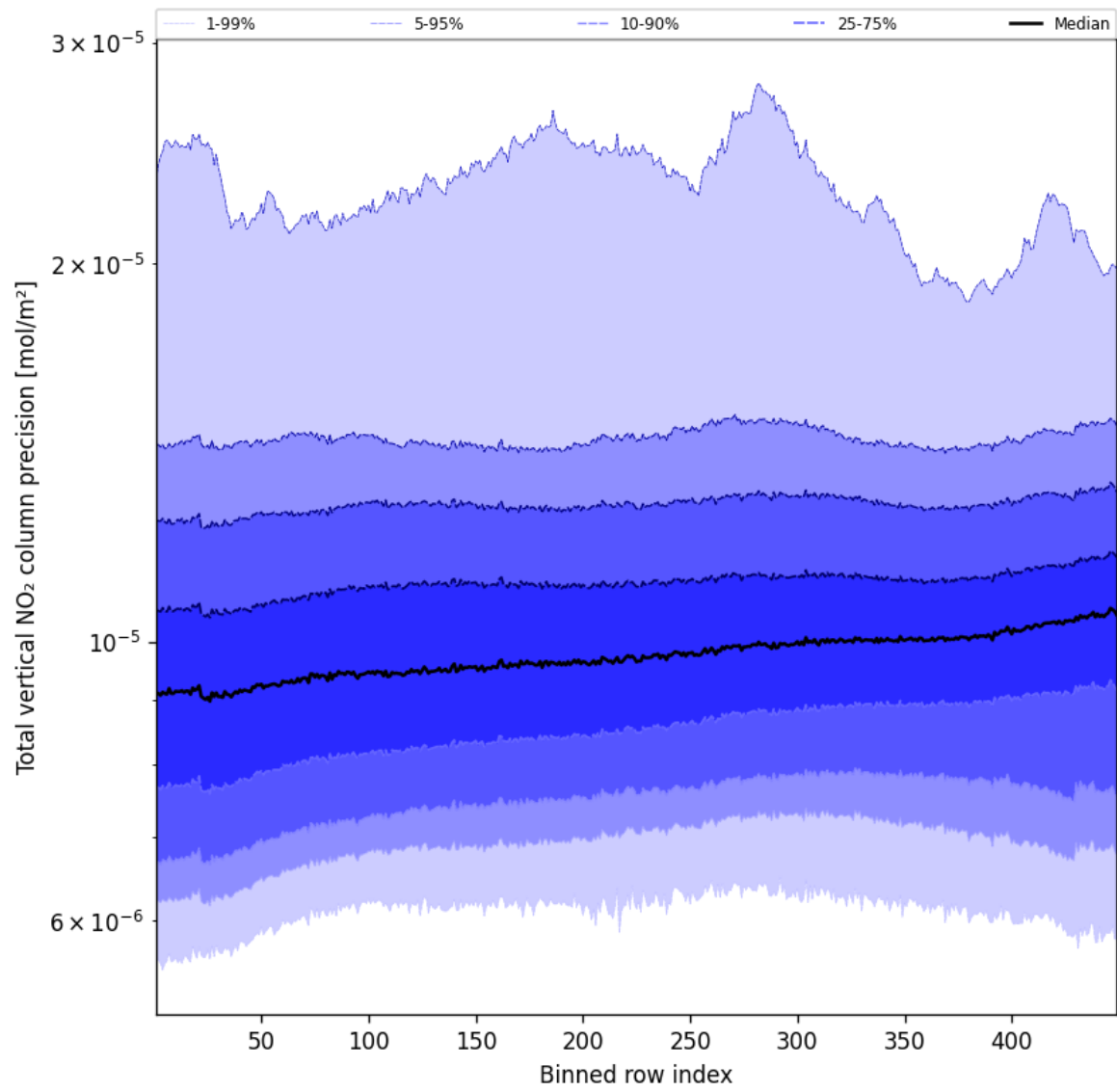
Figure 56: Along track statistics of “Total vertical NO 2 column precision” for 2025-03-30 to 2025-03-31
