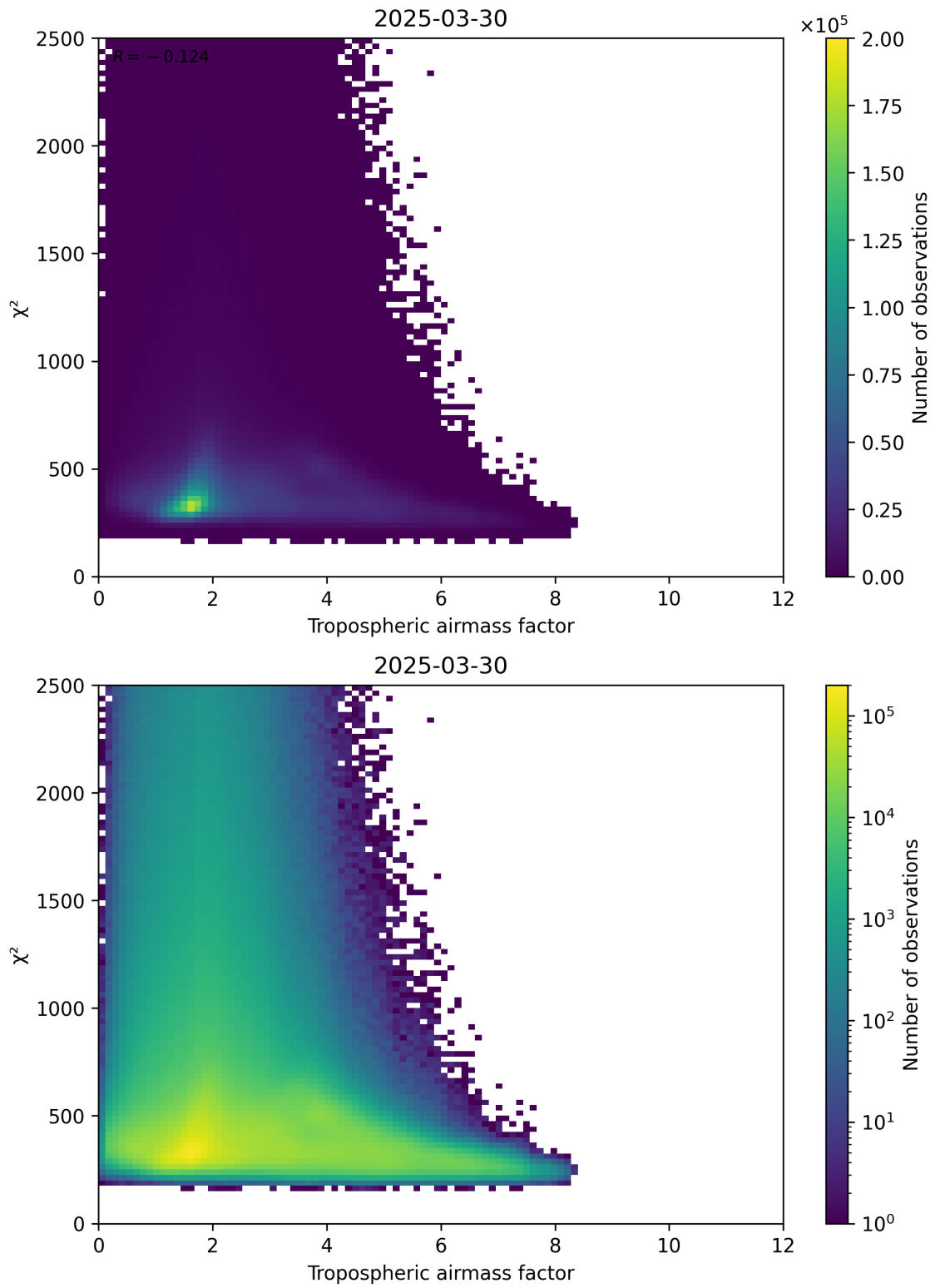
Figure 73: Scatter density plot of “Tropospheric airmass factor” against “ \chi^2 ” for 2025-03-30 to 2025-03-31.
