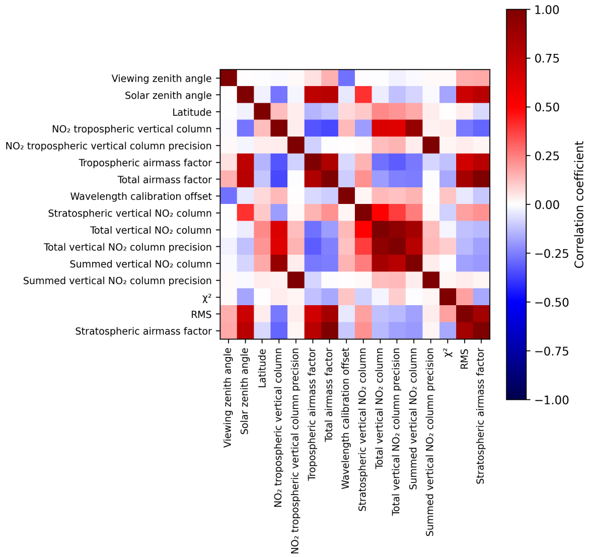
Figure 2: Map of correlation matrix for 2025-03-30 to 2025-03-31.
