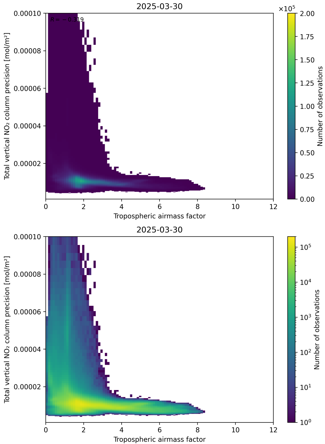
Figure 78: Scatter density plot of “Tropospheric air mass factor” against “Total vertical NO 2 column precision” for 2025-03-30 to 2025-03-31.
