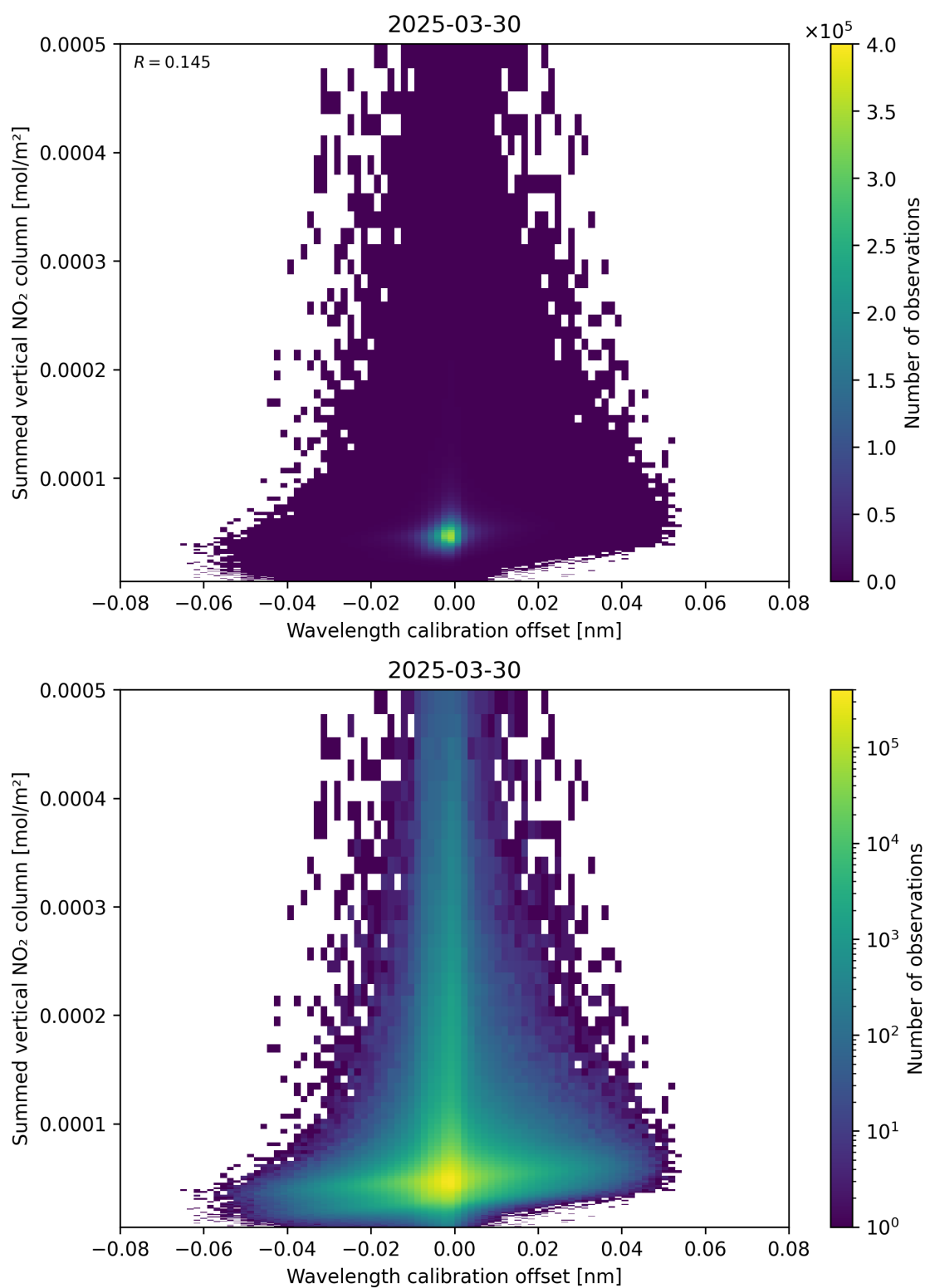
Figure 177: Scatter density plot of “Wavelength calibration offset” against “Summed vertical NO 2 column” for 2025-03-30 to 2025-03-31.
