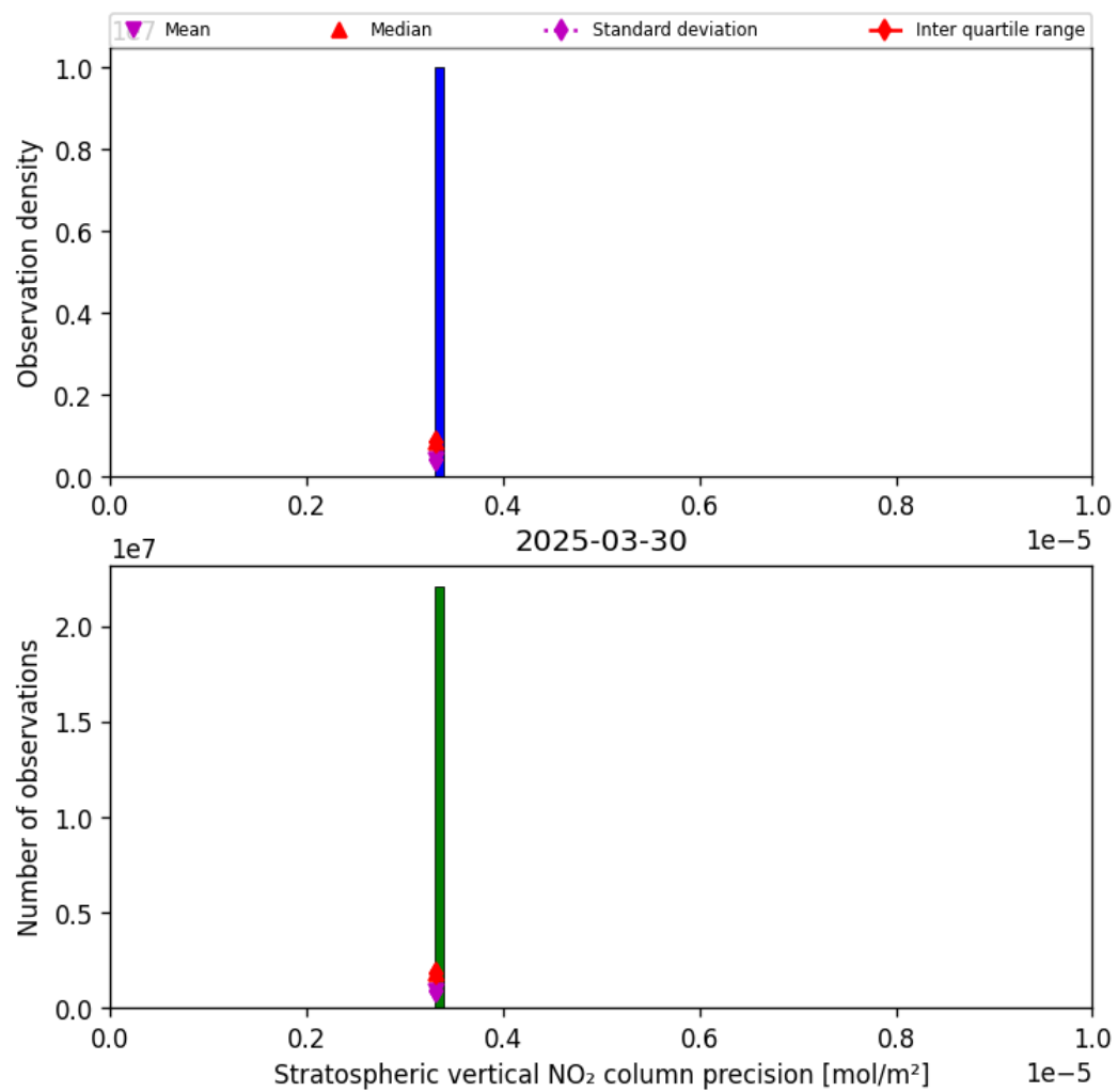
Figure 37: Histogram of “Stratospheric vertical NO 2 column precision” for 2025-03-30 to 2025-03-31
