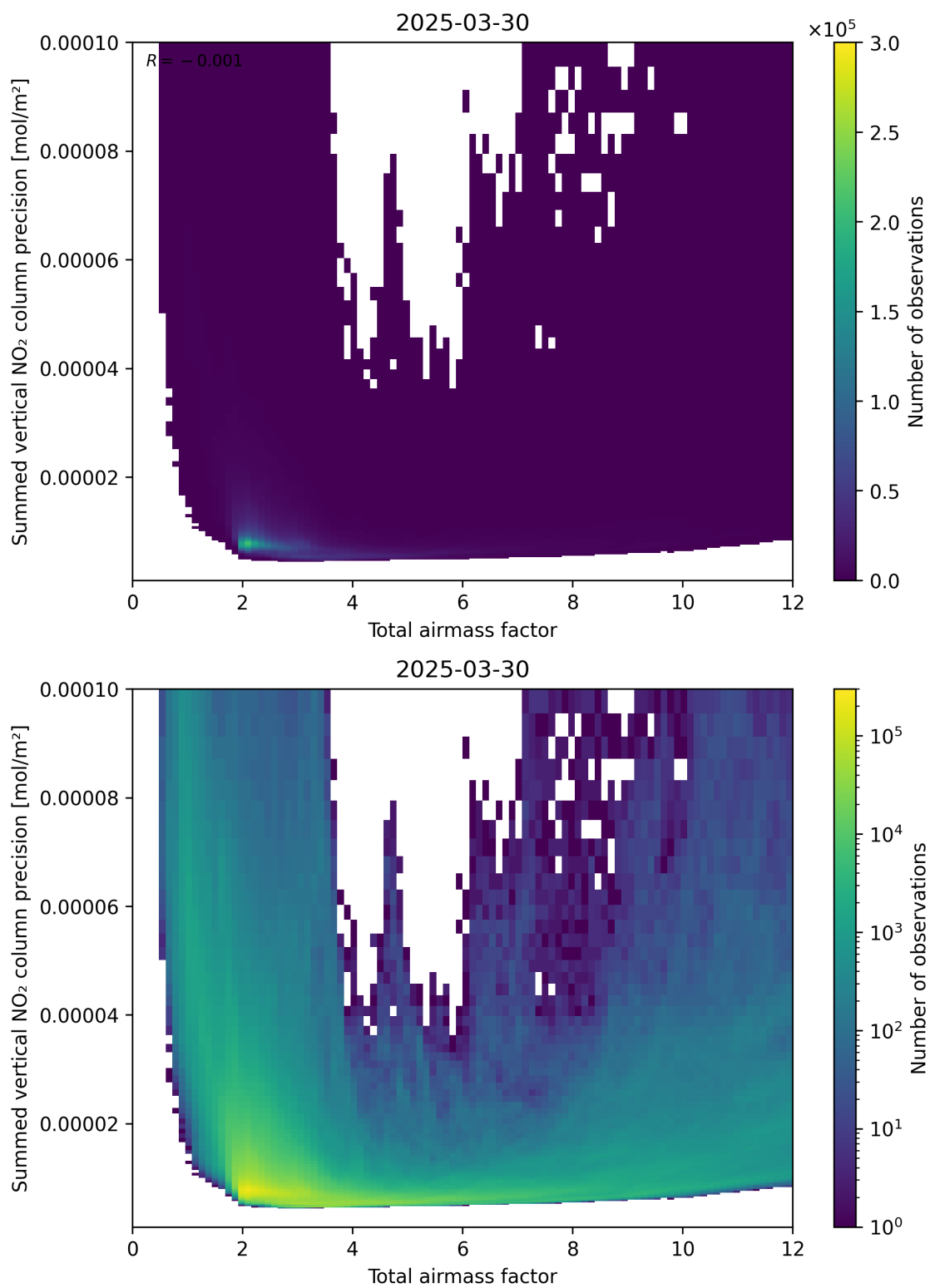
Figure 66: Scatter density plot of “Total airmass factor” against “Summed vertical NO 2 column precision” for 2025-03-30 to 2025-03-31.
