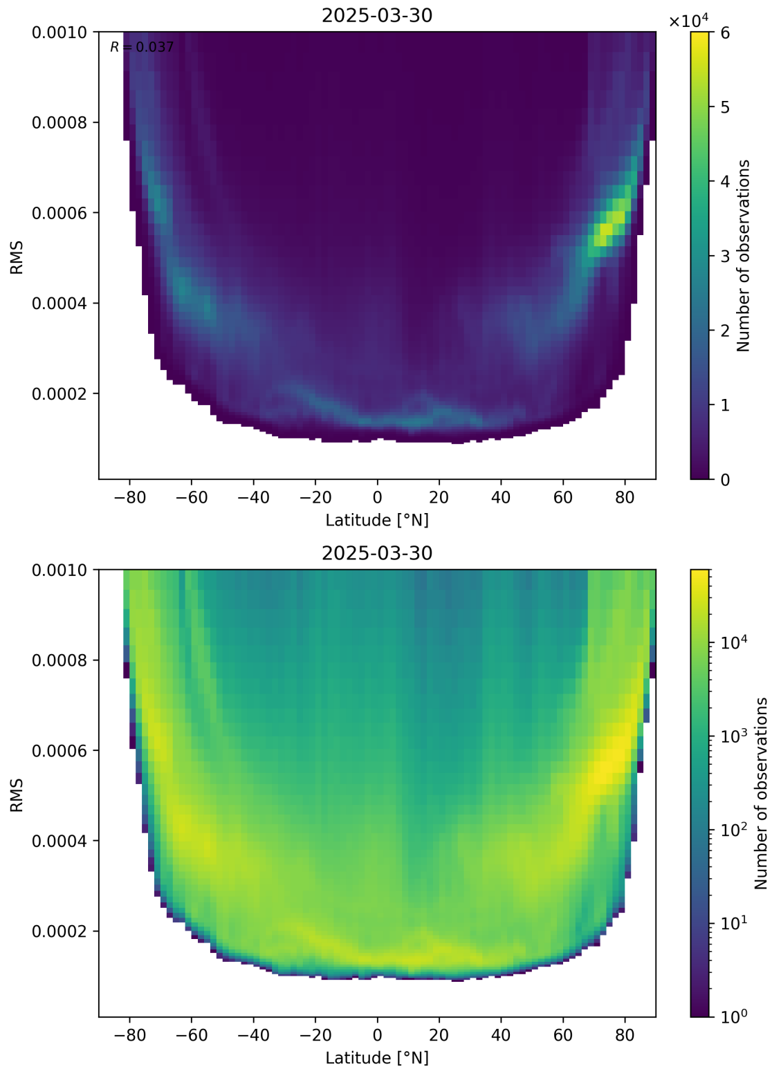
Figure 94: Scatter density plot of “Latitude” against “RMS” for 2025-03-30 to 2025-03-31.
