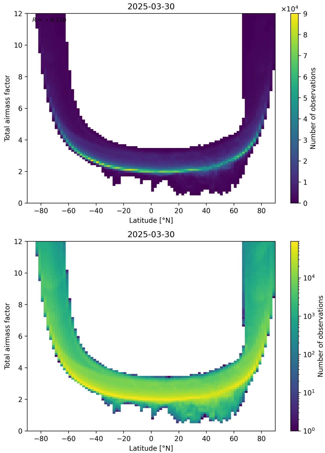
Figure 84: Scatter density plot of “Latitude” against “Total airmass factor” for 2025-03-30 to 2025-03-31.
