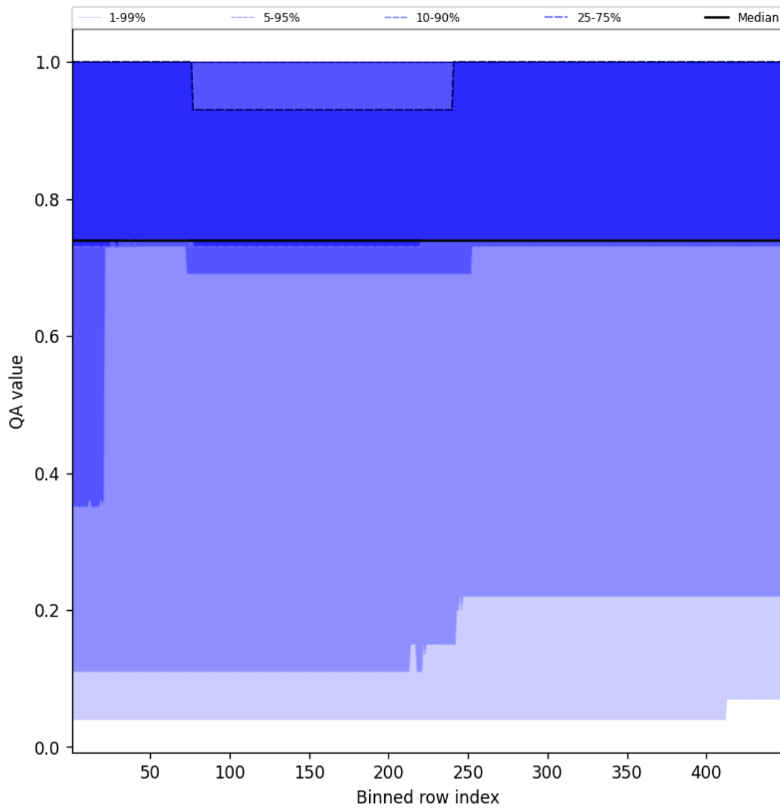
Figure 45: Along track statistics of "QA value" for 2025-03-30 to 2025-03-31
