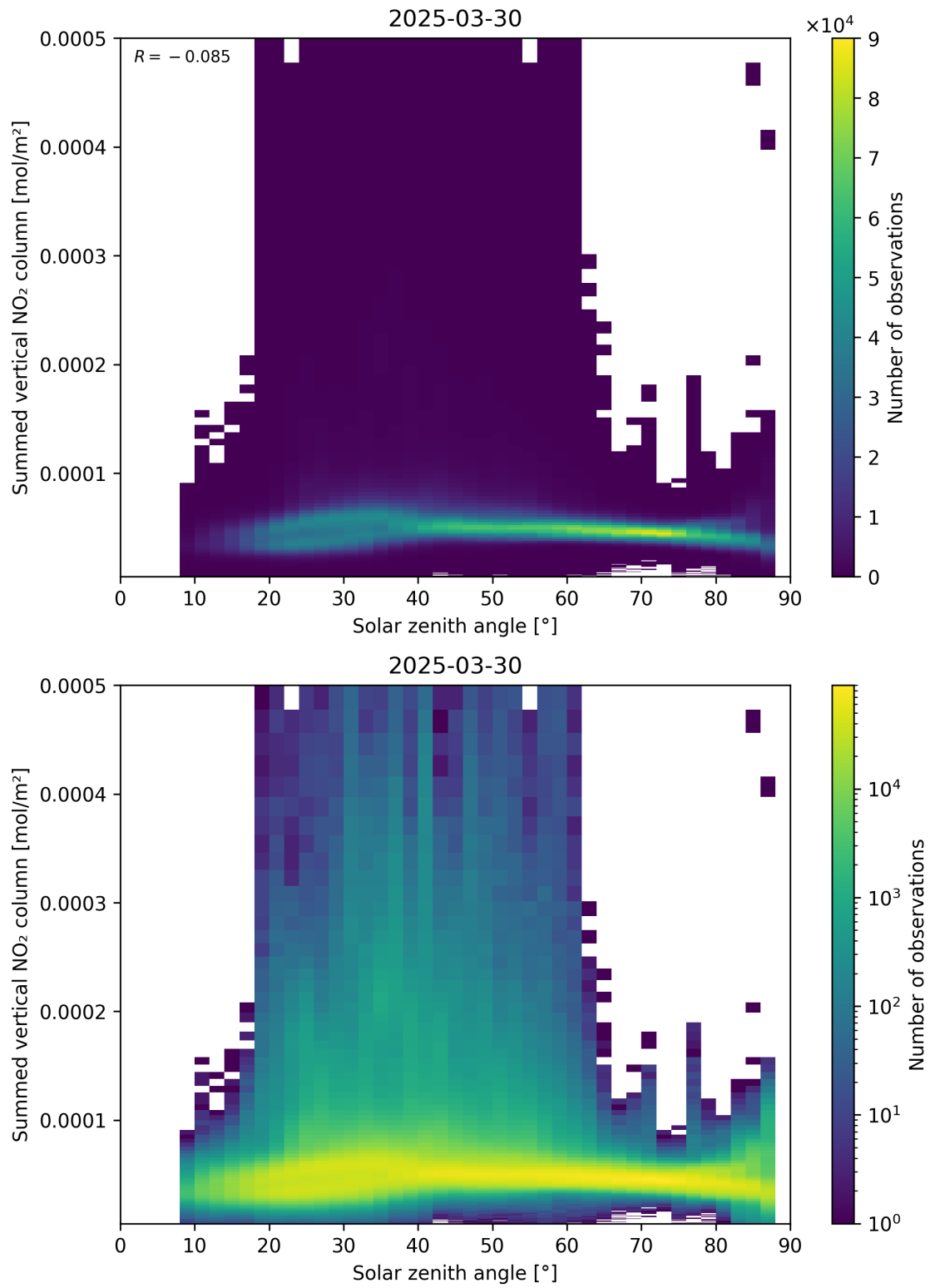
Figure 151: Scatter density plot of “Solar zenith angle” against “Summed vertical NO 2 column” for 2025-03-30 to 2025-03-31.
