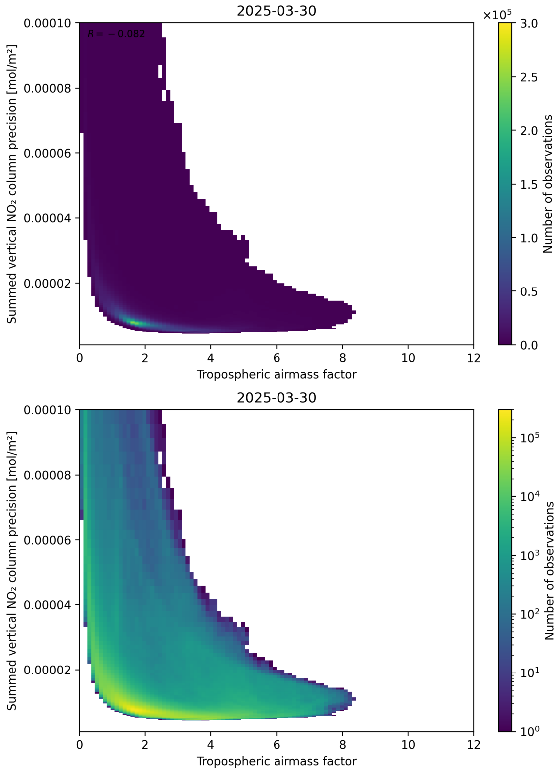
Figure 76: Scatter density plot of “Tropospheric airmass factor” against “Summed vertical NO 2 column precision” for 2025-03-30 to 2025-03-31.
