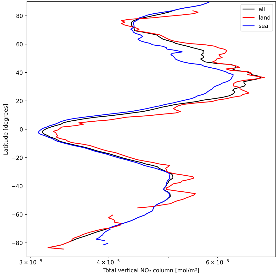
Figure 21: Zonal average of “Total vertical NO 2 column” for 2025-03-30 to 2025-03-31.
