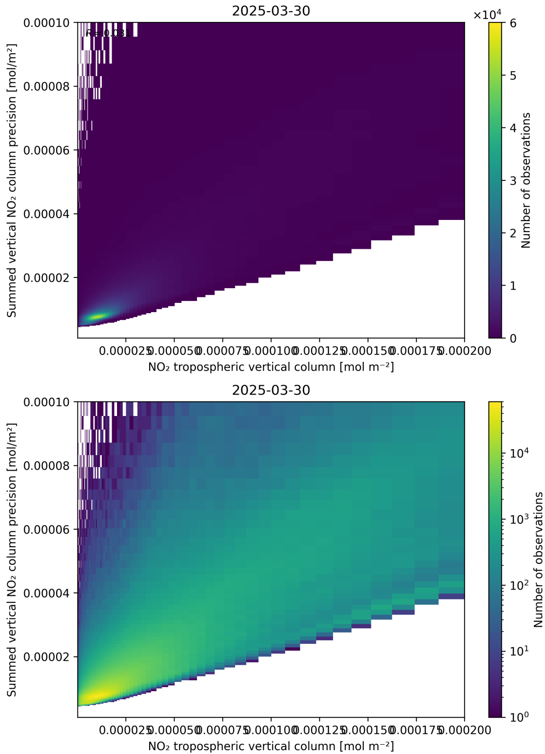
Figure 127: Scatter density plot of “NO 2 tropospheric vertical column” against “Summed vertical NO 2 column precision” for 2025-03-30 to 2025-03-31.
