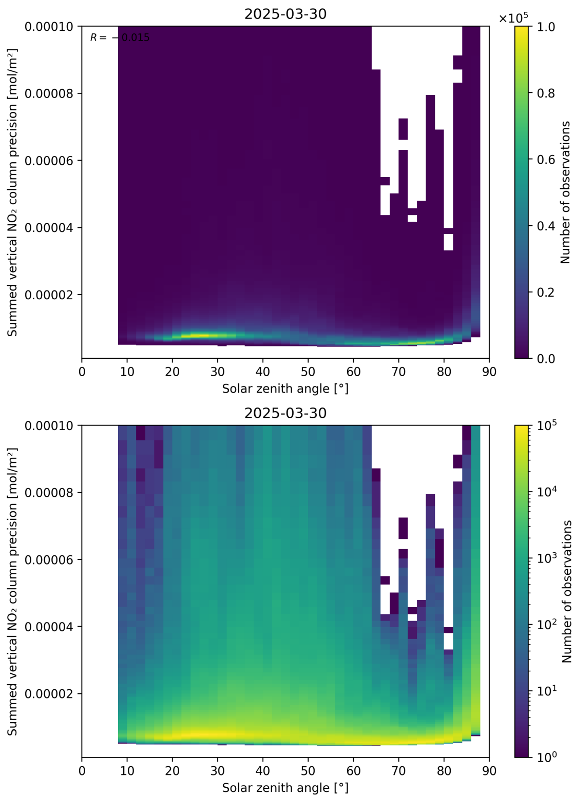
Figure 152: Scatter density plot of “Solar zenith angle” against “Summed vertical NO 2 column precision” for 2025-03-30 to 2025-03-31.
