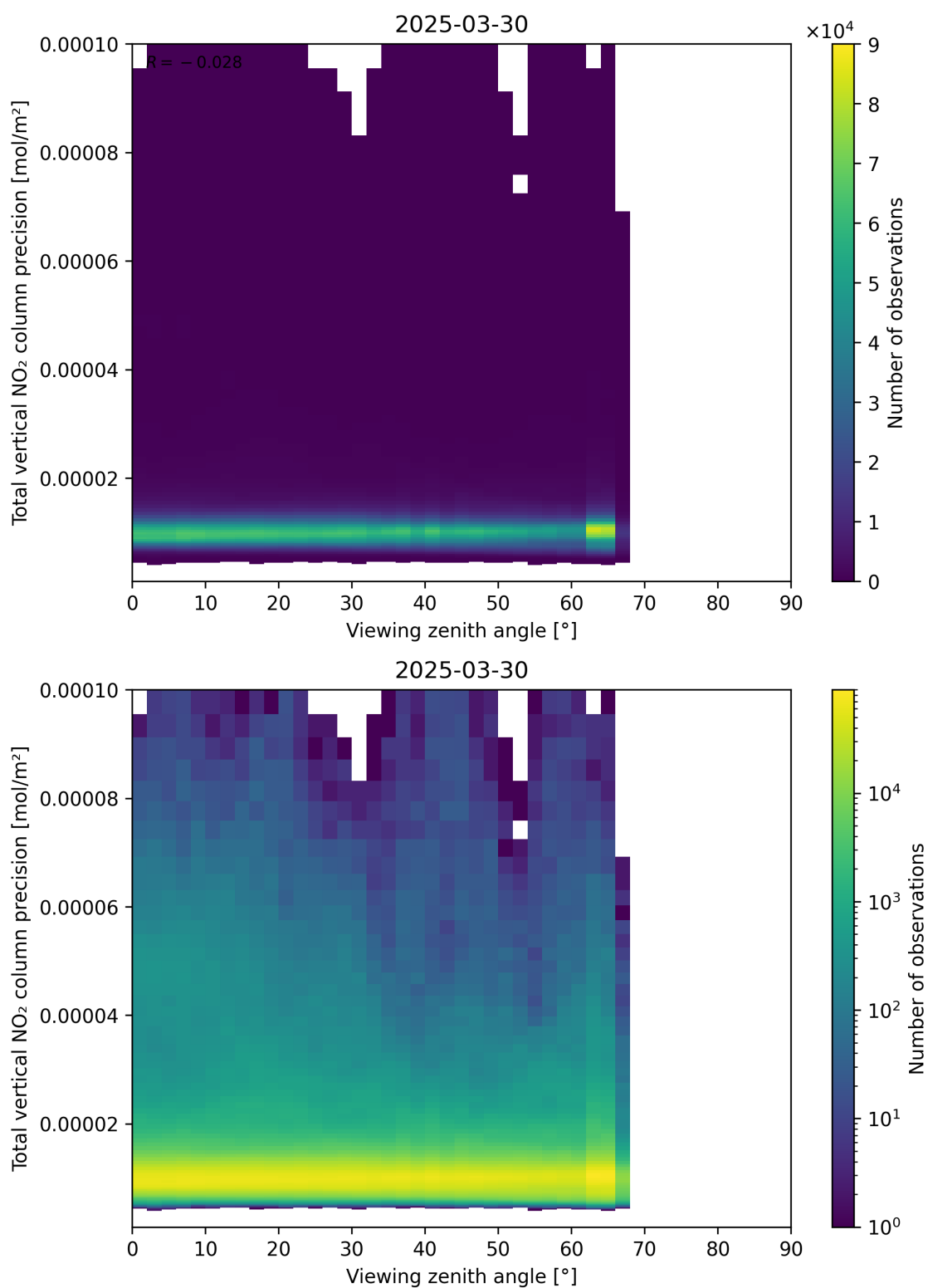
Figure 168: Scatter density plot of “Viewing zenith angle” against “Total vertical NO 2 column precision” for 2025-03-30 to 2025-03-31.
