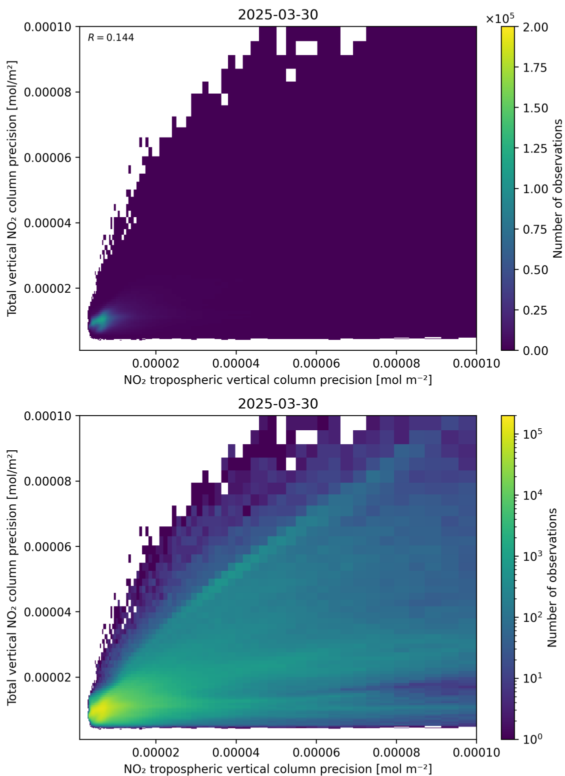
Figure 139: Scatter density plot of “NO 2 tropospheric vertical column precision” against “Total vertical NO 2 column precision” for 2025-03-30 to 2025-03-31.
