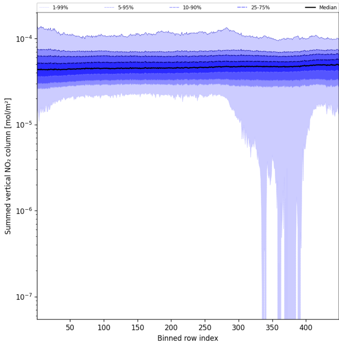
Figure 57: Along track statistics of “Summed vertical NO 2 column” for 2025-03-30 to 2025-03-31
