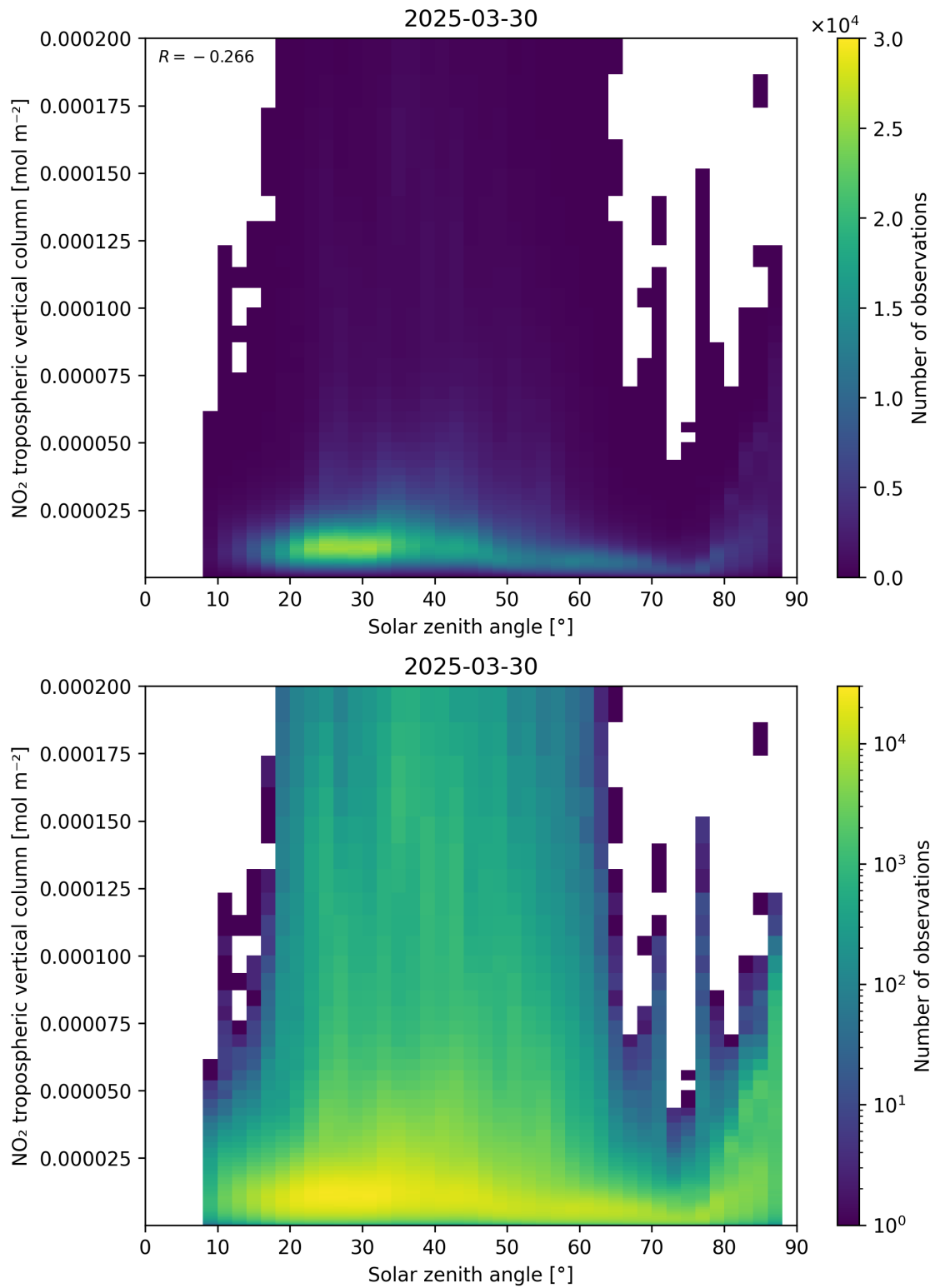
Figure 155: Scatter density plot of “Solar zenith angle” against “NO 2 tropospheric vertical column” for 2025-03-30 to 2025-03-31.
