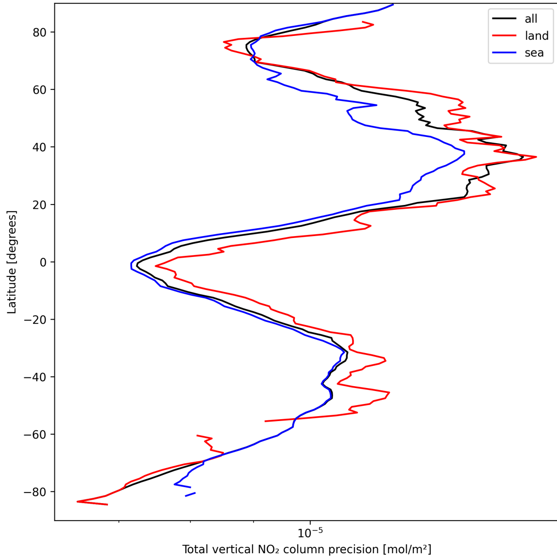
Figure 22: Zonal average of “Total vertical NO 2 column precision” for 2025-03-30 to 2025-03-31.
