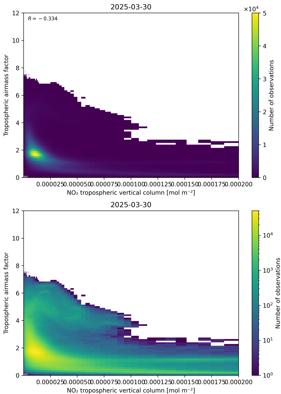
Figure 123: Scatter density plot of “NO 2 tropospheric vertical column” against “Tropospheric air mass factor” for 2025-03-30 to 2025-03-31.
