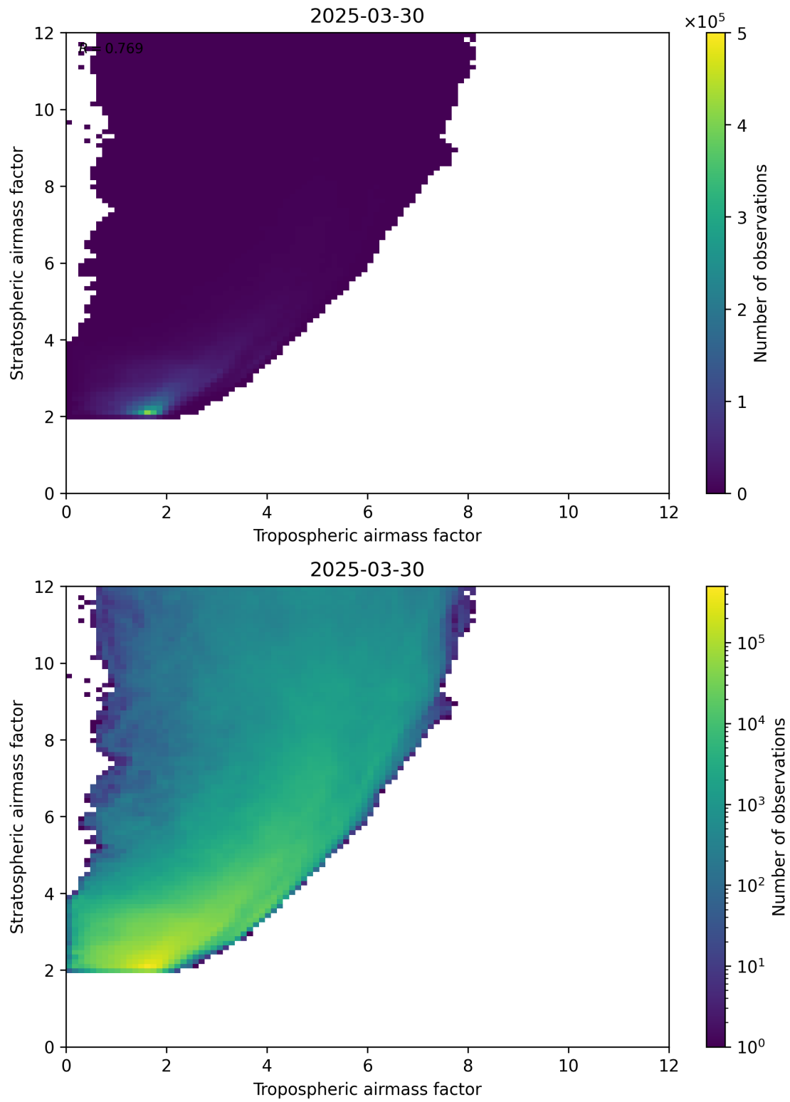
Figure 71: Scatter density plot of “Tropospheric airmass factor” against “Stratospheric airmass factor” for 2025-03-30 to 2025-03-31.
