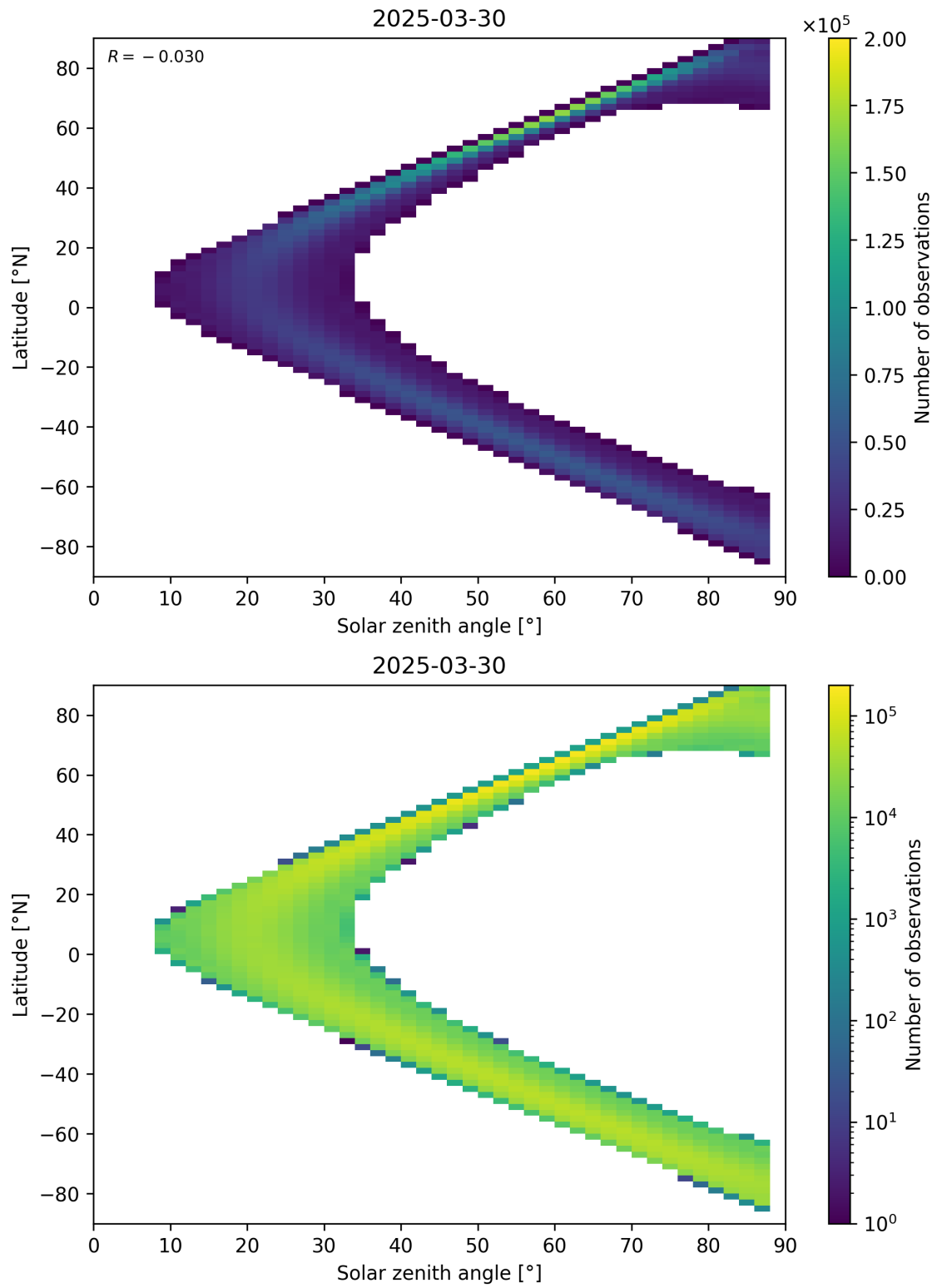
Figure 149: Scatter density plot of “Solar zenith angle” against “Latitude” for 2025-03-30 to 2025-03-31.
