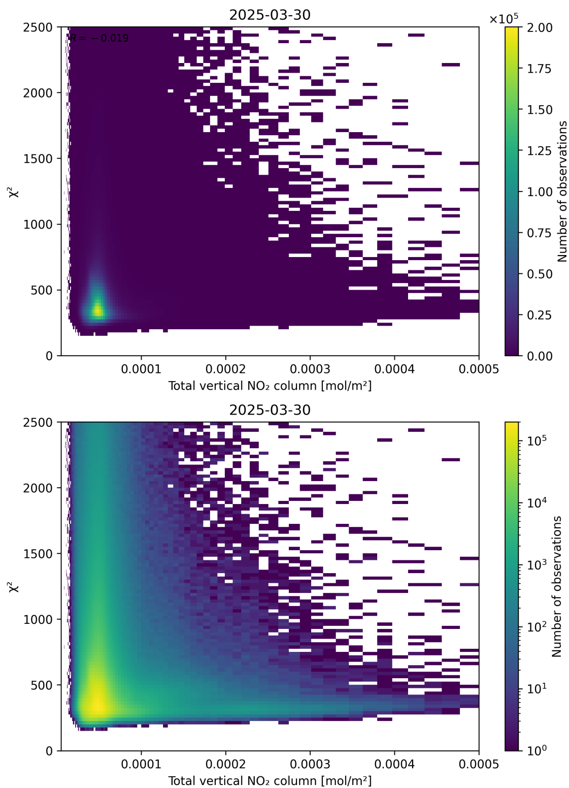
Figure 111: Scatter density plot of “Total vertical NO 2 column” against “ \chi^2 ” for 2025-03-30 to 2025-03-31.
