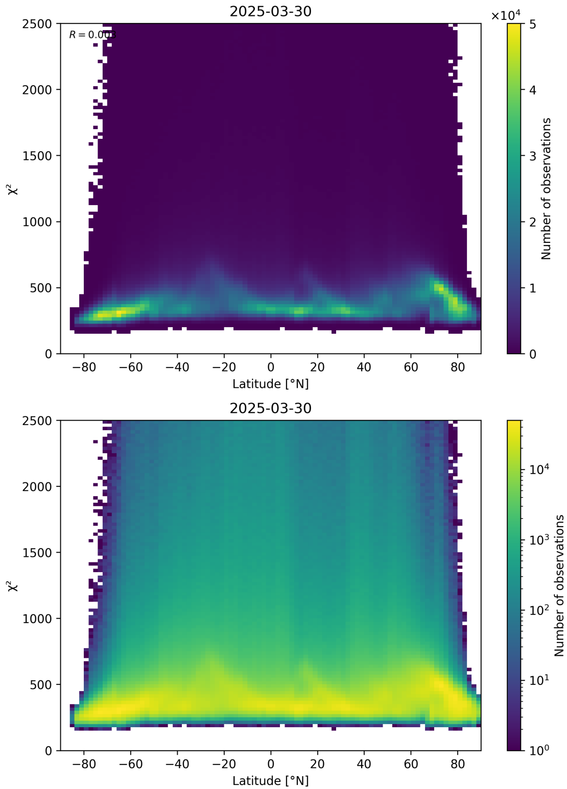
Figure 86: Scatter density plot of “Latitude” against “ \chi^2 ” for 2025-03-30 to 2025-03-31.
