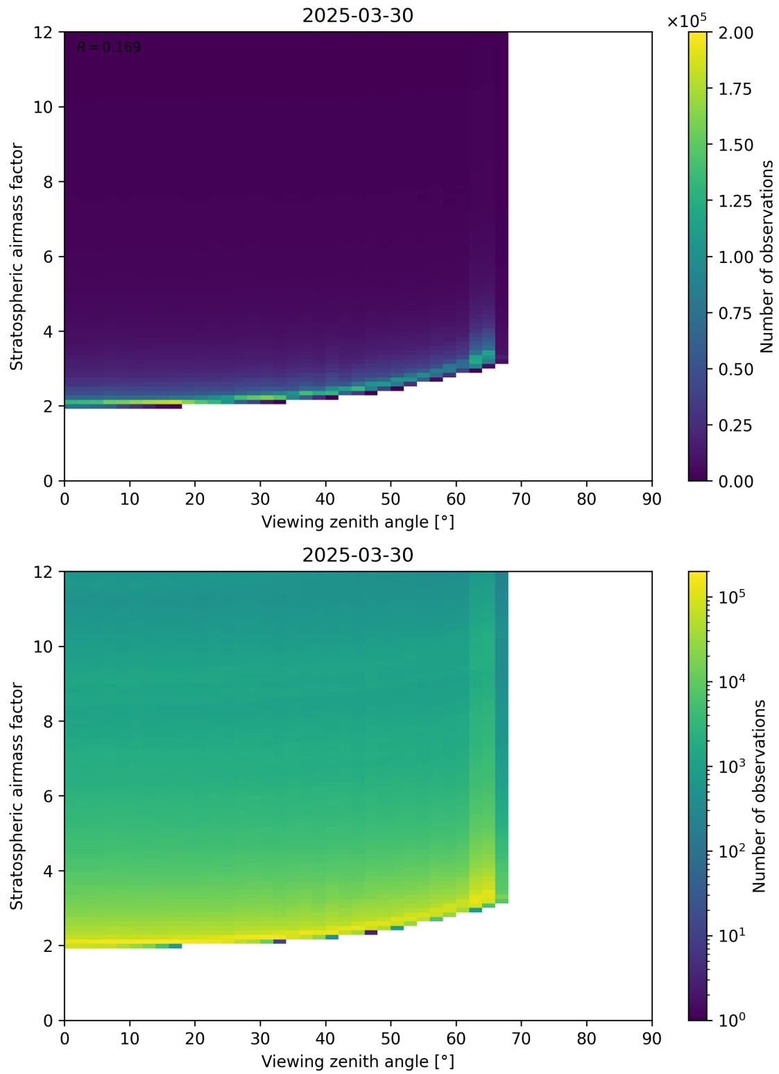
Figure 159: Scatter density plot of “Viewing zenith angle” against “Stratospheric airmass factor” for 2025-03-30 to 2025-03-31.
