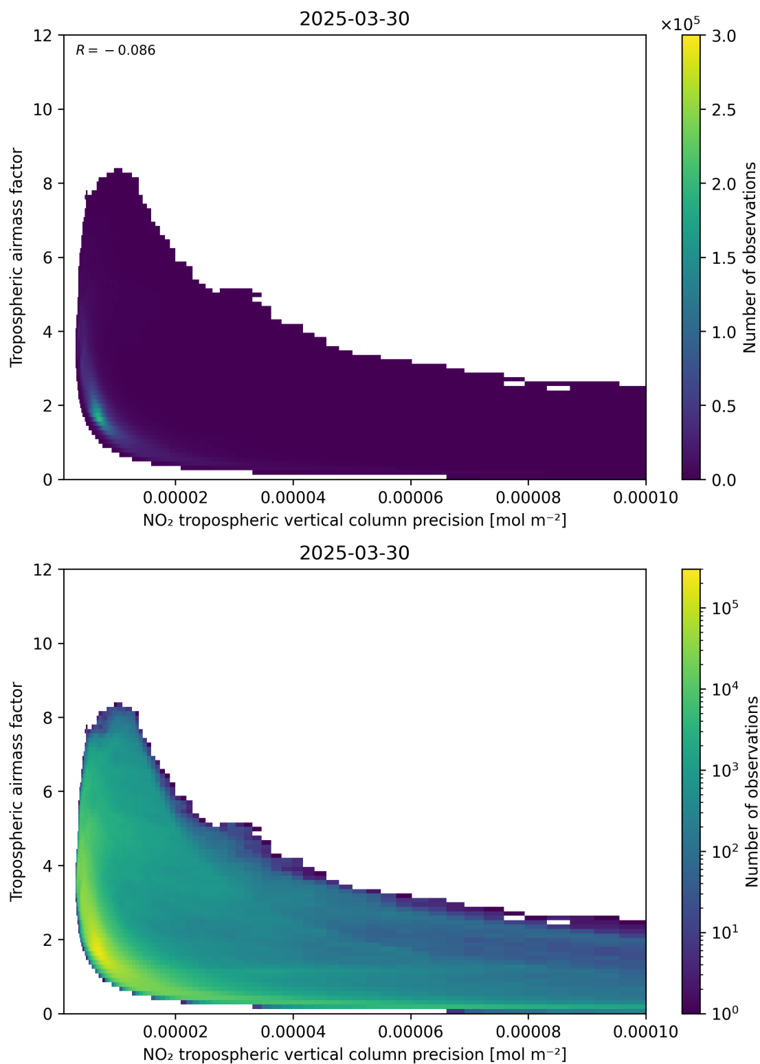
Figure 133: Scatter density plot of “NO 2 tropospheric vertical column precision” against “Tropospheric air mass factor” for 2025-03-30 to 2025-03-31.
