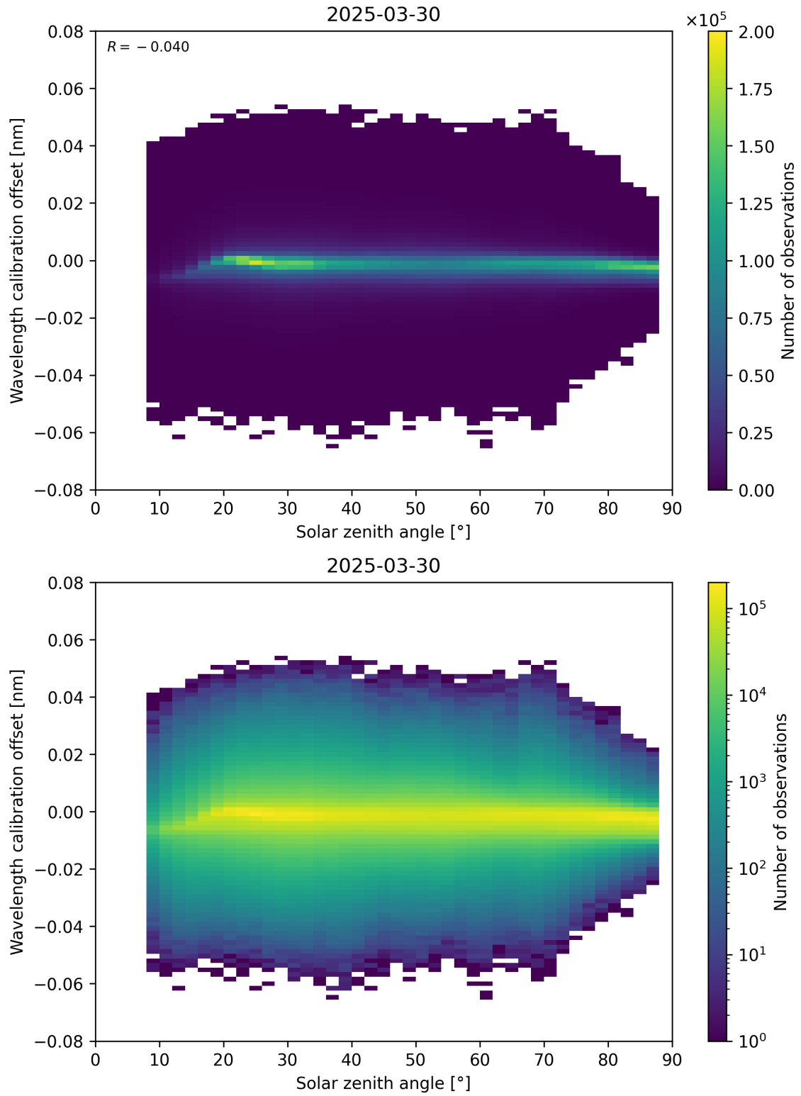
Figure 158: Scatter density plot of “Solar zenith angle” against “Wavelength calibration offset” for 2025-03-30 to 2025-03-31.
