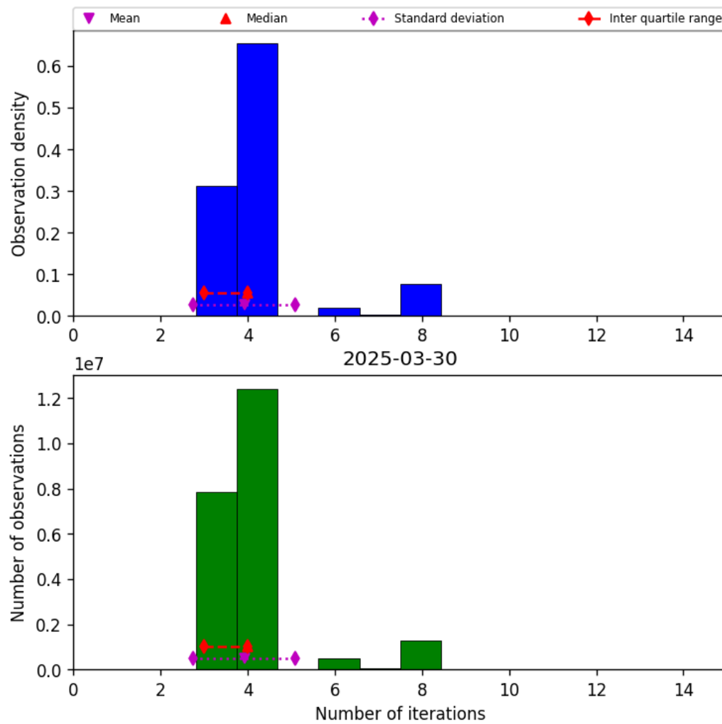
Figure 34: Histogram of “Number of iterations” for 2025-03-30 to 2025-03-31
