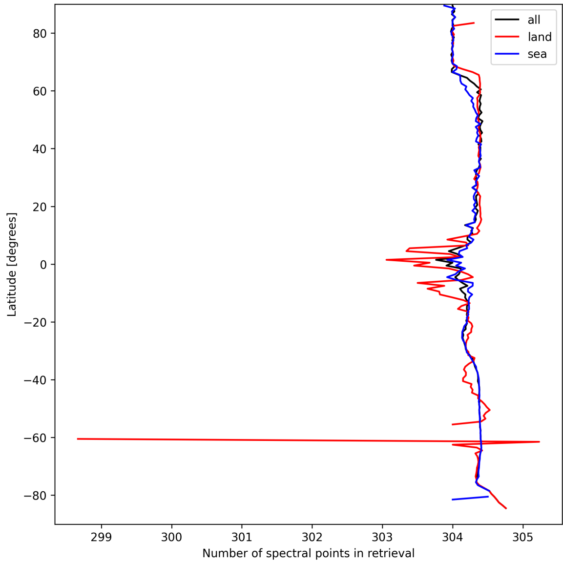
Figure 16: Zonal average of “Number of spectral points in retrieval” for 2025-03-30 to 2025-03-31.
