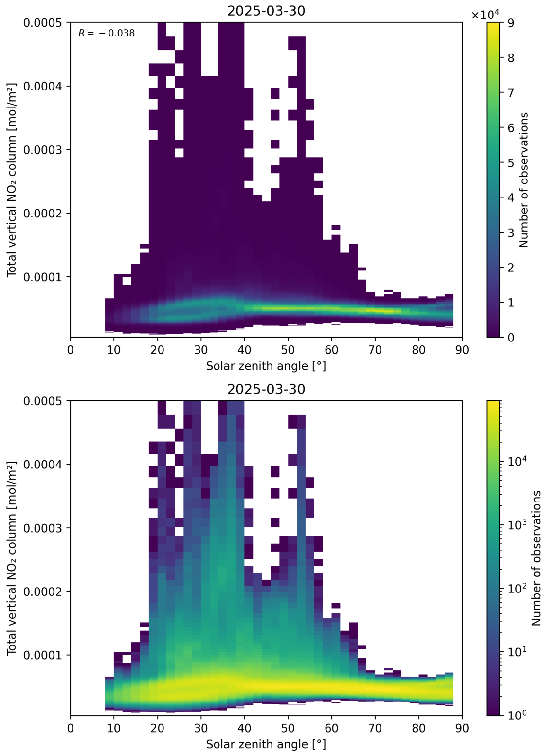
Figure 153: Scatter density plot of “Solar zenith angle” against “Total vertical NO 2 column” for 2025-03-30 to 2025-03-31.
