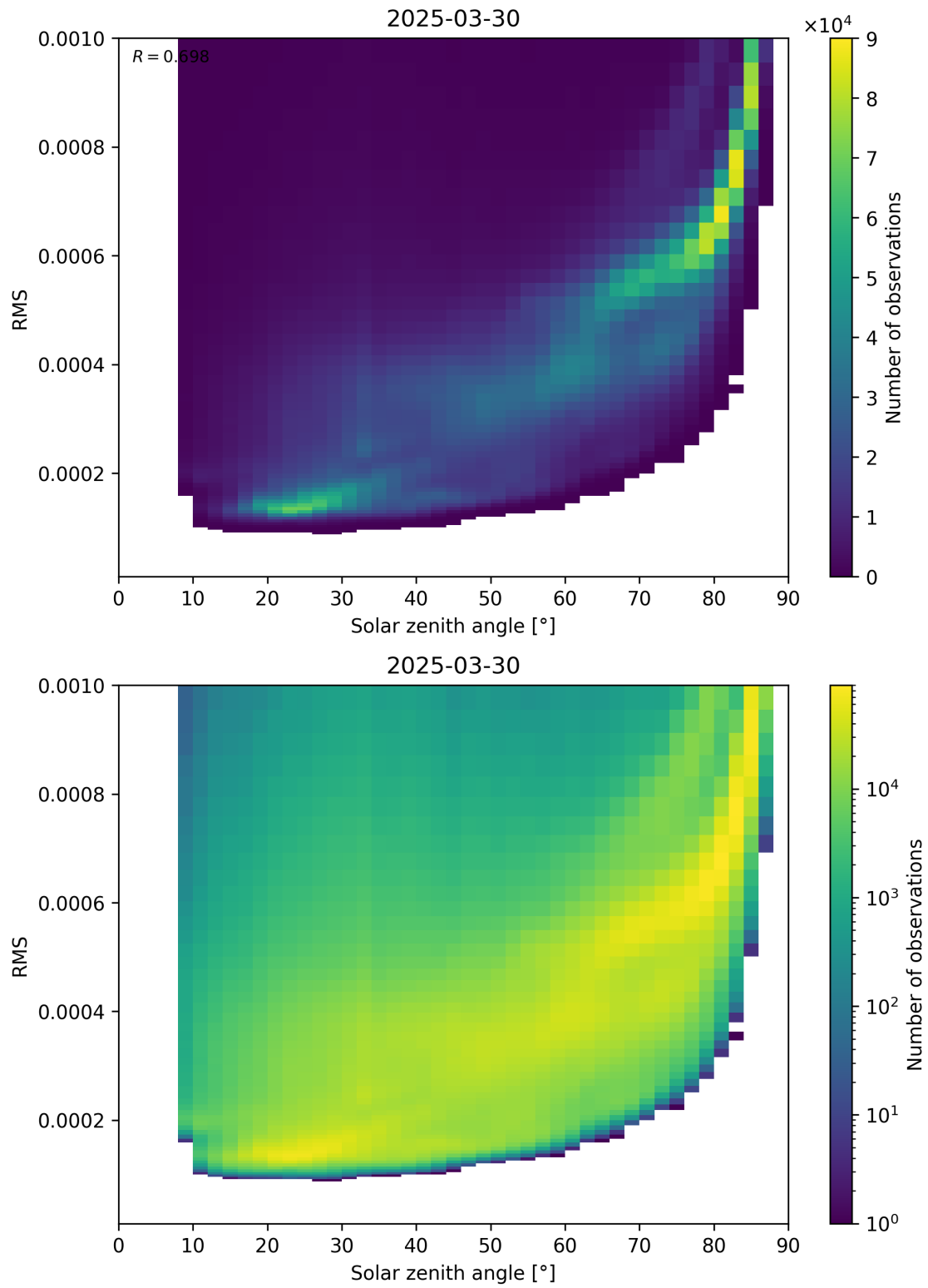
Figure 157: Scatter density plot of “Solar zenith angle” against “RMS” for 2025-03-30 to 2025-03-31.
