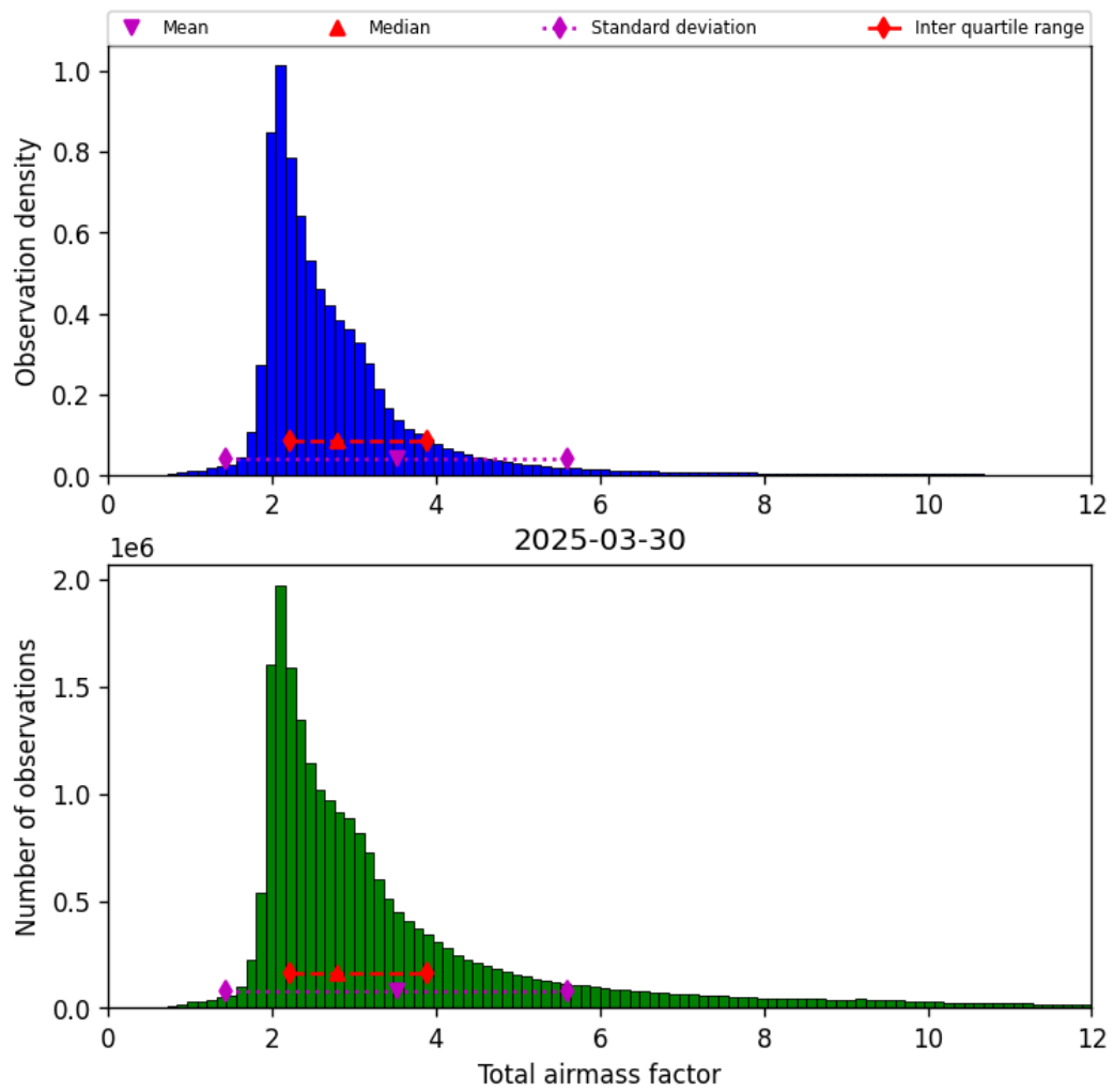
Figure 32: Histogram of “Total airmass factor” for 2025-03-30 to 2025-03-31
