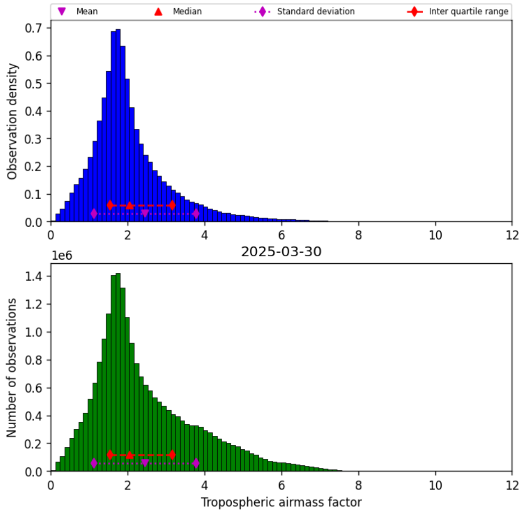
Figure 31: Histogram of “Tropospheric airmass factor” for 2025-03-30 to 2025-03-31
