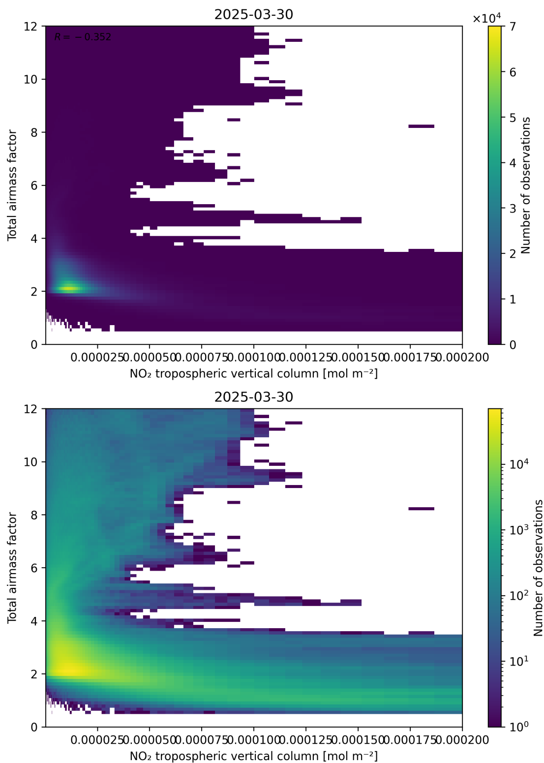
Figure 122: Scatter density plot of “NO 2 tropospheric vertical column” against “Total air mass factor” for 2025-03-30 to 2025-03-31.
