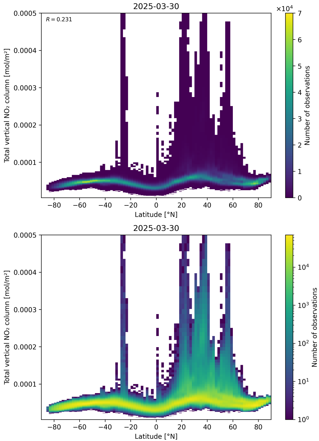
Figure 90: Scatter density plot of “Latitude” against “Total vertical \text{NO}_2 column” for 2025-03-30 to 2025-03-31.
