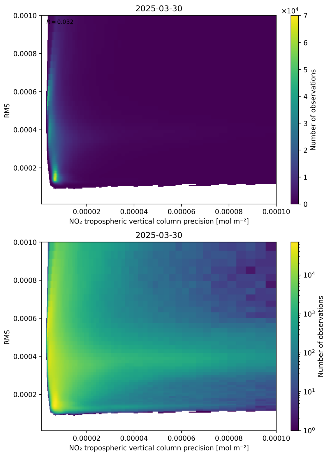
Figure 140: Scatter density plot of “NO 2 tropospheric vertical column precision” against “RMS” for 2025-03-30 to 2025-03-31.
