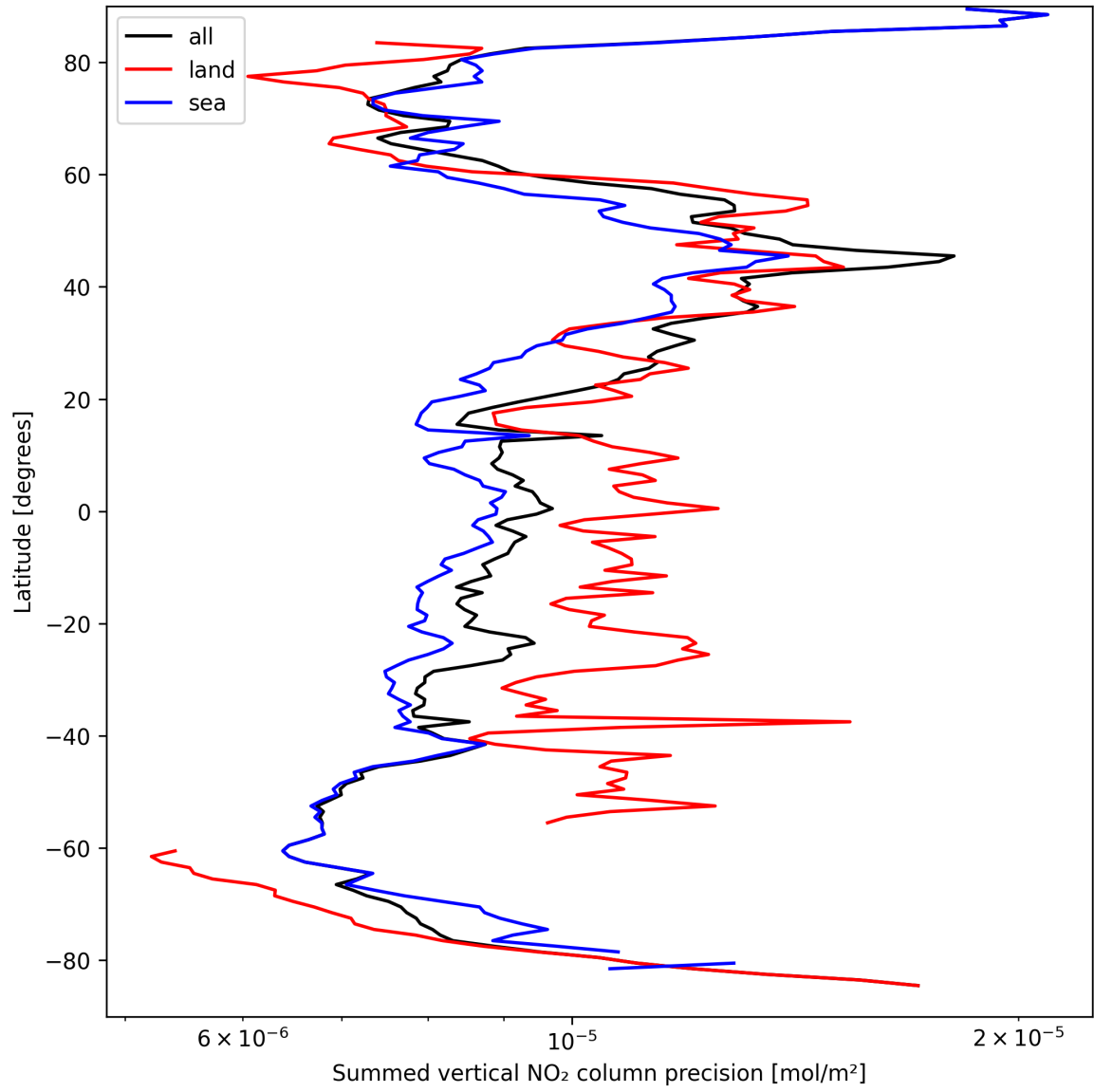
Figure 24: Zonal average of “Summed vertical NO 2 column precision” for 2025-03-30 to 2025-03-31.
