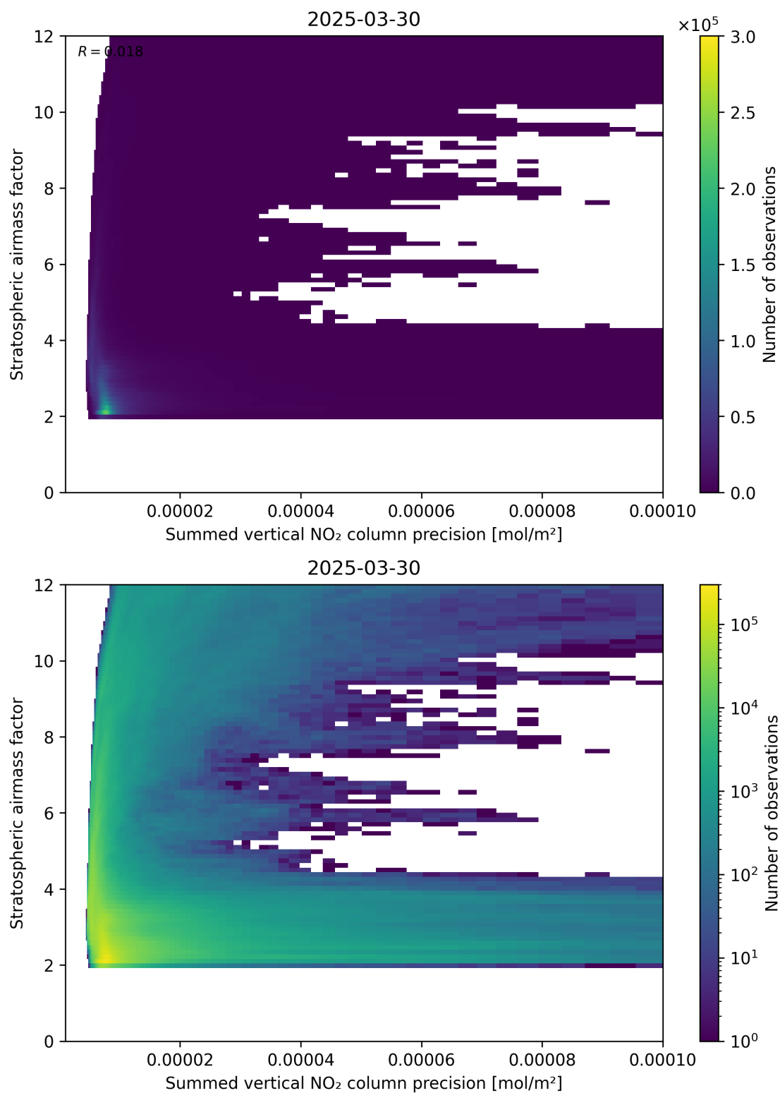
Figure 106: Scatter density plot of “Summed vertical NO 2 column precision” against “Stratospheric airmass factor” for 2025-03-30 to 2025-03-31.
