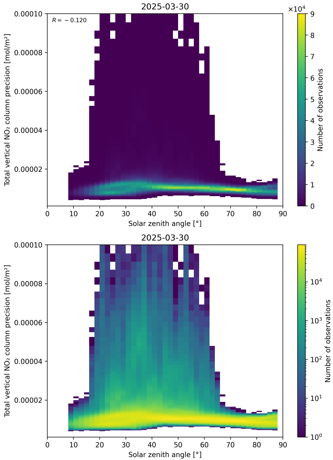
Figure 154: Scatter density plot of “Solar zenith angle” against “Total vertical NO 2 column precision” for 2025-03-30 to 2025-03-31.
