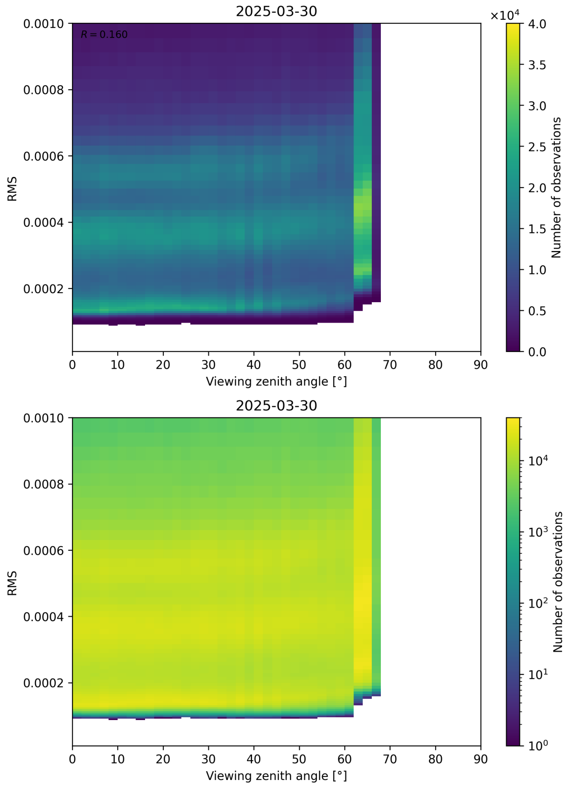
Figure 171: Scatter density plot of “Viewing zenith angle” against “RMS” for 2025-03-30 to 2025-03-31.
