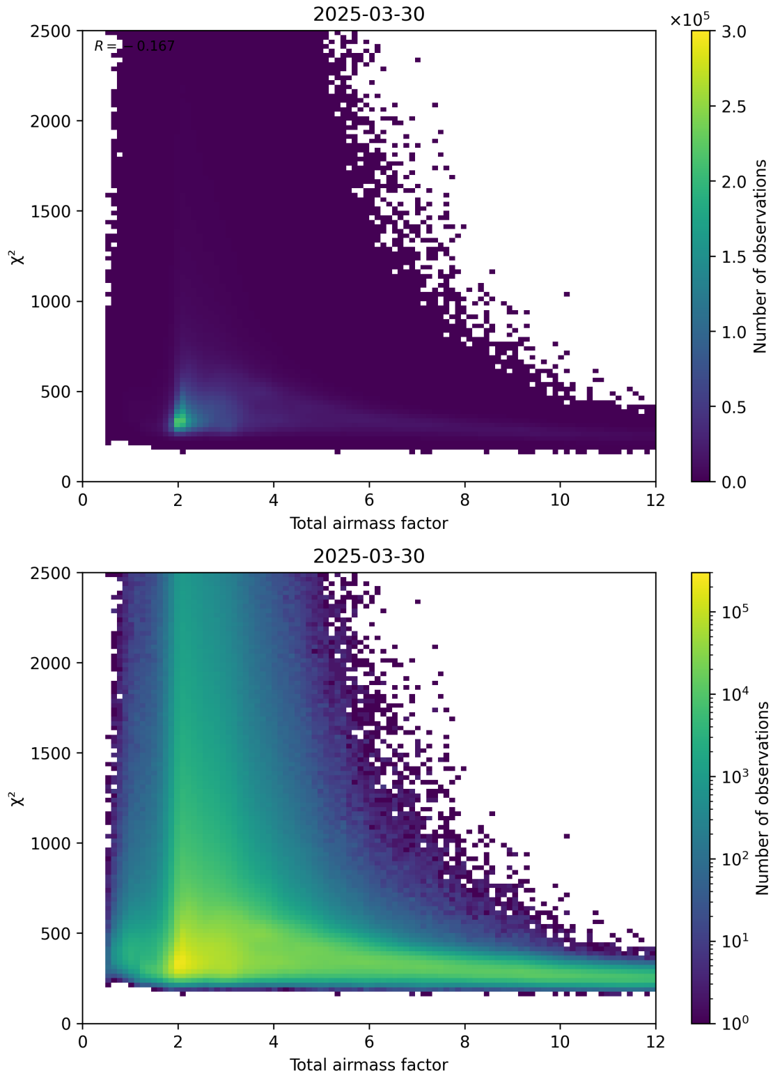
Figure 63: Scatter density plot of “Total airmass factor” against “ \chi^2 ” for 2025-03-30 to 2025-03-31.
