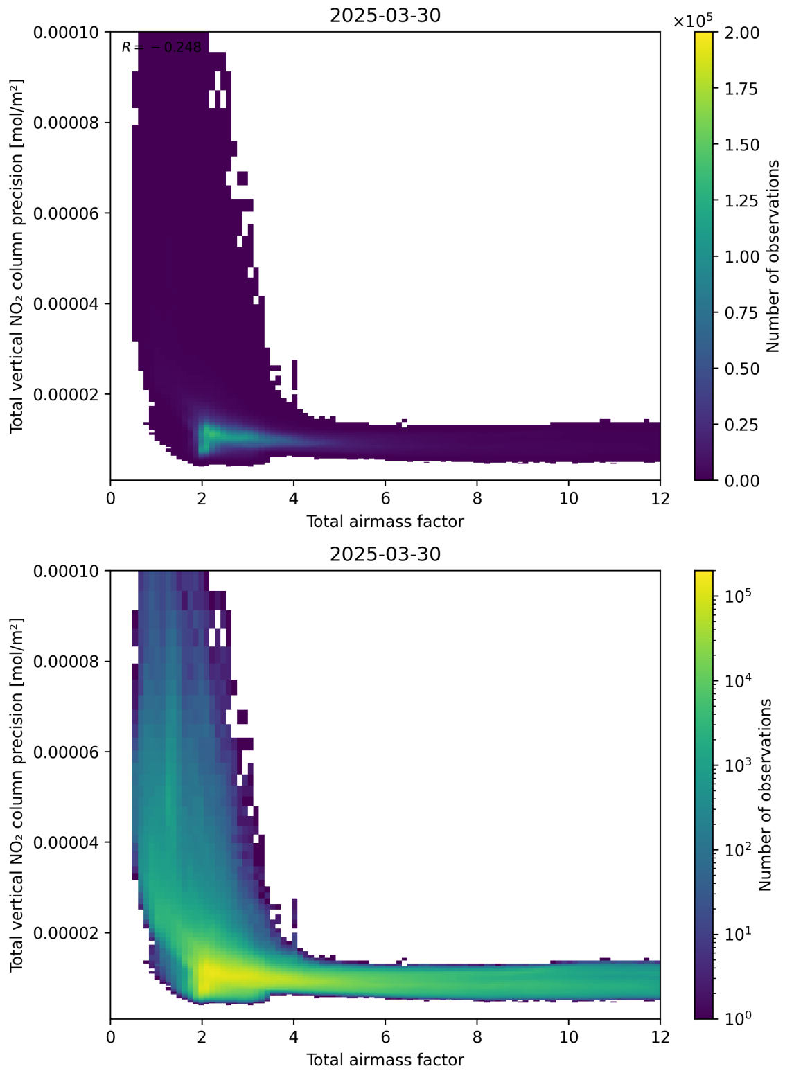
Figure 68: Scatter density plot of “Total airmass factor” against “Total vertical NO 2 column precision” for 2025-03-30 to 2025-03-31.
