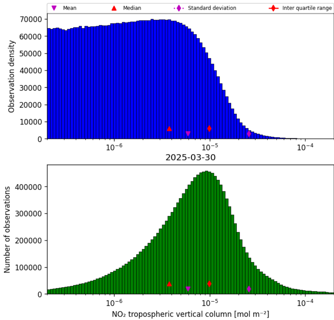
Figure 29: Histogram of “NO 2 tropospheric vertical column” for 2025-03-30 to 2025-03-31
