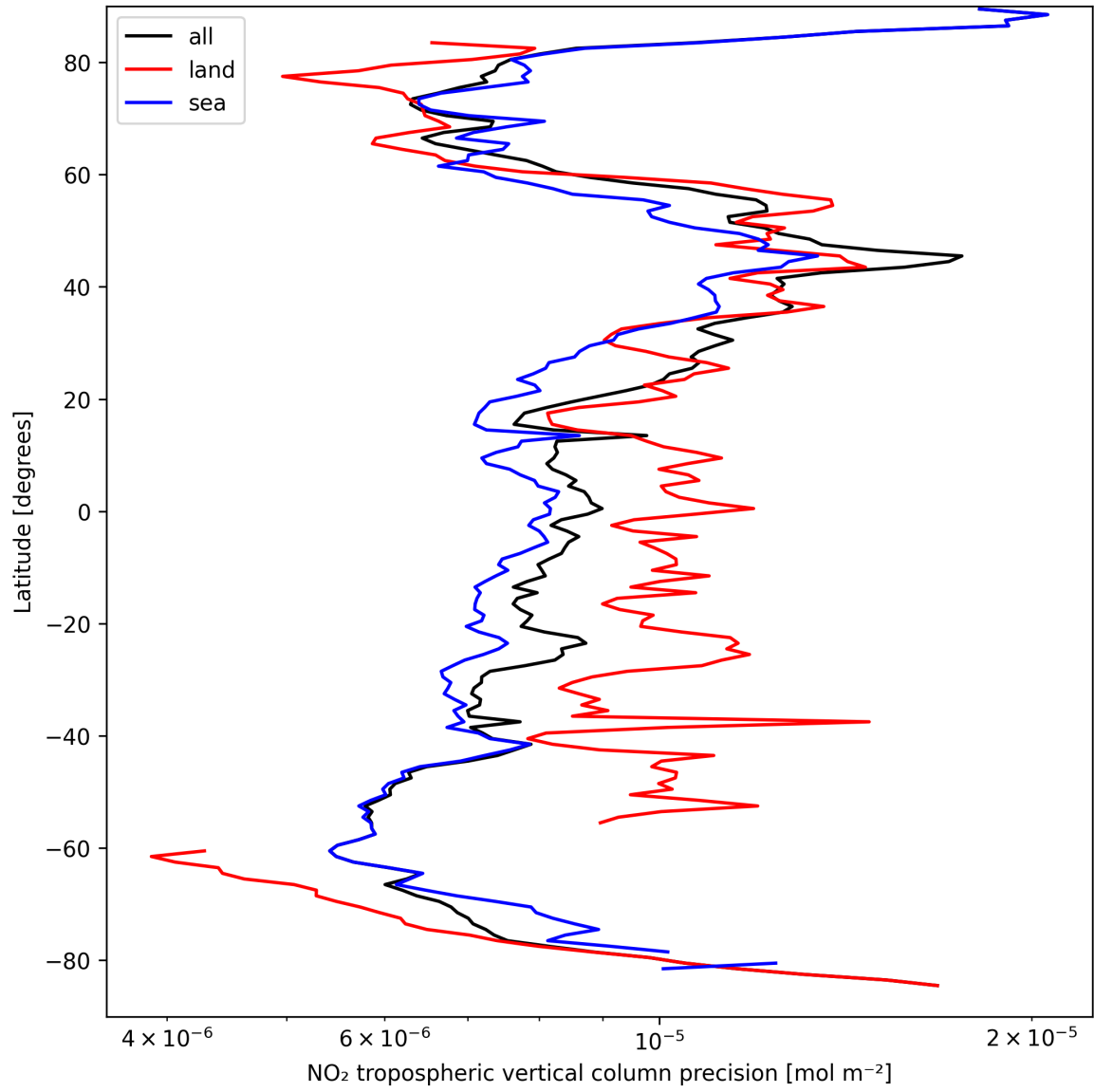
Figure 13: Zonal average of “NO 2 tropospheric vertical column precision” for 2025-03-30 to 2025-03-31.
