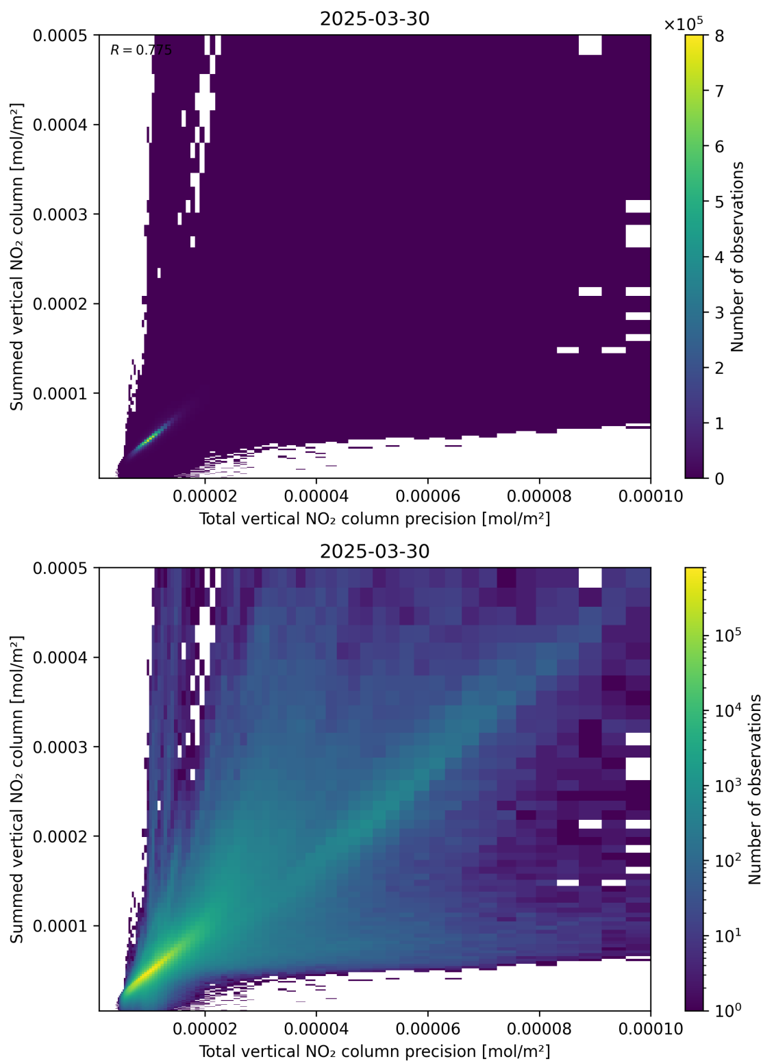
Figure 117: Scatter density plot of “Total vertical NO 2 column precision” against “Summed vertical NO 2 column” for 2025-03-30 to 2025-03-31.
