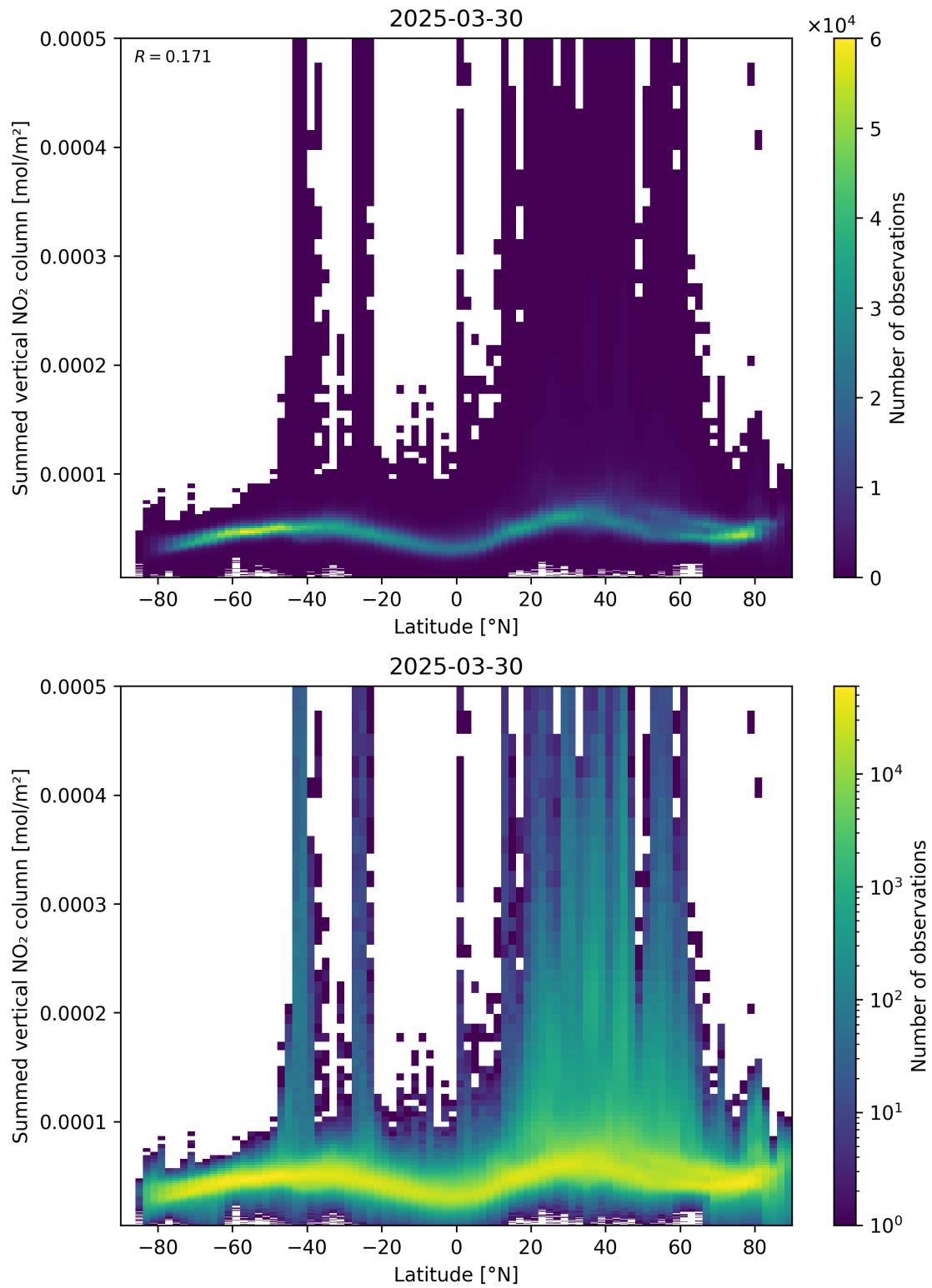
Figure 88: Scatter density plot of “Latitude” against “Summed vertical NO 2 column” for 2025-03-30 to 2025-03-31.
