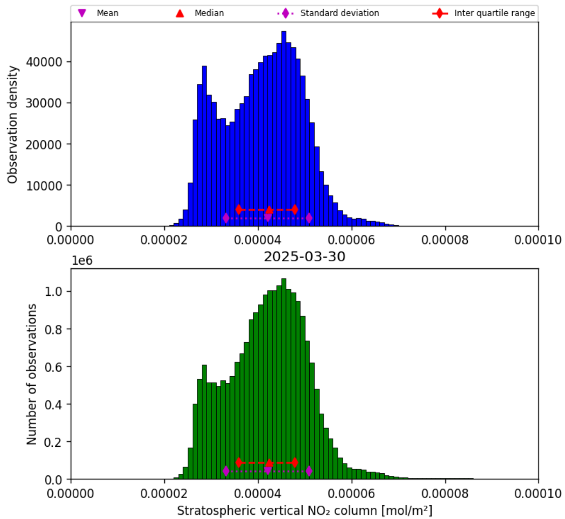
Figure 36: Histogram of “Stratospheric vertical NO 2 column” for 2025-03-30 to 2025-03-31
