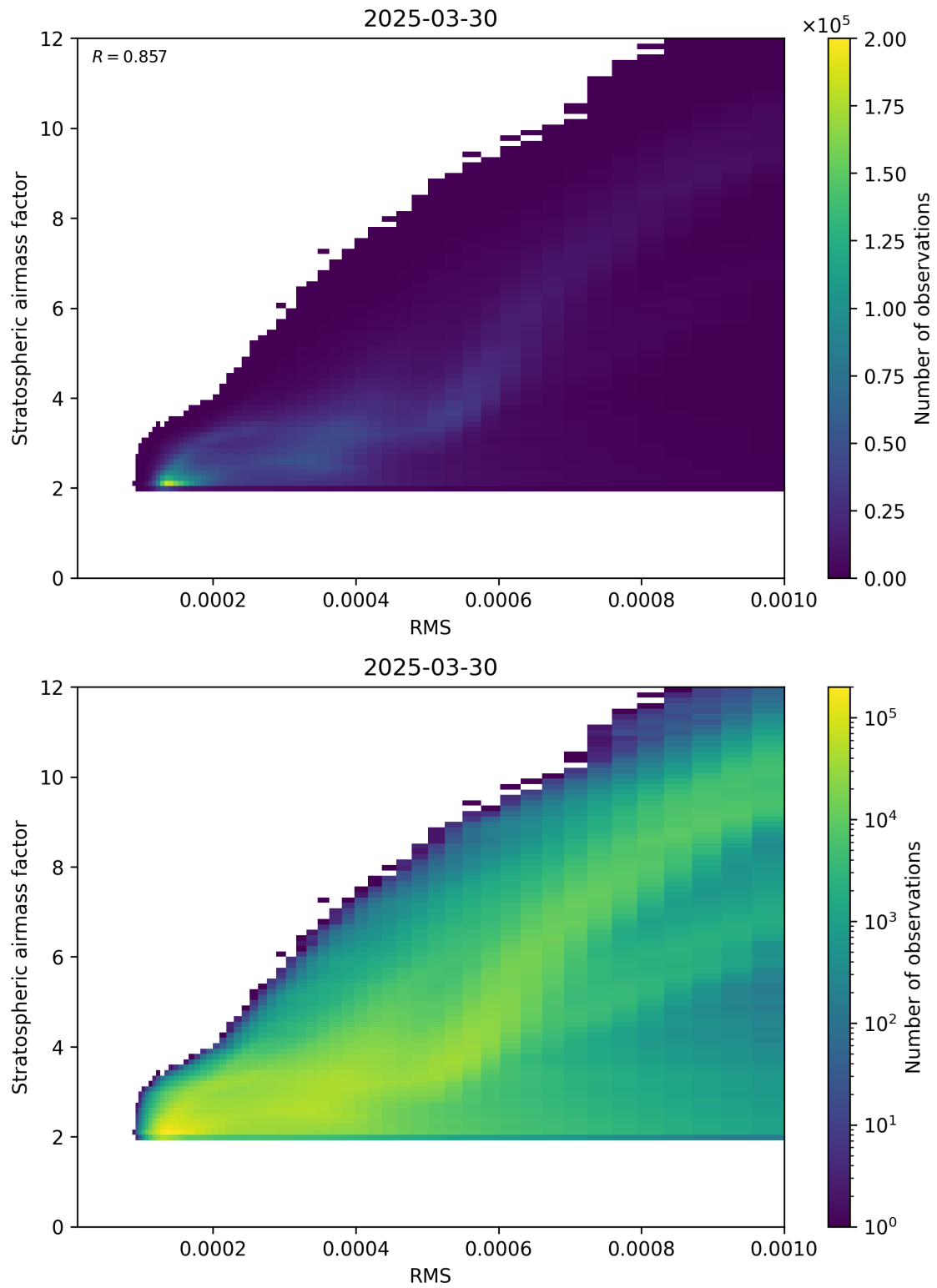
Figure 144: Scatter density plot of “RMS” against “Stratospheric airmass factor” for 2025-03-30 to 2025-03-31.
