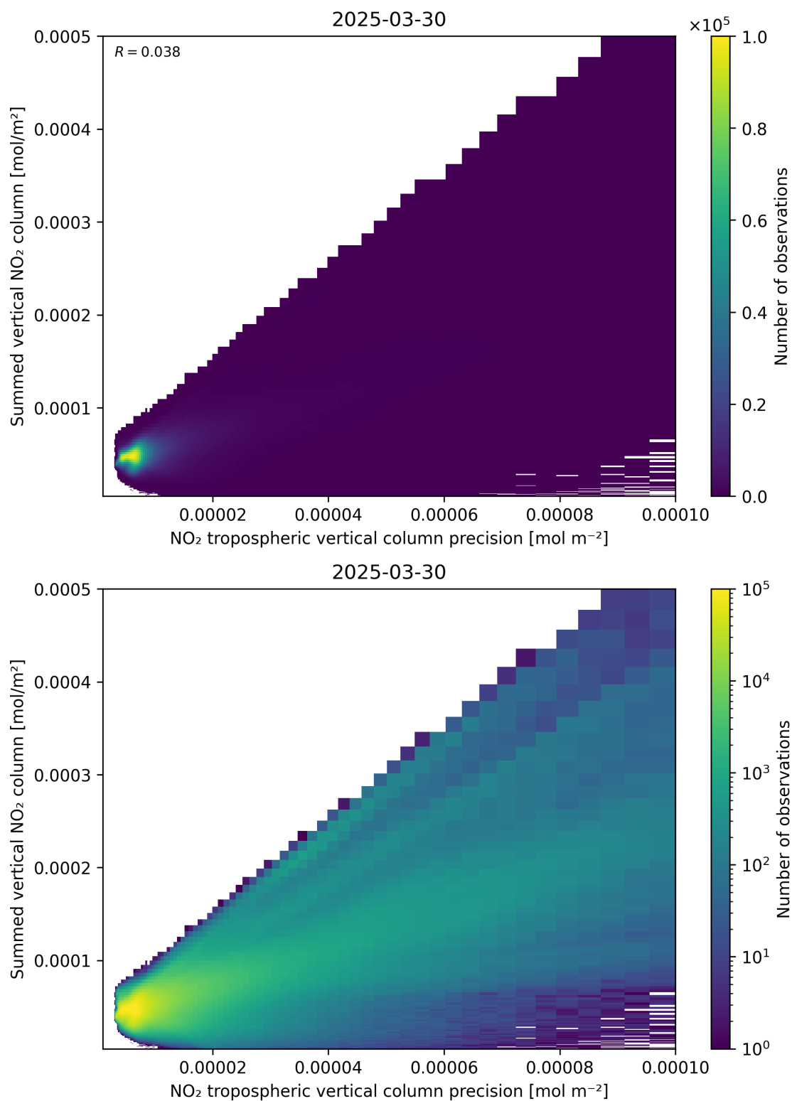
Figure 136: Scatter density plot of “NO 2 tropospheric vertical column precision” against “Summed vertical NO 2 column” for 2025-03-30 to 2025-03-31.
