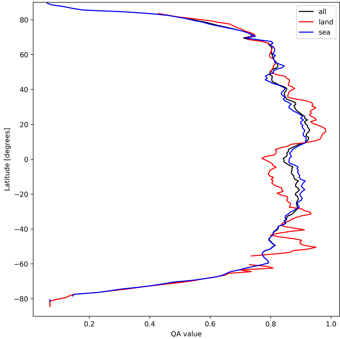
Figure 11: Zonal average of “QA value” for 2025-03-30 to 2025-03-31.
