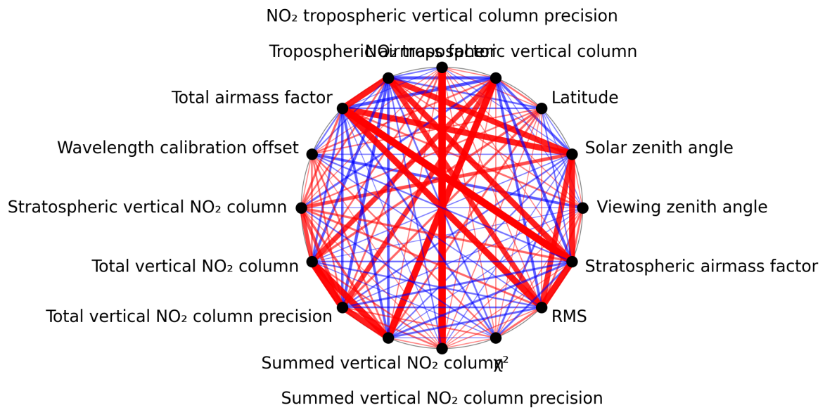
Figure 1: Map of correlation graph for 2025-03-30 to 2025-03-31.
