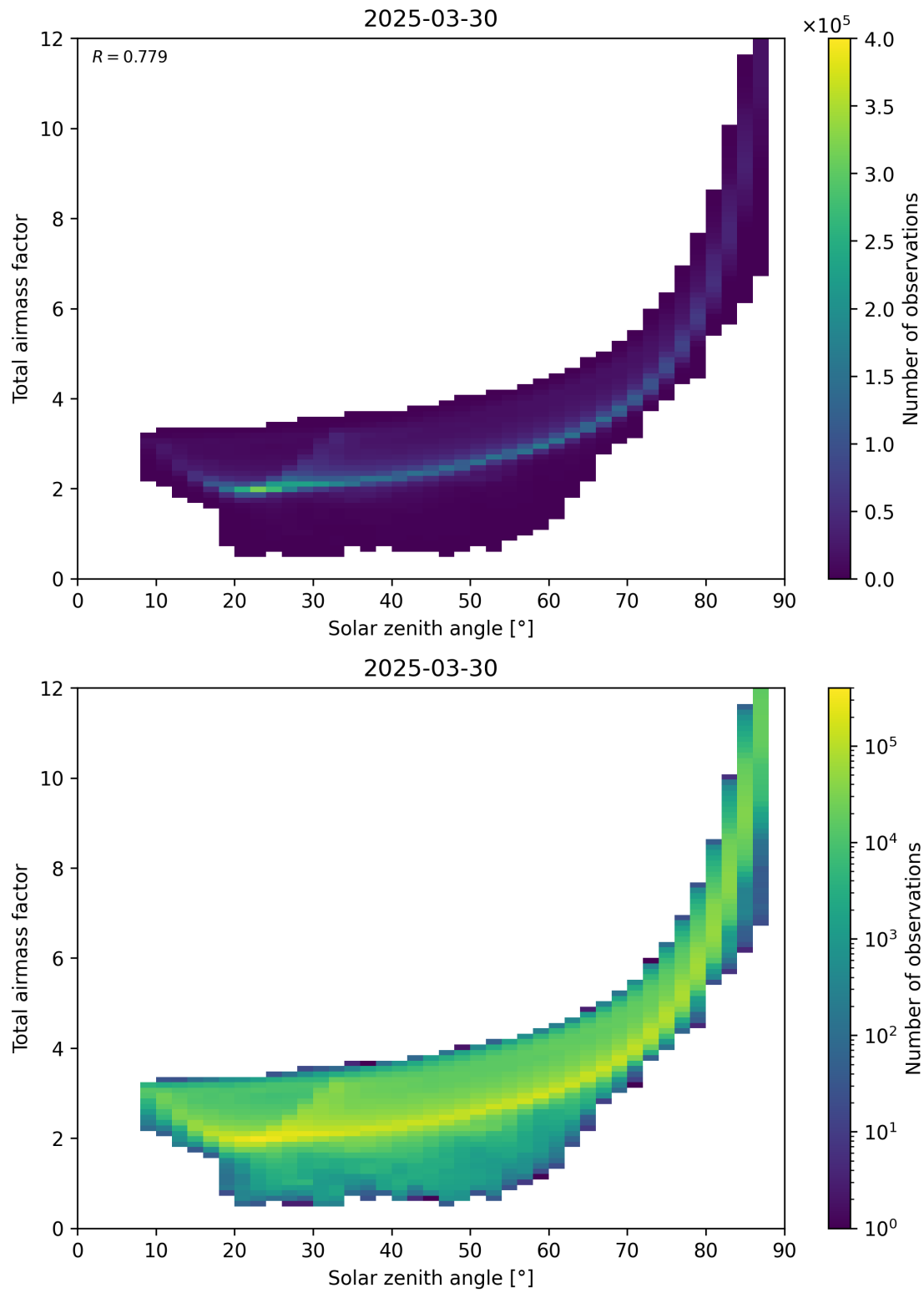
Figure 146: Scatter density plot of “Solar zenith angle” against “Total air mass factor” for 2025-03-30 to 2025-03-31.
