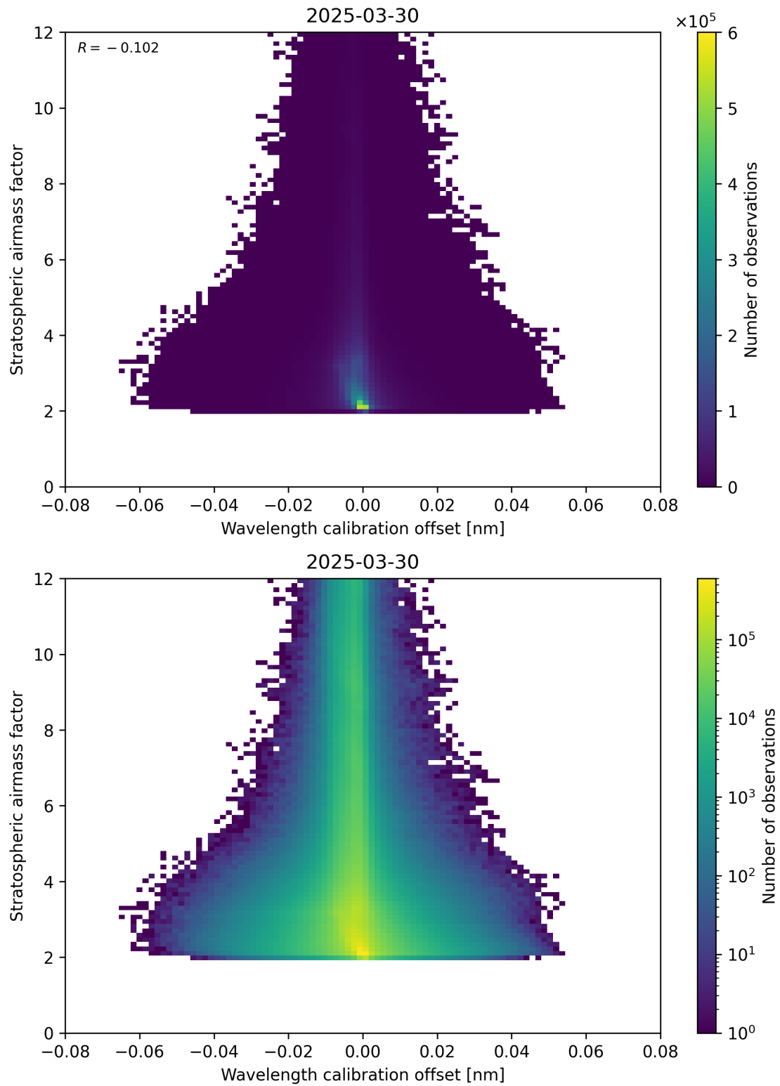
Figure 174: Scatter density plot of “Wavelength calibration offset” against “Stratospheric airmass factor” for 2025-03-30 to 2025-03-31.
