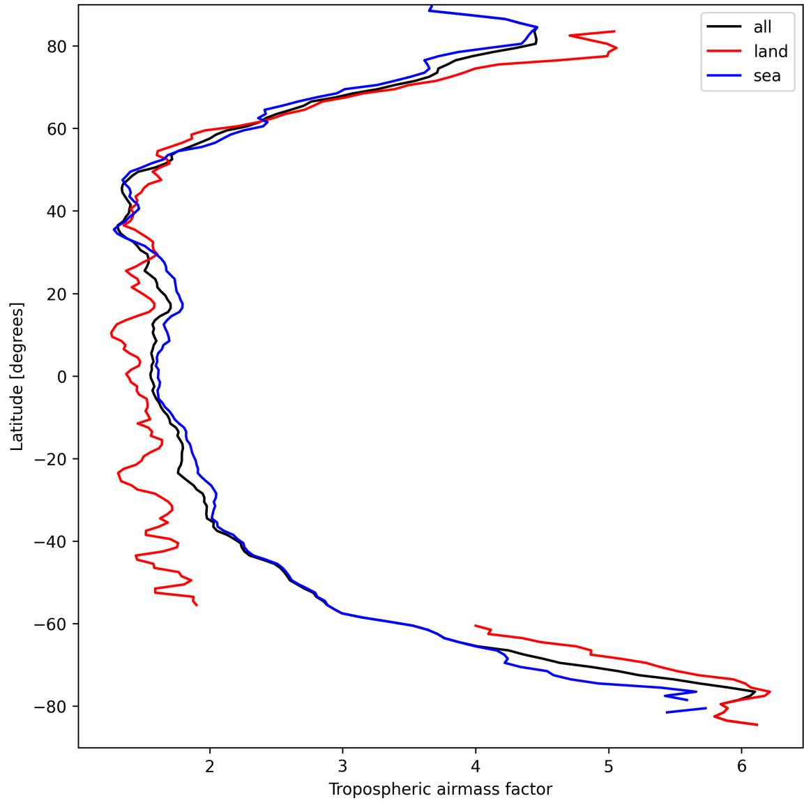
Figure 14: Zonal average of “Tropospheric airmass factor” for 2025-03-30 to 2025-03-31.
