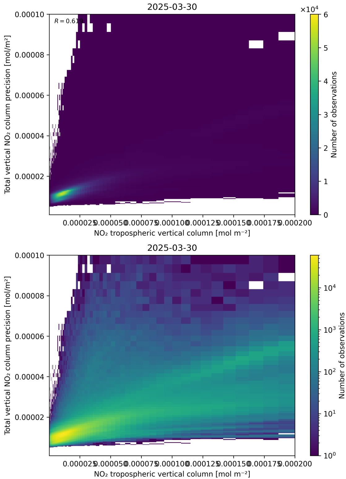
Figure 129: Scatter density plot of “NO 2 tropospheric vertical column” against “Total vertical NO 2 column precision” for 2025-03-30 to 2025-03-31.
