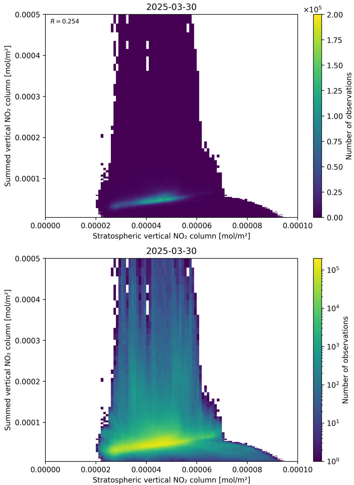
Figure 98: Scatter density plot of “Stratospheric vertical NO 2 column” against “Summed vertical NO 2 column” for 2025-03-30 to 2025-03-31.
