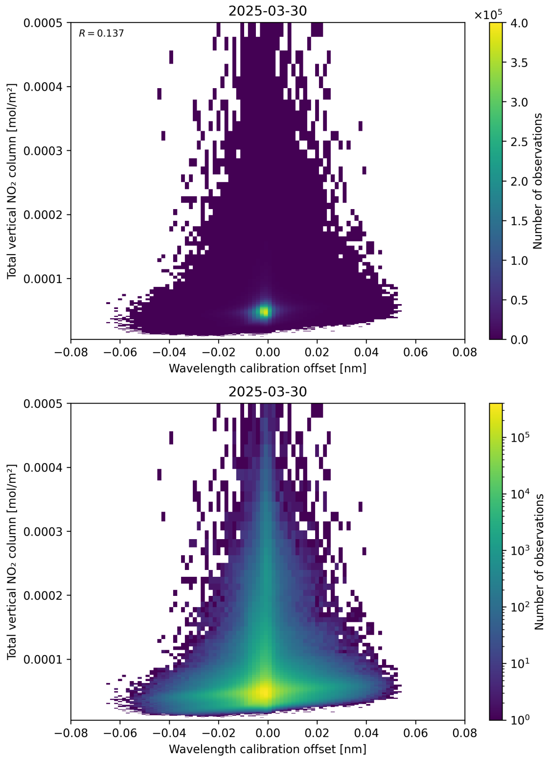
Figure 179: Scatter density plot of “Wavelength calibration offset” against “Total vertical NO 2 column” for 2025-03-30 to 2025-03-31.
