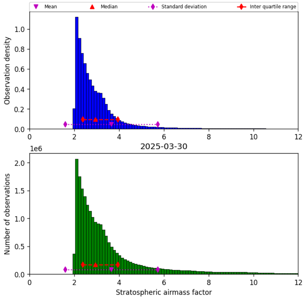
Figure 44: Histogram of “Stratospheric airmass factor” for 2025-03-30 to 2025-03-31
