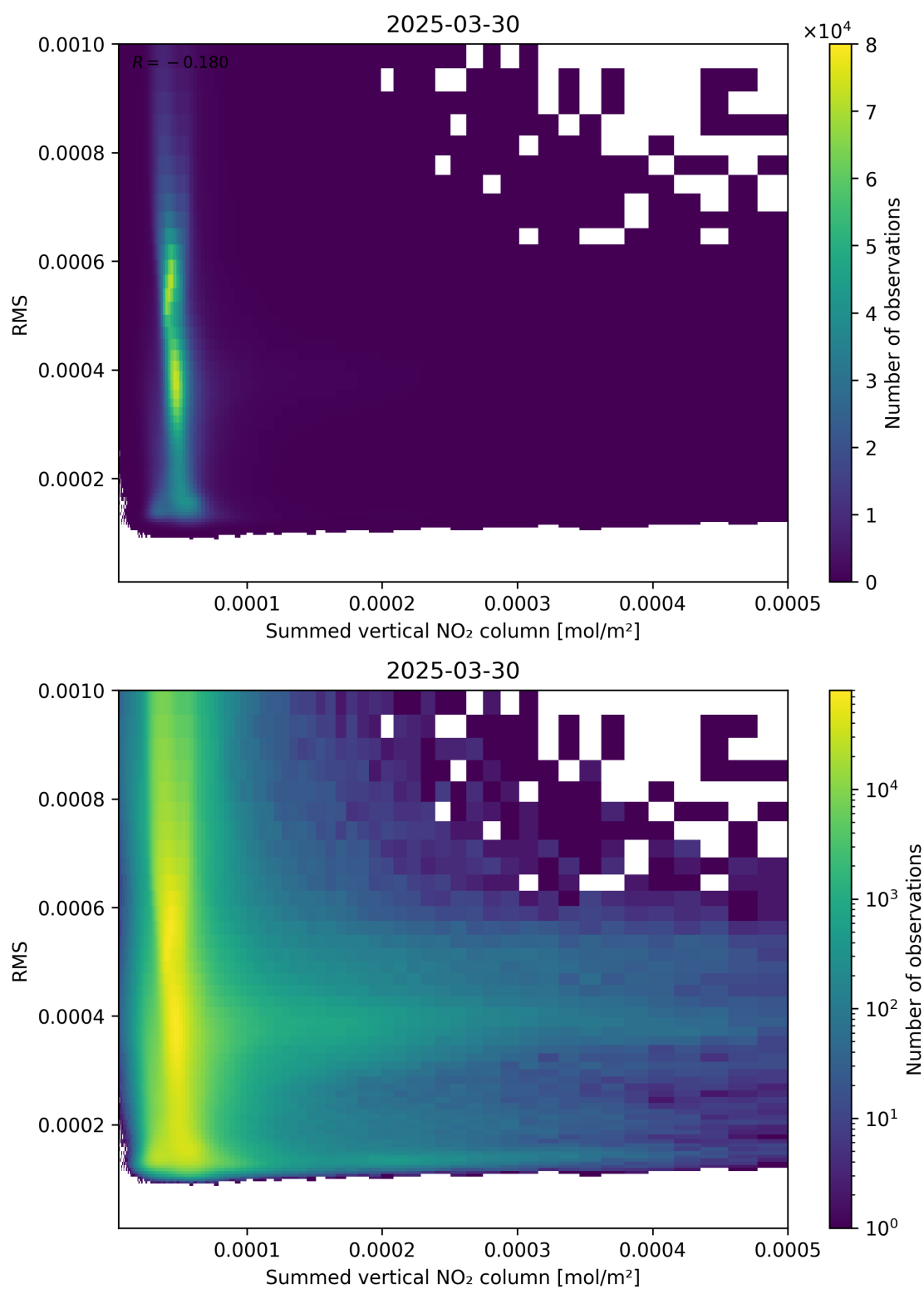
Figure 109: Scatter density plot of “Summed vertical NO 2 column” against “RMS” for 2025-03-30 to 2025-03-31.
