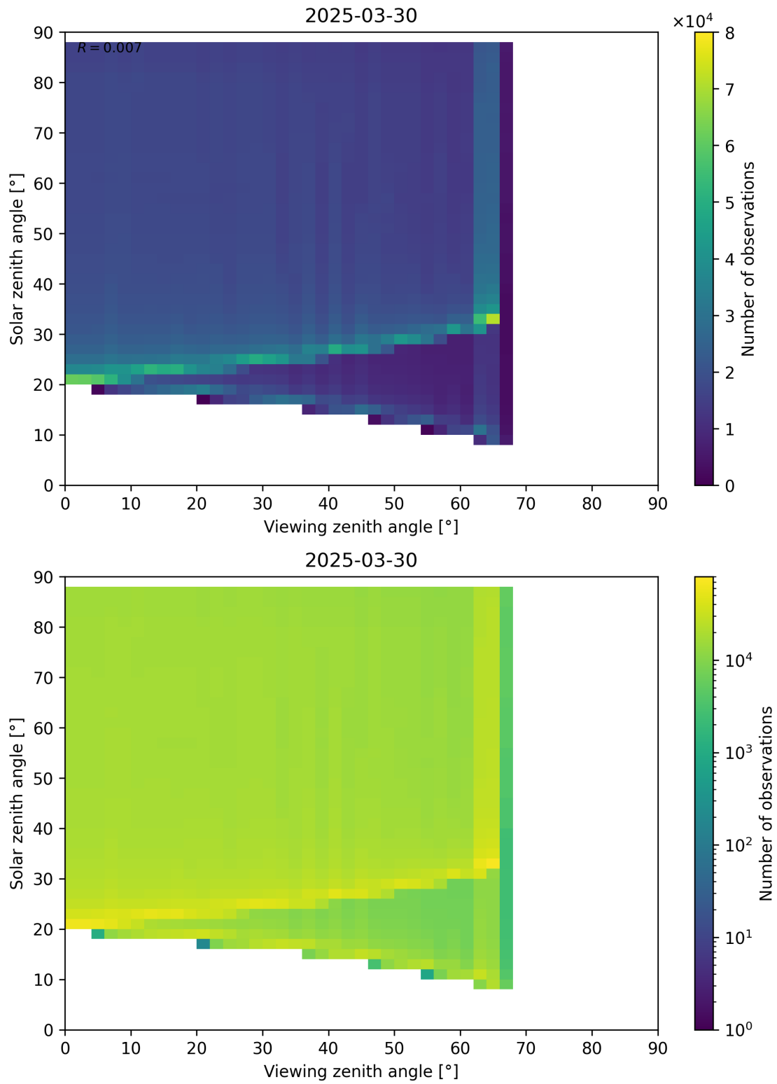
Figure 172: Scatter density plot of “Viewing zenith angle” against “Solar zenith angle” for 2025-03-30 to 2025-03-31.
