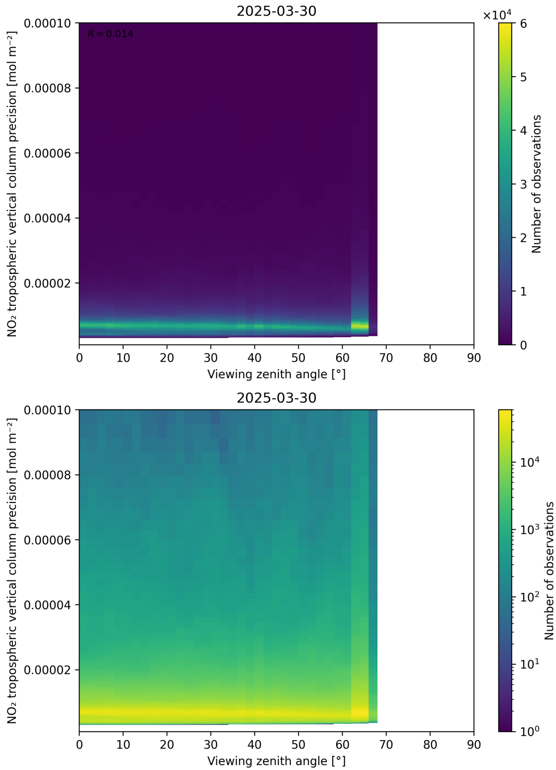
Figure 170: Scatter density plot of “Viewing zenith angle” against “NO 2 tropospheric vertical column precision” for 2025-03-30 to 2025-03-31.
