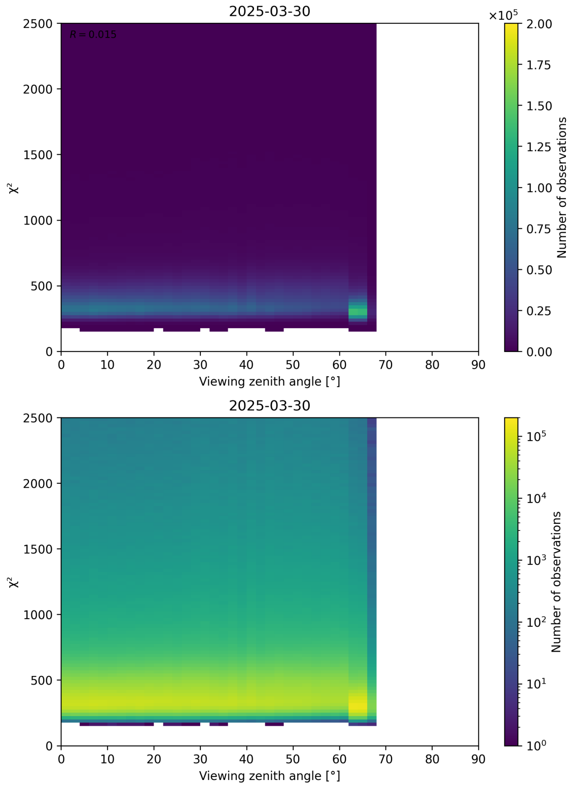
Figure 162: Scatter density plot of “Viewing zenith angle” against “ \chi^2 ” for 2025-03-30 to 2025-03-31.
