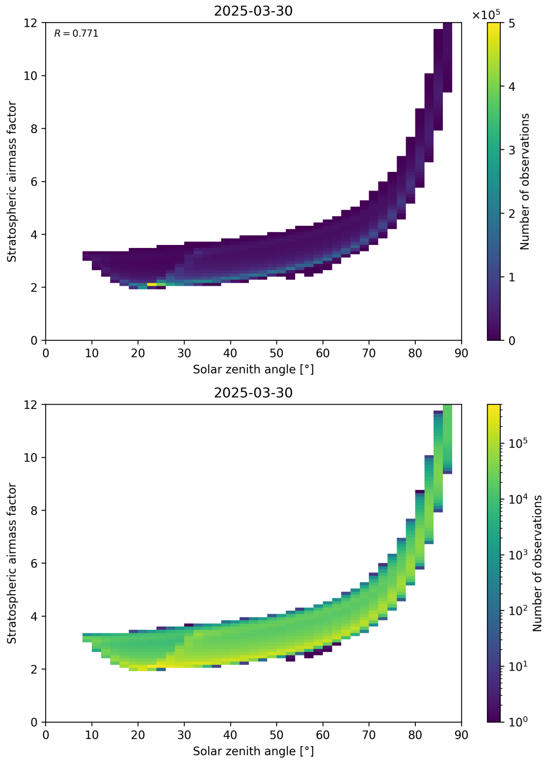
Figure 145: Scatter density plot of “Solar zenith angle” against “Stratospheric airmass factor” for 2025-03-30 to 2025-03-31.
