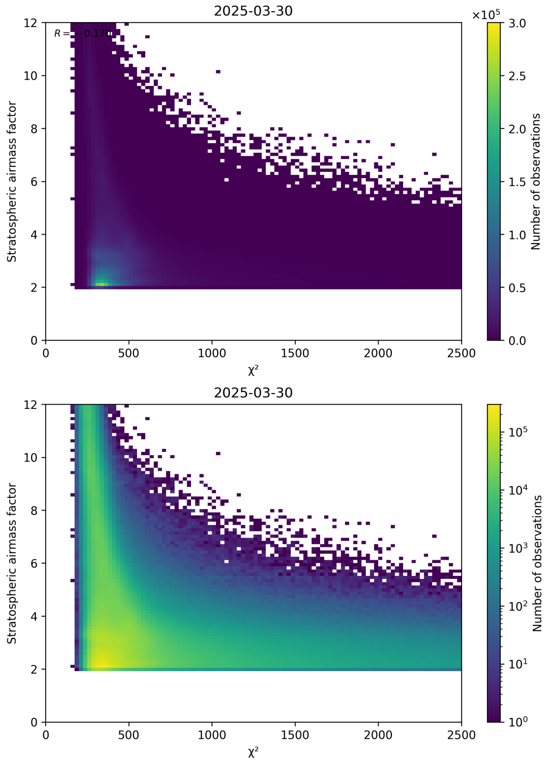
Figure 81: Scatter density plot of " \chi^2 " against "Stratospheric airmass factor" for 2025-03-30 to 2025-03-31.
