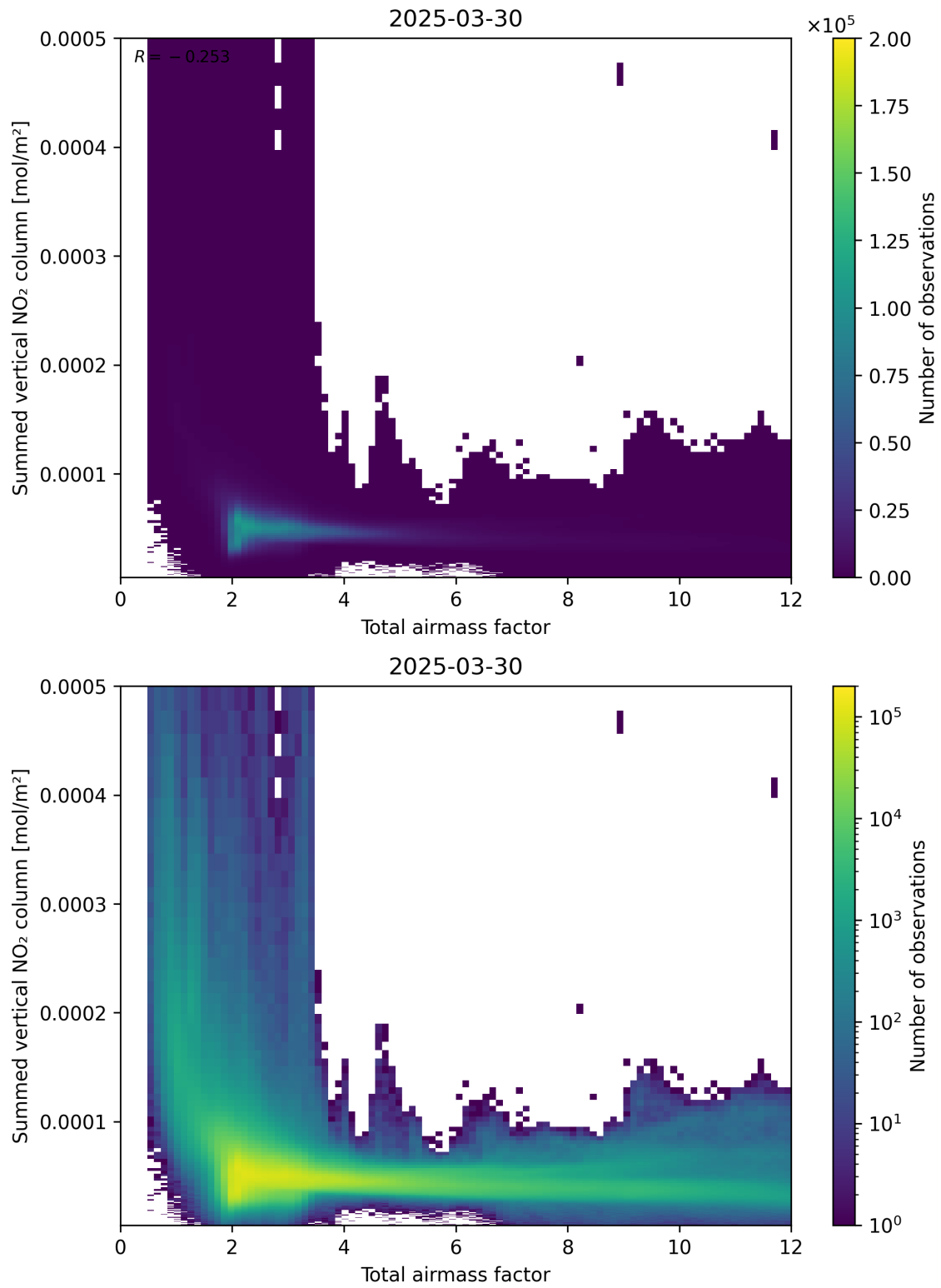
Figure 65: Scatter density plot of “Total airmass factor” against “Summed vertical NO 2 column” for 2025-03-30 to 2025-03-31.
