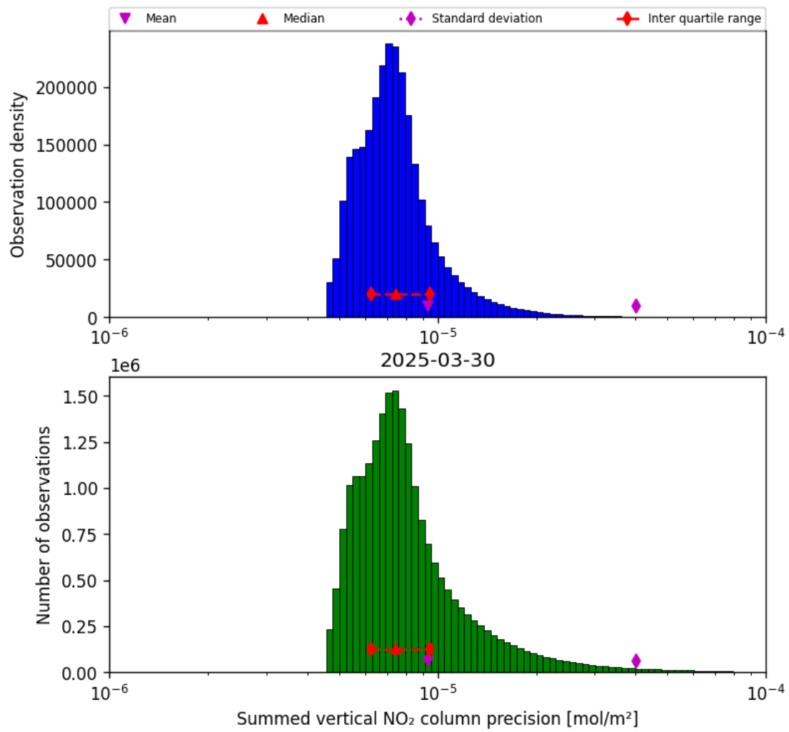
Figure 41: Histogram of “Summed vertical NO 2 column precision” for 2025-03-30 to 2025-03-31
