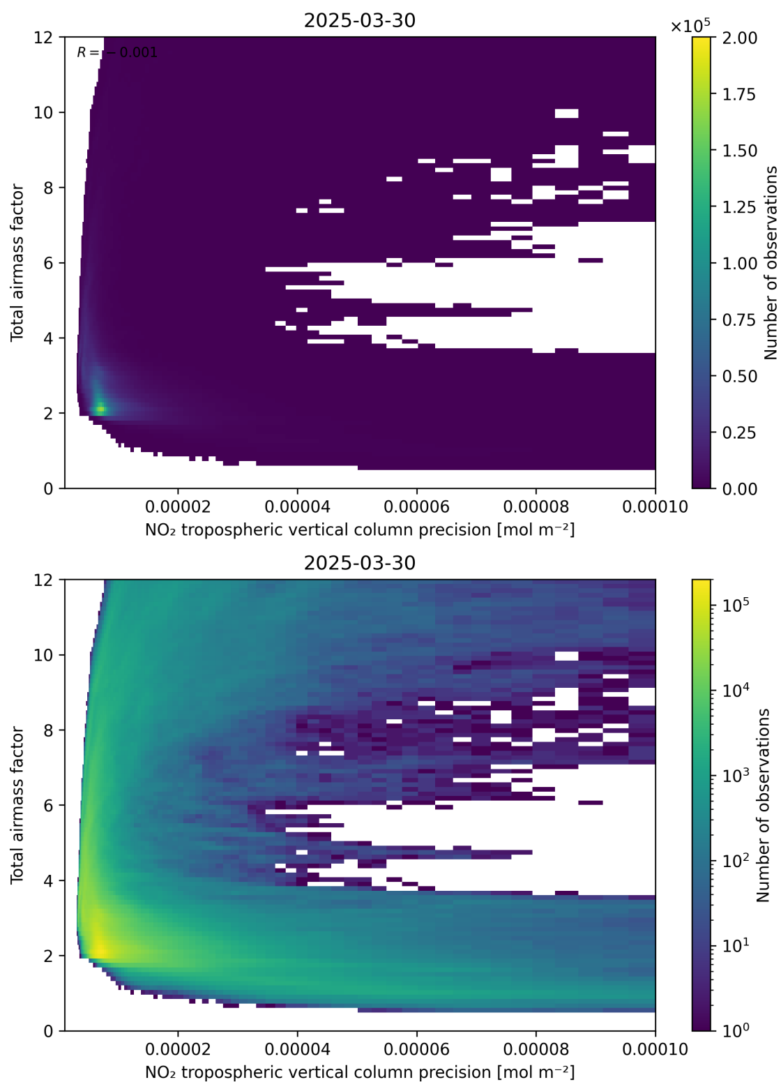
Figure 132: Scatter density plot of “NO 2 tropospheric vertical column precision” against “Total air mass factor” for 2025-03-30 to 2025-03-31.
