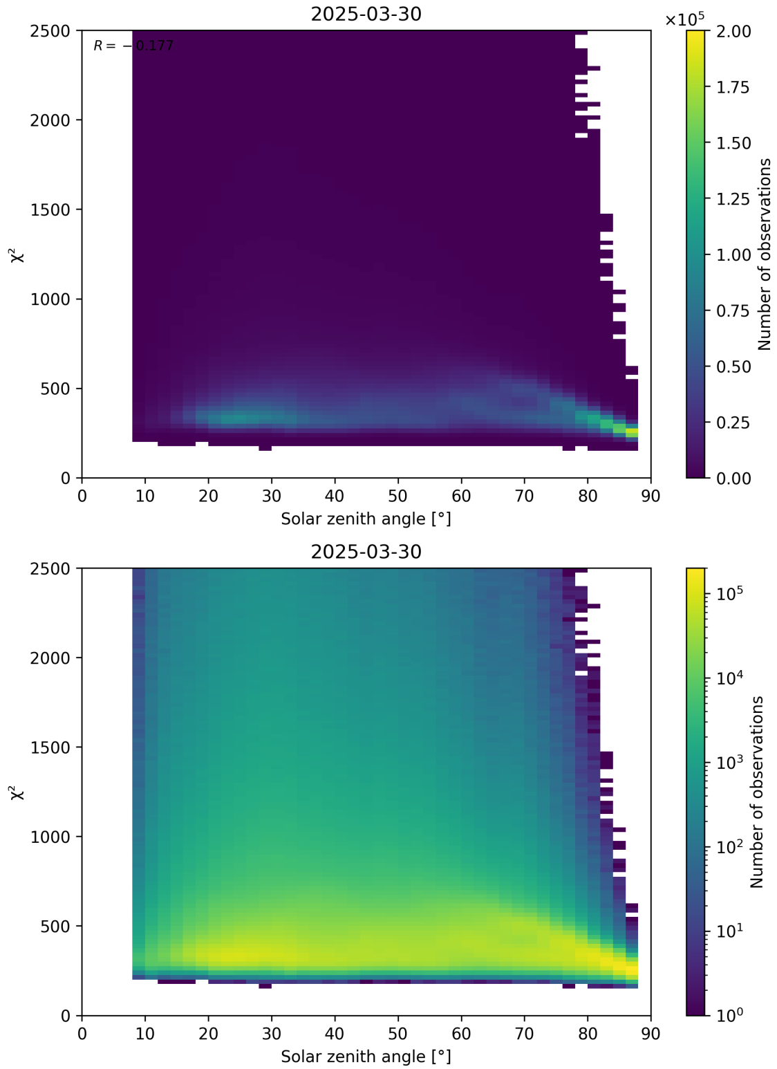
Figure 148: Scatter density plot of “Solar zenith angle” against “ \chi^2 ” for 2025-03-30 to 2025-03-31.
