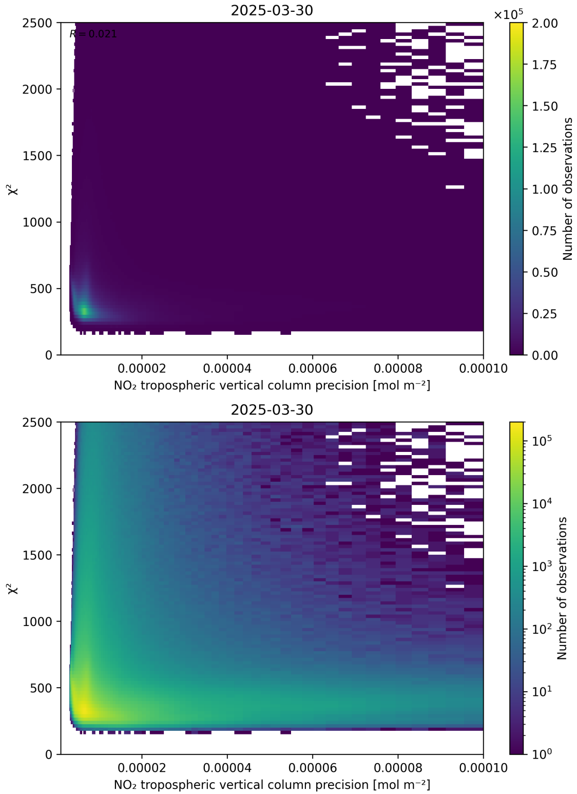
Figure 134: Scatter density plot of “NO 2 tropospheric vertical column precision” against “ \chi^2 ” for 2025-03-30 to 2025-03-31.
