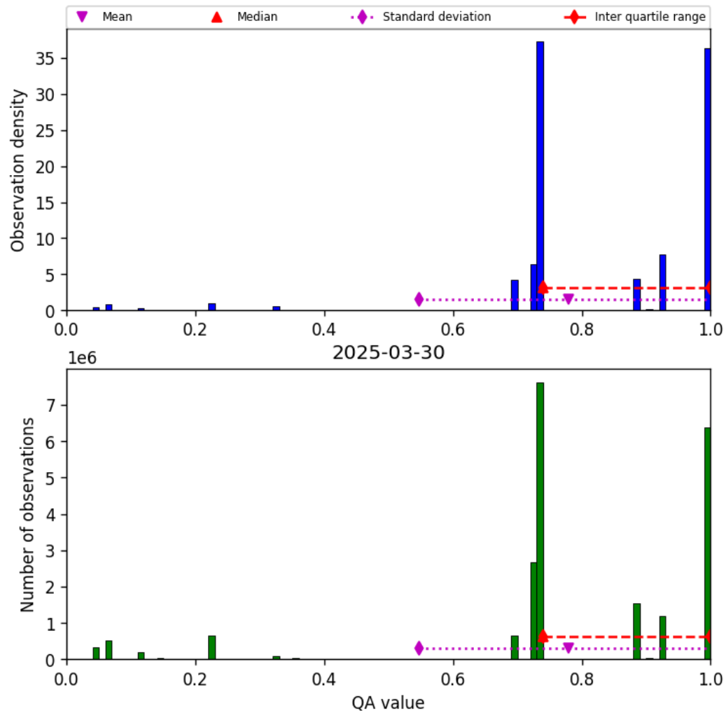
Figure 28: Histogram of “QA value” for 2025-03-30 to 2025-03-31
