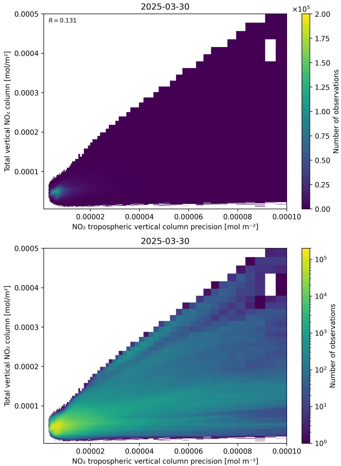
Figure 138: Scatter density plot of “NO 2 tropospheric vertical column precision” against “Total vertical NO 2 column” for 2025-03-30 to 2025-03-31.
