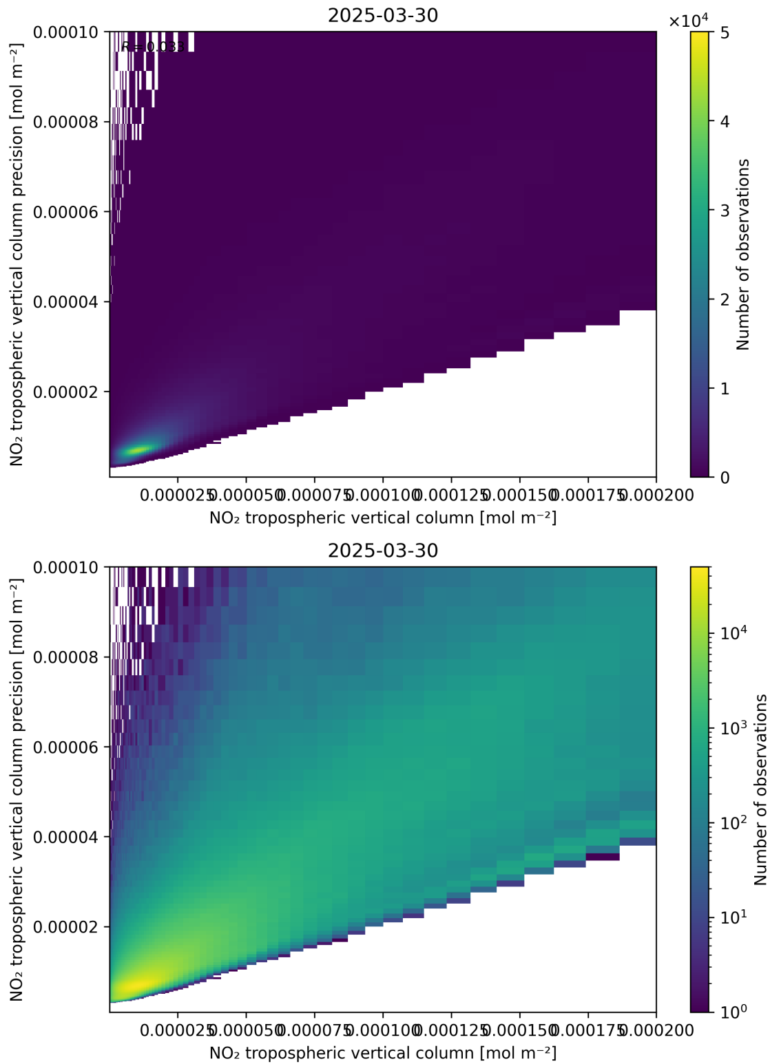
Figure 130: Scatter density plot of “NO 2 tropospheric vertical column” against “NO 2 tropospheric vertical column precision” for 2025-03-30 to 2025-03-31.
