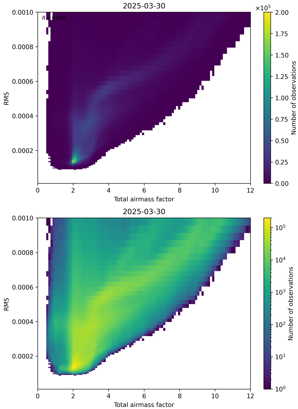
Figure 69: Scatter density plot of “Total airmass factor” against “RMS” for 2025-03-30 to 2025-03-31.
