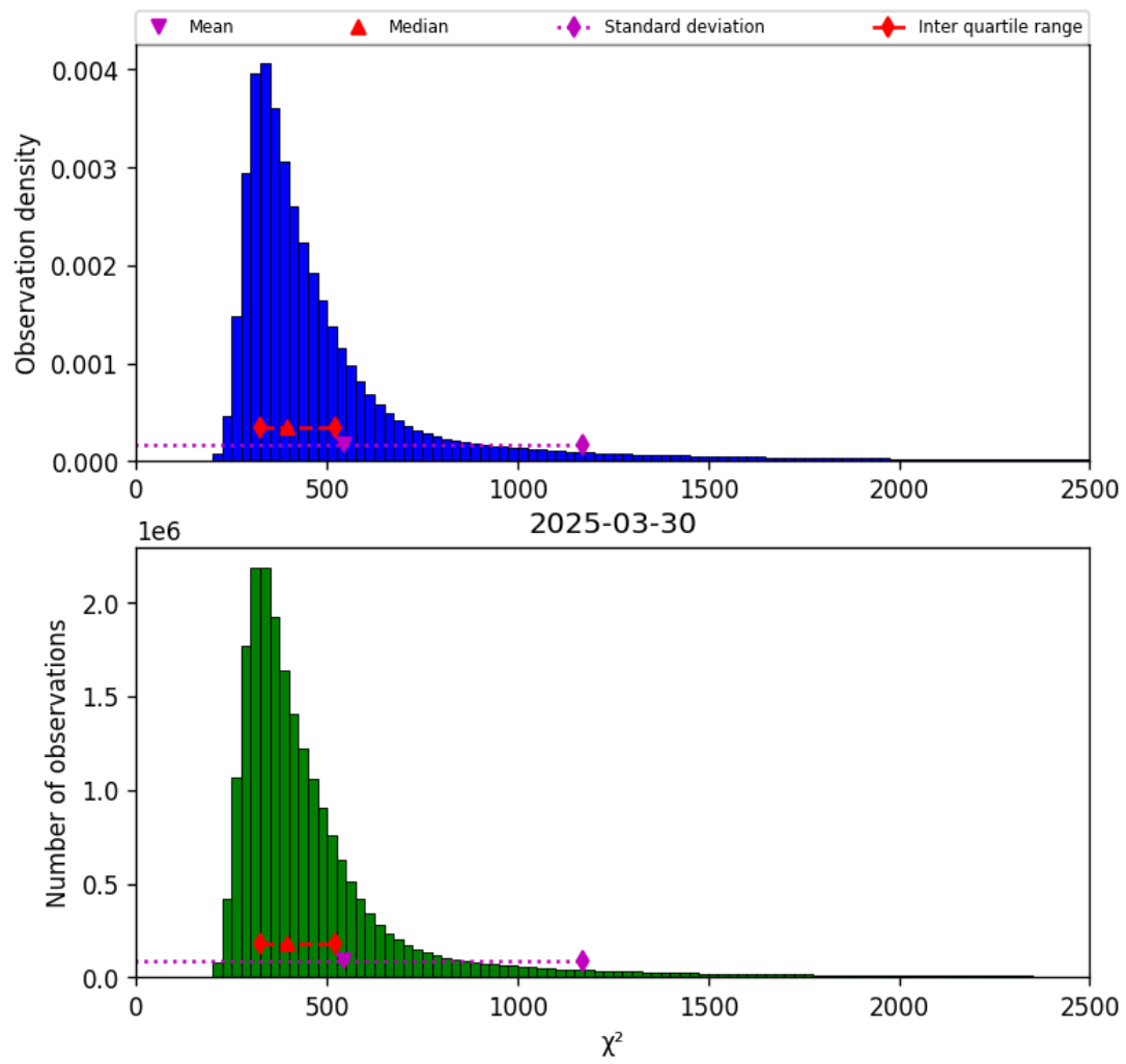
Figure 42: Histogram of “ \chi^2 ” for 2025-03-30 to 2025-03-31
