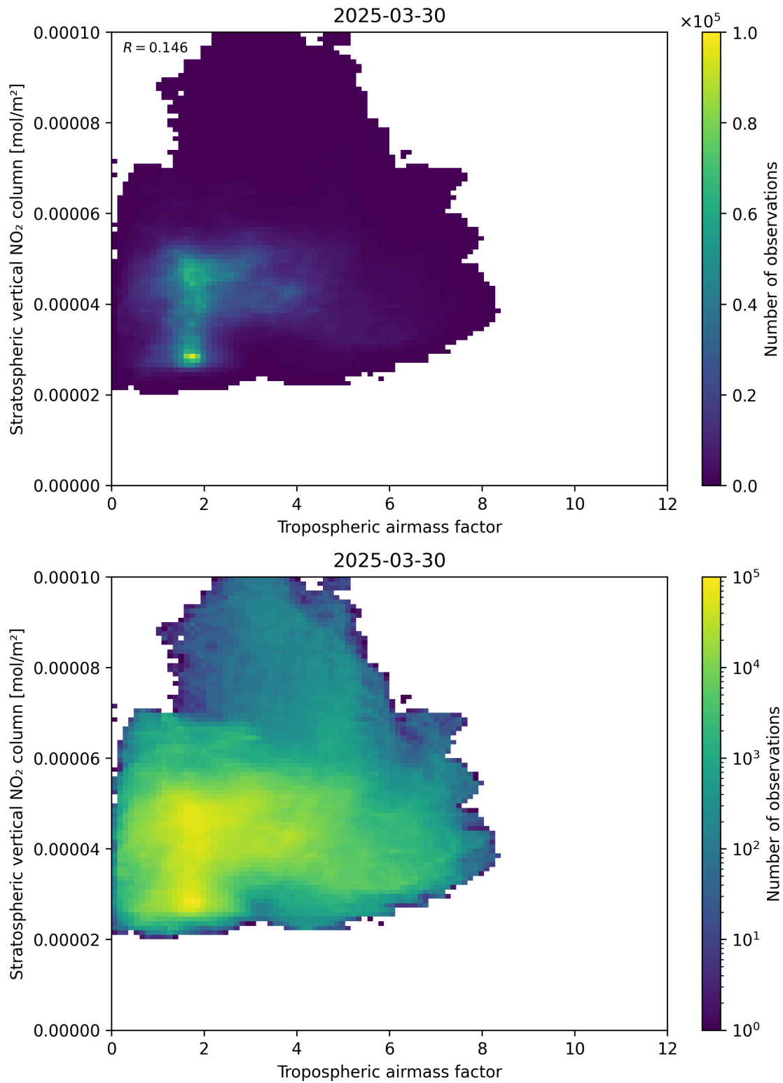
Figure 74: Scatter density plot of “Tropospheric air mass factor” against “Stratospheric vertical NO 2 column” for 2025-03-30 to 2025-03-31.
