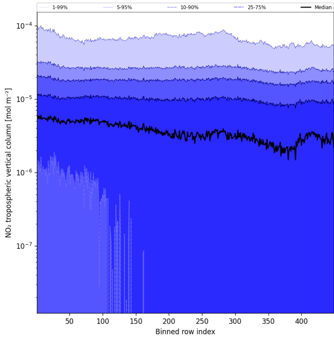
Figure 46: Along track statistics of “NO 2 tropospheric vertical column” for 2025-03-30 to 2025-03-31
