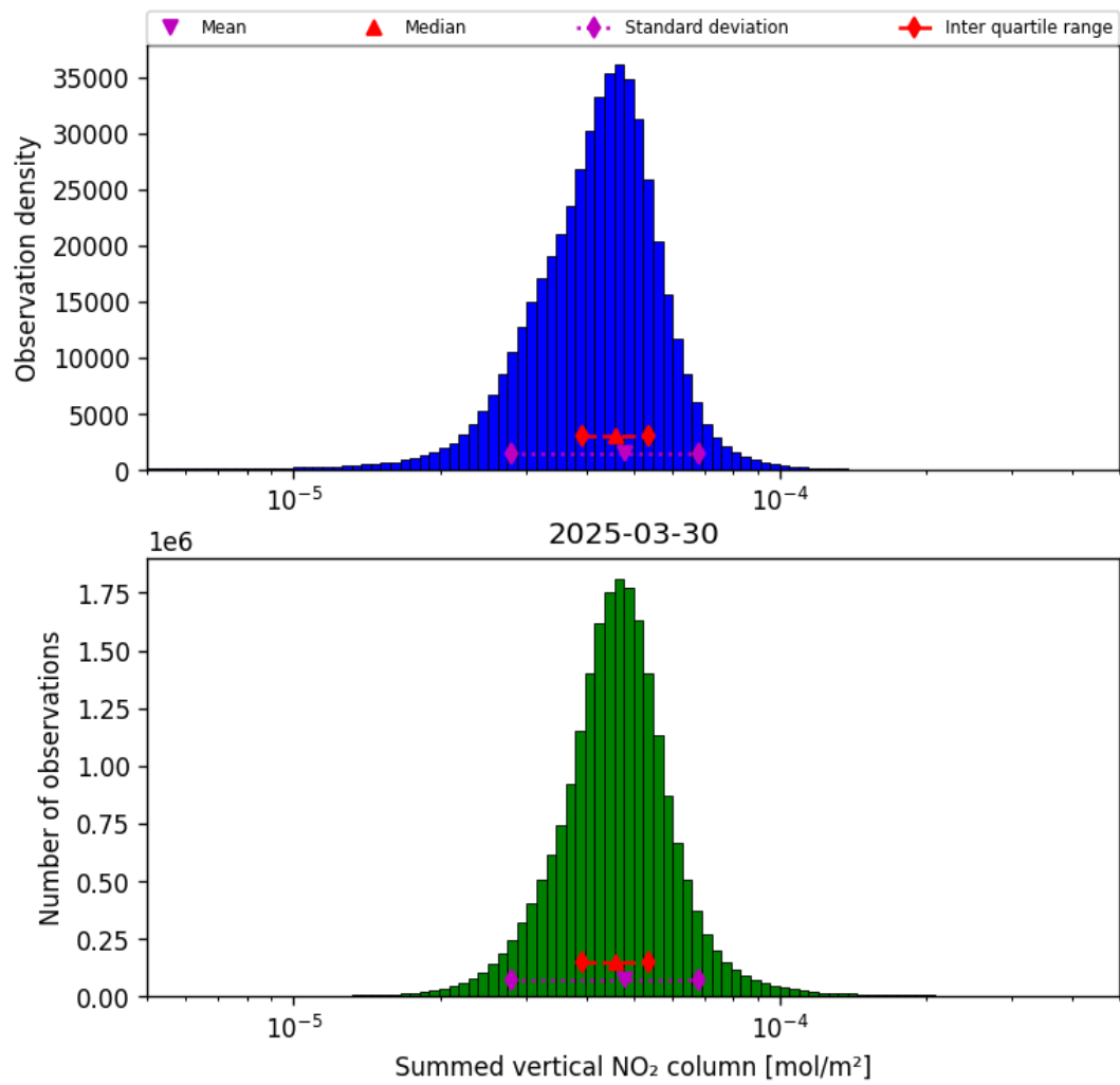
Figure 40: Histogram of “Summed vertical NO 2 column” for 2025-03-30 to 2025-03-31
