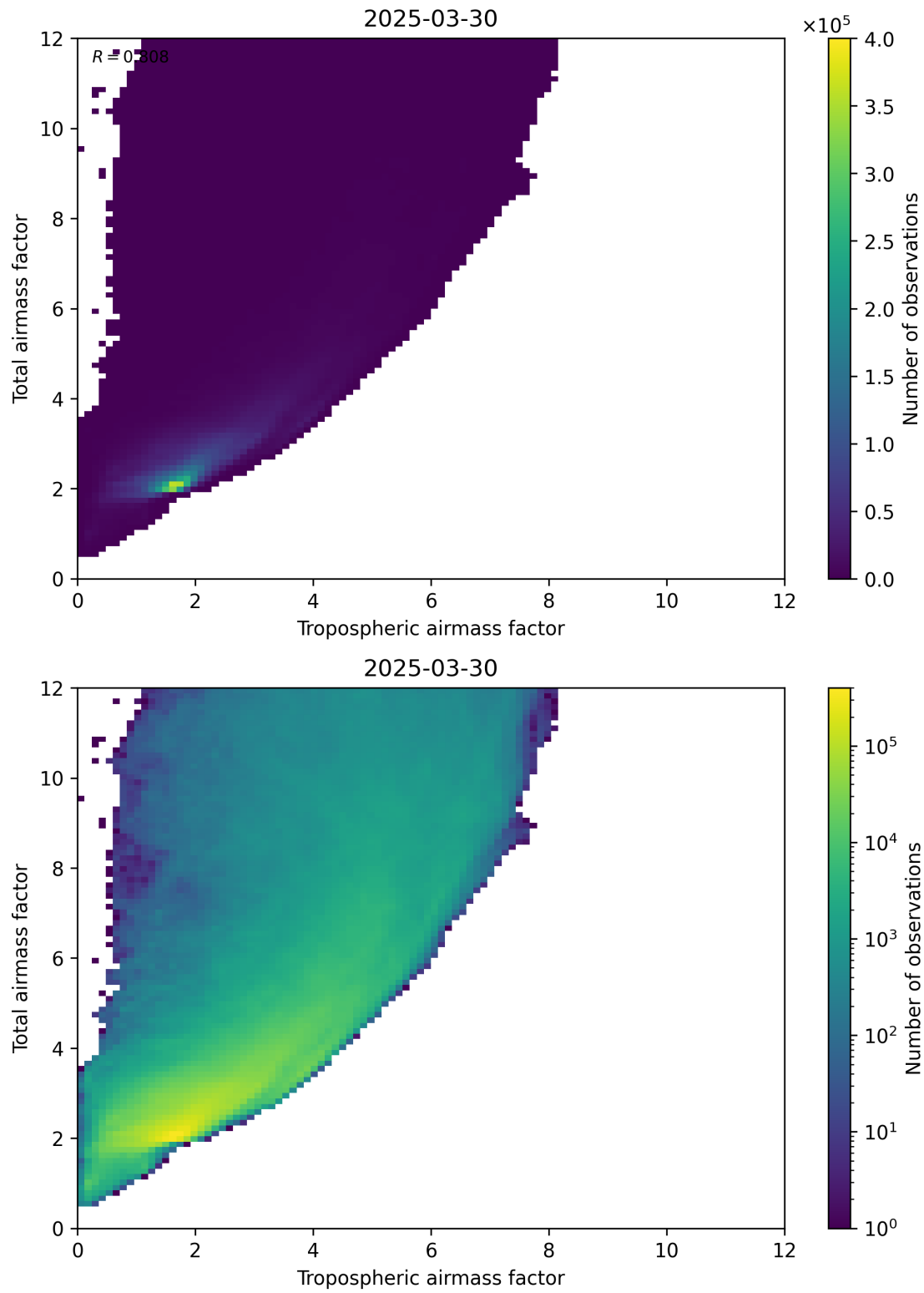
Figure 72: Scatter density plot of “Tropospheric airmass factor” against “Total airmass factor” for 2025-03-30 to 2025-03-31.
