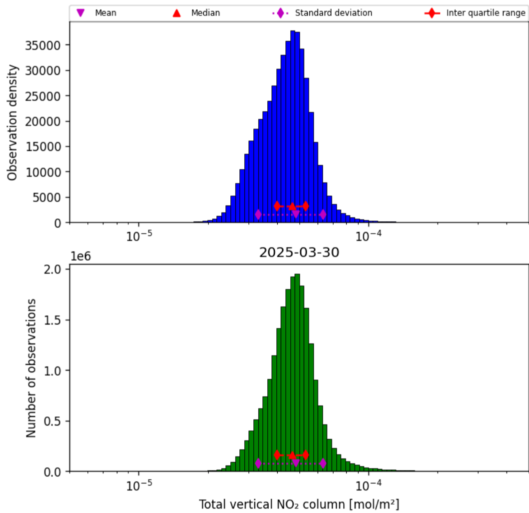
Figure 38: Histogram of “Total vertical NO 2 column” for 2025-03-30 to 2025-03-31
