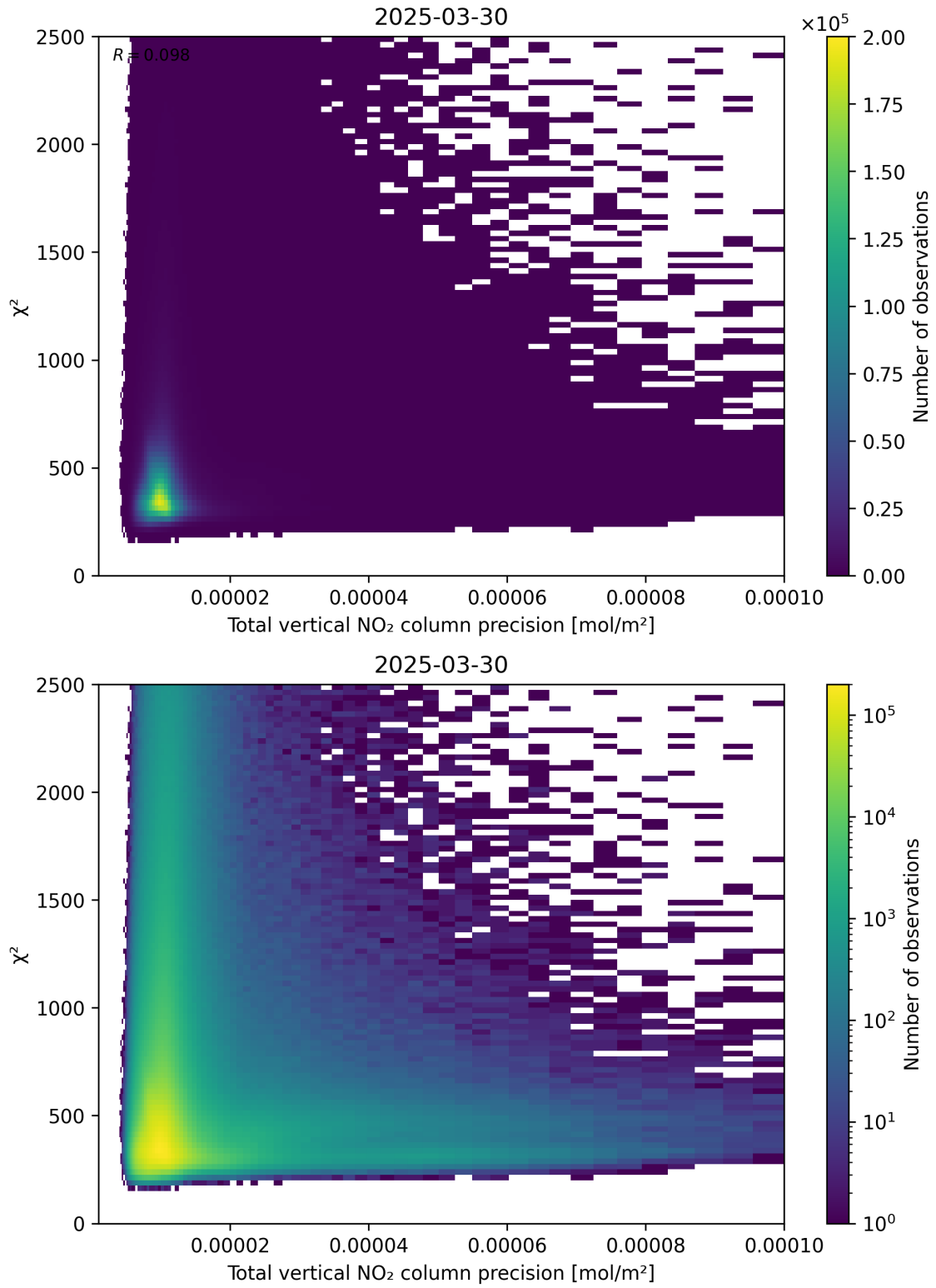
Figure 116: Scatter density plot of “Total vertical NO 2 column precision” against “ \chi^2 ” for 2025-03-30 to 2025-03-31.
