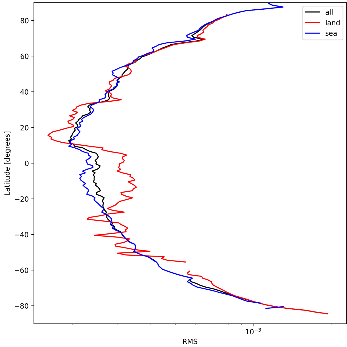
Figure 26: Zonal average of “RMS” for 2025-03-30 to 2025-03-31.
