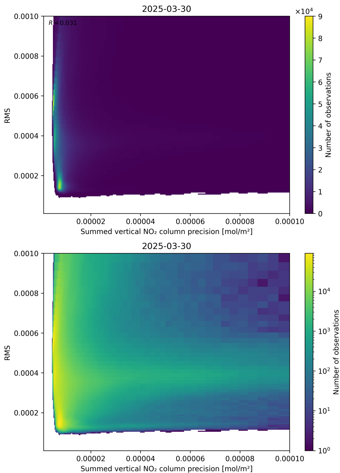
Figure 108: Scatter density plot of “Summed vertical NO 2 column precision” against “RMS” for 2025-03-30 to 2025-03-31.
