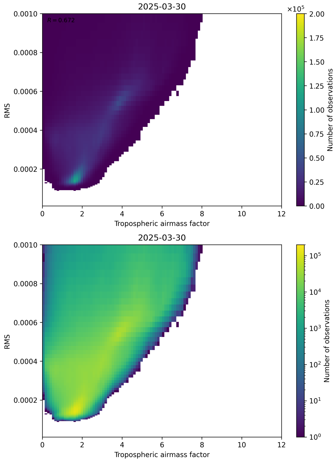
Figure 79: Scatter density plot of “Tropospheric airmass factor” against “RMS” for 2025-03-30 to 2025-03-31.
