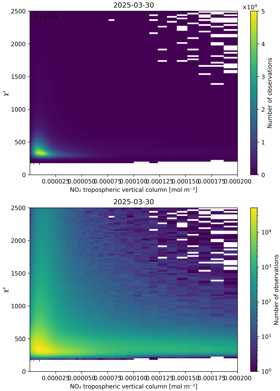
Figure 124: Scatter density plot of “NO 2 tropospheric vertical column” against “ \chi^2 ” for 2025-03-30 to 2025-03-31.
