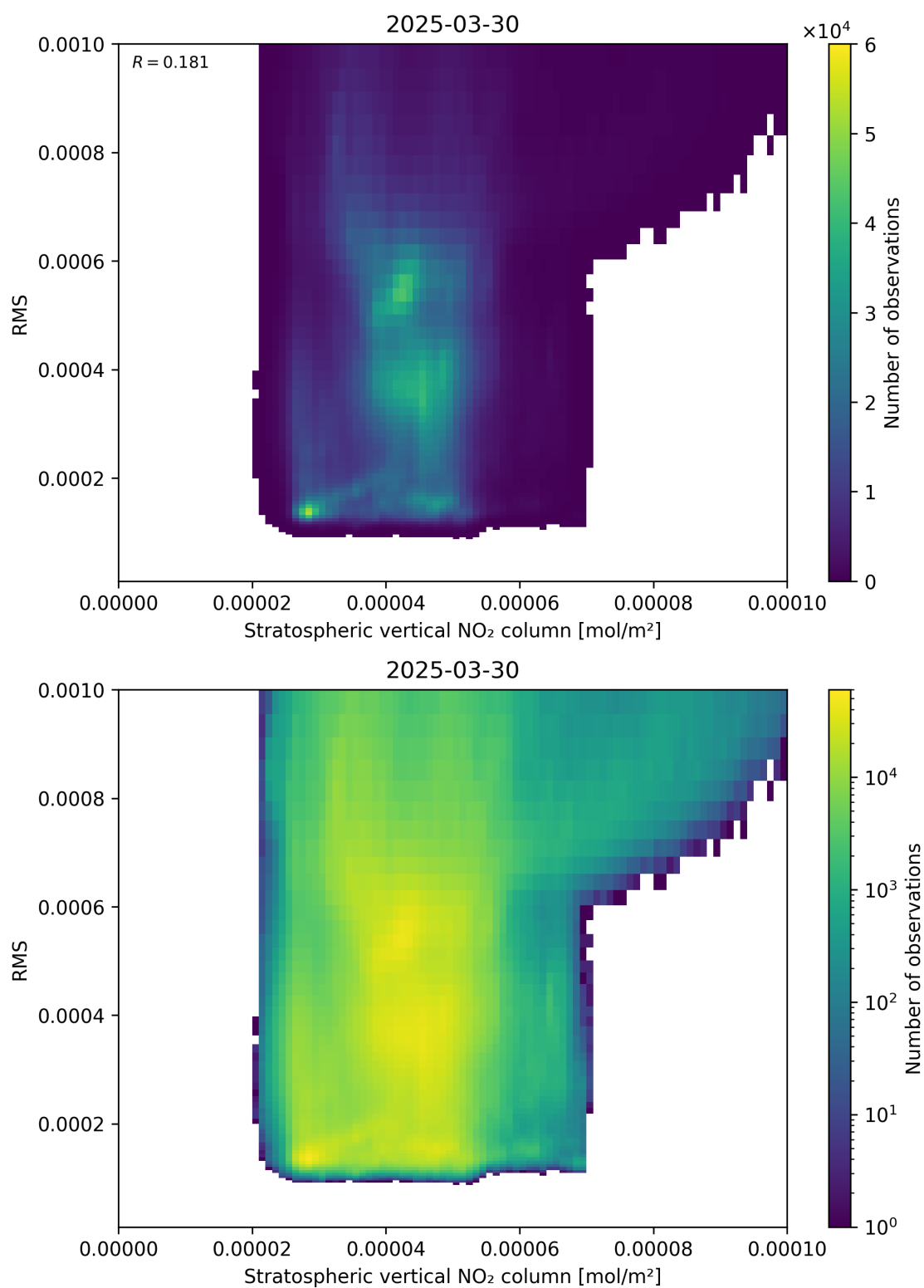
Figure 102: Scatter density plot of “Stratospheric vertical NO 2 column” against “RMS” for 2025-03-30 to 2025-03-31.
