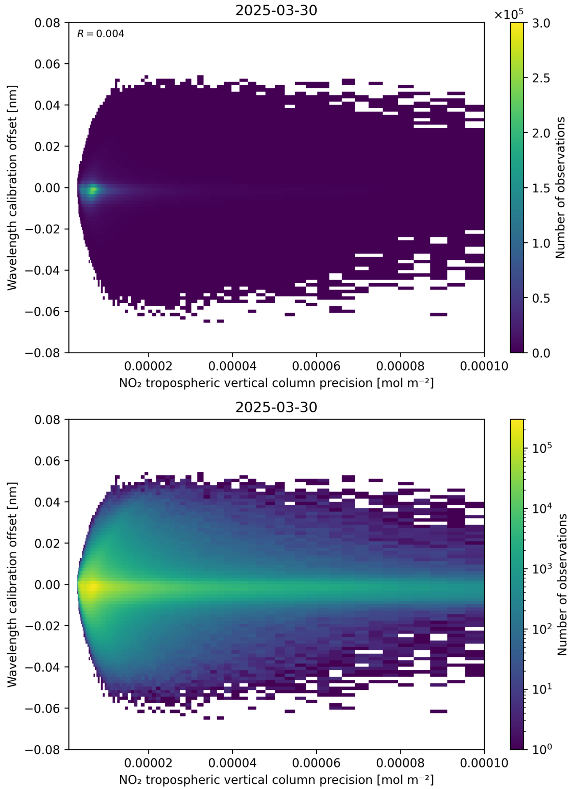
Figure 141: Scatter density plot of “NO 2 tropospheric vertical column precision” against “Wavelength calibration offset” for 2025-03-30 to 2025-03-31.
