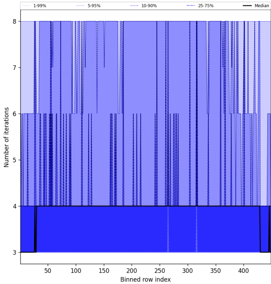
Figure 51: Along track statistics of “Number of iterations” for 2025-03-30 to 2025-03-31
