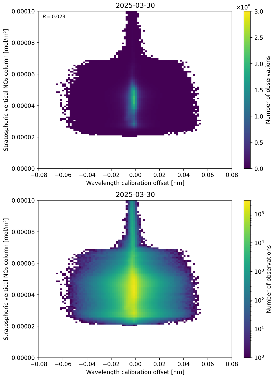
Figure 176: Scatter density plot of “Wavelength calibration offset” against “Stratospheric vertical NO 2 column” for 2025-03-30 to 2025-03-31.
