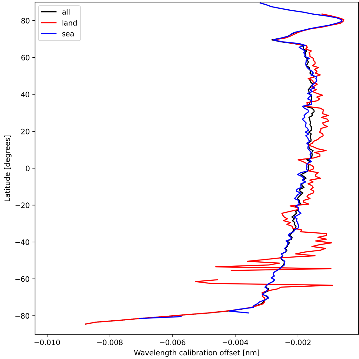
Figure 18: Zonal average of “Wavelength calibration offset” for 2025-03-30 to 2025-03-31.
