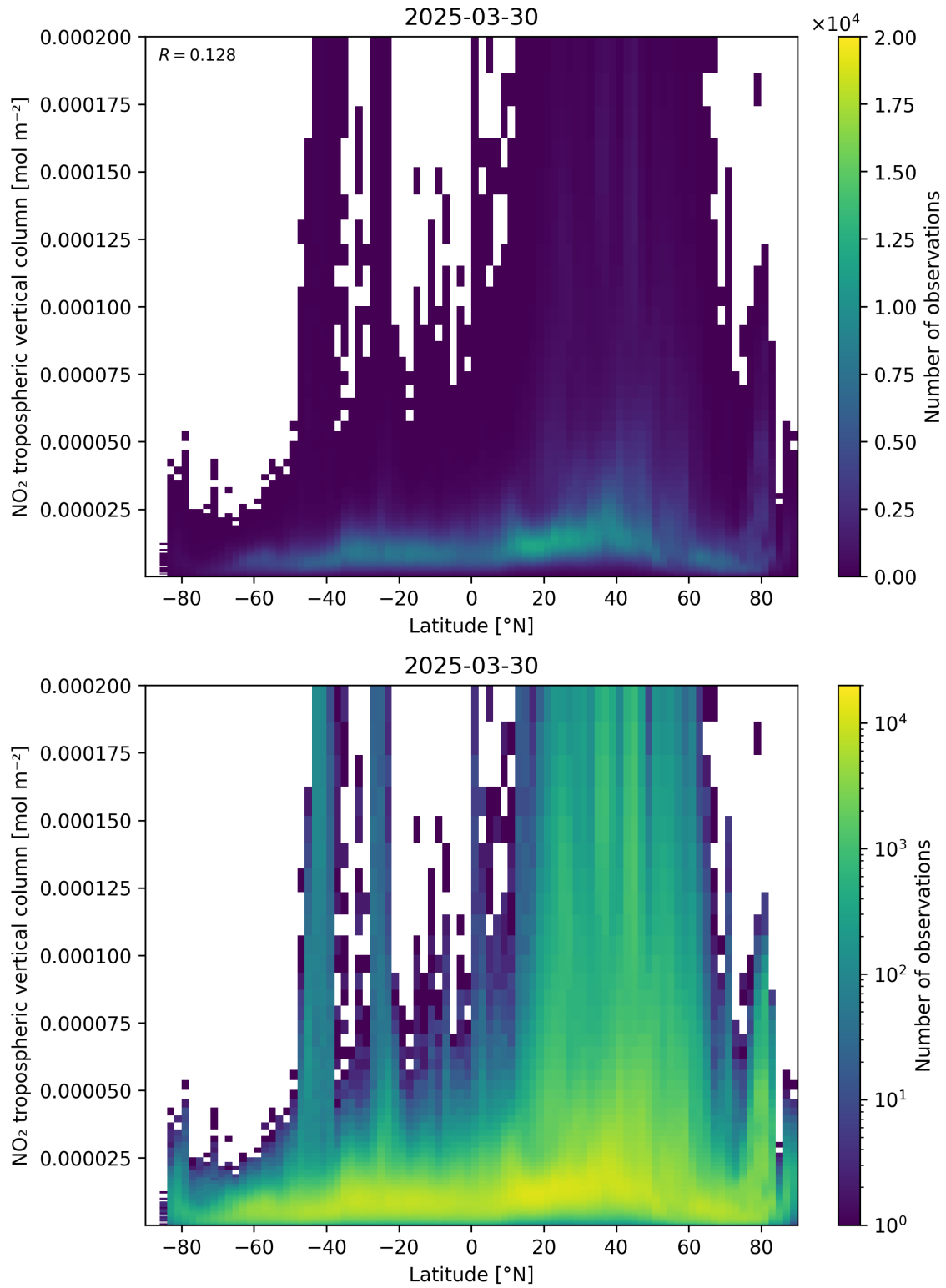
Figure 92: Scatter density plot of “Latitude” against “NO 2 tropospheric vertical column” for 2025-03-30 to 2025-03-31.
