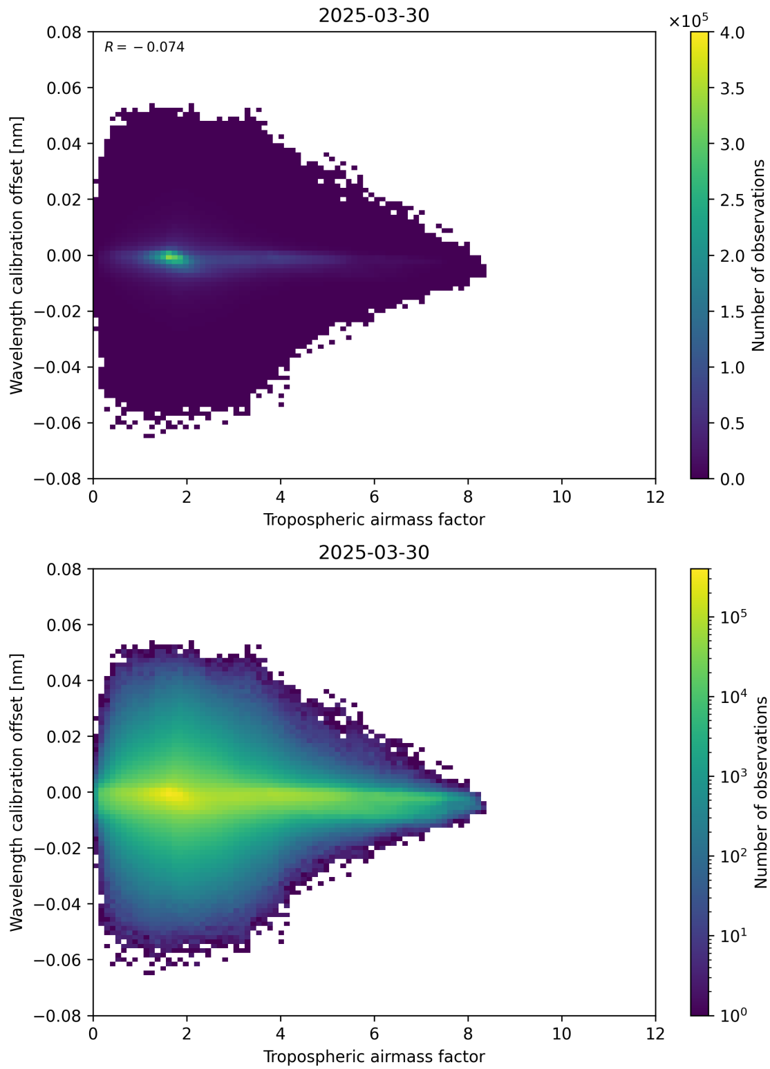
Figure 80: Scatter density plot of “Tropospheric airmass factor” against “Wavelength calibration offset” for 2025-03-30 to 2025-03-31.
