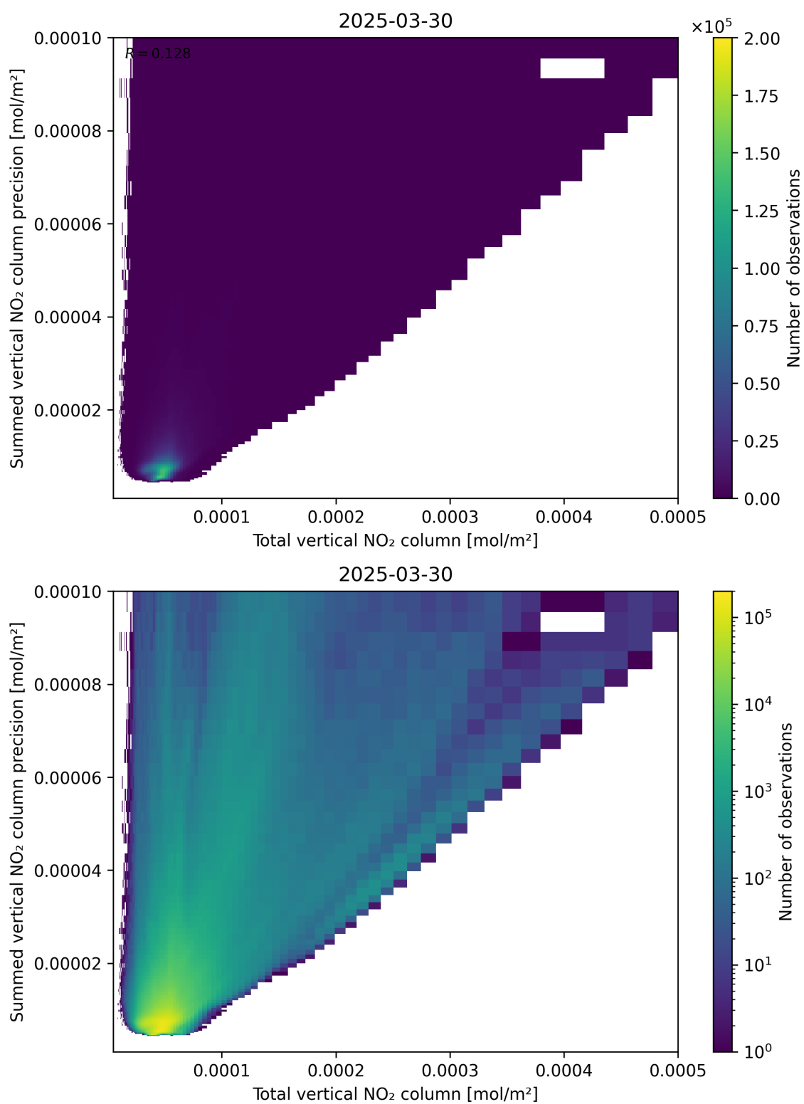
Figure 113: Scatter density plot of “Total vertical NO 2 column” against “Summed vertical NO 2 column precision” for 2025-03-30 to 2025-03-31.
