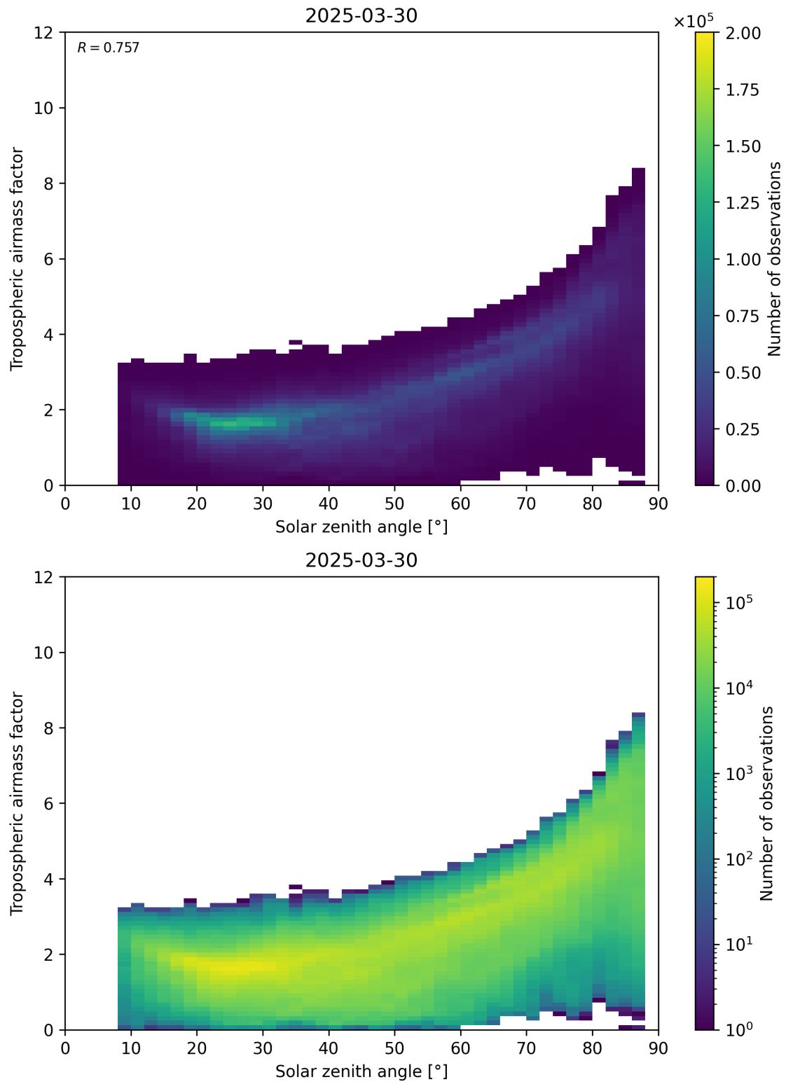
Figure 147: Scatter density plot of “Solar zenith angle” against “Tropospheric airmass factor” for 2025-03-30 to 2025-03-31.
