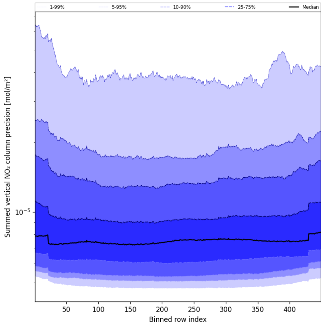
Figure 58: Along track statistics of “Summed vertical NO 2 column precision” for 2025-03-30 to 2025-03-31
