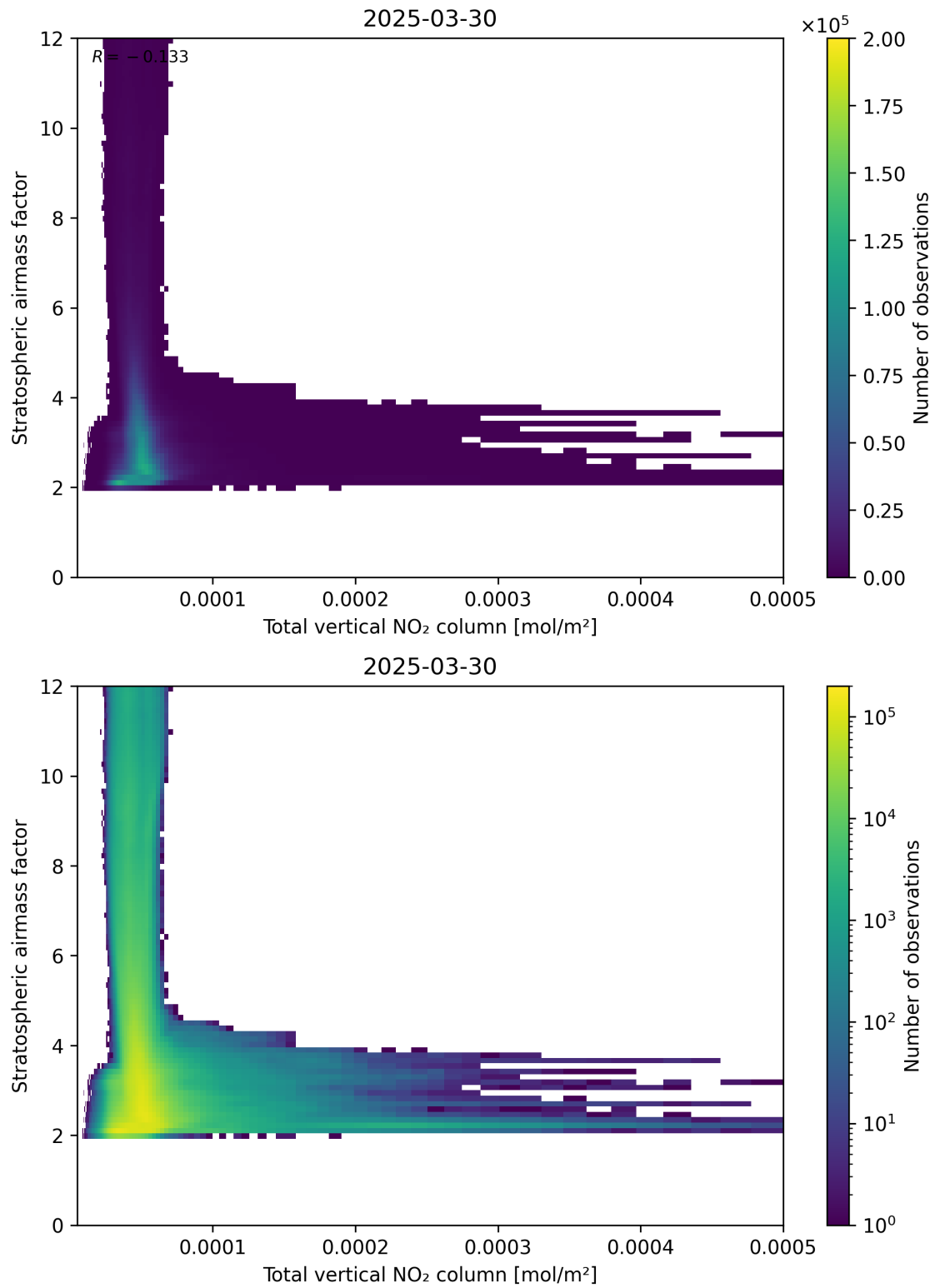
Figure 110: Scatter density plot of “Total vertical NO 2 column” against “Stratospheric airmass factor” for 2025-03-30 to 2025-03-31.
