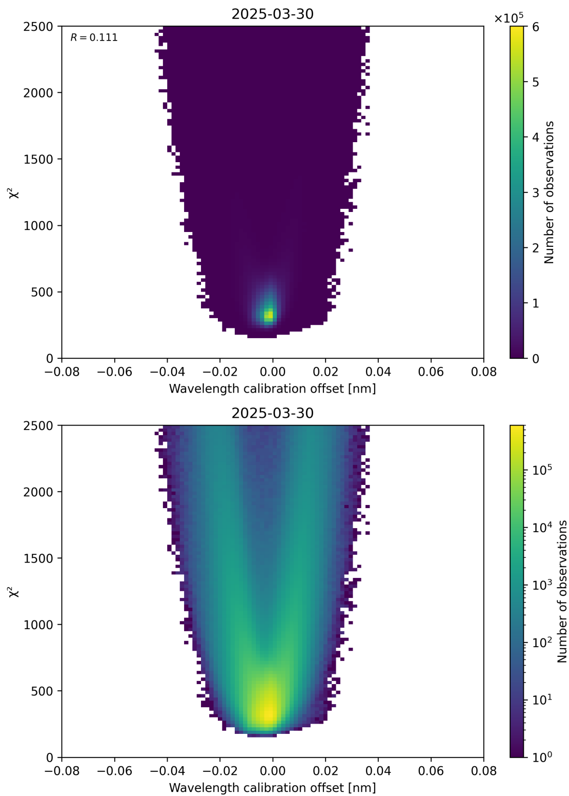
Figure 175: Scatter density plot of “Wavelength calibration offset” against “ \chi^2 ” for 2025-03-30 to 2025-03-31.
