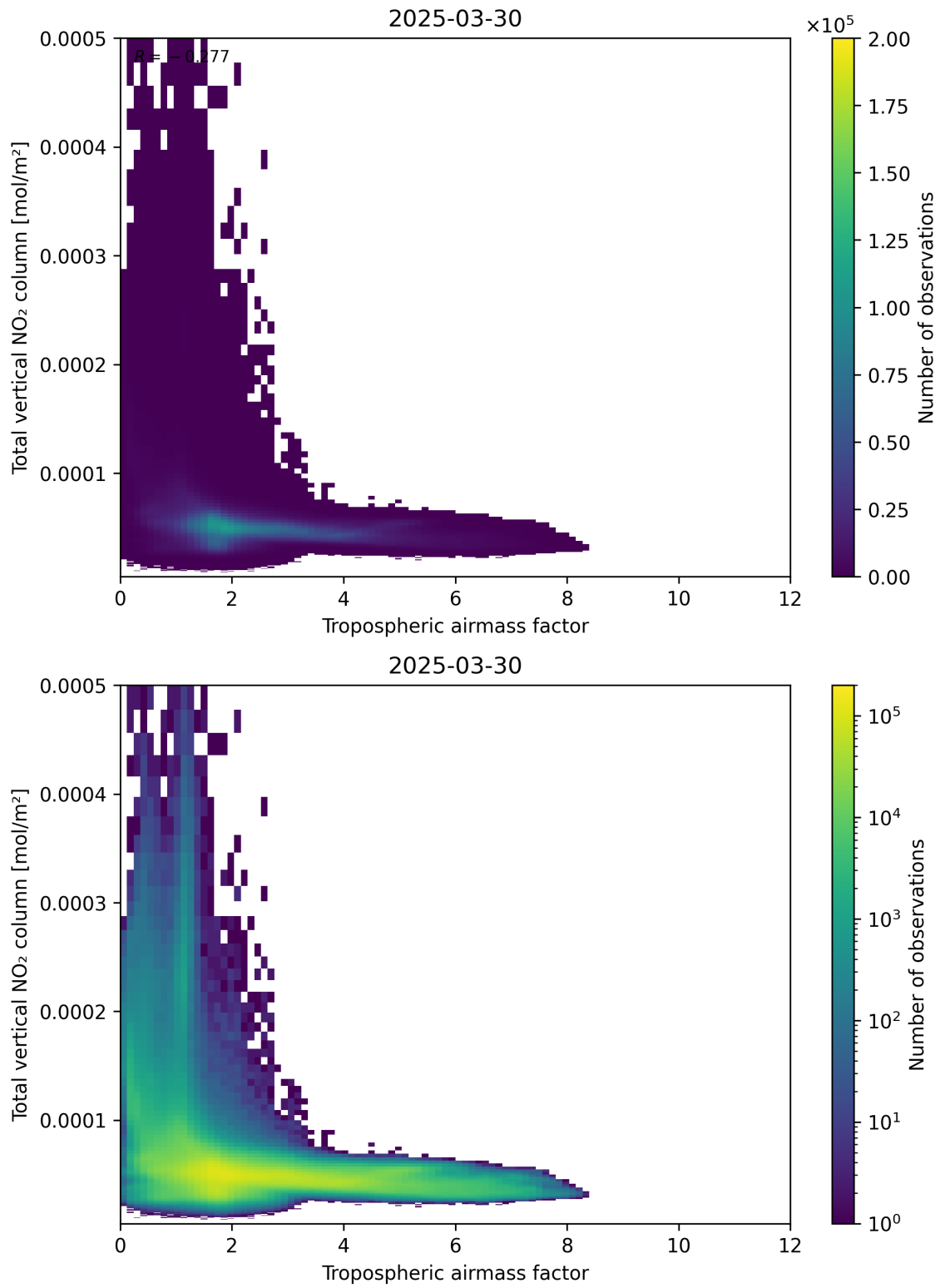
Figure 77: Scatter density plot of “Tropospheric airmass factor” against “Total vertical NO 2 column” for 2025-03-30 to 2025-03-31.
