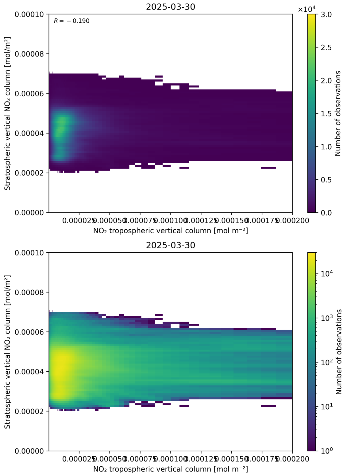
Figure 125: Scatter density plot of “NO 2 tropospheric vertical column” against “Stratospheric vertical NO 2 column” for 2025-03-30 to 2025-03-31.
