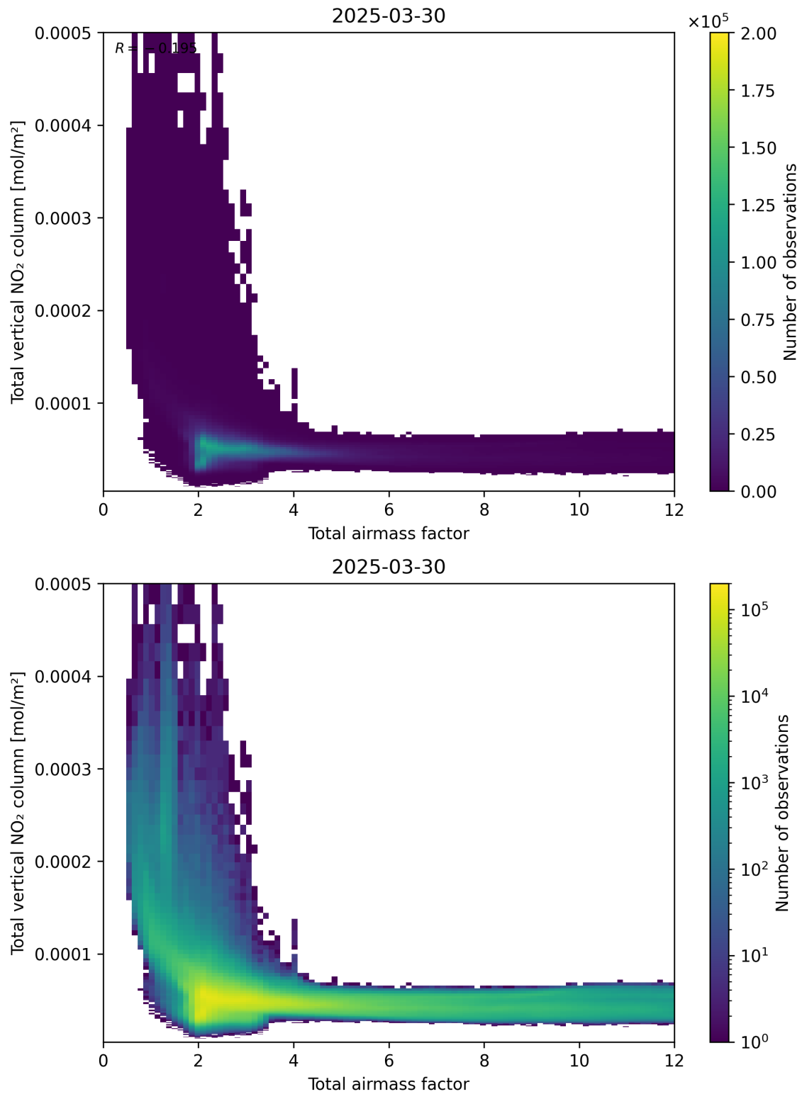
Figure 67: Scatter density plot of “Total airmass factor” against “Total vertical NO 2 column” for 2025-03-30 to 2025-03-31.
