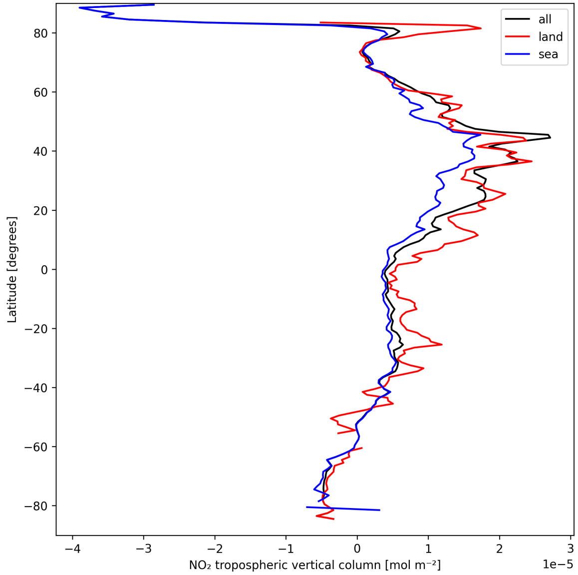
Figure 12: Zonal average of “NO 2 tropospheric vertical column” for 2025-03-30 to 2025-03-31.
