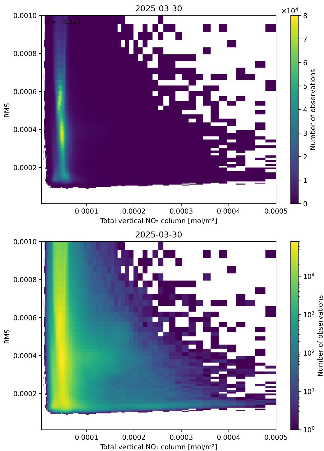
Figure 120: Scatter density plot of “Total vertical NO 2 column” against “RMS” for 2025-03-30 to 2025-03-31.
