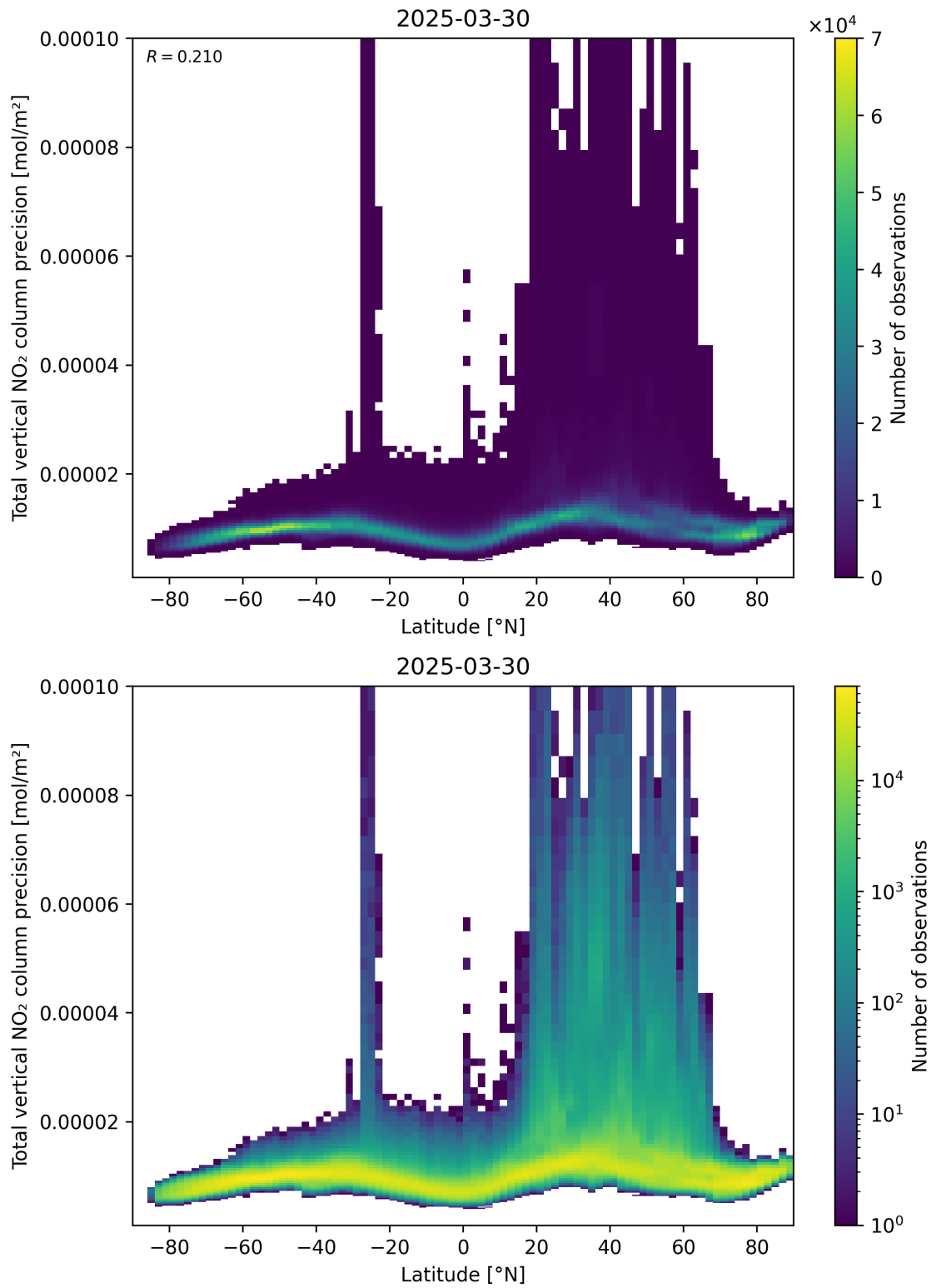
Figure 91: Scatter density plot of “Latitude” against “Total vertical NO 2 column precision” for 2025-03-30 to 2025-03-31.
