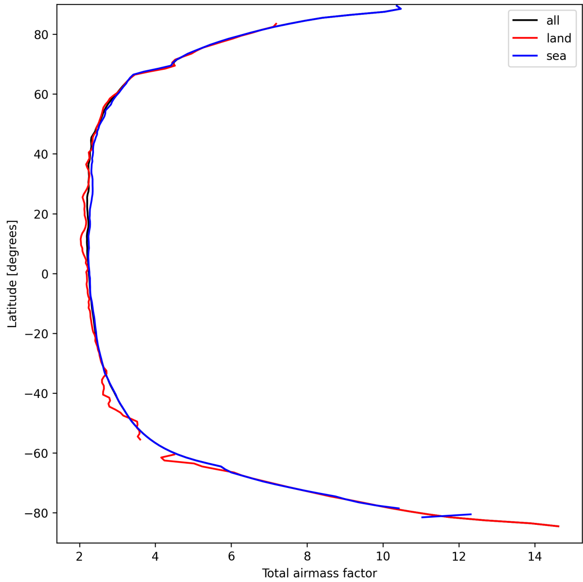
Figure 15: Zonal average of “Total airmass factor” for 2025-03-30 to 2025-03-31.
