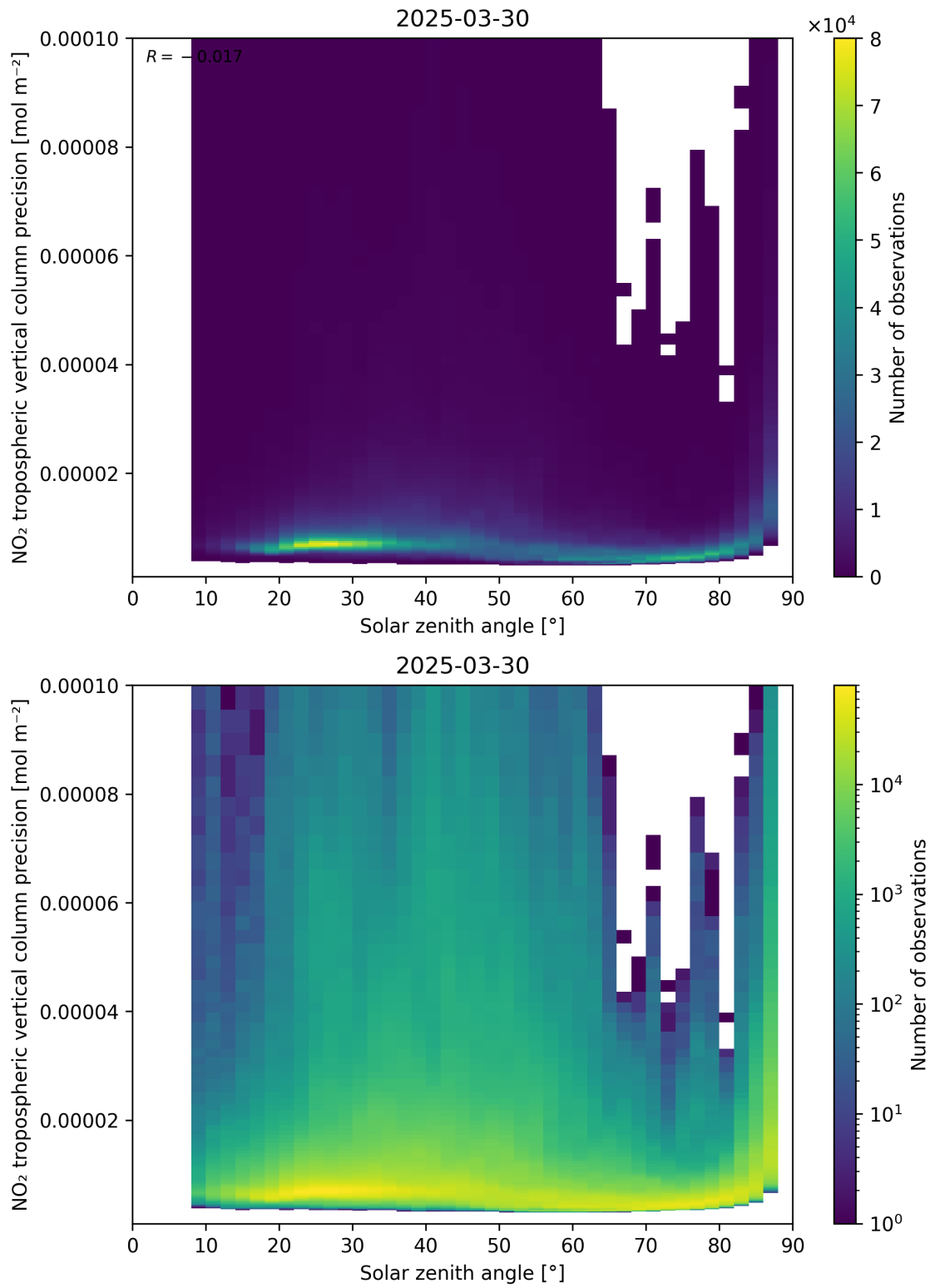
Figure 156: Scatter density plot of “Solar zenith angle” against “NO 2 tropospheric vertical column precision” for 2025-03-30 to 2025-03-31.
