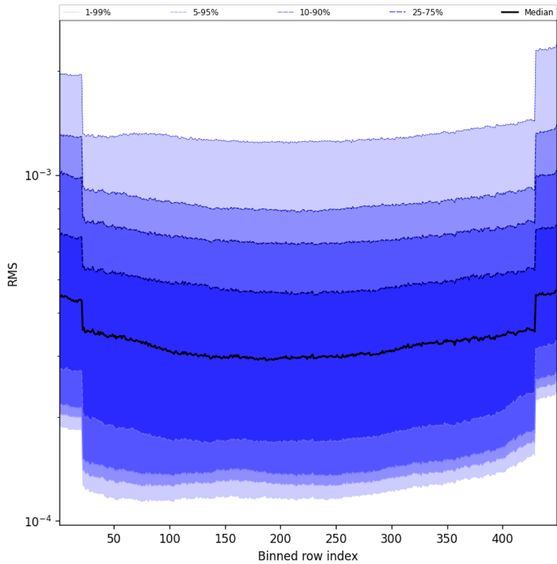
Figure 60: Along track statistics of “RMS” for 2025-03-30 to 2025-03-31
