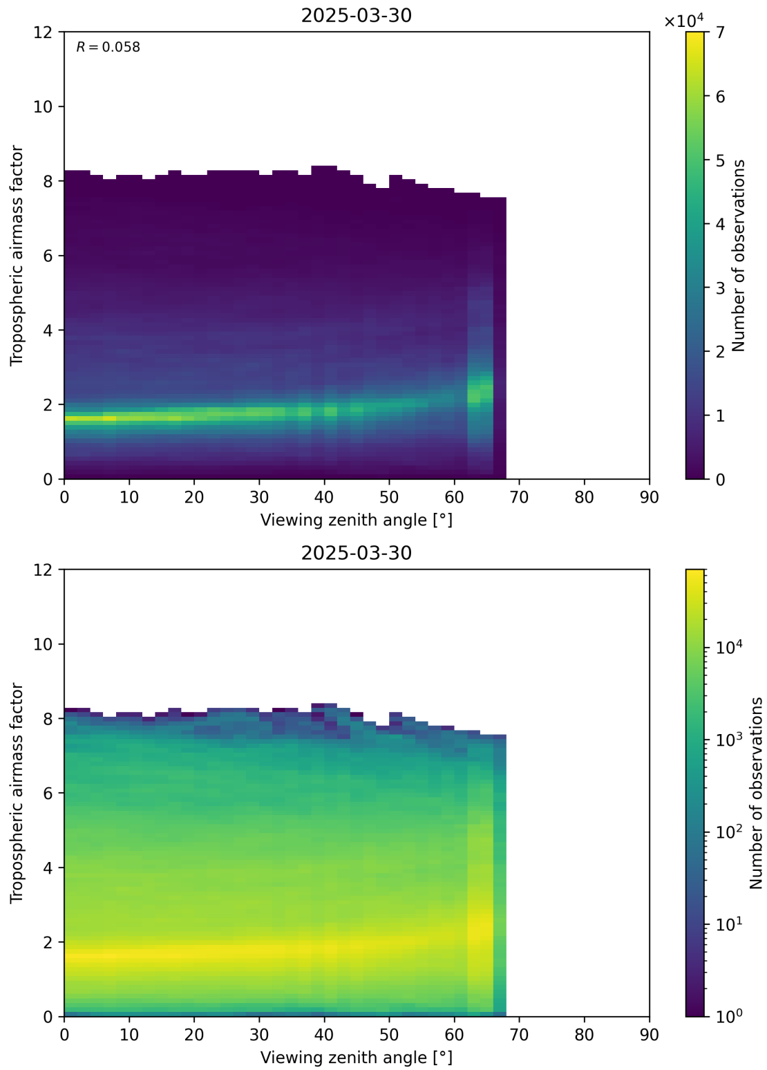
Figure 161: Scatter density plot of “Viewing zenith angle” against “Tropospheric airmass factor” for 2025-03-30 to 2025-03-31.
