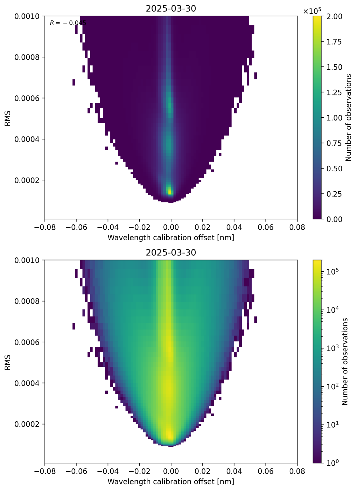
Figure 181: Scatter density plot of “Wavelength calibration offset” against “RMS” for 2025-03-30 to 2025-03-31.
