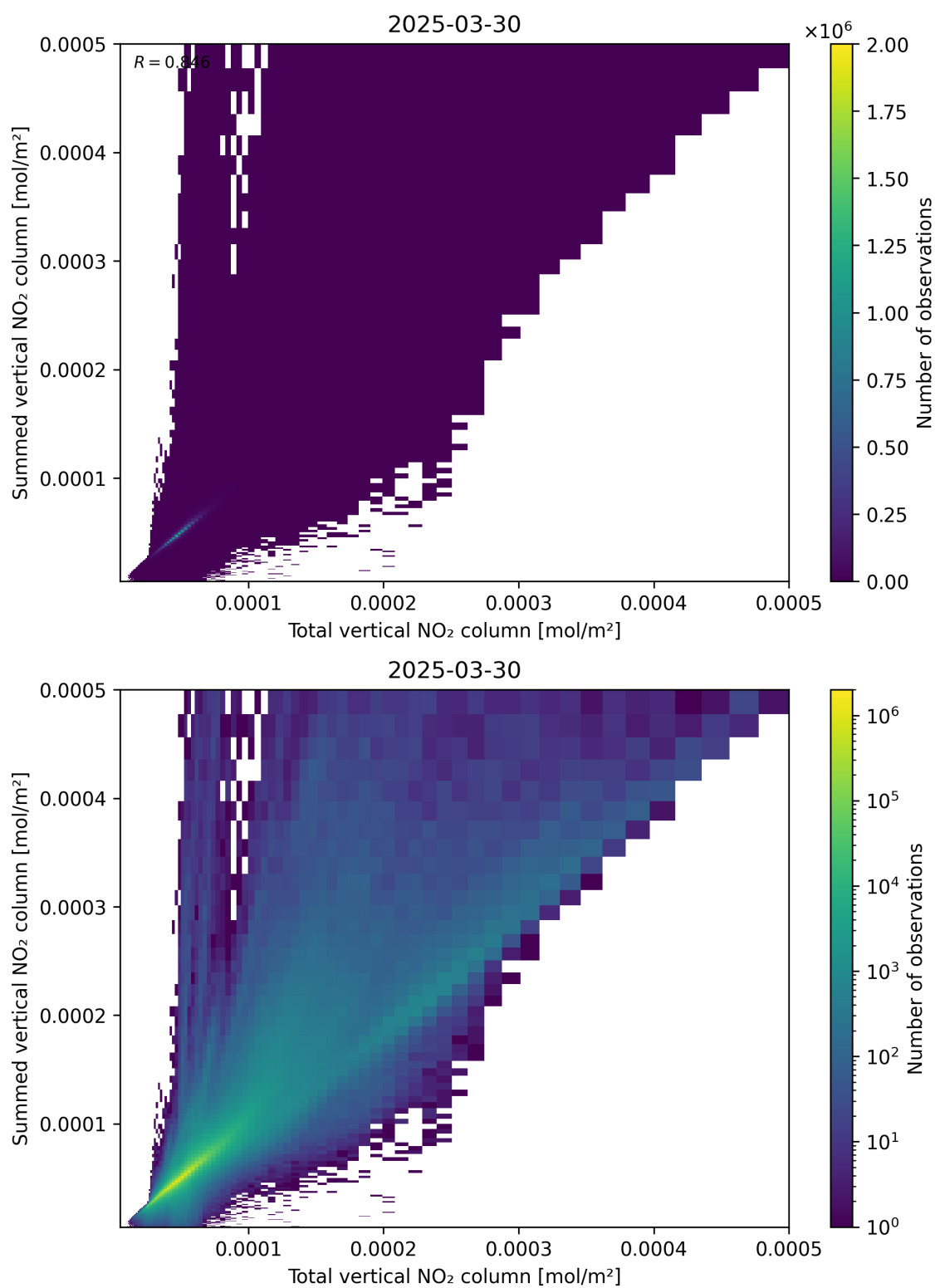
Figure 112: Scatter density plot of “Total vertical NO 2 column” against “Summed vertical NO 2 column” for 2025-03-30 to 2025-03-31.
