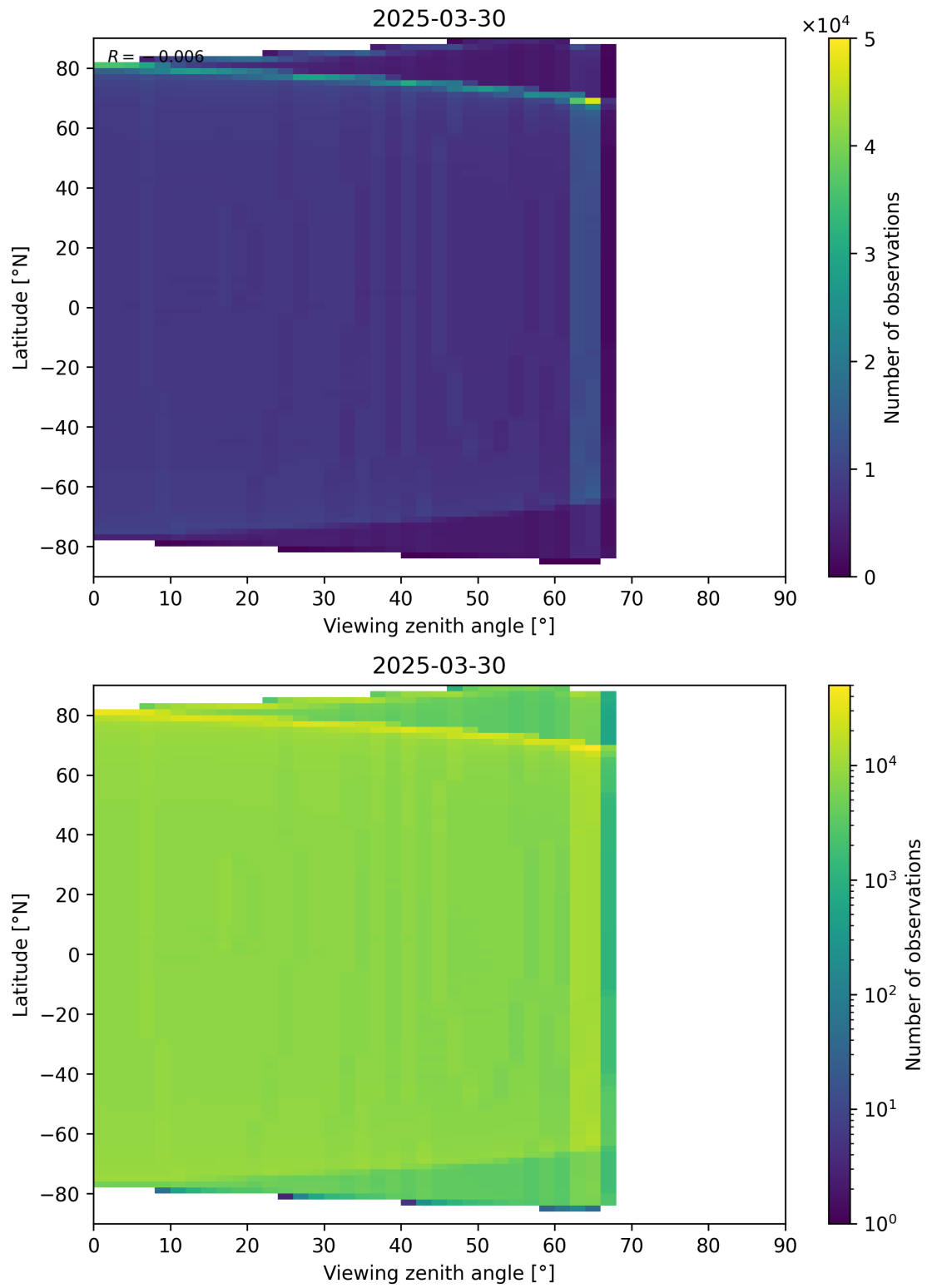
Figure 163: Scatter density plot of “Viewing zenith angle” against “Latitude” for 2025-03-30 to 2025-03-31.
