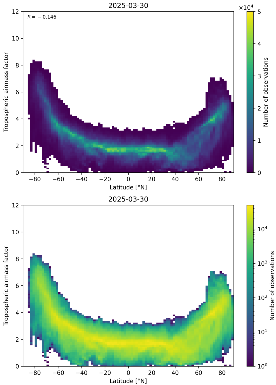
Figure 85: Scatter density plot of “Latitude” against “Tropospheric airmass factor” for 2025-03-30 to 2025-03-31.
