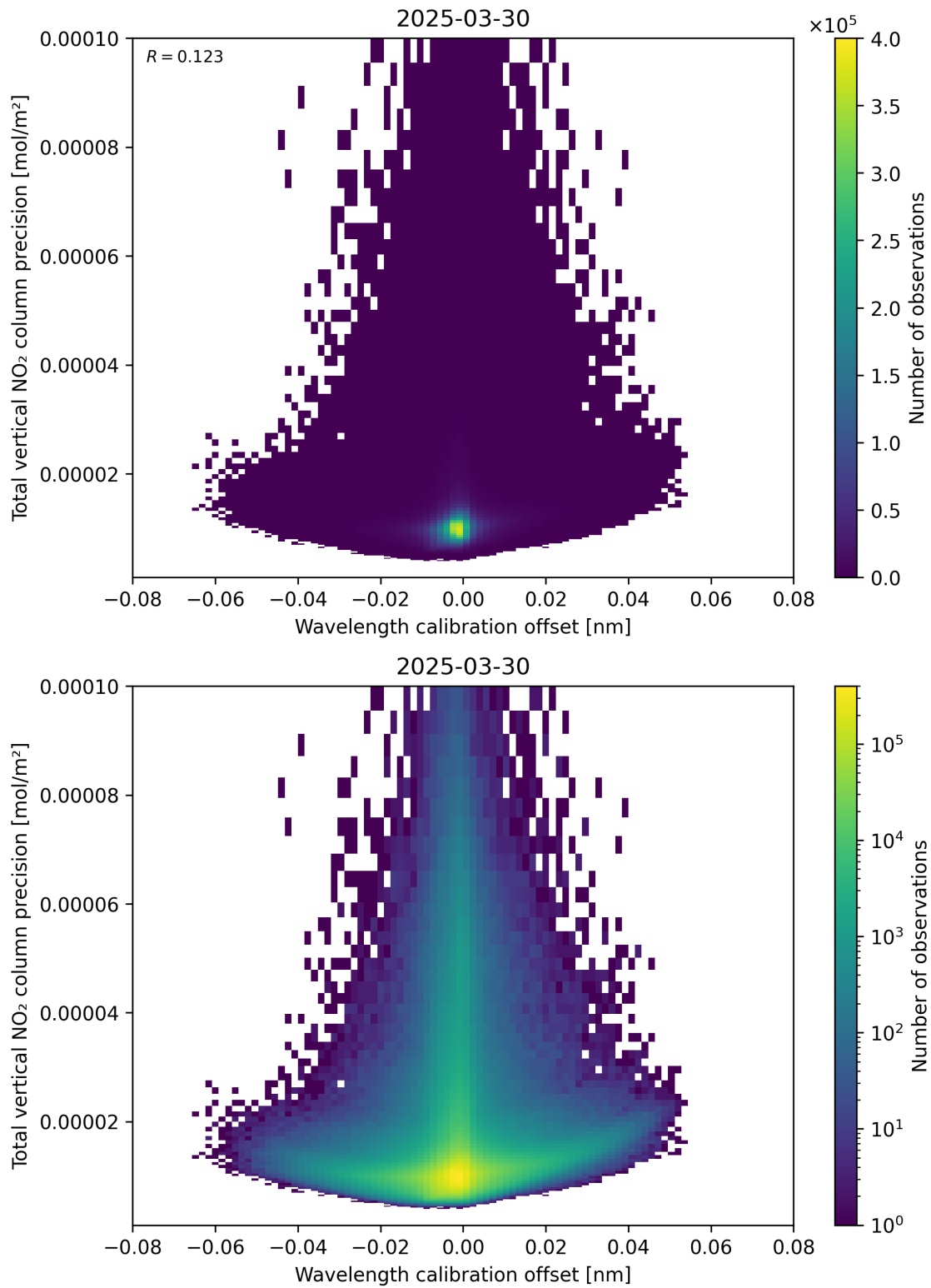
Figure 180: Scatter density plot of “Wavelength calibration offset” against “Total vertical NO 2 column precision” for 2025-03-30 to 2025-03-31.
