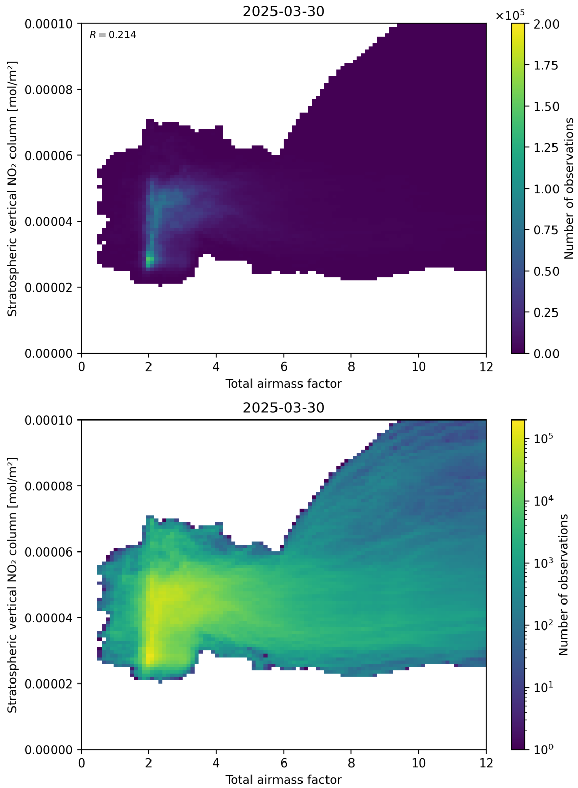
Figure 64: Scatter density plot of “Total airmass factor” against “Stratospheric vertical \text{NO}_2 column” for 2025-03-30 to 2025-03-31.
