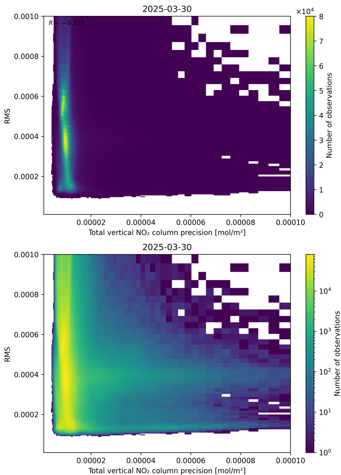
Figure 119: Scatter density plot of “Total vertical NO 2 column precision” against “RMS” for 2025-03-30 to 2025-03-31.
