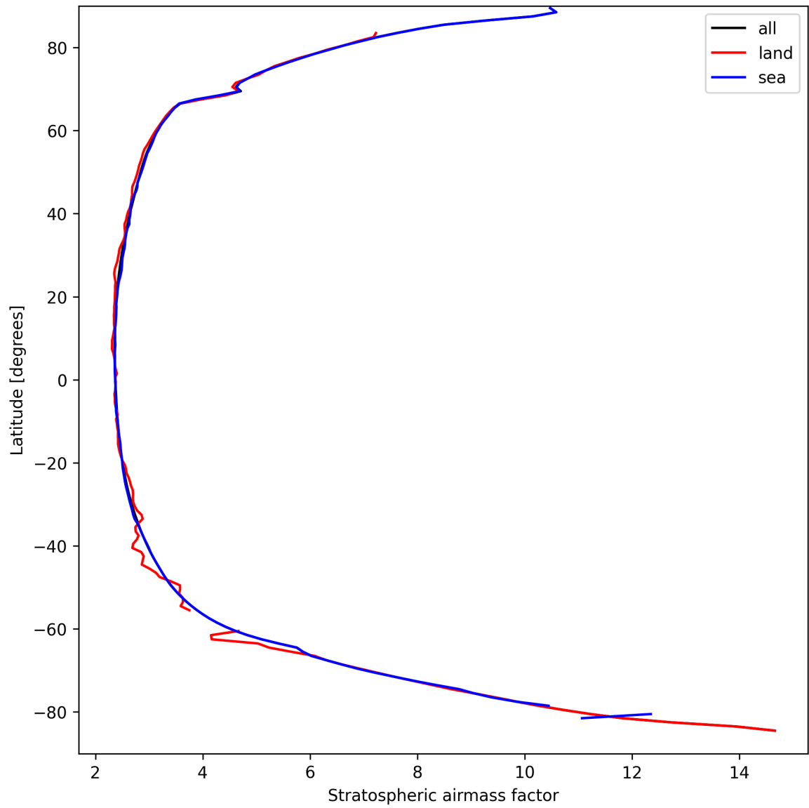
Figure 27: Zonal average of “Stratospheric airmass factor” for 2025-03-30 to 2025-03-31.
