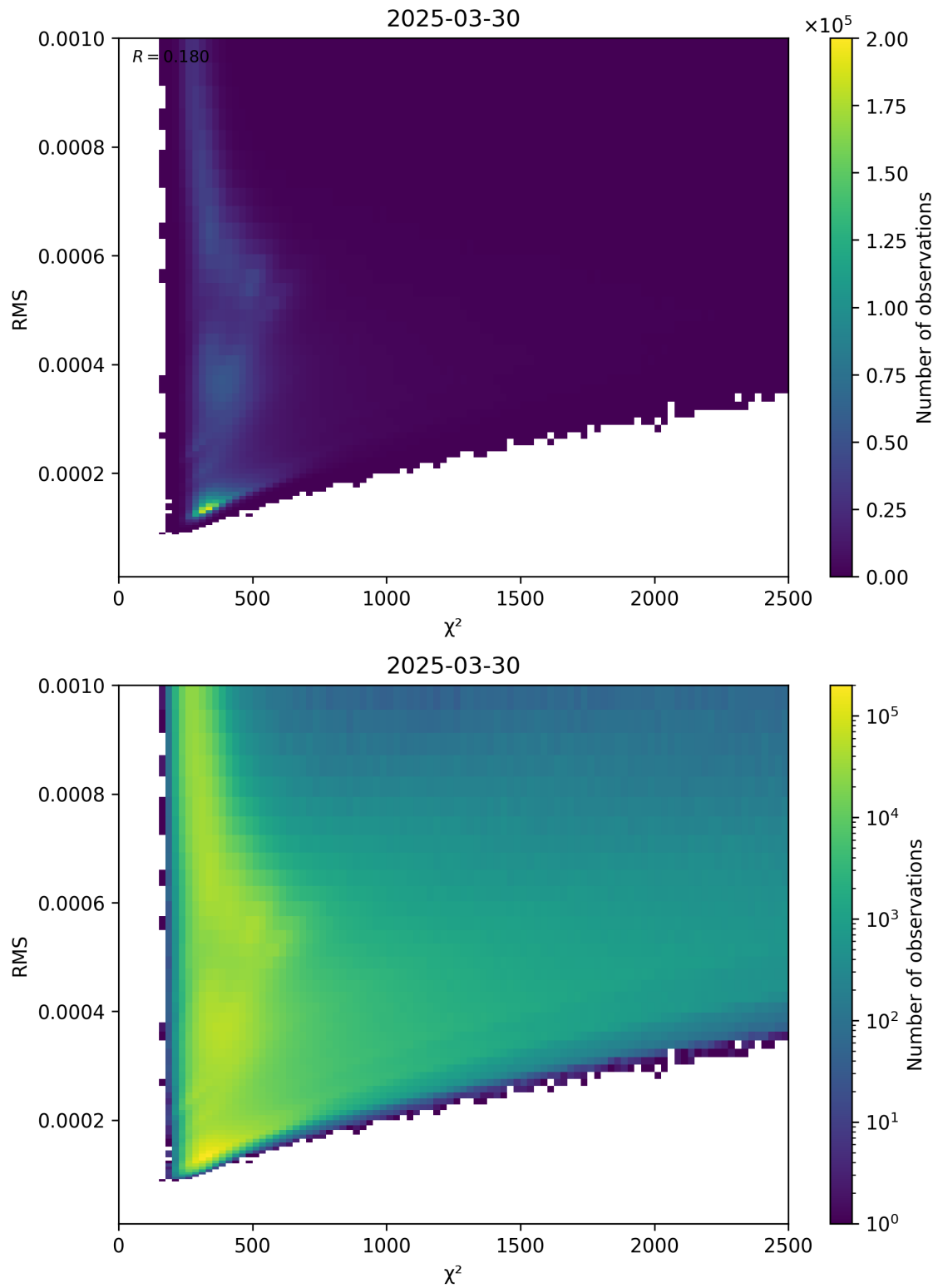
Figure 82: Scatter density plot of “ \chi^2 ” against “RMS” for 2025-03-30 to 2025-03-31.
