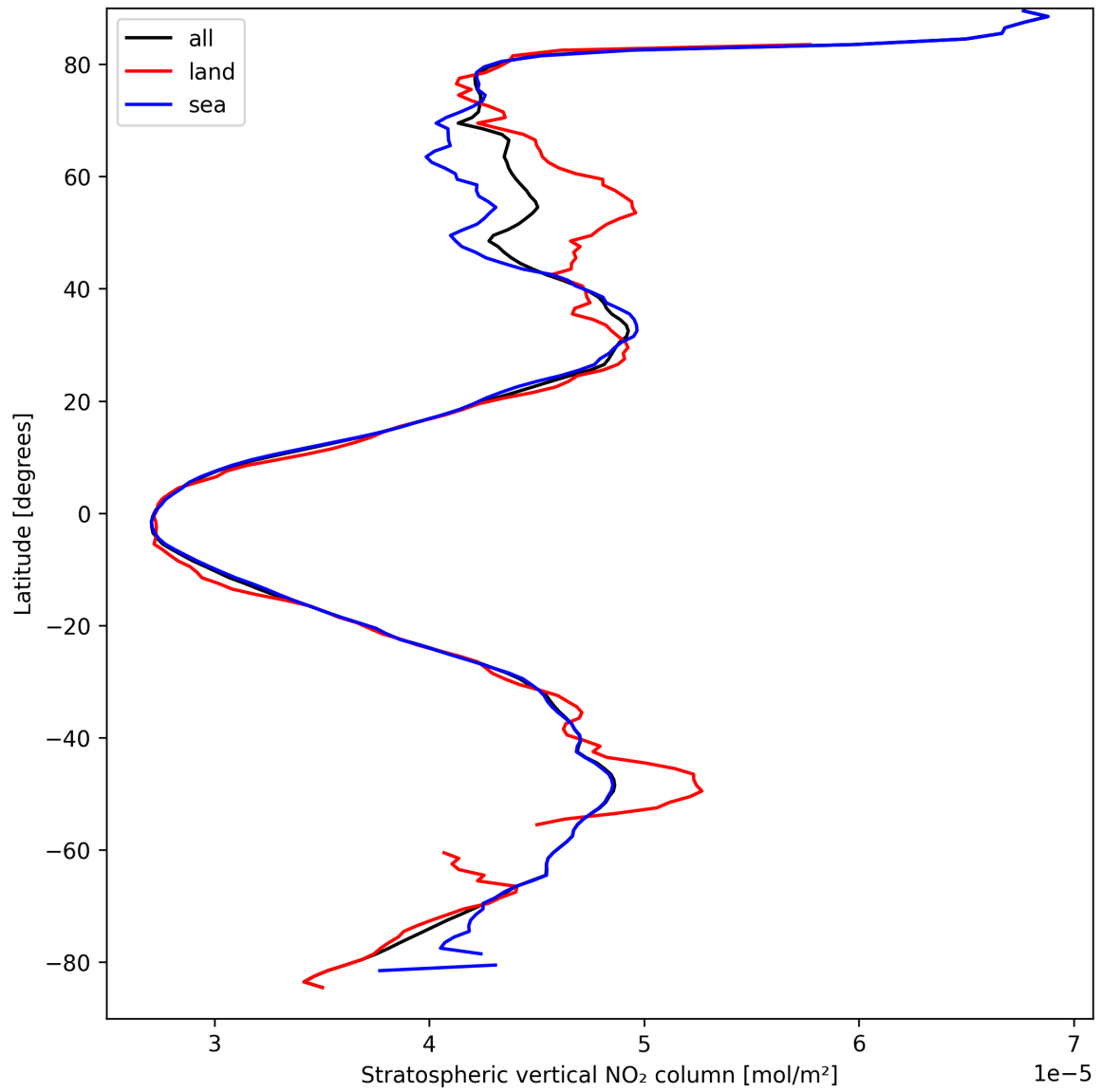
Figure 19: Zonal average of “Stratospheric vertical NO 2 column” for 2025-03-30 to 2025-03-31.
