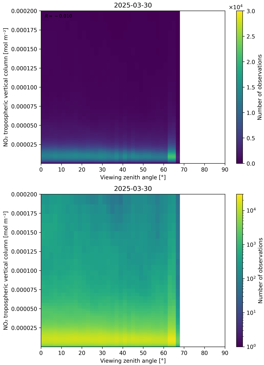
Figure 169: Scatter density plot of “Viewing zenith angle” against “NO 2 tropospheric vertical column” for 2025-03-30 to 2025-03-31.
