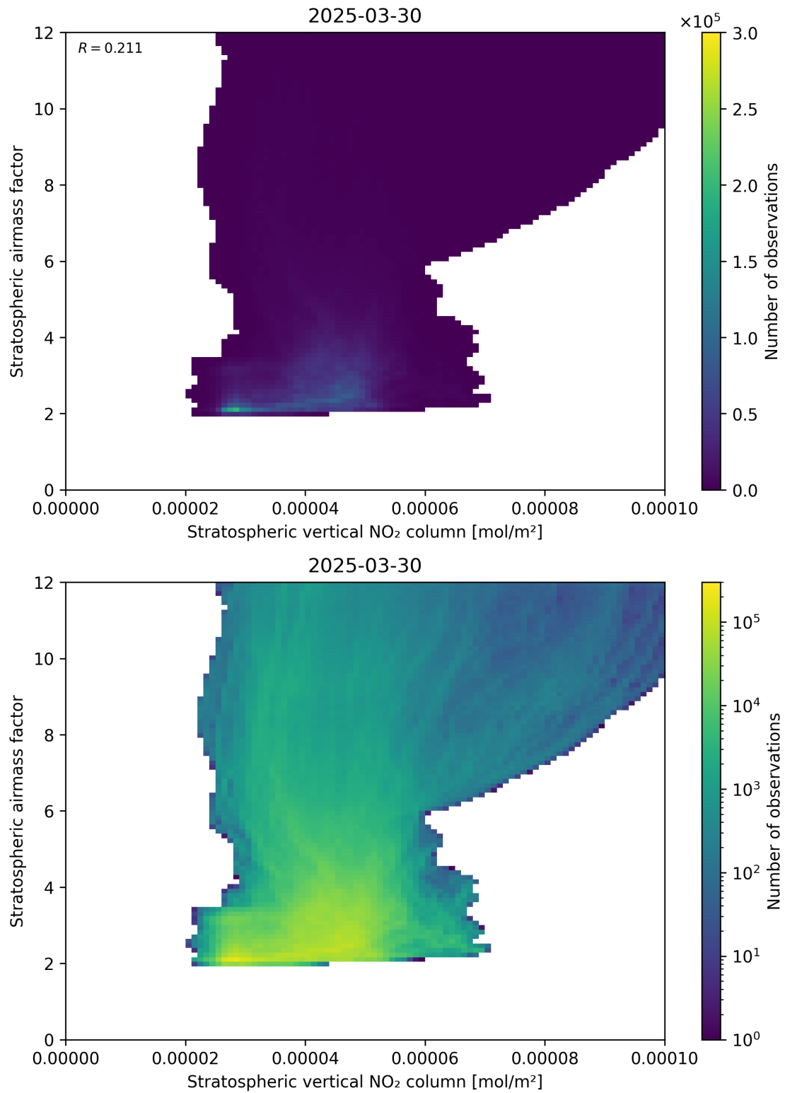
Figure 96: Scatter density plot of “Stratospheric vertical NO 2 column” against “Stratospheric airmass factor” for 2025-03-30 to 2025-03-31.
