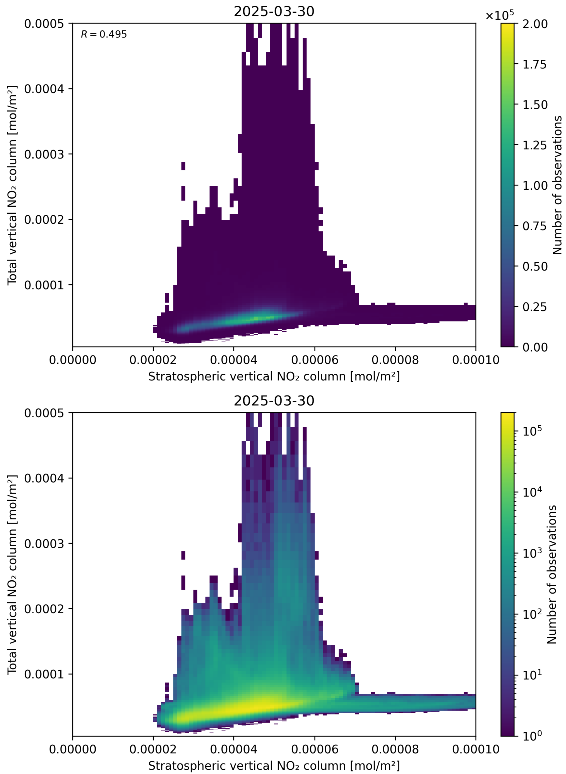
Figure 100: Scatter density plot of “Stratospheric vertical NO 2 column” against “Total vertical NO 2 column” for 2025-03-30 to 2025-03-31.
