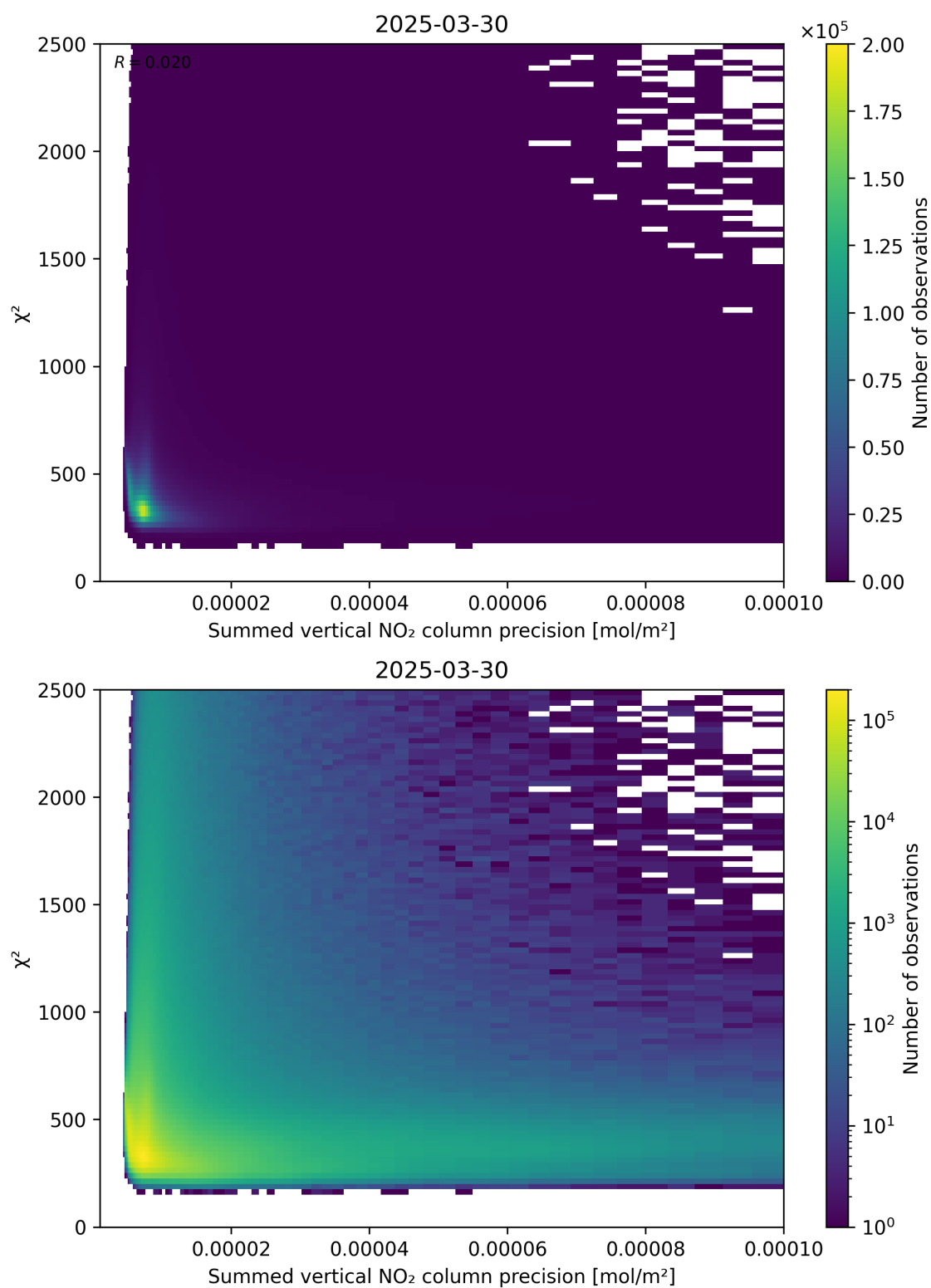
Figure 107: Scatter density plot of “Summed vertical NO 2 column precision” against “ \chi^2 ” for 2025-03-30 to 2025-03-31.
