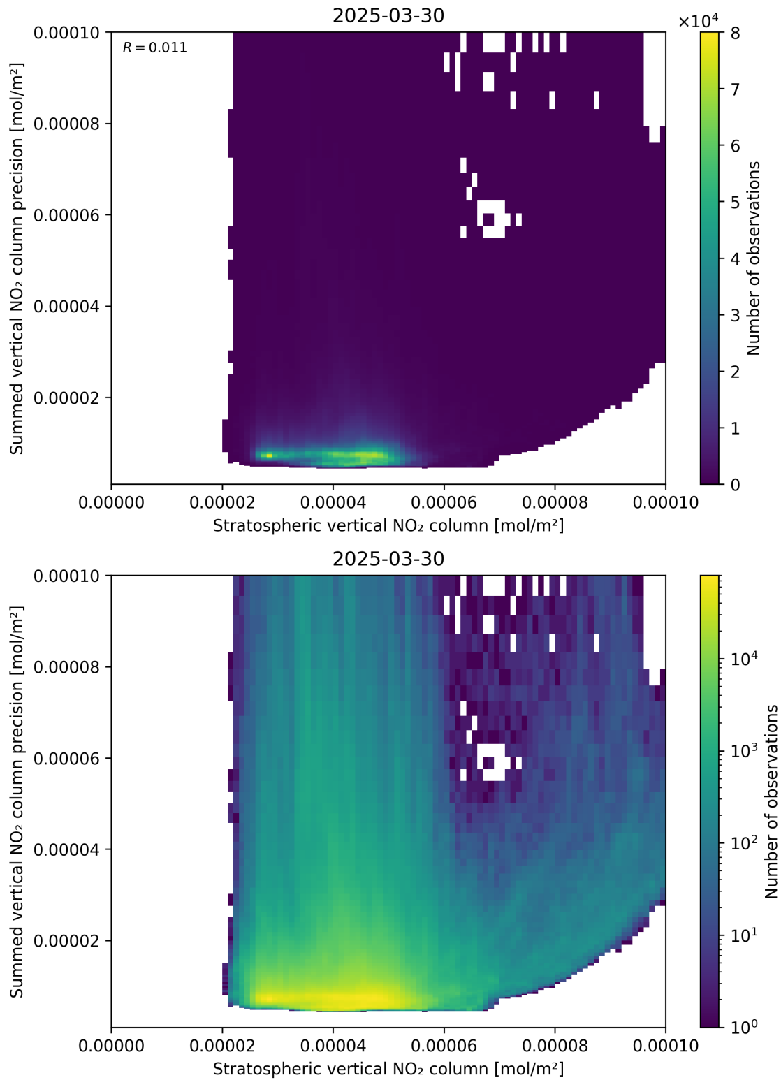
Figure 99: Scatter density plot of “Stratospheric vertical NO 2 column” against “Summed vertical NO 2 column precision” for 2025-03-30 to 2025-03-31.
