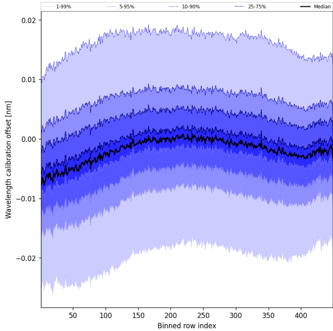
Figure 52: Along track statistics of “Wavelength calibration offset” for 2025-03-30 to 2025-03-31
