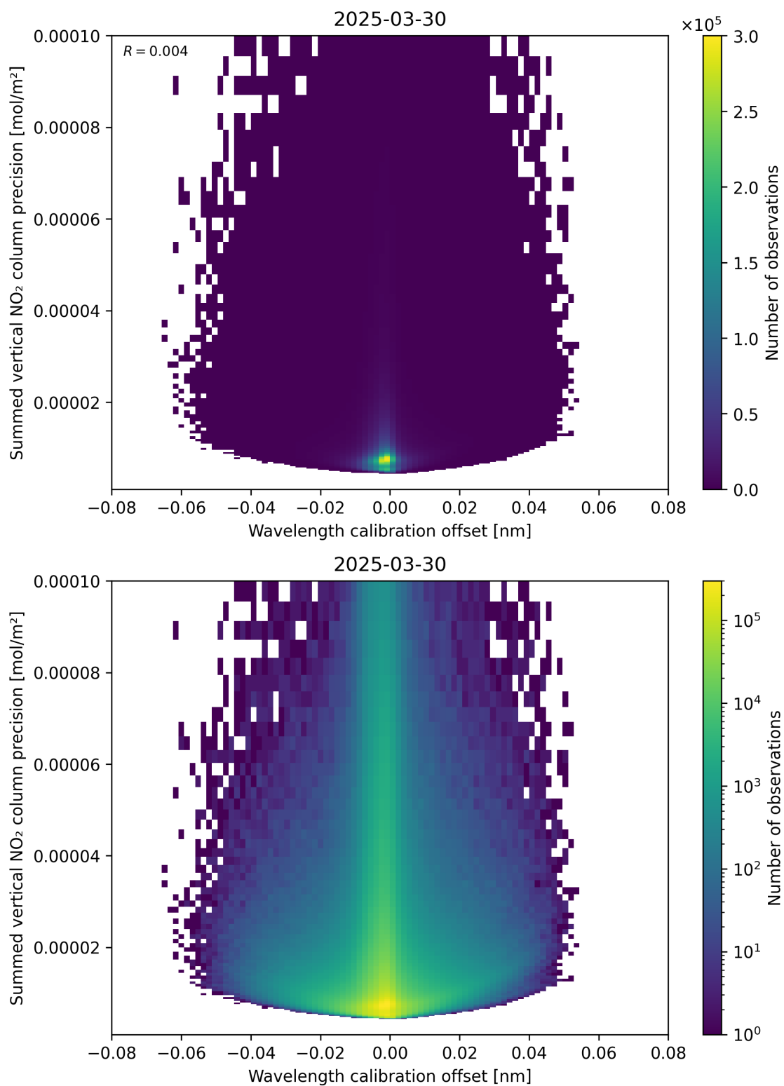
Figure 178: Scatter density plot of “Wavelength calibration offset” against “Summed vertical NO 2 column precision” for 2025-03-30 to 2025-03-31.
