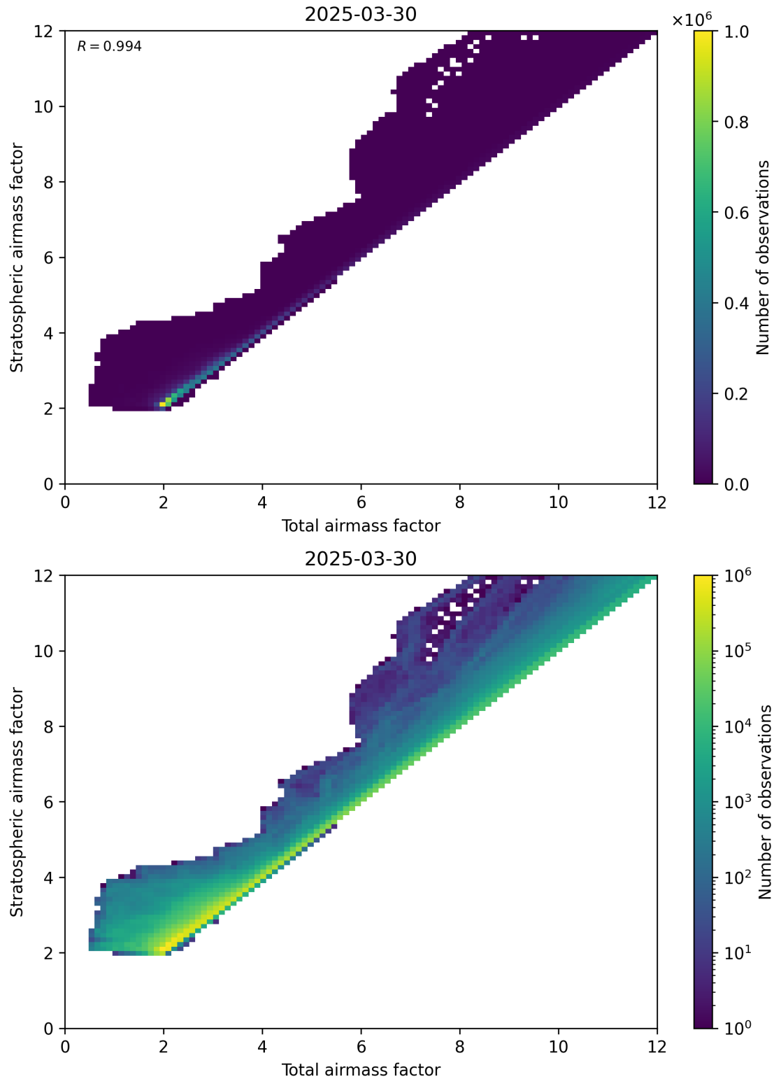
Figure 62: Scatter density plot of “Total airmass factor” against “Stratospheric airmass factor” for 2025-03-30 to 2025-03-31.
