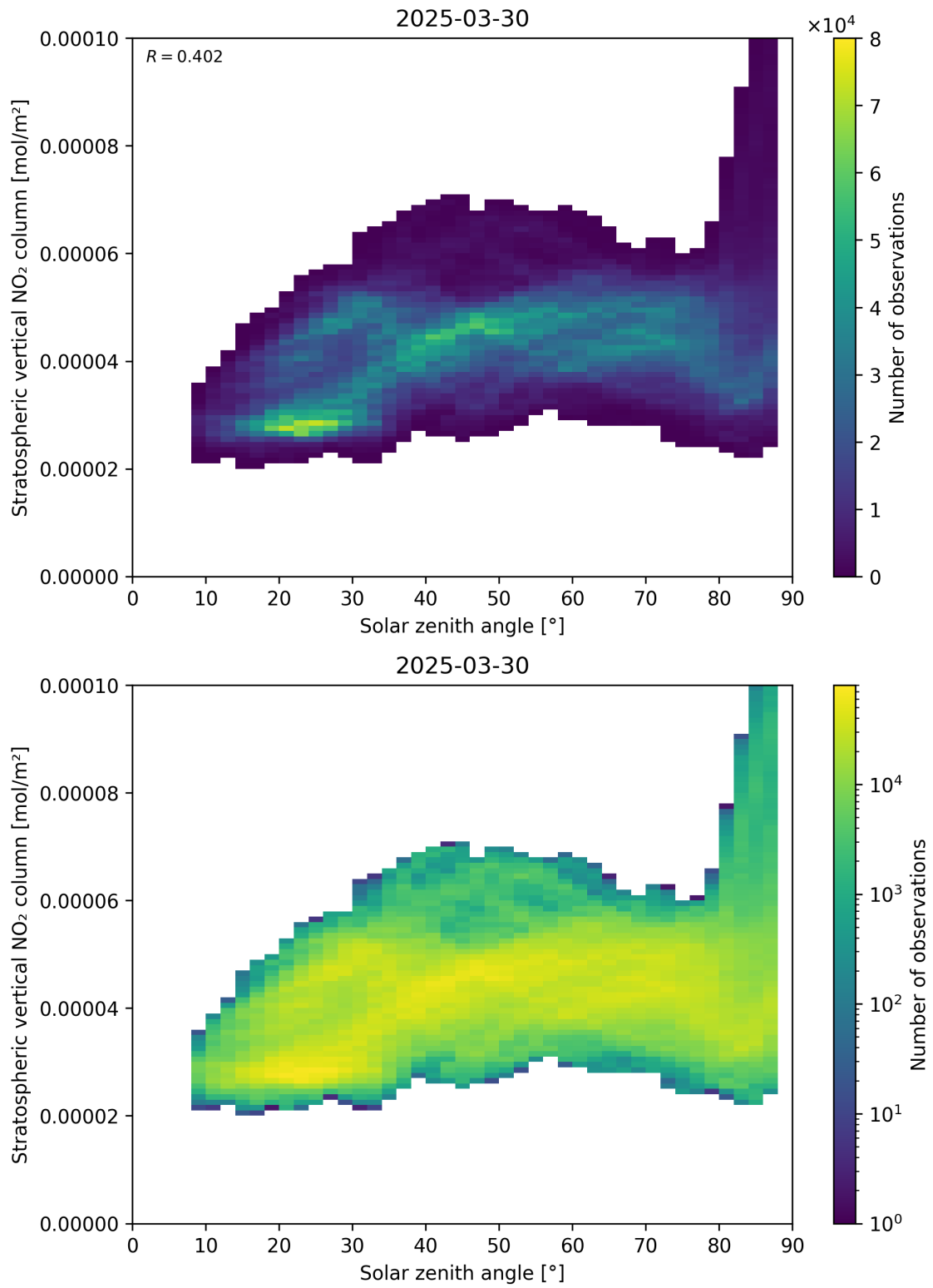
Figure 150: Scatter density plot of “Solar zenith angle” against “Stratospheric vertical NO 2 column” for 2025-03-30 to 2025-03-31.
