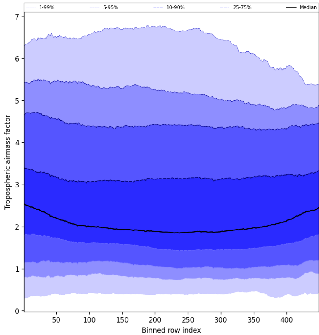
Figure 48: Along track statistics of “Tropospheric air mass factor” for 2025-03-30 to 2025-03-31
