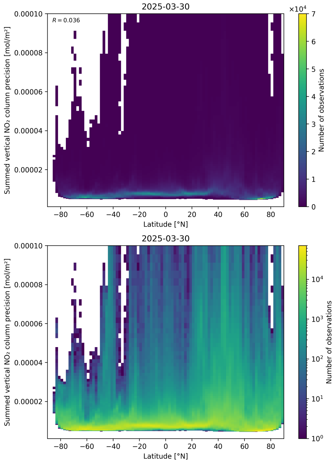
Figure 89: Scatter density plot of “Latitude” against “Summed vertical NO 2 column precision” for 2025-03-30 to 2025-03-31.
