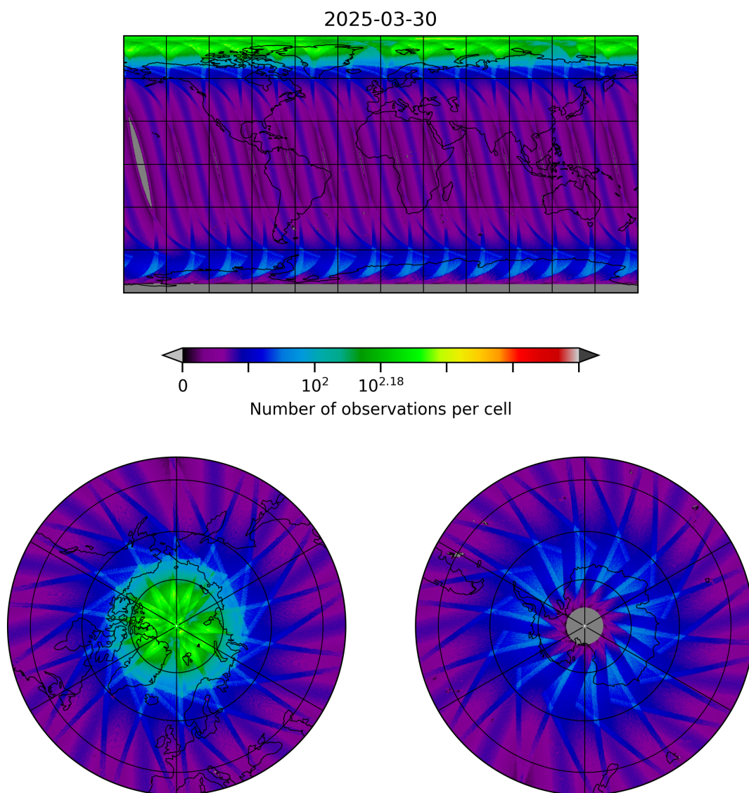
Figure 10: Map of the number of observations for 2025-03-30 to 2025-03-31
