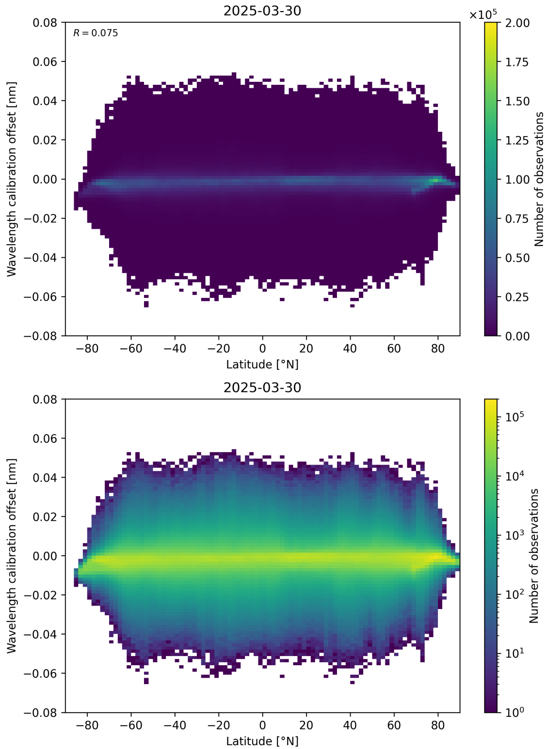
Figure 95: Scatter density plot of “Latitude” against “Wavelength calibration offset” for 2025-03-30 to 2025-03-31.
