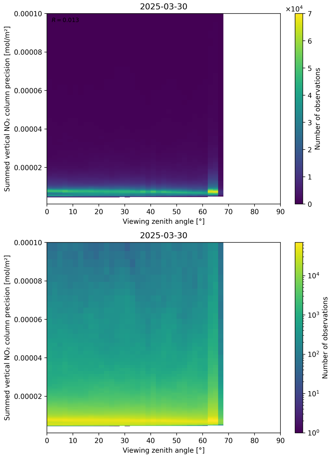
Figure 166: Scatter density plot of “Viewing zenith angle” against “Summed vertical NO 2 column precision” for 2025-03-30 to 2025-03-31.
