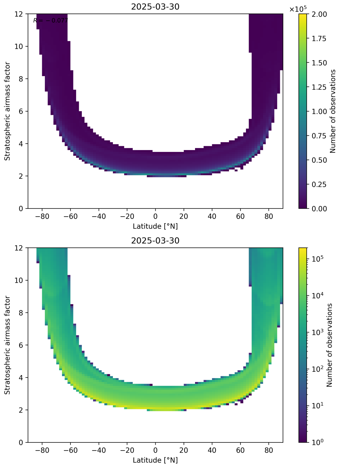
Figure 83: Scatter density plot of “Latitude” against “Stratospheric airmass factor” for 2025-03-30 to 2025-03-31.
