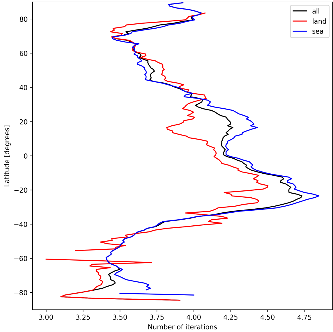
Figure 17: Zonal average of “Number of iterations” for 2025-03-30 to 2025-03-31.
