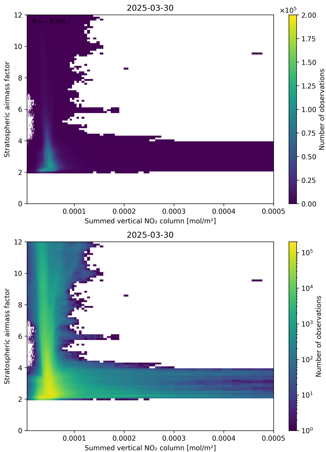
Figure 103: Scatter density plot of “Summed vertical NO 2 column” against “Stratospheric air mass factor” for 2025-03-30 to 2025-03-31.
