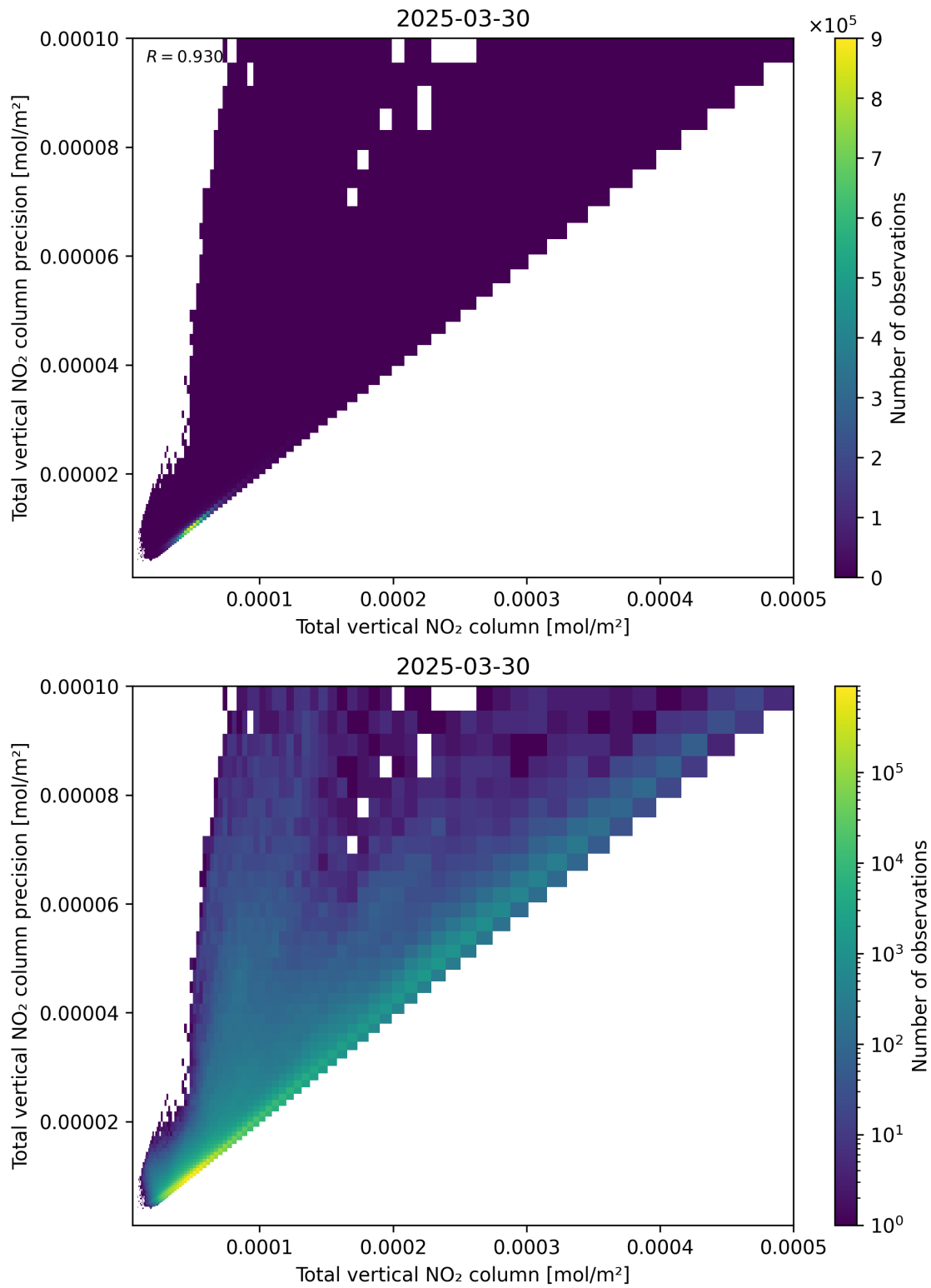
Figure 114: Scatter density plot of “Total vertical NO 2 column” against “Total vertical NO 2 column precision” for 2025-03-30 to 2025-03-31.
