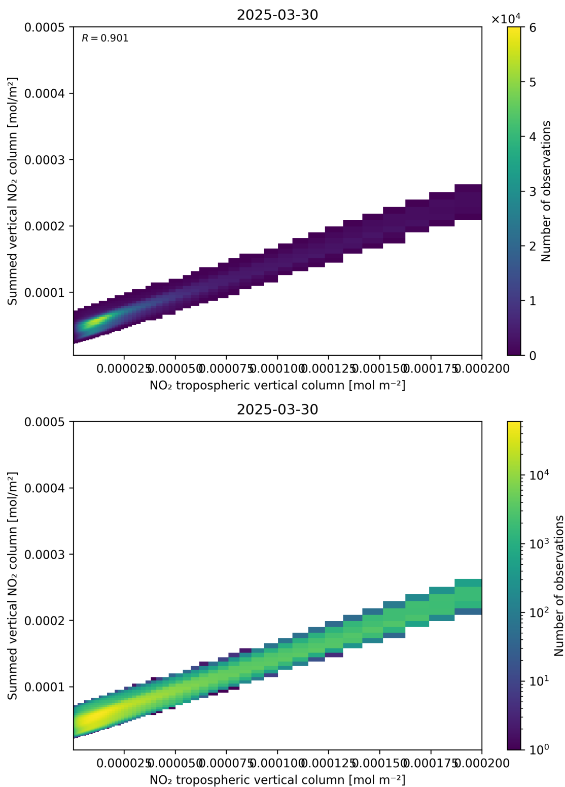
Figure 126: Scatter density plot of “NO 2 tropospheric vertical column” against “Summed vertical NO 2 column” for 2025-03-30 to 2025-03-31.
