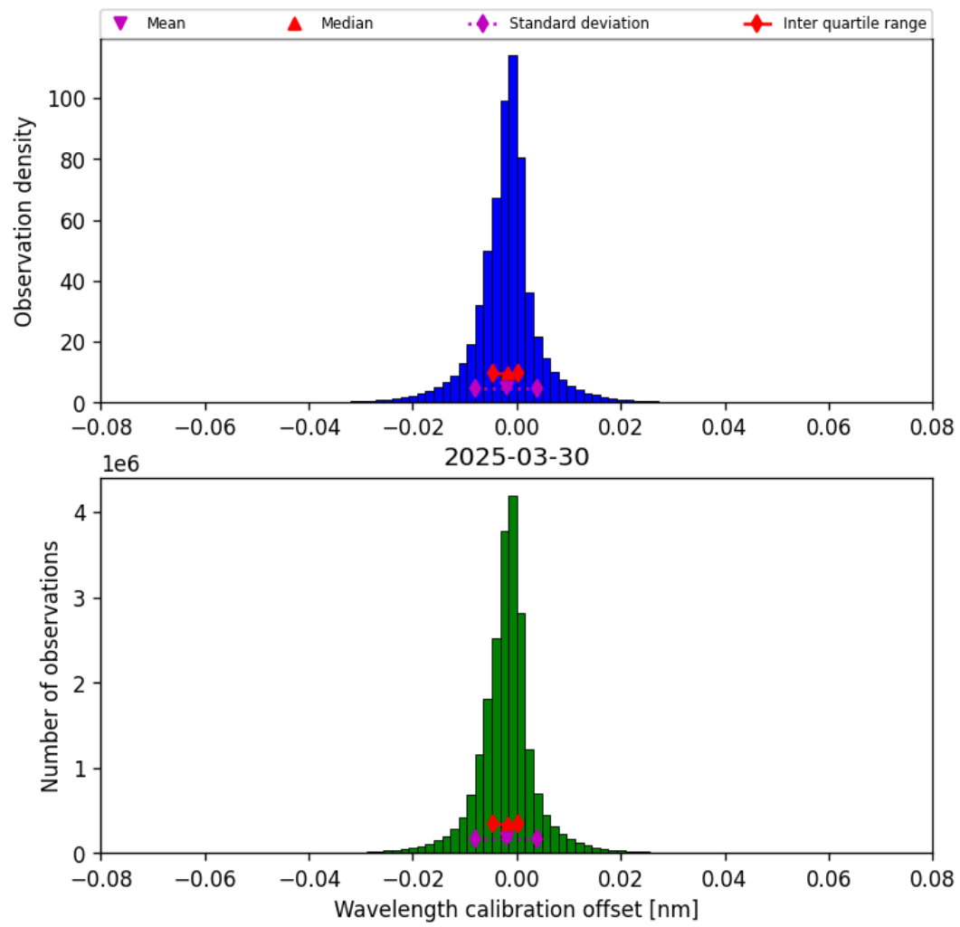
Figure 35: Histogram of “Wavelength calibration offset” for 2025-03-30 to 2025-03-31
