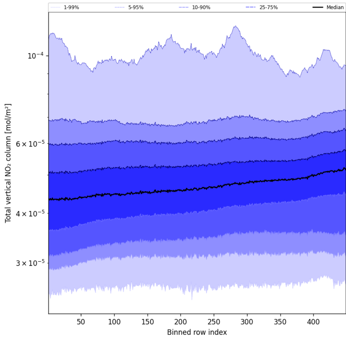
Figure 55: Along track statistics of “Total vertical NO 2 column” for 2025-03-30 to 2025-03-31
