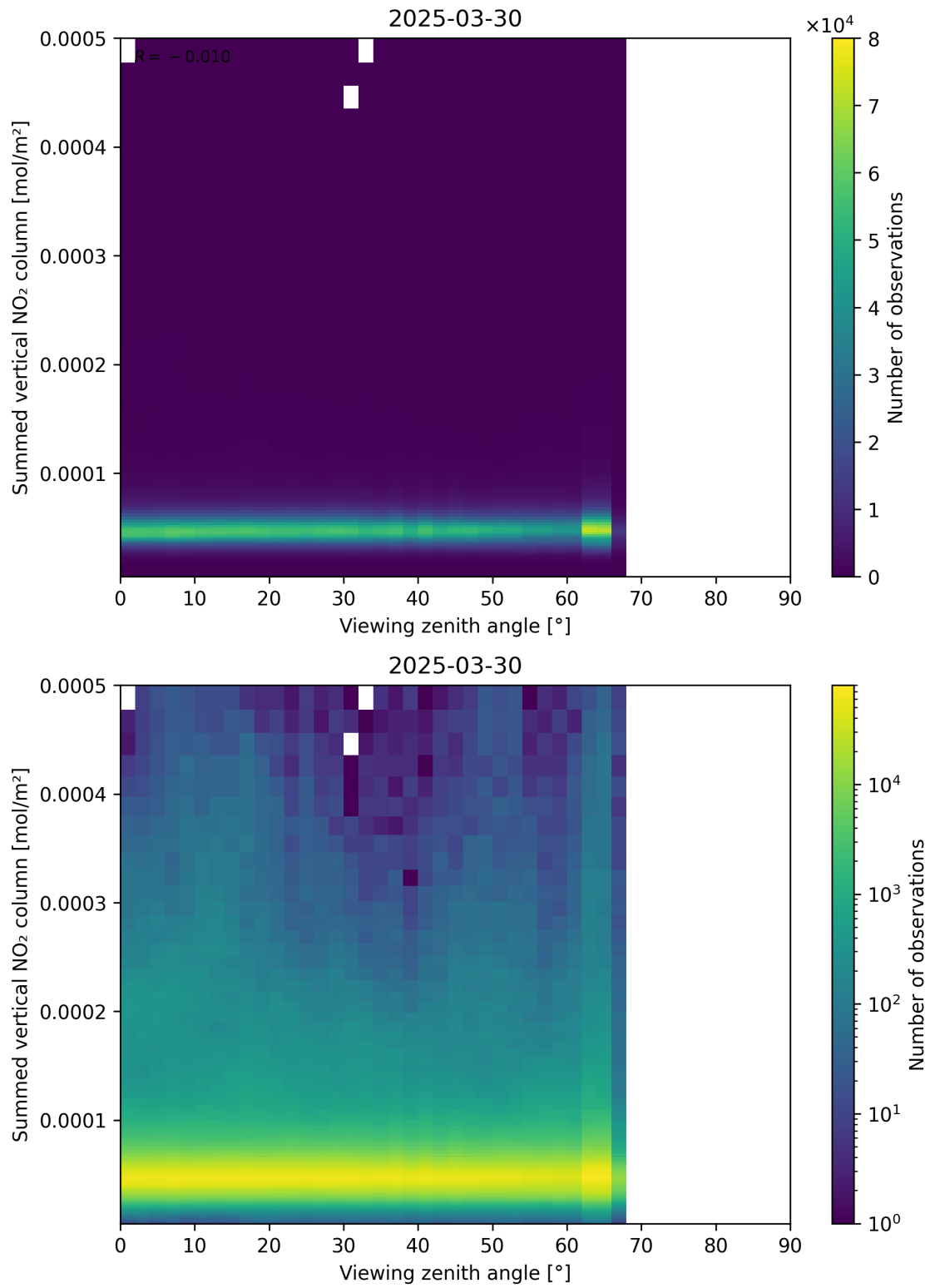
Figure 165: Scatter density plot of “Viewing zenith angle” against “Summed vertical NO 2 column” for 2025-03-30 to 2025-03-31.
