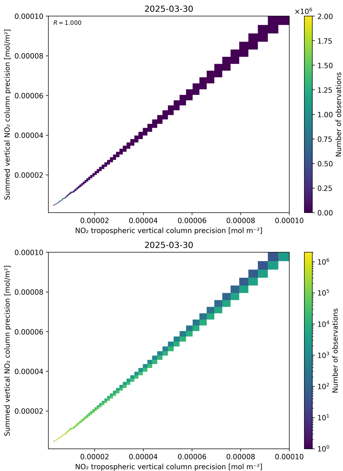
Figure 137: Scatter density plot of “NO 2 tropospheric vertical column precision” against “Summed vertical NO 2 column precision” for 2025-03-30 to 2025-03-31.
