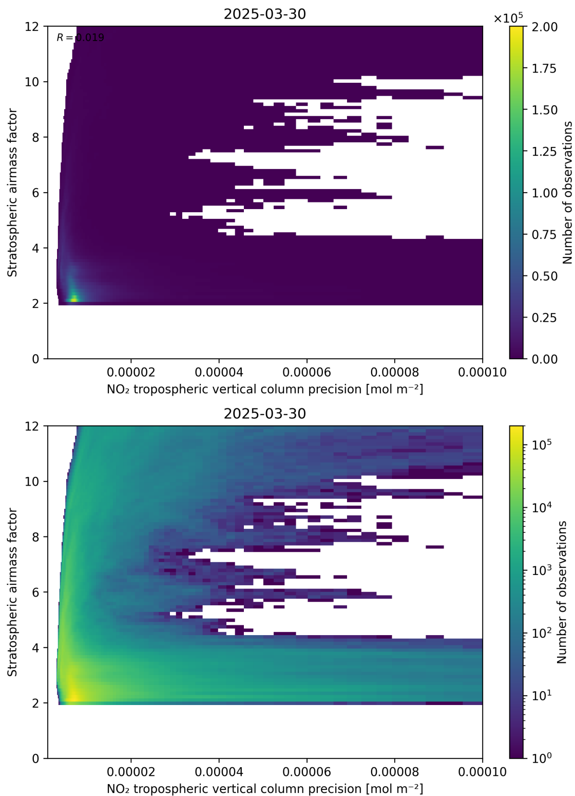
Figure 131: Scatter density plot of “NO 2 tropospheric vertical column precision” against “Stratospheric airmass factor” for 2025-03-30 to 2025-03-31.
