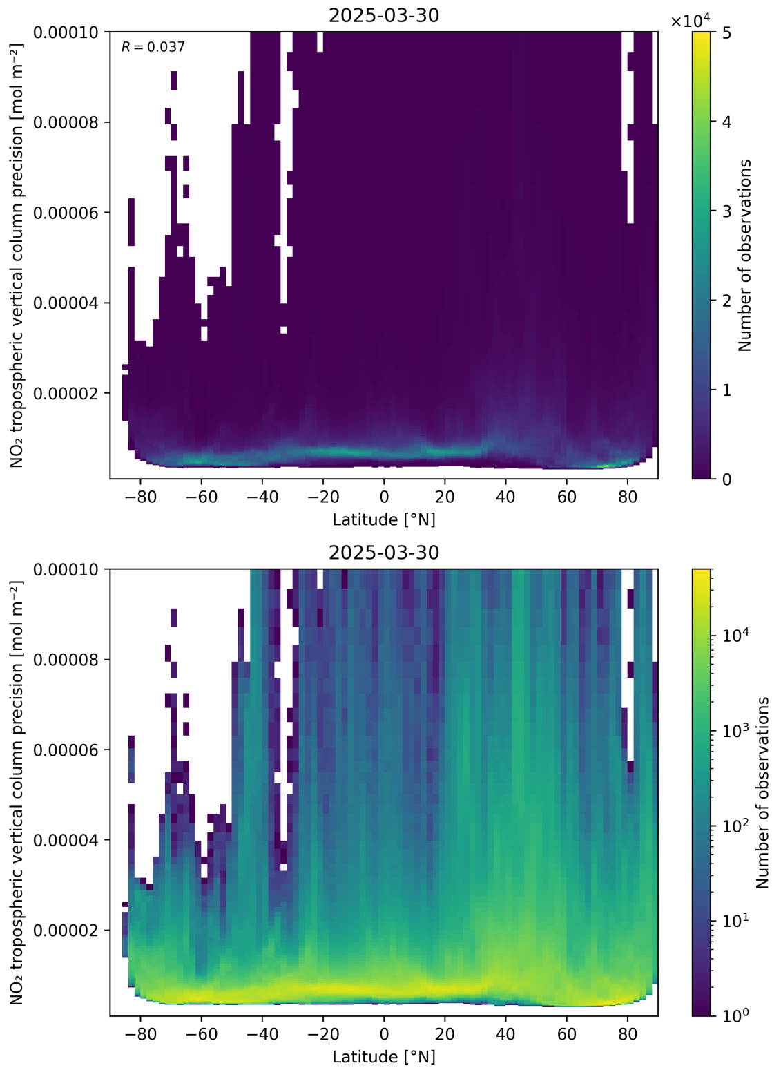
Figure 93: Scatter density plot of “Latitude” against “NO 2 tropospheric vertical column precision” for 2025-03-30 to 2025-03-31.
