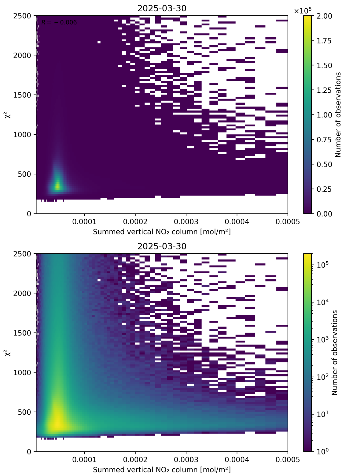
Figure 104: Scatter density plot of “Summed vertical NO 2 column” against “ \chi^2 ” for 2025-03-30 to 2025-03-31.
