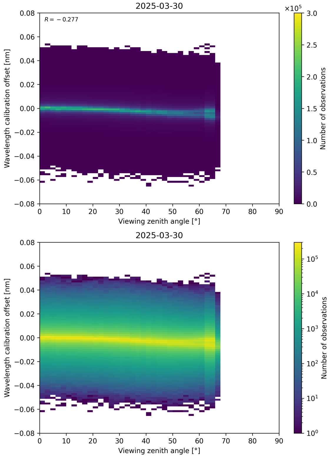
Figure 173: Scatter density plot of “Viewing zenith angle” against “Wavelength calibration offset” for 2025-03-30 to 2025-03-31.
