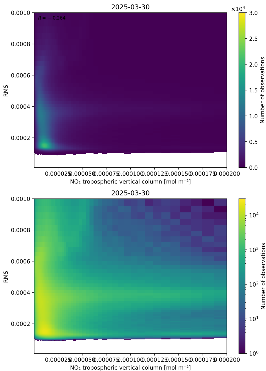
Figure 142: Scatter density plot of “NO 2 tropospheric vertical column” against “RMS” for 2025-03-30 to 2025-03-31.
