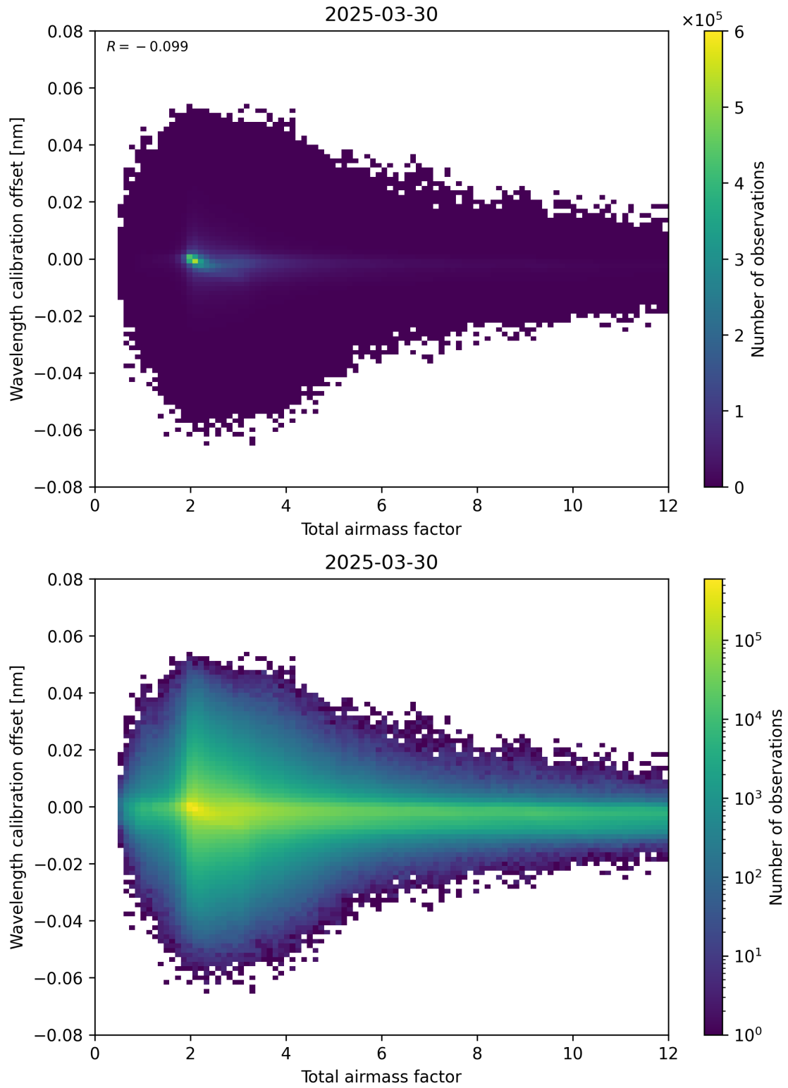
Figure 70: Scatter density plot of “Total airmass factor” against “Wavelength calibration offset” for 2025-03-30 to 2025-03-31.
