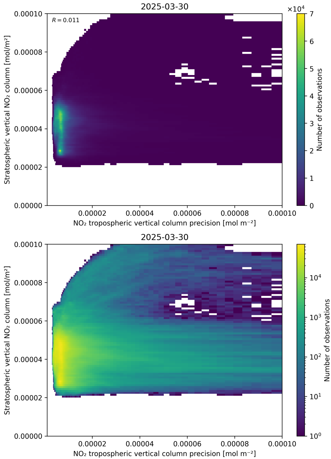
Figure 135: Scatter density plot of “NO 2 tropospheric vertical column precision” against “Stratospheric vertical NO 2 column” for 2025-03-30 to 2025-03-31.
