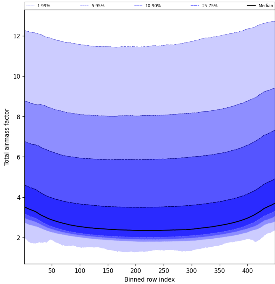
Figure 49: Along track statistics of “Total airmass factor” for 2025-03-30 to 2025-03-31
