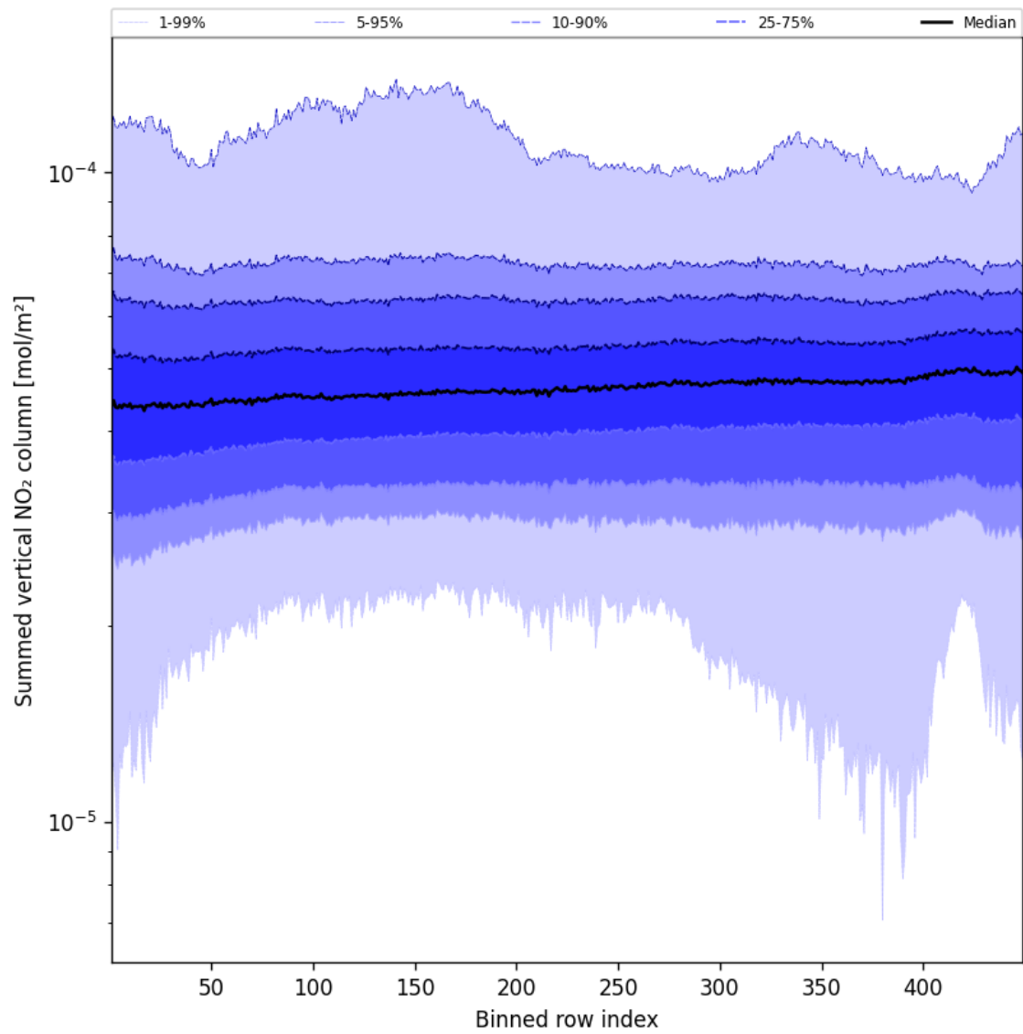
Figure 57: Along track statistics of “Summed vertical NO 2 column” for 2025-03-31 to 2025-03-31
