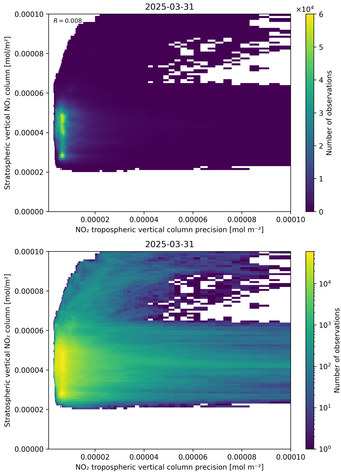
Figure 135: Scatter density plot of “NO 2 tropospheric vertical column precision” against “Stratospheric vertical NO 2 column” for 2025-03-31 to 2025-03-31.
