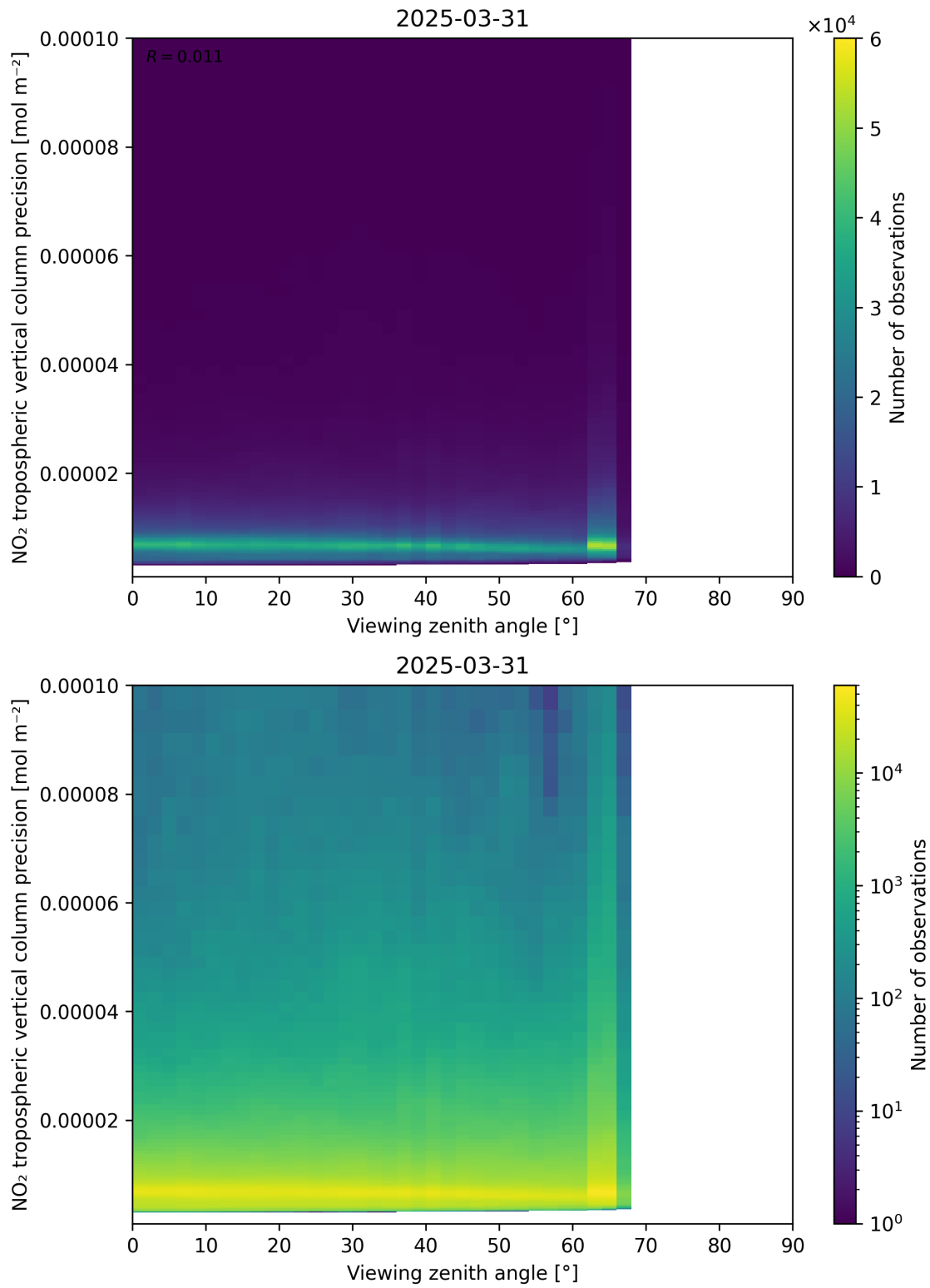
Figure 170: Scatter density plot of “Viewing zenith angle” against “NO 2 tropospheric vertical column precision” for 2025-03-31 to 2025-03-31.
