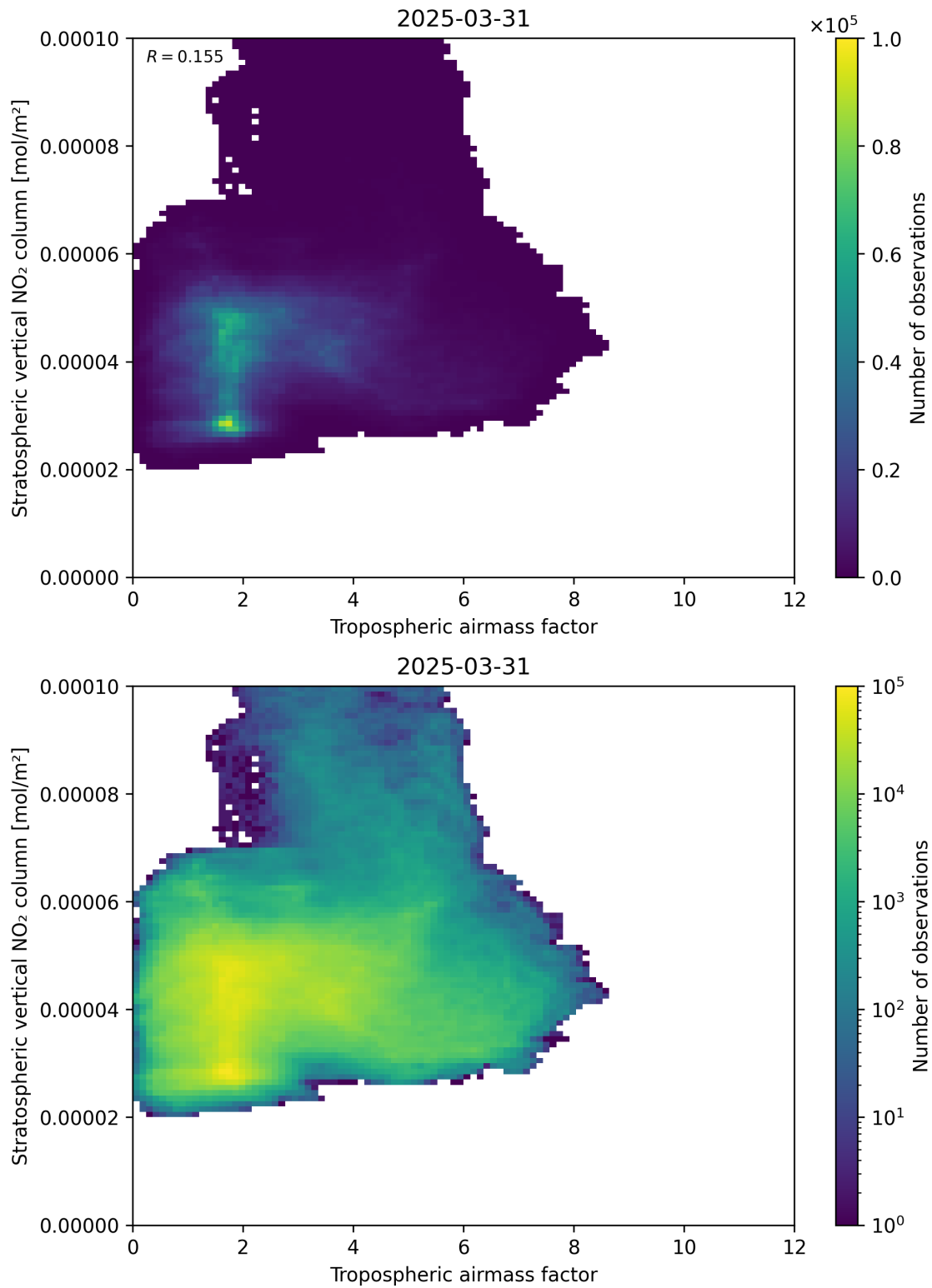
Figure 74: Scatter density plot of “Tropospheric air mass factor” against “Stratospheric vertical NO 2 column” for 2025-03-31 to 2025-03-31.
