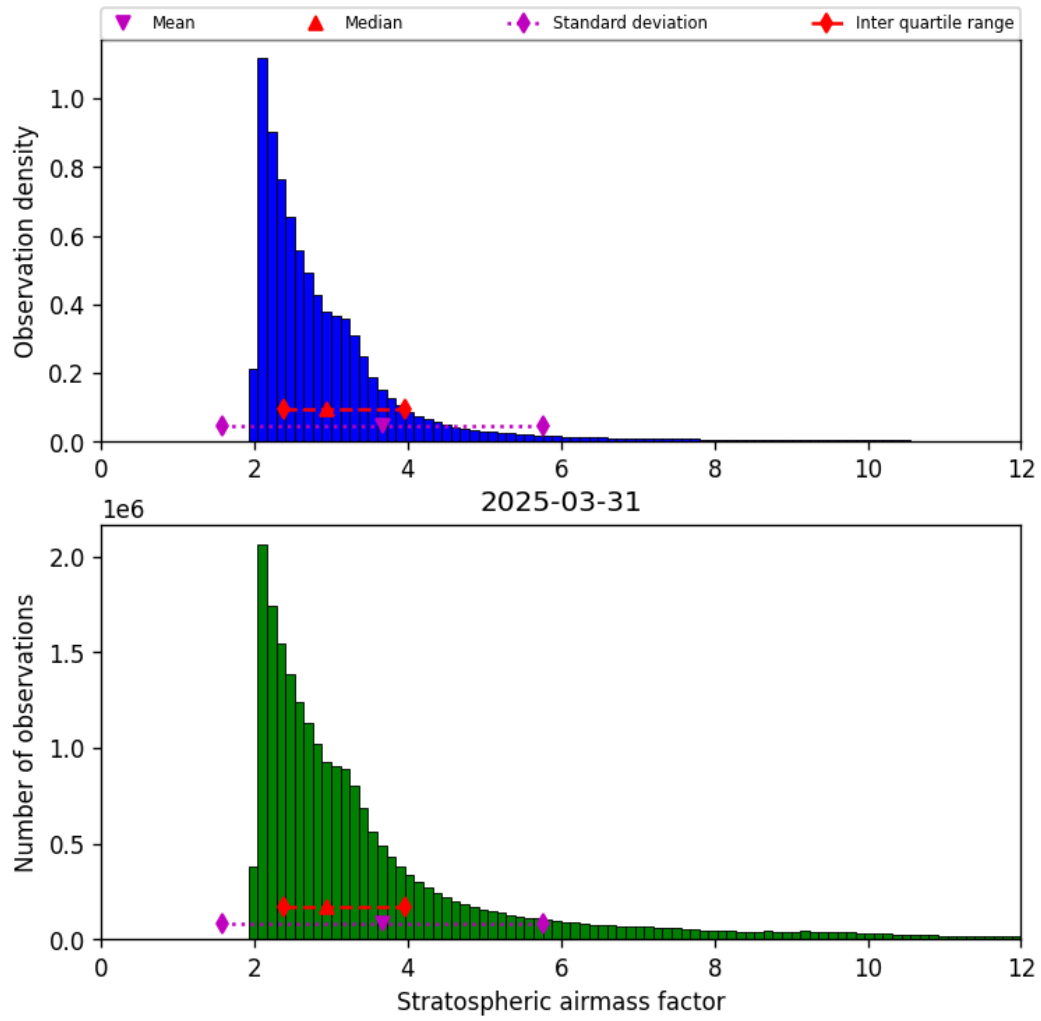
Figure 44: Histogram of “Stratospheric airmass factor” for 2025-03-31 to 2025-03-31
