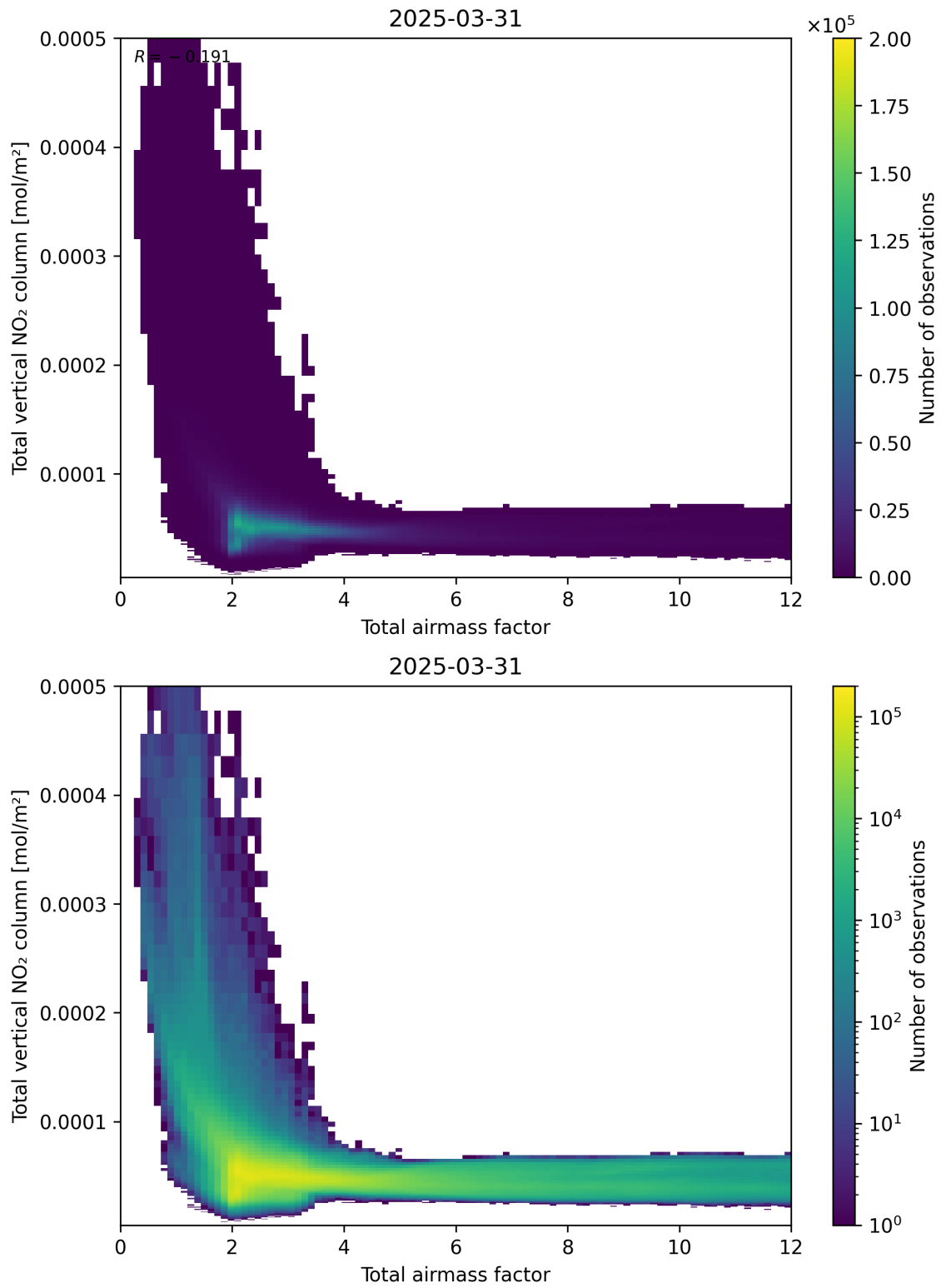
Figure 67: Scatter density plot of “Total airmass factor” against “Total vertical NO 2 column” for 2025-03-31 to 2025-03-31.
