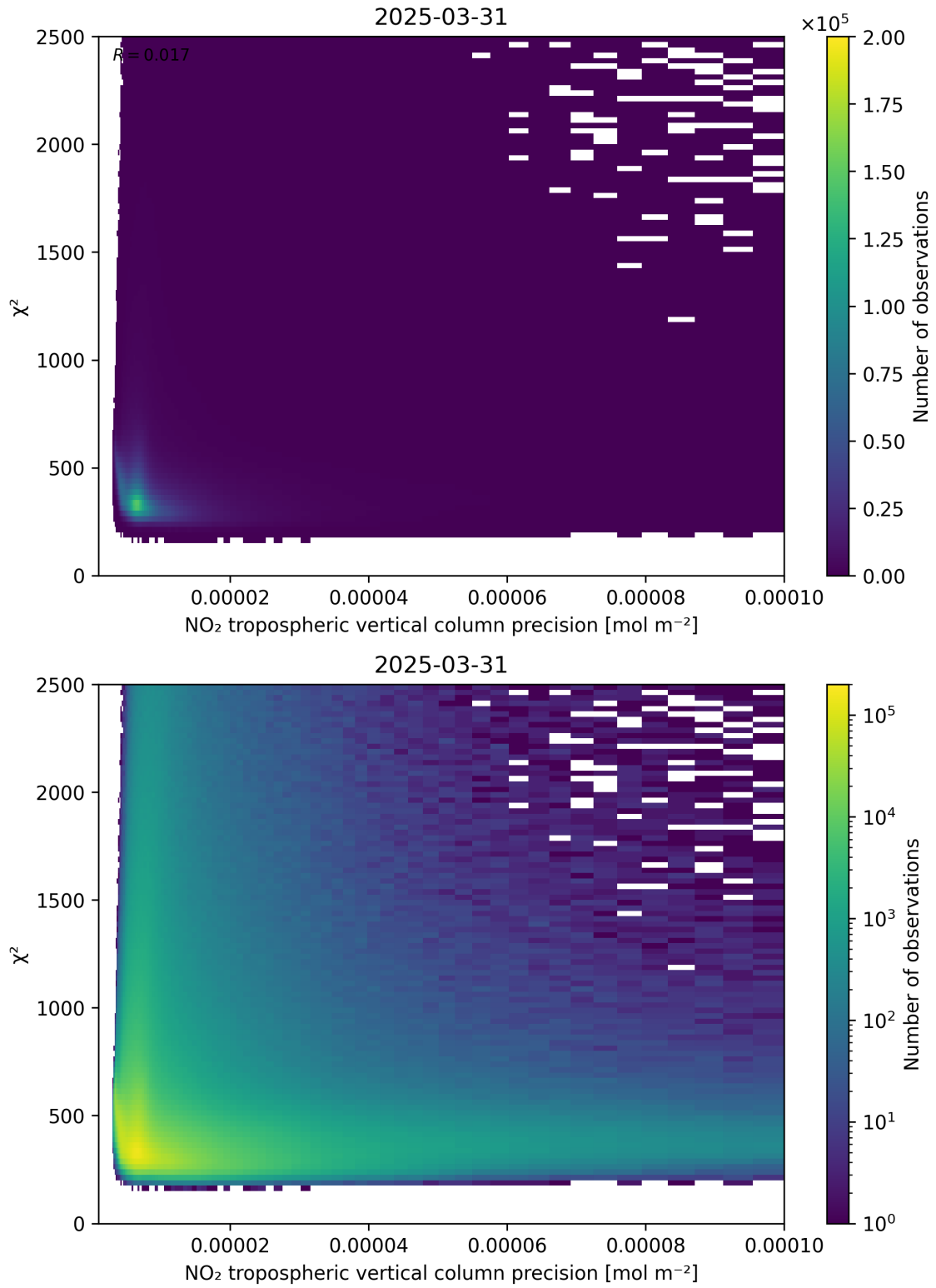
Figure 134: Scatter density plot of “NO 2 tropospheric vertical column precision” against “ \chi^2 ” for 2025-03-31 to 2025-03-31.
