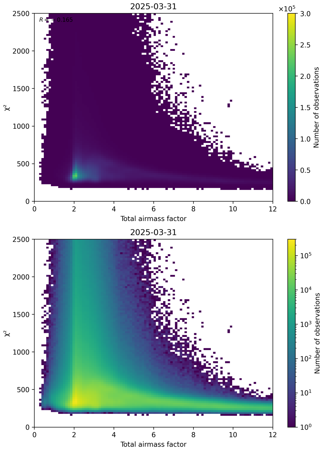
Figure 63: Scatter density plot of “Total airmass factor” against “ \chi^2 ” for 2025-03-31 to 2025-03-31.
