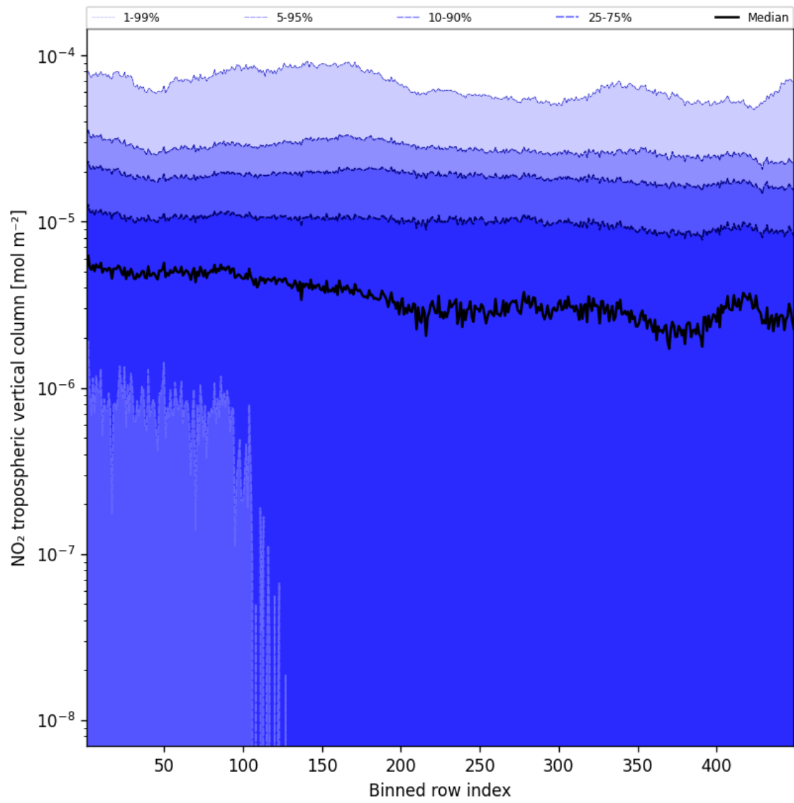
Figure 46: Along track statistics of “NO 2 tropospheric vertical column” for 2025-03-31 to 2025-03-31
