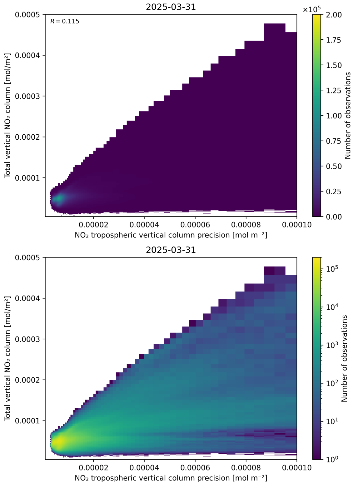
Figure 138: Scatter density plot of “NO 2 tropospheric vertical column precision” against “Total vertical NO 2 column” for 2025-03-31 to 2025-03-31.
