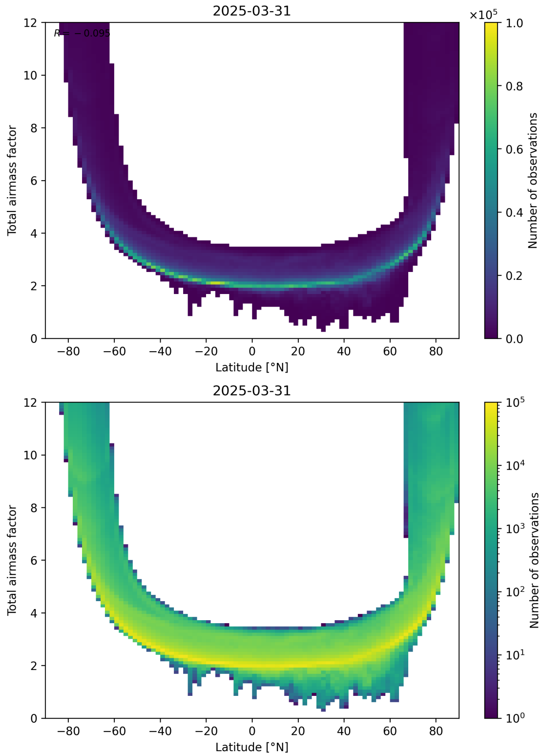
Figure 84: Scatter density plot of “Latitude” against “Total airmass factor” for 2025-03-31 to 2025-03-31.
