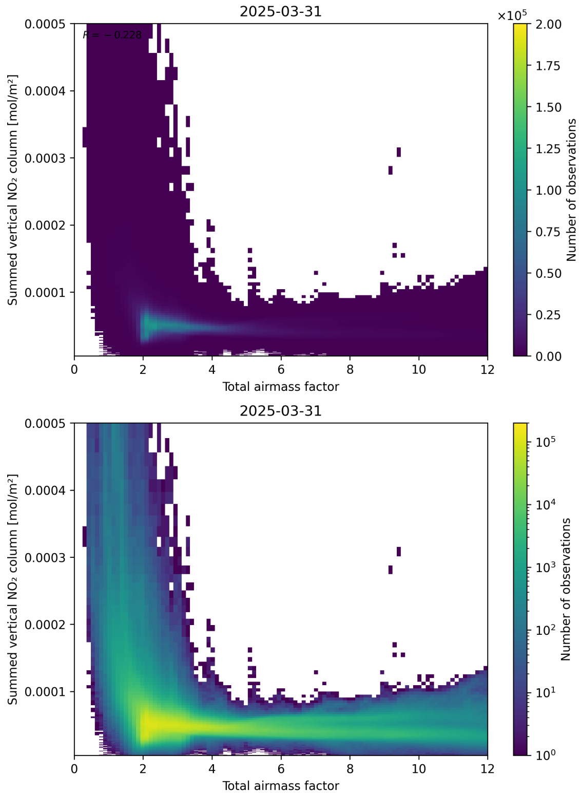
Figure 65: Scatter density plot of “Total airmass factor” against “Summed vertical NO 2 column” for 2025-03-31 to 2025-03-31.
