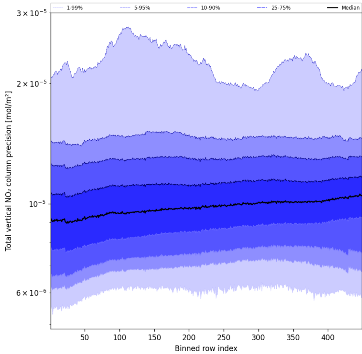
Figure 56: Along track statistics of “Total vertical NO 2 column precision” for 2025-03-31 to 2025-03-31
