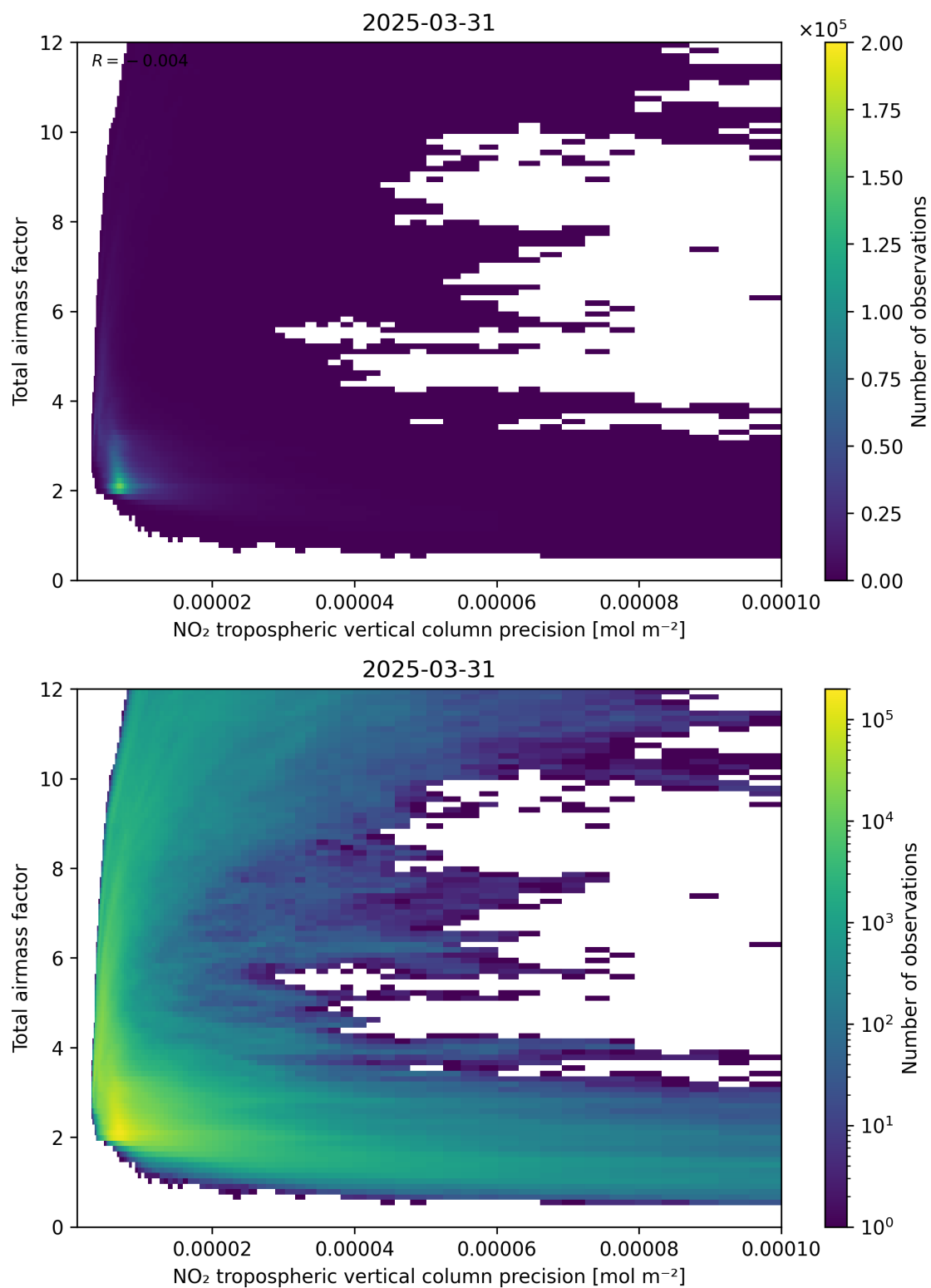
Figure 132: Scatter density plot of “NO 2 tropospheric vertical column precision” against “Total air mass factor” for 2025-03-31 to 2025-03-31.
