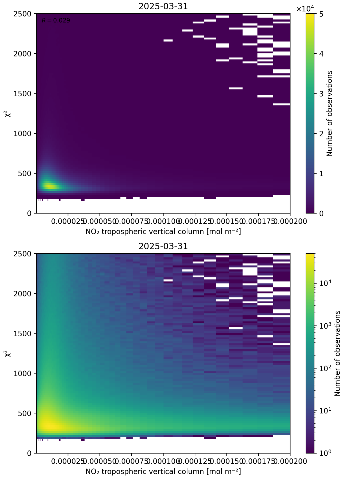
Figure 124: Scatter density plot of “NO 2 tropospheric vertical column” against “ \chi^2 ” for 2025-03-31 to 2025-03-31.
