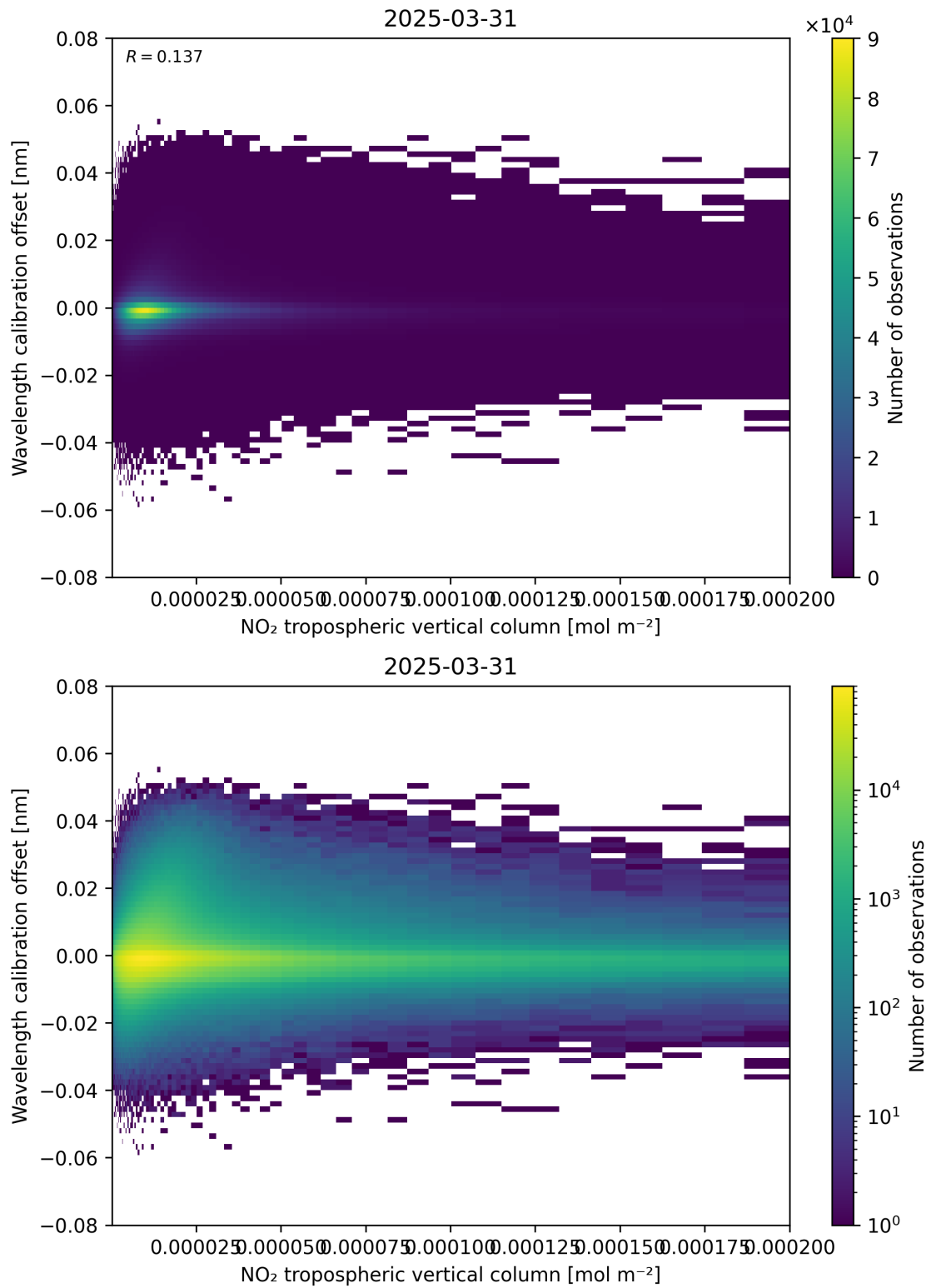
Figure 143: Scatter density plot of “NO 2 tropospheric vertical column” against “Wavelength calibration offset” for 2025-03-31 to 2025-03-31.
