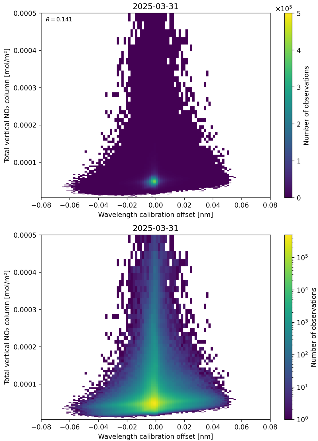
Figure 179: Scatter density plot of “Wavelength calibration offset” against “Total vertical NO 2 column” for 2025-03-31 to 2025-03-31.
