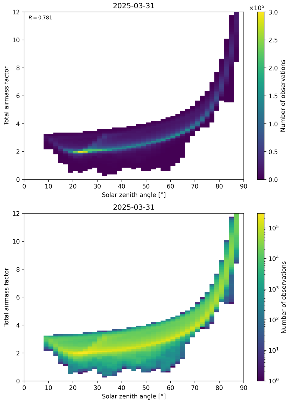
Figure 146: Scatter density plot of “Solar zenith angle” against “Total airmass factor” for 2025-03-31 to 2025-03-31.
