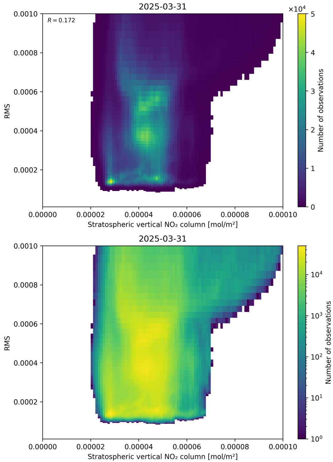
Figure 102: Scatter density plot of “Stratospheric vertical NO 2 column” against “RMS” for 2025-03-31 to 2025-03-31.
