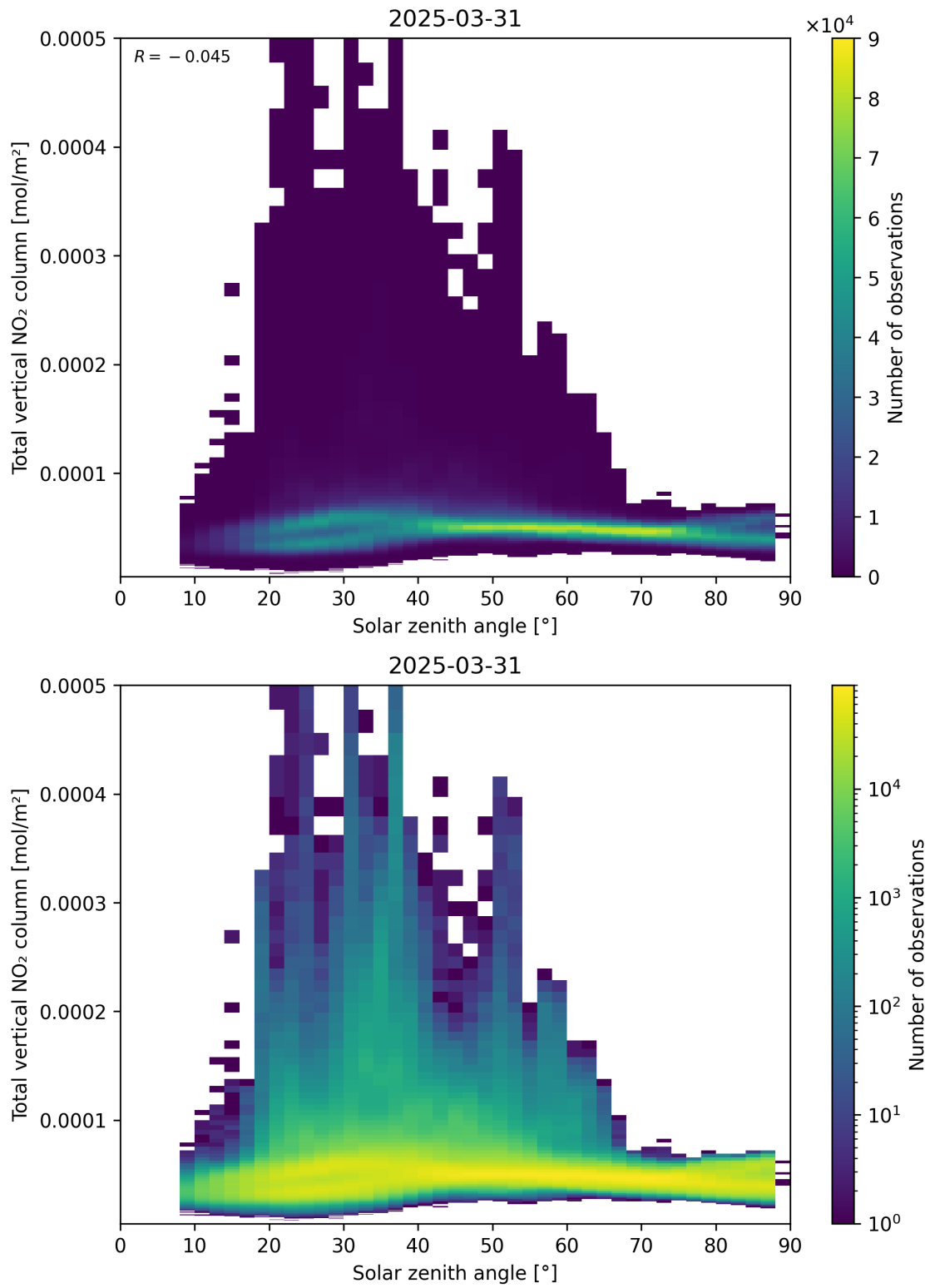
Figure 153: Scatter density plot of “Solar zenith angle” against “Total vertical NO 2 column” for 2025-03-31 to 2025-03-31.
