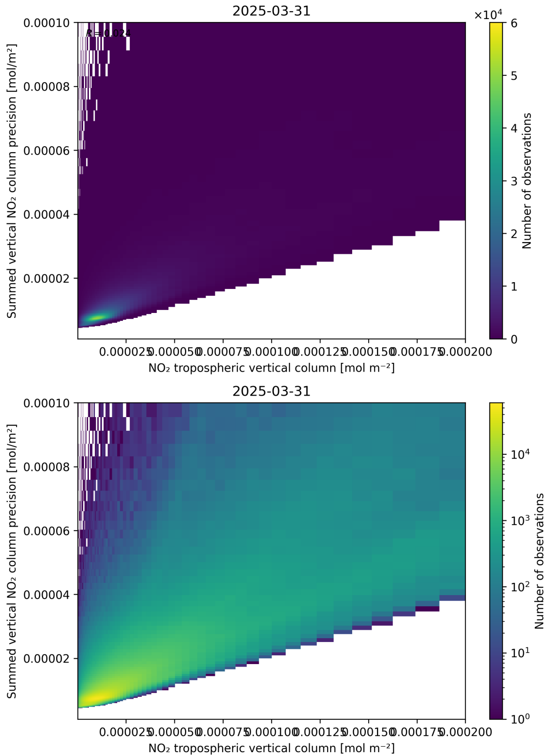
Figure 127: Scatter density plot of “NO 2 tropospheric vertical column” against “Summed vertical NO 2 column precision” for 2025-03-31 to 2025-03-31.
