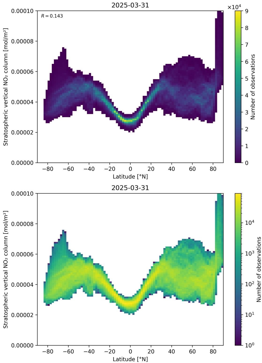
Figure 87: Scatter density plot of “Latitude” against “Stratospheric vertical NO 2 column” for 2025-03-31 to 2025-03-31.
