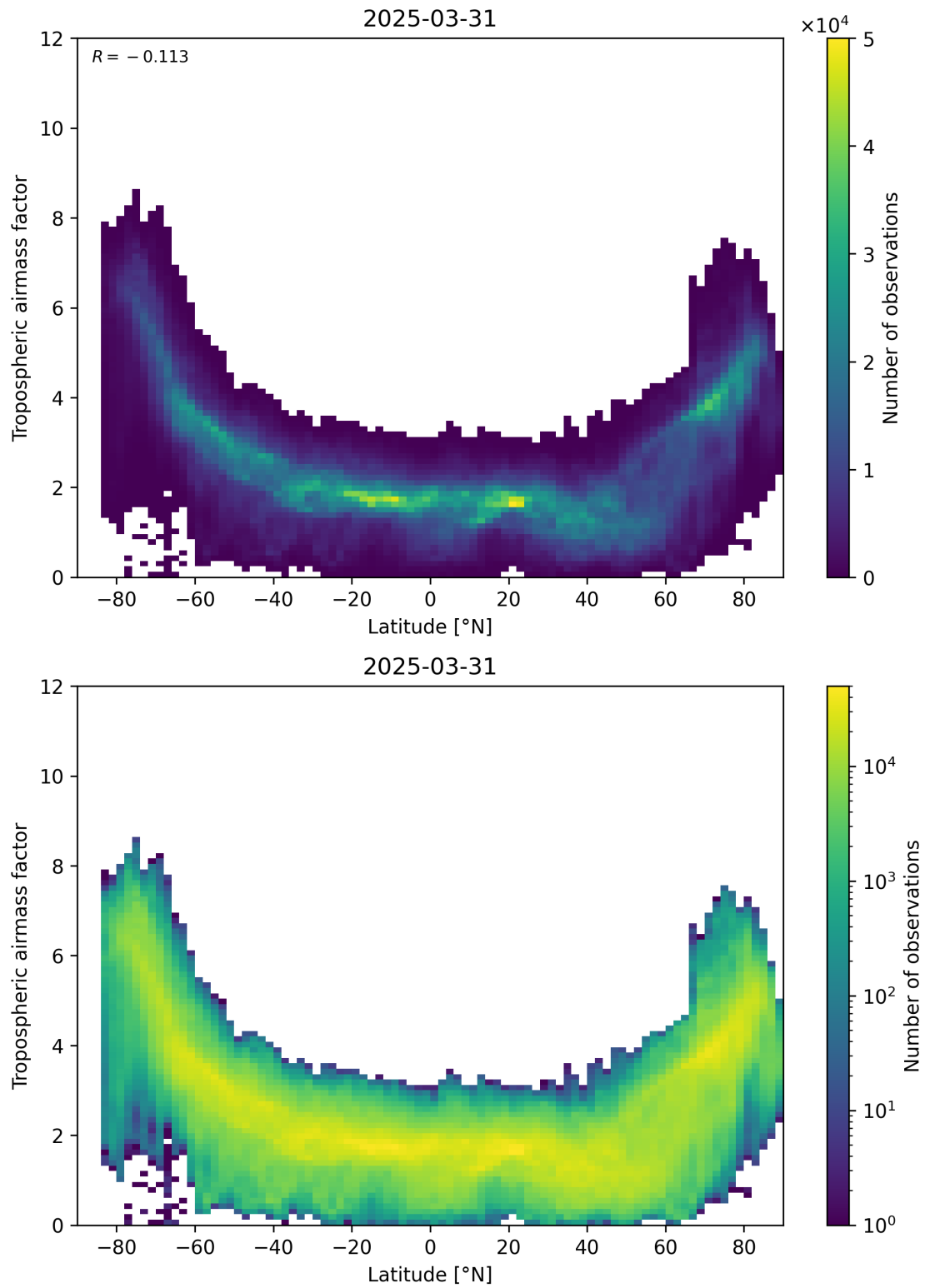
Figure 85: Scatter density plot of “Latitude” against “Tropospheric airmass factor” for 2025-03-31 to 2025-03-31.
