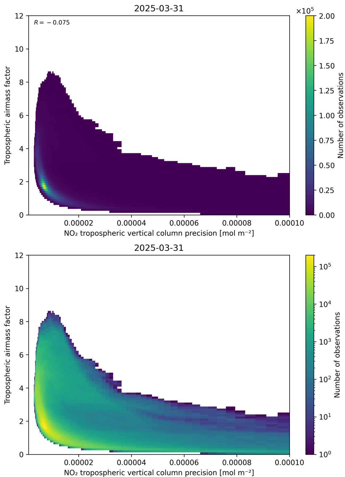
Figure 133: Scatter density plot of “NO 2 tropospheric vertical column precision” against “Tropospheric airmass factor” for 2025-03-31 to 2025-03-31.
