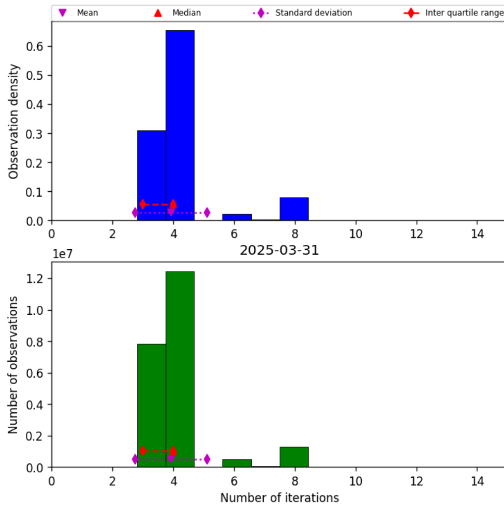
Figure 34: Histogram of “Number of iterations” for 2025-03-31 to 2025-03-31
