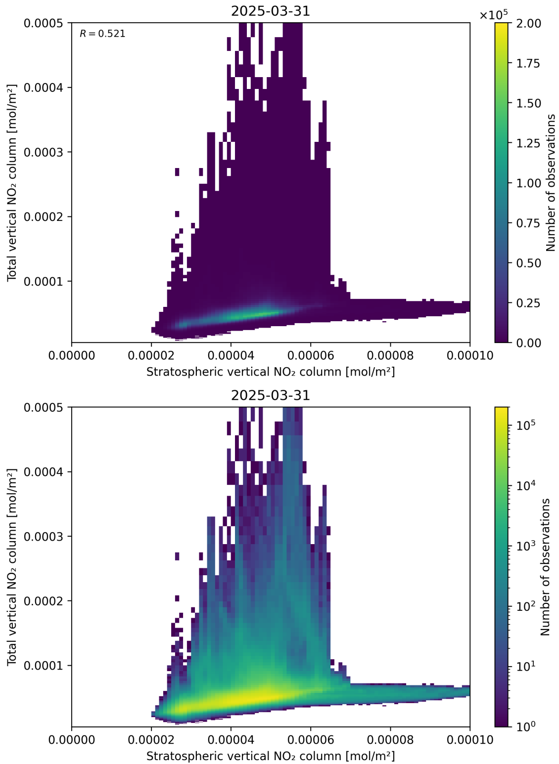
Figure 100: Scatter density plot of “Stratospheric vertical NO 2 column” against “Total vertical NO 2 column” for 2025-03-31 to 2025-03-31.
