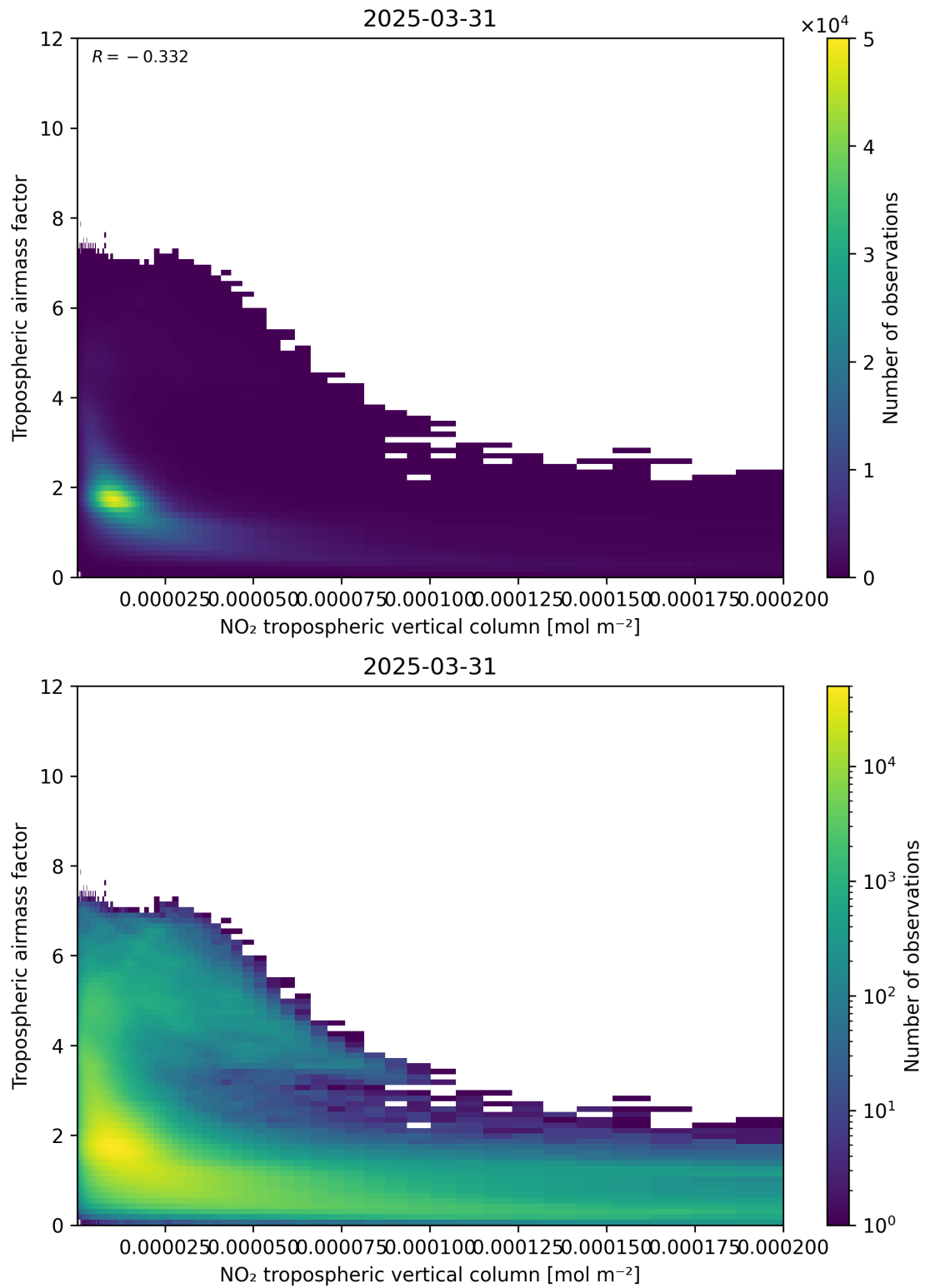
Figure 123: Scatter density plot of “NO 2 tropospheric vertical column” against “Tropospheric air mass factor” for 2025-03-31 to 2025-03-31.
