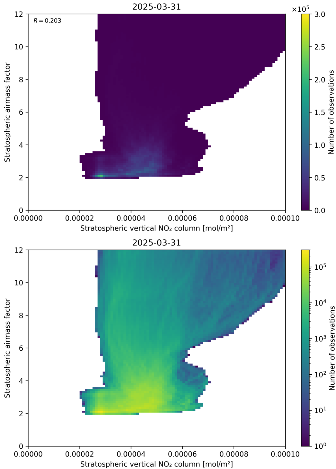
Figure 96: Scatter density plot of “Stratospheric vertical NO 2 column” against “Stratospheric airmass factor” for 2025-03-31 to 2025-03-31.
