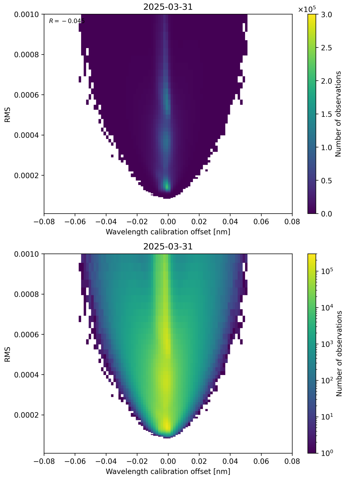
Figure 181: Scatter density plot of “Wavelength calibration offset” against “RMS” for 2025-03-31 to 2025-03-31.
