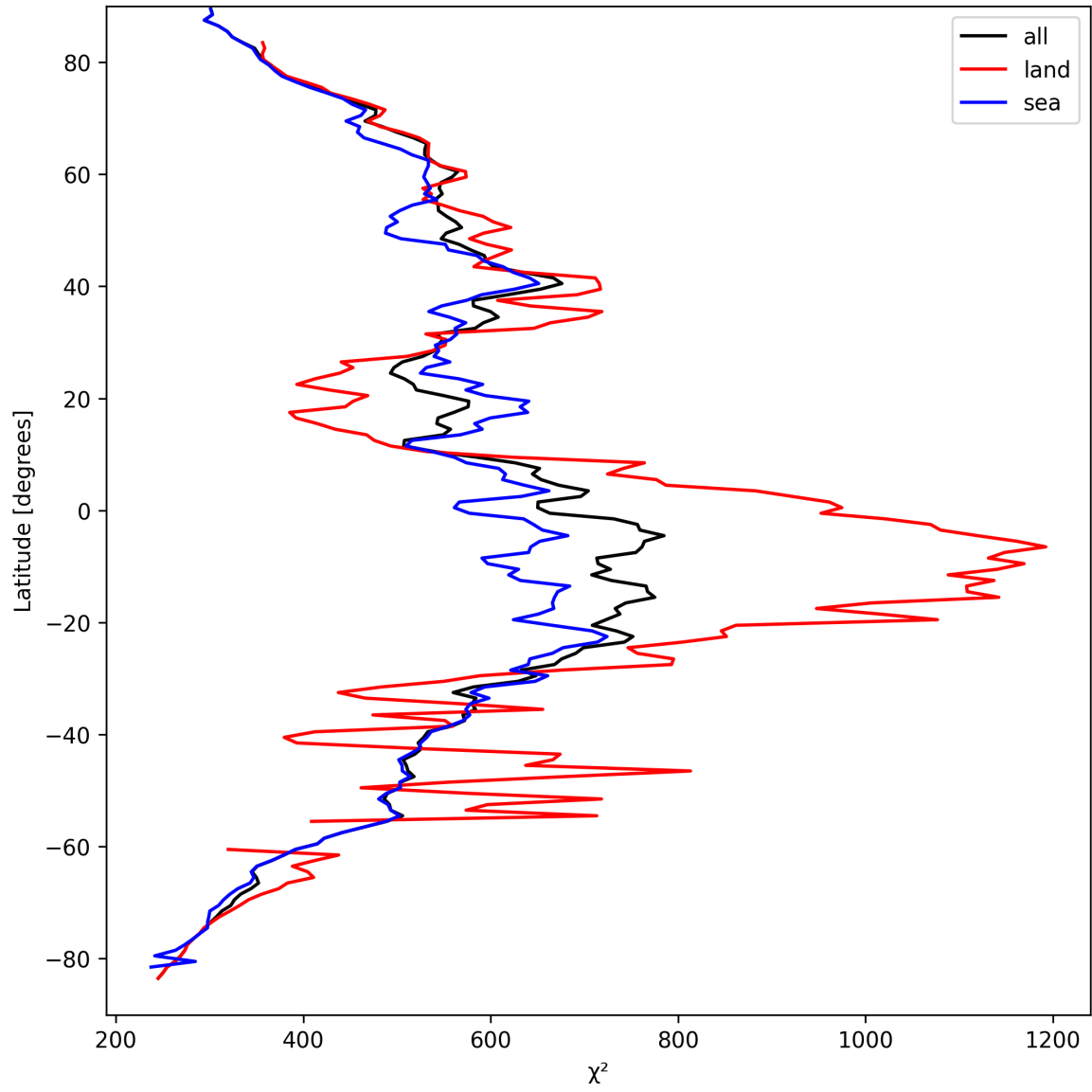
Figure 25: Zonal average of “ \chi^2 ” for 2025-03-31 to 2025-03-31.
