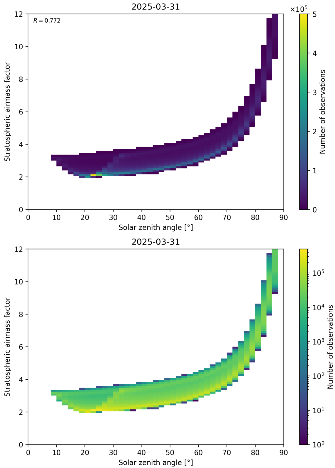
Figure 145: Scatter density plot of “Solar zenith angle” against “Stratospheric airmass factor” for 2025-03-31 to 2025-03-31.
