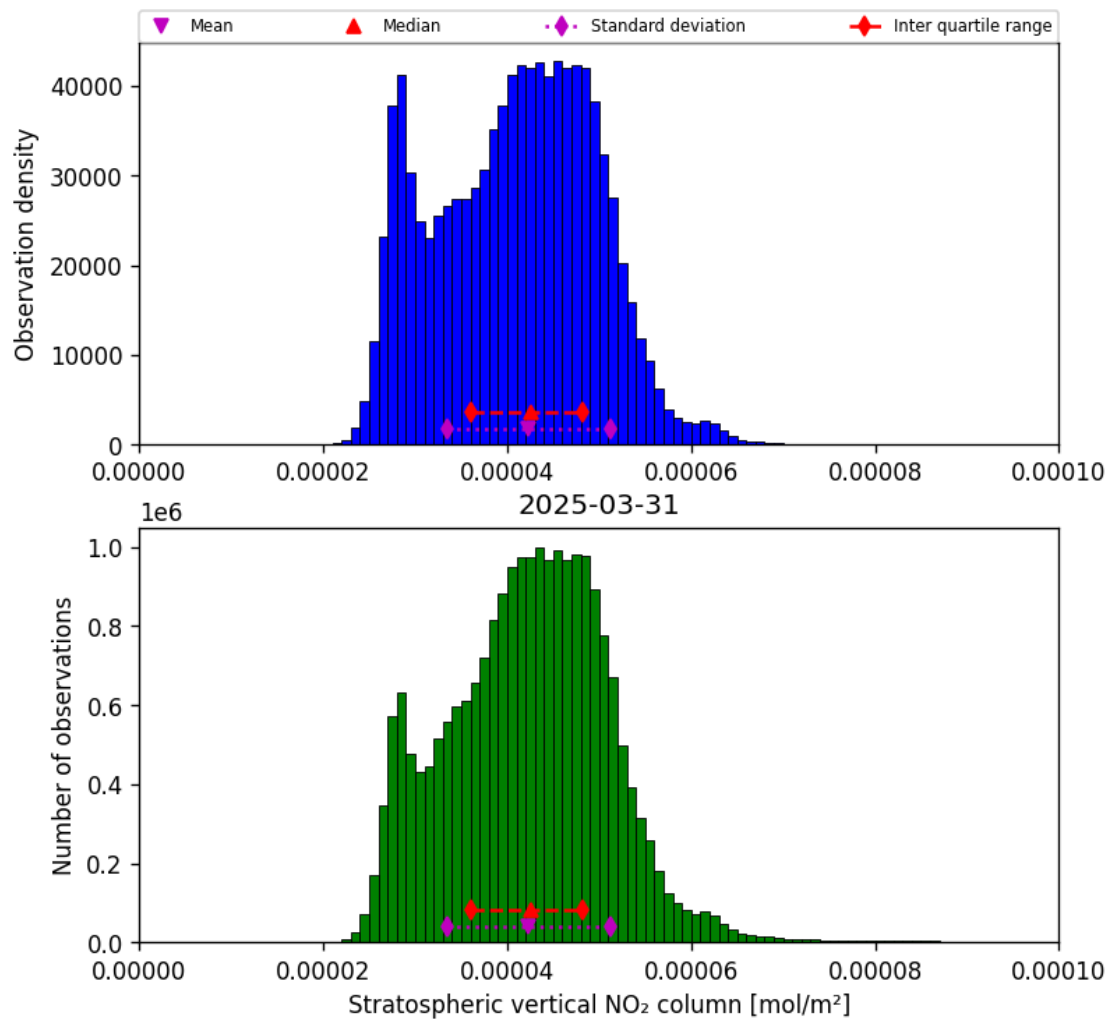
Figure 36: Histogram of “Stratospheric vertical NO 2 column” for 2025-03-31 to 2025-03-31
