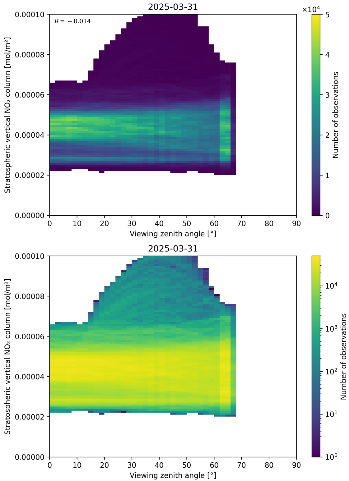
Figure 164: Scatter density plot of “Viewing zenith angle” against “Stratospheric vertical NO 2 column” for 2025-03-31 to 2025-03-31.
