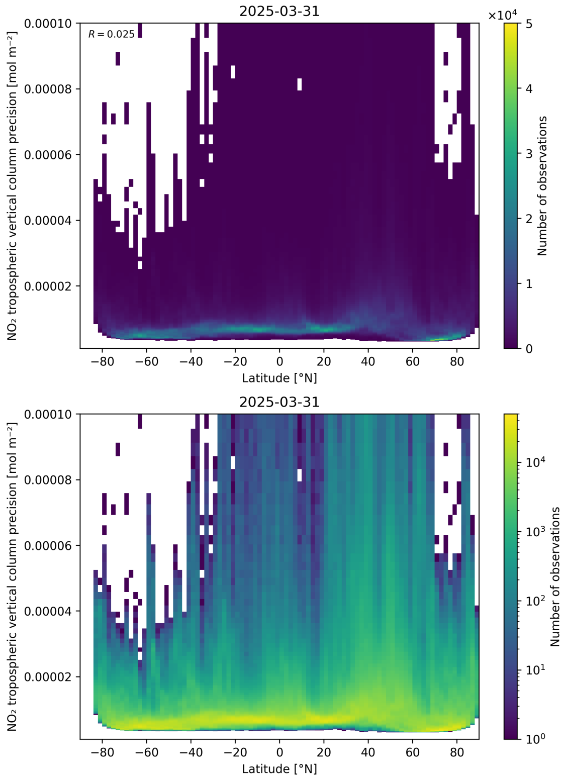
Figure 93: Scatter density plot of “Latitude” against “NO 2 tropospheric vertical column precision” for 2025-03-31 to 2025-03-31.
