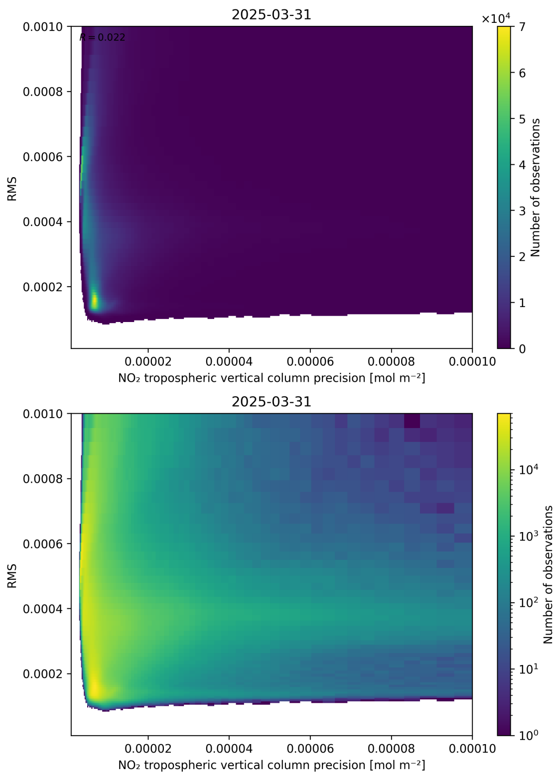
Figure 140: Scatter density plot of “NO 2 tropospheric vertical column precision” against “RMS” for 2025-03-31 to 2025-03-31.
