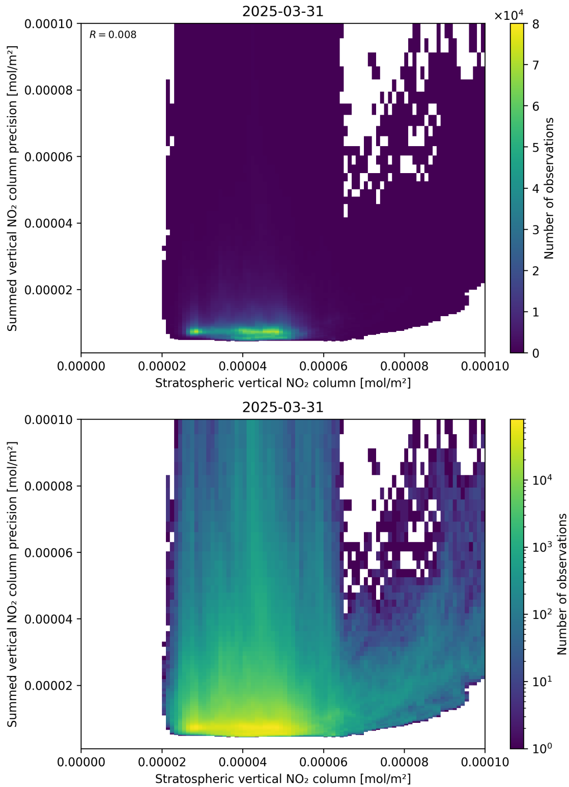
Figure 99: Scatter density plot of “Stratospheric vertical NO 2 column” against “Summed vertical NO 2 column precision” for 2025-03-31 to 2025-03-31.
