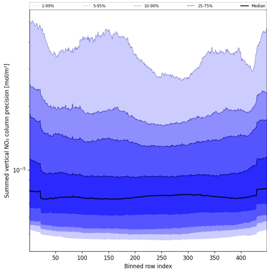
Figure 58: Along track statistics of “Summed vertical NO 2 column precision” for 2025-03-31 to 2025-03-31
