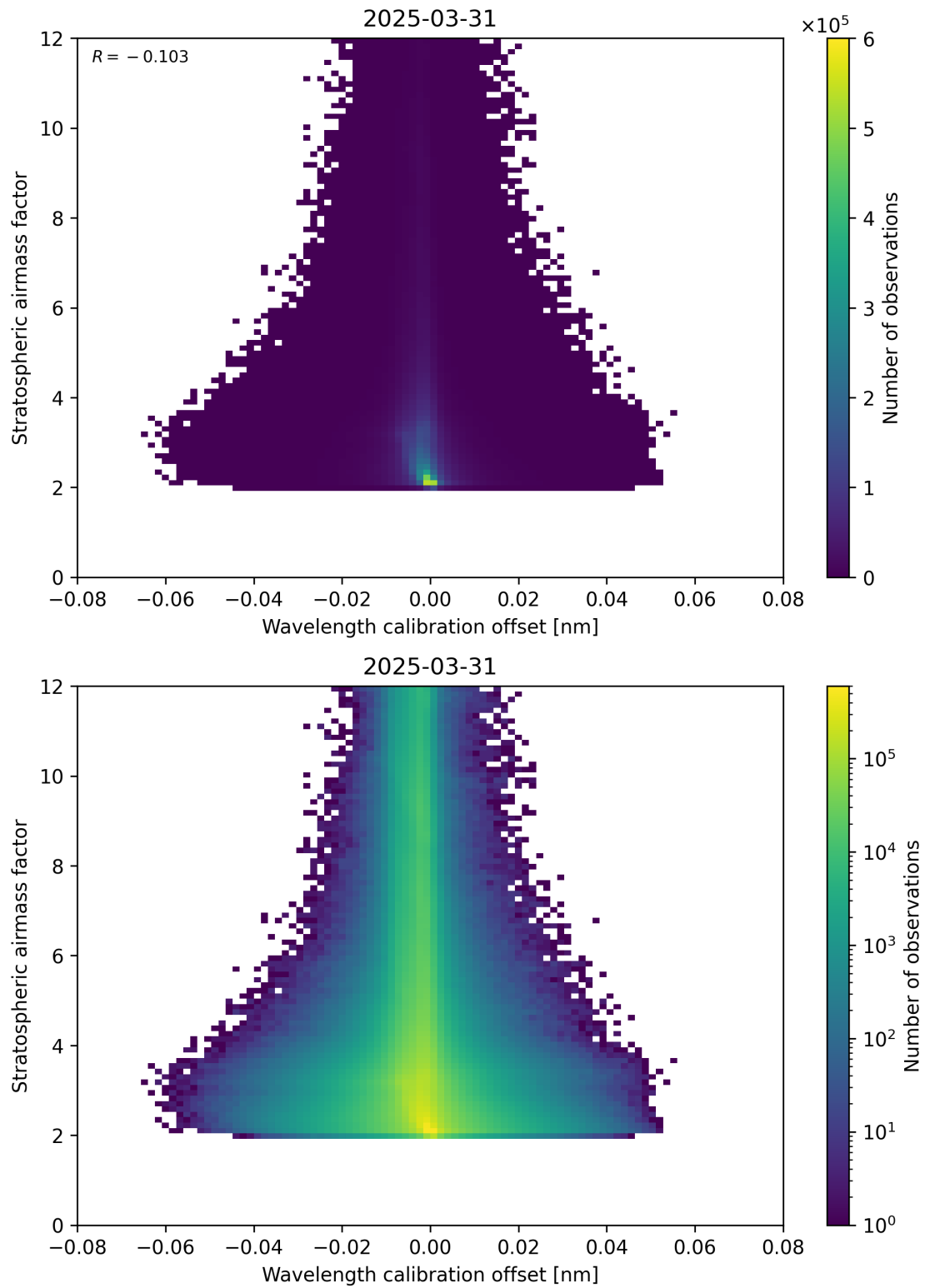
Figure 174: Scatter density plot of “Wavelength calibration offset” against “Stratospheric airmass factor” for 2025-03-31 to 2025-03-31.
