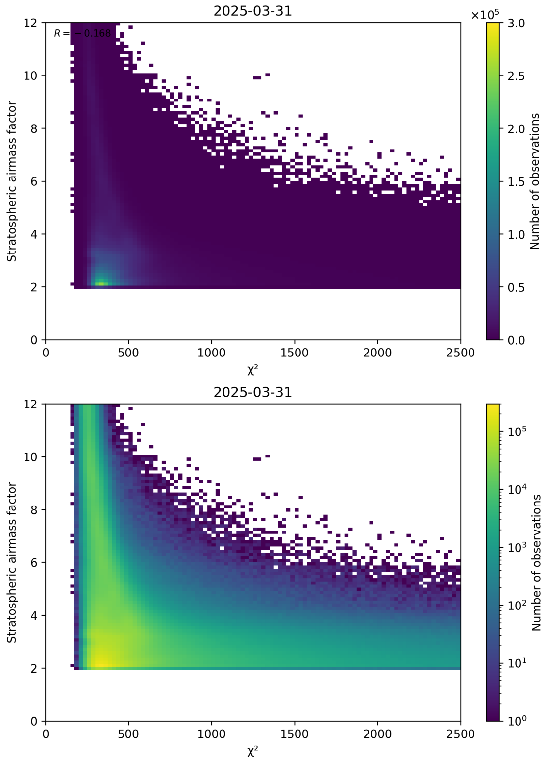
Figure 81: Scatter density plot of “ \chi^2 ” against “Stratospheric airmass factor” for 2025-03-31 to 2025-03-31.
