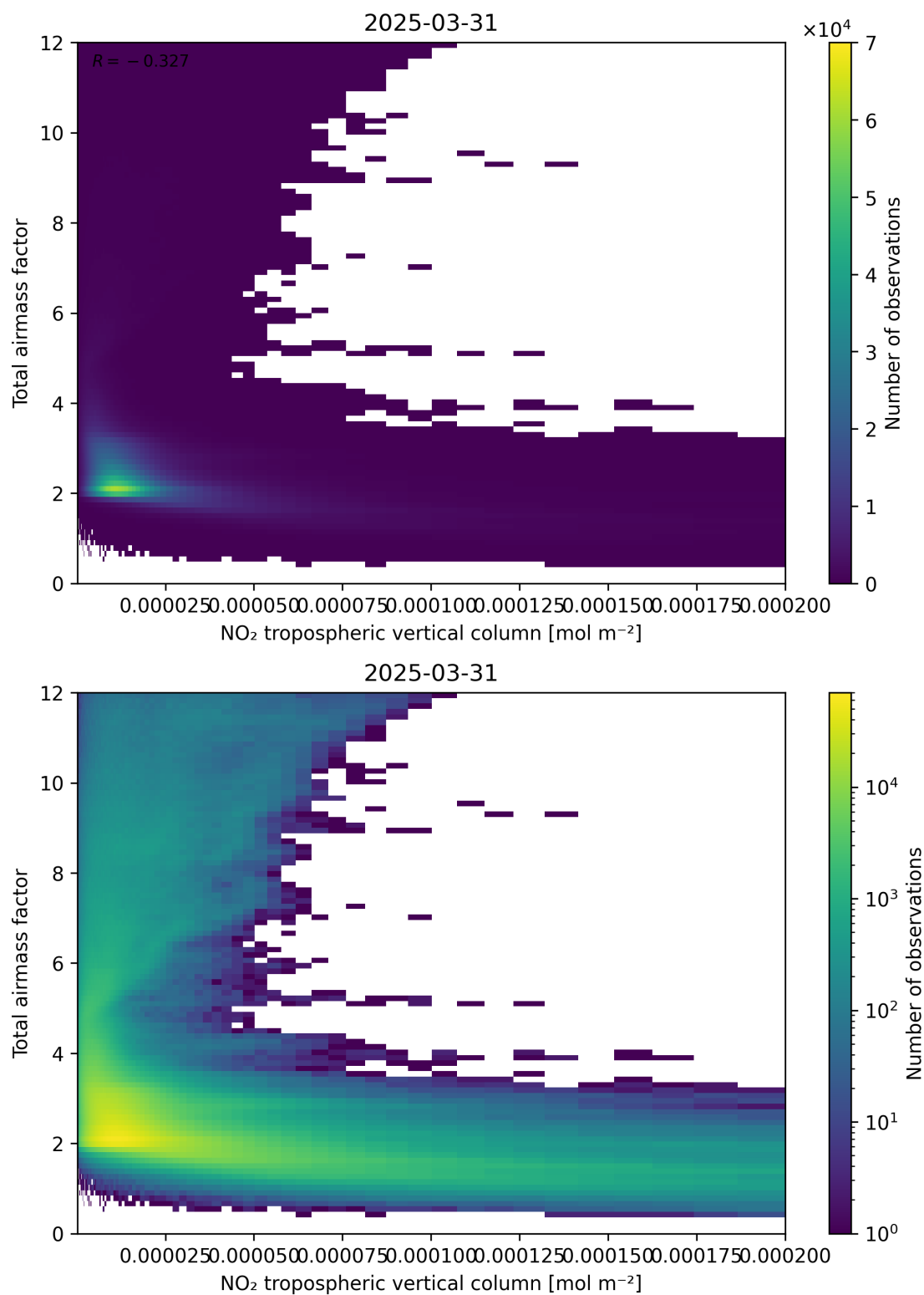
Figure 122: Scatter density plot of “NO 2 tropospheric vertical column” against “Total air mass factor” for 2025-03-31 to 2025-03-31.
