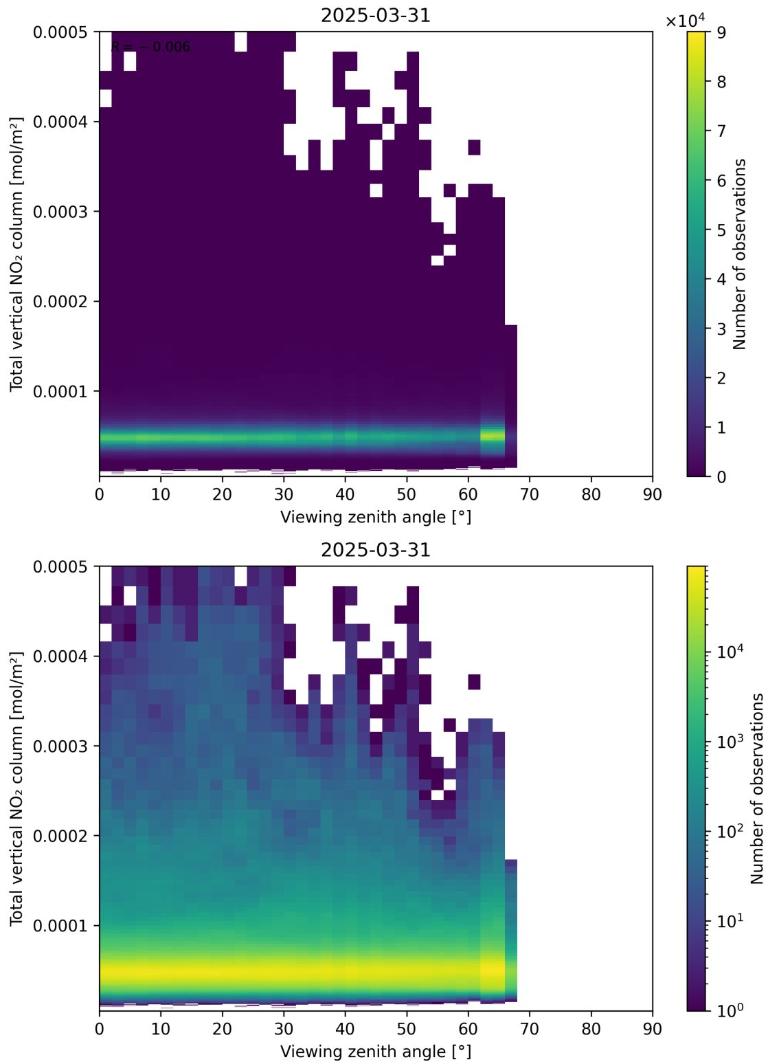
Figure 167: Scatter density plot of “Viewing zenith angle” against “Total vertical NO 2 column” for 2025-03-31 to 2025-03-31.
