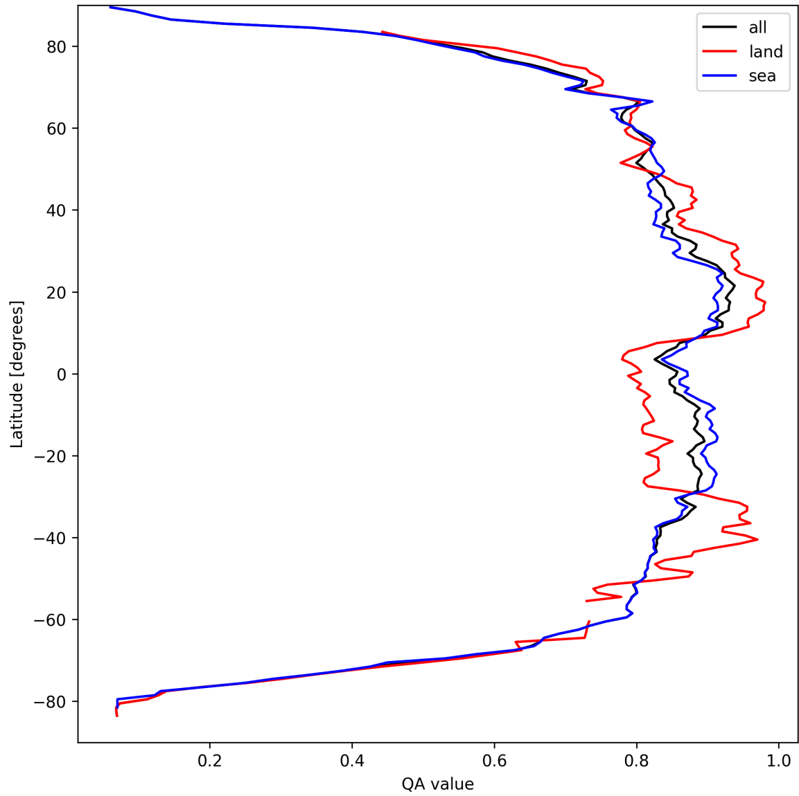
Figure 11: Zonal average of “QA value” for 2025-03-31 to 2025-03-31.
