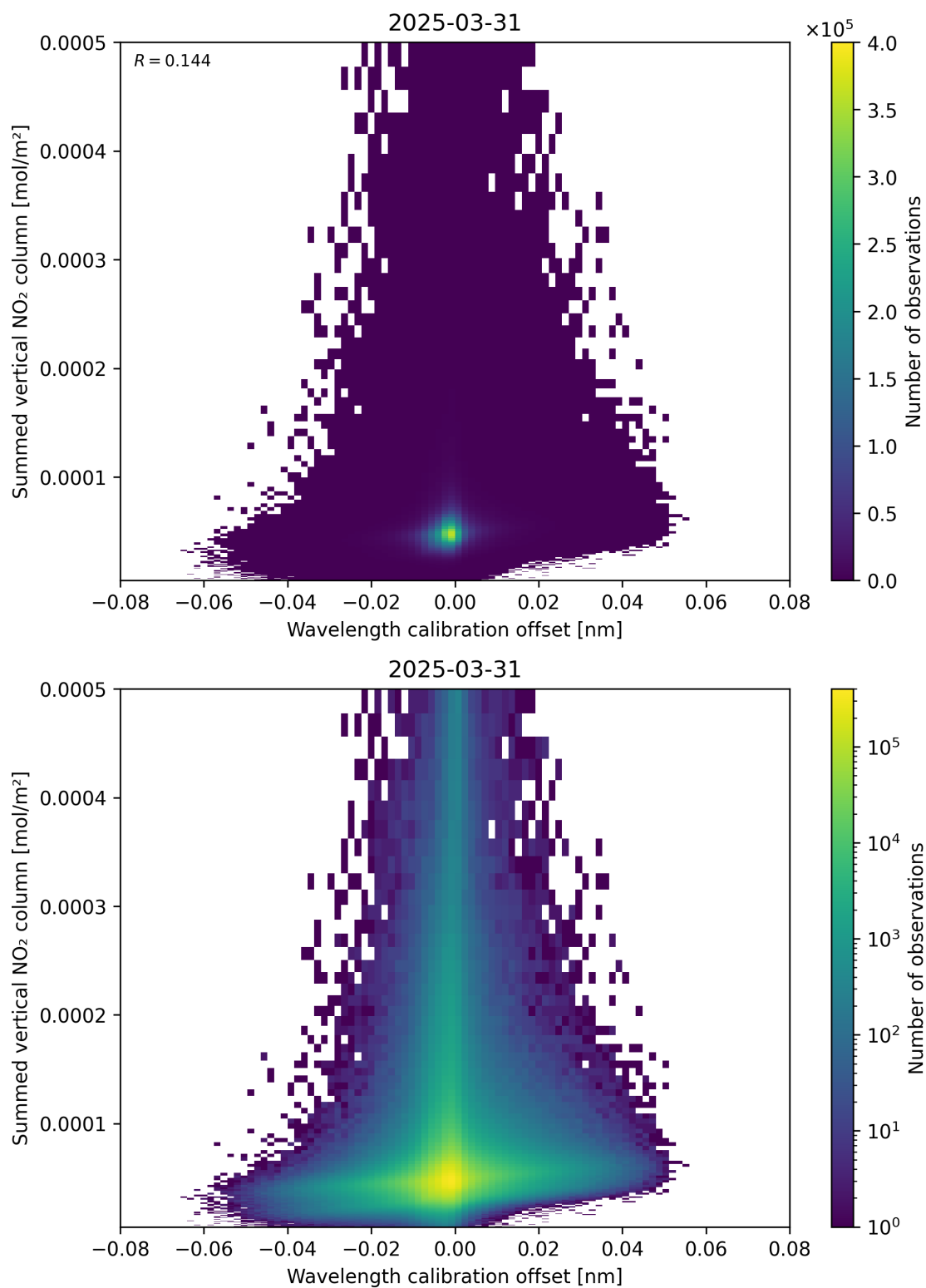
Figure 177: Scatter density plot of “Wavelength calibration offset” against “Summed vertical NO 2 column” for 2025-03-31 to 2025-03-31.
