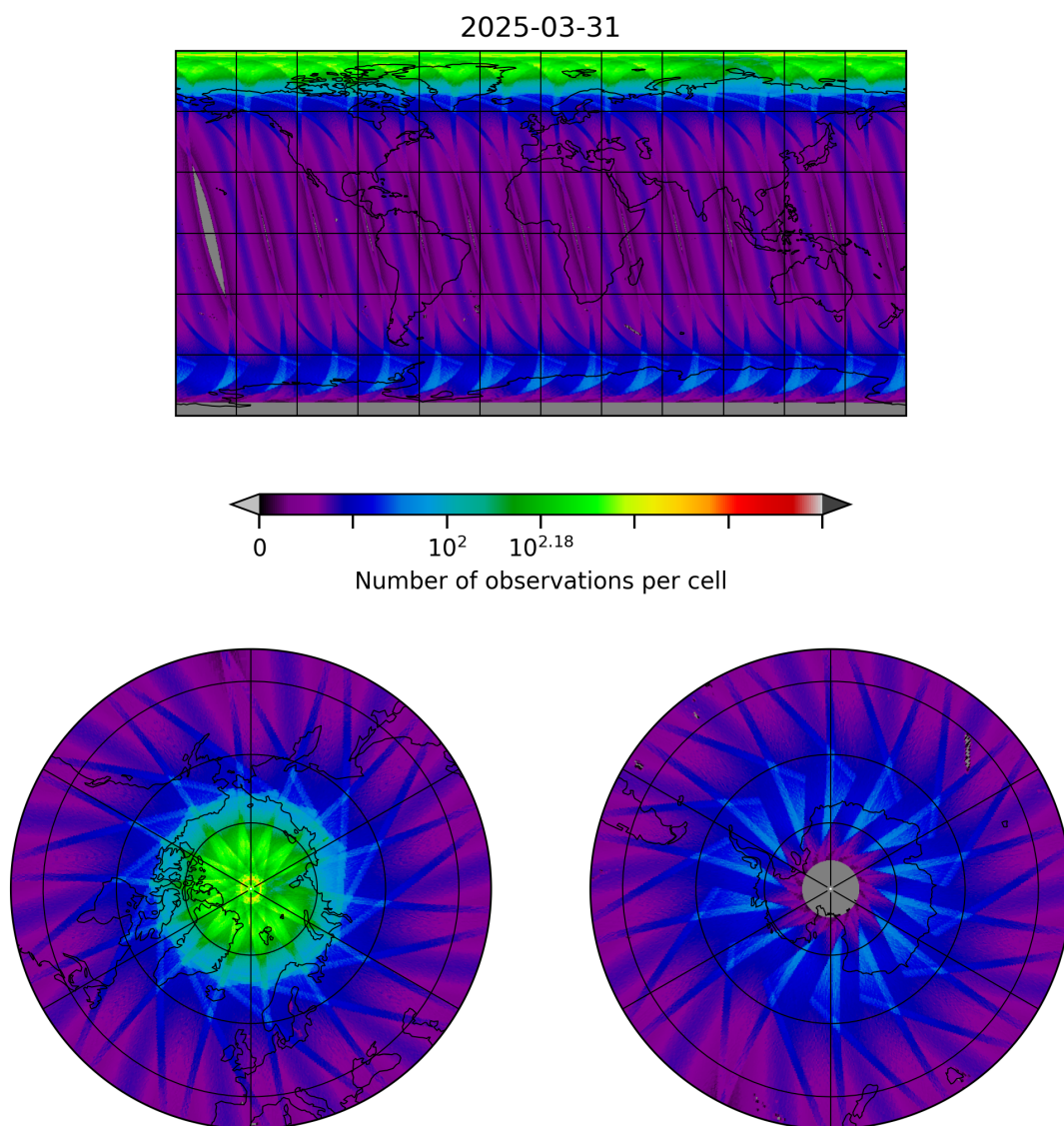
Figure 10: Map of the number of observations for 2025-03-31 to 2025-03-31
