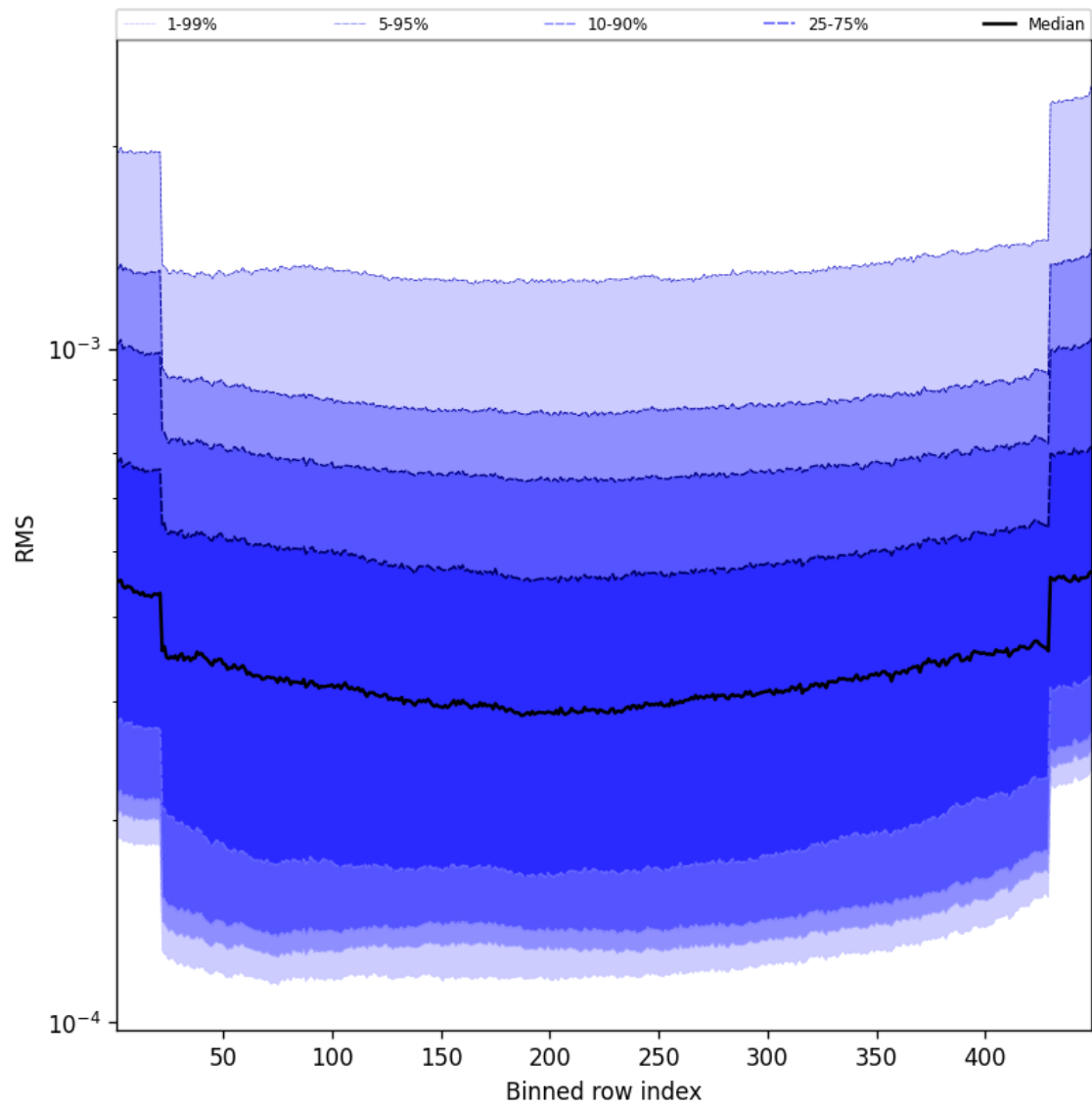
Figure 60: Along track statistics of “RMS” for 2025-03-31 to 2025-03-31
