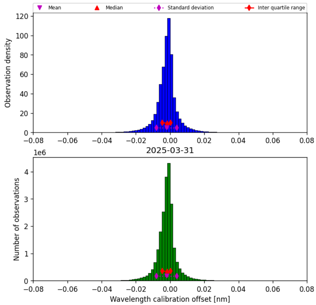
Figure 35: Histogram of “Wavelength calibration offset” for 2025-03-31 to 2025-03-31
