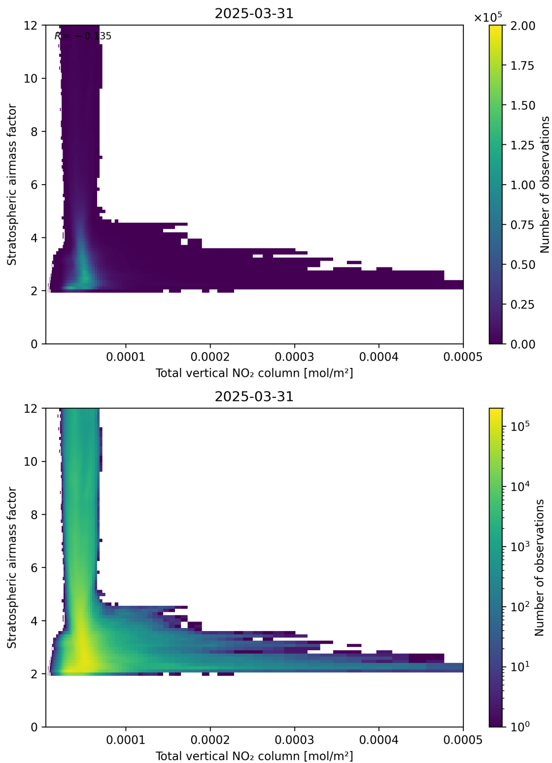
Figure 110: Scatter density plot of “Total vertical NO 2 column” against “Stratospheric airmass factor” for 2025-03-31 to 2025-03-31.
