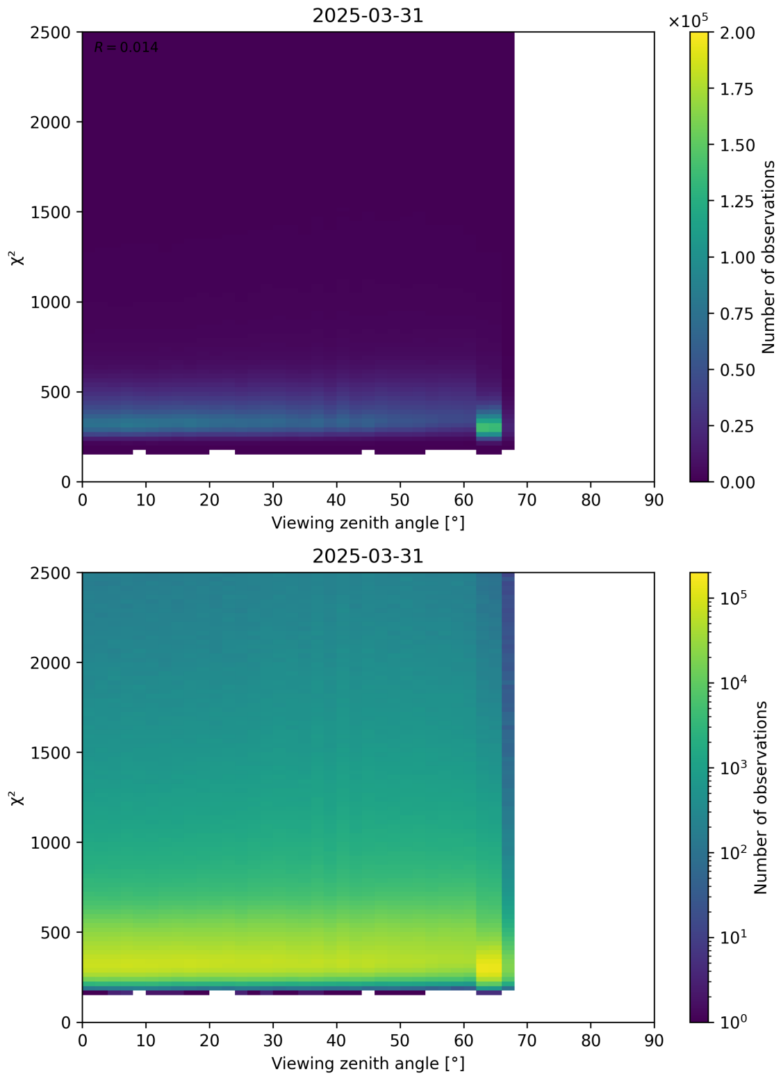
Figure 162: Scatter density plot of “Viewing zenith angle” against “ \chi^2 ” for 2025-03-31 to 2025-03-31.
