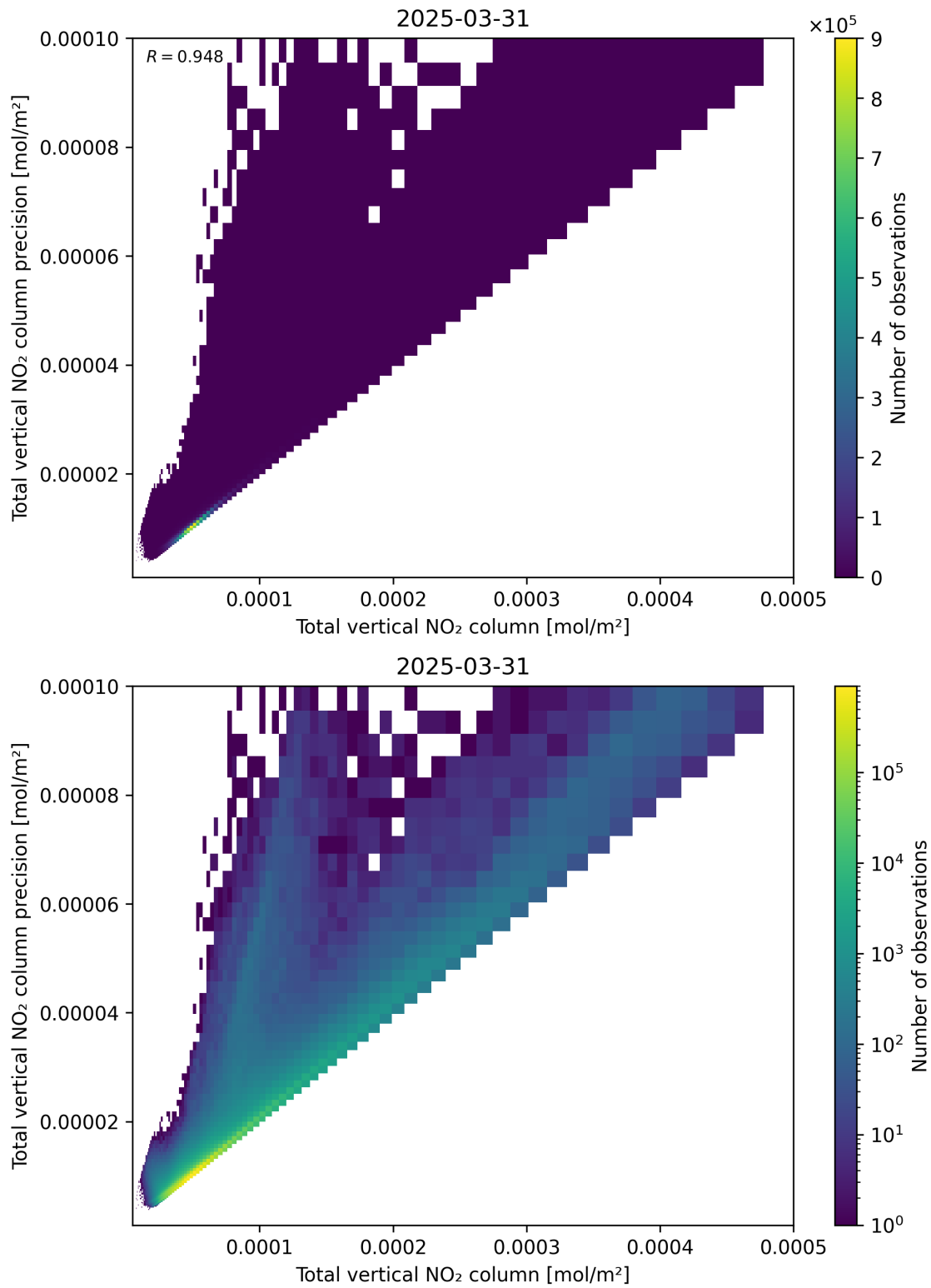
Figure 114: Scatter density plot of “Total vertical NO 2 column” against “Total vertical NO 2 column precision” for 2025-03-31 to 2025-03-31.
