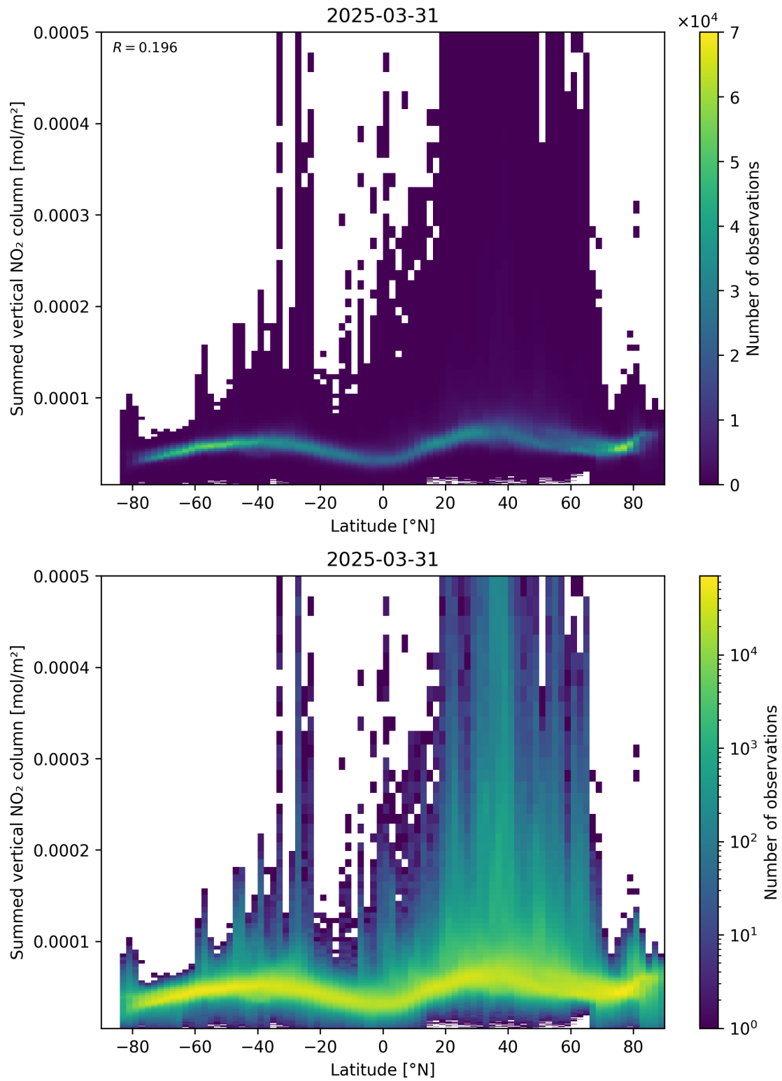
Figure 88: Scatter density plot of “Latitude” against “Summed vertical NO 2 column” for 2025-03-31 to 2025-03-31.
