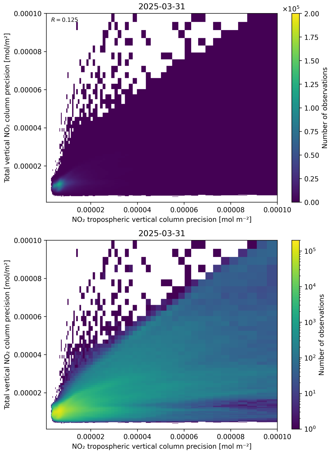
Figure 139: Scatter density plot of “NO 2 tropospheric vertical column precision” against “Total vertical NO 2 column precision” for 2025-03-31 to 2025-03-31.
