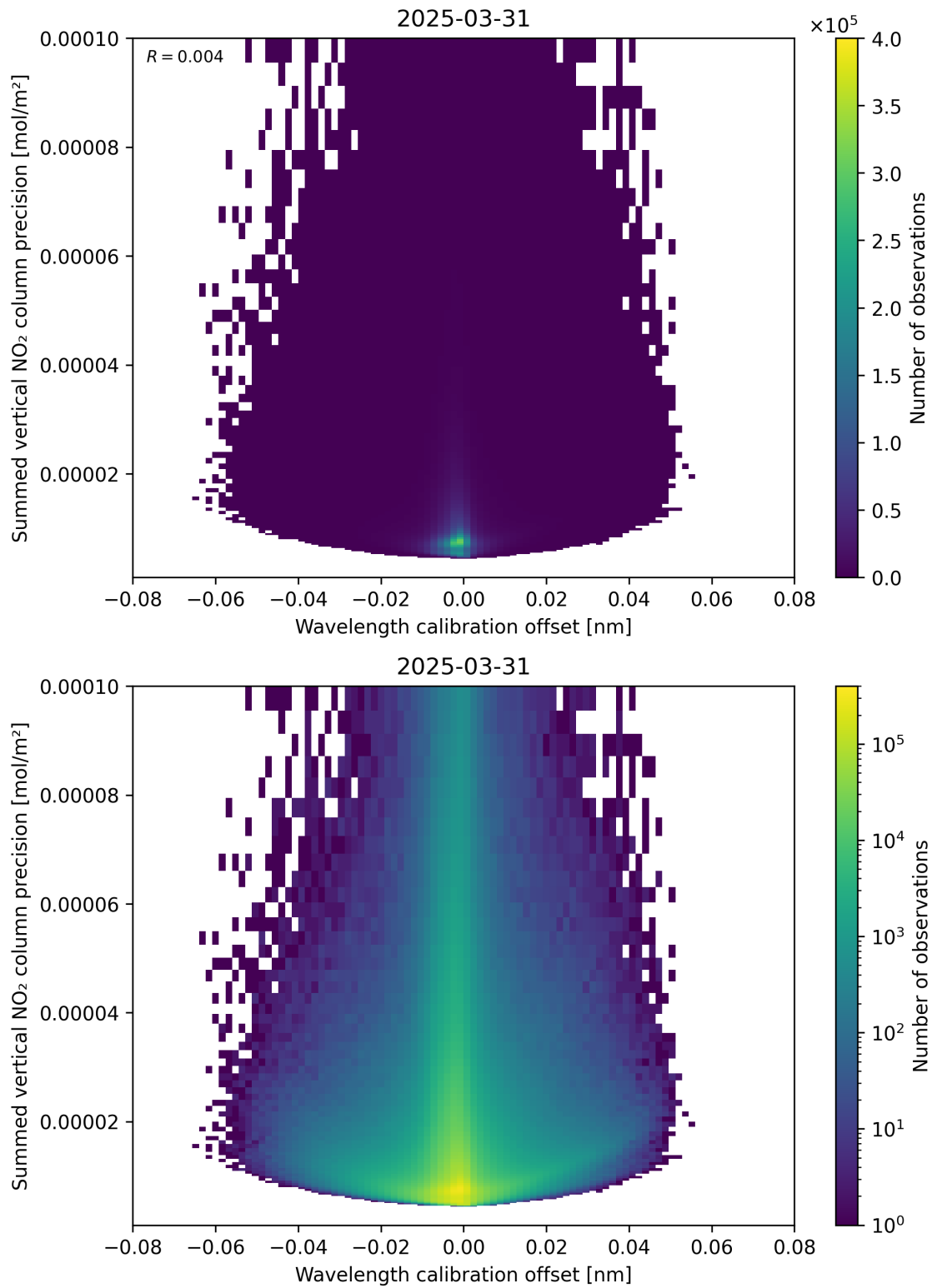
Figure 178: Scatter density plot of “Wavelength calibration offset” against “Summed vertical NO 2 column precision” for 2025-03-31 to 2025-03-31.
