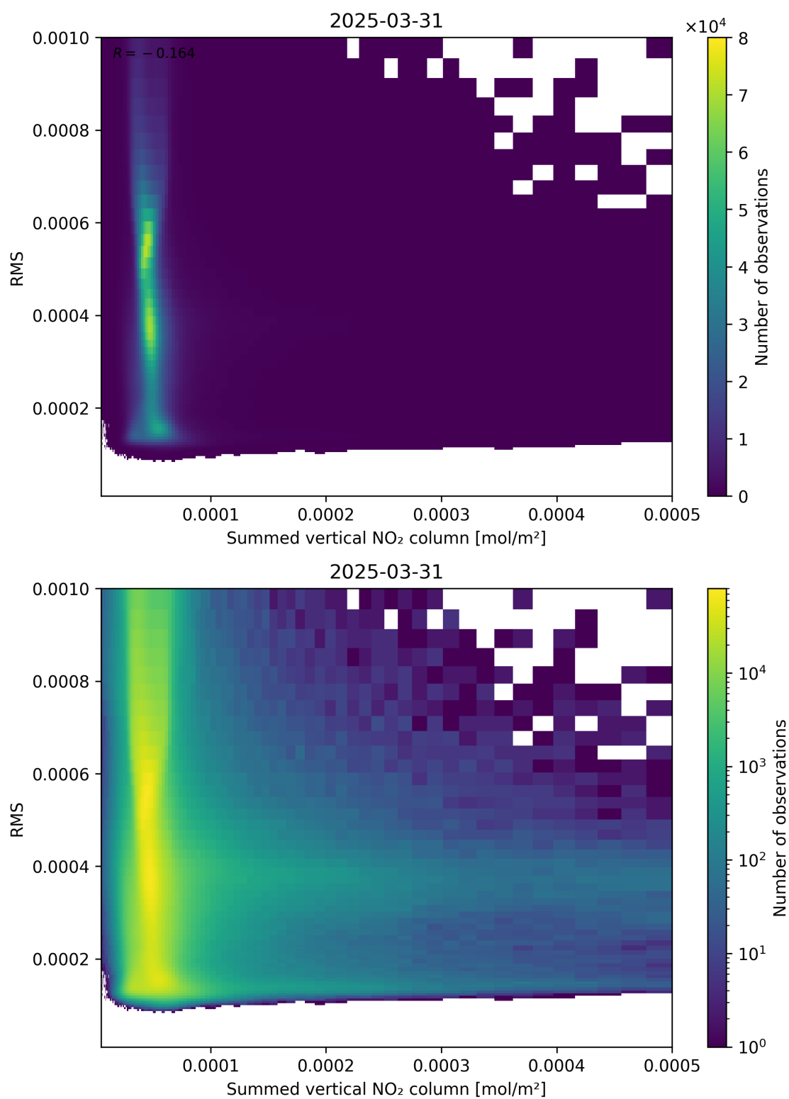
Figure 109: Scatter density plot of “Summed vertical NO 2 column” against “RMS” for 2025-03-31 to 2025-03-31.
