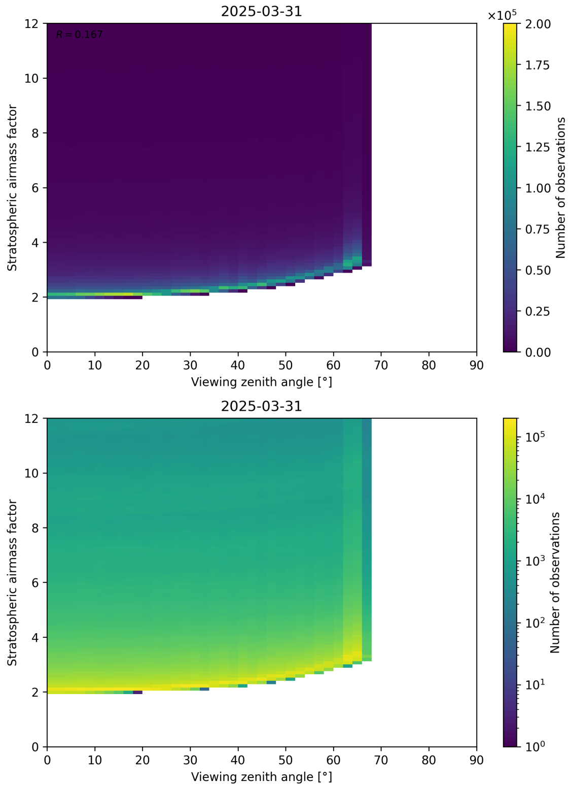
Figure 159: Scatter density plot of “Viewing zenith angle” against “Stratospheric airmass factor” for 2025-03-31 to 2025-03-31.
