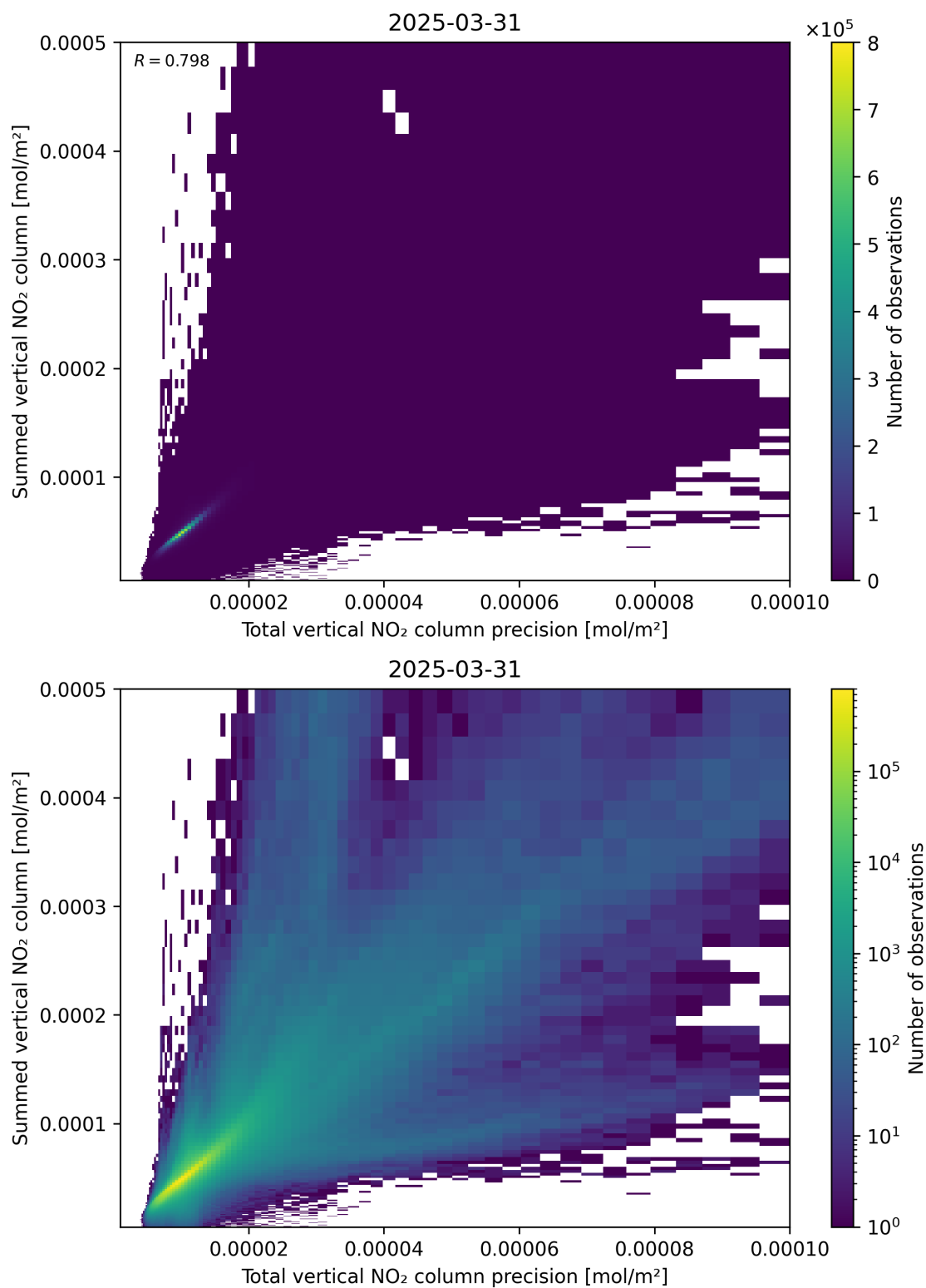
Figure 117: Scatter density plot of “Total vertical NO 2 column precision” against “Summed vertical NO 2 column” for 2025-03-31 to 2025-03-31.
