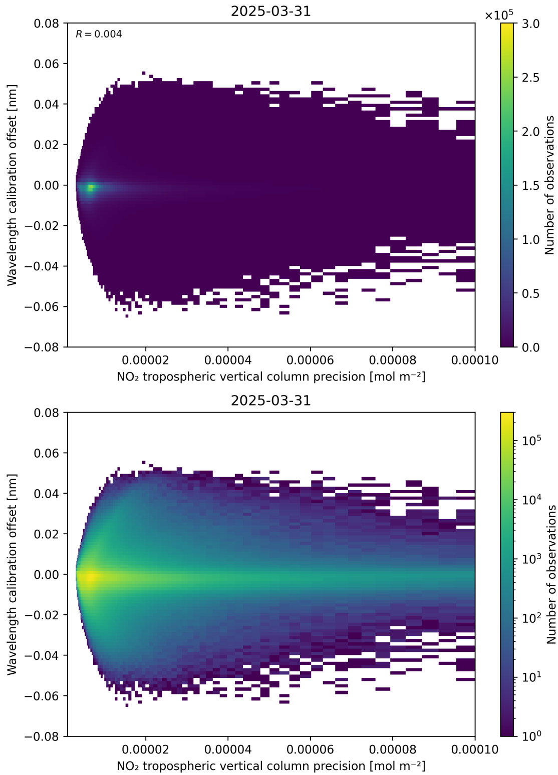
Figure 141: Scatter density plot of “NO 2 tropospheric vertical column precision” against “Wavelength calibration offset” for 2025-03-31 to 2025-03-31.
