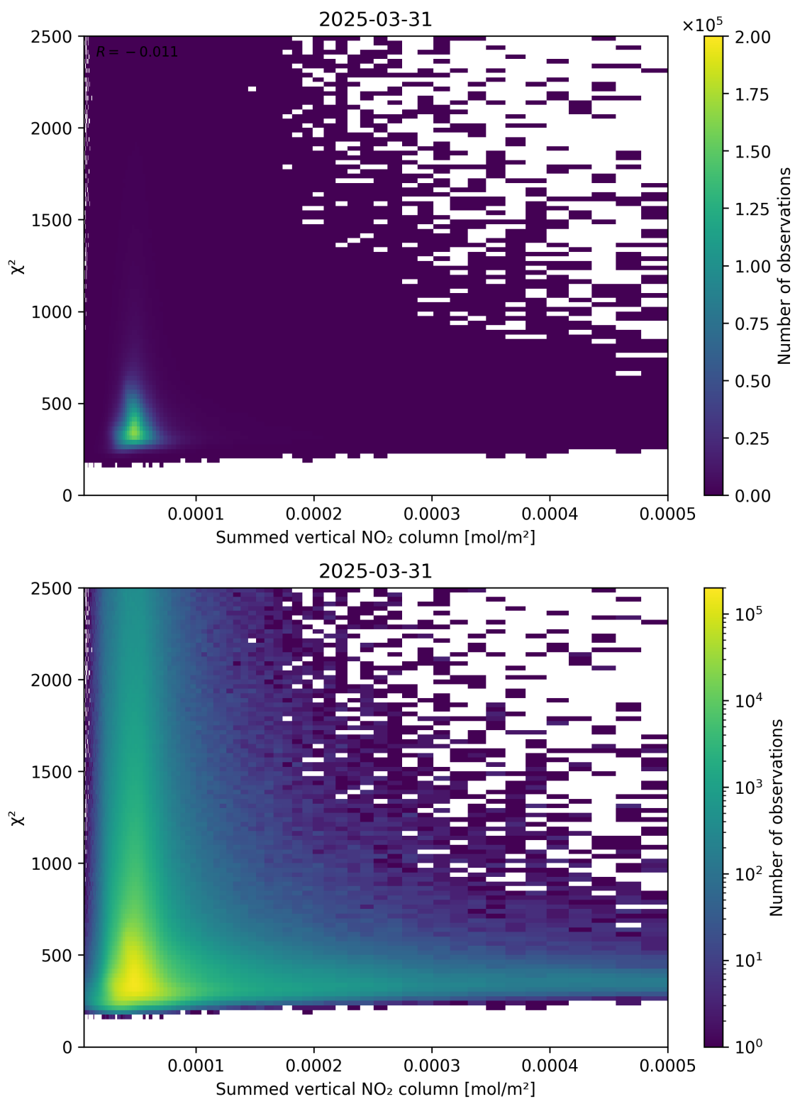
Figure 104: Scatter density plot of “Summed vertical NO 2 column” against “ \chi^2 ” for 2025-03-31 to 2025-03-31.
