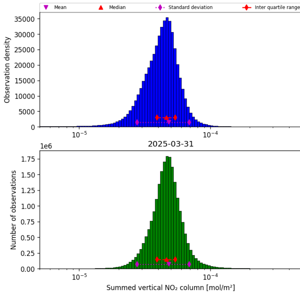
Figure 40: Histogram of "Summed vertical NO 2 column" for 2025-03-31 to 2025-03-31
