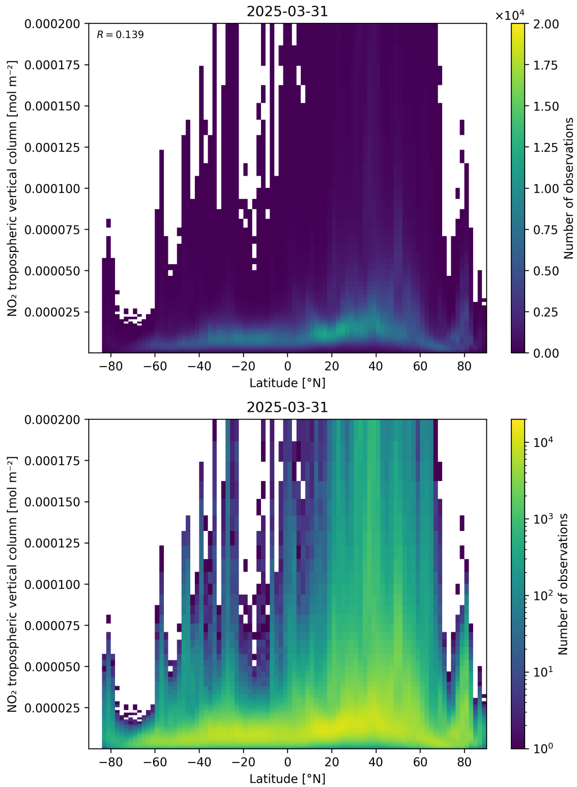
Figure 92: Scatter density plot of “Latitude” against “NO 2 tropospheric vertical column” for 2025-03-31 to 2025-03-31.
