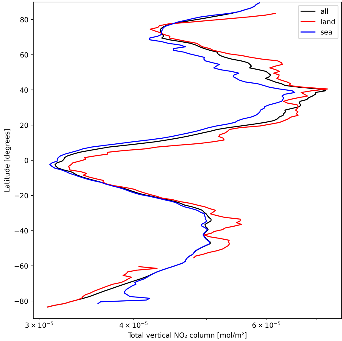
Figure 21: Zonal average of “Total vertical NO 2 column” for 2025-03-31 to 2025-03-31.
