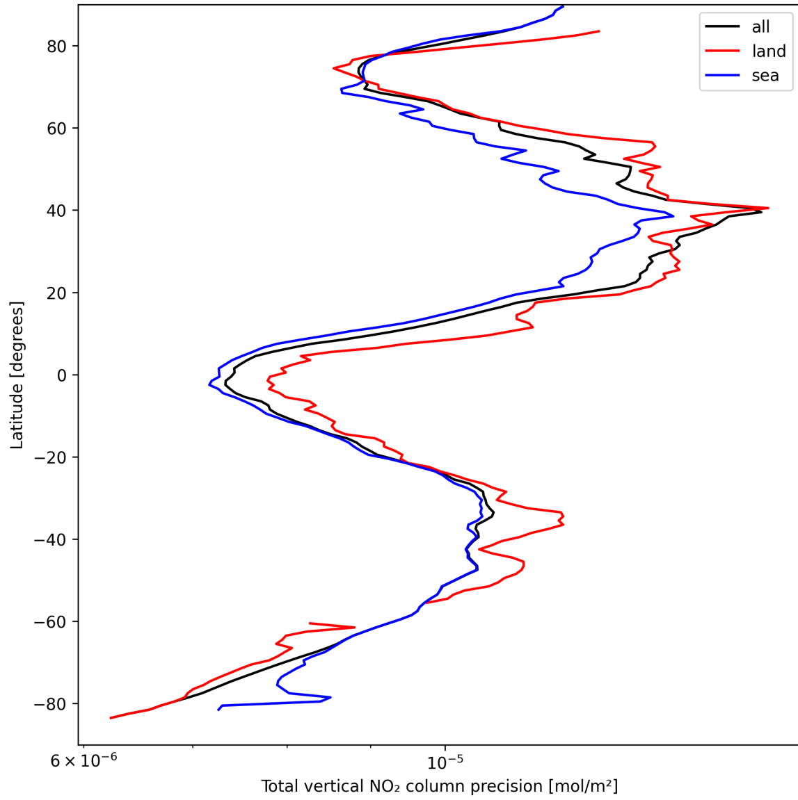
Figure 22: Zonal average of “Total vertical NO 2 column precision” for 2025-03-31 to 2025-03-31.
