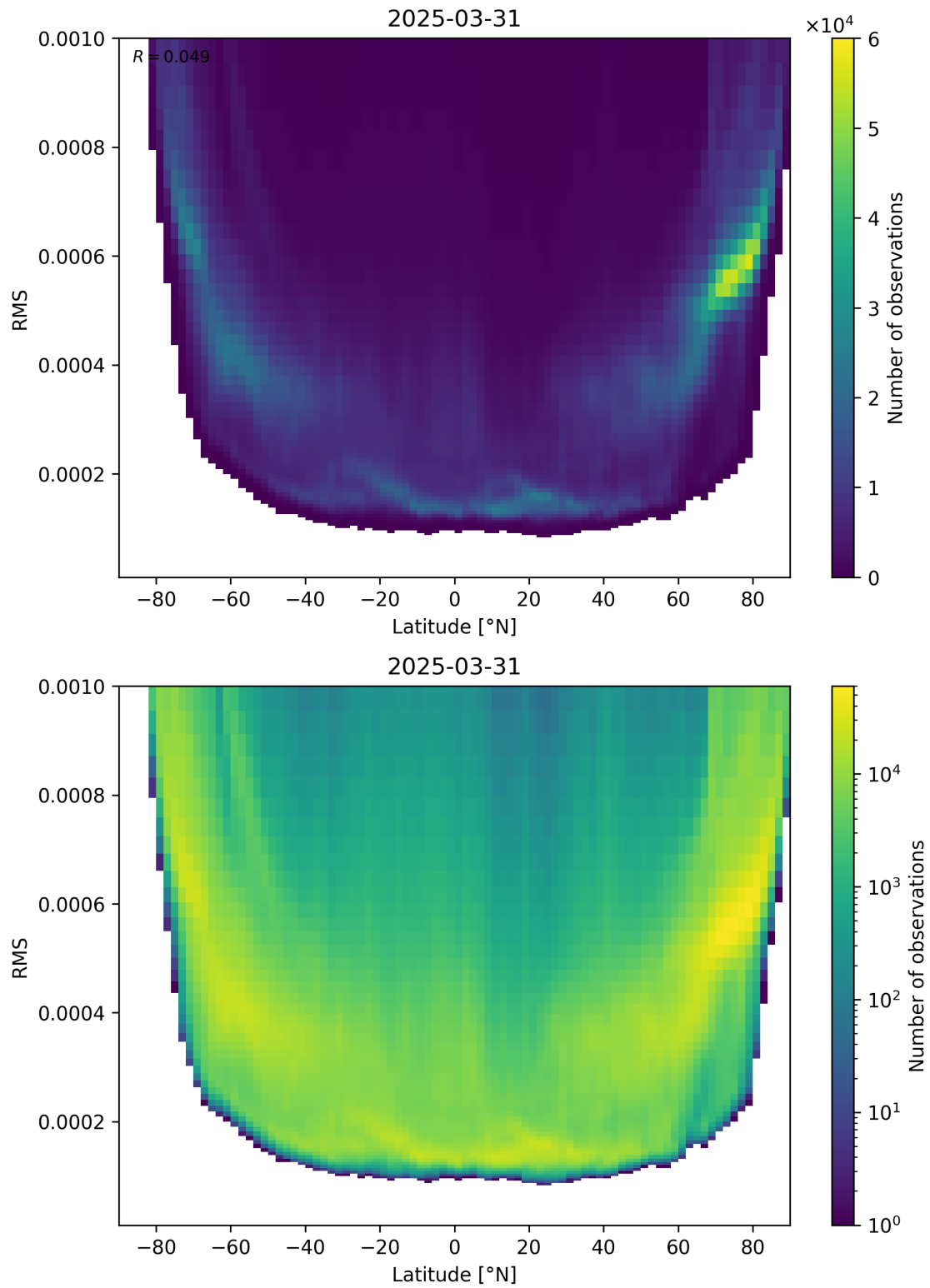
Figure 94: Scatter density plot of “Latitude” against “RMS” for 2025-03-31 to 2025-03-31.
