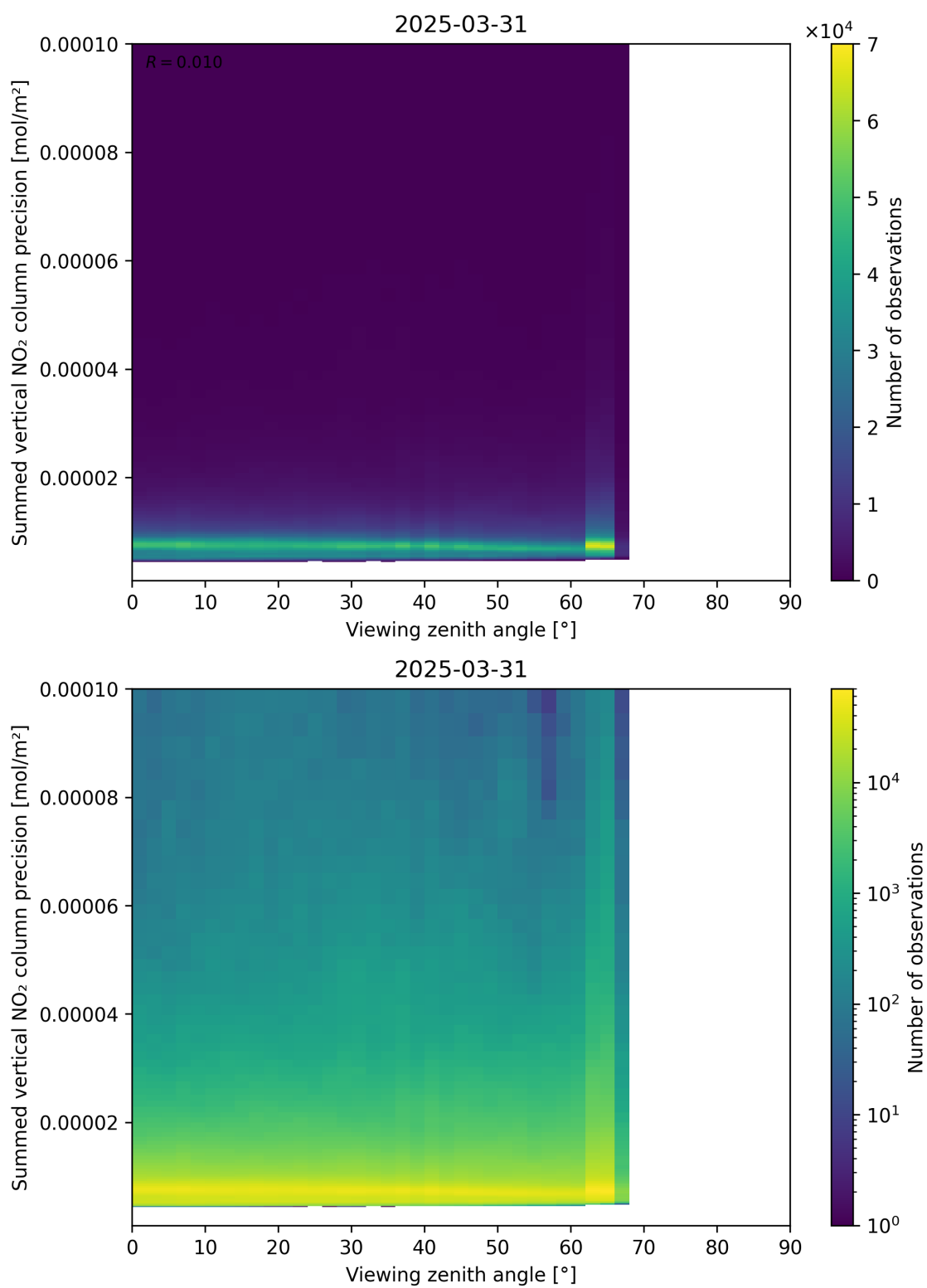
Figure 166: Scatter density plot of “Viewing zenith angle” against “Summed vertical NO 2 column precision” for 2025-03-31 to 2025-03-31.
