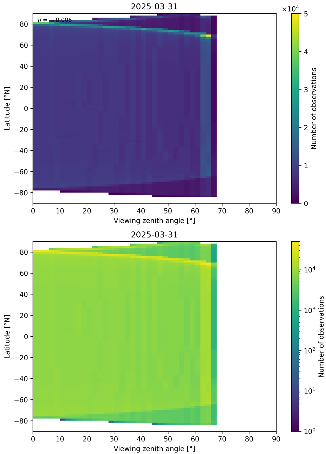
Figure 163: Scatter density plot of “Viewing zenith angle” against “Latitude” for 2025-03-31 to 2025-03-31.
