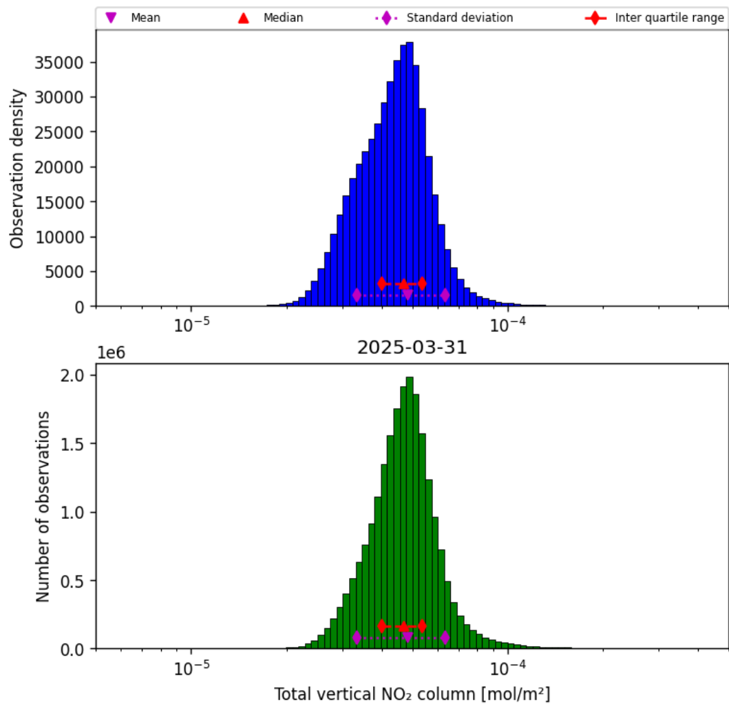
Figure 38: Histogram of “Total vertical NO 2 column” for 2025-03-31 to 2025-03-31
