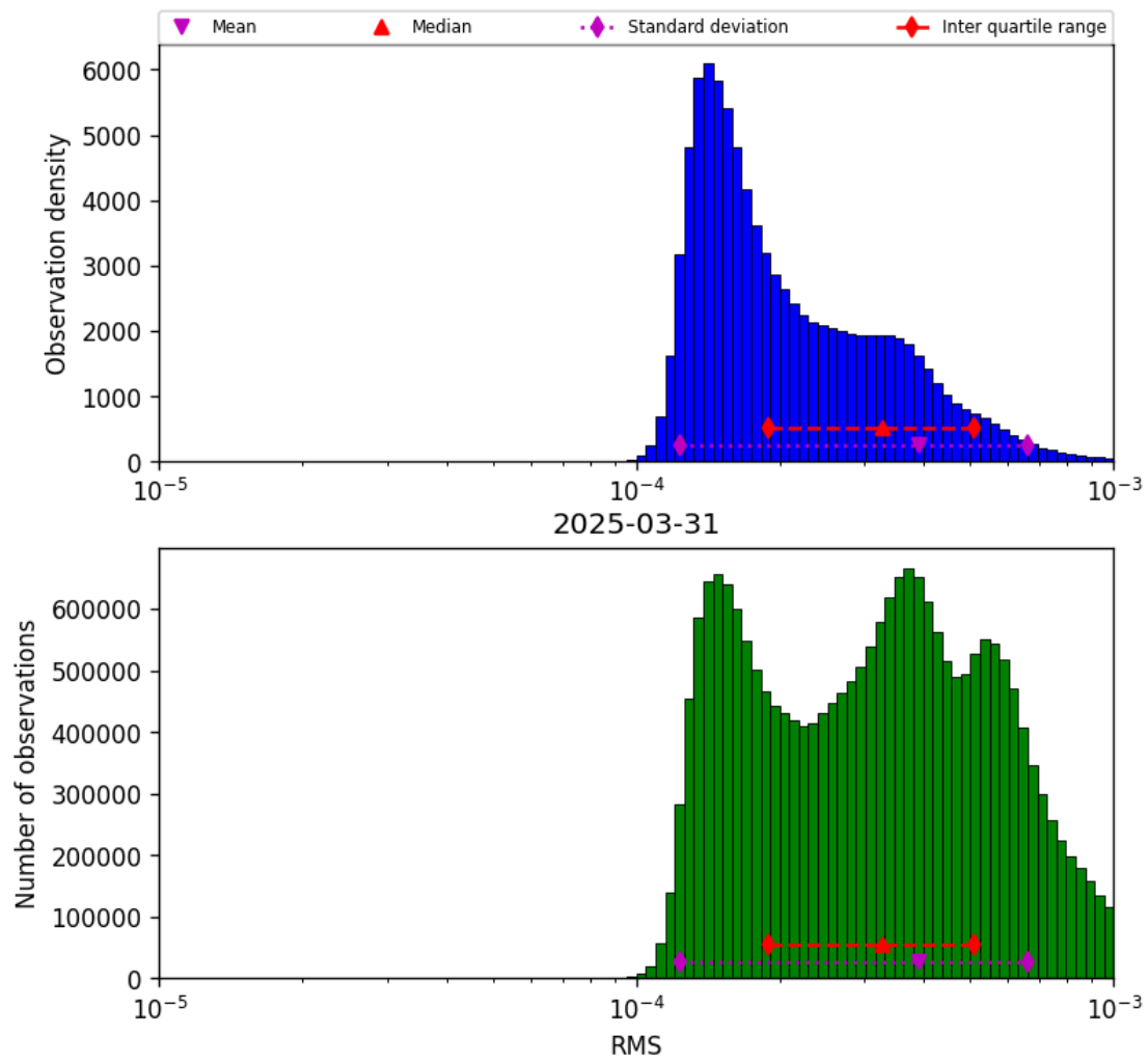
Figure 43: Histogram of “RMS” for 2025-03-31 to 2025-03-31
