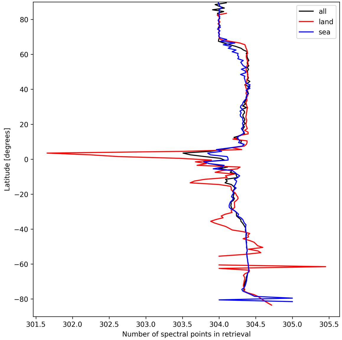
Figure 16: Zonal average of “Number of spectral points in retrieval” for 2025-03-31 to 2025-03-31.
