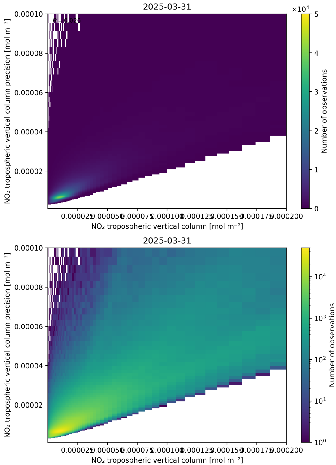
Figure 130: Scatter density plot of “NO 2 tropospheric vertical column” against “NO 2 tropospheric vertical column precision” for 2025-03-31 to 2025-03-31.
