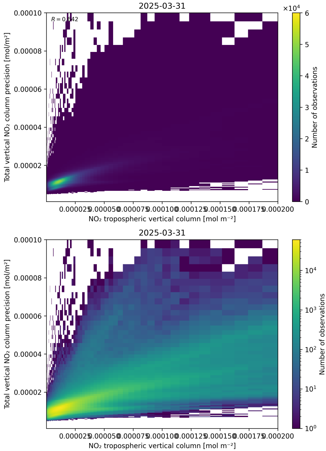
Figure 129: Scatter density plot of “NO 2 tropospheric vertical column” against “Total vertical NO 2 column precision” for 2025-03-31 to 2025-03-31.
