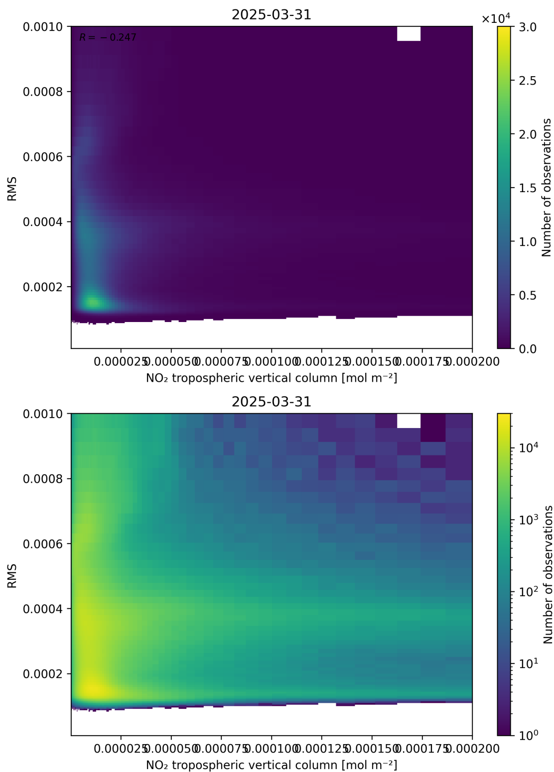
Figure 142: Scatter density plot of “NO 2 tropospheric vertical column” against “RMS” for 2025-03-31 to 2025-03-31.
