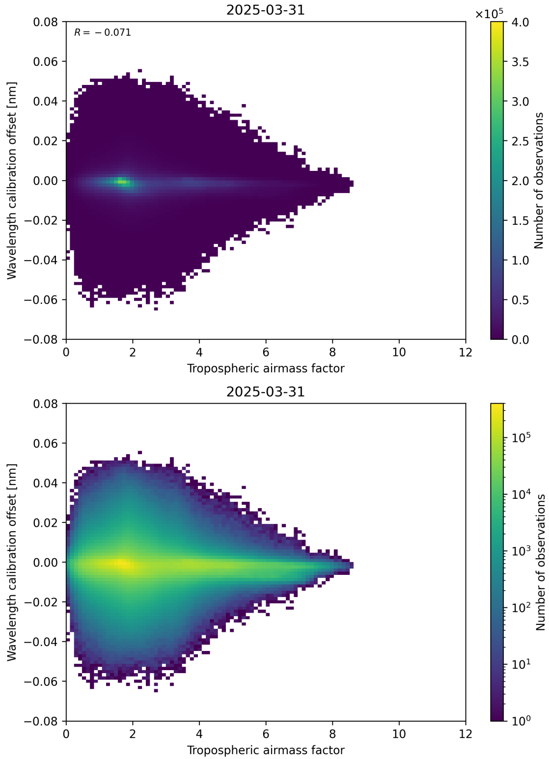
Figure 80: Scatter density plot of “Tropospheric airmass factor” against “Wavelength calibration offset” for 2025-03-31 to 2025-03-31.
