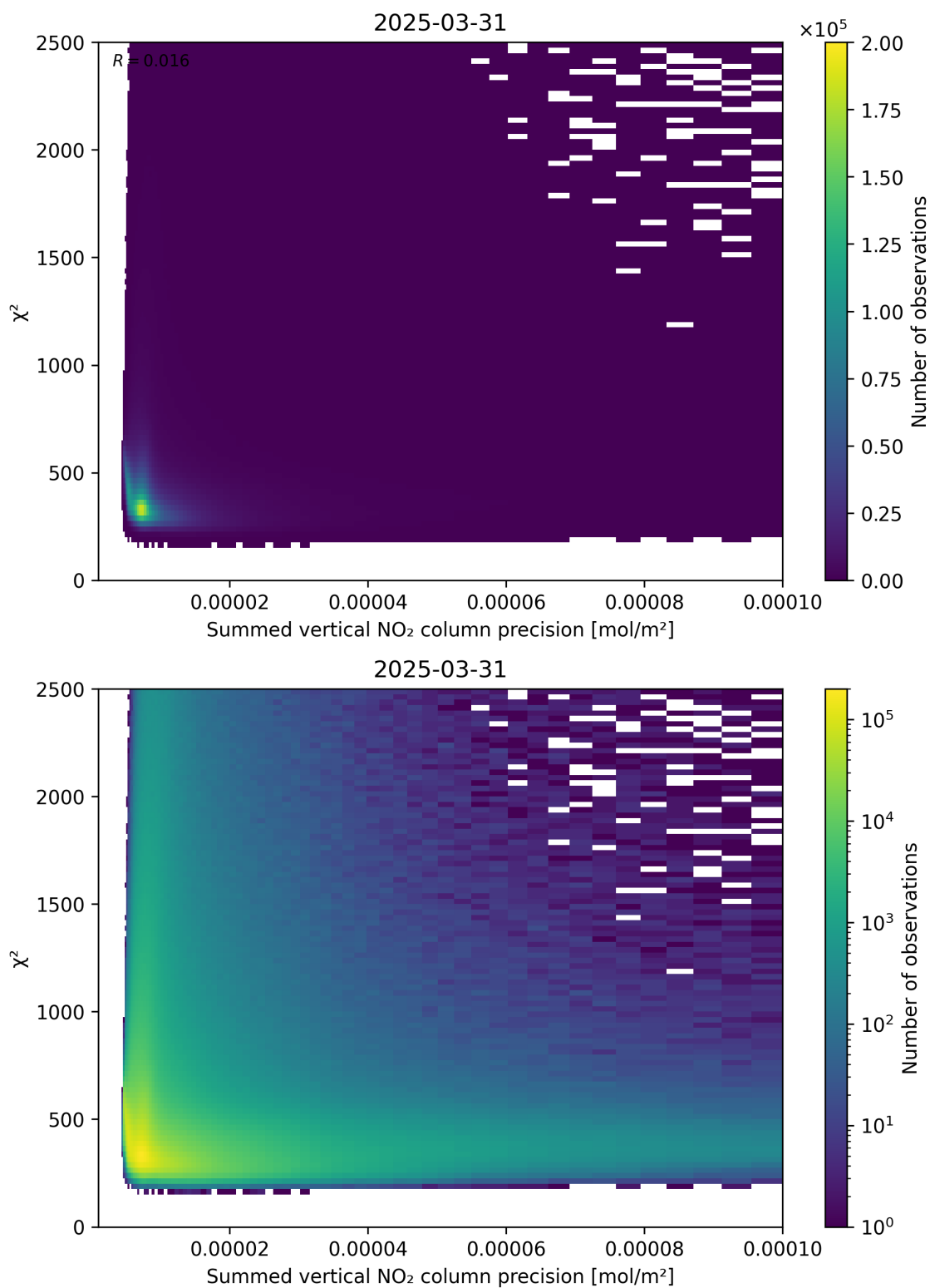
Figure 107: Scatter density plot of “Summed vertical NO 2 column precision” against “ \chi^2 ” for 2025-03-31 to 2025-03-31.
