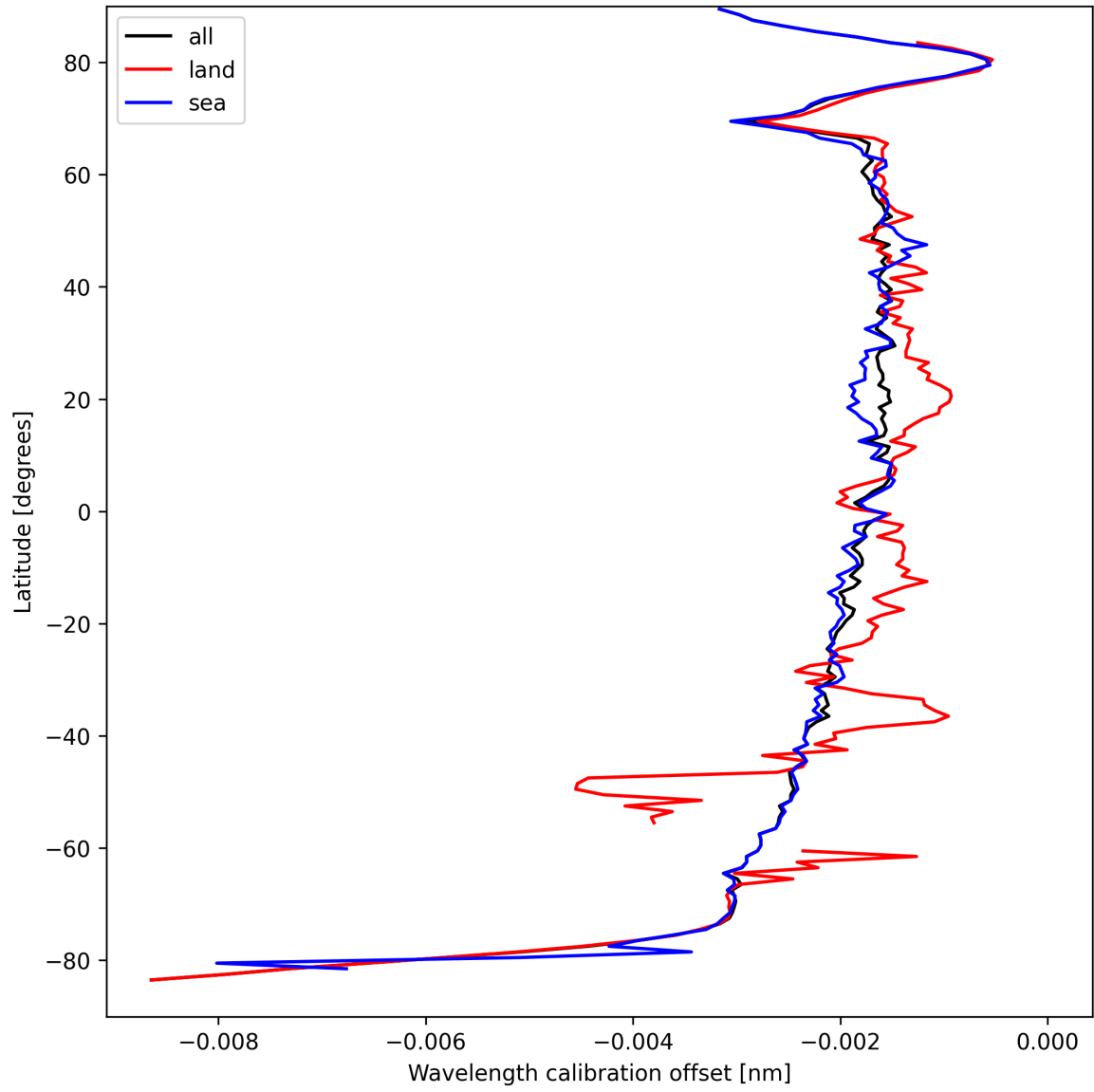
Figure 18: Zonal average of “Wavelength calibration offset” for 2025-03-31 to 2025-03-31.
