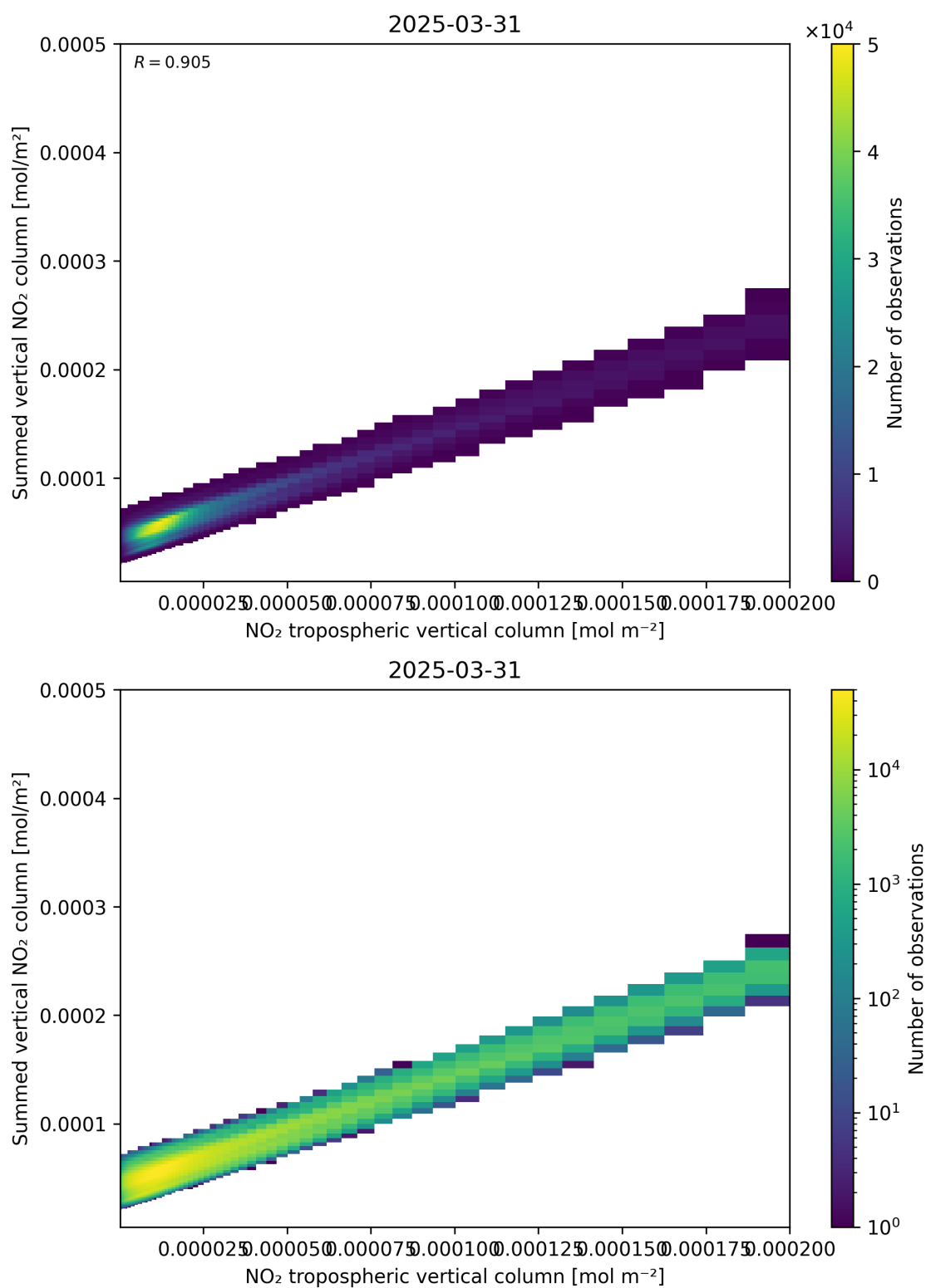
Figure 126: Scatter density plot of “NO 2 tropospheric vertical column” against “Summed vertical NO 2 column” for 2025-03-31 to 2025-03-31.
