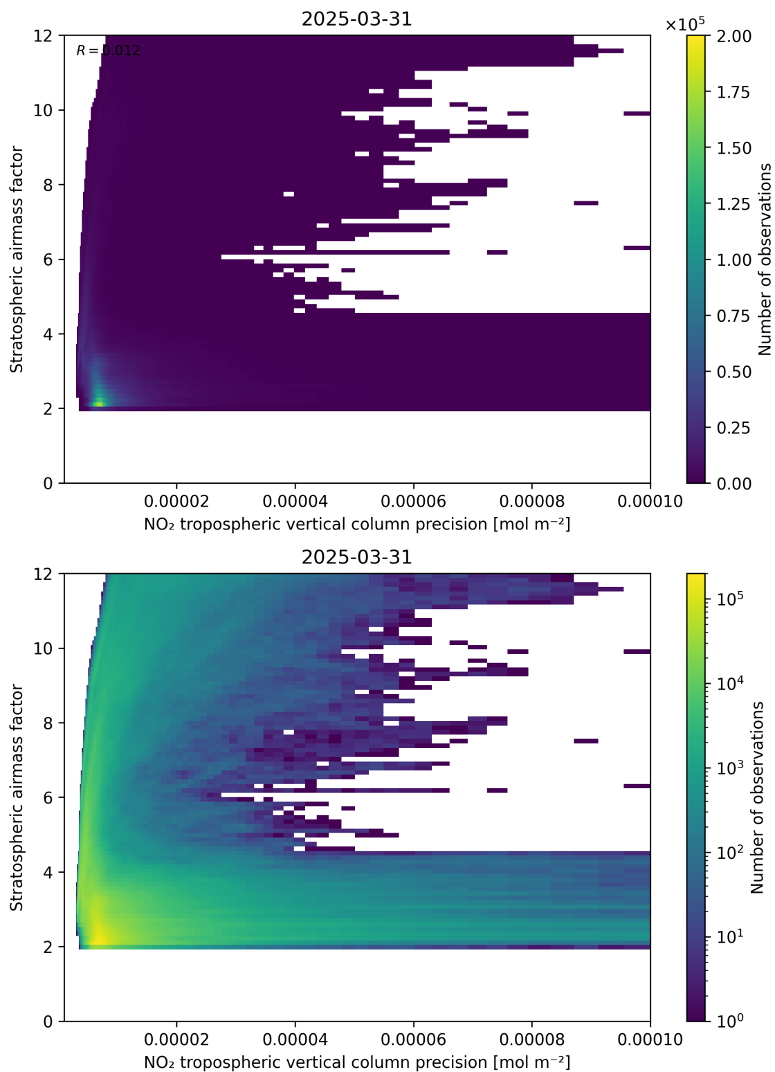
Figure 131: Scatter density plot of “NO 2 tropospheric vertical column precision” against “Stratospheric airmass factor” for 2025-03-31 to 2025-03-31.
