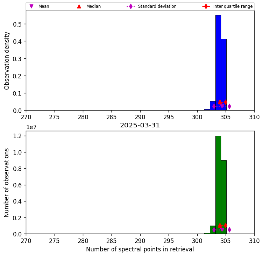
Figure 33: Histogram of “Number of spectral points in retrieval” for 2025-03-31 to 2025-03-31
