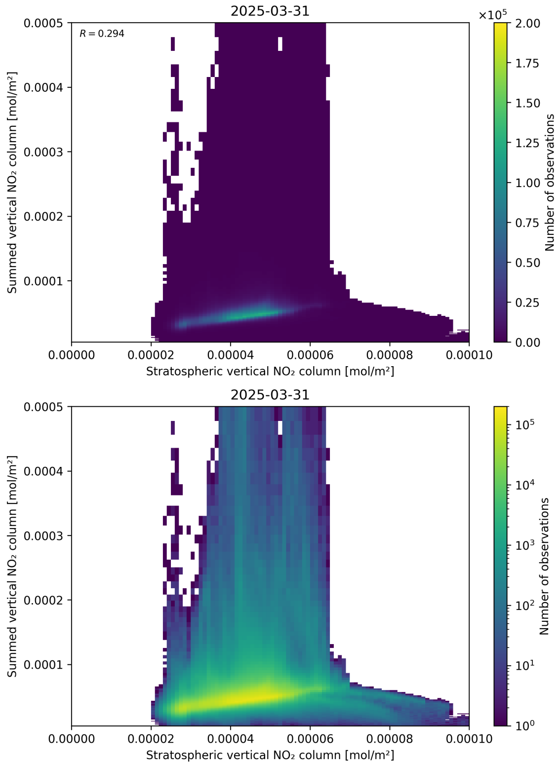
Figure 98: Scatter density plot of “Stratospheric vertical NO 2 column” against “Summed vertical NO 2 column” for 2025-03-31 to 2025-03-31.
