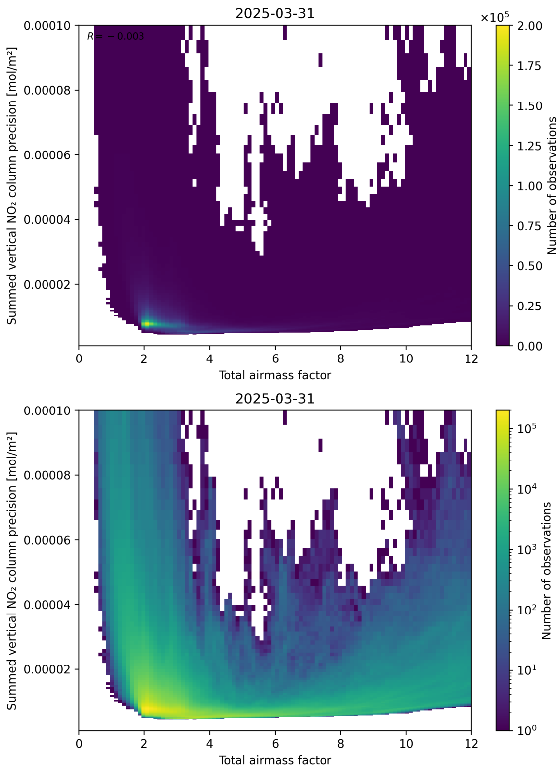
Figure 66: Scatter density plot of “Total airmass factor” against “Summed vertical NO 2 column precision” for 2025-03-31 to 2025-03-31.
