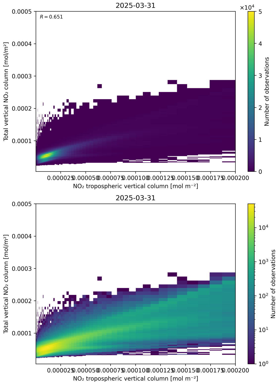
Figure 128: Scatter density plot of “NO 2 tropospheric vertical column” against “Total vertical NO 2 column” for 2025-03-31 to 2025-03-31.
