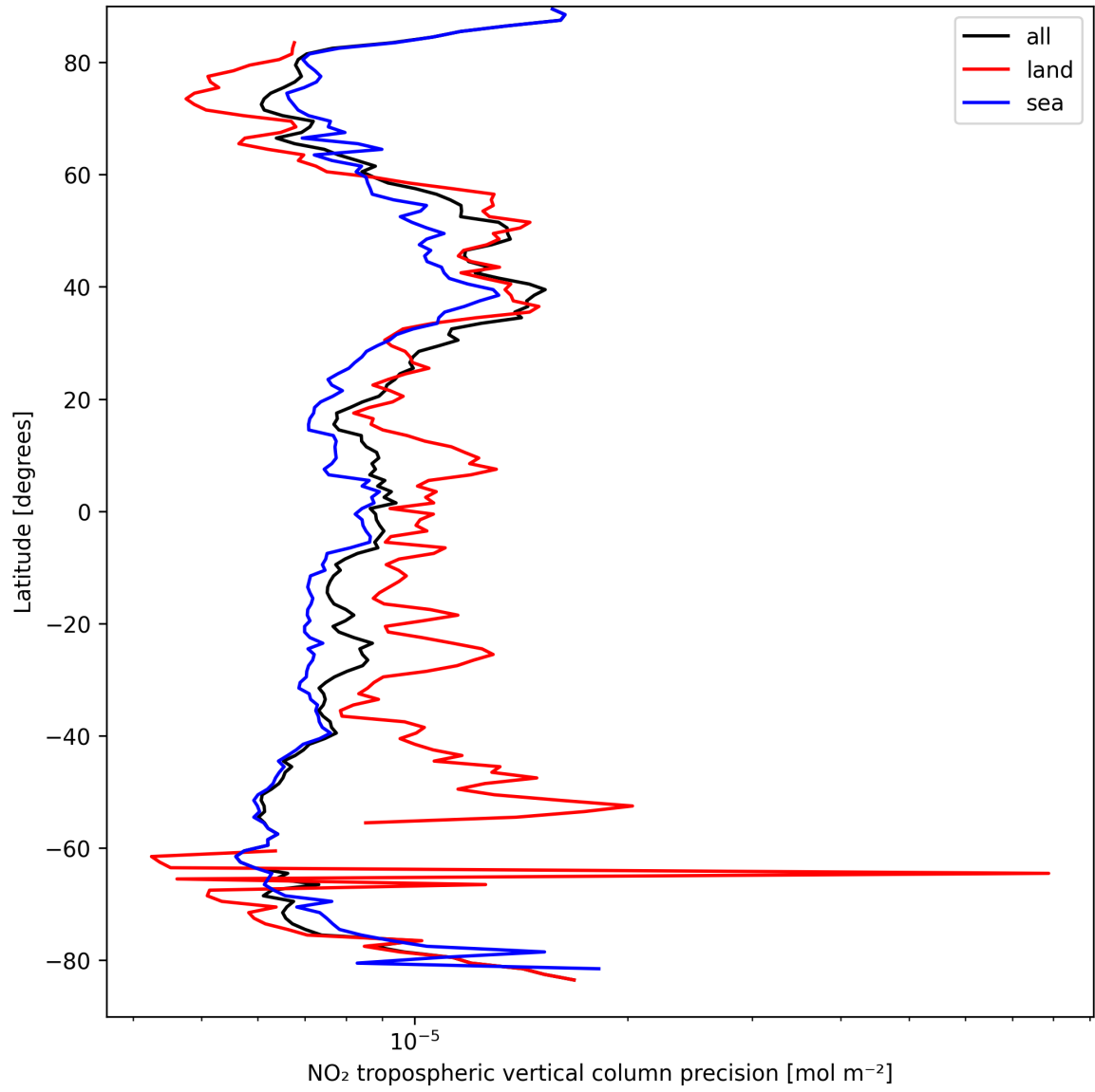
Figure 13: Zonal average of “NO 2 tropospheric vertical column precision” for 2025-03-31 to 2025-03-31.
