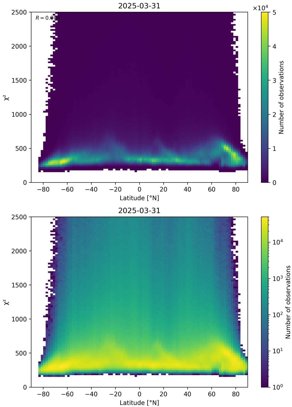
Figure 86: Scatter density plot of “Latitude” against “ \chi^2 ” for 2025-03-31 to 2025-03-31.
