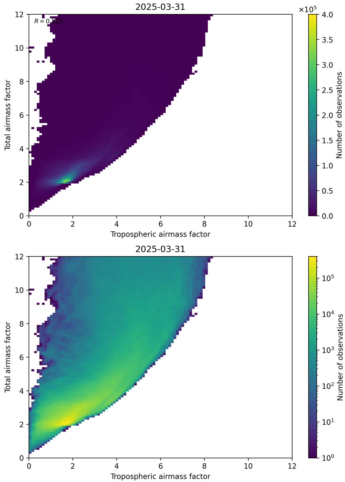
Figure 72: Scatter density plot of “Tropospheric airmass factor” against “Total airmass factor” for 2025-03-31 to 2025-03-31.
