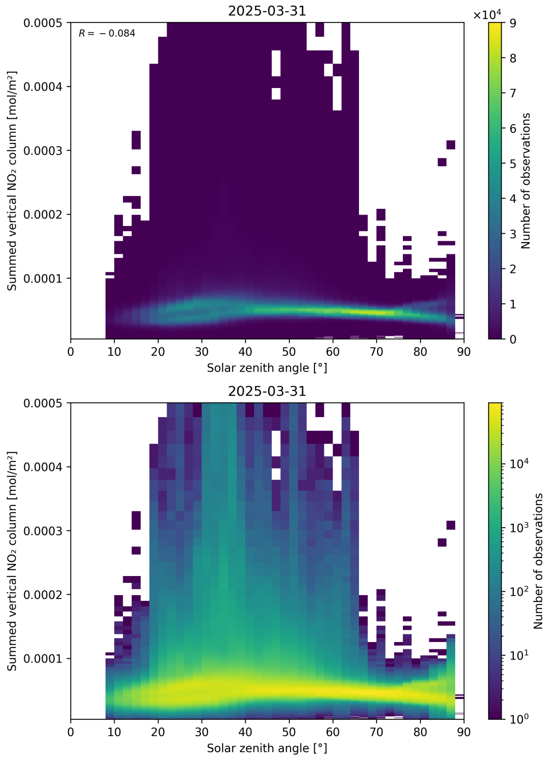
Figure 151: Scatter density plot of “Solar zenith angle” against “Summed vertical NO 2 column” for 2025-03-31 to 2025-03-31.
