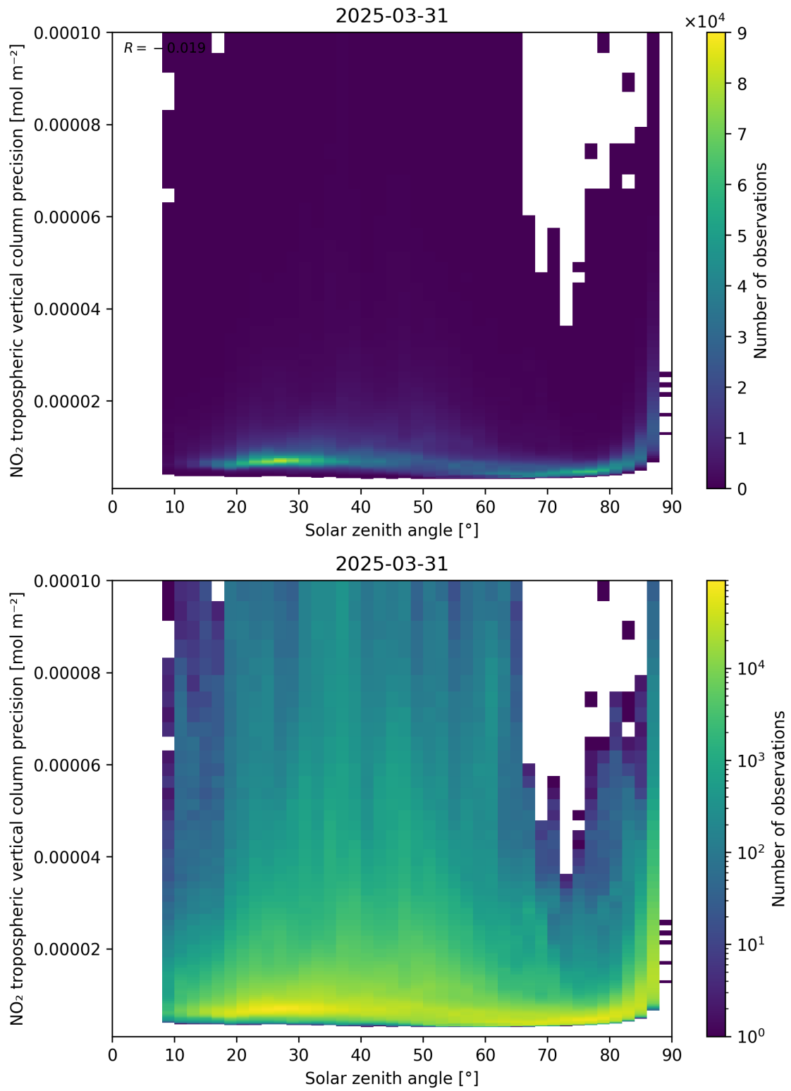
Figure 156: Scatter density plot of “Solar zenith angle” against “NO 2 tropospheric vertical column precision” for 2025-03-31 to 2025-03-31.
