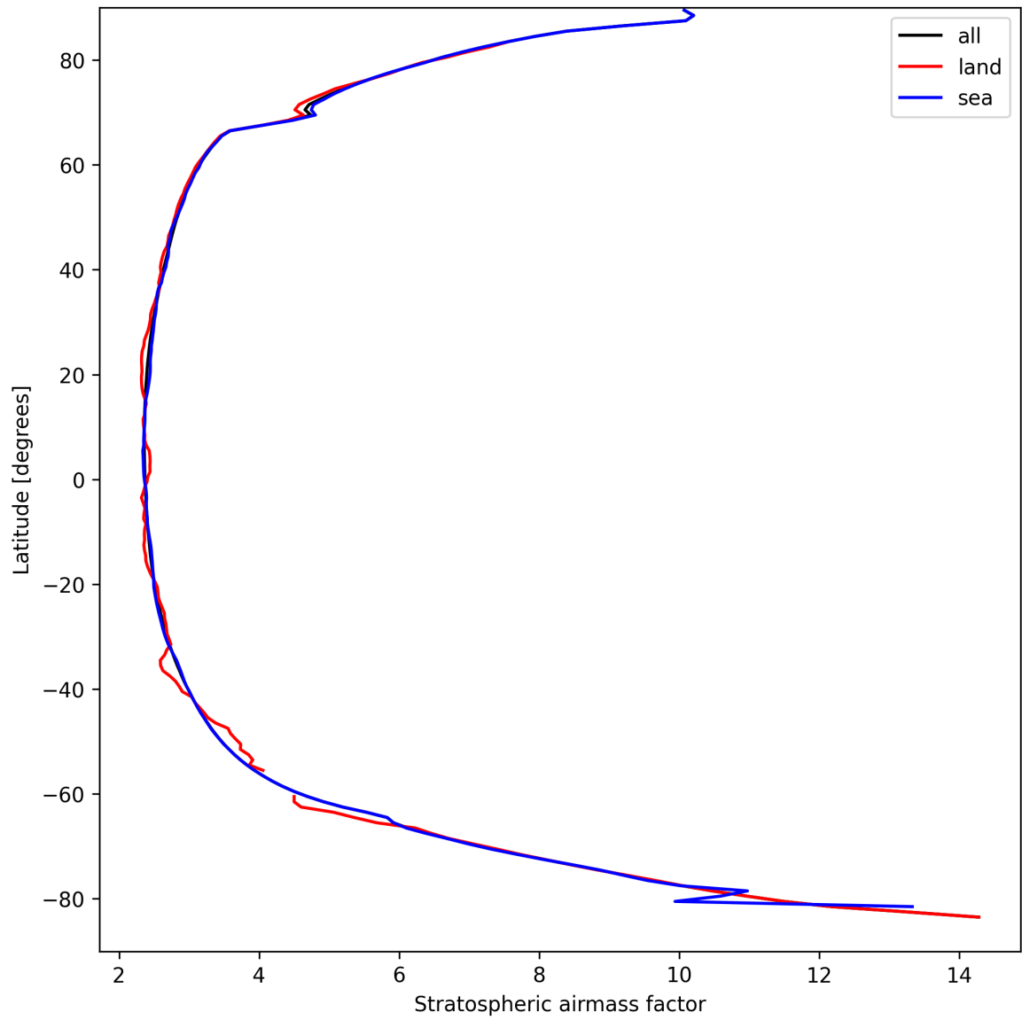
Figure 27: Zonal average of “Stratospheric air mass factor” for 2025-03-31 to 2025-03-31.
