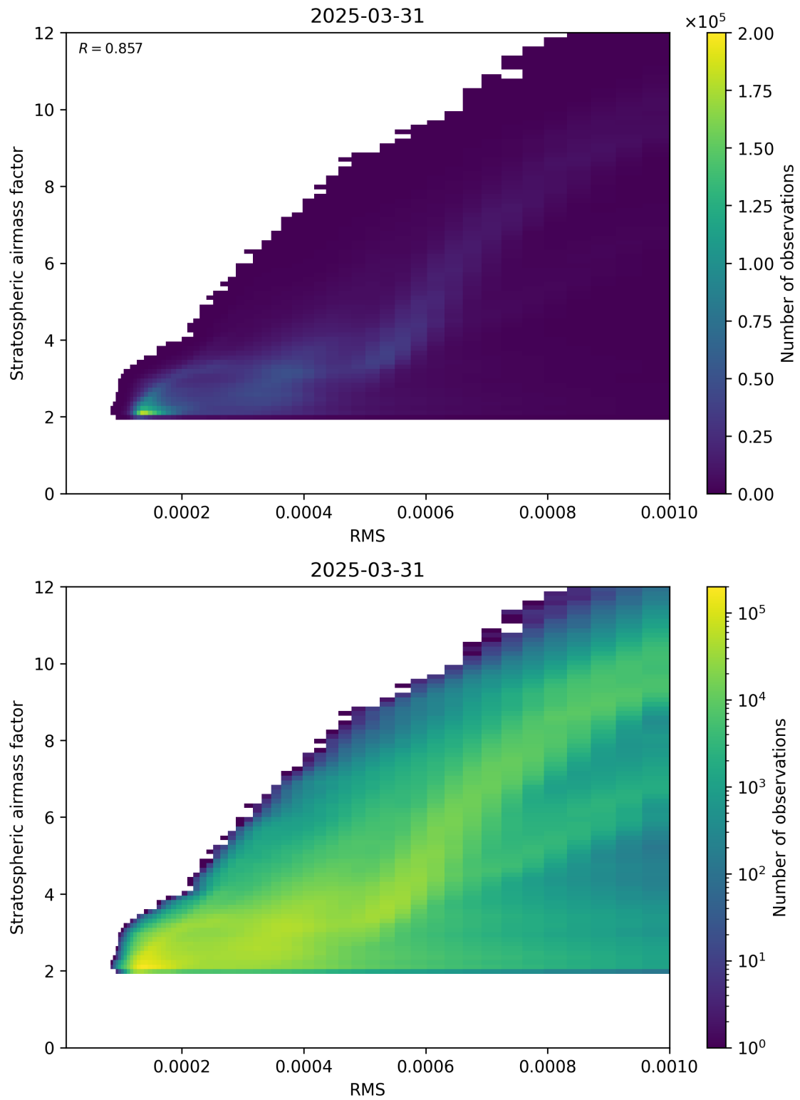
Figure 144: Scatter density plot of “RMS” against “Stratospheric airmass factor” for 2025-03-31 to 2025-03-31.
