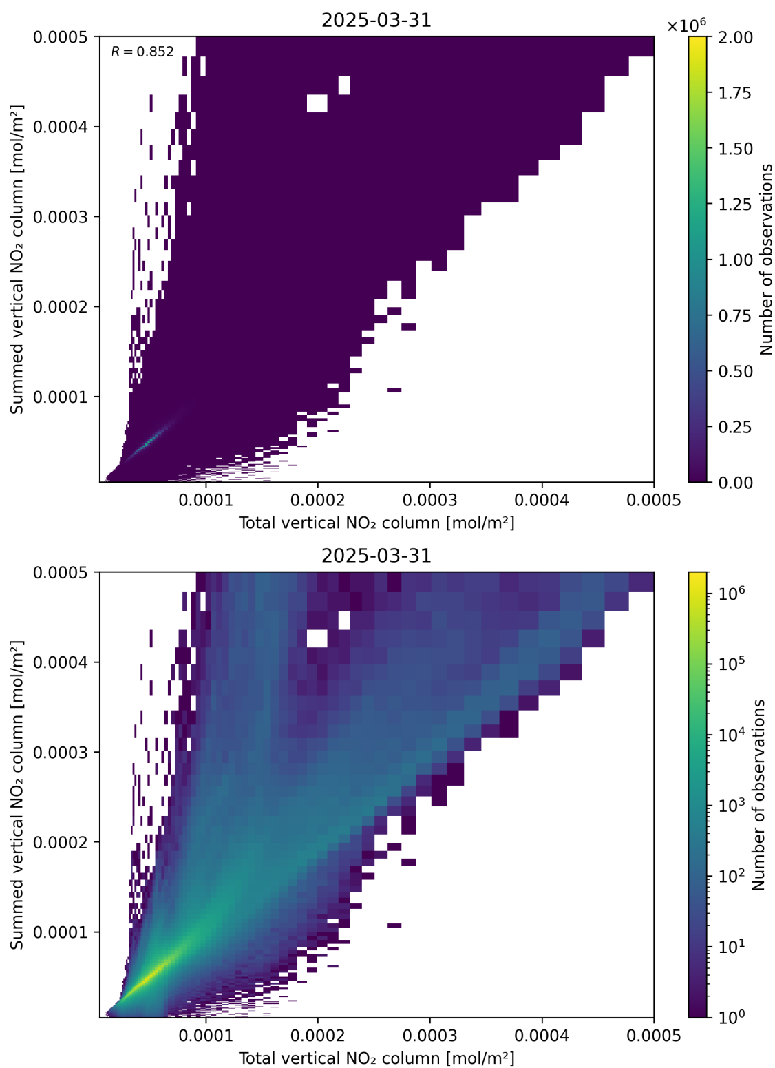
Figure 112: Scatter density plot of “Total vertical NO 2 column” against “Summed vertical NO 2 column” for 2025-03-31 to 2025-03-31.
