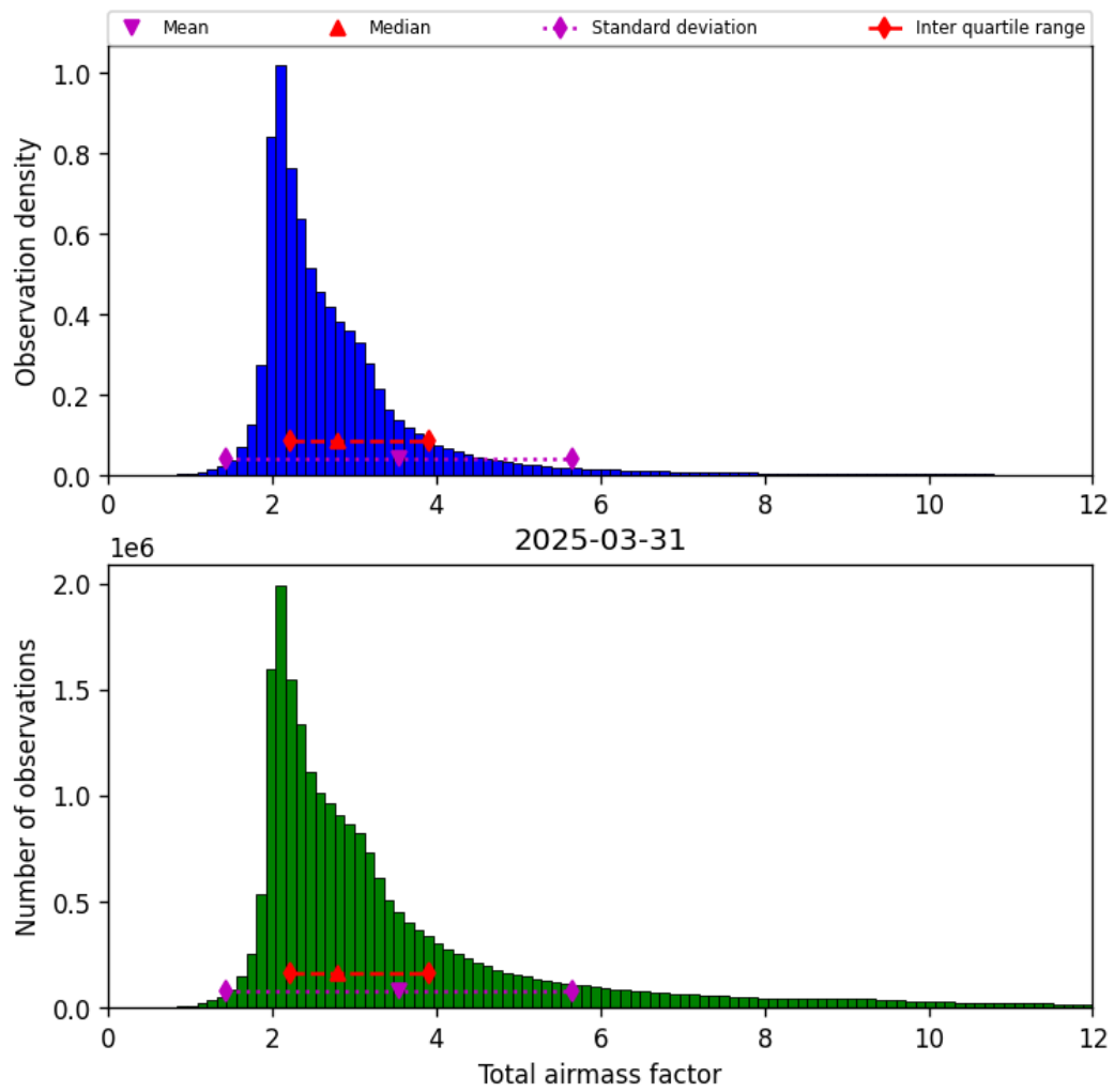
Figure 32: Histogram of “Total airmass factor” for 2025-03-31 to 2025-03-31
