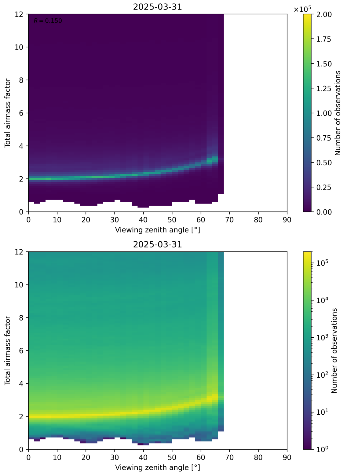
Figure 160: Scatter density plot of “Viewing zenith angle” against “Total airmass factor” for 2025-03-31 to 2025-03-31.
