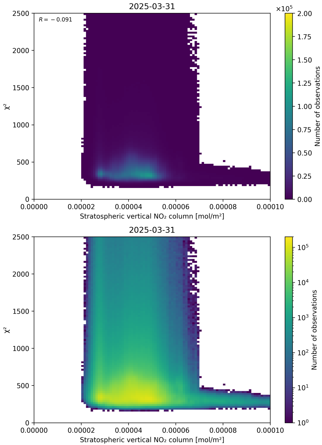
Figure 97: Scatter density plot of “Stratospheric vertical NO 2 column” against “ \chi^2 ” for 2025-03-31 to 2025-03-31.
