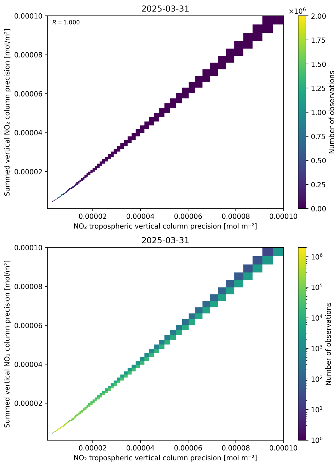
Figure 137: Scatter density plot of “NO 2 tropospheric vertical column precision” against “Summed vertical NO 2 column precision” for 2025-03-31 to 2025-03-31.
