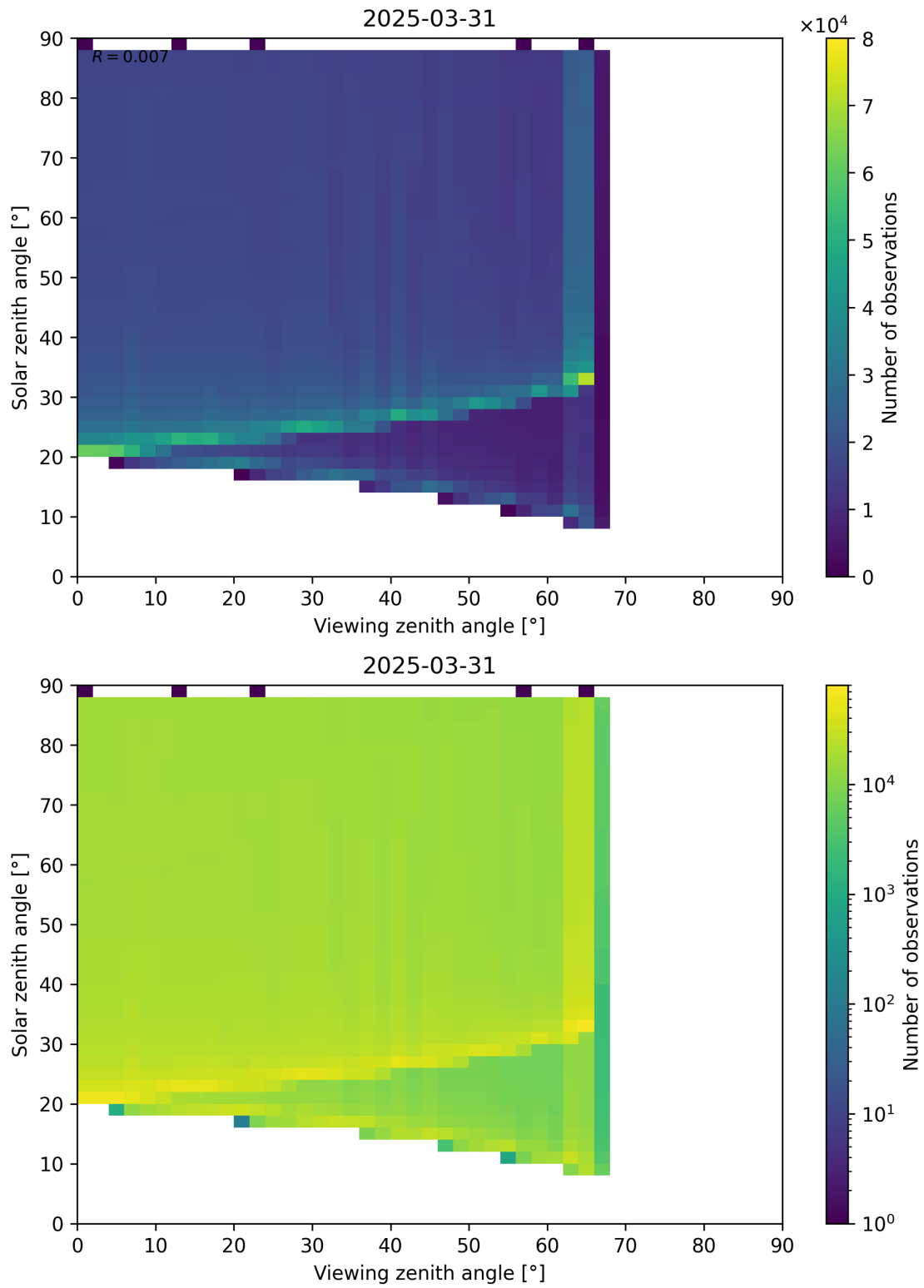
Figure 172: Scatter density plot of “Viewing zenith angle” against “Solar zenith angle” for 2025-03-31 to 2025-03-31.
