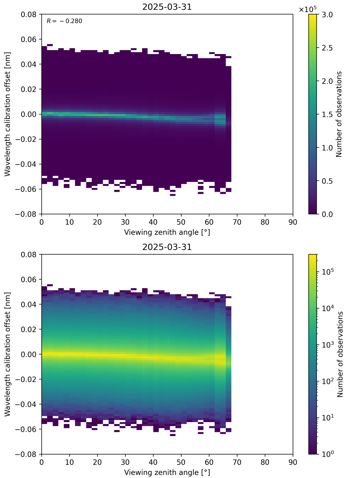
Figure 173: Scatter density plot of “Viewing zenith angle” against “Wavelength calibration offset” for 2025-03-31 to 2025-03-31.
