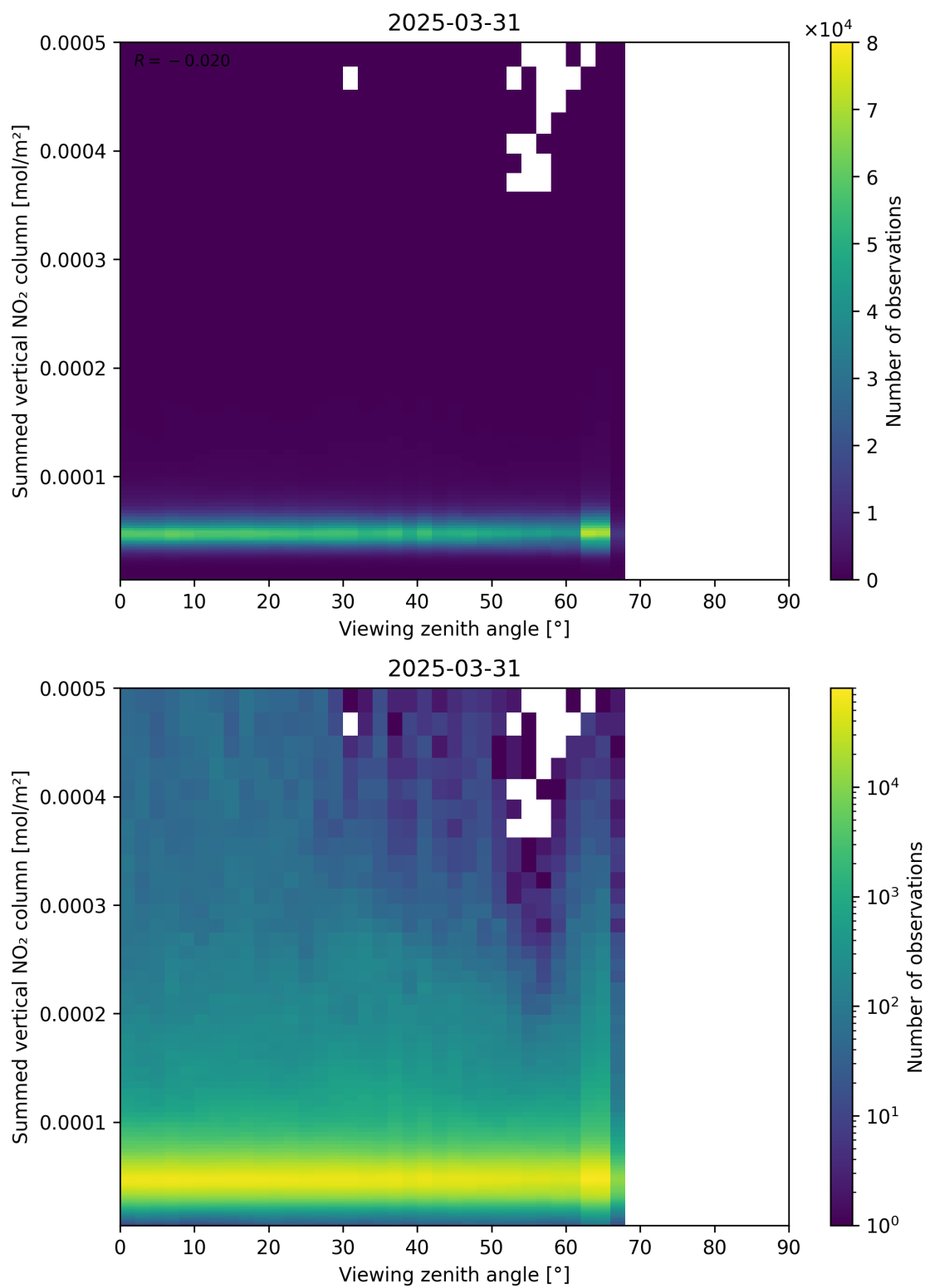
Figure 165: Scatter density plot of “Viewing zenith angle” against “Summed vertical NO 2 column” for 2025-03-31 to 2025-03-31.
