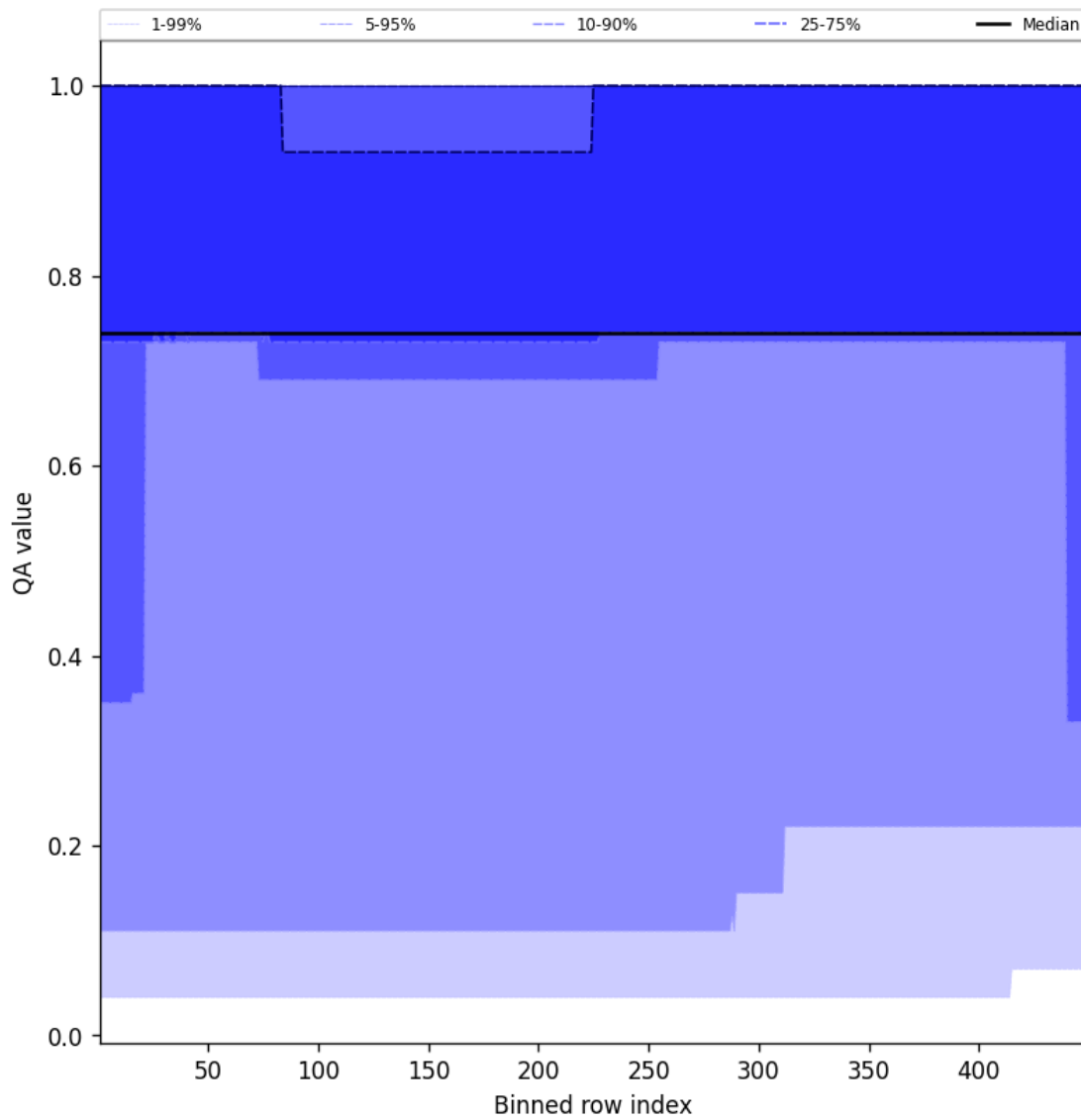
Figure 45: Along track statistics of “QA value” for 2025-03-31 to 2025-03-31
