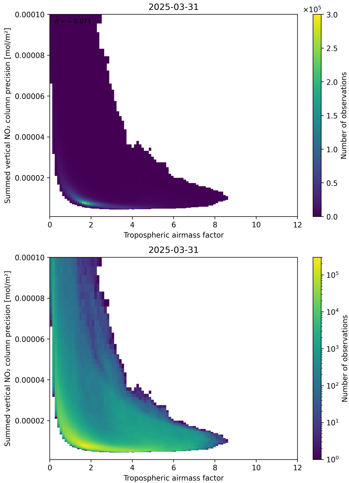
Figure 76: Scatter density plot of “Tropospheric airmass factor” against “Summed vertical NO 2 column precision” for 2025-03-31 to 2025-03-31.
