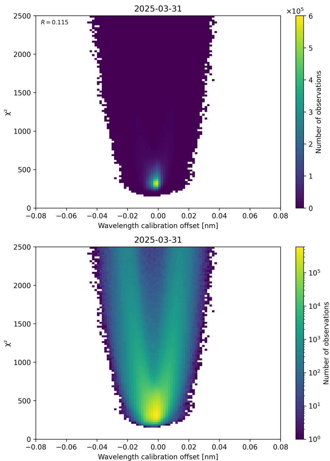
Figure 175: Scatter density plot of “Wavelength calibration offset” against “ \chi^2 ” for 2025-03-31 to 2025-03-31.
