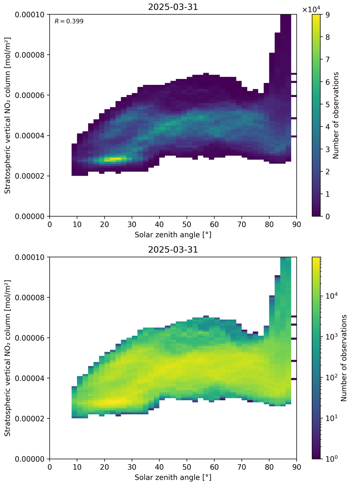
Figure 150: Scatter density plot of “Solar zenith angle” against “Stratospheric vertical NO 2 column” for 2025-03-31 to 2025-03-31.
