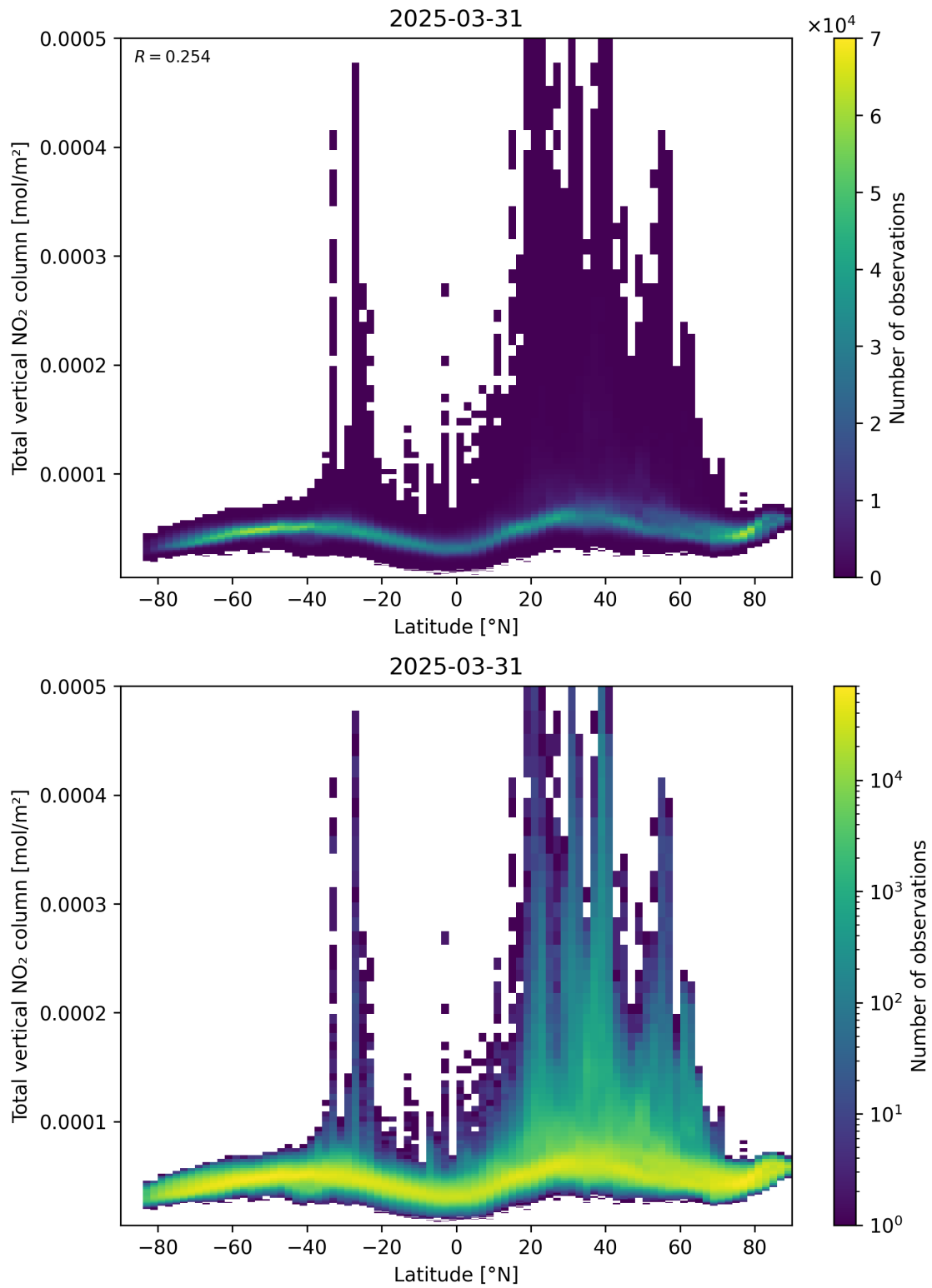
Figure 90: Scatter density plot of “Latitude” against “Total vertical NO 2 column” for 2025-03-31 to 2025-03-31.
