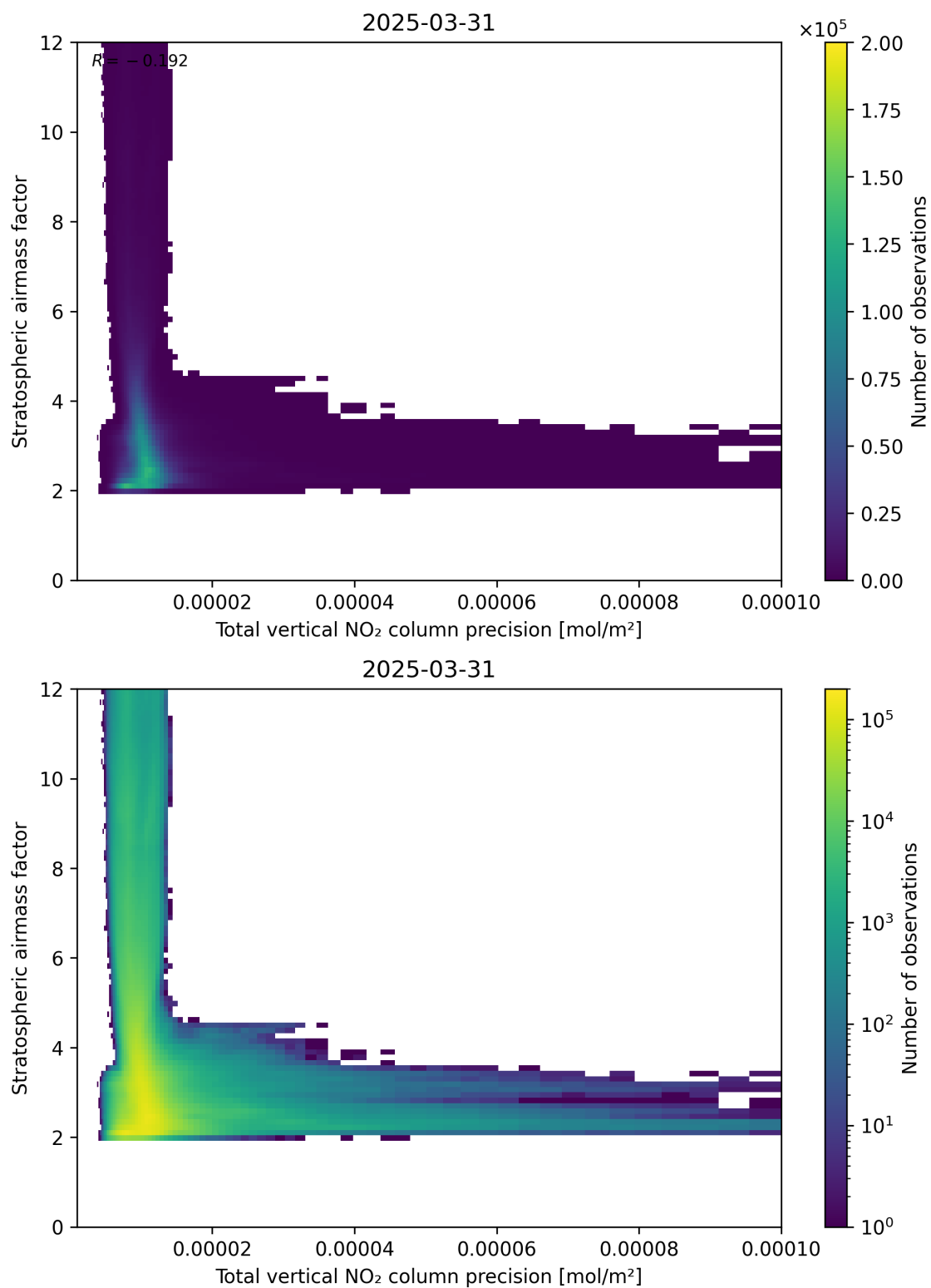
Figure 115: Scatter density plot of “Total vertical NO 2 column precision” against “Stratospheric air mass factor” for 2025-03-31 to 2025-03-31.
