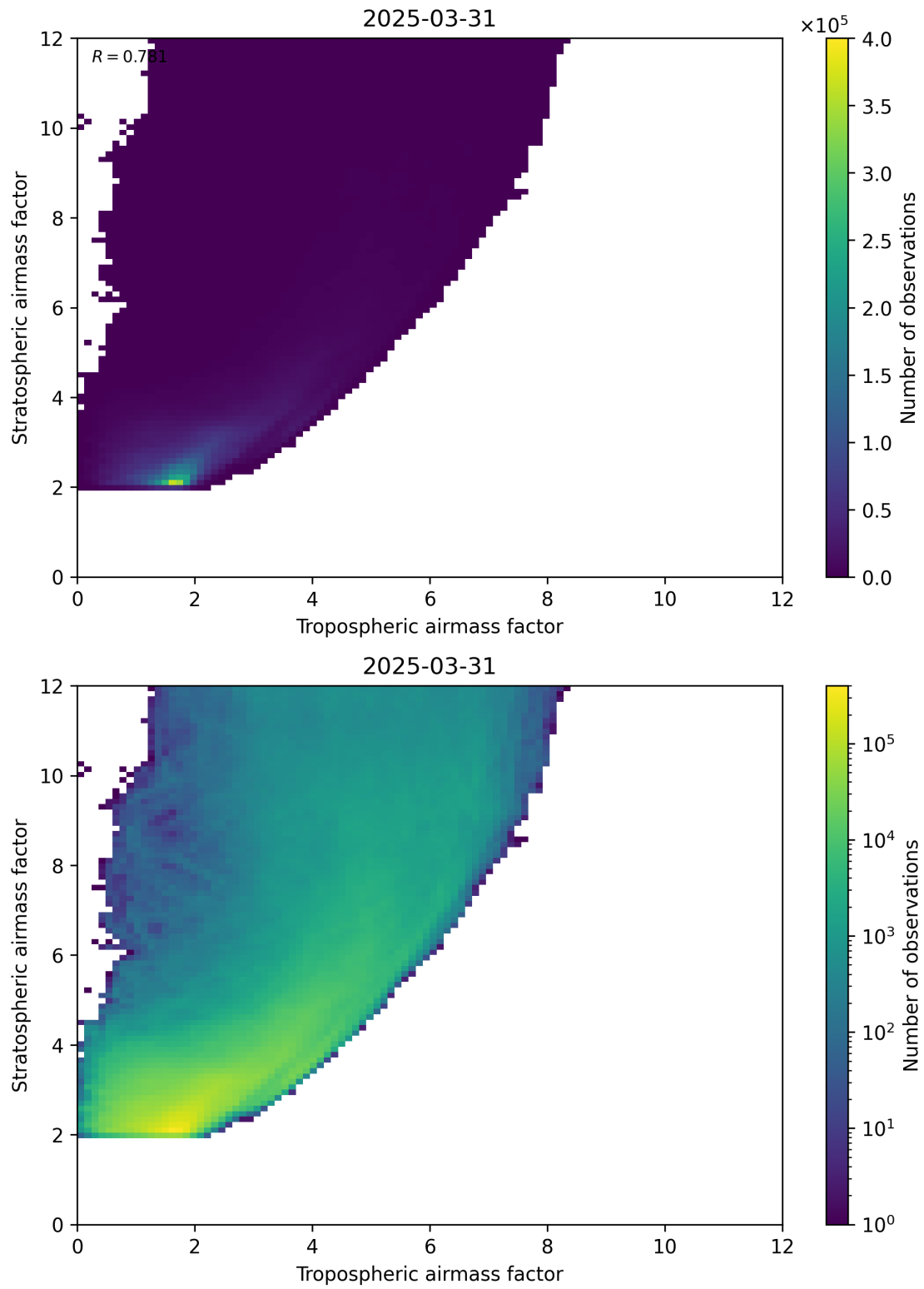
Figure 71: Scatter density plot of “Tropospheric airmass factor” against “Stratospheric airmass factor” for 2025-03-31 to 2025-03-31.
