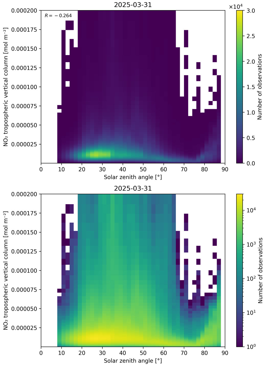
Figure 155: Scatter density plot of “Solar zenith angle” against “NO 2 tropospheric vertical column” for 2025-03-31 to 2025-03-31.
