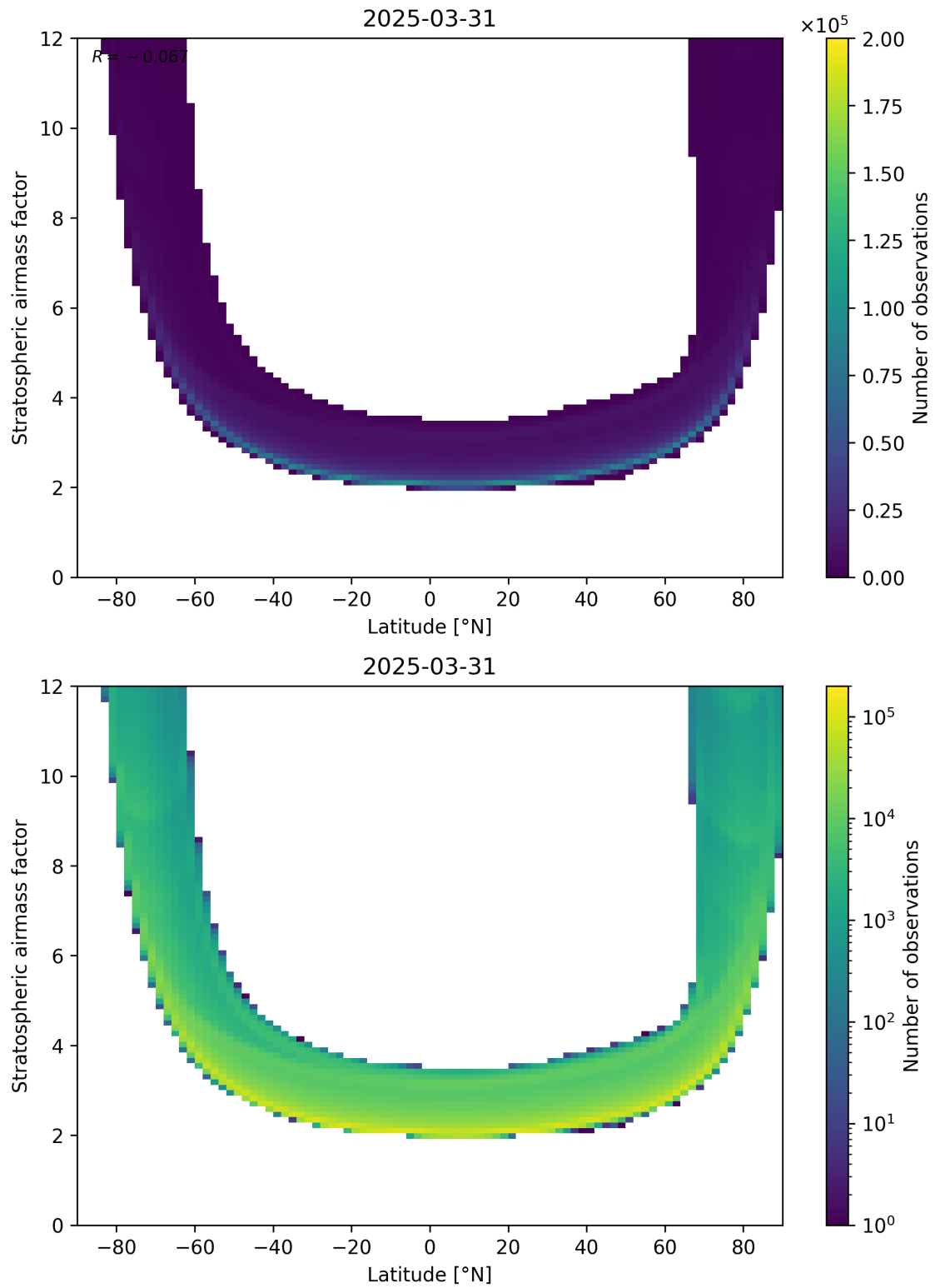
Figure 83: Scatter density plot of “Latitude” against “Stratospheric air mass factor” for 2025-03-31 to 2025-03-31.
