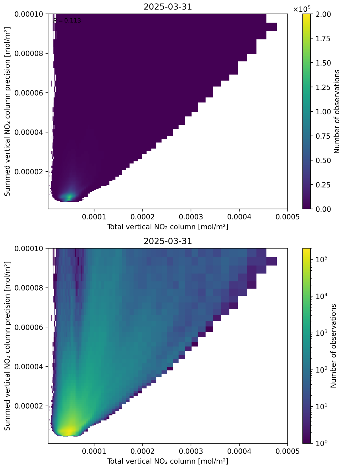
Figure 113: Scatter density plot of “Total vertical NO 2 column” against “Summed vertical NO 2 column precision” for 2025-03-31 to 2025-03-31.
