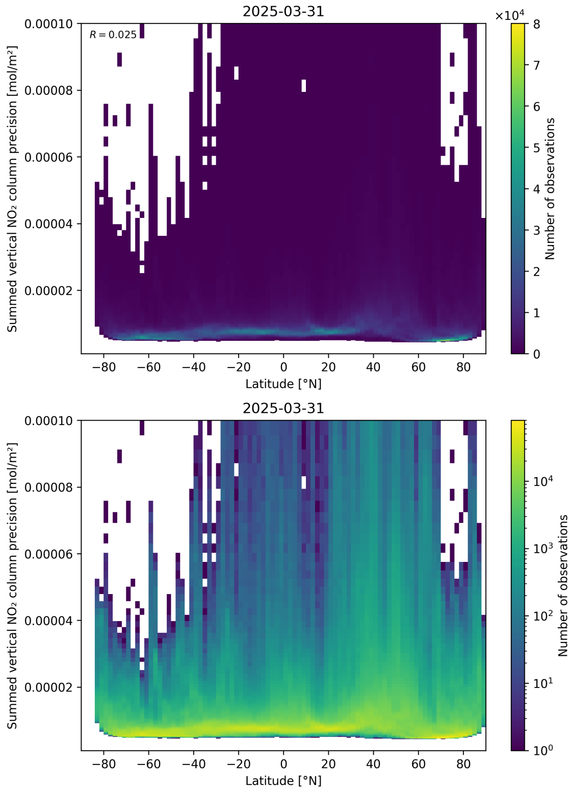
Figure 89: Scatter density plot of “Latitude” against “Summed vertical NO 2 column precision” for 2025-03-31 to 2025-03-31.
