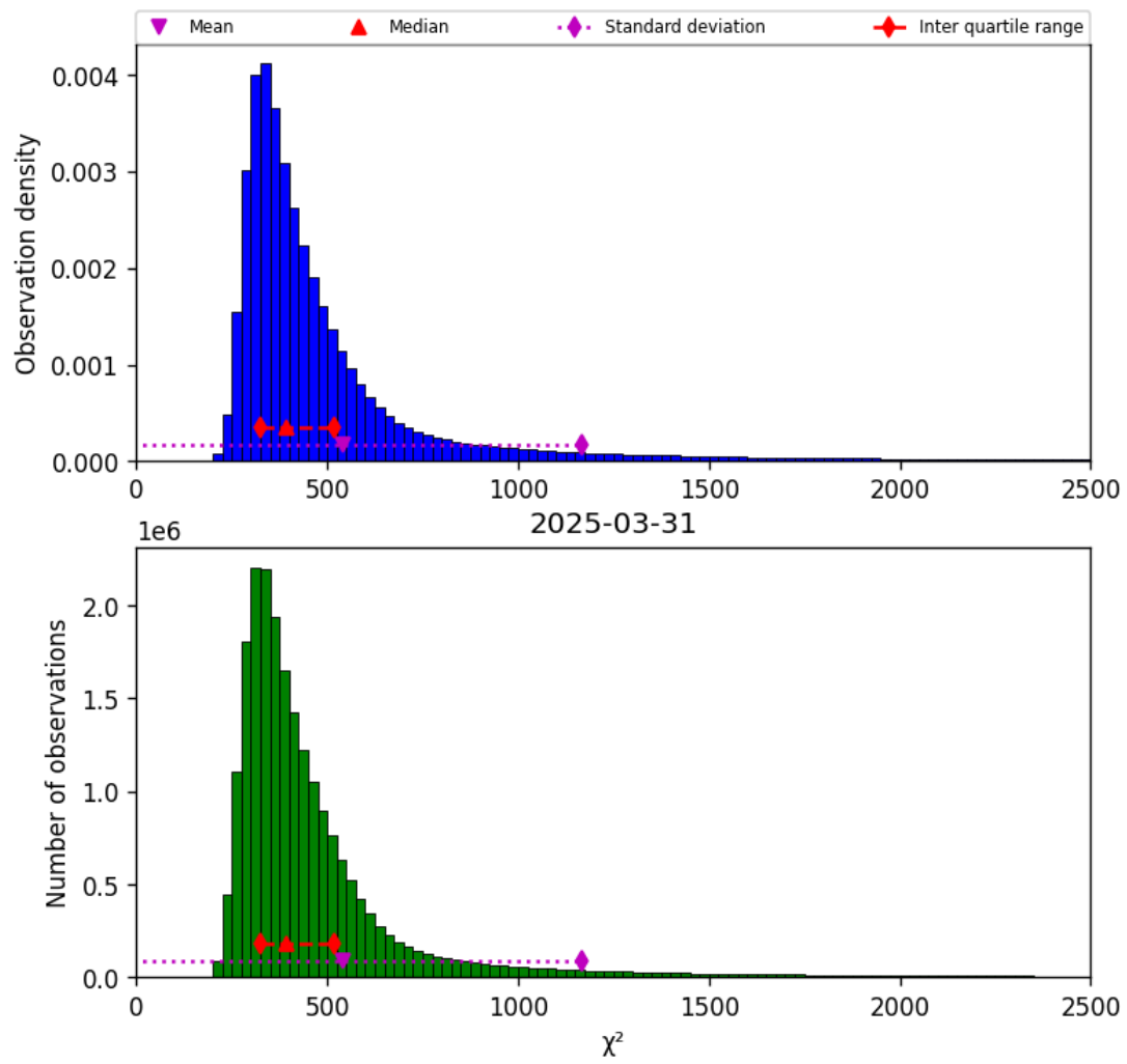
Figure 42: Histogram of “ \chi^2 ” for 2025-03-31 to 2025-03-31
