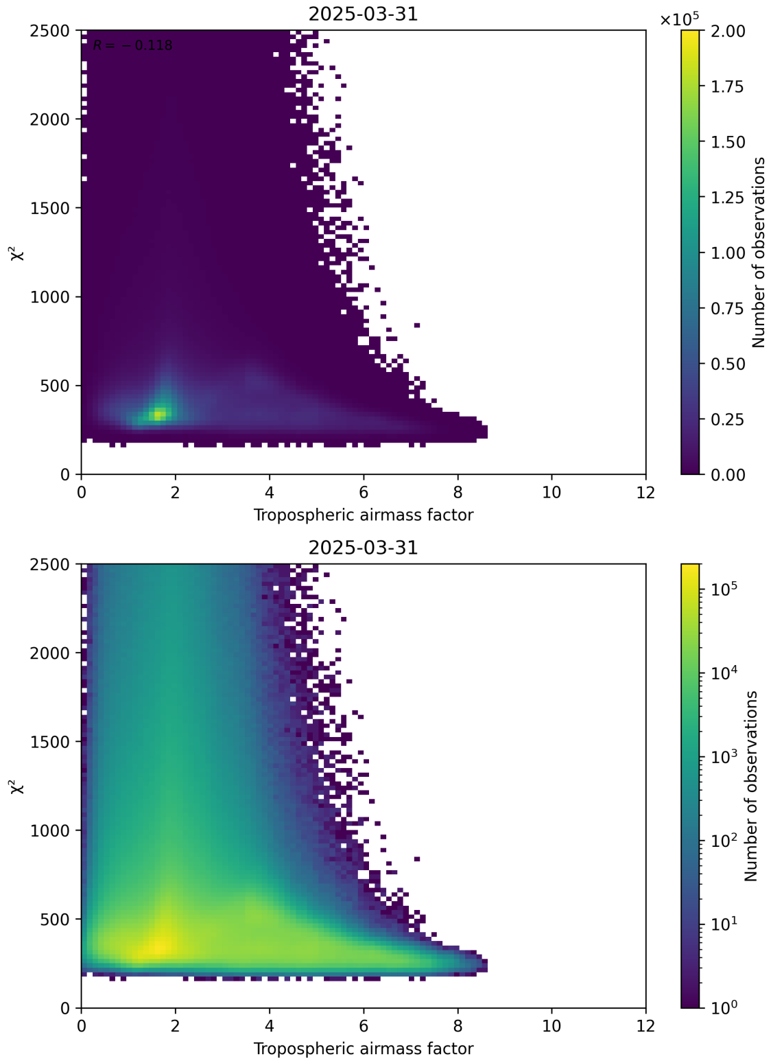
Figure 73: Scatter density plot of “Tropospheric airmass factor” against “ \chi^2 ” for 2025-03-31 to 2025-03-31.
