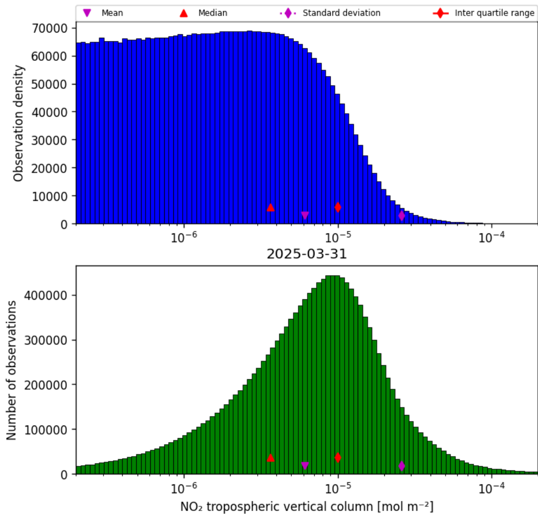
Figure 29: Histogram of “ \text{NO}_2 tropospheric vertical column” for 2025-03-31 to 2025-03-31
