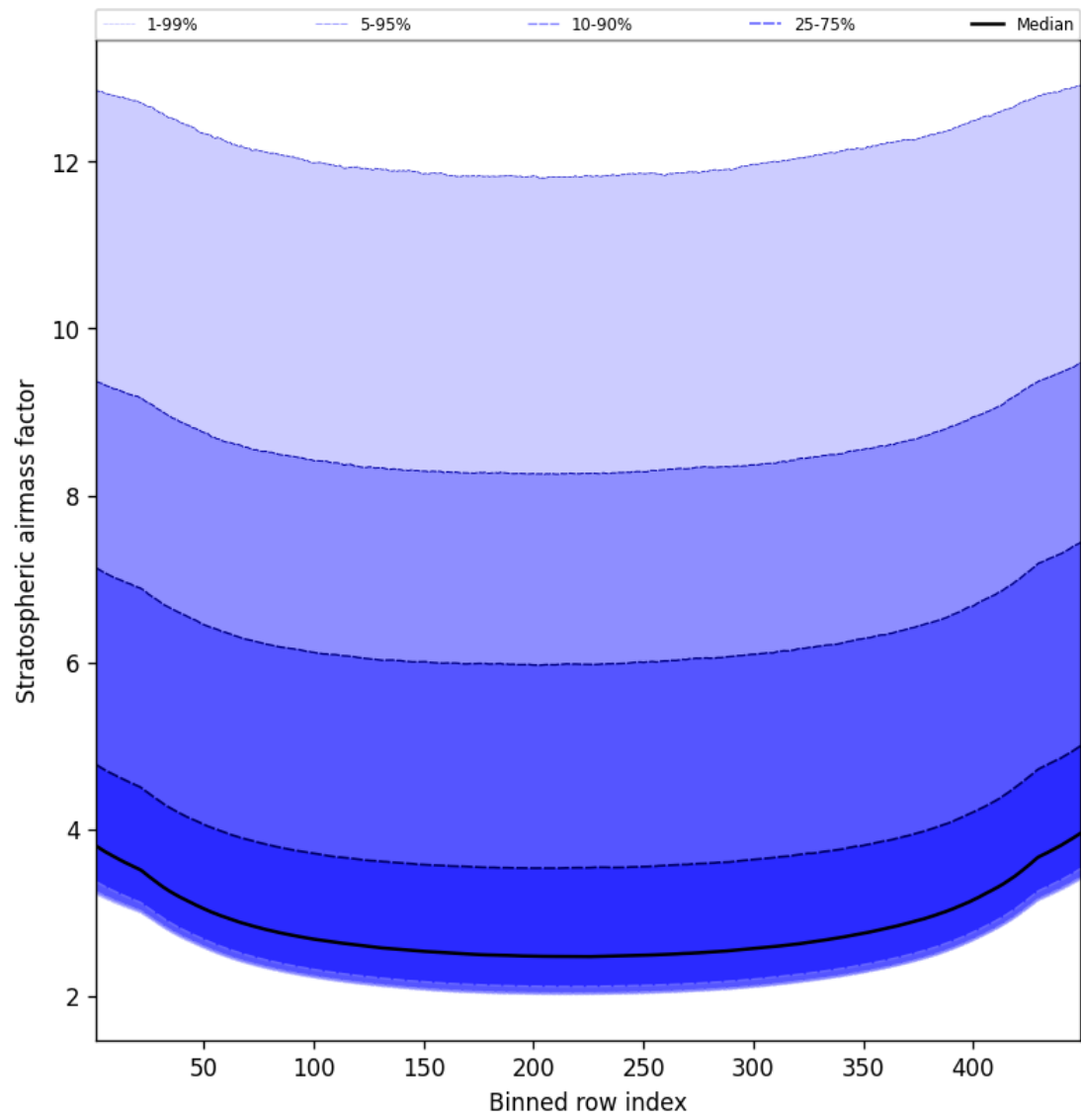
Figure 61: Along track statistics of “Stratospheric airmass factor” for 2025-03-31 to 2025-03-31
