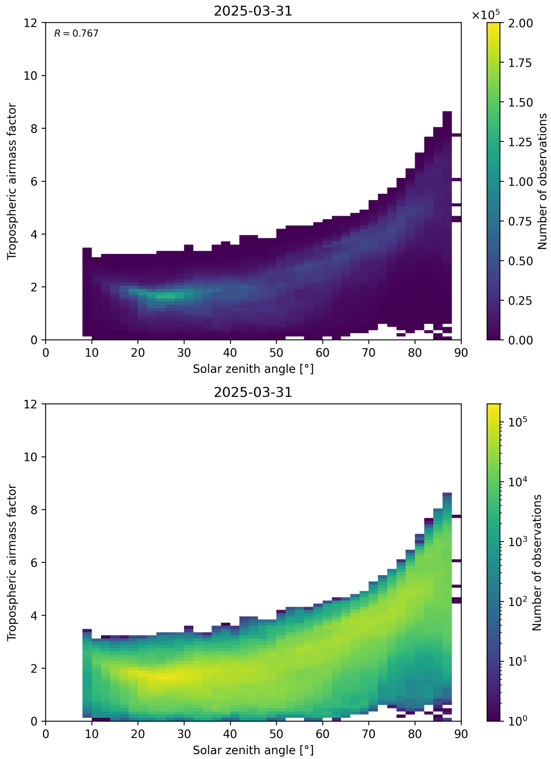
Figure 147: Scatter density plot of “Solar zenith angle” against “Tropospheric airmass factor” for 2025-03-31 to 2025-03-31.
