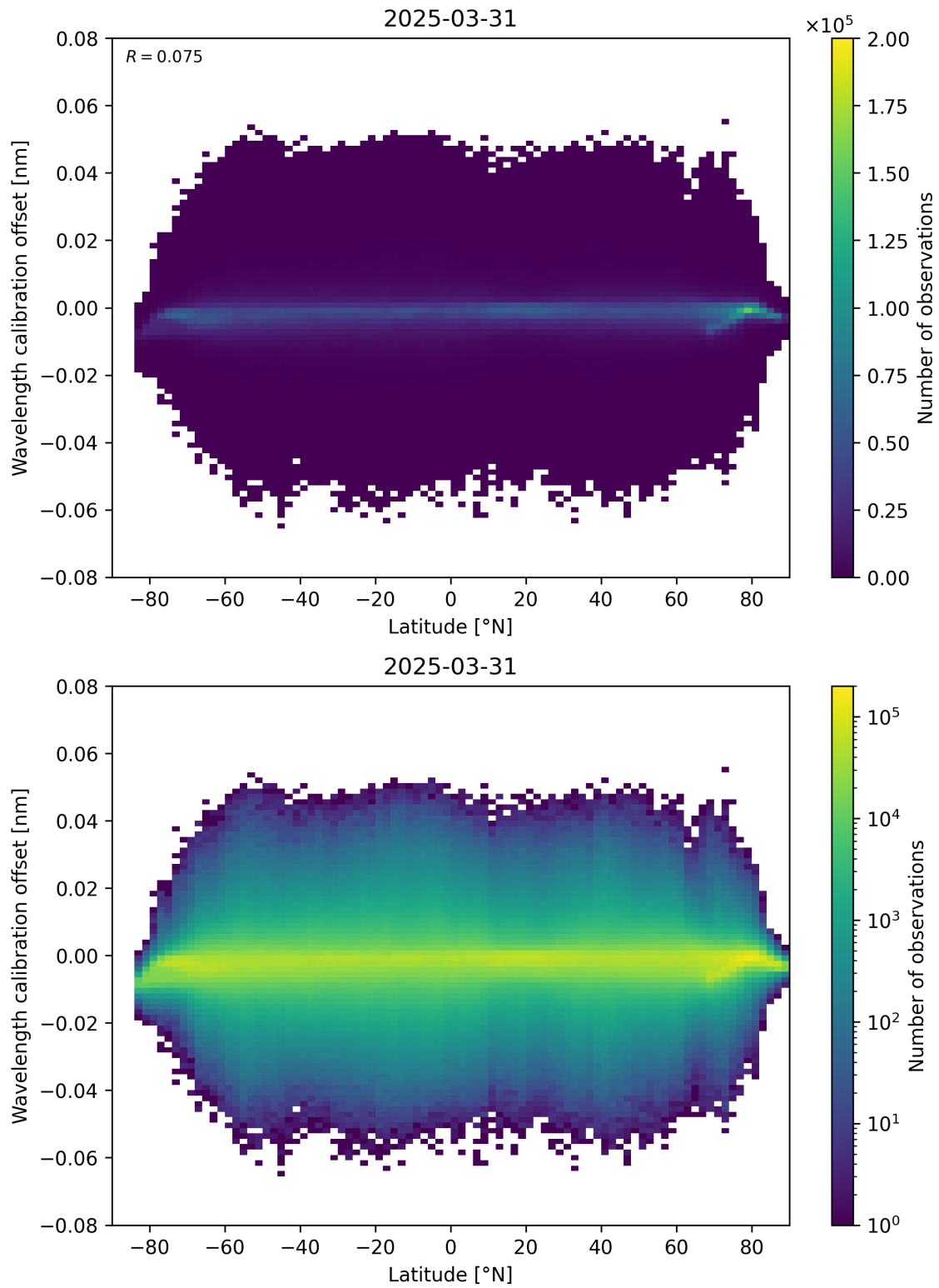
Figure 95: Scatter density plot of “Latitude” against “Wavelength calibration offset” for 2025-03-31 to 2025-03-31.
