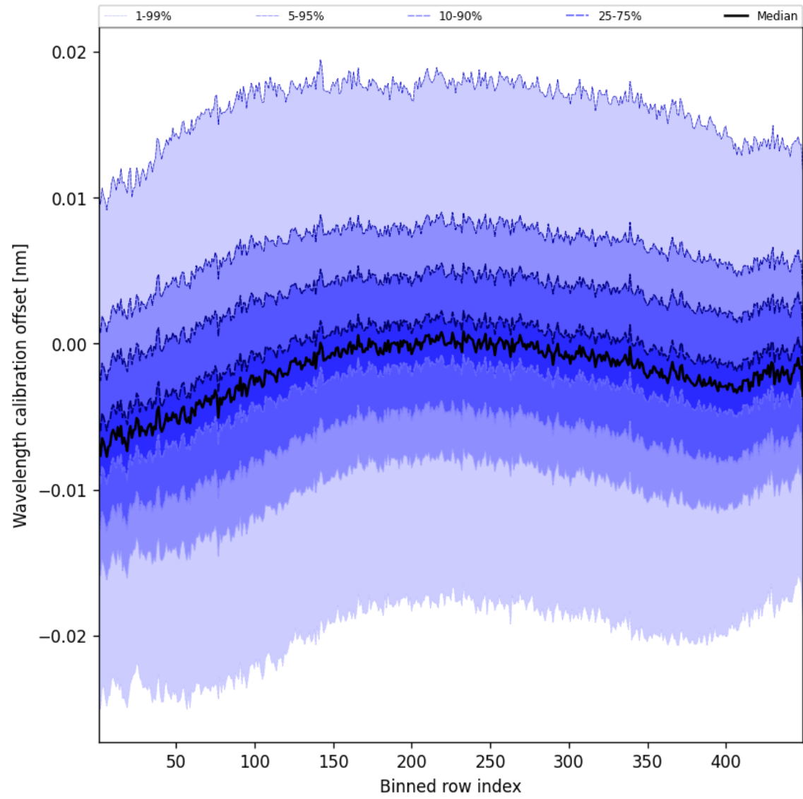
Figure 52: Along track statistics of “Wavelength calibration offset” for 2025-03-31 to 2025-03-31
