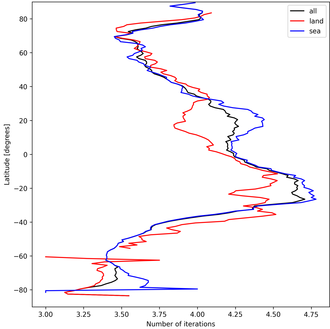
Figure 17: Zonal average of “Number of iterations” for 2025-03-31 to 2025-03-31.
