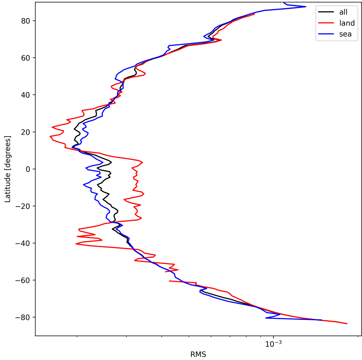
Figure 26: Zonal average of “RMS” for 2025-03-31 to 2025-03-31.
