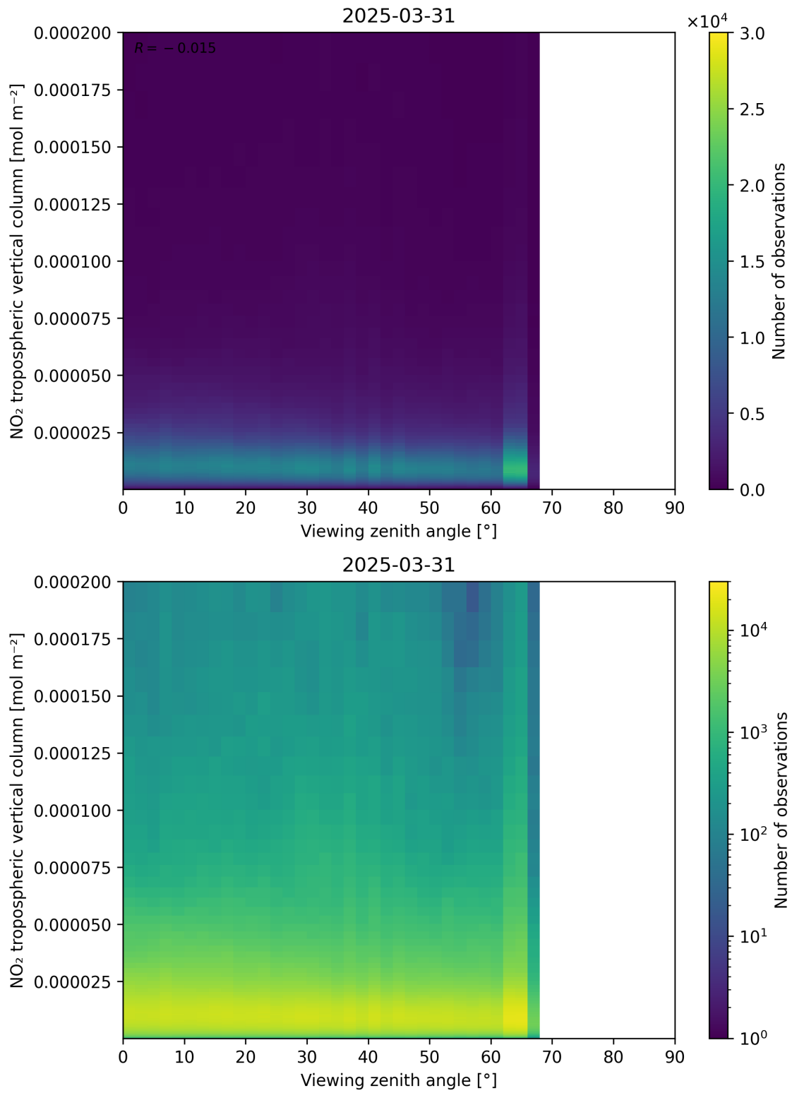
Figure 169: Scatter density plot of “Viewing zenith angle” against “NO 2 tropospheric vertical column” for 2025-03-31 to 2025-03-31.
