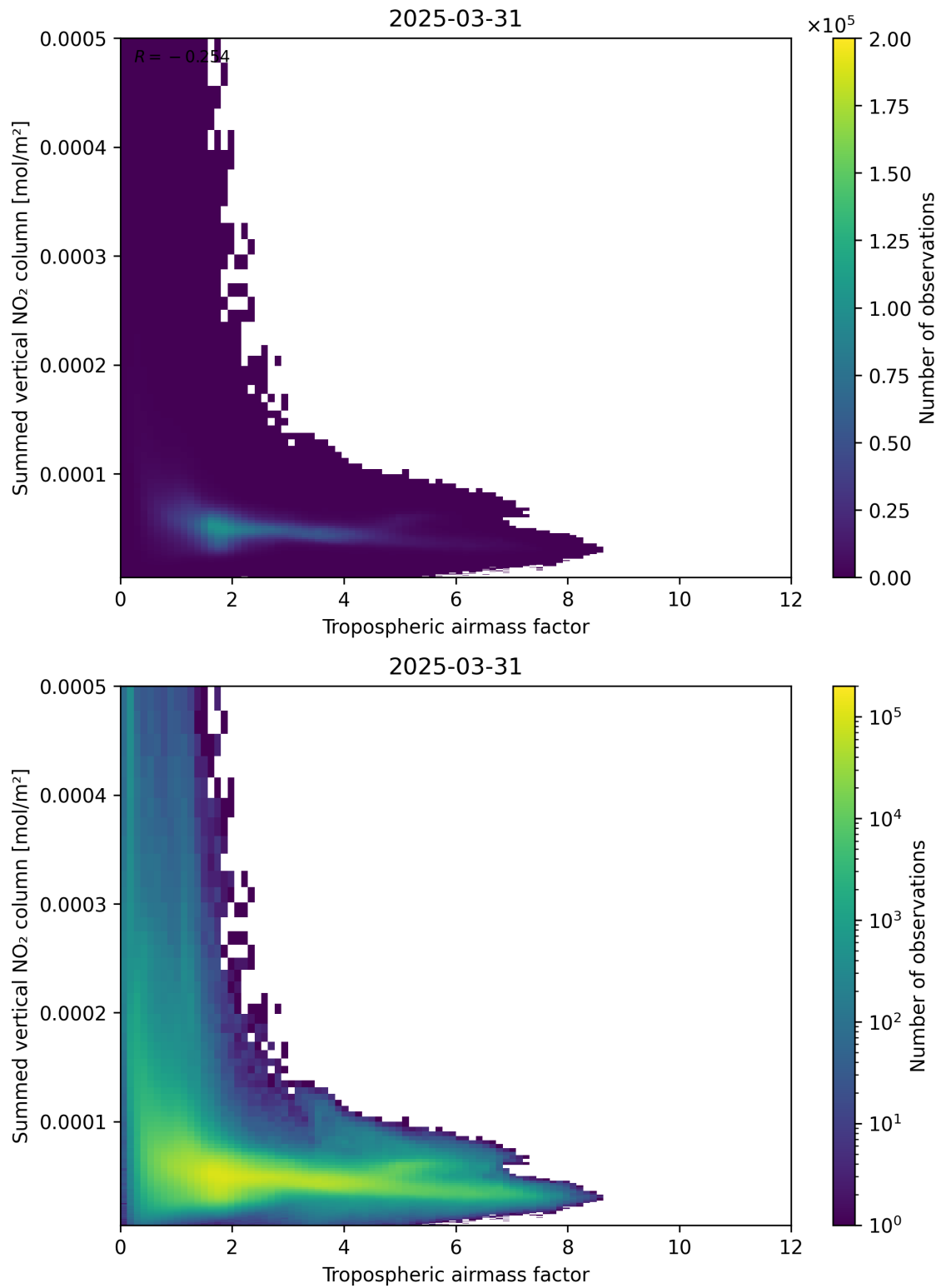
Figure 75: Scatter density plot of “Tropospheric air mass factor” against “Summed vertical NO 2 column” for 2025-03-31 to 2025-03-31.
