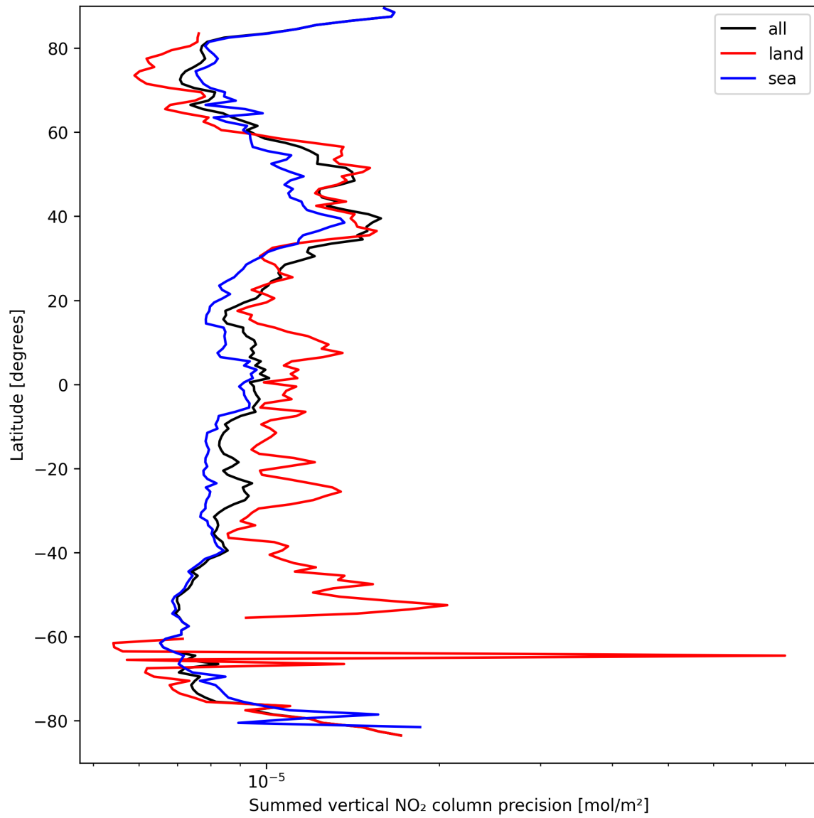
Figure 24: Zonal average of “Summed vertical NO 2 column precision” for 2025-03-31 to 2025-03-31.
