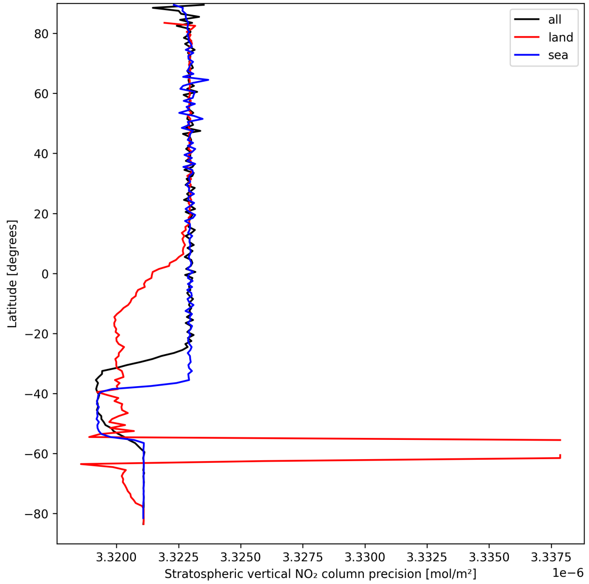
Figure 20: Zonal average of “Stratospheric vertical NO 2 column precision” for 2025-03-31 to 2025-03-31.
