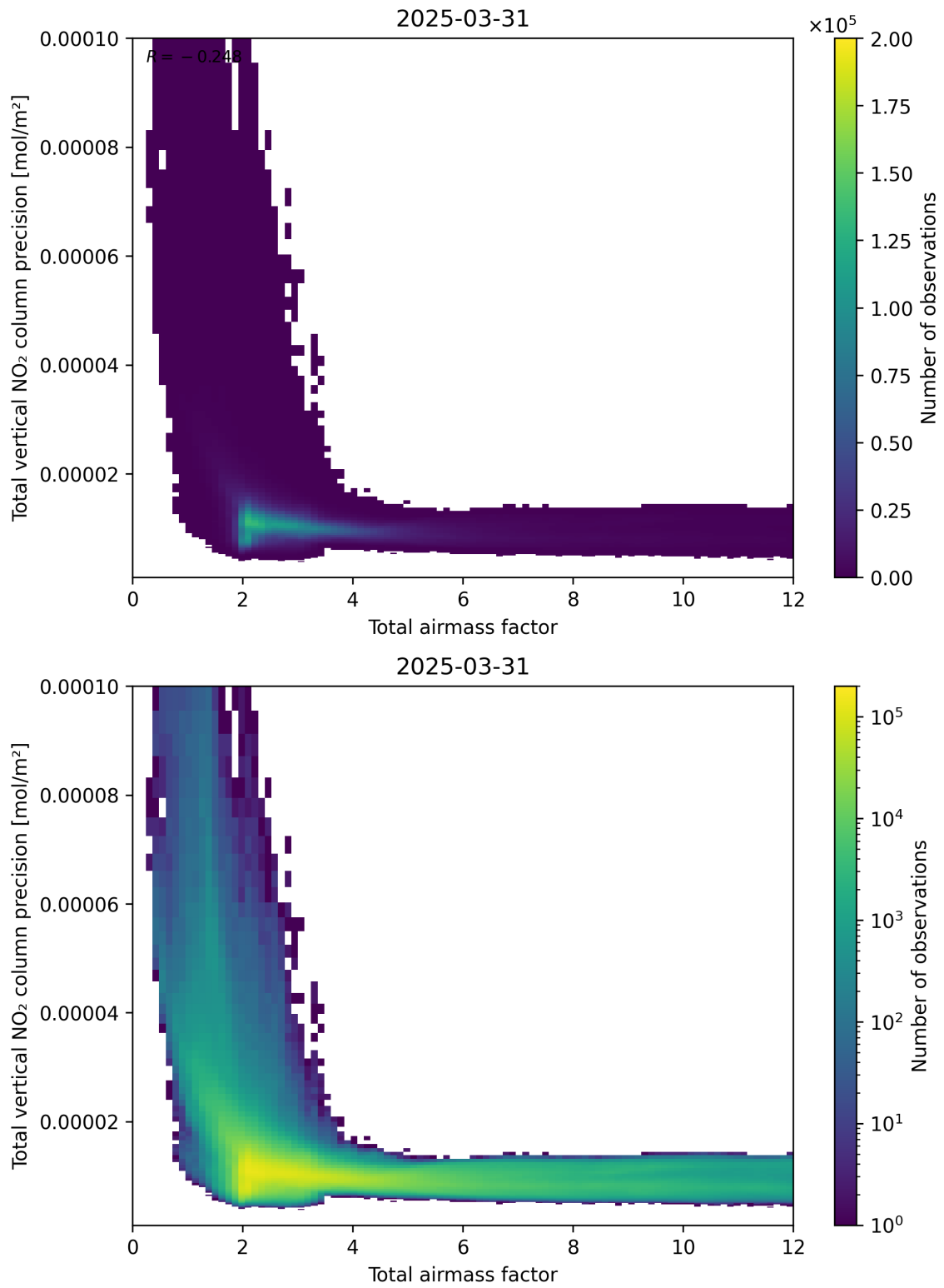
Figure 68: Scatter density plot of “Total airmass factor” against “Total vertical NO 2 column precision” for 2025-03-31 to 2025-03-31.
