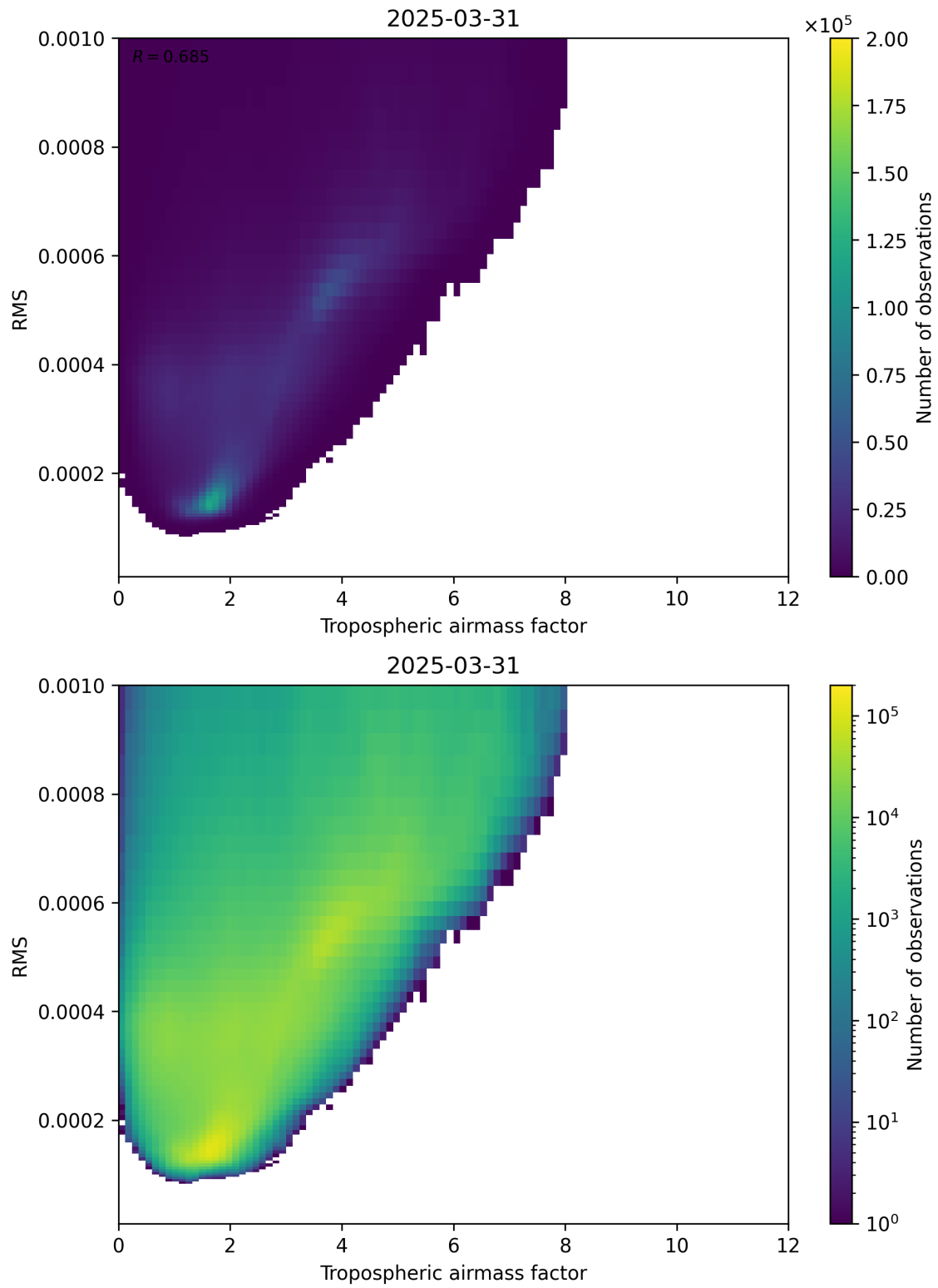
Figure 79: Scatter density plot of “Tropospheric airmass factor” against “RMS” for 2025-03-31 to 2025-03-31.
