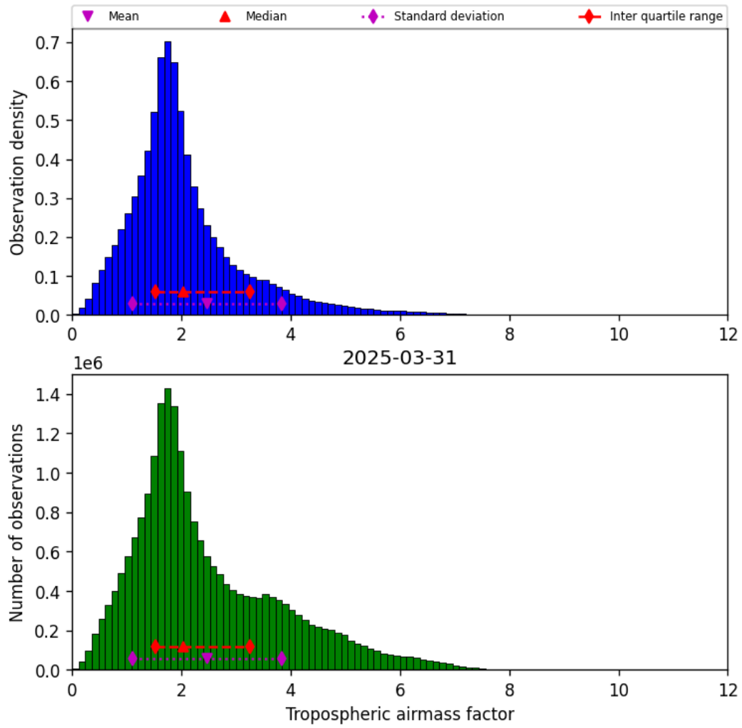
Figure 31: Histogram of “Tropospheric airmass factor” for 2025-03-31 to 2025-03-31
