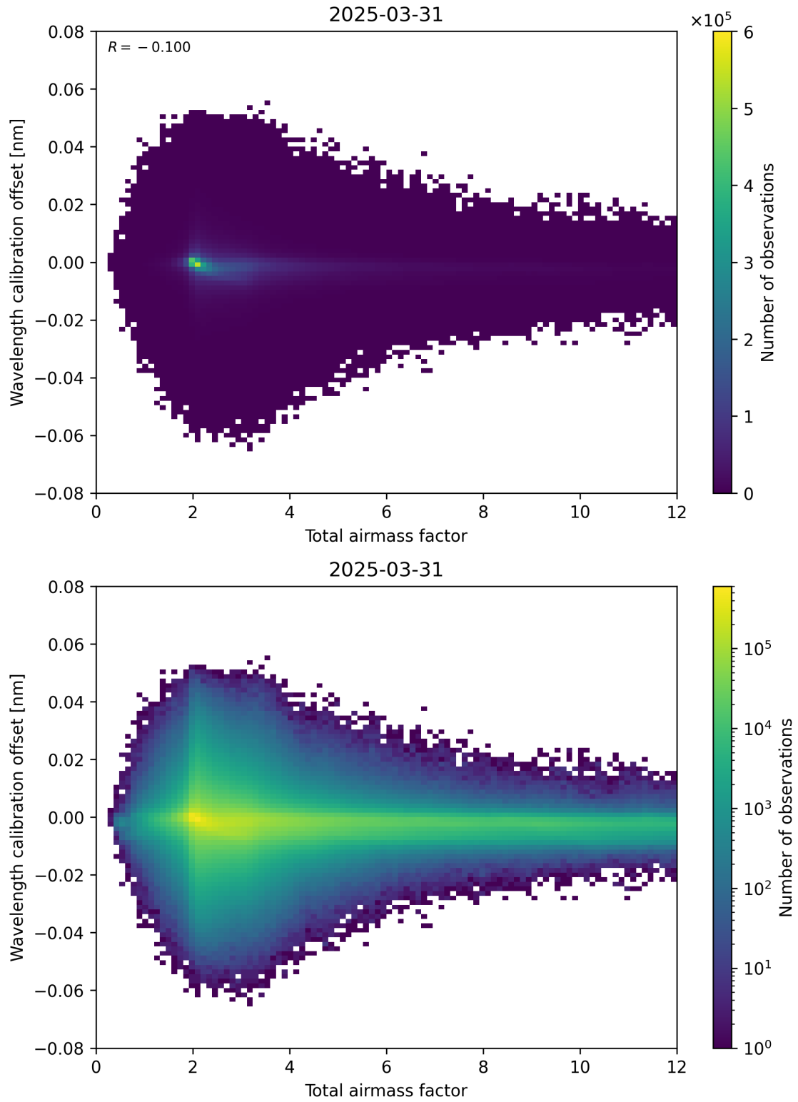
Figure 70: Scatter density plot of “Total airmass factor” against “Wavelength calibration offset” for 2025-03-31 to 2025-03-31.
