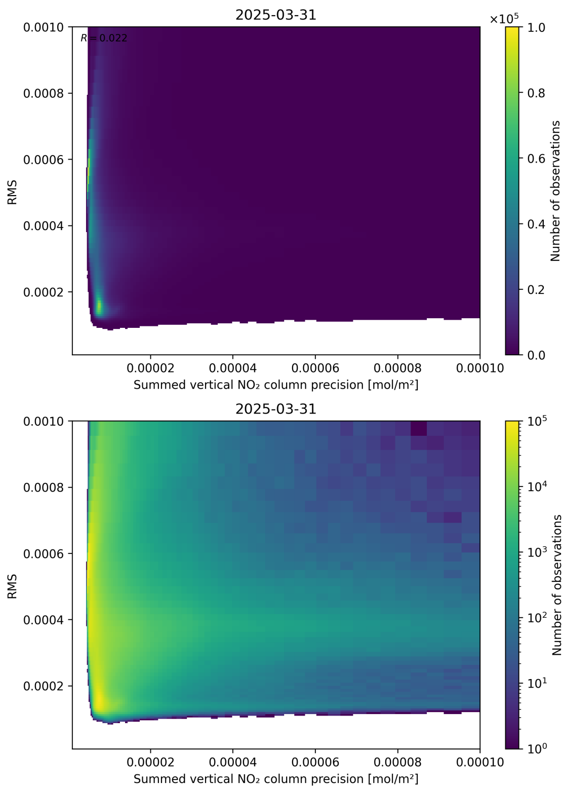
Figure 108: Scatter density plot of “Summed vertical NO 2 column precision” against “RMS” for 2025-03-31 to 2025-03-31.
