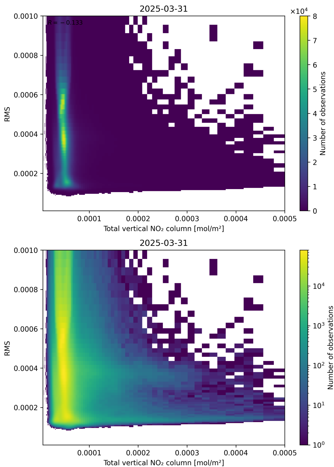
Figure 120: Scatter density plot of “Total vertical NO 2 column” against “RMS” for 2025-03-31 to 2025-03-31.
