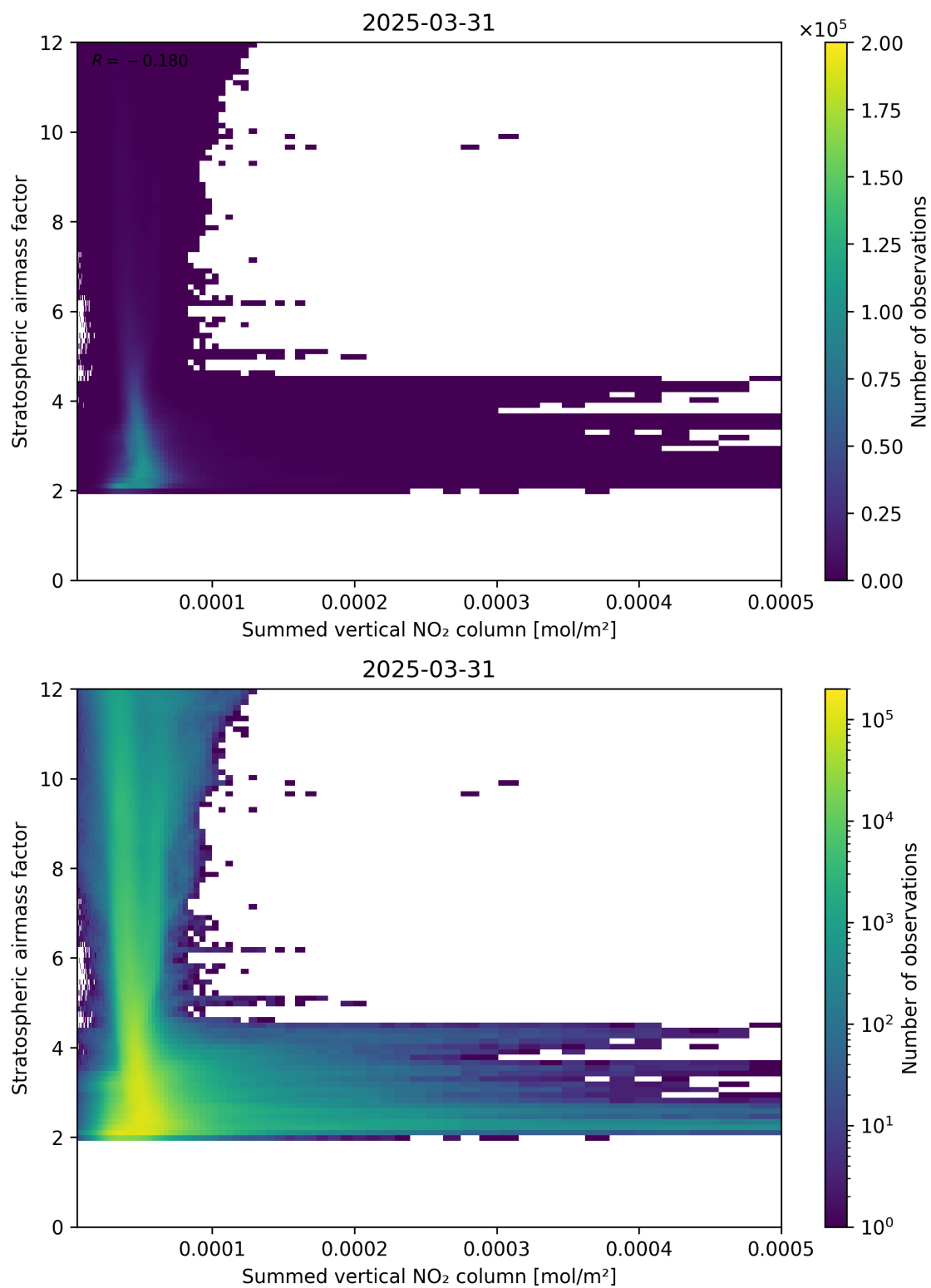
Figure 103: Scatter density plot of “Summed vertical NO 2 column” against “Stratospheric airmass factor” for 2025-03-31 to 2025-03-31.
