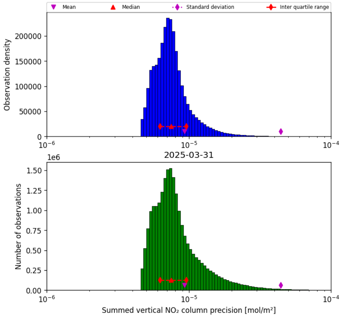
Figure 41: Histogram of "Summed vertical NO 2 column precision" for 2025-03-31 to 2025-03-31
