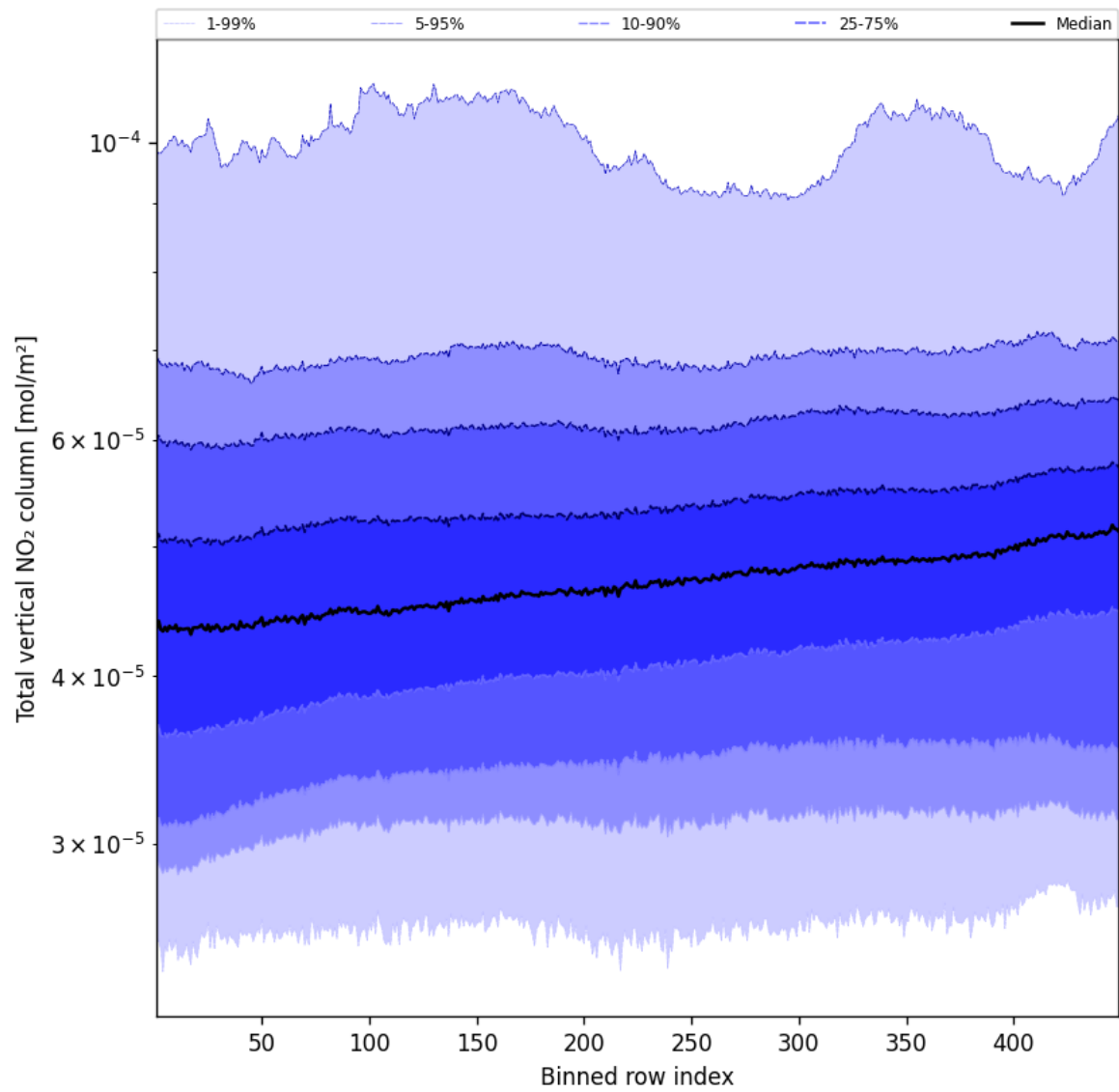
Figure 55: Along track statistics of “Total vertical NO 2 column” for 2025-03-31 to 2025-03-31
