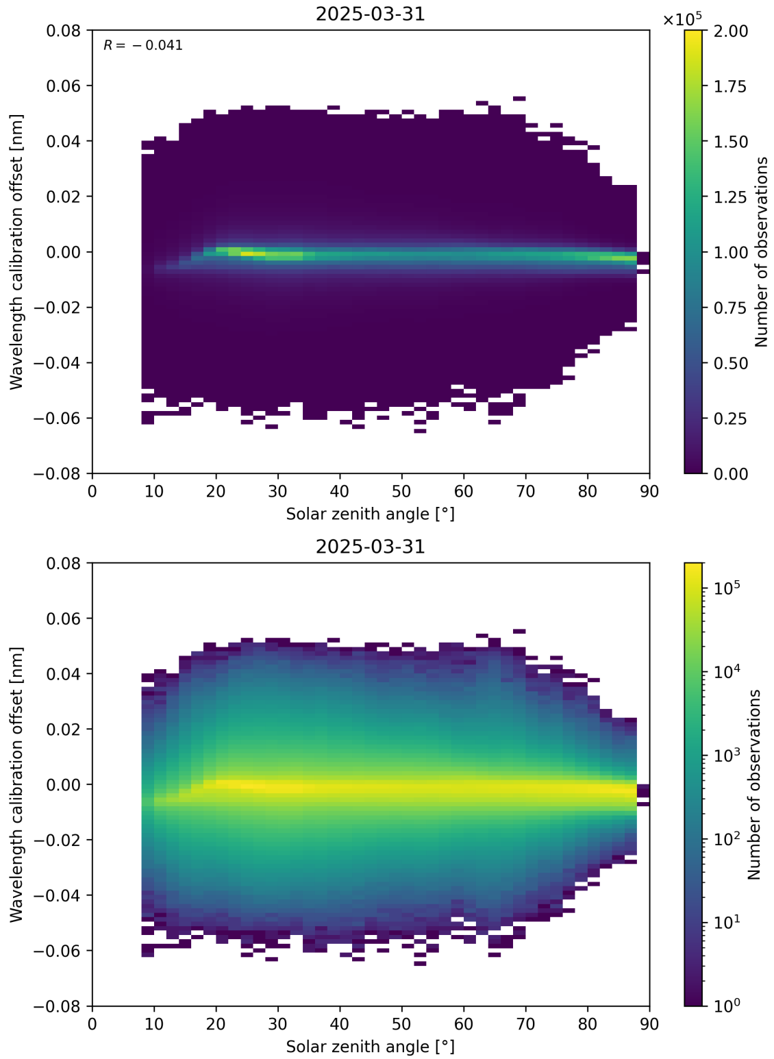
Figure 158: Scatter density plot of “Solar zenith angle” against “Wavelength calibration offset” for 2025-03-31 to 2025-03-31.
