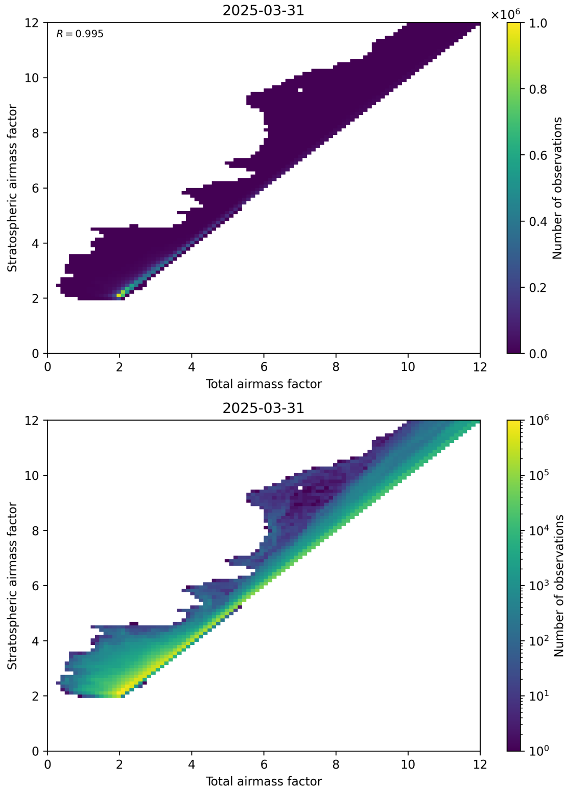
Figure 62: Scatter density plot of “Total airmass factor” against “Stratospheric airmass factor” for 2025-03-31 to 2025-03-31.
