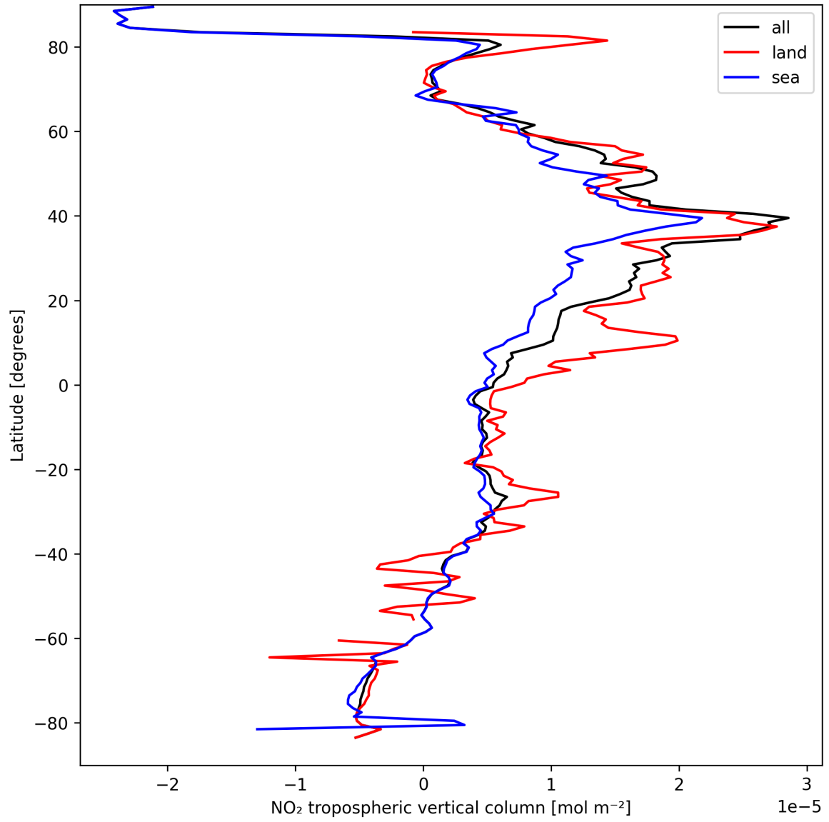
Figure 12: Zonal average of “NO 2 tropospheric vertical column” for 2025-03-31 to 2025-03-31.
