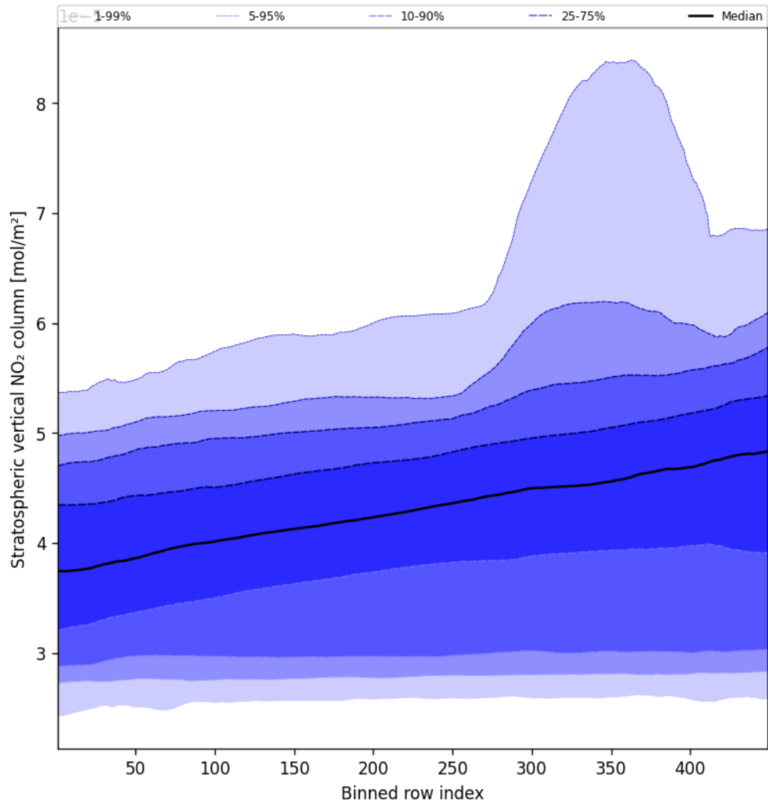
Figure 53: Along track statistics of “Stratospheric vertical NO 2 column” for 2025-03-31 to 2025-03-31
