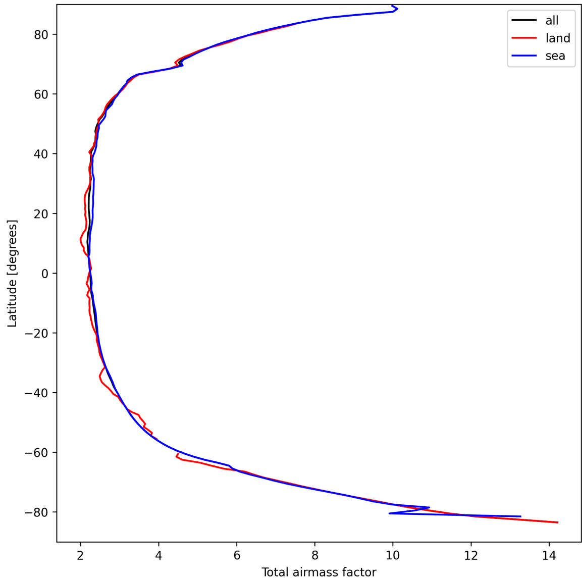
Figure 15: Zonal average of “Total airmass factor” for 2025-03-31 to 2025-03-31.
