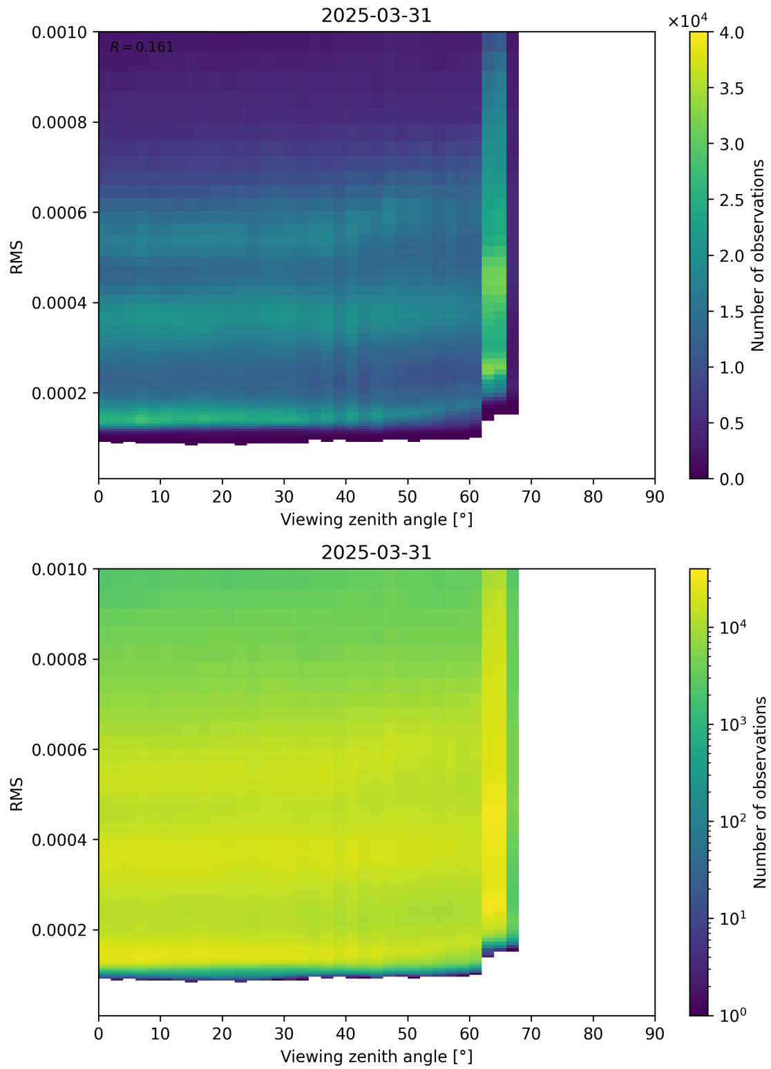
Figure 171: Scatter density plot of “Viewing zenith angle” against “RMS” for 2025-03-31 to 2025-03-31.
