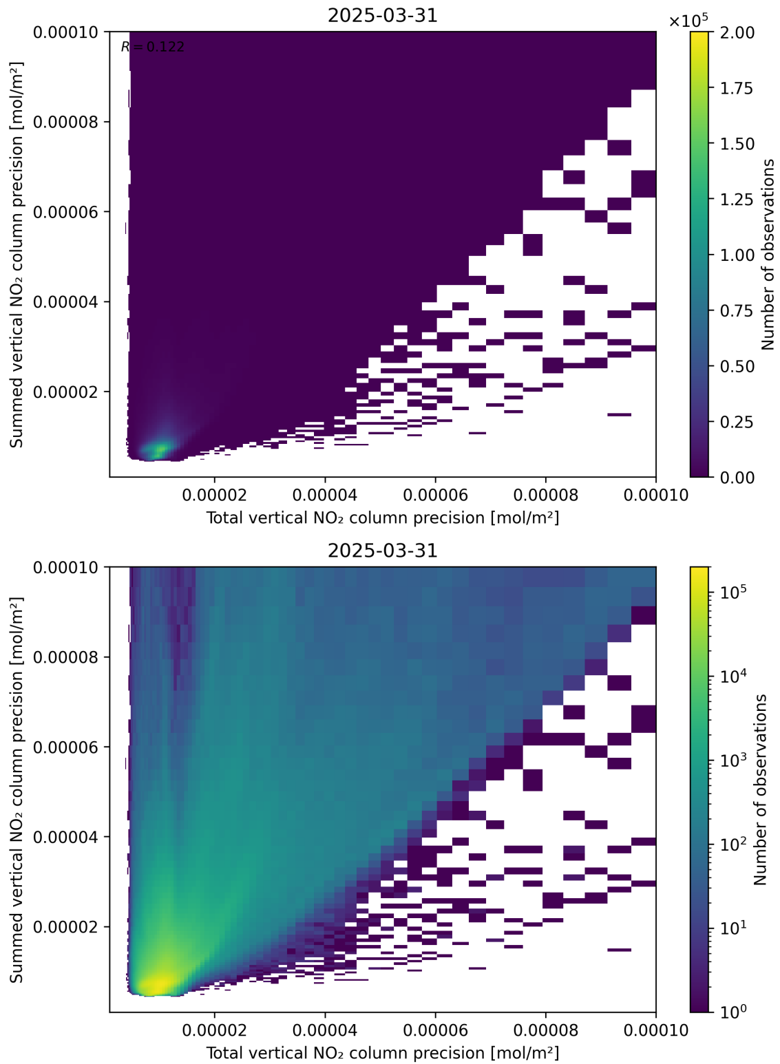
Figure 118: Scatter density plot of “Total vertical NO 2 column precision” against “Summed vertical NO 2 column precision” for 2025-03-31 to 2025-03-31.
