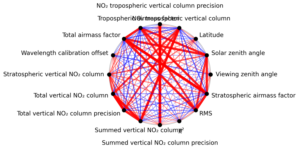
Figure 1: Map of correlation graph for 2025-03-31 to 2025-03-31.
