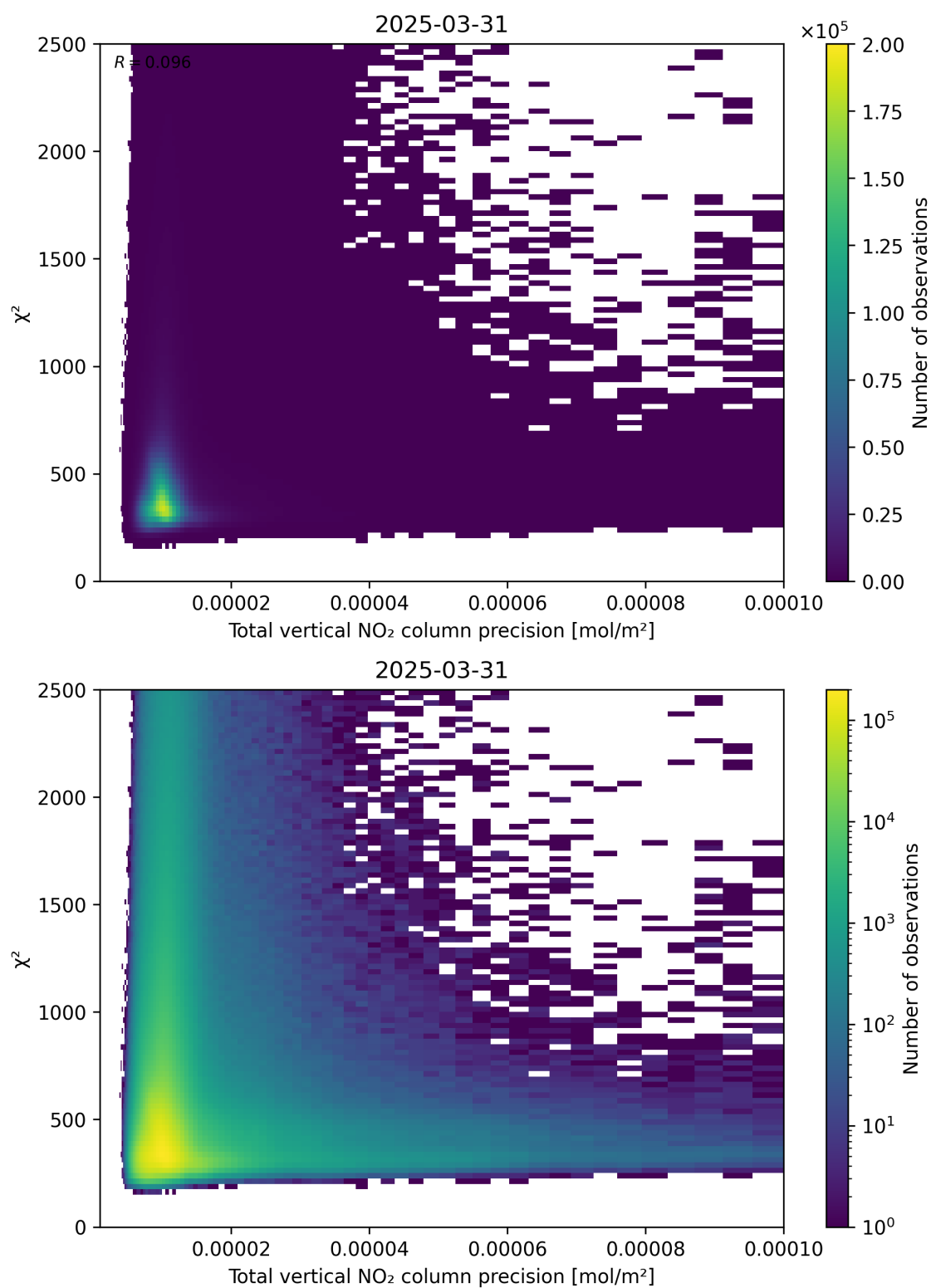
Figure 116: Scatter density plot of “Total vertical NO 2 column precision” against “ \chi^2 ” for 2025-03-31 to 2025-03-31.
