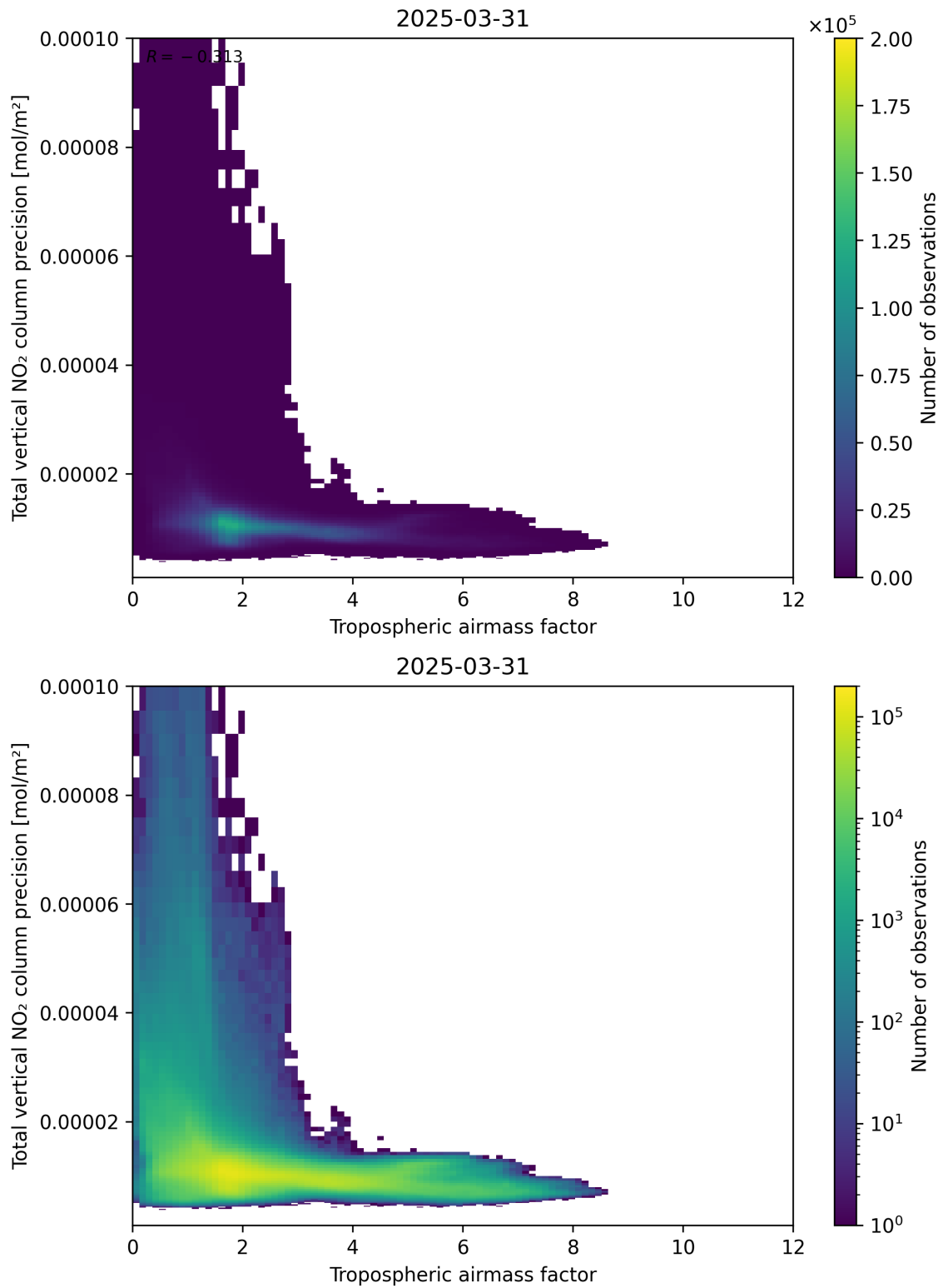
Figure 78: Scatter density plot of “Tropospheric air mass factor” against “Total vertical NO 2 column precision” for 2025-03-31 to 2025-03-31.
