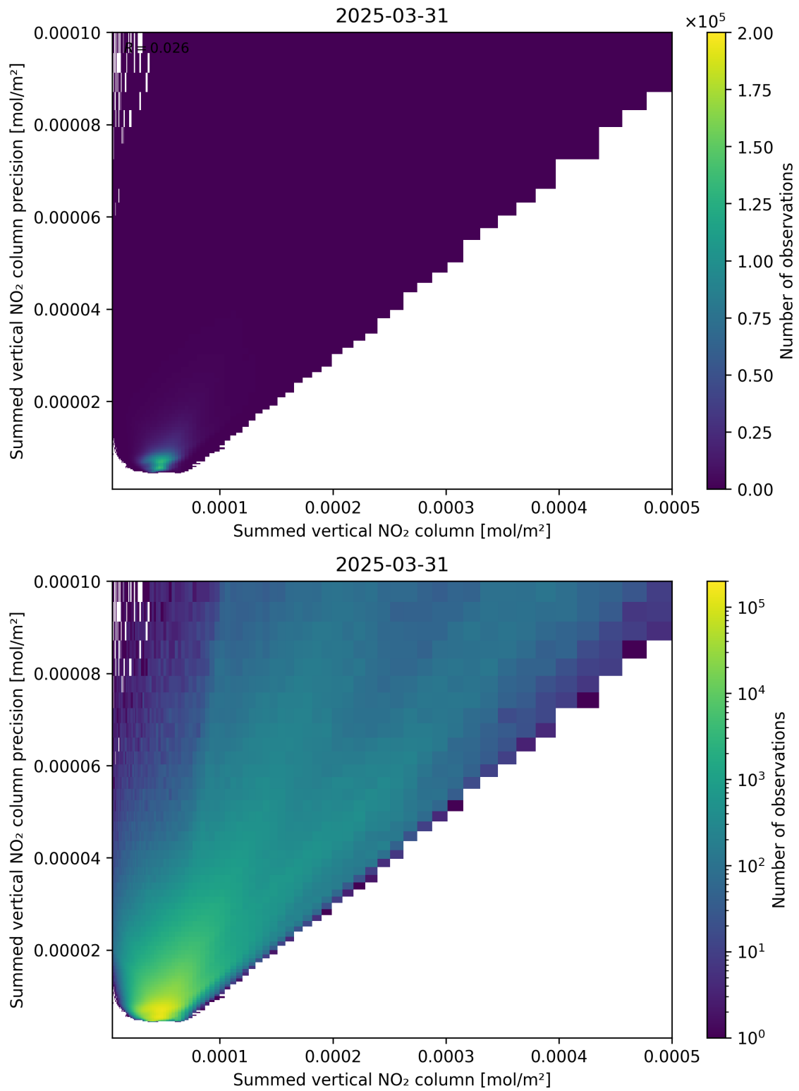
Figure 105: Scatter density plot of “Summed vertical NO 2 column” against “Summed vertical NO 2 column precision” for 2025-03-31 to 2025-03-31.
