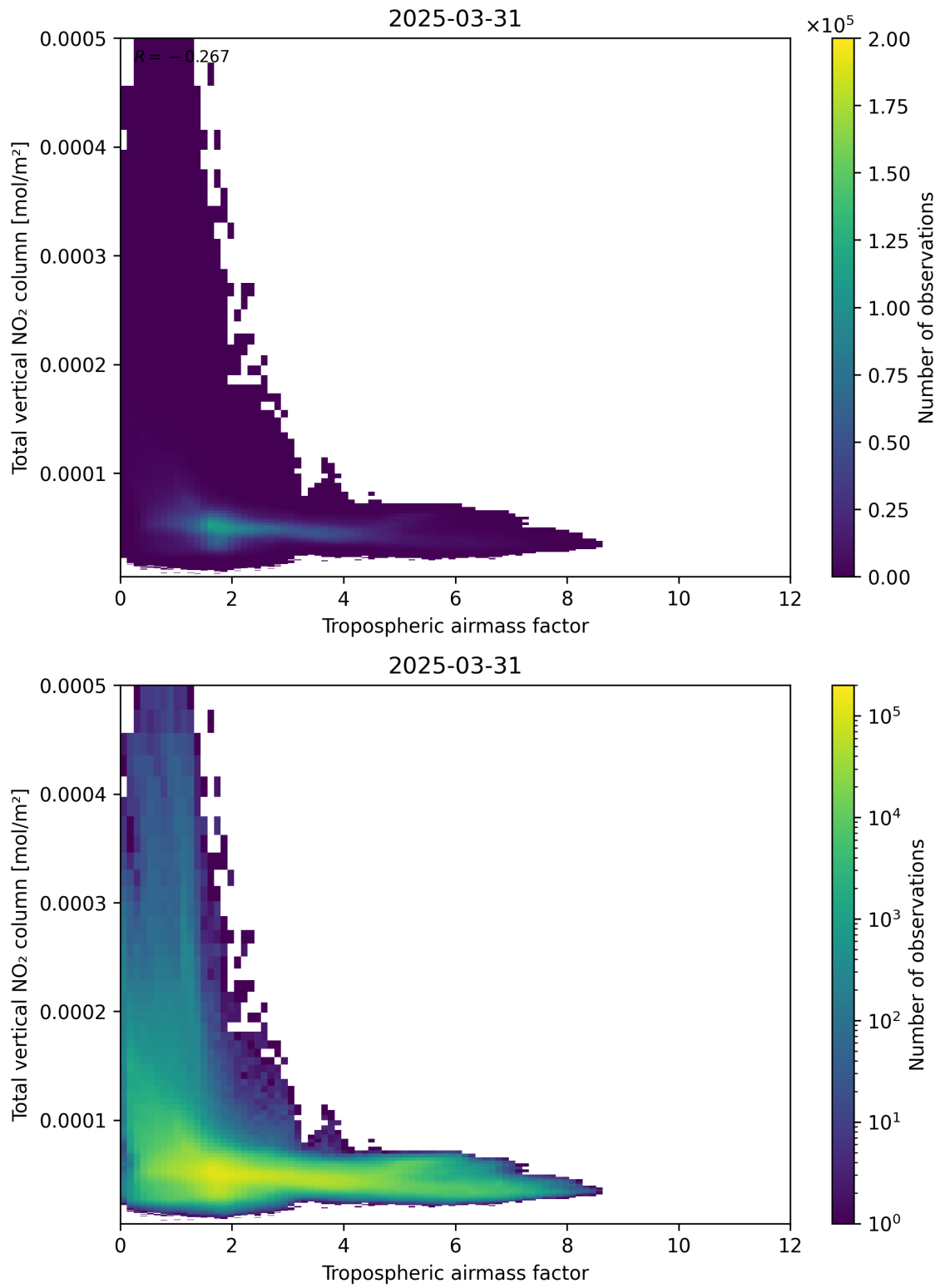
Figure 77: Scatter density plot of “Tropospheric airmass factor” against “Total vertical NO 2 column” for 2025-03-31 to 2025-03-31.
