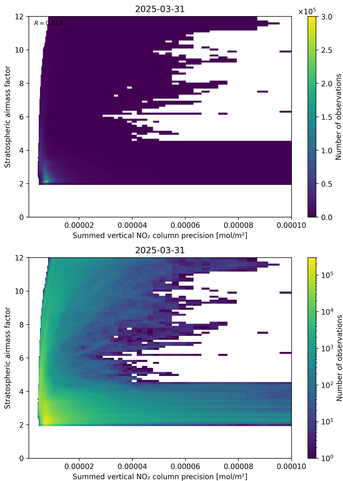
Figure 106: Scatter density plot of “Summed vertical NO 2 column precision” against “Stratospheric airmass factor” for 2025-03-31 to 2025-03-31.
