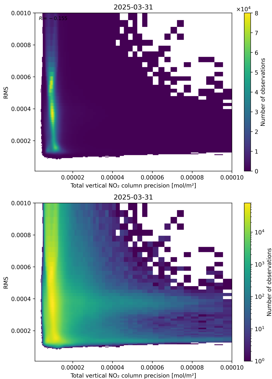
Figure 119: Scatter density plot of “Total vertical NO 2 column precision” against “RMS” for 2025-03-31 to 2025-03-31.
