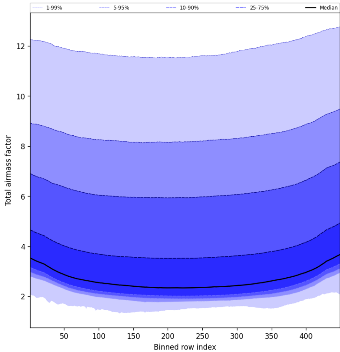
Figure 49: Along track statistics of “Total airmass factor” for 2025-03-31 to 2025-03-31
