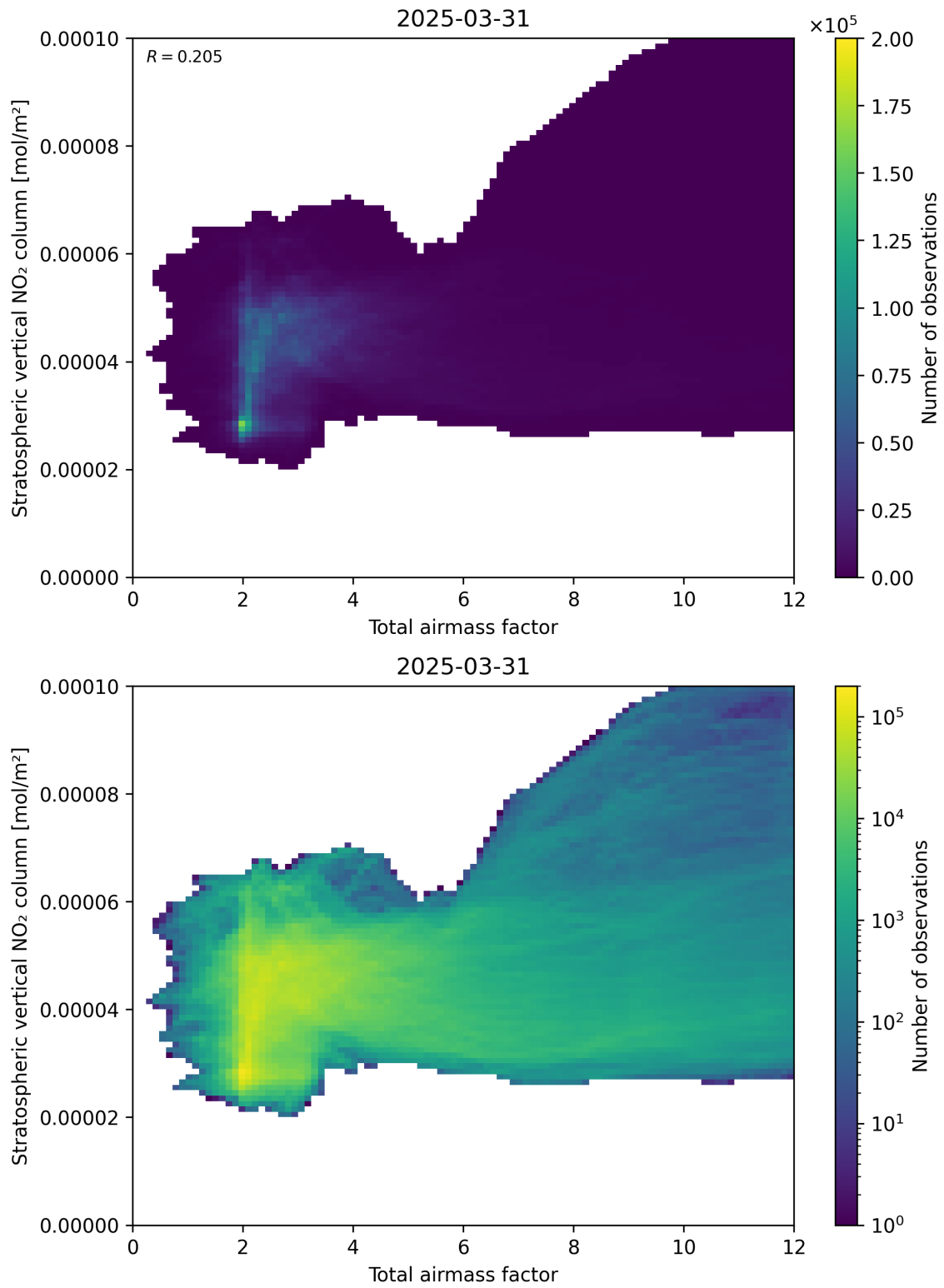
Figure 64: Scatter density plot of “Total airmass factor” against “Stratospheric vertical \text{NO}_2 column” for 2025-03-31 to 2025-03-31.
