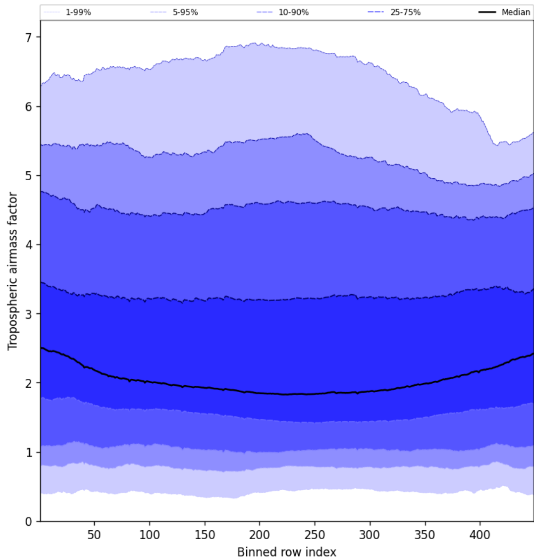
Figure 48: Along track statistics of “Tropospheric air mass factor” for 2025-03-31 to 2025-03-31
