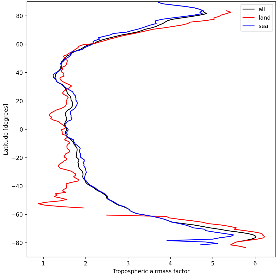
Figure 14: Zonal average of “Tropospheric airmass factor” for 2025-03-31 to 2025-03-31.
