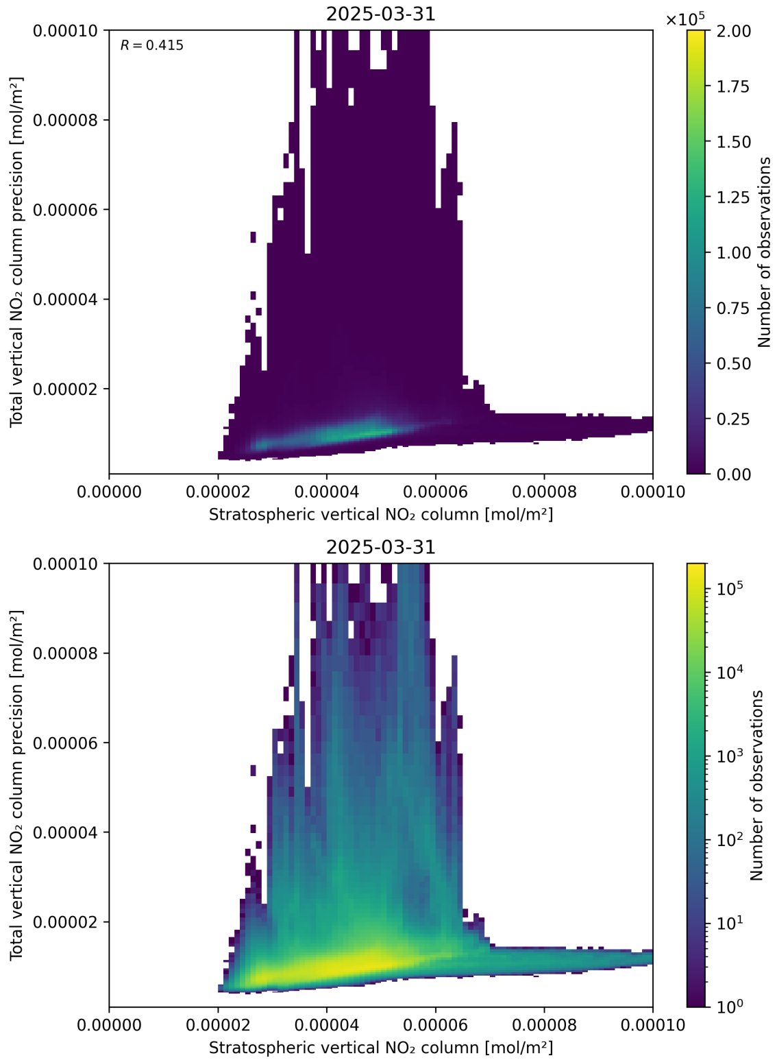
Figure 101: Scatter density plot of “Stratospheric vertical NO 2 column” against “Total vertical NO 2 column precision” for 2025-03-31 to 2025-03-31.
