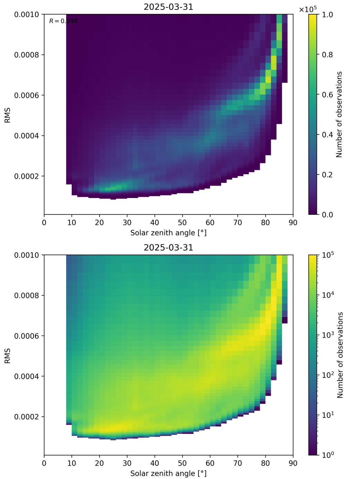
Figure 157: Scatter density plot of “Solar zenith angle” against “RMS” for 2025-03-31 to 2025-03-31.
