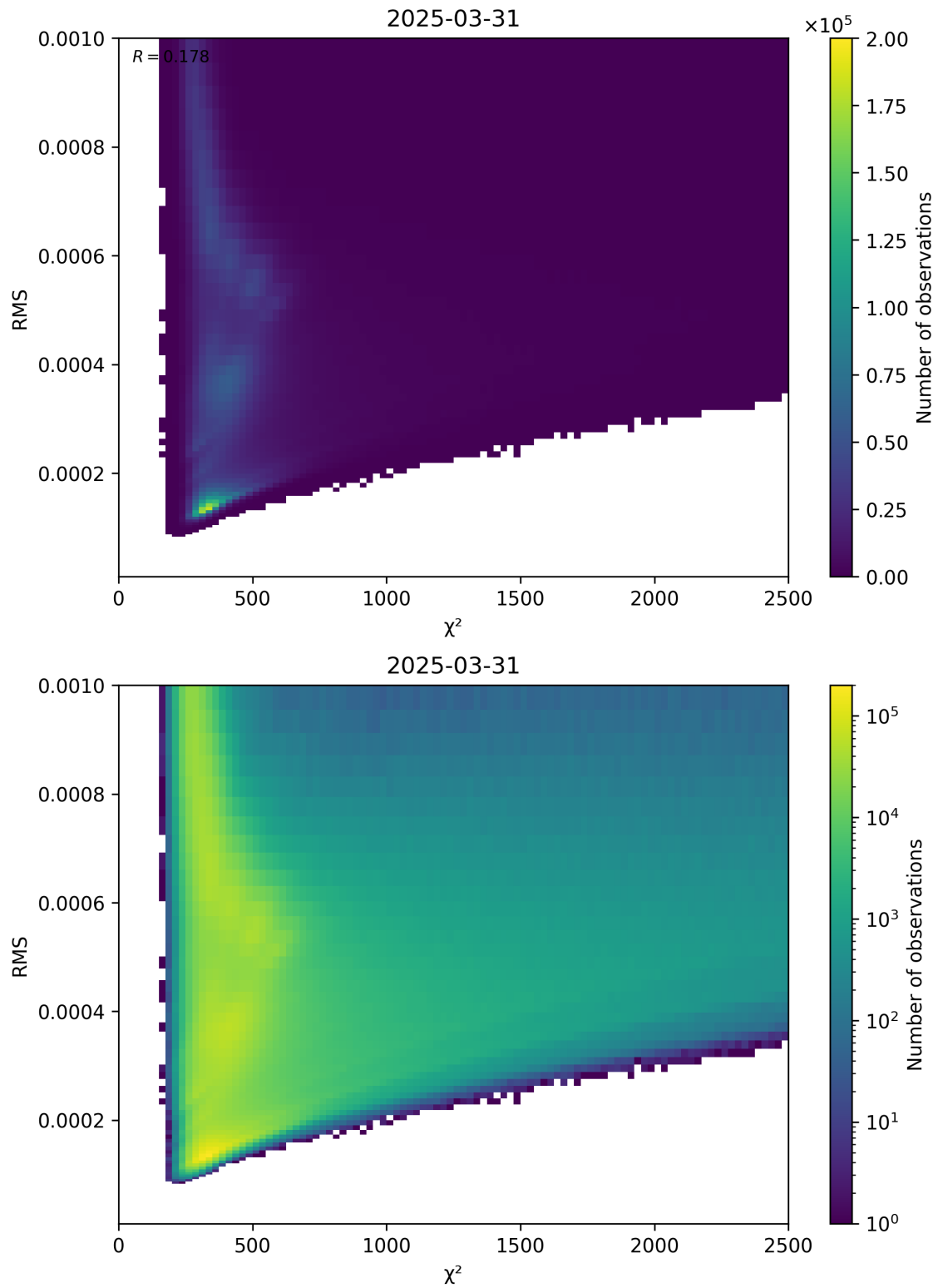
Figure 82: Scatter density plot of “ \chi^2 ” against “RMS” for 2025-03-31 to 2025-03-31.
