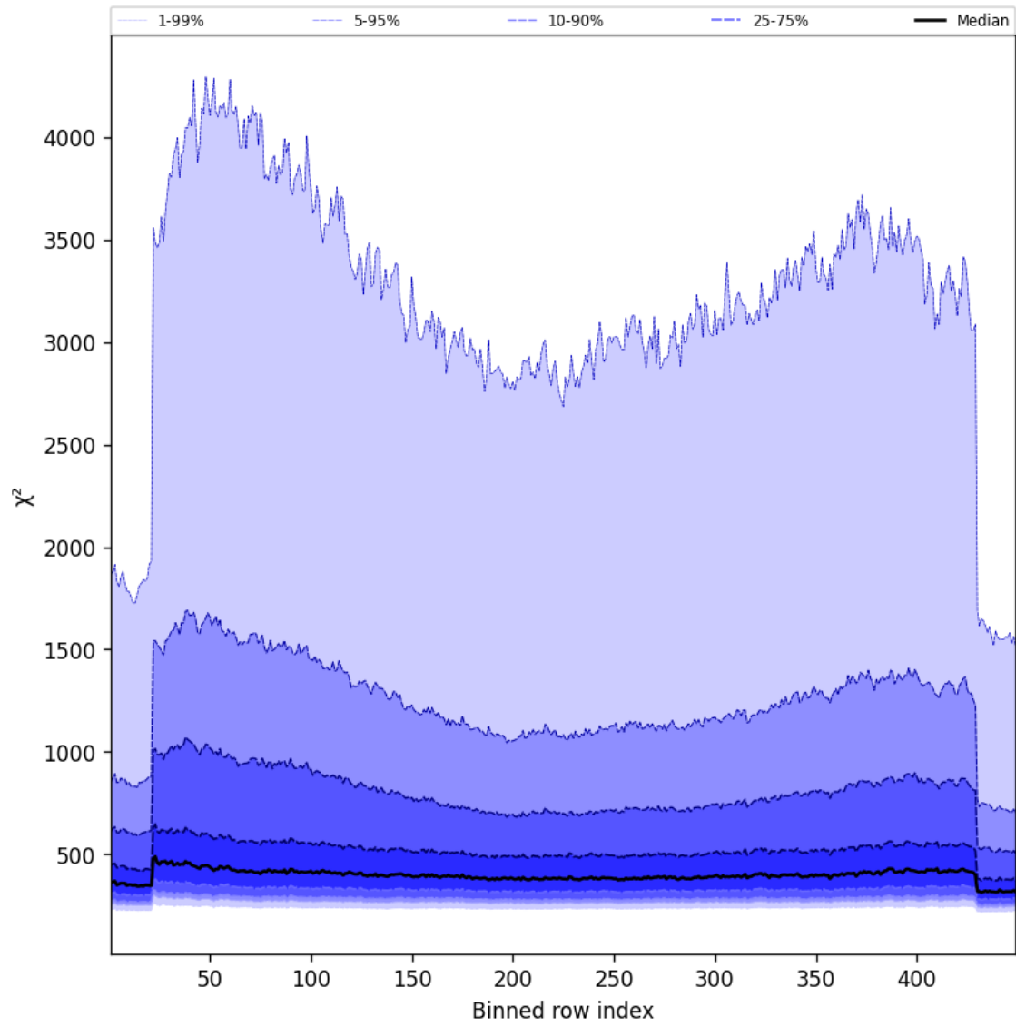
Figure 59: Along track statistics of “ \chi^2 ” for 2025-03-31 to 2025-03-31
