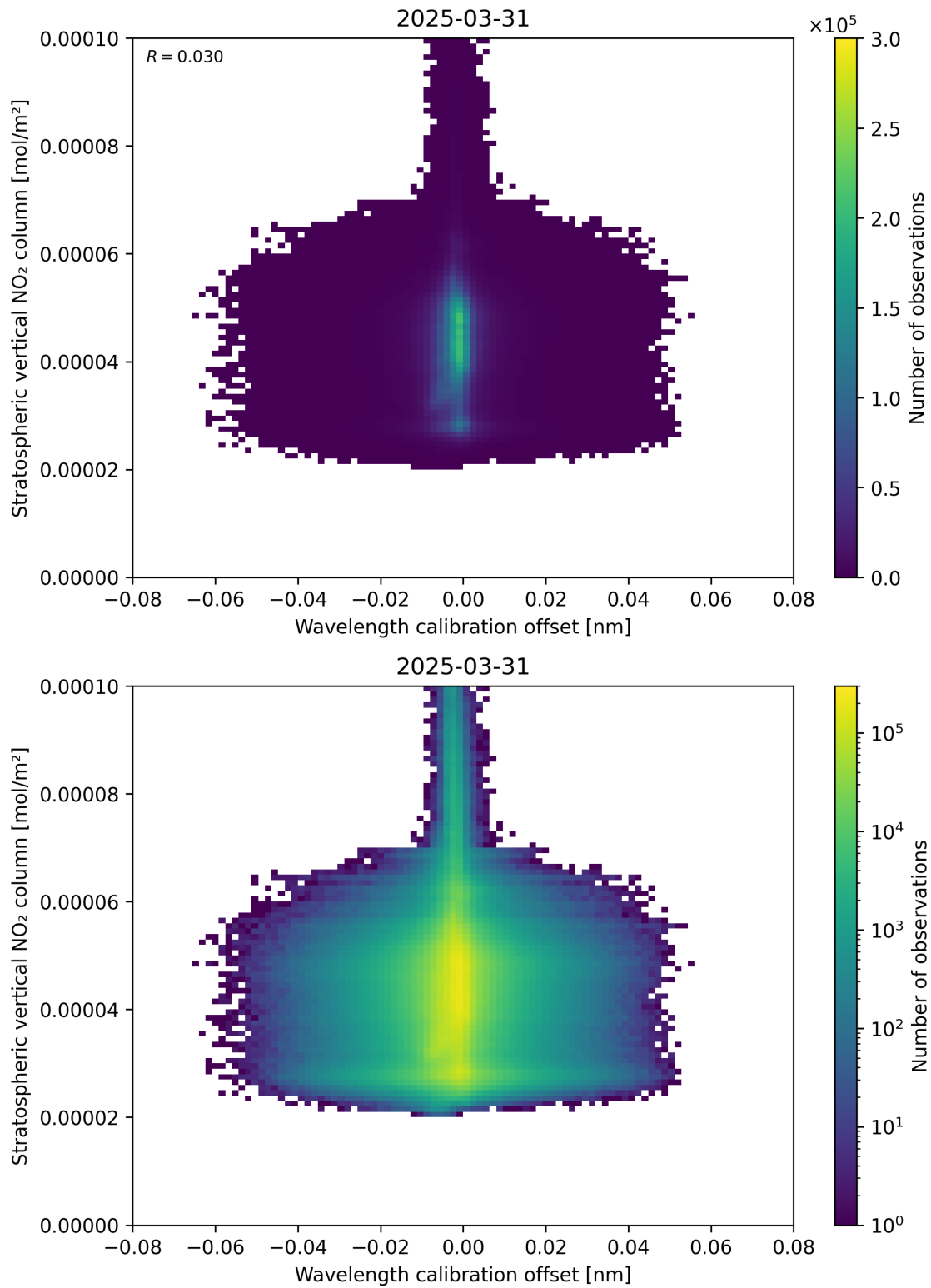
Figure 176: Scatter density plot of “Wavelength calibration offset” against “Stratospheric vertical NO 2 column” for 2025-03-31 to 2025-03-31.
