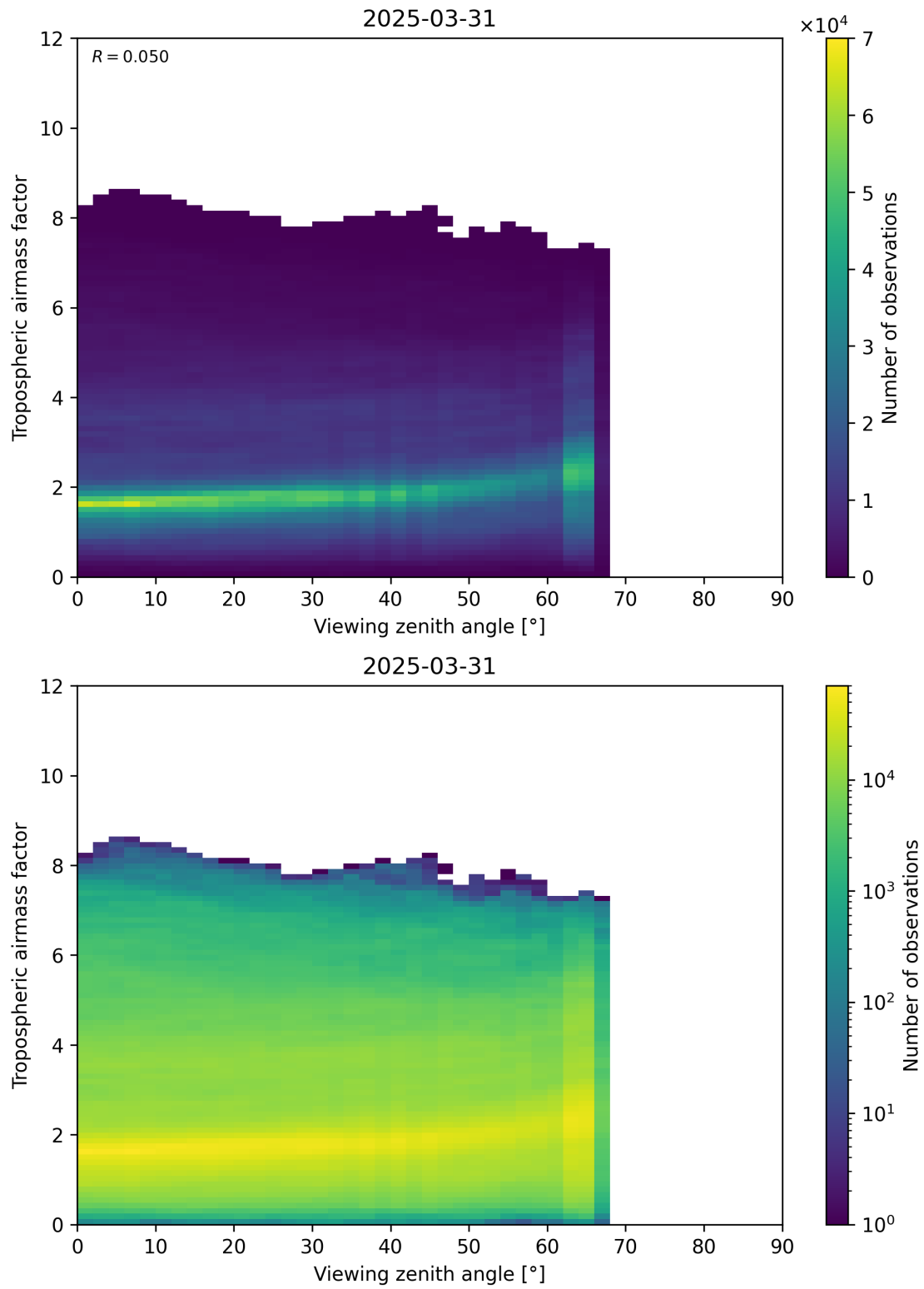
Figure 161: Scatter density plot of “Viewing zenith angle” against “Tropospheric airmass factor” for 2025-03-31 to 2025-03-31.
