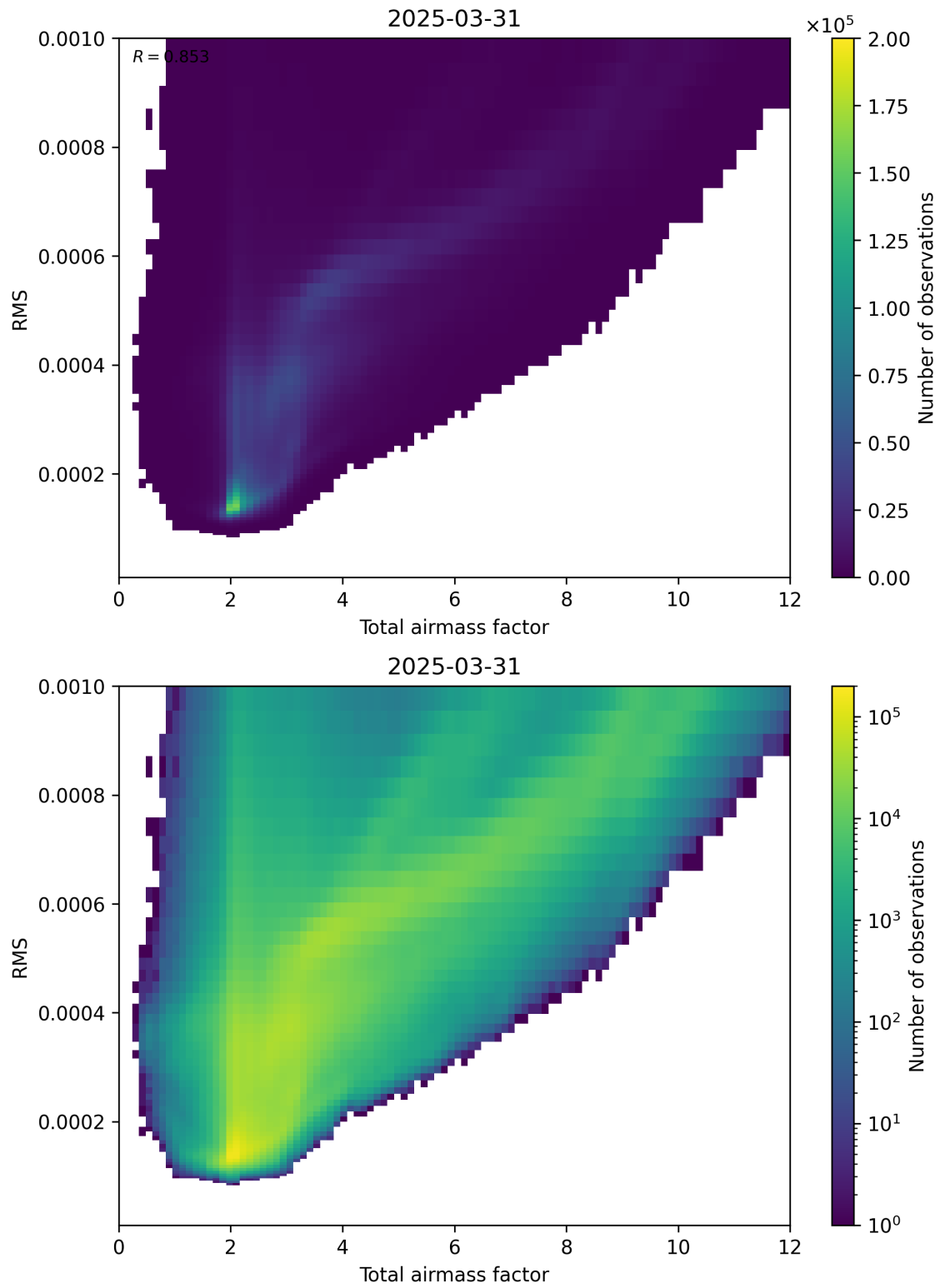
Figure 69: Scatter density plot of “Total airmass factor” against “RMS” for 2025-03-31 to 2025-03-31.
