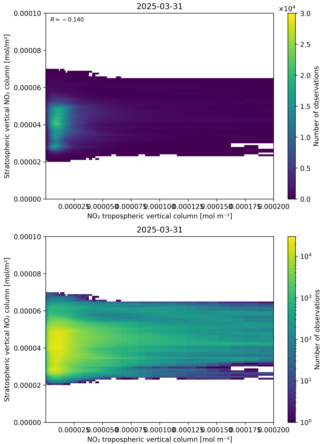
Figure 125: Scatter density plot of “NO 2 tropospheric vertical column” against “Stratospheric vertical NO 2 column” for 2025-03-31 to 2025-03-31.
