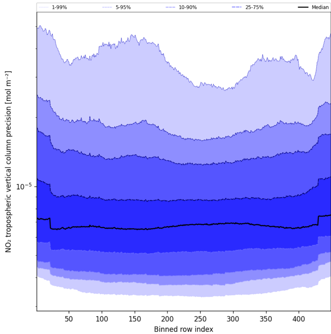
Figure 47: Along track statistics of “NO 2 tropospheric vertical column precision” for 2025-03-31 to 2025-03-31
