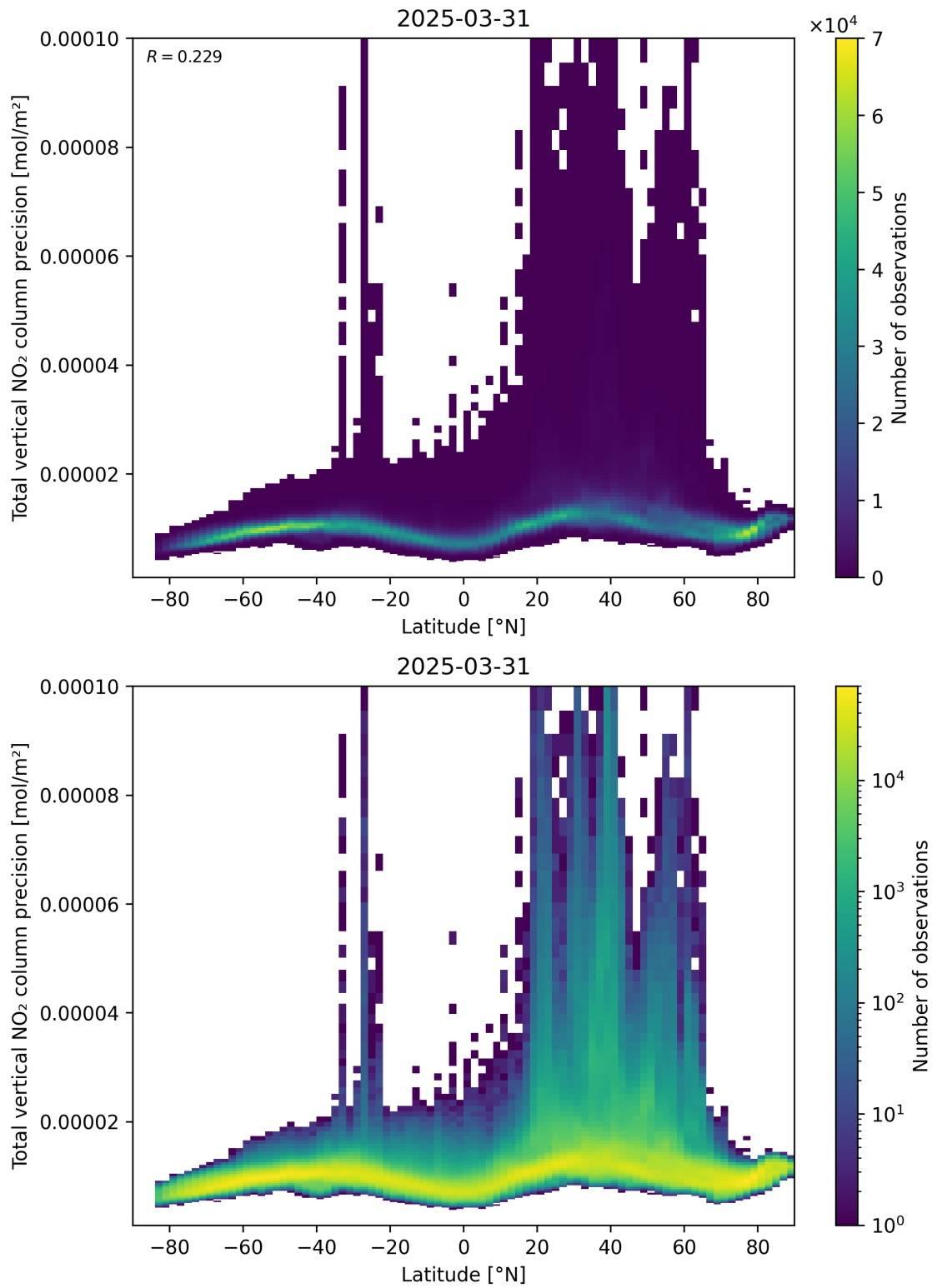
Figure 91: Scatter density plot of “Latitude” against “Total vertical NO 2 column precision” for 2025-03-31 to 2025-03-31.
