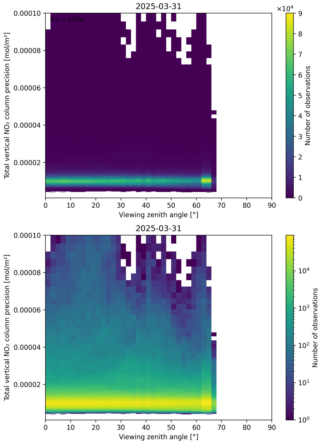
Figure 168: Scatter density plot of “Viewing zenith angle” against “Total vertical NO 2 column precision” for 2025-03-31 to 2025-03-31.
