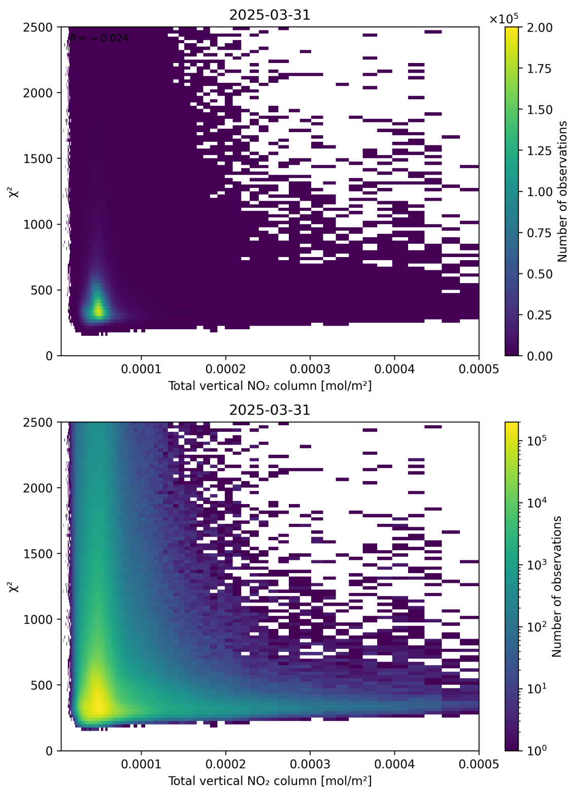
Figure 111: Scatter density plot of “Total vertical NO 2 column” against “ \chi^2 ” for 2025-03-31 to 2025-03-31.
