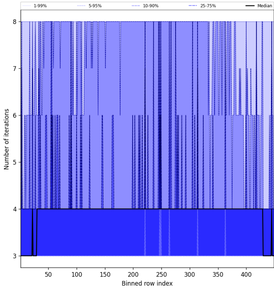
Figure 51: Along track statistics of “Number of iterations” for 2025-03-31 to 2025-03-31
