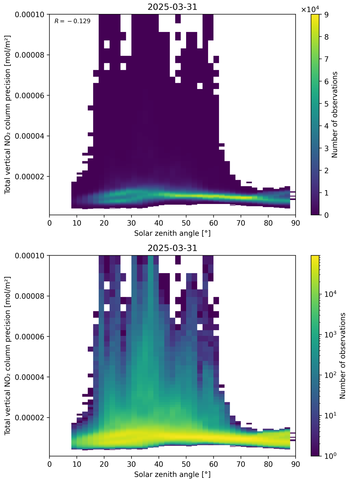
Figure 154: Scatter density plot of “Solar zenith angle” against “Total vertical NO 2 column precision” for 2025-03-31 to 2025-03-31.
