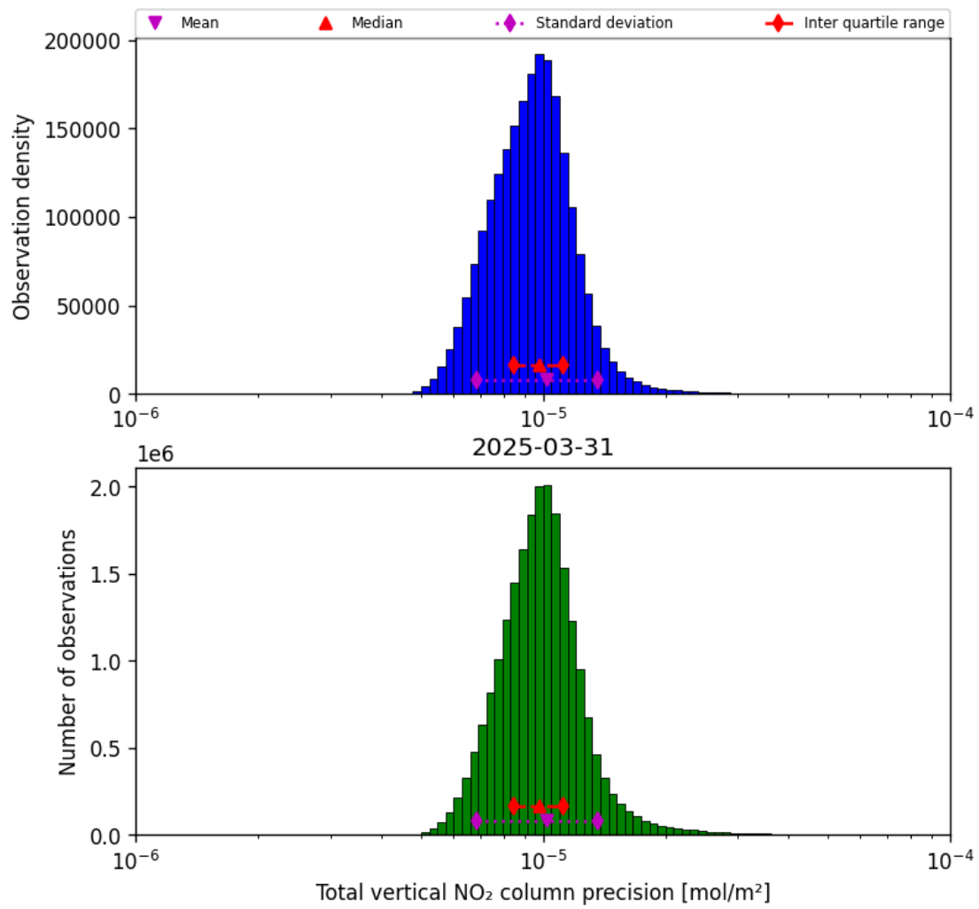
Figure 39: Histogram of "Total vertical NO 2 column precision" for 2025-03-31 to 2025-03-31
