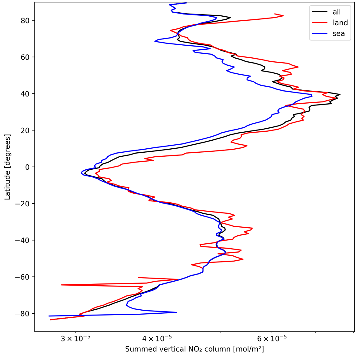
Figure 23: Zonal average of “Summed vertical NO 2 column” for 2025-03-31 to 2025-03-31.
