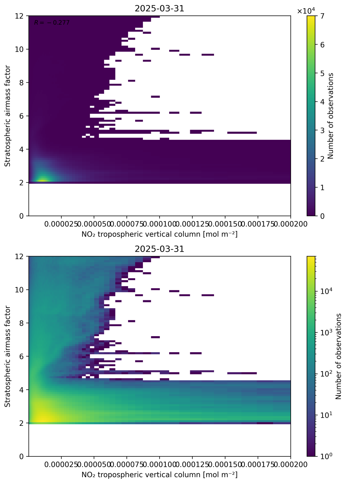
Figure 121: Scatter density plot of “NO 2 tropospheric vertical column” against “Stratospheric air mass factor” for 2025-03-31 to 2025-03-31.
