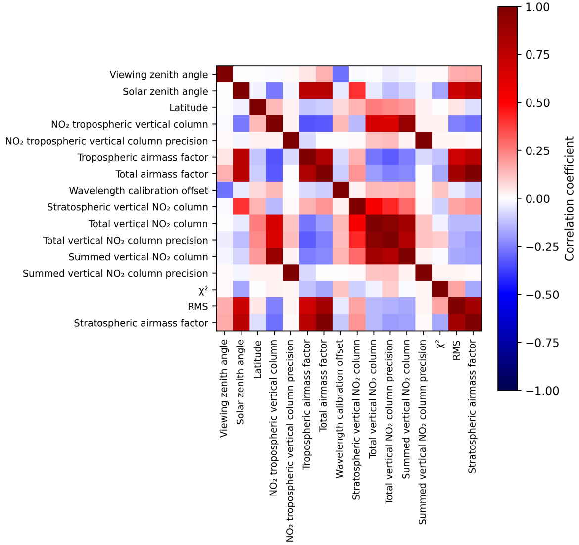
Figure 2: Map of correlation matrix for 2025-03-31 to 2025-03-31.
