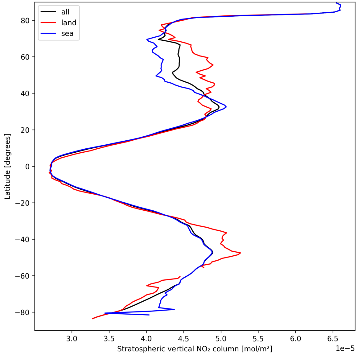
Figure 19: Zonal average of “Stratospheric vertical NO 2 column” for 2025-03-31 to 2025-03-31.
