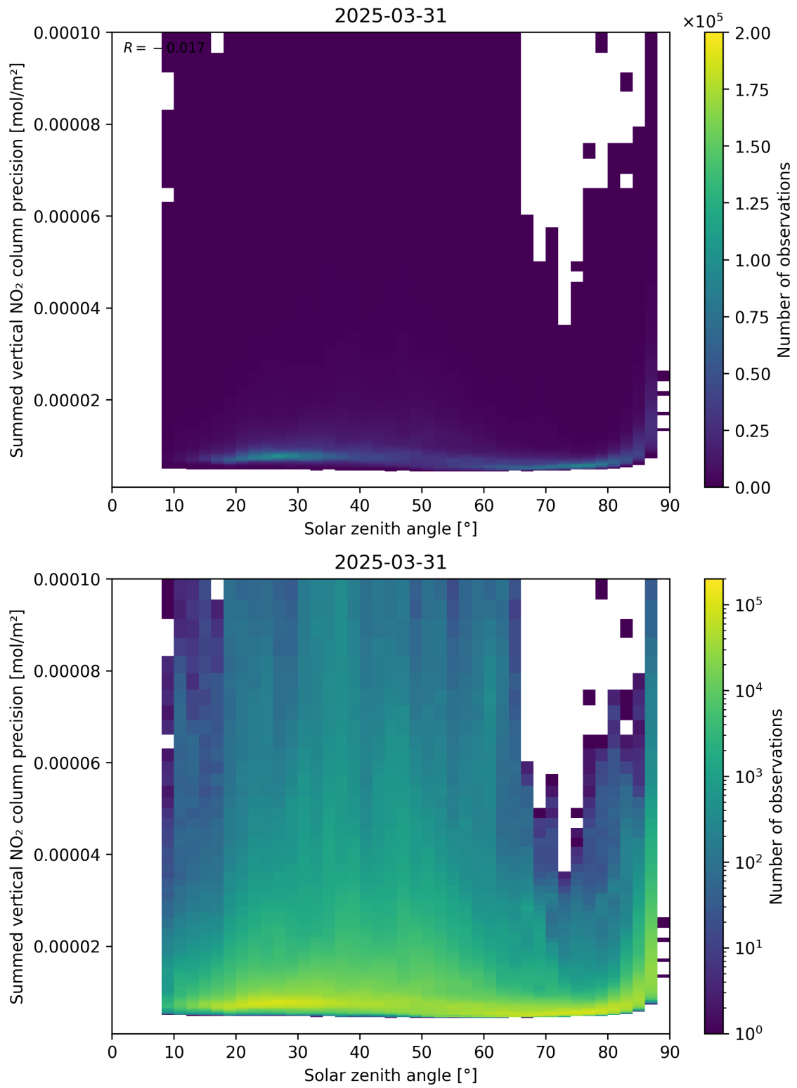
Figure 152: Scatter density plot of “Solar zenith angle” against “Summed vertical NO 2 column precision” for 2025-03-31 to 2025-03-31.
