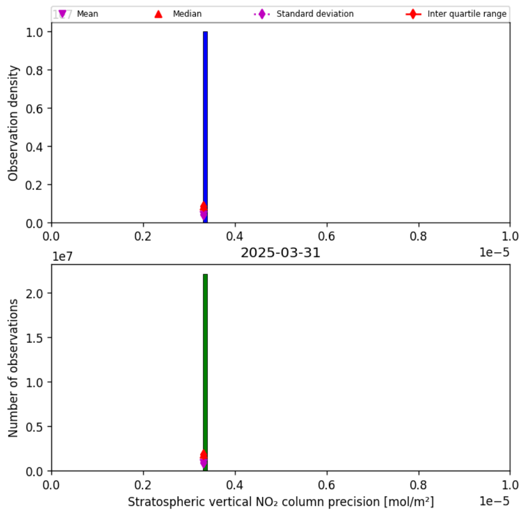
Figure 37: Histogram of “Stratospheric vertical NO 2 column precision” for 2025-03-31 to 2025-03-31
