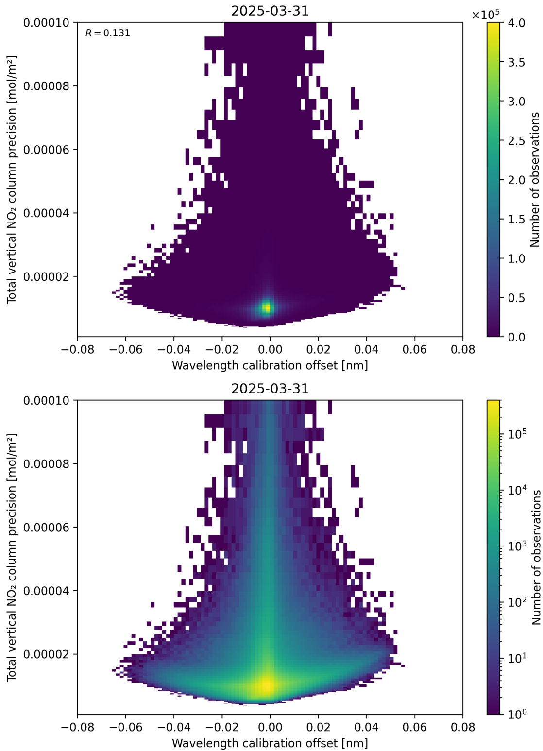
Figure 180: Scatter density plot of “Wavelength calibration offset” against “Total vertical NO 2 column precision” for 2025-03-31 to 2025-03-31.
