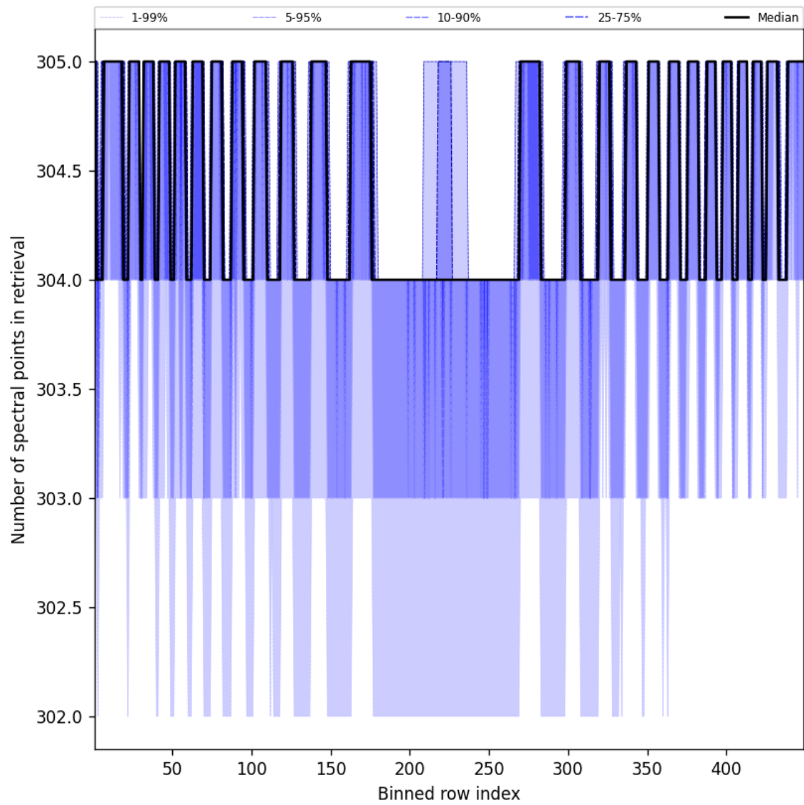
Figure 50: Along track statistics of “Number of spectral points in retrieval” for 2025-03-31 to 2025-03-31
