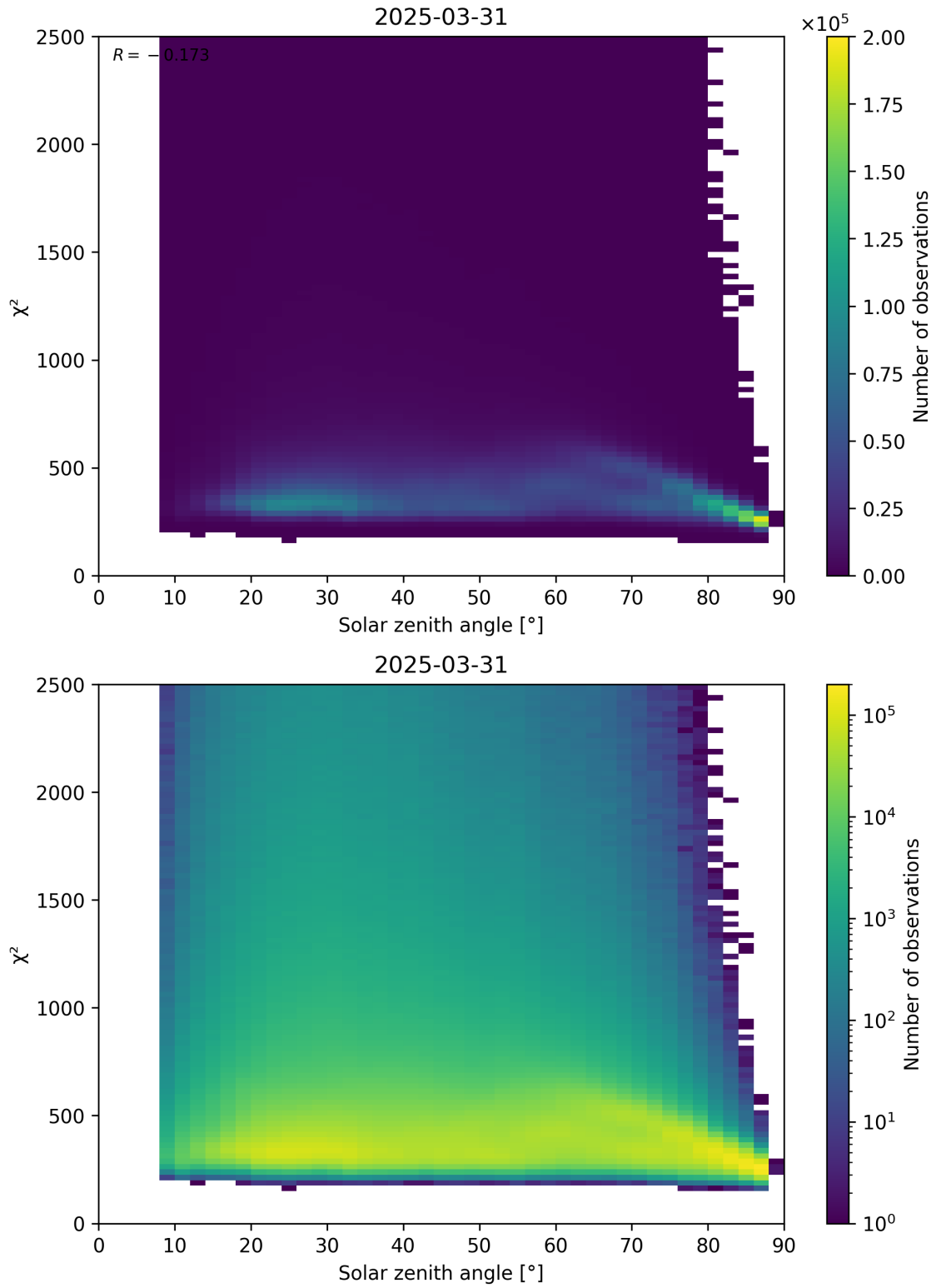
Figure 148: Scatter density plot of “Solar zenith angle” against “ \chi^2 ” for 2025-03-31 to 2025-03-31.
