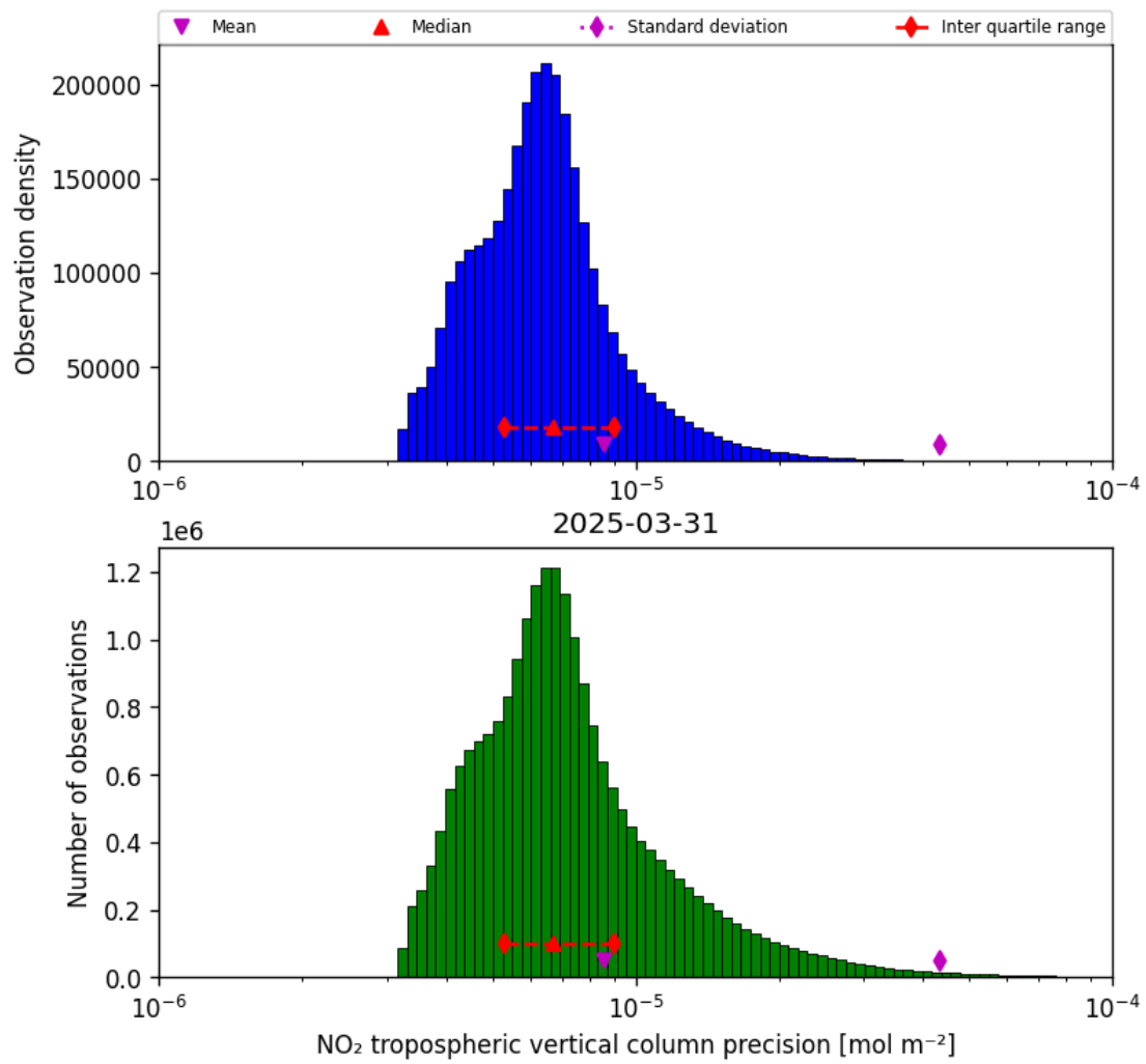
Figure 30: Histogram of “NO 2 tropospheric vertical column precision” for 2025-03-31 to 2025-03-31
