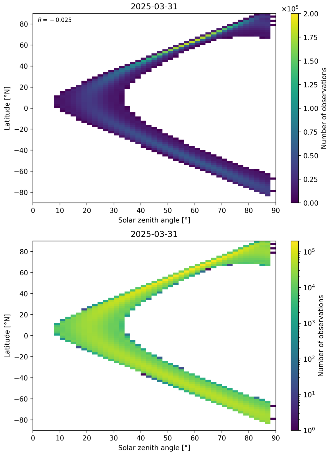
Figure 149: Scatter density plot of “Solar zenith angle” against “Latitude” for 2025-03-31 to 2025-03-31.
