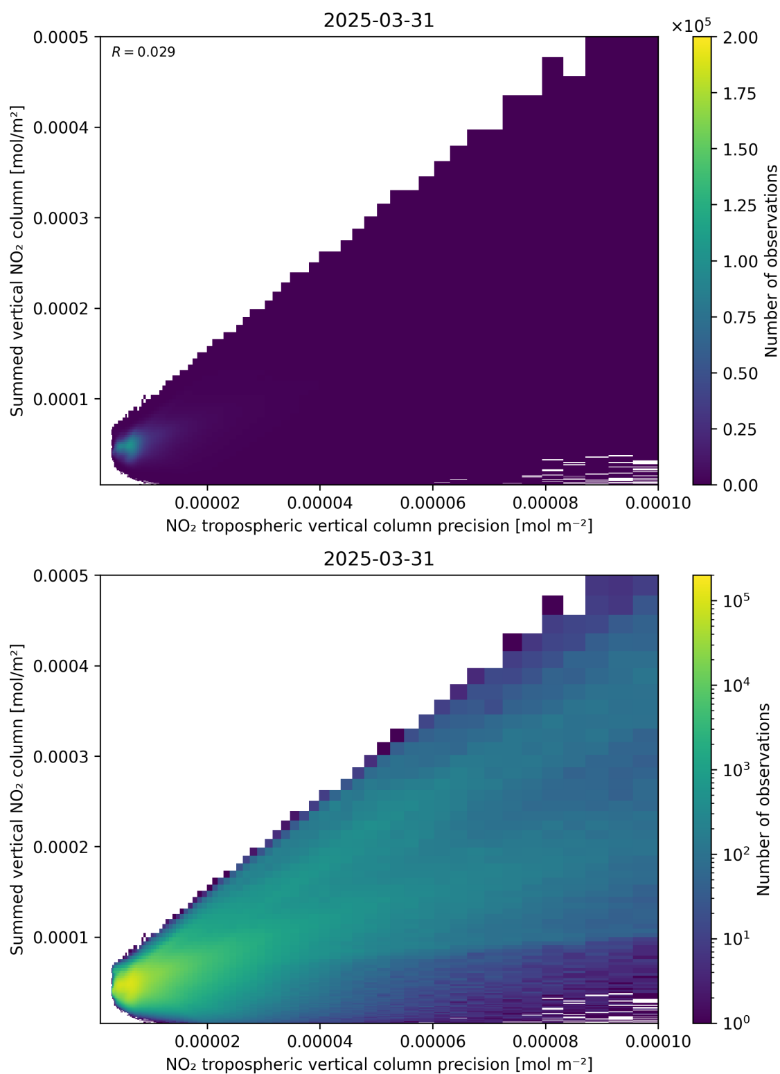
Figure 136: Scatter density plot of “NO 2 tropospheric vertical column precision” against “Summed vertical NO 2 column” for 2025-03-31 to 2025-03-31.
