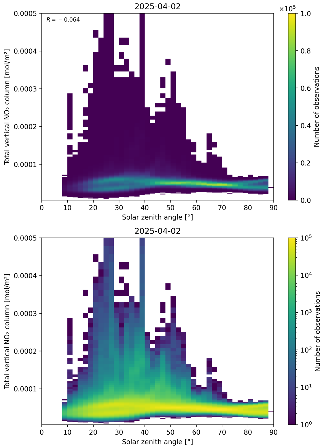
Figure 153: Scatter density plot of “Solar zenith angle” against “Total vertical NO 2 column” for 2025-04-02 to 2025-04-03.
