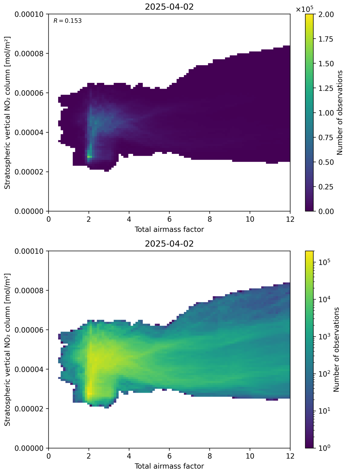
Figure 64: Scatter density plot of “Total airmass factor” against “Stratospheric vertical NO 2 column” for 2025-04-02 to 2025-04-03.
