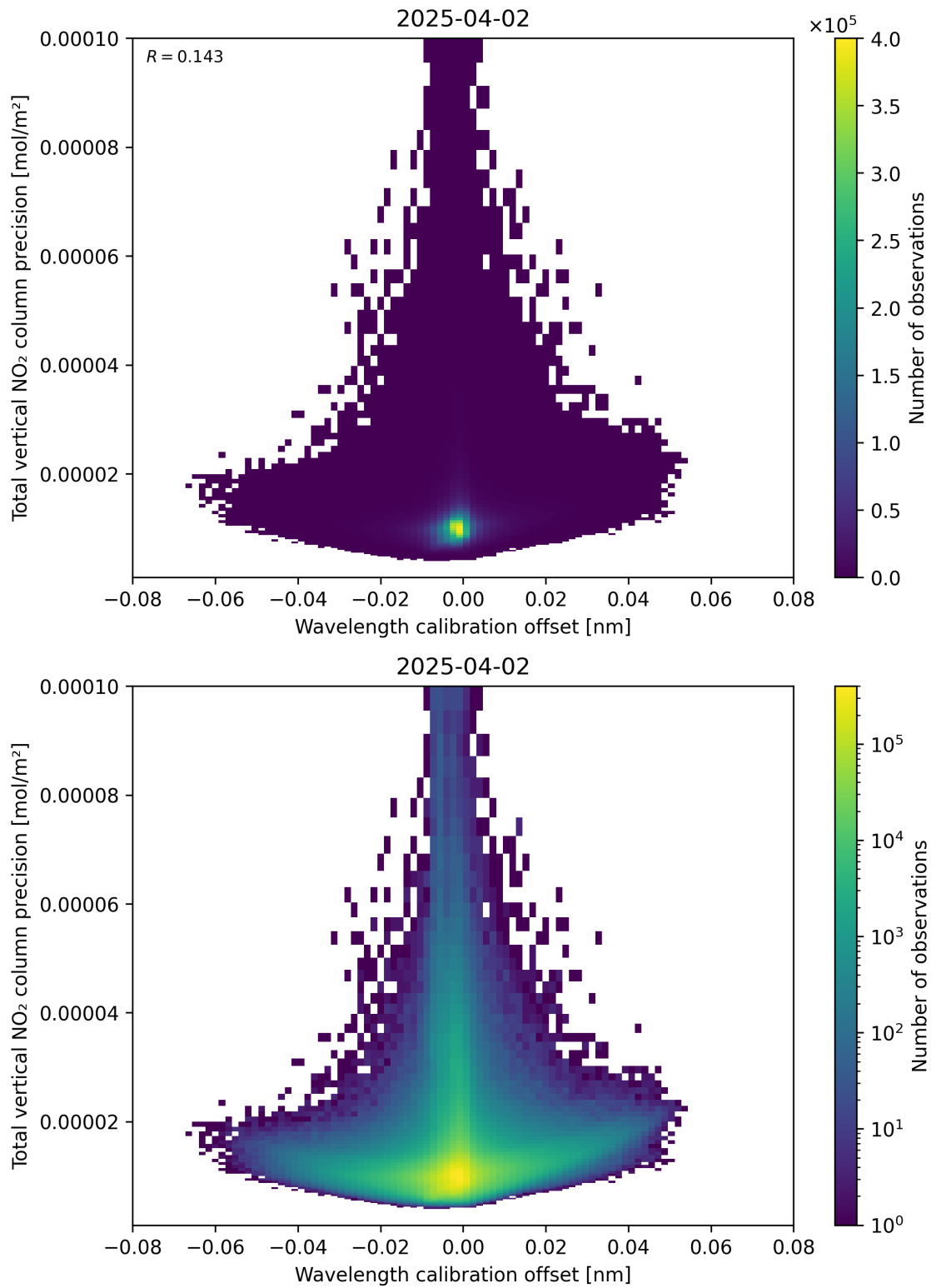
Figure 180: Scatter density plot of “Wavelength calibration offset” against “Total vertical NO 2 column precision” for 2025-04-02 to 2025-04-03.
