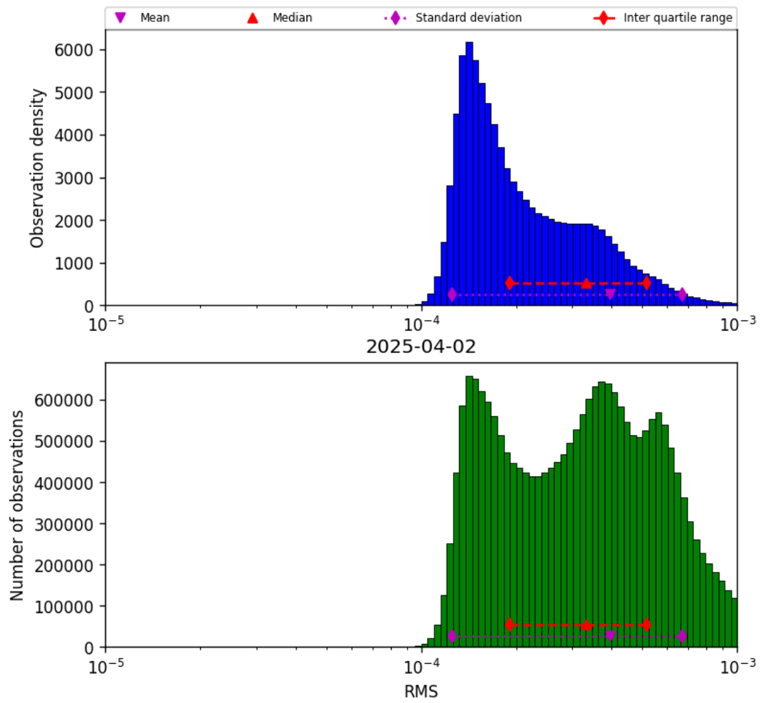
Figure 43: Histogram of “RMS” for 2025-04-02 to 2025-04-03
