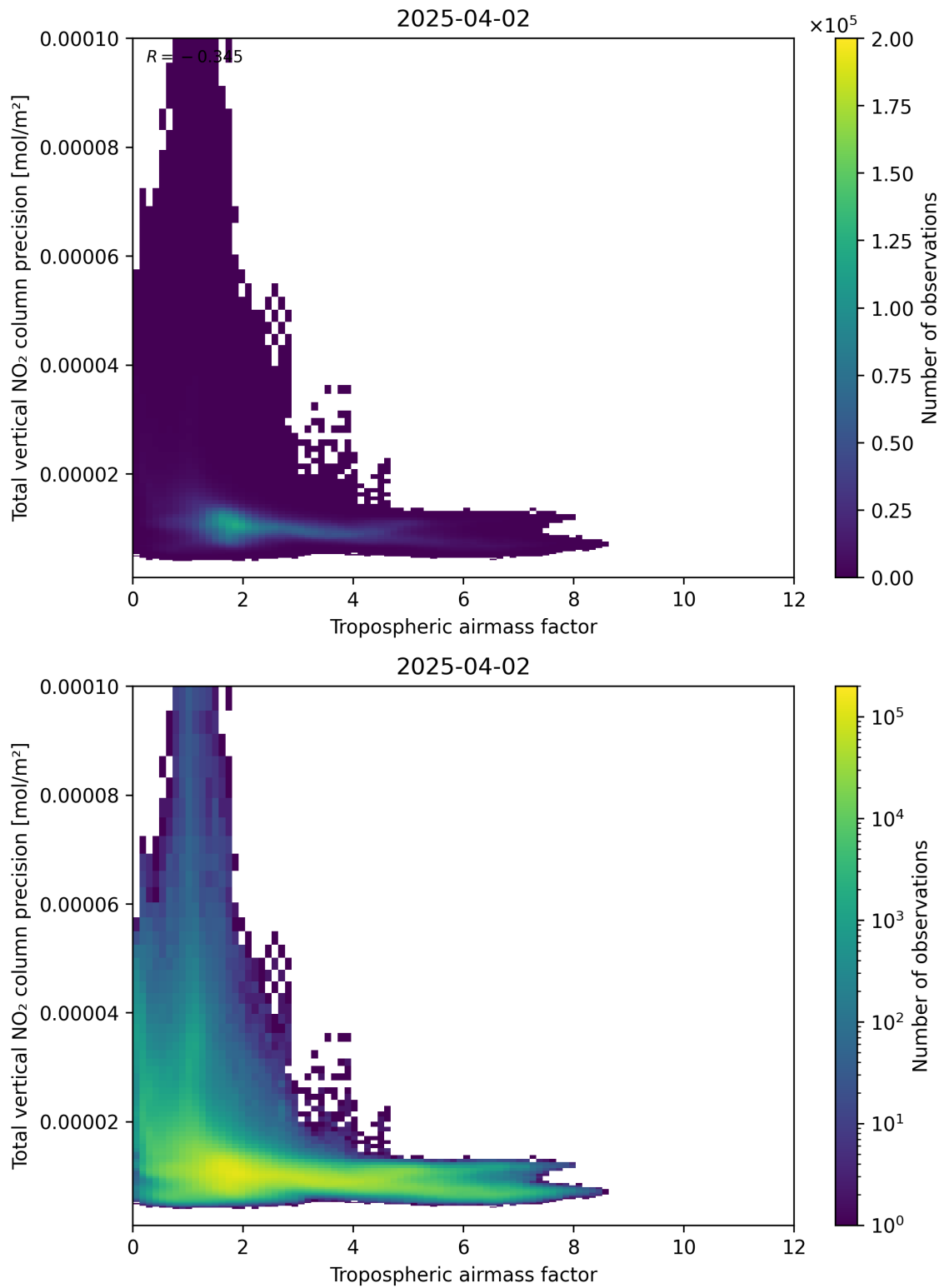
Figure 78: Scatter density plot of “Tropospheric airmass factor” against “Total vertical NO 2 column precision” for 2025-04-02 to 2025-04-03.
