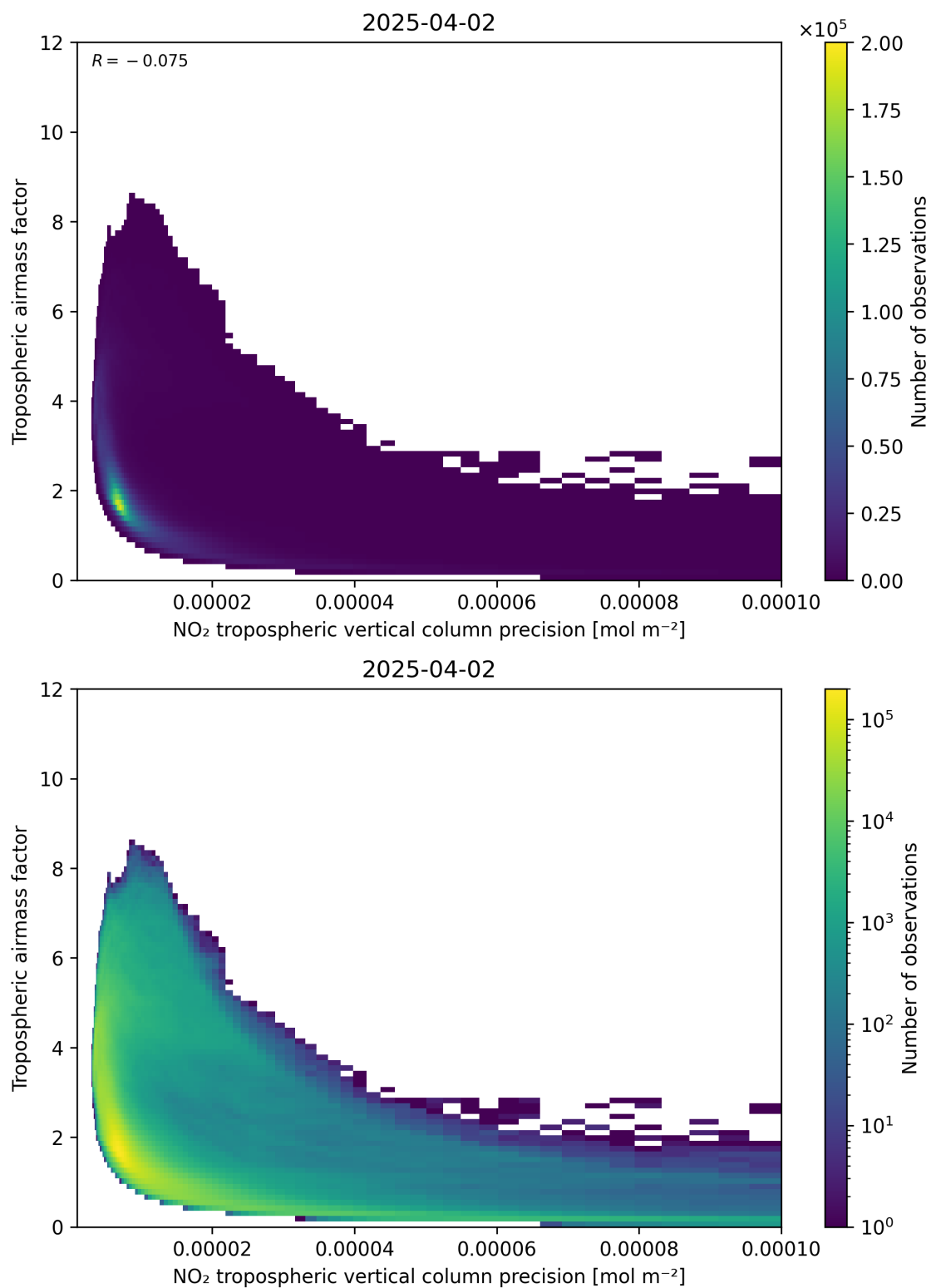
Figure 133: Scatter density plot of “NO 2 tropospheric vertical column precision” against “Tropospheric airmass factor” for 2025-04-02 to 2025-04-03.
