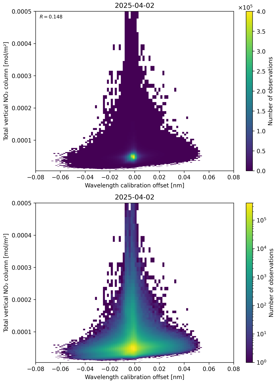
Figure 179: Scatter density plot of “Wavelength calibration offset” against “Total vertical NO 2 column” for 2025-04-02 to 2025-04-03.
