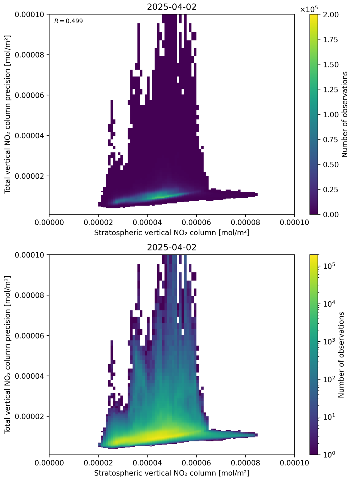
Figure 101: Scatter density plot of “Stratospheric vertical NO 2 column” against “Total vertical NO 2 column precision” for 2025-04-02 to 2025-04-03.
