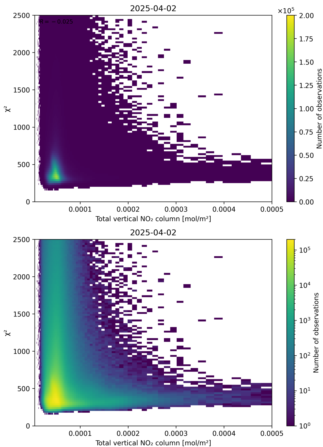
Figure 111: Scatter density plot of “Total vertical NO 2 column” against “ \chi^2 ” for 2025-04-02 to 2025-04-03.
