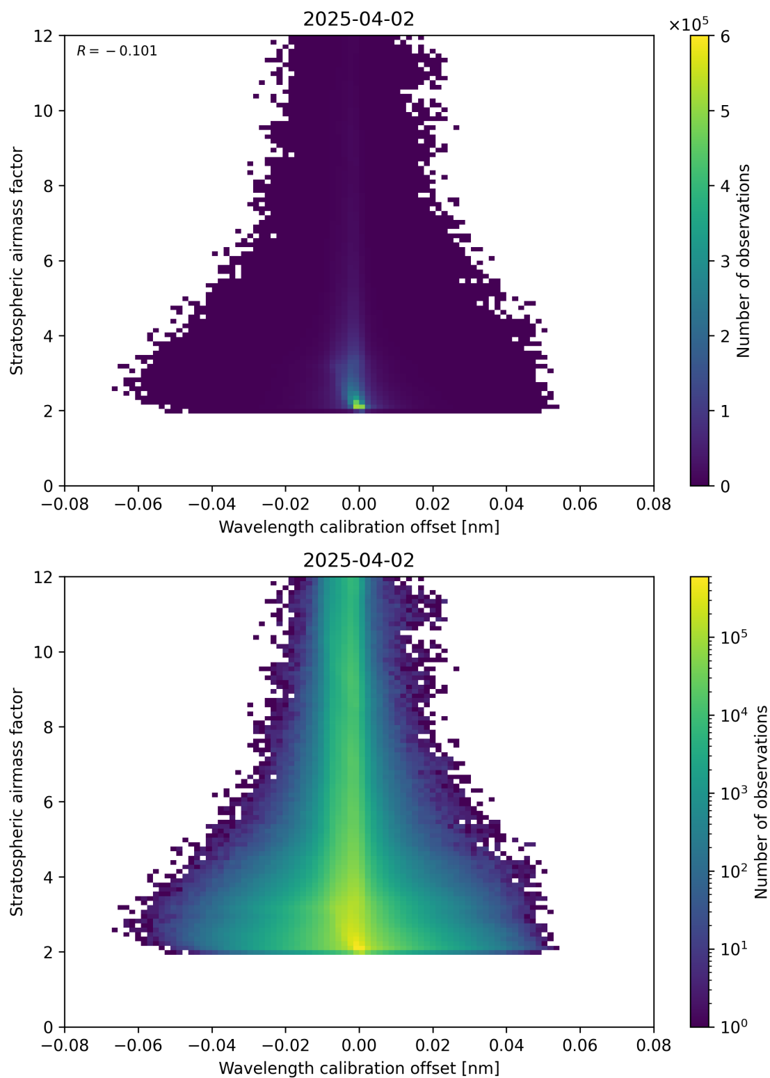
Figure 174: Scatter density plot of “Wavelength calibration offset” against “Stratospheric airmass factor” for 2025-04-02 to 2025-04-03.
