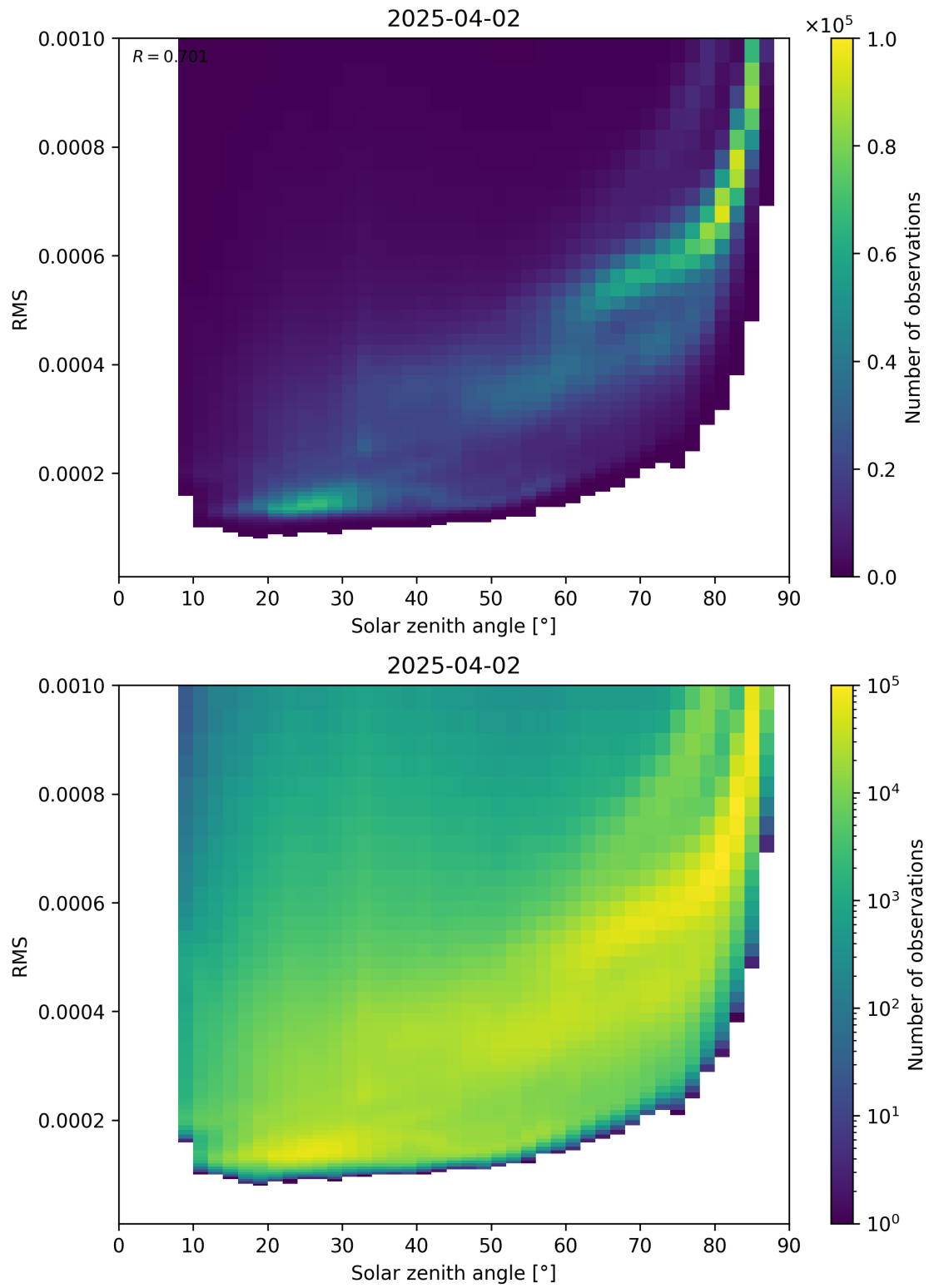
Figure 157: Scatter density plot of “Solar zenith angle” against “RMS” for 2025-04-02 to 2025-04-03.
