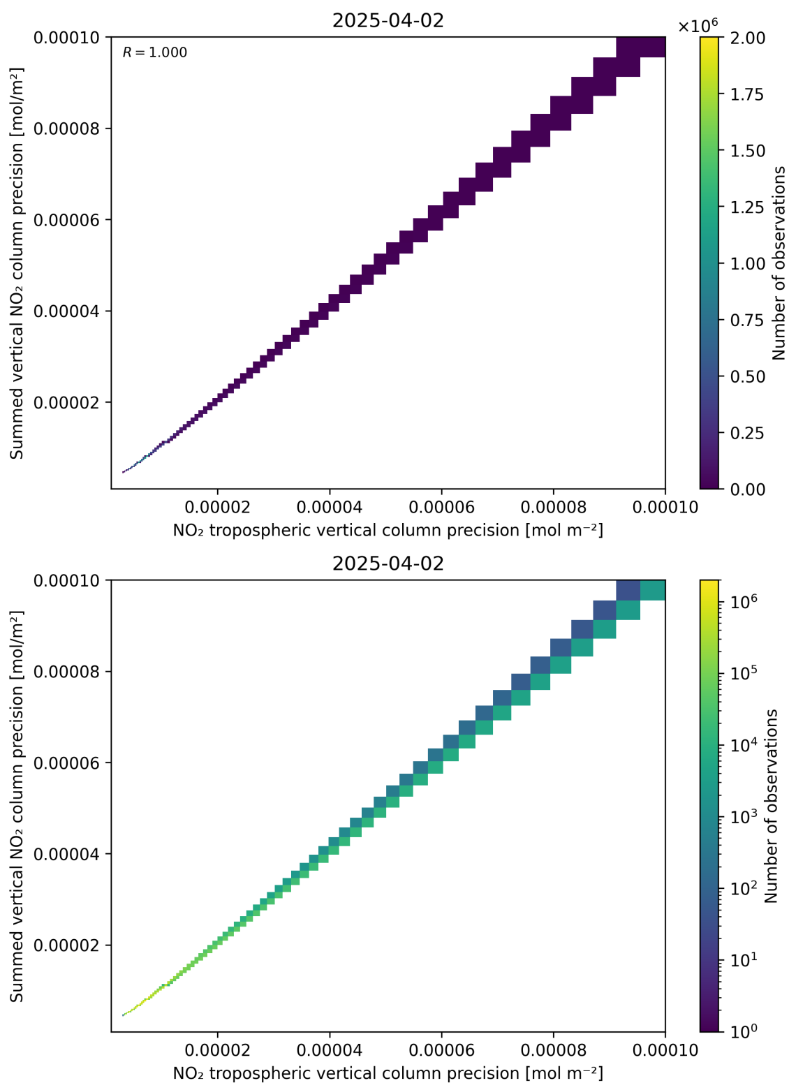
Figure 137: Scatter density plot of “NO 2 tropospheric vertical column precision” against “Summed vertical NO 2 column precision” for 2025-04-02 to 2025-04-03.
