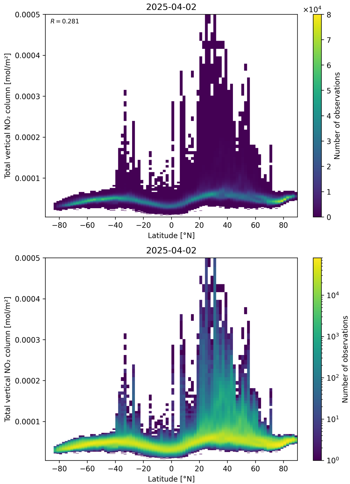
Figure 90: Scatter density plot of “Latitude” against “Total vertical NO 2 column” for 2025-04-02 to 2025-04-03.
