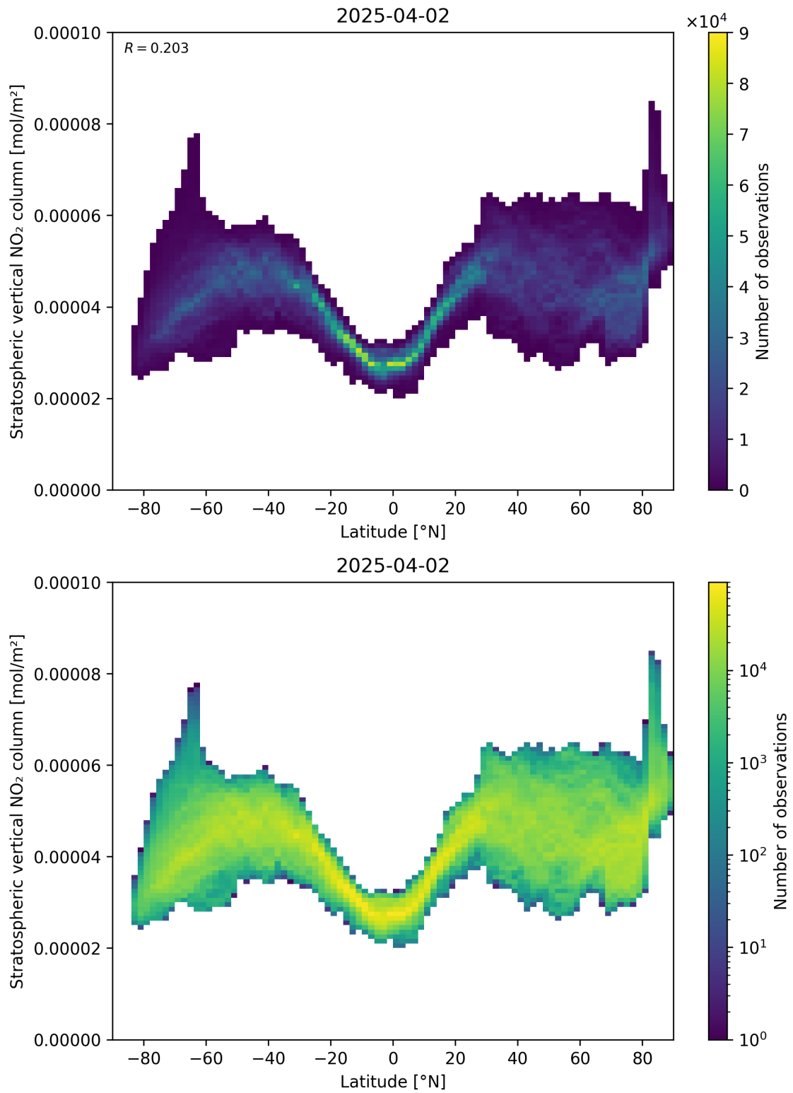
Figure 87: Scatter density plot of “Latitude” against “Stratospheric vertical NO 2 column” for 2025-04-02 to 2025-04-03.
