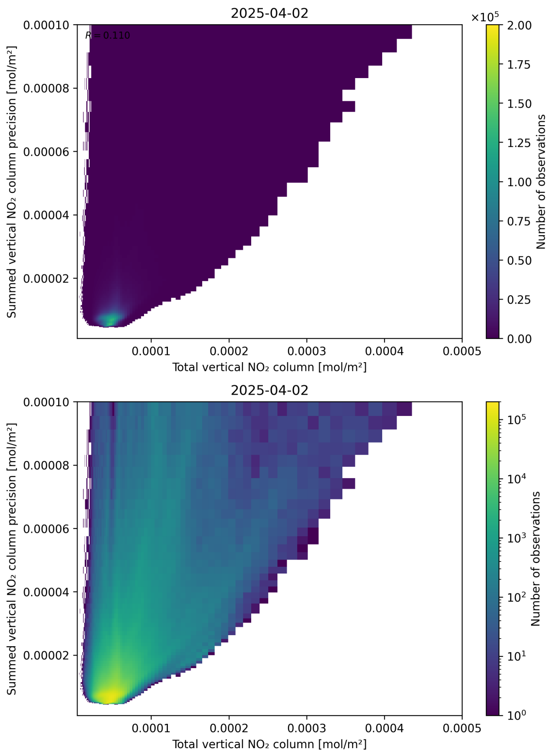
Figure 113: Scatter density plot of “Total vertical NO 2 column” against “Summed vertical NO 2 column precision” for 2025-04-02 to 2025-04-03.
