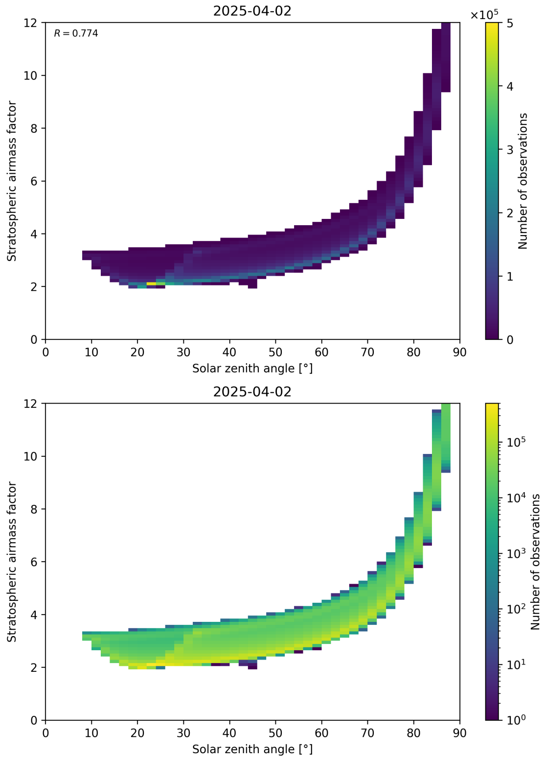
Figure 145: Scatter density plot of “Solar zenith angle” against “Stratospheric airmass factor” for 2025-04-02 to 2025-04-03.
