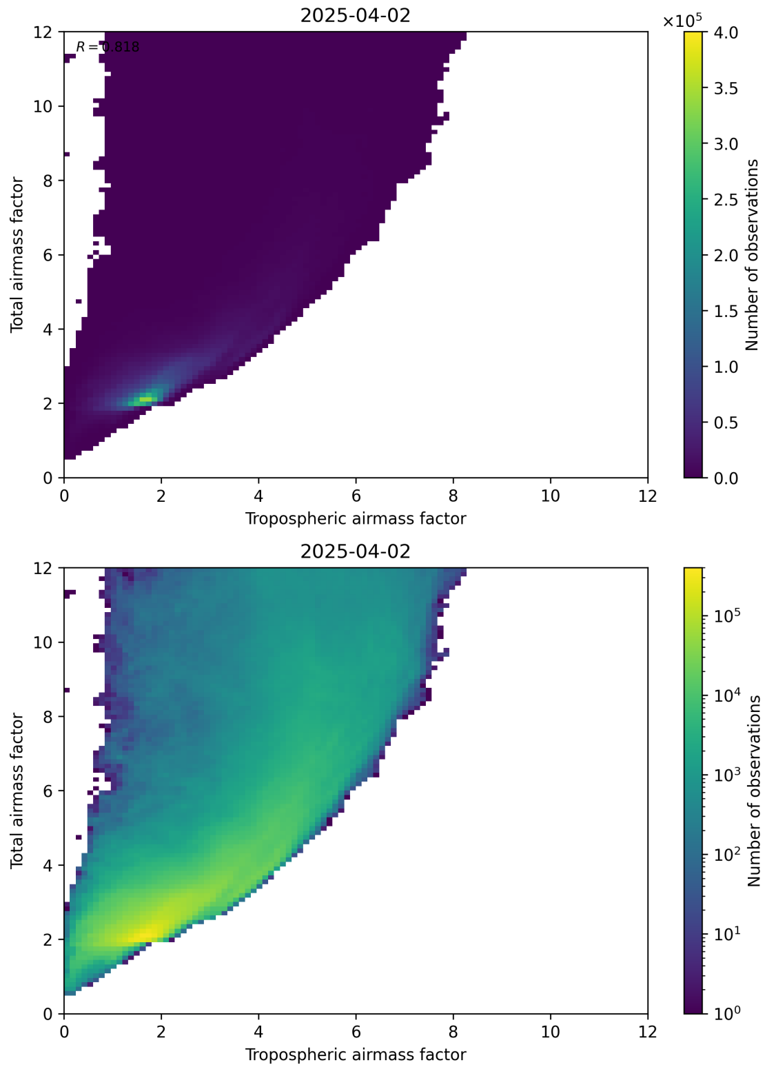
Figure 72: Scatter density plot of “Tropospheric airmass factor” against “Total airmass factor” for 2025-04-02 to 2025-04-03.
