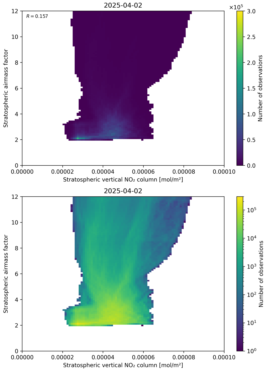
Figure 96: Scatter density plot of “Stratospheric vertical NO 2 column” against “Stratospheric airmass factor” for 2025-04-02 to 2025-04-03.
