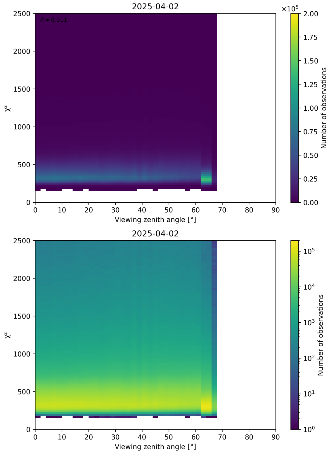
Figure 162: Scatter density plot of “Viewing zenith angle” against “ \chi^2 ” for 2025-04-02 to 2025-04-03.
