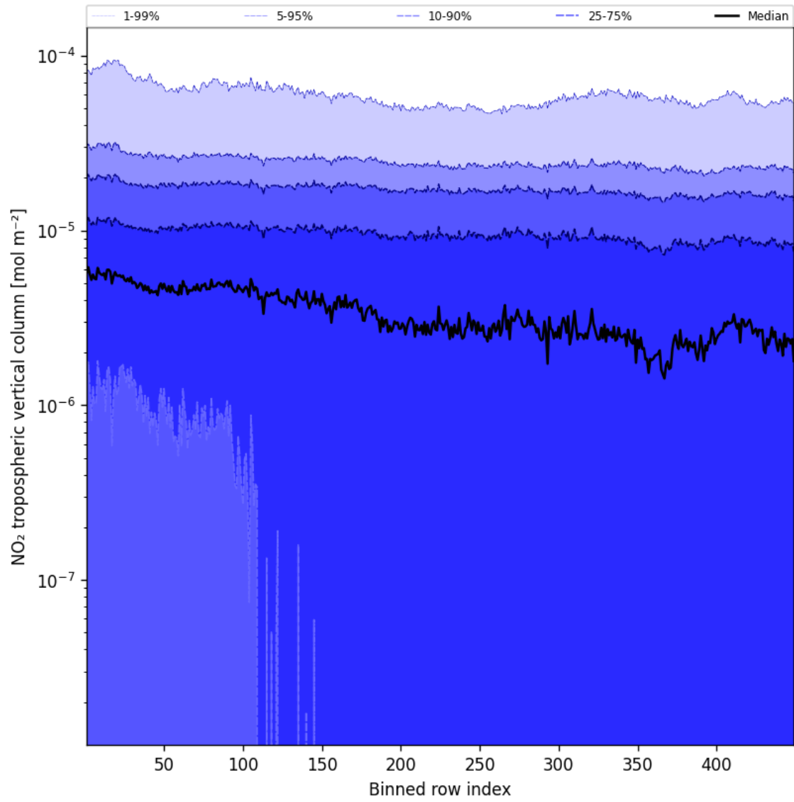
Figure 46: Along track statistics of “NO 2 tropospheric vertical column” for 2025-04-02 to 2025-04-03
