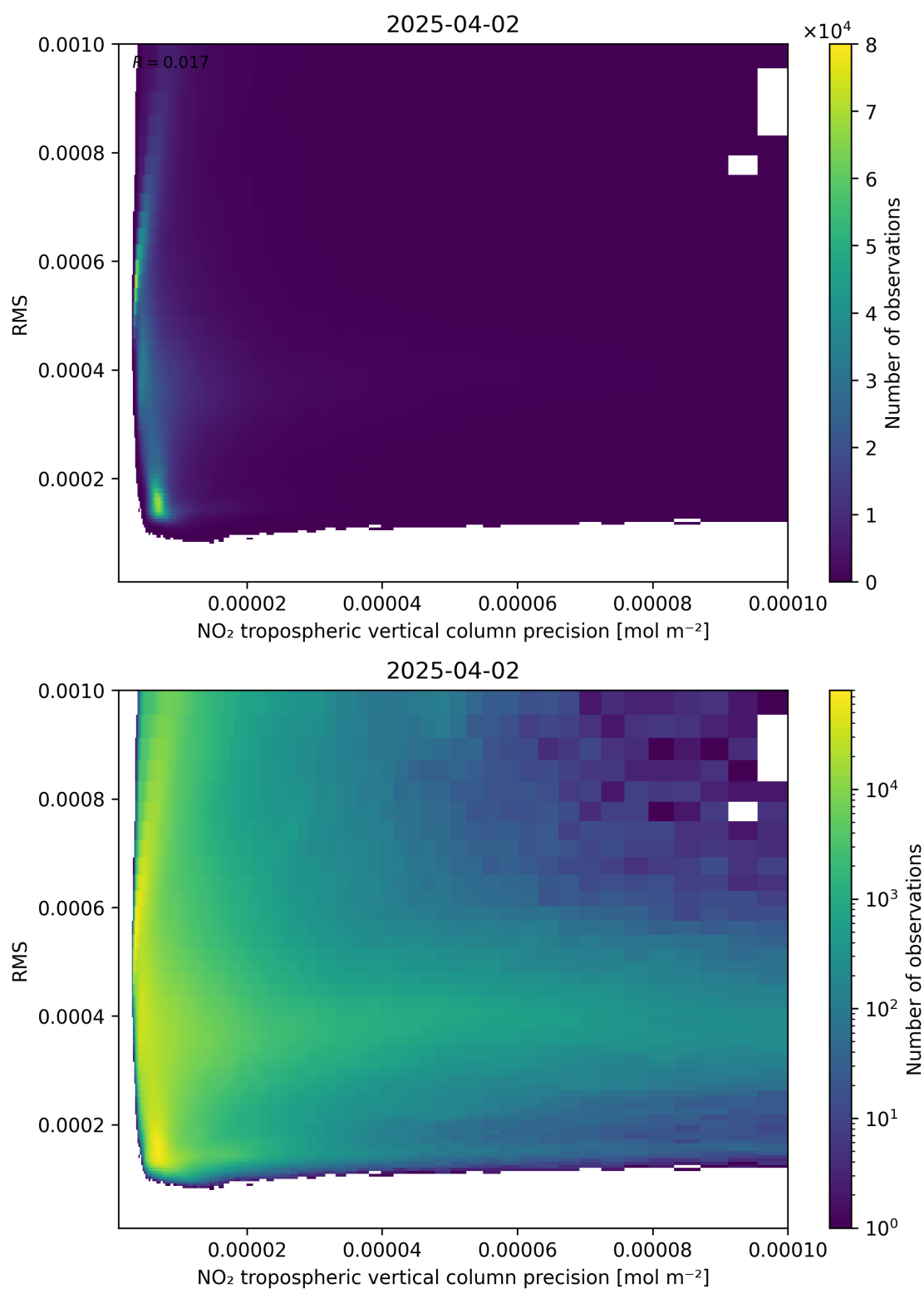
Figure 140: Scatter density plot of “NO 2 tropospheric vertical column precision” against “RMS” for 2025-04-02 to 2025-04-03.
