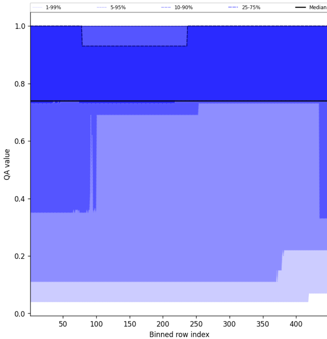
Figure 45: Along track statistics of “QA value” for 2025-04-02 to 2025-04-03
