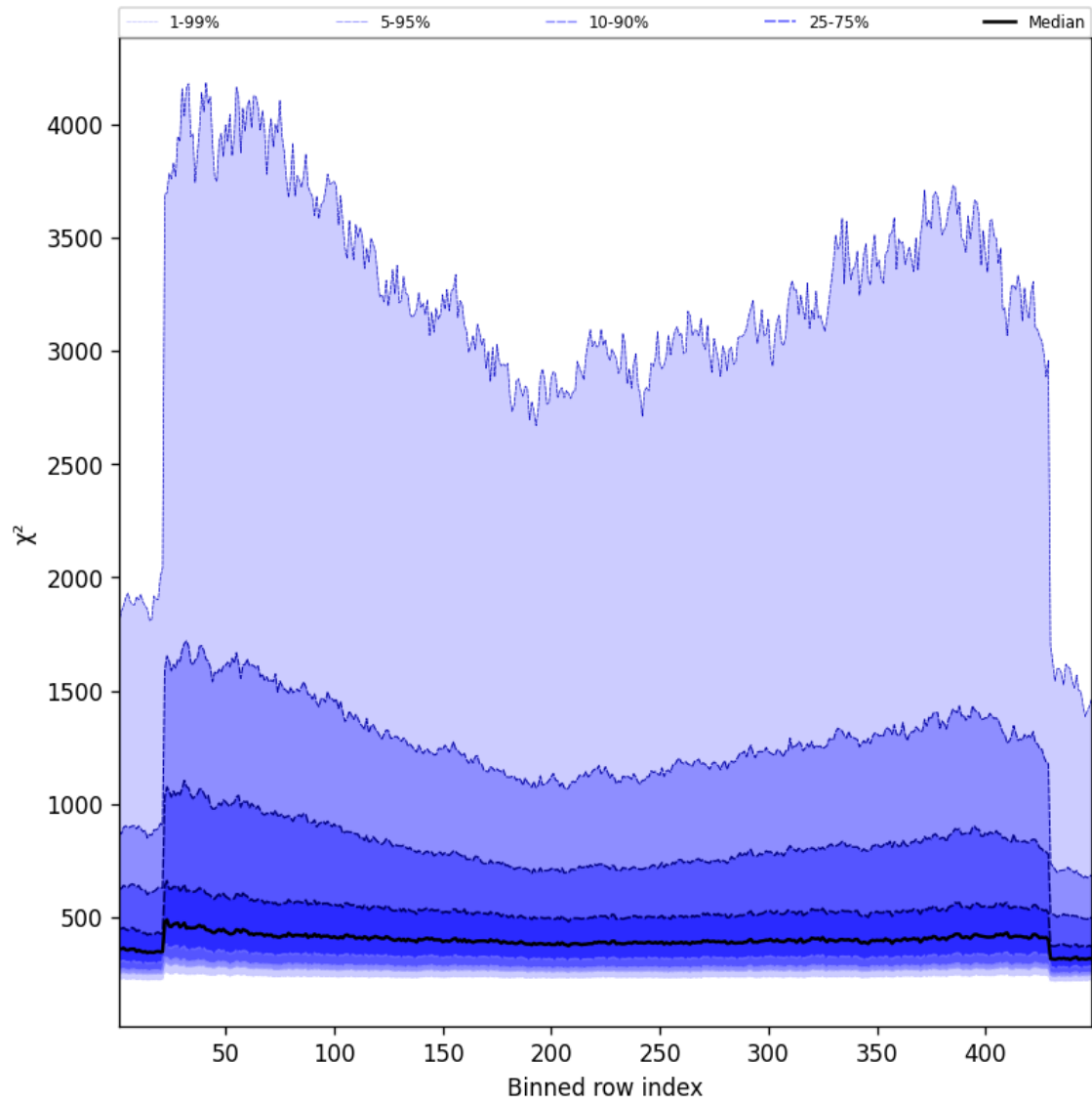
Figure 59: Along track statistics of “ \chi^2 ” for 2025-04-02 to 2025-04-03
