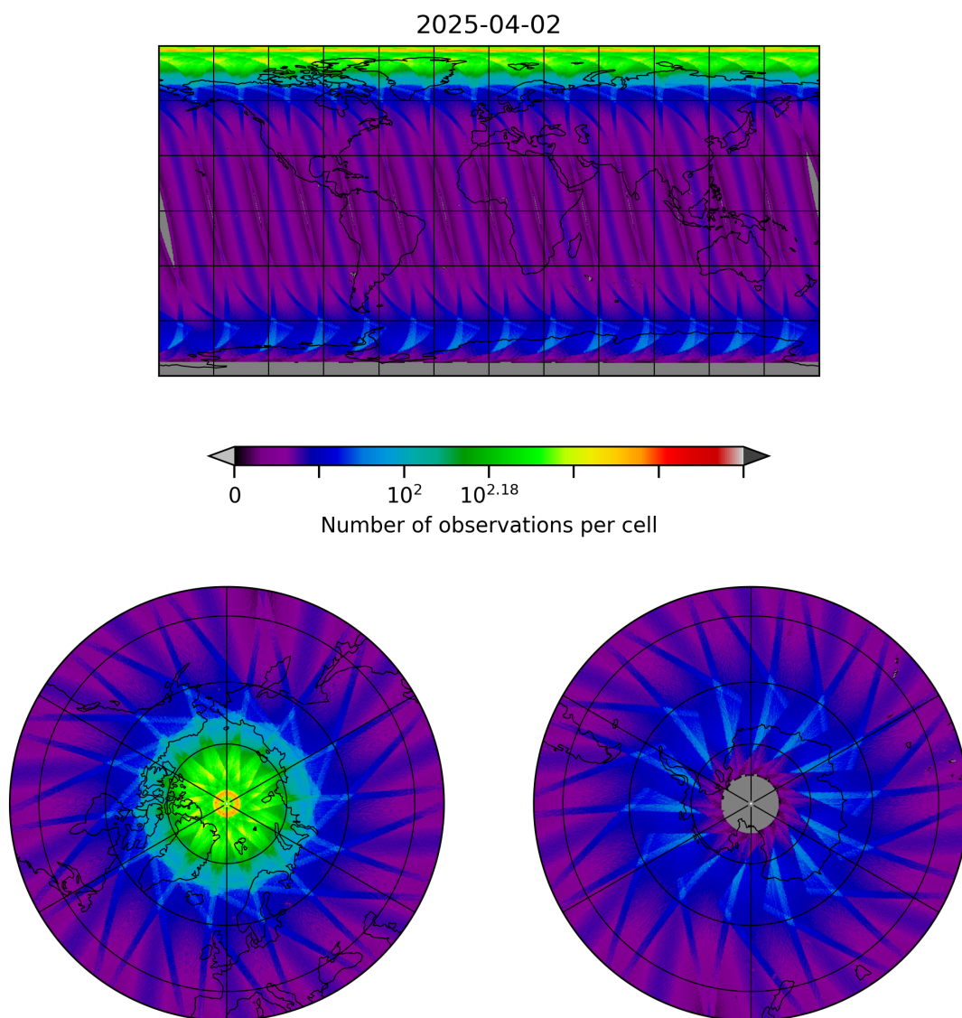
Figure 10: Map of the number of observations for 2025-04-02 to 2025-04-03
