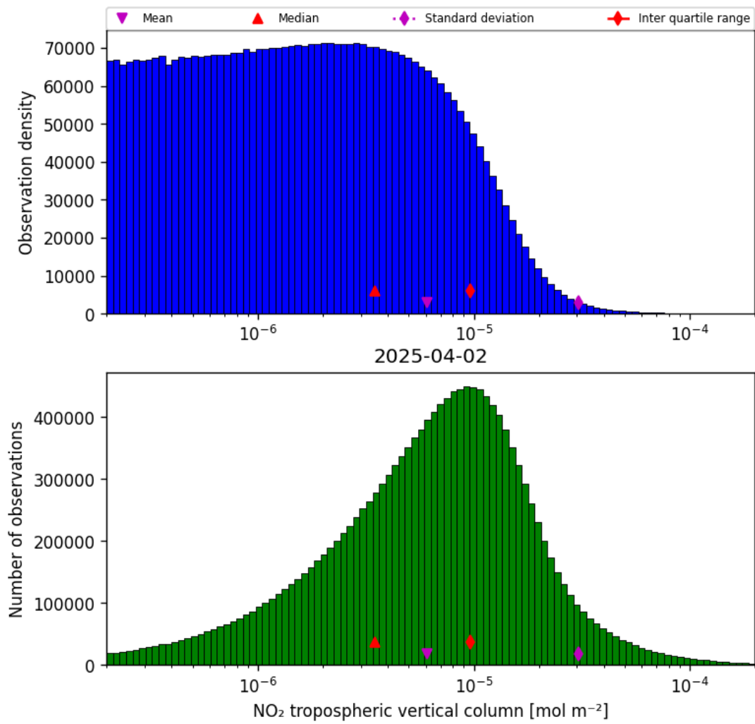
Figure 29: Histogram of “NO 2 tropospheric vertical column” for 2025-04-02 to 2025-04-03
