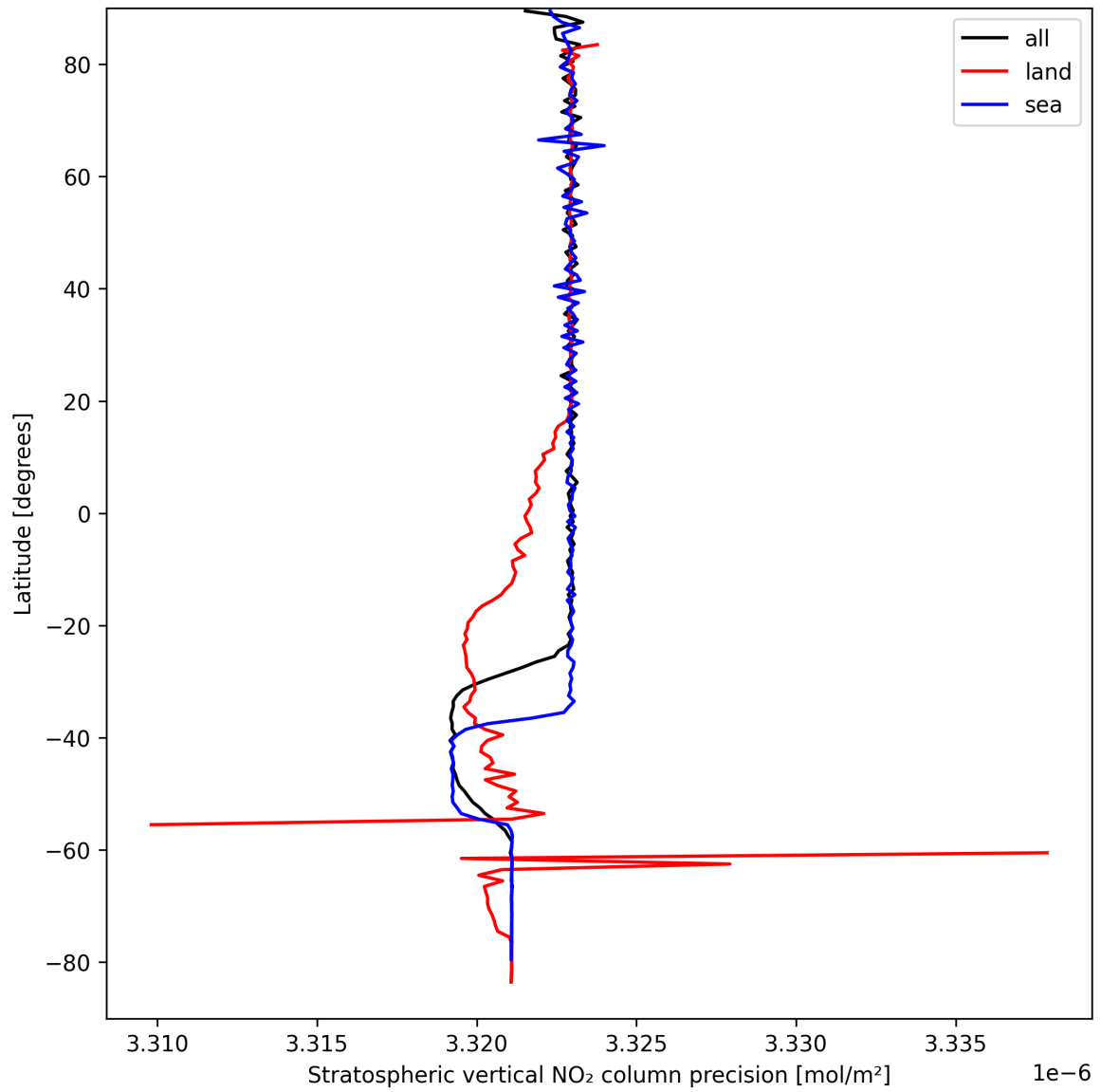
Figure 20: Zonal average of “Stratospheric vertical NO 2 column precision” for 2025-04-02 to 2025-04-03.
