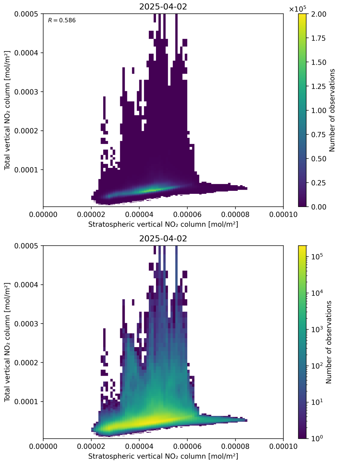
Figure 100: Scatter density plot of “Stratospheric vertical NO 2 column” against “Total vertical NO 2 column” for 2025-04-02 to 2025-04-03.
