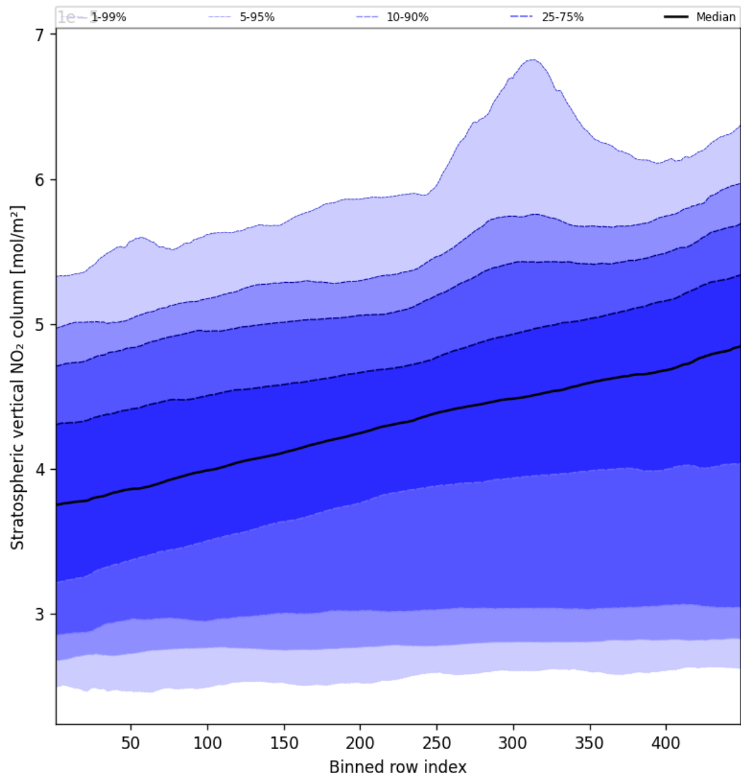
Figure 53: Along track statistics of “Stratospheric vertical NO 2 column” for 2025-04-02 to 2025-04-03
