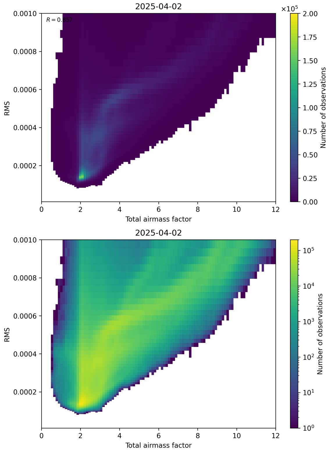
Figure 69: Scatter density plot of “Total airmass factor” against “RMS” for 2025-04-02 to 2025-04-03.
