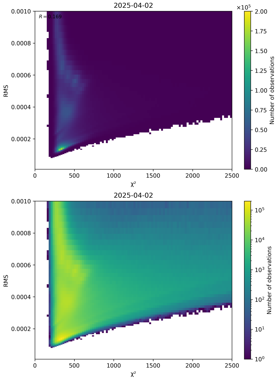
Figure 82: Scatter density plot of “ \chi^2 ” against “RMS” for 2025-04-02 to 2025-04-03.
