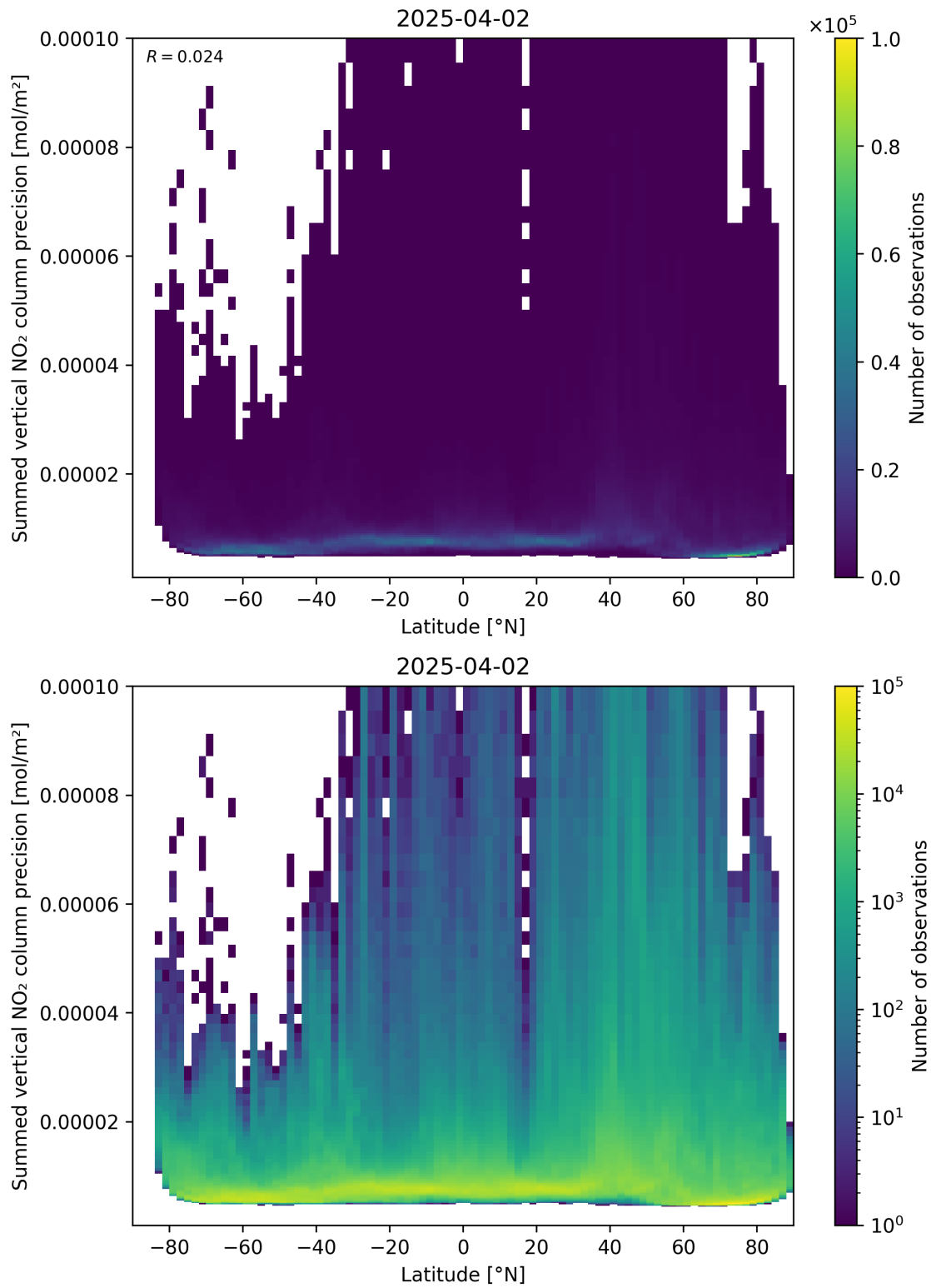
Figure 89: Scatter density plot of “Latitude” against “Summed vertical NO 2 column precision” for 2025-04-02 to 2025-04-03.
