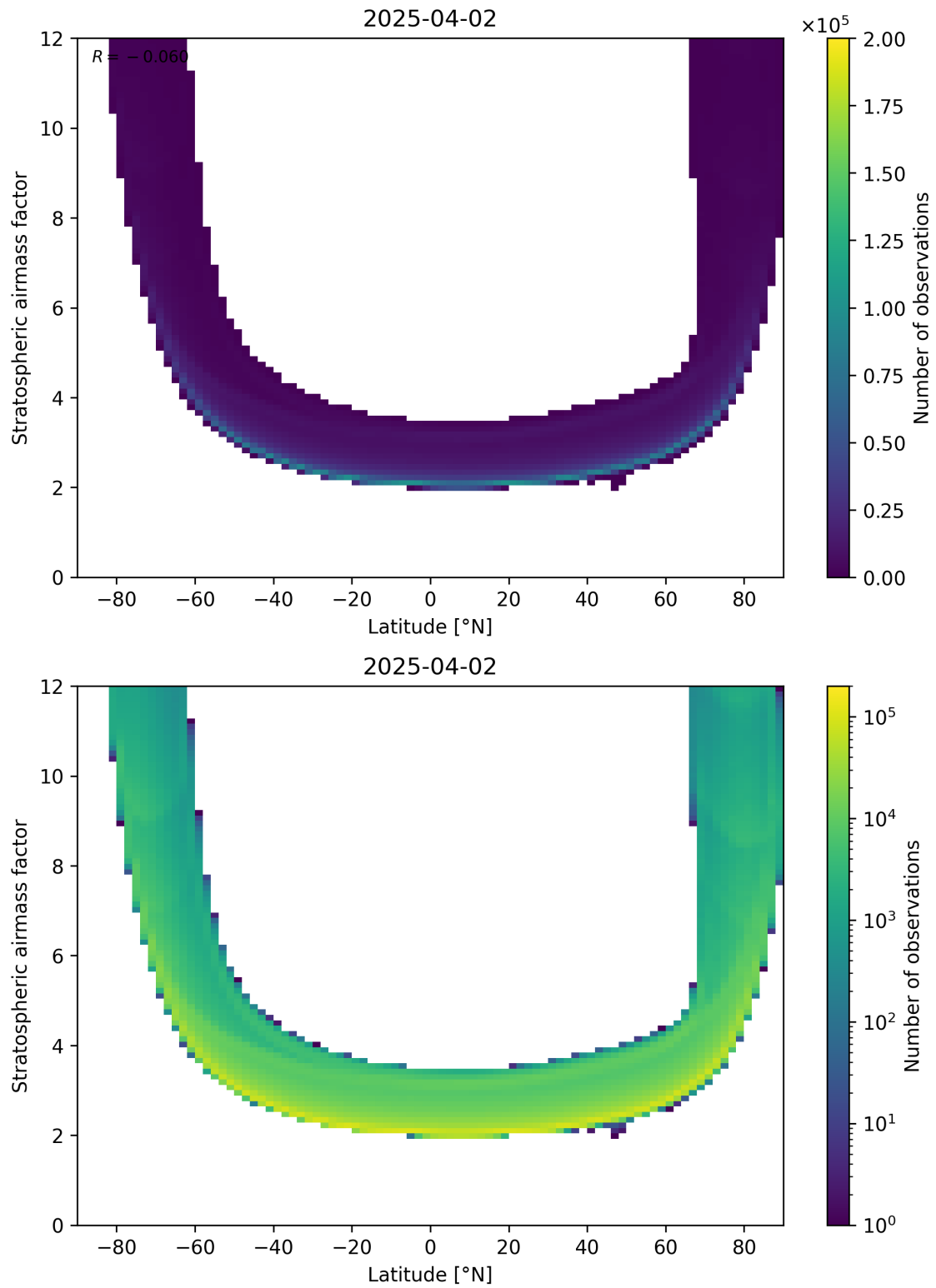
Figure 83: Scatter density plot of “Latitude” against “Stratospheric air mass factor” for 2025-04-02 to 2025-04-03.
