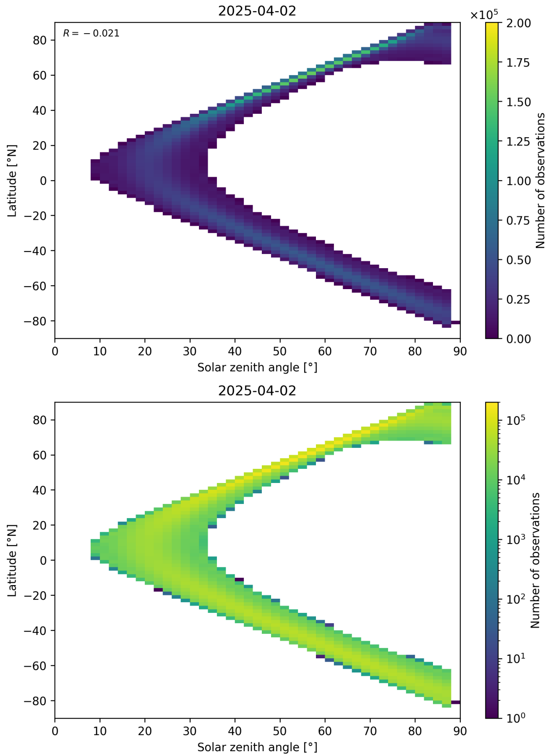
Figure 149: Scatter density plot of “Solar zenith angle” against “Latitude” for 2025-04-02 to 2025-04-03.
