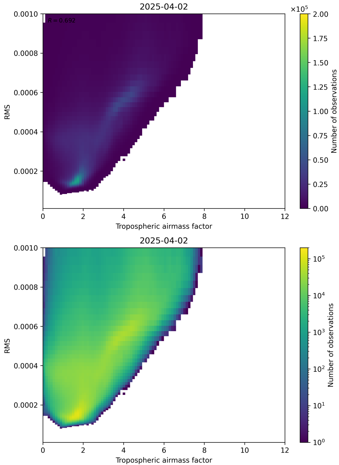
Figure 79: Scatter density plot of “Tropospheric airmass factor” against “RMS” for 2025-04-02 to 2025-04-03.
