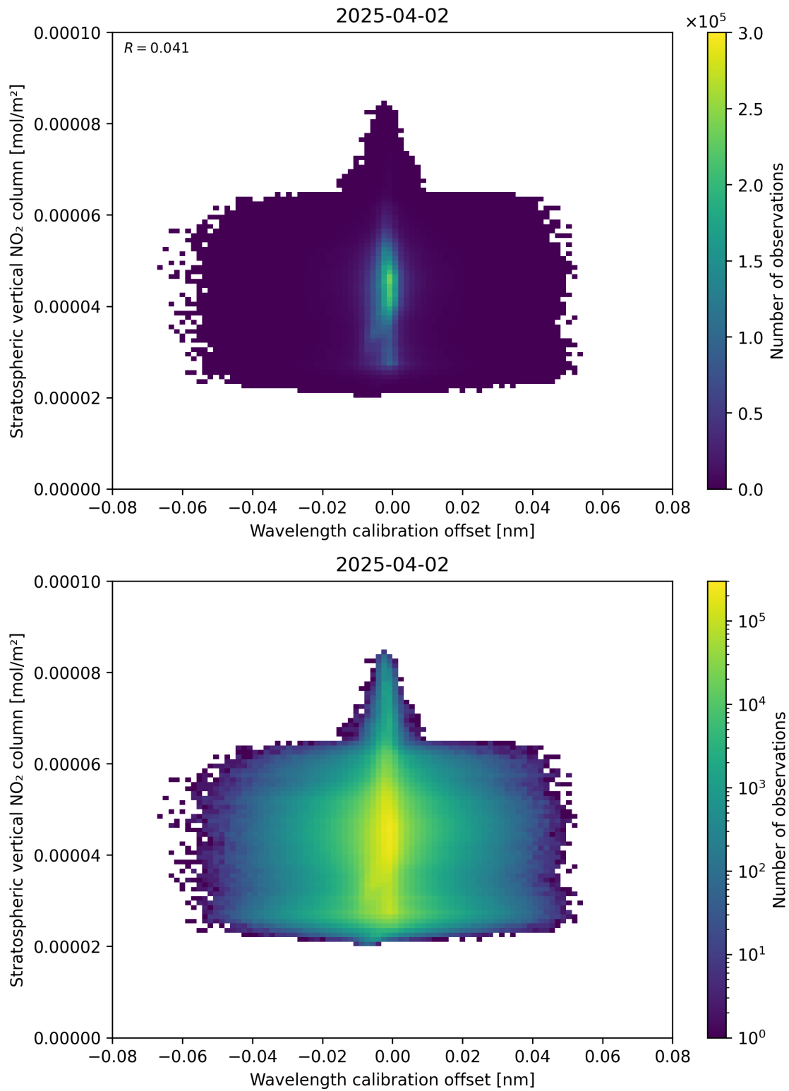
Figure 176: Scatter density plot of “Wavelength calibration offset” against “Stratospheric vertical NO 2 column” for 2025-04-02 to 2025-04-03.
