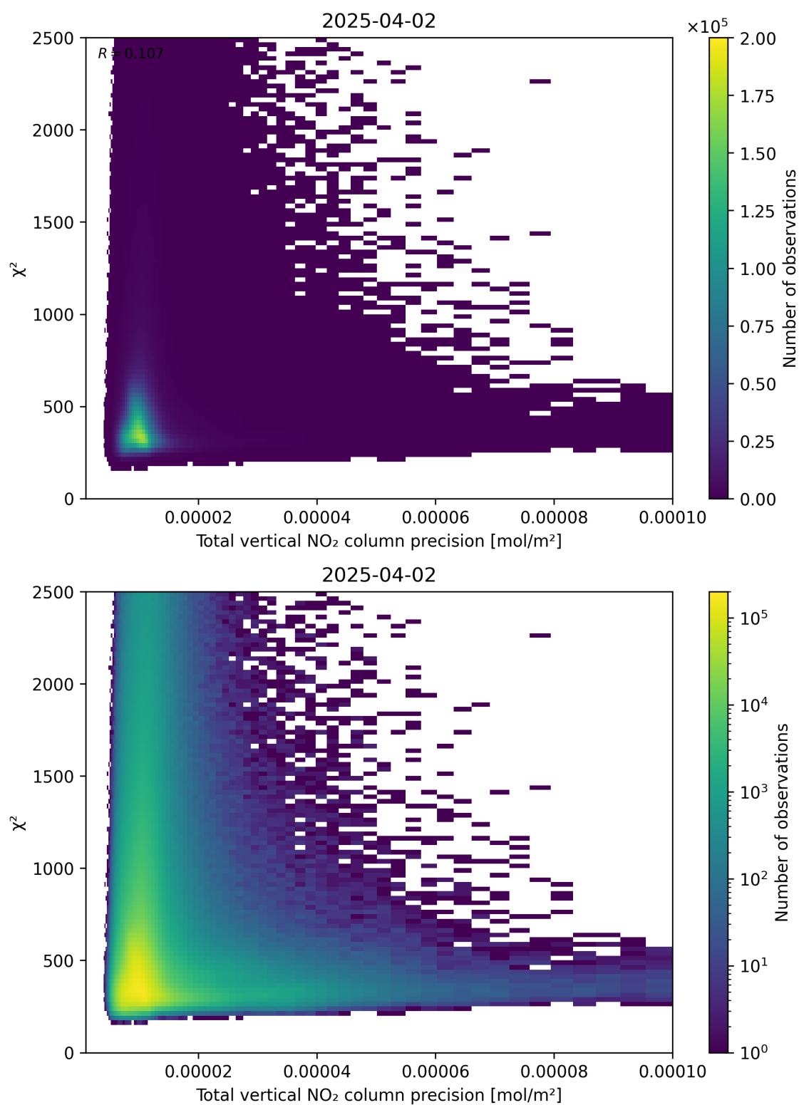
Figure 116: Scatter density plot of “Total vertical NO 2 column precision” against “ \chi^2 ” for 2025-04-02 to 2025-04-03.
