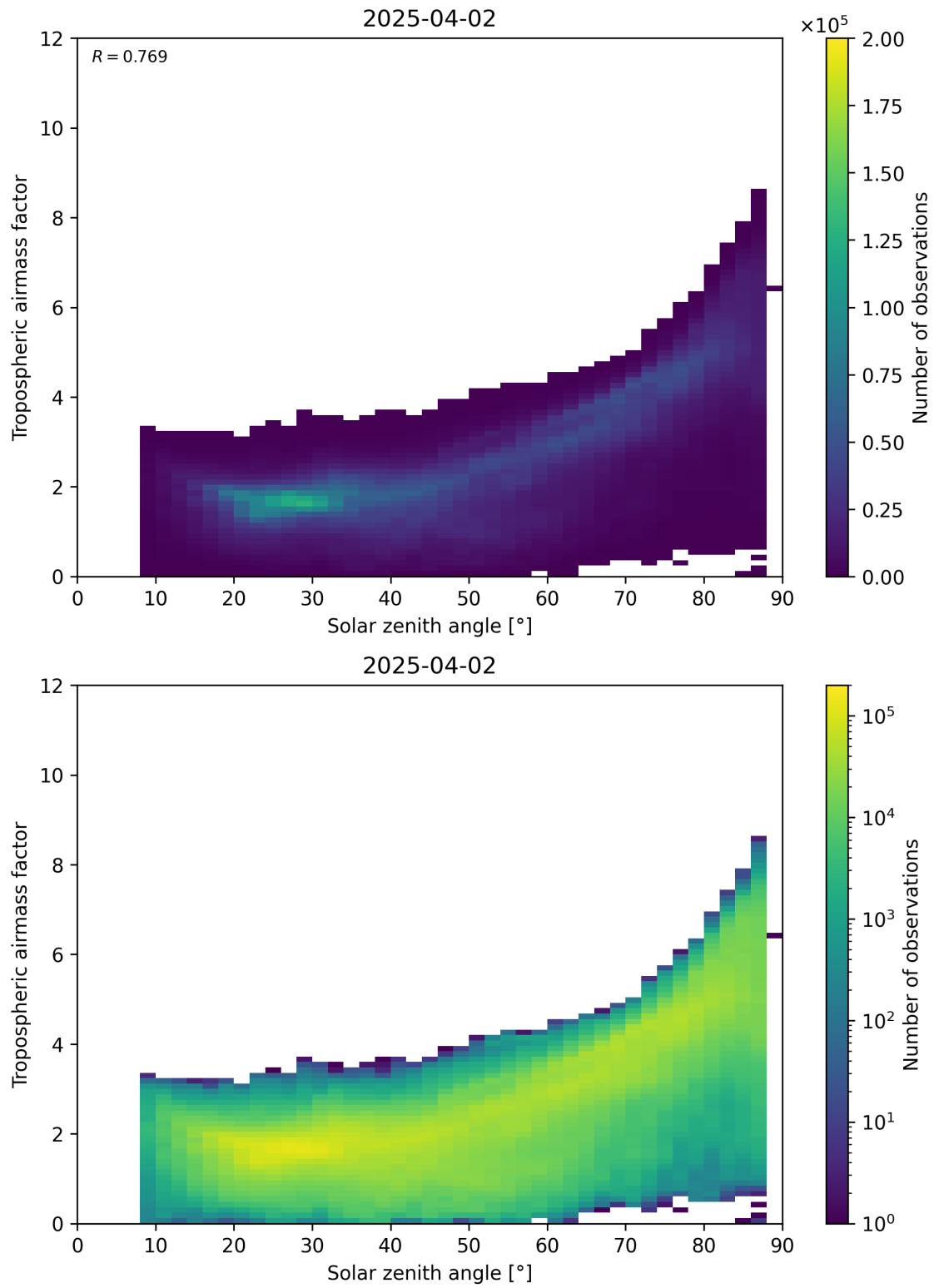
Figure 147: Scatter density plot of “Solar zenith angle” against “Tropospheric airmass factor” for 2025-04-02 to 2025-04-03.
