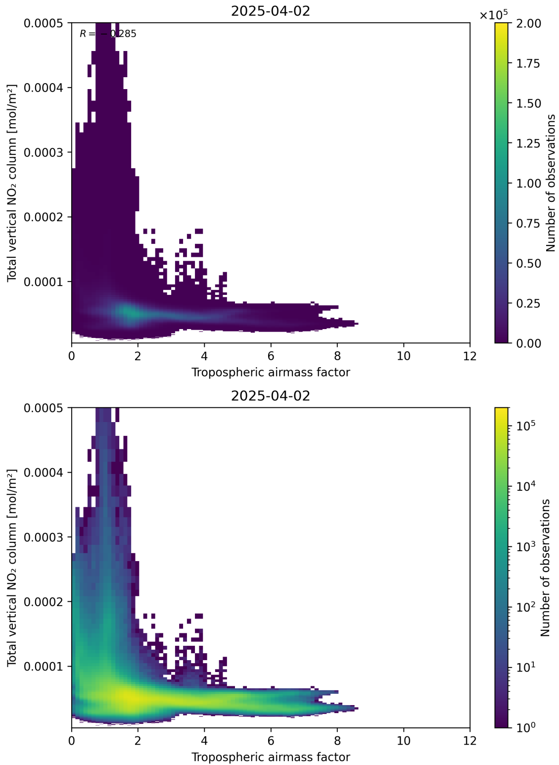
Figure 77: Scatter density plot of “Tropospheric airmass factor” against “Total vertical NO 2 column” for 2025-04-02 to 2025-04-03.
