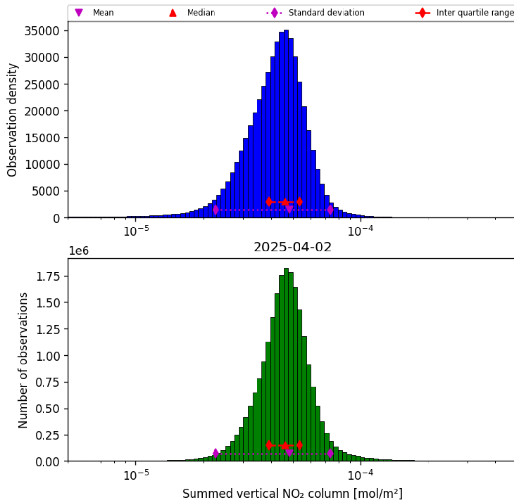
Figure 40: Histogram of “Summed vertical NO 2 column” for 2025-04-02 to 2025-04-03
