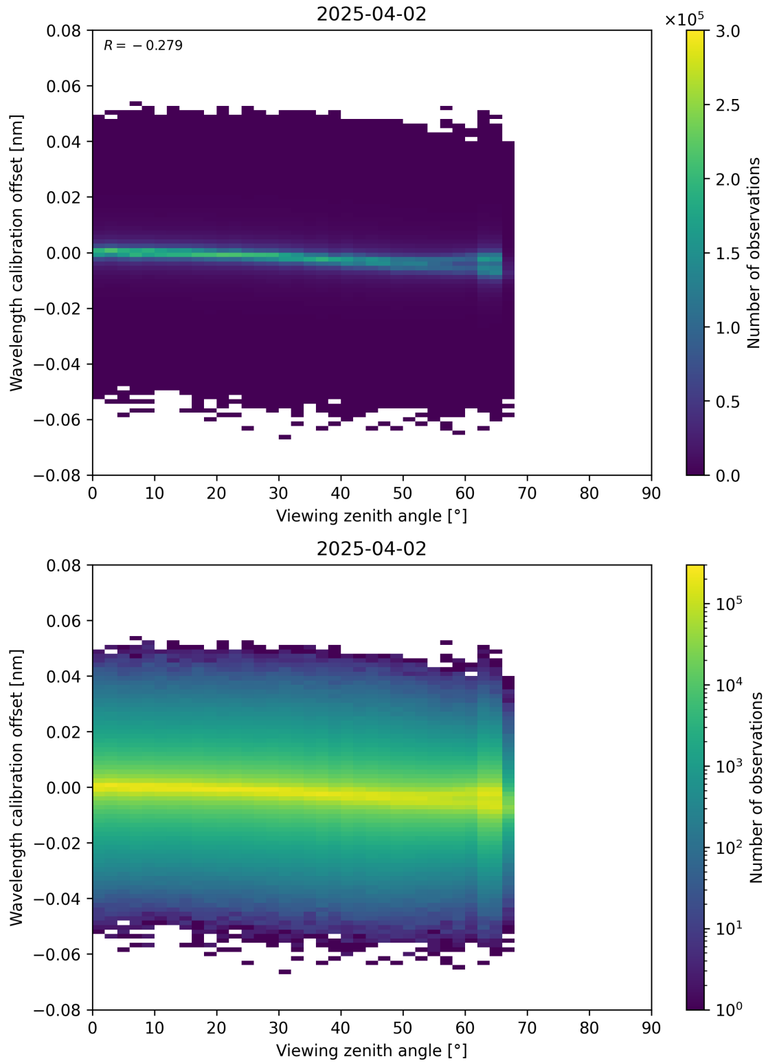
Figure 173: Scatter density plot of “Viewing zenith angle” against “Wavelength calibration offset” for 2025-04-02 to 2025-04-03.
