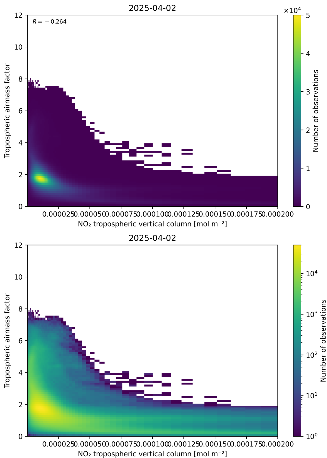
Figure 123: Scatter density plot of “NO 2 tropospheric vertical column” against “Tropospheric air mass factor” for 2025-04-02 to 2025-04-03.
