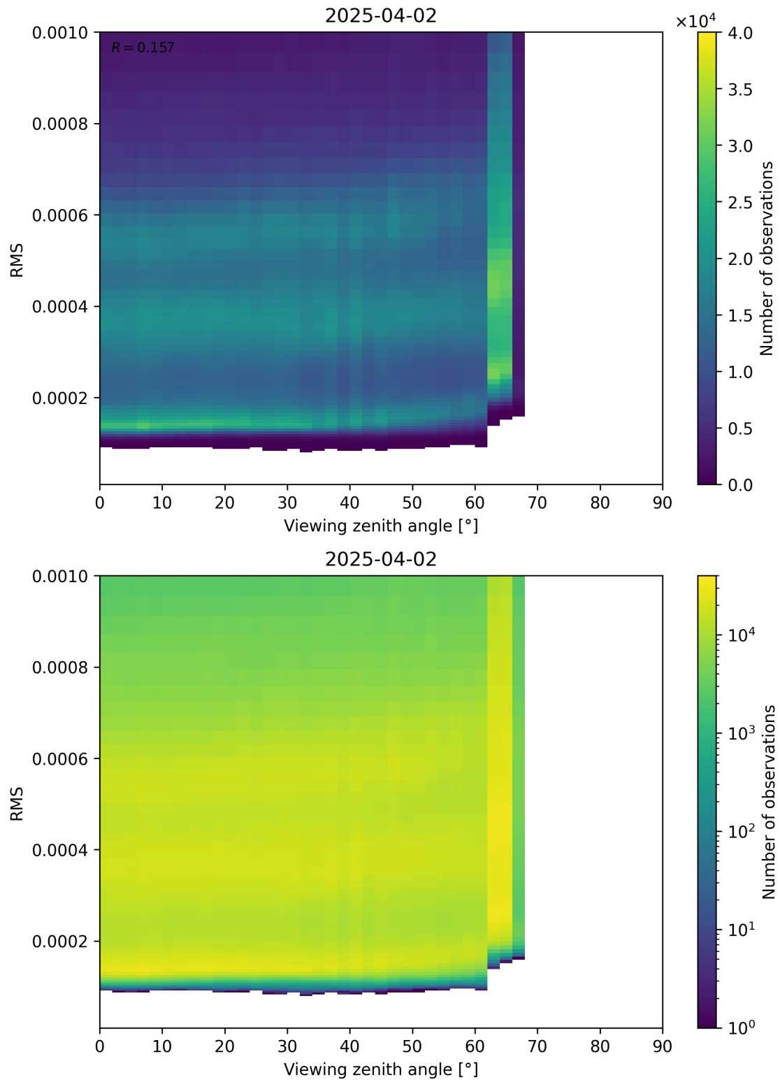
Figure 171: Scatter density plot of “Viewing zenith angle” against “RMS” for 2025-04-02 to 2025-04-03.
