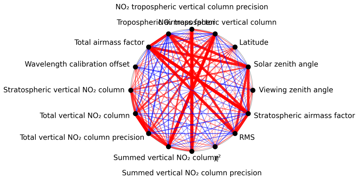
Figure 1: Map of correlation graph for 2025-04-02 to 2025-04-03.
