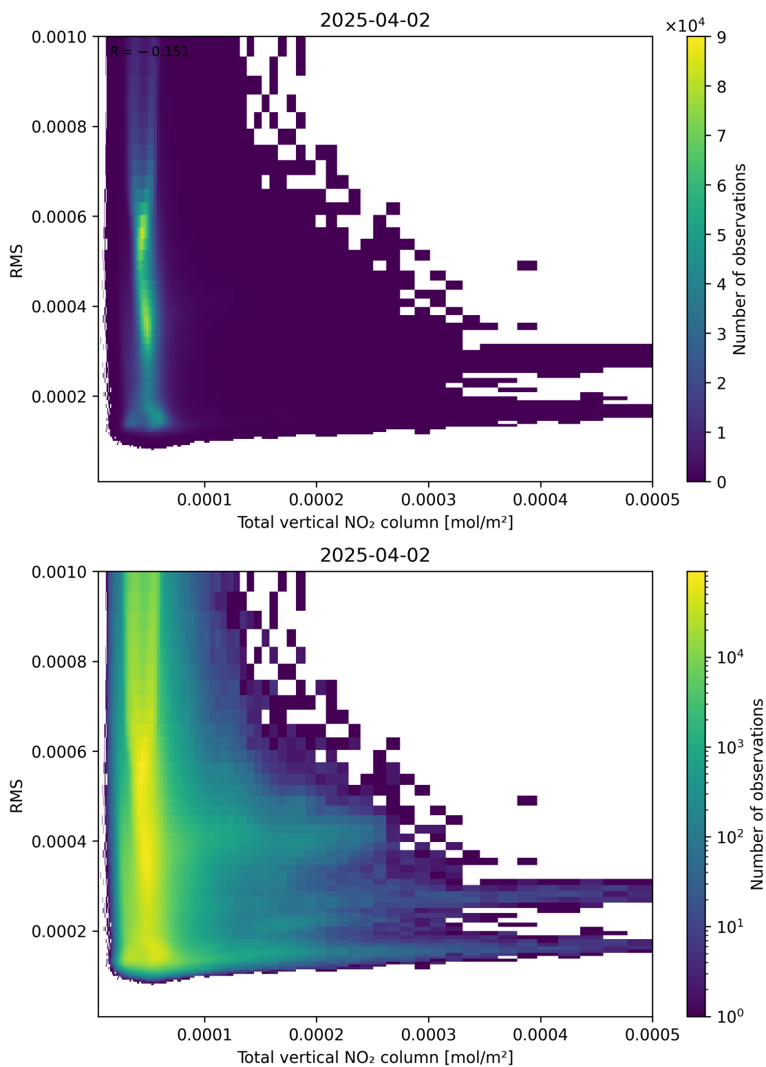
Figure 120: Scatter density plot of “Total vertical NO 2 column” against “RMS” for 2025-04-02 to 2025-04-03.
