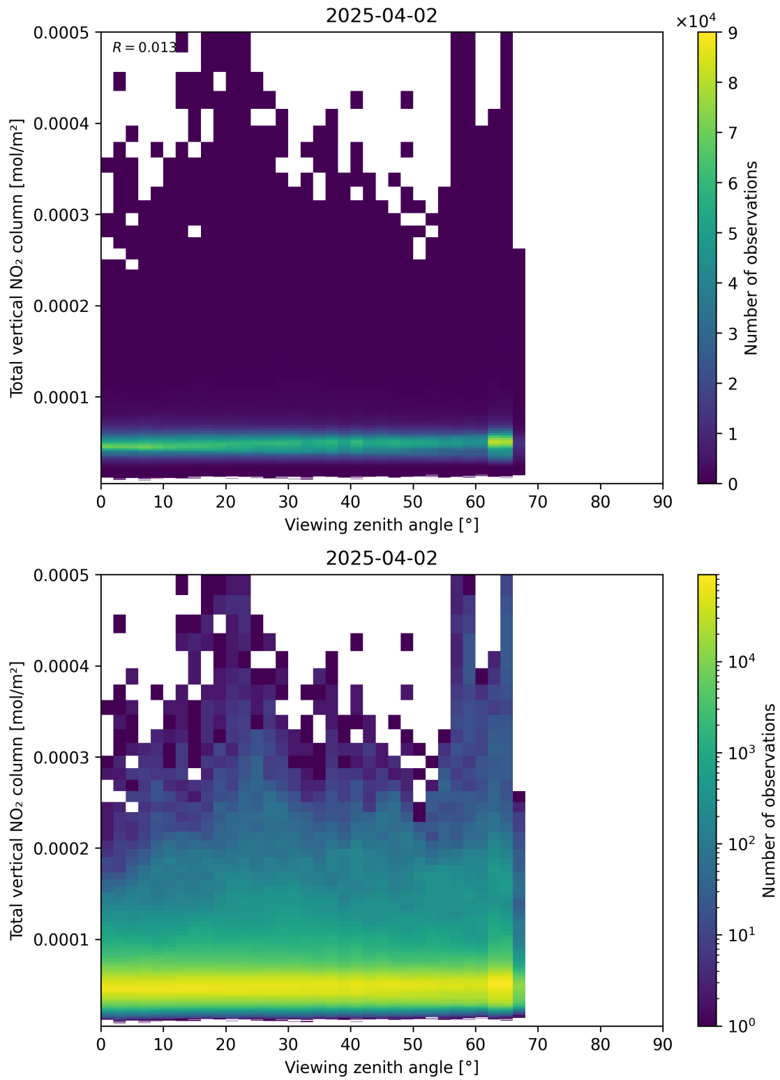
Figure 167: Scatter density plot of “Viewing zenith angle” against “Total vertical NO 2 column” for 2025-04-02 to 2025-04-03.
