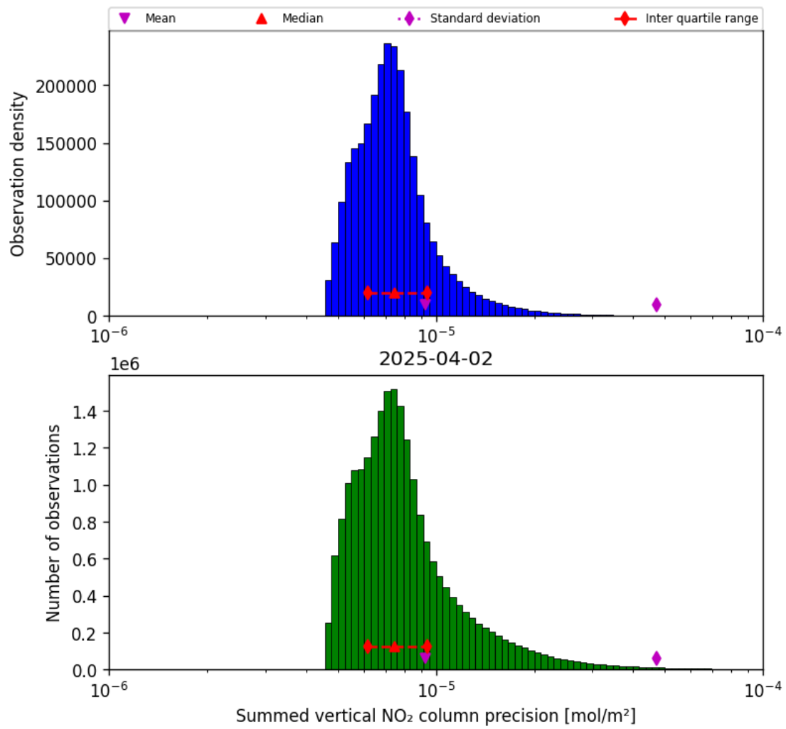
Figure 41: Histogram of “Summed vertical NO 2 column precision” for 2025-04-02 to 2025-04-03
