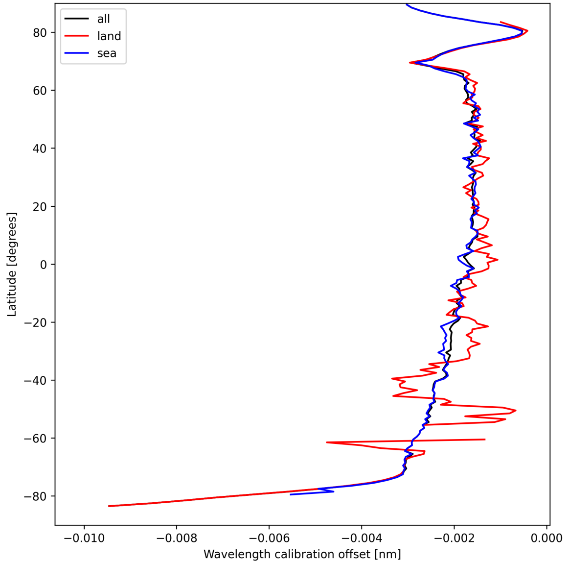
Figure 18: Zonal average of “Wavelength calibration offset” for 2025-04-02 to 2025-04-03.
