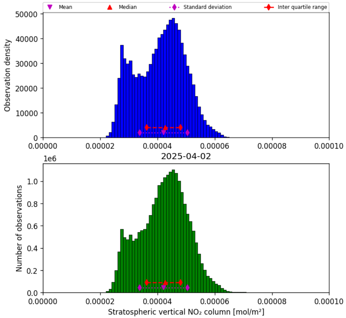
Figure 36: Histogram of “Stratospheric vertical NO 2 column” for 2025-04-02 to 2025-04-03
