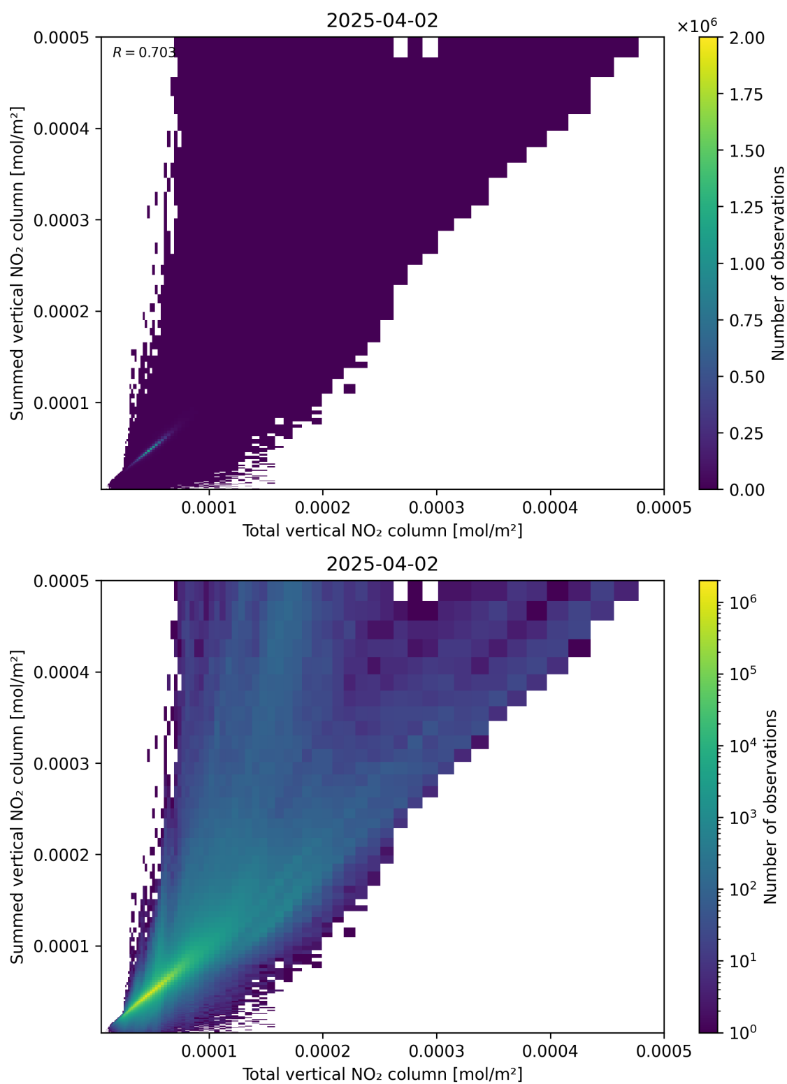
Figure 112: Scatter density plot of “Total vertical NO 2 column” against “Summed vertical NO 2 column” for 2025-04-02 to 2025-04-03.
