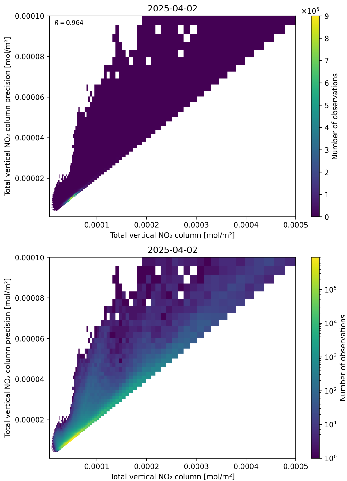
Figure 114: Scatter density plot of “Total vertical NO 2 column” against “Total vertical NO 2 column precision” for 2025-04-02 to 2025-04-03.
