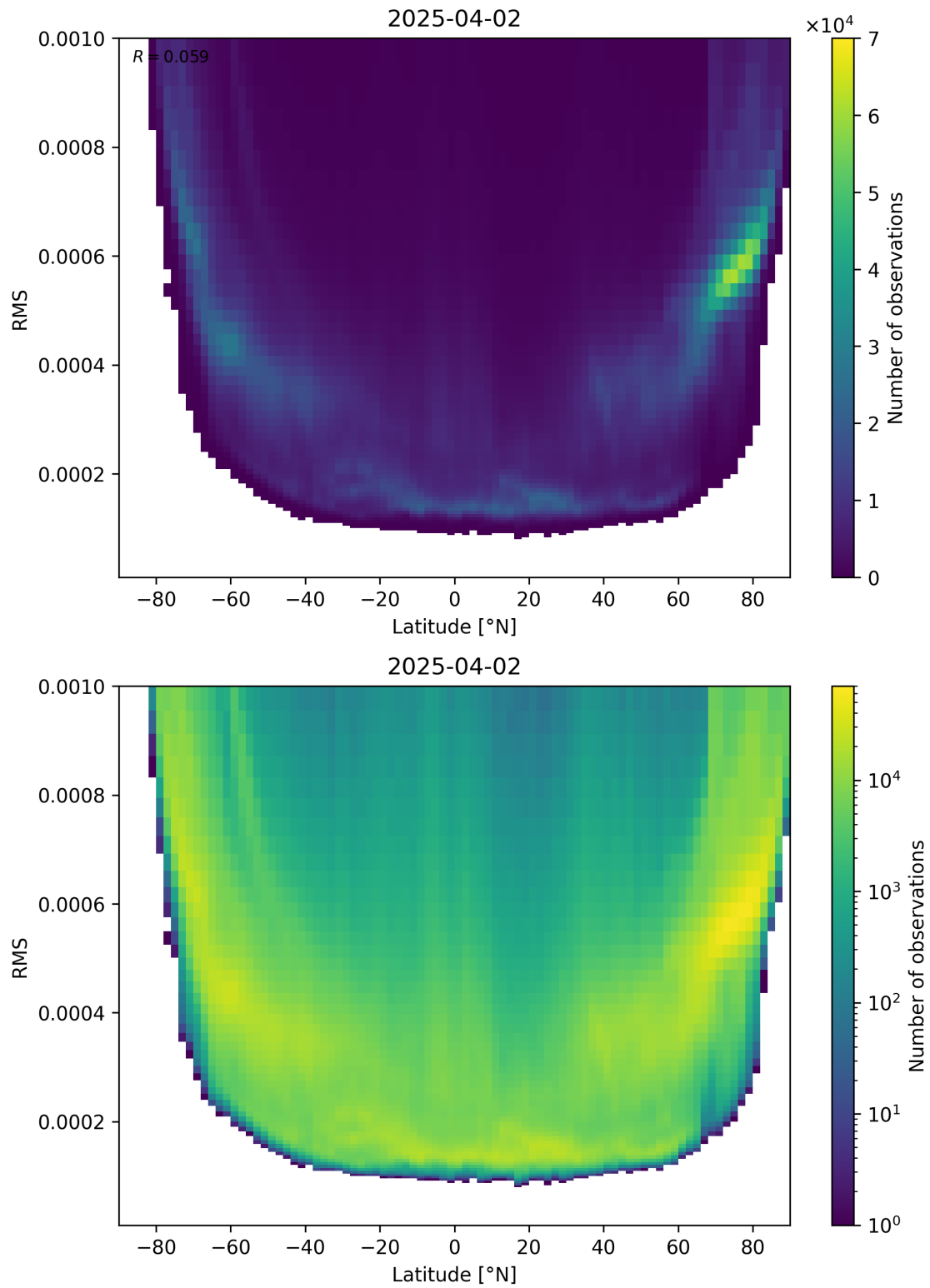
Figure 94: Scatter density plot of “Latitude” against “RMS” for 2025-04-02 to 2025-04-03.
