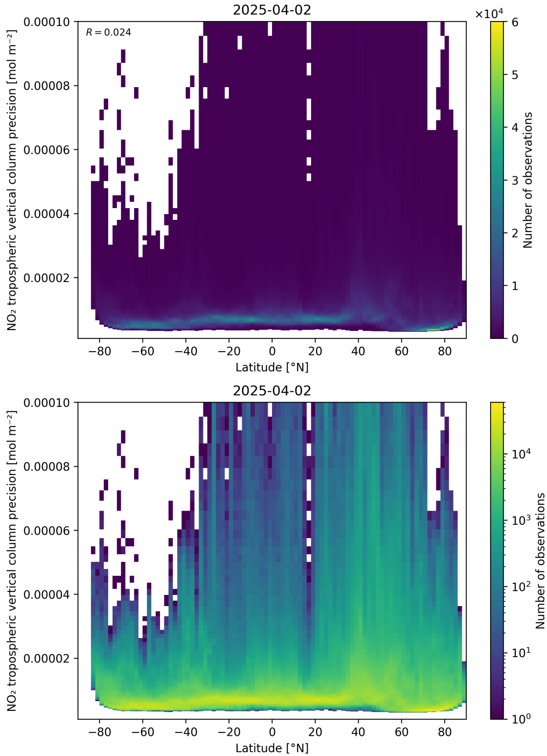
Figure 93: Scatter density plot of “Latitude” against “NO 2 tropospheric vertical column precision” for 2025-04-02 to 2025-04-03.
