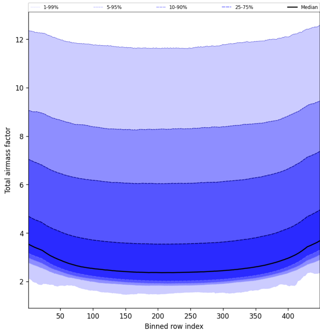
Figure 49: Along track statistics of “Total airmass factor” for 2025-04-02 to 2025-04-03
