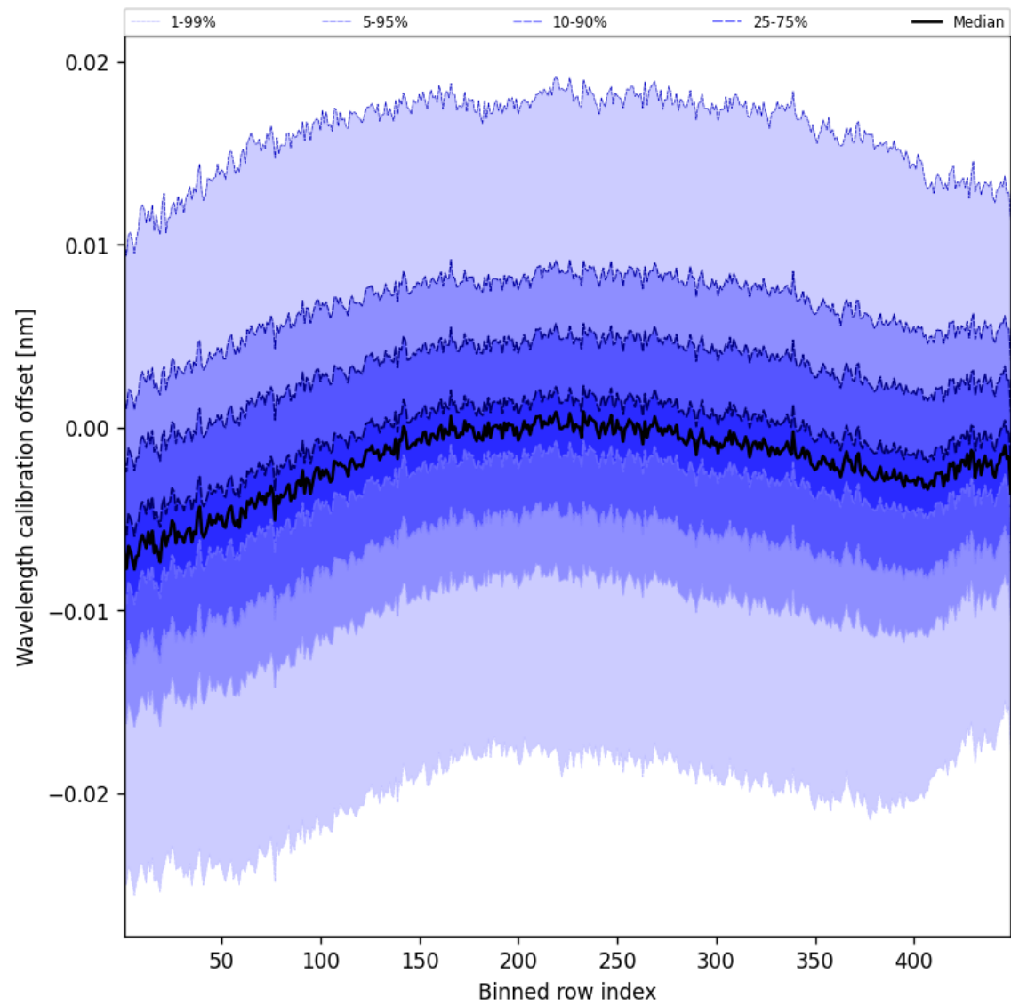
Figure 52: Along track statistics of “Wavelength calibration offset” for 2025-04-02 to 2025-04-03
