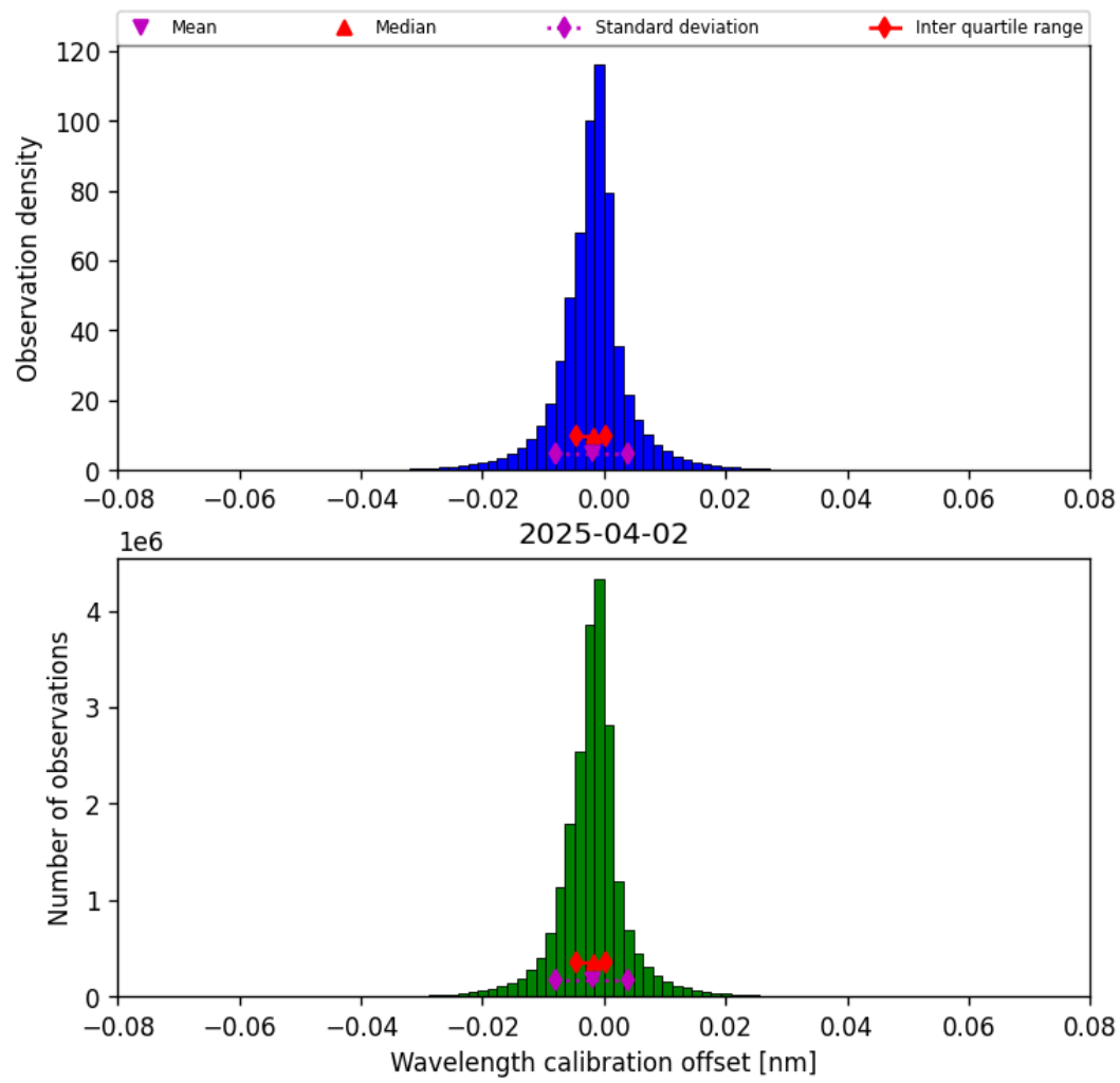
Figure 35: Histogram of “Wavelength calibration offset” for 2025-04-02 to 2025-04-03
