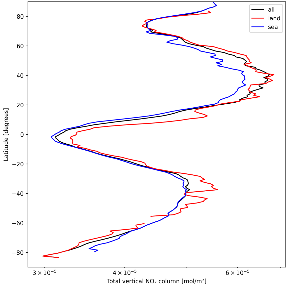
Figure 21: Zonal average of “Total vertical NO 2 column” for 2025-04-02 to 2025-04-03.
