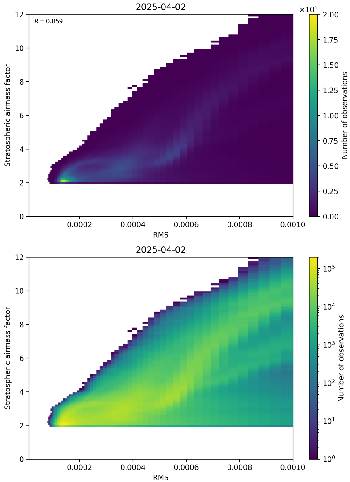
Figure 144: Scatter density plot of “RMS” against “Stratospheric airmass factor” for 2025-04-02 to 2025-04-03.
