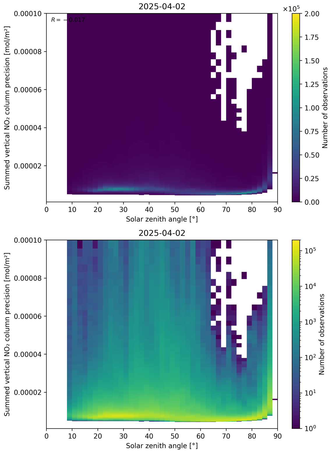
Figure 152: Scatter density plot of “Solar zenith angle” against “Summed vertical NO 2 column precision” for 2025-04-02 to 2025-04-03.
