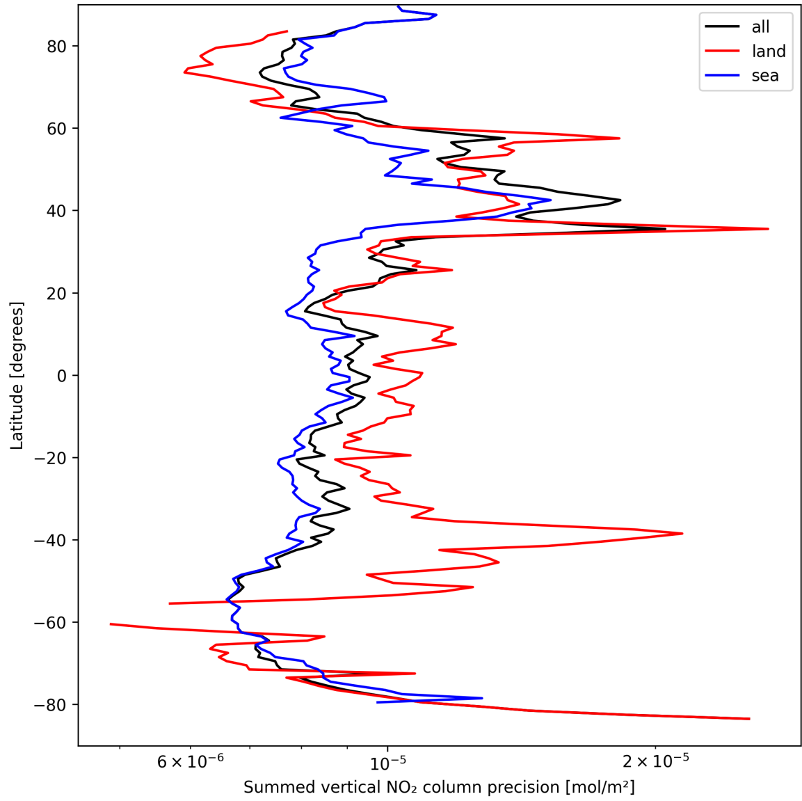
Figure 24: Zonal average of “Summed vertical NO 2 column precision” for 2025-04-02 to 2025-04-03.
