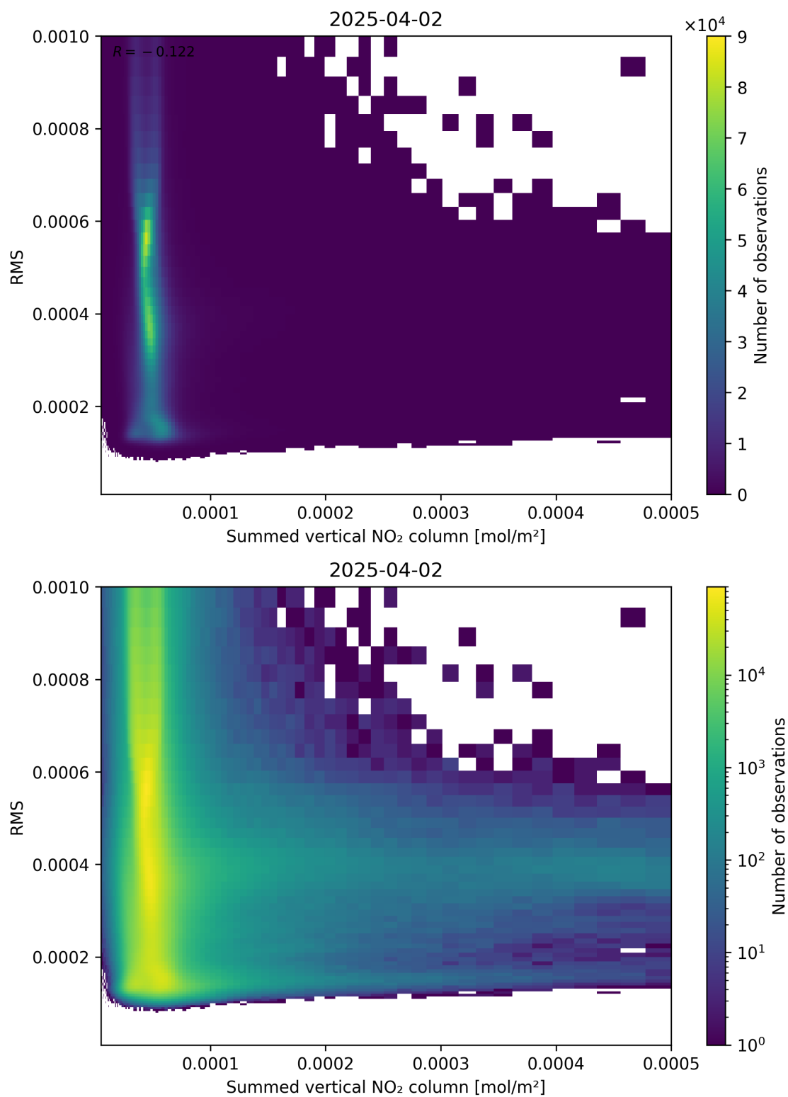
Figure 109: Scatter density plot of “Summed vertical NO 2 column” against “RMS” for 2025-04-02 to 2025-04-03.
