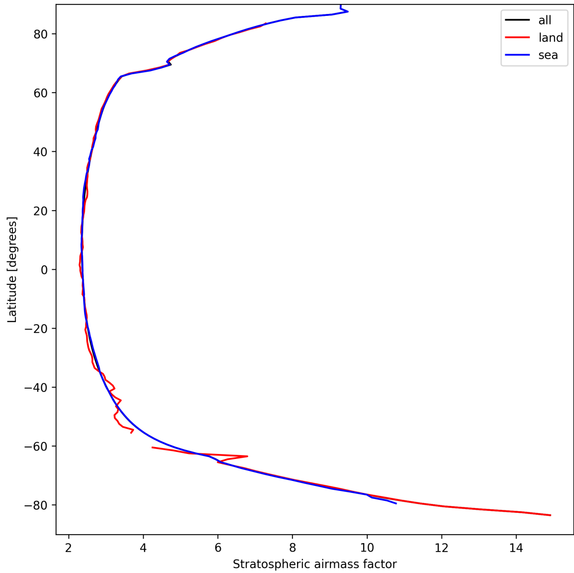
Figure 27: Zonal average of “Stratospheric air mass factor” for 2025-04-02 to 2025-04-03.
