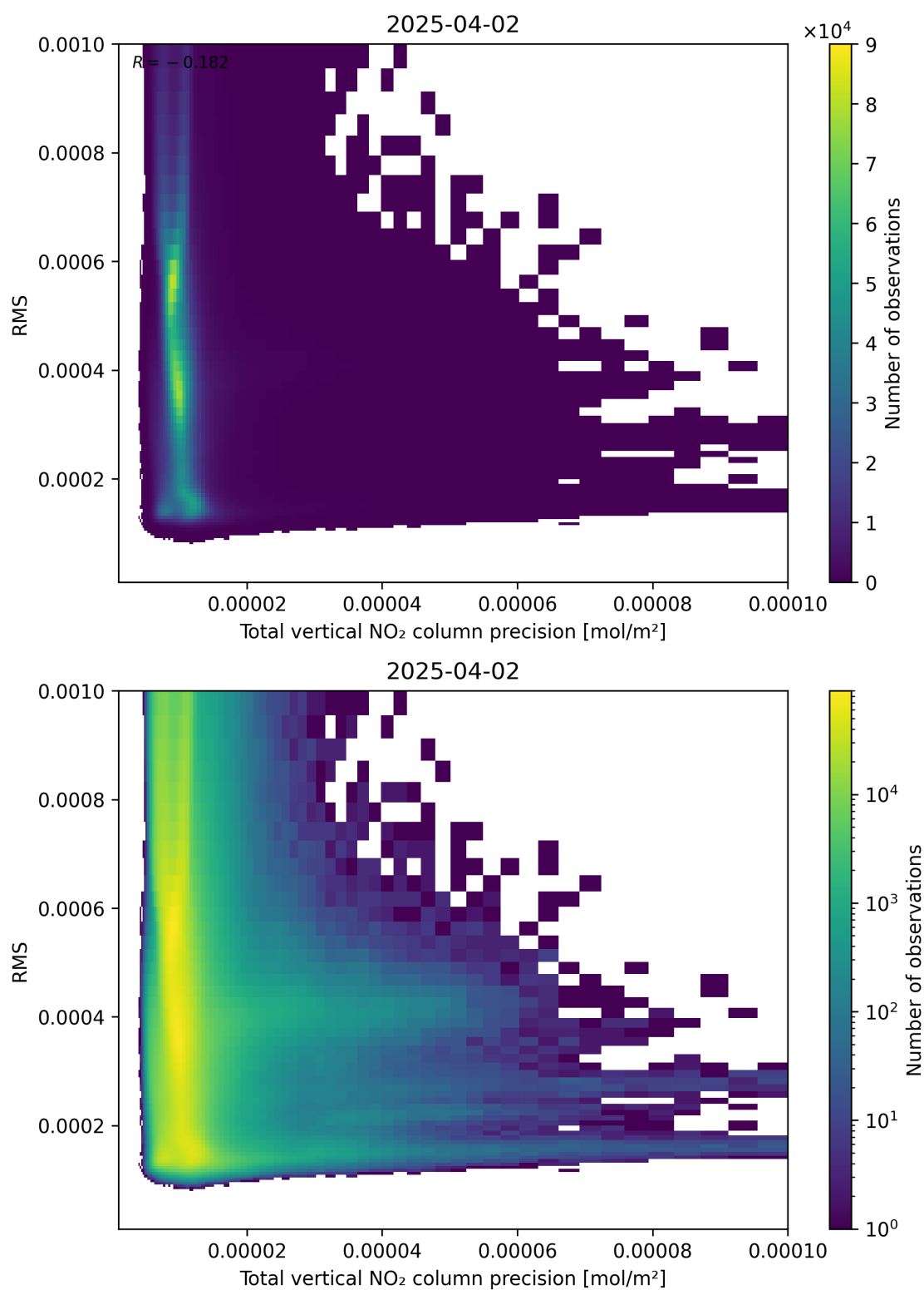
Figure 119: Scatter density plot of “Total vertical NO 2 column precision” against “RMS” for 2025-04-02 to 2025-04-03.
