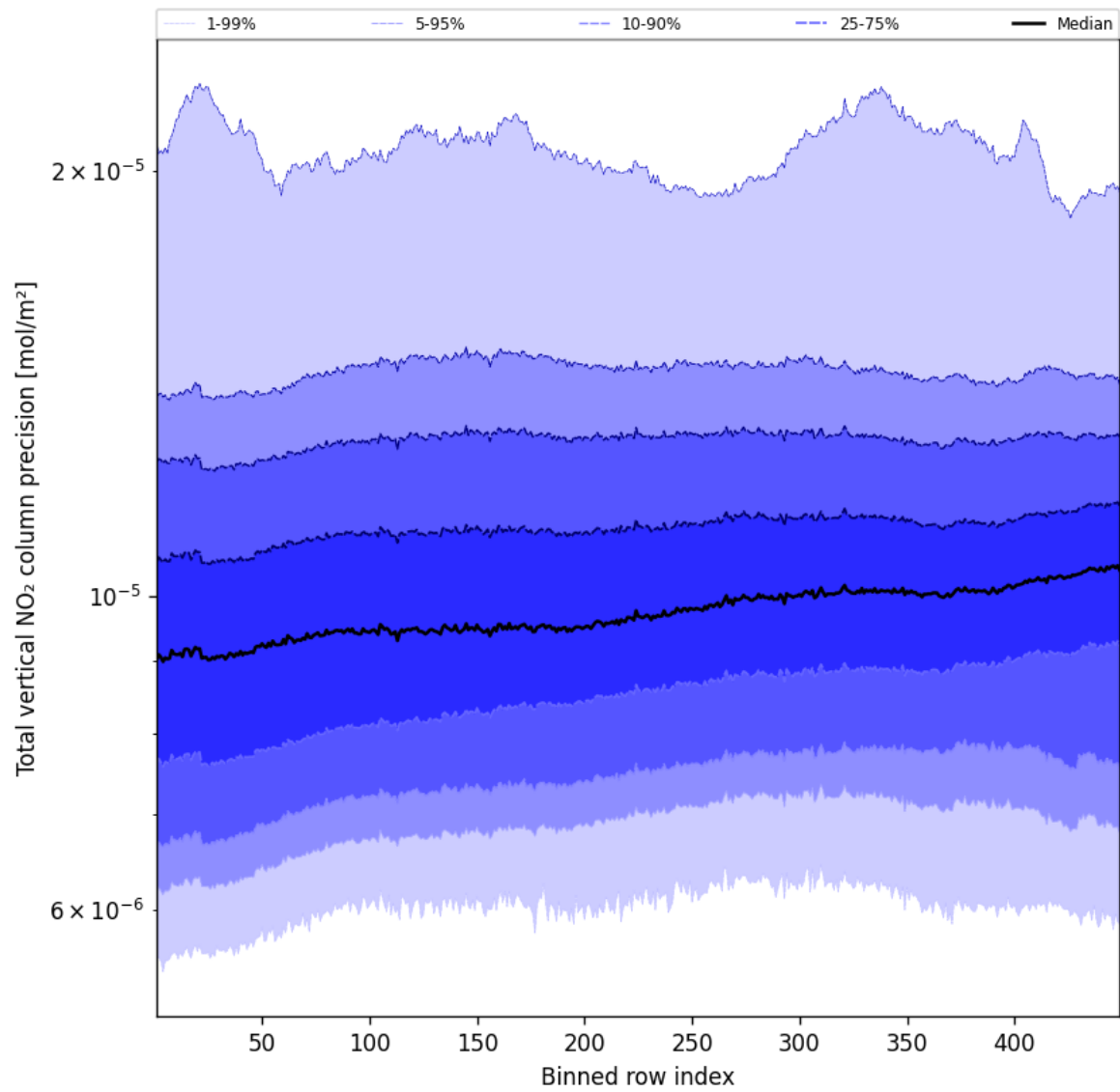
Figure 56: Along track statistics of “Total vertical NO 2 column precision” for 2025-04-02 to 2025-04-03
