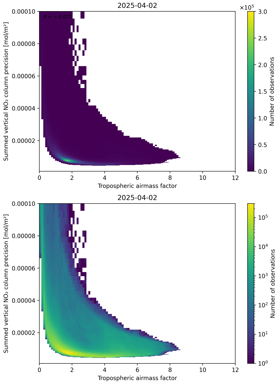
Figure 76: Scatter density plot of “Tropospheric air mass factor” against “Summed vertical NO 2 column precision” for 2025-04-02 to 2025-04-03.
