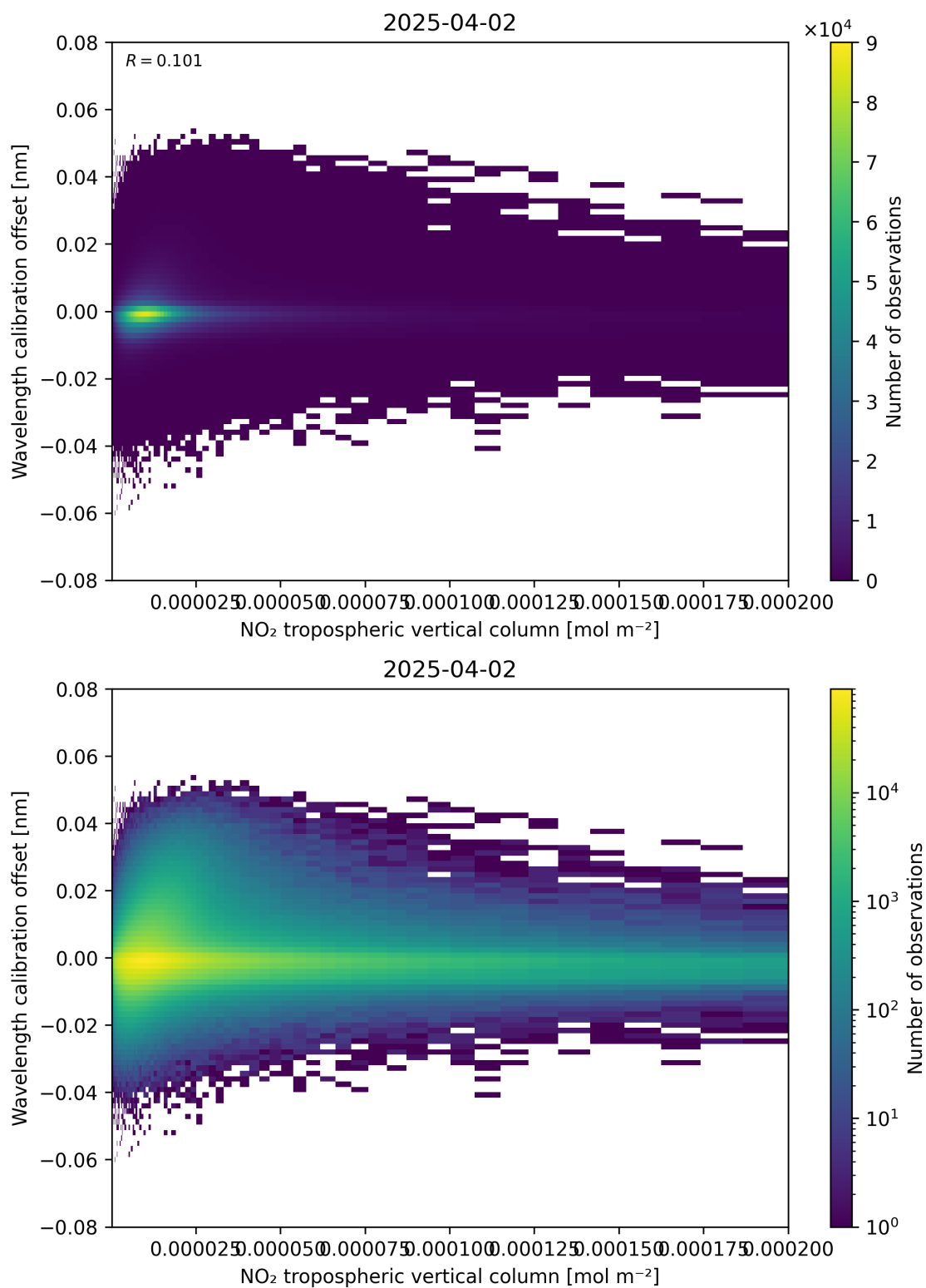
Figure 143: Scatter density plot of “NO 2 tropospheric vertical column” against “Wavelength calibration offset” for 2025-04-02 to 2025-04-03.
