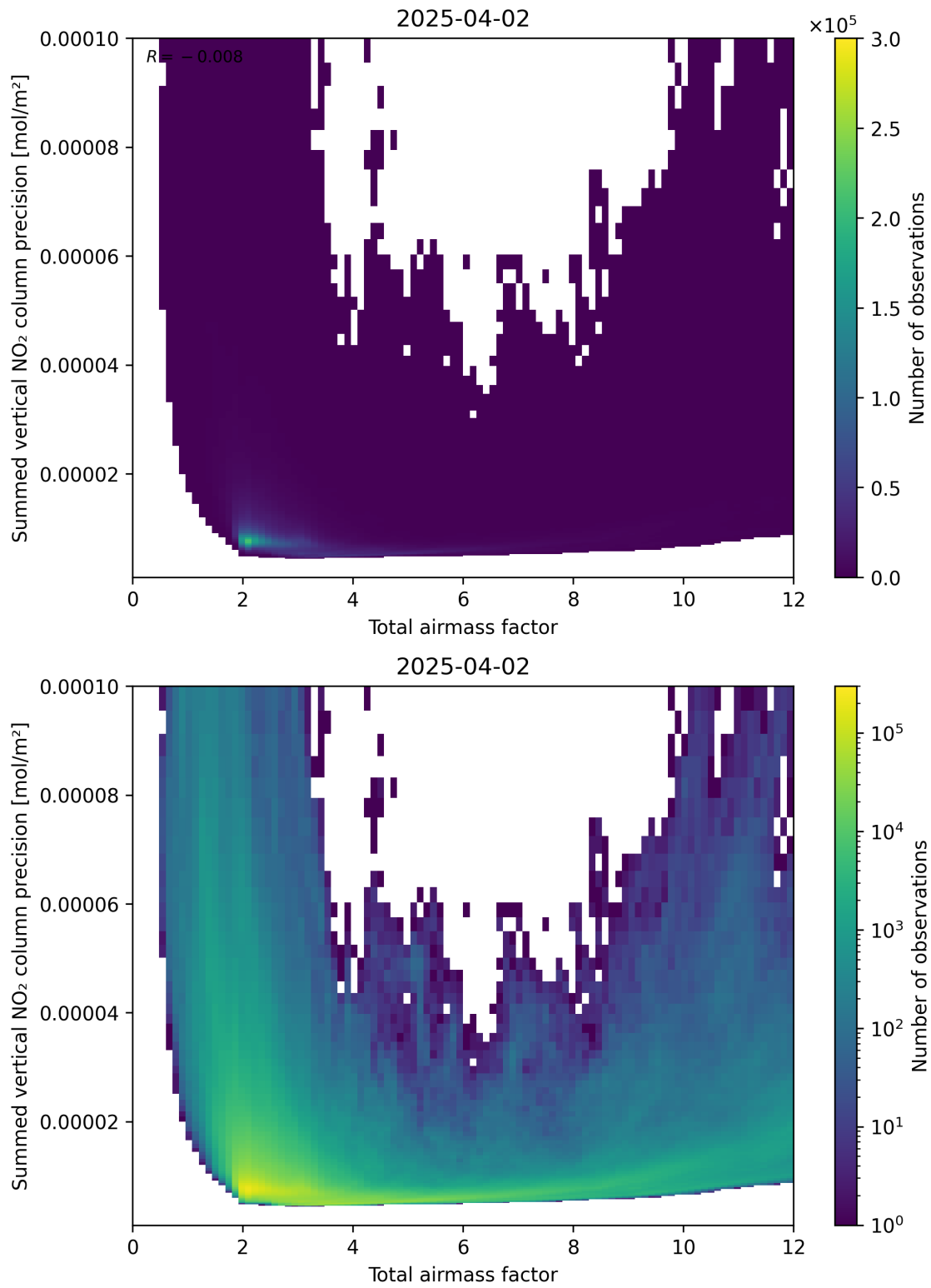
Figure 66: Scatter density plot of “Total airmass factor” against “Summed vertical NO 2 column precision” for 2025-04-02 to 2025-04-03.
