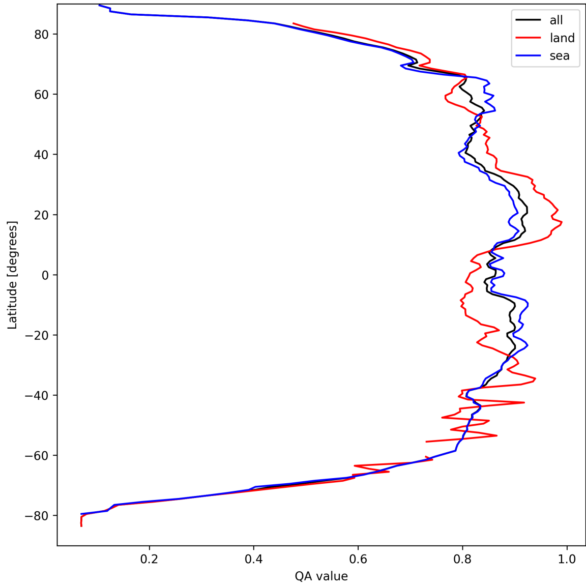
Figure 11: Zonal average of “QA value” for 2025-04-02 to 2025-04-03.
