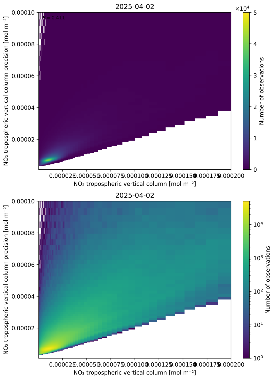
Figure 130: Scatter density plot of “NO 2 tropospheric vertical column” against “NO 2 tropospheric vertical column precision” for 2025-04-02 to 2025-04-03.
