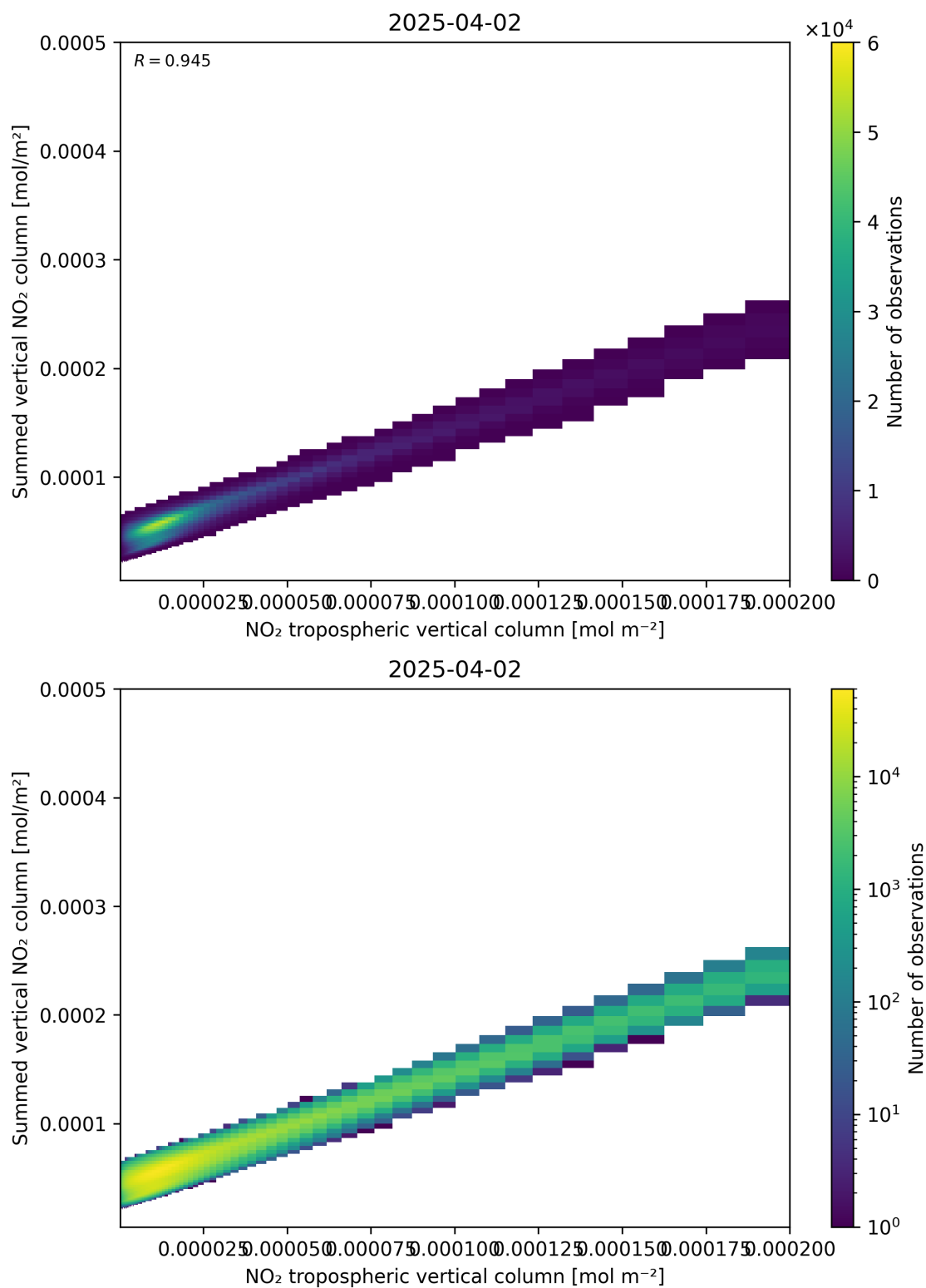
Figure 126: Scatter density plot of “NO 2 tropospheric vertical column” against “Summed vertical NO 2 column” for 2025-04-02 to 2025-04-03.
