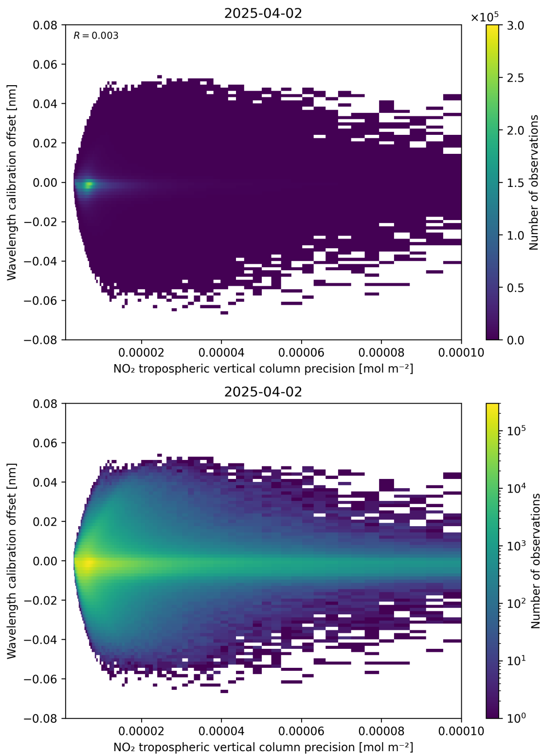
Figure 141: Scatter density plot of “NO 2 tropospheric vertical column precision” against “Wavelength calibration offset” for 2025-04-02 to 2025-04-03.
