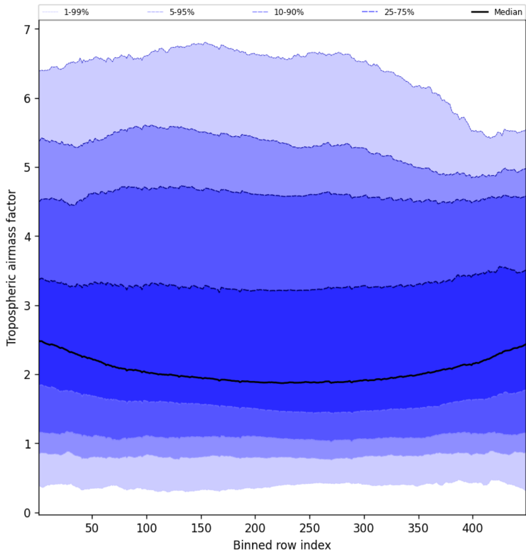
Figure 48: Along track statistics of “Tropospheric airmass factor” for 2025-04-02 to 2025-04-03
