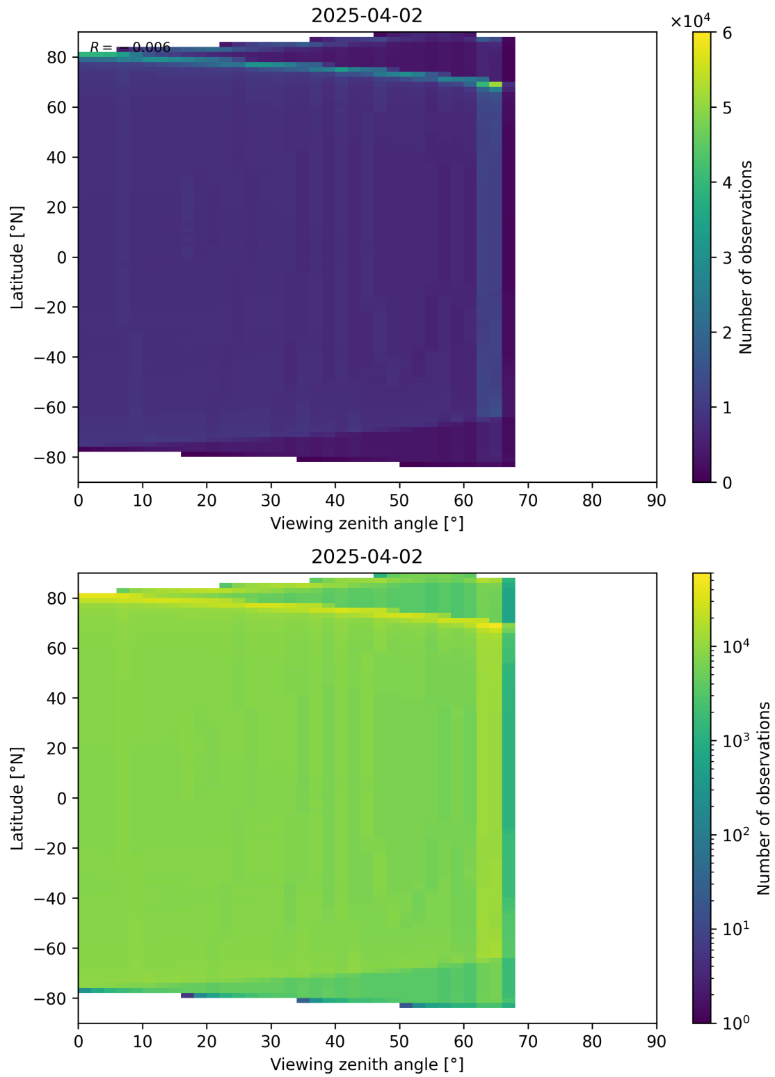
Figure 163: Scatter density plot of “Viewing zenith angle” against “Latitude” for 2025-04-02 to 2025-04-03.
