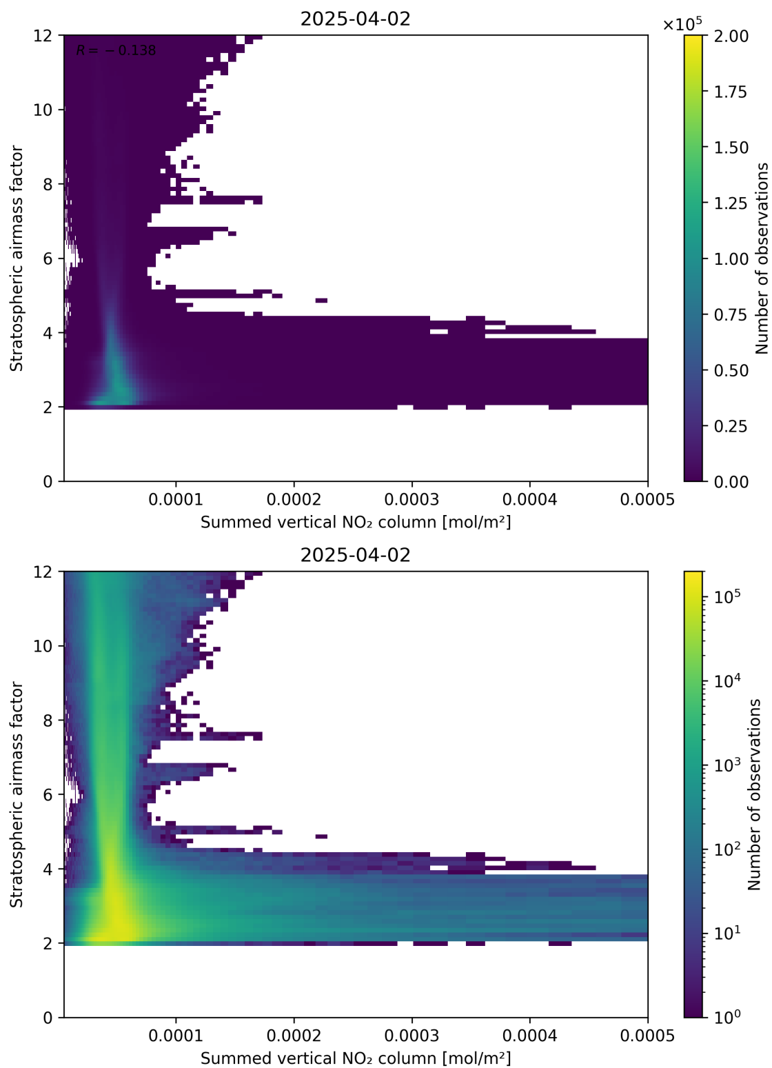
Figure 103: Scatter density plot of “Summed vertical NO 2 column” against “Stratospheric airmass factor” for 2025-04-02 to 2025-04-03.
