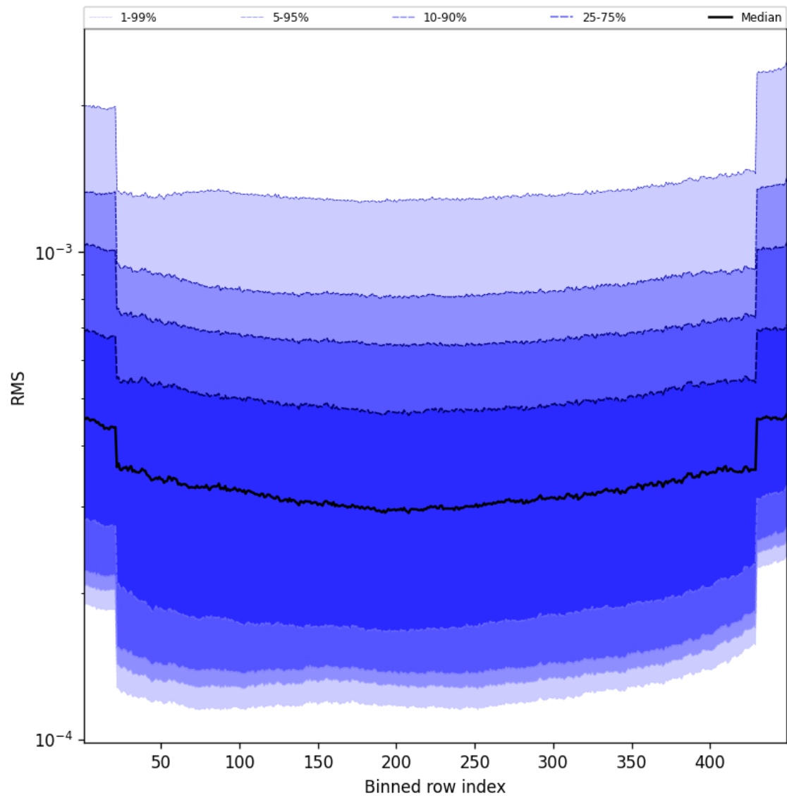
Figure 60: Along track statistics of “RMS” for 2025-04-02 to 2025-04-03
