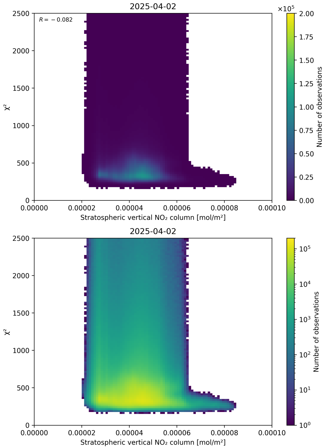
Figure 97: Scatter density plot of “Stratospheric vertical NO 2 column” against “ \chi^2 ” for 2025-04-02 to 2025-04-03.
