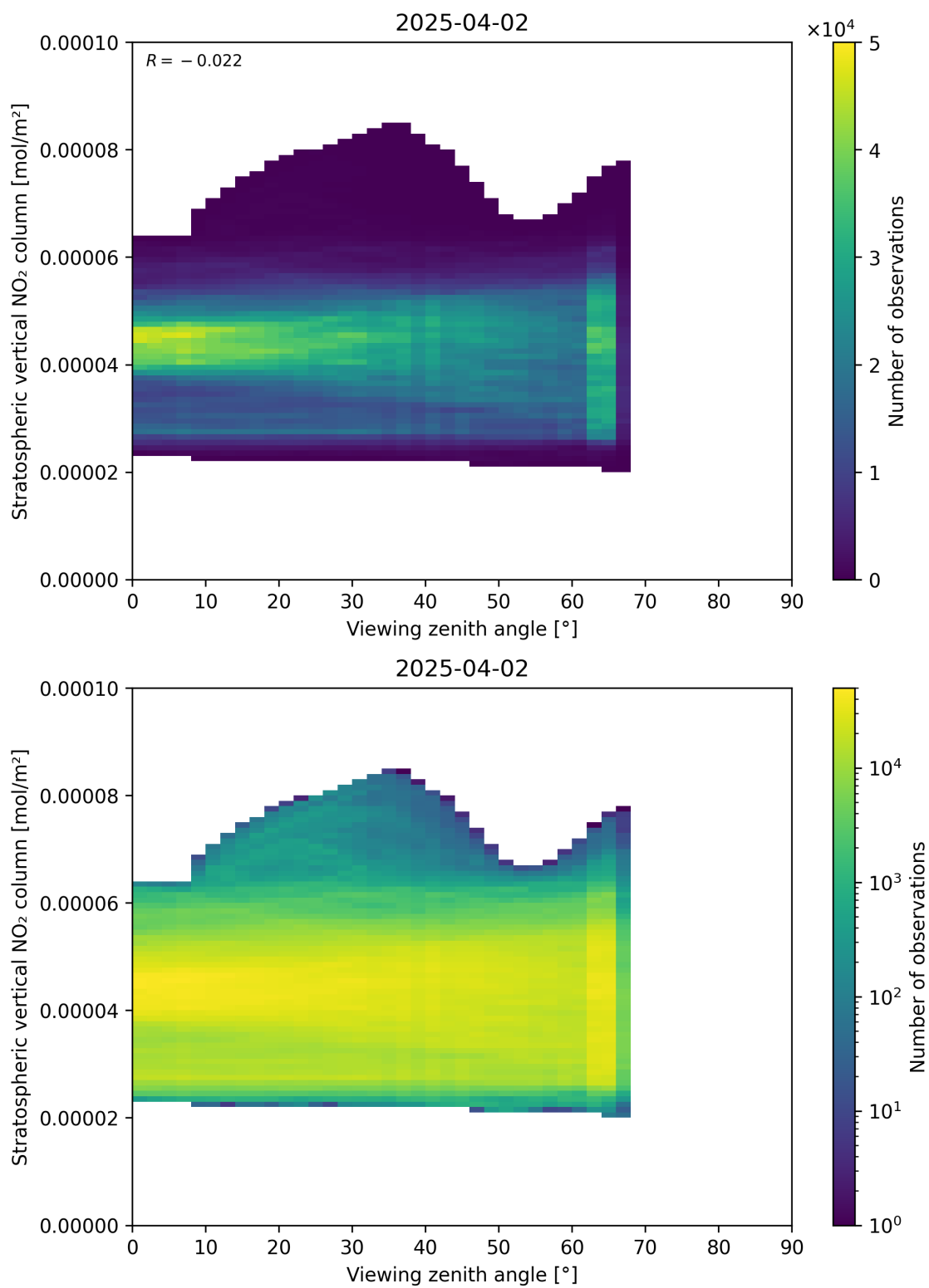
Figure 164: Scatter density plot of “Viewing zenith angle” against “Stratospheric vertical NO 2 column” for 2025-04-02 to 2025-04-03.
