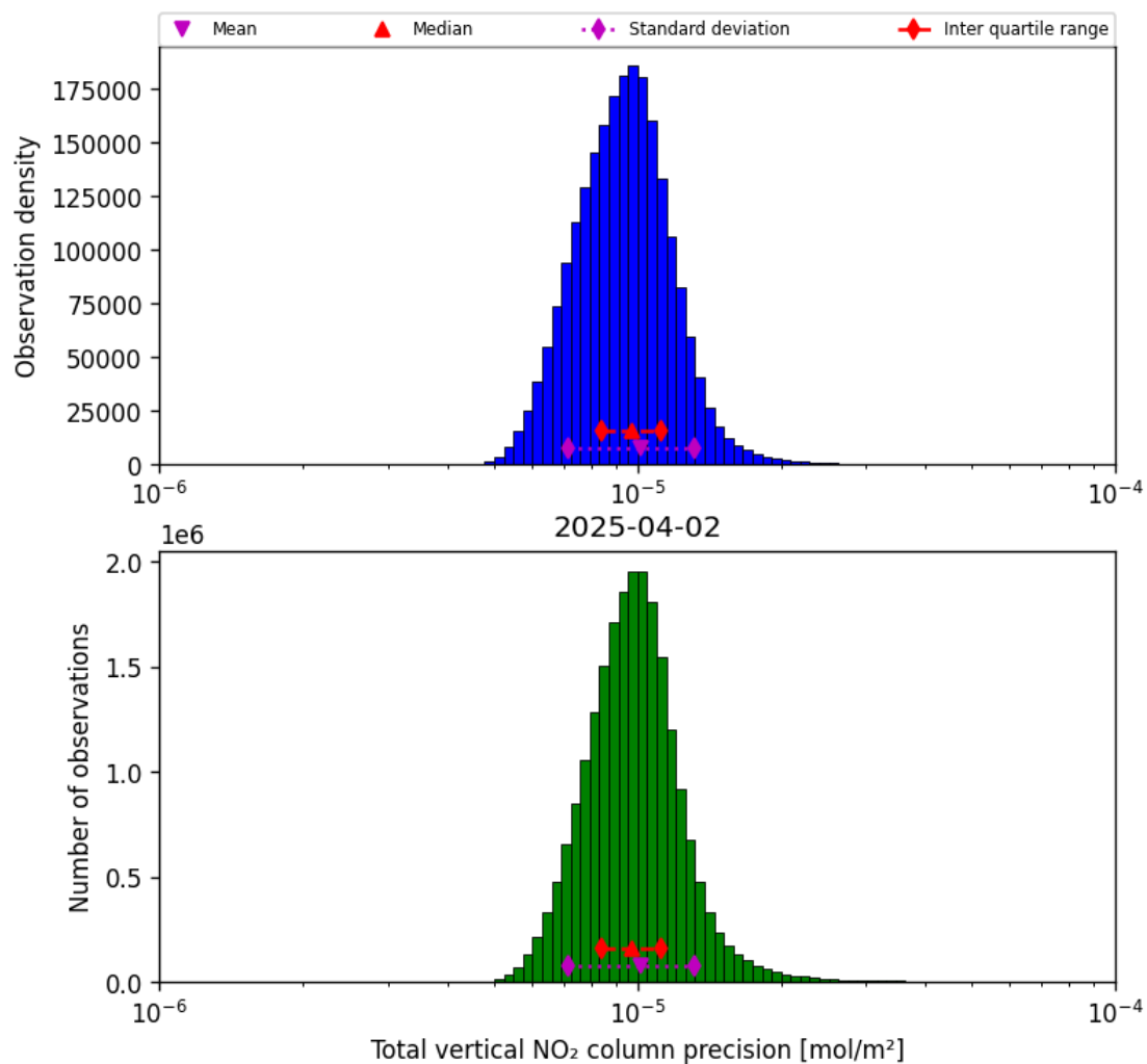
Figure 39: Histogram of “Total vertical NO 2 column precision” for 2025-04-02 to 2025-04-03
