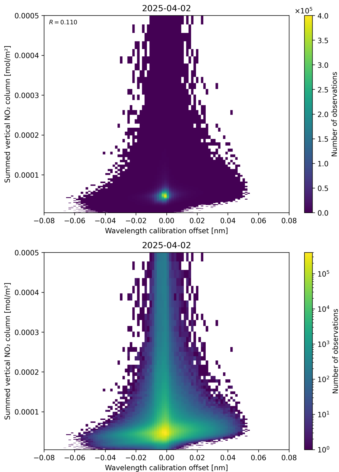
Figure 177: Scatter density plot of “Wavelength calibration offset” against “Summed vertical NO 2 column” for 2025-04-02 to 2025-04-03.
