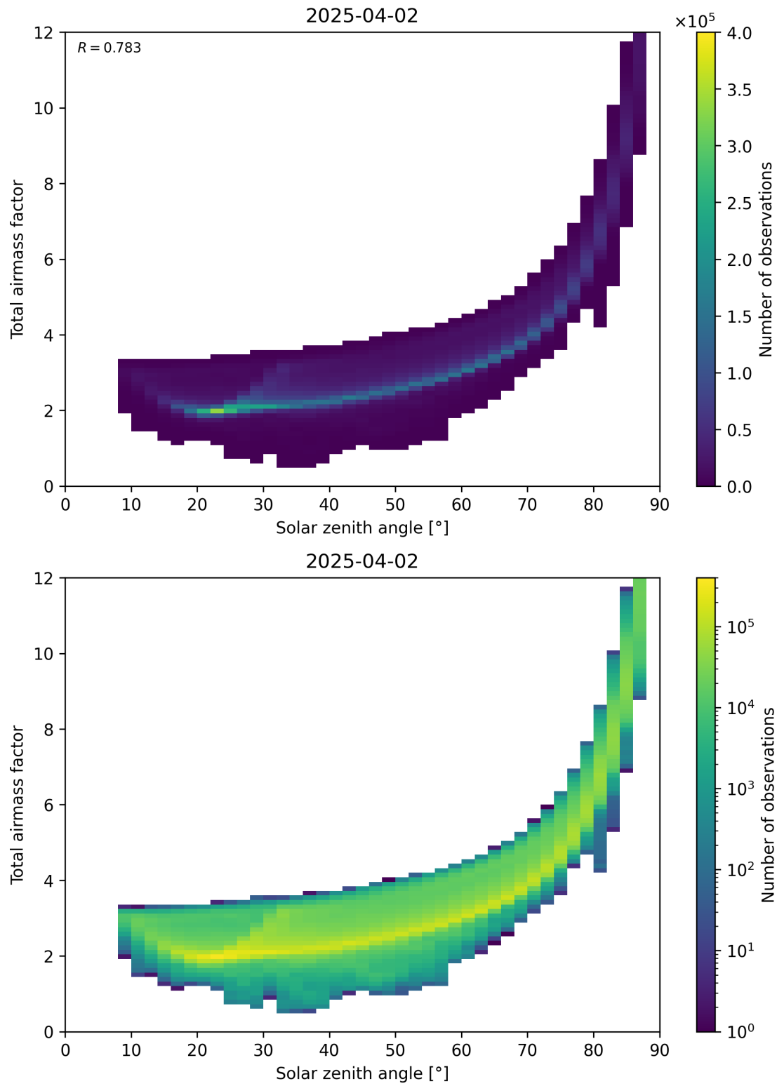
Figure 146: Scatter density plot of “Solar zenith angle” against “Total air mass factor” for 2025-04-02 to 2025-04-03.
