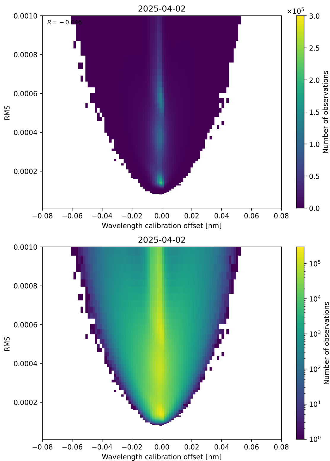
Figure 181: Scatter density plot of “Wavelength calibration offset” against “RMS” for 2025-04-02 to 2025-04-03.
