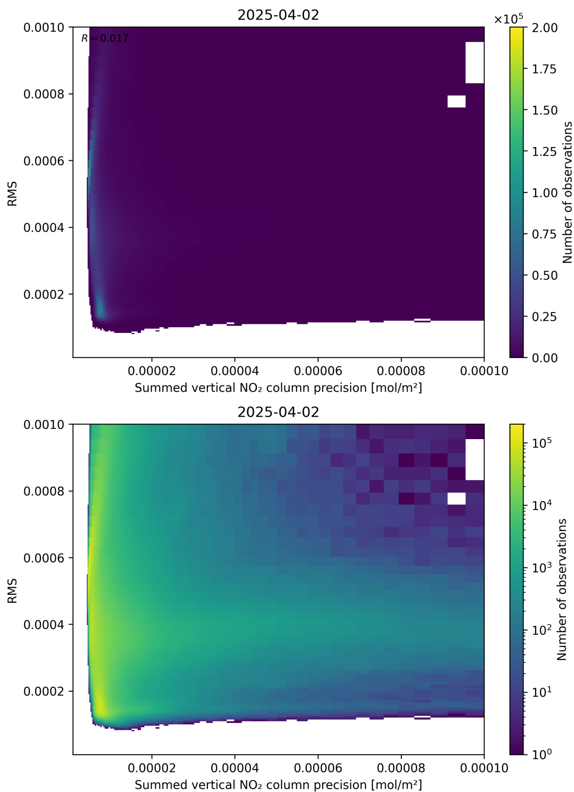
Figure 108: Scatter density plot of “Summed vertical NO 2 column precision” against “RMS” for 2025-04-02 to 2025-04-03.
