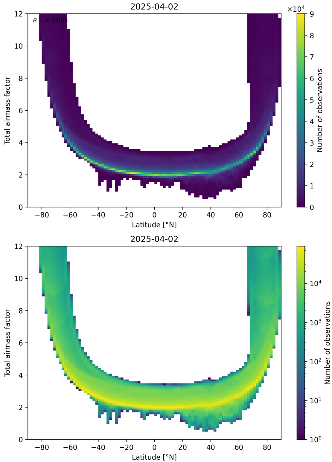
Figure 84: Scatter density plot of “Latitude” against “Total airmass factor” for 2025-04-02 to 2025-04-03.
