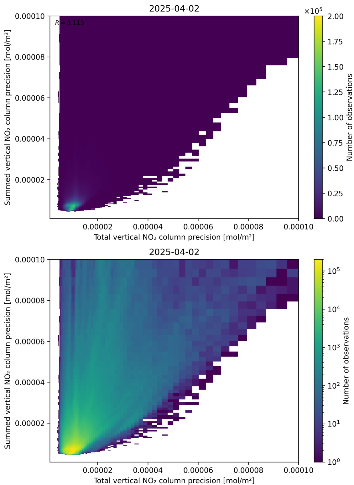
Figure 118: Scatter density plot of “Total vertical NO 2 column precision” against “Summed vertical NO 2 column precision” for 2025-04-02 to 2025-04-03.
