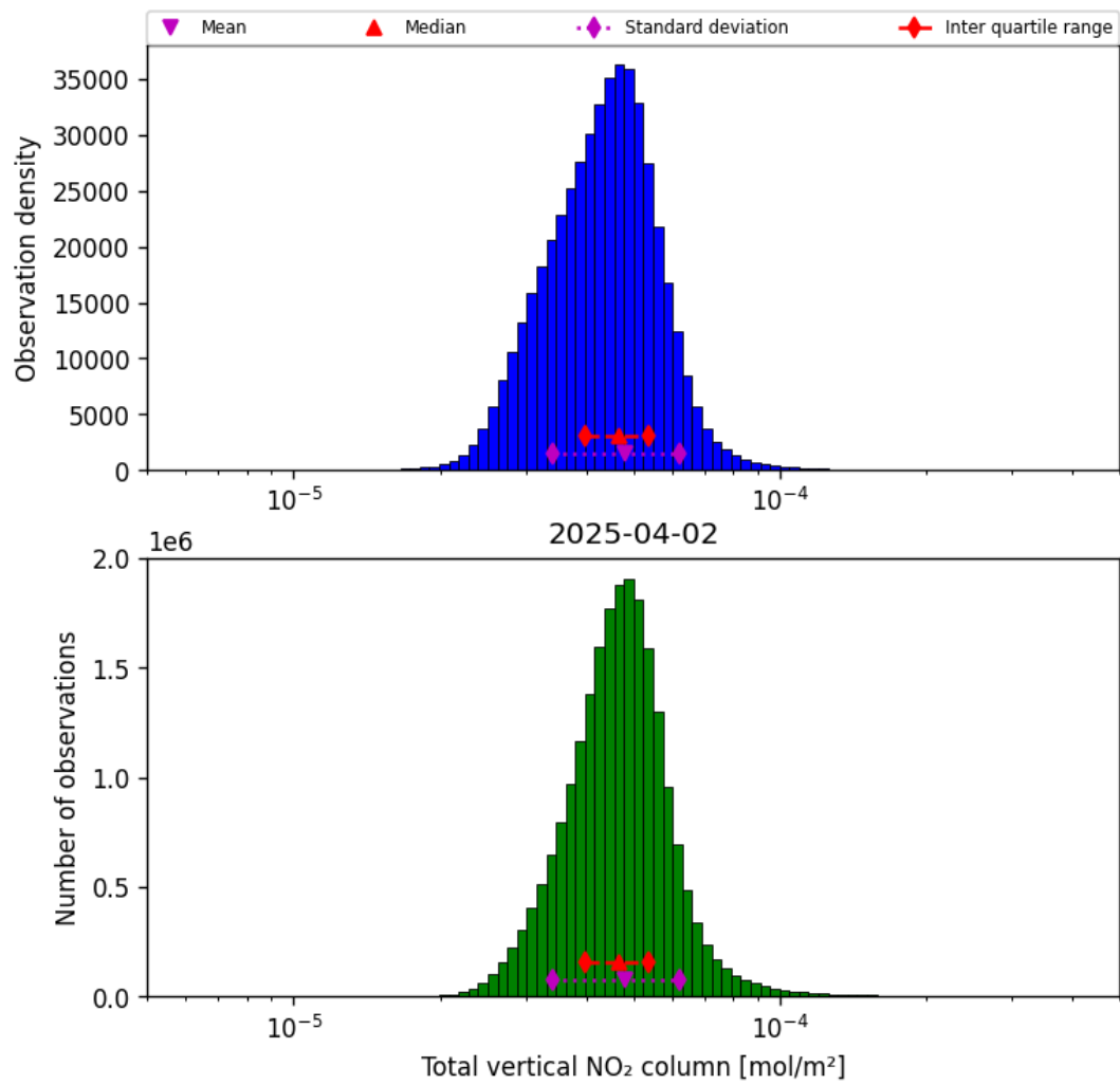
Figure 38: Histogram of “Total vertical NO 2 column” for 2025-04-02 to 2025-04-03
