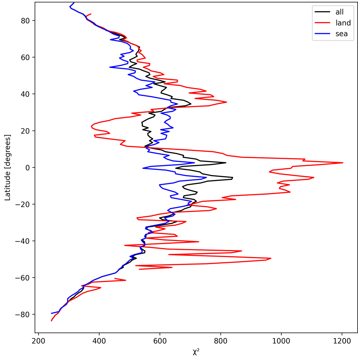
Figure 25: Zonal average of “ \chi^2 ” for 2025-04-02 to 2025-04-03.
