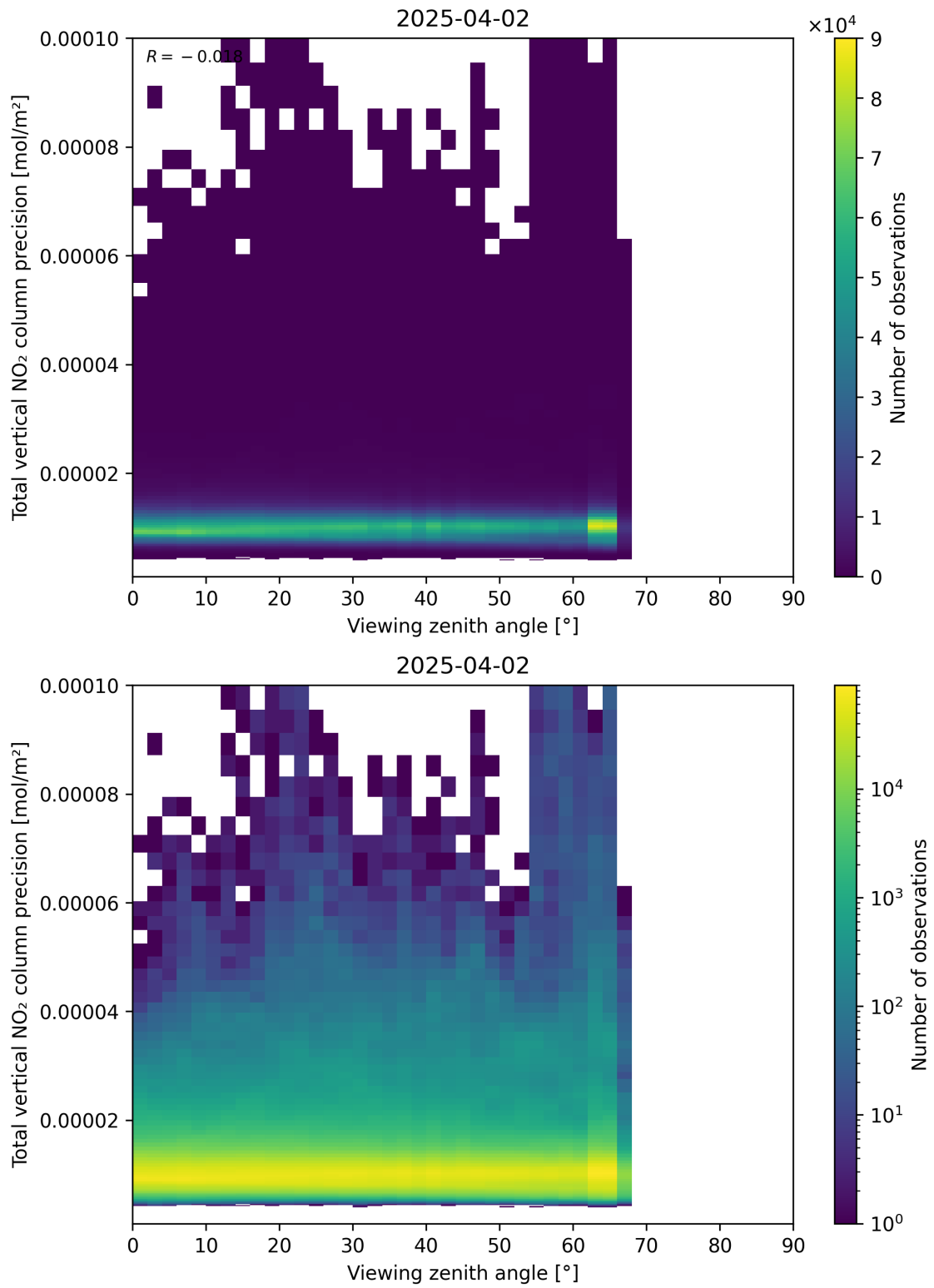
Figure 168: Scatter density plot of “Viewing zenith angle” against “Total vertical NO 2 column precision” for 2025-04-02 to 2025-04-03.
