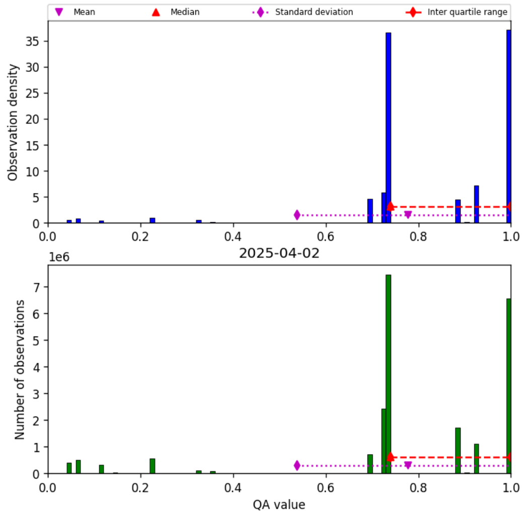
Figure 28: Histogram of “QA value” for 2025-04-02 to 2025-04-03
