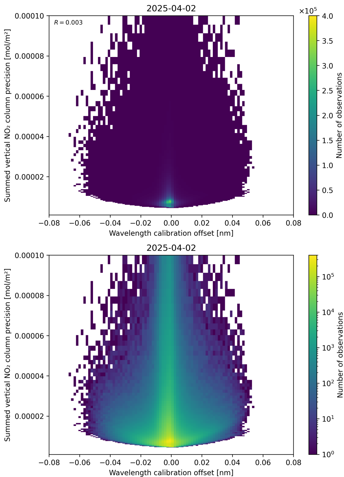
Figure 178: Scatter density plot of “Wavelength calibration offset” against “Summed vertical NO 2 column precision” for 2025-04-02 to 2025-04-03.
