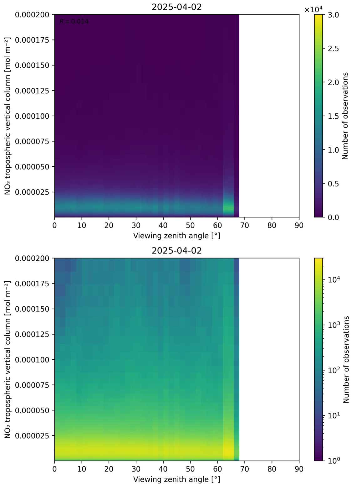
Figure 169: Scatter density plot of “Viewing zenith angle” against “NO 2 tropospheric vertical column” for 2025-04-02 to 2025-04-03.
