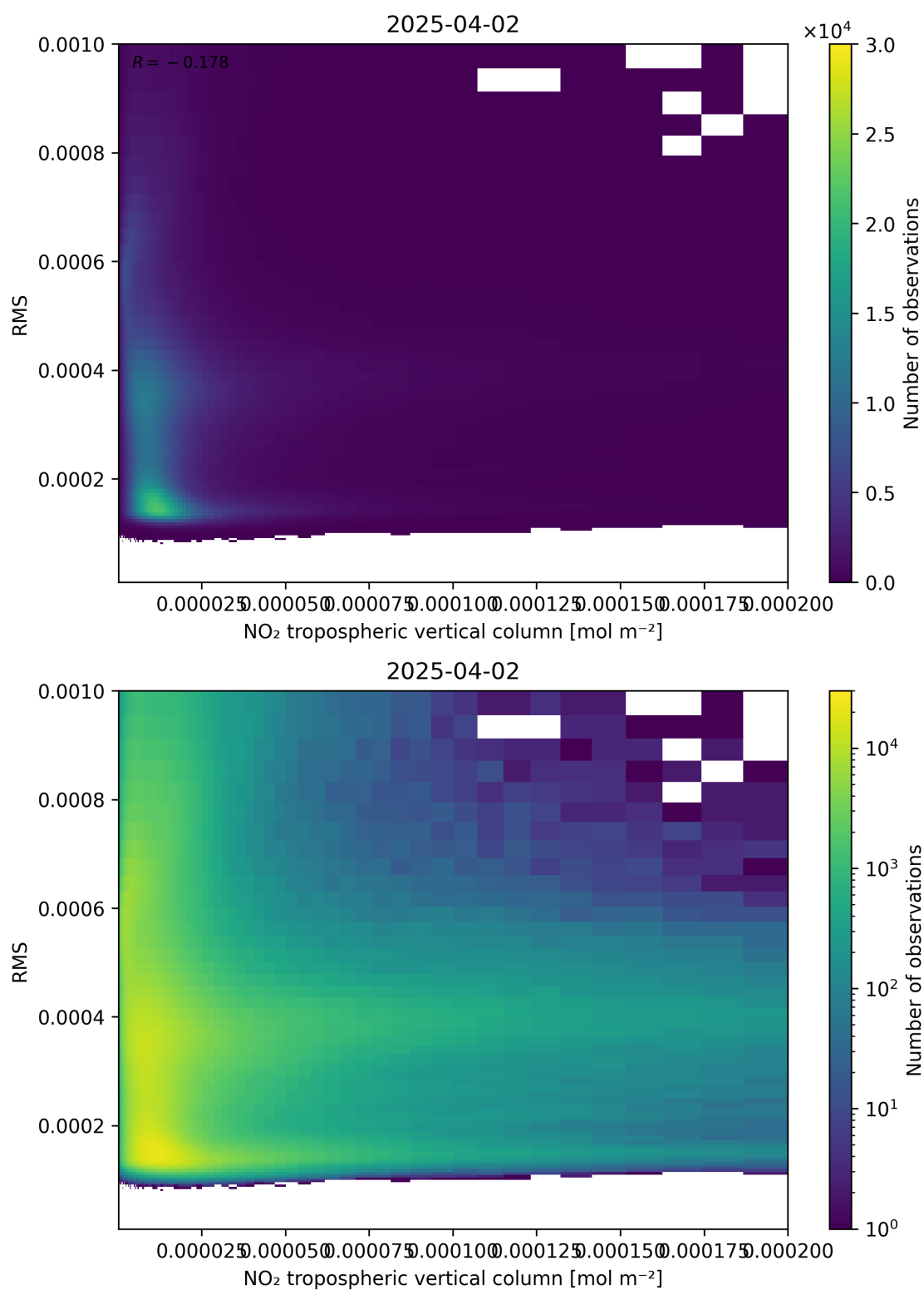
Figure 142: Scatter density plot of “NO 2 tropospheric vertical column” against “RMS” for 2025-04-02 to 2025-04-03.
