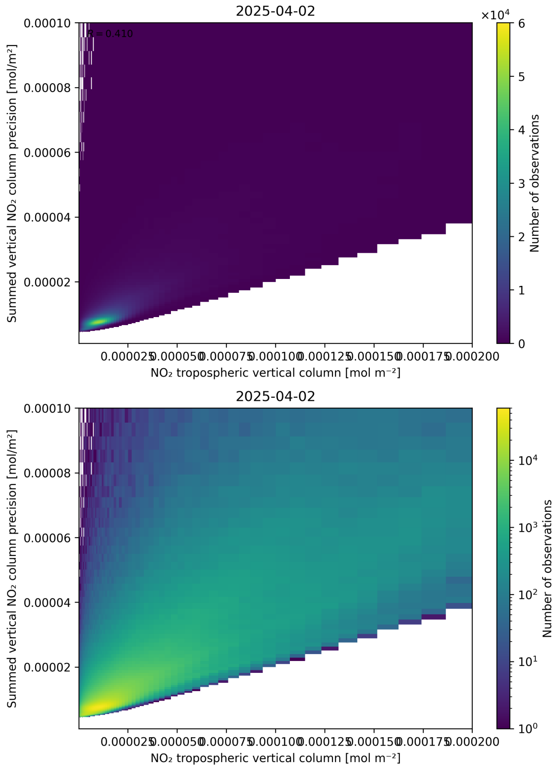
Figure 127: Scatter density plot of “NO 2 tropospheric vertical column” against “Summed vertical NO 2 column precision” for 2025-04-02 to 2025-04-03.
