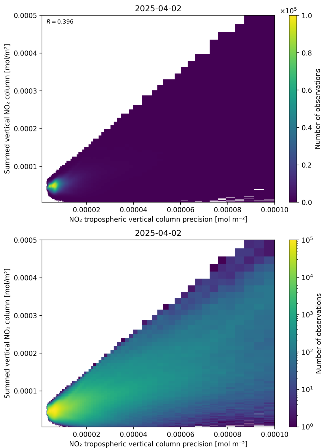
Figure 136: Scatter density plot of “NO 2 tropospheric vertical column precision” against “Summed vertical NO 2 column” for 2025-04-02 to 2025-04-03.
