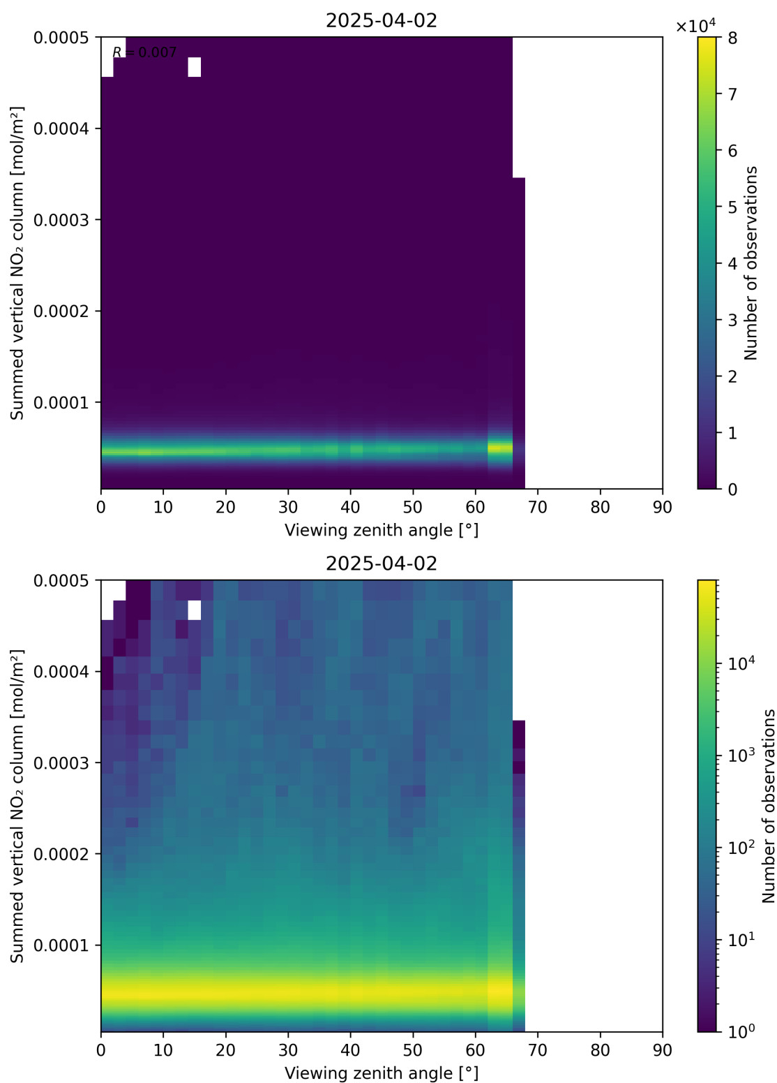
Figure 165: Scatter density plot of “Viewing zenith angle” against “Summed vertical NO 2 column” for 2025-04-02 to 2025-04-03.
