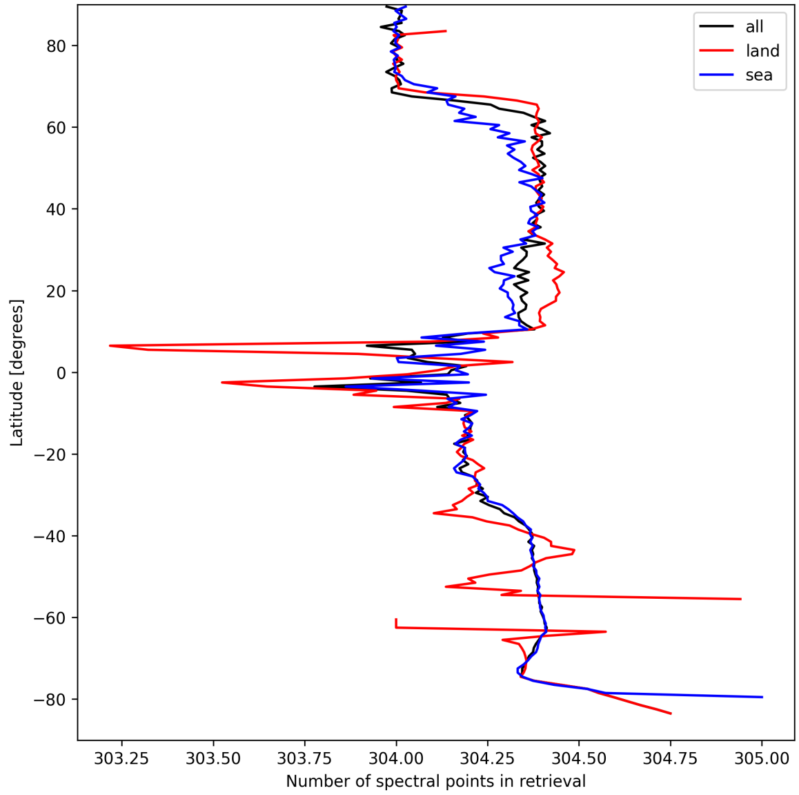
Figure 16: Zonal average of “Number of spectral points in retrieval” for 2025-04-02 to 2025-04-03.
