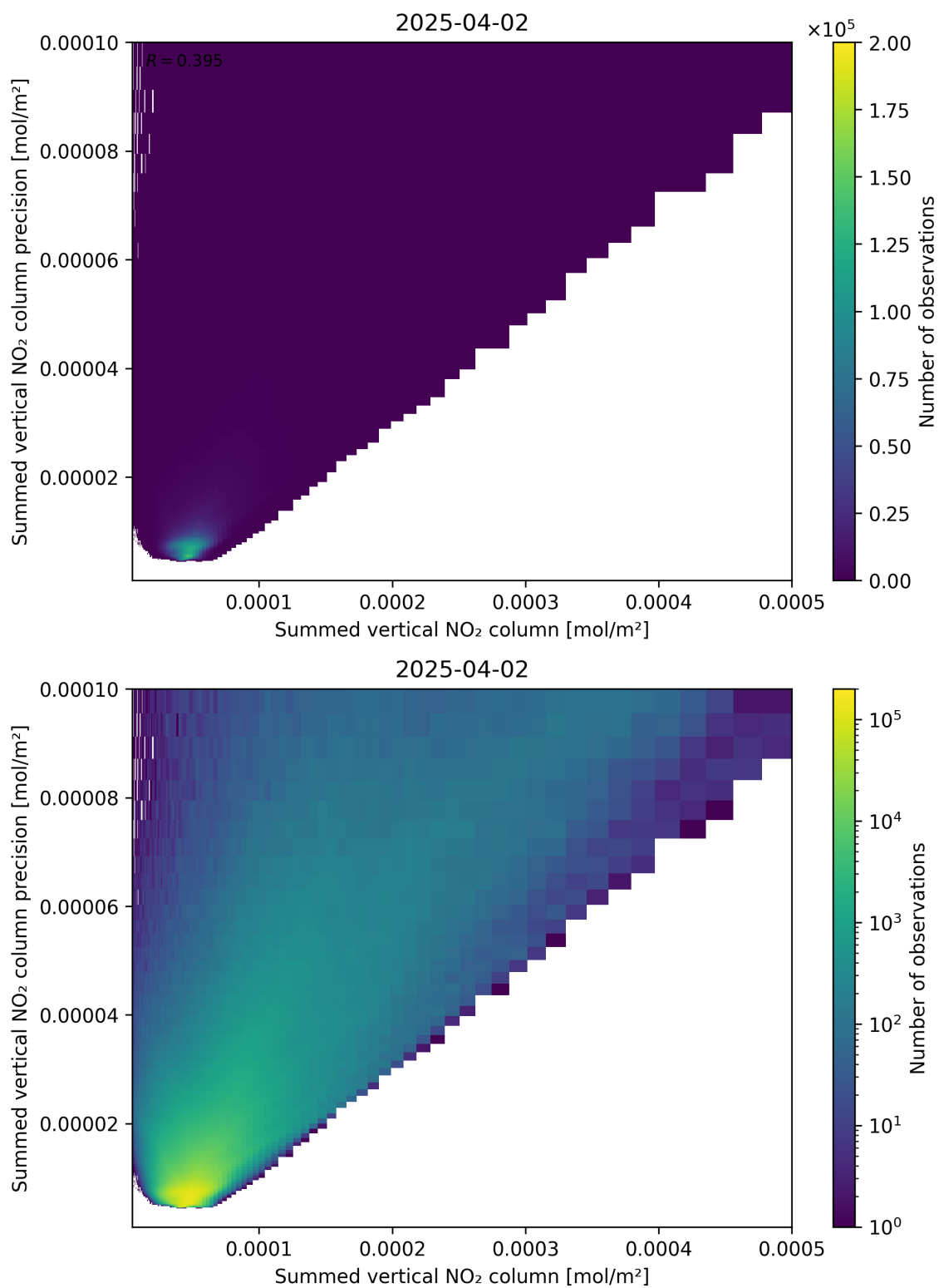
Figure 105: Scatter density plot of “Summed vertical NO 2 column” against “Summed vertical NO 2 column precision” for 2025-04-02 to 2025-04-03.
