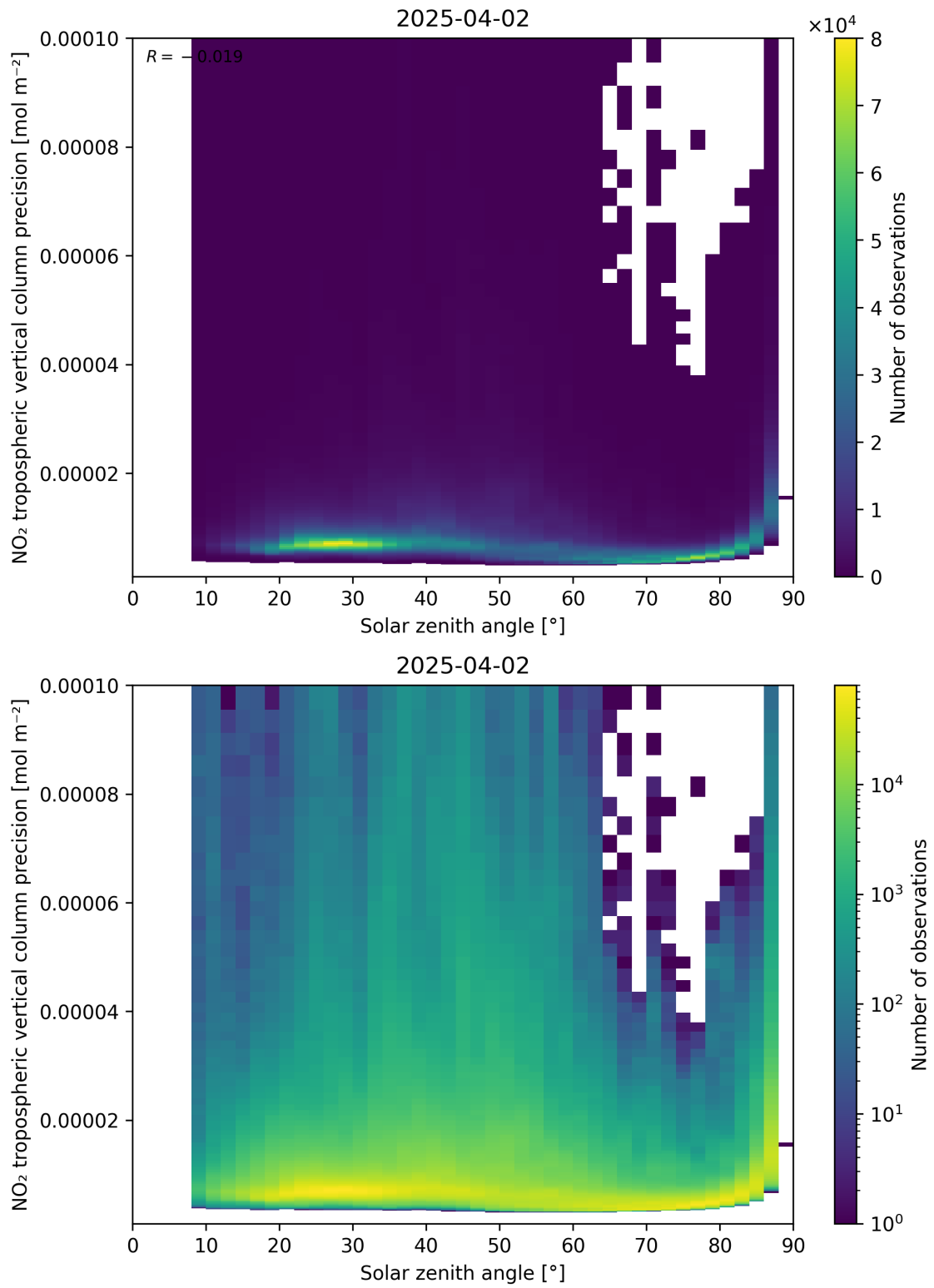
Figure 156: Scatter density plot of “Solar zenith angle” against “NO 2 tropospheric vertical column precision” for 2025-04-02 to 2025-04-03.
