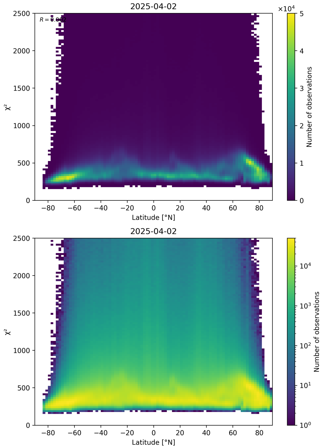
Figure 86: Scatter density plot of “Latitude” against “ \chi^2 ” for 2025-04-02 to 2025-04-03.
