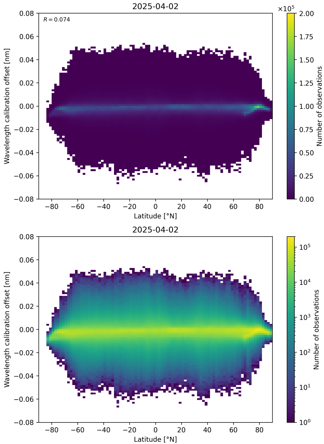
Figure 95: Scatter density plot of “Latitude” against “Wavelength calibration offset” for 2025-04-02 to 2025-04-03.
