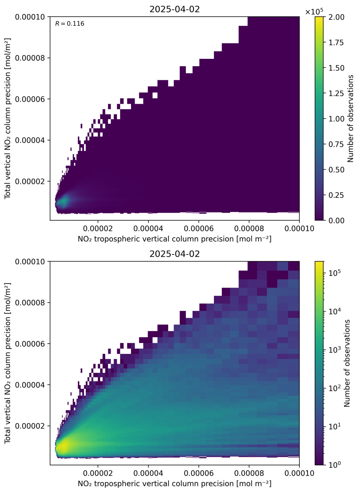
Figure 139: Scatter density plot of “NO 2 tropospheric vertical column precision” against “Total vertical NO 2 column precision” for 2025-04-02 to 2025-04-03.
