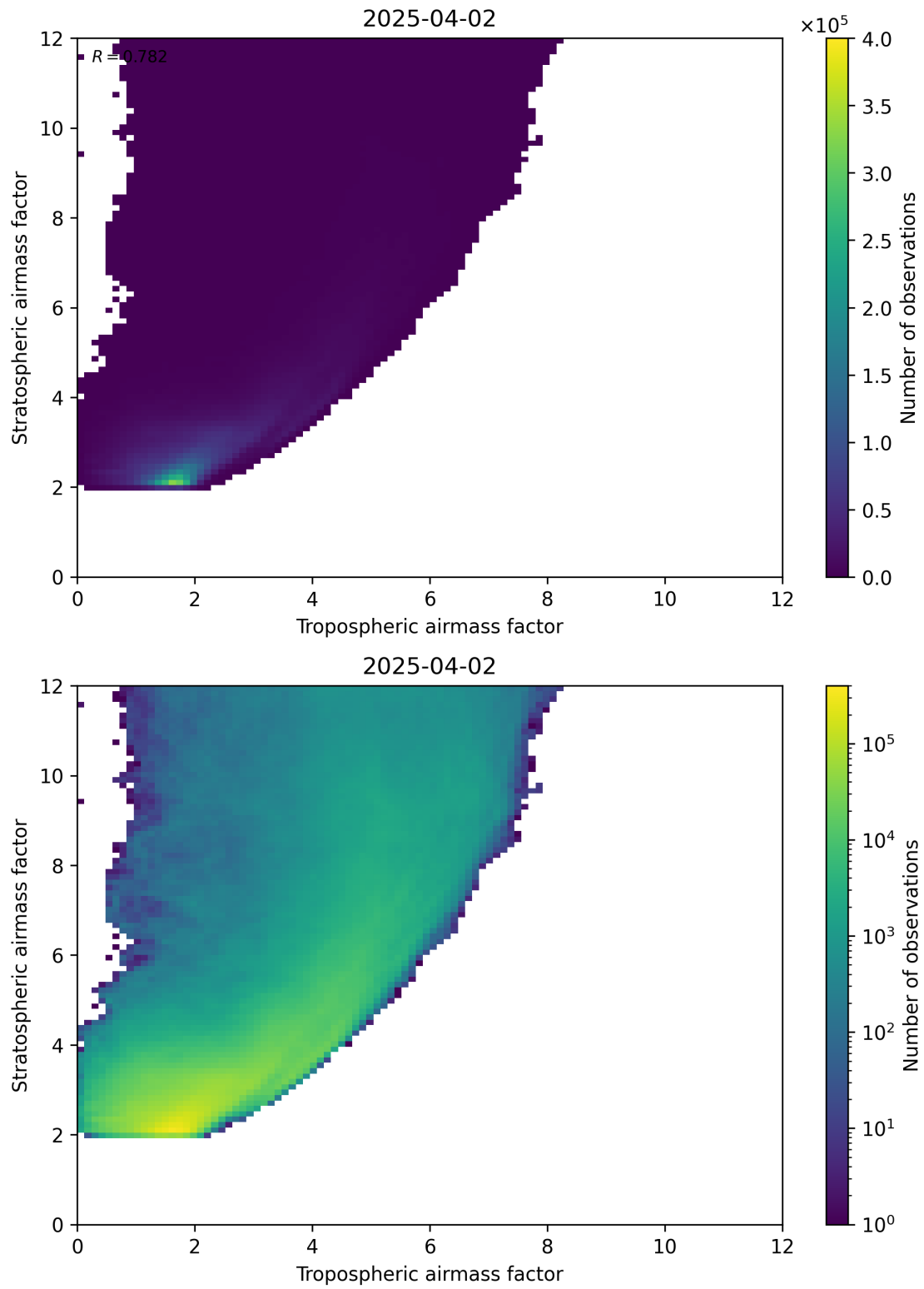
Figure 71: Scatter density plot of “Tropospheric airmass factor” against “Stratospheric airmass factor” for 2025-04-02 to 2025-04-03.
