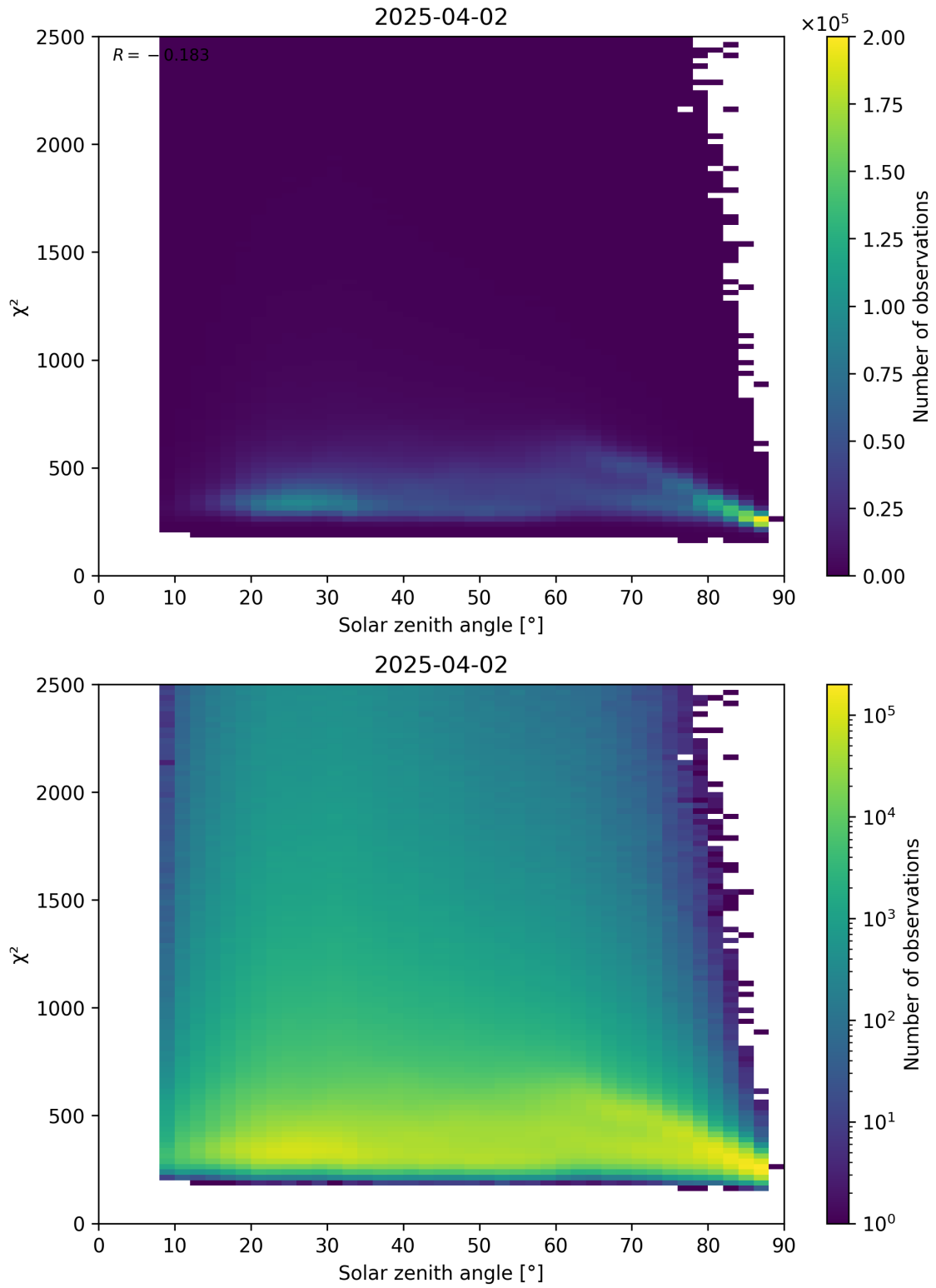
Figure 148: Scatter density plot of “Solar zenith angle” against “ \chi^2 ” for 2025-04-02 to 2025-04-03.
