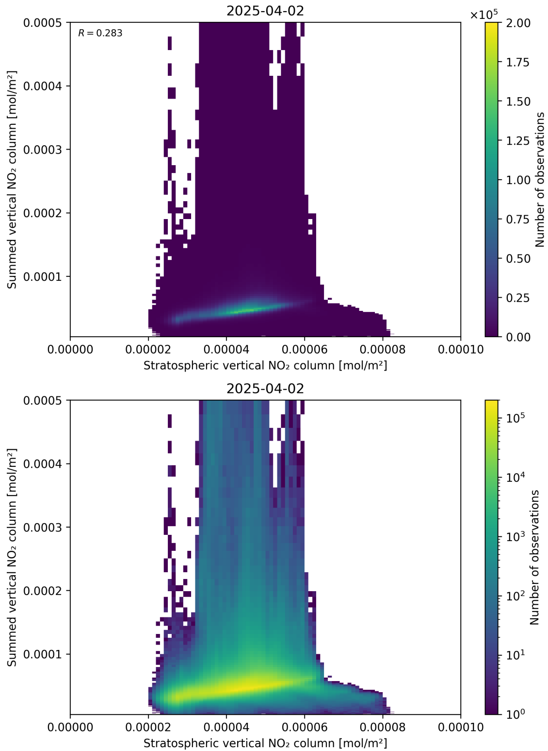
Figure 98: Scatter density plot of “Stratospheric vertical NO 2 column” against “Summed vertical NO 2 column” for 2025-04-02 to 2025-04-03.
