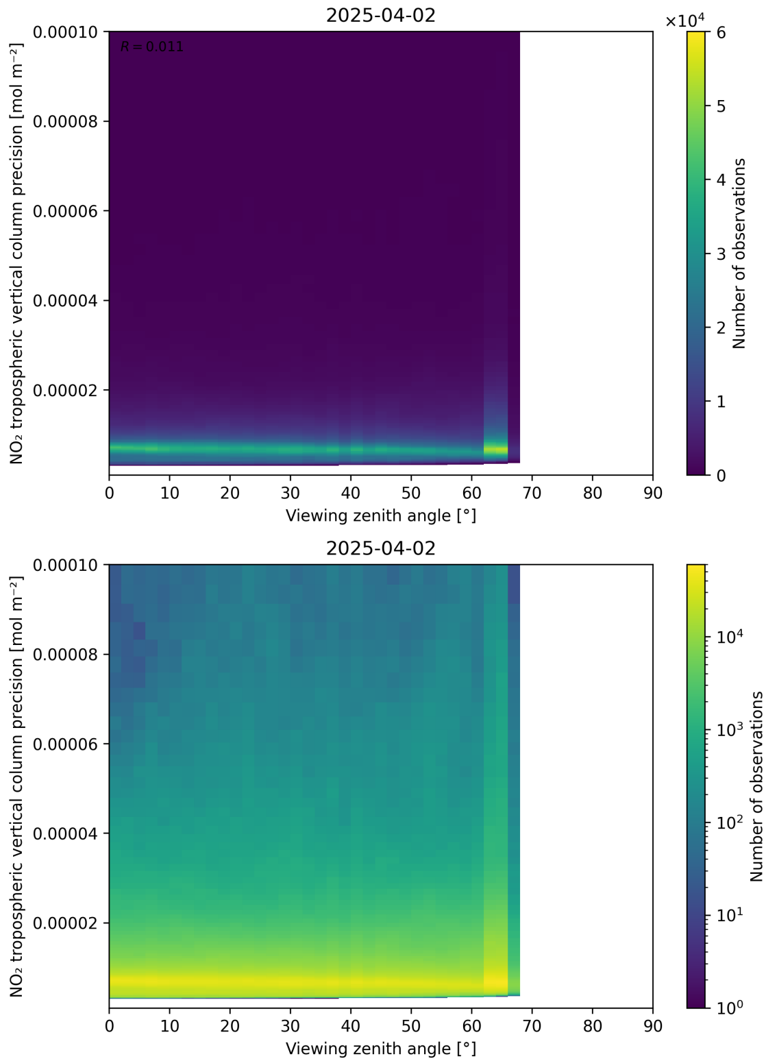
Figure 170: Scatter density plot of “Viewing zenith angle” against “NO 2 tropospheric vertical column precision” for 2025-04-02 to 2025-04-03.
