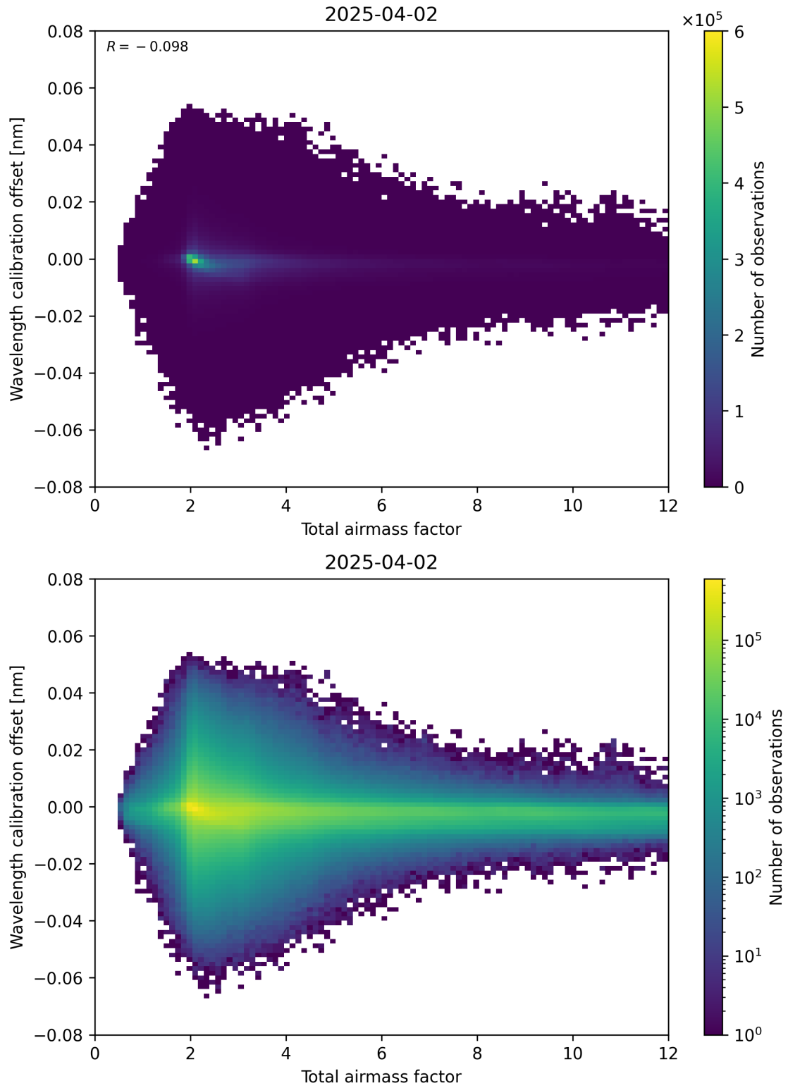
Figure 70: Scatter density plot of “Total airmass factor” against “Wavelength calibration offset” for 2025-04-02 to 2025-04-03.
