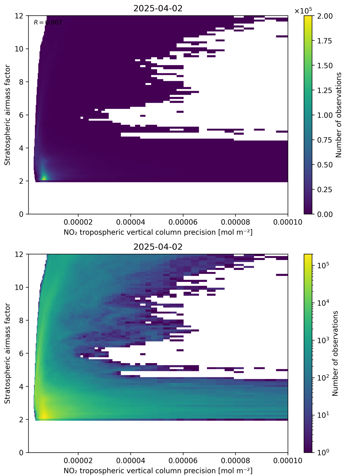
Figure 131: Scatter density plot of “NO 2 tropospheric vertical column precision” against “Stratospheric airmass factor” for 2025-04-02 to 2025-04-03.
