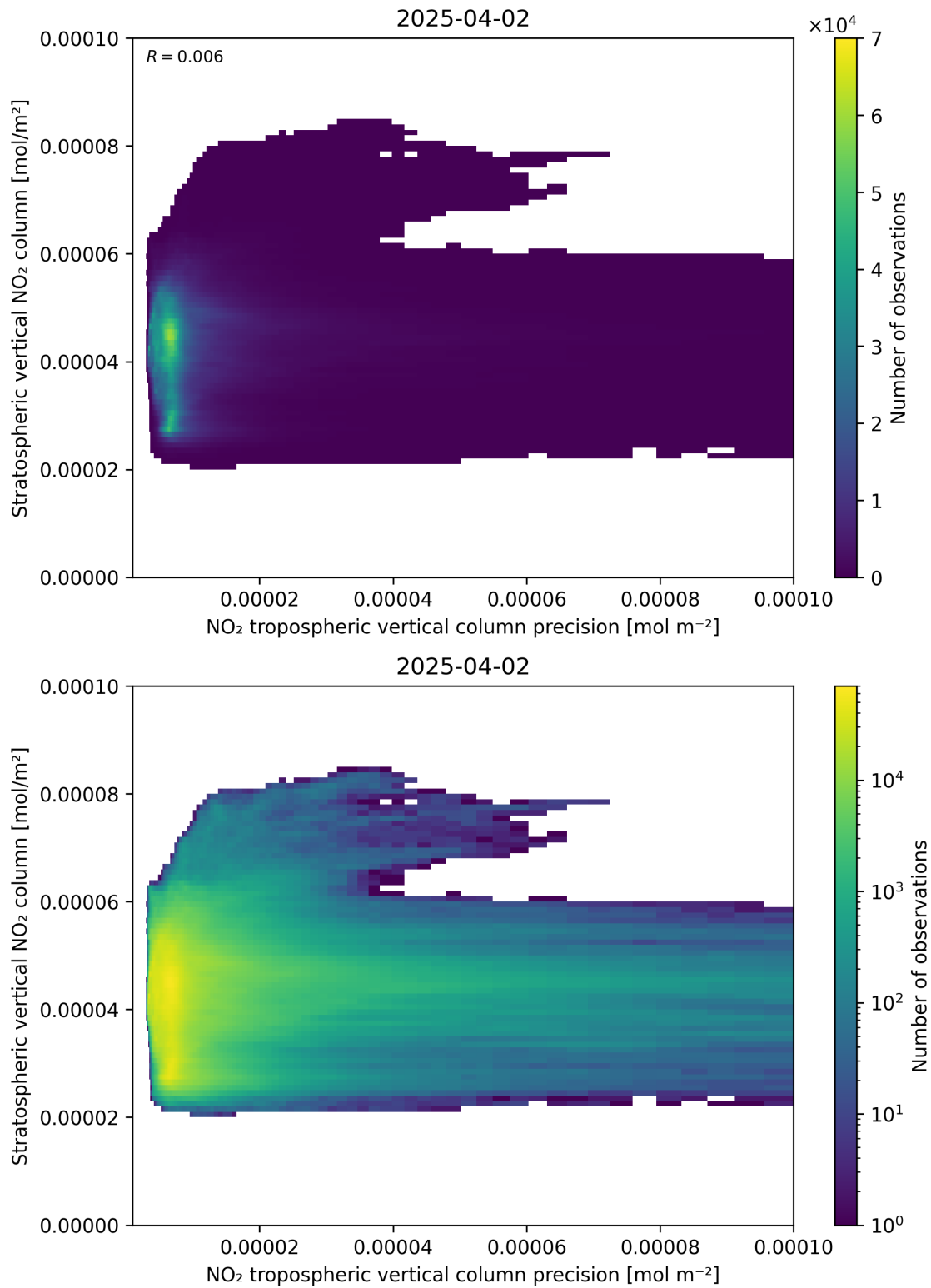
Figure 135: Scatter density plot of “NO 2 tropospheric vertical column precision” against “Stratospheric vertical NO 2 column” for 2025-04-02 to 2025-04-03.
