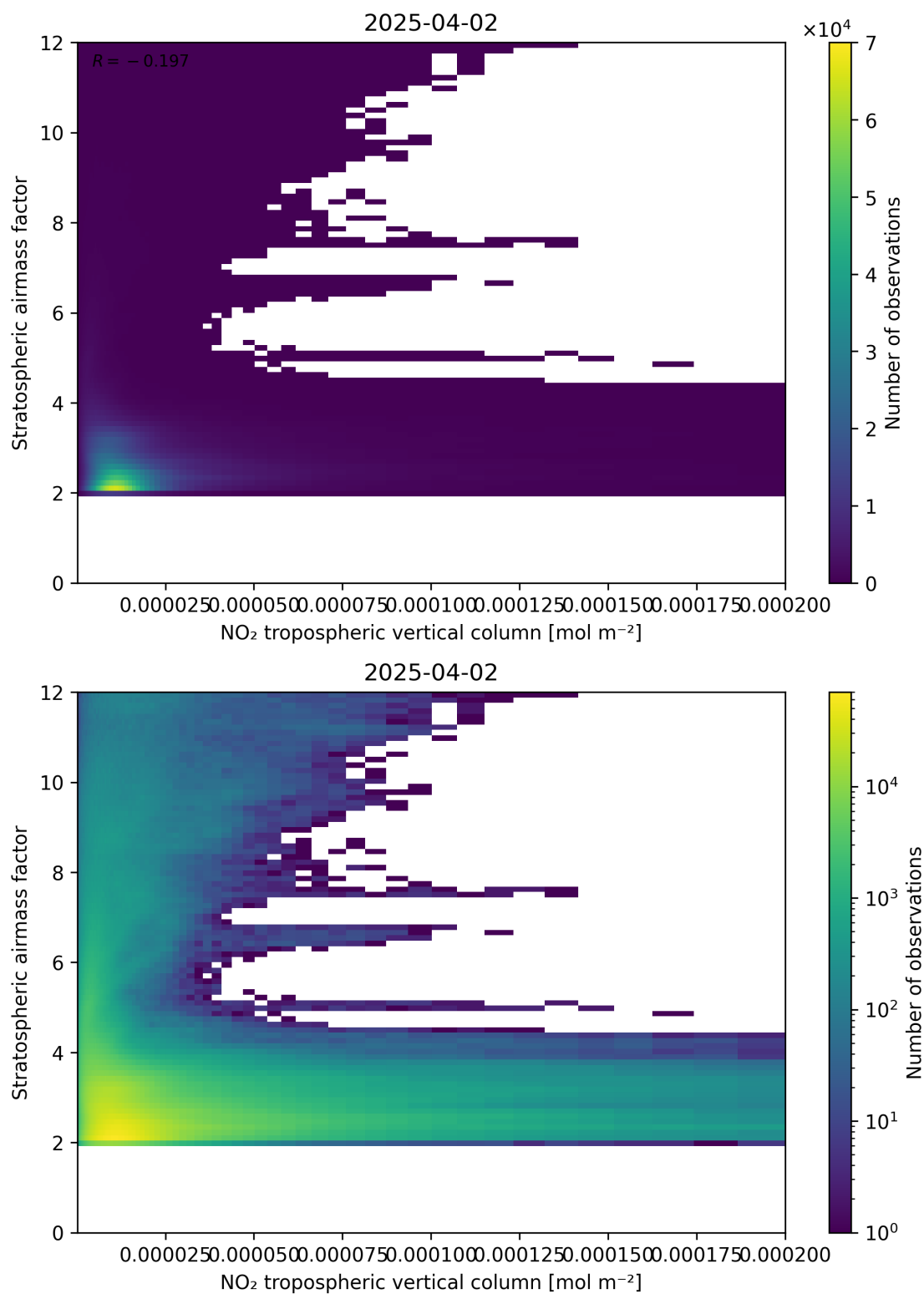
Figure 121: Scatter density plot of “NO 2 tropospheric vertical column” against “Stratospheric air mass factor” for 2025-04-02 to 2025-04-03.
