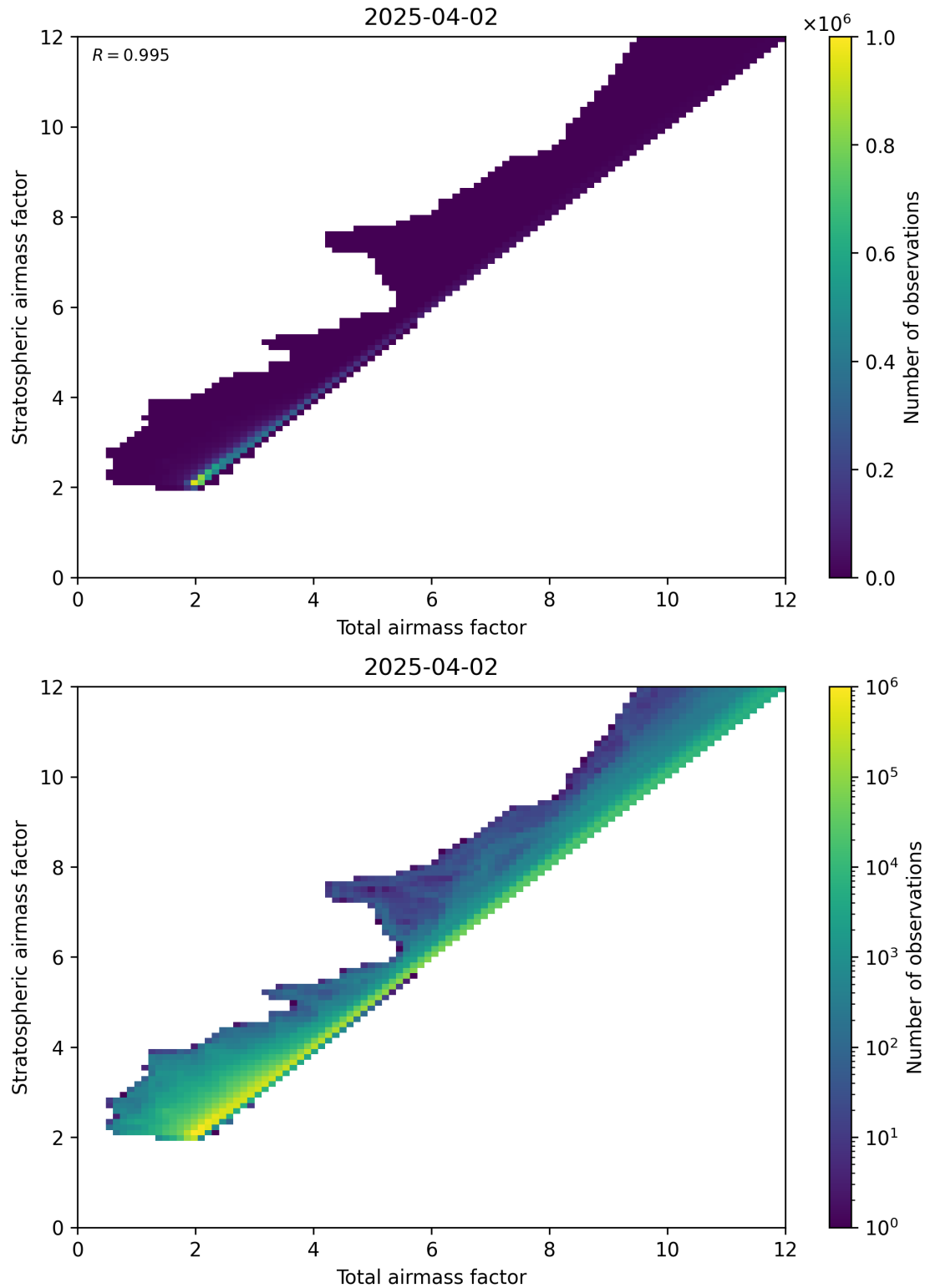
Figure 62: Scatter density plot of “Total airmass factor” against “Stratospheric airmass factor” for 2025-04-02 to 2025-04-03.
