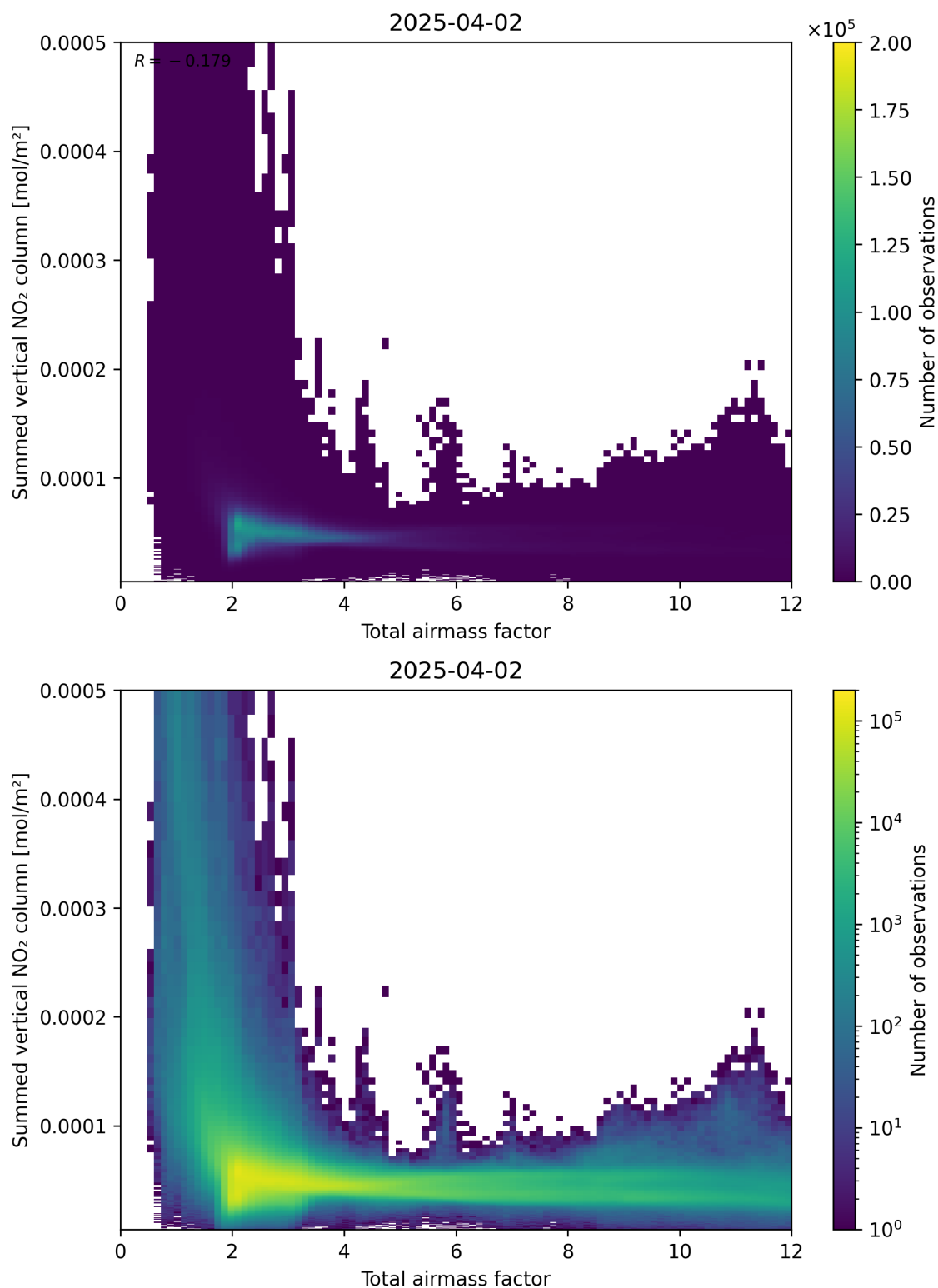
Figure 65: Scatter density plot of “Total airmass factor” against “Summed vertical NO 2 column” for 2025-04-02 to 2025-04-03.
