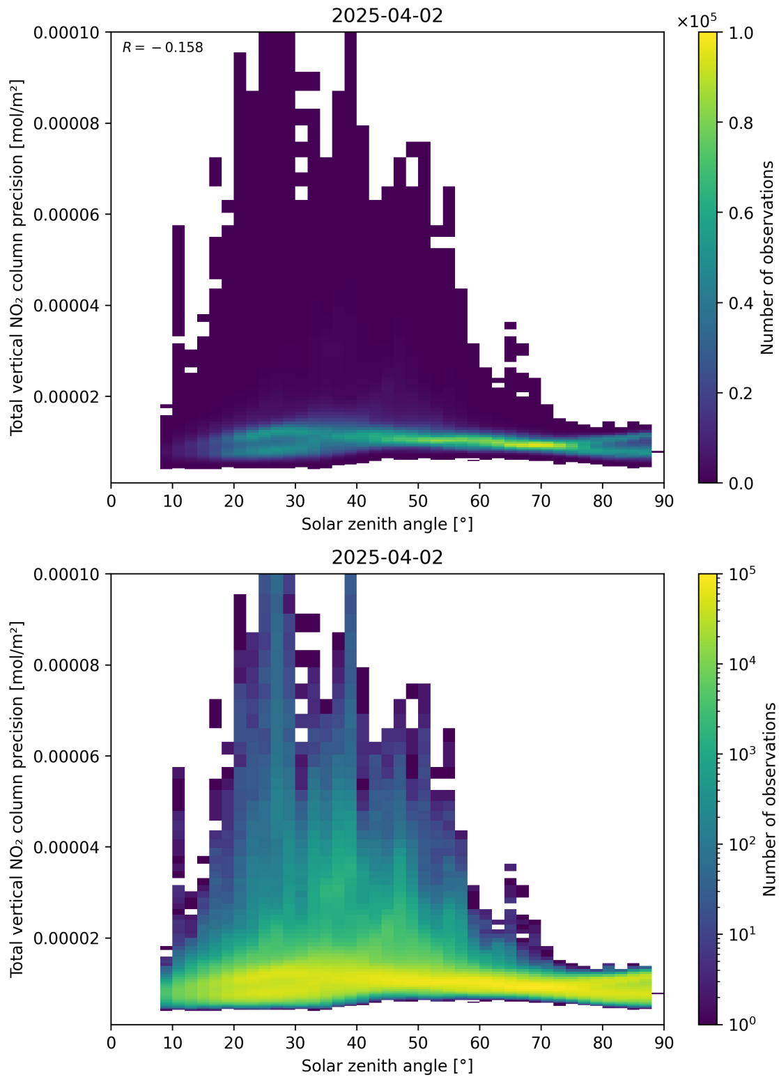
Figure 154: Scatter density plot of “Solar zenith angle” against “Total vertical NO 2 column precision” for 2025-04-02 to 2025-04-03.
