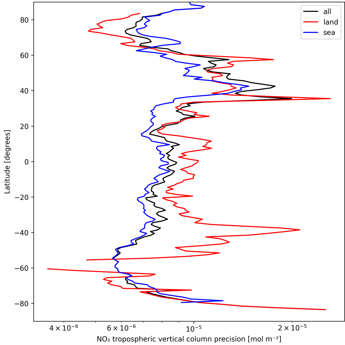
Figure 13: Zonal average of “NO 2 tropospheric vertical column precision” for 2025-04-02 to 2025-04-03.
