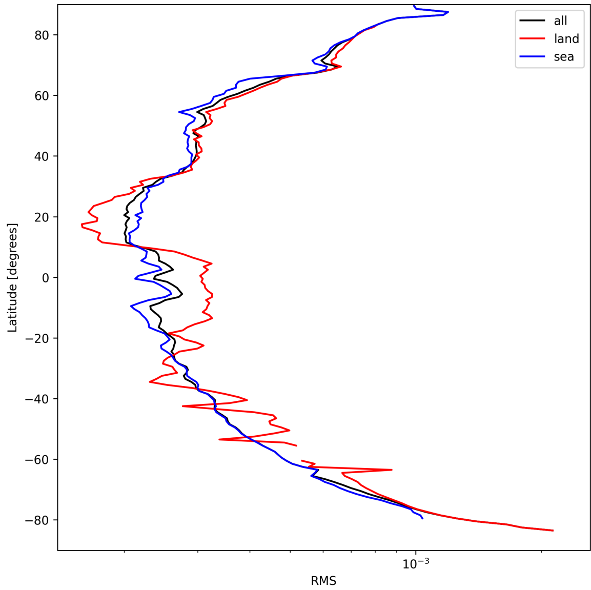
Figure 26: Zonal average of “RMS” for 2025-04-02 to 2025-04-03.
