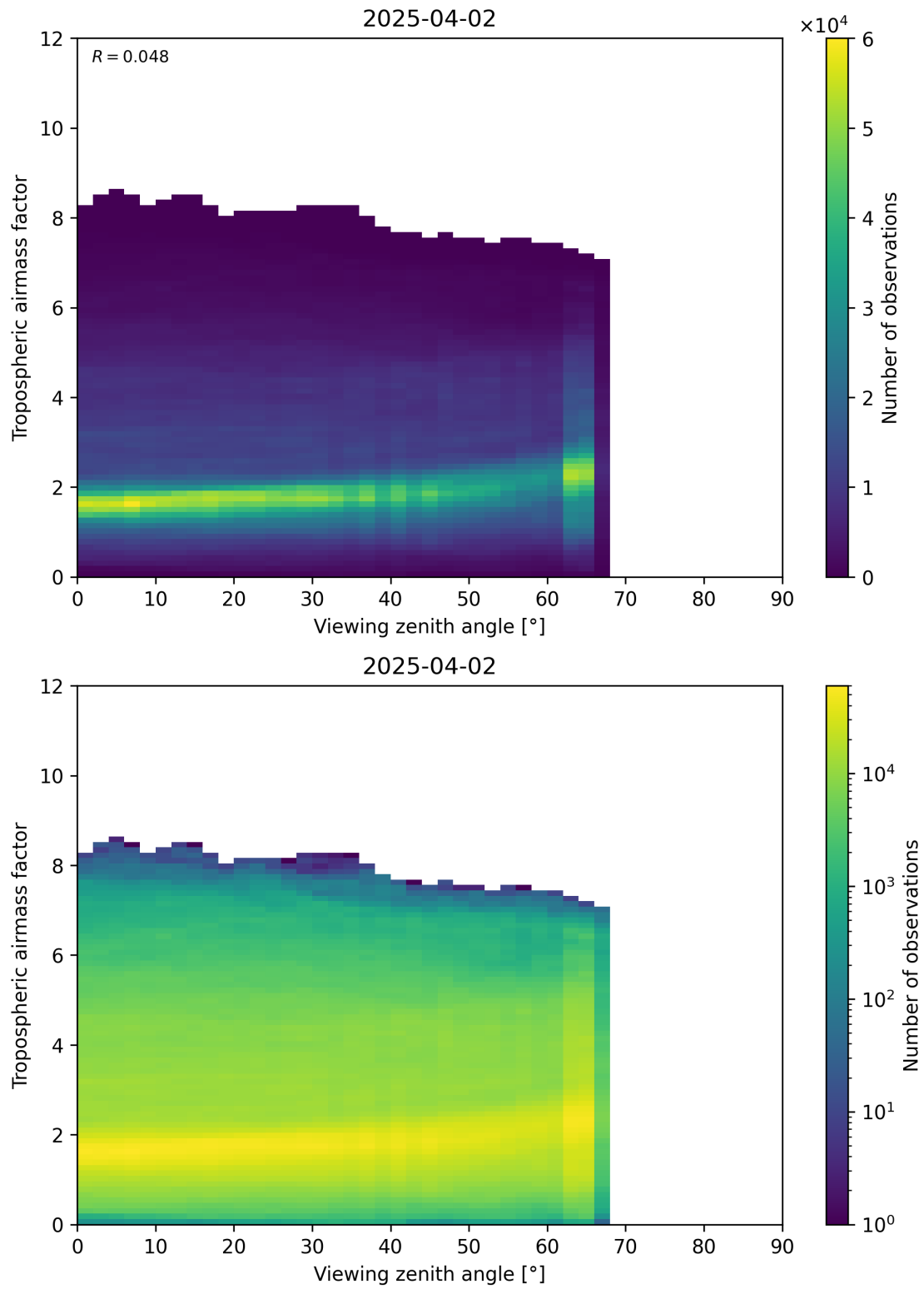
Figure 161: Scatter density plot of “Viewing zenith angle” against “Tropospheric airmass factor” for 2025-04-02 to 2025-04-03.
