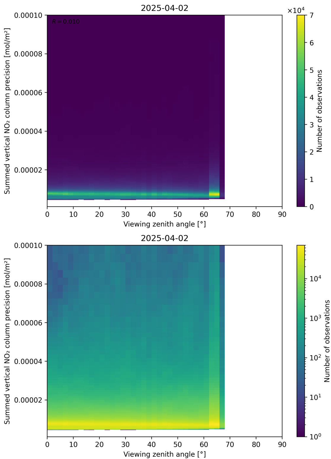
Figure 166: Scatter density plot of “Viewing zenith angle” against “Summed vertical NO 2 column precision” for 2025-04-02 to 2025-04-03.
