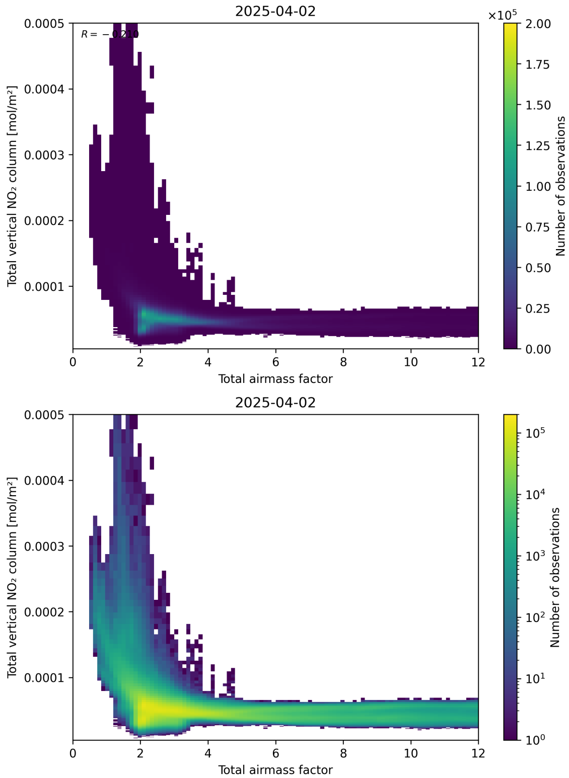
Figure 67: Scatter density plot of “Total airmass factor” against “Total vertical NO 2 column” for 2025-04-02 to 2025-04-03.
