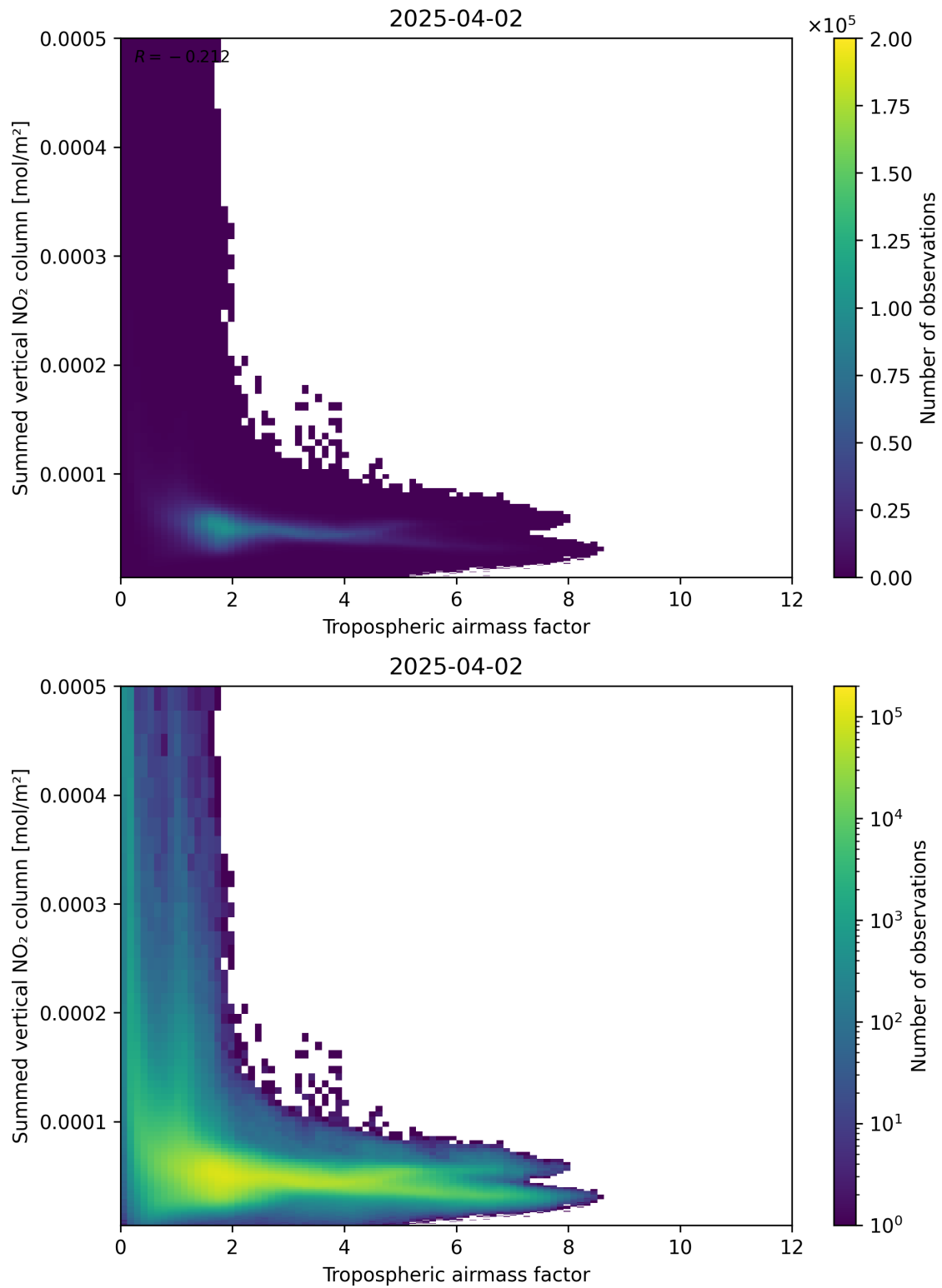
Figure 75: Scatter density plot of “Tropospheric airmass factor” against “Summed vertical NO 2 column” for 2025-04-02 to 2025-04-03.
