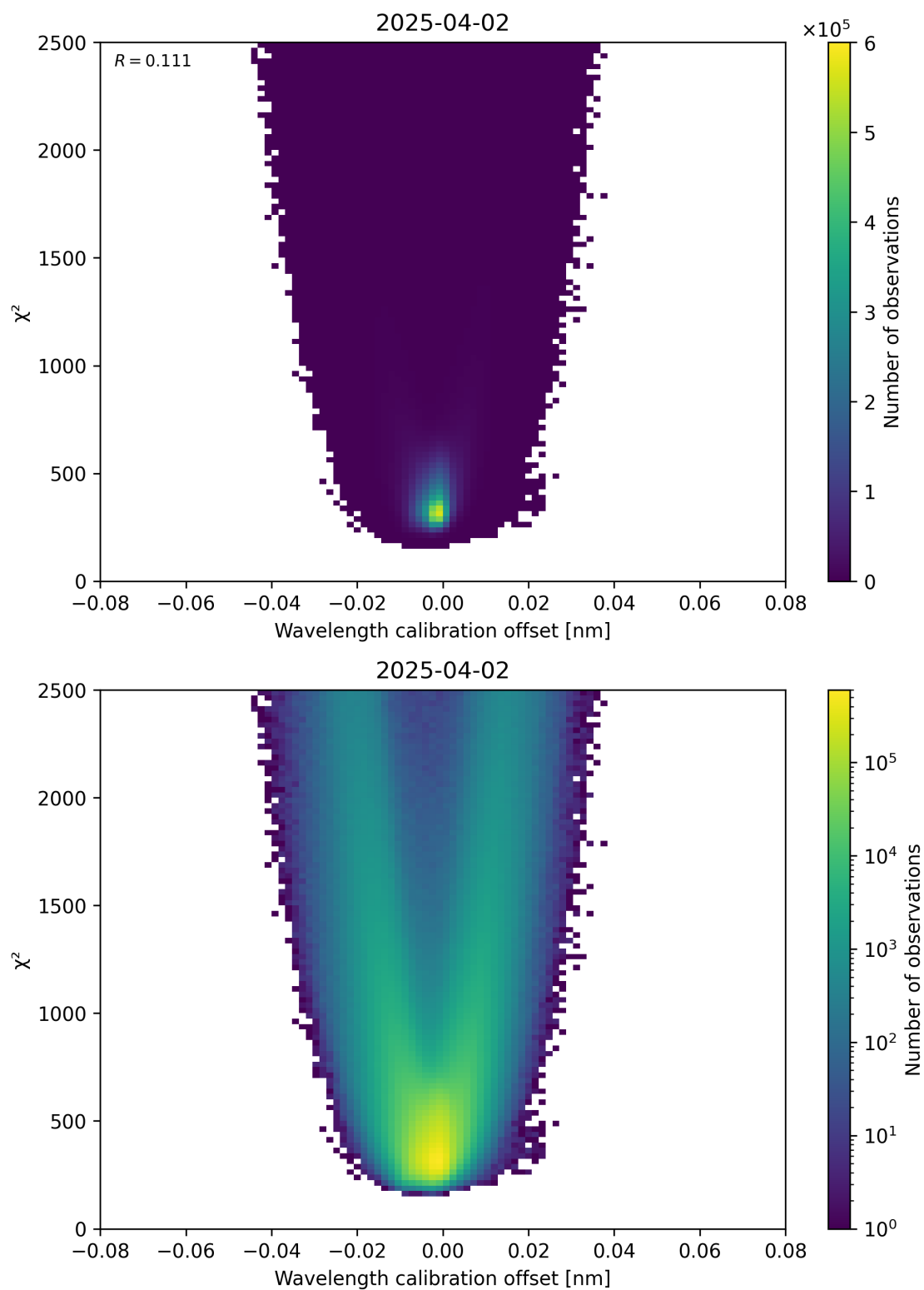
Figure 175: Scatter density plot of “Wavelength calibration offset” against “ \chi^2 ” for 2025-04-02 to 2025-04-03.
