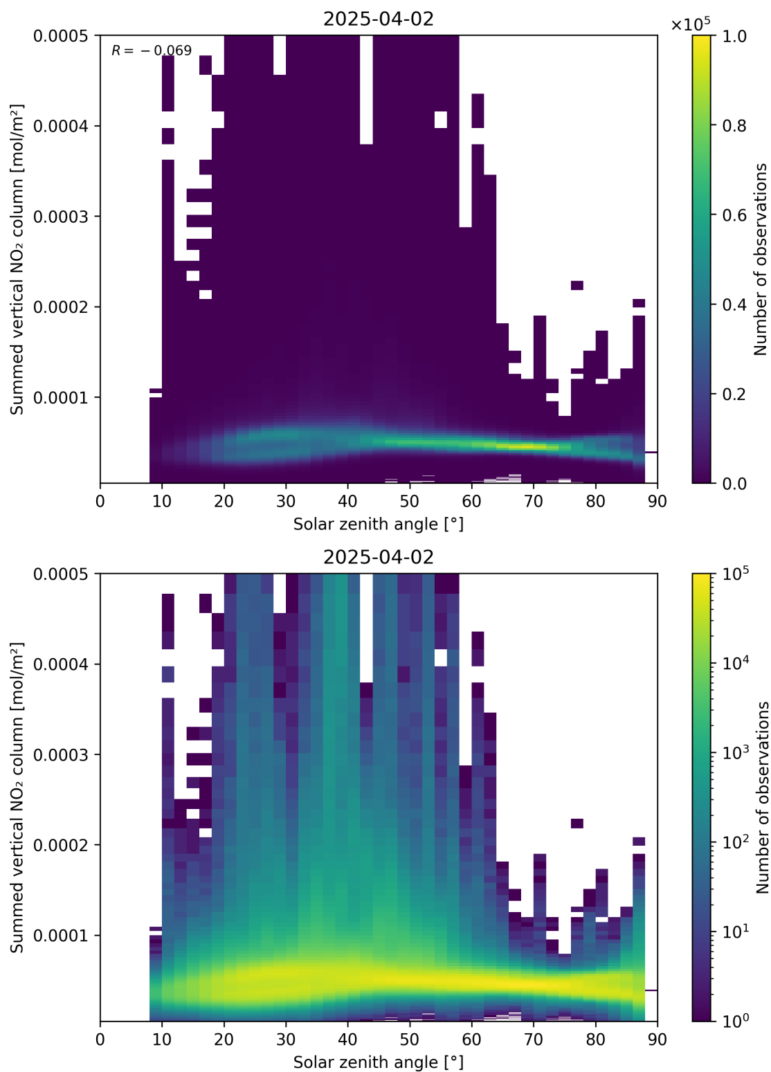
Figure 151: Scatter density plot of “Solar zenith angle” against “Summed vertical NO 2 column” for 2025-04-02 to 2025-04-03.
