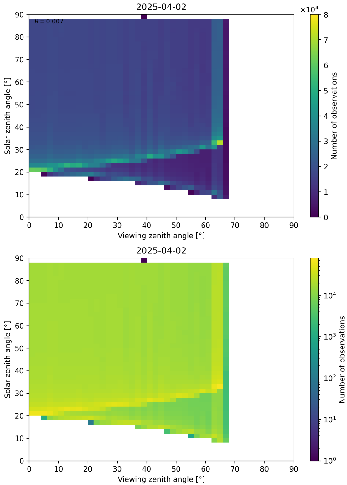
Figure 172: Scatter density plot of “Viewing zenith angle” against “Solar zenith angle” for 2025-04-02 to 2025-04-03.
