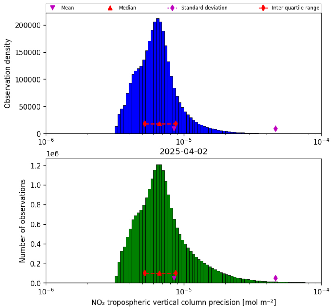
Figure 30: Histogram of “NO 2 tropospheric vertical column precision” for 2025-04-02 to 2025-04-03
