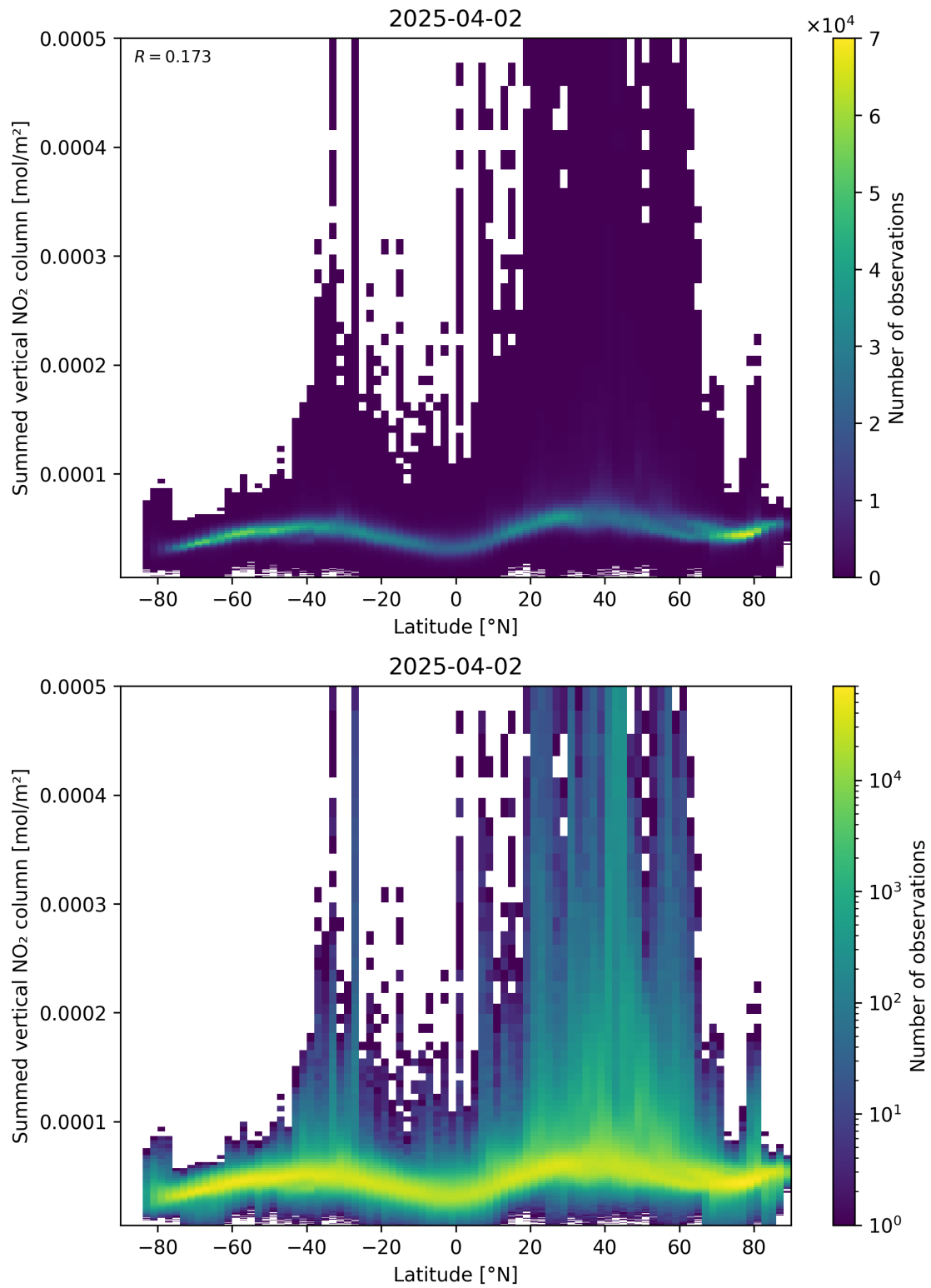
Figure 88: Scatter density plot of “Latitude” against “Summed vertical NO 2 column” for 2025-04-02 to 2025-04-03.
