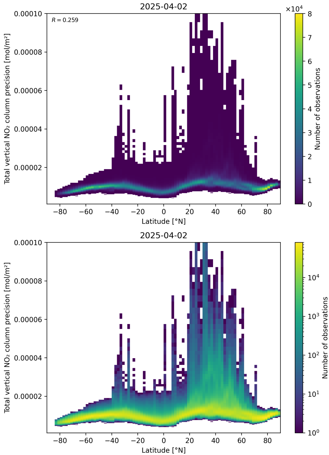
Figure 91: Scatter density plot of “Latitude” against “Total vertical NO 2 column precision” for 2025-04-02 to 2025-04-03.
