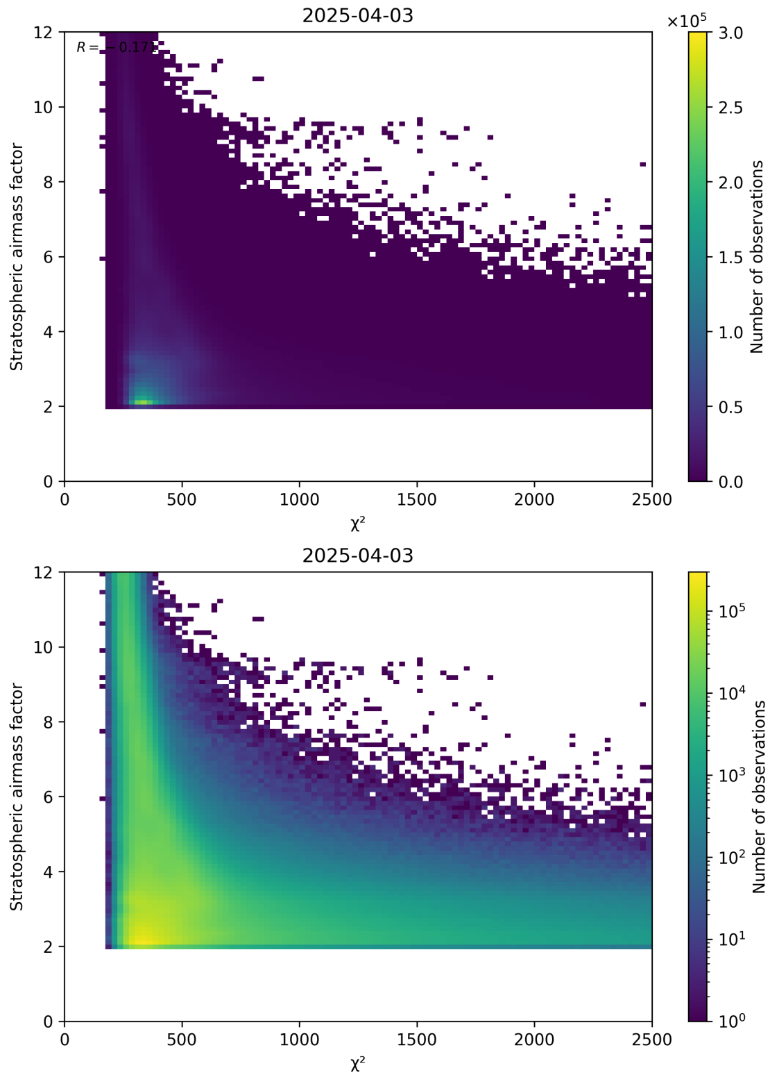
Figure 81: Scatter density plot of “ \chi^2 ” against “Stratospheric airmass factor” for 2025-04-03 to 2025-04-04.
