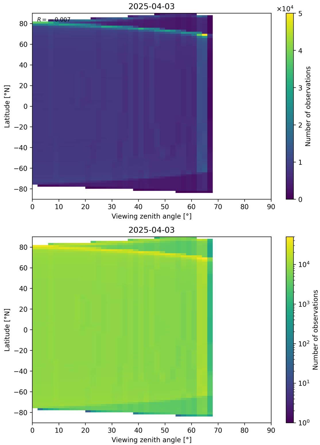
Figure 163: Scatter density plot of “Viewing zenith angle” against “Latitude” for 2025-04-03 to 2025-04-04.
