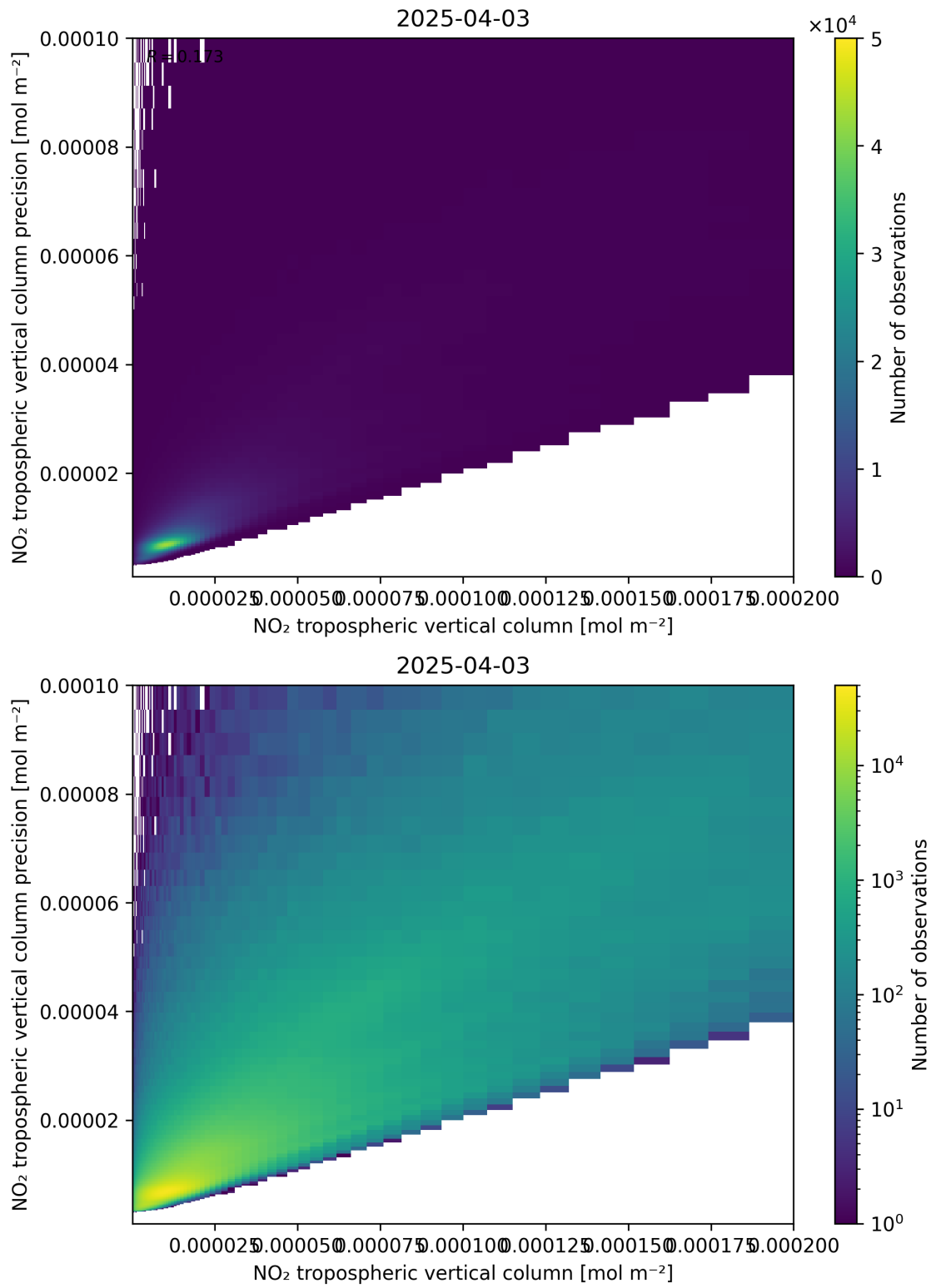
Figure 130: Scatter density plot of “NO 2 tropospheric vertical column” against “NO 2 tropospheric vertical column precision” for 2025-04-03 to 2025-04-04.
