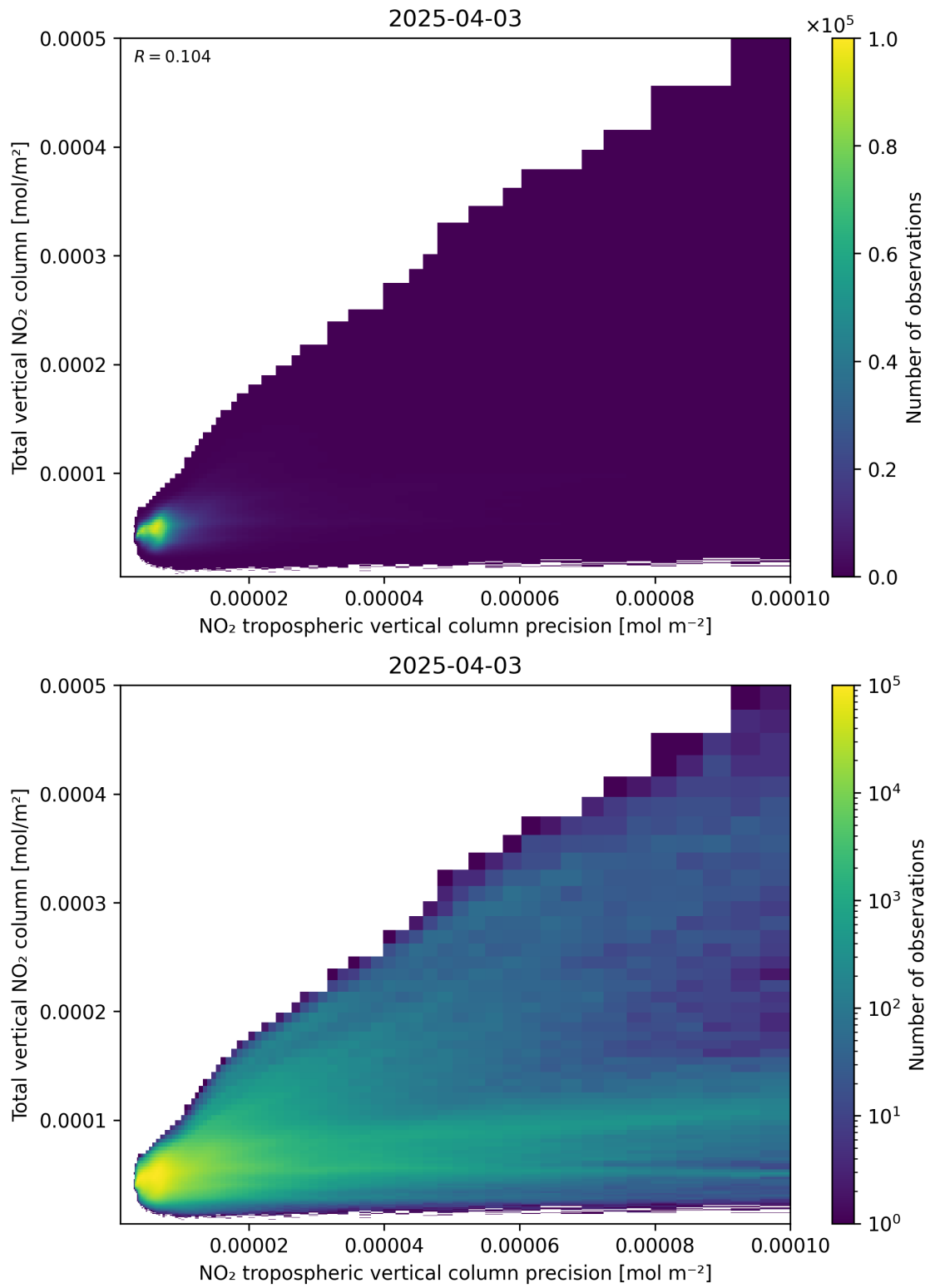
Figure 138: Scatter density plot of “NO 2 tropospheric vertical column precision” against “Total vertical NO 2 column” for 2025-04-03 to 2025-04-04.
