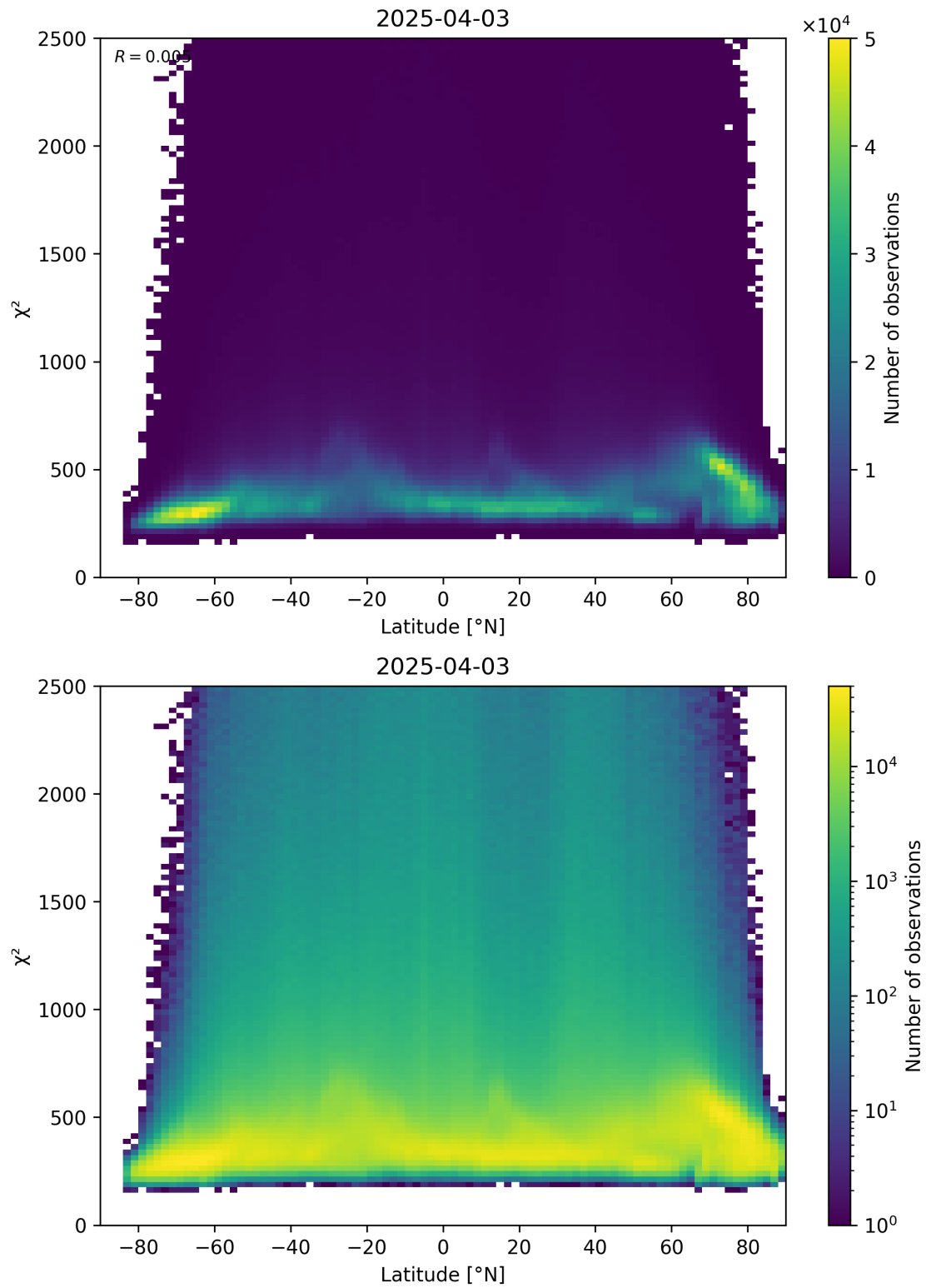
Figure 86: Scatter density plot of “Latitude” against “ \chi^2 ” for 2025-04-03 to 2025-04-04.
