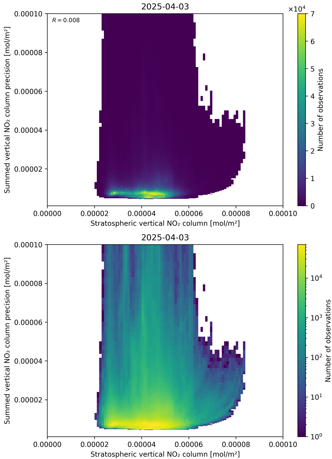
Figure 99: Scatter density plot of “Stratospheric vertical NO 2 column” against “Summed vertical NO 2 column precision” for 2025-04-03 to 2025-04-04.
