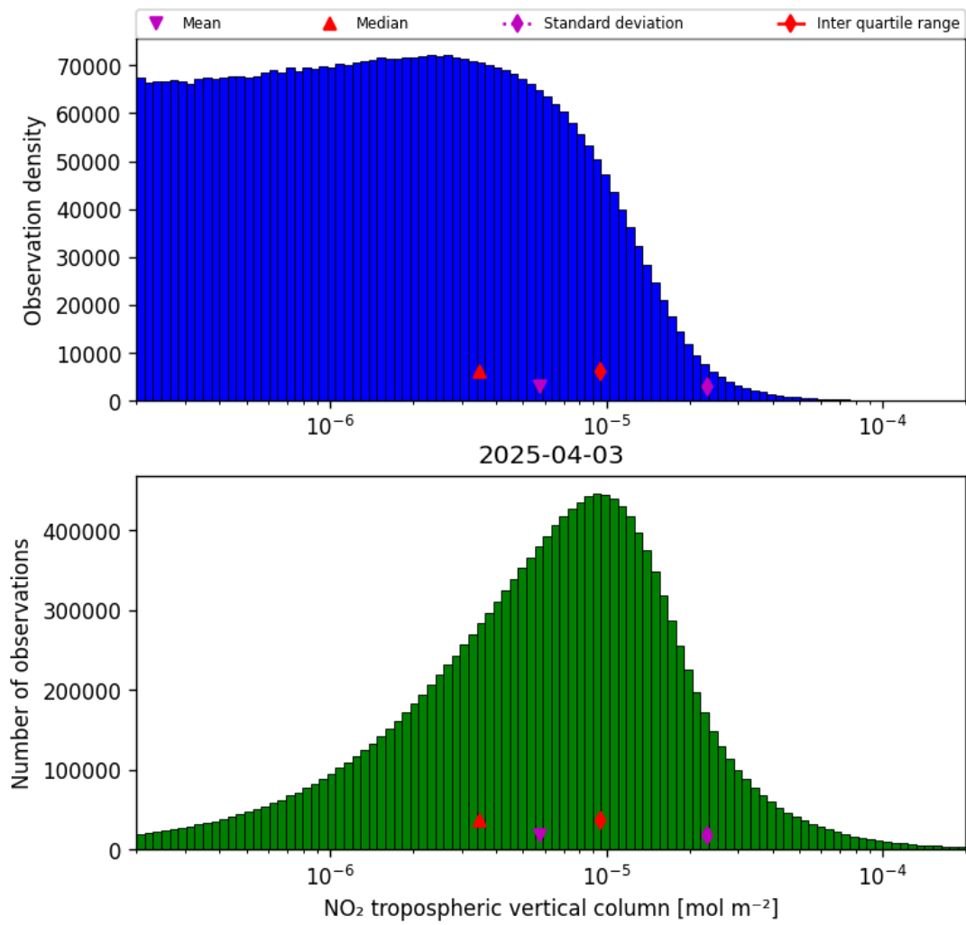
Figure 29: Histogram of “NO 2 tropospheric vertical column” for 2025-04-03 to 2025-04-04
