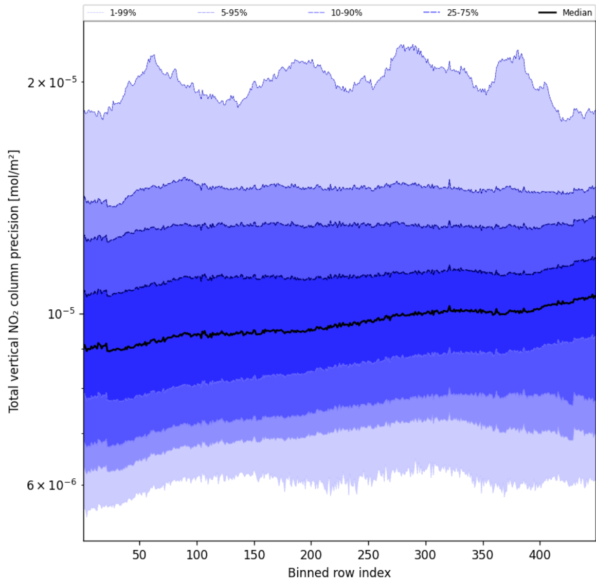
Figure 56: Along track statistics of “Total vertical NO 2 column precision” for 2025-04-03 to 2025-04-04
