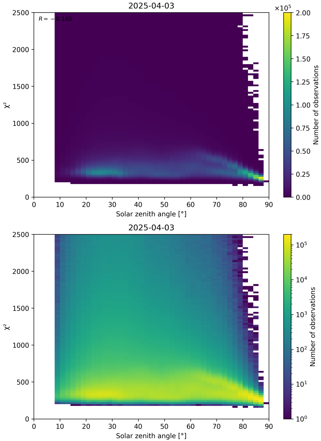
Figure 148: Scatter density plot of “Solar zenith angle” against “ \chi^2 ” for 2025-04-03 to 2025-04-04.
