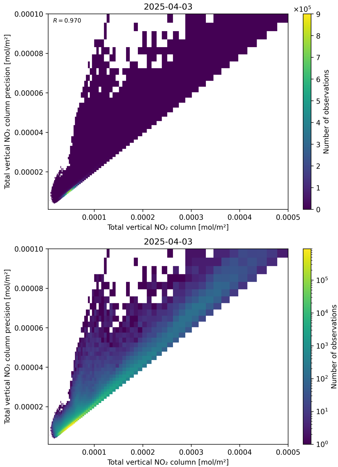
Figure 114: Scatter density plot of “Total vertical NO 2 column” against “Total vertical NO 2 column precision” for 2025-04-03 to 2025-04-04.
