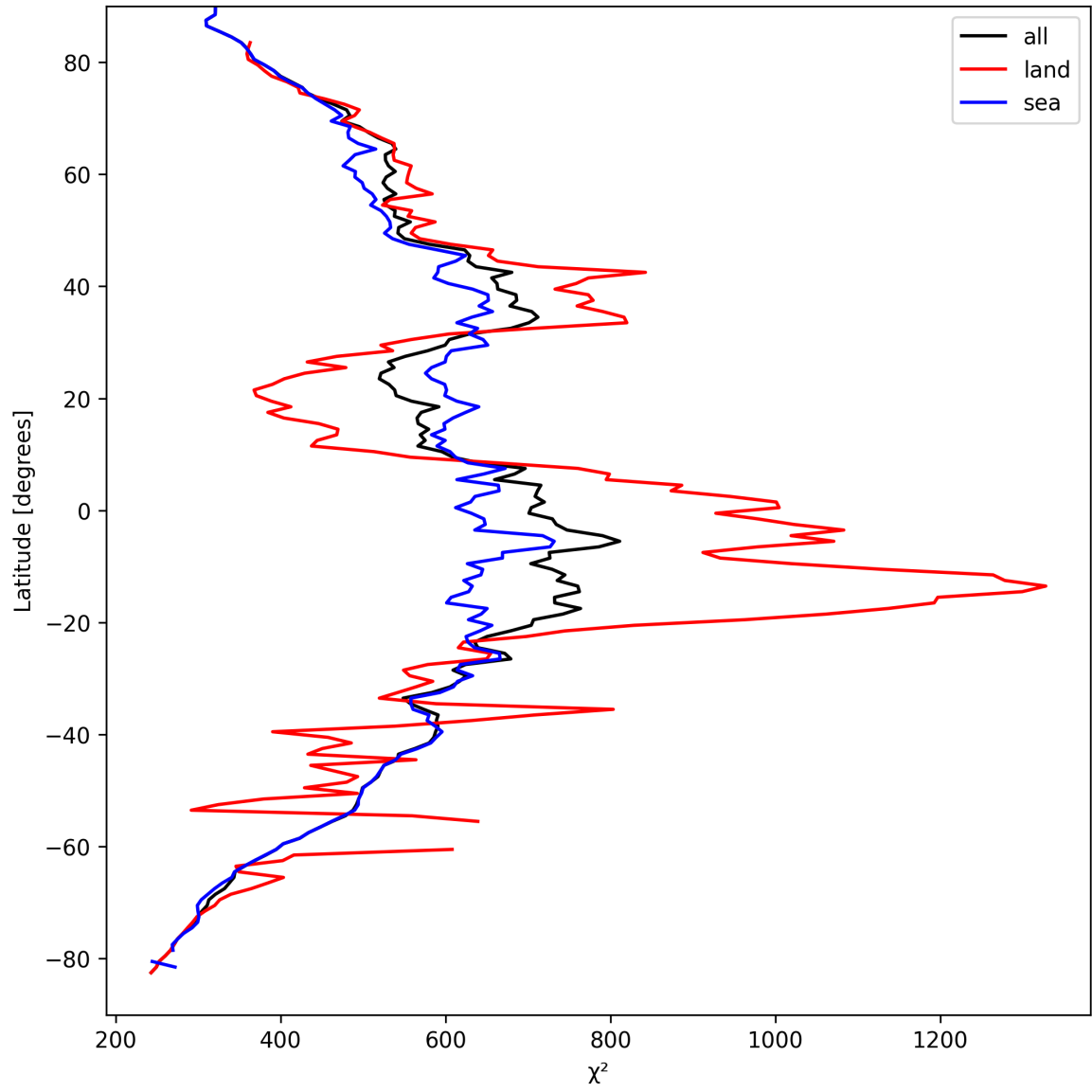
Figure 25: Zonal average of “ \chi^2 ” for 2025-04-03 to 2025-04-04.
