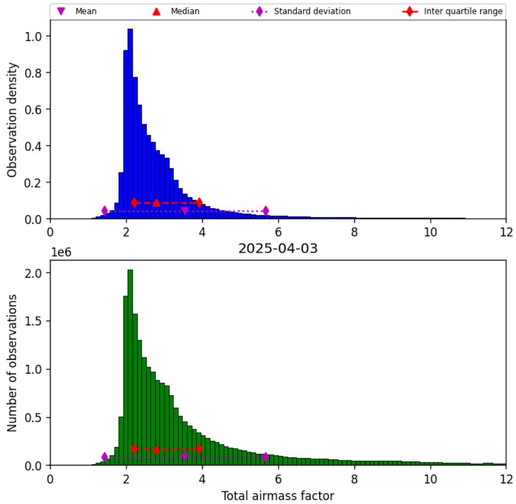
Figure 32: Histogram of “Total airmass factor” for 2025-04-03 to 2025-04-04
