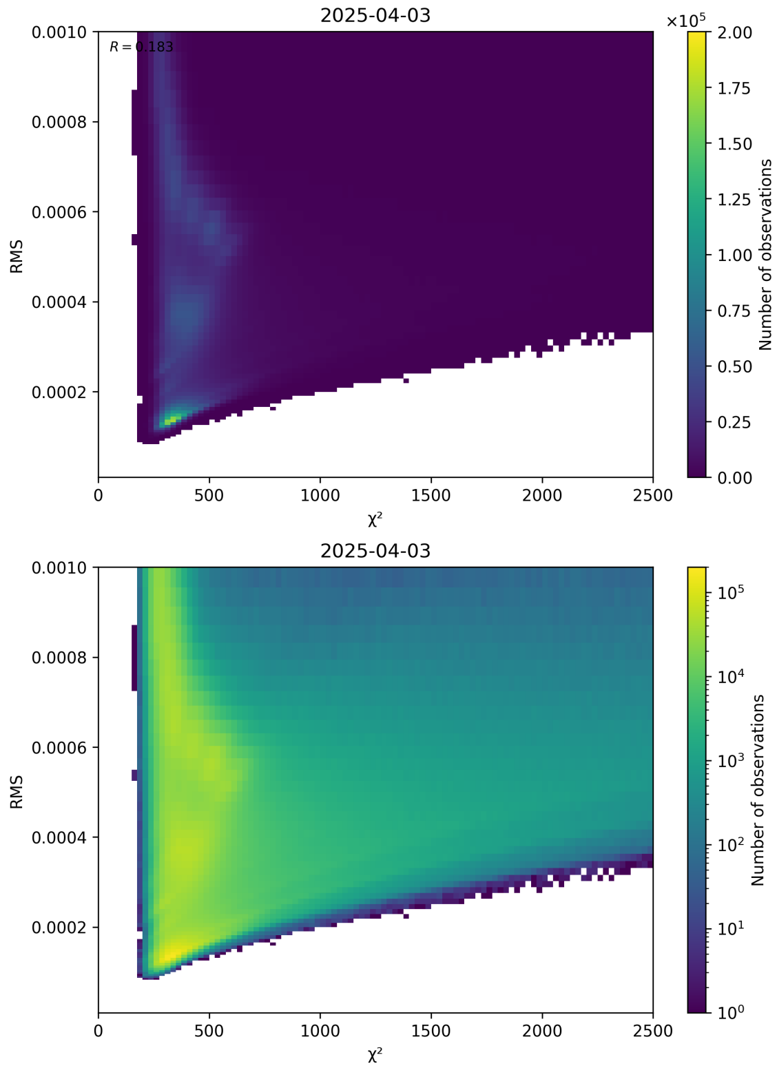
Figure 82: Scatter density plot of “ \chi^2 ” against “RMS” for 2025-04-03 to 2025-04-04.
