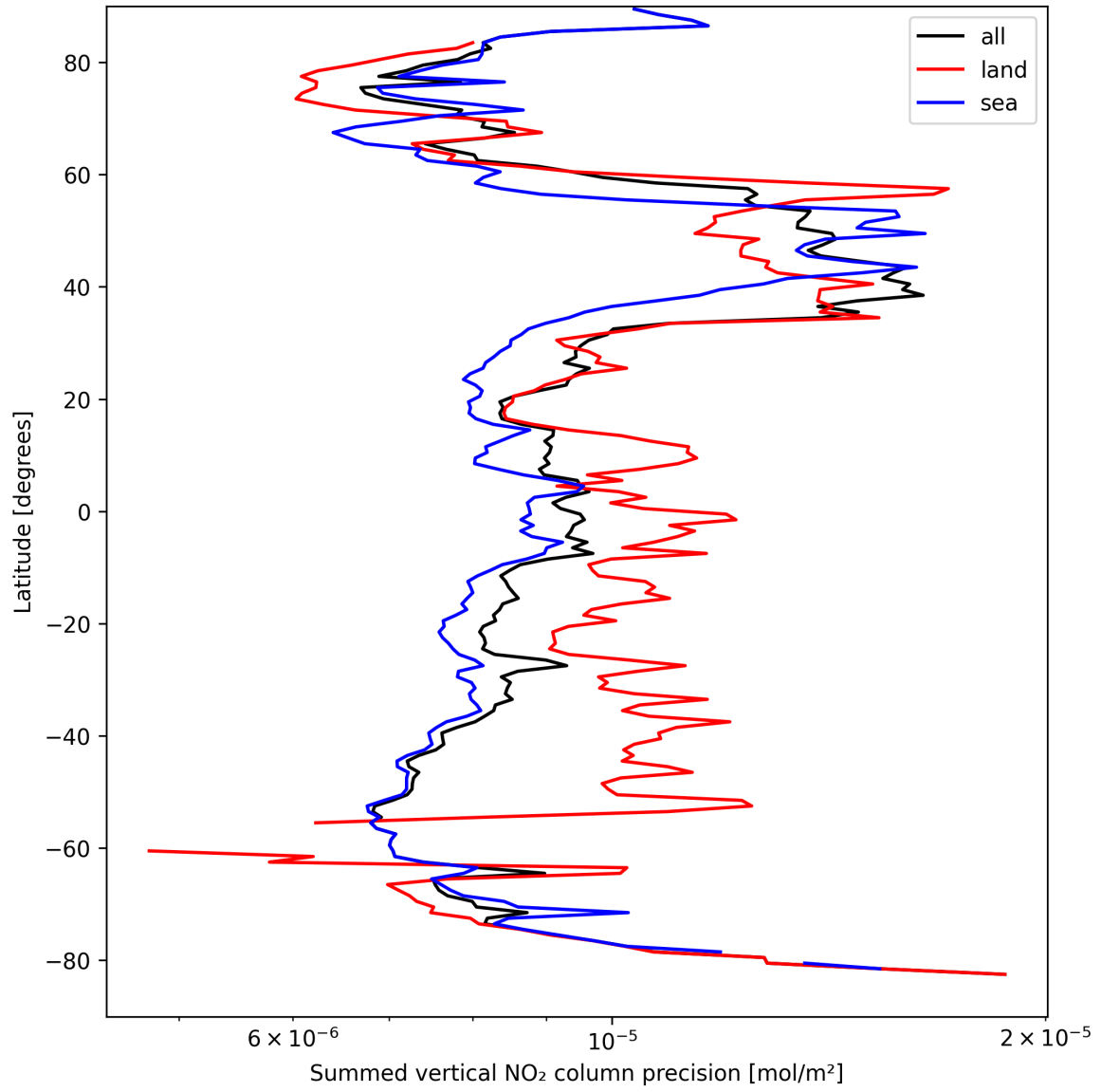
Figure 24: Zonal average of “Summed vertical NO 2 column precision” for 2025-04-03 to 2025-04-04.
