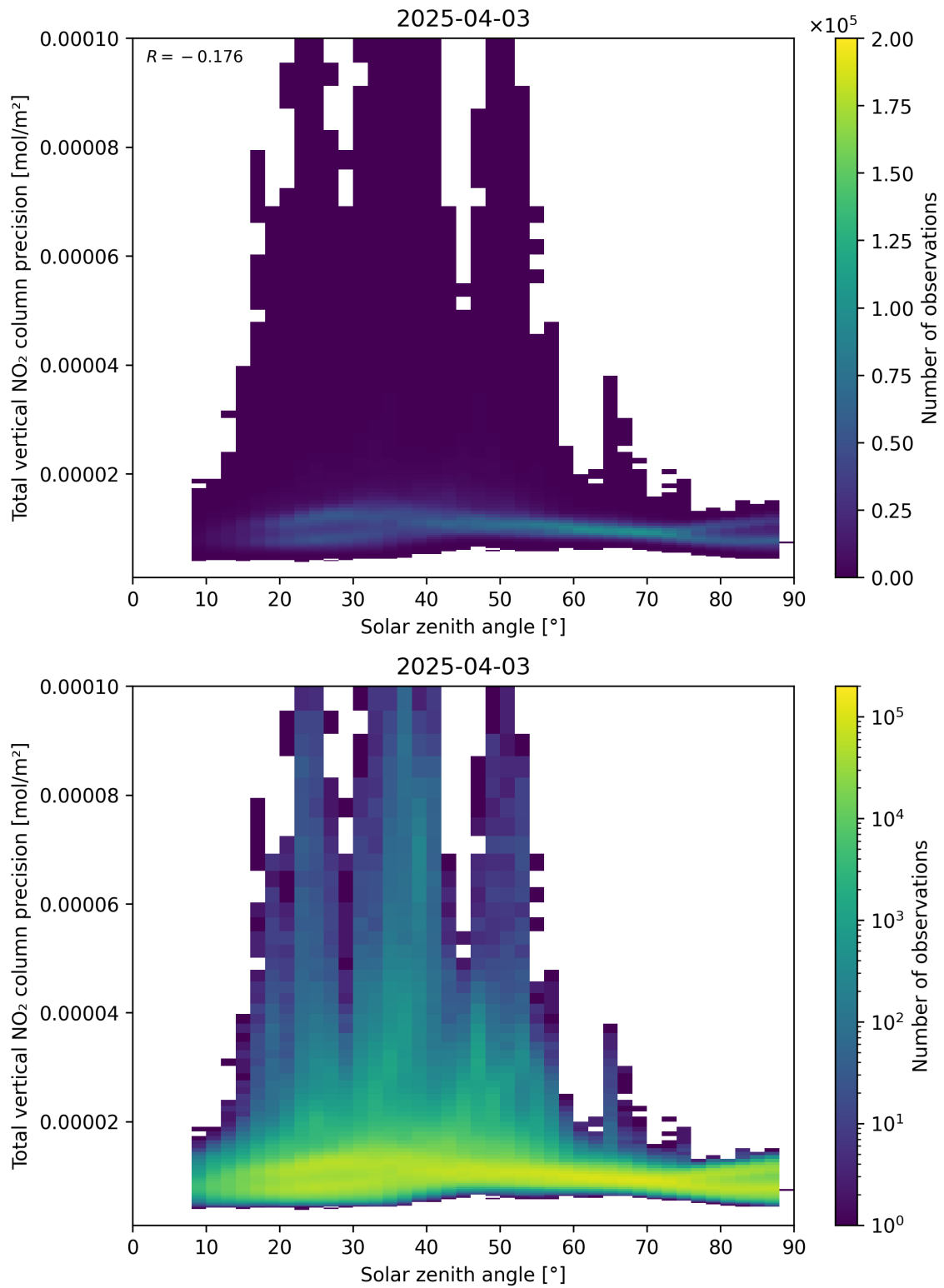
Figure 154: Scatter density plot of “Solar zenith angle” against “Total vertical NO 2 column precision” for 2025-04-03 to 2025-04-04.
