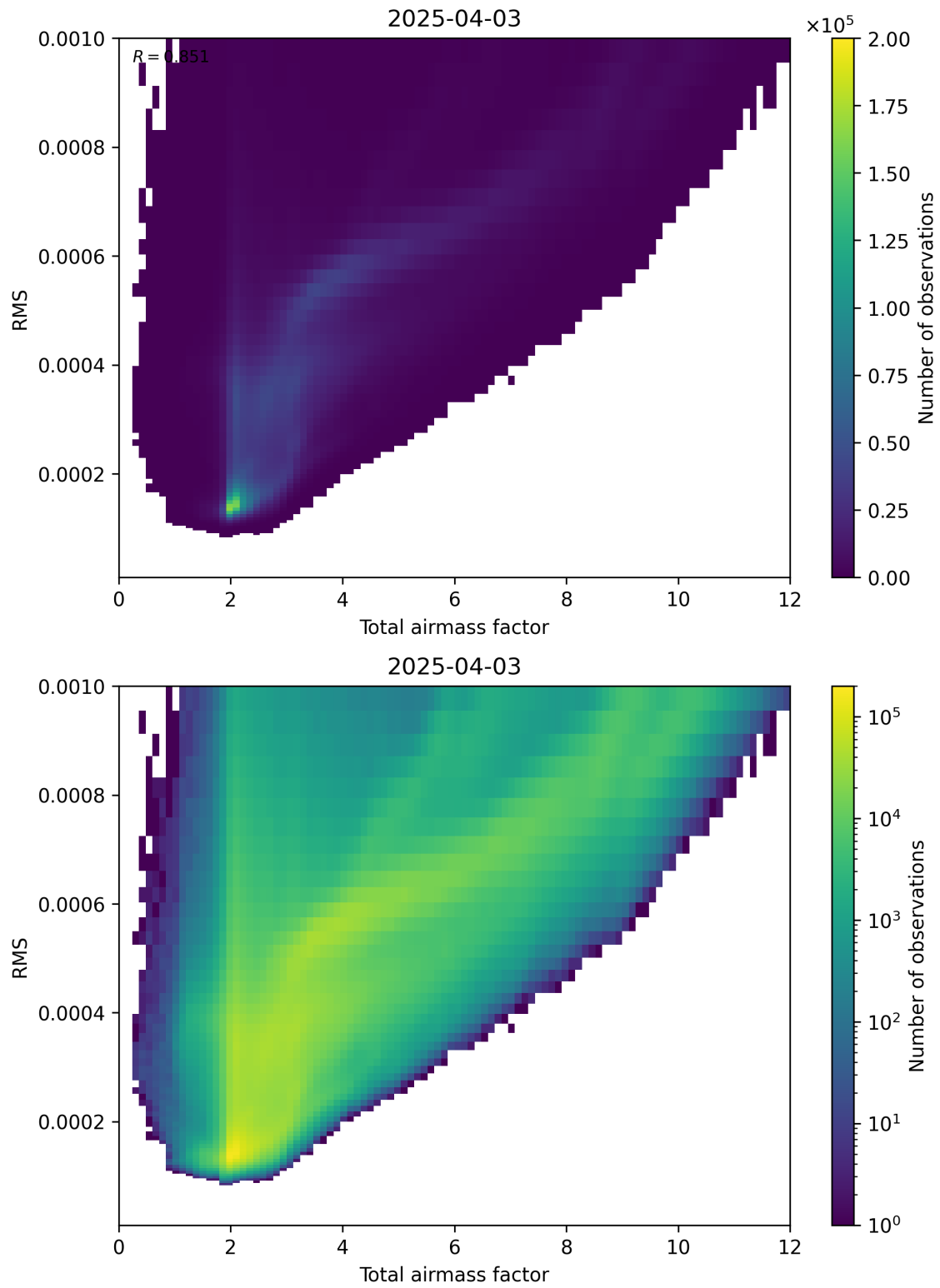
Figure 69: Scatter density plot of “Total airmass factor” against “RMS” for 2025-04-03 to 2025-04-04.
