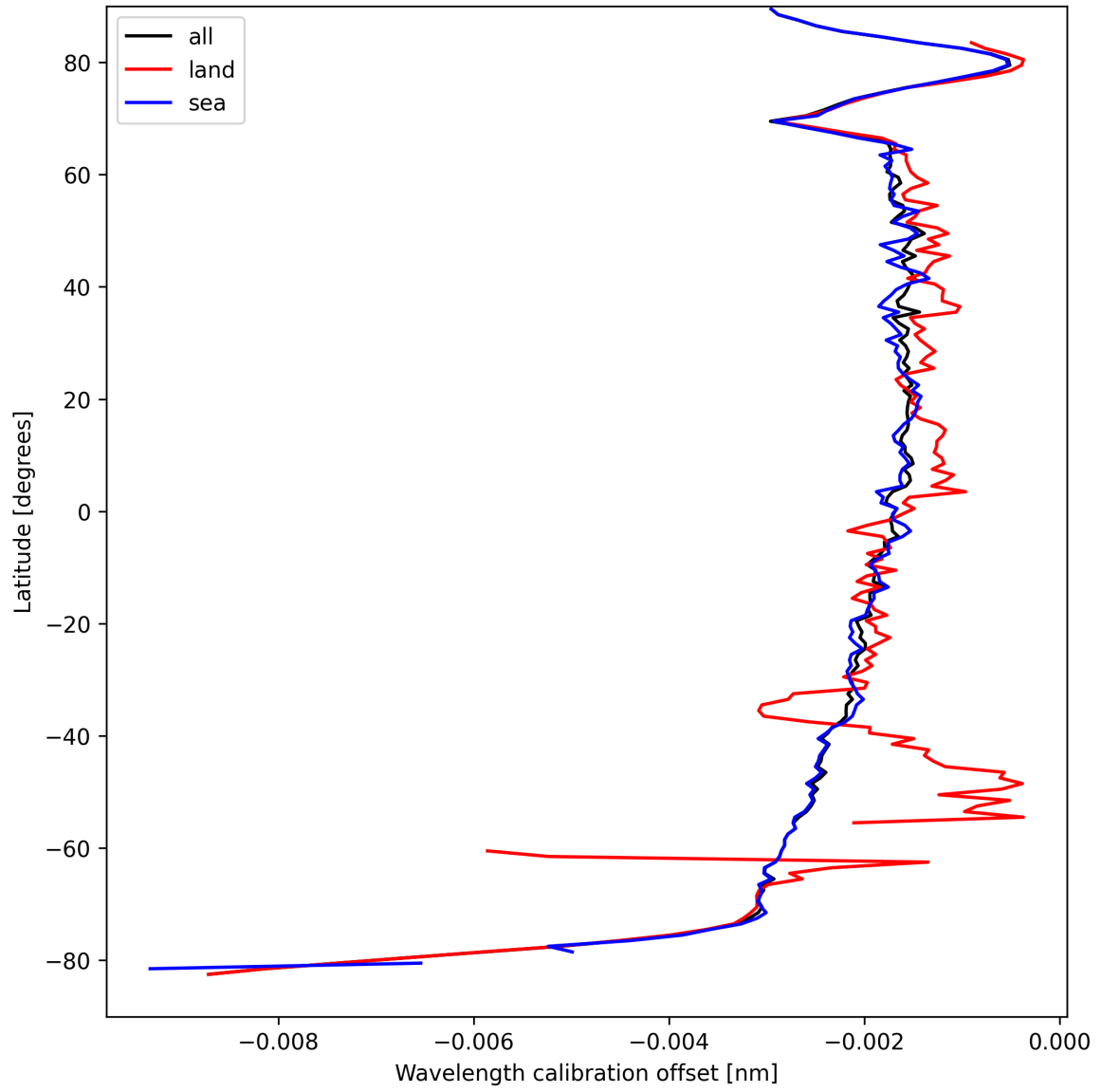
Figure 18: Zonal average of “Wavelength calibration offset” for 2025-04-03 to 2025-04-04.
