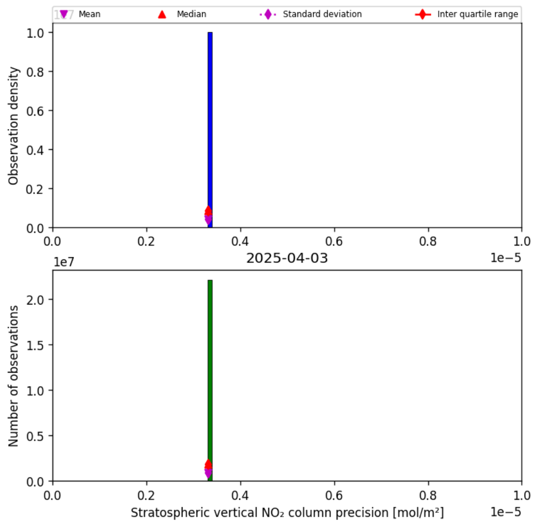
Figure 37: Histogram of “Stratospheric vertical NO 2 column precision” for 2025-04-03 to 2025-04-04
