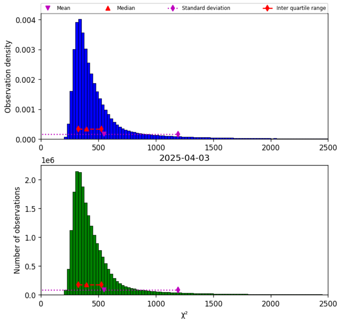
Figure 42: Histogram of “ \chi^2 ” for 2025-04-03 to 2025-04-04
