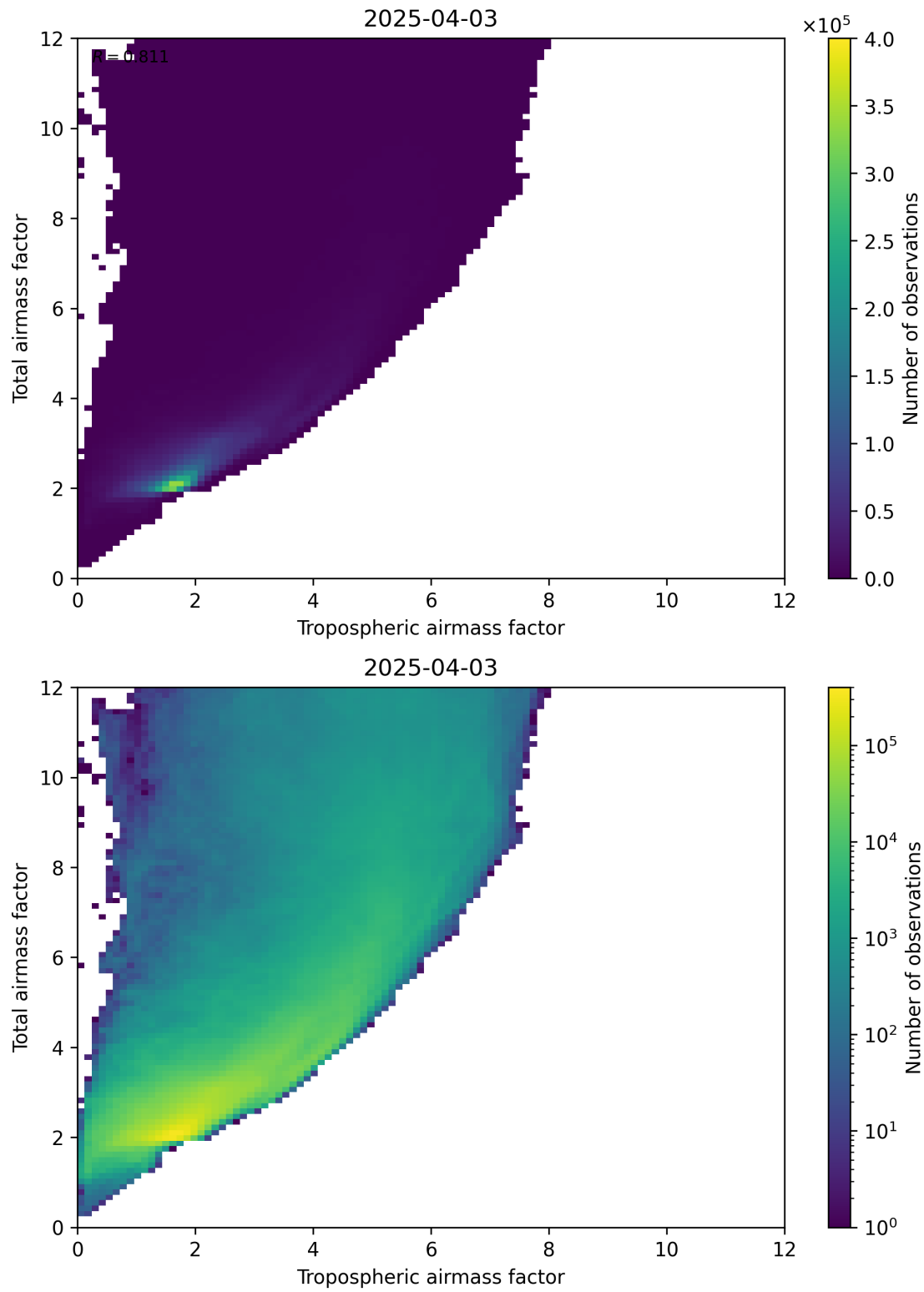
Figure 72: Scatter density plot of “Tropospheric airmass factor” against “Total airmass factor” for 2025-04-03 to 2025-04-04.
