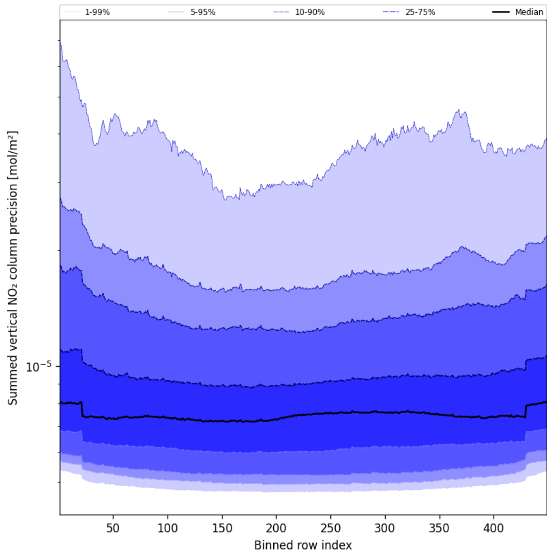
Figure 58: Along track statistics of “Summed vertical NO 2 column precision” for 2025-04-03 to 2025-04-04
