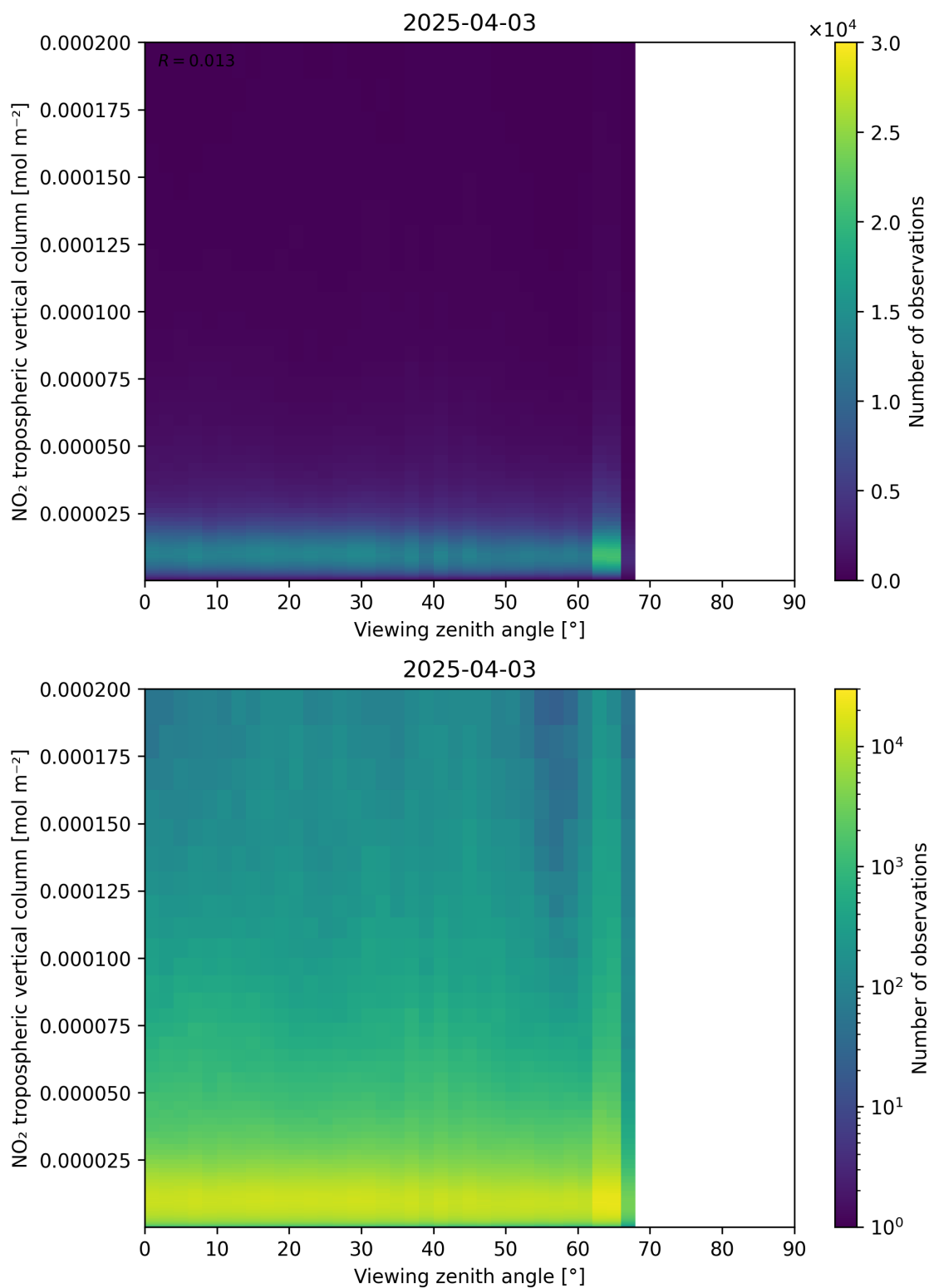
Figure 169: Scatter density plot of “Viewing zenith angle” against “NO 2 tropospheric vertical column” for 2025-04-03 to 2025-04-04.
