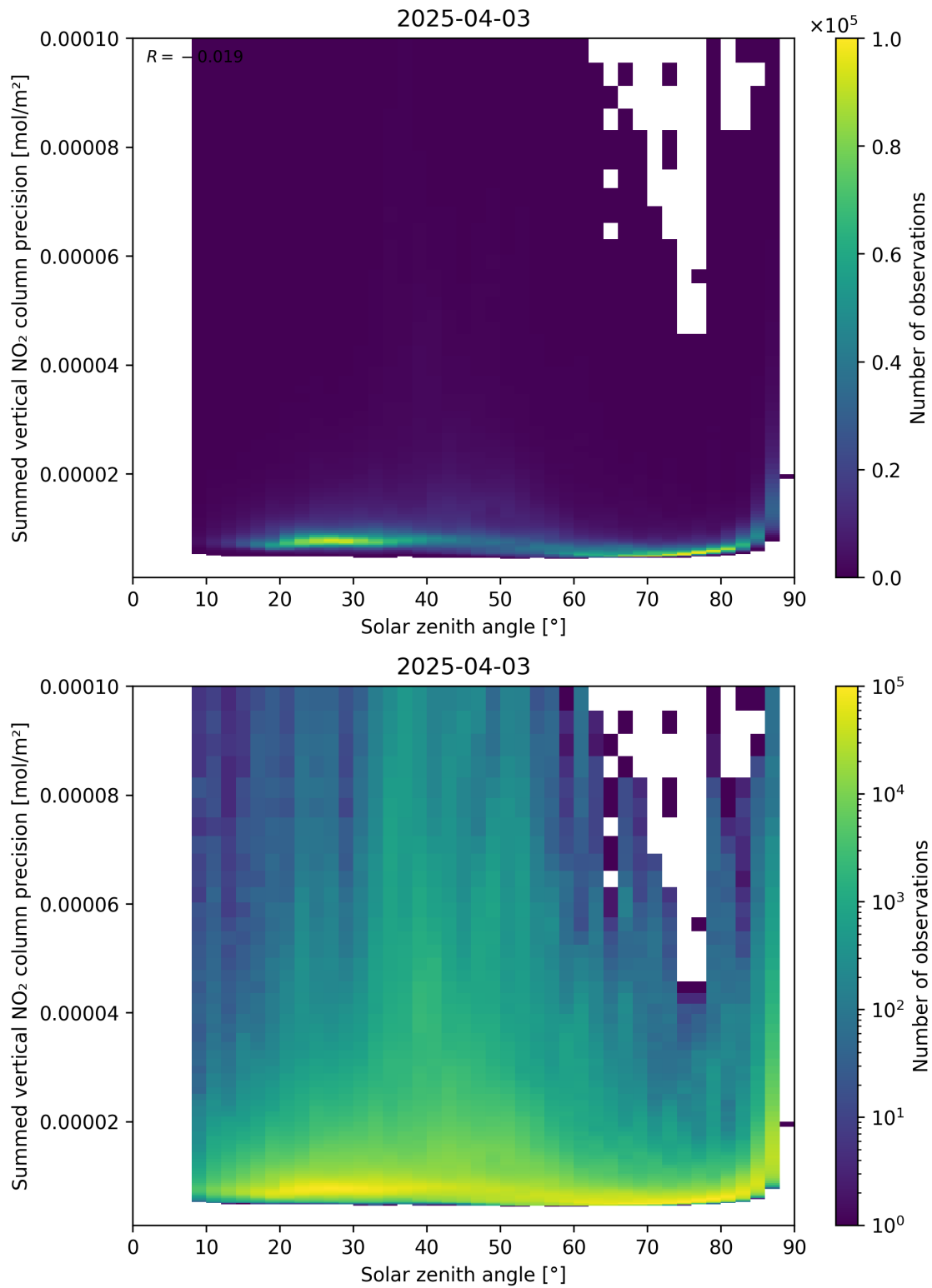
Figure 152: Scatter density plot of “Solar zenith angle” against “Summed vertical NO 2 column precision” for 2025-04-03 to 2025-04-04.
