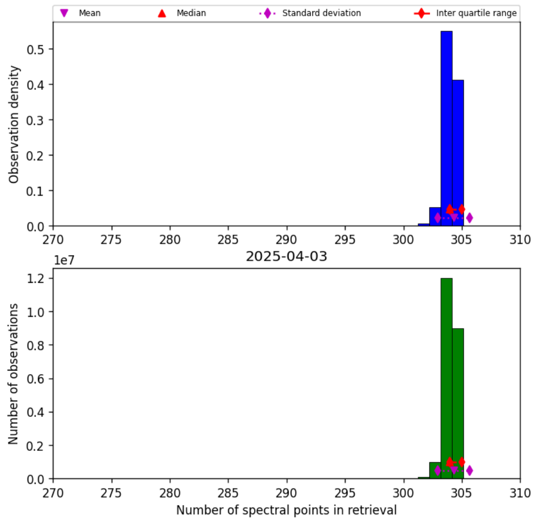
Figure 33: Histogram of “Number of spectral points in retrieval” for 2025-04-03 to 2025-04-04
