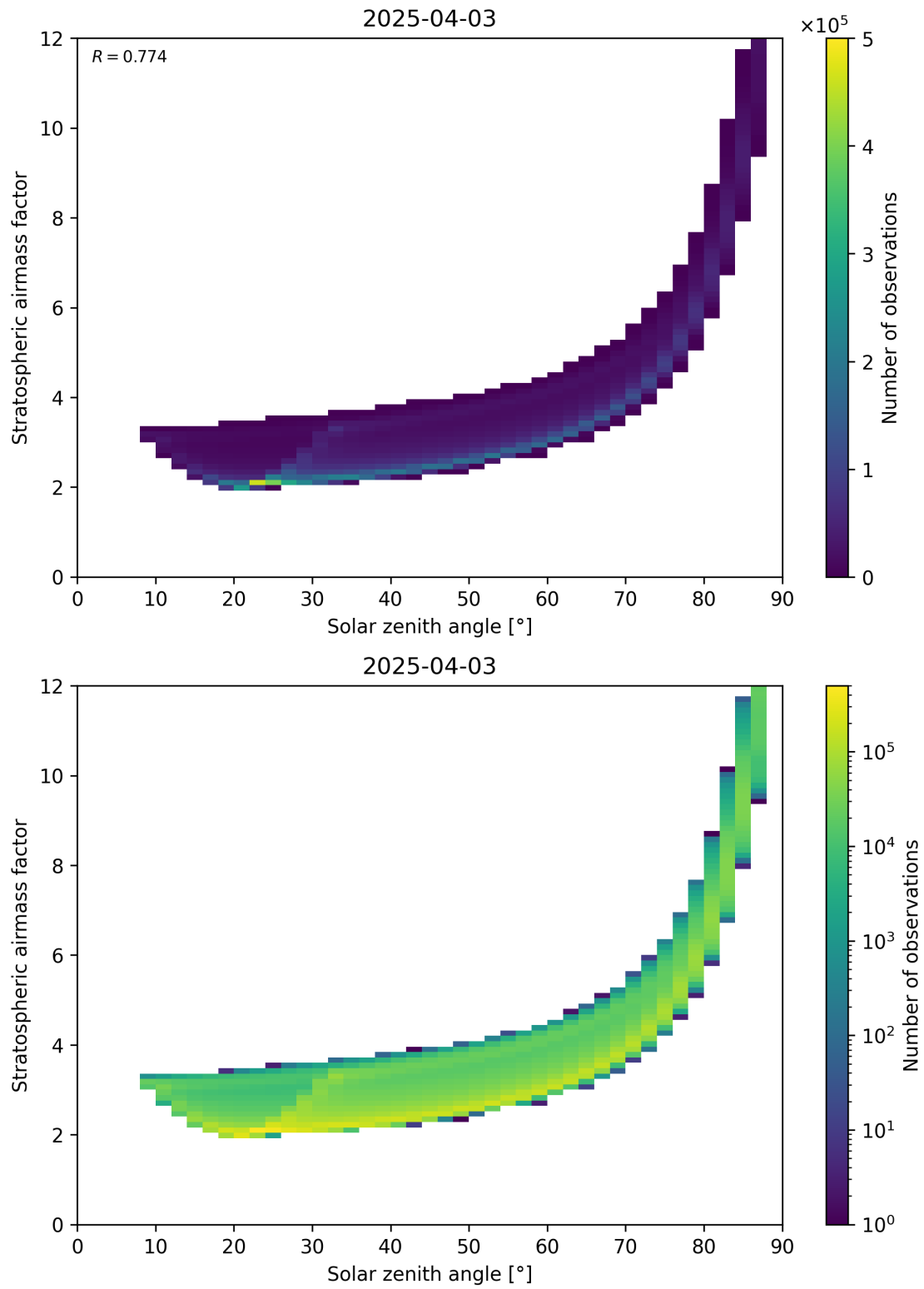
Figure 145: Scatter density plot of “Solar zenith angle” against “Stratospheric airmass factor” for 2025-04-03 to 2025-04-04.
