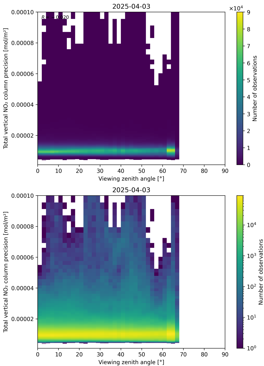
Figure 168: Scatter density plot of “Viewing zenith angle” against “Total vertical NO 2 column precision” for 2025-04-03 to 2025-04-04.
