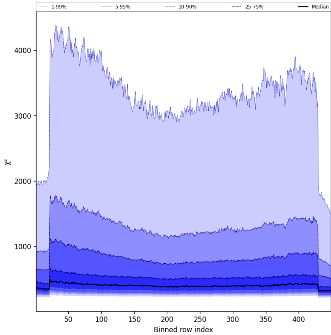
Figure 59: Along track statistics of “ \chi^2 ” for 2025-04-03 to 2025-04-04
