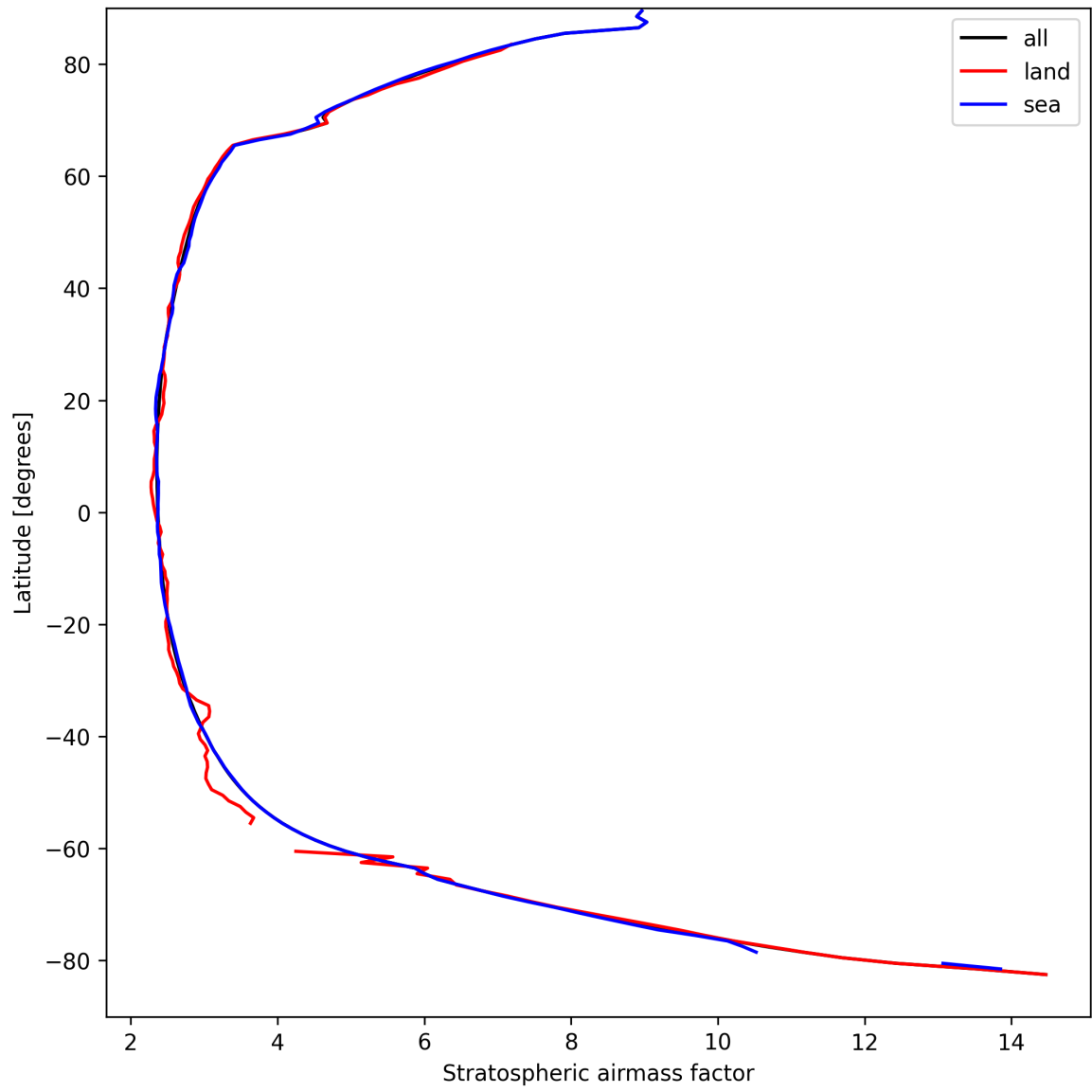
Figure 27: Zonal average of “Stratospheric airmass factor” for 2025-04-03 to 2025-04-04.
