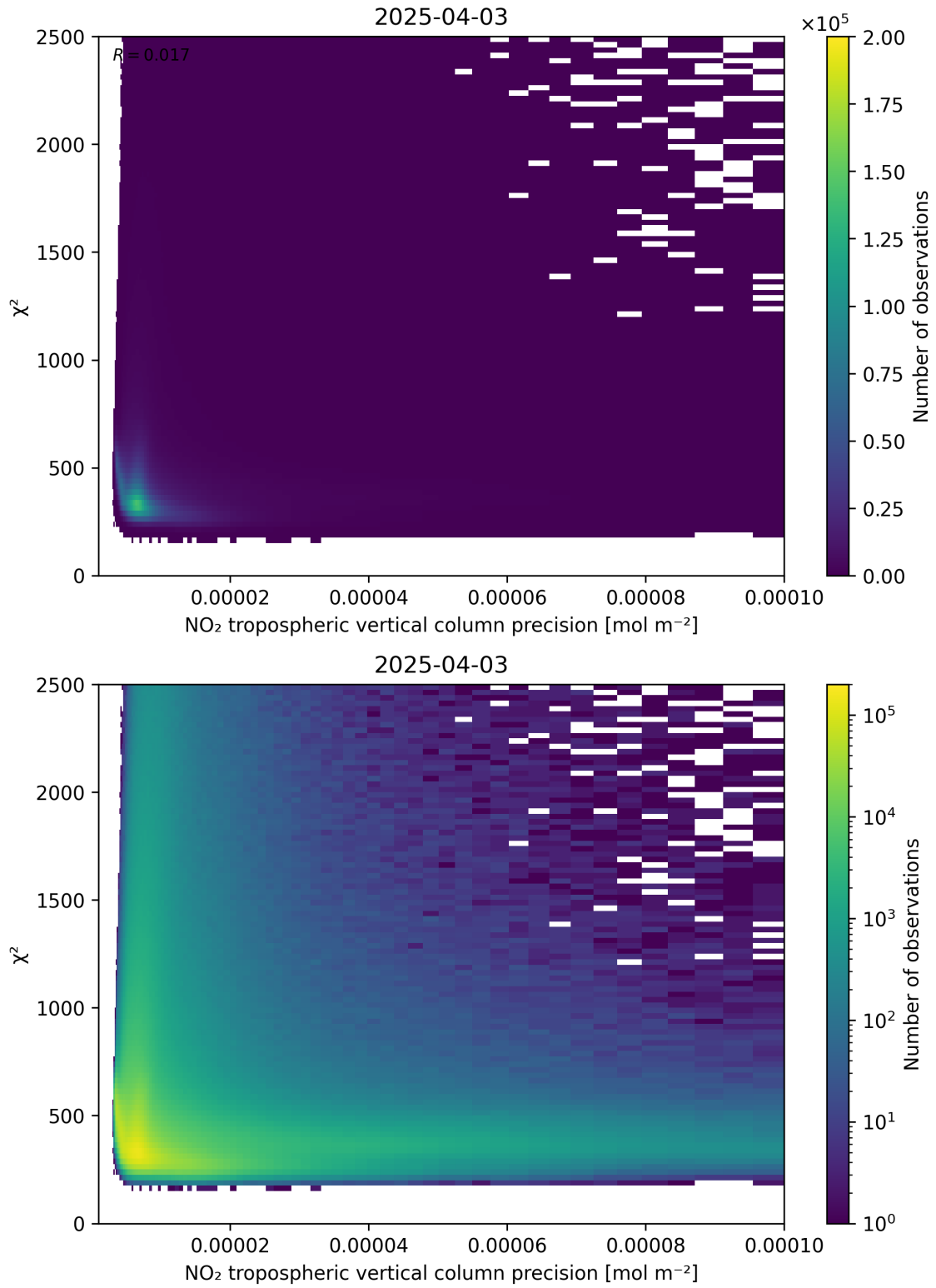
Figure 134: Scatter density plot of “NO 2 tropospheric vertical column precision” against “ \chi^2 ” for 2025-04-03 to 2025-04-04.
