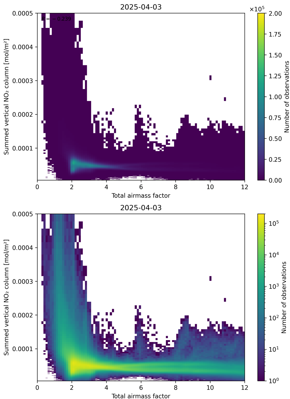
Figure 65: Scatter density plot of “Total airmass factor” against “Summed vertical NO 2 column” for 2025-04-03 to 2025-04-04.
