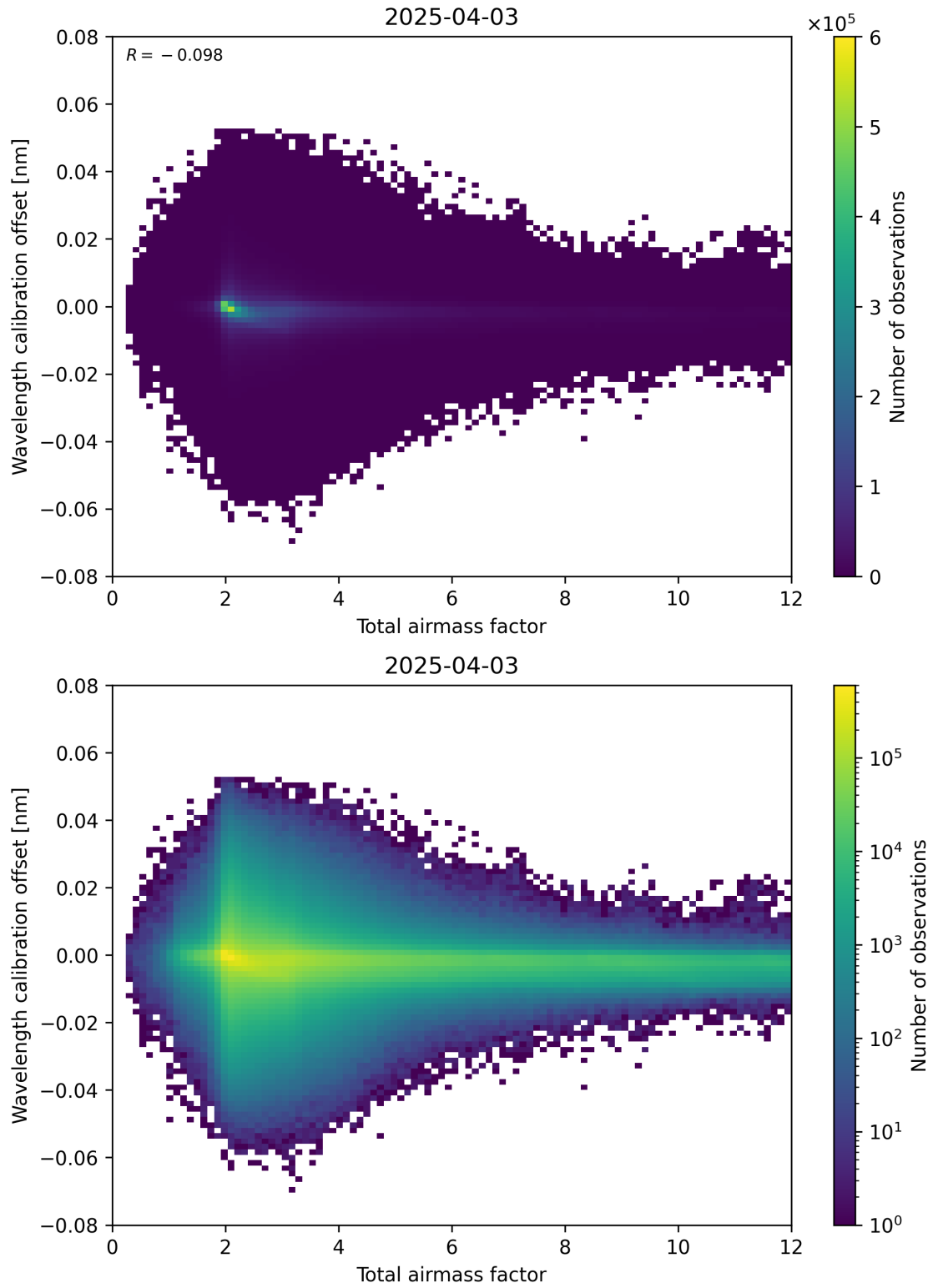
Figure 70: Scatter density plot of “Total airmass factor” against “Wavelength calibration offset” for 2025-04-03 to 2025-04-04.
