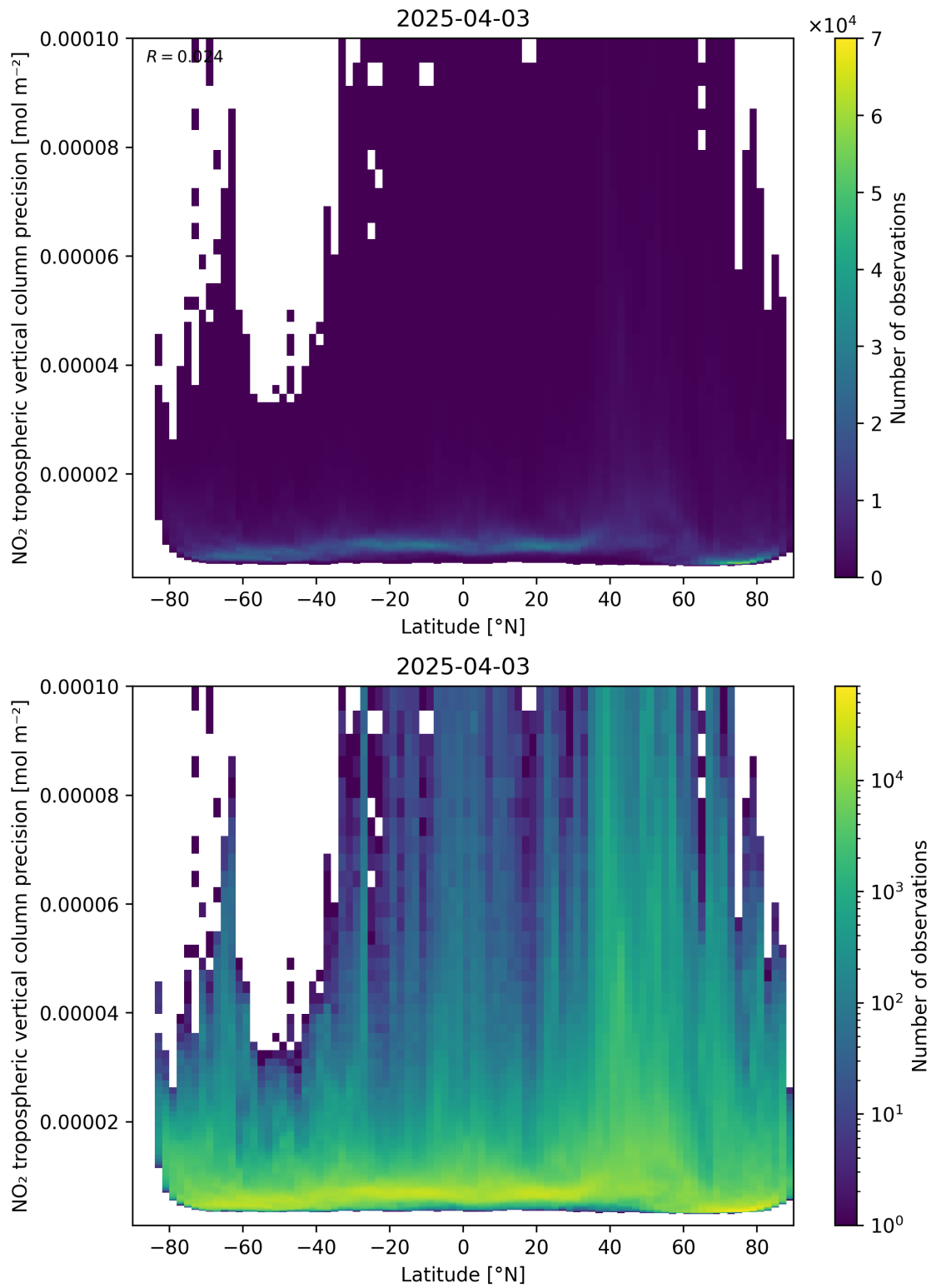
Figure 93: Scatter density plot of “Latitude” against “NO 2 tropospheric vertical column precision” for 2025-04-03 to 2025-04-04.
