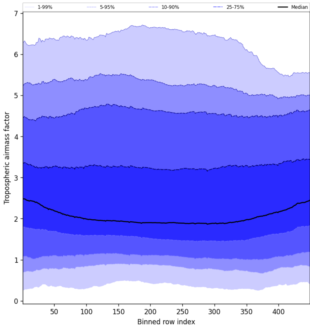
Figure 48: Along track statistics of “Tropospheric air mass factor” for 2025-04-03 to 2025-04-04
