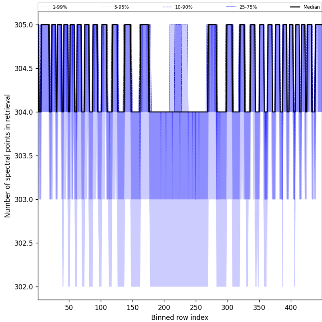
Figure 50: Along track statistics of “Number of spectral points in retrieval” for 2025-04-03 to 2025-04-04
