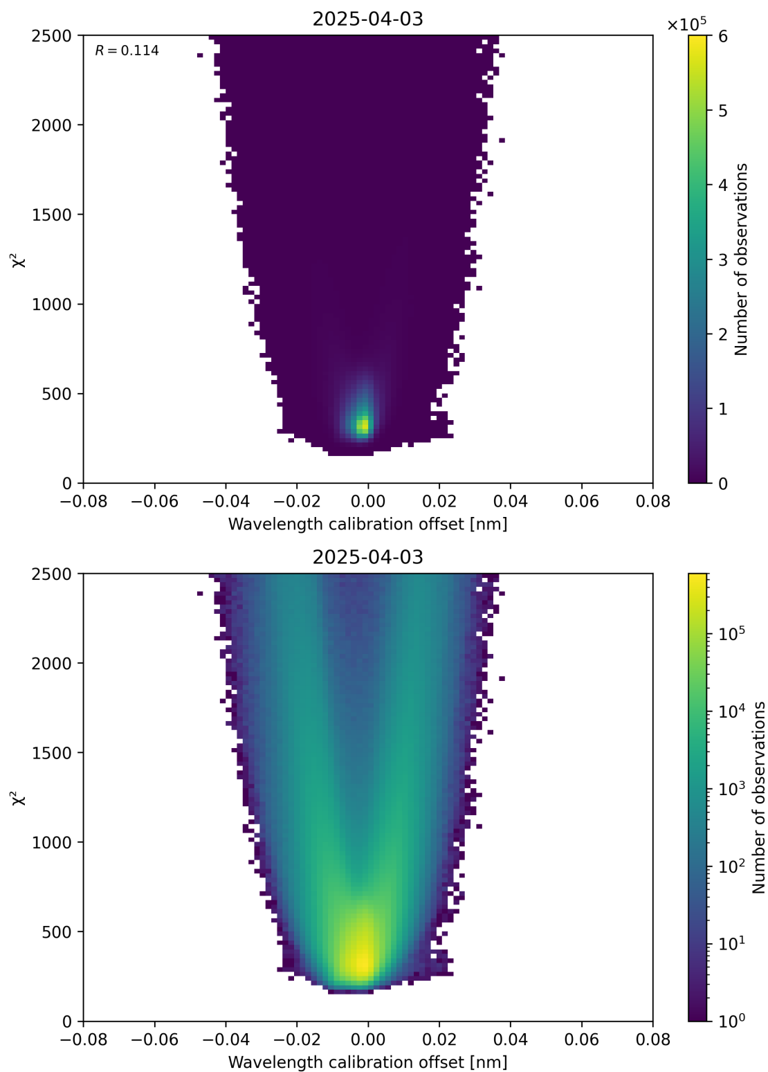
Figure 175: Scatter density plot of “Wavelength calibration offset” against “ \chi^2 ” for 2025-04-03 to 2025-04-04.
