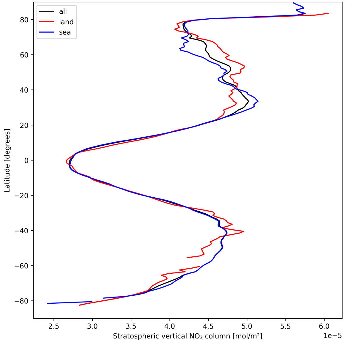
Figure 19: Zonal average of “Stratospheric vertical NO 2 column” for 2025-04-03 to 2025-04-04.
