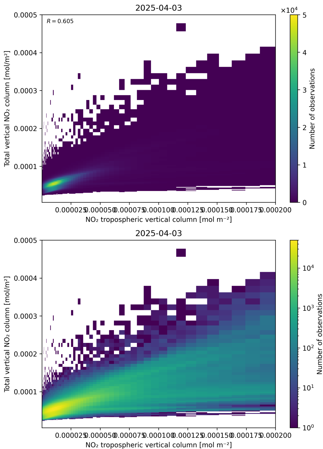
Figure 128: Scatter density plot of “NO 2 tropospheric vertical column” against “Total vertical NO 2 column” for 2025-04-03 to 2025-04-04.
