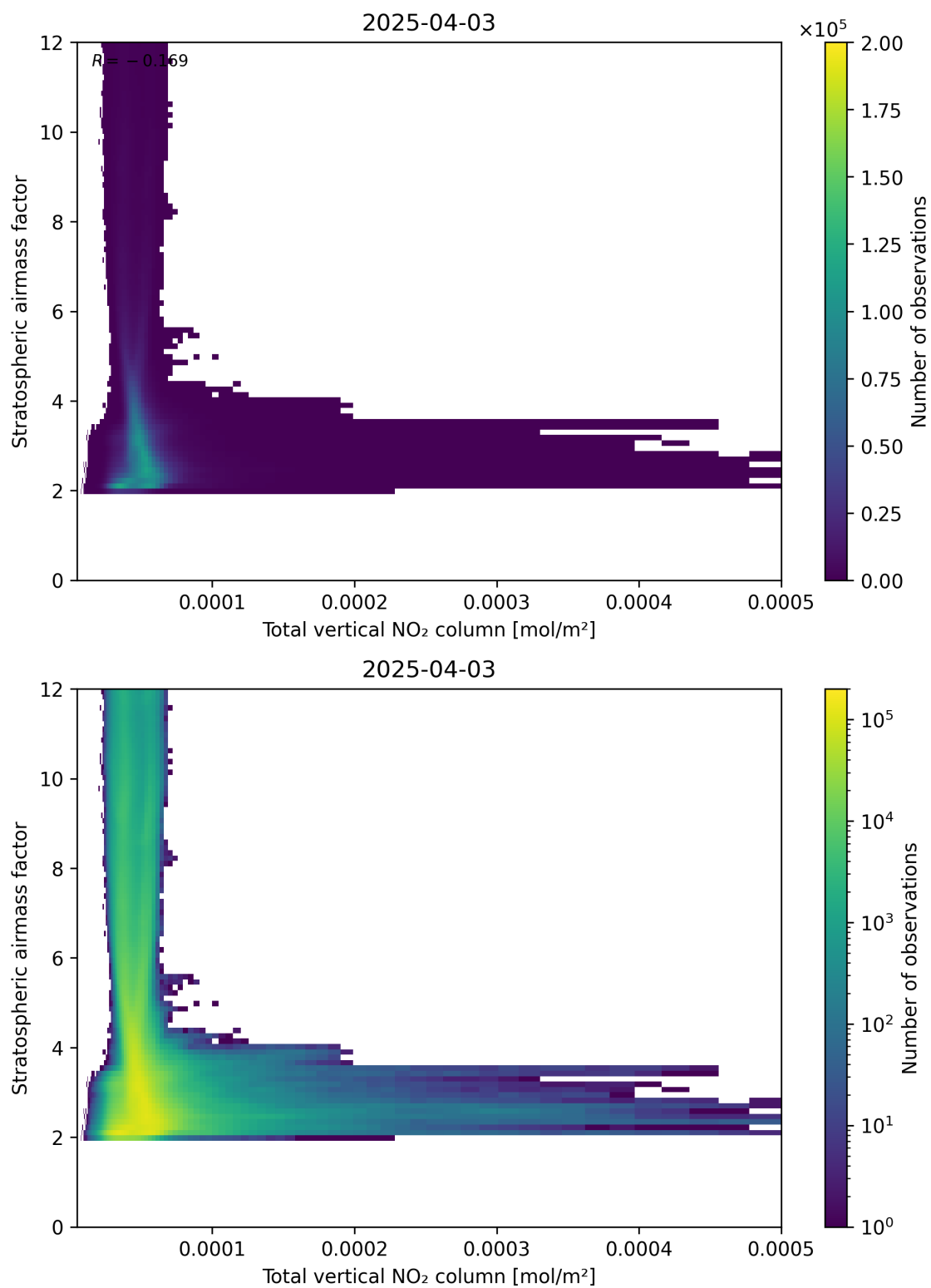
Figure 110: Scatter density plot of “Total vertical NO 2 column” against “Stratospheric airmass factor” for 2025-04-03 to 2025-04-04.
