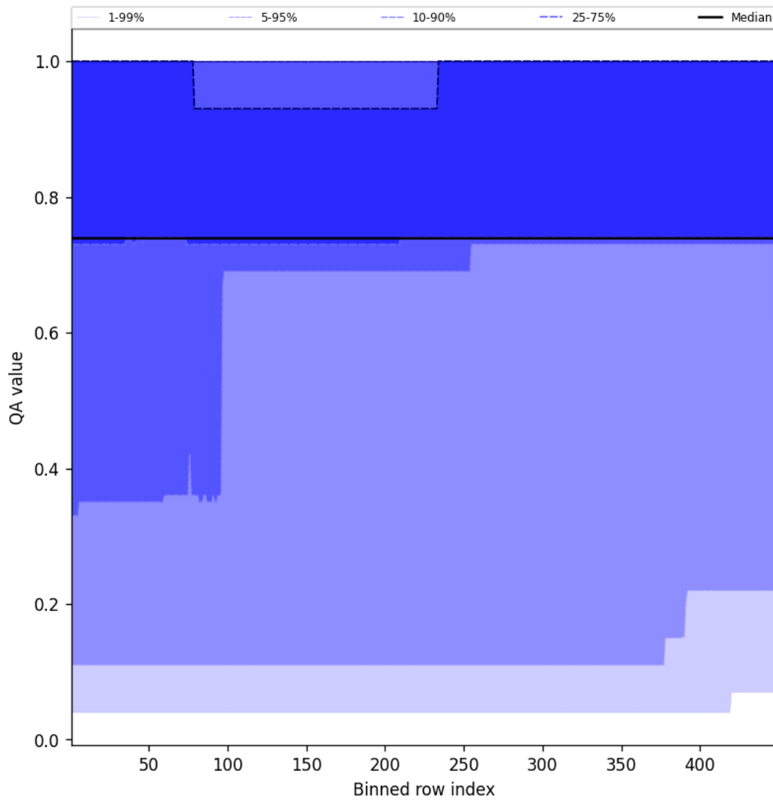
Figure 45: Along track statistics of “QA value” for 2025-04-03 to 2025-04-04
