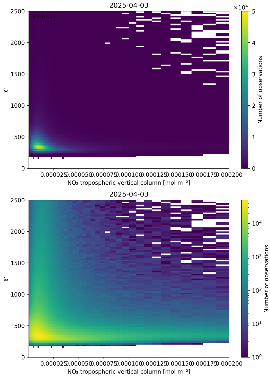
Figure 124: Scatter density plot of “NO 2 tropospheric vertical column” against “ \chi^2 ” for 2025-04-03 to 2025-04-04.
