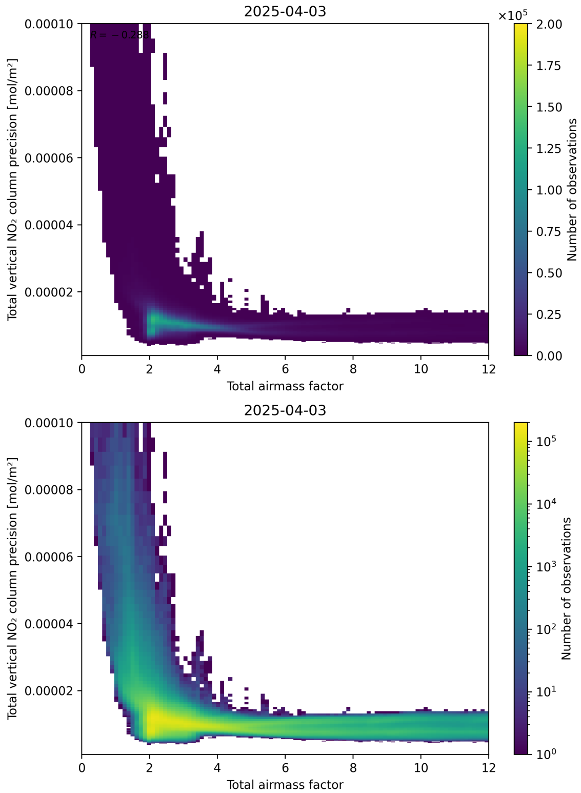
Figure 68: Scatter density plot of “Total airmass factor” against “Total vertical NO 2 column precision” for 2025-04-03 to 2025-04-04.
