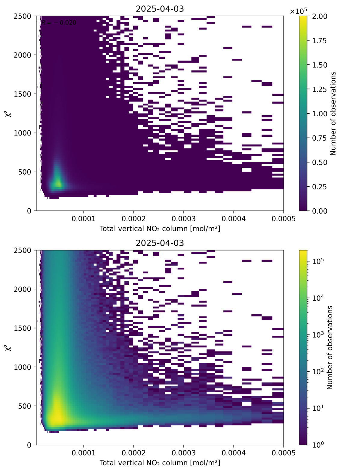
Figure 111: Scatter density plot of “Total vertical NO 2 column” against “ \chi^2 ” for 2025-04-03 to 2025-04-04.
