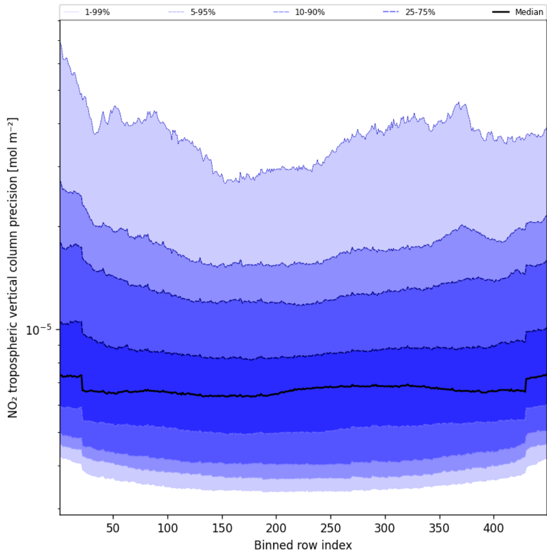
Figure 47: Along track statistics of “NO 2 tropospheric vertical column precision” for 2025-04-03 to 2025-04-04
