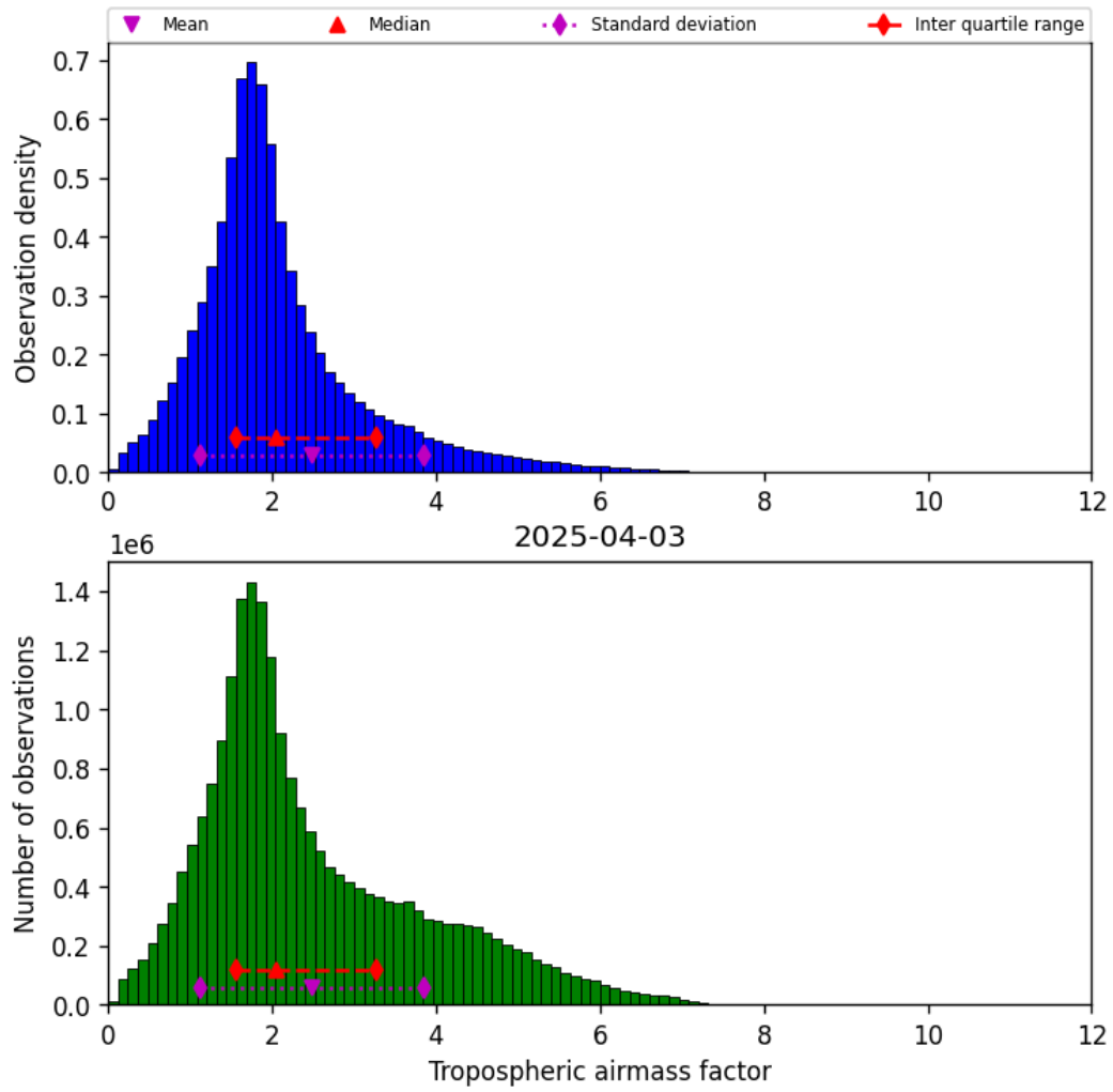
Figure 31: Histogram of “Tropospheric airmass factor” for 2025-04-03 to 2025-04-04
