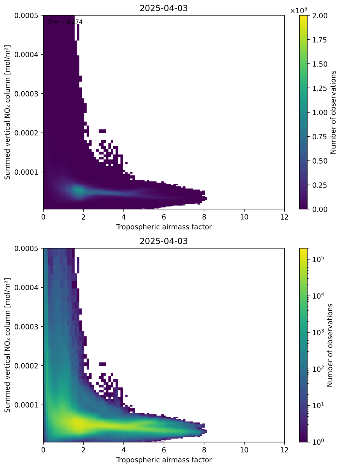
Figure 75: Scatter density plot of “Tropospheric air mass factor” against “Summed vertical NO 2 column” for 2025-04-03 to 2025-04-04.
