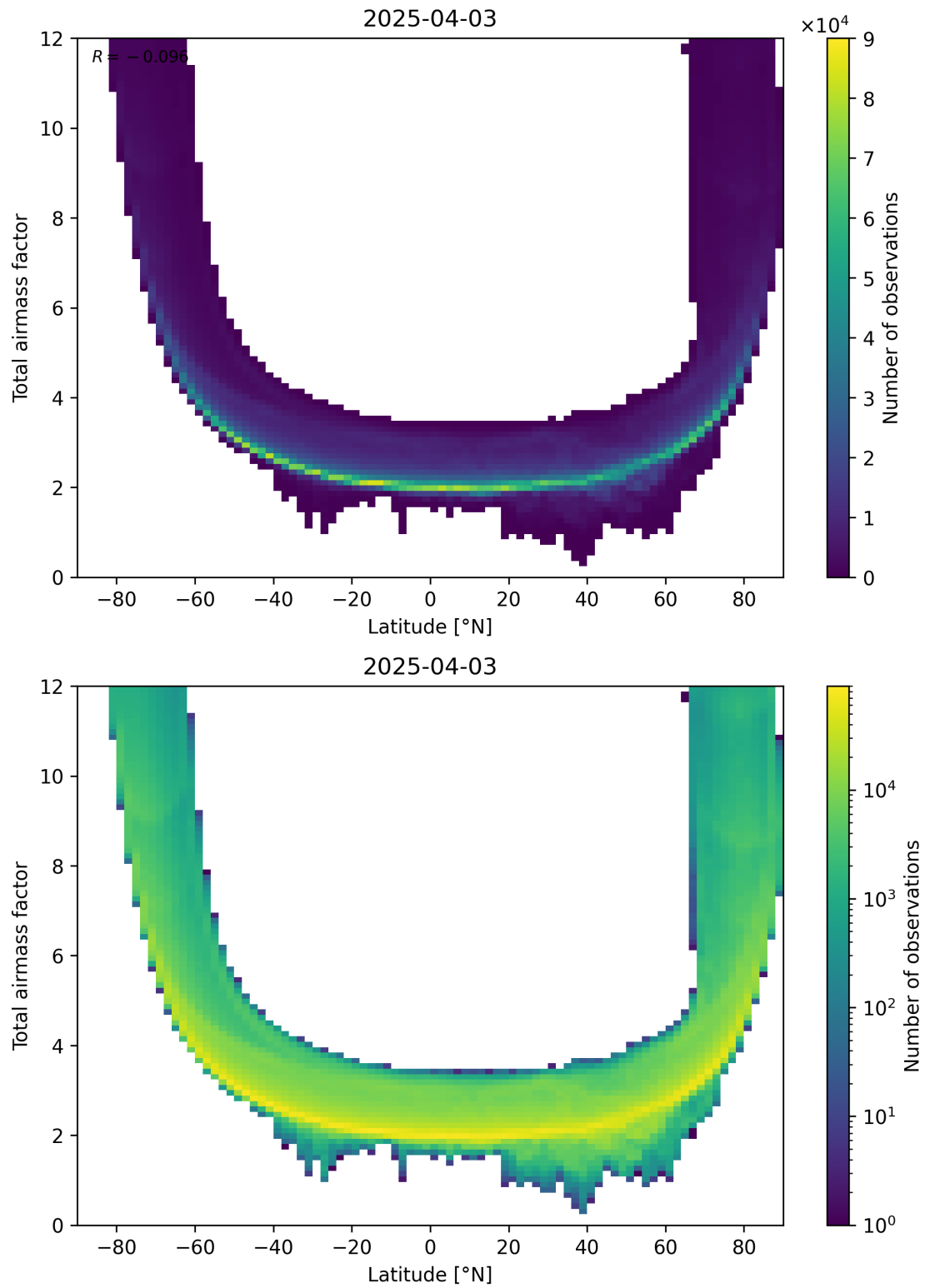
Figure 84: Scatter density plot of “Latitude” against “Total airmass factor” for 2025-04-03 to 2025-04-04.
