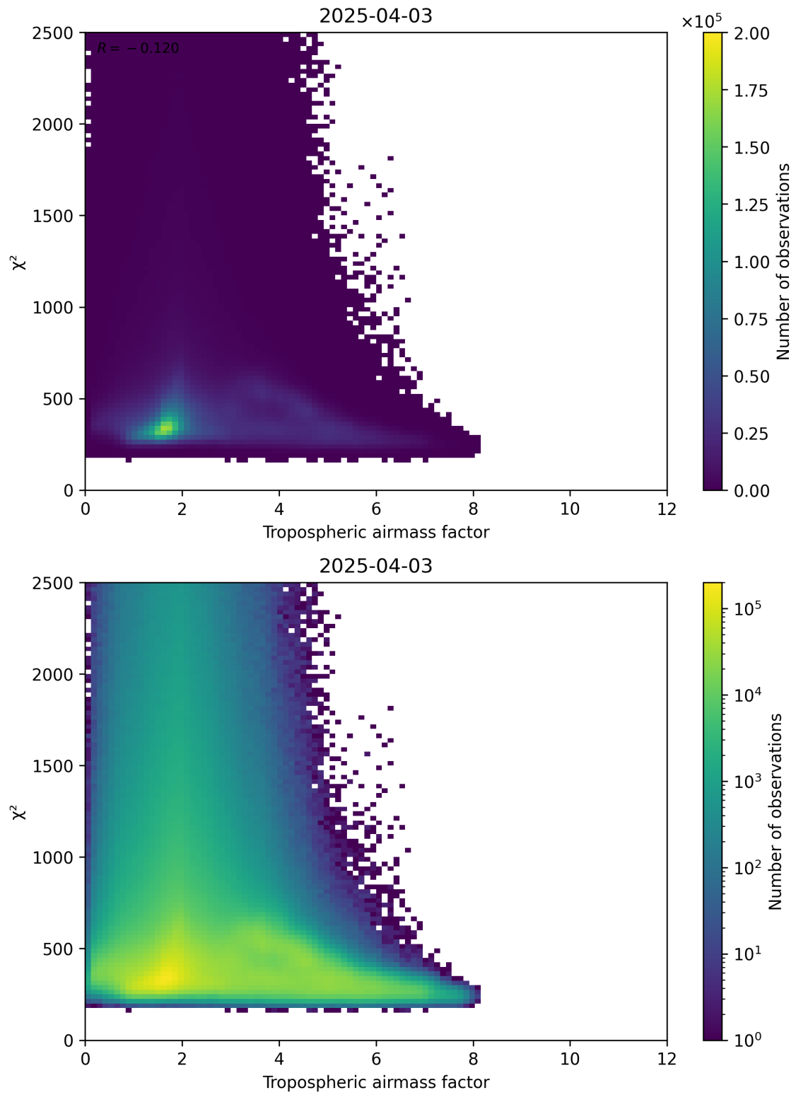
Figure 73: Scatter density plot of “Tropospheric airmass factor” against “ \chi^2 ” for 2025-04-03 to 2025-04-04.
