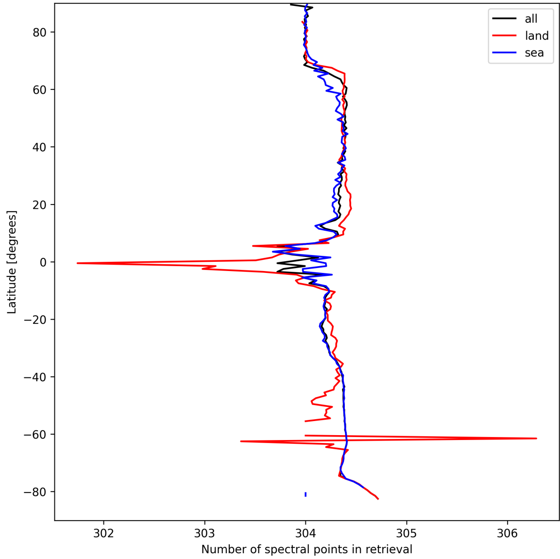
Figure 16: Zonal average of “Number of spectral points in retrieval” for 2025-04-03 to 2025-04-04.
