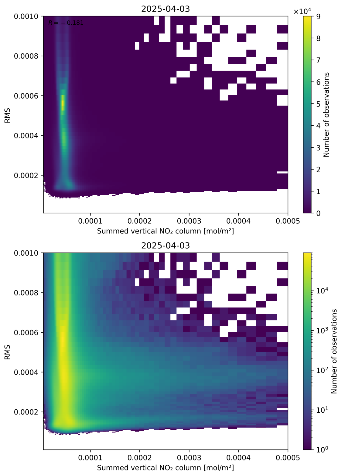
Figure 109: Scatter density plot of “Summed vertical NO 2 column” against “RMS” for 2025-04-03 to 2025-04-04.
