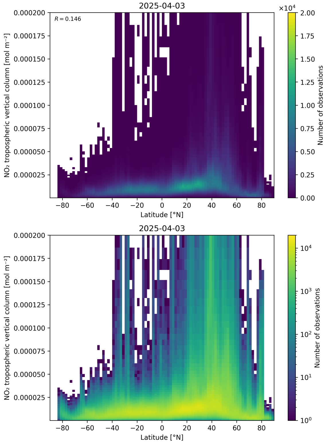
Figure 92: Scatter density plot of “Latitude” against “NO 2 tropospheric vertical column” for 2025-04-03 to 2025-04-04.
