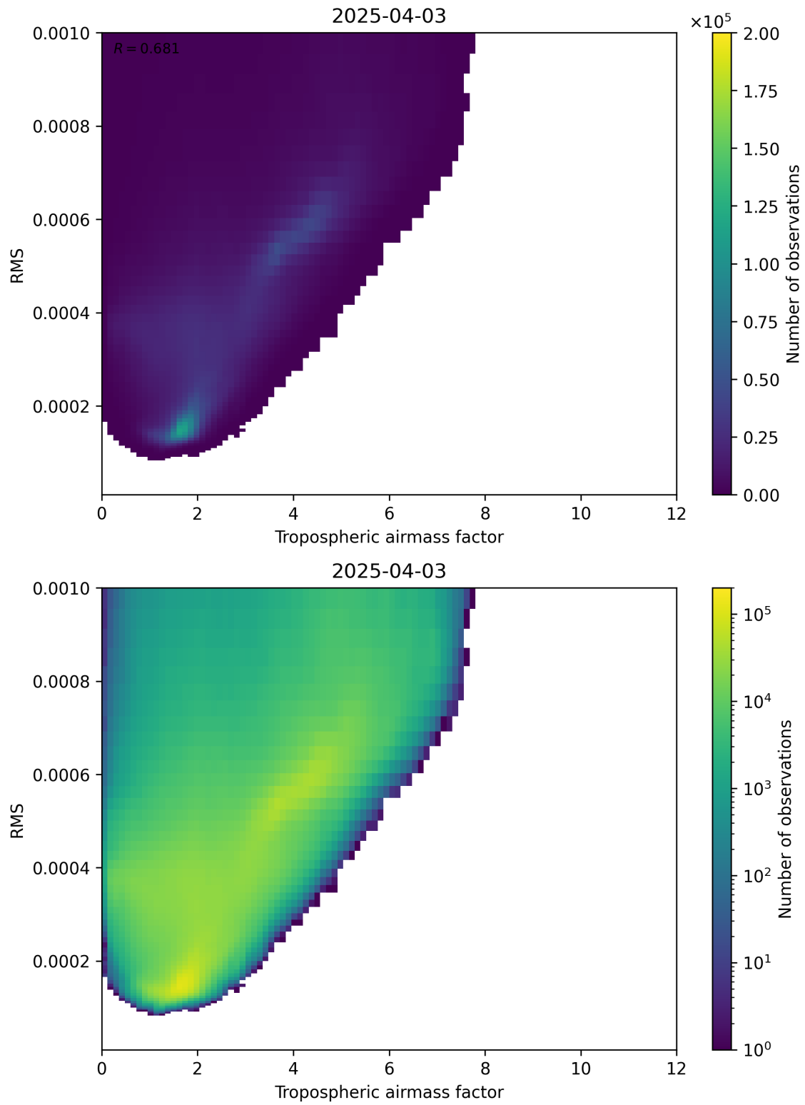
Figure 79: Scatter density plot of “Tropospheric airmass factor” against “RMS” for 2025-04-03 to 2025-04-04.
