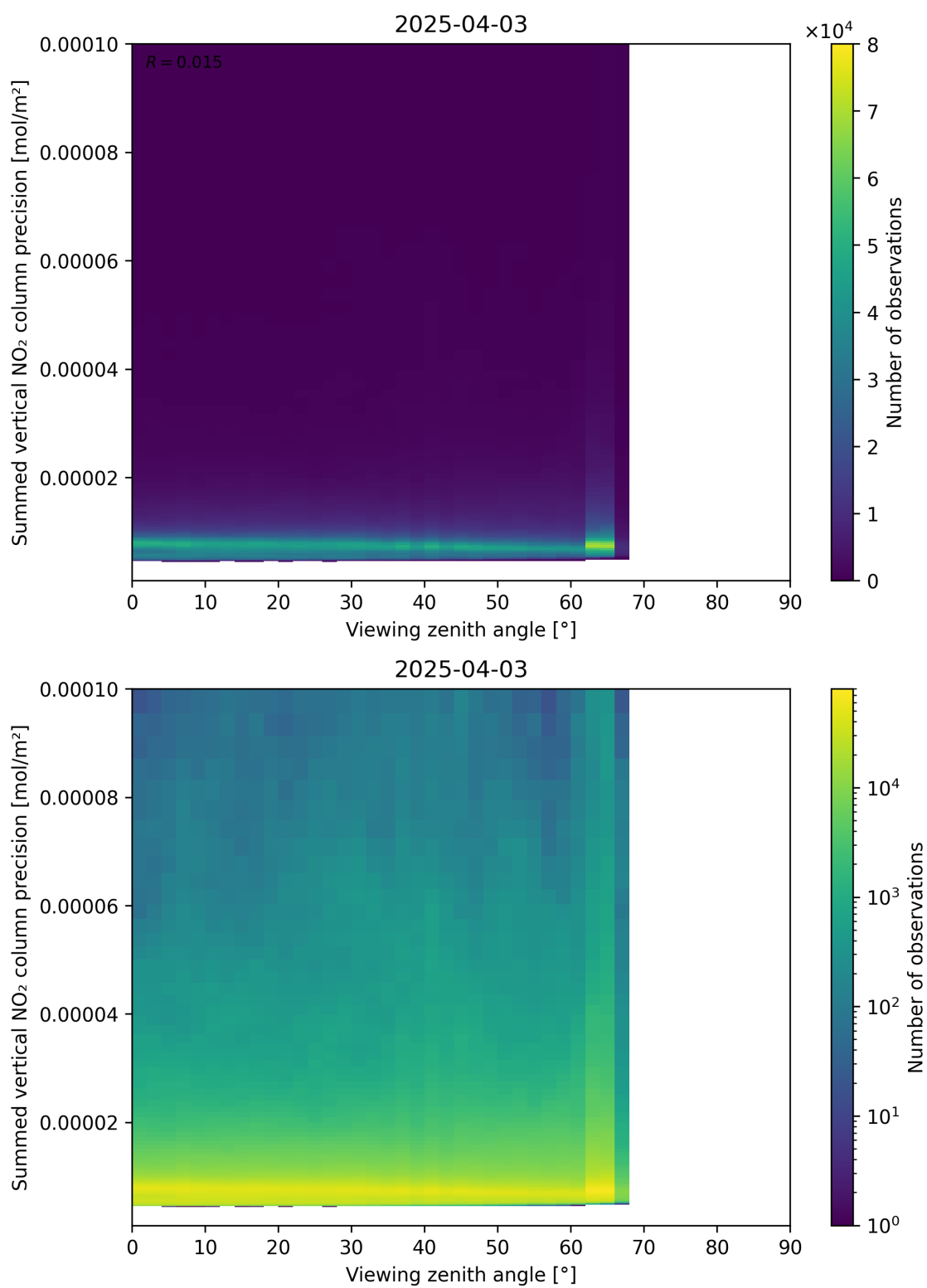
Figure 166: Scatter density plot of “Viewing zenith angle” against “Summed vertical NO 2 column precision” for 2025-04-03 to 2025-04-04.
