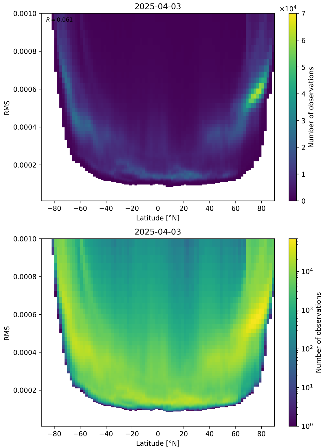
Figure 94: Scatter density plot of “Latitude” against “RMS” for 2025-04-03 to 2025-04-04.
