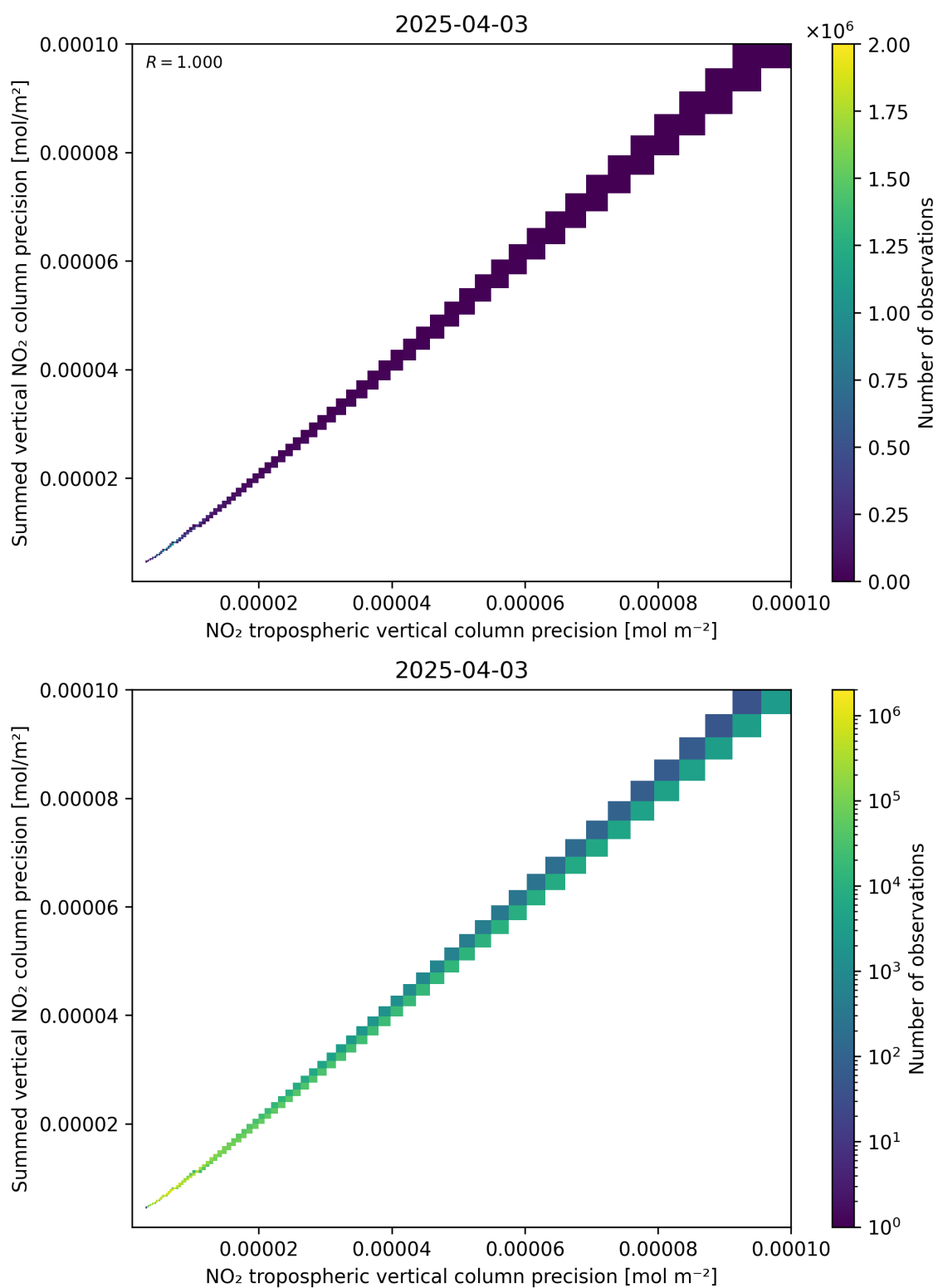
Figure 137: Scatter density plot of “NO 2 tropospheric vertical column precision” against “Summed vertical NO 2 column precision” for 2025-04-03 to 2025-04-04.
