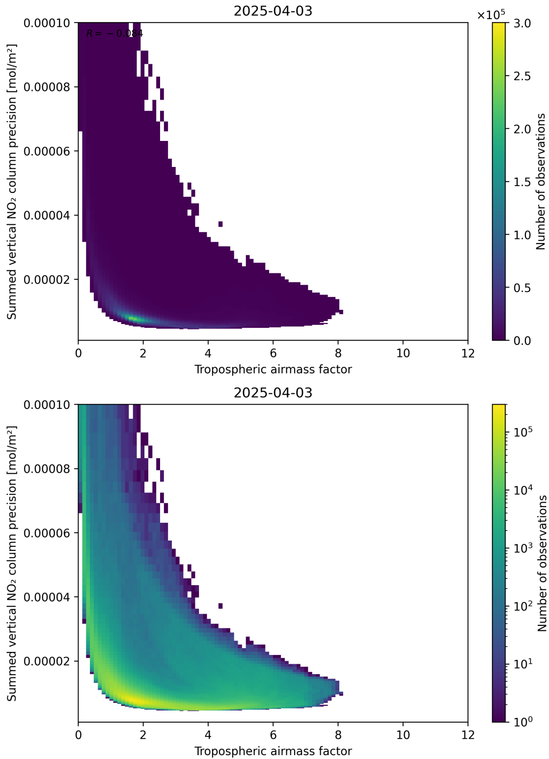
Figure 76: Scatter density plot of “Tropospheric air mass factor” against “Summed vertical NO 2 column precision” for 2025-04-03 to 2025-04-04.
