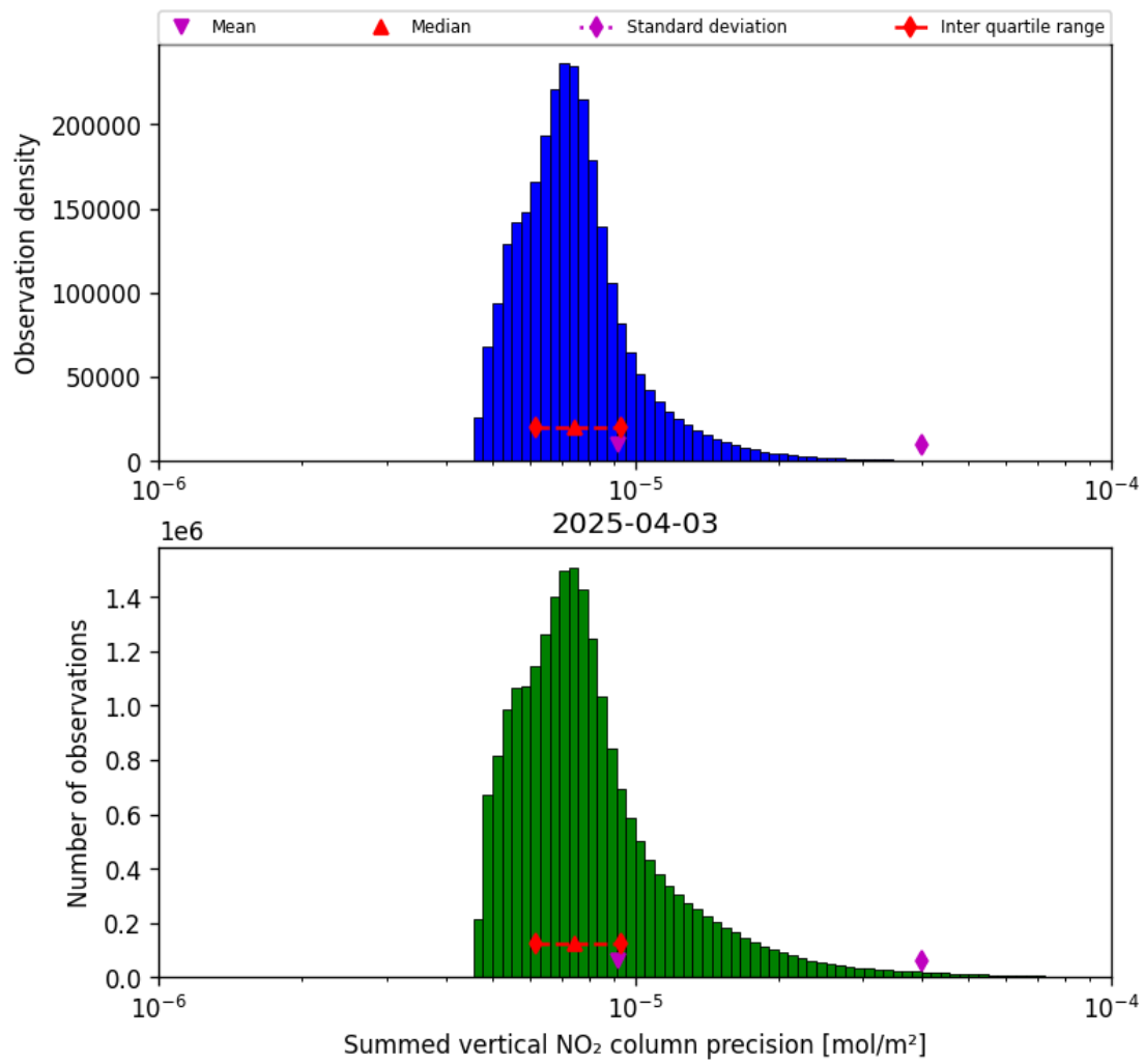
Figure 41: Histogram of "Summed vertical NO 2 column precision" for 2025-04-03 to 2025-04-04
