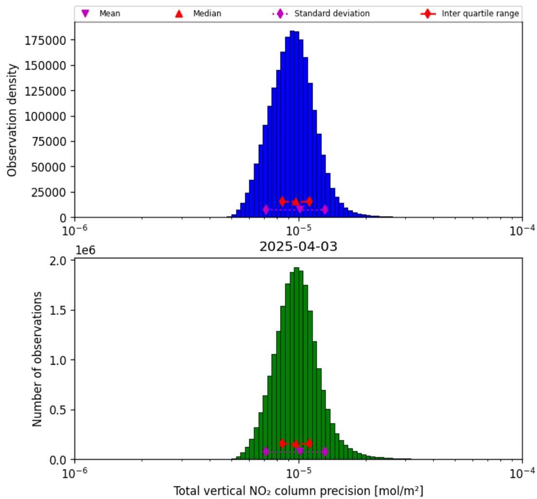
Figure 39: Histogram of “Total vertical NO 2 column precision” for 2025-04-03 to 2025-04-04
