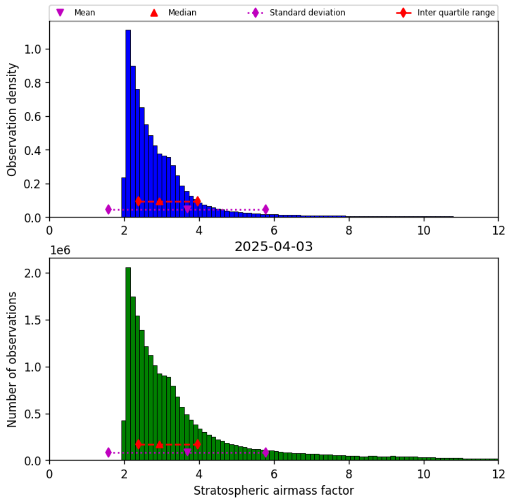
Figure 44: Histogram of “Stratospheric airmass factor” for 2025-04-03 to 2025-04-04
