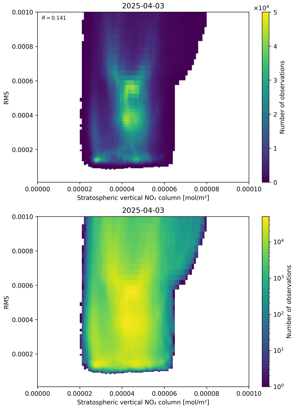
Figure 102: Scatter density plot of “Stratospheric vertical NO 2 column” against “RMS” for 2025-04-03 to 2025-04-04.
