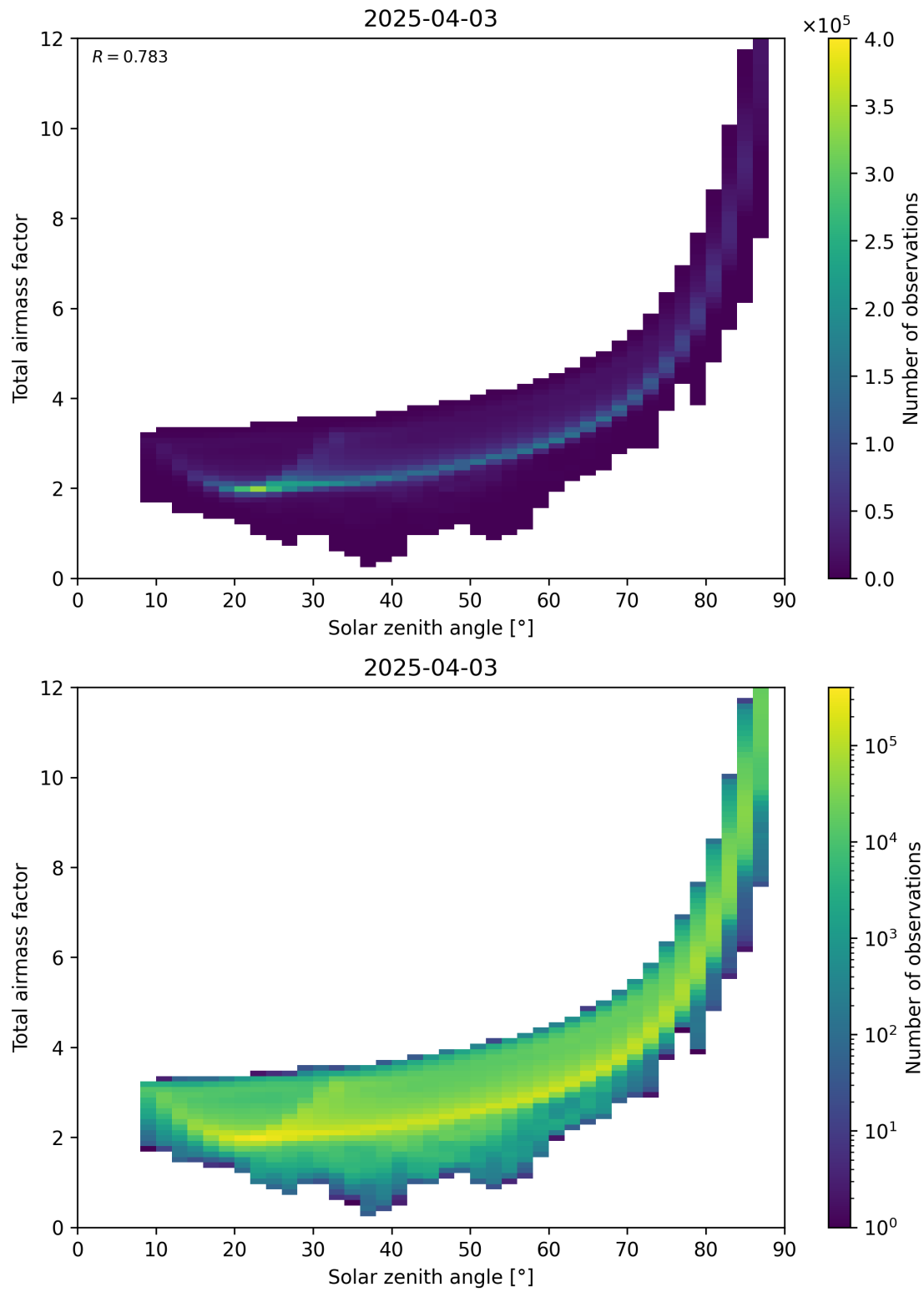
Figure 146: Scatter density plot of “Solar zenith angle” against “Total air mass factor” for 2025-04-03 to 2025-04-04.
