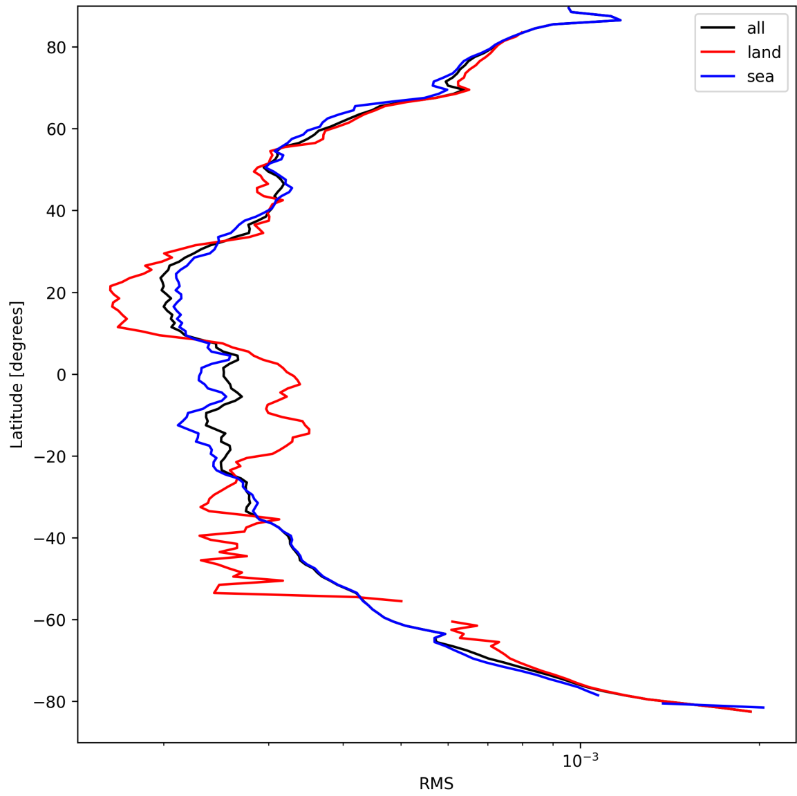
Figure 26: Zonal average of “RMS” for 2025-04-03 to 2025-04-04.
