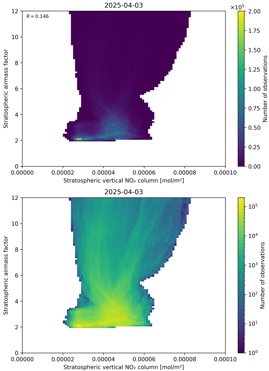
Figure 96: Scatter density plot of “Stratospheric vertical NO 2 column” against “Stratospheric airmass factor” for 2025-04-03 to 2025-04-04.
