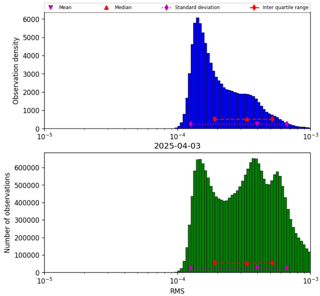
Figure 43: Histogram of “RMS” for 2025-04-03 to 2025-04-04
