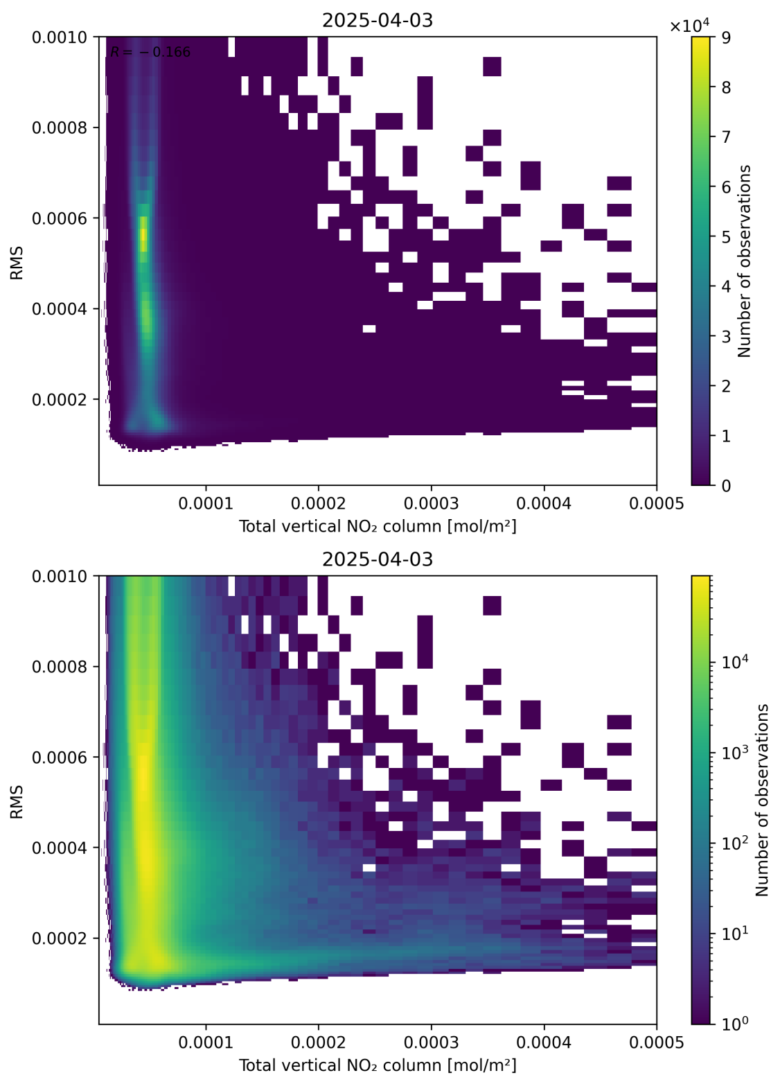
Figure 120: Scatter density plot of “Total vertical NO 2 column” against “RMS” for 2025-04-03 to 2025-04-04.
