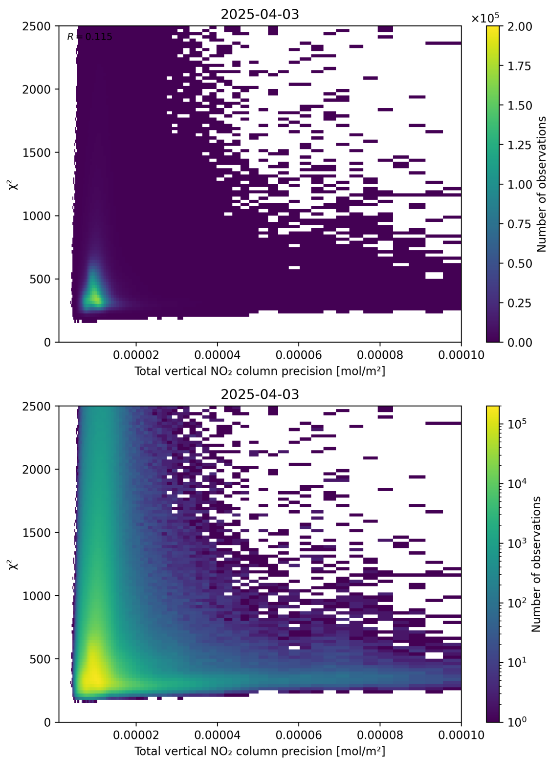
Figure 116: Scatter density plot of “Total vertical NO 2 column precision” against “ \chi^2 ” for 2025-04-03 to 2025-04-04.
