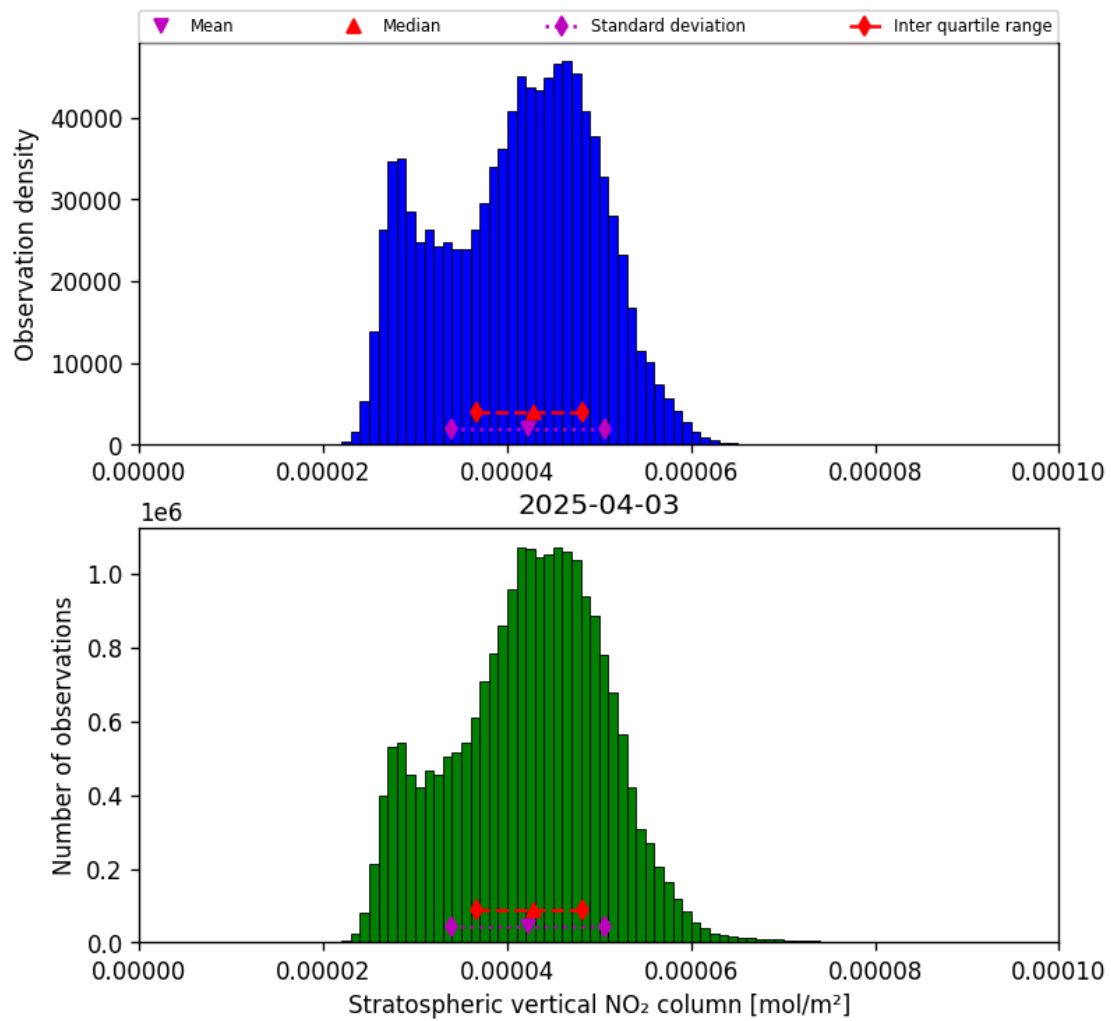
Figure 36: Histogram of “Stratospheric vertical NO 2 column” for 2025-04-03 to 2025-04-04
