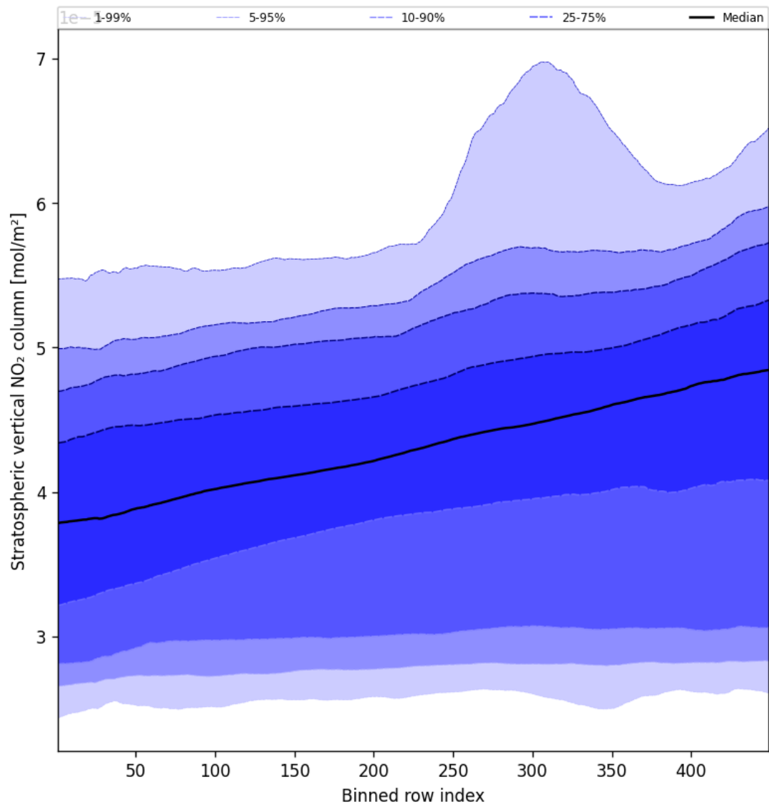
Figure 53: Along track statistics of “Stratospheric vertical NO 2 column” for 2025-04-03 to 2025-04-04
