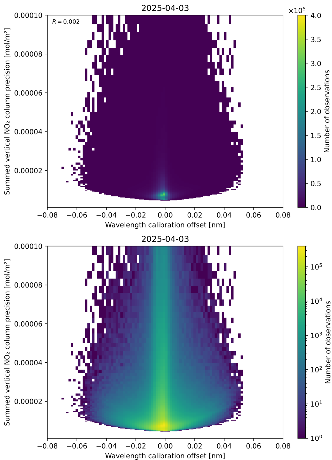
Figure 178: Scatter density plot of “Wavelength calibration offset” against “Summed vertical NO 2 column precision” for 2025-04-03 to 2025-04-04.
