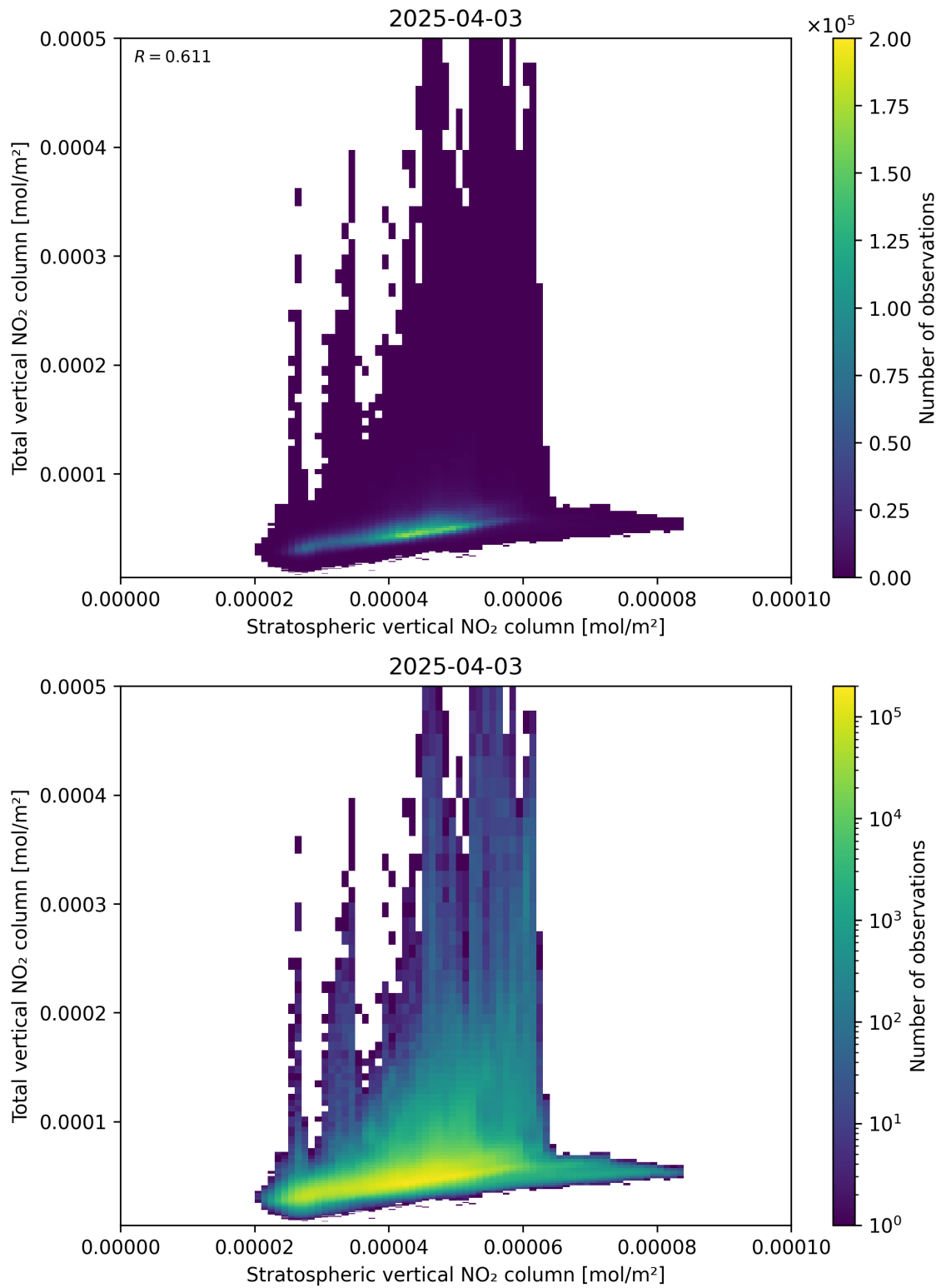
Figure 100: Scatter density plot of “Stratospheric vertical NO 2 column” against “Total vertical NO 2 column” for 2025-04-03 to 2025-04-04.
