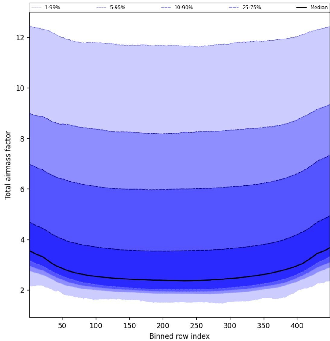
Figure 49: Along track statistics of “Total airmass factor” for 2025-04-03 to 2025-04-04
