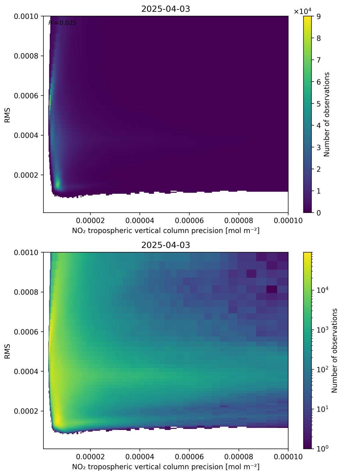
Figure 140: Scatter density plot of “NO 2 tropospheric vertical column precision” against “RMS” for 2025-04-03 to 2025-04-04.
