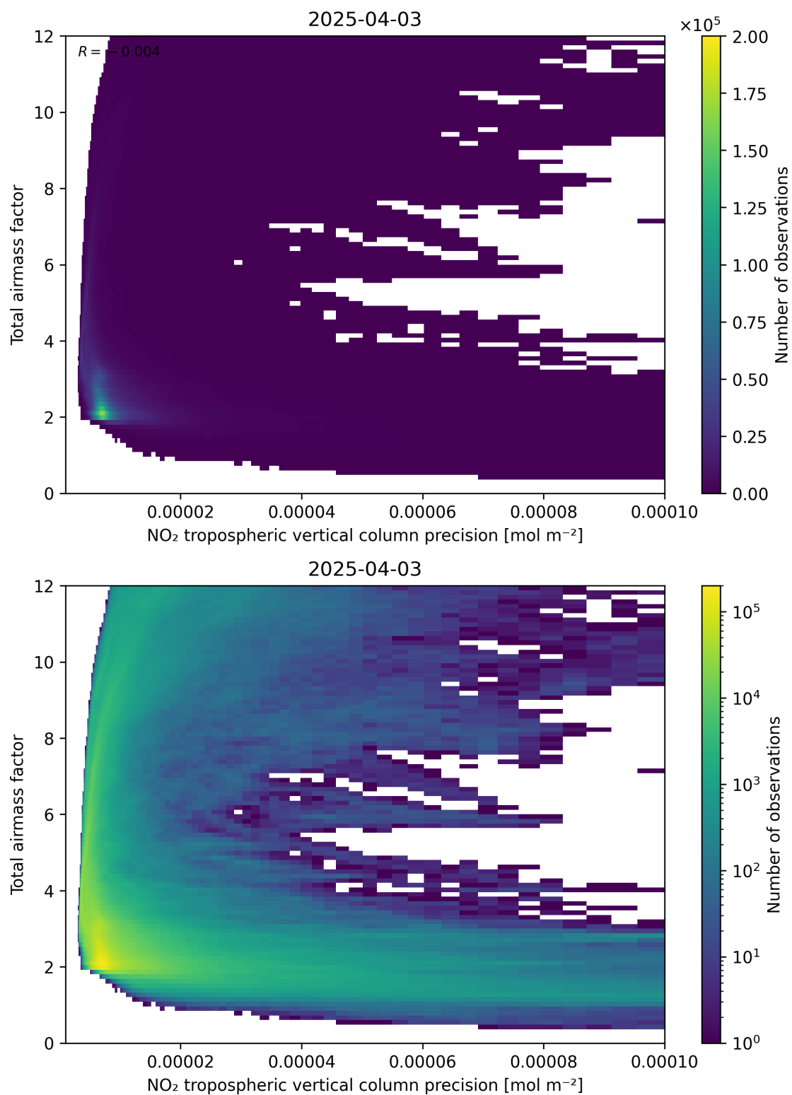
Figure 132: Scatter density plot of “NO 2 tropospheric vertical column precision” against “Total air mass factor” for 2025-04-03 to 2025-04-04.
