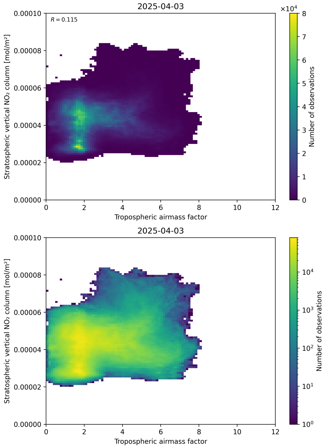
Figure 74: Scatter density plot of “Tropospheric air mass factor” against “Stratospheric vertical NO 2 column” for 2025-04-03 to 2025-04-04.
