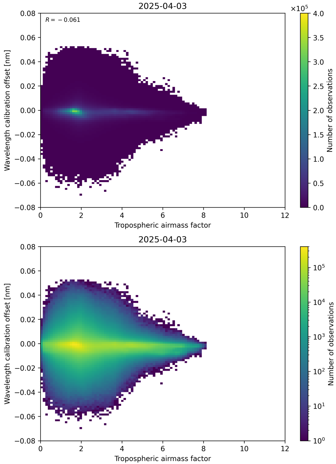
Figure 80: Scatter density plot of “Tropospheric airmass factor” against “Wavelength calibration offset” for 2025-04-03 to 2025-04-04.
