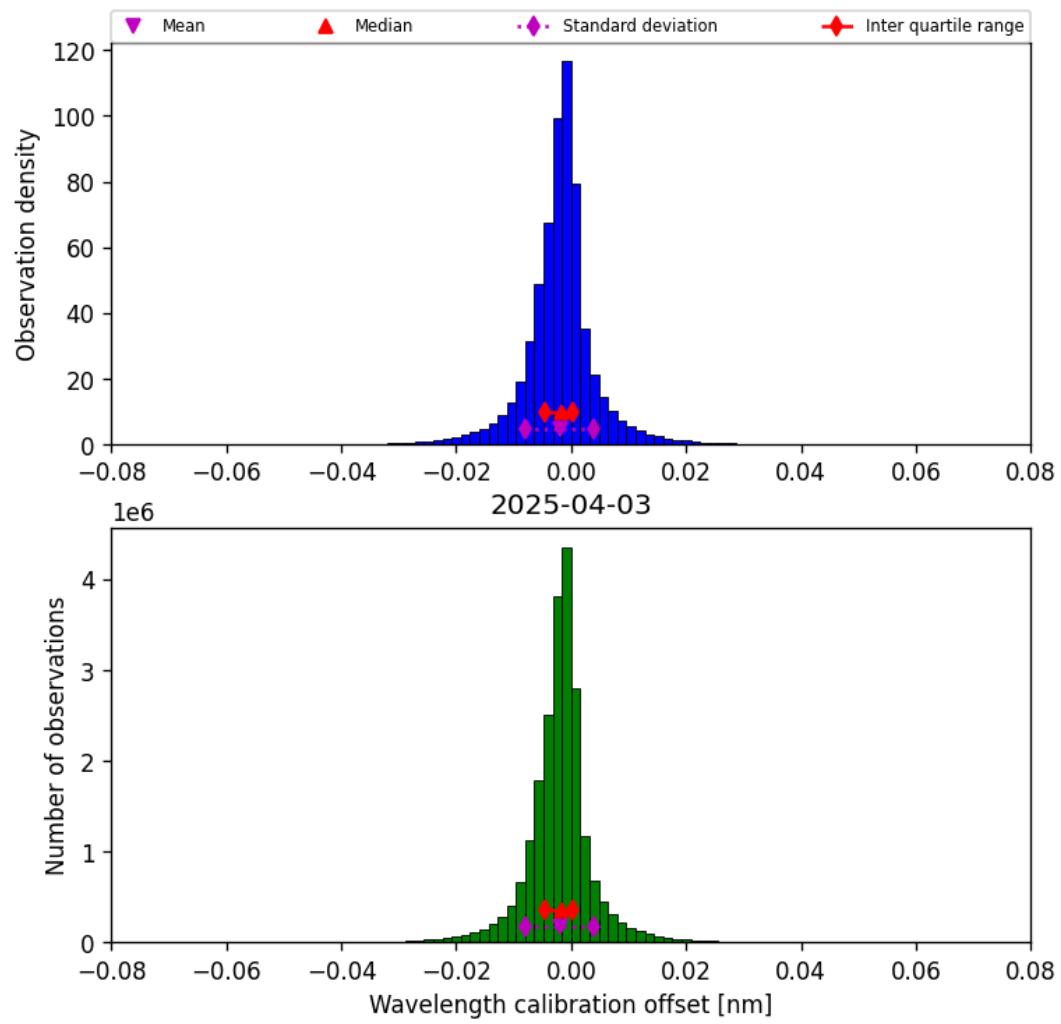
Figure 35: Histogram of “Wavelength calibration offset” for 2025-04-03 to 2025-04-04
