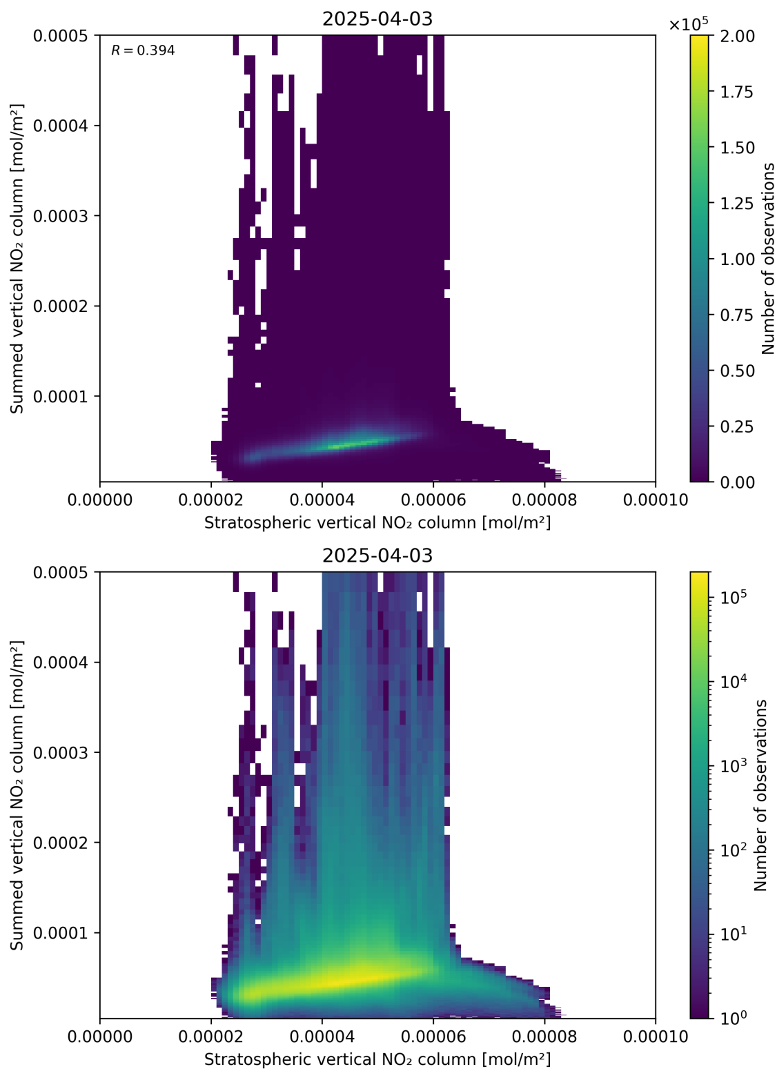
Figure 98: Scatter density plot of “Stratospheric vertical NO 2 column” against “Summed vertical NO 2 column” for 2025-04-03 to 2025-04-04.
