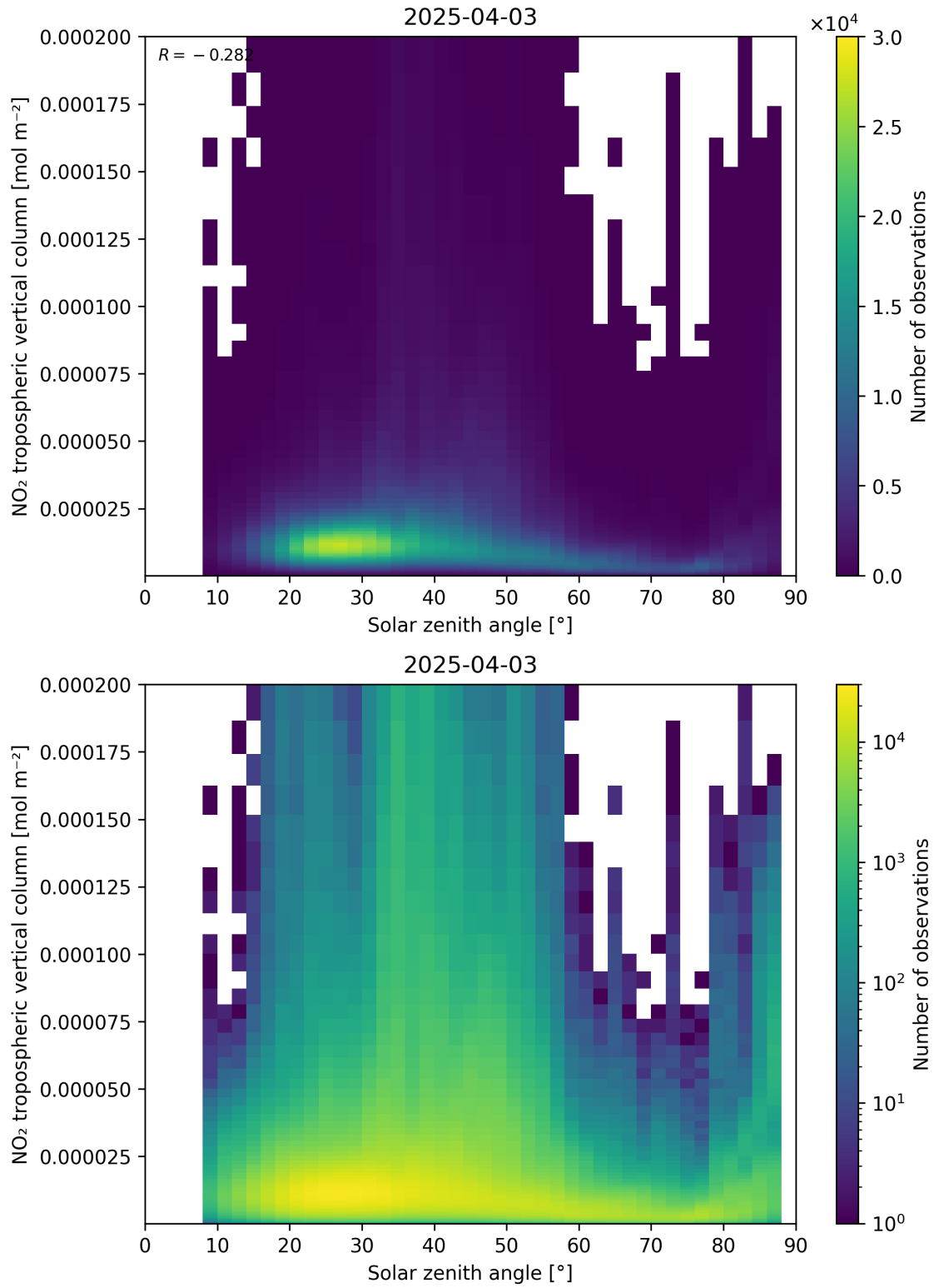
Figure 155: Scatter density plot of “Solar zenith angle” against “NO 2 tropospheric vertical column” for 2025-04-03 to 2025-04-04.
