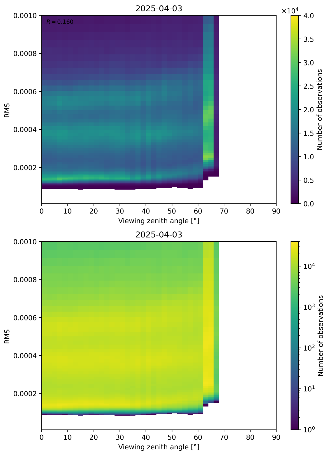
Figure 171: Scatter density plot of “Viewing zenith angle” against “RMS” for 2025-04-03 to 2025-04-04.
