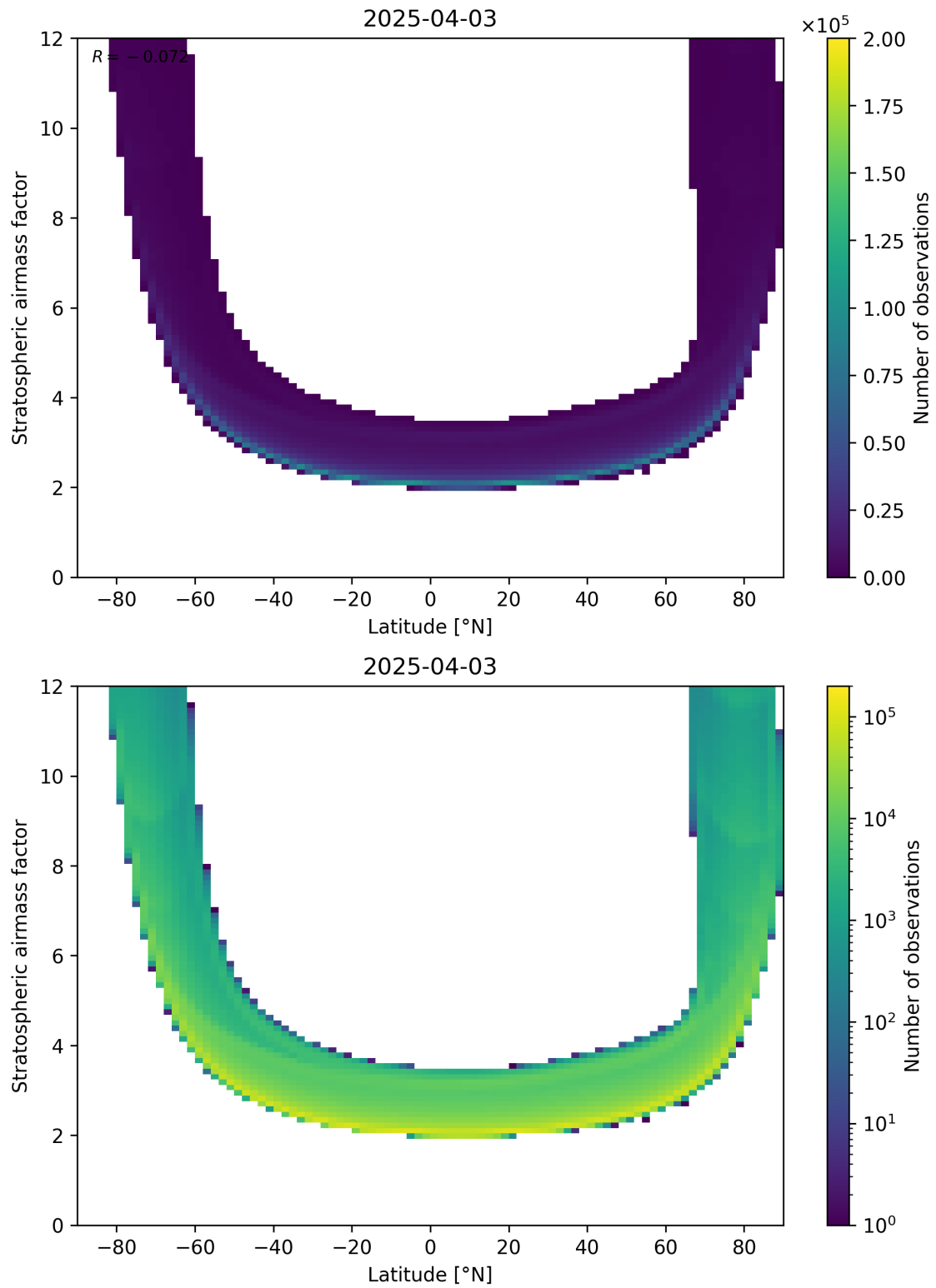
Figure 83: Scatter density plot of “Latitude” against “Stratospheric air mass factor” for 2025-04-03 to 2025-04-04.
