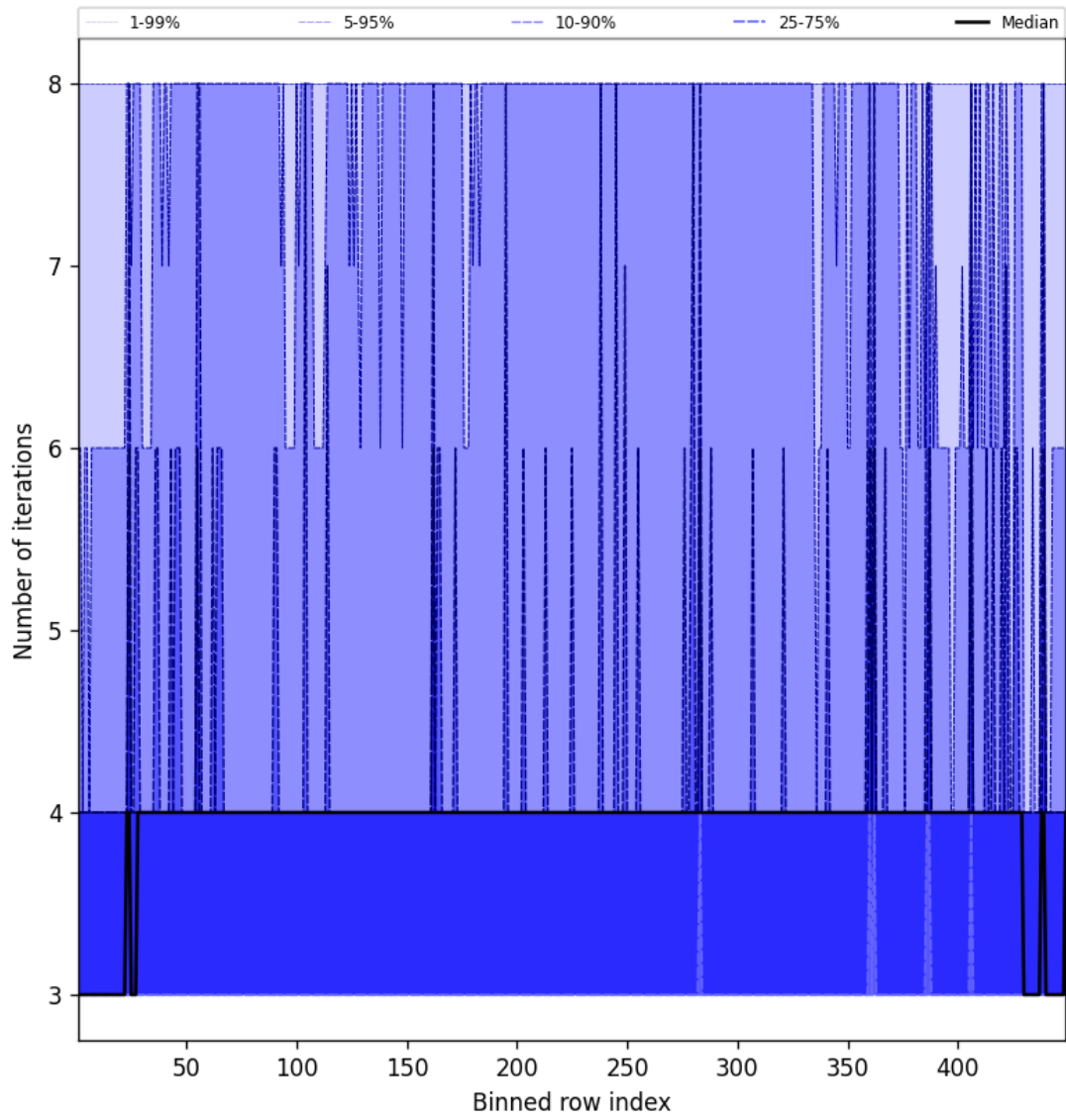
Figure 51: Along track statistics of “Number of iterations” for 2025-04-03 to 2025-04-04
