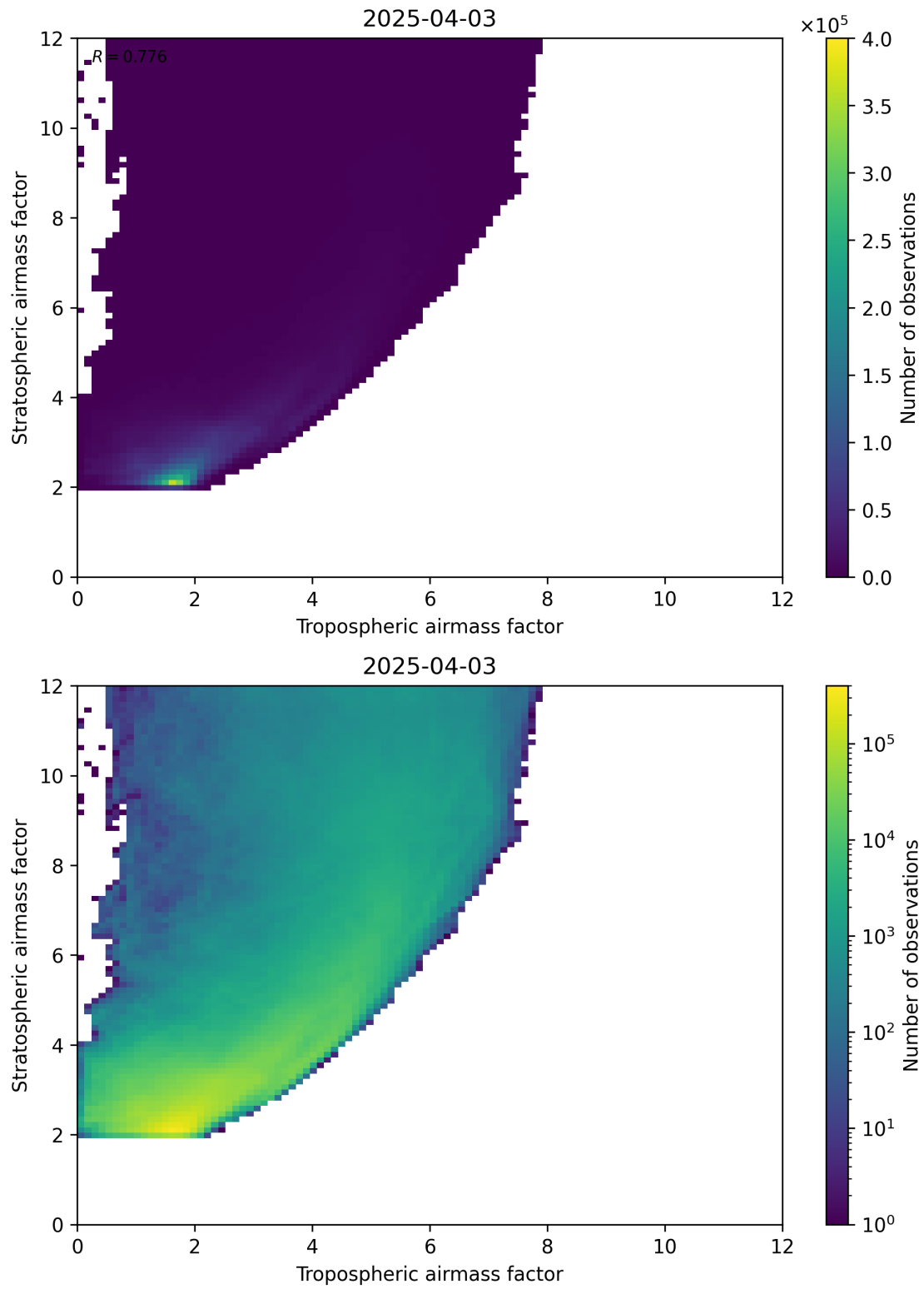
Figure 71: Scatter density plot of “Tropospheric airmass factor” against “Stratospheric airmass factor” for 2025-04-03 to 2025-04-04.
