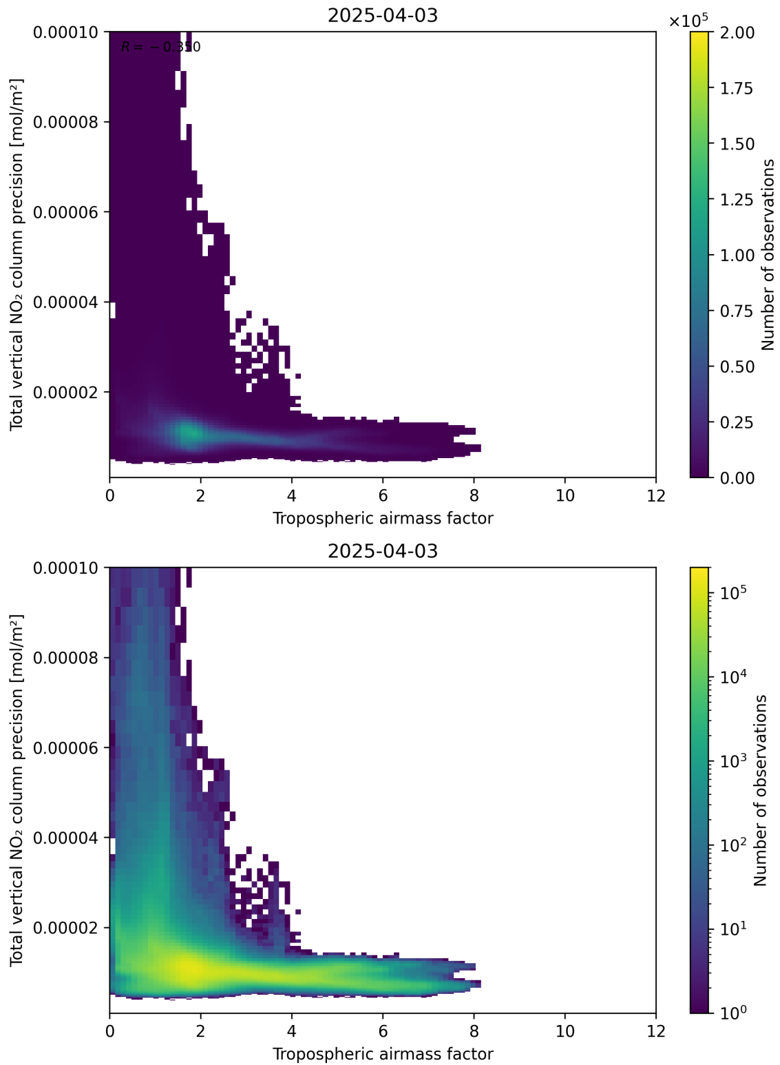
Figure 78: Scatter density plot of “Tropospheric airmass factor” against “Total vertical NO 2 column precision” for 2025-04-03 to 2025-04-04.
