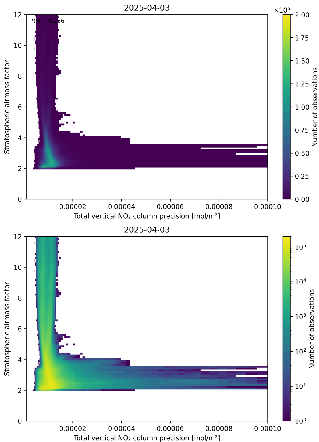
Figure 115: Scatter density plot of “Total vertical NO 2 column precision” against “Stratospheric air mass factor” for 2025-04-03 to 2025-04-04.
