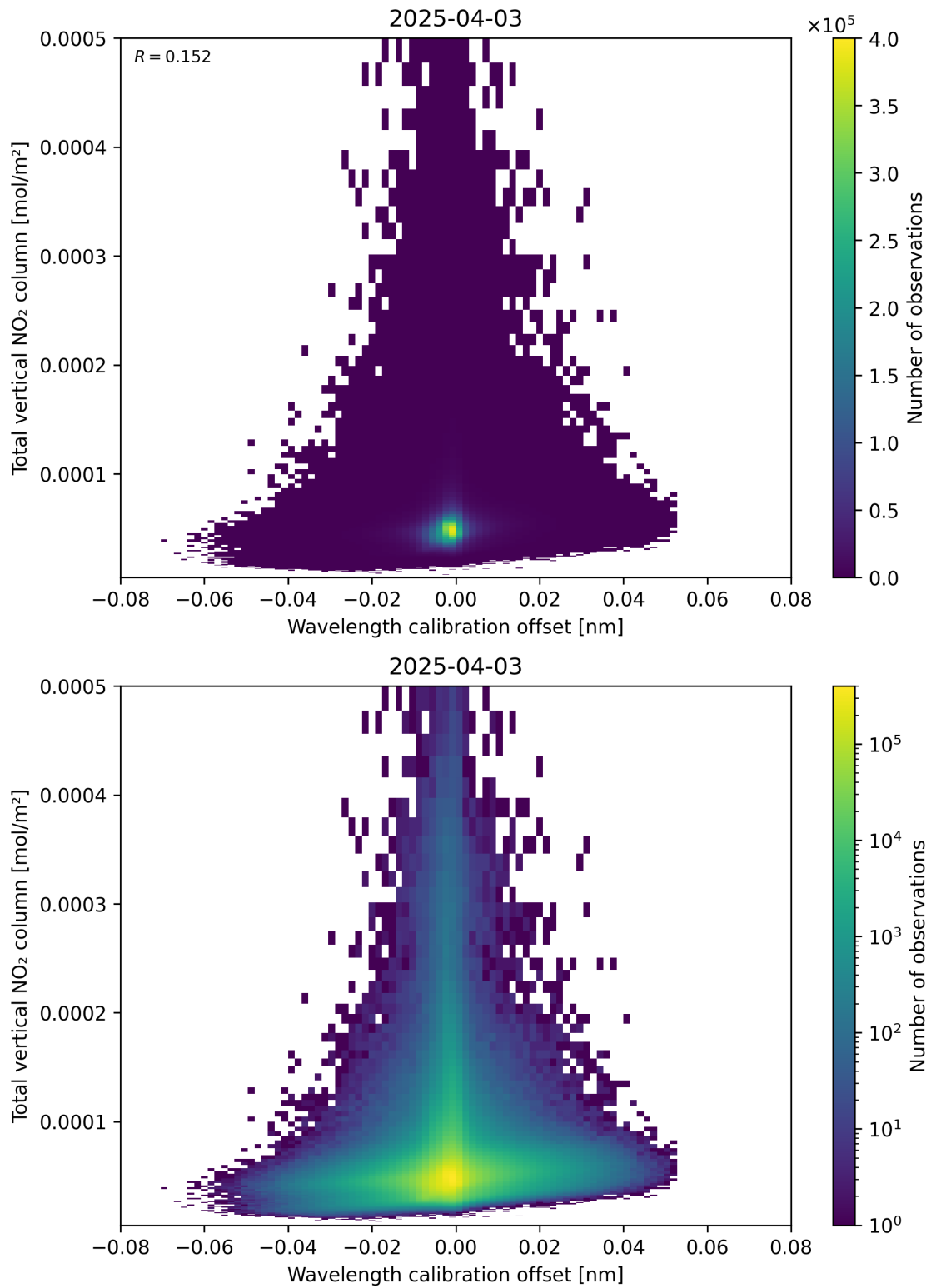
Figure 179: Scatter density plot of “Wavelength calibration offset” against “Total vertical NO 2 column” for 2025-04-03 to 2025-04-04.
