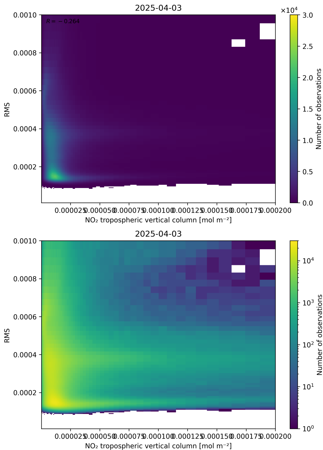
Figure 142: Scatter density plot of “NO 2 tropospheric vertical column” against “RMS” for 2025-04-03 to 2025-04-04.
