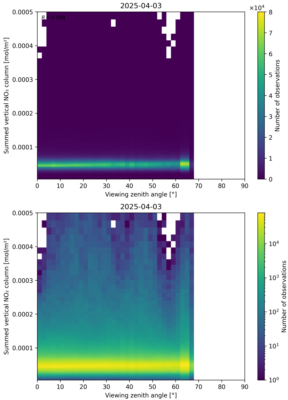
Figure 165: Scatter density plot of “Viewing zenith angle” against “Summed vertical NO 2 column” for 2025-04-03 to 2025-04-04.
