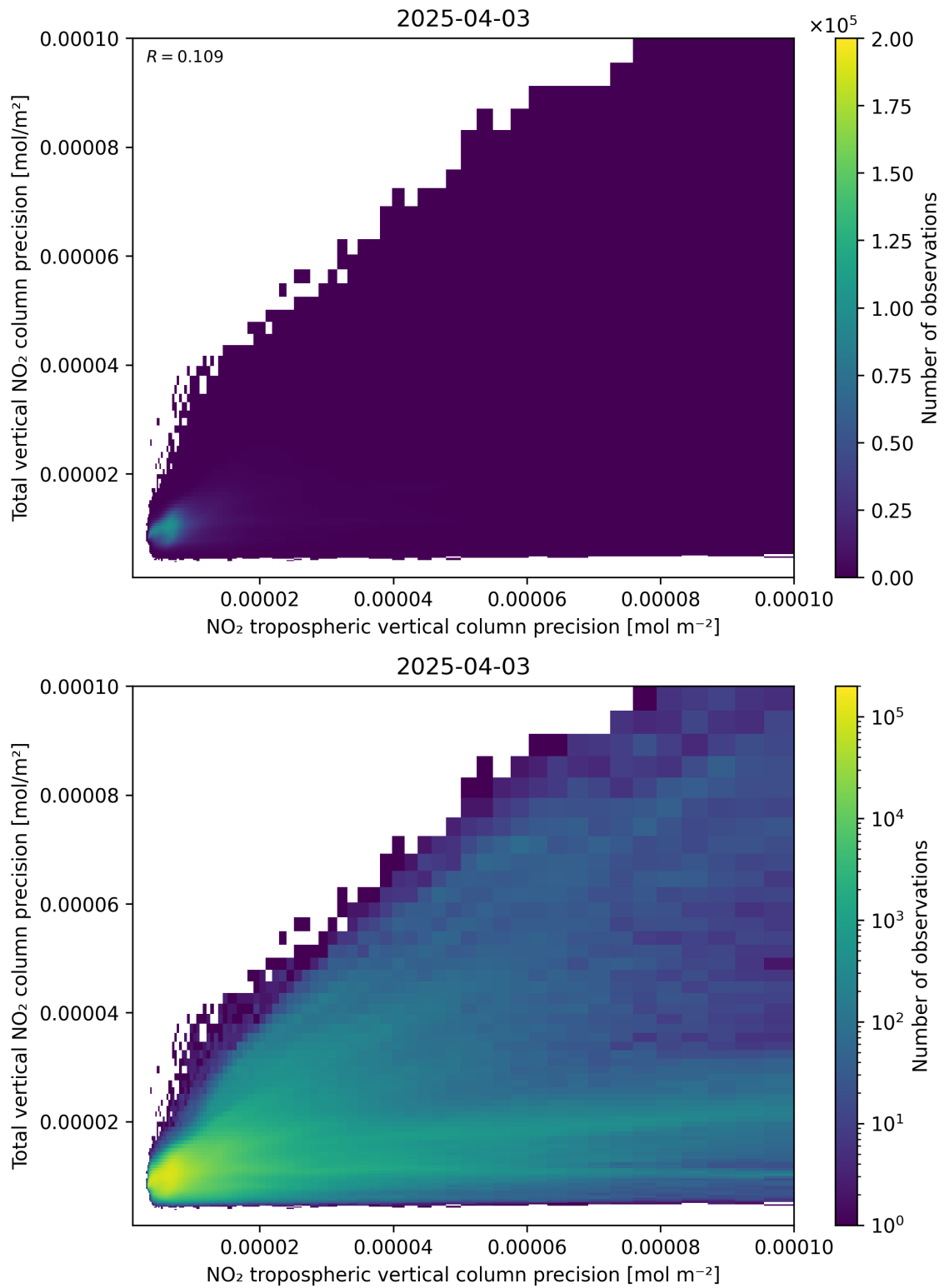
Figure 139: Scatter density plot of “NO 2 tropospheric vertical column precision” against “Total vertical NO 2 column precision” for 2025-04-03 to 2025-04-04.
