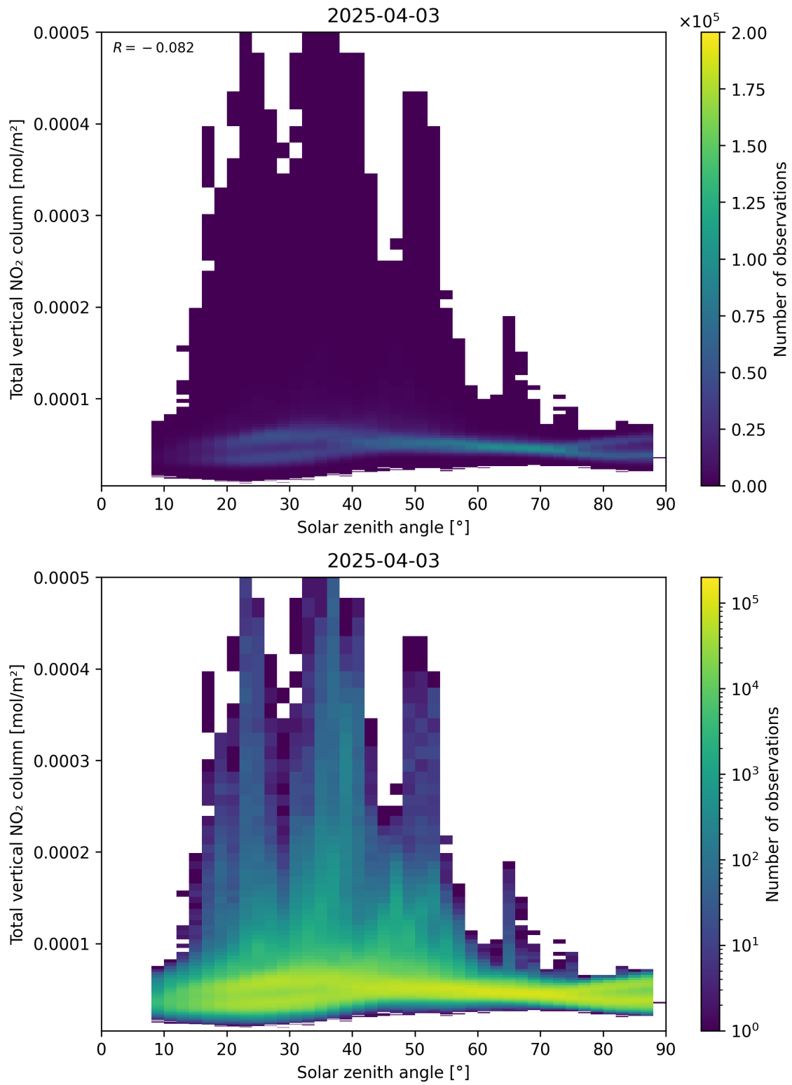
Figure 153: Scatter density plot of “Solar zenith angle” against “Total vertical NO 2 column” for 2025-04-03 to 2025-04-04.
