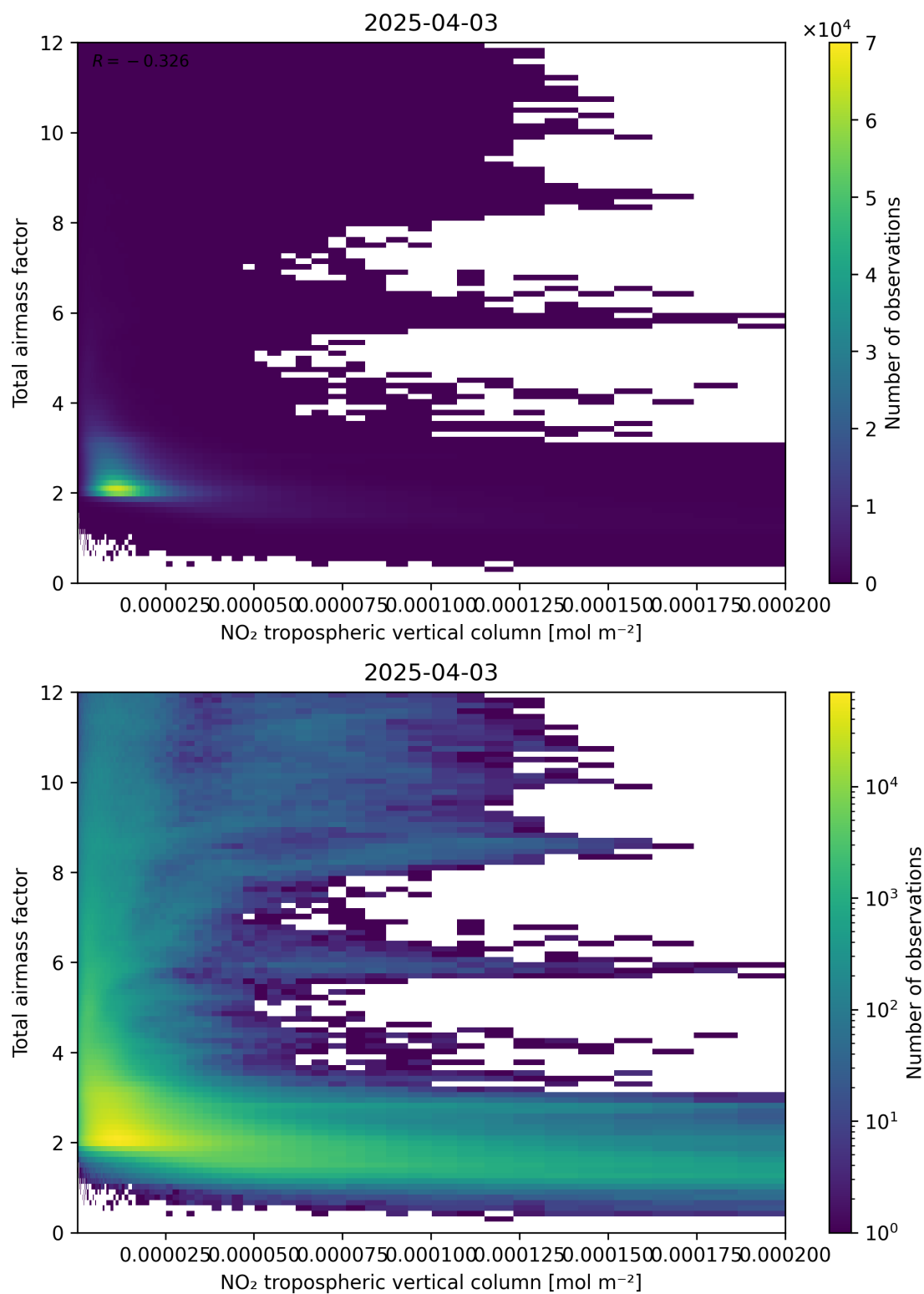
Figure 122: Scatter density plot of “NO 2 tropospheric vertical column” against “Total air mass factor” for 2025-04-03 to 2025-04-04.
