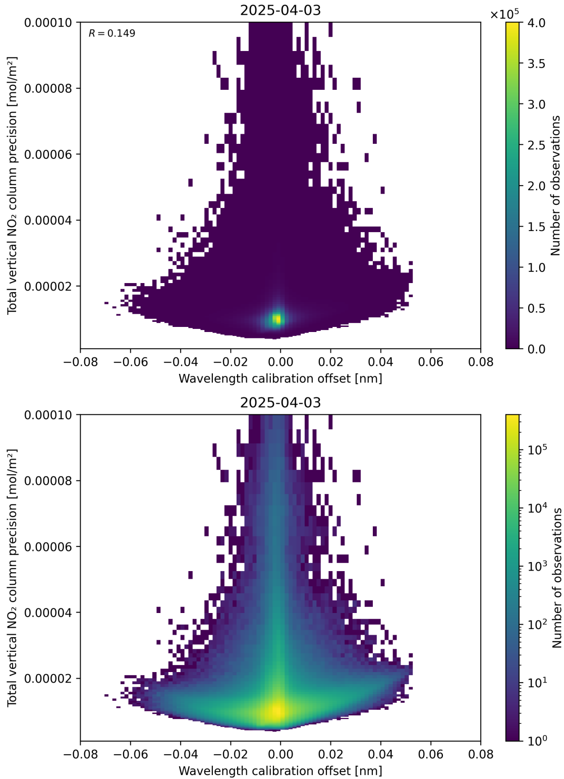
Figure 180: Scatter density plot of “Wavelength calibration offset” against “Total vertical NO 2 column precision” for 2025-04-03 to 2025-04-04.
