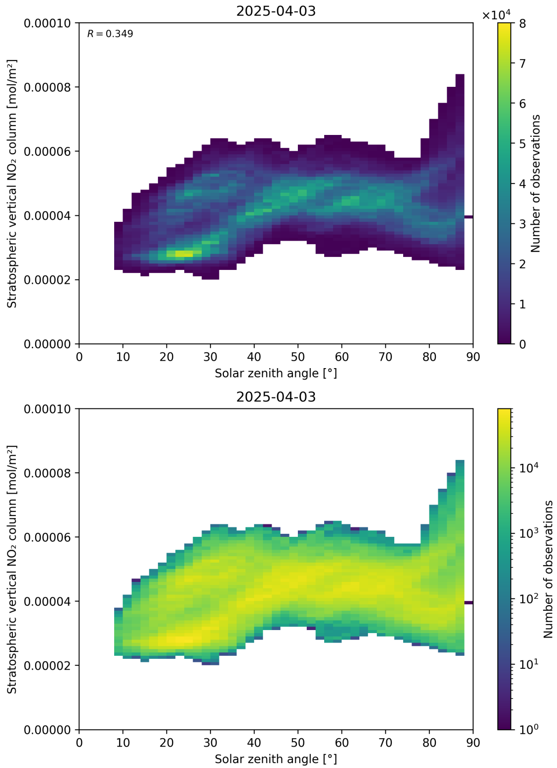
Figure 150: Scatter density plot of “Solar zenith angle” against “Stratospheric vertical NO 2 column” for 2025-04-03 to 2025-04-04.
