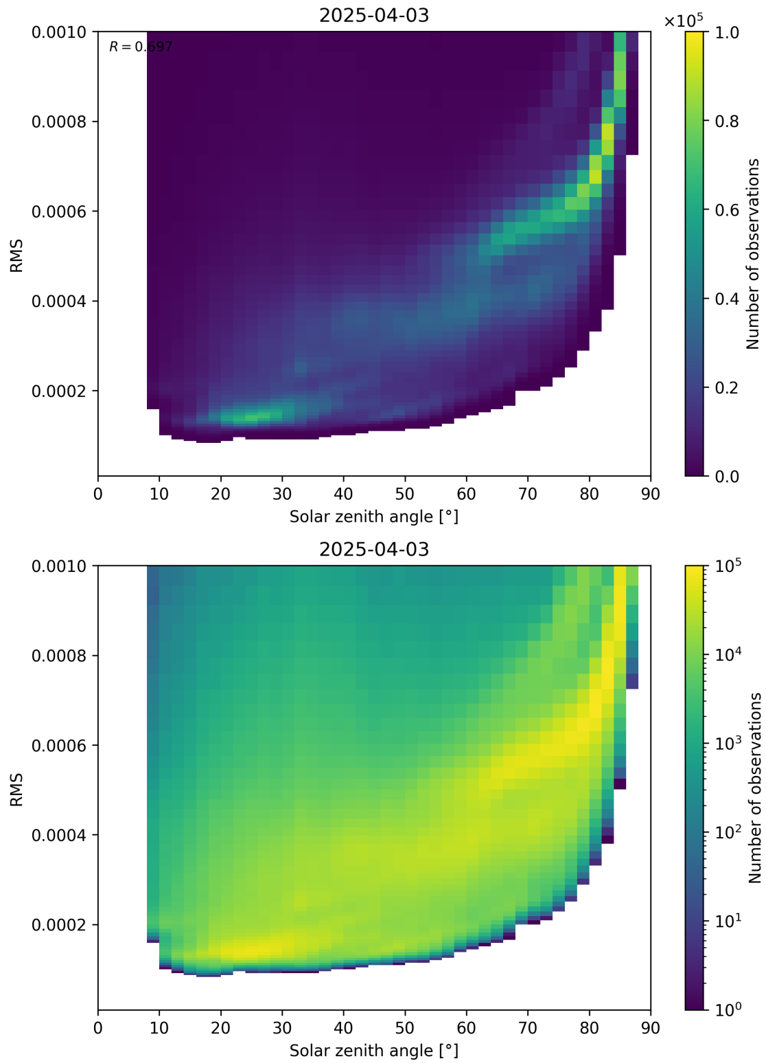
Figure 157: Scatter density plot of “Solar zenith angle” against “RMS” for 2025-04-03 to 2025-04-04.
