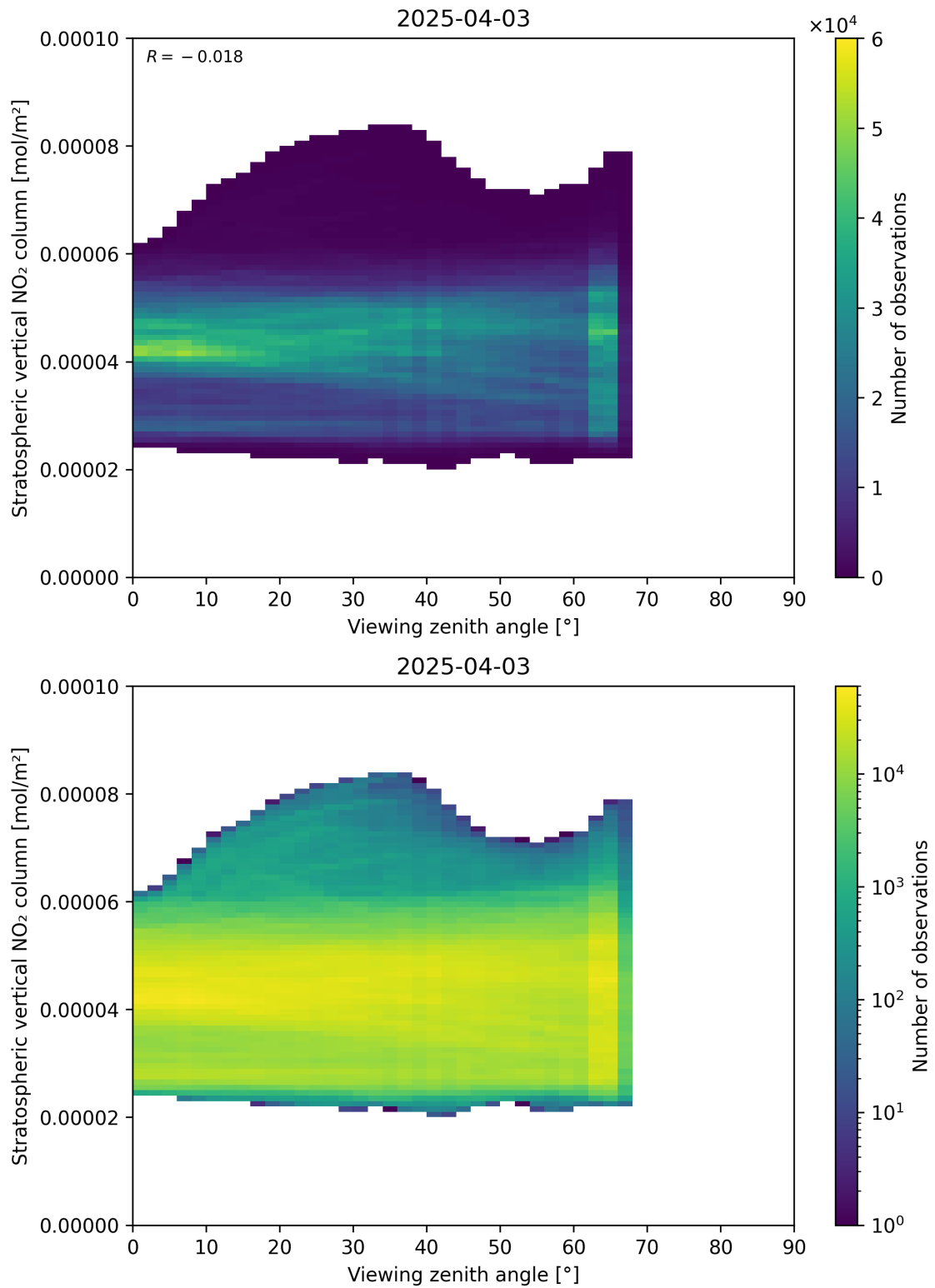
Figure 164: Scatter density plot of “Viewing zenith angle” against “Stratospheric vertical NO 2 column” for 2025-04-03 to 2025-04-04.
