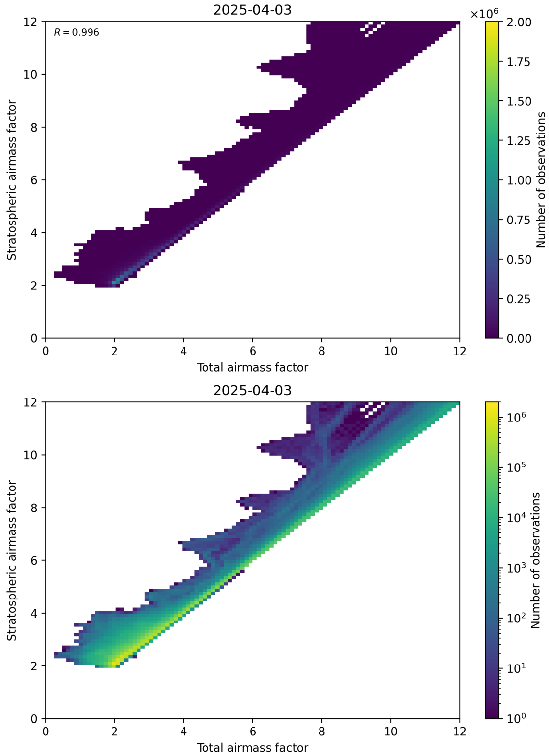
Figure 62: Scatter density plot of “Total airmass factor” against “Stratospheric airmass factor” for 2025-04-03 to 2025-04-04.
