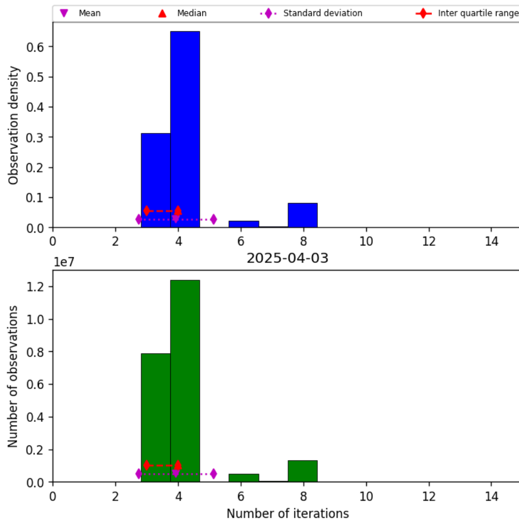
Figure 34: Histogram of “Number of iterations” for 2025-04-03 to 2025-04-04
