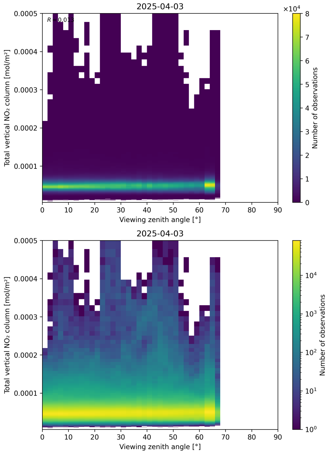
Figure 167: Scatter density plot of “Viewing zenith angle” against “Total vertical NO 2 column” for 2025-04-03 to 2025-04-04.
