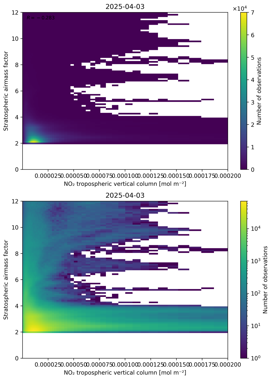
Figure 121: Scatter density plot of “NO 2 tropospheric vertical column” against “Stratospheric air mass factor” for 2025-04-03 to 2025-04-04.
