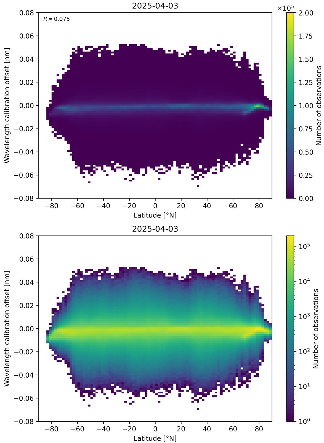
Figure 95: Scatter density plot of “Latitude” against “Wavelength calibration offset” for 2025-04-03 to 2025-04-04.
