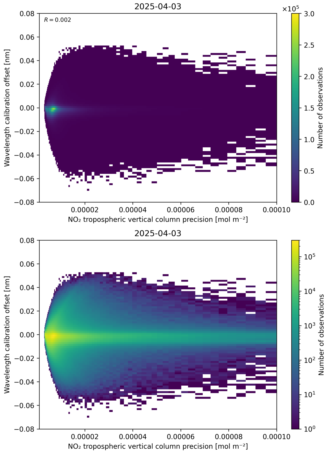
Figure 141: Scatter density plot of “NO 2 tropospheric vertical column precision” against “Wavelength calibration offset” for 2025-04-03 to 2025-04-04.
