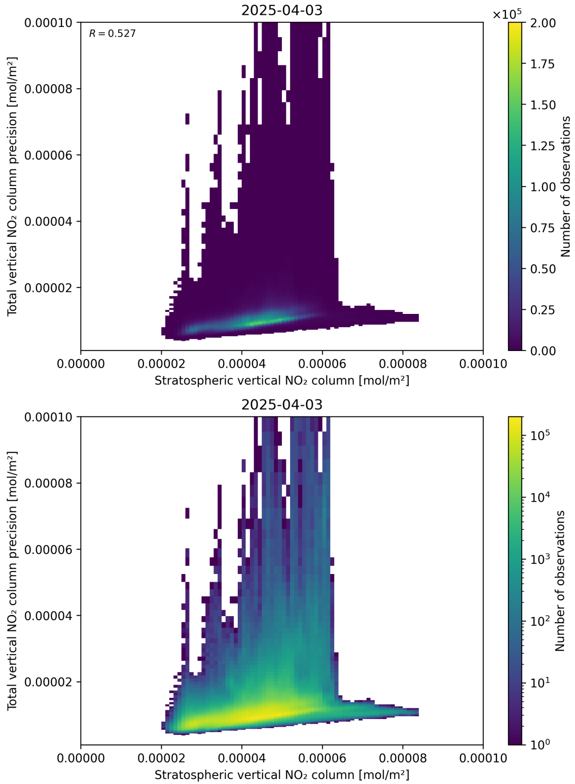
Figure 101: Scatter density plot of “Stratospheric vertical NO 2 column” against “Total vertical NO 2 column precision” for 2025-04-03 to 2025-04-04.
