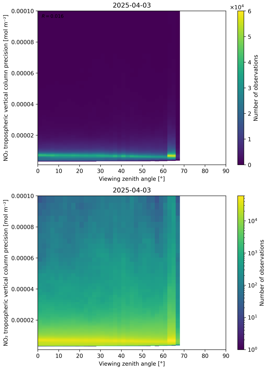
Figure 170: Scatter density plot of “Viewing zenith angle” against “NO 2 tropospheric vertical column precision” for 2025-04-03 to 2025-04-04.
