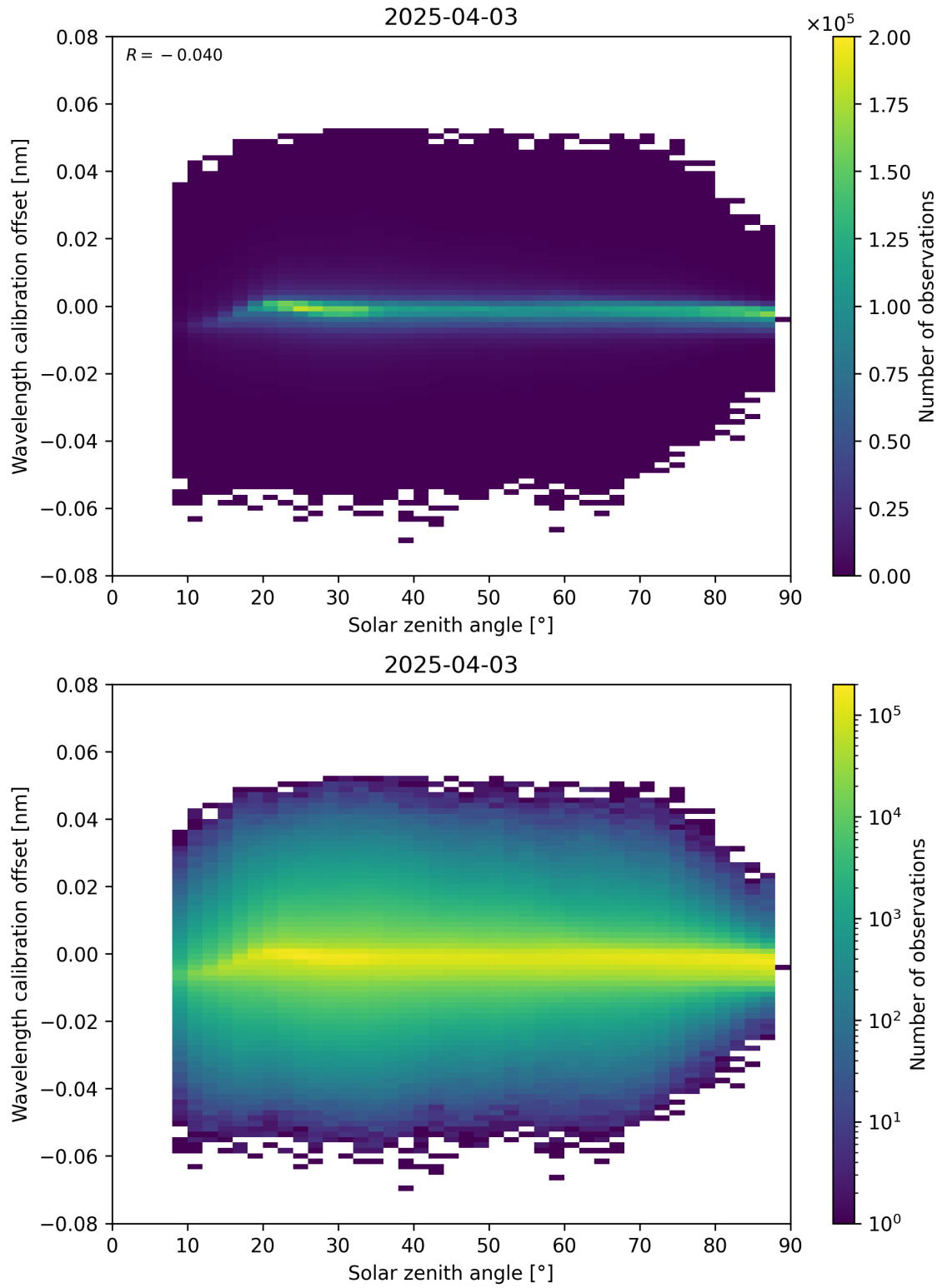
Figure 158: Scatter density plot of “Solar zenith angle” against “Wavelength calibration offset” for 2025-04-03 to 2025-04-04.
