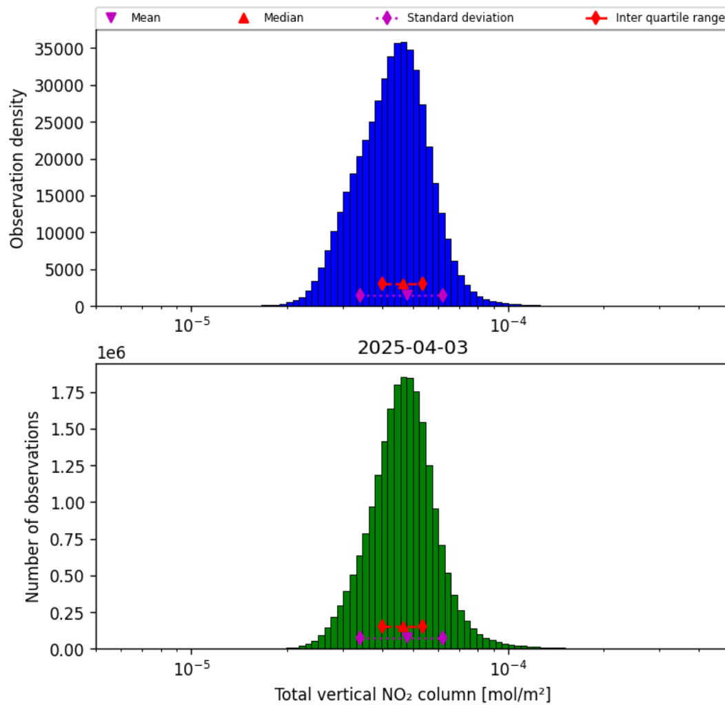
Figure 38: Histogram of “Total vertical NO 2 column” for 2025-04-03 to 2025-04-04
