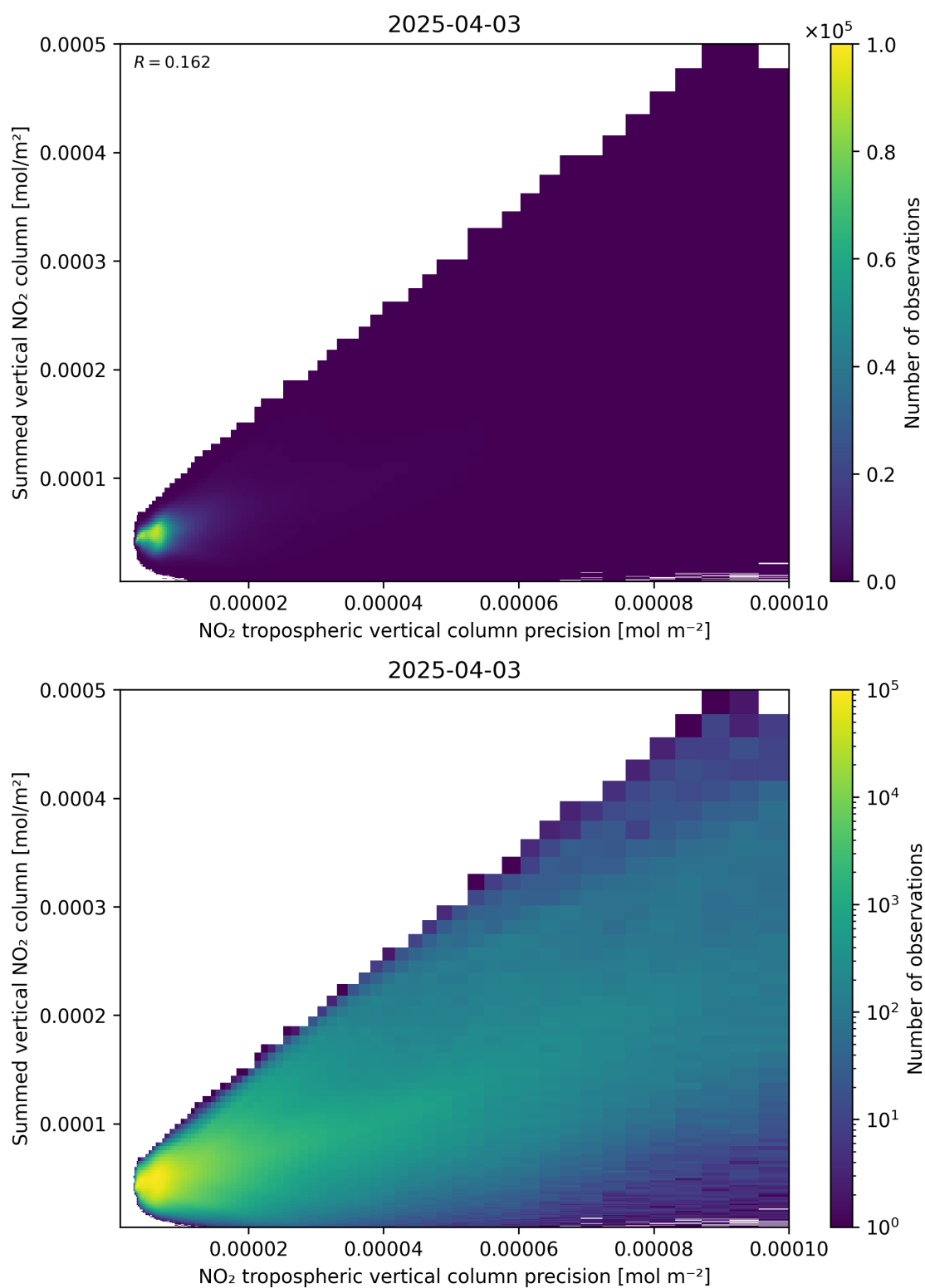
Figure 136: Scatter density plot of “NO 2 tropospheric vertical column precision” against “Summed vertical NO 2 column” for 2025-04-03 to 2025-04-04.
