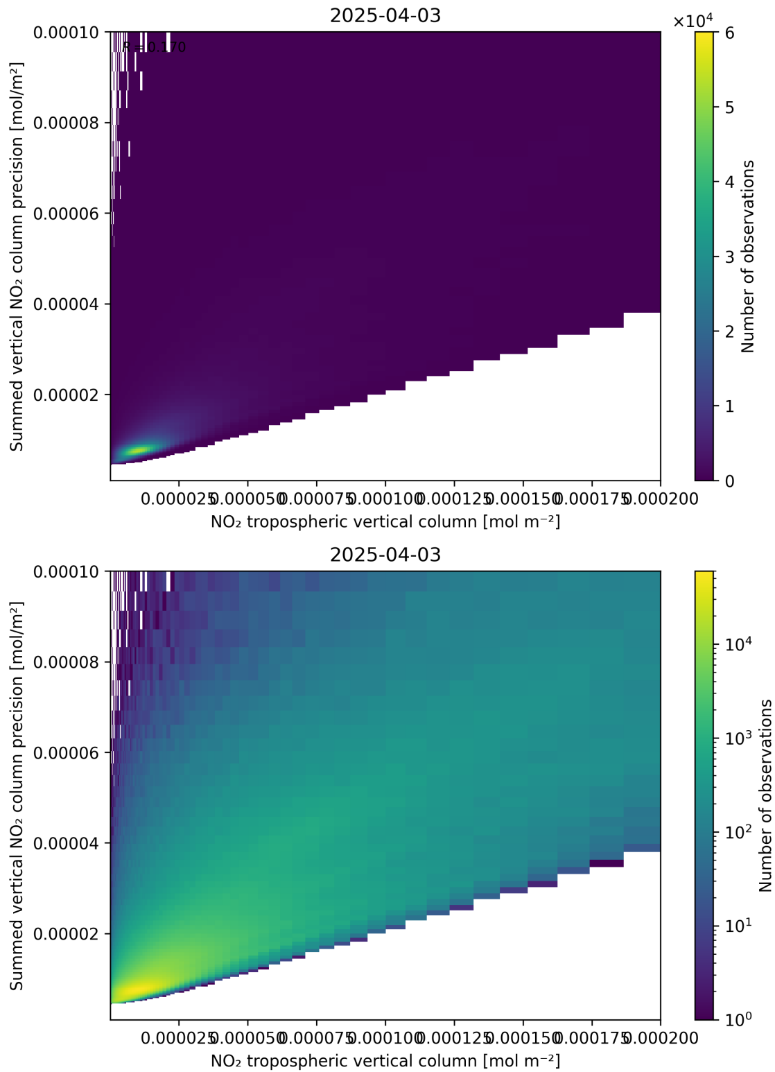
Figure 127: Scatter density plot of “NO 2 tropospheric vertical column” against “Summed vertical NO 2 column precision” for 2025-04-03 to 2025-04-04.
