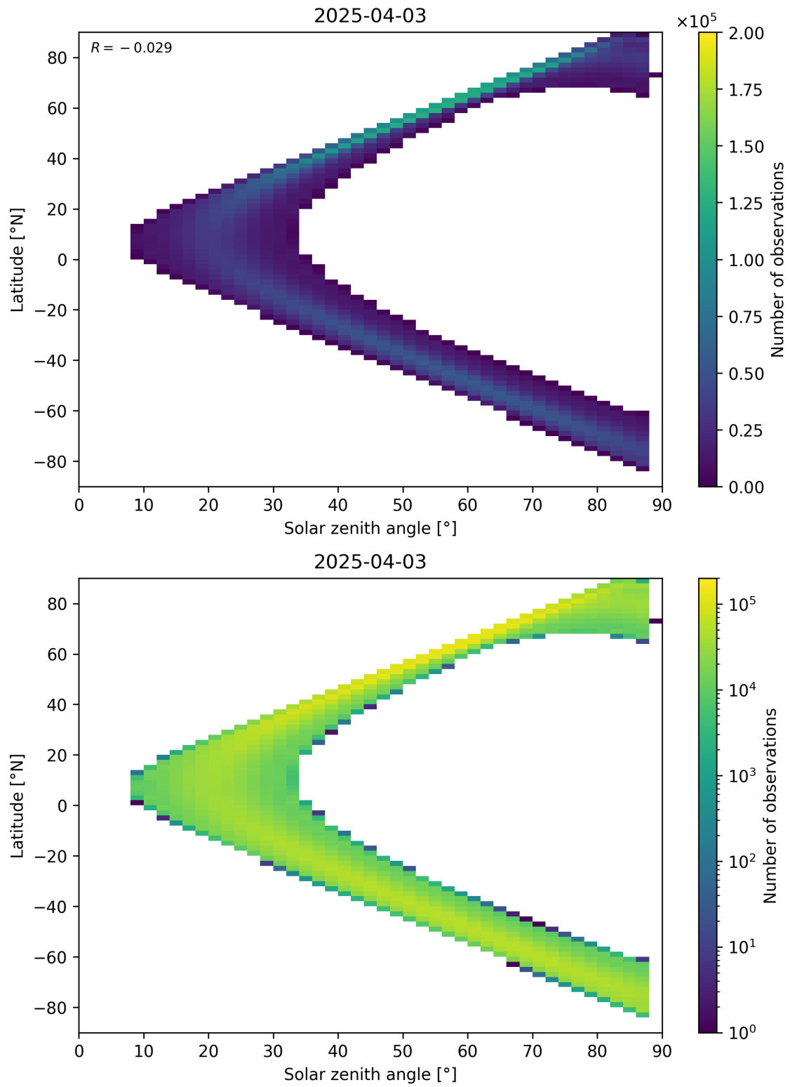
Figure 149: Scatter density plot of “Solar zenith angle” against “Latitude” for 2025-04-03 to 2025-04-04.
