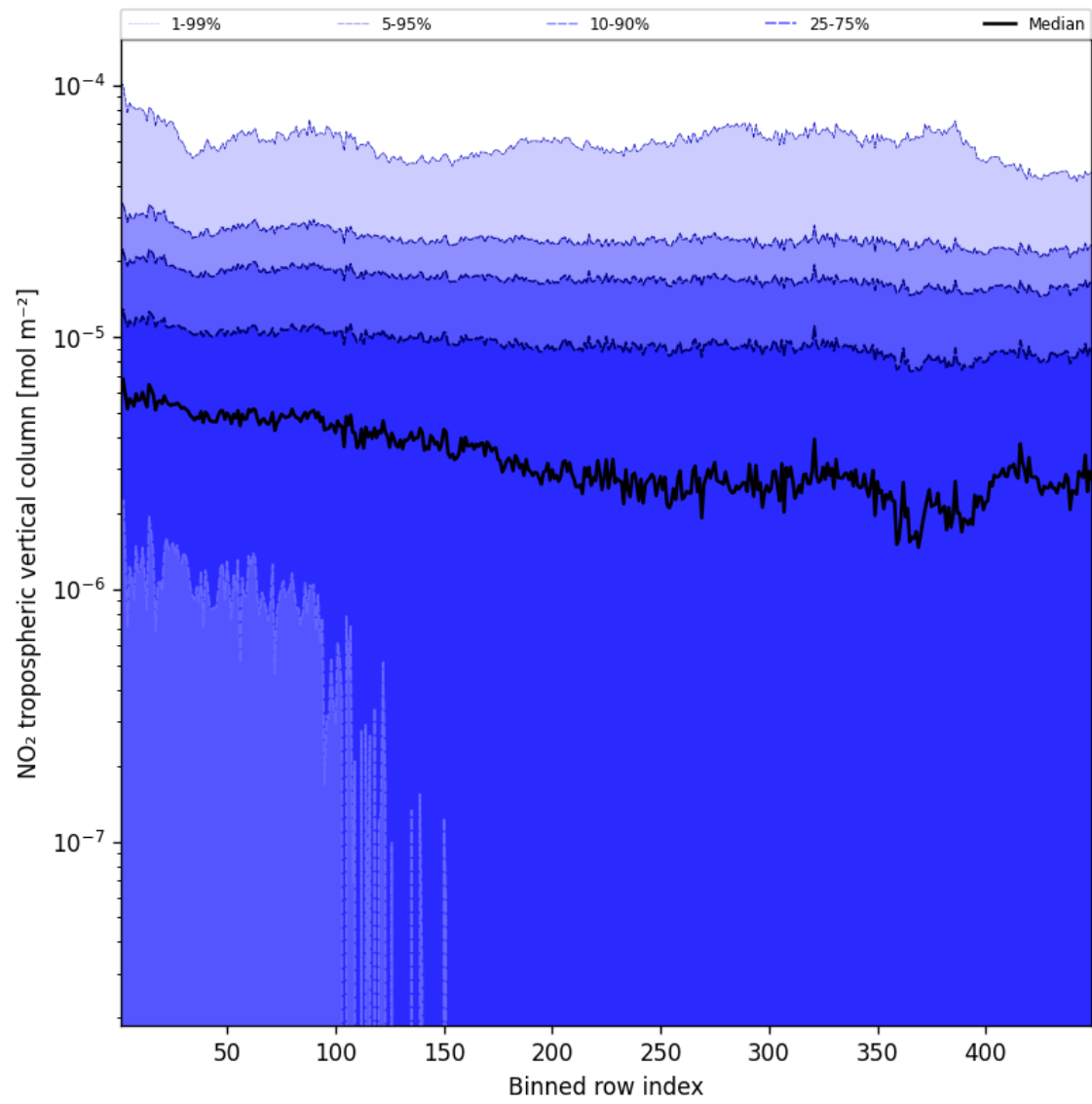
Figure 46: Along track statistics of “NO 2 tropospheric vertical column” for 2025-04-03 to 2025-04-04
