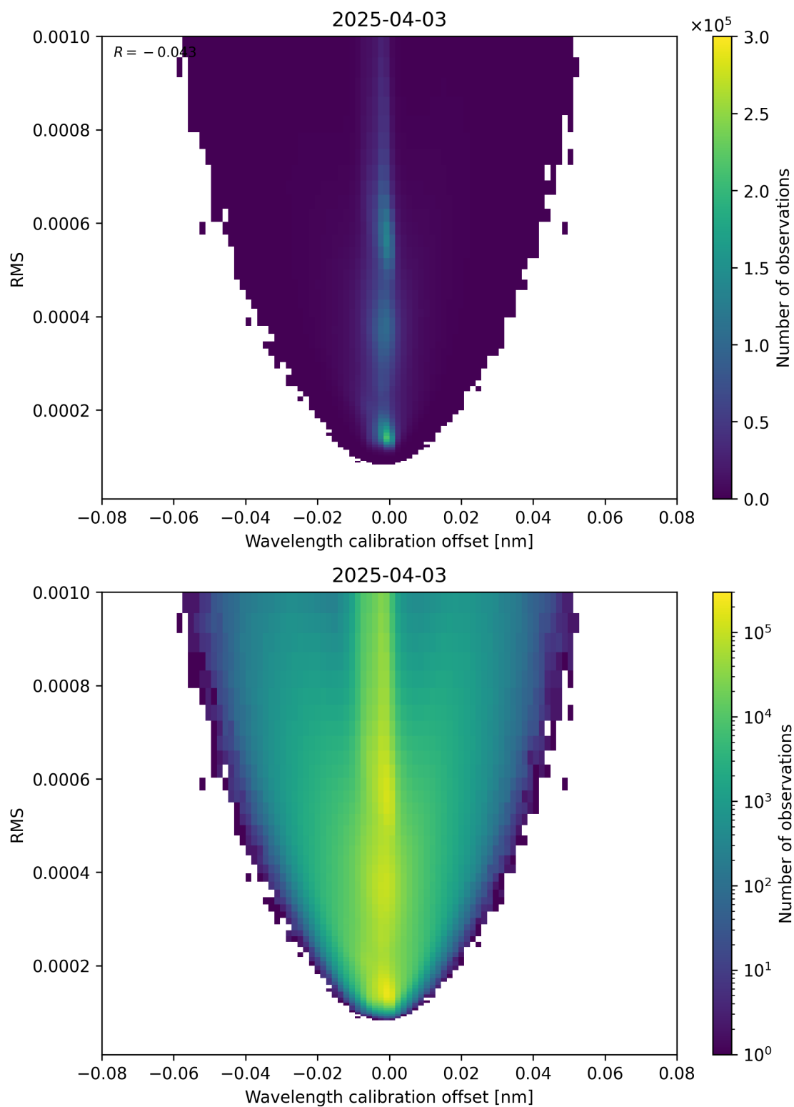
Figure 181: Scatter density plot of “Wavelength calibration offset” against “RMS” for 2025-04-03 to 2025-04-04.
