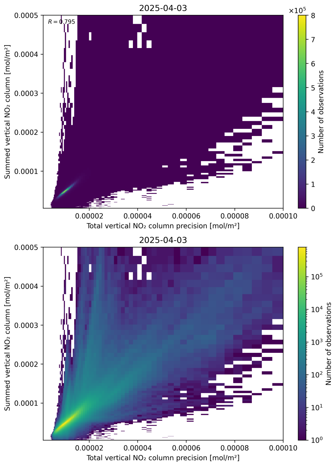
Figure 117: Scatter density plot of “Total vertical NO 2 column precision” against “Summed vertical NO 2 column” for 2025-04-03 to 2025-04-04.
