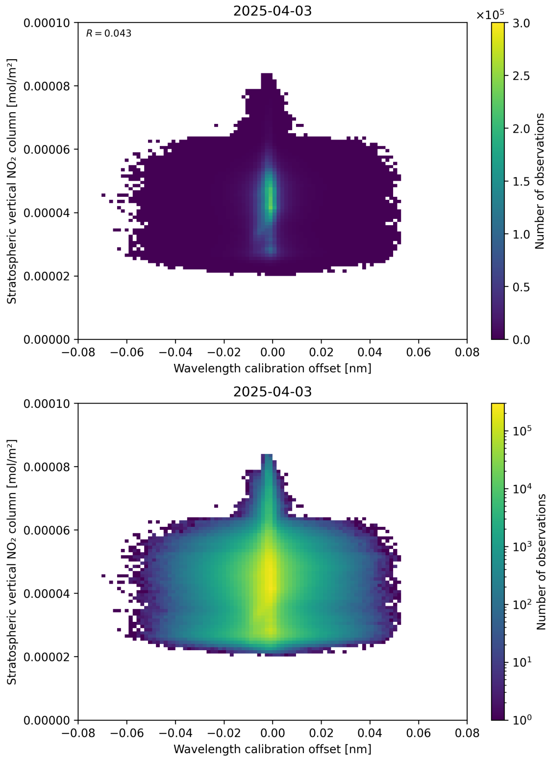
Figure 176: Scatter density plot of “Wavelength calibration offset” against “Stratospheric vertical NO 2 column” for 2025-04-03 to 2025-04-04.
