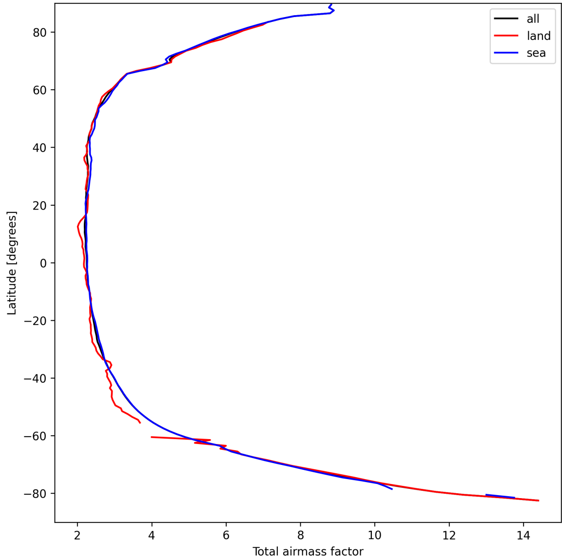
Figure 15: Zonal average of “Total airmass factor” for 2025-04-03 to 2025-04-04.
