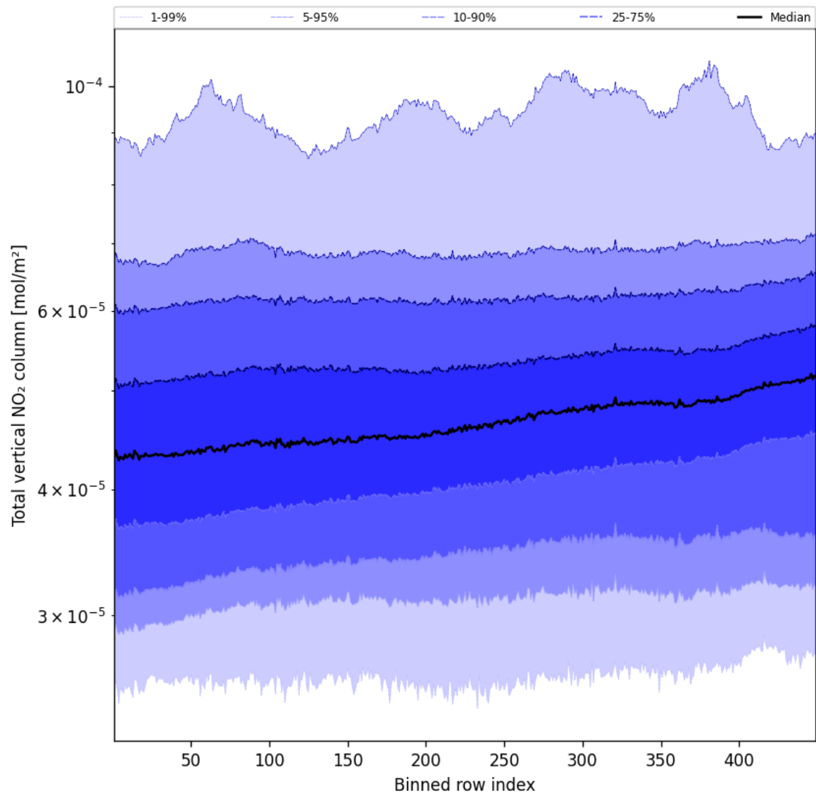
Figure 55: Along track statistics of “Total vertical NO 2 column” for 2025-04-03 to 2025-04-04
