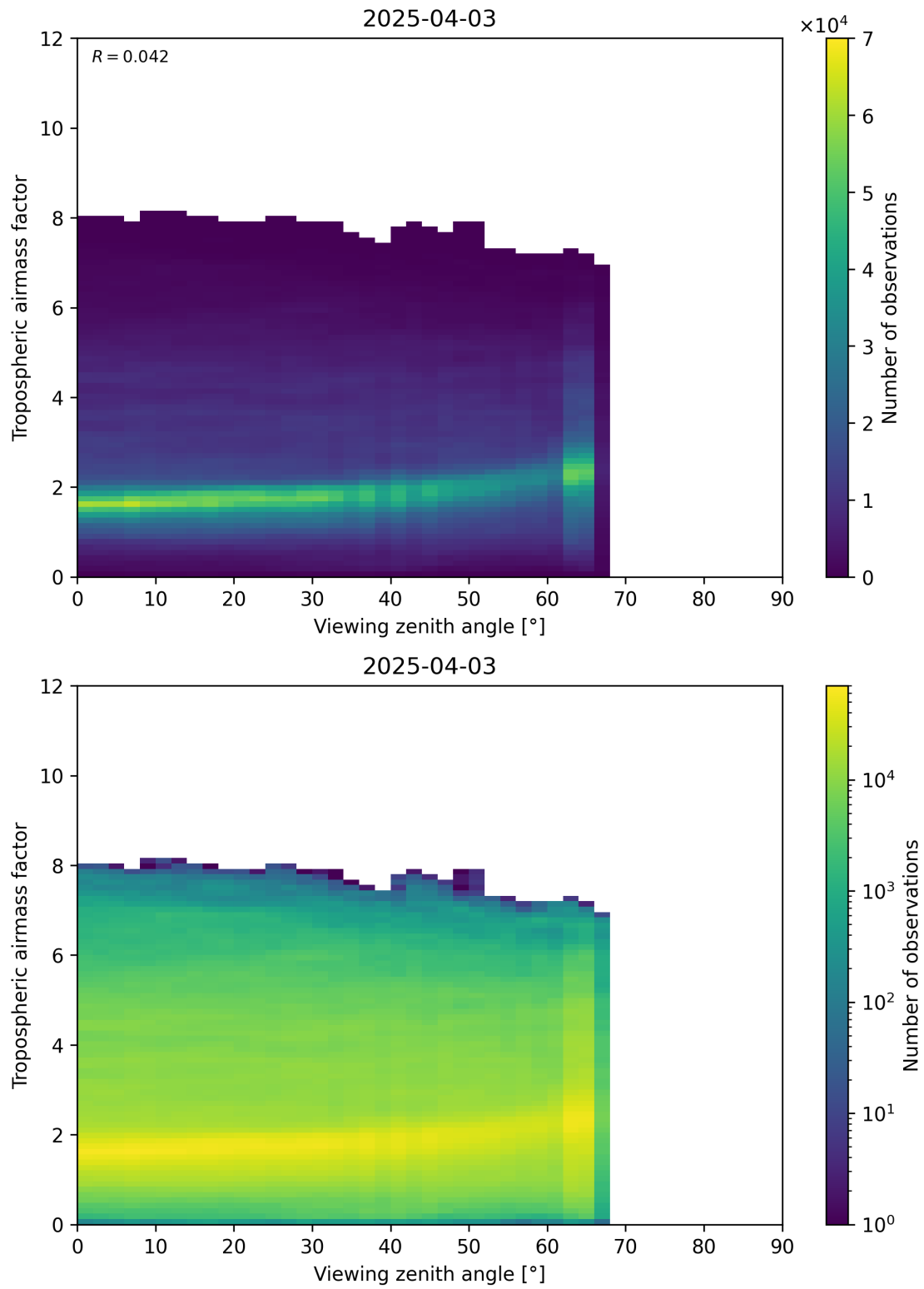
Figure 161: Scatter density plot of “Viewing zenith angle” against “Tropospheric airmass factor” for 2025-04-03 to 2025-04-04.
