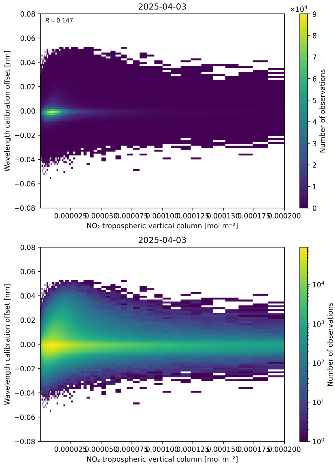
Figure 143: Scatter density plot of “NO 2 tropospheric vertical column” against “Wavelength calibration offset” for 2025-04-03 to 2025-04-04.
