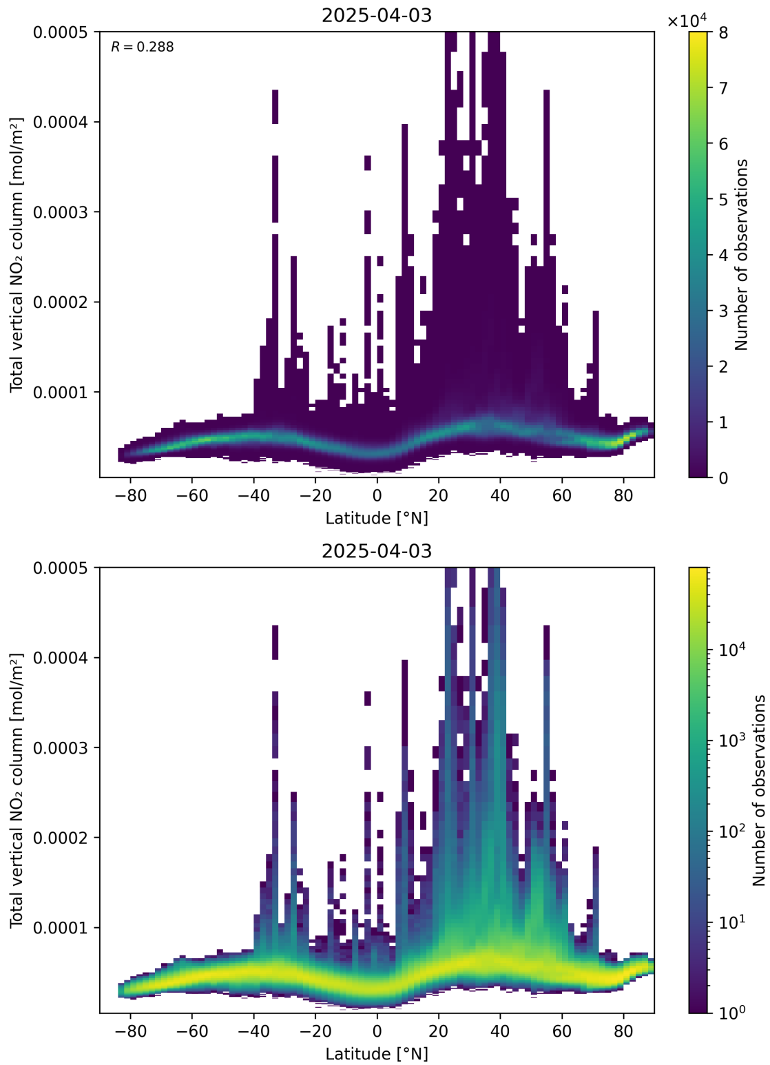
Figure 90: Scatter density plot of “Latitude” against “Total vertical NO 2 column” for 2025-04-03 to 2025-04-04.
