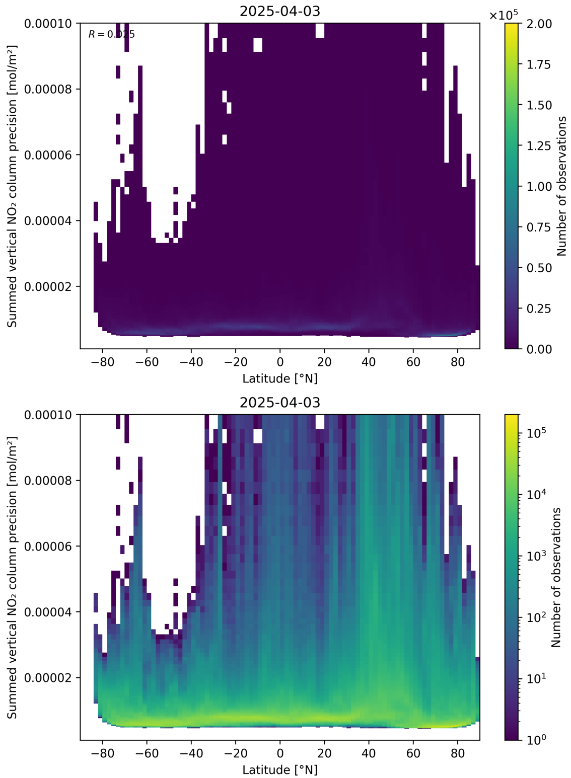
Figure 89: Scatter density plot of “Latitude” against “Summed vertical NO 2 column precision” for 2025-04-03 to 2025-04-04.
