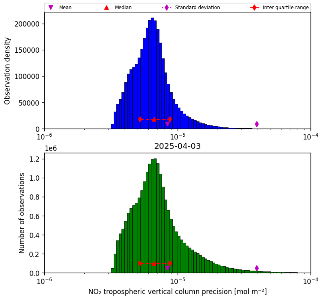
Figure 30: Histogram of “NO 2 tropospheric vertical column precision” for 2025-04-03 to 2025-04-04
