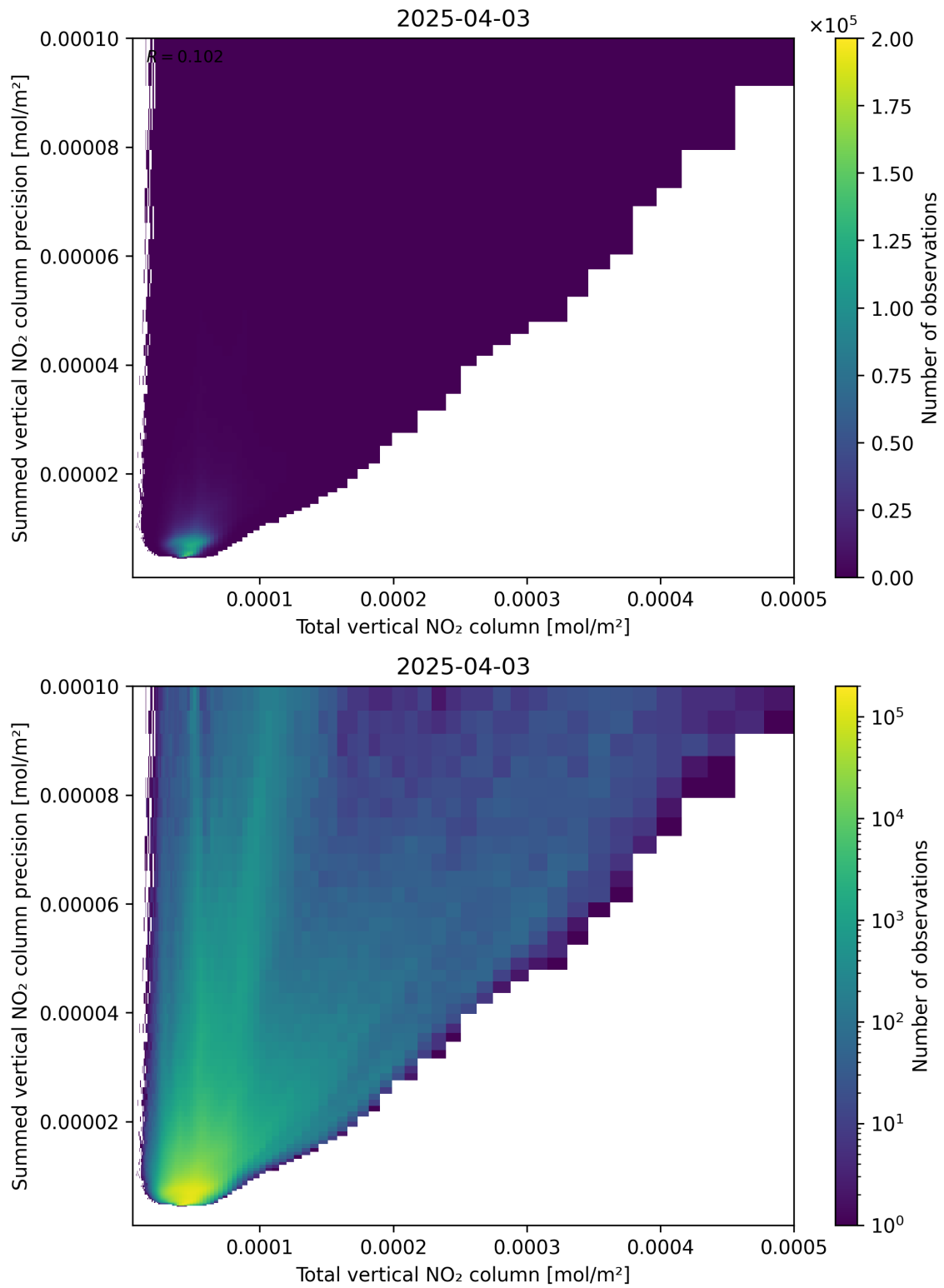
Figure 113: Scatter density plot of “Total vertical NO 2 column” against “Summed vertical NO 2 column precision” for 2025-04-03 to 2025-04-04.
