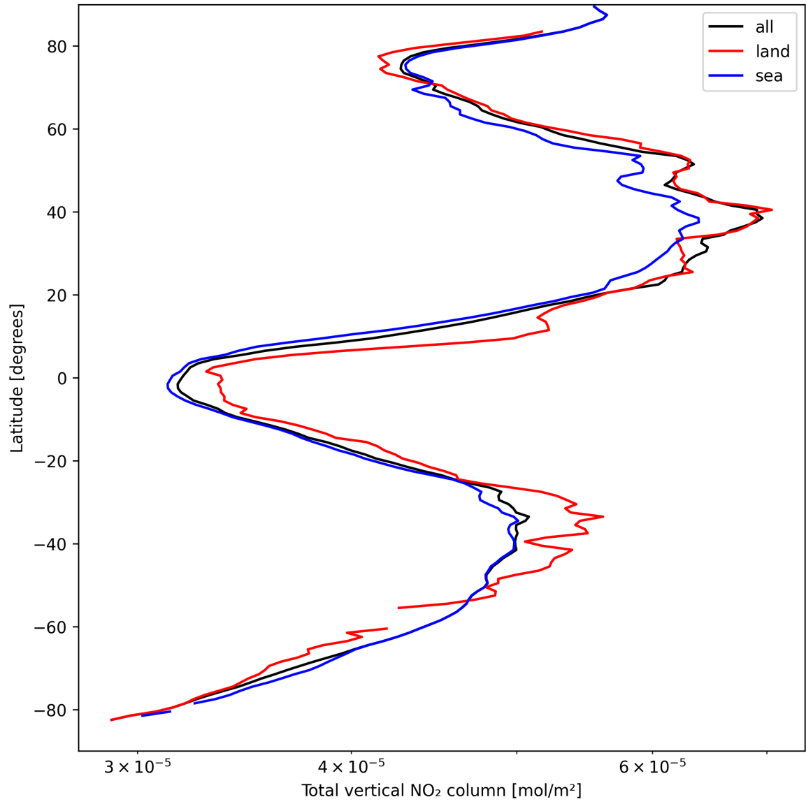
Figure 21: Zonal average of “Total vertical NO 2 column” for 2025-04-03 to 2025-04-04.
