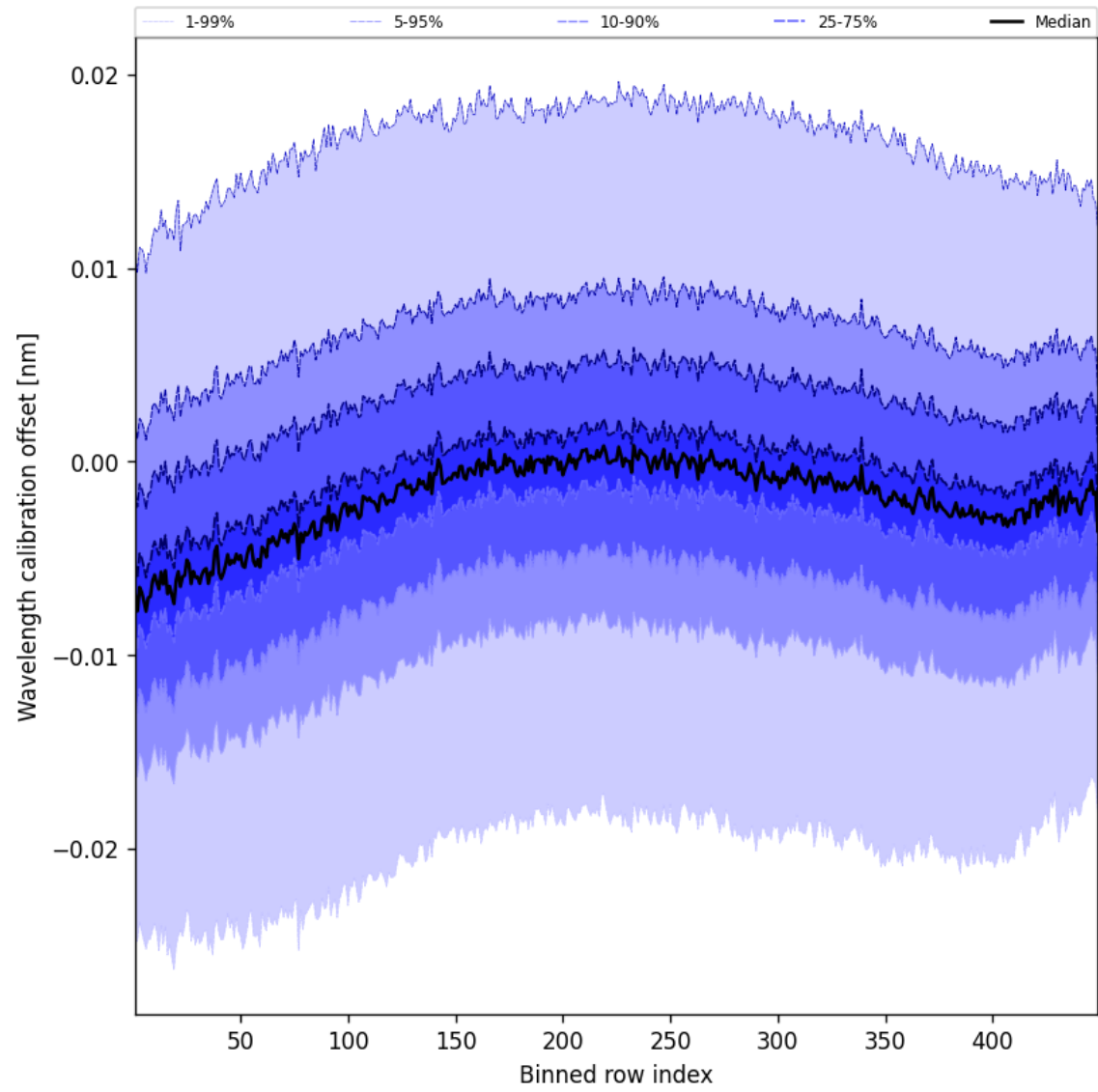
Figure 52: Along track statistics of “Wavelength calibration offset” for 2025-04-03 to 2025-04-04
