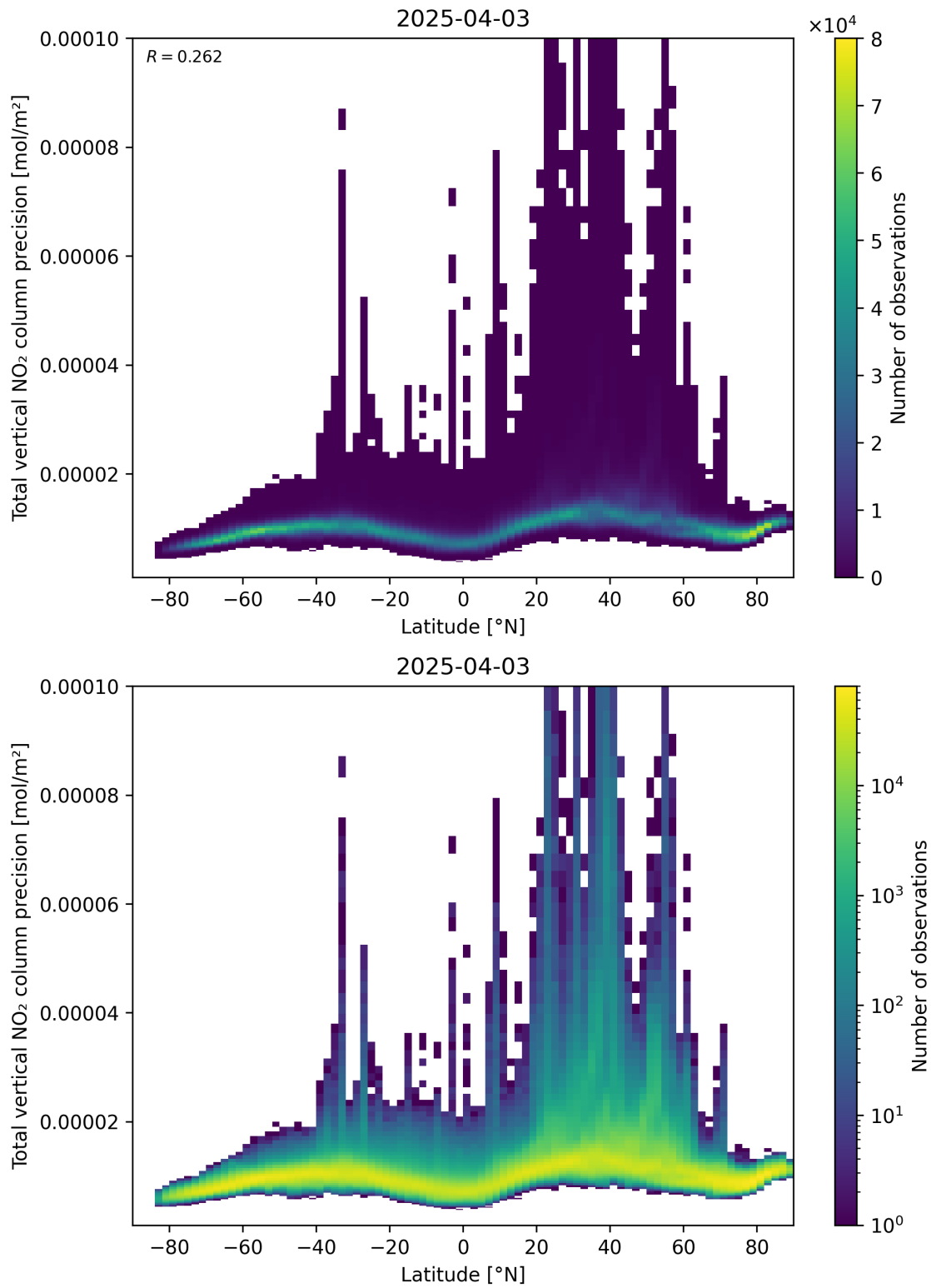
Figure 91: Scatter density plot of “Latitude” against “Total vertical NO 2 column precision” for 2025-04-03 to 2025-04-04.
