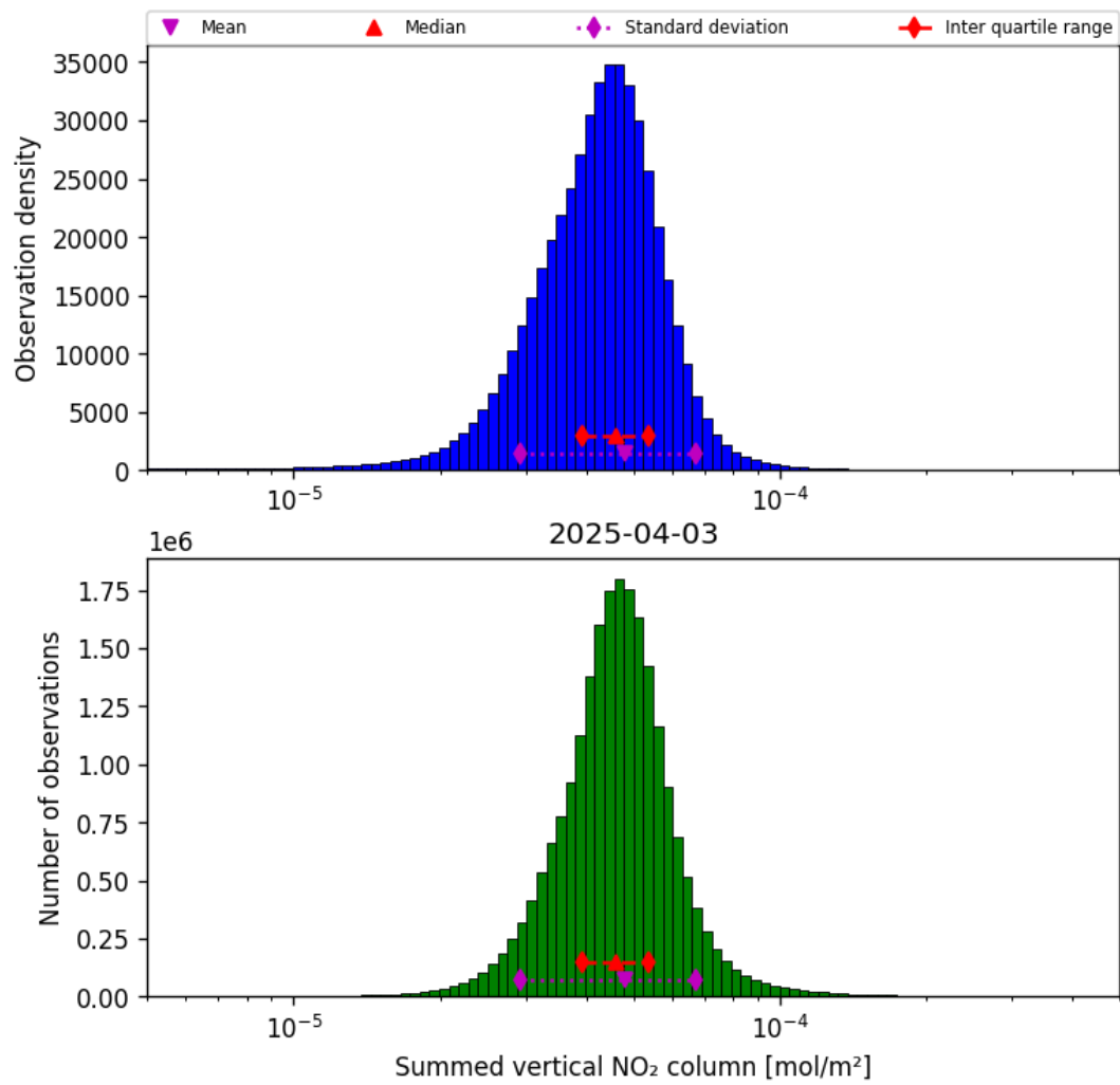
Figure 40: Histogram of “Summed vertical NO 2 column” for 2025-04-03 to 2025-04-04
