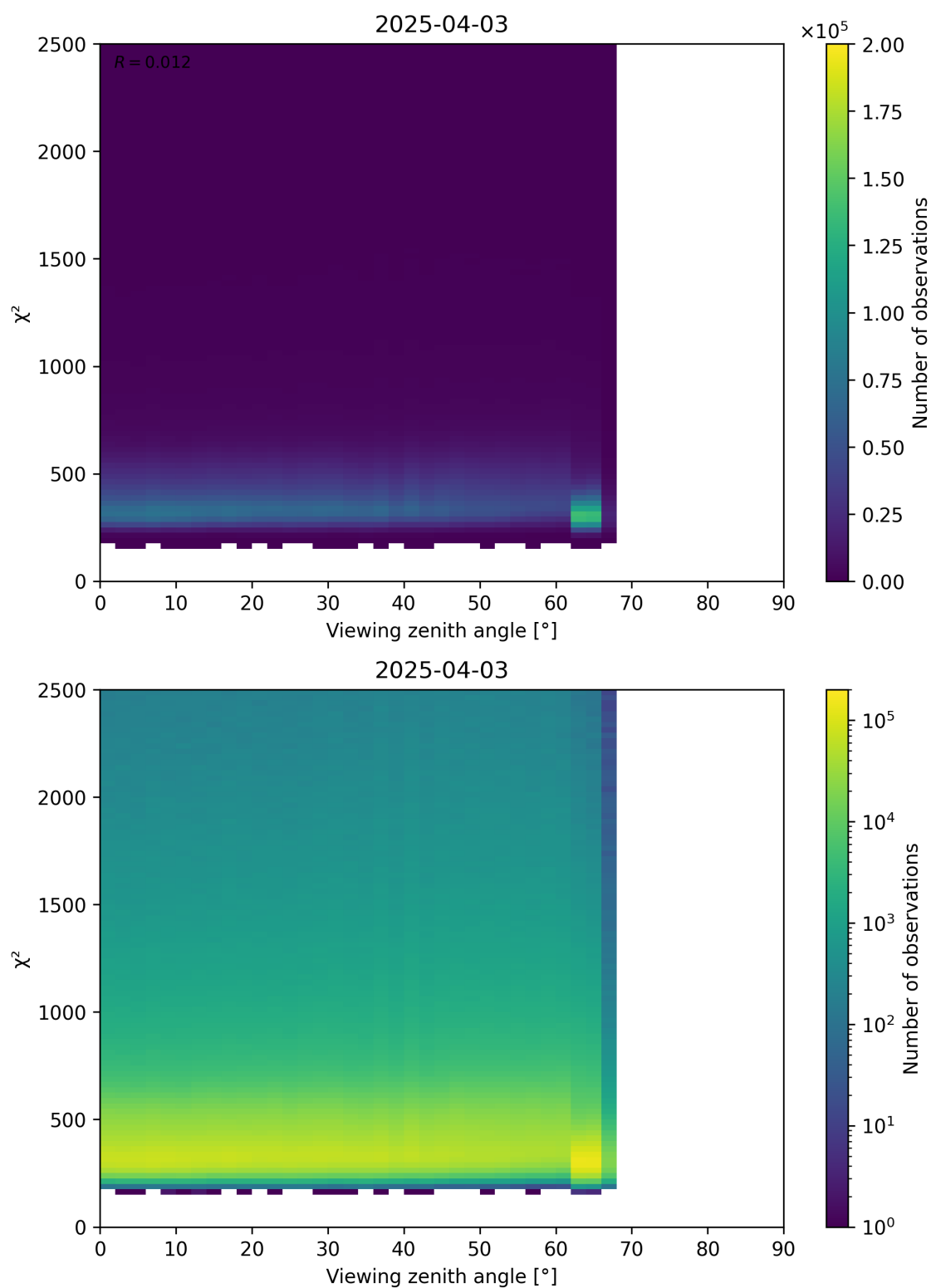
Figure 162: Scatter density plot of “Viewing zenith angle” against “ \chi^2 ” for 2025-04-03 to 2025-04-04.
