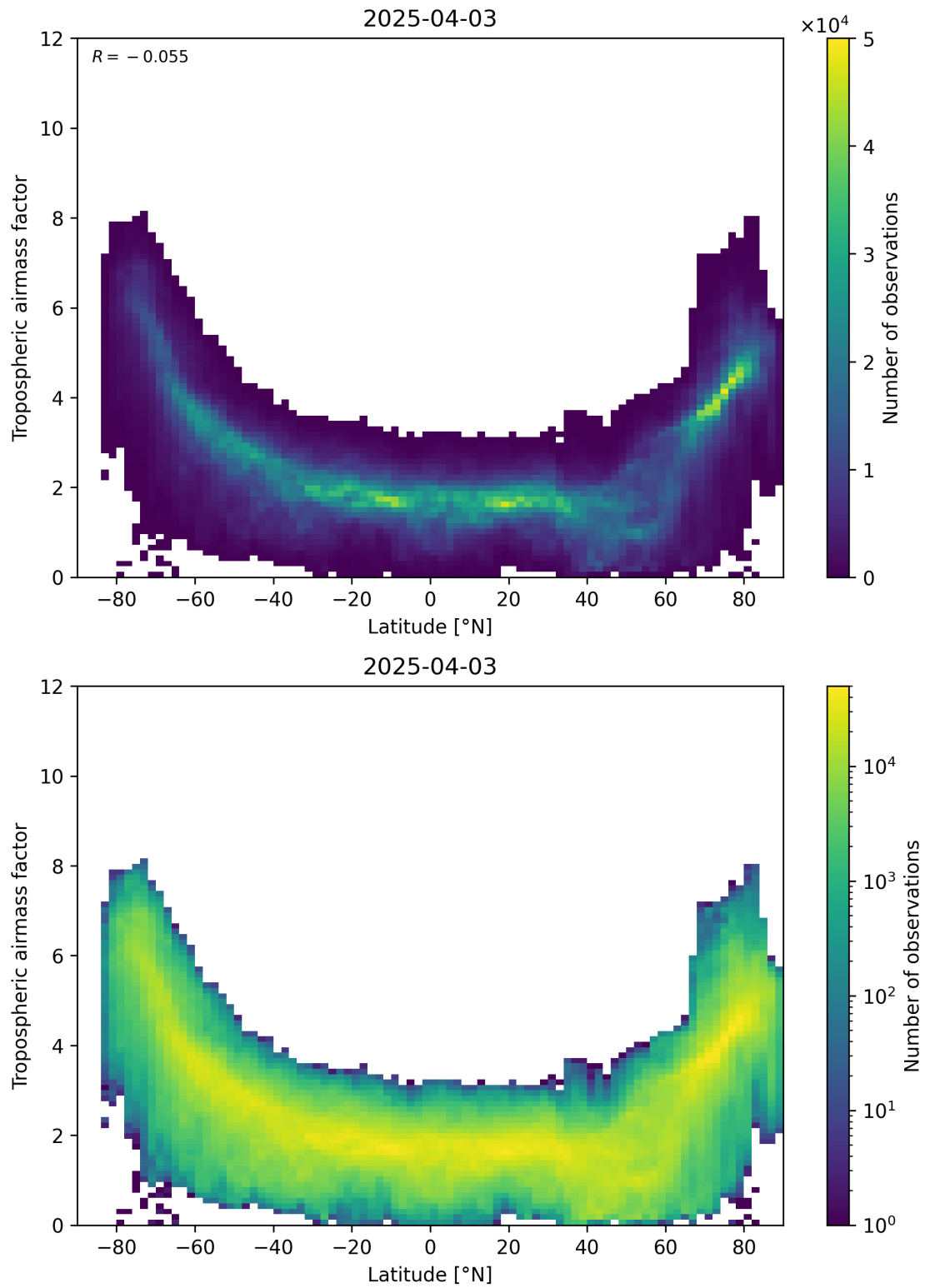
Figure 85: Scatter density plot of “Latitude” against “Tropospheric airmass factor” for 2025-04-03 to 2025-04-04.
