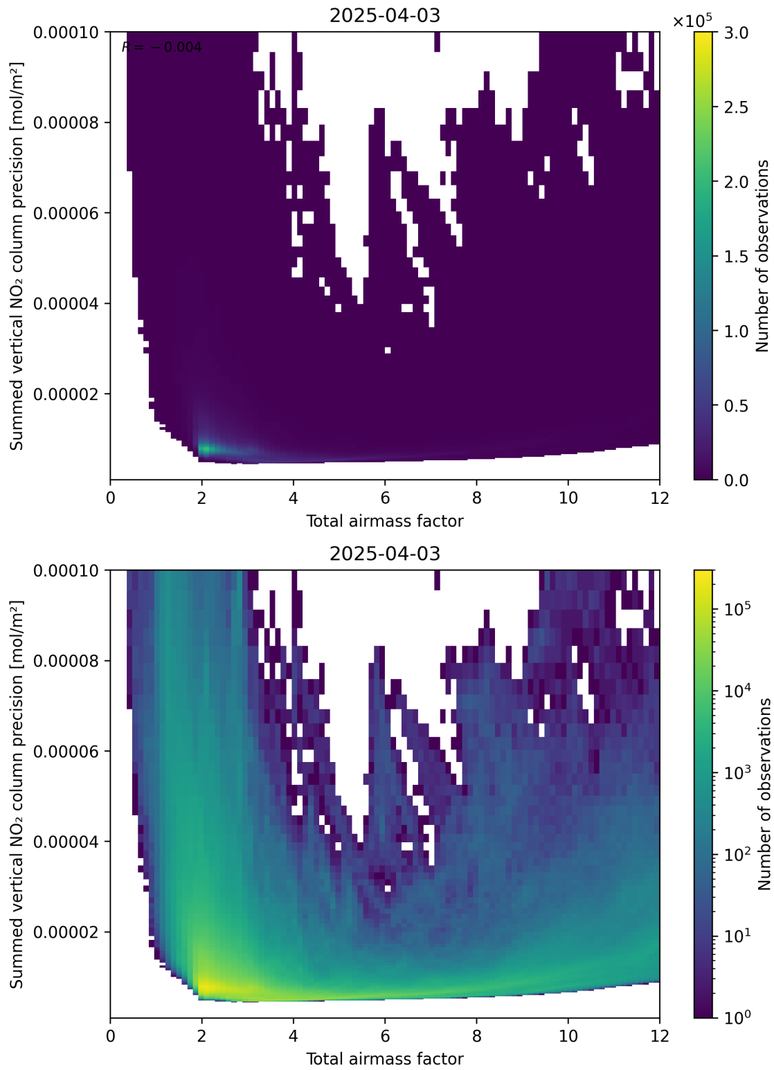
Figure 66: Scatter density plot of “Total airmass factor” against “Summed vertical NO 2 column precision” for 2025-04-03 to 2025-04-04.
