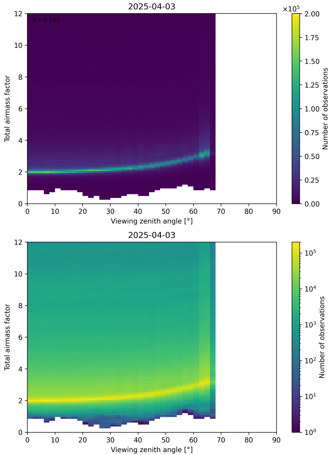
Figure 160: Scatter density plot of “Viewing zenith angle” against “Total airmass factor” for 2025-04-03 to 2025-04-04.
