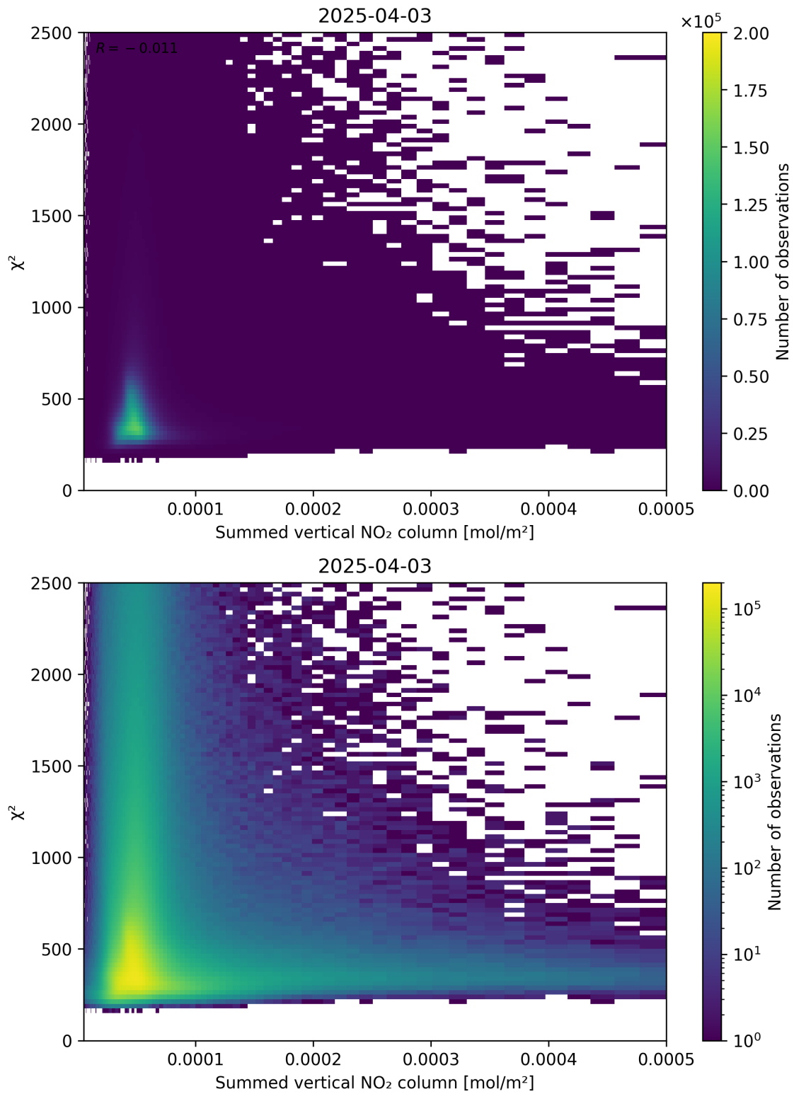
Figure 104: Scatter density plot of “Summed vertical NO 2 column” against “ \chi^2 ” for 2025-04-03 to 2025-04-04.
