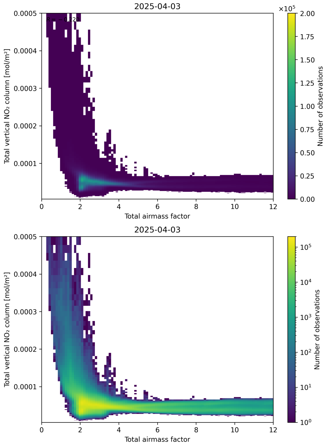
Figure 67: Scatter density plot of “Total airmass factor” against “Total vertical NO 2 column” for 2025-04-03 to 2025-04-04.
