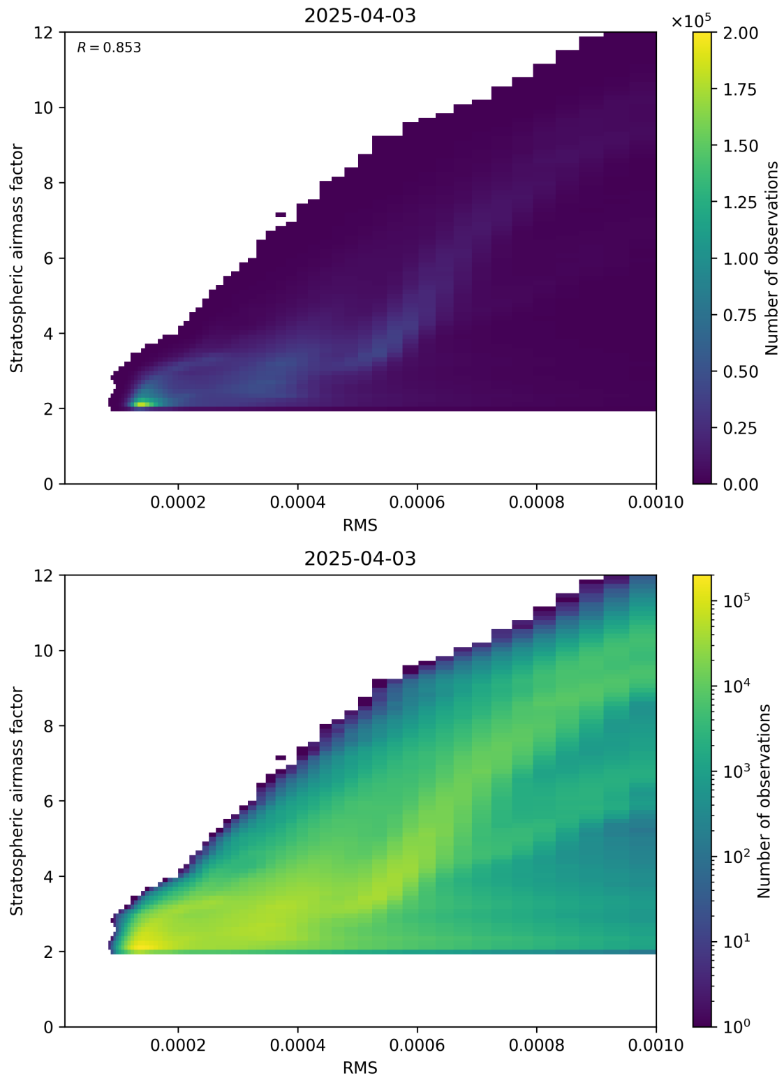
Figure 144: Scatter density plot of “RMS” against “Stratospheric airmass factor” for 2025-04-03 to 2025-04-04.
