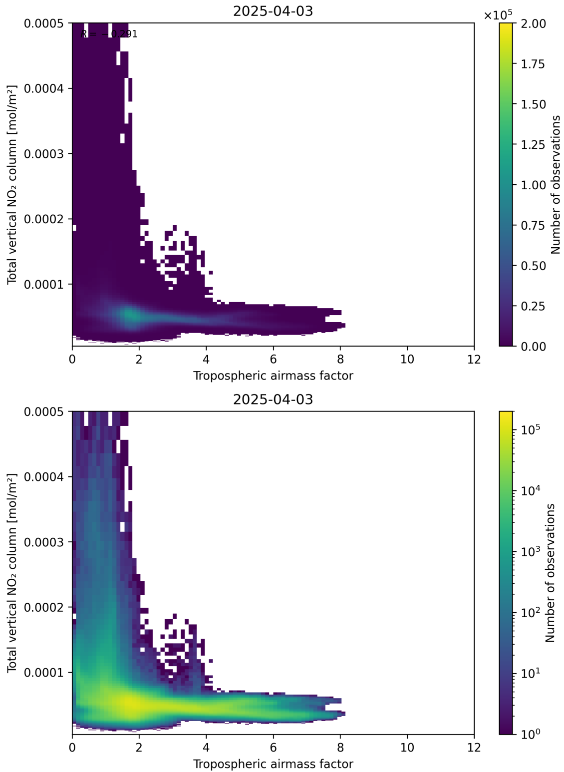
Figure 77: Scatter density plot of “Tropospheric airmass factor” against “Total vertical NO 2 column” for 2025-04-03 to 2025-04-04.
