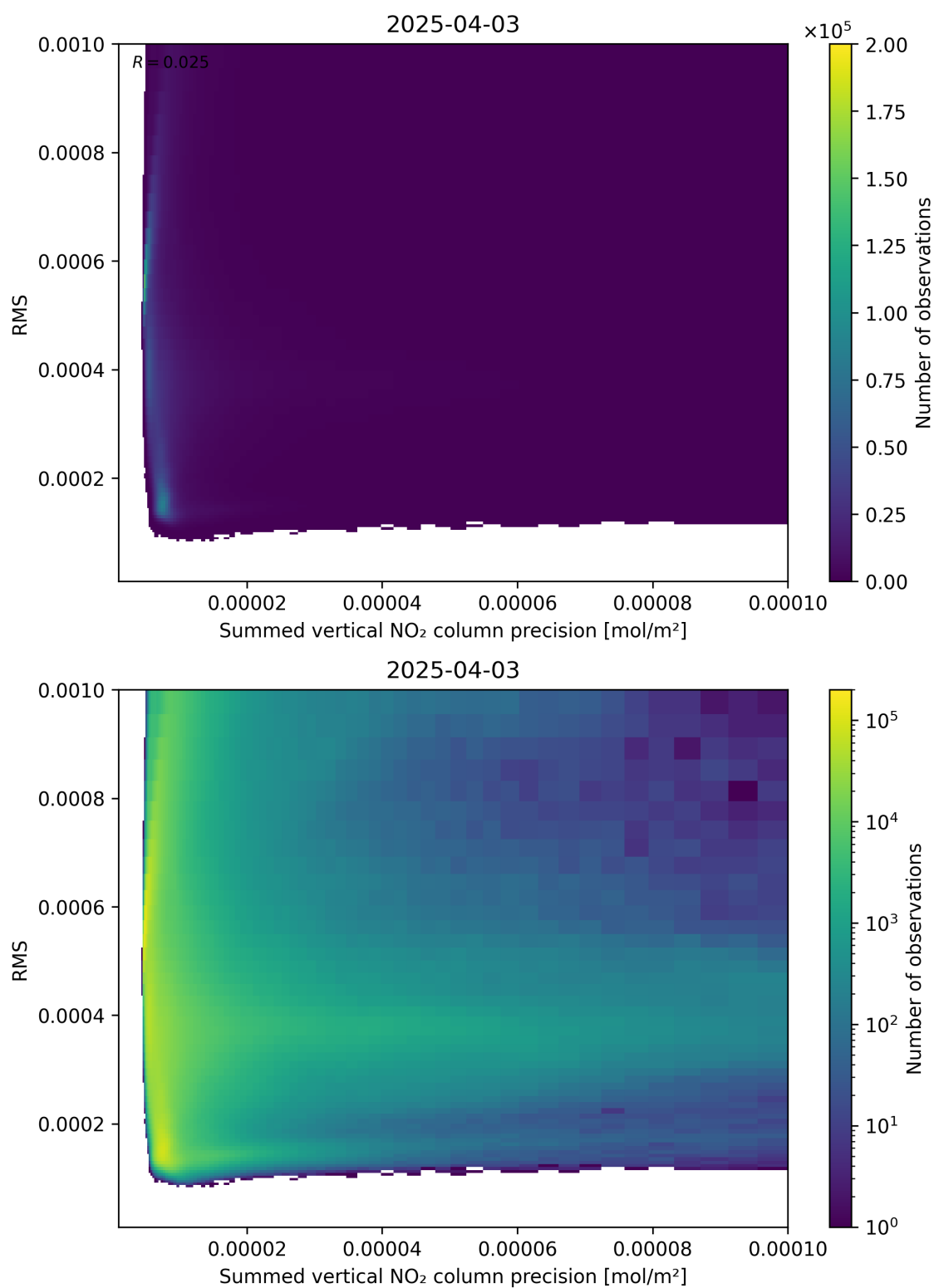
Figure 108: Scatter density plot of “Summed vertical NO 2 column precision” against “RMS” for 2025-04-03 to 2025-04-04.
