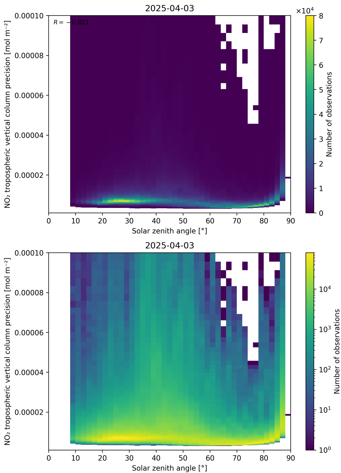
Figure 156: Scatter density plot of “Solar zenith angle” against “NO 2 tropospheric vertical column precision” for 2025-04-03 to 2025-04-04.
