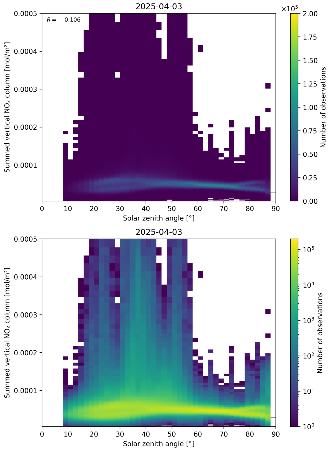
Figure 151: Scatter density plot of “Solar zenith angle” against “Summed vertical NO 2 column” for 2025-04-03 to 2025-04-04.
