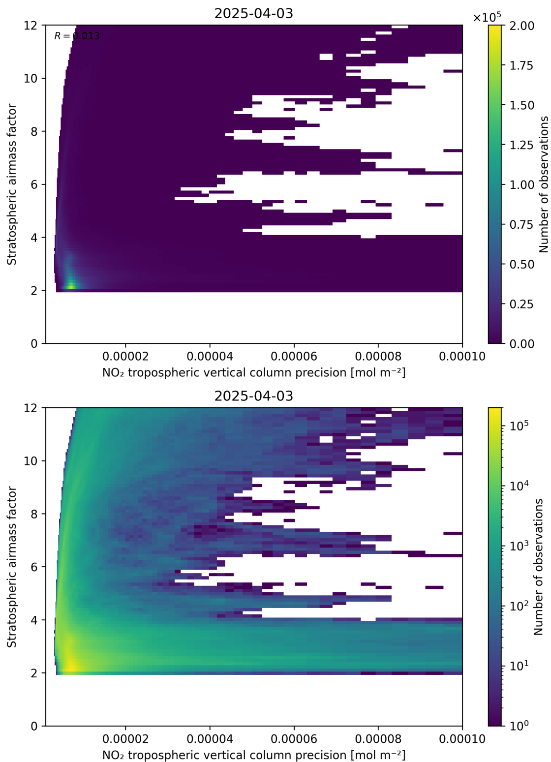
Figure 131: Scatter density plot of “NO 2 tropospheric vertical column precision” against “Stratospheric airmass factor” for 2025-04-03 to 2025-04-04.
