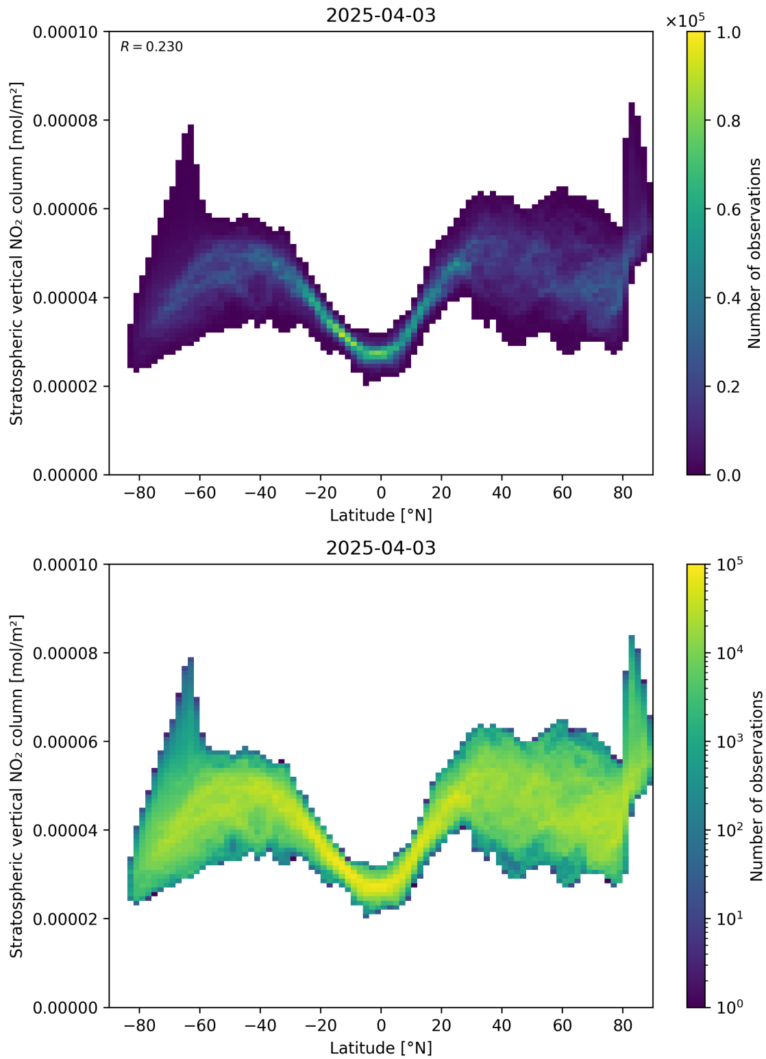
Figure 87: Scatter density plot of “Latitude” against “Stratospheric vertical NO 2 column” for 2025-04-03 to 2025-04-04.
