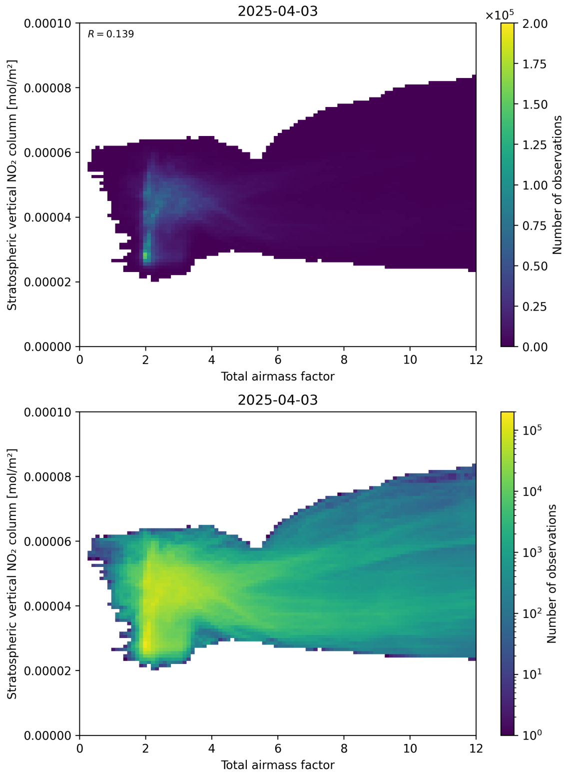
Figure 64: Scatter density plot of “Total airmass factor” against “Stratospheric vertical NO 2 column” for 2025-04-03 to 2025-04-04.
