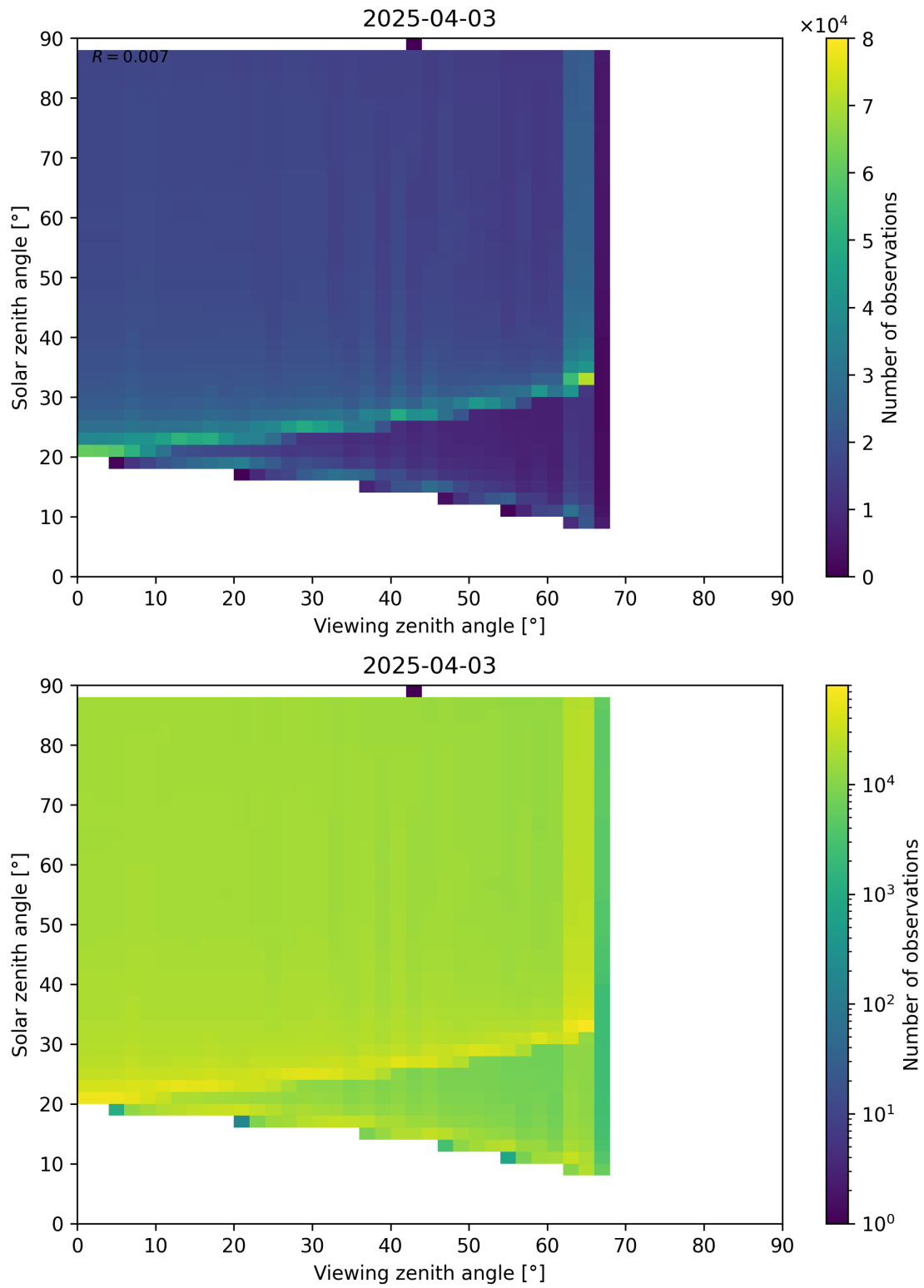
Figure 172: Scatter density plot of “Viewing zenith angle” against “Solar zenith angle” for 2025-04-03 to 2025-04-04.
