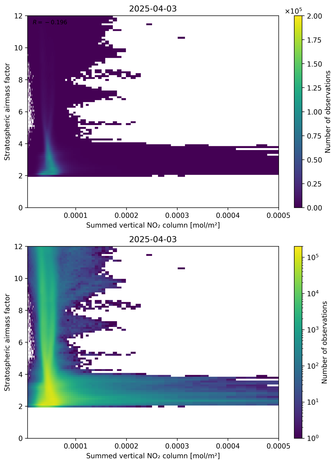
Figure 103: Scatter density plot of “Summed vertical NO 2 column” against “Stratospheric air mass factor” for 2025-04-03 to 2025-04-04.
