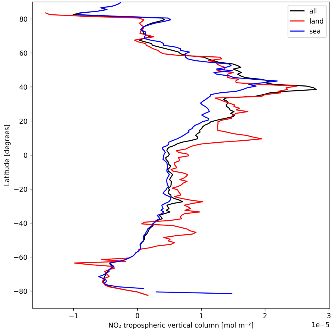
Figure 12: Zonal average of “NO 2 tropospheric vertical column” for 2025-04-03 to 2025-04-04.
