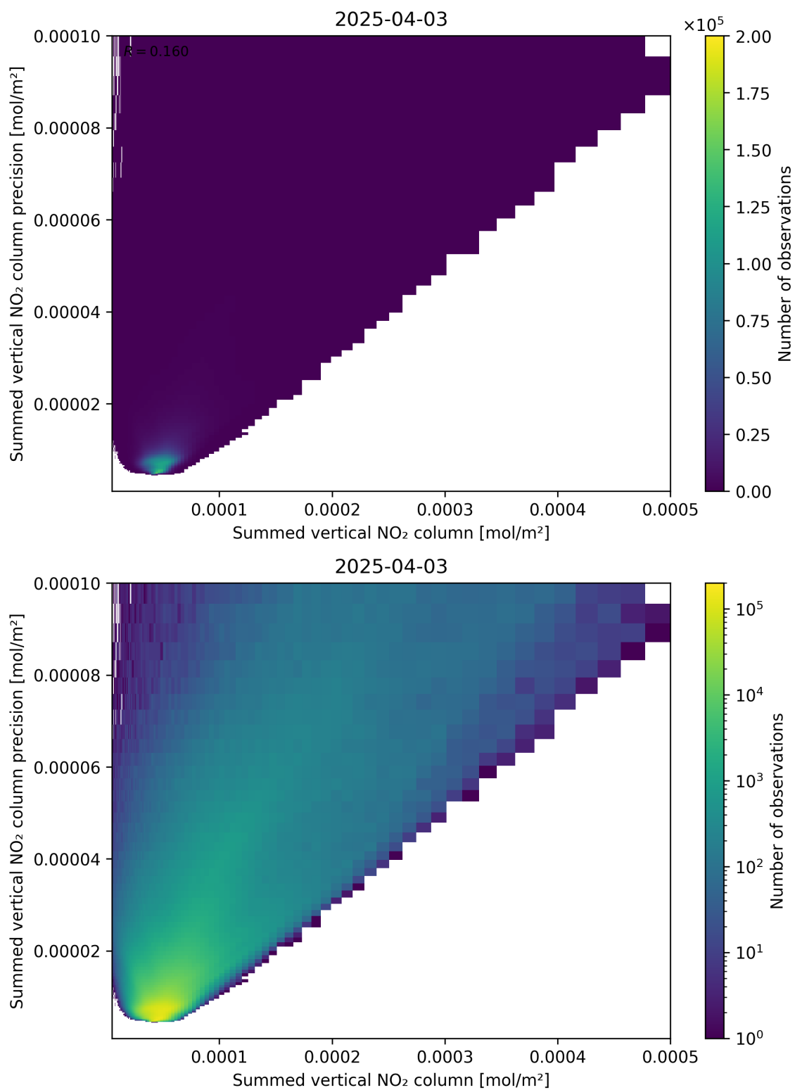
Figure 105: Scatter density plot of “Summed vertical NO 2 column” against “Summed vertical NO 2 column precision” for 2025-04-03 to 2025-04-04.
