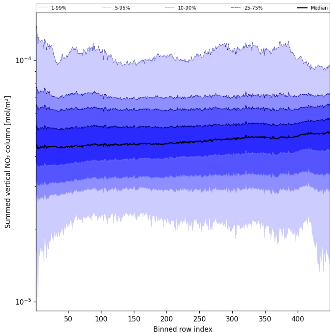
Figure 57: Along track statistics of “Summed vertical NO 2 column” for 2025-04-03 to 2025-04-04
