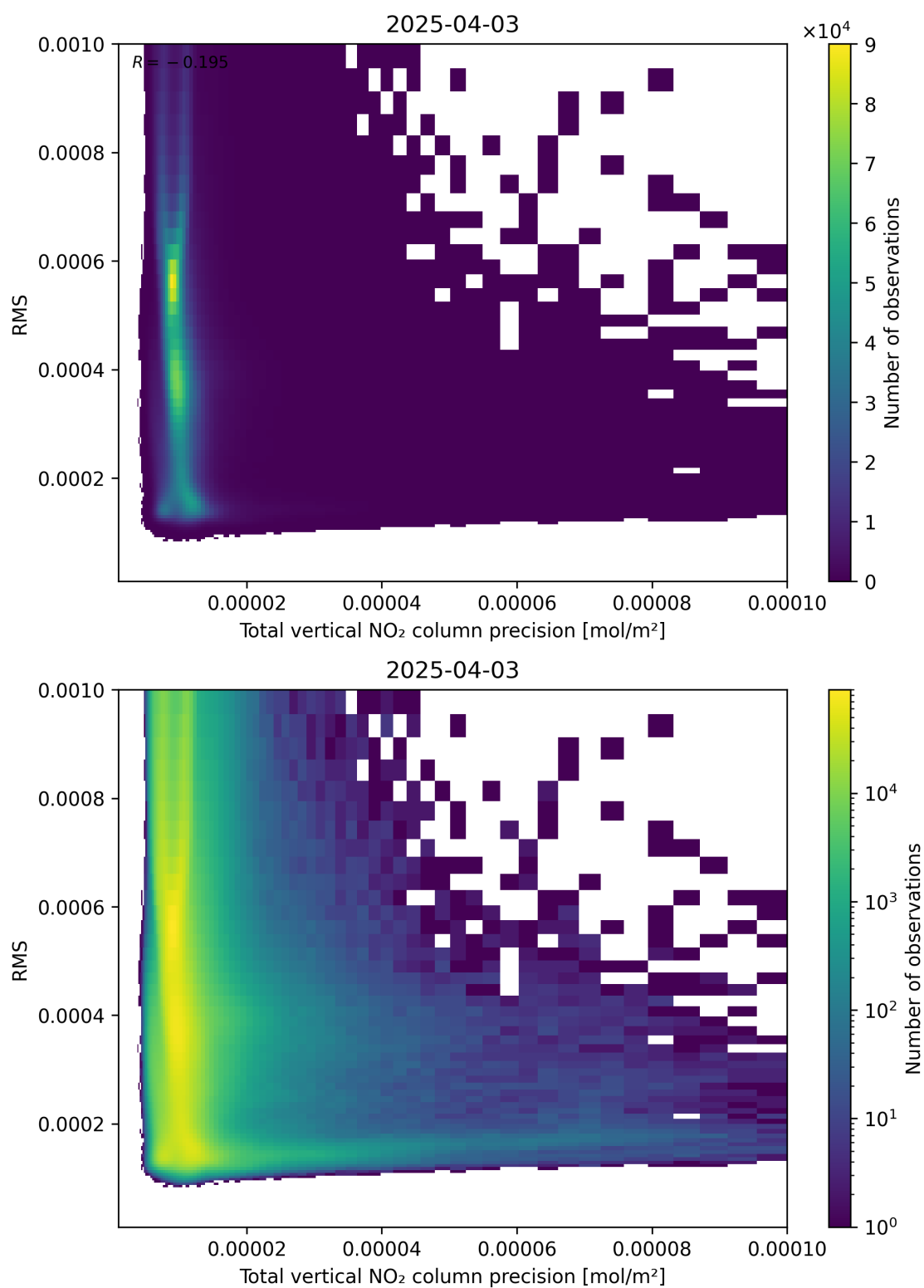
Figure 119: Scatter density plot of “Total vertical NO 2 column precision” against “RMS” for 2025-04-03 to 2025-04-04.
