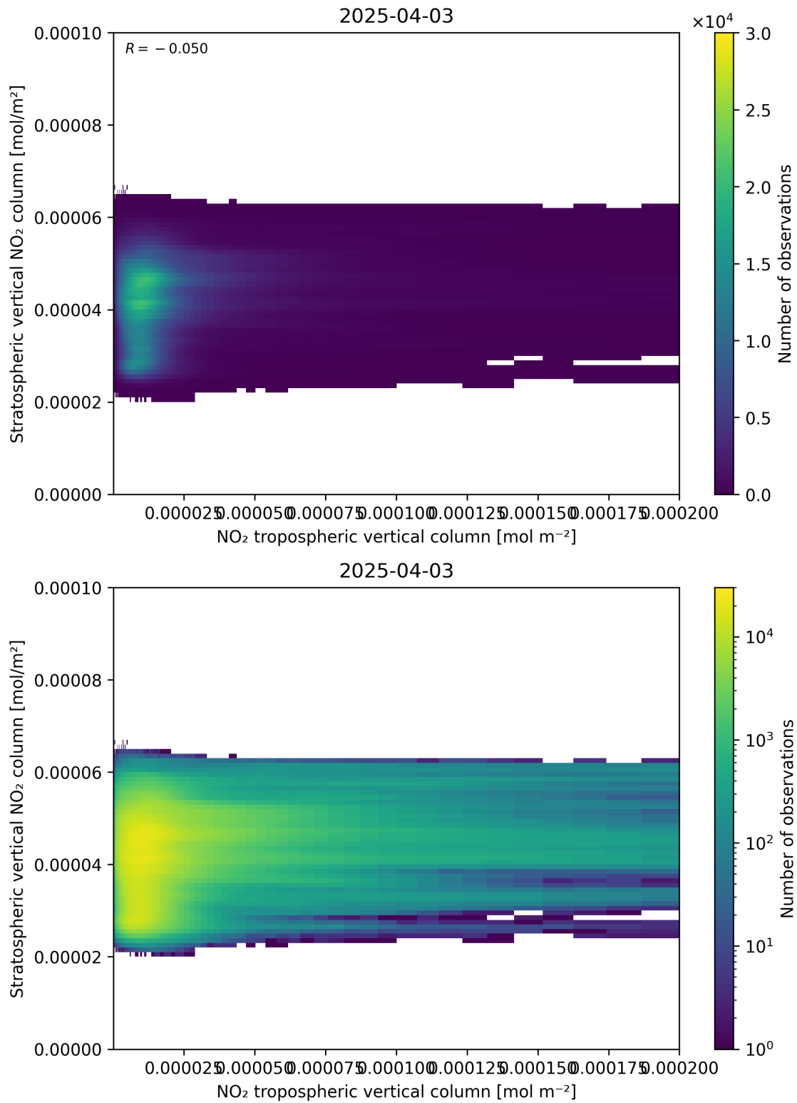
Figure 125: Scatter density plot of “NO 2 tropospheric vertical column” against “Stratospheric vertical NO 2 column” for 2025-04-03 to 2025-04-04.
