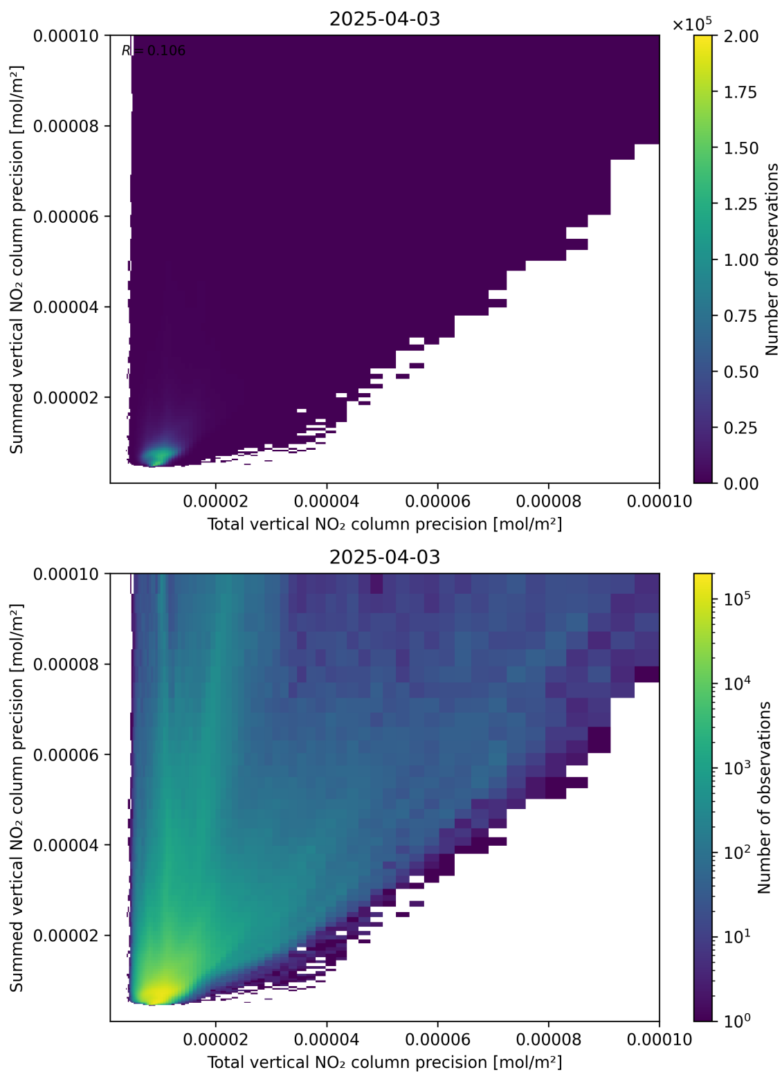
Figure 118: Scatter density plot of “Total vertical NO 2 column precision” against “Summed vertical NO 2 column precision” for 2025-04-03 to 2025-04-04.
