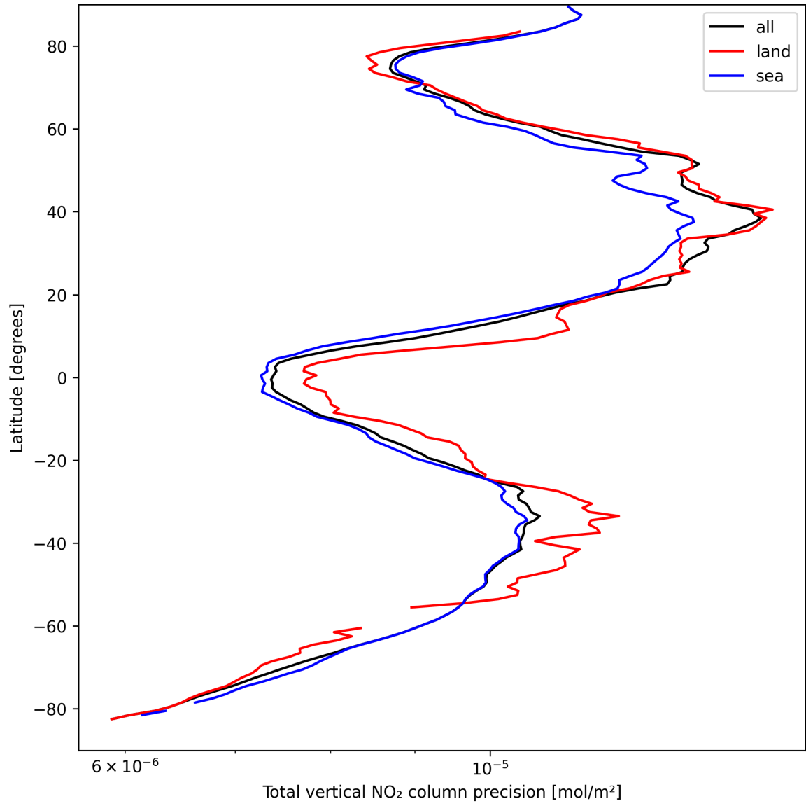
Figure 22: Zonal average of “Total vertical NO 2 column precision” for 2025-04-03 to 2025-04-04.
