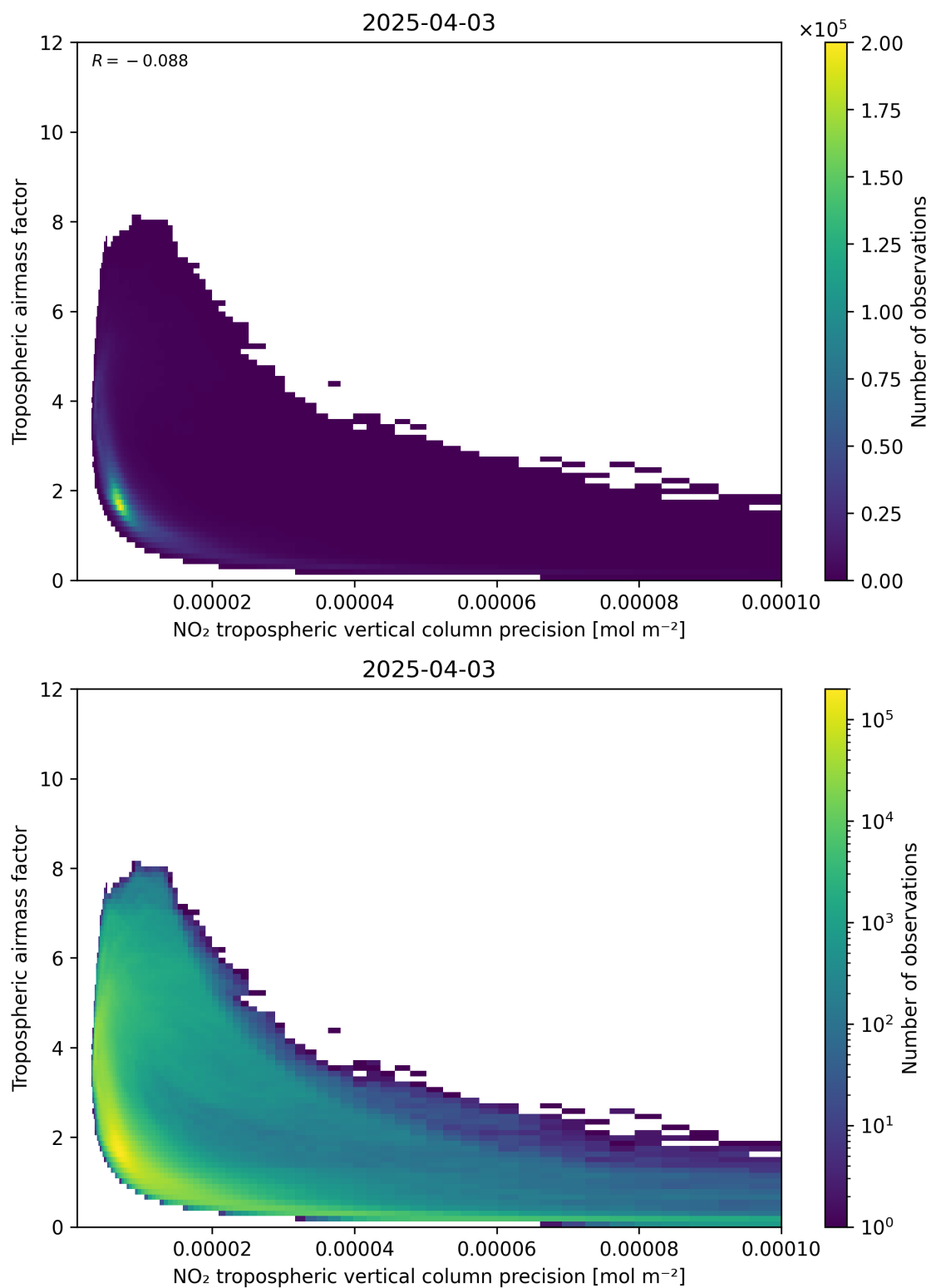
Figure 133: Scatter density plot of “NO 2 tropospheric vertical column precision” against “Tropospheric airmass factor” for 2025-04-03 to 2025-04-04.
