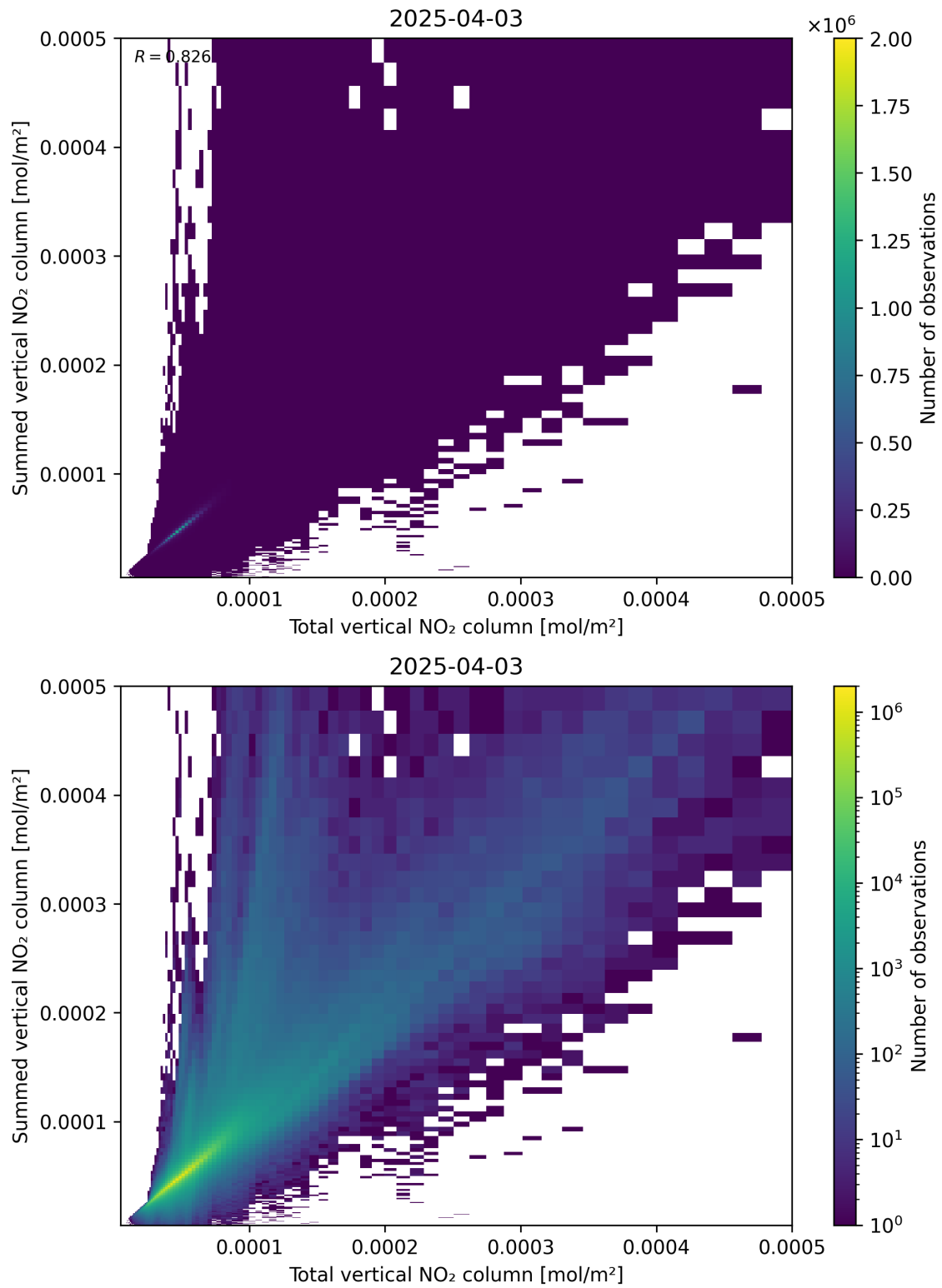
Figure 112: Scatter density plot of “Total vertical NO 2 column” against “Summed vertical NO 2 column” for 2025-04-03 to 2025-04-04.
