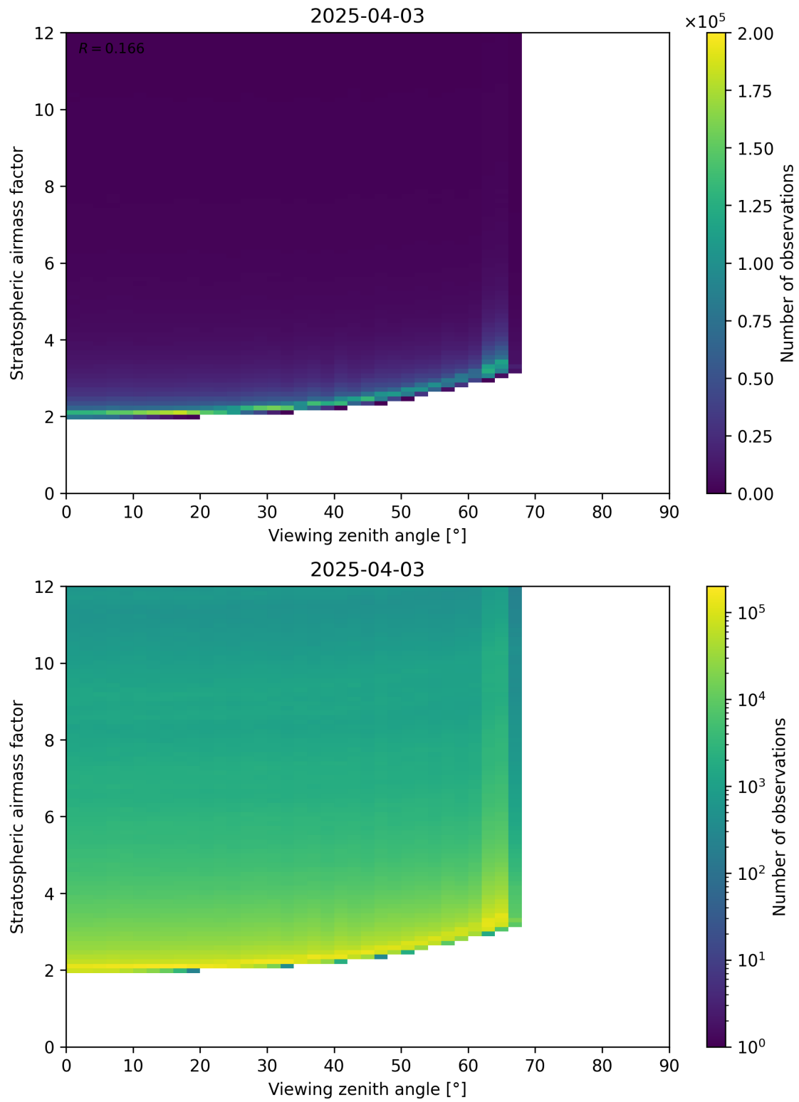
Figure 159: Scatter density plot of “Viewing zenith angle” against “Stratospheric airmass factor” for 2025-04-03 to 2025-04-04.
