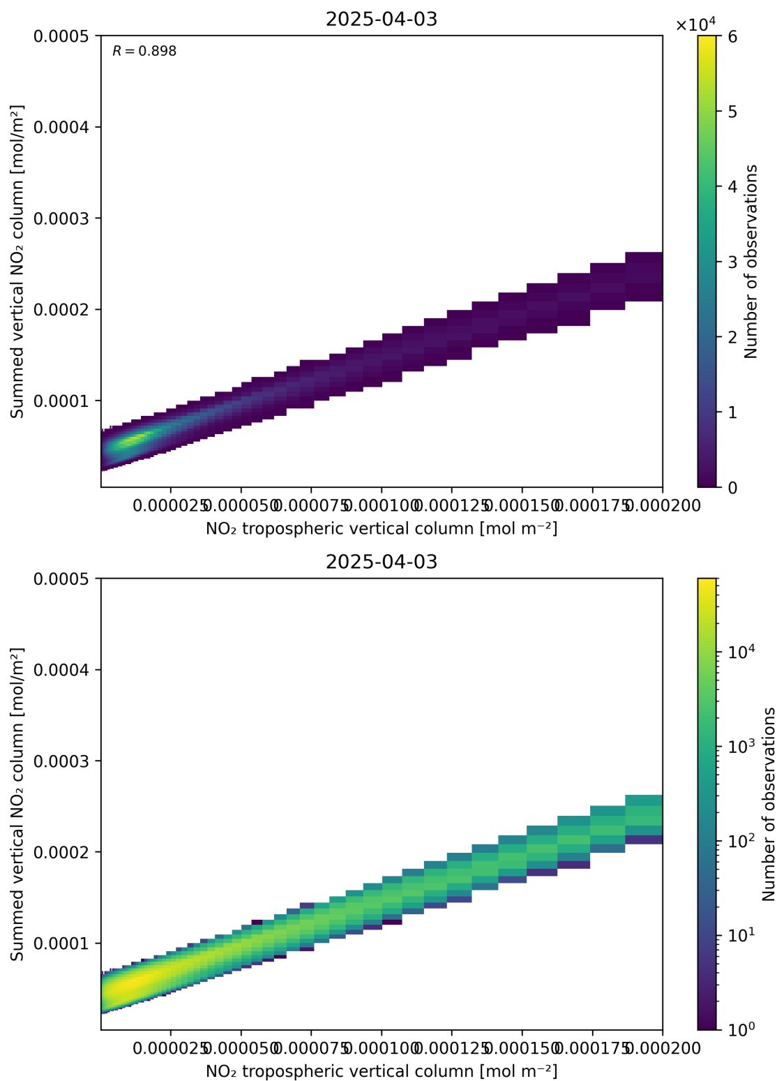
Figure 126: Scatter density plot of “NO 2 tropospheric vertical column” against “Summed vertical NO 2 column” for 2025-04-03 to 2025-04-04.
