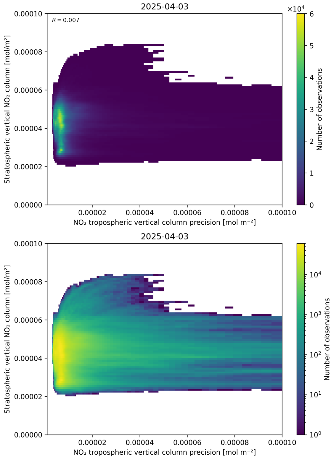
Figure 135: Scatter density plot of “NO 2 tropospheric vertical column precision” against “Stratospheric vertical NO 2 column” for 2025-04-03 to 2025-04-04.
