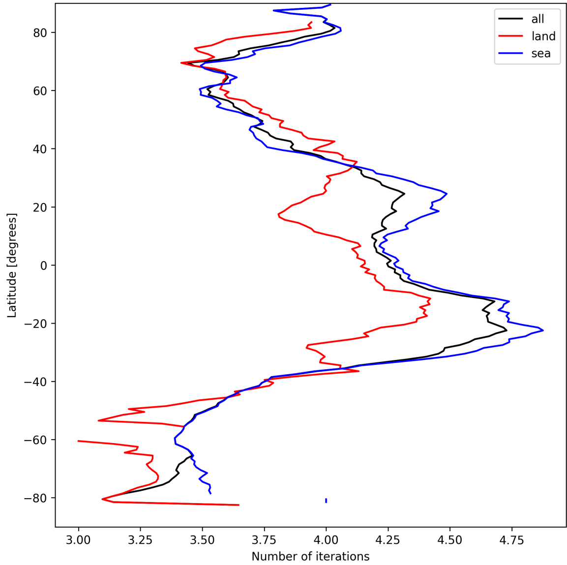
Figure 17: Zonal average of “Number of iterations” for 2025-04-03 to 2025-04-04.
