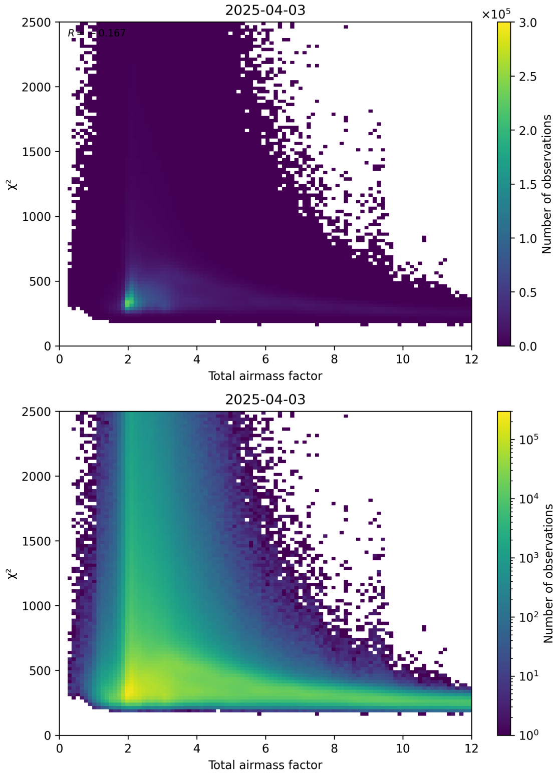
Figure 63: Scatter density plot of “Total airmass factor” against “ \chi^2 ” for 2025-04-03 to 2025-04-04.
