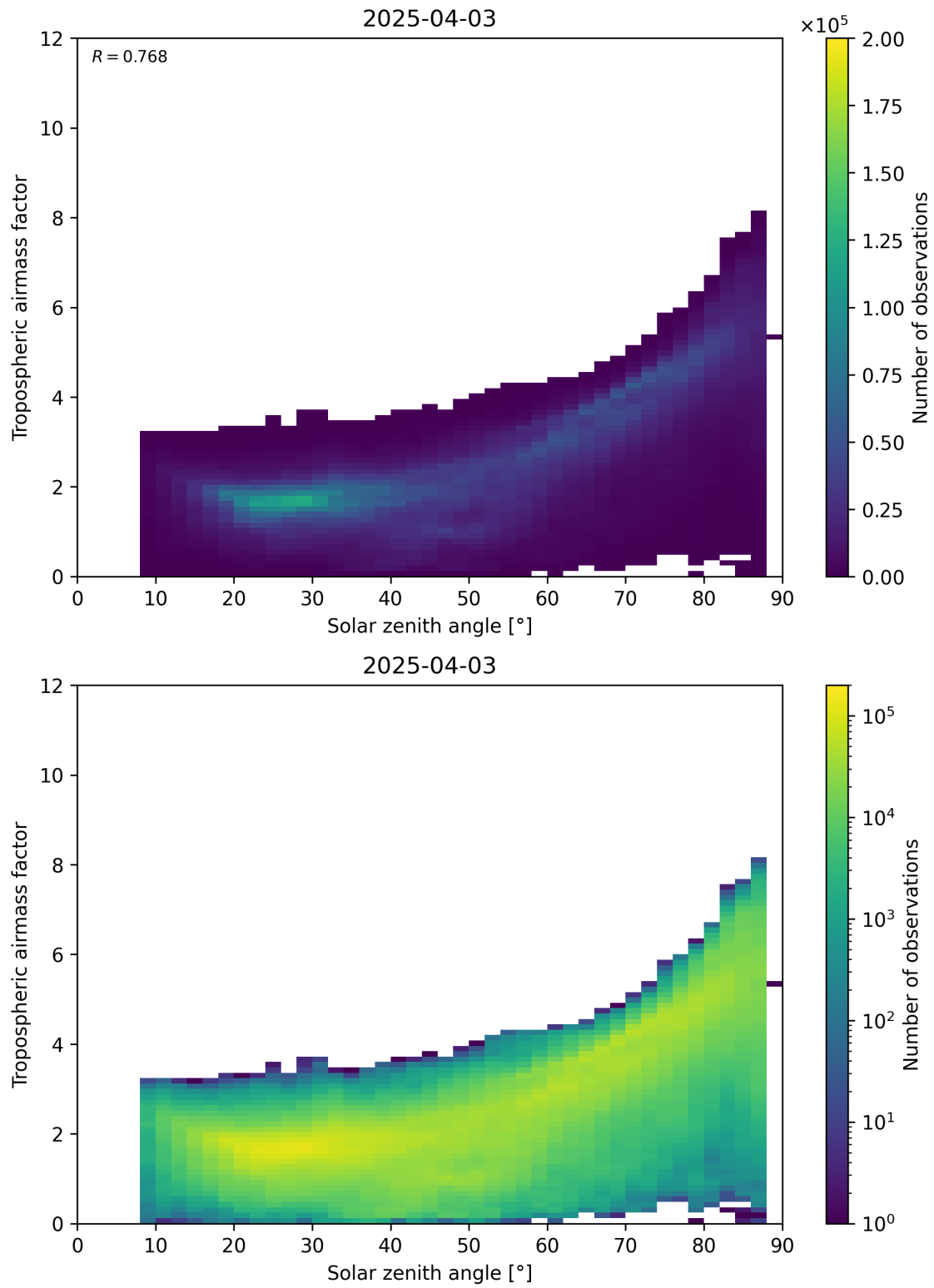
Figure 147: Scatter density plot of “Solar zenith angle” against “Tropospheric airmass factor” for 2025-04-03 to 2025-04-04.
