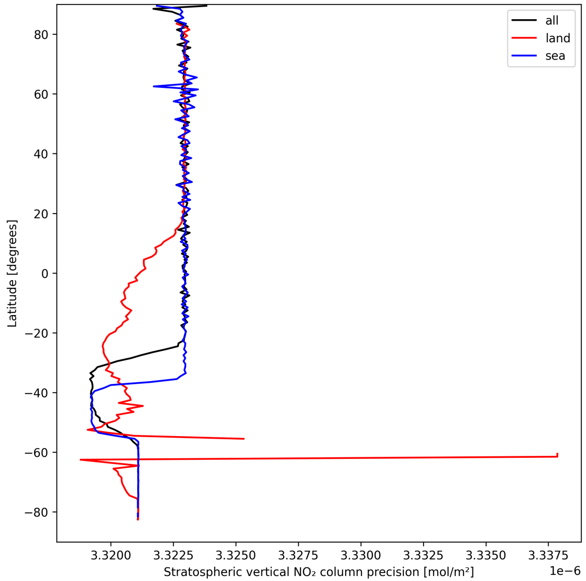
Figure 20: Zonal average of “Stratospheric vertical NO 2 column precision” for 2025-04-03 to 2025-04-04.
