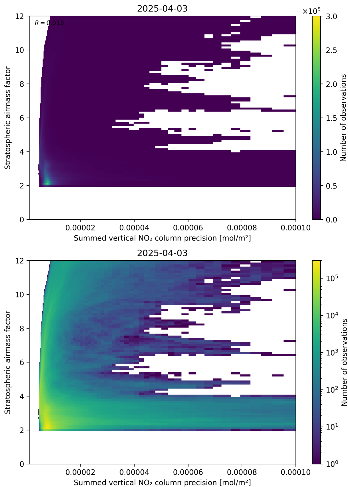
Figure 106: Scatter density plot of “Summed vertical NO 2 column precision” against “Stratospheric airmass factor” for 2025-04-03 to 2025-04-04.
