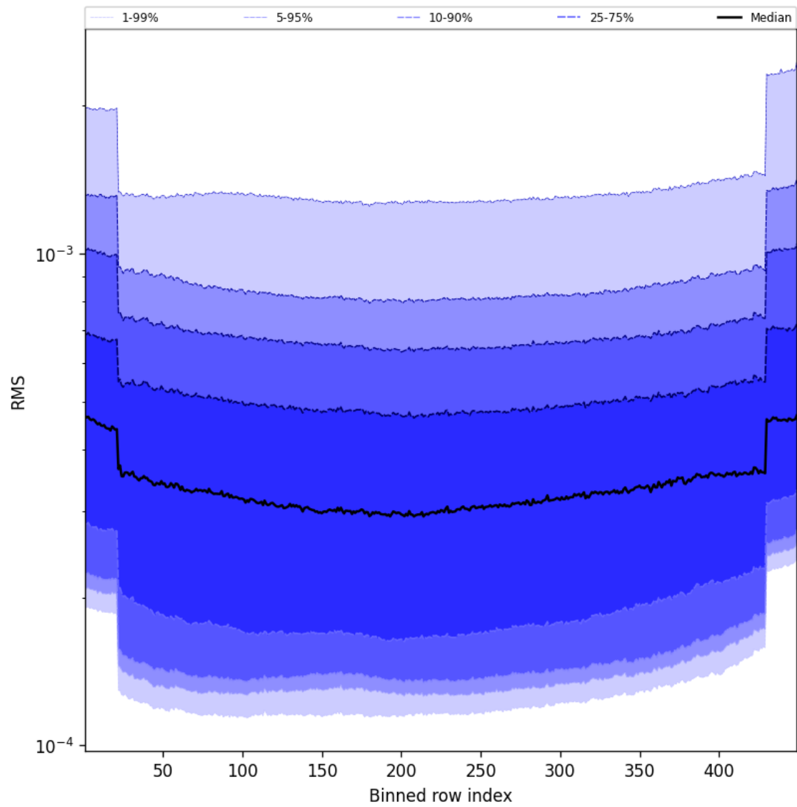
Figure 60: Along track statistics of “RMS” for 2025-04-03 to 2025-04-04
