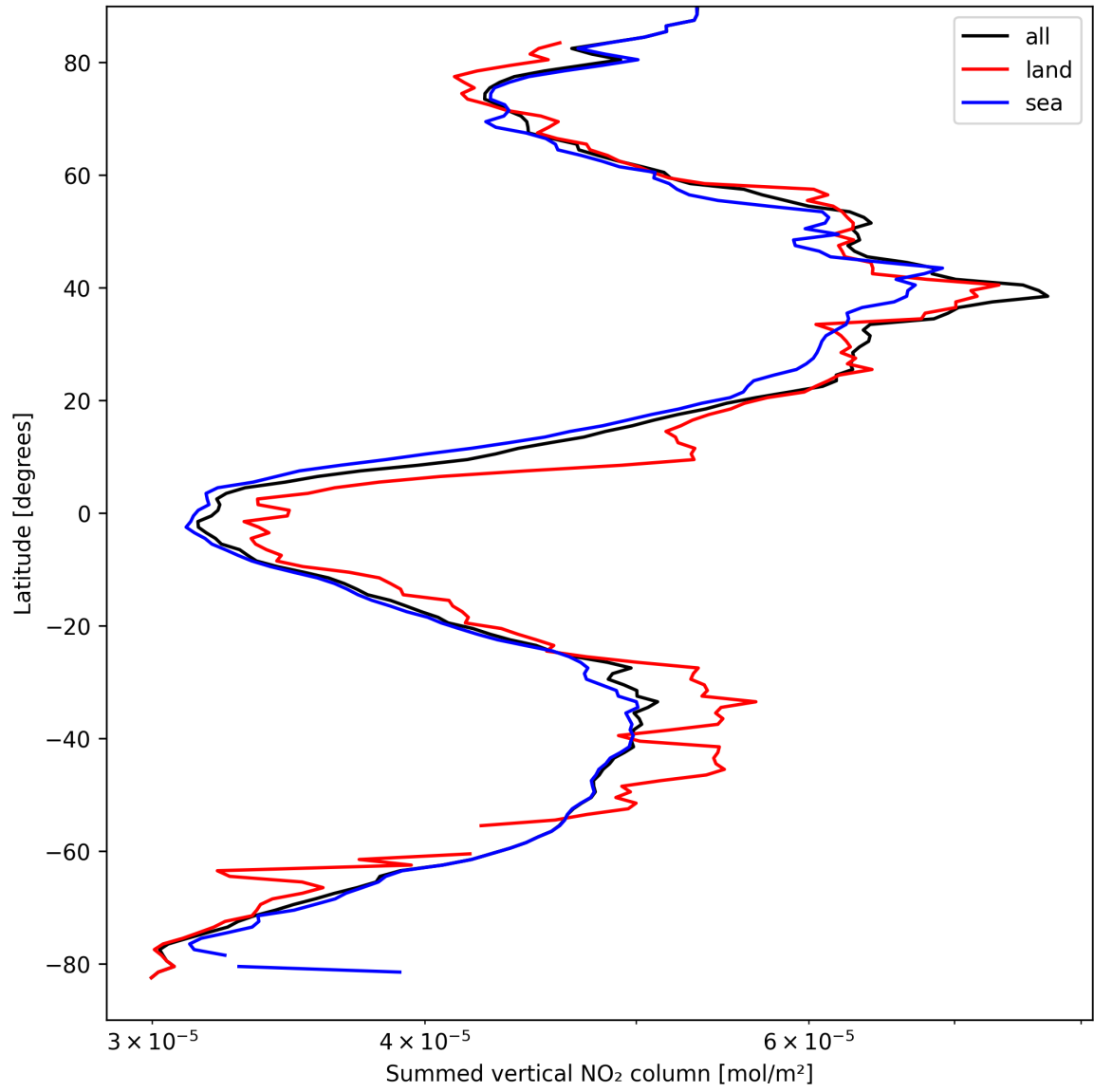
Figure 23: Zonal average of “Summed vertical NO 2 column” for 2025-04-03 to 2025-04-04.
