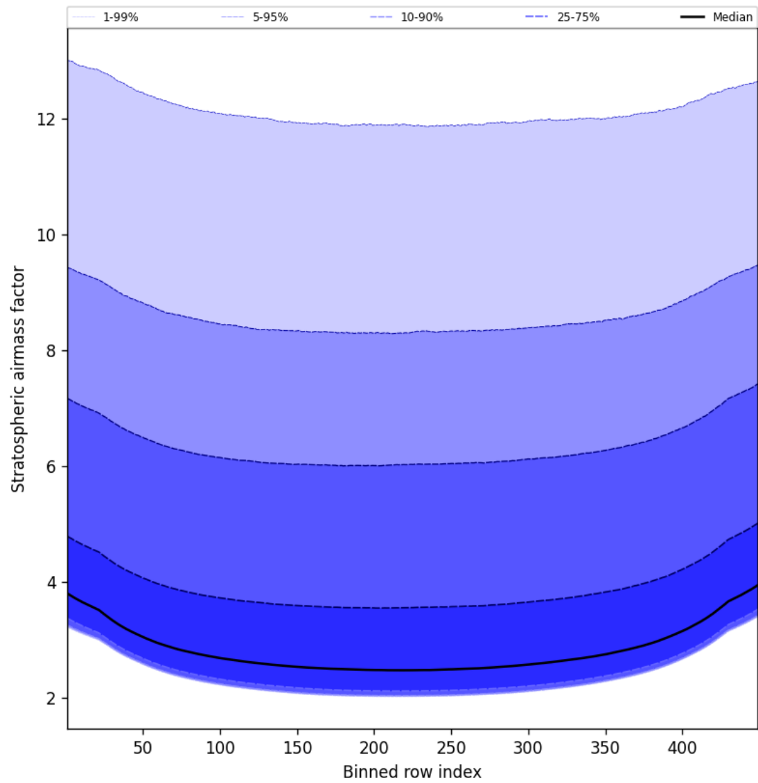
Figure 61: Along track statistics of “Stratospheric airmass factor” for 2025-04-03 to 2025-04-04
