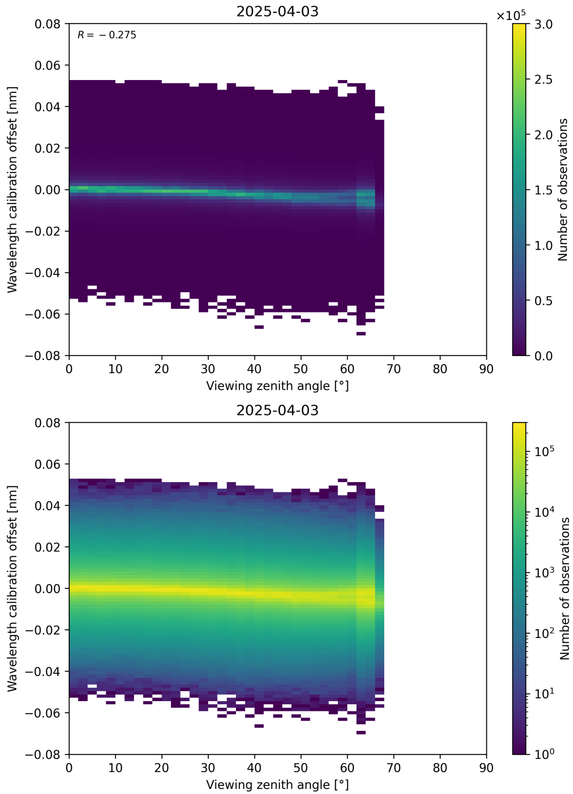
Figure 173: Scatter density plot of “Viewing zenith angle” against “Wavelength calibration offset” for 2025-04-03 to 2025-04-04.
