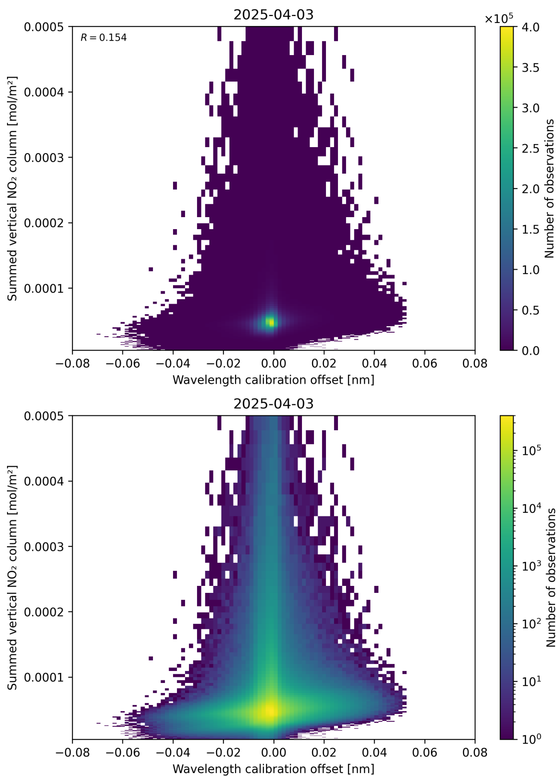
Figure 177: Scatter density plot of “Wavelength calibration offset” against “Summed vertical NO 2 column” for 2025-04-03 to 2025-04-04.
