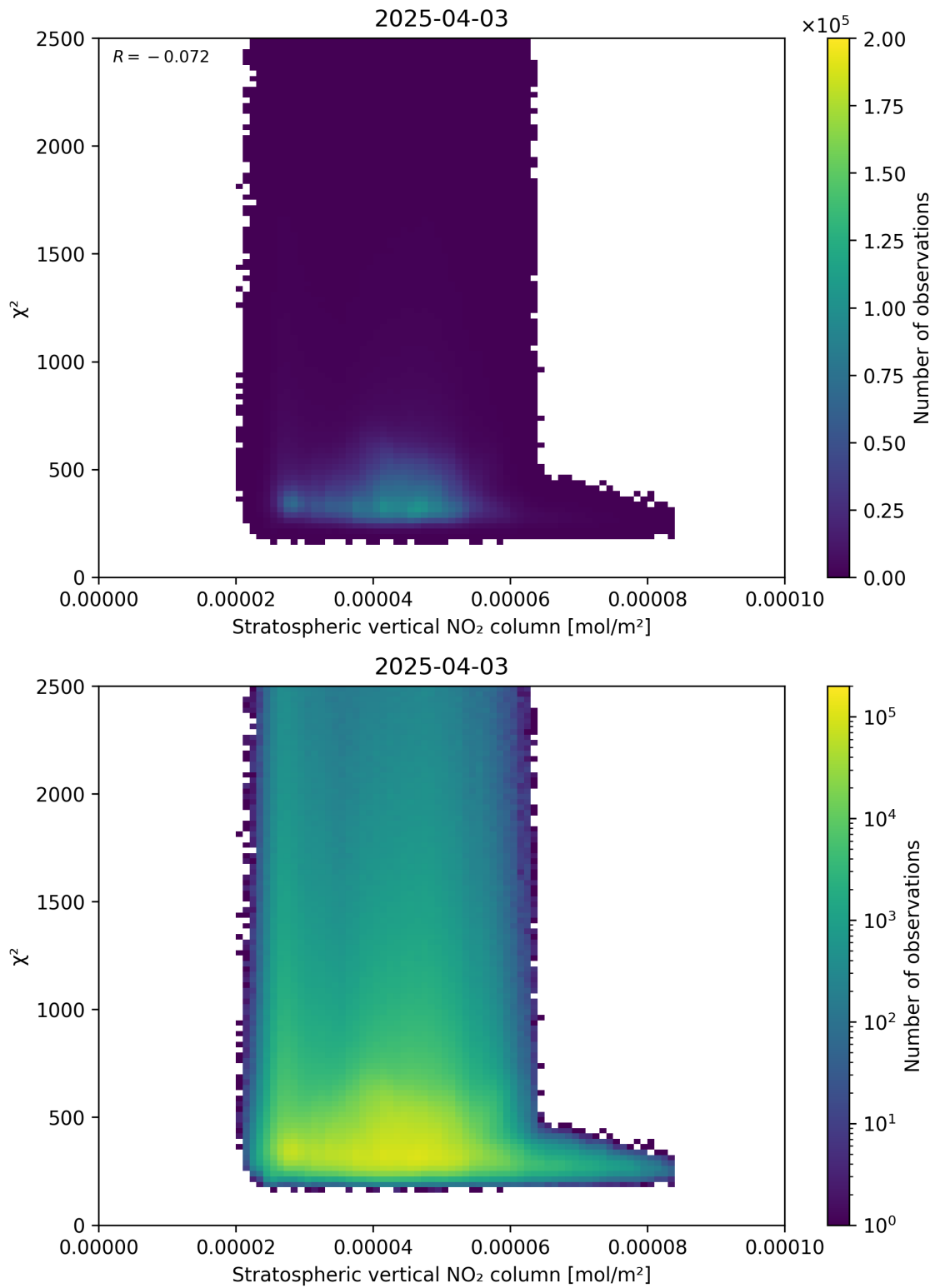
Figure 97: Scatter density plot of “Stratospheric vertical NO 2 column” against “ \chi^2 ” for 2025-04-03 to 2025-04-04.
