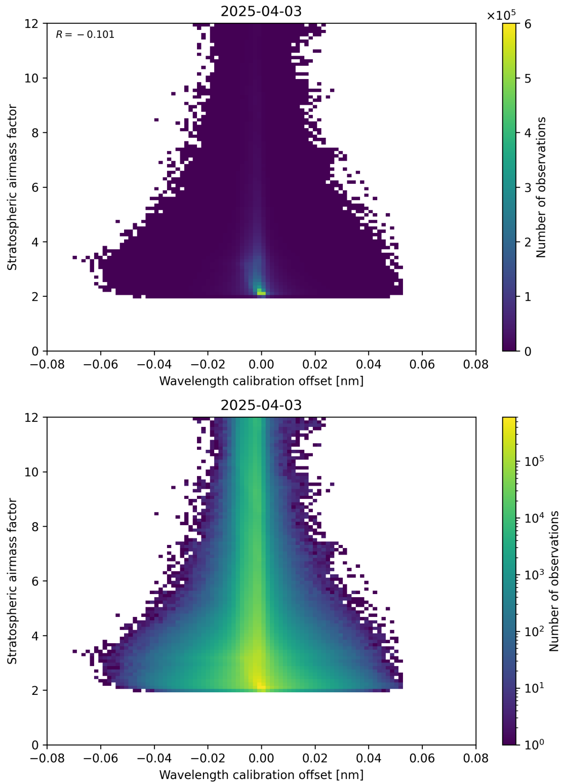
Figure 174: Scatter density plot of “Wavelength calibration offset” against “Stratospheric airmass factor” for 2025-04-03 to 2025-04-04.
