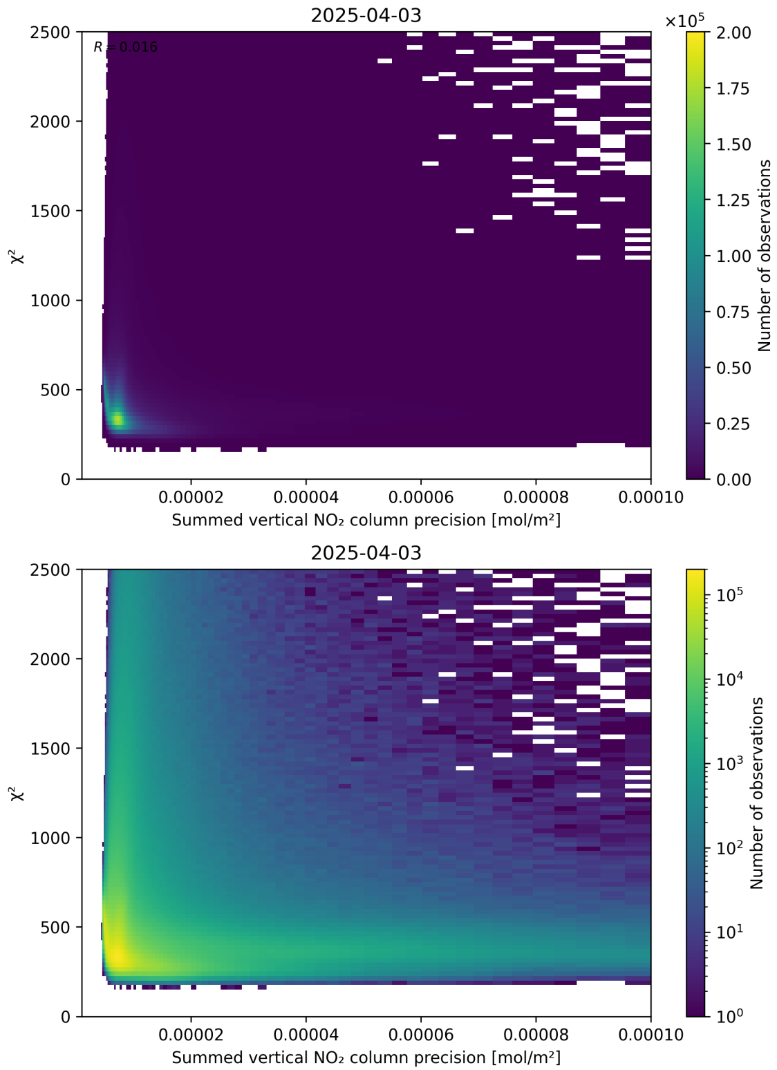
Figure 107: Scatter density plot of “Summed vertical NO 2 column precision” against “ \chi^2 ” for 2025-04-03 to 2025-04-04.
