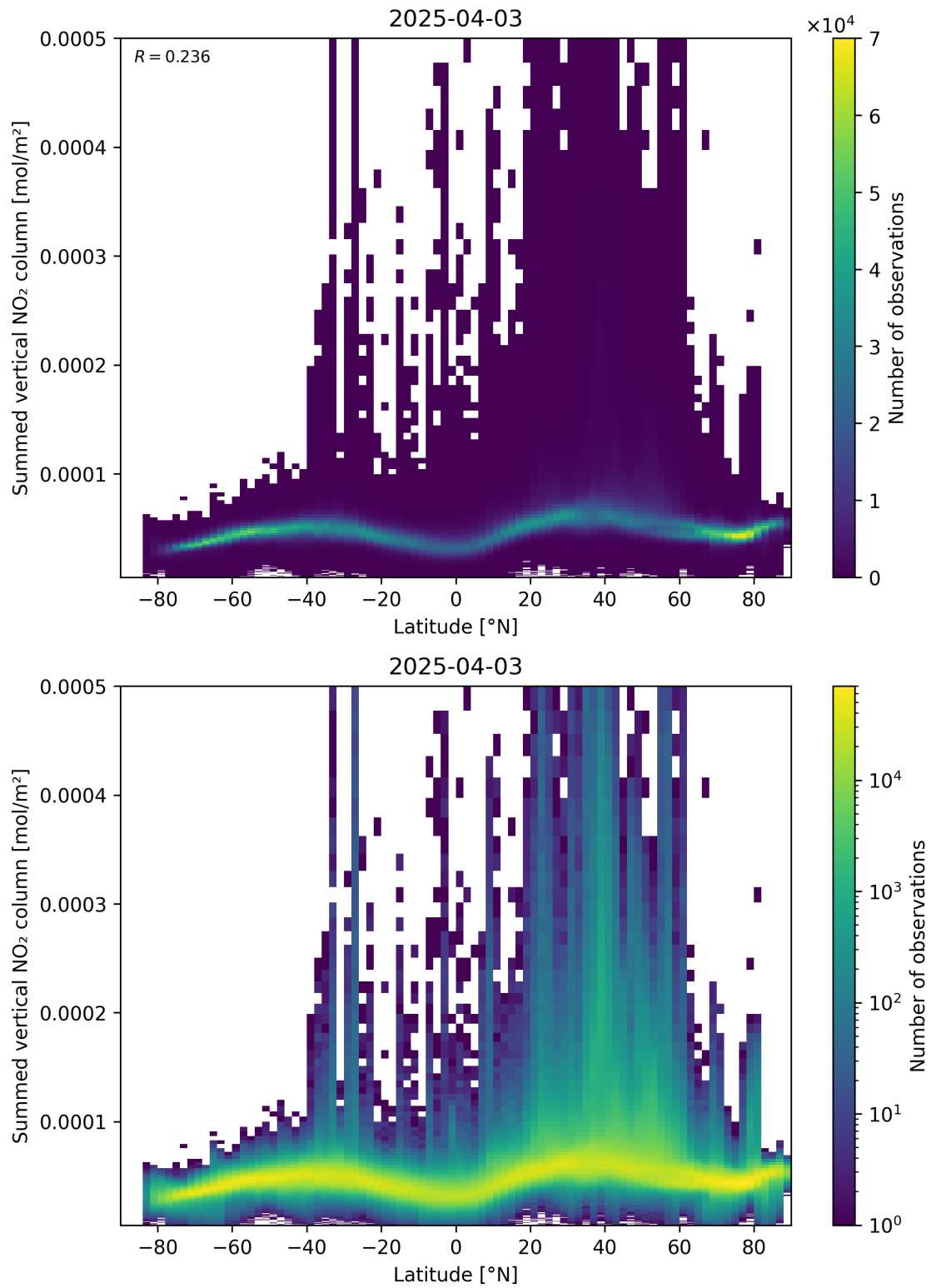
Figure 88: Scatter density plot of “Latitude” against “Summed vertical NO 2 column” for 2025-04-03 to 2025-04-04.
