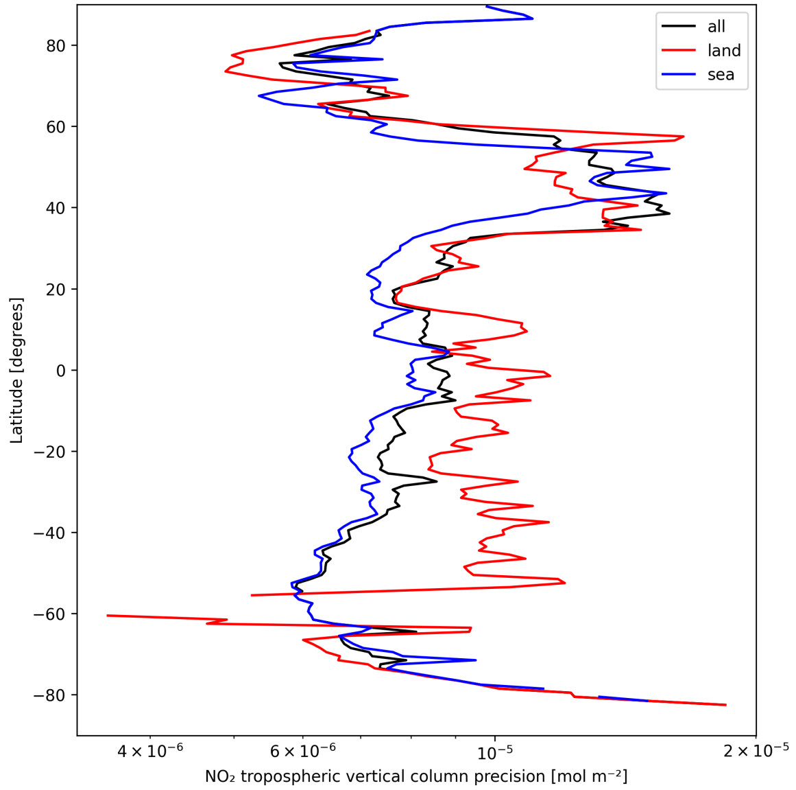
Figure 13: Zonal average of “NO 2 tropospheric vertical column precision” for 2025-04-03 to 2025-04-04.
