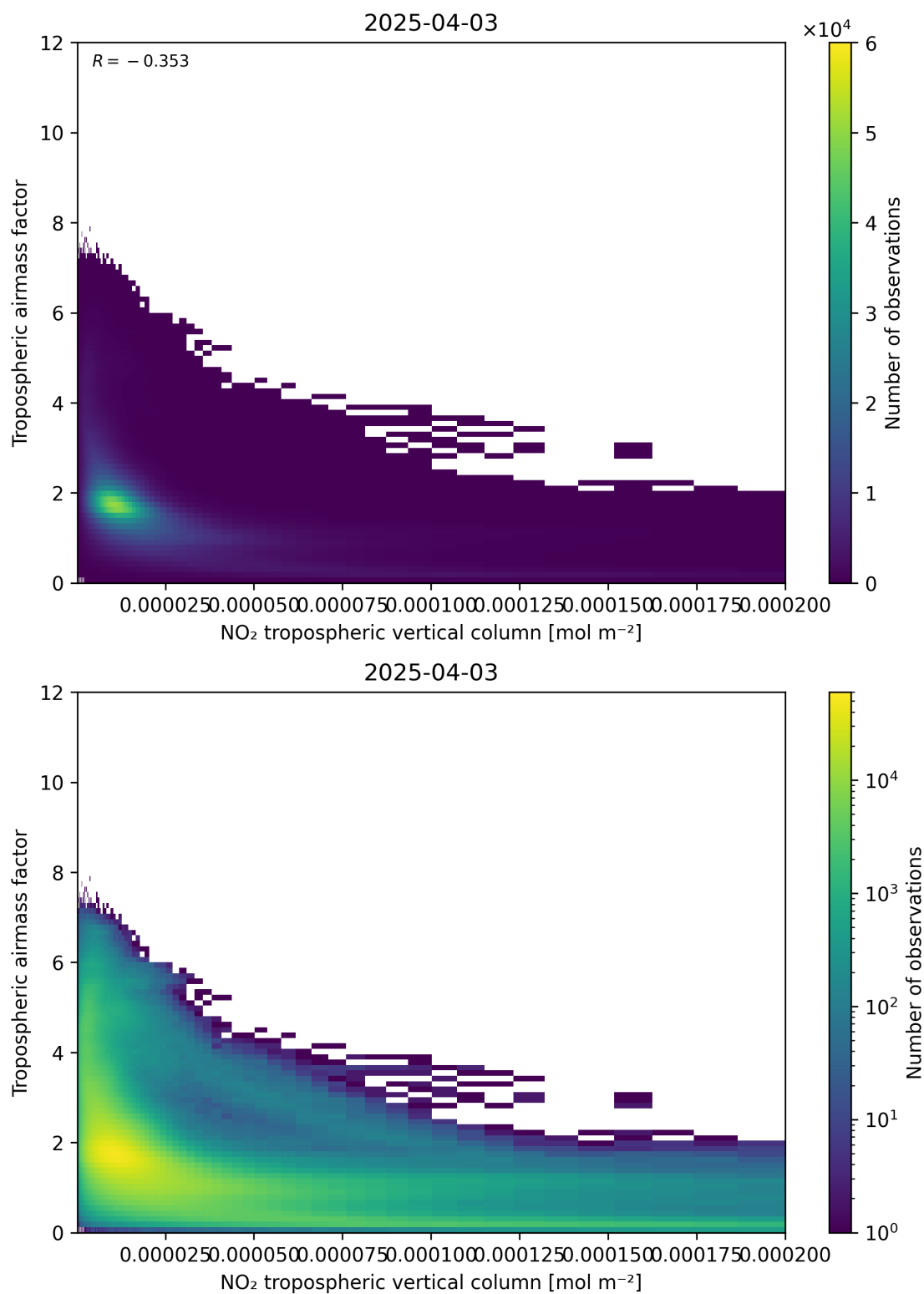
Figure 123: Scatter density plot of “NO 2 tropospheric vertical column” against “Tropospheric air mass factor” for 2025-04-03 to 2025-04-04.
