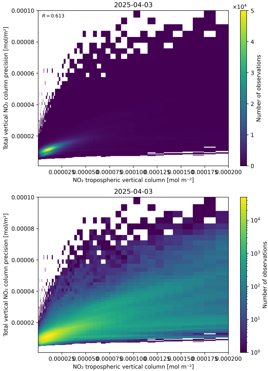
Figure 129: Scatter density plot of “NO 2 tropospheric vertical column” against “Total vertical NO 2 column precision” for 2025-04-03 to 2025-04-04.
