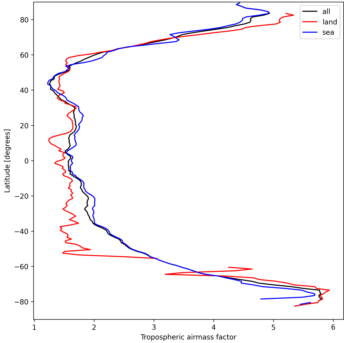
Figure 14: Zonal average of “Tropospheric air mass factor” for 2025-04-03 to 2025-04-04.
