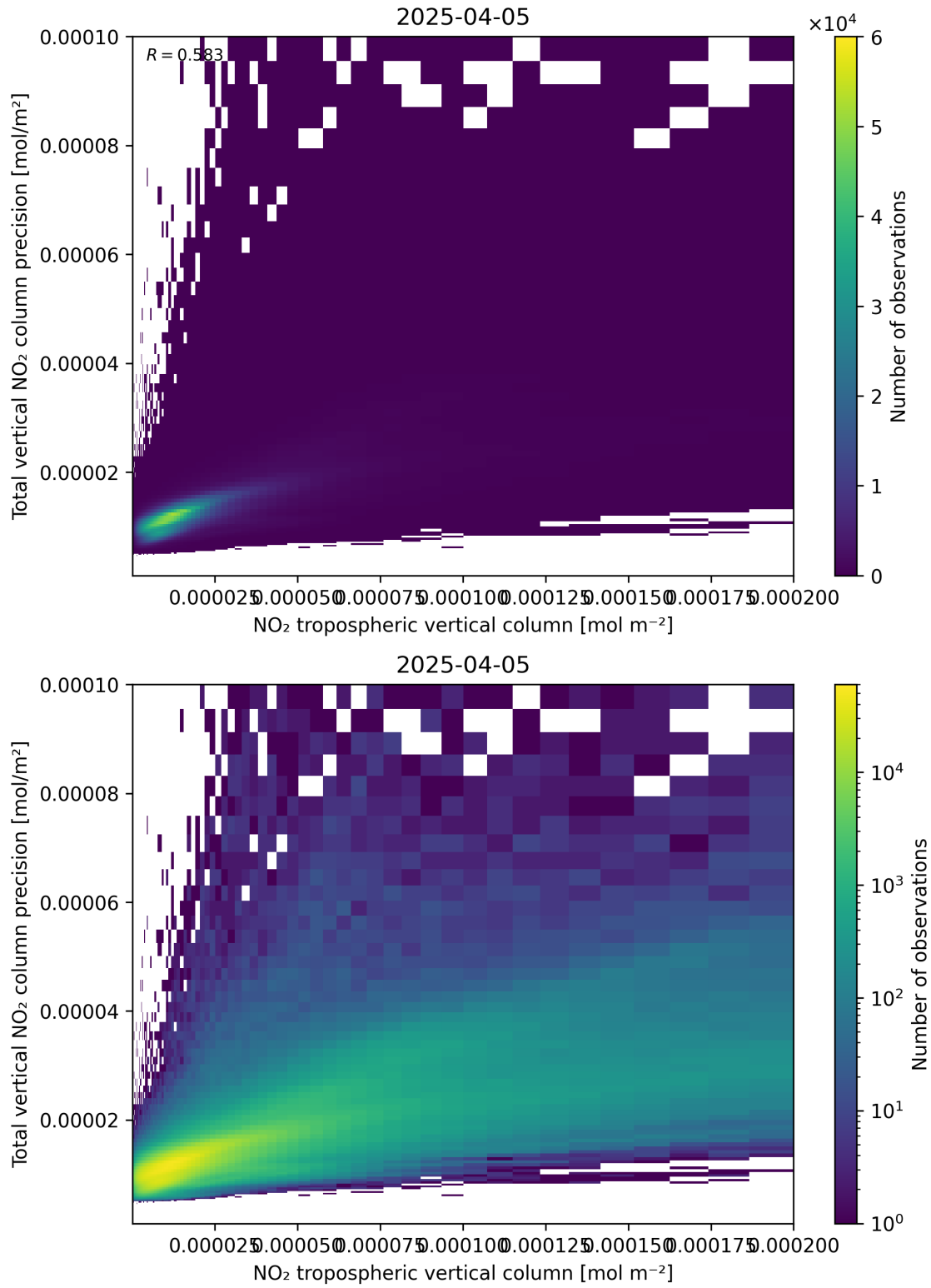
Figure 129: Scatter density plot of “NO 2 tropospheric vertical column” against “Total vertical NO 2 column precision” for 2025-04-05 to 2025-04-06.
