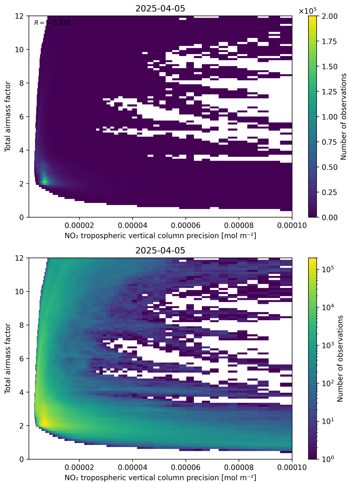
Figure 132: Scatter density plot of “NO 2 tropospheric vertical column precision” against “Total air mass factor” for 2025-04-05 to 2025-04-06.
