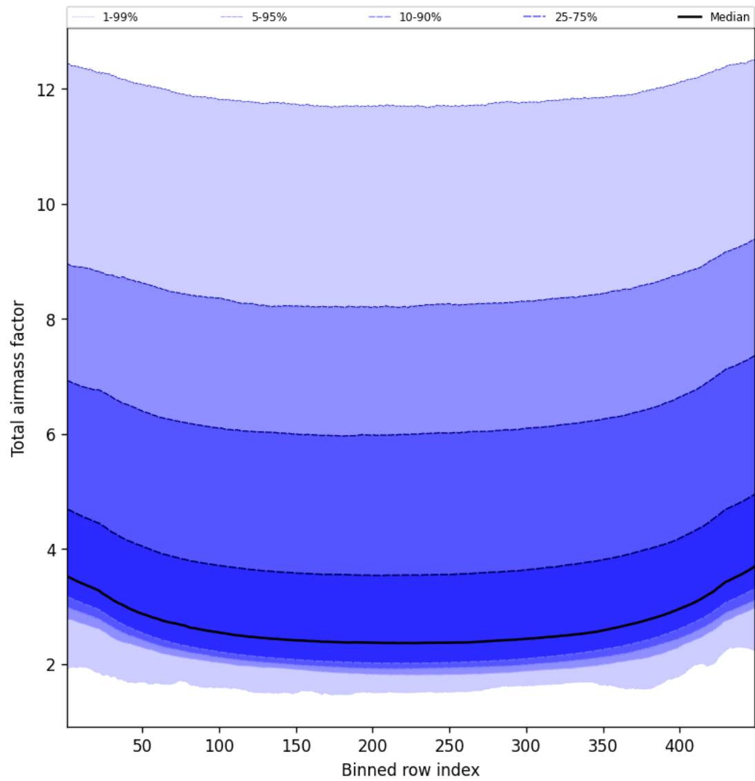
Figure 49: Along track statistics of “Total airmass factor” for 2025-04-05 to 2025-04-06
