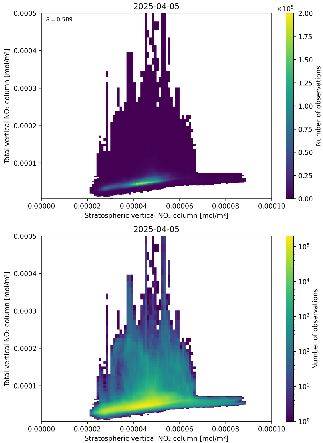
Figure 100: Scatter density plot of “Stratospheric vertical NO 2 column” against “Total vertical NO 2 column” for 2025-04-05 to 2025-04-06.
