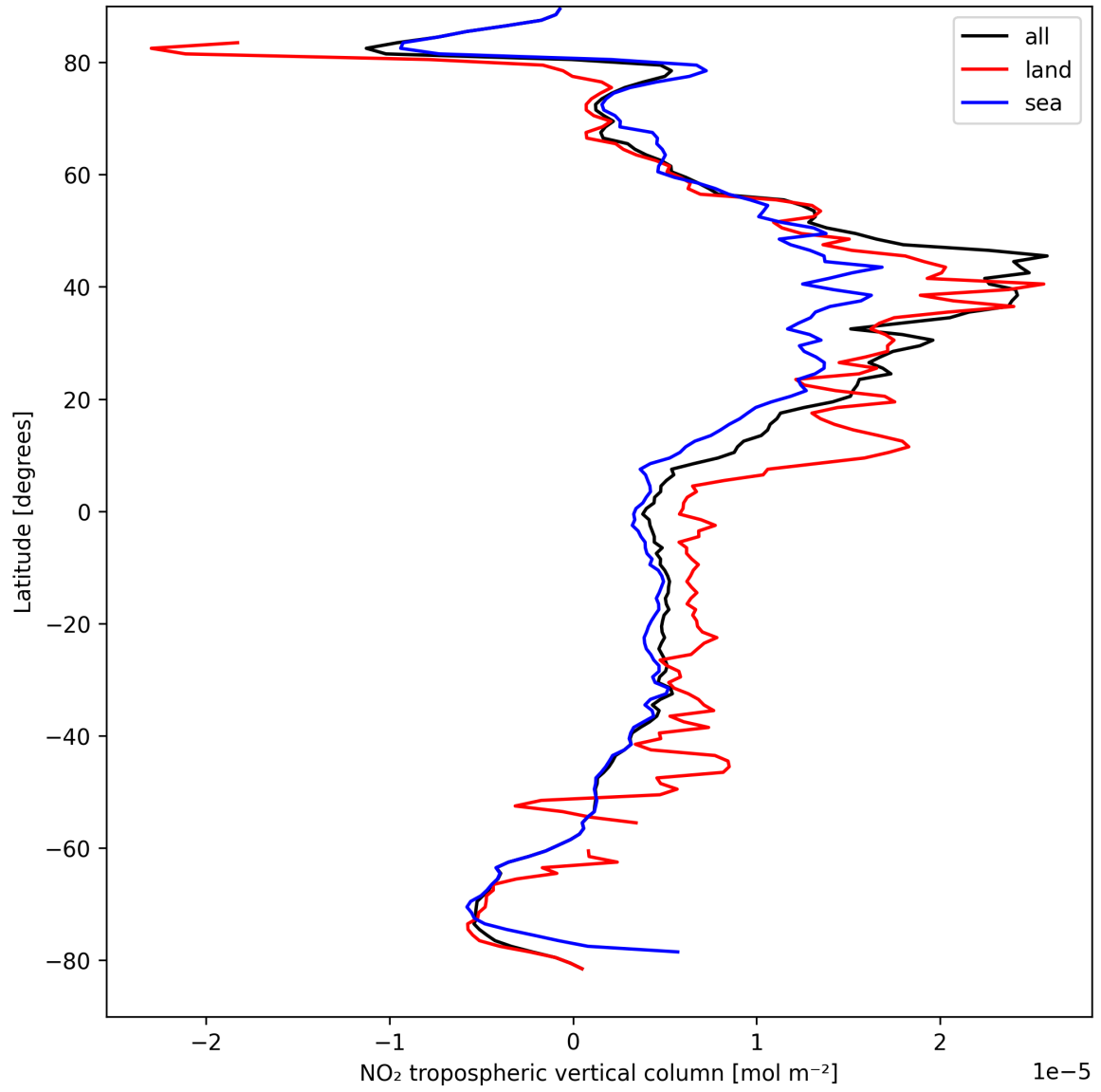
Figure 12: Zonal average of “NO 2 tropospheric vertical column” for 2025-04-05 to 2025-04-06.
