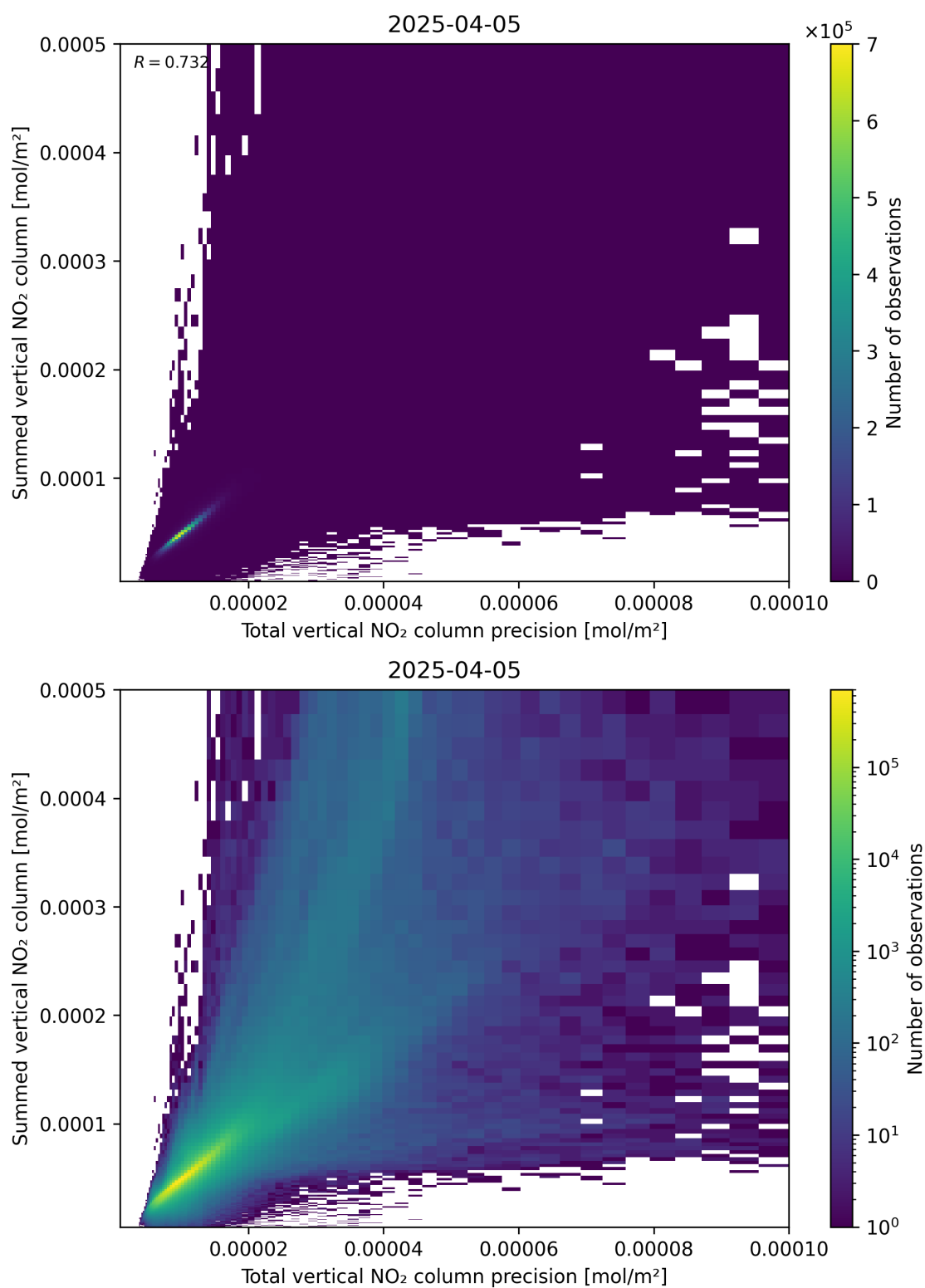
Figure 117: Scatter density plot of “Total vertical NO 2 column precision” against “Summed vertical NO 2 column” for 2025-04-05 to 2025-04-06.
