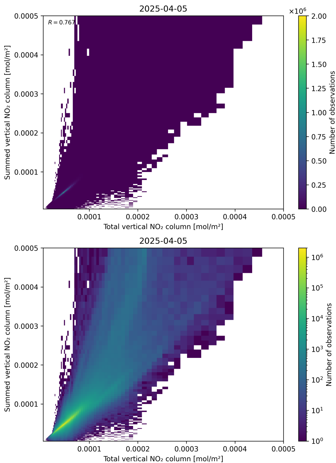
Figure 112: Scatter density plot of “Total vertical NO 2 column” against “Summed vertical NO 2 column” for 2025-04-05 to 2025-04-06.
