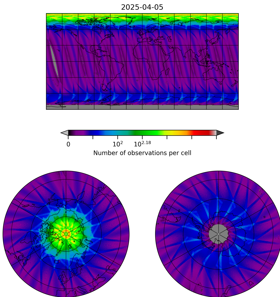
Figure 10: Map of the number of observations for 2025-04-05 to 2025-04-06
