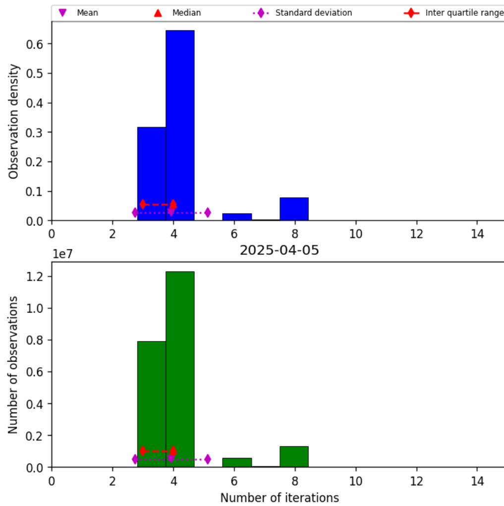
Figure 34: Histogram of “Number of iterations” for 2025-04-05 to 2025-04-06
