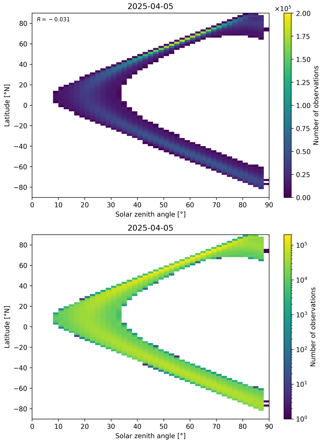
Figure 149: Scatter density plot of “Solar zenith angle” against “Latitude” for 2025-04-05 to 2025-04-06.
