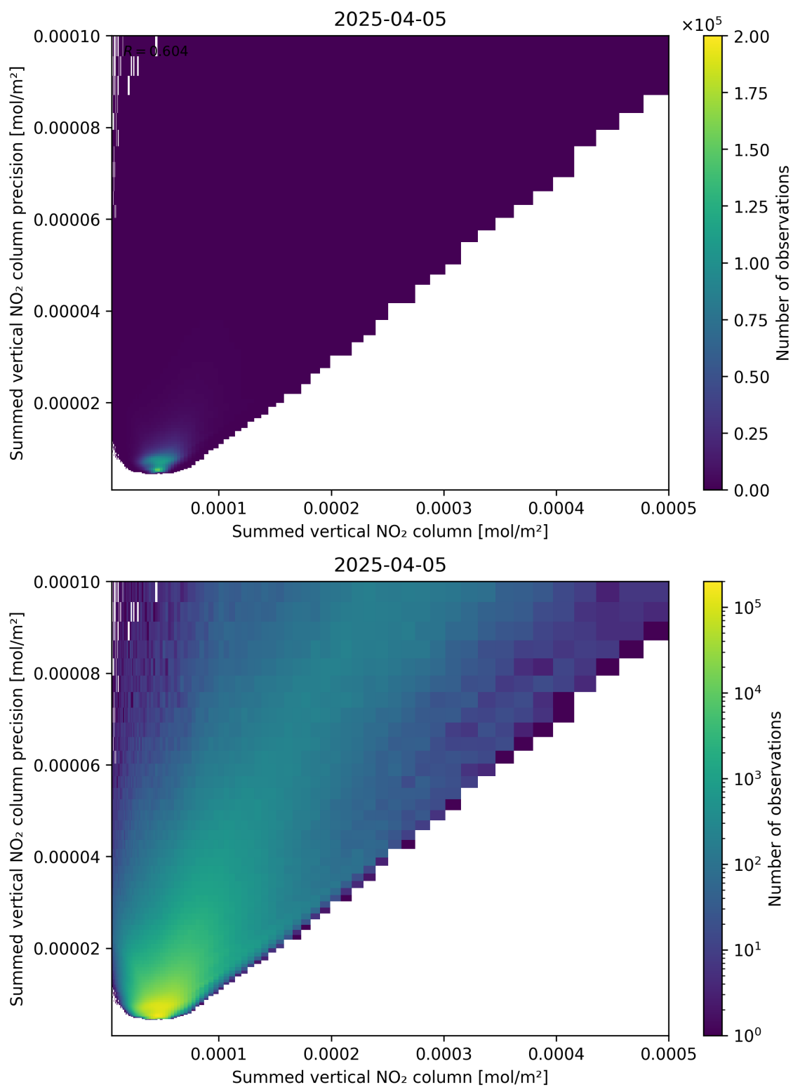
Figure 105: Scatter density plot of “Summed vertical NO 2 column” against “Summed vertical NO 2 column precision” for 2025-04-05 to 2025-04-06.
