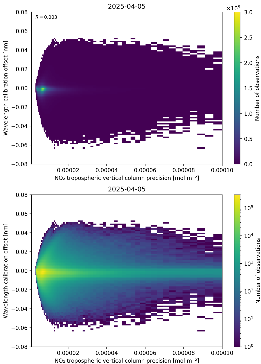
Figure 141: Scatter density plot of “NO 2 tropospheric vertical column precision” against “Wavelength calibration offset” for 2025-04-05 to 2025-04-06.
