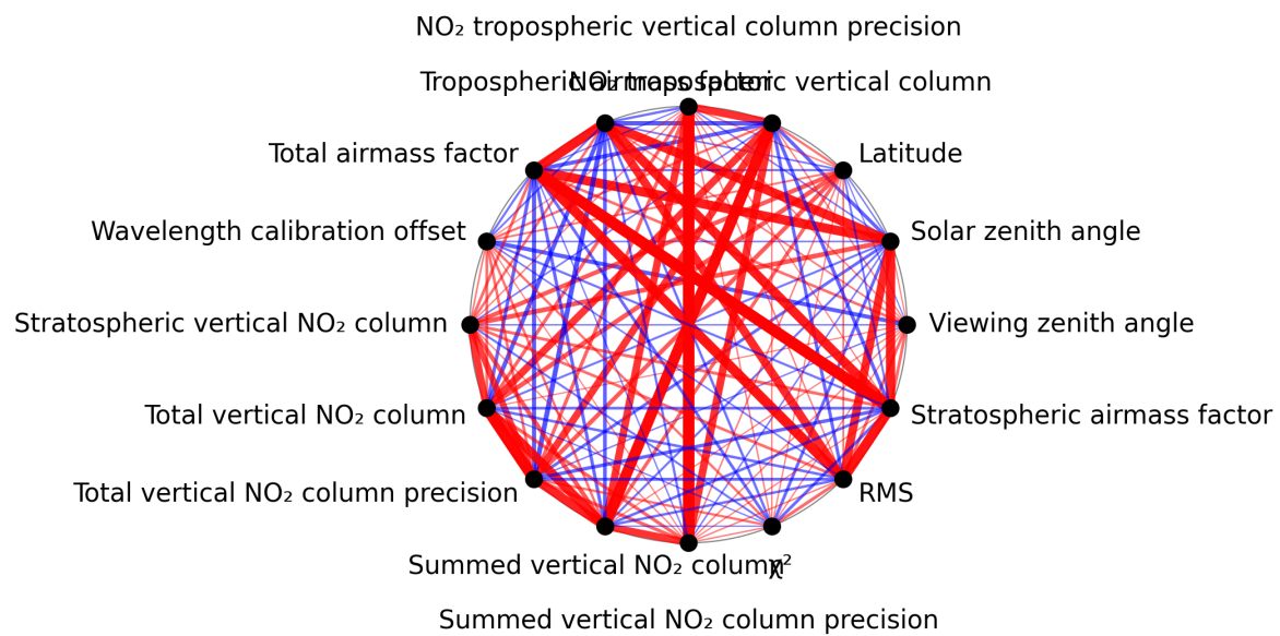
Figure 1: Map of correlation graph for 2025-04-05 to 2025-04-06.
