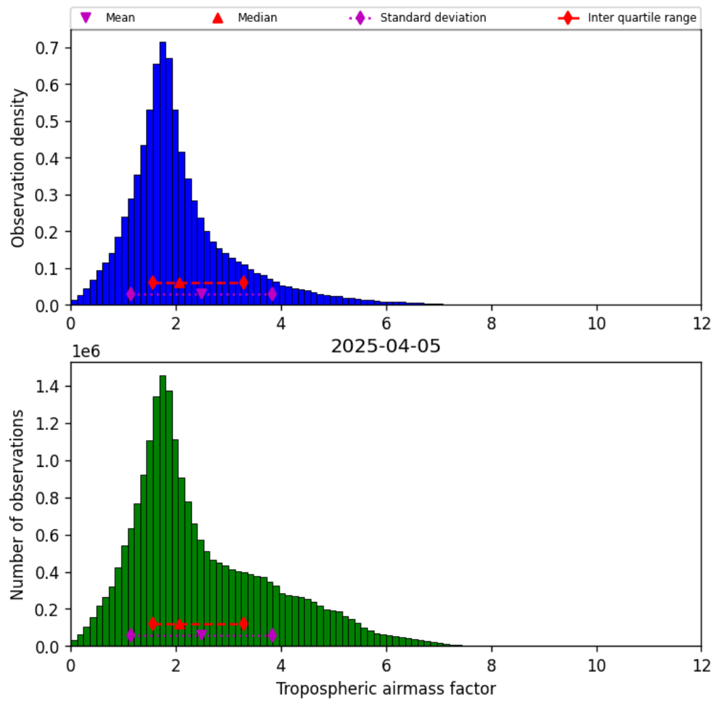
Figure 31: Histogram of “Tropospheric airmass factor” for 2025-04-05 to 2025-04-06
