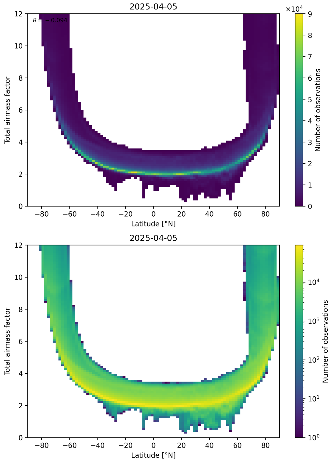
Figure 84: Scatter density plot of “Latitude” against “Total airmass factor” for 2025-04-05 to 2025-04-06.
