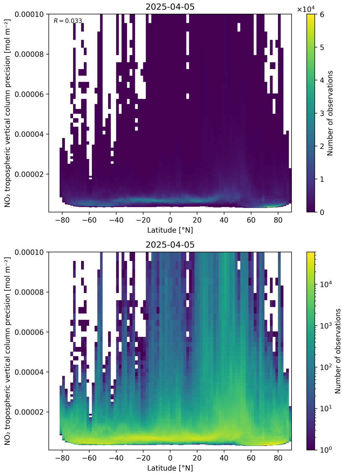
Figure 93: Scatter density plot of “Latitude” against “NO 2 tropospheric vertical column precision” for 2025-04-05 to 2025-04-06.
