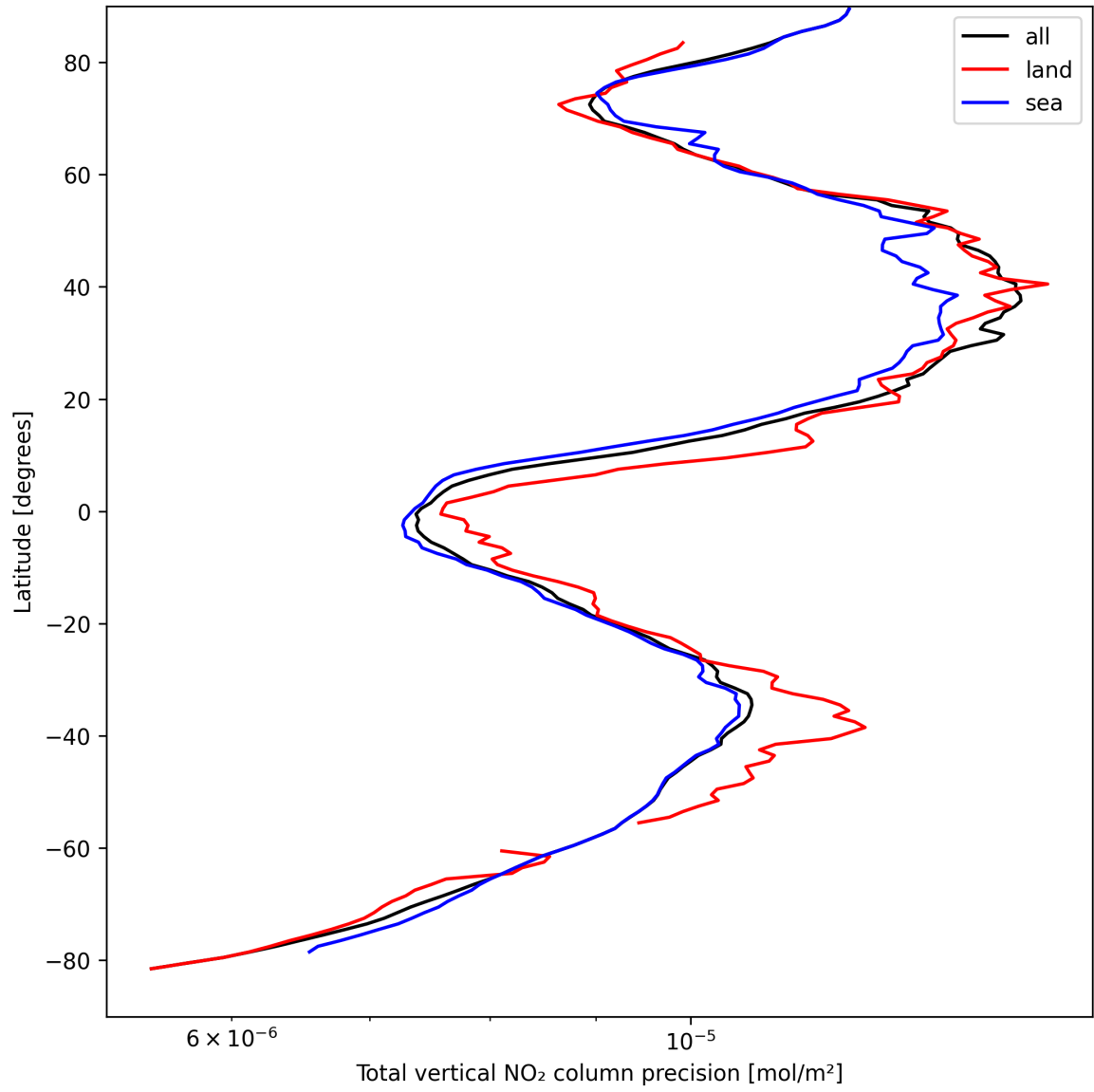
Figure 22: Zonal average of “Total vertical NO 2 column precision” for 2025-04-05 to 2025-04-06.
