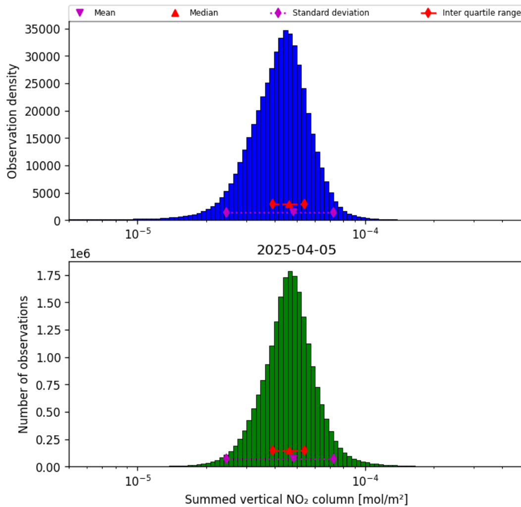
Figure 40: Histogram of “Summed vertical NO 2 column” for 2025-04-05 to 2025-04-06
