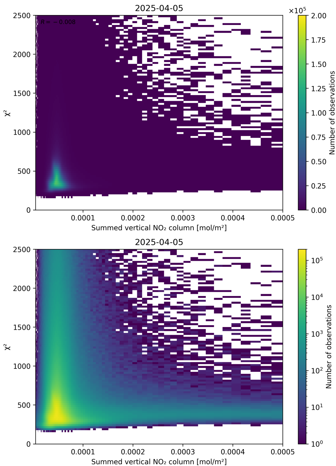
Figure 104: Scatter density plot of “Summed vertical NO 2 column” against “ \chi^2 ” for 2025-04-05 to 2025-04-06.
