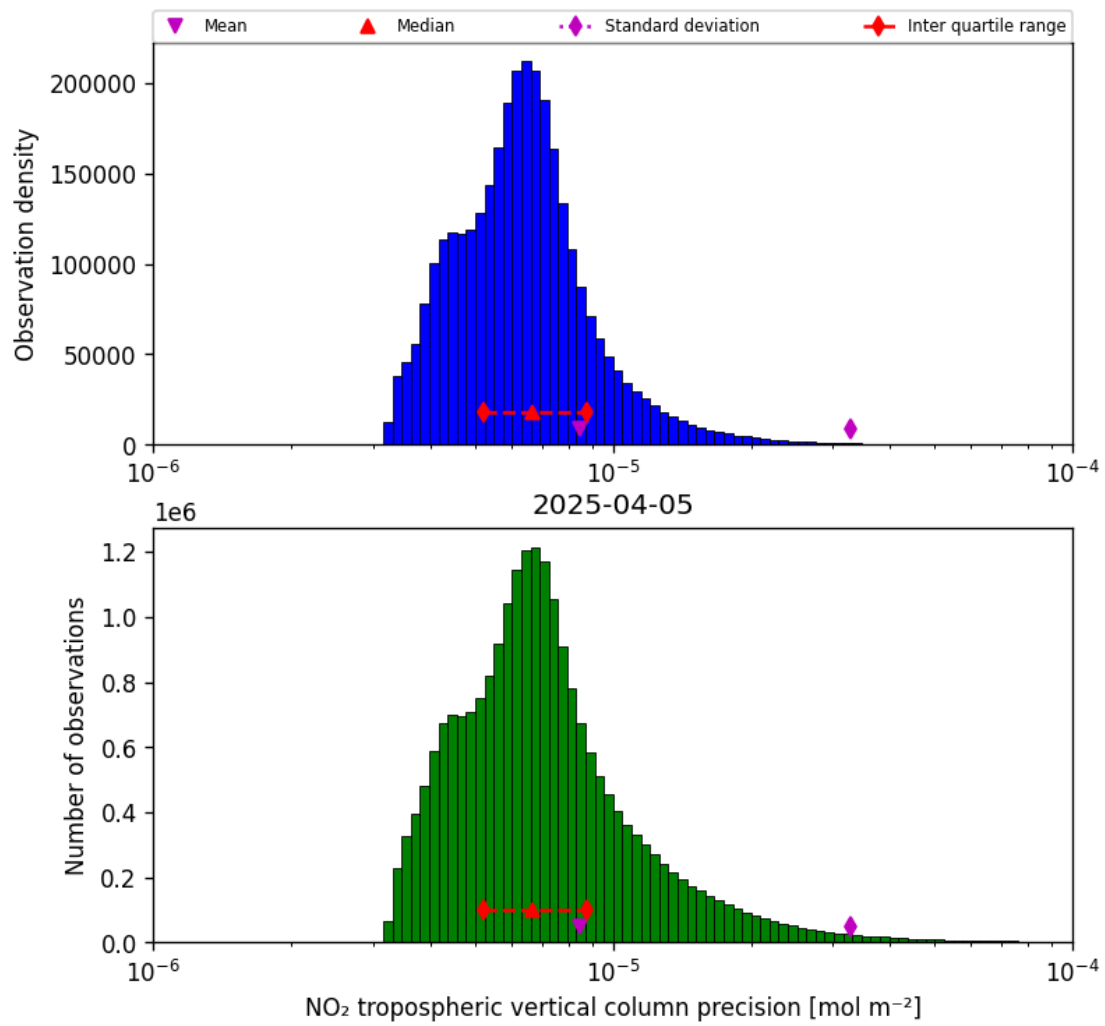
Figure 30: Histogram of “NO 2 tropospheric vertical column precision” for 2025-04-05 to 2025-04-06
