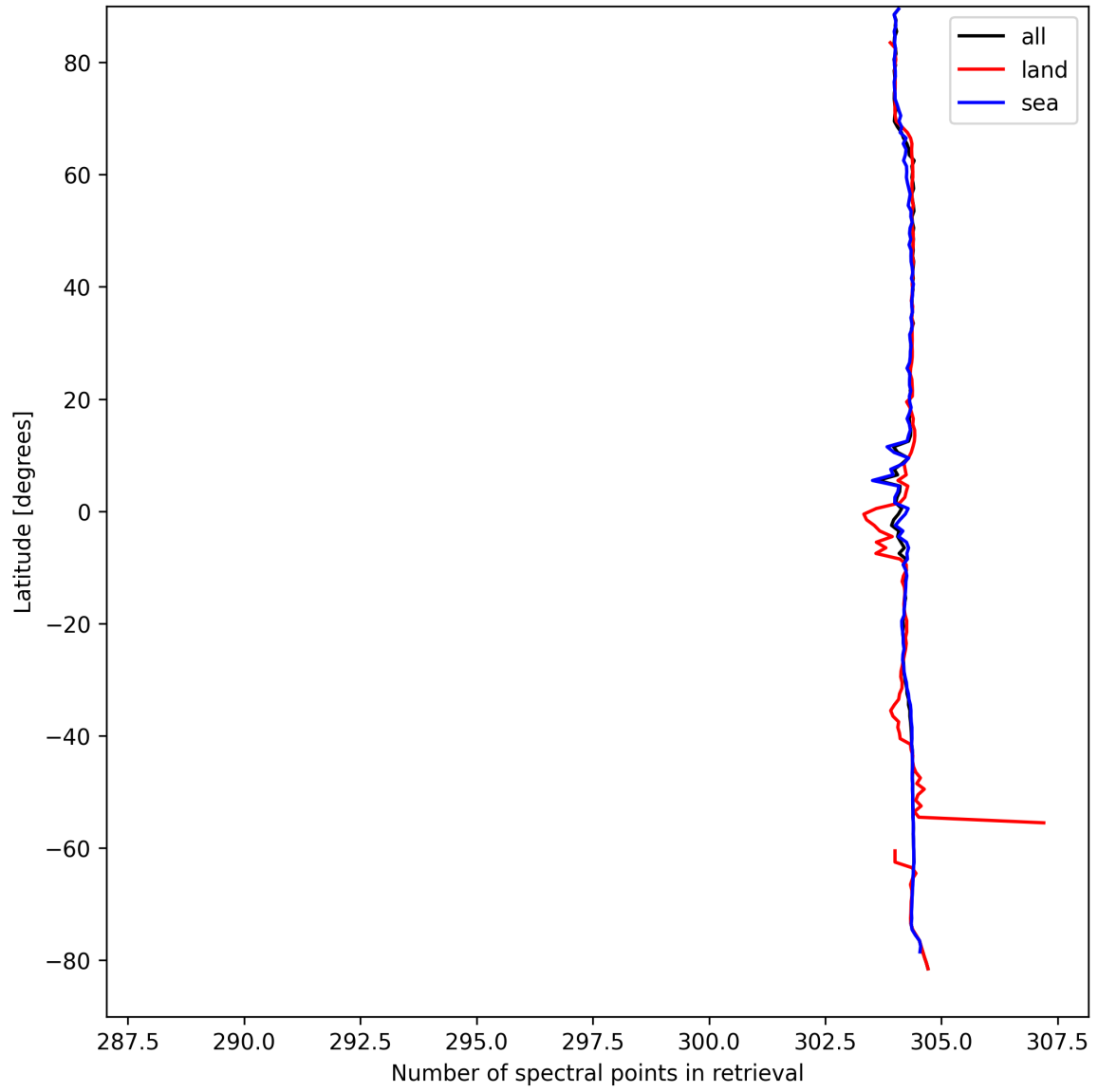
Figure 16: Zonal average of “Number of spectral points in retrieval” for 2025-04-05 to 2025-04-06.
