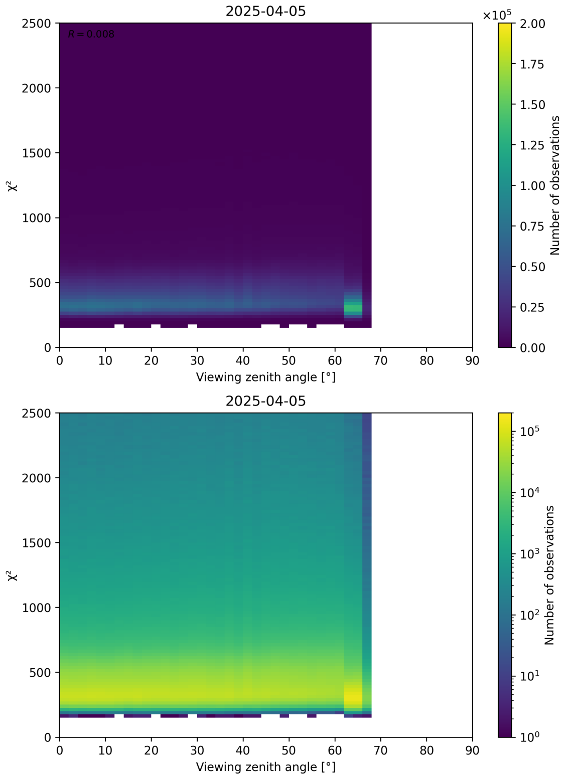
Figure 162: Scatter density plot of “Viewing zenith angle” against “ \chi^2 ” for 2025-04-05 to 2025-04-06.
