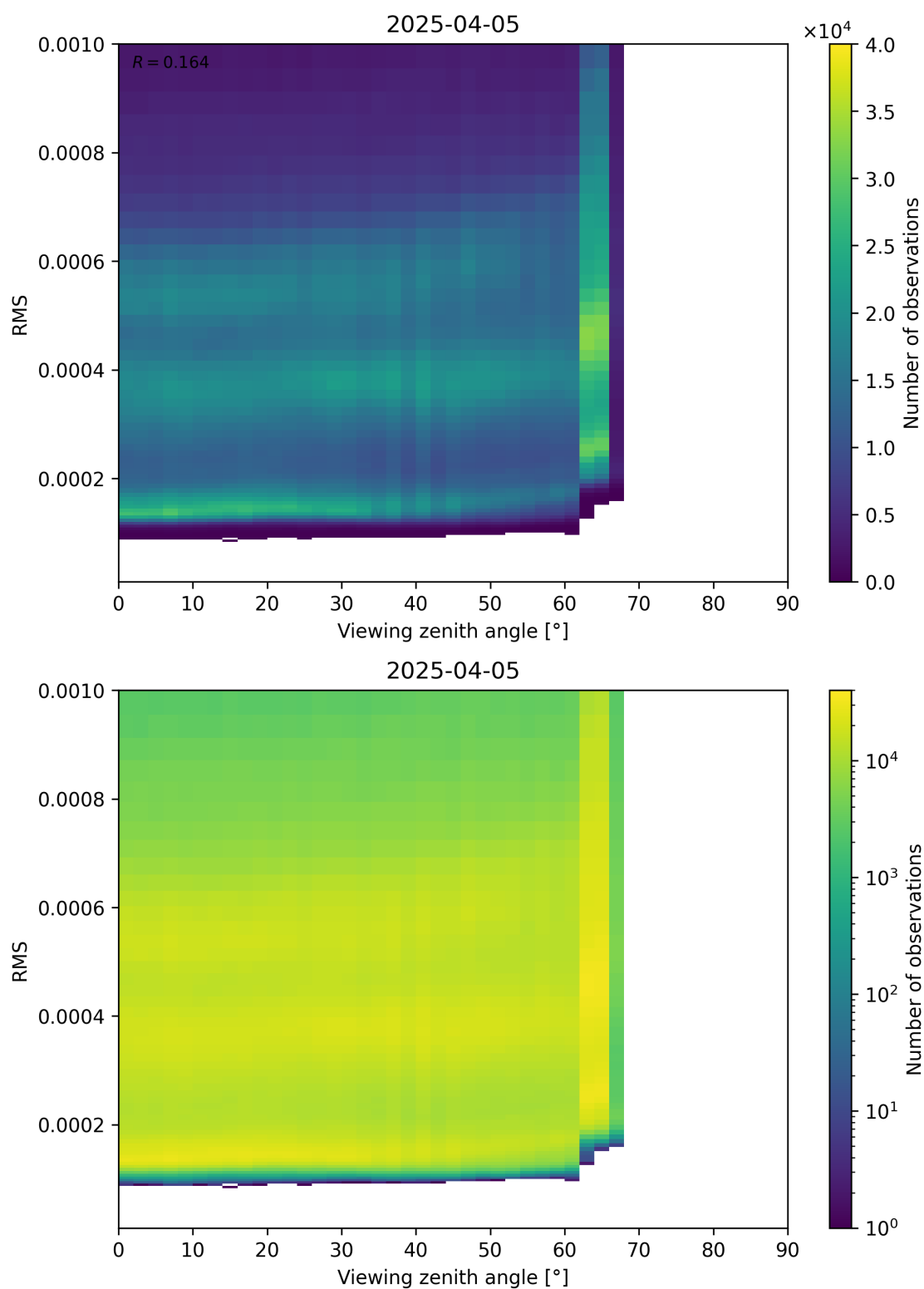
Figure 171: Scatter density plot of “Viewing zenith angle” against “RMS” for 2025-04-05 to 2025-04-06.
