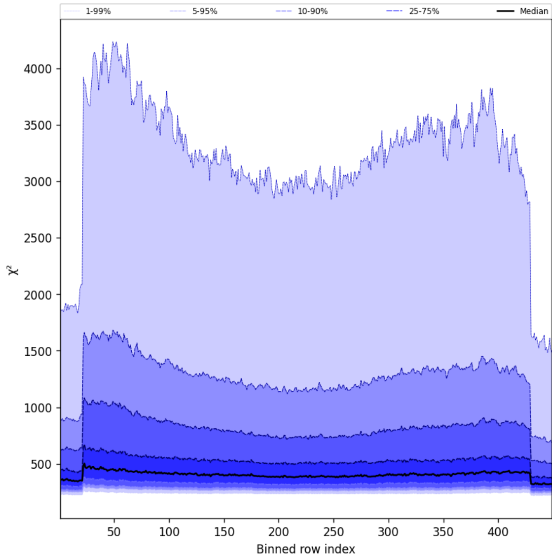
Figure 59: Along track statistics of “ \chi^2 ” for 2025-04-05 to 2025-04-06
