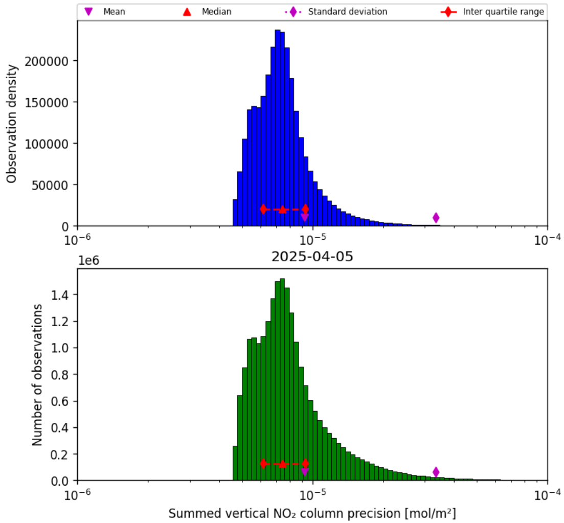
Figure 41: Histogram of "Summed vertical NO 2 column precision" for 2025-04-05 to 2025-04-06
