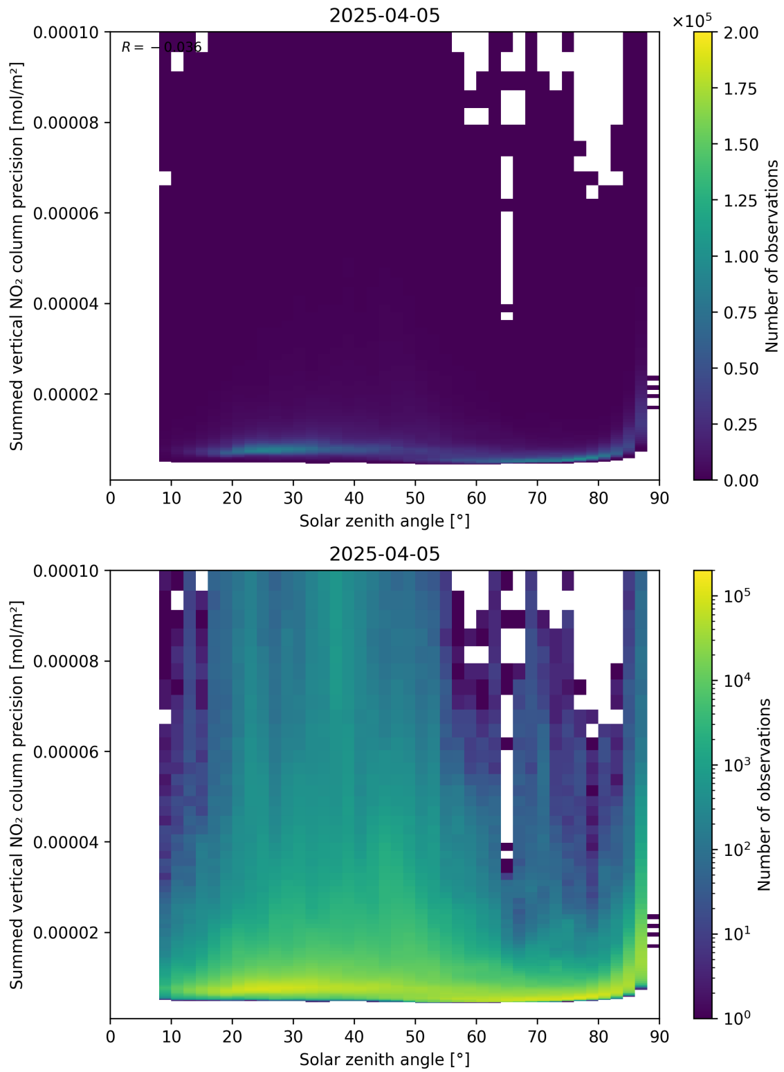
Figure 152: Scatter density plot of “Solar zenith angle” against “Summed vertical NO 2 column precision” for 2025-04-05 to 2025-04-06.
