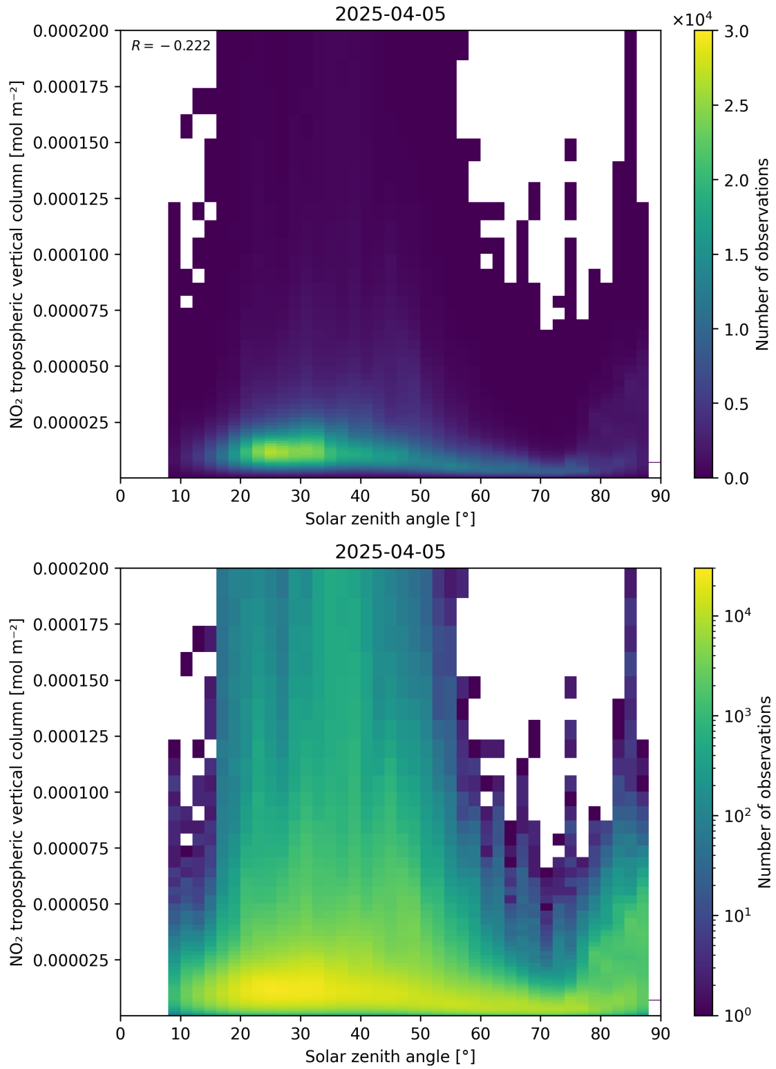
Figure 155: Scatter density plot of “Solar zenith angle” against “NO 2 tropospheric vertical column” for 2025-04-05 to 2025-04-06.
