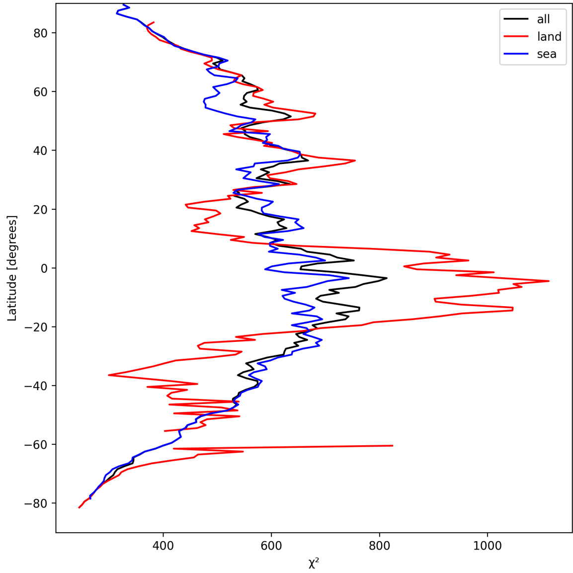
Figure 25: Zonal average of “ \chi^2 ” for 2025-04-05 to 2025-04-06.
