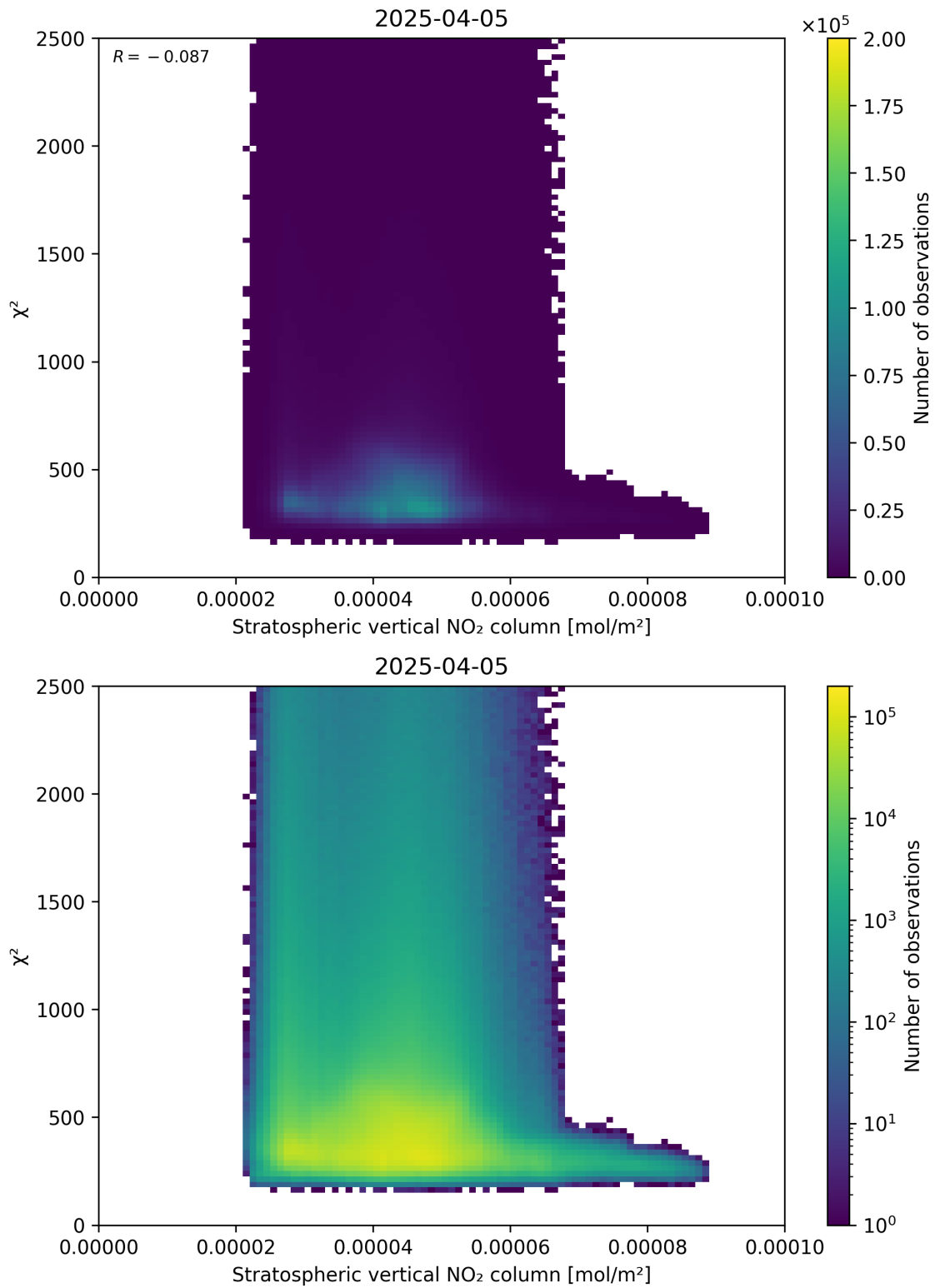
Figure 97: Scatter density plot of “Stratospheric vertical NO 2 column” against “ \chi^2 ” for 2025-04-05 to 2025-04-06.
