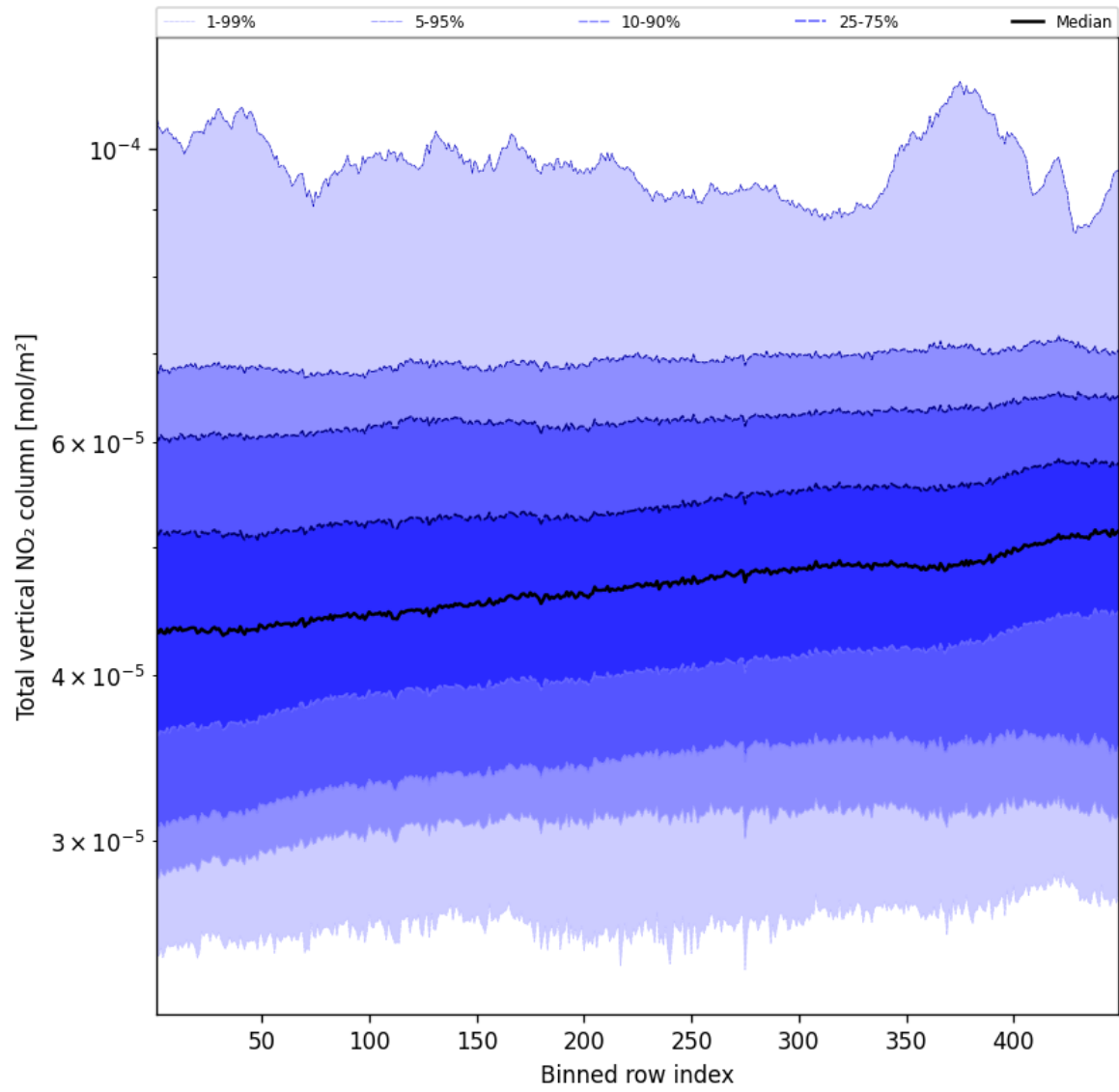
Figure 55: Along track statistics of “Total vertical NO 2 column” for 2025-04-05 to 2025-04-06
