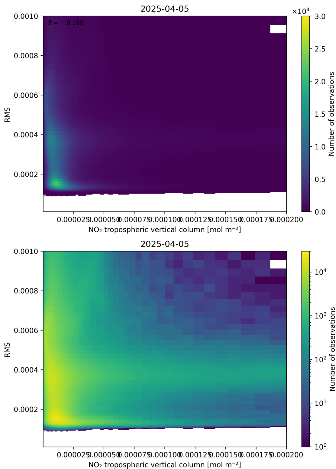
Figure 142: Scatter density plot of “NO 2 tropospheric vertical column” against “RMS” for 2025-04-05 to 2025-04-06.
