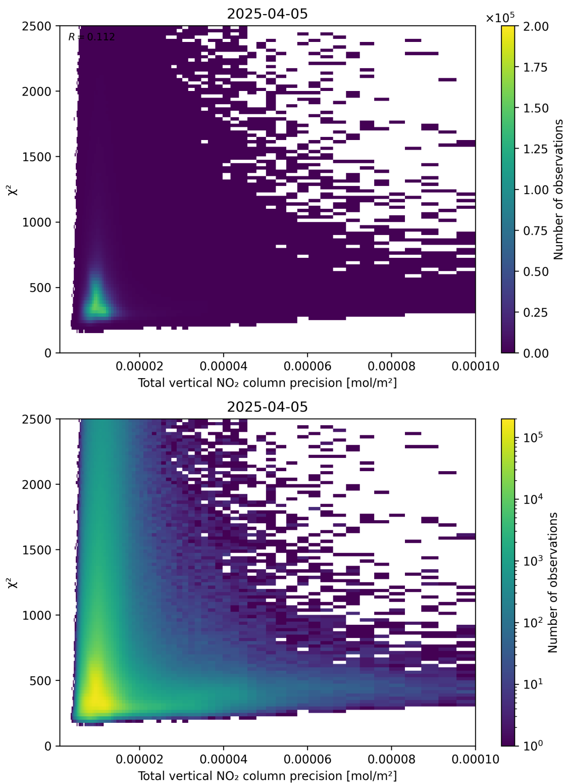
Figure 116: Scatter density plot of “Total vertical NO 2 column precision” against “ \chi^2 ” for 2025-04-05 to 2025-04-06.
