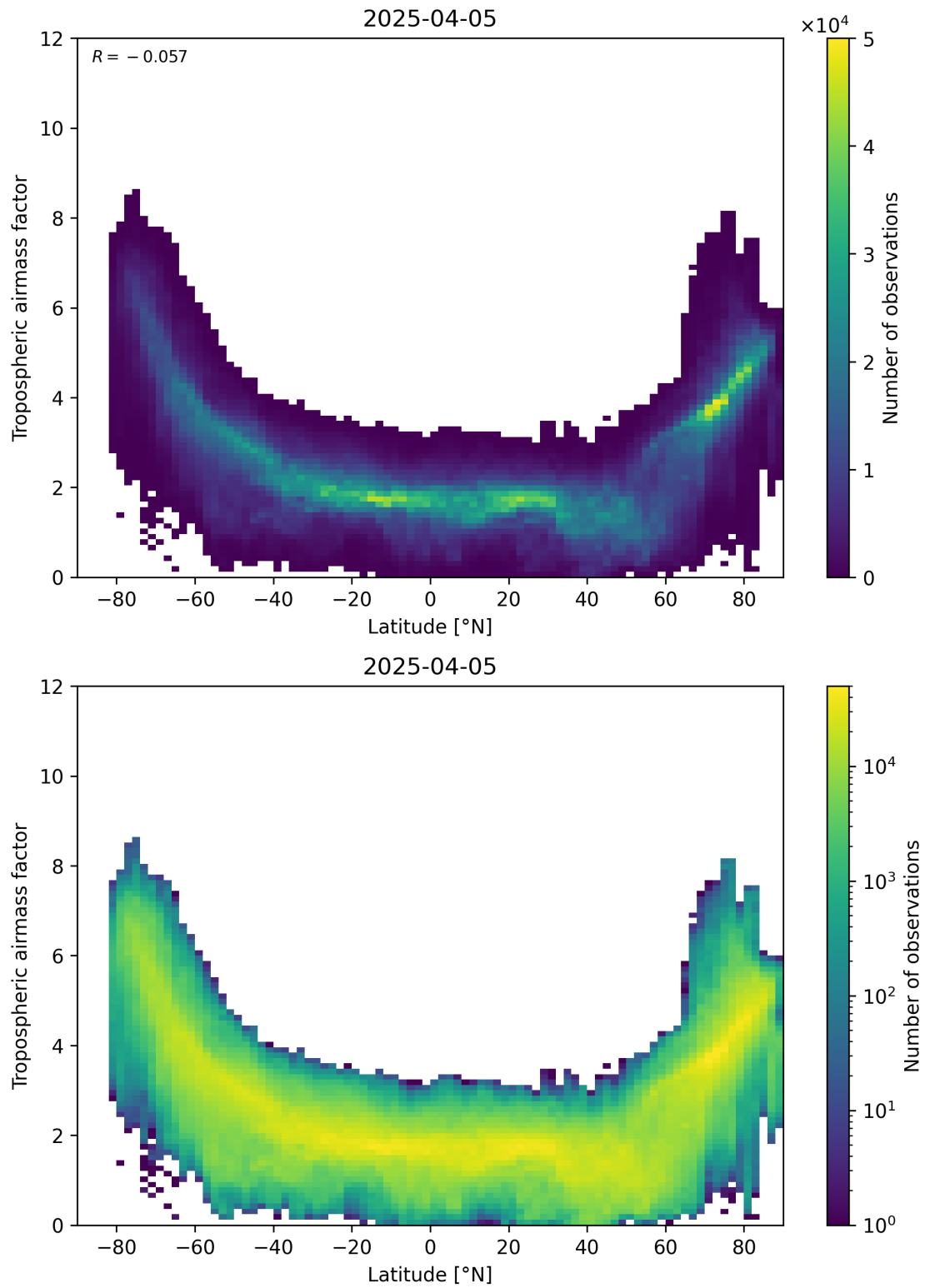
Figure 85: Scatter density plot of “Latitude” against “Tropospheric airmass factor” for 2025-04-05 to 2025-04-06.
