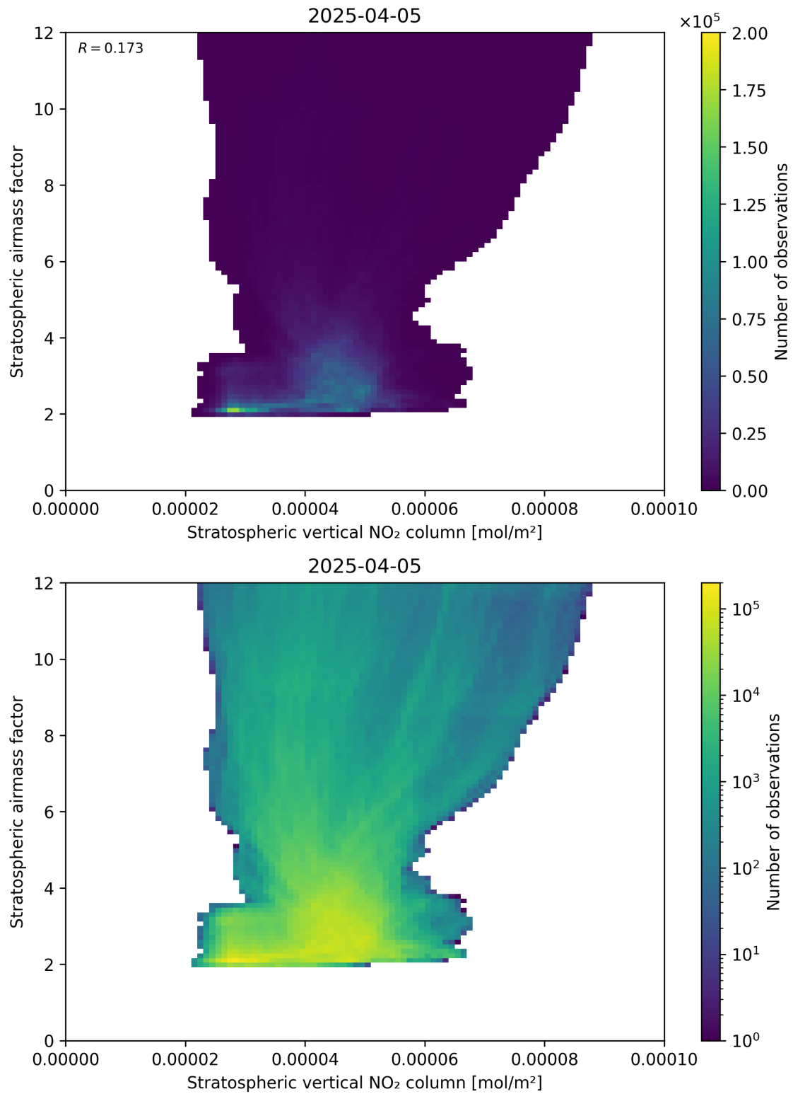
Figure 96: Scatter density plot of “Stratospheric vertical NO 2 column” against “Stratospheric airmass factor” for 2025-04-05 to 2025-04-06.
