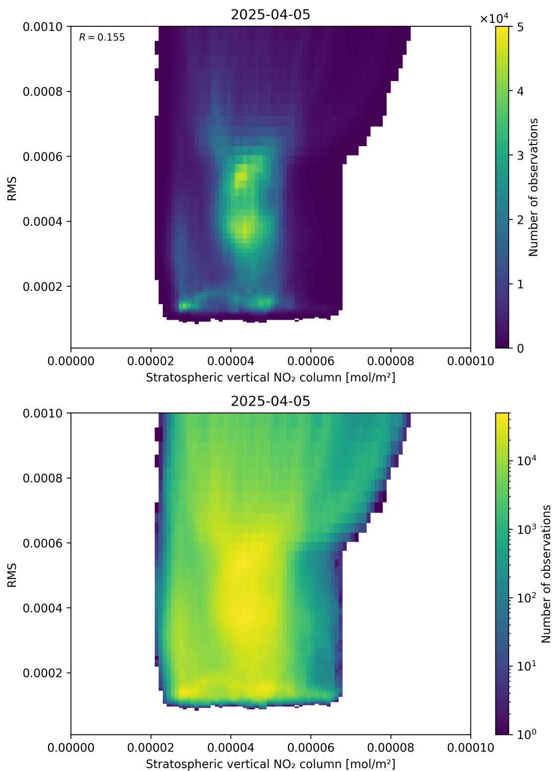
Figure 102: Scatter density plot of “Stratospheric vertical NO 2 column” against “RMS” for 2025-04-05 to 2025-04-06.
