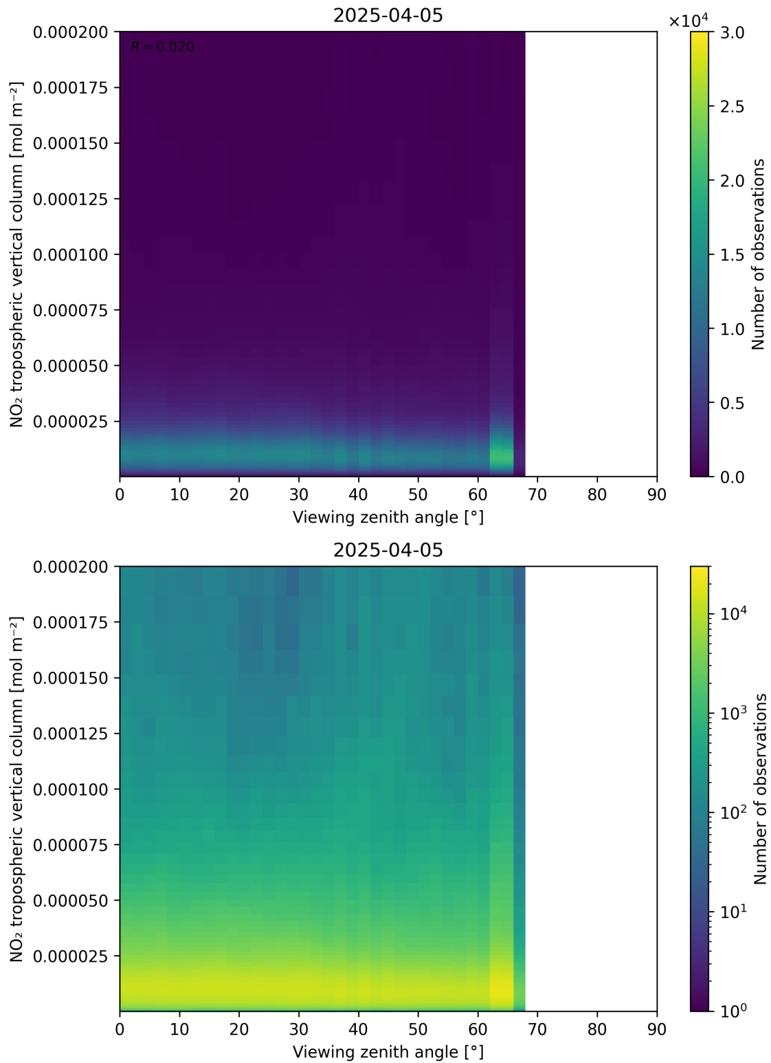
Figure 169: Scatter density plot of “Viewing zenith angle” against “NO 2 tropospheric vertical column” for 2025-04-05 to 2025-04-06.
