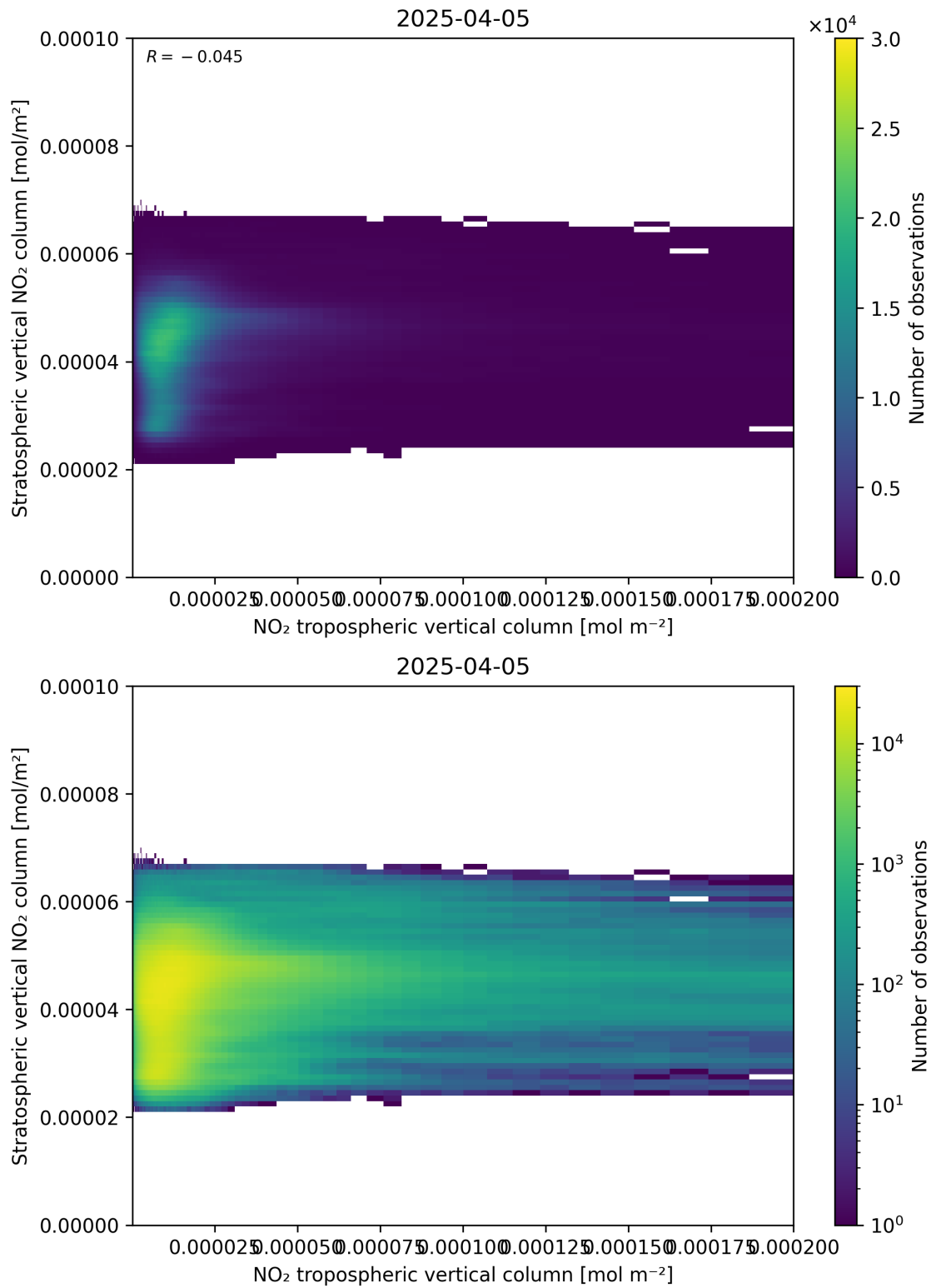
Figure 125: Scatter density plot of “NO 2 tropospheric vertical column” against “Stratospheric vertical NO 2 column” for 2025-04-05 to 2025-04-06.
