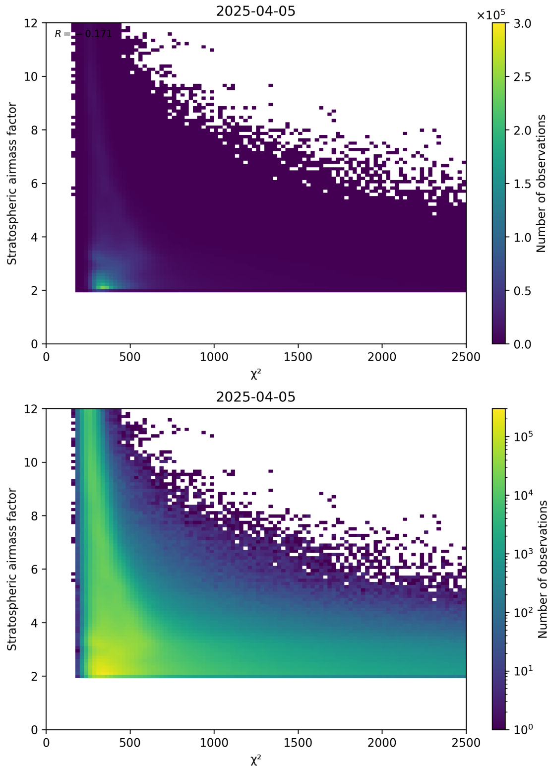
Figure 81: Scatter density plot of “ \chi^2 ” against “Stratospheric airmass factor” for 2025-04-05 to 2025-04-06.
