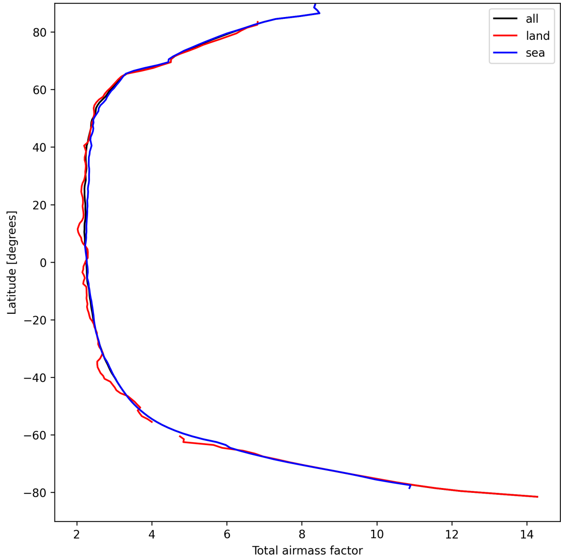
Figure 15: Zonal average of “Total airmass factor” for 2025-04-05 to 2025-04-06.
