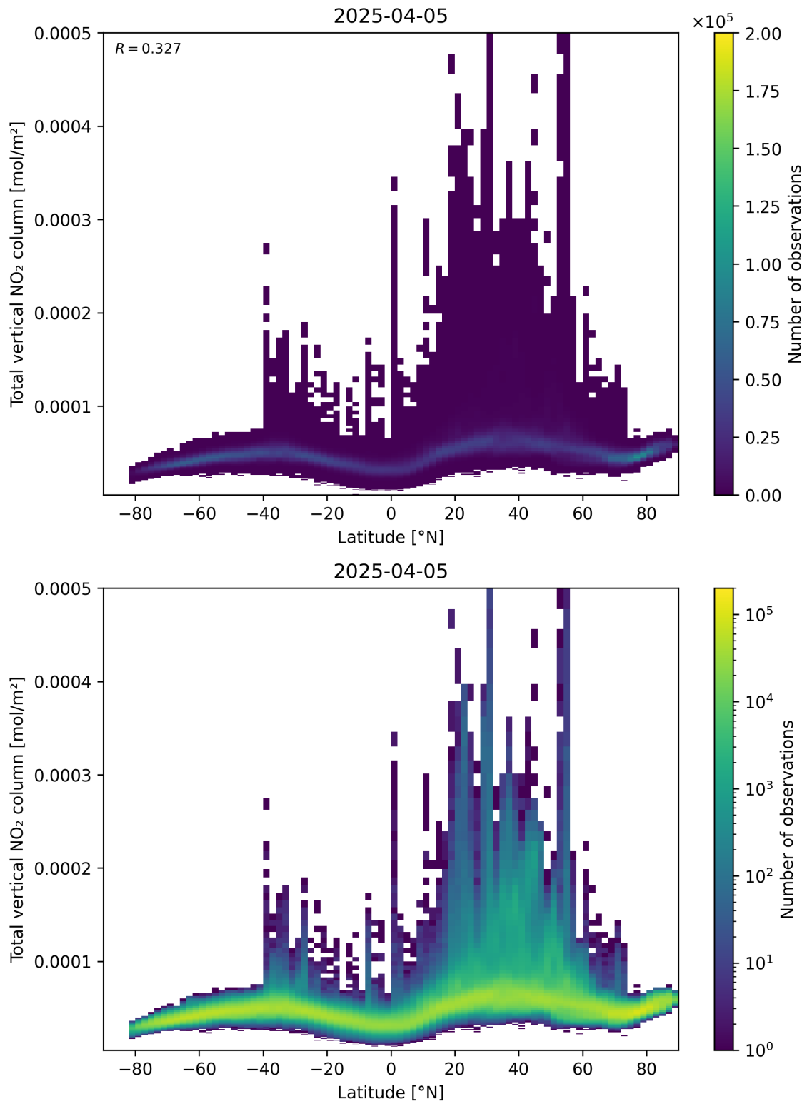
Figure 90: Scatter density plot of “Latitude” against “Total vertical NO 2 column” for 2025-04-05 to 2025-04-06.
