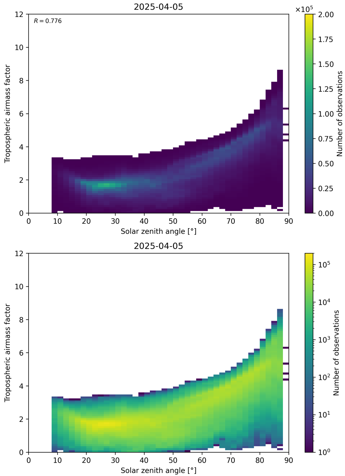
Figure 147: Scatter density plot of “Solar zenith angle” against “Tropospheric airmass factor” for 2025-04-05 to 2025-04-06.
