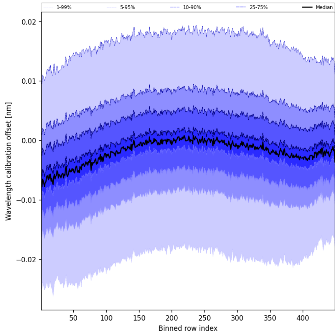
Figure 52: Along track statistics of “Wavelength calibration offset” for 2025-04-05 to 2025-04-06
