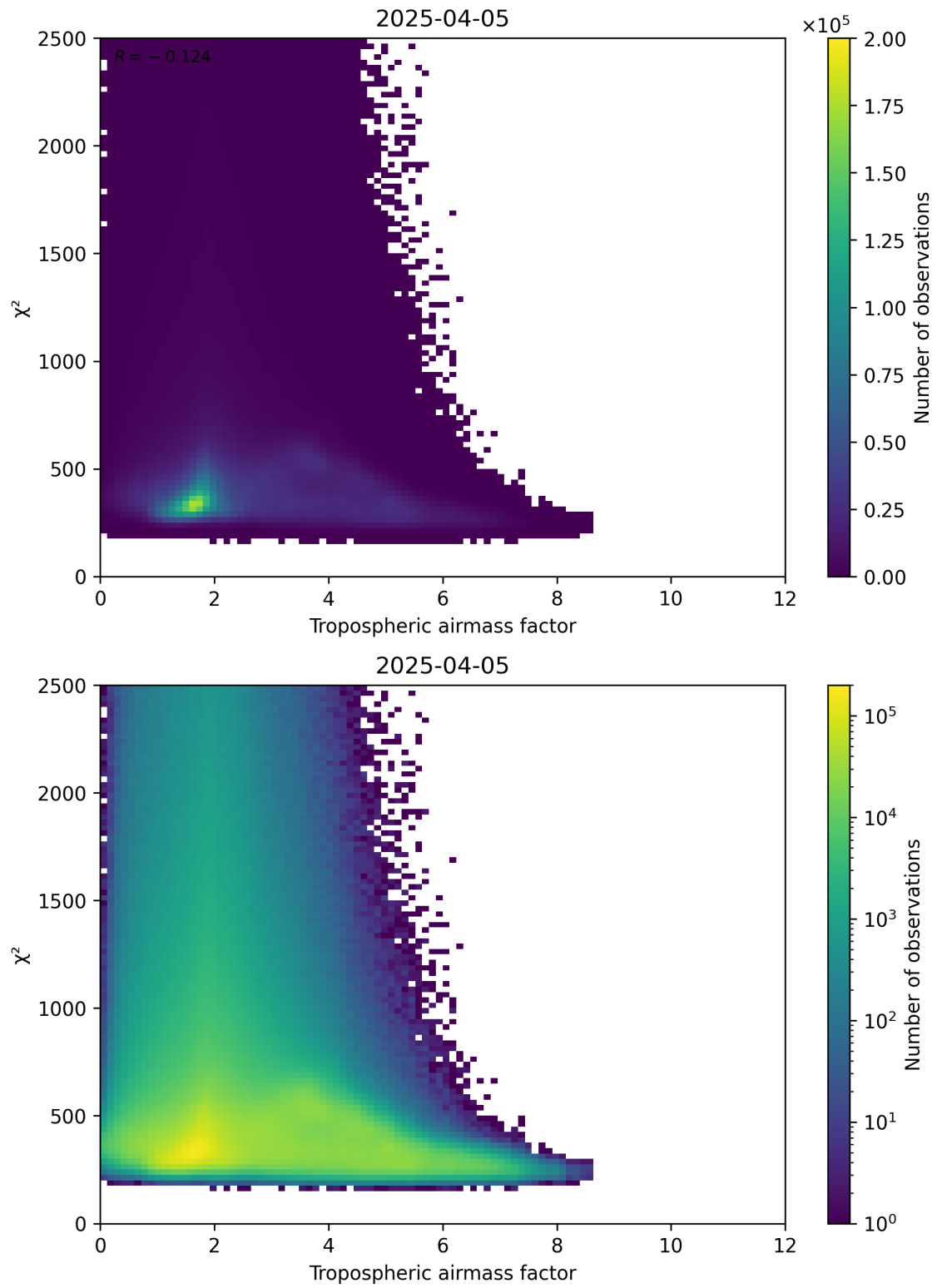
Figure 73: Scatter density plot of “Tropospheric airmass factor” against “ \chi^2 ” for 2025-04-05 to 2025-04-06.
