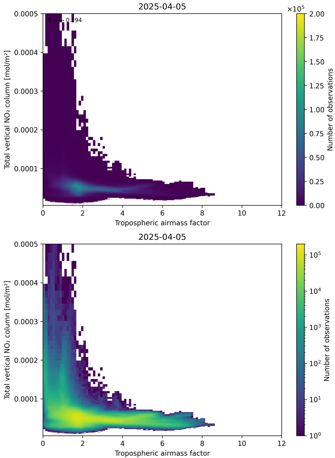
Figure 77: Scatter density plot of “Tropospheric airmass factor” against “Total vertical NO 2 column” for 2025-04-05 to 2025-04-06.
