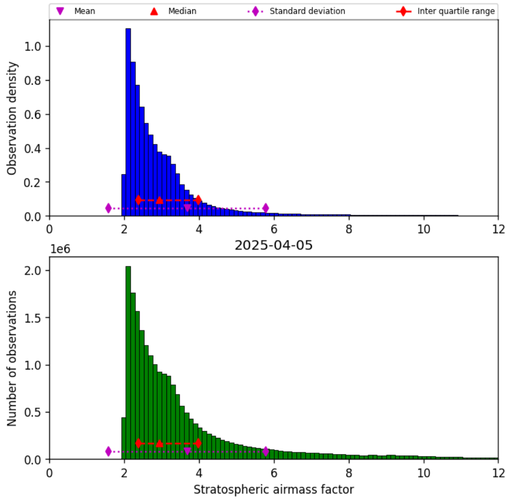
Figure 44: Histogram of “Stratospheric airmass factor” for 2025-04-05 to 2025-04-06
