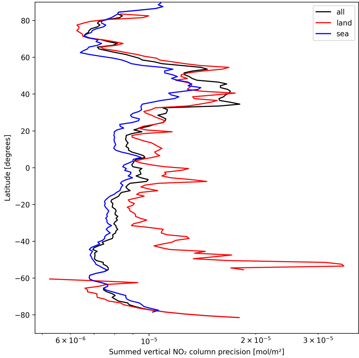
Figure 24: Zonal average of “Summed vertical NO 2 column precision” for 2025-04-05 to 2025-04-06.
