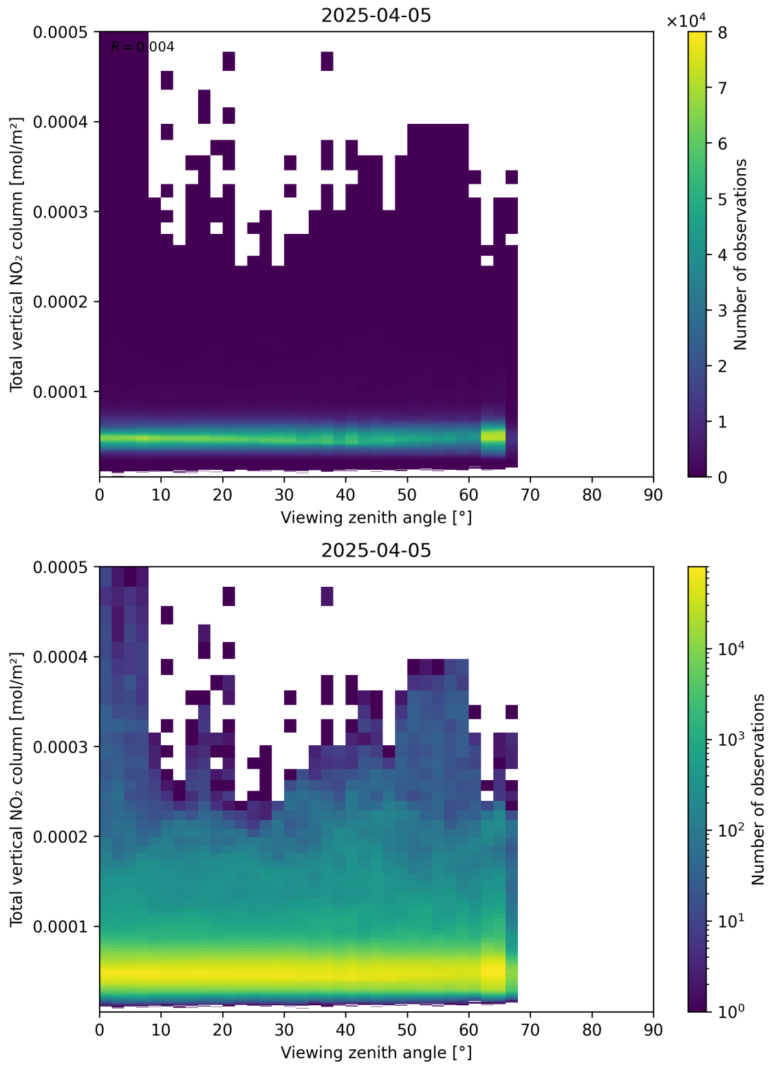
Figure 167: Scatter density plot of “Viewing zenith angle” against “Total vertical NO 2 column” for 2025-04-05 to 2025-04-06.
