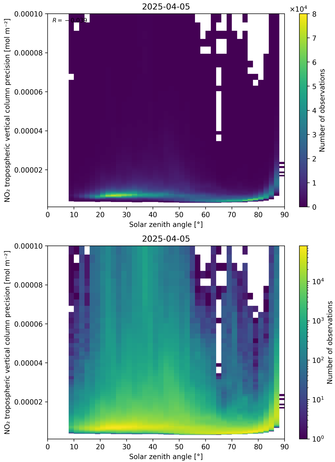
Figure 156: Scatter density plot of “Solar zenith angle” against “NO 2 tropospheric vertical column precision” for 2025-04-05 to 2025-04-06.
