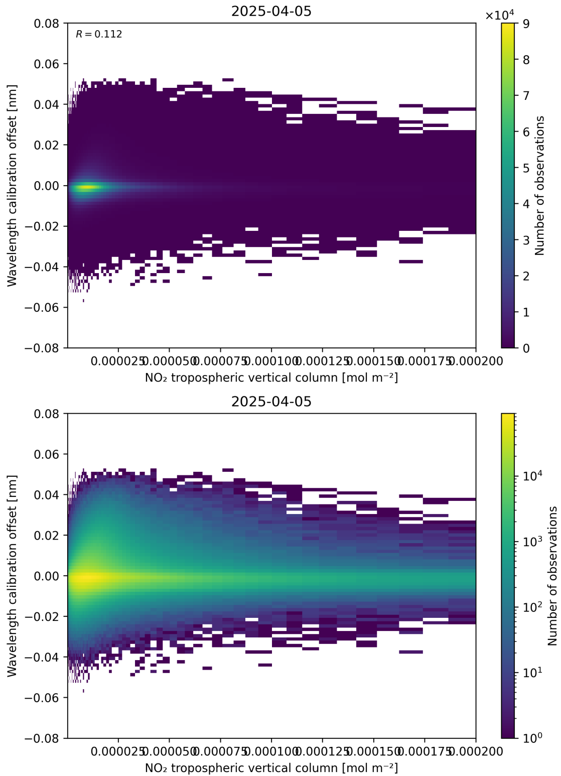
Figure 143: Scatter density plot of “NO 2 tropospheric vertical column” against “Wavelength calibration offset” for 2025-04-05 to 2025-04-06.
