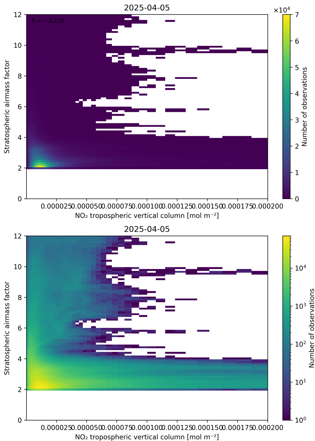
Figure 121: Scatter density plot of “NO 2 tropospheric vertical column” against “Stratospheric air mass factor” for 2025-04-05 to 2025-04-06.
