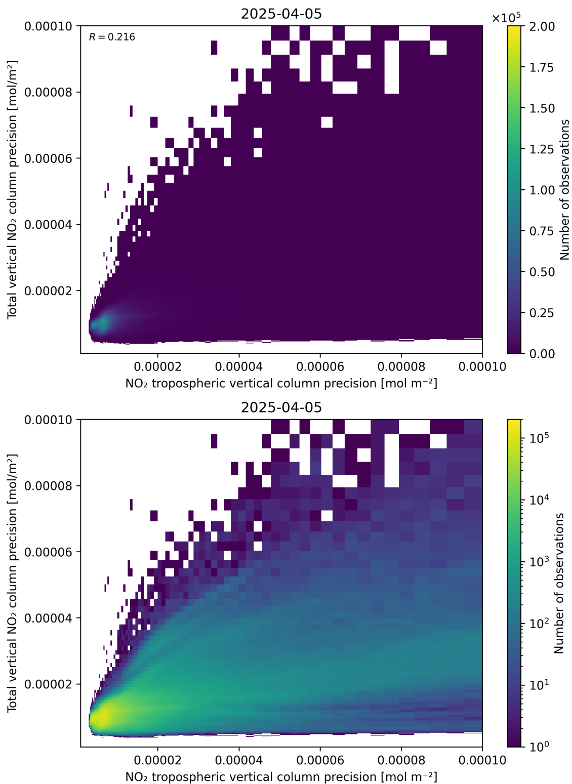
Figure 139: Scatter density plot of “NO 2 tropospheric vertical column precision” against “Total vertical NO 2 column precision” for 2025-04-05 to 2025-04-06.
