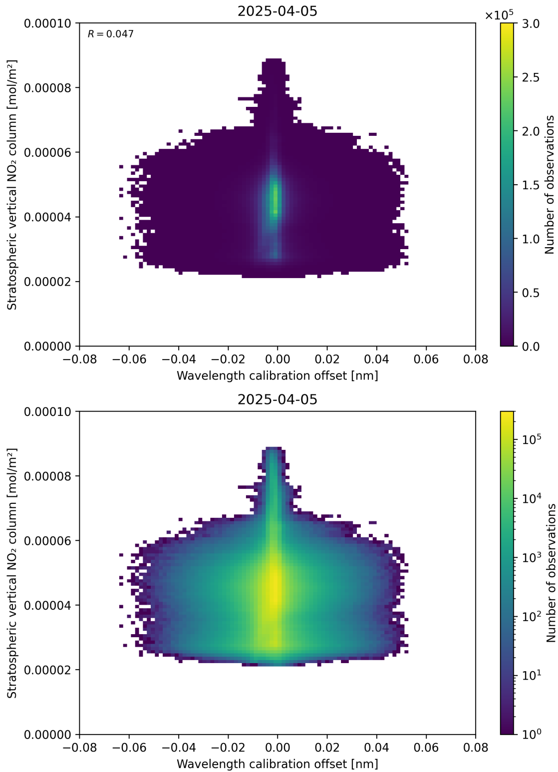
Figure 176: Scatter density plot of “Wavelength calibration offset” against “Stratospheric vertical NO 2 column” for 2025-04-05 to 2025-04-06.
