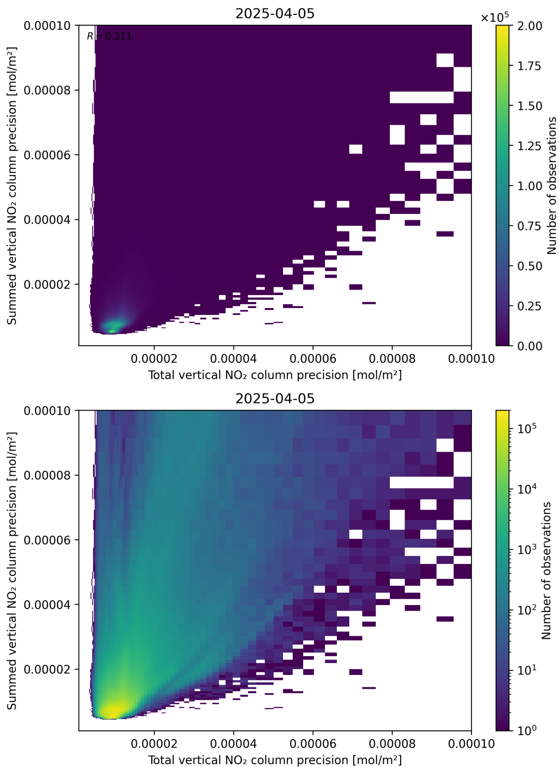
Figure 118: Scatter density plot of “Total vertical NO 2 column precision” against “Summed vertical NO 2 column precision” for 2025-04-05 to 2025-04-06.
