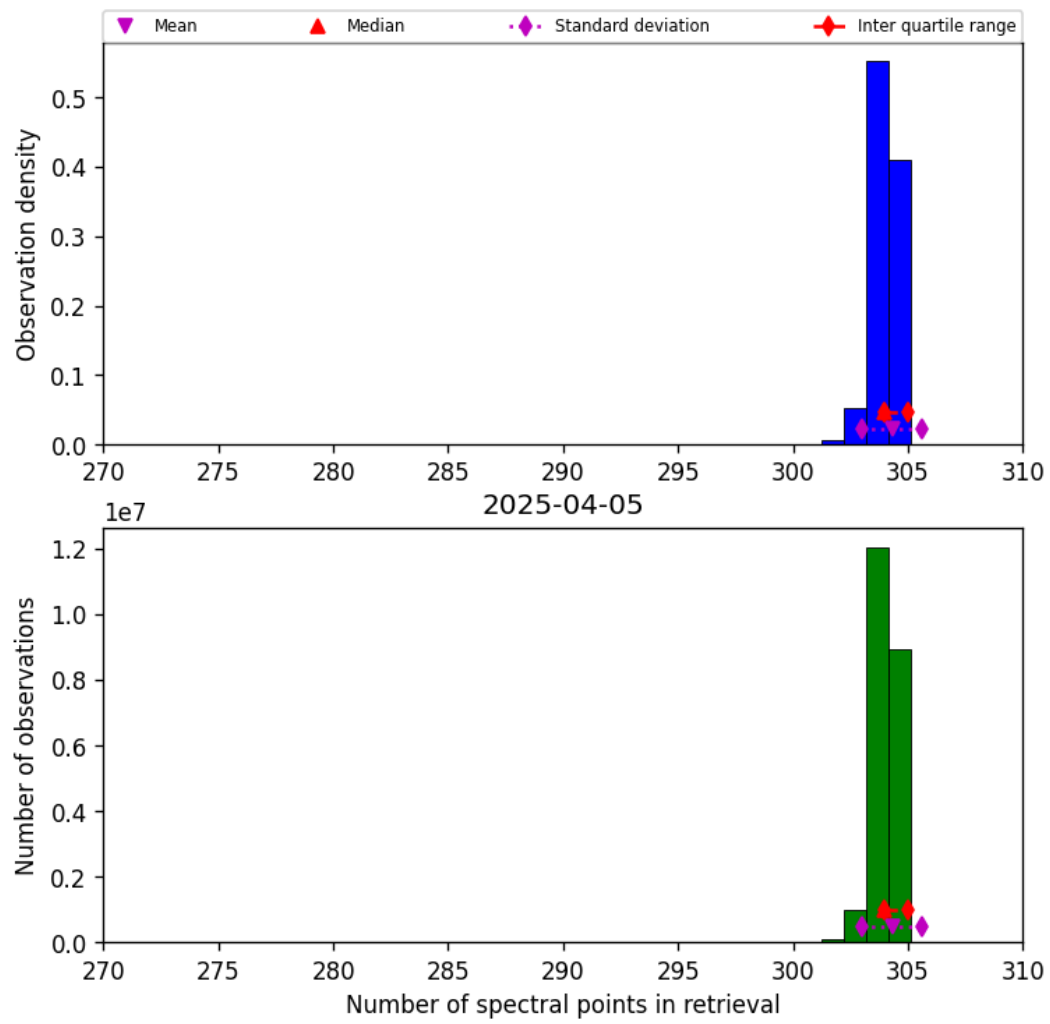
Figure 33: Histogram of “Number of spectral points in retrieval” for 2025-04-05 to 2025-04-06
