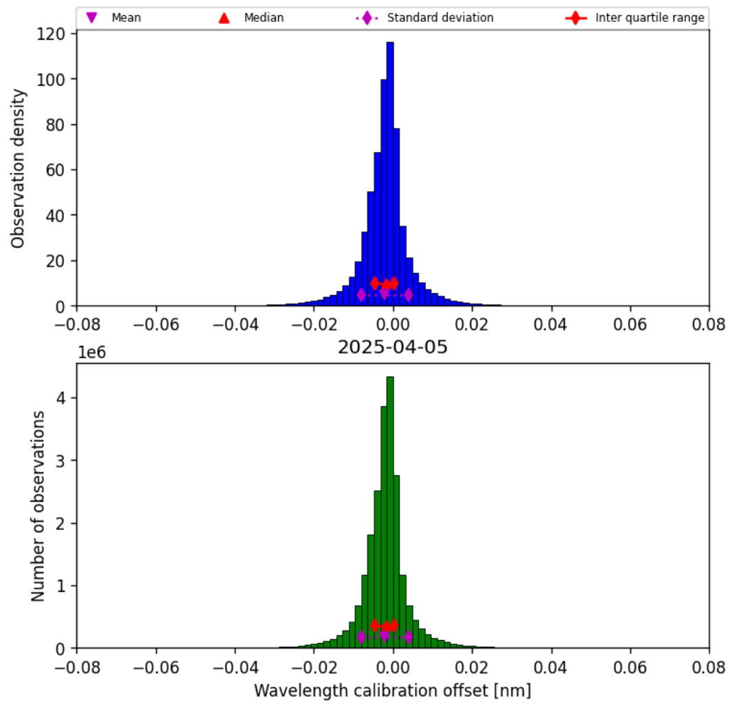
Figure 35: Histogram of “Wavelength calibration offset” for 2025-04-05 to 2025-04-06
