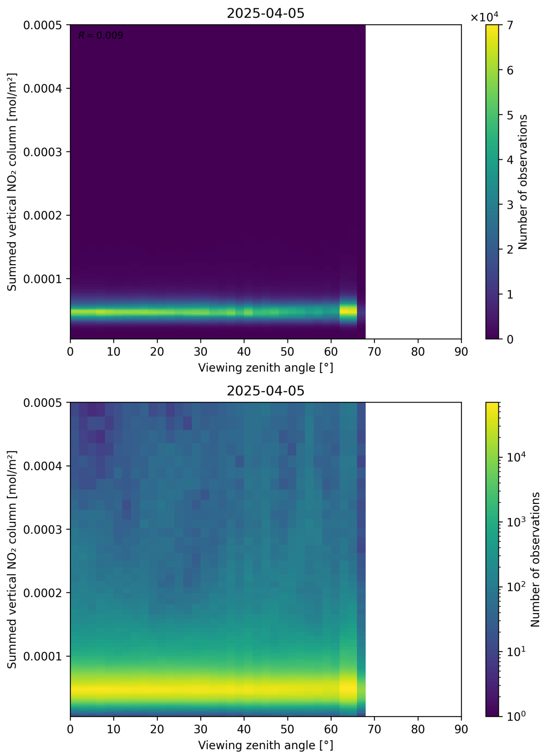
Figure 165: Scatter density plot of “Viewing zenith angle” against “Summed vertical NO 2 column” for 2025-04-05 to 2025-04-06.
