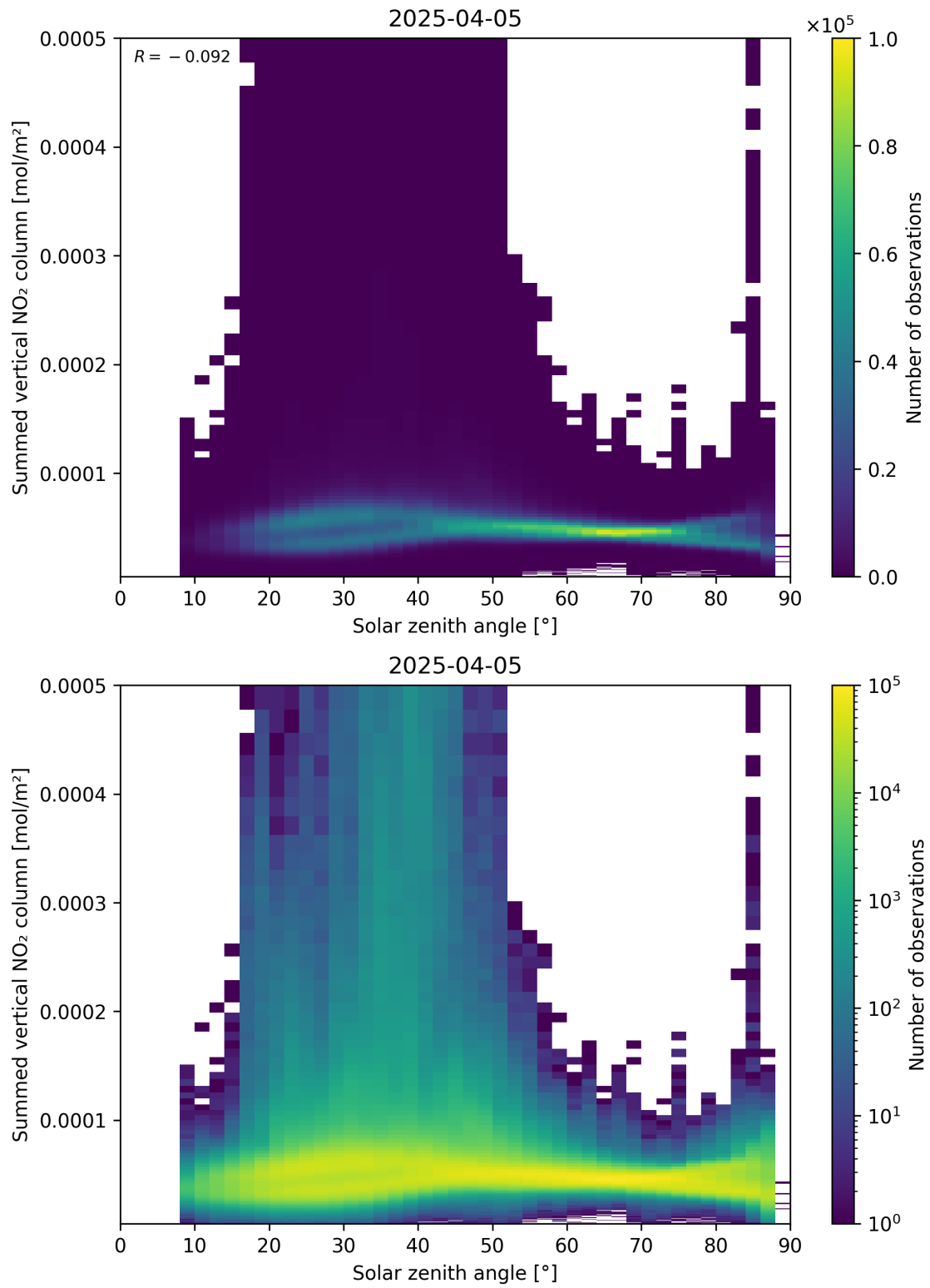
Figure 151: Scatter density plot of “Solar zenith angle” against “Summed vertical NO 2 column” for 2025-04-05 to 2025-04-06.
