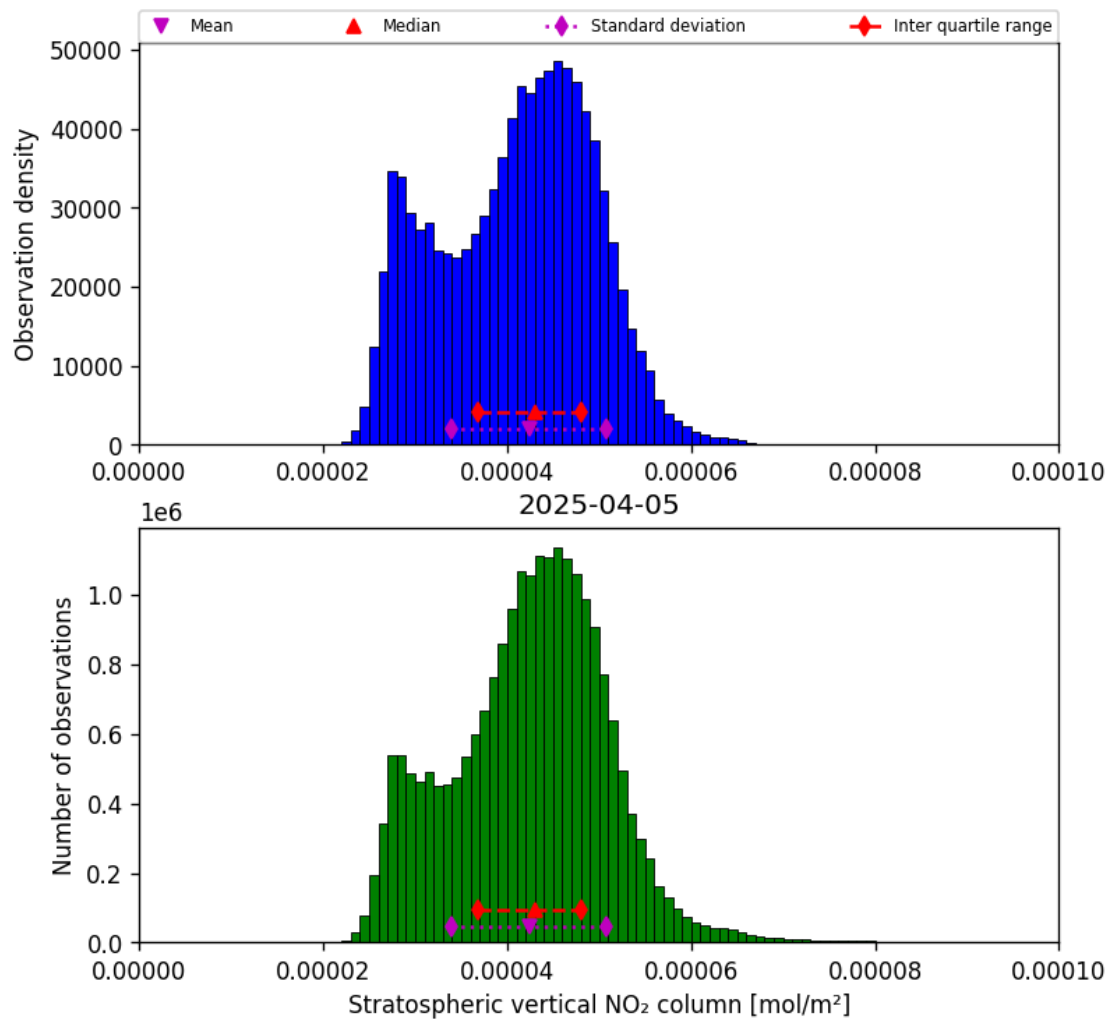
Figure 36: Histogram of “Stratospheric vertical NO 2 column” for 2025-04-05 to 2025-04-06
