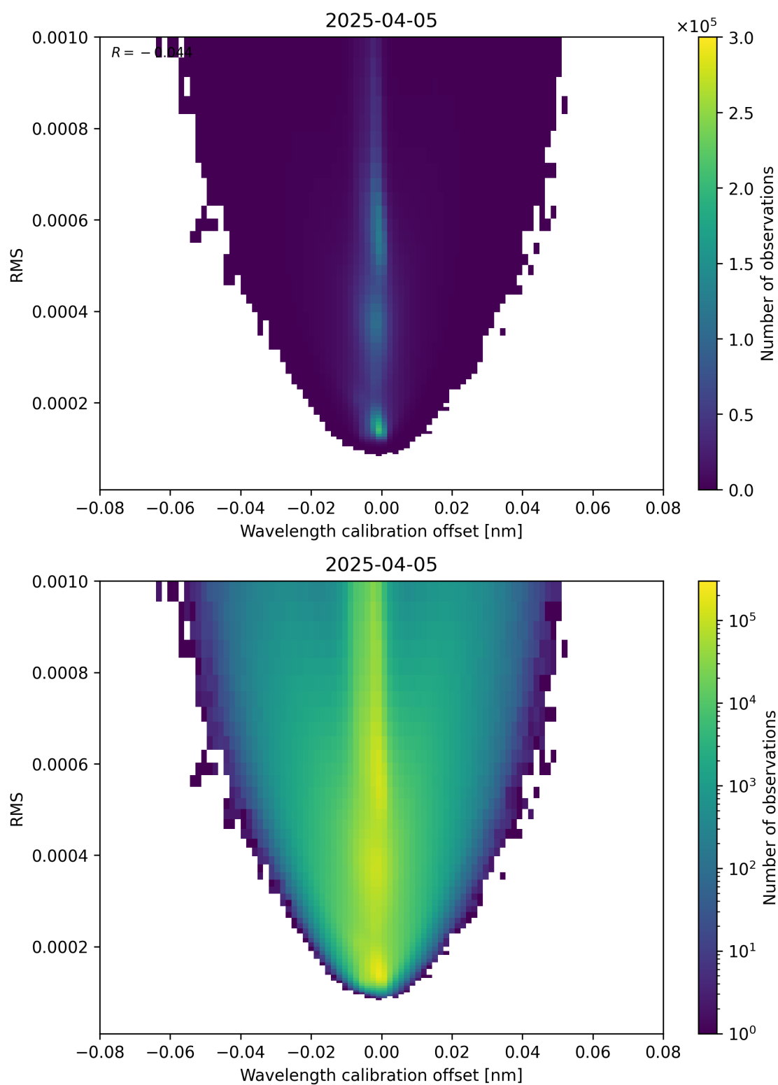
Figure 181: Scatter density plot of “Wavelength calibration offset” against “RMS” for 2025-04-05 to 2025-04-06.
