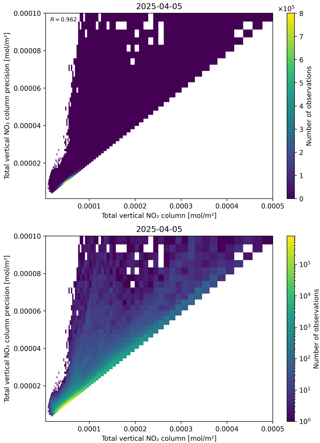
Figure 114: Scatter density plot of “Total vertical NO 2 column” against “Total vertical NO 2 column precision” for 2025-04-05 to 2025-04-06.
