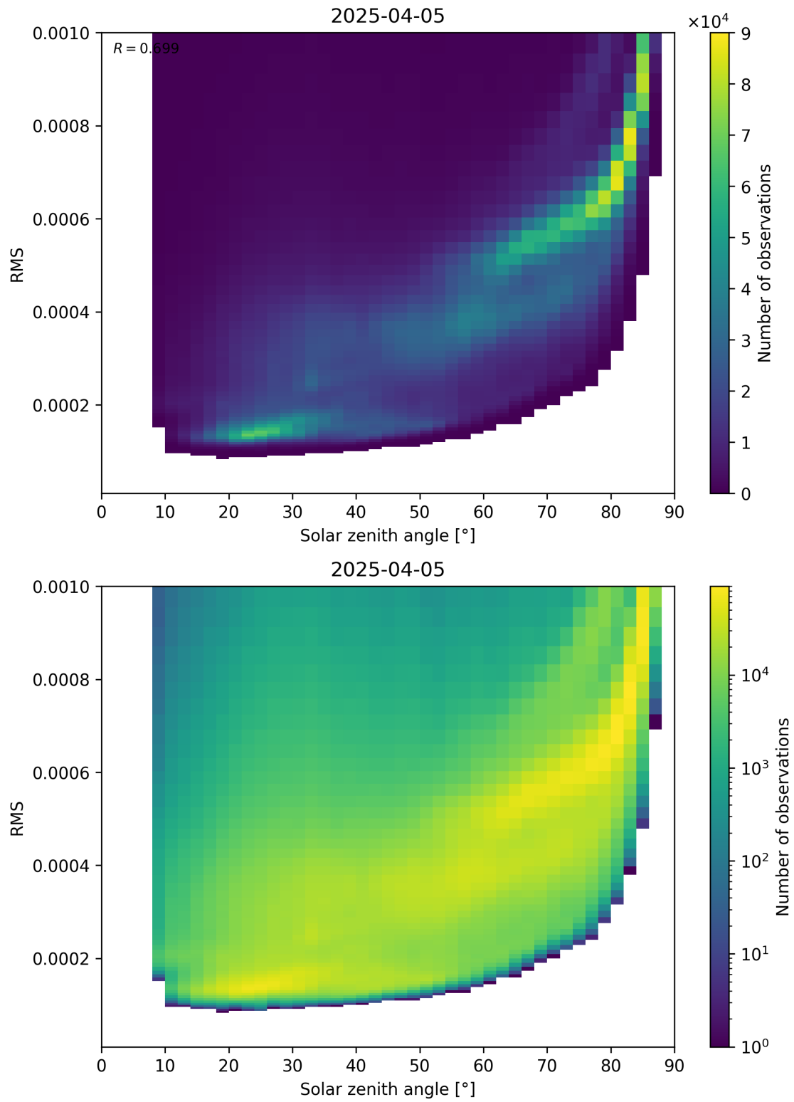
Figure 157: Scatter density plot of “Solar zenith angle” against “RMS” for 2025-04-05 to 2025-04-06.
