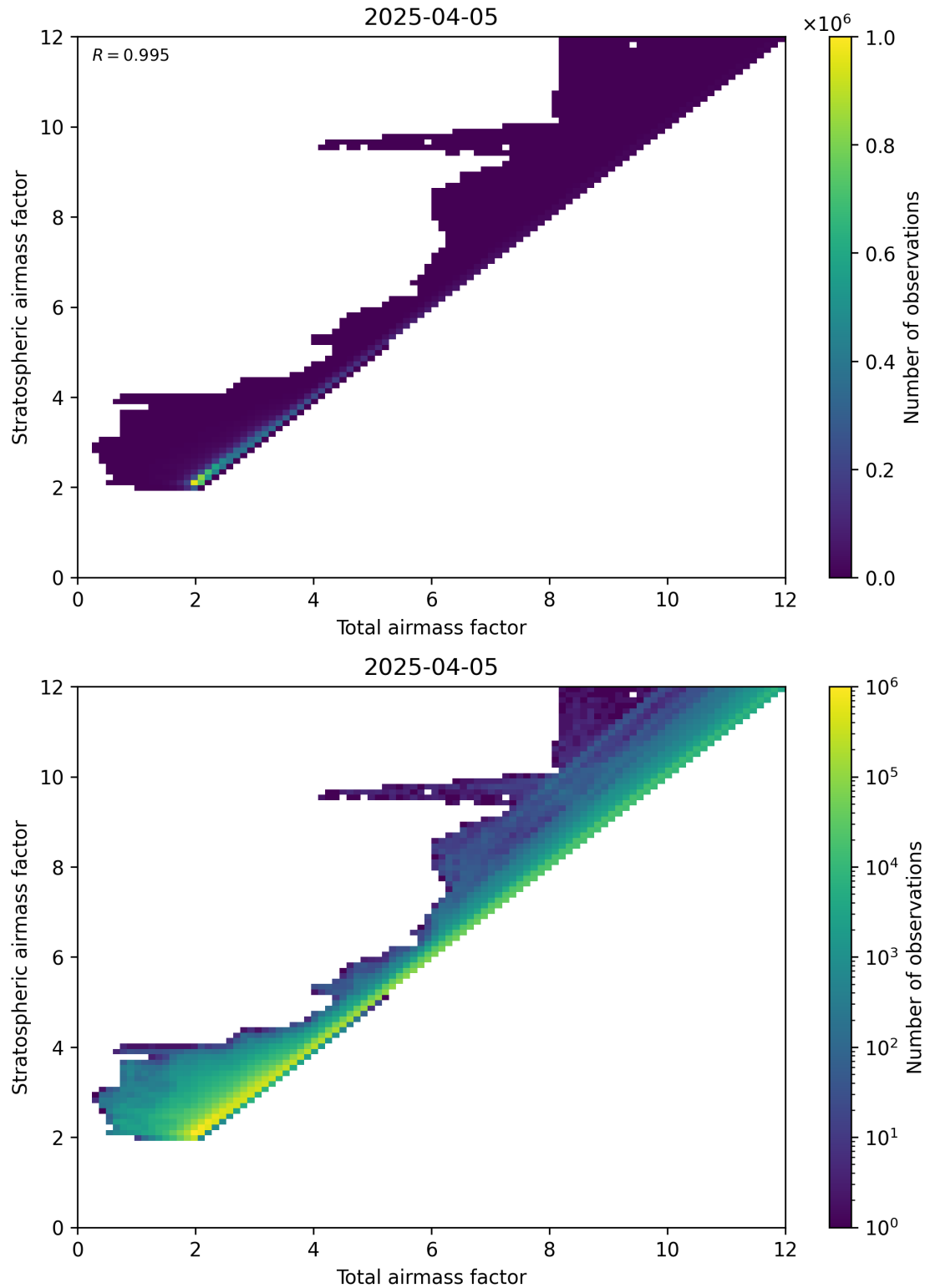
Figure 62: Scatter density plot of “Total airmass factor” against “Stratospheric airmass factor” for 2025-04-05 to 2025-04-06.
