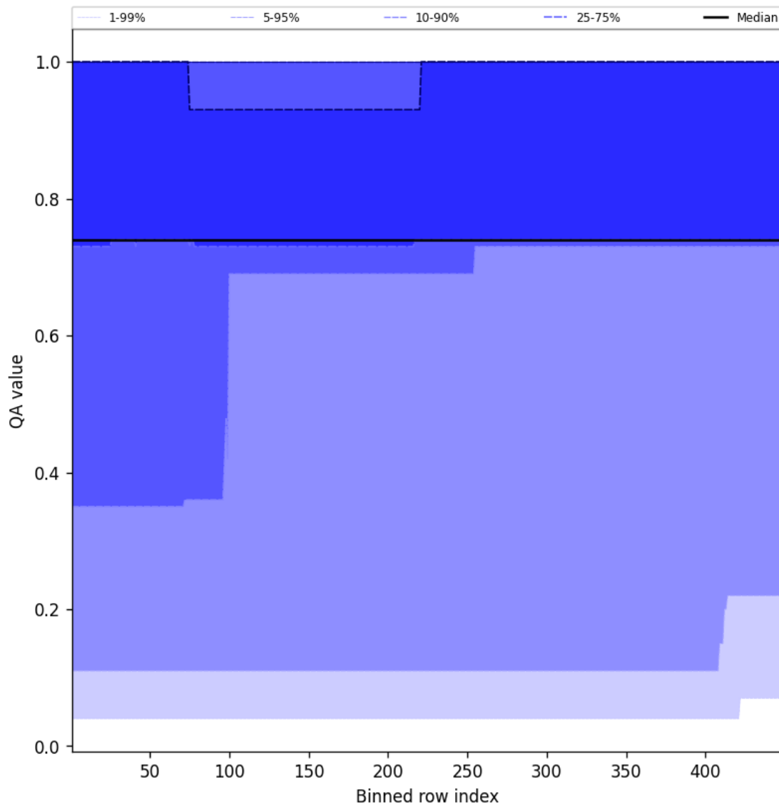
Figure 45: Along track statistics of “QA value” for 2025-04-05 to 2025-04-06
