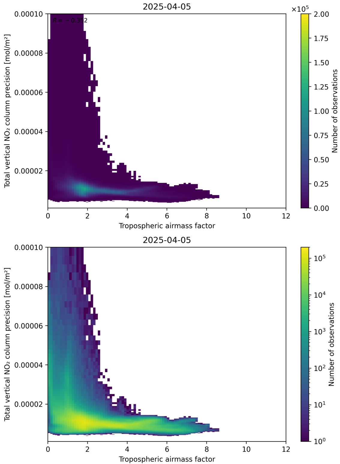
Figure 78: Scatter density plot of “Tropospheric air mass factor” against “Total vertical NO 2 column precision” for 2025-04-05 to 2025-04-06.
