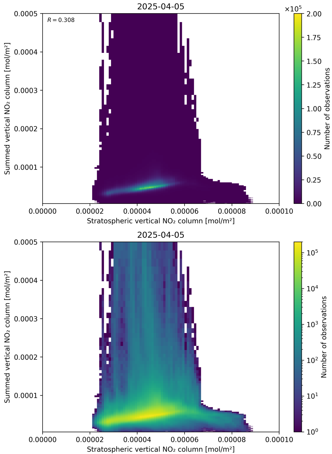
Figure 98: Scatter density plot of “Stratospheric vertical NO 2 column” against “Summed vertical NO 2 column” for 2025-04-05 to 2025-04-06.
