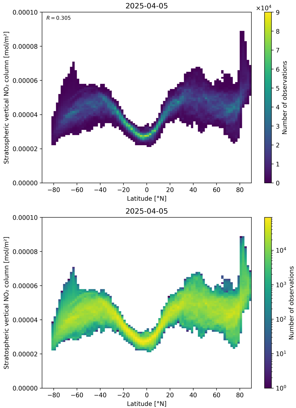
Figure 87: Scatter density plot of “Latitude” against “Stratospheric vertical \text{NO}_2 column” for 2025-04-05 to 2025-04-06.
