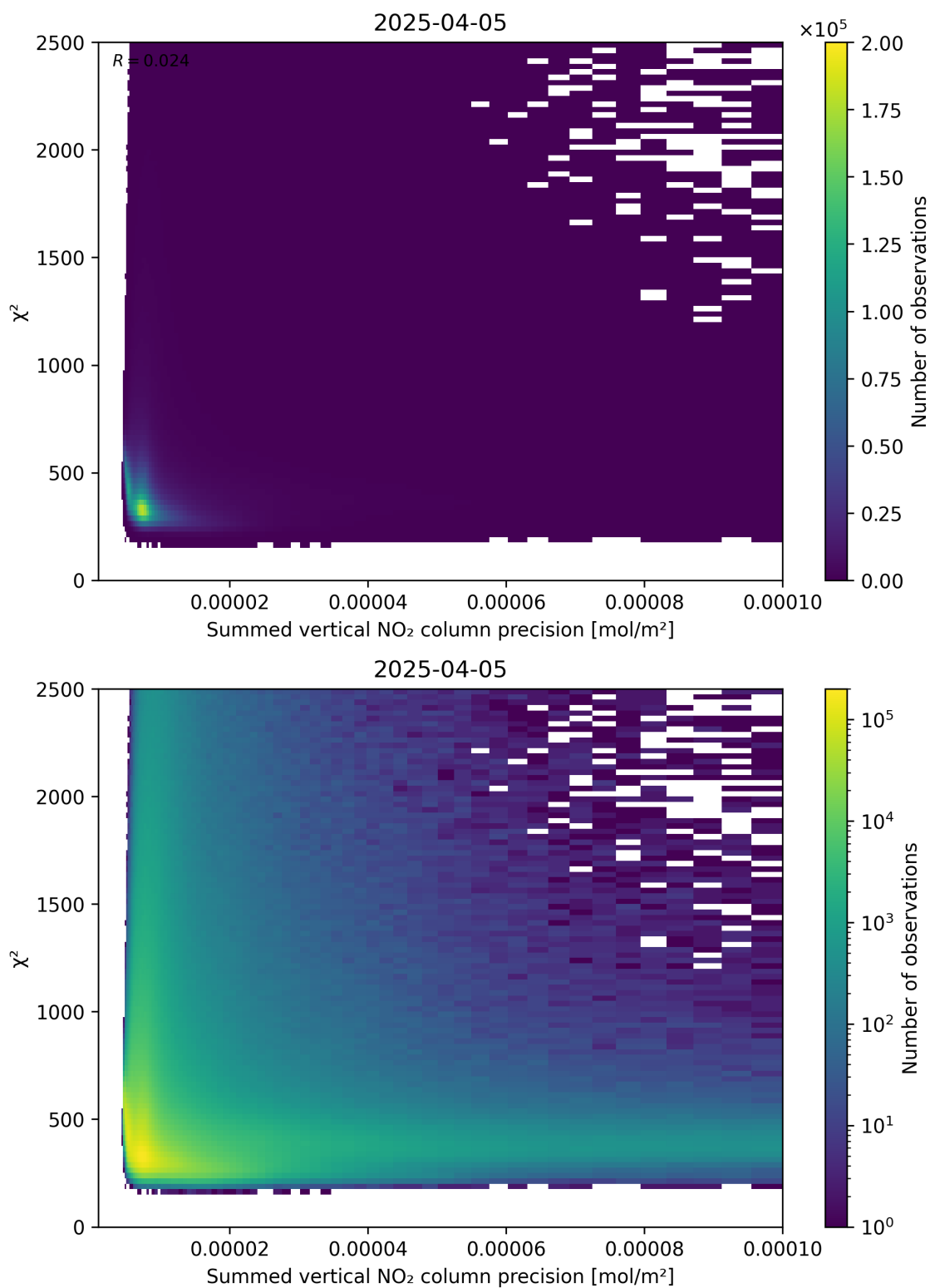
Figure 107: Scatter density plot of “Summed vertical NO 2 column precision” against “ \chi^2 ” for 2025-04-05 to 2025-04-06.
