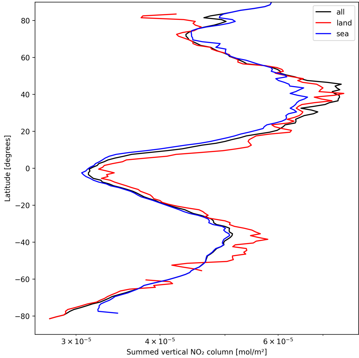
Figure 23: Zonal average of “Summed vertical NO 2 column” for 2025-04-05 to 2025-04-06.
