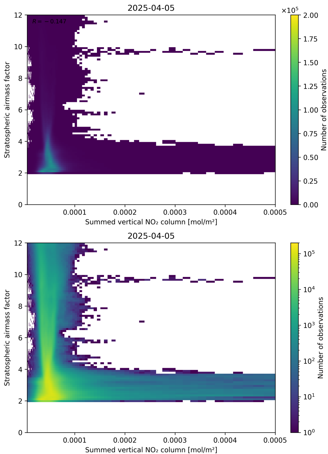
Figure 103: Scatter density plot of “Summed vertical NO 2 column” against “Stratospheric air mass factor” for 2025-04-05 to 2025-04-06.
