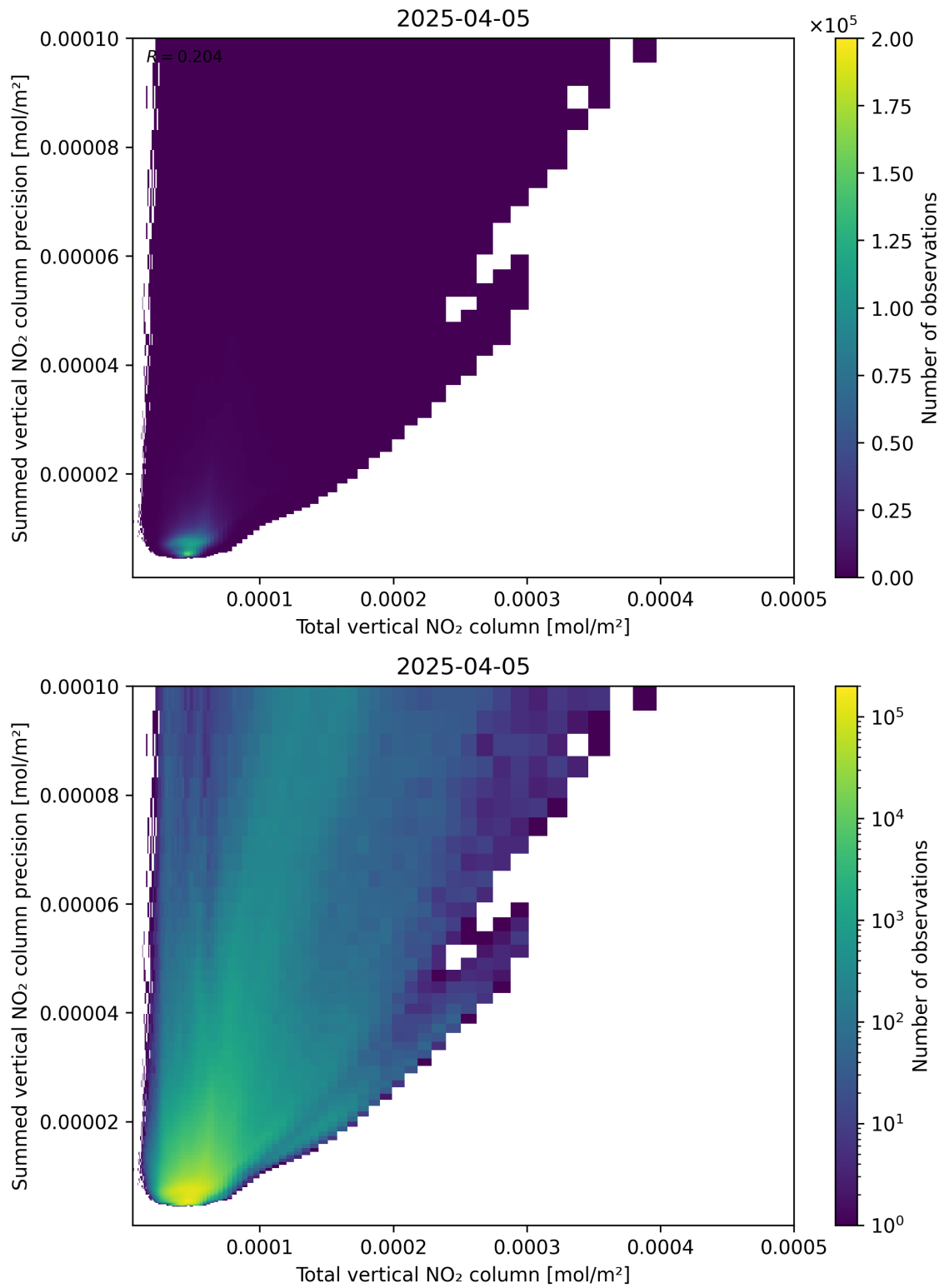
Figure 113: Scatter density plot of “Total vertical NO 2 column” against “Summed vertical NO 2 column precision” for 2025-04-05 to 2025-04-06.
