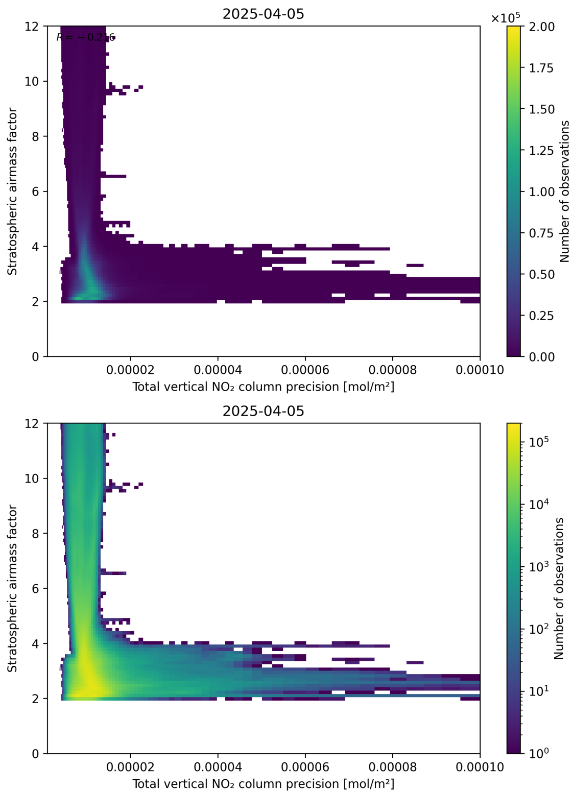
Figure 115: Scatter density plot of “Total vertical NO 2 column precision” against “Stratospheric air mass factor” for 2025-04-05 to 2025-04-06.
