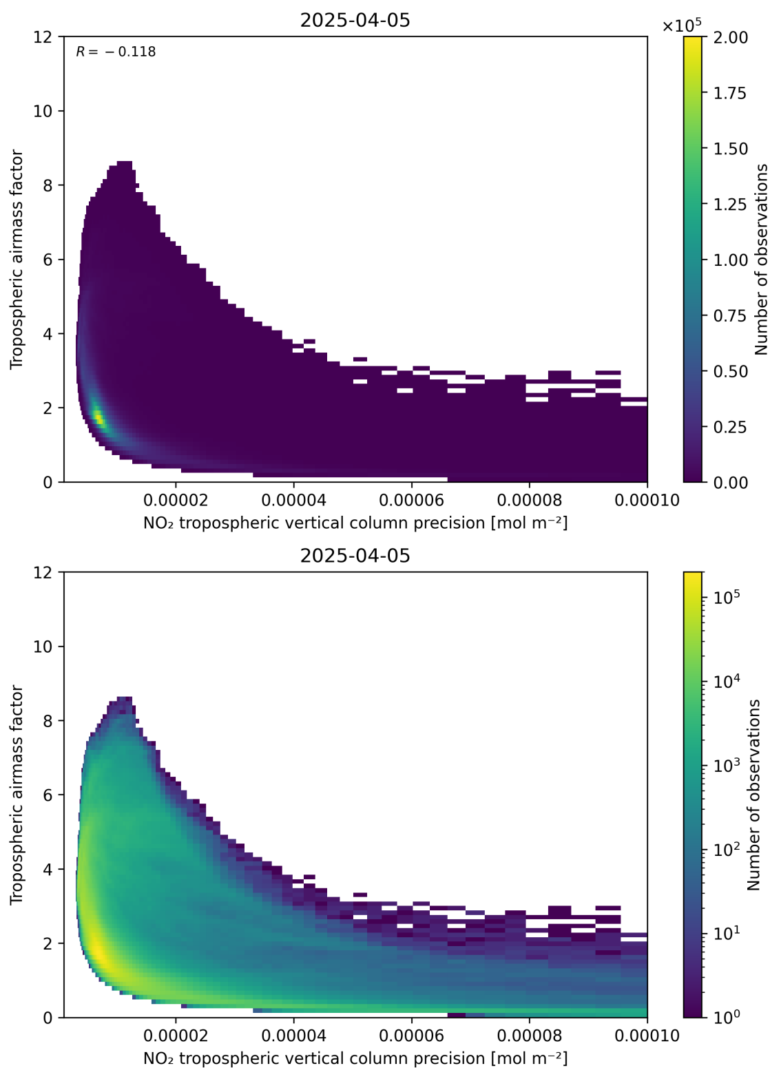
Figure 133: Scatter density plot of “NO 2 tropospheric vertical column precision” against “Tropospheric airmass factor” for 2025-04-05 to 2025-04-06.
