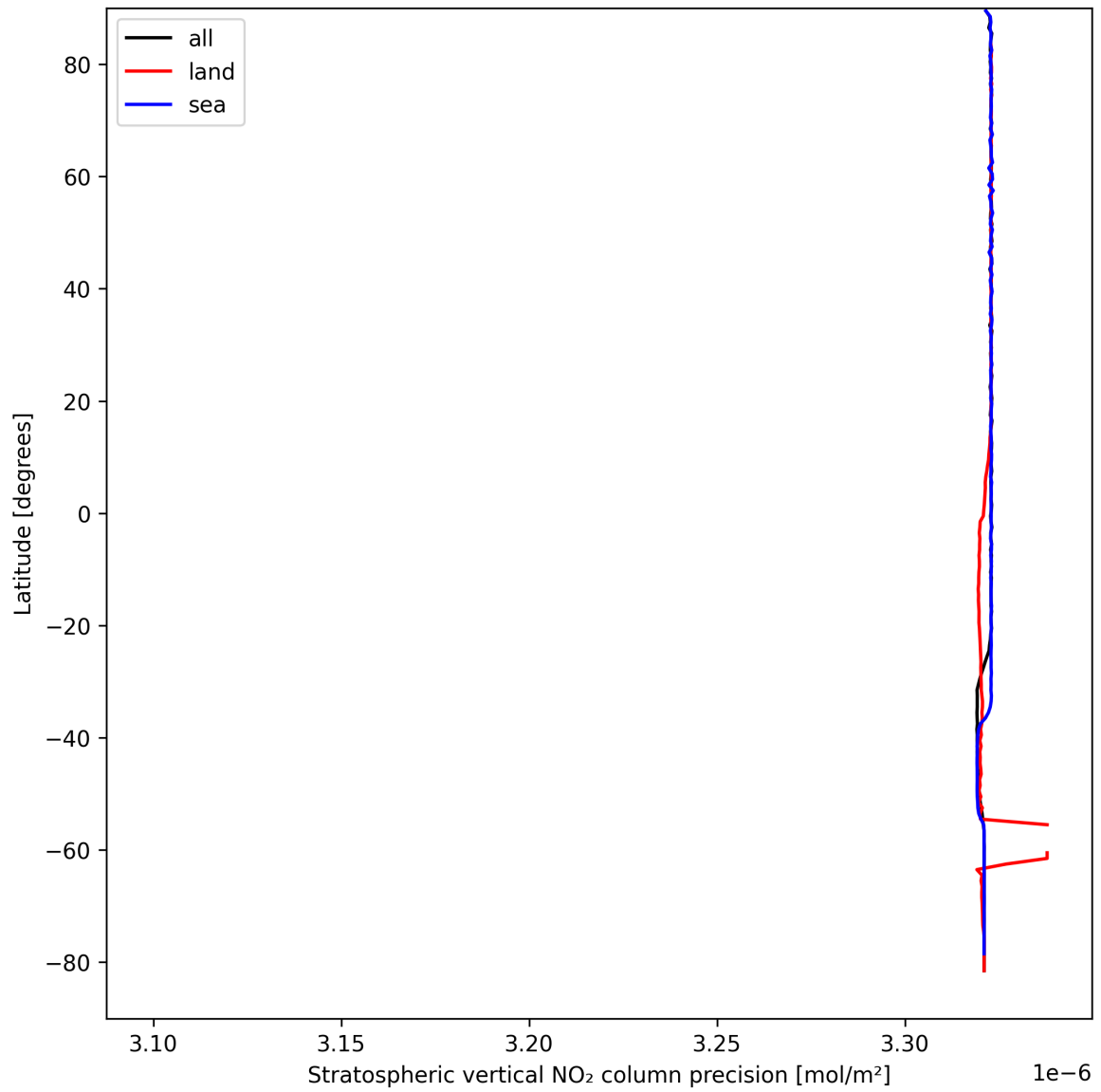
Figure 20: Zonal average of “Stratospheric vertical NO 2 column precision” for 2025-04-05 to 2025-04-06.
