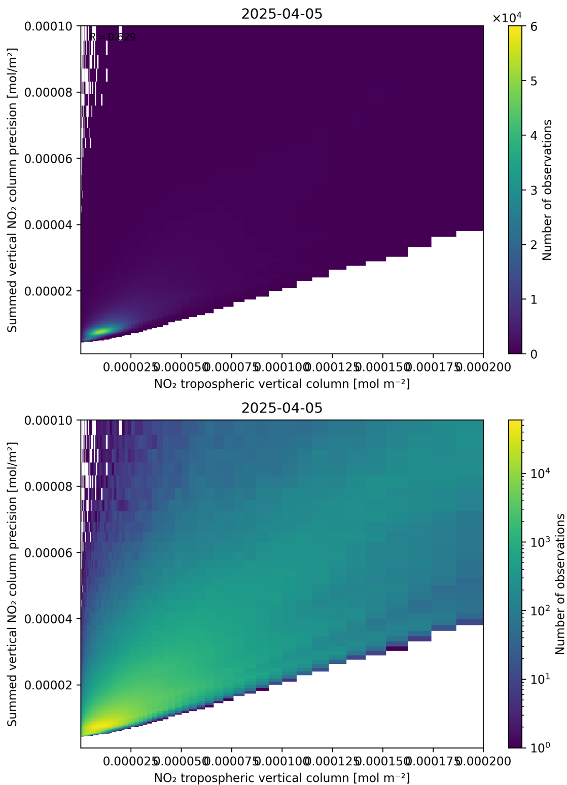
Figure 127: Scatter density plot of “NO 2 tropospheric vertical column” against “Summed vertical NO 2 column precision” for 2025-04-05 to 2025-04-06.
