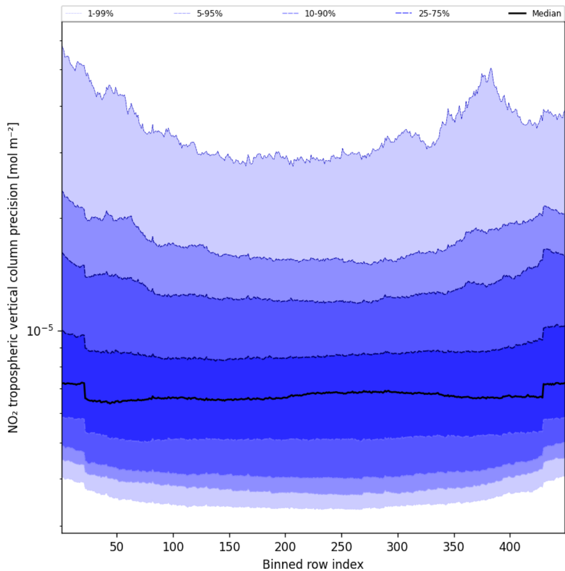
Figure 47: Along track statistics of “NO 2 tropospheric vertical column precision” for 2025-04-05 to 2025-04-06
