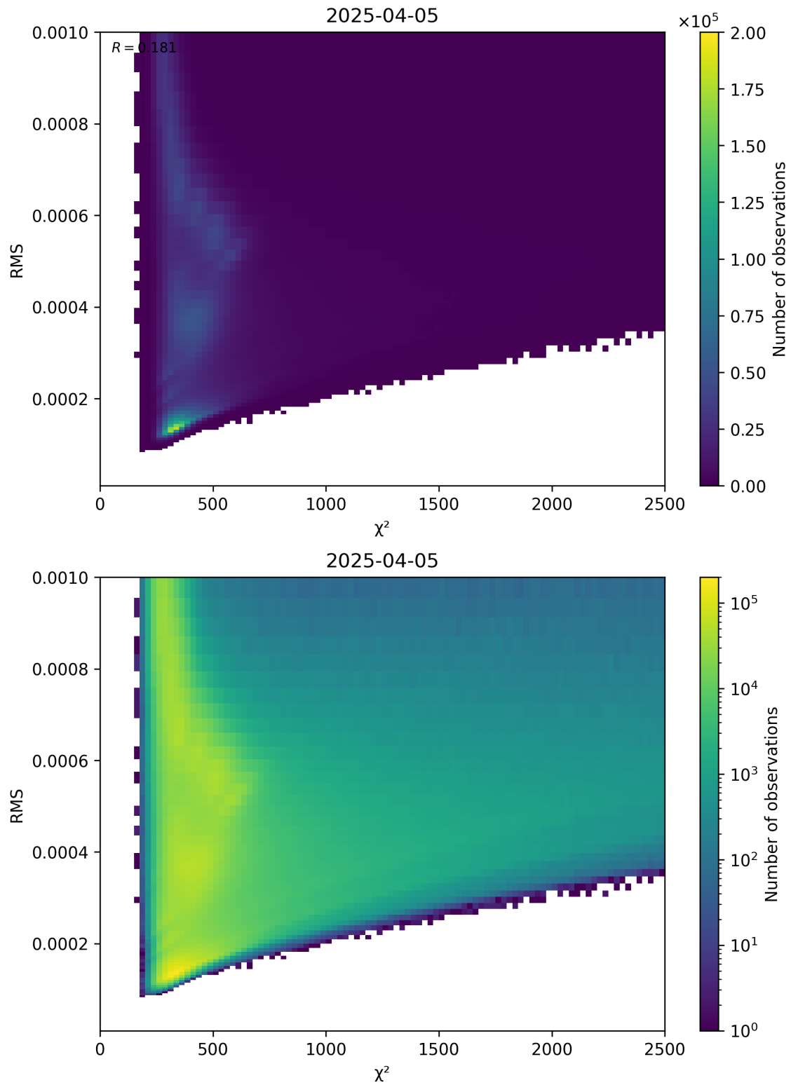
Figure 82: Scatter density plot of “ \chi^2 ” against “RMS” for 2025-04-05 to 2025-04-06.
