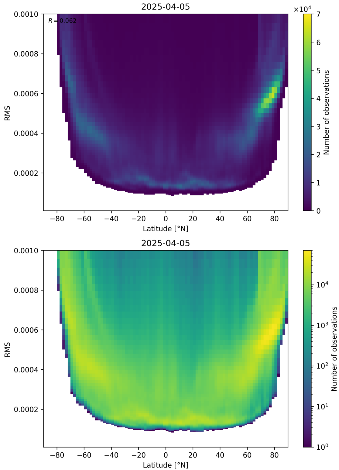
Figure 94: Scatter density plot of “Latitude” against “RMS” for 2025-04-05 to 2025-04-06.
