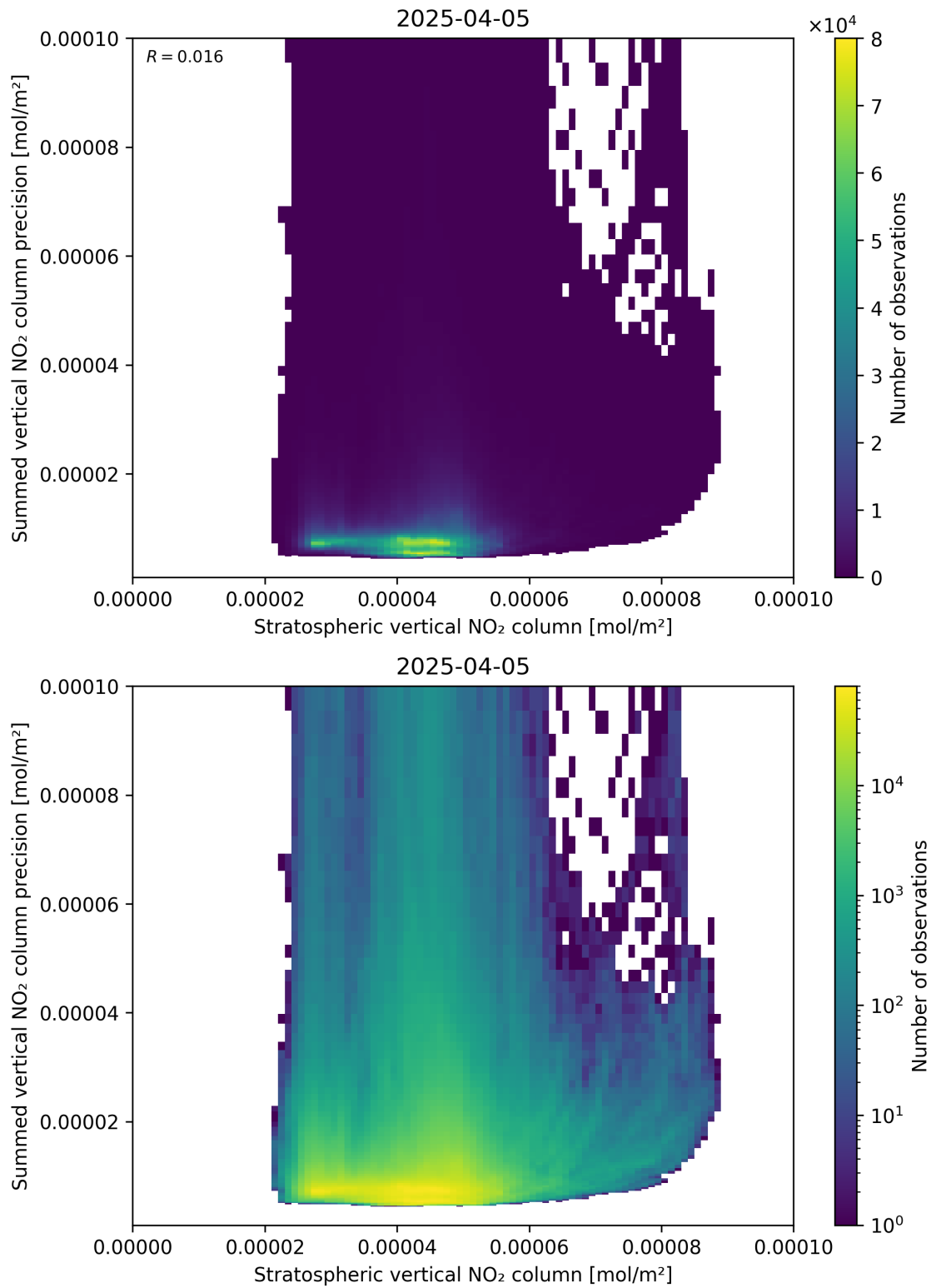
Figure 99: Scatter density plot of “Stratospheric vertical NO 2 column” against “Summed vertical NO 2 column precision” for 2025-04-05 to 2025-04-06.
