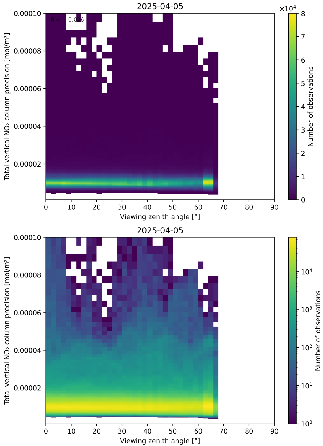
Figure 168: Scatter density plot of “Viewing zenith angle” against “Total vertical NO 2 column precision” for 2025-04-05 to 2025-04-06.
