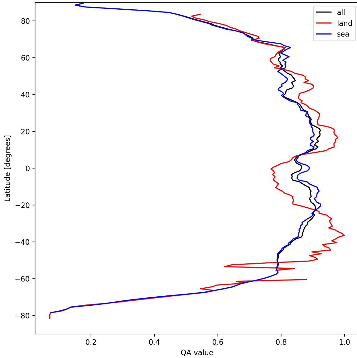
Figure 11: Zonal average of “QA value” for 2025-04-05 to 2025-04-06.
