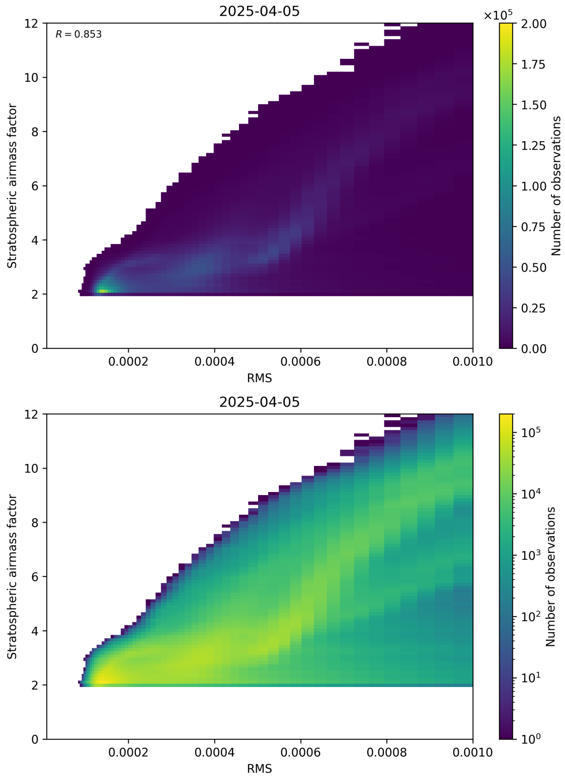
Figure 144: Scatter density plot of “RMS” against “Stratospheric airmass factor” for 2025-04-05 to 2025-04-06.
