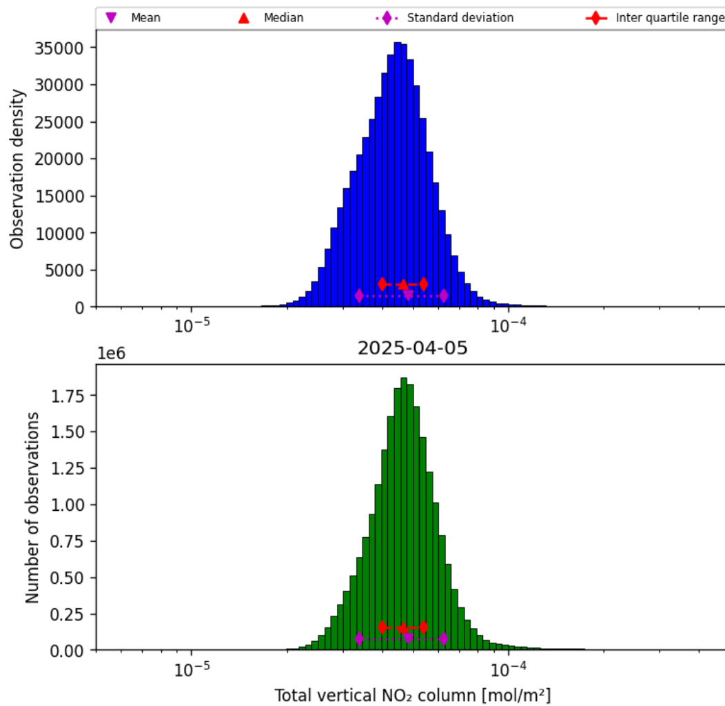
Figure 38: Histogram of “Total vertical NO 2 column” for 2025-04-05 to 2025-04-06
