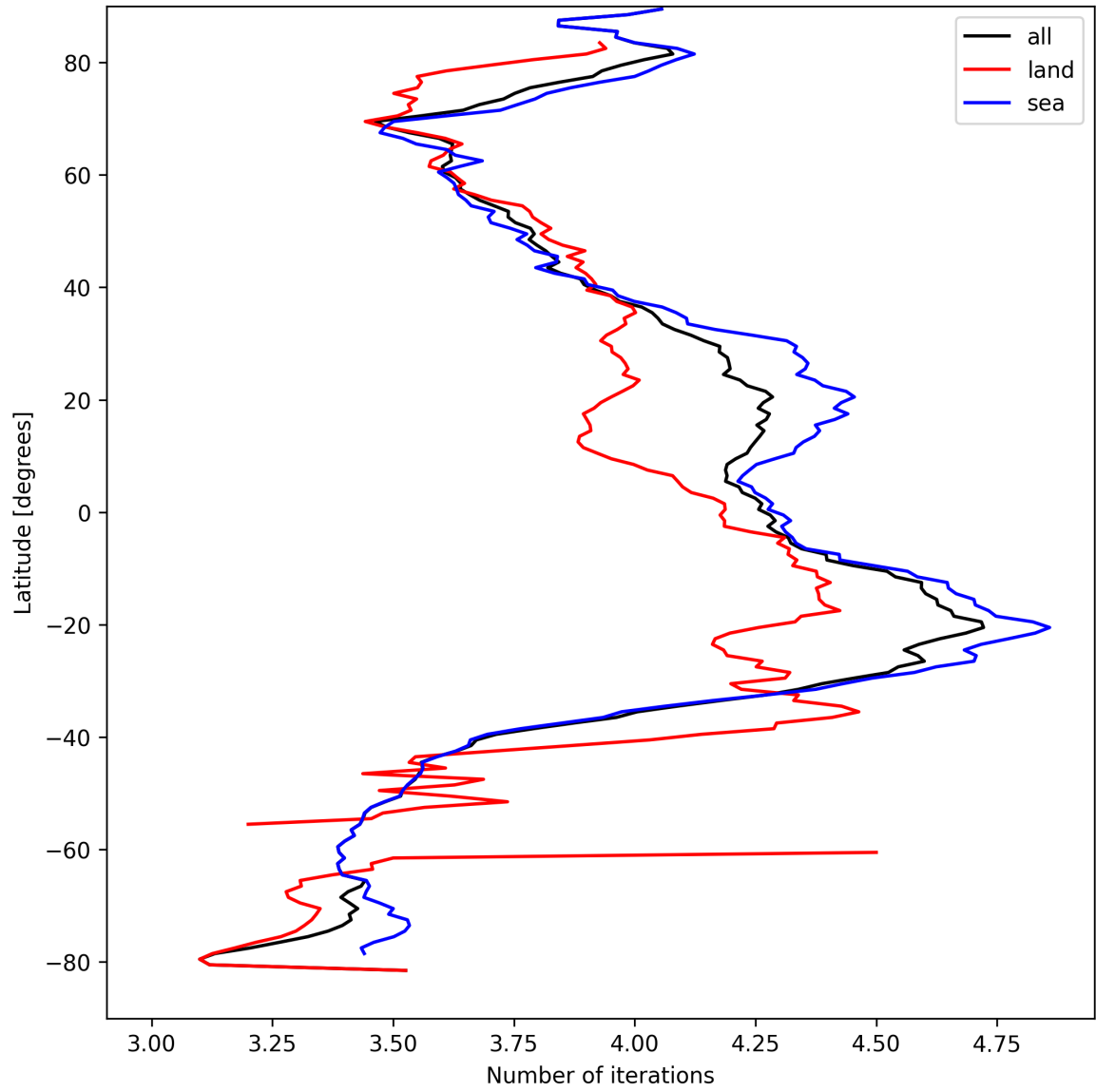
Figure 17: Zonal average of “Number of iterations” for 2025-04-05 to 2025-04-06.
