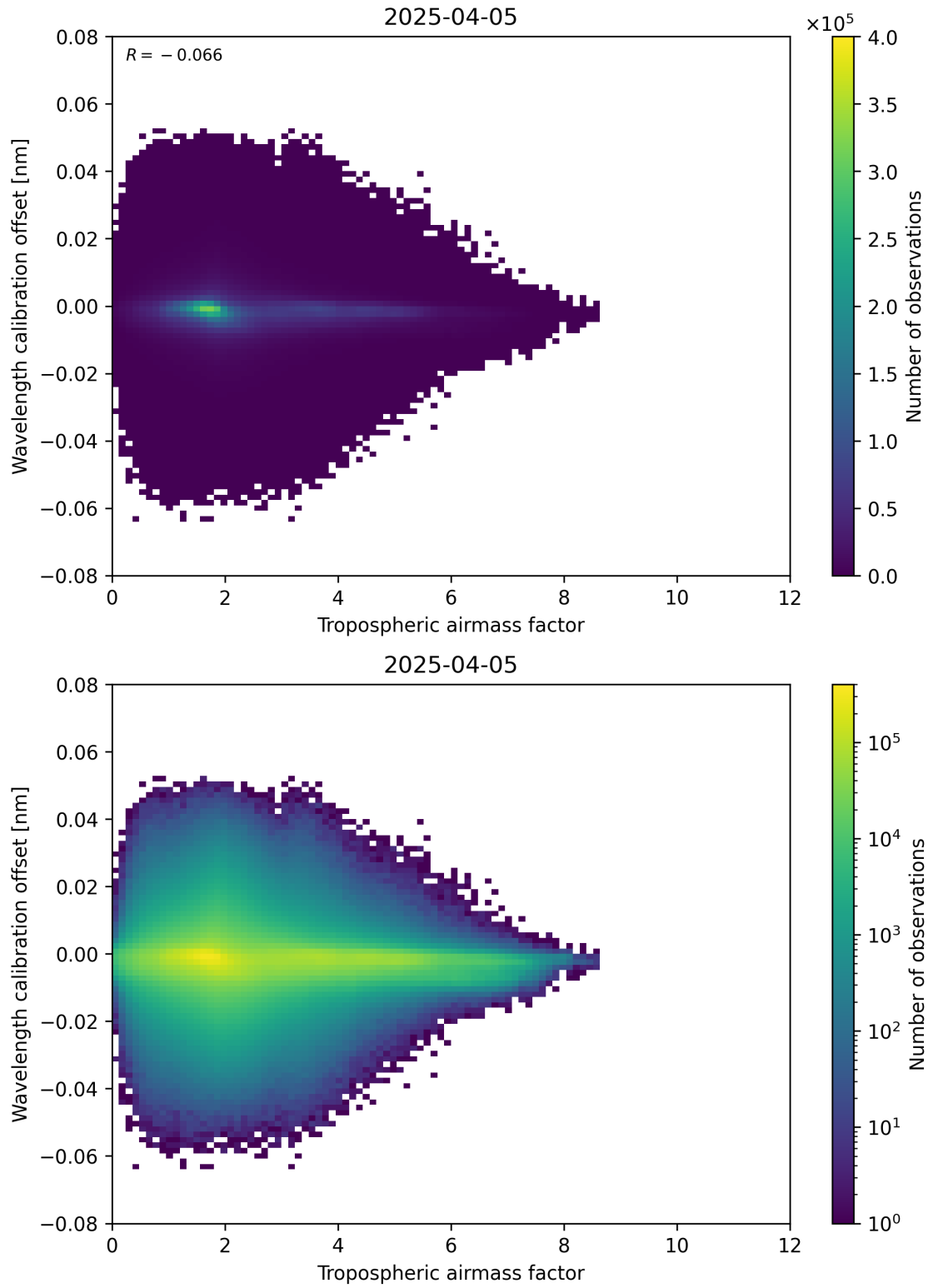
Figure 80: Scatter density plot of “Tropospheric airmass factor” against “Wavelength calibration offset” for 2025-04-05 to 2025-04-06.
