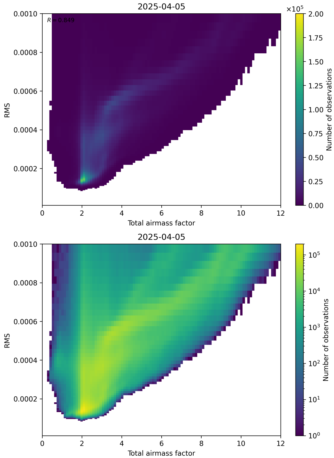
Figure 69: Scatter density plot of “Total airmass factor” against “RMS” for 2025-04-05 to 2025-04-06.
