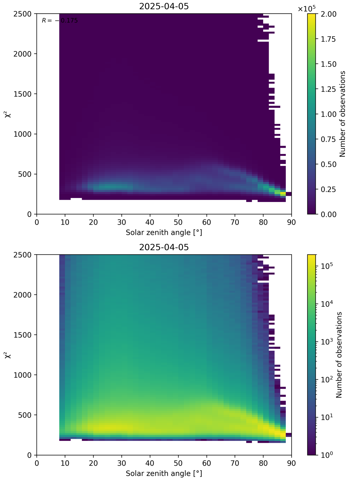
Figure 148: Scatter density plot of “Solar zenith angle” against “ \chi^2 ” for 2025-04-05 to 2025-04-06.
