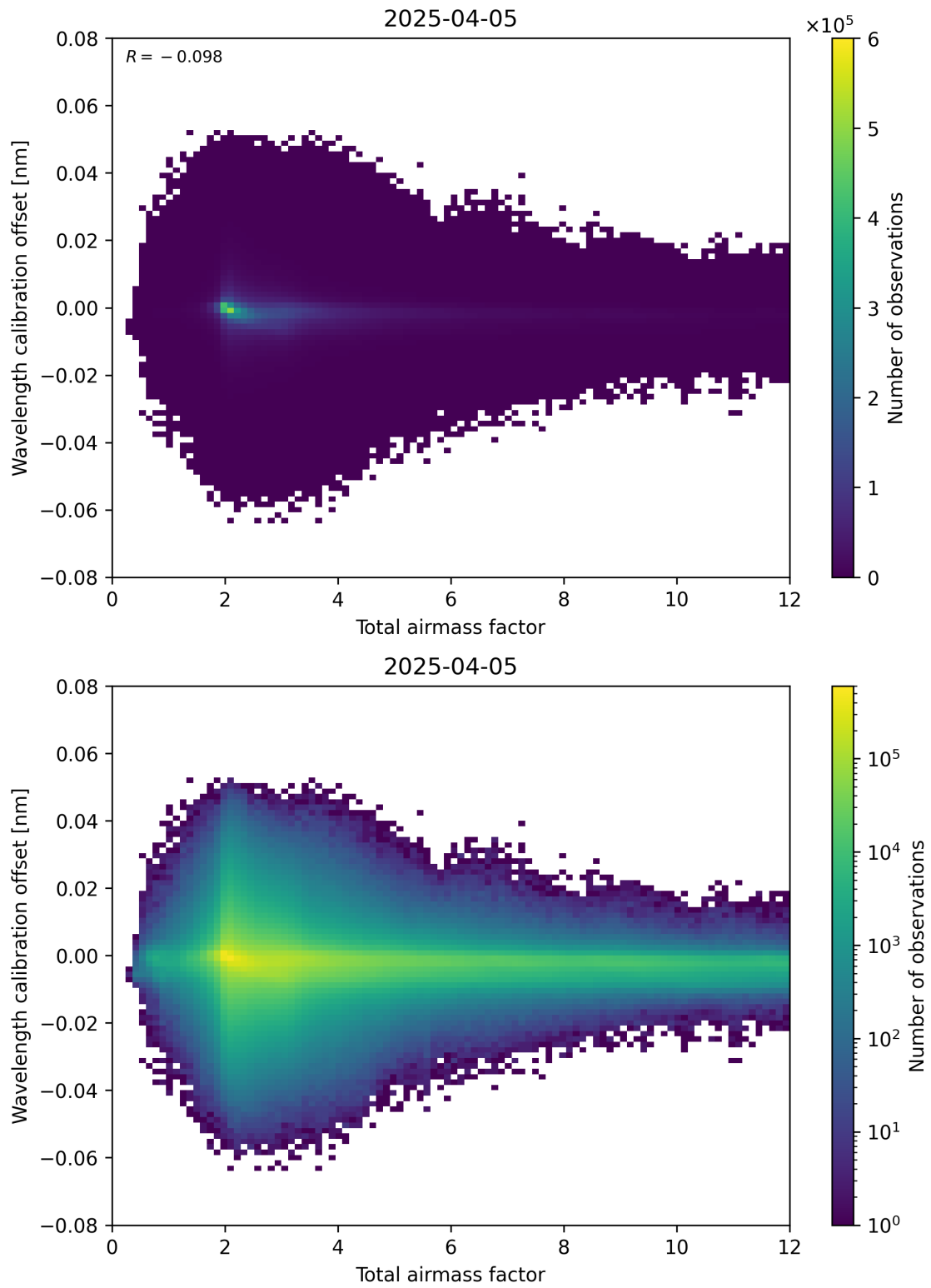
Figure 70: Scatter density plot of “Total airmass factor” against “Wavelength calibration offset” for 2025-04-05 to 2025-04-06.
