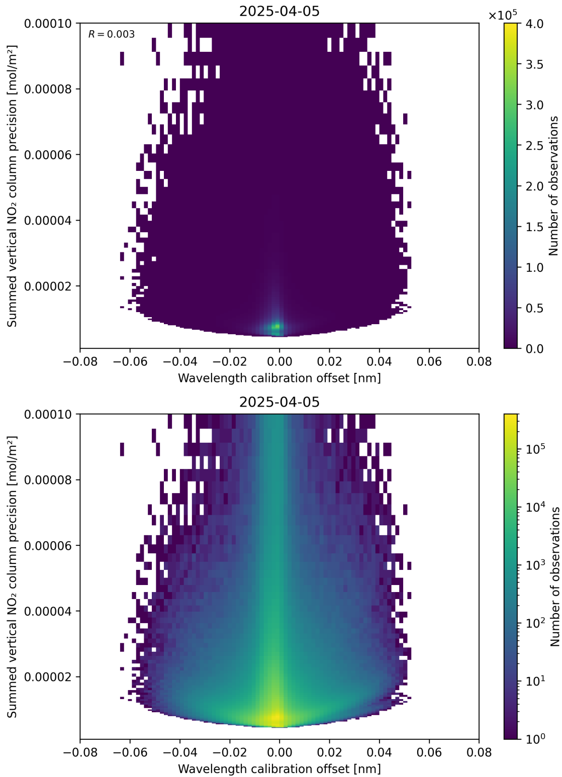
Figure 178: Scatter density plot of “Wavelength calibration offset” against “Summed vertical NO 2 column precision” for 2025-04-05 to 2025-04-06.
