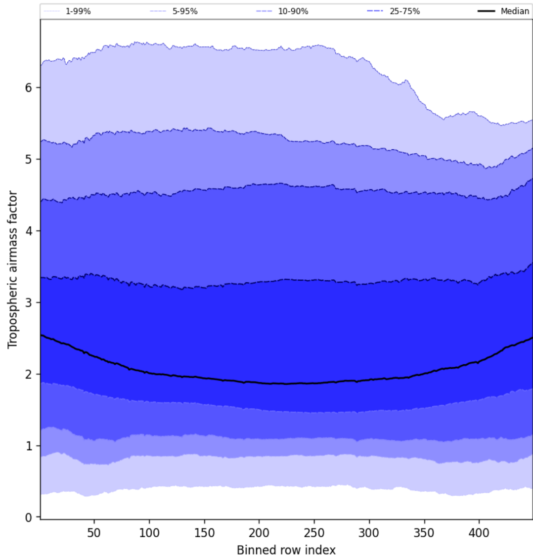
Figure 48: Along track statistics of “Tropospheric air mass factor” for 2025-04-05 to 2025-04-06
