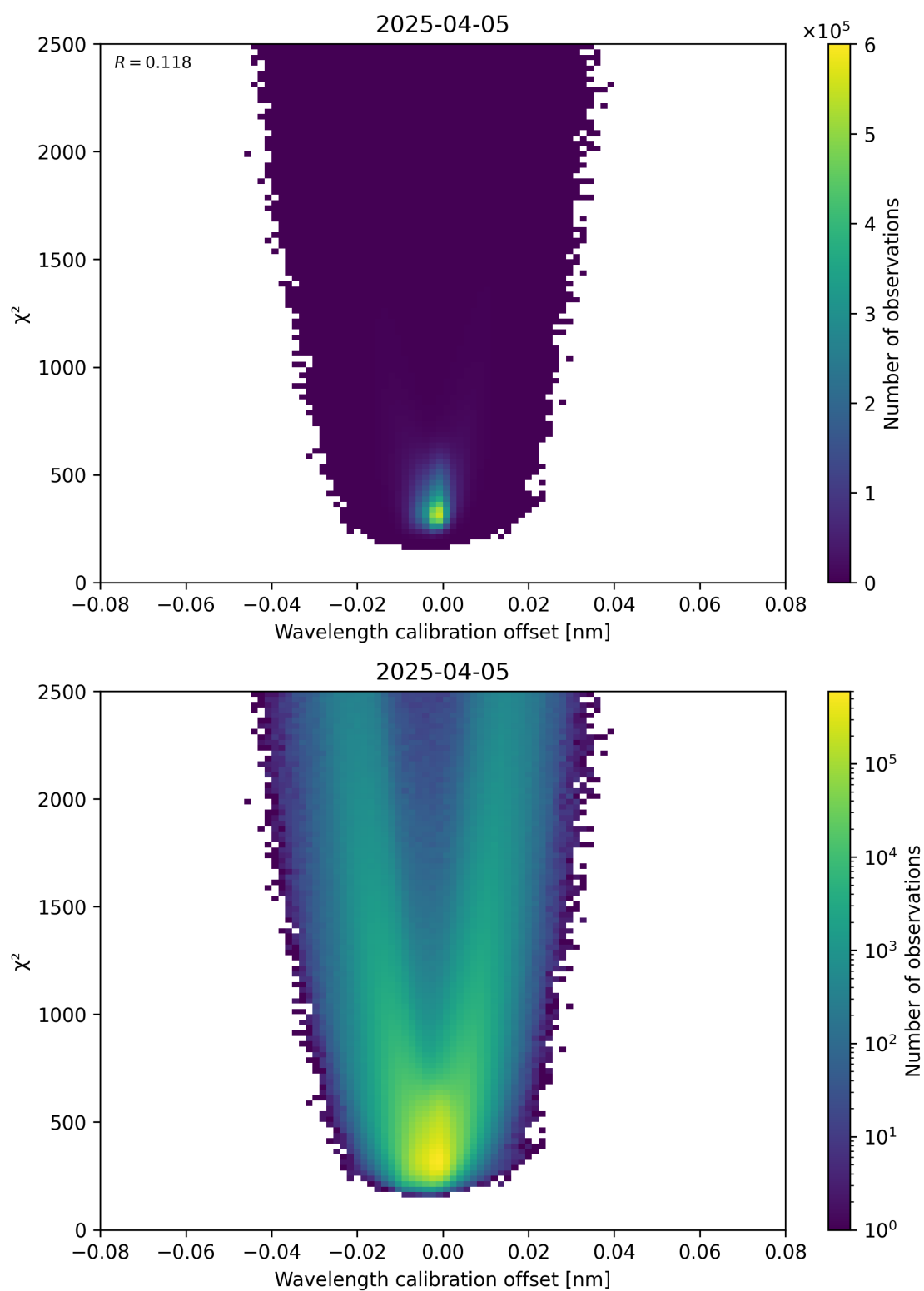
Figure 175: Scatter density plot of “Wavelength calibration offset” against “ \chi^2 ” for 2025-04-05 to 2025-04-06.
