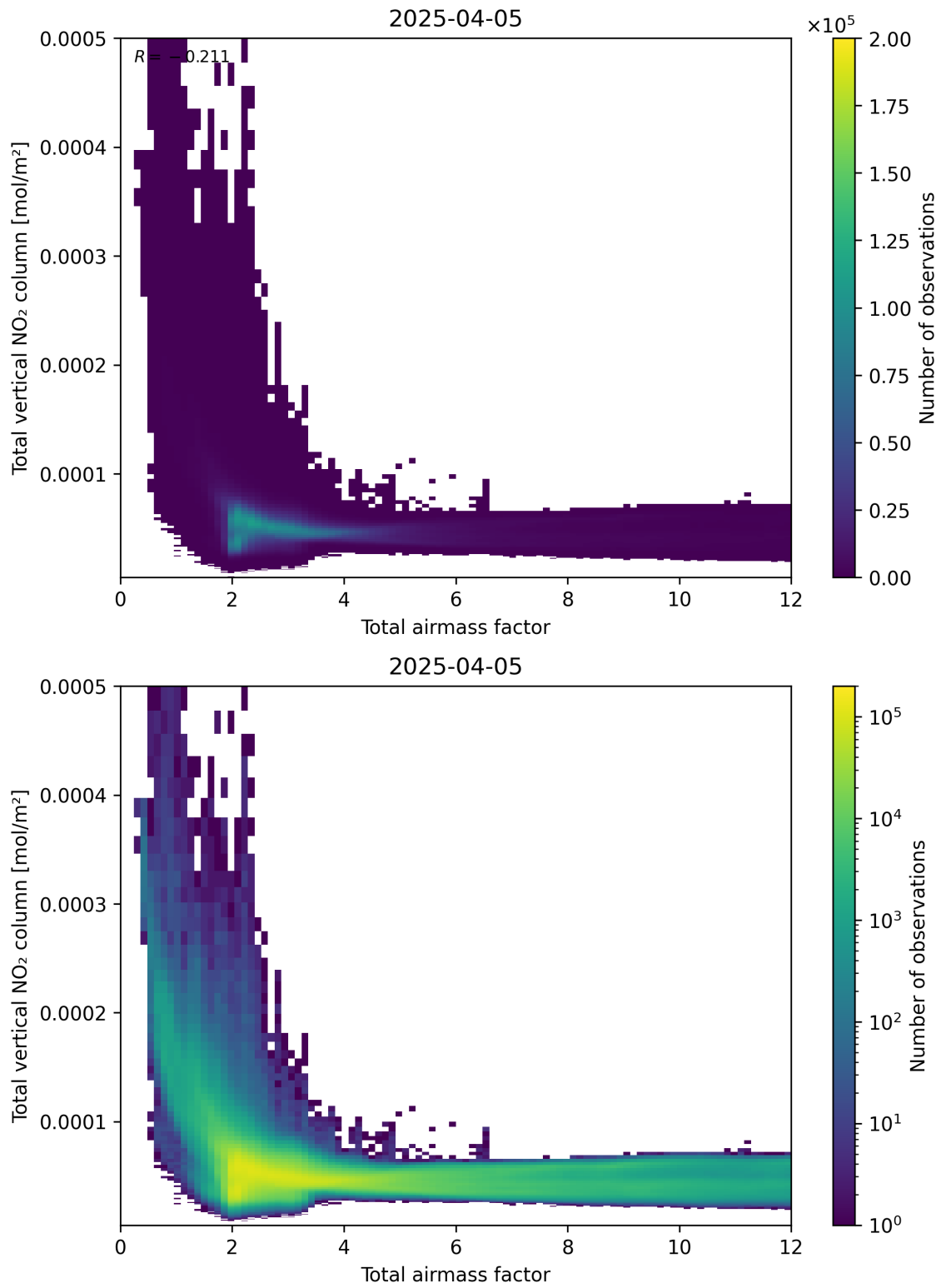
Figure 67: Scatter density plot of “Total airmass factor” against “Total vertical NO 2 column” for 2025-04-05 to 2025-04-06.
