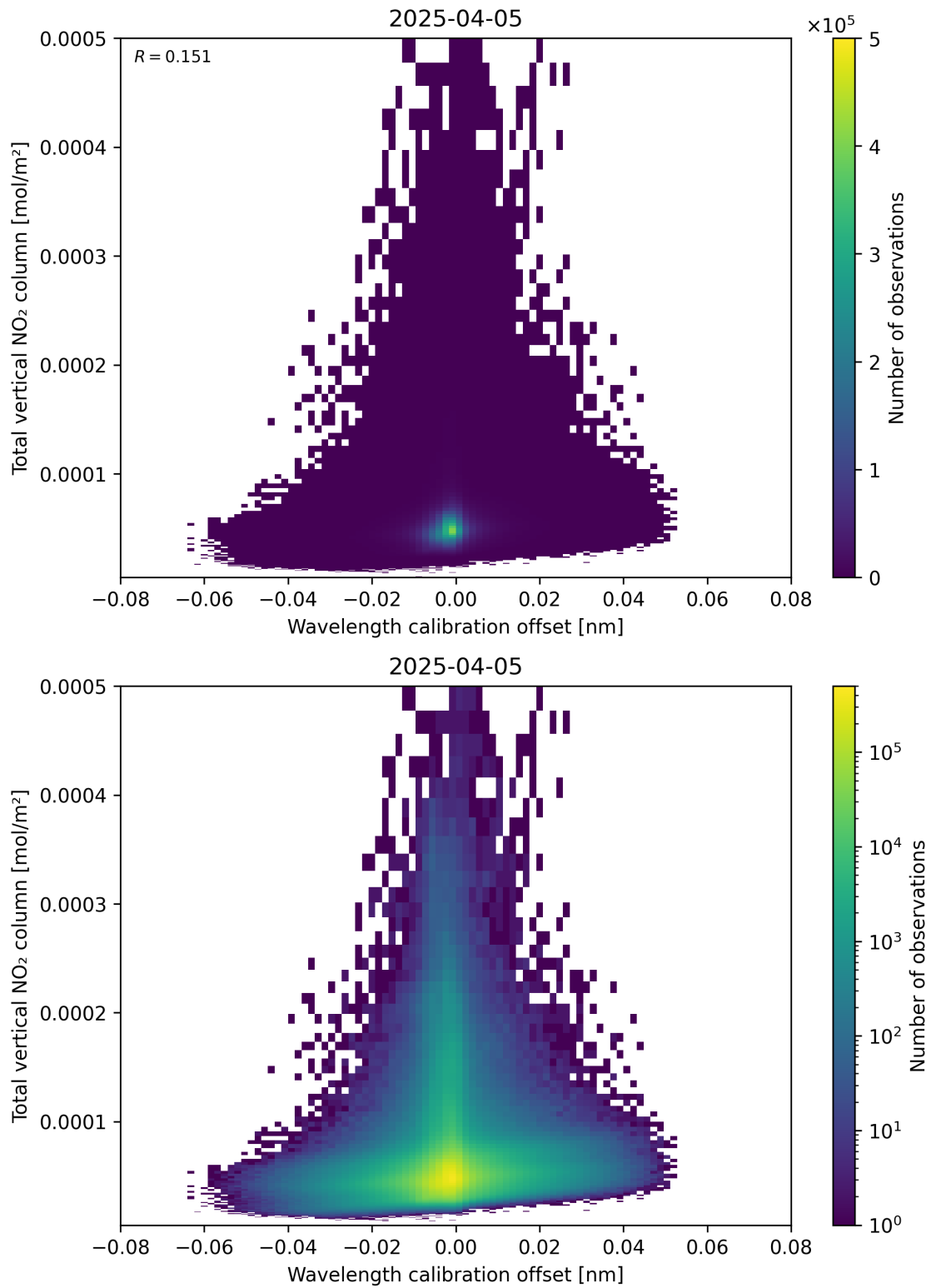
Figure 179: Scatter density plot of “Wavelength calibration offset” against “Total vertical NO 2 column” for 2025-04-05 to 2025-04-06.
