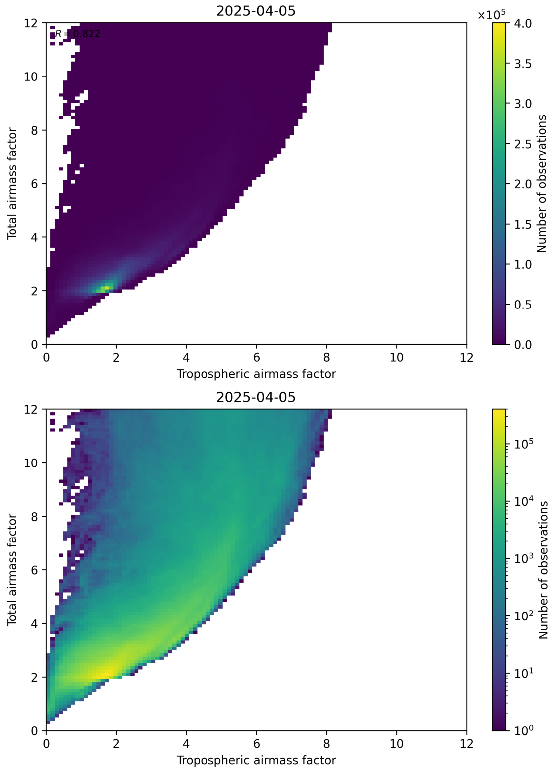
Figure 72: Scatter density plot of “Tropospheric airmass factor” against “Total airmass factor” for 2025-04-05 to 2025-04-06.
