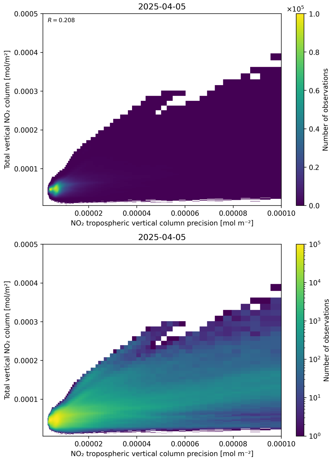
Figure 138: Scatter density plot of “NO 2 tropospheric vertical column precision” against “Total vertical NO 2 column” for 2025-04-05 to 2025-04-06.
