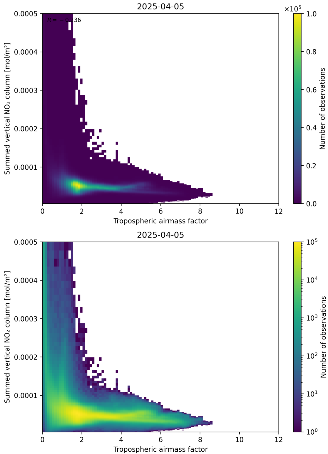
Figure 75: Scatter density plot of “Tropospheric airmass factor” against “Summed vertical NO 2 column” for 2025-04-05 to 2025-04-06.
