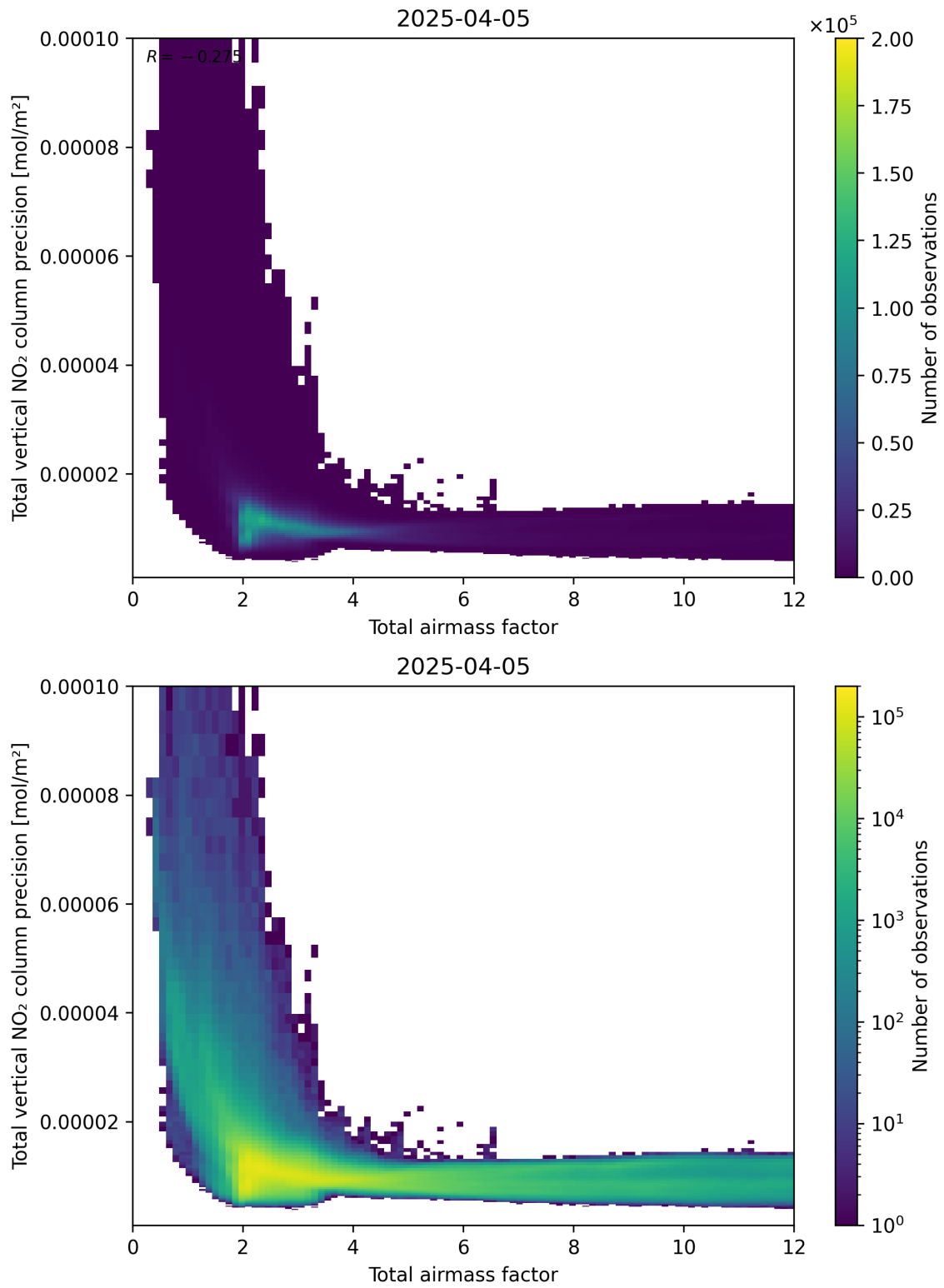
Figure 68: Scatter density plot of “Total airmass factor” against “Total vertical NO 2 column precision” for 2025-04-05 to 2025-04-06.
