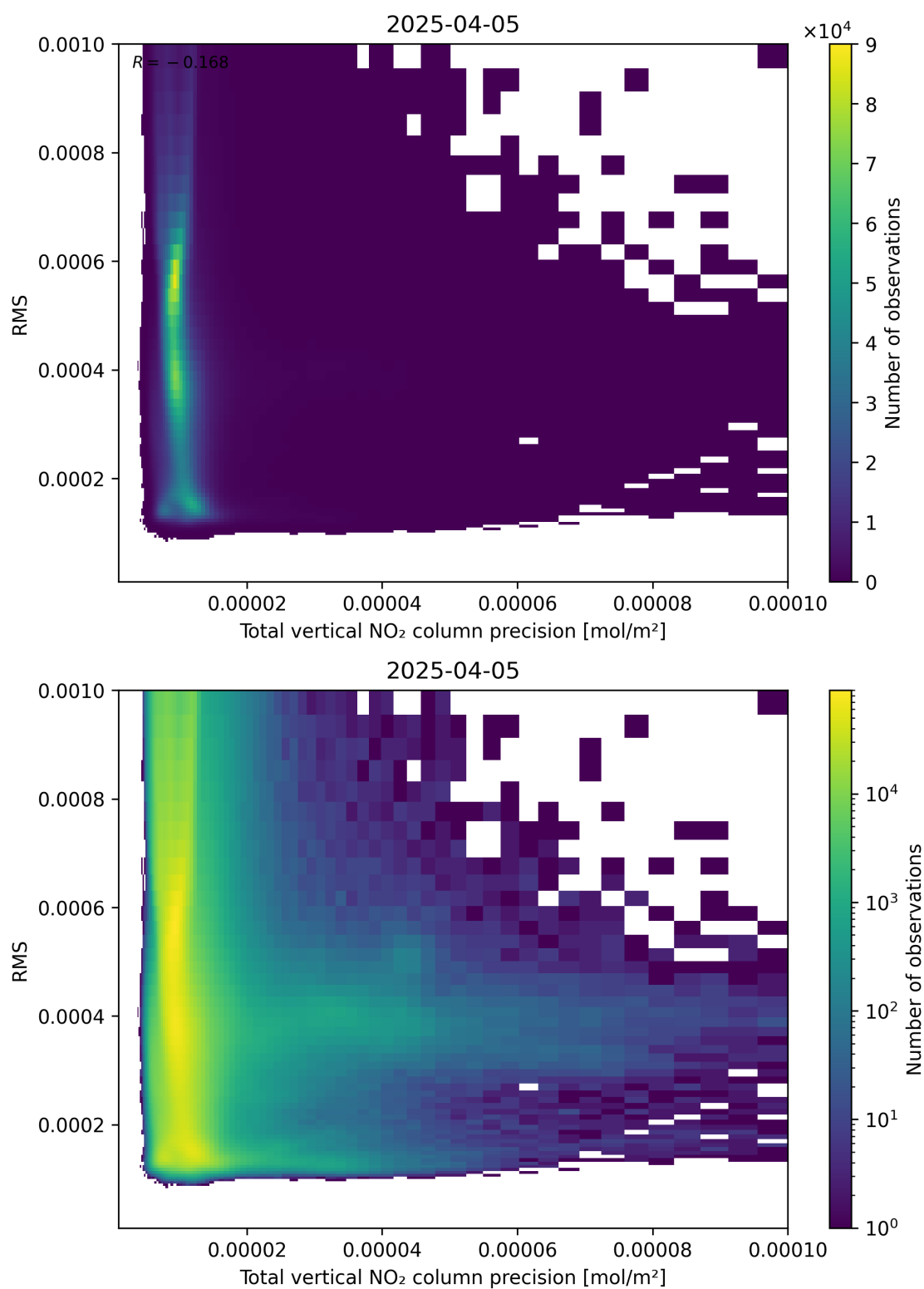
Figure 119: Scatter density plot of “Total vertical NO 2 column precision” against “RMS” for 2025-04-05 to 2025-04-06.
