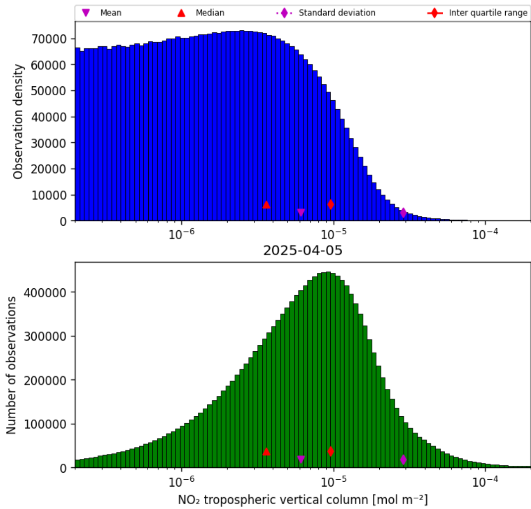
Figure 29: Histogram of “NO 2 tropospheric vertical column” for 2025-04-05 to 2025-04-06
