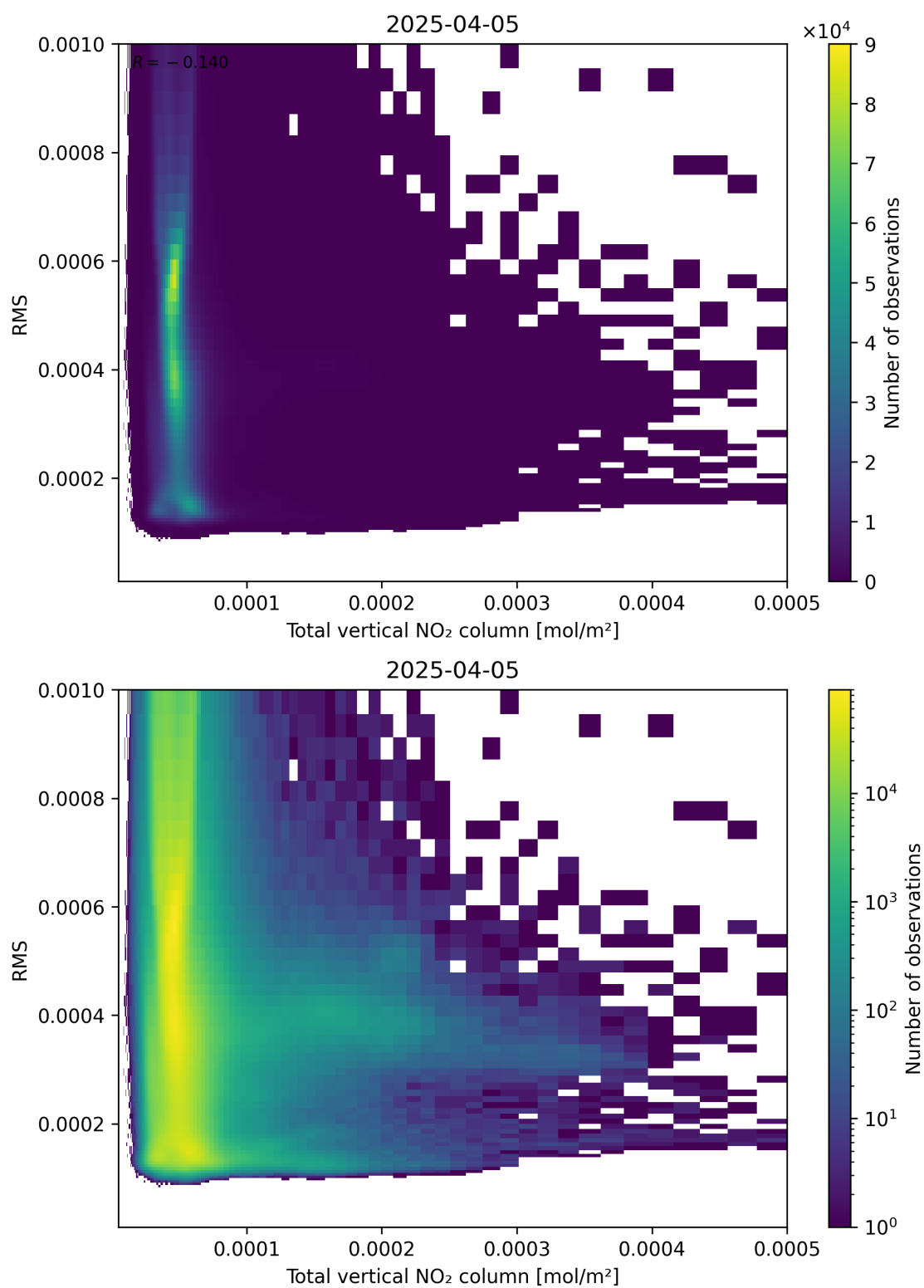
Figure 120: Scatter density plot of “Total vertical NO 2 column” against “RMS” for 2025-04-05 to 2025-04-06.
