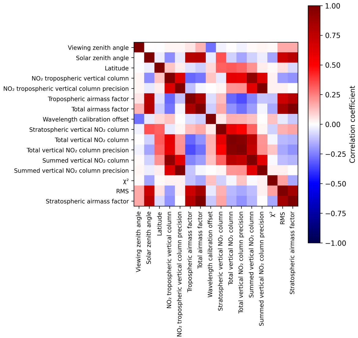
Figure 2: Map of correlation matrix for 2025-04-05 to 2025-04-06.
