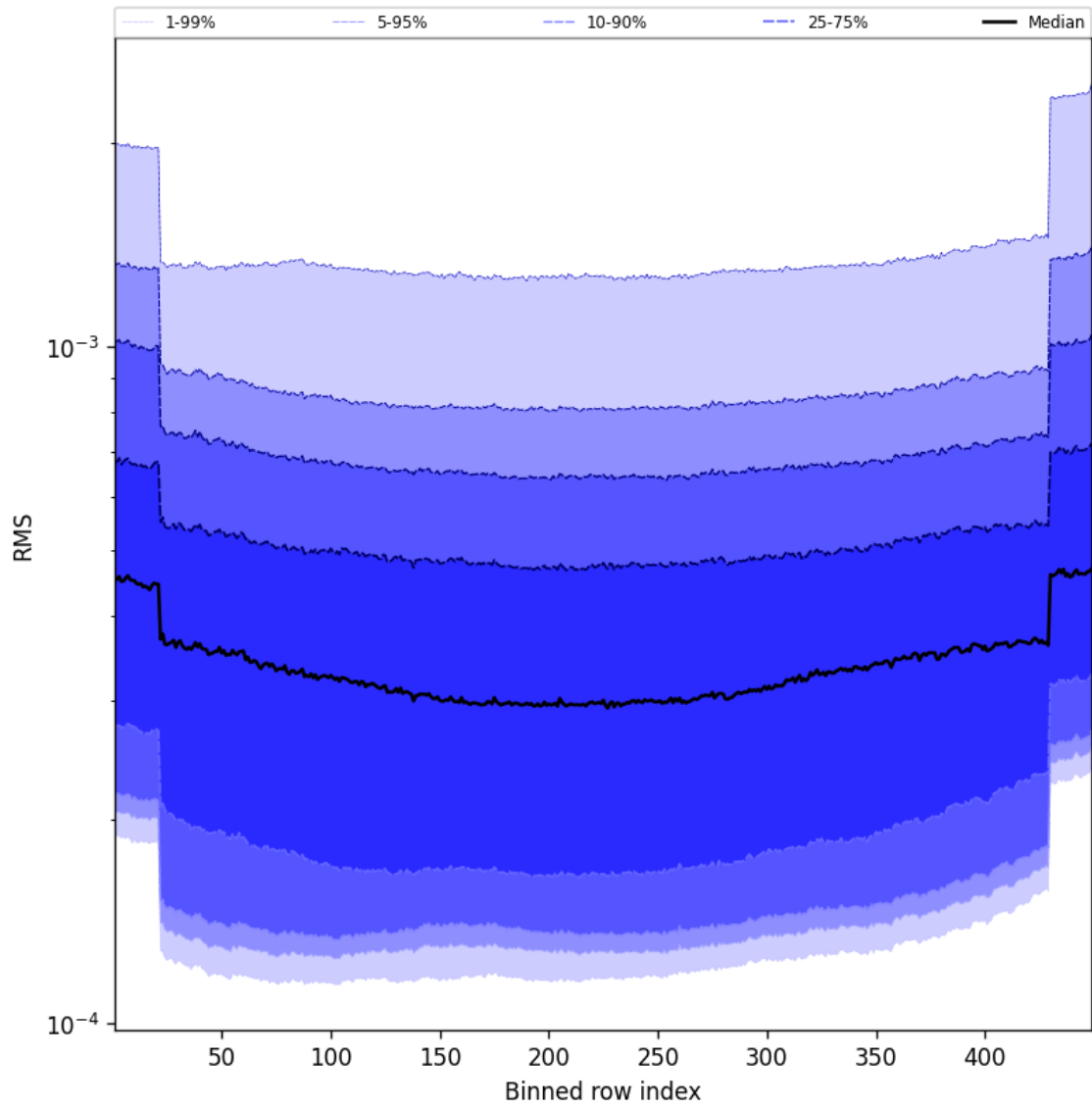
Figure 60: Along track statistics of “RMS” for 2025-04-05 to 2025-04-06
