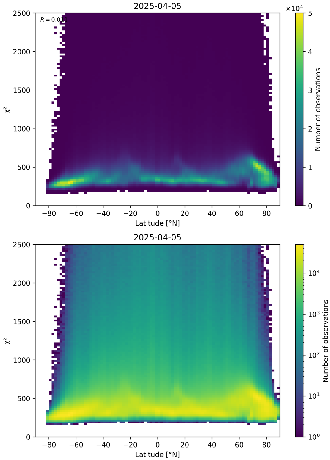
Figure 86: Scatter density plot of “Latitude” against “ \chi^2 ” for 2025-04-05 to 2025-04-06.
