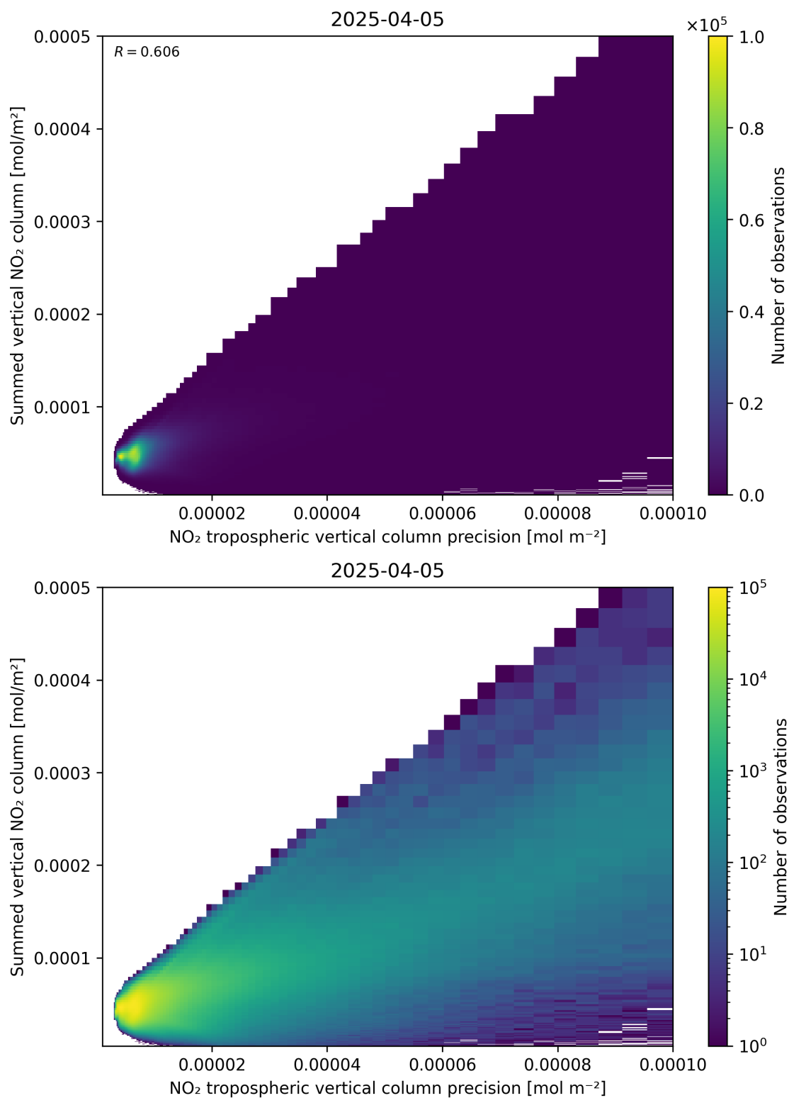
Figure 136: Scatter density plot of “NO 2 tropospheric vertical column precision” against “Summed vertical NO 2 column” for 2025-04-05 to 2025-04-06.
