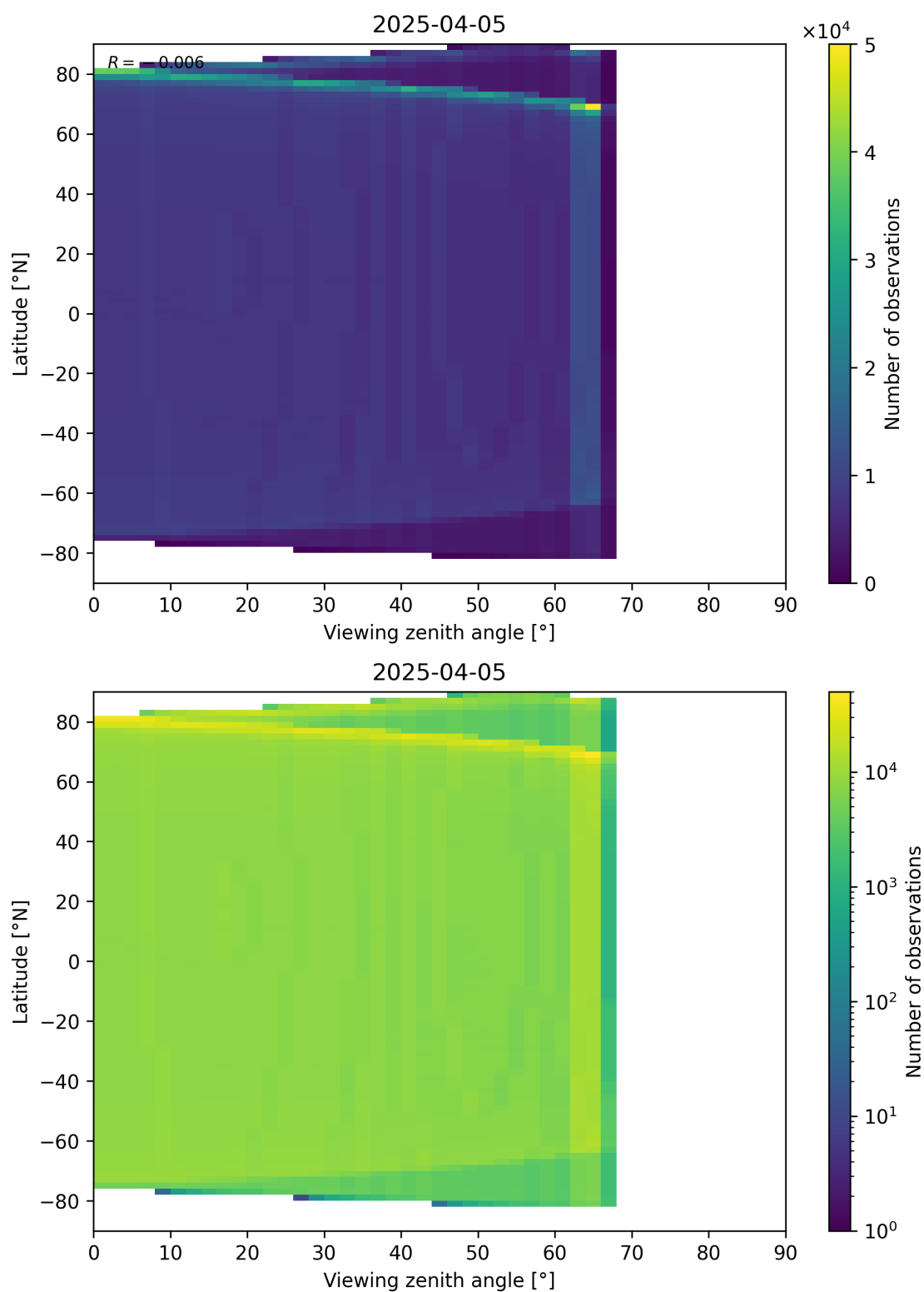
Figure 163: Scatter density plot of “Viewing zenith angle” against “Latitude” for 2025-04-05 to 2025-04-06.
