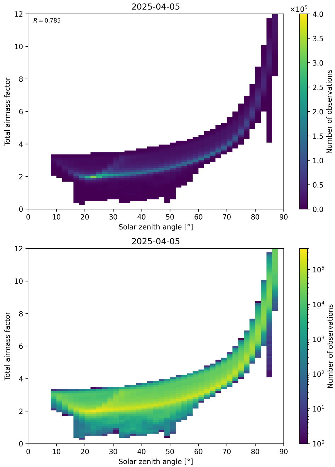
Figure 146: Scatter density plot of “Solar zenith angle” against “Total air mass factor” for 2025-04-05 to 2025-04-06.
