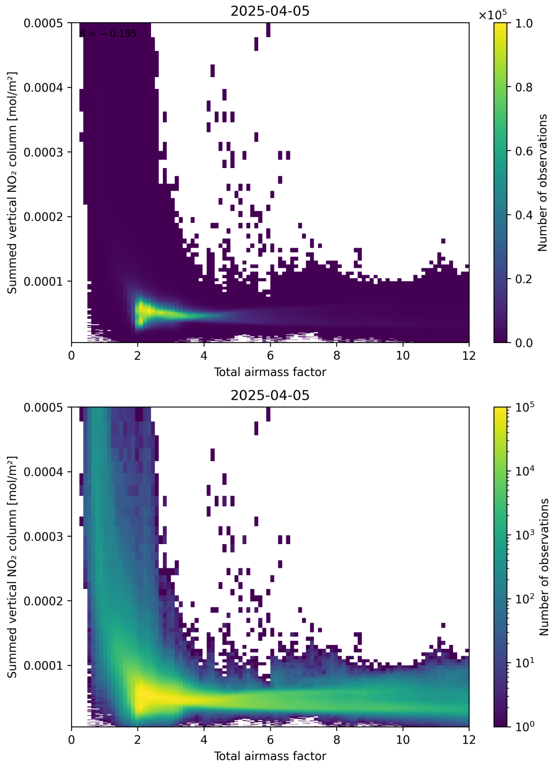
Figure 65: Scatter density plot of “Total airmass factor” against “Summed vertical NO 2 column” for 2025-04-05 to 2025-04-06.
