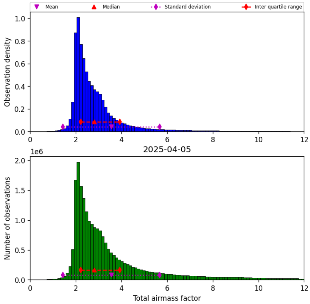
Figure 32: Histogram of “Total airmass factor” for 2025-04-05 to 2025-04-06
