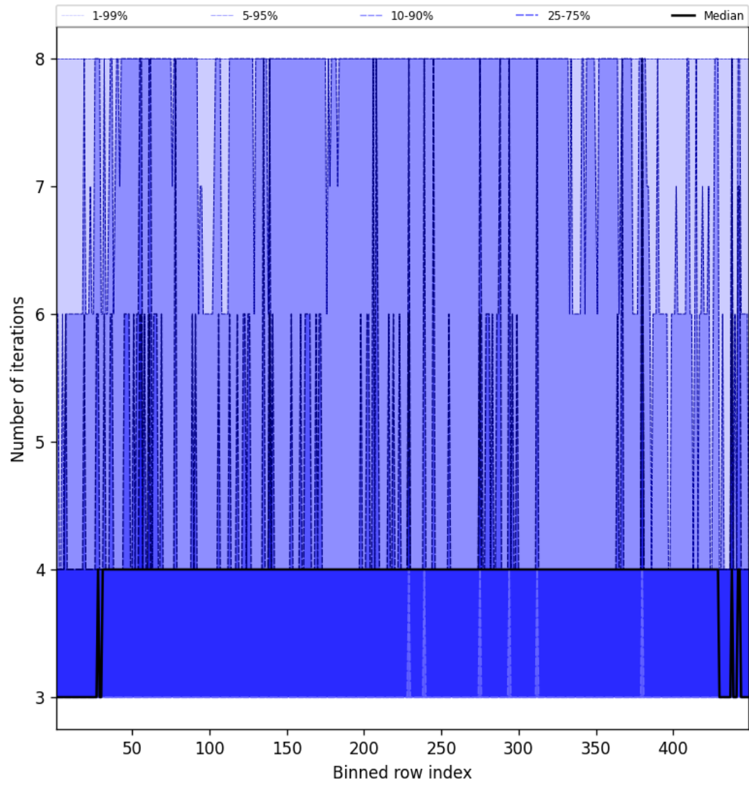
Figure 51: Along track statistics of “Number of iterations” for 2025-04-05 to 2025-04-06
