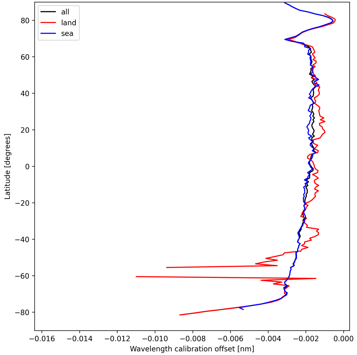
Figure 18: Zonal average of “Wavelength calibration offset” for 2025-04-05 to 2025-04-06.
