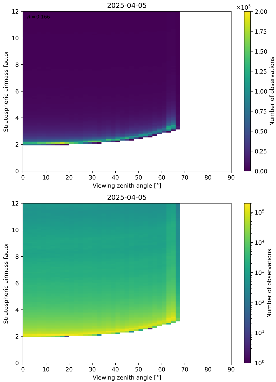
Figure 159: Scatter density plot of “Viewing zenith angle” against “Stratospheric airmass factor” for 2025-04-05 to 2025-04-06.
