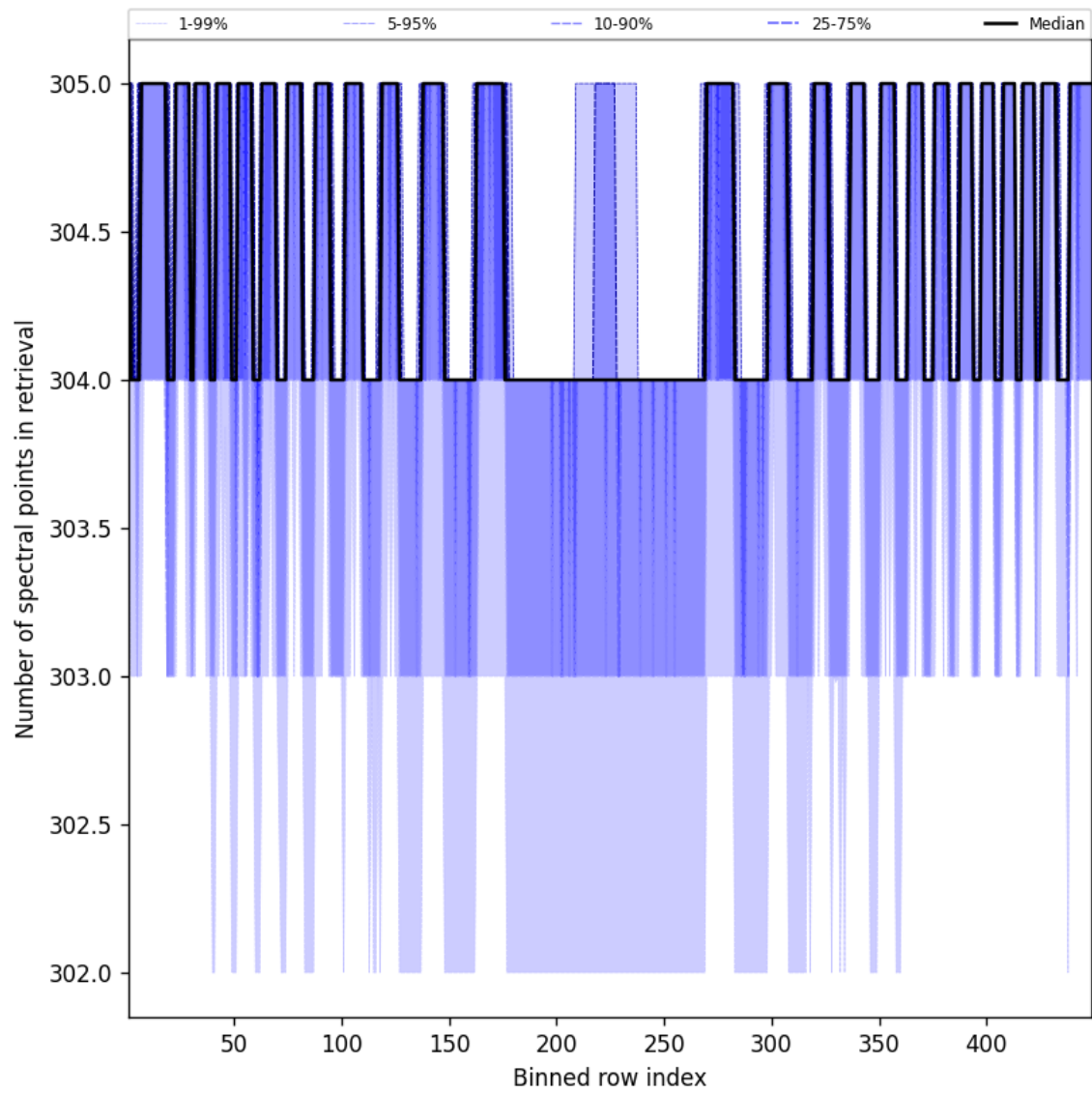
Figure 50: Along track statistics of “Number of spectral points in retrieval” for 2025-04-05 to 2025-04-06
