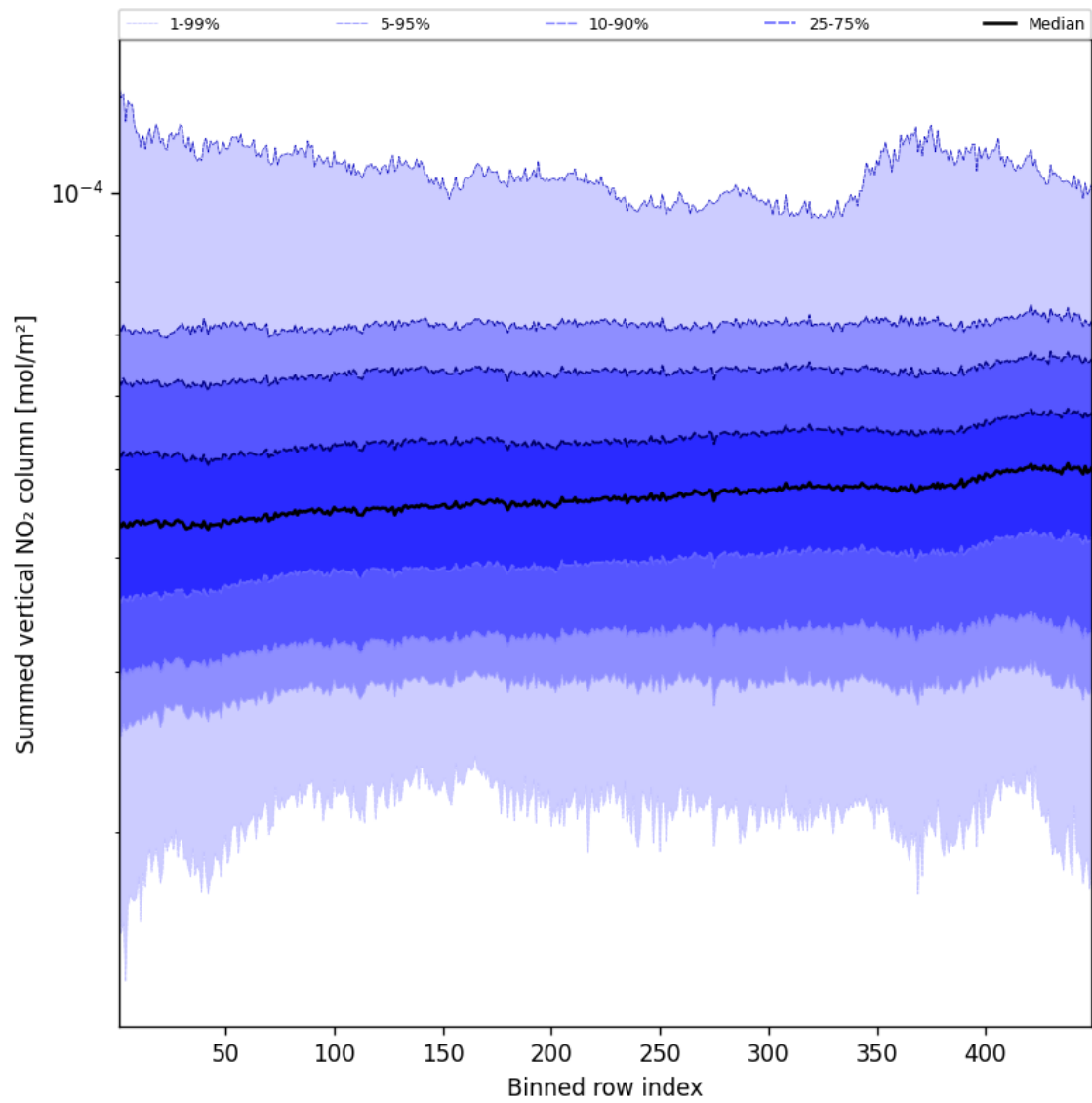
Figure 57: Along track statistics of “Summed vertical NO 2 column” for 2025-04-05 to 2025-04-06
