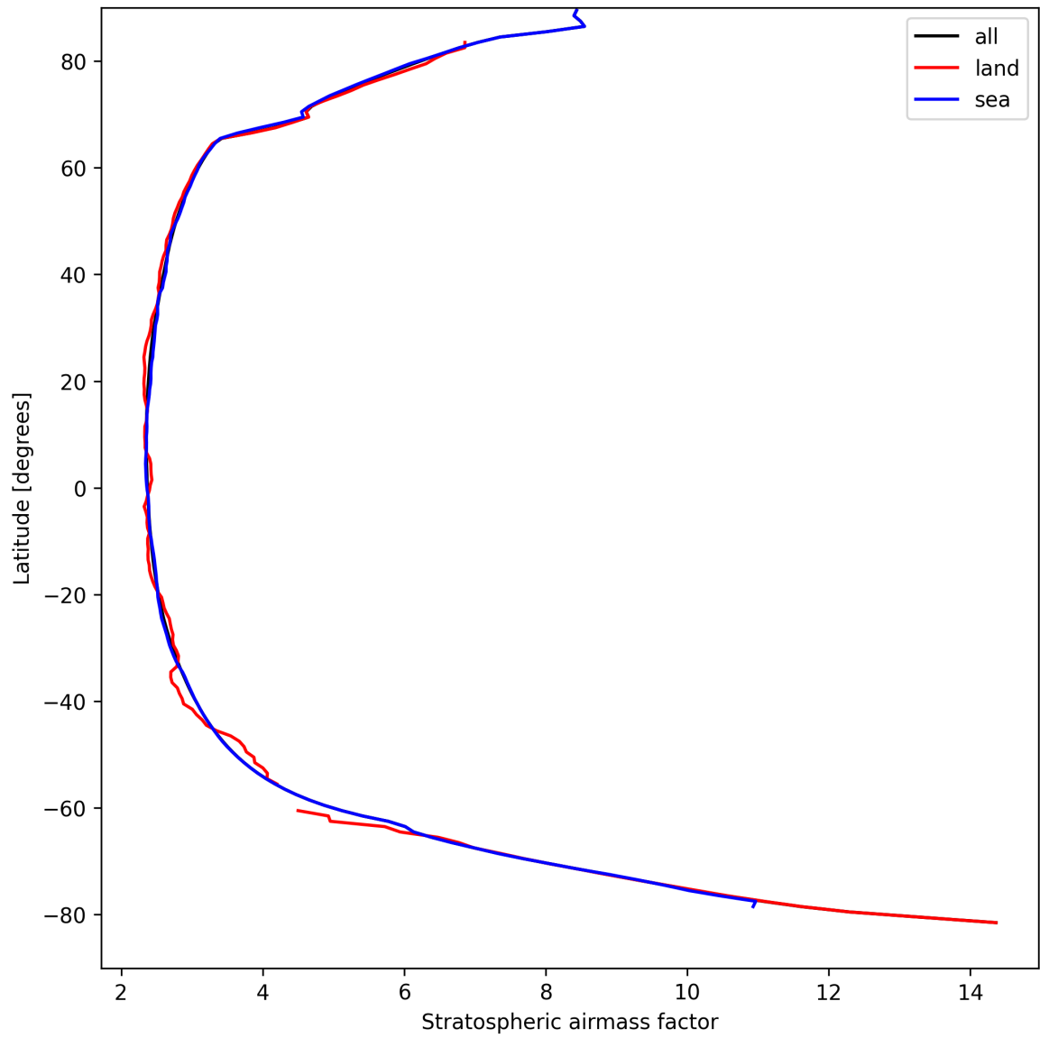
Figure 27: Zonal average of “Stratospheric airmass factor” for 2025-04-05 to 2025-04-06.
