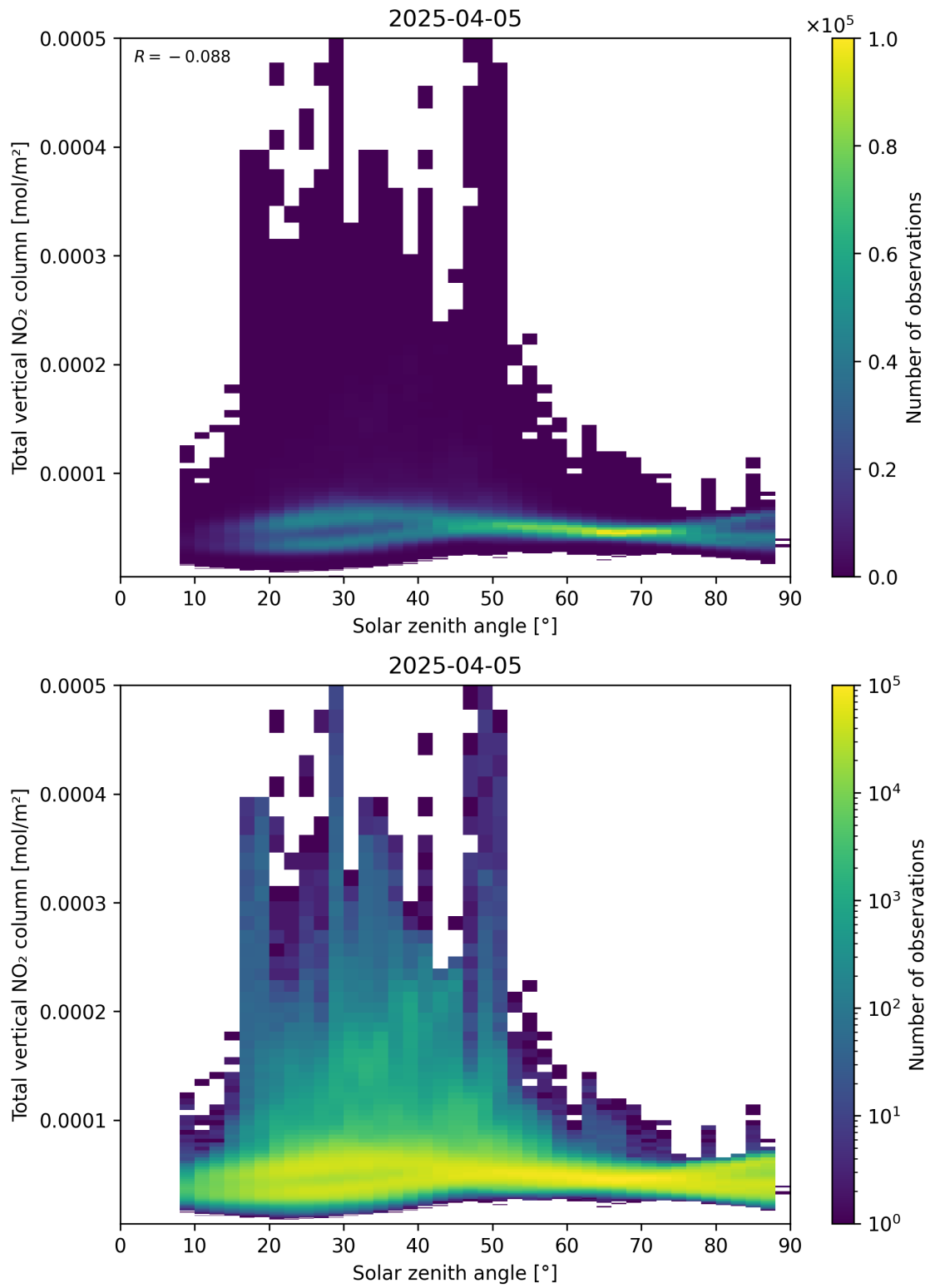
Figure 153: Scatter density plot of “Solar zenith angle” against “Total vertical NO 2 column” for 2025-04-05 to 2025-04-06.
