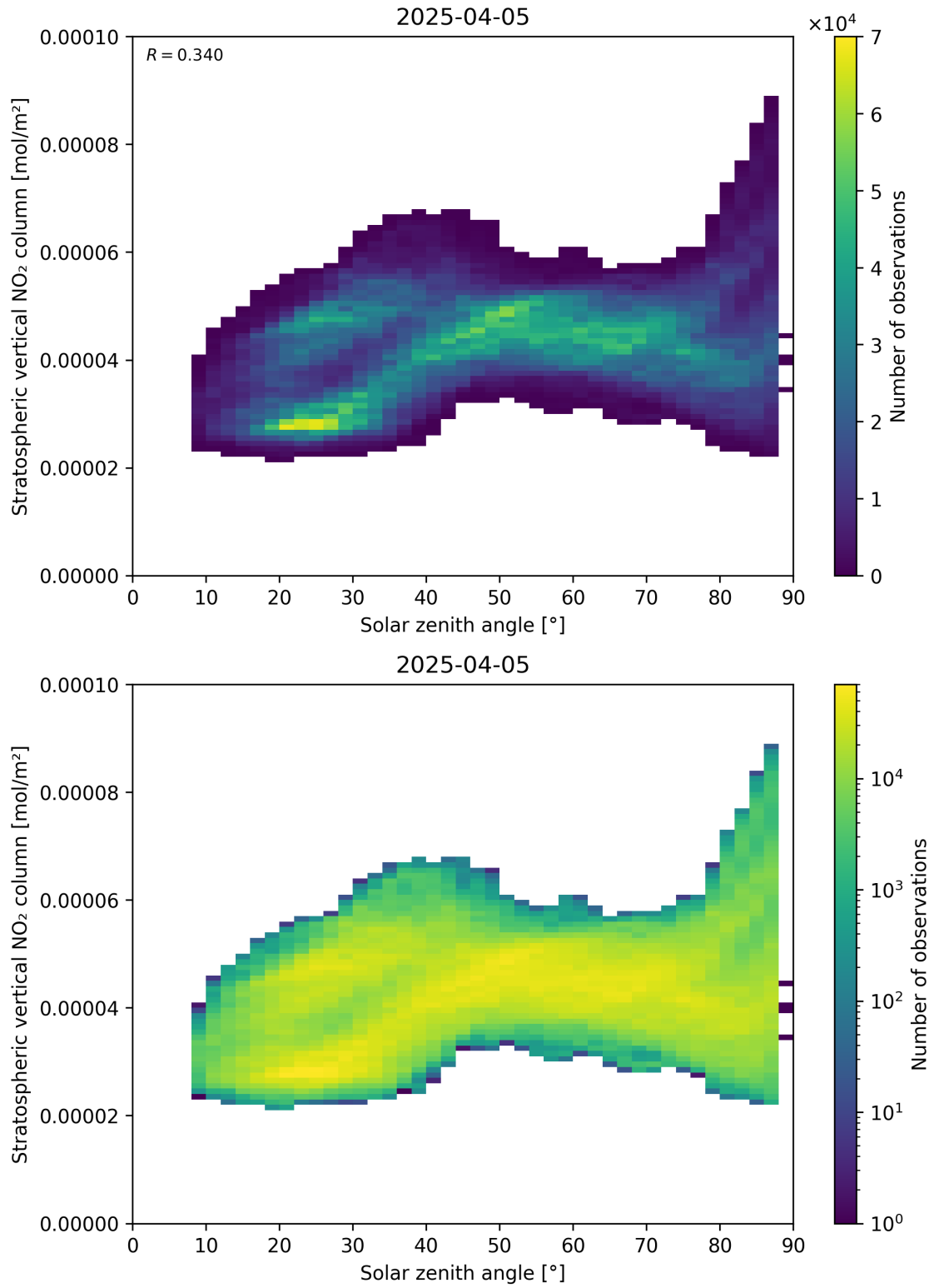
Figure 150: Scatter density plot of “Solar zenith angle” against “Stratospheric vertical NO 2 column” for 2025-04-05 to 2025-04-06.
