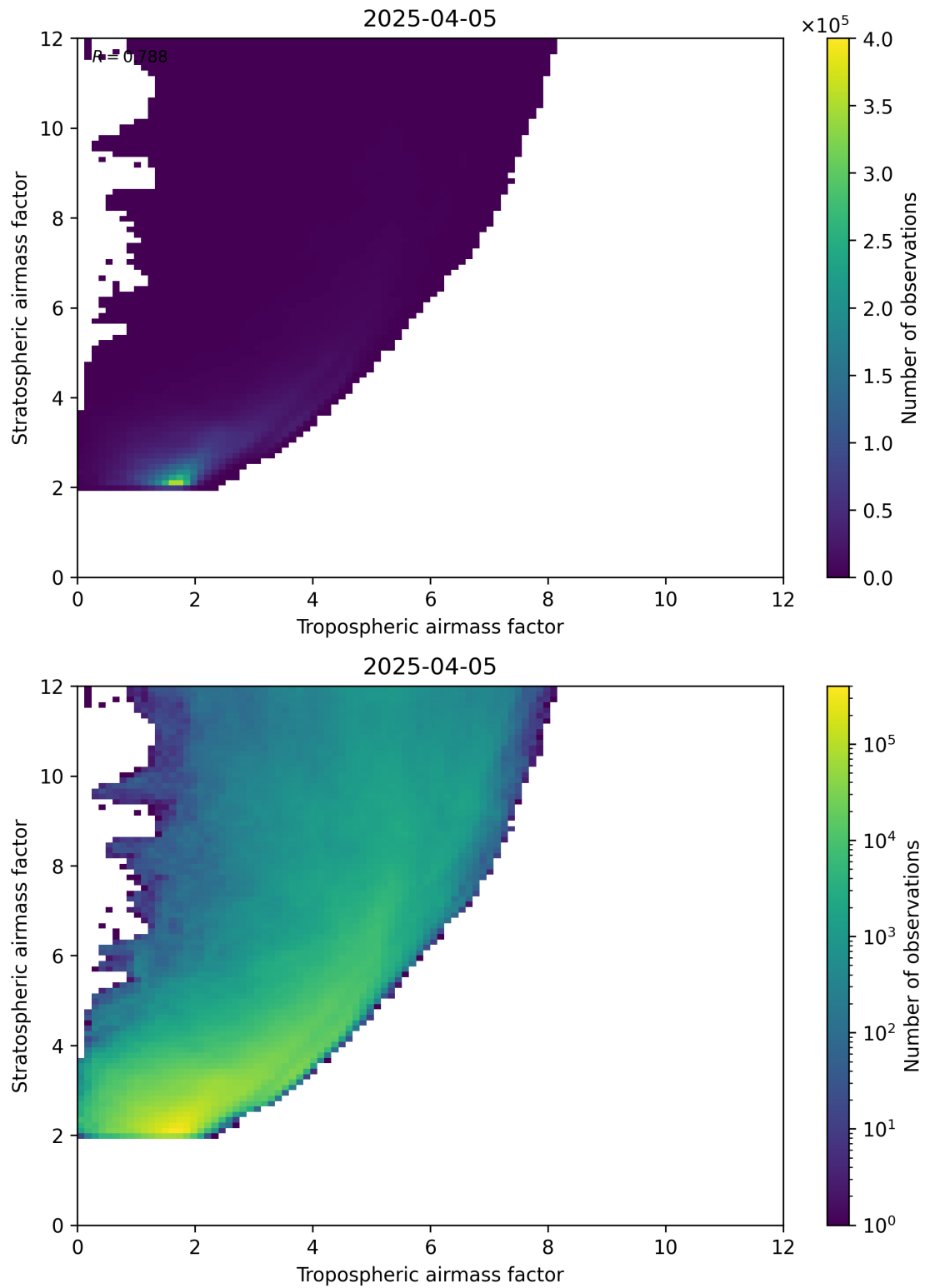
Figure 71: Scatter density plot of “Tropospheric airmass factor” against “Stratospheric airmass factor” for 2025-04-05 to 2025-04-06.
