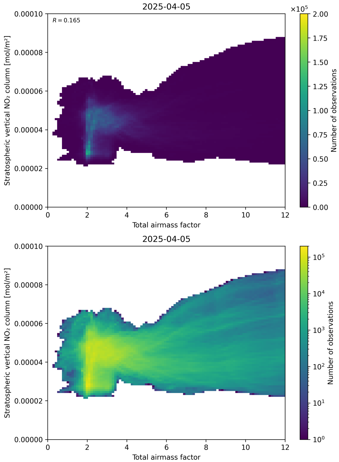
Figure 64: Scatter density plot of “Total air mass factor” against “Stratospheric vertical \text{NO}_2 column” for 2025-04-05 to 2025-04-06.
