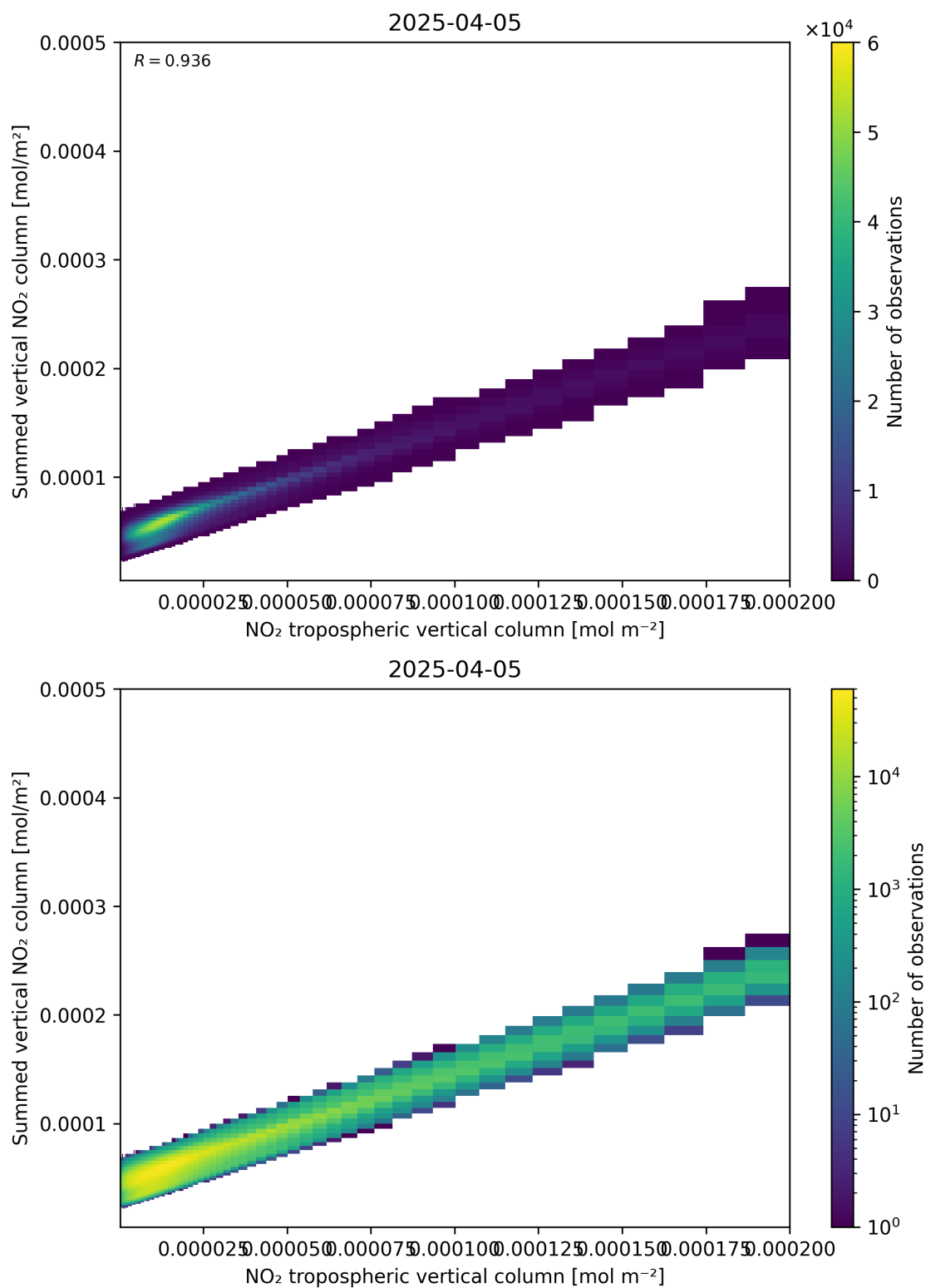
Figure 126: Scatter density plot of “NO 2 tropospheric vertical column” against “Summed vertical NO 2 column” for 2025-04-05 to 2025-04-06.
