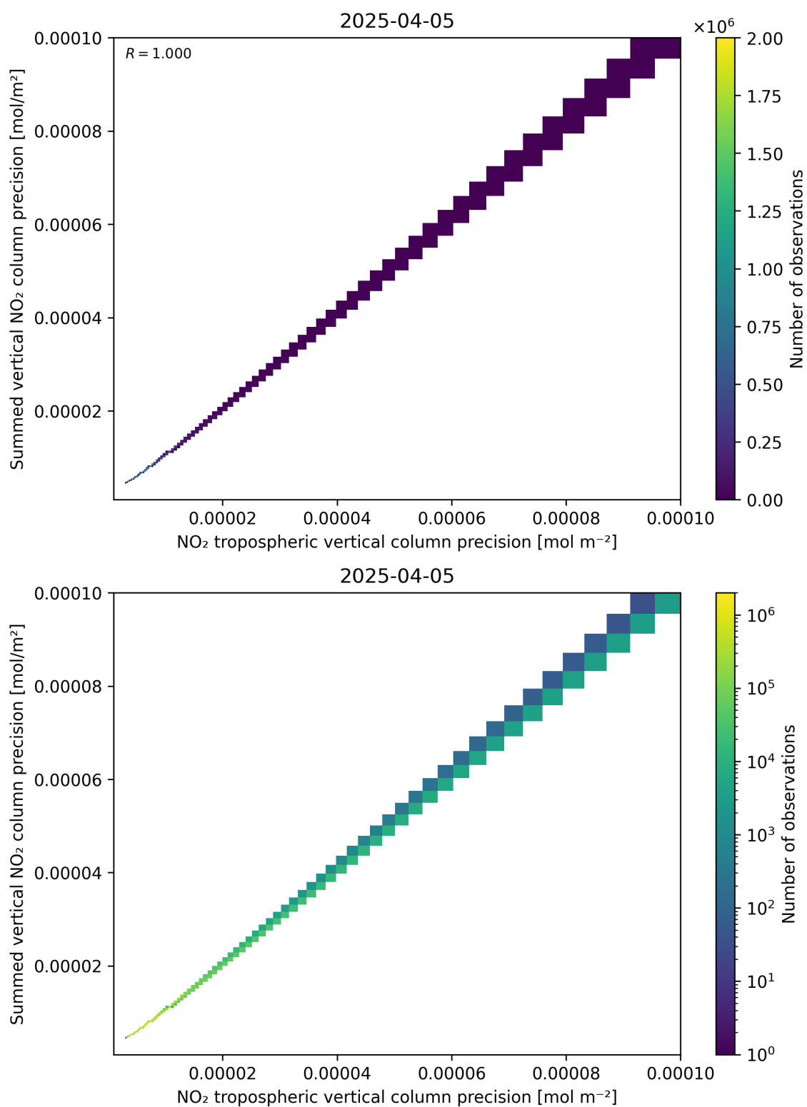
Figure 137: Scatter density plot of “NO 2 tropospheric vertical column precision” against “Summed vertical NO 2 column precision” for 2025-04-05 to 2025-04-06.
