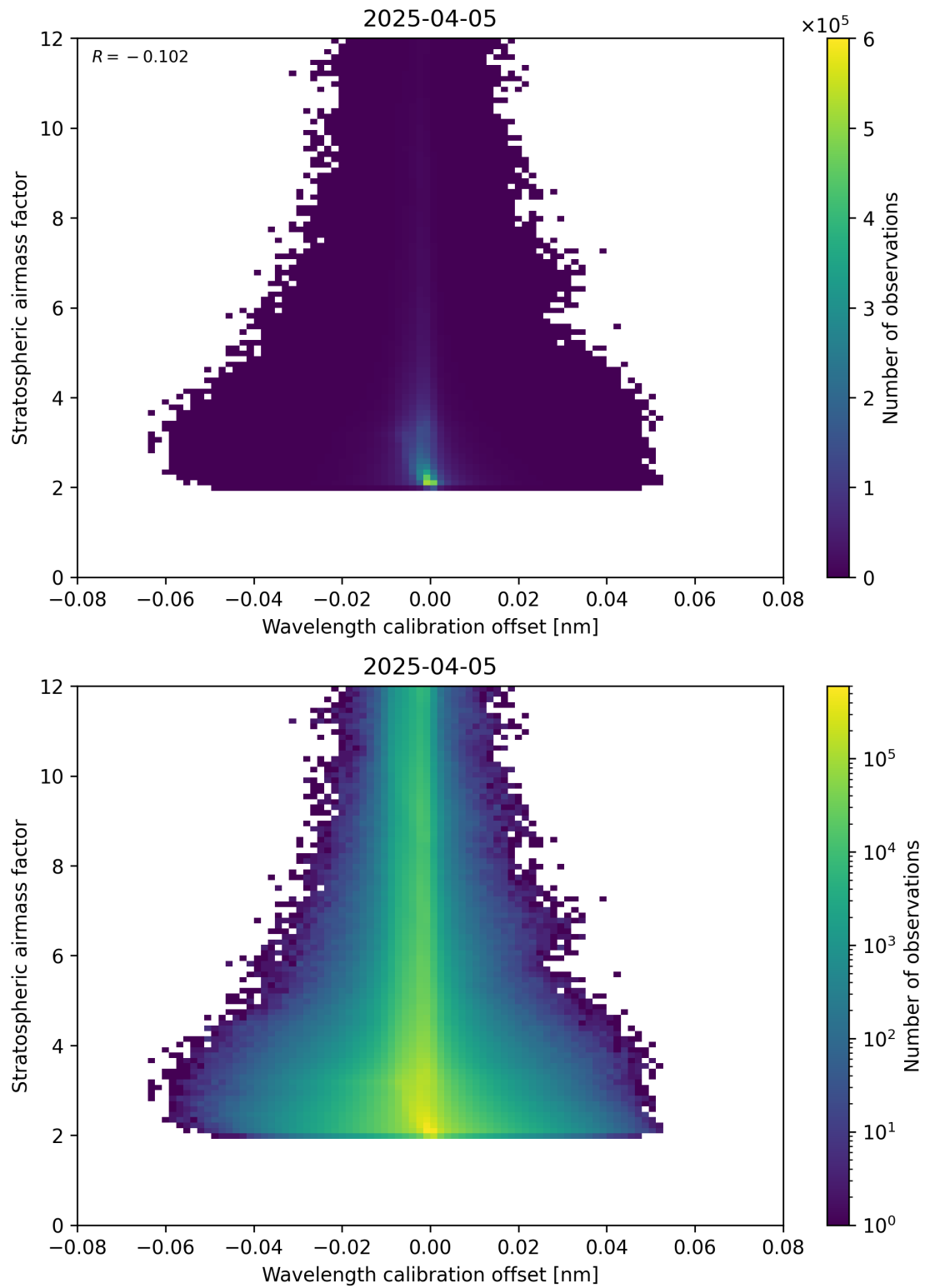
Figure 174: Scatter density plot of “Wavelength calibration offset” against “Stratospheric airmass factor” for 2025-04-05 to 2025-04-06.
