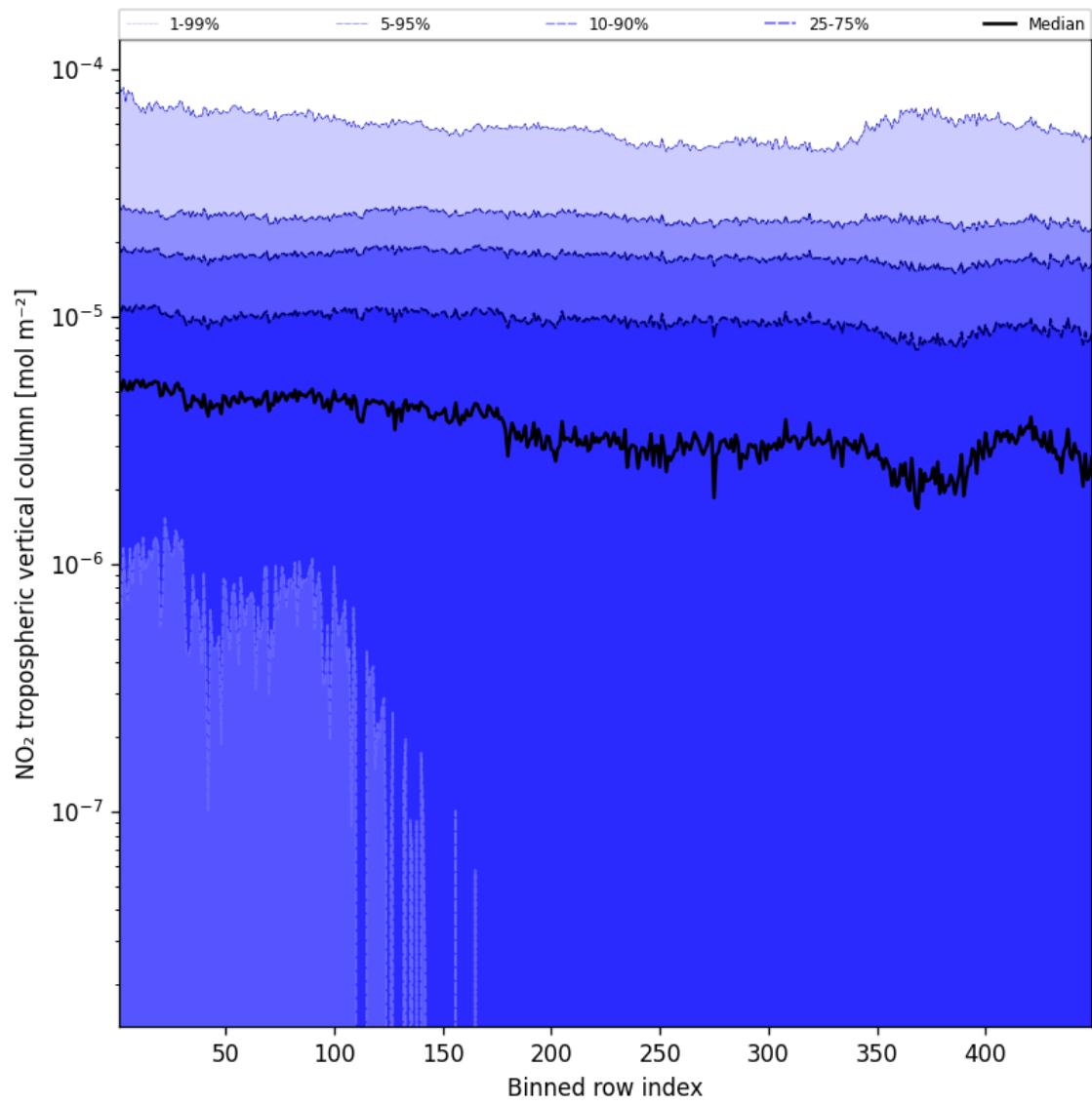
Figure 46: Along track statistics of “NO 2 tropospheric vertical column” for 2025-04-05 to 2025-04-06
