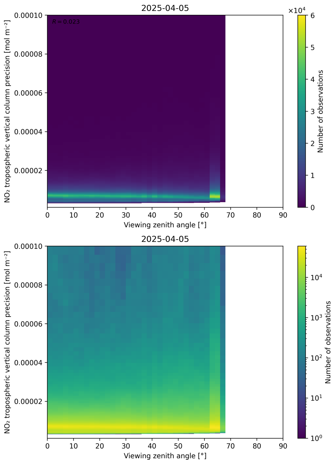
Figure 170: Scatter density plot of “Viewing zenith angle” against “NO 2 tropospheric vertical column precision” for 2025-04-05 to 2025-04-06.
