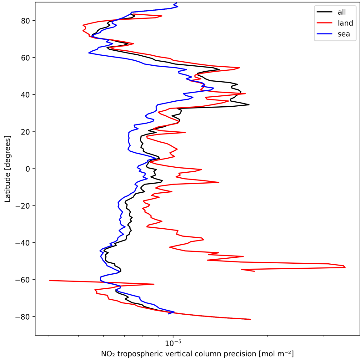
Figure 13: Zonal average of “NO 2 tropospheric vertical column precision” for 2025-04-05 to 2025-04-06.
