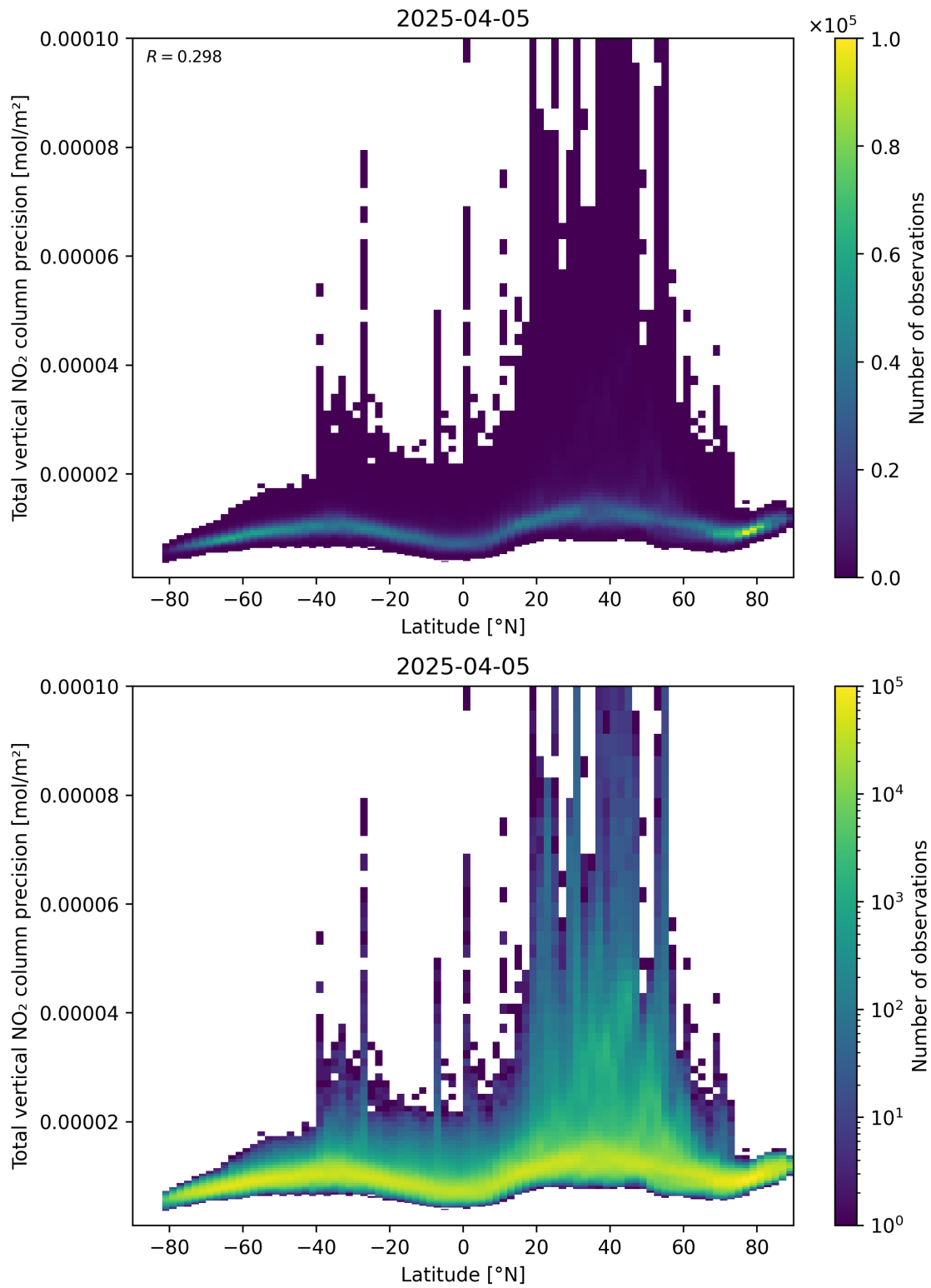
Figure 91: Scatter density plot of “Latitude” against “Total vertical NO 2 column precision” for 2025-04-05 to 2025-04-06.
