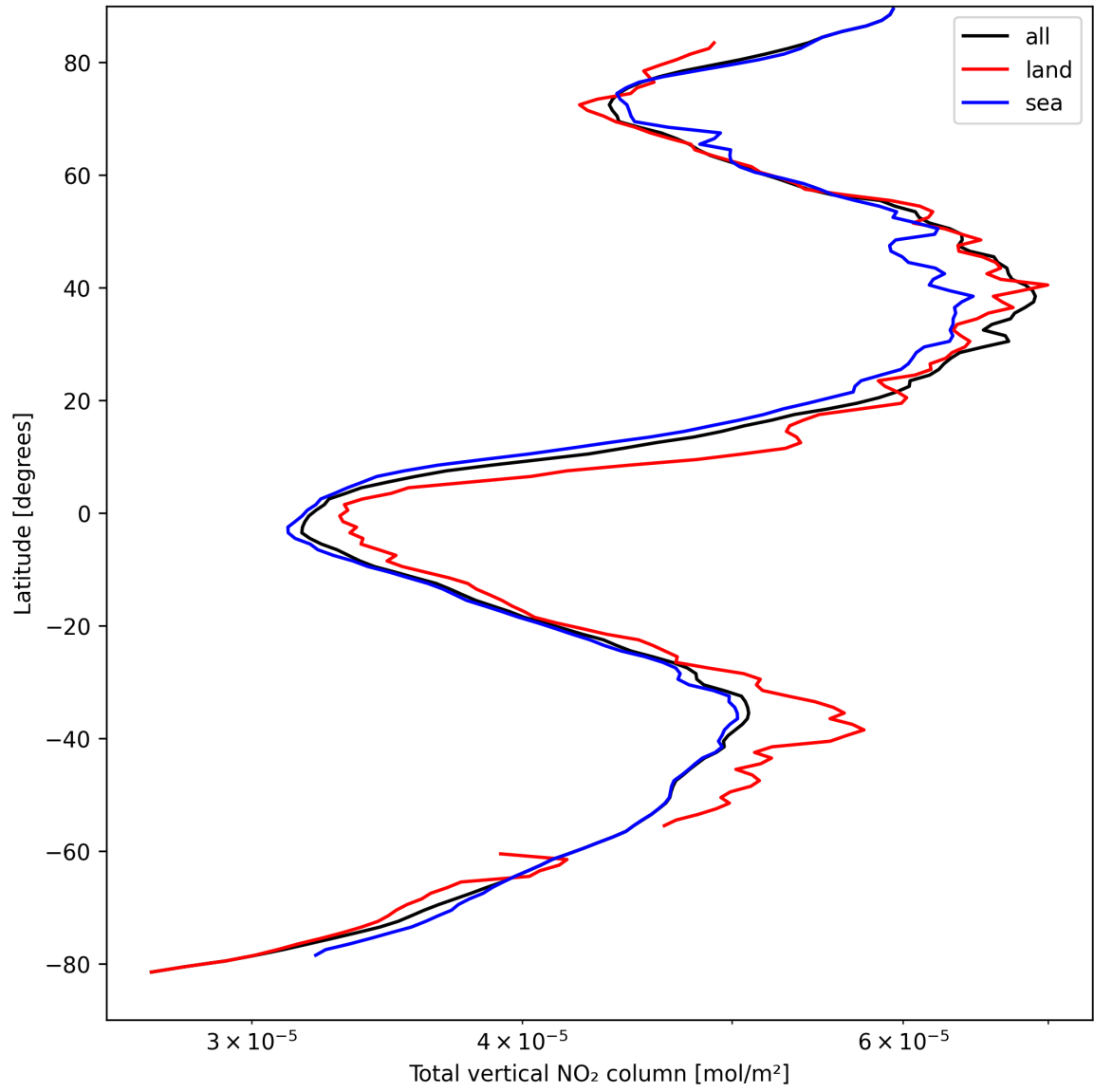
Figure 21: Zonal average of “Total vertical NO 2 column” for 2025-04-05 to 2025-04-06.
