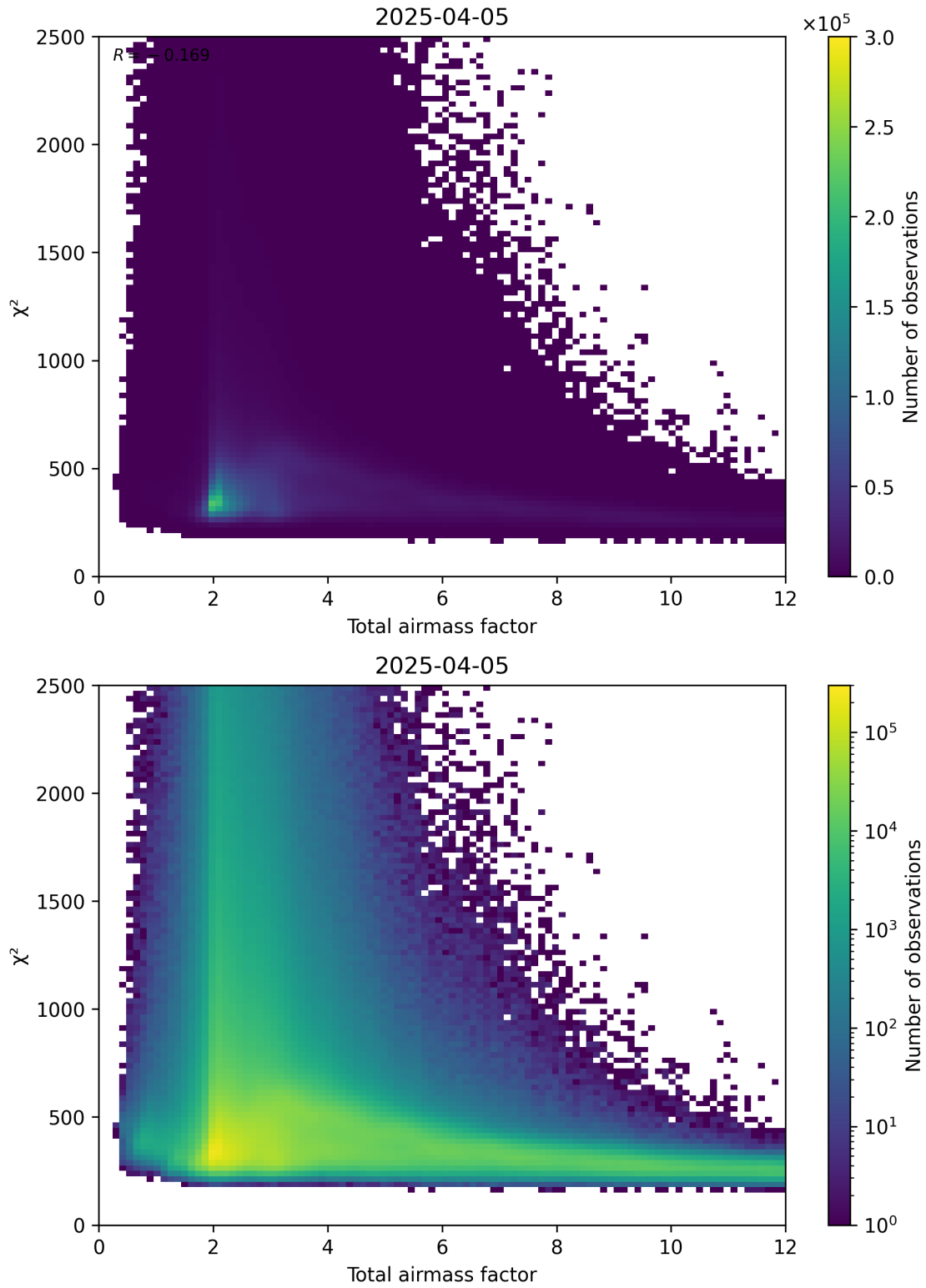
Figure 63: Scatter density plot of “Total airmass factor” against “ \chi^2 ” for 2025-04-05 to 2025-04-06.
