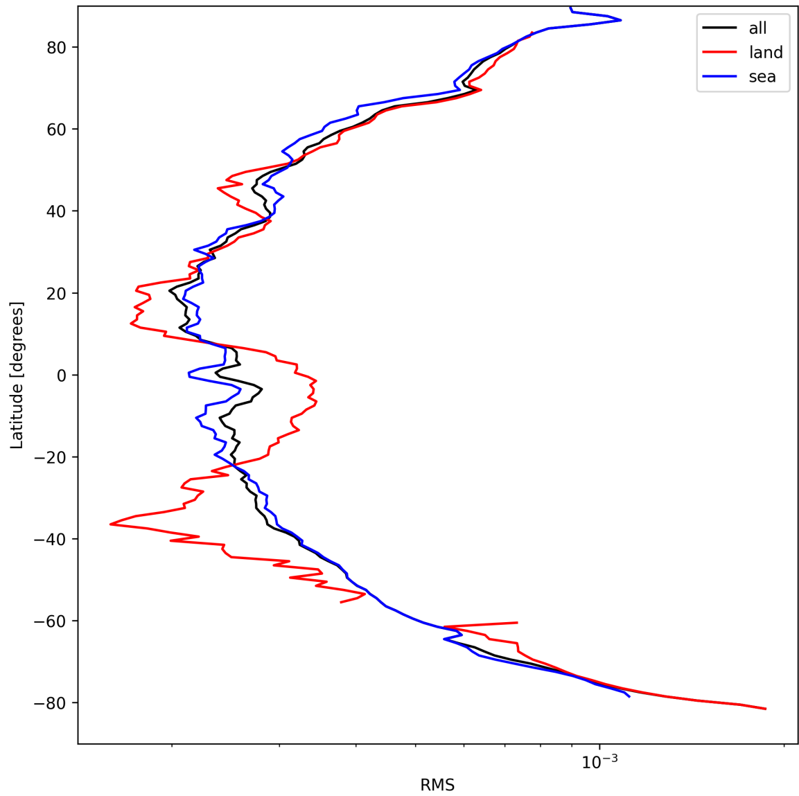
Figure 26: Zonal average of “RMS” for 2025-04-05 to 2025-04-06.
