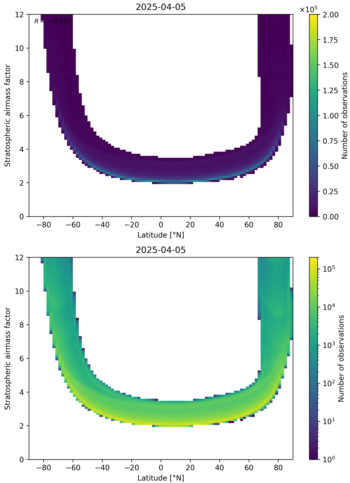
Figure 83: Scatter density plot of “Latitude” against “Stratospheric air mass factor” for 2025-04-05 to 2025-04-06.
