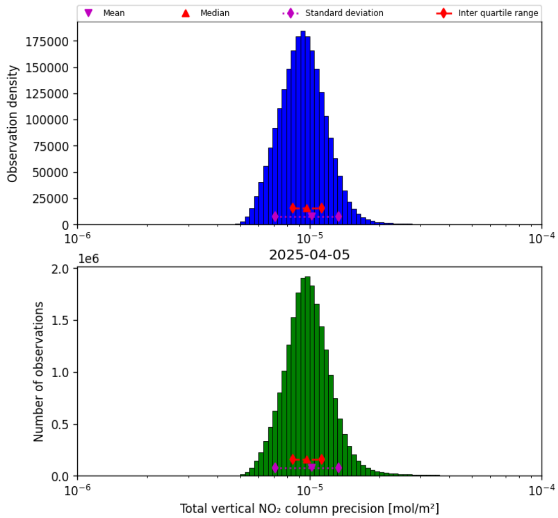
Figure 39: Histogram of “Total vertical NO 2 column precision” for 2025-04-05 to 2025-04-06
