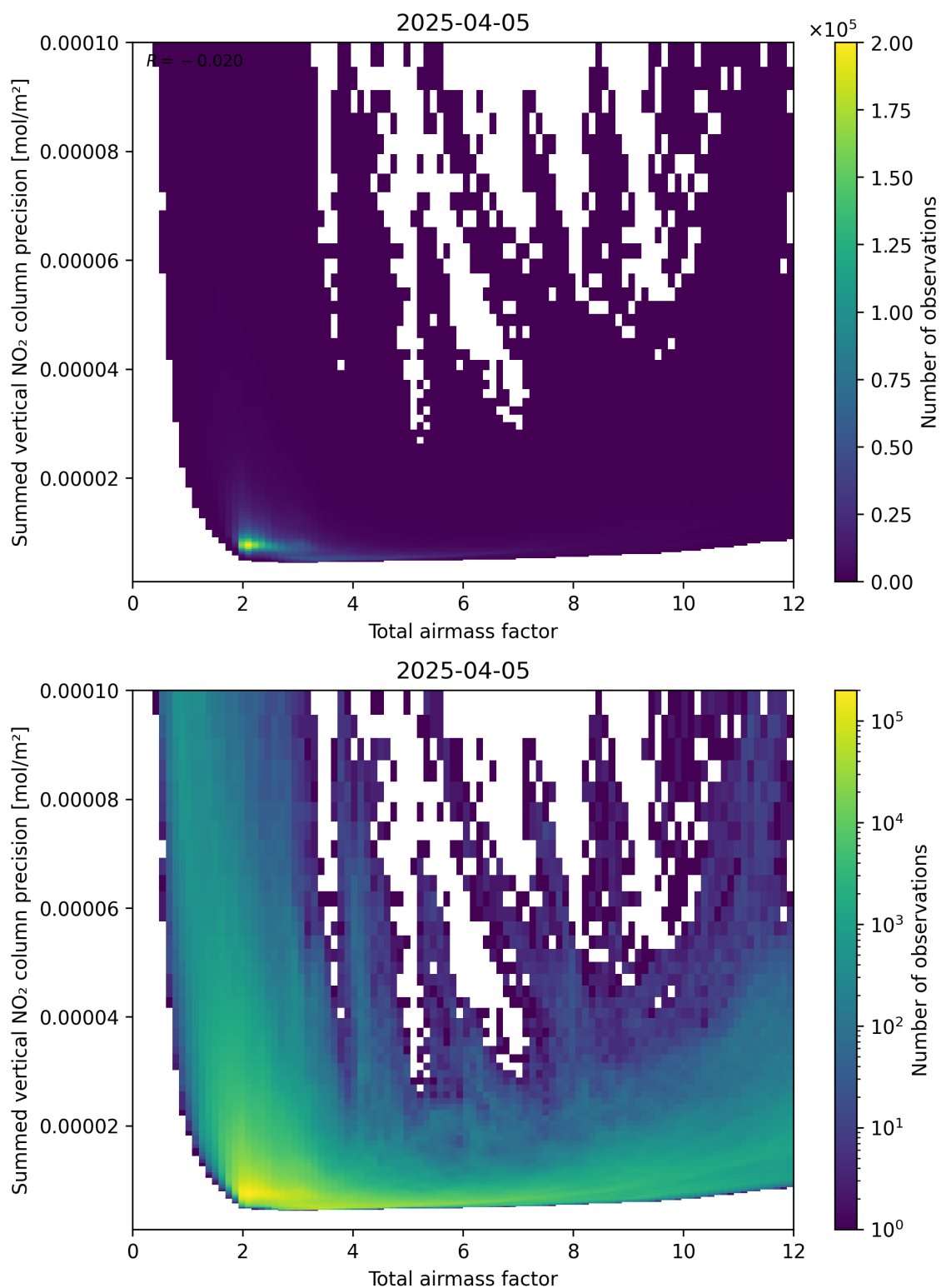
Figure 66: Scatter density plot of “Total airmass factor” against “Summed vertical NO 2 column precision” for 2025-04-05 to 2025-04-06.
