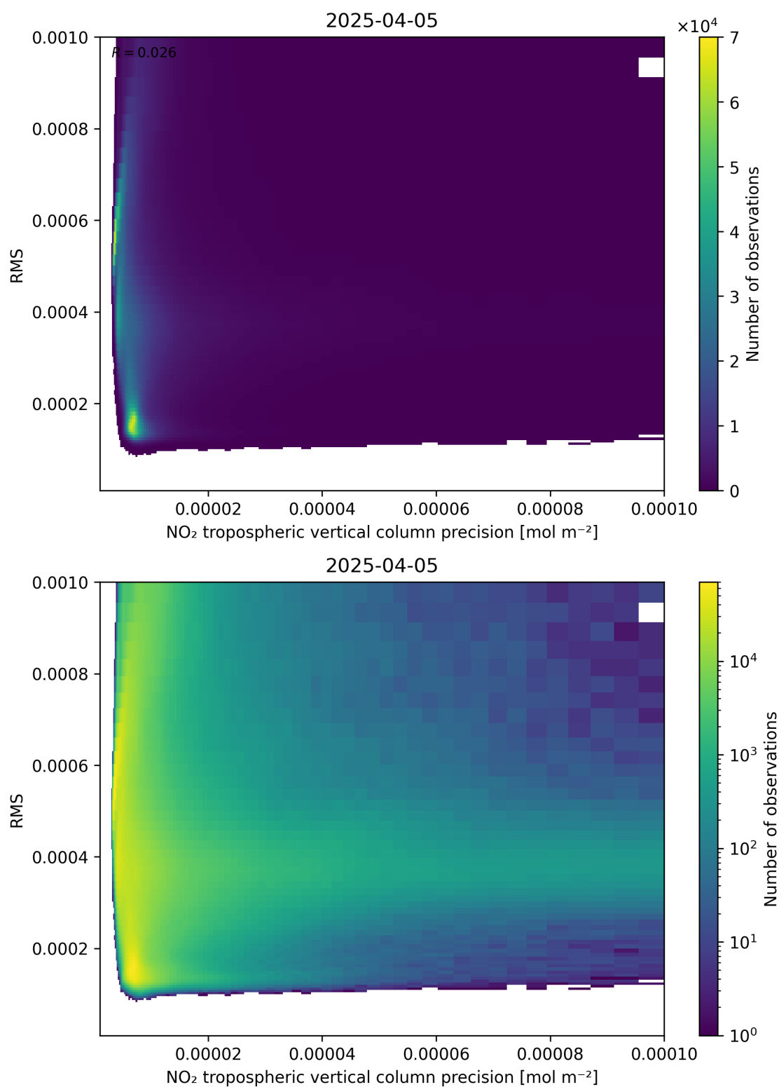
Figure 140: Scatter density plot of “NO 2 tropospheric vertical column precision” against “RMS” for 2025-04-05 to 2025-04-06.
