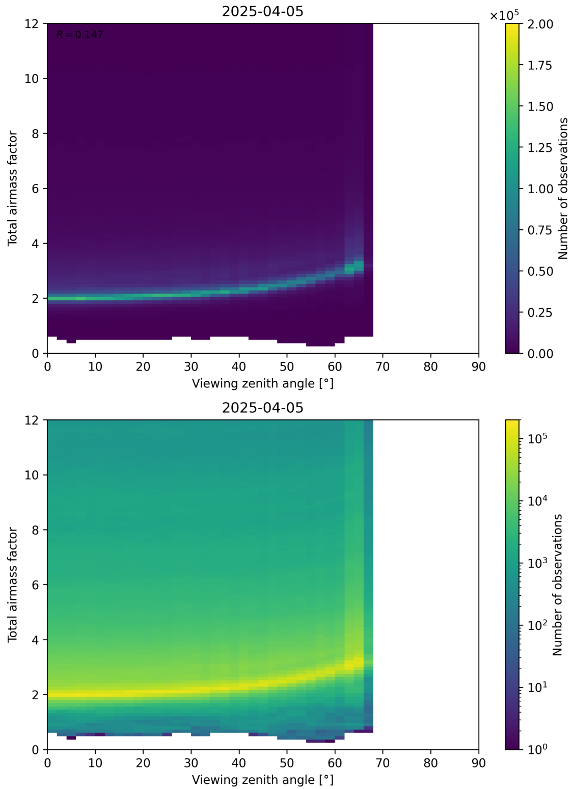
Figure 160: Scatter density plot of “Viewing zenith angle” against “Total airmass factor” for 2025-04-05 to 2025-04-06.
