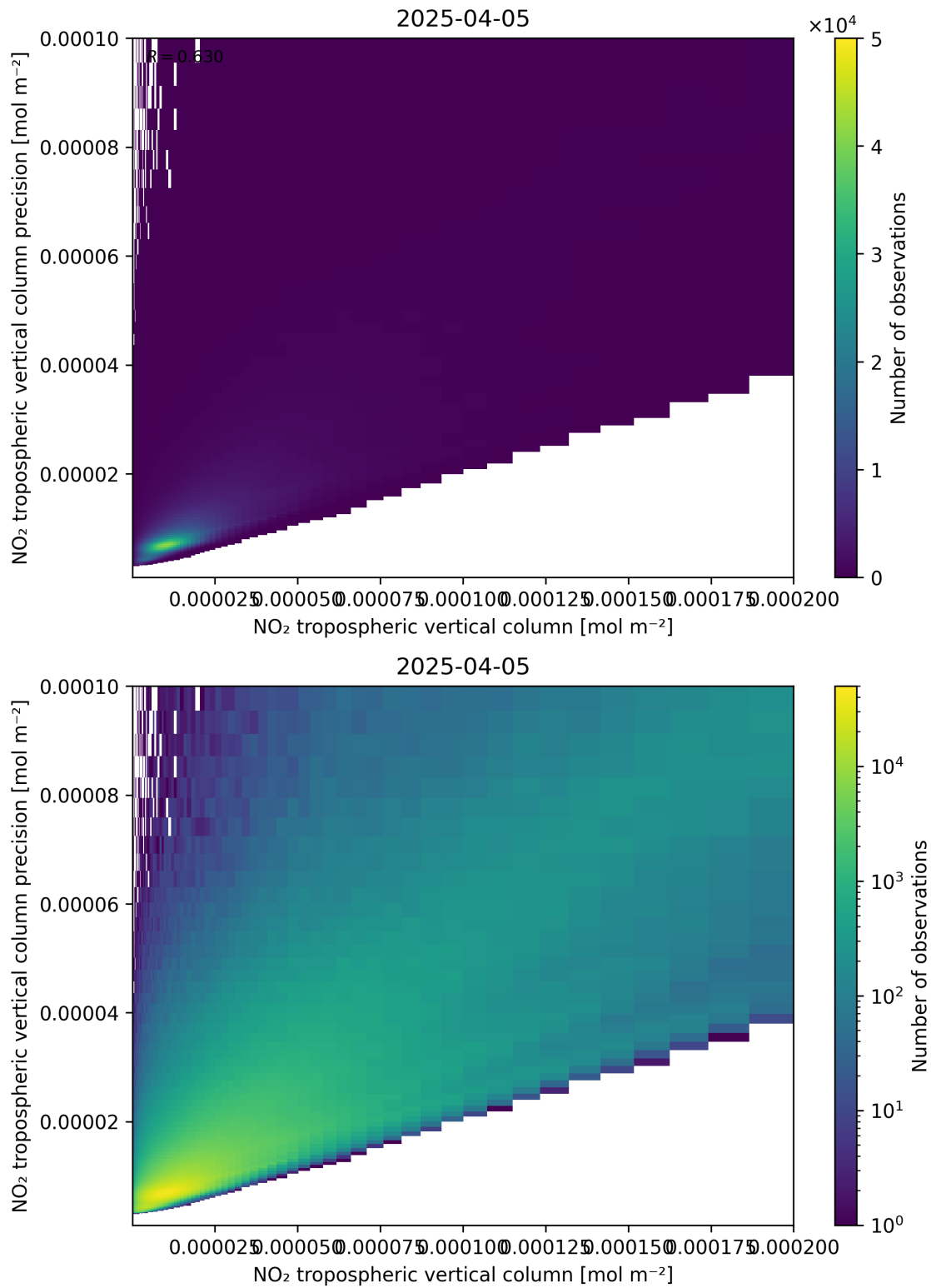
Figure 130: Scatter density plot of “NO 2 tropospheric vertical column” against “NO 2 tropospheric vertical column precision” for 2025-04-05 to 2025-04-06.
