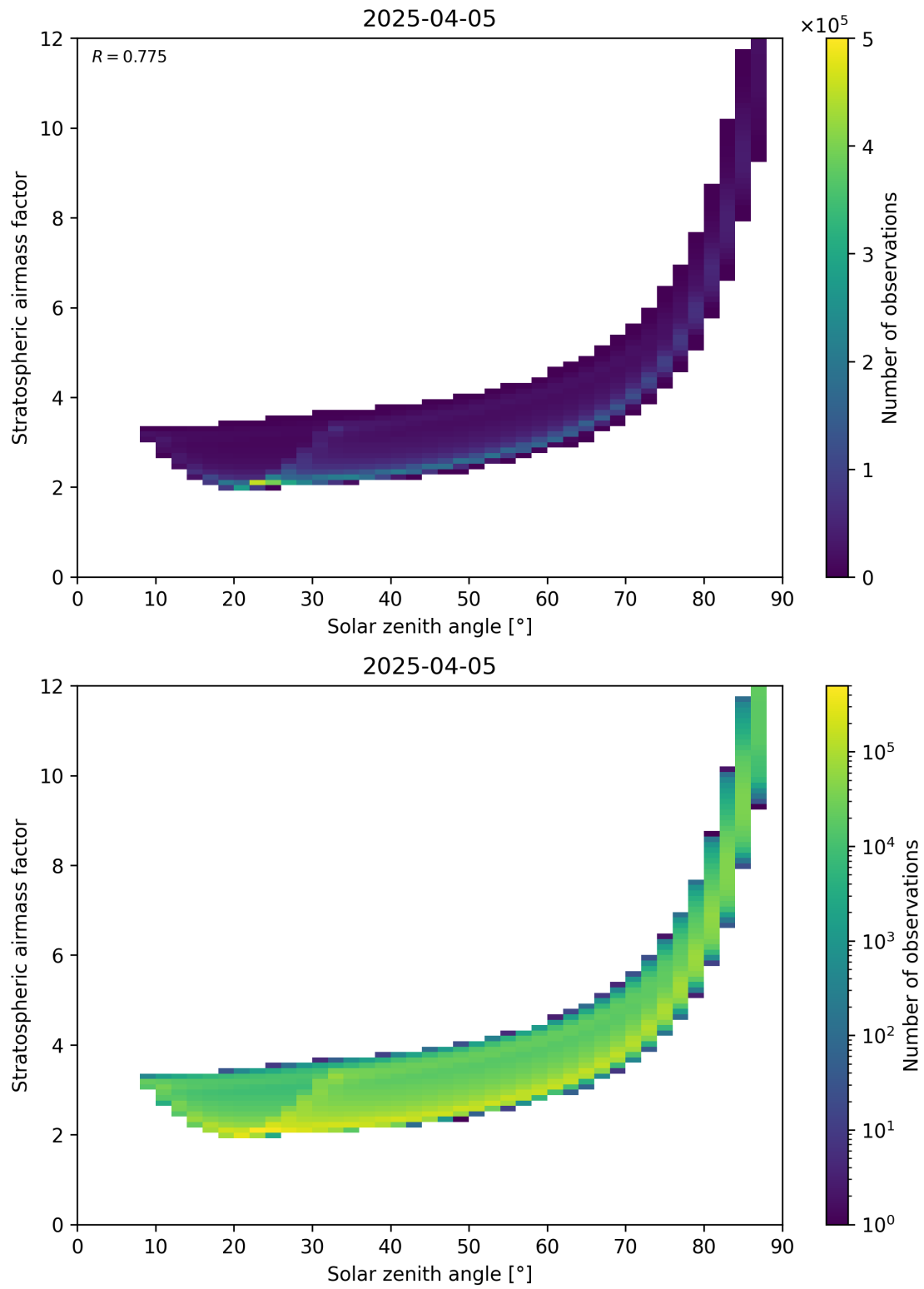
Figure 145: Scatter density plot of “Solar zenith angle” against “Stratospheric airmass factor” for 2025-04-05 to 2025-04-06.
