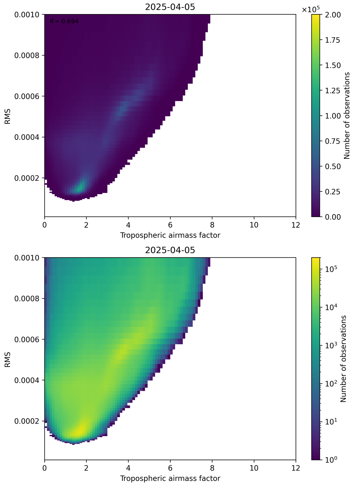
Figure 79: Scatter density plot of “Tropospheric airmass factor” against “RMS” for 2025-04-05 to 2025-04-06.
