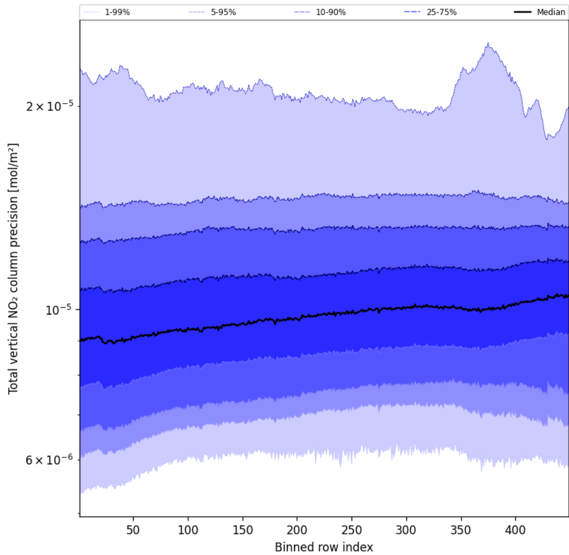
Figure 56: Along track statistics of “Total vertical NO 2 column precision” for 2025-04-05 to 2025-04-06
