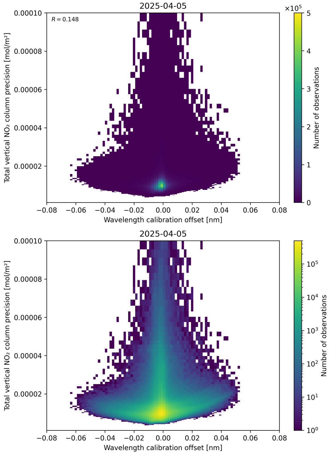
Figure 180: Scatter density plot of “Wavelength calibration offset” against “Total vertical NO 2 column precision” for 2025-04-05 to 2025-04-06.
