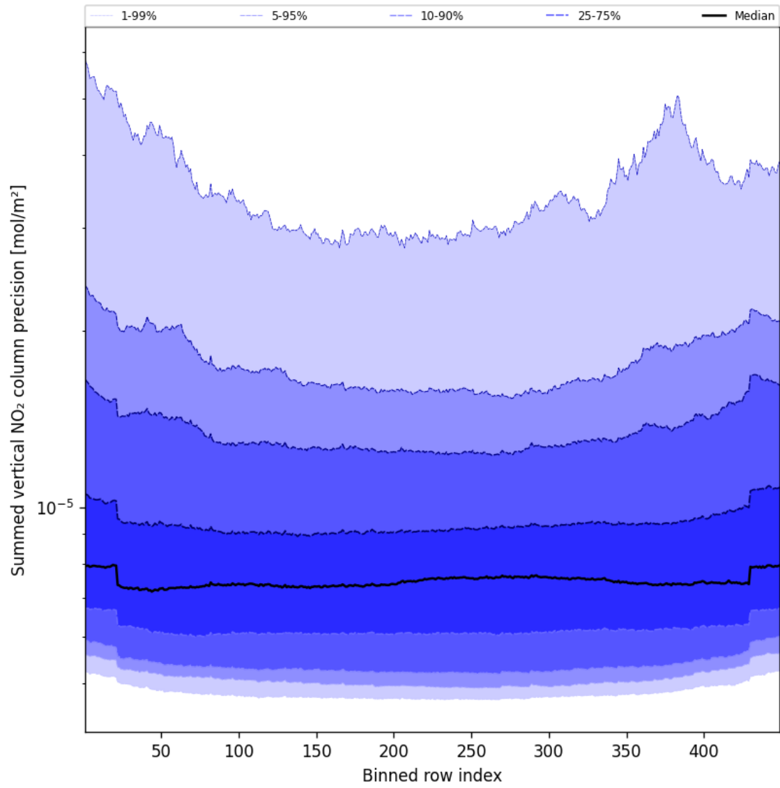
Figure 58: Along track statistics of “Summed vertical NO 2 column precision” for 2025-04-05 to 2025-04-06
