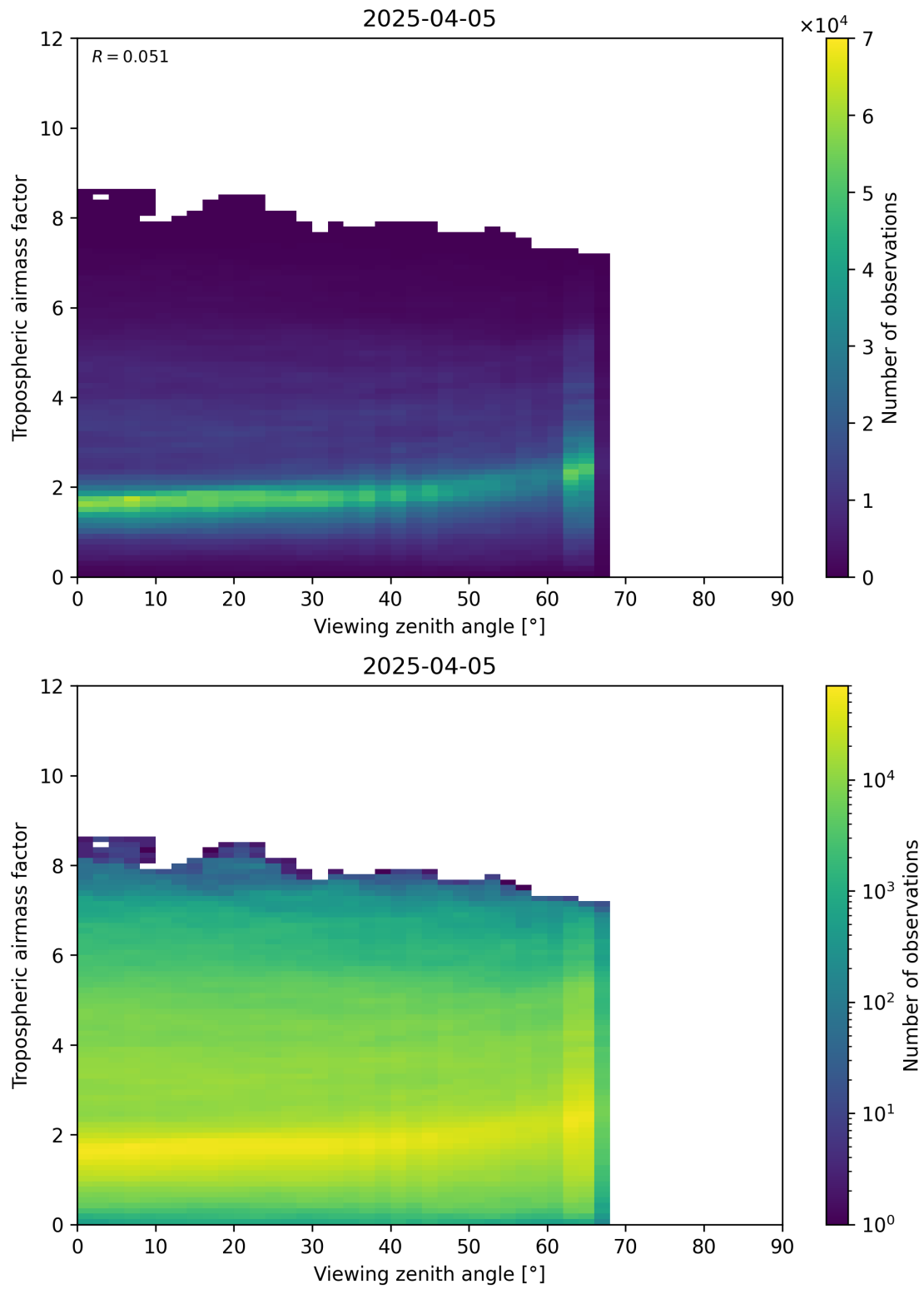
Figure 161: Scatter density plot of “Viewing zenith angle” against “Tropospheric airmass factor” for 2025-04-05 to 2025-04-06.
