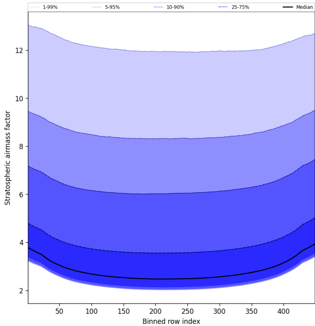
Figure 61: Along track statistics of “Stratospheric airmass factor” for 2025-04-05 to 2025-04-06
