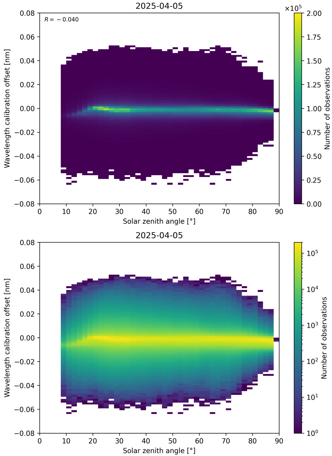
Figure 158: Scatter density plot of “Solar zenith angle” against “Wavelength calibration offset” for 2025-04-05 to 2025-04-06.
