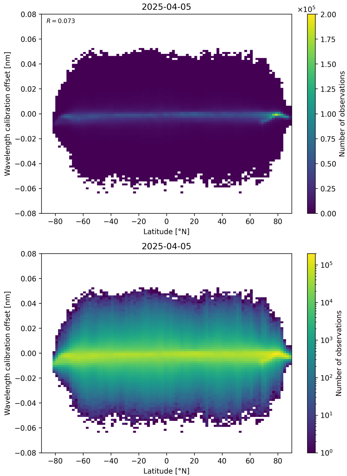
Figure 95: Scatter density plot of “Latitude” against “Wavelength calibration offset” for 2025-04-05 to 2025-04-06.
