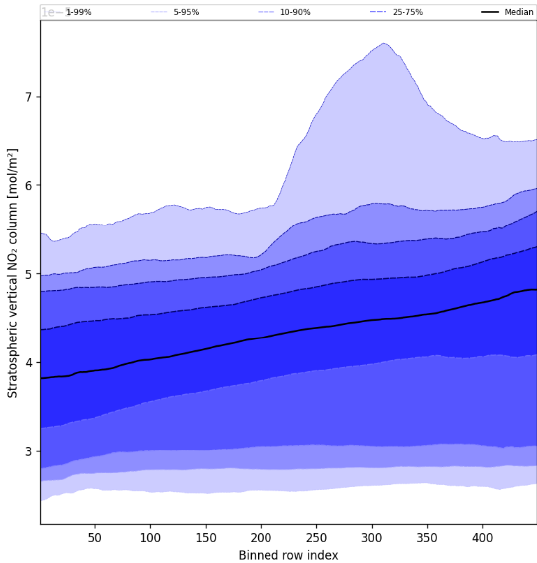
Figure 53: Along track statistics of “Stratospheric vertical NO 2 column” for 2025-04-05 to 2025-04-06
