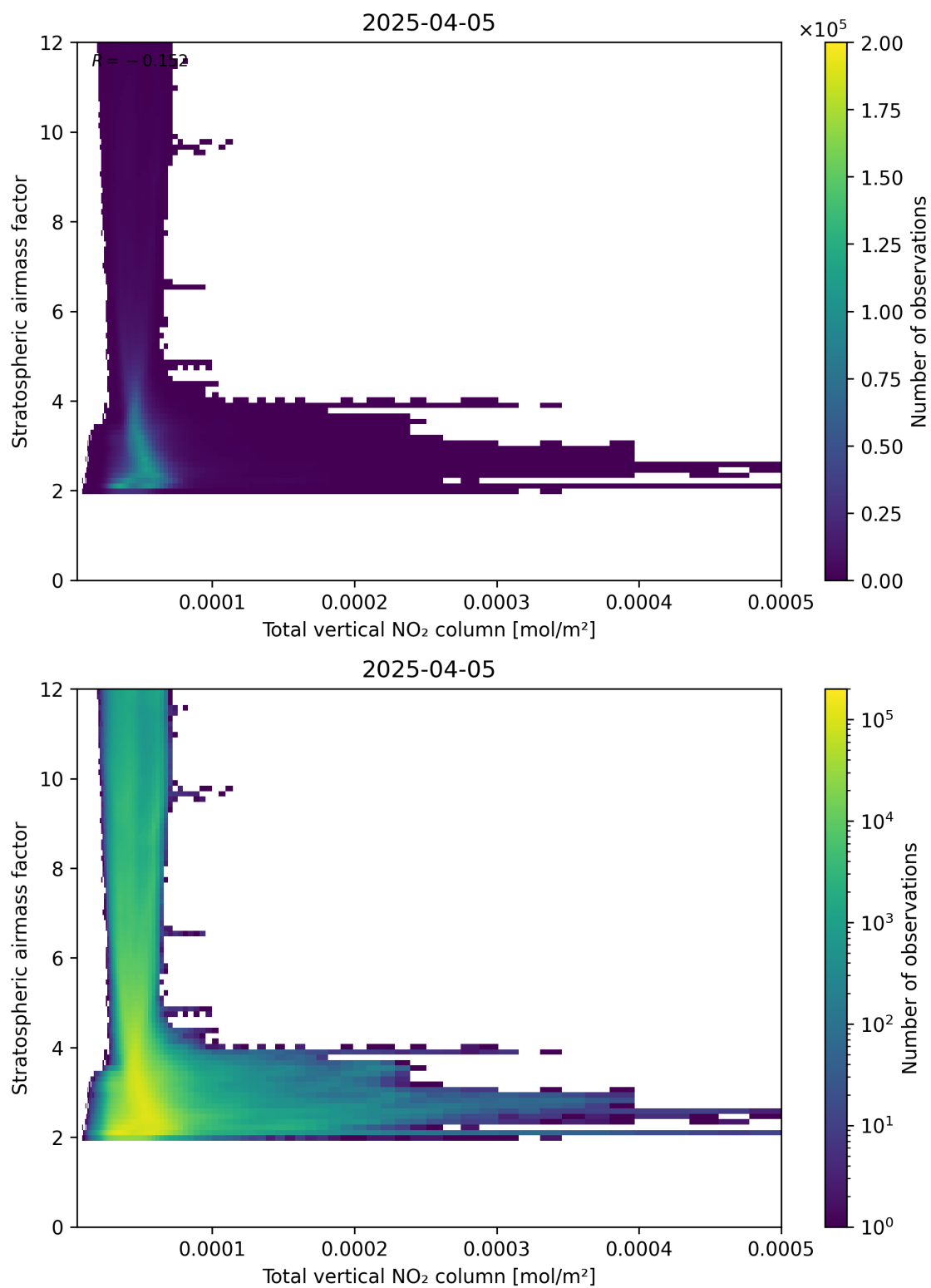
Figure 110: Scatter density plot of “Total vertical NO 2 column” against “Stratospheric airmass factor” for 2025-04-05 to 2025-04-06.
