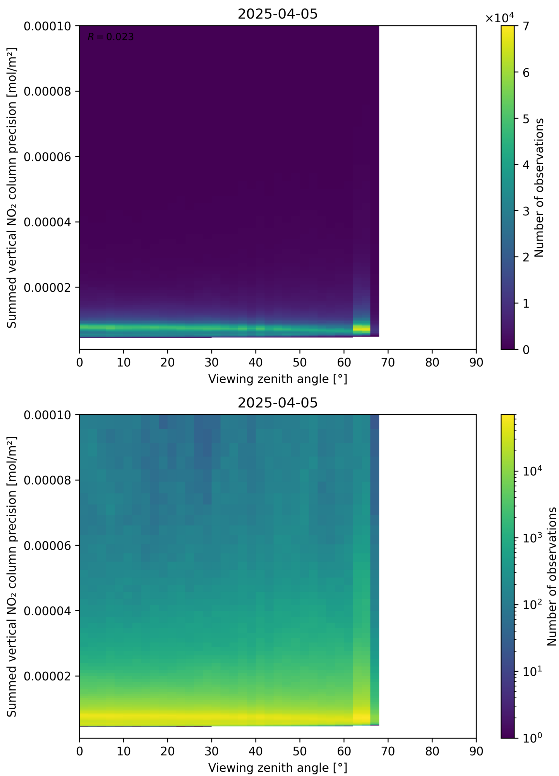
Figure 166: Scatter density plot of “Viewing zenith angle” against “Summed vertical NO 2 column precision” for 2025-04-05 to 2025-04-06.
