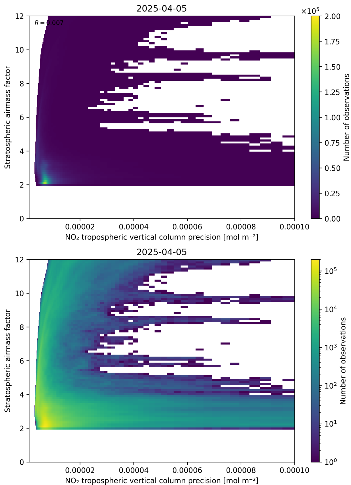
Figure 131: Scatter density plot of “NO 2 tropospheric vertical column precision” against “Stratospheric airmass factor” for 2025-04-05 to 2025-04-06.
