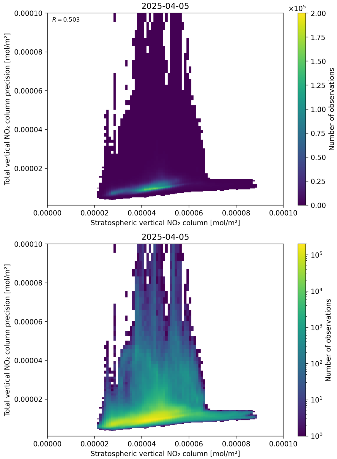
Figure 101: Scatter density plot of “Stratospheric vertical NO 2 column” against “Total vertical NO 2 column precision” for 2025-04-05 to 2025-04-06.
