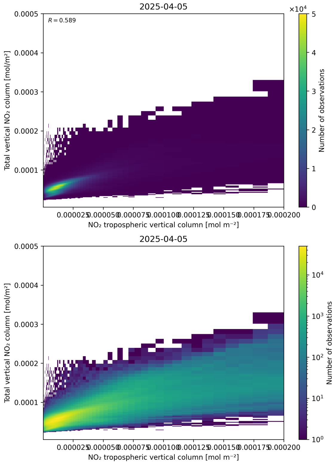
Figure 128: Scatter density plot of “NO 2 tropospheric vertical column” against “Total vertical NO 2 column” for 2025-04-05 to 2025-04-06.
