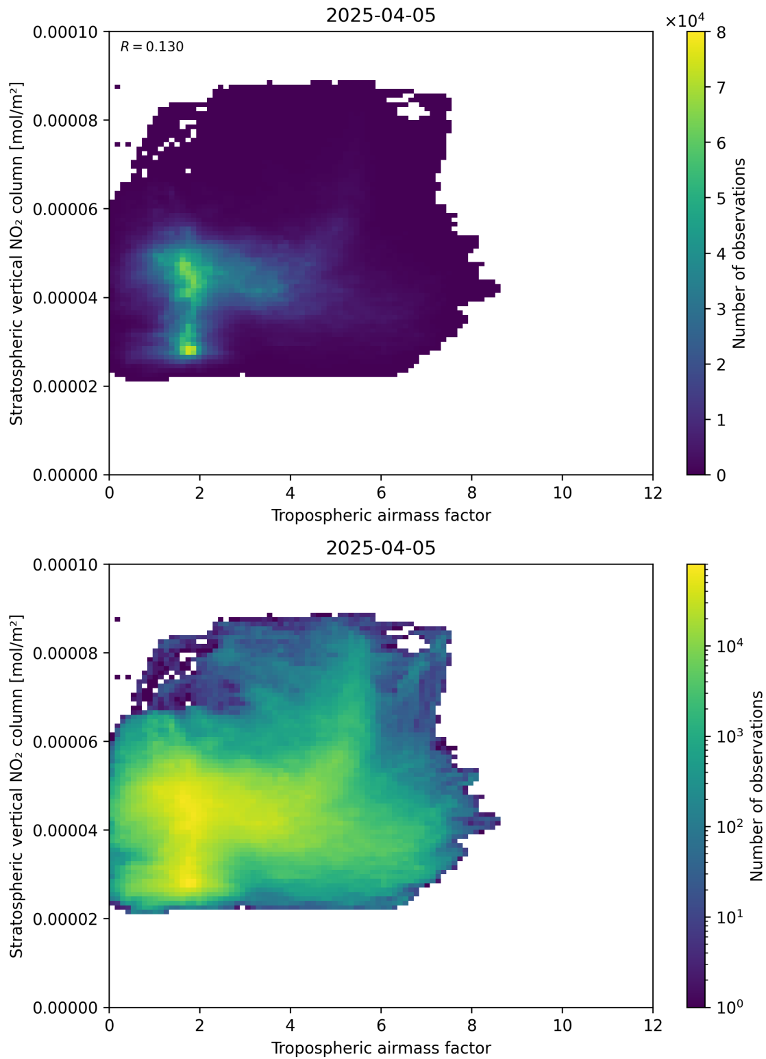
Figure 74: Scatter density plot of “Tropospheric airmass factor” against “Stratospheric vertical NO 2 column” for 2025-04-05 to 2025-04-06.
