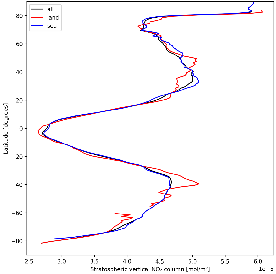
Figure 19: Zonal average of “Stratospheric vertical NO 2 column” for 2025-04-05 to 2025-04-06.
