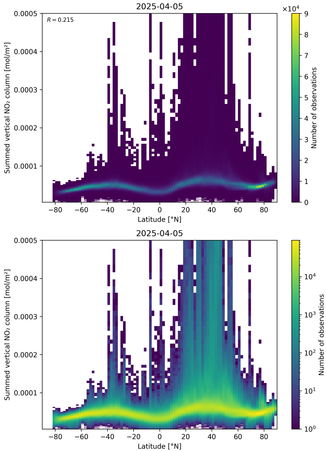
Figure 88: Scatter density plot of “Latitude” against “Summed vertical NO 2 column” for 2025-04-05 to 2025-04-06.
