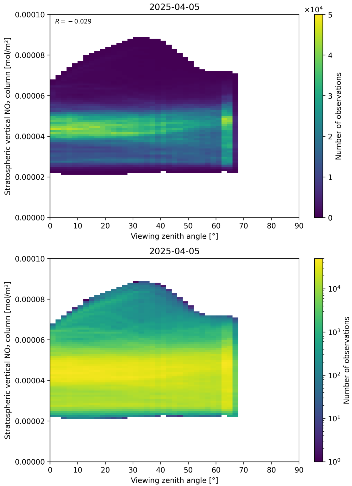
Figure 164: Scatter density plot of “Viewing zenith angle” against “Stratospheric vertical NO 2 column” for 2025-04-05 to 2025-04-06.
