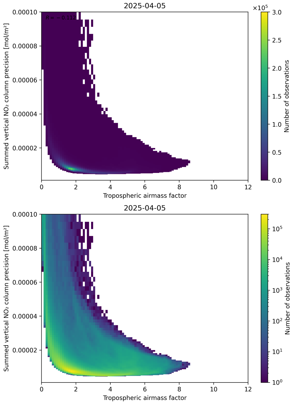
Figure 76: Scatter density plot of “Tropospheric airmass factor” against “Summed vertical NO 2 column precision” for 2025-04-05 to 2025-04-06.
