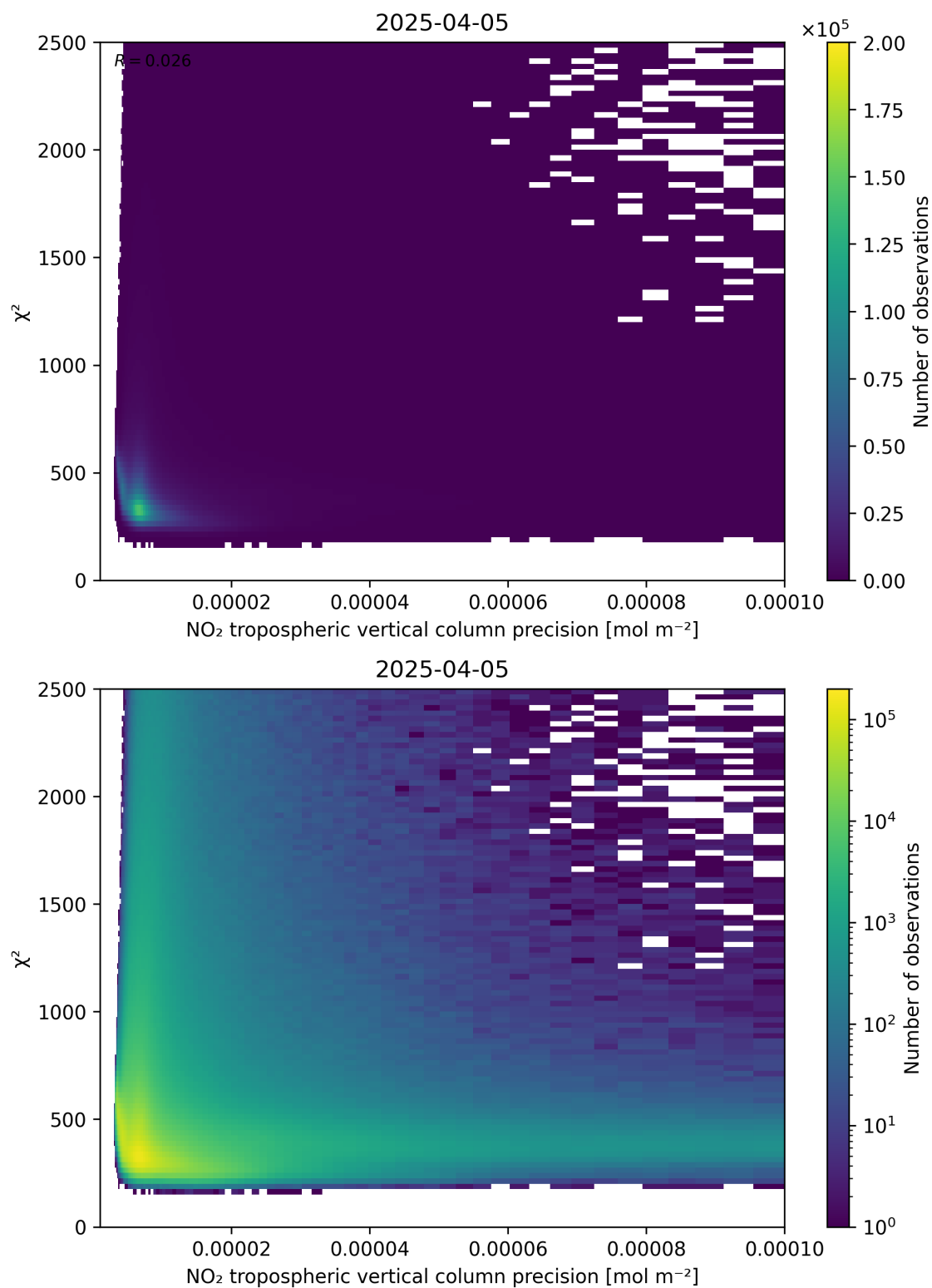
Figure 134: Scatter density plot of “NO 2 tropospheric vertical column precision” against “ \chi^2 ” for 2025-04-05 to 2025-04-06.
