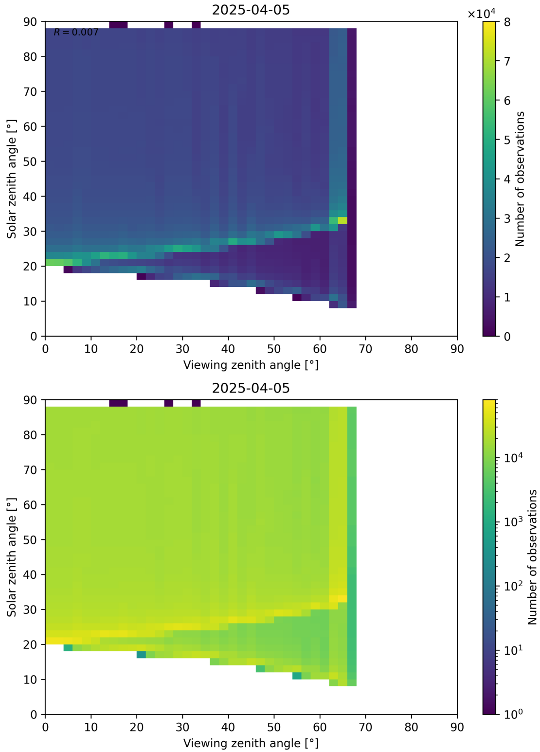
Figure 172: Scatter density plot of “Viewing zenith angle” against “Solar zenith angle” for 2025-04-05 to 2025-04-06.
