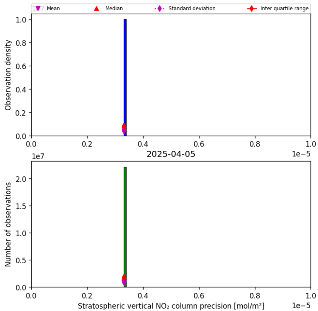
Figure 37: Histogram of “Stratospheric vertical NO 2 column precision” for 2025-04-05 to 2025-04-06
