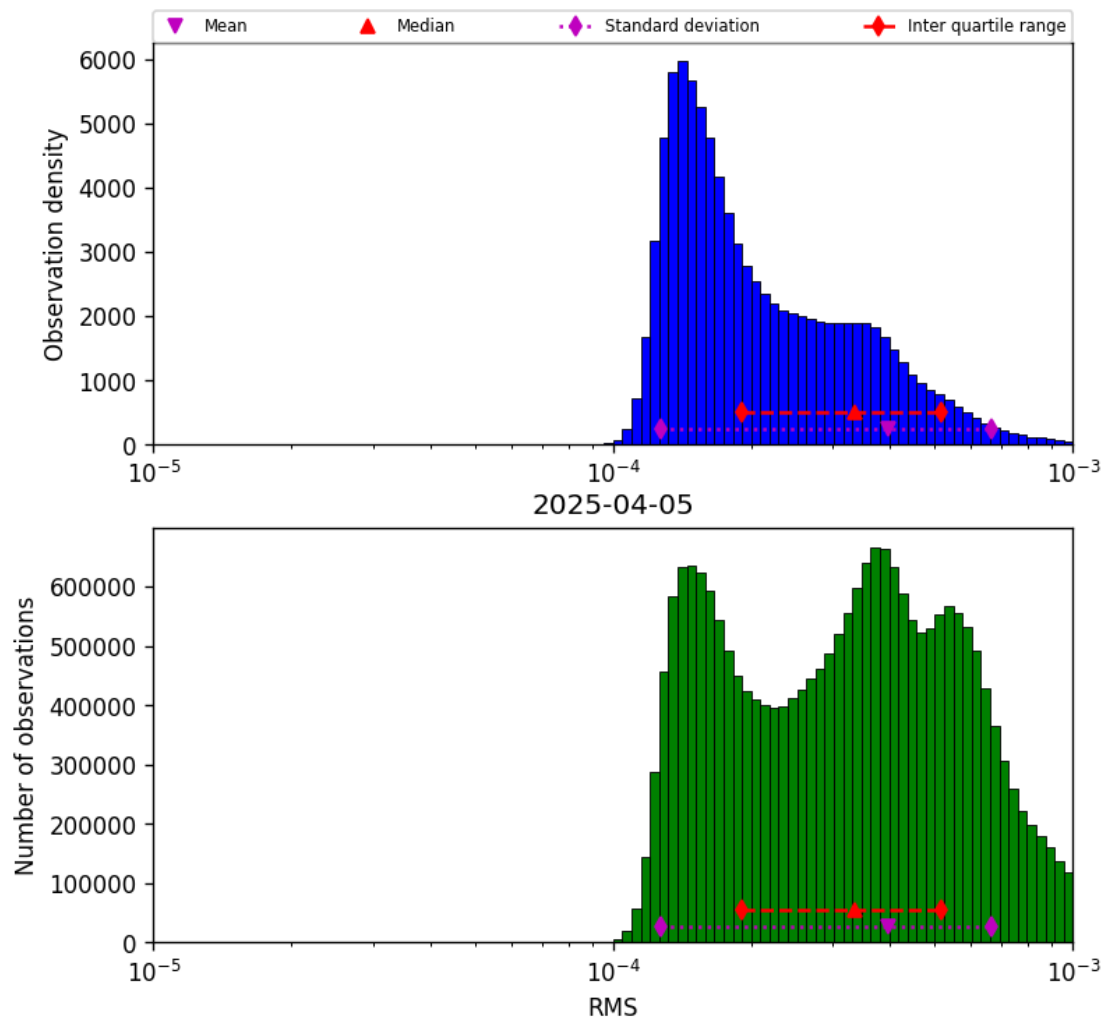
Figure 43: Histogram of “RMS” for 2025-04-05 to 2025-04-06
