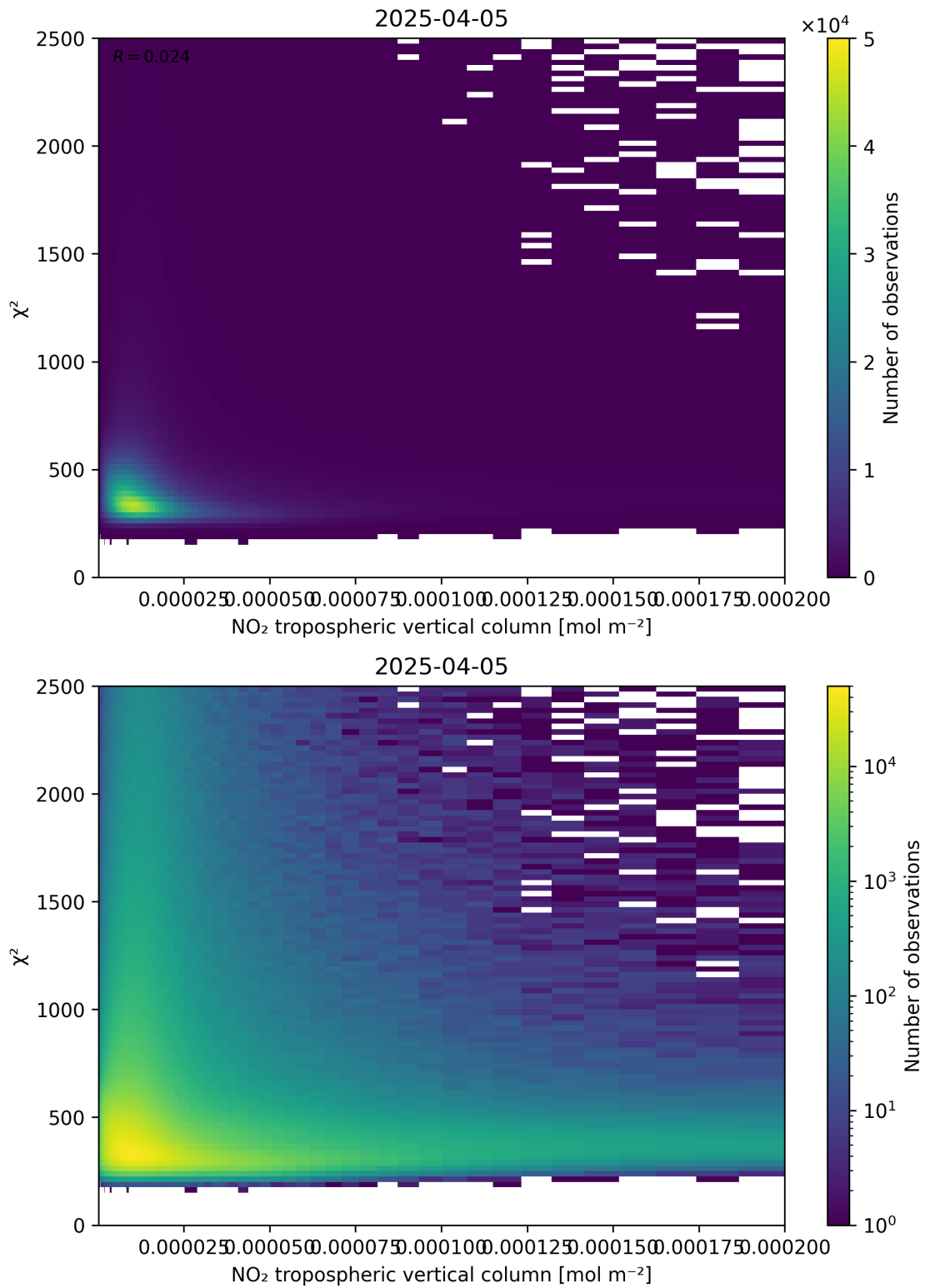
Figure 124: Scatter density plot of “NO 2 tropospheric vertical column” against “ \chi^2 ” for 2025-04-05 to 2025-04-06.
