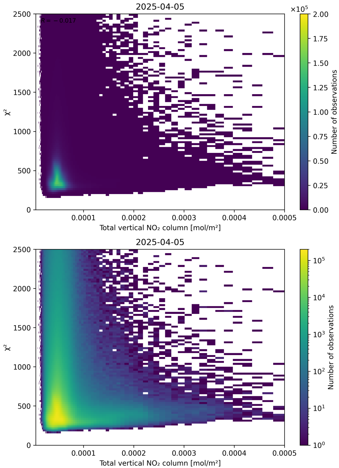
Figure 111: Scatter density plot of “Total vertical NO 2 column” against “ \chi^2 ” for 2025-04-05 to 2025-04-06.
