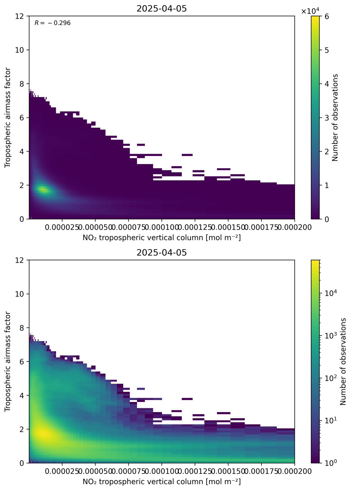
Figure 123: Scatter density plot of “NO 2 tropospheric vertical column” against “Tropospheric air mass factor” for 2025-04-05 to 2025-04-06.
