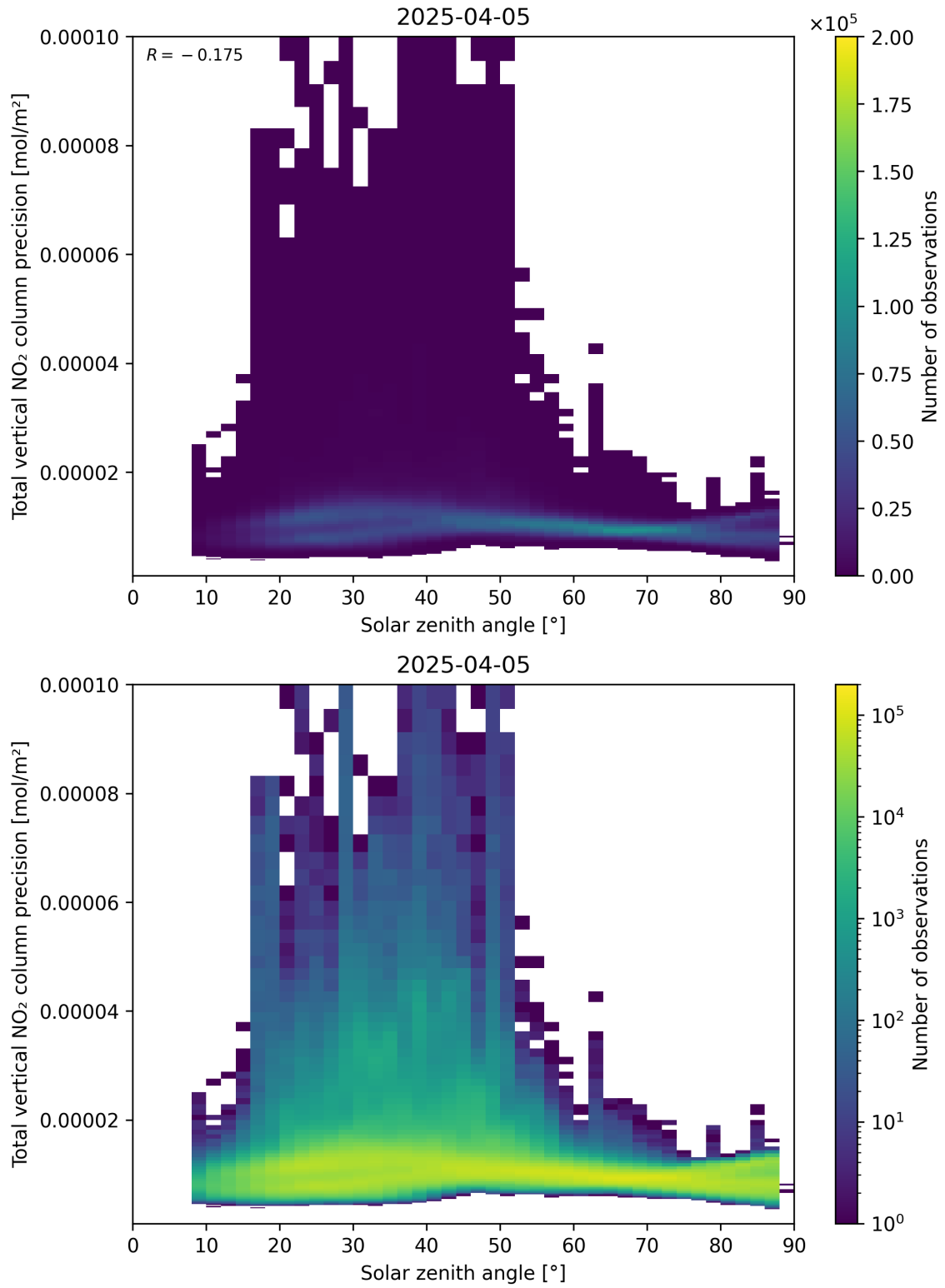
Figure 154: Scatter density plot of “Solar zenith angle” against “Total vertical NO 2 column precision” for 2025-04-05 to 2025-04-06.
