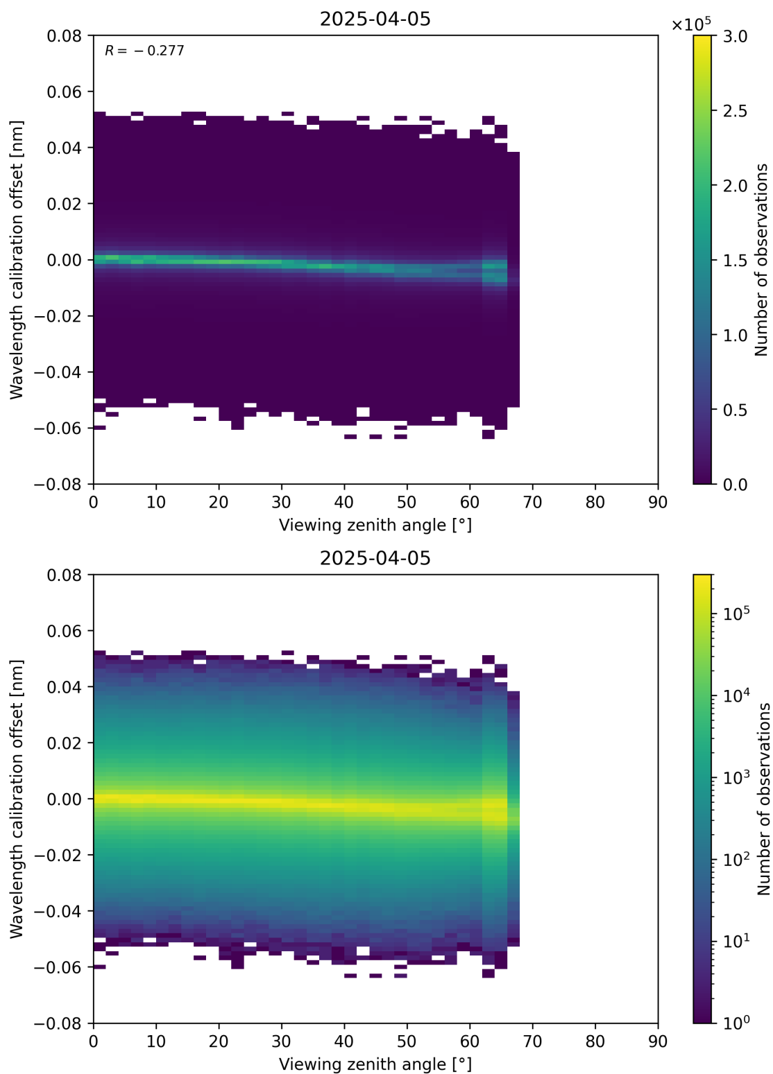
Figure 173: Scatter density plot of “Viewing zenith angle” against “Wavelength calibration offset” for 2025-04-05 to 2025-04-06.
