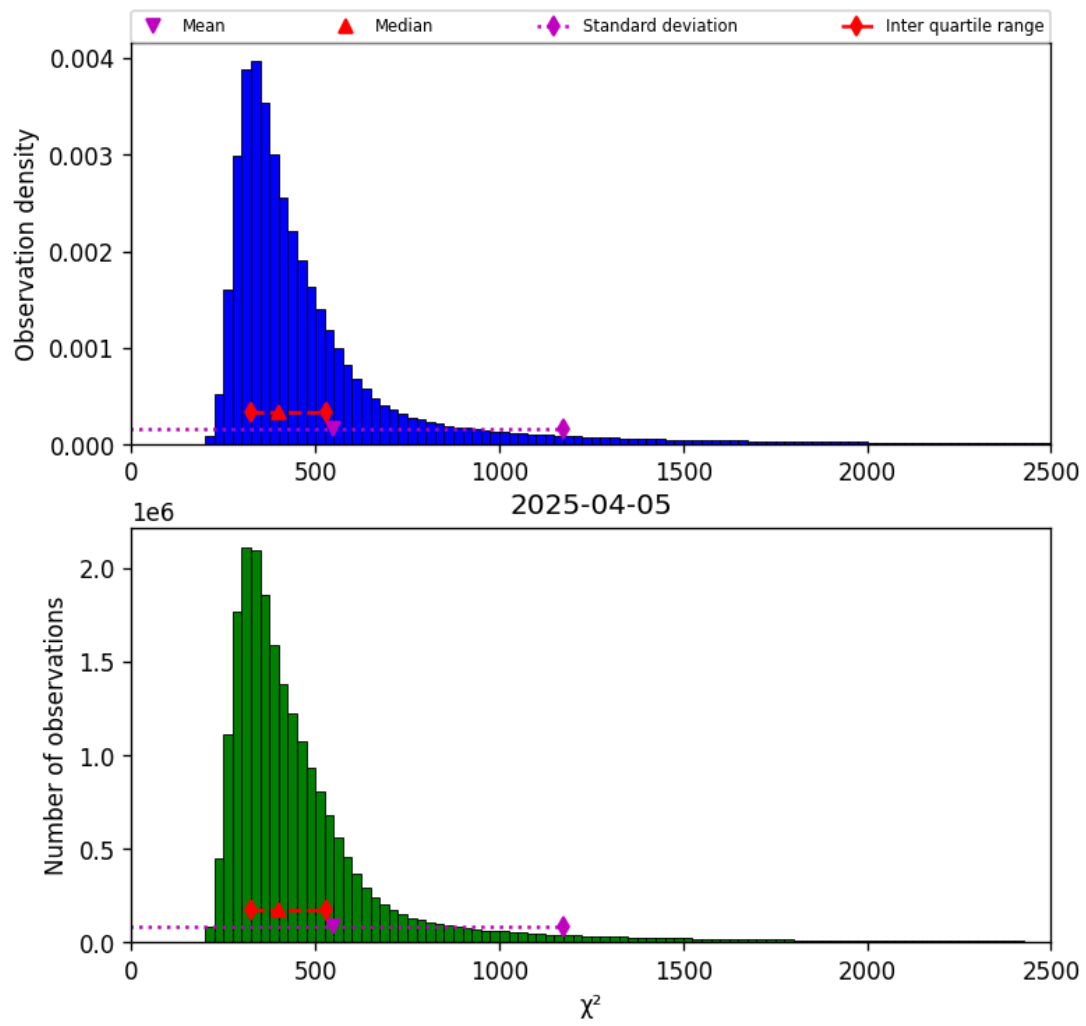
Figure 42: Histogram of “ \chi^2 ” for 2025-04-05 to 2025-04-06
