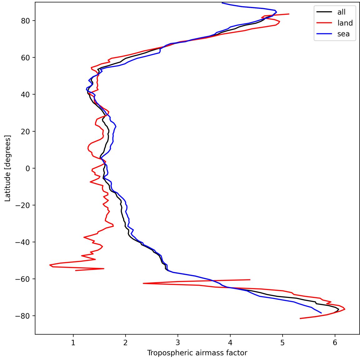
Figure 14: Zonal average of “Tropospheric air mass factor” for 2025-04-05 to 2025-04-06.
