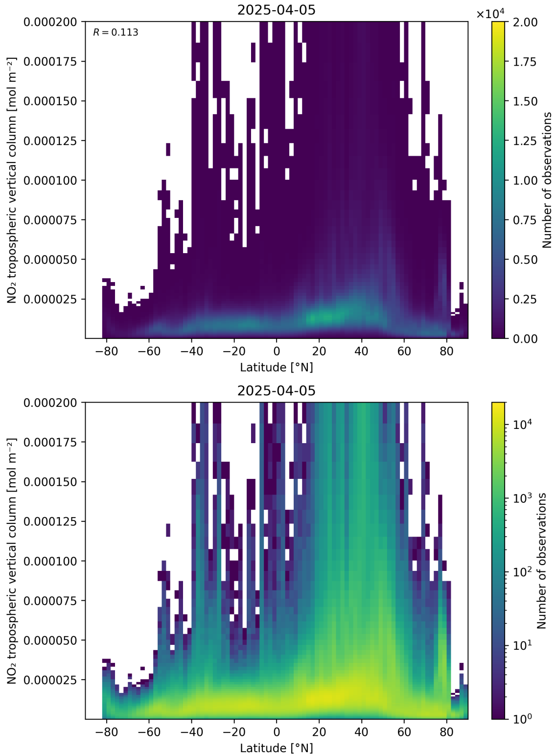
Figure 92: Scatter density plot of “Latitude” against “NO 2 tropospheric vertical column” for 2025-04-05 to 2025-04-06.
