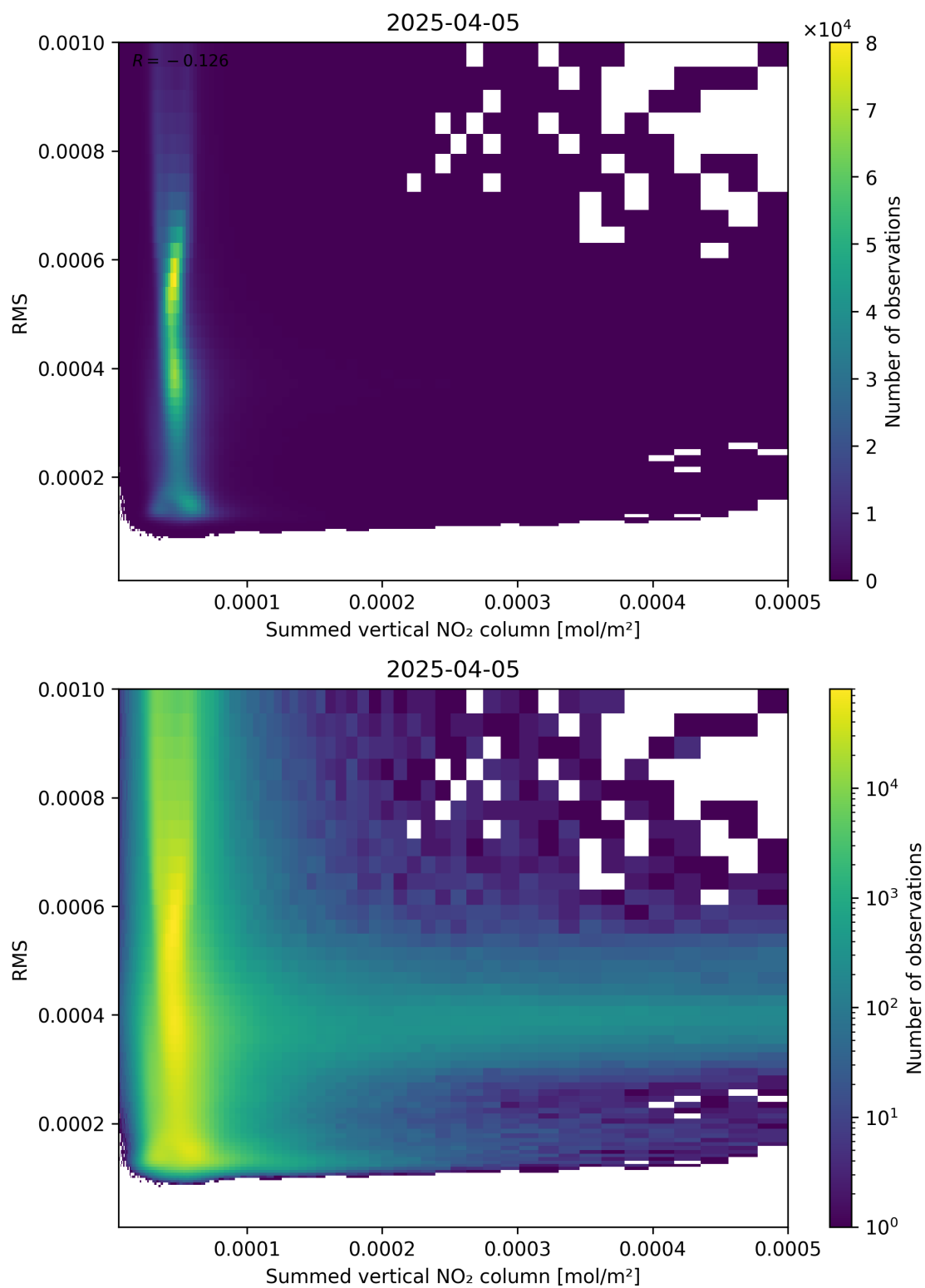
Figure 109: Scatter density plot of “Summed vertical NO 2 column” against “RMS” for 2025-04-05 to 2025-04-06.
