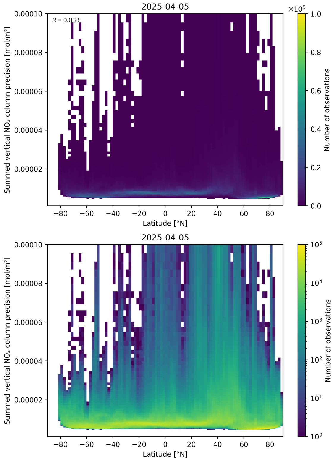
Figure 89: Scatter density plot of “Latitude” against “Summed vertical NO 2 column precision” for 2025-04-05 to 2025-04-06.
