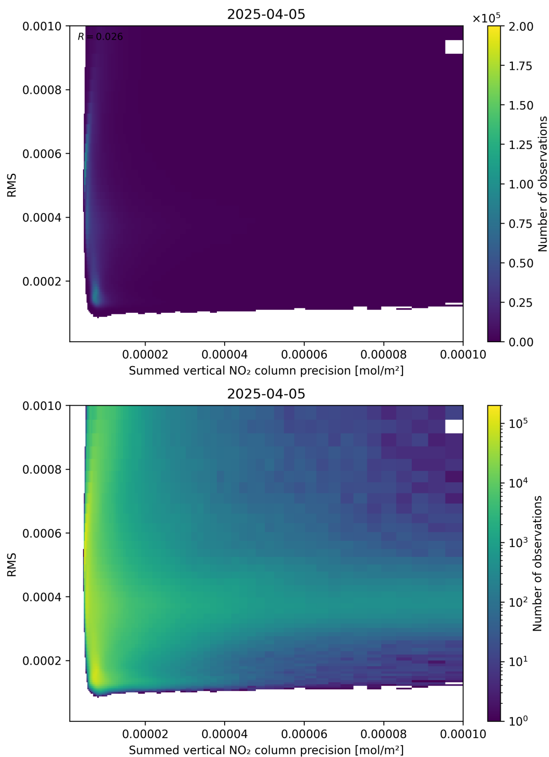
Figure 108: Scatter density plot of “Summed vertical NO 2 column precision” against “RMS” for 2025-04-05 to 2025-04-06.
