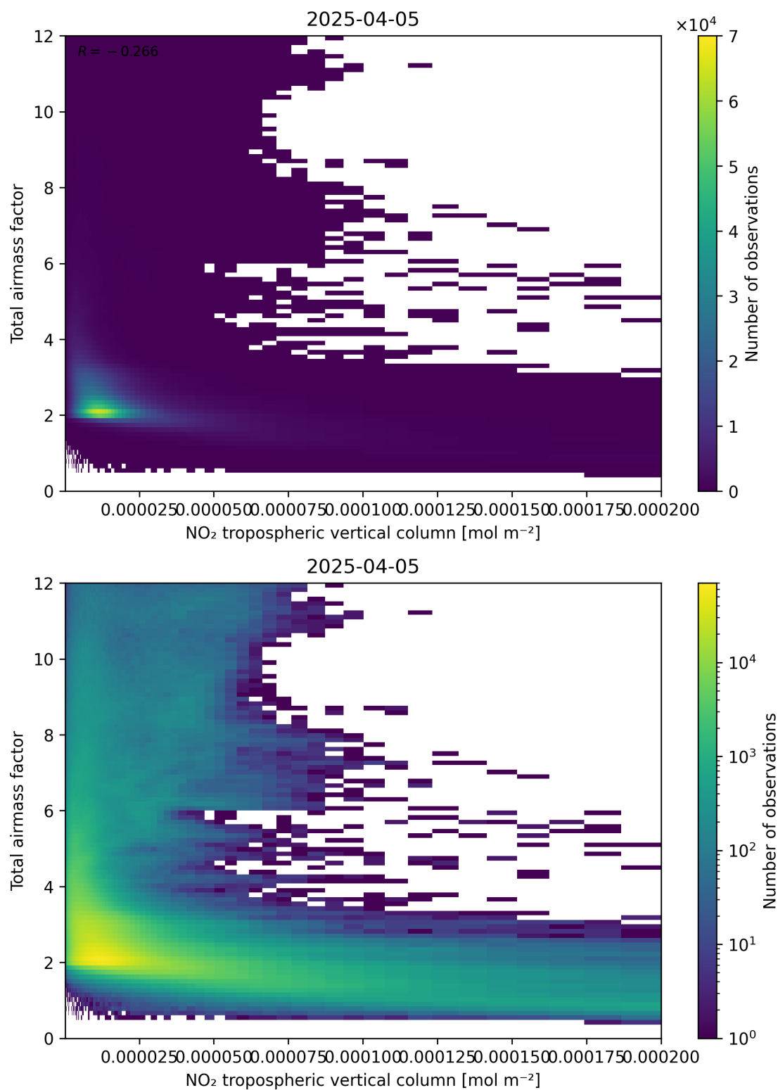
Figure 122: Scatter density plot of “NO 2 tropospheric vertical column” against “Total air mass factor” for 2025-04-05 to 2025-04-06.
