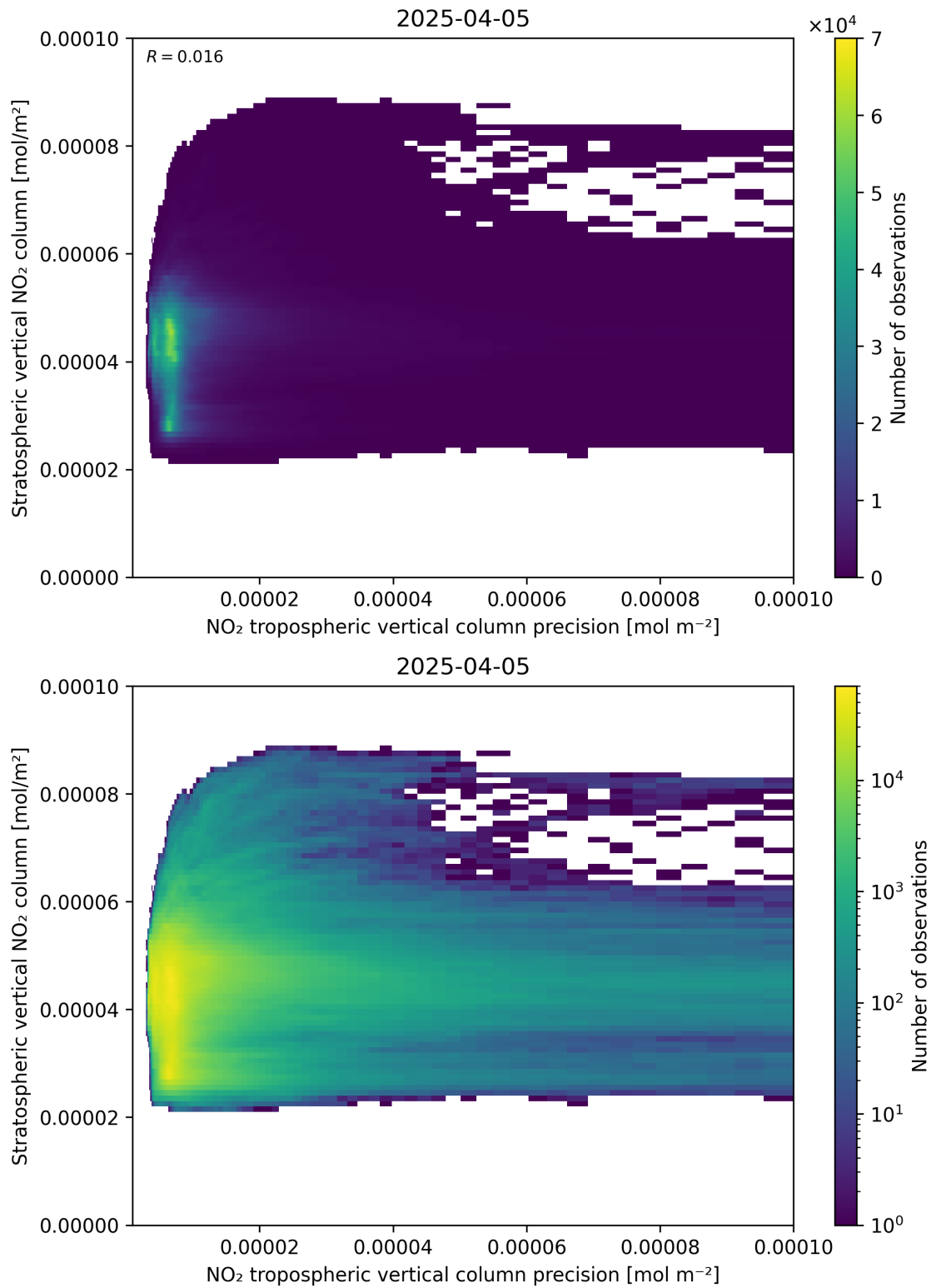
Figure 135: Scatter density plot of “NO 2 tropospheric vertical column precision” against “Stratospheric vertical NO 2 column” for 2025-04-05 to 2025-04-06.
