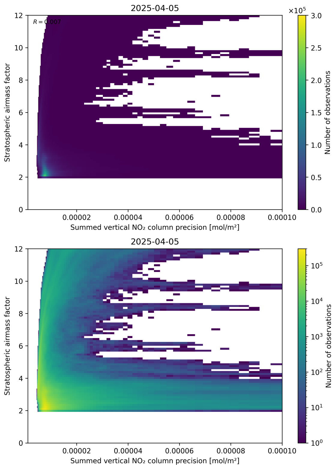
Figure 106: Scatter density plot of “Summed vertical NO 2 column precision” against “Stratospheric airmass factor” for 2025-04-05 to 2025-04-06.
