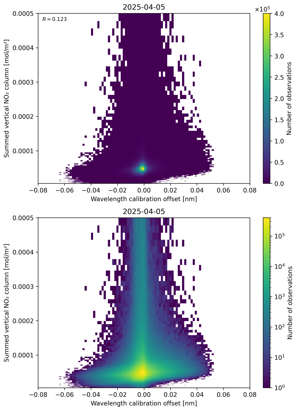
Figure 177: Scatter density plot of “Wavelength calibration offset” against “Summed vertical NO 2 column” for 2025-04-05 to 2025-04-06.
