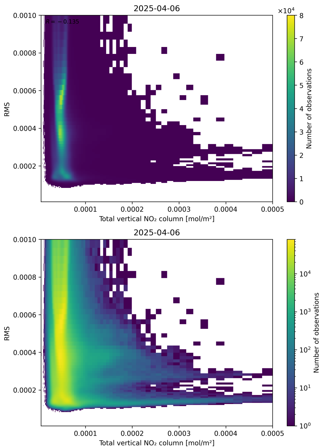
Figure 120: Scatter density plot of “Total vertical NO 2 column” against “RMS” for 2025-04-06 to 2025-04-06.
