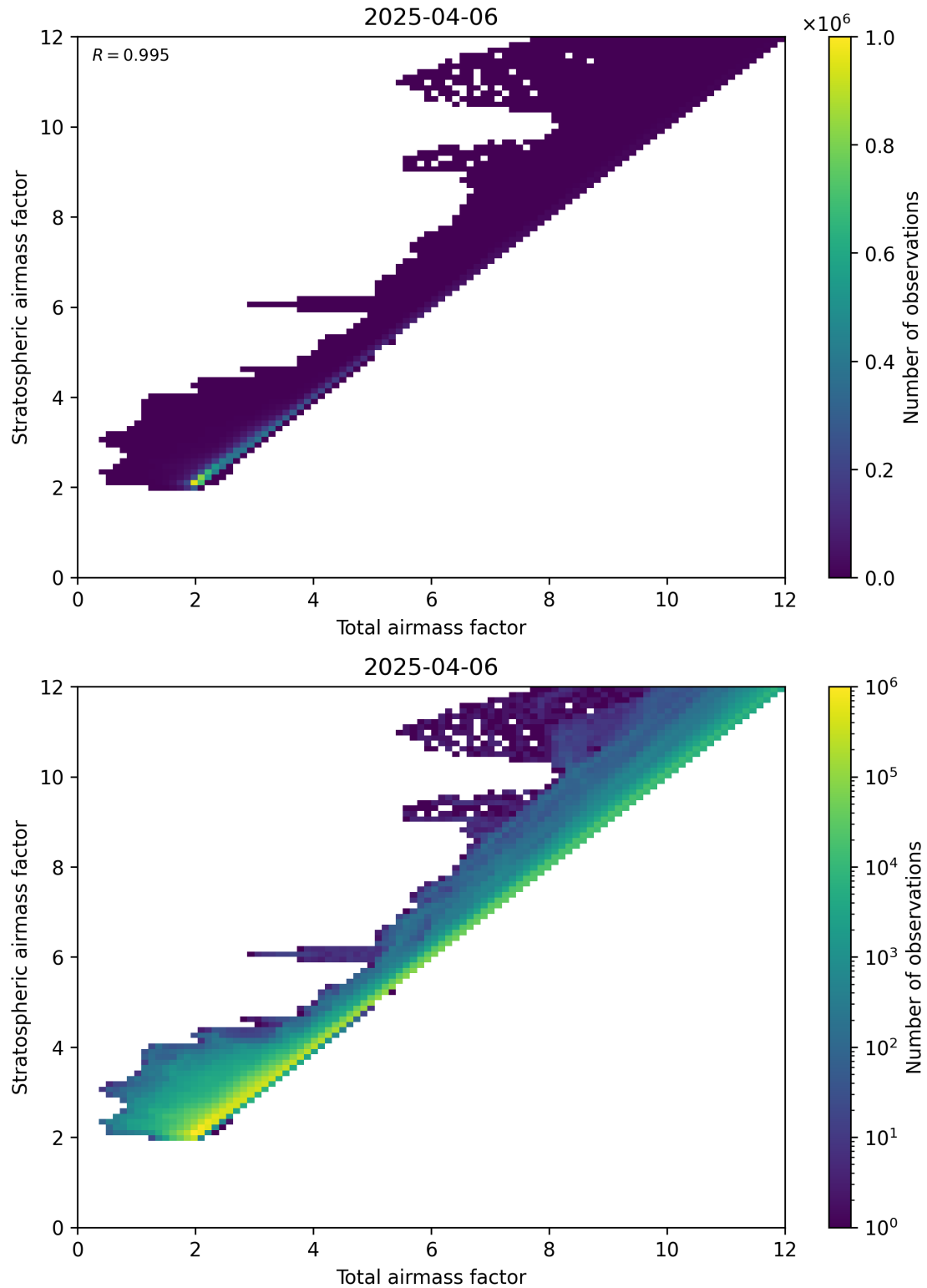
Figure 62: Scatter density plot of “Total airmass factor” against “Stratospheric airmass factor” for 2025-04-06 to 2025-04-06.
