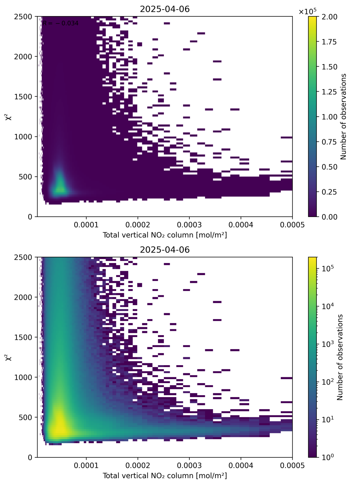
Figure 111: Scatter density plot of “Total vertical NO 2 column” against “ \chi^2 ” for 2025-04-06 to 2025-04-06.
