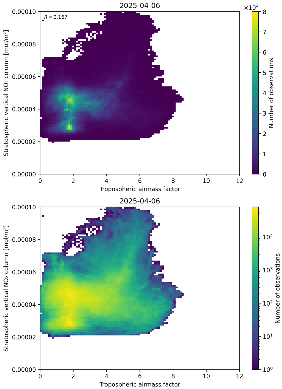
Figure 74: Scatter density plot of “Tropospheric air mass factor” against “Stratospheric vertical NO 2 column” for 2025-04-06 to 2025-04-06.
