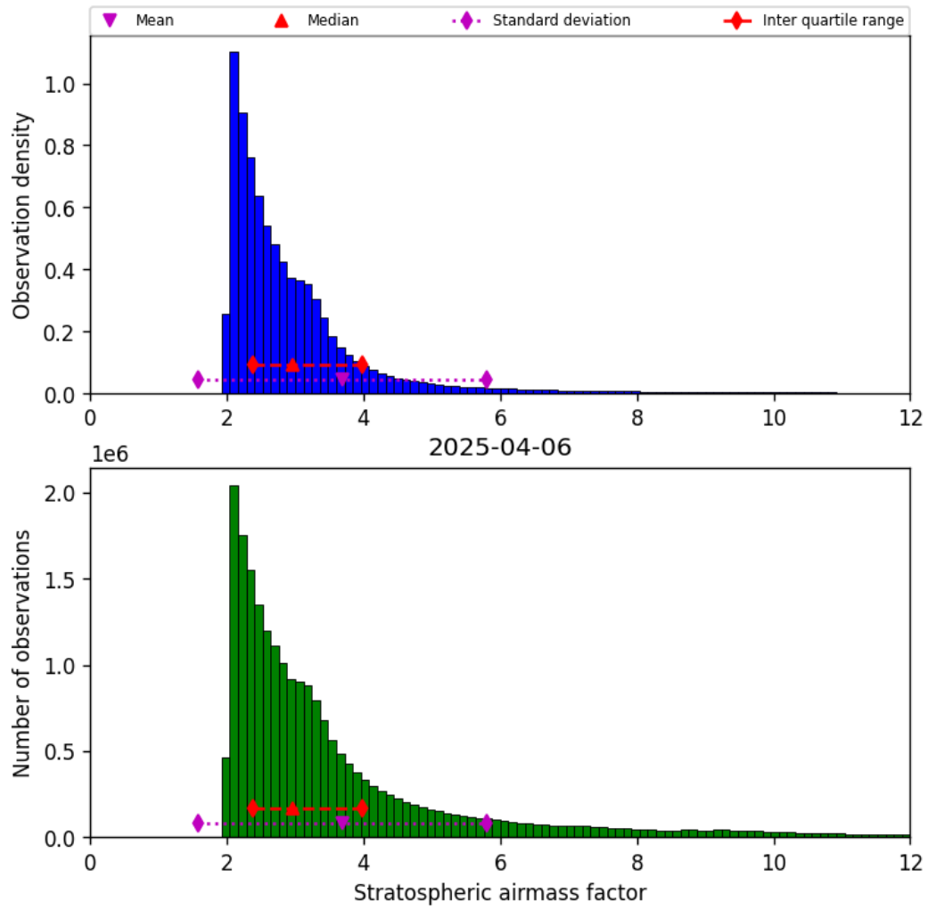
Figure 44: Histogram of “Stratospheric airmass factor” for 2025-04-06 to 2025-04-06
