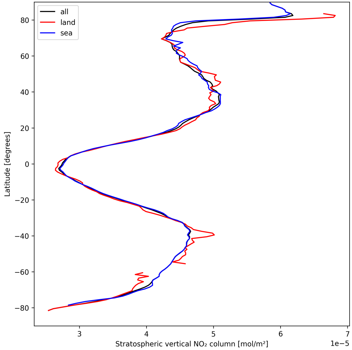
Figure 19: Zonal average of “Stratospheric vertical NO 2 column” for 2025-04-06 to 2025-04-06.
