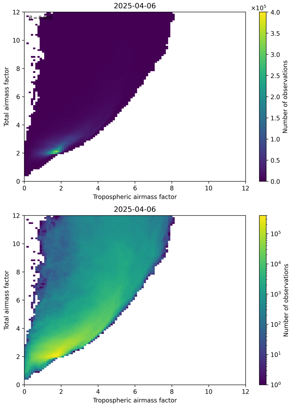
Figure 72: Scatter density plot of “Tropospheric airmass factor” against “Total airmass factor” for 2025-04-06 to 2025-04-06.
