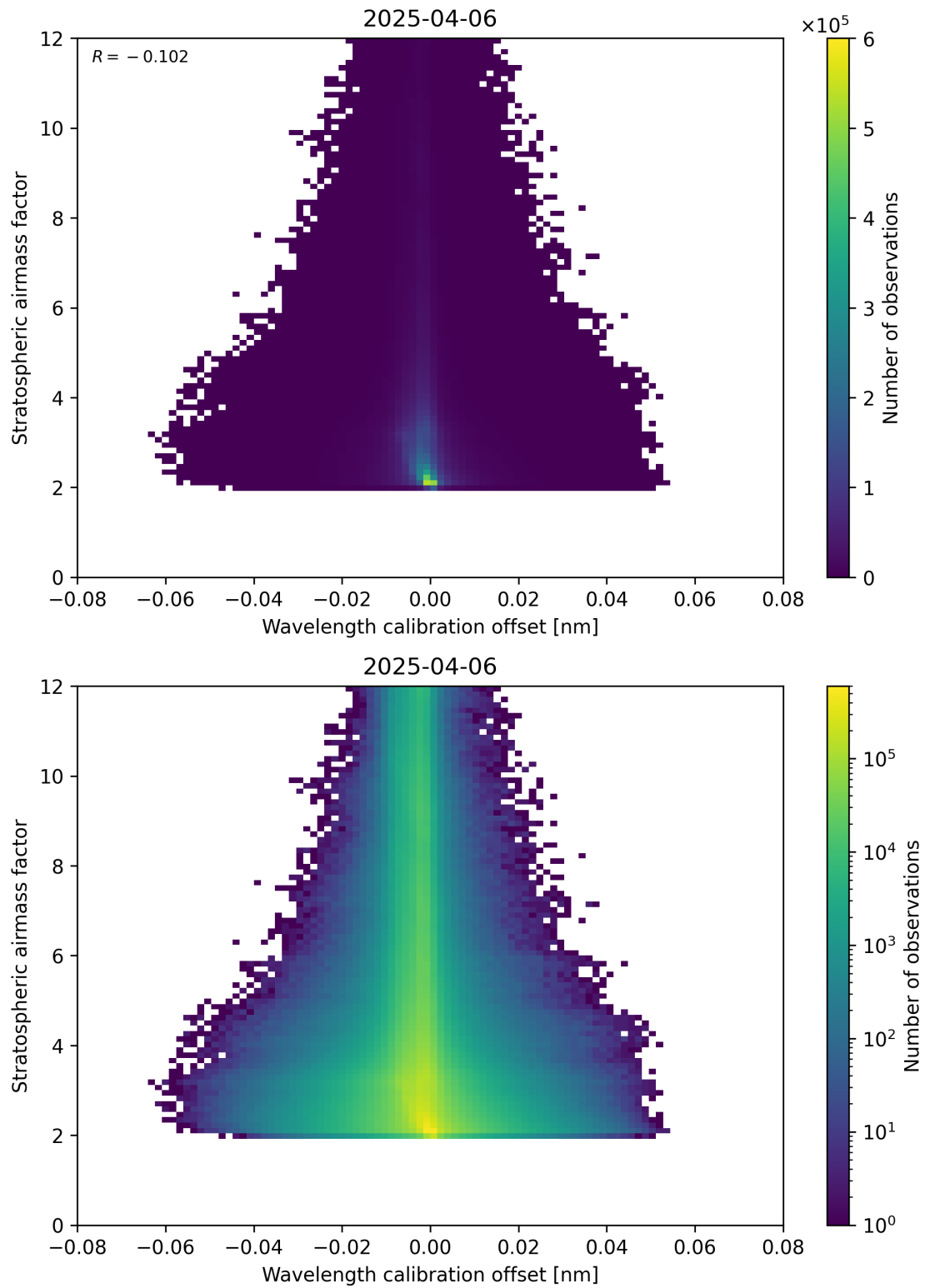
Figure 174: Scatter density plot of “Wavelength calibration offset” against “Stratospheric airmass factor” for 2025-04-06 to 2025-04-06.
