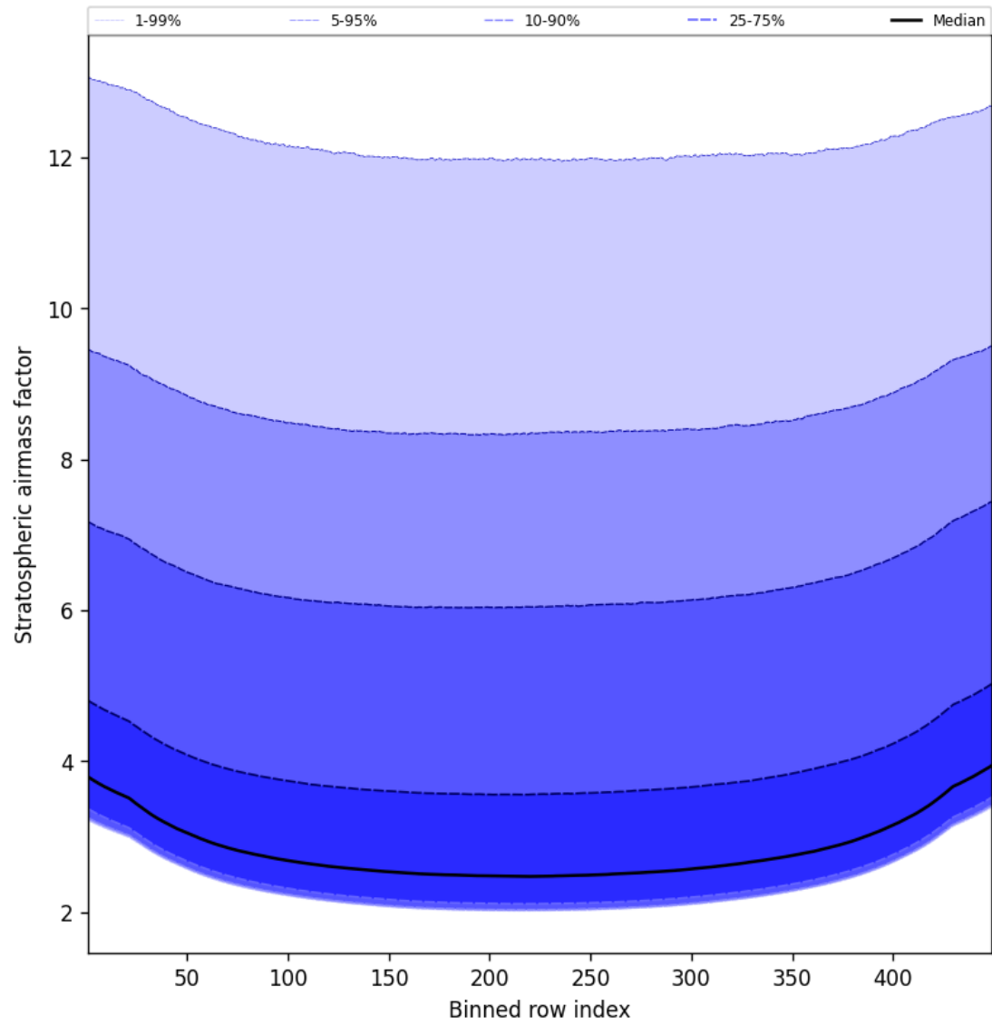
Figure 61: Along track statistics of “Stratospheric airmass factor” for 2025-04-06 to 2025-04-06
