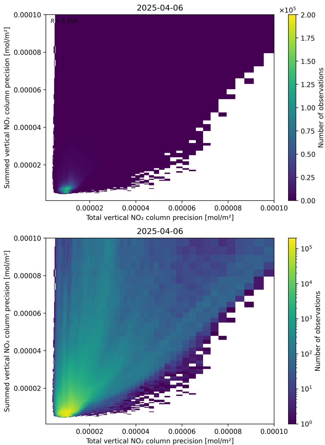
Figure 118: Scatter density plot of “Total vertical NO 2 column precision” against “Summed vertical NO 2 column precision” for 2025-04-06 to 2025-04-06.
