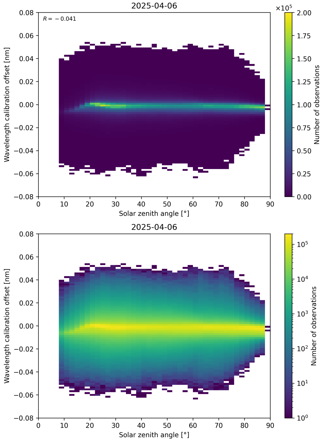
Figure 158: Scatter density plot of “Solar zenith angle” against “Wavelength calibration offset” for 2025-04-06 to 2025-04-06.
