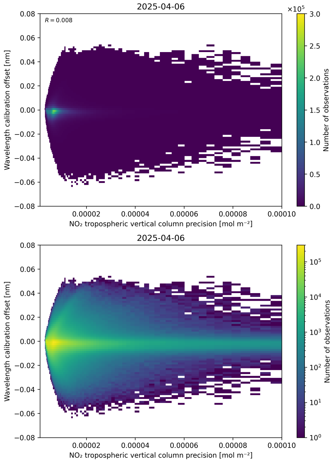
Figure 141: Scatter density plot of “NO 2 tropospheric vertical column precision” against “Wavelength calibration offset” for 2025-04-06 to 2025-04-06.
