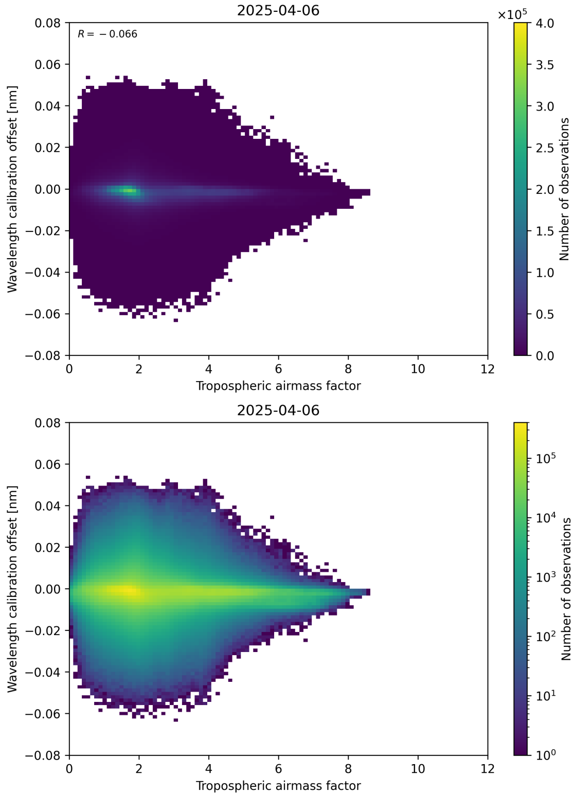
Figure 80: Scatter density plot of “Tropospheric airmass factor” against “Wavelength calibration offset” for 2025-04-06 to 2025-04-06.
