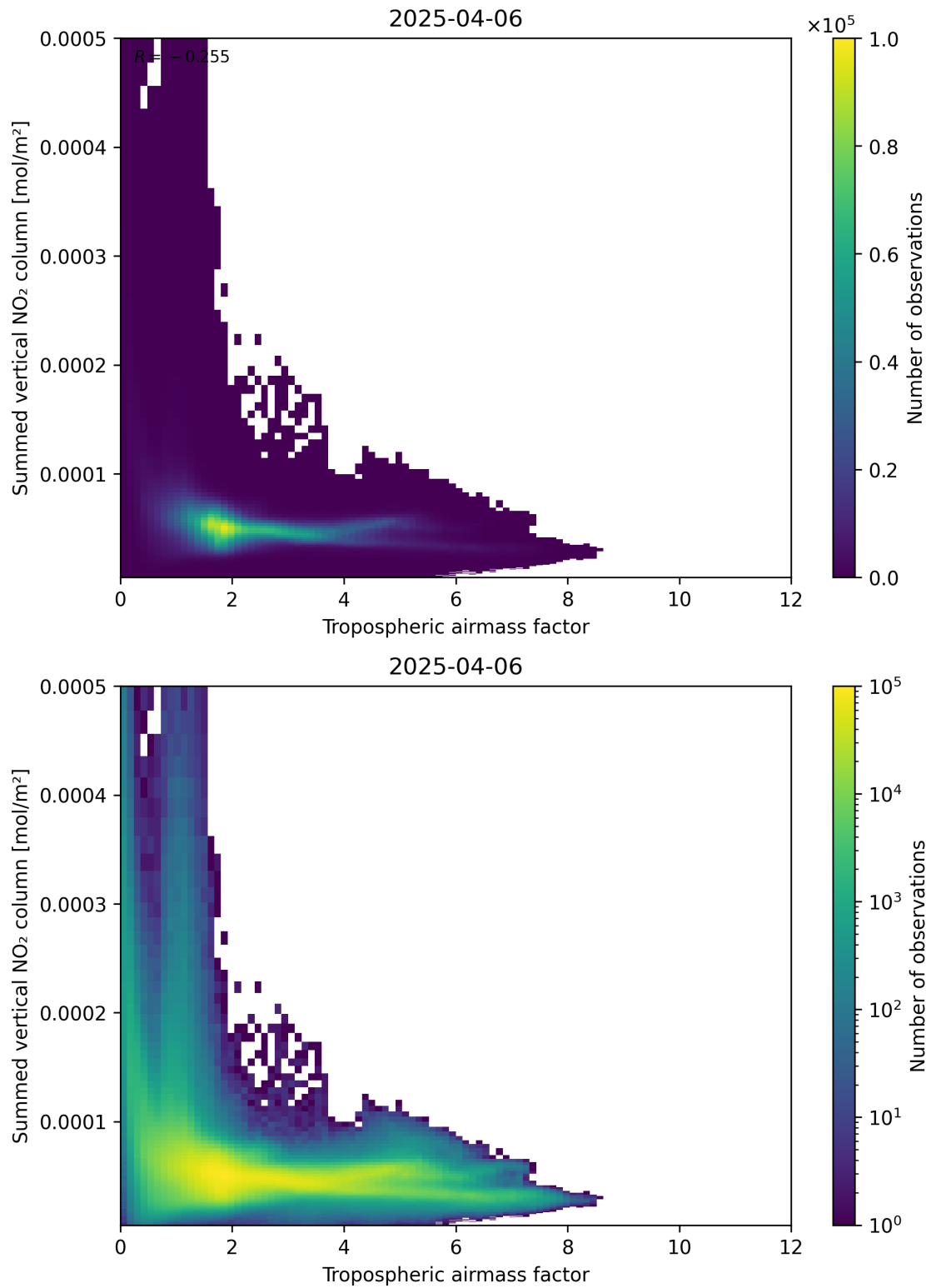
Figure 75: Scatter density plot of “Tropospheric airmass factor” against “Summed vertical NO 2 column” for 2025-04-06 to 2025-04-06.
