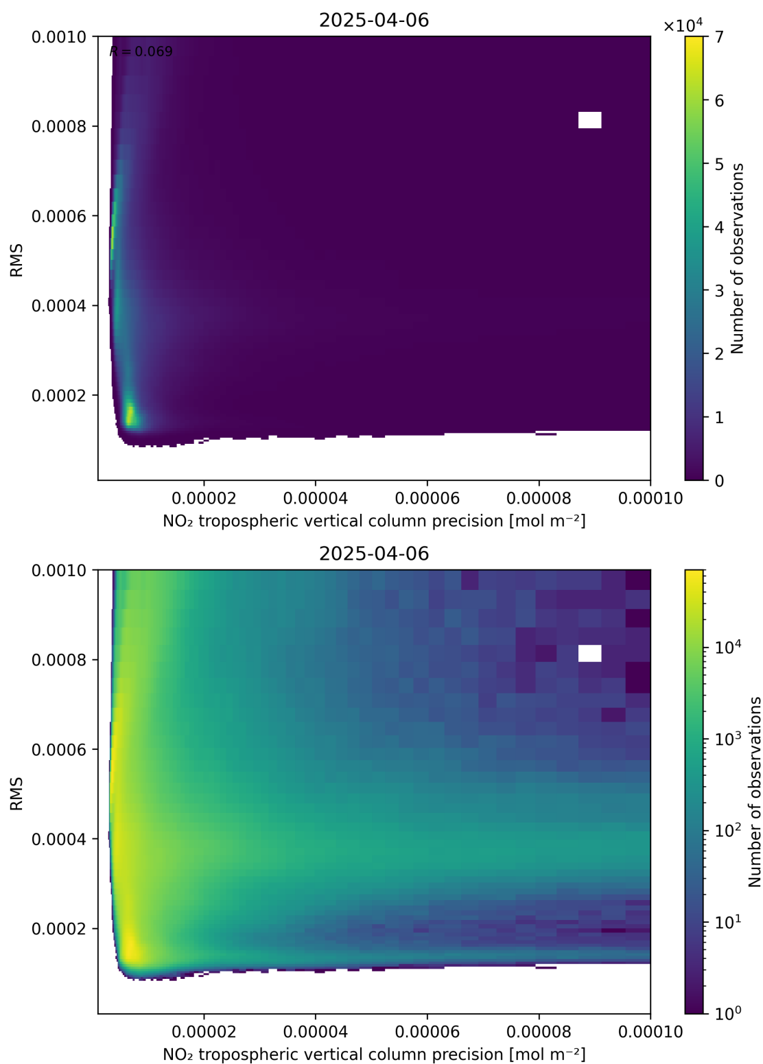
Figure 140: Scatter density plot of “NO 2 tropospheric vertical column precision” against “RMS” for 2025-04-06 to 2025-04-06.
