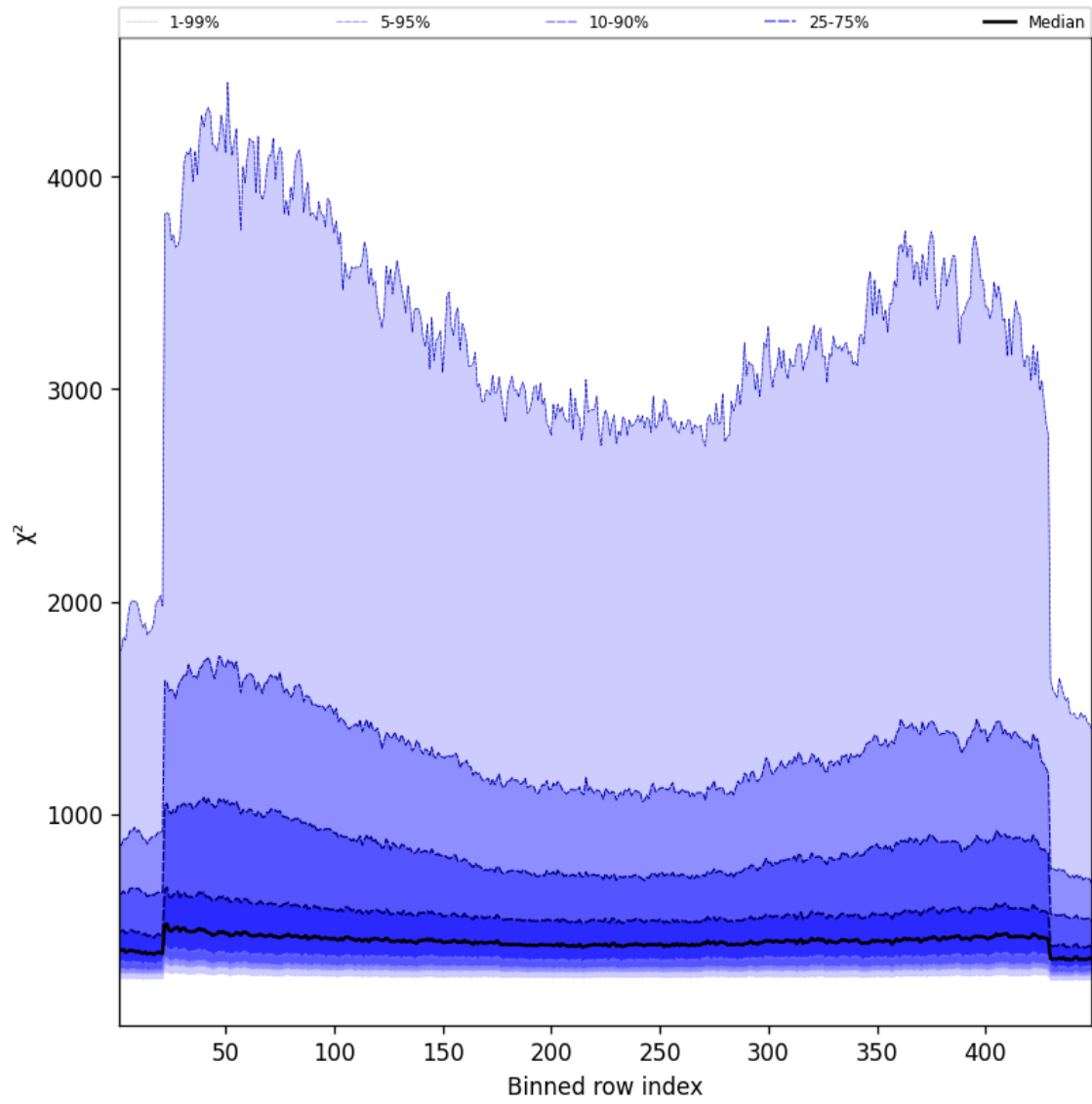
Figure 59: Along track statistics of “ \chi^2 ” for 2025-04-06 to 2025-04-06
