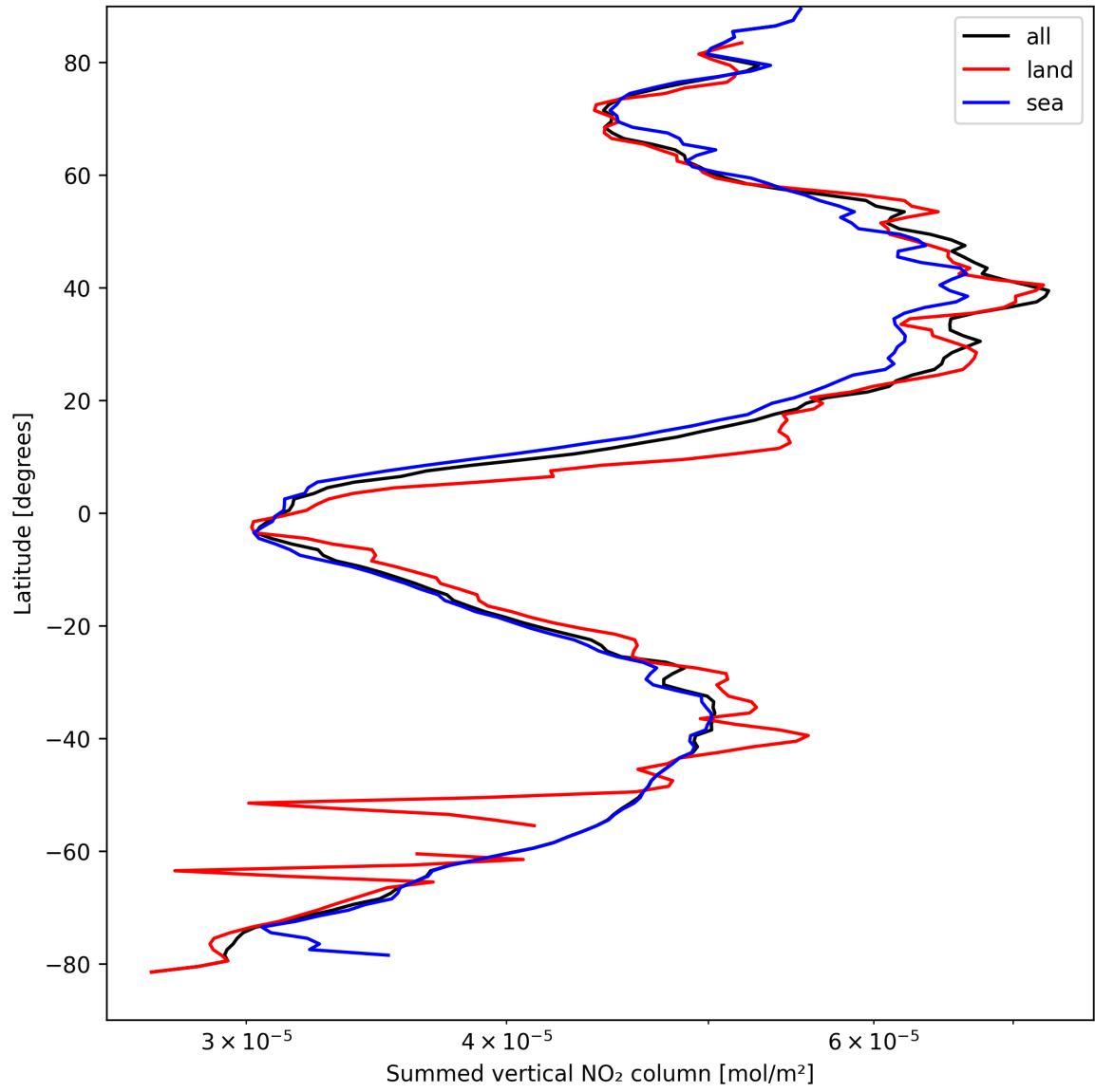
Figure 23: Zonal average of “Summed vertical NO 2 column” for 2025-04-06 to 2025-04-06.
