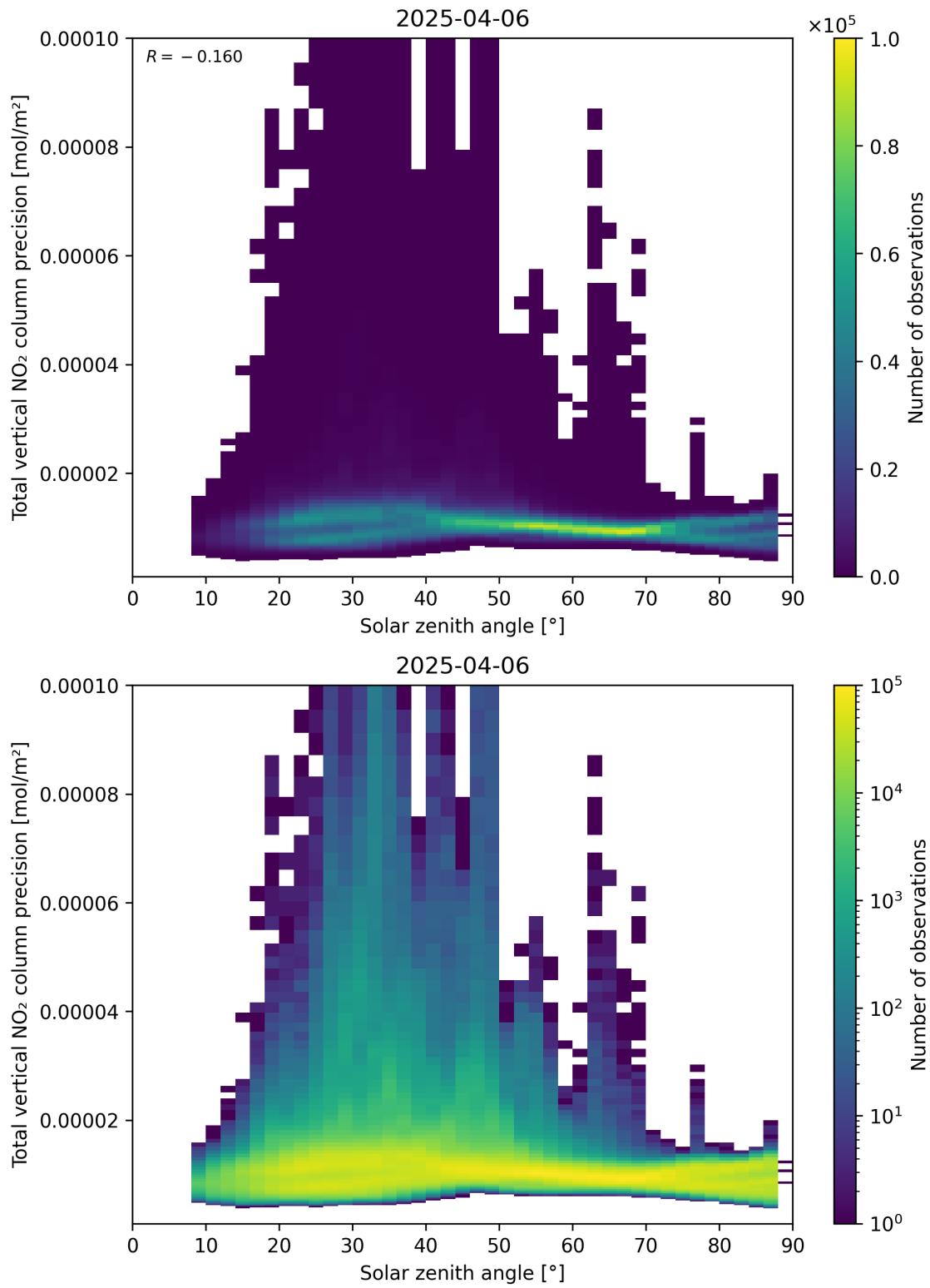
Figure 154: Scatter density plot of “Solar zenith angle” against “Total vertical NO 2 column precision” for 2025-04-06 to 2025-04-06.
