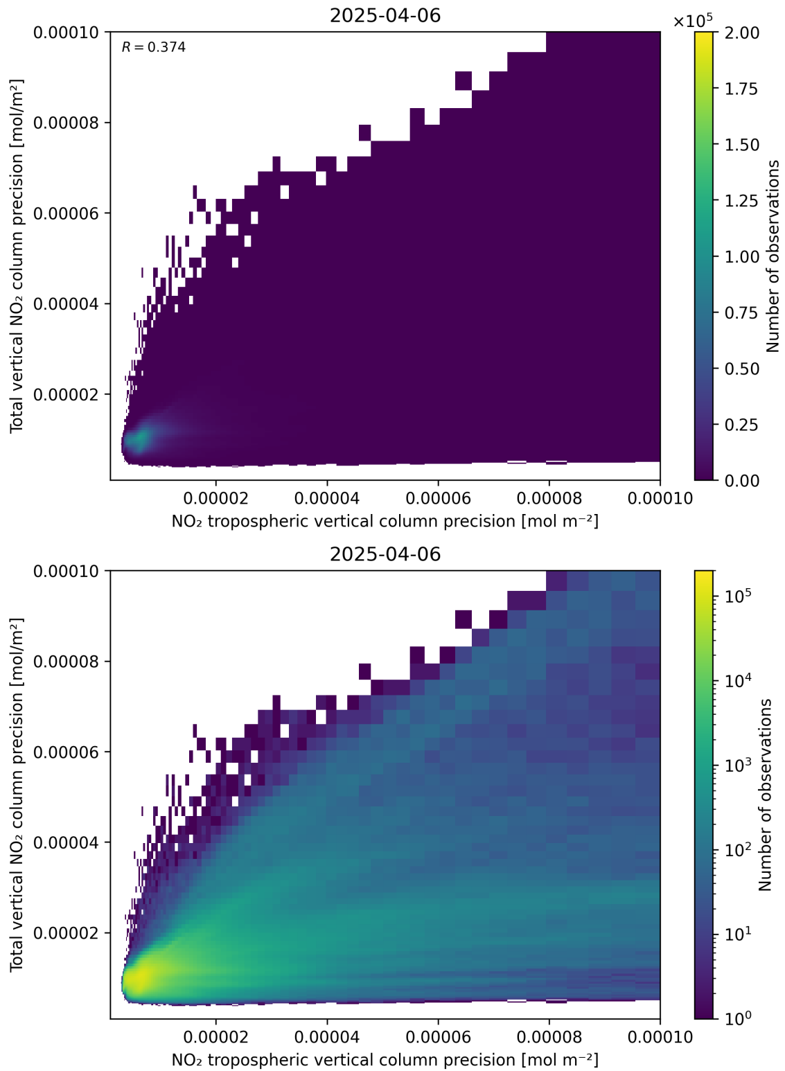
Figure 139: Scatter density plot of “NO 2 tropospheric vertical column precision” against “Total vertical NO 2 column precision” for 2025-04-06 to 2025-04-06.
