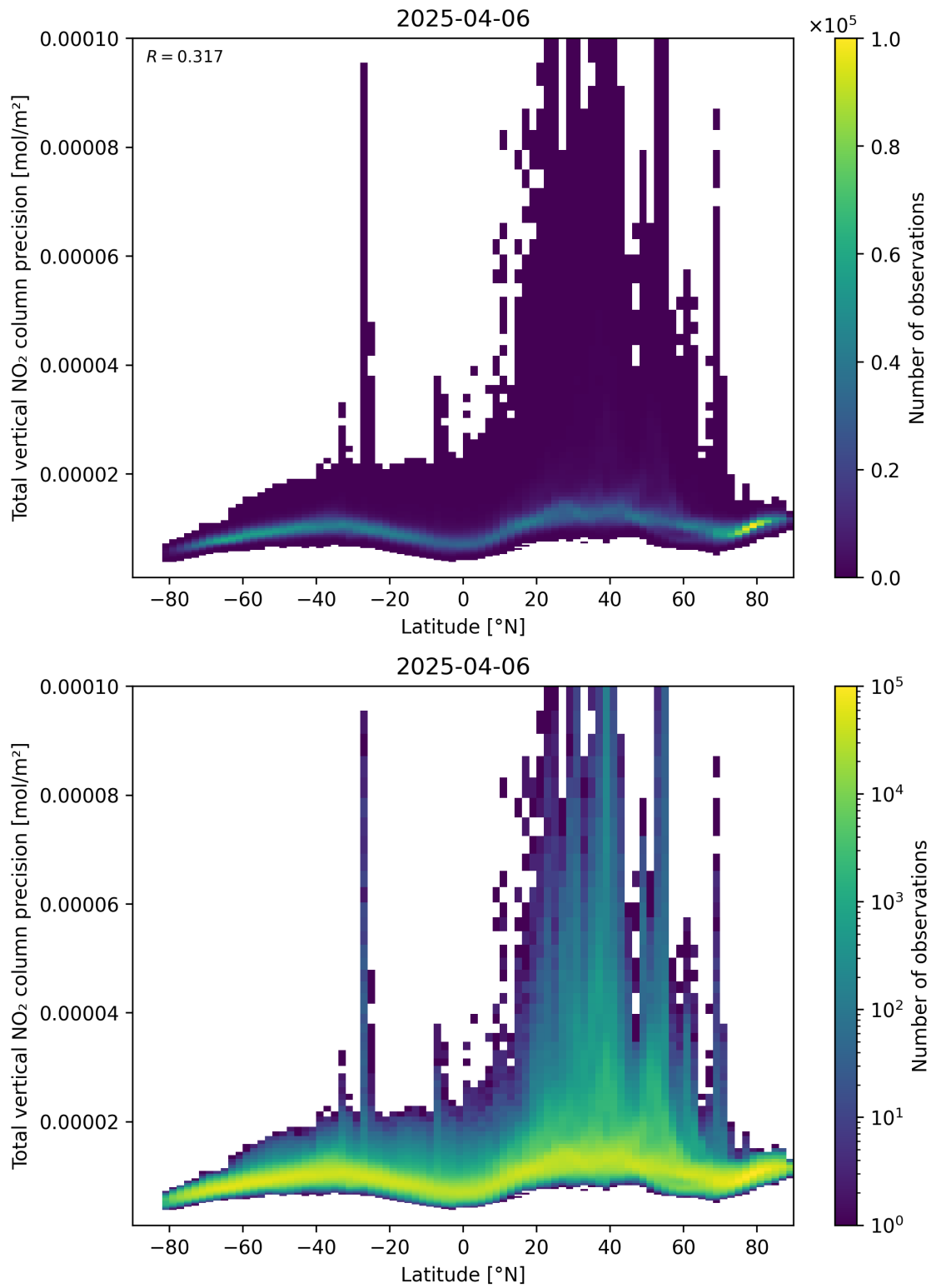
Figure 91: Scatter density plot of “Latitude” against “Total vertical NO 2 column precision” for 2025-04-06 to 2025-04-06.
