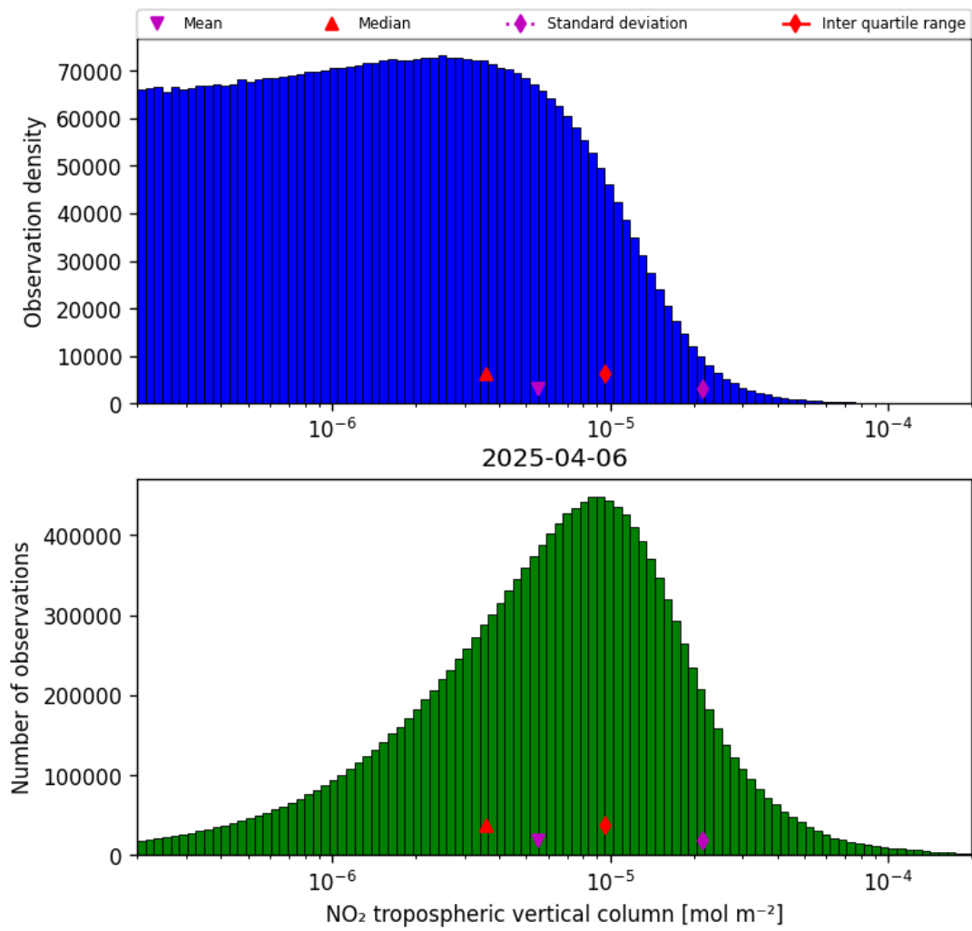
Figure 29: Histogram of “NO 2 tropospheric vertical column” for 2025-04-06 to 2025-04-06
