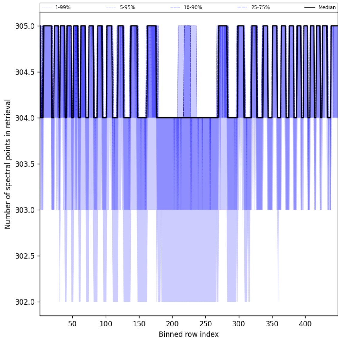
Figure 50: Along track statistics of “Number of spectral points in retrieval” for 2025-04-06 to 2025-04-06
