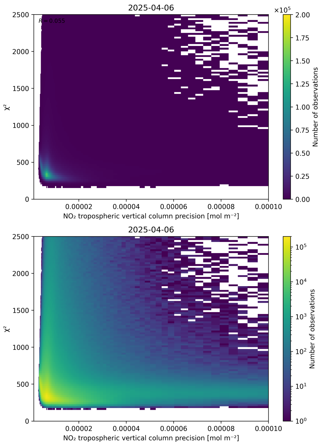
Figure 134: Scatter density plot of “NO 2 tropospheric vertical column precision” against “ \chi^2 ” for 2025-04-06 to 2025-04-06.
