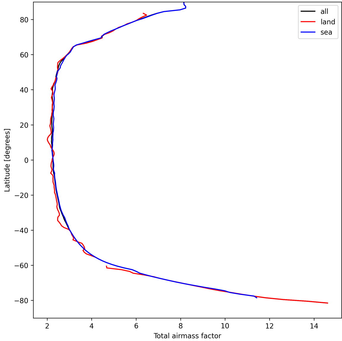
Figure 15: Zonal average of “Total airmass factor” for 2025-04-06 to 2025-04-06.
