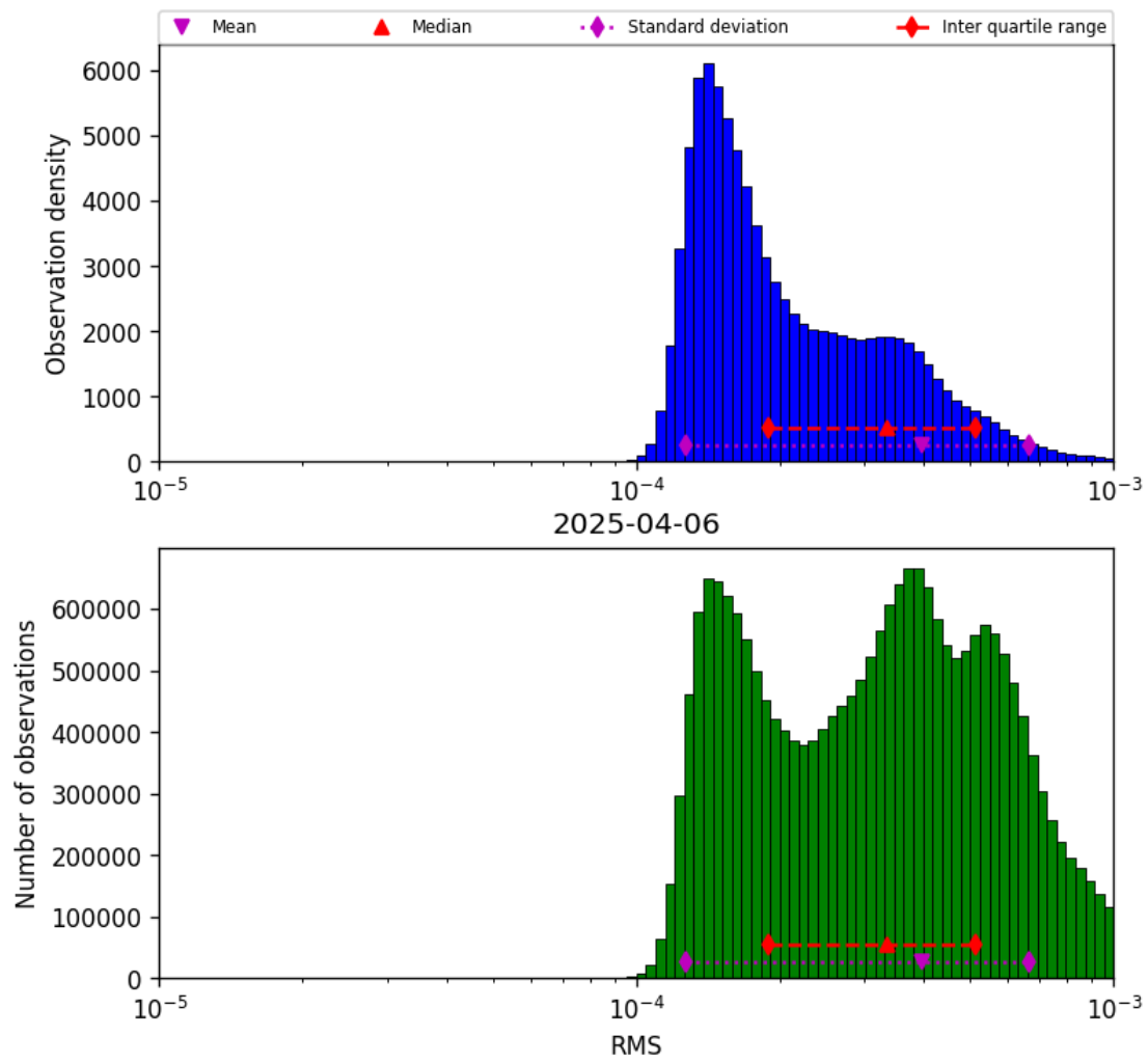
Figure 43: Histogram of “RMS” for 2025-04-06 to 2025-04-06
