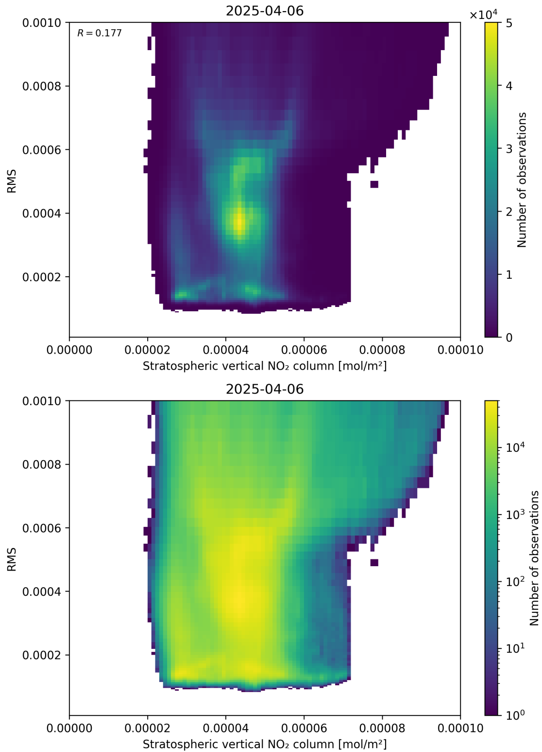
Figure 102: Scatter density plot of “Stratospheric vertical NO 2 column” against “RMS” for 2025-04-06 to 2025-04-06.
