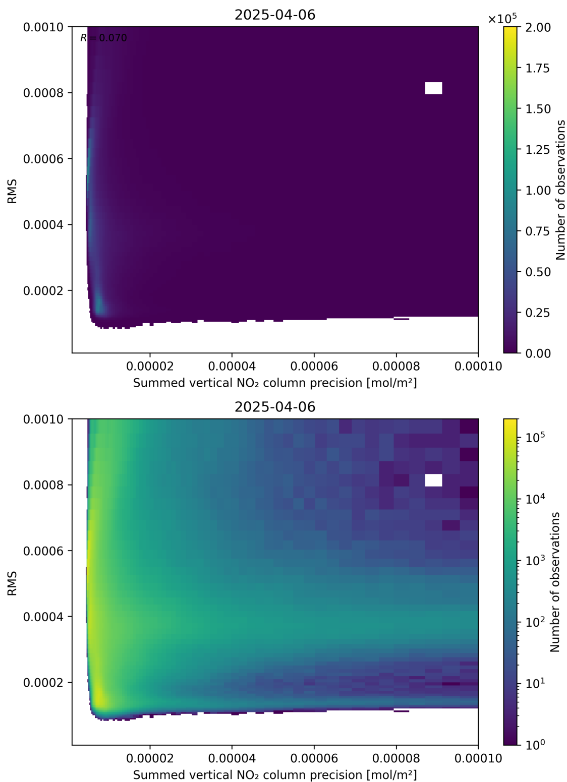
Figure 108: Scatter density plot of “Summed vertical NO 2 column precision” against “RMS” for 2025-04-06 to 2025-04-06.
