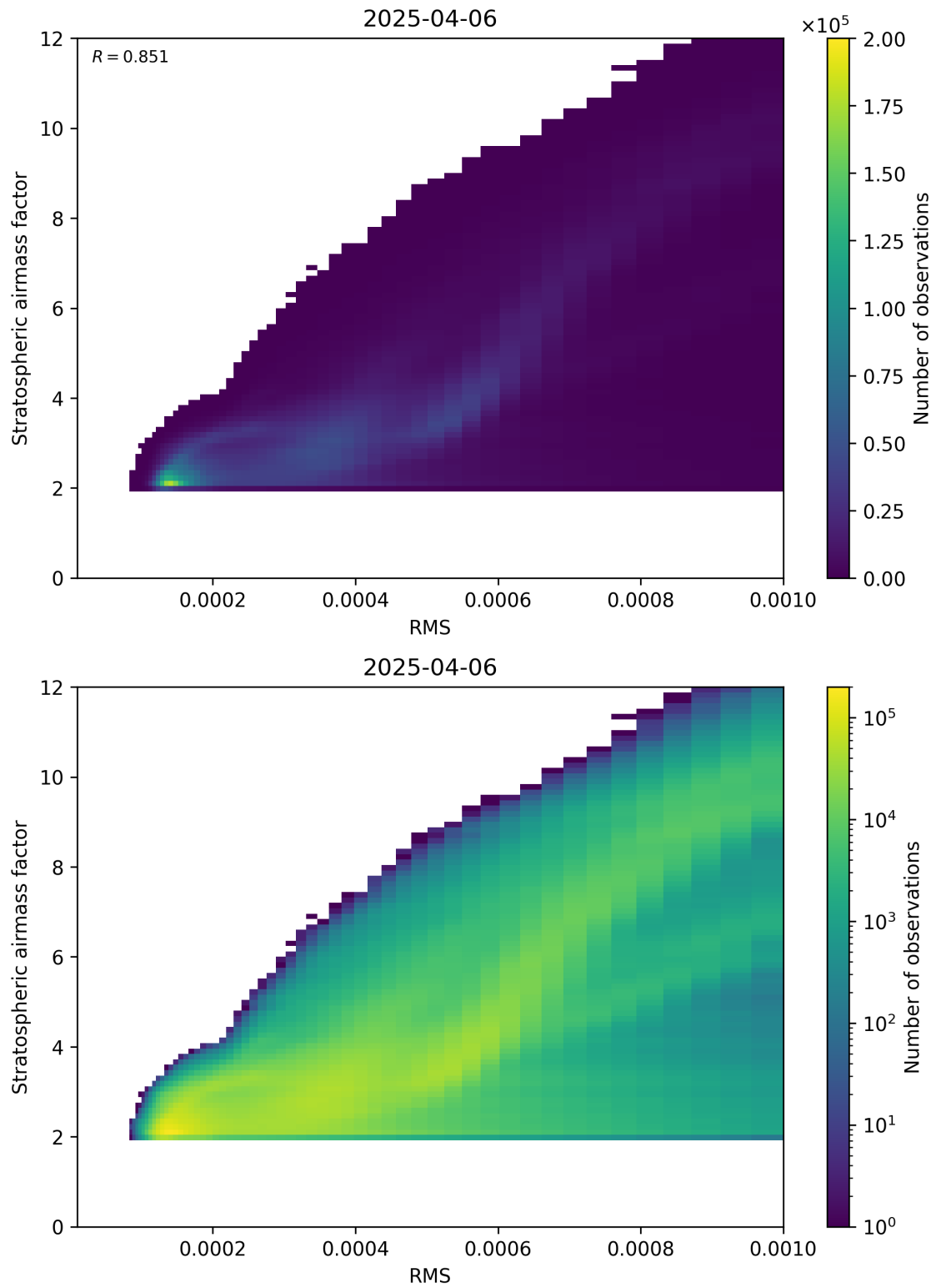
Figure 144: Scatter density plot of “RMS” against “Stratospheric airmass factor” for 2025-04-06 to 2025-04-06.
