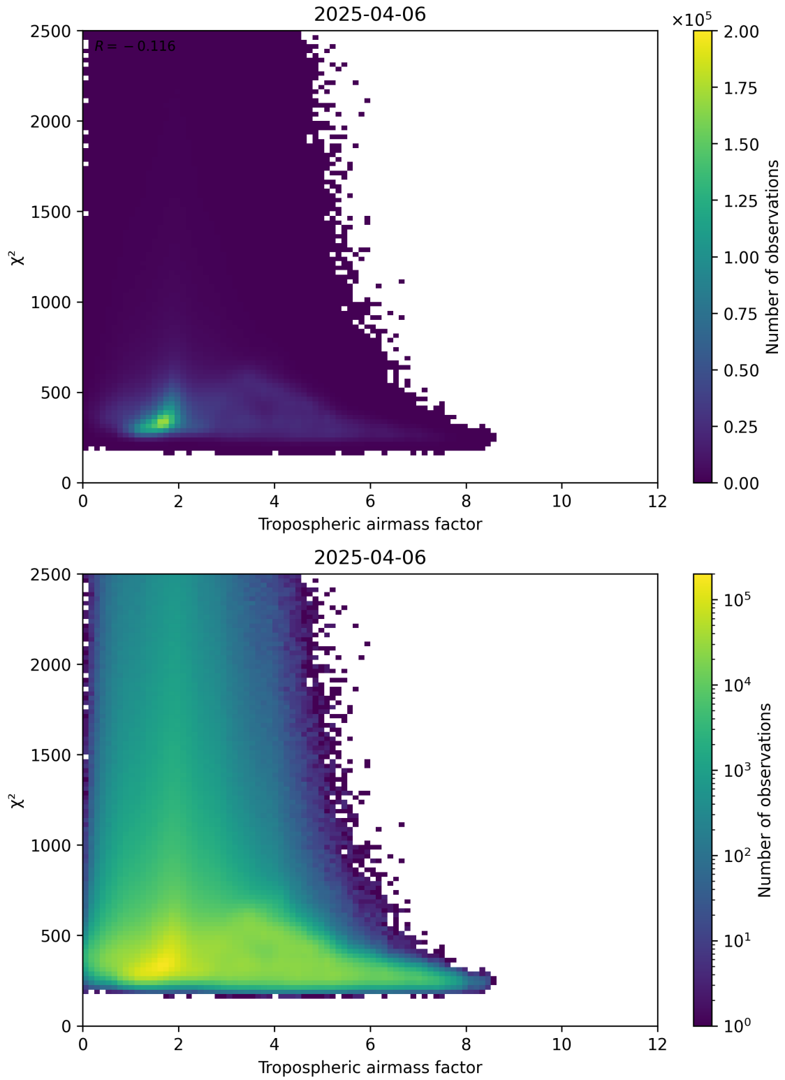
Figure 73: Scatter density plot of “Tropospheric airmass factor” against “ \chi^2 ” for 2025-04-06 to 2025-04-06.
