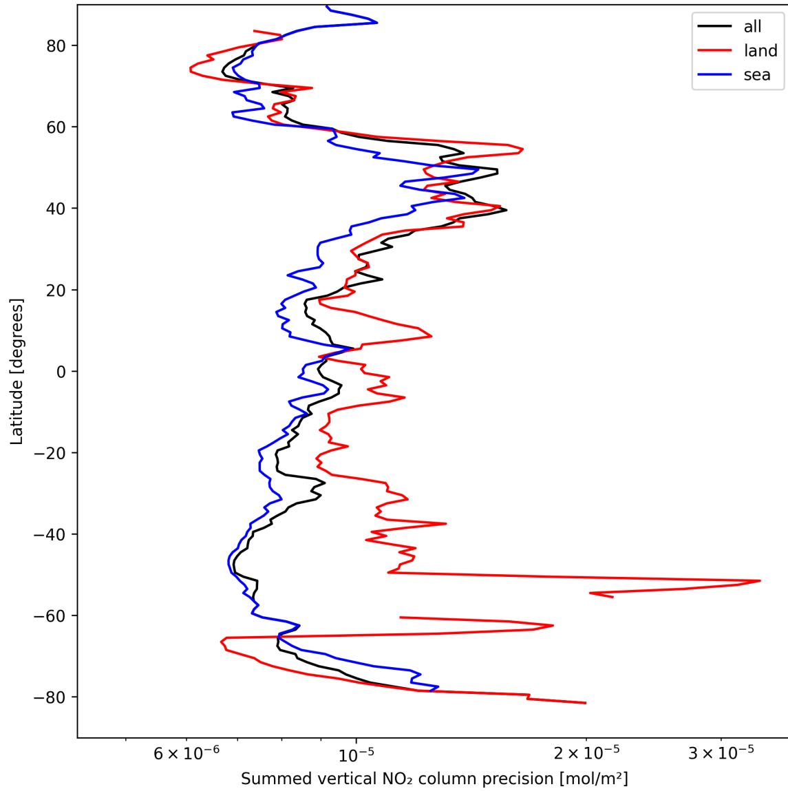
Figure 24: Zonal average of “Summed vertical NO 2 column precision” for 2025-04-06 to 2025-04-06.
