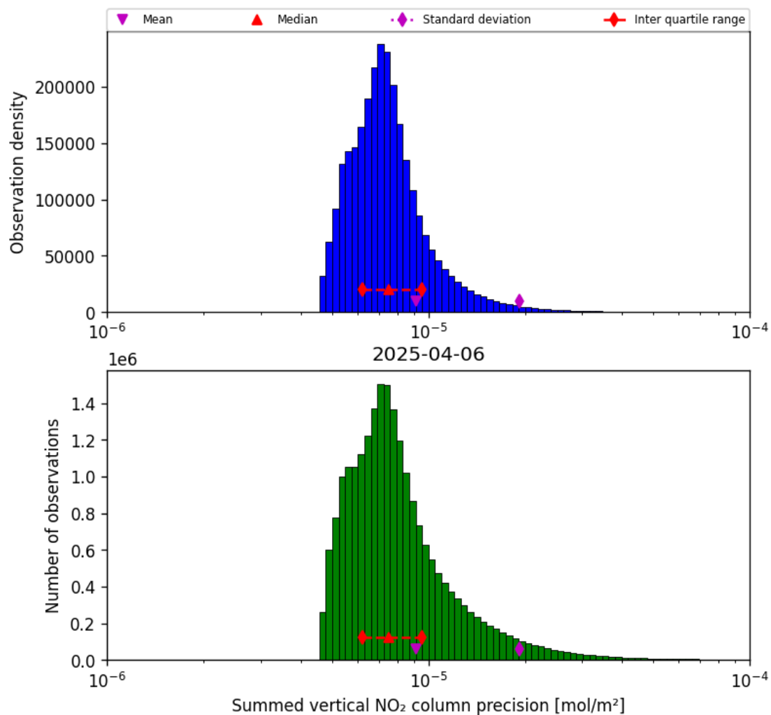
Figure 41: Histogram of "Summed vertical NO 2 column precision" for 2025-04-06 to 2025-04-06
