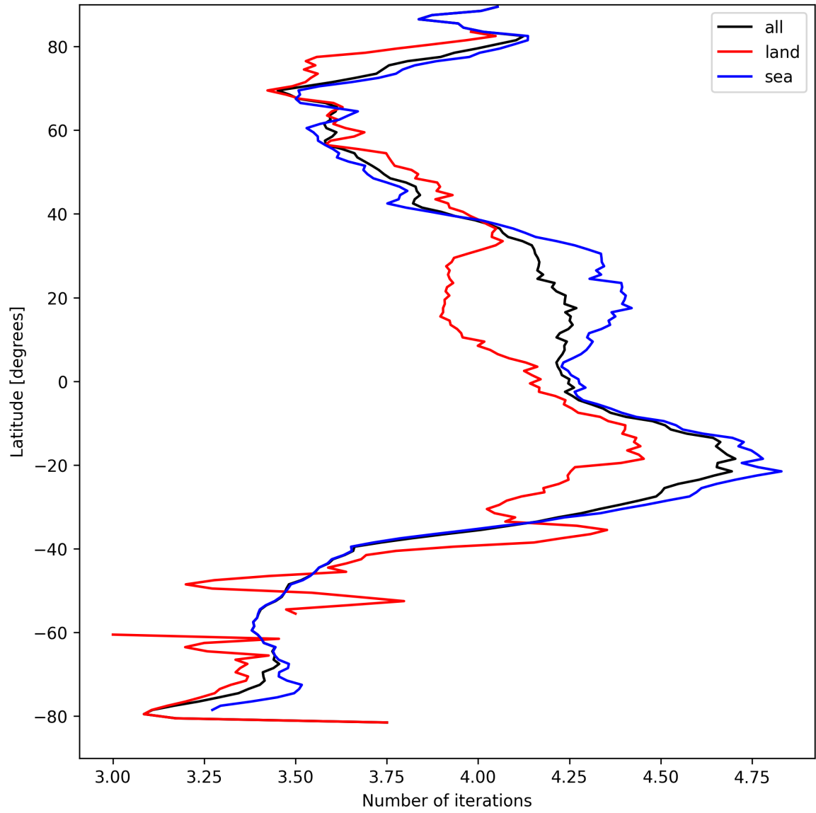
Figure 17: Zonal average of “Number of iterations” for 2025-04-06 to 2025-04-06.
