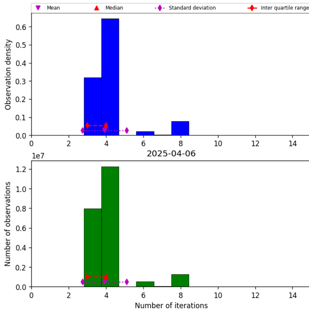
Figure 34: Histogram of “Number of iterations” for 2025-04-06 to 2025-04-06
