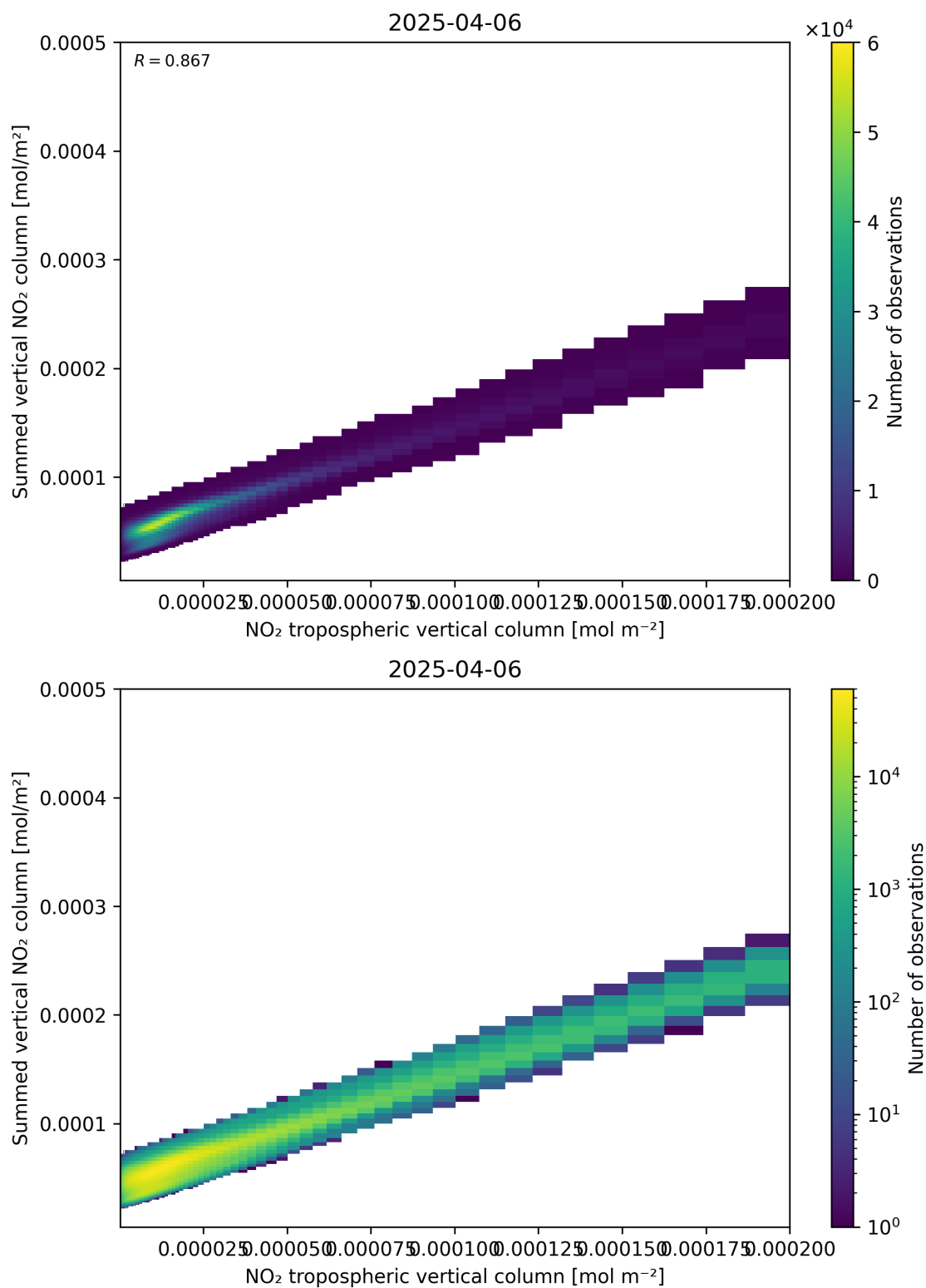
Figure 126: Scatter density plot of “NO 2 tropospheric vertical column” against “Summed vertical NO 2 column” for 2025-04-06 to 2025-04-06.
