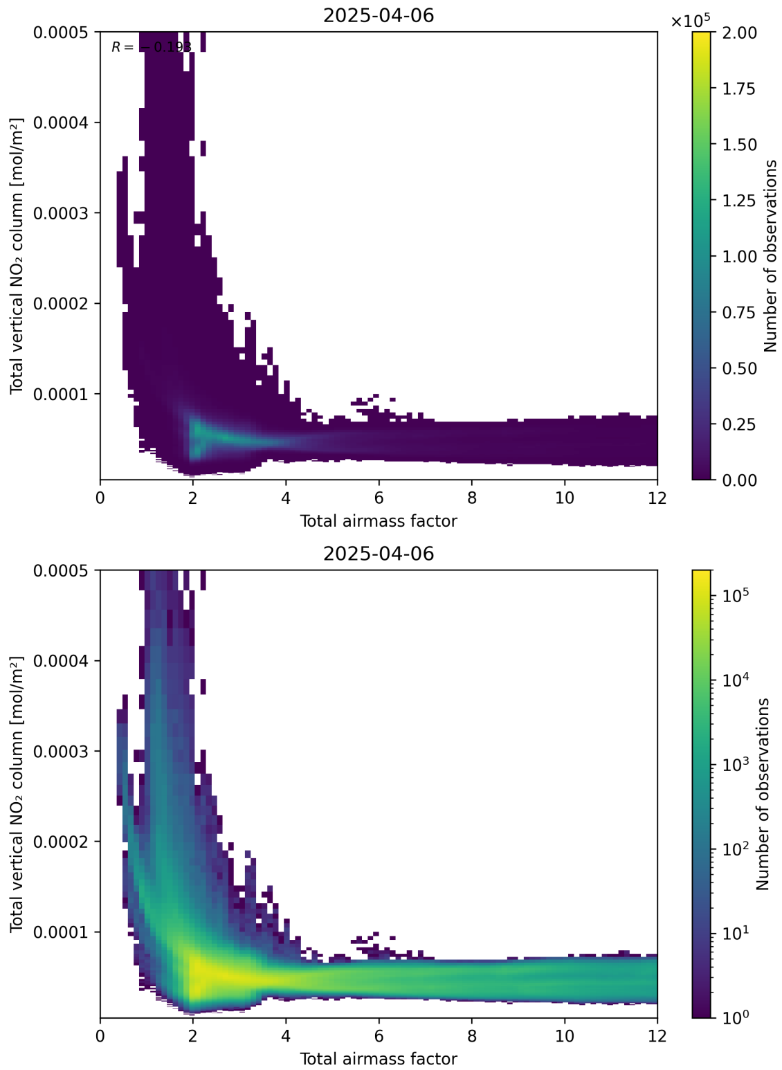
Figure 67: Scatter density plot of “Total airmass factor” against “Total vertical NO 2 column” for 2025-04-06 to 2025-04-06.
