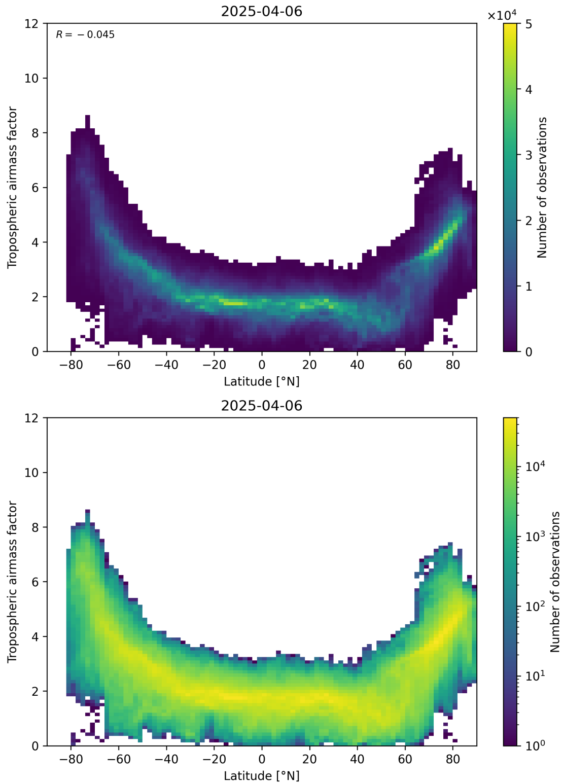
Figure 85: Scatter density plot of “Latitude” against “Tropospheric airmass factor” for 2025-04-06 to 2025-04-06.
