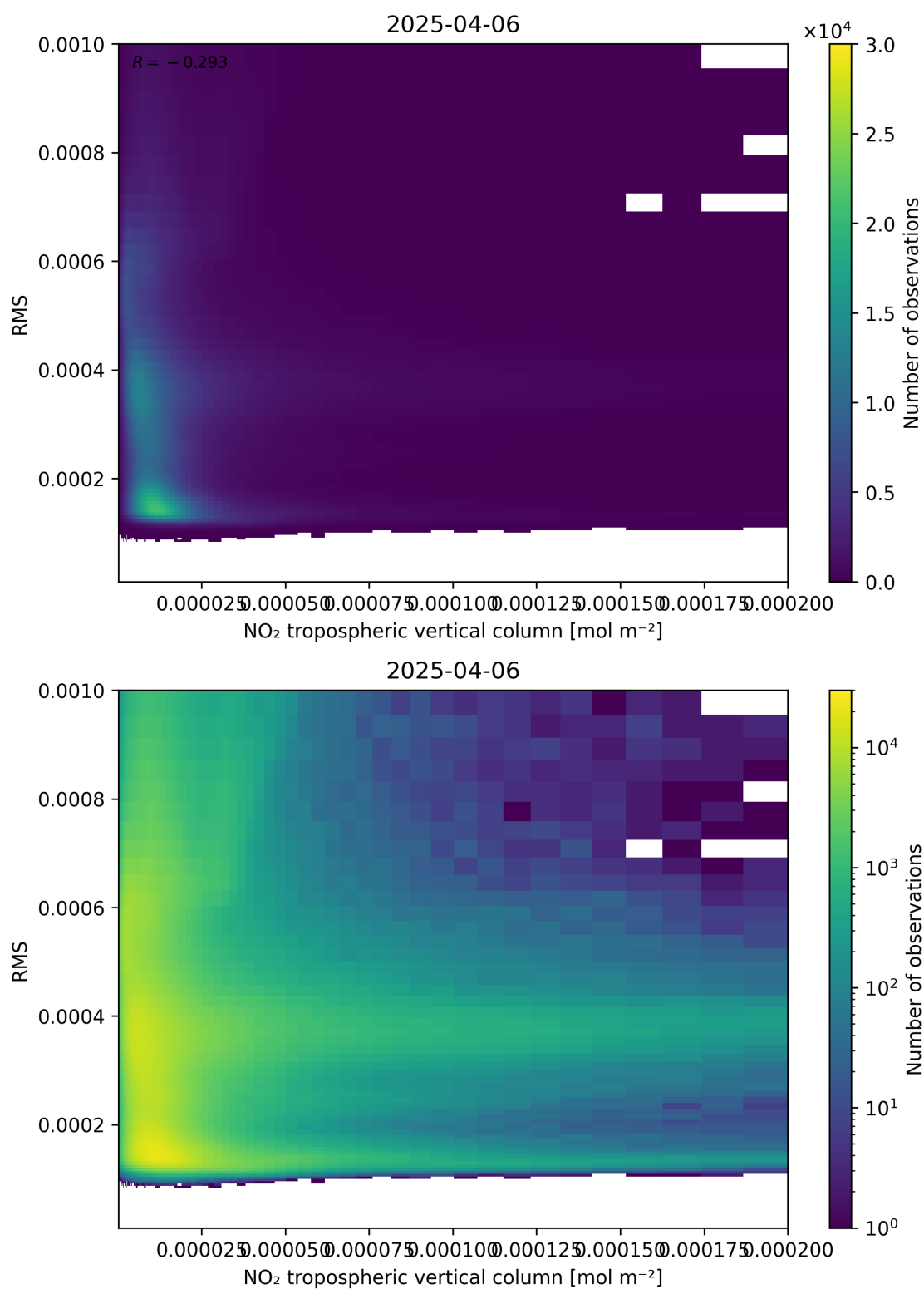
Figure 142: Scatter density plot of “NO 2 tropospheric vertical column” against “RMS” for 2025-04-06 to 2025-04-06.
