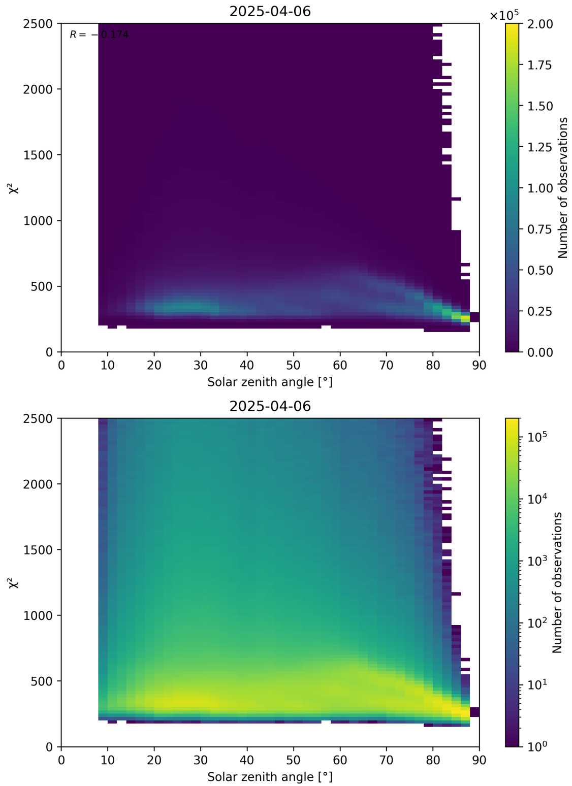
Figure 148: Scatter density plot of “Solar zenith angle” against “ \chi^2 ” for 2025-04-06 to 2025-04-06.
