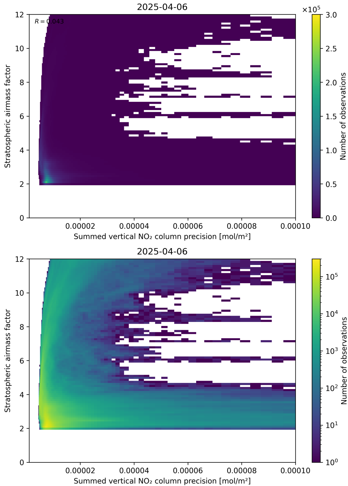
Figure 106: Scatter density plot of “Summed vertical NO 2 column precision” against “Stratospheric airmass factor” for 2025-04-06 to 2025-04-06.
