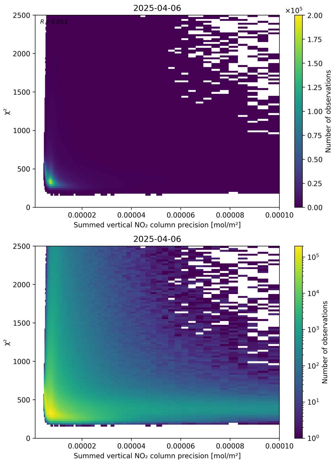
Figure 107: Scatter density plot of “Summed vertical NO 2 column precision” against “ \chi^2 ” for 2025-04-06 to 2025-04-06.
