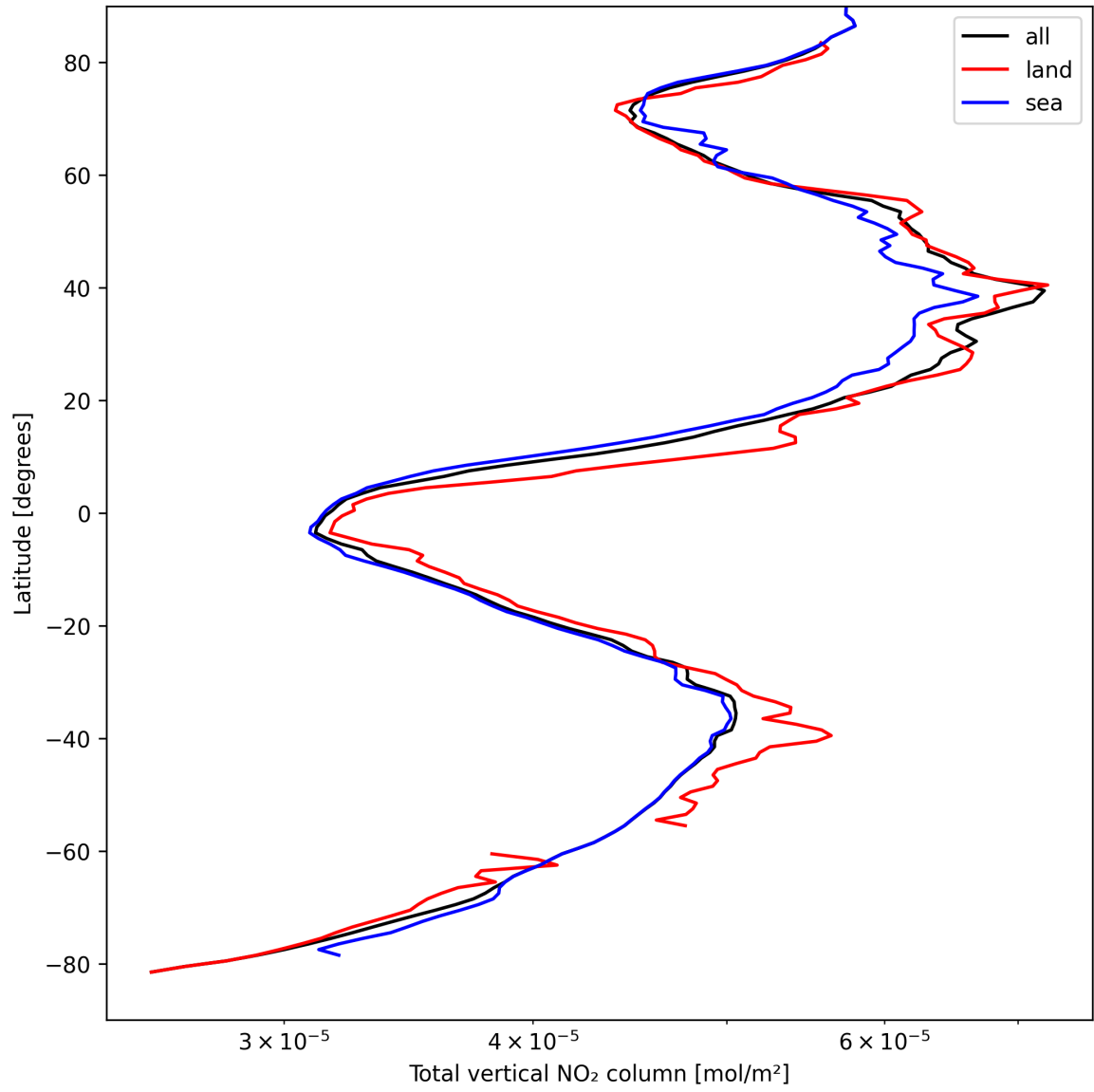
Figure 21: Zonal average of “Total vertical NO 2 column” for 2025-04-06 to 2025-04-06.
