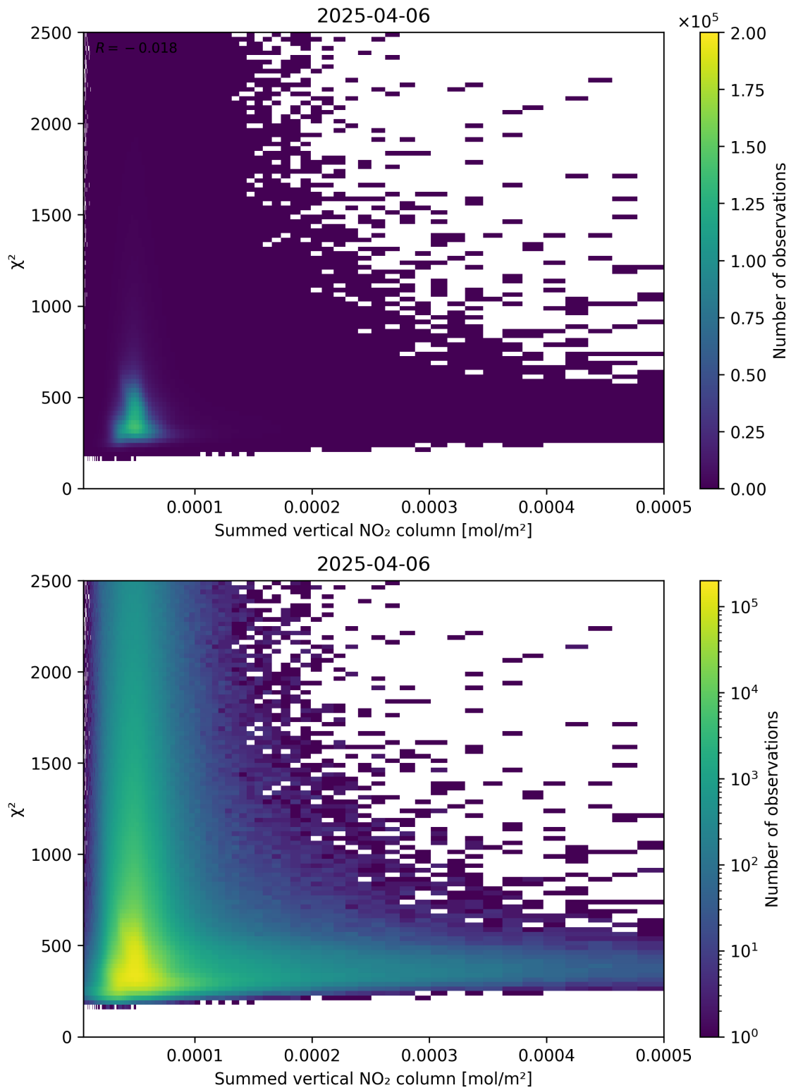
Figure 104: Scatter density plot of “Summed vertical NO 2 column” against “ \chi^2 ” for 2025-04-06 to 2025-04-06.
