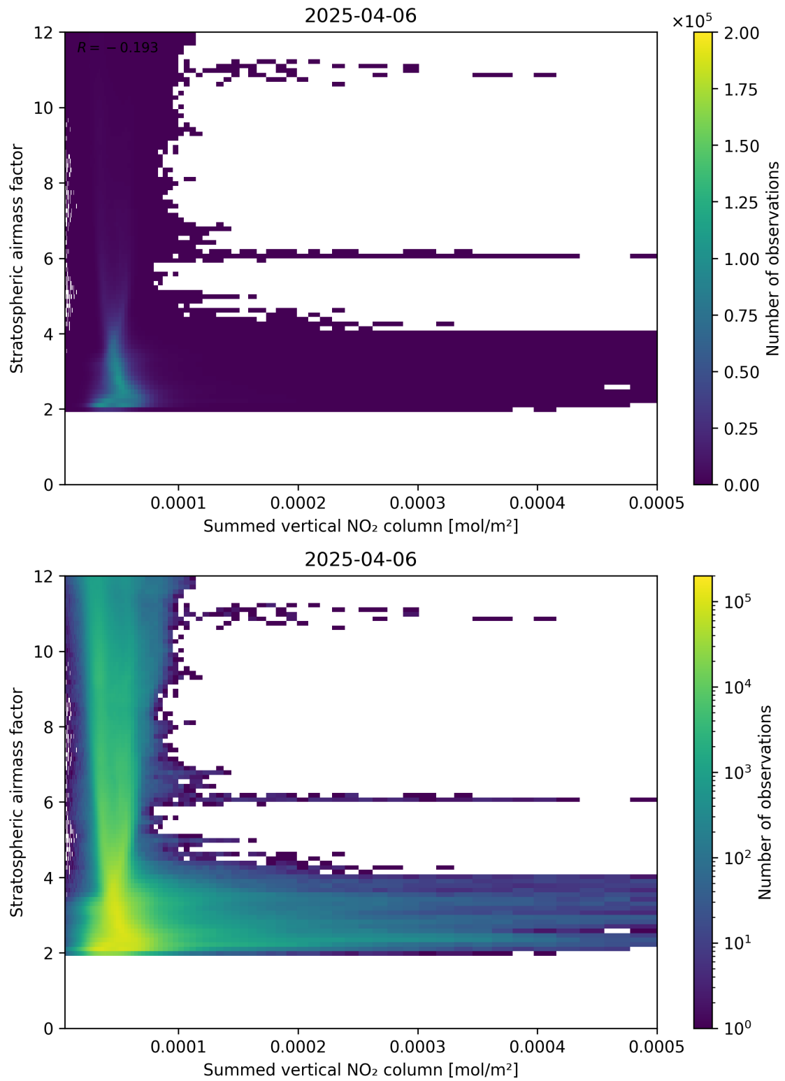
Figure 103: Scatter density plot of “Summed vertical NO 2 column” against “Stratospheric airmass factor” for 2025-04-06 to 2025-04-06.
