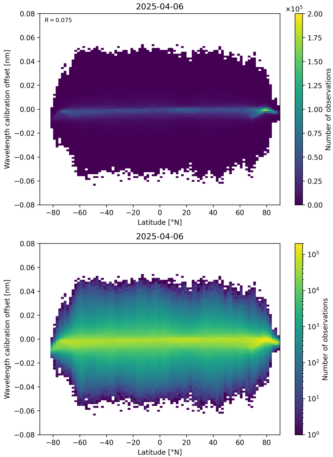
Figure 95: Scatter density plot of “Latitude” against “Wavelength calibration offset” for 2025-04-06 to 2025-04-06.
