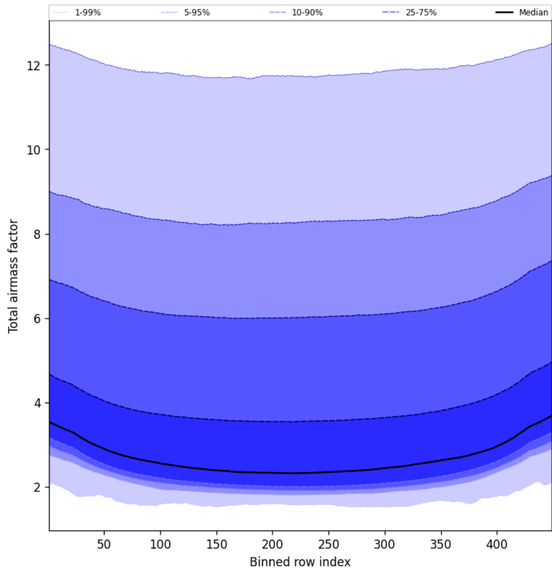
Figure 49: Along track statistics of “Total airmass factor” for 2025-04-06 to 2025-04-06
