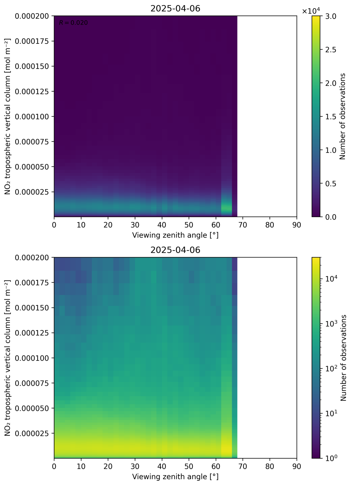
Figure 169: Scatter density plot of “Viewing zenith angle” against “NO 2 tropospheric vertical column” for 2025-04-06 to 2025-04-06.
