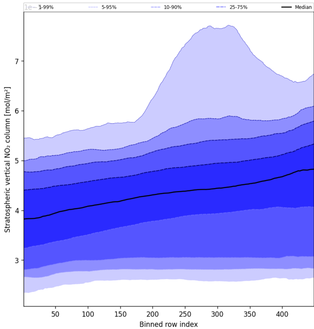
Figure 53: Along track statistics of “Stratospheric vertical NO 2 column” for 2025-04-06 to 2025-04-06
