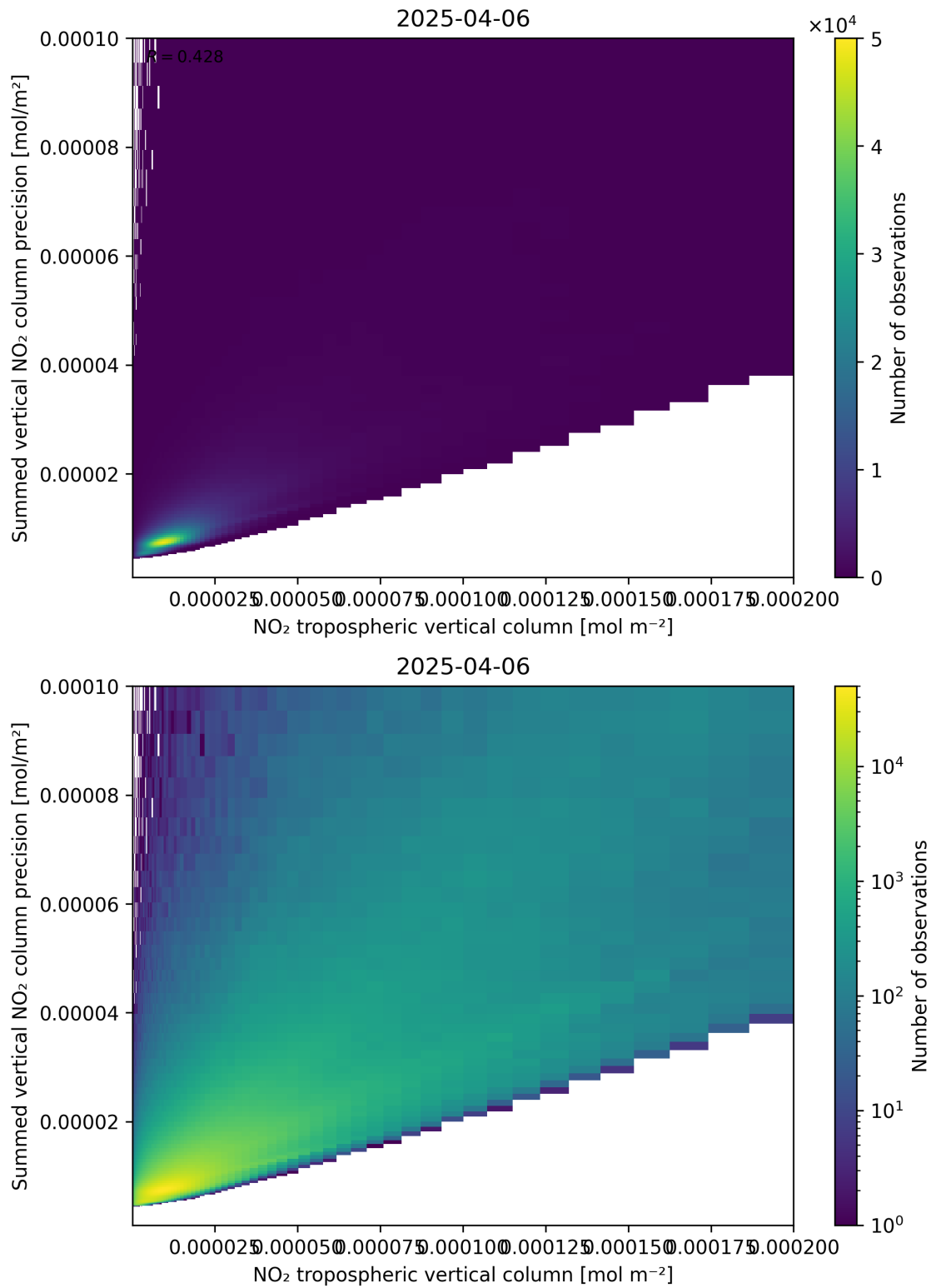
Figure 127: Scatter density plot of “NO 2 tropospheric vertical column” against “Summed vertical NO 2 column precision” for 2025-04-06 to 2025-04-06.
