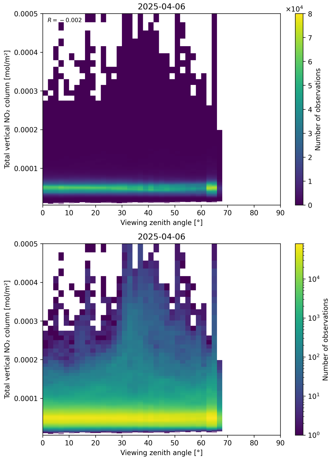
Figure 167: Scatter density plot of “Viewing zenith angle” against “Total vertical NO 2 column” for 2025-04-06 to 2025-04-06.
