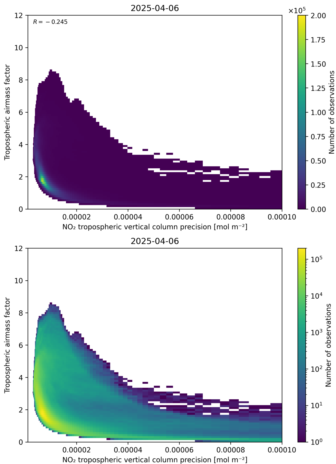
Figure 133: Scatter density plot of “NO 2 tropospheric vertical column precision” against “Tropospheric air mass factor” for 2025-04-06 to 2025-04-06.
