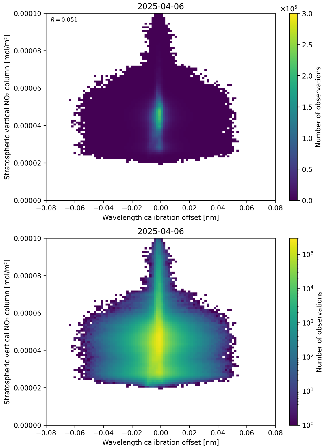
Figure 176: Scatter density plot of “Wavelength calibration offset” against “Stratospheric vertical NO 2 column” for 2025-04-06 to 2025-04-06.
