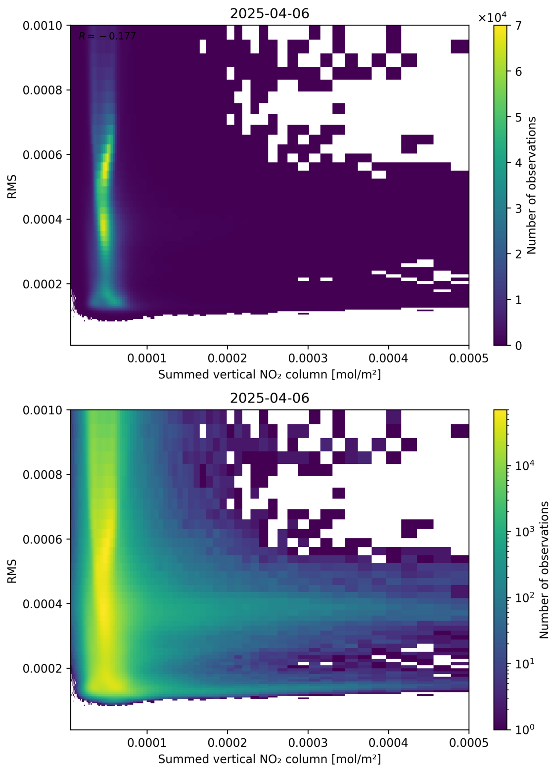
Figure 109: Scatter density plot of “Summed vertical NO 2 column” against “RMS” for 2025-04-06 to 2025-04-06.
