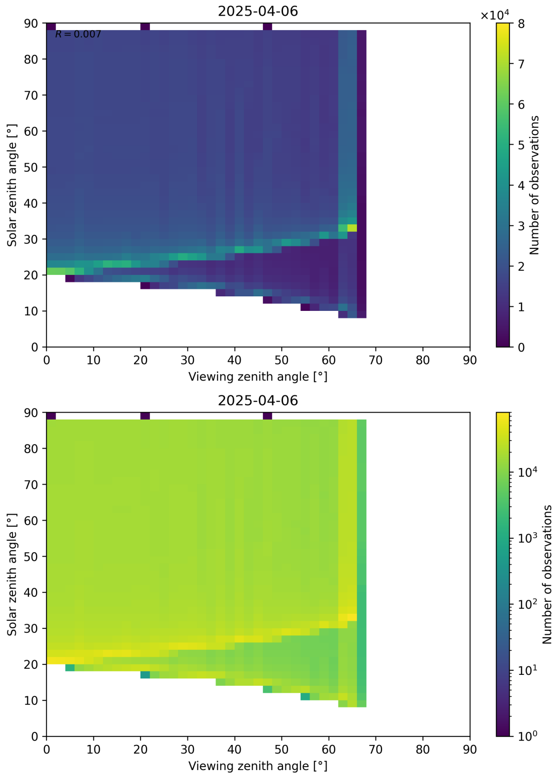
Figure 172: Scatter density plot of “Viewing zenith angle” against “Solar zenith angle” for 2025-04-06 to 2025-04-06.
