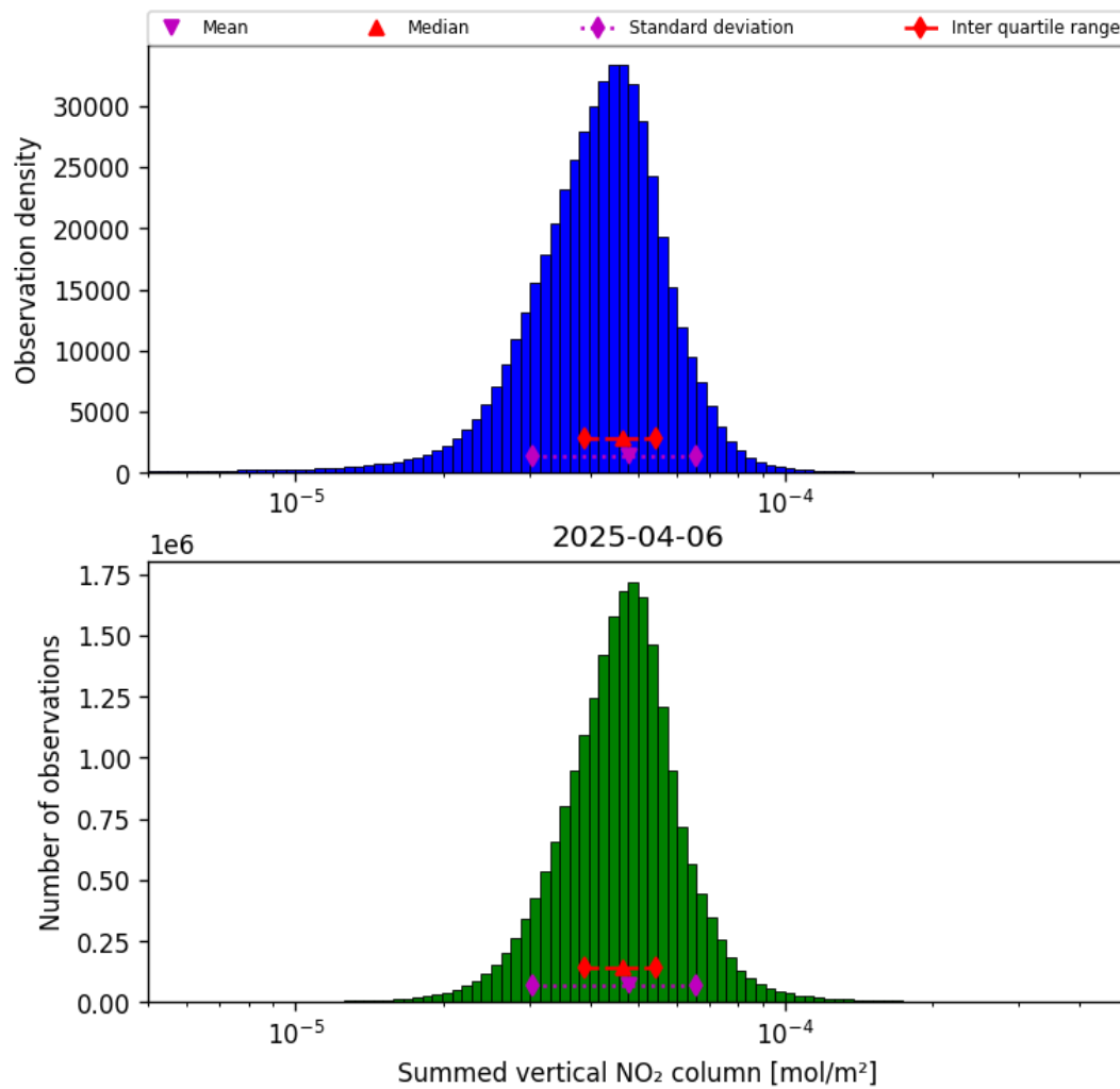
Figure 40: Histogram of “Summed vertical NO 2 column” for 2025-04-06 to 2025-04-06
