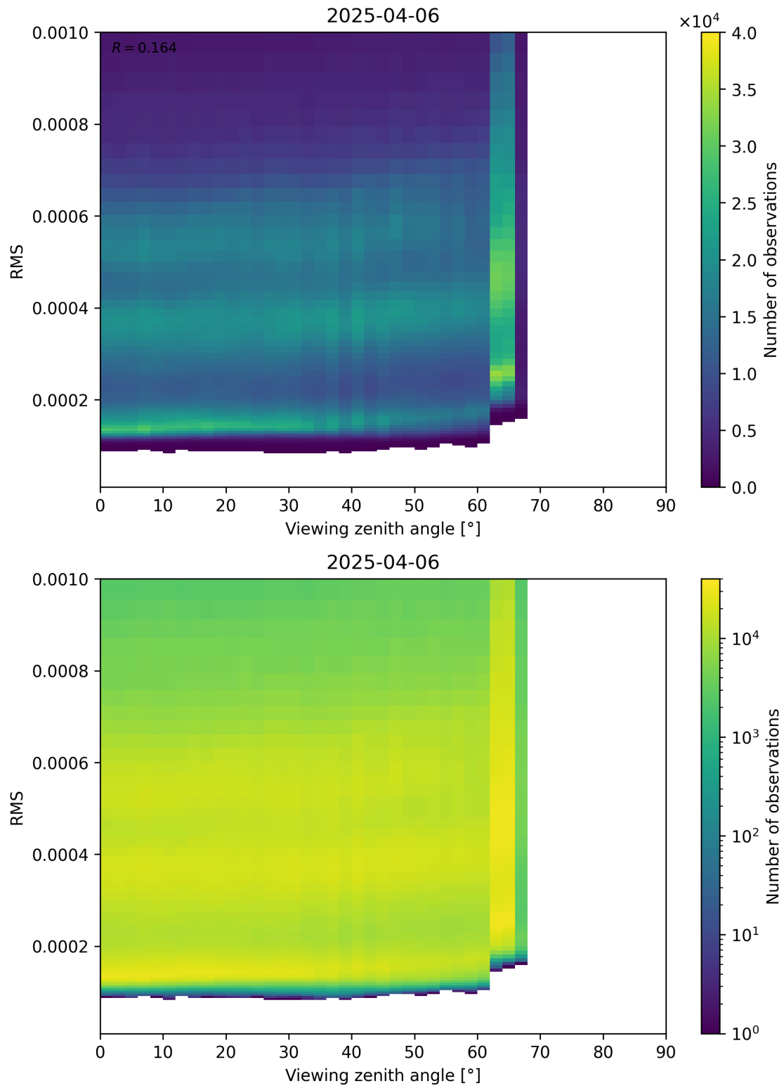
Figure 171: Scatter density plot of “Viewing zenith angle” against “RMS” for 2025-04-06 to 2025-04-06.
