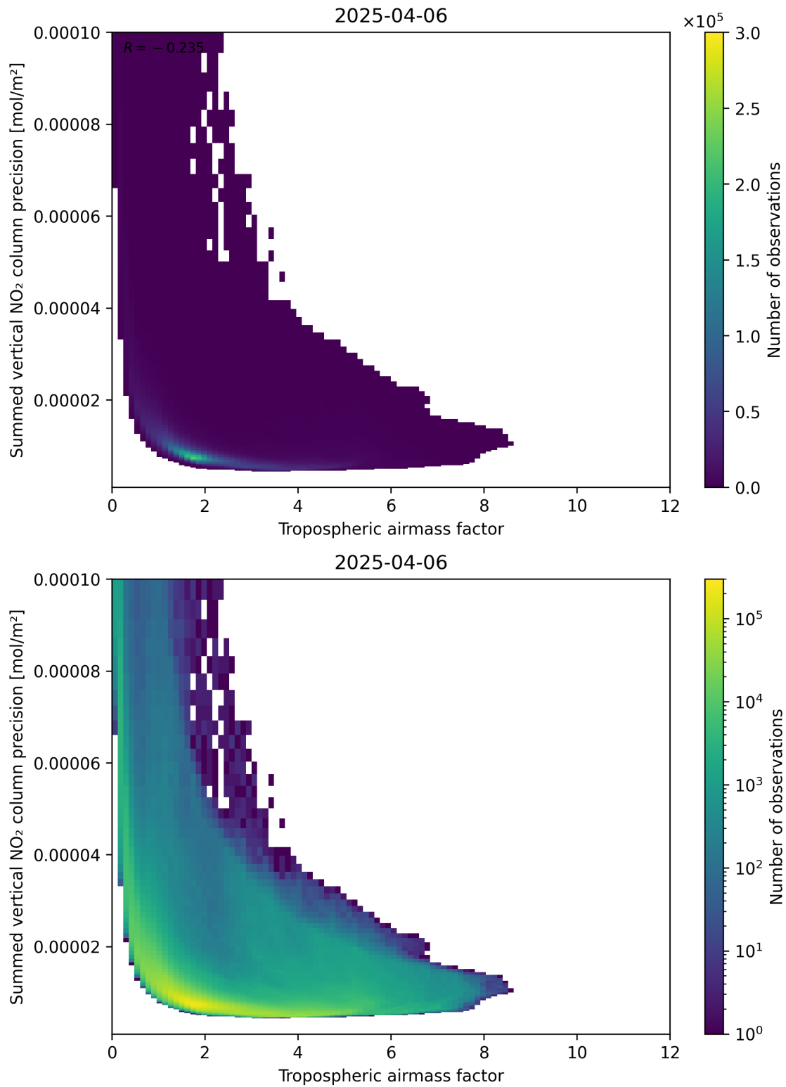
Figure 76: Scatter density plot of “Tropospheric air mass factor” against “Summed vertical NO 2 column precision” for 2025-04-06 to 2025-04-06.
