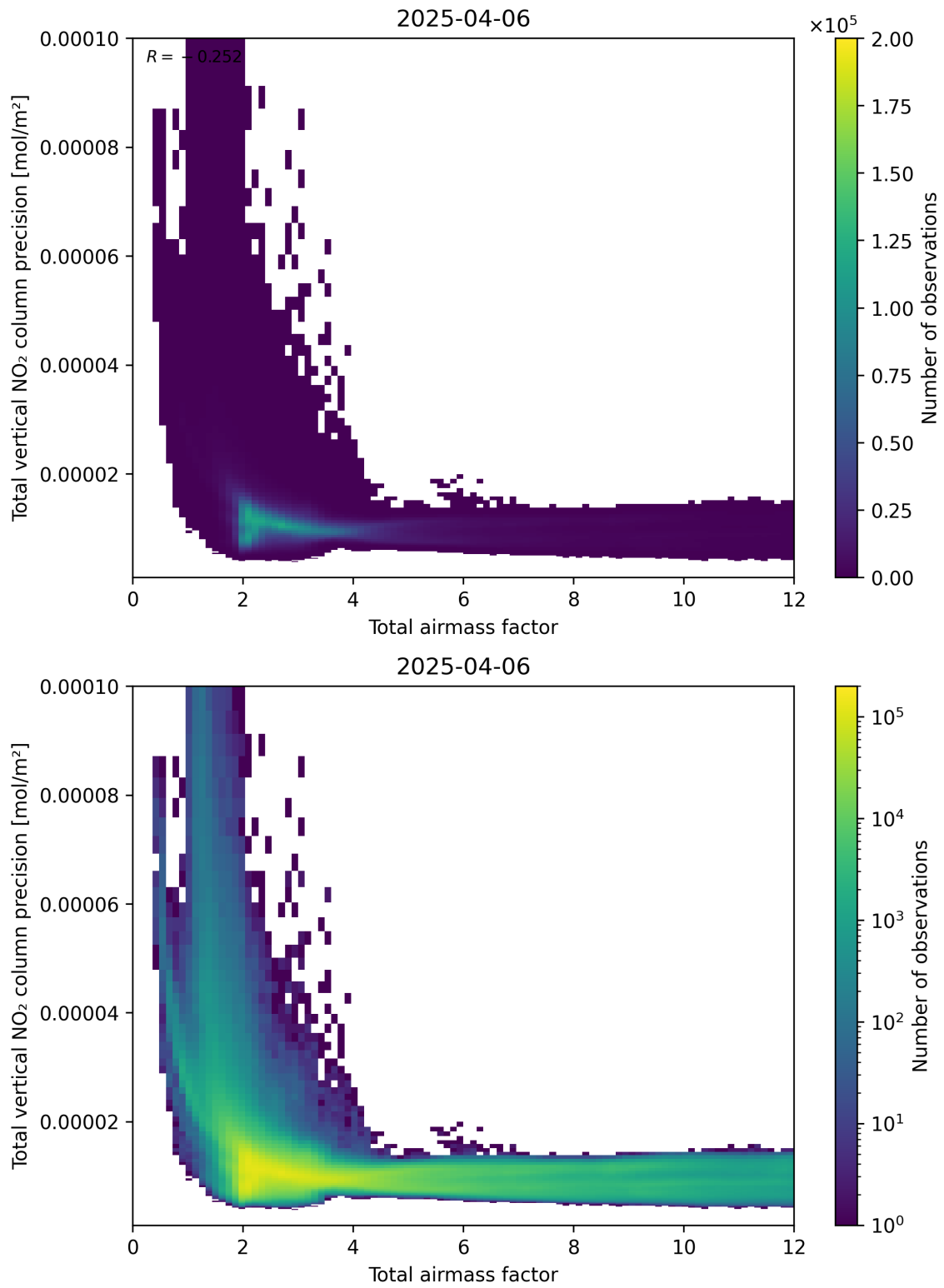
Figure 68: Scatter density plot of “Total airmass factor” against “Total vertical NO 2 column precision” for 2025-04-06 to 2025-04-06.
