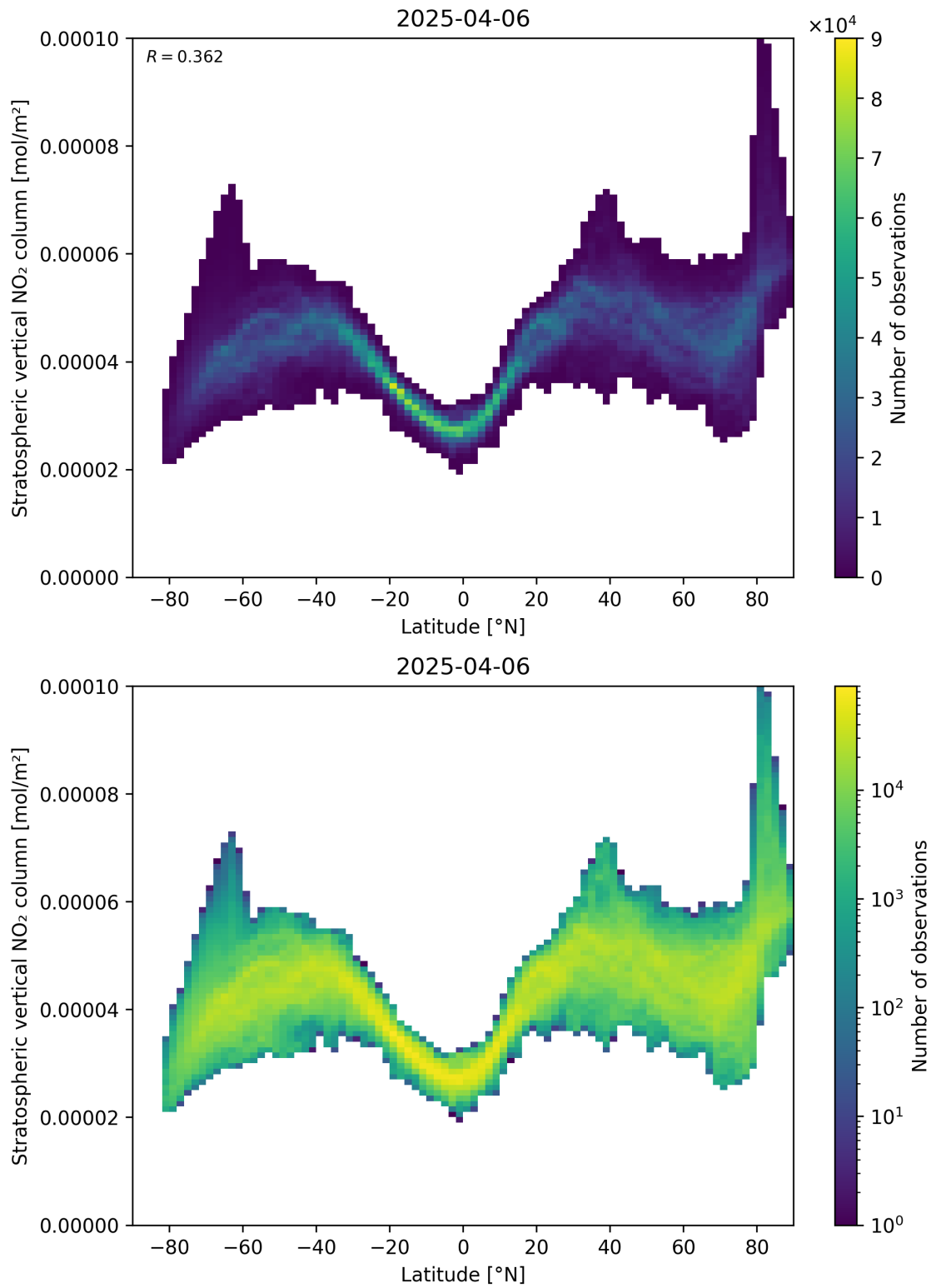
Figure 87: Scatter density plot of “Latitude” against “Stratospheric vertical \text{NO}_2 column” for 2025-04-06 to 2025-04-06.
