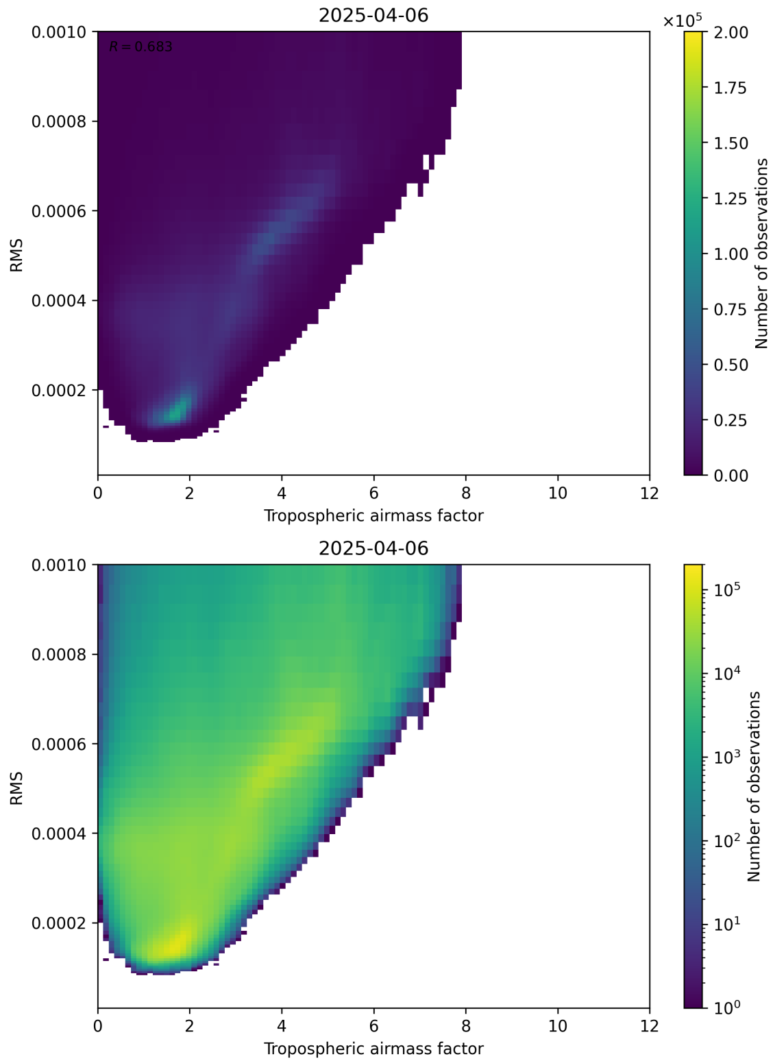
Figure 79: Scatter density plot of “Tropospheric airmass factor” against “RMS” for 2025-04-06 to 2025-04-06.
