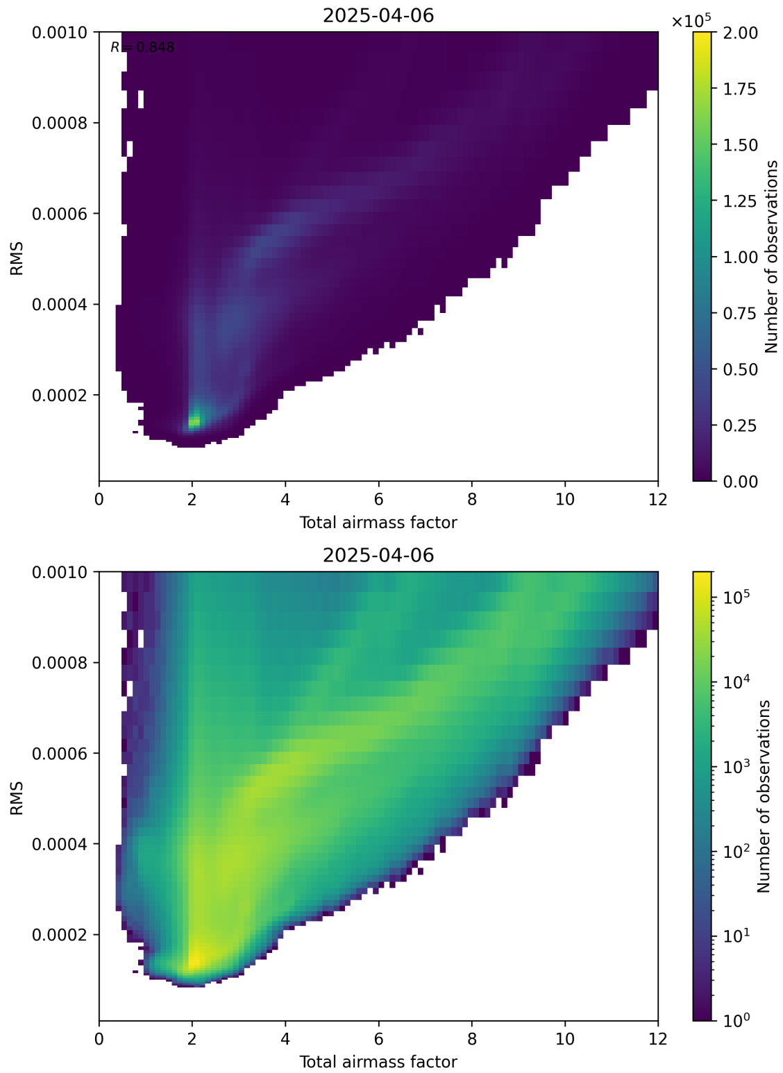
Figure 69: Scatter density plot of “Total airmass factor” against “RMS” for 2025-04-06 to 2025-04-06.
