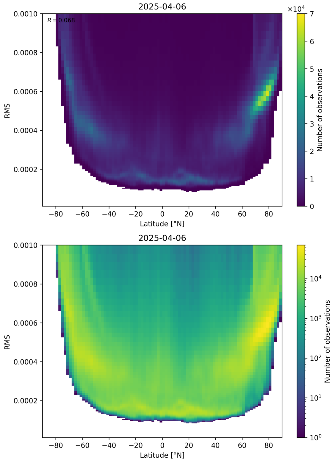
Figure 94: Scatter density plot of “Latitude” against “RMS” for 2025-04-06 to 2025-04-06.
