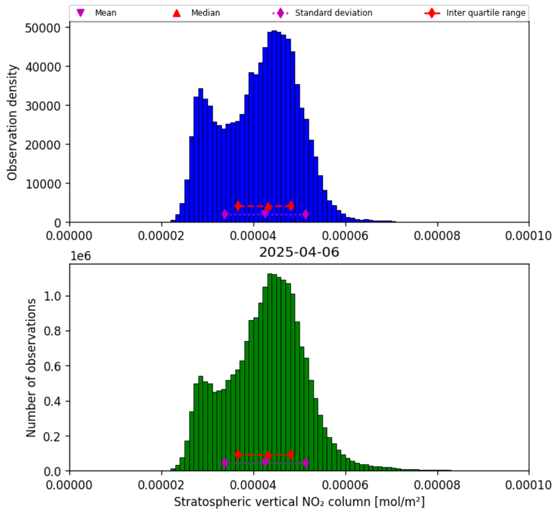
Figure 36: Histogram of “Stratospheric vertical NO 2 column” for 2025-04-06 to 2025-04-06
