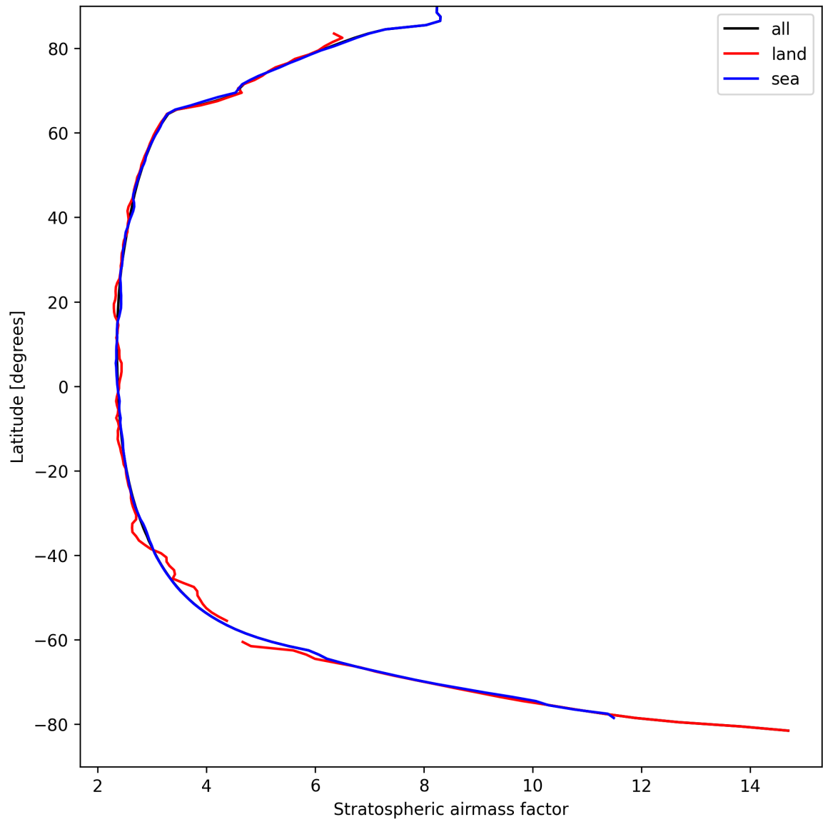
Figure 27: Zonal average of “Stratospheric air mass factor” for 2025-04-06 to 2025-04-06.
