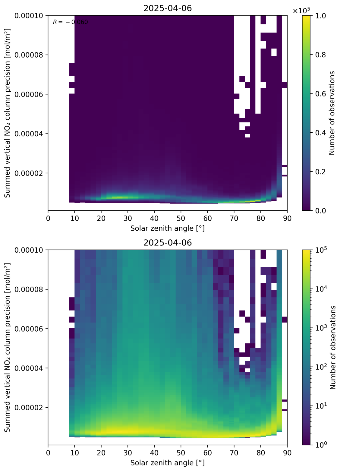
Figure 152: Scatter density plot of “Solar zenith angle” against “Summed vertical NO 2 column precision” for 2025-04-06 to 2025-04-06.
