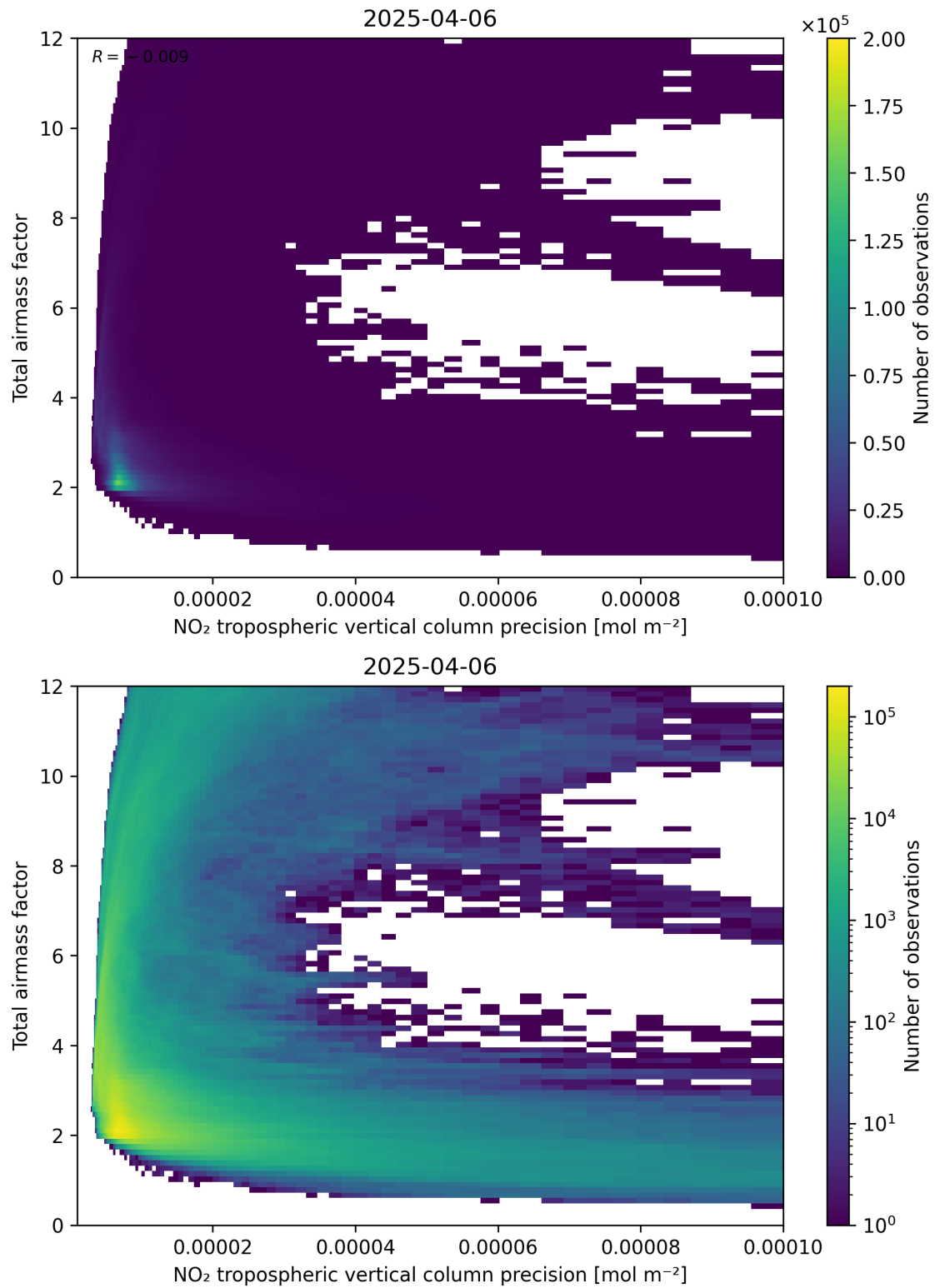
Figure 132: Scatter density plot of “NO 2 tropospheric vertical column precision” against “Total air mass factor” for 2025-04-06 to 2025-04-06.
