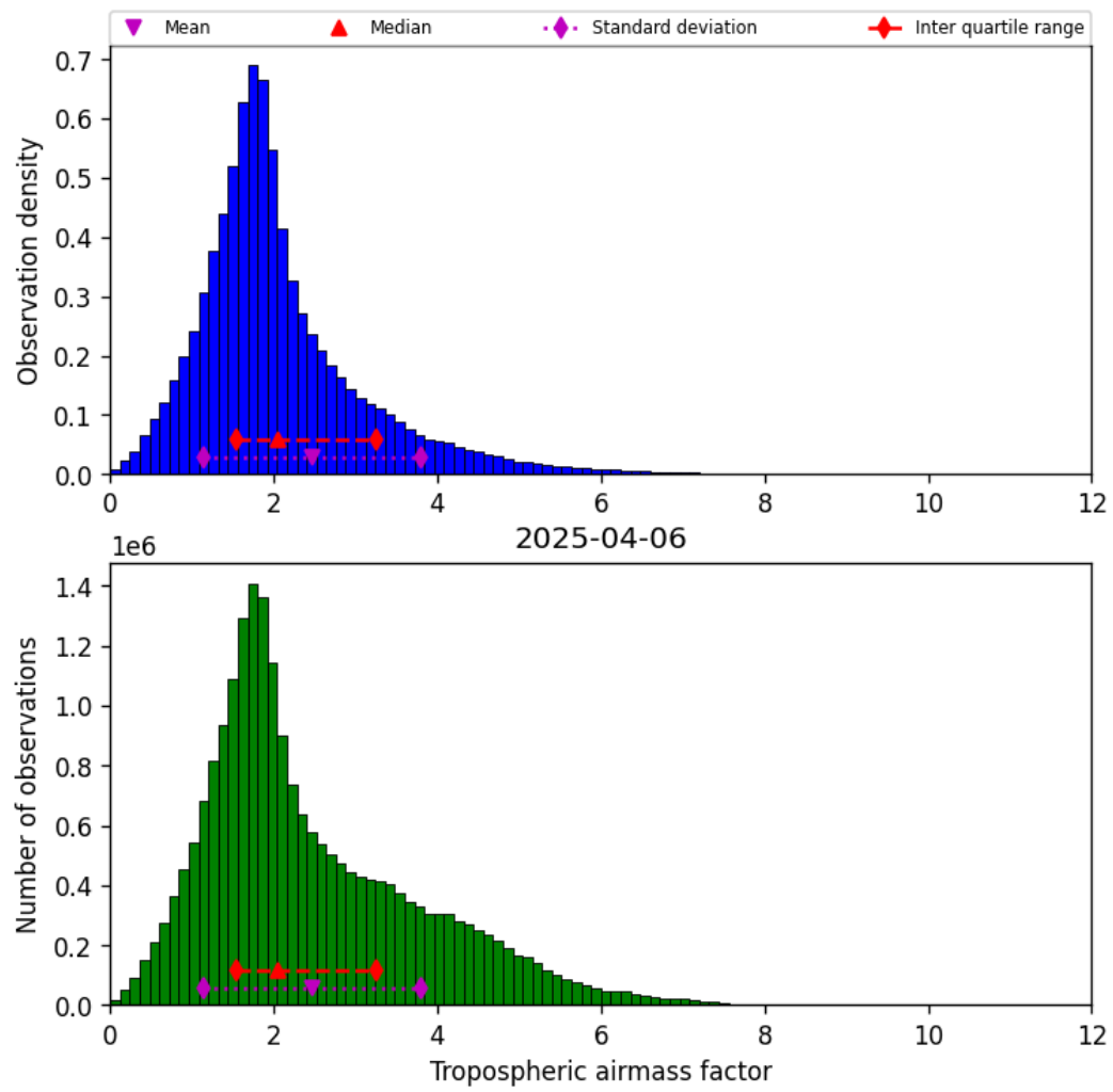
Figure 31: Histogram of “Tropospheric airmass factor” for 2025-04-06 to 2025-04-06
