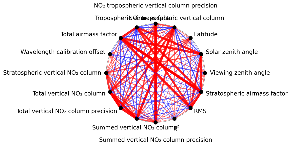
Figure 1: Map of correlation graph for 2025-04-06 to 2025-04-06.
