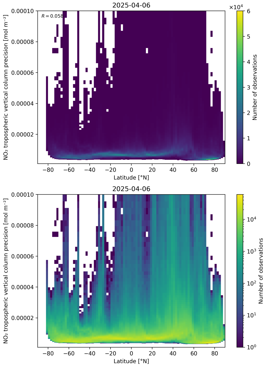
Figure 93: Scatter density plot of “Latitude” against “NO 2 tropospheric vertical column precision” for 2025-04-06 to 2025-04-06.
