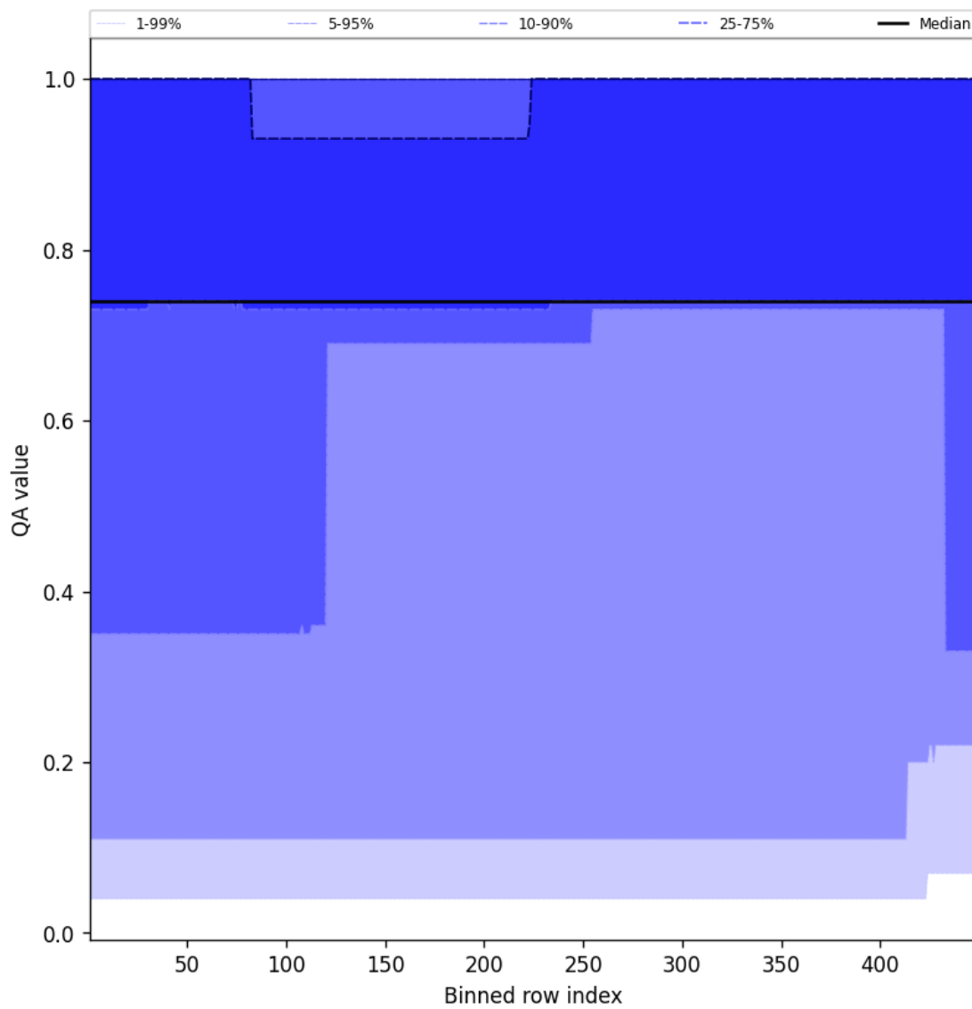
Figure 45: Along track statistics of “QA value” for 2025-04-06 to 2025-04-06
