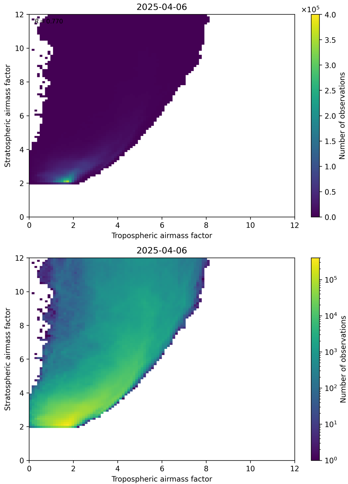
Figure 71: Scatter density plot of “Tropospheric airmass factor” against “Stratospheric airmass factor” for 2025-04-06 to 2025-04-06.
