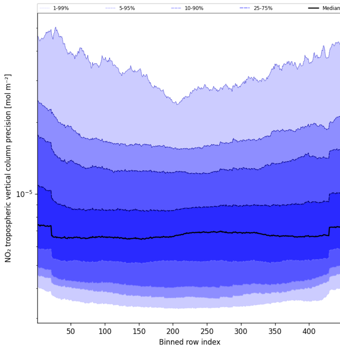
Figure 47: Along track statistics of “NO 2 tropospheric vertical column precision” for 2025-04-06 to 2025-04-06
