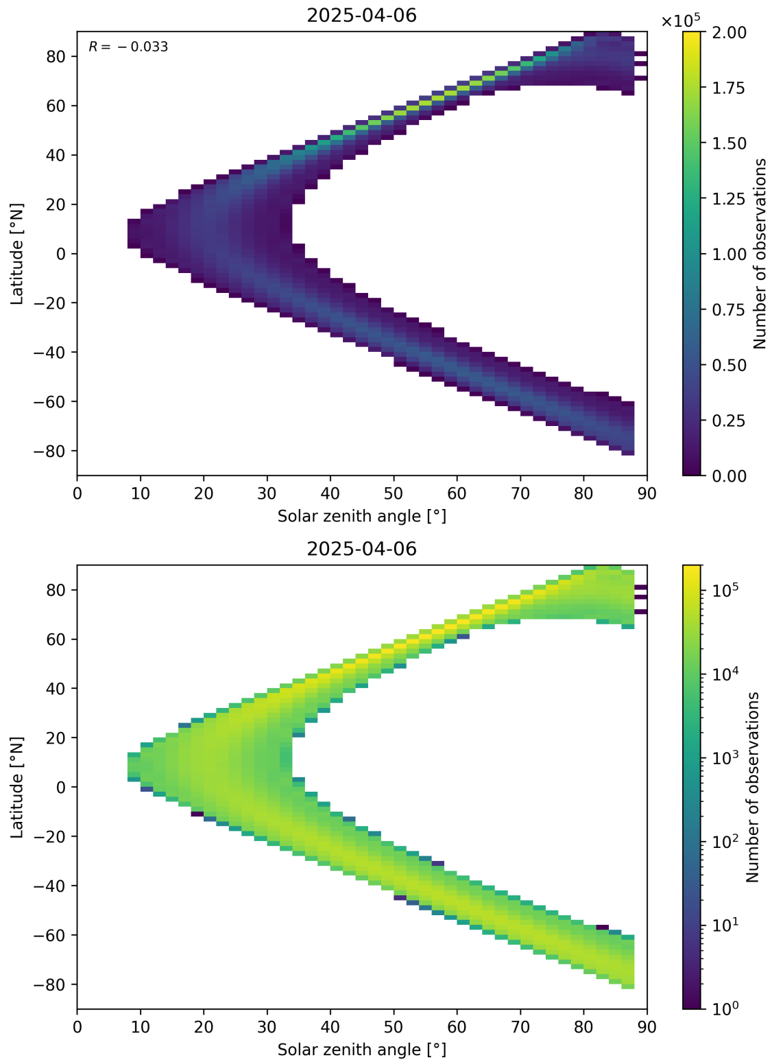
Figure 149: Scatter density plot of “Solar zenith angle” against “Latitude” for 2025-04-06 to 2025-04-06.
