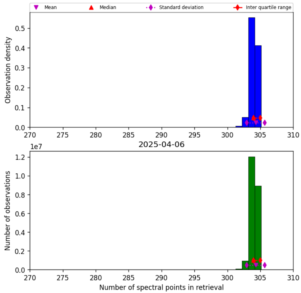
Figure 33: Histogram of “Number of spectral points in retrieval” for 2025-04-06 to 2025-04-06
