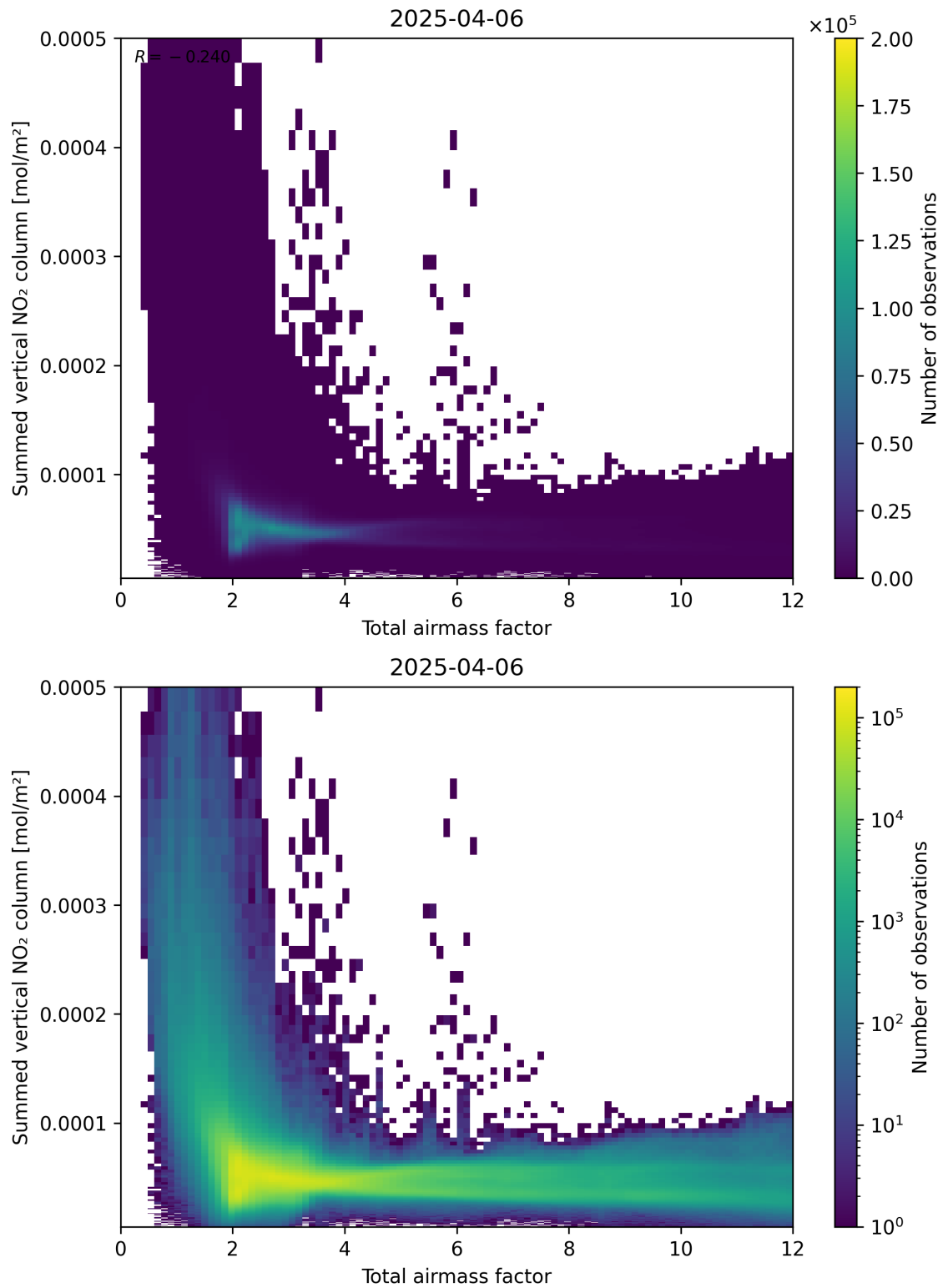
Figure 65: Scatter density plot of “Total airmass factor” against “Summed vertical NO 2 column” for 2025-04-06 to 2025-04-06.
