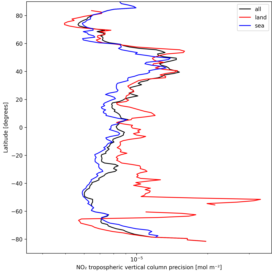
Figure 13: Zonal average of "NO 2 tropospheric vertical column precision" for 2025-04-06 to 2025-04-06.
