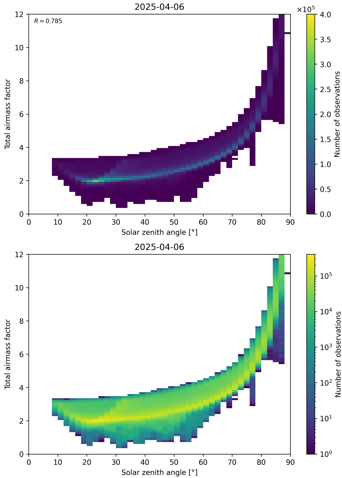
Figure 146: Scatter density plot of “Solar zenith angle” against “Total air mass factor” for 2025-04-06 to 2025-04-06.
