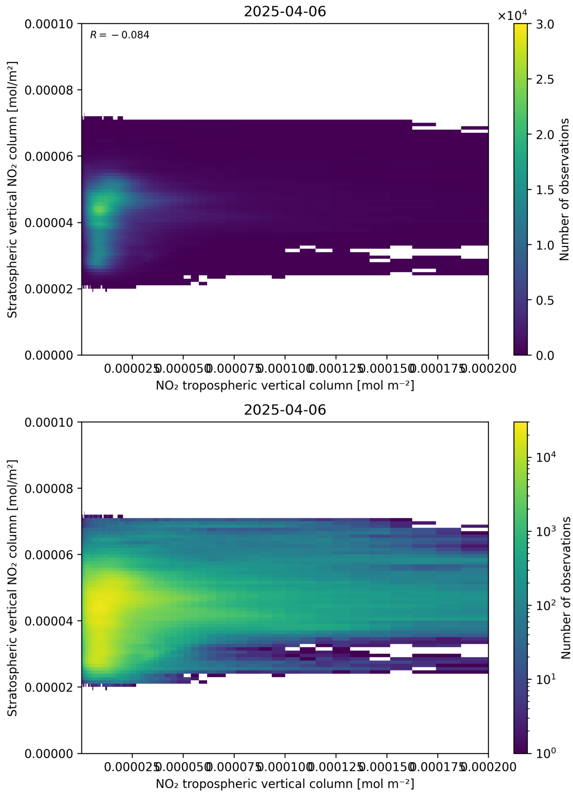
Figure 125: Scatter density plot of “NO 2 tropospheric vertical column” against “Stratospheric vertical NO 2 column” for 2025-04-06 to 2025-04-06.
