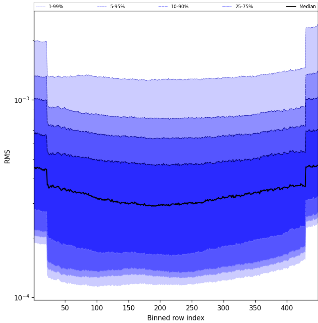
Figure 60: Along track statistics of “RMS” for 2025-04-06 to 2025-04-06
