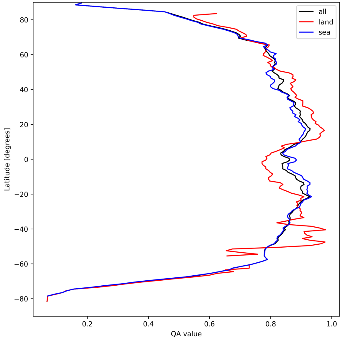
Figure 11: Zonal average of “QA value” for 2025-04-06 to 2025-04-06.
