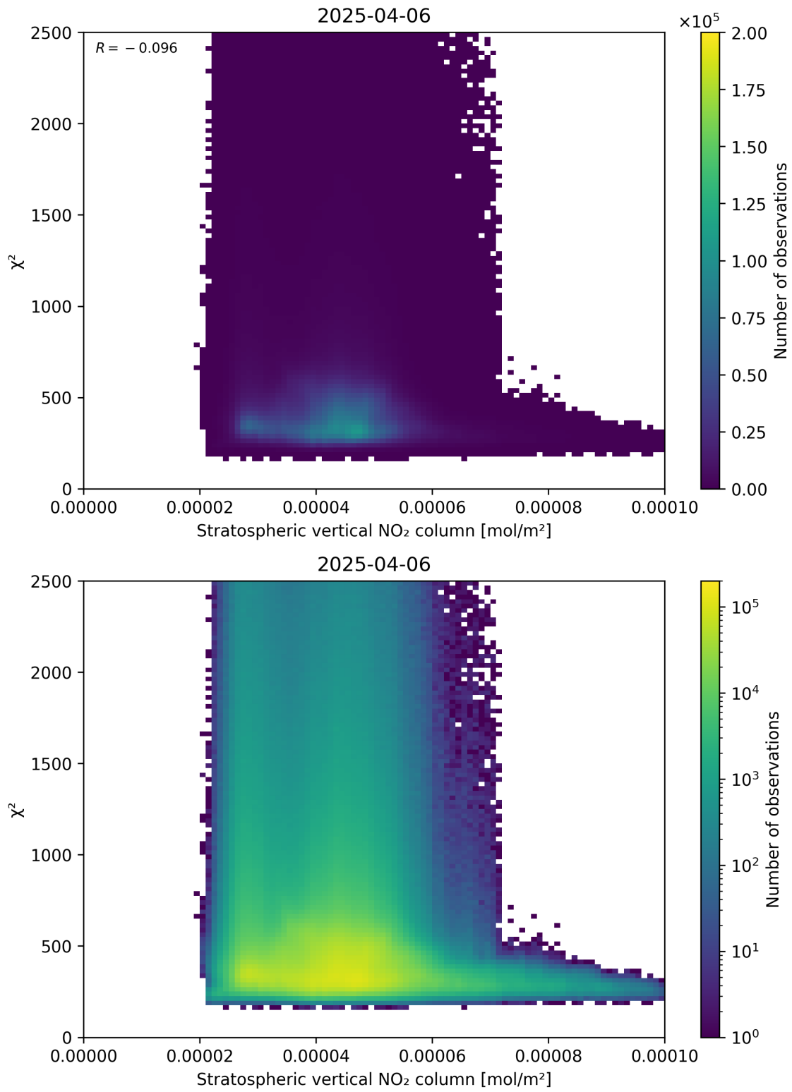
Figure 97: Scatter density plot of “Stratospheric vertical NO 2 column” against “ \chi^2 ” for 2025-04-06 to 2025-04-06.
