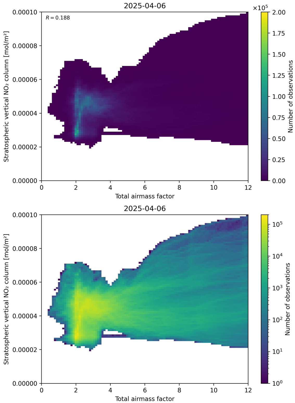
Figure 64: Scatter density plot of “Total airmass factor” against “Stratospheric vertical \text{NO}_2 column” for 2025-04-06 to 2025-04-06.
