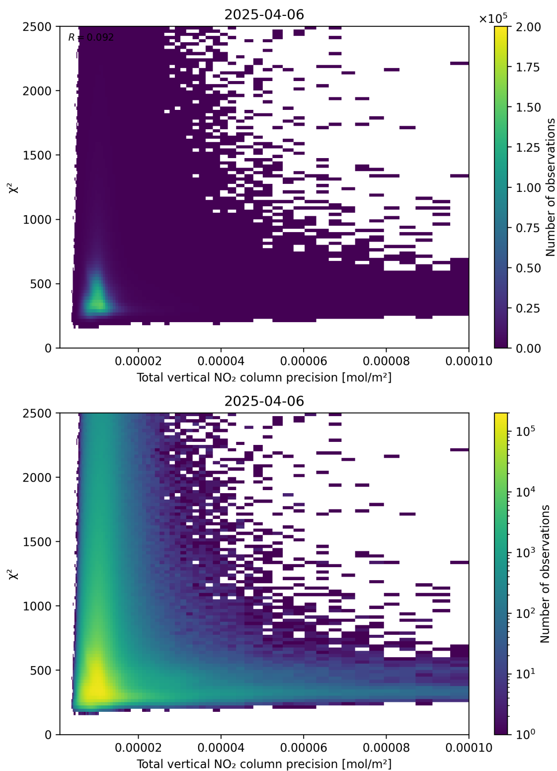
Figure 116: Scatter density plot of “Total vertical NO 2 column precision” against “ \chi^2 ” for 2025-04-06 to 2025-04-06.
