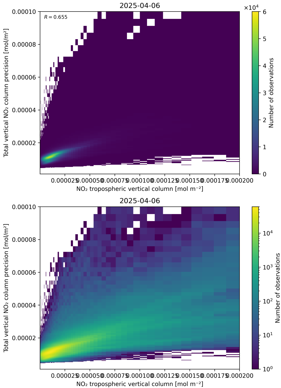
Figure 129: Scatter density plot of “NO 2 tropospheric vertical column” against “Total vertical NO 2 column precision” for 2025-04-06 to 2025-04-06.
