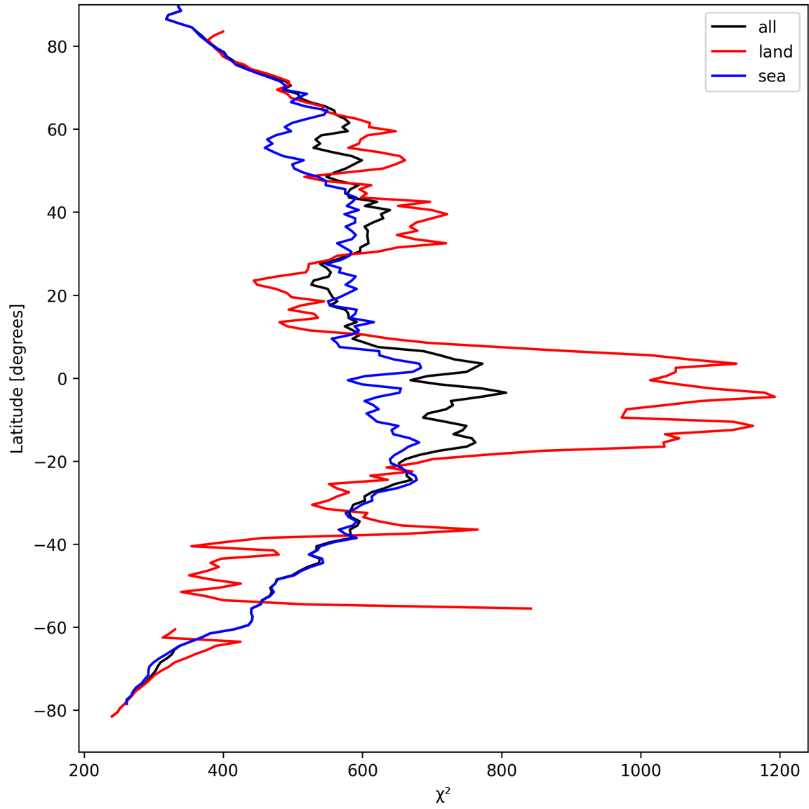
Figure 25: Zonal average of “ \chi^2 ” for 2025-04-06 to 2025-04-06.
