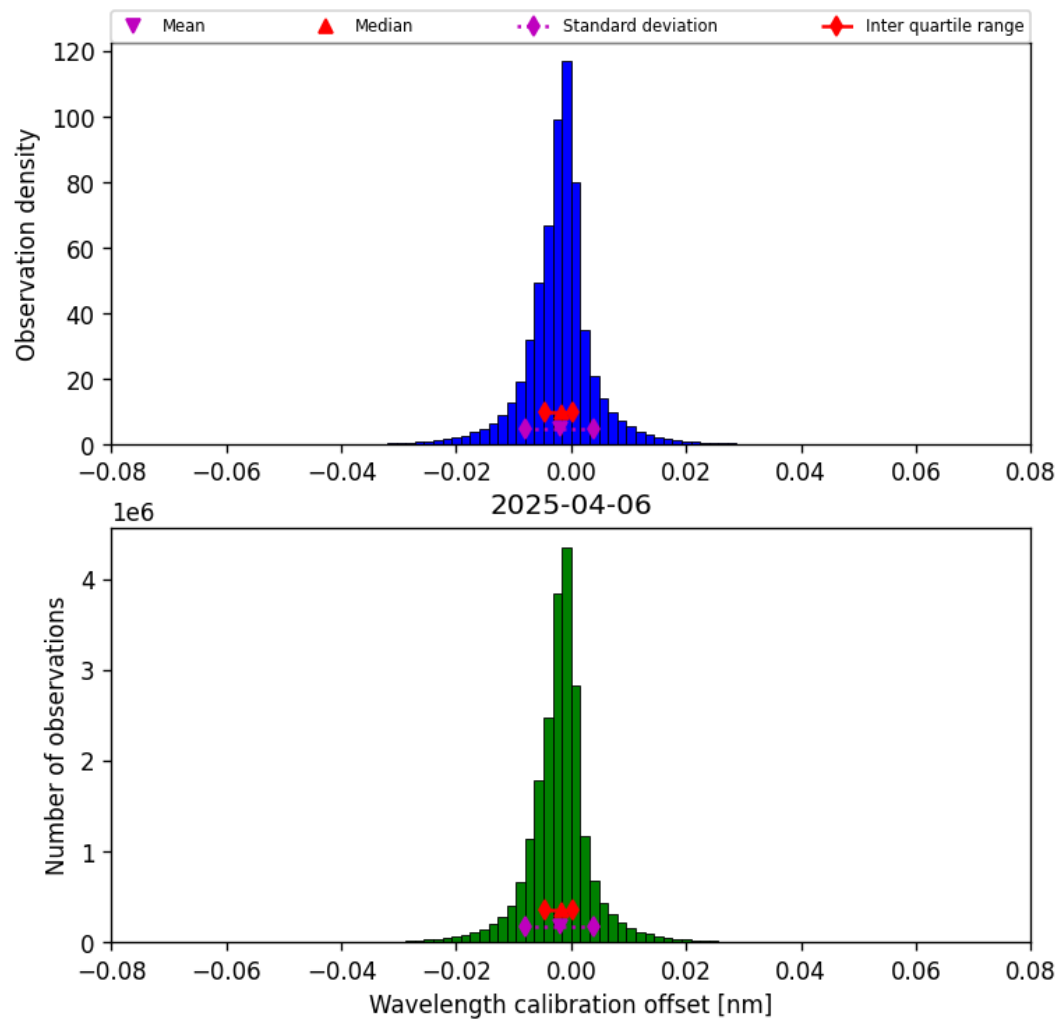
Figure 35: Histogram of “Wavelength calibration offset” for 2025-04-06 to 2025-04-06
