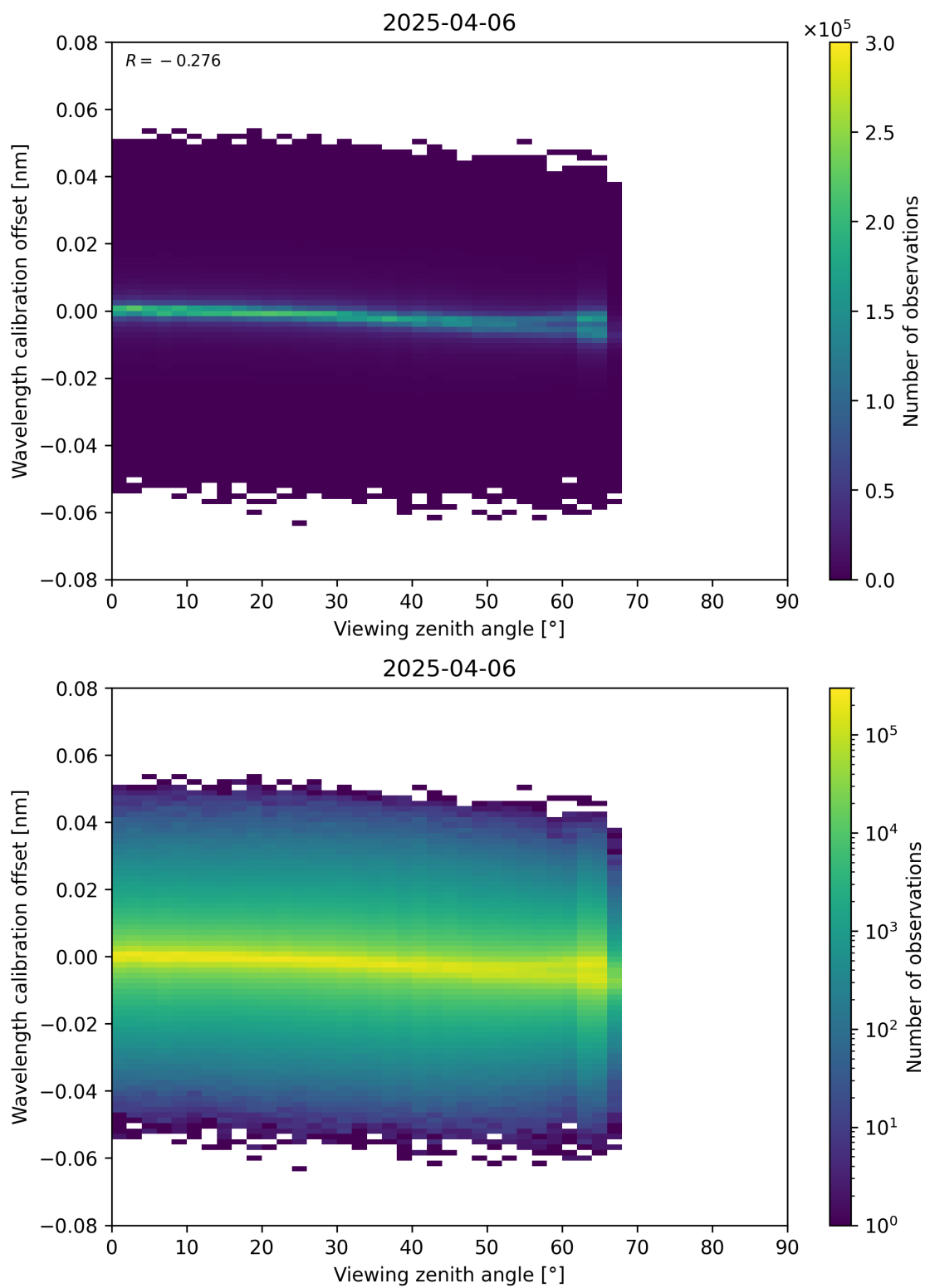
Figure 173: Scatter density plot of “Viewing zenith angle” against “Wavelength calibration offset” for 2025-04-06 to 2025-04-06.
