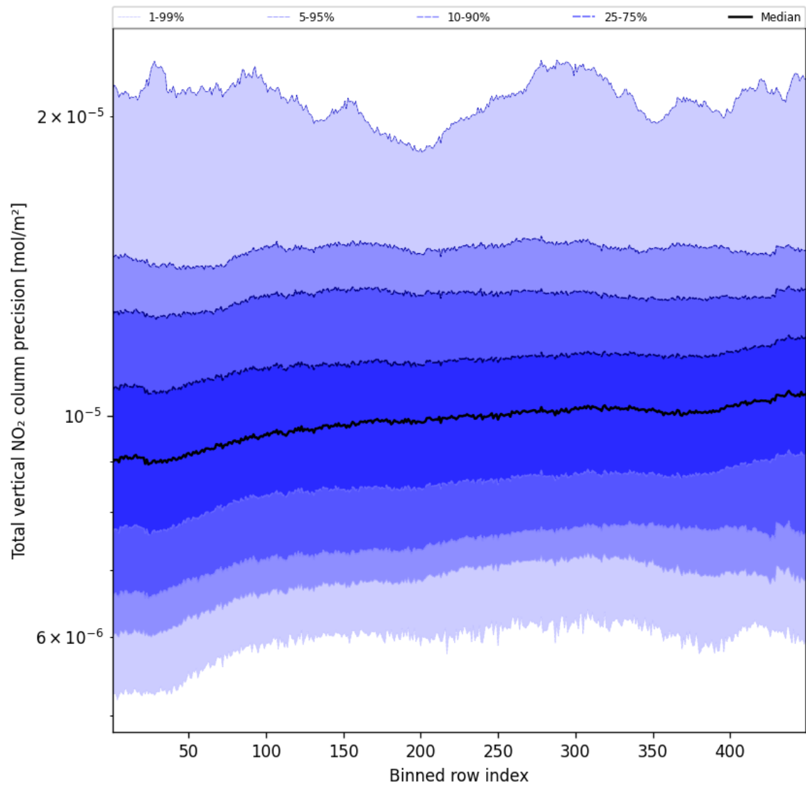
Figure 56: Along track statistics of “Total vertical NO 2 column precision” for 2025-04-06 to 2025-04-06
