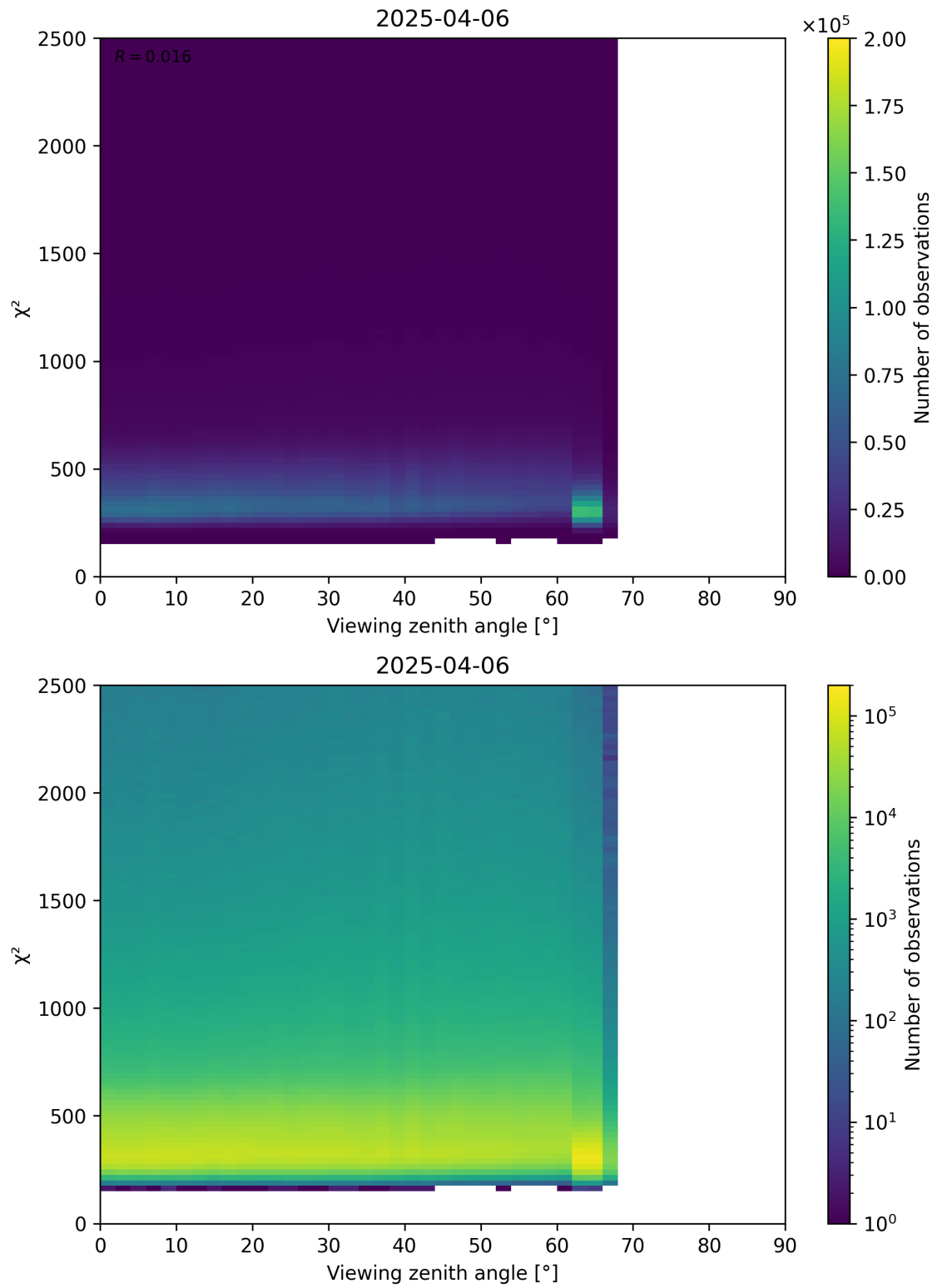
Figure 162: Scatter density plot of “Viewing zenith angle” against “ \chi^2 ” for 2025-04-06 to 2025-04-06.
