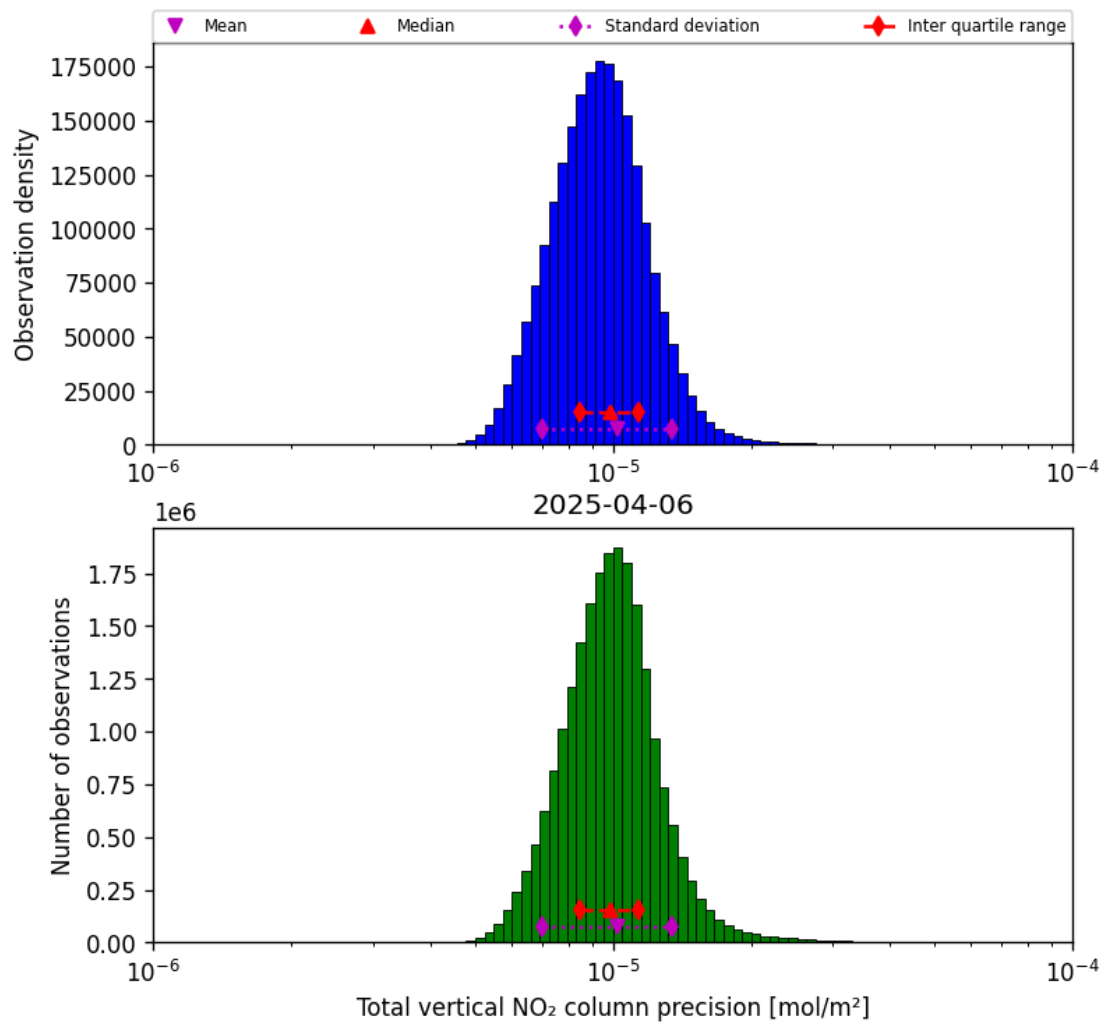
Figure 39: Histogram of "Total vertical NO 2 column precision" for 2025-04-06 to 2025-04-06
