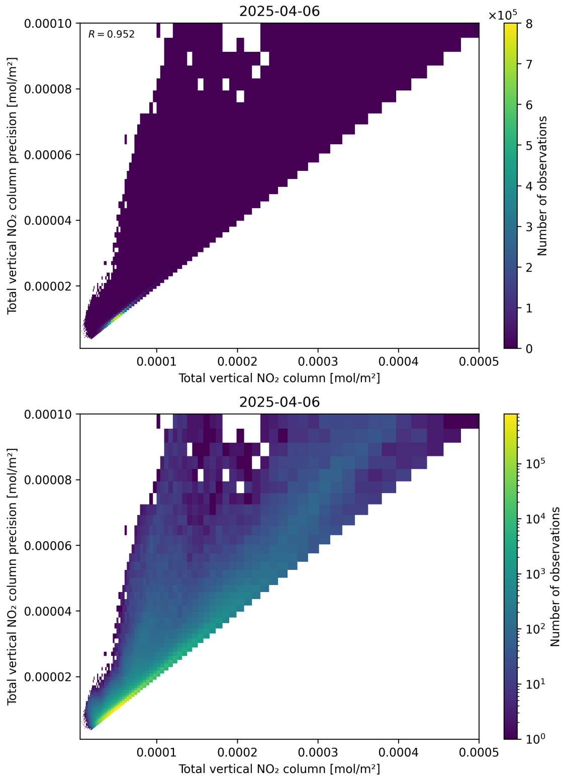
Figure 114: Scatter density plot of “Total vertical NO 2 column” against “Total vertical NO 2 column precision” for 2025-04-06 to 2025-04-06.
