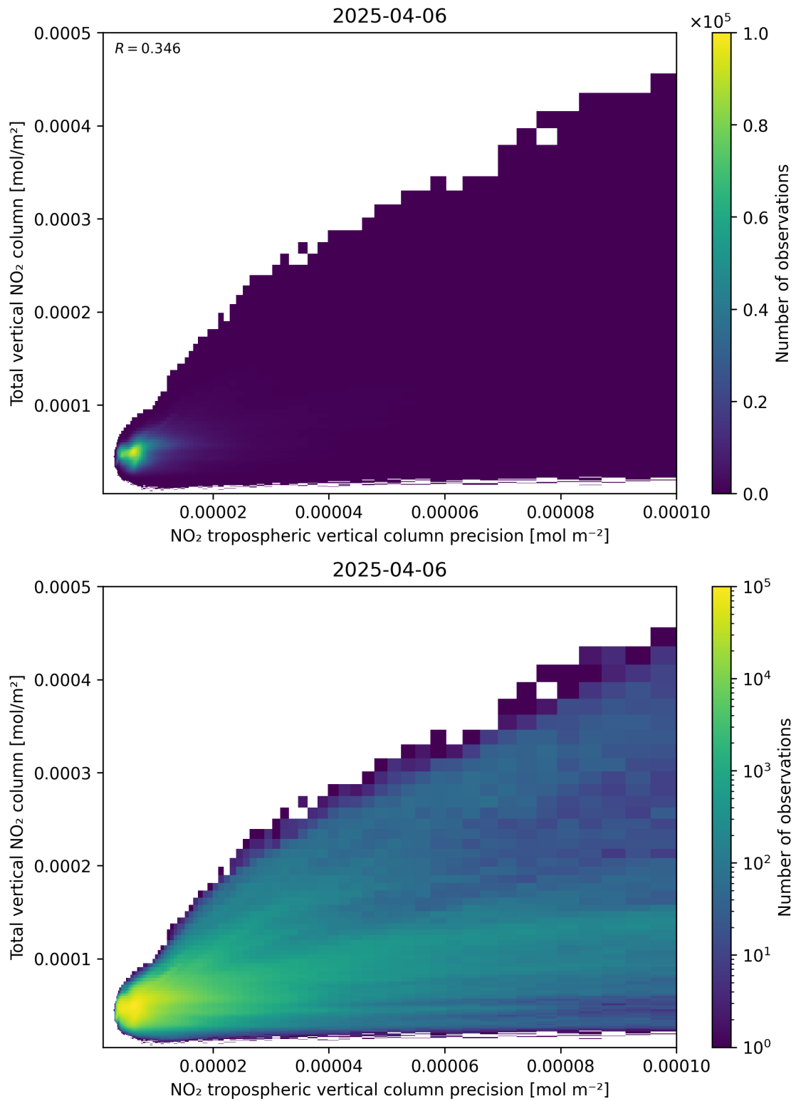
Figure 138: Scatter density plot of “NO 2 tropospheric vertical column precision” against “Total vertical NO 2 column” for 2025-04-06 to 2025-04-06.
