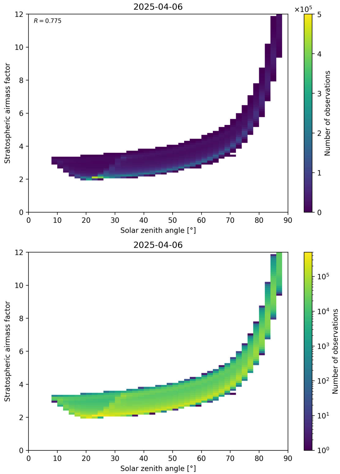
Figure 145: Scatter density plot of “Solar zenith angle” against “Stratospheric airmass factor” for 2025-04-06 to 2025-04-06.
