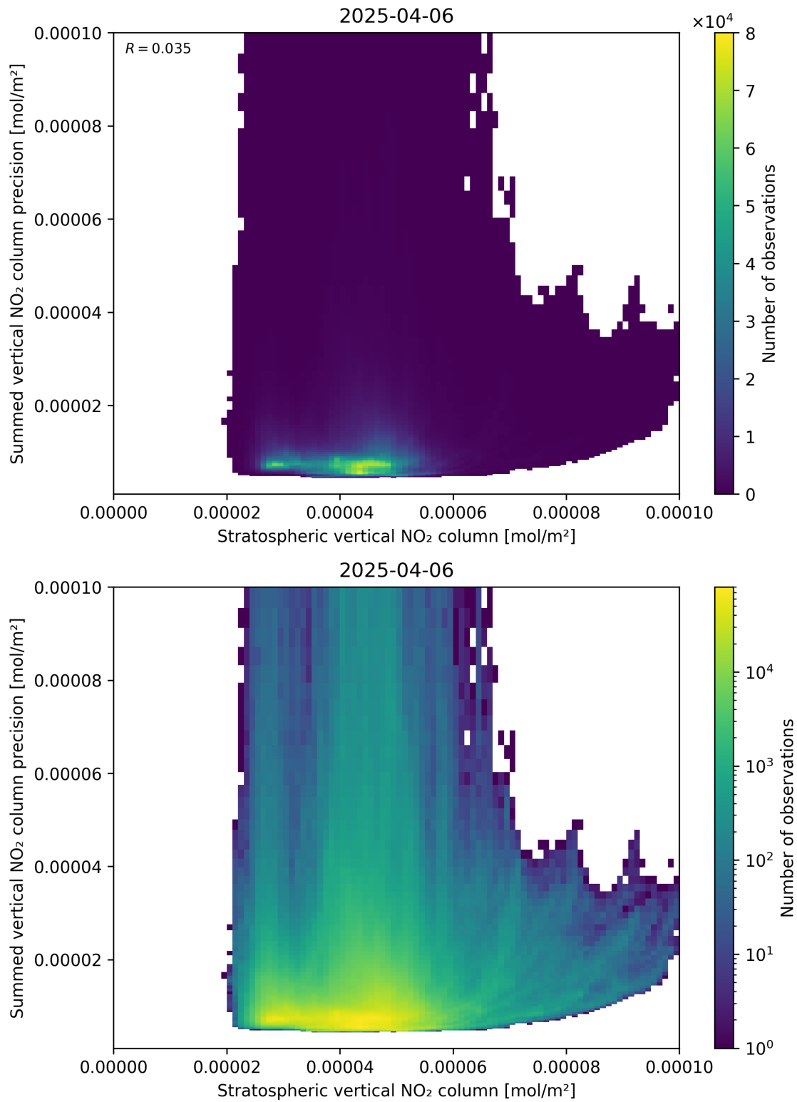
Figure 99: Scatter density plot of “Stratospheric vertical NO 2 column” against “Summed vertical NO 2 column precision” for 2025-04-06 to 2025-04-06.
