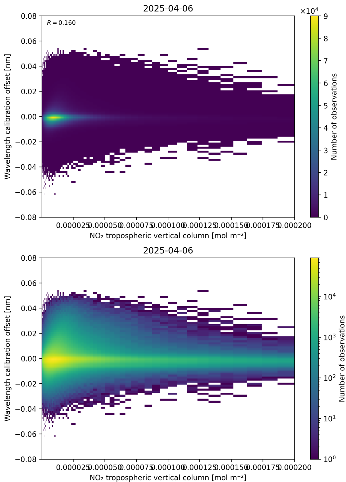
Figure 143: Scatter density plot of “NO 2 tropospheric vertical column” against “Wavelength calibration offset” for 2025-04-06 to 2025-04-06.
