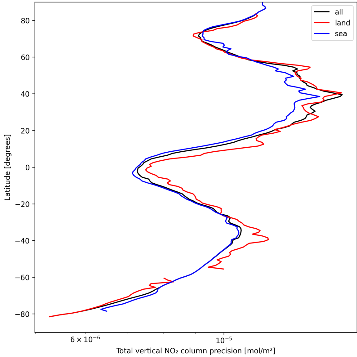
Figure 22: Zonal average of “Total vertical NO 2 column precision” for 2025-04-06 to 2025-04-06.
