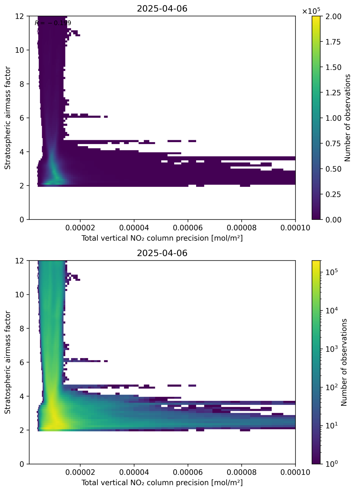
Figure 115: Scatter density plot of “Total vertical NO 2 column precision” against “Stratospheric air mass factor” for 2025-04-06 to 2025-04-06.
