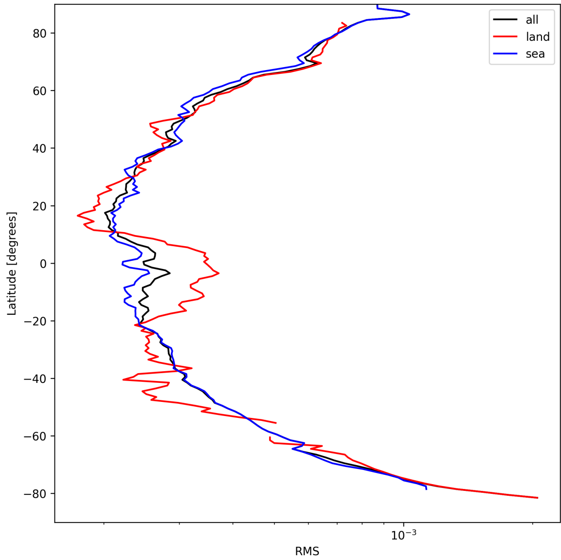
Figure 26: Zonal average of “RMS” for 2025-04-06 to 2025-04-06.
