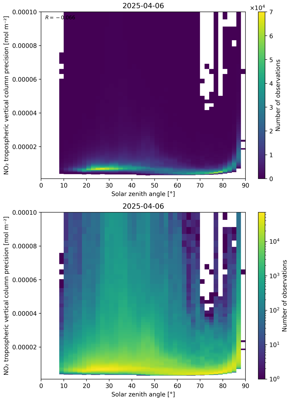
Figure 156: Scatter density plot of “Solar zenith angle” against “NO 2 tropospheric vertical column precision” for 2025-04-06 to 2025-04-06.
