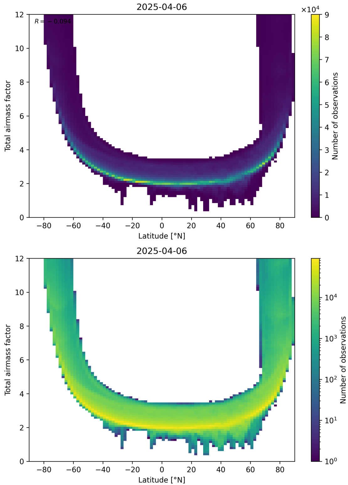
Figure 84: Scatter density plot of “Latitude” against “Total airmass factor” for 2025-04-06 to 2025-04-06.
