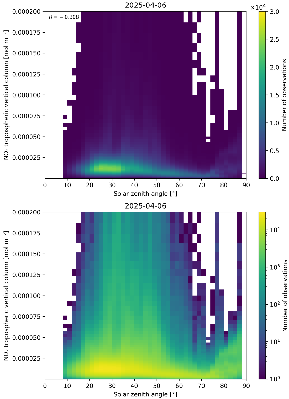
Figure 155: Scatter density plot of “Solar zenith angle” against “NO 2 tropospheric vertical column” for 2025-04-06 to 2025-04-06.
