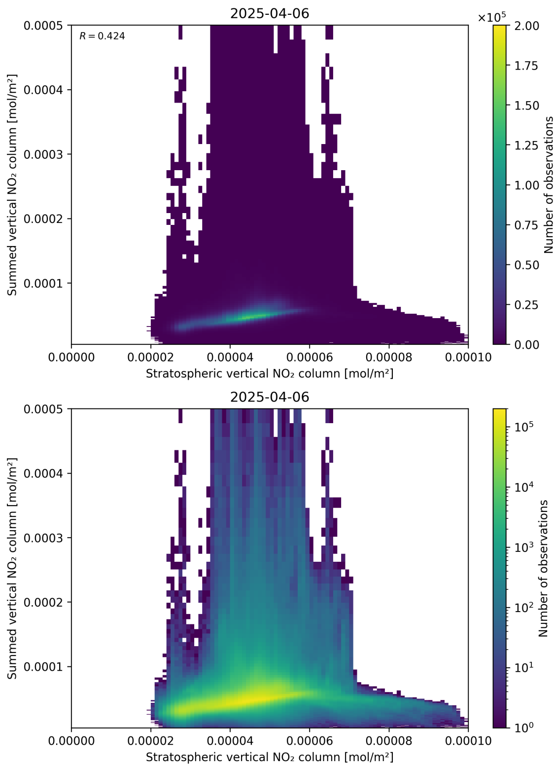
Figure 98: Scatter density plot of “Stratospheric vertical NO 2 column” against “Summed vertical NO 2 column” for 2025-04-06 to 2025-04-06.
