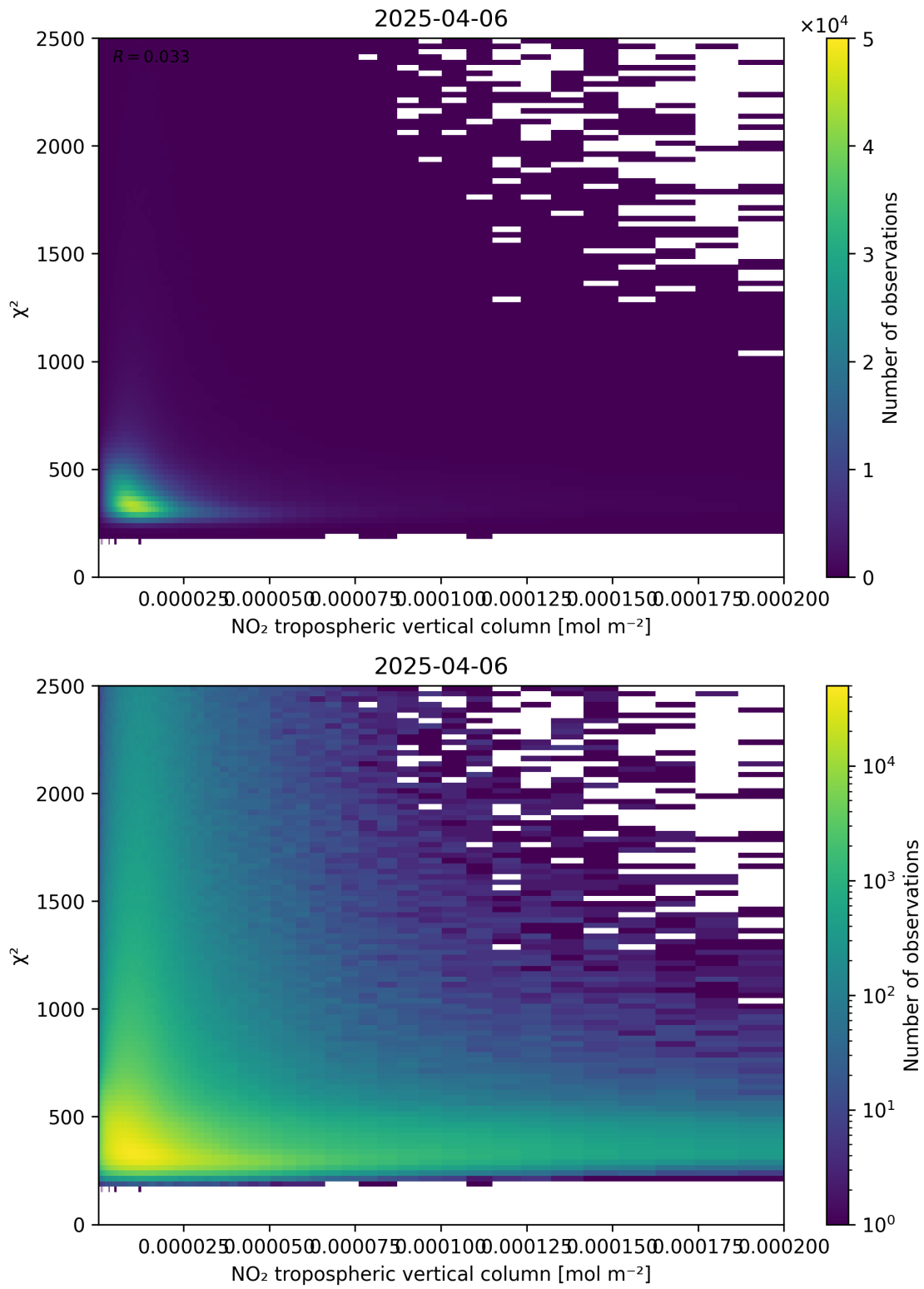
Figure 124: Scatter density plot of “NO 2 tropospheric vertical column” against “ \chi^2 ” for 2025-04-06 to 2025-04-06.
