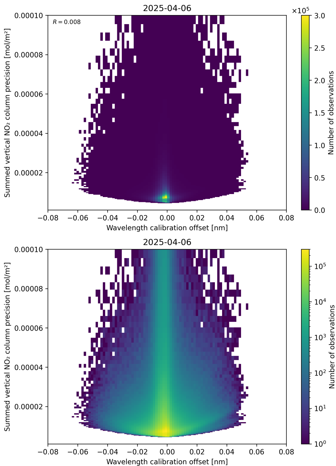
Figure 178: Scatter density plot of “Wavelength calibration offset” against “Summed vertical NO 2 column precision” for 2025-04-06 to 2025-04-06.
