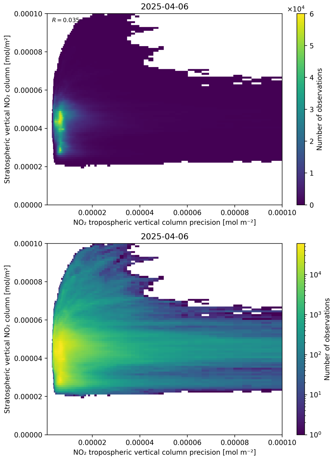
Figure 135: Scatter density plot of “NO 2 tropospheric vertical column precision” against “Stratospheric vertical NO 2 column” for 2025-04-06 to 2025-04-06.
