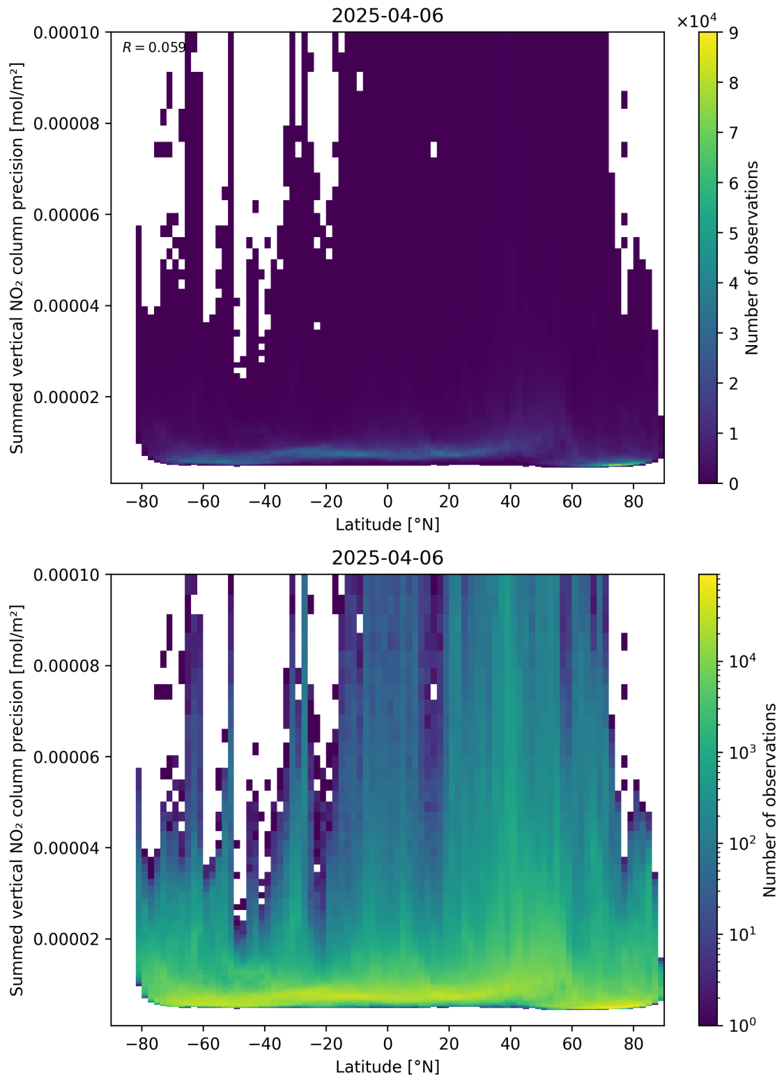
Figure 89: Scatter density plot of “Latitude” against “Summed vertical NO 2 column precision” for 2025-04-06 to 2025-04-06.
