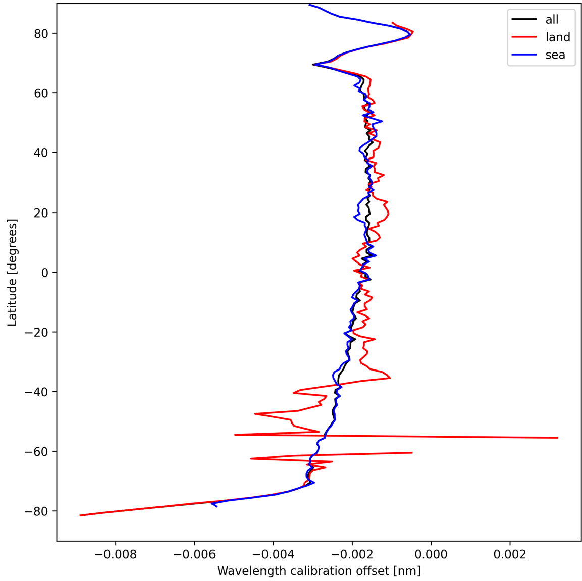
Figure 18: Zonal average of “Wavelength calibration offset” for 2025-04-06 to 2025-04-06.
