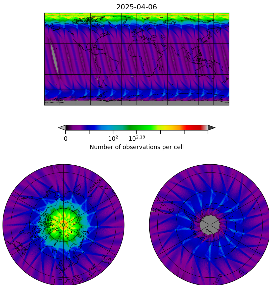
Figure 10: Map of the number of observations for 2025-04-06 to 2025-04-06
