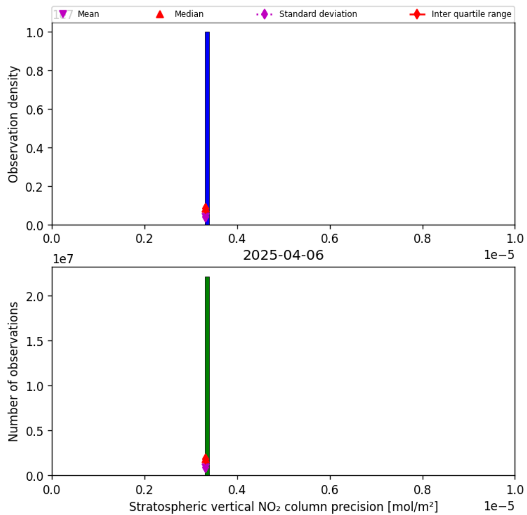
Figure 37: Histogram of “Stratospheric vertical NO 2 column precision” for 2025-04-06 to 2025-04-06
