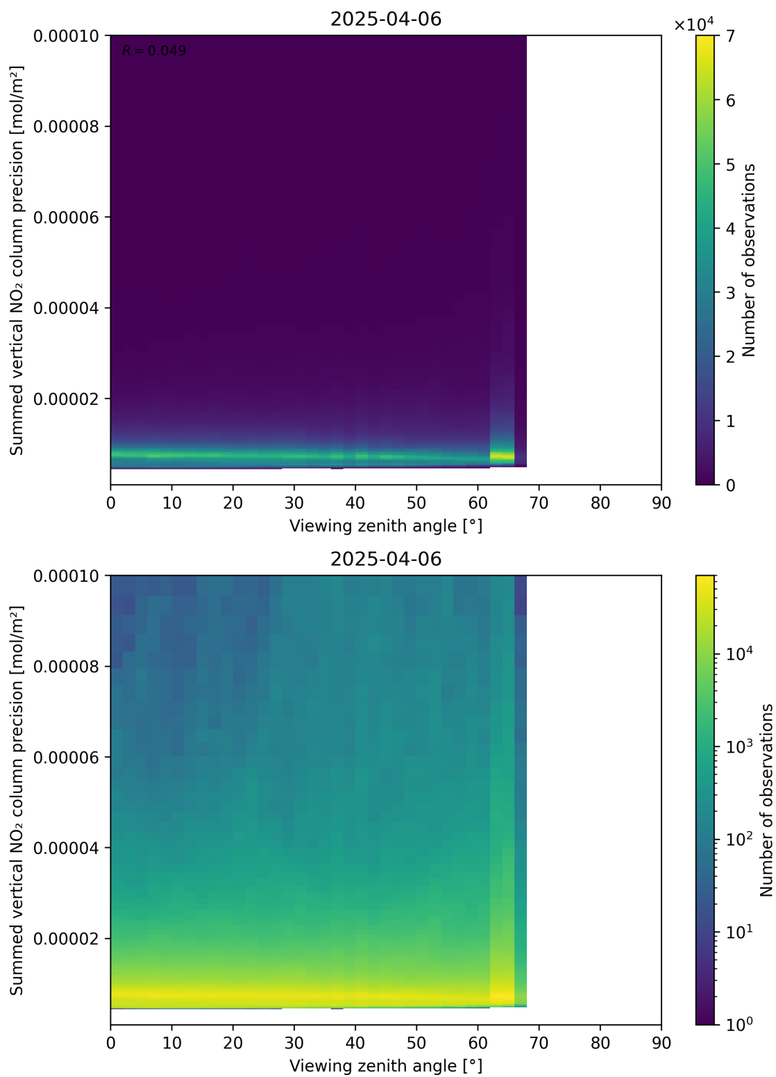
Figure 166: Scatter density plot of “Viewing zenith angle” against “Summed vertical NO 2 column precision” for 2025-04-06 to 2025-04-06.
