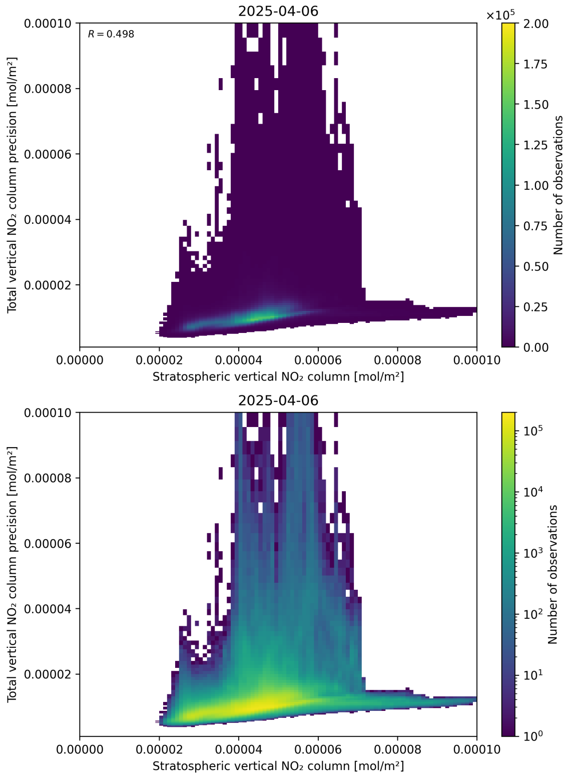
Figure 101: Scatter density plot of “Stratospheric vertical NO 2 column” against “Total vertical NO 2 column precision” for 2025-04-06 to 2025-04-06.
