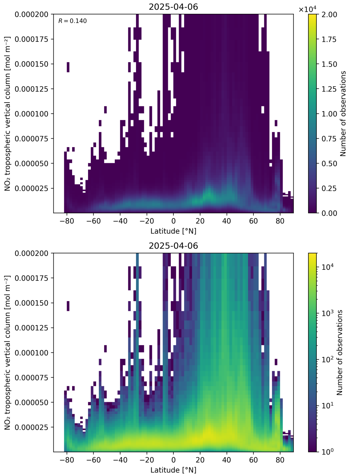
Figure 92: Scatter density plot of “Latitude” against “NO 2 tropospheric vertical column” for 2025-04-06 to 2025-04-06.
