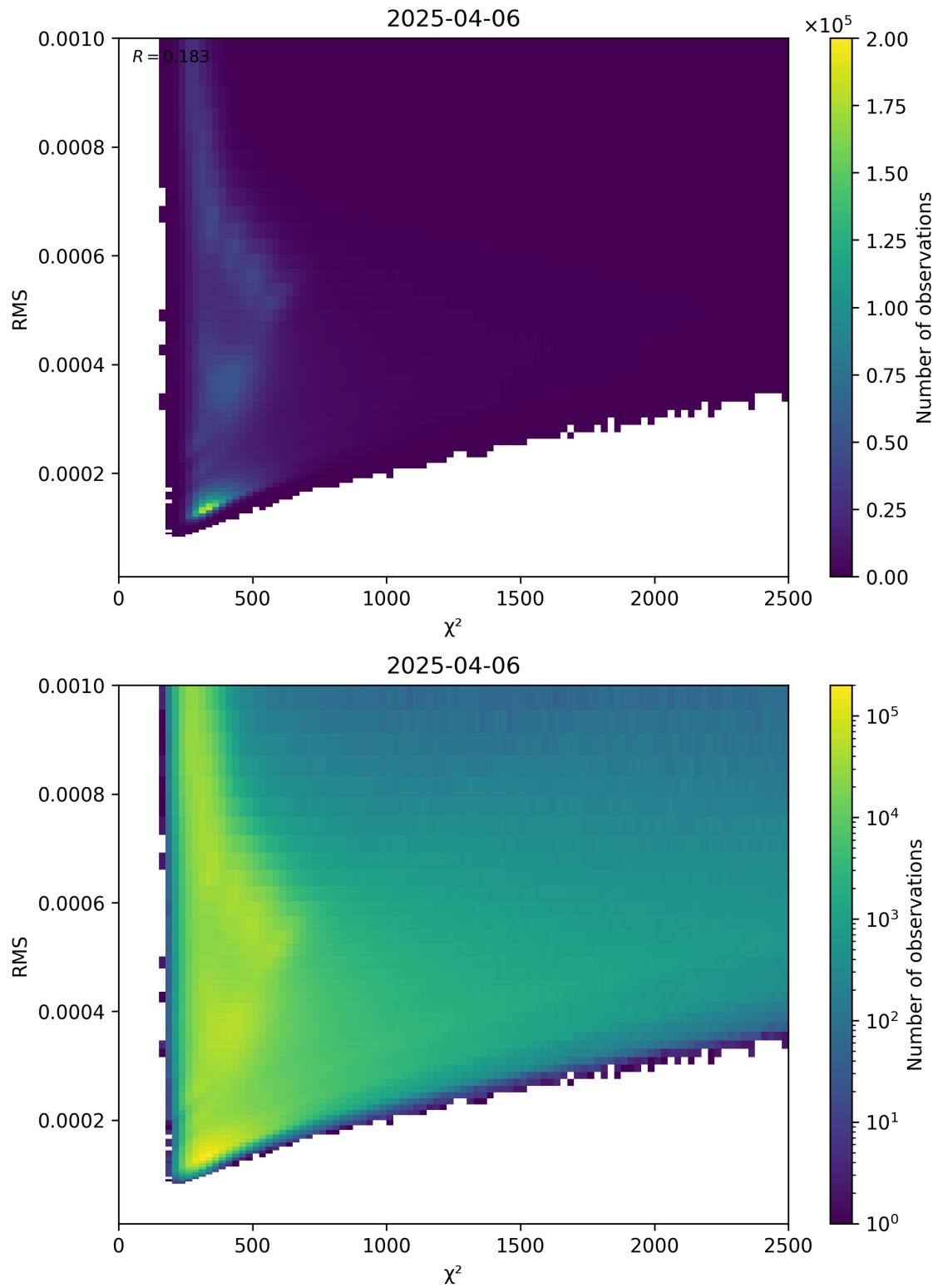
Figure 82: Scatter density plot of “ \chi^2 ” against “RMS” for 2025-04-06 to 2025-04-06.
