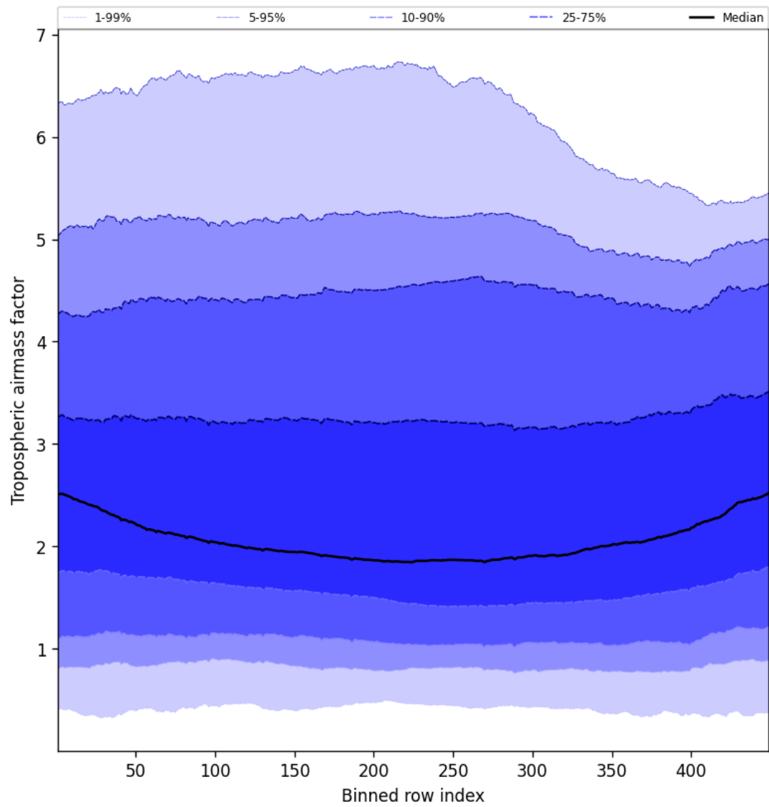
Figure 48: Along track statistics of “Tropospheric airmass factor” for 2025-04-06 to 2025-04-06
