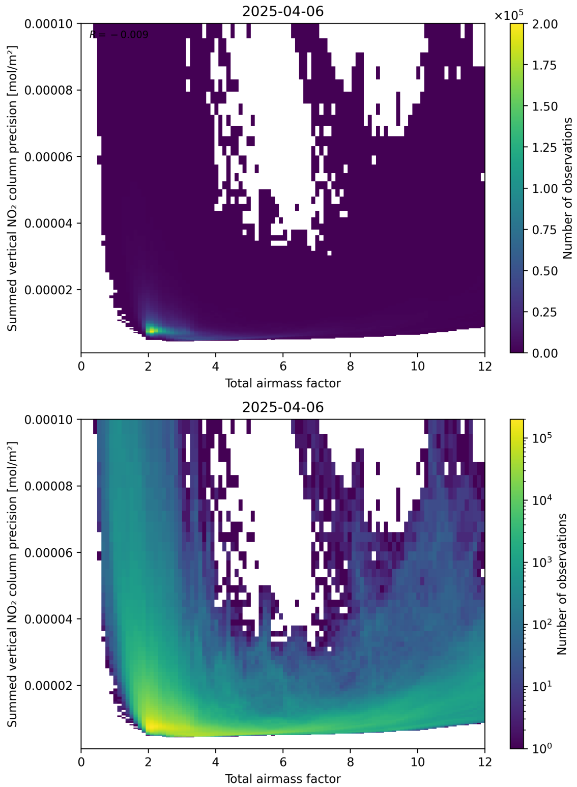
Figure 66: Scatter density plot of “Total airmass factor” against “Summed vertical NO 2 column precision” for 2025-04-06 to 2025-04-06.
