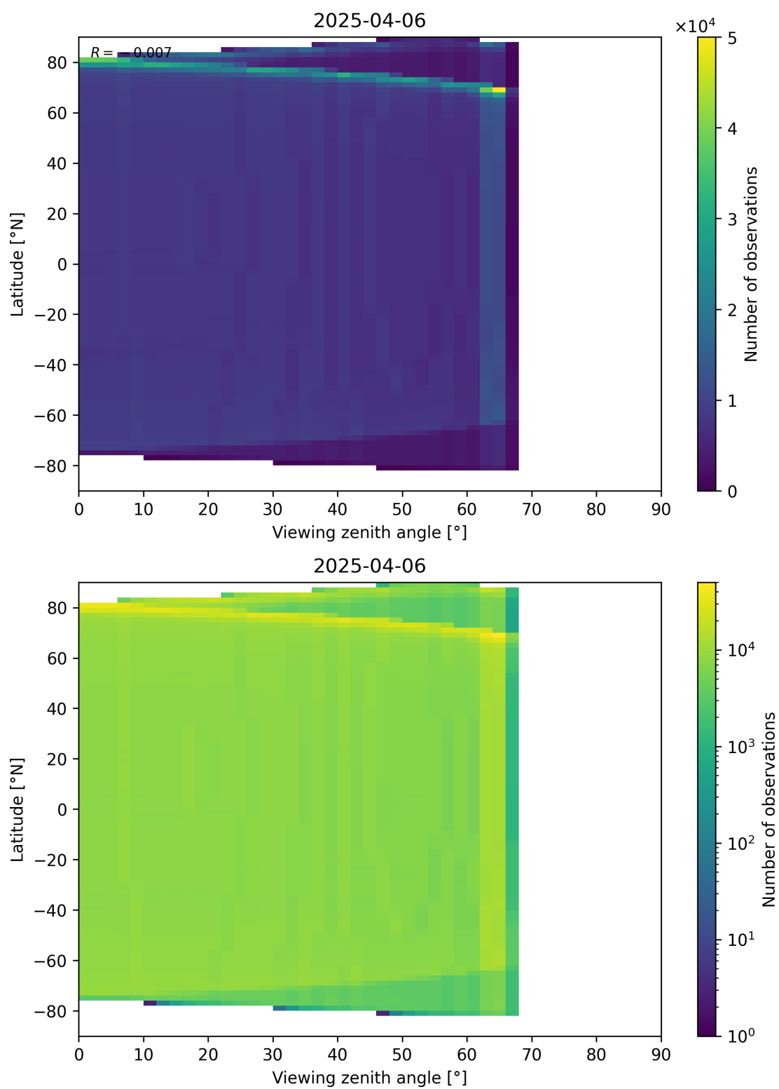
Figure 163: Scatter density plot of “Viewing zenith angle” against “Latitude” for 2025-04-06 to 2025-04-06.
