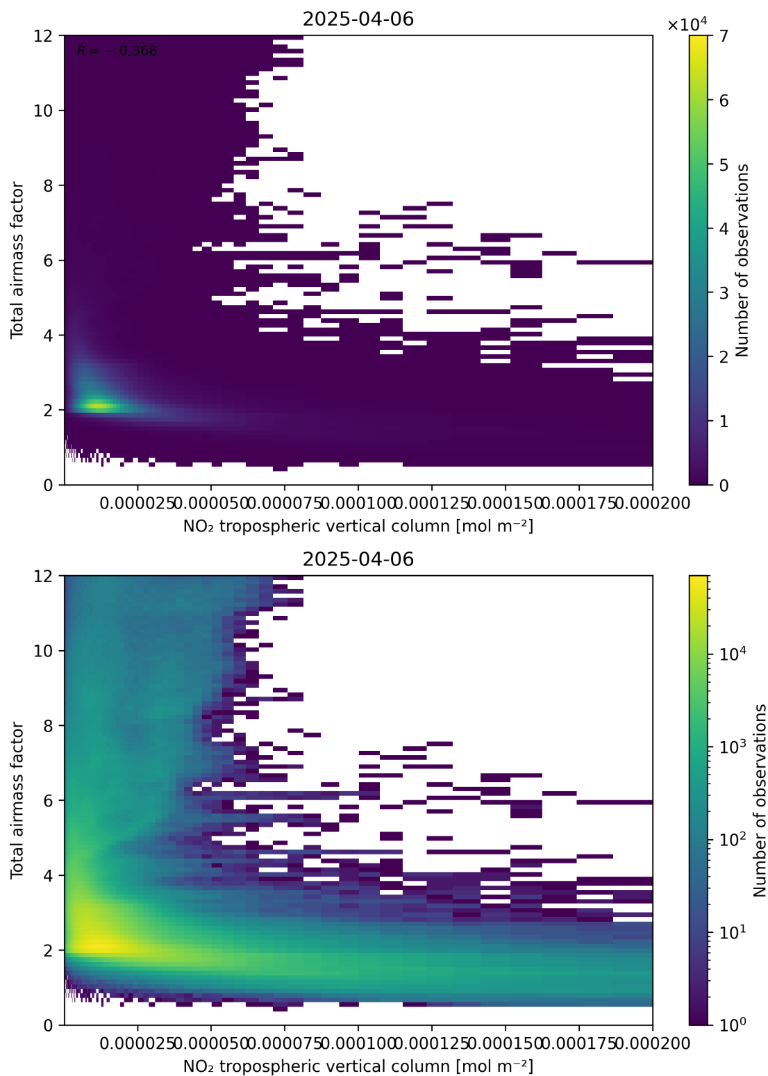
Figure 122: Scatter density plot of “NO 2 tropospheric vertical column” against “Total air mass factor” for 2025-04-06 to 2025-04-06.
