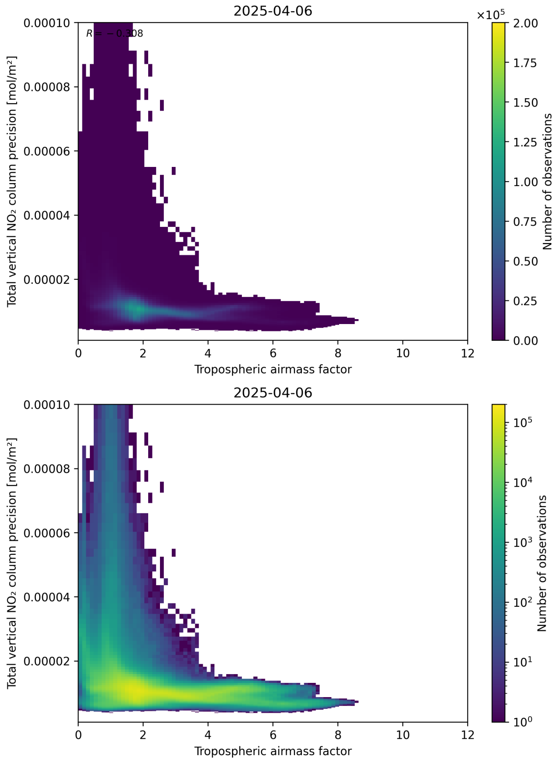
Figure 78: Scatter density plot of “Tropospheric air mass factor” against “Total vertical NO 2 column precision” for 2025-04-06 to 2025-04-06.
