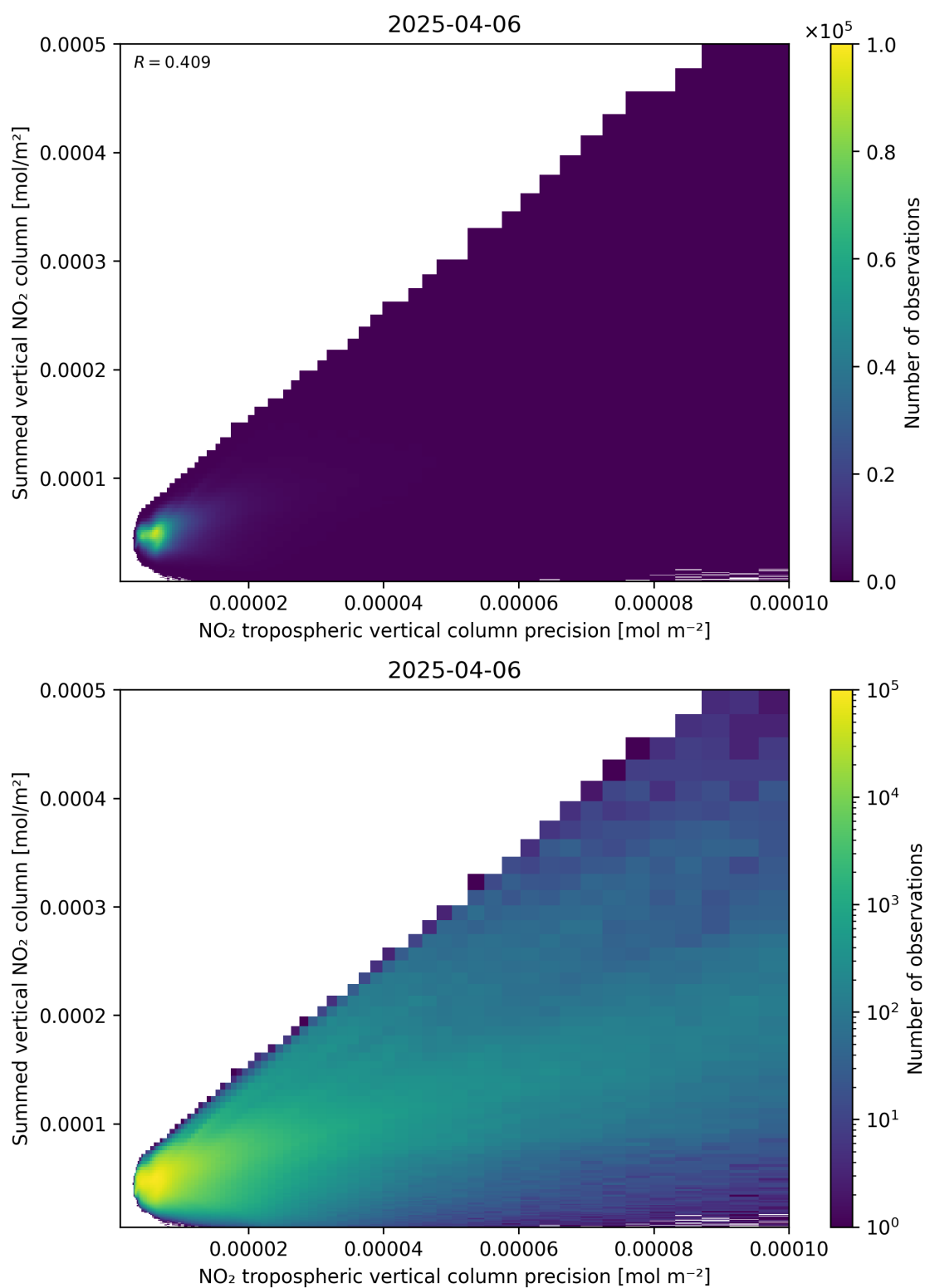
Figure 136: Scatter density plot of “NO 2 tropospheric vertical column precision” against “Summed vertical NO 2 column” for 2025-04-06 to 2025-04-06.
