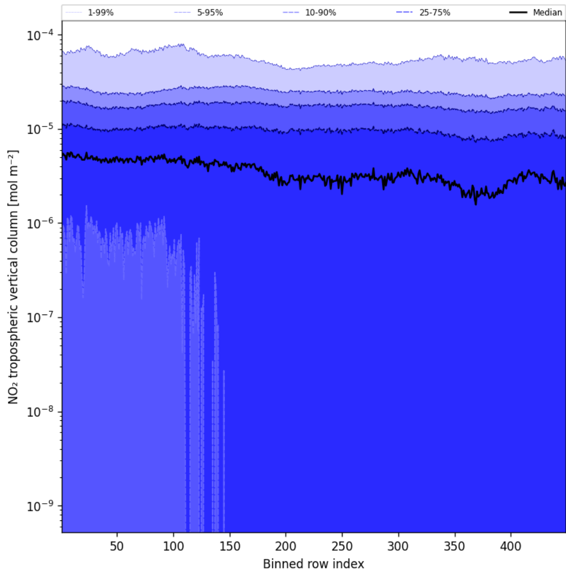
Figure 46: Along track statistics of “NO 2 tropospheric vertical column” for 2025-04-06 to 2025-04-06
