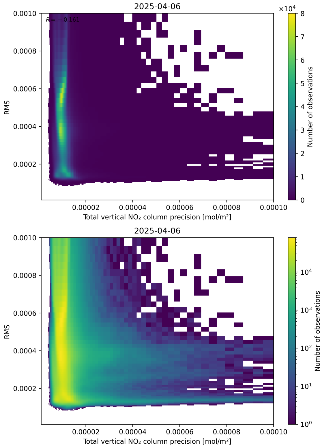
Figure 119: Scatter density plot of “Total vertical NO 2 column precision” against “RMS” for 2025-04-06 to 2025-04-06.
