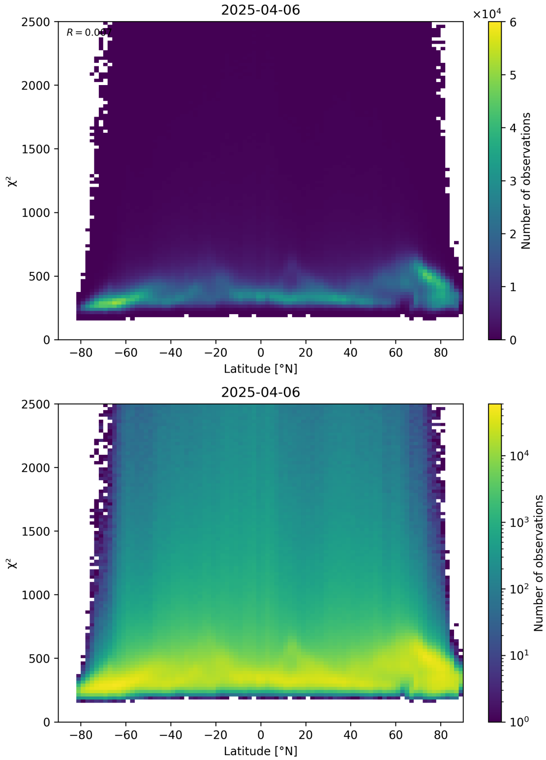
Figure 86: Scatter density plot of “Latitude” against “ \chi^2 ” for 2025-04-06 to 2025-04-06.
