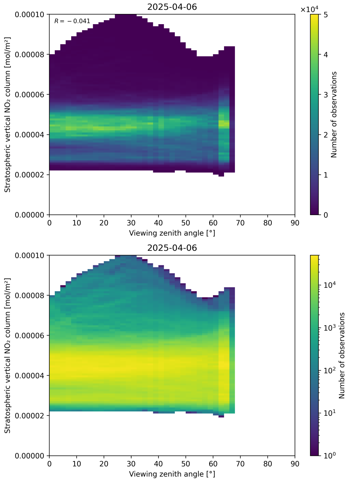
Figure 164: Scatter density plot of “Viewing zenith angle” against “Stratospheric vertical NO 2 column” for 2025-04-06 to 2025-04-06.
