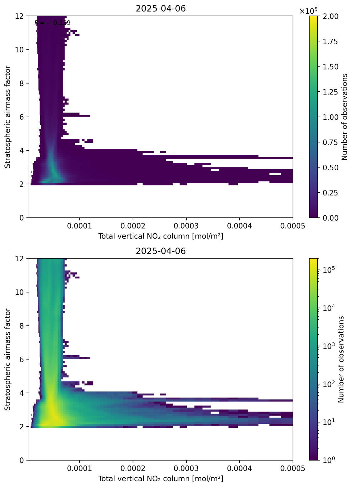
Figure 110: Scatter density plot of “Total vertical NO 2 column” against “Stratospheric airmass factor” for 2025-04-06 to 2025-04-06.
