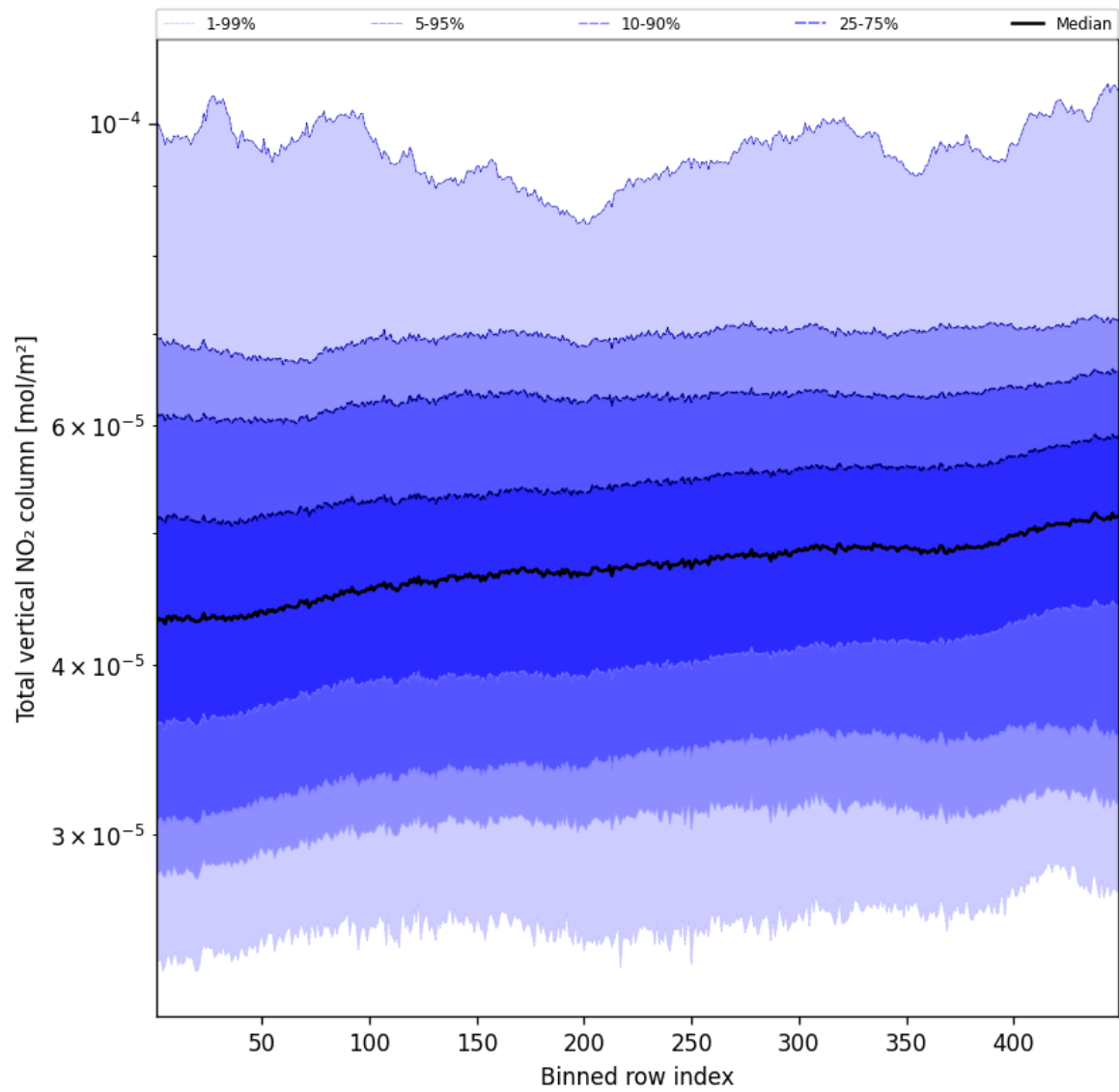
Figure 55: Along track statistics of “Total vertical NO 2 column” for 2025-04-06 to 2025-04-06
