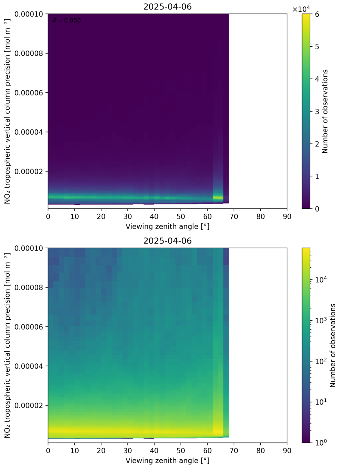
Figure 170: Scatter density plot of “Viewing zenith angle” against “NO 2 tropospheric vertical column precision” for 2025-04-06 to 2025-04-06.
