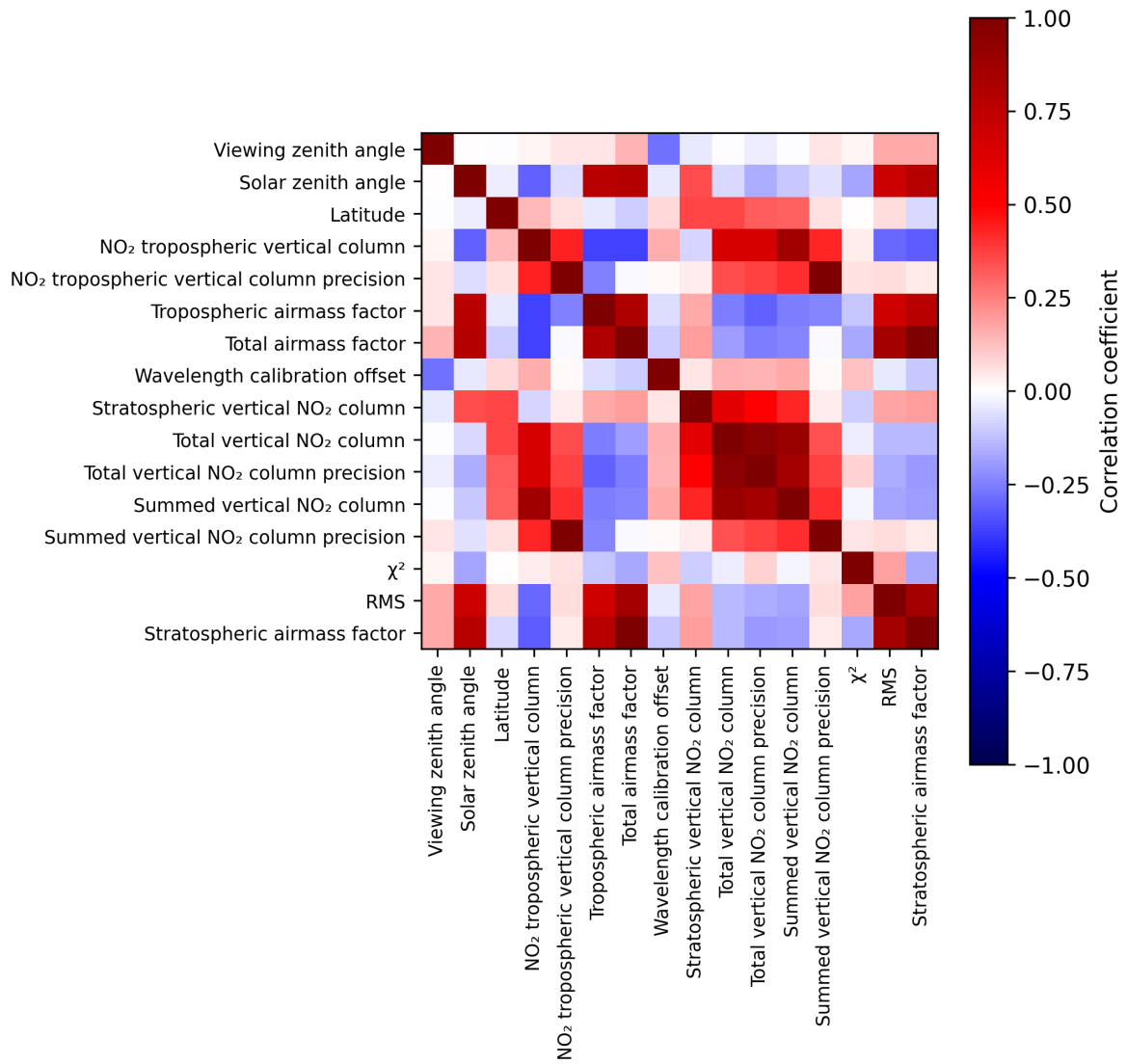
Figure 2: Map of correlation matrix for 2025-04-06 to 2025-04-06.
