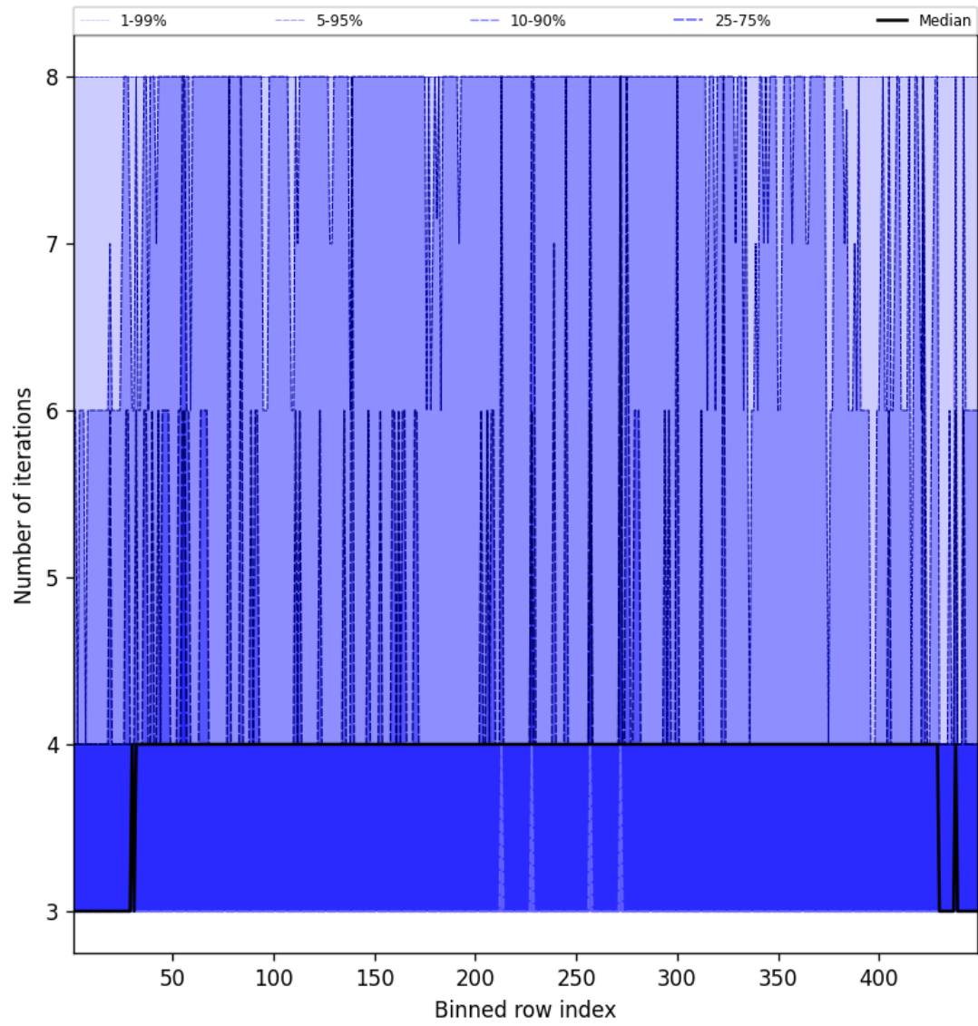
Figure 51: Along track statistics of “Number of iterations” for 2025-04-06 to 2025-04-06
