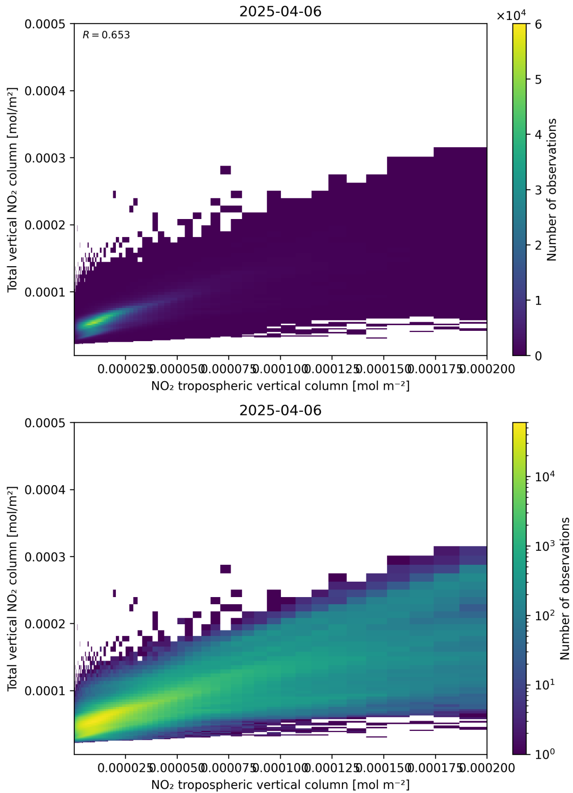
Figure 128: Scatter density plot of “NO 2 tropospheric vertical column” against “Total vertical NO 2 column” for 2025-04-06 to 2025-04-06.
