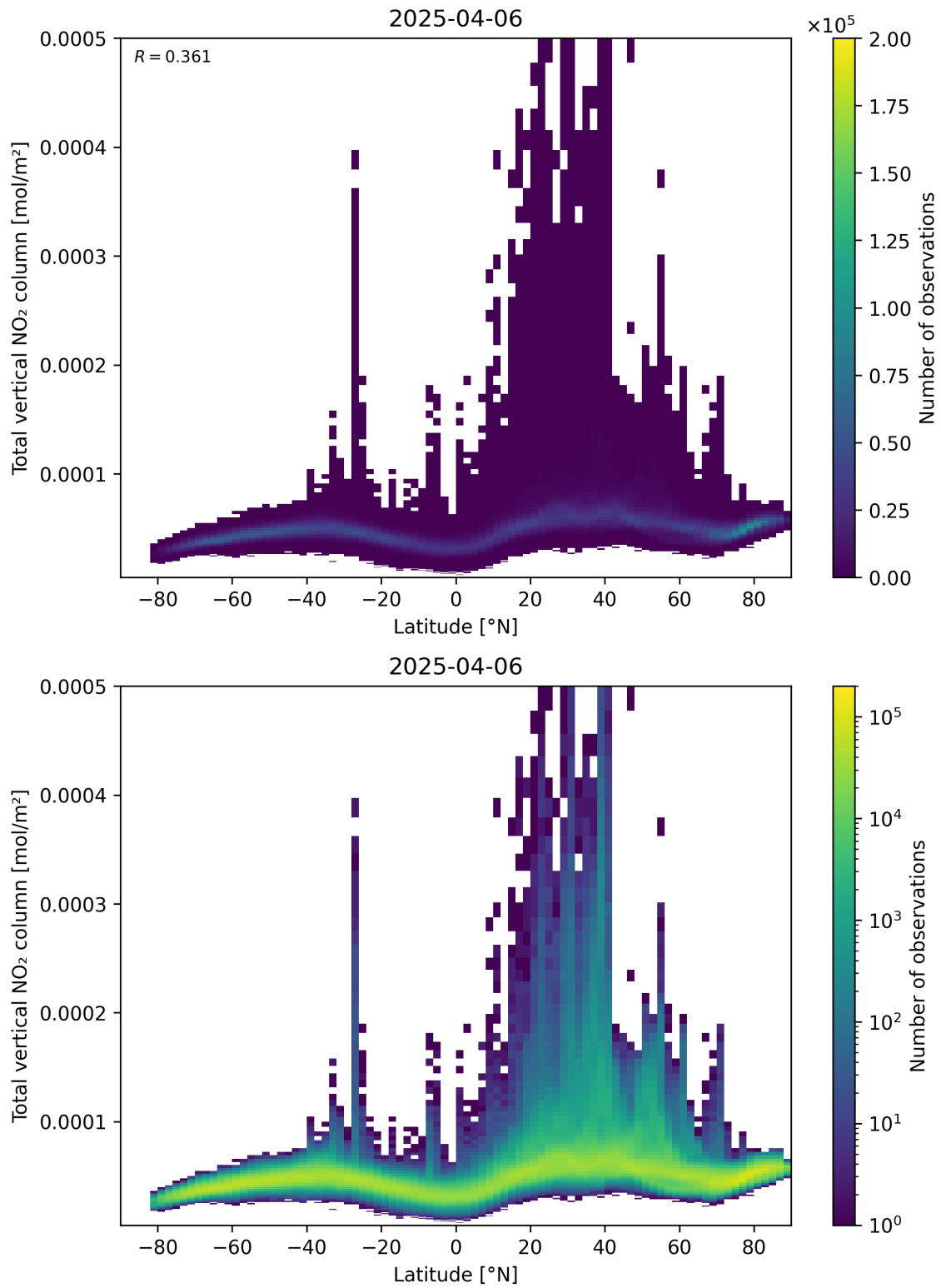
Figure 90: Scatter density plot of “Latitude” against “Total vertical NO 2 column” for 2025-04-06 to 2025-04-06.
