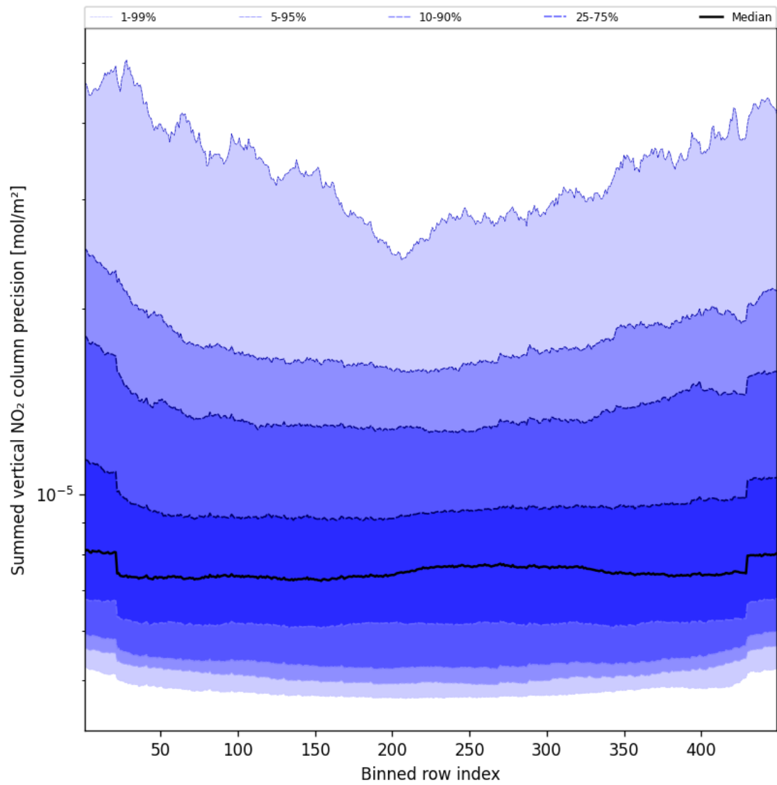
Figure 58: Along track statistics of “Summed vertical NO 2 column precision” for 2025-04-06 to 2025-04-06
