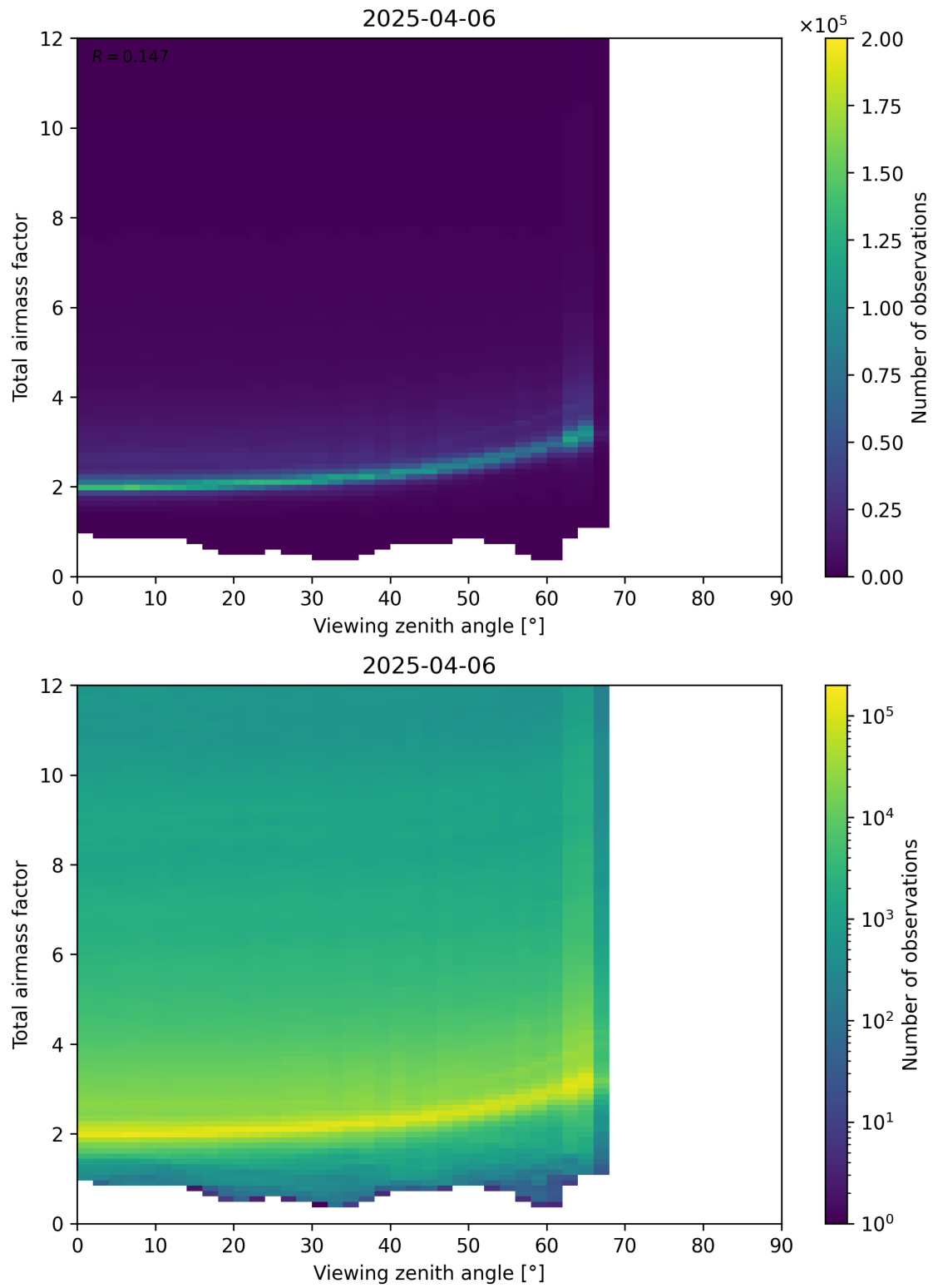
Figure 160: Scatter density plot of “Viewing zenith angle” against “Total airmass factor” for 2025-04-06 to 2025-04-06.
