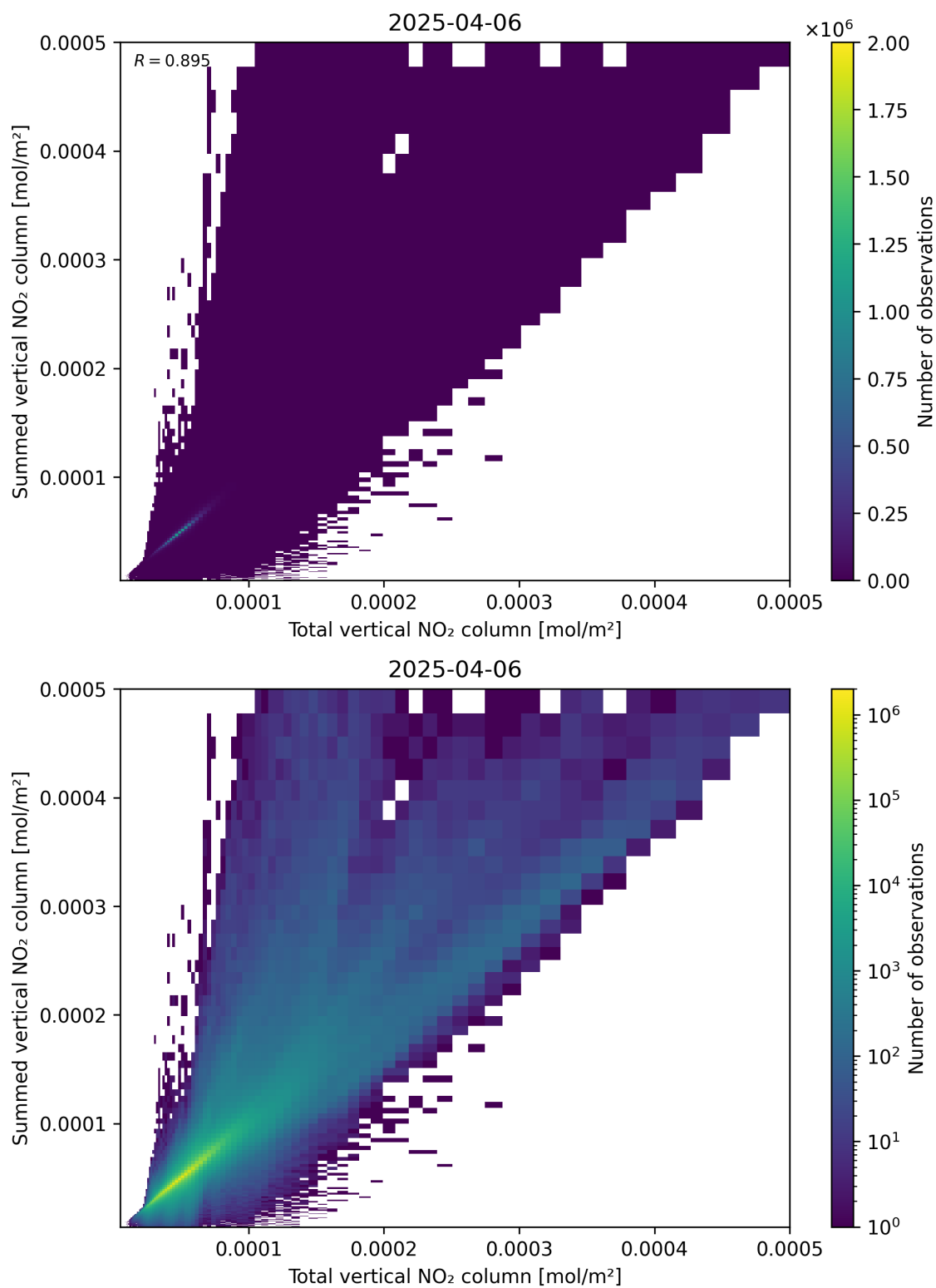
Figure 112: Scatter density plot of “Total vertical NO 2 column” against “Summed vertical NO 2 column” for 2025-04-06 to 2025-04-06.
