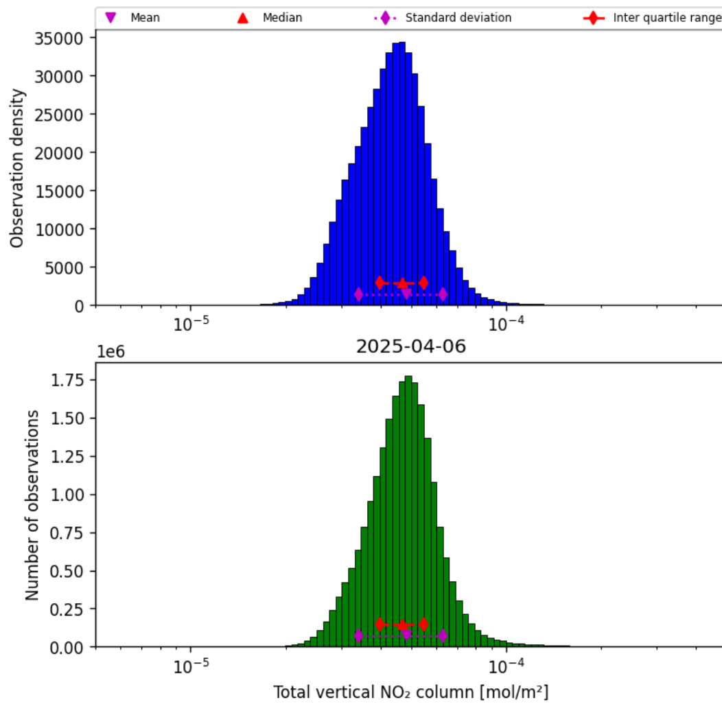
Figure 38: Histogram of “Total vertical NO 2 column” for 2025-04-06 to 2025-04-06
