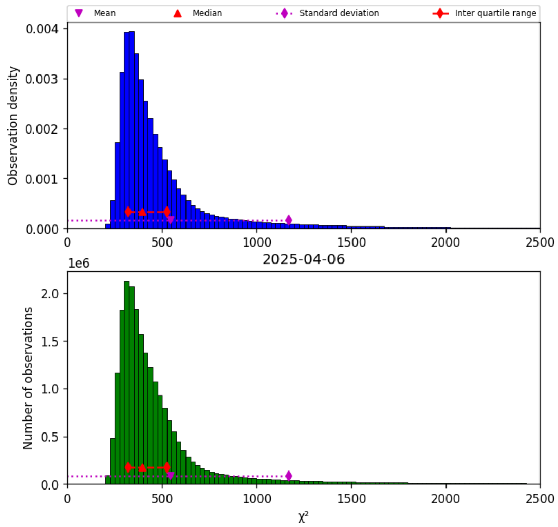
Figure 42: Histogram of “ \chi^2 ” for 2025-04-06 to 2025-04-06
