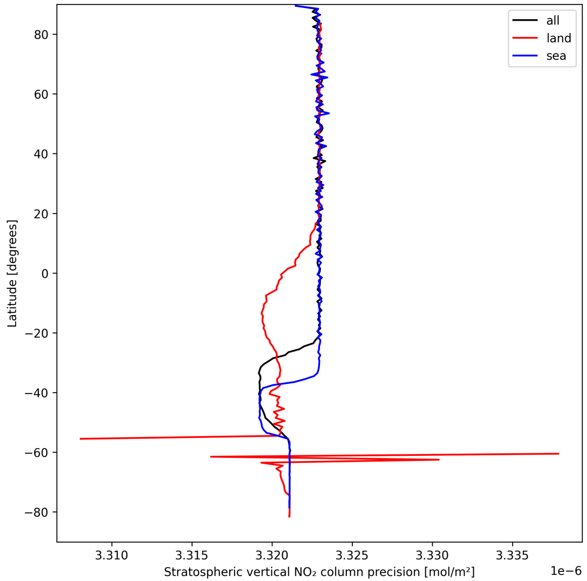
Figure 20: Zonal average of “Stratospheric vertical NO 2 column precision” for 2025-04-06 to 2025-04-06.
