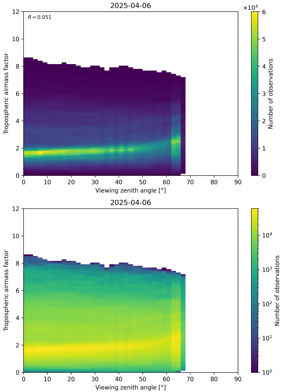
Figure 161: Scatter density plot of “Viewing zenith angle” against “Tropospheric airmass factor” for 2025-04-06 to 2025-04-06.
