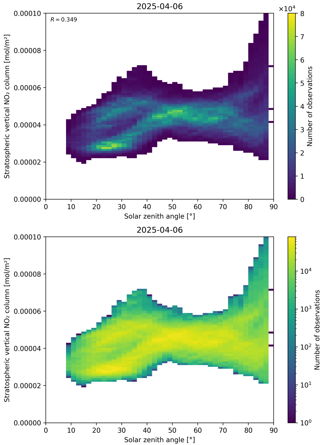
Figure 150: Scatter density plot of “Solar zenith angle” against “Stratospheric vertical NO 2 column” for 2025-04-06 to 2025-04-06.
