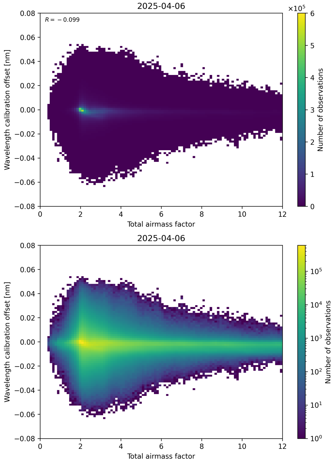
Figure 70: Scatter density plot of “Total airmass factor” against “Wavelength calibration offset” for 2025-04-06 to 2025-04-06.
