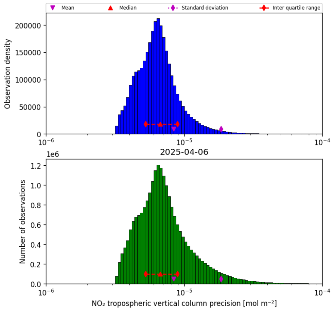
Figure 30: Histogram of “NO 2 tropospheric vertical column precision” for 2025-04-06 to 2025-04-06
