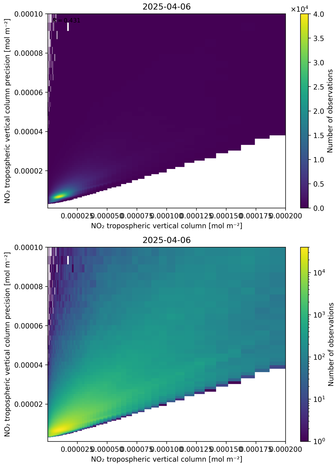
Figure 130: Scatter density plot of “NO 2 tropospheric vertical column” against “NO 2 tropospheric vertical column precision” for 2025-04-06 to 2025-04-06.
