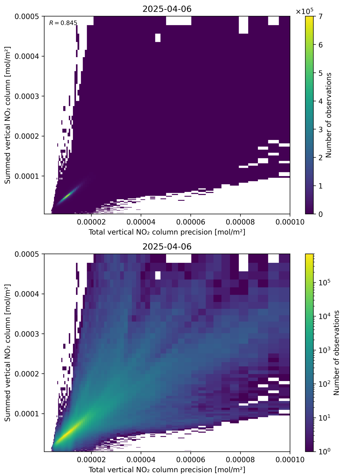
Figure 117: Scatter density plot of “Total vertical NO 2 column precision” against “Summed vertical NO 2 column” for 2025-04-06 to 2025-04-06.
