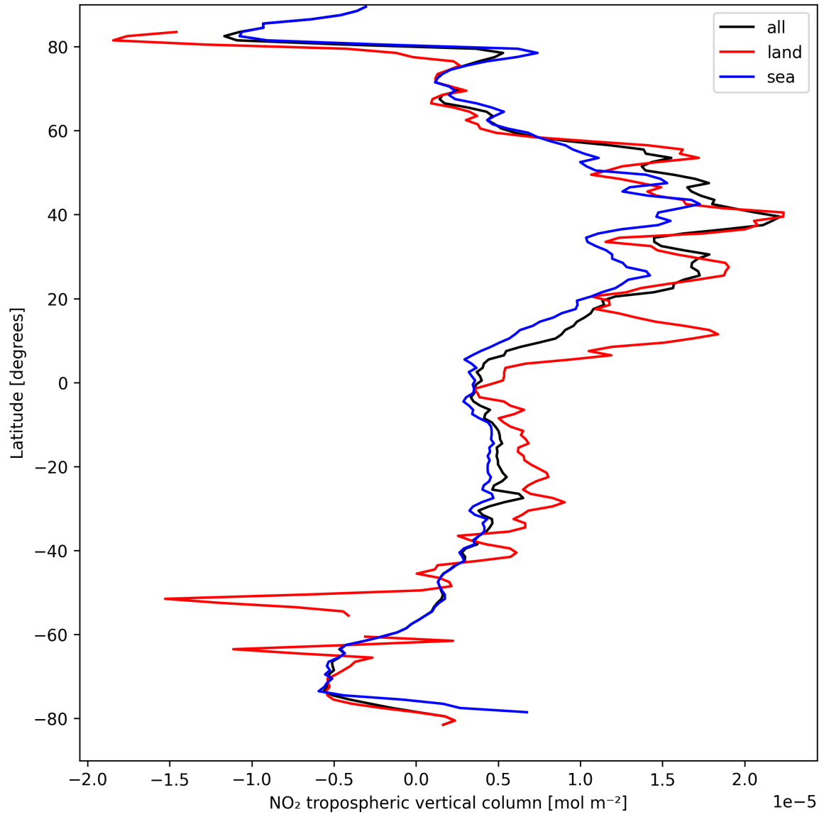
Figure 12: Zonal average of “NO 2 tropospheric vertical column” for 2025-04-06 to 2025-04-06.
