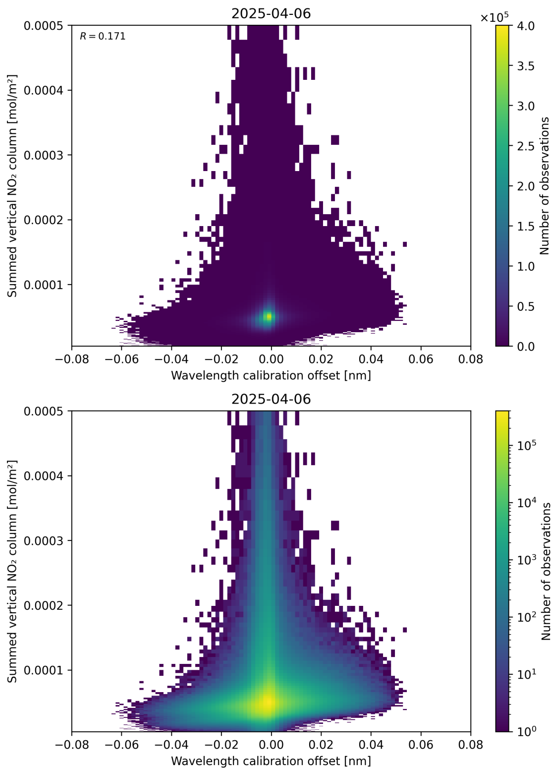
Figure 177: Scatter density plot of “Wavelength calibration offset” against “Summed vertical NO 2 column” for 2025-04-06 to 2025-04-06.
