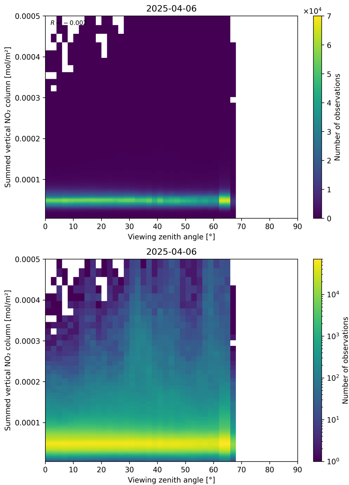
Figure 165: Scatter density plot of “Viewing zenith angle” against “Summed vertical NO 2 column” for 2025-04-06 to 2025-04-06.
