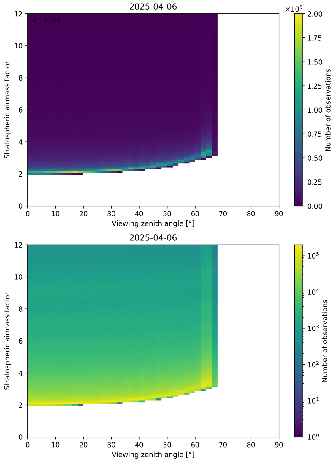
Figure 159: Scatter density plot of “Viewing zenith angle” against “Stratospheric airmass factor” for 2025-04-06 to 2025-04-06.
