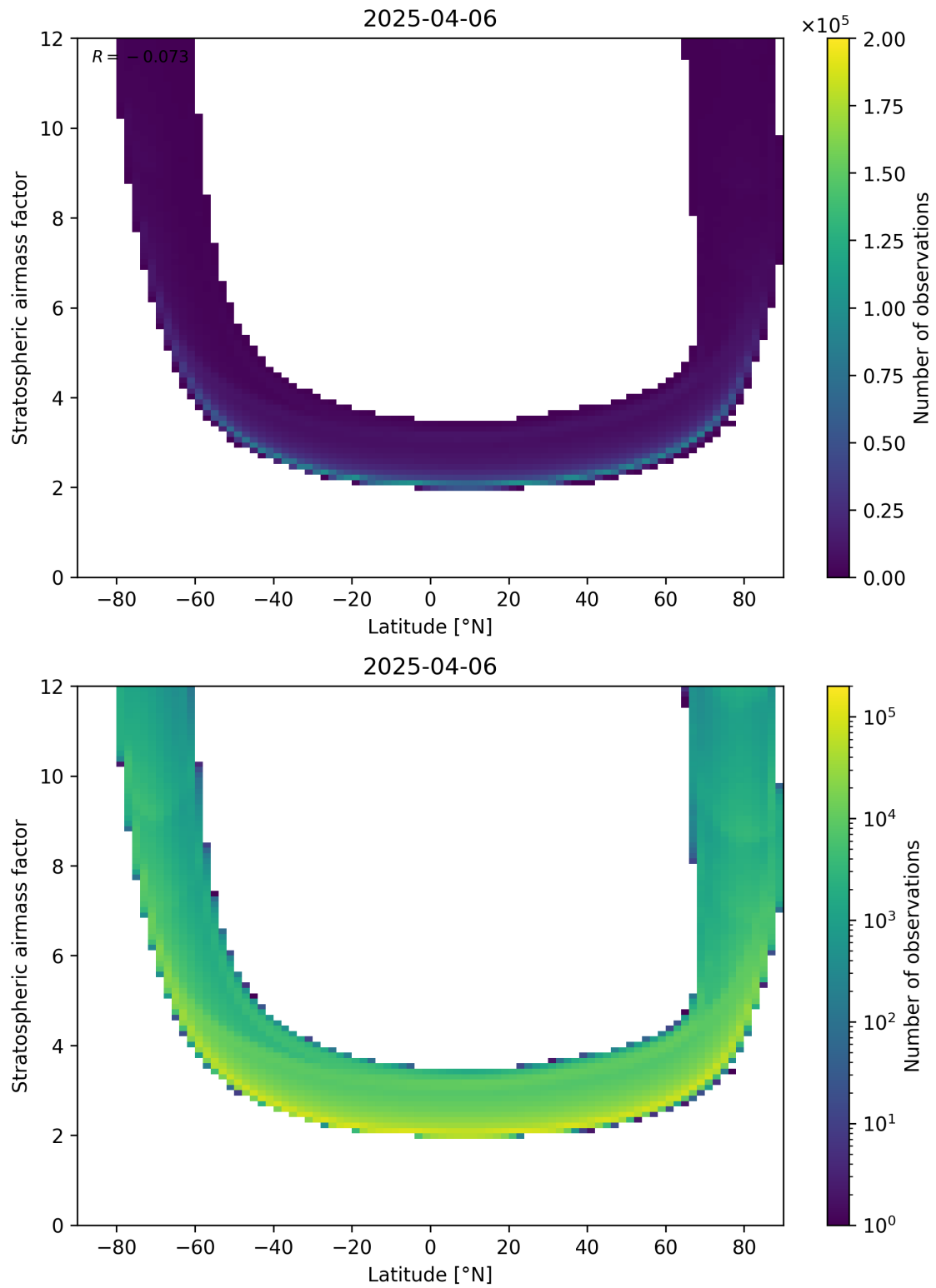
Figure 83: Scatter density plot of “Latitude” against “Stratospheric air mass factor” for 2025-04-06 to 2025-04-06.
