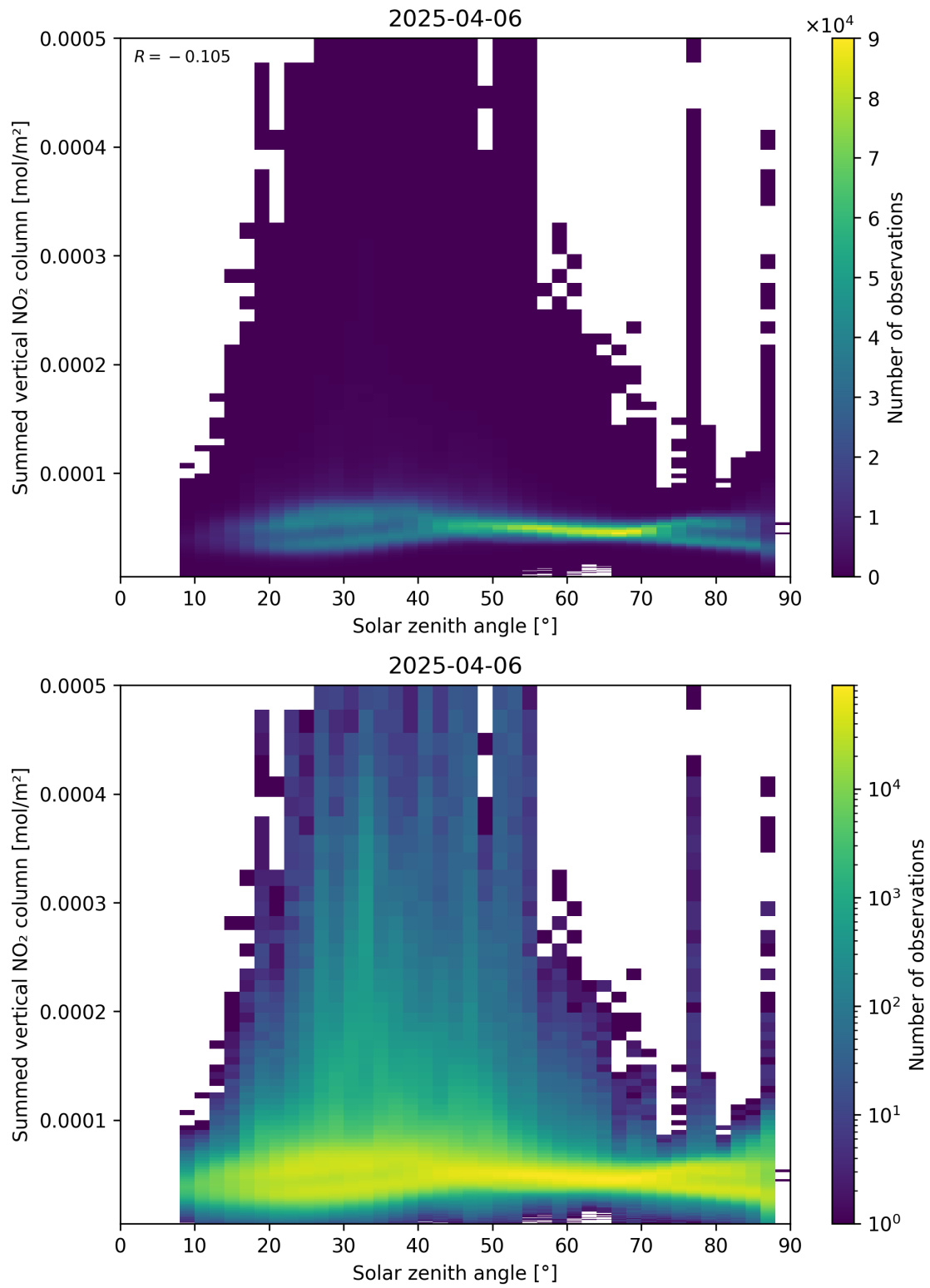
Figure 151: Scatter density plot of “Solar zenith angle” against “Summed vertical NO 2 column” for 2025-04-06 to 2025-04-06.
