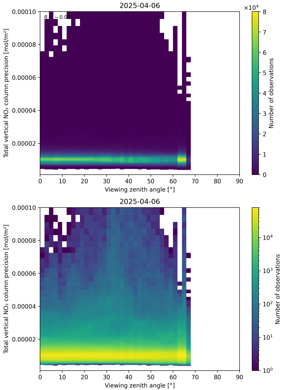
Figure 168: Scatter density plot of “Viewing zenith angle” against “Total vertical NO 2 column precision” for 2025-04-06 to 2025-04-06.
