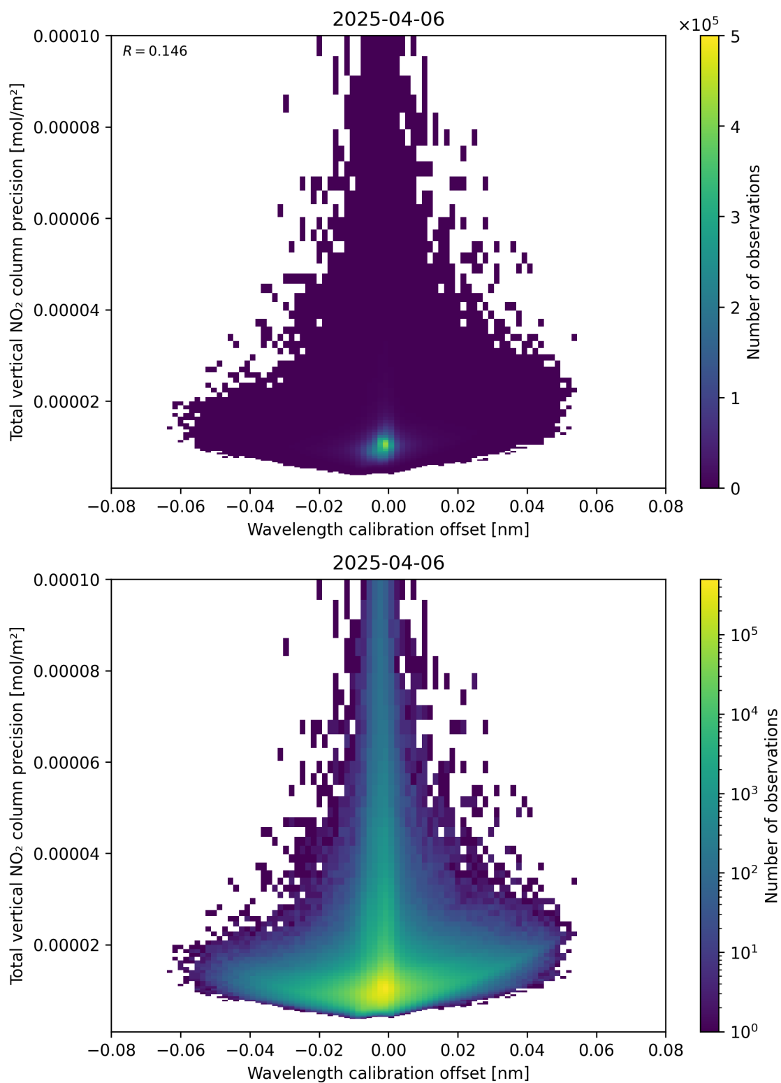
Figure 180: Scatter density plot of “Wavelength calibration offset” against “Total vertical NO 2 column precision” for 2025-04-06 to 2025-04-06.
