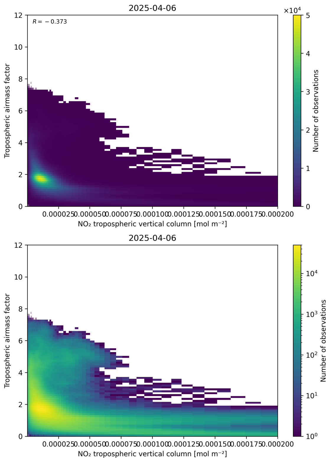
Figure 123: Scatter density plot of “NO 2 tropospheric vertical column” against “Tropospheric air mass factor” for 2025-04-06 to 2025-04-06.
