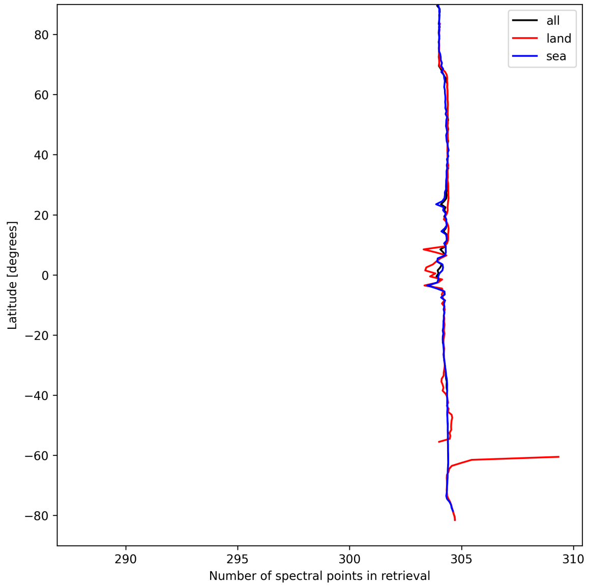
Figure 16: Zonal average of “Number of spectral points in retrieval” for 2025-04-06 to 2025-04-06.
