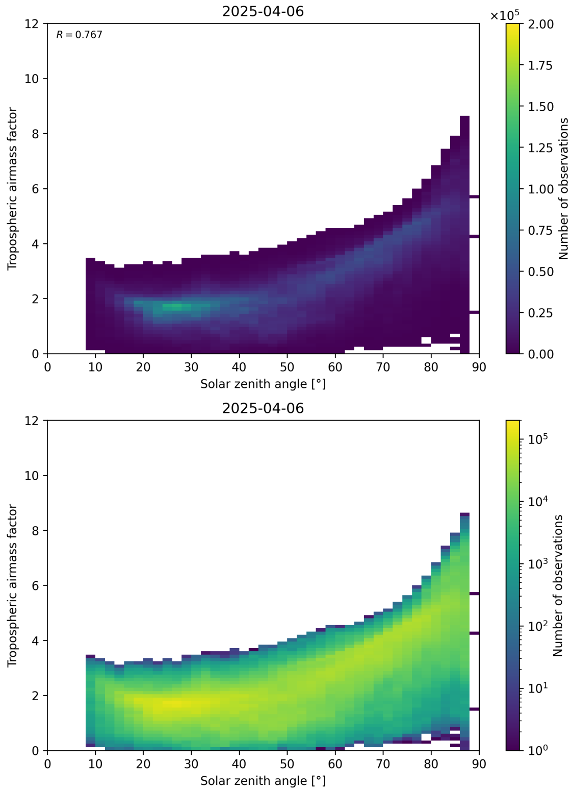
Figure 147: Scatter density plot of “Solar zenith angle” against “Tropospheric airmass factor” for 2025-04-06 to 2025-04-06.
