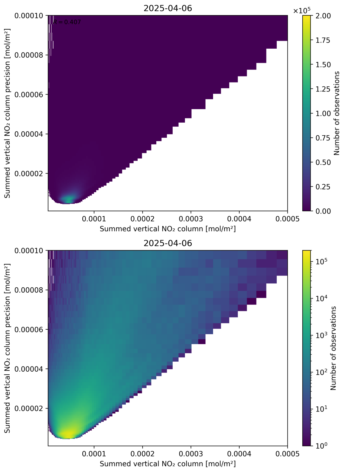
Figure 105: Scatter density plot of “Summed vertical NO 2 column” against “Summed vertical NO 2 column precision” for 2025-04-06 to 2025-04-06.
