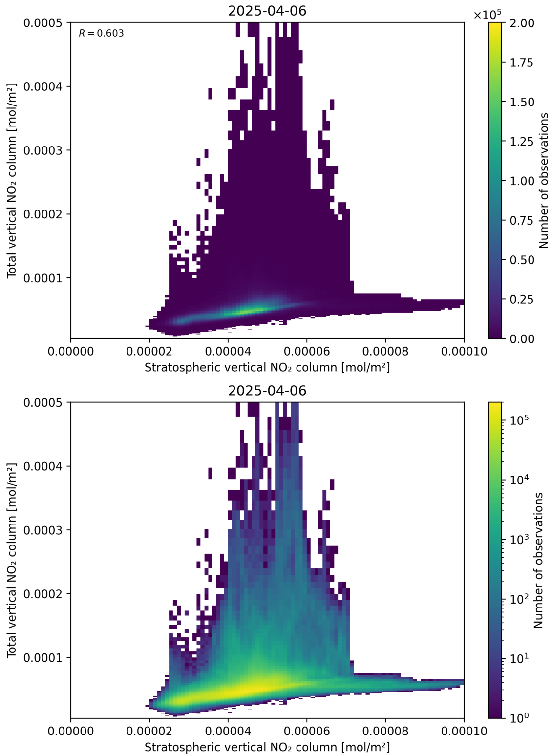
Figure 100: Scatter density plot of “Stratospheric vertical NO 2 column” against “Total vertical NO 2 column” for 2025-04-06 to 2025-04-06.
