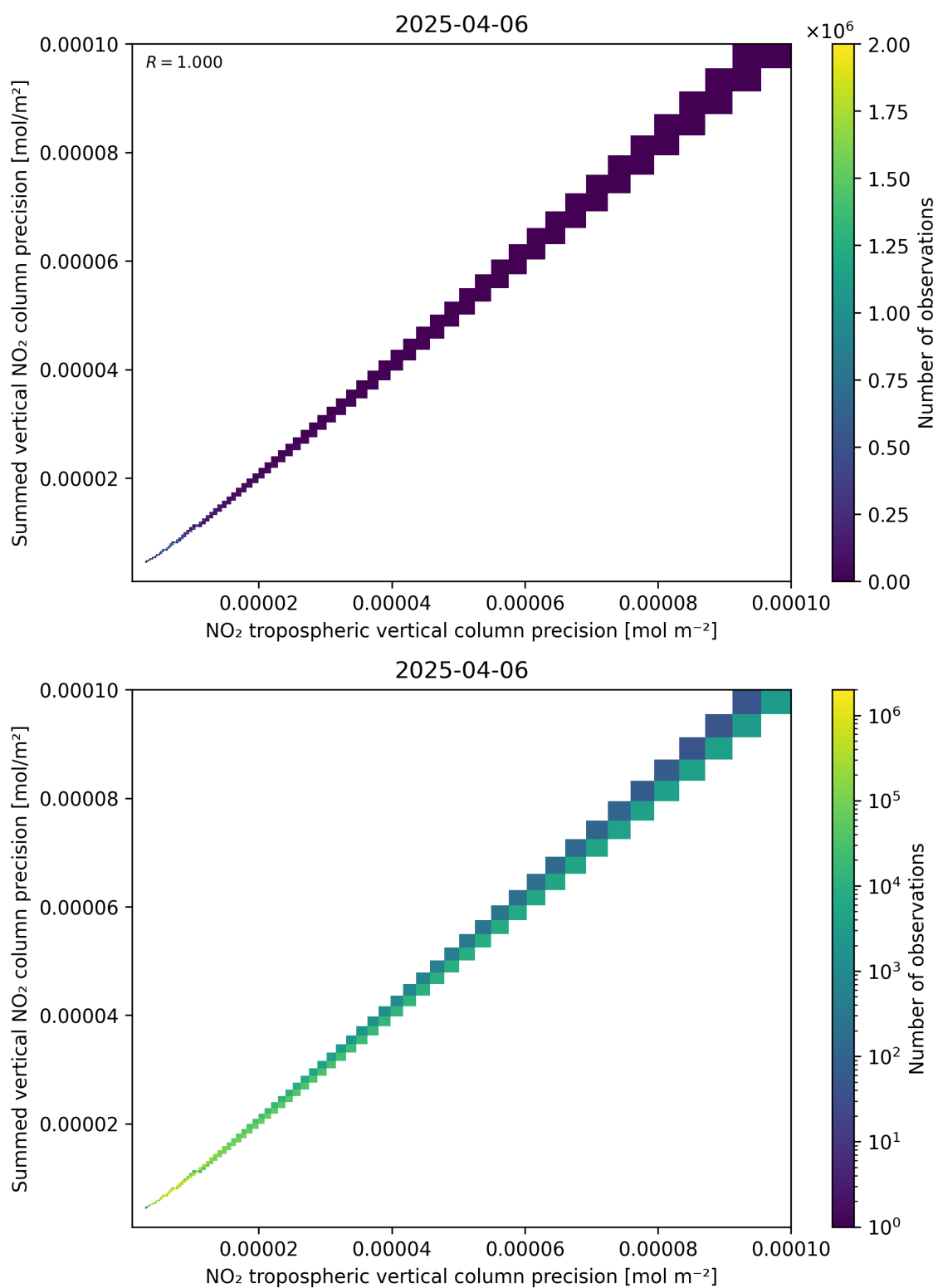
Figure 137: Scatter density plot of “NO 2 tropospheric vertical column precision” against “Summed vertical NO 2 column precision” for 2025-04-06 to 2025-04-06.
