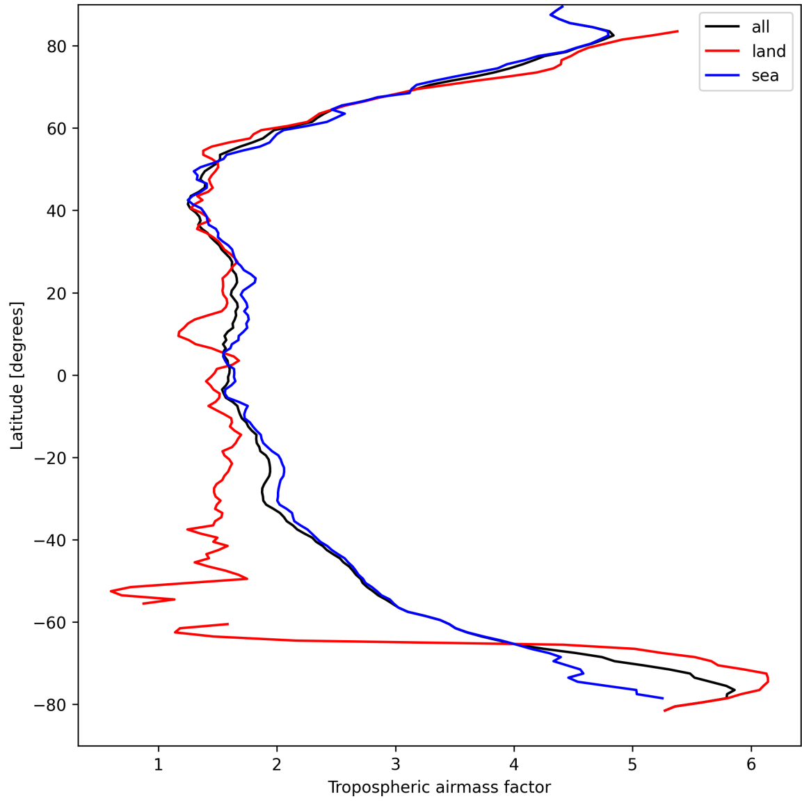
Figure 14: Zonal average of “Tropospheric air mass factor” for 2025-04-06 to 2025-04-06.
