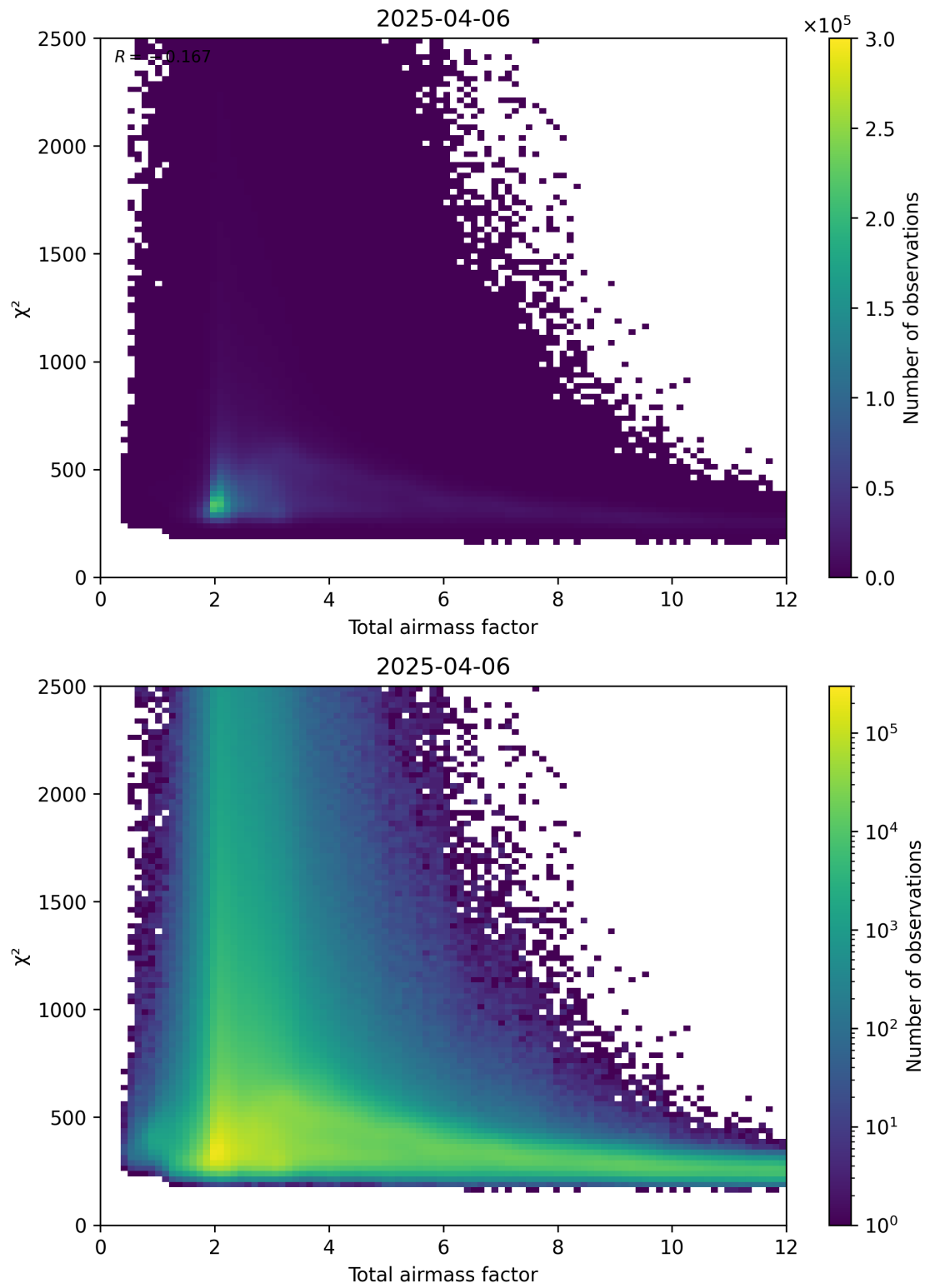
Figure 63: Scatter density plot of “Total airmass factor” against “ \chi^2 ” for 2025-04-06 to 2025-04-06.
