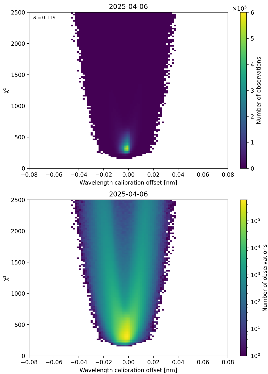
Figure 175: Scatter density plot of “Wavelength calibration offset” against “ \chi^2 ” for 2025-04-06 to 2025-04-06.
