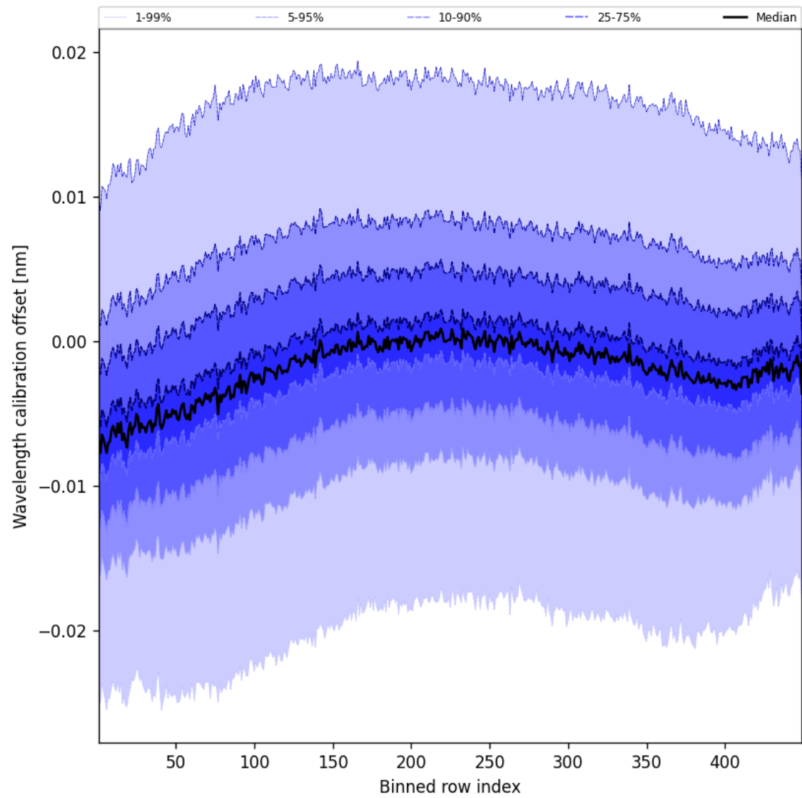
Figure 52: Along track statistics of “Wavelength calibration offset” for 2025-04-06 to 2025-04-06
