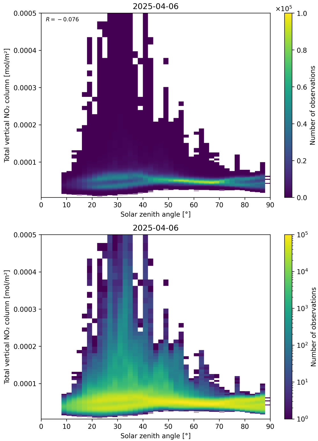
Figure 153: Scatter density plot of “Solar zenith angle” against “Total vertical NO 2 column” for 2025-04-06 to 2025-04-06.
