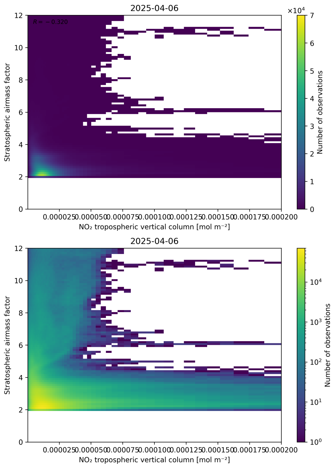
Figure 121: Scatter density plot of “NO 2 tropospheric vertical column” against “Stratospheric air mass factor” for 2025-04-06 to 2025-04-06.
