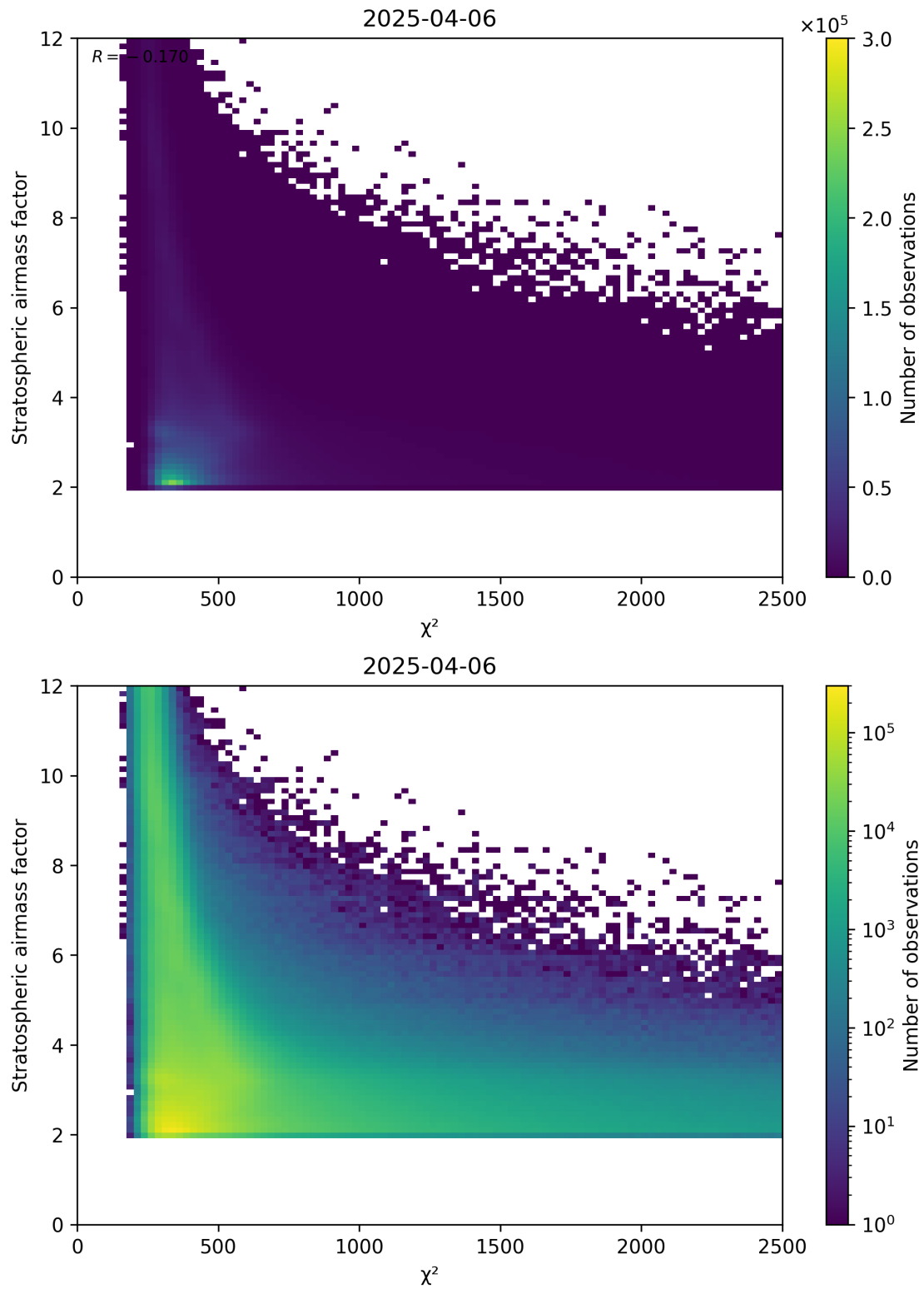
Figure 81: Scatter density plot of “ \chi^2 ” against “Stratospheric airmass factor” for 2025-04-06 to 2025-04-06.
