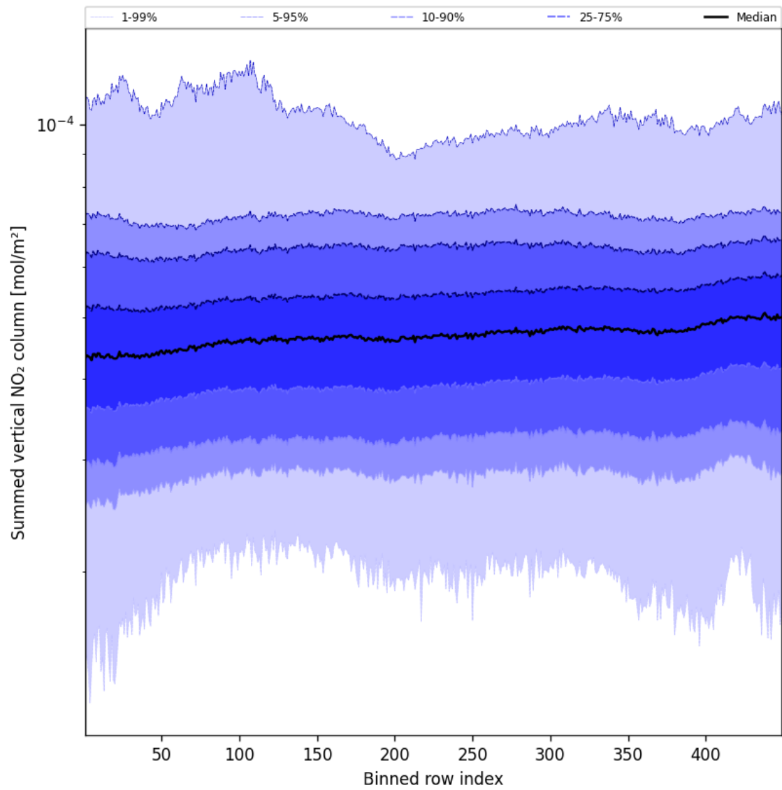
Figure 57: Along track statistics of “Summed vertical NO 2 column” for 2025-04-06 to 2025-04-06
