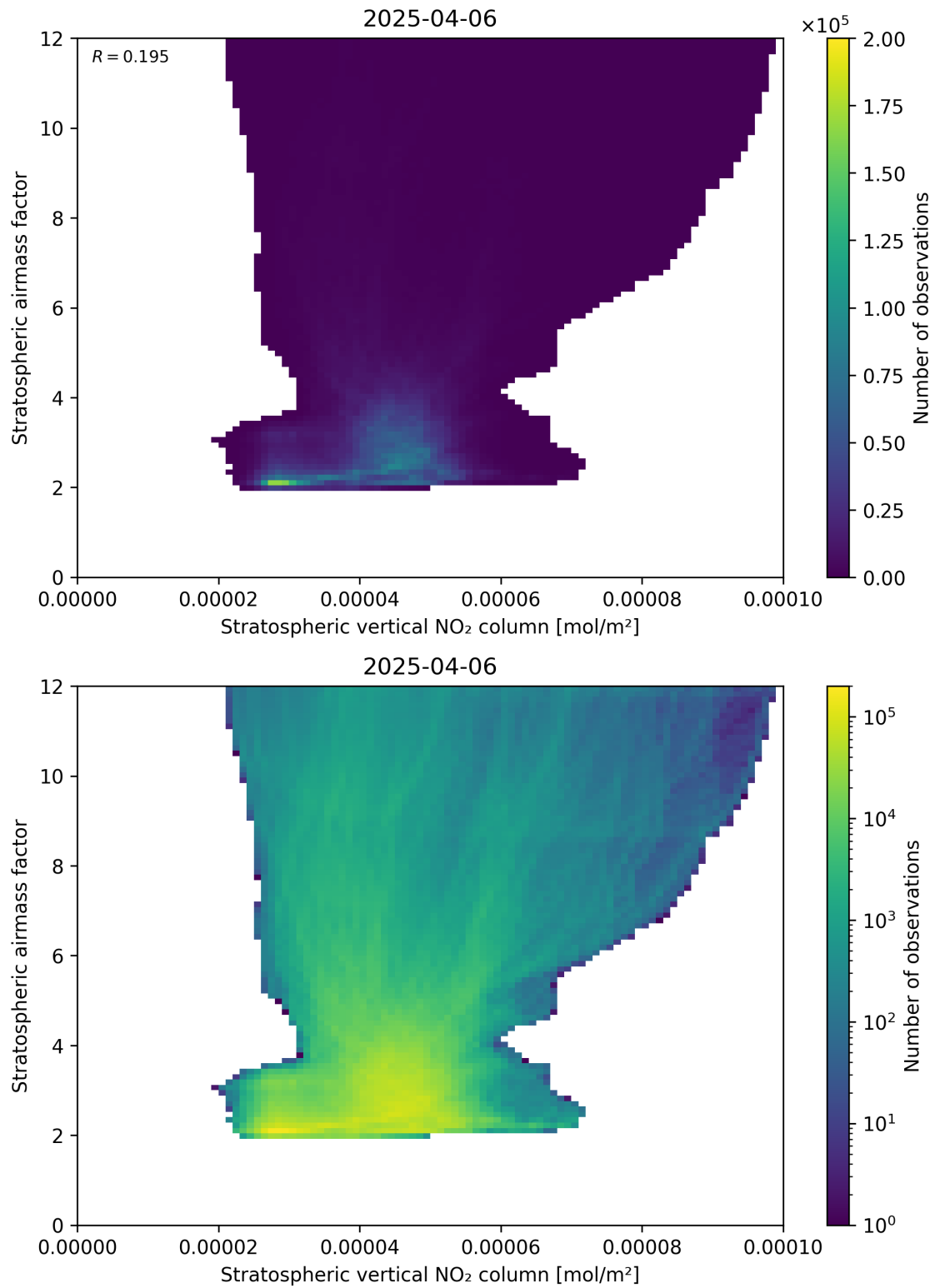
Figure 96: Scatter density plot of “Stratospheric vertical NO 2 column” against “Stratospheric airmass factor” for 2025-04-06 to 2025-04-06.
