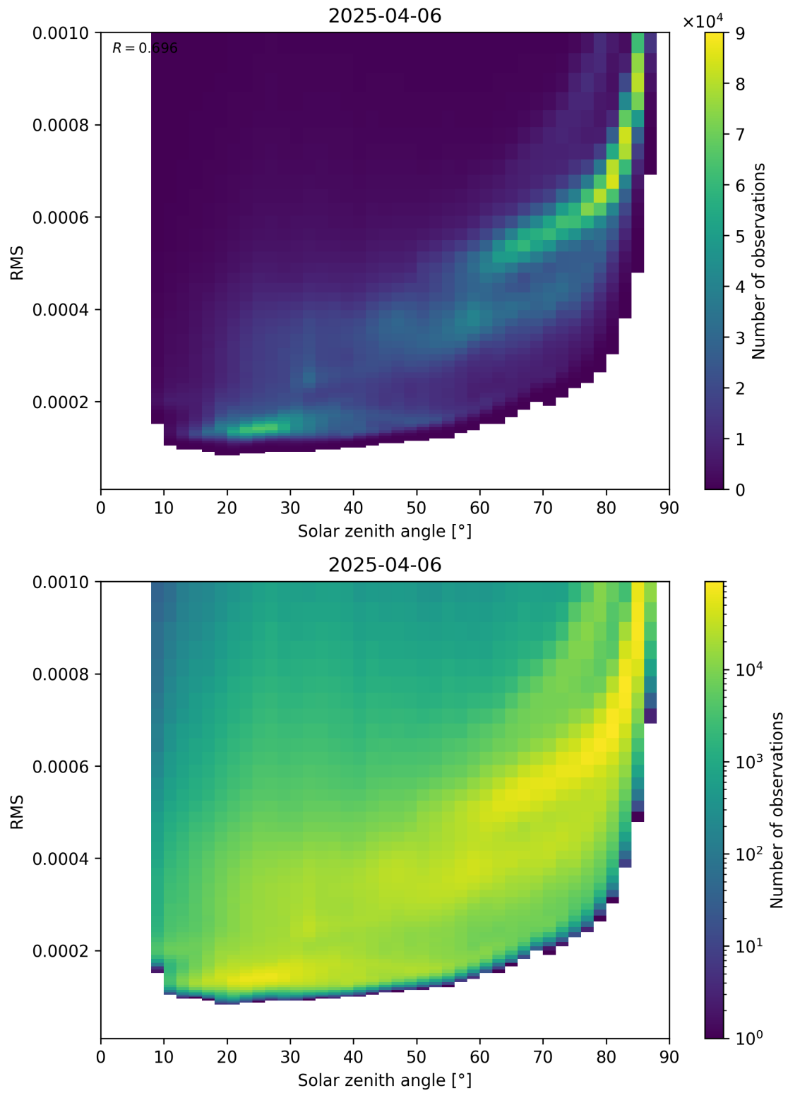
Figure 157: Scatter density plot of “Solar zenith angle” against “RMS” for 2025-04-06 to 2025-04-06.
