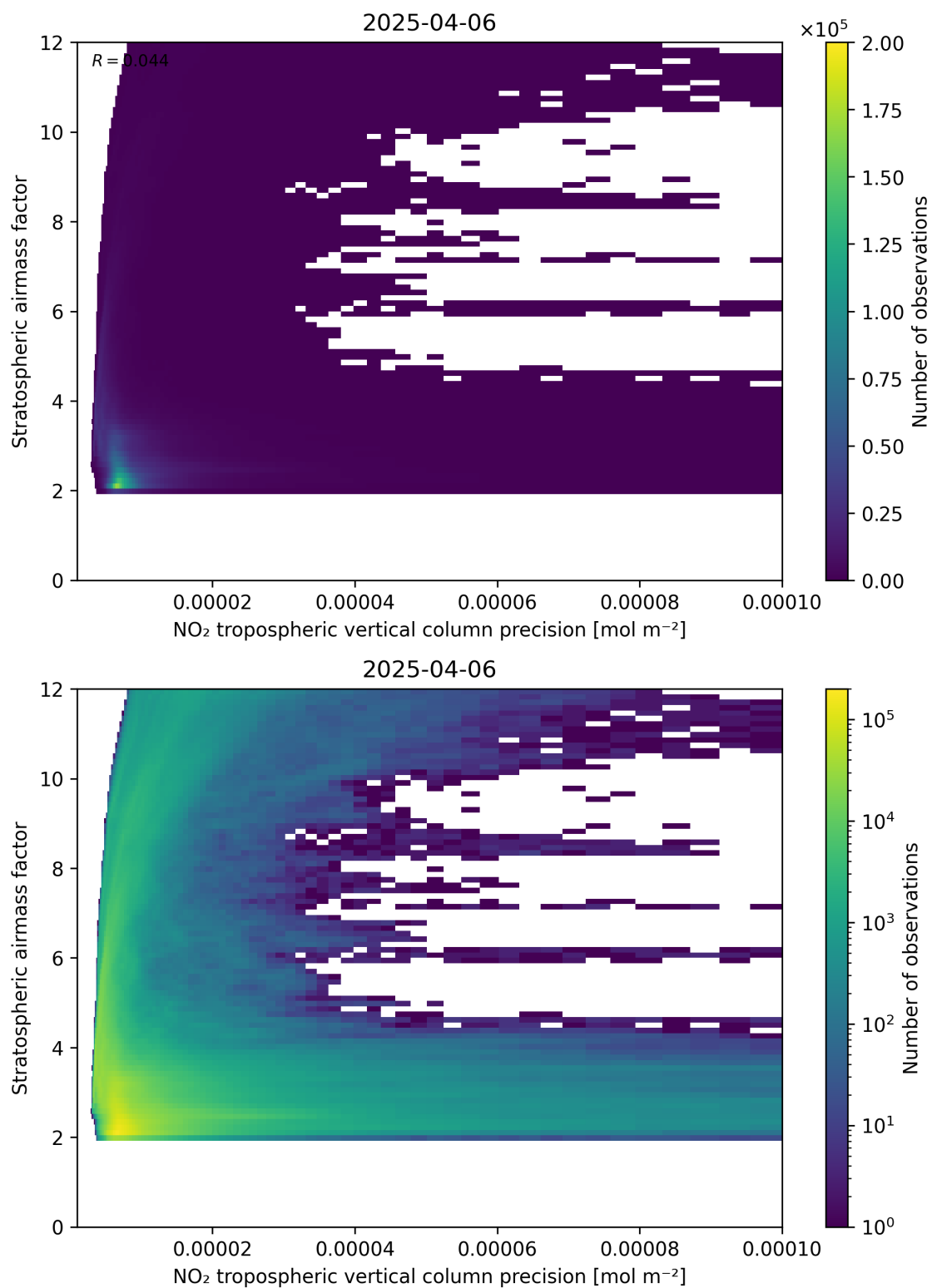
Figure 131: Scatter density plot of “NO 2 tropospheric vertical column precision” against “Stratospheric airmass factor” for 2025-04-06 to 2025-04-06.
