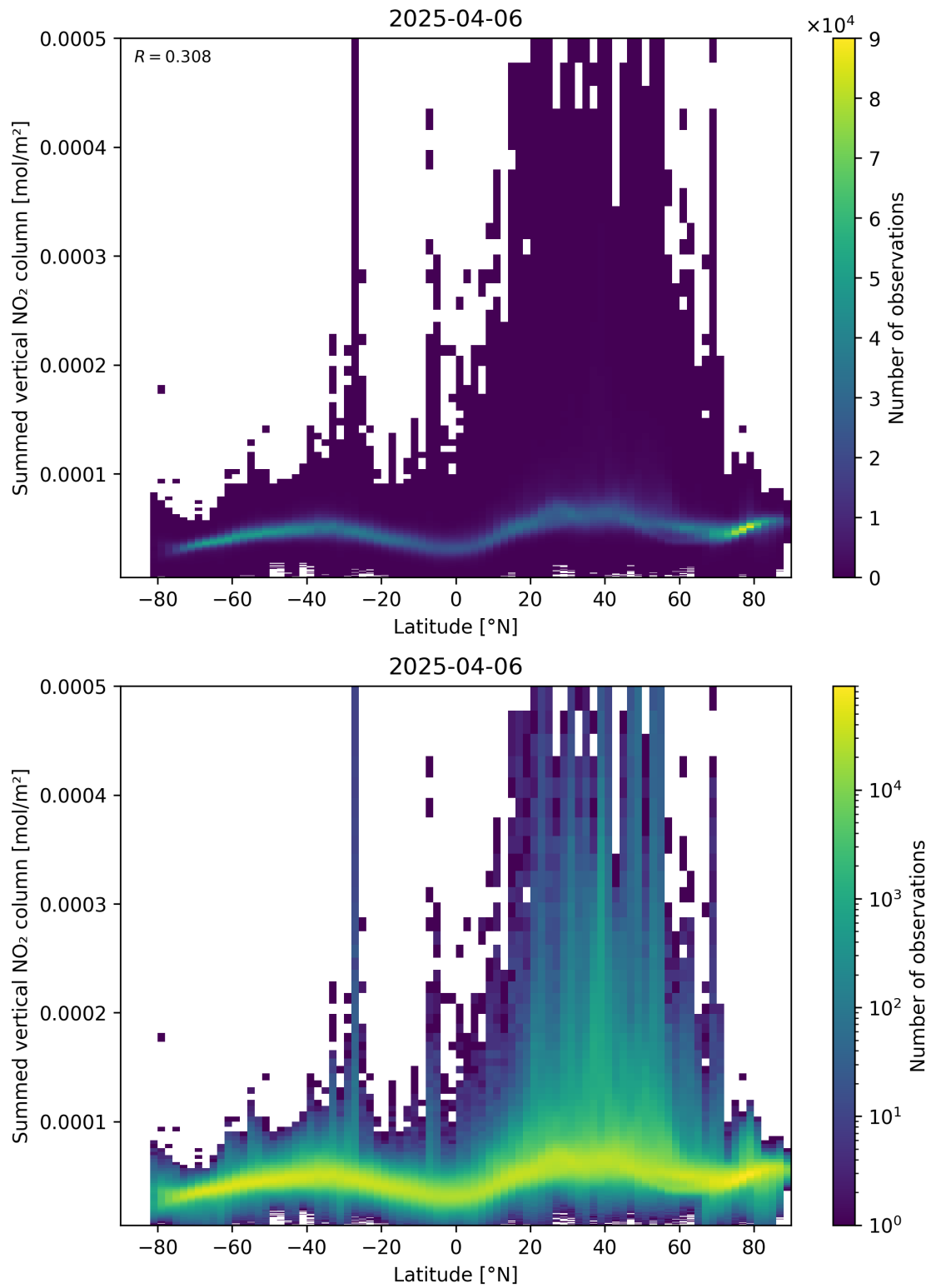
Figure 88: Scatter density plot of “Latitude” against “Summed vertical NO 2 column” for 2025-04-06 to 2025-04-06.
