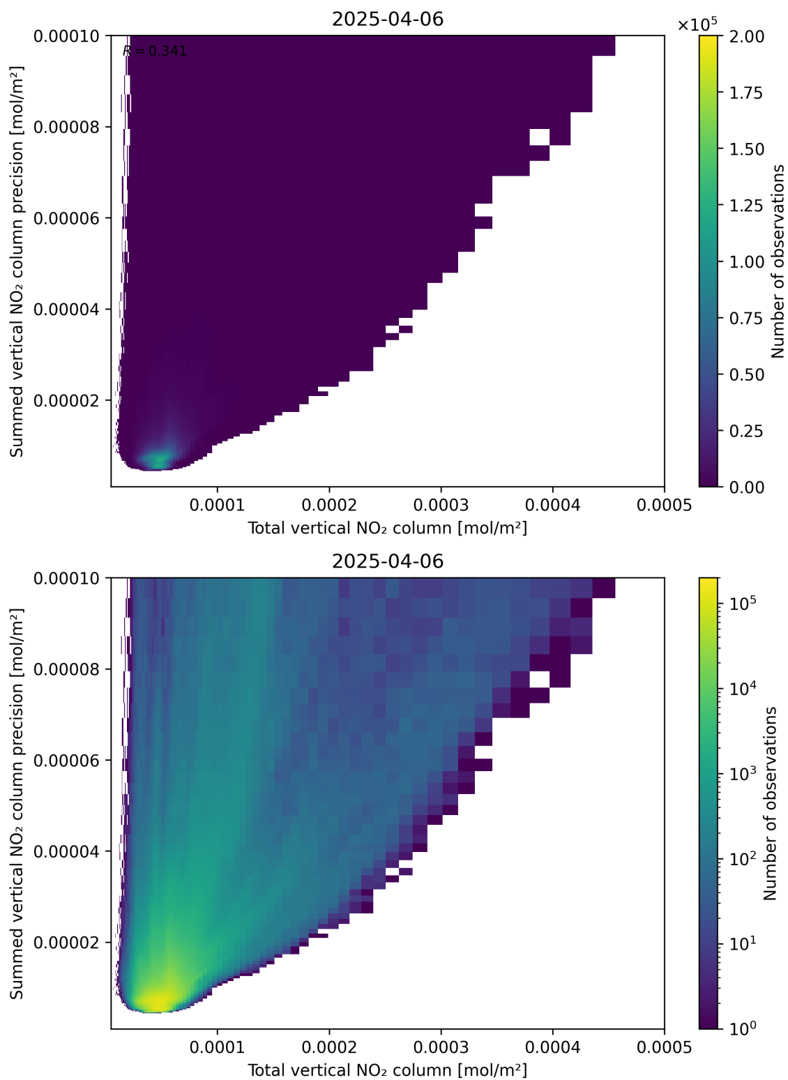
Figure 113: Scatter density plot of “Total vertical NO 2 column” against “Summed vertical NO 2 column precision” for 2025-04-06 to 2025-04-06.
