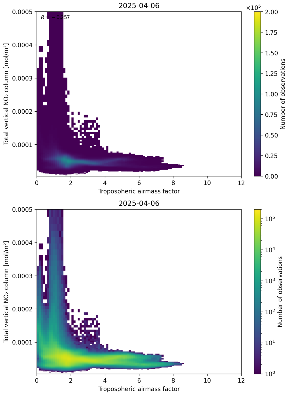
Figure 77: Scatter density plot of “Tropospheric airmass factor” against “Total vertical NO 2 column” for 2025-04-06 to 2025-04-06.
