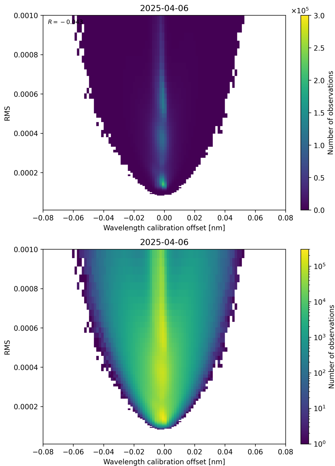
Figure 181: Scatter density plot of “Wavelength calibration offset” against “RMS” for 2025-04-06 to 2025-04-06.
