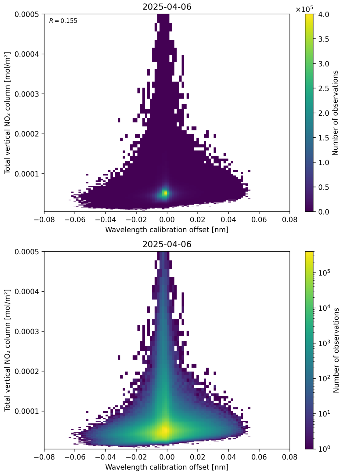
Figure 179: Scatter density plot of “Wavelength calibration offset” against “Total vertical NO 2 column” for 2025-04-06 to 2025-04-06.
