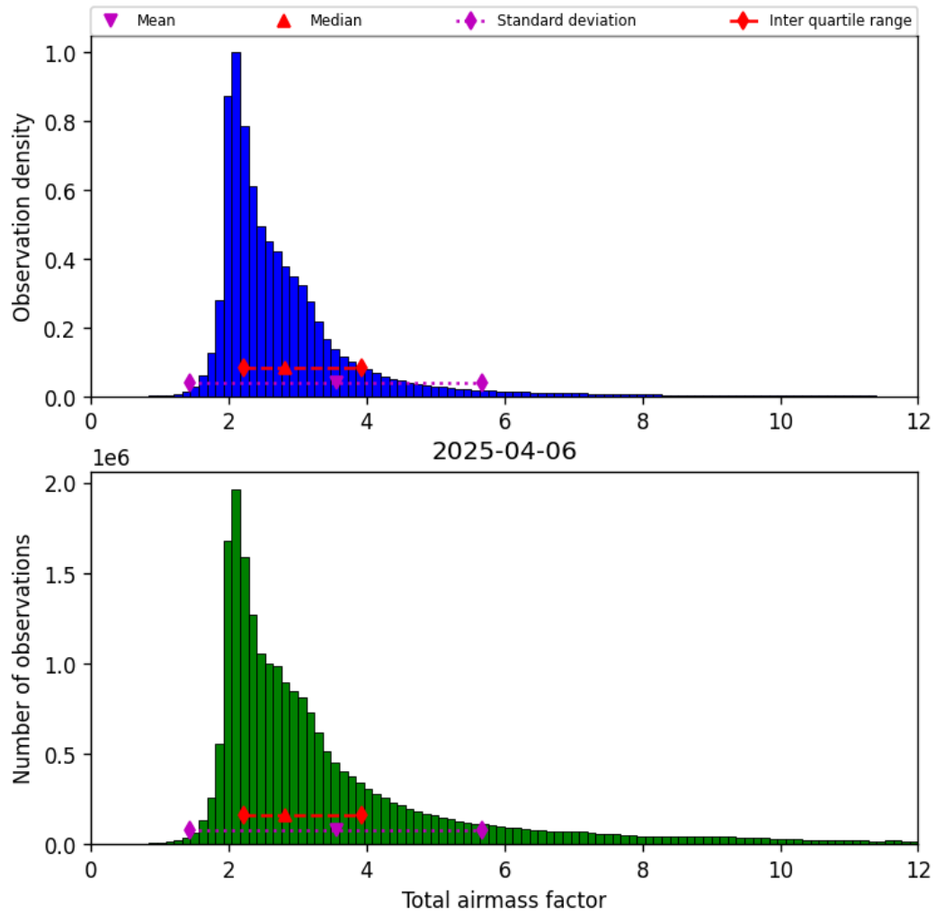
Figure 32: Histogram of “Total airmass factor” for 2025-04-06 to 2025-04-06
