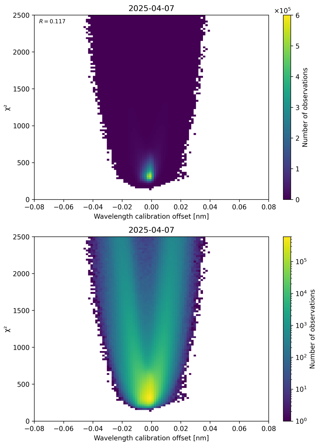
Figure 175: Scatter density plot of “Wavelength calibration offset” against “ \chi^2 ” for 2025-04-07 to 2025-04-08.
