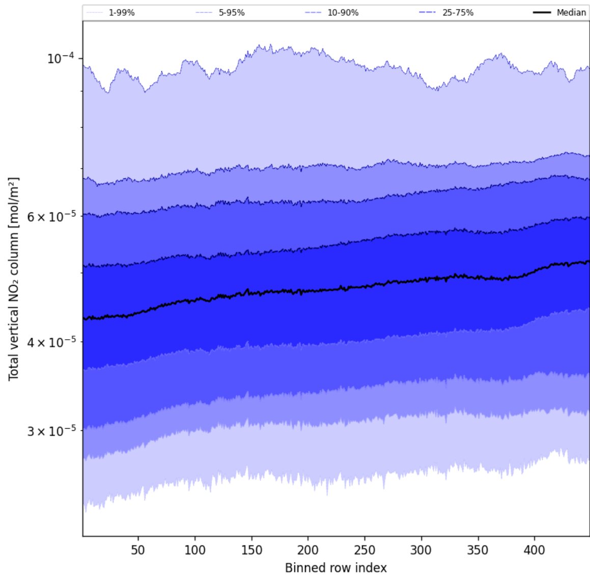
Figure 55: Along track statistics of “Total vertical NO 2 column” for 2025-04-07 to 2025-04-08
