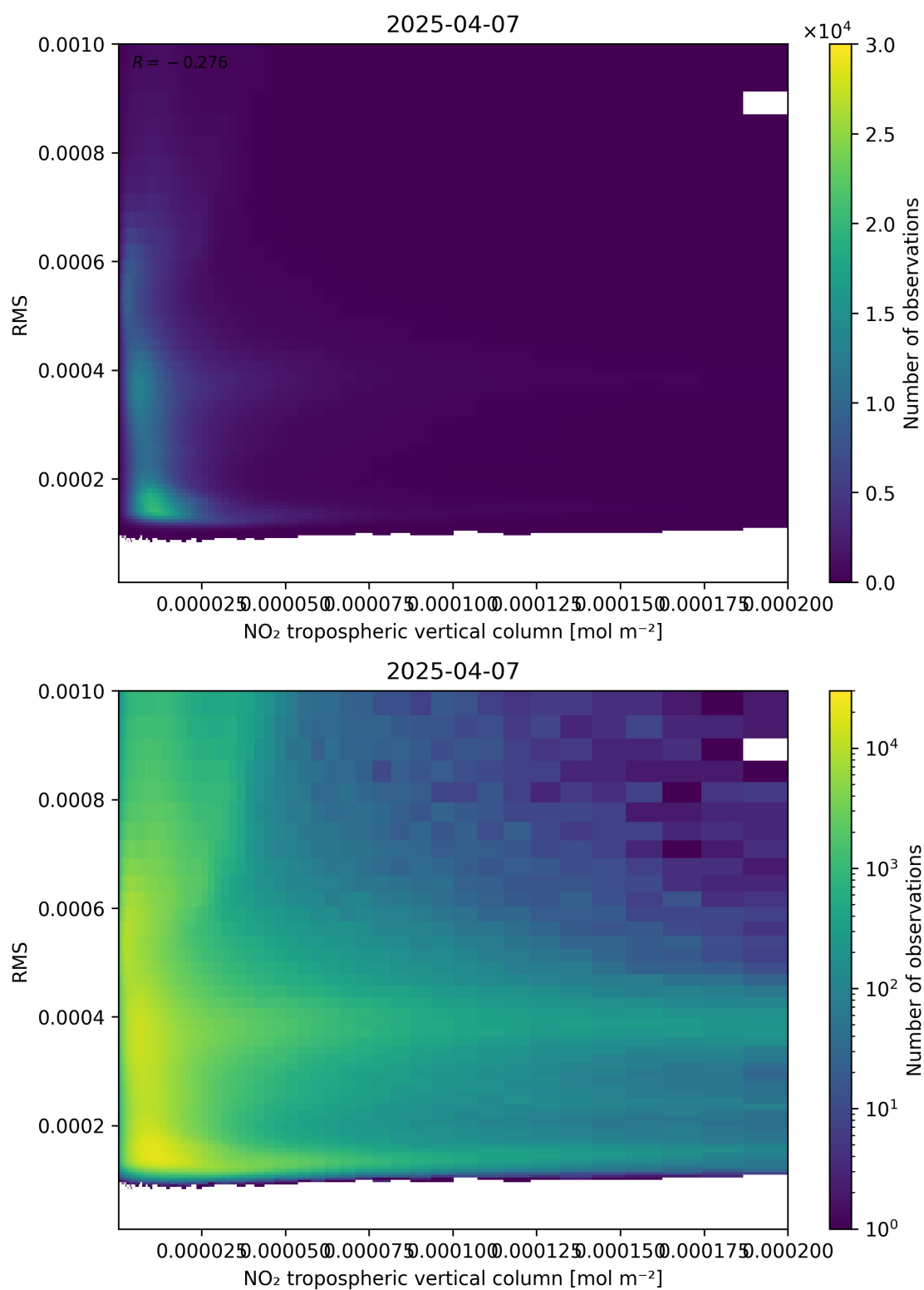
Figure 142: Scatter density plot of “NO 2 tropospheric vertical column” against “RMS” for 2025-04-07 to 2025-04-08.
