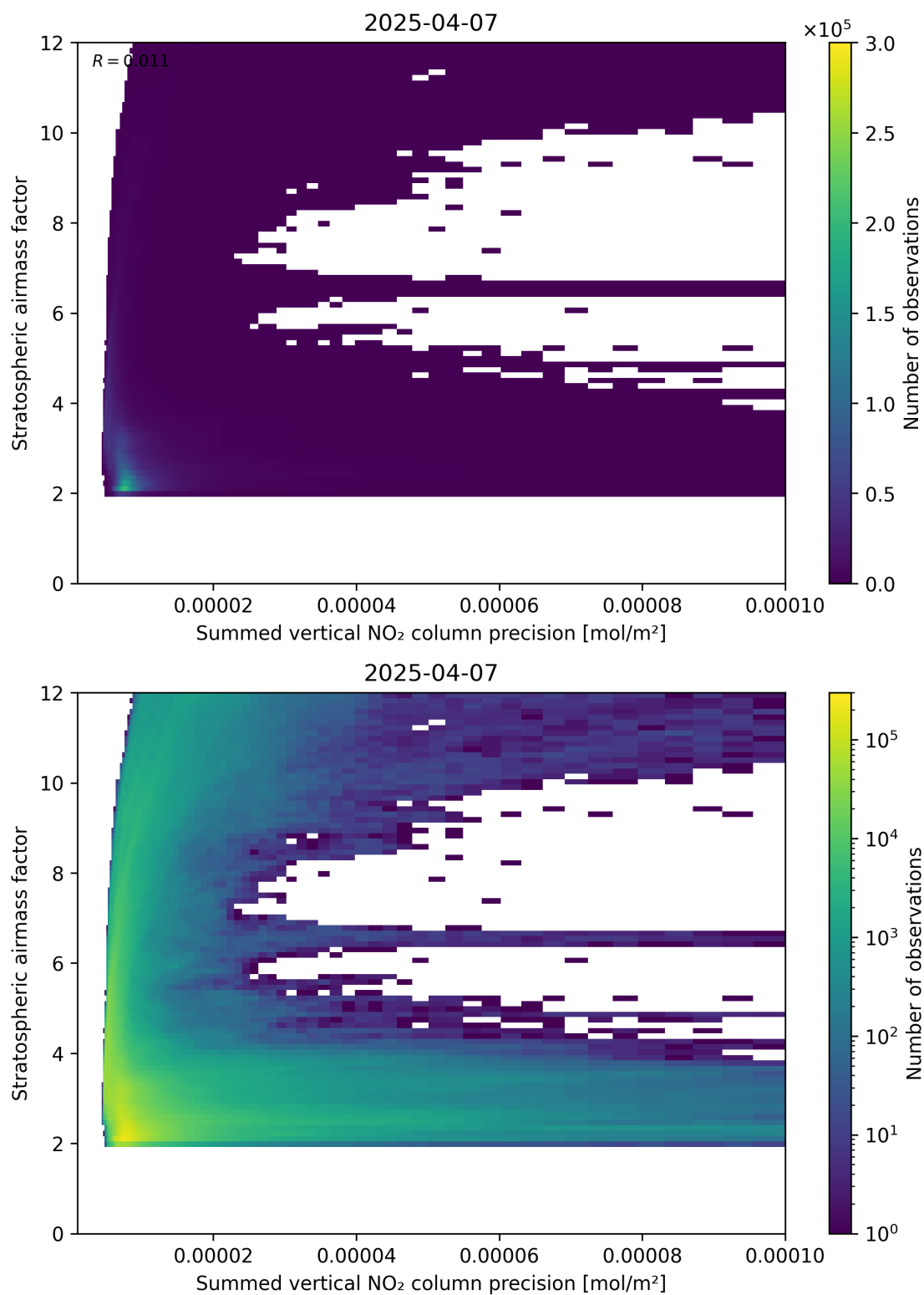
Figure 106: Scatter density plot of “Summed vertical NO 2 column precision” against “Stratospheric airmass factor” for 2025-04-07 to 2025-04-08.
