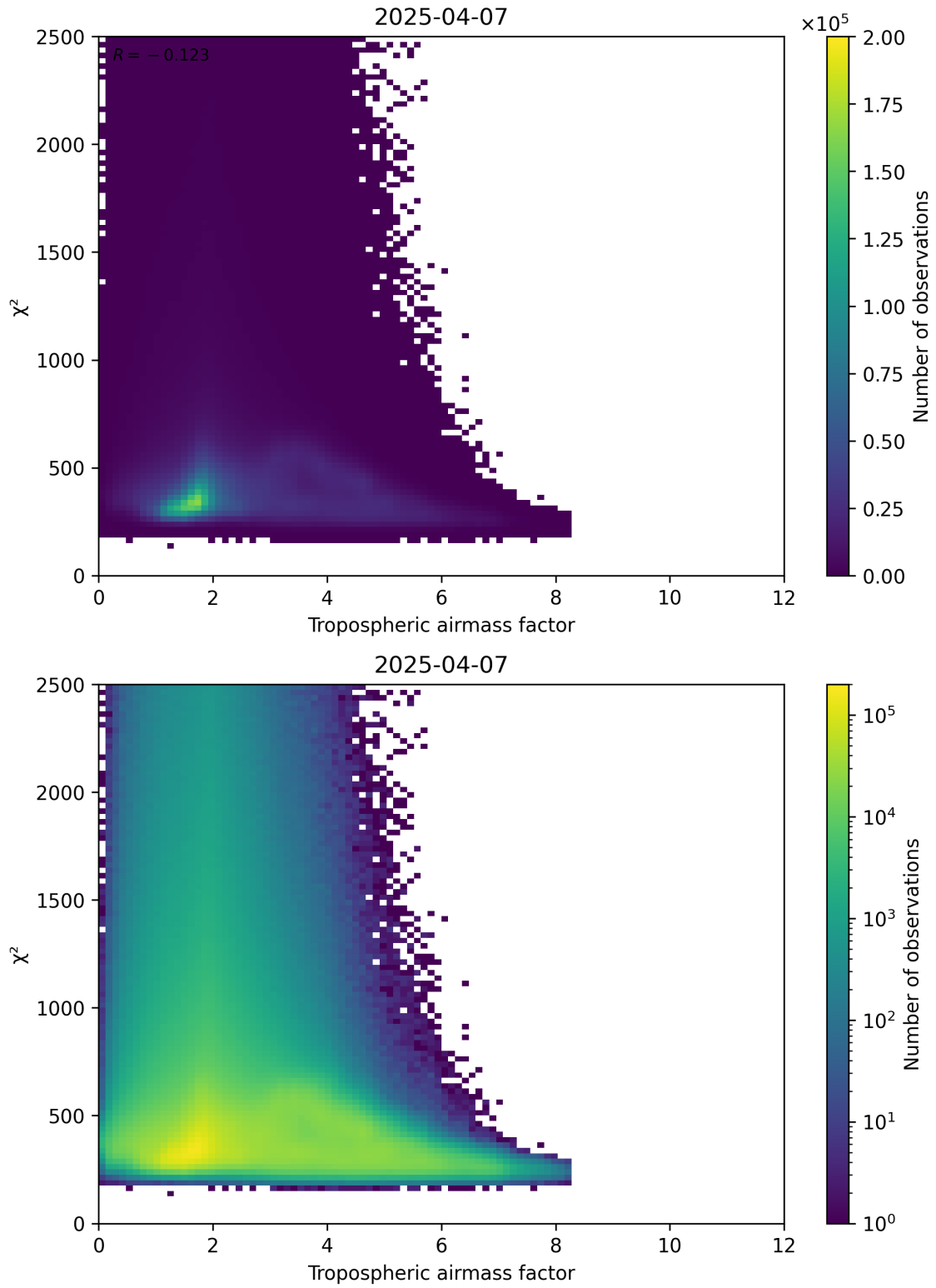
Figure 73: Scatter density plot of “Tropospheric airmass factor” against “ \chi^2 ” for 2025-04-07 to 2025-04-08.
