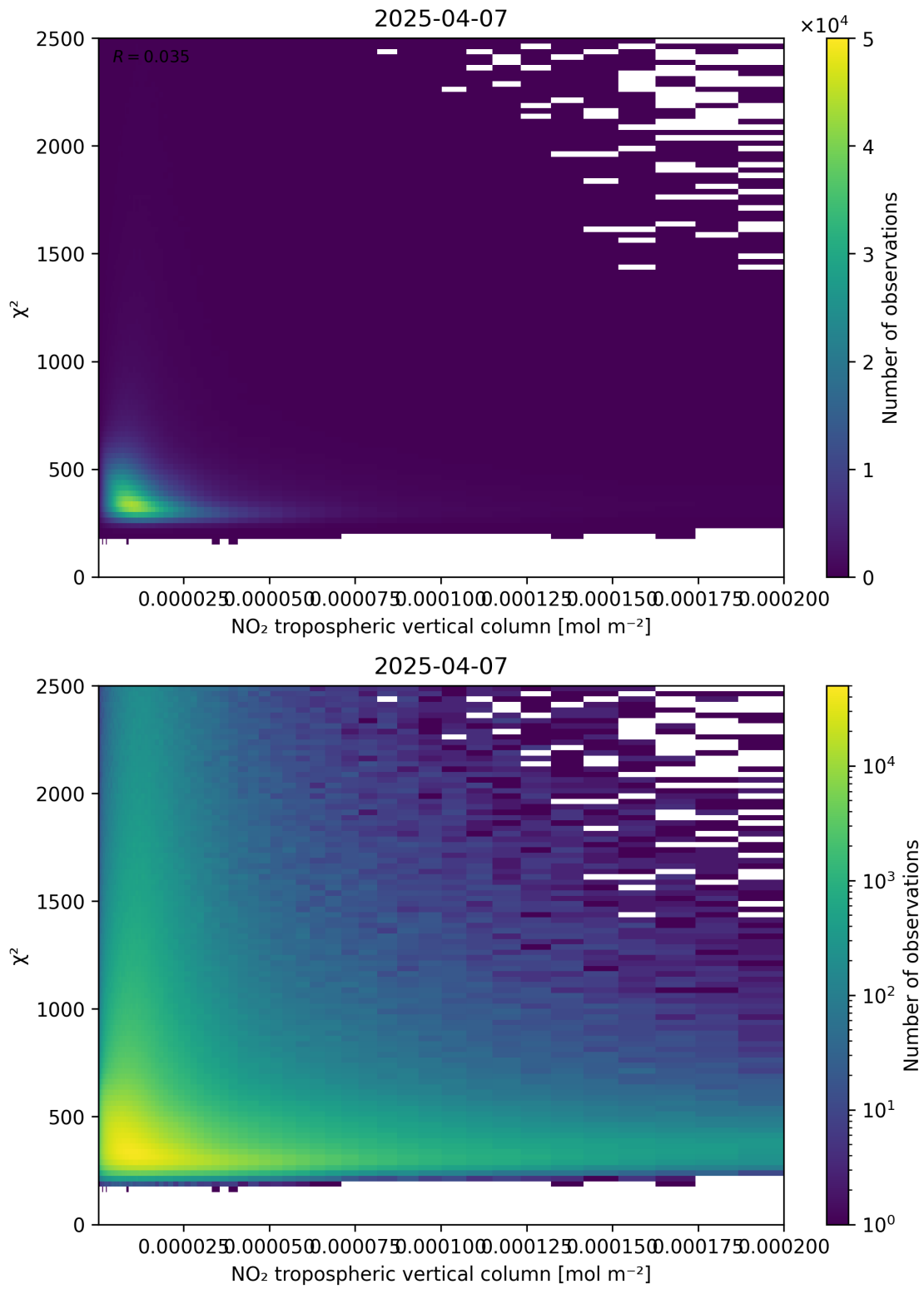
Figure 124: Scatter density plot of “NO 2 tropospheric vertical column” against “ \chi^2 ” for 2025-04-07 to 2025-04-08.
