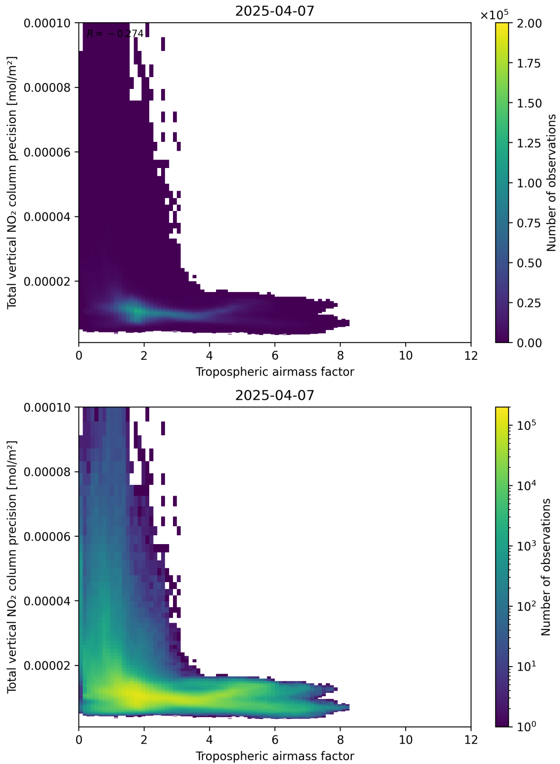
Figure 78: Scatter density plot of “Tropospheric airmass factor” against “Total vertical NO 2 column precision” for 2025-04-07 to 2025-04-08.
