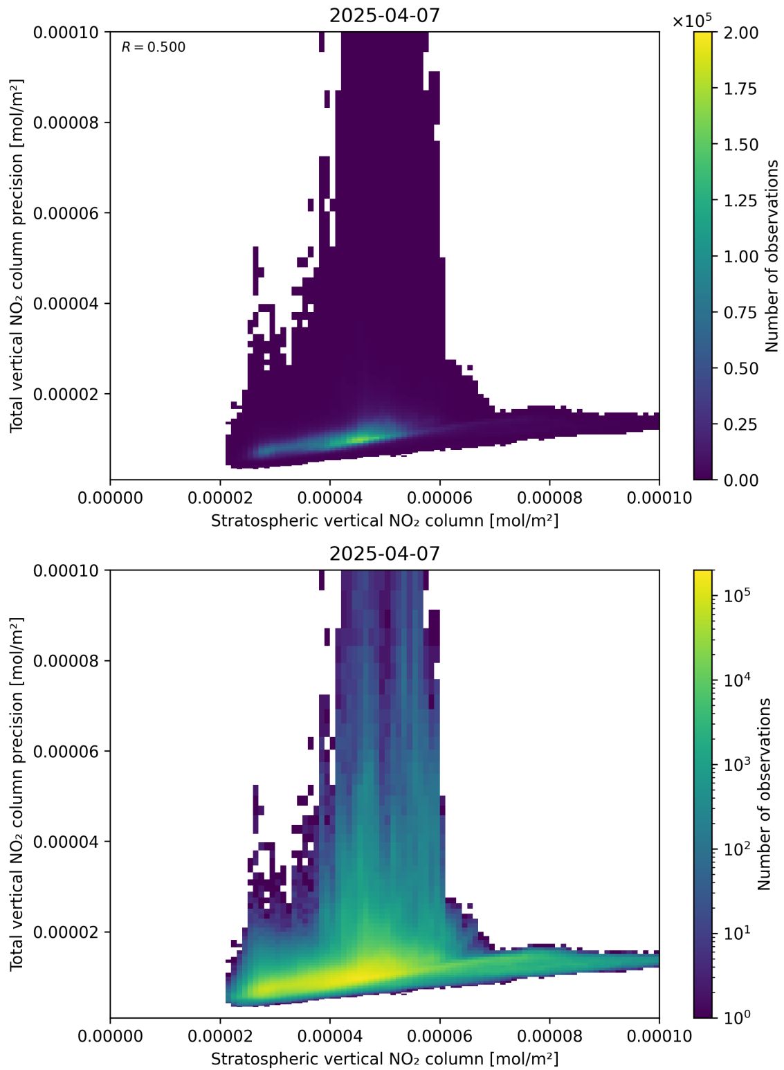
Figure 101: Scatter density plot of “Stratospheric vertical NO 2 column” against “Total vertical NO 2 column precision” for 2025-04-07 to 2025-04-08.
