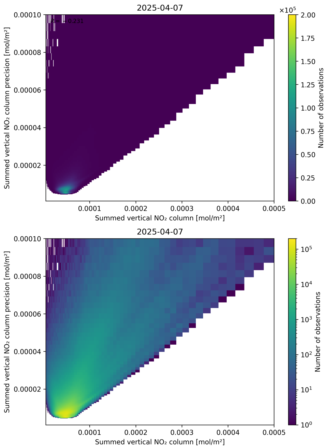
Figure 105: Scatter density plot of “Summed vertical NO 2 column” against “Summed vertical NO 2 column precision” for 2025-04-07 to 2025-04-08.
