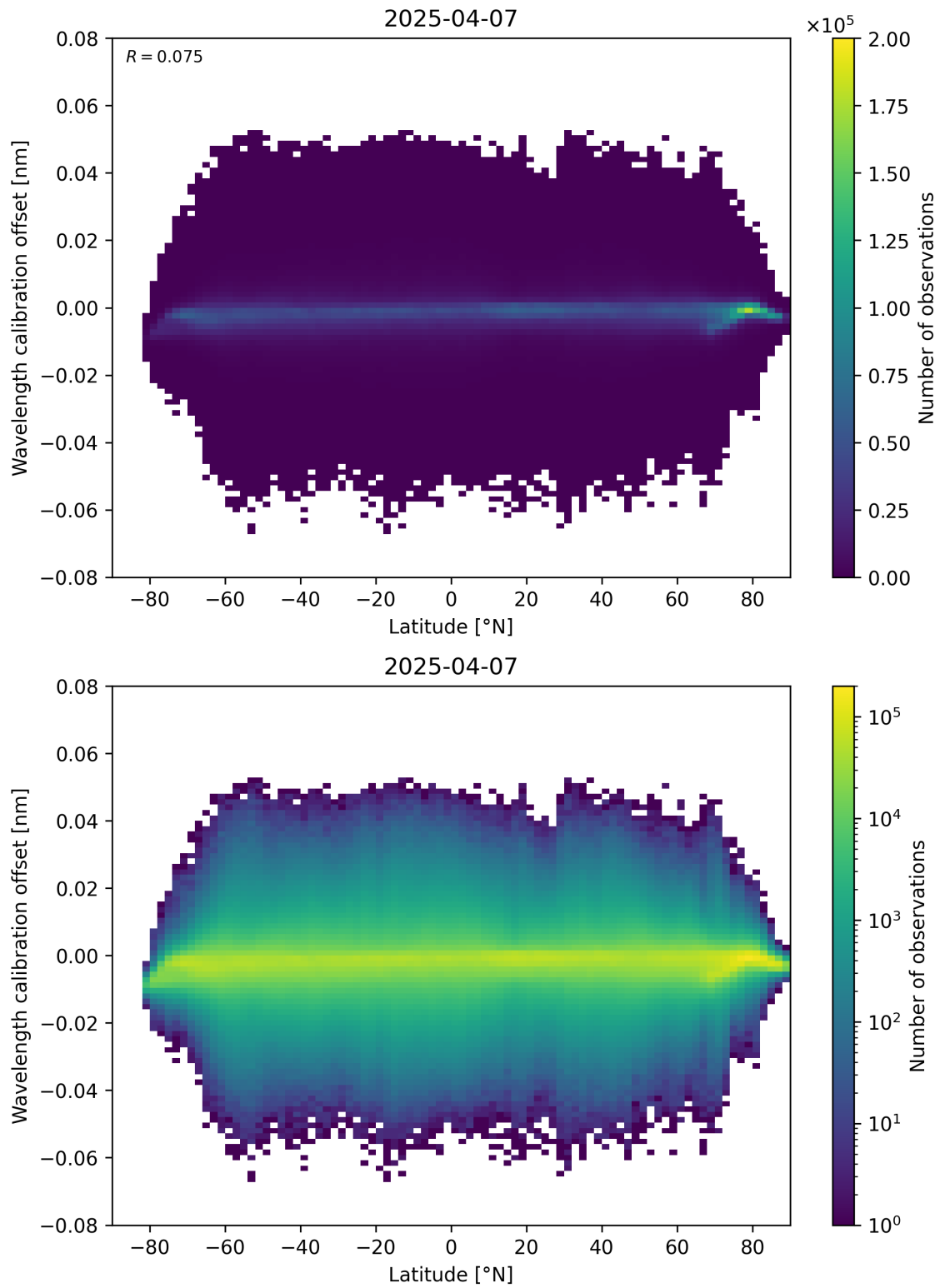
Figure 95: Scatter density plot of “Latitude” against “Wavelength calibration offset” for 2025-04-07 to 2025-04-08.
