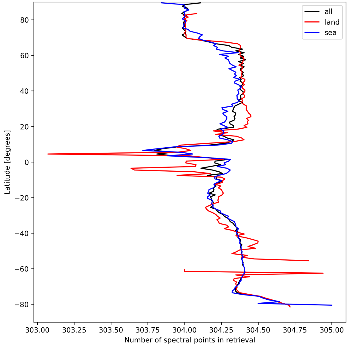
Figure 16: Zonal average of “Number of spectral points in retrieval” for 2025-04-07 to 2025-04-08.
