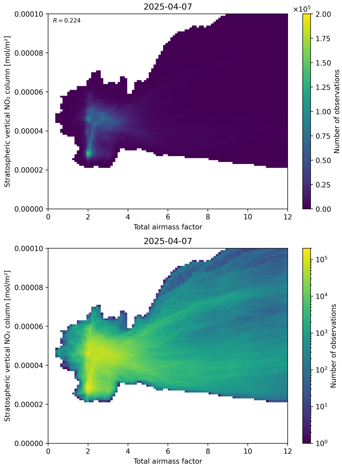
Figure 64: Scatter density plot of “Total airmass factor” against “Stratospheric vertical \text{NO}_2 column” for 2025-04-07 to 2025-04-08.
