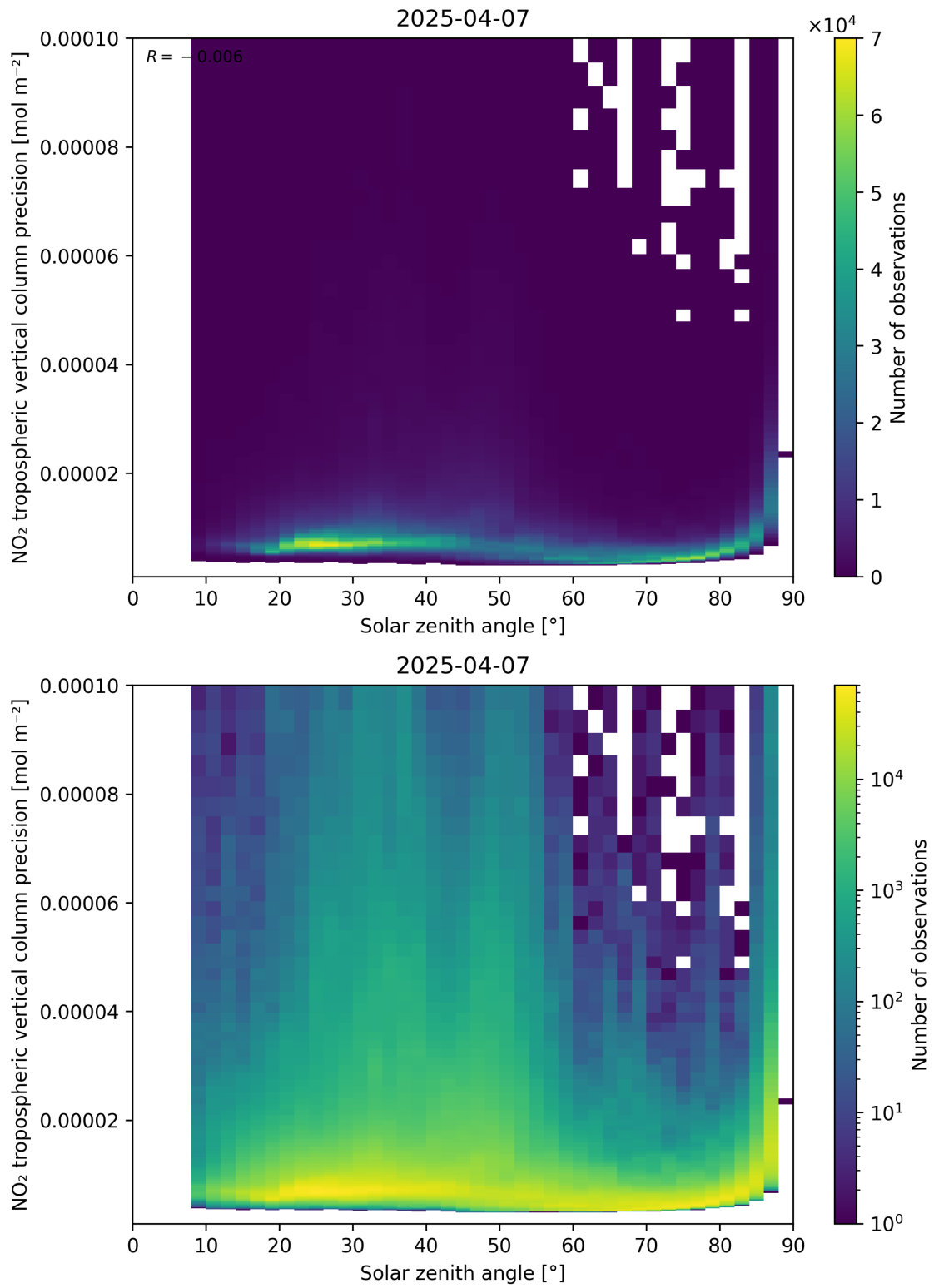
Figure 156: Scatter density plot of “Solar zenith angle” against “NO 2 tropospheric vertical column precision” for 2025-04-07 to 2025-04-08.
