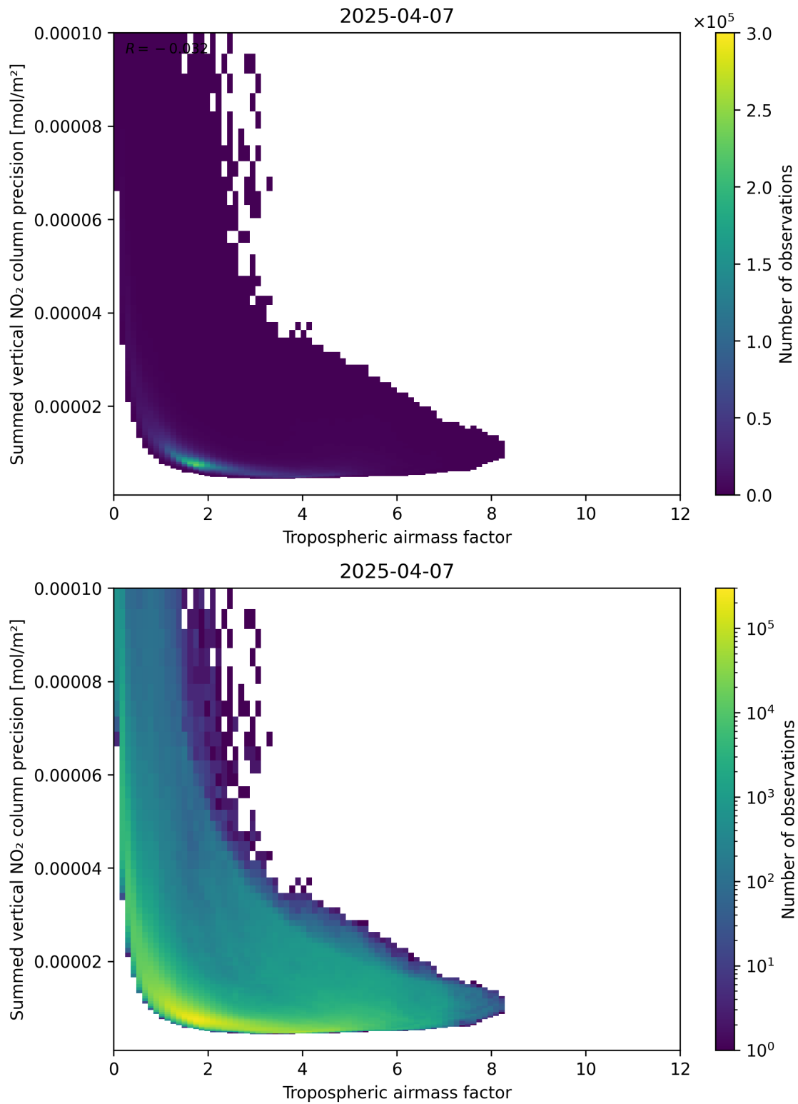
Figure 76: Scatter density plot of “Tropospheric air mass factor” against “Summed vertical NO 2 column precision” for 2025-04-07 to 2025-04-08.
