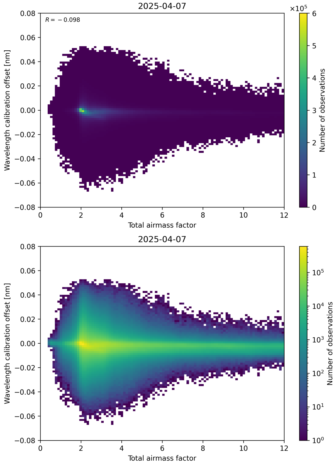
Figure 70: Scatter density plot of “Total airmass factor” against “Wavelength calibration offset” for 2025-04-07 to 2025-04-08.
