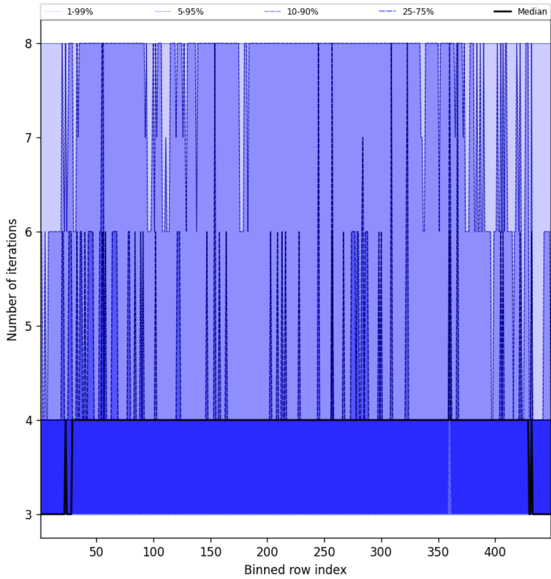
Figure 51: Along track statistics of “Number of iterations” for 2025-04-07 to 2025-04-08
