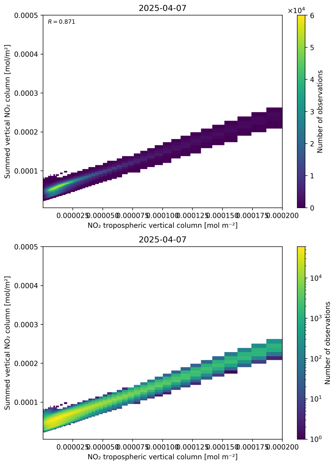
Figure 126: Scatter density plot of “NO 2 tropospheric vertical column” against “Summed vertical NO 2 column” for 2025-04-07 to 2025-04-08.
