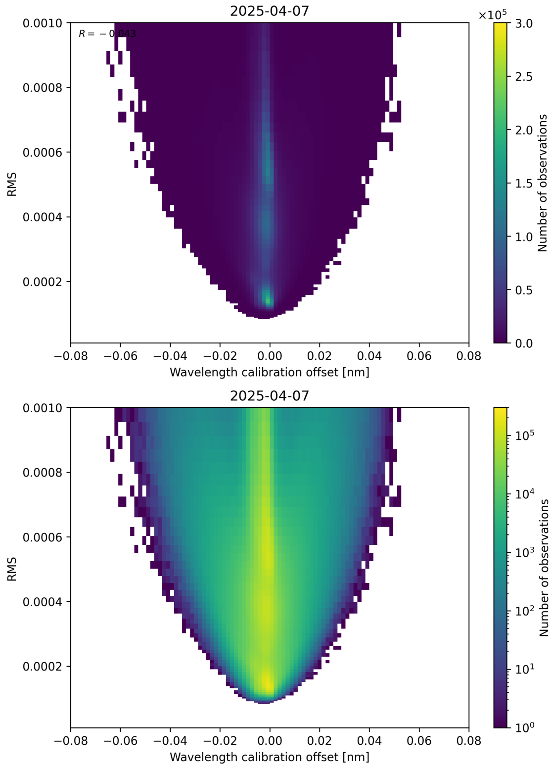
Figure 181: Scatter density plot of “Wavelength calibration offset” against “RMS” for 2025-04-07 to 2025-04-08.
