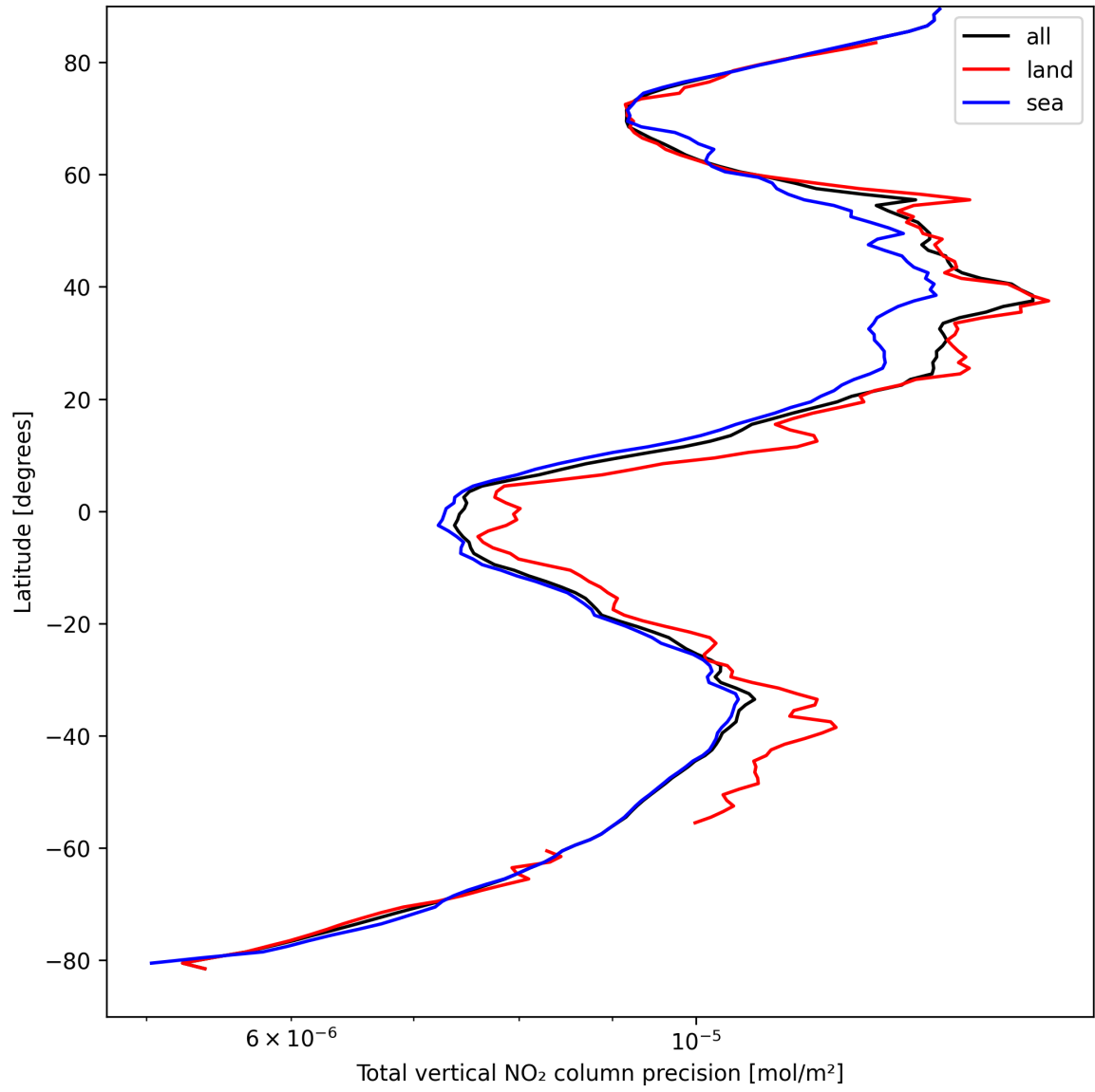
Figure 22: Zonal average of “Total vertical NO 2 column precision” for 2025-04-07 to 2025-04-08.
