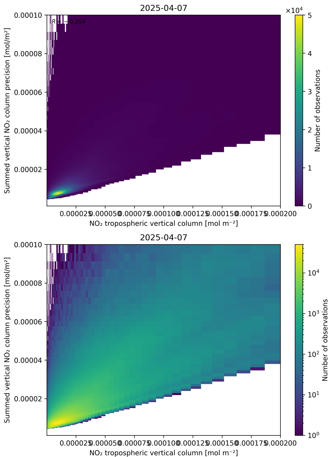
Figure 127: Scatter density plot of “NO 2 tropospheric vertical column” against “Summed vertical NO 2 column precision” for 2025-04-07 to 2025-04-08.
