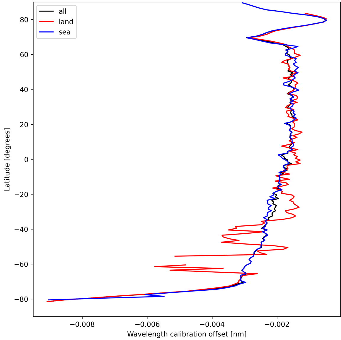
Figure 18: Zonal average of “Wavelength calibration offset” for 2025-04-07 to 2025-04-08.
