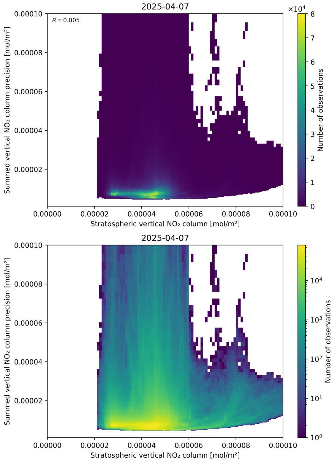
Figure 99: Scatter density plot of “Stratospheric vertical NO 2 column” against “Summed vertical NO 2 column precision” for 2025-04-07 to 2025-04-08.
