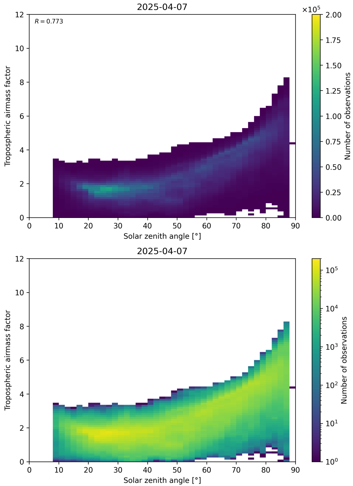
Figure 147: Scatter density plot of “Solar zenith angle” against “Tropospheric airmass factor” for 2025-04-07 to 2025-04-08.
