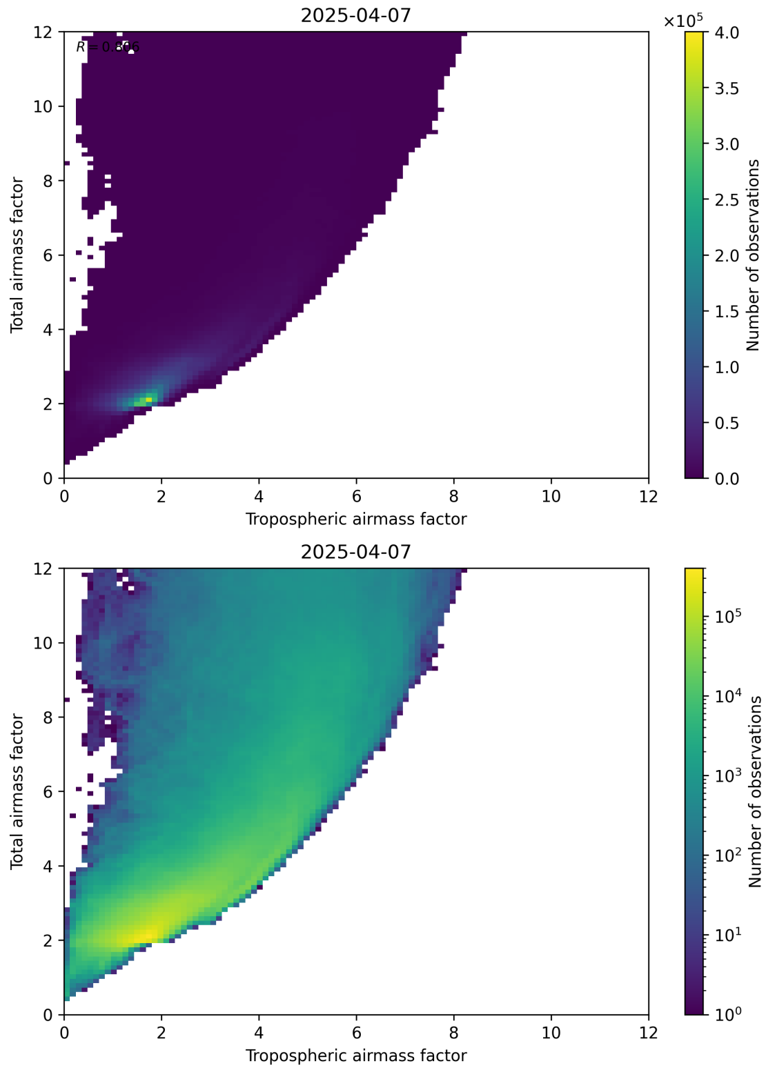
Figure 72: Scatter density plot of “Tropospheric airmass factor” against “Total airmass factor” for 2025-04-07 to 2025-04-08.
