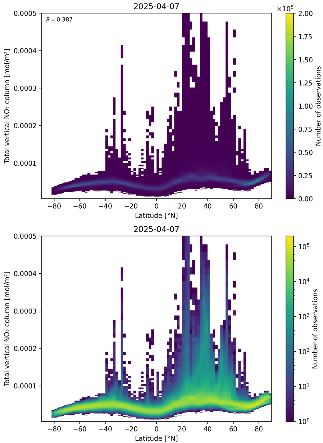
Figure 90: Scatter density plot of “Latitude” against “Total vertical NO 2 column” for 2025-04-07 to 2025-04-08.
