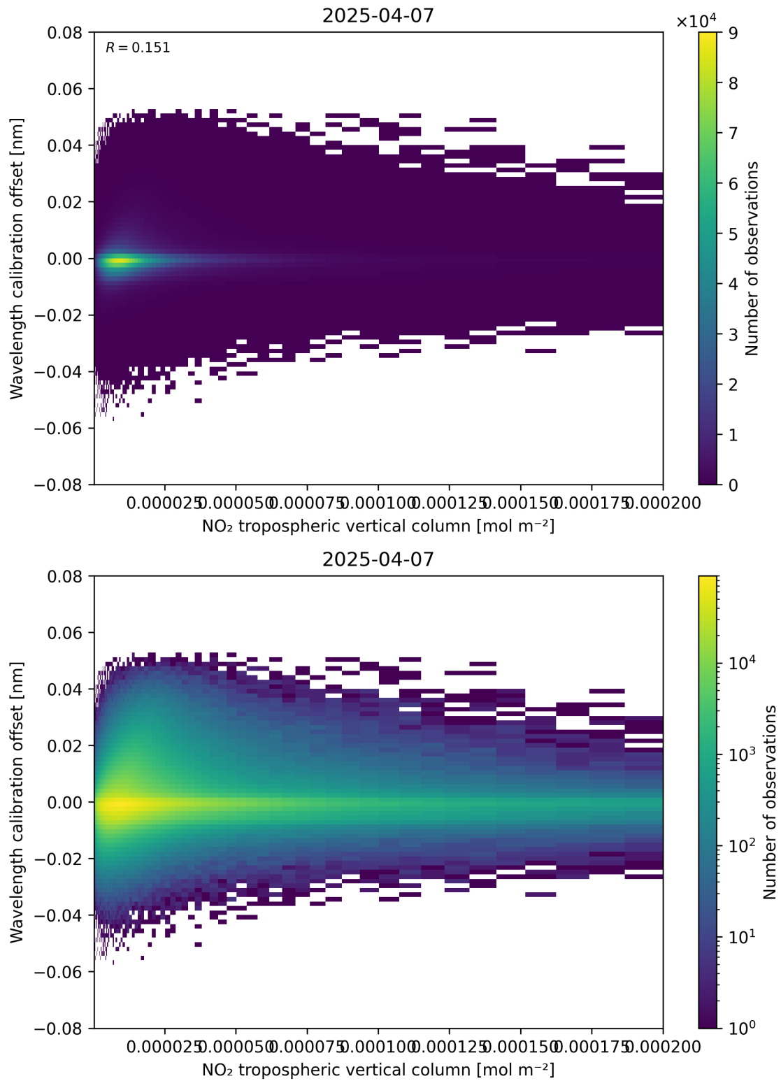
Figure 143: Scatter density plot of “NO 2 tropospheric vertical column” against “Wavelength calibration offset” for 2025-04-07 to 2025-04-08.
