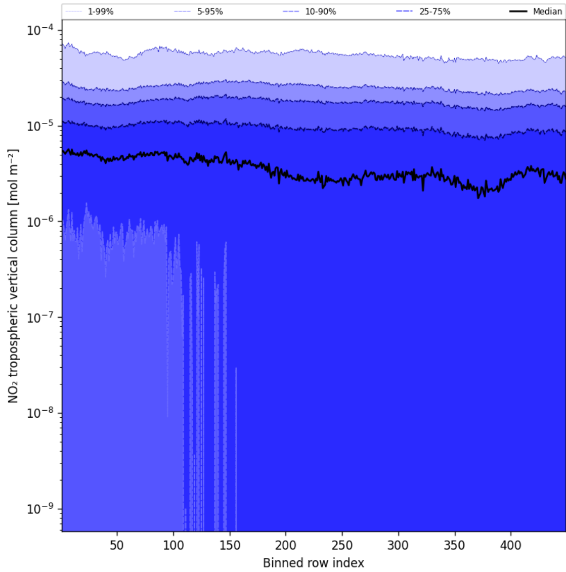
Figure 46: Along track statistics of “NO 2 tropospheric vertical column” for 2025-04-07 to 2025-04-08
