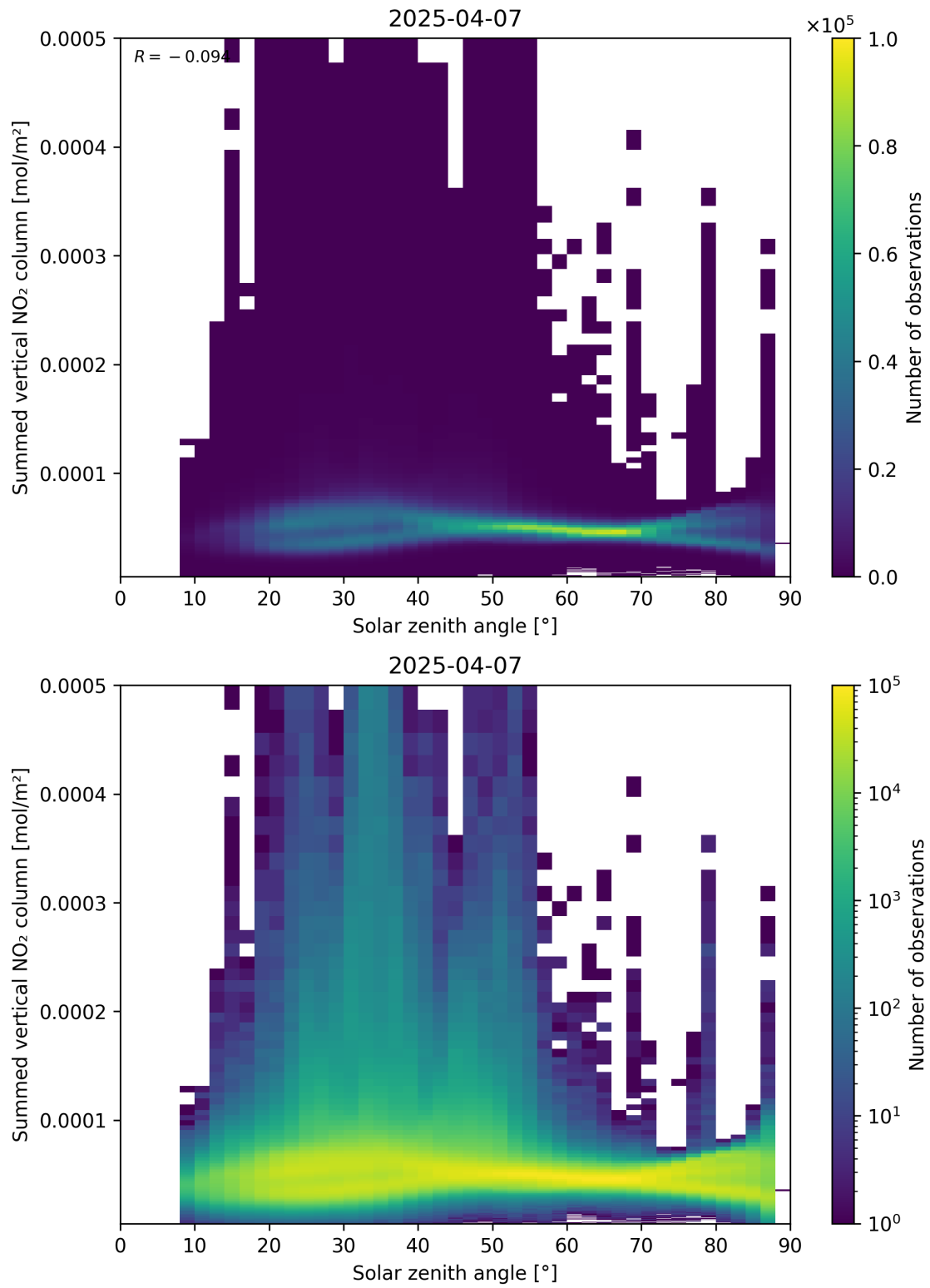
Figure 151: Scatter density plot of “Solar zenith angle” against “Summed vertical NO 2 column” for 2025-04-07 to 2025-04-08.
