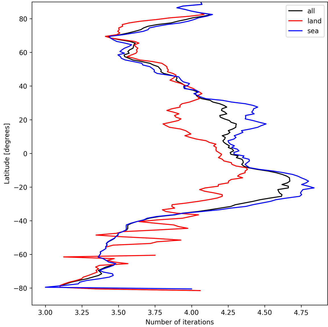
Figure 17: Zonal average of “Number of iterations” for 2025-04-07 to 2025-04-08.
