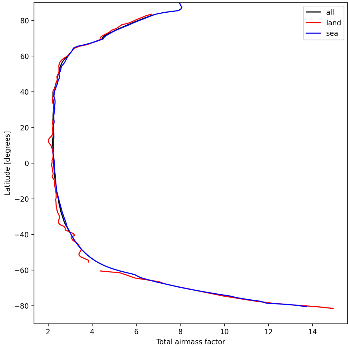
Figure 15: Zonal average of “Total airmass factor” for 2025-04-07 to 2025-04-08.
