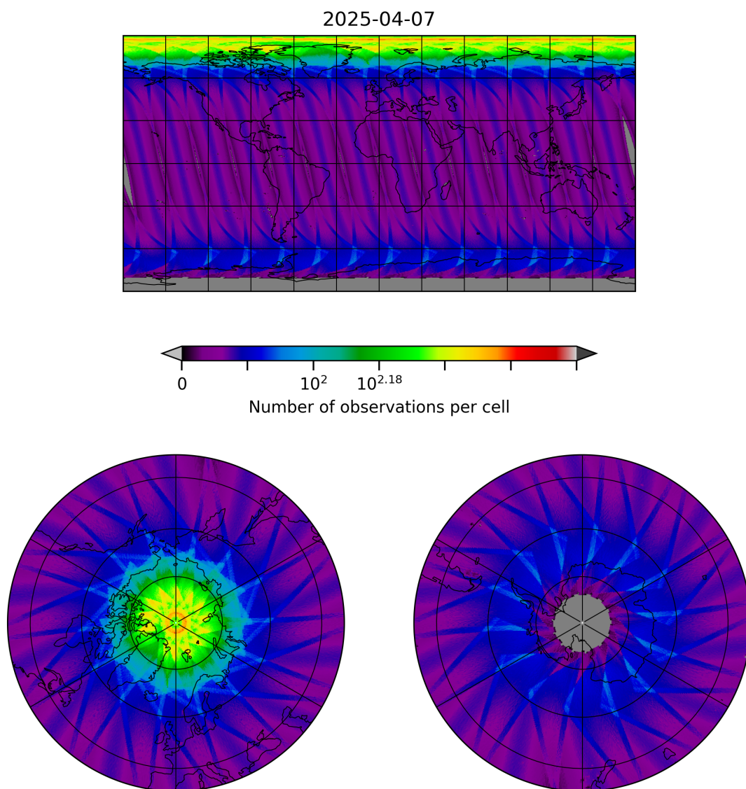
Figure 10: Map of the number of observations for 2025-04-07 to 2025-04-08
