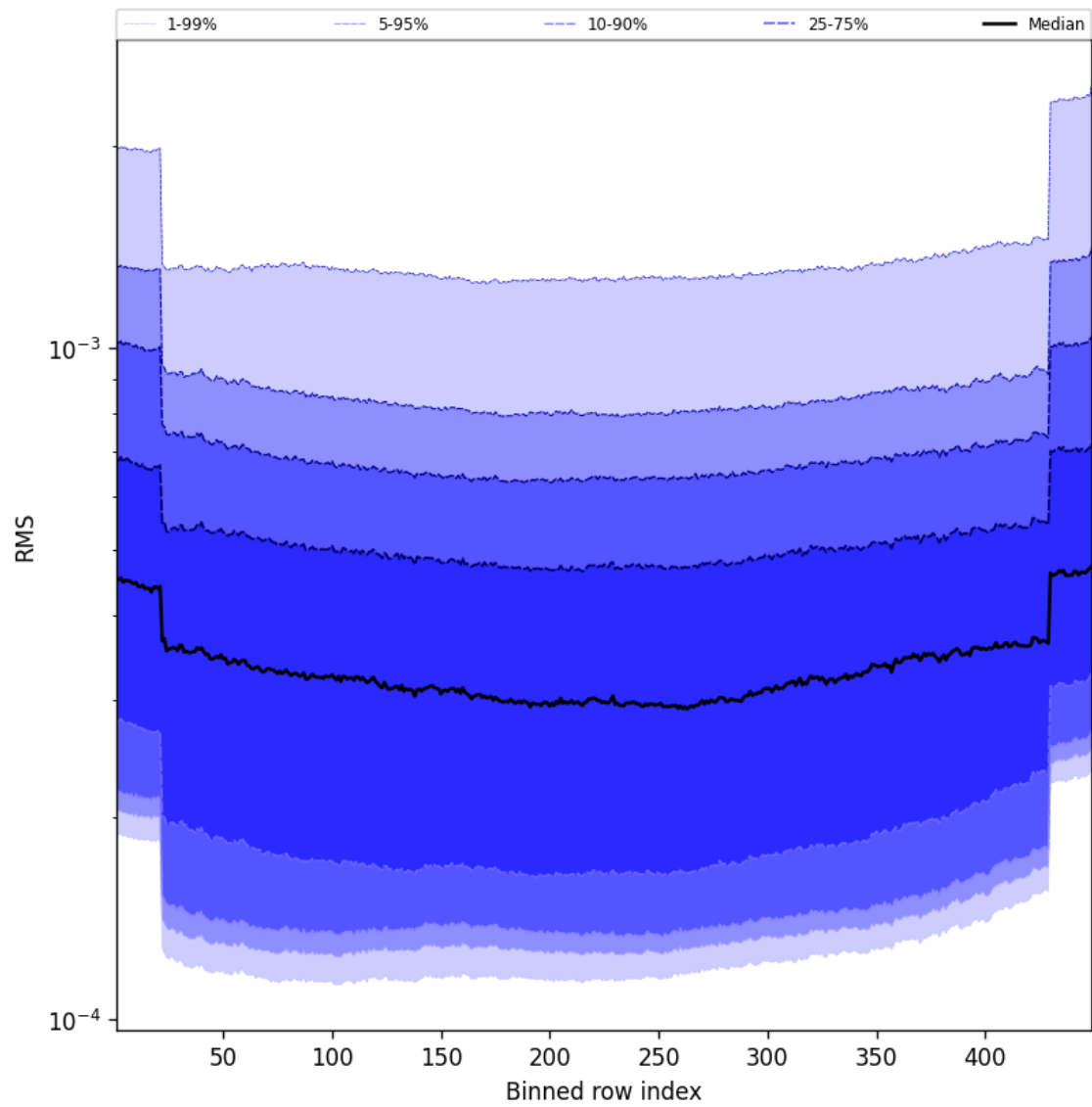
Figure 60: Along track statistics of “RMS” for 2025-04-07 to 2025-04-08
