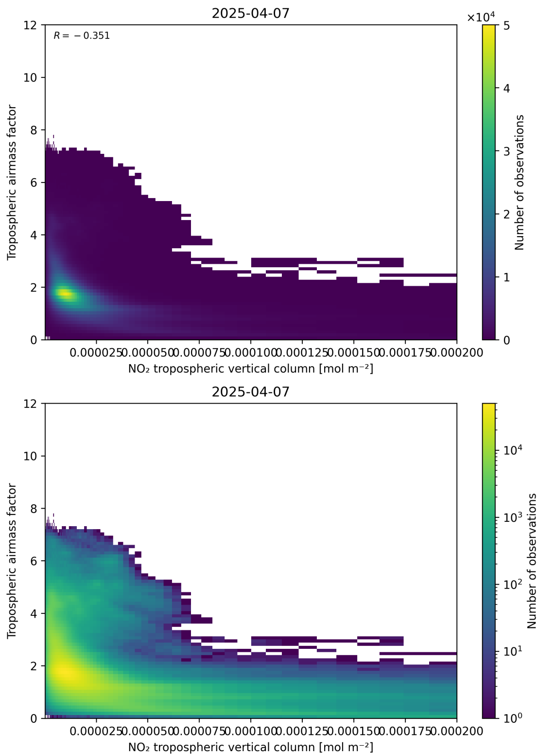
Figure 123: Scatter density plot of “NO 2 tropospheric vertical column” against “Tropospheric airmass factor” for 2025-04-07 to 2025-04-08.
