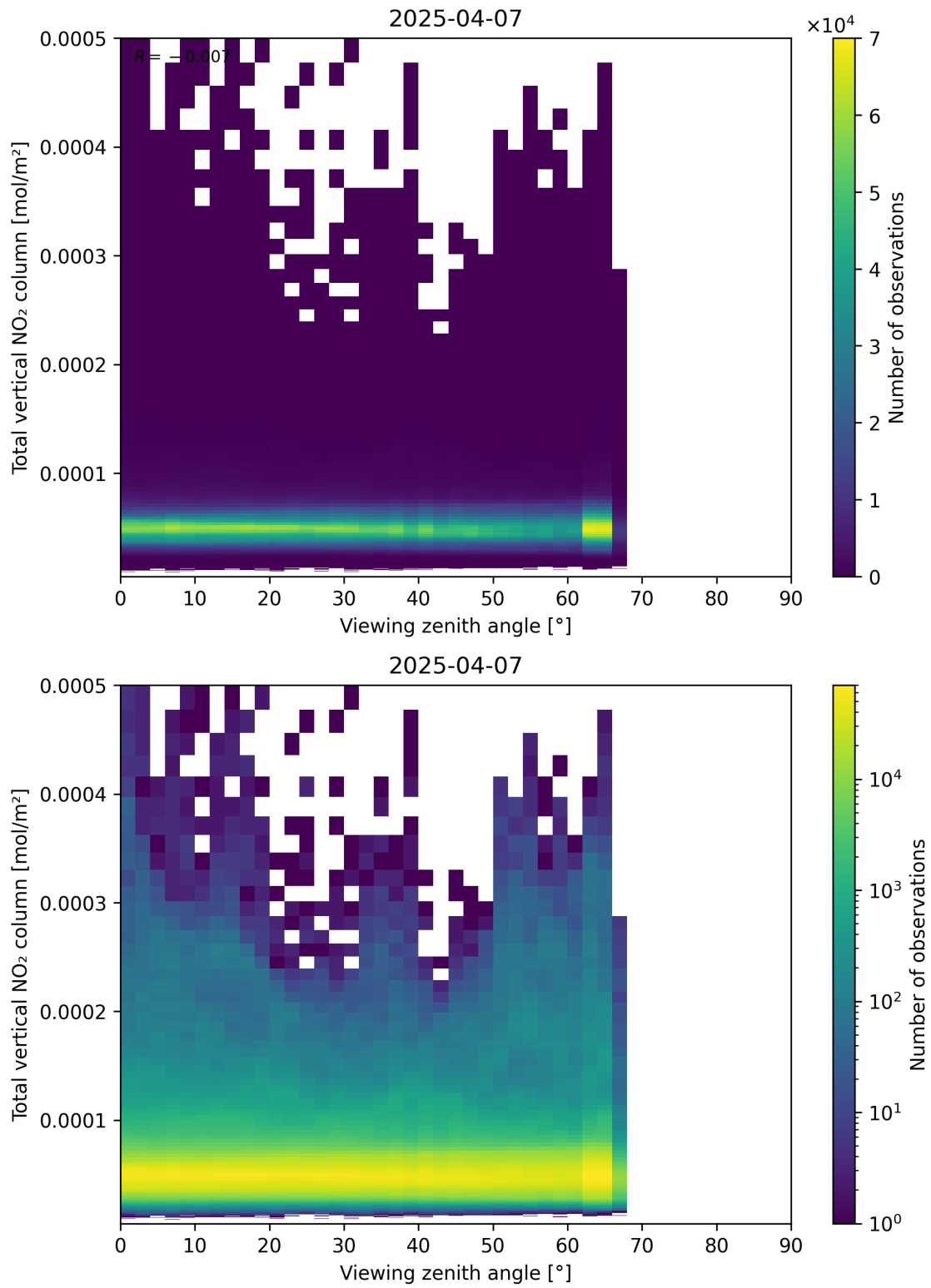
Figure 167: Scatter density plot of “Viewing zenith angle” against “Total vertical NO 2 column” for 2025-04-07 to 2025-04-08.
