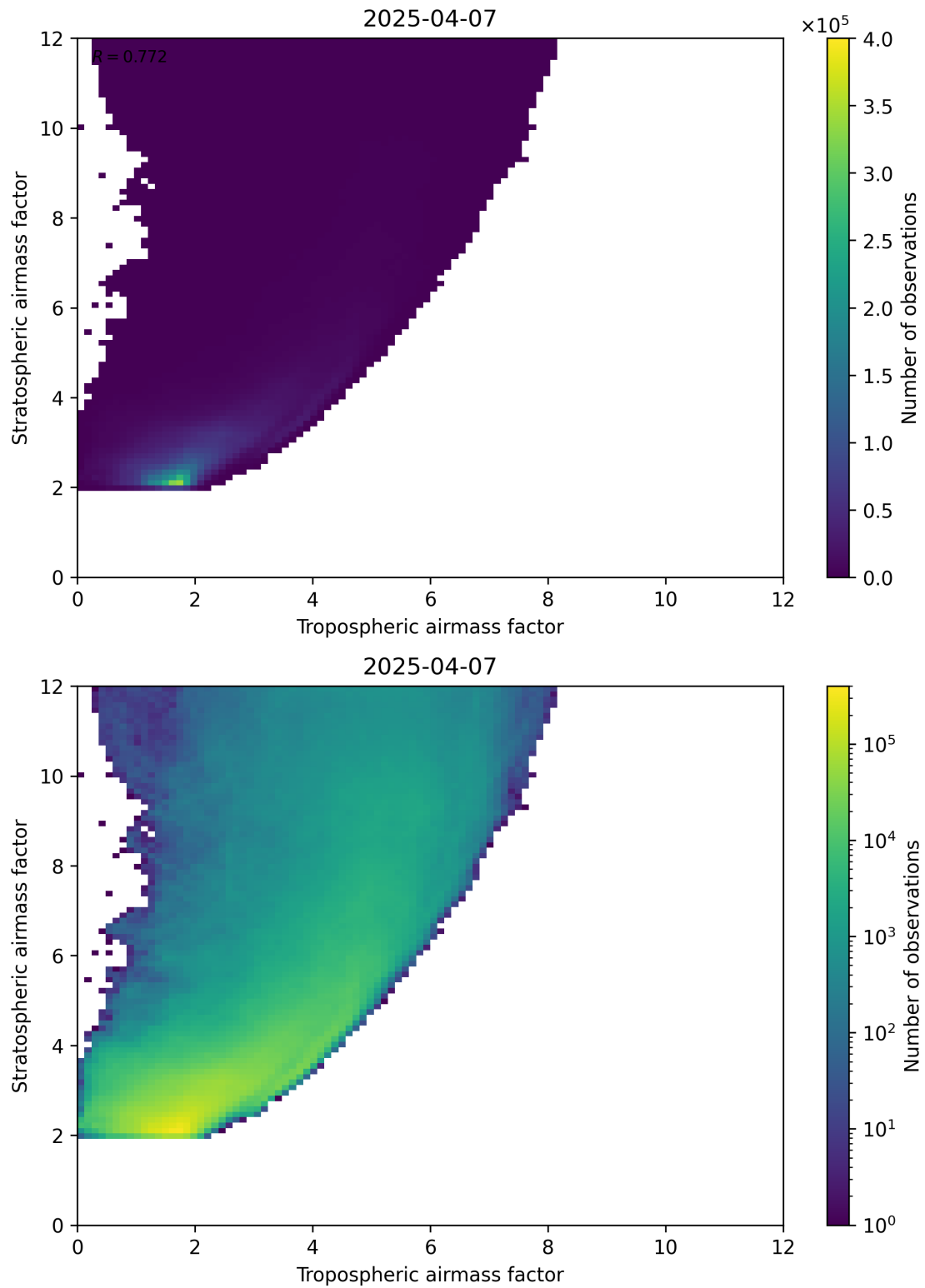
Figure 71: Scatter density plot of “Tropospheric airmass factor” against “Stratospheric airmass factor” for 2025-04-07 to 2025-04-08.
