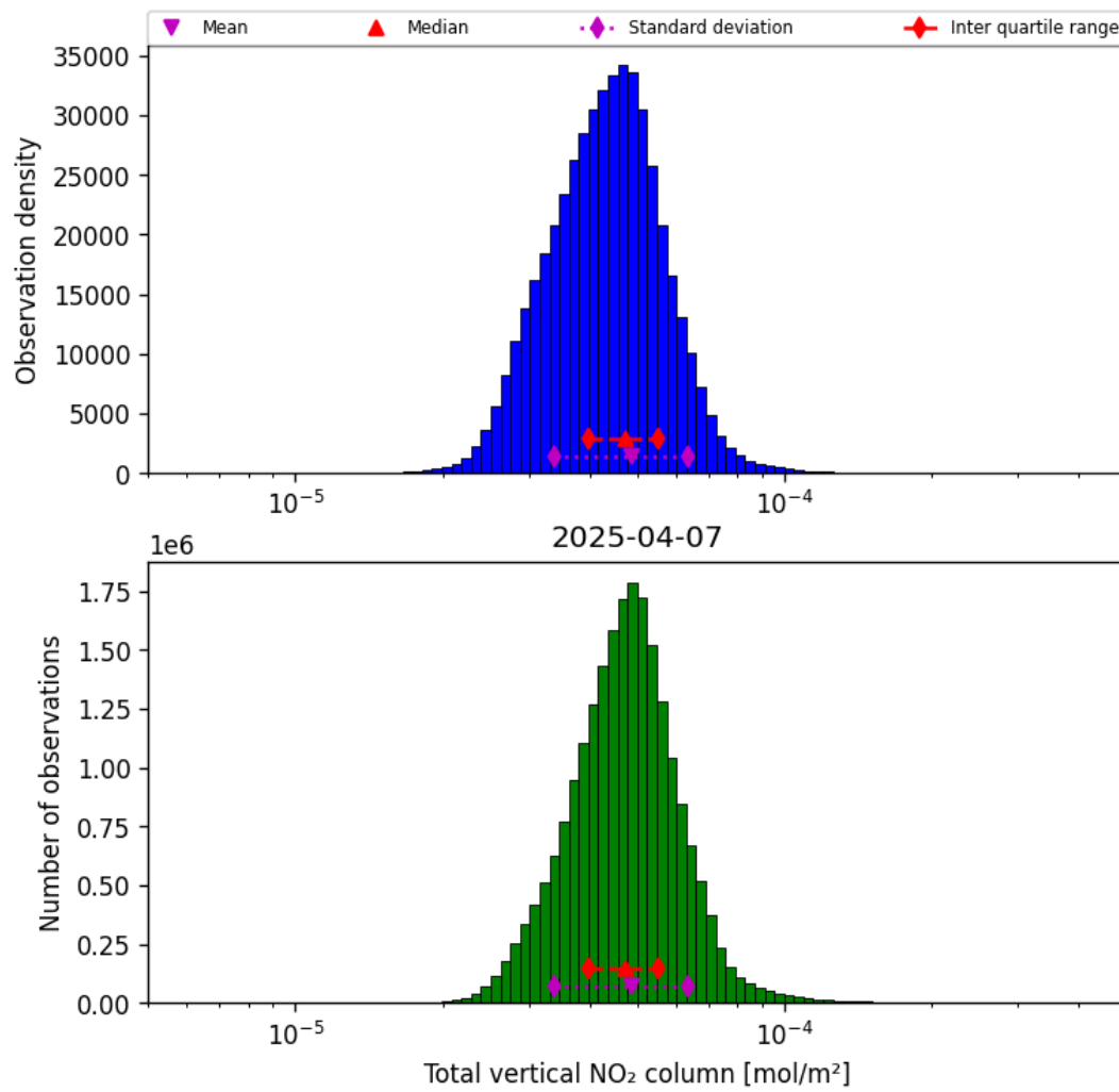
Figure 38: Histogram of “Total vertical NO 2 column” for 2025-04-07 to 2025-04-08
