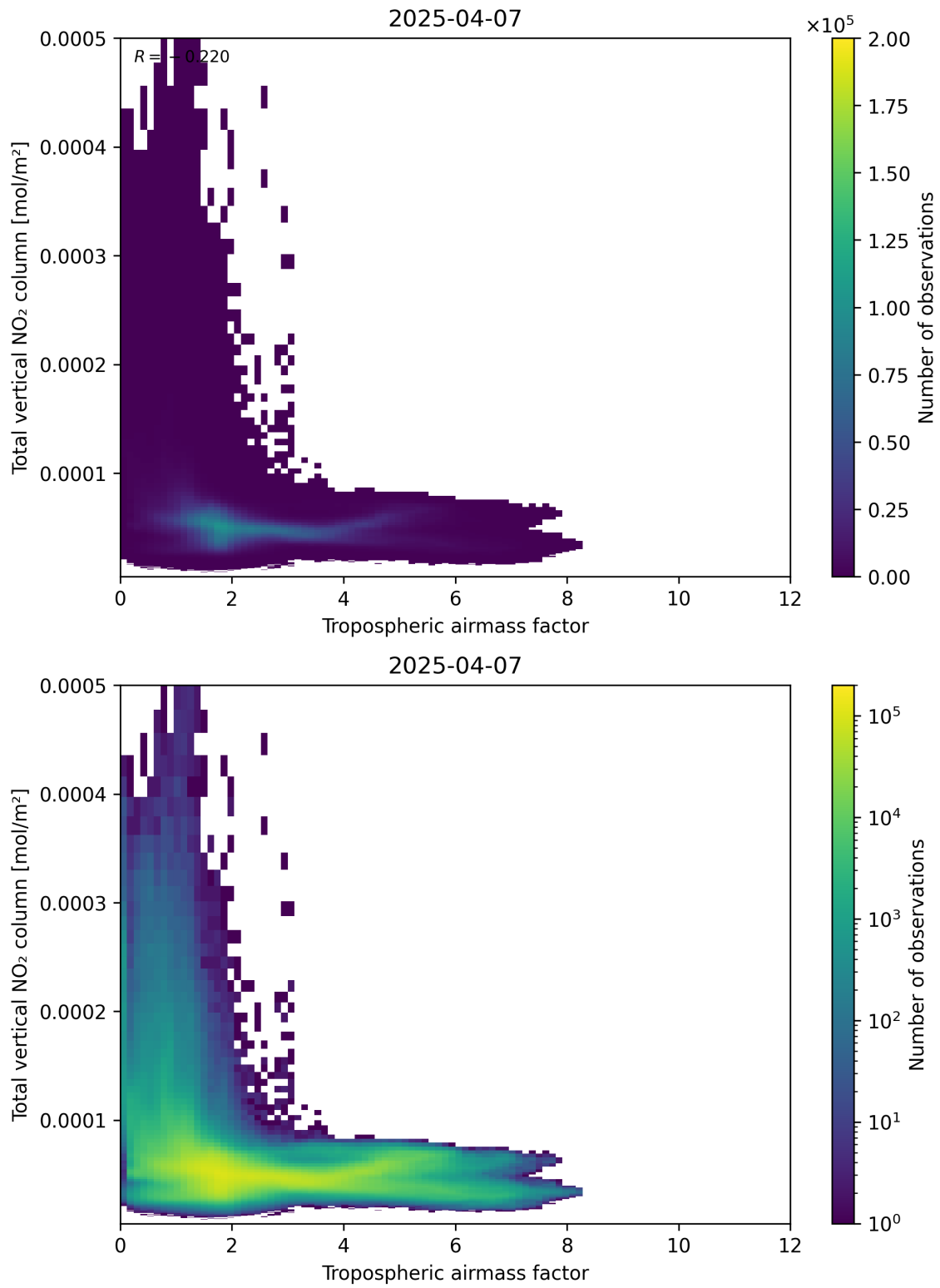
Figure 77: Scatter density plot of “Tropospheric airmass factor” against “Total vertical NO 2 column” for 2025-04-07 to 2025-04-08.
