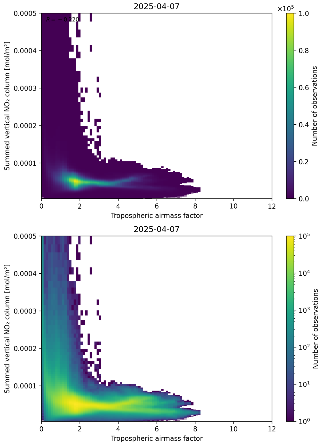
Figure 75: Scatter density plot of “Tropospheric air mass factor” against “Summed vertical NO 2 column” for 2025-04-07 to 2025-04-08.
