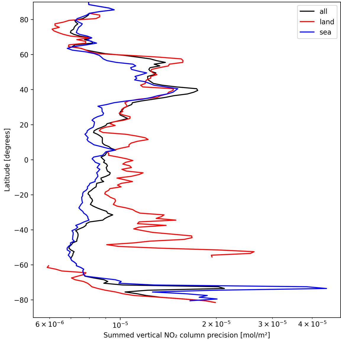
Figure 24: Zonal average of “Summed vertical NO 2 column precision” for 2025-04-07 to 2025-04-08.
