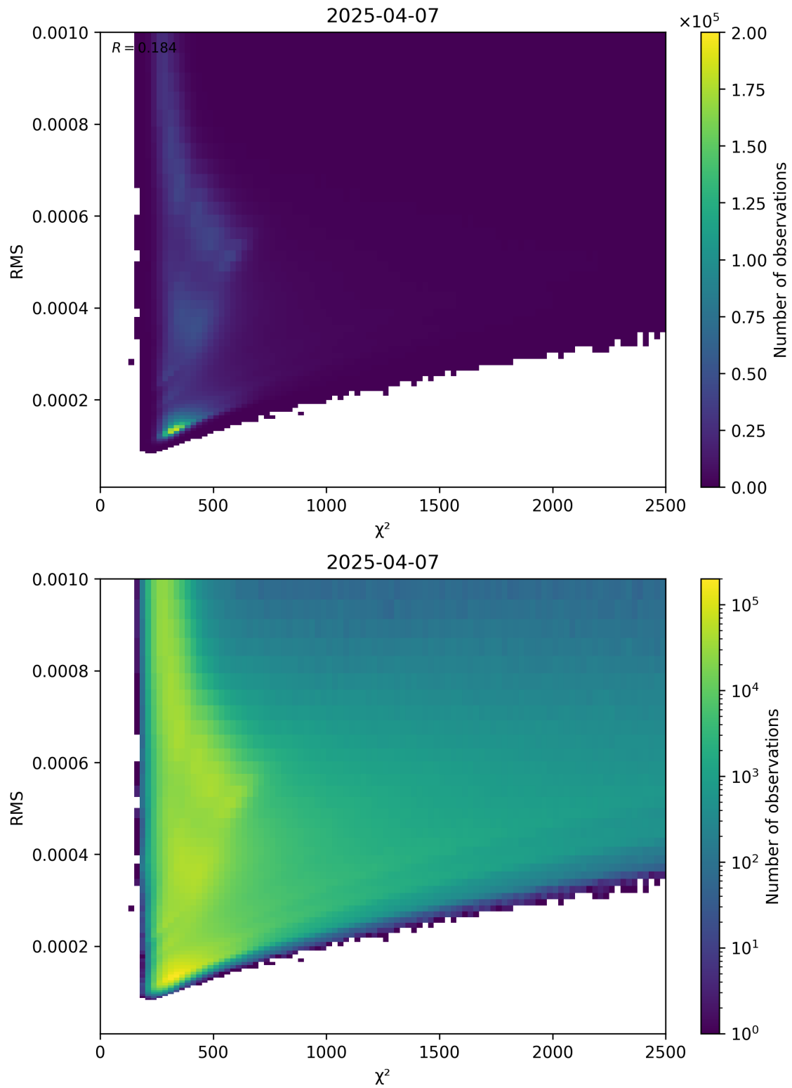
Figure 82: Scatter density plot of “ \chi^2 ” against “RMS” for 2025-04-07 to 2025-04-08.
