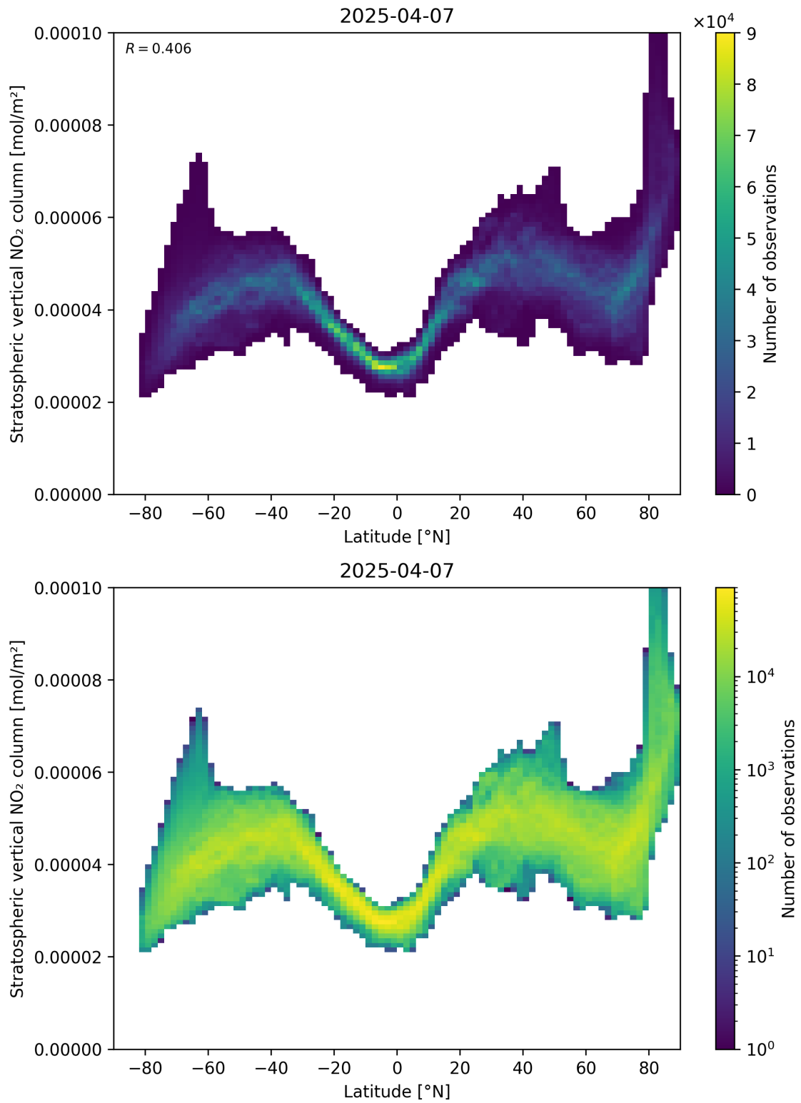
Figure 87: Scatter density plot of “Latitude” against “Stratospheric vertical NO 2 column” for 2025-04-07 to 2025-04-08.
