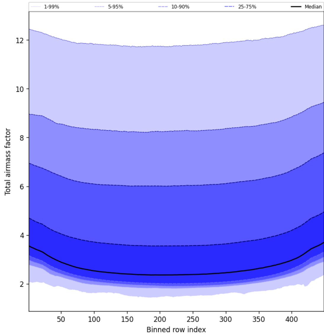
Figure 49: Along track statistics of “Total airmass factor” for 2025-04-07 to 2025-04-08
