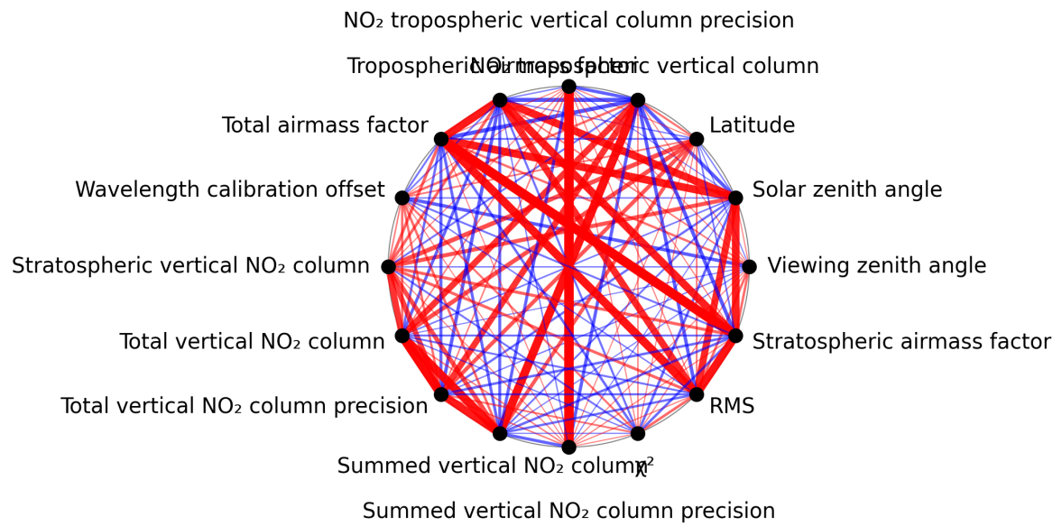
Figure 1: Map of correlation graph for 2025-04-07 to 2025-04-08.
