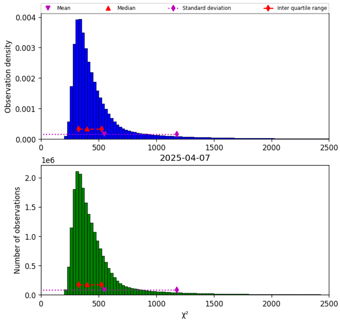
Figure 42: Histogram of “ \chi^2 ” for 2025-04-07 to 2025-04-08
