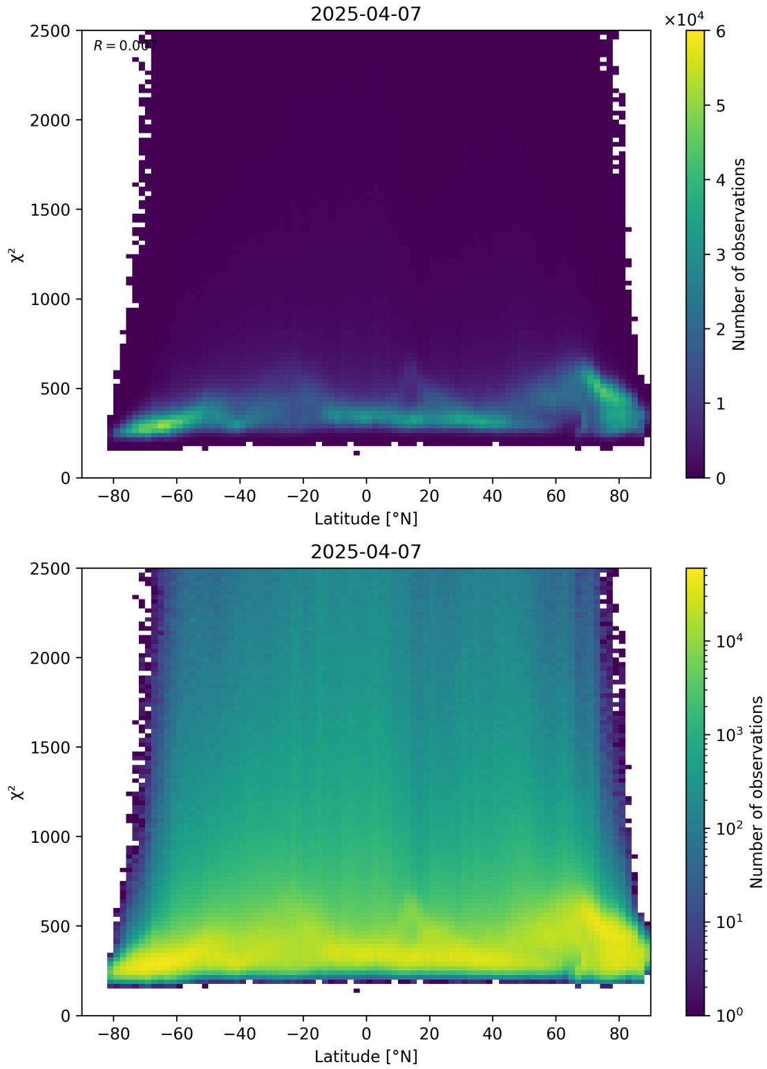
Figure 86: Scatter density plot of “Latitude” against “ \chi^2 ” for 2025-04-07 to 2025-04-08.
