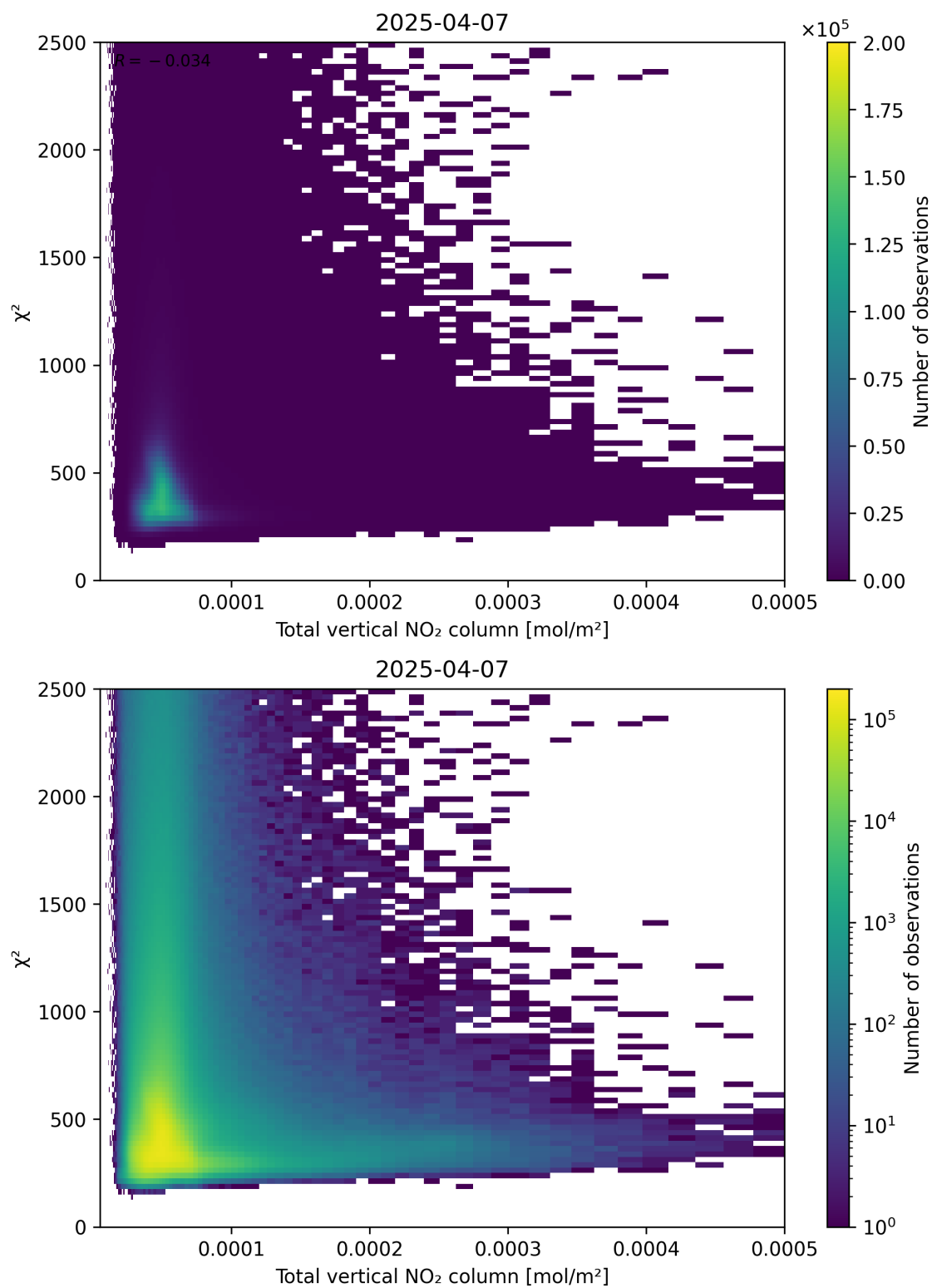
Figure 111: Scatter density plot of “Total vertical NO 2 column” against “ \chi^2 ” for 2025-04-07 to 2025-04-08.
