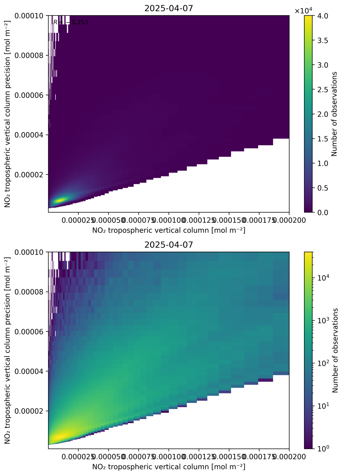
Figure 130: Scatter density plot of “NO 2 tropospheric vertical column” against “NO 2 tropospheric vertical column precision” for 2025-04-07 to 2025-04-08.
