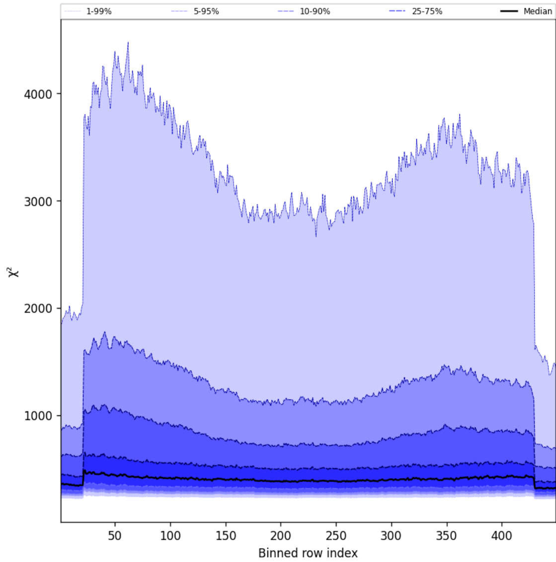
Figure 59: Along track statistics of “ \chi^2 ” for 2025-04-07 to 2025-04-08
