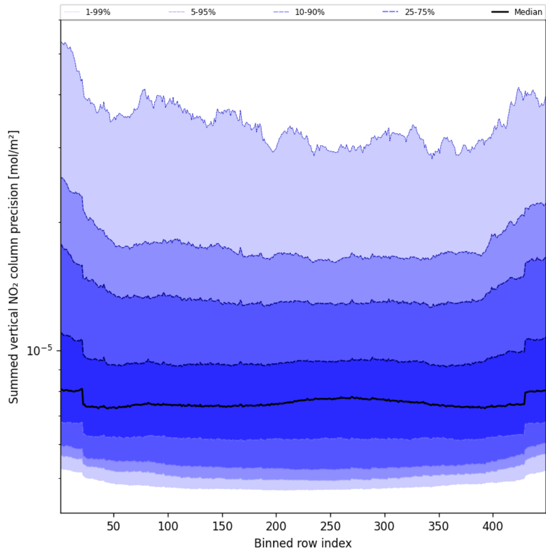
Figure 58: Along track statistics of “Summed vertical NO 2 column precision” for 2025-04-07 to 2025-04-08
