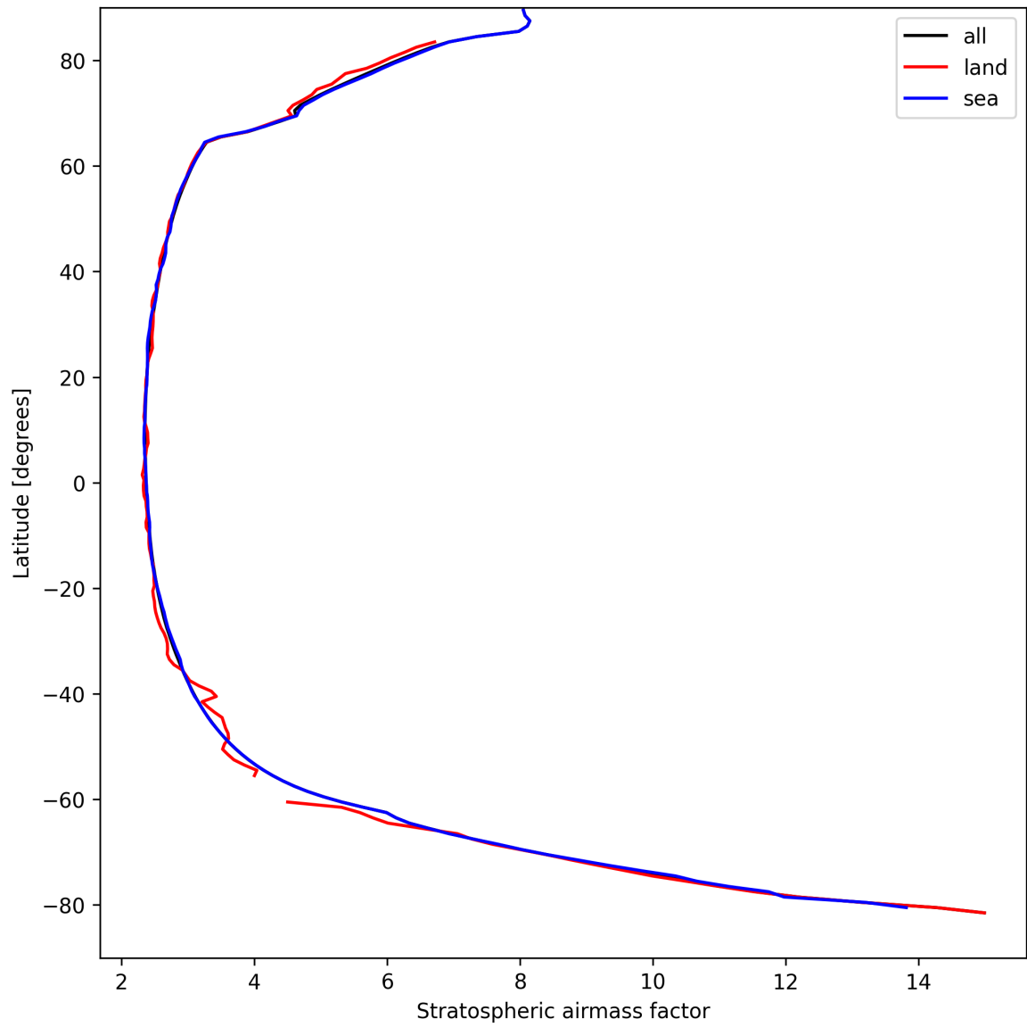
Figure 27: Zonal average of “Stratospheric air mass factor” for 2025-04-07 to 2025-04-08.
