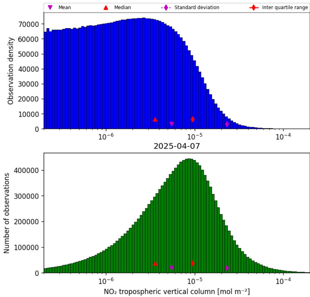
Figure 29: Histogram of “NO 2 tropospheric vertical column” for 2025-04-07 to 2025-04-08
