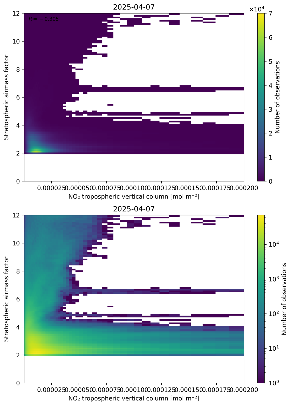
Figure 121: Scatter density plot of “NO 2 tropospheric vertical column” against “Stratospheric air mass factor” for 2025-04-07 to 2025-04-08.
