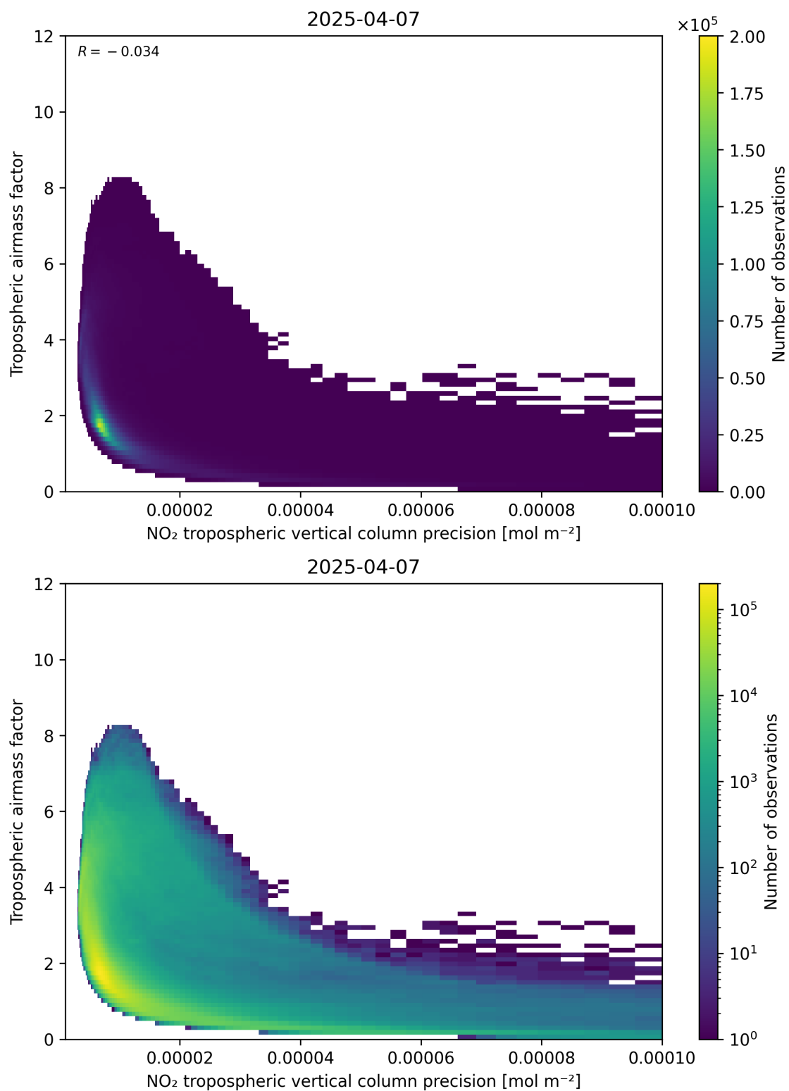
Figure 133: Scatter density plot of “NO 2 tropospheric vertical column precision” against “Tropospheric airmass factor” for 2025-04-07 to 2025-04-08.
