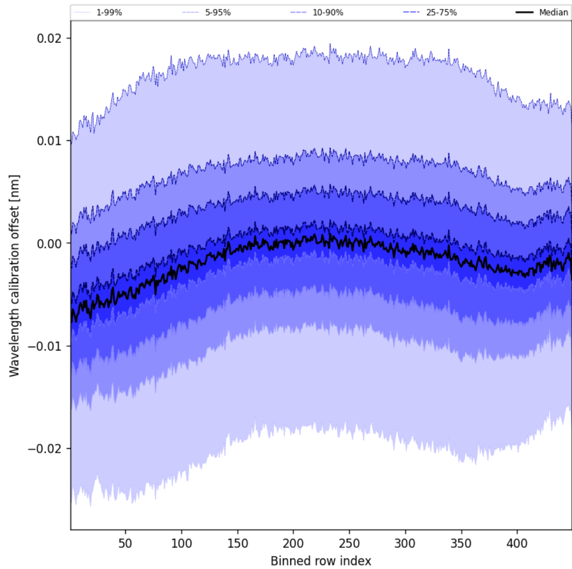
Figure 52: Along track statistics of “Wavelength calibration offset” for 2025-04-07 to 2025-04-08
