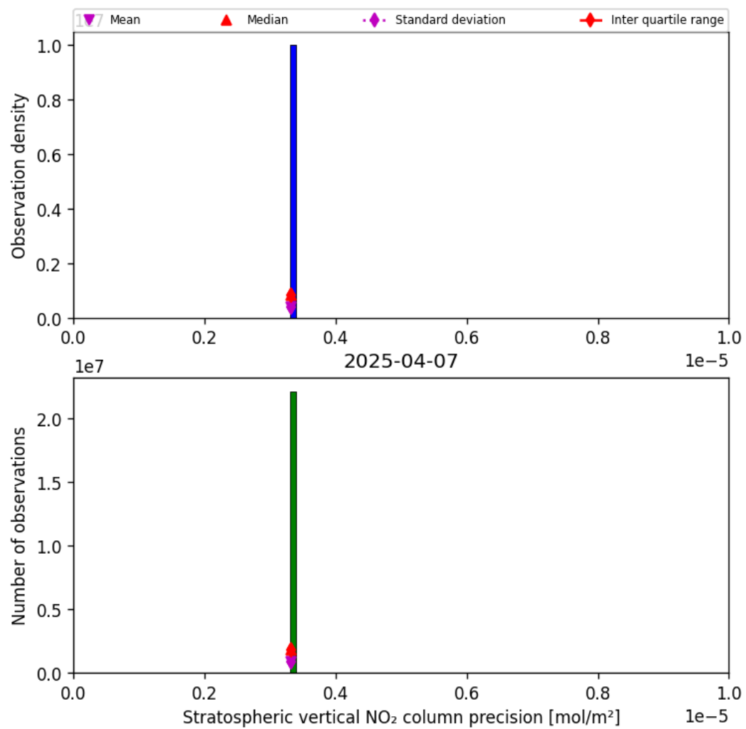
Figure 37: Histogram of “Stratospheric vertical NO 2 column precision” for 2025-04-07 to 2025-04-08
