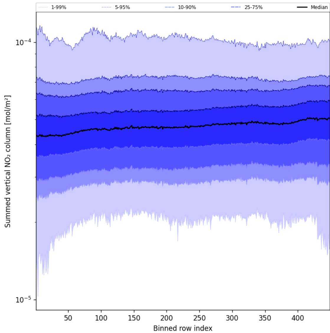
Figure 57: Along track statistics of “Summed vertical NO 2 column” for 2025-04-07 to 2025-04-08
