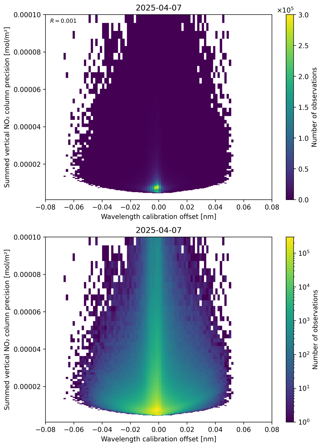
Figure 178: Scatter density plot of “Wavelength calibration offset” against “Summed vertical NO 2 column precision” for 2025-04-07 to 2025-04-08.
