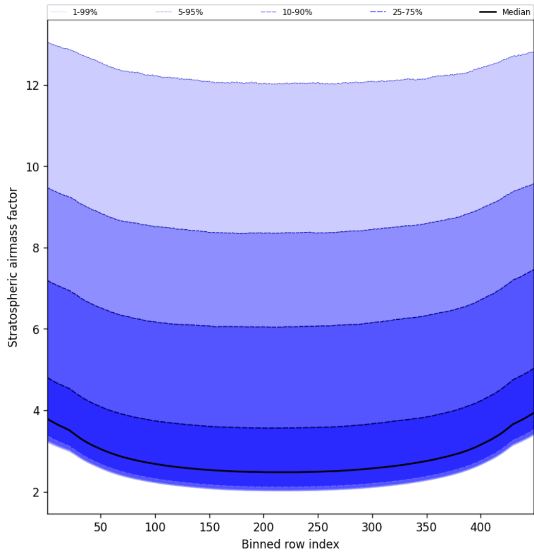
Figure 61: Along track statistics of “Stratospheric air mass factor” for 2025-04-07 to 2025-04-08
