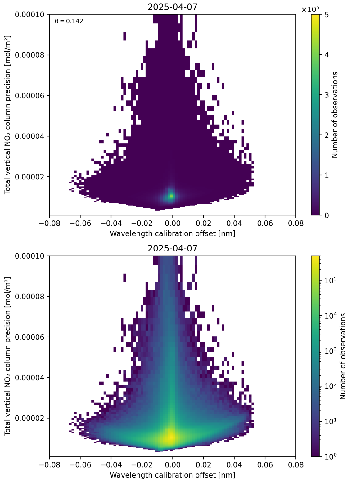
Figure 180: Scatter density plot of “Wavelength calibration offset” against “Total vertical NO 2 column precision” for 2025-04-07 to 2025-04-08.
