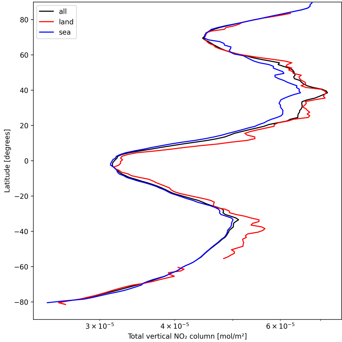
Figure 21: Zonal average of “Total vertical NO 2 column” for 2025-04-07 to 2025-04-08.
