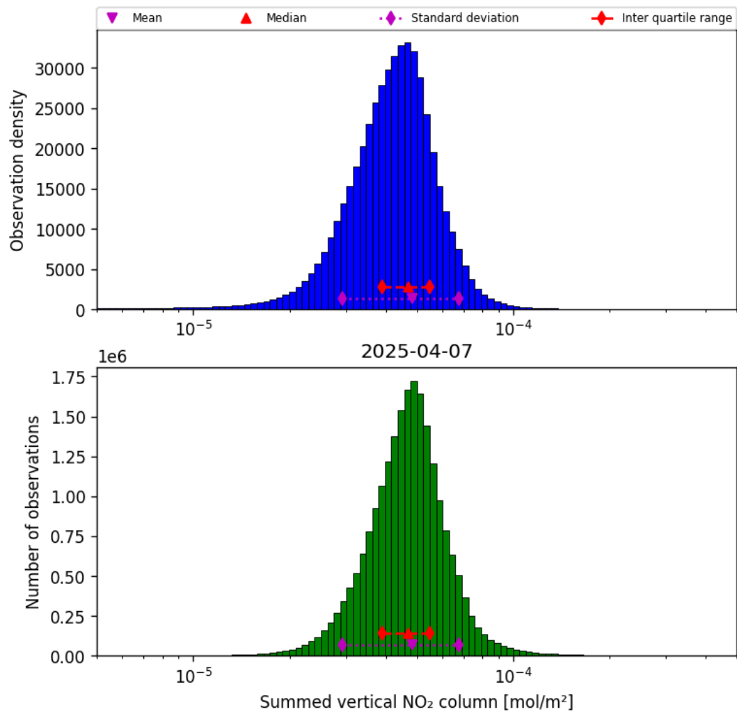
Figure 40: Histogram of “Summed vertical NO 2 column” for 2025-04-07 to 2025-04-08
