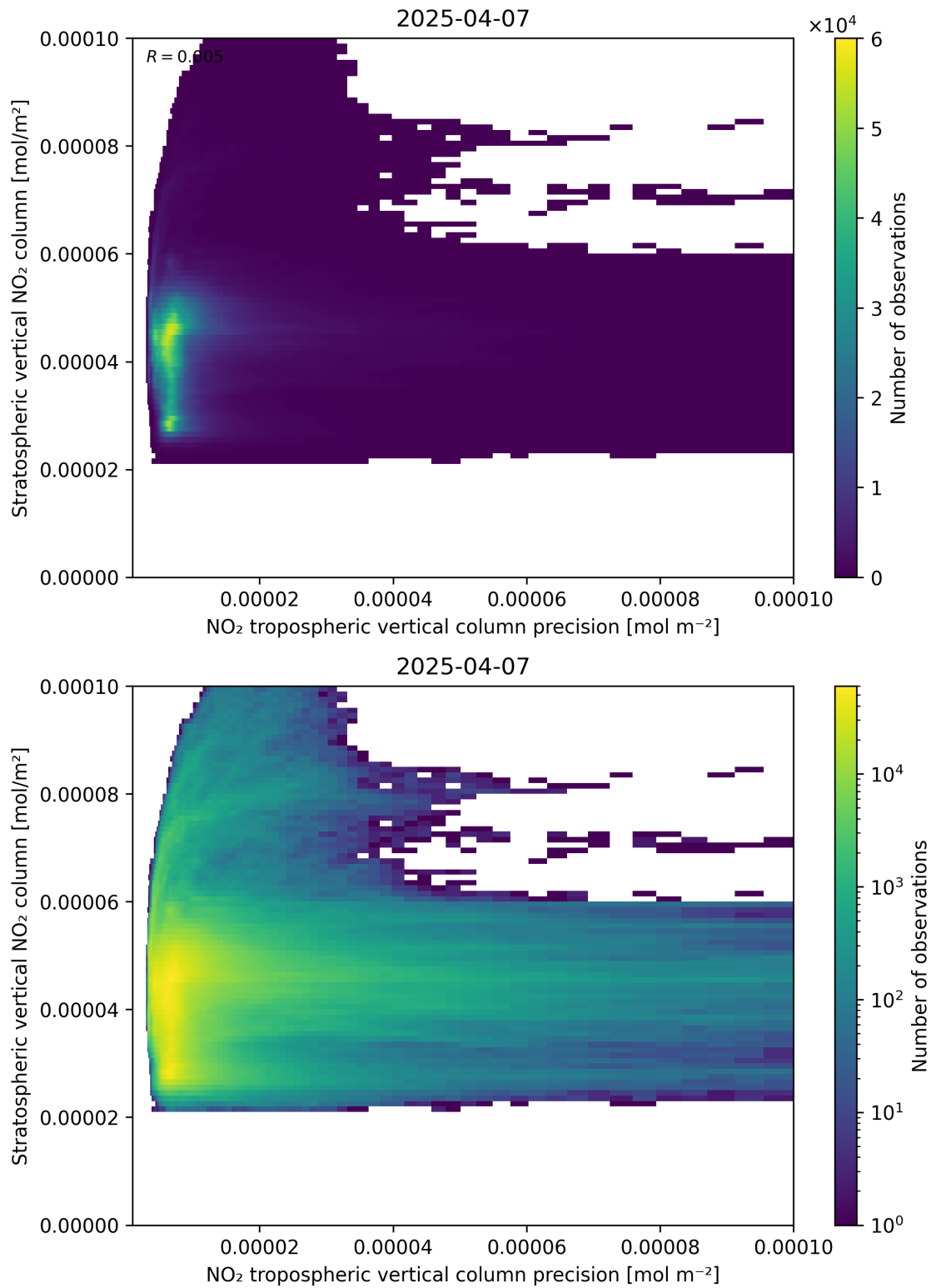
Figure 135: Scatter density plot of “NO 2 tropospheric vertical column precision” against “Stratospheric vertical NO 2 column” for 2025-04-07 to 2025-04-08.
