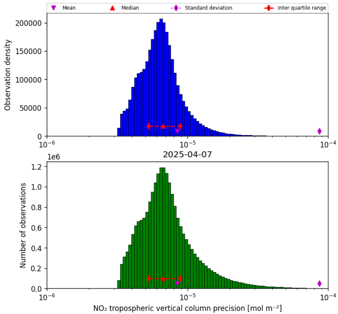
Figure 30: Histogram of “NO 2 tropospheric vertical column precision” for 2025-04-07 to 2025-04-08
