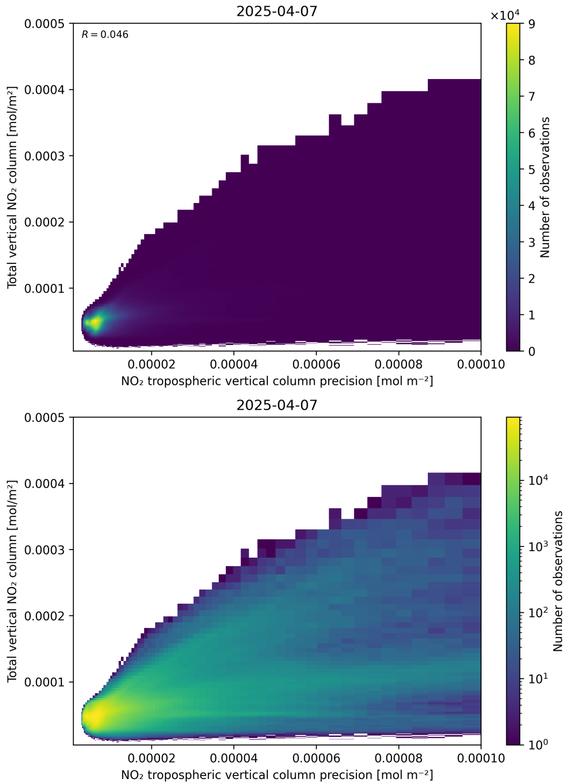
Figure 138: Scatter density plot of “NO 2 tropospheric vertical column precision” against “Total vertical NO 2 column” for 2025-04-07 to 2025-04-08.
