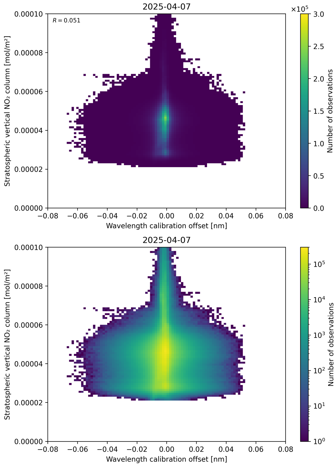
Figure 176: Scatter density plot of “Wavelength calibration offset” against “Stratospheric vertical NO 2 column” for 2025-04-07 to 2025-04-08.
