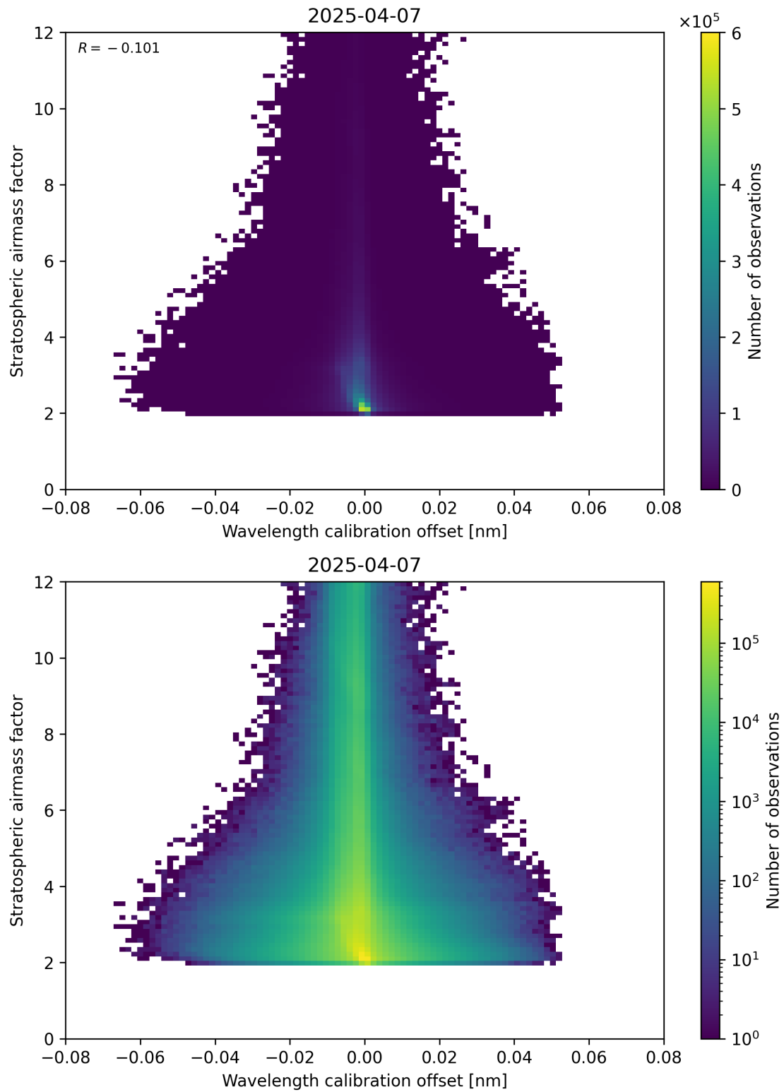
Figure 174: Scatter density plot of “Wavelength calibration offset” against “Stratospheric airmass factor” for 2025-04-07 to 2025-04-08.
