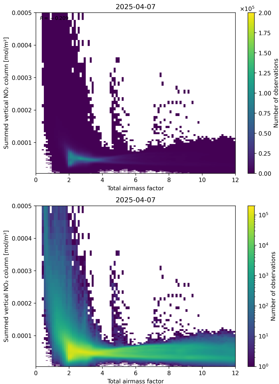
Figure 65: Scatter density plot of “Total airmass factor” against “Summed vertical NO 2 column” for 2025-04-07 to 2025-04-08.
