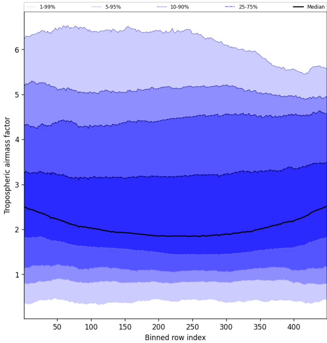
Figure 48: Along track statistics of “Tropospheric airmass factor” for 2025-04-07 to 2025-04-08
