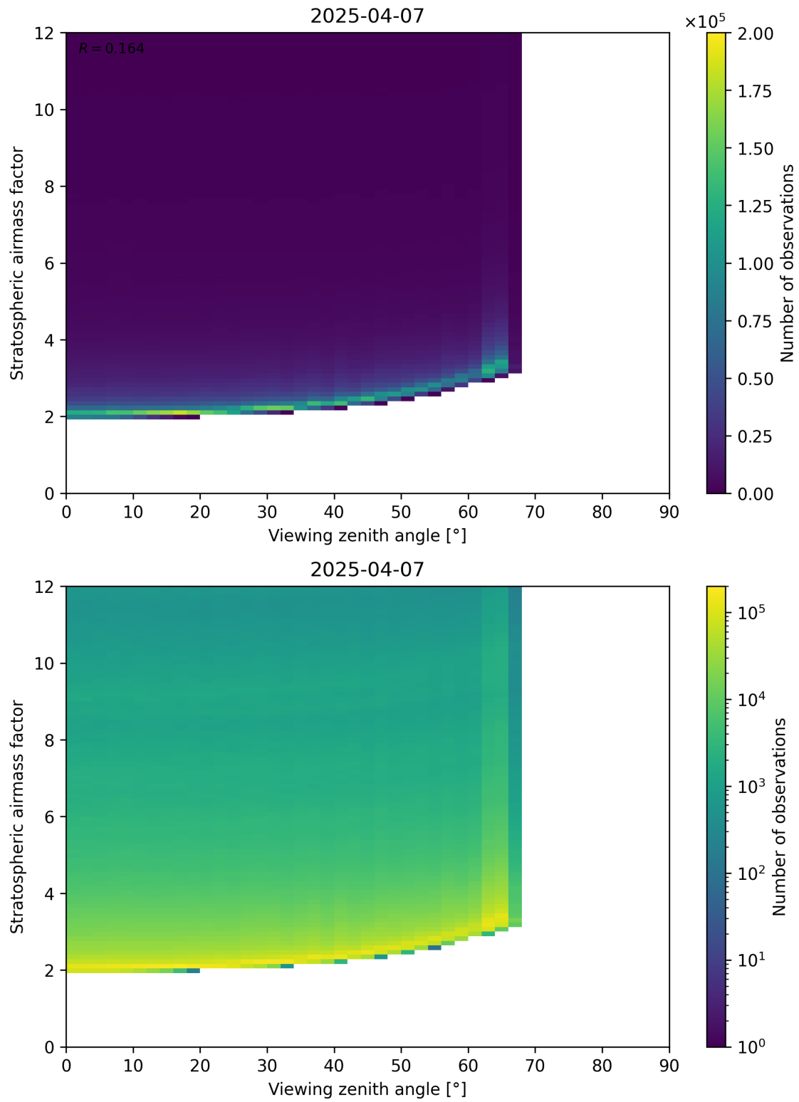
Figure 159: Scatter density plot of “Viewing zenith angle” against “Stratospheric airmass factor” for 2025-04-07 to 2025-04-08.
