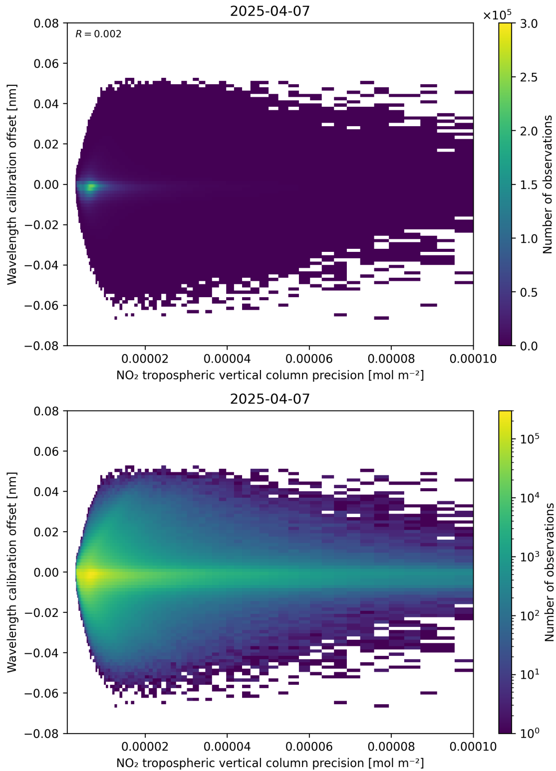
Figure 141: Scatter density plot of “NO 2 tropospheric vertical column precision” against “Wavelength calibration offset” for 2025-04-07 to 2025-04-08.
