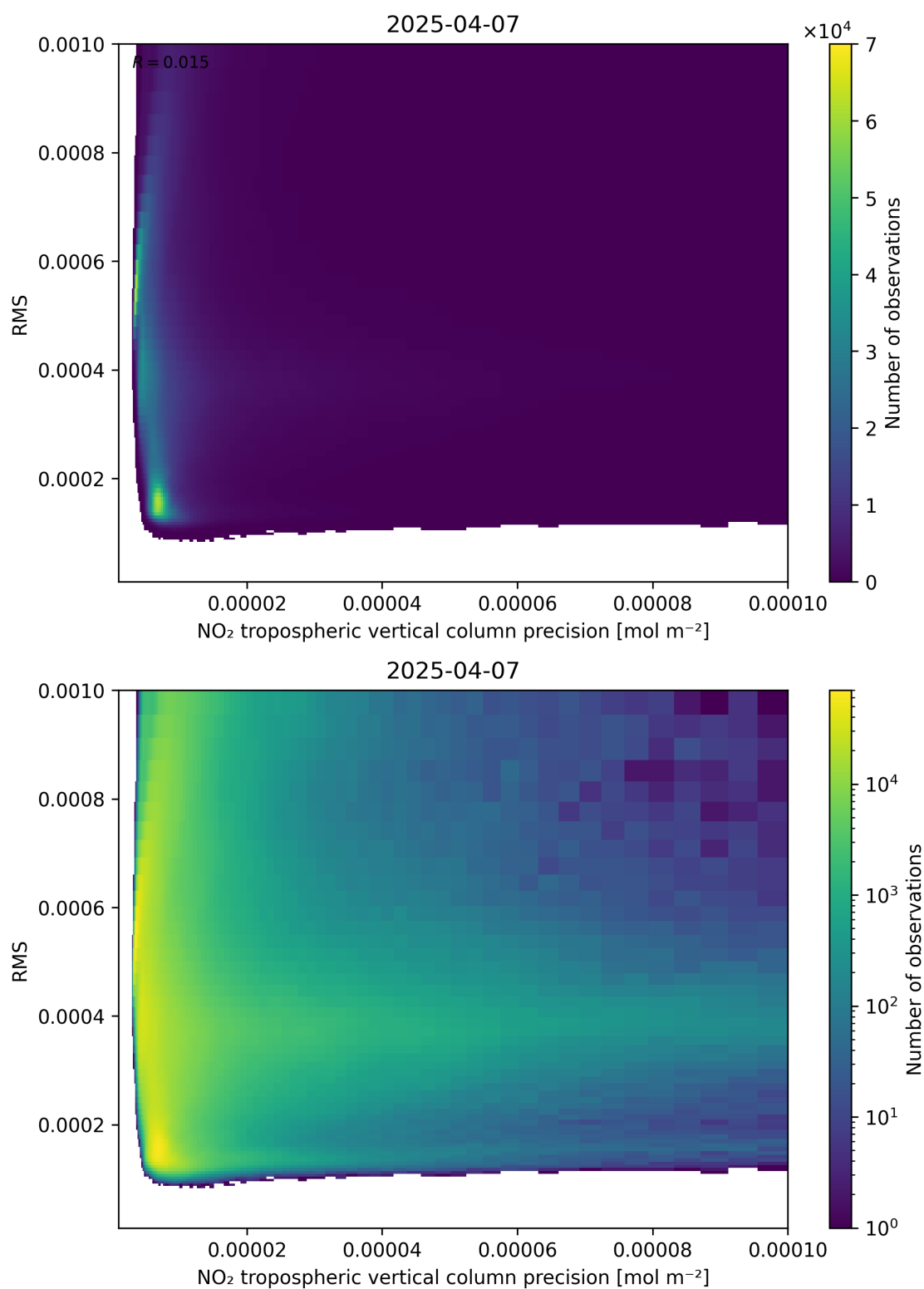
Figure 140: Scatter density plot of “NO 2 tropospheric vertical column precision” against “RMS” for 2025-04-07 to 2025-04-08.
