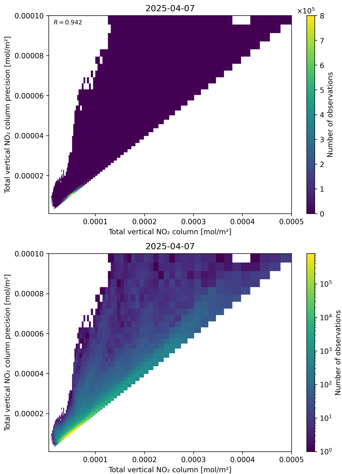
Figure 114: Scatter density plot of “Total vertical NO 2 column” against “Total vertical NO 2 column precision” for 2025-04-07 to 2025-04-08.
