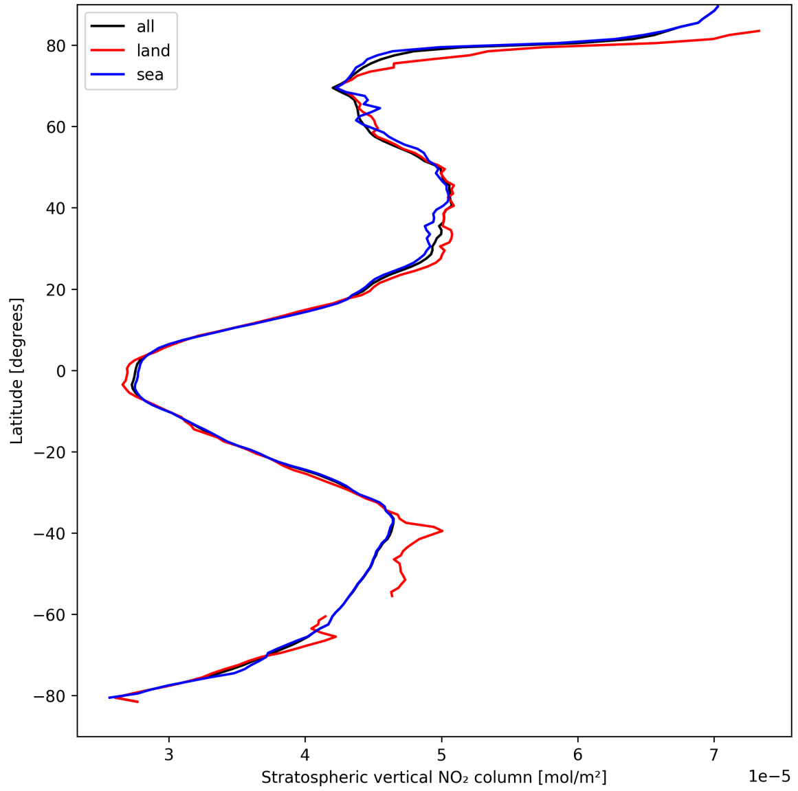
Figure 19: Zonal average of “Stratospheric vertical NO 2 column” for 2025-04-07 to 2025-04-08.
