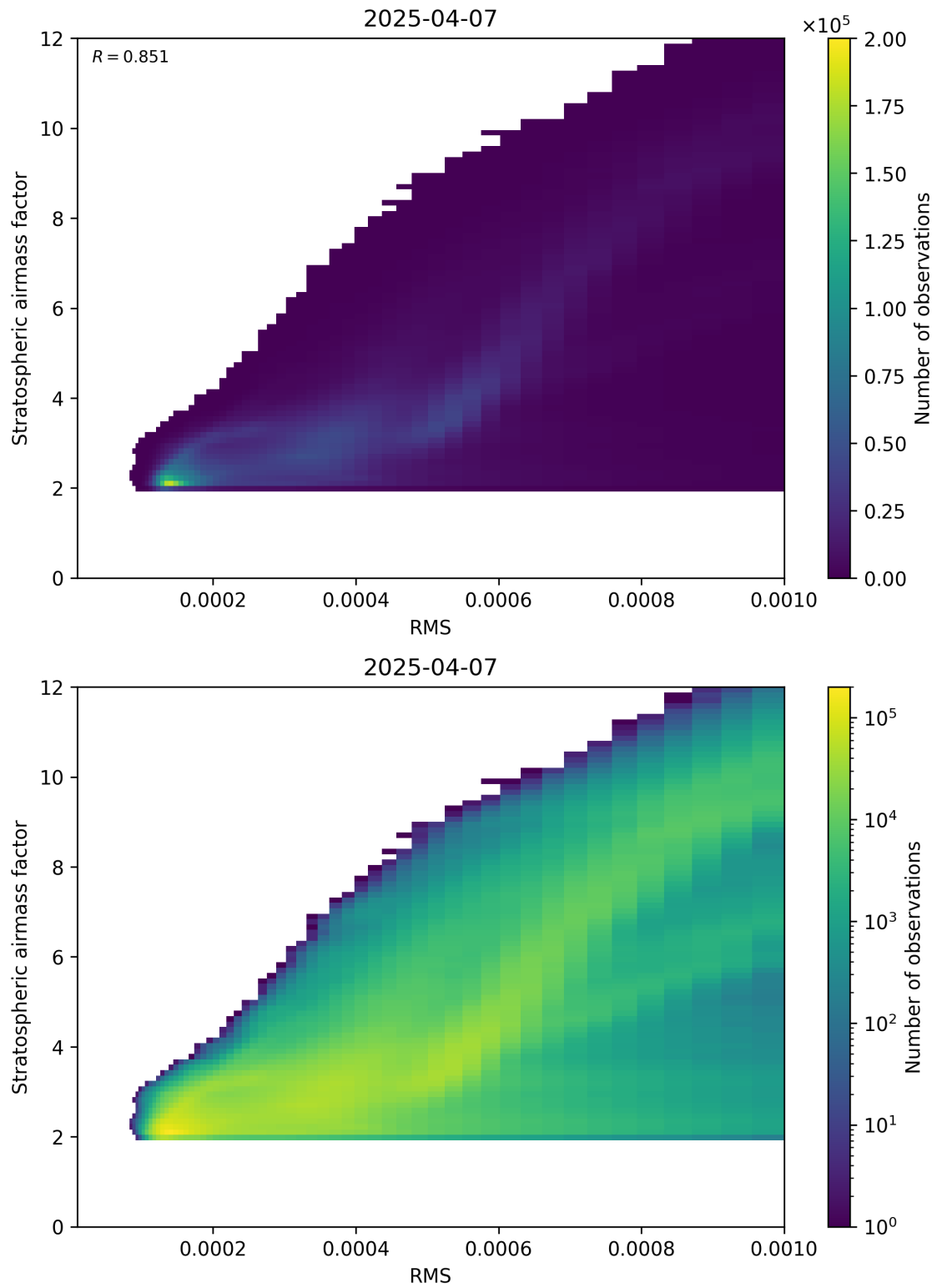
Figure 144: Scatter density plot of “RMS” against “Stratospheric airmass factor” for 2025-04-07 to 2025-04-08.
