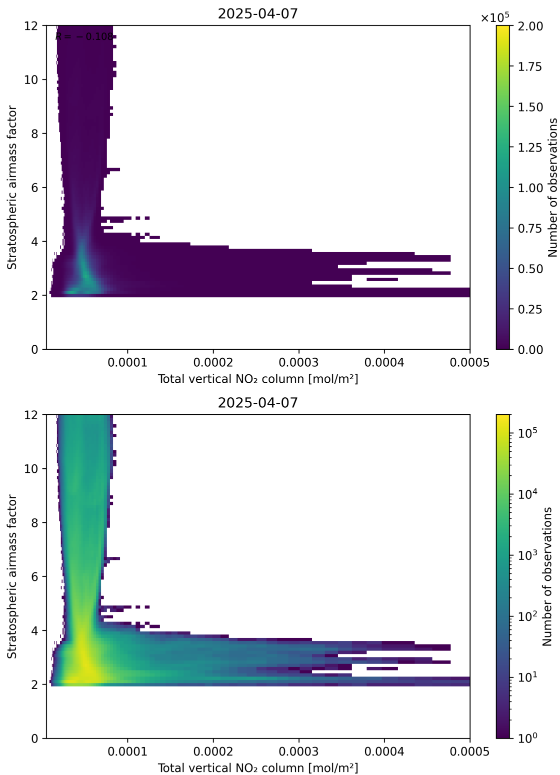
Figure 110: Scatter density plot of “Total vertical NO 2 column” against “Stratospheric airmass factor” for 2025-04-07 to 2025-04-08.
