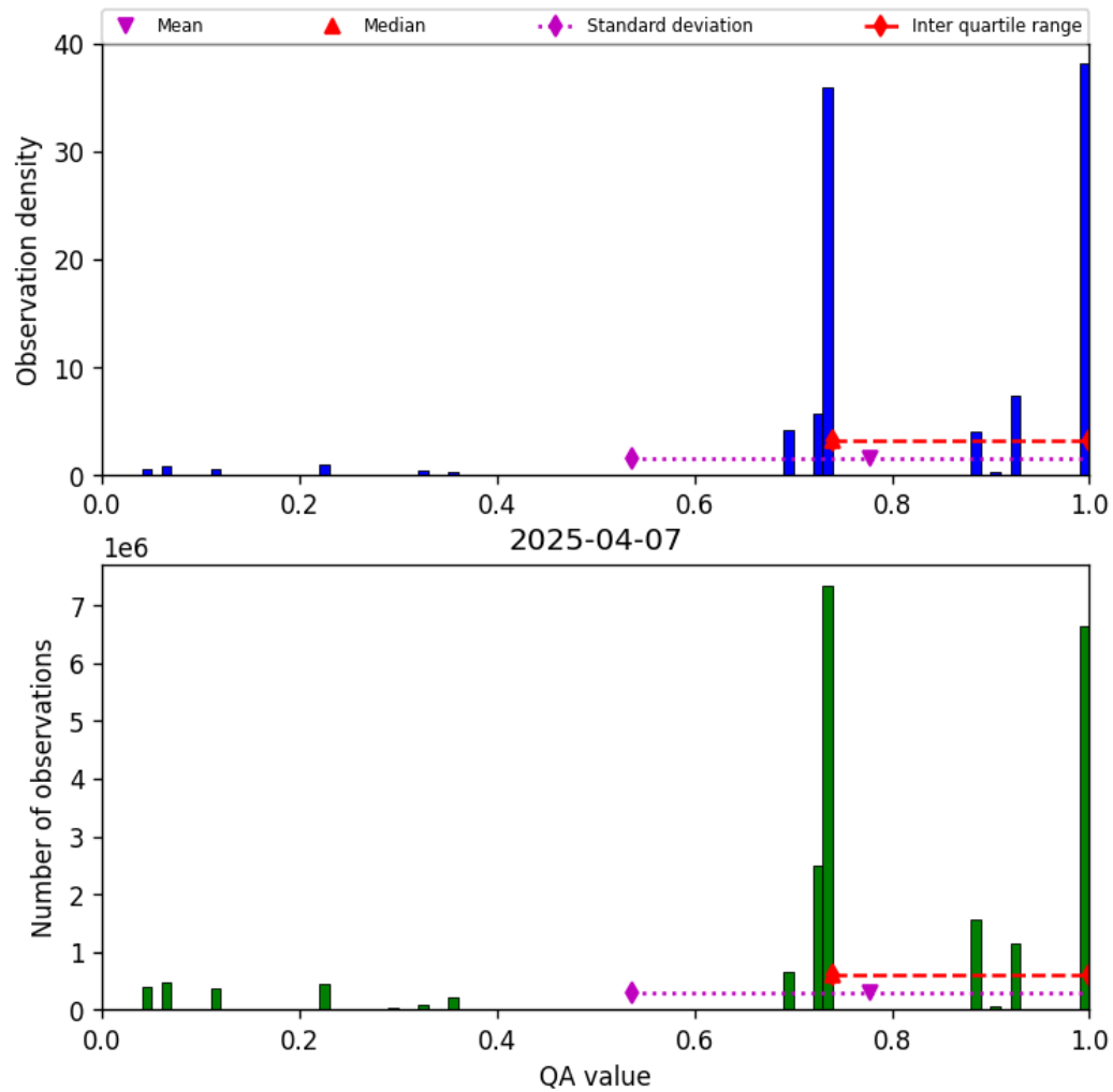
Figure 28: Histogram of “QA value” for 2025-04-07 to 2025-04-08
