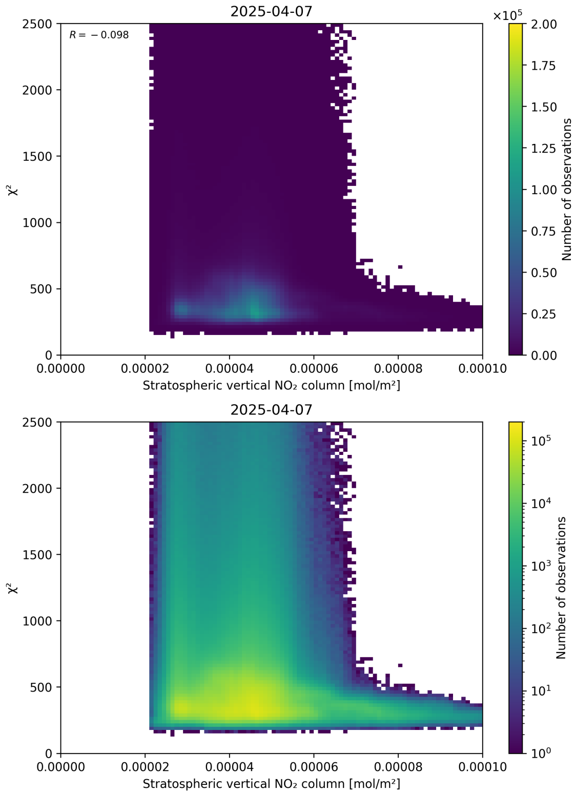
Figure 97: Scatter density plot of “Stratospheric vertical NO 2 column” against “ \chi^2 ” for 2025-04-07 to 2025-04-08.
