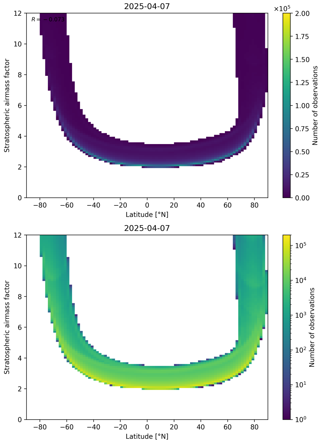
Figure 83: Scatter density plot of “Latitude” against “Stratospheric air mass factor” for 2025-04-07 to 2025-04-08.
