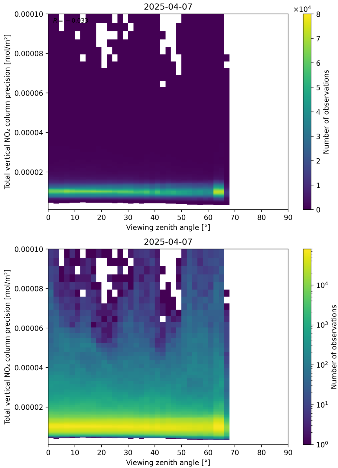
Figure 168: Scatter density plot of “Viewing zenith angle” against “Total vertical NO 2 column precision” for 2025-04-07 to 2025-04-08.
