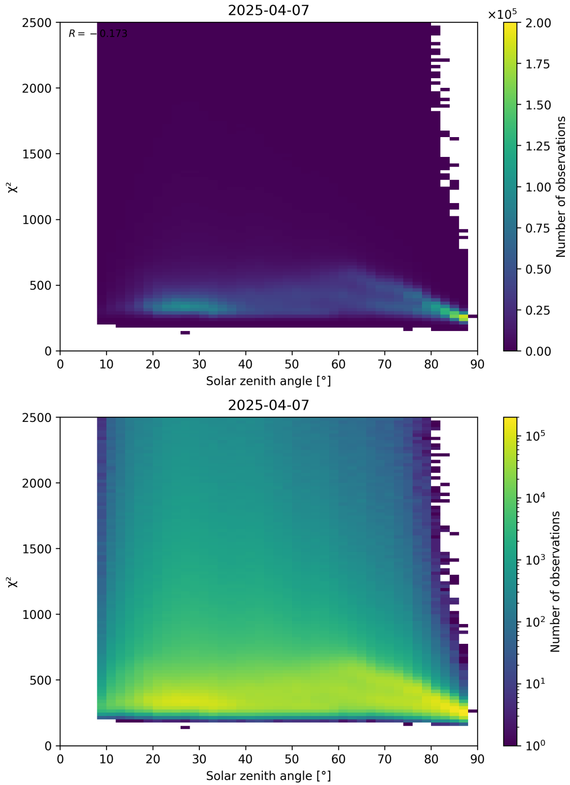
Figure 148: Scatter density plot of “Solar zenith angle” against “ \chi^2 ” for 2025-04-07 to 2025-04-08.
