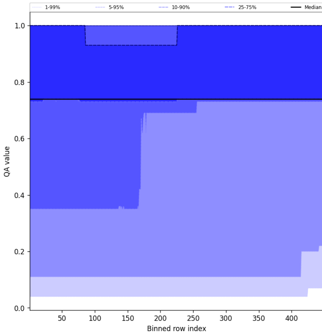
Figure 45: Along track statistics of “QA value” for 2025-04-07 to 2025-04-08
