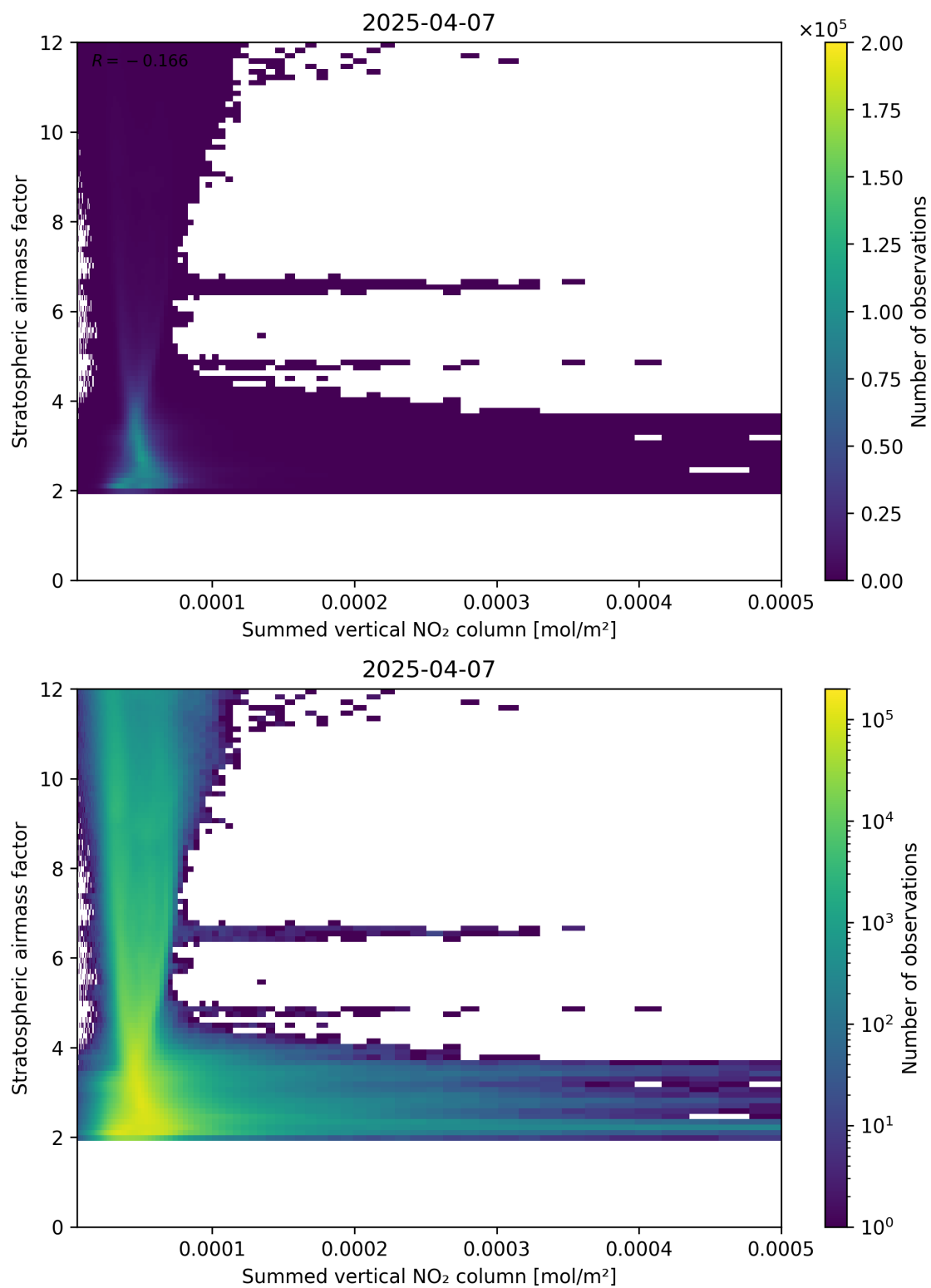
Figure 103: Scatter density plot of “Summed vertical NO 2 column” against “Stratospheric airmass factor” for 2025-04-07 to 2025-04-08.
