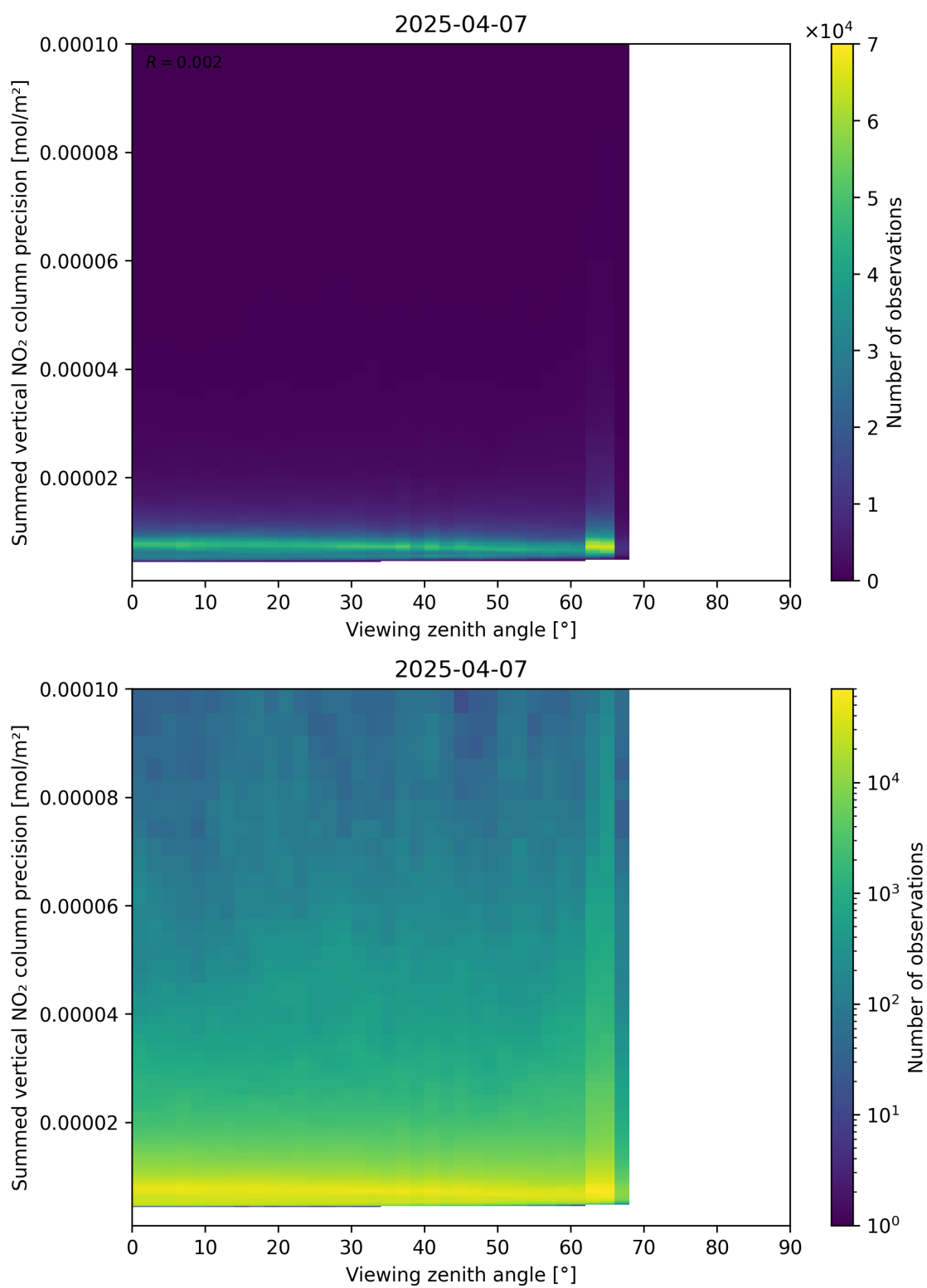
Figure 166: Scatter density plot of “Viewing zenith angle” against “Summed vertical NO 2 column precision” for 2025-04-07 to 2025-04-08.
