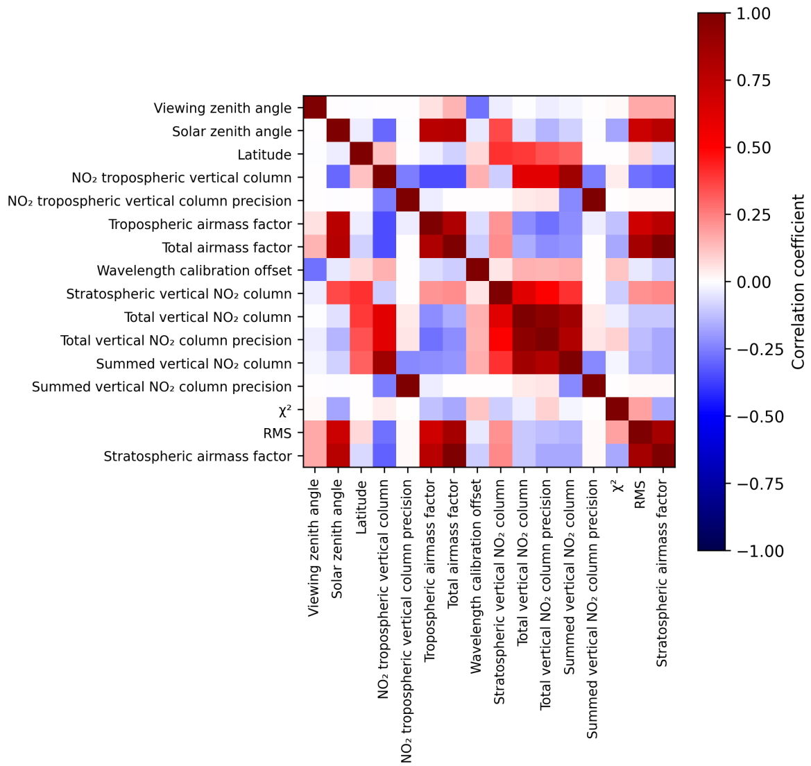
Figure 2: Map of correlation matrix for 2025-04-07 to 2025-04-08.
