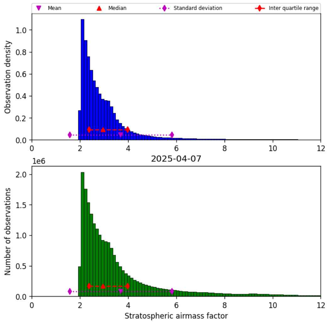
Figure 44: Histogram of “Stratospheric airmass factor” for 2025-04-07 to 2025-04-08
