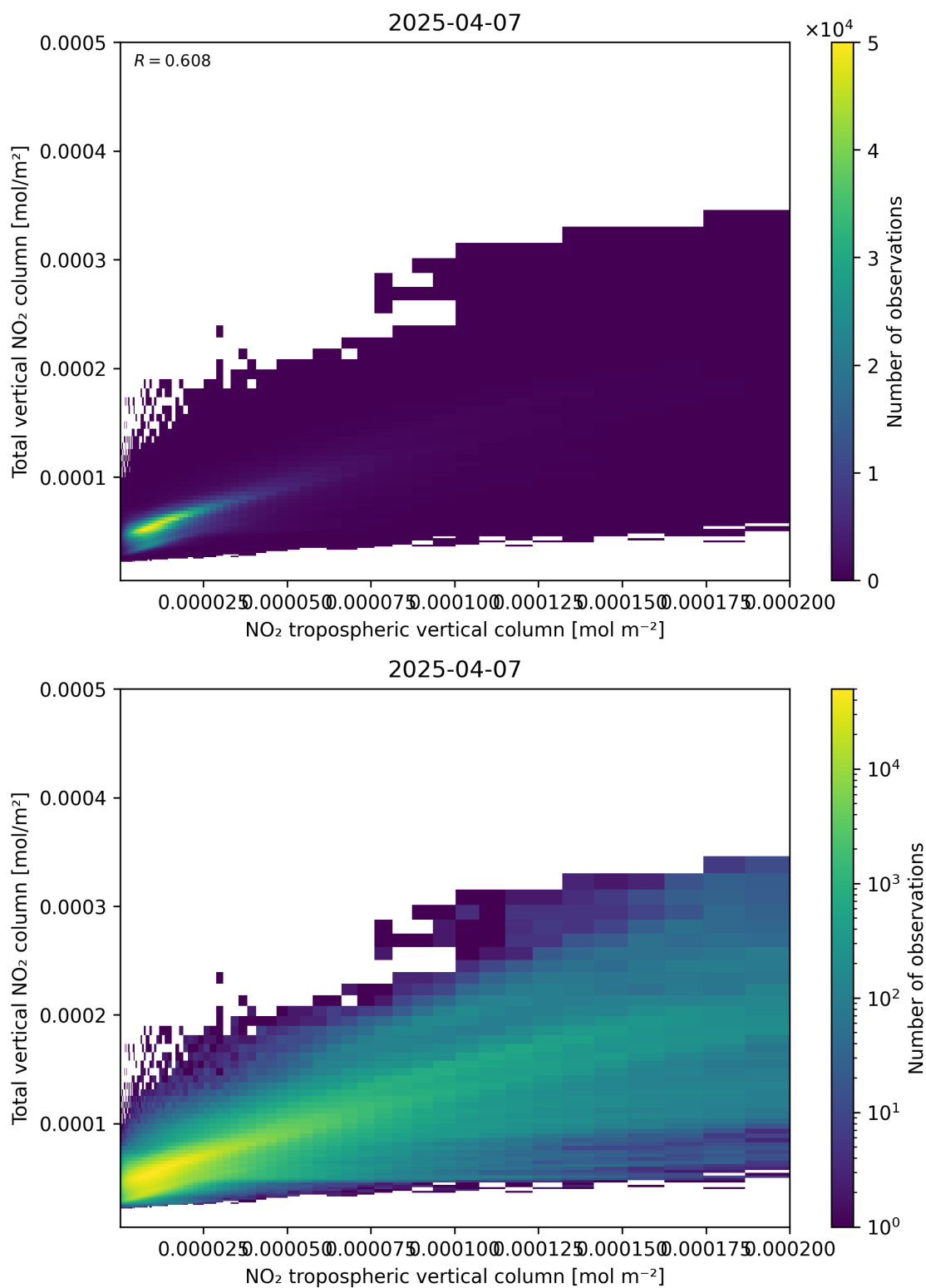
Figure 128: Scatter density plot of “NO 2 tropospheric vertical column” against “Total vertical NO 2 column” for 2025-04-07 to 2025-04-08.
