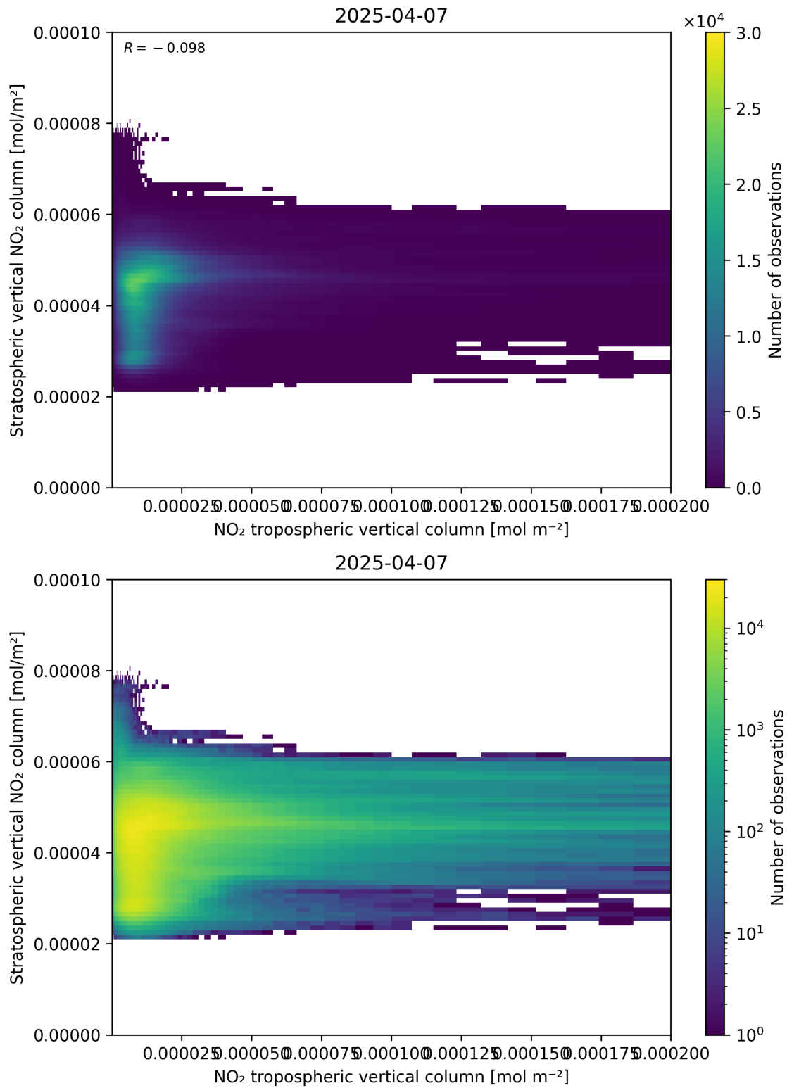
Figure 125: Scatter density plot of “NO 2 tropospheric vertical column” against “Stratospheric vertical NO 2 column” for 2025-04-07 to 2025-04-08.
