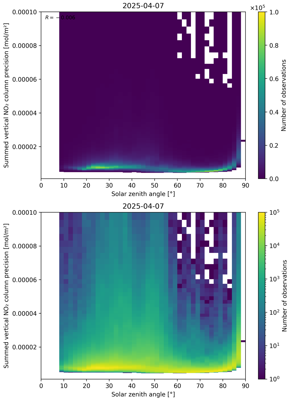
Figure 152: Scatter density plot of “Solar zenith angle” against “Summed vertical NO 2 column precision” for 2025-04-07 to 2025-04-08.
