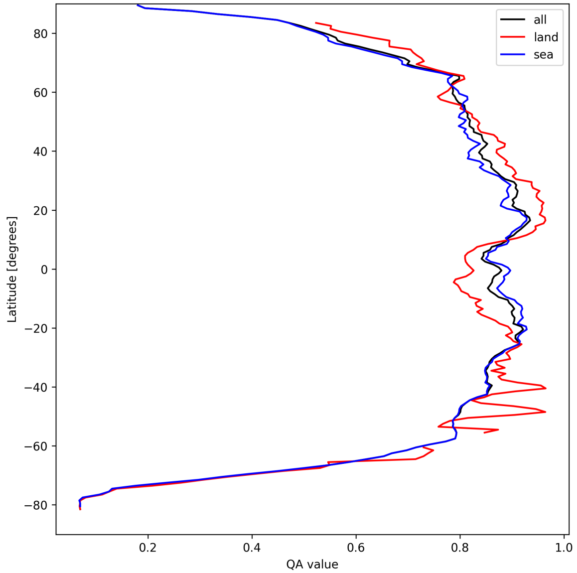
Figure 11: Zonal average of “QA value” for 2025-04-07 to 2025-04-08.
