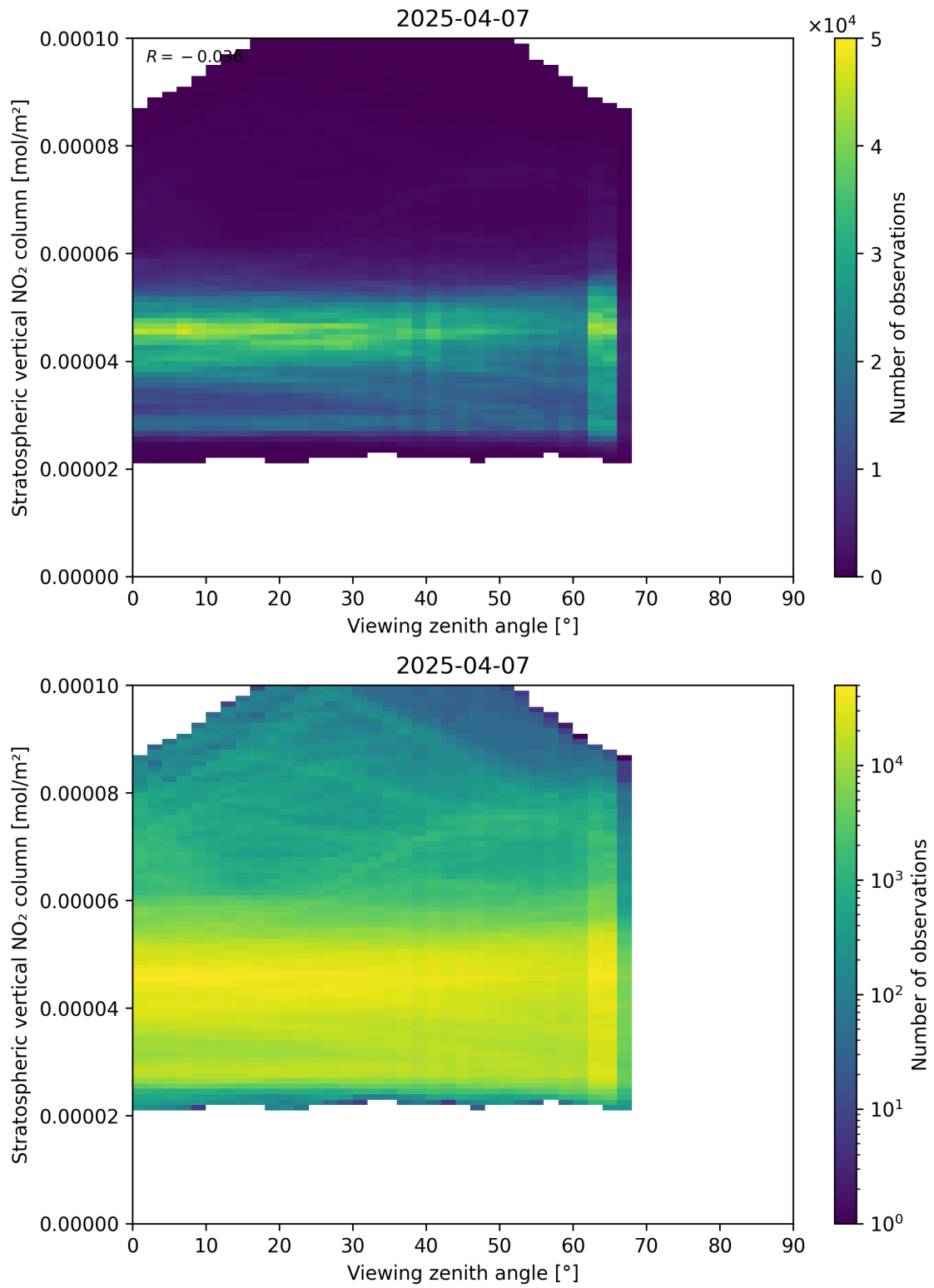
Figure 164: Scatter density plot of “Viewing zenith angle” against “Stratospheric vertical NO 2 column” for 2025-04-07 to 2025-04-08.
