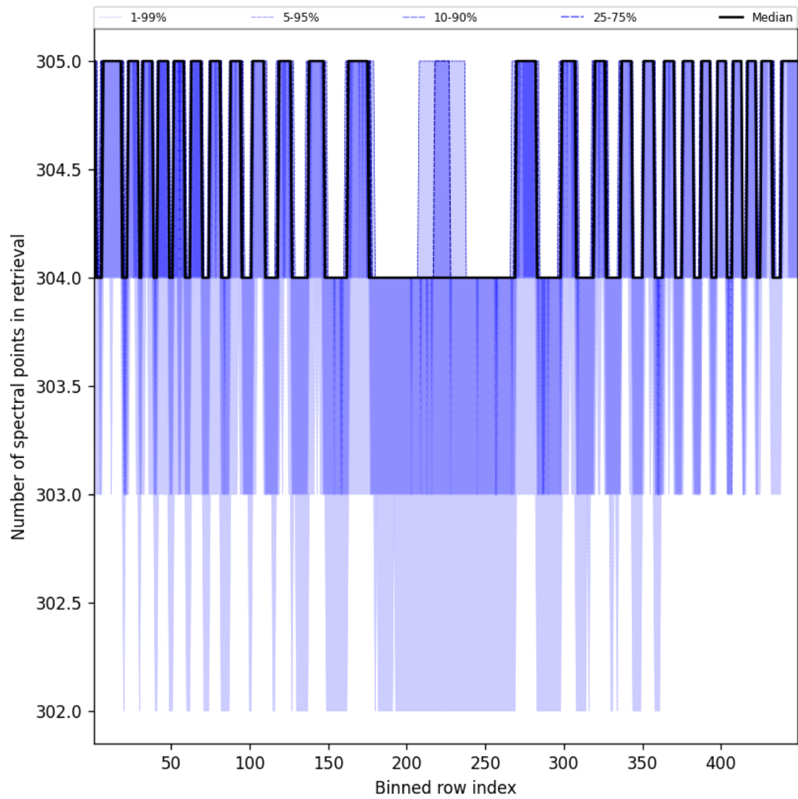
Figure 50: Along track statistics of “Number of spectral points in retrieval” for 2025-04-07 to 2025-04-08
