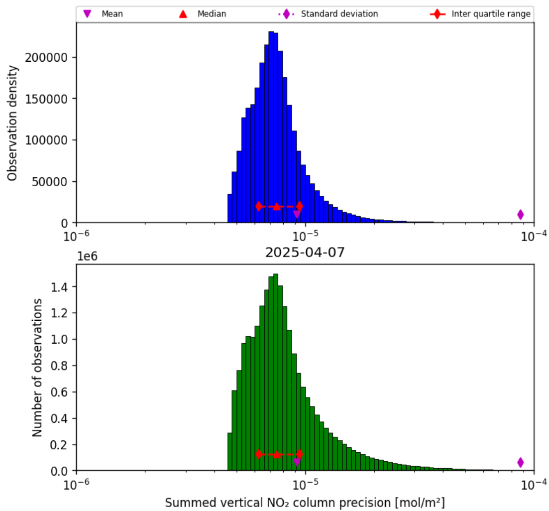
Figure 41: Histogram of “Summed vertical NO 2 column precision” for 2025-04-07 to 2025-04-08
