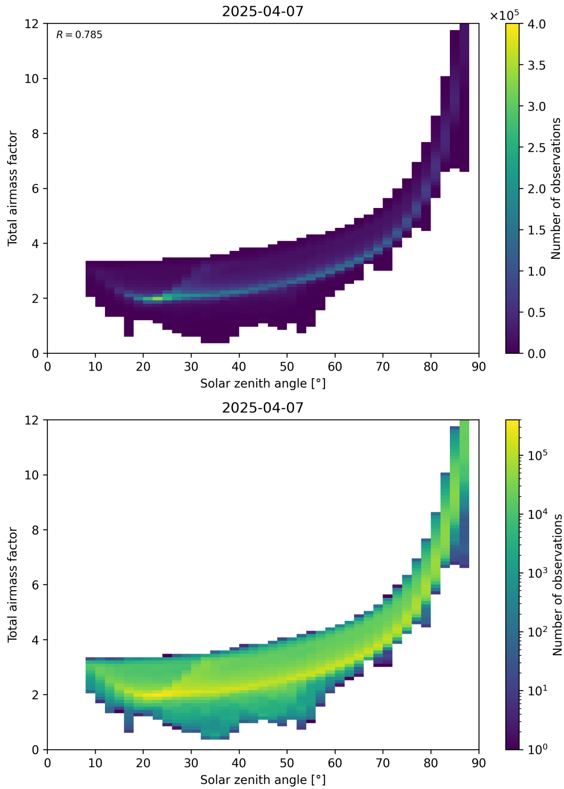
Figure 146: Scatter density plot of “Solar zenith angle” against “Total air mass factor” for 2025-04-07 to 2025-04-08.
