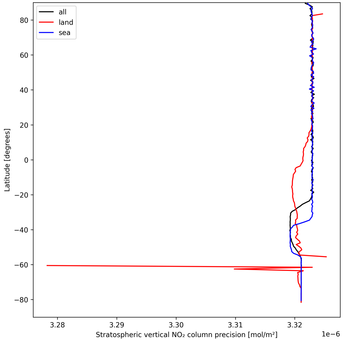
Figure 20: Zonal average of “Stratospheric vertical NO 2 column precision” for 2025-04-07 to 2025-04-08.
