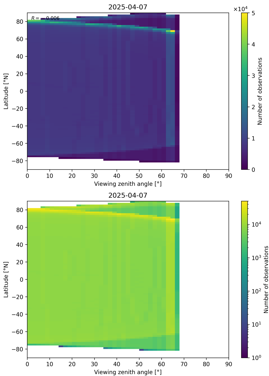
Figure 163: Scatter density plot of “Viewing zenith angle” against “Latitude” for 2025-04-07 to 2025-04-08.
