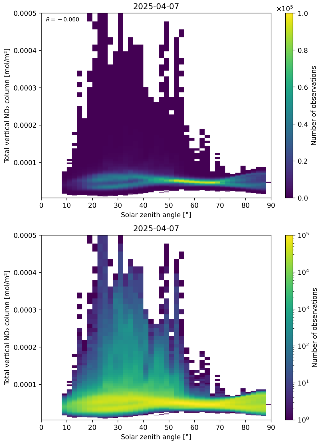
Figure 153: Scatter density plot of “Solar zenith angle” against “Total vertical NO 2 column” for 2025-04-07 to 2025-04-08.
