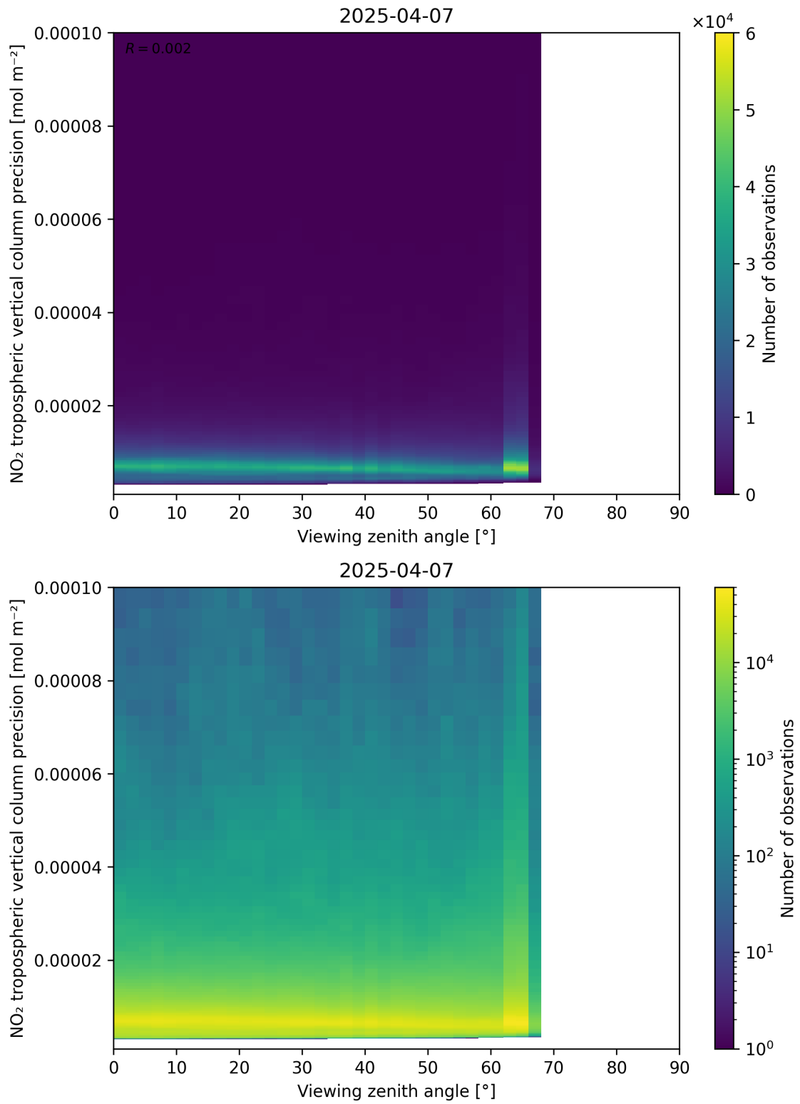
Figure 170: Scatter density plot of “Viewing zenith angle” against “NO 2 tropospheric vertical column precision” for 2025-04-07 to 2025-04-08.
