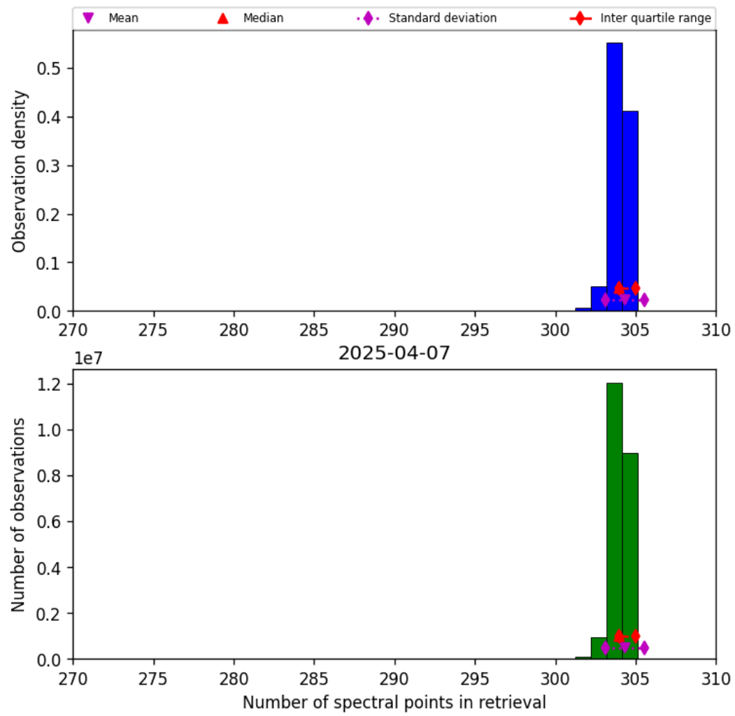
Figure 33: Histogram of “Number of spectral points in retrieval” for 2025-04-07 to 2025-04-08
