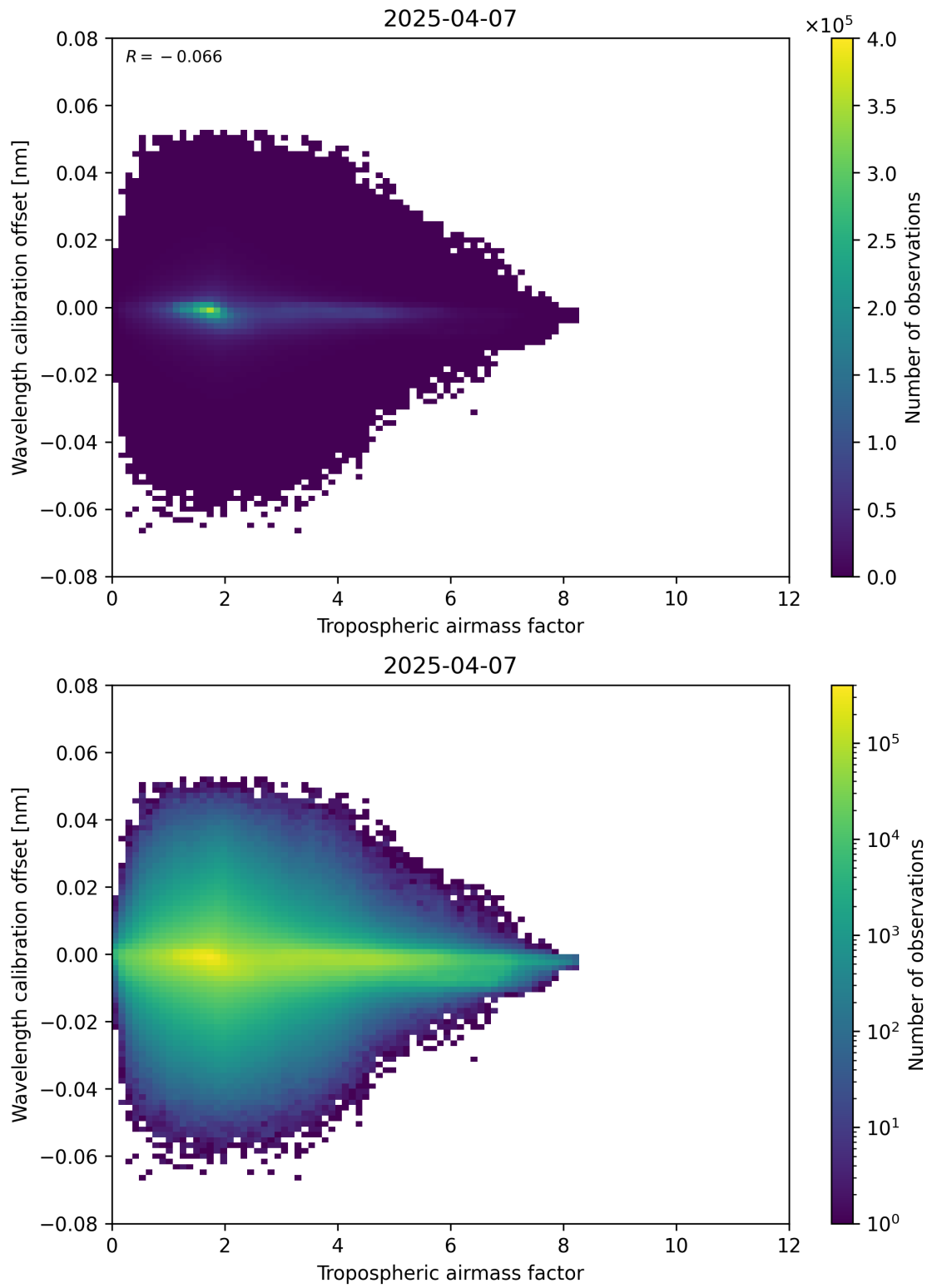
Figure 80: Scatter density plot of “Tropospheric airmass factor” against “Wavelength calibration offset” for 2025-04-07 to 2025-04-08.
