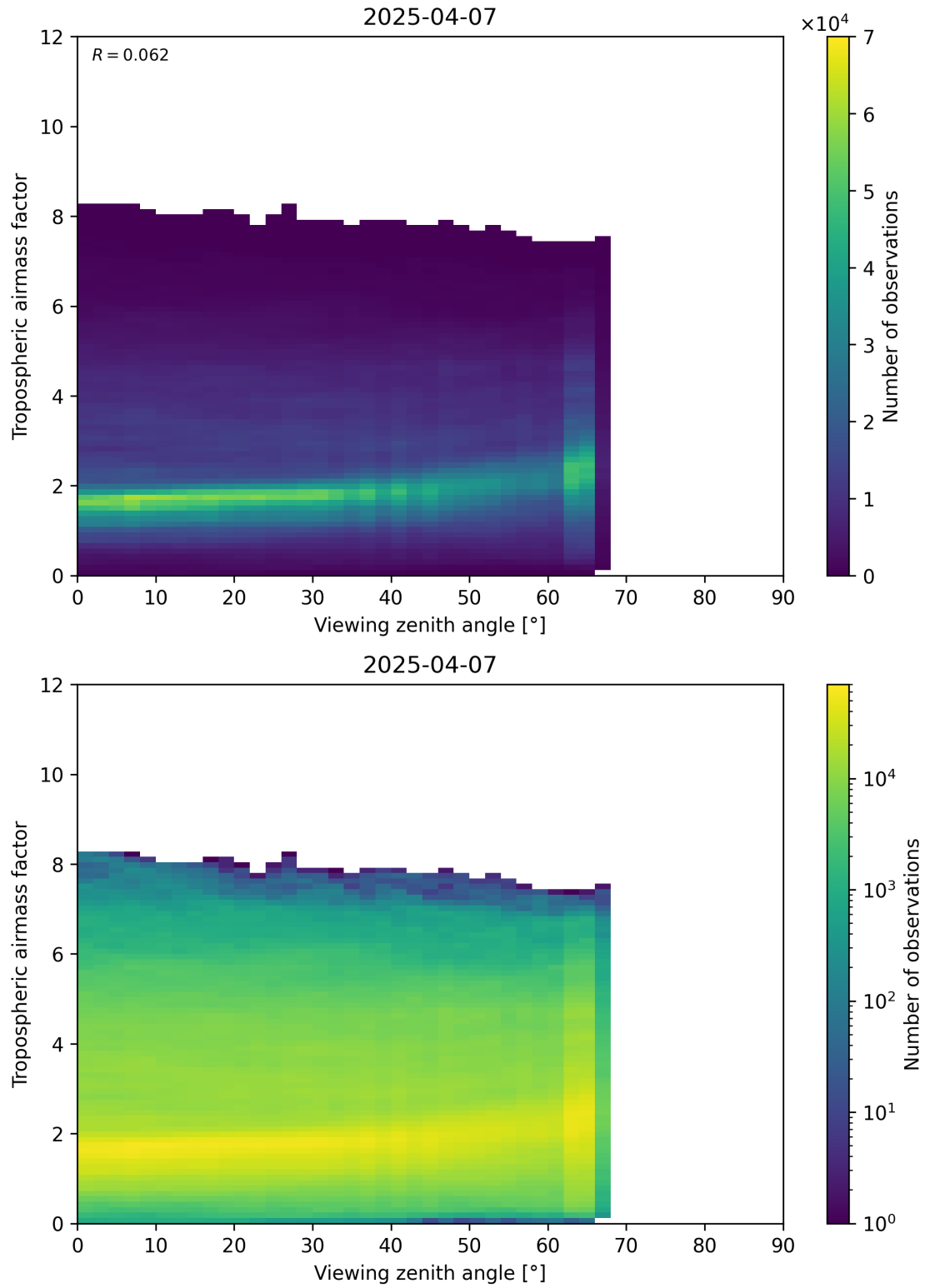
Figure 161: Scatter density plot of “Viewing zenith angle” against “Tropospheric airmass factor” for 2025-04-07 to 2025-04-08.
