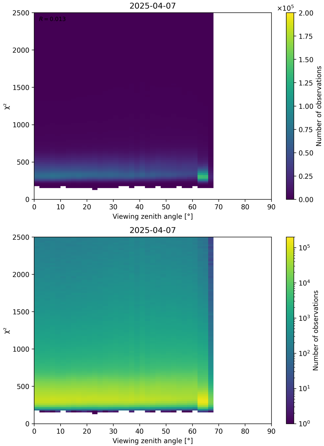
Figure 162: Scatter density plot of “Viewing zenith angle” against “ \chi^2 ” for 2025-04-07 to 2025-04-08.
