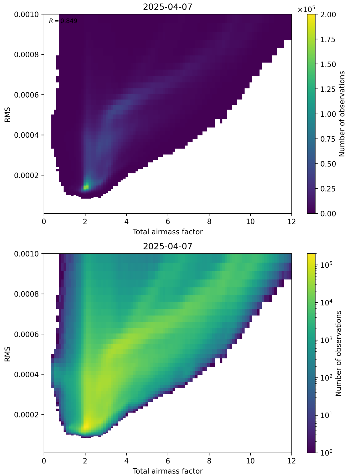
Figure 69: Scatter density plot of “Total airmass factor” against “RMS” for 2025-04-07 to 2025-04-08.
