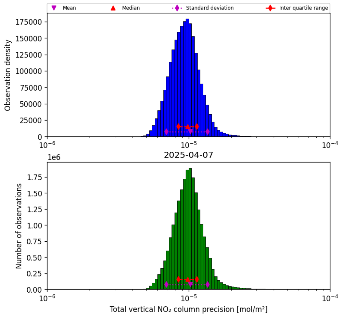
Figure 39: Histogram of “Total vertical NO 2 column precision” for 2025-04-07 to 2025-04-08
