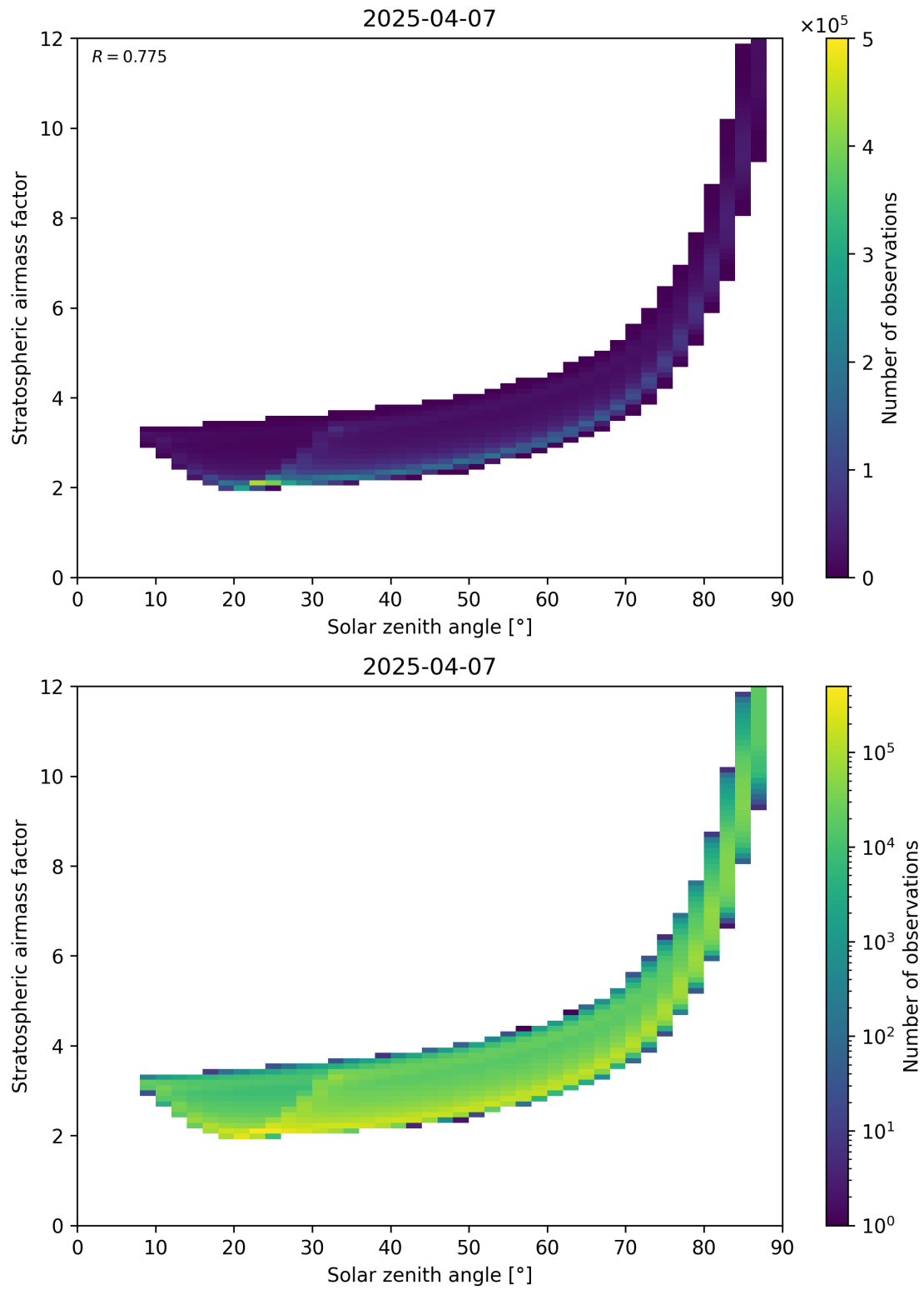
Figure 145: Scatter density plot of “Solar zenith angle” against “Stratospheric airmass factor” for 2025-04-07 to 2025-04-08.
