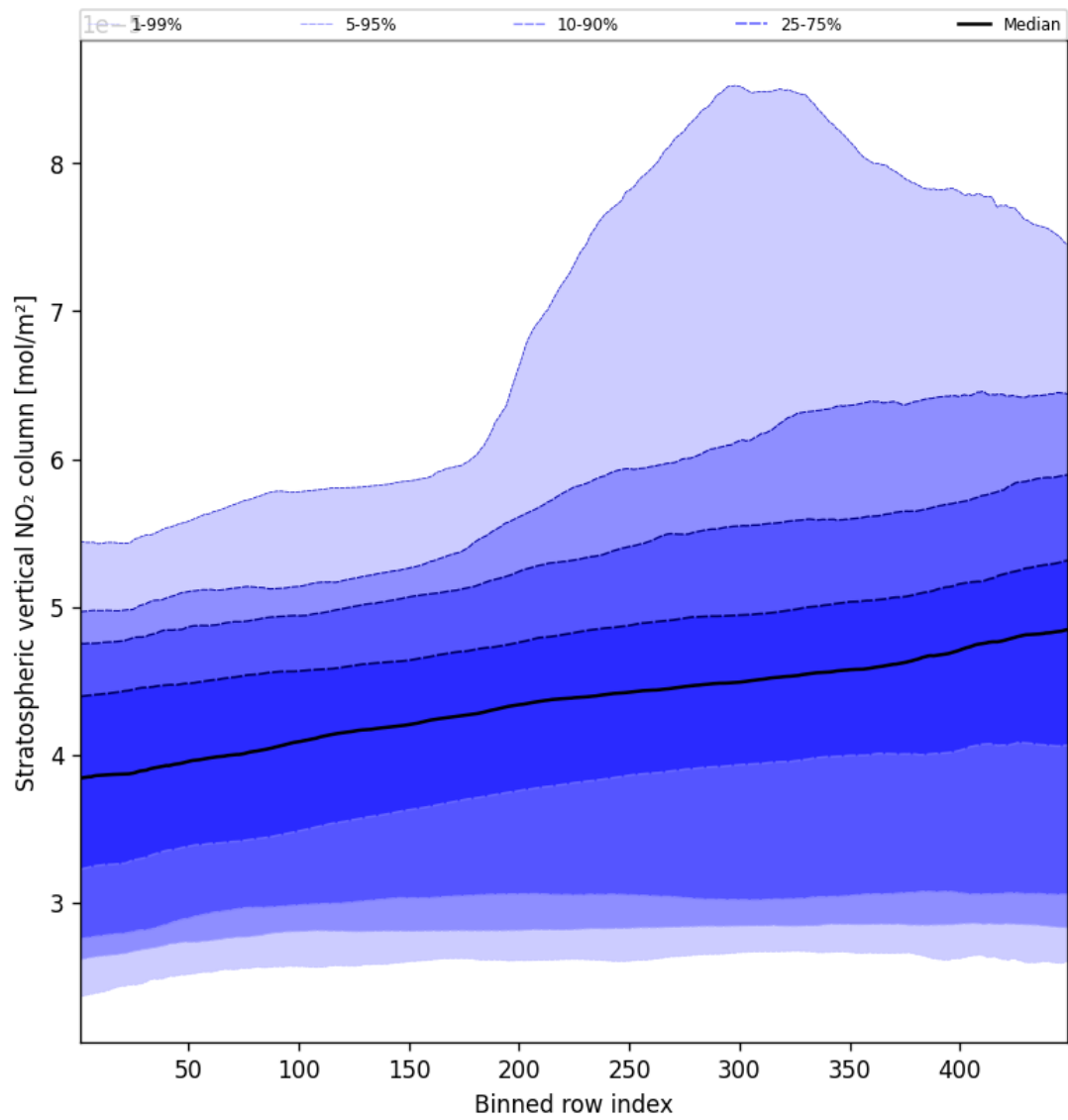
Figure 53: Along track statistics of “Stratospheric vertical NO 2 column” for 2025-04-07 to 2025-04-08
