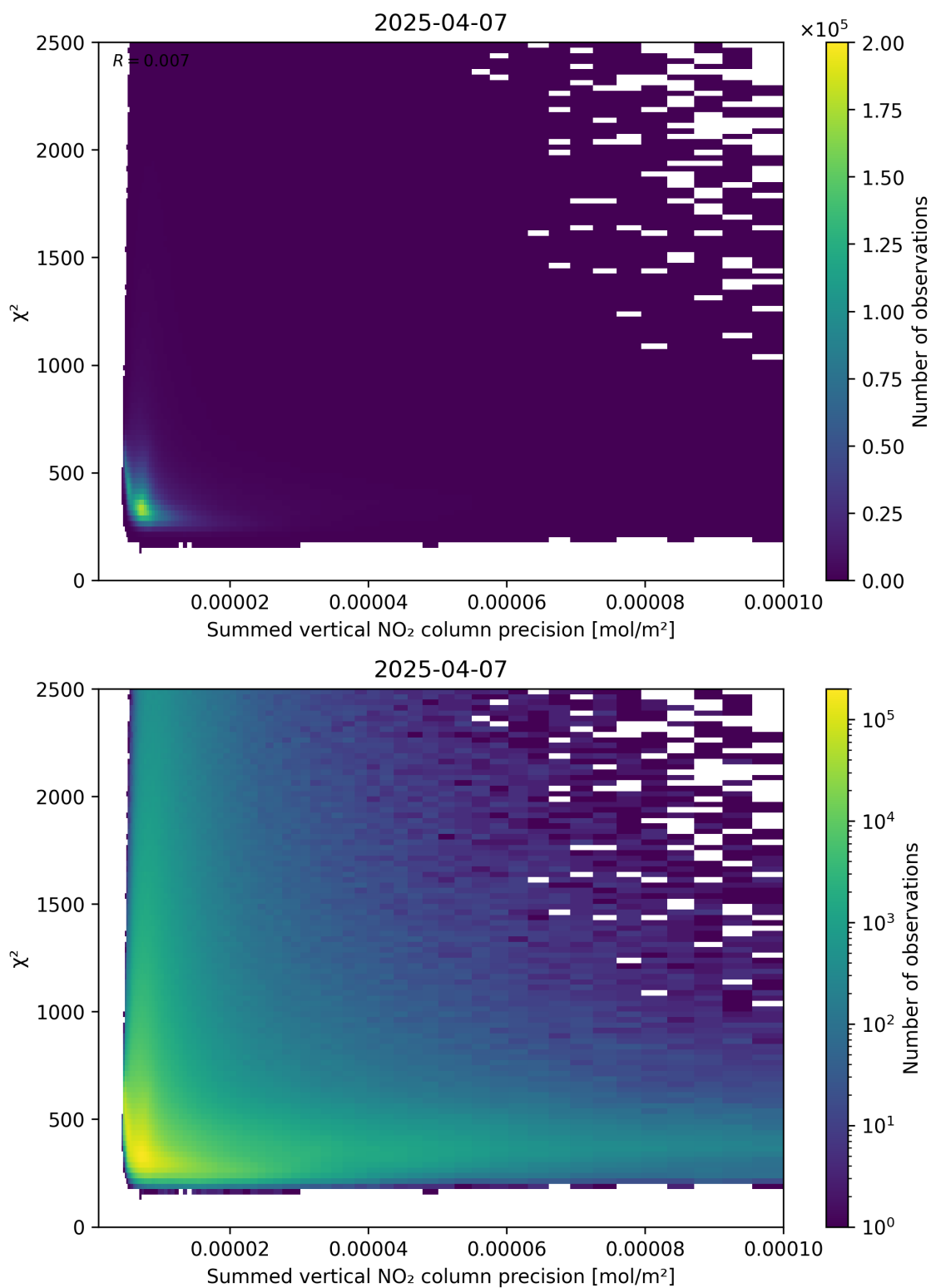
Figure 107: Scatter density plot of “Summed vertical NO 2 column precision” against “ \chi^2 ” for 2025-04-07 to 2025-04-08.
