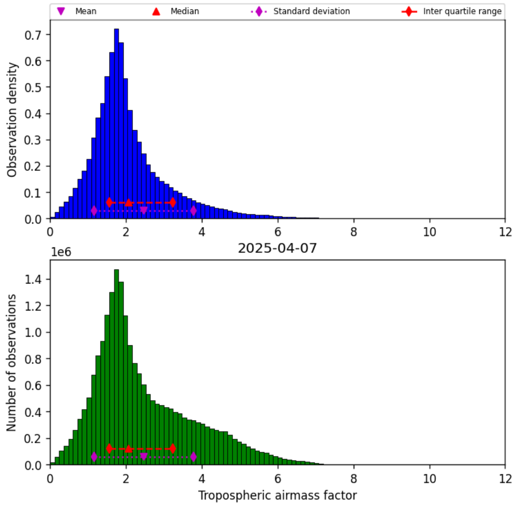
Figure 31: Histogram of “Tropospheric airmass factor” for 2025-04-07 to 2025-04-08
