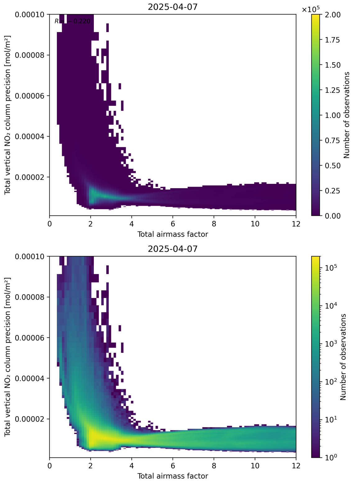
Figure 68: Scatter density plot of “Total airmass factor” against “Total vertical NO 2 column precision” for 2025-04-07 to 2025-04-08.
