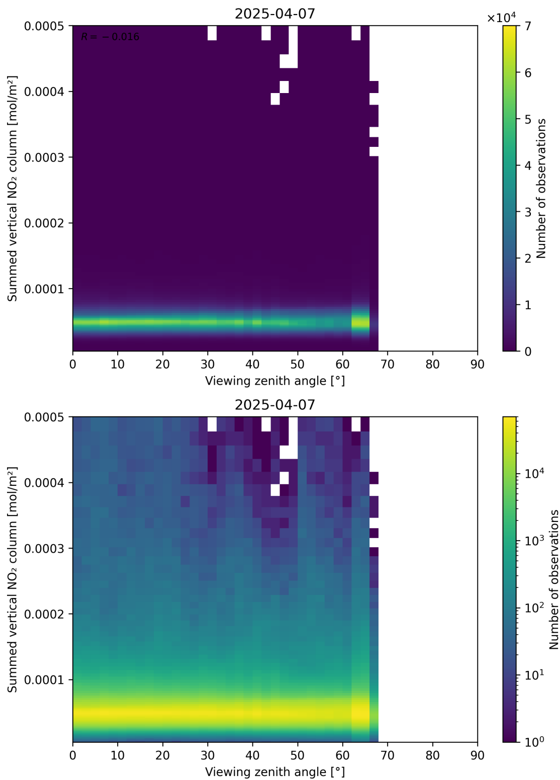
Figure 165: Scatter density plot of “Viewing zenith angle” against “Summed vertical NO 2 column” for 2025-04-07 to 2025-04-08.
