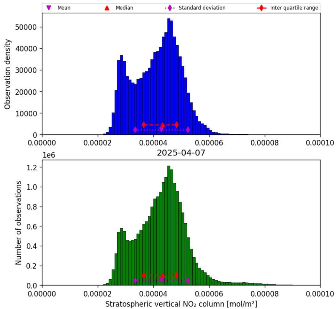
Figure 36: Histogram of “Stratospheric vertical NO 2 column” for 2025-04-07 to 2025-04-08
