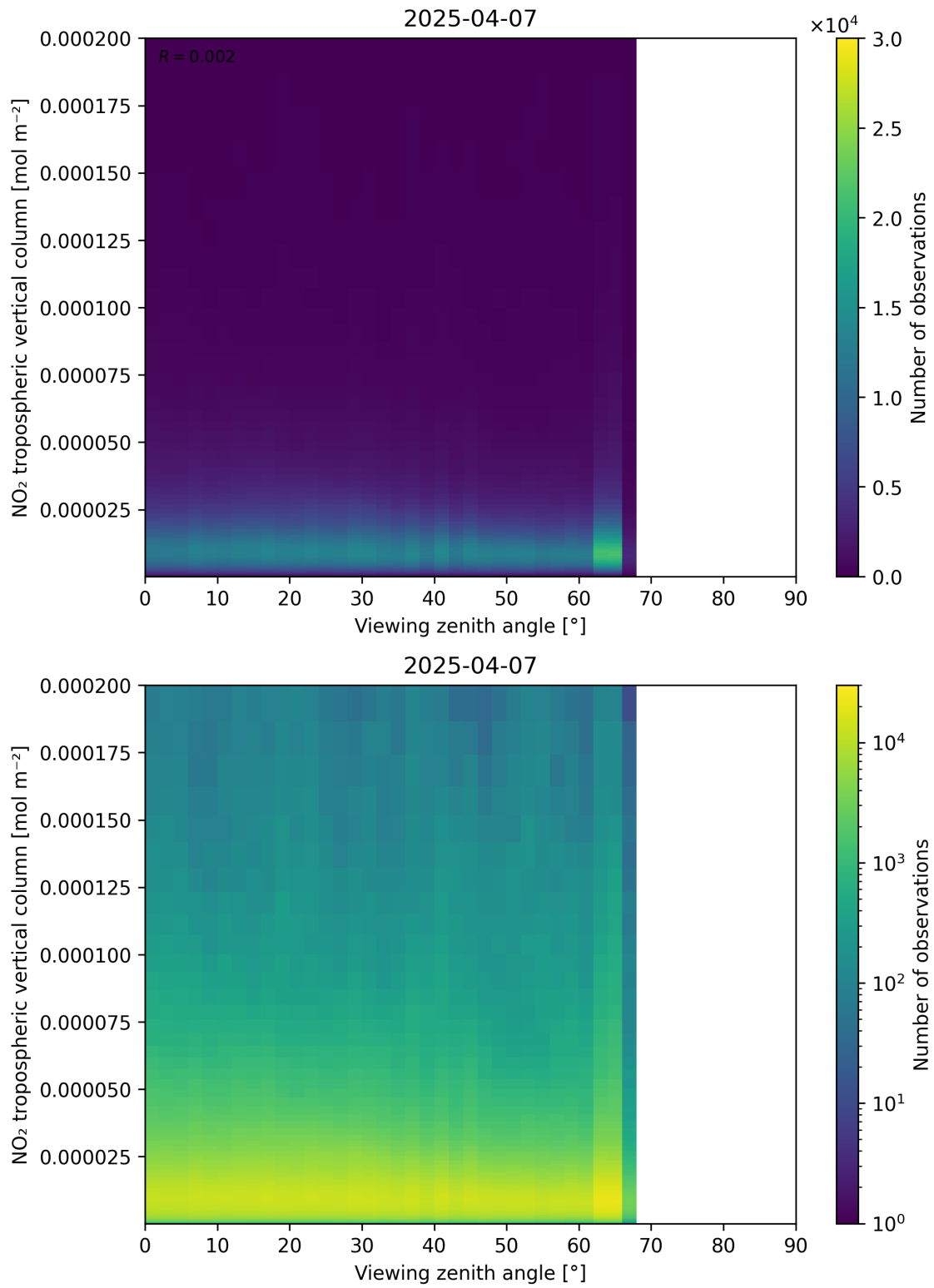
Figure 169: Scatter density plot of “Viewing zenith angle” against “NO 2 tropospheric vertical column” for 2025-04-07 to 2025-04-08.
