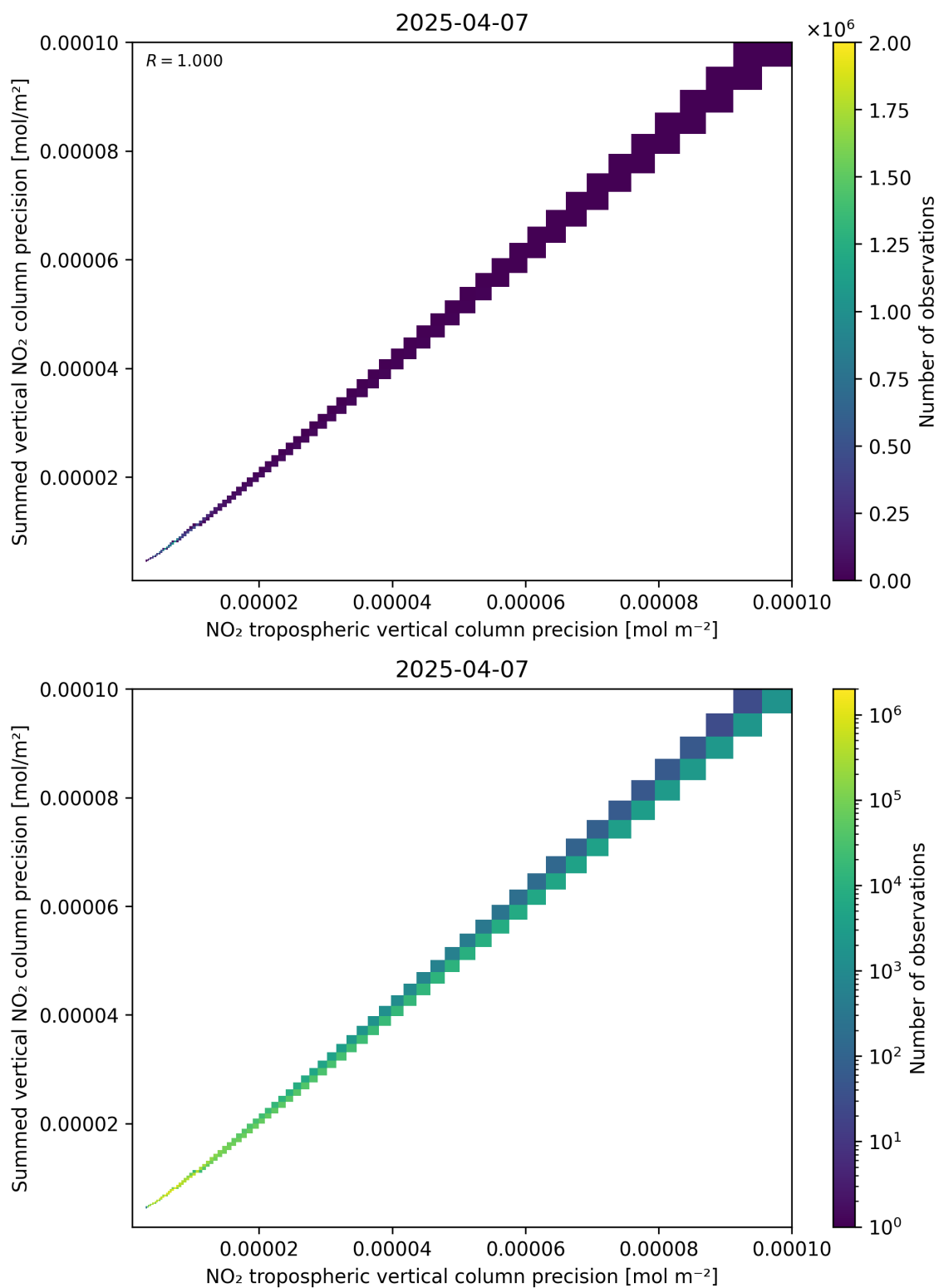
Figure 137: Scatter density plot of “NO 2 tropospheric vertical column precision” against “Summed vertical NO 2 column precision” for 2025-04-07 to 2025-04-08.
