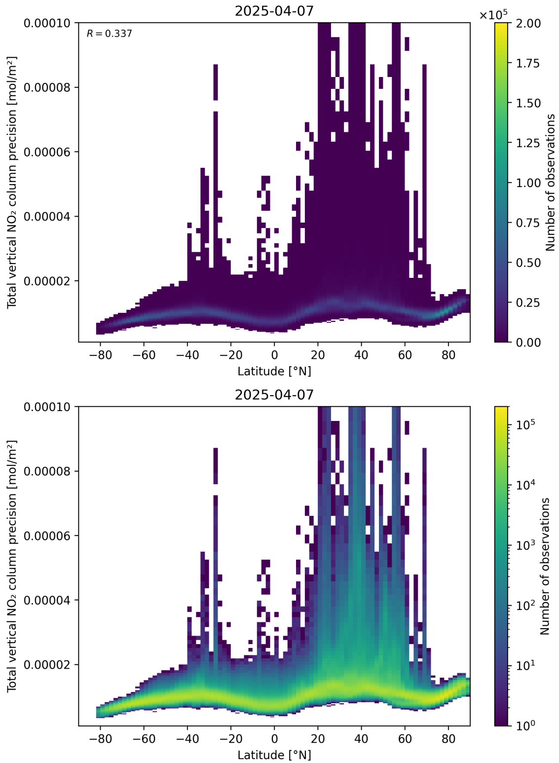
Figure 91: Scatter density plot of “Latitude” against “Total vertical NO 2 column precision” for 2025-04-07 to 2025-04-08.
