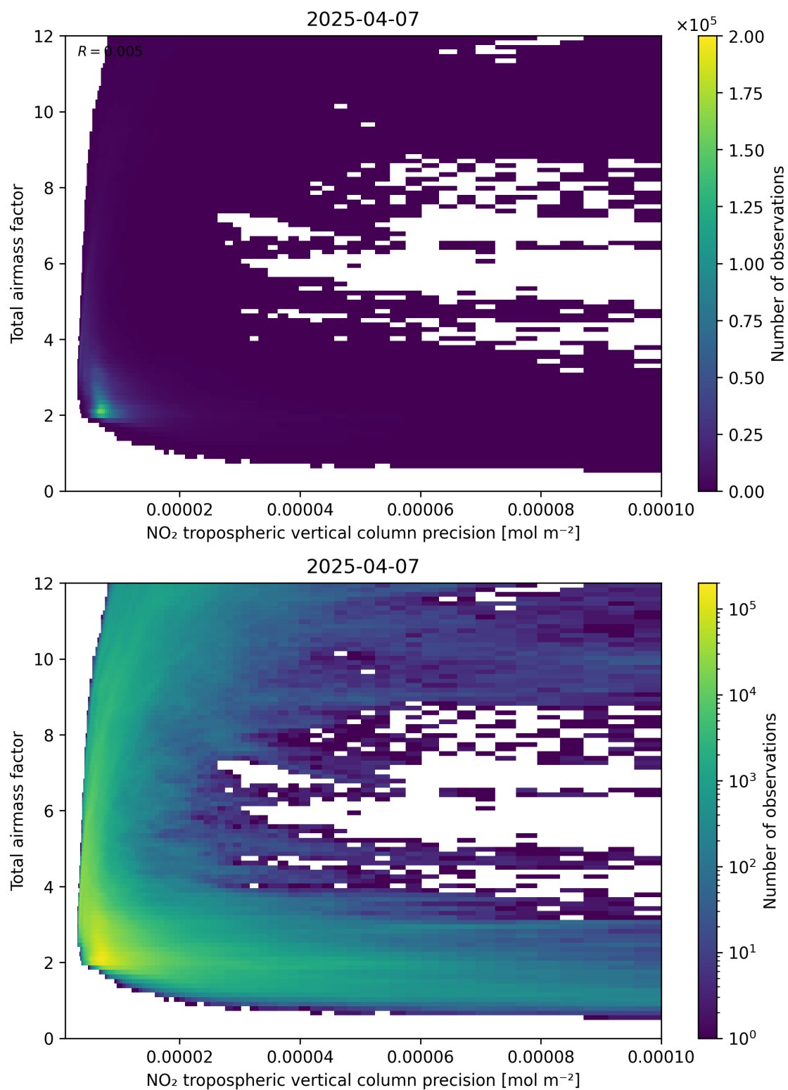
Figure 132: Scatter density plot of “NO 2 tropospheric vertical column precision” against “Total air mass factor” for 2025-04-07 to 2025-04-08.
