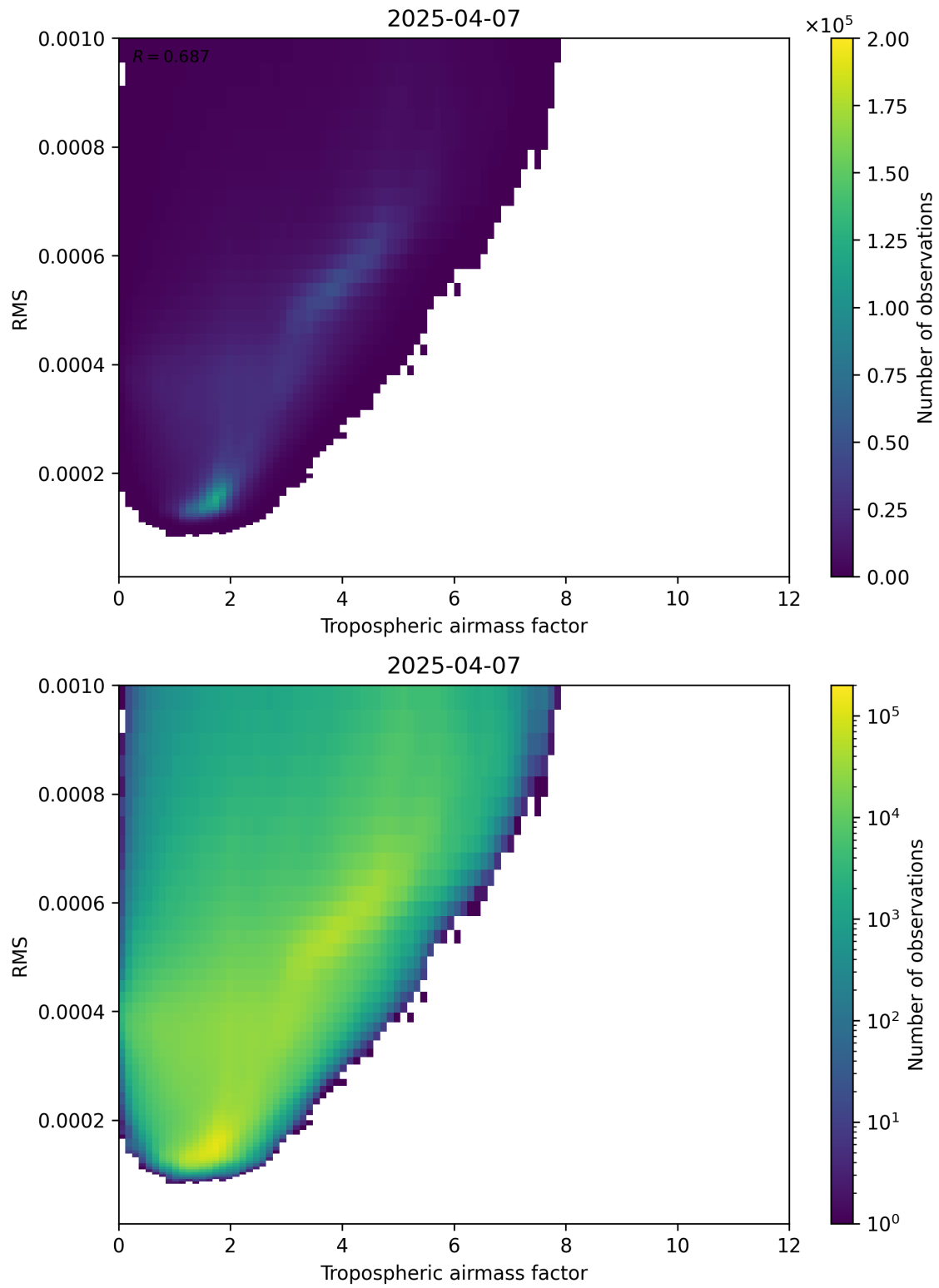
Figure 79: Scatter density plot of “Tropospheric airmass factor” against “RMS” for 2025-04-07 to 2025-04-08.
