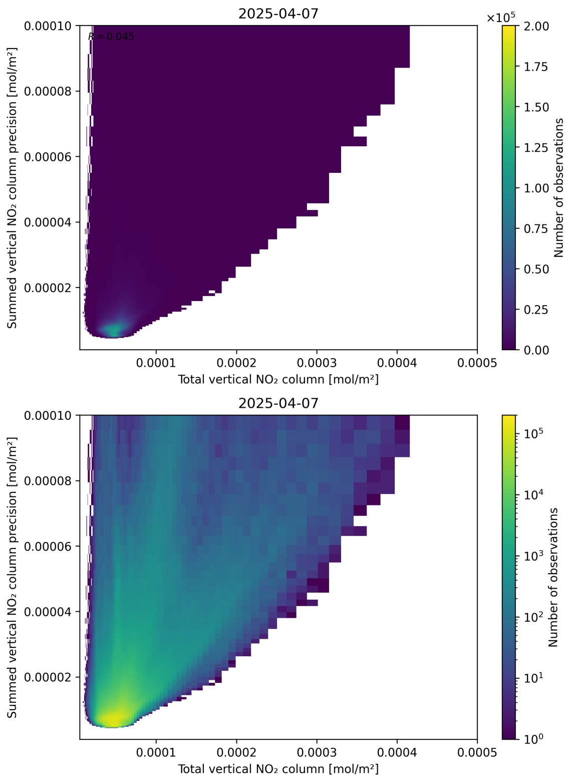
Figure 113: Scatter density plot of “Total vertical NO 2 column” against “Summed vertical NO 2 column precision” for 2025-04-07 to 2025-04-08.
