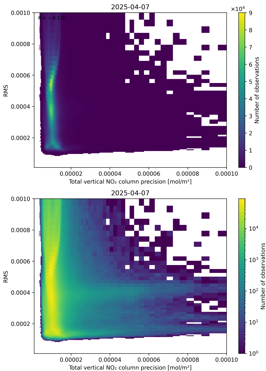
Figure 119: Scatter density plot of “Total vertical NO 2 column precision” against “RMS” for 2025-04-07 to 2025-04-08.
