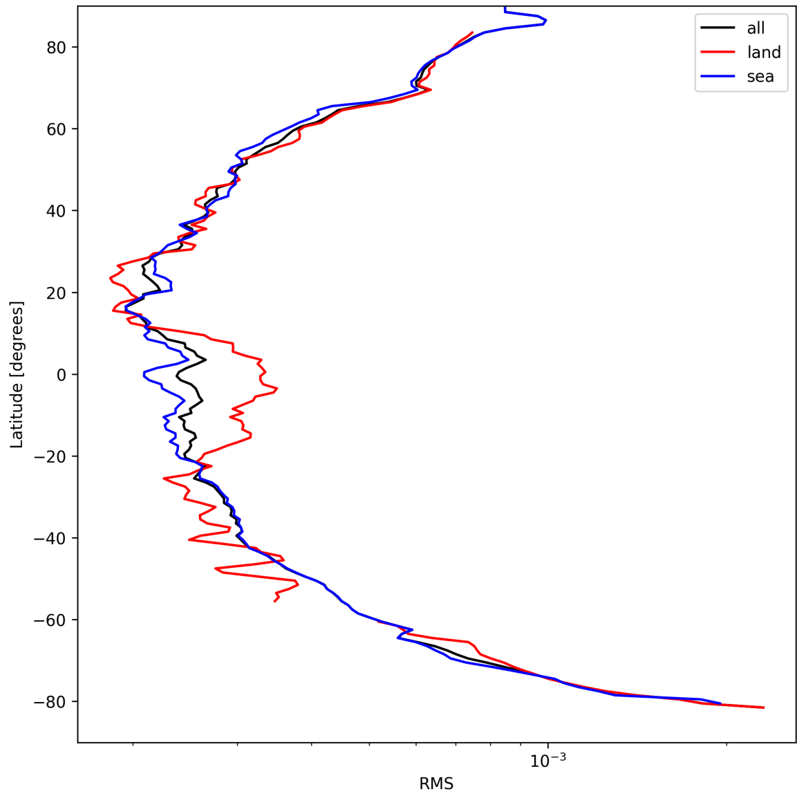
Figure 26: Zonal average of “RMS” for 2025-04-07 to 2025-04-08.
