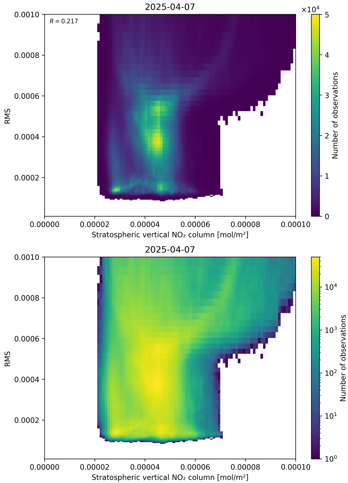
Figure 102: Scatter density plot of “Stratospheric vertical NO 2 column” against “RMS” for 2025-04-07 to 2025-04-08.
