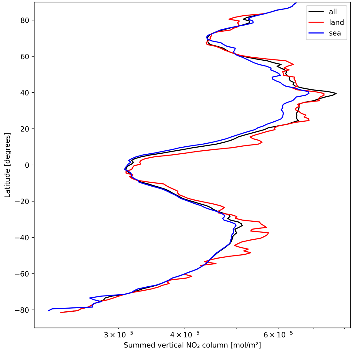
Figure 23: Zonal average of “Summed vertical NO 2 column” for 2025-04-07 to 2025-04-08.
