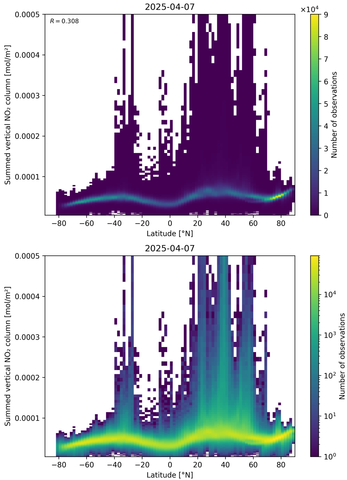
Figure 88: Scatter density plot of “Latitude” against “Summed vertical NO 2 column” for 2025-04-07 to 2025-04-08.
