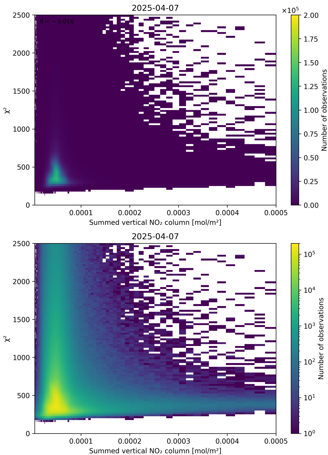
Figure 104: Scatter density plot of “Summed vertical NO 2 column” against “ \chi^2 ” for 2025-04-07 to 2025-04-08.
