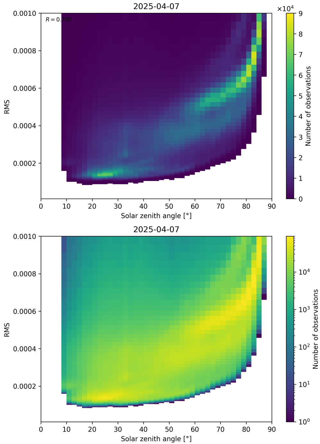
Figure 157: Scatter density plot of “Solar zenith angle” against “RMS” for 2025-04-07 to 2025-04-08.
