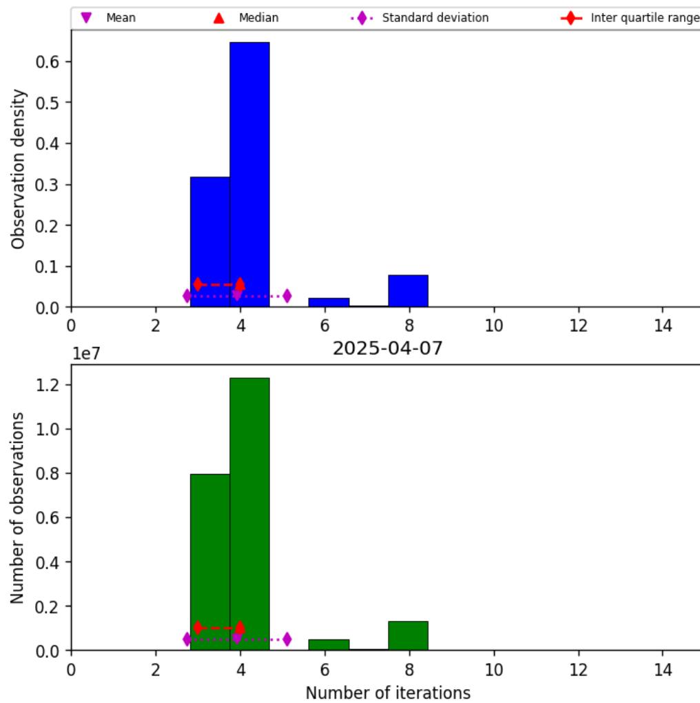
Figure 34: Histogram of “Number of iterations” for 2025-04-07 to 2025-04-08
