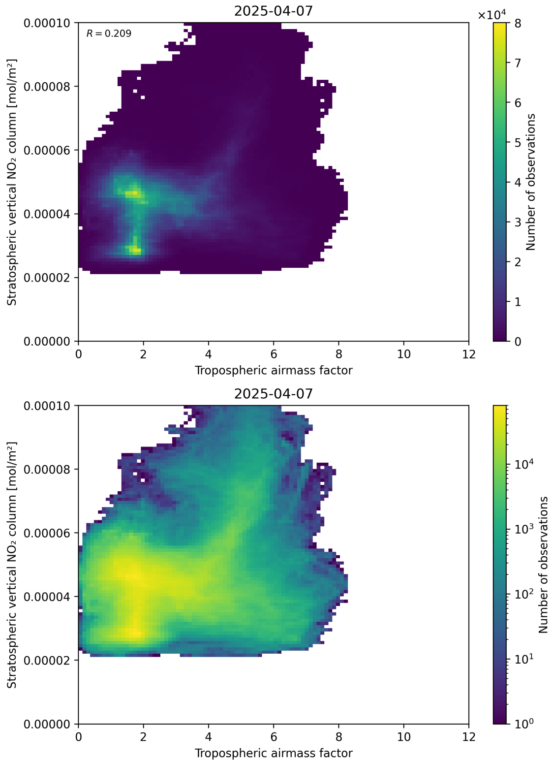
Figure 74: Scatter density plot of “Tropospheric air mass factor” against “Stratospheric vertical NO 2 column” for 2025-04-07 to 2025-04-08.
