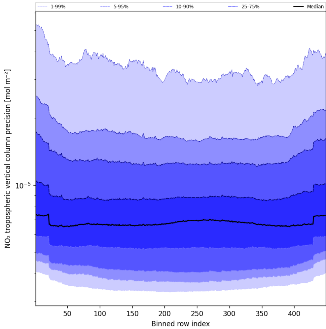
Figure 47: Along track statistics of “NO 2 tropospheric vertical column precision” for 2025-04-07 to 2025-04-08
