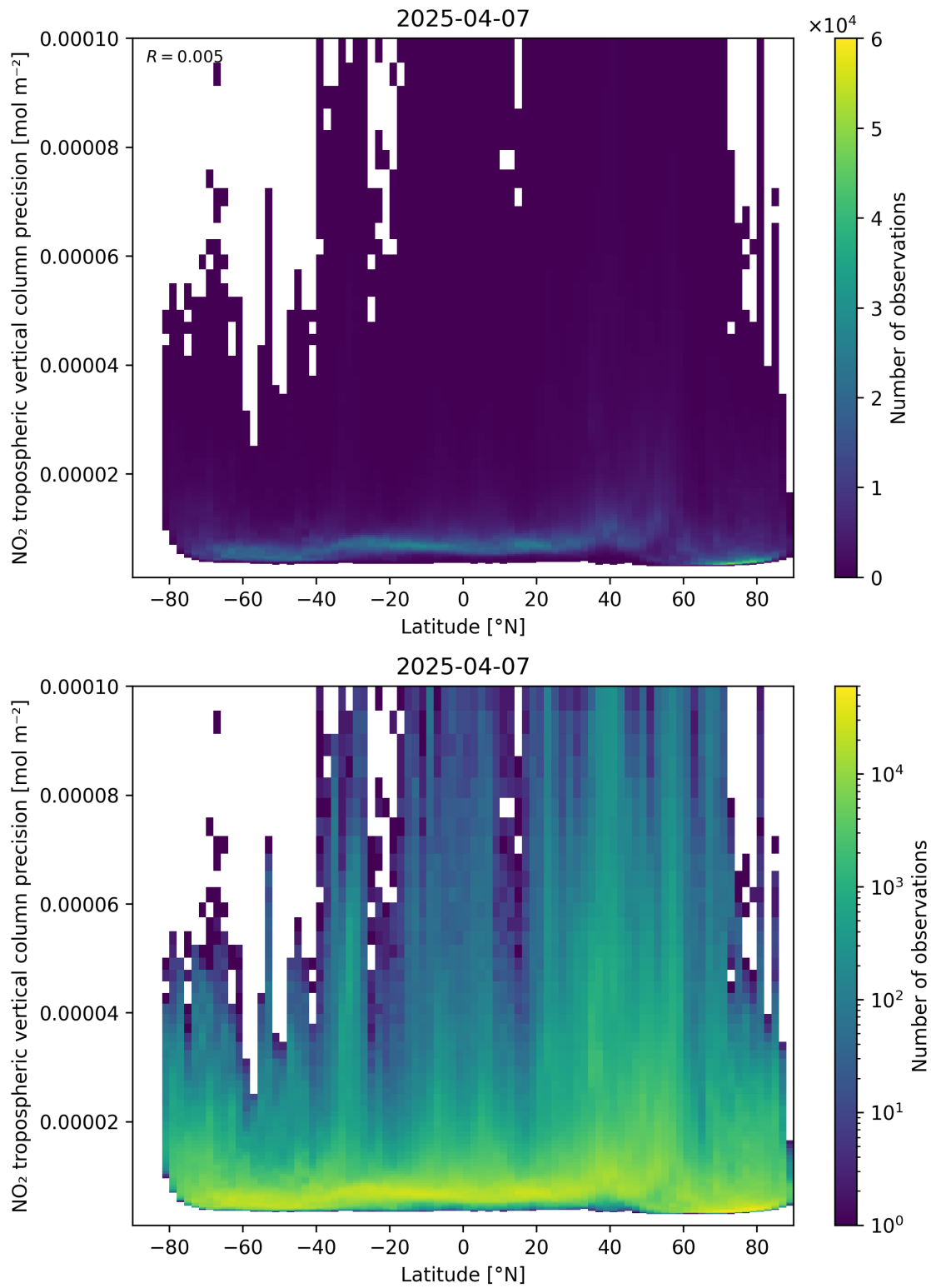
Figure 93: Scatter density plot of “Latitude” against “NO 2 tropospheric vertical column precision” for 2025-04-07 to 2025-04-08.
