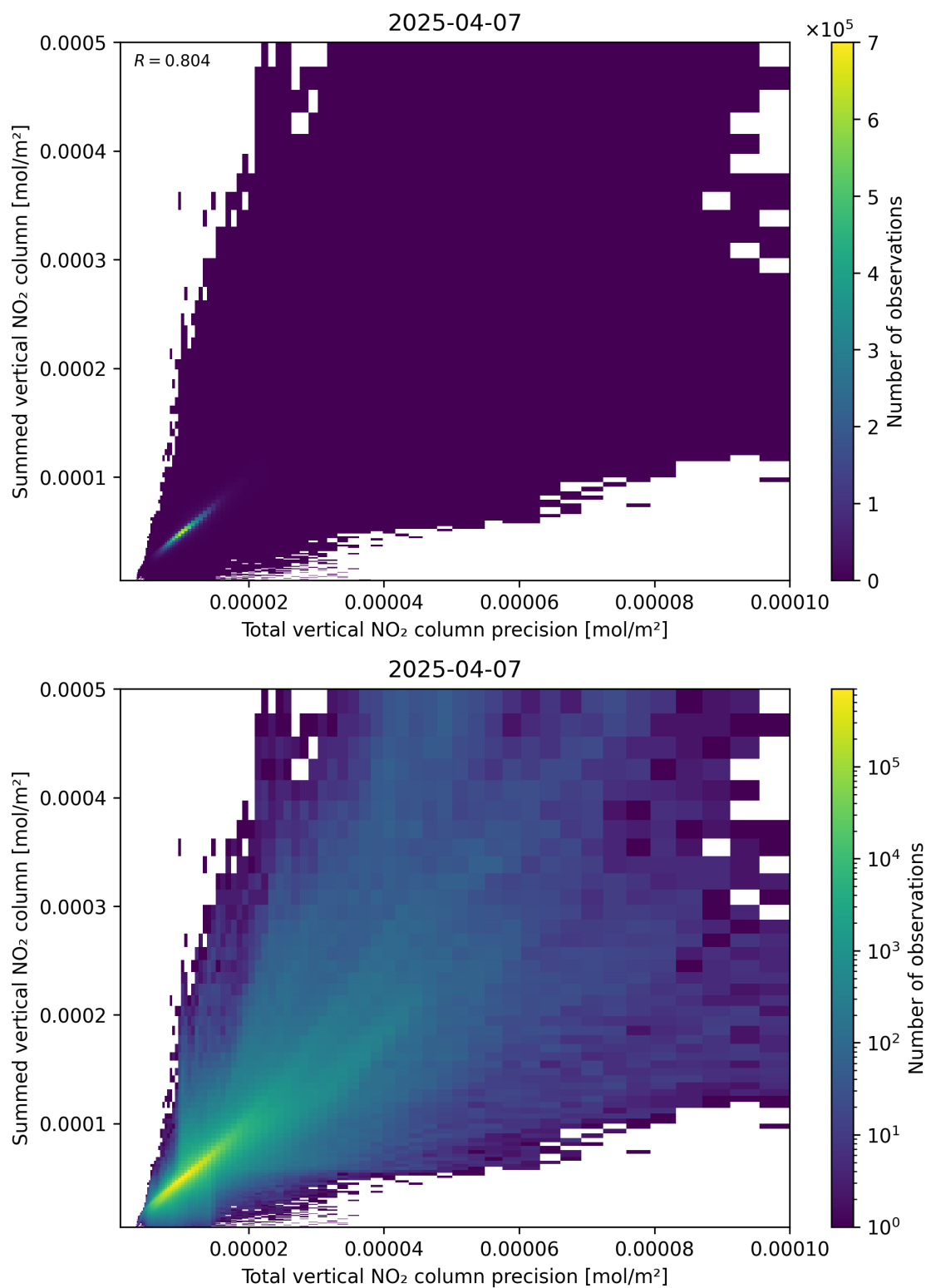
Figure 117: Scatter density plot of “Total vertical NO 2 column precision” against “Summed vertical NO 2 column” for 2025-04-07 to 2025-04-08.
