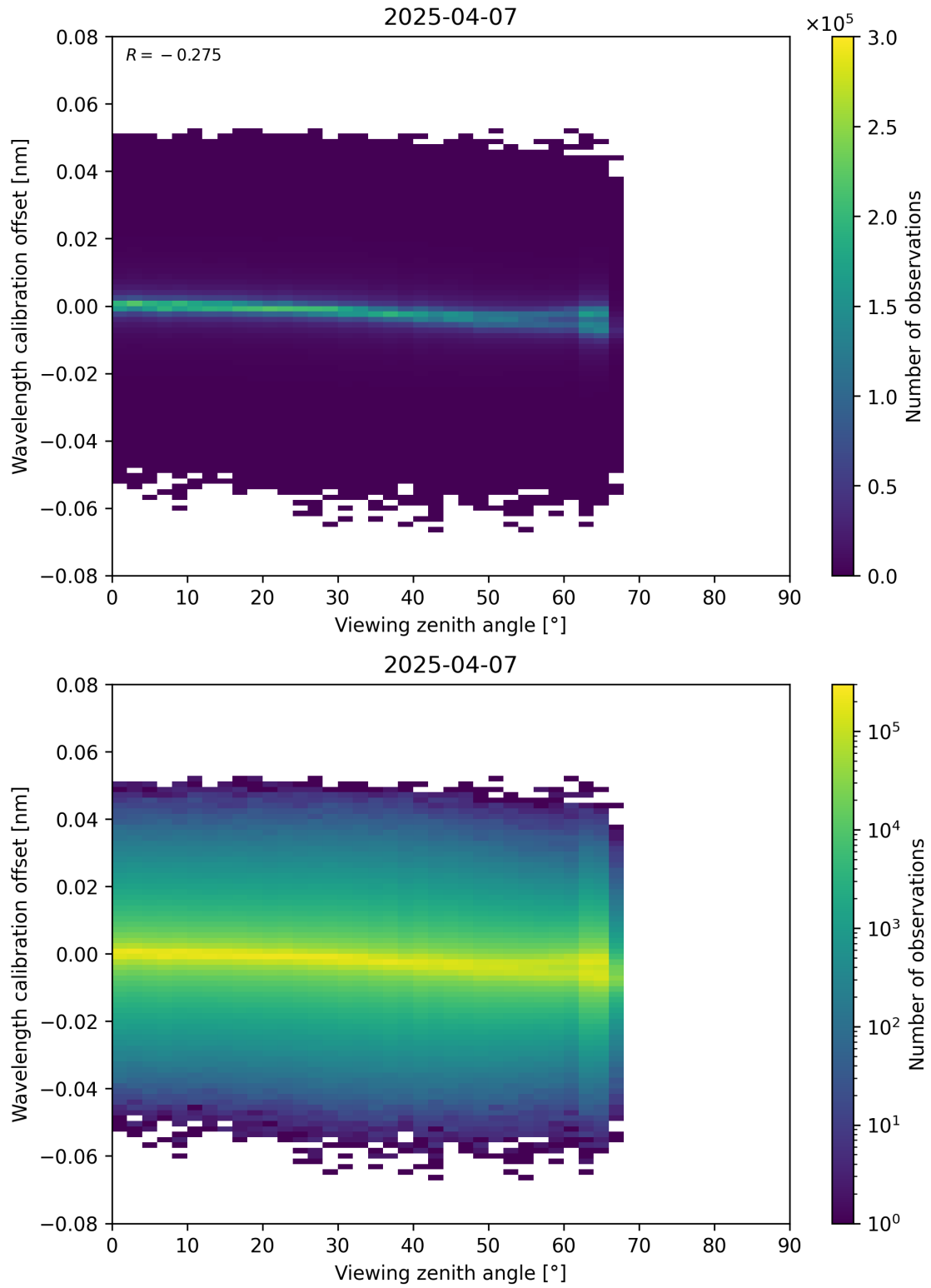
Figure 173: Scatter density plot of “Viewing zenith angle” against “Wavelength calibration offset” for 2025-04-07 to 2025-04-08.
