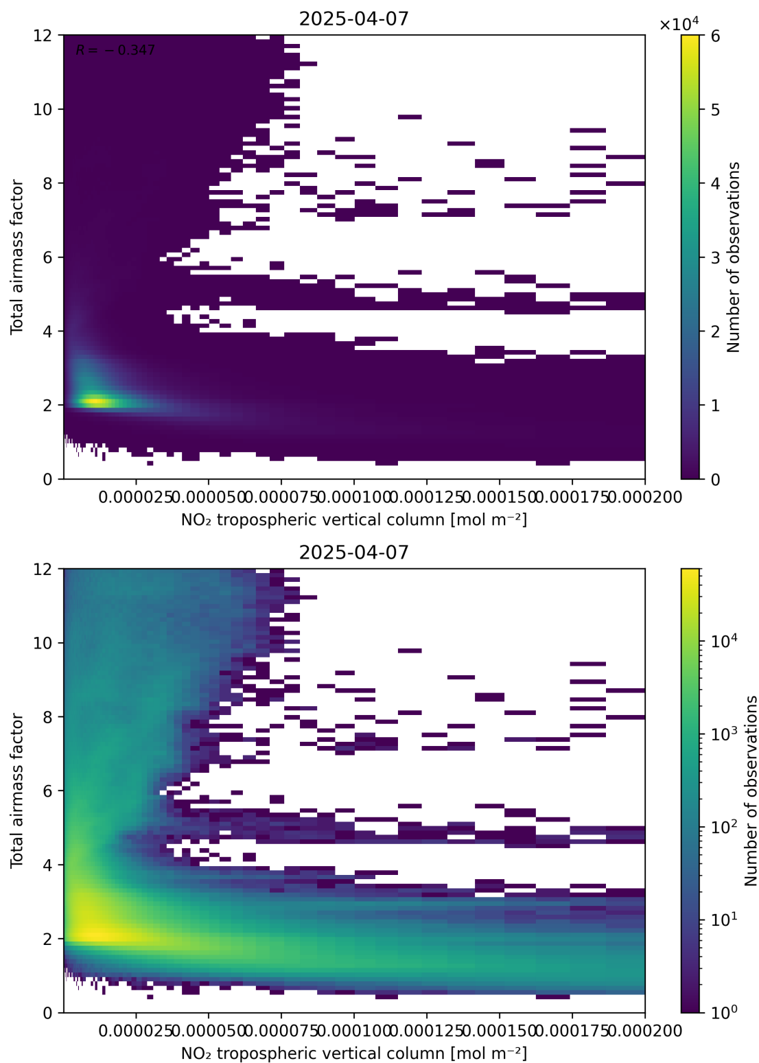
Figure 122: Scatter density plot of “NO 2 tropospheric vertical column” against “Total air mass factor” for 2025-04-07 to 2025-04-08.
