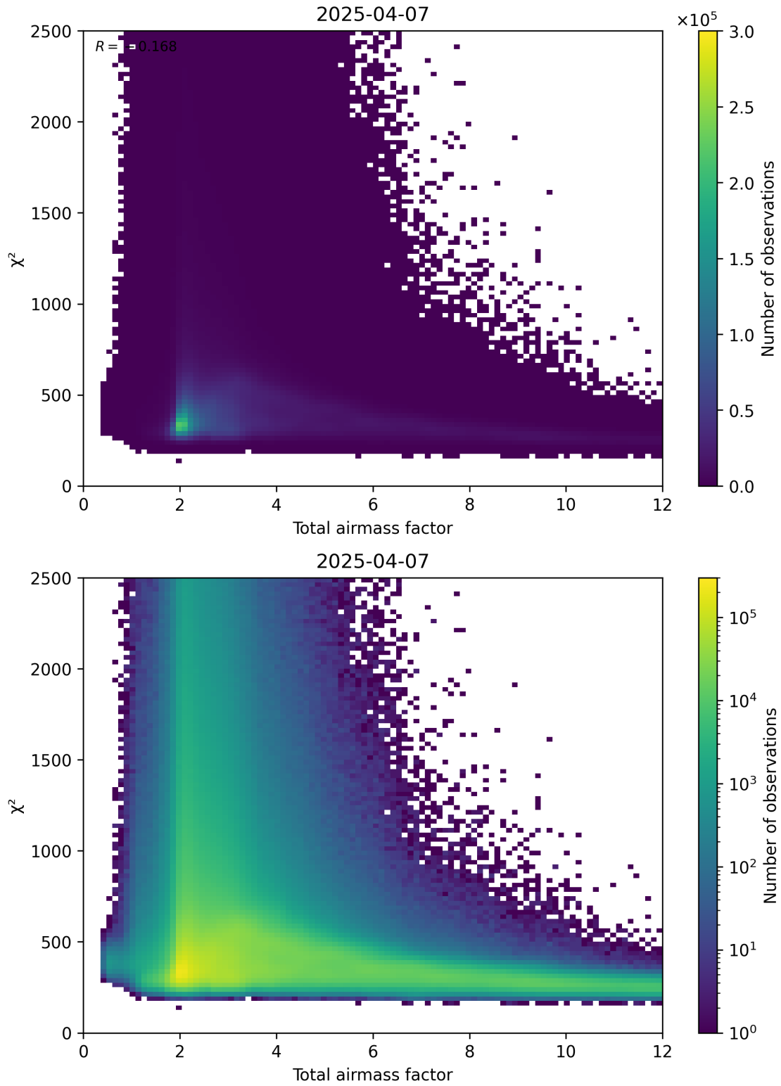
Figure 63: Scatter density plot of “Total airmass factor” against “ \chi^2 ” for 2025-04-07 to 2025-04-08.
