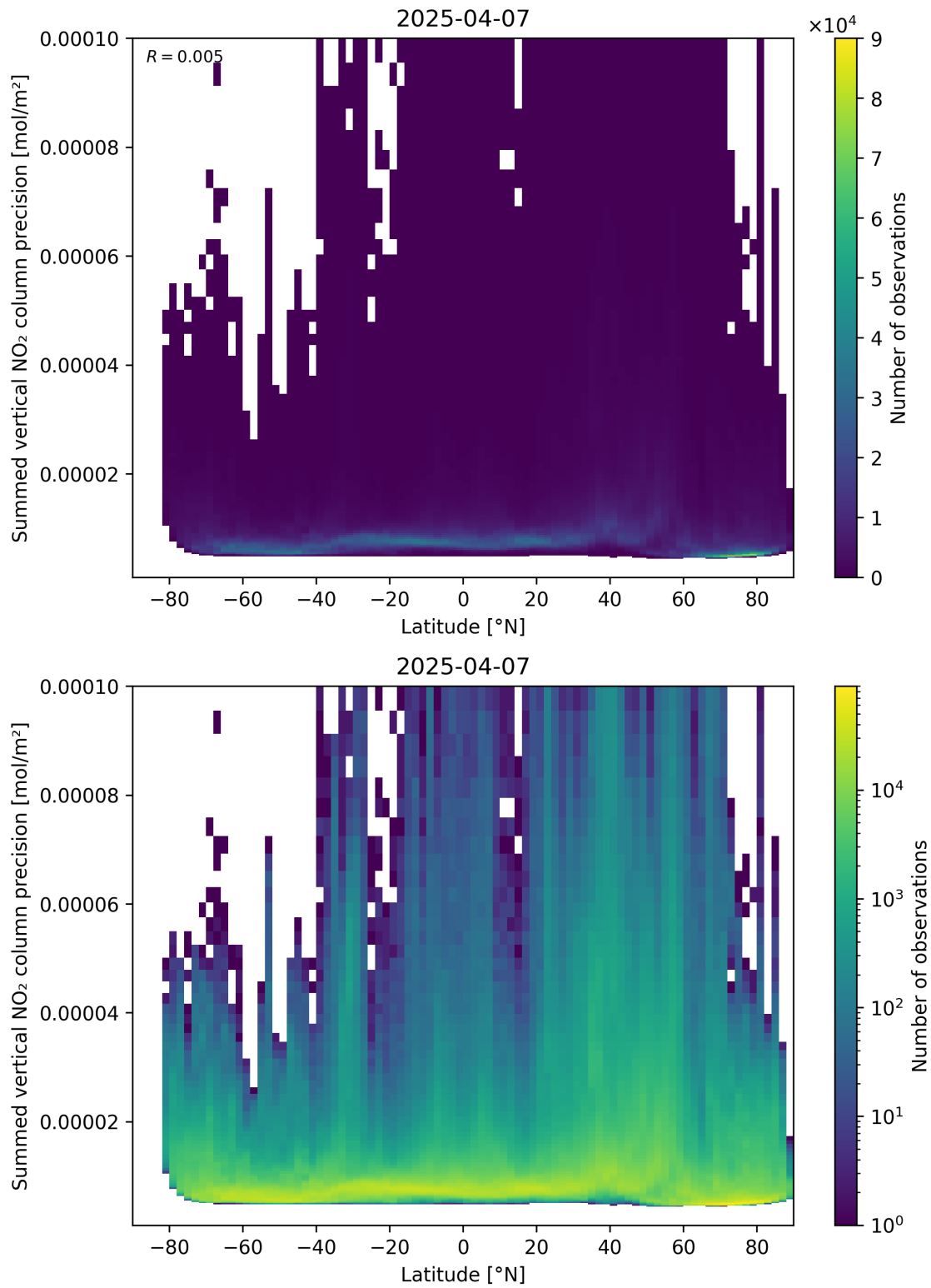
Figure 89: Scatter density plot of “Latitude” against “Summed vertical NO 2 column precision” for 2025-04-07 to 2025-04-08.
