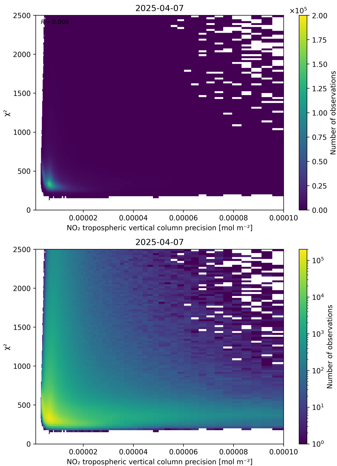
Figure 134: Scatter density plot of “NO 2 tropospheric vertical column precision” against “ \chi^2 ” for 2025-04-07 to 2025-04-08.
