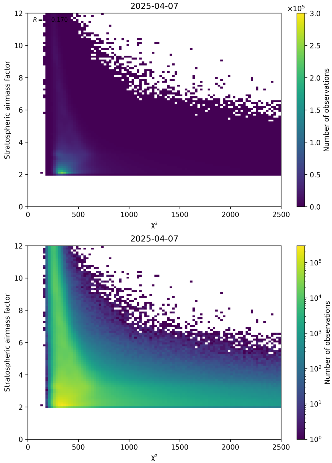
Figure 81: Scatter density plot of “ \chi^2 ” against “Stratospheric airmass factor” for 2025-04-07 to 2025-04-08.
