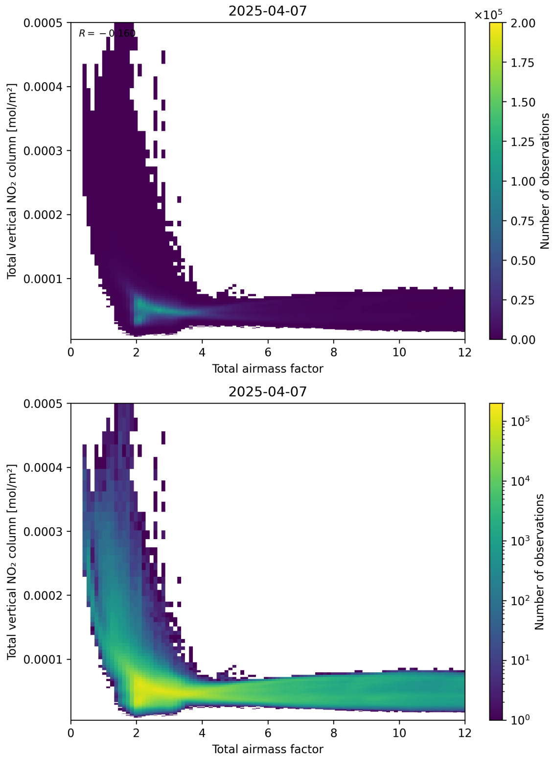
Figure 67: Scatter density plot of “Total airmass factor” against “Total vertical NO 2 column” for 2025-04-07 to 2025-04-08.
