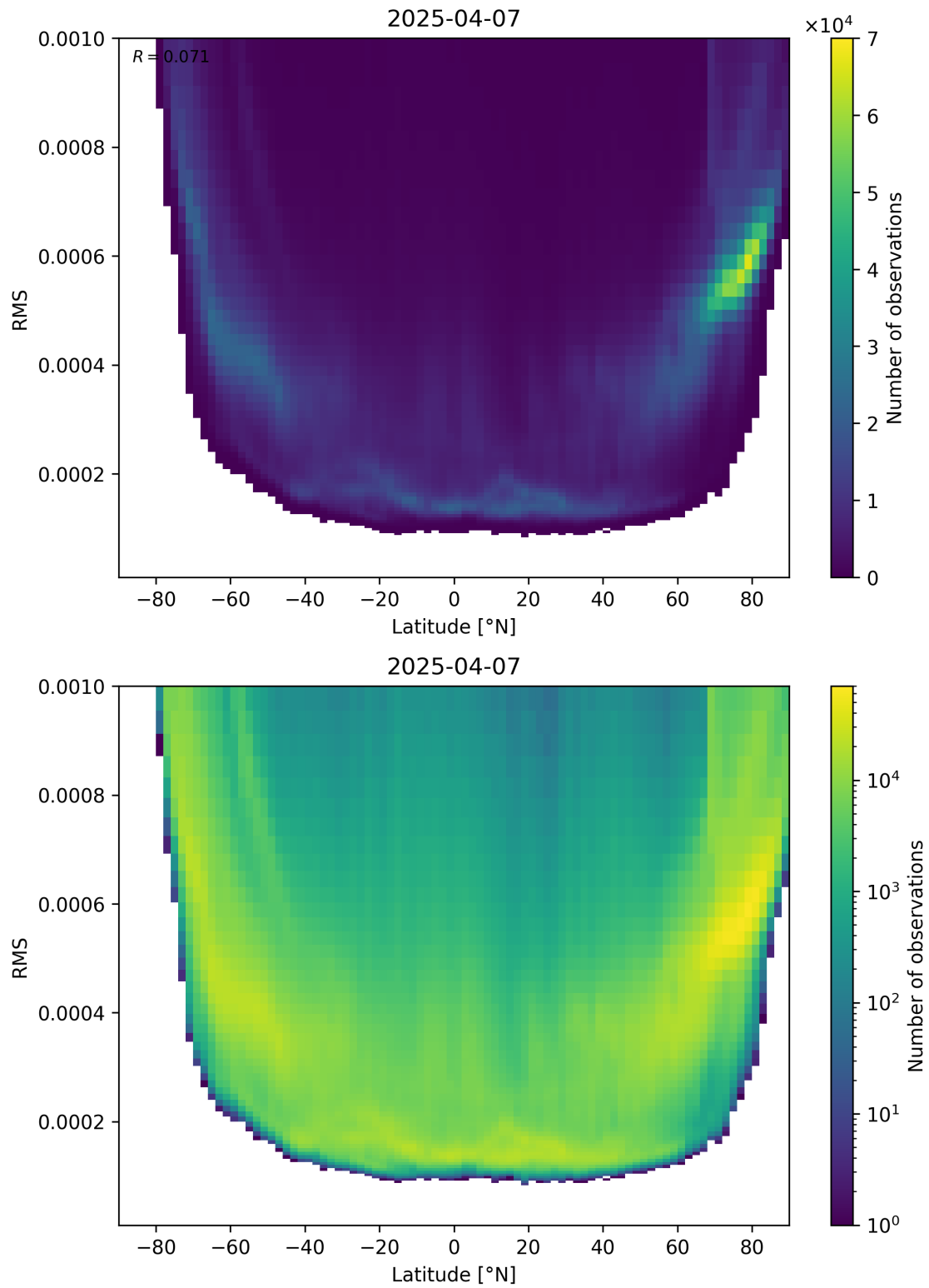
Figure 94: Scatter density plot of “Latitude” against “RMS” for 2025-04-07 to 2025-04-08.
