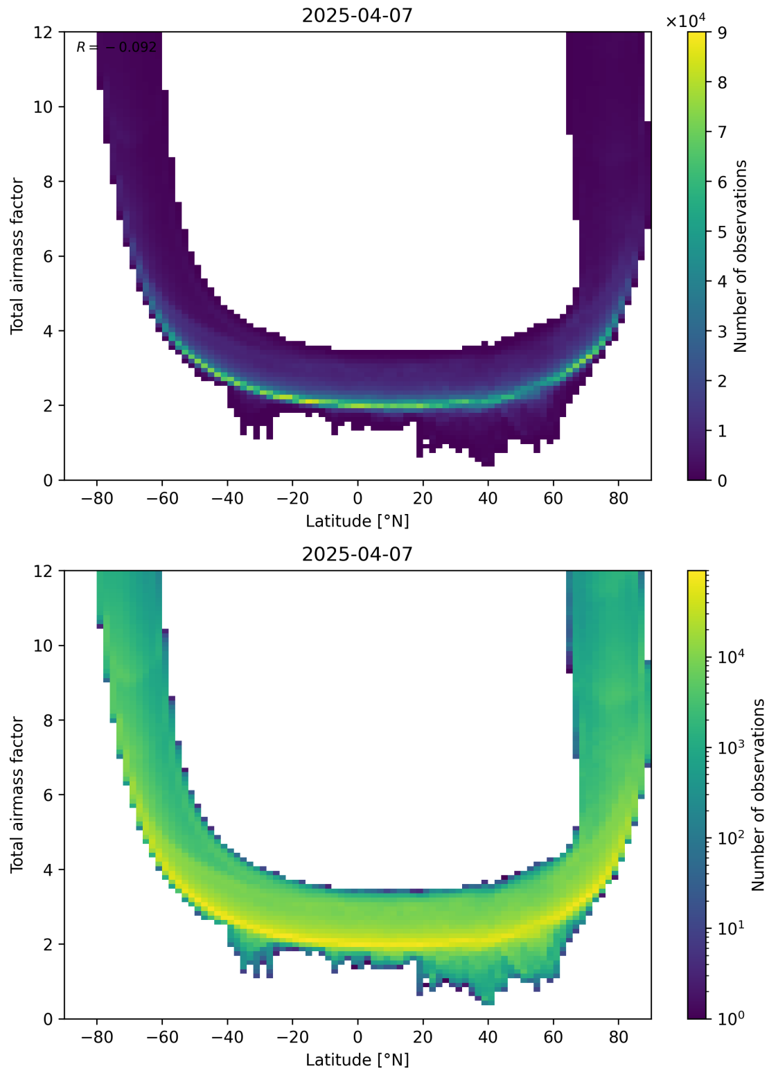
Figure 84: Scatter density plot of “Latitude” against “Total airmass factor” for 2025-04-07 to 2025-04-08.
