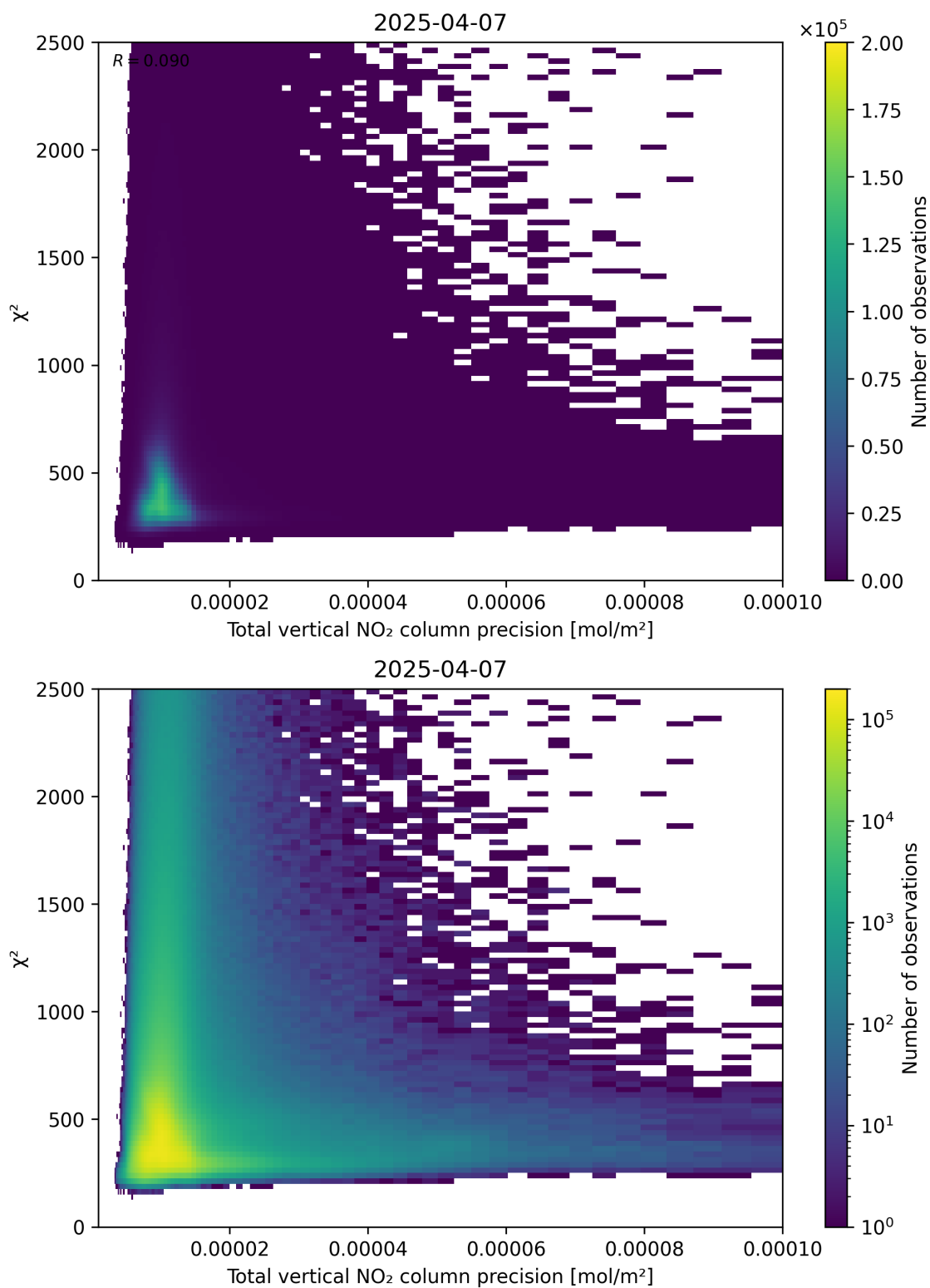
Figure 116: Scatter density plot of “Total vertical NO 2 column precision” against “ \chi^2 ” for 2025-04-07 to 2025-04-08.
