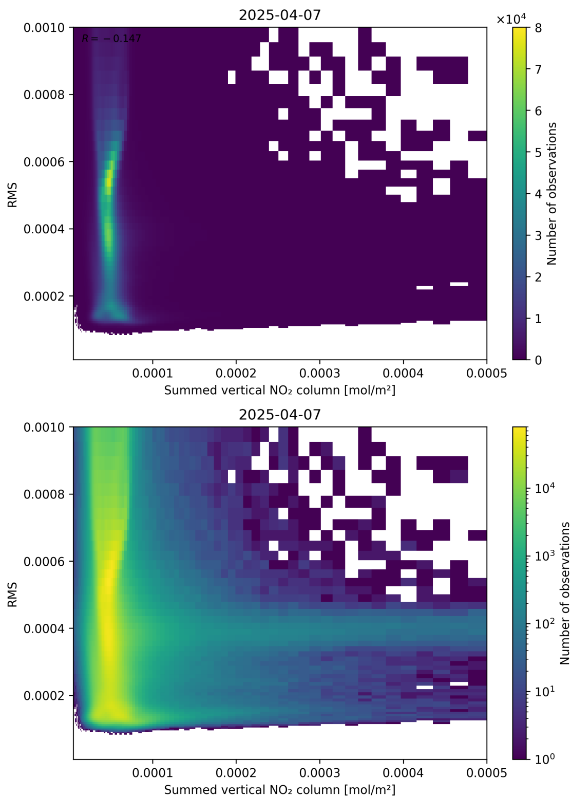
Figure 109: Scatter density plot of “Summed vertical NO 2 column” against “RMS” for 2025-04-07 to 2025-04-08.
