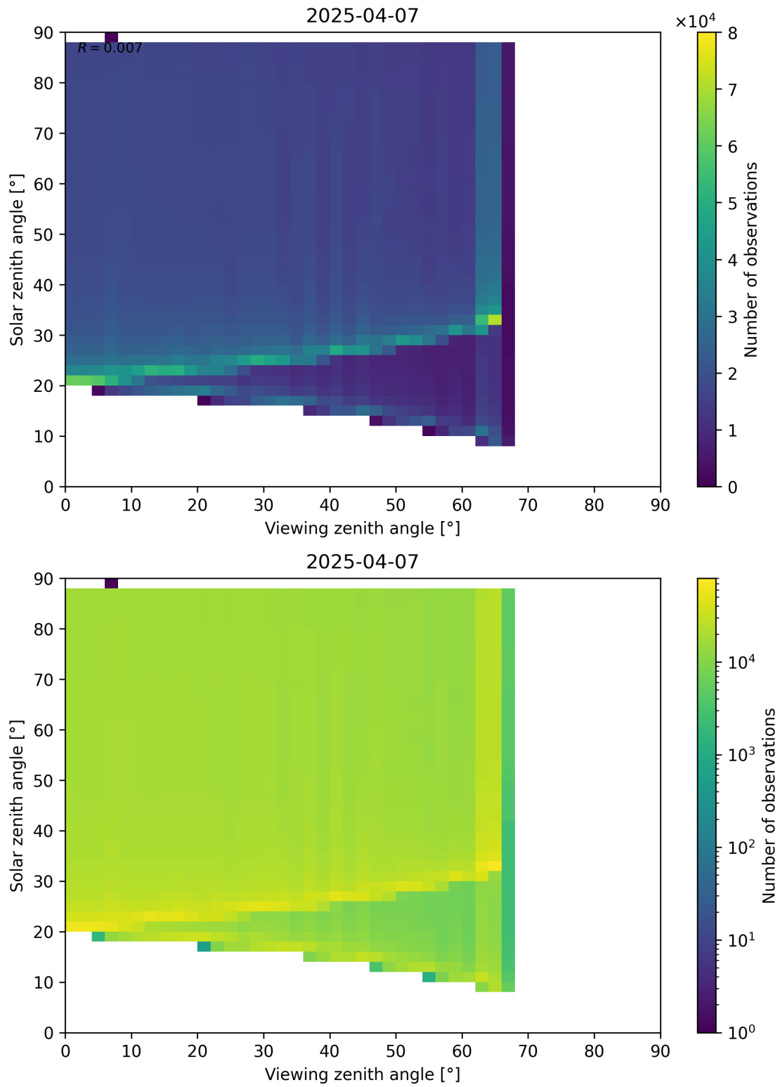
Figure 172: Scatter density plot of “Viewing zenith angle” against “Solar zenith angle” for 2025-04-07 to 2025-04-08.
