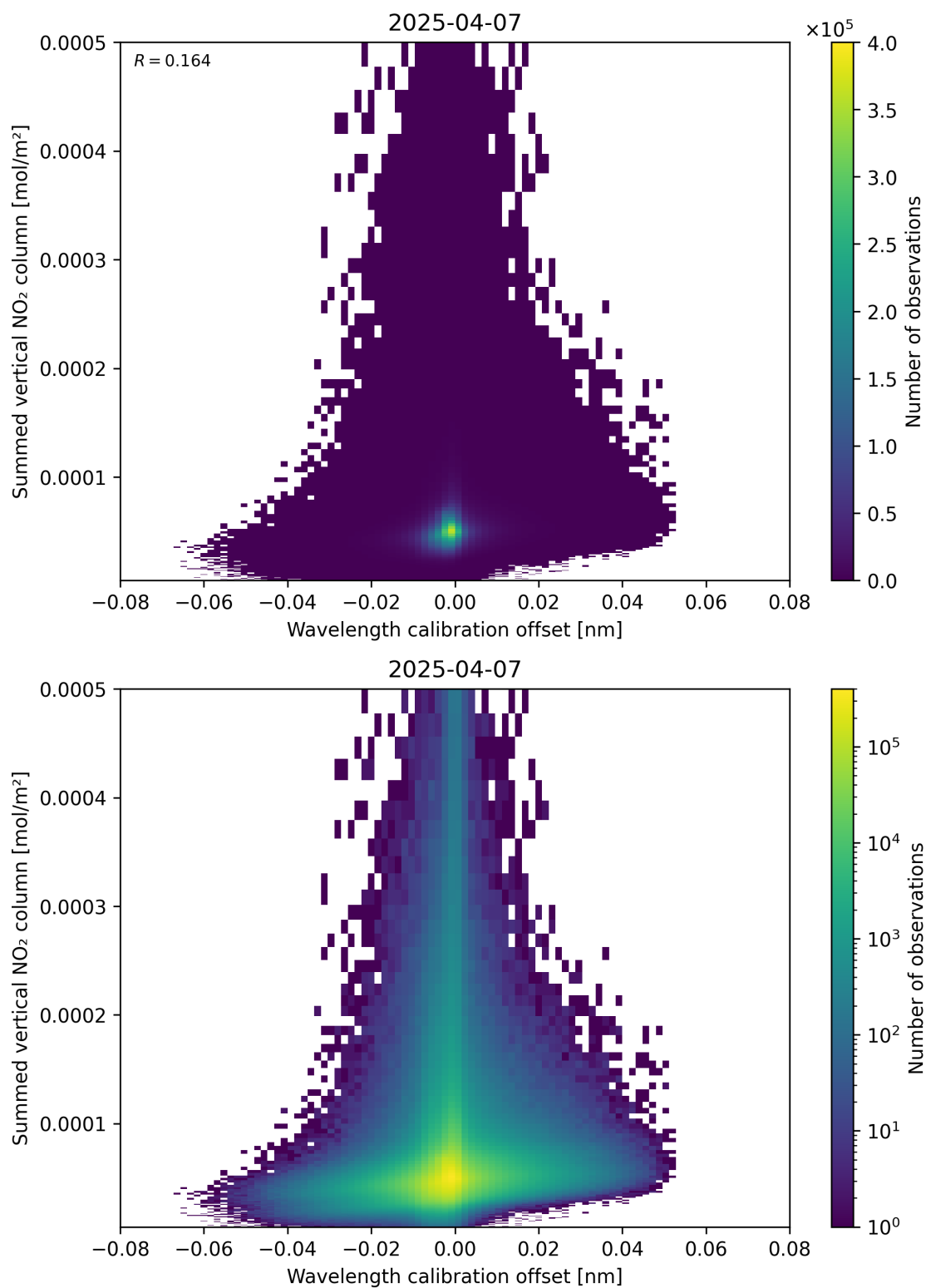
Figure 177: Scatter density plot of “Wavelength calibration offset” against “Summed vertical NO 2 column” for 2025-04-07 to 2025-04-08.
