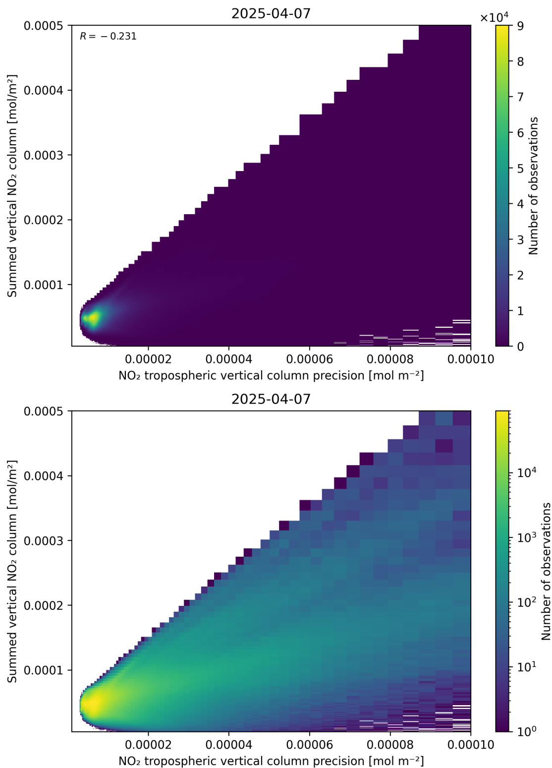
Figure 136: Scatter density plot of “NO 2 tropospheric vertical column precision” against “Summed vertical NO 2 column” for 2025-04-07 to 2025-04-08.
