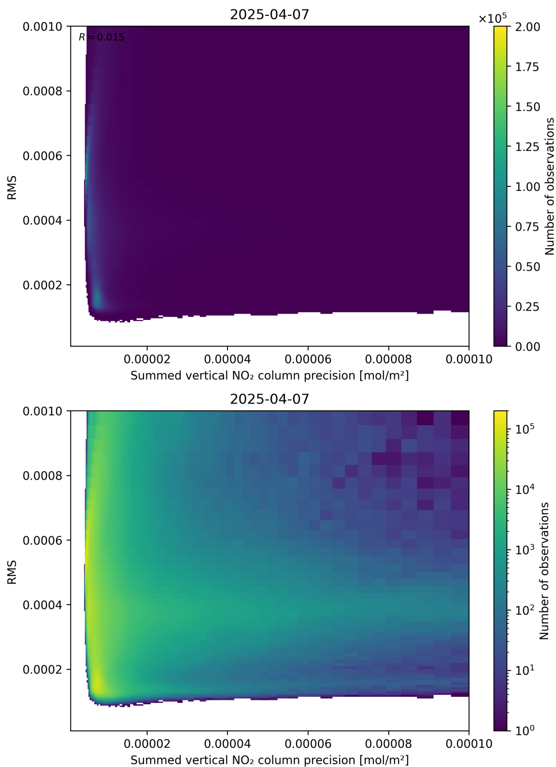
Figure 108: Scatter density plot of “Summed vertical NO 2 column precision” against “RMS” for 2025-04-07 to 2025-04-08.
