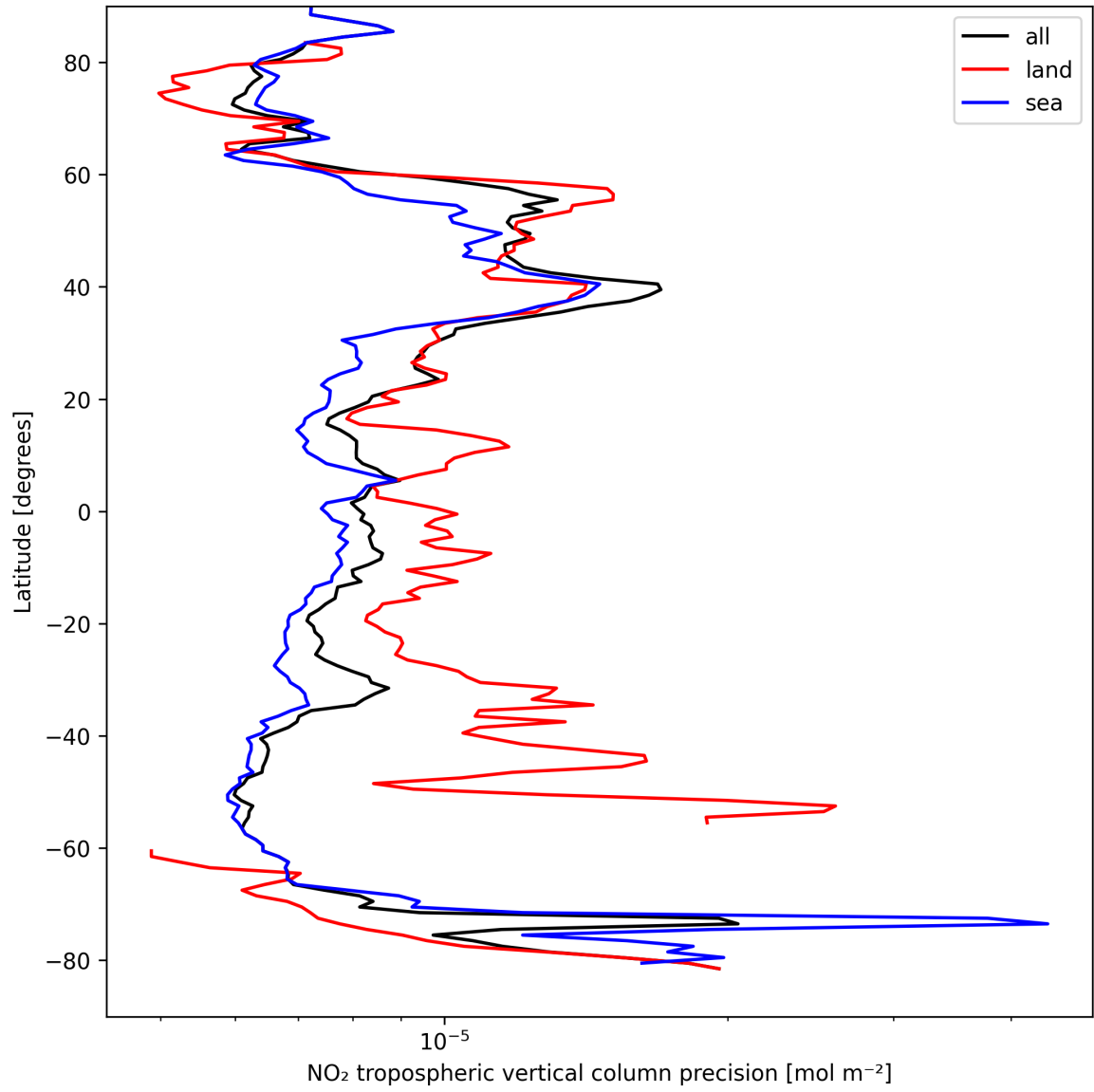
Figure 13: Zonal average of "NO 2 tropospheric vertical column precision" for 2025-04-07 to 2025-04-08.
