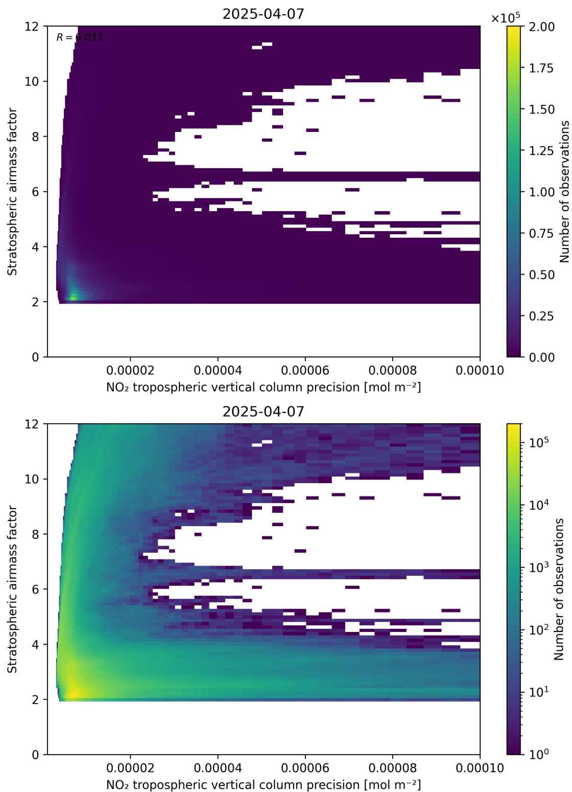
Figure 131: Scatter density plot of “NO 2 tropospheric vertical column precision” against “Stratospheric airmass factor” for 2025-04-07 to 2025-04-08.
