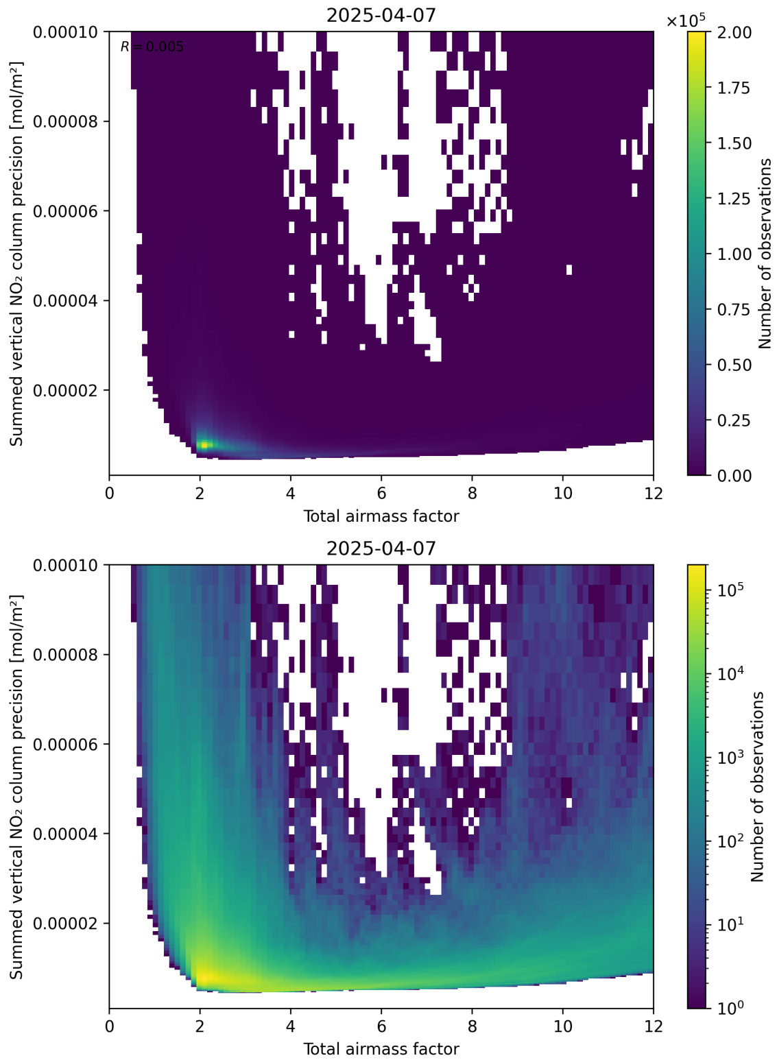
Figure 66: Scatter density plot of “Total airmass factor” against “Summed vertical NO 2 column precision” for 2025-04-07 to 2025-04-08.
