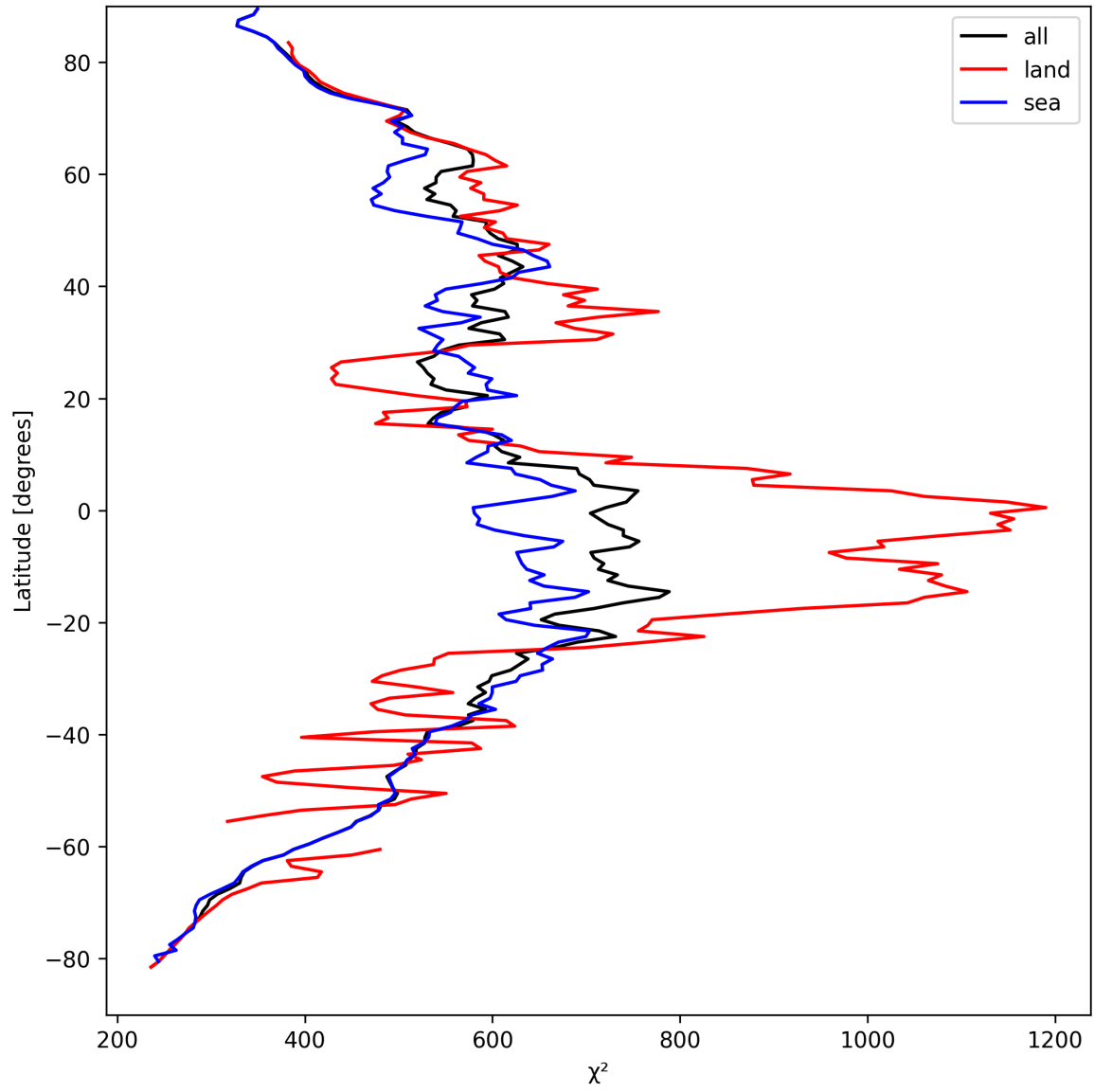
Figure 25: Zonal average of “ \chi^2 ” for 2025-04-07 to 2025-04-08.
