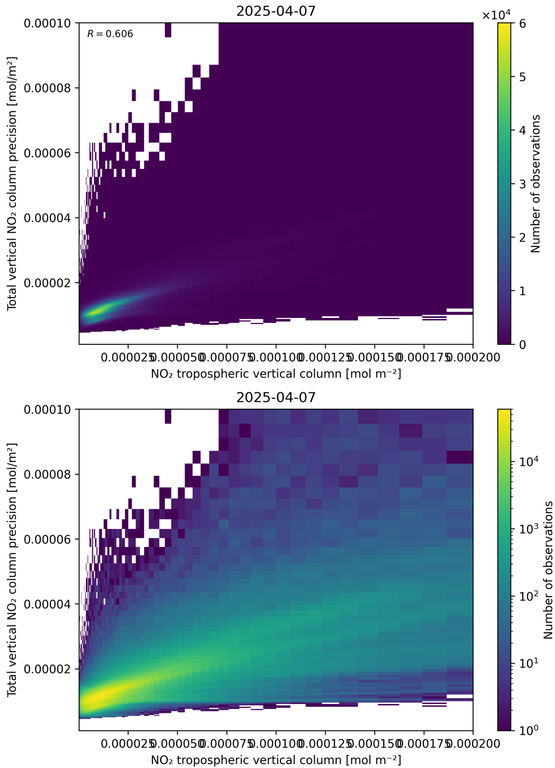
Figure 129: Scatter density plot of “NO 2 tropospheric vertical column” against “Total vertical NO 2 column precision” for 2025-04-07 to 2025-04-08.
