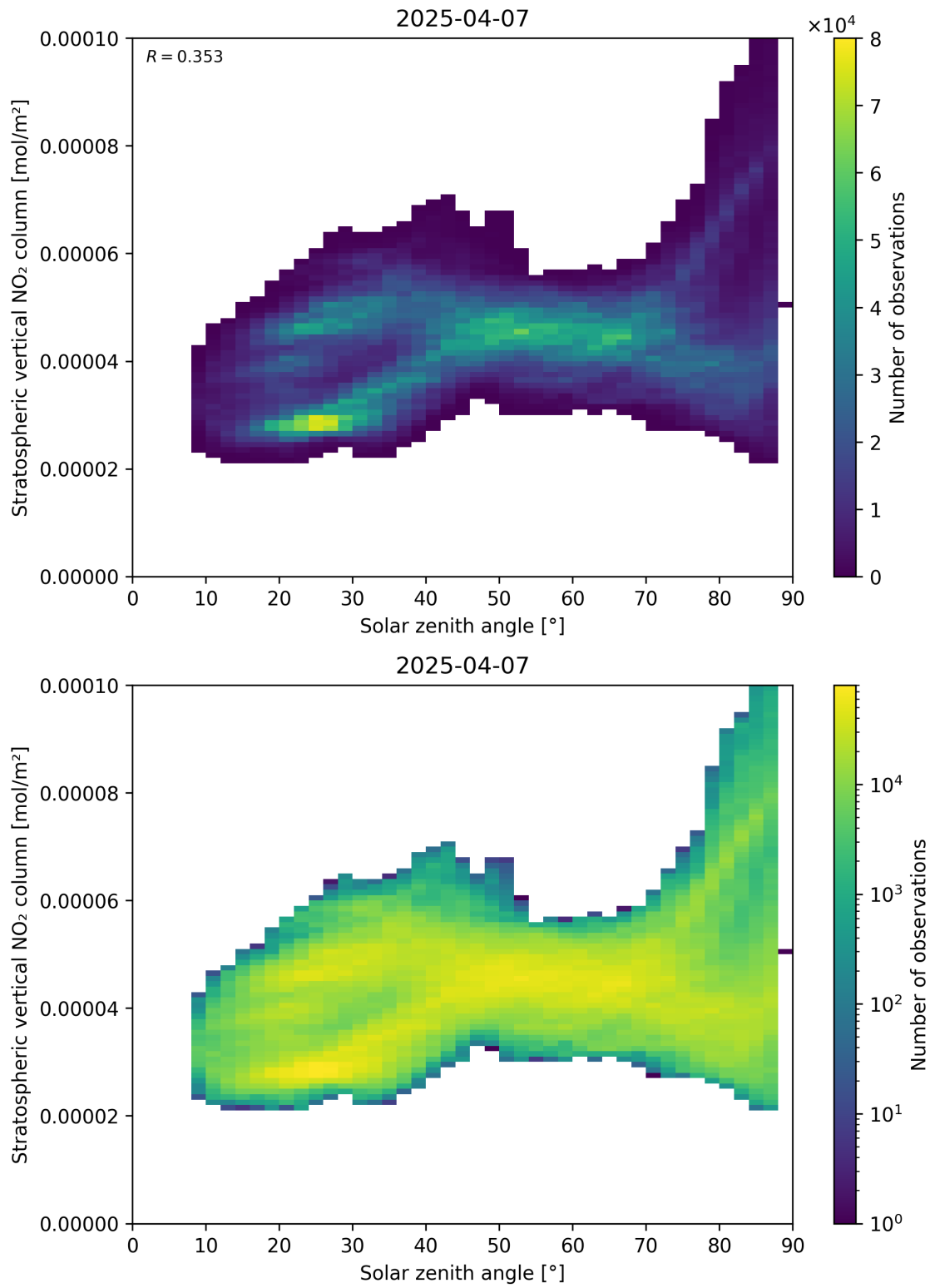
Figure 150: Scatter density plot of “Solar zenith angle” against “Stratospheric vertical NO 2 column” for 2025-04-07 to 2025-04-08.
