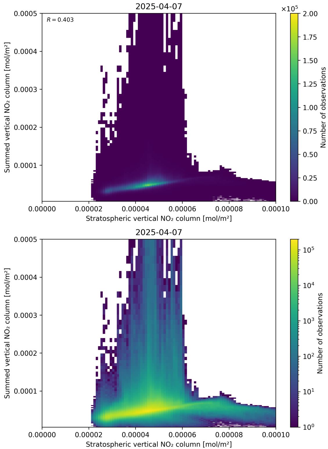
Figure 98: Scatter density plot of “Stratospheric vertical NO 2 column” against “Summed vertical NO 2 column” for 2025-04-07 to 2025-04-08.
