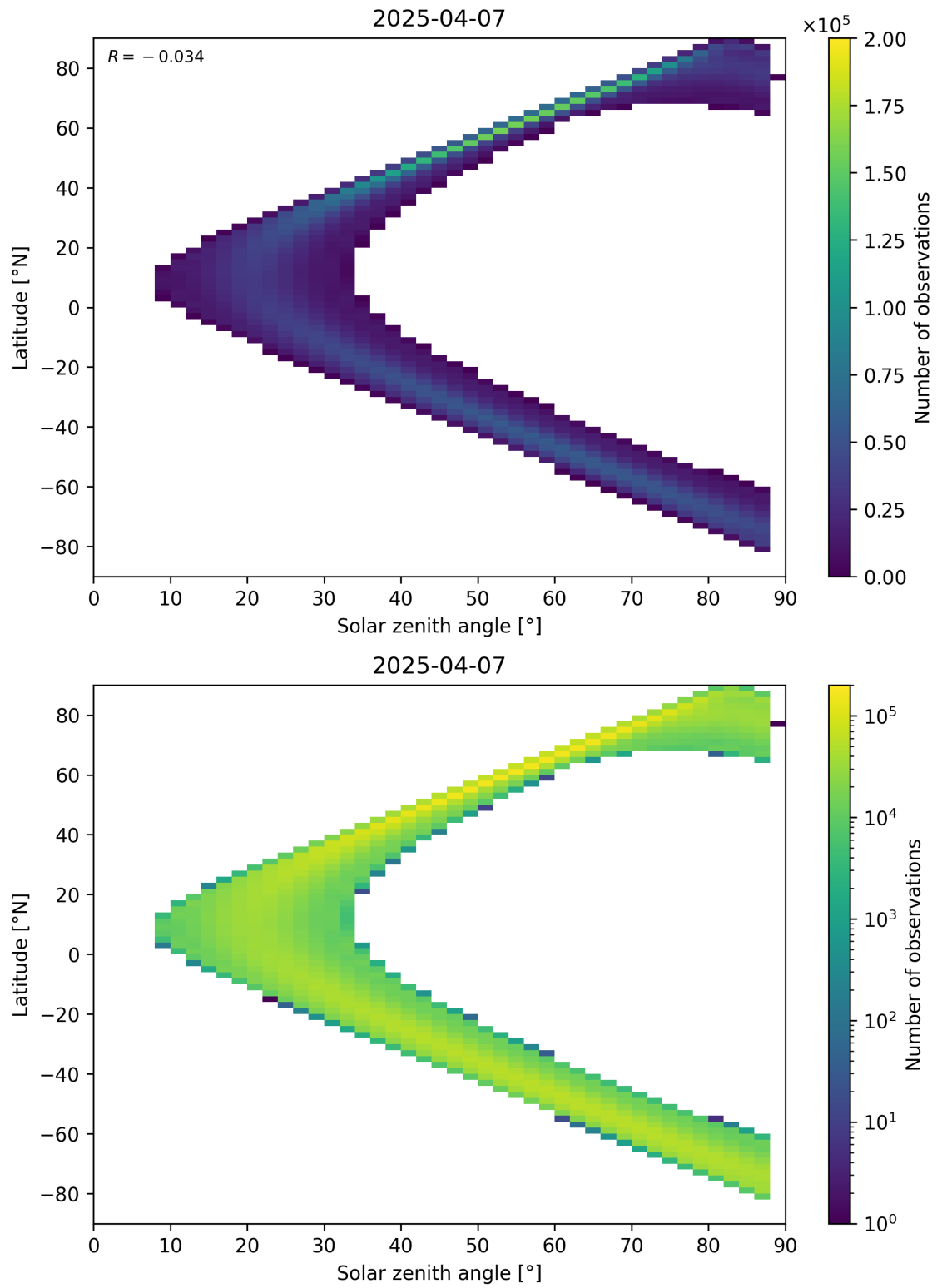
Figure 149: Scatter density plot of “Solar zenith angle” against “Latitude” for 2025-04-07 to 2025-04-08.
