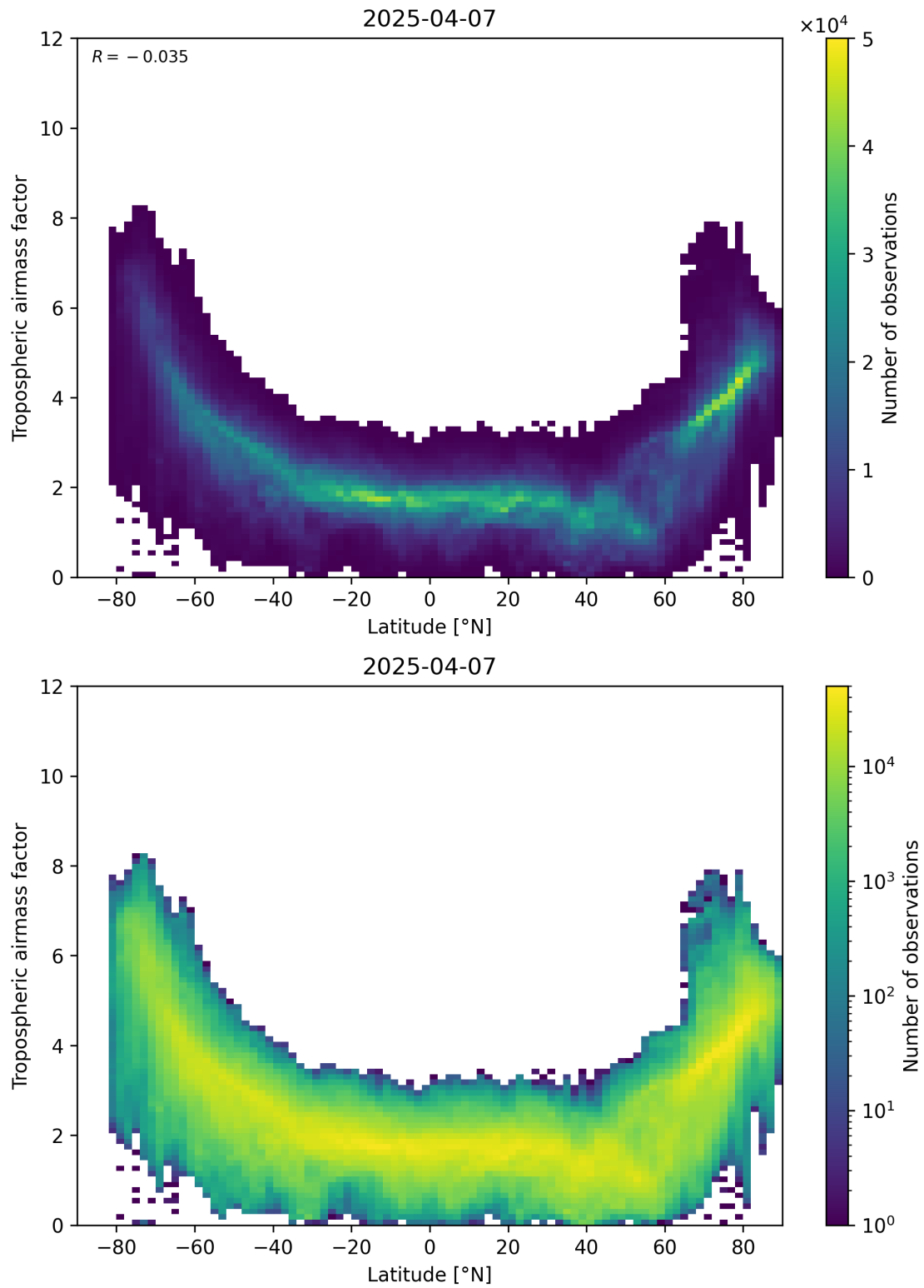
Figure 85: Scatter density plot of “Latitude” against “Tropospheric airmass factor” for 2025-04-07 to 2025-04-08.
