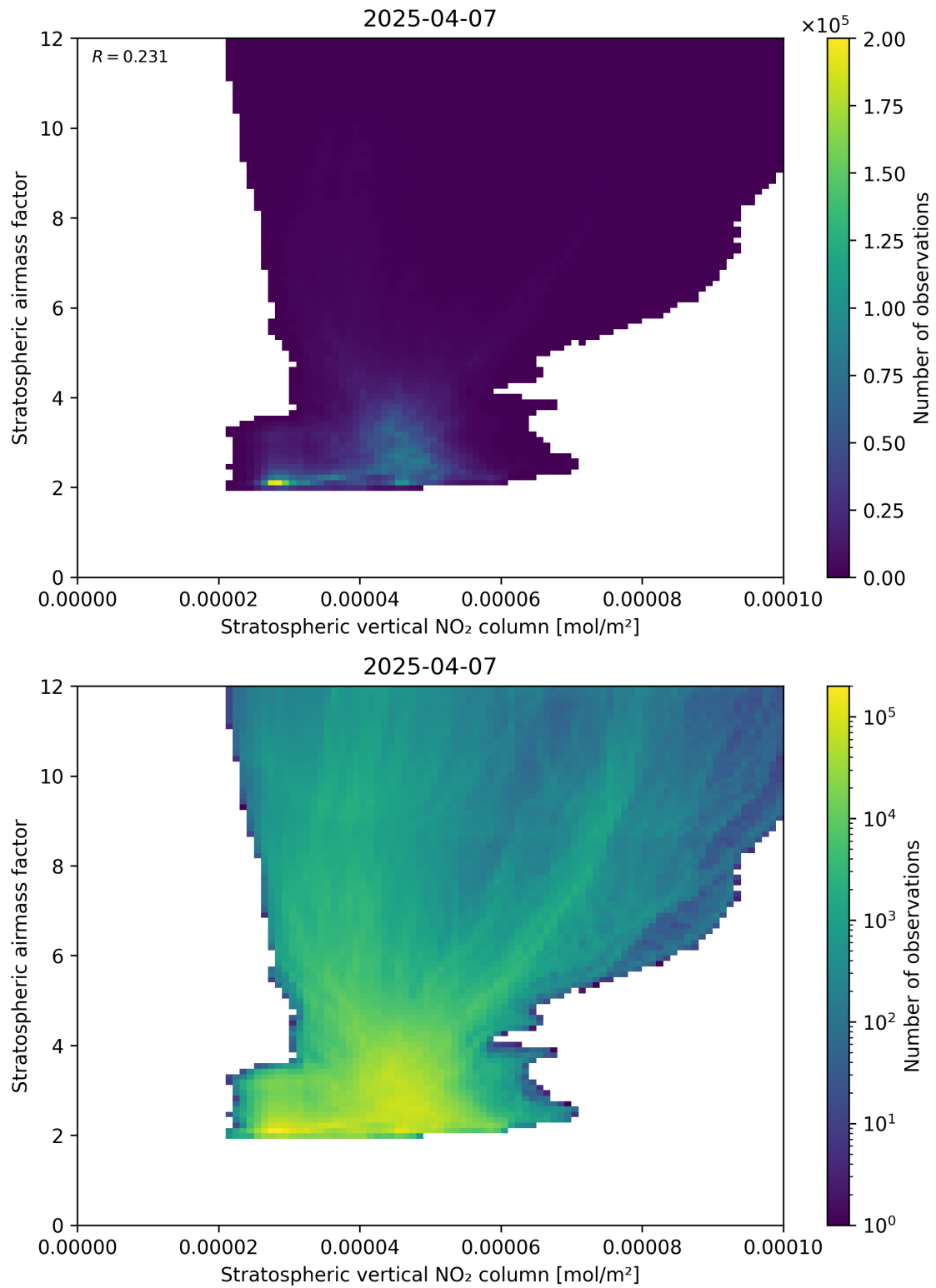
Figure 96: Scatter density plot of “Stratospheric vertical NO 2 column” against “Stratospheric airmass factor” for 2025-04-07 to 2025-04-08.
