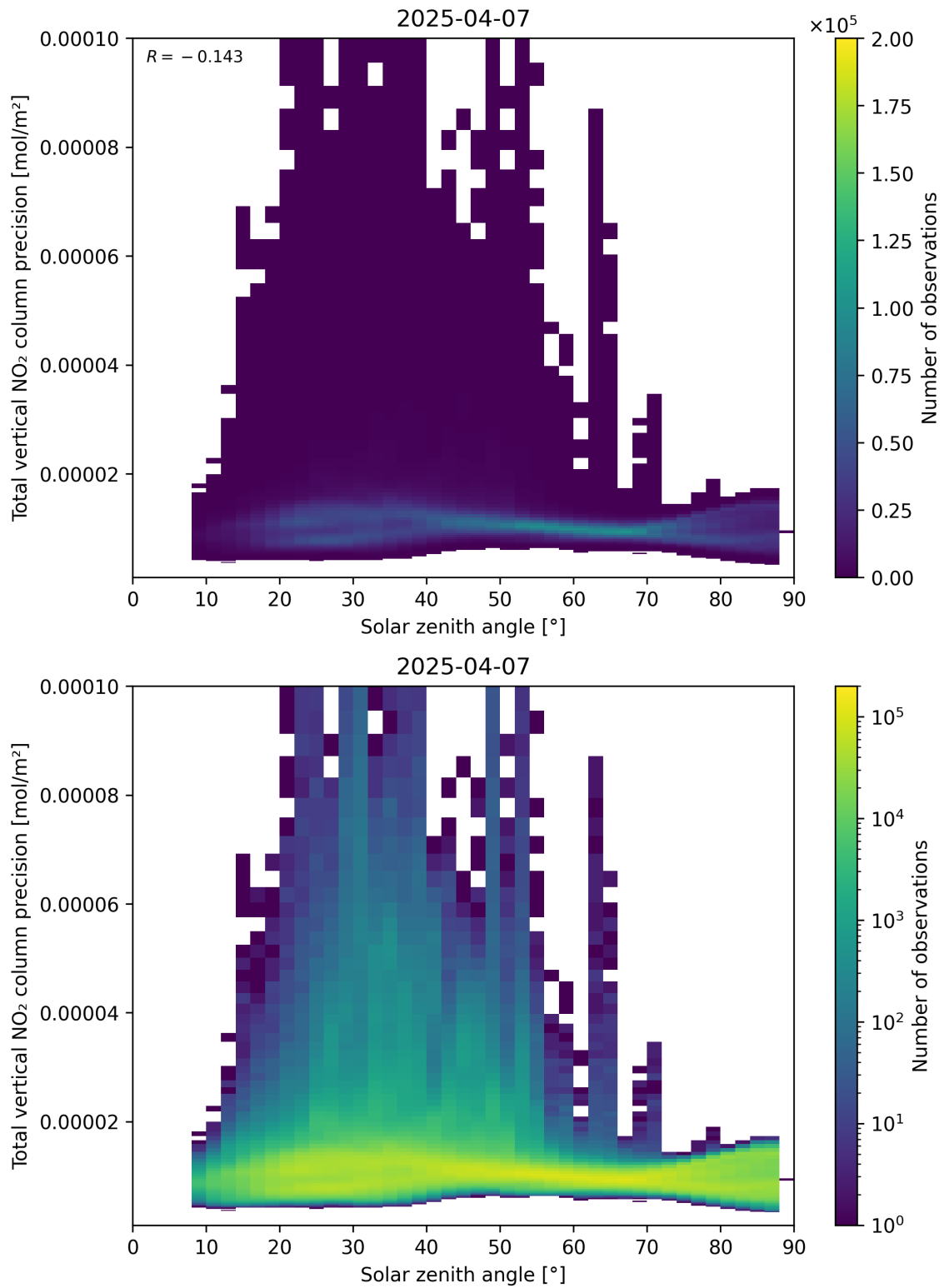
Figure 154: Scatter density plot of “Solar zenith angle” against “Total vertical NO 2 column precision” for 2025-04-07 to 2025-04-08.
