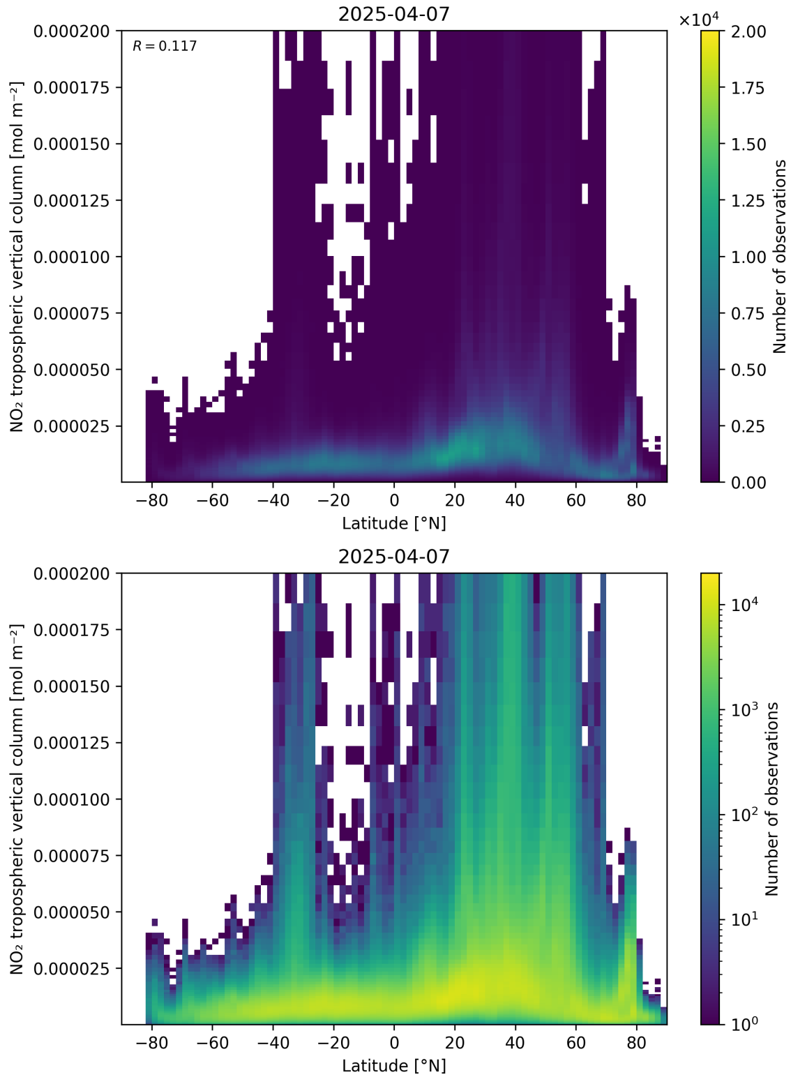
Figure 92: Scatter density plot of “Latitude” against “NO 2 tropospheric vertical column” for 2025-04-07 to 2025-04-08.
