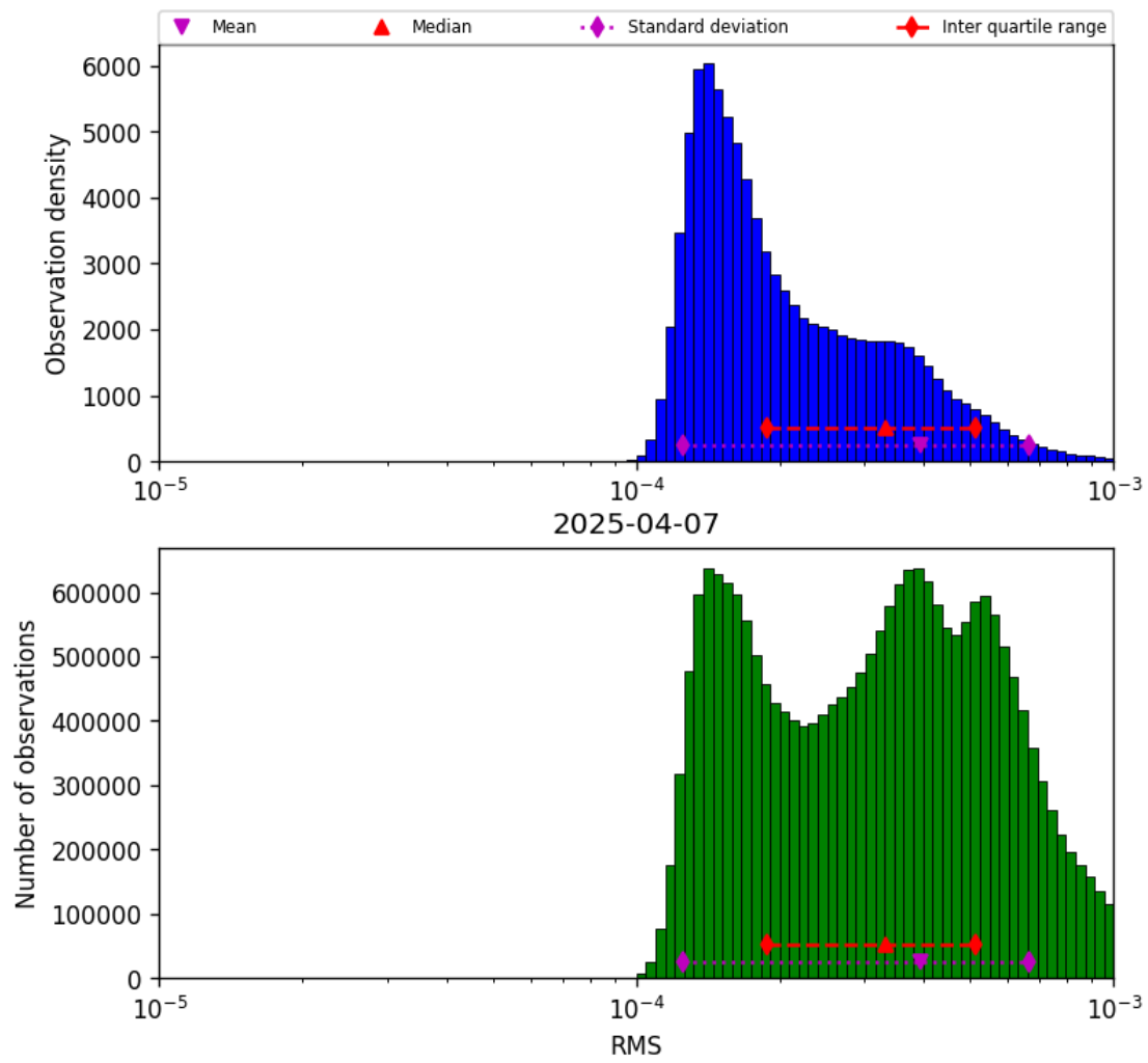
Figure 43: Histogram of “RMS” for 2025-04-07 to 2025-04-08
