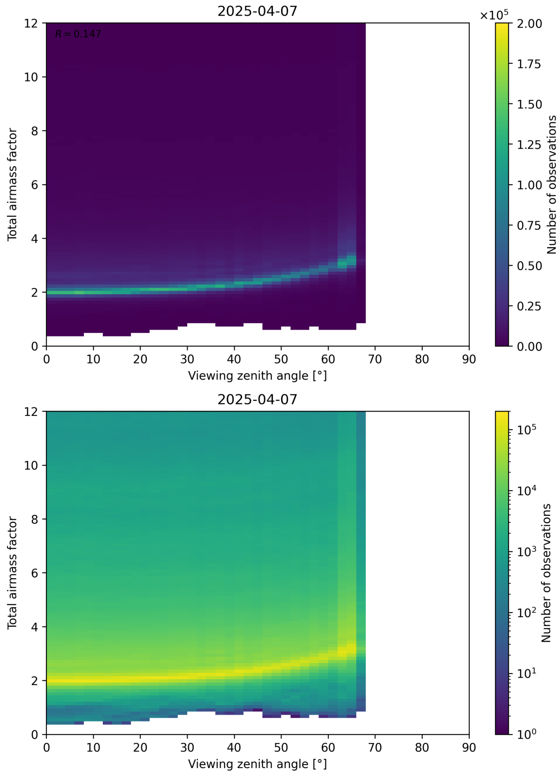
Figure 160: Scatter density plot of “Viewing zenith angle” against “Total airmass factor” for 2025-04-07 to 2025-04-08.
