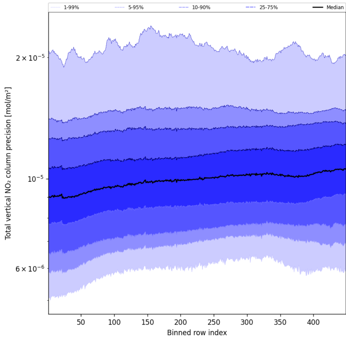
Figure 56: Along track statistics of “Total vertical NO 2 column precision” for 2025-04-07 to 2025-04-08
