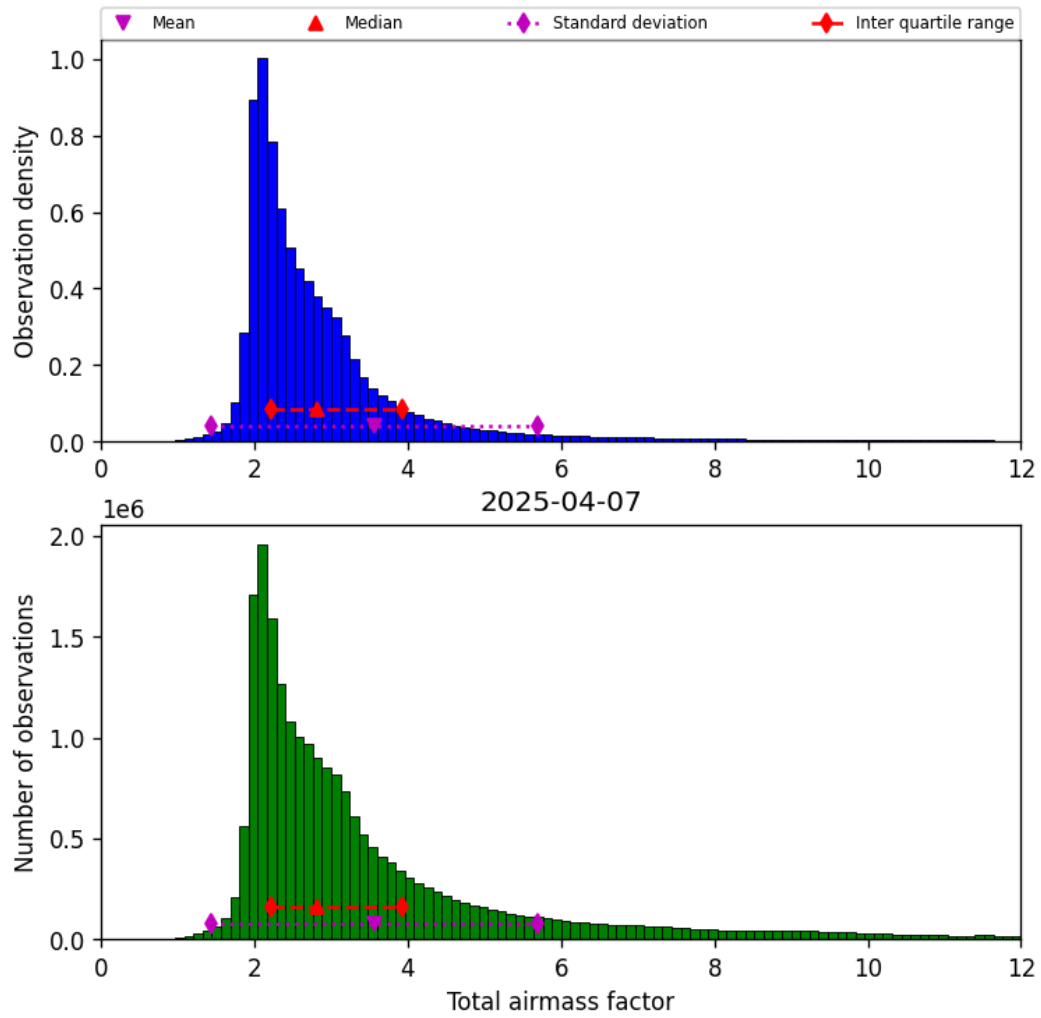
Figure 32: Histogram of “Total airmass factor” for 2025-04-07 to 2025-04-08
