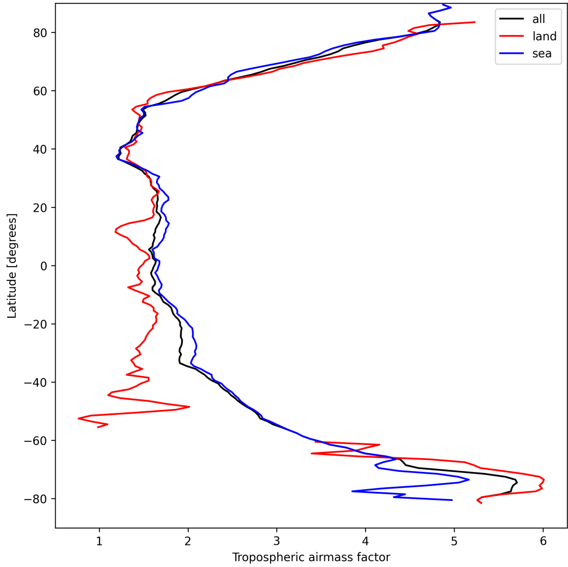
Figure 14: Zonal average of “Tropospheric air mass factor” for 2025-04-07 to 2025-04-08.
