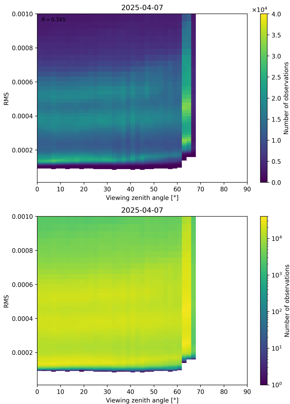
Figure 171: Scatter density plot of “Viewing zenith angle” against “RMS” for 2025-04-07 to 2025-04-08.
