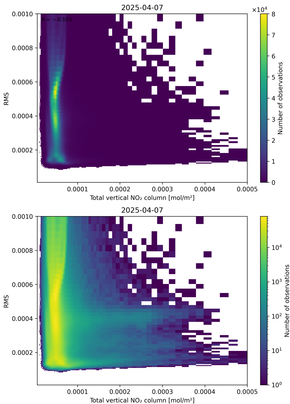
Figure 120: Scatter density plot of “Total vertical NO 2 column” against “RMS” for 2025-04-07 to 2025-04-08.
