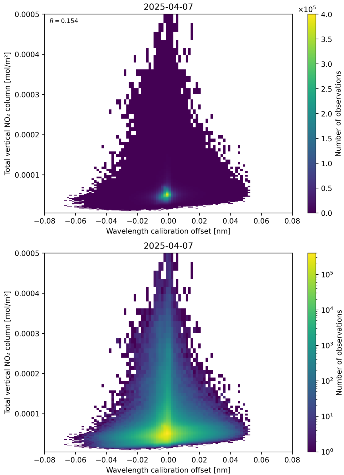
Figure 179: Scatter density plot of “Wavelength calibration offset” against “Total vertical NO 2 column” for 2025-04-07 to 2025-04-08.
