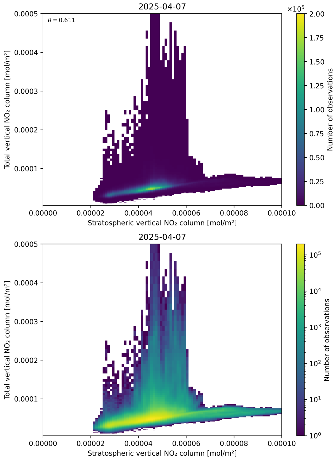
Figure 100: Scatter density plot of “Stratospheric vertical NO 2 column” against “Total vertical NO 2 column” for 2025-04-07 to 2025-04-08.
