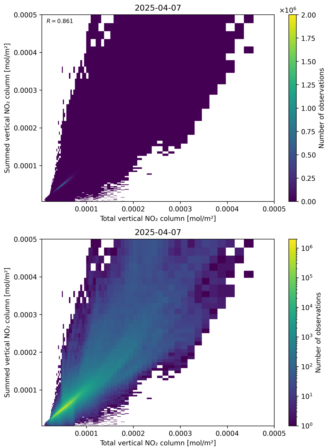
Figure 112: Scatter density plot of “Total vertical NO 2 column” against “Summed vertical NO 2 column” for 2025-04-07 to 2025-04-08.
