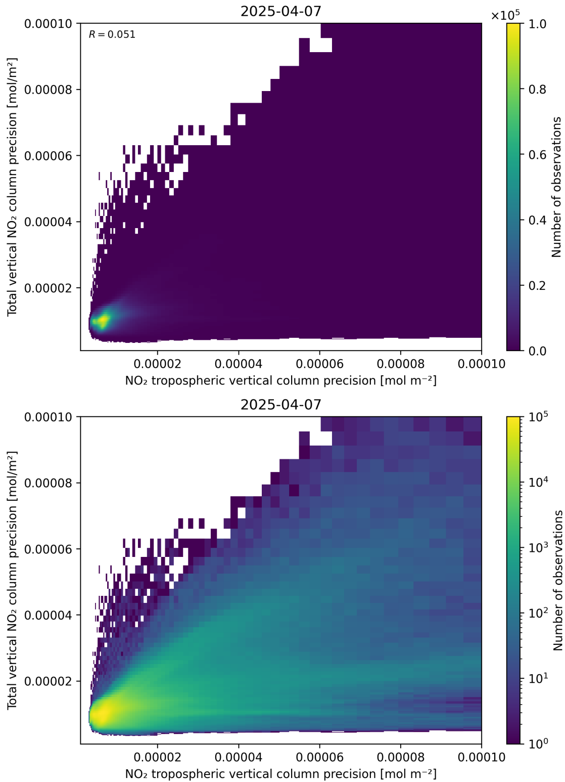
Figure 139: Scatter density plot of “NO 2 tropospheric vertical column precision” against “Total vertical NO 2 column precision” for 2025-04-07 to 2025-04-08.
