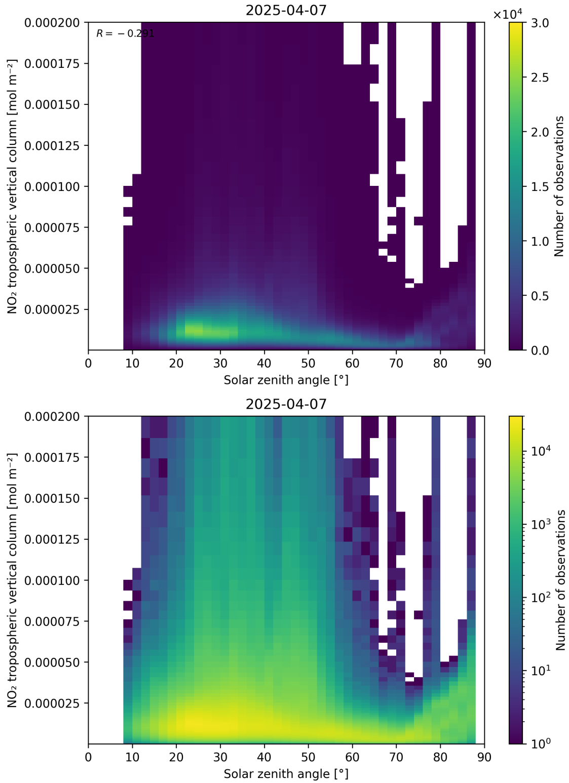
Figure 155: Scatter density plot of “Solar zenith angle” against “NO 2 tropospheric vertical column” for 2025-04-07 to 2025-04-08.
