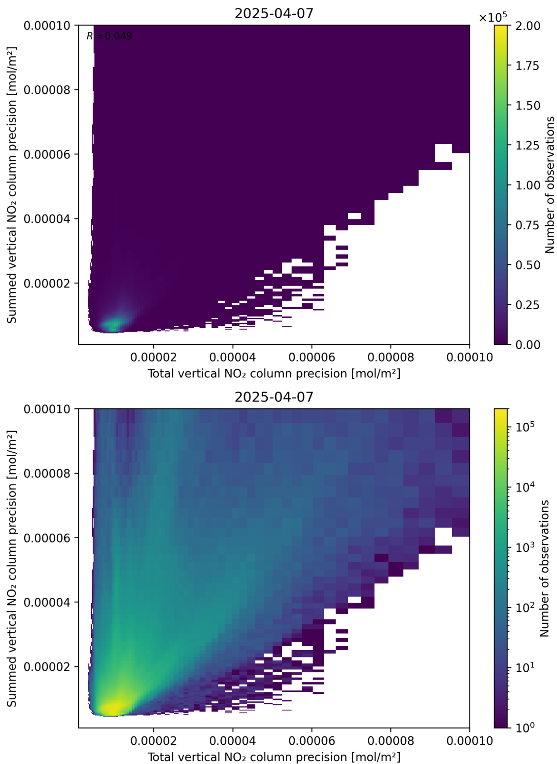
Figure 118: Scatter density plot of “Total vertical NO 2 column precision” against “Summed vertical NO 2 column precision” for 2025-04-07 to 2025-04-08.
