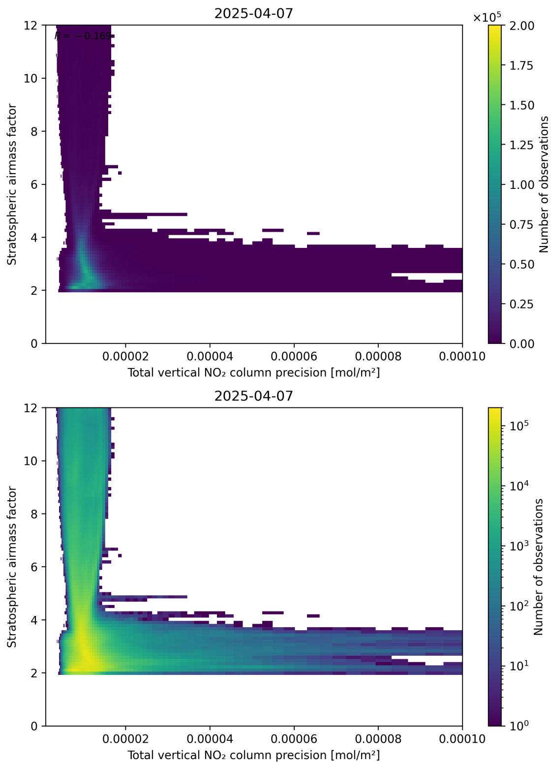
Figure 115: Scatter density plot of “Total vertical NO 2 column precision” against “Stratospheric air mass factor” for 2025-04-07 to 2025-04-08.
