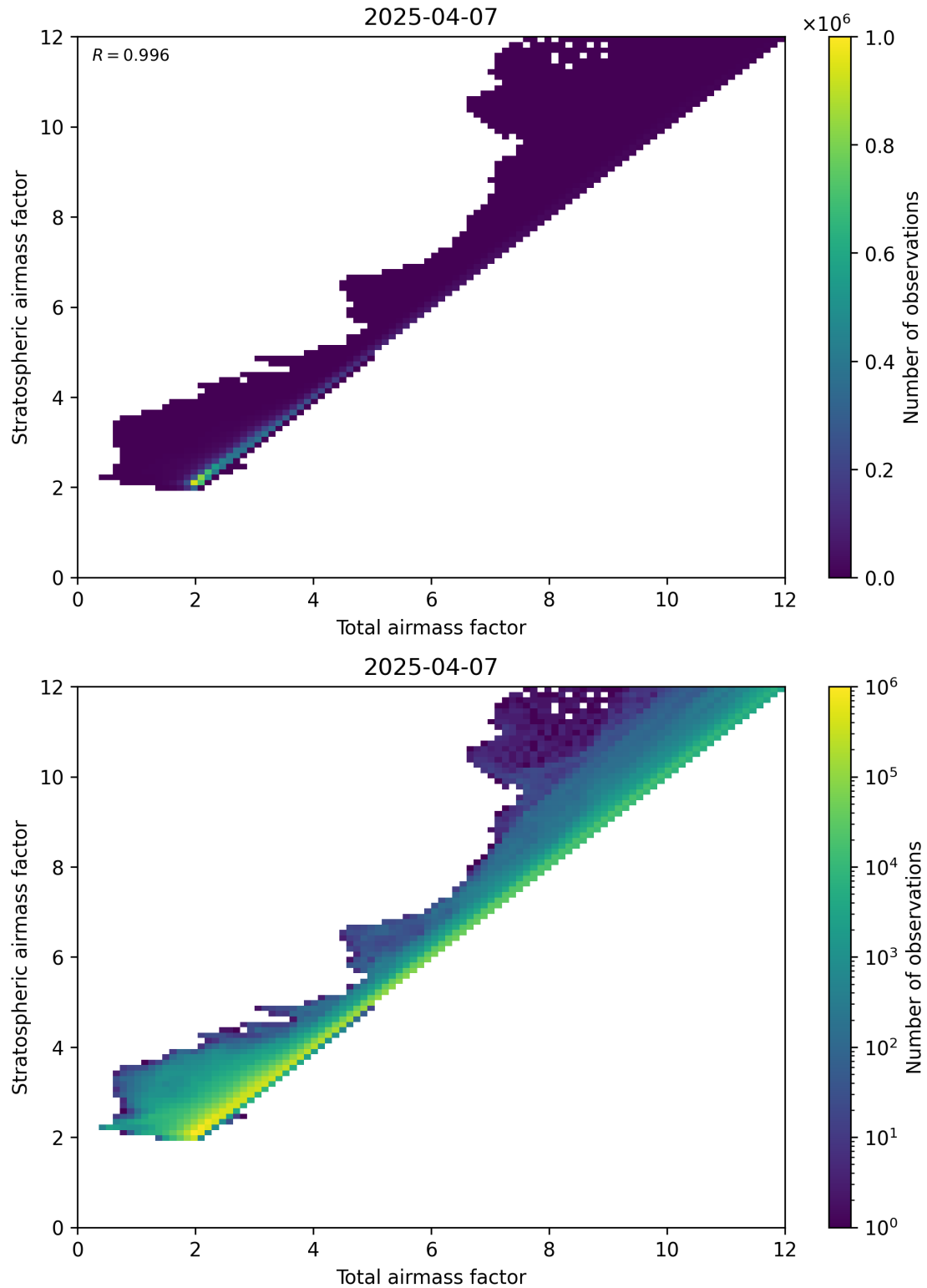
Figure 62: Scatter density plot of “Total airmass factor” against “Stratospheric airmass factor” for 2025-04-07 to 2025-04-08.
