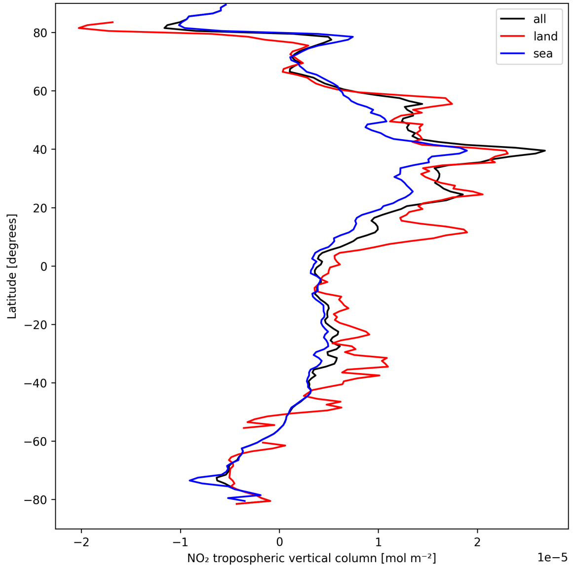
Figure 12: Zonal average of “NO 2 tropospheric vertical column” for 2025-04-07 to 2025-04-08.
