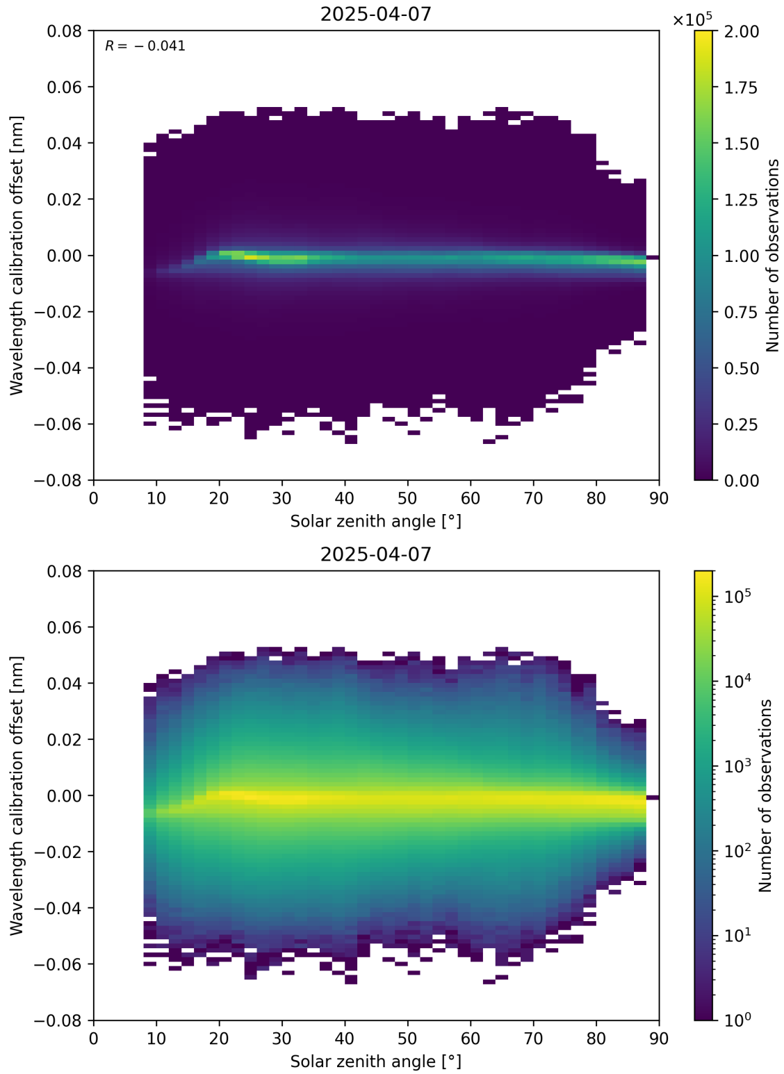
Figure 158: Scatter density plot of “Solar zenith angle” against “Wavelength calibration offset” for 2025-04-07 to 2025-04-08.
