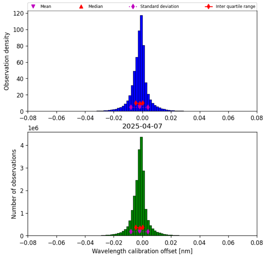
Figure 35: Histogram of “Wavelength calibration offset” for 2025-04-07 to 2025-04-08
