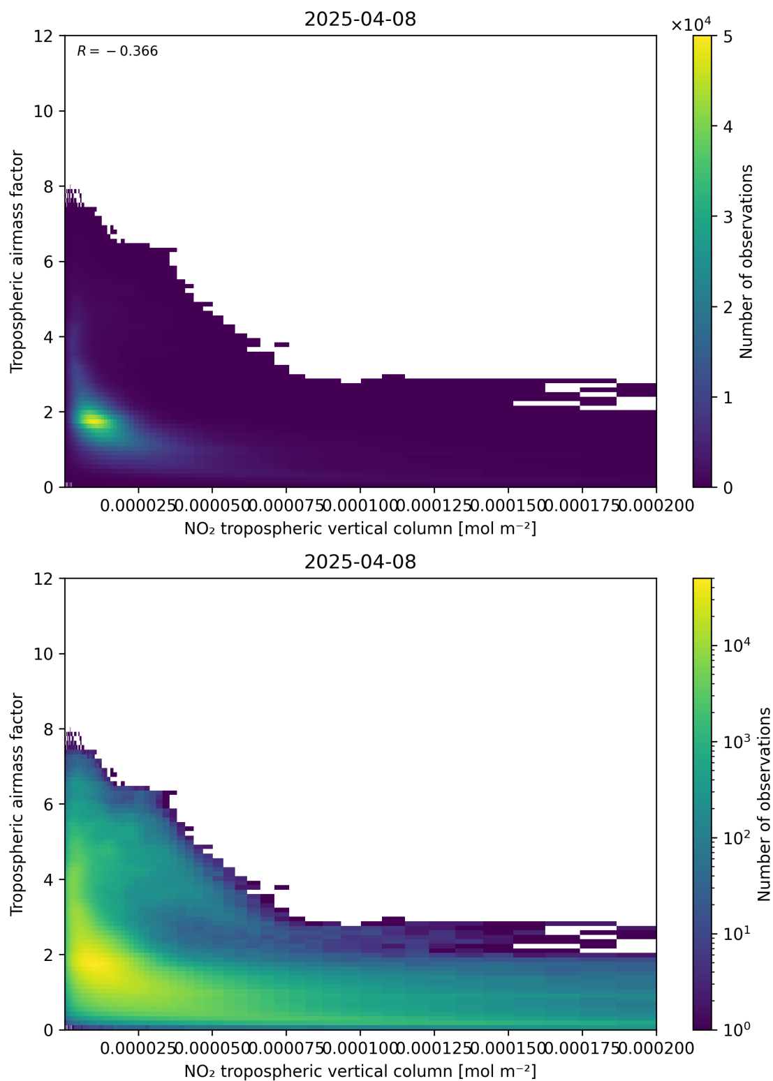
Figure 123: Scatter density plot of “NO 2 tropospheric vertical column” against “Tropospheric air mass factor” for 2025-04-08 to 2025-04-09.
