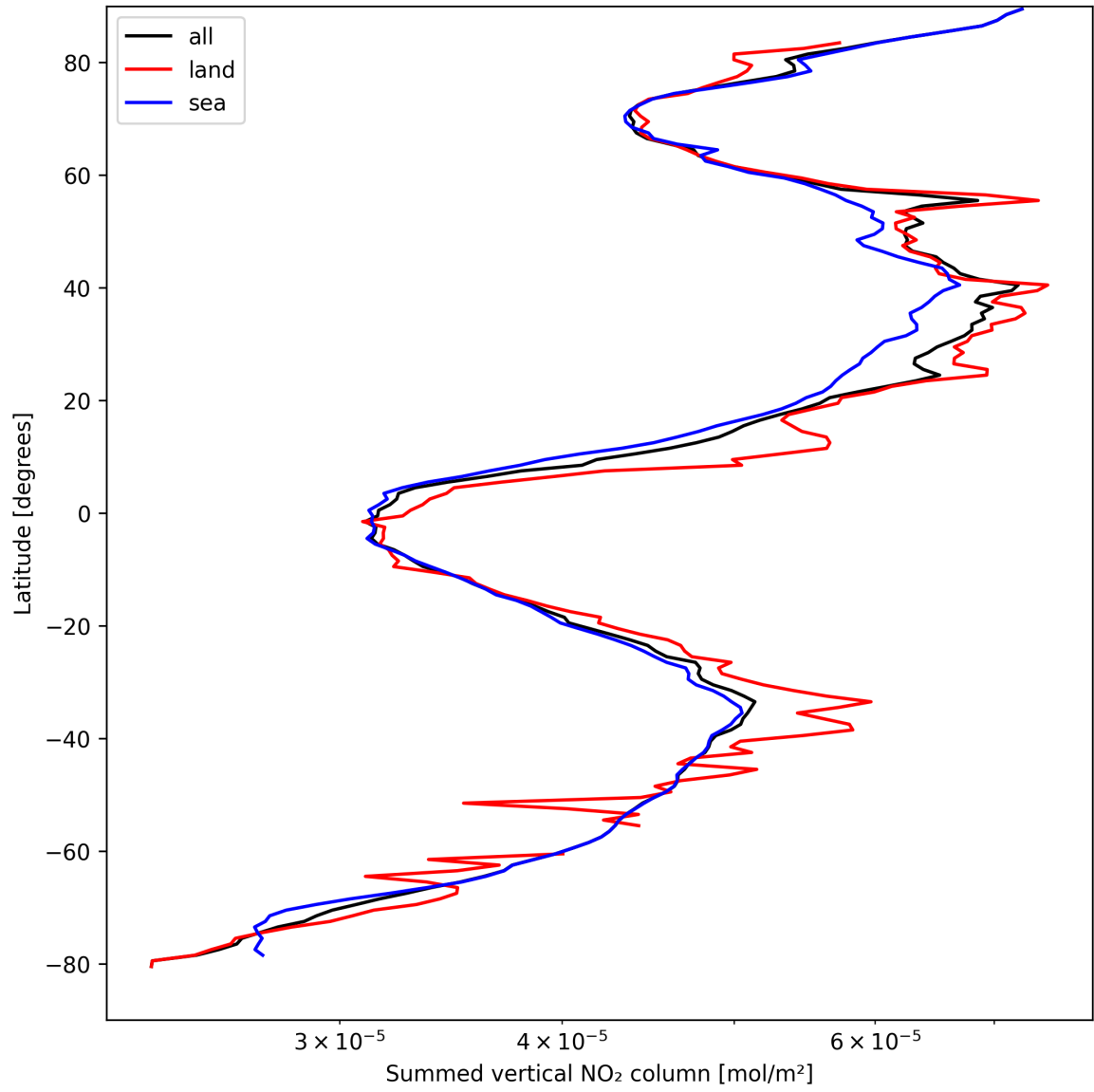
Figure 23: Zonal average of “Summed vertical NO 2 column” for 2025-04-08 to 2025-04-09.
