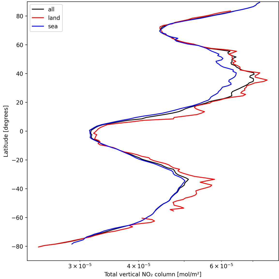
Figure 21: Zonal average of “Total vertical NO 2 column” for 2025-04-08 to 2025-04-09.
