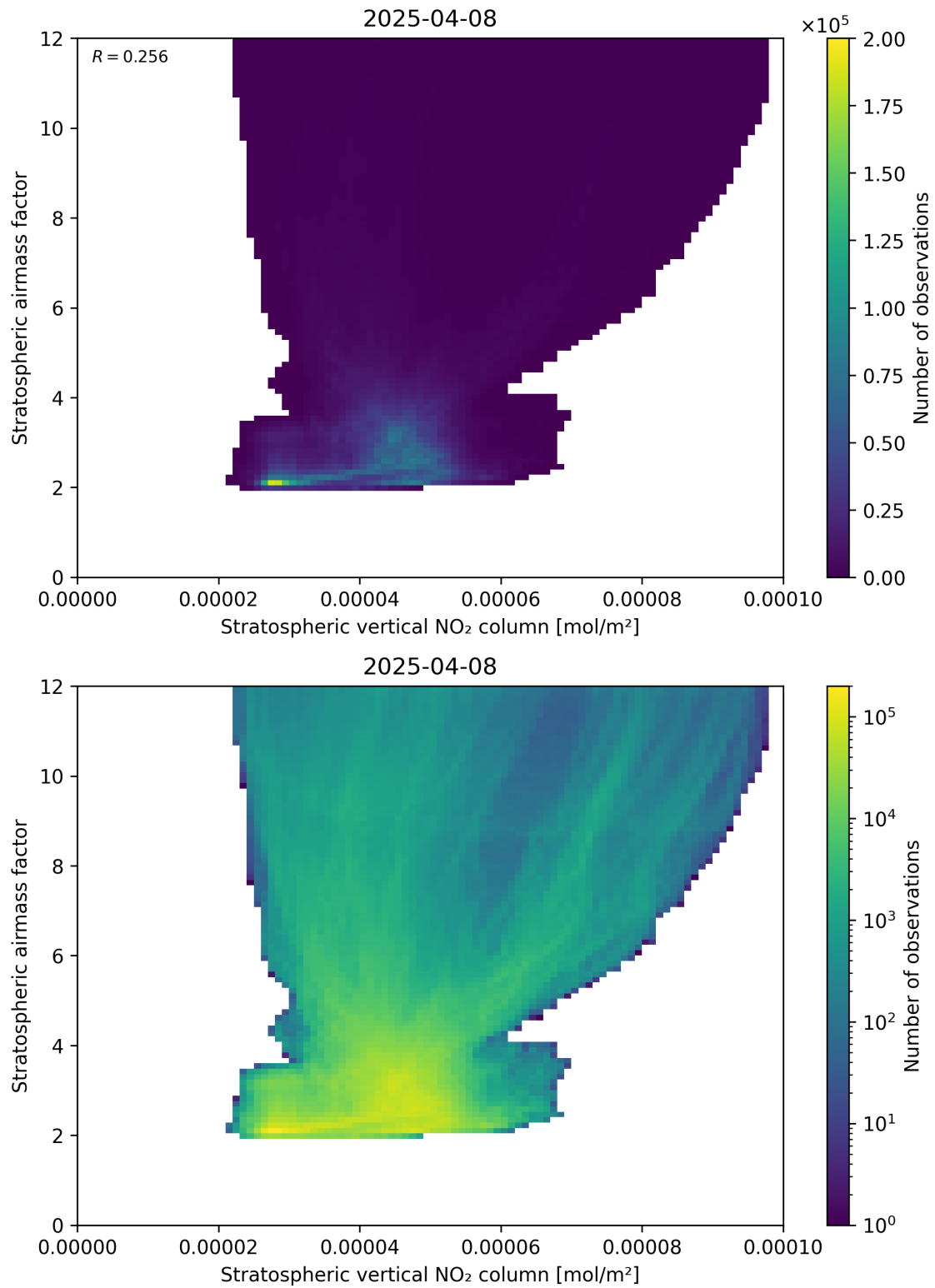
Figure 96: Scatter density plot of “Stratospheric vertical NO 2 column” against “Stratospheric airmass factor” for 2025-04-08 to 2025-04-09.
