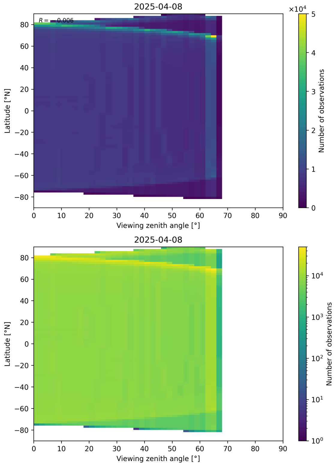
Figure 163: Scatter density plot of “Viewing zenith angle” against “Latitude” for 2025-04-08 to 2025-04-09.
