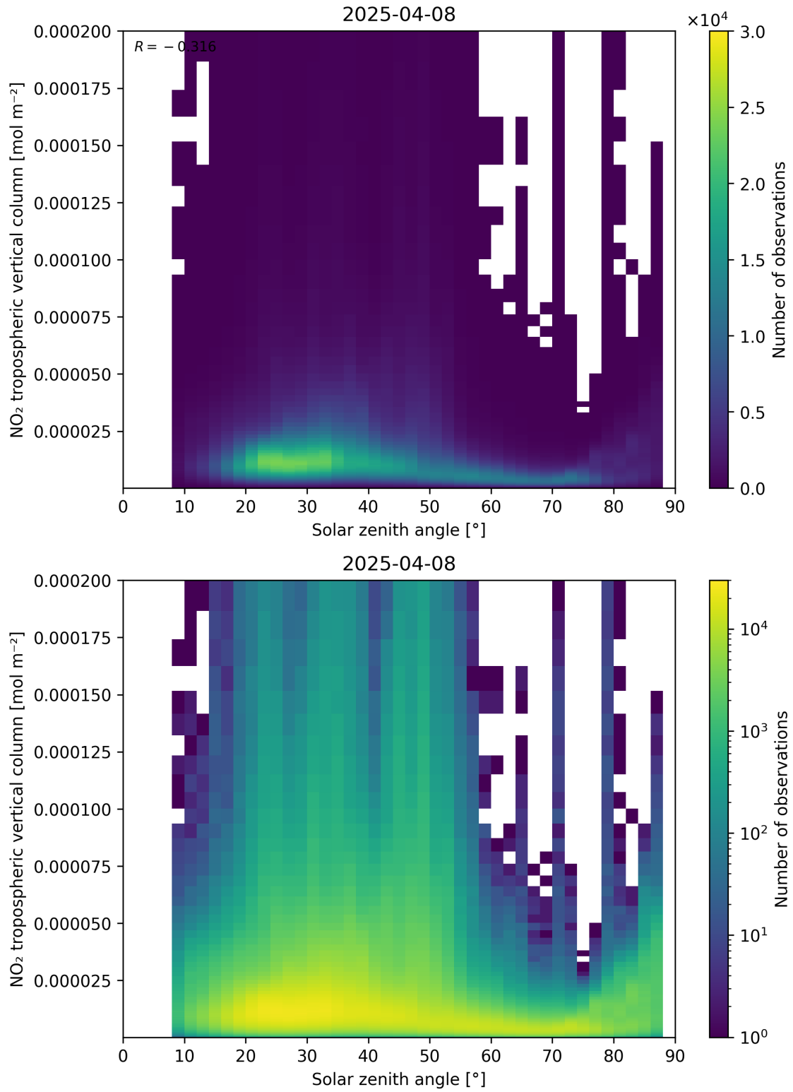
Figure 155: Scatter density plot of “Solar zenith angle” against “NO 2 tropospheric vertical column” for 2025-04-08 to 2025-04-09.
