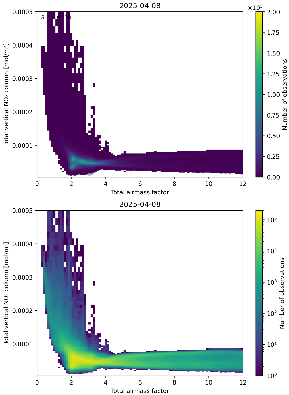
Figure 67: Scatter density plot of “Total airmass factor” against “Total vertical NO 2 column” for 2025-04-08 to 2025-04-09.
