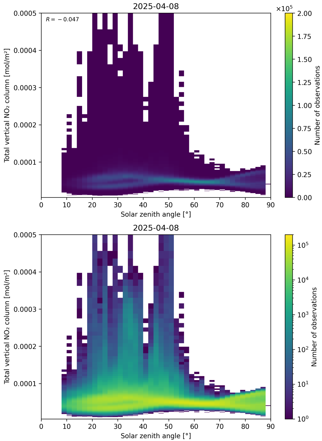
Figure 153: Scatter density plot of “Solar zenith angle” against “Total vertical NO 2 column” for 2025-04-08 to 2025-04-09.
