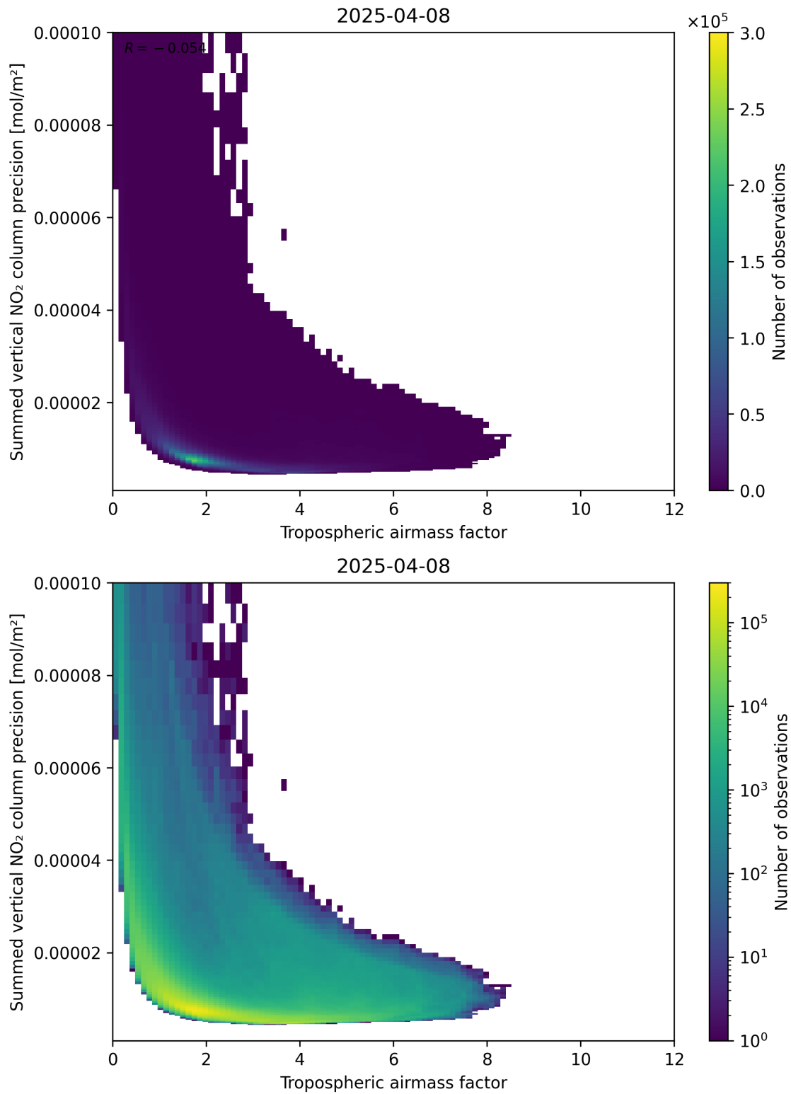
Figure 76: Scatter density plot of “Tropospheric air mass factor” against “Summed vertical NO 2 column precision” for 2025-04-08 to 2025-04-09.
