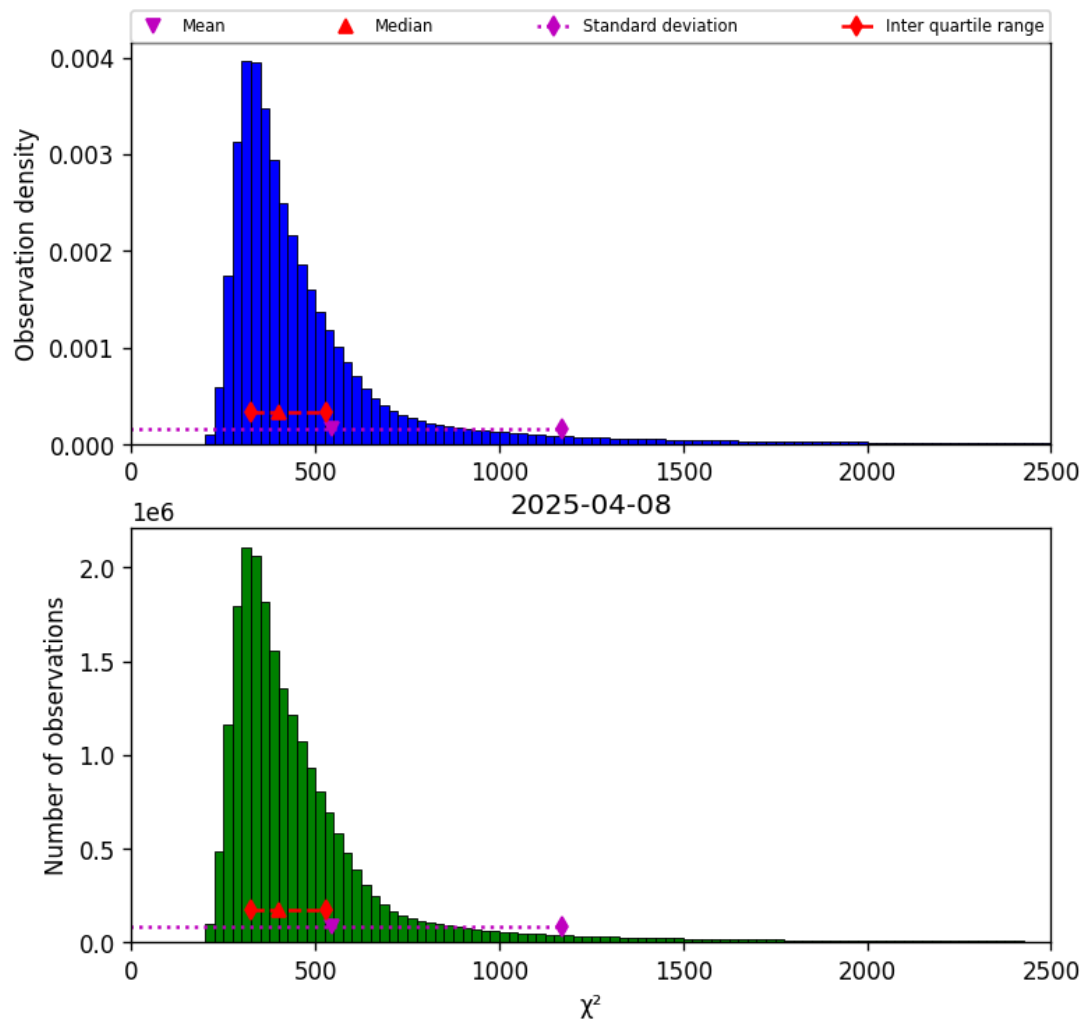
Figure 42: Histogram of “ \chi^2 ” for 2025-04-08 to 2025-04-09
