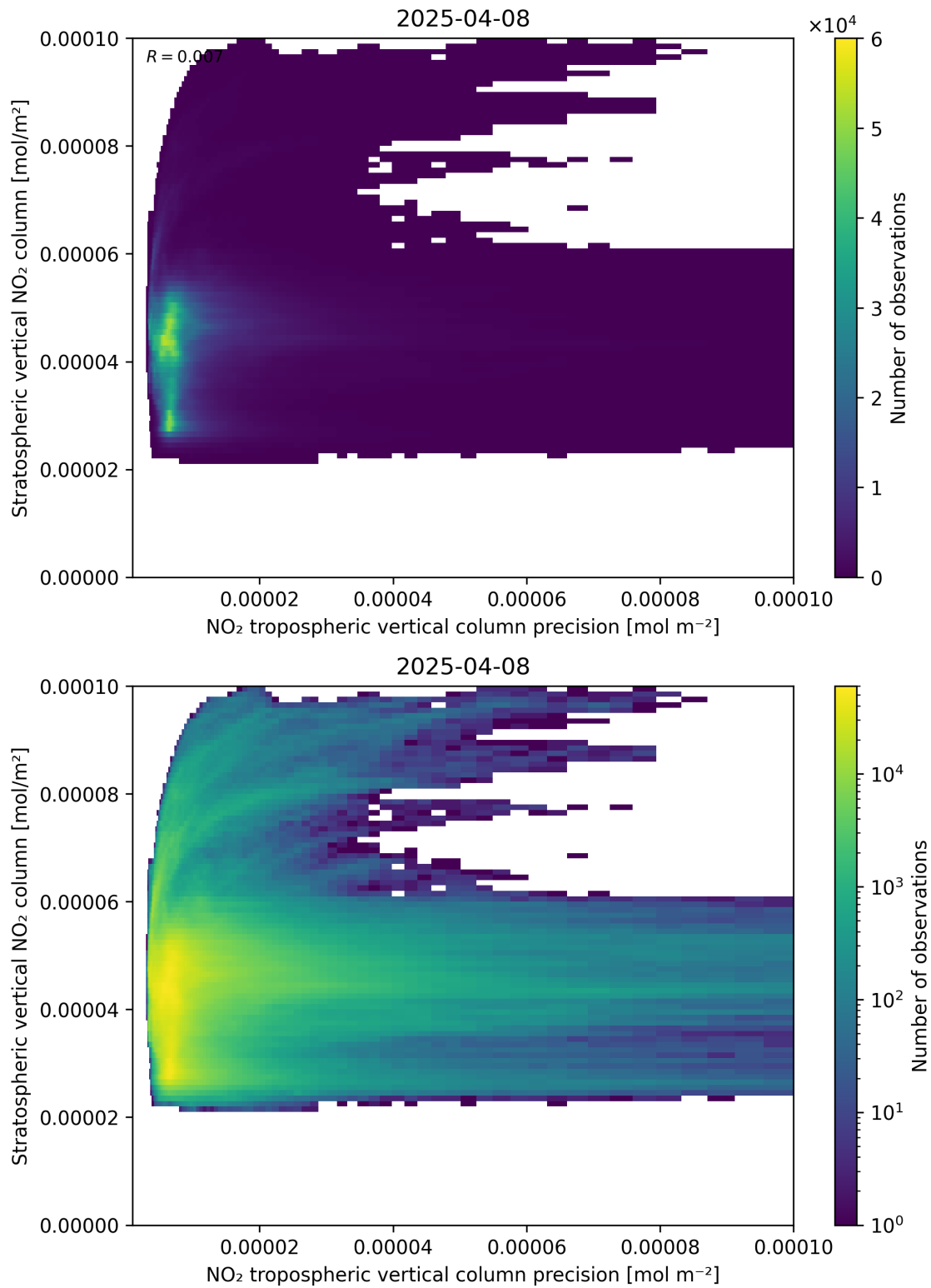
Figure 135: Scatter density plot of “NO 2 tropospheric vertical column precision” against “Stratospheric vertical NO 2 column” for 2025-04-08 to 2025-04-09.
