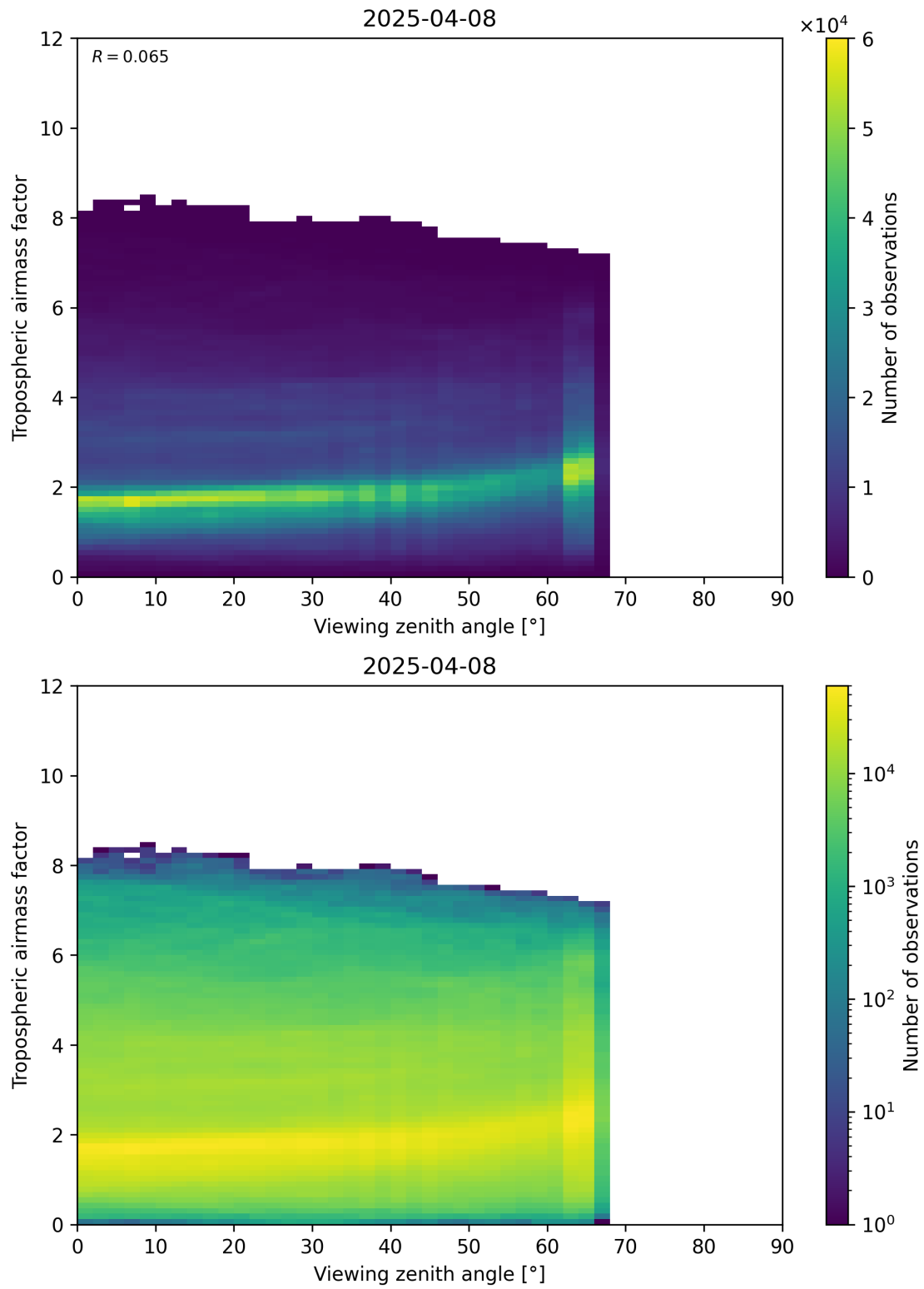
Figure 161: Scatter density plot of “Viewing zenith angle” against “Tropospheric airmass factor” for 2025-04-08 to 2025-04-09.
