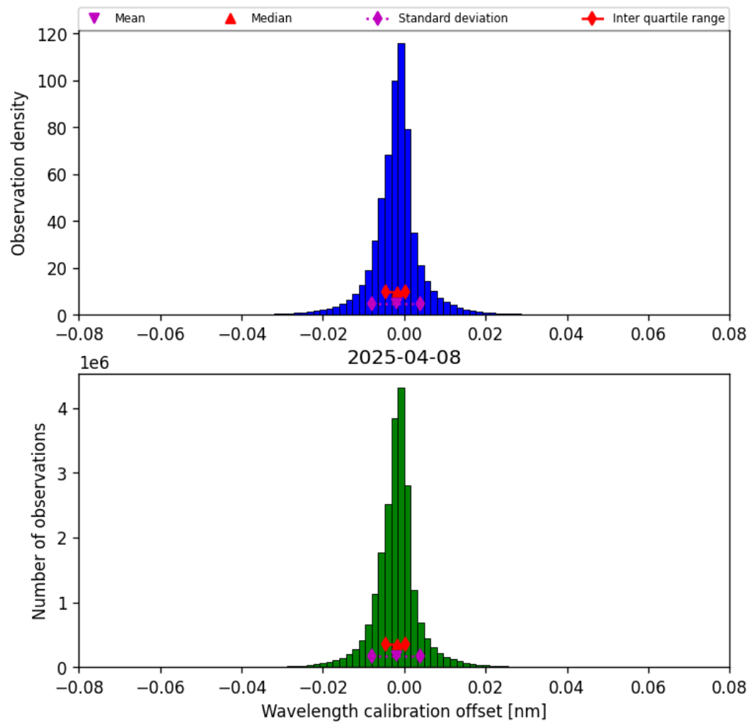
Figure 35: Histogram of “Wavelength calibration offset” for 2025-04-08 to 2025-04-09
