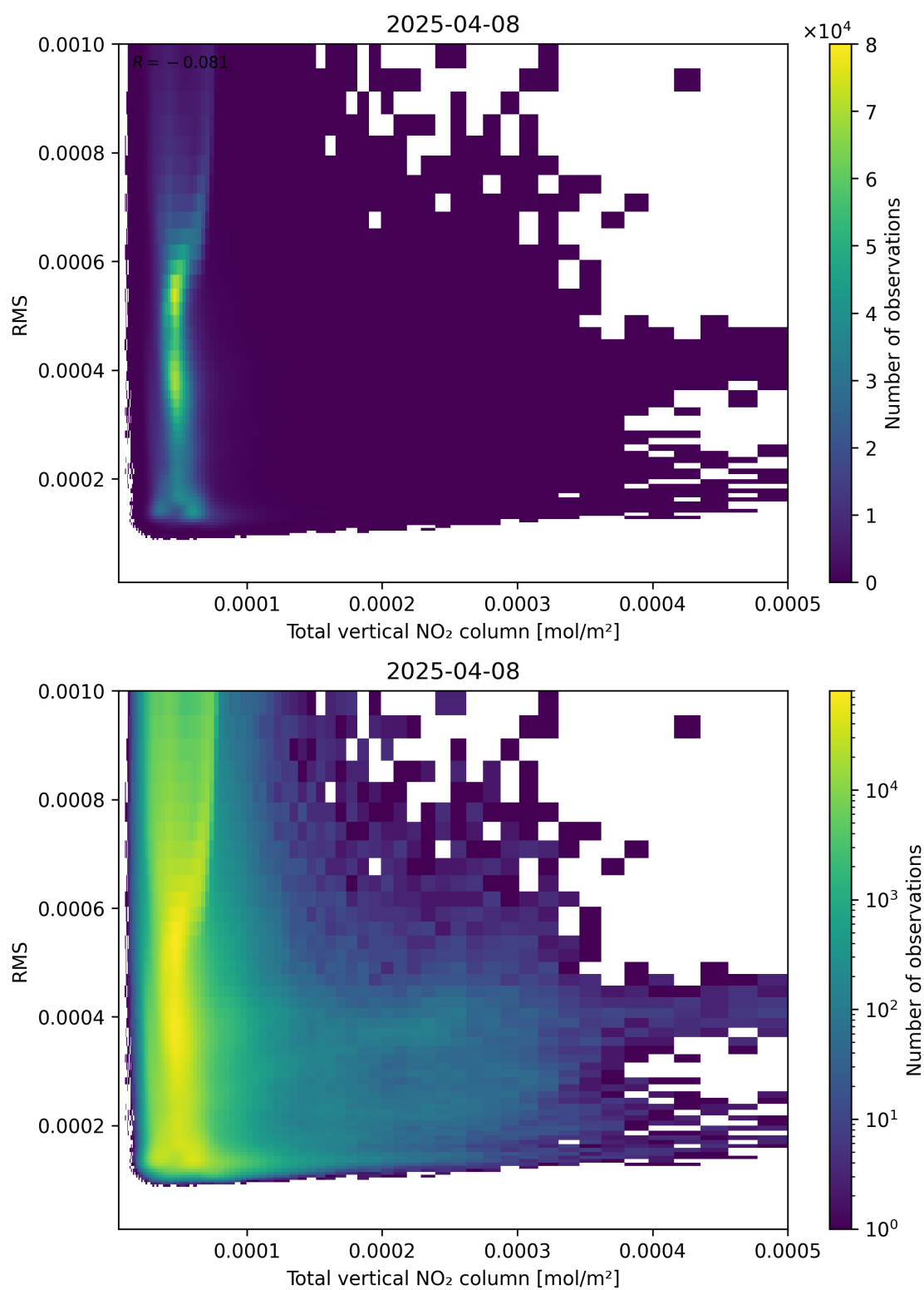
Figure 120: Scatter density plot of “Total vertical NO 2 column” against “RMS” for 2025-04-08 to 2025-04-09.
