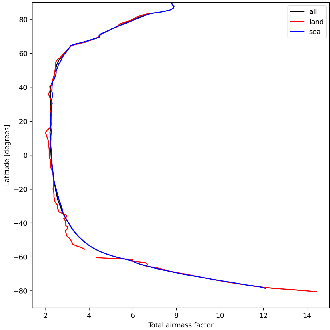
Figure 15: Zonal average of “Total airmass factor” for 2025-04-08 to 2025-04-09.
