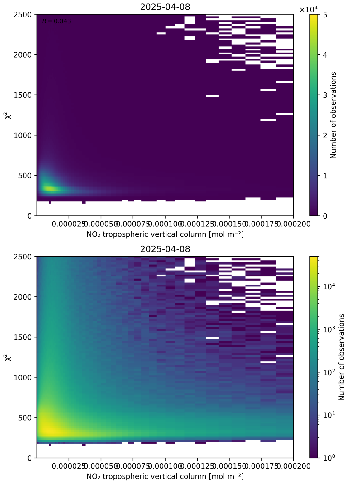
Figure 124: Scatter density plot of “NO 2 tropospheric vertical column” against “ \chi^2 ” for 2025-04-08 to 2025-04-09.
