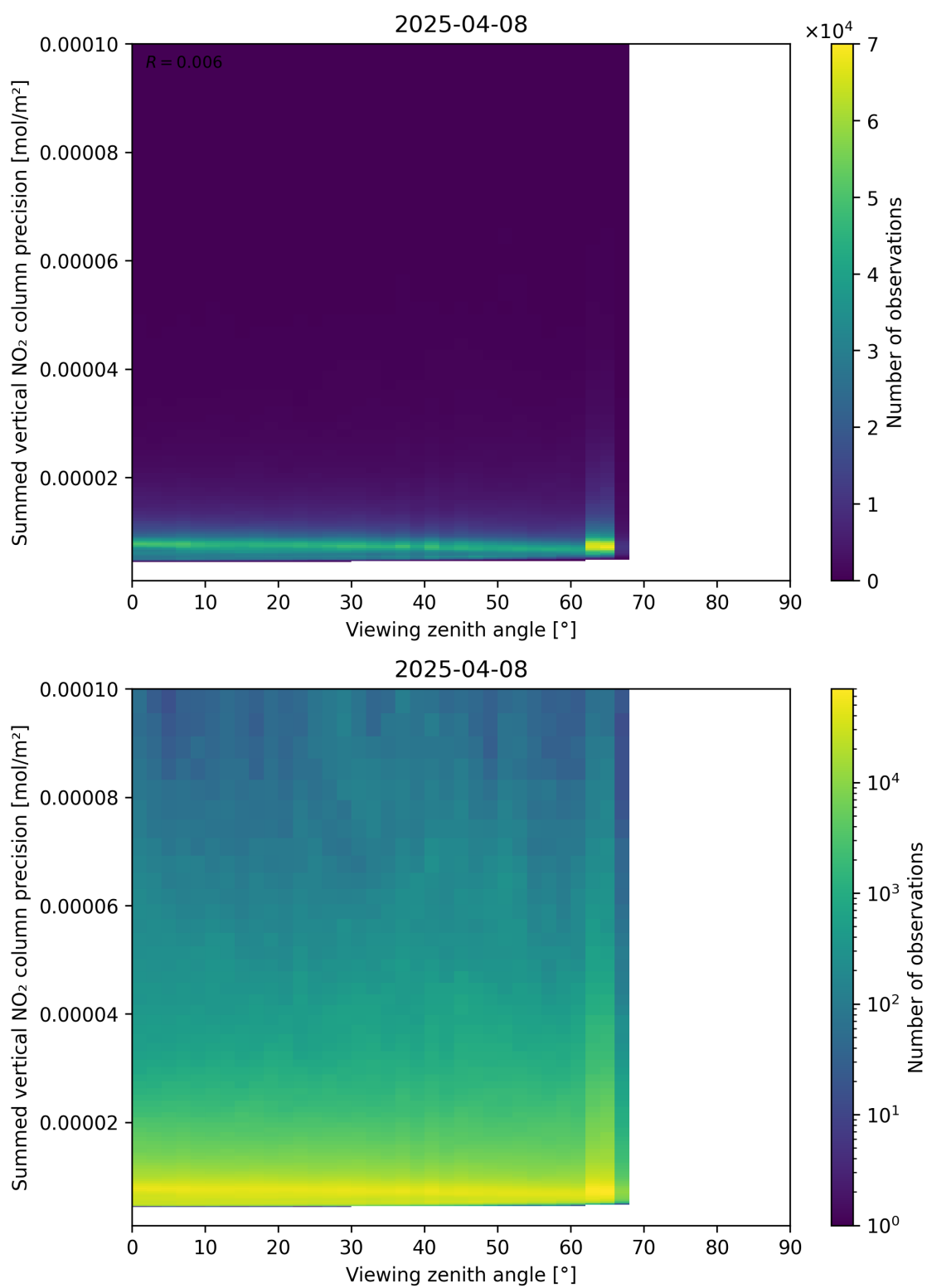
Figure 166: Scatter density plot of “Viewing zenith angle” against “Summed vertical NO 2 column precision” for 2025-04-08 to 2025-04-09.
