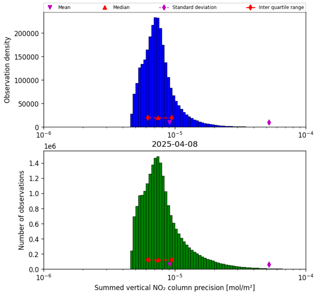
Figure 41: Histogram of “Summed vertical NO 2 column precision” for 2025-04-08 to 2025-04-09
