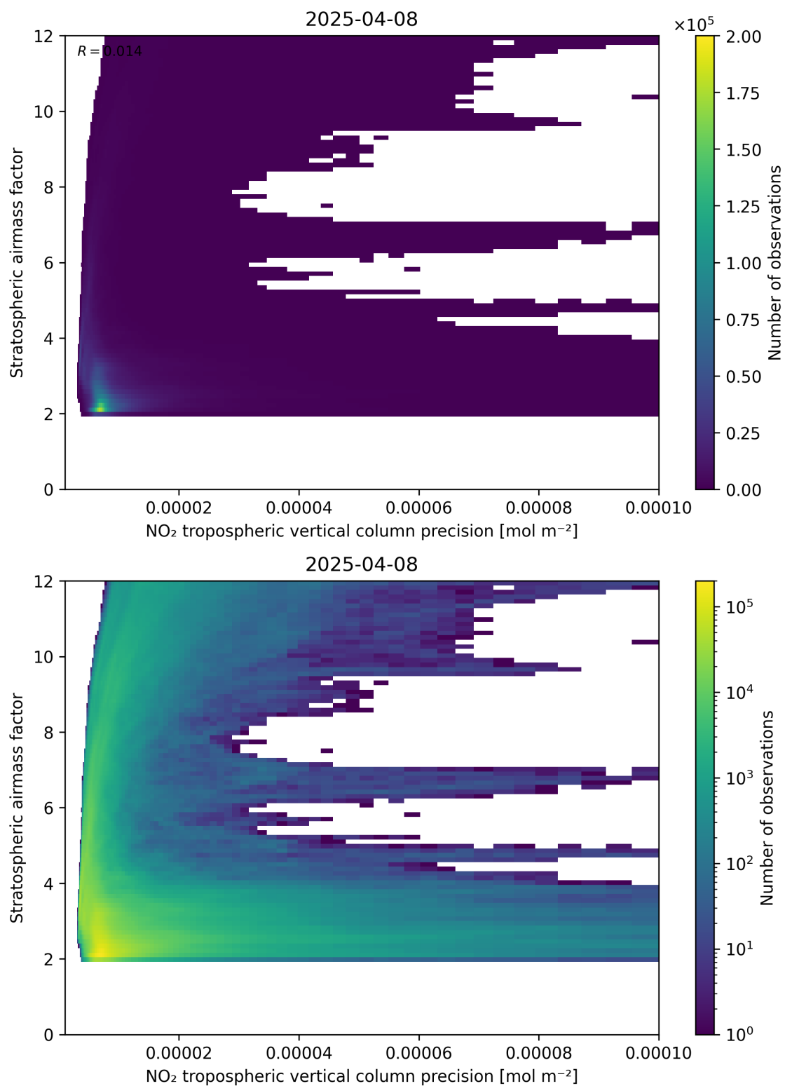
Figure 131: Scatter density plot of “NO 2 tropospheric vertical column precision” against “Stratospheric airmass factor” for 2025-04-08 to 2025-04-09.
