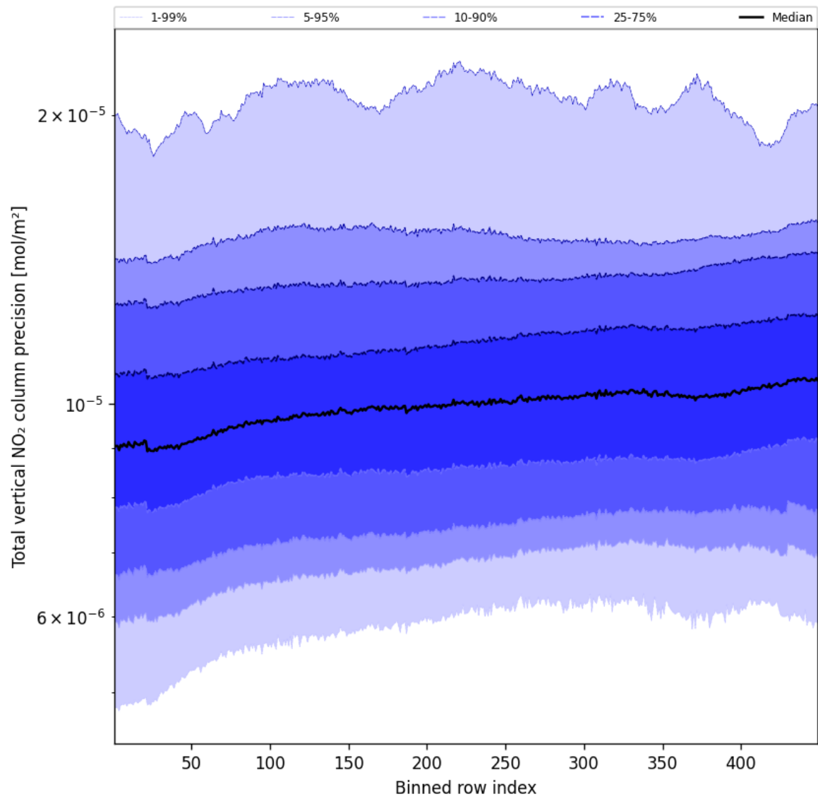
Figure 56: Along track statistics of “Total vertical NO 2 column precision” for 2025-04-08 to 2025-04-09
