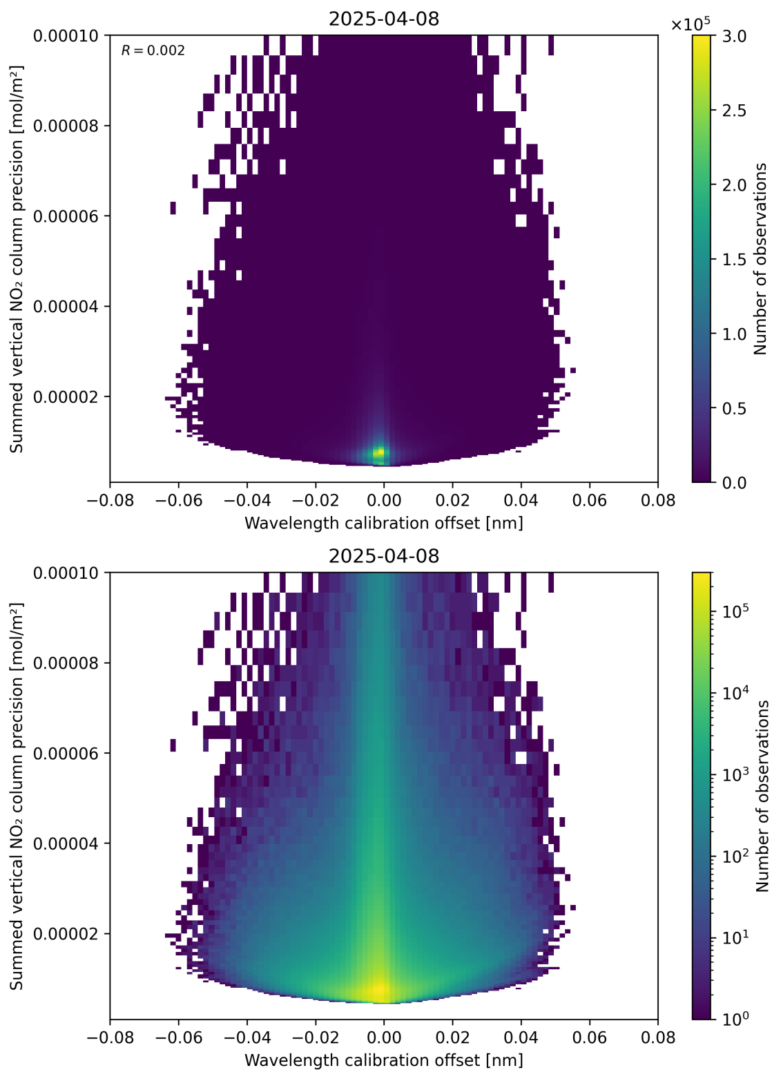
Figure 178: Scatter density plot of “Wavelength calibration offset” against “Summed vertical NO 2 column precision” for 2025-04-08 to 2025-04-09.
