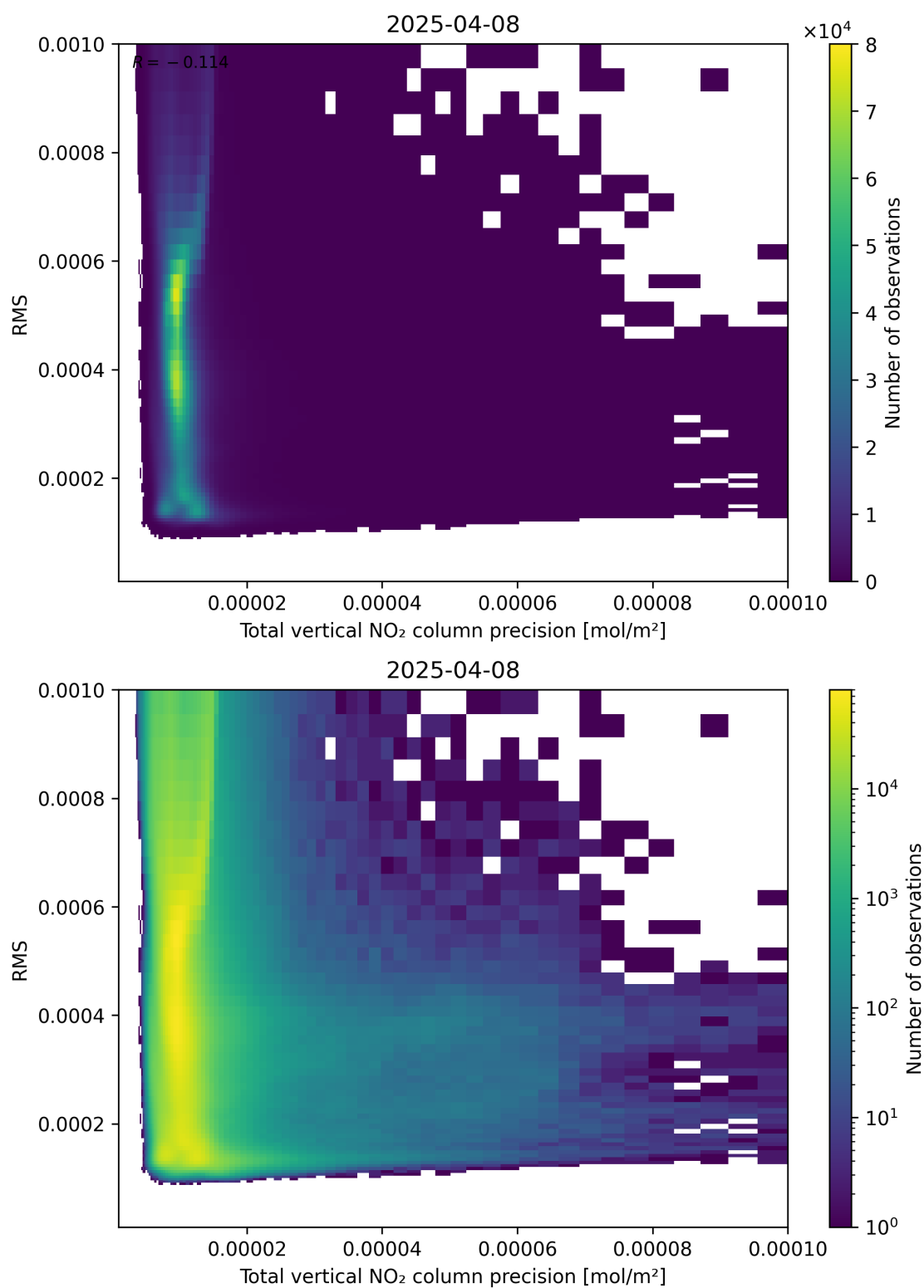
Figure 119: Scatter density plot of “Total vertical NO 2 column precision” against “RMS” for 2025-04-08 to 2025-04-09.
