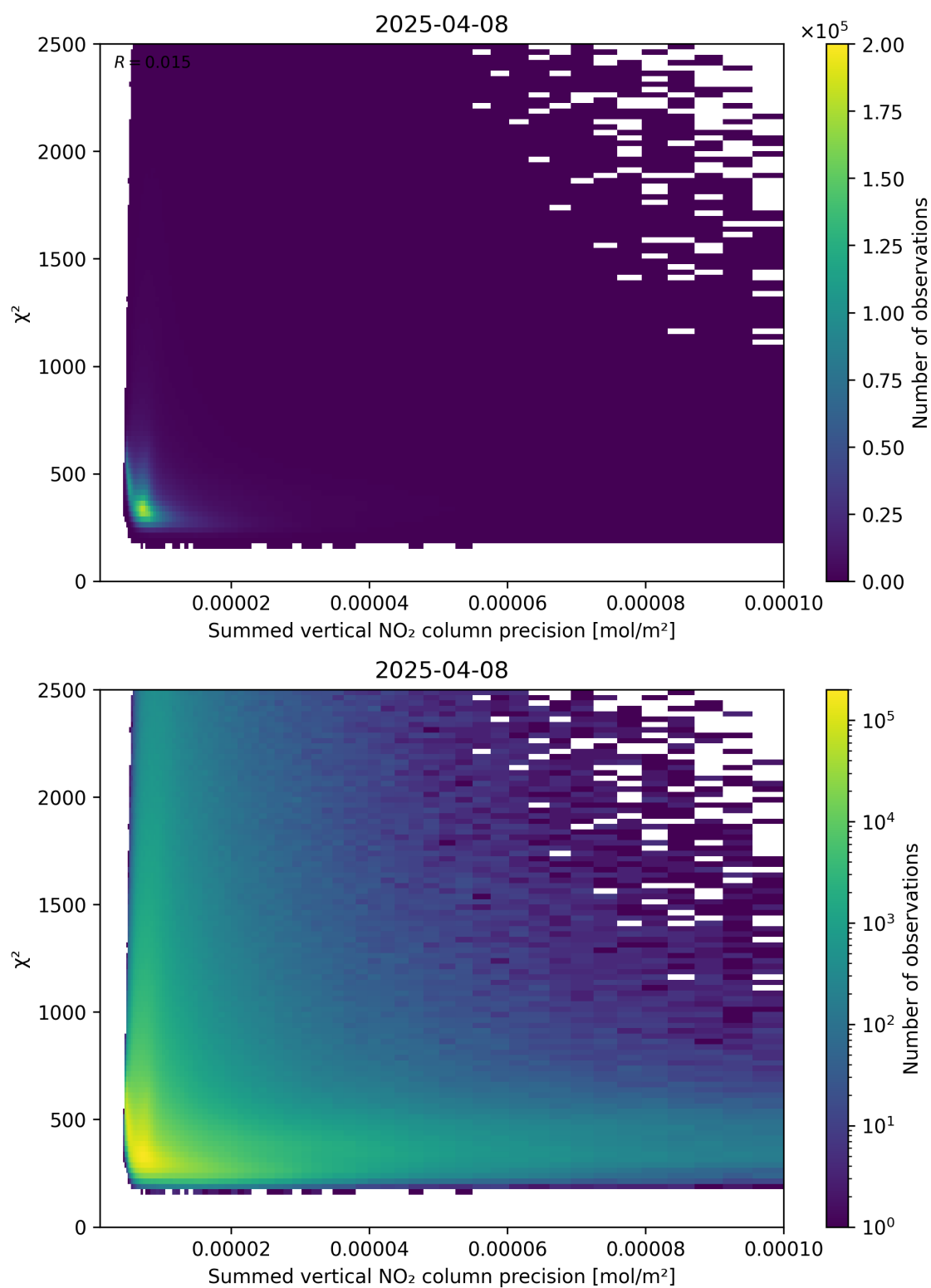
Figure 107: Scatter density plot of “Summed vertical NO 2 column precision” against “ \chi^2 ” for 2025-04-08 to 2025-04-09.
