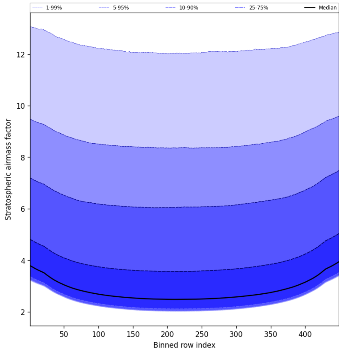
Figure 61: Along track statistics of “Stratospheric airmass factor” for 2025-04-08 to 2025-04-09
