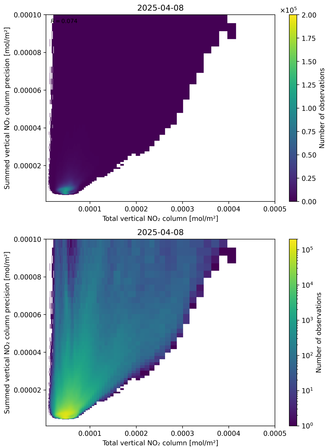
Figure 113: Scatter density plot of “Total vertical NO 2 column” against “Summed vertical NO 2 column precision” for 2025-04-08 to 2025-04-09.
