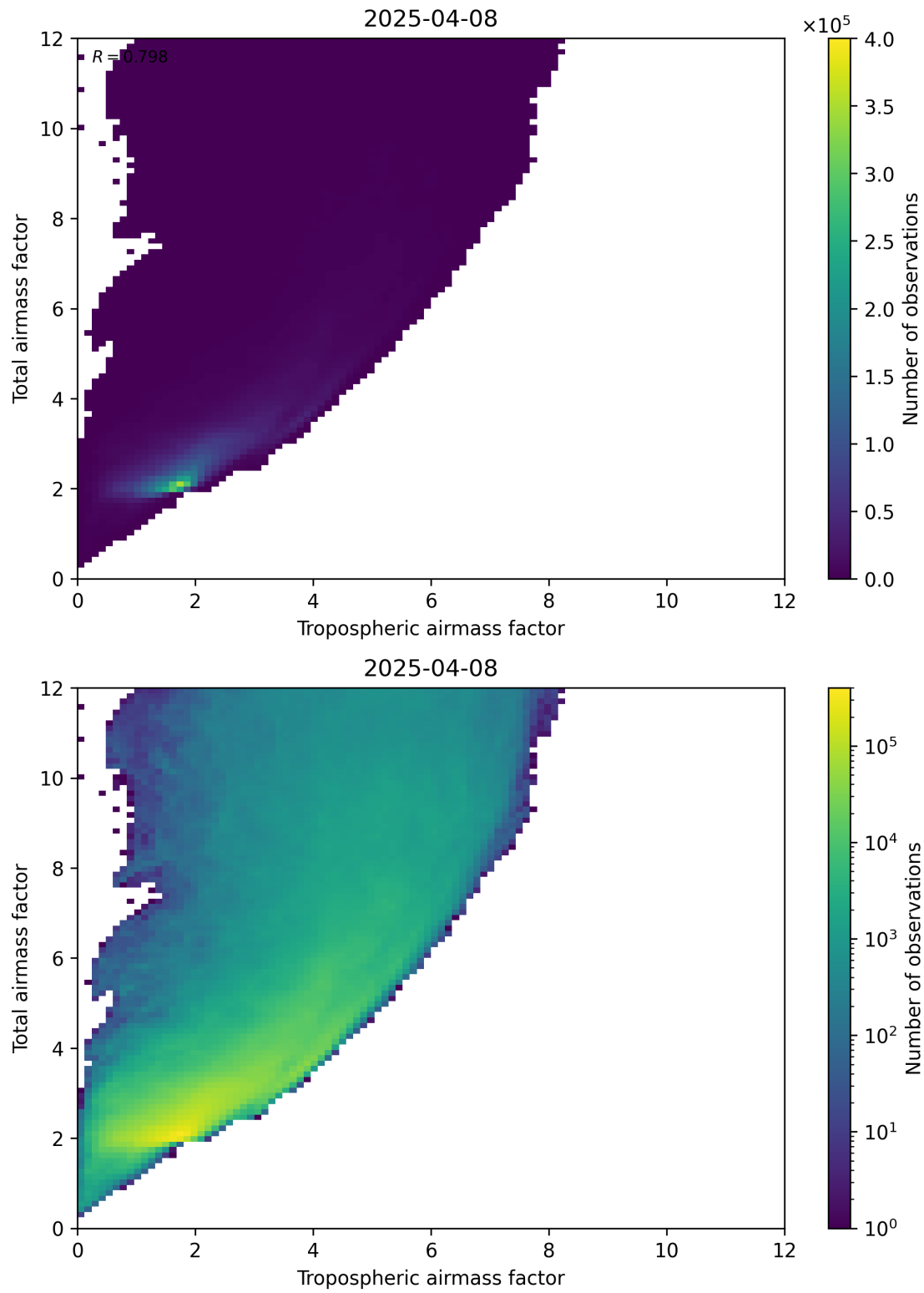
Figure 72: Scatter density plot of “Tropospheric airmass factor” against “Total airmass factor” for 2025-04-08 to 2025-04-09.
