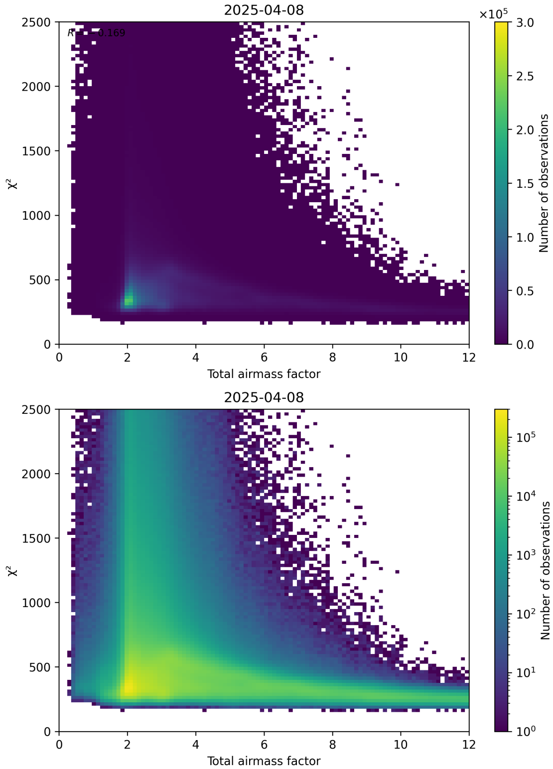
Figure 63: Scatter density plot of “Total airmass factor” against “ \chi^2 ” for 2025-04-08 to 2025-04-09.
