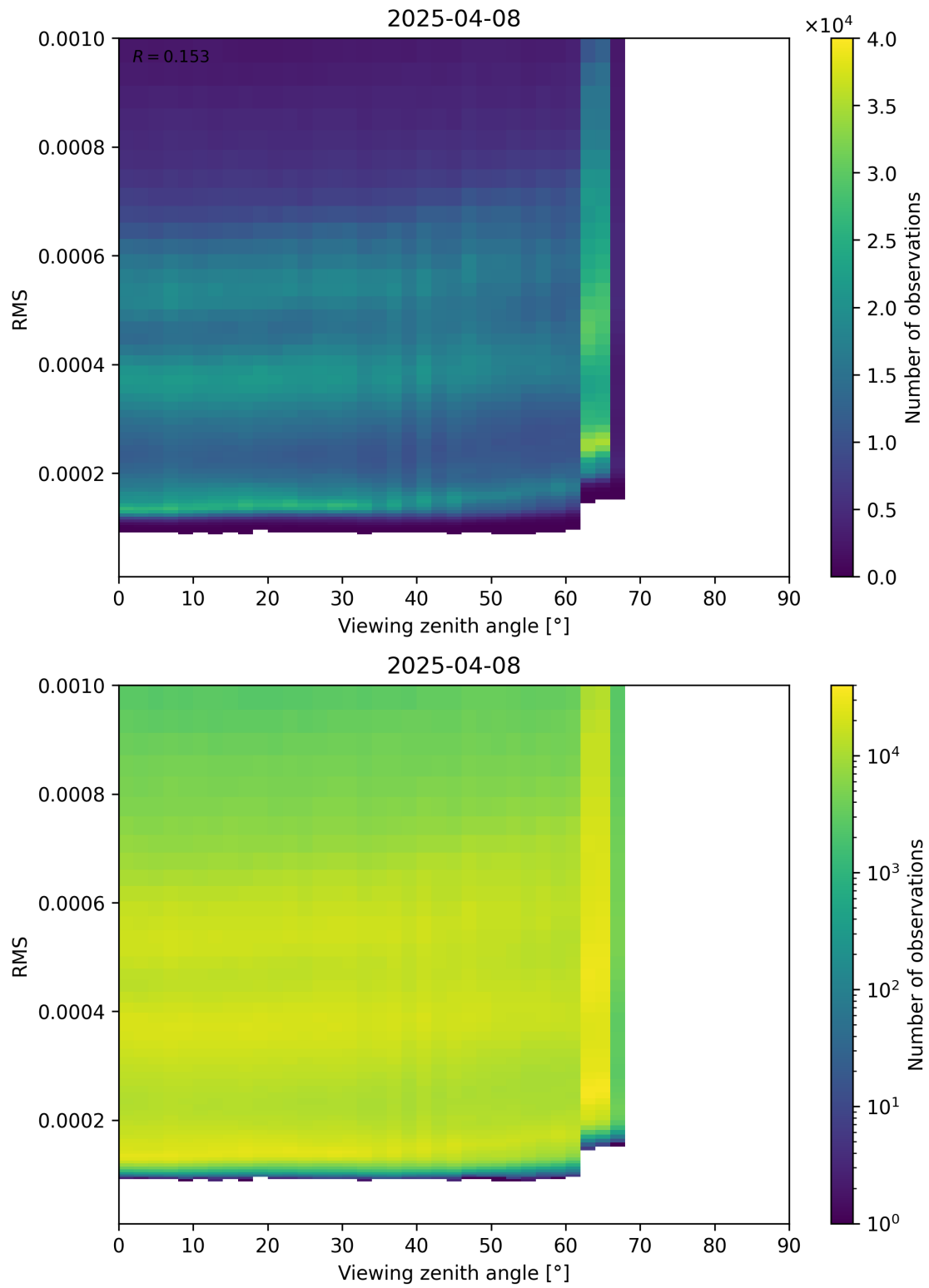
Figure 171: Scatter density plot of “Viewing zenith angle” against “RMS” for 2025-04-08 to 2025-04-09.
