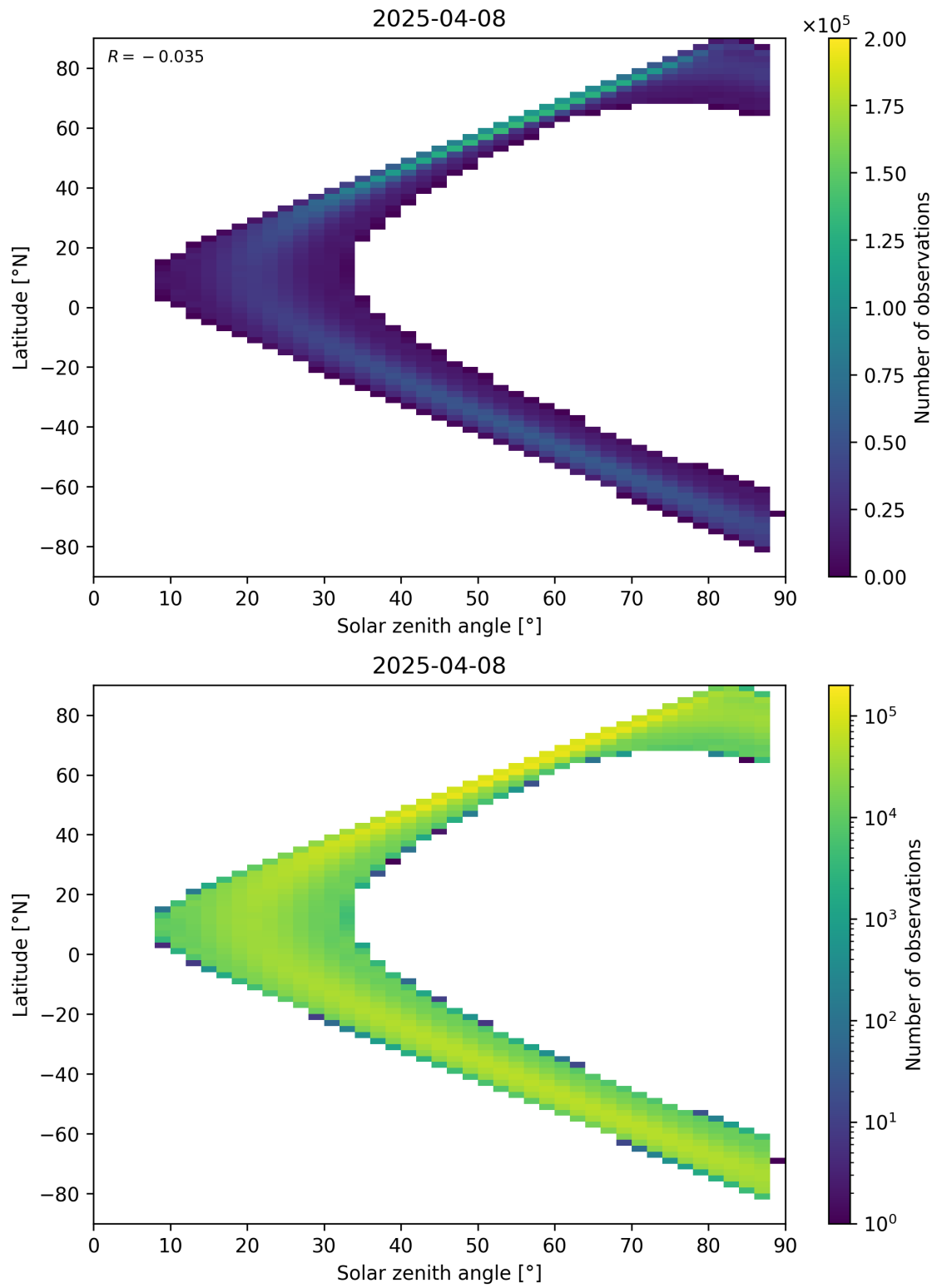
Figure 149: Scatter density plot of “Solar zenith angle” against “Latitude” for 2025-04-08 to 2025-04-09.
