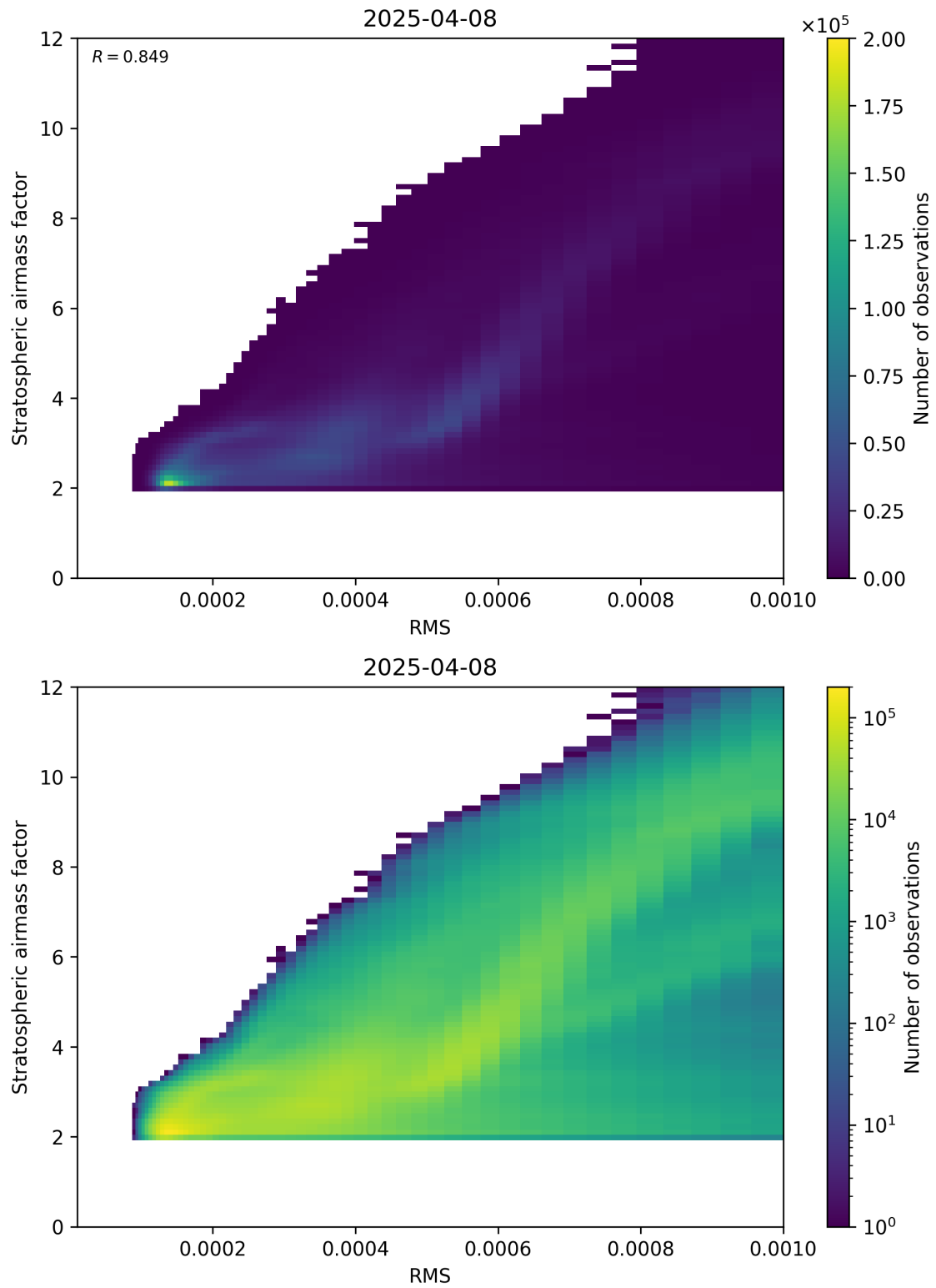
Figure 144: Scatter density plot of “RMS” against “Stratospheric airmass factor” for 2025-04-08 to 2025-04-09.
