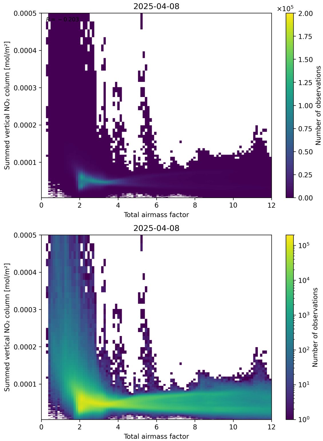
Figure 65: Scatter density plot of “Total airmass factor” against “Summed vertical NO 2 column” for 2025-04-08 to 2025-04-09.
