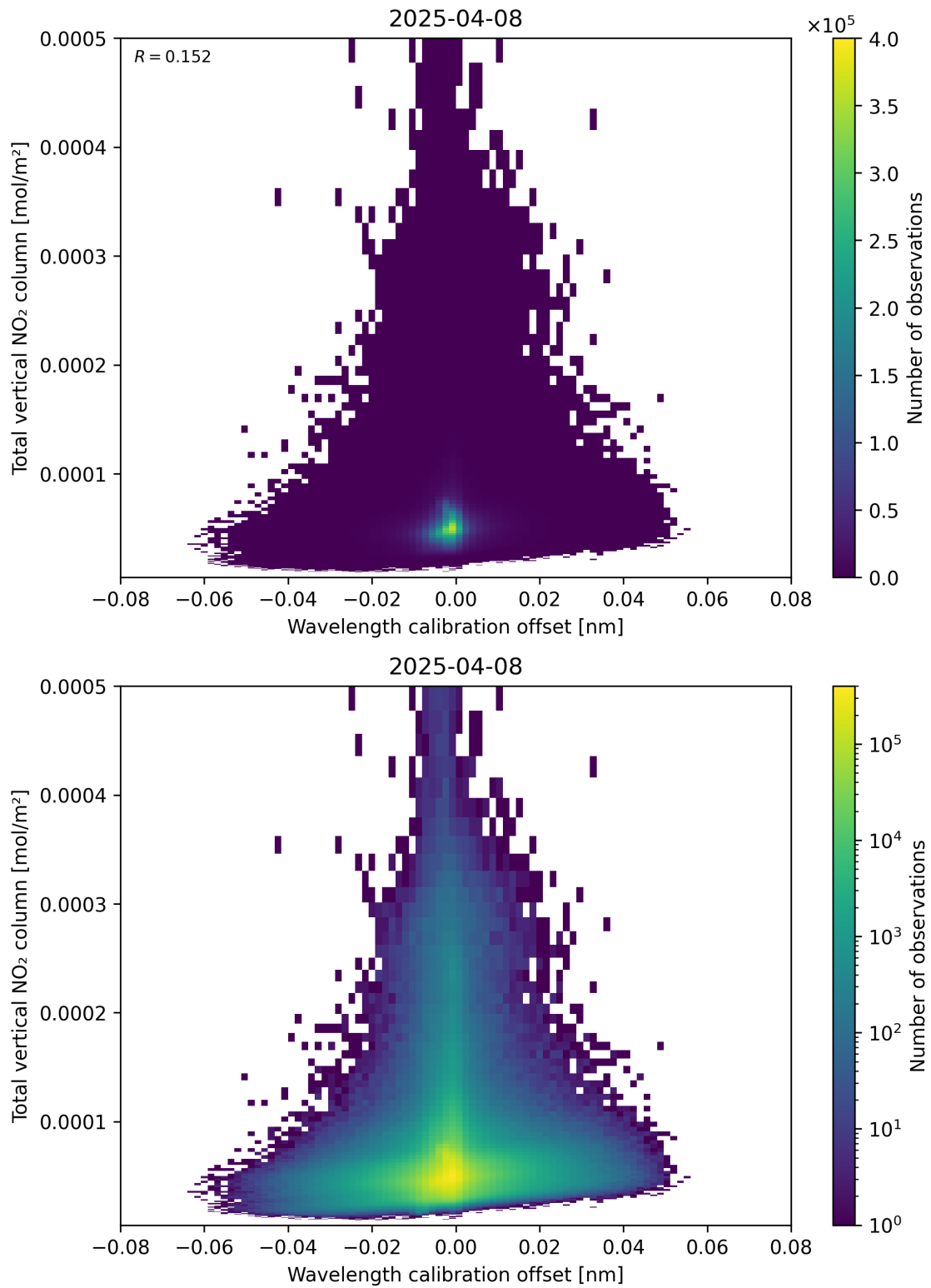
Figure 179: Scatter density plot of “Wavelength calibration offset” against “Total vertical NO 2 column” for 2025-04-08 to 2025-04-09.
