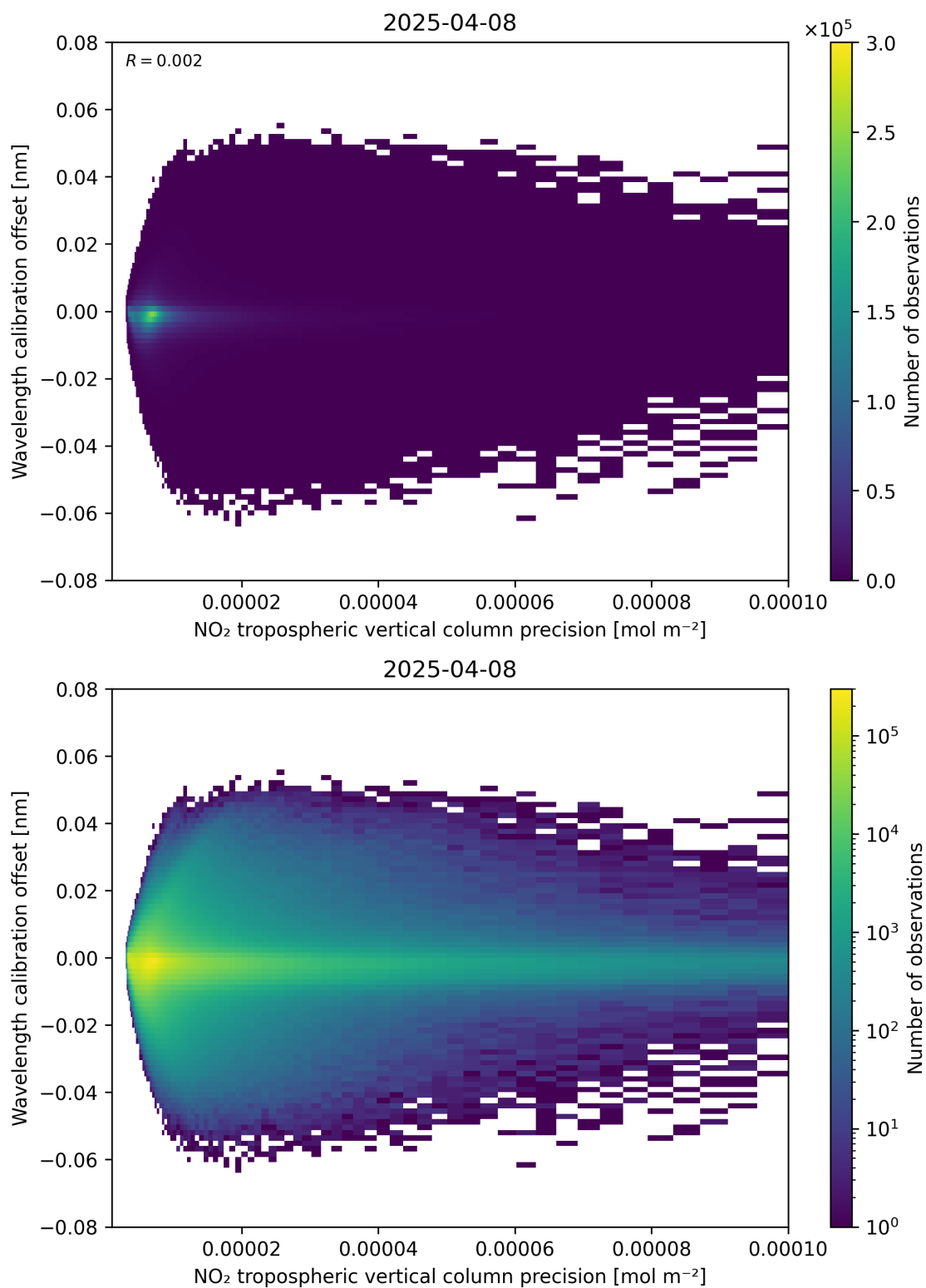
Figure 141: Scatter density plot of “NO 2 tropospheric vertical column precision” against “Wavelength calibration offset” for 2025-04-08 to 2025-04-09.
