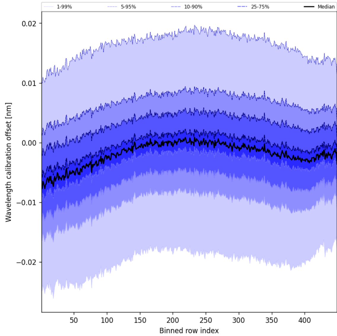
Figure 52: Along track statistics of “Wavelength calibration offset” for 2025-04-08 to 2025-04-09
