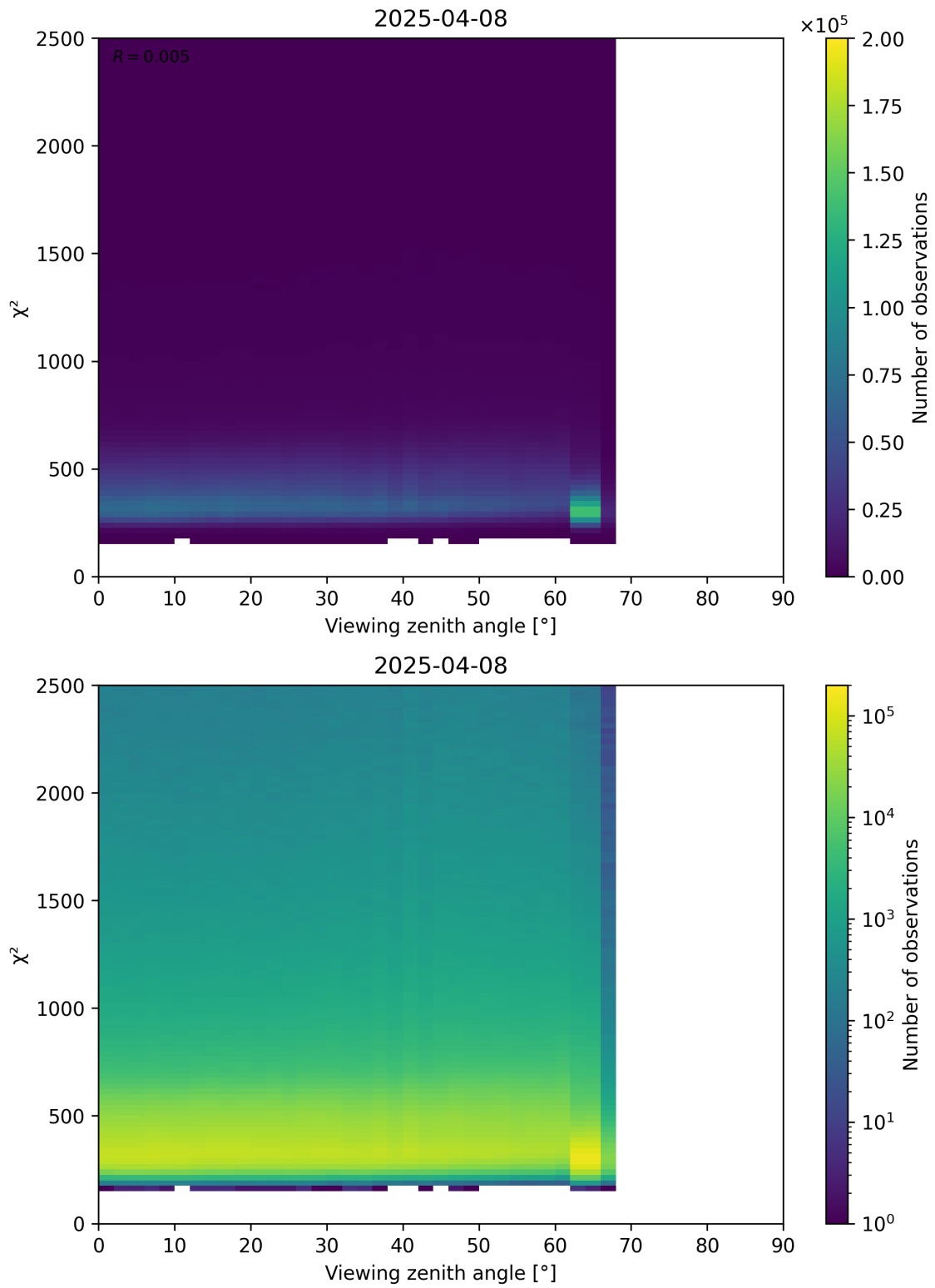
Figure 162: Scatter density plot of “Viewing zenith angle” against “ \chi^2 ” for 2025-04-08 to 2025-04-09.
