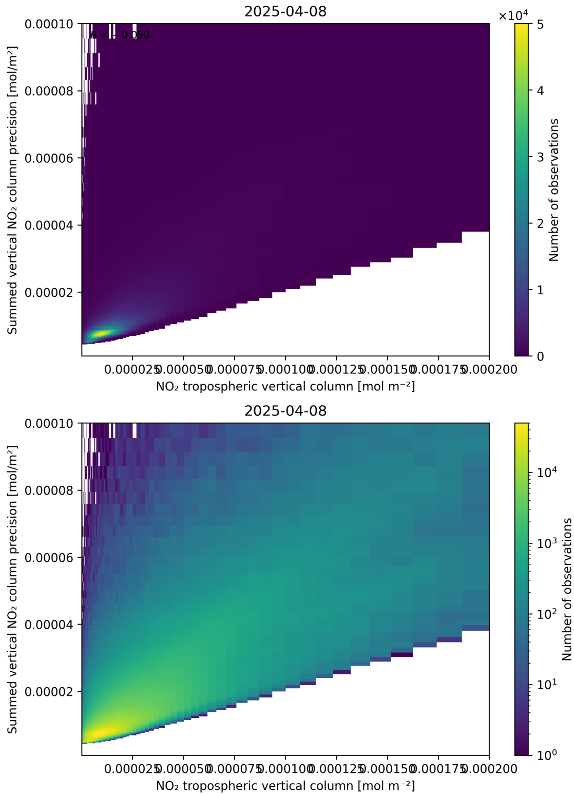
Figure 127: Scatter density plot of “NO 2 tropospheric vertical column” against “Summed vertical NO 2 column precision” for 2025-04-08 to 2025-04-09.
