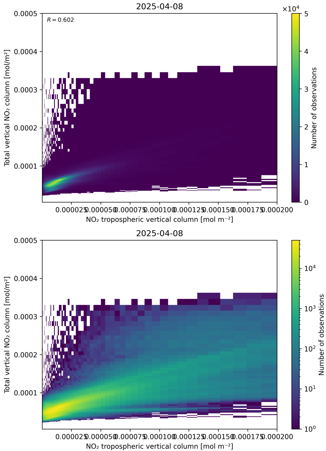
Figure 128: Scatter density plot of “NO 2 tropospheric vertical column” against “Total vertical NO 2 column” for 2025-04-08 to 2025-04-09.
