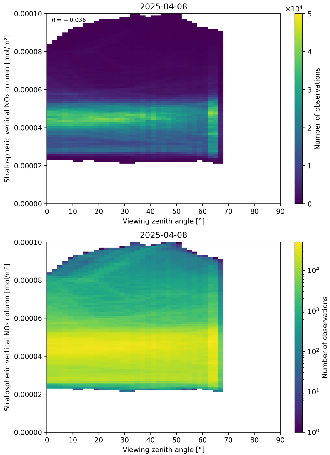
Figure 164: Scatter density plot of “Viewing zenith angle” against “Stratospheric vertical NO 2 column” for 2025-04-08 to 2025-04-09.
