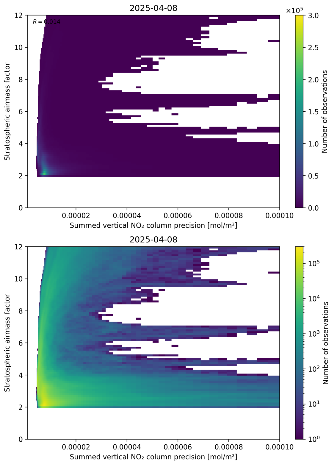
Figure 106: Scatter density plot of “Summed vertical NO 2 column precision” against “Stratospheric airmass factor” for 2025-04-08 to 2025-04-09.
