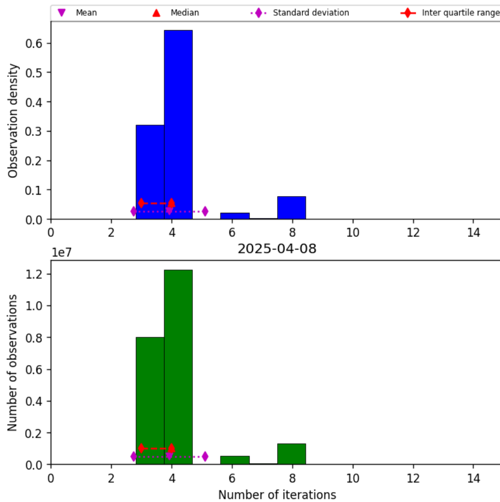
Figure 34: Histogram of “Number of iterations” for 2025-04-08 to 2025-04-09
