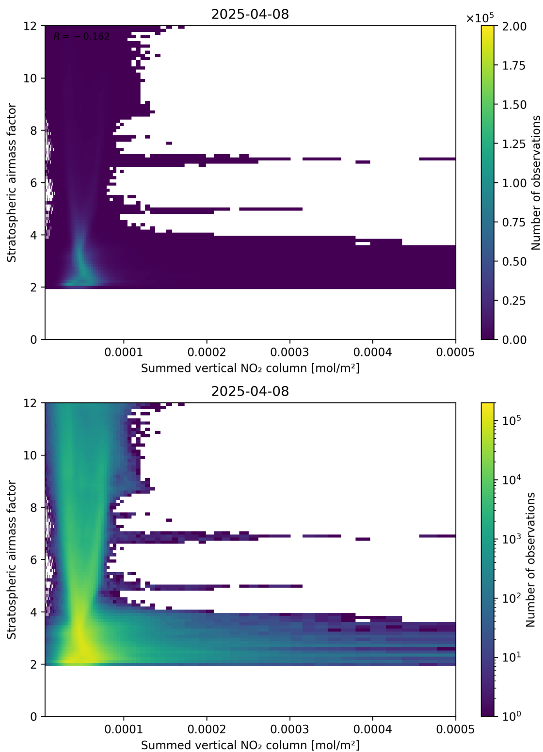
Figure 103: Scatter density plot of “Summed vertical NO 2 column” against “Stratospheric air mass factor” for 2025-04-08 to 2025-04-09.
