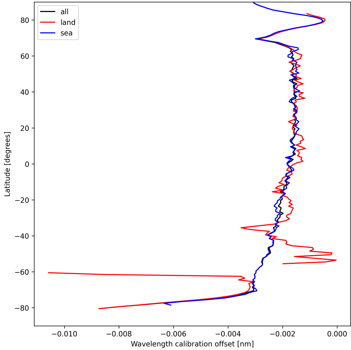
Figure 18: Zonal average of “Wavelength calibration offset” for 2025-04-08 to 2025-04-09.
