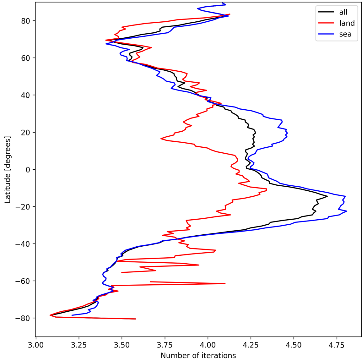
Figure 17: Zonal average of “Number of iterations” for 2025-04-08 to 2025-04-09.
