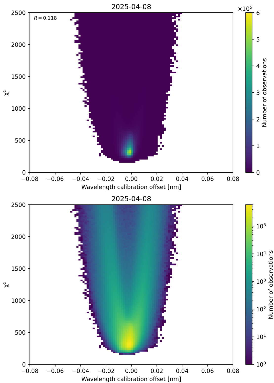
Figure 175: Scatter density plot of “Wavelength calibration offset” against “ \chi^2 ” for 2025-04-08 to 2025-04-09.
