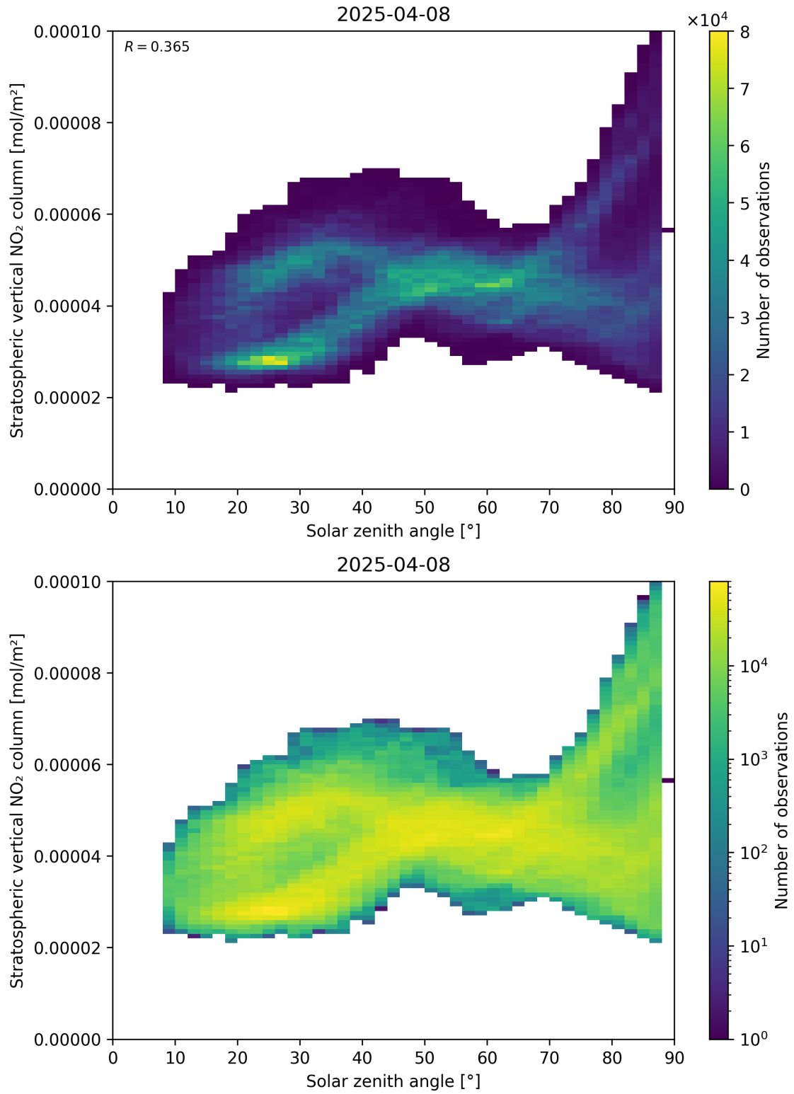
Figure 150: Scatter density plot of “Solar zenith angle” against “Stratospheric vertical NO 2 column” for 2025-04-08 to 2025-04-09.
