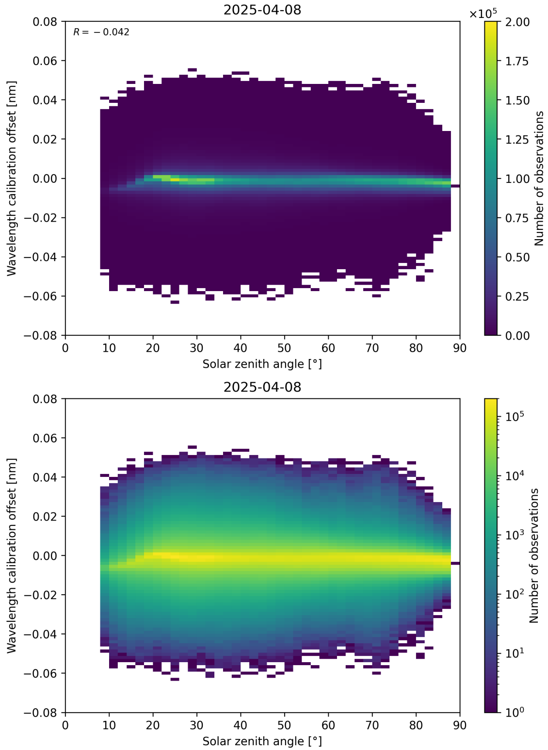
Figure 158: Scatter density plot of “Solar zenith angle” against “Wavelength calibration offset” for 2025-04-08 to 2025-04-09.
