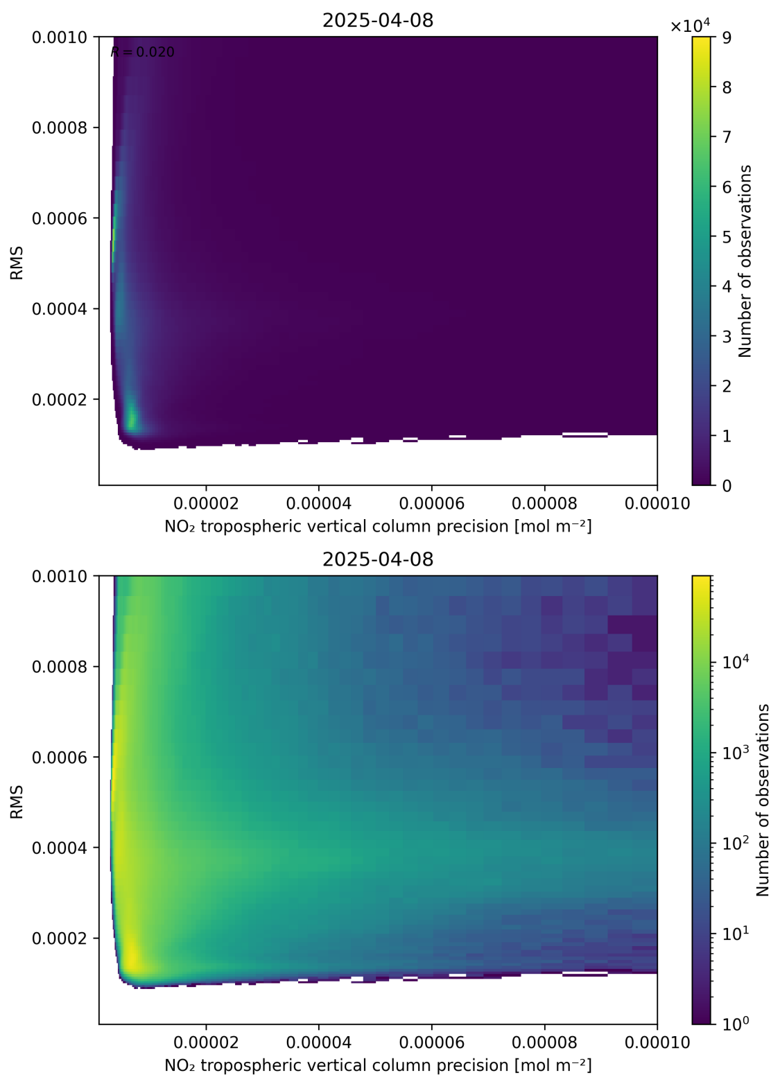
Figure 140: Scatter density plot of “NO 2 tropospheric vertical column precision” against “RMS” for 2025-04-08 to 2025-04-09.
