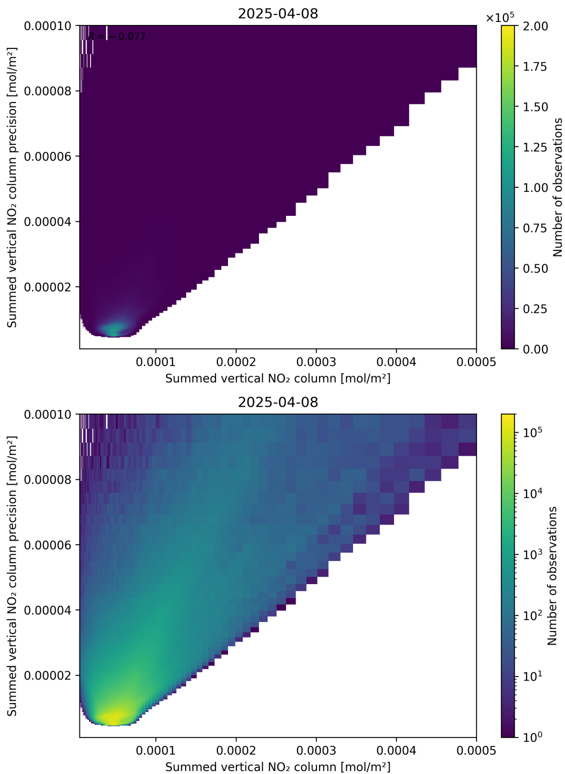
Figure 105: Scatter density plot of “Summed vertical NO 2 column” against “Summed vertical NO 2 column precision” for 2025-04-08 to 2025-04-09.
