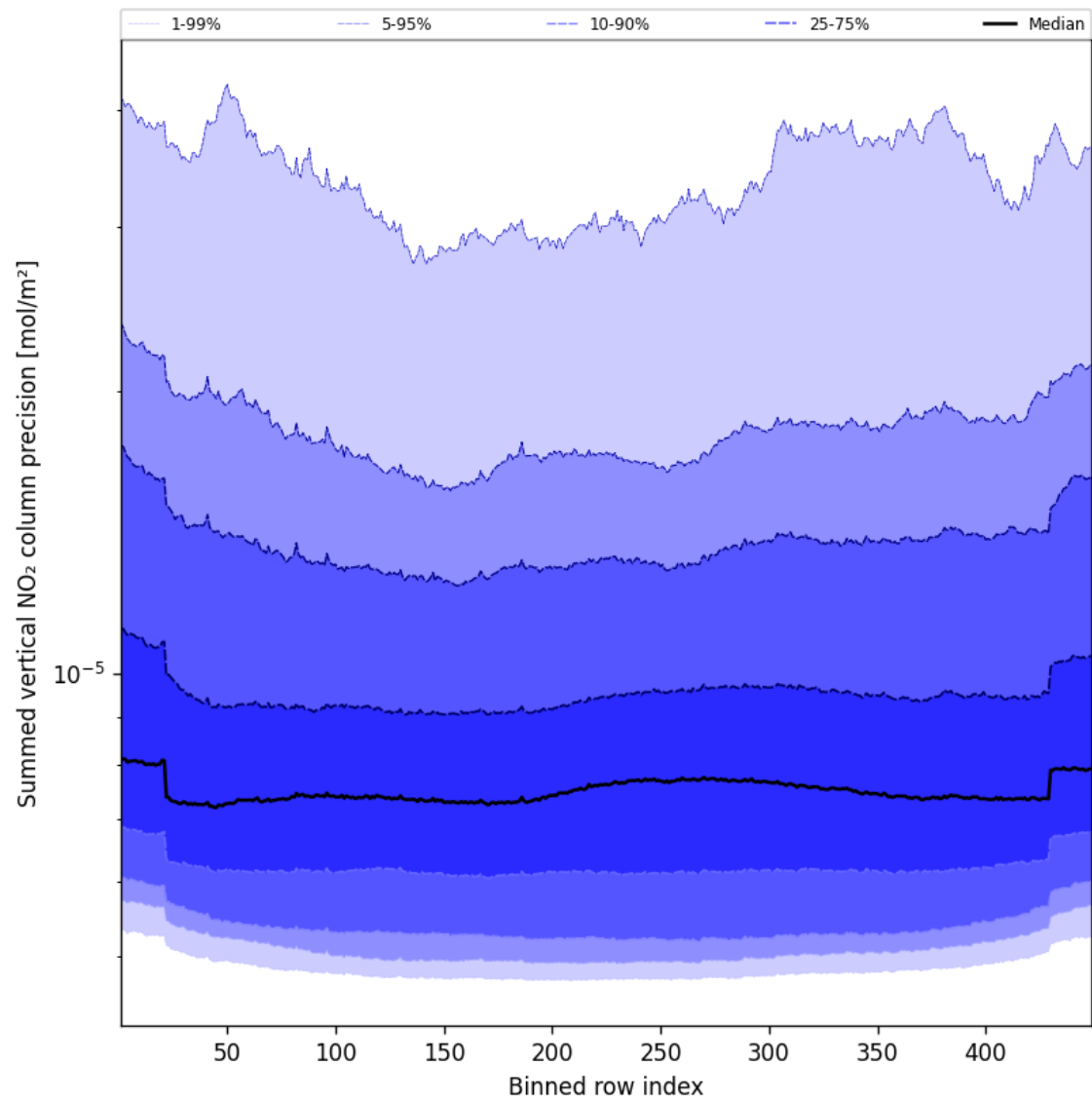
Figure 58: Along track statistics of “Summed vertical NO 2 column precision” for 2025-04-08 to 2025-04-09
