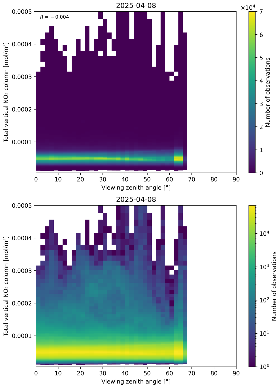
Figure 167: Scatter density plot of “Viewing zenith angle” against “Total vertical NO 2 column” for 2025-04-08 to 2025-04-09.
