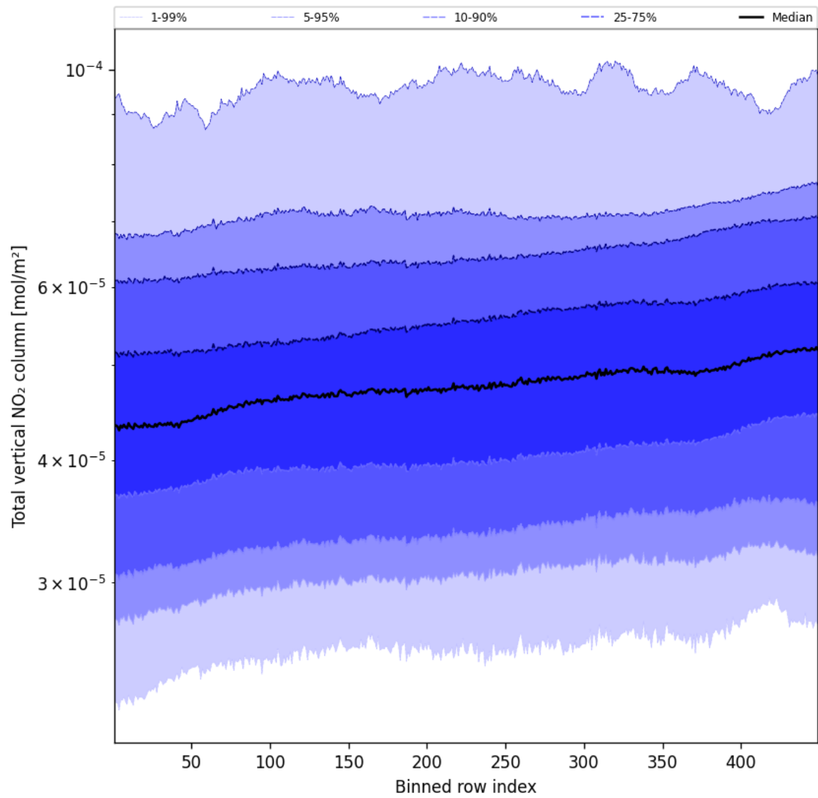
Figure 55: Along track statistics of “Total vertical NO 2 column” for 2025-04-08 to 2025-04-09
