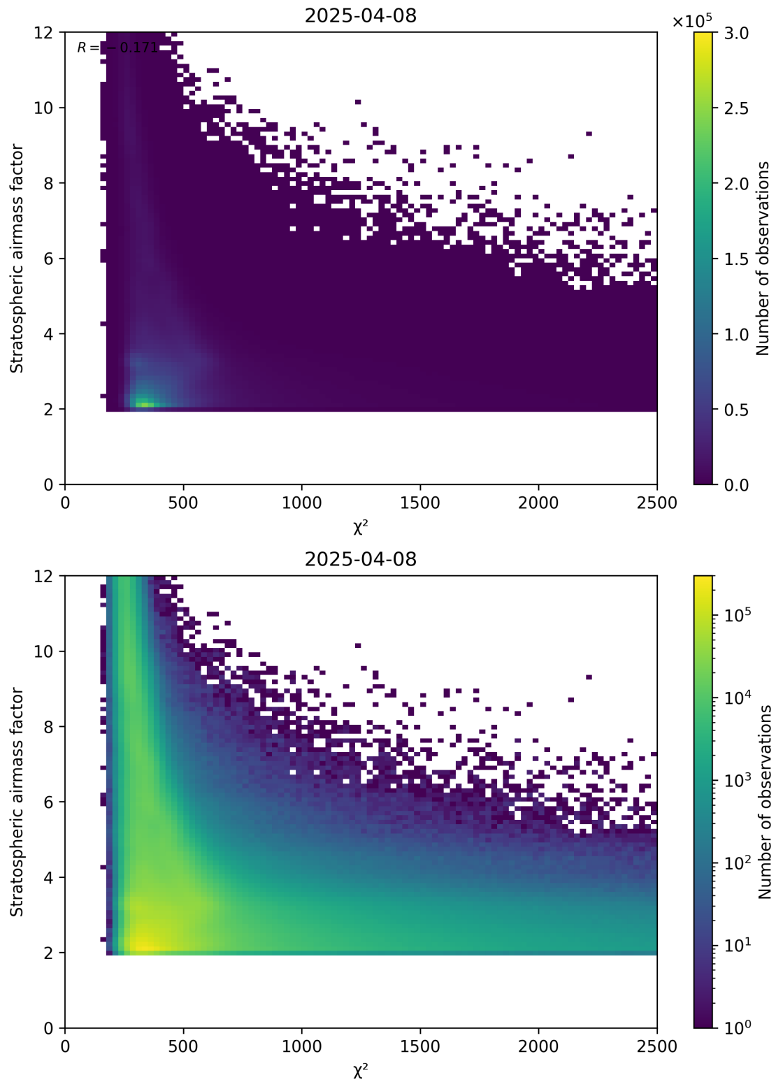
Figure 81: Scatter density plot of “ \chi^2 ” against “Stratospheric airmass factor” for 2025-04-08 to 2025-04-09.
