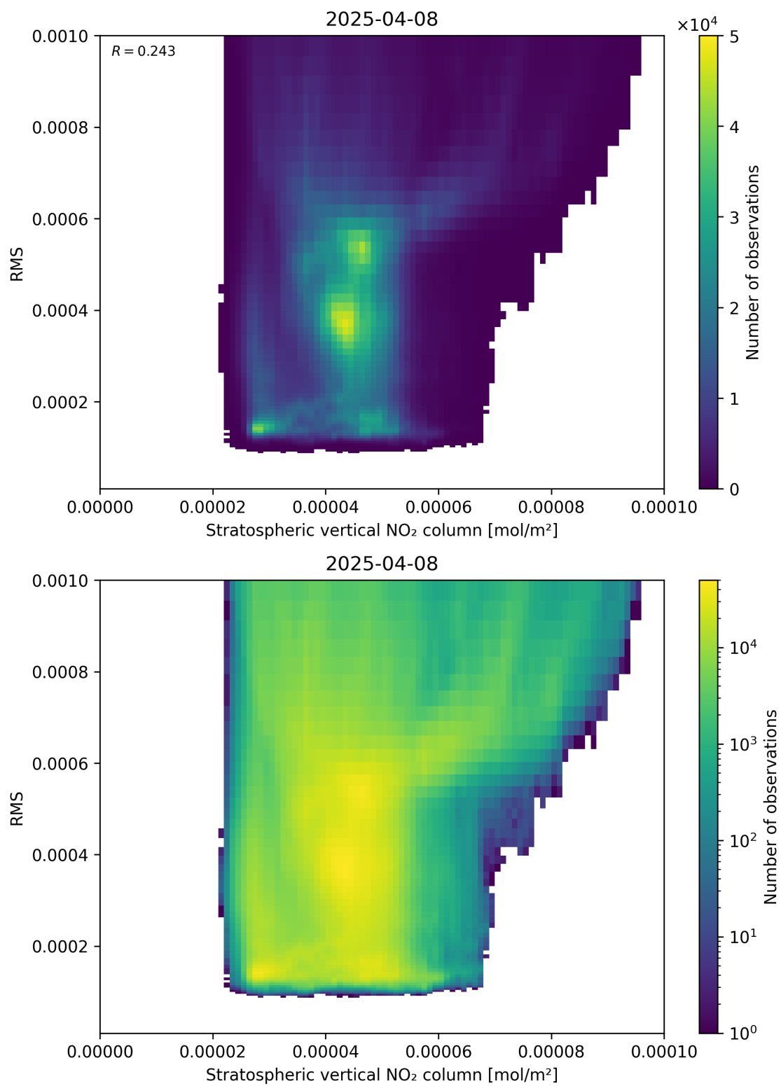
Figure 102: Scatter density plot of “Stratospheric vertical NO 2 column” against “RMS” for 2025-04-08 to 2025-04-09.
