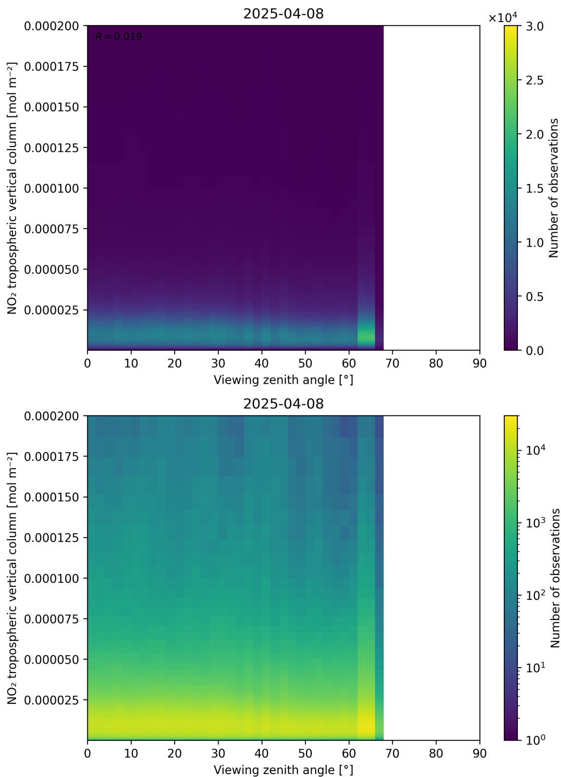
Figure 169: Scatter density plot of “Viewing zenith angle” against “NO 2 tropospheric vertical column” for 2025-04-08 to 2025-04-09.
