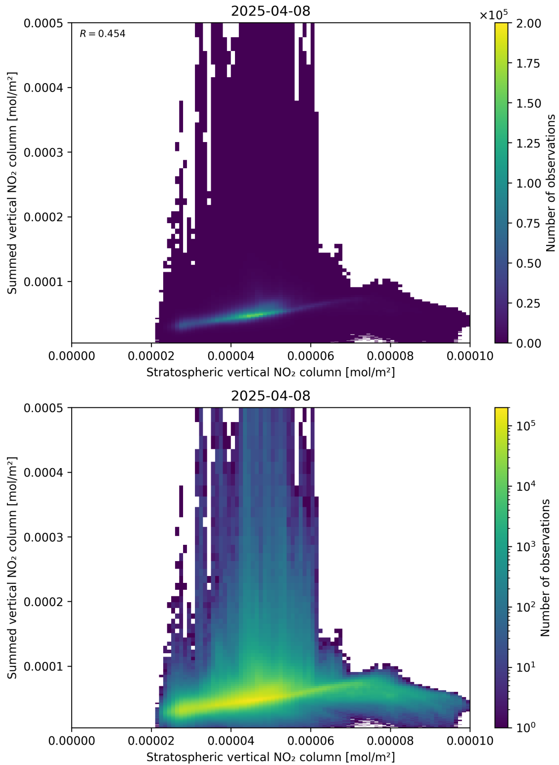
Figure 98: Scatter density plot of “Stratospheric vertical NO 2 column” against “Summed vertical NO 2 column” for 2025-04-08 to 2025-04-09.
