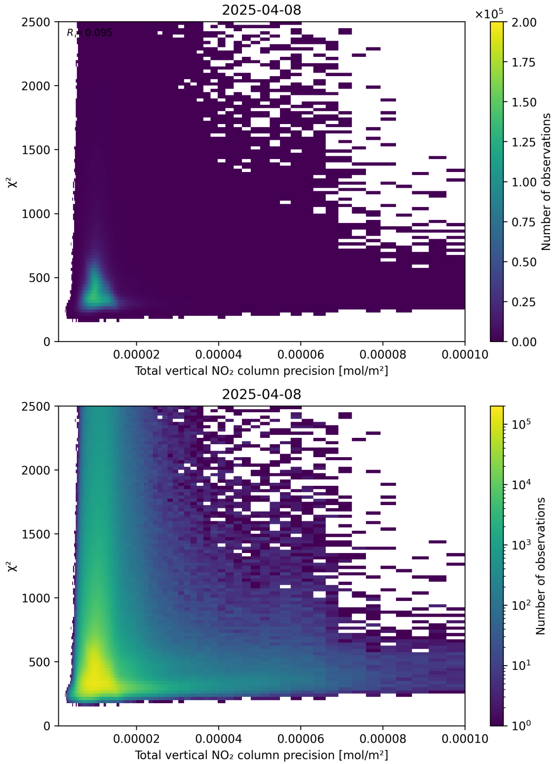
Figure 116: Scatter density plot of “Total vertical NO 2 column precision” against “ \chi^2 ” for 2025-04-08 to 2025-04-09.
