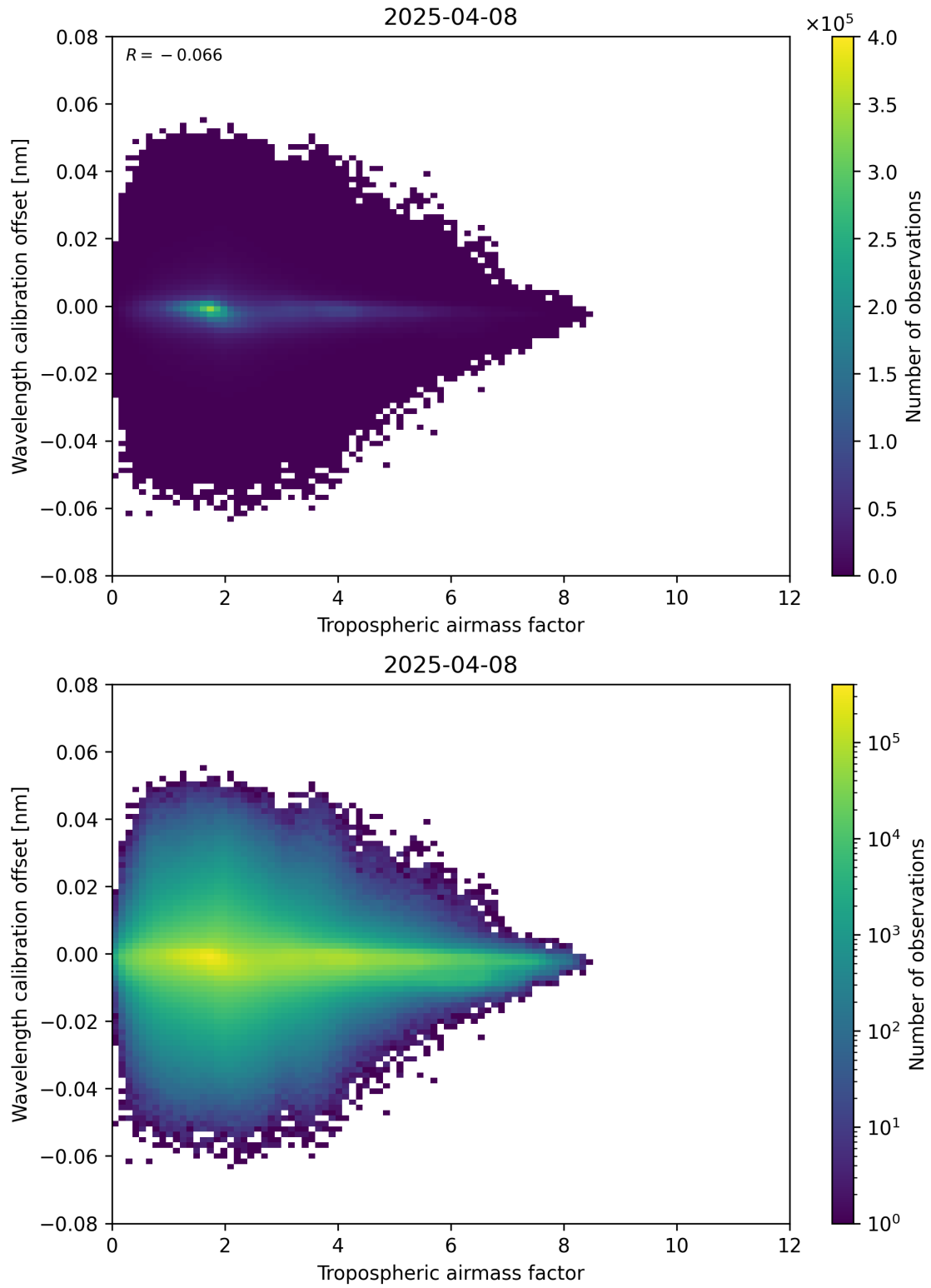
Figure 80: Scatter density plot of “Tropospheric airmass factor” against “Wavelength calibration offset” for 2025-04-08 to 2025-04-09.
