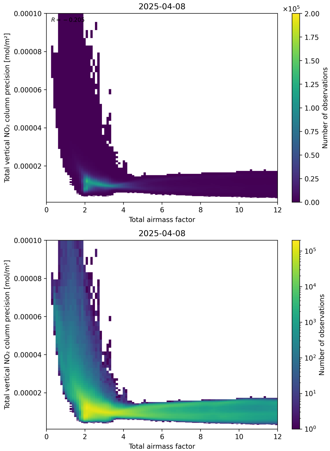
Figure 68: Scatter density plot of “Total airmass factor” against “Total vertical NO 2 column precision” for 2025-04-08 to 2025-04-09.
