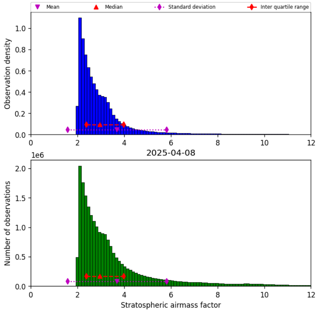
Figure 44: Histogram of “Stratospheric airmass factor” for 2025-04-08 to 2025-04-09
