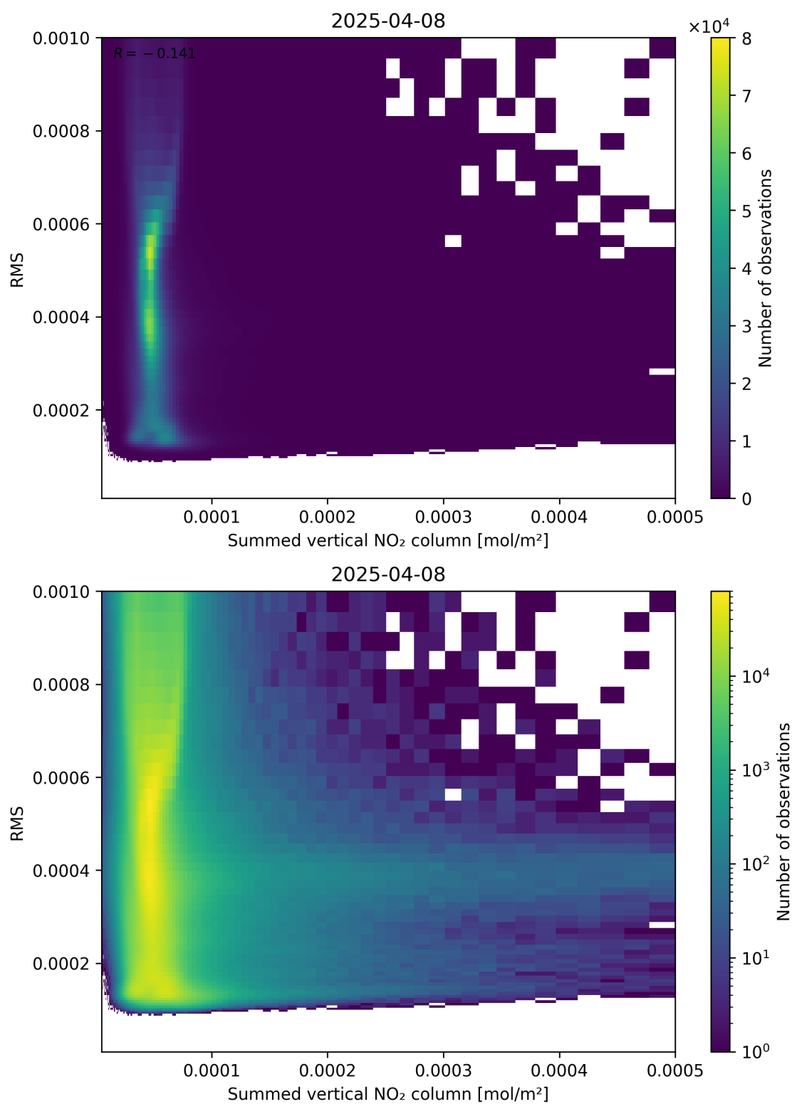
Figure 109: Scatter density plot of “Summed vertical NO 2 column” against “RMS” for 2025-04-08 to 2025-04-09.
