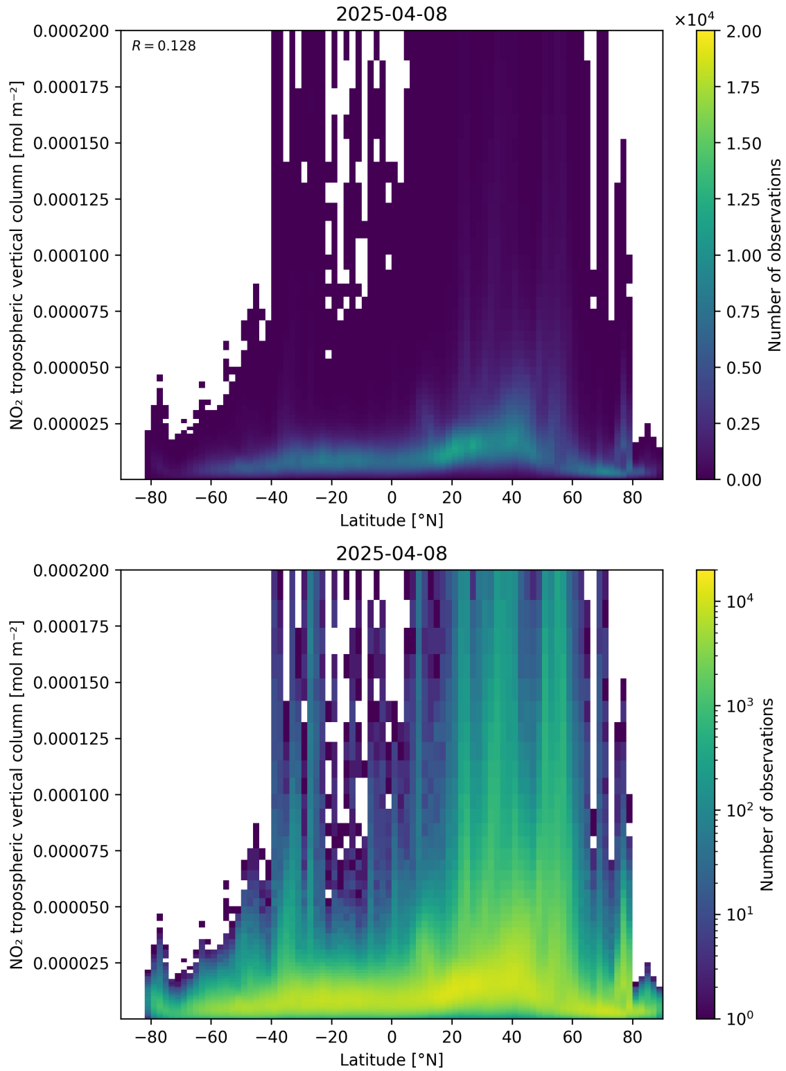
Figure 92: Scatter density plot of “Latitude” against “NO 2 tropospheric vertical column” for 2025-04-08 to 2025-04-09.
