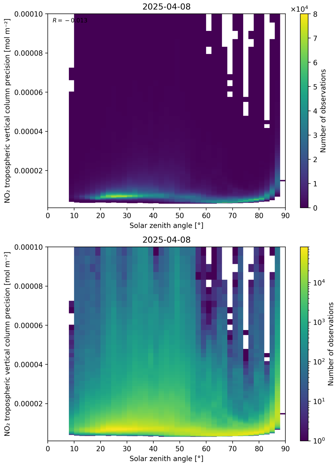
Figure 156: Scatter density plot of “Solar zenith angle” against “NO 2 tropospheric vertical column precision” for 2025-04-08 to 2025-04-09.
