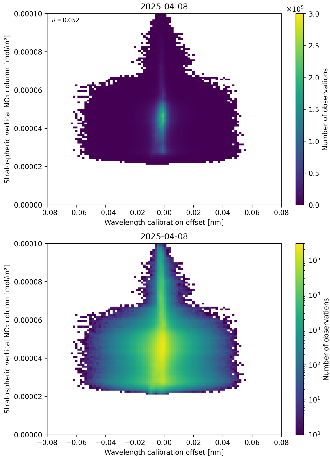
Figure 176: Scatter density plot of “Wavelength calibration offset” against “Stratospheric vertical NO 2 column” for 2025-04-08 to 2025-04-09.
