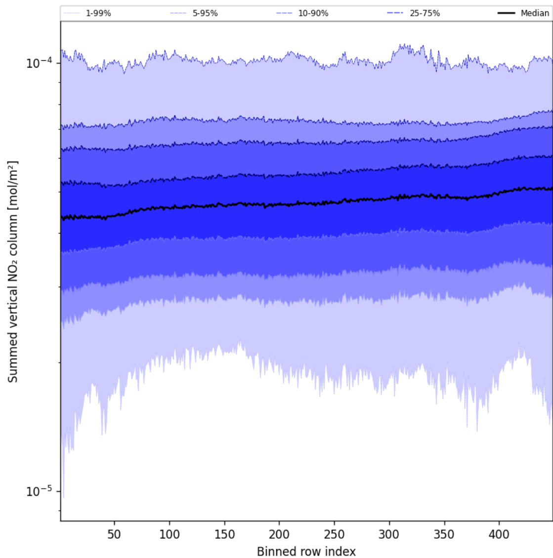
Figure 57: Along track statistics of “Summed vertical NO 2 column” for 2025-04-08 to 2025-04-09
