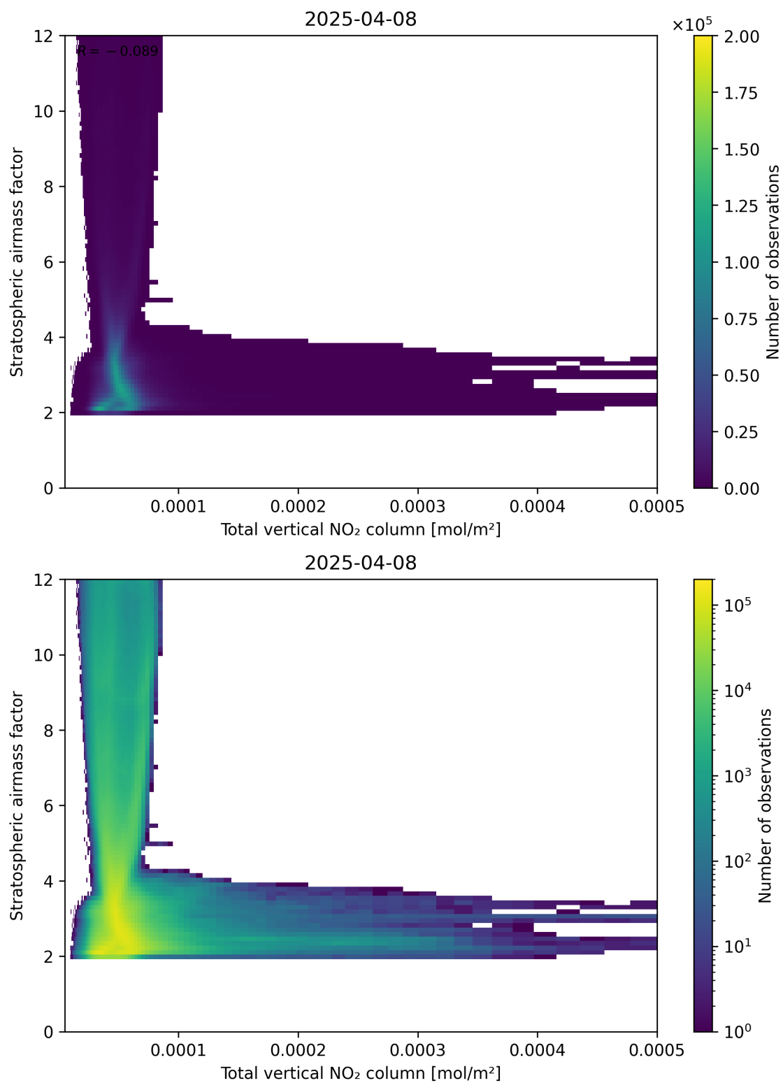
Figure 110: Scatter density plot of “Total vertical NO 2 column” against “Stratospheric airmass factor” for 2025-04-08 to 2025-04-09.
