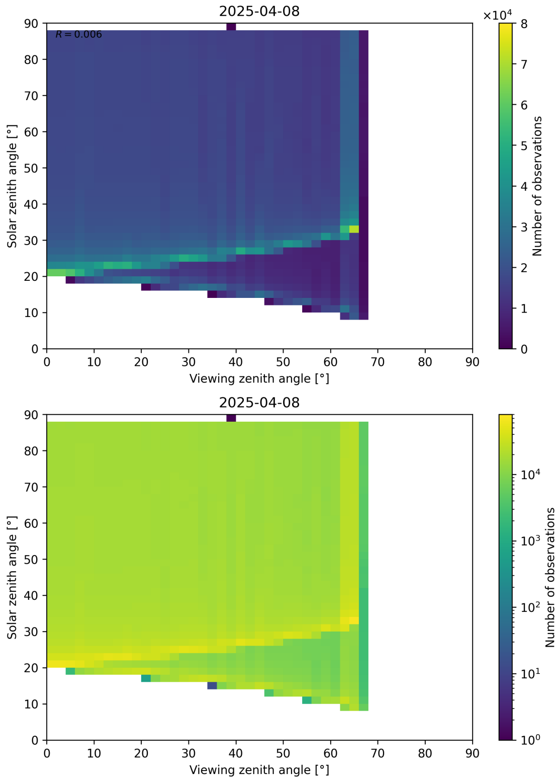
Figure 172: Scatter density plot of “Viewing zenith angle” against “Solar zenith angle” for 2025-04-08 to 2025-04-09.
