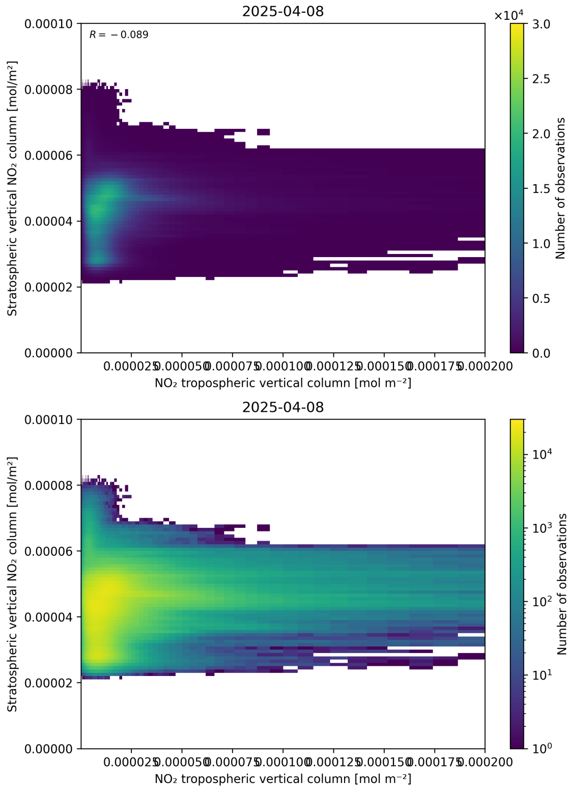
Figure 125: Scatter density plot of “NO 2 tropospheric vertical column” against “Stratospheric vertical NO 2 column” for 2025-04-08 to 2025-04-09.
