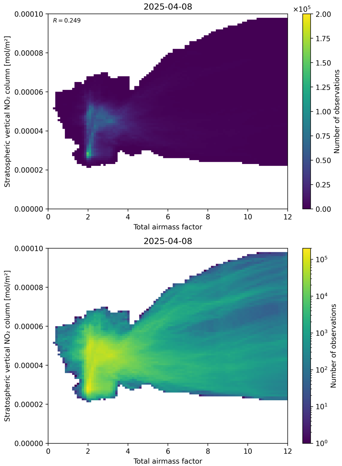
Figure 64: Scatter density plot of “Total airmass factor” against “Stratospheric vertical NO 2 column” for 2025-04-08 to 2025-04-09.
