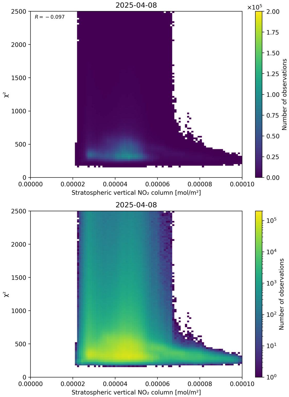
Figure 97: Scatter density plot of “Stratospheric vertical NO 2 column” against “ \chi^2 ” for 2025-04-08 to 2025-04-09.
