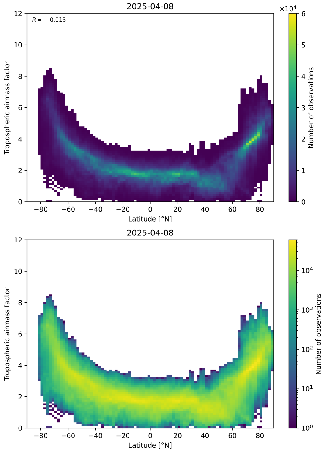
Figure 85: Scatter density plot of “Latitude” against “Tropospheric air mass factor” for 2025-04-08 to 2025-04-09.
