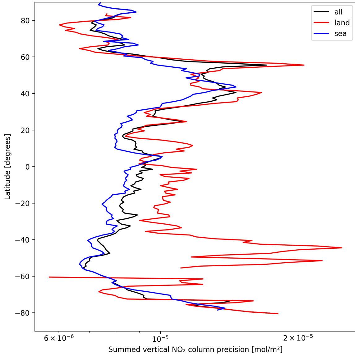
Figure 24: Zonal average of “Summed vertical NO 2 column precision” for 2025-04-08 to 2025-04-09.
