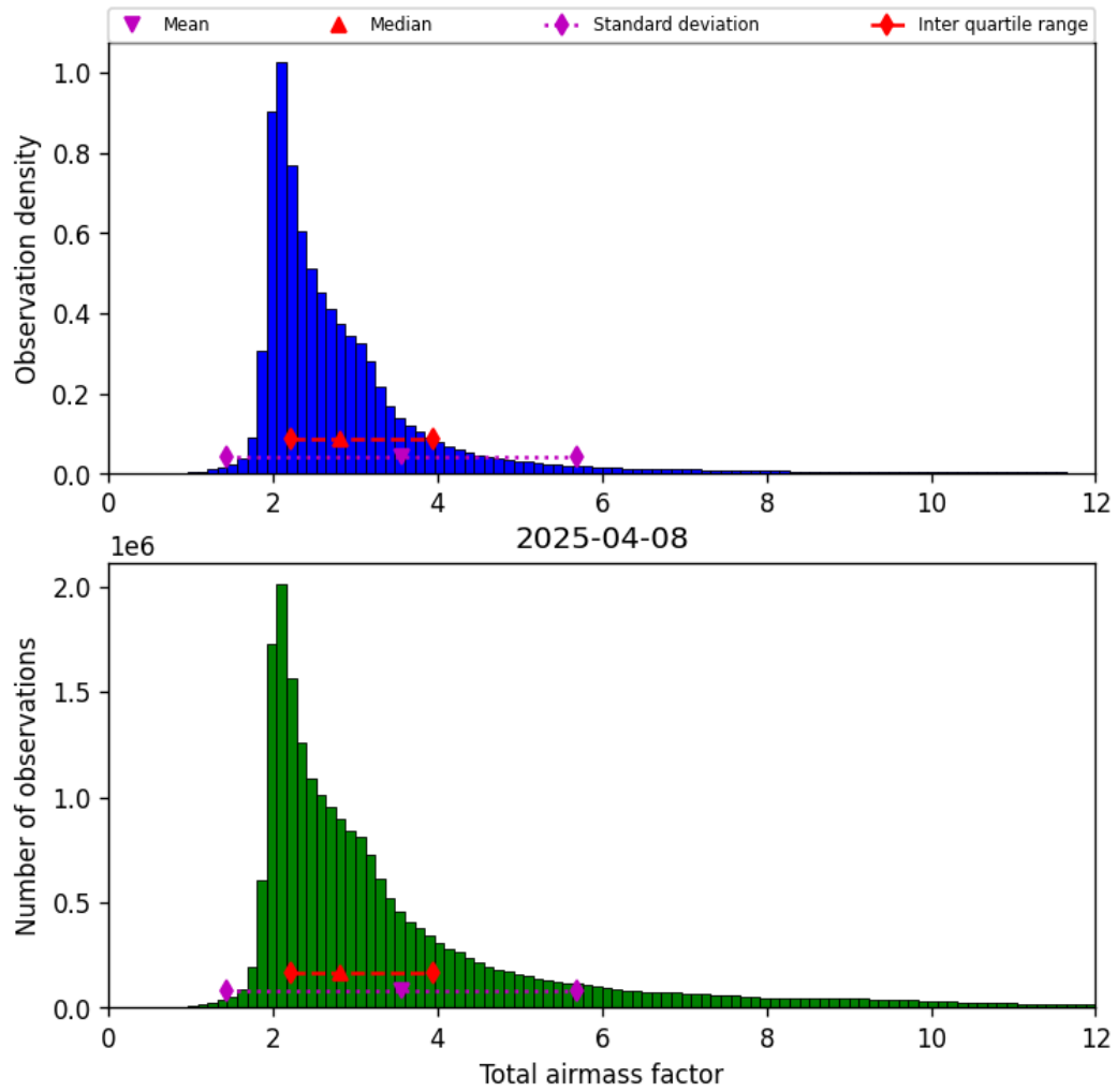
Figure 32: Histogram of “Total airmass factor” for 2025-04-08 to 2025-04-09
