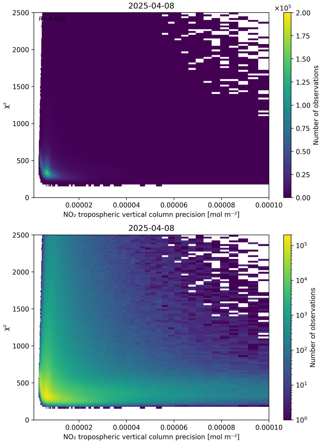
Figure 134: Scatter density plot of “NO 2 tropospheric vertical column precision” against “ \chi^2 ” for 2025-04-08 to 2025-04-09.
