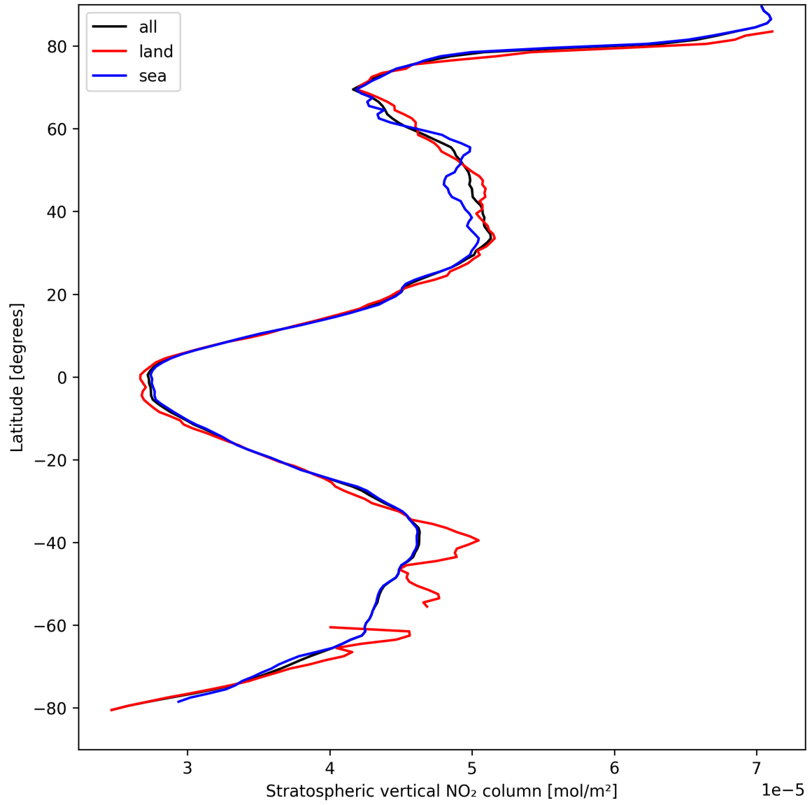
Figure 19: Zonal average of “Stratospheric vertical NO 2 column” for 2025-04-08 to 2025-04-09.
