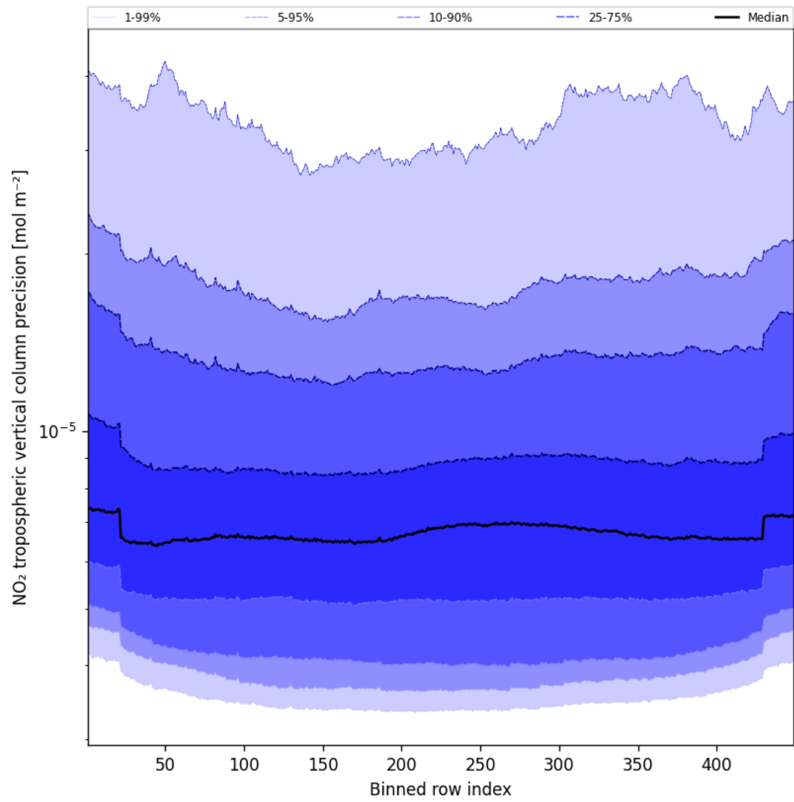
Figure 47: Along track statistics of “NO 2 tropospheric vertical column precision” for 2025-04-08 to 2025-04-09
