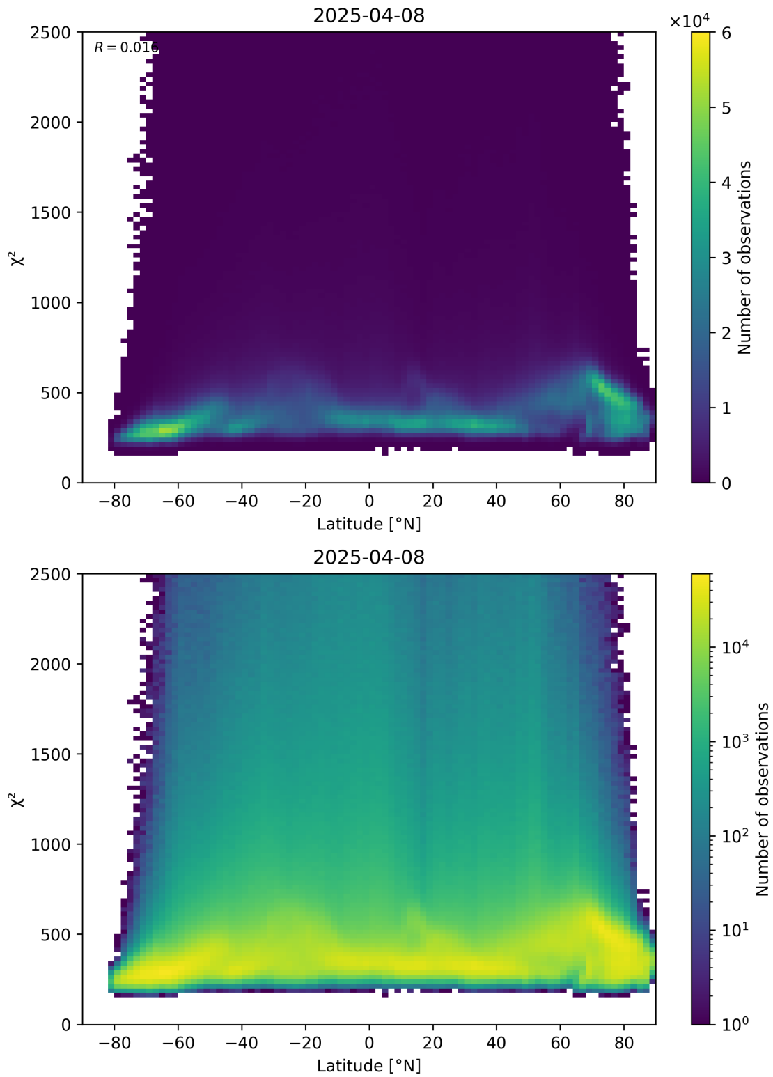
Figure 86: Scatter density plot of “Latitude” against “ \chi^2 ” for 2025-04-08 to 2025-04-09.
