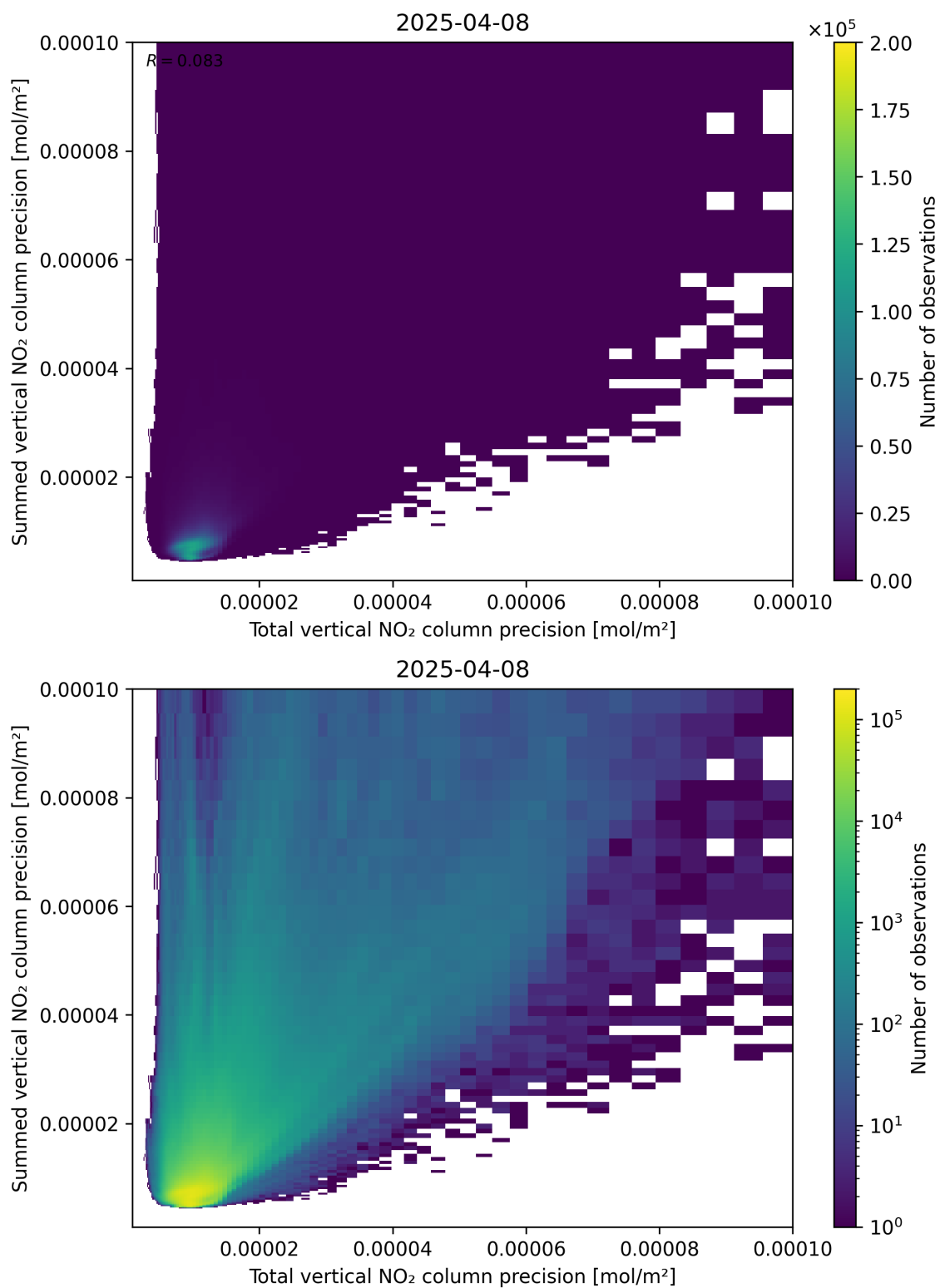
Figure 118: Scatter density plot of “Total vertical NO 2 column precision” against “Summed vertical NO 2 column precision” for 2025-04-08 to 2025-04-09.
