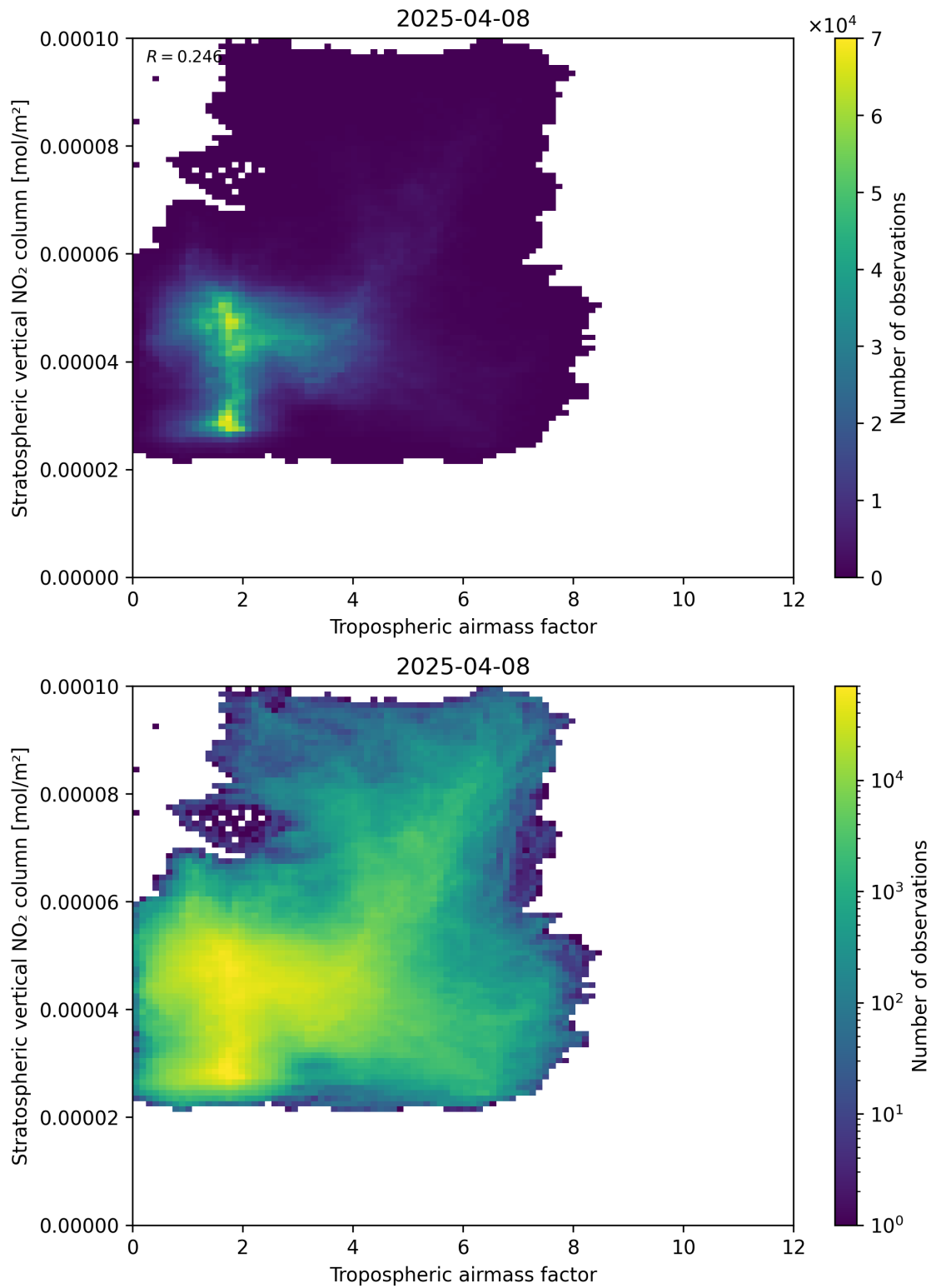
Figure 74: Scatter density plot of “Tropospheric air mass factor” against “Stratospheric vertical NO 2 column” for 2025-04-08 to 2025-04-09.
