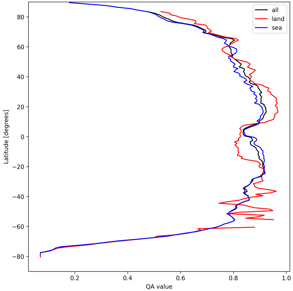
Figure 11: Zonal average of “QA value” for 2025-04-08 to 2025-04-09.
