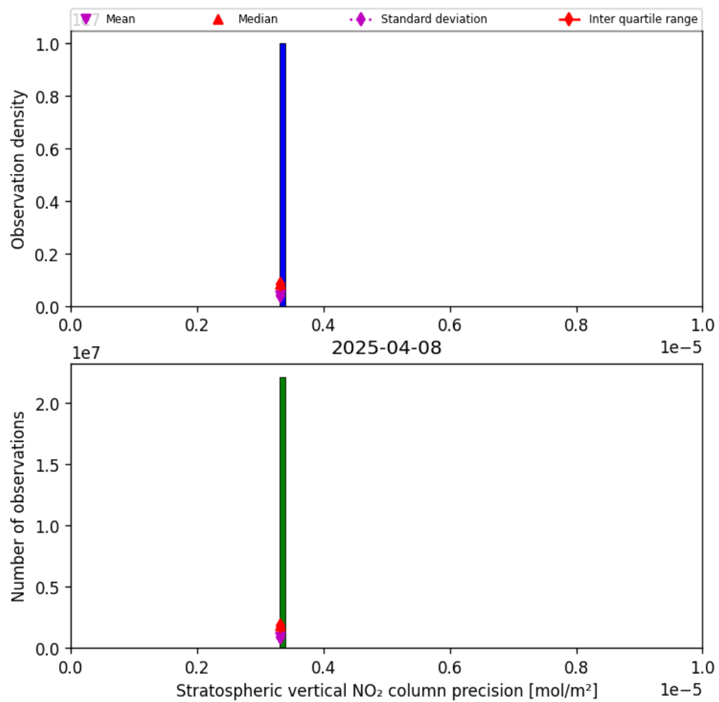
Figure 37: Histogram of “Stratospheric vertical NO 2 column precision” for 2025-04-08 to 2025-04-09
