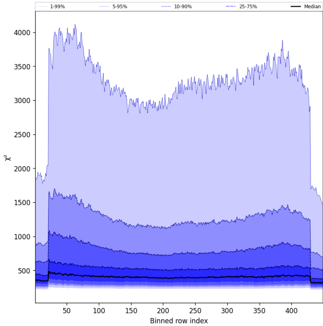
Figure 59: Along track statistics of “ \chi^2 ” for 2025-04-08 to 2025-04-09
