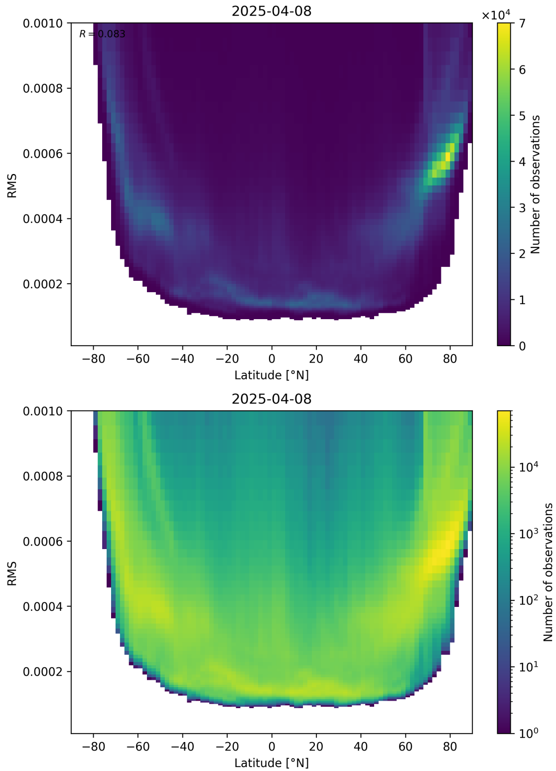
Figure 94: Scatter density plot of “Latitude” against “RMS” for 2025-04-08 to 2025-04-09.
