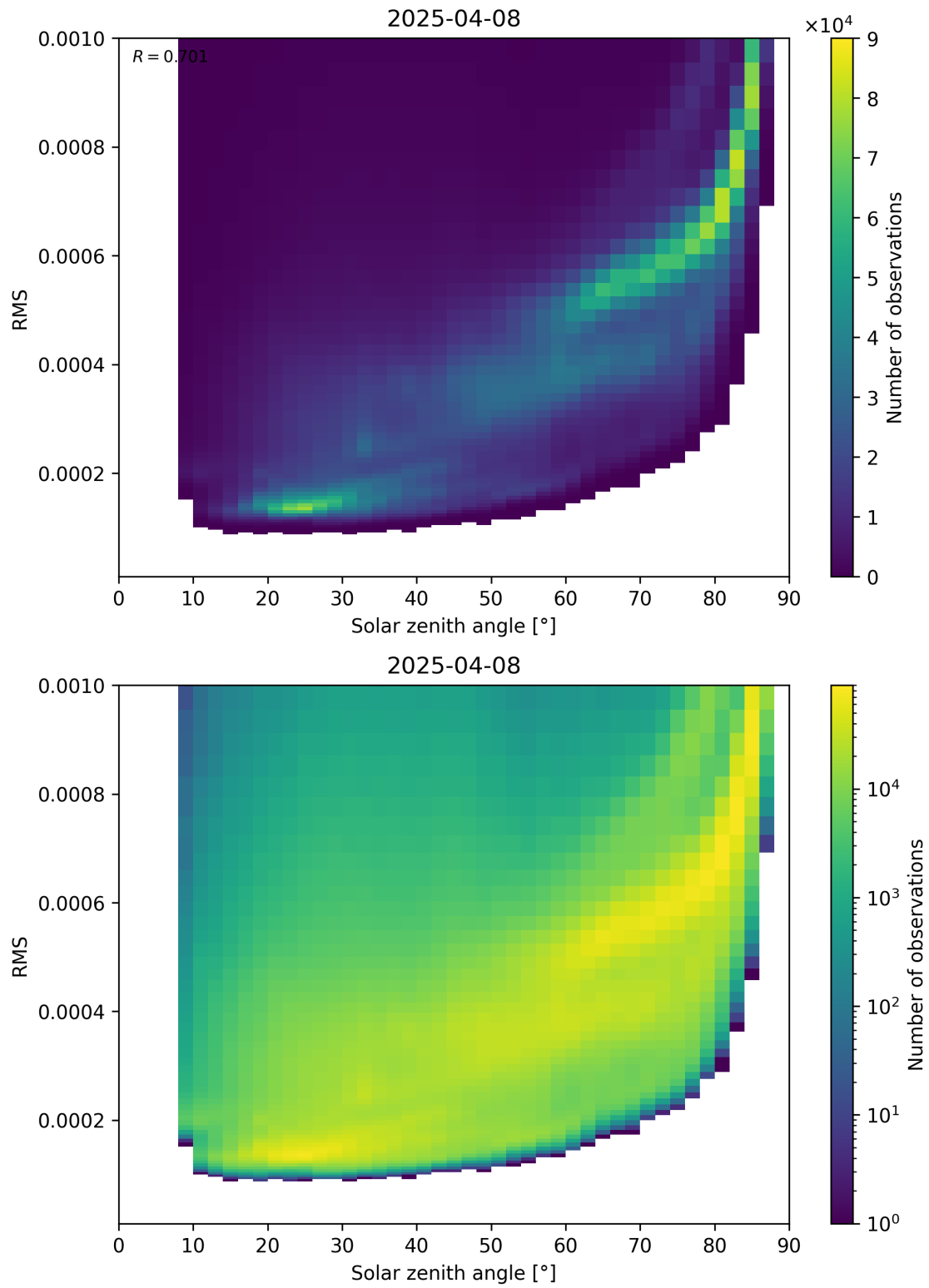
Figure 157: Scatter density plot of “Solar zenith angle” against “RMS” for 2025-04-08 to 2025-04-09.
