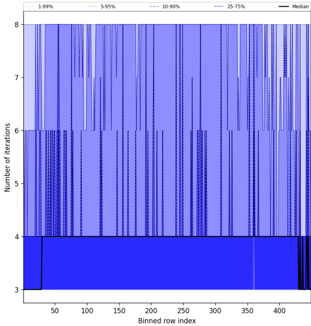
Figure 51: Along track statistics of “Number of iterations” for 2025-04-08 to 2025-04-09
