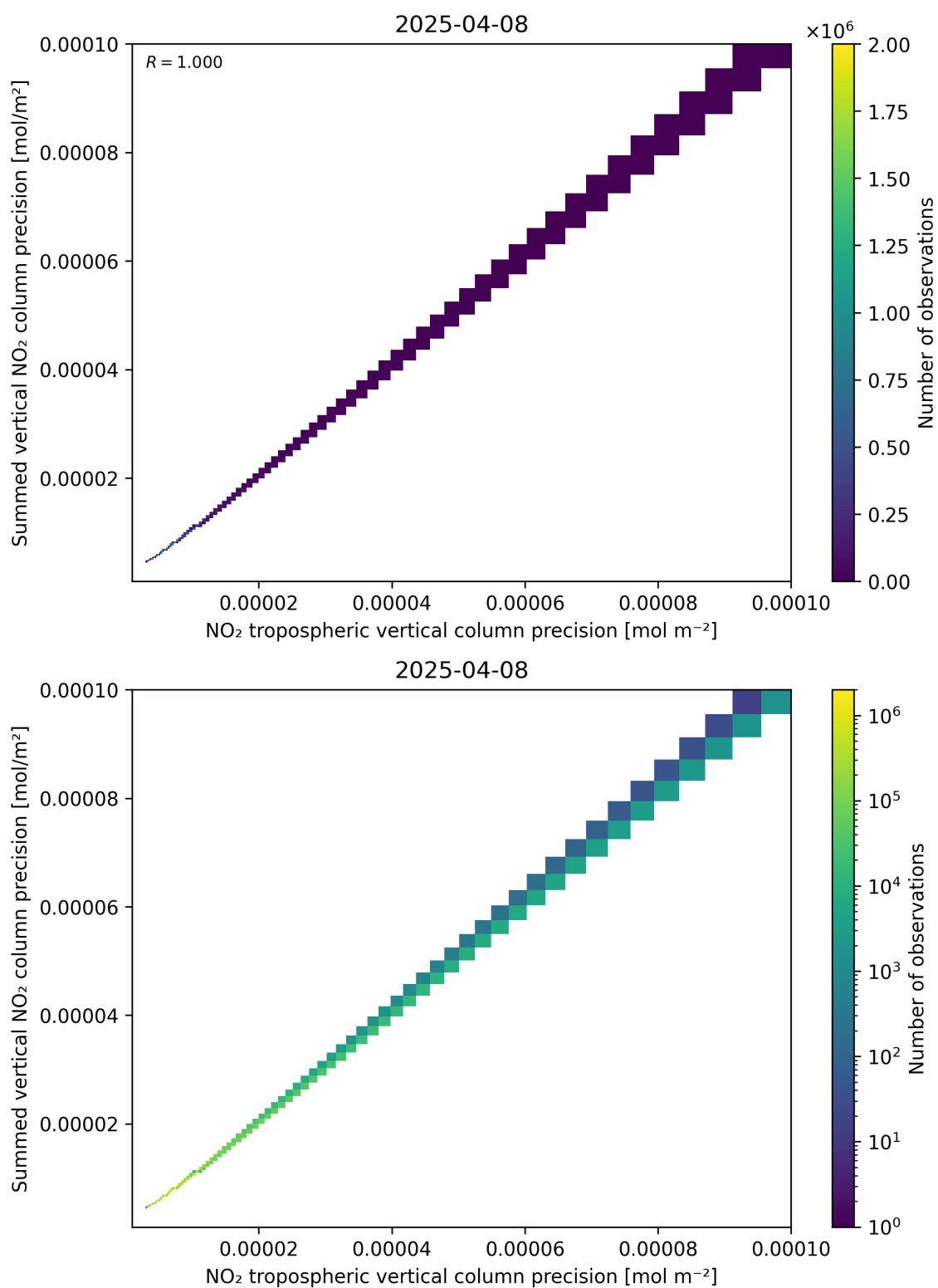
Figure 137: Scatter density plot of “NO 2 tropospheric vertical column precision” against “Summed vertical NO 2 column precision” for 2025-04-08 to 2025-04-09.
