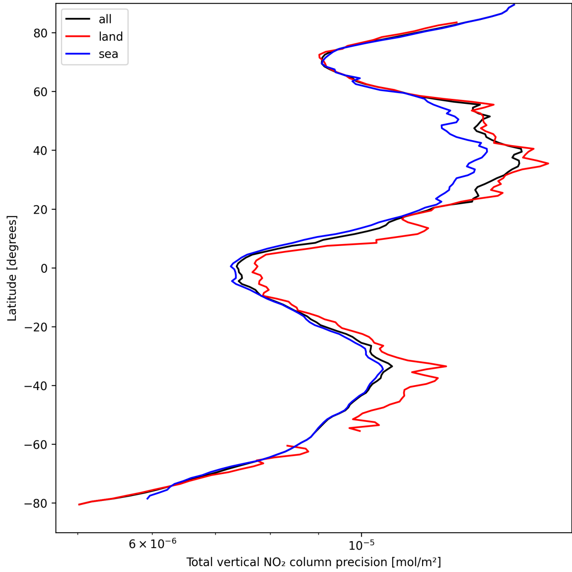
Figure 22: Zonal average of “Total vertical NO 2 column precision” for 2025-04-08 to 2025-04-09.
