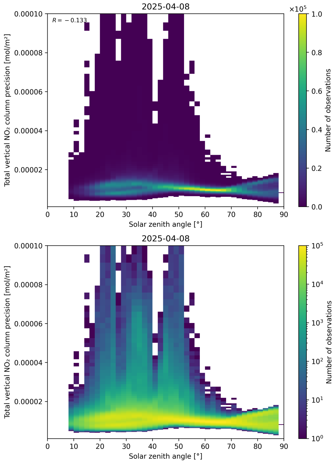
Figure 154: Scatter density plot of “Solar zenith angle” against “Total vertical NO 2 column precision” for 2025-04-08 to 2025-04-09.
