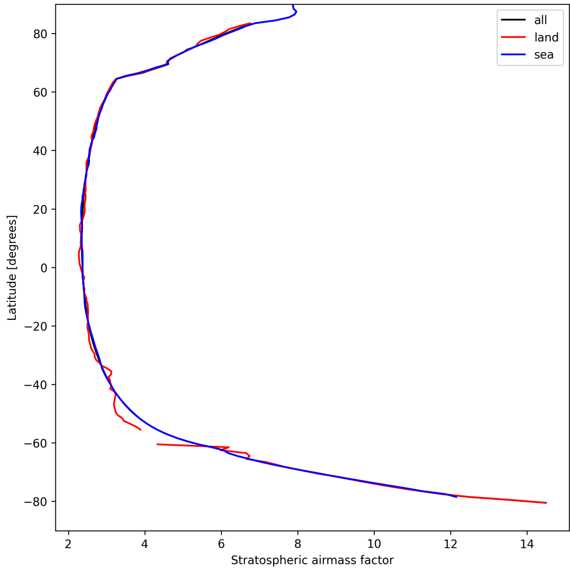
Figure 27: Zonal average of “Stratospheric airmass factor” for 2025-04-08 to 2025-04-09.
