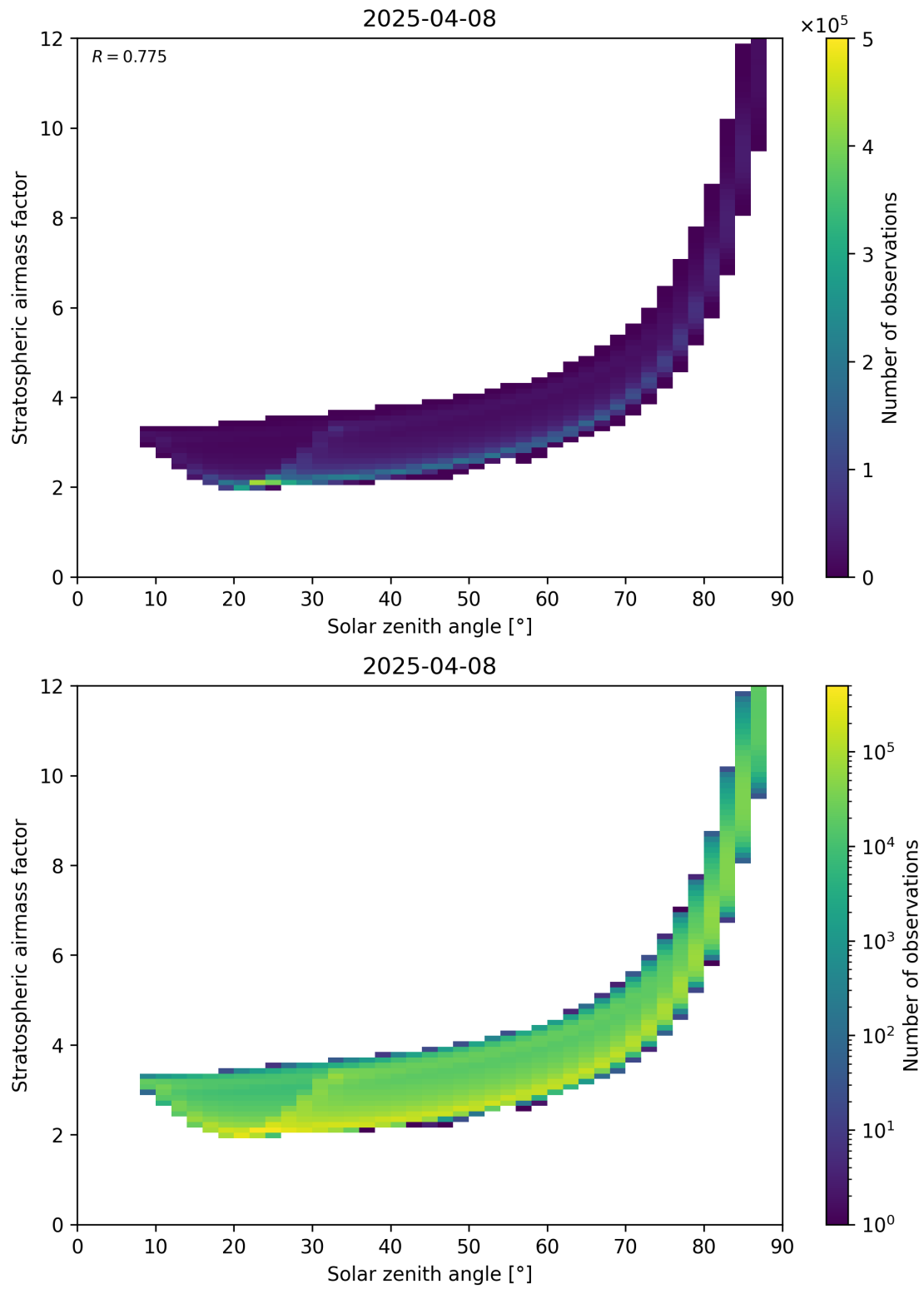
Figure 145: Scatter density plot of “Solar zenith angle” against “Stratospheric airmass factor” for 2025-04-08 to 2025-04-09.
