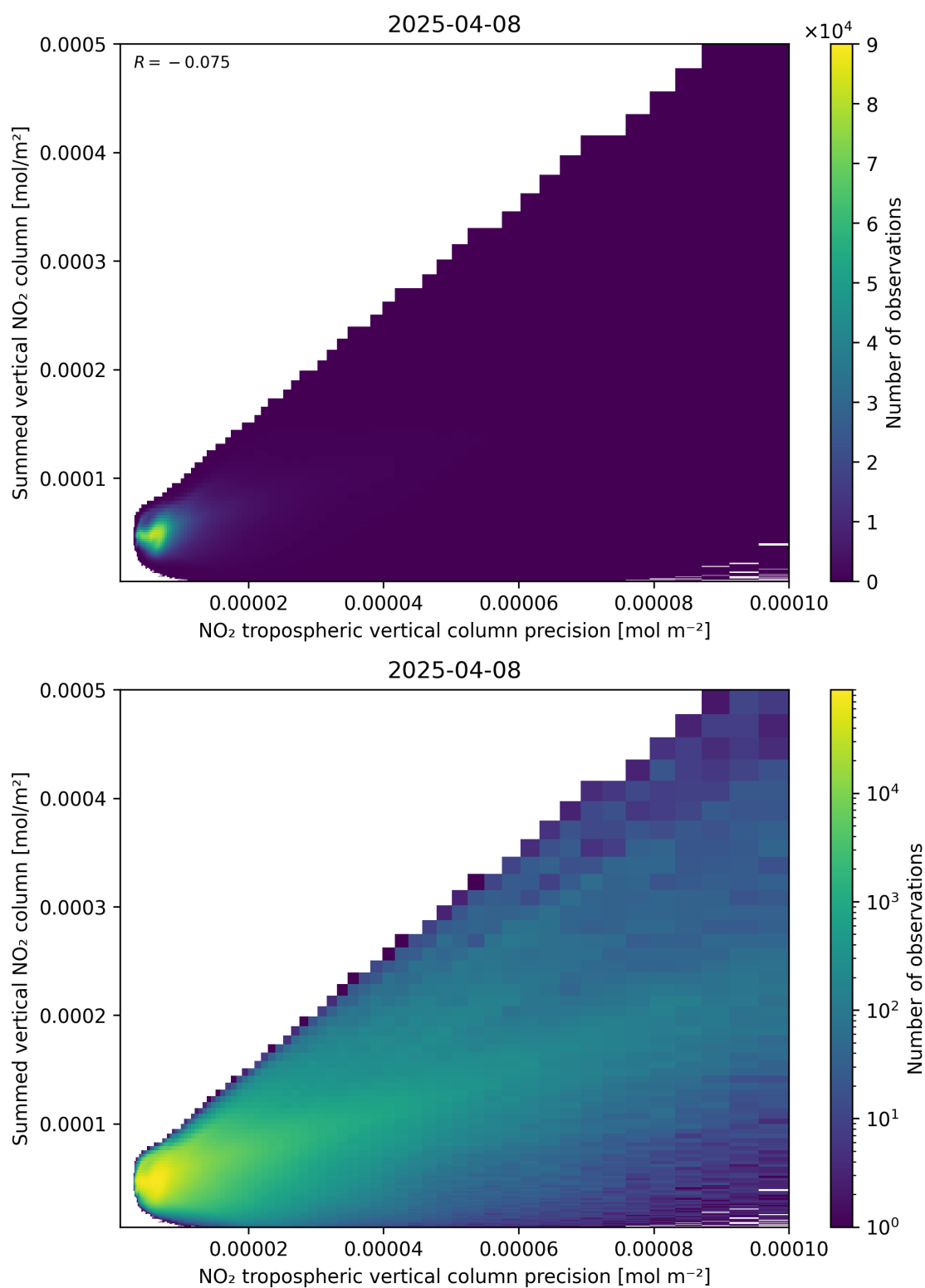
Figure 136: Scatter density plot of “NO 2 tropospheric vertical column precision” against “Summed vertical NO 2 column” for 2025-04-08 to 2025-04-09.
