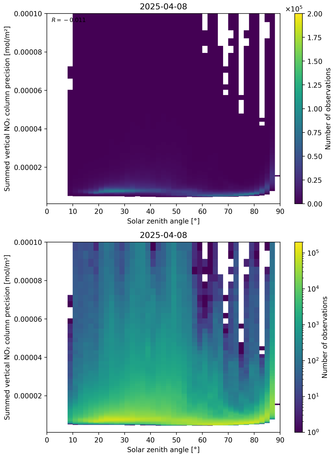
Figure 152: Scatter density plot of “Solar zenith angle” against “Summed vertical NO 2 column precision” for 2025-04-08 to 2025-04-09.
