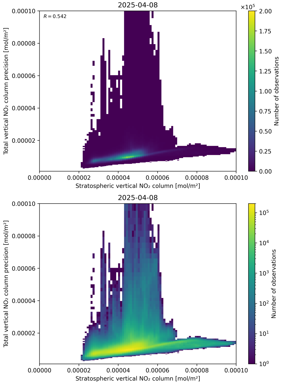
Figure 101: Scatter density plot of “Stratospheric vertical NO 2 column” against “Total vertical NO 2 column precision” for 2025-04-08 to 2025-04-09.
