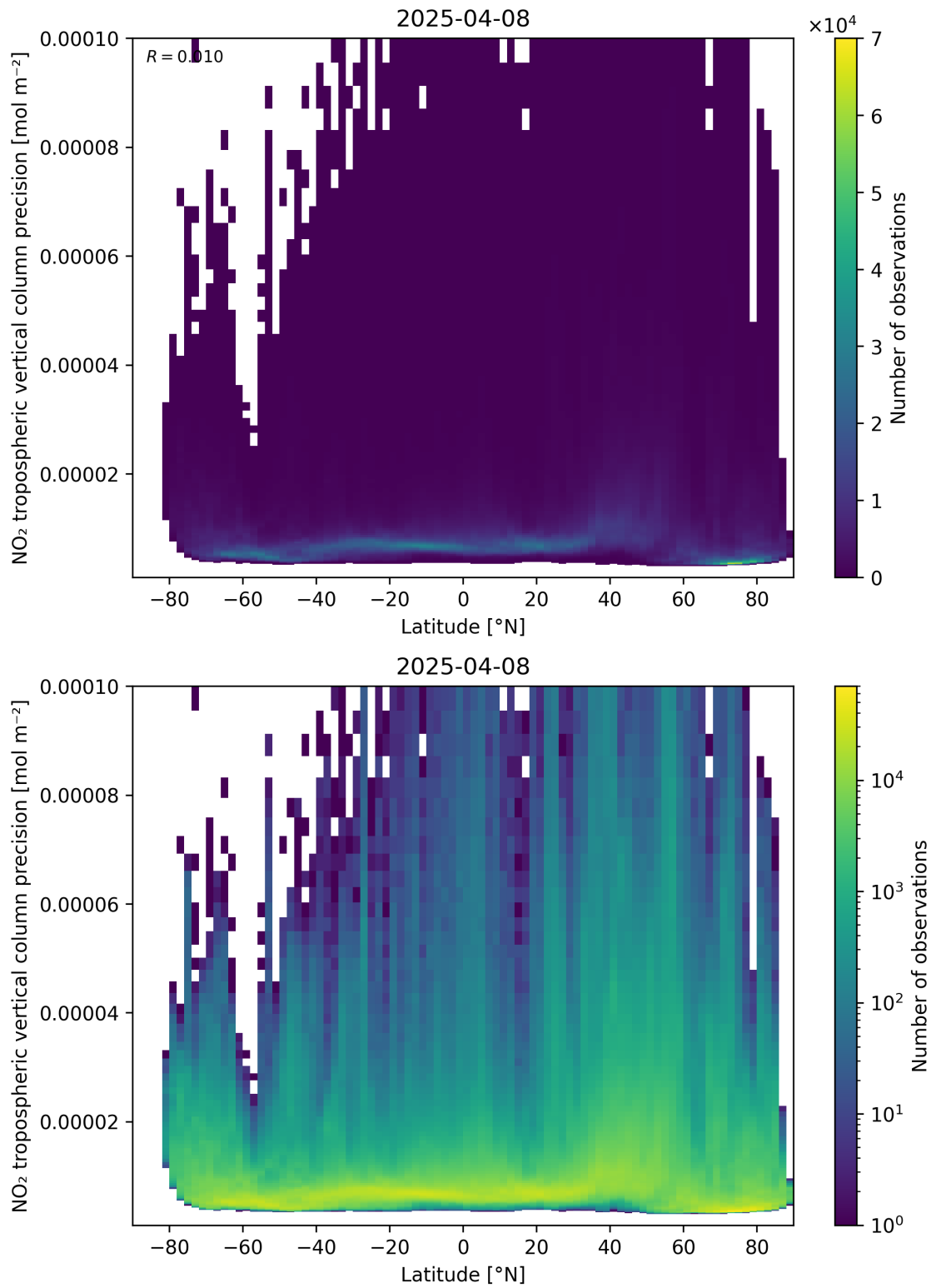
Figure 93: Scatter density plot of “Latitude” against “NO 2 tropospheric vertical column precision” for 2025-04-08 to 2025-04-09.
