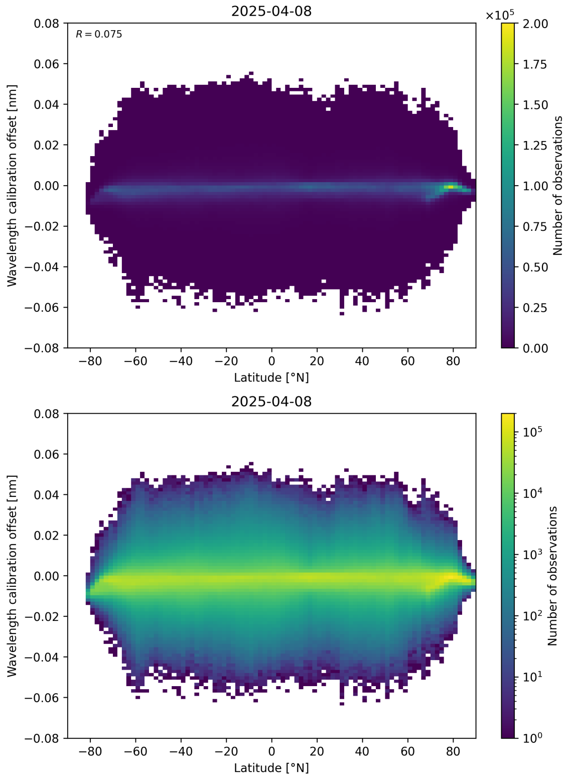
Figure 95: Scatter density plot of “Latitude” against “Wavelength calibration offset” for 2025-04-08 to 2025-04-09.
