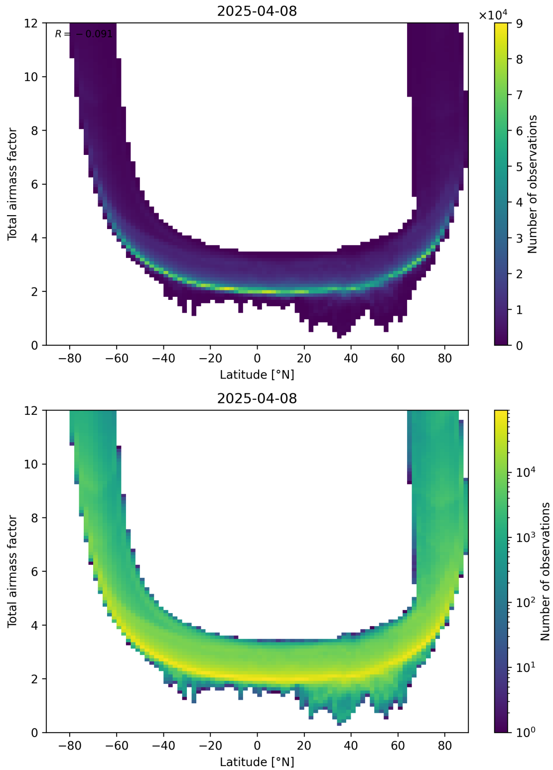
Figure 84: Scatter density plot of “Latitude” against “Total airmass factor” for 2025-04-08 to 2025-04-09.
