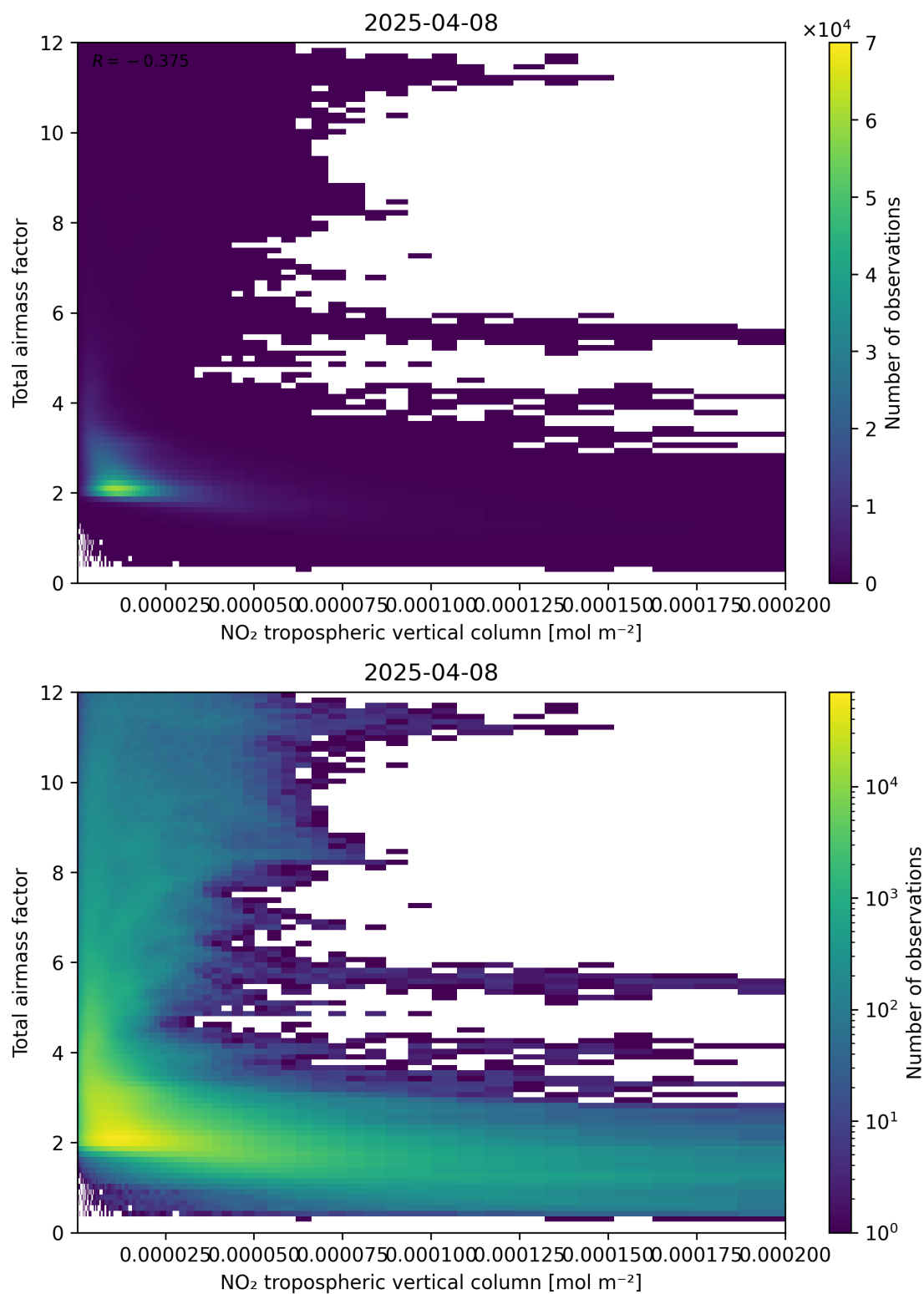
Figure 122: Scatter density plot of “NO 2 tropospheric vertical column” against “Total air mass factor” for 2025-04-08 to 2025-04-09.
