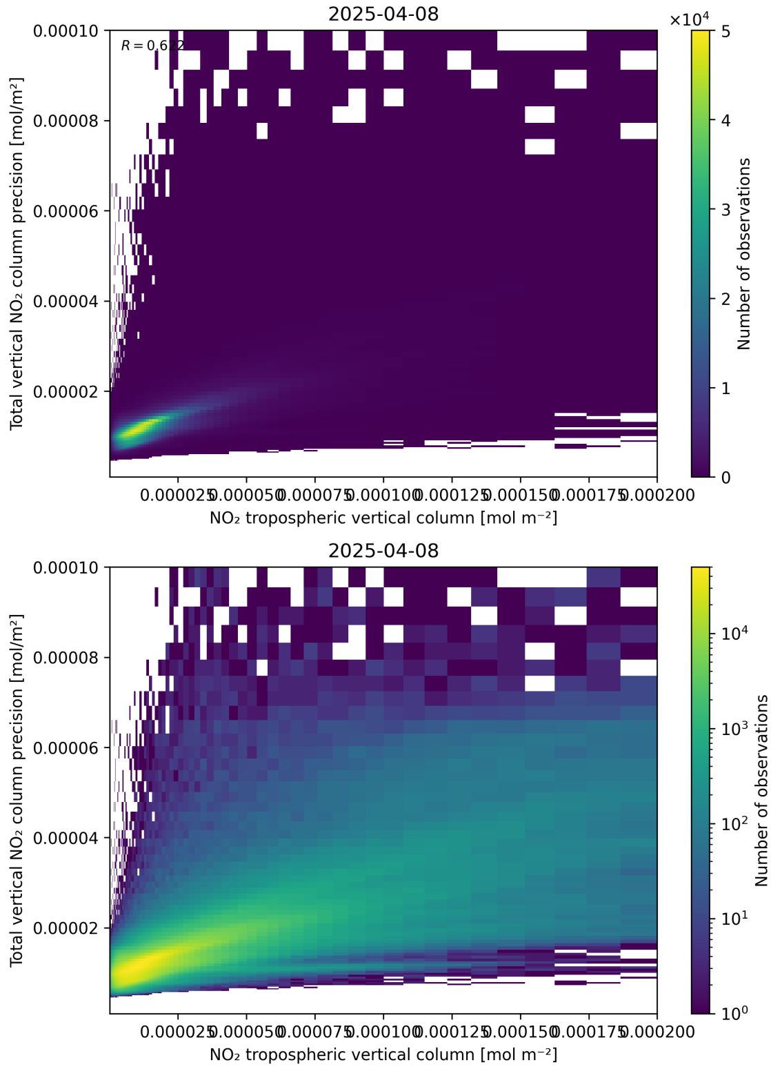
Figure 129: Scatter density plot of “NO 2 tropospheric vertical column” against “Total vertical NO 2 column precision” for 2025-04-08 to 2025-04-09.
