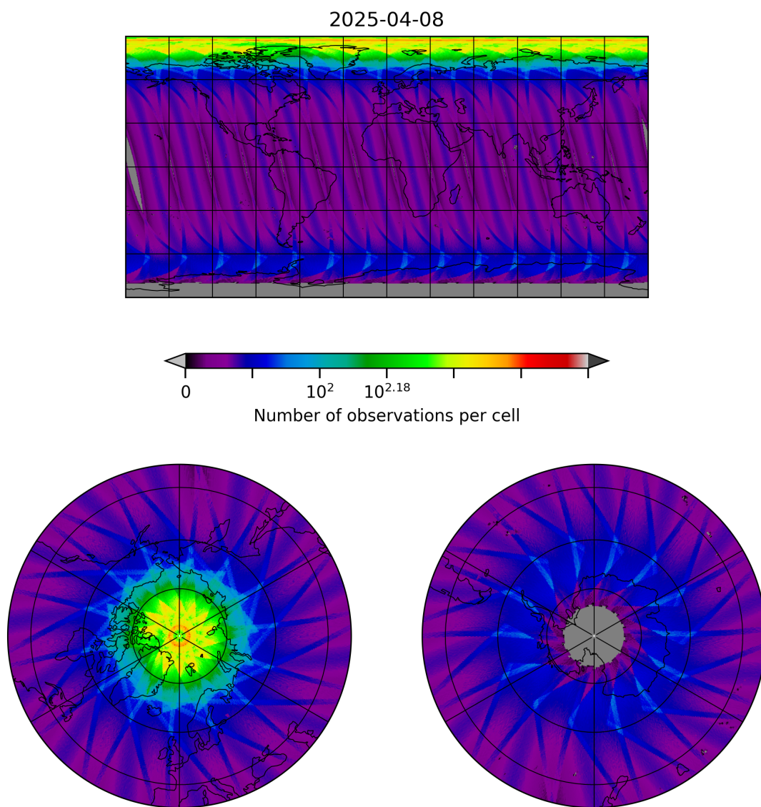
Figure 10: Map of the number of observations for 2025-04-08 to 2025-04-09
