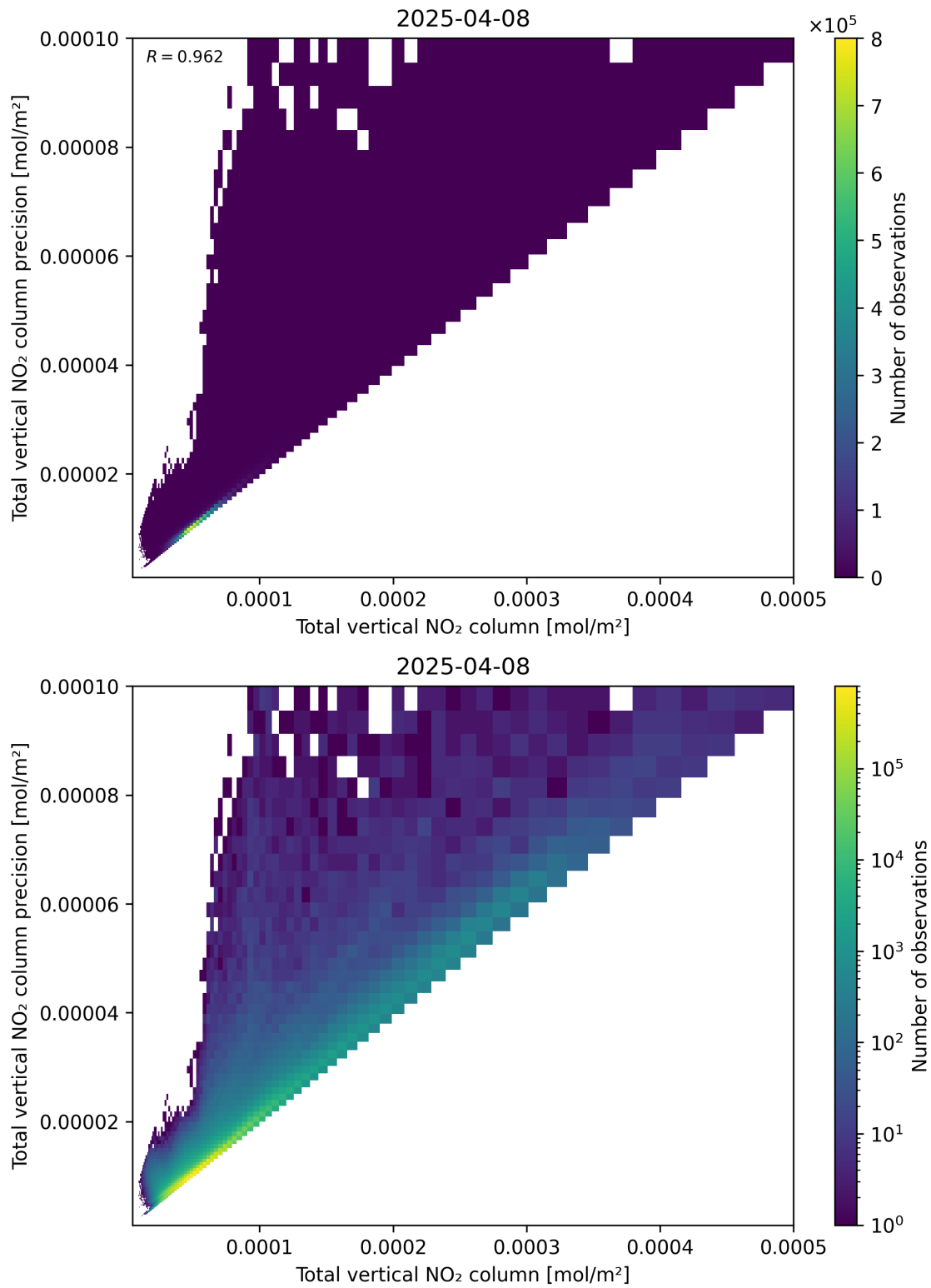
Figure 114: Scatter density plot of “Total vertical NO 2 column” against “Total vertical NO 2 column precision” for 2025-04-08 to 2025-04-09.
