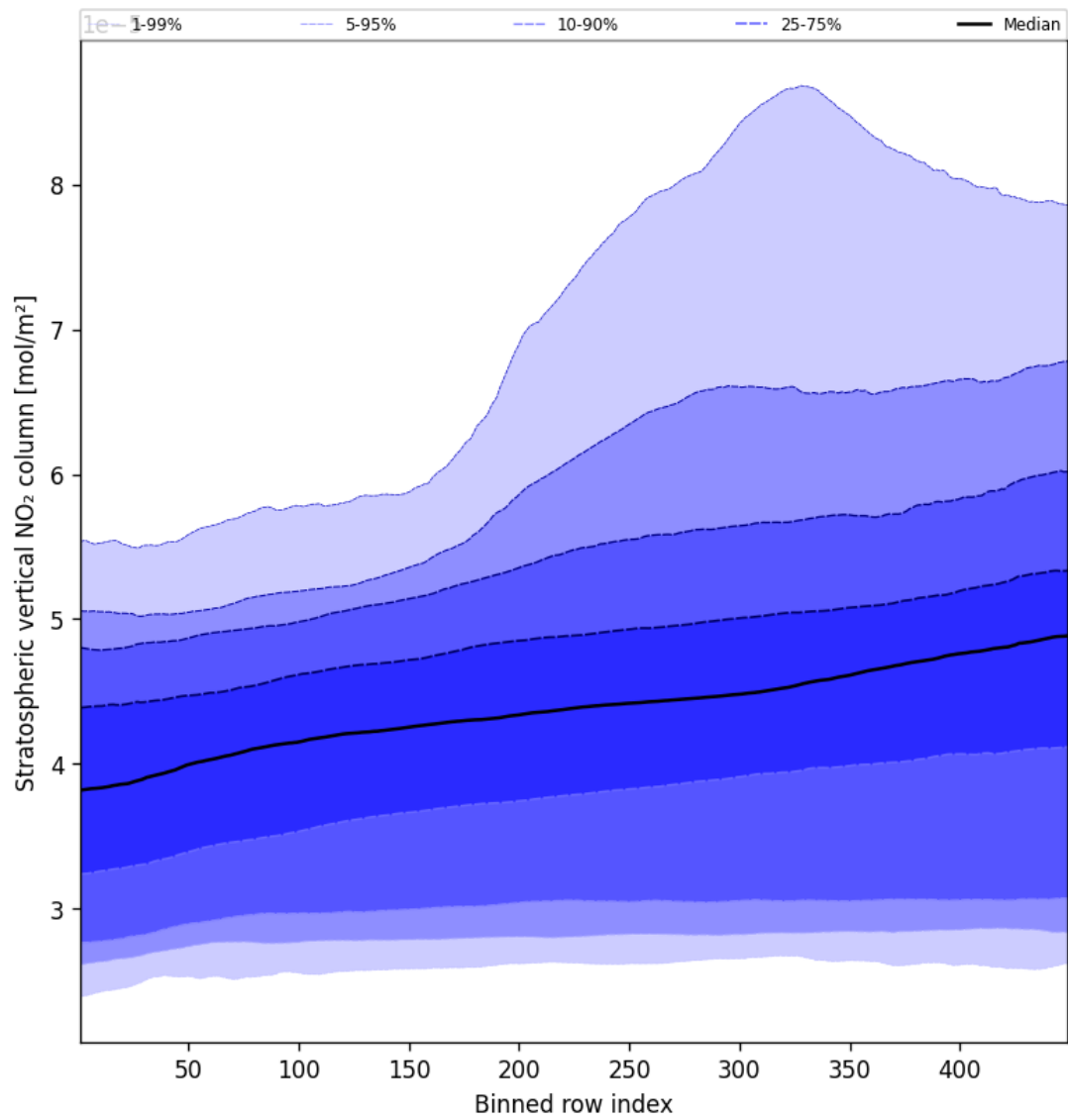
Figure 53: Along track statistics of “Stratospheric vertical NO 2 column” for 2025-04-08 to 2025-04-09
