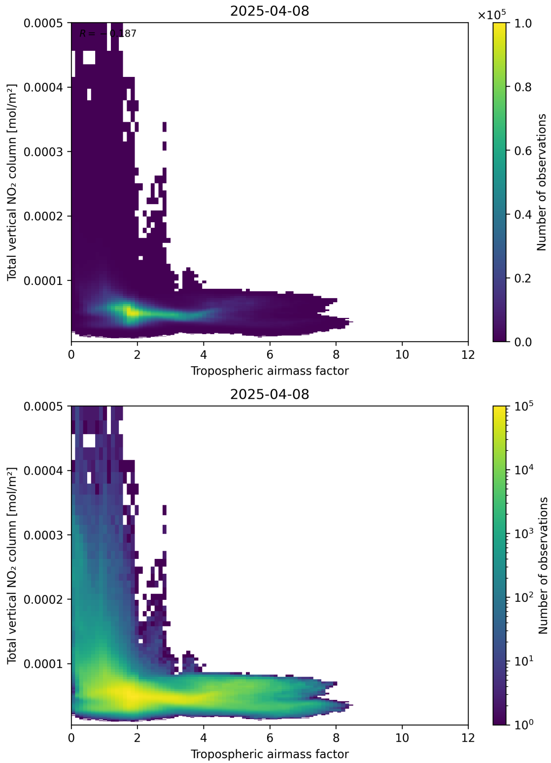
Figure 77: Scatter density plot of “Tropospheric airmass factor” against “Total vertical NO 2 column” for 2025-04-08 to 2025-04-09.
