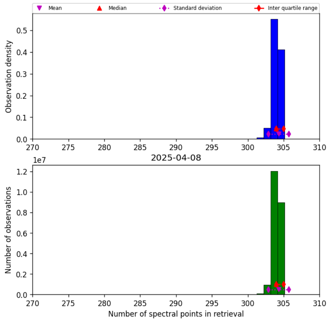
Figure 33: Histogram of “Number of spectral points in retrieval” for 2025-04-08 to 2025-04-09
