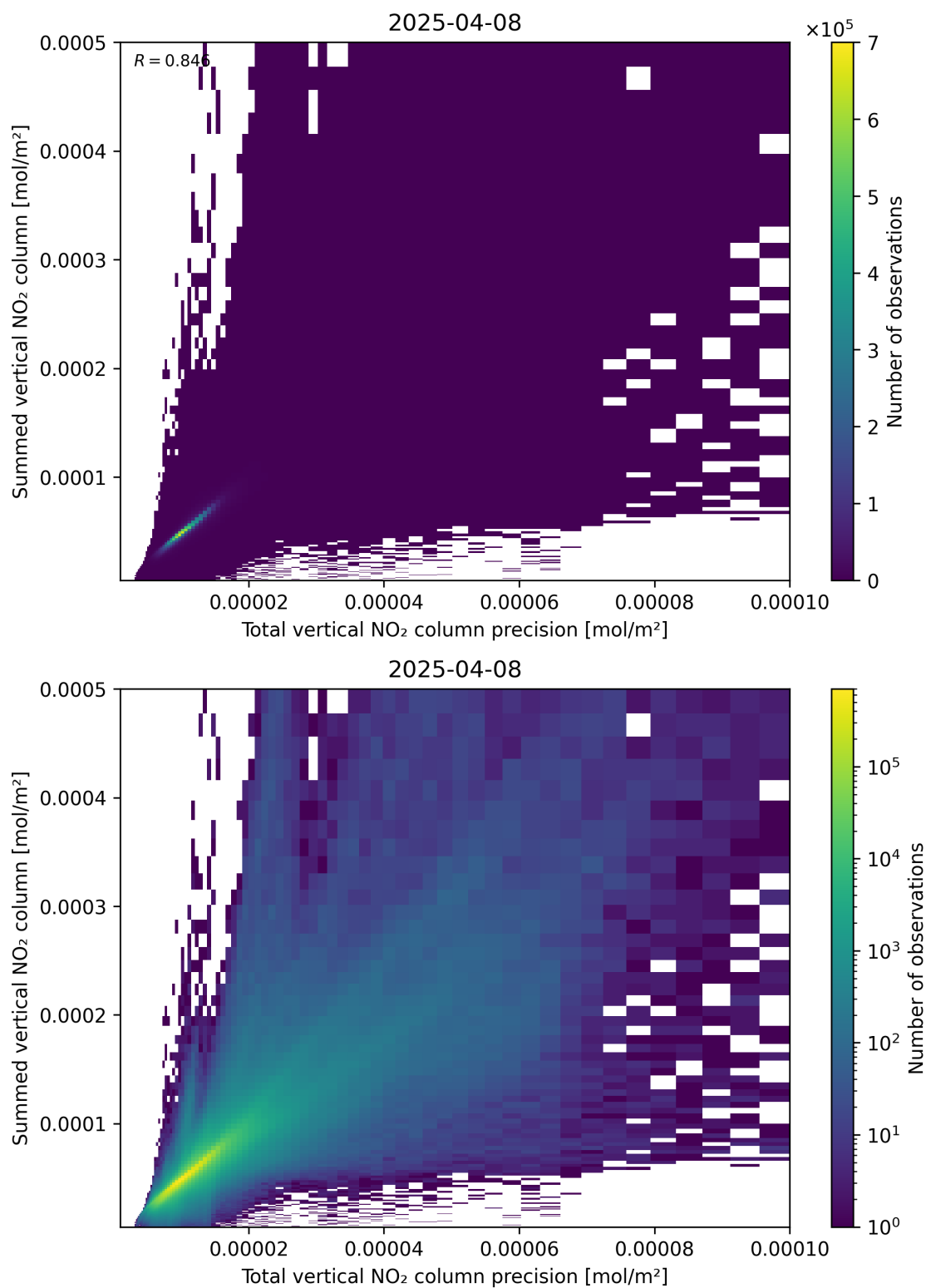
Figure 117: Scatter density plot of “Total vertical NO 2 column precision” against “Summed vertical NO 2 column” for 2025-04-08 to 2025-04-09.
