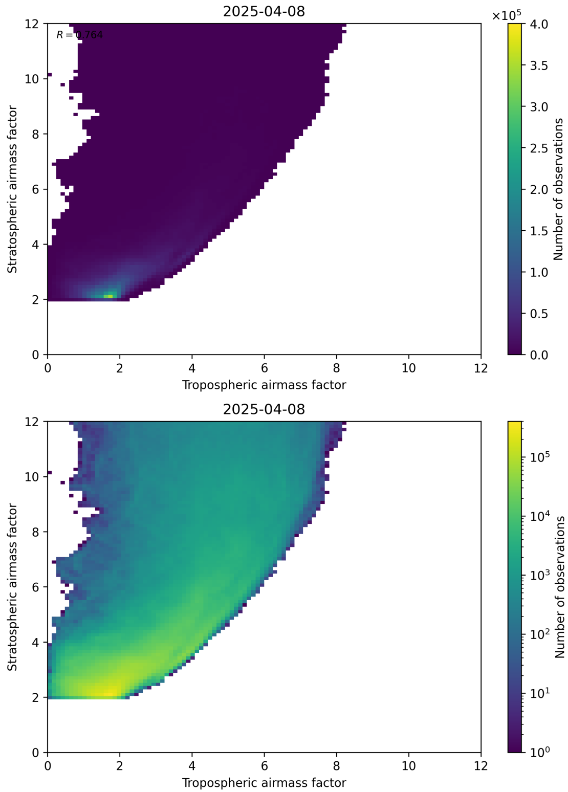
Figure 71: Scatter density plot of “Tropospheric airmass factor” against “Stratospheric airmass factor” for 2025-04-08 to 2025-04-09.
