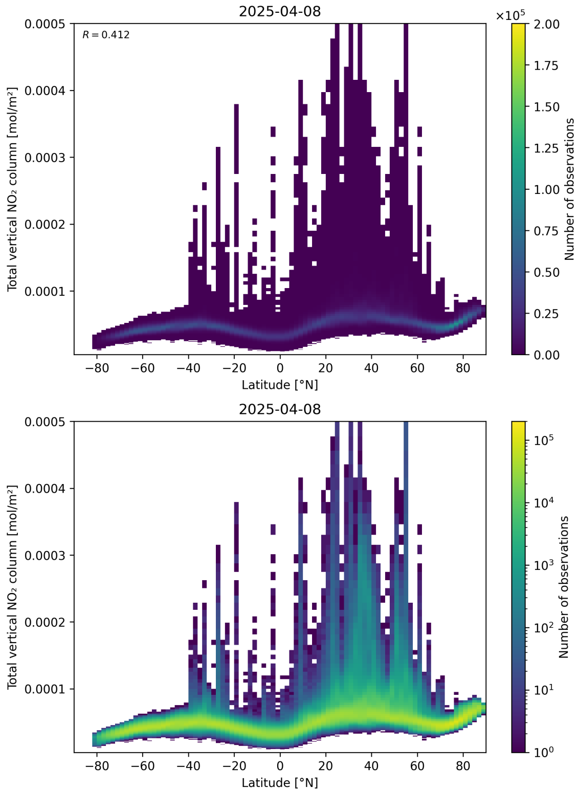
Figure 90: Scatter density plot of “Latitude” against “Total vertical NO 2 column” for 2025-04-08 to 2025-04-09.
