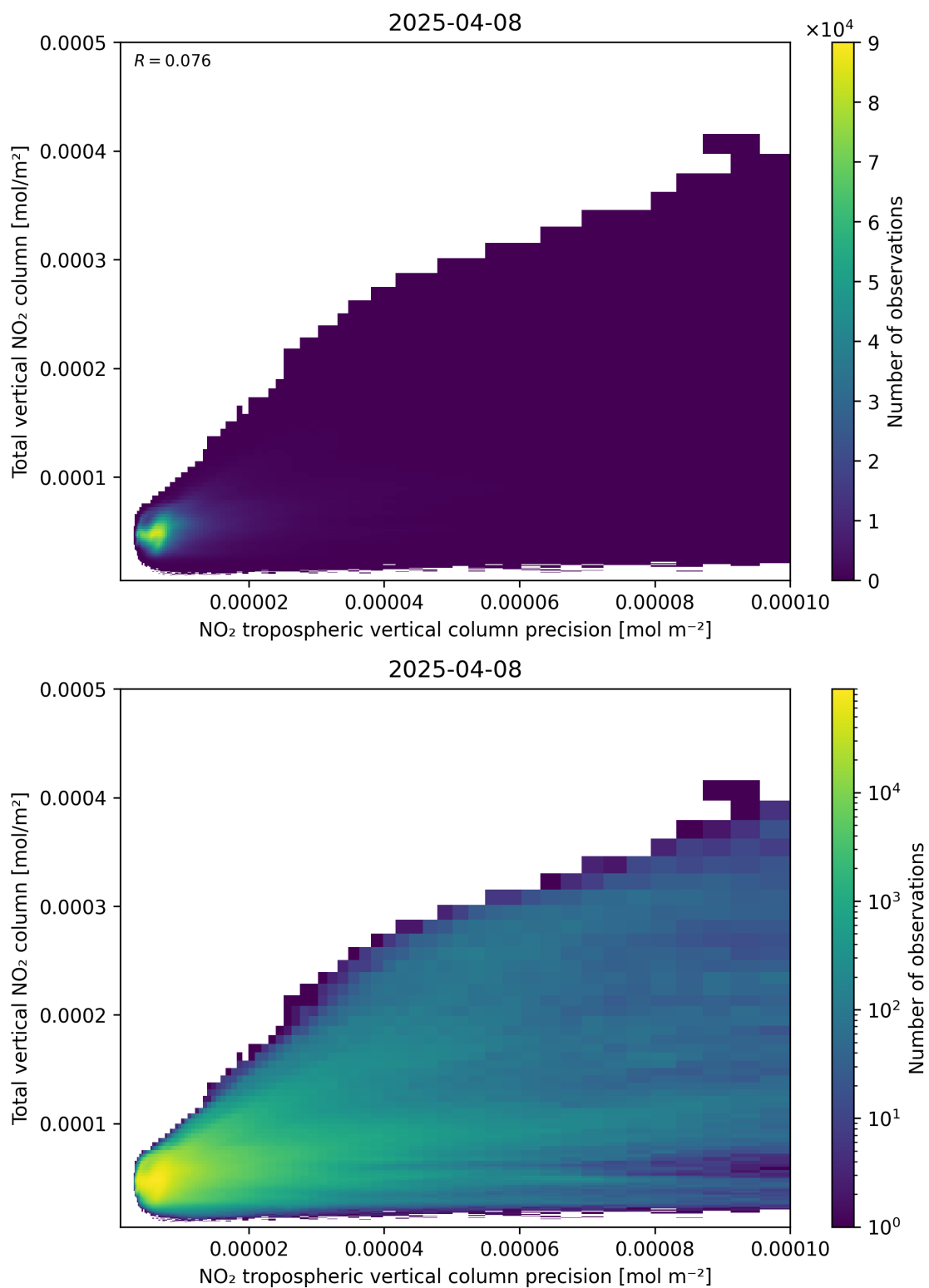
Figure 138: Scatter density plot of “NO 2 tropospheric vertical column precision” against “Total vertical NO 2 column” for 2025-04-08 to 2025-04-09.
