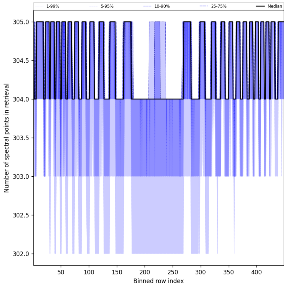
Figure 50: Along track statistics of “Number of spectral points in retrieval” for 2025-04-08 to 2025-04-09
