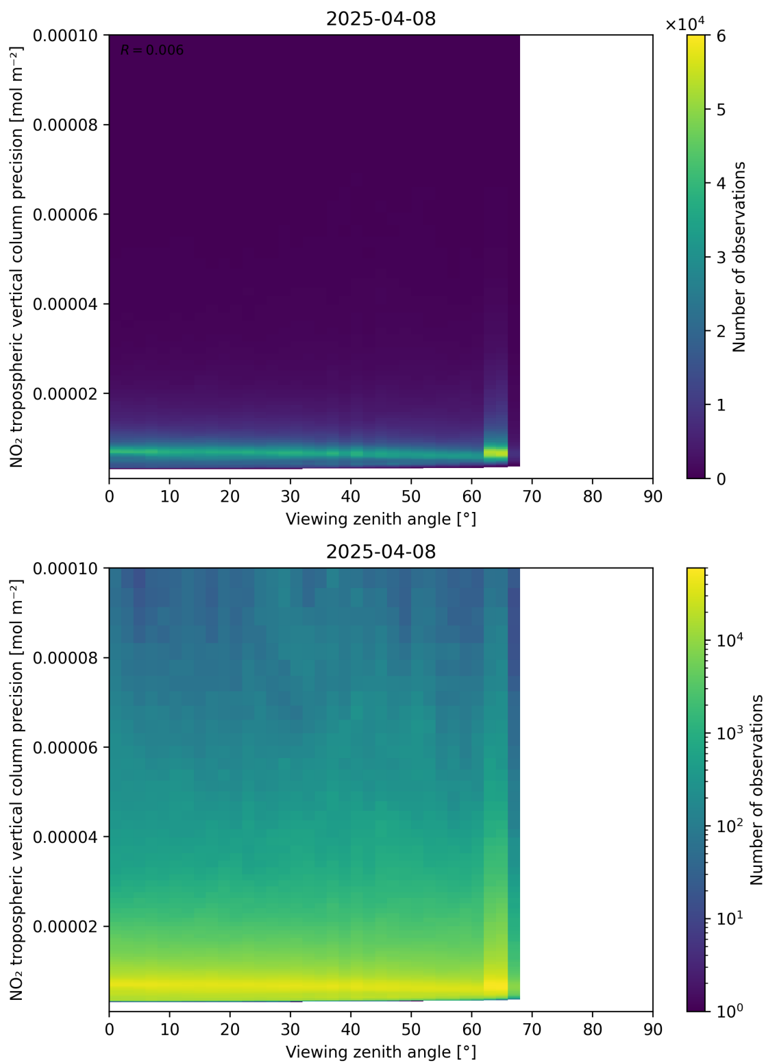
Figure 170: Scatter density plot of “Viewing zenith angle” against “NO 2 tropospheric vertical column precision” for 2025-04-08 to 2025-04-09.
