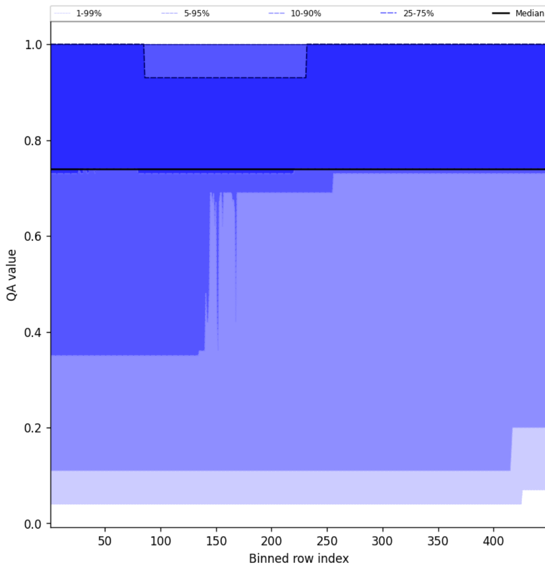
Figure 45: Along track statistics of “QA value” for 2025-04-08 to 2025-04-09
