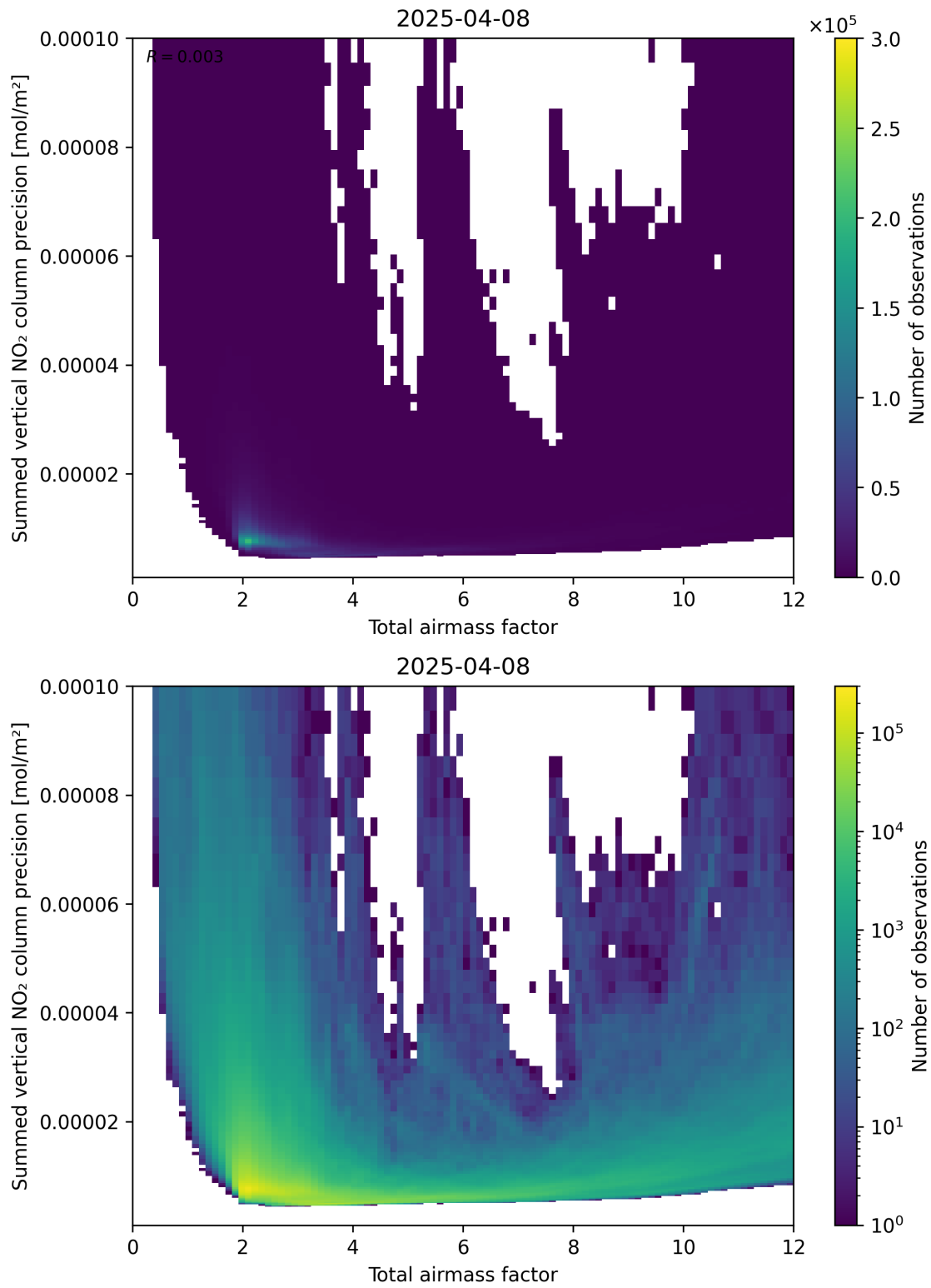
Figure 66: Scatter density plot of “Total airmass factor” against “Summed vertical NO 2 column precision” for 2025-04-08 to 2025-04-09.
