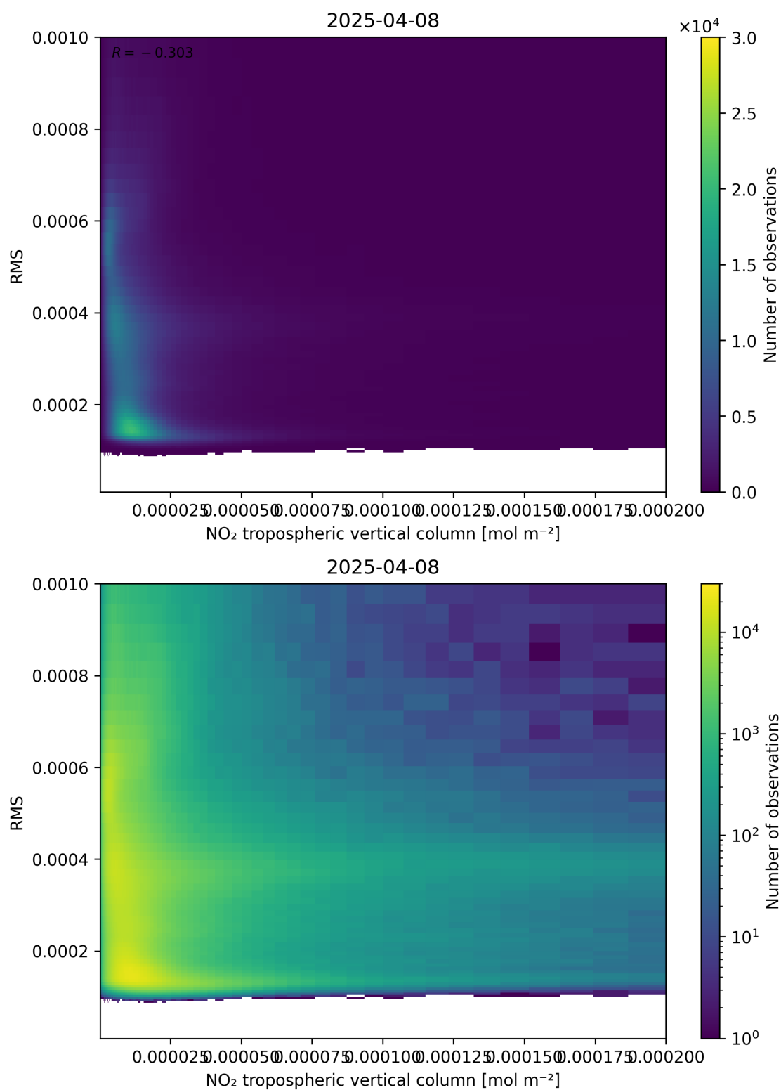
Figure 142: Scatter density plot of “NO 2 tropospheric vertical column” against “RMS” for 2025-04-08 to 2025-04-09.
