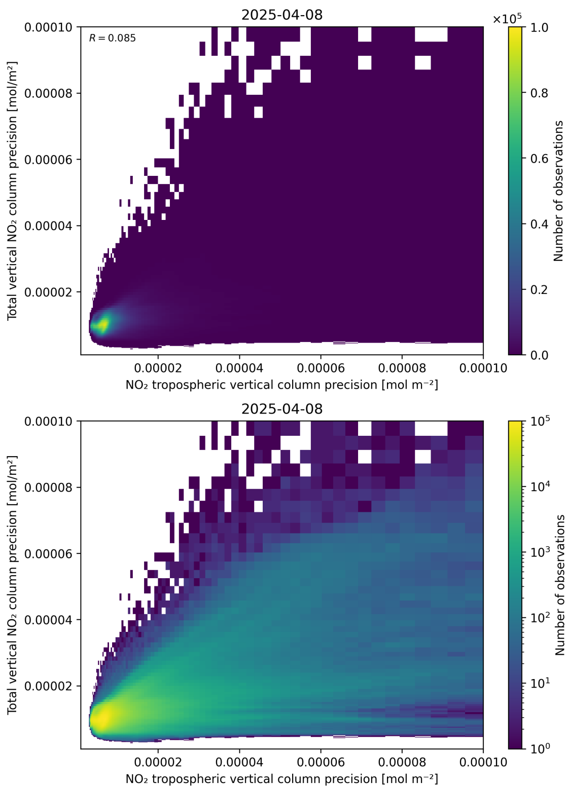
Figure 139: Scatter density plot of “NO 2 tropospheric vertical column precision” against “Total vertical NO 2 column precision” for 2025-04-08 to 2025-04-09.
