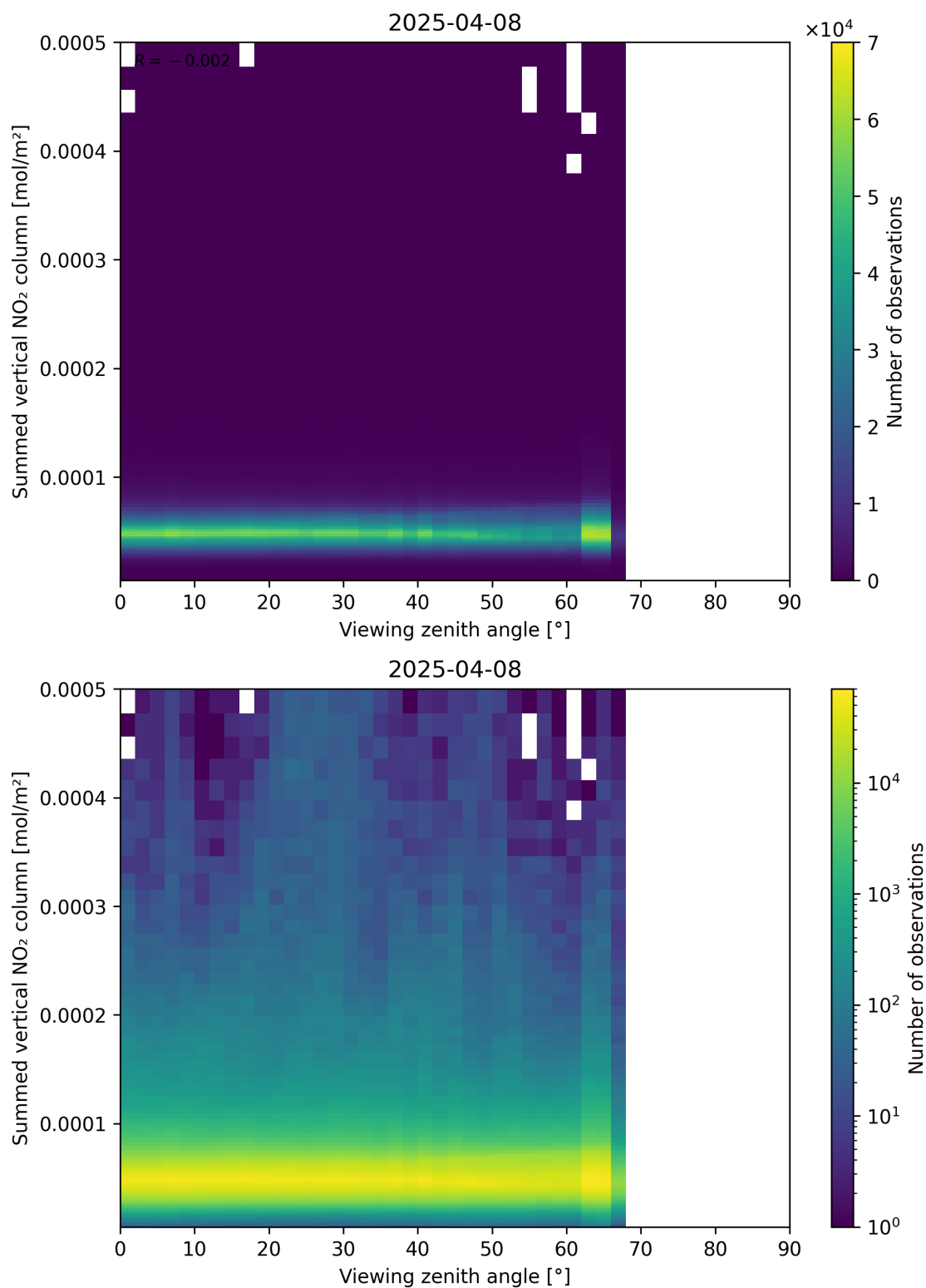
Figure 165: Scatter density plot of “Viewing zenith angle” against “Summed vertical NO 2 column” for 2025-04-08 to 2025-04-09.
