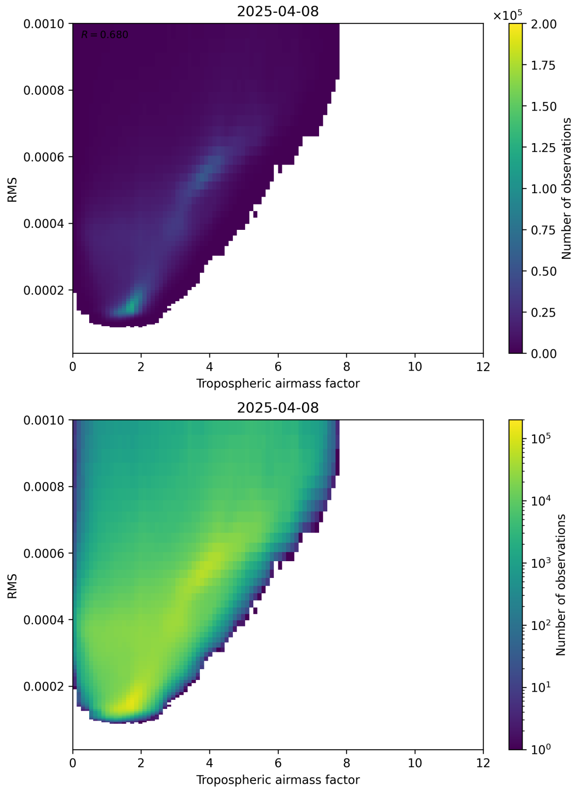
Figure 79: Scatter density plot of “Tropospheric airmass factor” against “RMS” for 2025-04-08 to 2025-04-09.
