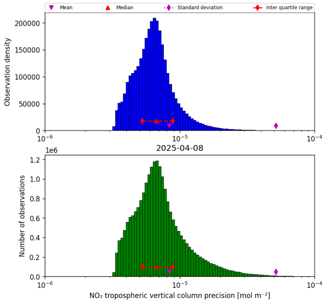
Figure 30: Histogram of “NO 2 tropospheric vertical column precision” for 2025-04-08 to 2025-04-09
