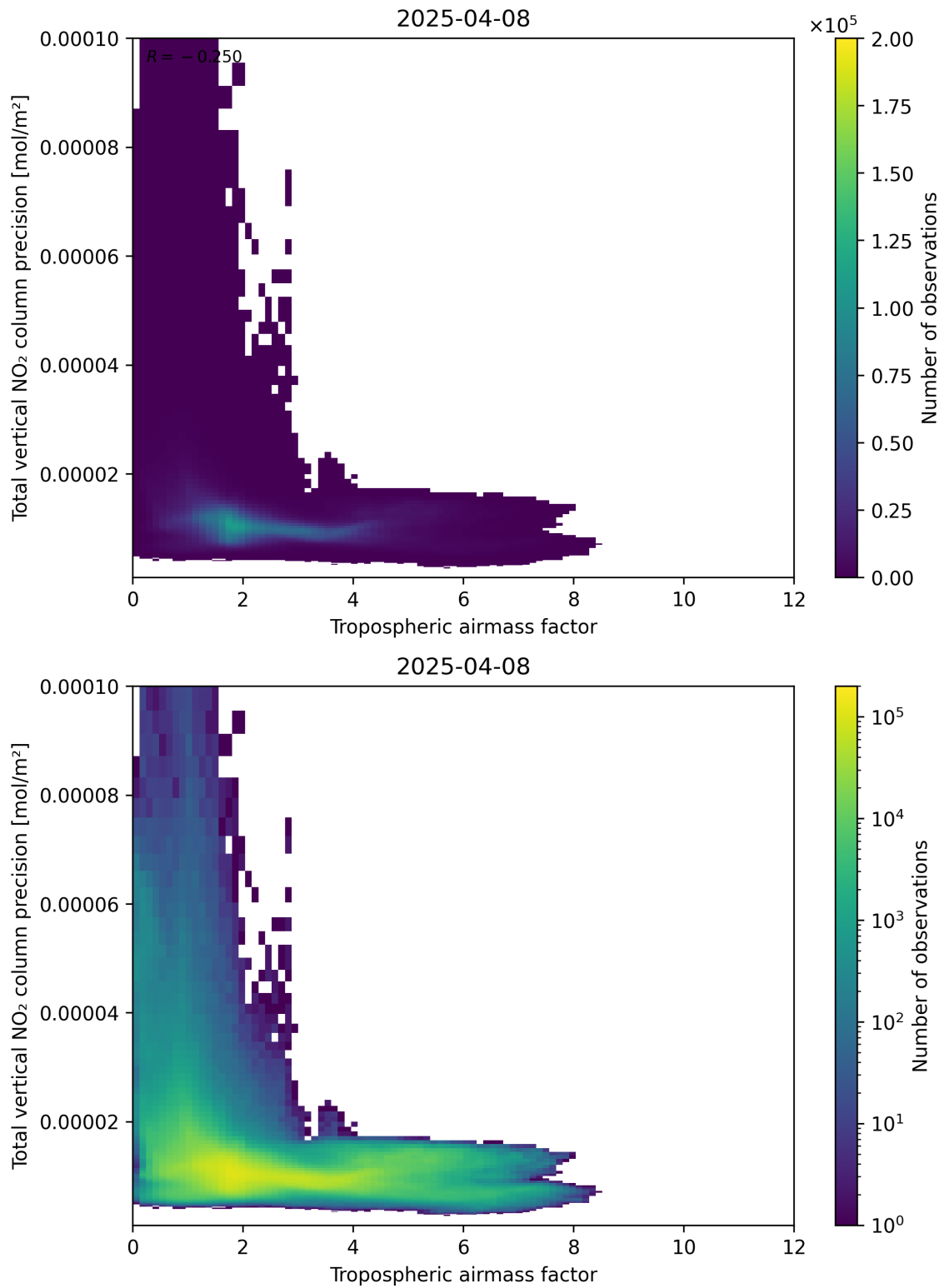
Figure 78: Scatter density plot of “Tropospheric airmass factor” against “Total vertical NO 2 column precision” for 2025-04-08 to 2025-04-09.
