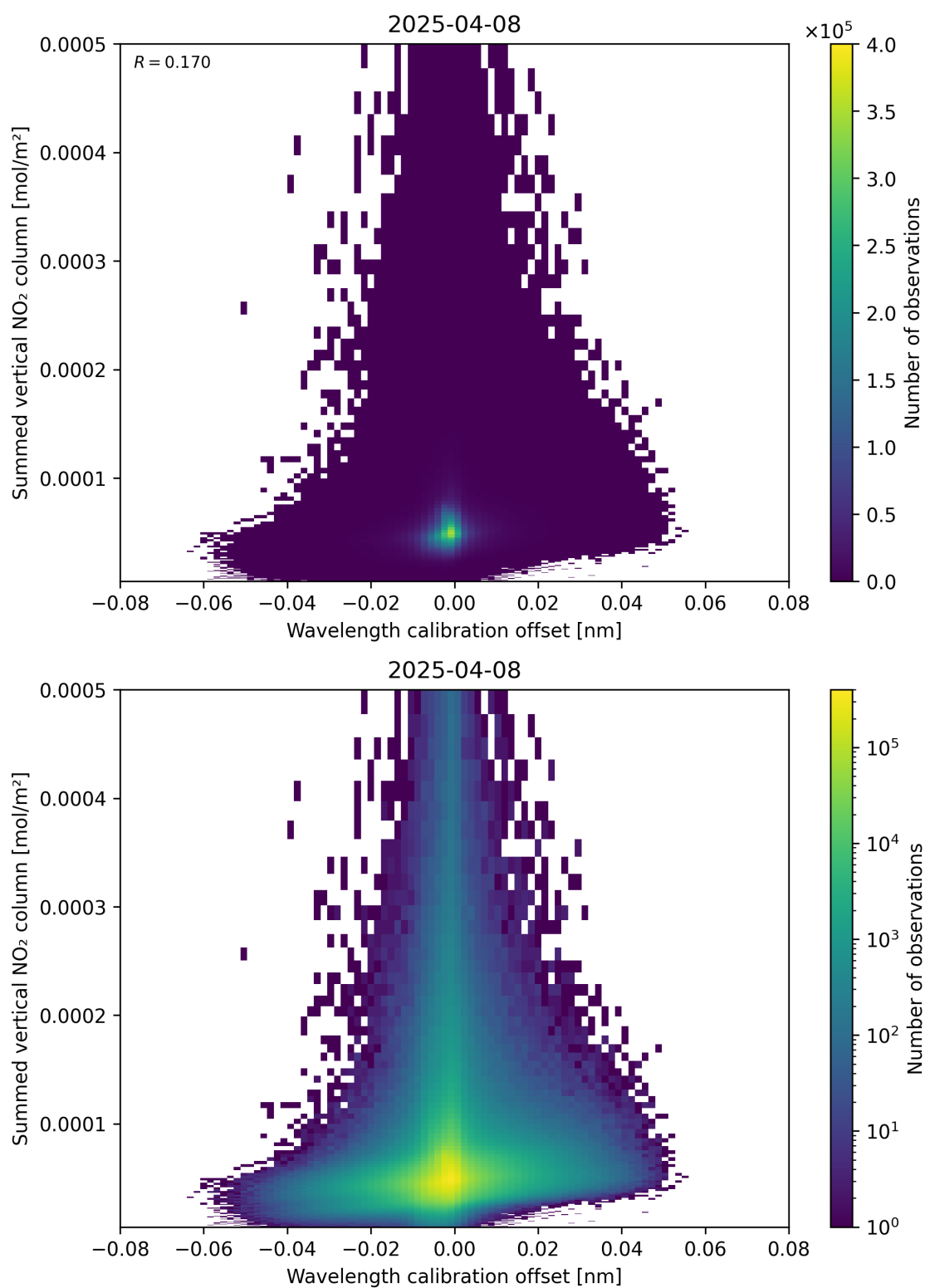
Figure 177: Scatter density plot of “Wavelength calibration offset” against “Summed vertical NO 2 column” for 2025-04-08 to 2025-04-09.
