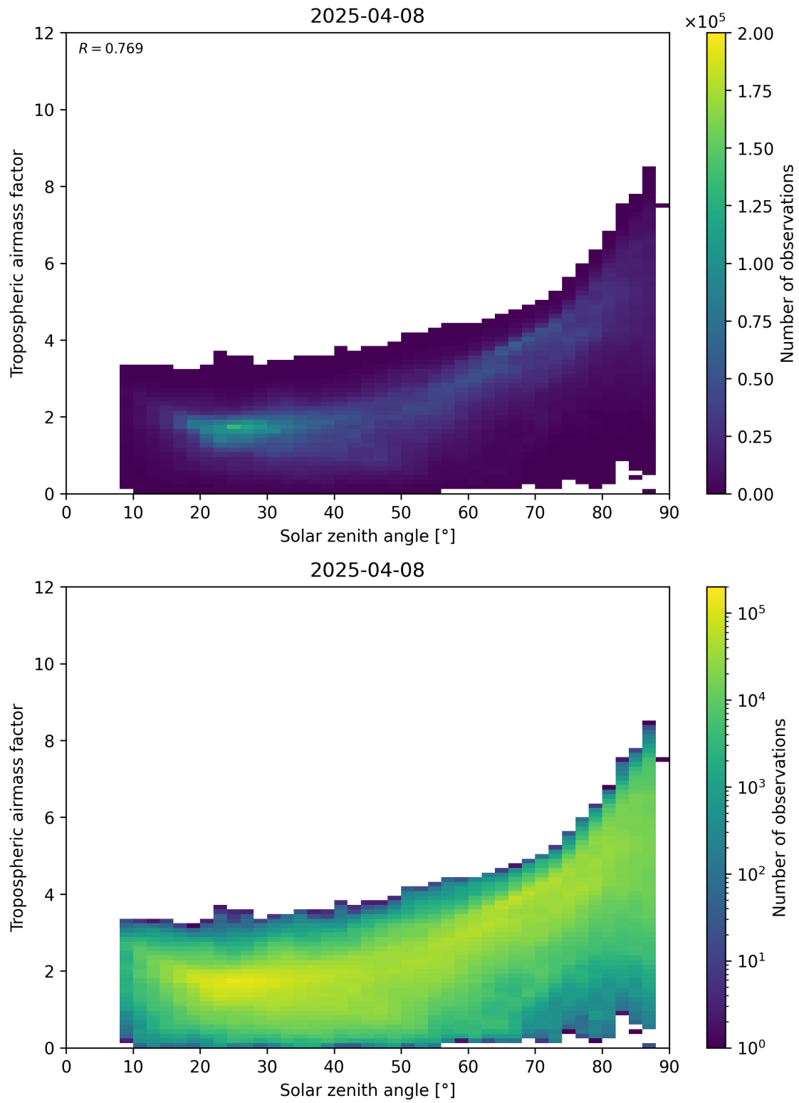
Figure 147: Scatter density plot of “Solar zenith angle” against “Tropospheric airmass factor” for 2025-04-08 to 2025-04-09.
