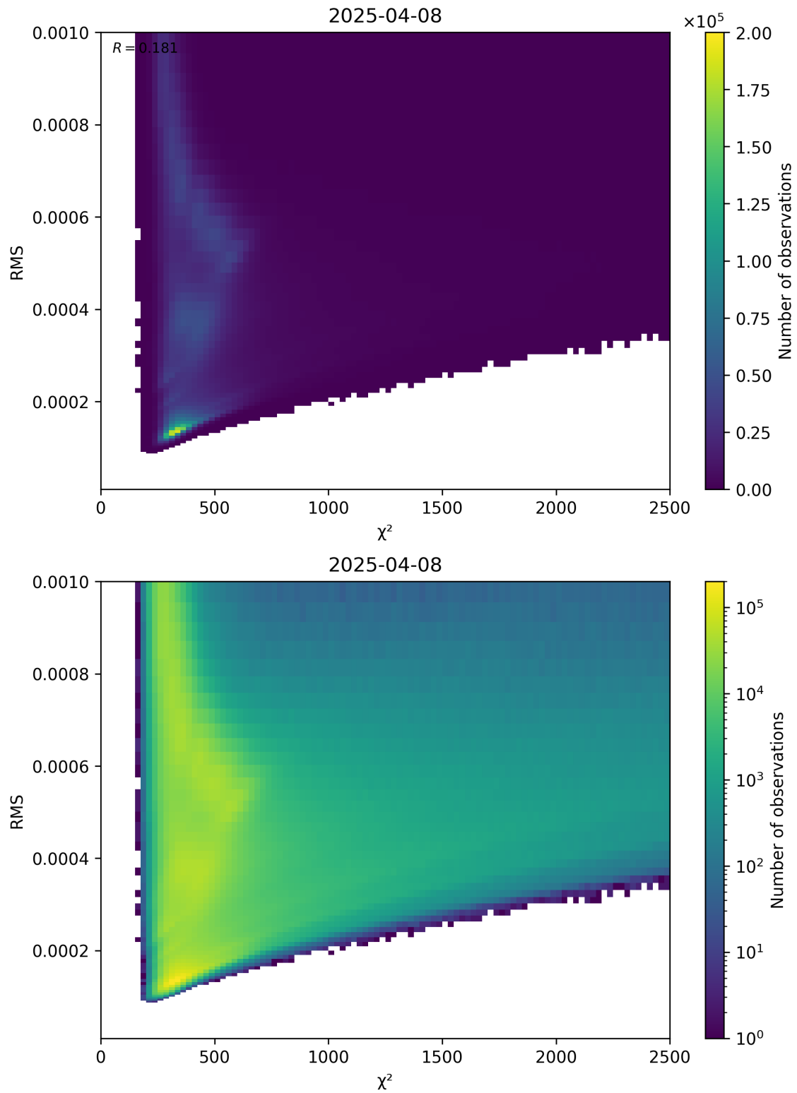
Figure 82: Scatter density plot of “ \chi^2 ” against “RMS” for 2025-04-08 to 2025-04-09.
