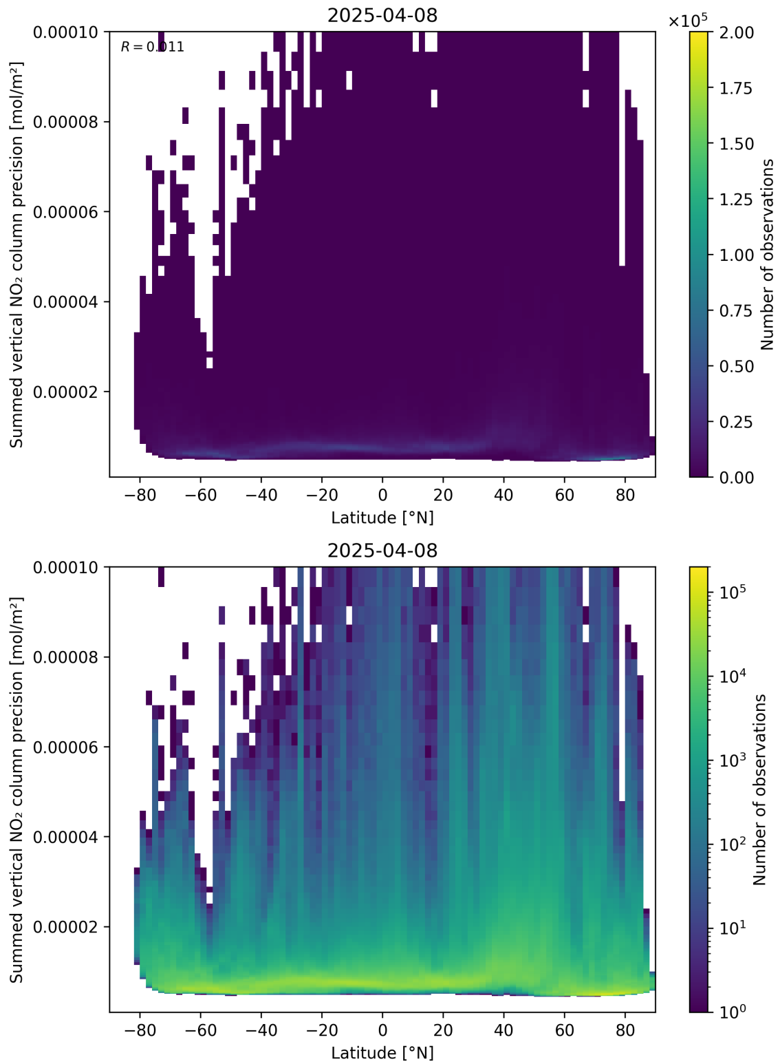
Figure 89: Scatter density plot of “Latitude” against “Summed vertical NO 2 column precision” for 2025-04-08 to 2025-04-09.
