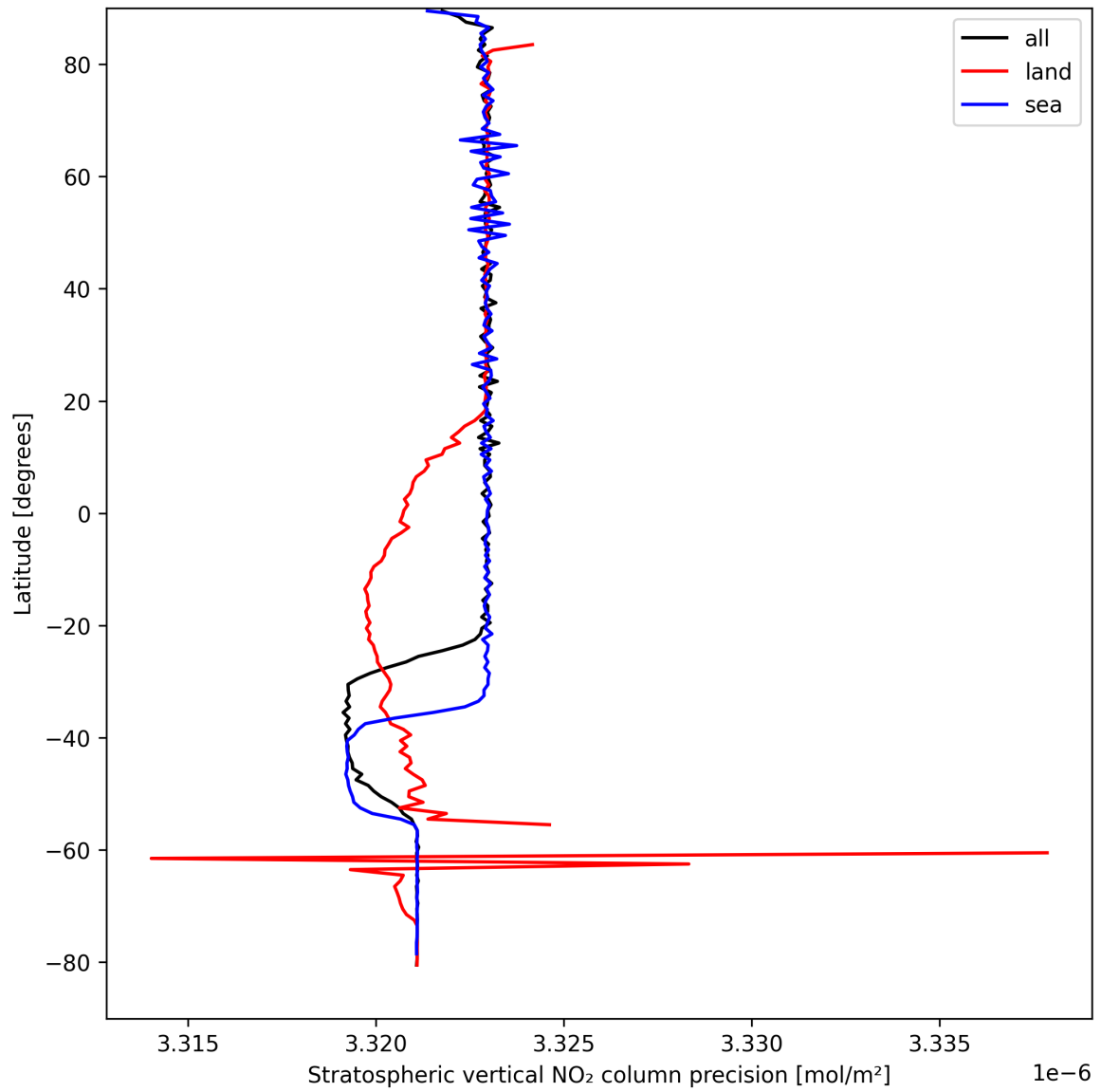
Figure 20: Zonal average of “Stratospheric vertical NO 2 column precision” for 2025-04-08 to 2025-04-09.
