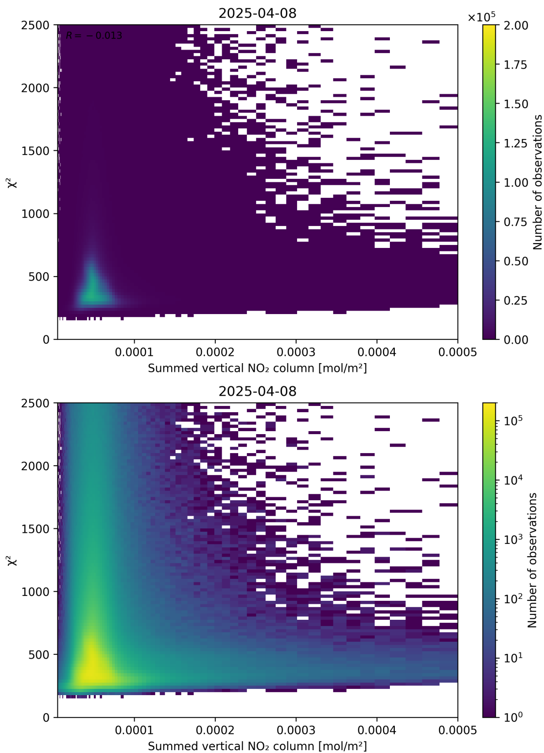
Figure 104: Scatter density plot of “Summed vertical NO 2 column” against “ \chi^2 ” for 2025-04-08 to 2025-04-09.
