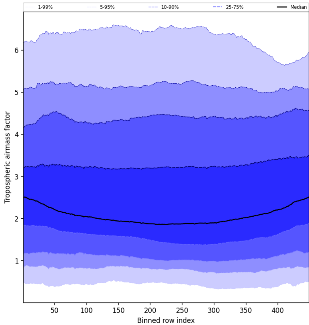
Figure 48: Along track statistics of “Tropospheric airmass factor” for 2025-04-08 to 2025-04-09
