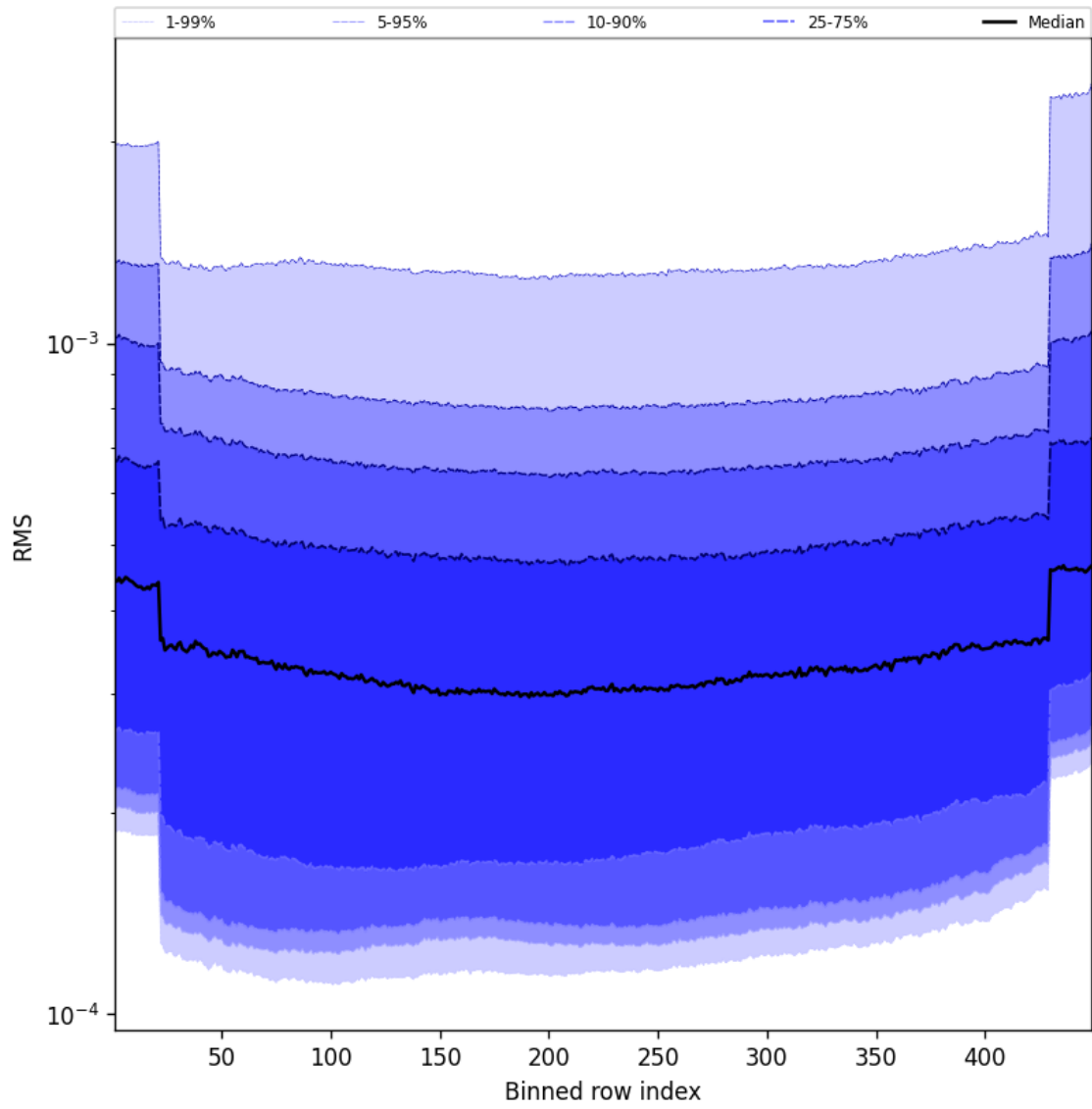
Figure 60: Along track statistics of “RMS” for 2025-04-08 to 2025-04-09
