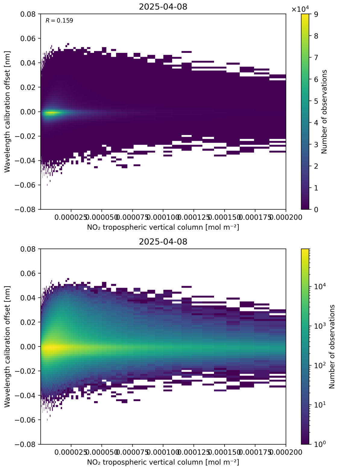
Figure 143: Scatter density plot of “NO 2 tropospheric vertical column” against “Wavelength calibration offset” for 2025-04-08 to 2025-04-09.
