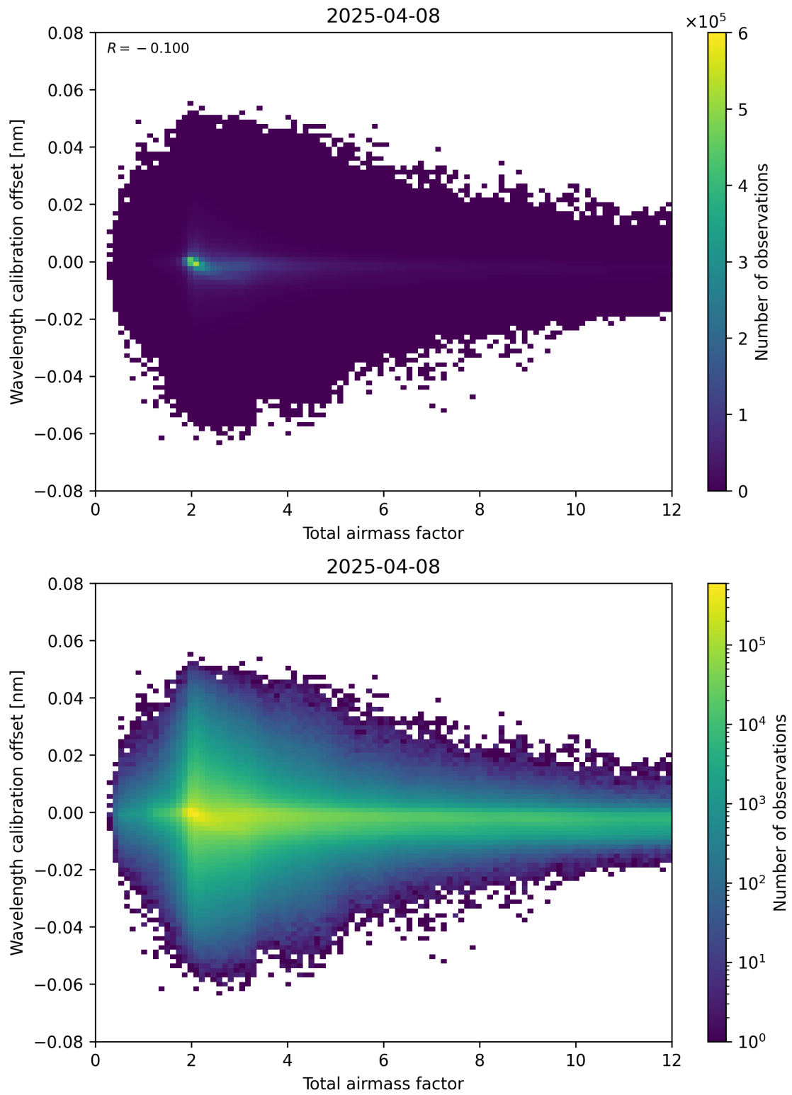
Figure 70: Scatter density plot of “Total airmass factor” against “Wavelength calibration offset” for 2025-04-08 to 2025-04-09.
