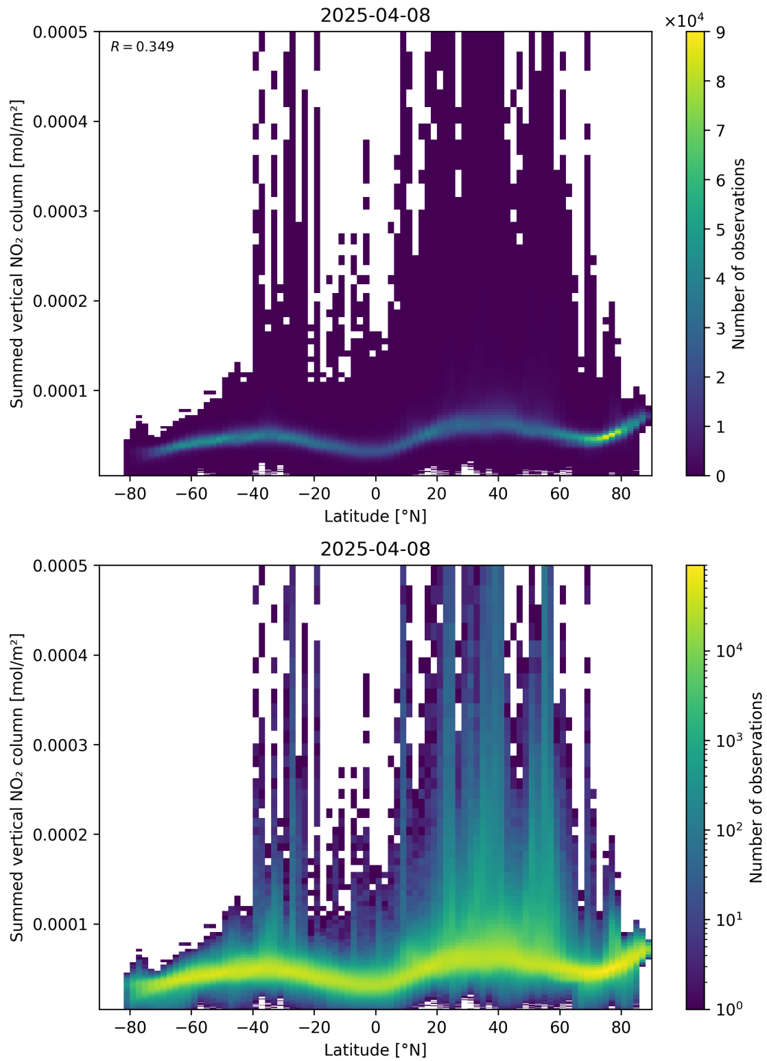
Figure 88: Scatter density plot of “Latitude” against “Summed vertical NO 2 column” for 2025-04-08 to 2025-04-09.
