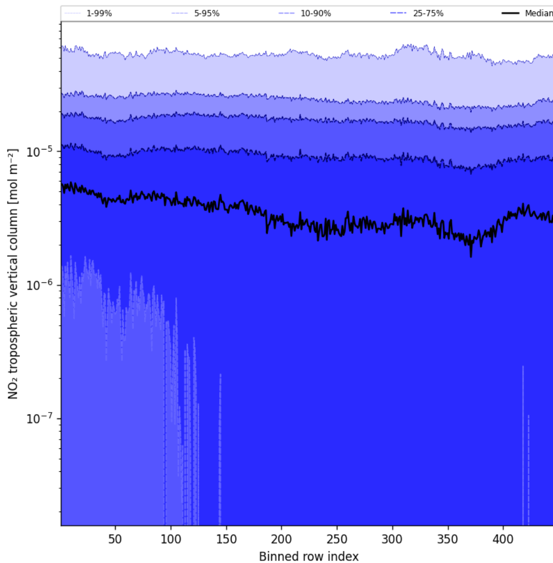
Figure 46: Along track statistics of “NO 2 tropospheric vertical column” for 2025-04-08 to 2025-04-09
