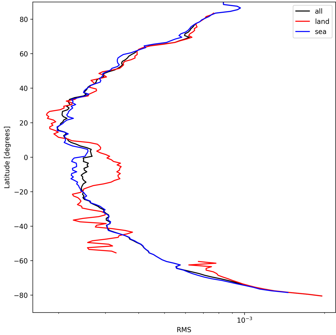
Figure 26: Zonal average of “RMS” for 2025-04-08 to 2025-04-09.
