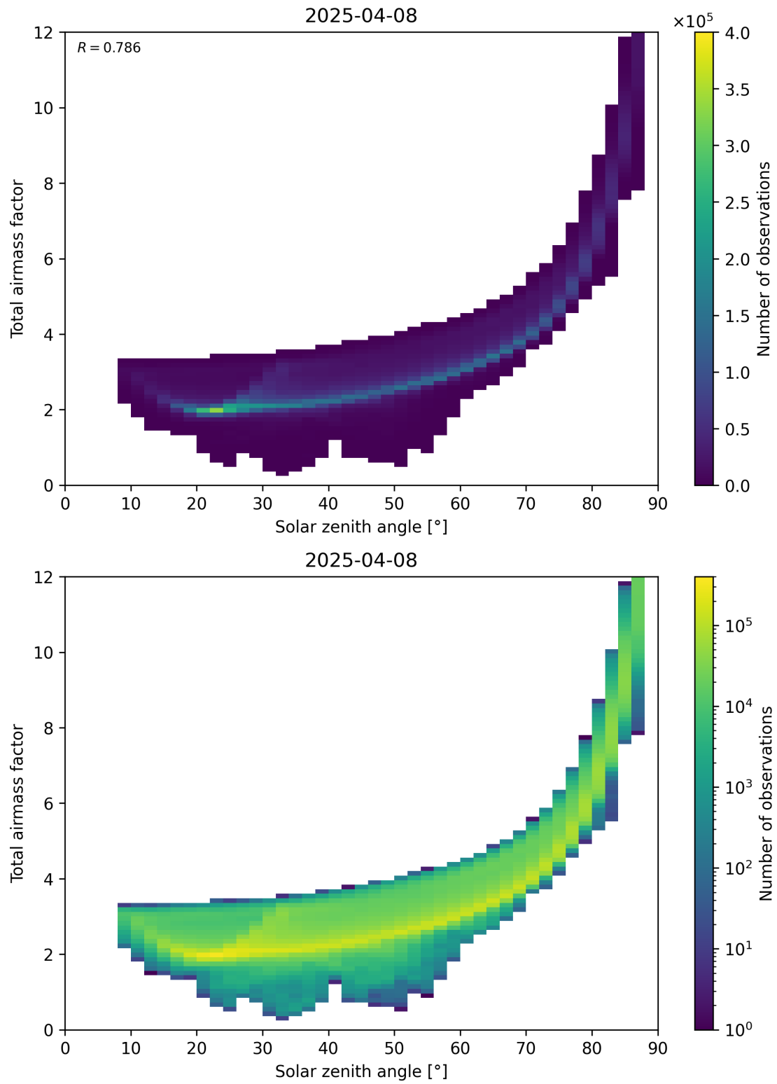
Figure 146: Scatter density plot of “Solar zenith angle” against “Total airmass factor” for 2025-04-08 to 2025-04-09.
