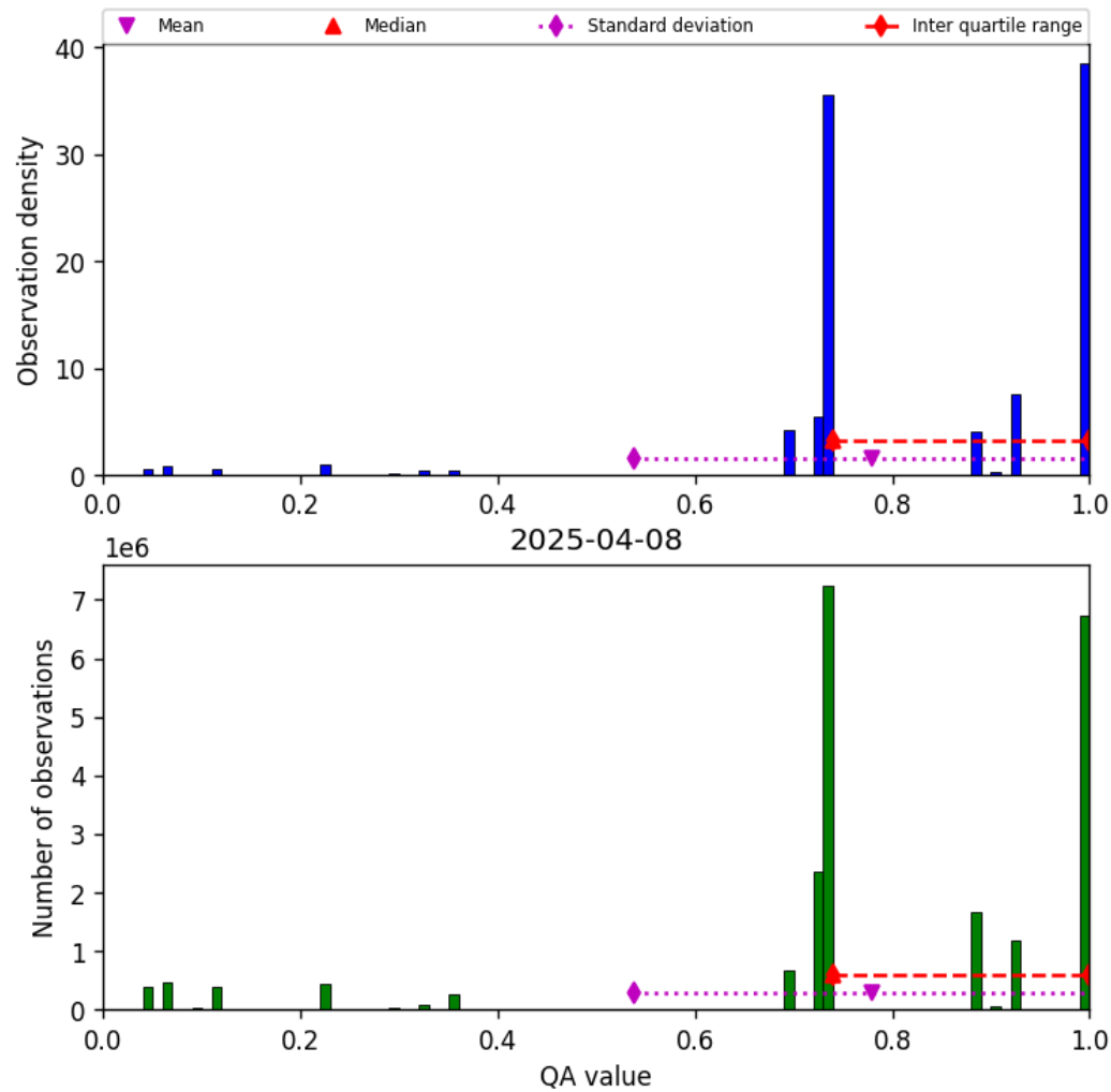
Figure 28: Histogram of “QA value” for 2025-04-08 to 2025-04-09
