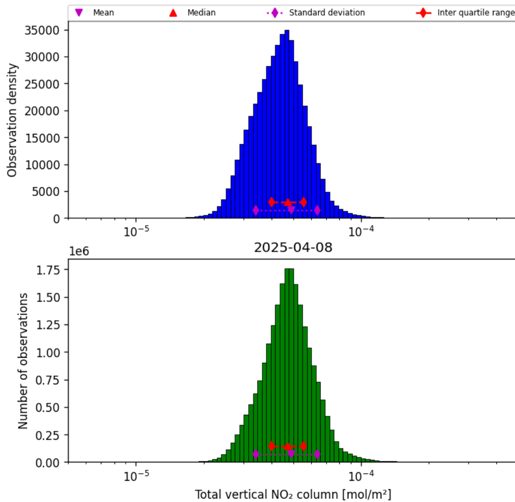
Figure 38: Histogram of “Total vertical NO 2 column” for 2025-04-08 to 2025-04-09
