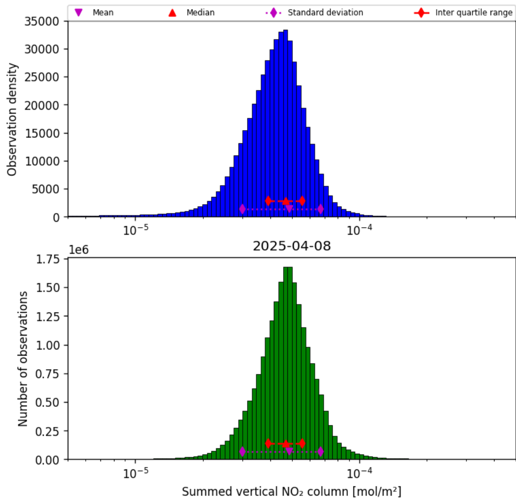
Figure 40: Histogram of “Summed vertical NO 2 column” for 2025-04-08 to 2025-04-09
