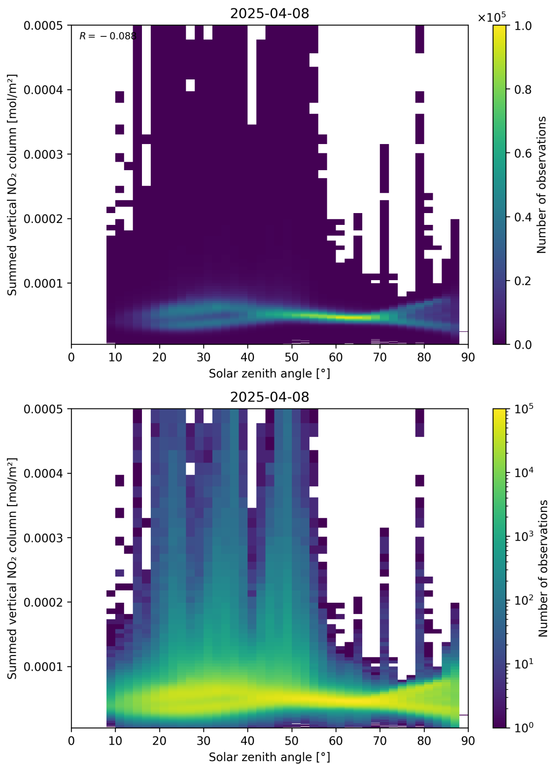
Figure 151: Scatter density plot of “Solar zenith angle” against “Summed vertical NO 2 column” for 2025-04-08 to 2025-04-09.
