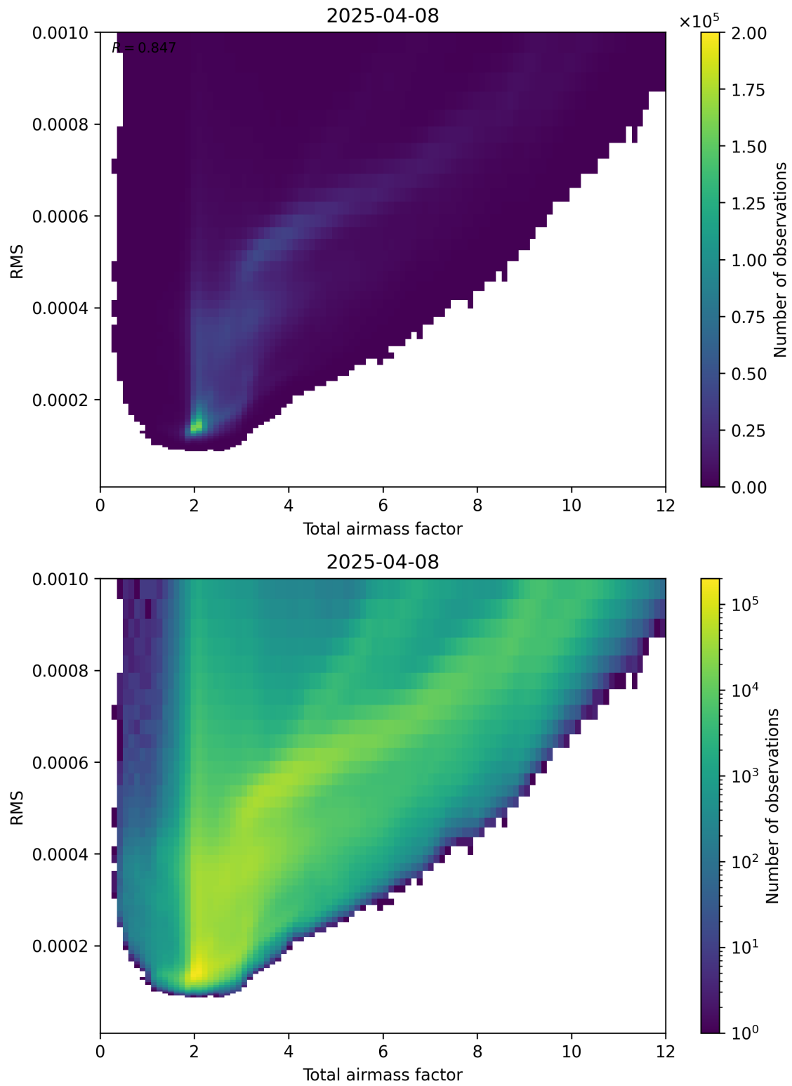
Figure 69: Scatter density plot of “Total airmass factor” against “RMS” for 2025-04-08 to 2025-04-09.
