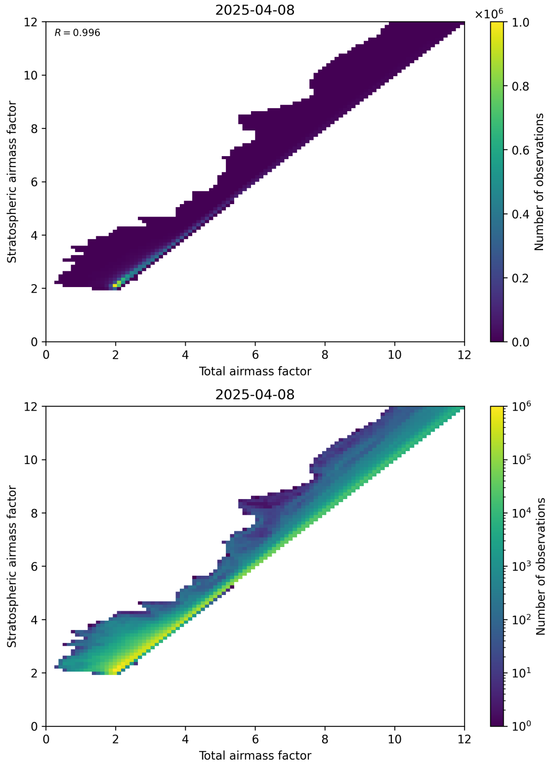
Figure 62: Scatter density plot of “Total airmass factor” against “Stratospheric airmass factor” for 2025-04-08 to 2025-04-09.
