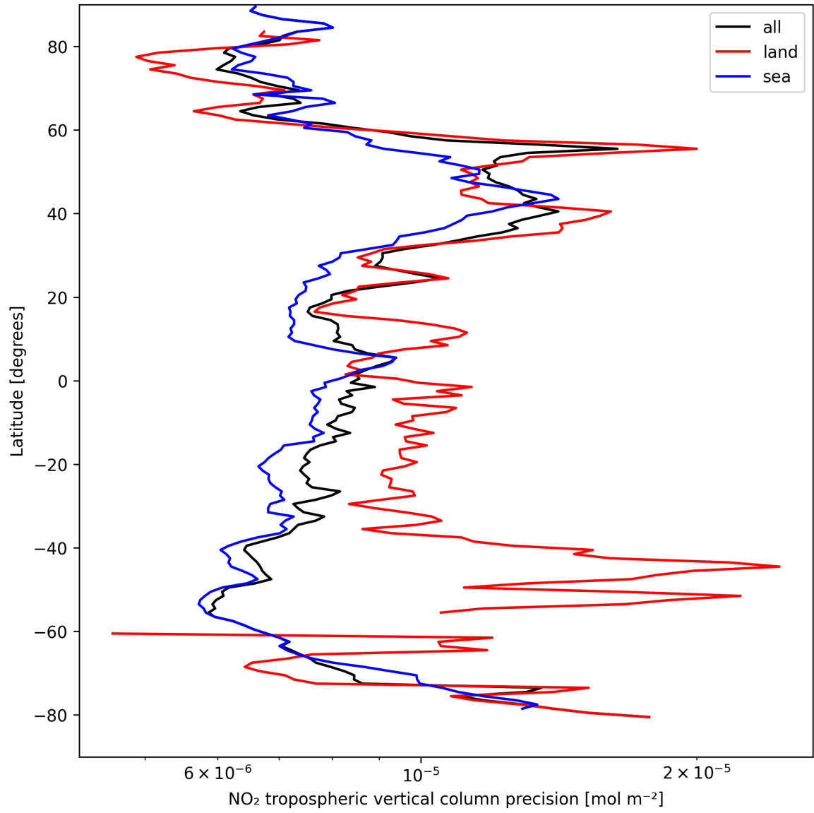
Figure 13: Zonal average of “NO 2 tropospheric vertical column precision” for 2025-04-08 to 2025-04-09.
