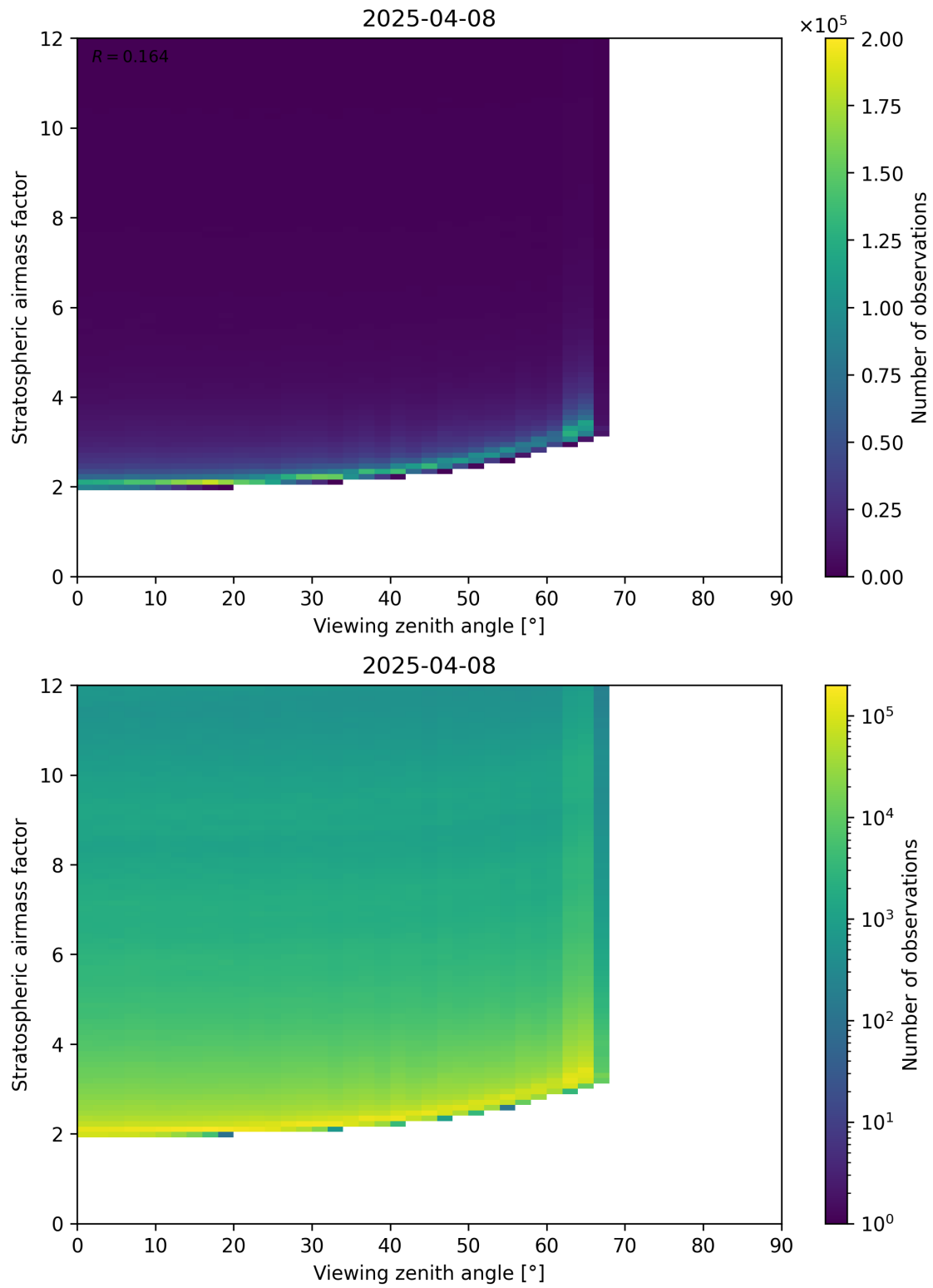
Figure 159: Scatter density plot of “Viewing zenith angle” against “Stratospheric airmass factor” for 2025-04-08 to 2025-04-09.
