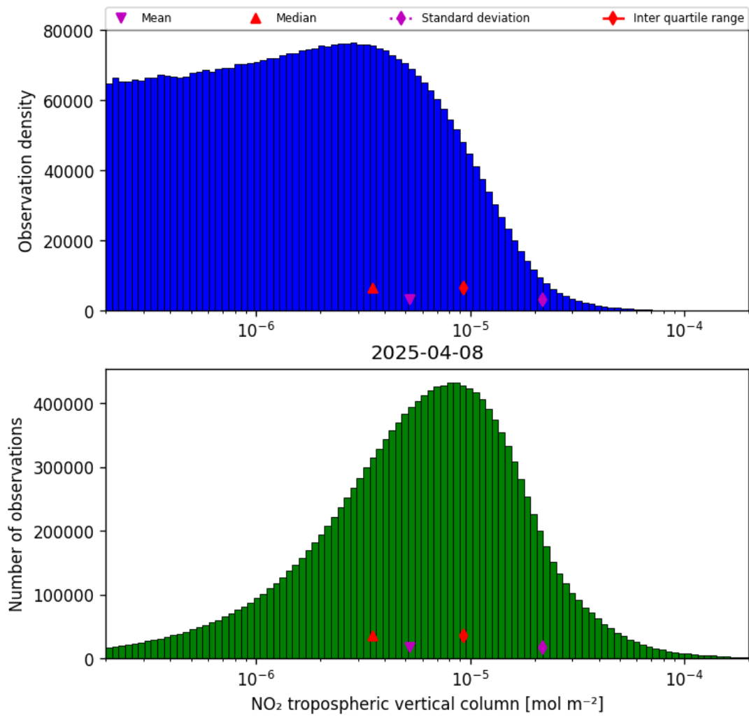
Figure 29: Histogram of “NO 2 tropospheric vertical column” for 2025-04-08 to 2025-04-09
