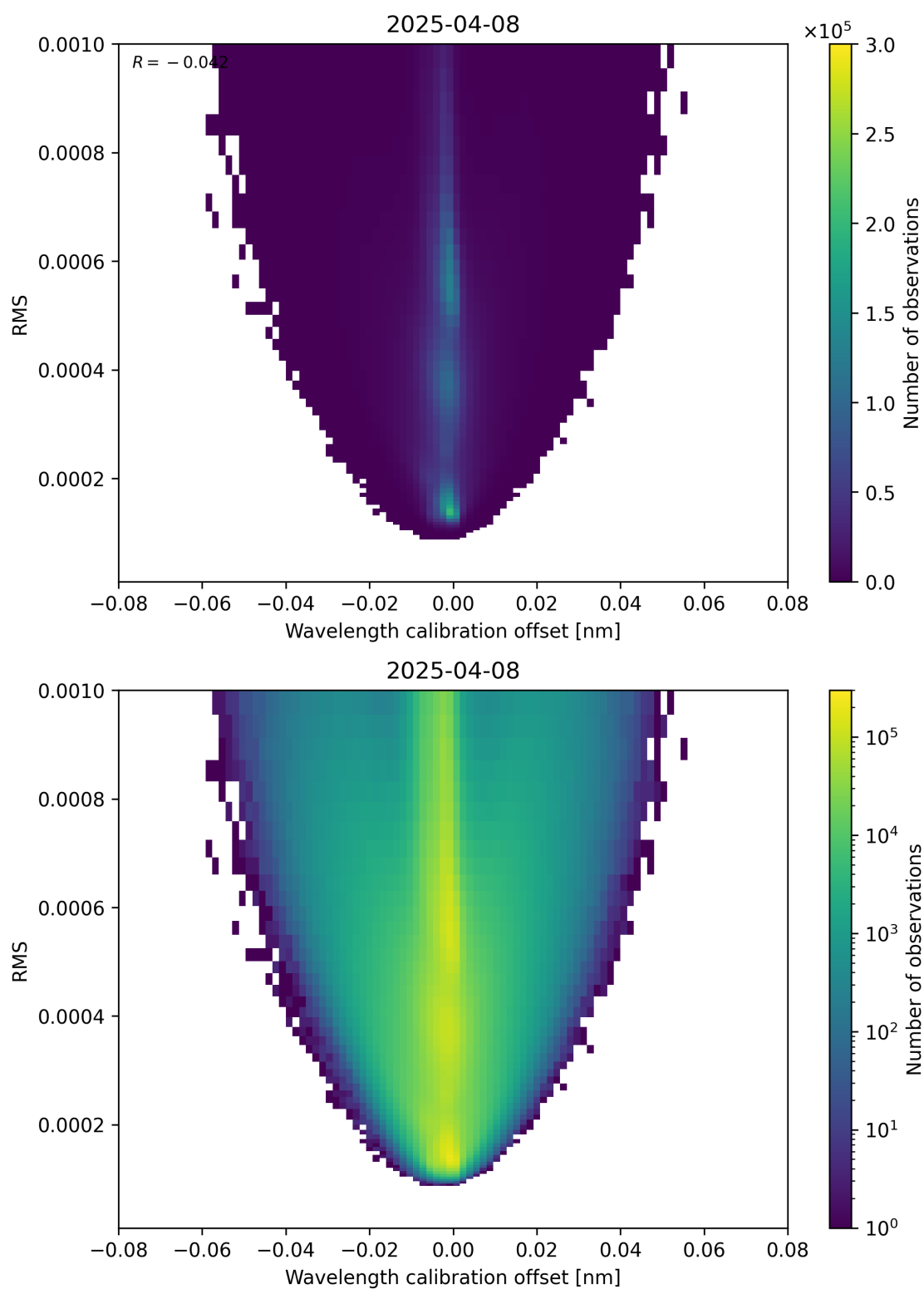
Figure 181: Scatter density plot of “Wavelength calibration offset” against “RMS” for 2025-04-08 to 2025-04-09.
