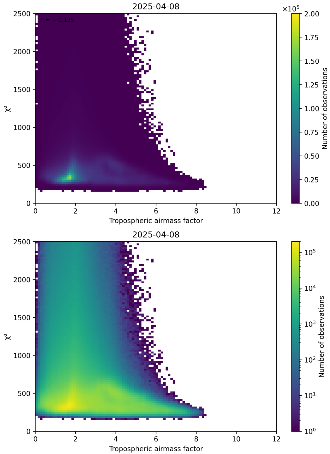
Figure 73: Scatter density plot of “Tropospheric airmass factor” against “ \chi^2 ” for 2025-04-08 to 2025-04-09.
