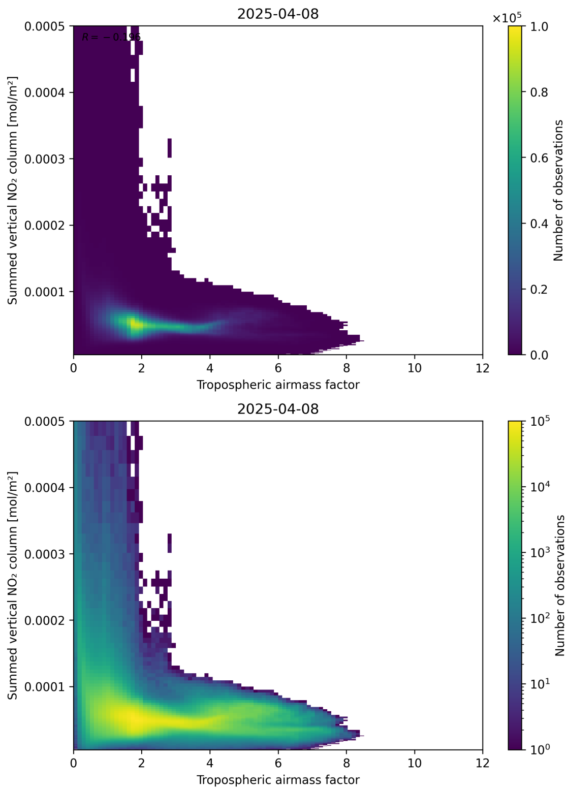
Figure 75: Scatter density plot of “Tropospheric air mass factor” against “Summed vertical NO 2 column” for 2025-04-08 to 2025-04-09.
