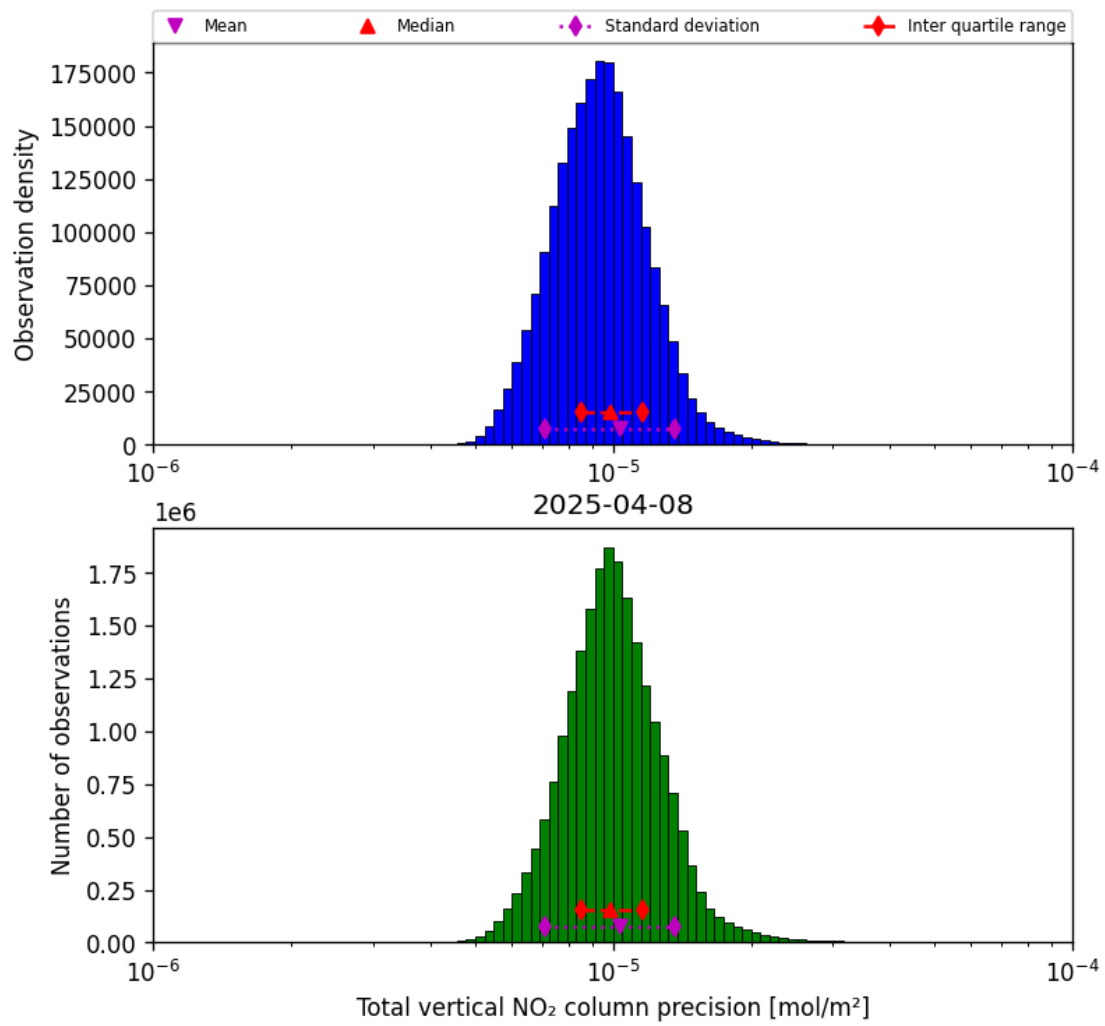
Figure 39: Histogram of “Total vertical NO 2 column precision” for 2025-04-08 to 2025-04-09
