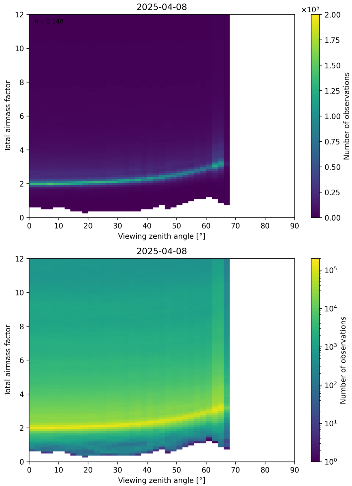
Figure 160: Scatter density plot of “Viewing zenith angle” against “Total airmass factor” for 2025-04-08 to 2025-04-09.
