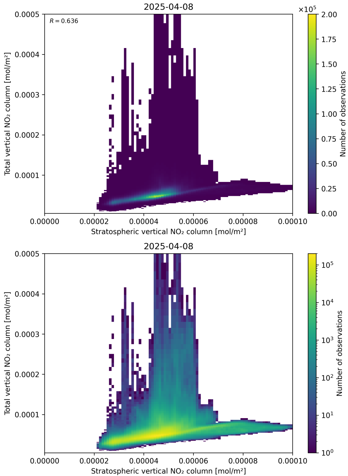
Figure 100: Scatter density plot of “Stratospheric vertical NO 2 column” against “Total vertical NO 2 column” for 2025-04-08 to 2025-04-09.
