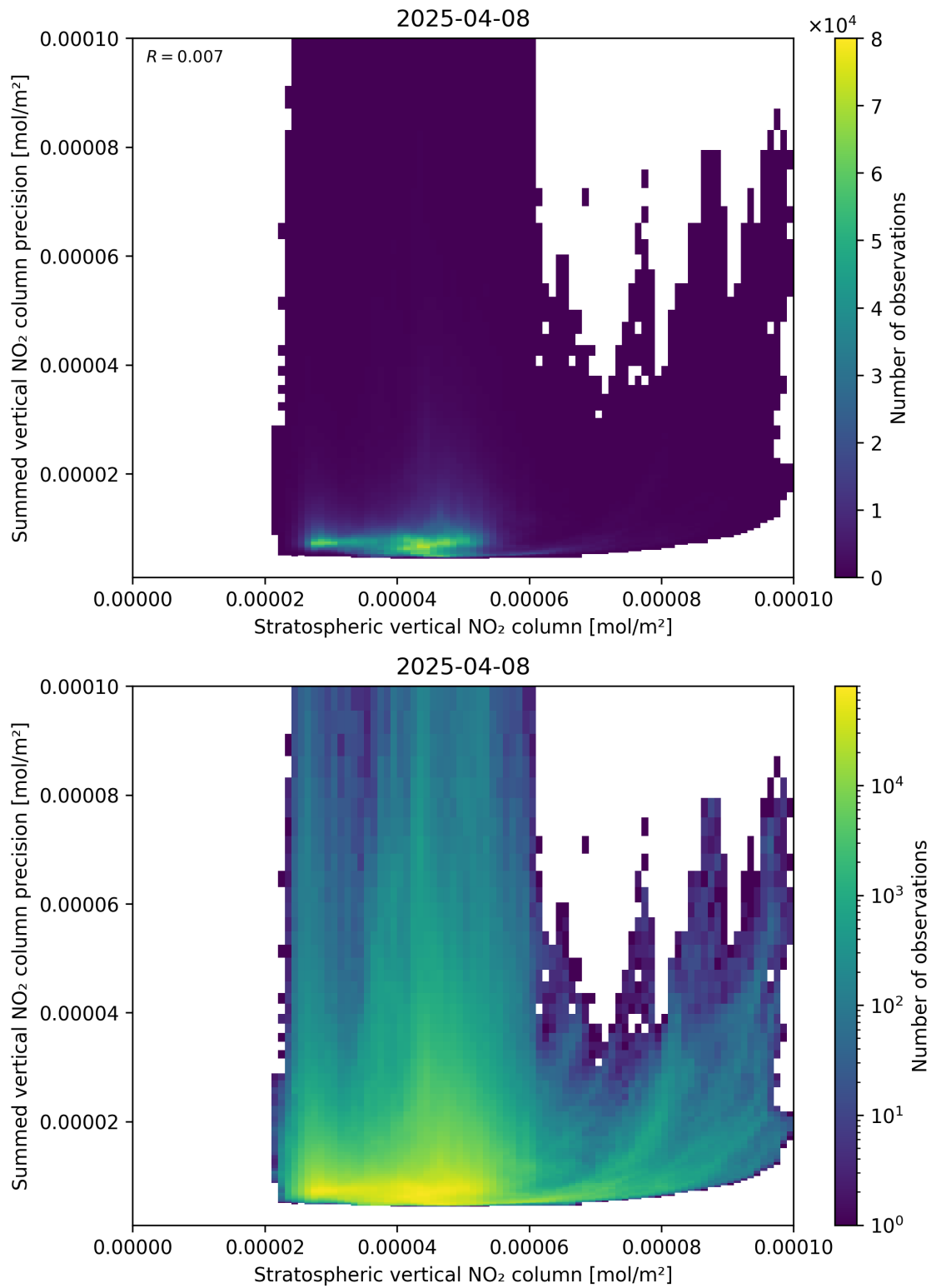
Figure 99: Scatter density plot of “Stratospheric vertical NO 2 column” against “Summed vertical NO 2 column precision” for 2025-04-08 to 2025-04-09.
