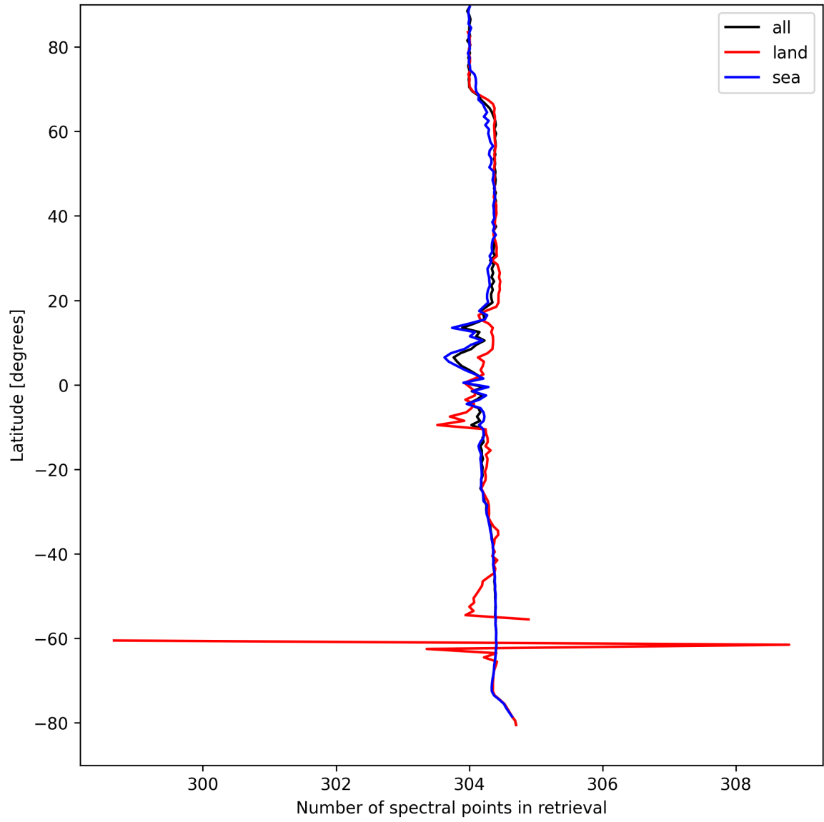
Figure 16: Zonal average of “Number of spectral points in retrieval” for 2025-04-08 to 2025-04-09.
