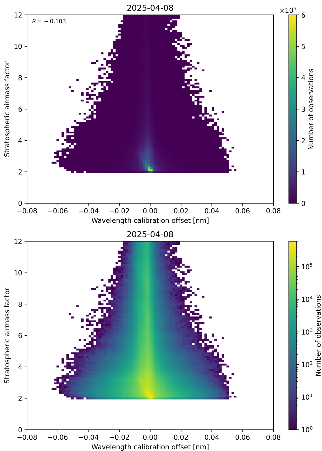
Figure 174: Scatter density plot of “Wavelength calibration offset” against “Stratospheric air mass factor” for 2025-04-08 to 2025-04-09.
