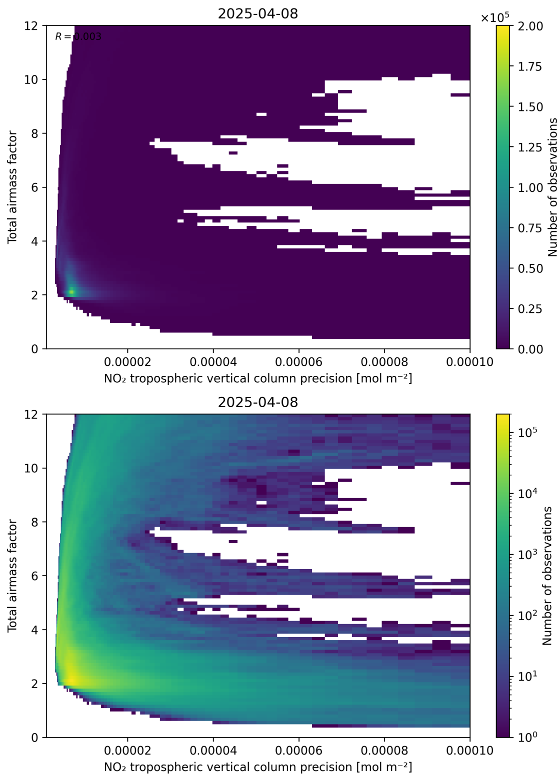
Figure 132: Scatter density plot of “NO 2 tropospheric vertical column precision” against “Total air mass factor” for 2025-04-08 to 2025-04-09.
