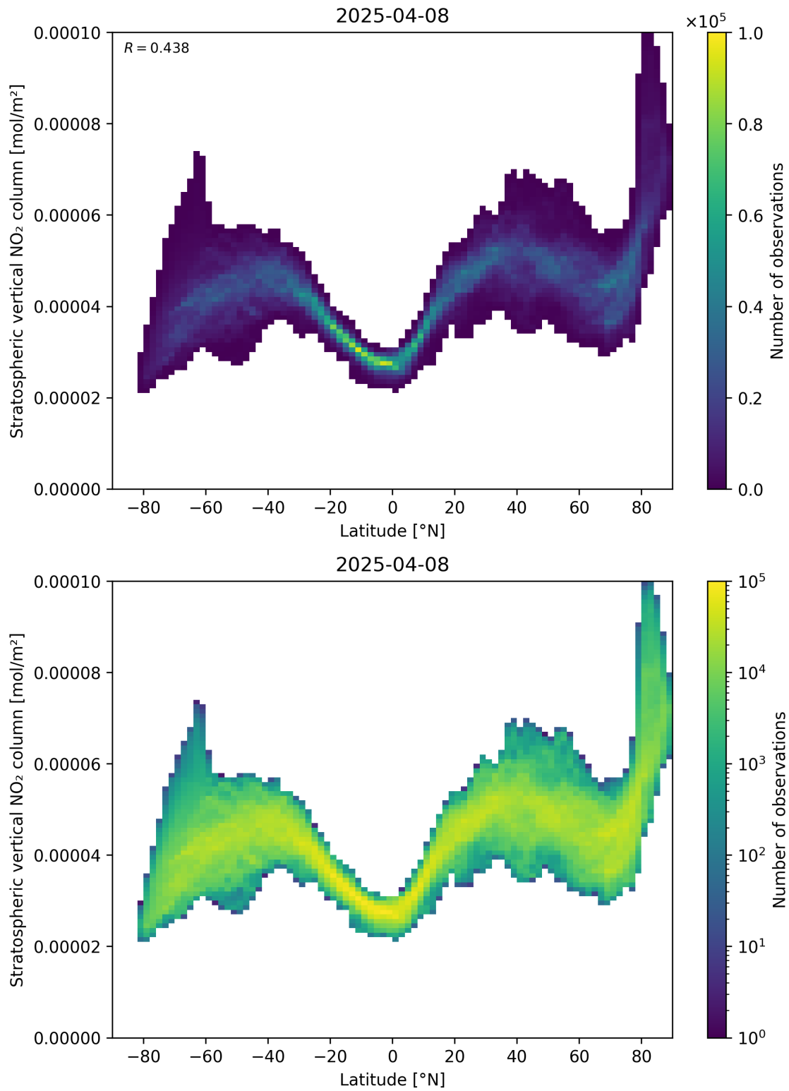
Figure 87: Scatter density plot of “Latitude” against “Stratospheric vertical NO 2 column” for 2025-04-08 to 2025-04-09.
