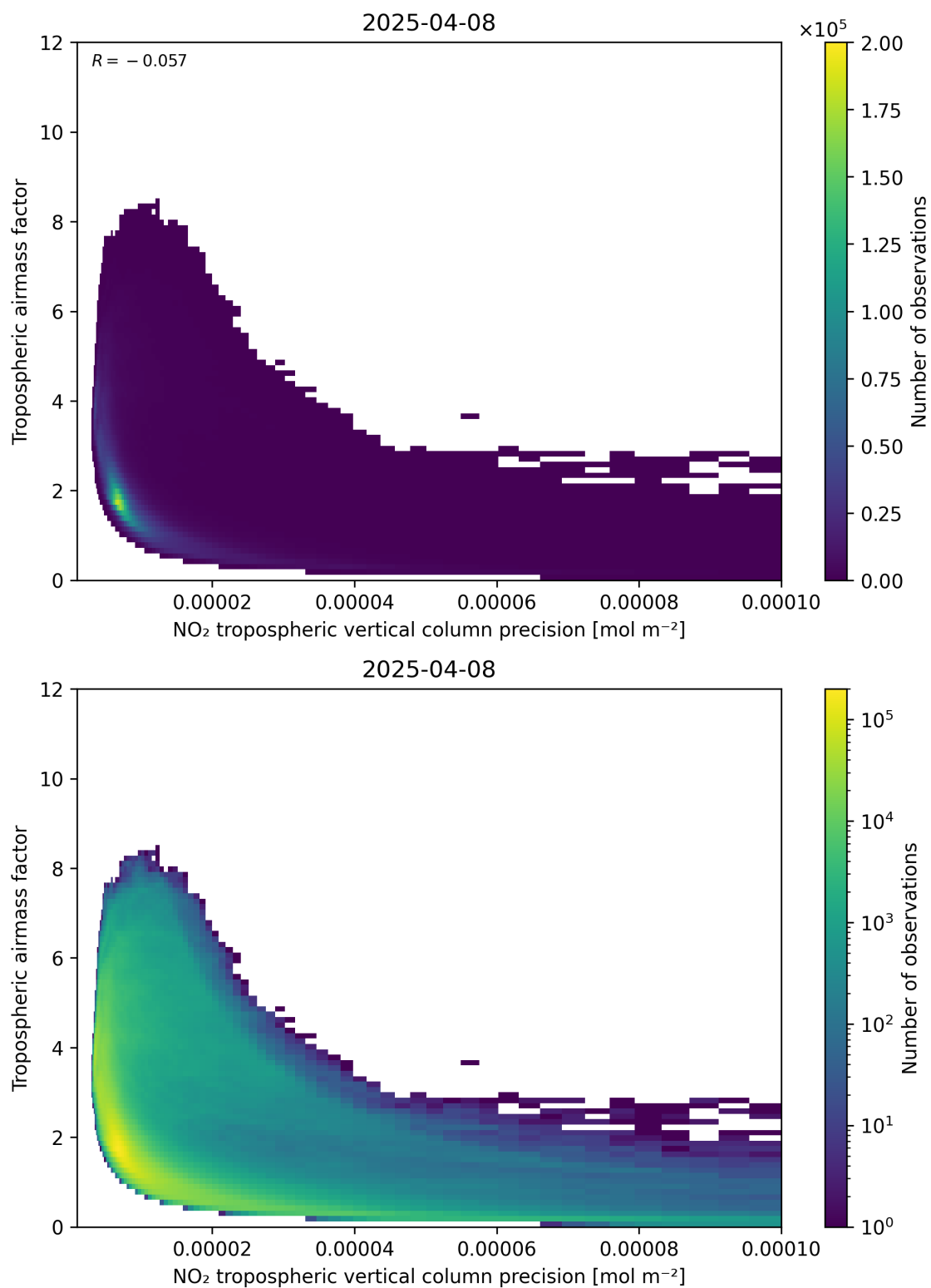
Figure 133: Scatter density plot of “NO 2 tropospheric vertical column precision” against “Tropospheric air mass factor” for 2025-04-08 to 2025-04-09.
