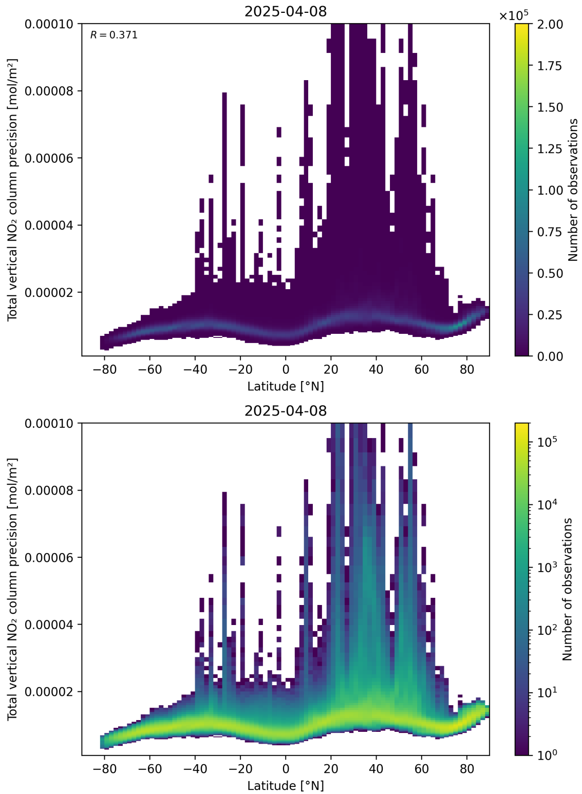
Figure 91: Scatter density plot of “Latitude” against “Total vertical NO 2 column precision” for 2025-04-08 to 2025-04-09.
