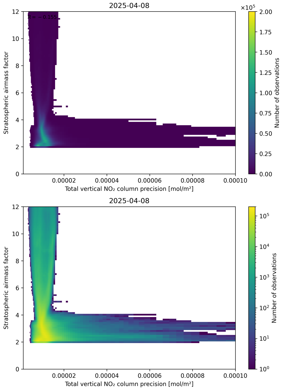
Figure 115: Scatter density plot of “Total vertical NO 2 column precision” against “Stratospheric air mass factor” for 2025-04-08 to 2025-04-09.
