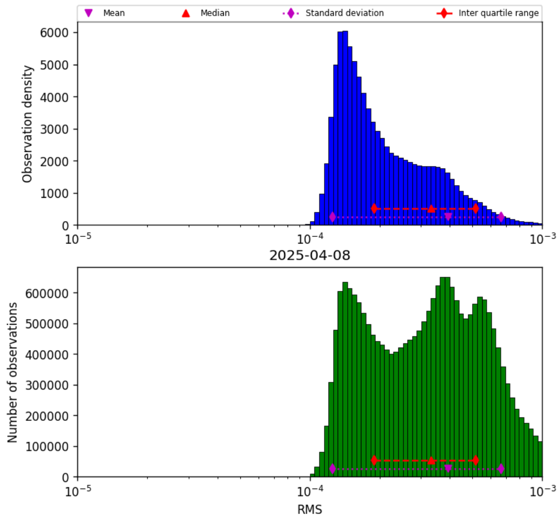
Figure 43: Histogram of “RMS” for 2025-04-08 to 2025-04-09
