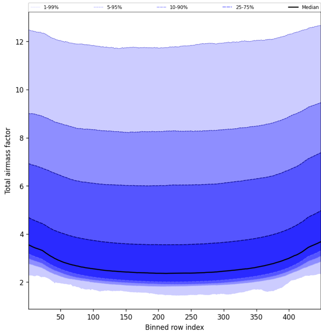
Figure 49: Along track statistics of “Total airmass factor” for 2025-04-08 to 2025-04-09
