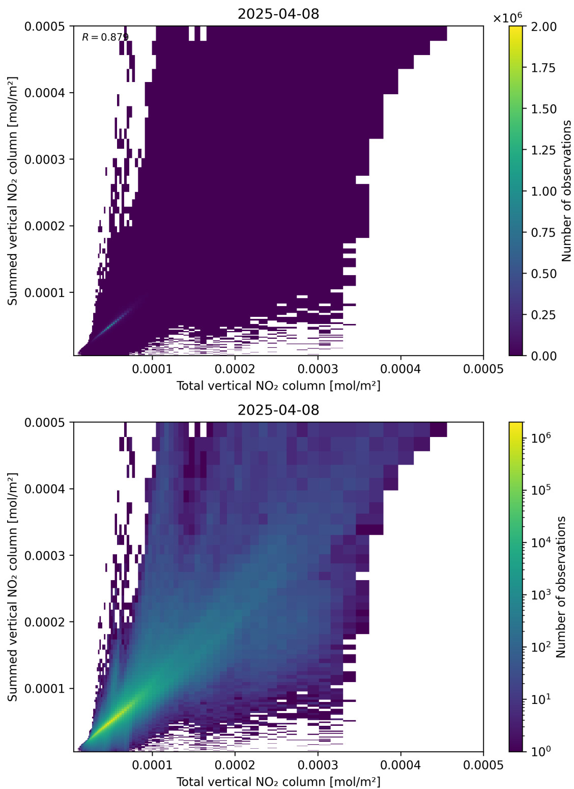
Figure 112: Scatter density plot of “Total vertical NO 2 column” against “Summed vertical NO 2 column” for 2025-04-08 to 2025-04-09.
