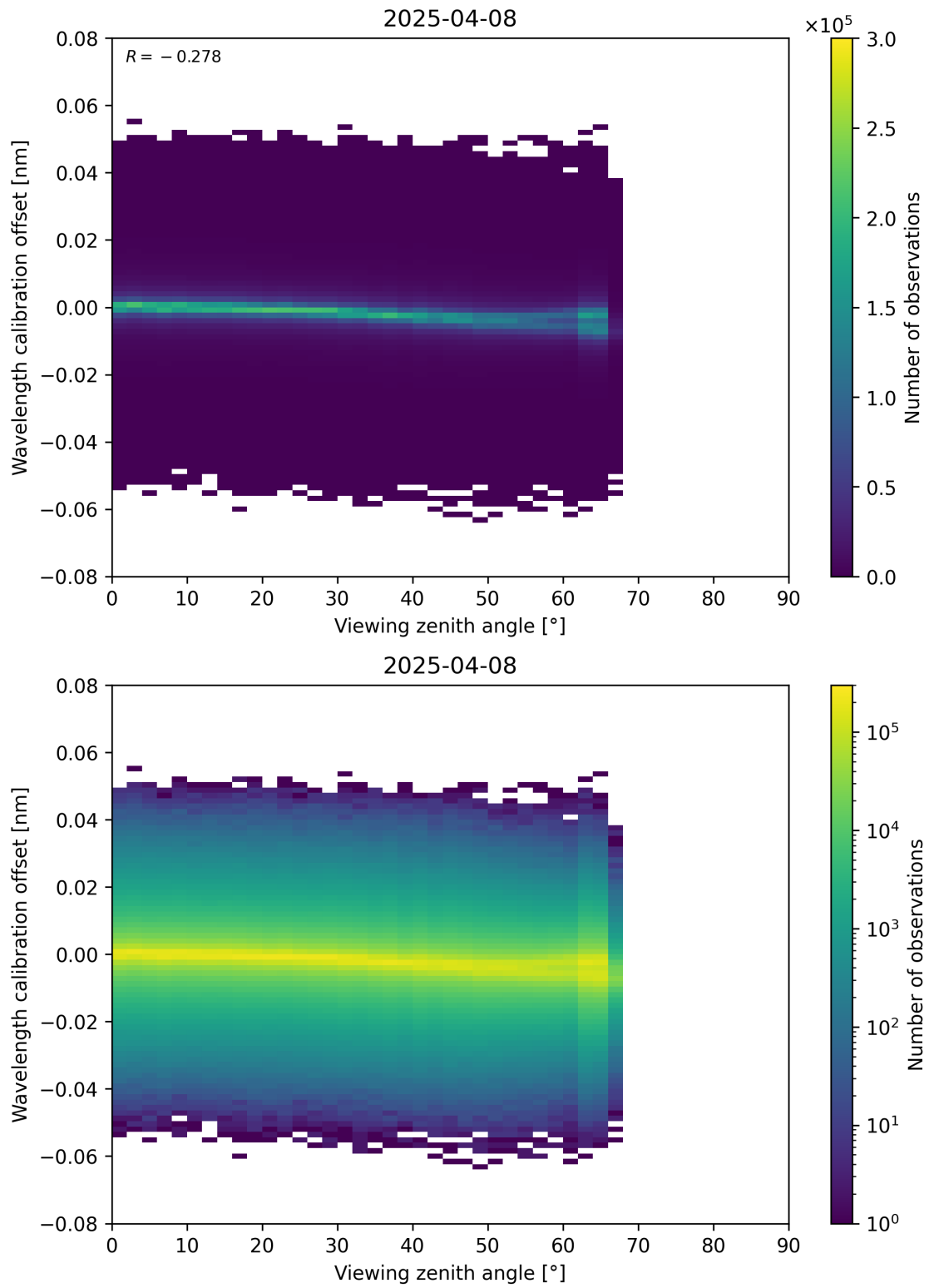
Figure 173: Scatter density plot of “Viewing zenith angle” against “Wavelength calibration offset” for 2025-04-08 to 2025-04-09.
