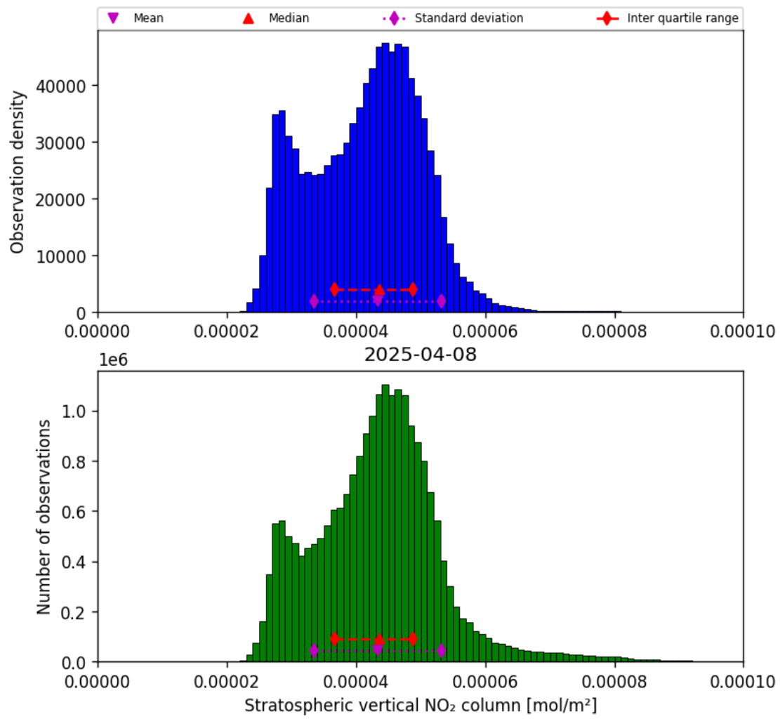
Figure 36: Histogram of “Stratospheric vertical NO 2 column” for 2025-04-08 to 2025-04-09
