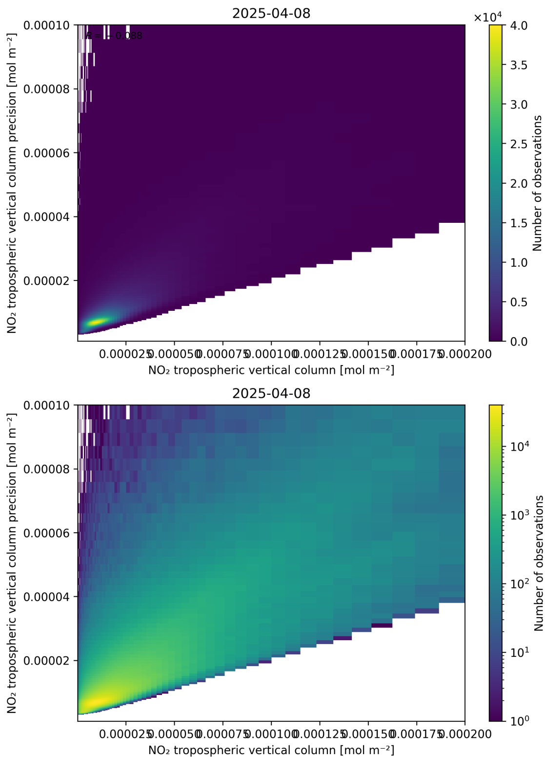
Figure 130: Scatter density plot of “NO 2 tropospheric vertical column” against “NO 2 tropospheric vertical column precision” for 2025-04-08 to 2025-04-09.
