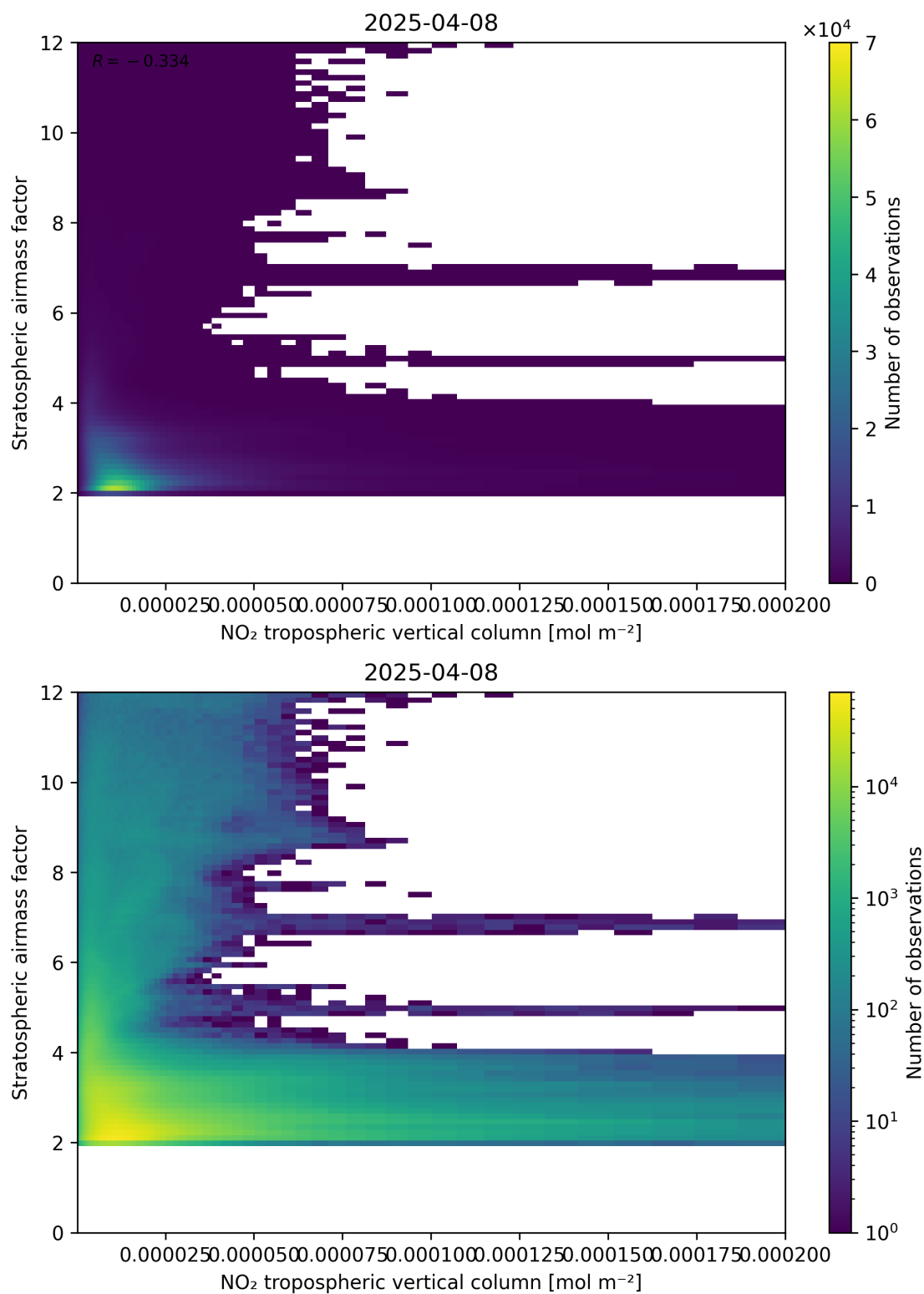
Figure 121: Scatter density plot of “NO 2 tropospheric vertical column” against “Stratospheric airmass factor” for 2025-04-08 to 2025-04-09.
