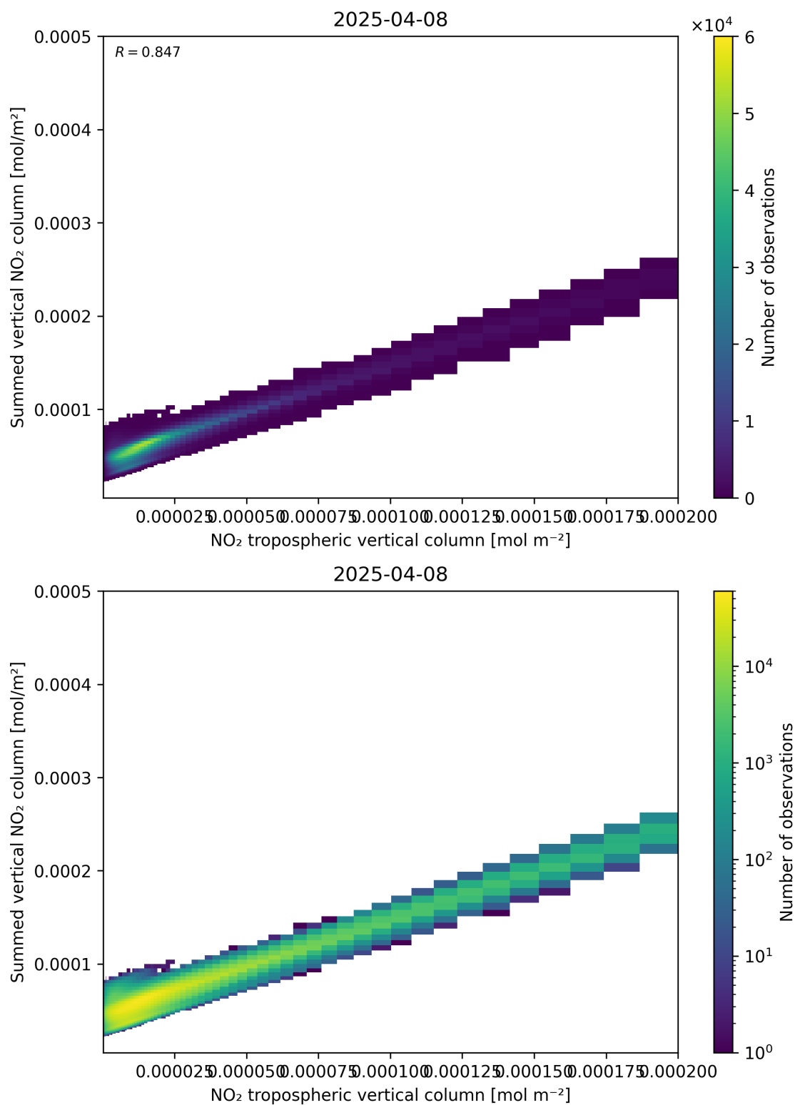
Figure 126: Scatter density plot of “NO 2 tropospheric vertical column” against “Summed vertical NO 2 column” for 2025-04-08 to 2025-04-09.
