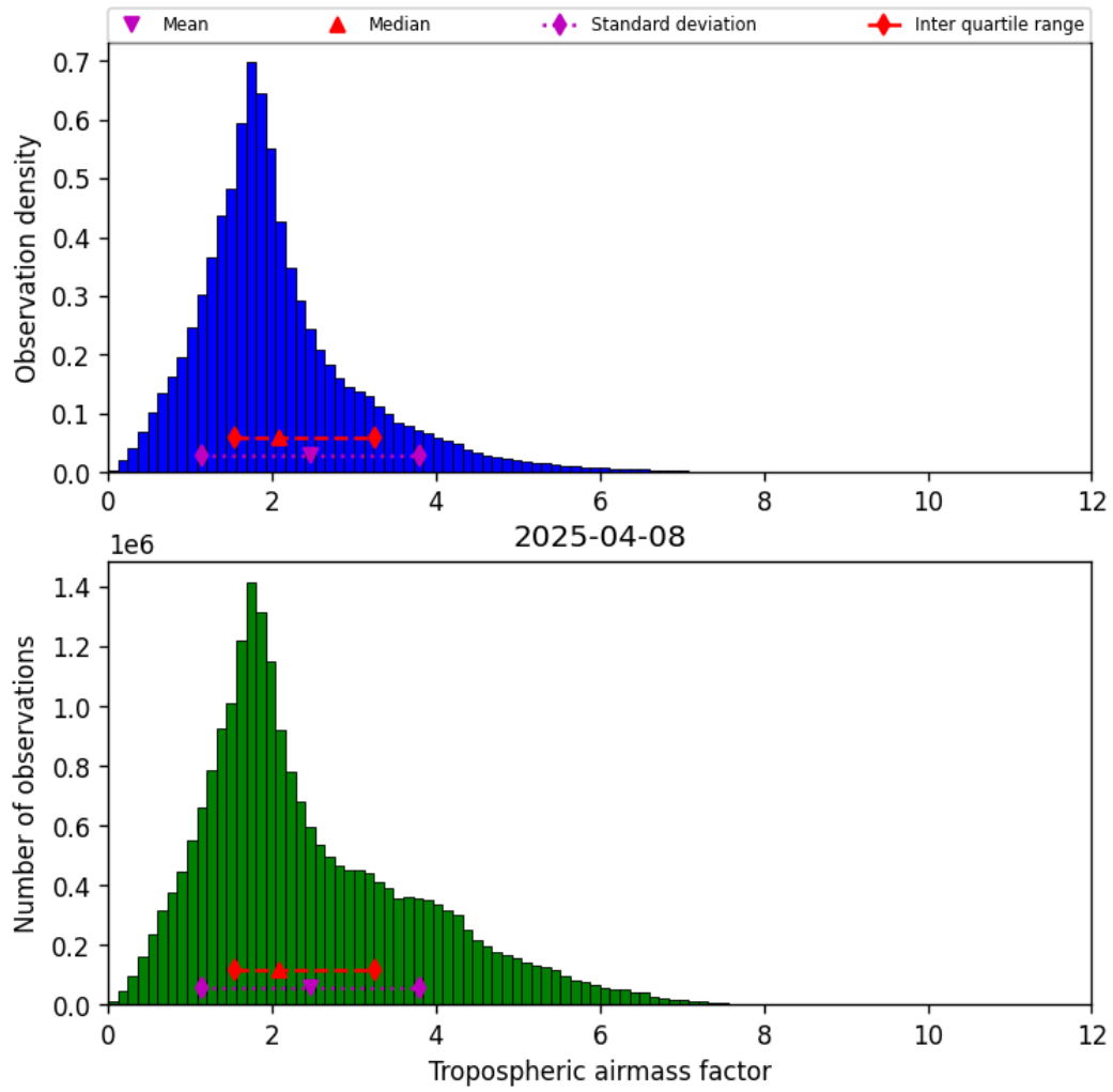
Figure 31: Histogram of “Tropospheric airmass factor” for 2025-04-08 to 2025-04-09
