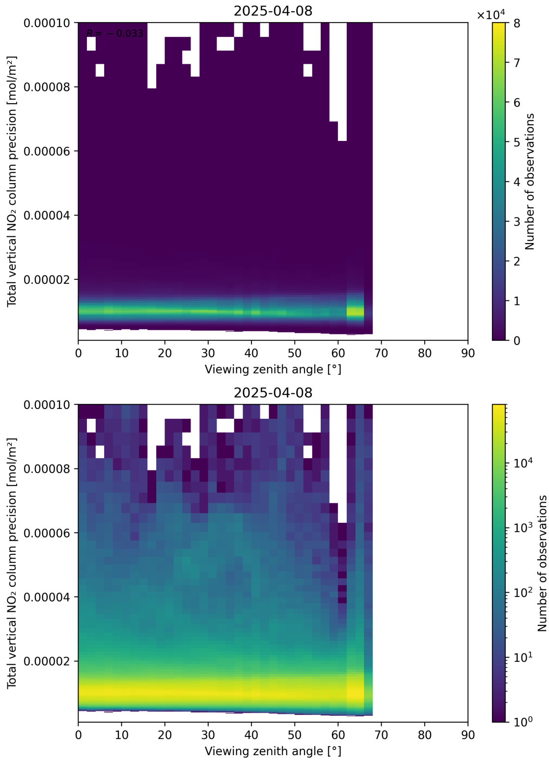
Figure 168: Scatter density plot of “Viewing zenith angle” against “Total vertical NO 2 column precision” for 2025-04-08 to 2025-04-09.
