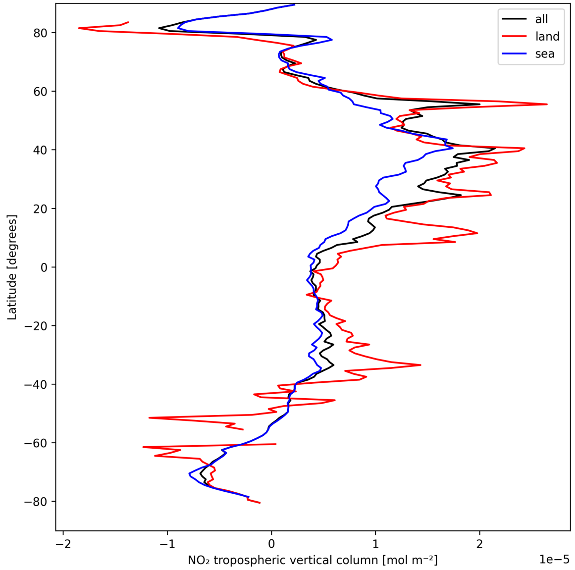
Figure 12: Zonal average of “NO 2 tropospheric vertical column” for 2025-04-08 to 2025-04-09.
