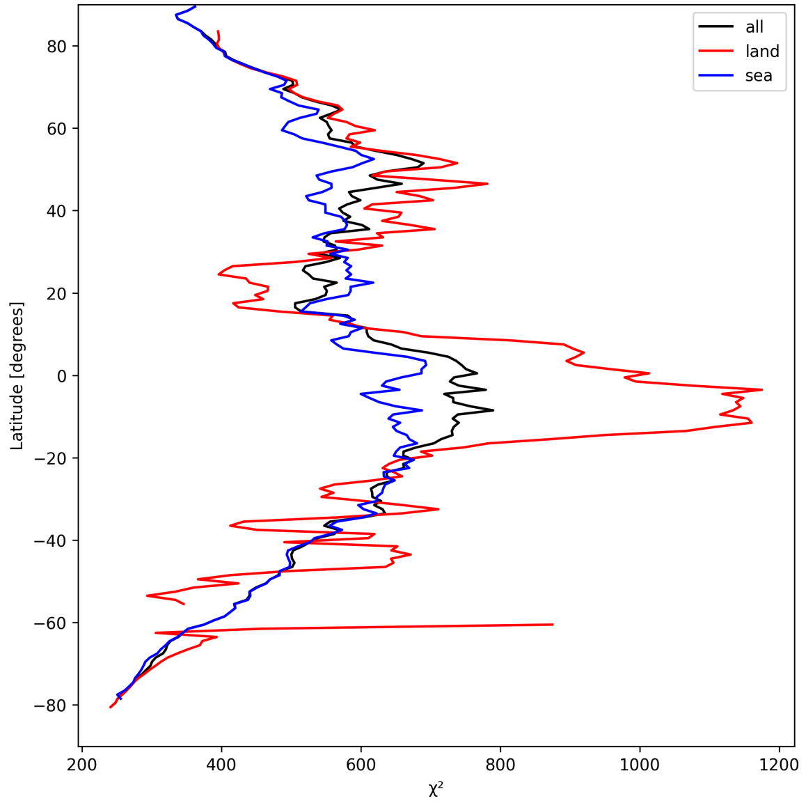
Figure 25: Zonal average of “ \chi^2 ” for 2025-04-08 to 2025-04-09.
