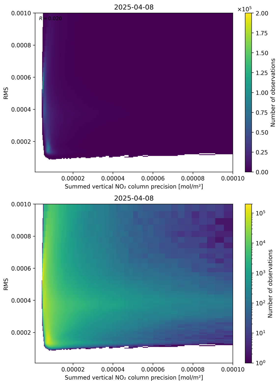
Figure 108: Scatter density plot of “Summed vertical NO 2 column precision” against “RMS” for 2025-04-08 to 2025-04-09.
