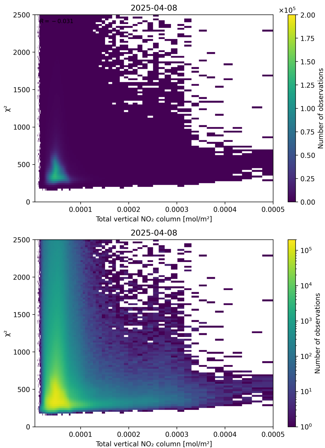
Figure 111: Scatter density plot of “Total vertical NO 2 column” against “ \chi^2 ” for 2025-04-08 to 2025-04-09.
