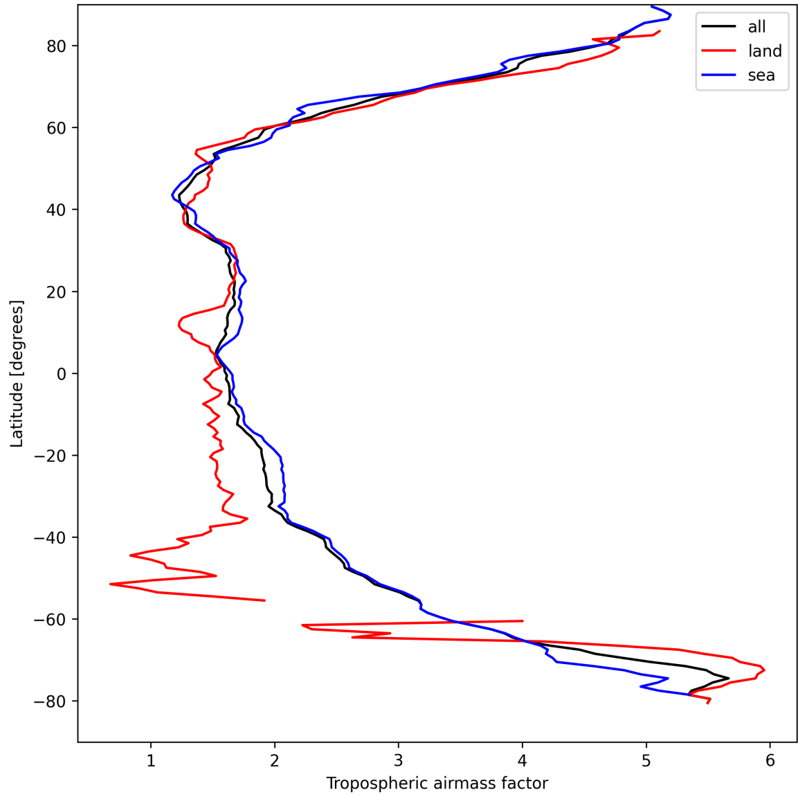
Figure 14: Zonal average of “Tropospheric air mass factor” for 2025-04-08 to 2025-04-09.
