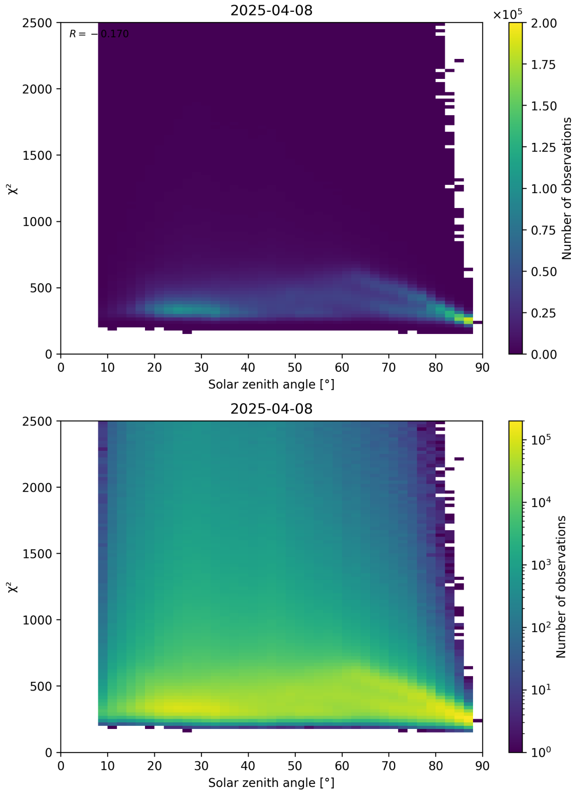
Figure 148: Scatter density plot of “Solar zenith angle” against “ \chi^2 ” for 2025-04-08 to 2025-04-09.
