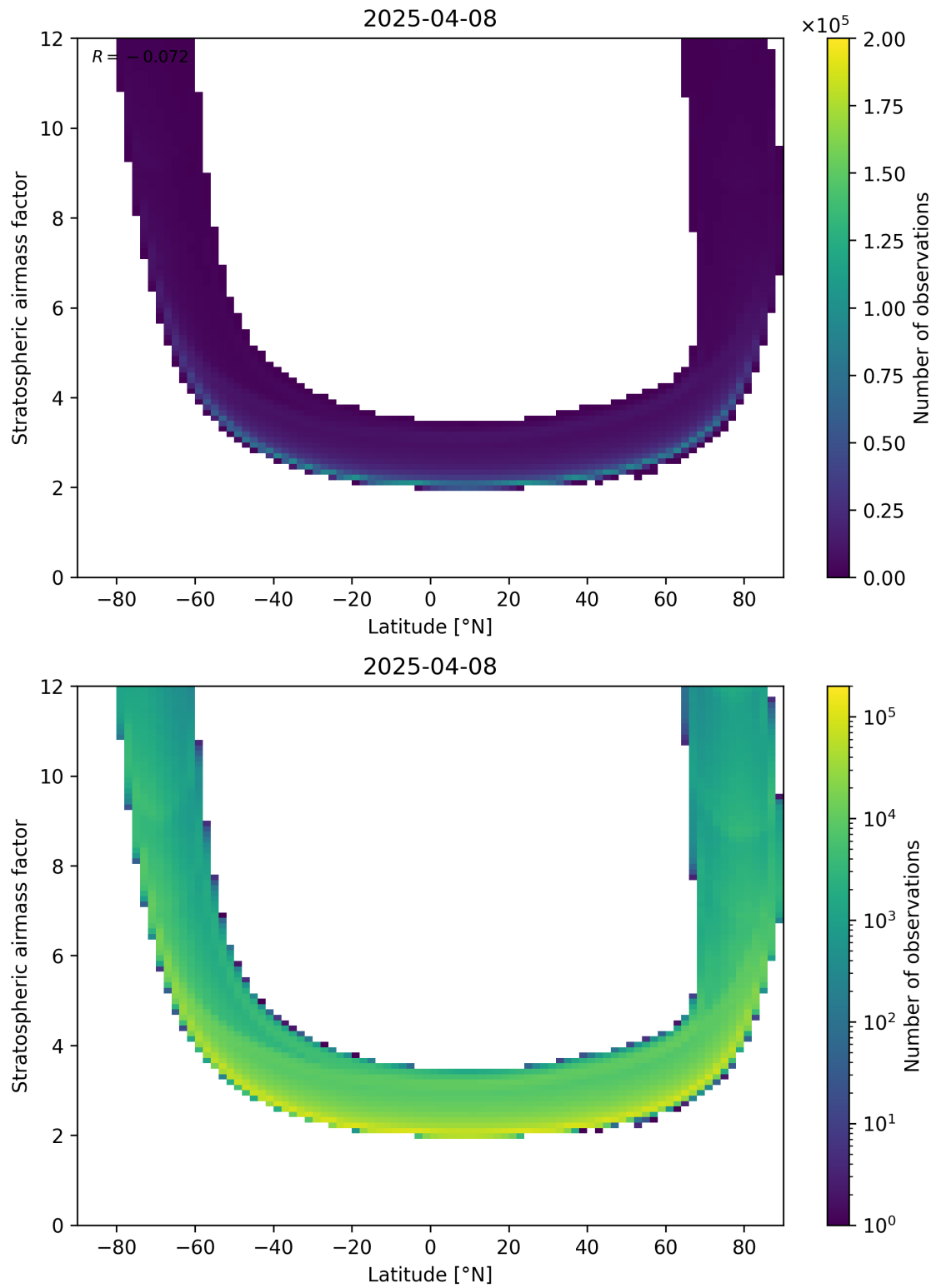
Figure 83: Scatter density plot of “Latitude” against “Stratospheric air mass factor” for 2025-04-08 to 2025-04-09.
