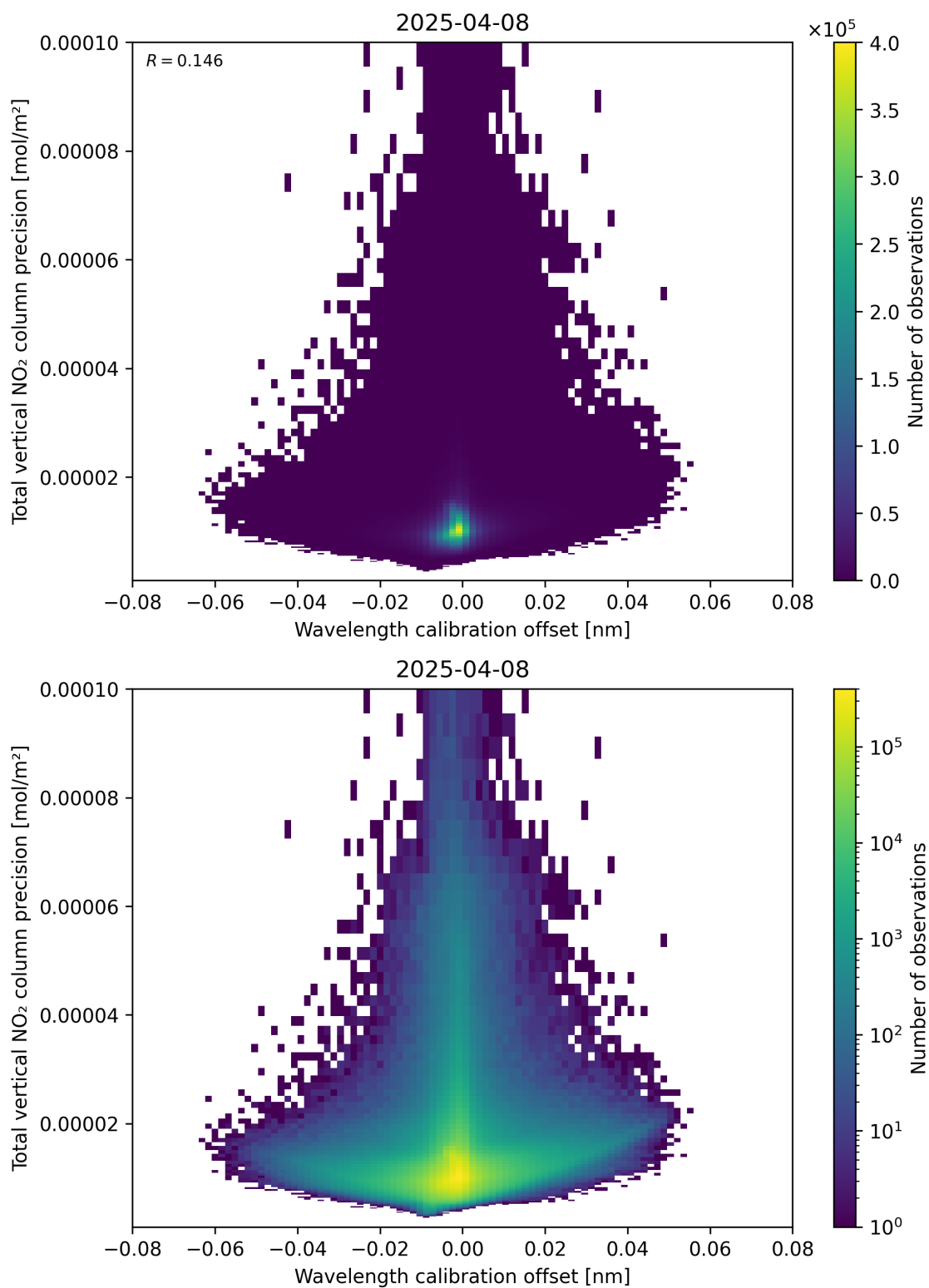
Figure 180: Scatter density plot of “Wavelength calibration offset” against “Total vertical NO 2 column precision” for 2025-04-08 to 2025-04-09.
