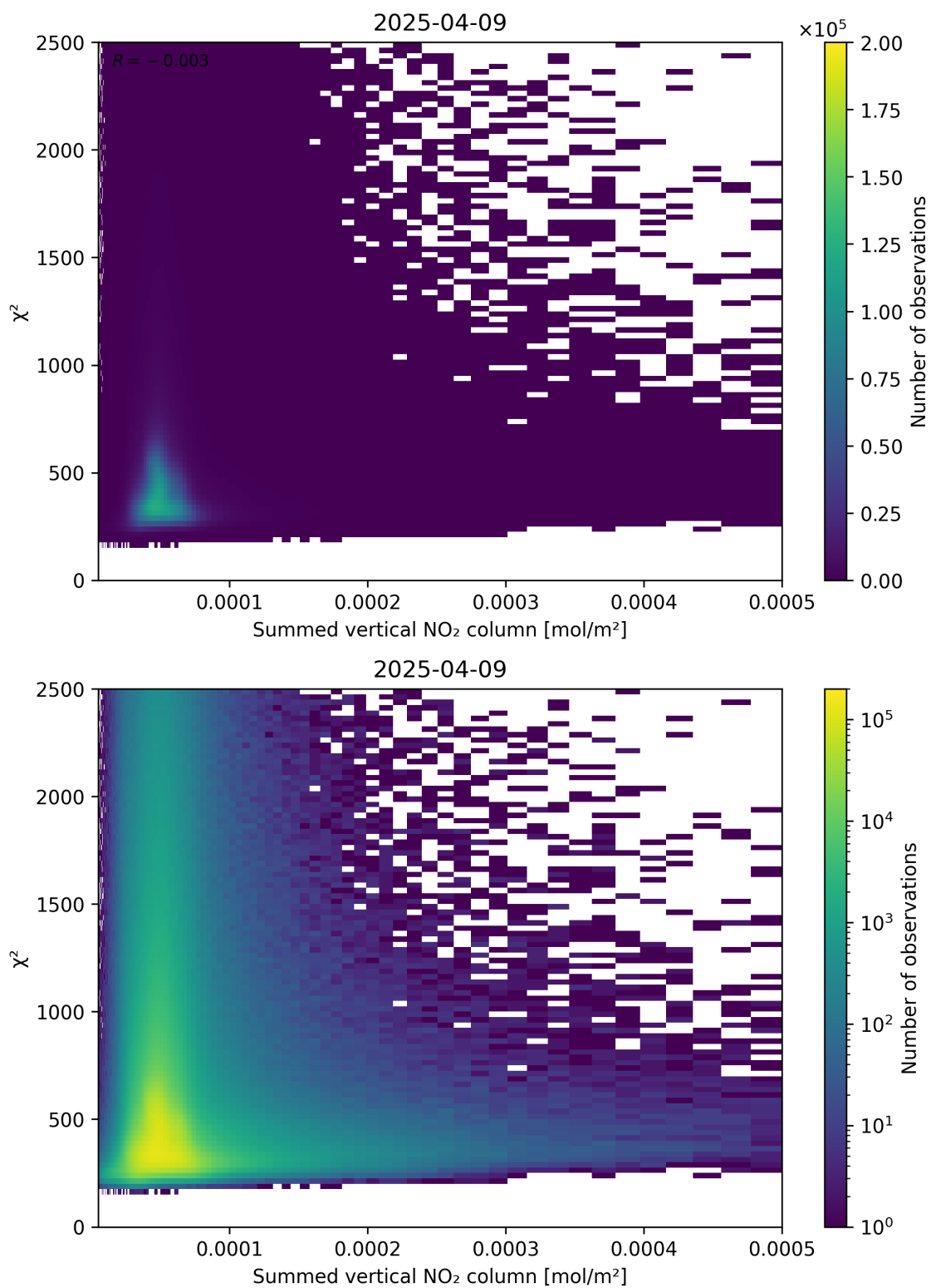
Figure 104: Scatter density plot of “Summed vertical NO 2 column” against “ \chi^2 ” for 2025-04-09 to 2025-04-10.
