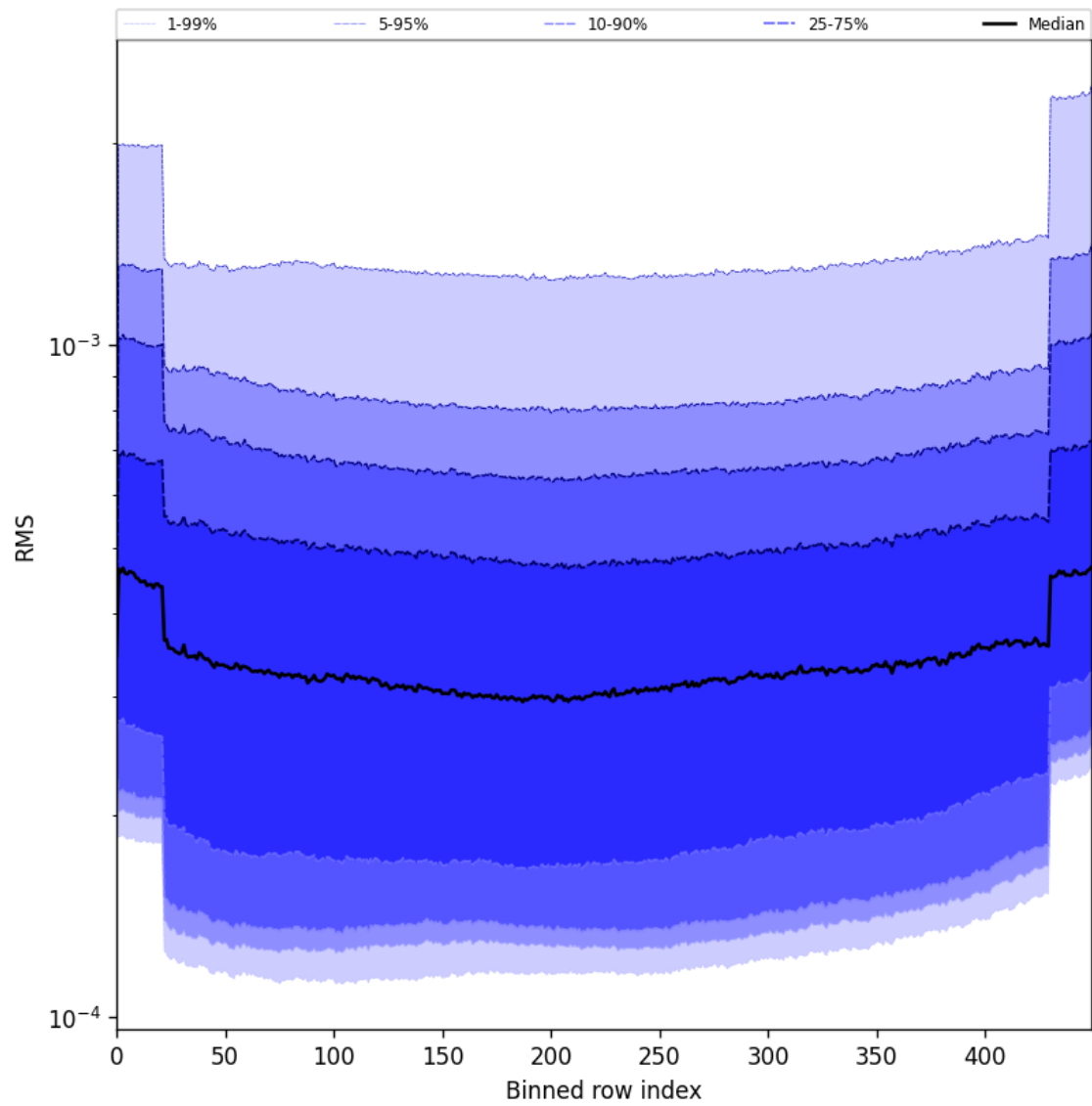
Figure 60: Along track statistics of “RMS” for 2025-04-09 to 2025-04-10
