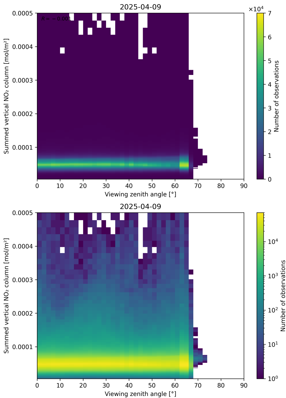
Figure 165: Scatter density plot of “Viewing zenith angle” against “Summed vertical NO 2 column” for 2025-04-09 to 2025-04-10.
