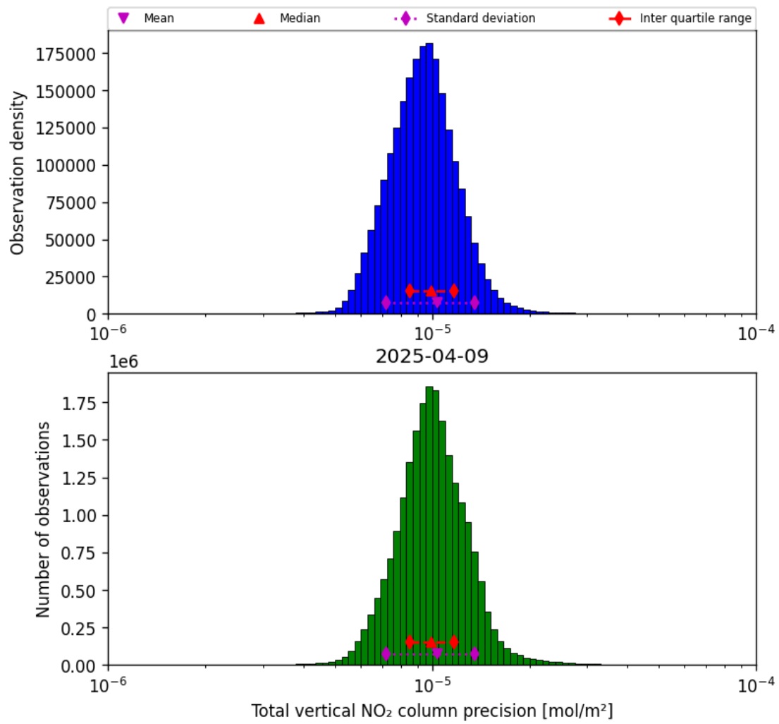
Figure 39: Histogram of “Total vertical NO 2 column precision” for 2025-04-09 to 2025-04-10
