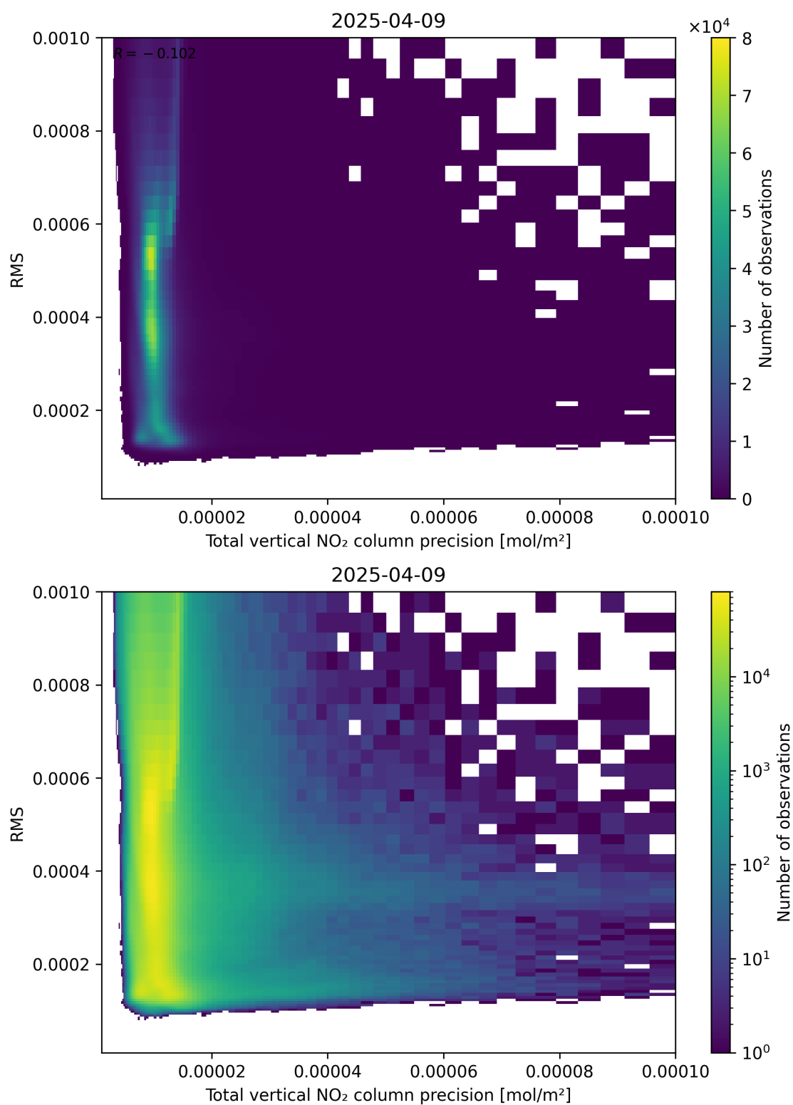
Figure 119: Scatter density plot of “Total vertical NO 2 column precision” against “RMS” for 2025-04-09 to 2025-04-10.
