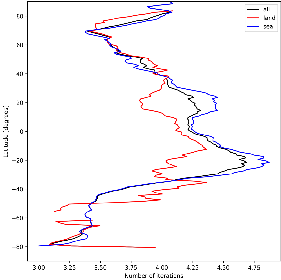
Figure 17: Zonal average of “Number of iterations” for 2025-04-09 to 2025-04-10.
