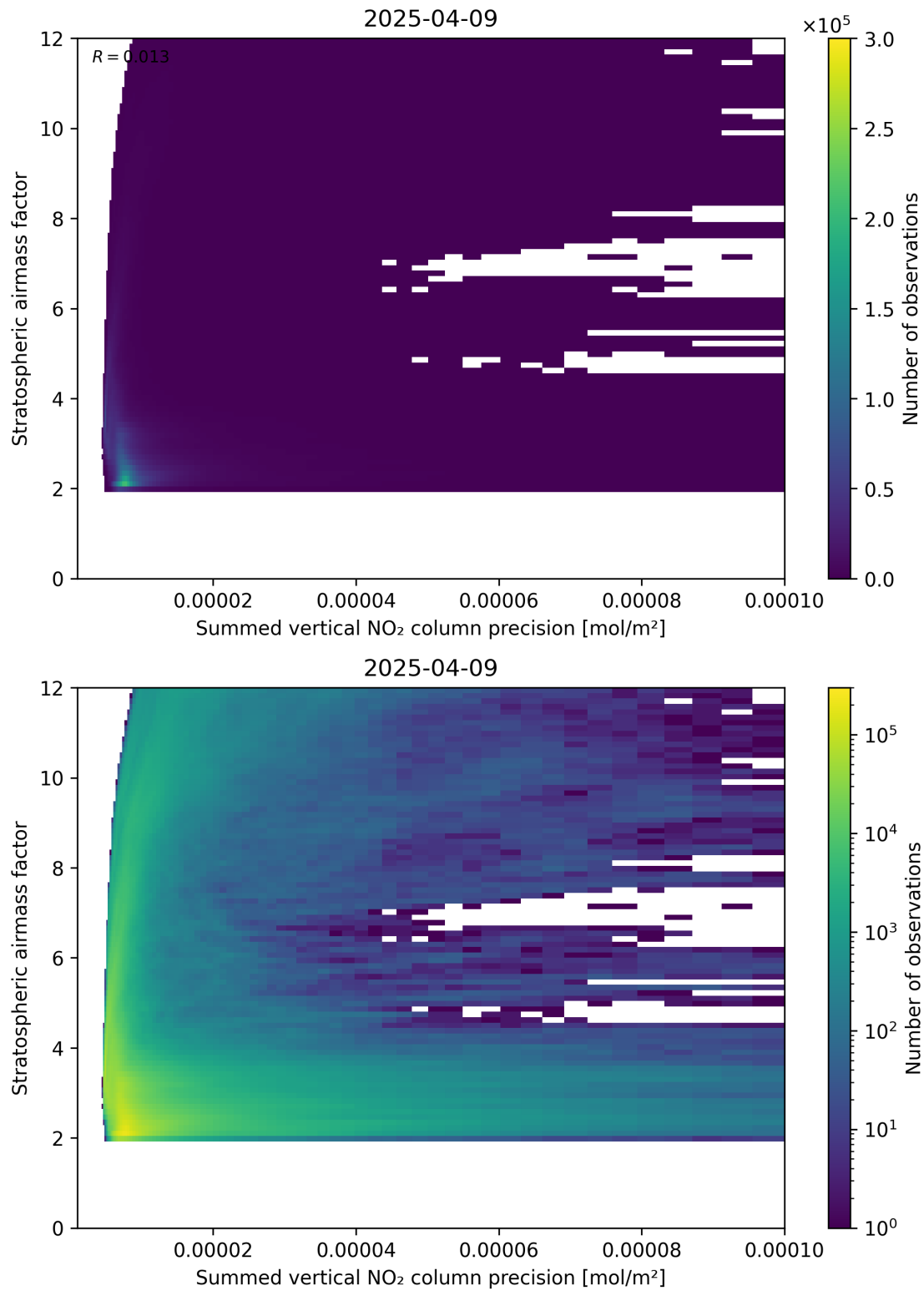
Figure 106: Scatter density plot of “Summed vertical NO 2 column precision” against “Stratospheric airmass factor” for 2025-04-09 to 2025-04-10.
