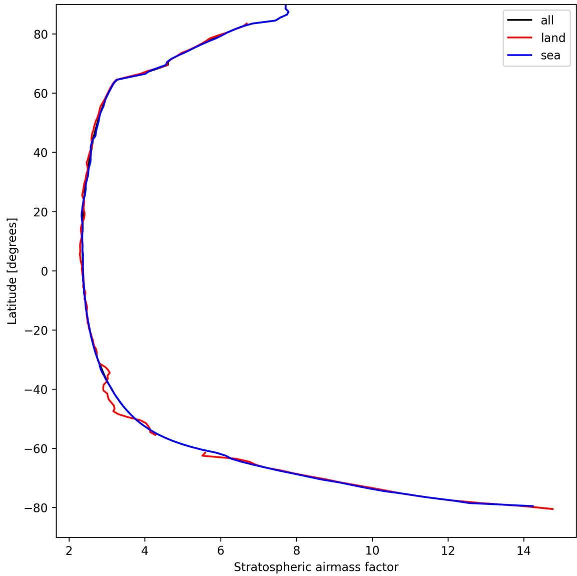
Figure 27: Zonal average of “Stratospheric air mass factor” for 2025-04-09 to 2025-04-10.
