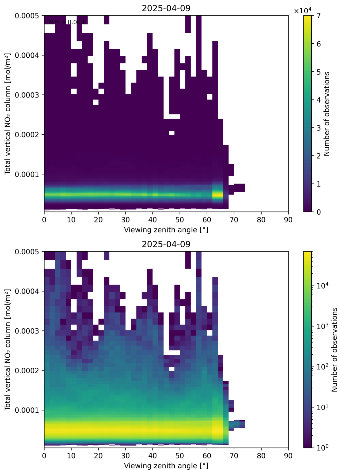
Figure 167: Scatter density plot of “Viewing zenith angle” against “Total vertical NO 2 column” for 2025-04-09 to 2025-04-10.
