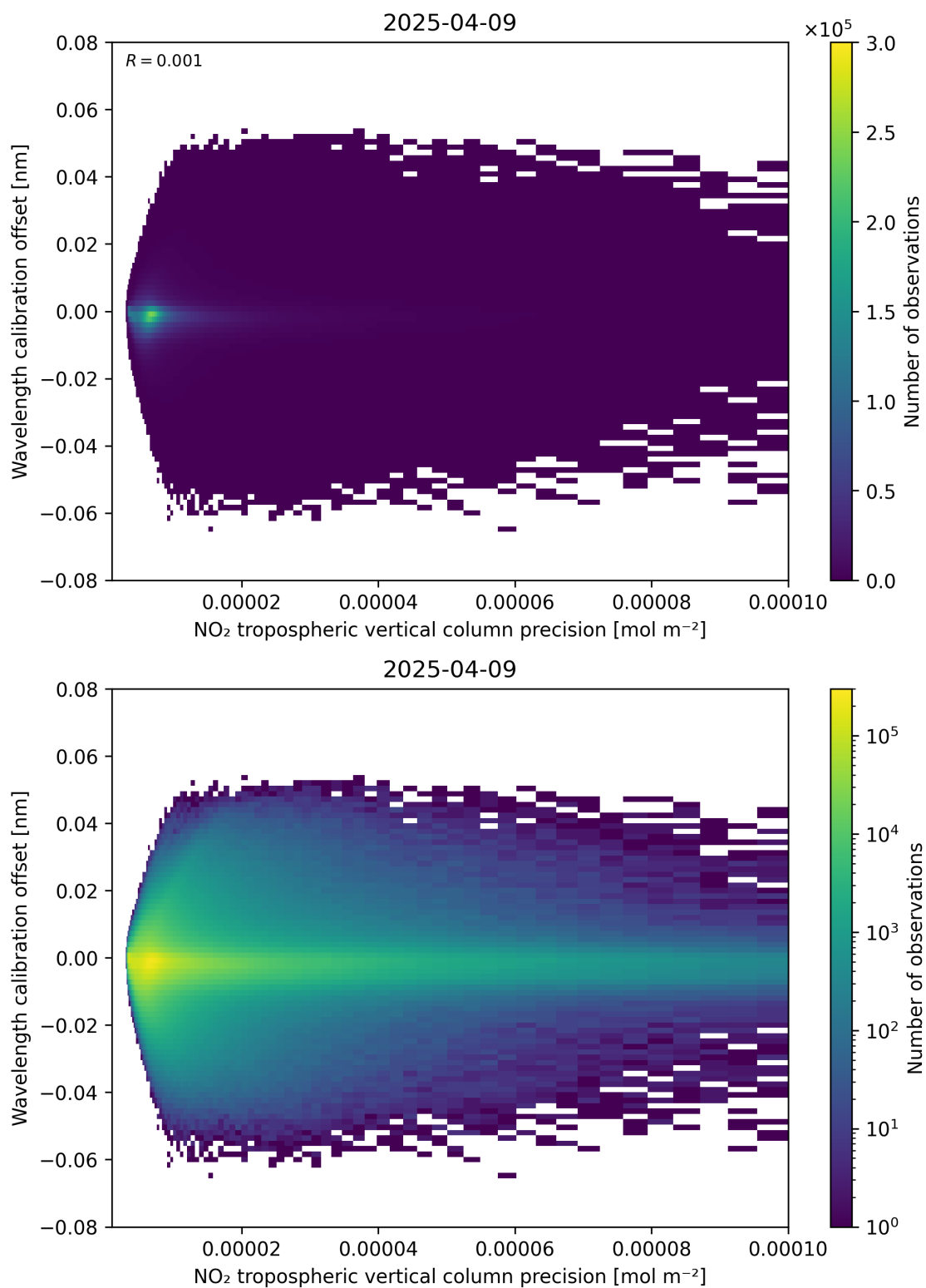
Figure 141: Scatter density plot of “NO 2 tropospheric vertical column precision” against “Wavelength calibration offset” for 2025-04-09 to 2025-04-10.
