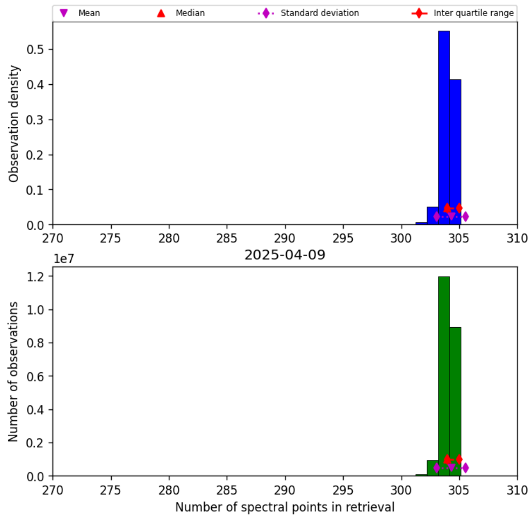
Figure 33: Histogram of “Number of spectral points in retrieval” for 2025-04-09 to 2025-04-10
