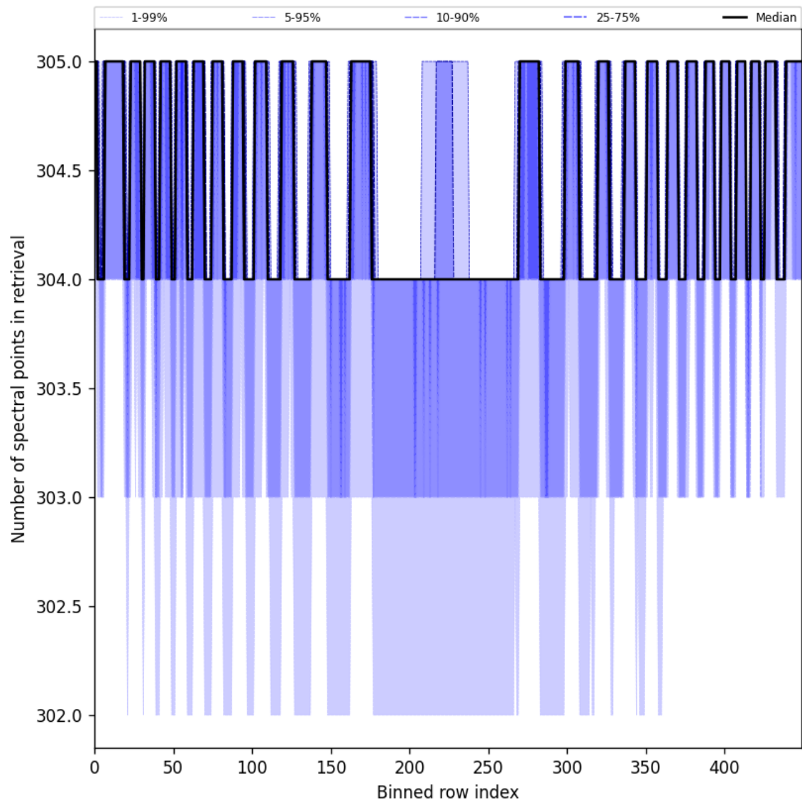
Figure 50: Along track statistics of “Number of spectral points in retrieval” for 2025-04-09 to 2025-04-10
