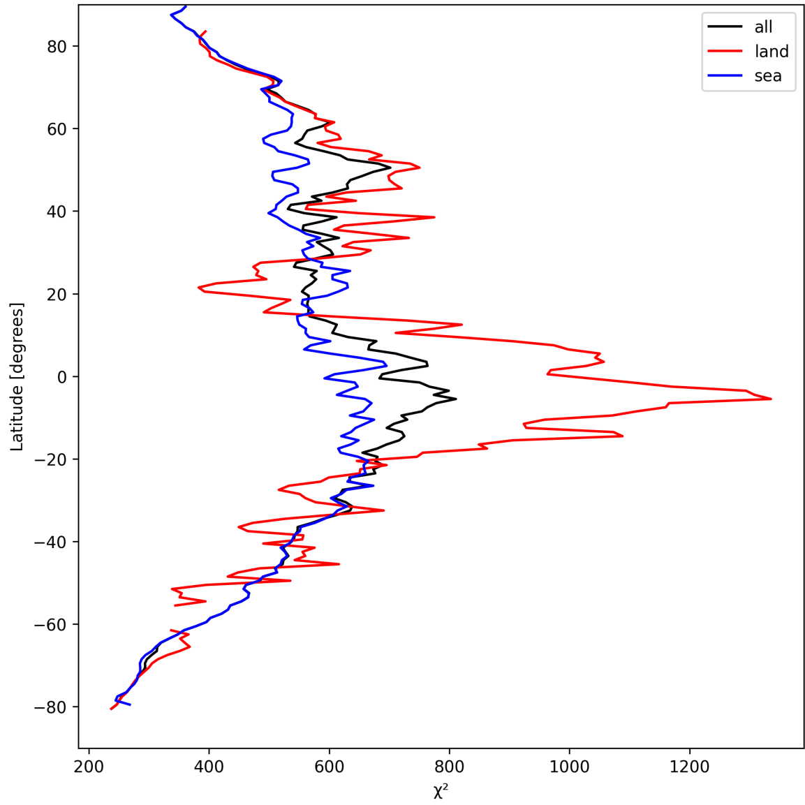
Figure 25: Zonal average of “ \chi^2 ” for 2025-04-09 to 2025-04-10.
