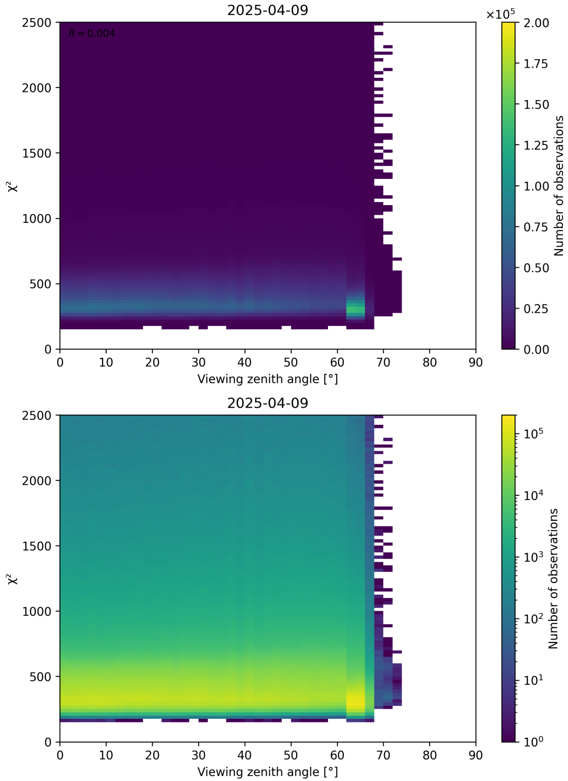
Figure 162: Scatter density plot of “Viewing zenith angle” against “ \chi^2 ” for 2025-04-09 to 2025-04-10.
