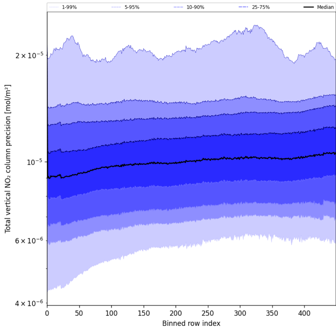
Figure 56: Along track statistics of “Total vertical NO 2 column precision” for 2025-04-09 to 2025-04-10
