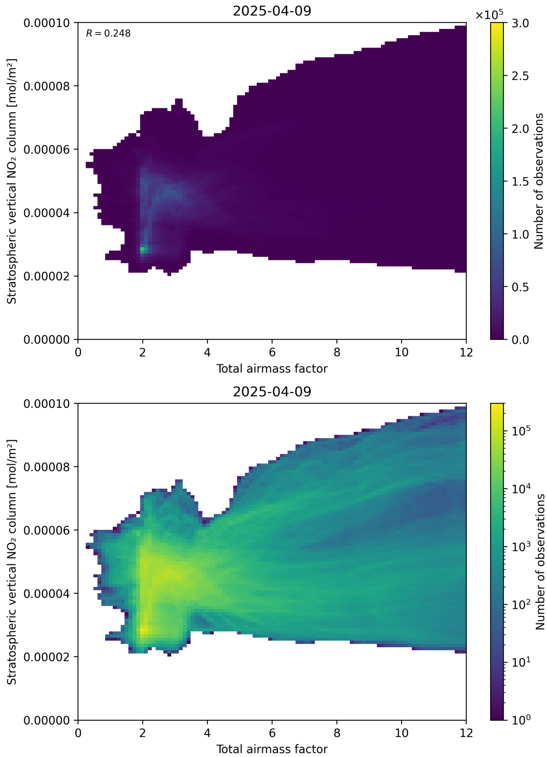
Figure 64: Scatter density plot of “Total airmass factor” against “Stratospheric vertical \text{NO}_2 column” for 2025-04-09 to 2025-04-10.
