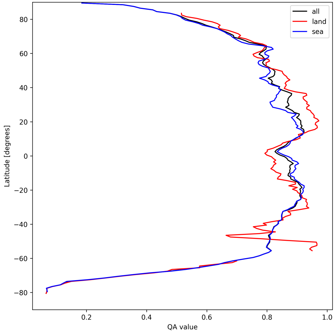
Figure 11: Zonal average of “QA value” for 2025-04-09 to 2025-04-10.
