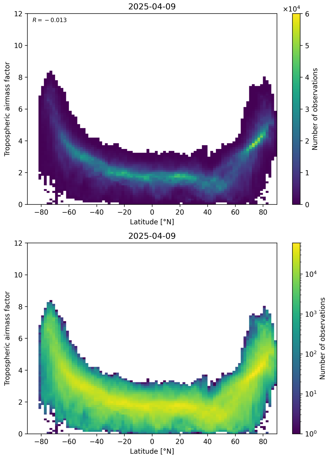
Figure 85: Scatter density plot of “Latitude” against “Tropospheric airmass factor” for 2025-04-09 to 2025-04-10.
