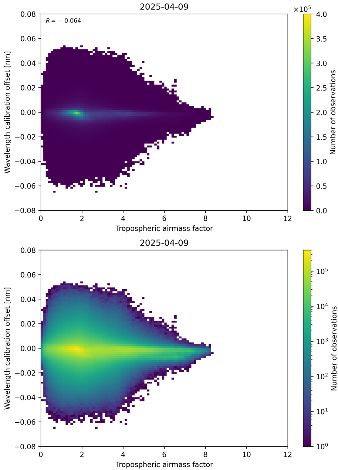
Figure 80: Scatter density plot of “Tropospheric airmass factor” against “Wavelength calibration offset” for 2025-04-09 to 2025-04-10.
