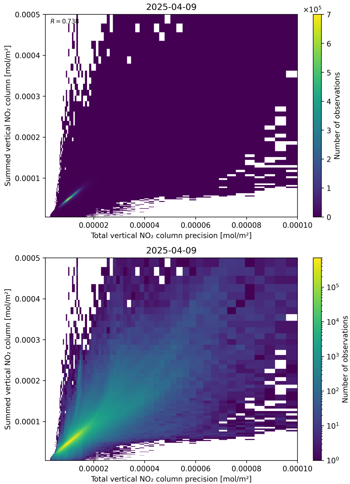
Figure 117: Scatter density plot of “Total vertical NO 2 column precision” against “Summed vertical NO 2 column” for 2025-04-09 to 2025-04-10.
