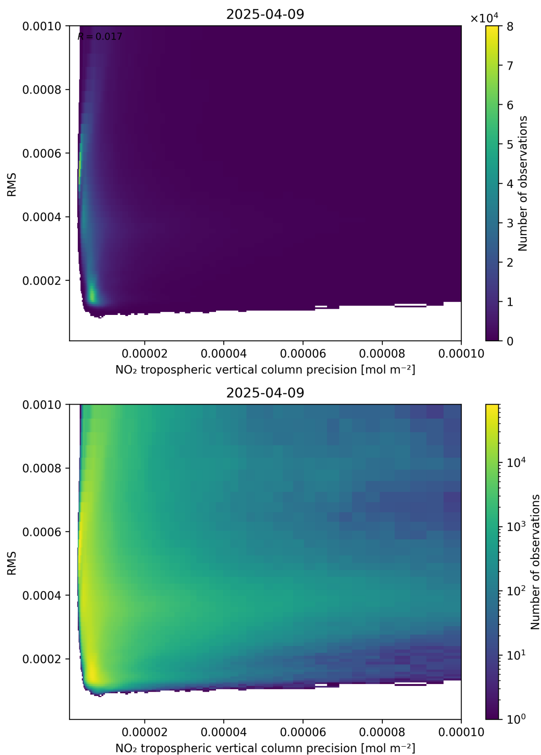
Figure 140: Scatter density plot of “NO 2 tropospheric vertical column precision” against “RMS” for 2025-04-09 to 2025-04-10.
