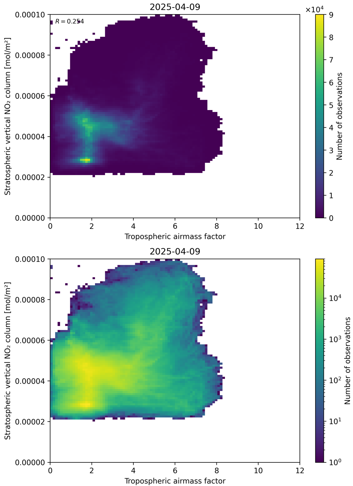
Figure 74: Scatter density plot of “Tropospheric air mass factor” against “Stratospheric vertical NO 2 column” for 2025-04-09 to 2025-04-10.
