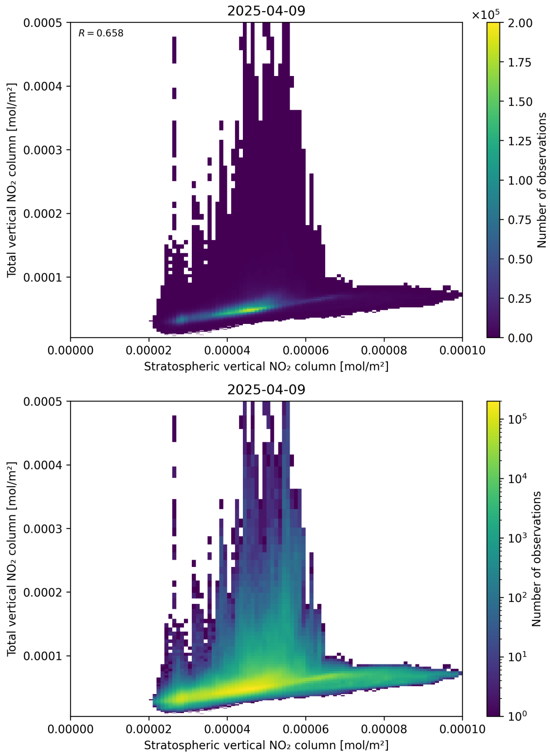
Figure 100: Scatter density plot of “Stratospheric vertical NO 2 column” against “Total vertical NO 2 column” for 2025-04-09 to 2025-04-10.
