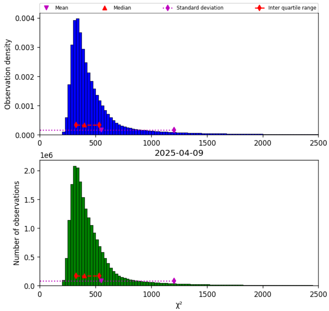
Figure 42: Histogram of “ \chi^2 ” for 2025-04-09 to 2025-04-10
