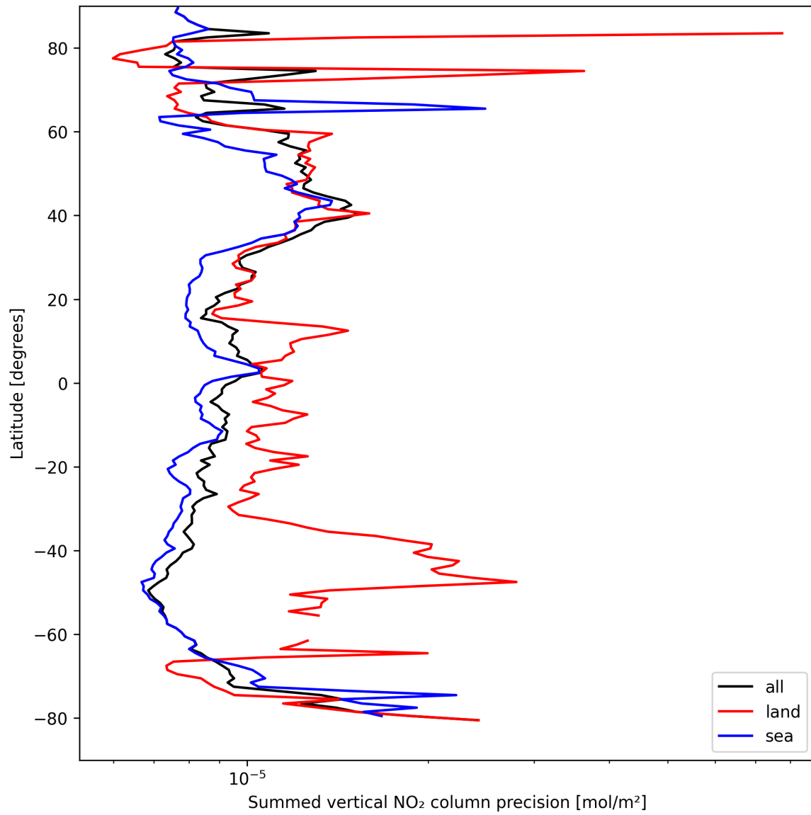
Figure 24: Zonal average of “Summed vertical NO 2 column precision” for 2025-04-09 to 2025-04-10.
