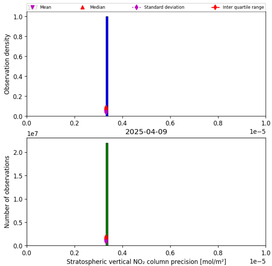
Figure 37: Histogram of “Stratospheric vertical NO 2 column precision” for 2025-04-09 to 2025-04-10
