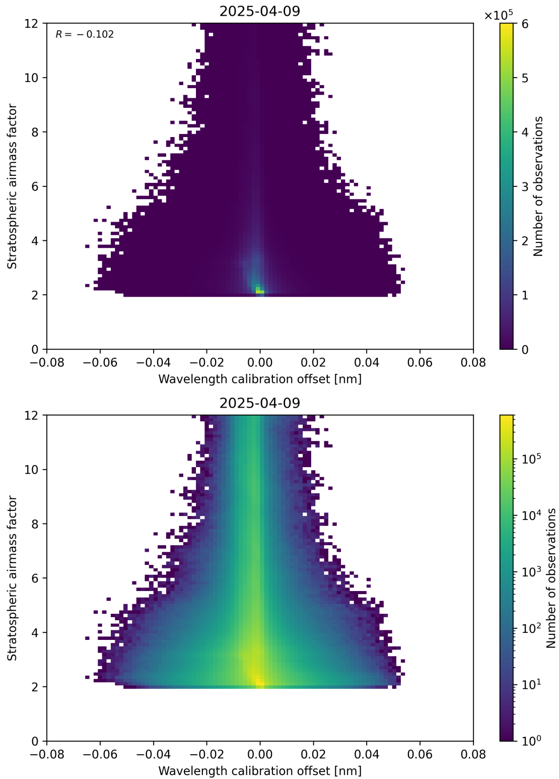
Figure 174: Scatter density plot of “Wavelength calibration offset” against “Stratospheric airmass factor” for 2025-04-09 to 2025-04-10.
