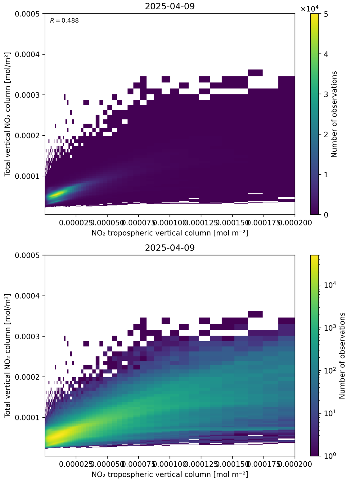
Figure 128: Scatter density plot of “NO 2 tropospheric vertical column” against “Total vertical NO 2 column” for 2025-04-09 to 2025-04-10.
