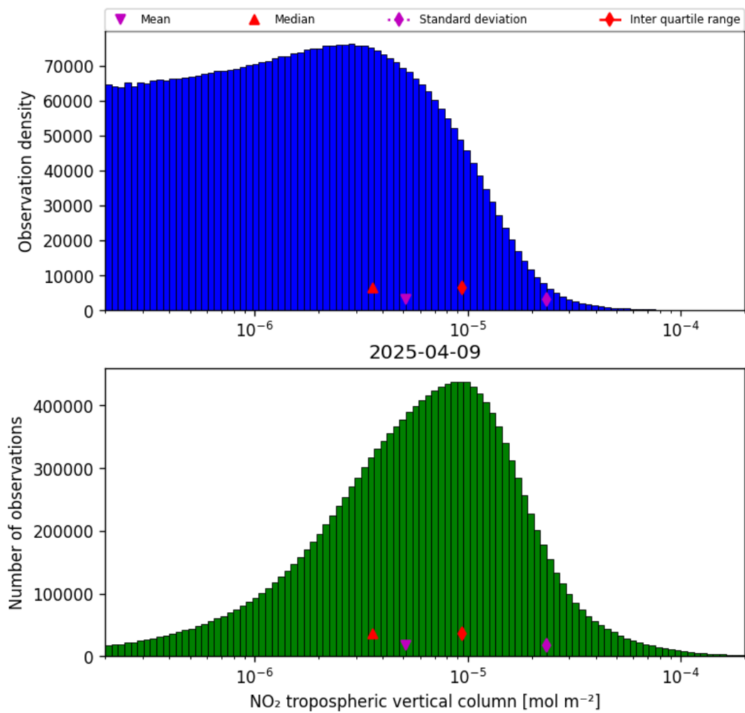
Figure 29: Histogram of “NO 2 tropospheric vertical column” for 2025-04-09 to 2025-04-10
