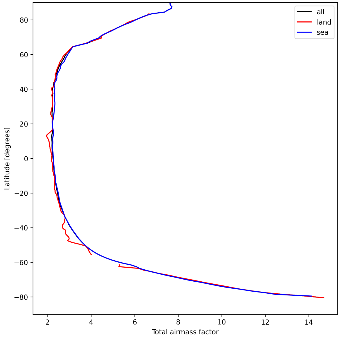
Figure 15: Zonal average of “Total airmass factor” for 2025-04-09 to 2025-04-10.
