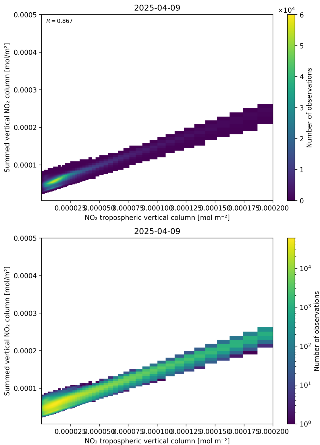
Figure 126: Scatter density plot of “NO 2 tropospheric vertical column” against “Summed vertical NO 2 column” for 2025-04-09 to 2025-04-10.
