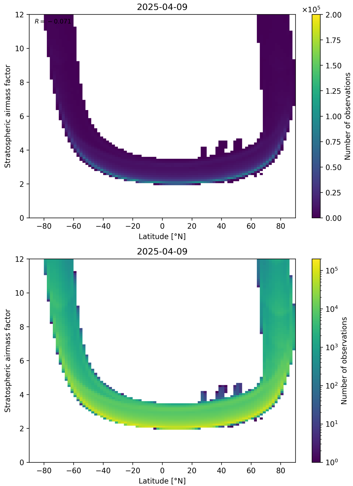
Figure 83: Scatter density plot of “Latitude” against “Stratospheric air mass factor” for 2025-04-09 to 2025-04-10.
