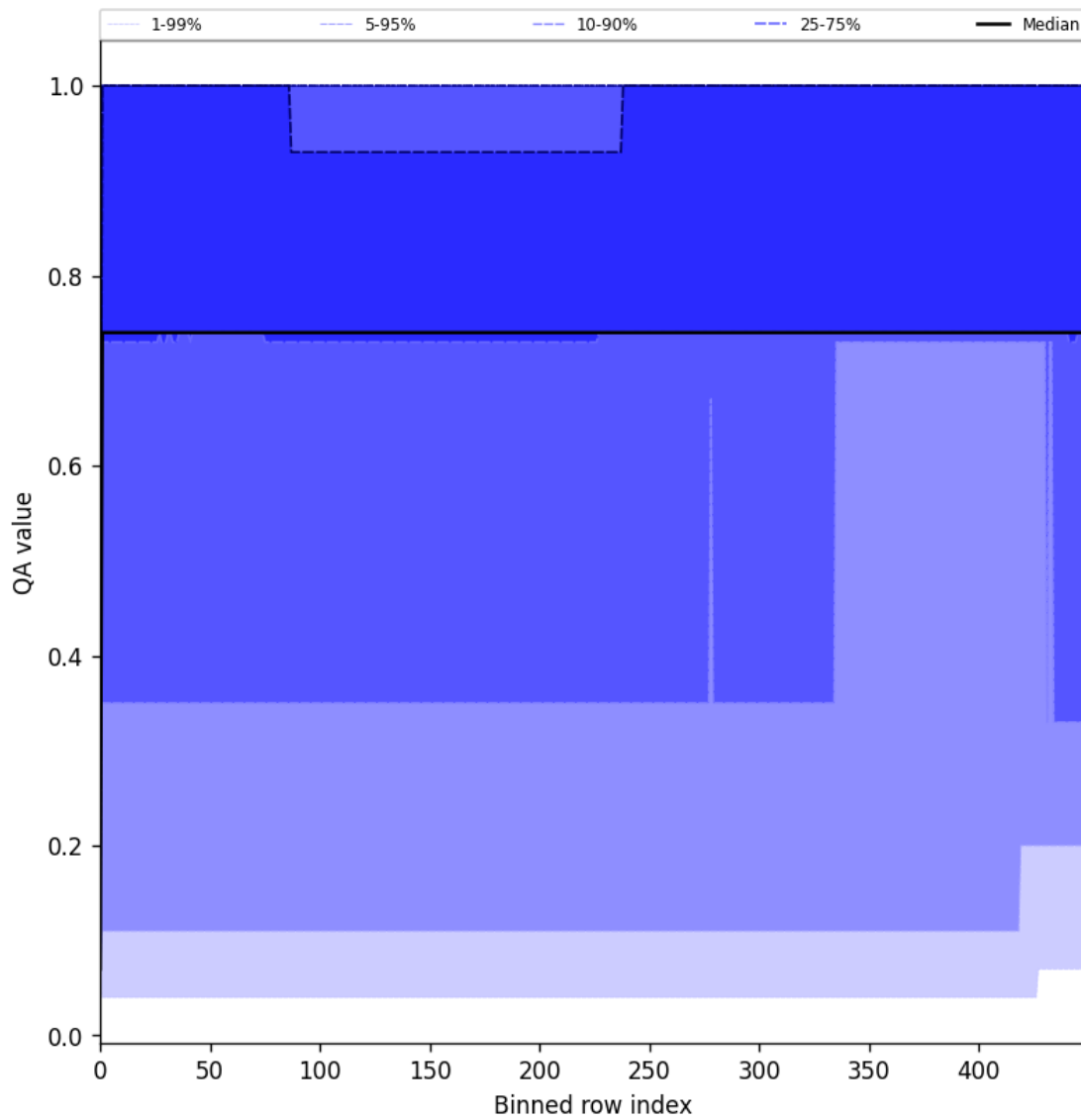
Figure 45: Along track statistics of “QA value” for 2025-04-09 to 2025-04-10
