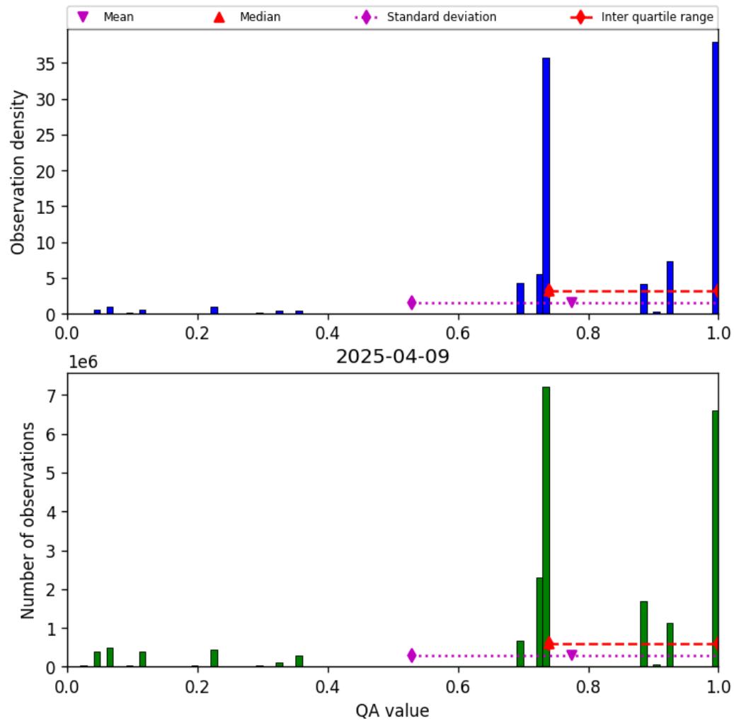
Figure 28: Histogram of “QA value” for 2025-04-09 to 2025-04-10
