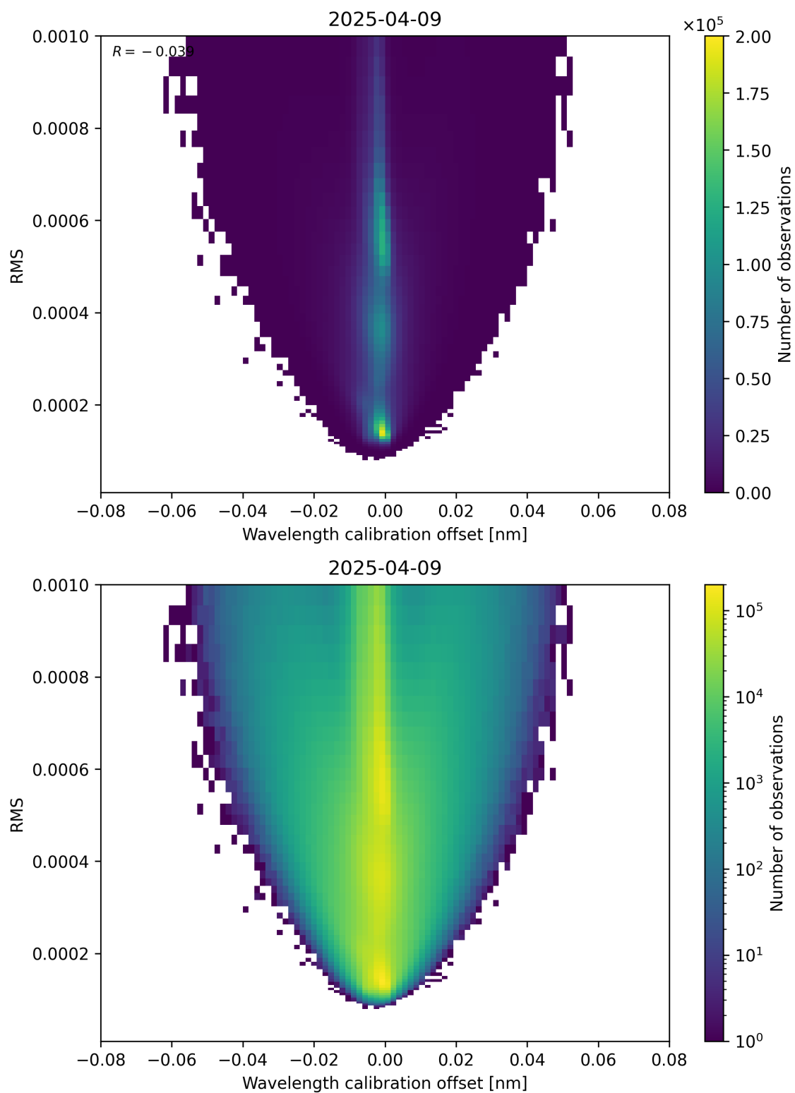
Figure 181: Scatter density plot of “Wavelength calibration offset” against “RMS” for 2025-04-09 to 2025-04-10.
