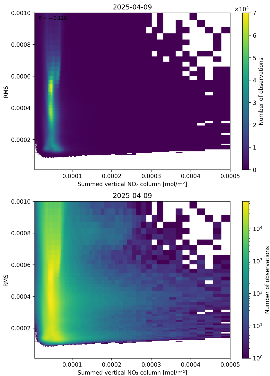
Figure 109: Scatter density plot of “Summed vertical NO 2 column” against “RMS” for 2025-04-09 to 2025-04-10.
