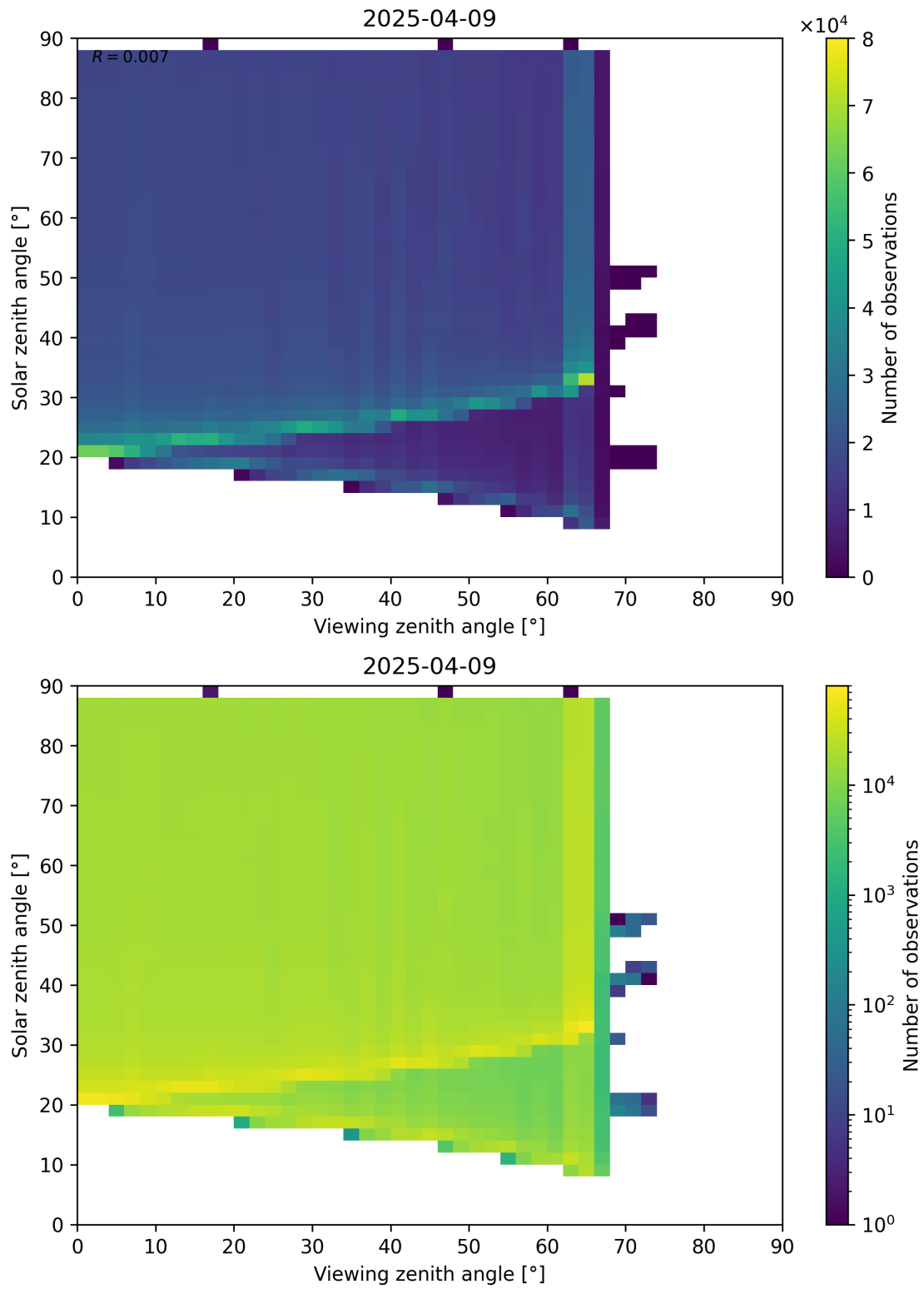
Figure 172: Scatter density plot of “Viewing zenith angle” against “Solar zenith angle” for 2025-04-09 to 2025-04-10.
