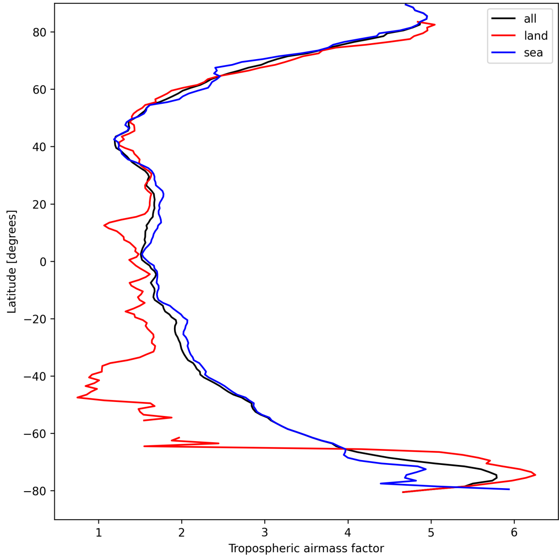
Figure 14: Zonal average of “Tropospheric airmass factor” for 2025-04-09 to 2025-04-10.
