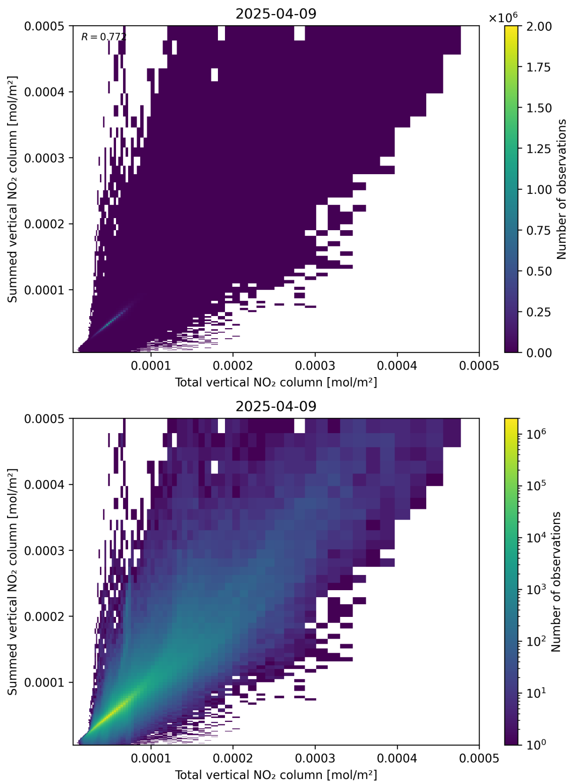
Figure 112: Scatter density plot of “Total vertical NO 2 column” against “Summed vertical NO 2 column” for 2025-04-09 to 2025-04-10.
