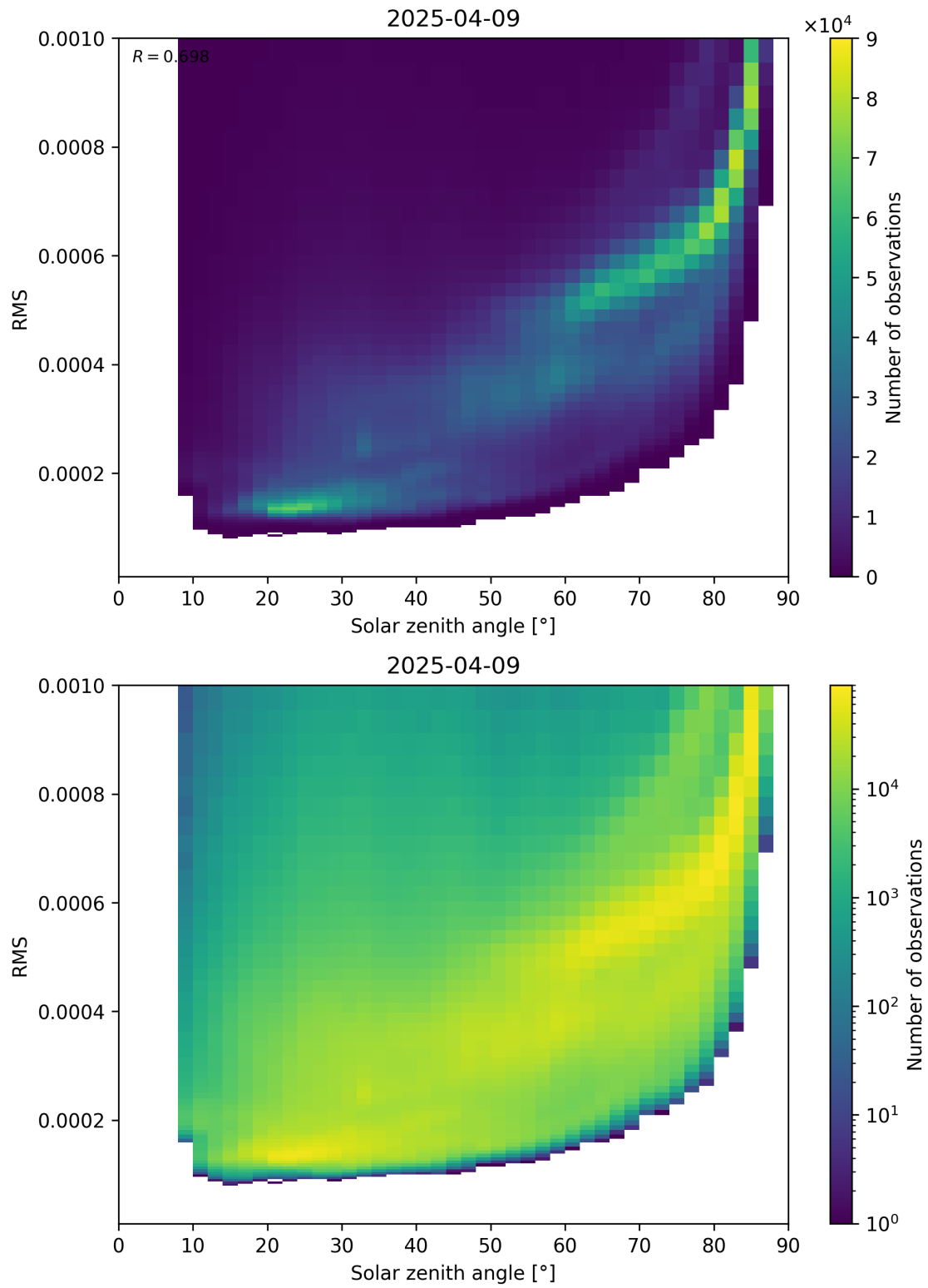
Figure 157: Scatter density plot of “Solar zenith angle” against “RMS” for 2025-04-09 to 2025-04-10.
