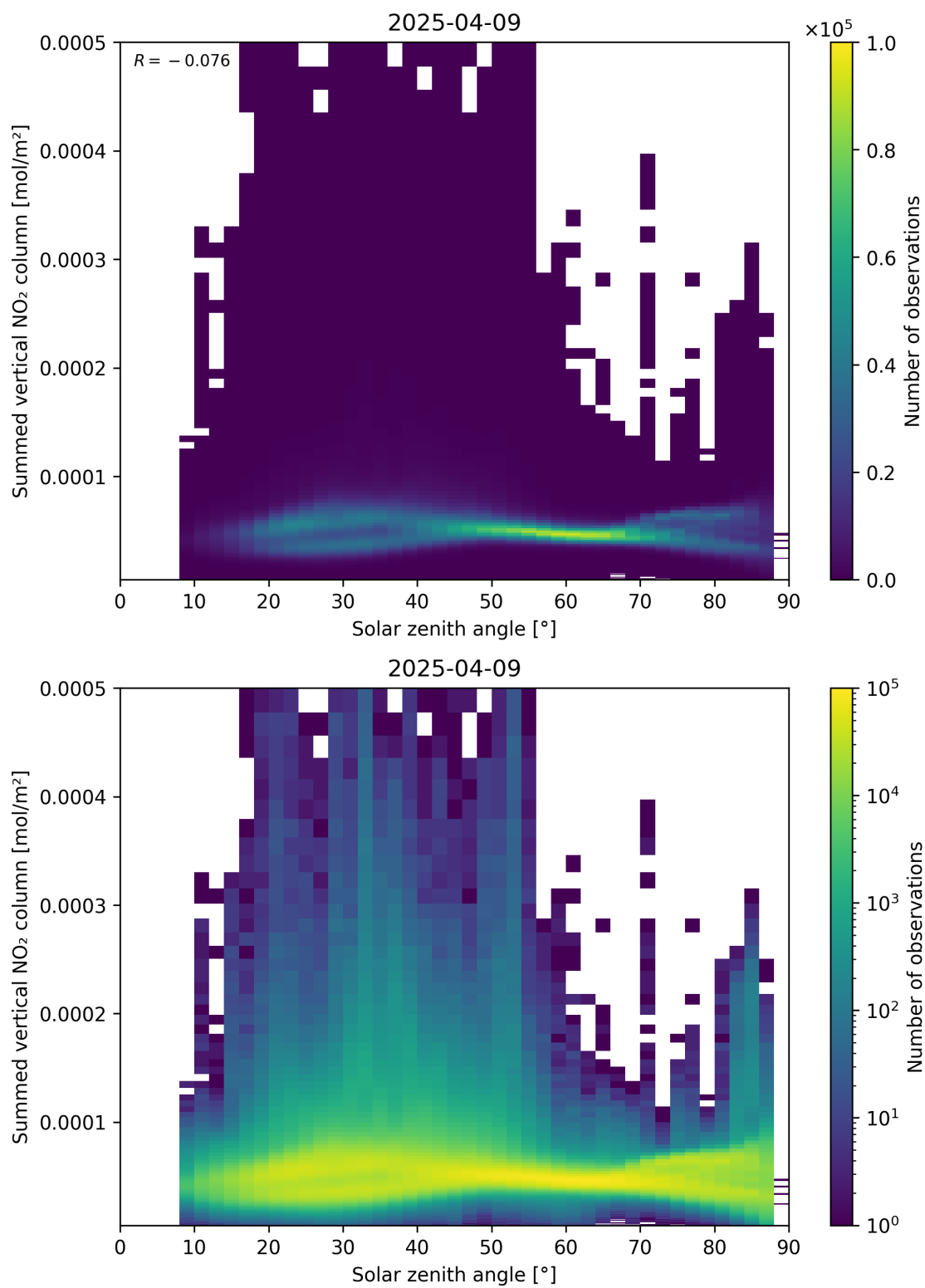
Figure 151: Scatter density plot of “Solar zenith angle” against “Summed vertical NO 2 column” for 2025-04-09 to 2025-04-10.
