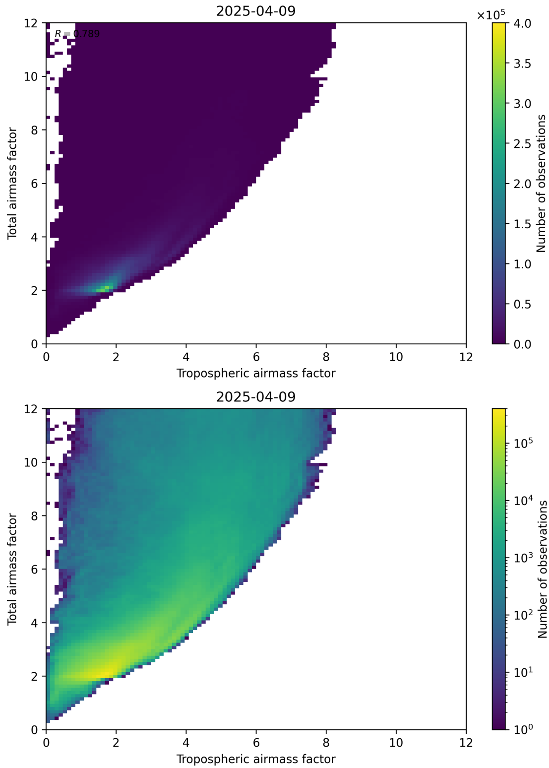
Figure 72: Scatter density plot of “Tropospheric airmass factor” against “Total airmass factor” for 2025-04-09 to 2025-04-10.
