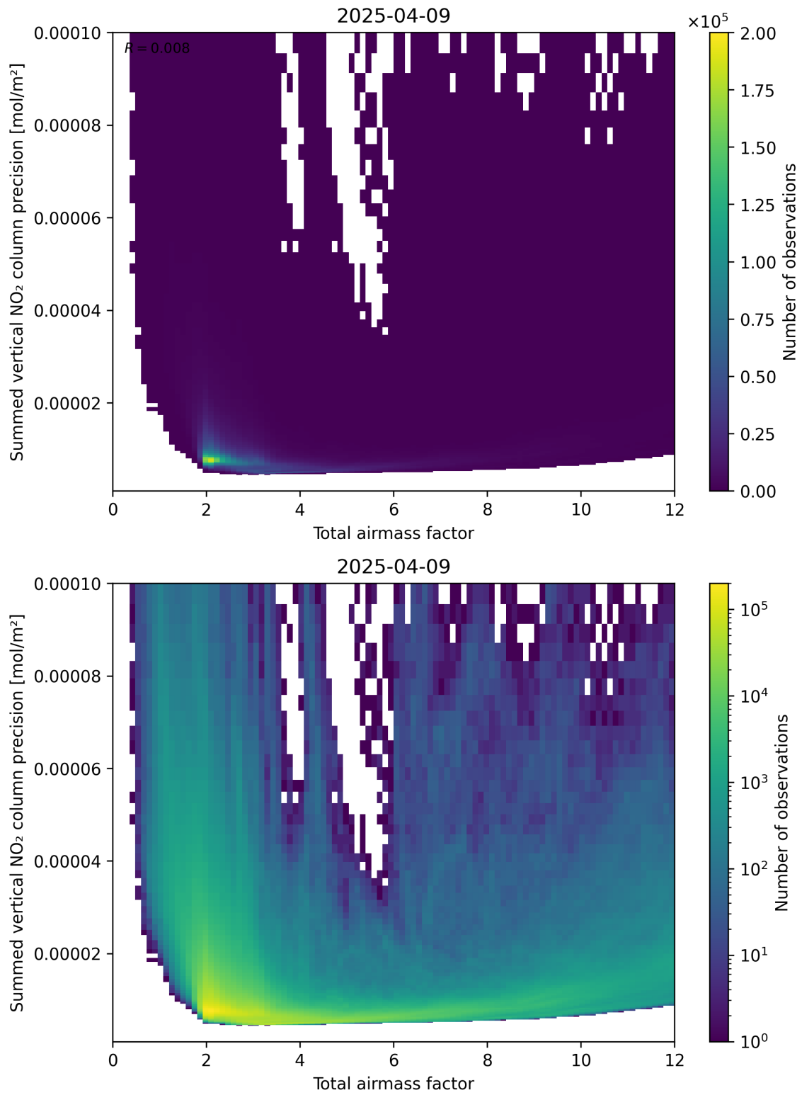
Figure 66: Scatter density plot of “Total airmass factor” against “Summed vertical NO 2 column precision” for 2025-04-09 to 2025-04-10.
