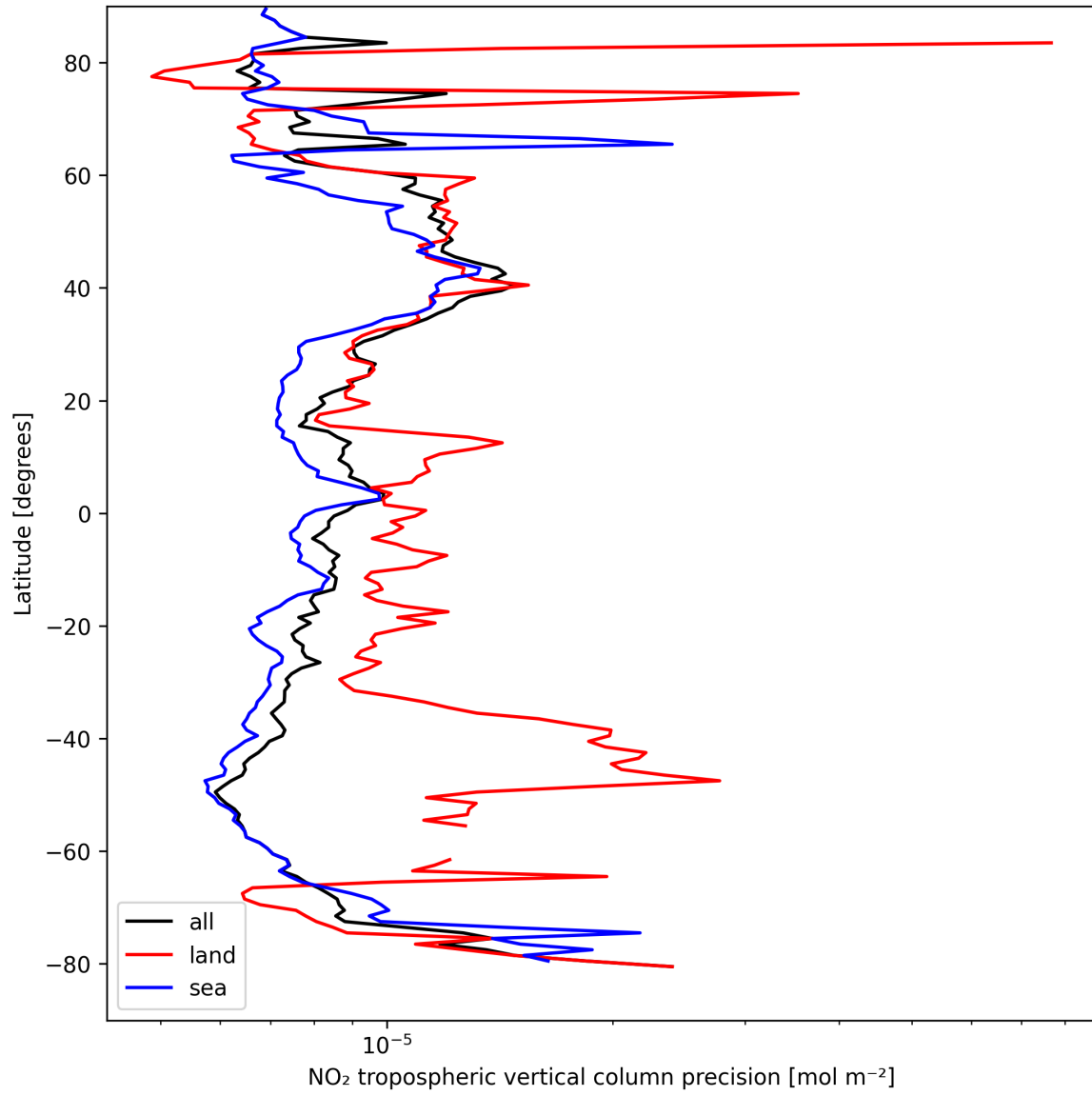
Figure 13: Zonal average of “NO 2 tropospheric vertical column precision” for 2025-04-09 to 2025-04-10.
