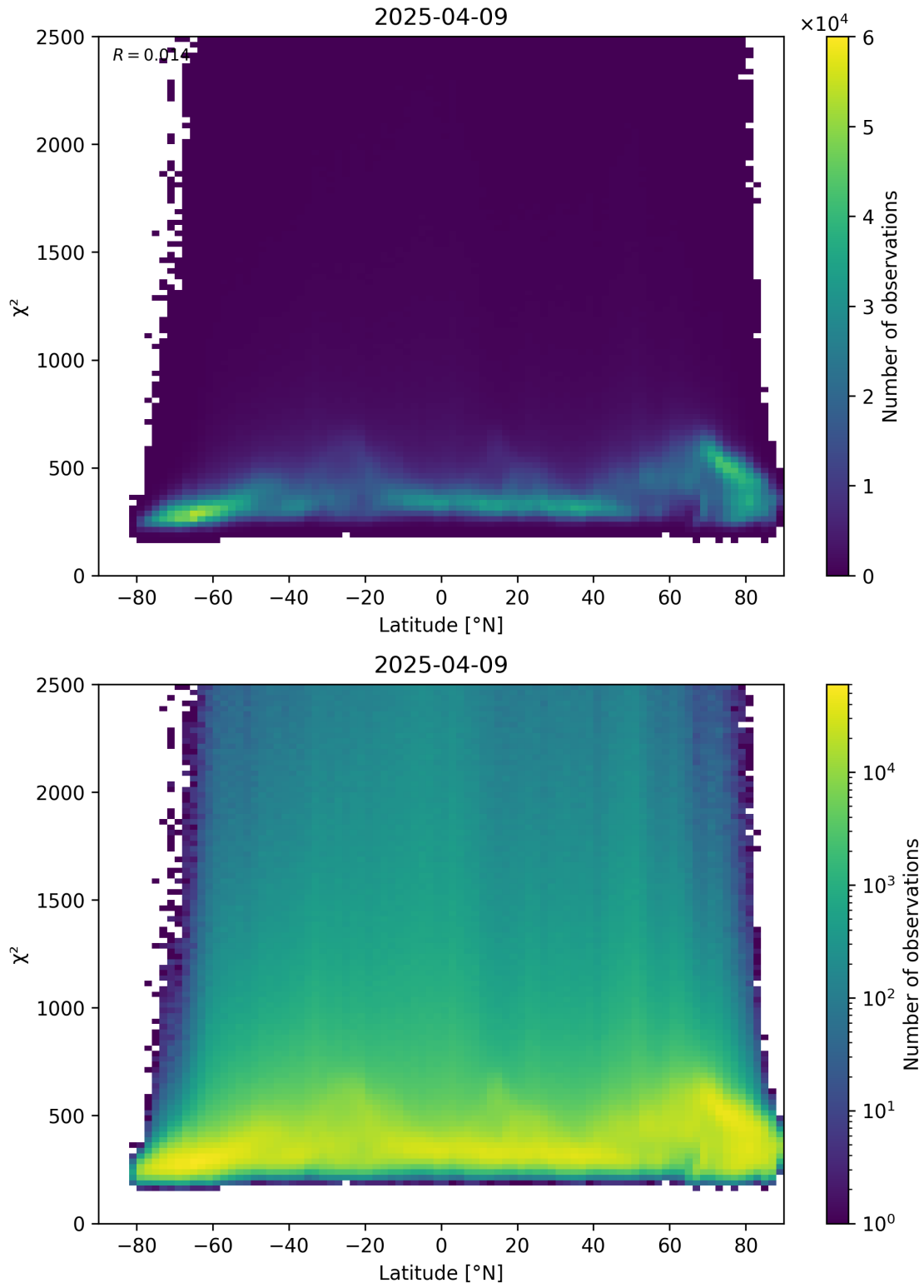
Figure 86: Scatter density plot of “Latitude” against “ \chi^2 ” for 2025-04-09 to 2025-04-10.
