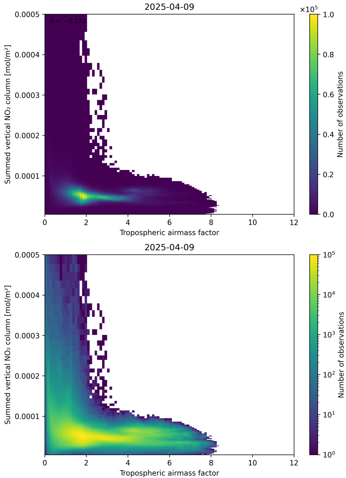
Figure 75: Scatter density plot of “Tropospheric air mass factor” against “Summed vertical NO 2 column” for 2025-04-09 to 2025-04-10.
