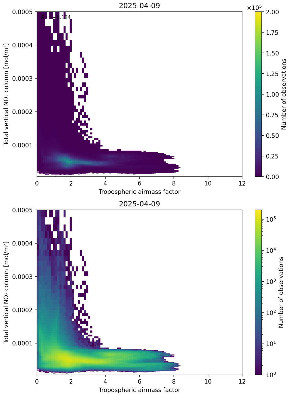
Figure 77: Scatter density plot of “Tropospheric airmass factor” against “Total vertical \text{NO}_2 column” for 2025-04-09 to 2025-04-10.
