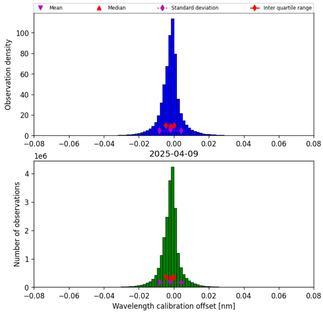
Figure 35: Histogram of “Wavelength calibration offset” for 2025-04-09 to 2025-04-10
