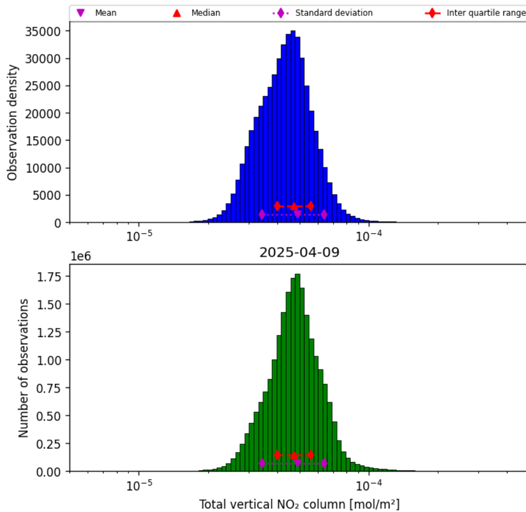
Figure 38: Histogram of “Total vertical NO 2 column” for 2025-04-09 to 2025-04-10
