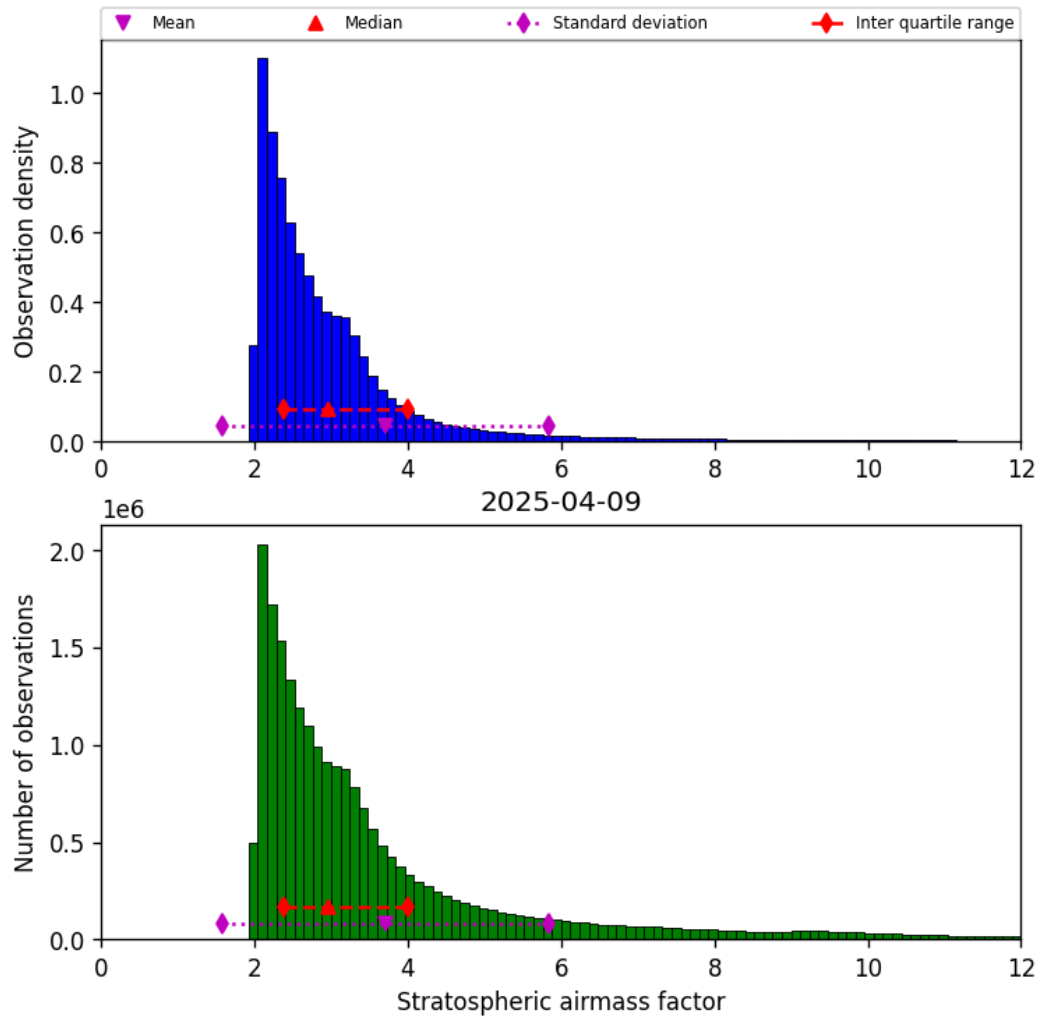
Figure 44: Histogram of “Stratospheric airmass factor” for 2025-04-09 to 2025-04-10
