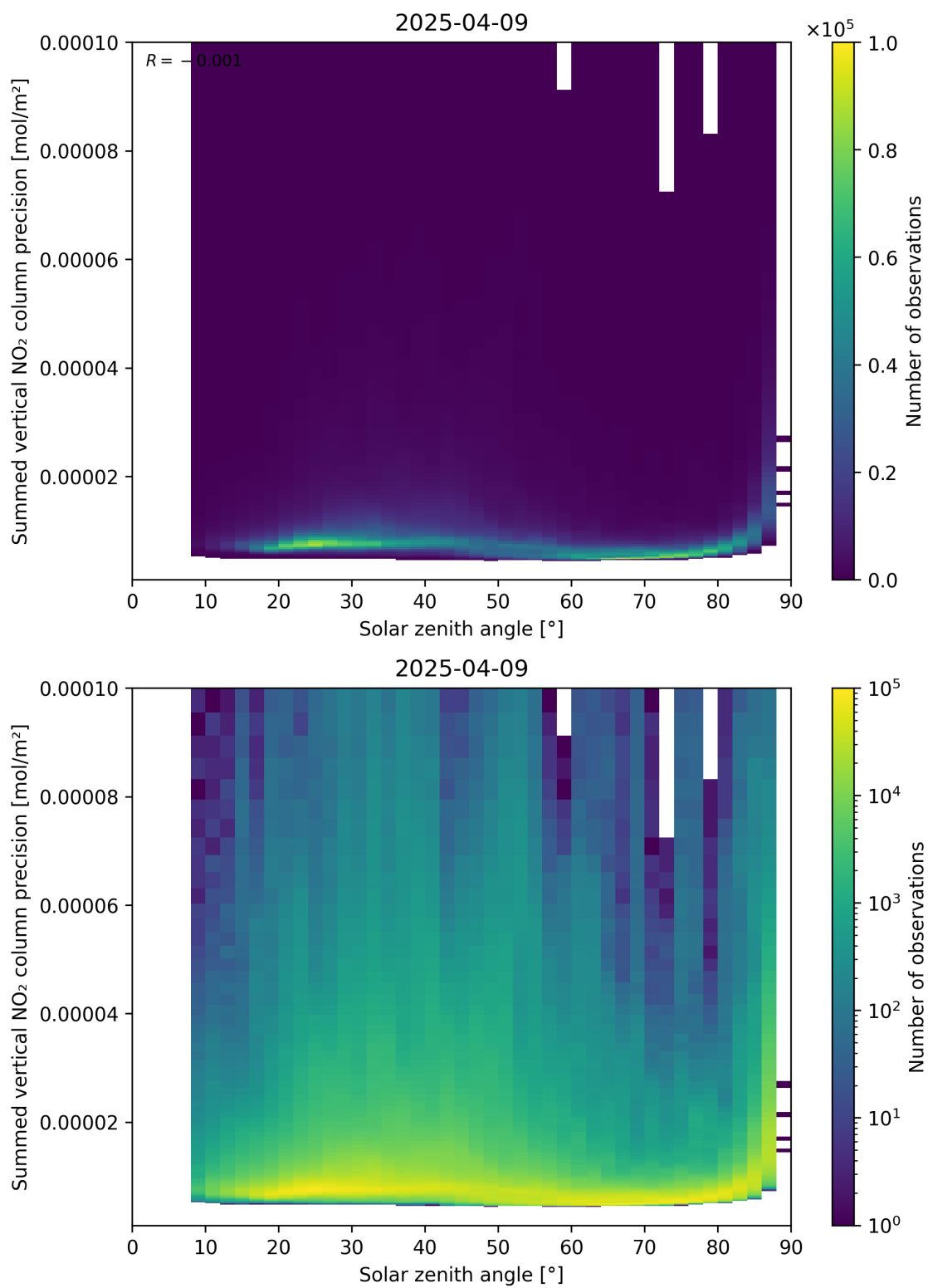
Figure 152: Scatter density plot of “Solar zenith angle” against “Summed vertical NO 2 column precision” for 2025-04-09 to 2025-04-10.
