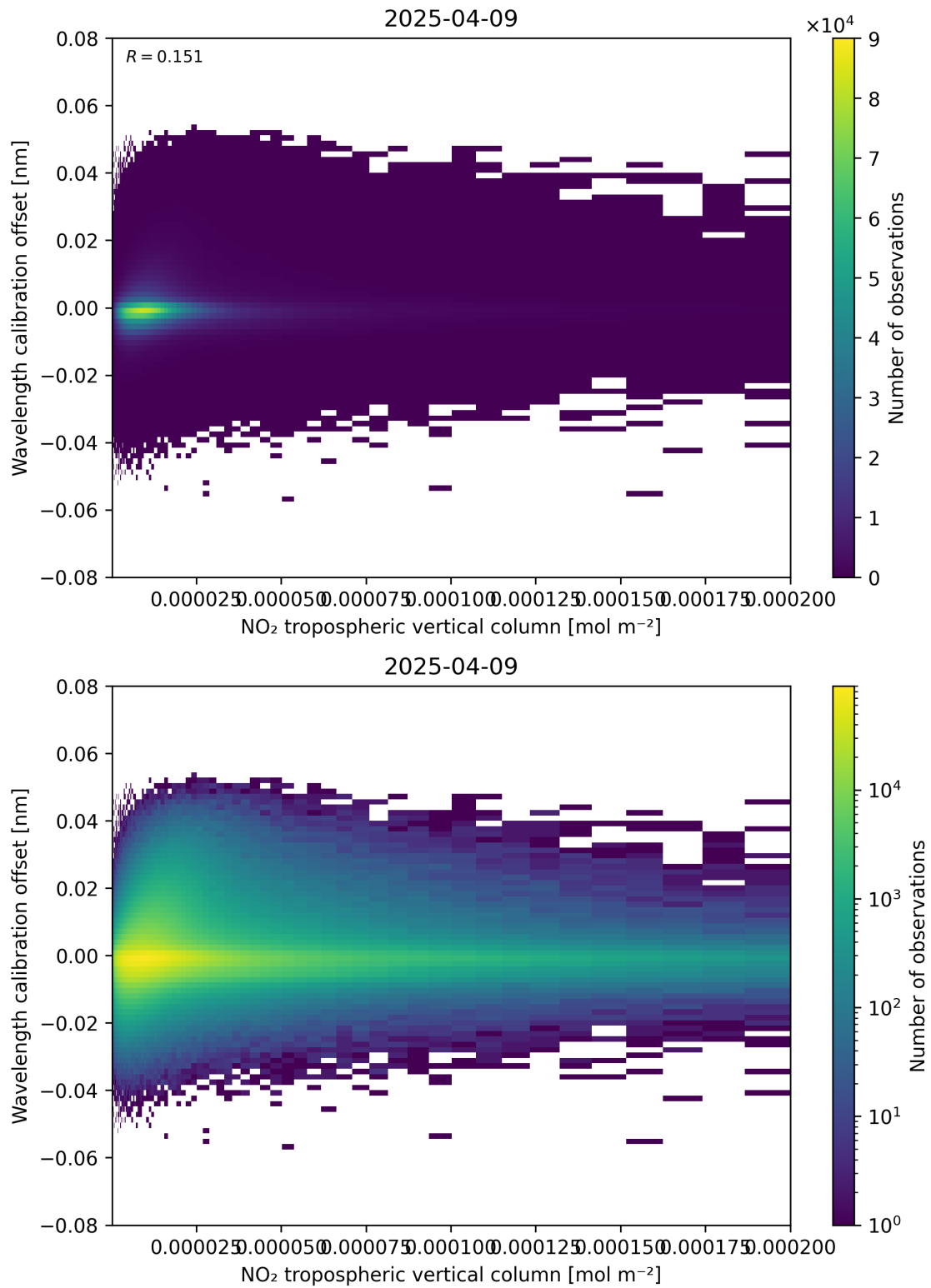
Figure 143: Scatter density plot of “NO 2 tropospheric vertical column” against “Wavelength calibration offset” for 2025-04-09 to 2025-04-10.
