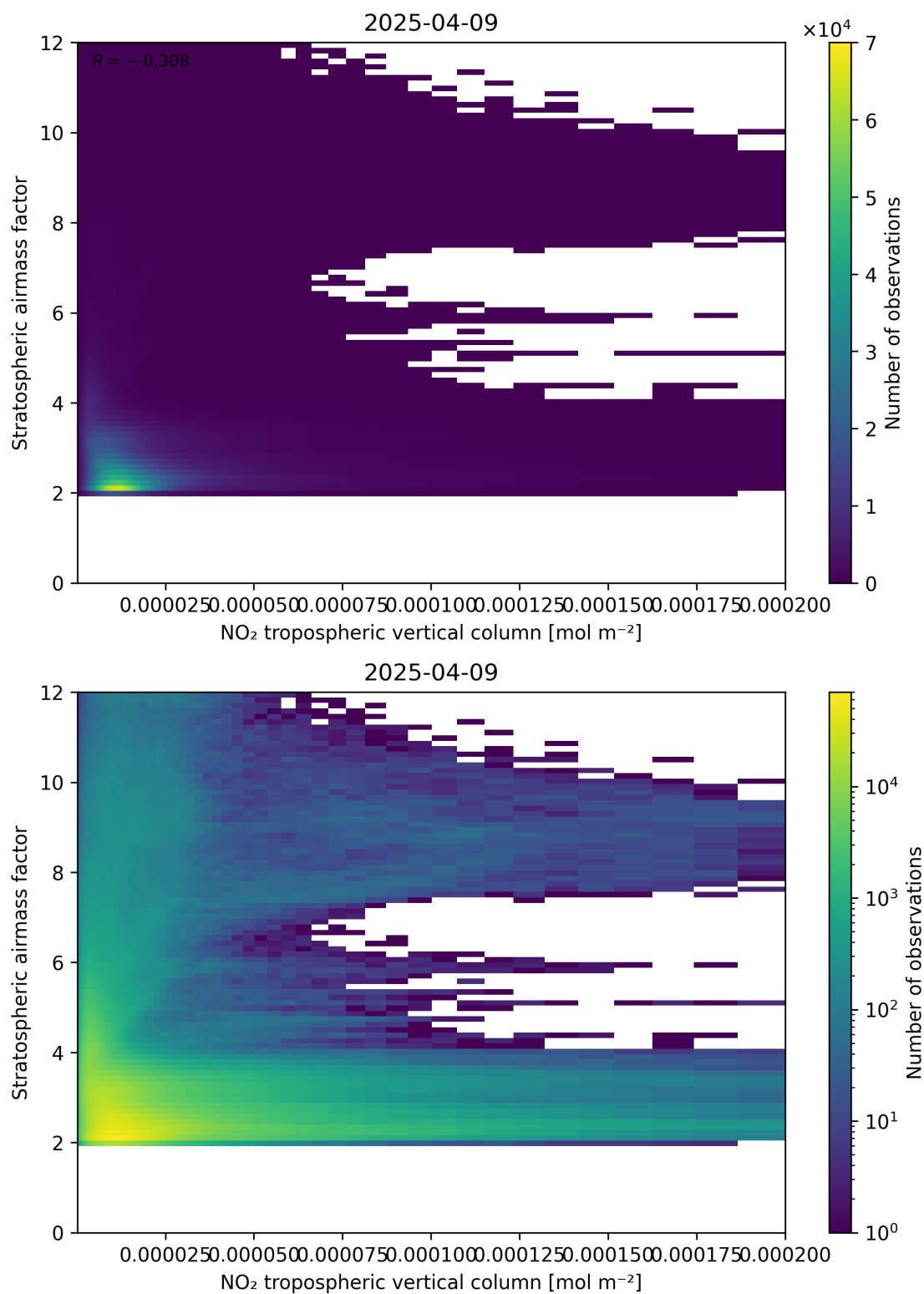
Figure 121: Scatter density plot of “NO 2 tropospheric vertical column” against “Stratospheric air mass factor” for 2025-04-09 to 2025-04-10.
