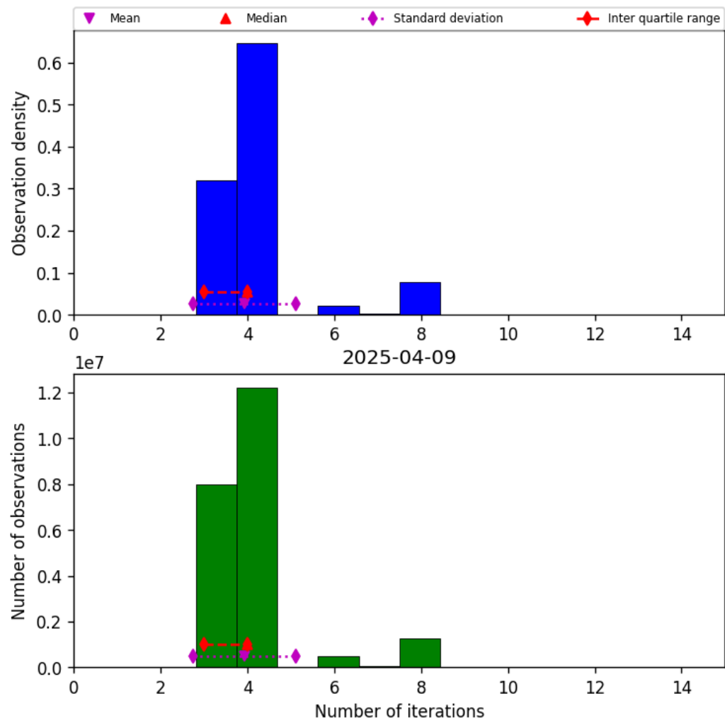
Figure 34: Histogram of “Number of iterations” for 2025-04-09 to 2025-04-10
