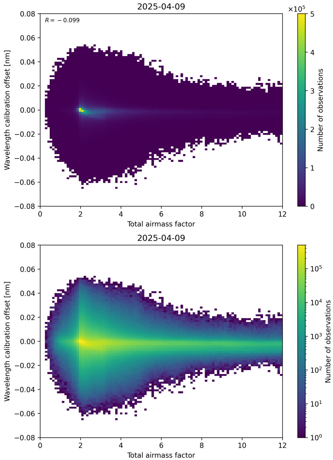
Figure 70: Scatter density plot of “Total airmass factor” against “Wavelength calibration offset” for 2025-04-09 to 2025-04-10.
