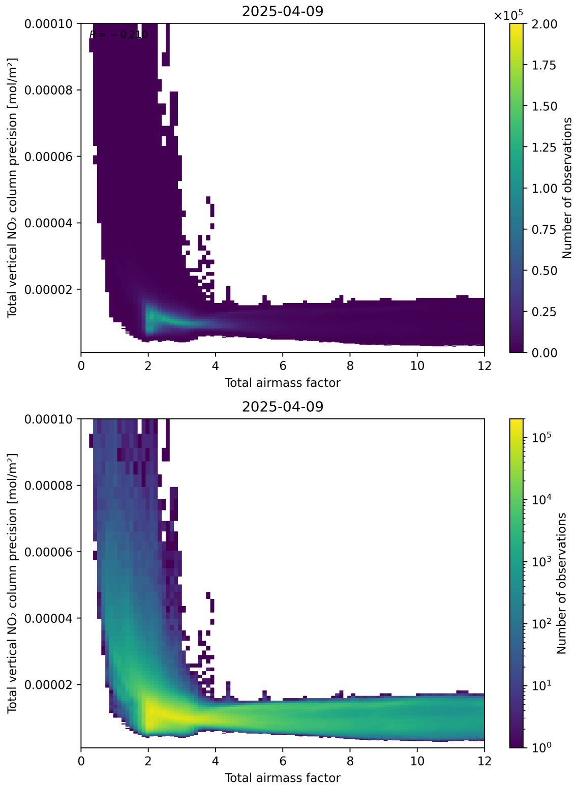
Figure 68: Scatter density plot of “Total airmass factor” against “Total vertical NO 2 column precision” for 2025-04-09 to 2025-04-10.
