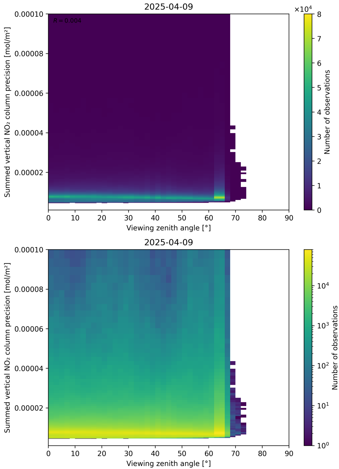
Figure 166: Scatter density plot of “Viewing zenith angle” against “Summed vertical NO 2 column precision” for 2025-04-09 to 2025-04-10.
