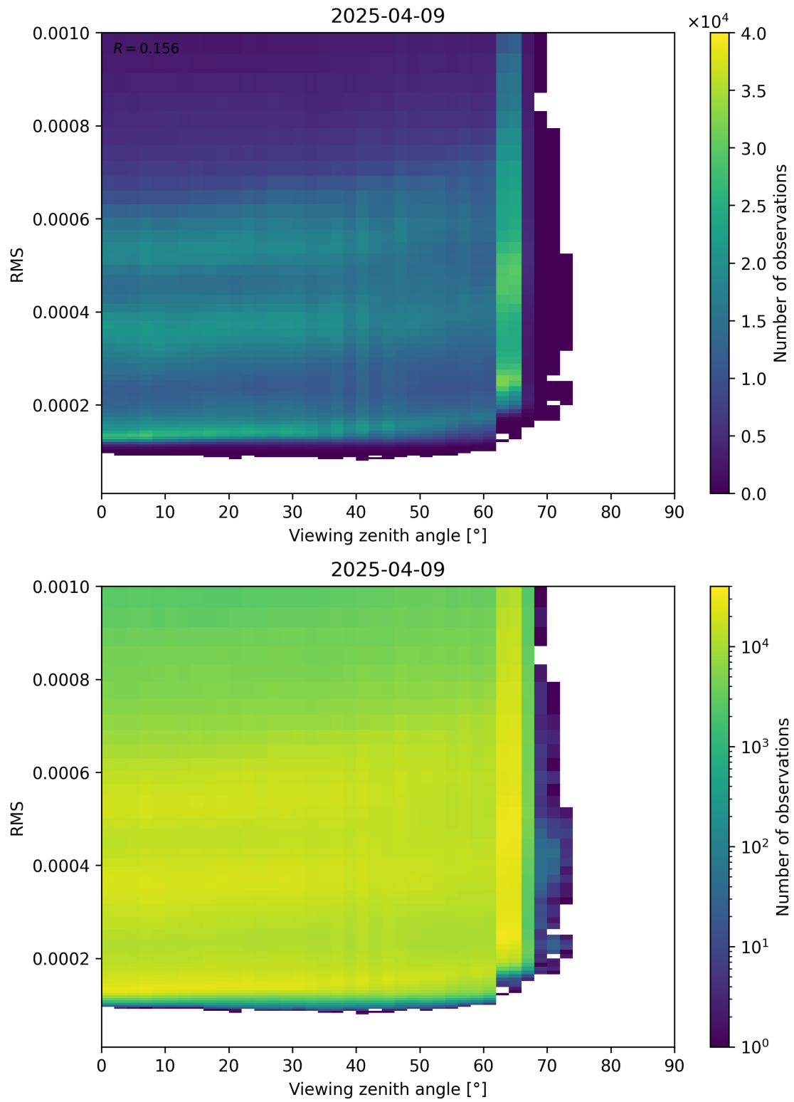
Figure 171: Scatter density plot of “Viewing zenith angle” against “RMS” for 2025-04-09 to 2025-04-10.
