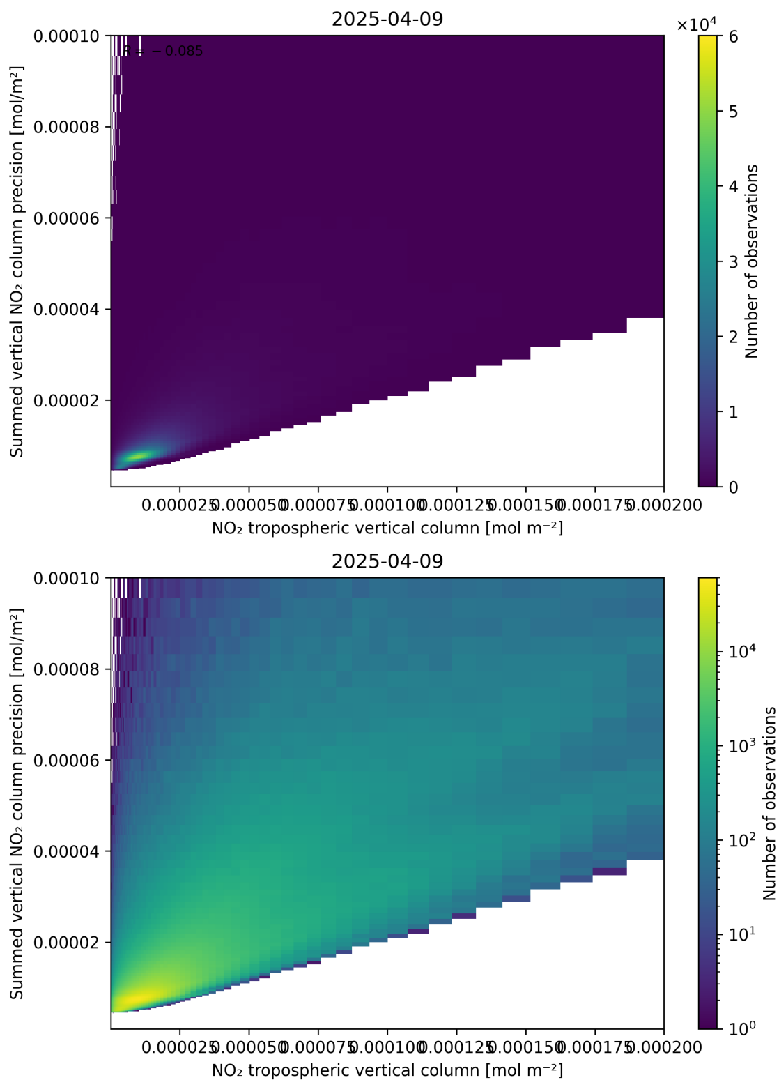
Figure 127: Scatter density plot of “NO 2 tropospheric vertical column” against “Summed vertical NO 2 column precision” for 2025-04-09 to 2025-04-10.
