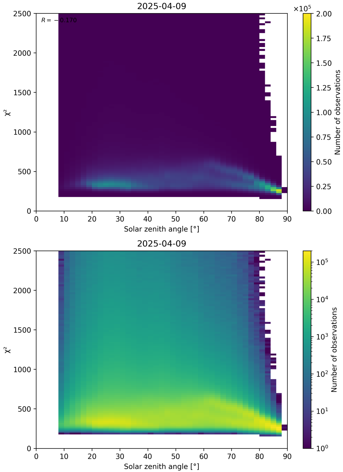
Figure 148: Scatter density plot of “Solar zenith angle” against “ \chi^2 ” for 2025-04-09 to 2025-04-10.
