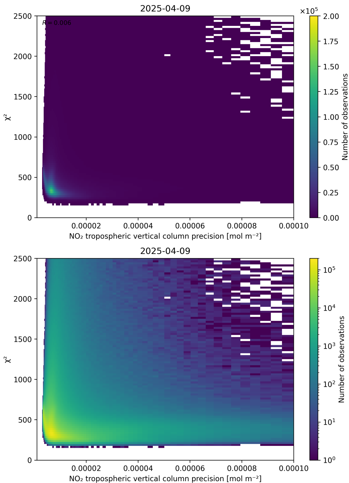
Figure 134: Scatter density plot of “NO 2 tropospheric vertical column precision” against “ \chi^2 ” for 2025-04-09 to 2025-04-10.
