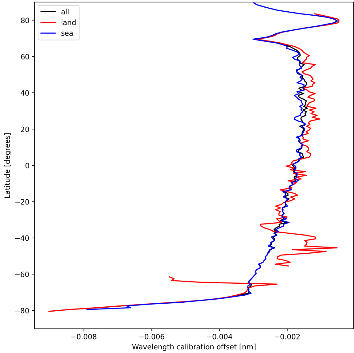
Figure 18: Zonal average of “Wavelength calibration offset” for 2025-04-09 to 2025-04-10.
