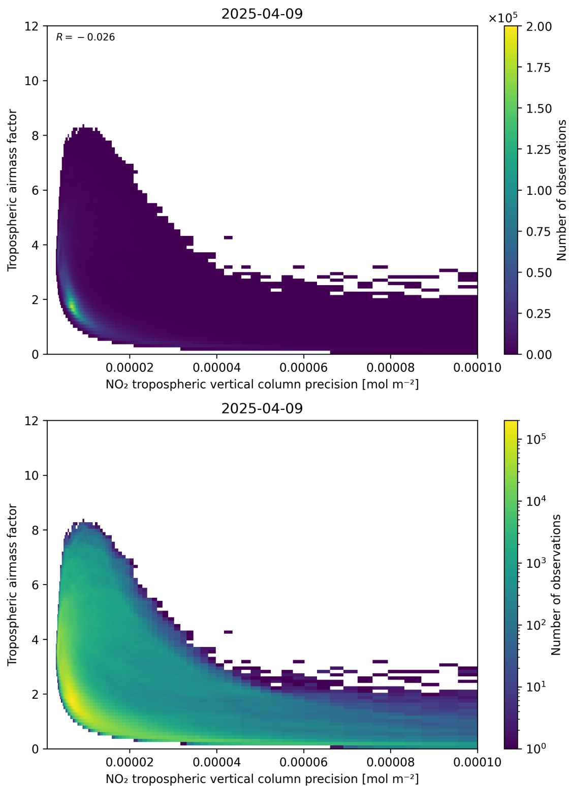
Figure 133: Scatter density plot of “NO 2 tropospheric vertical column precision” against “Tropospheric air mass factor” for 2025-04-09 to 2025-04-10.
