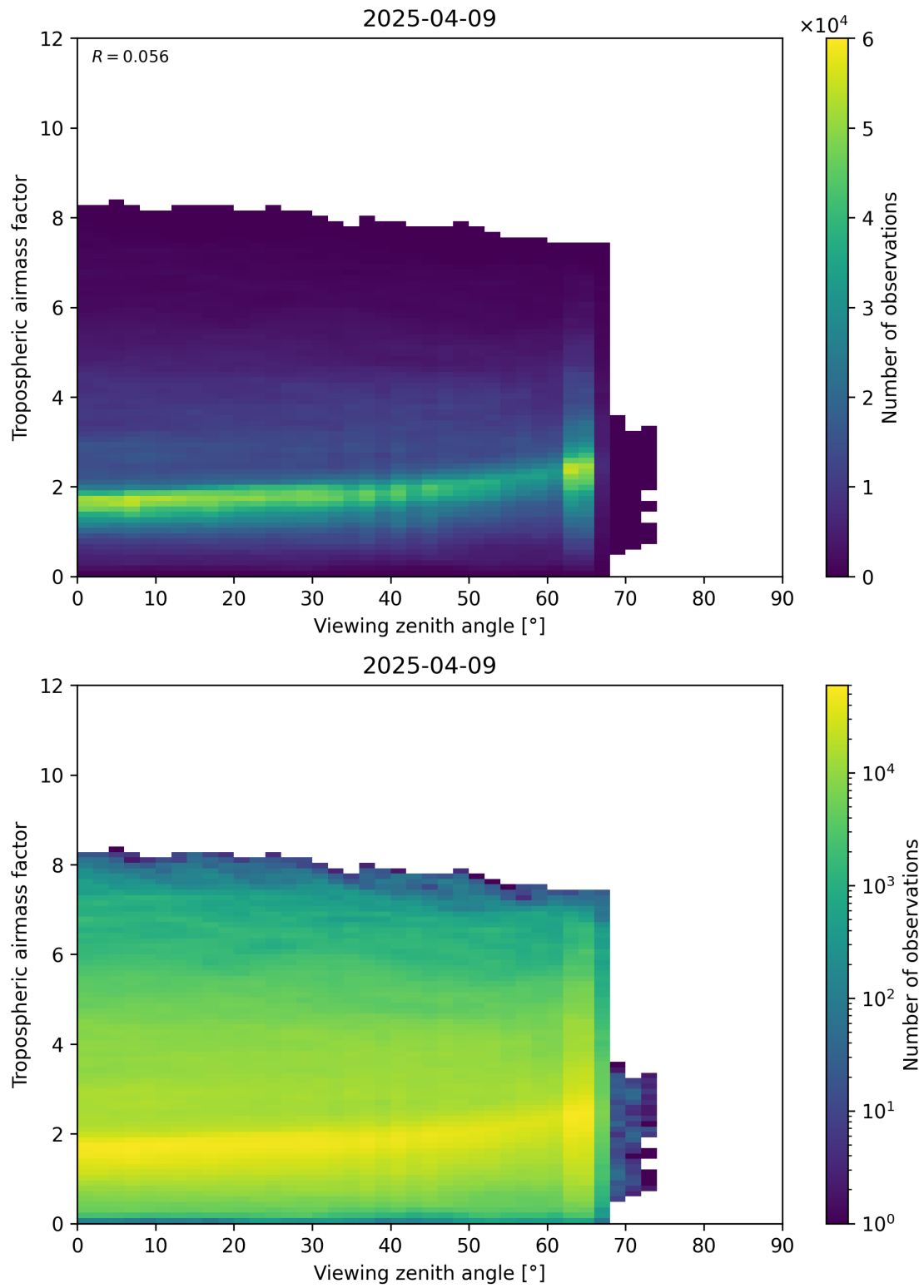
Figure 161: Scatter density plot of “Viewing zenith angle” against “Tropospheric airmass factor” for 2025-04-09 to 2025-04-10.
