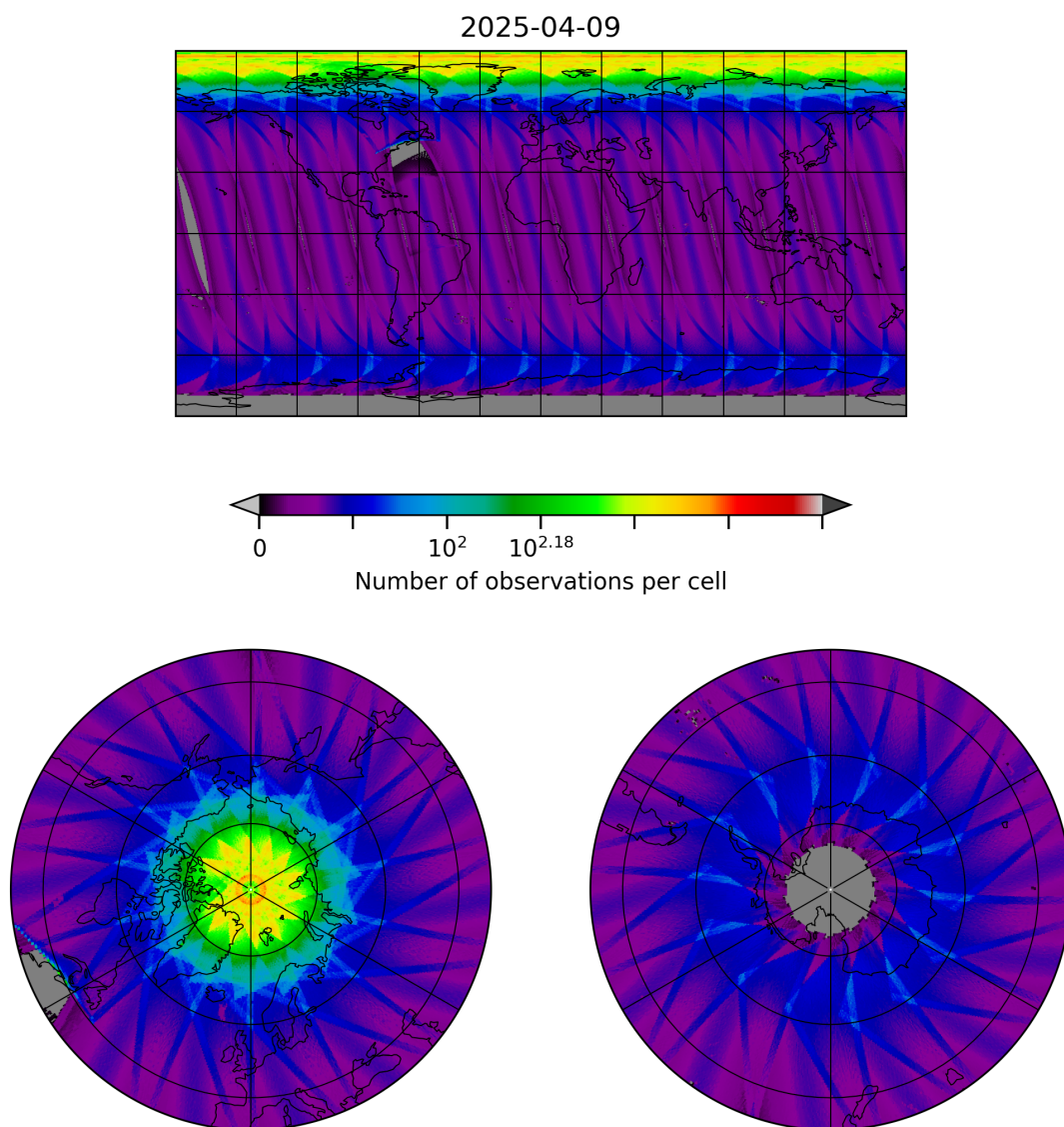
Figure 10: Map of the number of observations for 2025-04-09 to 2025-04-10
