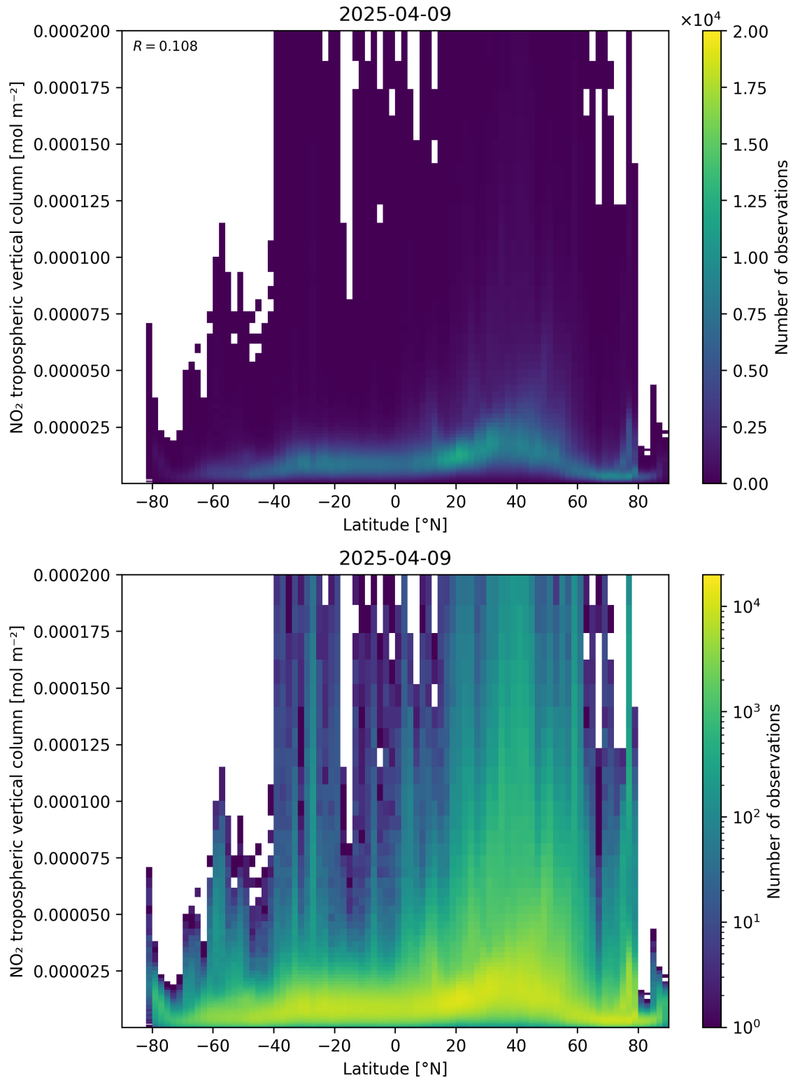
Figure 92: Scatter density plot of “Latitude” against “NO 2 tropospheric vertical column” for 2025-04-09 to 2025-04-10.
