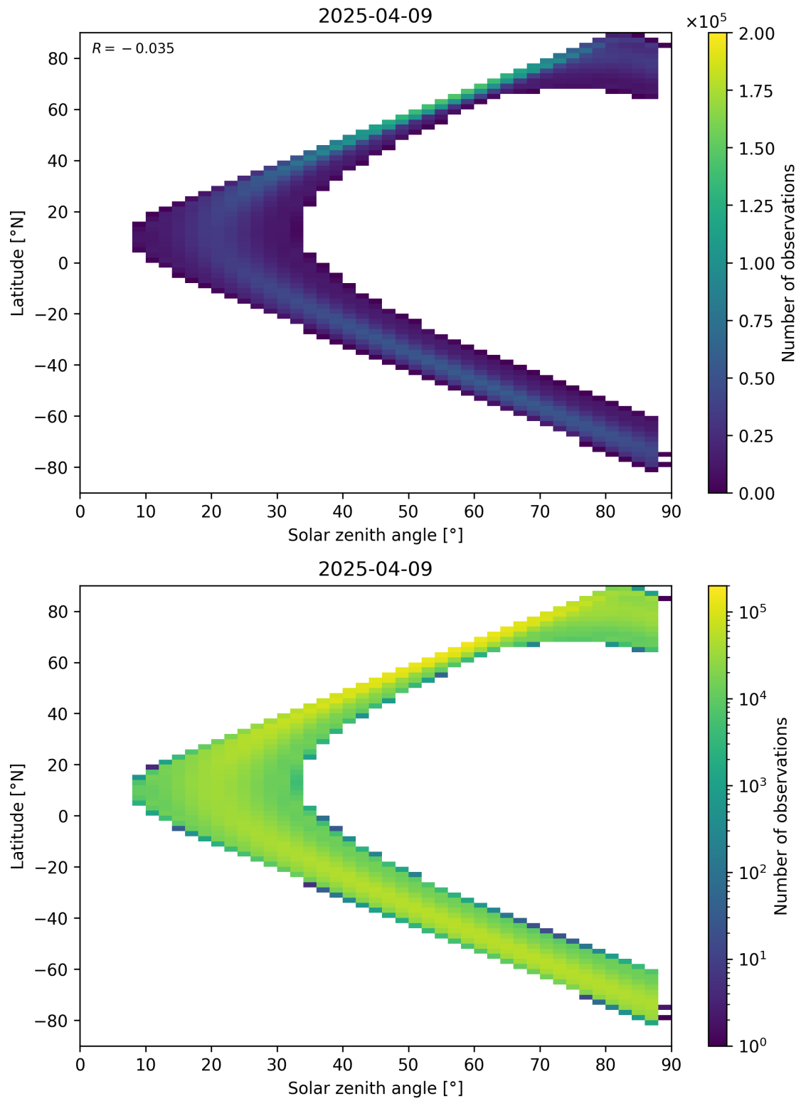
Figure 149: Scatter density plot of “Solar zenith angle” against “Latitude” for 2025-04-09 to 2025-04-10.
