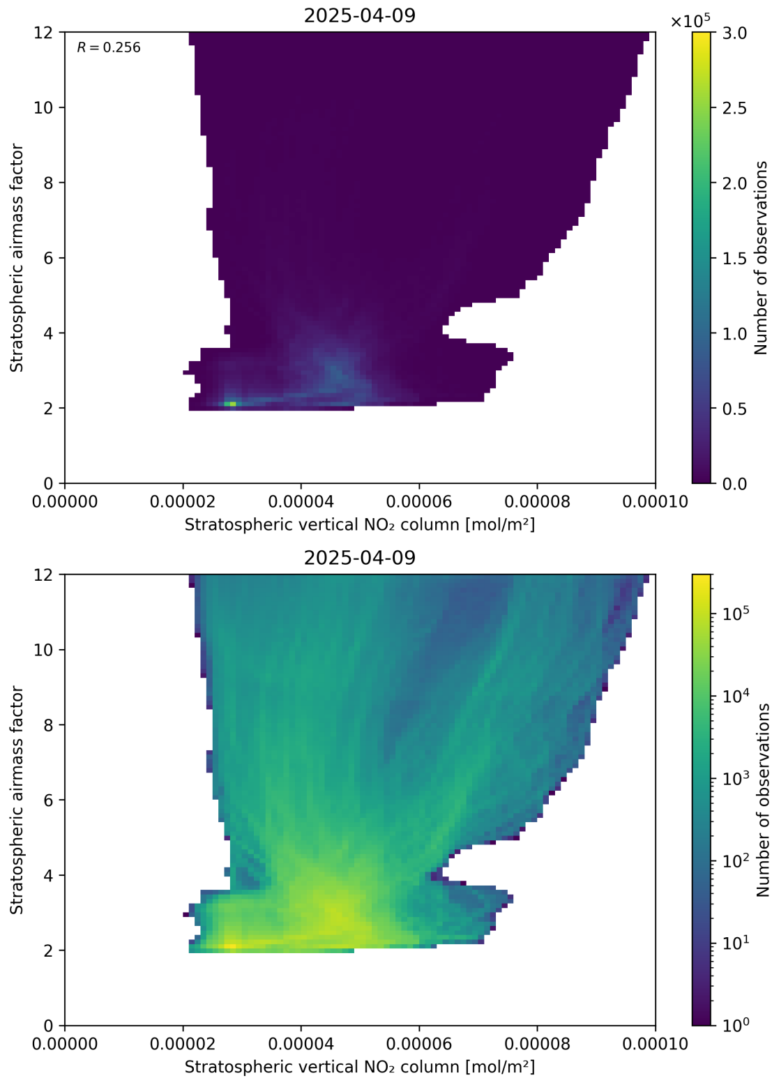
Figure 96: Scatter density plot of “Stratospheric vertical NO 2 column” against “Stratospheric airmass factor” for 2025-04-09 to 2025-04-10.
