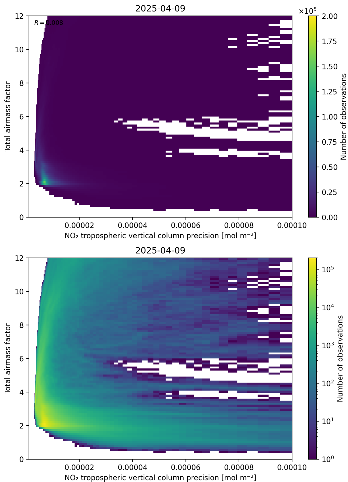
Figure 132: Scatter density plot of “NO 2 tropospheric vertical column precision” against “Total air mass factor” for 2025-04-09 to 2025-04-10.
