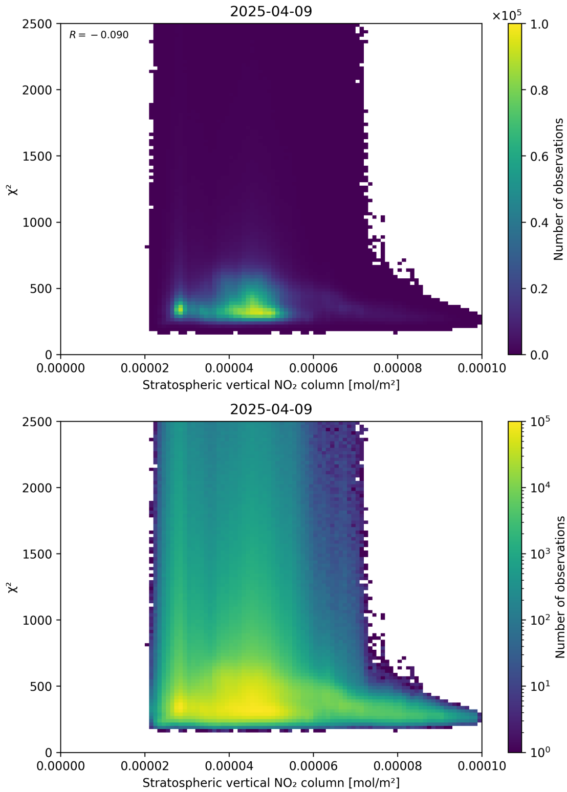
Figure 97: Scatter density plot of “Stratospheric vertical NO 2 column” against “ \chi^2 ” for 2025-04-09 to 2025-04-10.
