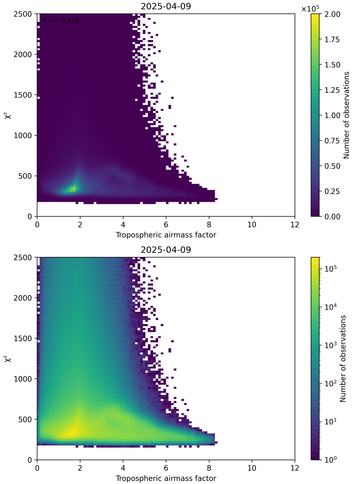
Figure 73: Scatter density plot of “Tropospheric airmass factor” against “ \chi^2 ” for 2025-04-09 to 2025-04-10.
