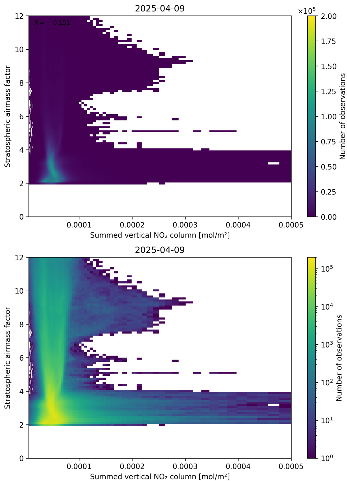
Figure 103: Scatter density plot of “Summed vertical NO 2 column” against “Stratospheric airmass factor” for 2025-04-09 to 2025-04-10.
