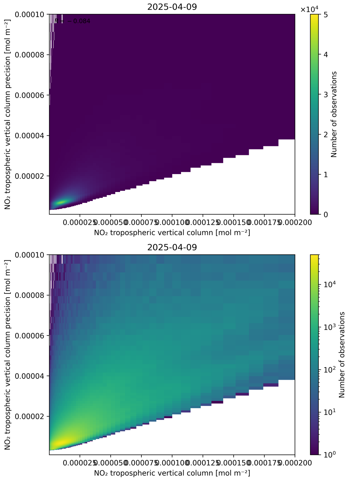
Figure 130: Scatter density plot of “NO 2 tropospheric vertical column” against “NO 2 tropospheric vertical column precision” for 2025-04-09 to 2025-04-10.
