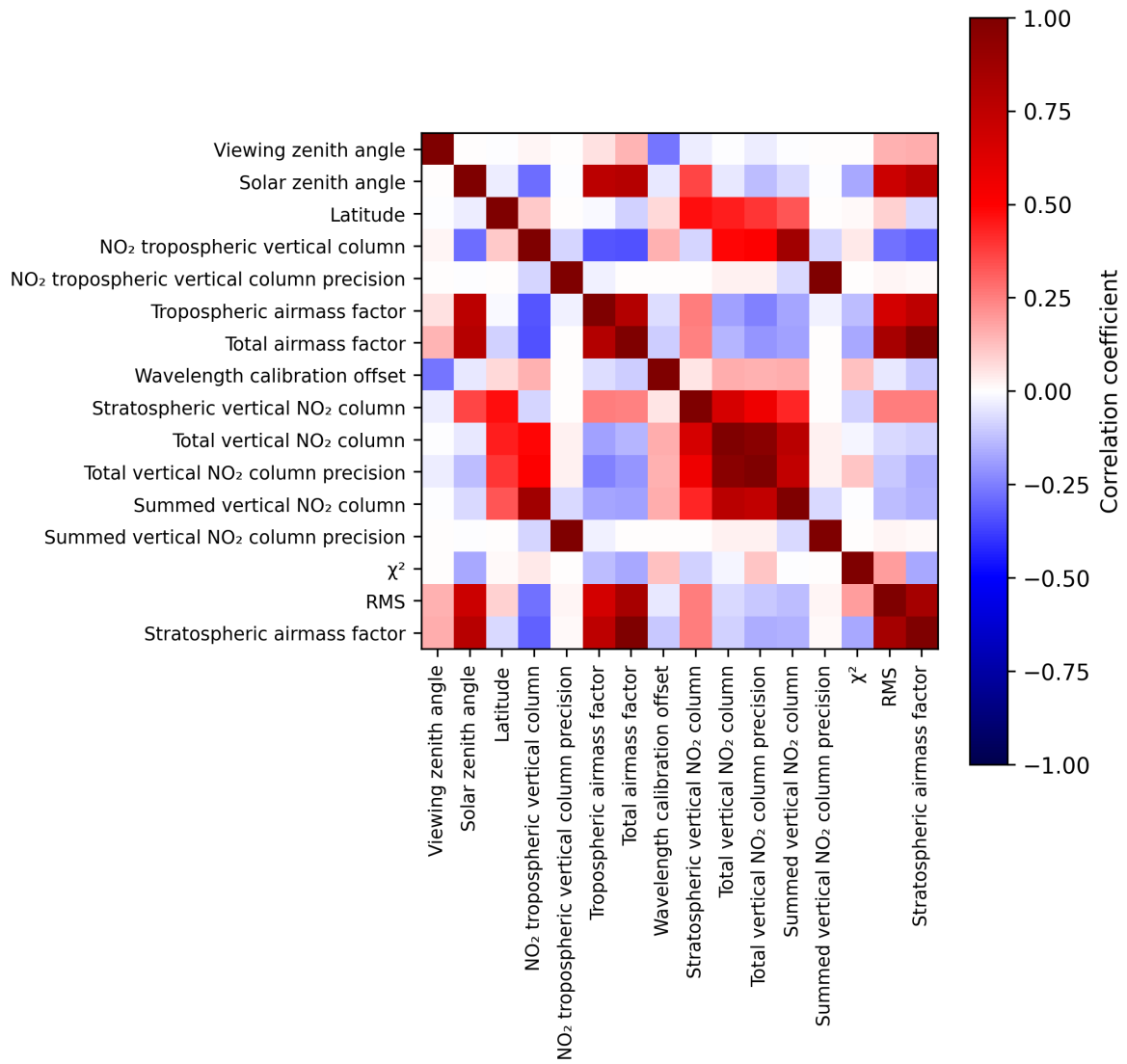
Figure 2: Map of correlation matrix for 2025-04-09 to 2025-04-10.
