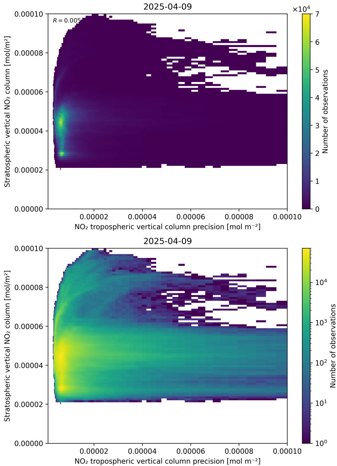
Figure 135: Scatter density plot of “NO 2 tropospheric vertical column precision” against “Stratospheric vertical NO 2 column” for 2025-04-09 to 2025-04-10.
