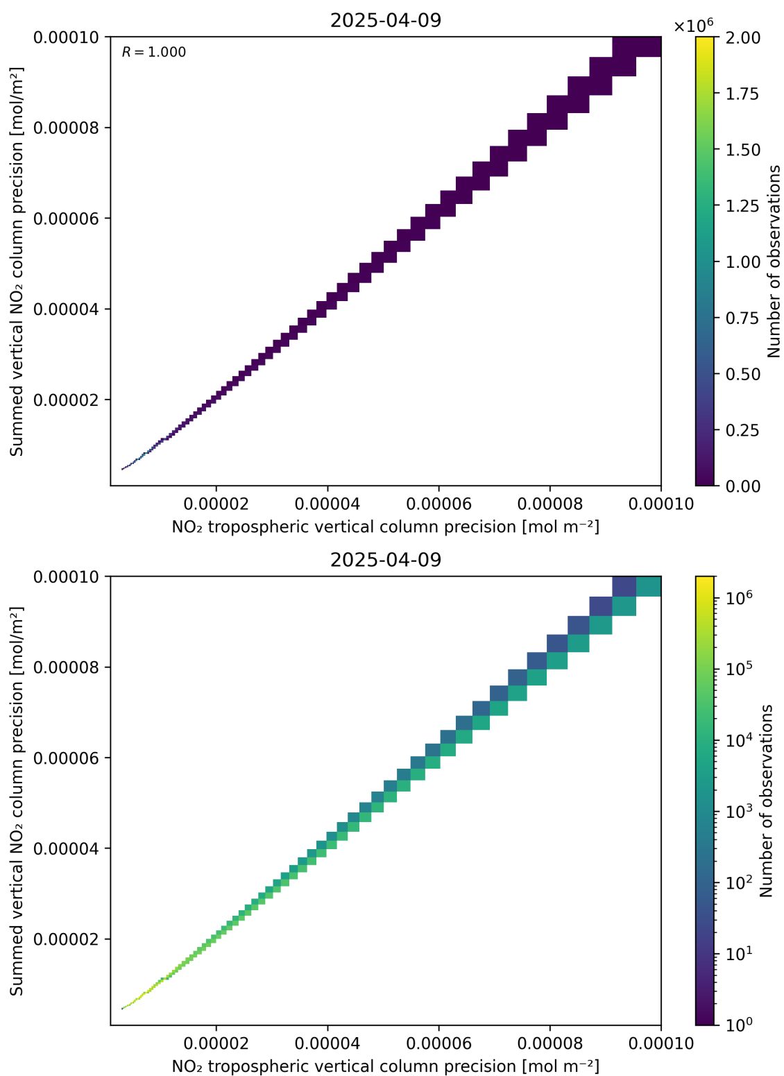
Figure 137: Scatter density plot of “NO 2 tropospheric vertical column precision” against “Summed vertical NO 2 column precision” for 2025-04-09 to 2025-04-10.
