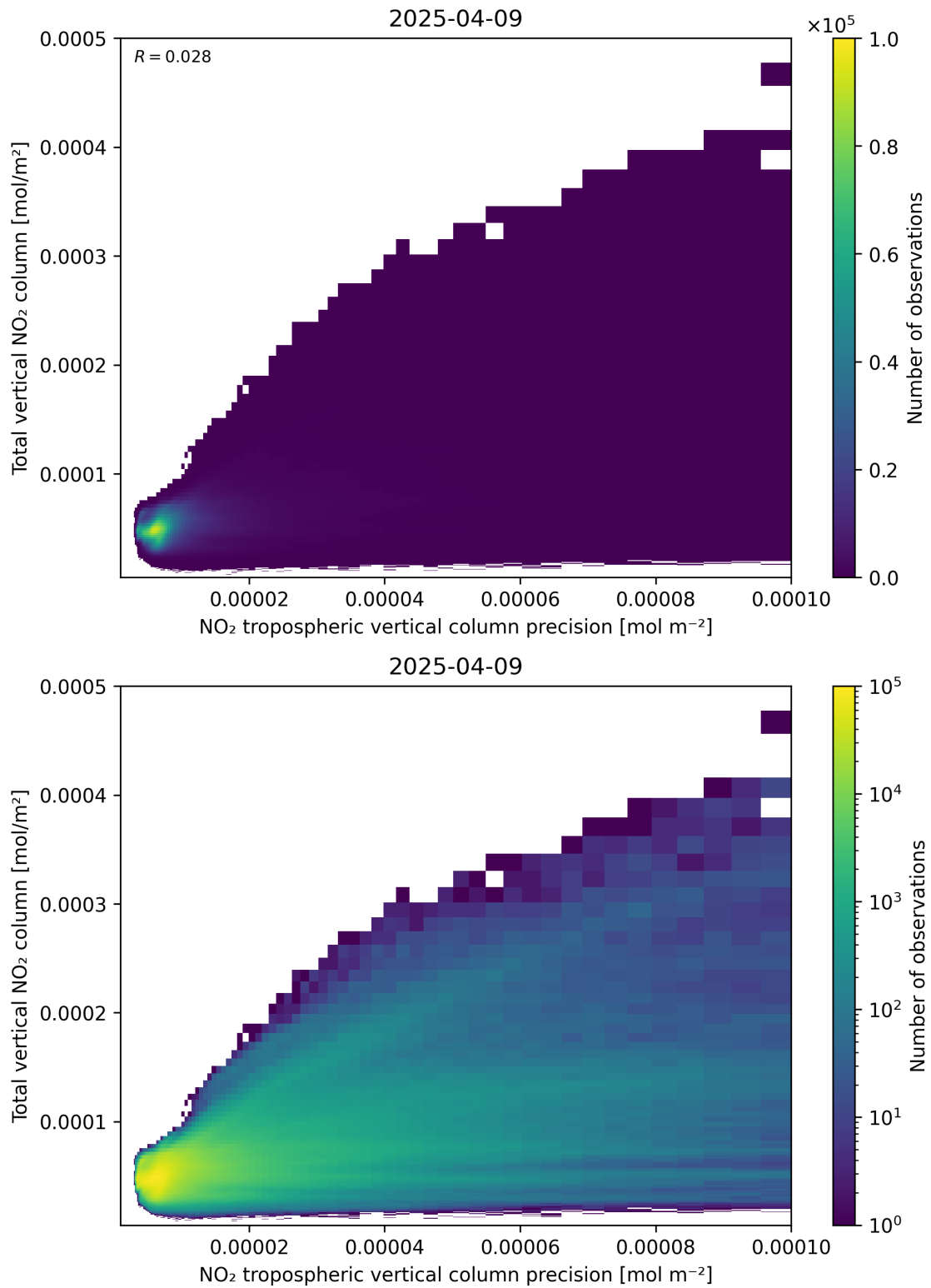
Figure 138: Scatter density plot of “NO 2 tropospheric vertical column precision” against “Total vertical NO 2 column” for 2025-04-09 to 2025-04-10.
