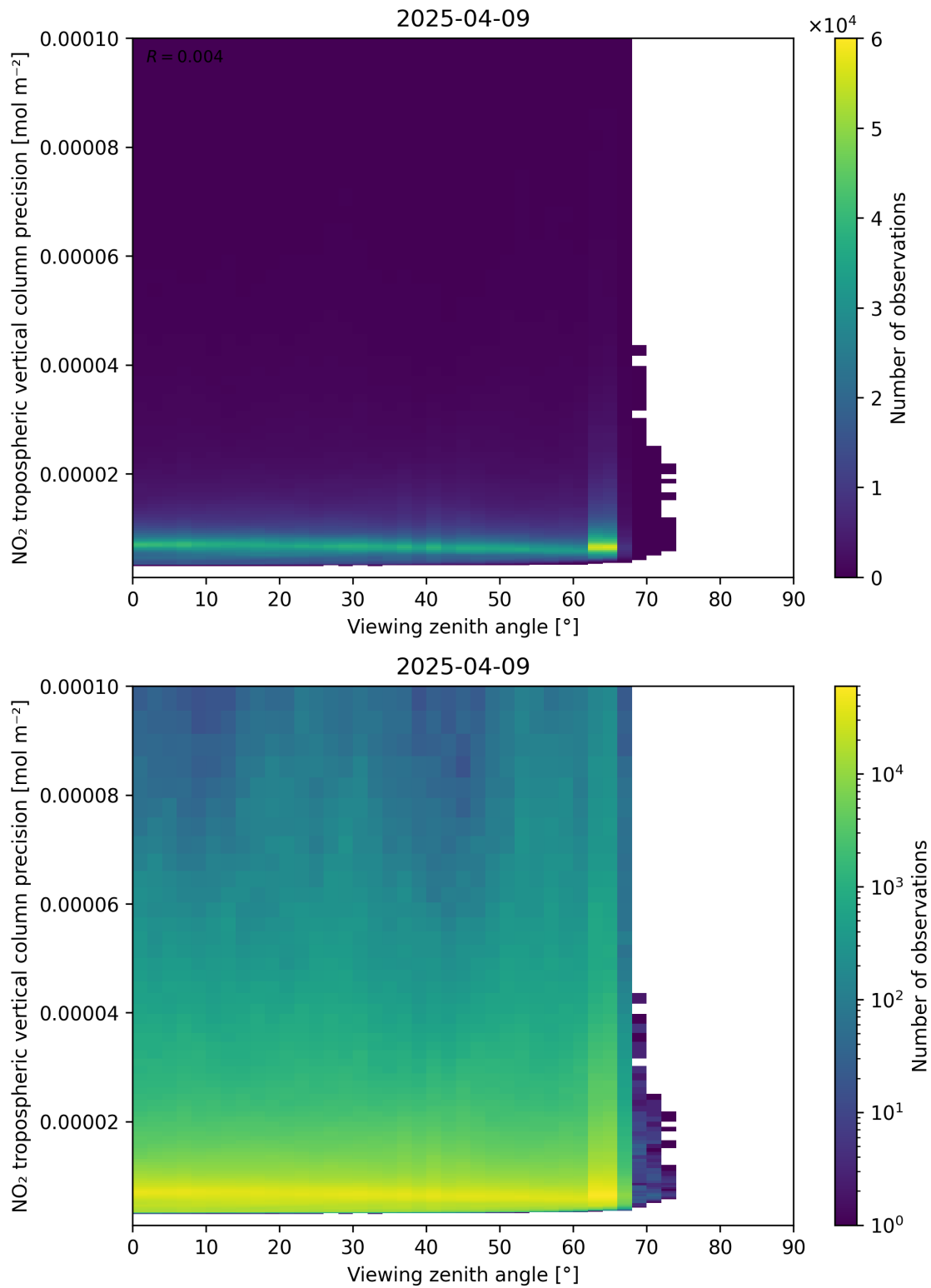
Figure 170: Scatter density plot of “Viewing zenith angle” against “NO 2 tropospheric vertical column precision” for 2025-04-09 to 2025-04-10.
