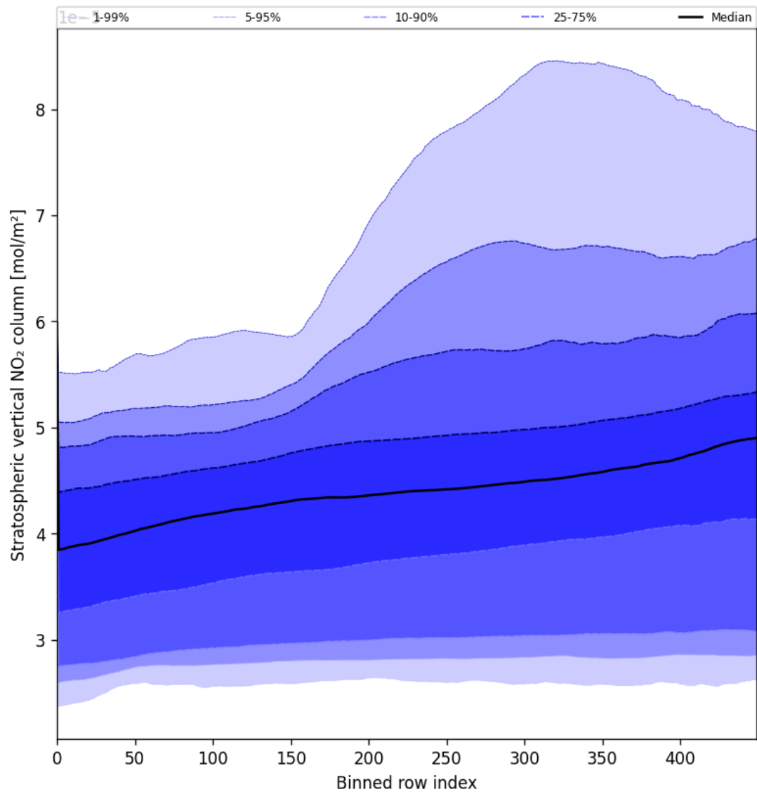
Figure 53: Along track statistics of “Stratospheric vertical NO 2 column” for 2025-04-09 to 2025-04-10
