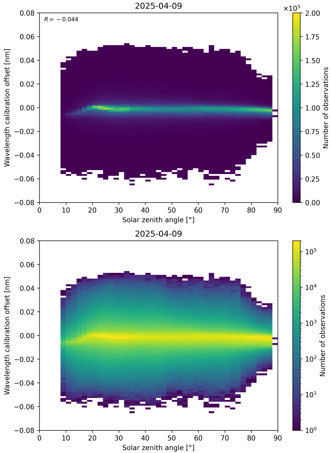
Figure 158: Scatter density plot of “Solar zenith angle” against “Wavelength calibration offset” for 2025-04-09 to 2025-04-10.
