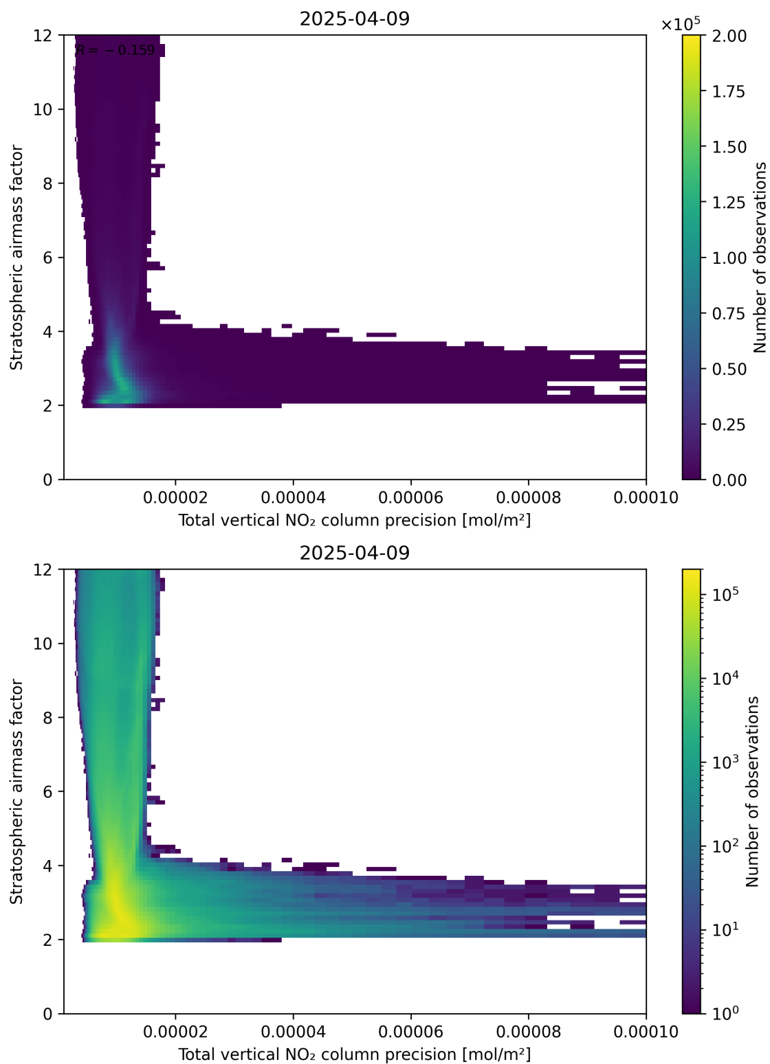
Figure 115: Scatter density plot of “Total vertical NO 2 column precision” against “Stratospheric air mass factor” for 2025-04-09 to 2025-04-10.
