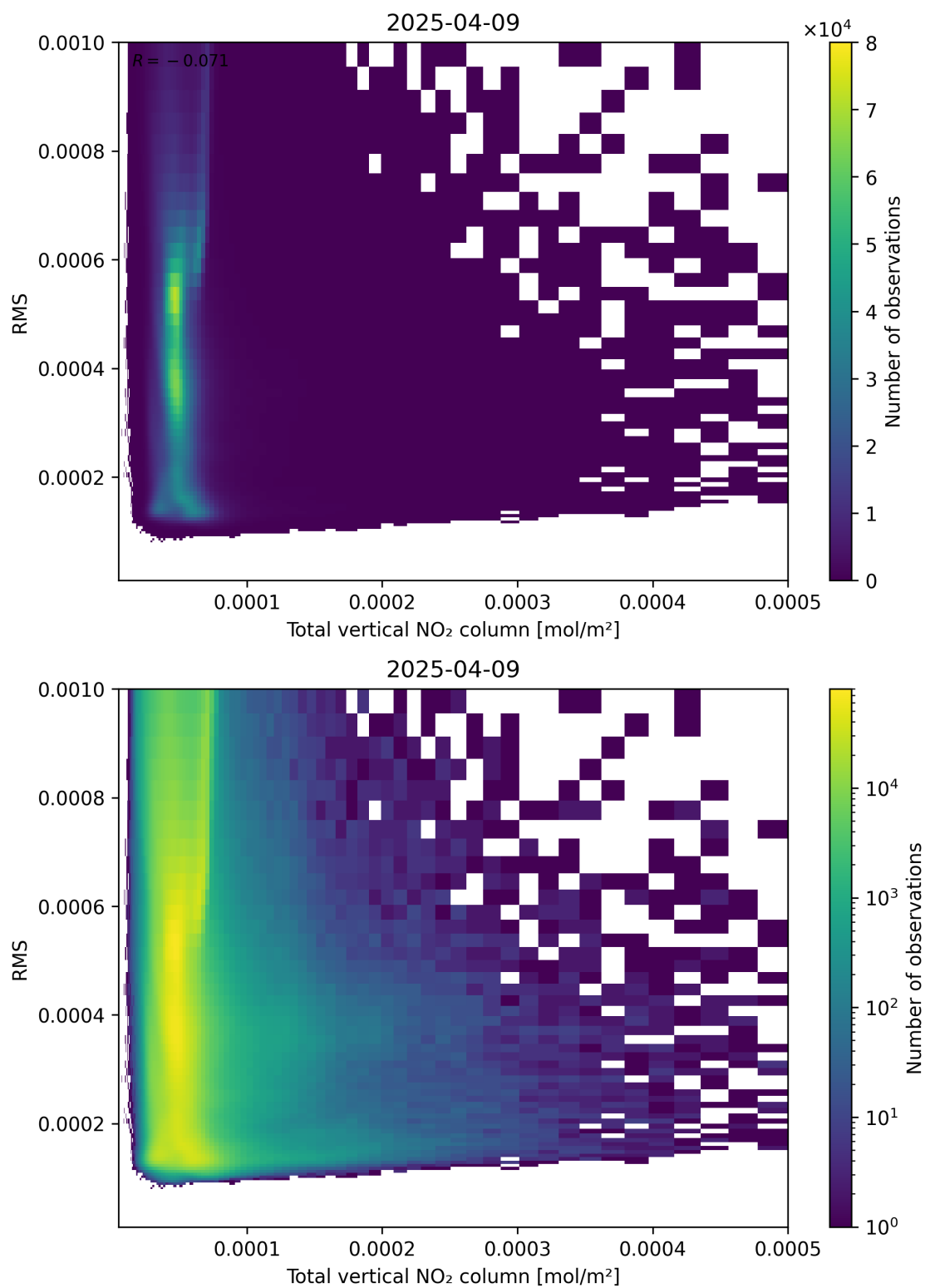
Figure 120: Scatter density plot of “Total vertical NO 2 column” against “RMS” for 2025-04-09 to 2025-04-10.
