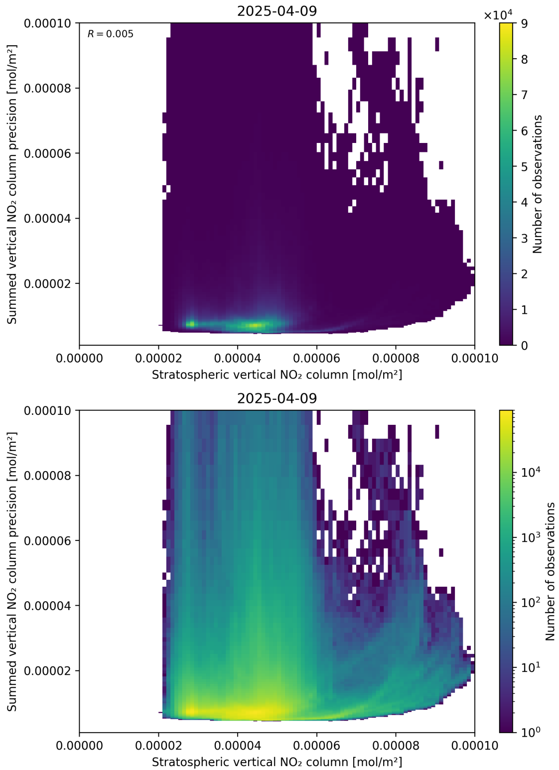
Figure 99: Scatter density plot of “Stratospheric vertical NO 2 column” against “Summed vertical NO 2 column precision” for 2025-04-09 to 2025-04-10.
