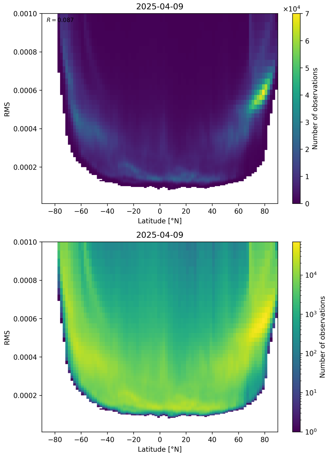
Figure 94: Scatter density plot of “Latitude” against “RMS” for 2025-04-09 to 2025-04-10.
