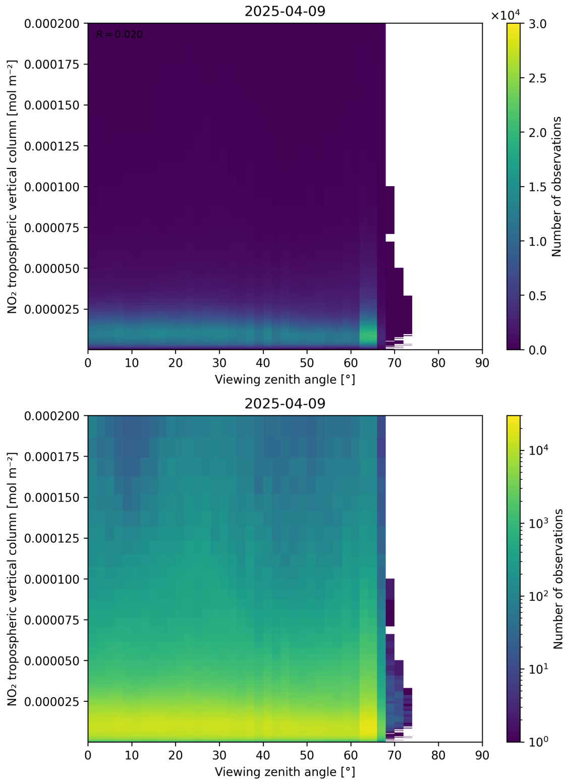
Figure 169: Scatter density plot of “Viewing zenith angle” against “NO 2 tropospheric vertical column” for 2025-04-09 to 2025-04-10.
