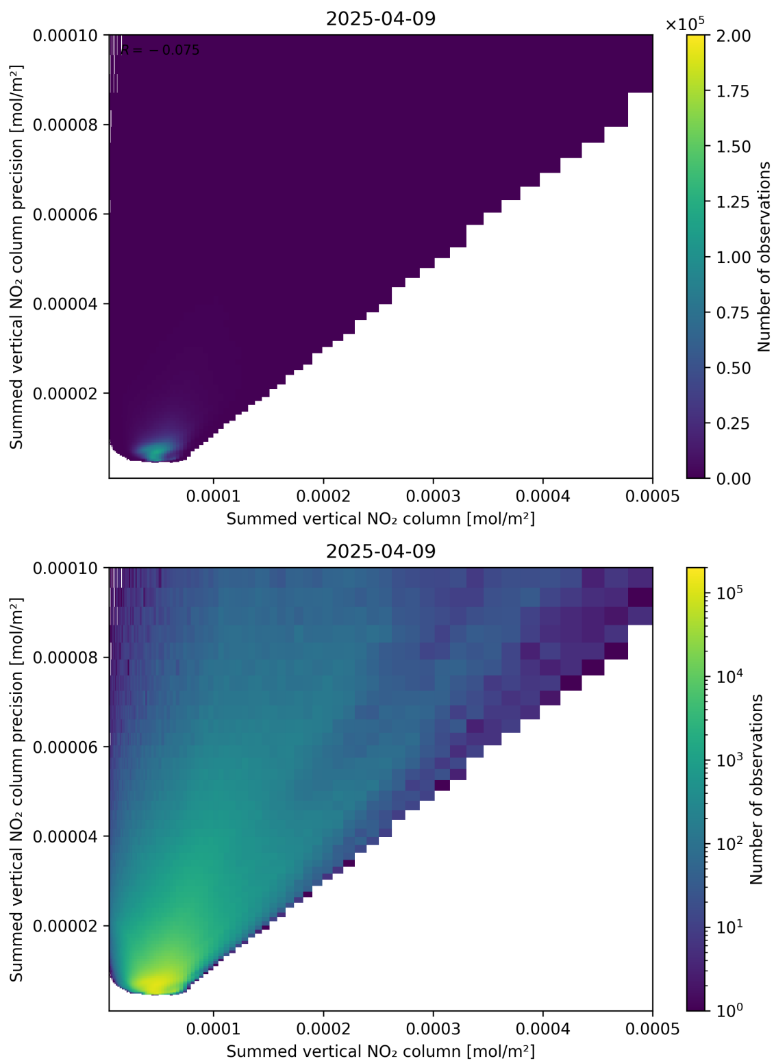
Figure 105: Scatter density plot of “Summed vertical NO 2 column” against “Summed vertical NO 2 column precision” for 2025-04-09 to 2025-04-10.
