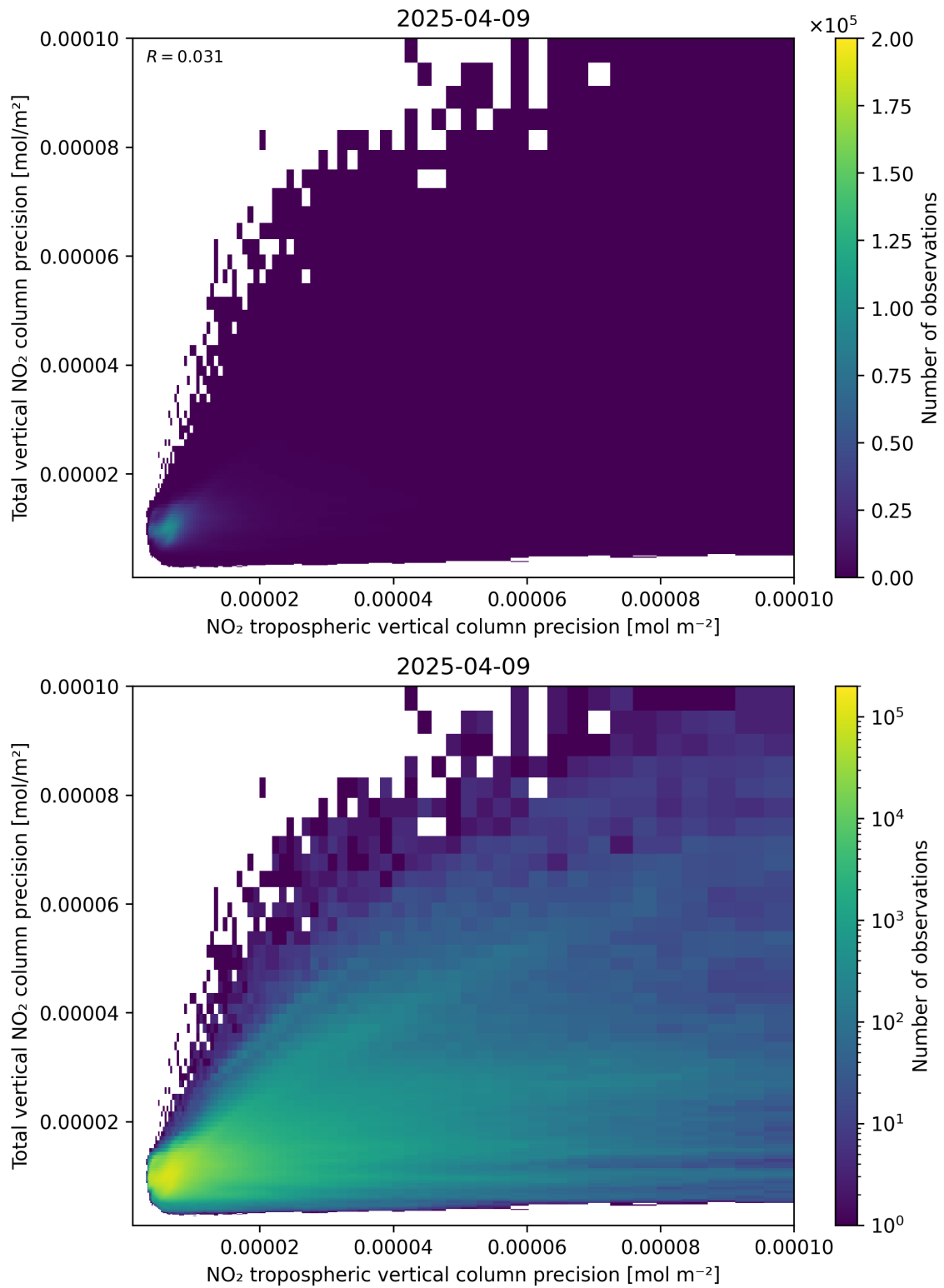
Figure 139: Scatter density plot of “NO 2 tropospheric vertical column precision” against “Total vertical NO 2 column precision” for 2025-04-09 to 2025-04-10.
