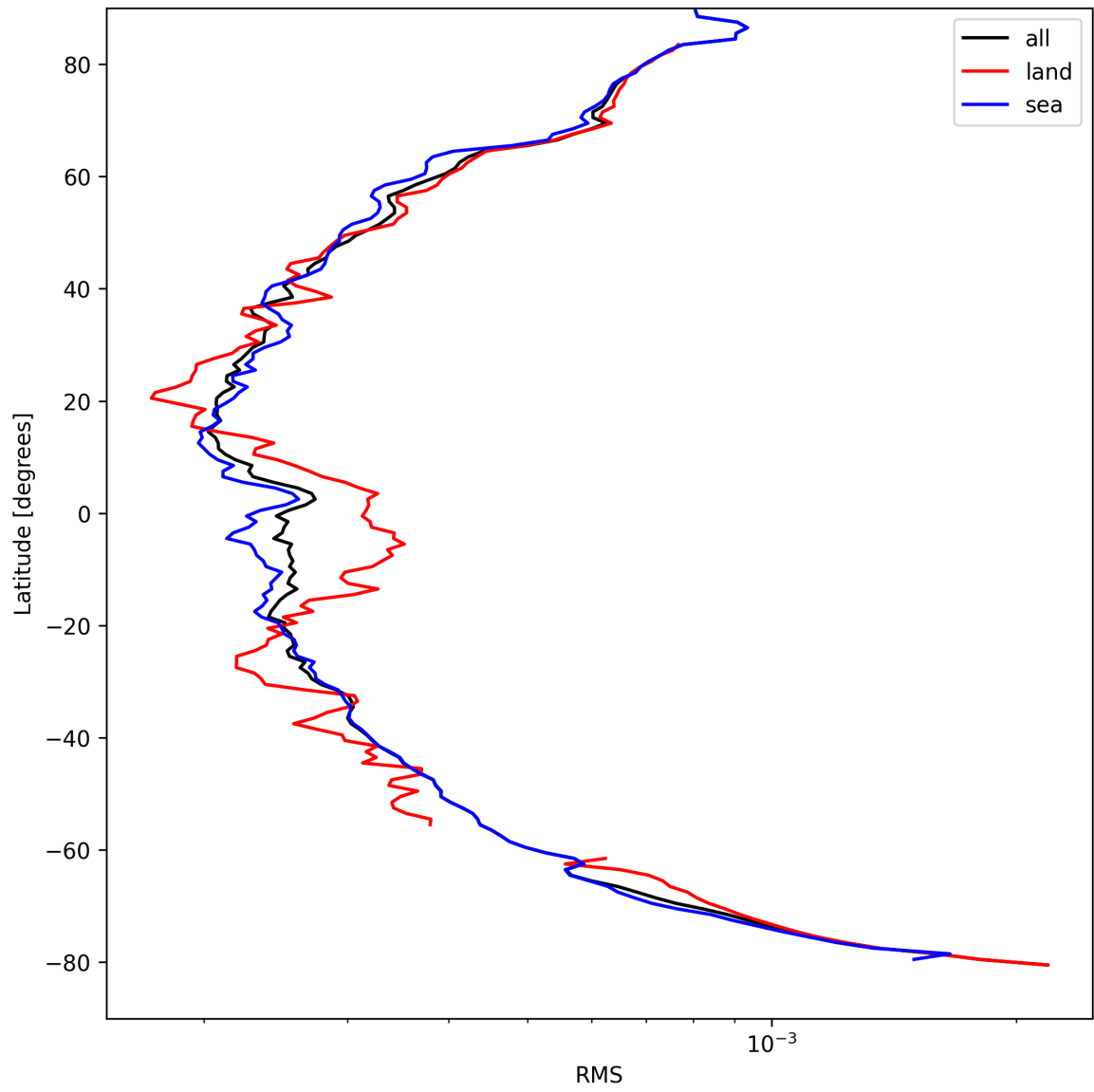
Figure 26: Zonal average of “RMS” for 2025-04-09 to 2025-04-10.
