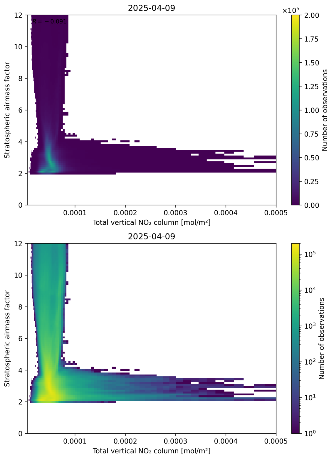
Figure 110: Scatter density plot of “Total vertical NO 2 column” against “Stratospheric airmass factor” for 2025-04-09 to 2025-04-10.
