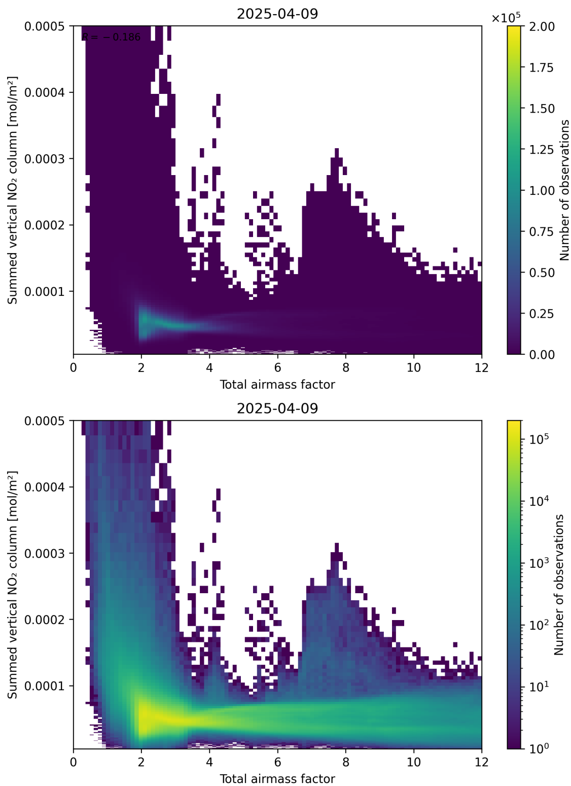
Figure 65: Scatter density plot of “Total airmass factor” against “Summed vertical NO 2 column” for 2025-04-09 to 2025-04-10.
