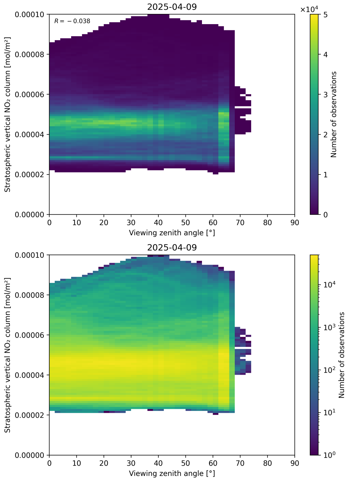
Figure 164: Scatter density plot of “Viewing zenith angle” against “Stratospheric vertical NO 2 column” for 2025-04-09 to 2025-04-10.
