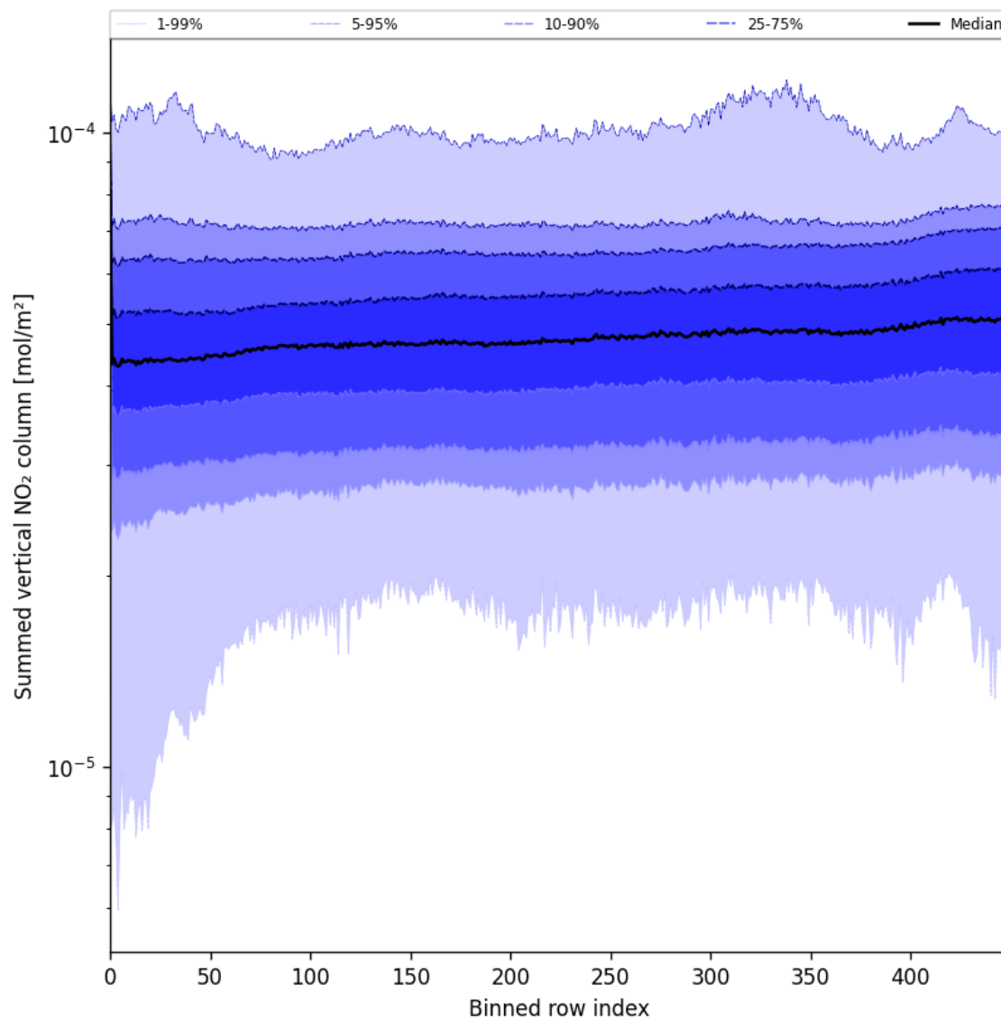
Figure 57: Along track statistics of “Summed vertical NO 2 column” for 2025-04-09 to 2025-04-10
