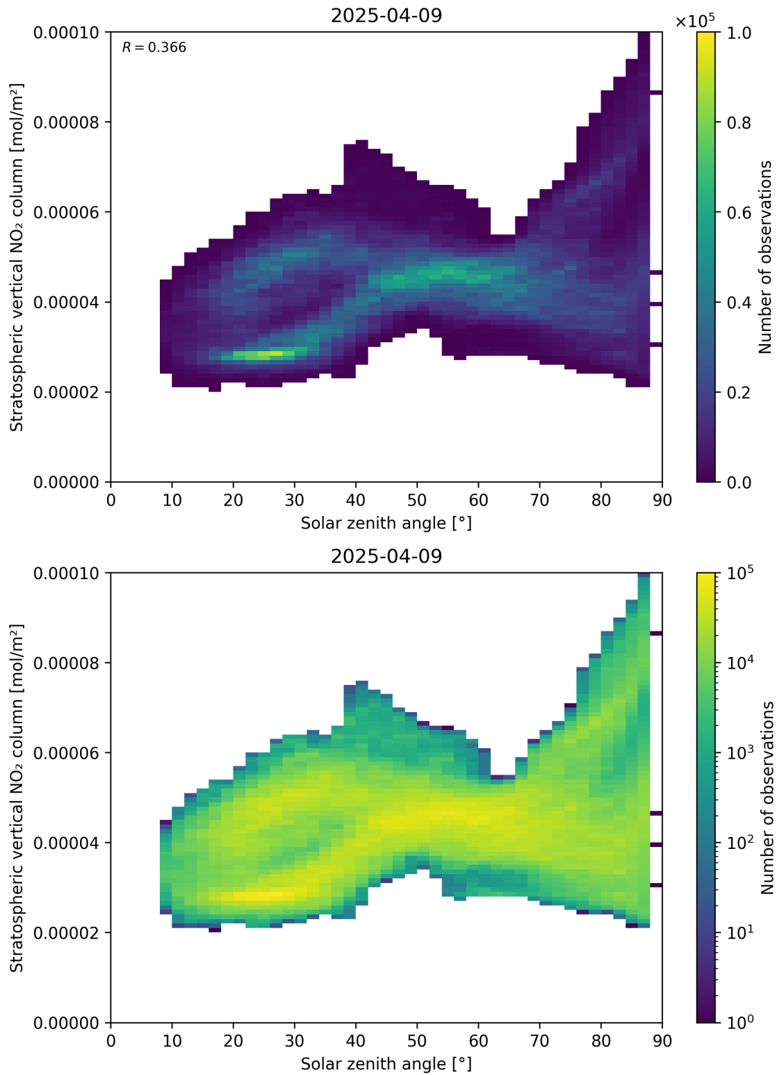
Figure 150: Scatter density plot of “Solar zenith angle” against “Stratospheric vertical NO 2 column” for 2025-04-09 to 2025-04-10.
