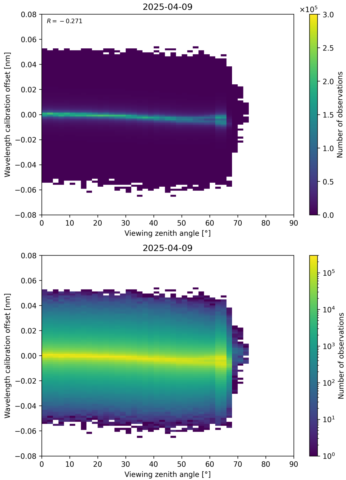
Figure 173: Scatter density plot of “Viewing zenith angle” against “Wavelength calibration offset” for 2025-04-09 to 2025-04-10.
