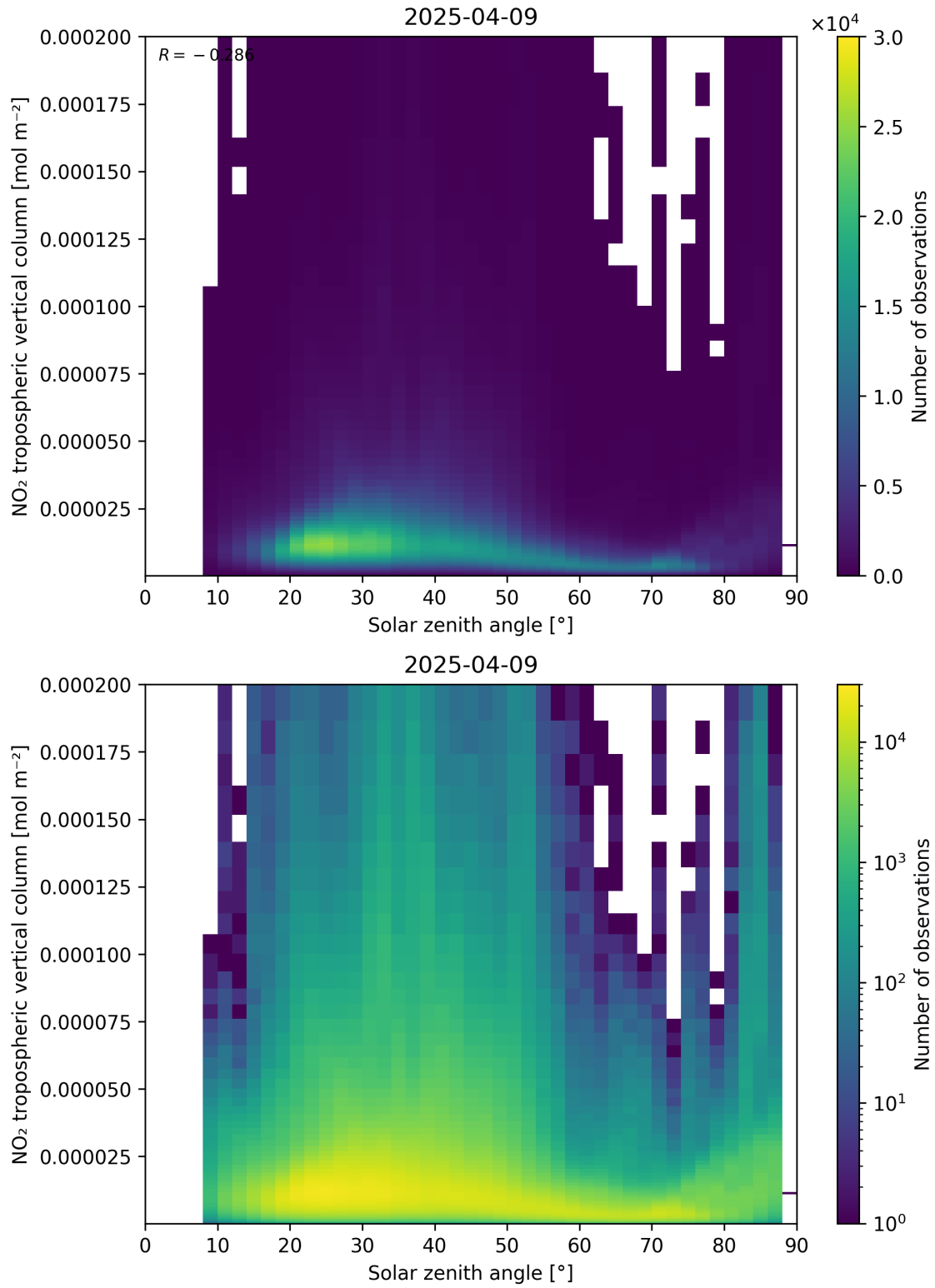
Figure 155: Scatter density plot of “Solar zenith angle” against “NO 2 tropospheric vertical column” for 2025-04-09 to 2025-04-10.
