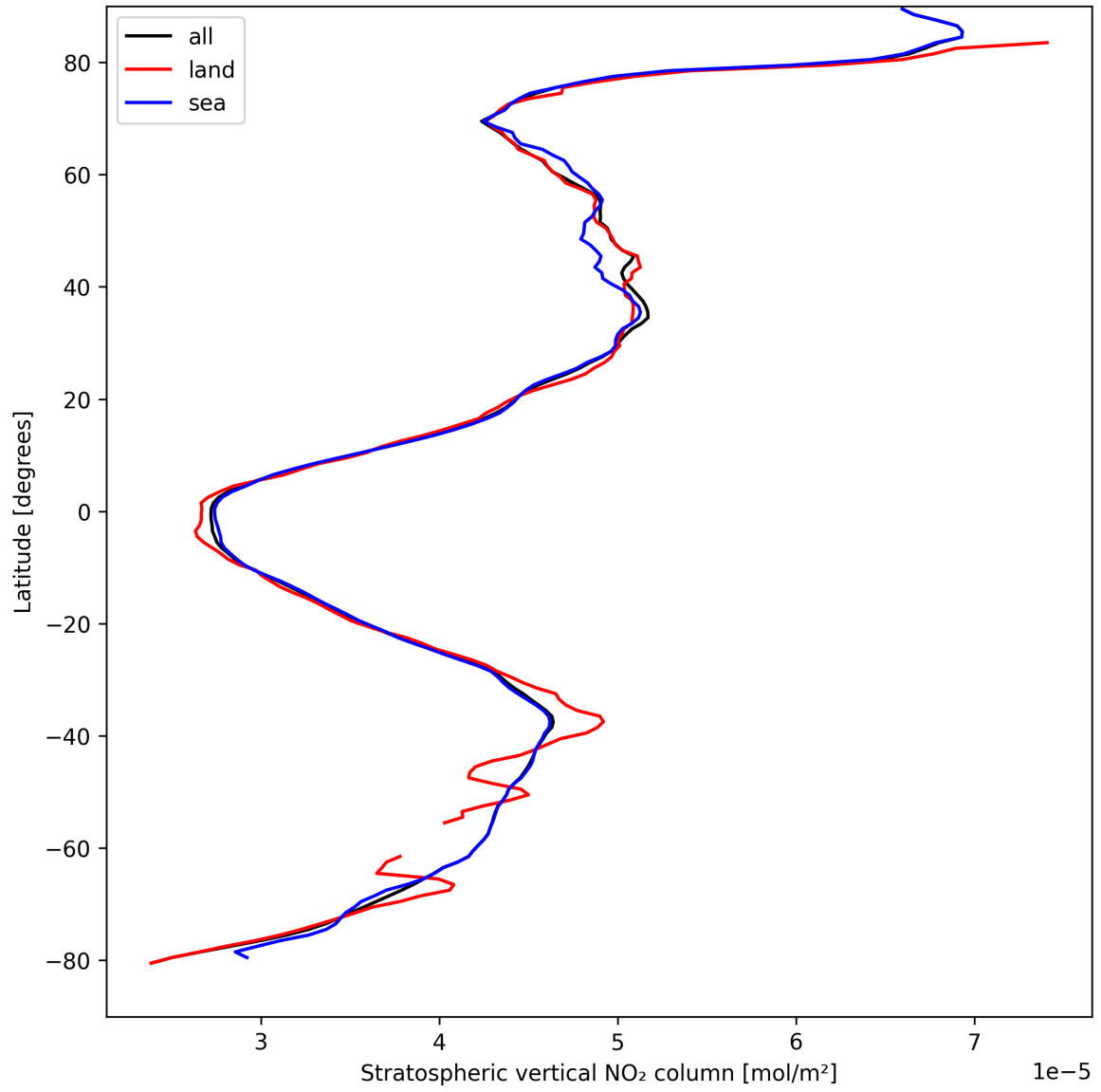
Figure 19: Zonal average of “Stratospheric vertical NO 2 column” for 2025-04-09 to 2025-04-10.
