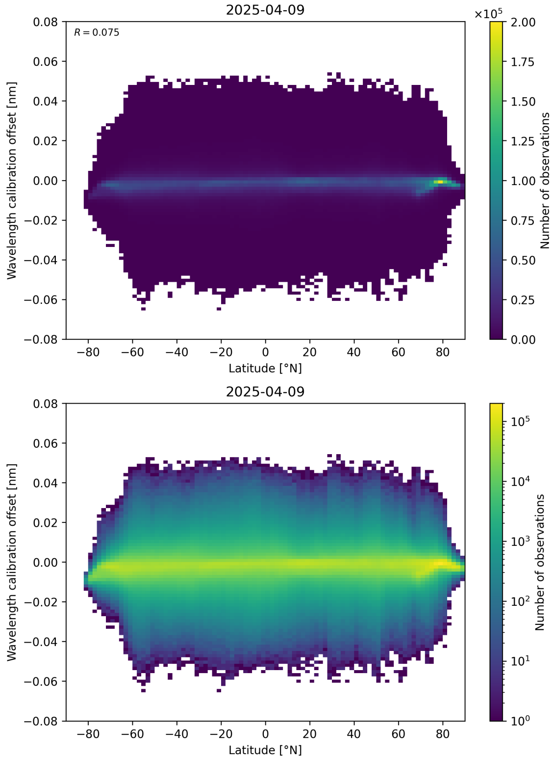
Figure 95: Scatter density plot of “Latitude” against “Wavelength calibration offset” for 2025-04-09 to 2025-04-10.
