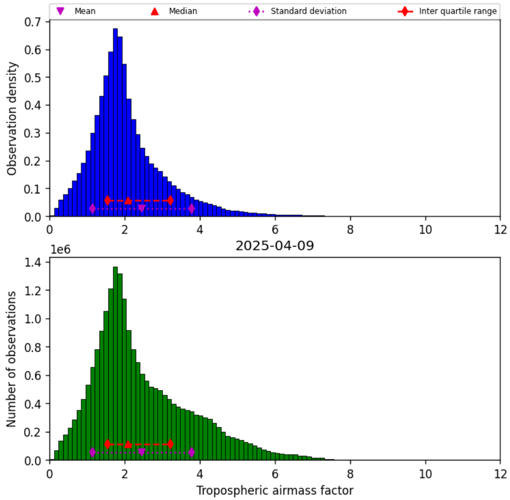
Figure 31: Histogram of “Tropospheric airmass factor” for 2025-04-09 to 2025-04-10
