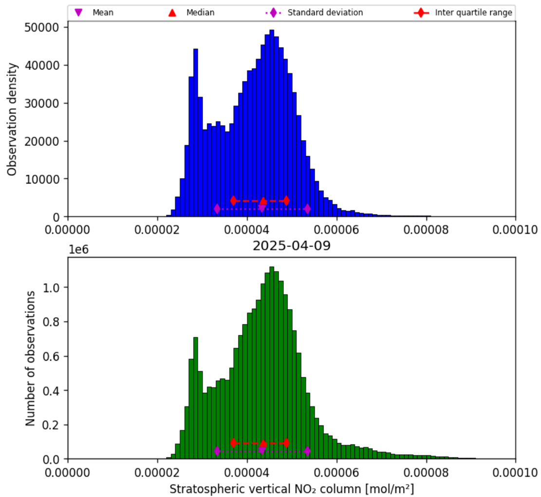
Figure 36: Histogram of “Stratospheric vertical NO 2 column” for 2025-04-09 to 2025-04-10
