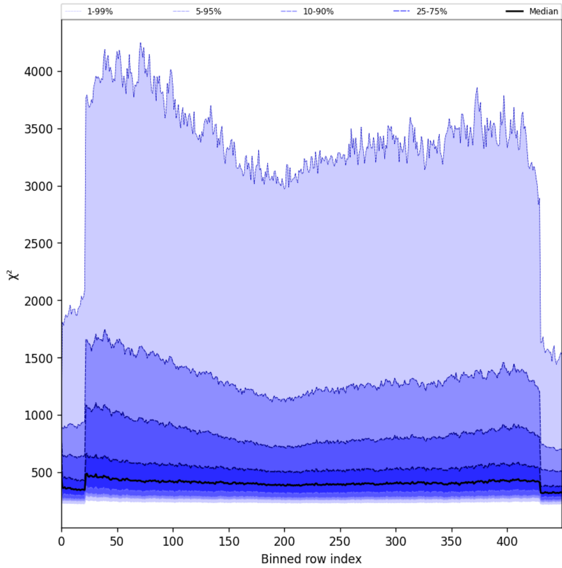
Figure 59: Along track statistics of “ \chi^2 ” for 2025-04-09 to 2025-04-10
