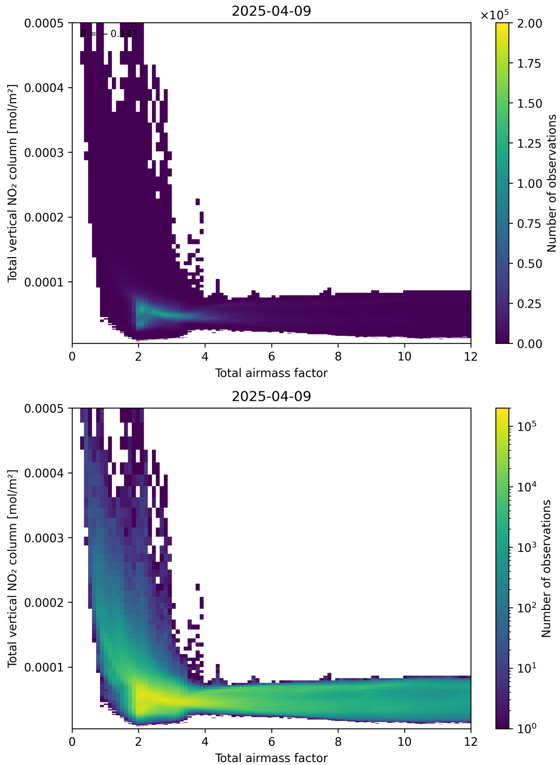
Figure 67: Scatter density plot of “Total airmass factor” against “Total vertical NO 2 column” for 2025-04-09 to 2025-04-10.
