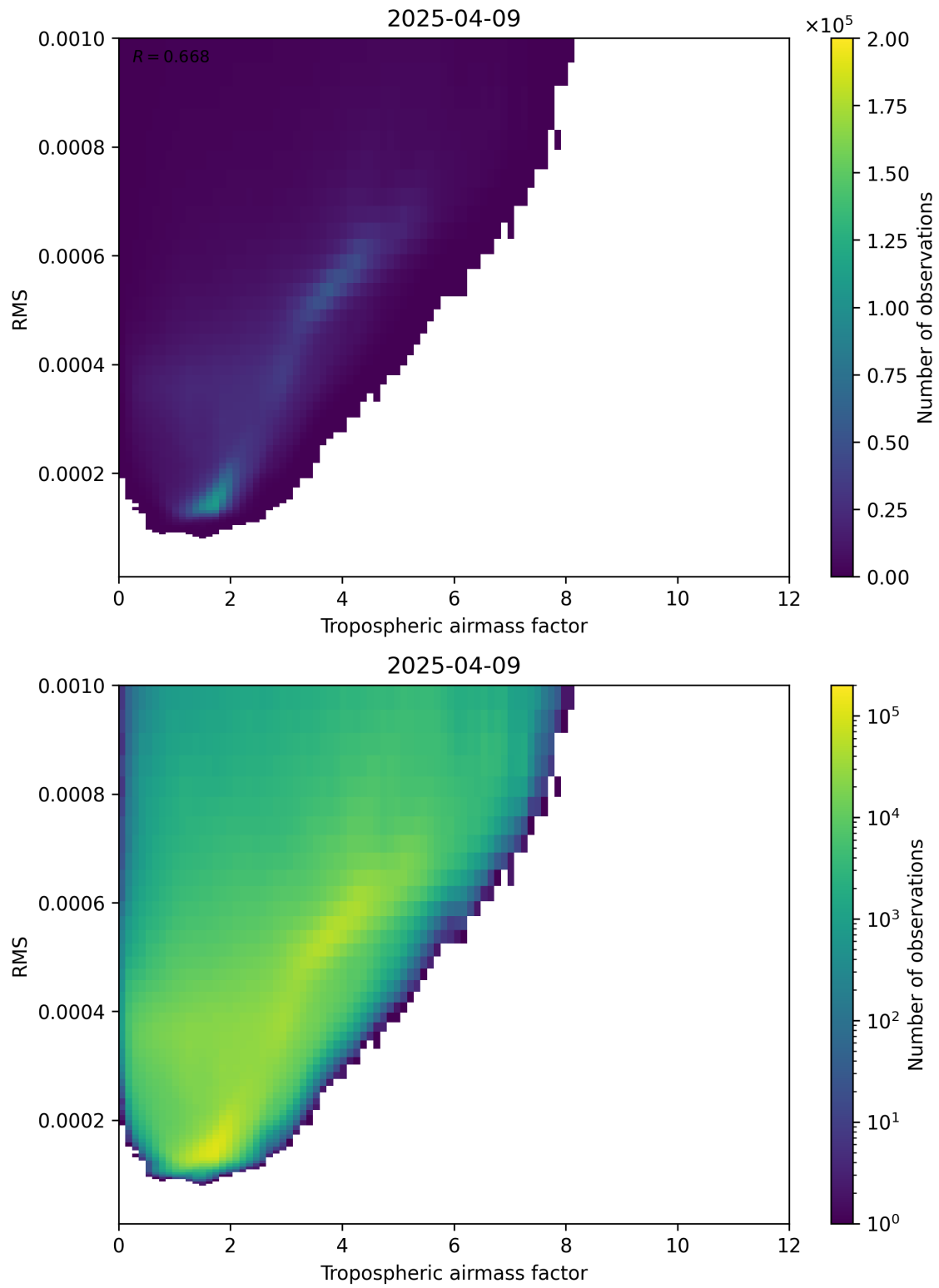
Figure 79: Scatter density plot of “Tropospheric airmass factor” against “RMS” for 2025-04-09 to 2025-04-10.
