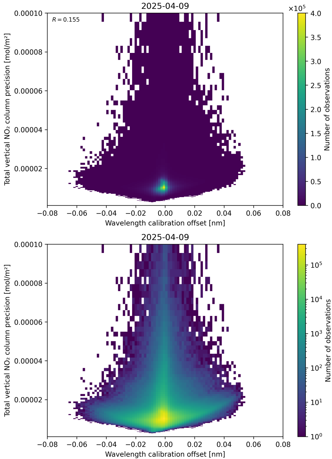
Figure 180: Scatter density plot of “Wavelength calibration offset” against “Total vertical NO 2 column precision” for 2025-04-09 to 2025-04-10.
