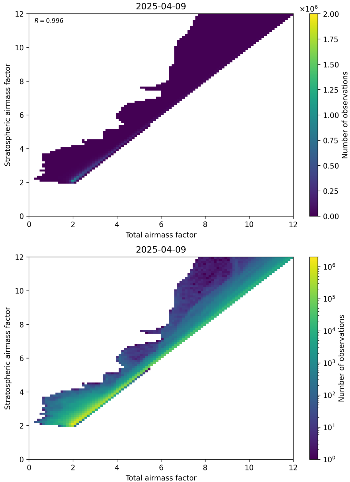
Figure 62: Scatter density plot of “Total airmass factor” against “Stratospheric airmass factor” for 2025-04-09 to 2025-04-10.
