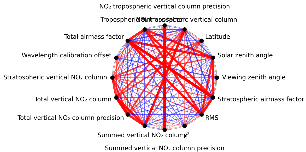
Figure 1: Map of correlation graph for 2025-04-09 to 2025-04-10.
