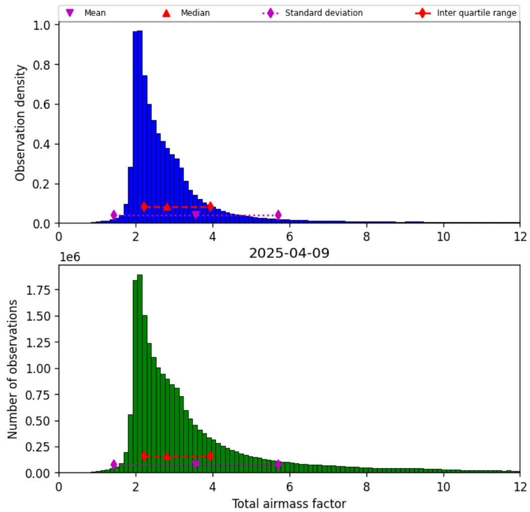
Figure 32: Histogram of “Total airmass factor” for 2025-04-09 to 2025-04-10
