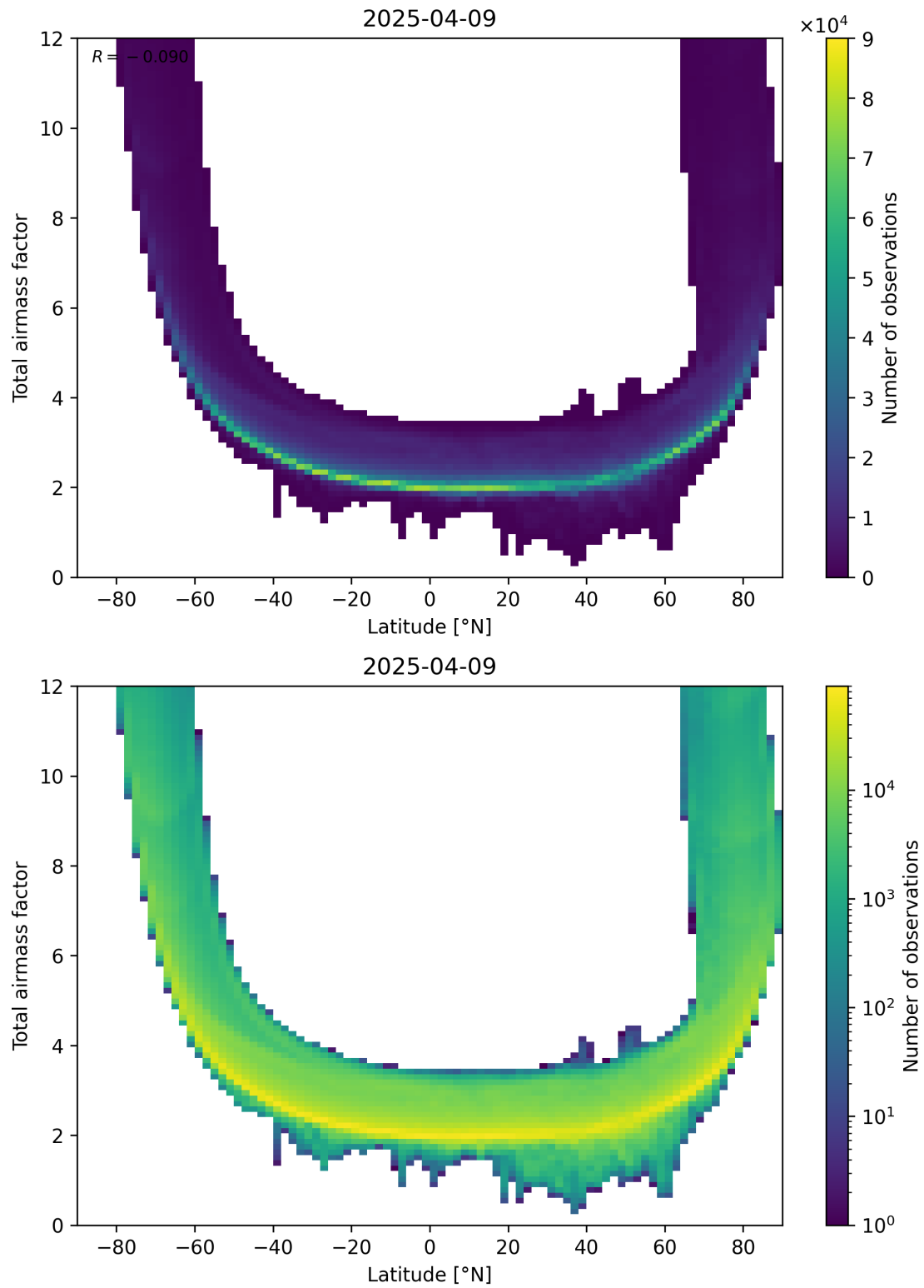
Figure 84: Scatter density plot of “Latitude” against “Total airmass factor” for 2025-04-09 to 2025-04-10.
