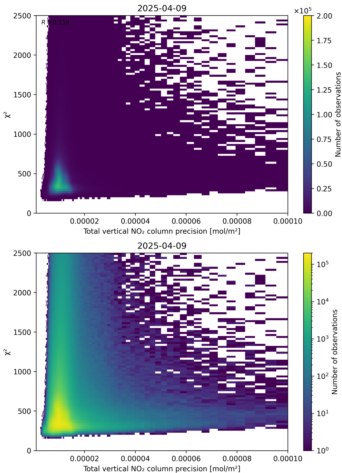
Figure 116: Scatter density plot of “Total vertical NO 2 column precision” against “ \chi^2 ” for 2025-04-09 to 2025-04-10.
