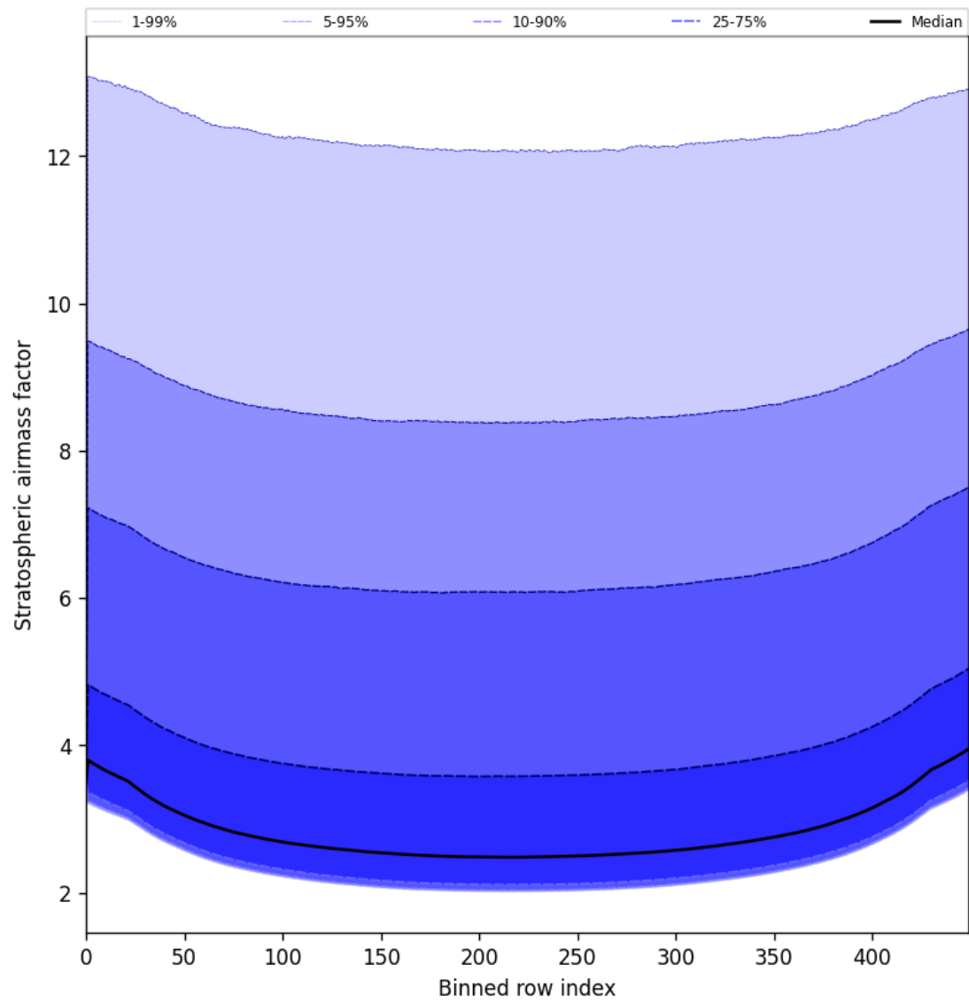
Figure 61: Along track statistics of “Stratospheric airmass factor” for 2025-04-09 to 2025-04-10
