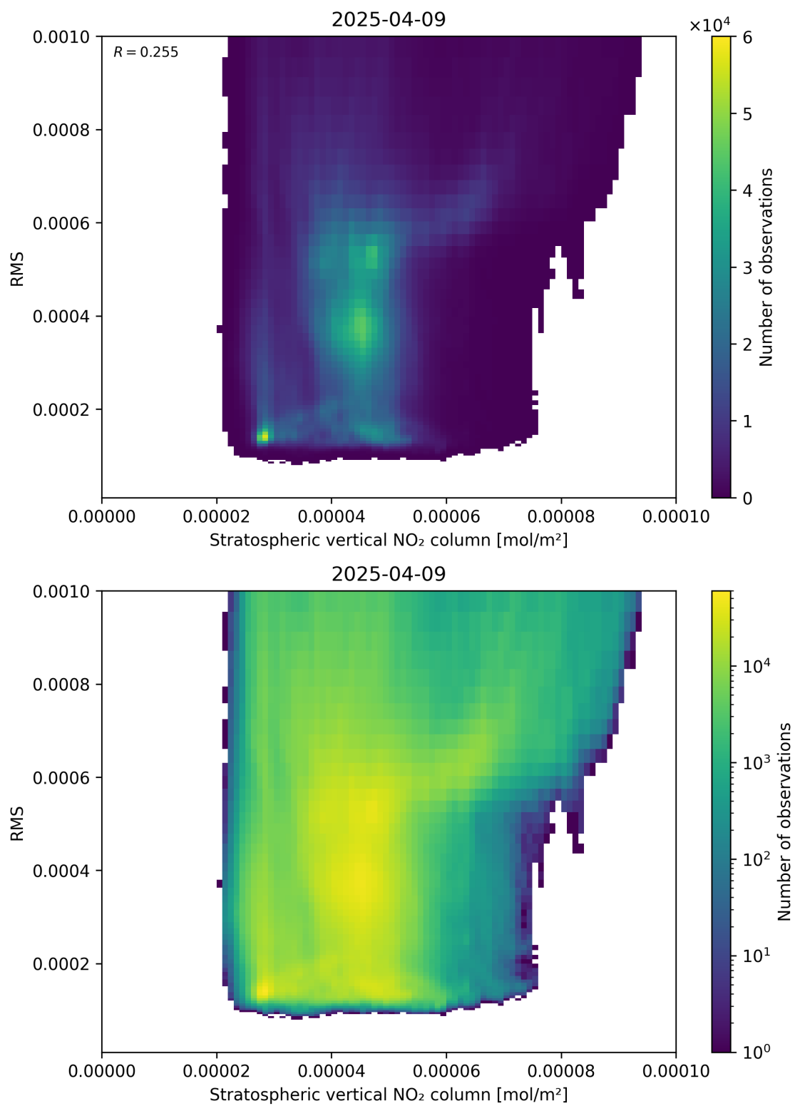
Figure 102: Scatter density plot of “Stratospheric vertical NO 2 column” against “RMS” for 2025-04-09 to 2025-04-10.
