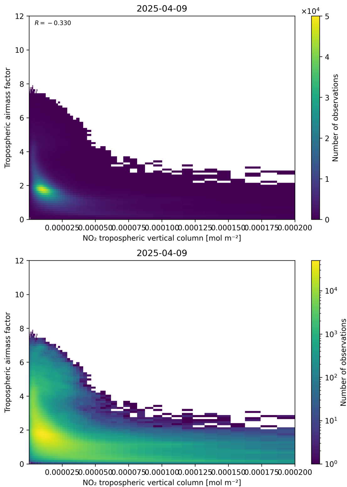
Figure 123: Scatter density plot of “NO 2 tropospheric vertical column” against “Tropospheric air mass factor” for 2025-04-09 to 2025-04-10.
