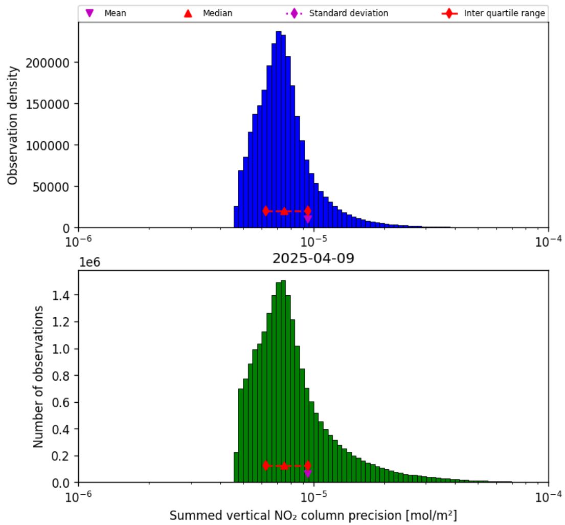
Figure 41: Histogram of "Summed vertical NO 2 column precision" for 2025-04-09 to 2025-04-10
