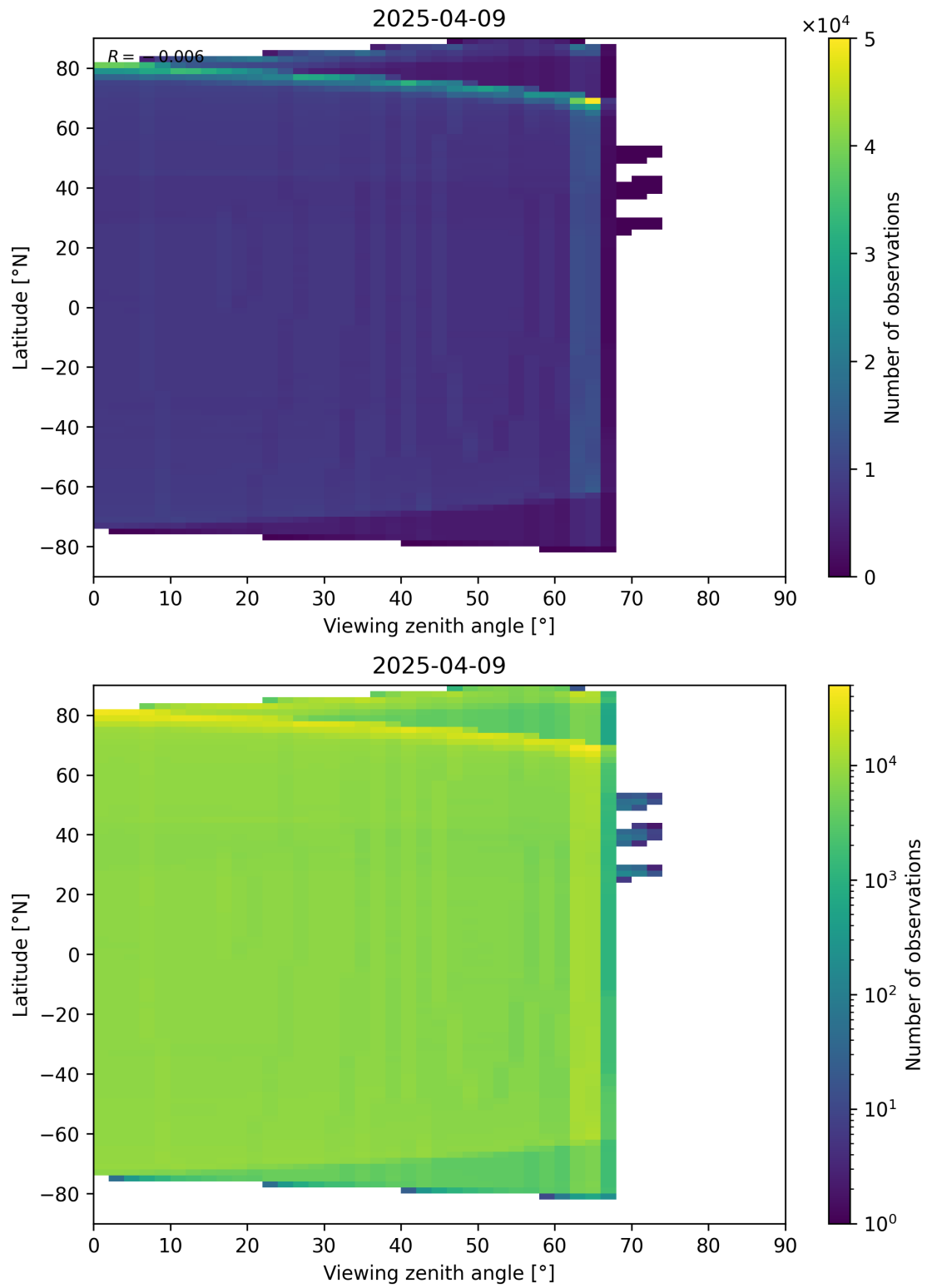
Figure 163: Scatter density plot of “Viewing zenith angle” against “Latitude” for 2025-04-09 to 2025-04-10.
