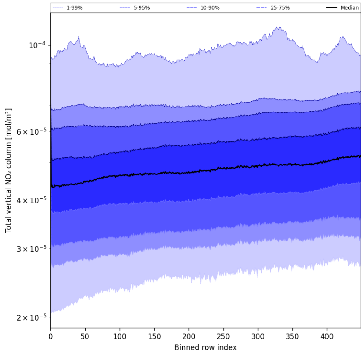
Figure 55: Along track statistics of “Total vertical NO 2 column” for 2025-04-09 to 2025-04-10
