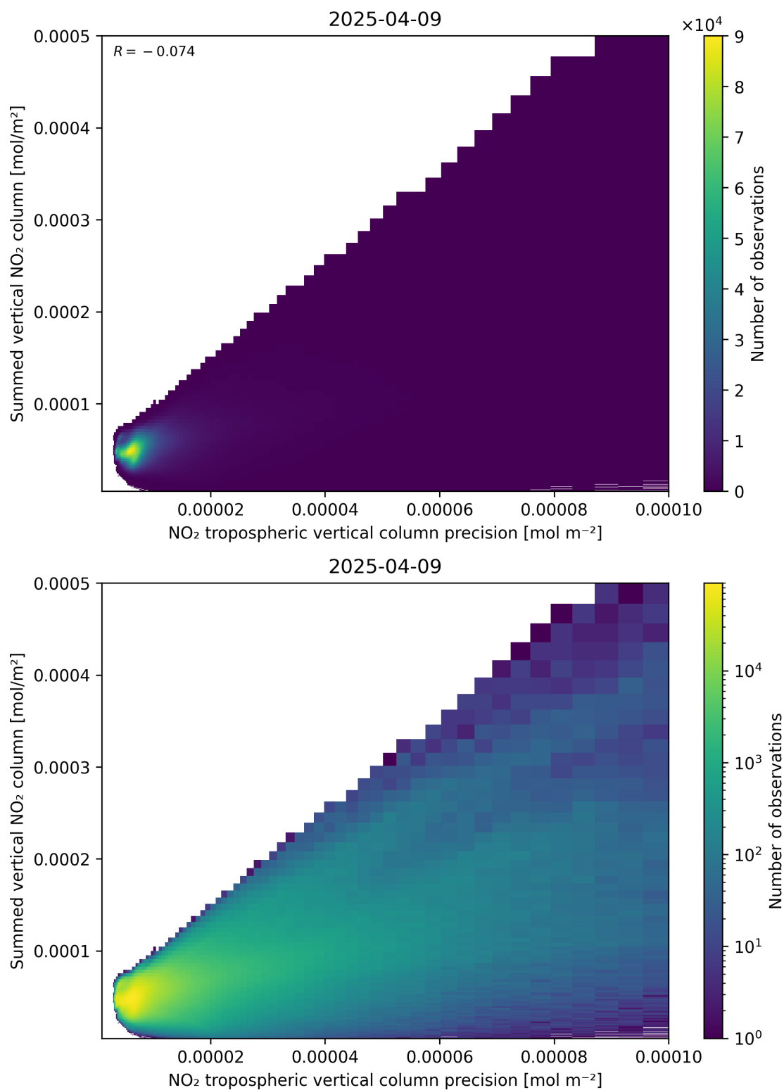
Figure 136: Scatter density plot of “NO 2 tropospheric vertical column precision” against “Summed vertical NO 2 column” for 2025-04-09 to 2025-04-10.
