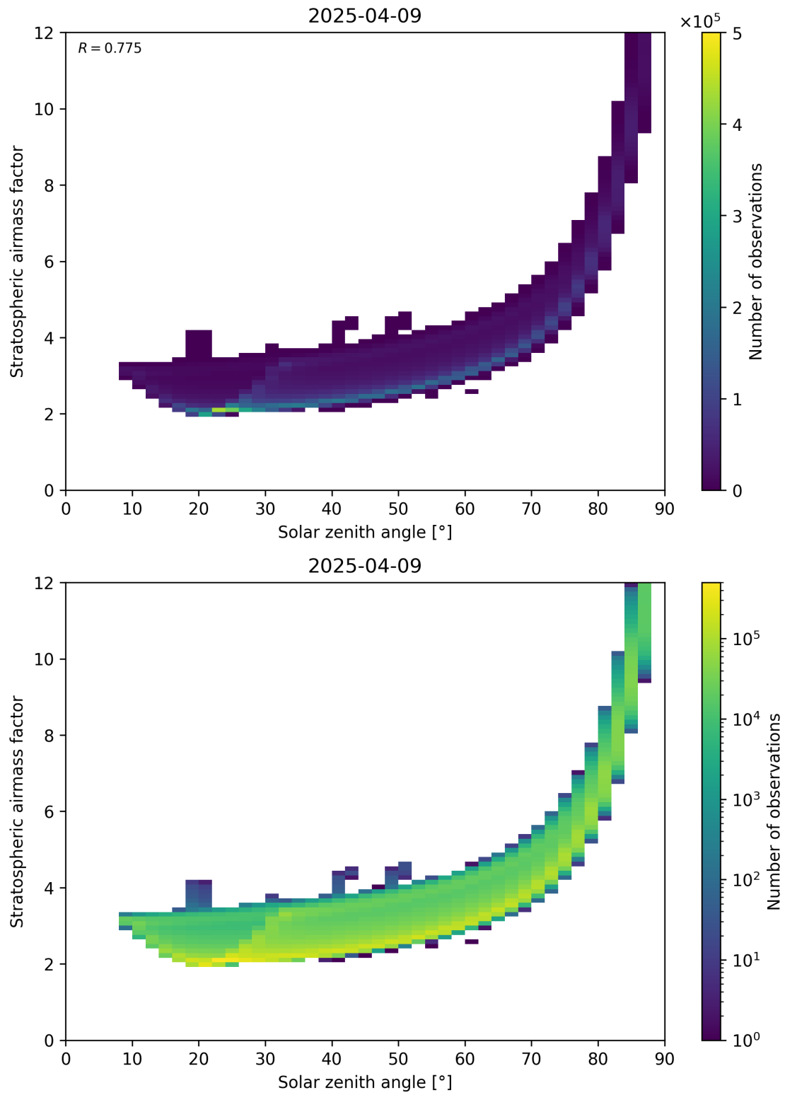
Figure 145: Scatter density plot of “Solar zenith angle” against “Stratospheric airmass factor” for 2025-04-09 to 2025-04-10.
