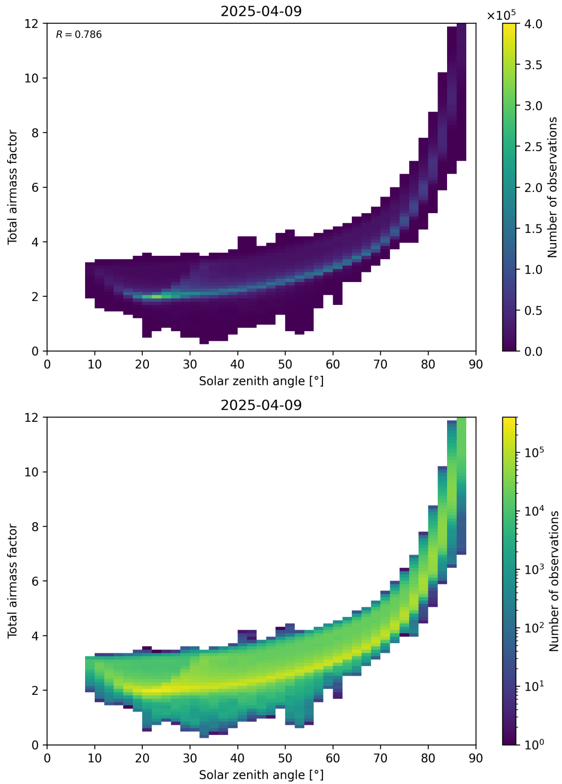
Figure 146: Scatter density plot of “Solar zenith angle” against “Total airmass factor” for 2025-04-09 to 2025-04-10.
