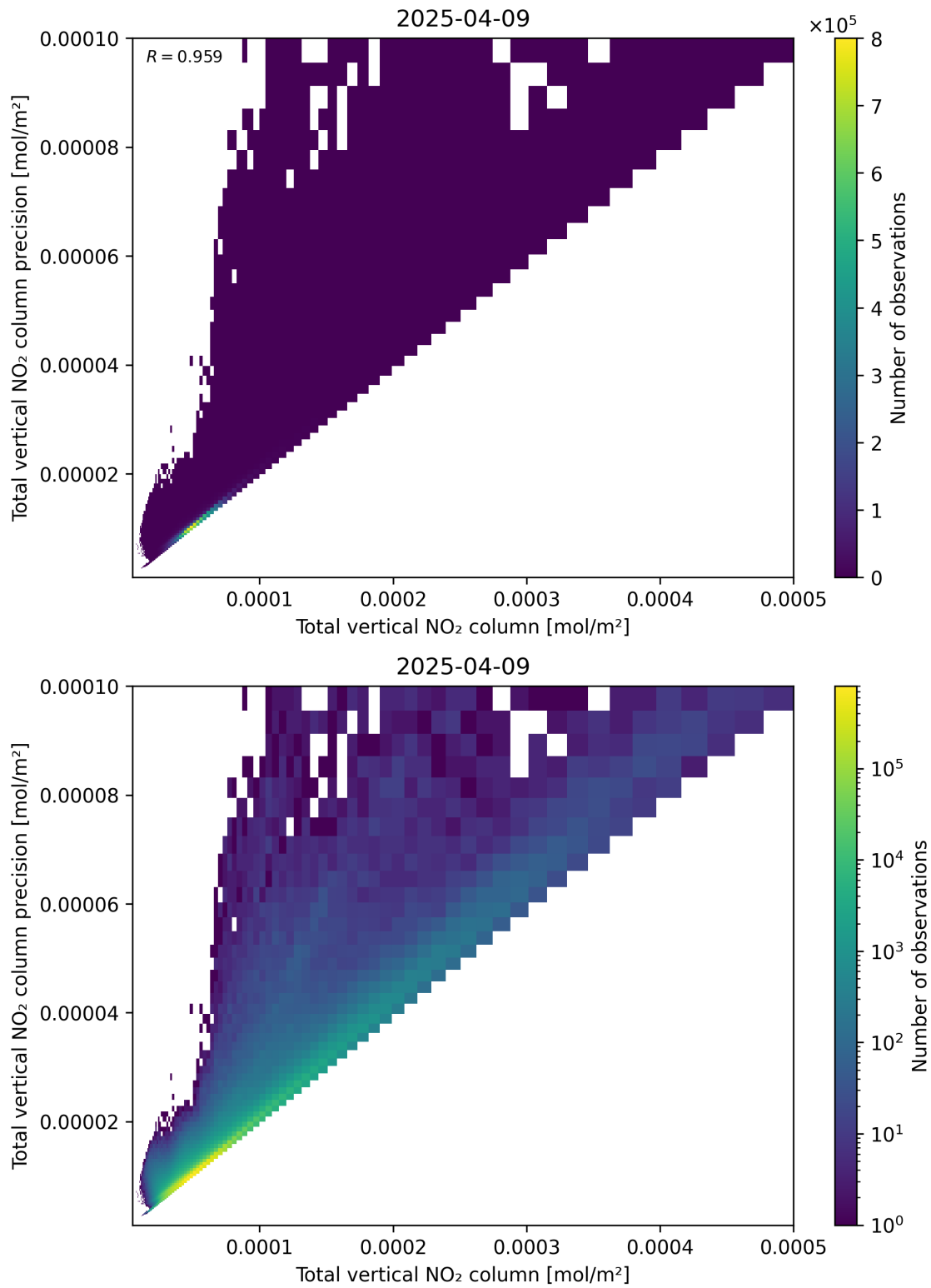
Figure 114: Scatter density plot of “Total vertical NO 2 column” against “Total vertical NO 2 column precision” for 2025-04-09 to 2025-04-10.
