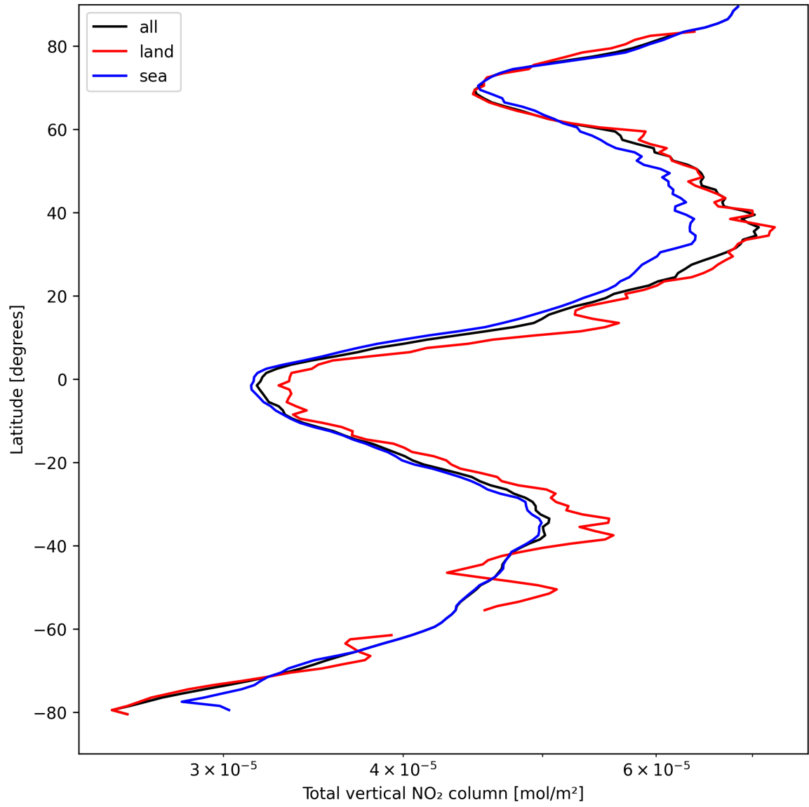
Figure 21: Zonal average of “Total vertical NO 2 column” for 2025-04-09 to 2025-04-10.
