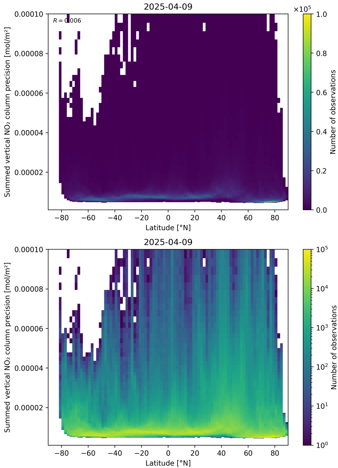
Figure 89: Scatter density plot of “Latitude” against “Summed vertical NO 2 column precision” for 2025-04-09 to 2025-04-10.
