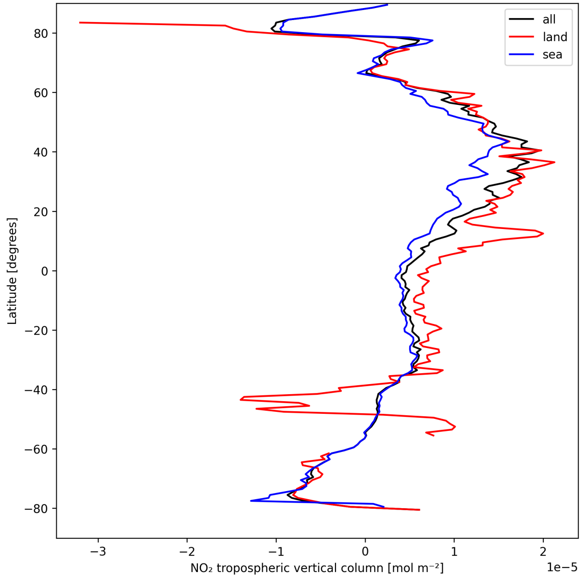
Figure 12: Zonal average of “NO 2 tropospheric vertical column” for 2025-04-09 to 2025-04-10.
