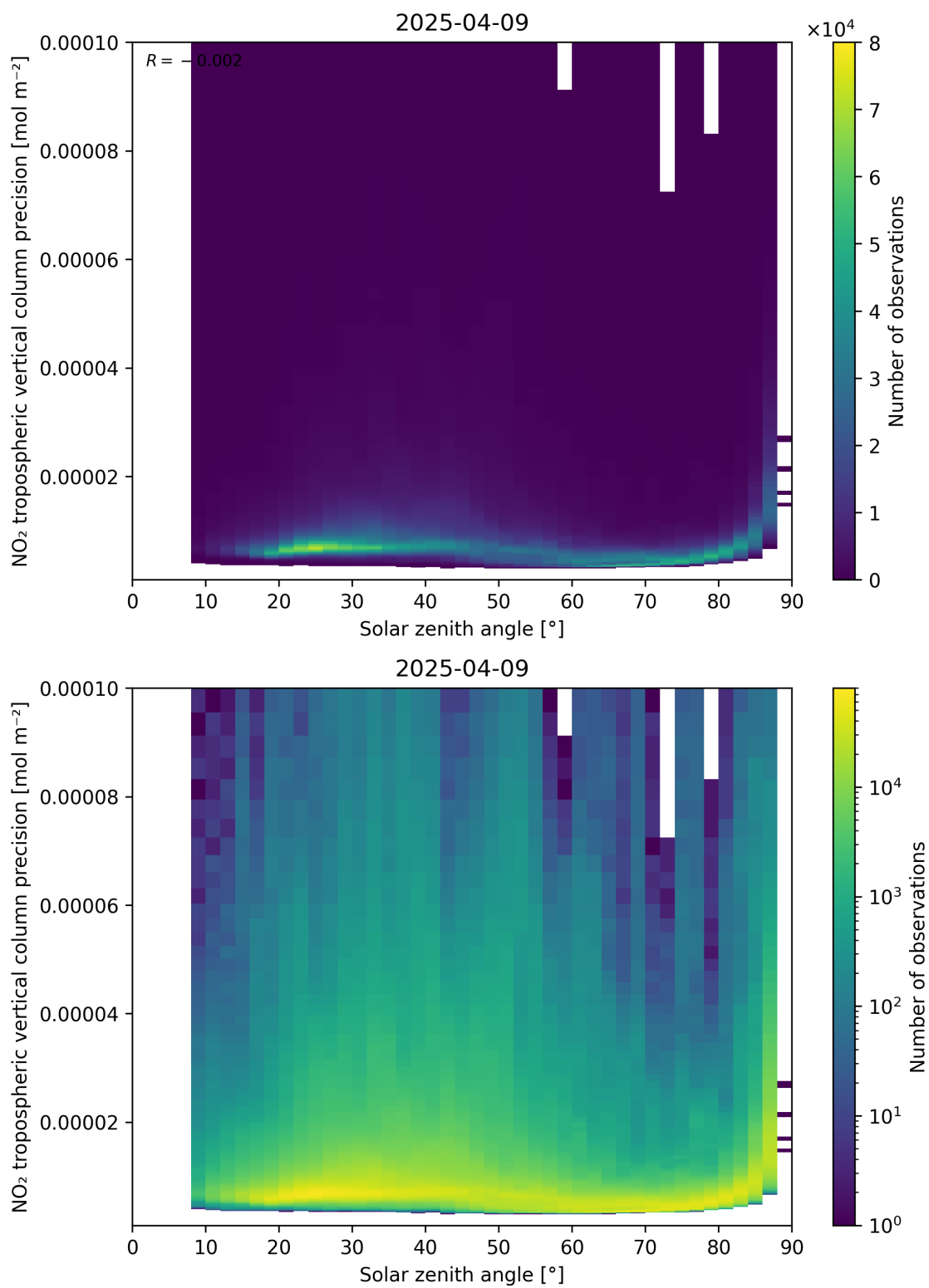
Figure 156: Scatter density plot of “Solar zenith angle” against “NO 2 tropospheric vertical column precision” for 2025-04-09 to 2025-04-10.
