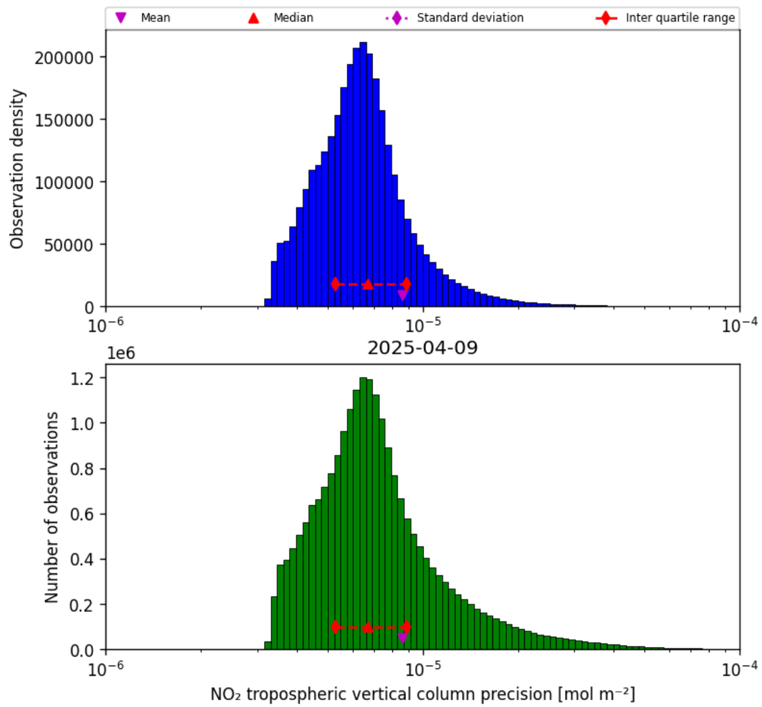
Figure 30: Histogram of “NO 2 tropospheric vertical column precision” for 2025-04-09 to 2025-04-10
