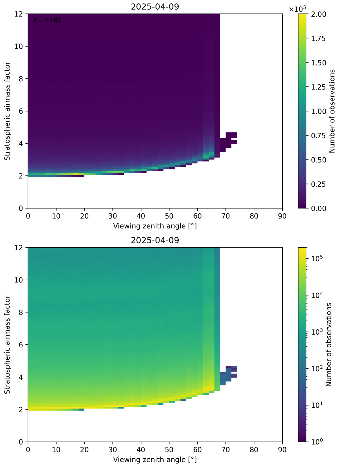
Figure 159: Scatter density plot of “Viewing zenith angle” against “Stratospheric airmass factor” for 2025-04-09 to 2025-04-10.
