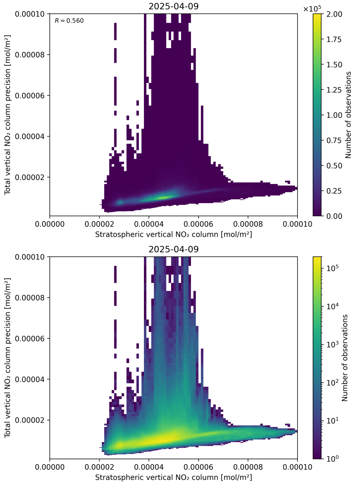
Figure 101: Scatter density plot of “Stratospheric vertical NO 2 column” against “Total vertical NO 2 column precision” for 2025-04-09 to 2025-04-10.
