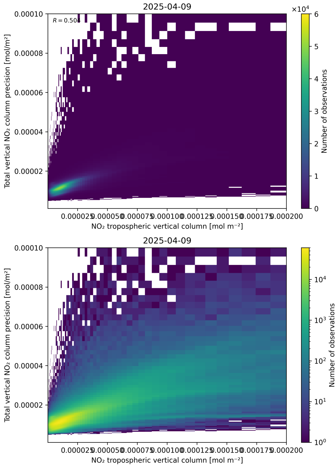
Figure 129: Scatter density plot of “NO 2 tropospheric vertical column” against “Total vertical NO 2 column precision” for 2025-04-09 to 2025-04-10.
