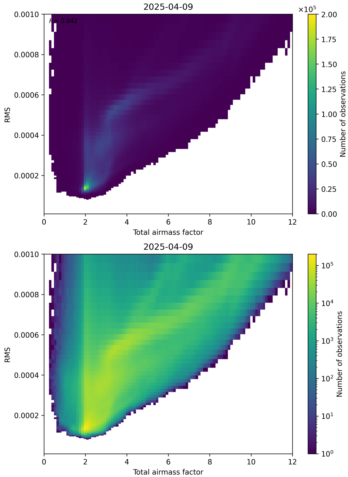
Figure 69: Scatter density plot of “Total airmass factor” against “RMS” for 2025-04-09 to 2025-04-10.
