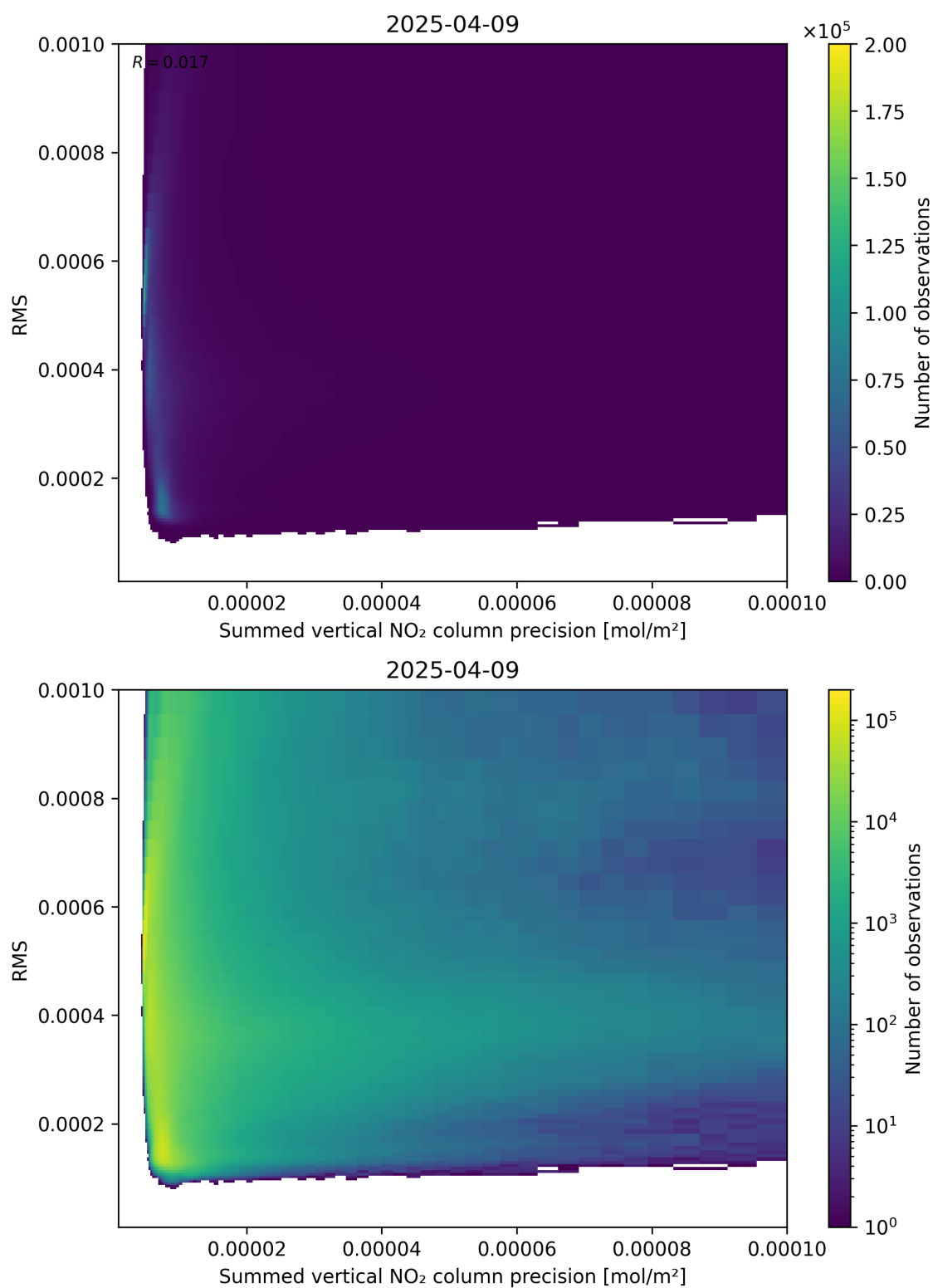
Figure 108: Scatter density plot of “Summed vertical NO 2 column precision” against “RMS” for 2025-04-09 to 2025-04-10.
