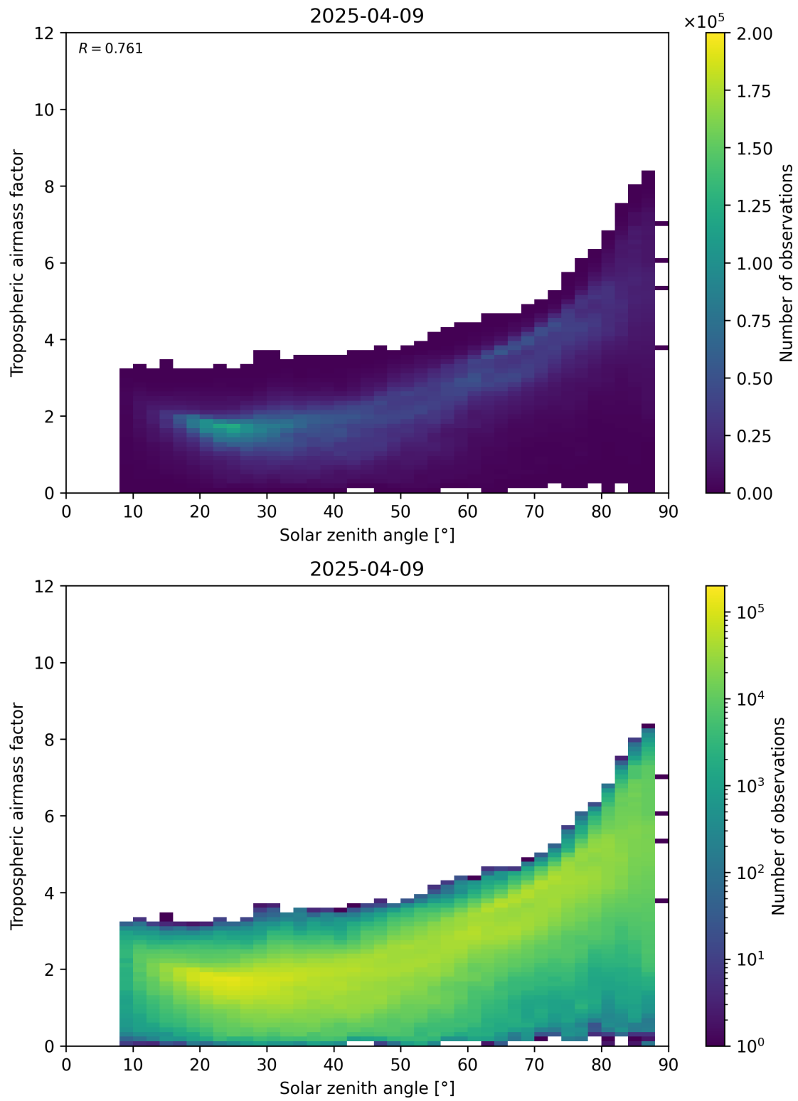
Figure 147: Scatter density plot of “Solar zenith angle” against “Tropospheric airmass factor” for 2025-04-09 to 2025-04-10.
