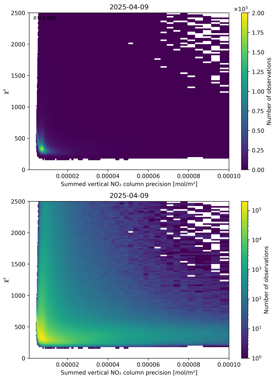
Figure 107: Scatter density plot of “Summed vertical NO 2 column precision” against “ \chi^2 ” for 2025-04-09 to 2025-04-10.
