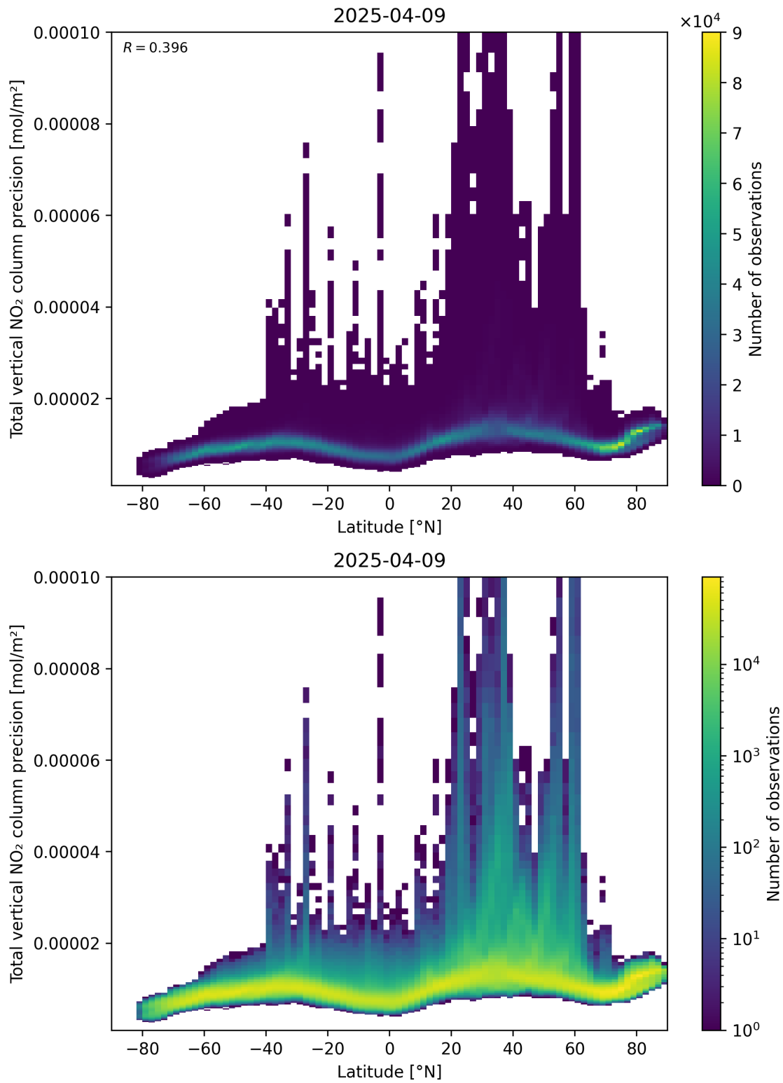
Figure 91: Scatter density plot of “Latitude” against “Total vertical NO 2 column precision” for 2025-04-09 to 2025-04-10.
