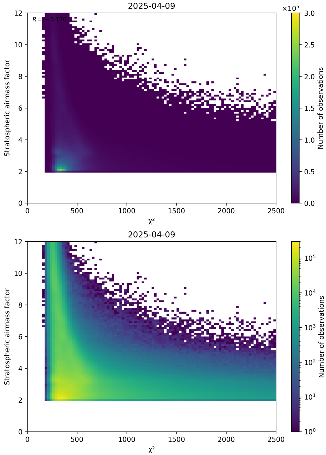
Figure 81: Scatter density plot of “ \chi^2 ” against “Stratospheric airmass factor” for 2025-04-09 to 2025-04-10.
