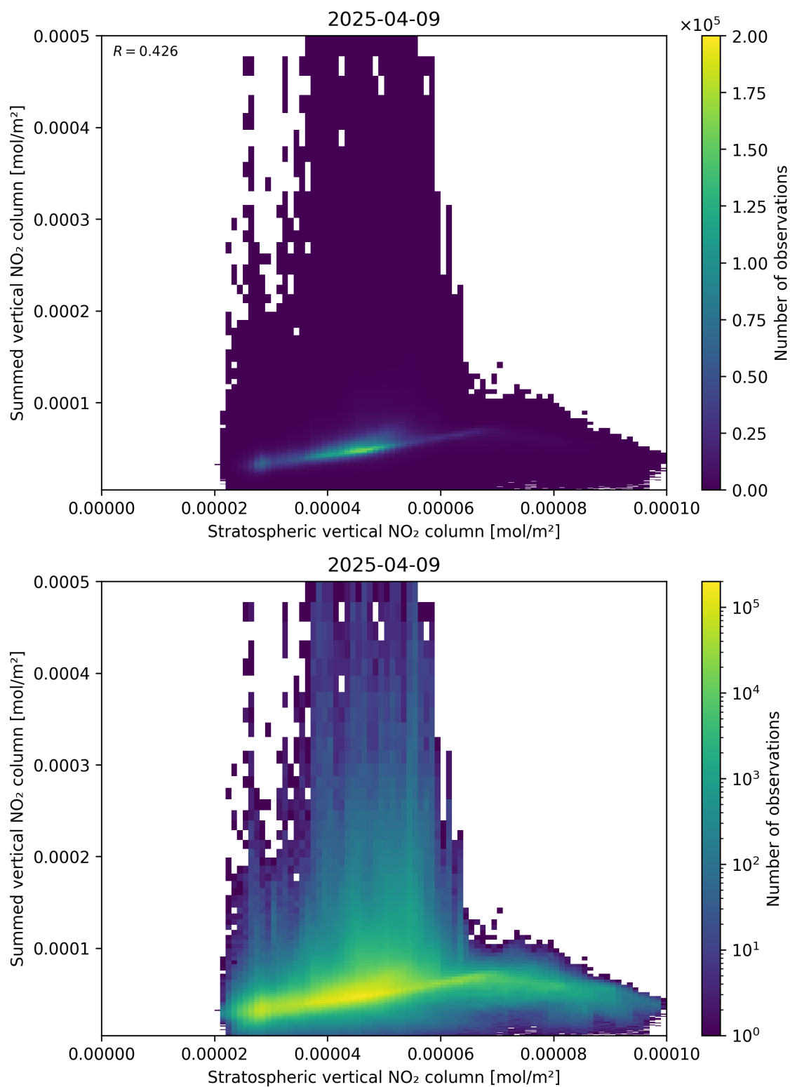
Figure 98: Scatter density plot of “Stratospheric vertical NO 2 column” against “Summed vertical NO 2 column” for 2025-04-09 to 2025-04-10.
