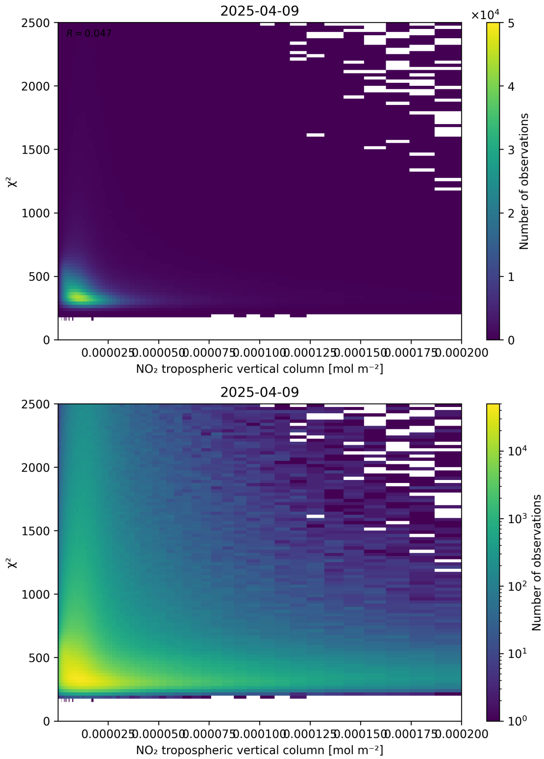
Figure 124: Scatter density plot of “NO 2 tropospheric vertical column” against “ \chi^2 ” for 2025-04-09 to 2025-04-10.
