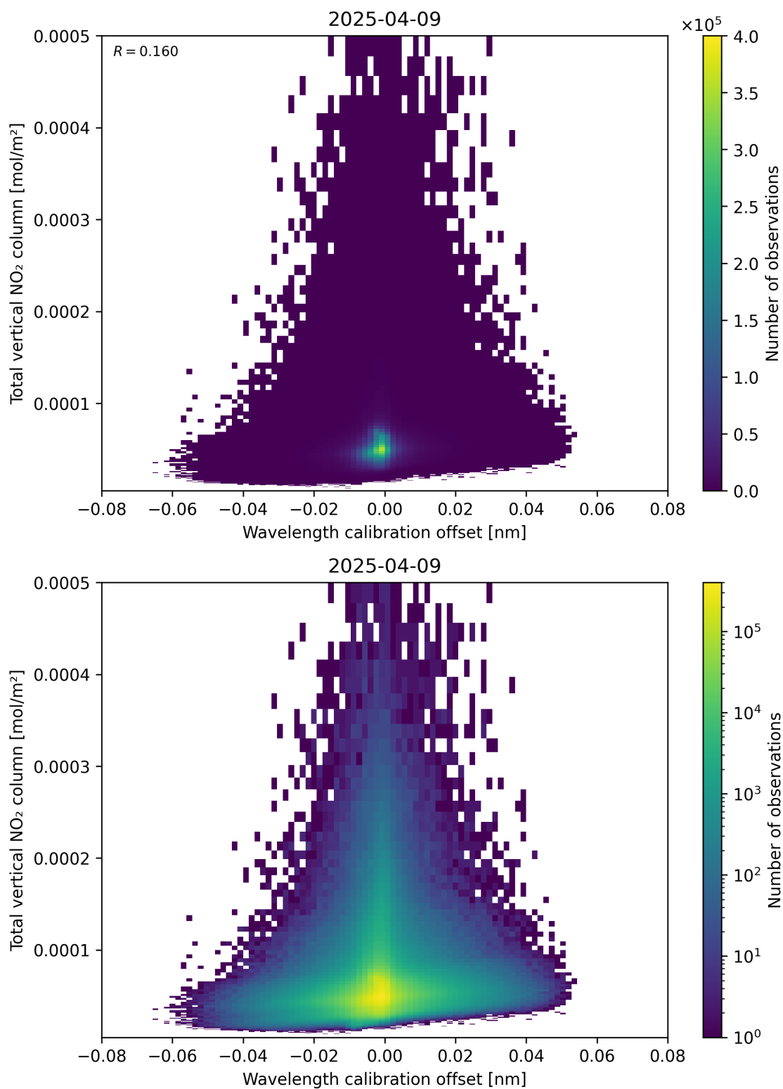
Figure 179: Scatter density plot of “Wavelength calibration offset” against “Total vertical NO 2 column” for 2025-04-09 to 2025-04-10.
