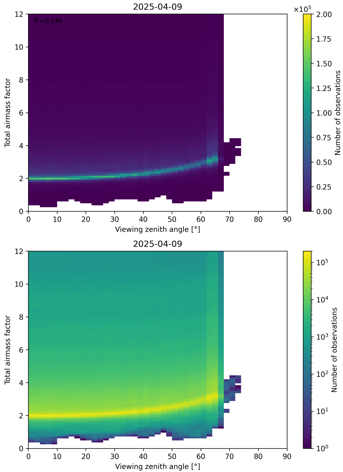
Figure 160: Scatter density plot of “Viewing zenith angle” against “Total airmass factor” for 2025-04-09 to 2025-04-10.
