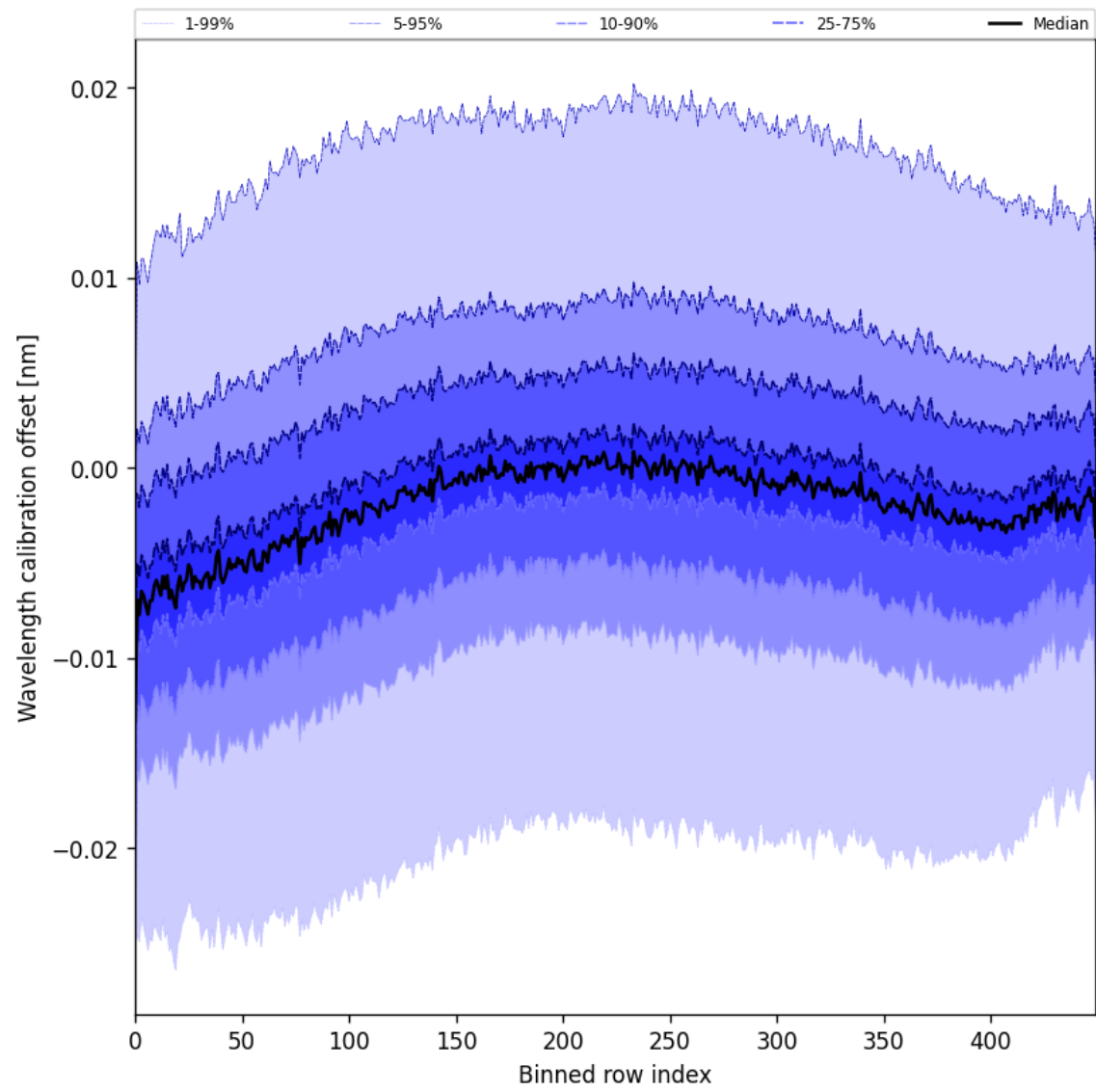
Figure 52: Along track statistics of “Wavelength calibration offset” for 2025-04-09 to 2025-04-10
