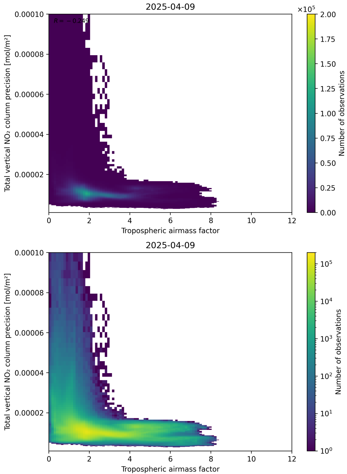
Figure 78: Scatter density plot of “Tropospheric air mass factor” against “Total vertical NO 2 column precision” for 2025-04-09 to 2025-04-10.
