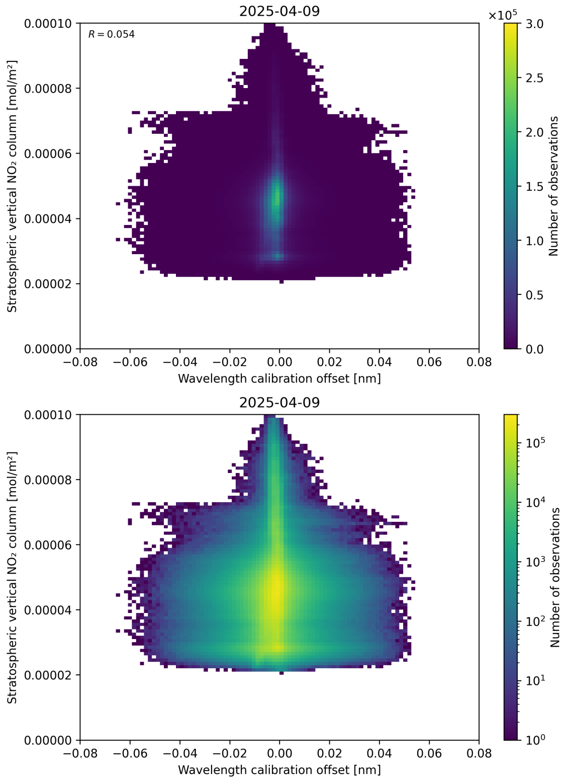
Figure 176: Scatter density plot of “Wavelength calibration offset” against “Stratospheric vertical NO 2 column” for 2025-04-09 to 2025-04-10.
