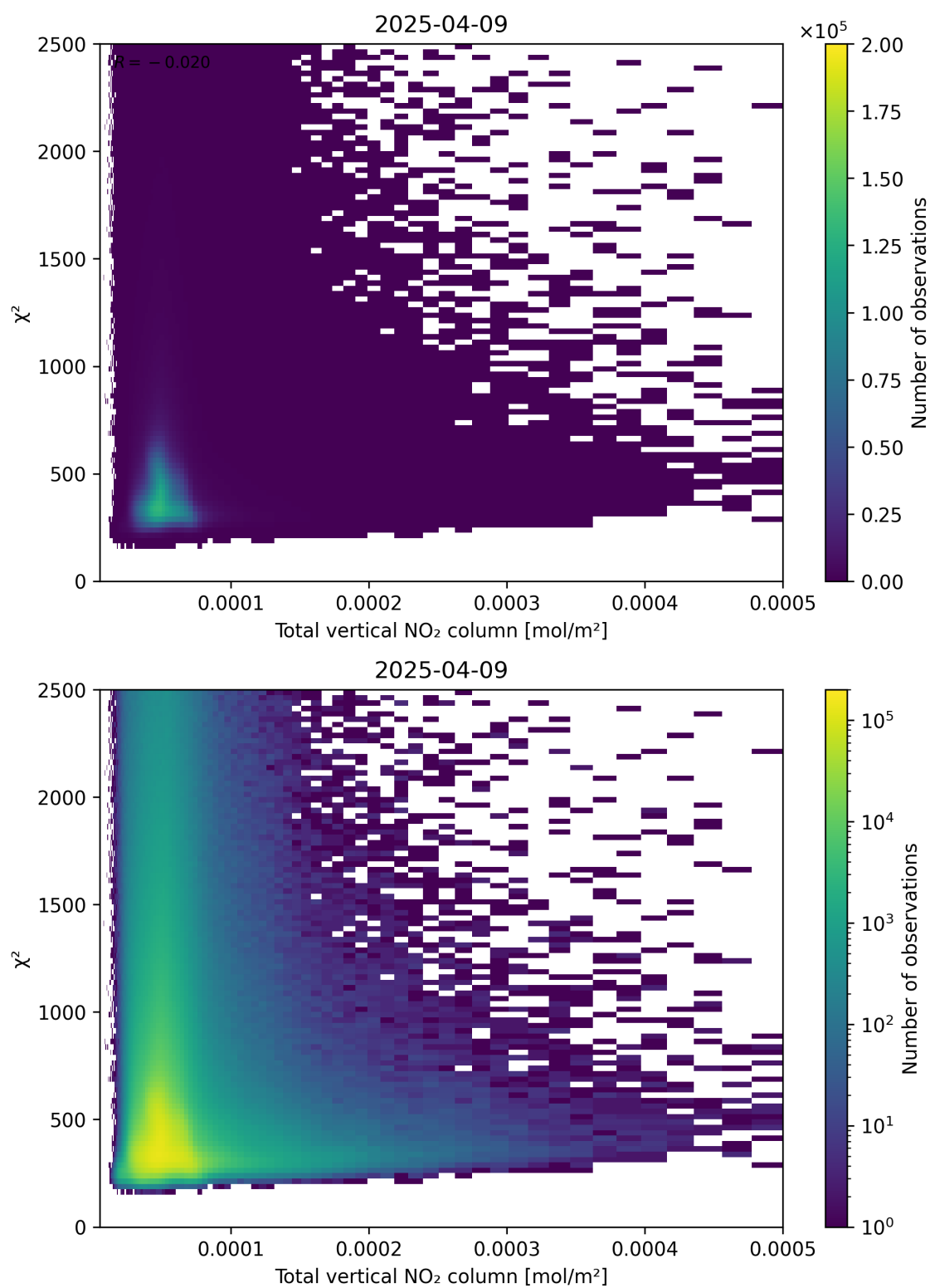
Figure 111: Scatter density plot of “Total vertical NO 2 column” against “ \chi^2 ” for 2025-04-09 to 2025-04-10.
