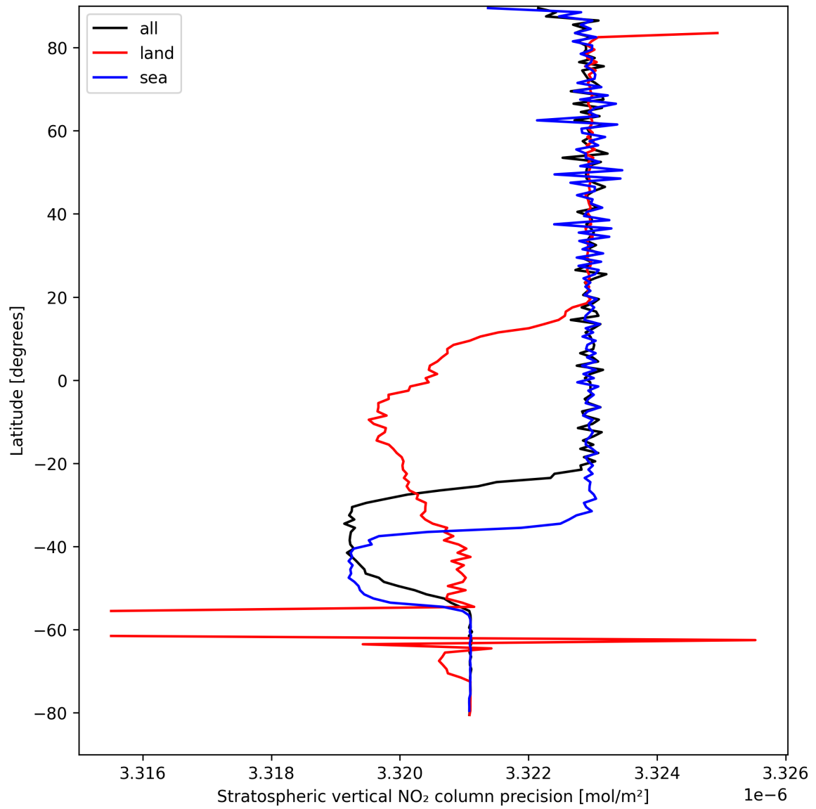
Figure 20: Zonal average of “Stratospheric vertical NO 2 column precision” for 2025-04-09 to 2025-04-10.
