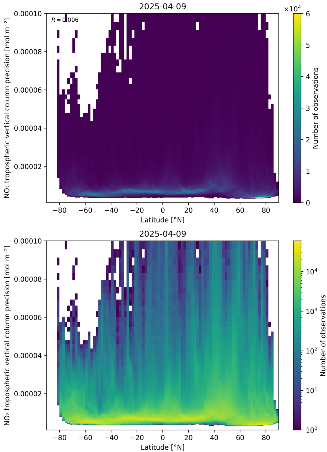
Figure 93: Scatter density plot of “Latitude” against “NO 2 tropospheric vertical column precision” for 2025-04-09 to 2025-04-10.
