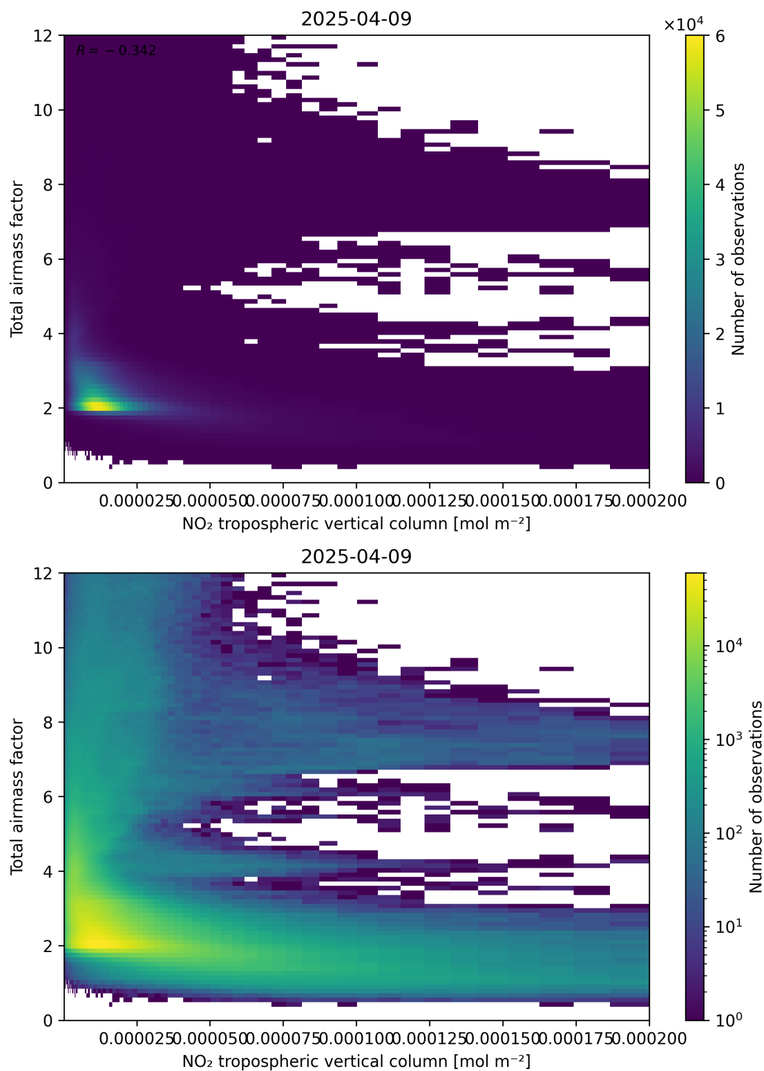
Figure 122: Scatter density plot of “NO 2 tropospheric vertical column” against “Total air mass factor” for 2025-04-09 to 2025-04-10.
