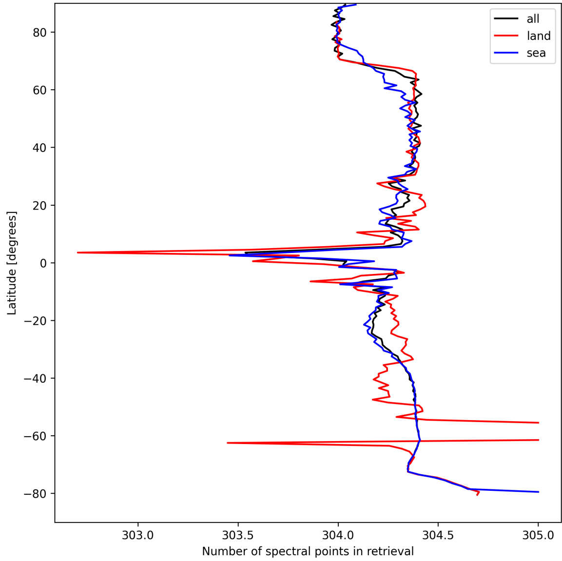
Figure 16: Zonal average of “Number of spectral points in retrieval” for 2025-04-09 to 2025-04-10.
