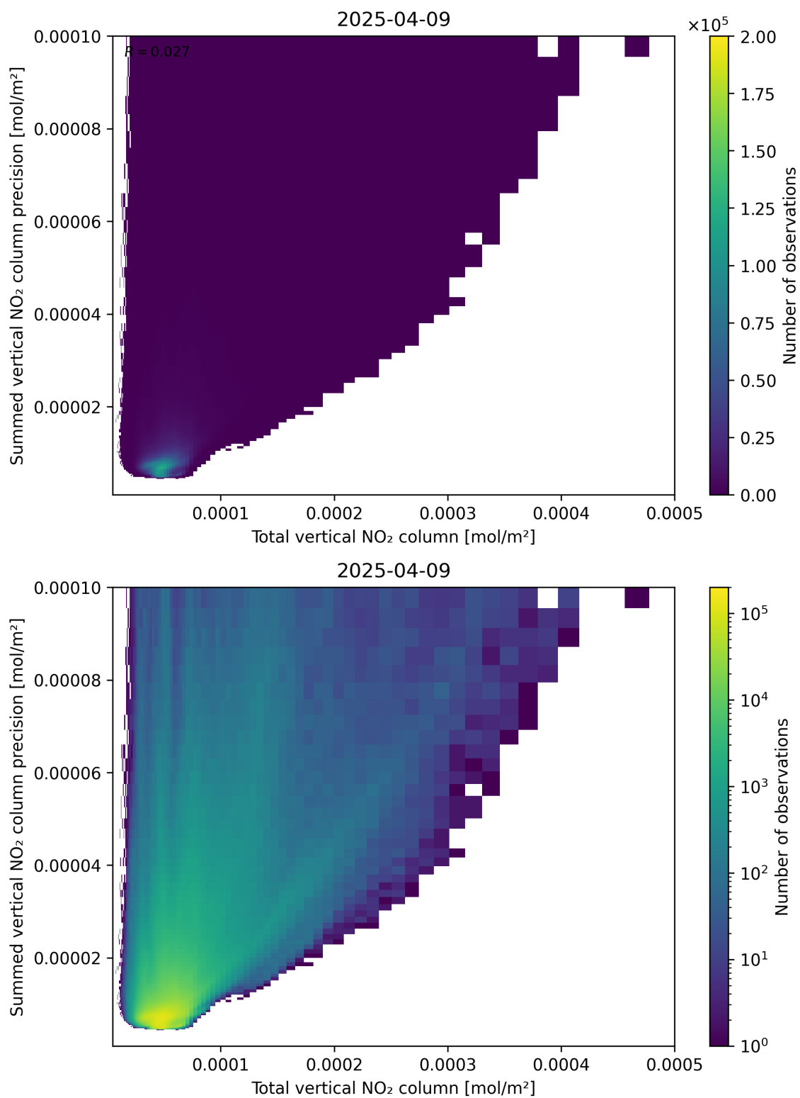
Figure 113: Scatter density plot of “Total vertical NO 2 column” against “Summed vertical NO 2 column precision” for 2025-04-09 to 2025-04-10.
