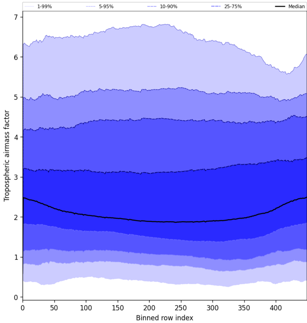
Figure 48: Along track statistics of “Tropospheric airmass factor” for 2025-04-09 to 2025-04-10
