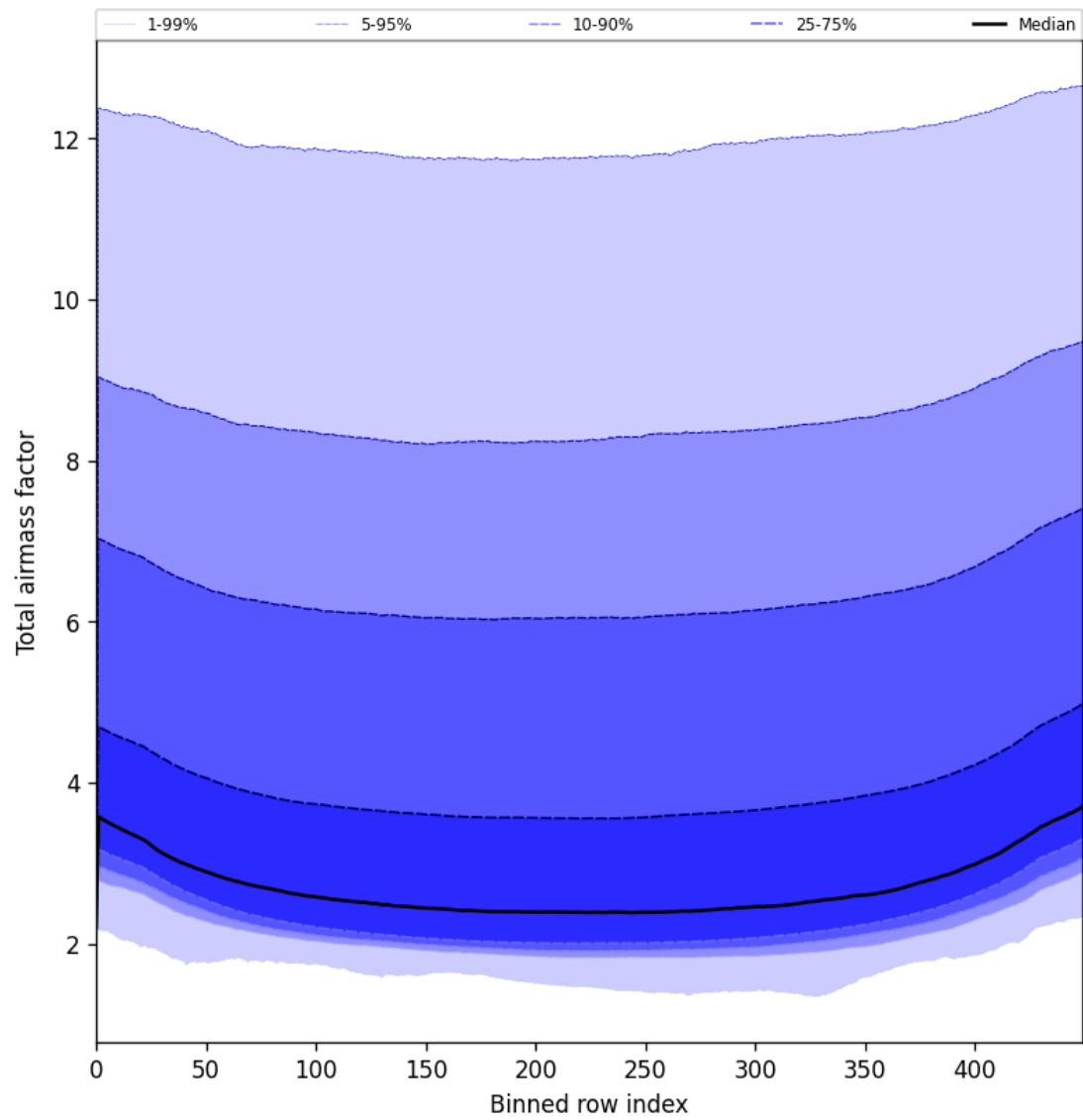
Figure 49: Along track statistics of “Total airmass factor” for 2025-04-09 to 2025-04-10
