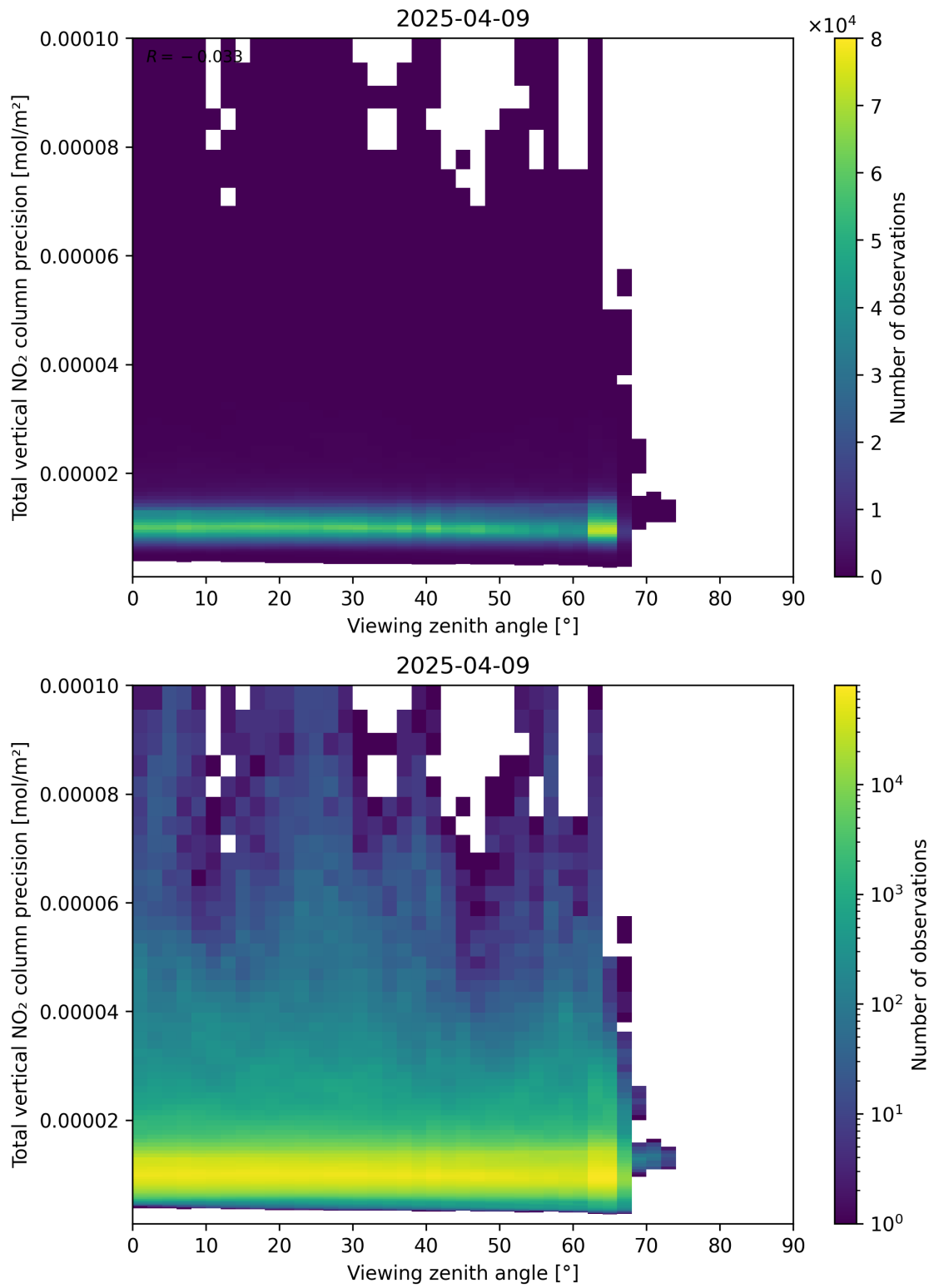
Figure 168: Scatter density plot of “Viewing zenith angle” against “Total vertical NO 2 column precision” for 2025-04-09 to 2025-04-10.
