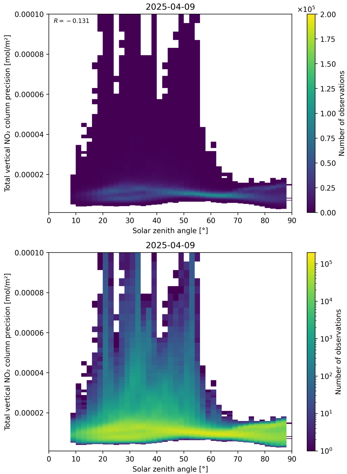
Figure 154: Scatter density plot of “Solar zenith angle” against “Total vertical NO 2 column precision” for 2025-04-09 to 2025-04-10.
