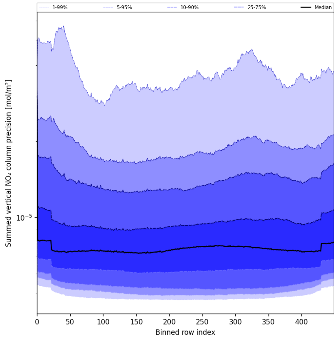
Figure 58: Along track statistics of “Summed vertical NO 2 column precision” for 2025-04-09 to 2025-04-10
