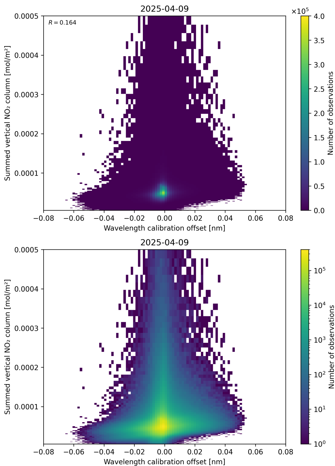
Figure 177: Scatter density plot of “Wavelength calibration offset” against “Summed vertical NO 2 column” for 2025-04-09 to 2025-04-10.
