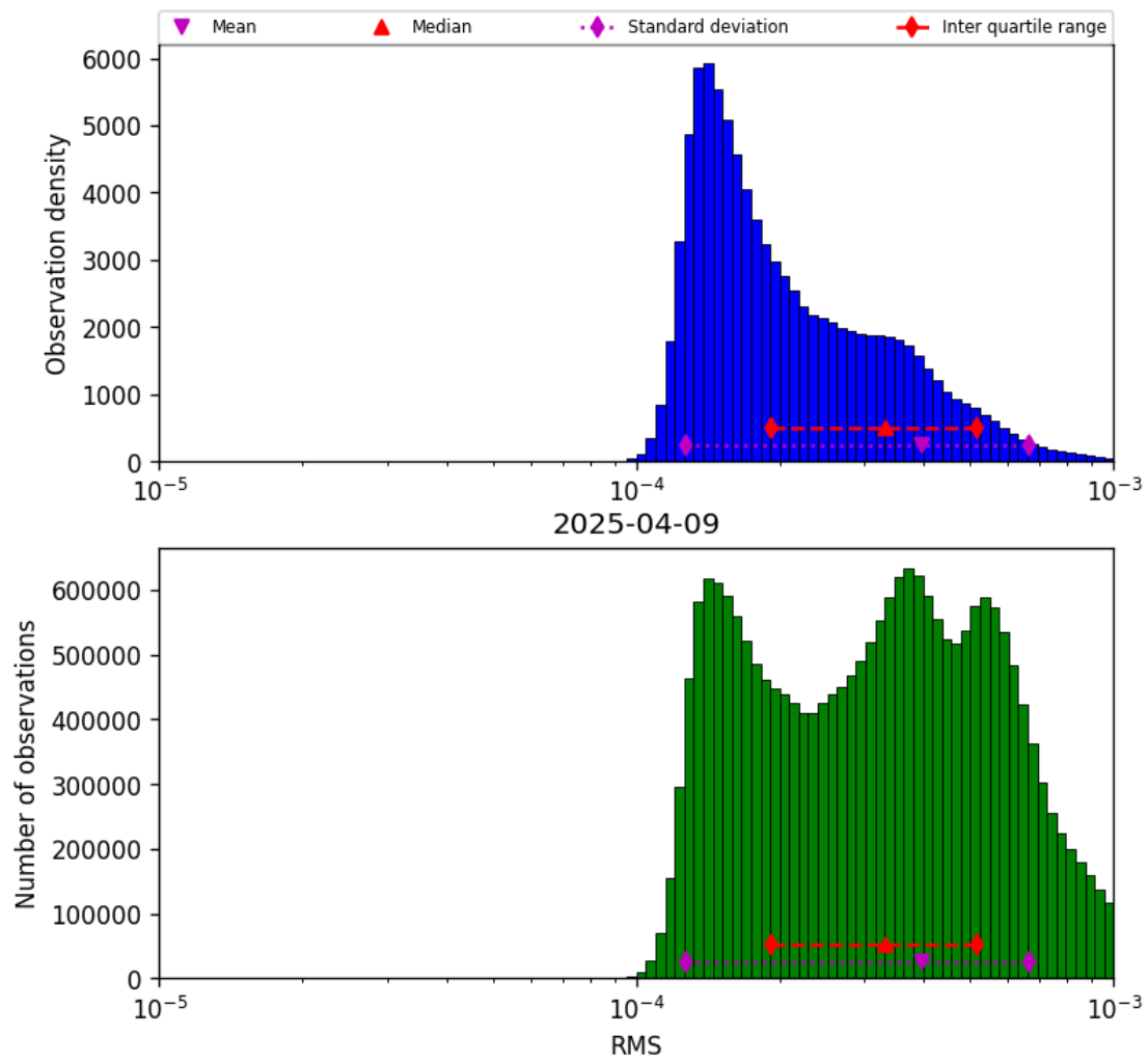
Figure 43: Histogram of “RMS” for 2025-04-09 to 2025-04-10
