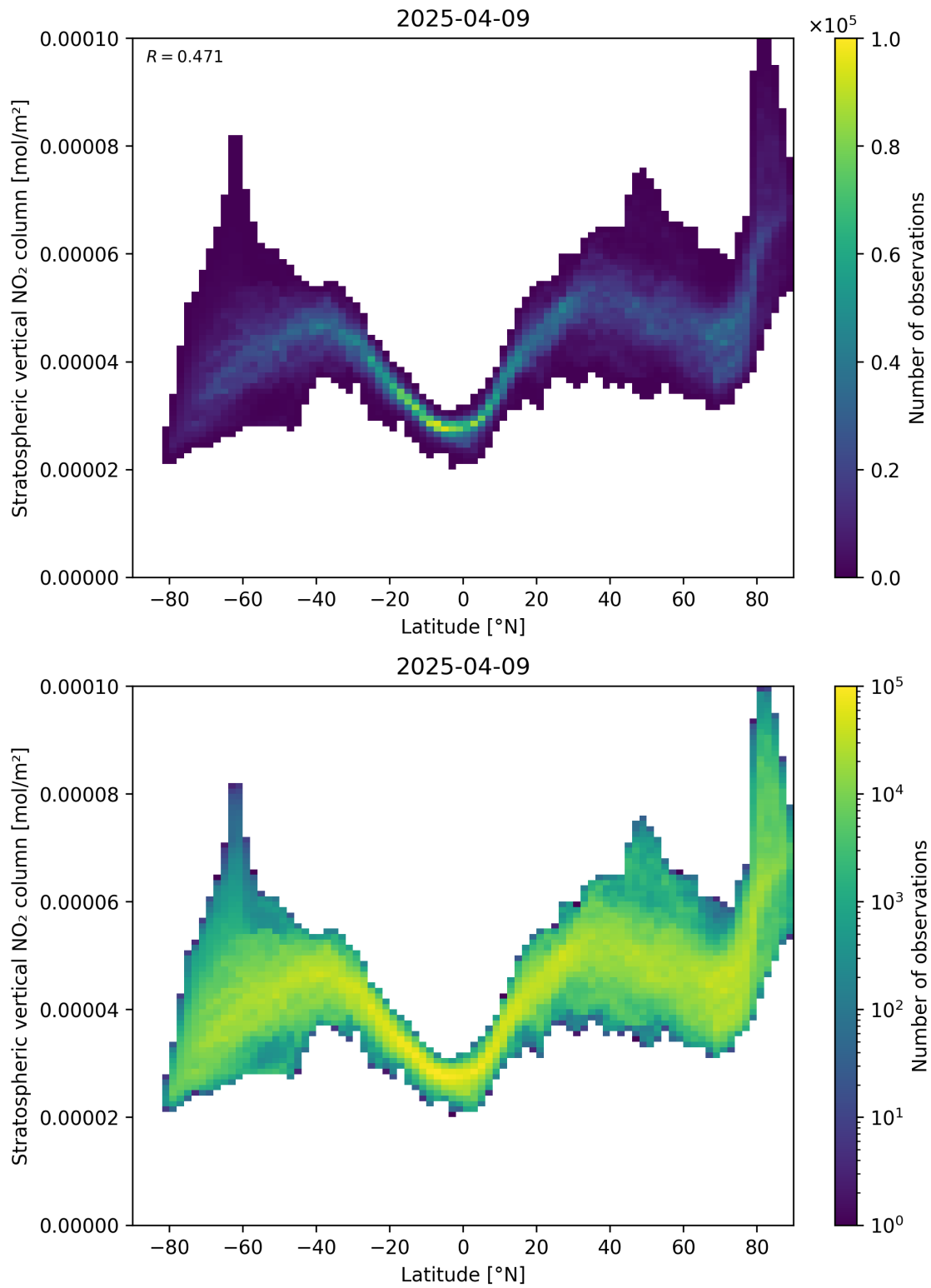
Figure 87: Scatter density plot of “Latitude” against “Stratospheric vertical \text{NO}_2 column” for 2025-04-09 to 2025-04-10.
