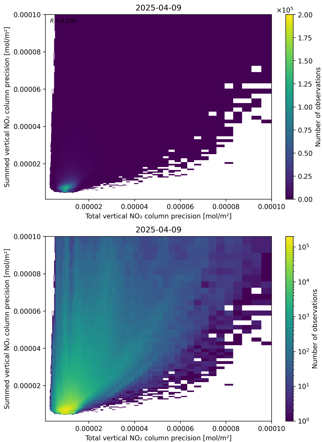
Figure 118: Scatter density plot of “Total vertical NO 2 column precision” against “Summed vertical NO 2 column precision” for 2025-04-09 to 2025-04-10.
