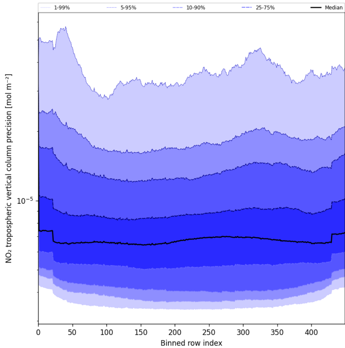
Figure 47: Along track statistics of “NO 2 tropospheric vertical column precision” for 2025-04-09 to 2025-04-10
