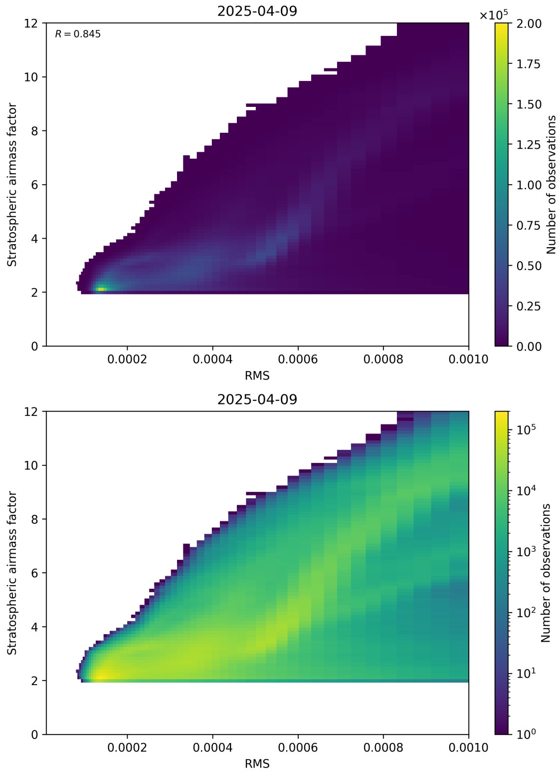
Figure 144: Scatter density plot of “RMS” against “Stratospheric airmass factor” for 2025-04-09 to 2025-04-10.
