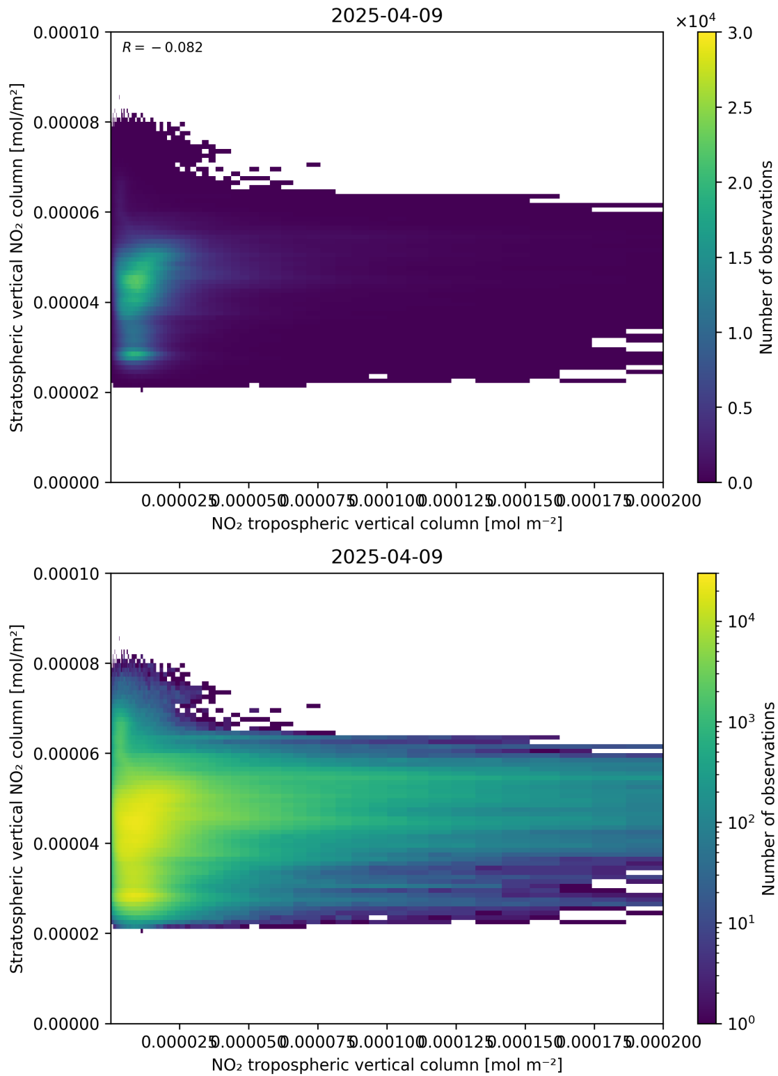
Figure 125: Scatter density plot of “NO 2 tropospheric vertical column” against “Stratospheric vertical NO 2 column” for 2025-04-09 to 2025-04-10.
