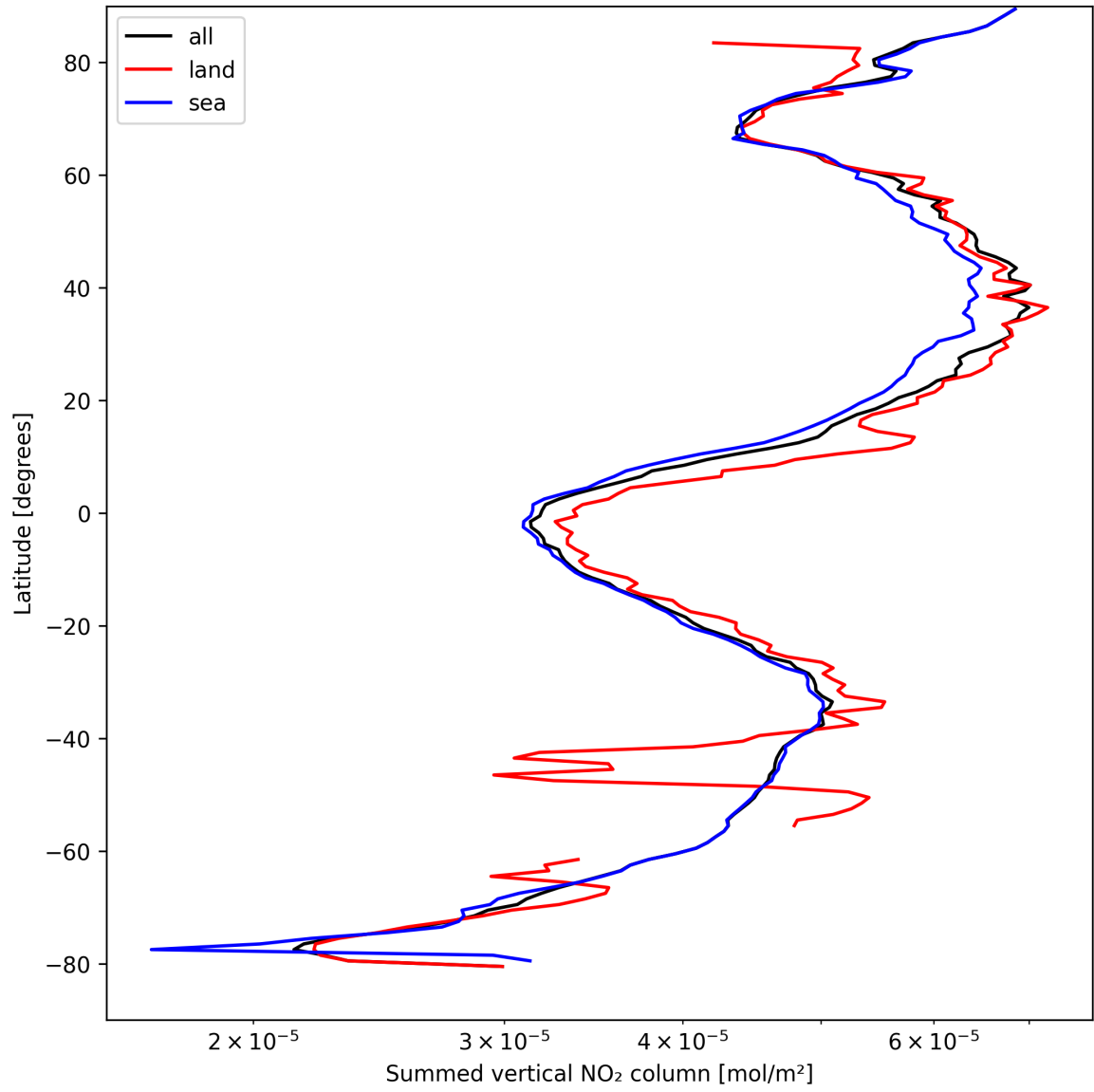
Figure 23: Zonal average of “Summed vertical NO 2 column” for 2025-04-09 to 2025-04-10.
