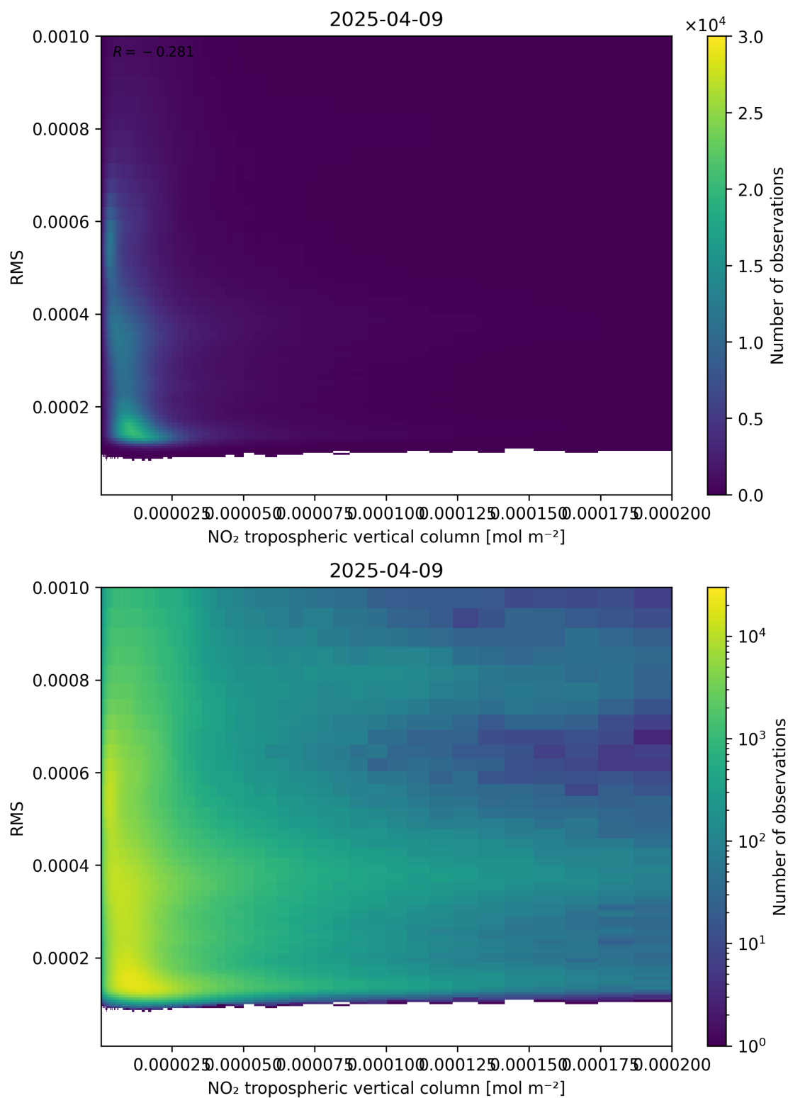
Figure 142: Scatter density plot of “NO 2 tropospheric vertical column” against “RMS” for 2025-04-09 to 2025-04-10.
