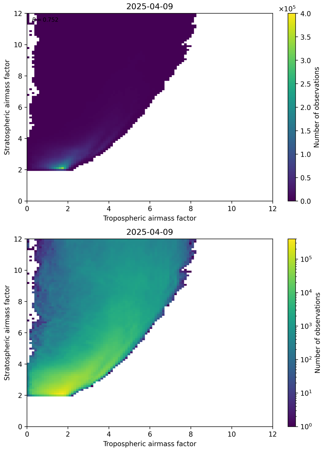
Figure 71: Scatter density plot of “Tropospheric airmass factor” against “Stratospheric airmass factor” for 2025-04-09 to 2025-04-10.
