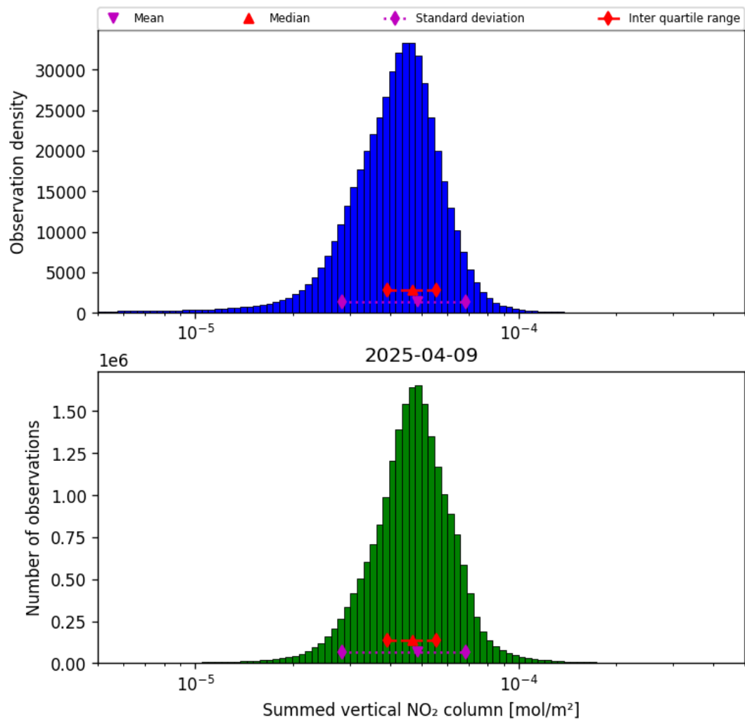
Figure 40: Histogram of “Summed vertical NO 2 column” for 2025-04-09 to 2025-04-10
