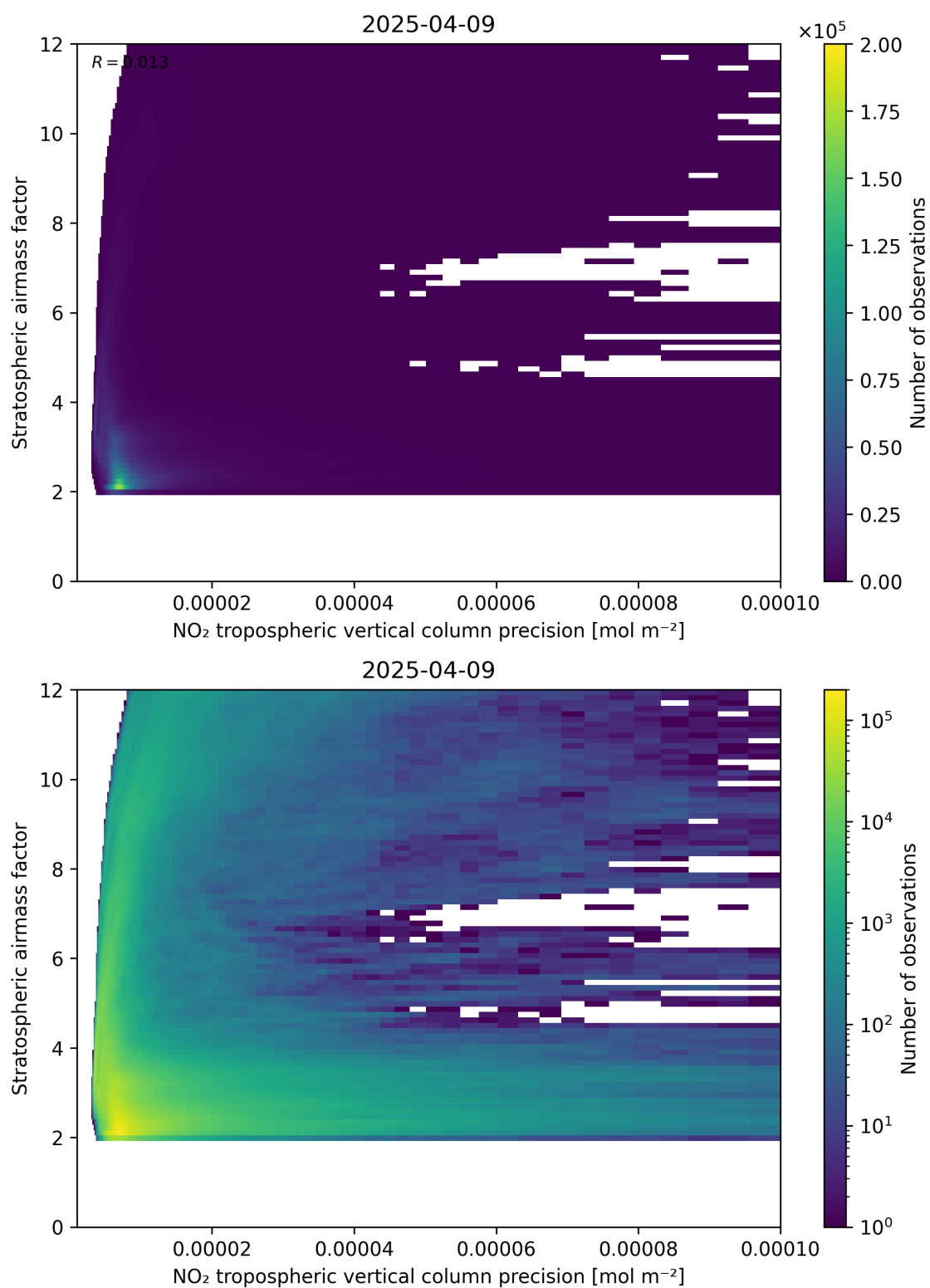
Figure 131: Scatter density plot of “NO 2 tropospheric vertical column precision” against “Stratospheric airmass factor” for 2025-04-09 to 2025-04-10.
