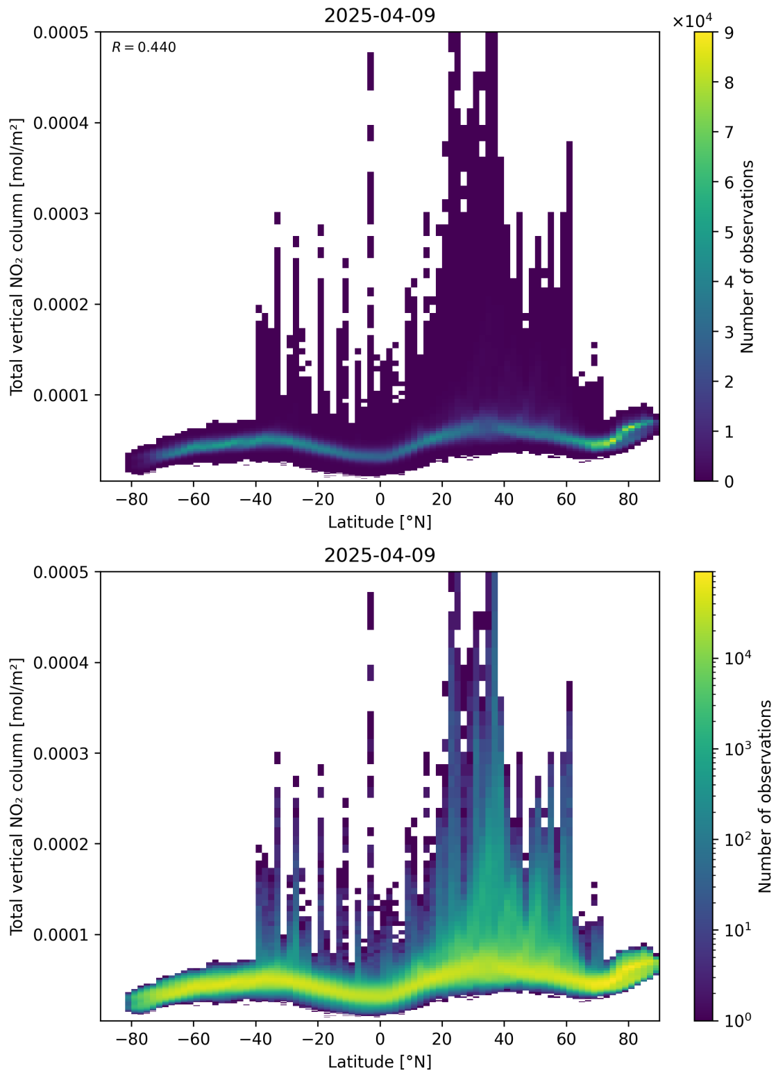
Figure 90: Scatter density plot of “Latitude” against “Total vertical NO 2 column” for 2025-04-09 to 2025-04-10.
