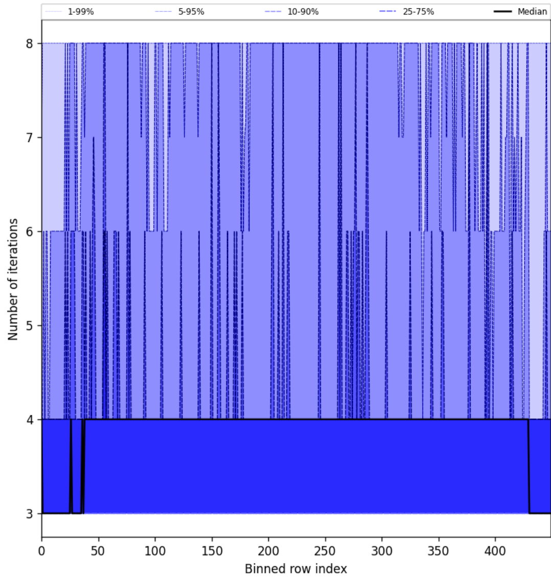
Figure 51: Along track statistics of “Number of iterations” for 2025-04-09 to 2025-04-10
