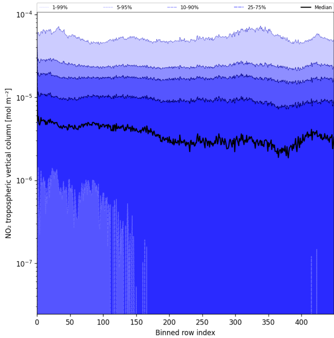
Figure 46: Along track statistics of “NO 2 tropospheric vertical column” for 2025-04-09 to 2025-04-10
