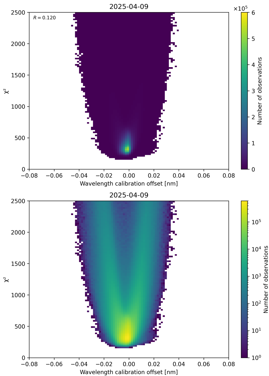
Figure 175: Scatter density plot of “Wavelength calibration offset” against “ \chi^2 ” for 2025-04-09 to 2025-04-10.
