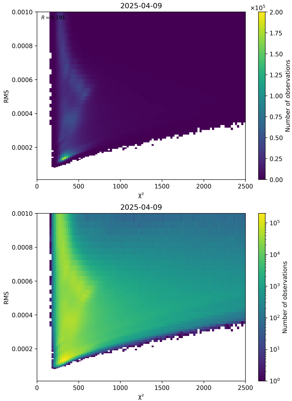
Figure 82: Scatter density plot of “ \chi^2 ” against “RMS” for 2025-04-09 to 2025-04-10.
