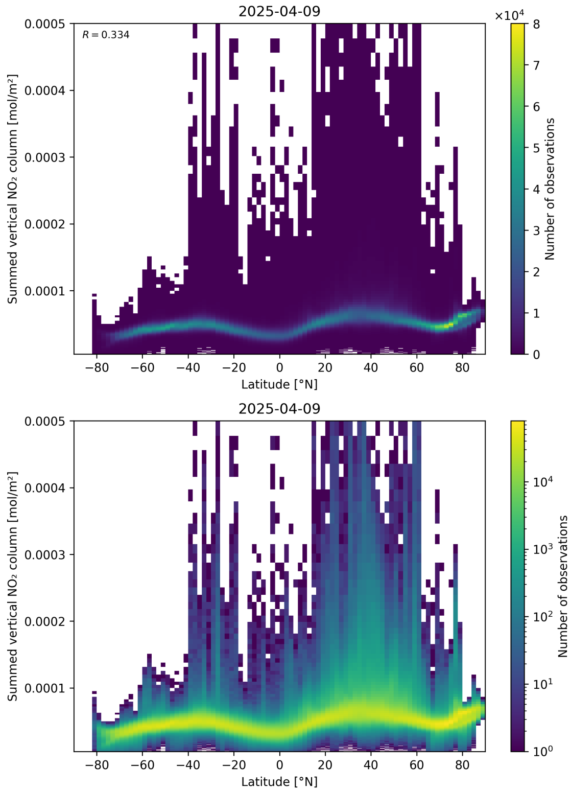
Figure 88: Scatter density plot of “Latitude” against “Summed vertical NO 2 column” for 2025-04-09 to 2025-04-10.
