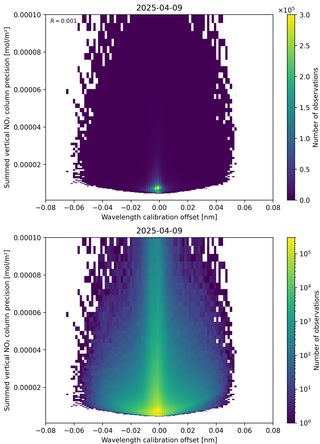
Figure 178: Scatter density plot of “Wavelength calibration offset” against “Summed vertical NO 2 column precision” for 2025-04-09 to 2025-04-10.
