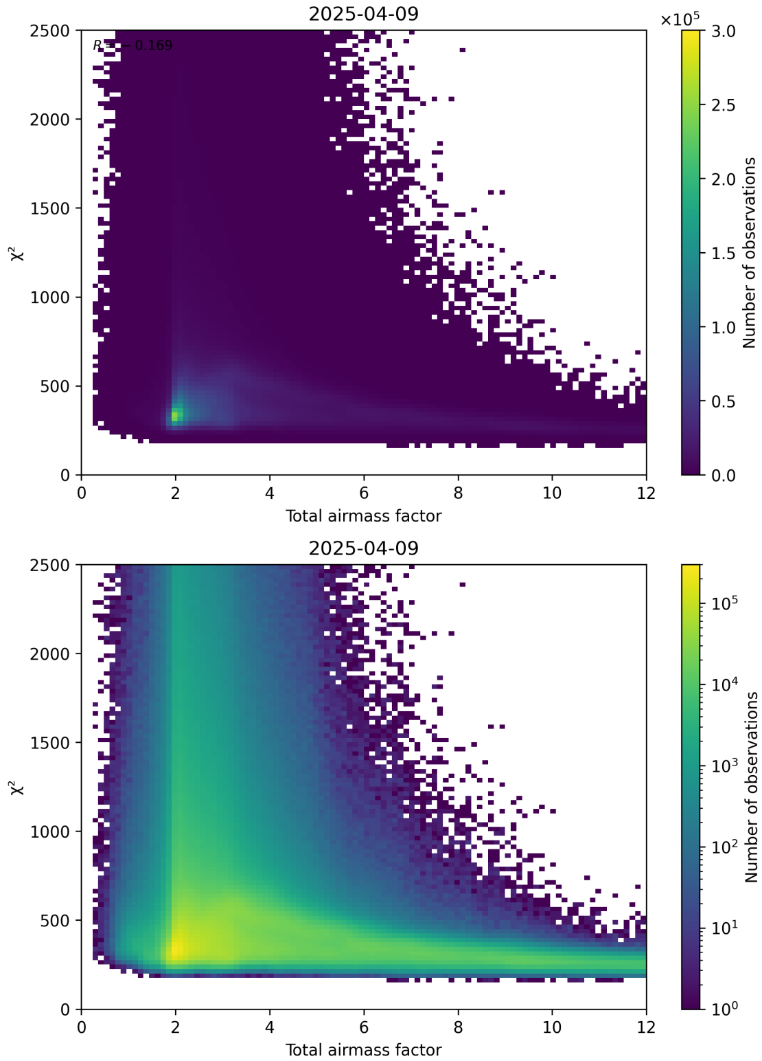
Figure 63: Scatter density plot of “Total airmass factor” against “ \chi^2 ” for 2025-04-09 to 2025-04-10.
