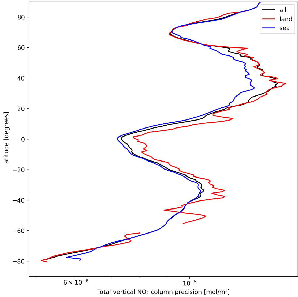
Figure 22: Zonal average of “Total vertical NO 2 column precision” for 2025-04-09 to 2025-04-10.
