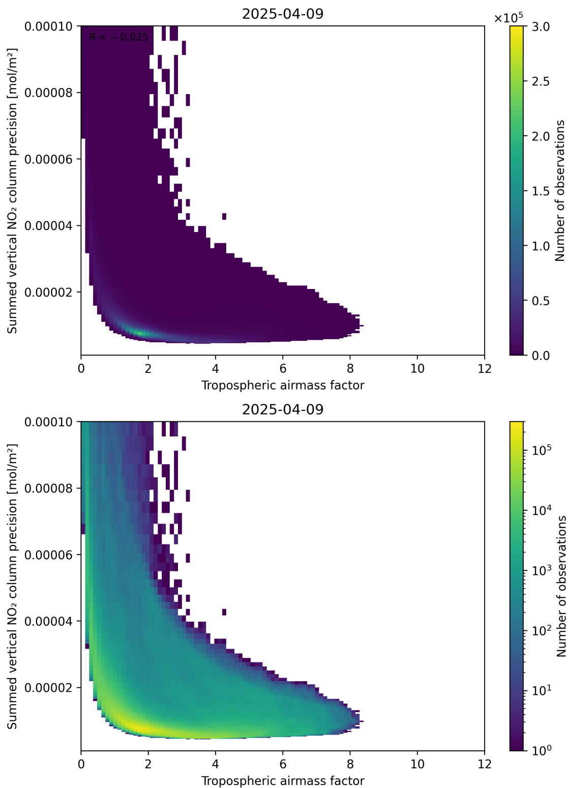
Figure 76: Scatter density plot of “Tropospheric air mass factor” against “Summed vertical NO 2 column precision” for 2025-04-09 to 2025-04-10.
