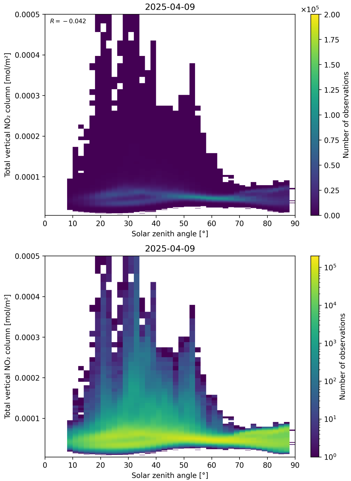
Figure 153: Scatter density plot of “Solar zenith angle” against “Total vertical NO 2 column” for 2025-04-09 to 2025-04-10.
