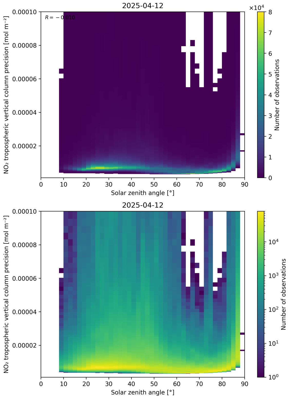
Figure 156: Scatter density plot of “Solar zenith angle” against “NO 2 tropospheric vertical column precision” for 2025-04-12 to 2025-04-13.
