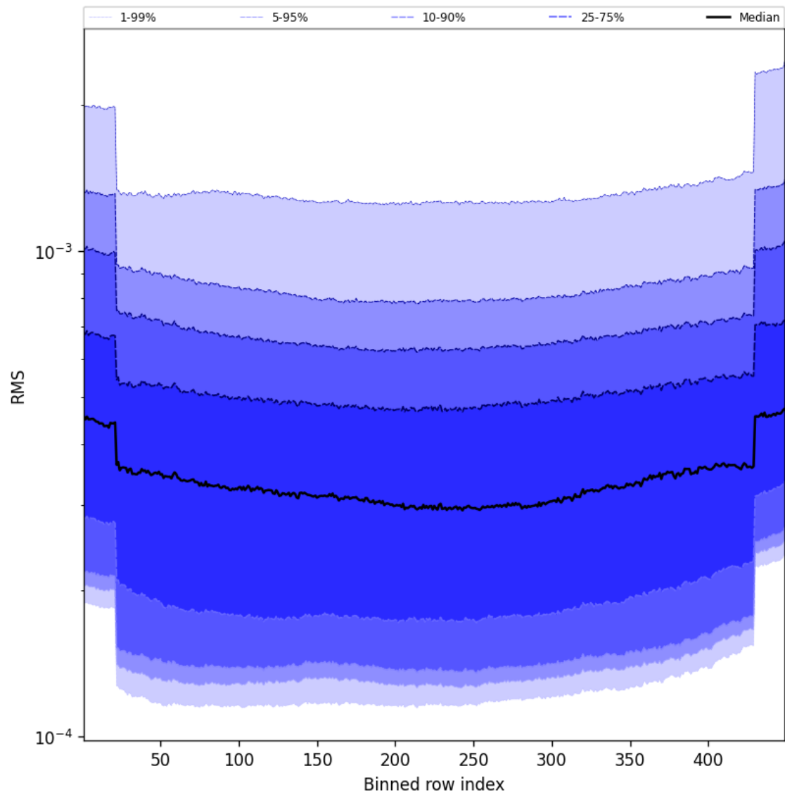
Figure 60: Along track statistics of “RMS” for 2025-04-12 to 2025-04-13
