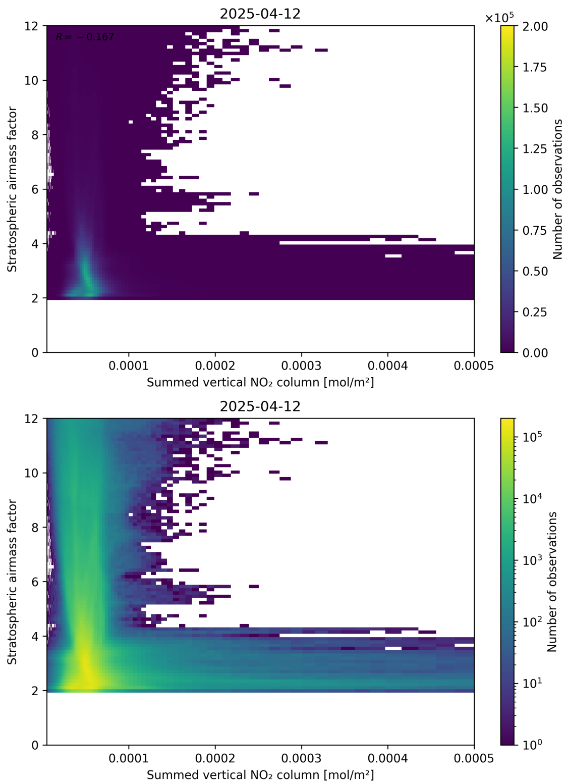
Figure 103: Scatter density plot of “Summed vertical NO 2 column” against “Stratospheric airmass factor” for 2025-04-12 to 2025-04-13.
