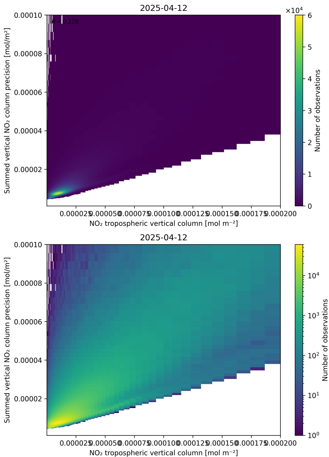
Figure 127: Scatter density plot of “NO 2 tropospheric vertical column” against “Summed vertical NO 2 column precision” for 2025-04-12 to 2025-04-13.
