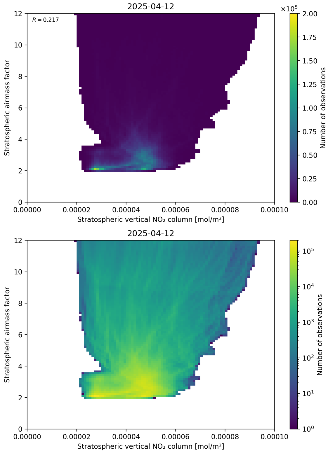
Figure 96: Scatter density plot of “Stratospheric vertical NO 2 column” against “Stratospheric airmass factor” for 2025-04-12 to 2025-04-13.
