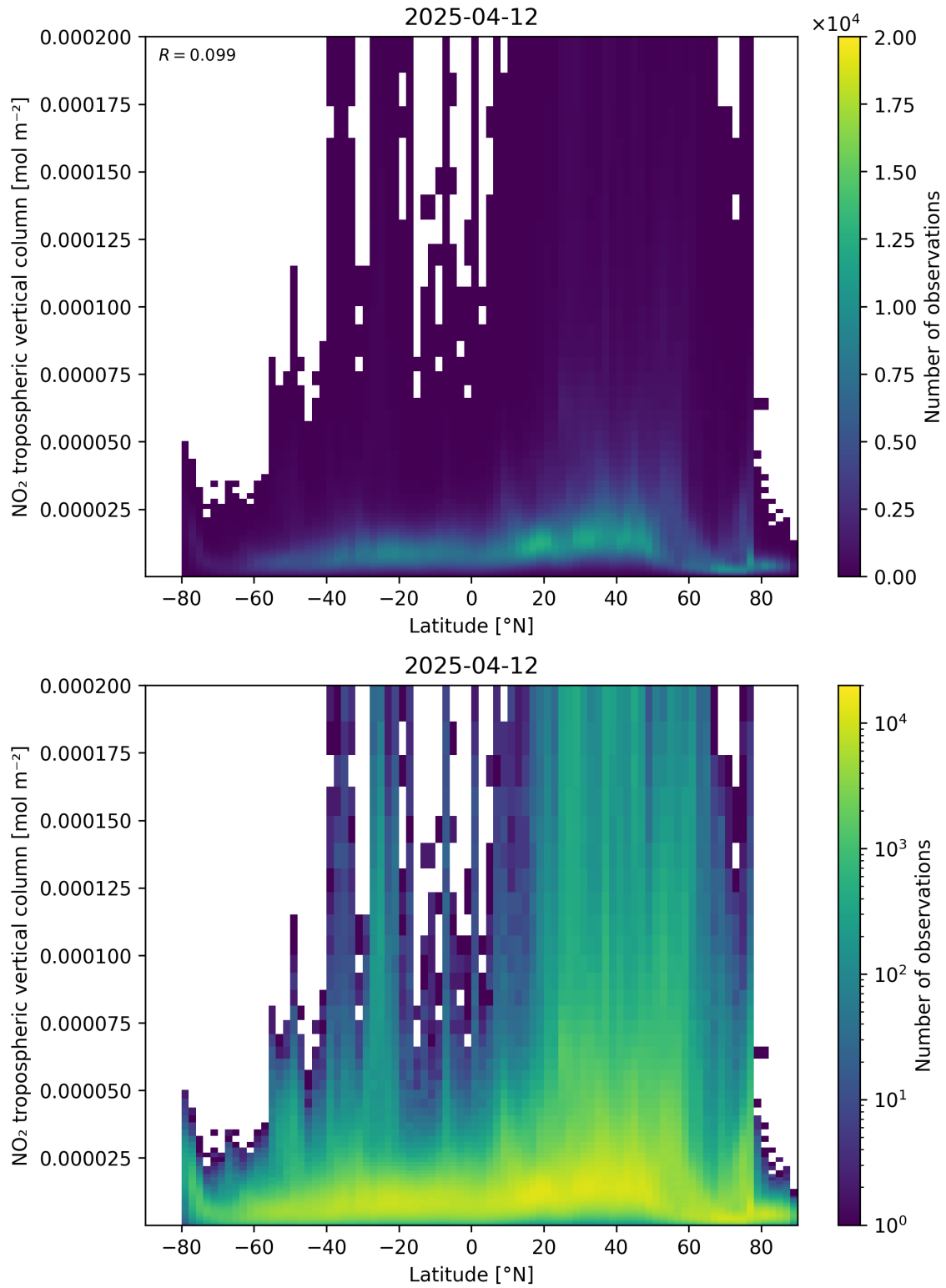
Figure 92: Scatter density plot of “Latitude” against “NO 2 tropospheric vertical column” for 2025-04-12 to 2025-04-13.
