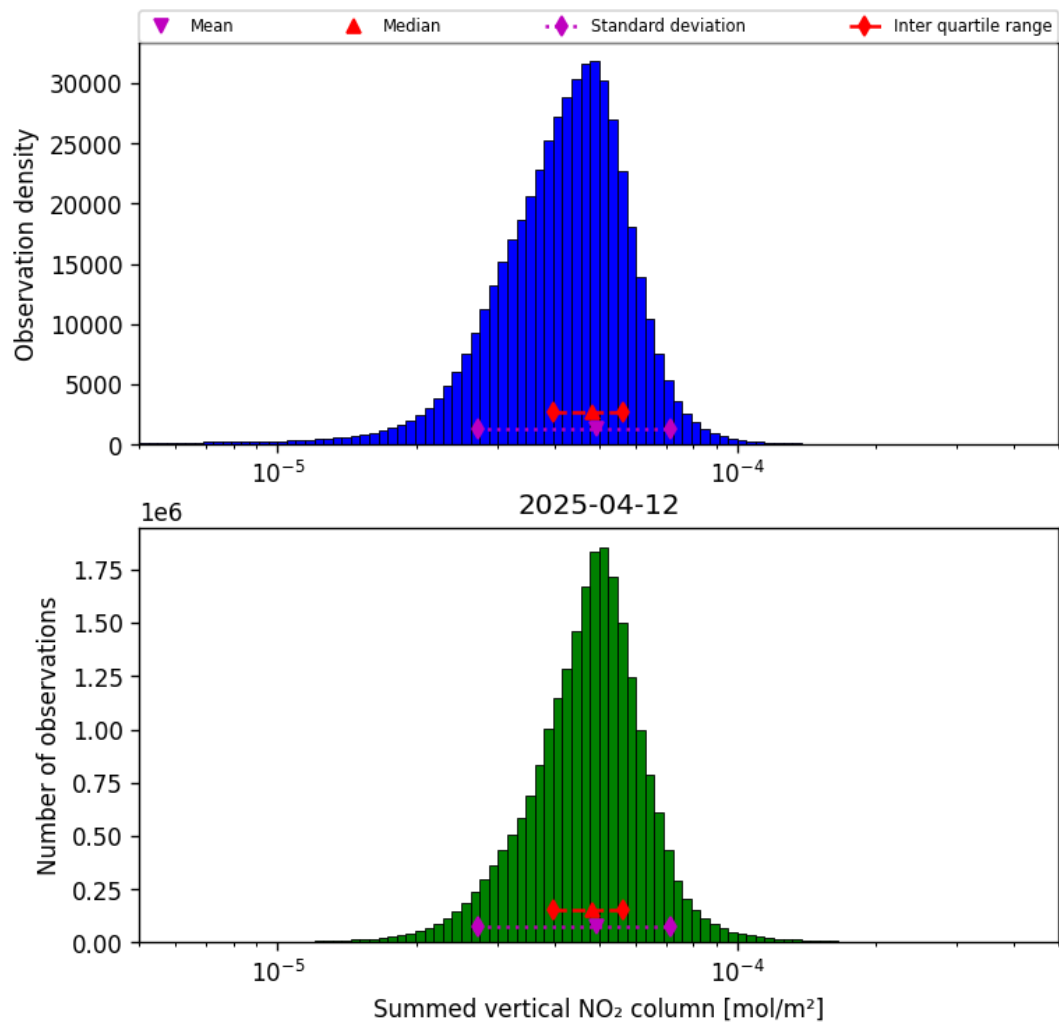
Figure 40: Histogram of “Summed vertical NO 2 column” for 2025-04-12 to 2025-04-13
