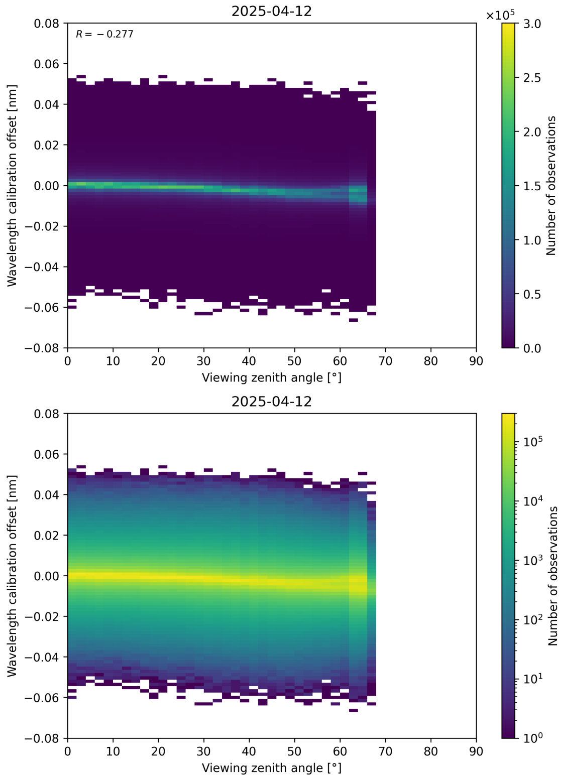
Figure 173: Scatter density plot of “Viewing zenith angle” against “Wavelength calibration offset” for 2025-04-12 to 2025-04-13.
