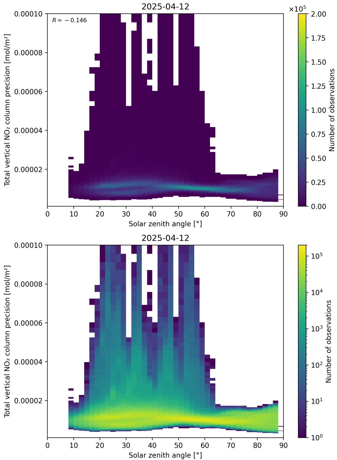
Figure 154: Scatter density plot of “Solar zenith angle” against “Total vertical NO 2 column precision” for 2025-04-12 to 2025-04-13.
