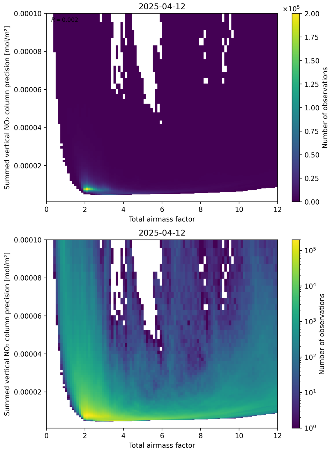
Figure 66: Scatter density plot of “Total airmass factor” against “Summed vertical NO 2 column precision” for 2025-04-12 to 2025-04-13.
