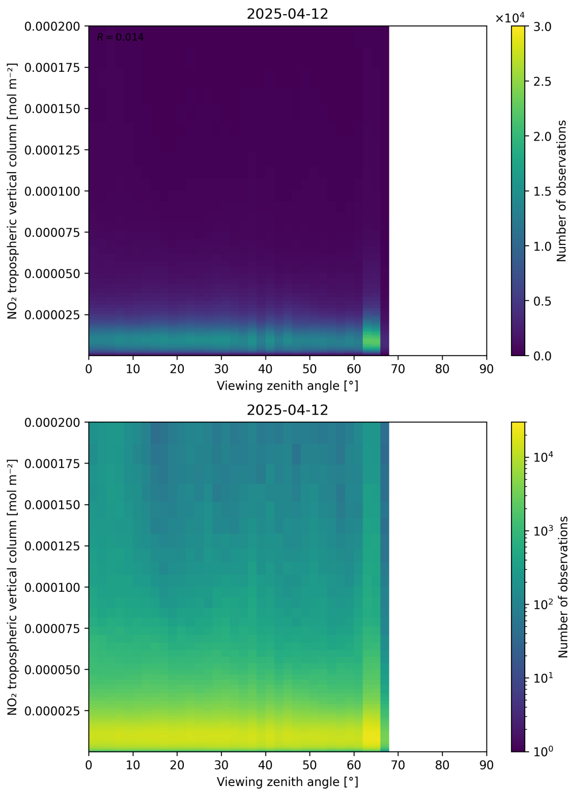
Figure 169: Scatter density plot of “Viewing zenith angle” against “NO 2 tropospheric vertical column” for 2025-04-12 to 2025-04-13.
