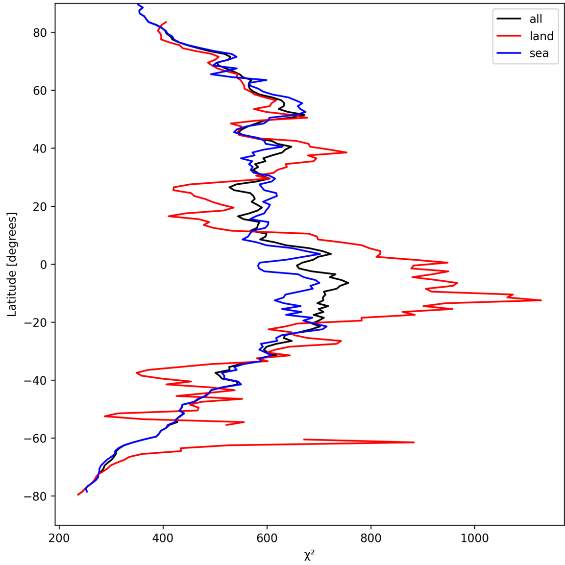
Figure 25: Zonal average of “ \chi^2 ” for 2025-04-12 to 2025-04-13.
