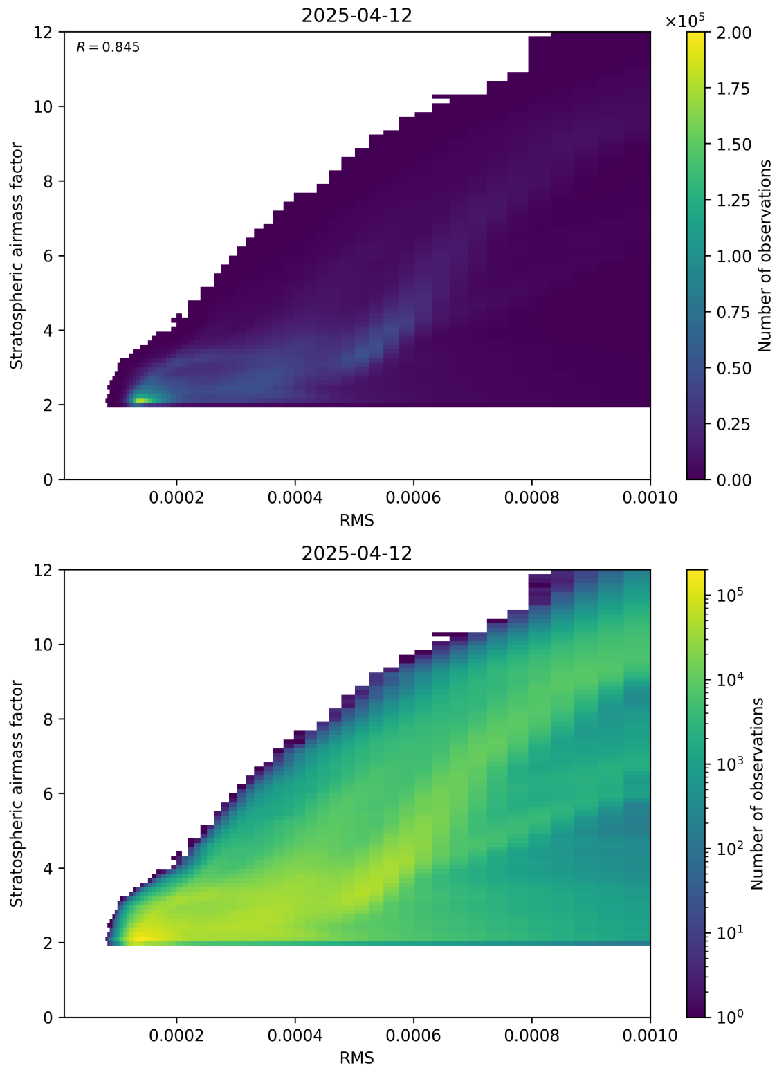
Figure 144: Scatter density plot of “RMS” against “Stratospheric airmass factor” for 2025-04-12 to 2025-04-13.
