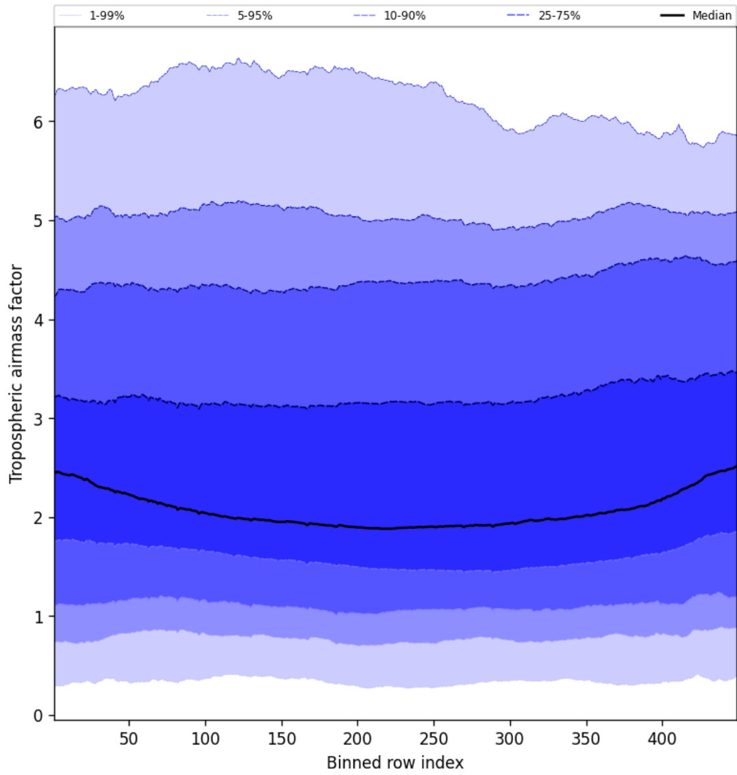
Figure 48: Along track statistics of “Tropospheric airmass factor” for 2025-04-12 to 2025-04-13
