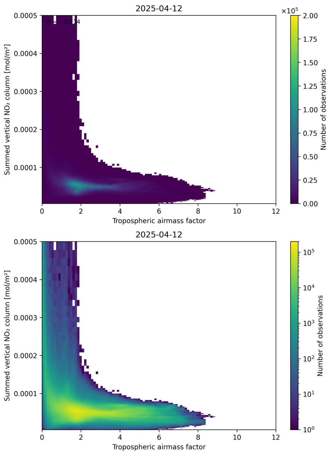
Figure 75: Scatter density plot of “Tropospheric air mass factor” against “Summed vertical NO 2 column” for 2025-04-12 to 2025-04-13.
