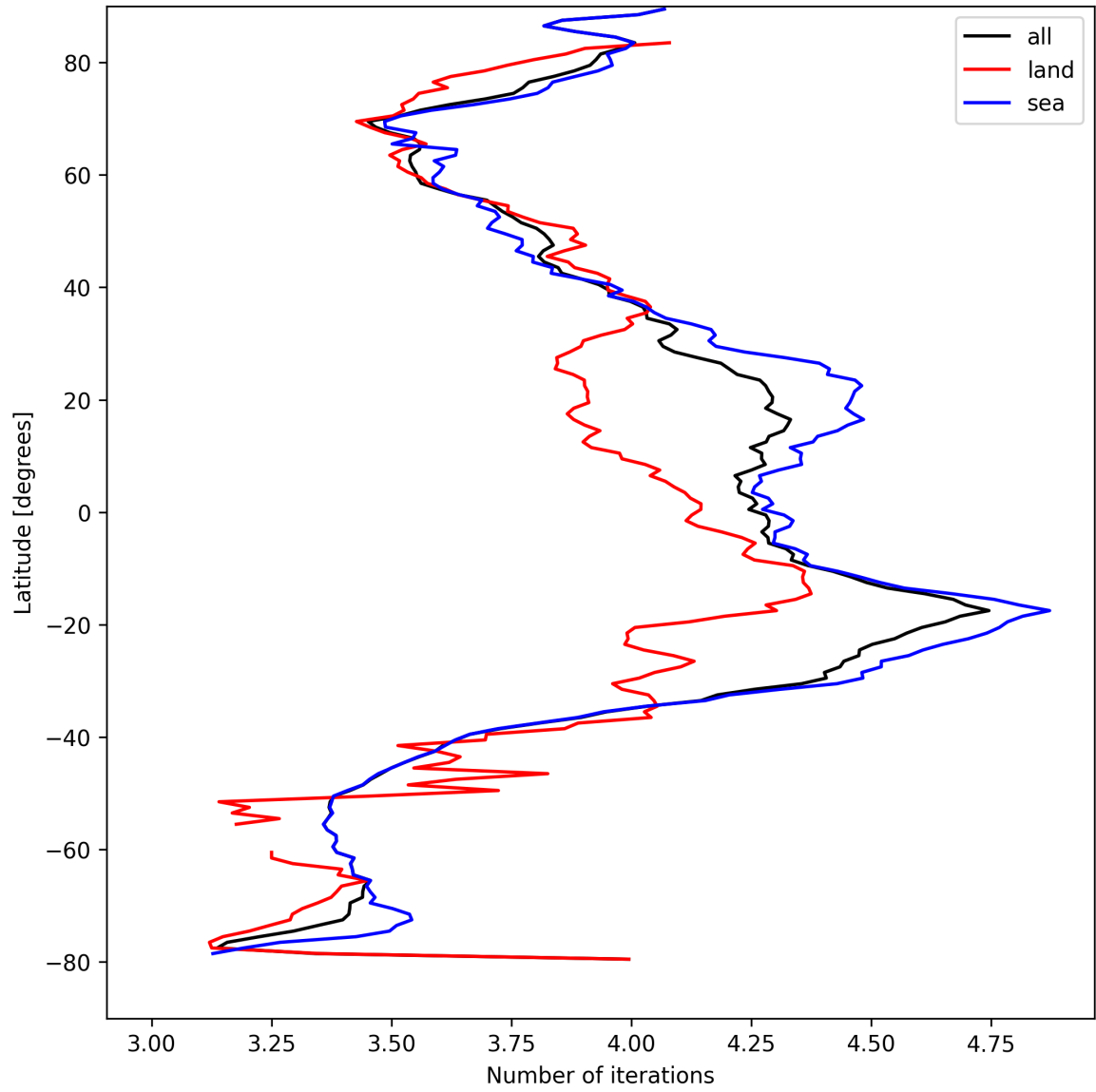
Figure 17: Zonal average of “Number of iterations” for 2025-04-12 to 2025-04-13.
