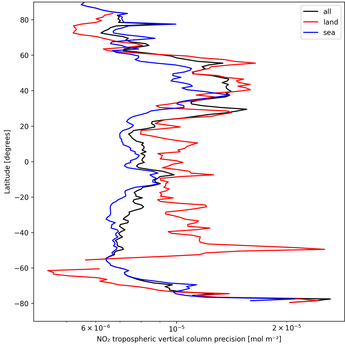
Figure 13: Zonal average of “NO 2 tropospheric vertical column precision” for 2025-04-12 to 2025-04-13.
