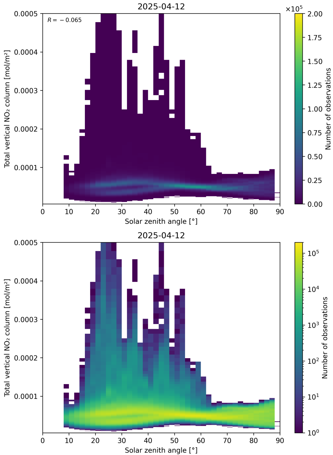
Figure 153: Scatter density plot of “Solar zenith angle” against “Total vertical NO 2 column” for 2025-04-12 to 2025-04-13.
