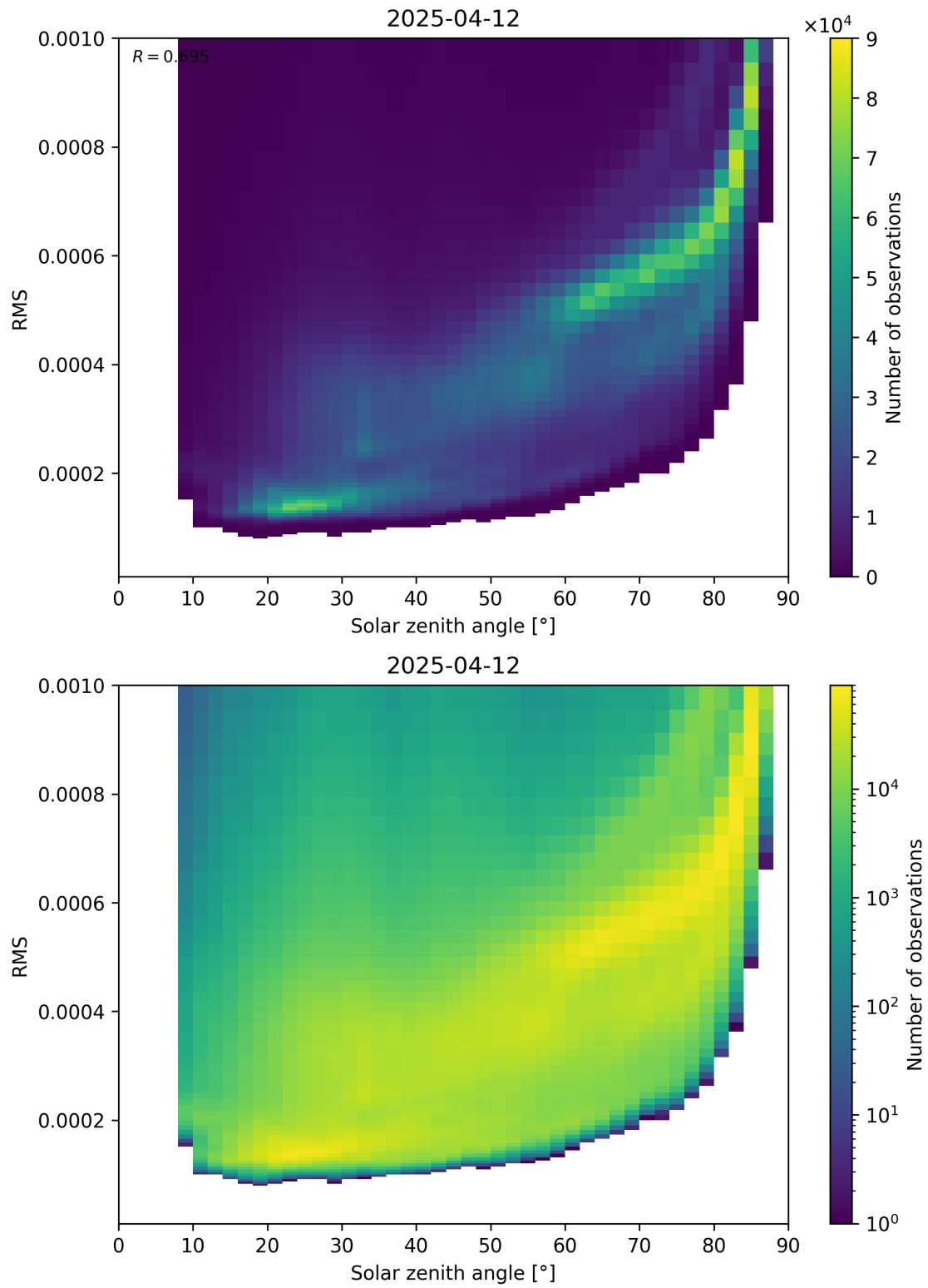
Figure 157: Scatter density plot of “Solar zenith angle” against “RMS” for 2025-04-12 to 2025-04-13.
