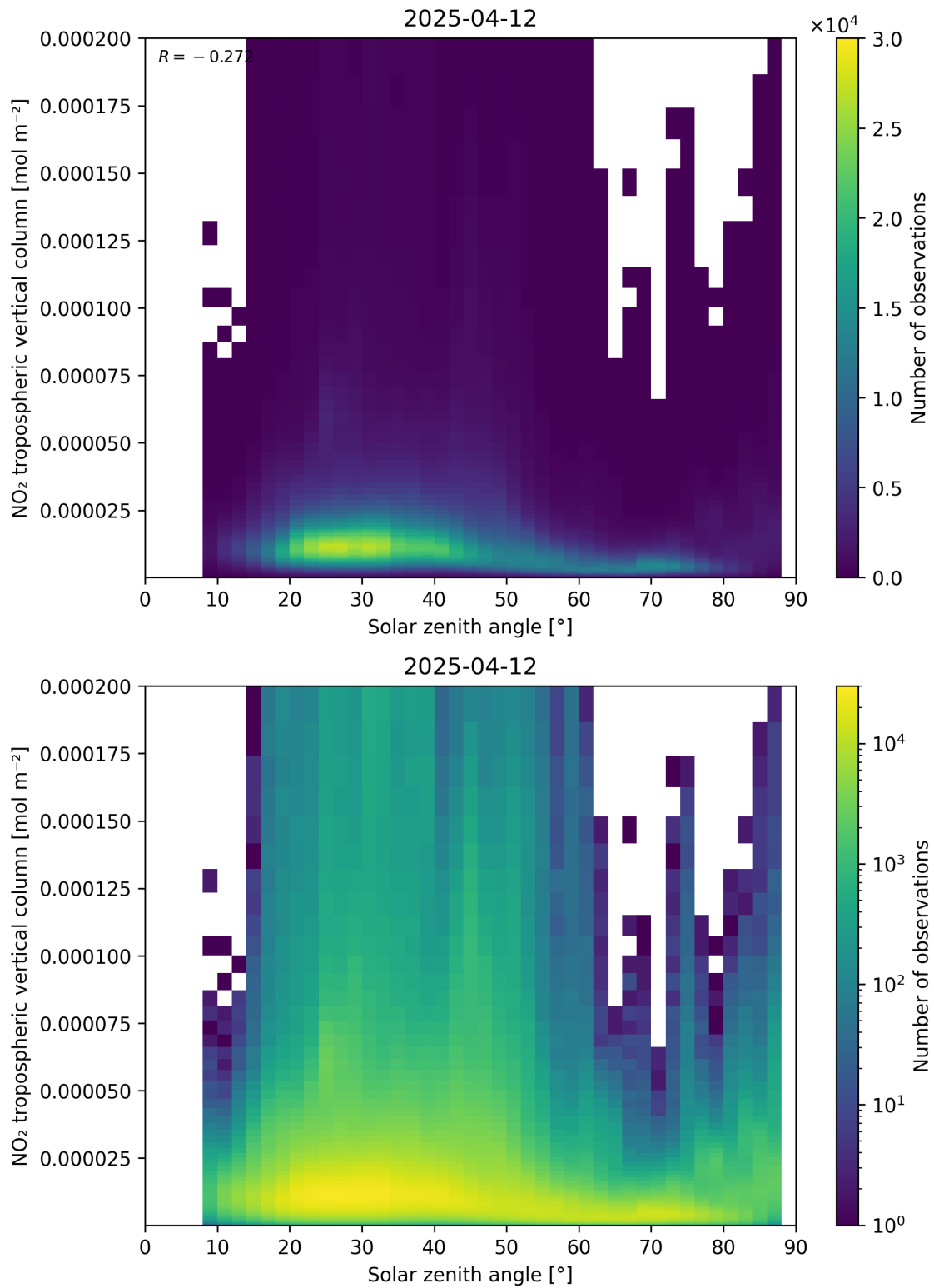
Figure 155: Scatter density plot of “Solar zenith angle” against “NO 2 tropospheric vertical column” for 2025-04-12 to 2025-04-13.
