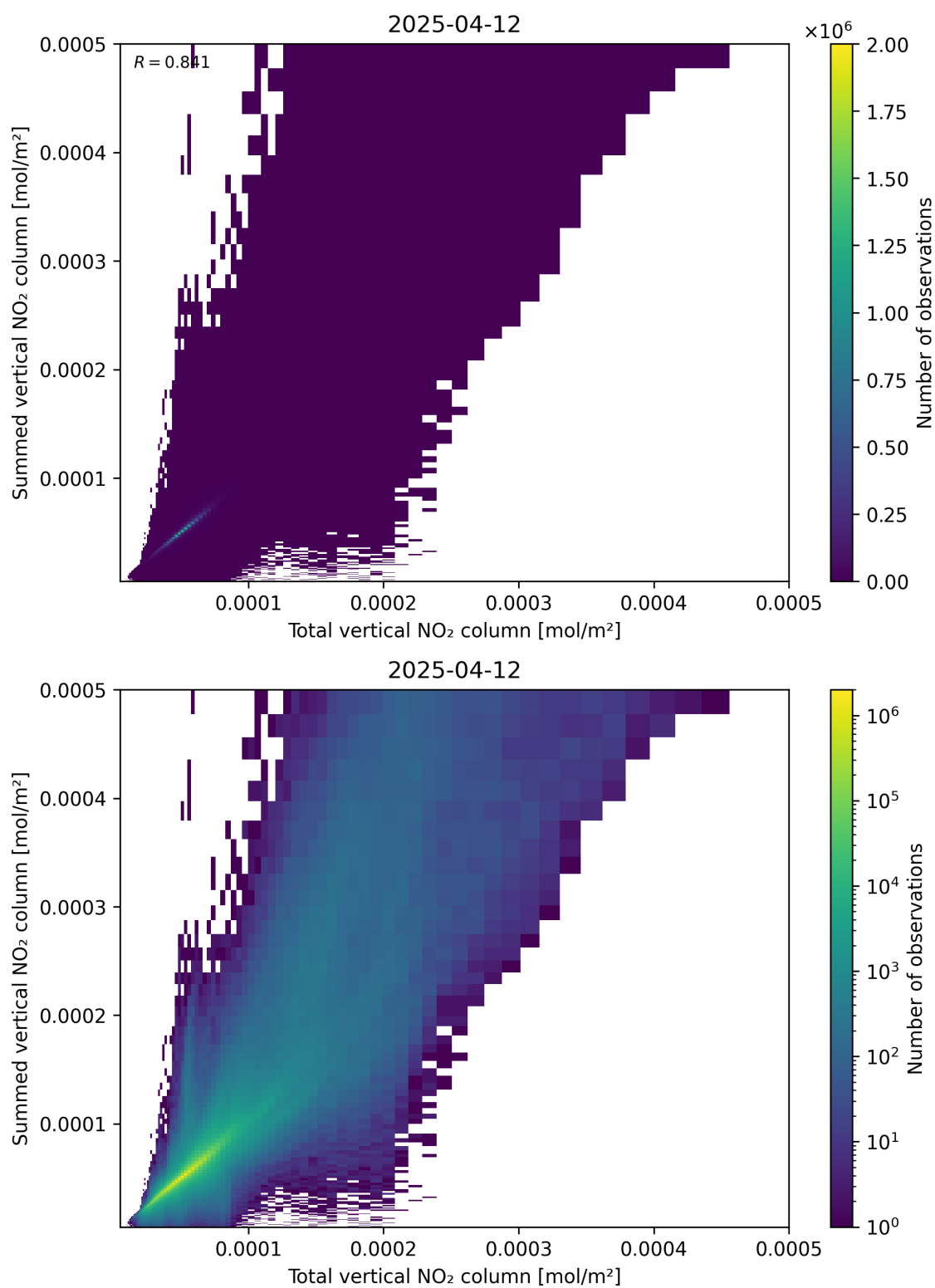
Figure 112: Scatter density plot of “Total vertical NO 2 column” against “Summed vertical NO 2 column” for 2025-04-12 to 2025-04-13.
