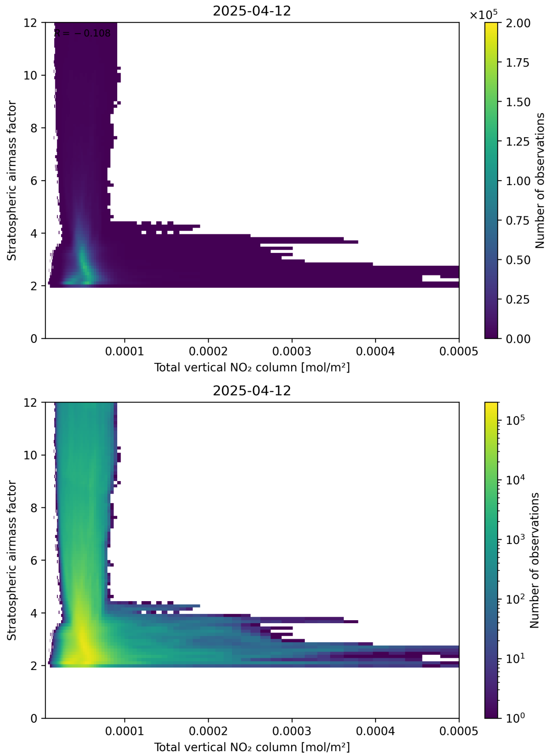
Figure 110: Scatter density plot of “Total vertical NO 2 column” against “Stratospheric air mass factor” for 2025-04-12 to 2025-04-13.
