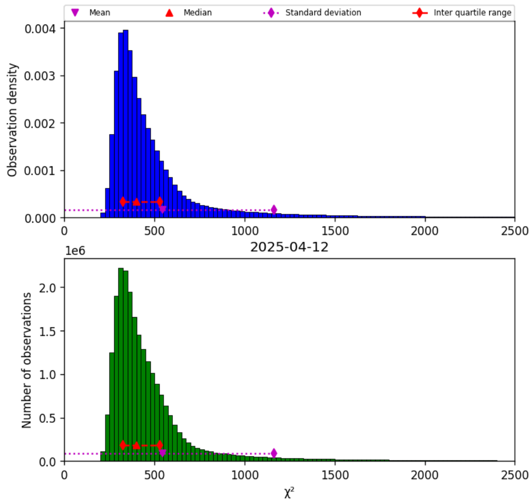
Figure 42: Histogram of “ \chi^2 ” for 2025-04-12 to 2025-04-13
