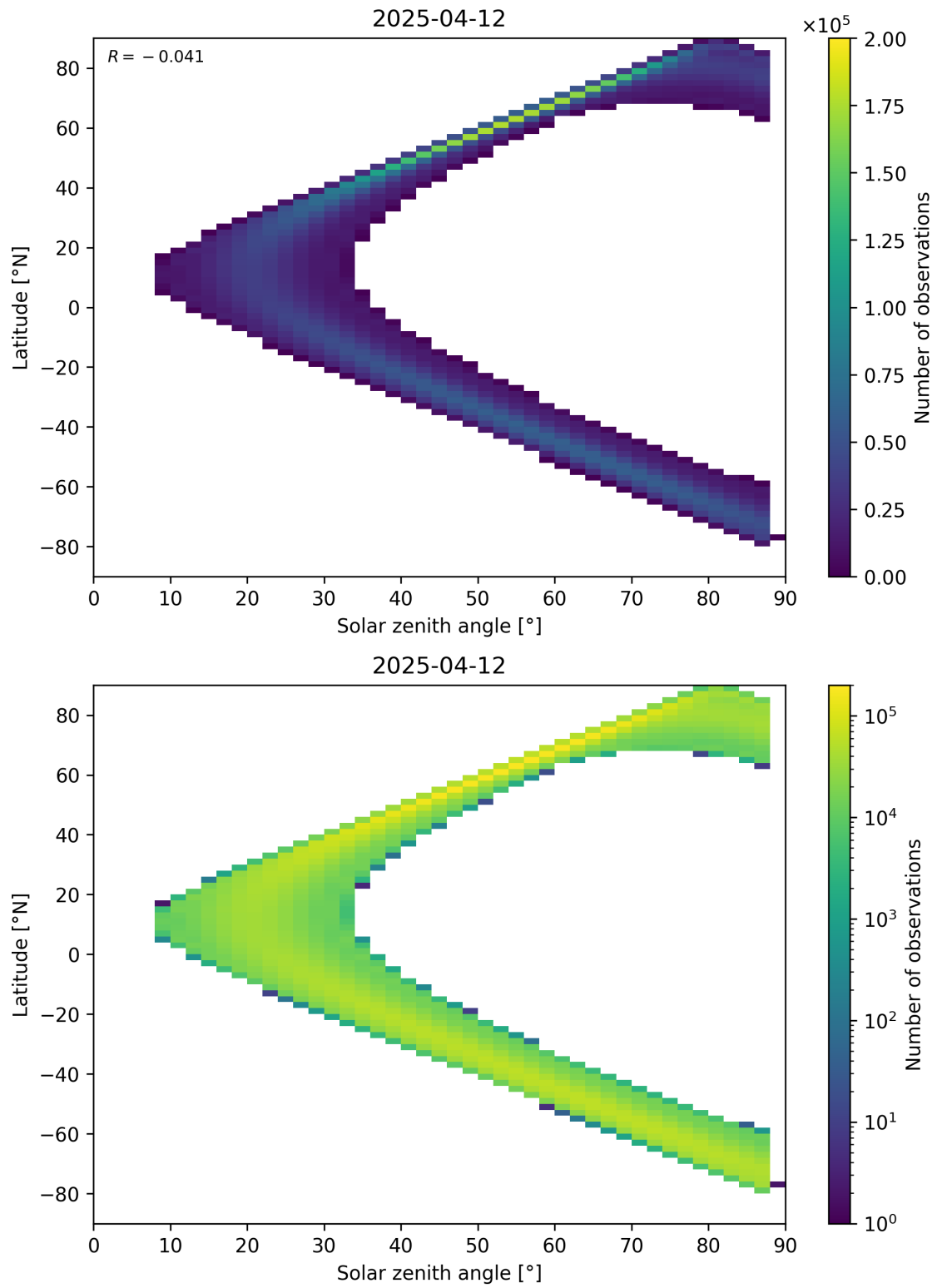
Figure 149: Scatter density plot of “Solar zenith angle” against “Latitude” for 2025-04-12 to 2025-04-13.
