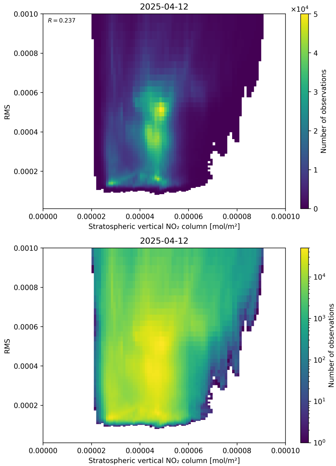
Figure 102: Scatter density plot of “Stratospheric vertical NO 2 column” against “RMS” for 2025-04-12 to 2025-04-13.
