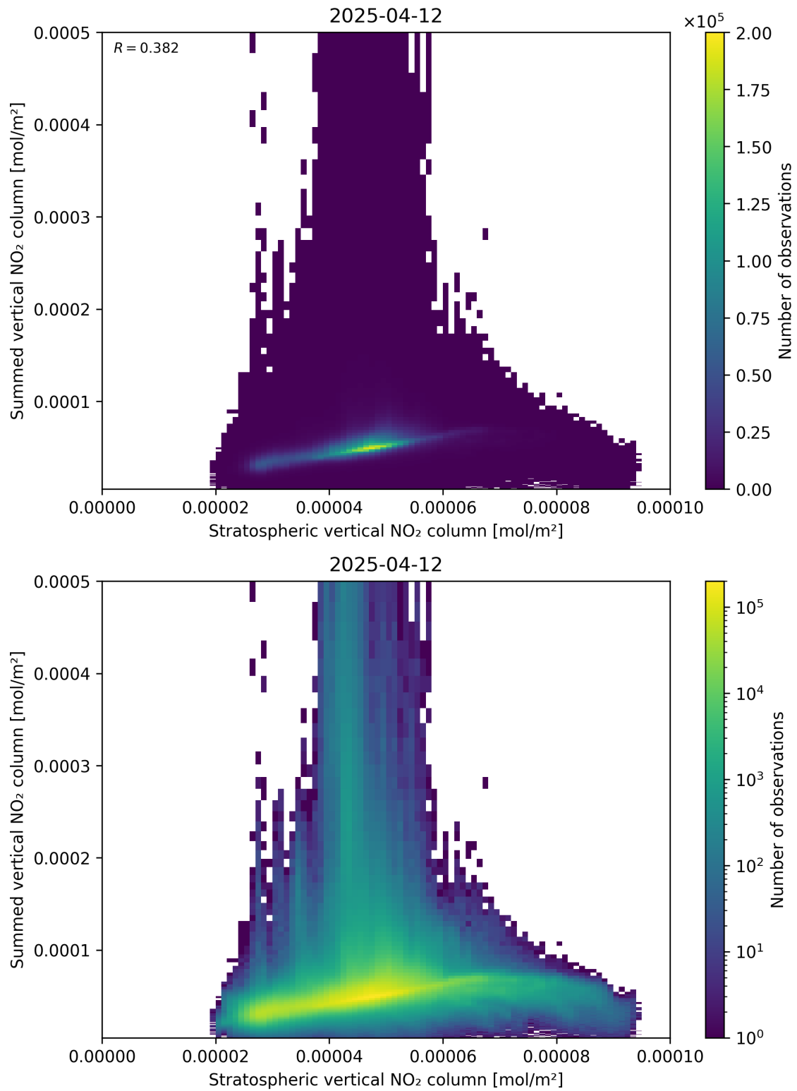
Figure 98: Scatter density plot of “Stratospheric vertical NO 2 column” against “Summed vertical NO 2 column” for 2025-04-12 to 2025-04-13.
