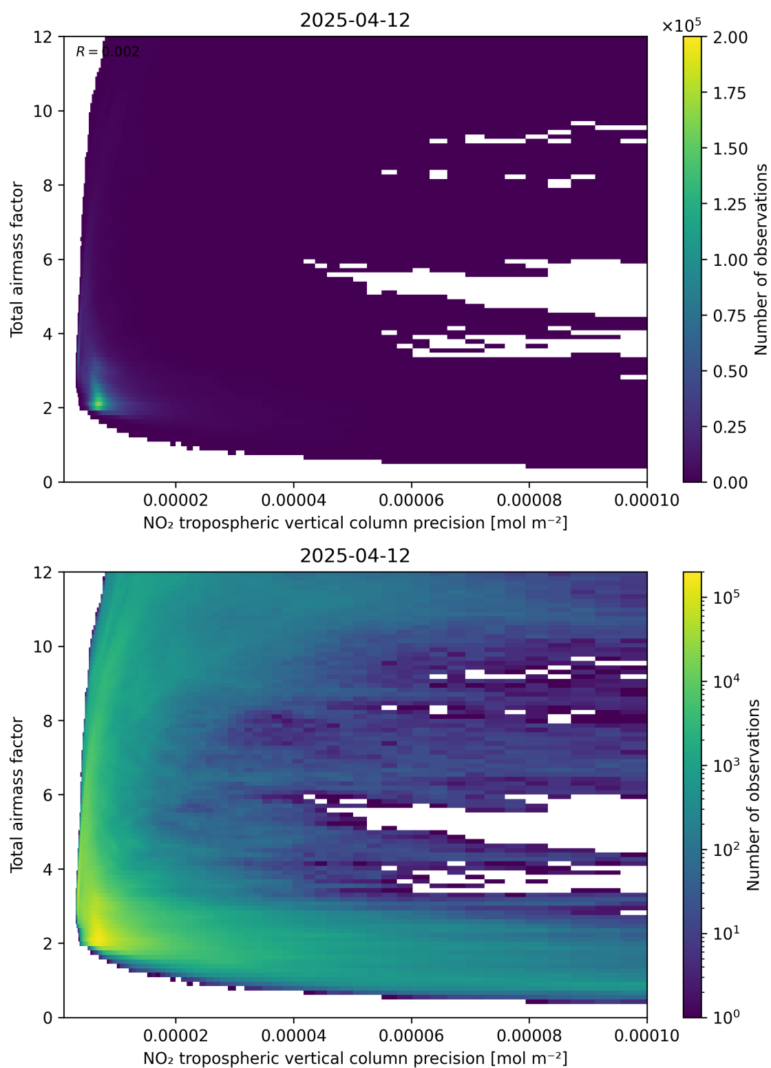
Figure 132: Scatter density plot of “NO 2 tropospheric vertical column precision” against “Total air mass factor” for 2025-04-12 to 2025-04-13.
