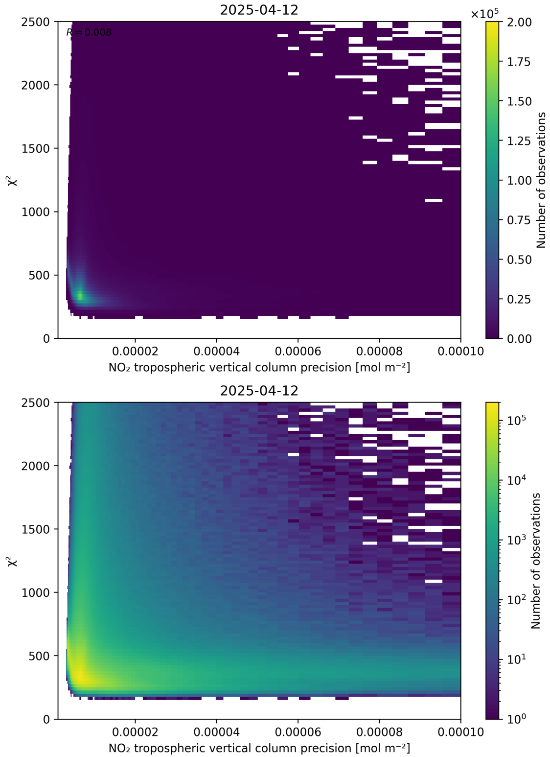
Figure 134: Scatter density plot of “NO 2 tropospheric vertical column precision” against “ \chi^2 ” for 2025-04-12 to 2025-04-13.
