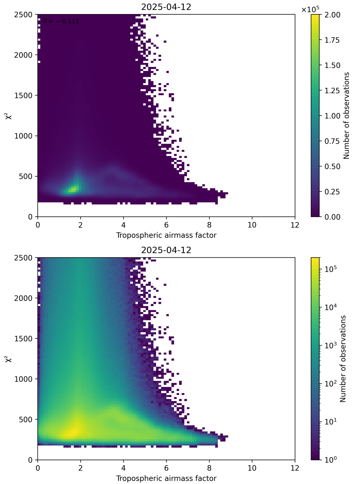
Figure 73: Scatter density plot of “Tropospheric airmass factor” against “ \chi^2 ” for 2025-04-12 to 2025-04-13.
