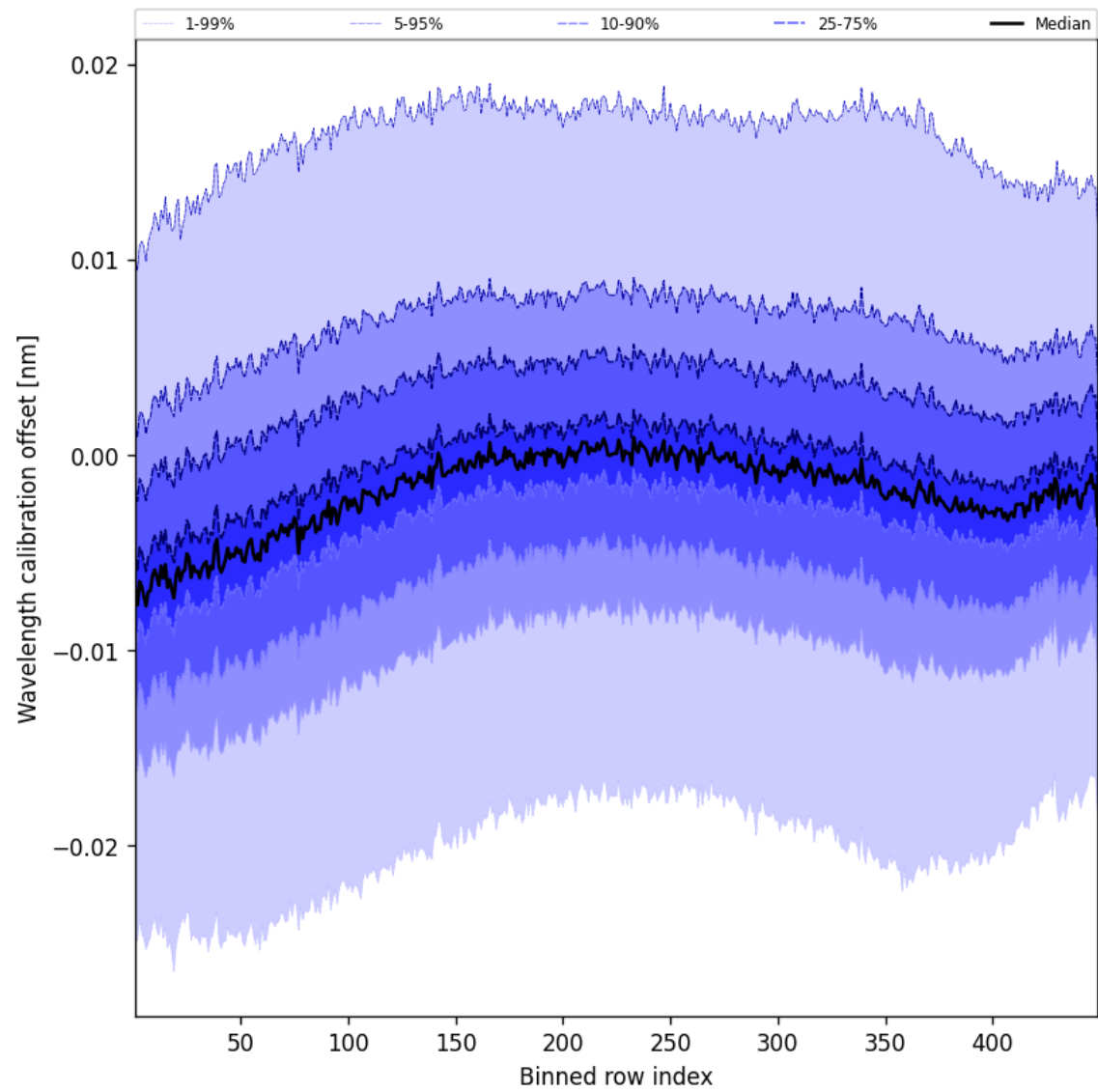
Figure 52: Along track statistics of “Wavelength calibration offset” for 2025-04-12 to 2025-04-13
