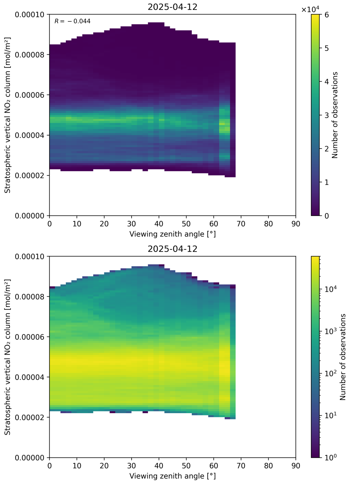
Figure 164: Scatter density plot of “Viewing zenith angle” against “Stratospheric vertical NO 2 column” for 2025-04-12 to 2025-04-13.
