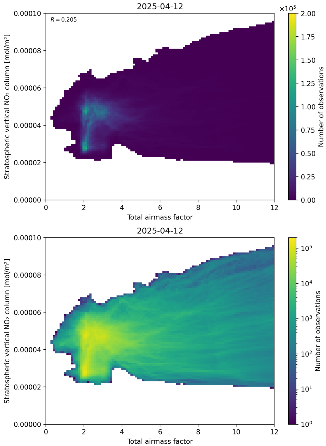
Figure 64: Scatter density plot of “Total airmass factor” against “Stratospheric vertical \text{NO}_2 column” for 2025-04-12 to 2025-04-13.
