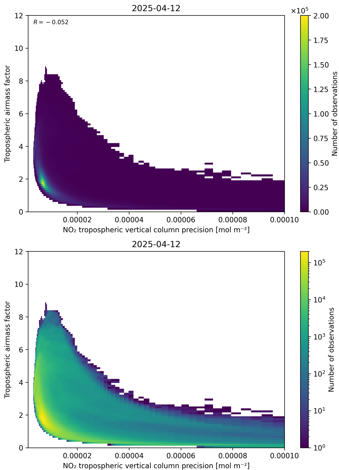
Figure 133: Scatter density plot of “NO 2 tropospheric vertical column precision” against “Tropospheric air mass factor” for 2025-04-12 to 2025-04-13.
