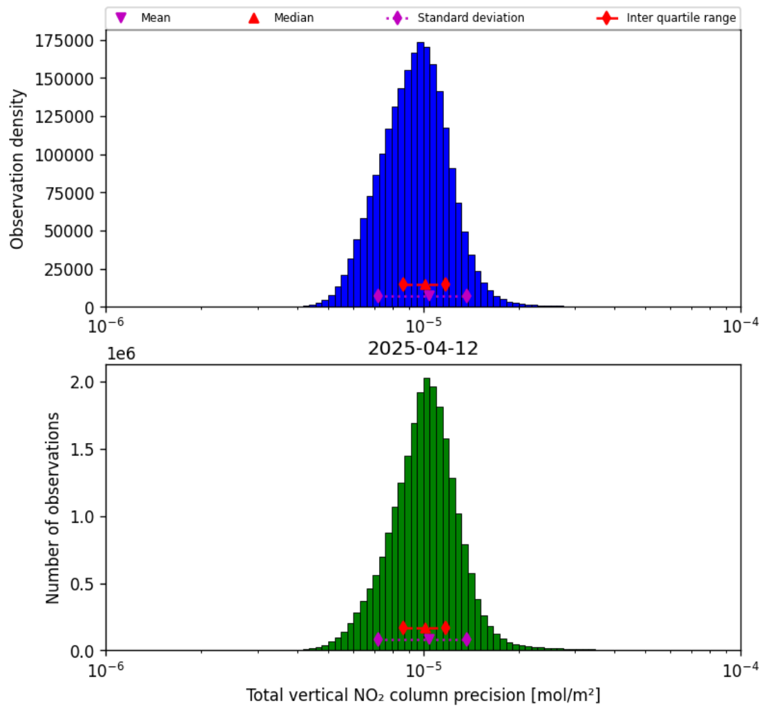
Figure 39: Histogram of “Total vertical NO 2 column precision” for 2025-04-12 to 2025-04-13
