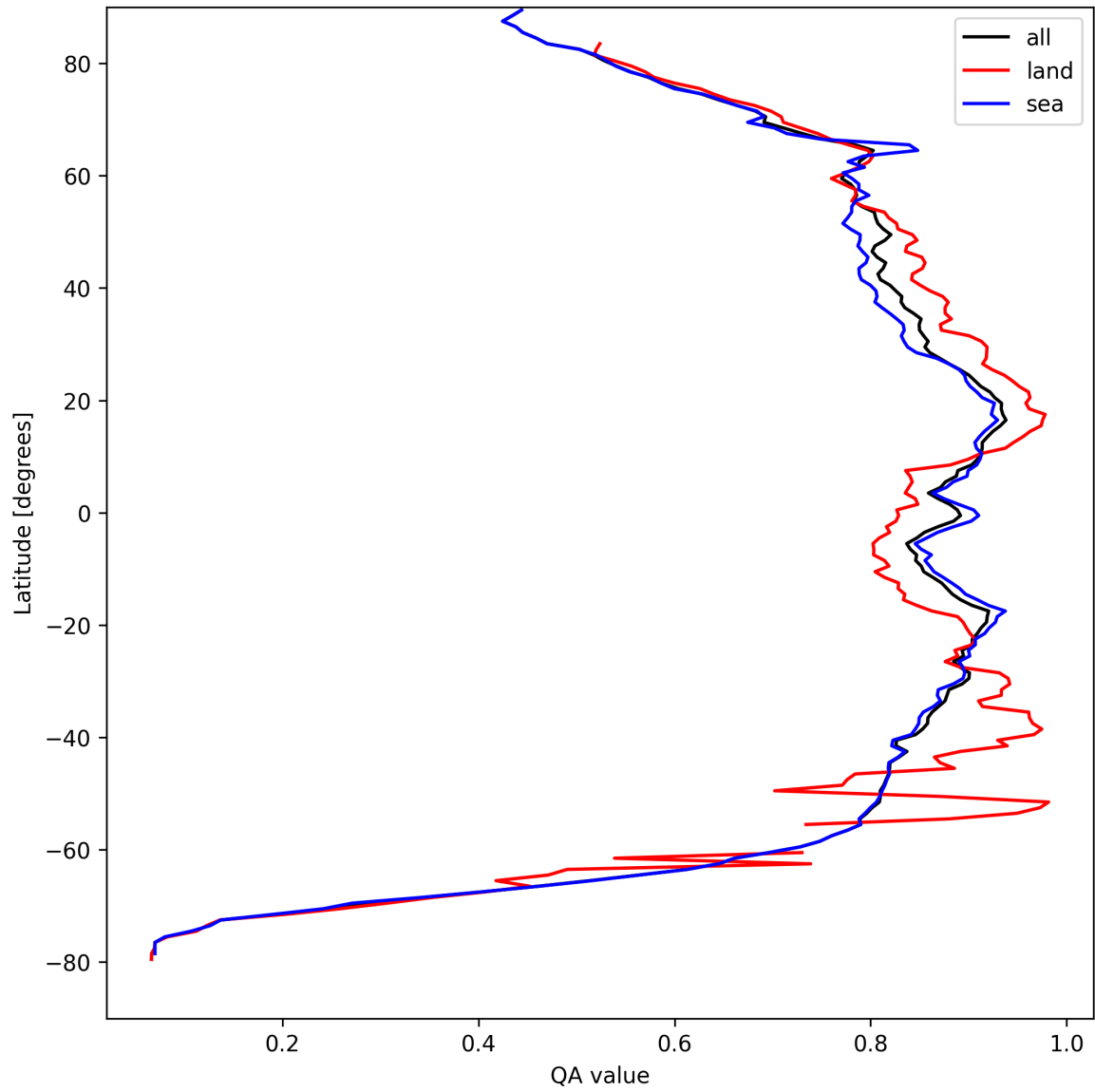
Figure 11: Zonal average of “QA value” for 2025-04-12 to 2025-04-13.
