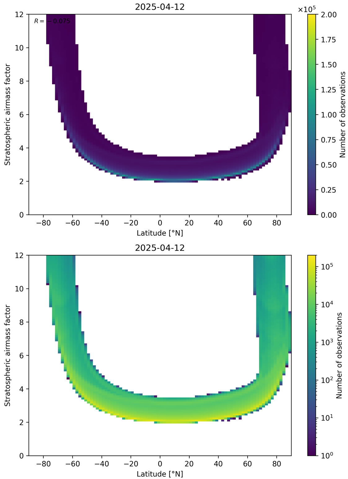
Figure 83: Scatter density plot of “Latitude” against “Stratospheric air mass factor” for 2025-04-12 to 2025-04-13.
