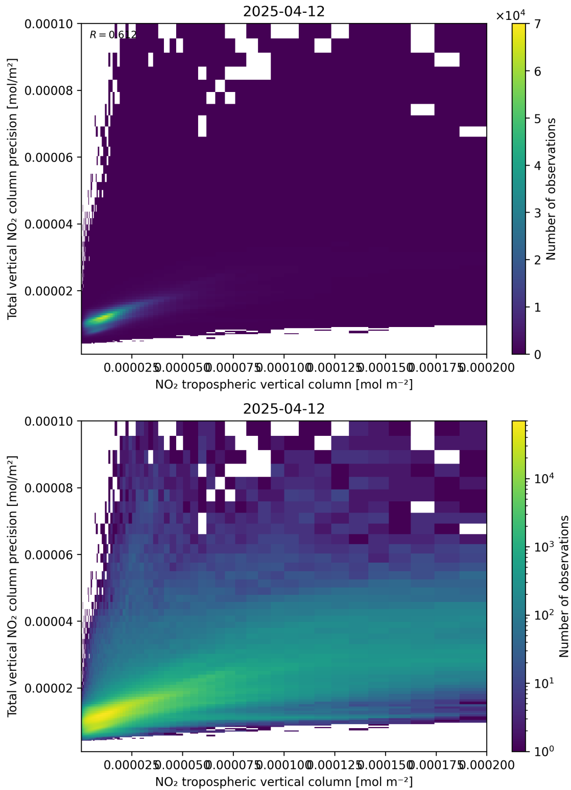
Figure 129: Scatter density plot of “NO 2 tropospheric vertical column” against “Total vertical NO 2 column precision” for 2025-04-12 to 2025-04-13.
