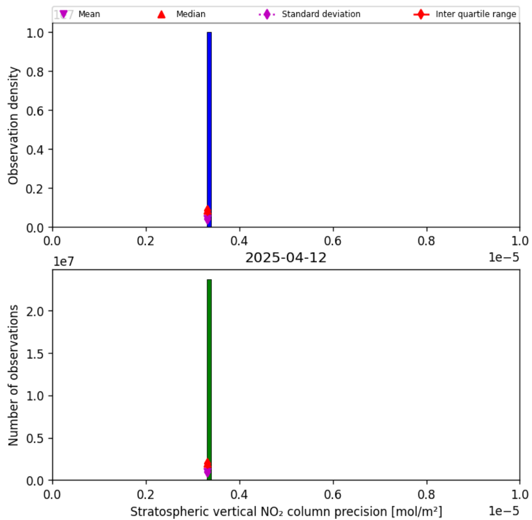
Figure 37: Histogram of “Stratospheric vertical NO 2 column precision” for 2025-04-12 to 2025-04-13
