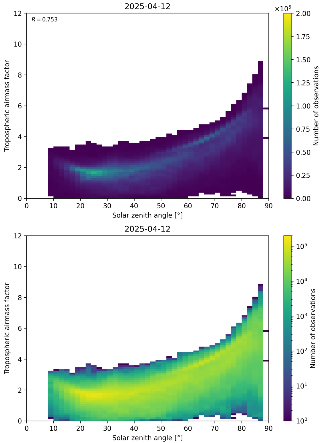
Figure 147: Scatter density plot of “Solar zenith angle” against “Tropospheric airmass factor” for 2025-04-12 to 2025-04-13.
