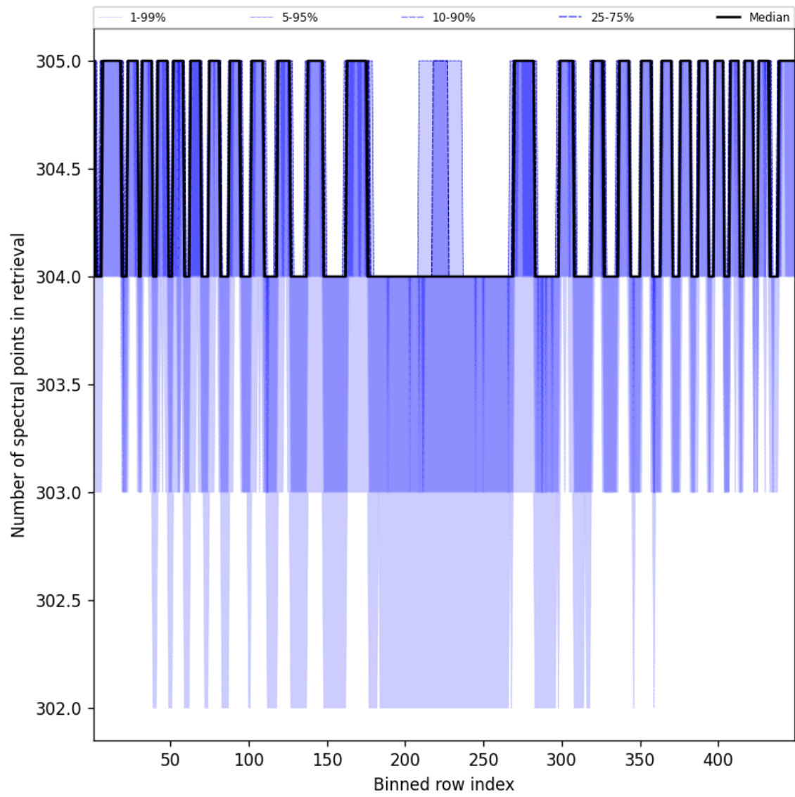
Figure 50: Along track statistics of “Number of spectral points in retrieval” for 2025-04-12 to 2025-04-13
