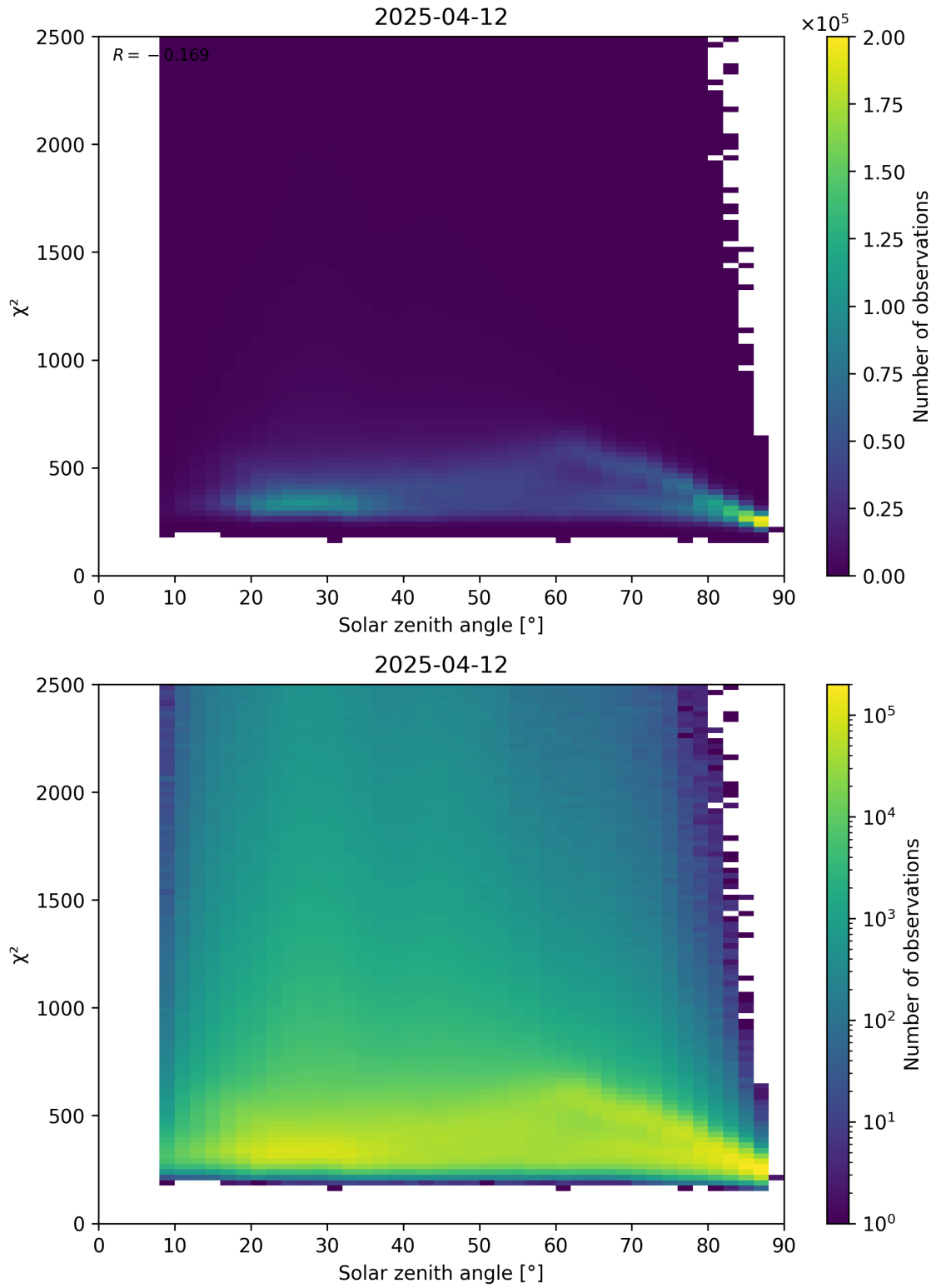
Figure 148: Scatter density plot of “Solar zenith angle” against “ \chi^2 ” for 2025-04-12 to 2025-04-13.
