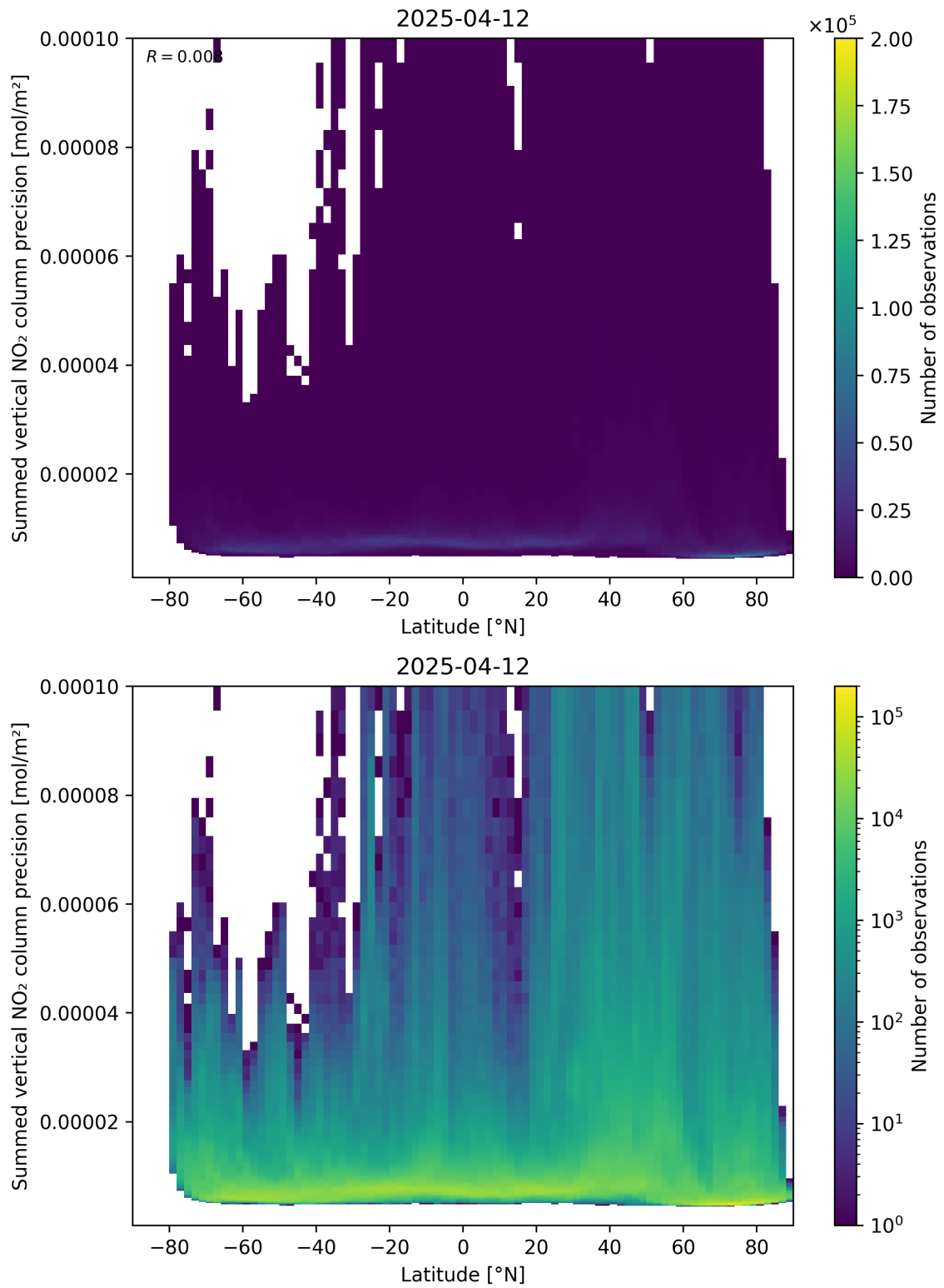
Figure 89: Scatter density plot of “Latitude” against “Summed vertical NO 2 column precision” for 2025-04-12 to 2025-04-13.
