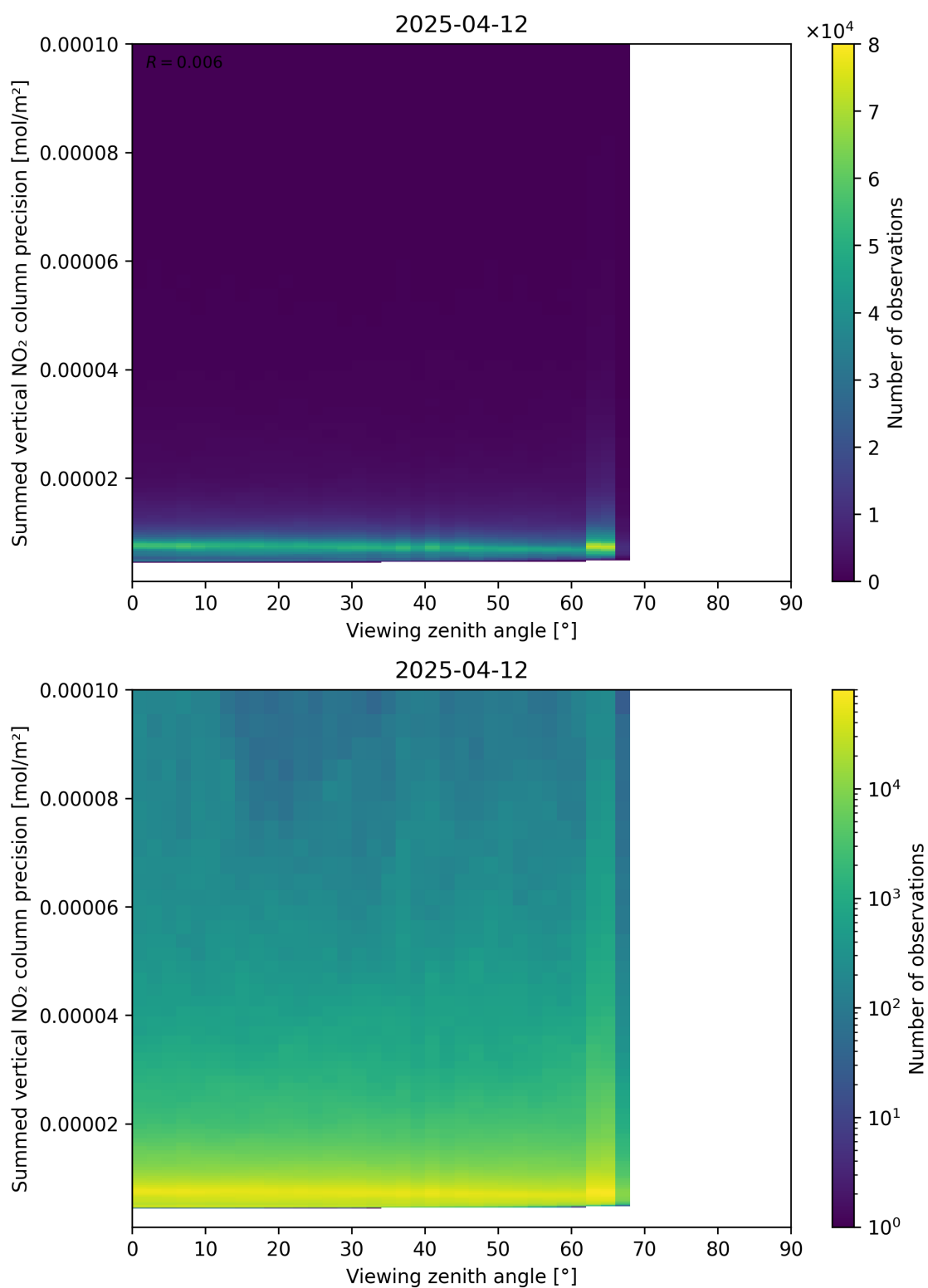
Figure 166: Scatter density plot of “Viewing zenith angle” against “Summed vertical NO 2 column precision” for 2025-04-12 to 2025-04-13.
