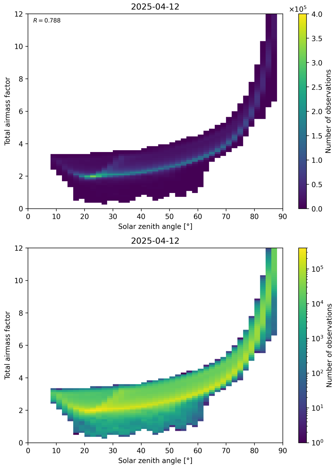
Figure 146: Scatter density plot of “Solar zenith angle” against “Total airmass factor” for 2025-04-12 to 2025-04-13.
