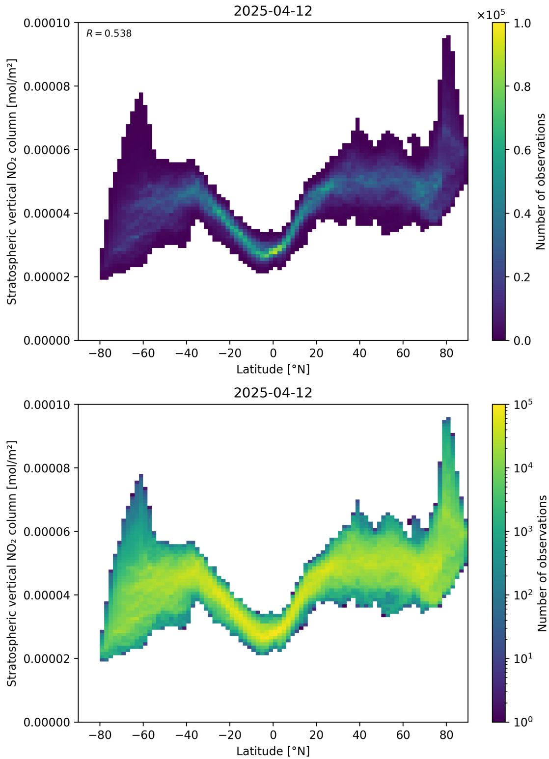
Figure 87: Scatter density plot of “Latitude” against “Stratospheric vertical \text{NO}_2 column” for 2025-04-12 to 2025-04-13.
