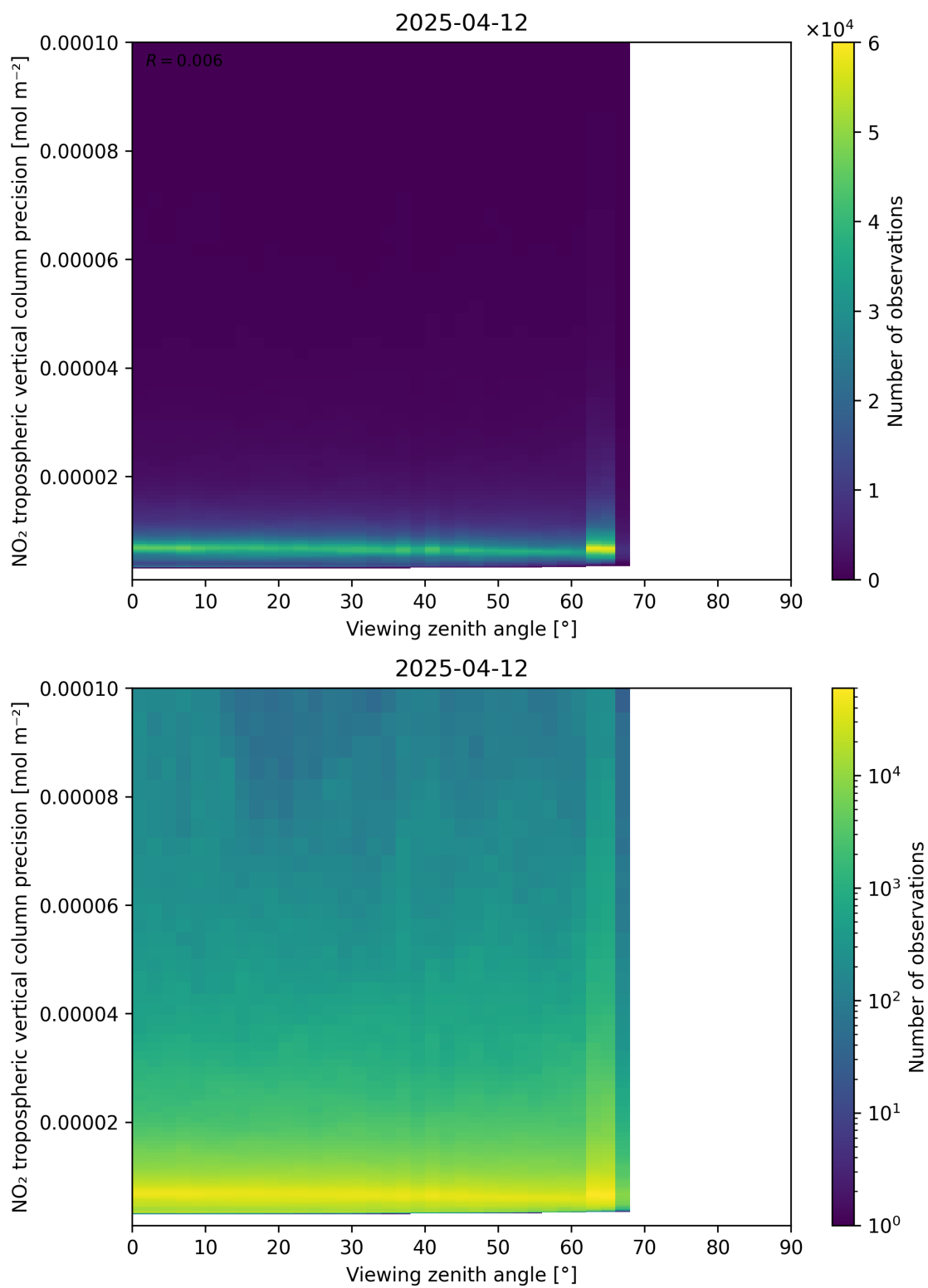
Figure 170: Scatter density plot of “Viewing zenith angle” against “NO 2 tropospheric vertical column precision” for 2025-04-12 to 2025-04-13.
