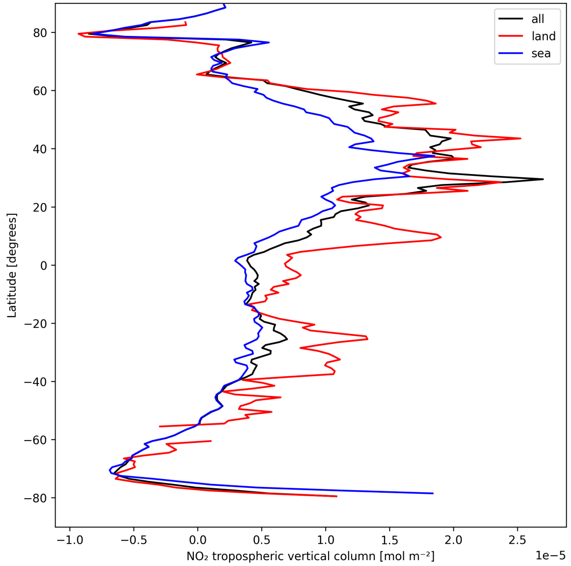
Figure 12: Zonal average of “NO 2 tropospheric vertical column” for 2025-04-12 to 2025-04-13.
