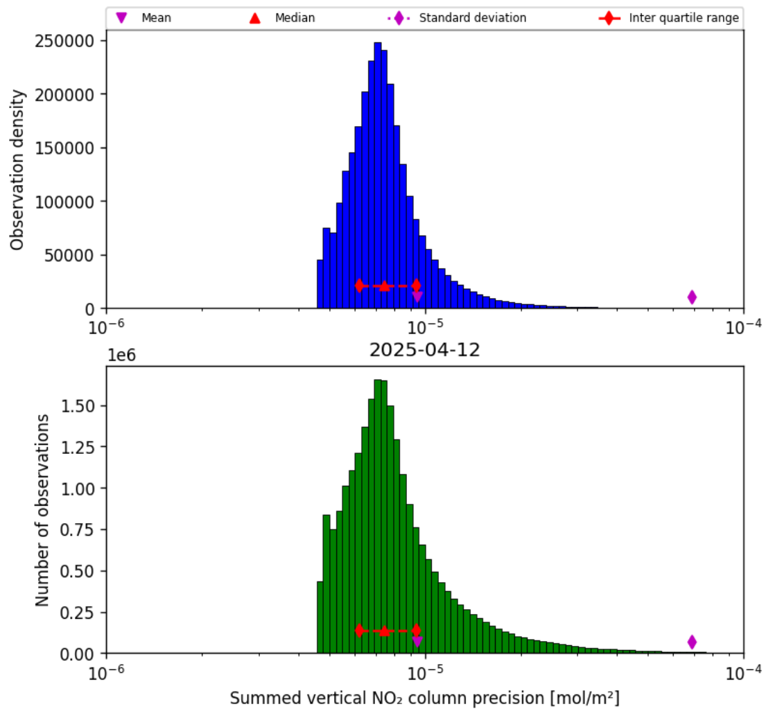
Figure 41: Histogram of “Summed vertical NO 2 column precision” for 2025-04-12 to 2025-04-13
