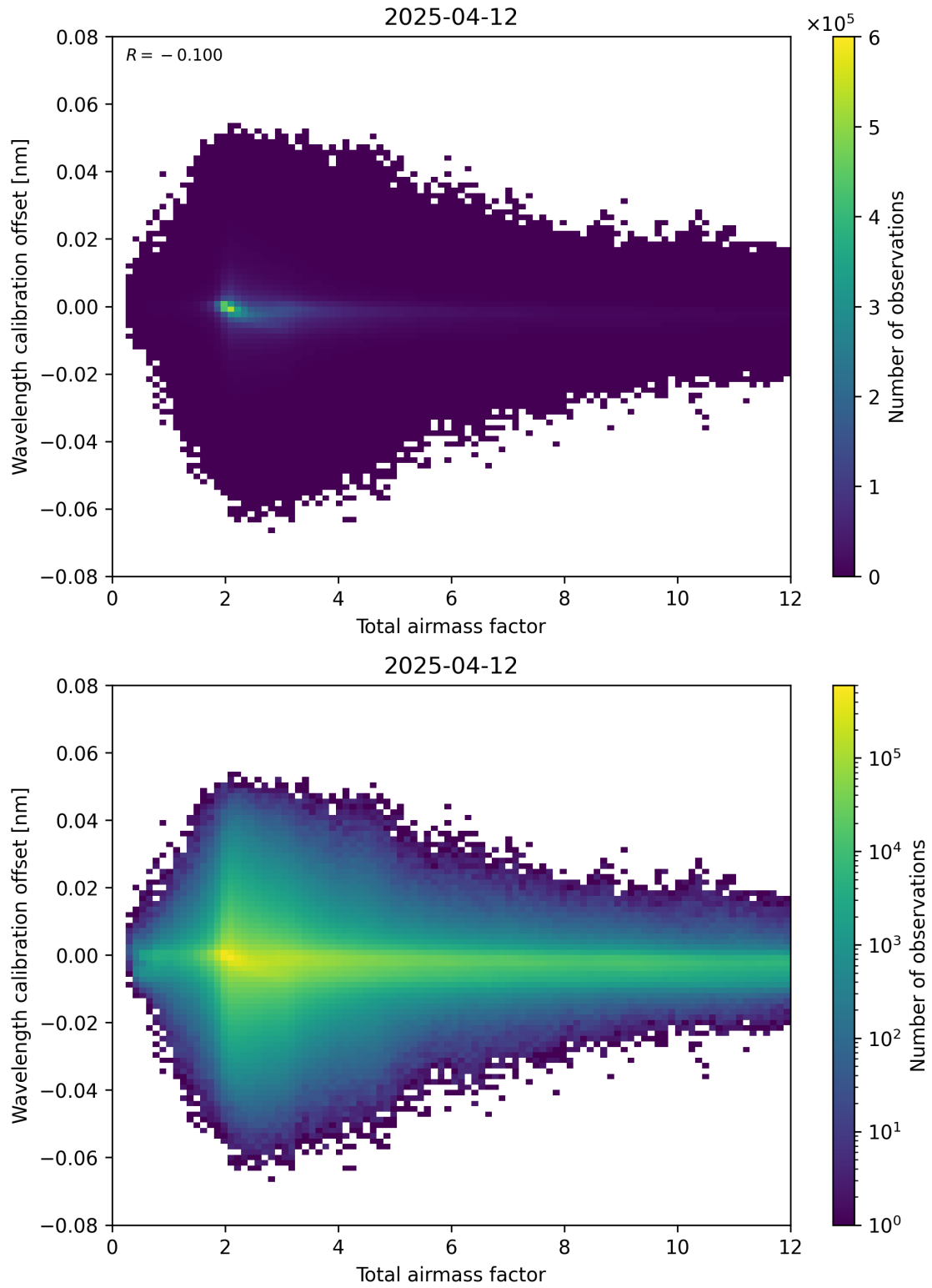
Figure 70: Scatter density plot of “Total airmass factor” against “Wavelength calibration offset” for 2025-04-12 to 2025-04-13.
