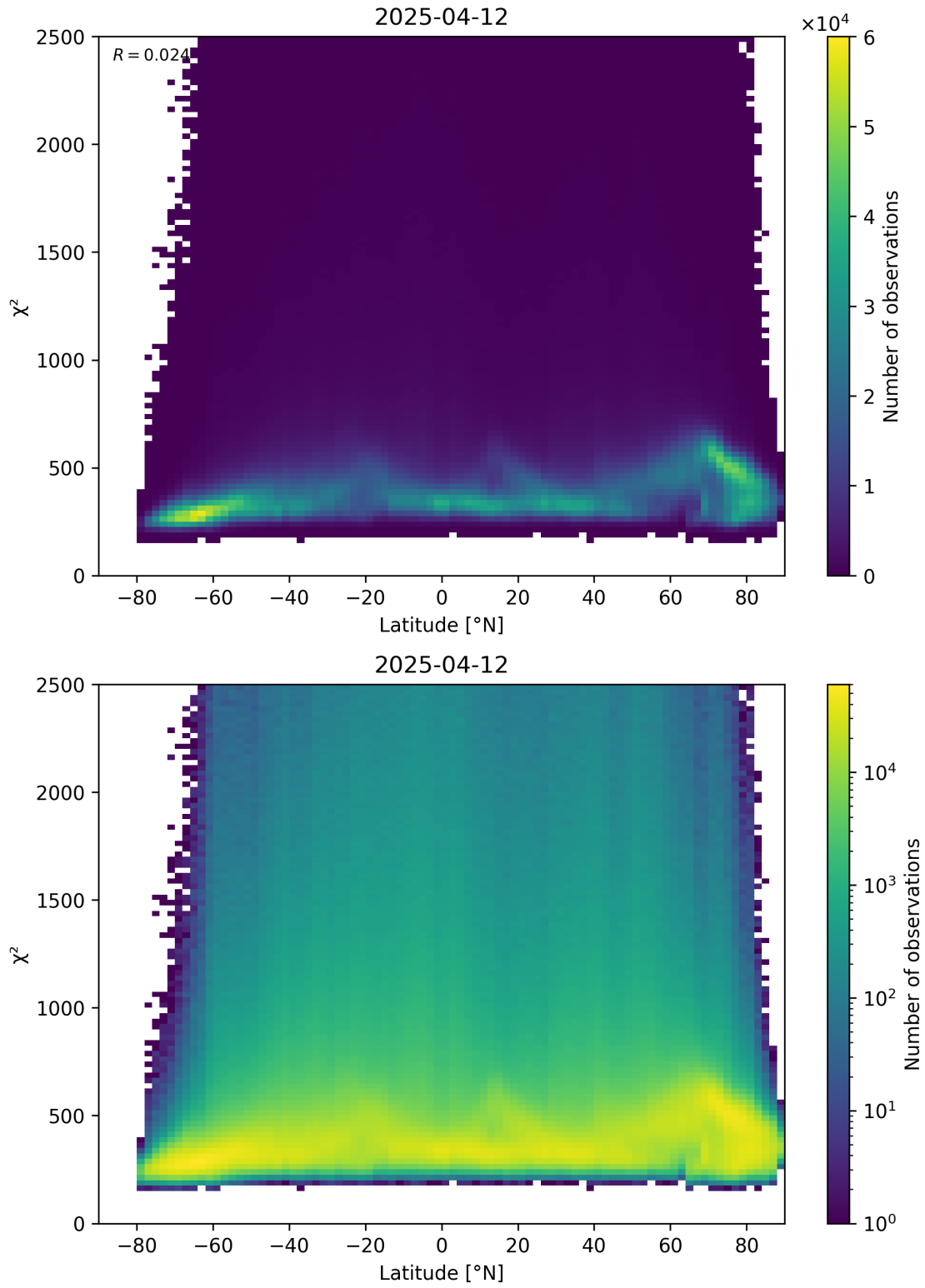
Figure 86: Scatter density plot of “Latitude” against “ \chi^2 ” for 2025-04-12 to 2025-04-13.
