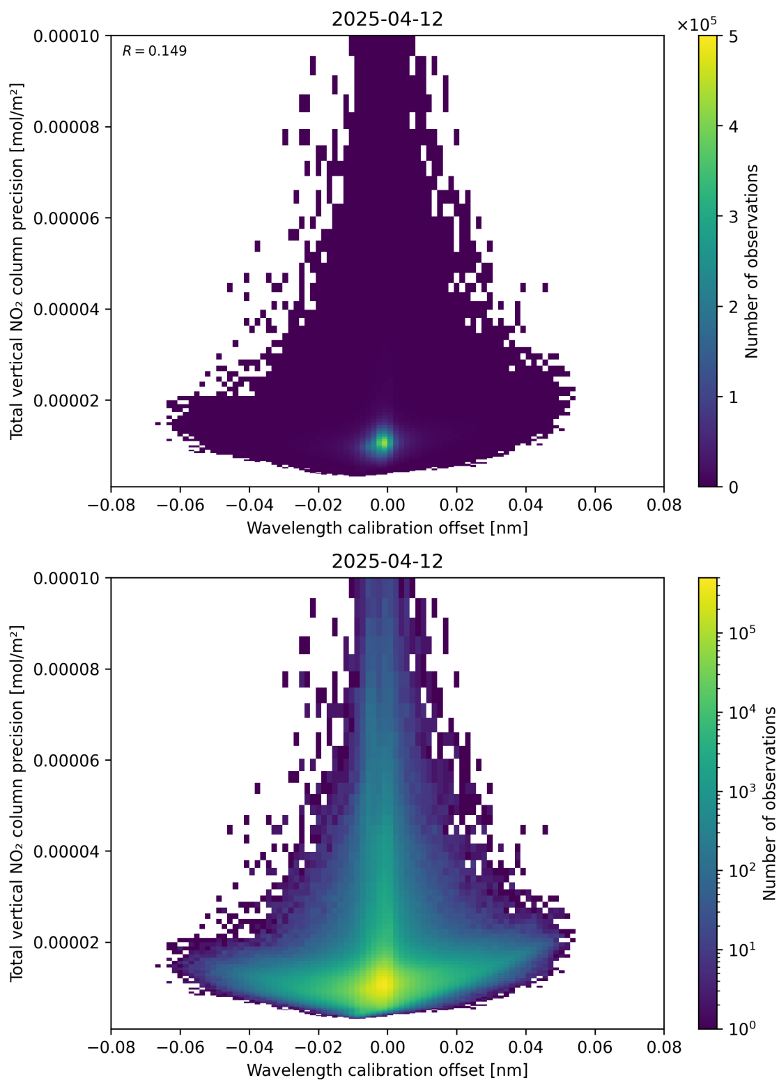
Figure 180: Scatter density plot of “Wavelength calibration offset” against “Total vertical NO 2 column precision” for 2025-04-12 to 2025-04-13.
