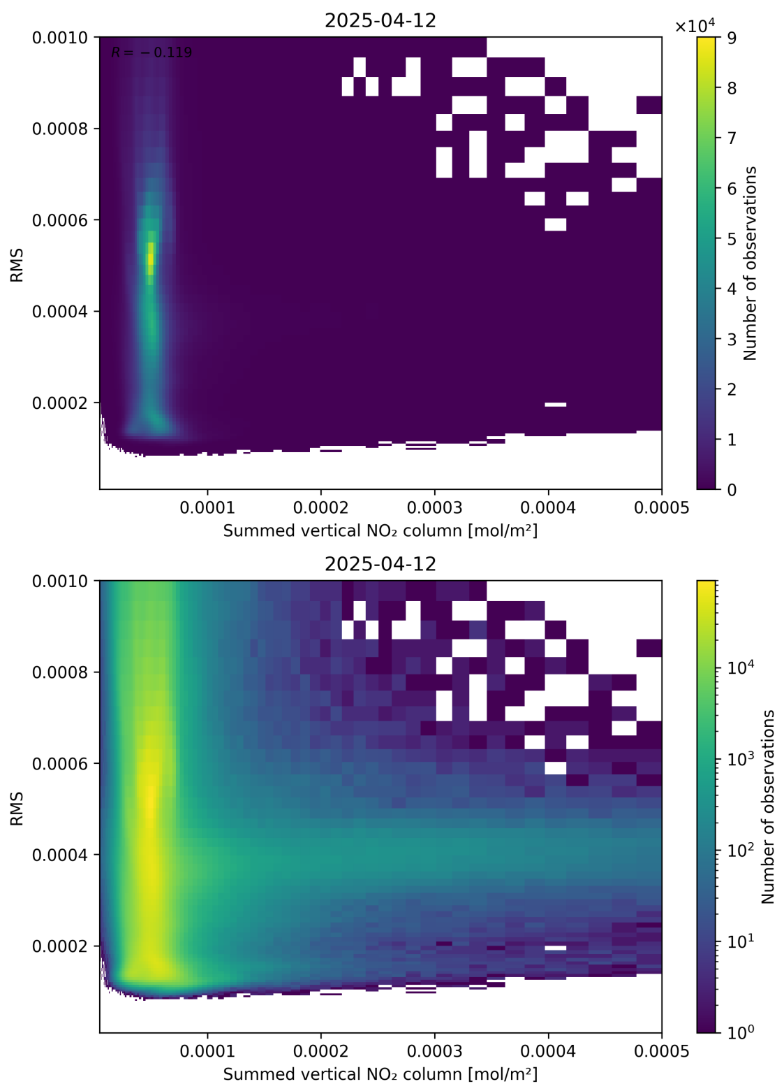
Figure 109: Scatter density plot of “Summed vertical NO 2 column” against “RMS” for 2025-04-12 to 2025-04-13.
