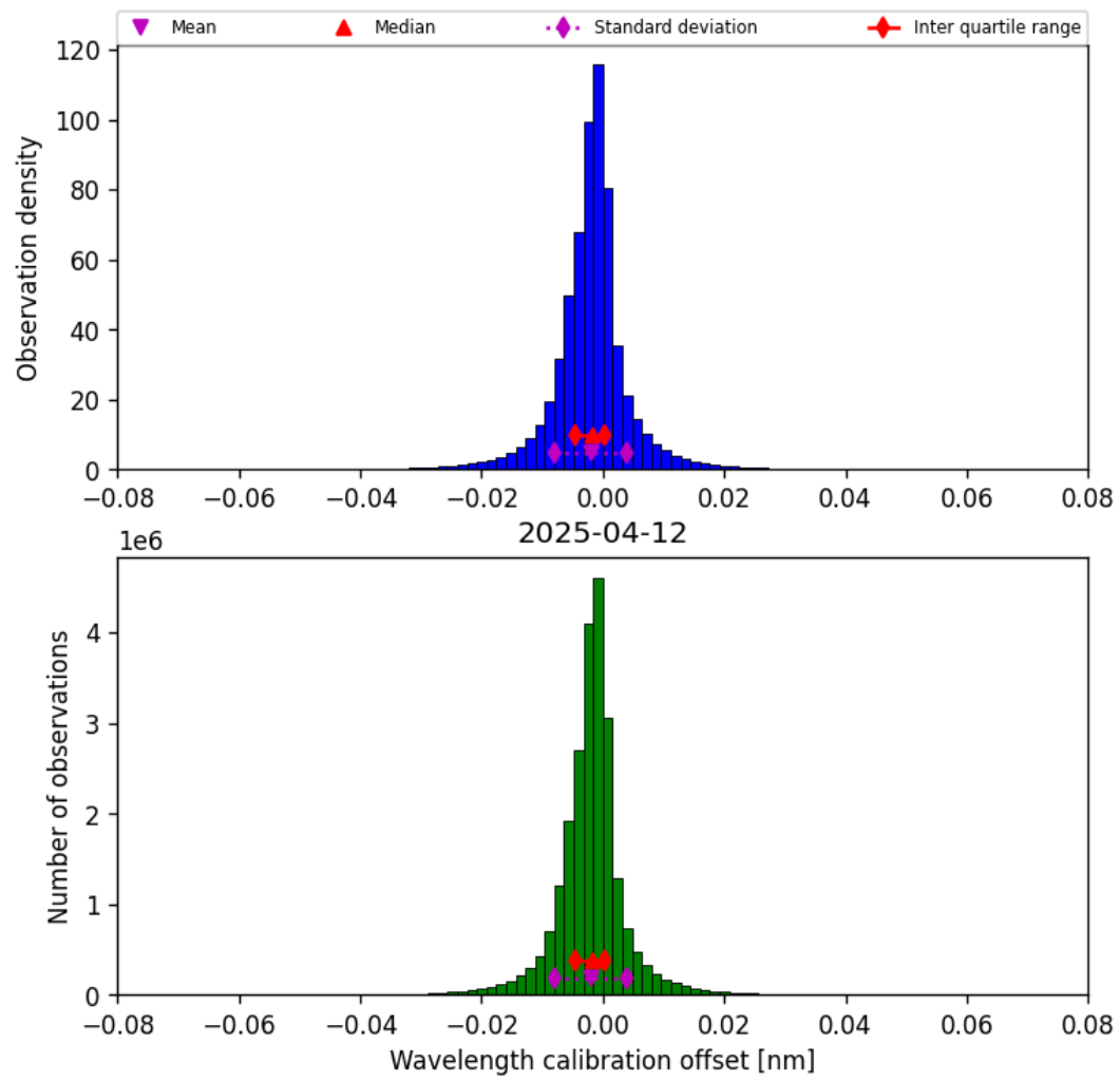
Figure 35: Histogram of “Wavelength calibration offset” for 2025-04-12 to 2025-04-13
