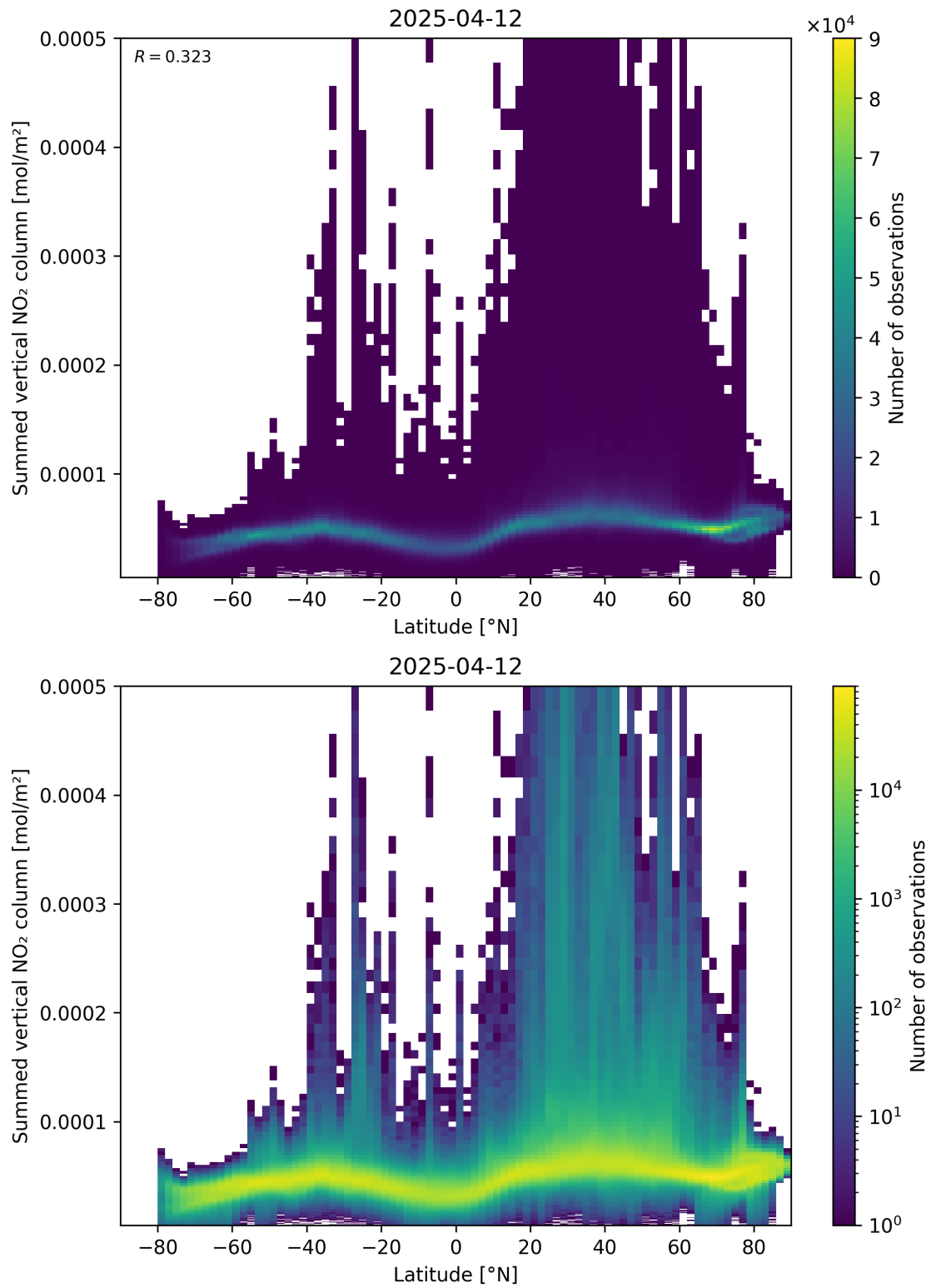
Figure 88: Scatter density plot of “Latitude” against “Summed vertical NO 2 column” for 2025-04-12 to 2025-04-13.
