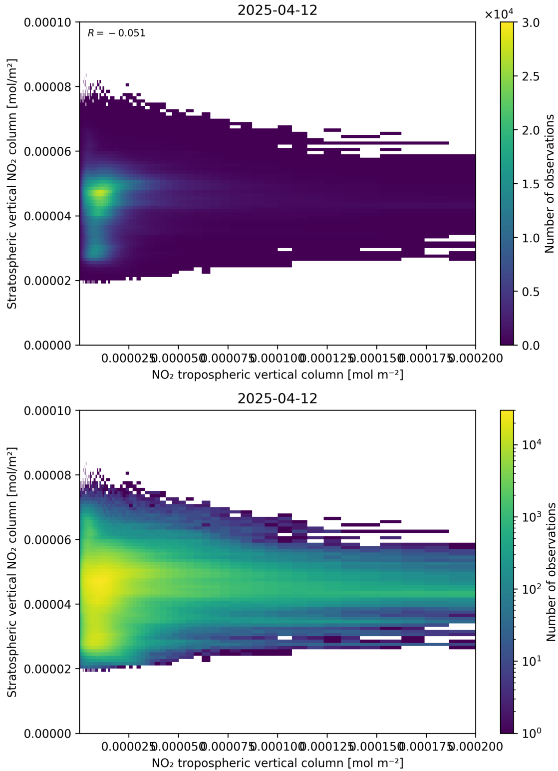
Figure 125: Scatter density plot of “NO 2 tropospheric vertical column” against “Stratospheric vertical NO 2 column” for 2025-04-12 to 2025-04-13.
