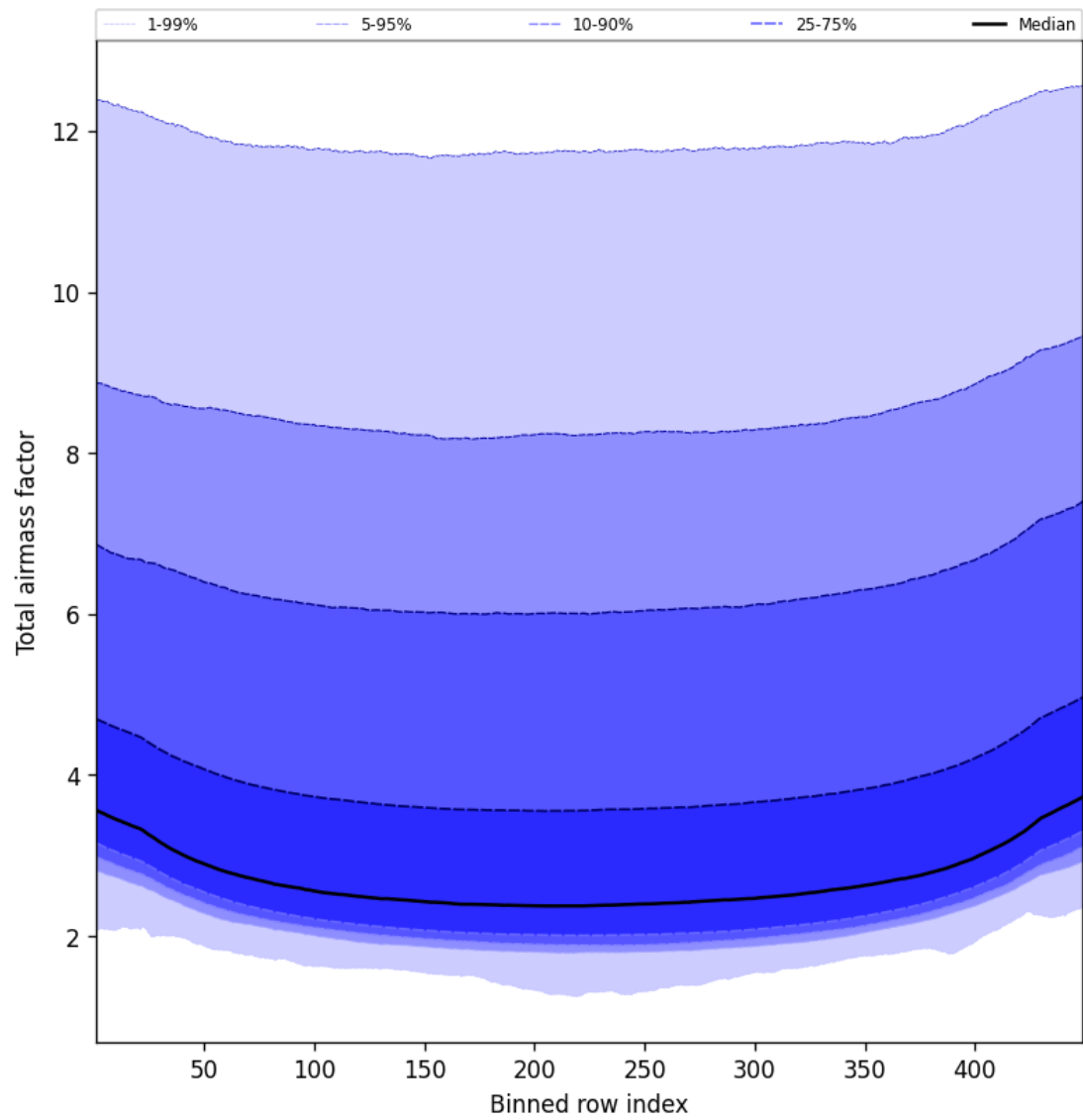
Figure 49: Along track statistics of “Total airmass factor” for 2025-04-12 to 2025-04-13
