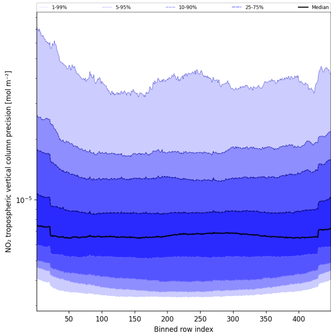
Figure 47: Along track statistics of “NO 2 tropospheric vertical column precision” for 2025-04-12 to 2025-04-13
