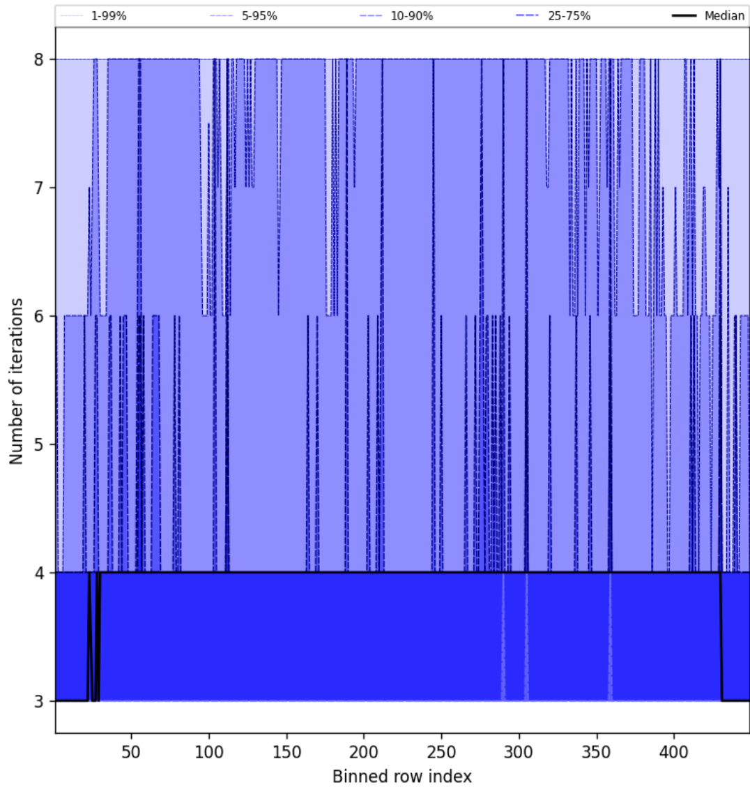
Figure 51: Along track statistics of “Number of iterations” for 2025-04-12 to 2025-04-13
