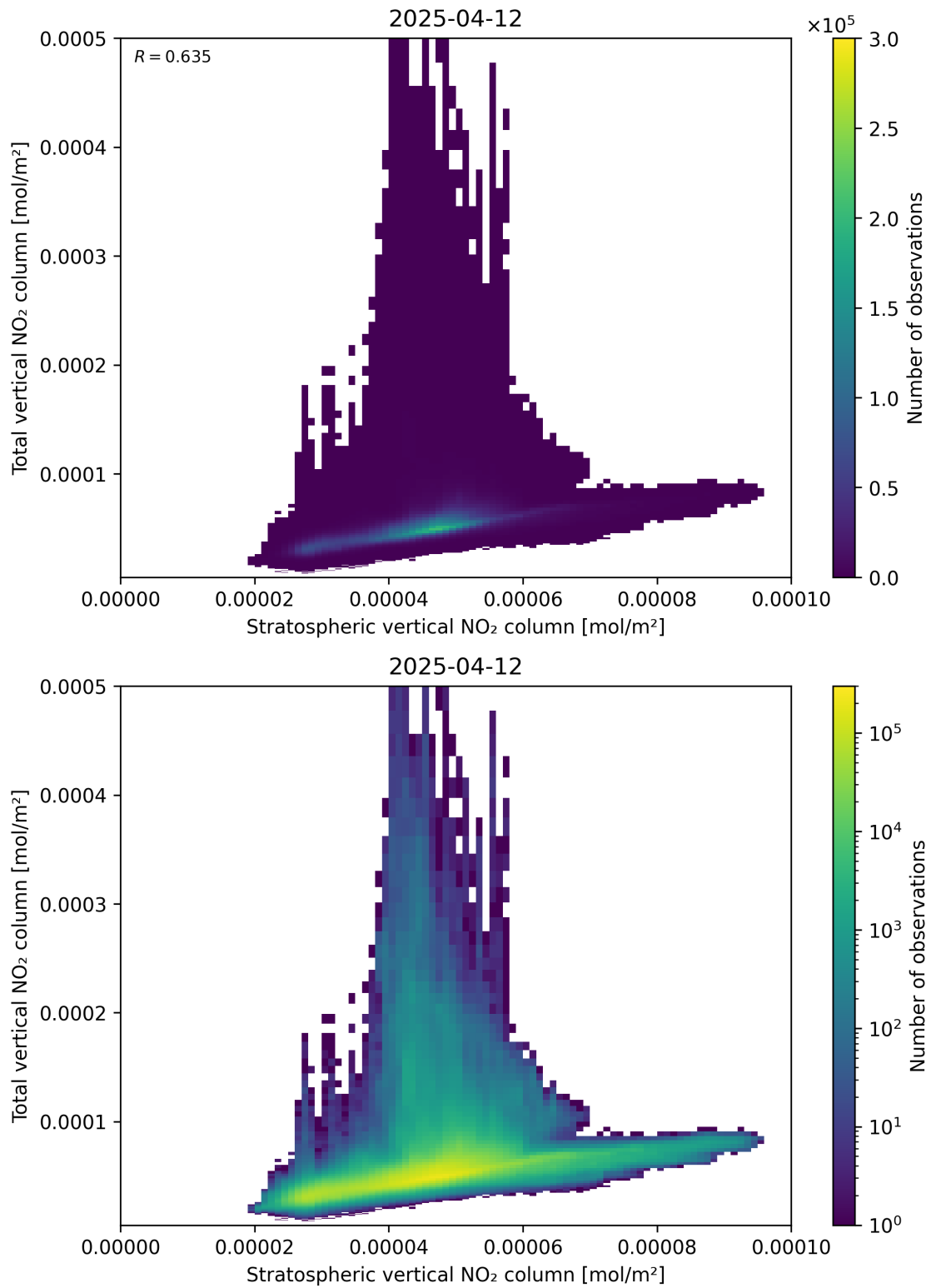
Figure 100: Scatter density plot of “Stratospheric vertical NO 2 column” against “Total vertical NO 2 column” for 2025-04-12 to 2025-04-13.
