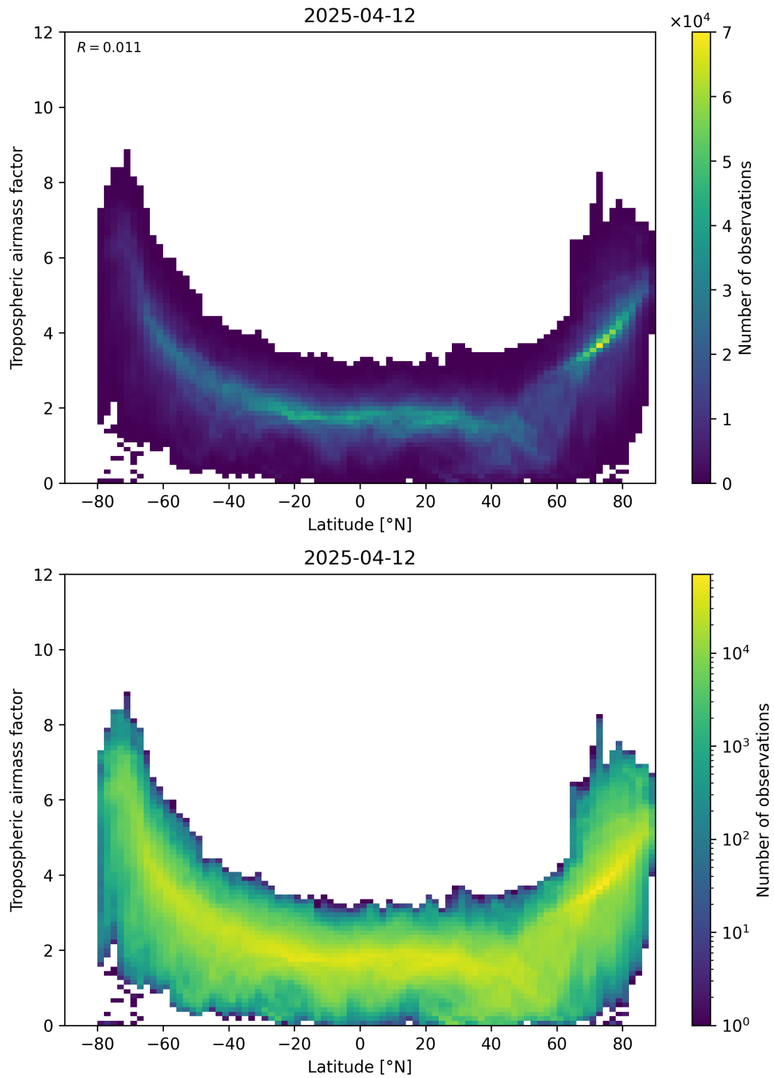
Figure 85: Scatter density plot of “Latitude” against “Tropospheric air mass factor” for 2025-04-12 to 2025-04-13.
