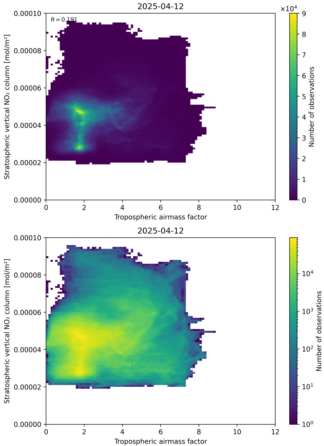
Figure 74: Scatter density plot of “Tropospheric air mass factor” against “Stratospheric vertical NO 2 column” for 2025-04-12 to 2025-04-13.
