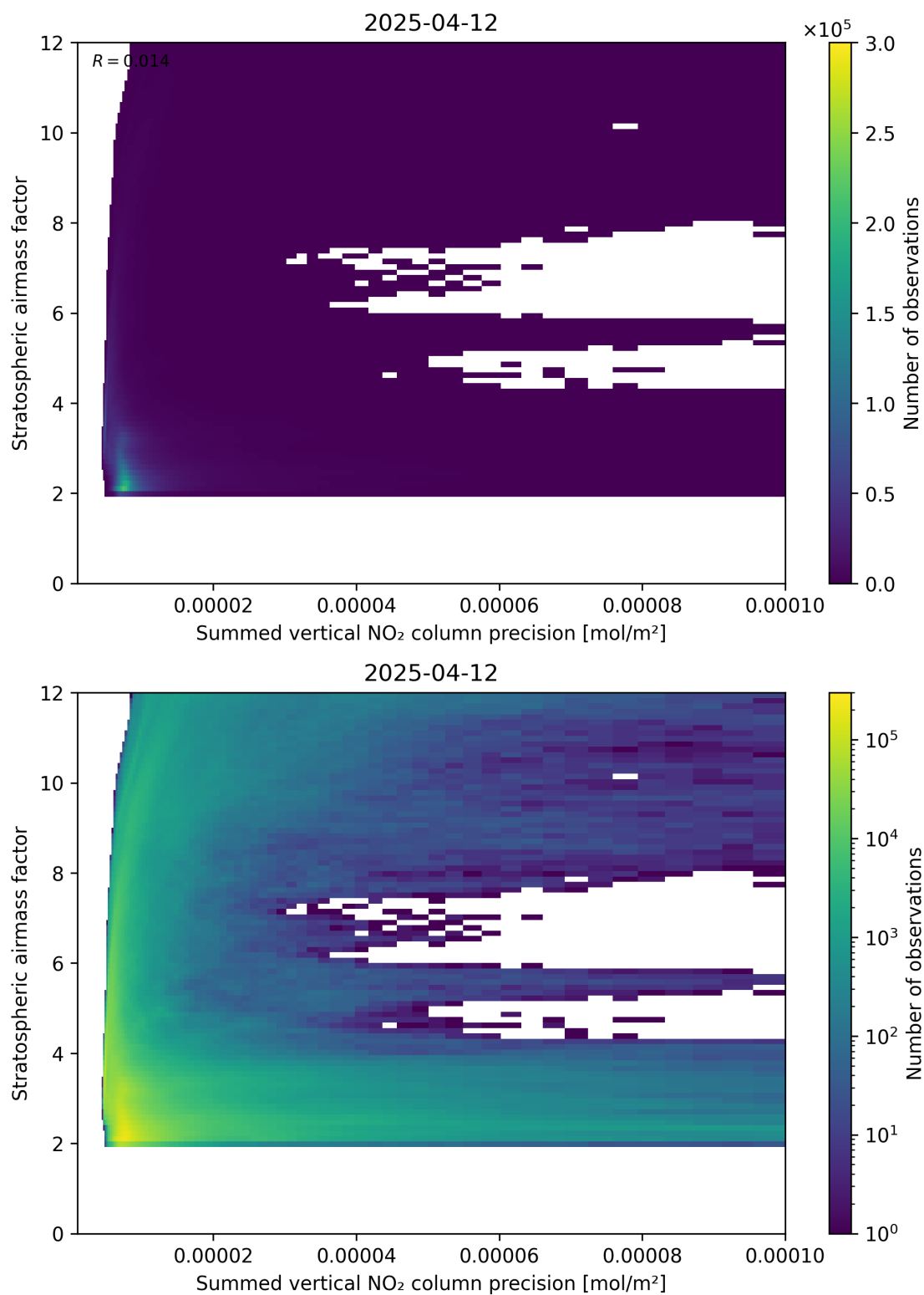
Figure 106: Scatter density plot of “Summed vertical NO 2 column precision” against “Stratospheric airmass factor” for 2025-04-12 to 2025-04-13.
