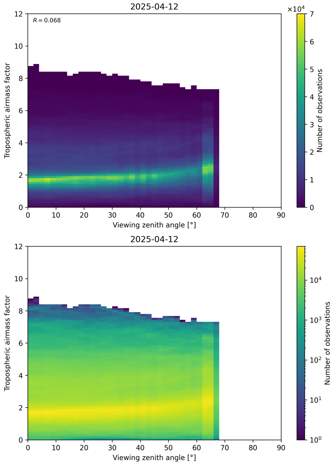
Figure 161: Scatter density plot of “Viewing zenith angle” against “Tropospheric airmass factor” for 2025-04-12 to 2025-04-13.
