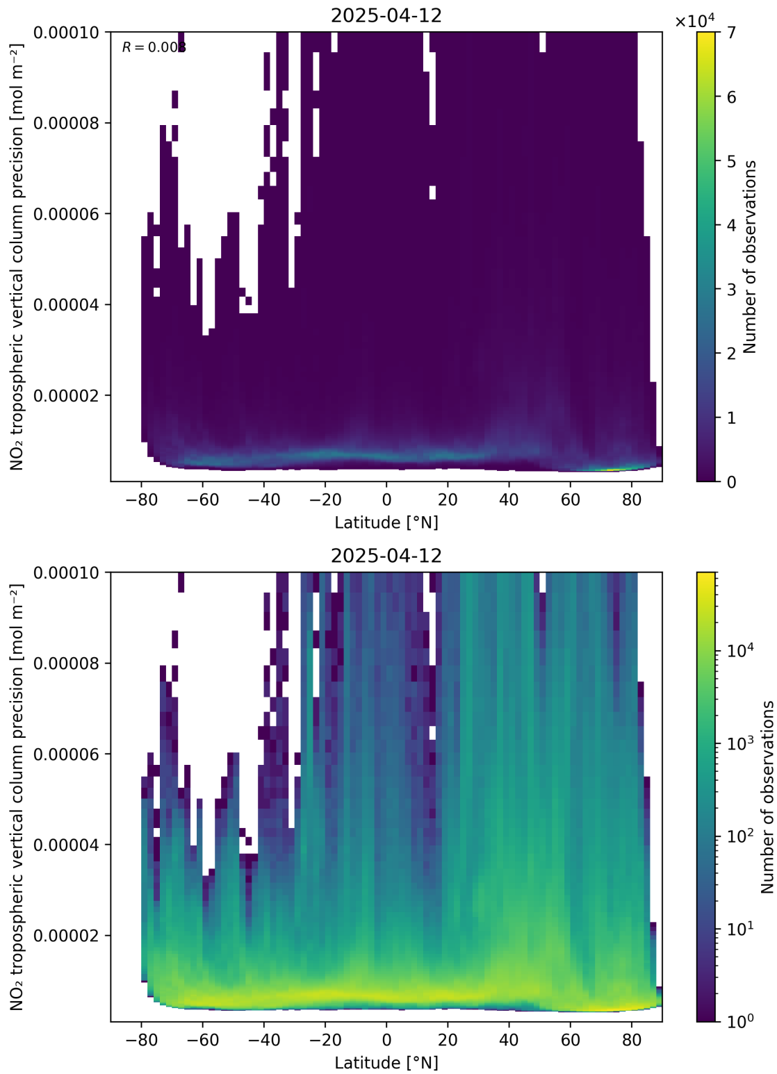
Figure 93: Scatter density plot of “Latitude” against “NO 2 tropospheric vertical column precision” for 2025-04-12 to 2025-04-13.
