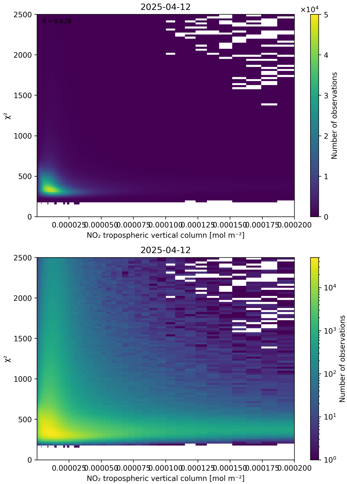
Figure 124: Scatter density plot of “NO 2 tropospheric vertical column” against “ \chi^2 ” for 2025-04-12 to 2025-04-13.
