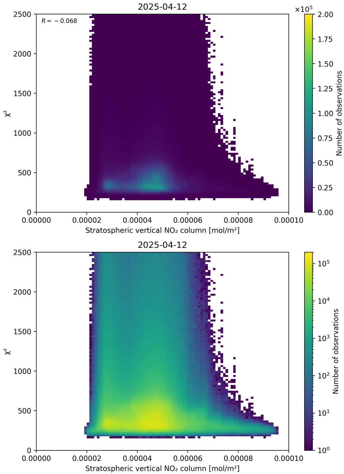
Figure 97: Scatter density plot of “Stratospheric vertical NO 2 column” against “ \chi^2 ” for 2025-04-12 to 2025-04-13.
