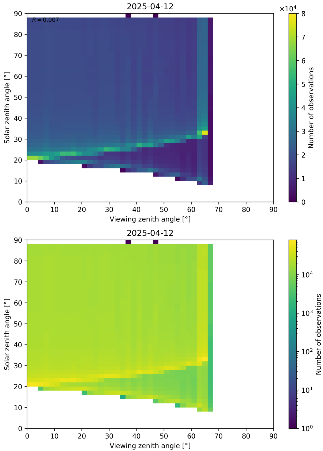
Figure 172: Scatter density plot of “Viewing zenith angle” against “Solar zenith angle” for 2025-04-12 to 2025-04-13.
