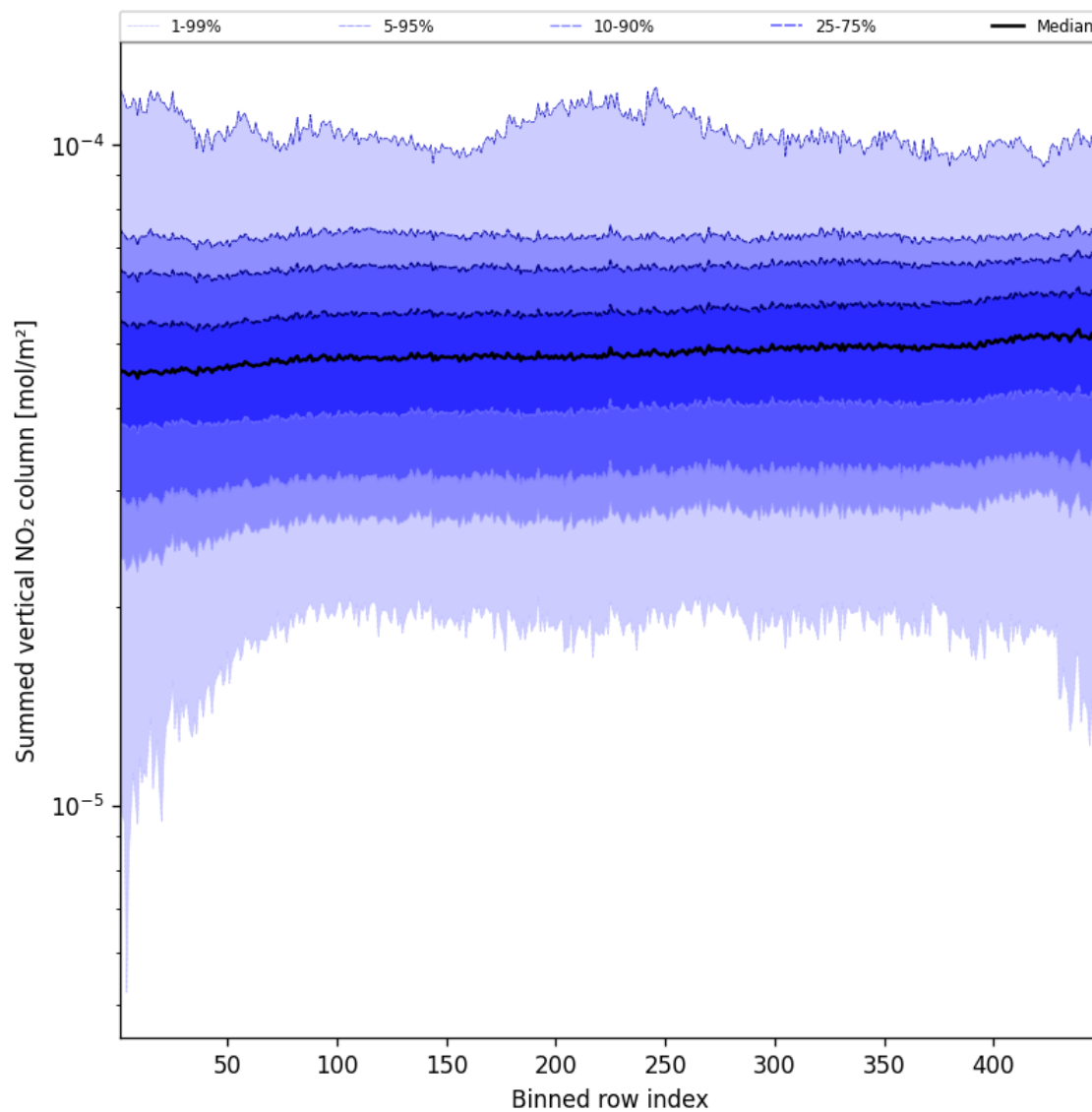
Figure 57: Along track statistics of “Summed vertical NO 2 column” for 2025-04-12 to 2025-04-13
