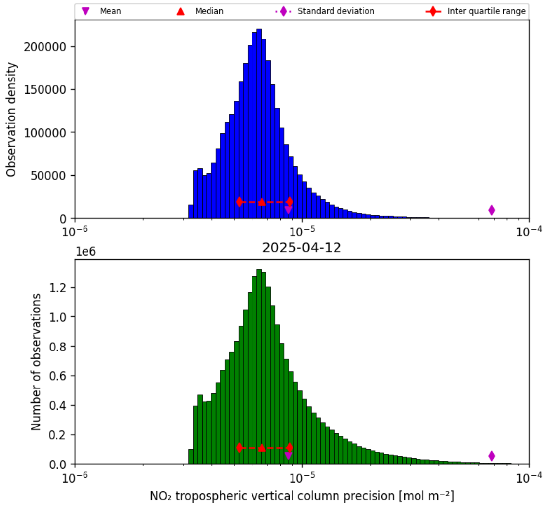
Figure 30: Histogram of “NO 2 tropospheric vertical column precision” for 2025-04-12 to 2025-04-13
