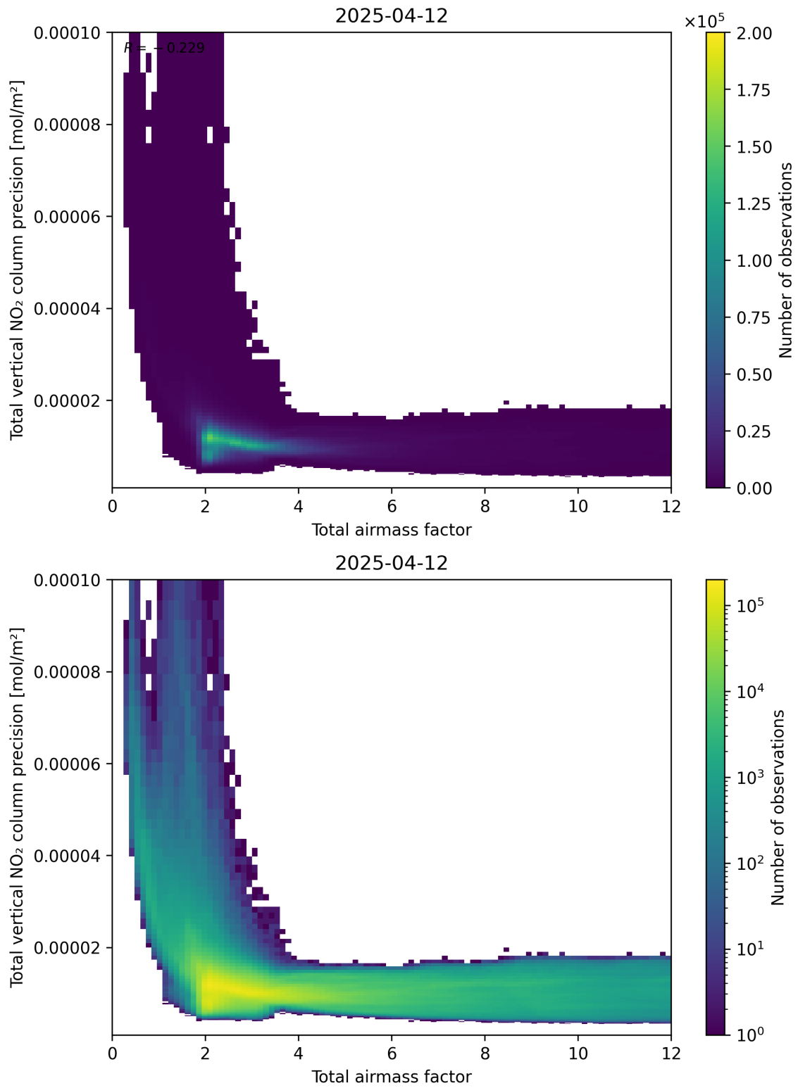
Figure 68: Scatter density plot of “Total airmass factor” against “Total vertical NO 2 column precision” for 2025-04-12 to 2025-04-13.
