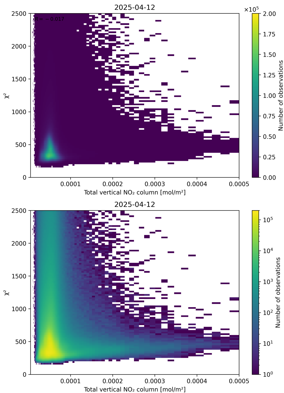
Figure 111: Scatter density plot of “Total vertical NO 2 column” against “ \chi^2 ” for 2025-04-12 to 2025-04-13.
