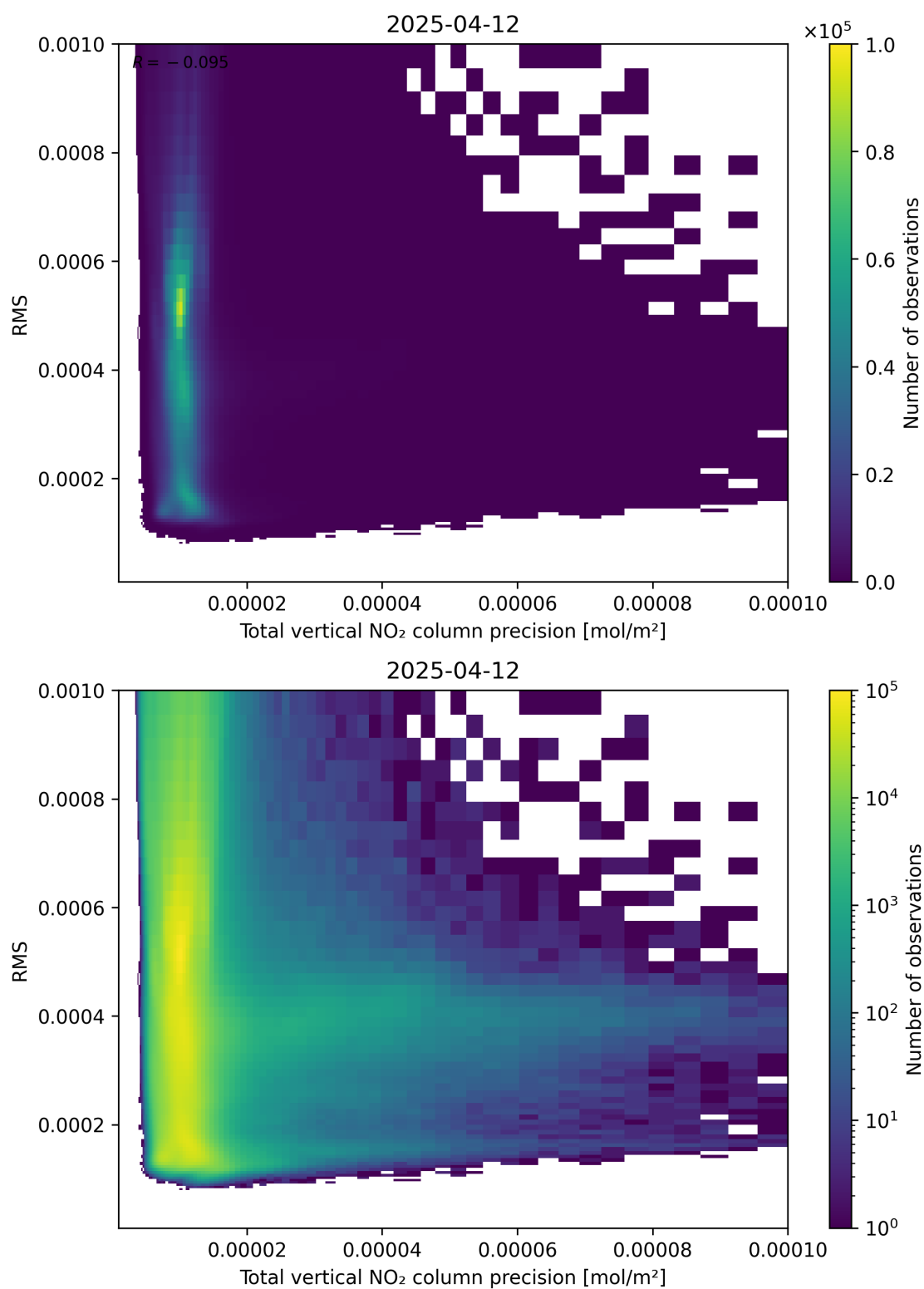
Figure 119: Scatter density plot of “Total vertical NO 2 column precision” against “RMS” for 2025-04-12 to 2025-04-13.
