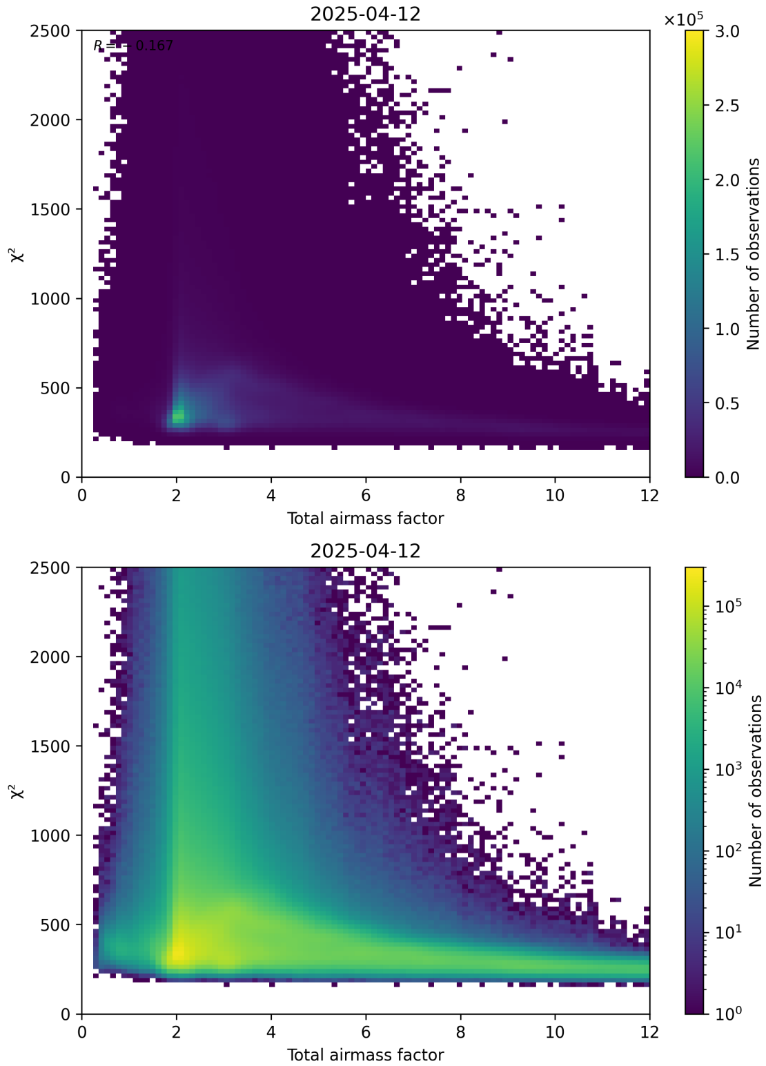
Figure 63: Scatter density plot of “Total airmass factor” against “ \chi^2 ” for 2025-04-12 to 2025-04-13.
