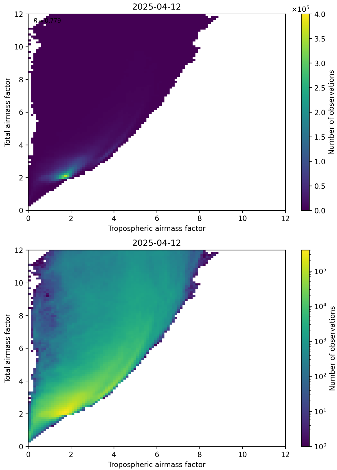
Figure 72: Scatter density plot of “Tropospheric airmass factor” against “Total airmass factor” for 2025-04-12 to 2025-04-13.
