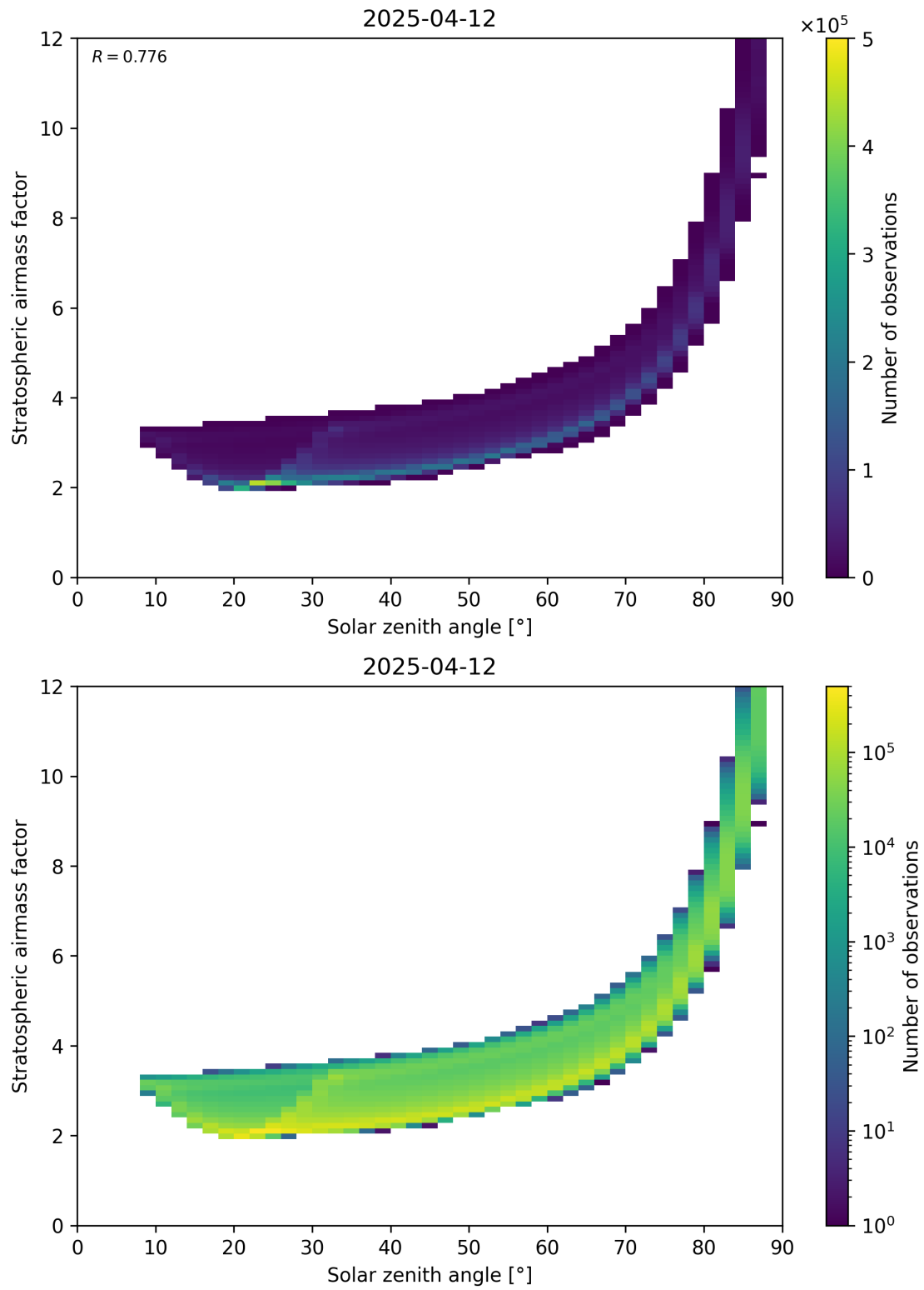
Figure 145: Scatter density plot of “Solar zenith angle” against “Stratospheric airmass factor” for 2025-04-12 to 2025-04-13.
