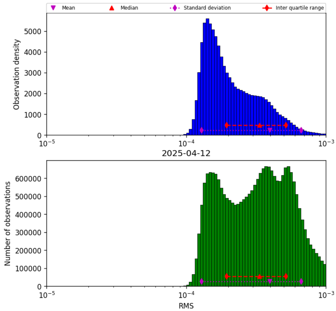
Figure 43: Histogram of “RMS” for 2025-04-12 to 2025-04-13
