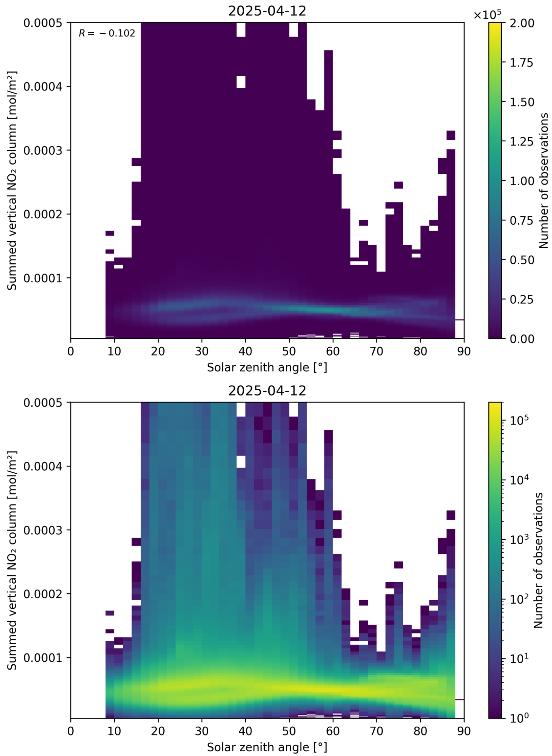
Figure 151: Scatter density plot of “Solar zenith angle” against “Summed vertical NO 2 column” for 2025-04-12 to 2025-04-13.
