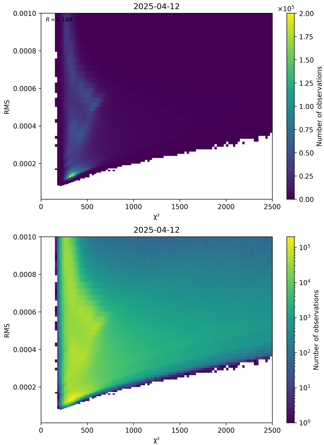
Figure 82: Scatter density plot of “ \chi^2 ” against “RMS” for 2025-04-12 to 2025-04-13.
