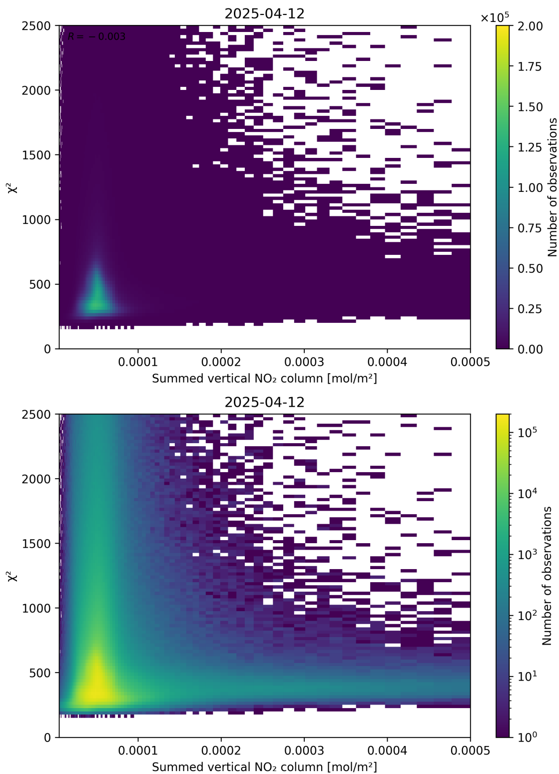
Figure 104: Scatter density plot of “Summed vertical NO 2 column” against “ \chi^2 ” for 2025-04-12 to 2025-04-13.
