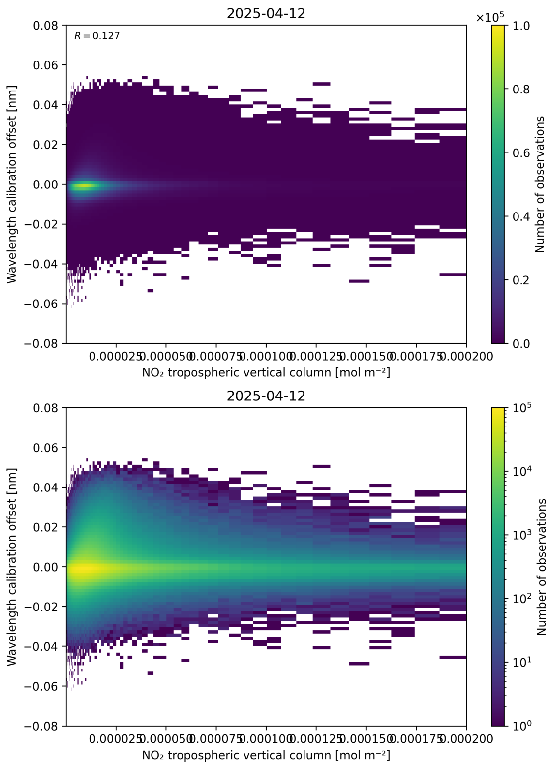
Figure 143: Scatter density plot of “NO 2 tropospheric vertical column” against “Wavelength calibration offset” for 2025-04-12 to 2025-04-13.
