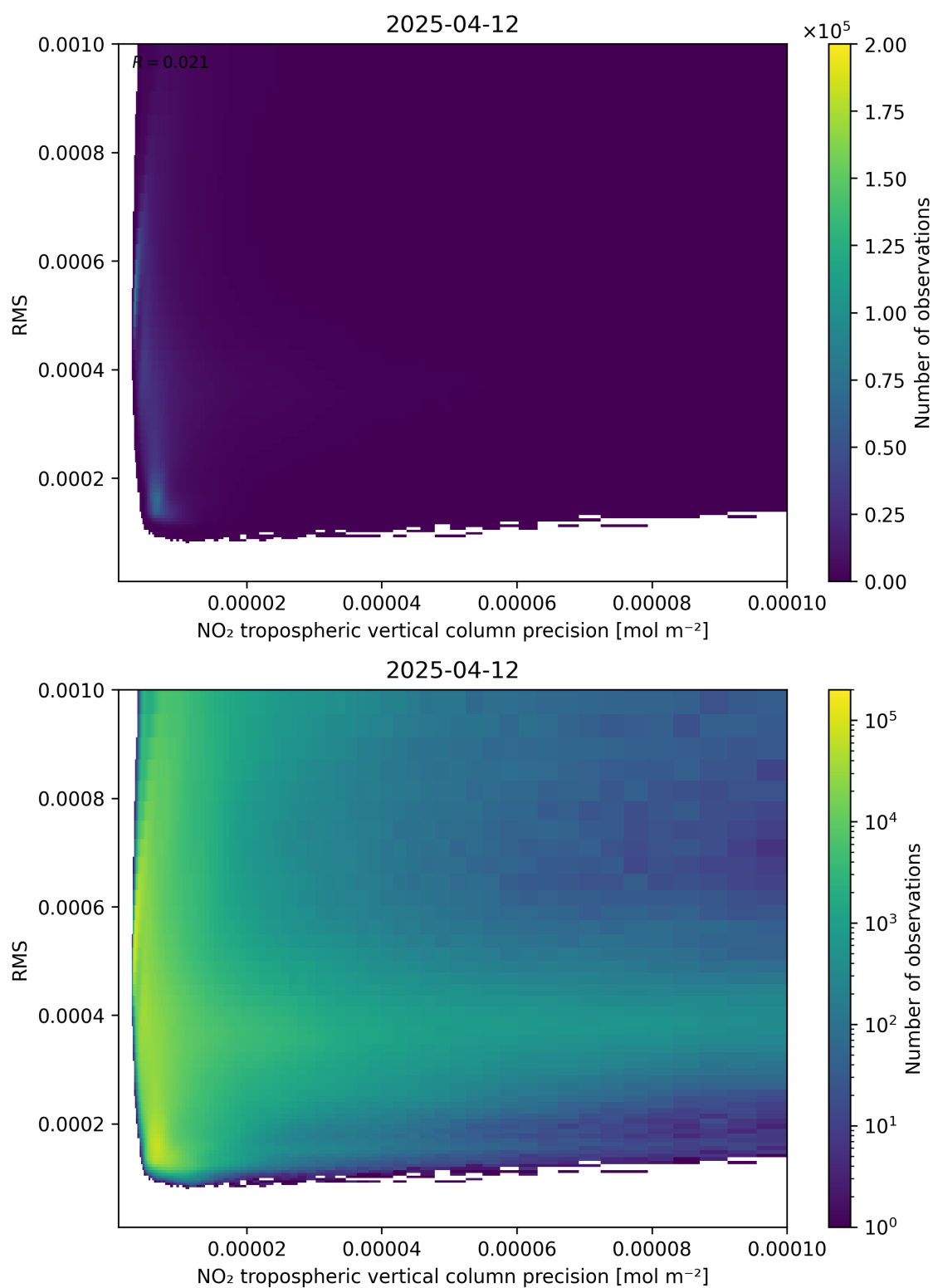
Figure 140: Scatter density plot of “NO 2 tropospheric vertical column precision” against “RMS” for 2025-04-12 to 2025-04-13.
