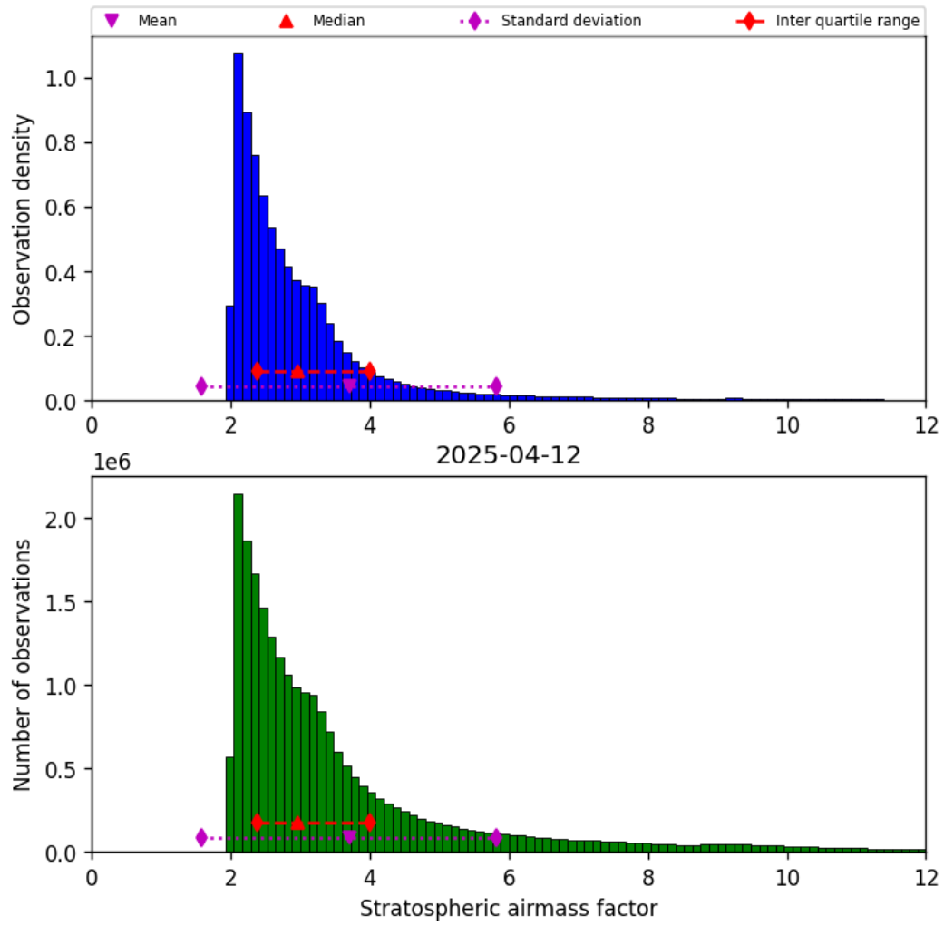
Figure 44: Histogram of “Stratospheric airmass factor” for 2025-04-12 to 2025-04-13
