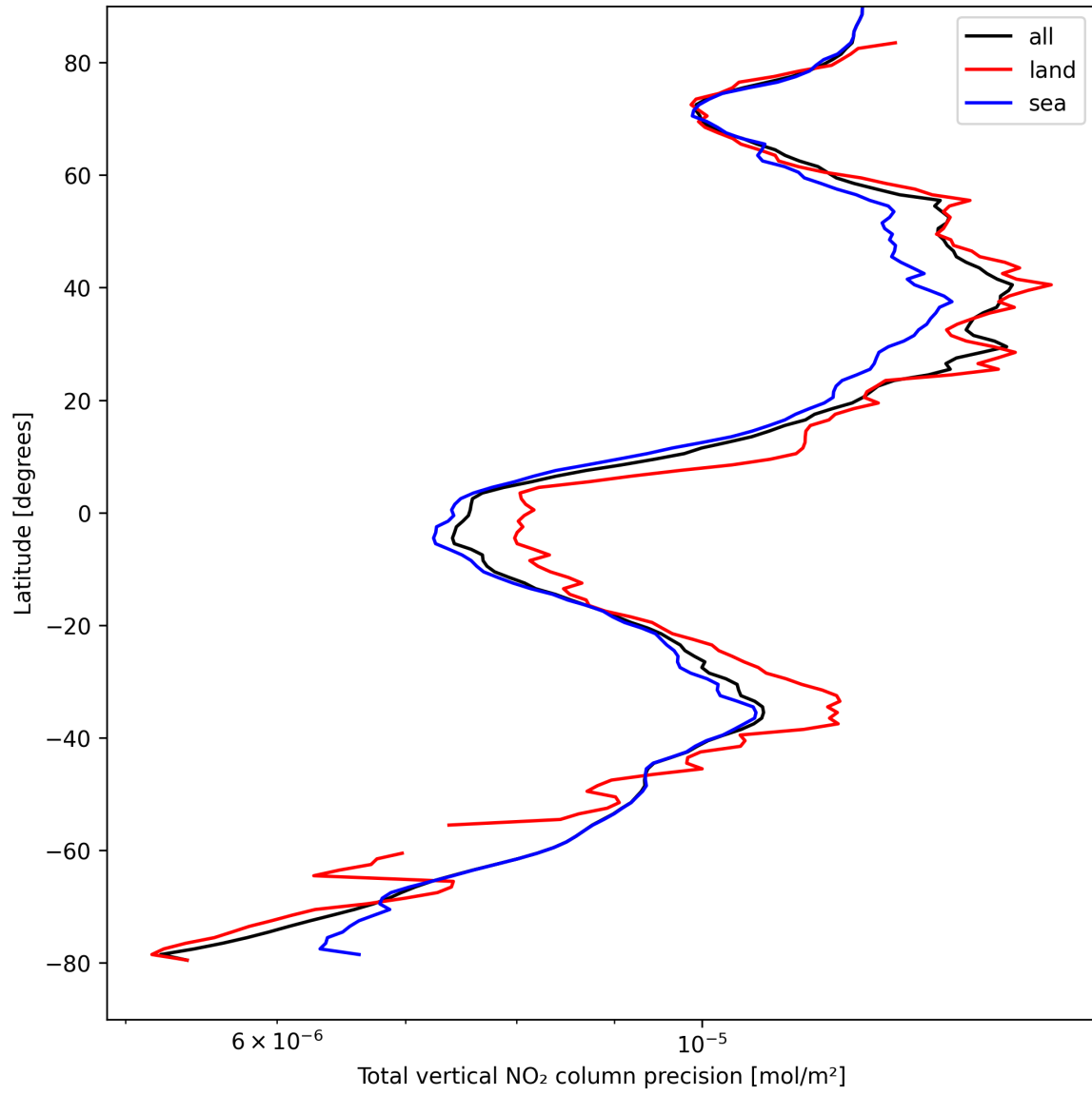
Figure 22: Zonal average of “Total vertical NO 2 column precision” for 2025-04-12 to 2025-04-13.
