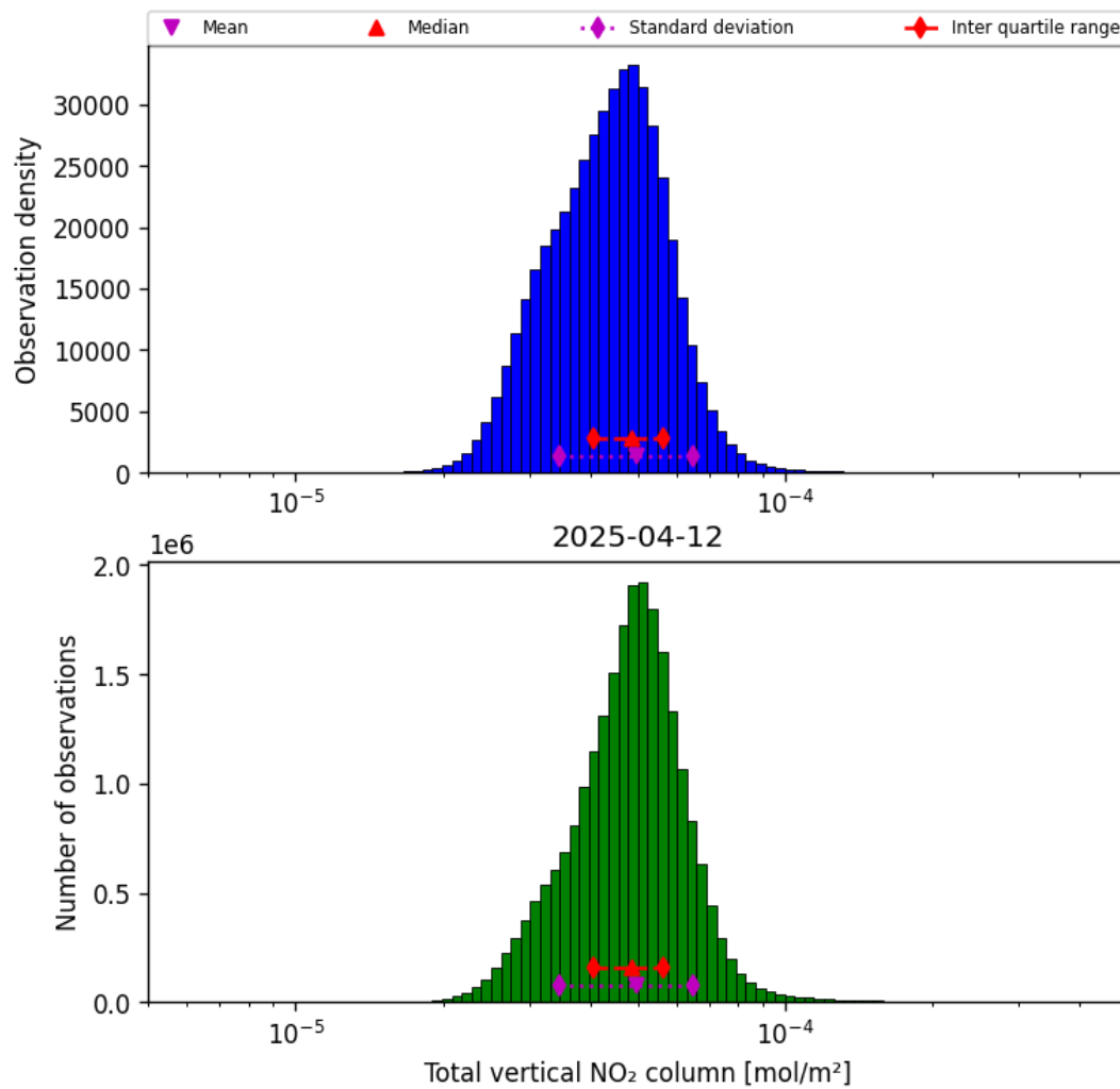
Figure 38: Histogram of “Total vertical NO 2 column” for 2025-04-12 to 2025-04-13
