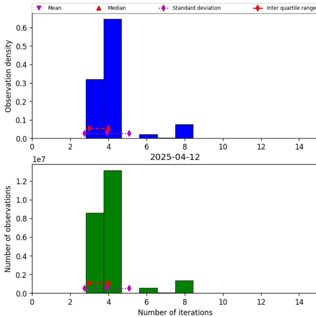
Figure 34: Histogram of “Number of iterations” for 2025-04-12 to 2025-04-13
