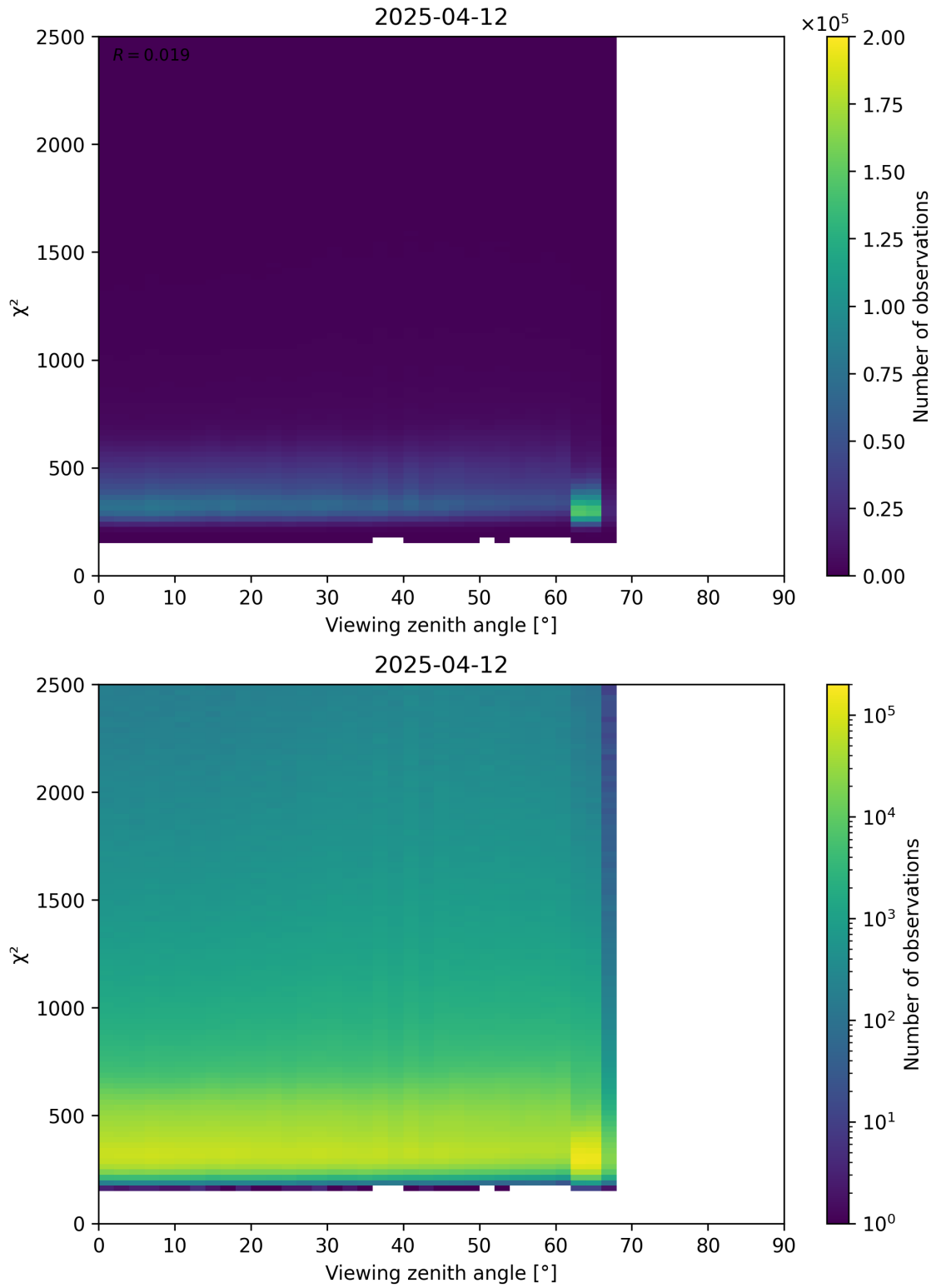
Figure 162: Scatter density plot of “Viewing zenith angle” against “ \chi^2 ” for 2025-04-12 to 2025-04-13.
