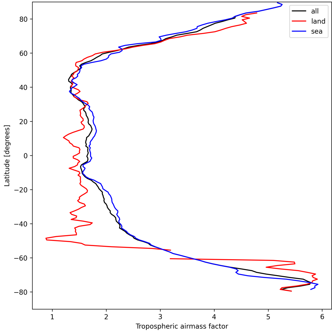
Figure 14: Zonal average of “Tropospheric airmass factor” for 2025-04-12 to 2025-04-13.
