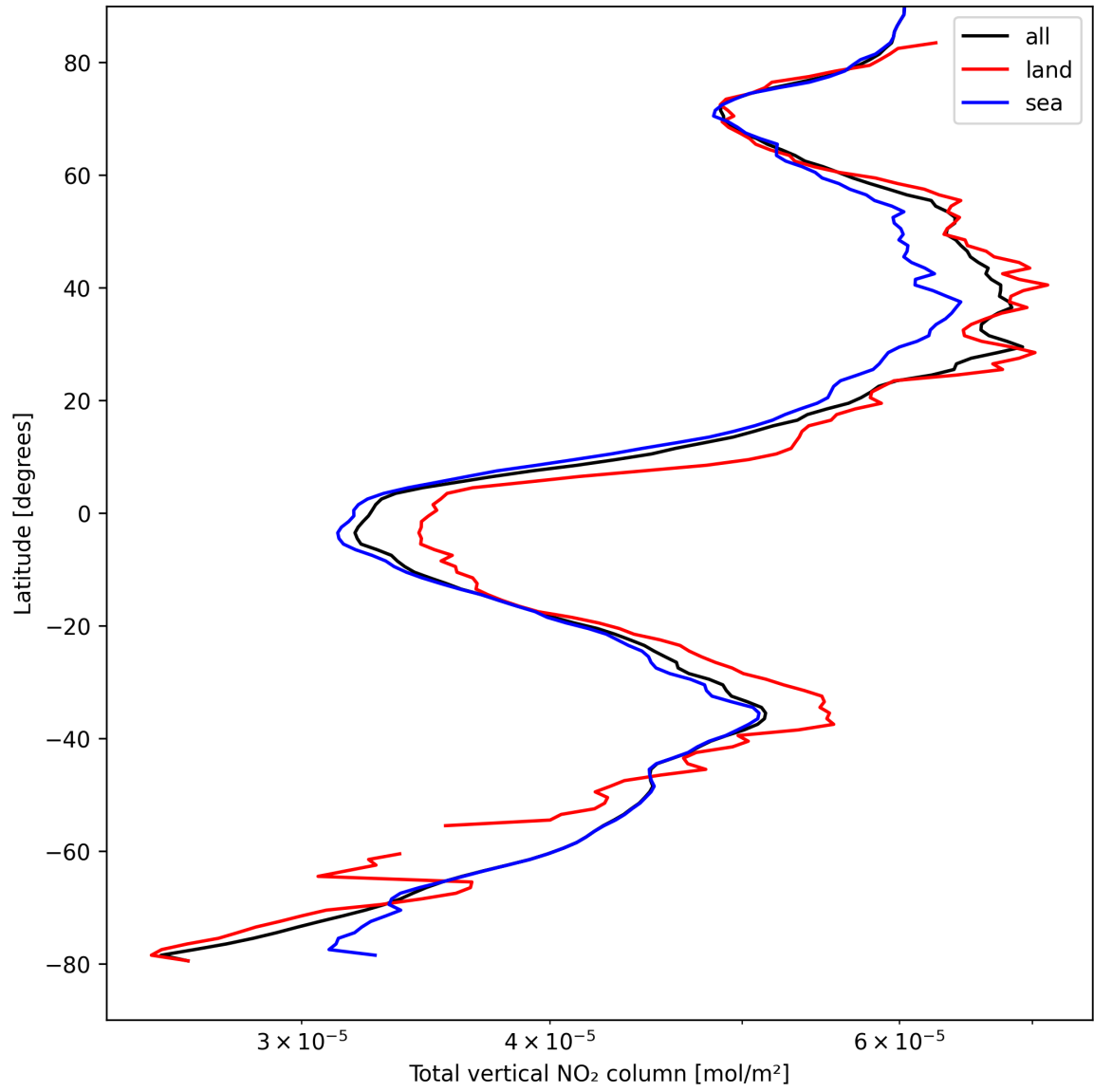
Figure 21: Zonal average of “Total vertical NO 2 column” for 2025-04-12 to 2025-04-13.
