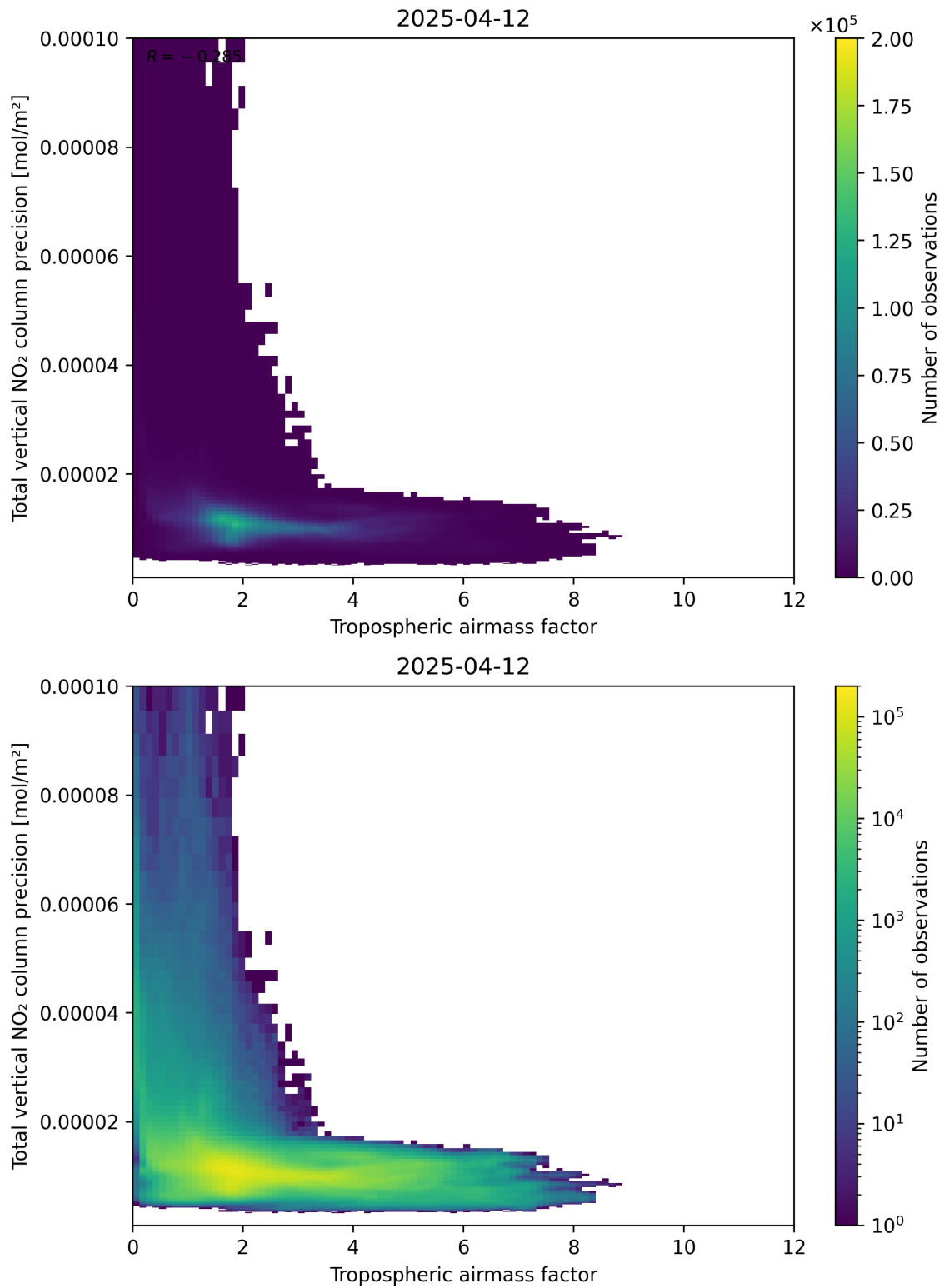
Figure 78: Scatter density plot of “Tropospheric airmass factor” against “Total vertical NO 2 column precision” for 2025-04-12 to 2025-04-13.
