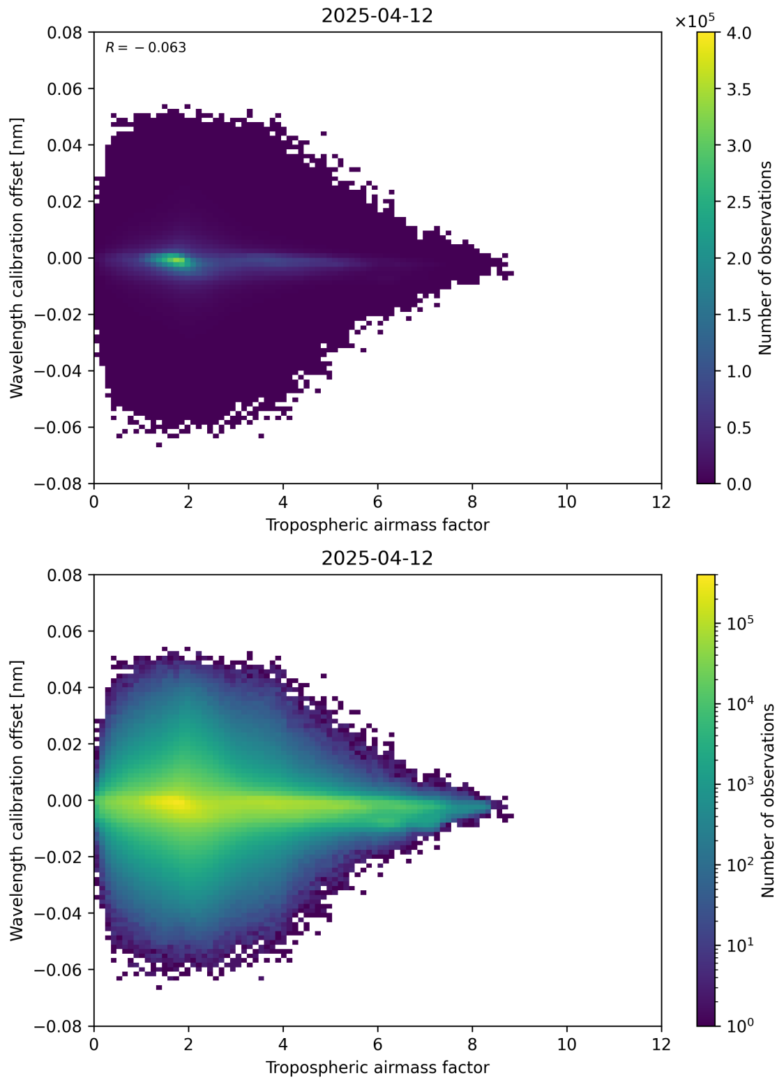
Figure 80: Scatter density plot of “Tropospheric airmass factor” against “Wavelength calibration offset” for 2025-04-12 to 2025-04-13.
