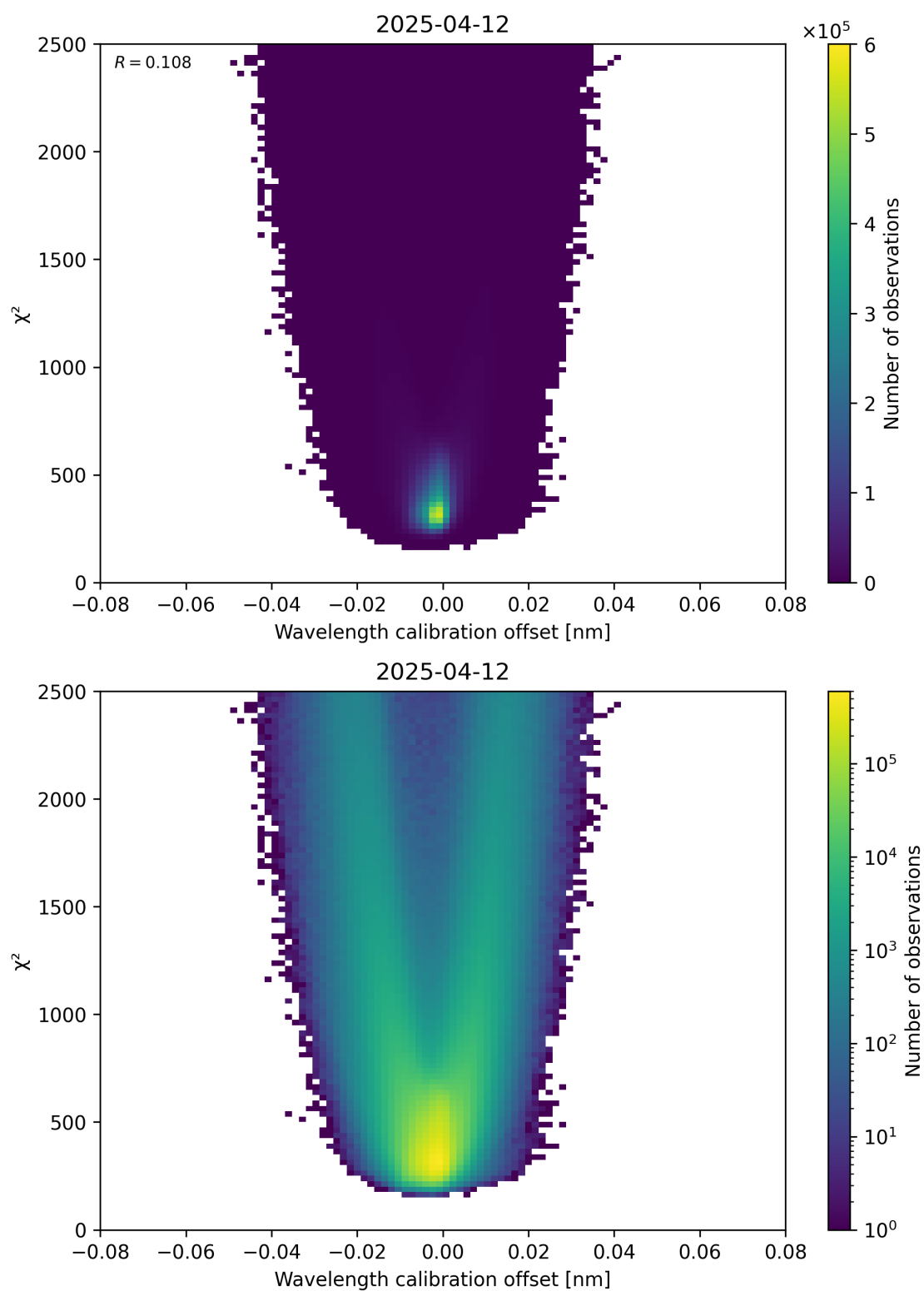
Figure 175: Scatter density plot of “Wavelength calibration offset” against “ \chi^2 ” for 2025-04-12 to 2025-04-13.
