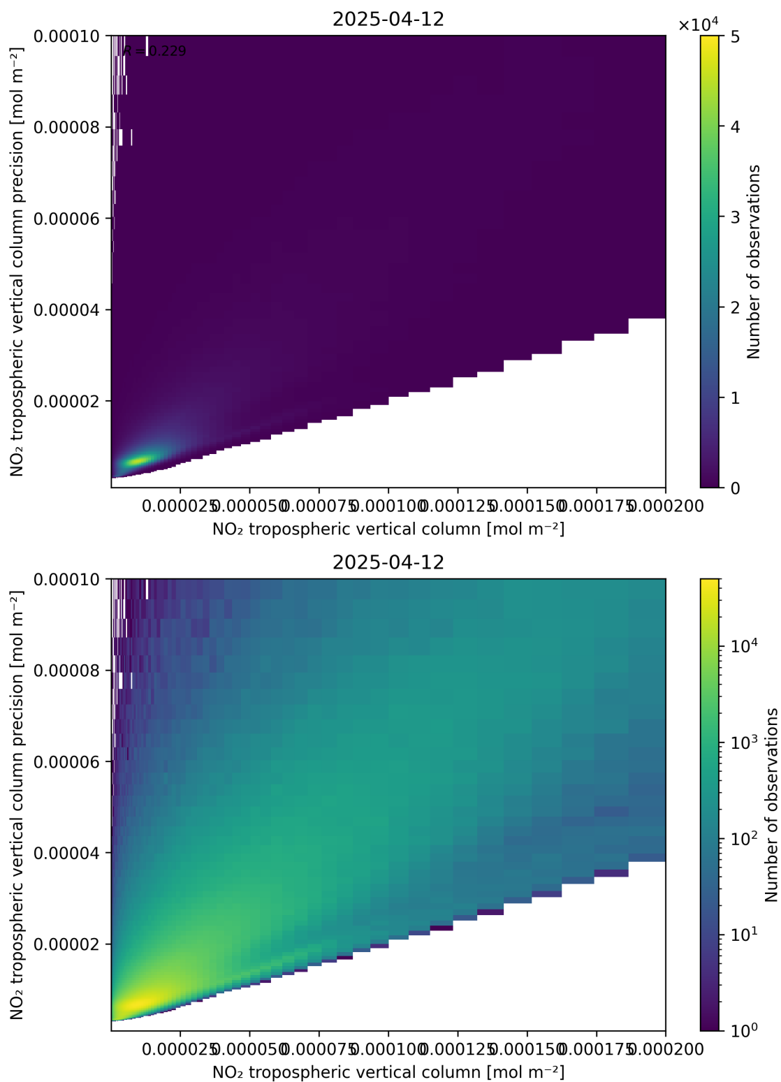
Figure 130: Scatter density plot of “NO 2 tropospheric vertical column” against “NO 2 tropospheric vertical column precision” for 2025-04-12 to 2025-04-13.
