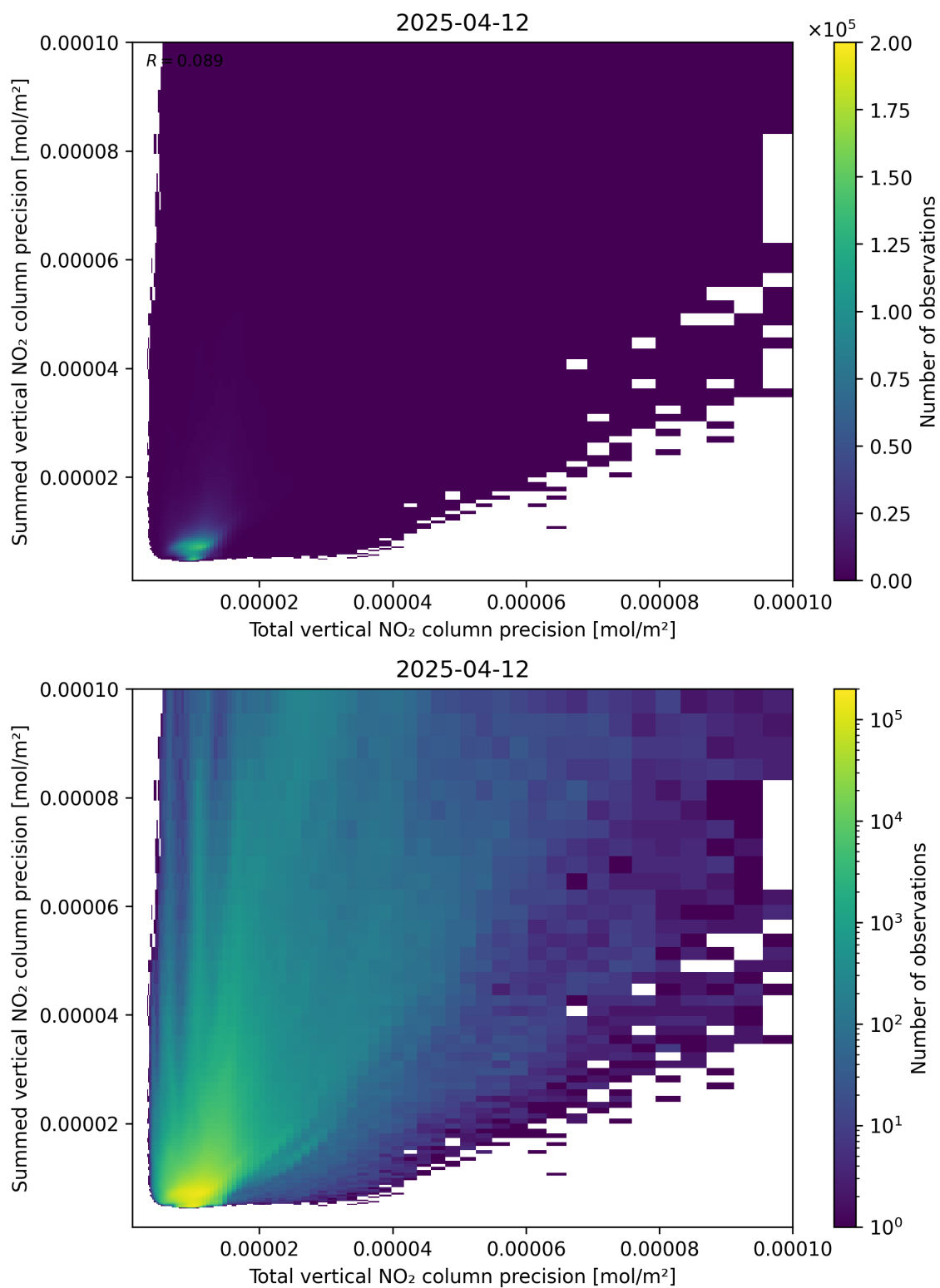
Figure 118: Scatter density plot of “Total vertical NO 2 column precision” against “Summed vertical NO 2 column precision” for 2025-04-12 to 2025-04-13.
