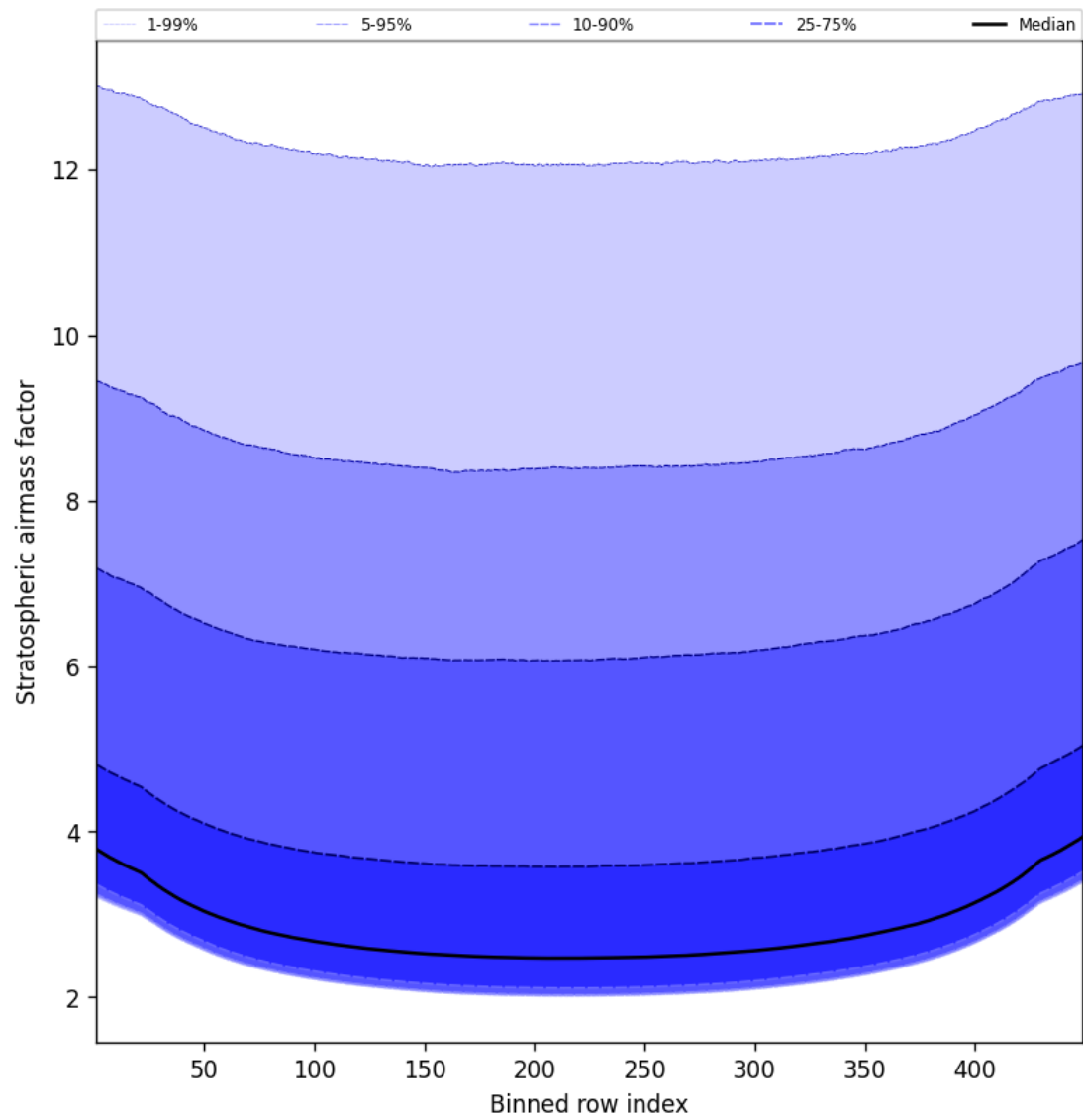
Figure 61: Along track statistics of “Stratospheric air mass factor” for 2025-04-12 to 2025-04-13
