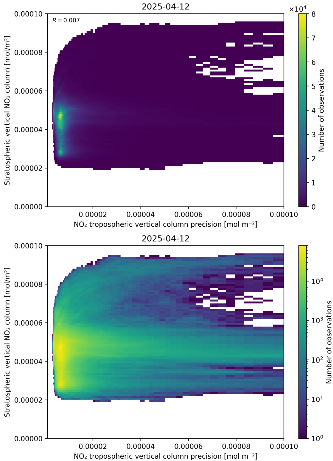
Figure 135: Scatter density plot of “NO 2 tropospheric vertical column precision” against “Stratospheric vertical NO 2 column” for 2025-04-12 to 2025-04-13.
