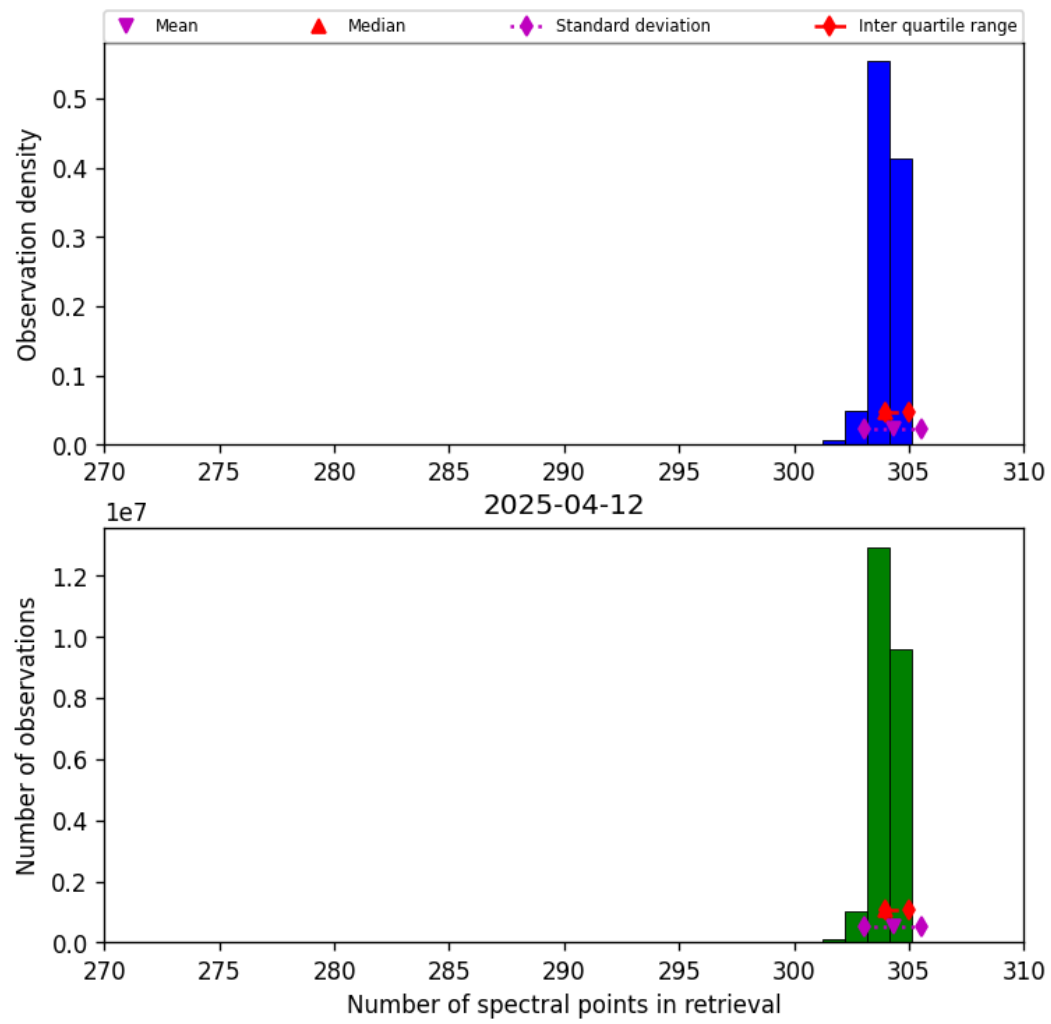
Figure 33: Histogram of “Number of spectral points in retrieval” for 2025-04-12 to 2025-04-13
