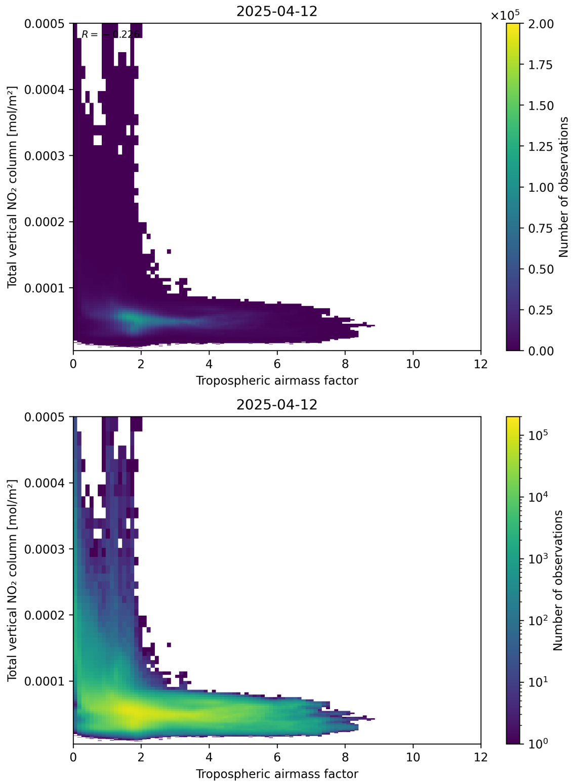
Figure 77: Scatter density plot of “Tropospheric airmass factor” against “Total vertical NO 2 column” for 2025-04-12 to 2025-04-13.
