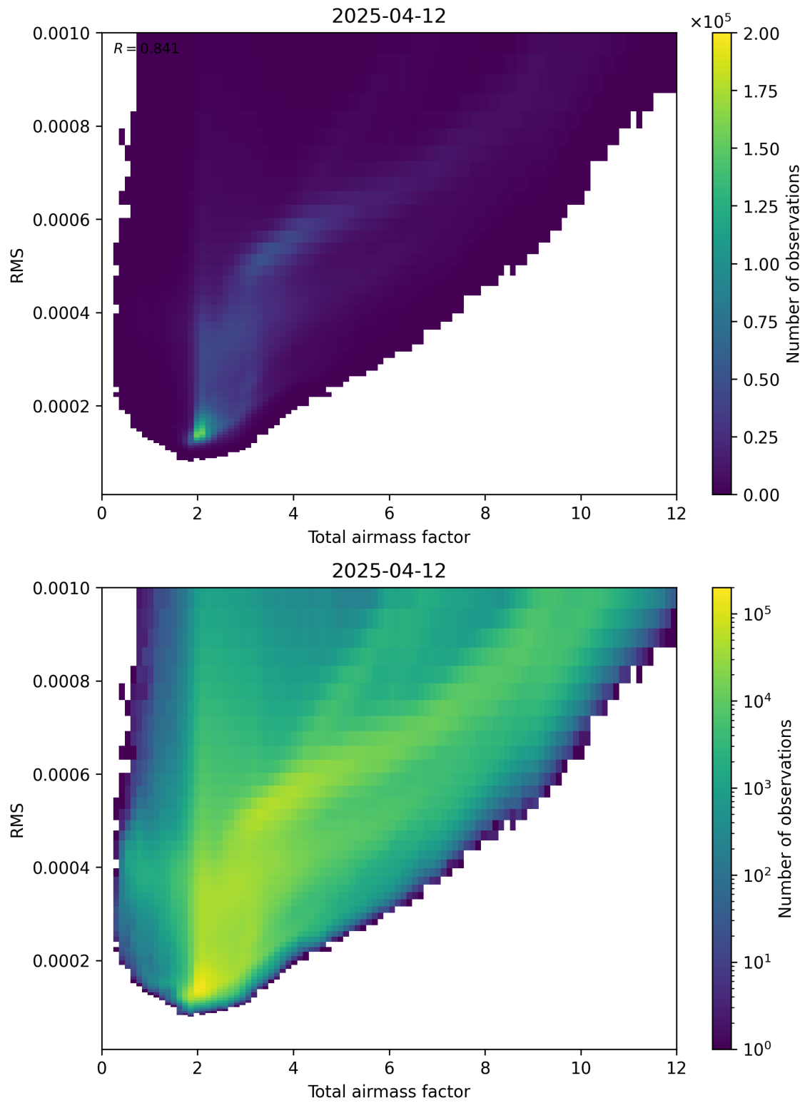
Figure 69: Scatter density plot of “Total airmass factor” against “RMS” for 2025-04-12 to 2025-04-13.
