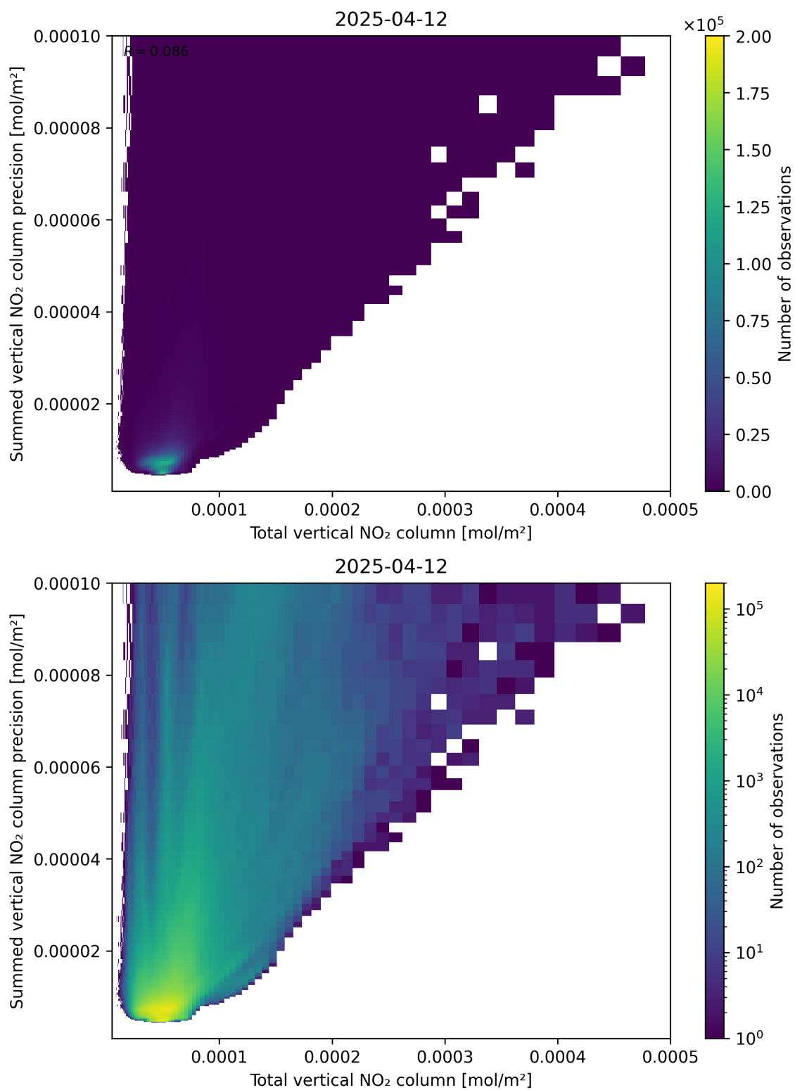
Figure 113: Scatter density plot of “Total vertical NO 2 column” against “Summed vertical NO 2 column precision” for 2025-04-12 to 2025-04-13.
