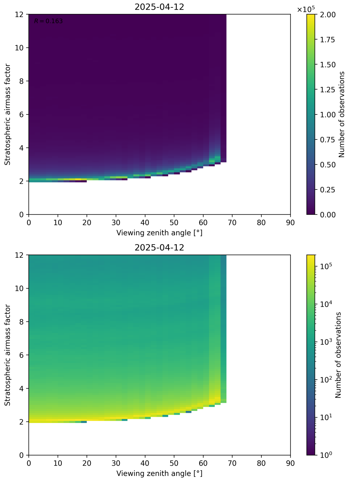
Figure 159: Scatter density plot of “Viewing zenith angle” against “Stratospheric airmass factor” for 2025-04-12 to 2025-04-13.
