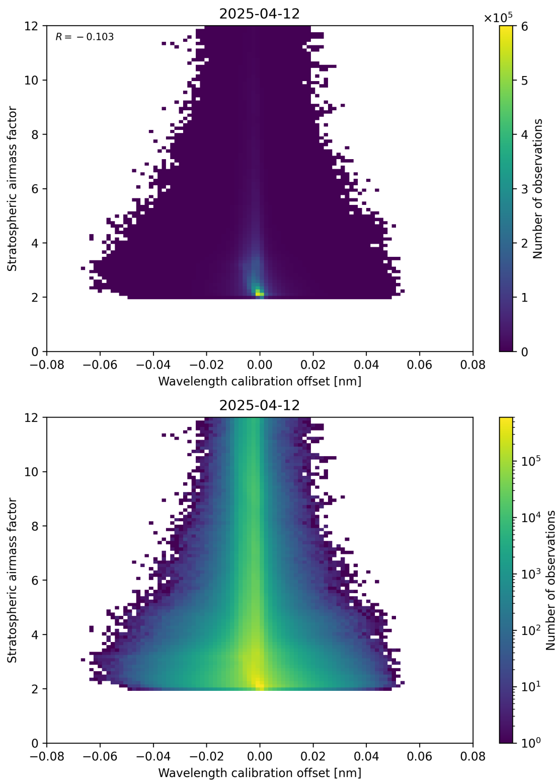
Figure 174: Scatter density plot of “Wavelength calibration offset” against “Stratospheric airmass factor” for 2025-04-12 to 2025-04-13.
