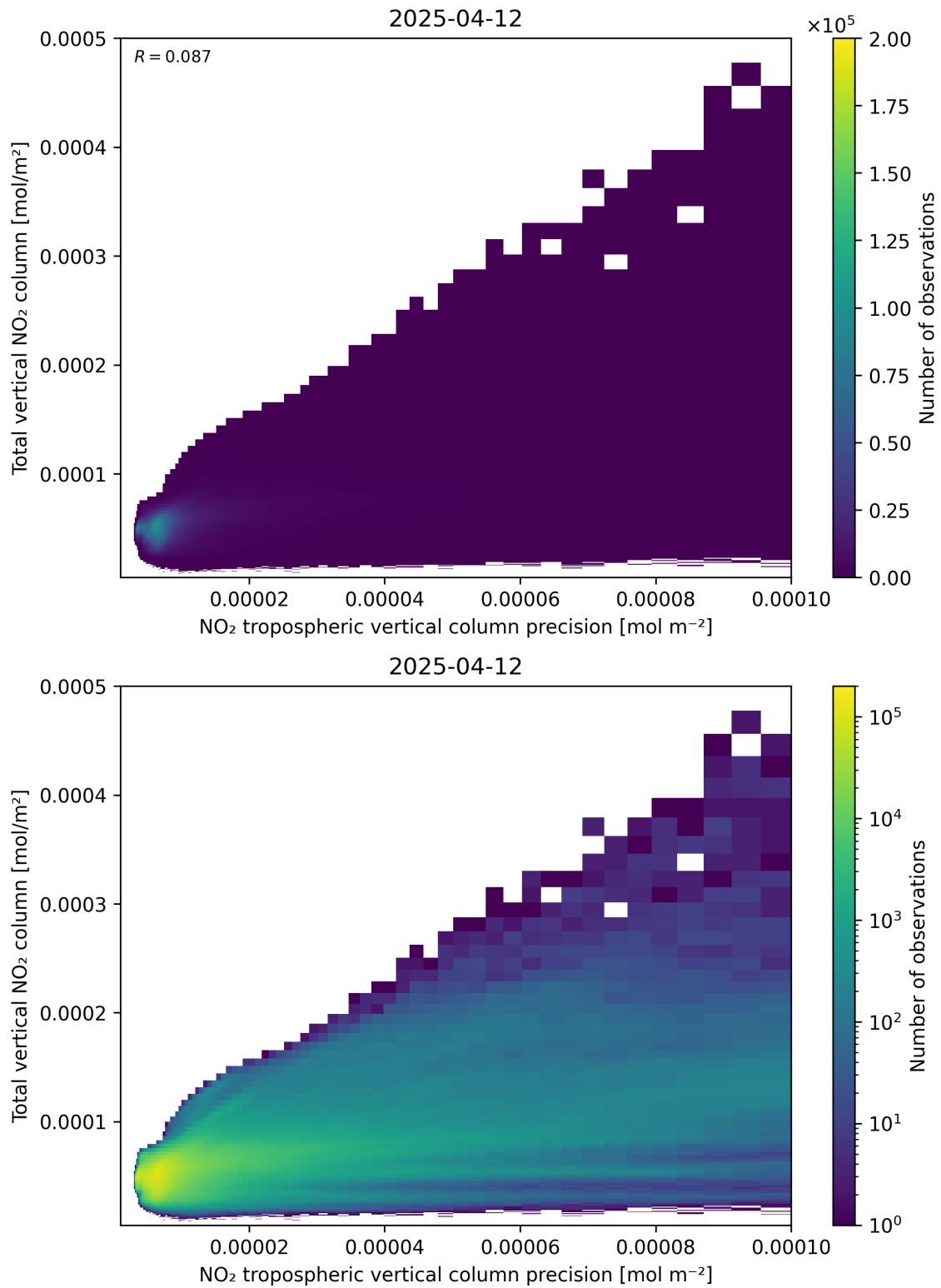
Figure 138: Scatter density plot of “NO 2 tropospheric vertical column precision” against “Total vertical NO 2 column” for 2025-04-12 to 2025-04-13.
