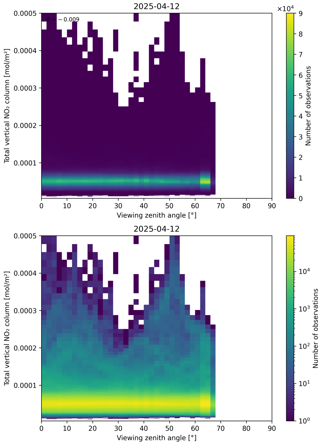
Figure 167: Scatter density plot of “Viewing zenith angle” against “Total vertical NO 2 column” for 2025-04-12 to 2025-04-13.
