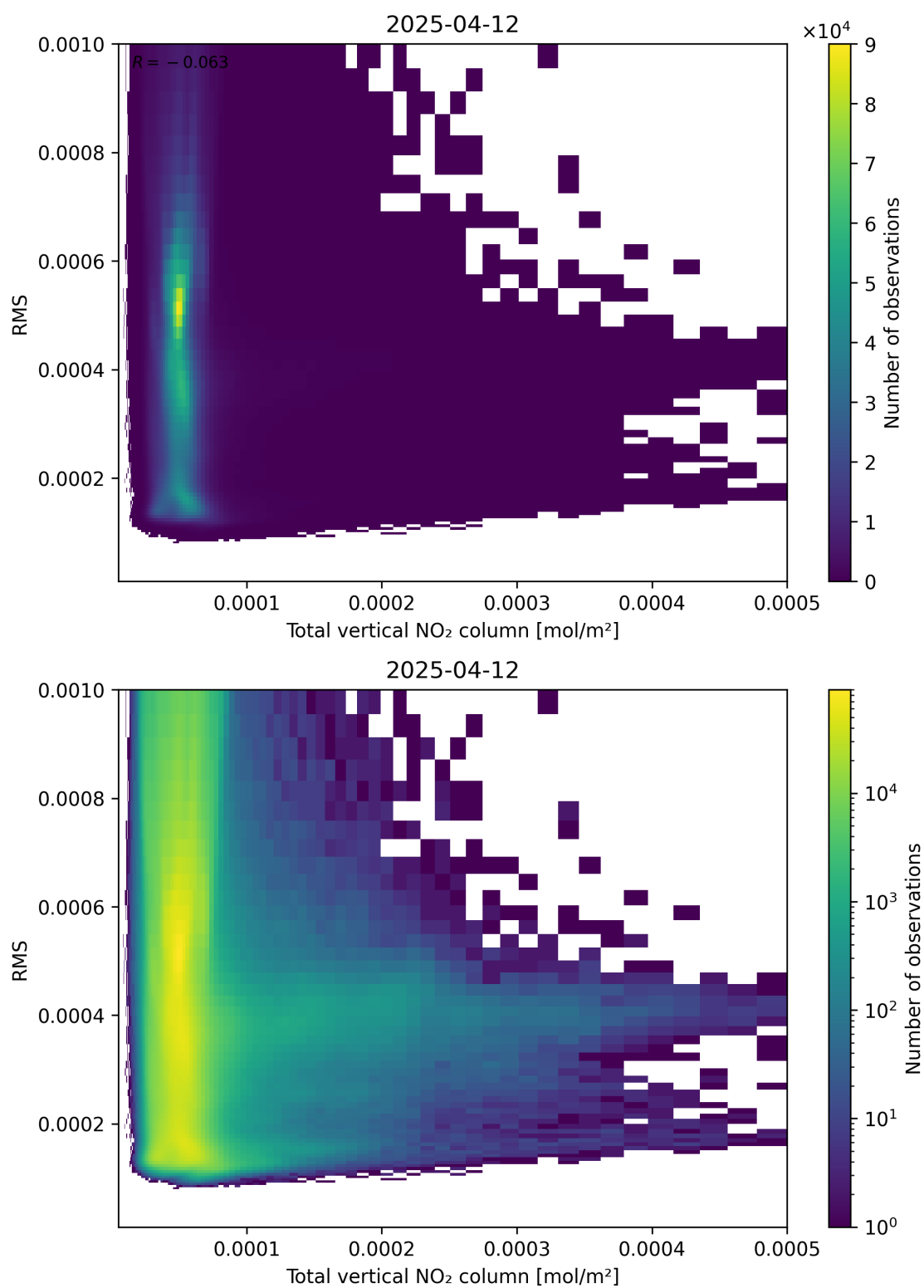
Figure 120: Scatter density plot of “Total vertical NO 2 column” against “RMS” for 2025-04-12 to 2025-04-13.
