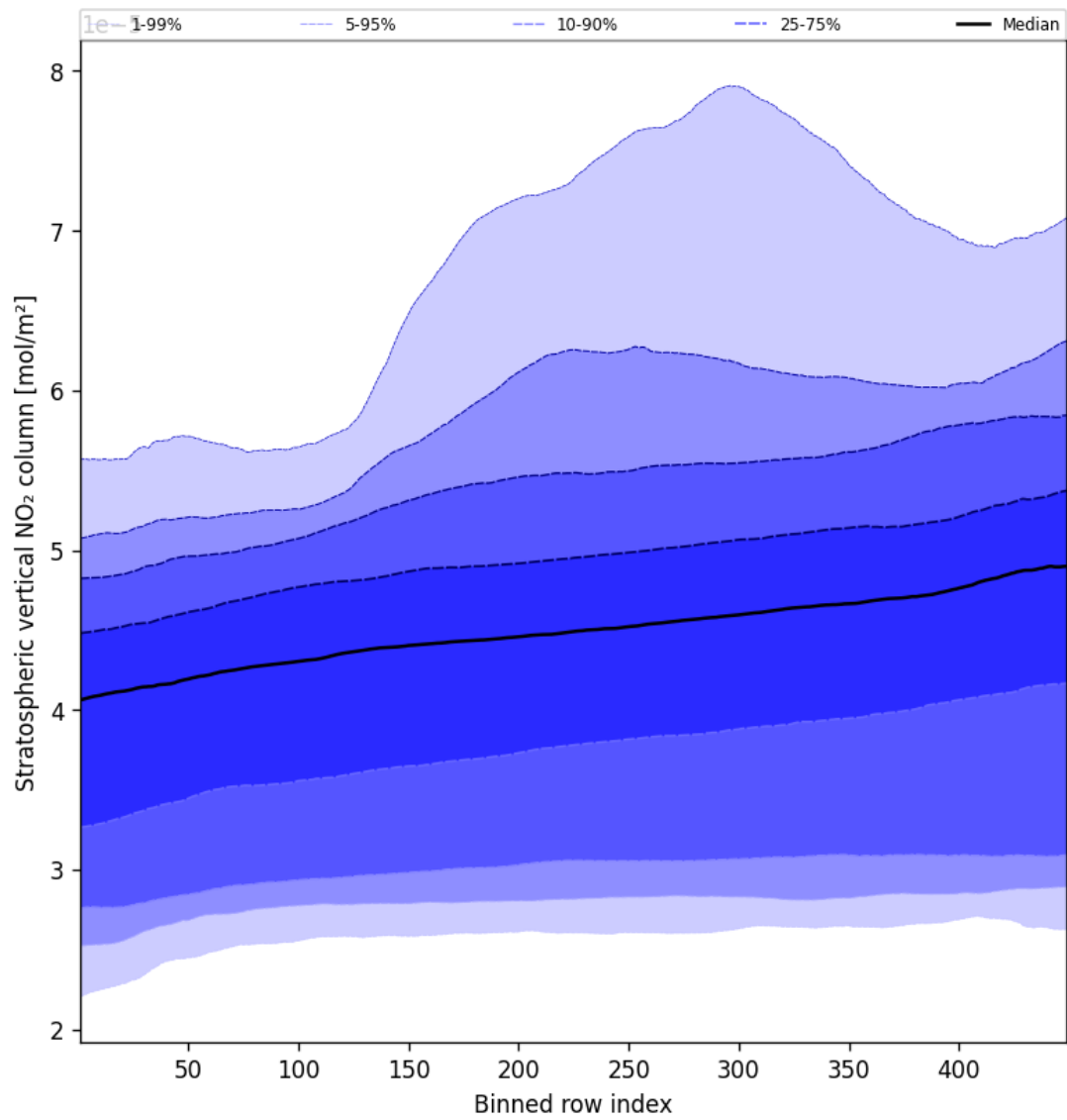
Figure 53: Along track statistics of “Stratospheric vertical NO 2 column” for 2025-04-12 to 2025-04-13
