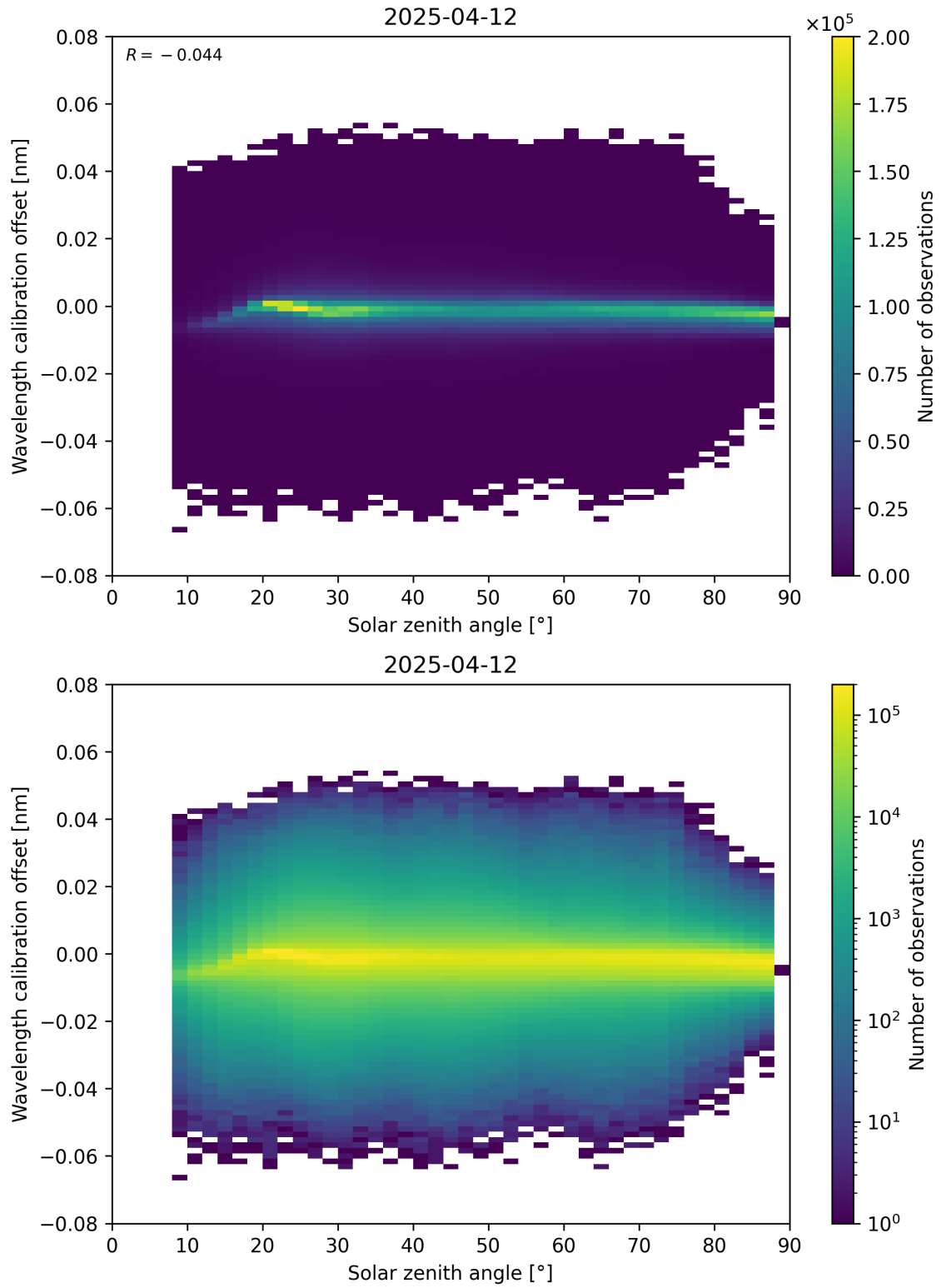
Figure 158: Scatter density plot of “Solar zenith angle” against “Wavelength calibration offset” for 2025-04-12 to 2025-04-13.
