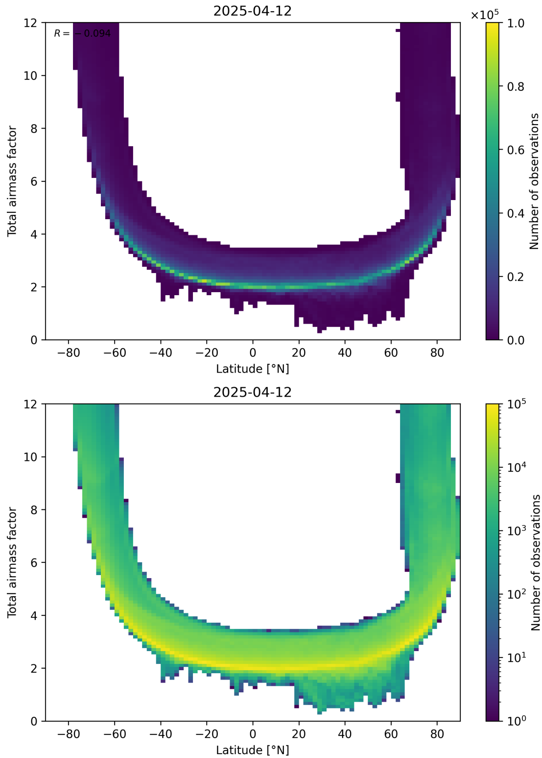
Figure 84: Scatter density plot of “Latitude” against “Total airmass factor” for 2025-04-12 to 2025-04-13.
