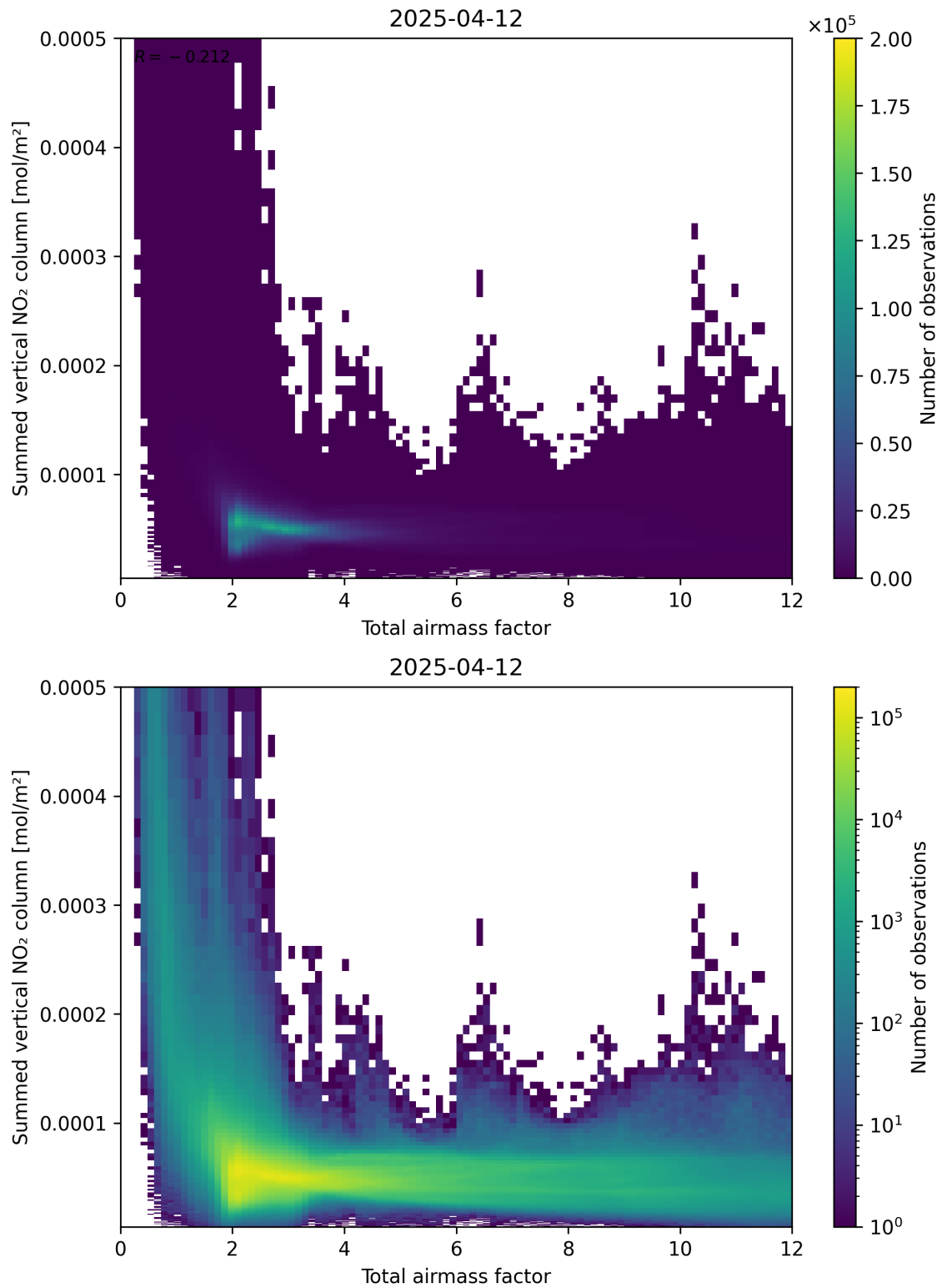
Figure 65: Scatter density plot of “Total airmass factor” against “Summed vertical NO 2 column” for 2025-04-12 to 2025-04-13.
