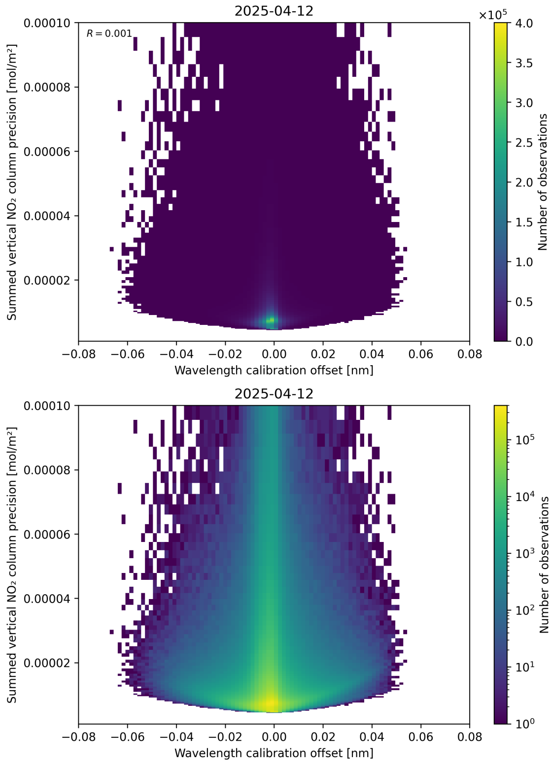
Figure 178: Scatter density plot of “Wavelength calibration offset” against “Summed vertical NO 2 column precision” for 2025-04-12 to 2025-04-13.
