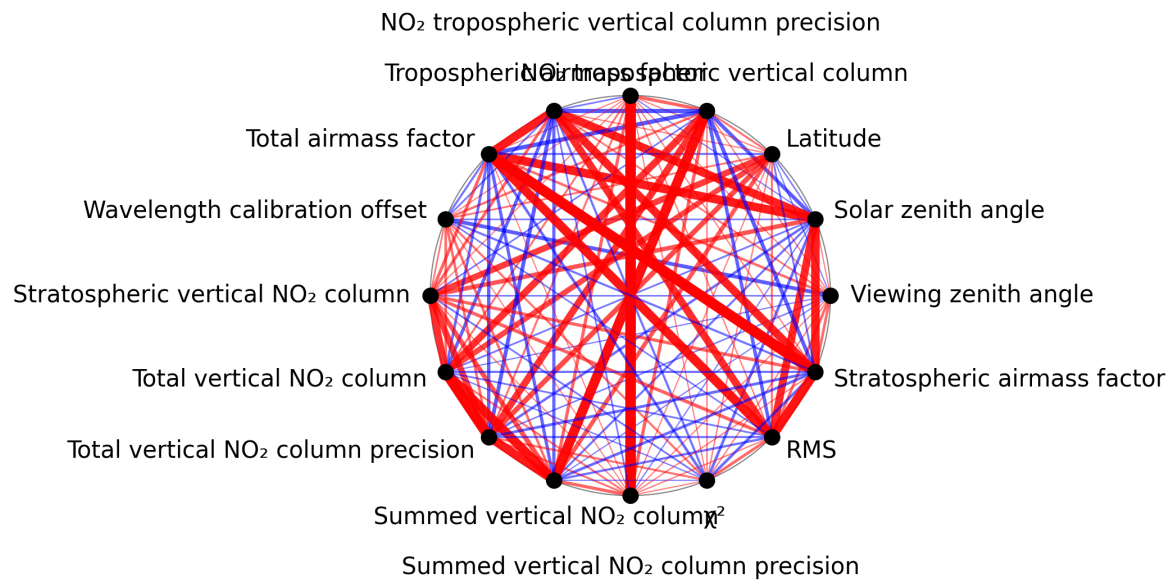
Figure 1: Map of correlation graph for 2025-04-12 to 2025-04-13.
