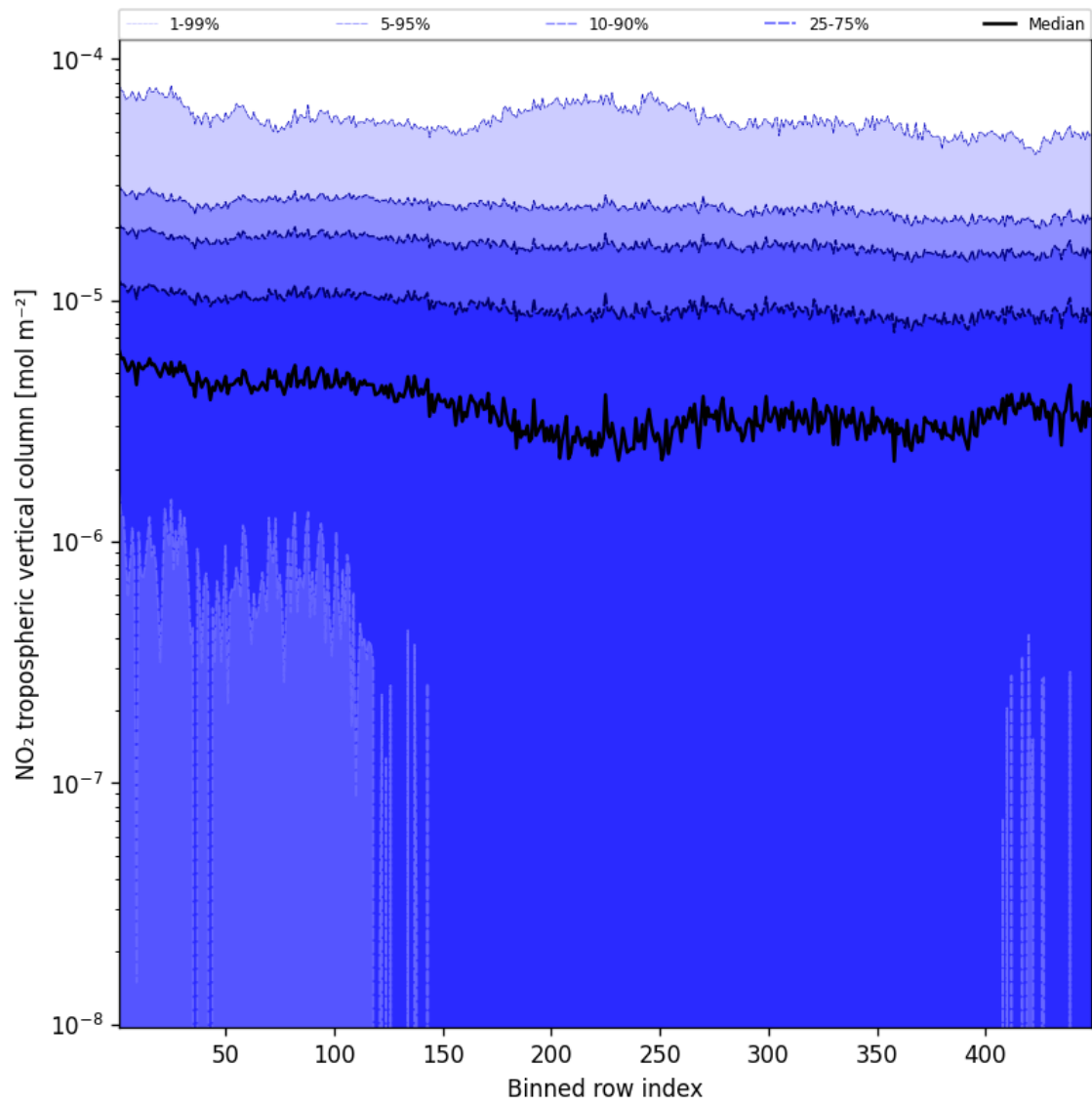
Figure 46: Along track statistics of “NO 2 tropospheric vertical column” for 2025-04-12 to 2025-04-13
