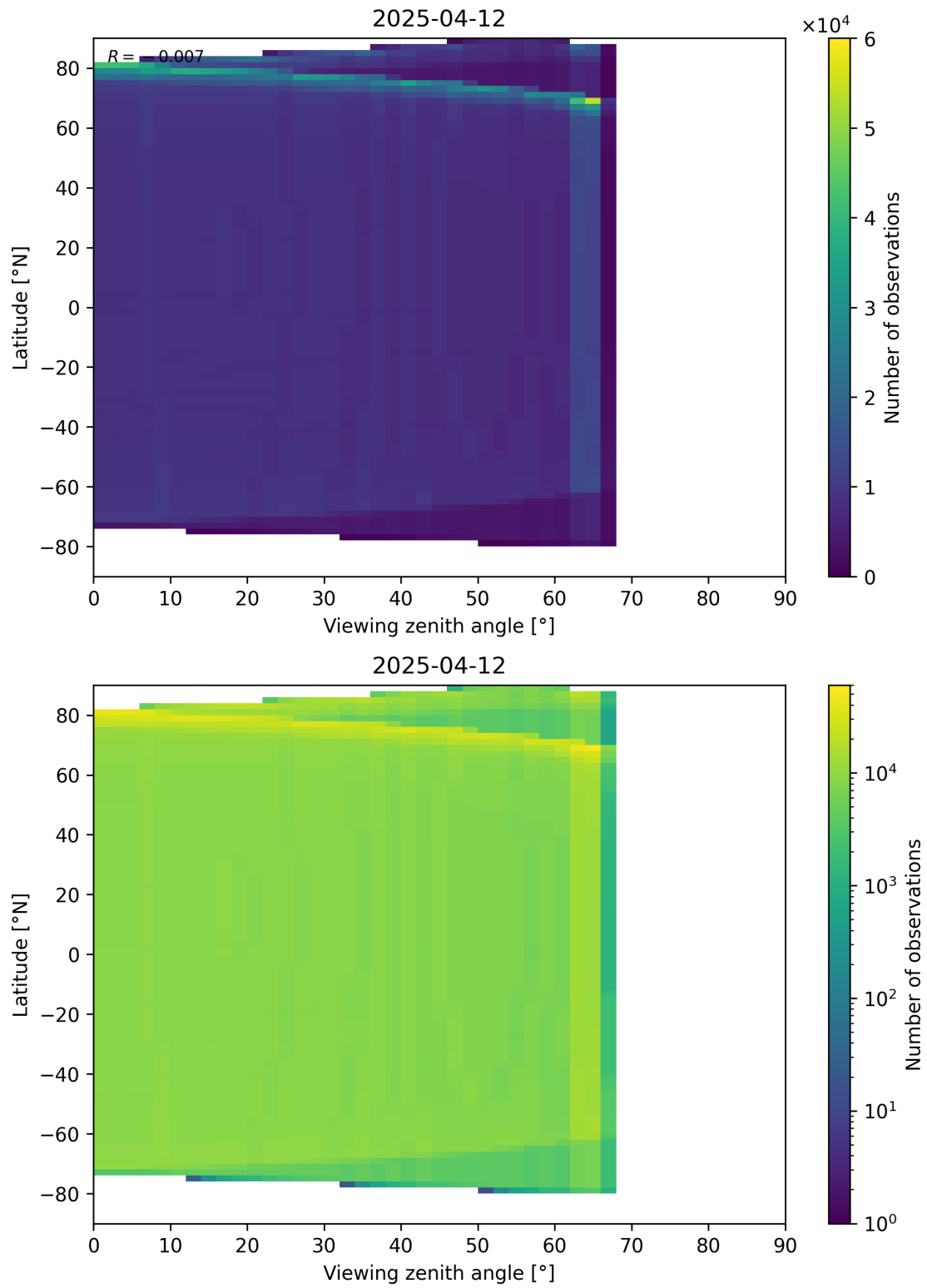
Figure 163: Scatter density plot of “Viewing zenith angle” against “Latitude” for 2025-04-12 to 2025-04-13.
