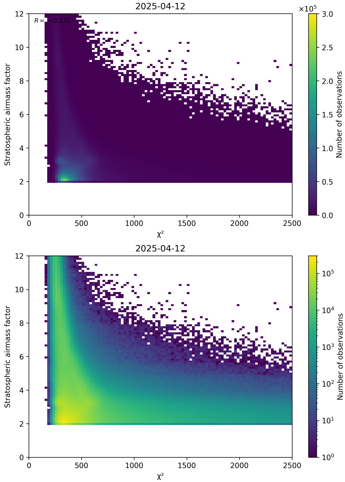
Figure 81: Scatter density plot of “ \chi^2 ” against “Stratospheric airmass factor” for 2025-04-12 to 2025-04-13.
