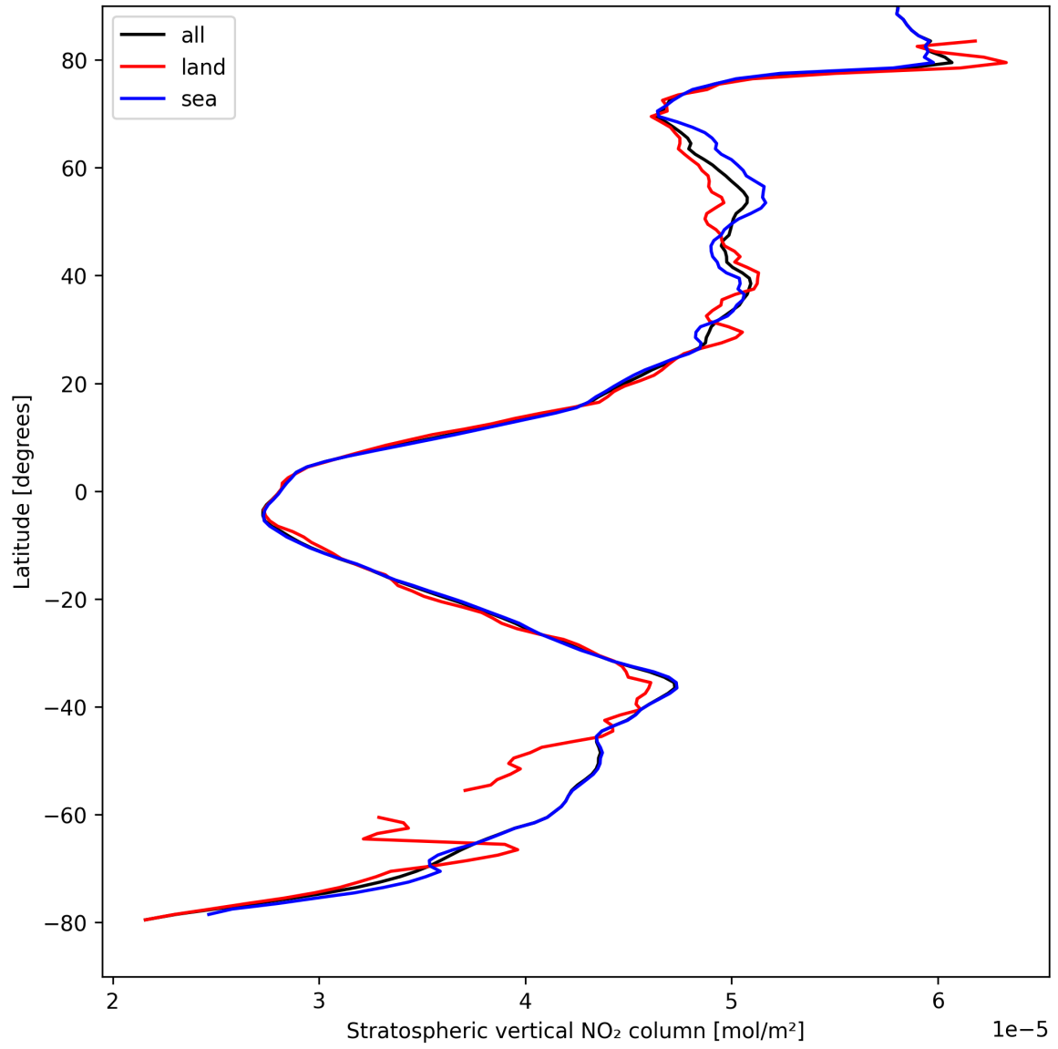
Figure 19: Zonal average of “Stratospheric vertical NO 2 column” for 2025-04-12 to 2025-04-13.
