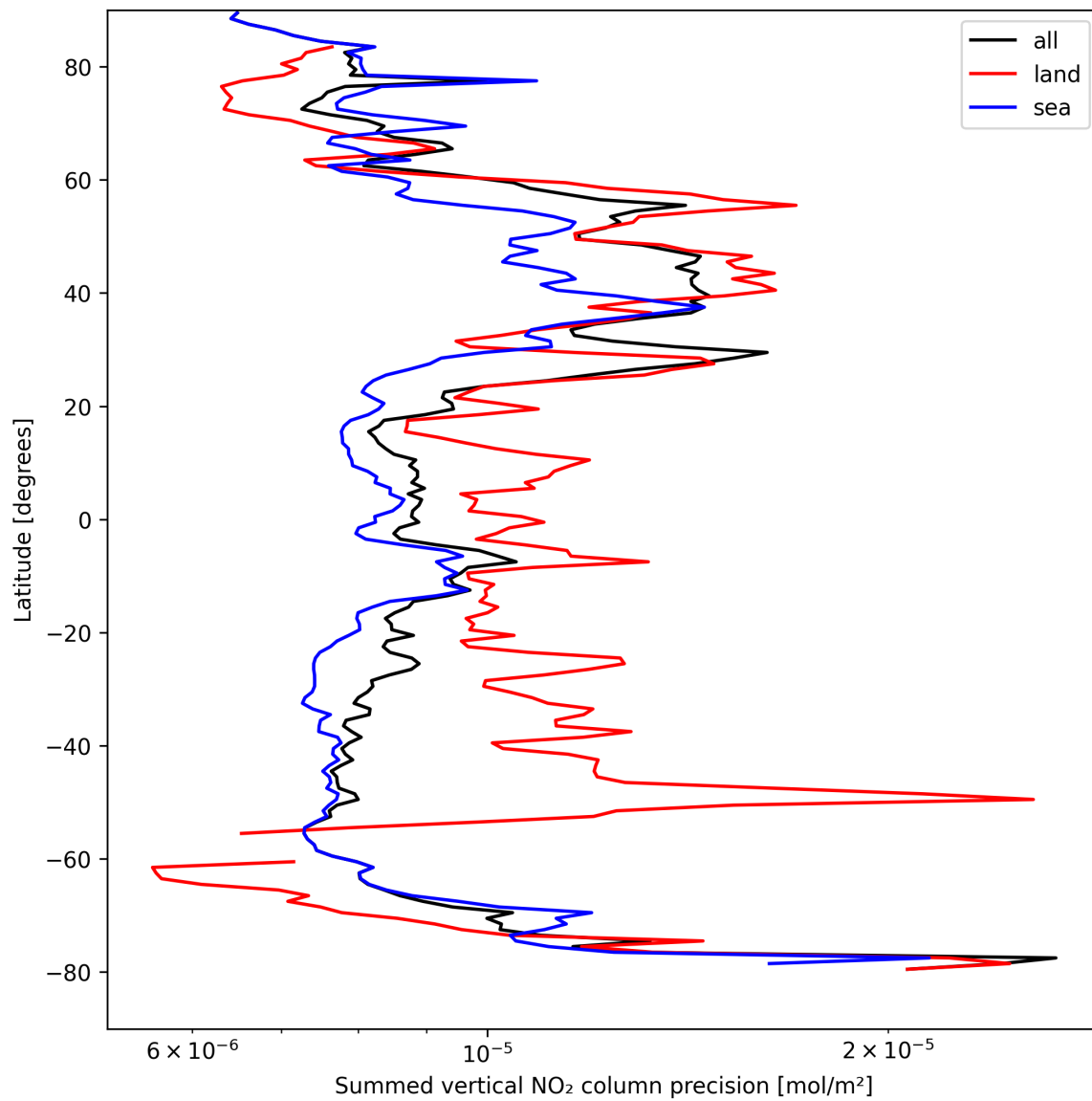
Figure 24: Zonal average of “Summed vertical NO 2 column precision” for 2025-04-12 to 2025-04-13.
