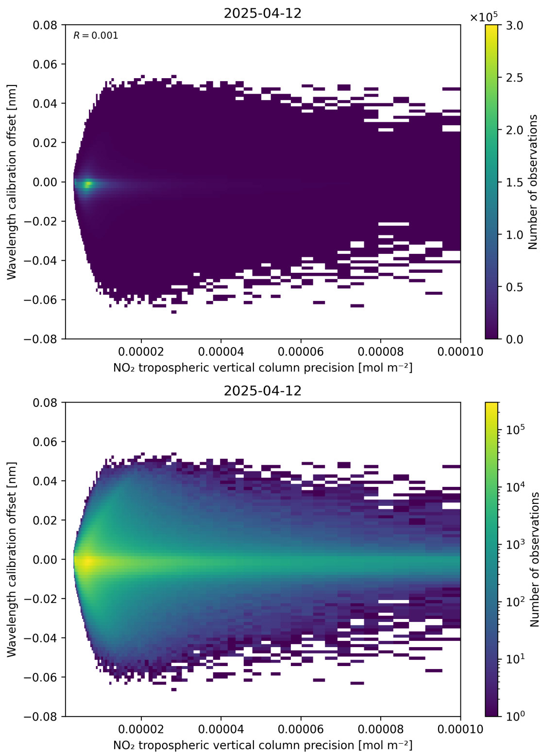
Figure 141: Scatter density plot of “NO 2 tropospheric vertical column precision” against “Wavelength calibration offset” for 2025-04-12 to 2025-04-13.
