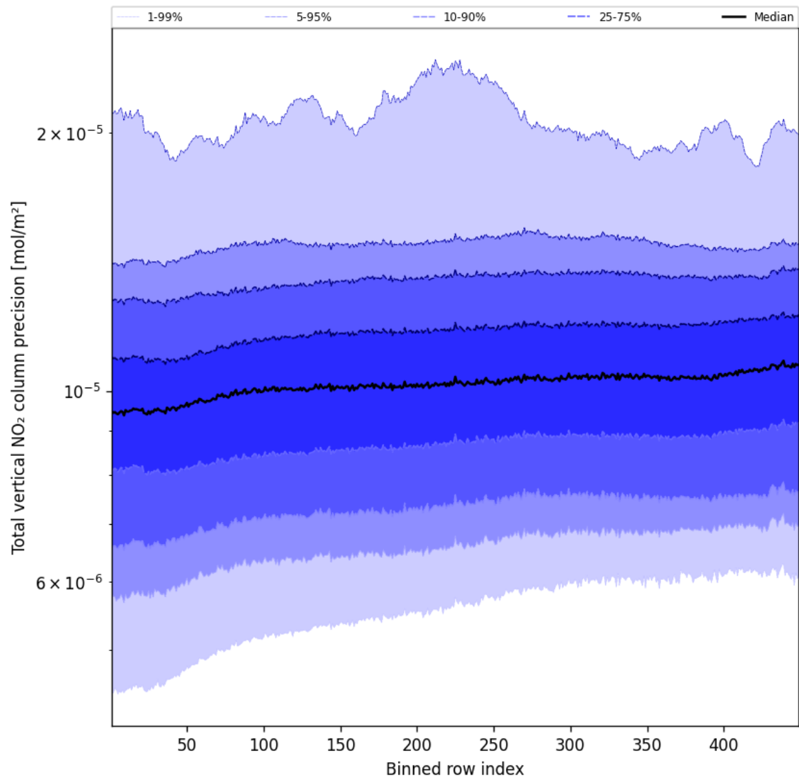
Figure 56: Along track statistics of “Total vertical NO 2 column precision” for 2025-04-12 to 2025-04-13
