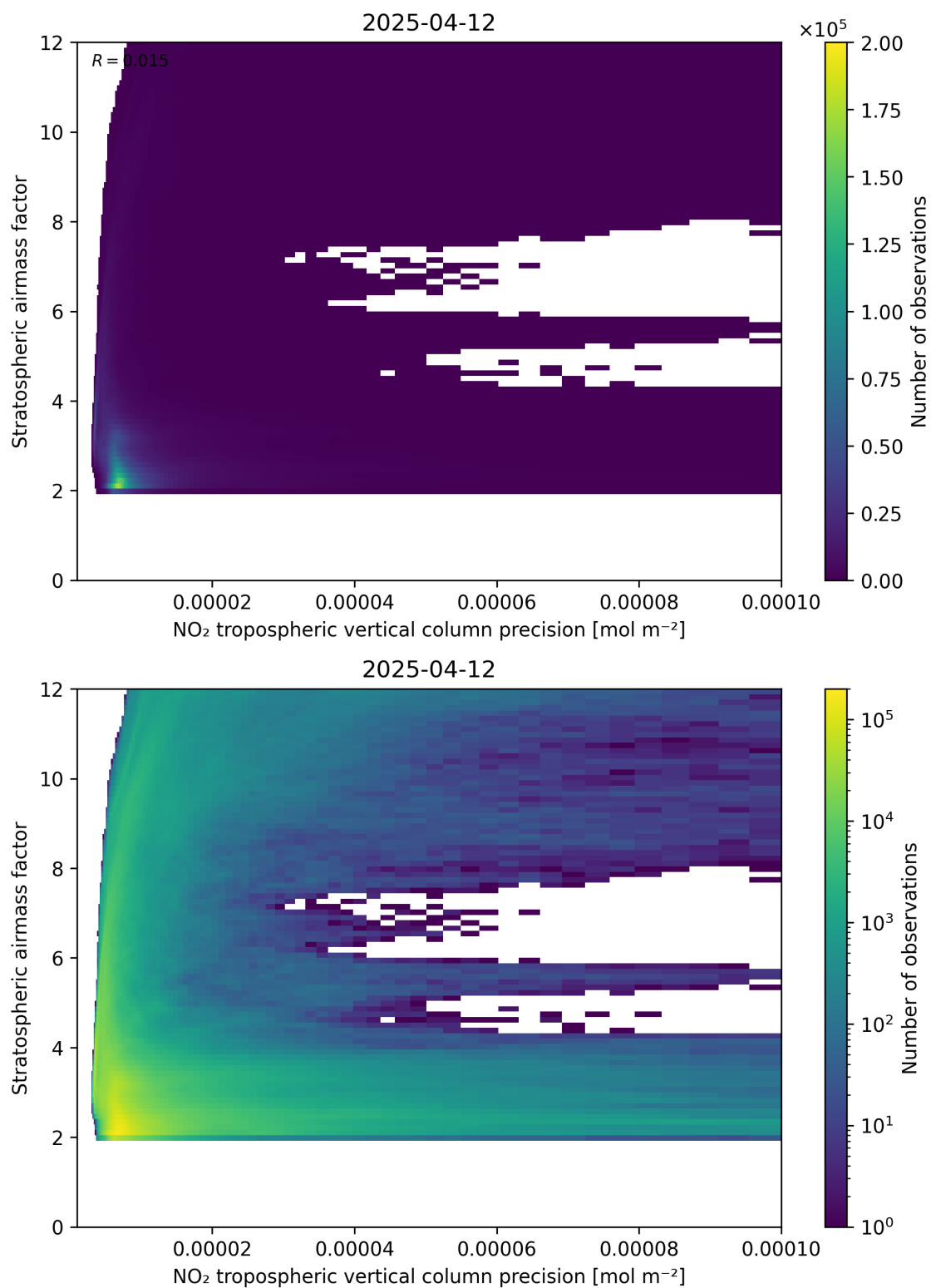
Figure 131: Scatter density plot of “NO 2 tropospheric vertical column precision” against “Stratospheric airmass factor” for 2025-04-12 to 2025-04-13.
