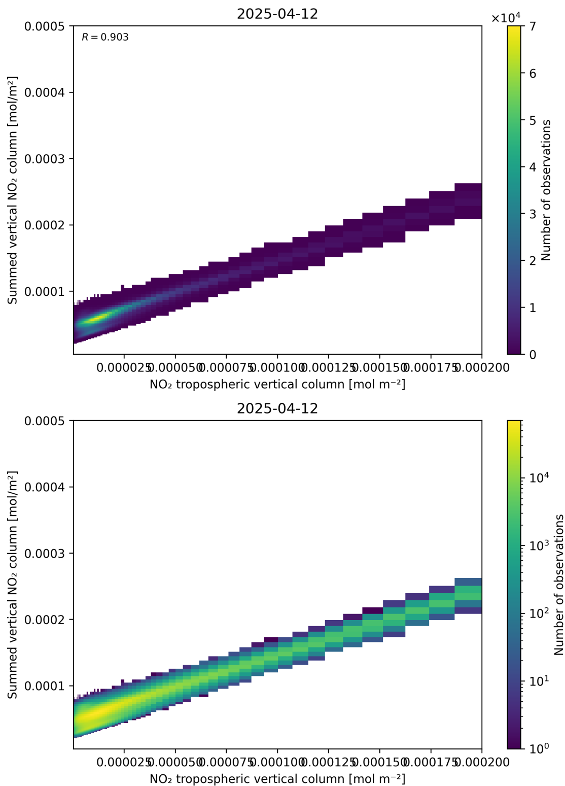
Figure 126: Scatter density plot of “NO 2 tropospheric vertical column” against “Summed vertical NO 2 column” for 2025-04-12 to 2025-04-13.
