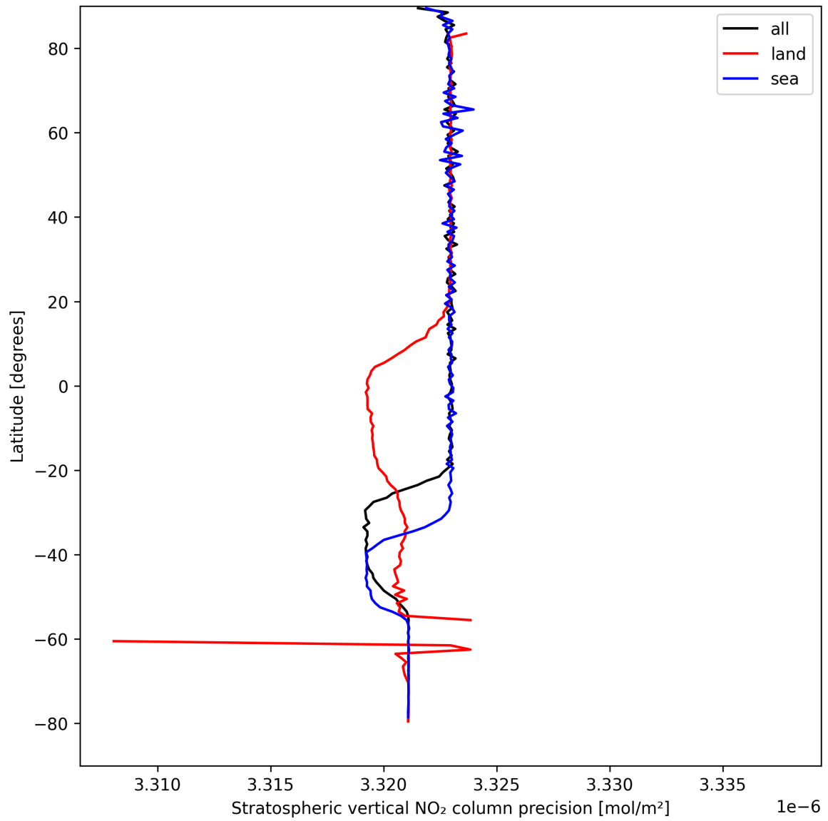
Figure 20: Zonal average of “Stratospheric vertical NO 2 column precision” for 2025-04-12 to 2025-04-13.
