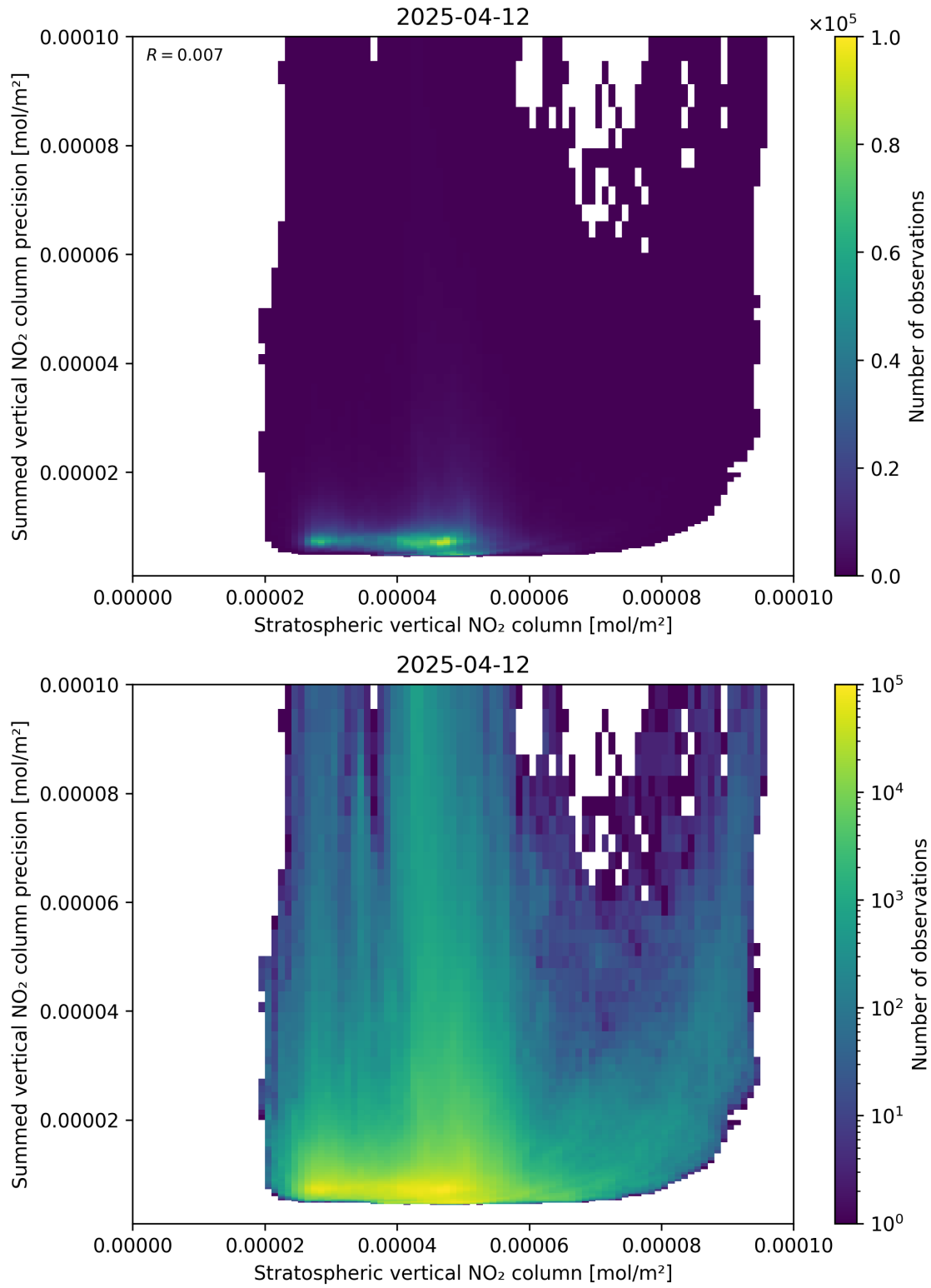
Figure 99: Scatter density plot of “Stratospheric vertical NO 2 column” against “Summed vertical NO 2 column precision” for 2025-04-12 to 2025-04-13.
