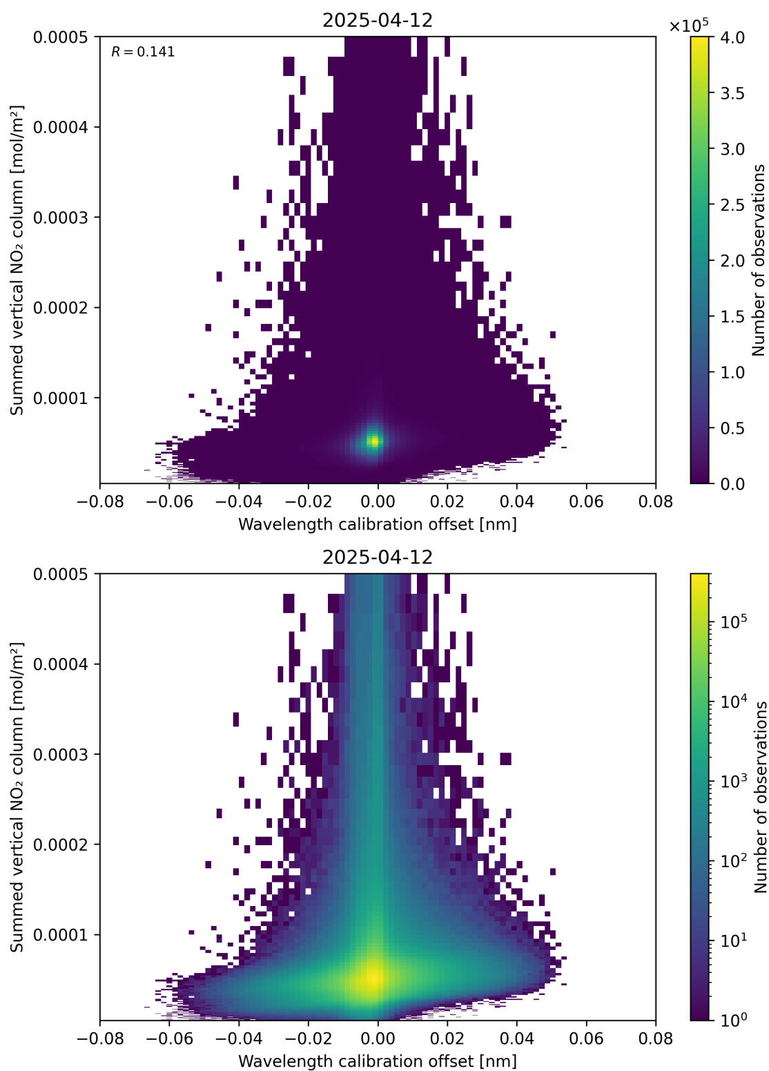
Figure 177: Scatter density plot of “Wavelength calibration offset” against “Summed vertical NO 2 column” for 2025-04-12 to 2025-04-13.
