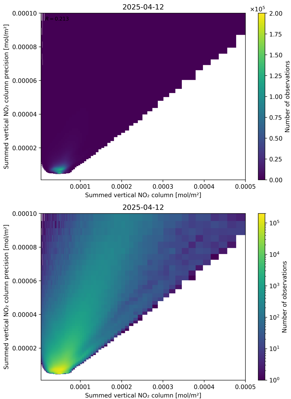
Figure 105: Scatter density plot of “Summed vertical NO 2 column” against “Summed vertical NO 2 column precision” for 2025-04-12 to 2025-04-13.
