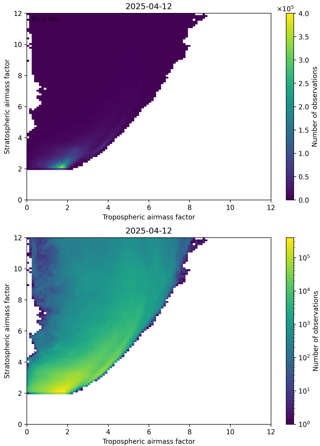
Figure 71: Scatter density plot of “Tropospheric airmass factor” against “Stratospheric airmass factor” for 2025-04-12 to 2025-04-13.
