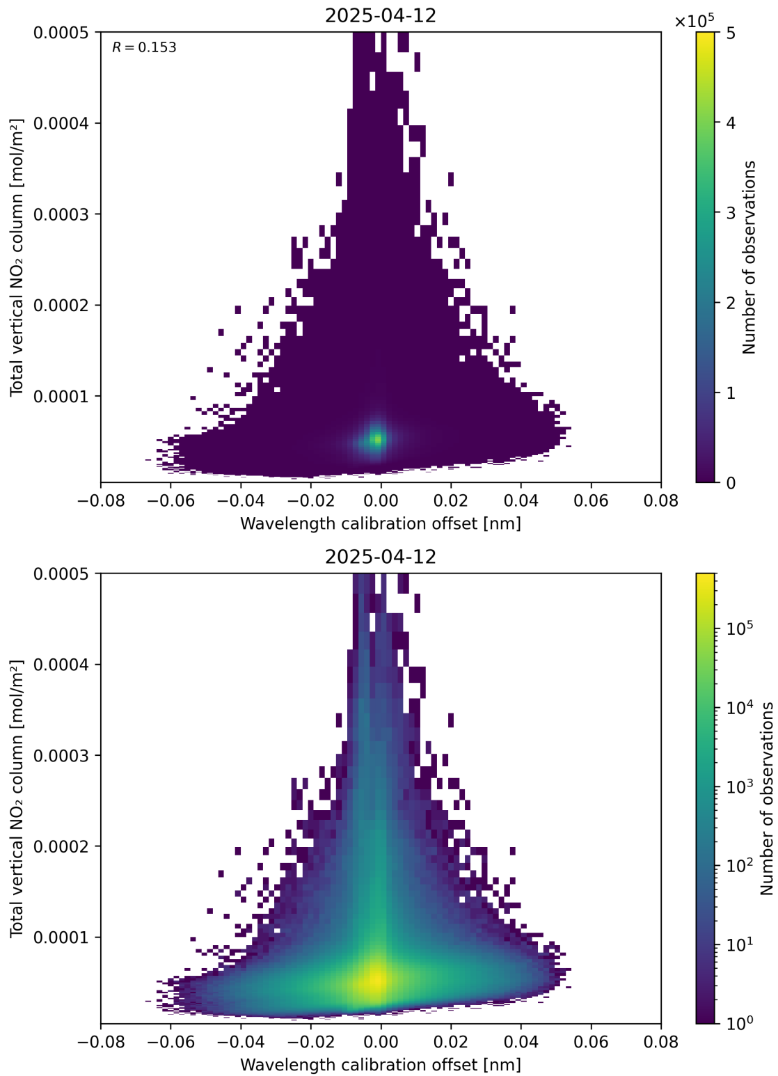
Figure 179: Scatter density plot of “Wavelength calibration offset” against “Total vertical NO 2 column” for 2025-04-12 to 2025-04-13.
