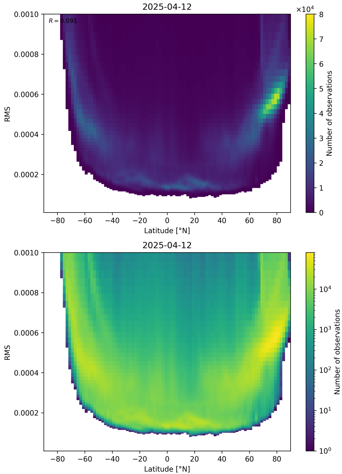
Figure 94: Scatter density plot of “Latitude” against “RMS” for 2025-04-12 to 2025-04-13.
