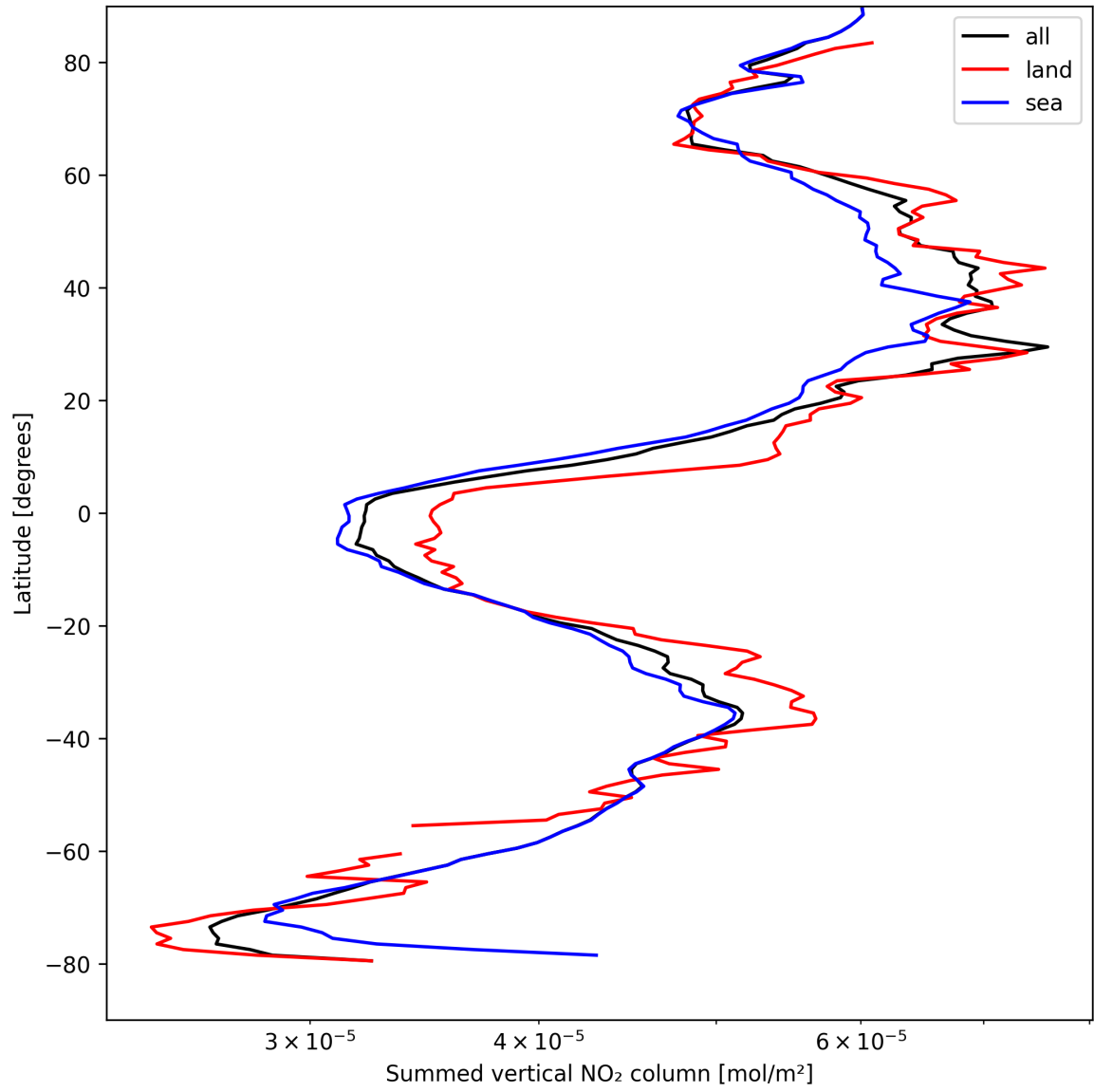
Figure 23: Zonal average of “Summed vertical NO 2 column” for 2025-04-12 to 2025-04-13.
