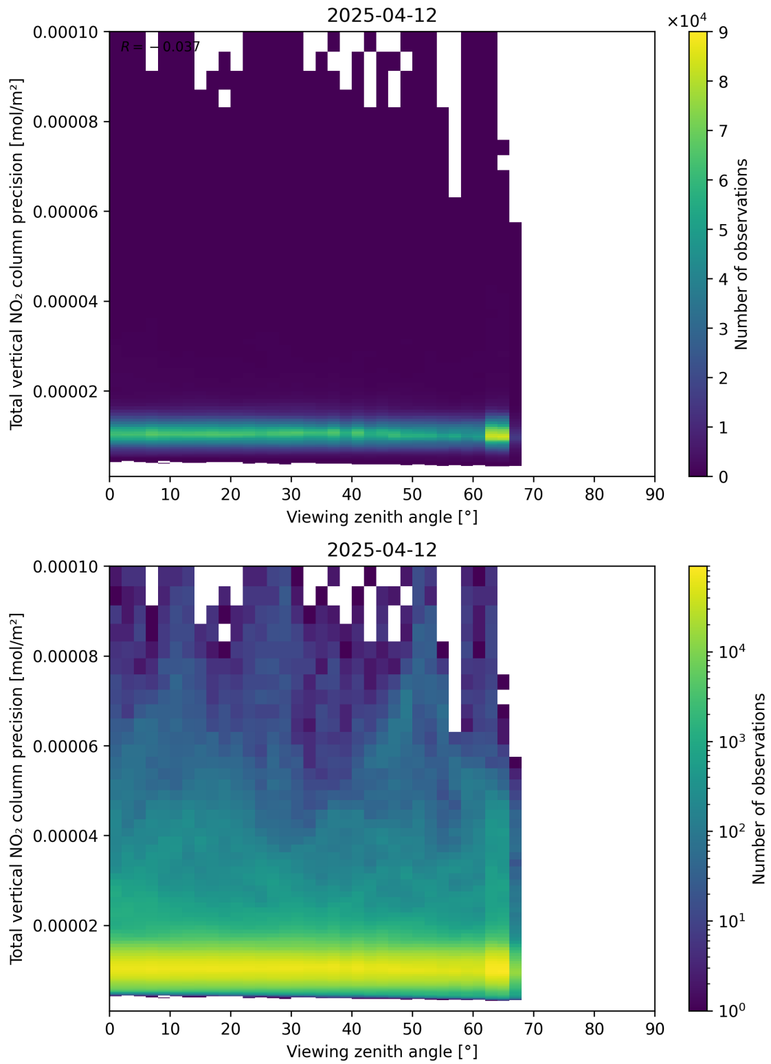
Figure 168: Scatter density plot of “Viewing zenith angle” against “Total vertical NO 2 column precision” for 2025-04-12 to 2025-04-13.
