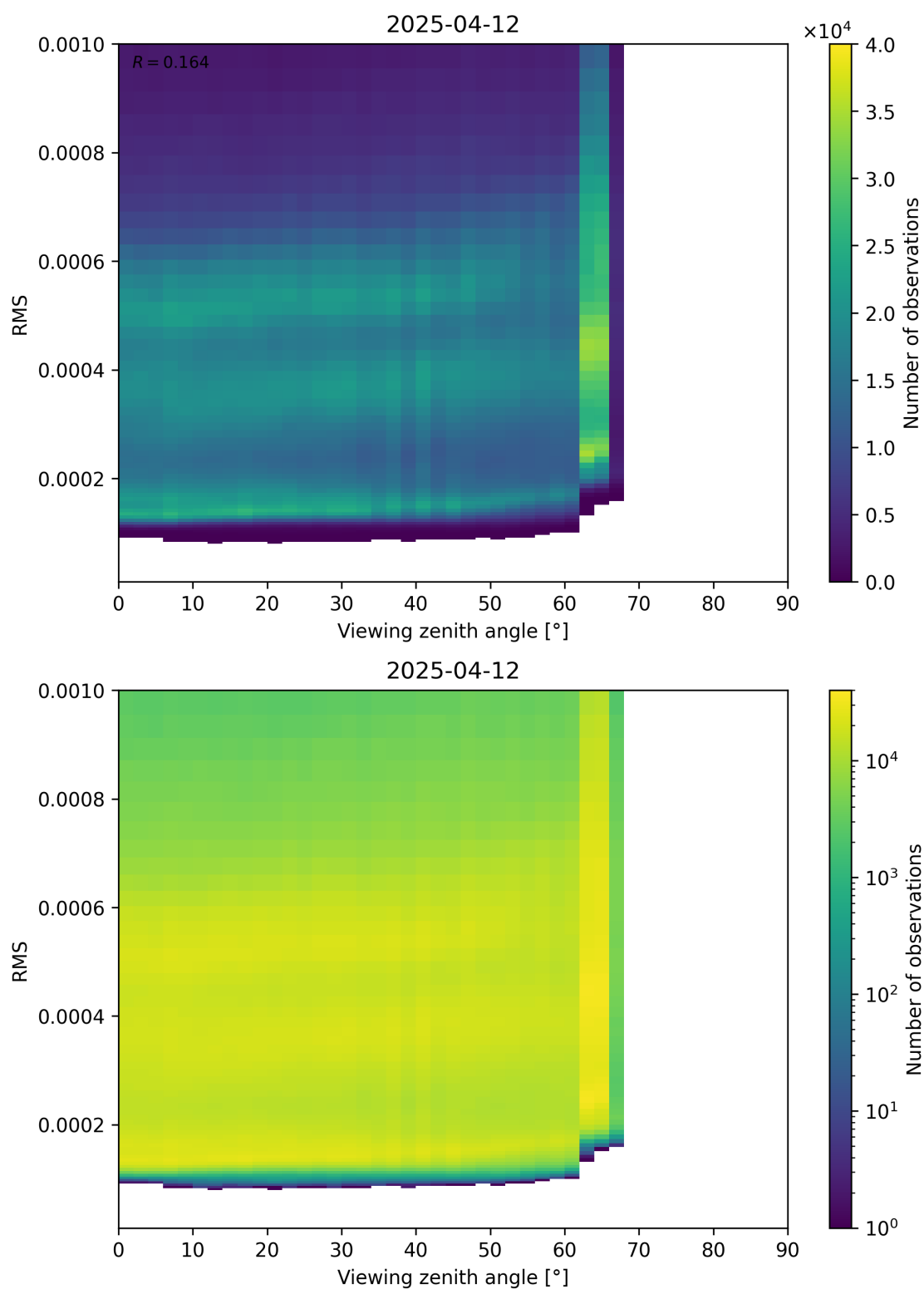
Figure 171: Scatter density plot of “Viewing zenith angle” against “RMS” for 2025-04-12 to 2025-04-13.
