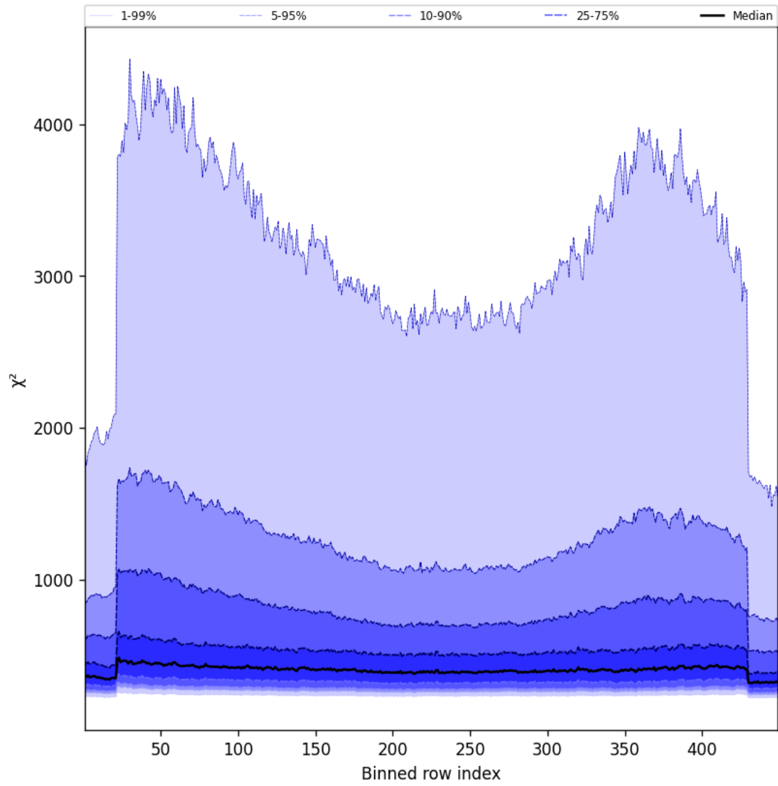
Figure 59: Along track statistics of “ \chi^2 ” for 2025-04-12 to 2025-04-13
