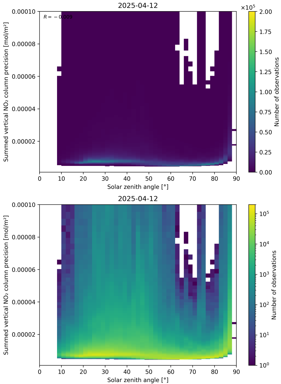
Figure 152: Scatter density plot of “Solar zenith angle” against “Summed vertical NO 2 column precision” for 2025-04-12 to 2025-04-13.
