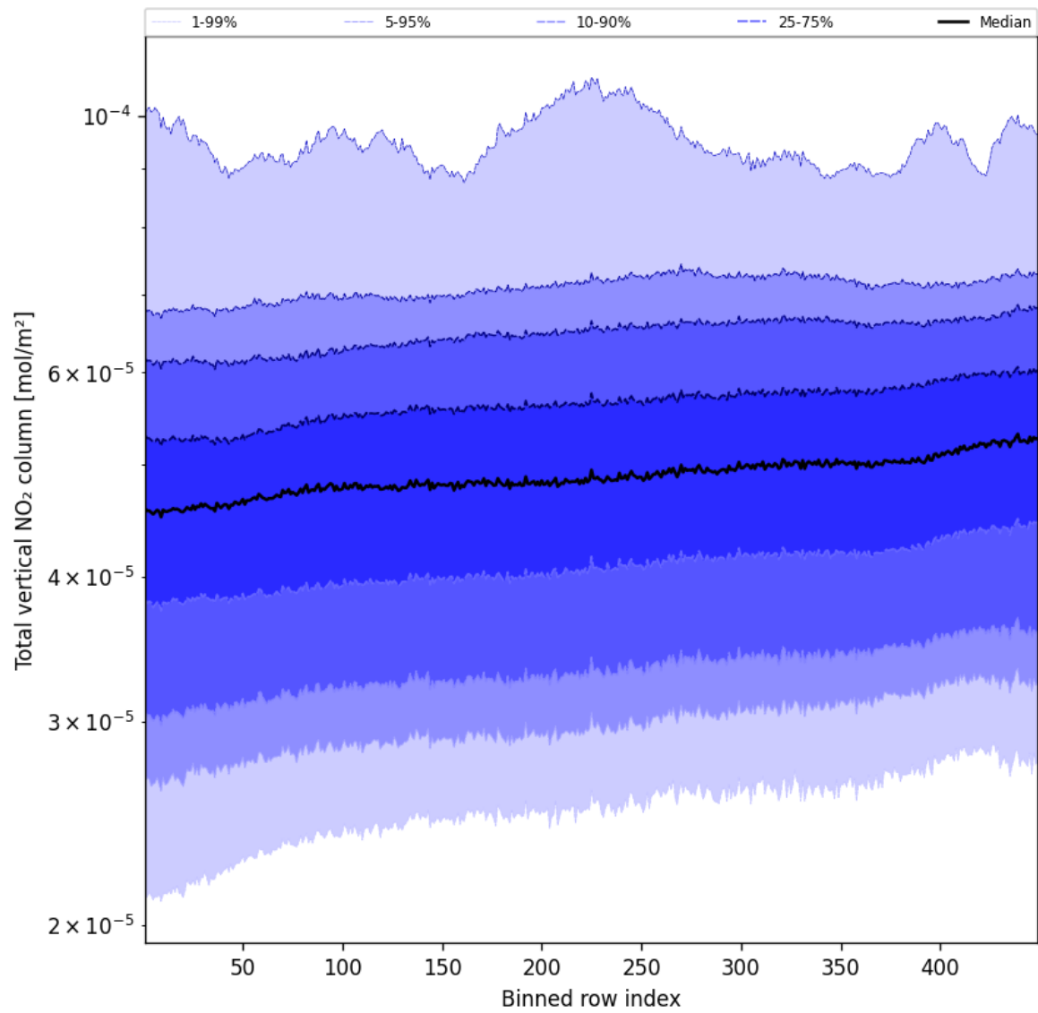
Figure 55: Along track statistics of “Total vertical NO 2 column” for 2025-04-12 to 2025-04-13
