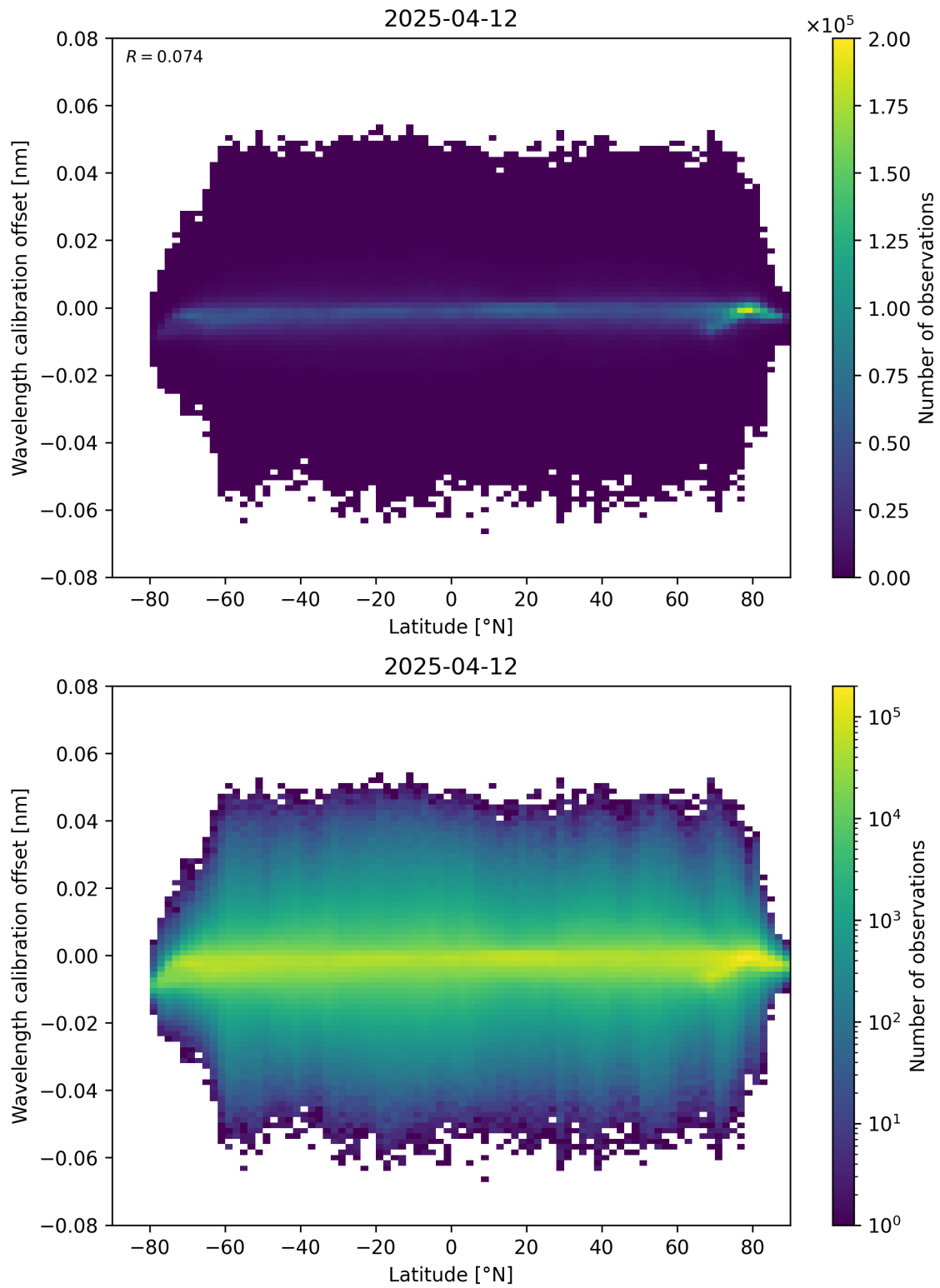
Figure 95: Scatter density plot of “Latitude” against “Wavelength calibration offset” for 2025-04-12 to 2025-04-13.
