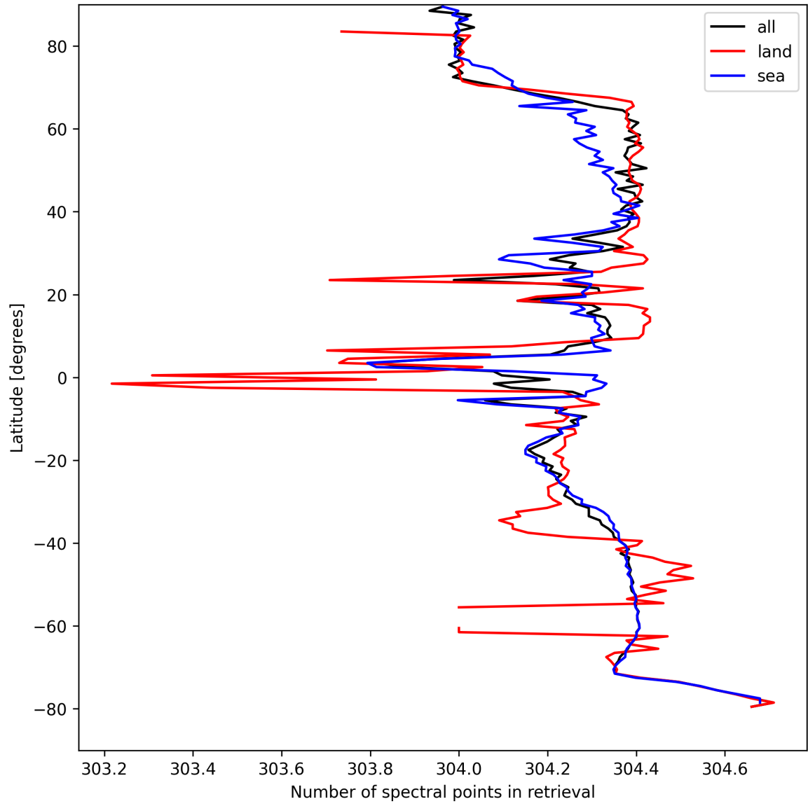
Figure 16: Zonal average of “Number of spectral points in retrieval” for 2025-04-12 to 2025-04-13.
