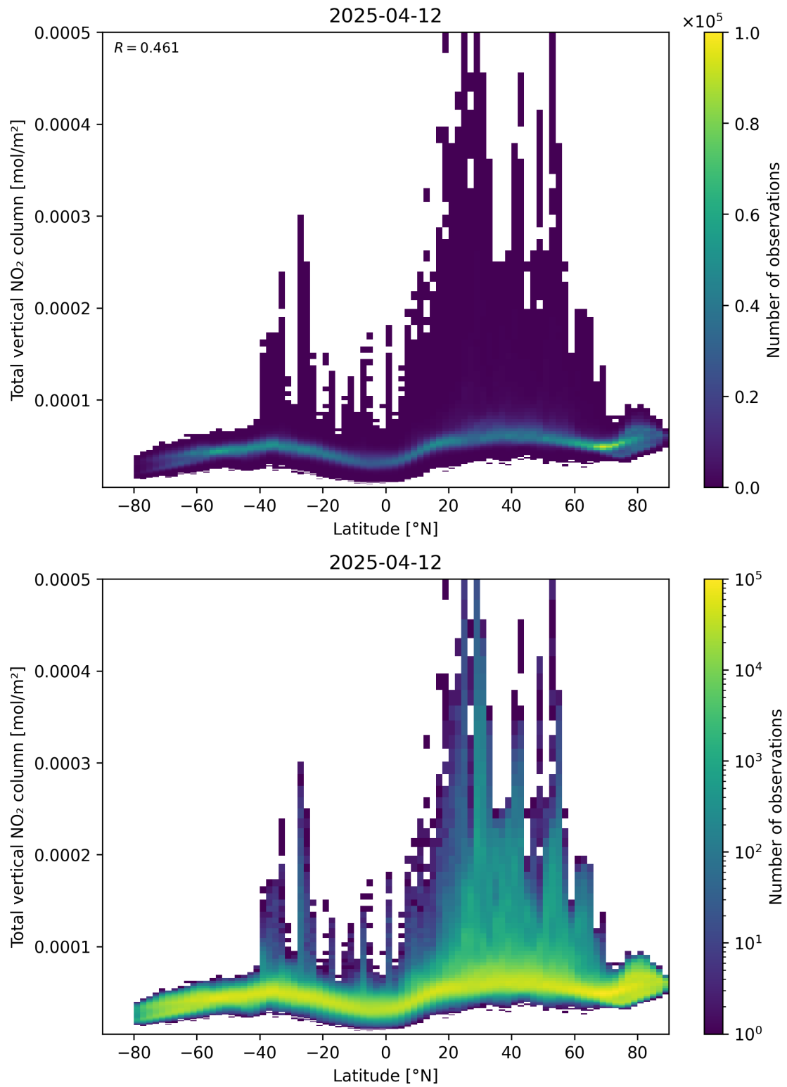
Figure 90: Scatter density plot of “Latitude” against “Total vertical NO 2 column” for 2025-04-12 to 2025-04-13.
