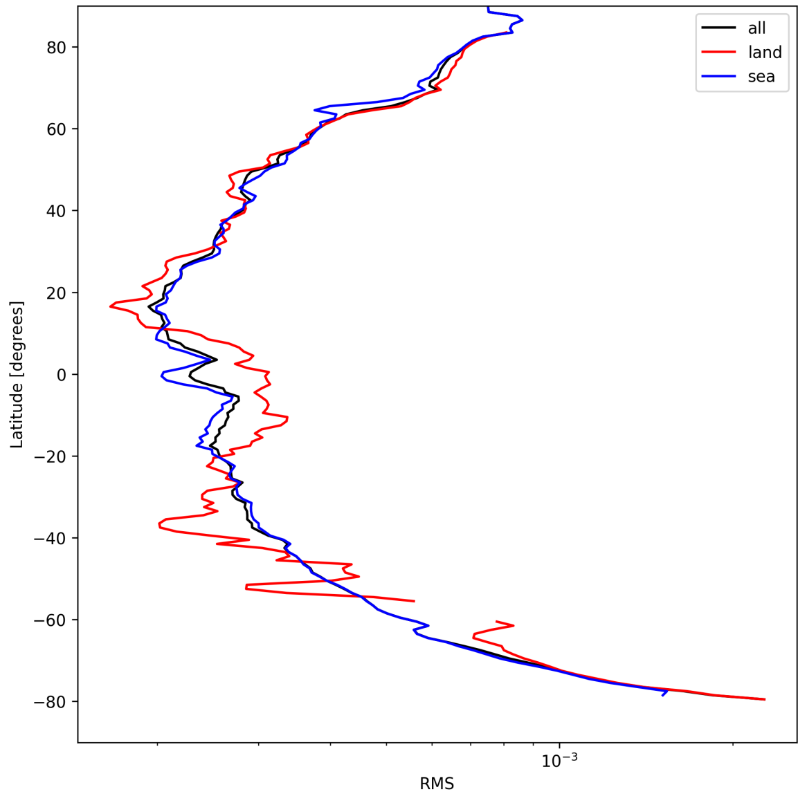
Figure 26: Zonal average of “RMS” for 2025-04-12 to 2025-04-13.
