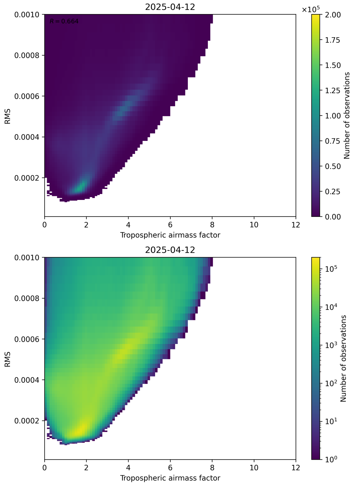
Figure 79: Scatter density plot of “Tropospheric airmass factor” against “RMS” for 2025-04-12 to 2025-04-13.
