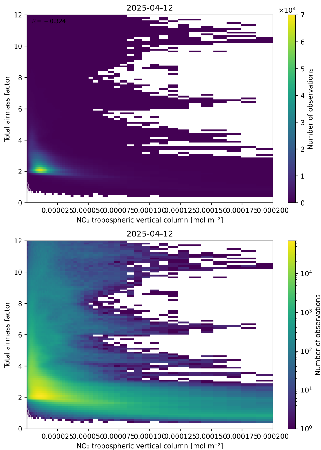
Figure 122: Scatter density plot of “NO 2 tropospheric vertical column” against “Total airmass factor” for 2025-04-12 to 2025-04-13.
