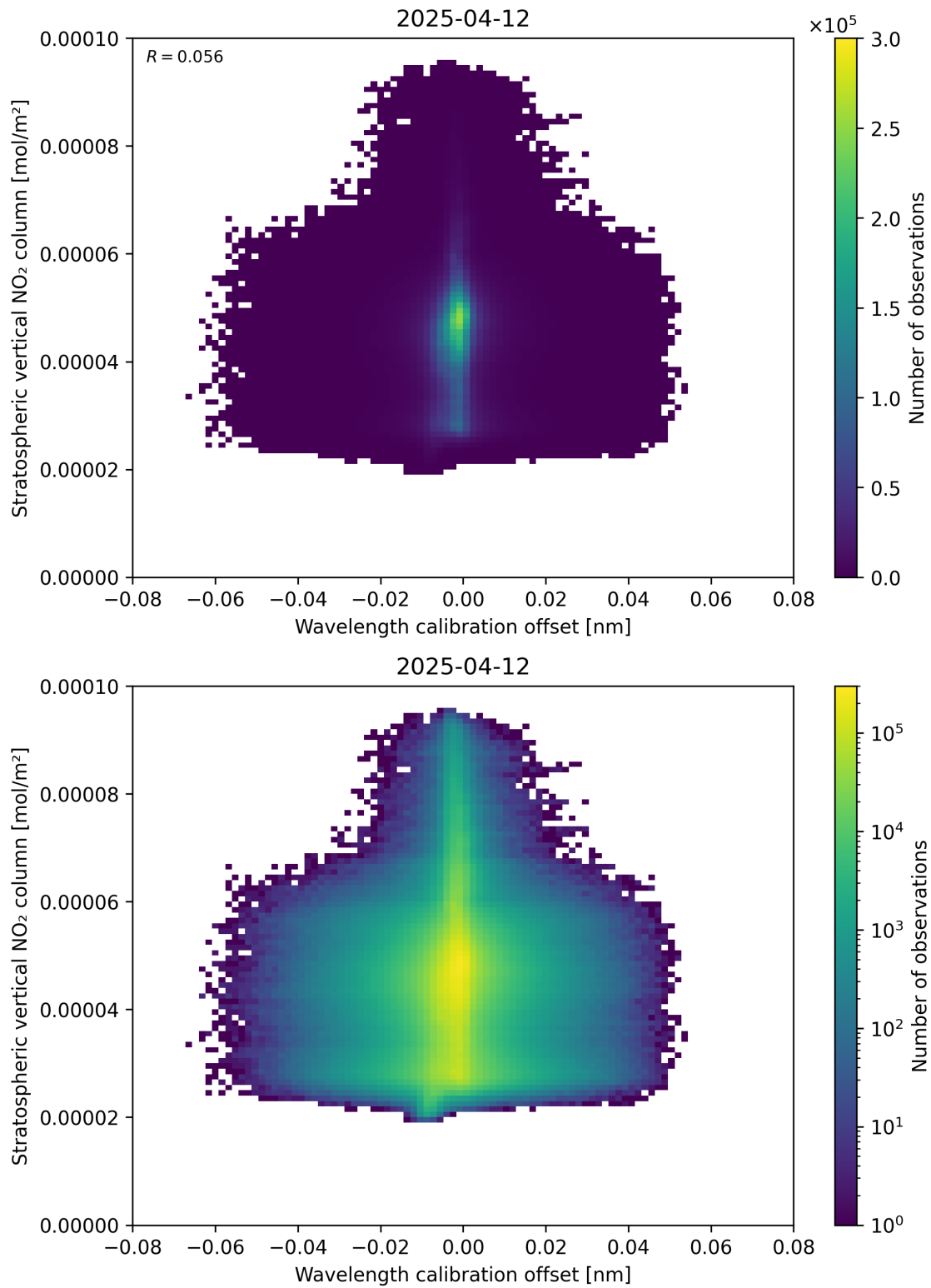
Figure 176: Scatter density plot of “Wavelength calibration offset” against “Stratospheric vertical NO 2 column” for 2025-04-12 to 2025-04-13.
