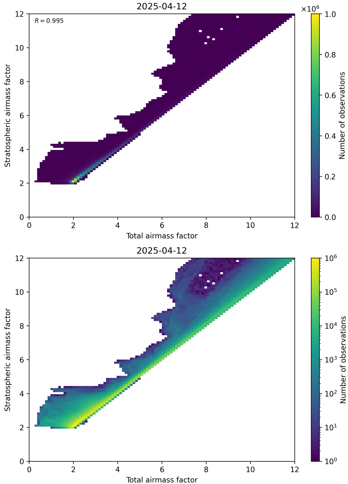
Figure 62: Scatter density plot of “Total airmass factor” against “Stratospheric airmass factor” for 2025-04-12 to 2025-04-13.
