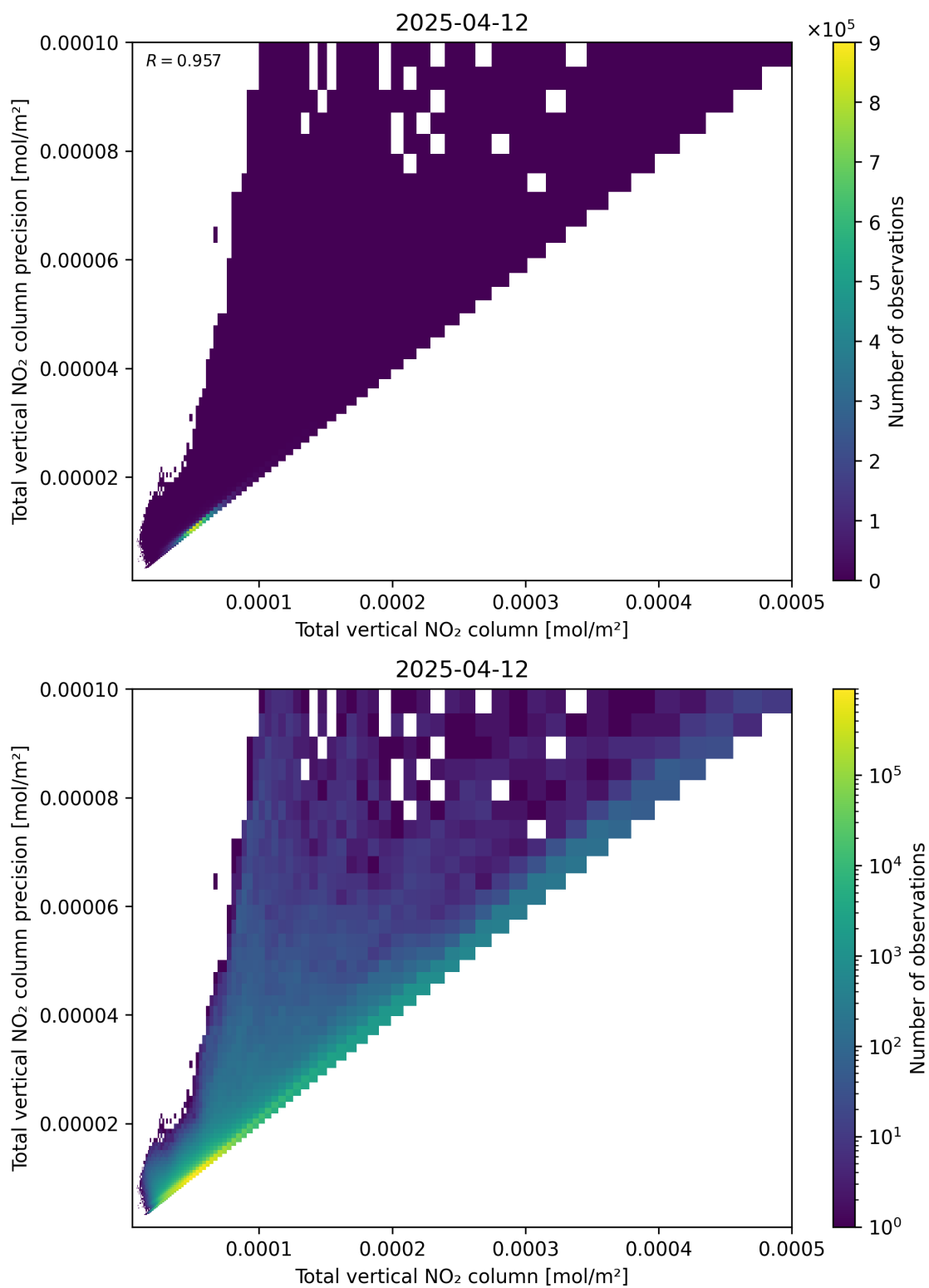
Figure 114: Scatter density plot of “Total vertical NO 2 column” against “Total vertical NO 2 column precision” for 2025-04-12 to 2025-04-13.
