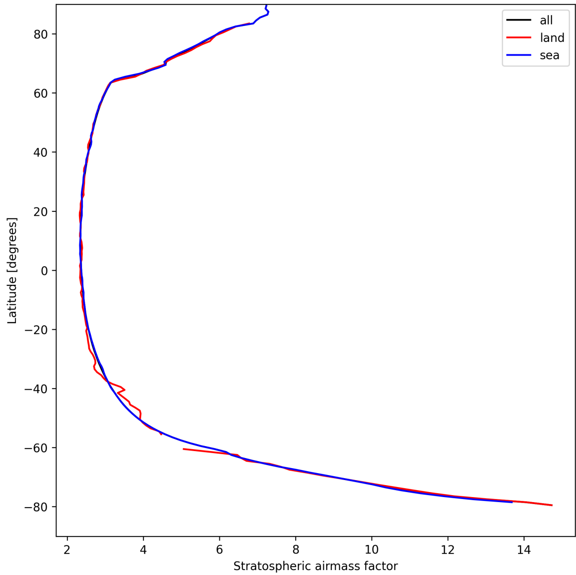
Figure 27: Zonal average of “Stratospheric air mass factor” for 2025-04-12 to 2025-04-13.
