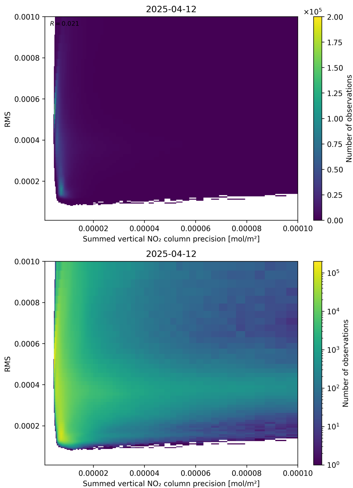
Figure 108: Scatter density plot of “Summed vertical NO 2 column precision” against “RMS” for 2025-04-12 to 2025-04-13.
