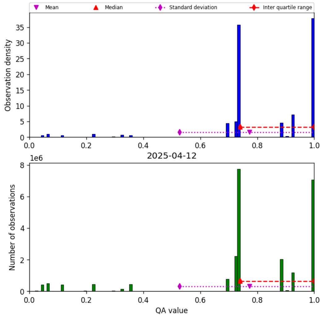
Figure 28: Histogram of “QA value” for 2025-04-12 to 2025-04-13
