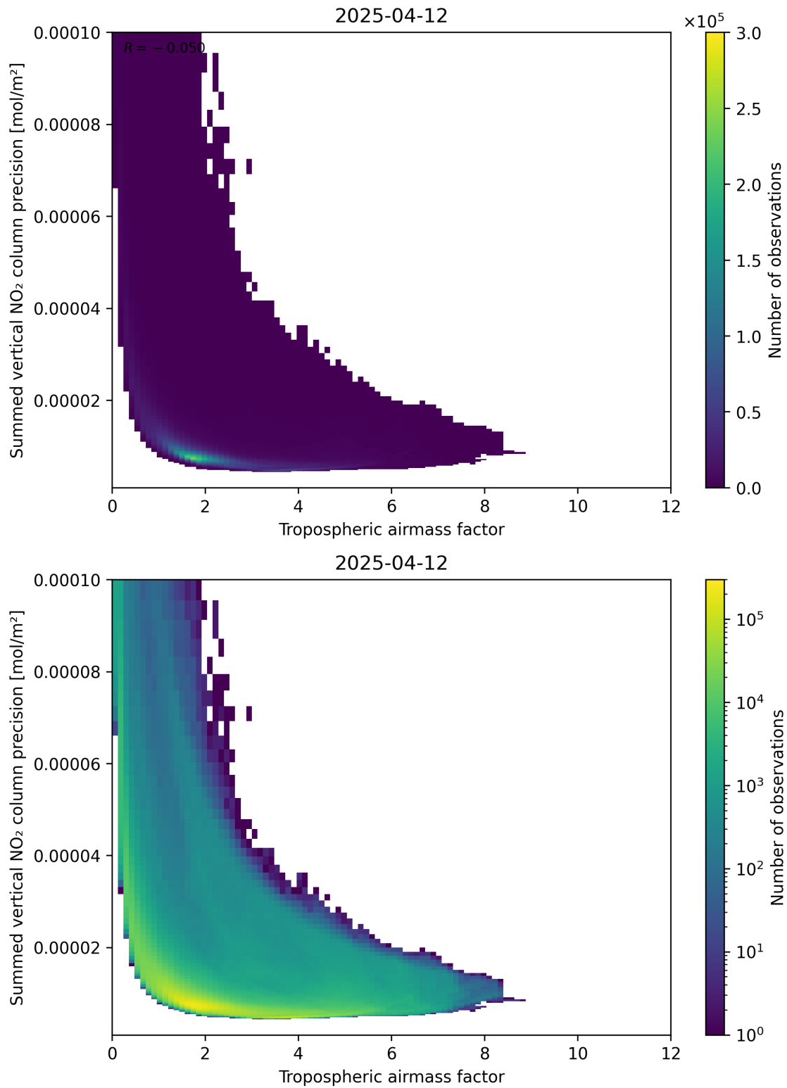
Figure 76: Scatter density plot of “Tropospheric air mass factor” against “Summed vertical NO 2 column precision” for 2025-04-12 to 2025-04-13.
