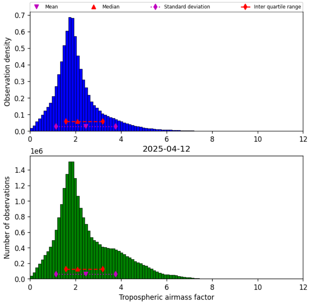
Figure 31: Histogram of “Tropospheric airmass factor” for 2025-04-12 to 2025-04-13
