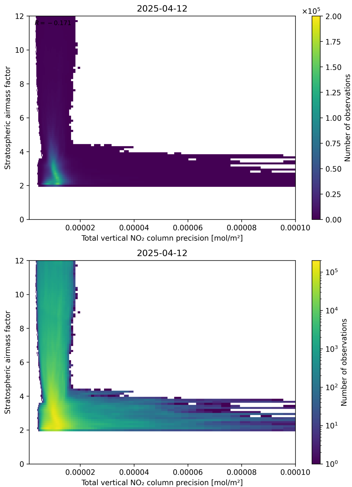
Figure 115: Scatter density plot of “Total vertical NO 2 column precision” against “Stratospheric air mass factor” for 2025-04-12 to 2025-04-13.
