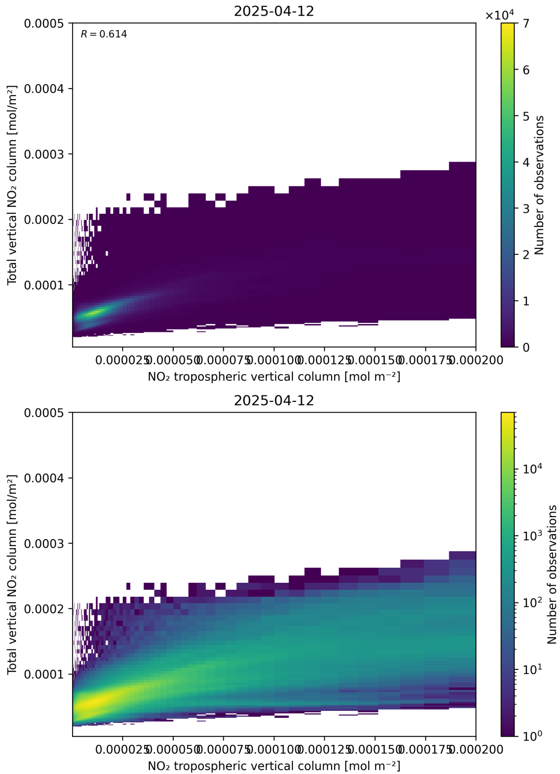
Figure 128: Scatter density plot of “NO 2 tropospheric vertical column” against “Total vertical NO 2 column” for 2025-04-12 to 2025-04-13.
