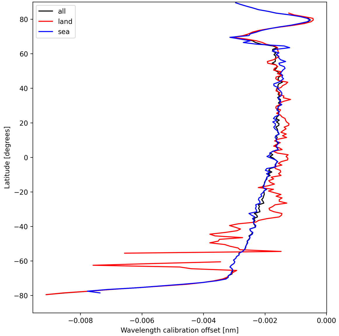
Figure 18: Zonal average of “Wavelength calibration offset” for 2025-04-12 to 2025-04-13.
