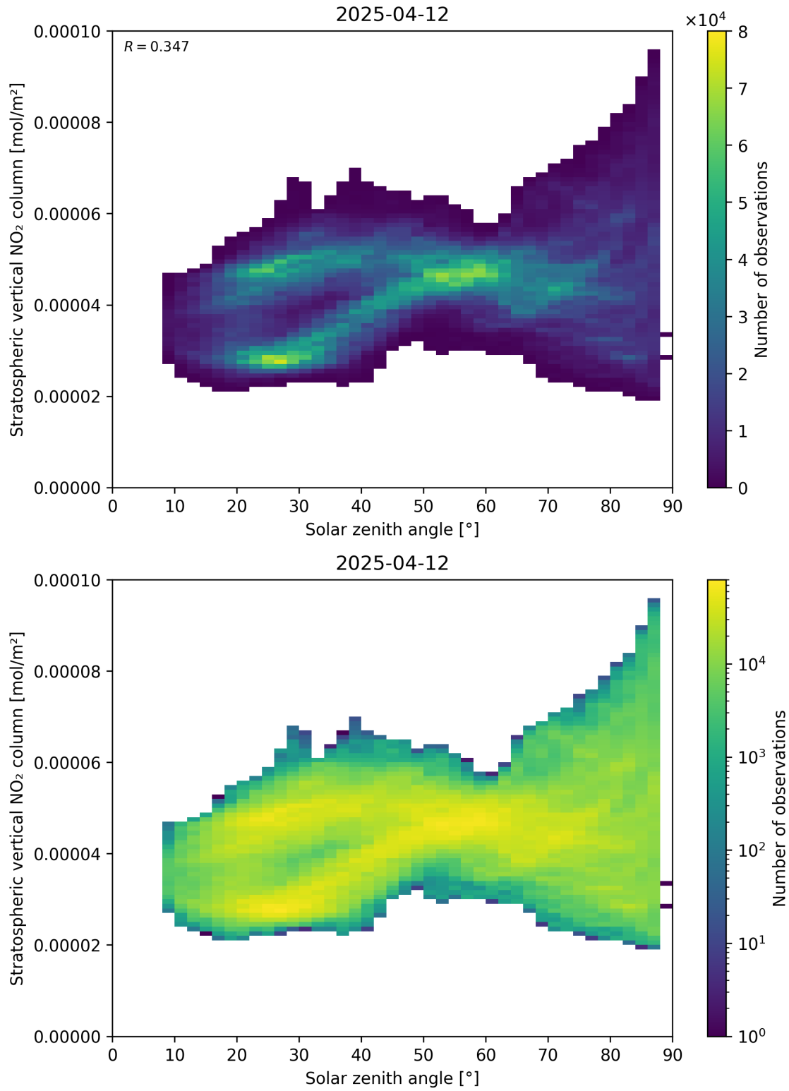
Figure 150: Scatter density plot of “Solar zenith angle” against “Stratospheric vertical NO 2 column” for 2025-04-12 to 2025-04-13.
