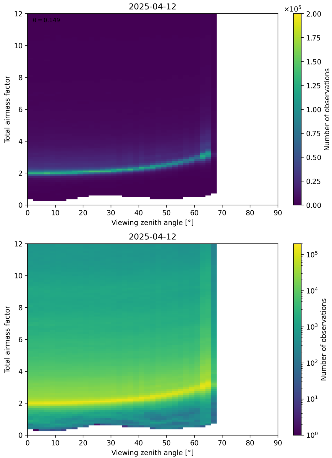
Figure 160: Scatter density plot of “Viewing zenith angle” against “Total airmass factor” for 2025-04-12 to 2025-04-13.
