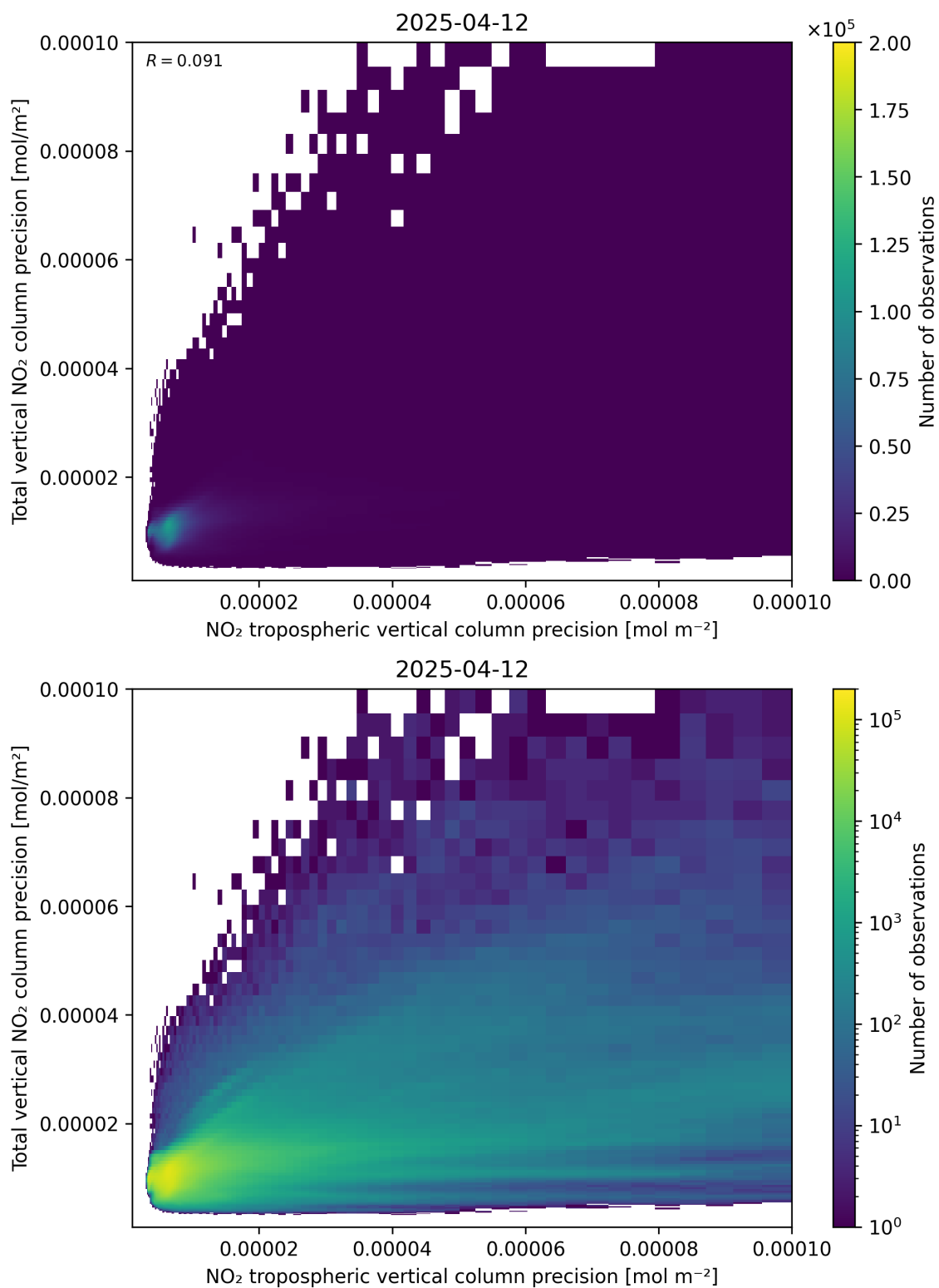
Figure 139: Scatter density plot of “NO 2 tropospheric vertical column precision” against “Total vertical NO 2 column precision” for 2025-04-12 to 2025-04-13.
