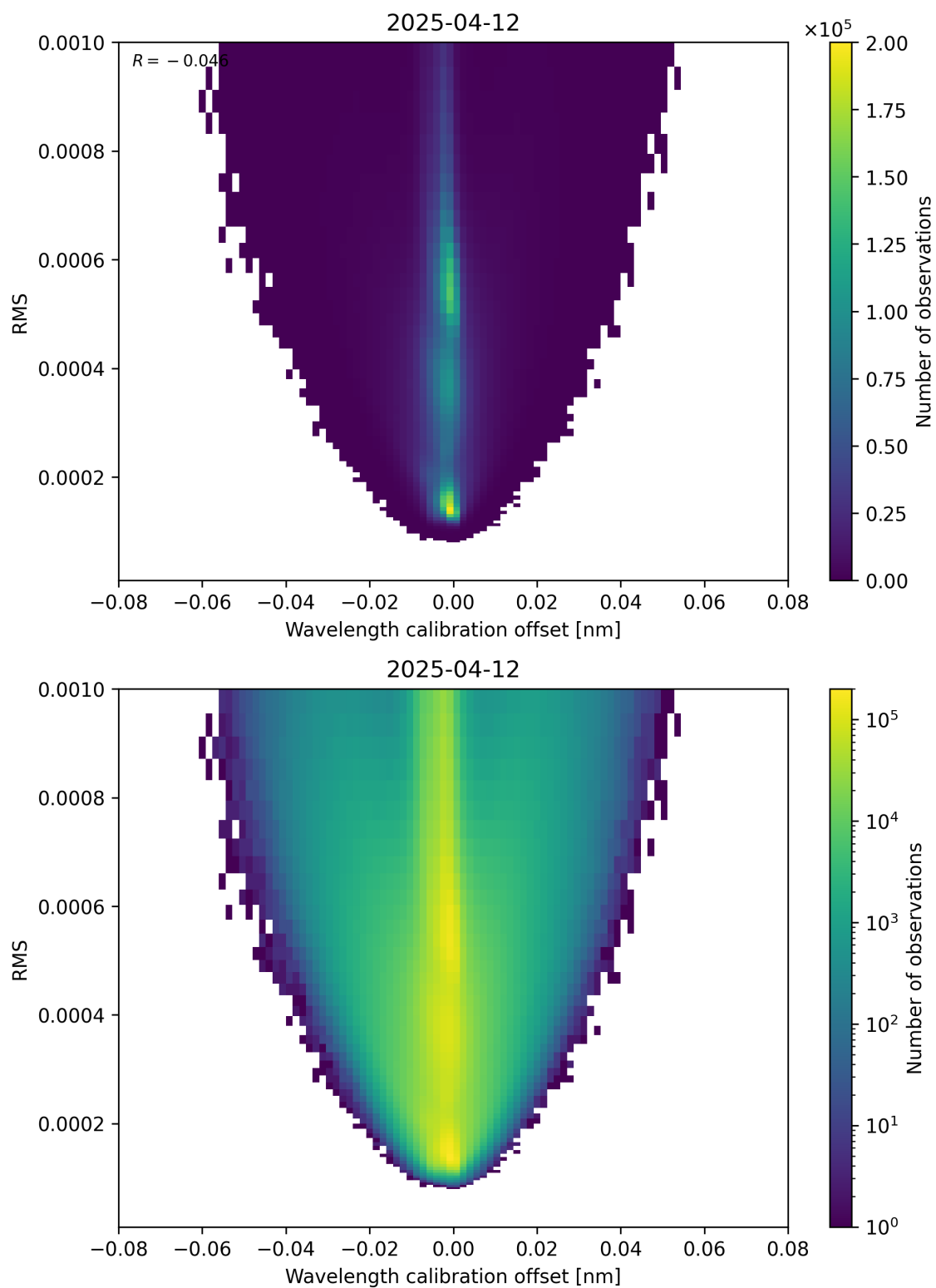
Figure 181: Scatter density plot of “Wavelength calibration offset” against “RMS” for 2025-04-12 to 2025-04-13.
