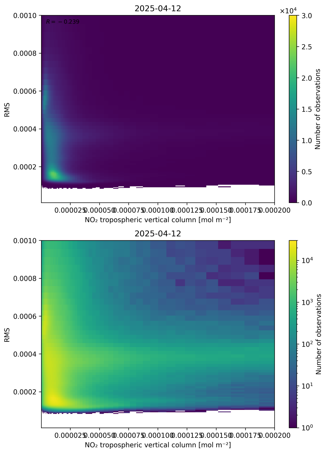
Figure 142: Scatter density plot of “NO 2 tropospheric vertical column” against “RMS” for 2025-04-12 to 2025-04-13.
