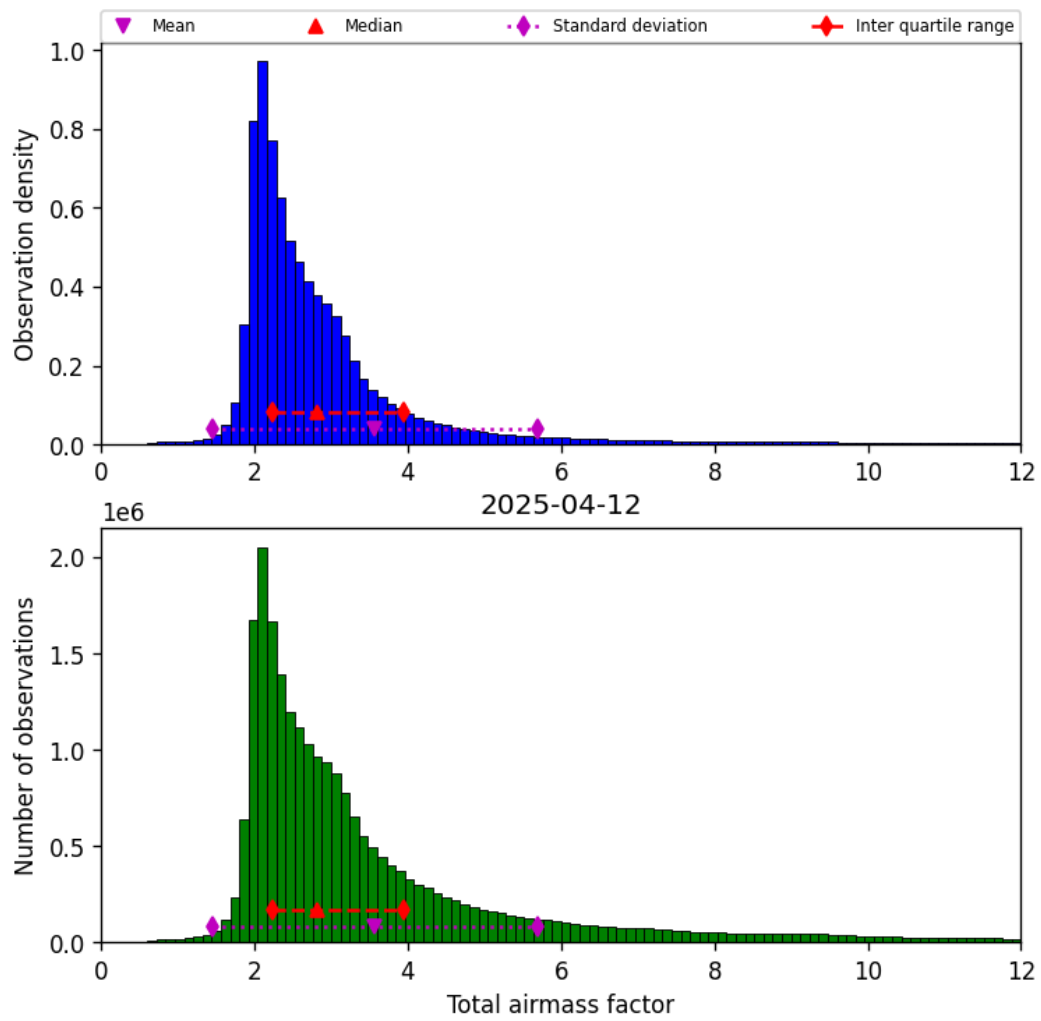
Figure 32: Histogram of “Total airmass factor” for 2025-04-12 to 2025-04-13
