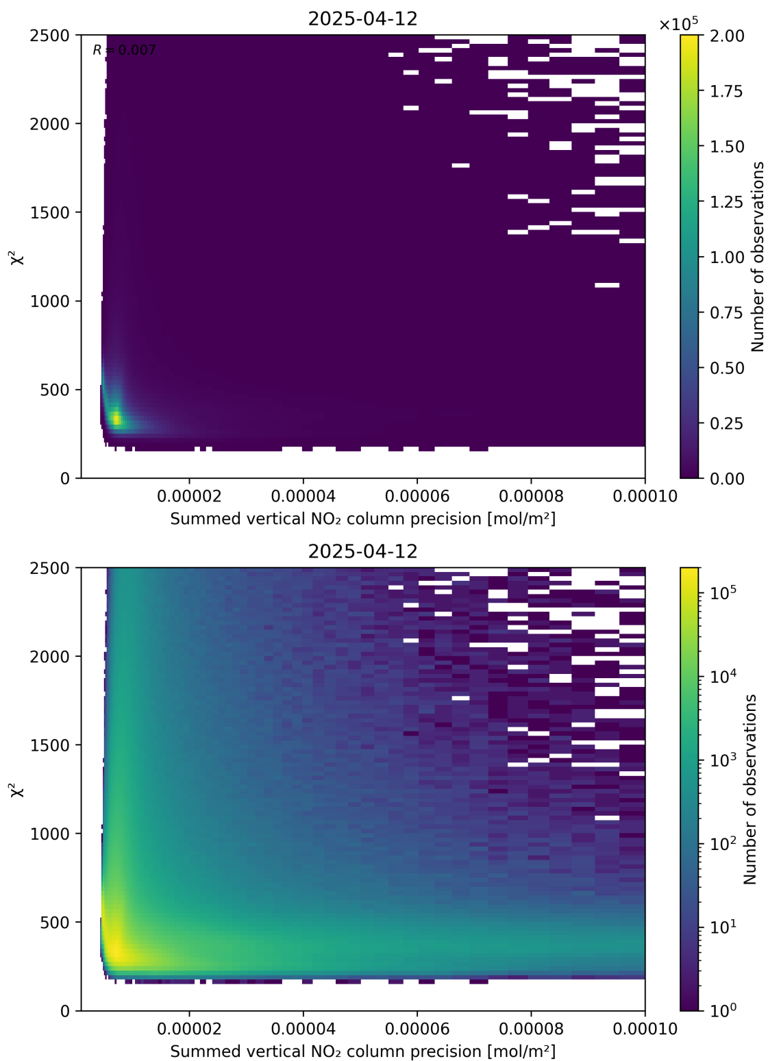
Figure 107: Scatter density plot of “Summed vertical NO 2 column precision” against “ \chi^2 ” for 2025-04-12 to 2025-04-13.
