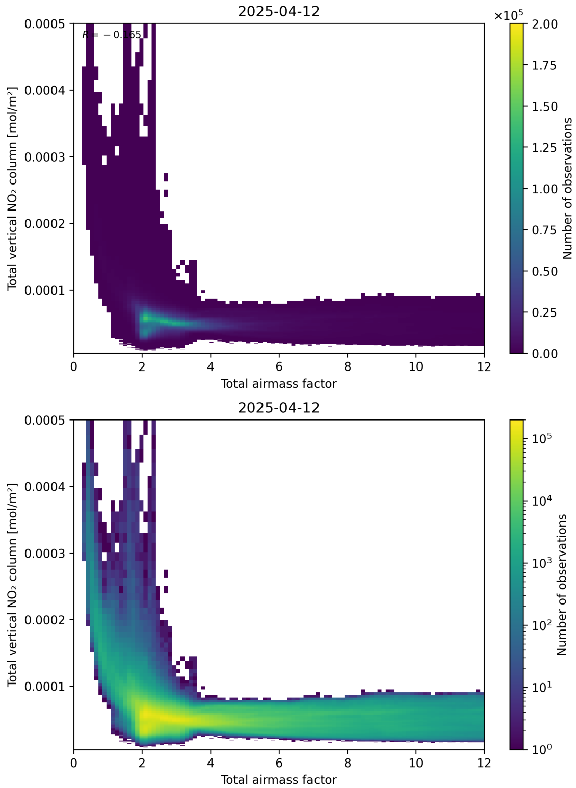
Figure 67: Scatter density plot of “Total airmass factor” against “Total vertical NO 2 column” for 2025-04-12 to 2025-04-13.
