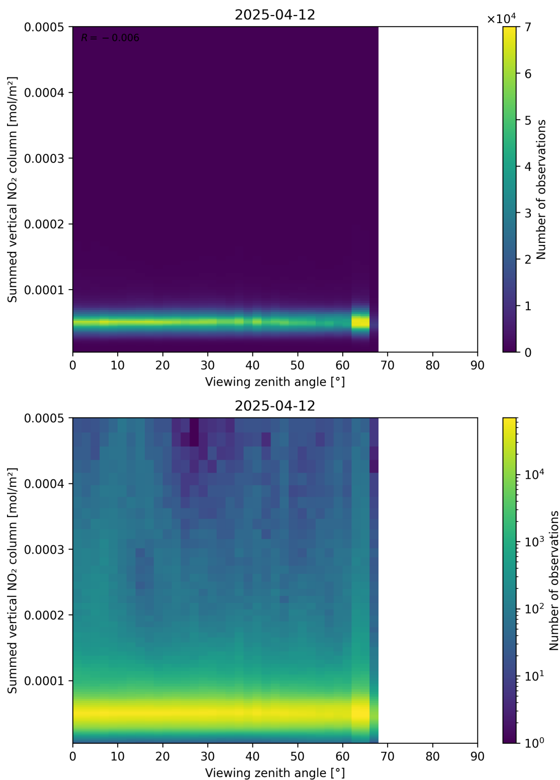
Figure 165: Scatter density plot of “Viewing zenith angle” against “Summed vertical NO 2 column” for 2025-04-12 to 2025-04-13.
