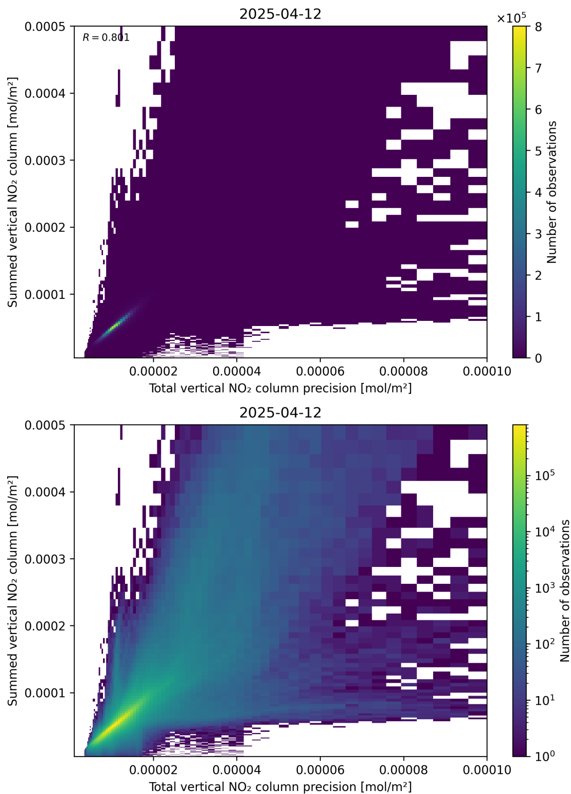
Figure 117: Scatter density plot of “Total vertical NO 2 column precision” against “Summed vertical NO 2 column” for 2025-04-12 to 2025-04-13.
