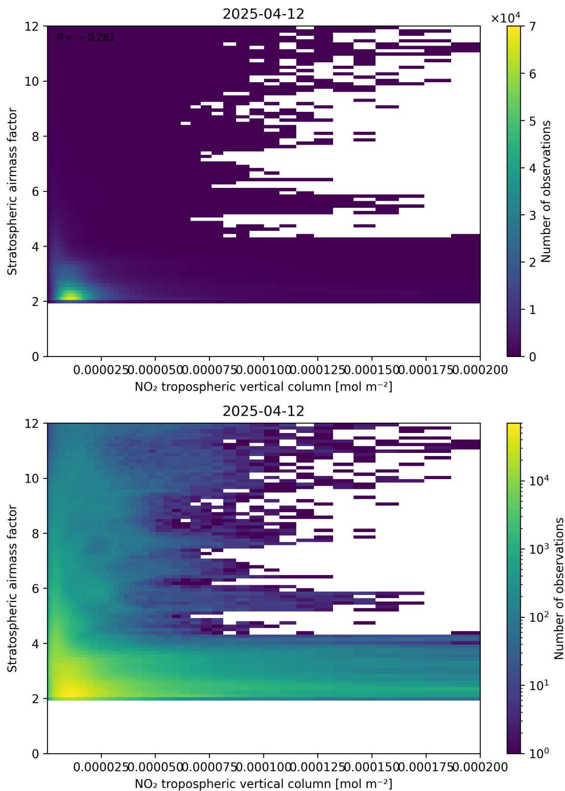
Figure 121: Scatter density plot of “NO 2 tropospheric vertical column” against “Stratospheric air mass factor” for 2025-04-12 to 2025-04-13.
