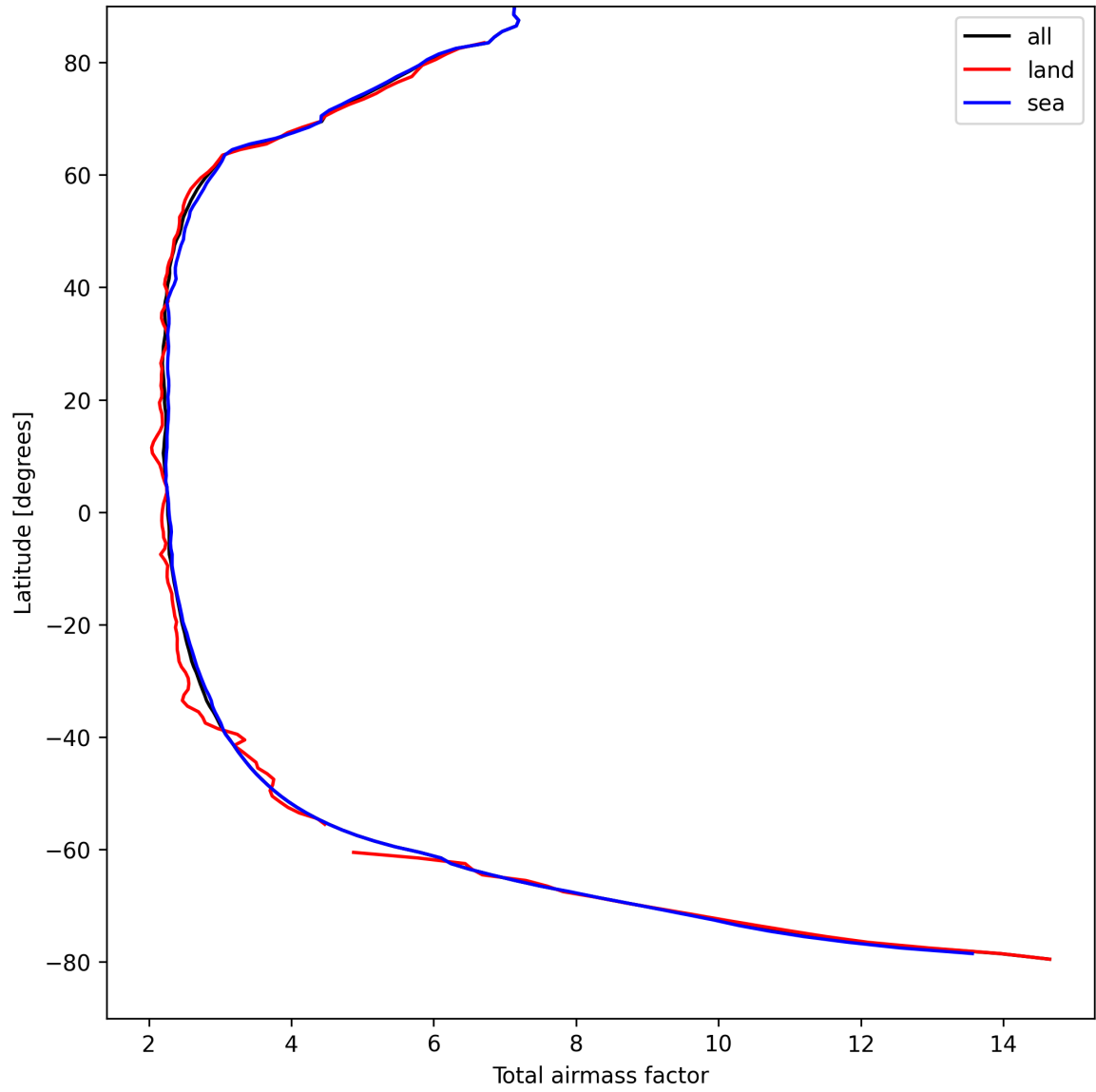
Figure 15: Zonal average of “Total airmass factor” for 2025-04-12 to 2025-04-13.
