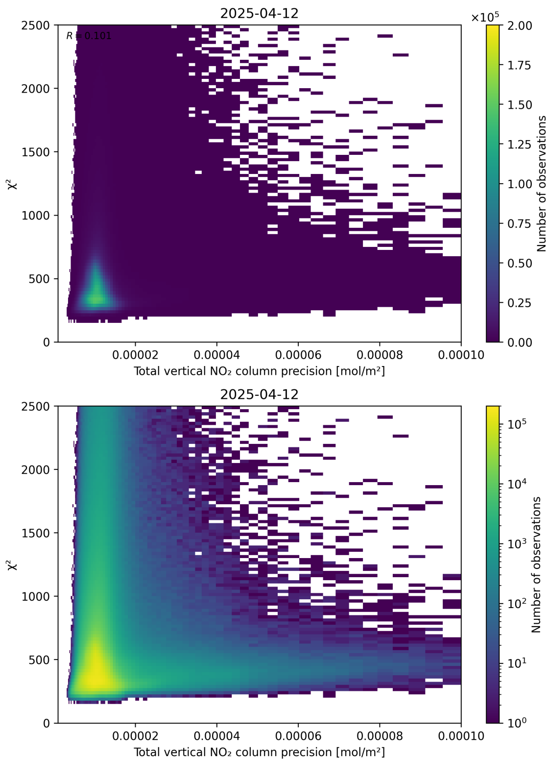
Figure 116: Scatter density plot of “Total vertical NO 2 column precision” against “ \chi^2 ” for 2025-04-12 to 2025-04-13.
