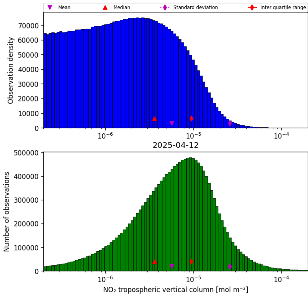
Figure 29: Histogram of “NO 2 tropospheric vertical column” for 2025-04-12 to 2025-04-13
