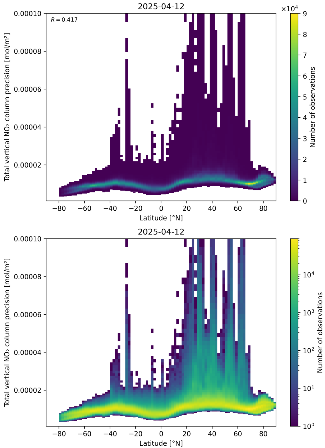
Figure 91: Scatter density plot of “Latitude” against “Total vertical NO 2 column precision” for 2025-04-12 to 2025-04-13.
