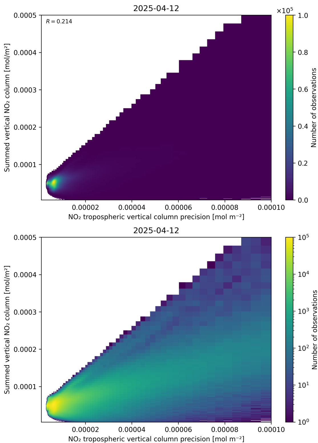
Figure 136: Scatter density plot of “NO 2 tropospheric vertical column precision” against “Summed vertical NO 2 column” for 2025-04-12 to 2025-04-13.
