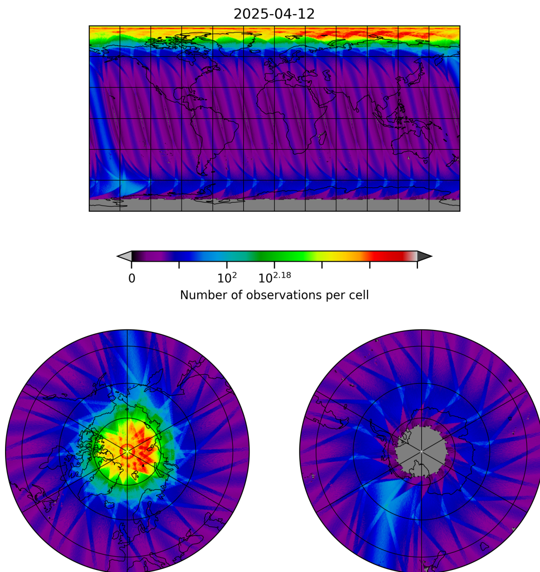
Figure 10: Map of the number of observations for 2025-04-12 to 2025-04-13
