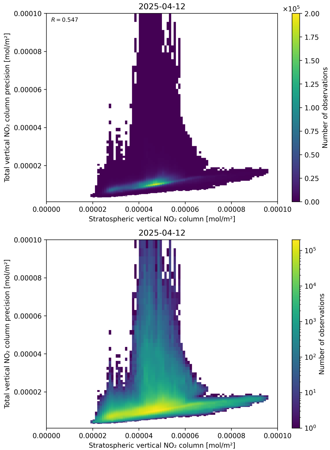
Figure 101: Scatter density plot of “Stratospheric vertical NO 2 column” against “Total vertical NO 2 column precision” for 2025-04-12 to 2025-04-13.
