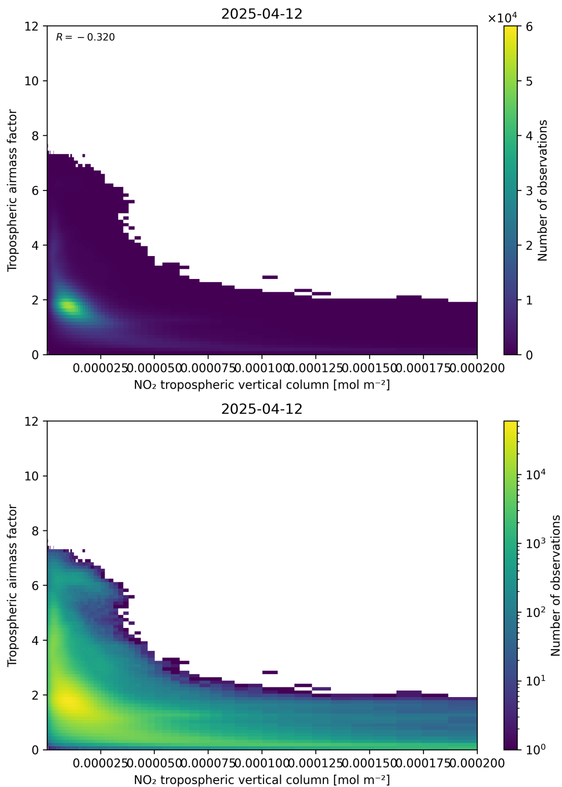
Figure 123: Scatter density plot of “NO 2 tropospheric vertical column” against “Tropospheric air mass factor” for 2025-04-12 to 2025-04-13.
