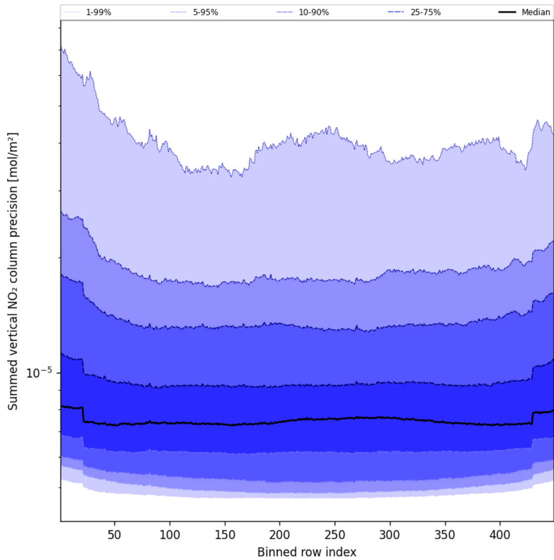
Figure 58: Along track statistics of “Summed vertical NO 2 column precision” for 2025-04-12 to 2025-04-13
