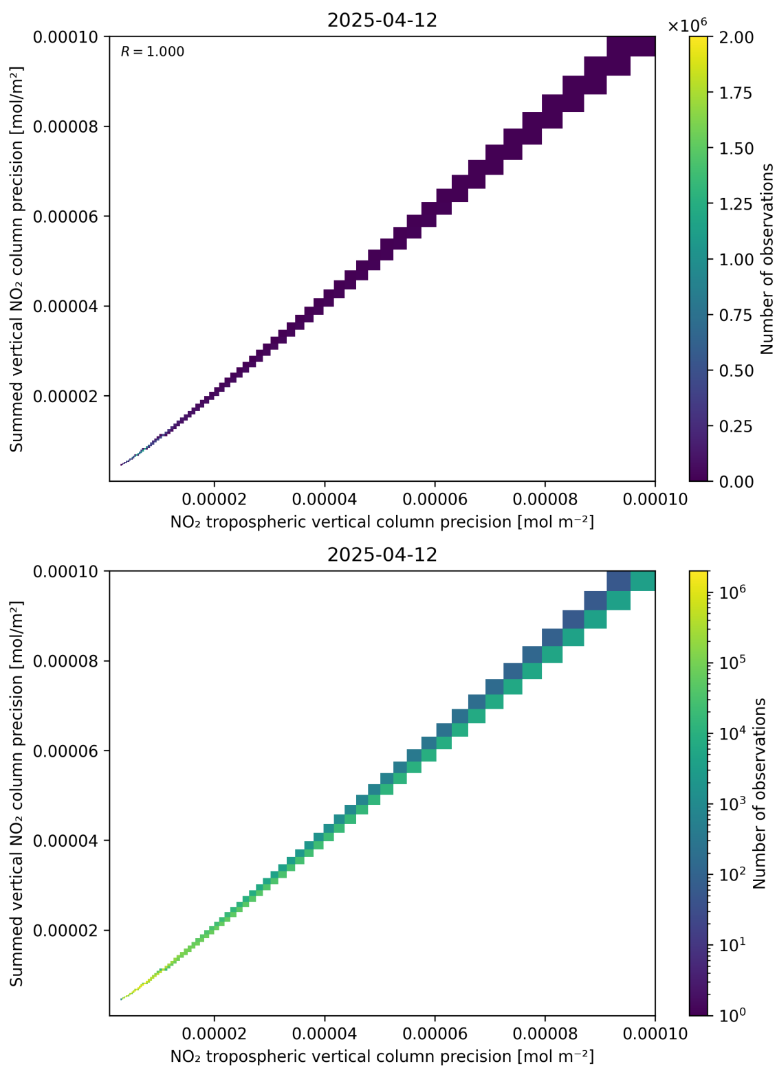
Figure 137: Scatter density plot of “NO 2 tropospheric vertical column precision” against “Summed vertical NO 2 column precision” for 2025-04-12 to 2025-04-13.
