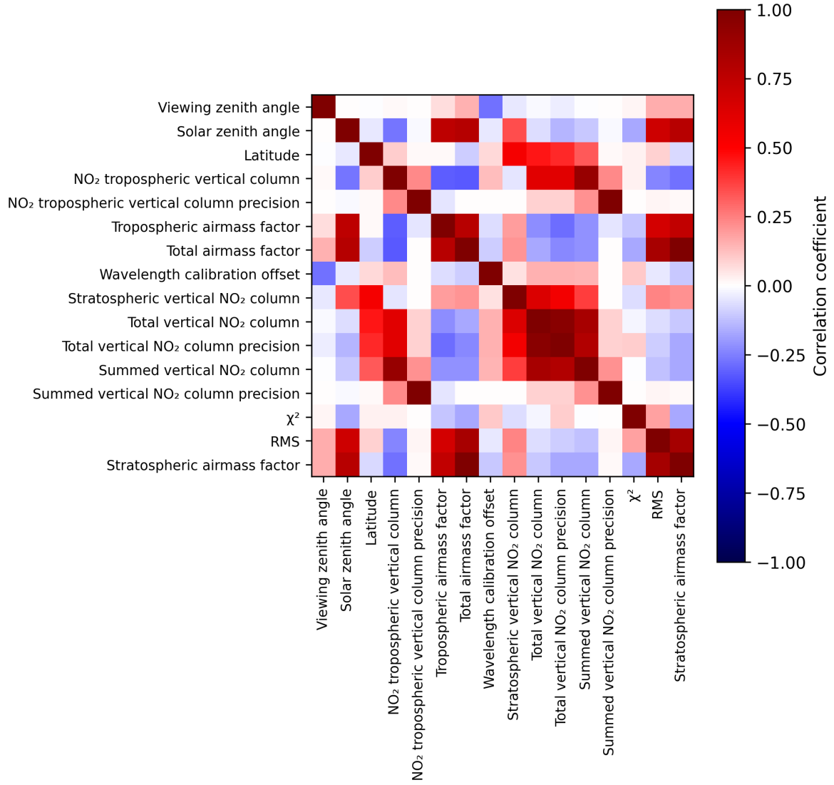
Figure 2: Map of correlation matrix for 2025-04-12 to 2025-04-13.
