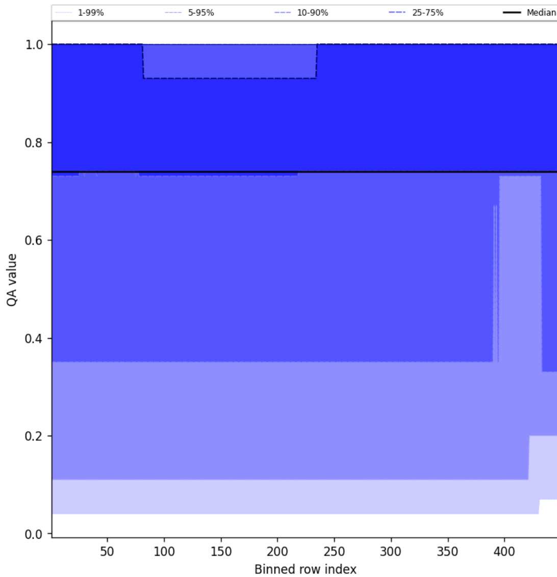
Figure 45: Along track statistics of “QA value” for 2025-04-12 to 2025-04-13
