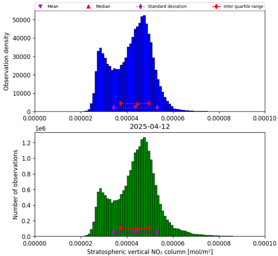
Figure 36: Histogram of “Stratospheric vertical NO 2 column” for 2025-04-12 to 2025-04-13
