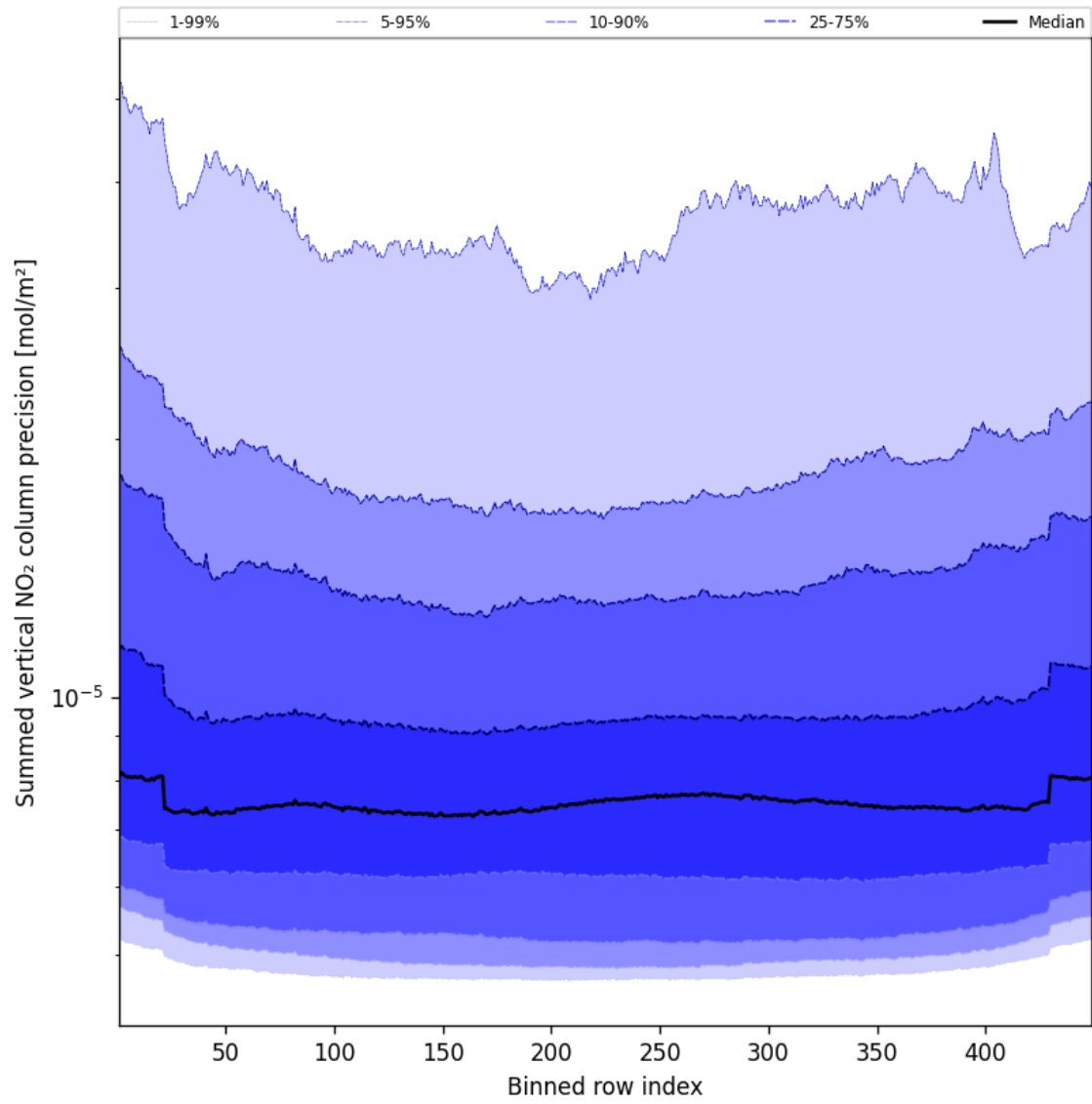
Figure 58: Along track statistics of “Summed vertical NO 2 column precision” for 2025-04-13 to 2025-04-14
