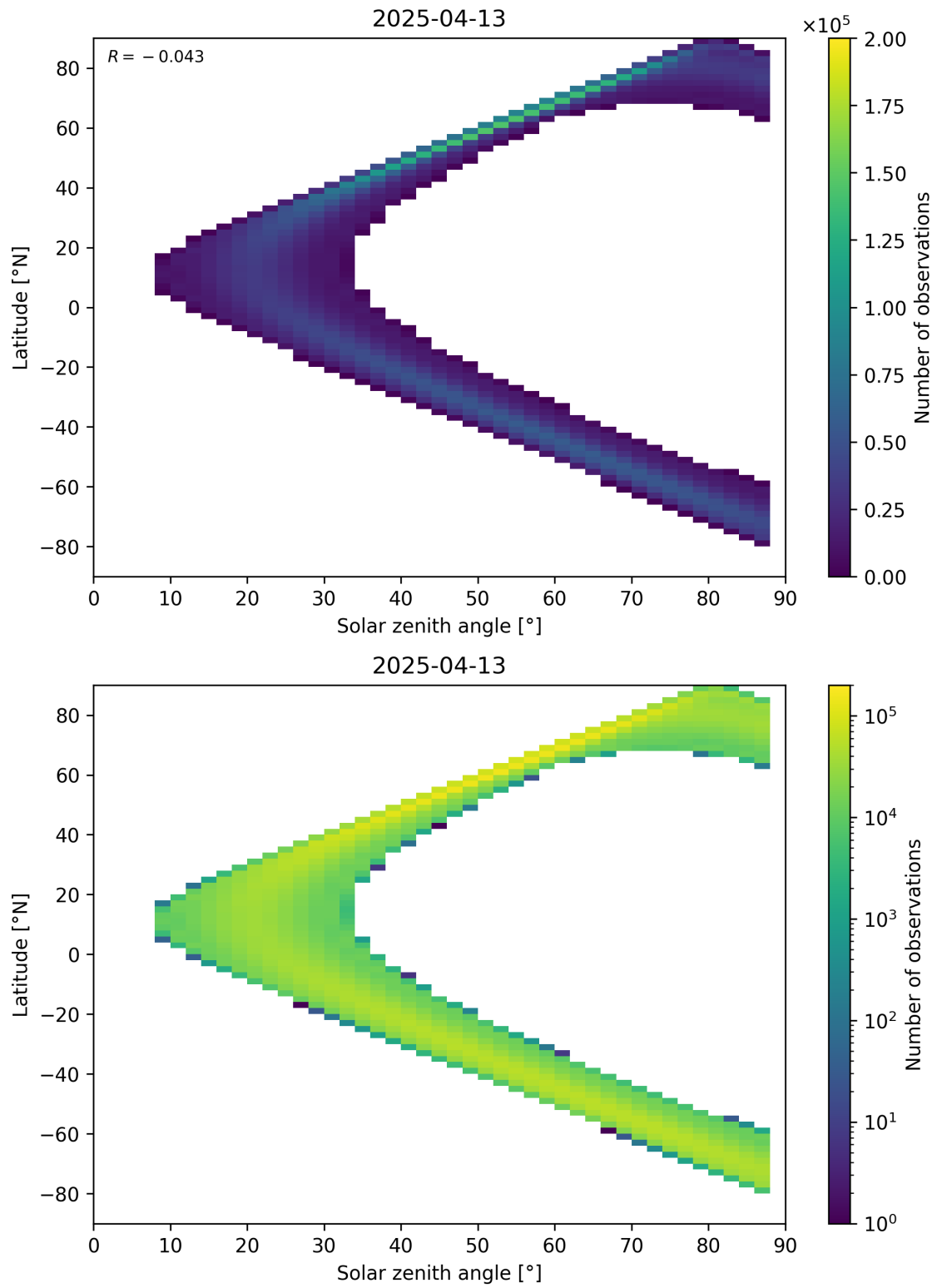
Figure 149: Scatter density plot of “Solar zenith angle” against “Latitude” for 2025-04-13 to 2025-04-14.
