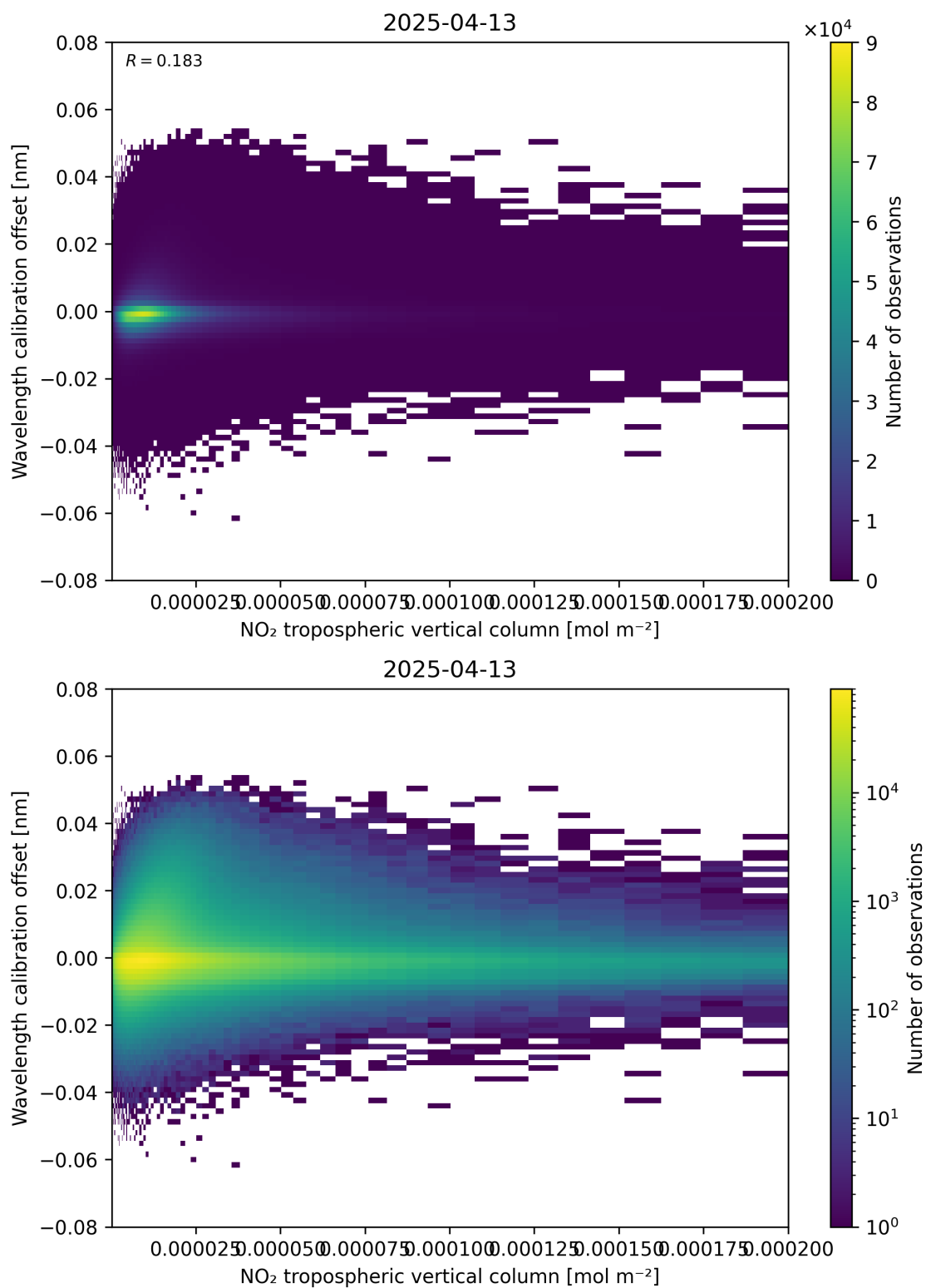
Figure 143: Scatter density plot of “NO 2 tropospheric vertical column” against “Wavelength calibration offset” for 2025-04-13 to 2025-04-14.
