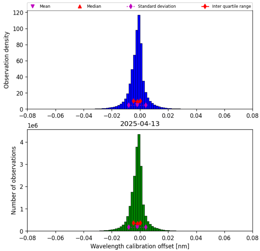
Figure 35: Histogram of “Wavelength calibration offset” for 2025-04-13 to 2025-04-14
