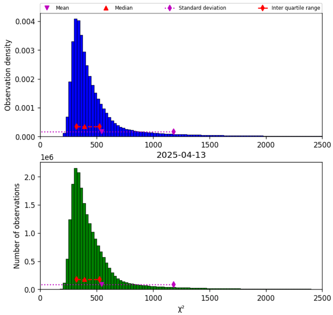
Figure 42: Histogram of “ \chi^2 ” for 2025-04-13 to 2025-04-14
