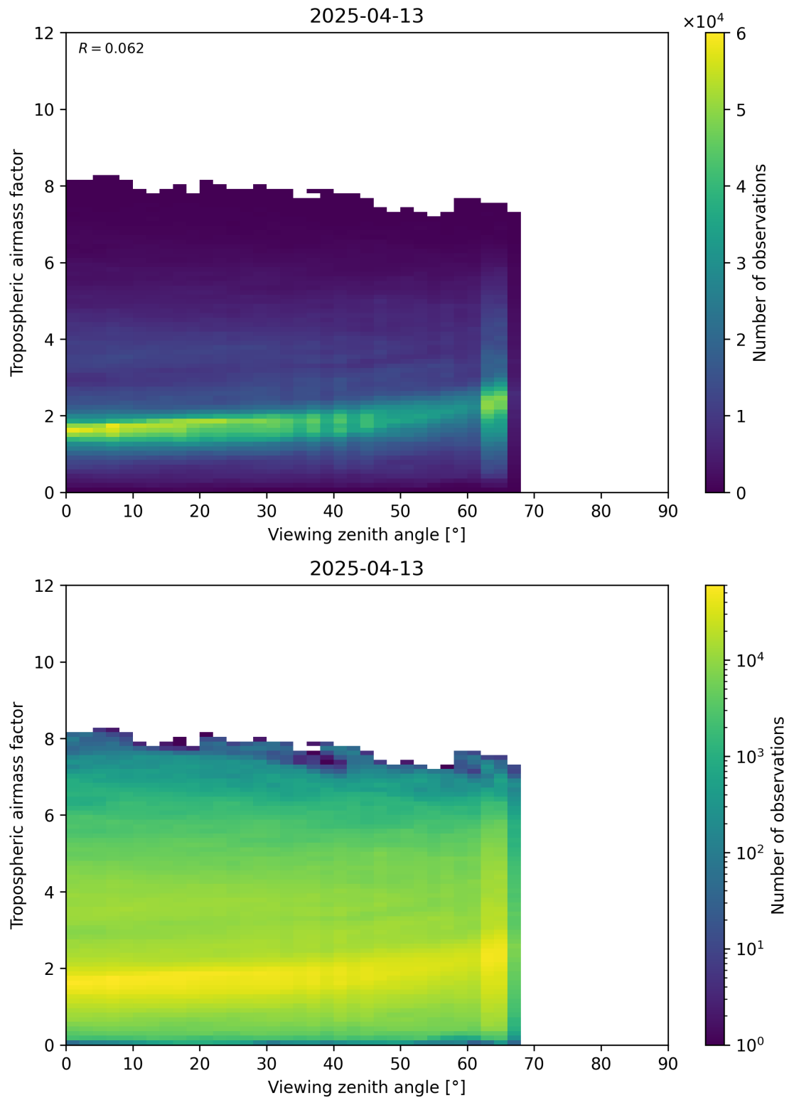
Figure 161: Scatter density plot of “Viewing zenith angle” against “Tropospheric airmass factor” for 2025-04-13 to 2025-04-14.
