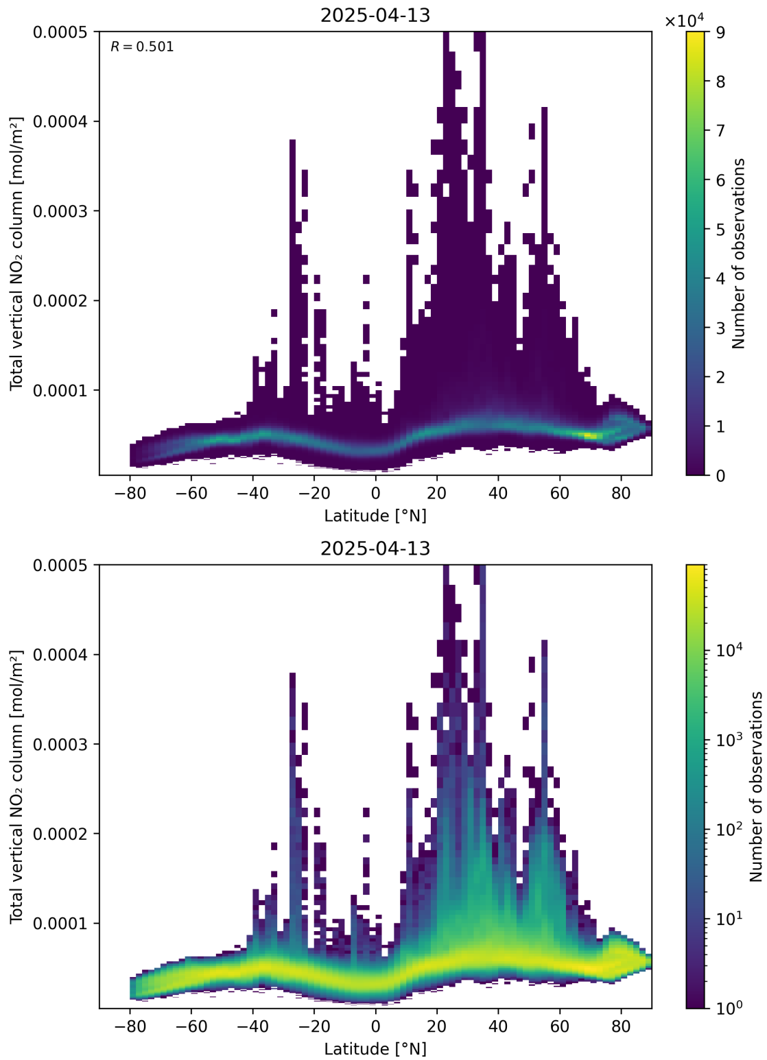
Figure 90: Scatter density plot of “Latitude” against “Total vertical NO 2 column” for 2025-04-13 to 2025-04-14.
