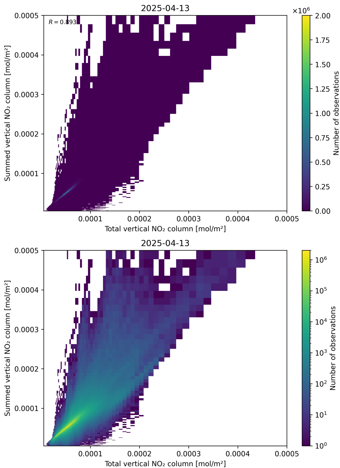
Figure 112: Scatter density plot of “Total vertical NO 2 column” against “Summed vertical NO 2 column” for 2025-04-13 to 2025-04-14.
