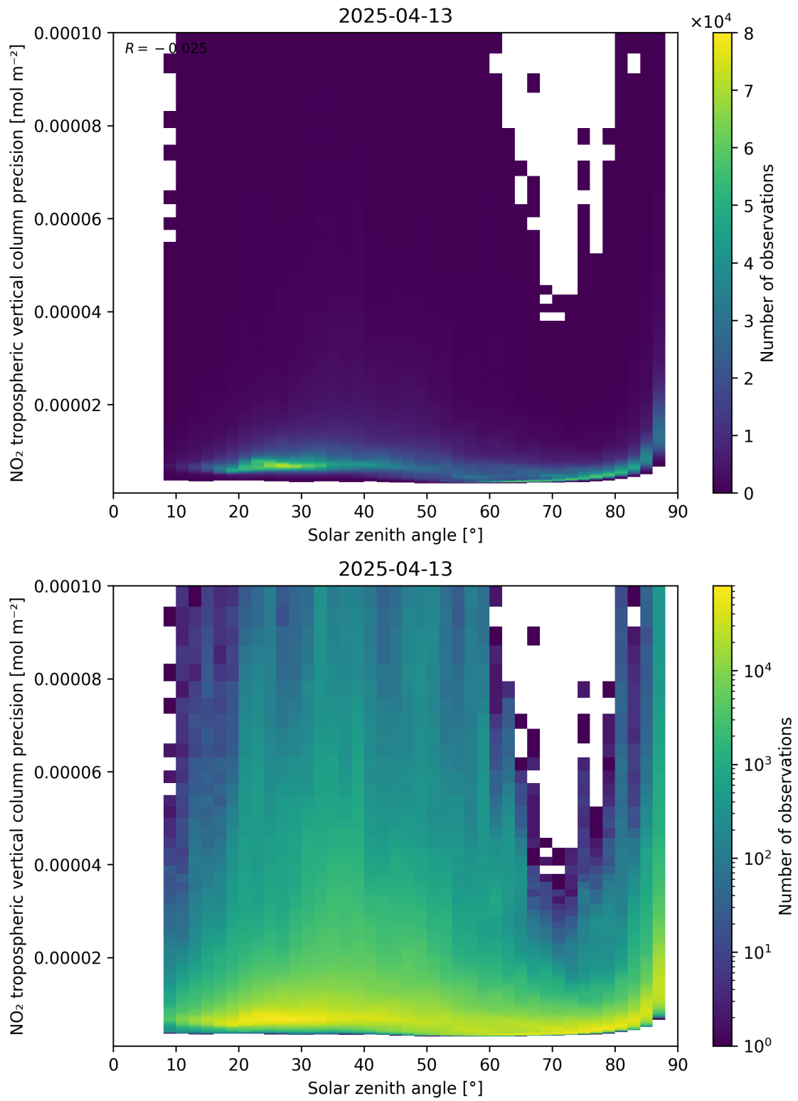
Figure 156: Scatter density plot of “Solar zenith angle” against “NO 2 tropospheric vertical column precision” for 2025-04-13 to 2025-04-14.
