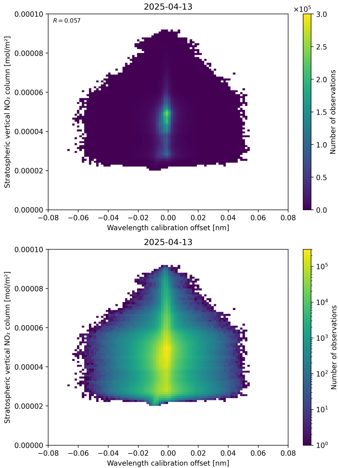
Figure 176: Scatter density plot of “Wavelength calibration offset” against “Stratospheric vertical NO 2 column” for 2025-04-13 to 2025-04-14.
