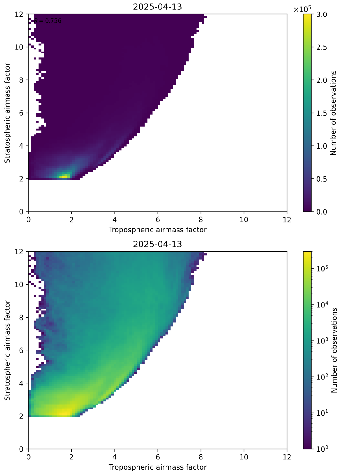
Figure 71: Scatter density plot of “Tropospheric airmass factor” against “Stratospheric airmass factor” for 2025-04-13 to 2025-04-14.
