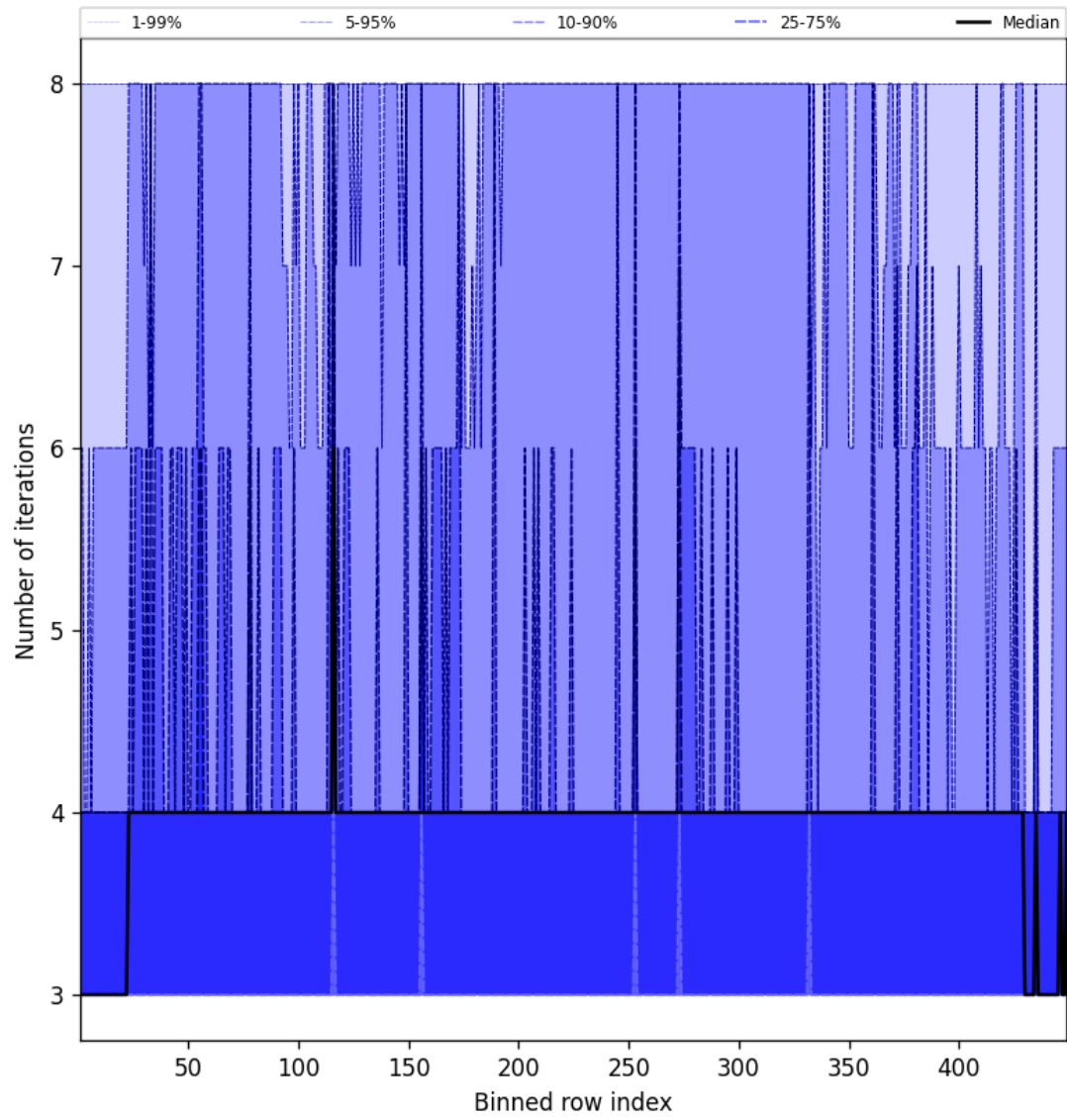
Figure 51: Along track statistics of “Number of iterations” for 2025-04-13 to 2025-04-14
