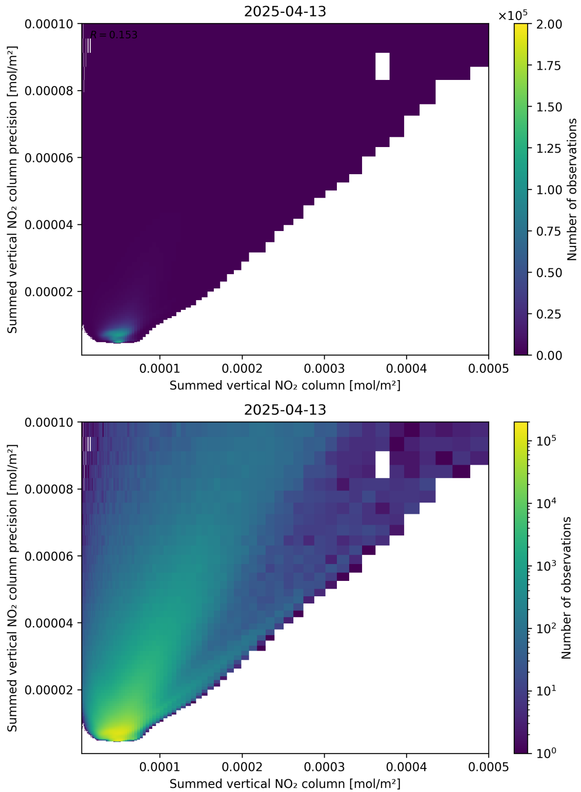
Figure 105: Scatter density plot of “Summed vertical NO 2 column” against “Summed vertical NO 2 column precision” for 2025-04-13 to 2025-04-14.
