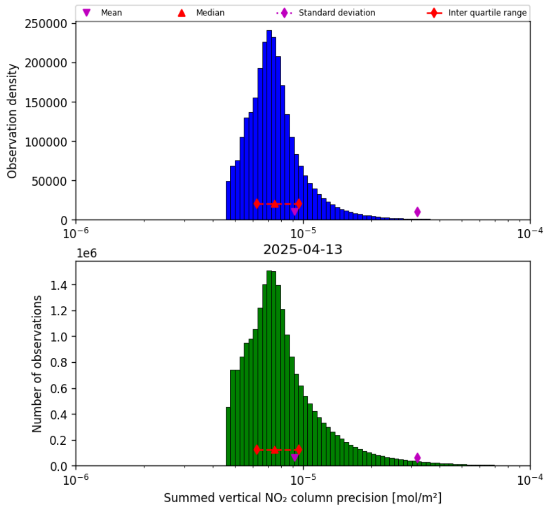
Figure 41: Histogram of "Summed vertical NO 2 column precision" for 2025-04-13 to 2025-04-14
