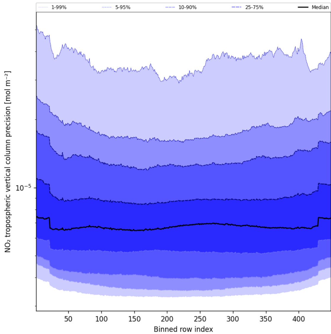
Figure 47: Along track statistics of “NO 2 tropospheric vertical column precision” for 2025-04-13 to 2025-04-14
