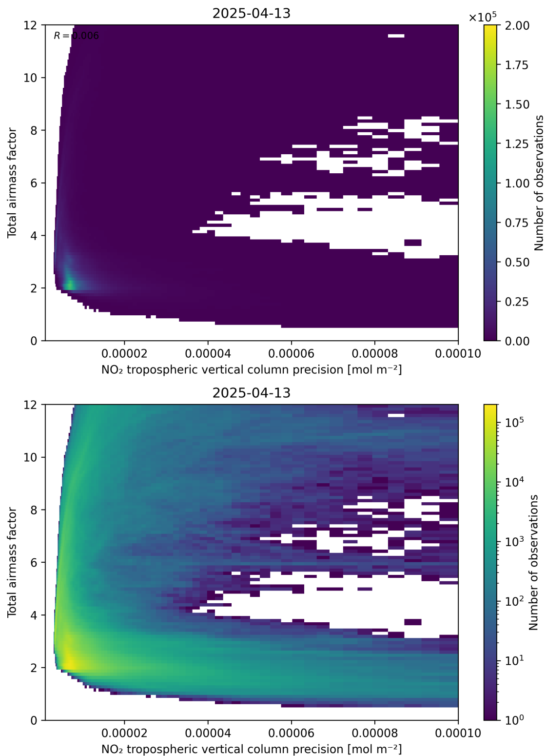
Figure 132: Scatter density plot of “NO 2 tropospheric vertical column precision” against “Total air mass factor” for 2025-04-13 to 2025-04-14.
