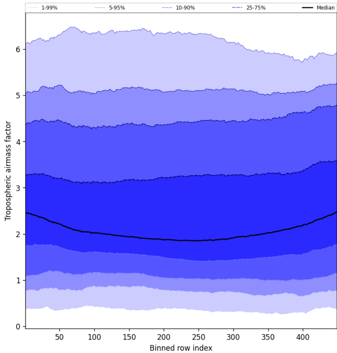
Figure 48: Along track statistics of “Tropospheric air mass factor” for 2025-04-13 to 2025-04-14
