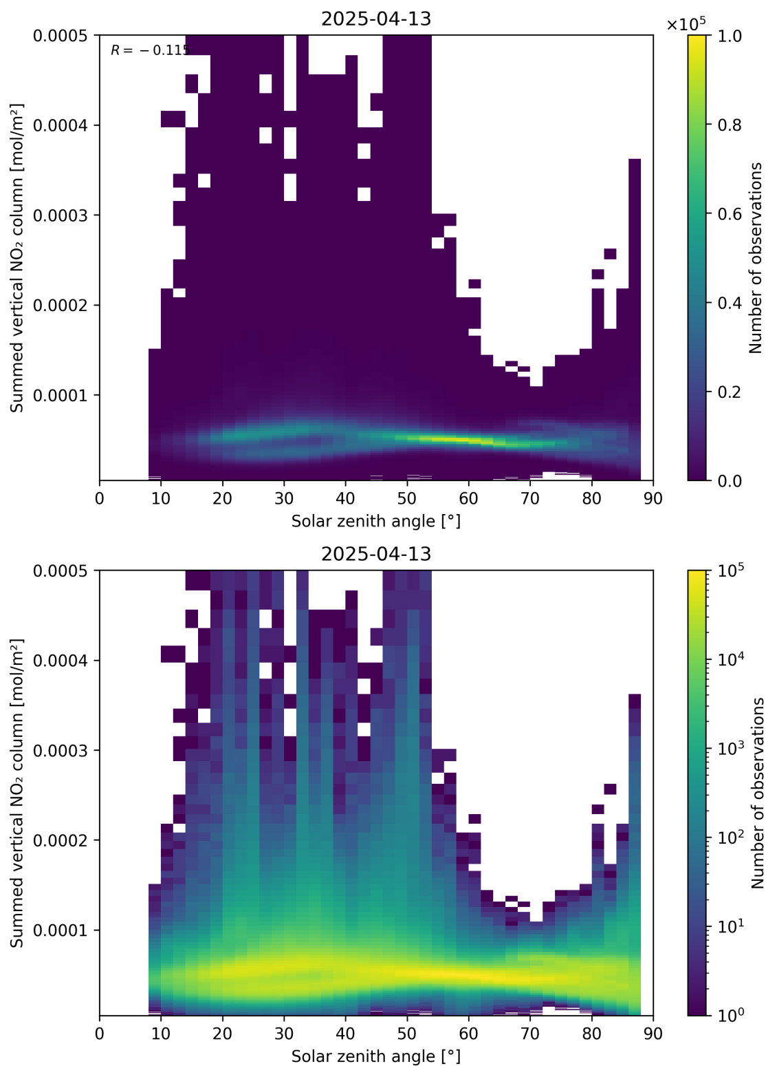
Figure 151: Scatter density plot of “Solar zenith angle” against “Summed vertical NO 2 column” for 2025-04-13 to 2025-04-14.
