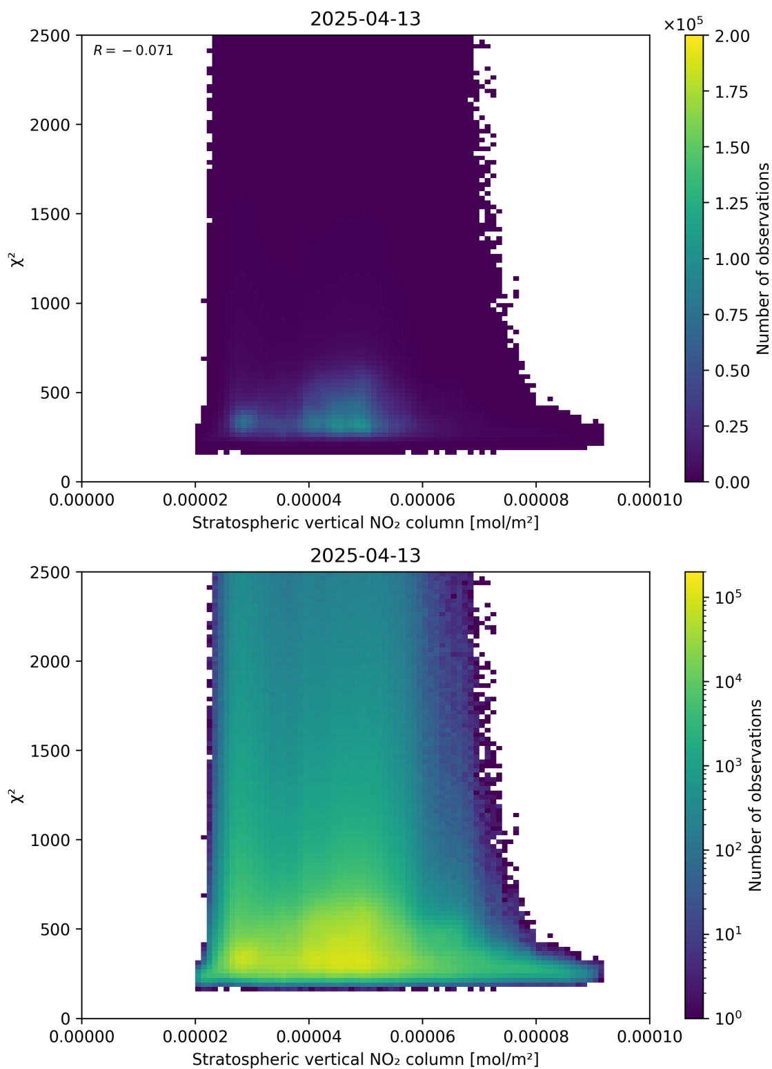
Figure 97: Scatter density plot of “Stratospheric vertical NO 2 column” against “ \chi^2 ” for 2025-04-13 to 2025-04-14.
