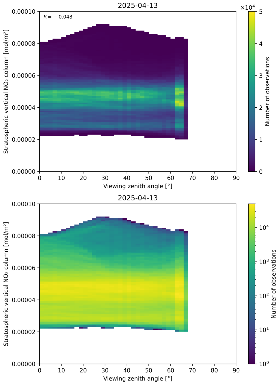
Figure 164: Scatter density plot of “Viewing zenith angle” against “Stratospheric vertical NO 2 column” for 2025-04-13 to 2025-04-14.
