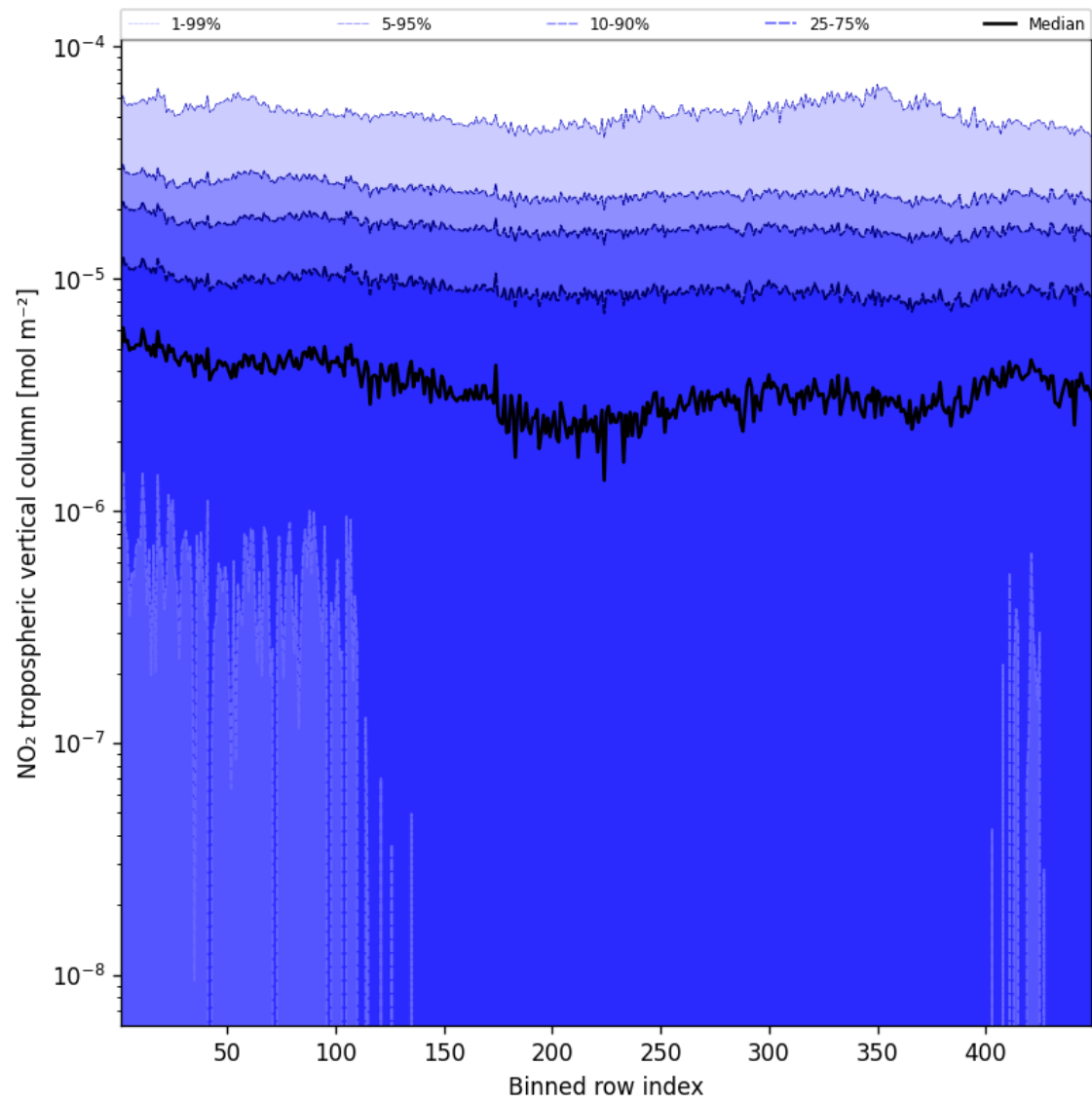
Figure 46: Along track statistics of “NO 2 tropospheric vertical column” for 2025-04-13 to 2025-04-14
