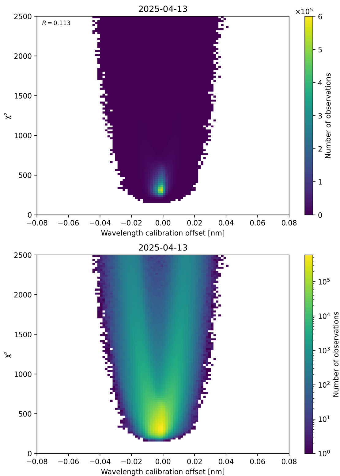
Figure 175: Scatter density plot of “Wavelength calibration offset” against “ \chi^2 ” for 2025-04-13 to 2025-04-14.
