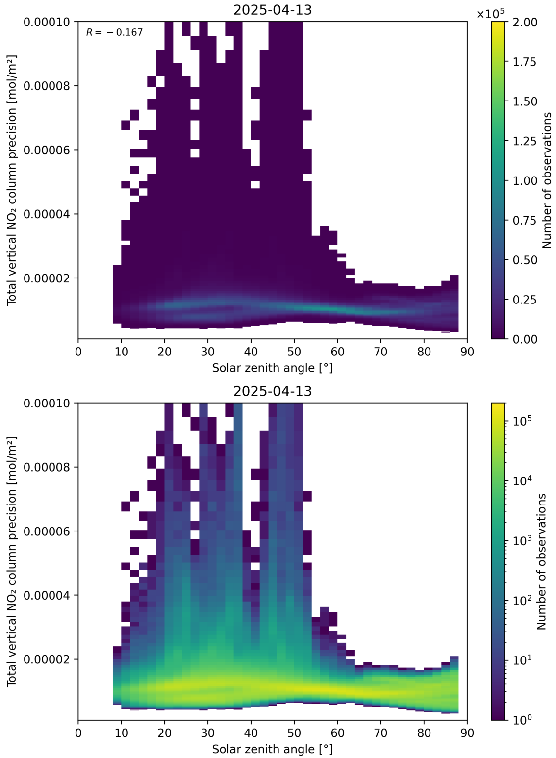
Figure 154: Scatter density plot of “Solar zenith angle” against “Total vertical NO 2 column precision” for 2025-04-13 to 2025-04-14.
