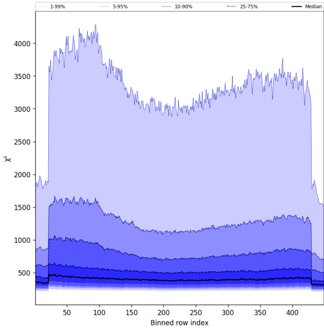
Figure 59: Along track statistics of “ \chi^2 ” for 2025-04-13 to 2025-04-14
