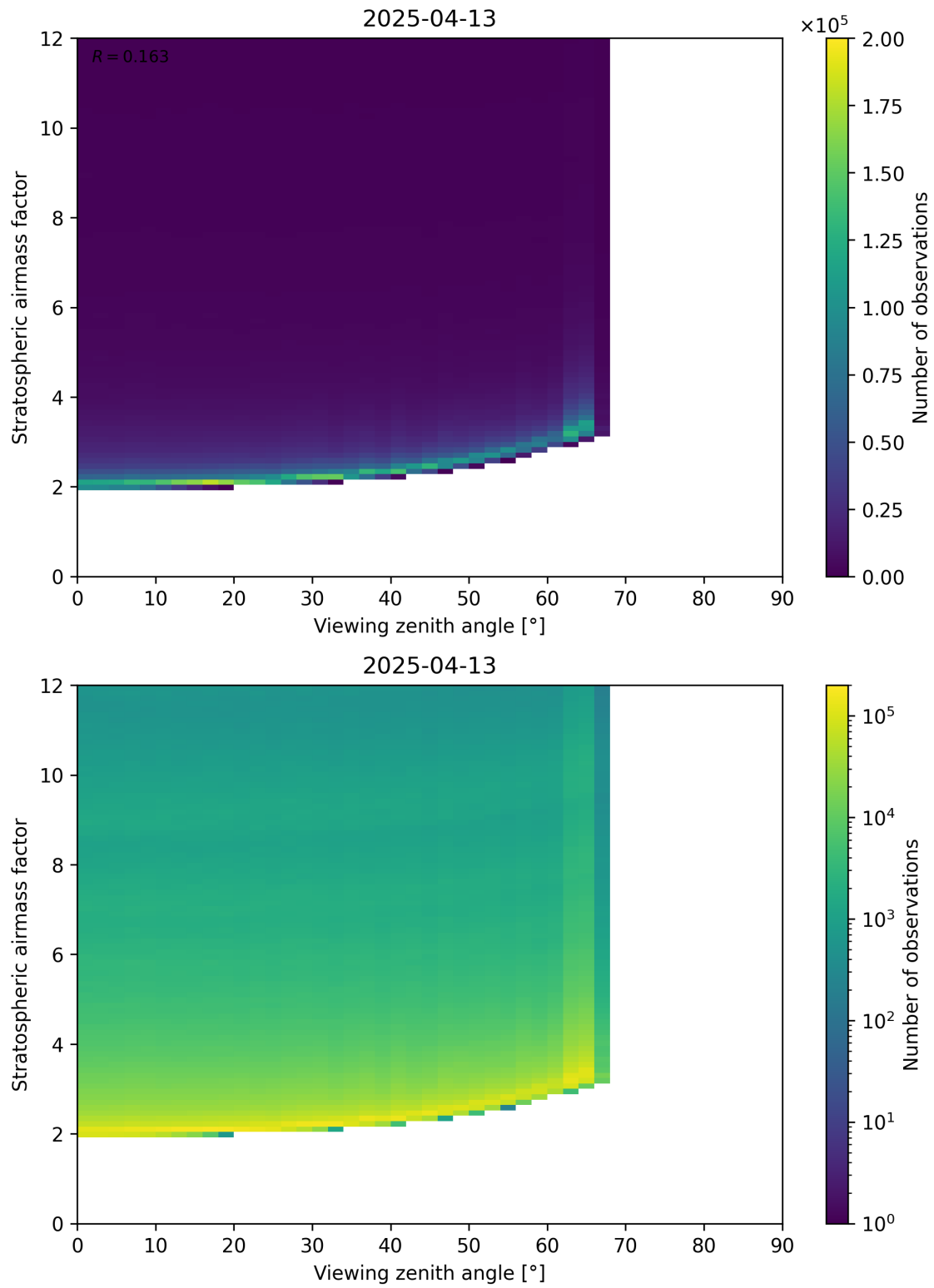
Figure 159: Scatter density plot of “Viewing zenith angle” against “Stratospheric airmass factor” for 2025-04-13 to 2025-04-14.
