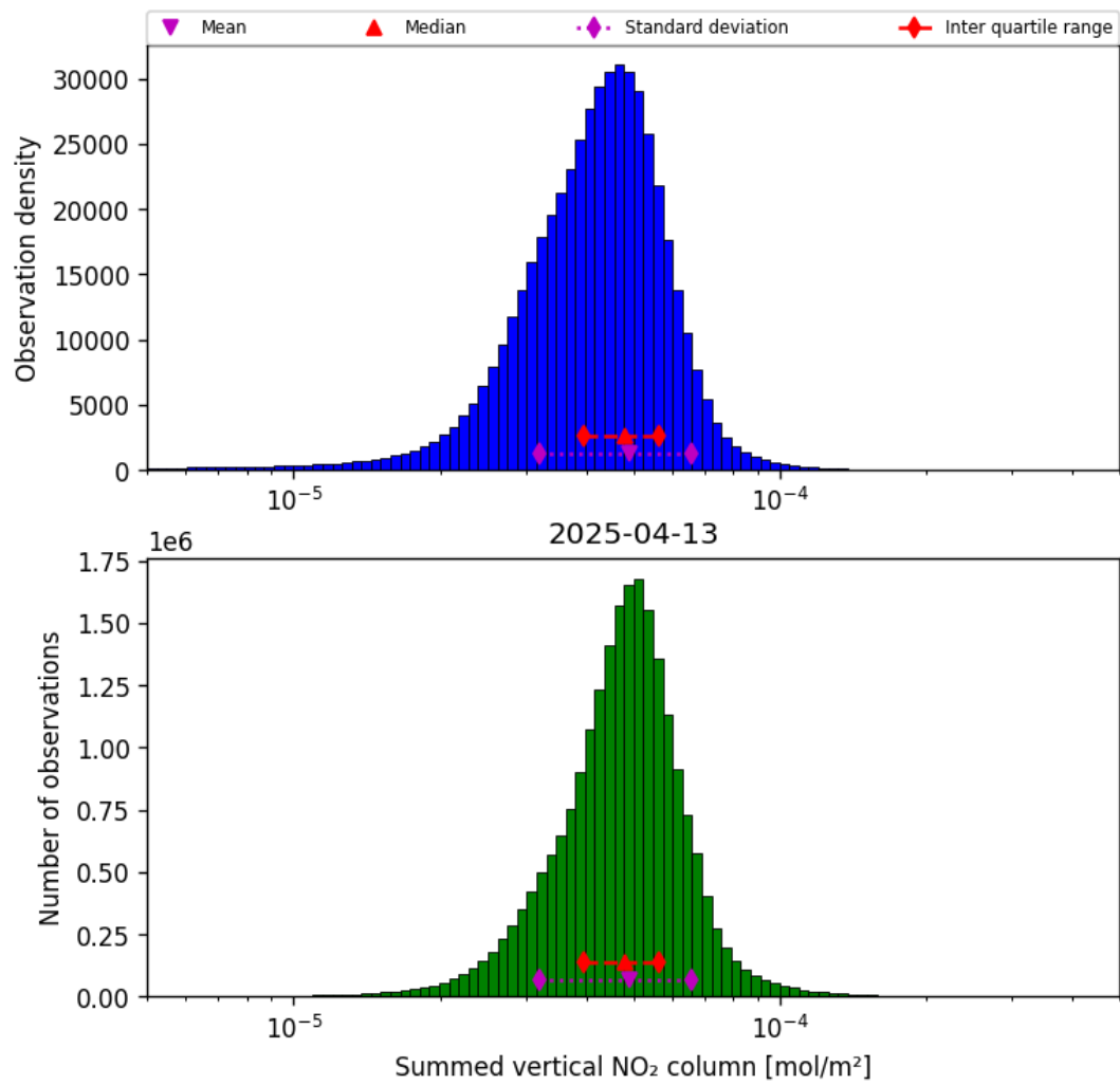
Figure 40: Histogram of “Summed vertical NO 2 column” for 2025-04-13 to 2025-04-14
