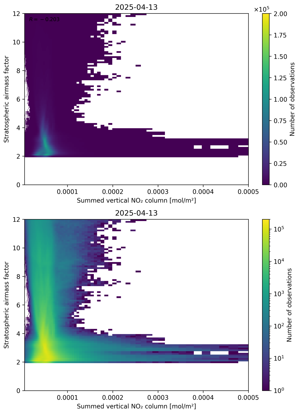
Figure 103: Scatter density plot of “Summed vertical NO 2 column” against “Stratospheric airmass factor” for 2025-04-13 to 2025-04-14.
