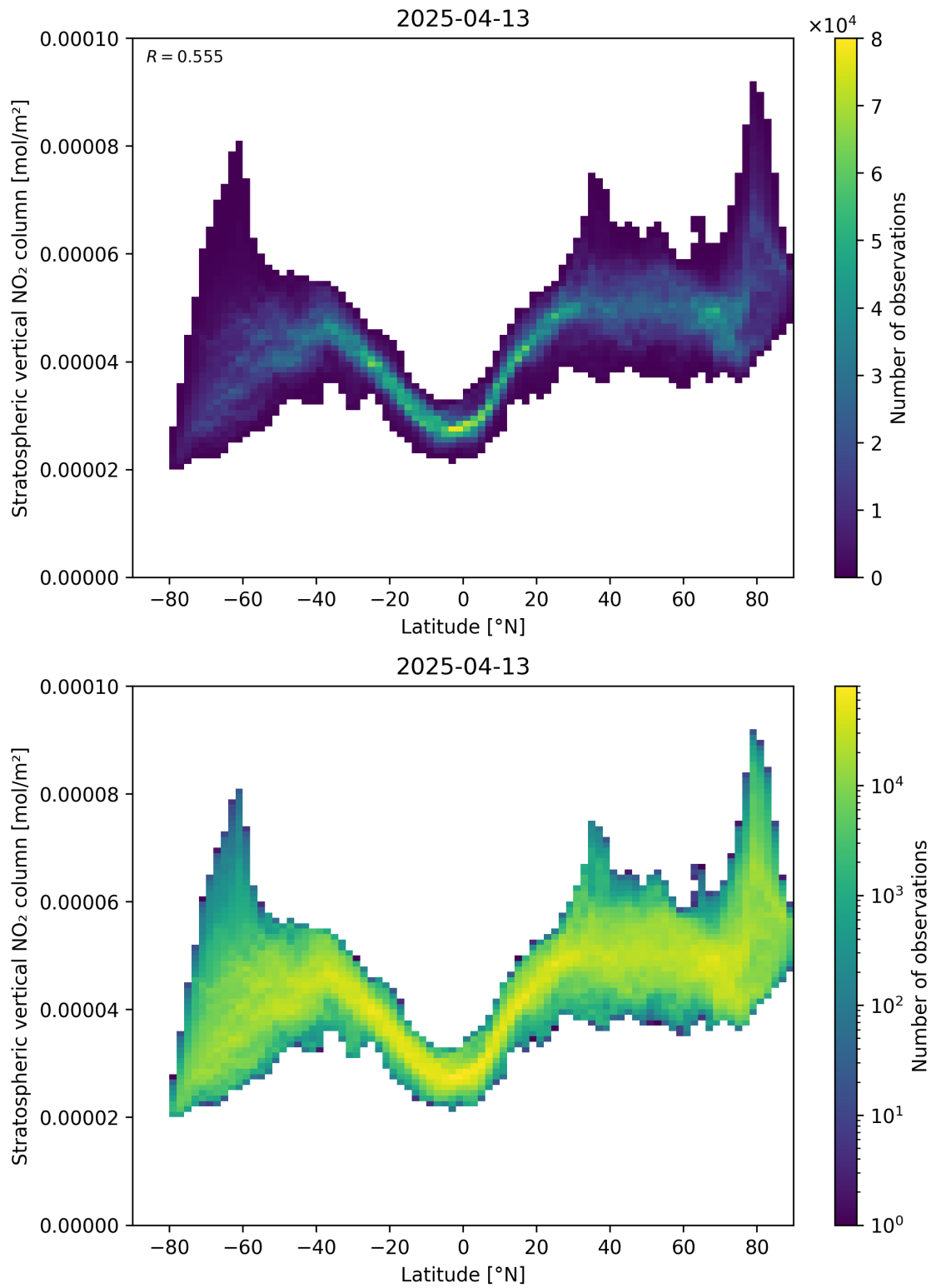
Figure 87: Scatter density plot of “Latitude” against “Stratospheric vertical NO 2 column” for 2025-04-13 to 2025-04-14.
