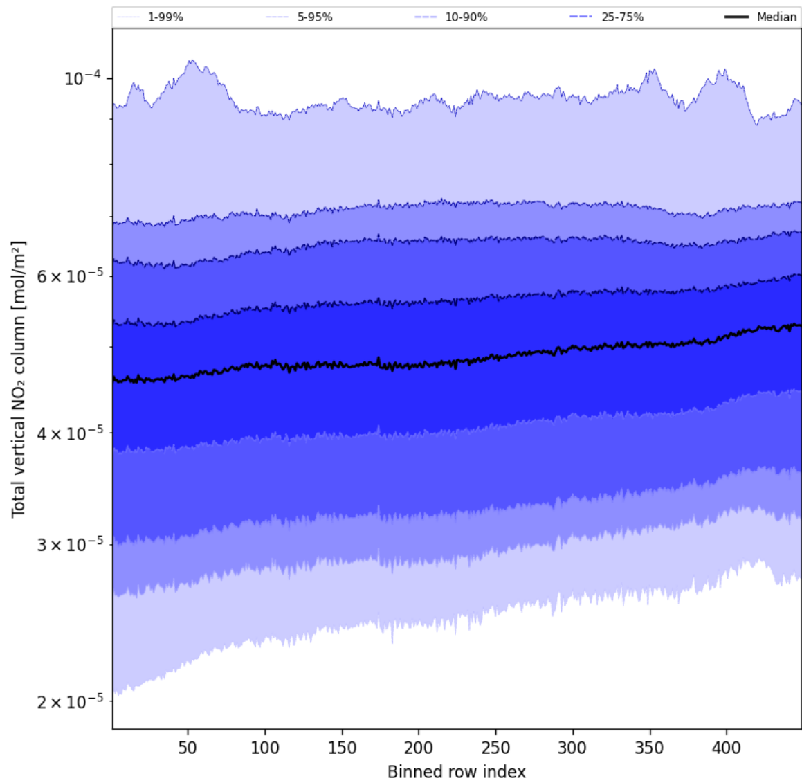
Figure 55: Along track statistics of “Total vertical NO 2 column” for 2025-04-13 to 2025-04-14
