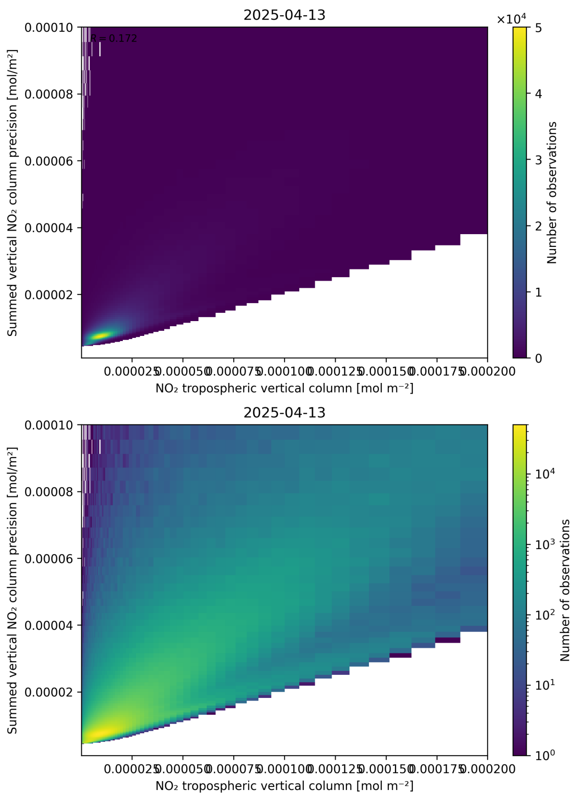
Figure 127: Scatter density plot of “NO 2 tropospheric vertical column” against “Summed vertical NO 2 column precision” for 2025-04-13 to 2025-04-14.
