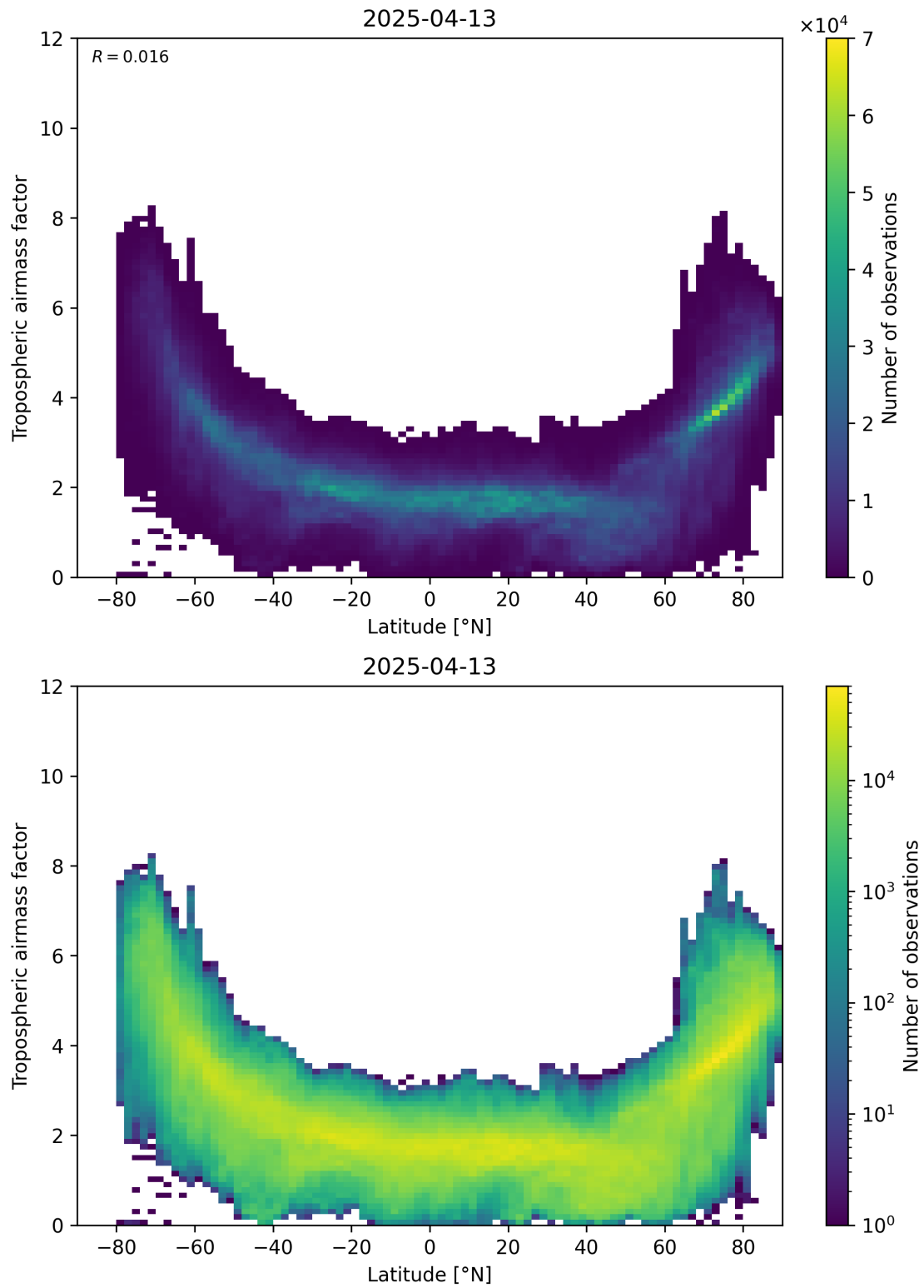
Figure 85: Scatter density plot of “Latitude” against “Tropospheric airmass factor” for 2025-04-13 to 2025-04-14.
