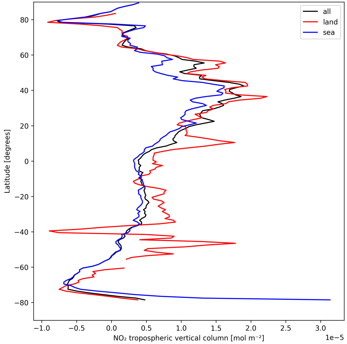
Figure 12: Zonal average of “NO 2 tropospheric vertical column” for 2025-04-13 to 2025-04-14.
