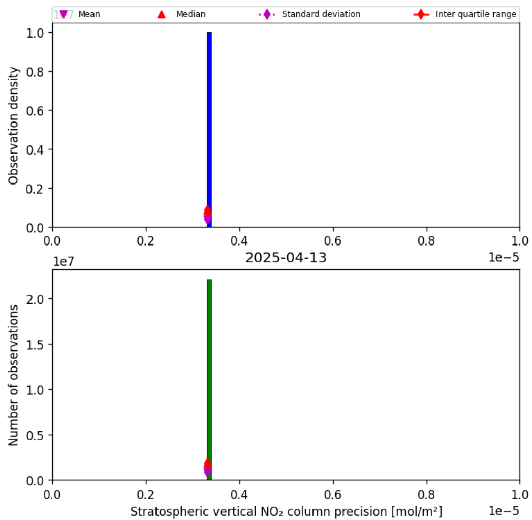
Figure 37: Histogram of “Stratospheric vertical NO 2 column precision” for 2025-04-13 to 2025-04-14
