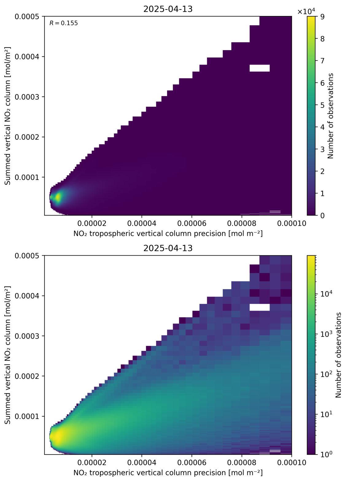
Figure 136: Scatter density plot of “NO 2 tropospheric vertical column precision” against “Summed vertical NO 2 column” for 2025-04-13 to 2025-04-14.
