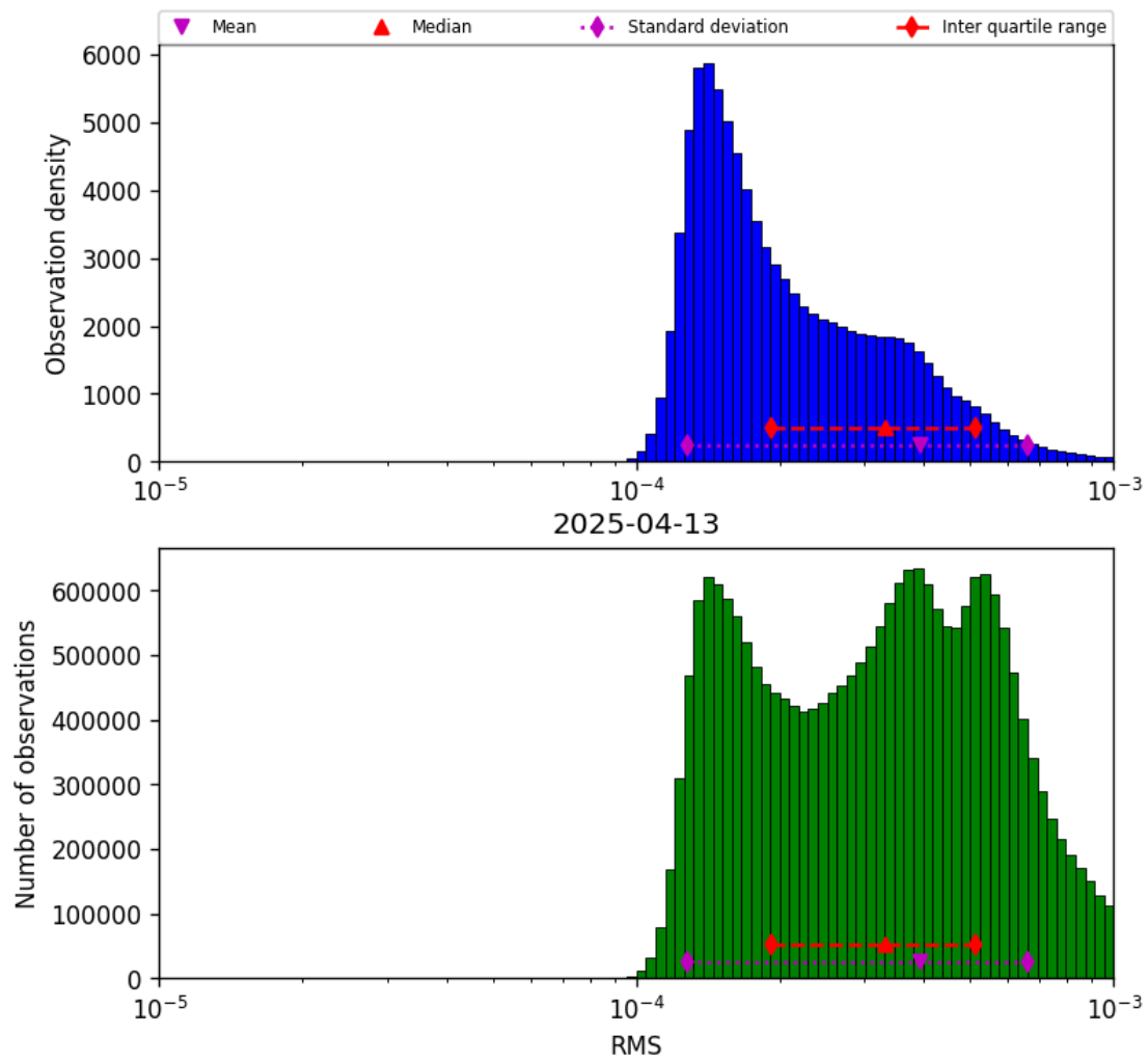
Figure 43: Histogram of “RMS” for 2025-04-13 to 2025-04-14
