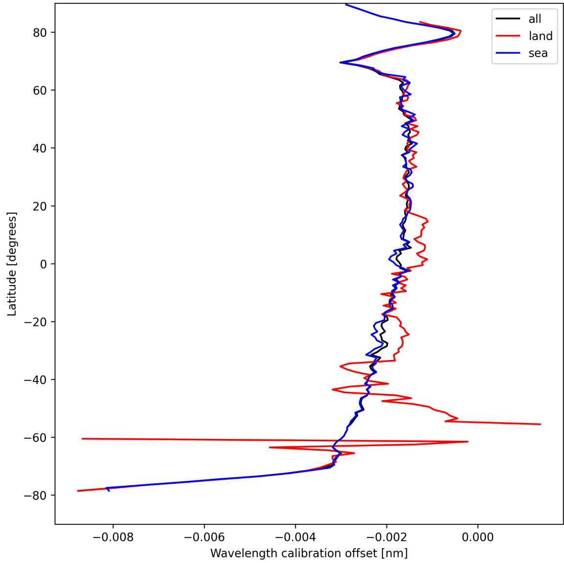
Figure 18: Zonal average of “Wavelength calibration offset” for 2025-04-13 to 2025-04-14.
