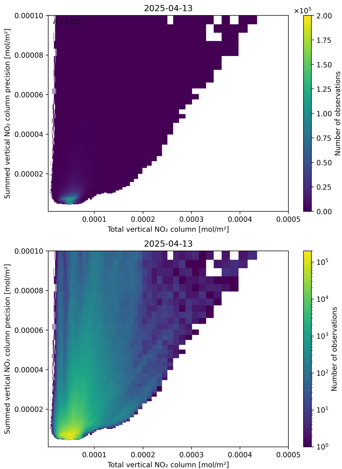
Figure 113: Scatter density plot of “Total vertical NO 2 column” against “Summed vertical NO 2 column precision” for 2025-04-13 to 2025-04-14.
