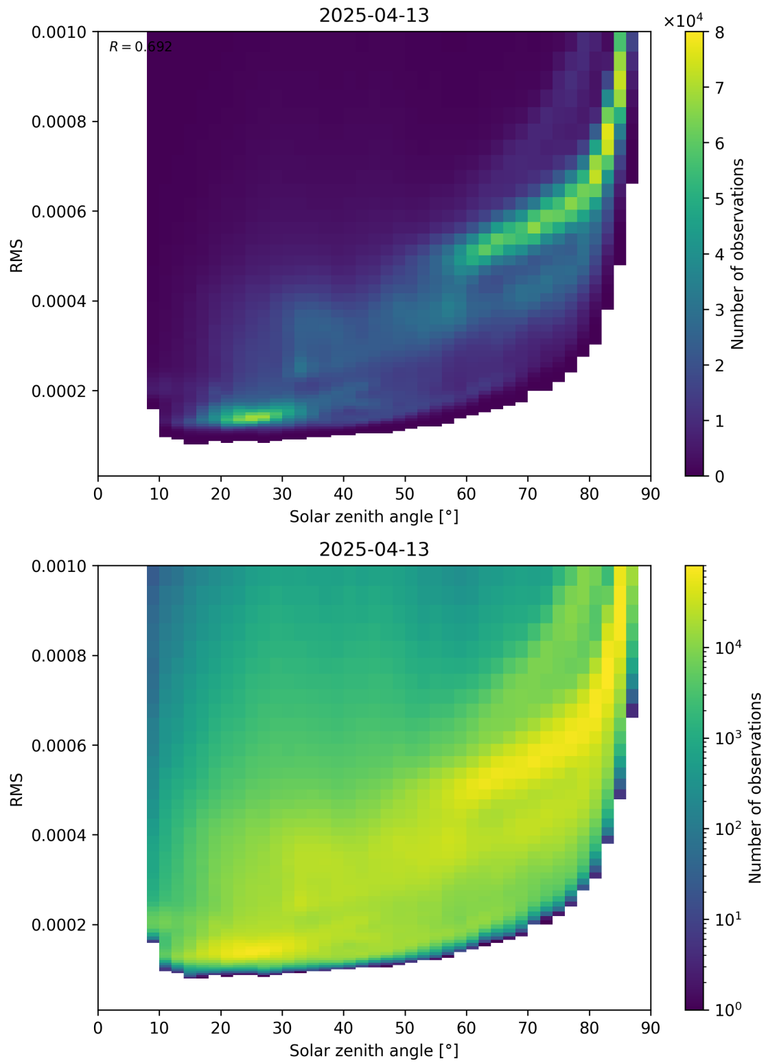
Figure 157: Scatter density plot of “Solar zenith angle” against “RMS” for 2025-04-13 to 2025-04-14.
