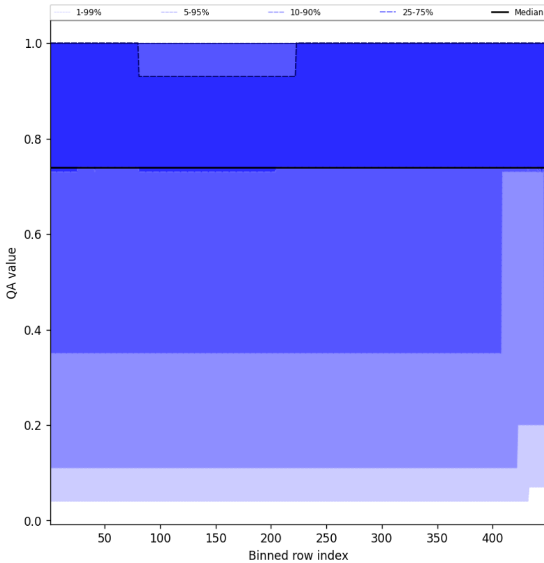
Figure 45: Along track statistics of “QA value” for 2025-04-13 to 2025-04-14
