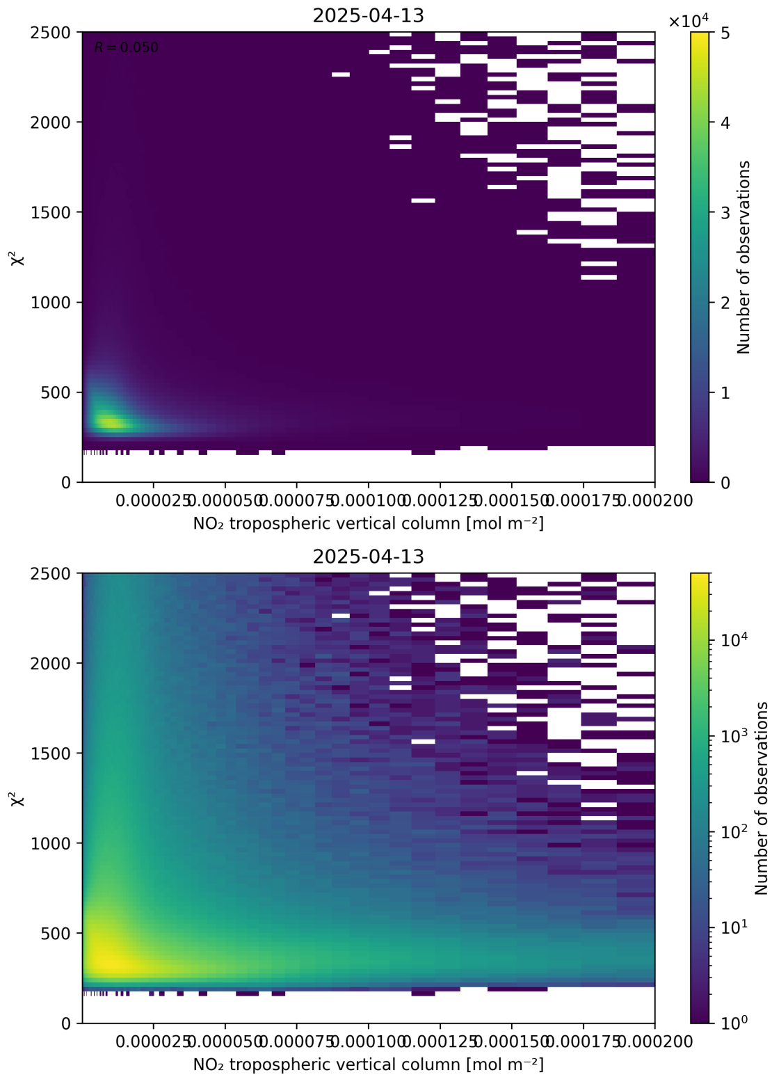
Figure 124: Scatter density plot of “NO 2 tropospheric vertical column” against “ \chi^2 ” for 2025-04-13 to 2025-04-14.
