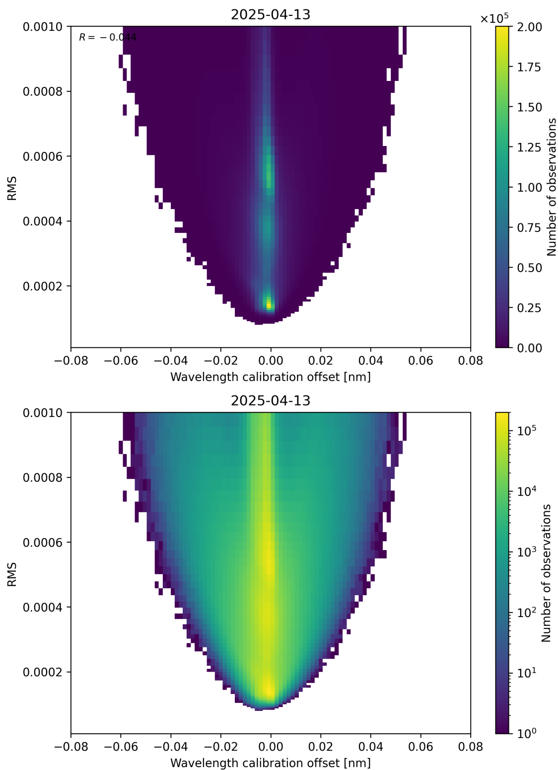
Figure 181: Scatter density plot of “Wavelength calibration offset” against “RMS” for 2025-04-13 to 2025-04-14.
