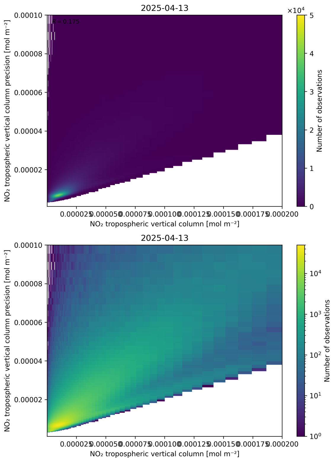
Figure 130: Scatter density plot of “NO 2 tropospheric vertical column” against “NO 2 tropospheric vertical column precision” for 2025-04-13 to 2025-04-14.
