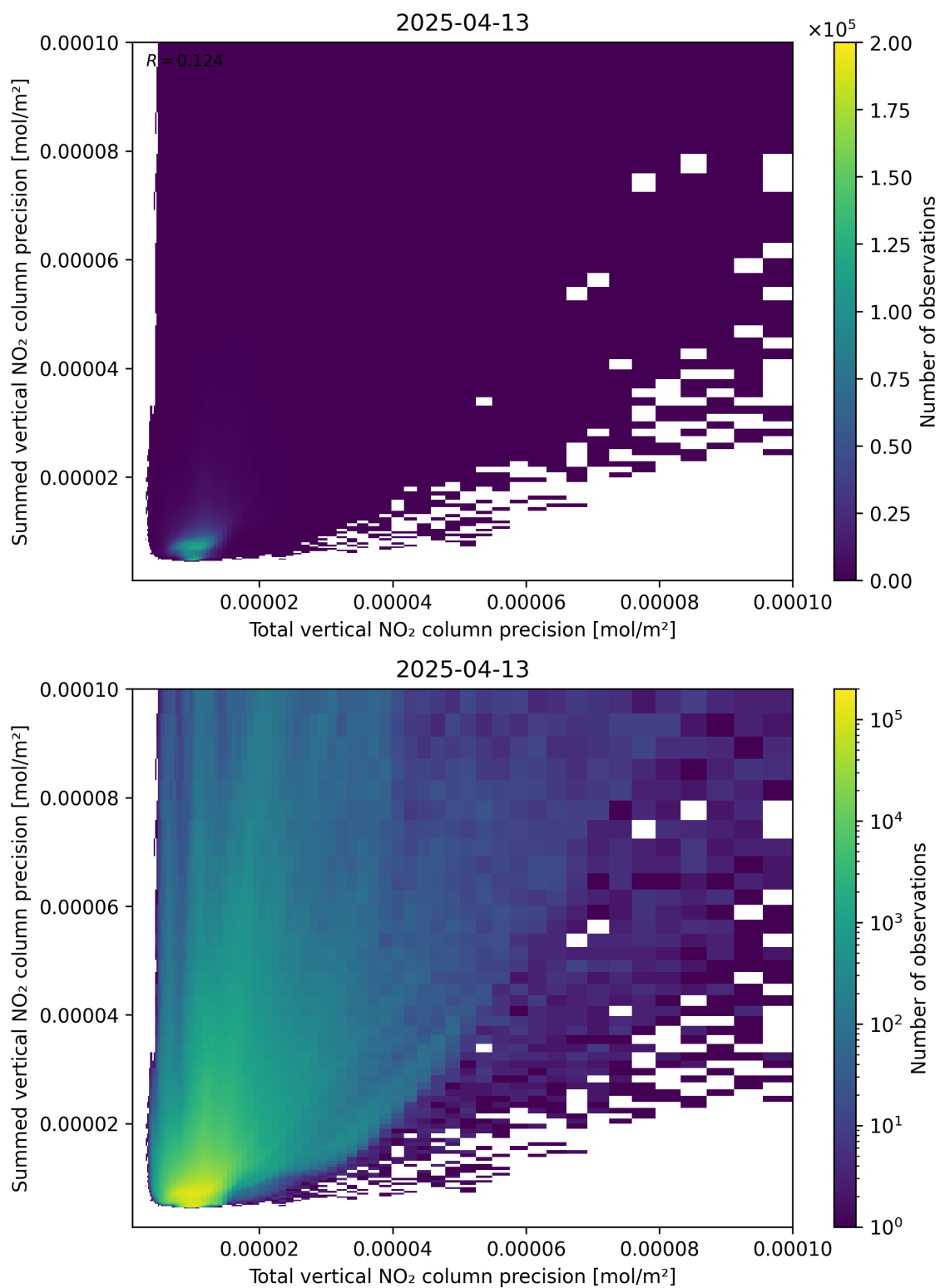
Figure 118: Scatter density plot of “Total vertical NO 2 column precision” against “Summed vertical NO 2 column precision” for 2025-04-13 to 2025-04-14.
