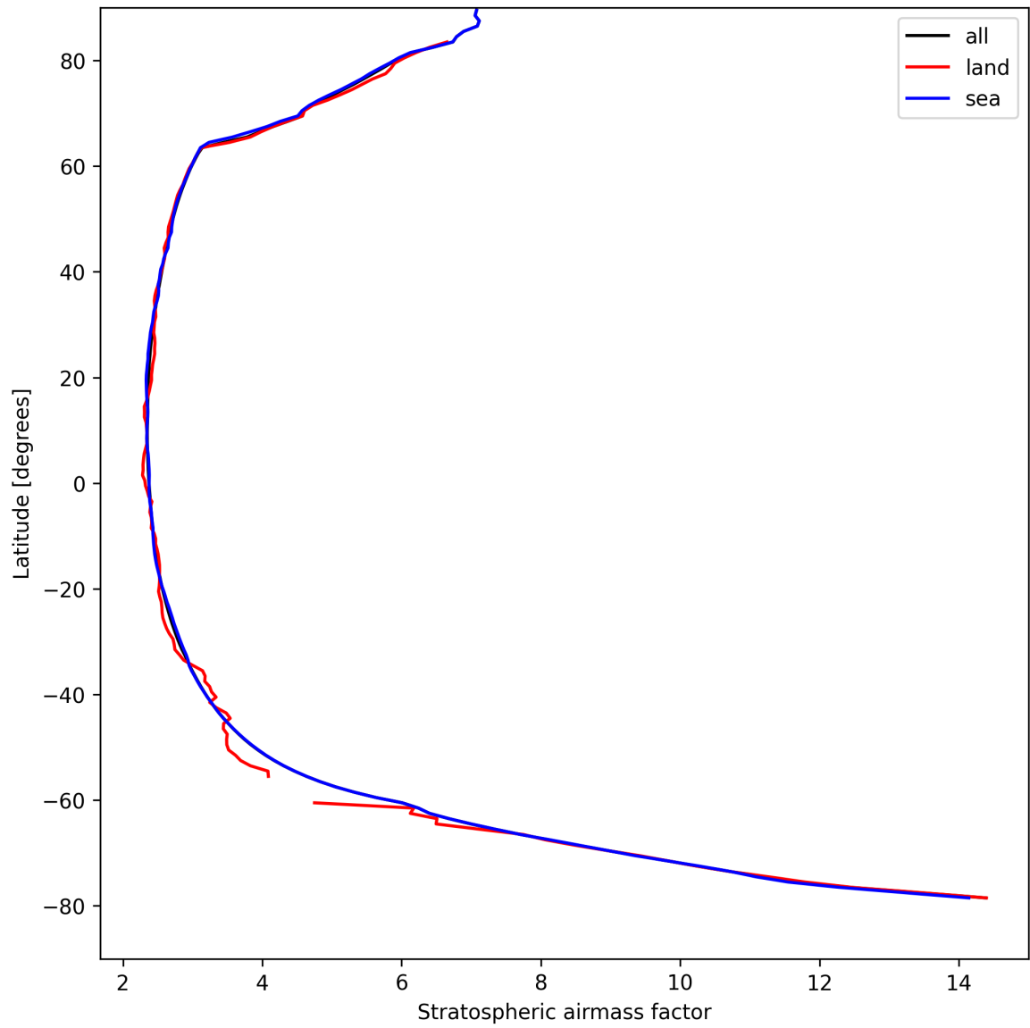
Figure 27: Zonal average of “Stratospheric air mass factor” for 2025-04-13 to 2025-04-14.
