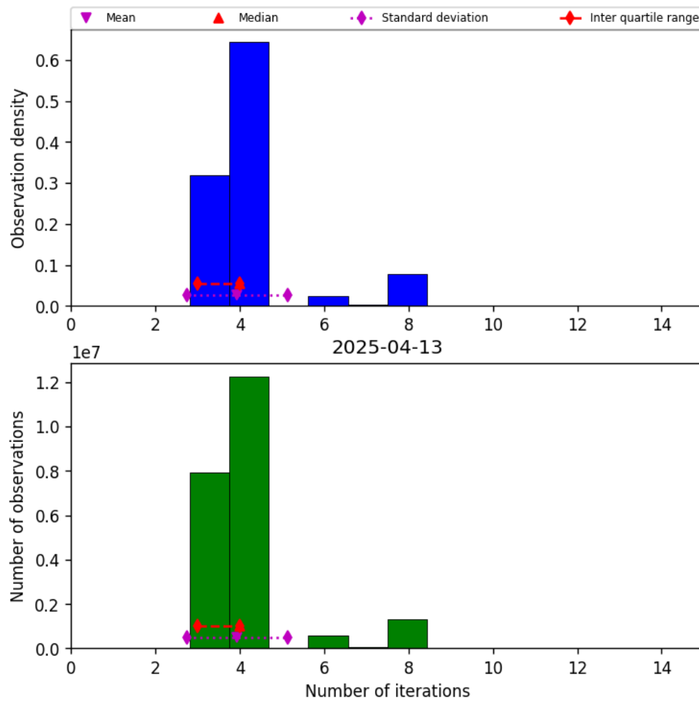
Figure 34: Histogram of “Number of iterations” for 2025-04-13 to 2025-04-14
