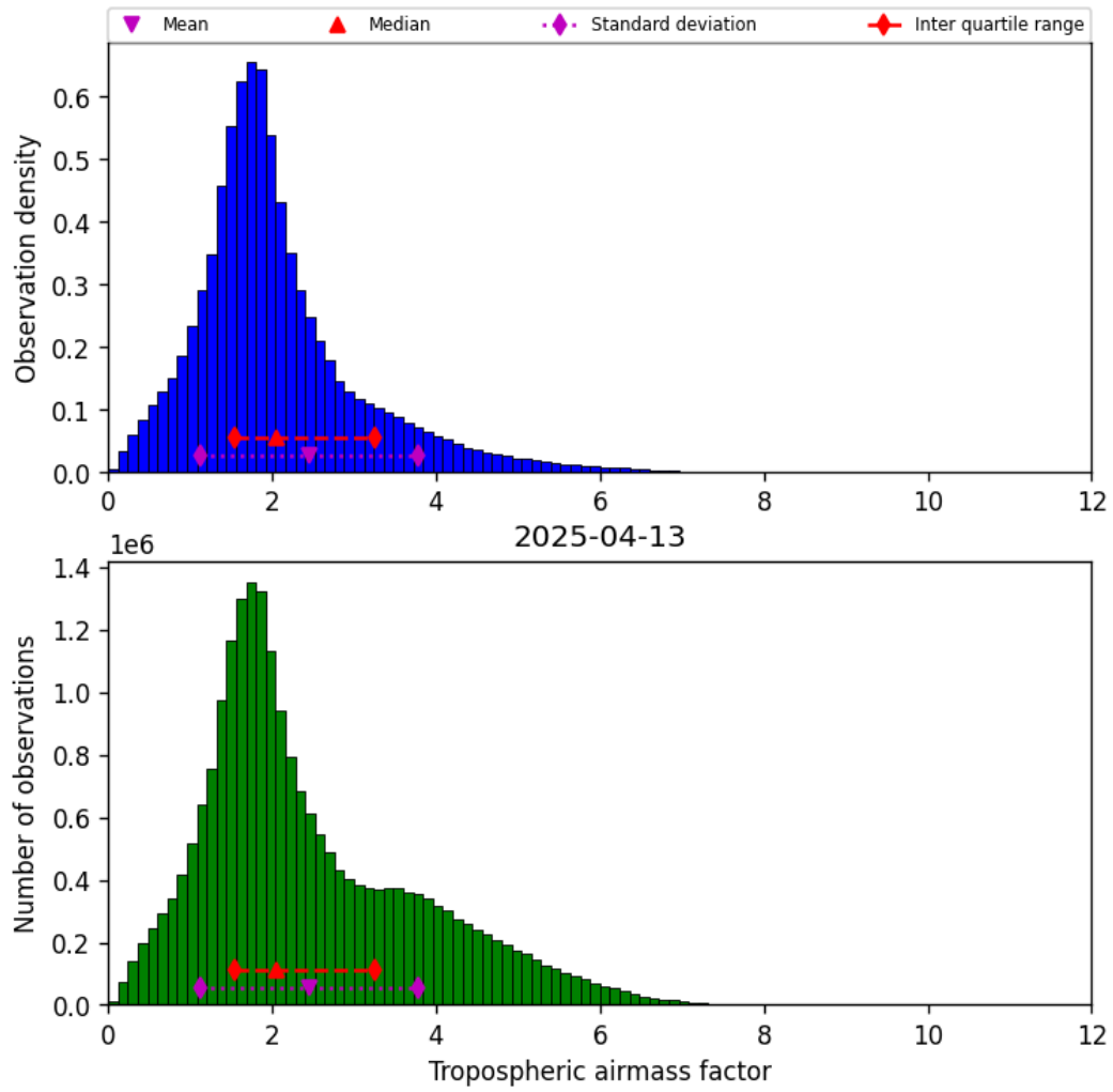
Figure 31: Histogram of “Tropospheric airmass factor” for 2025-04-13 to 2025-04-14
