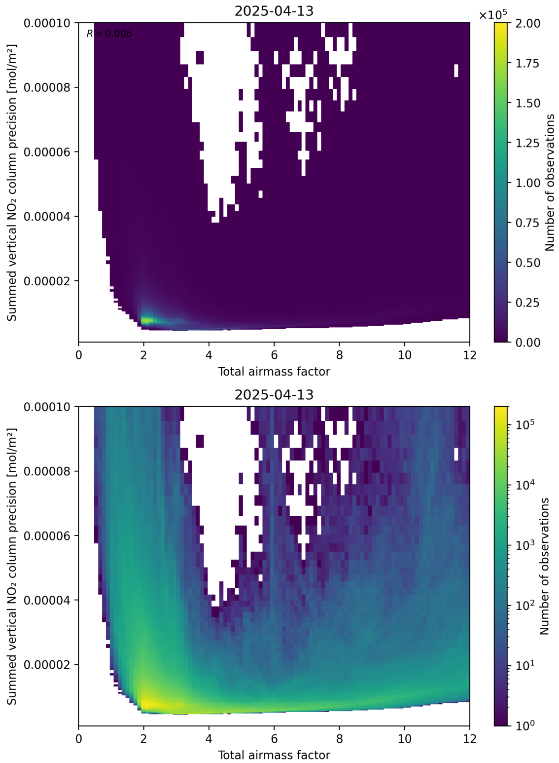
Figure 66: Scatter density plot of “Total airmass factor” against “Summed vertical NO 2 column precision” for 2025-04-13 to 2025-04-14.
