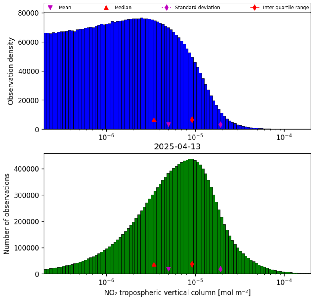
Figure 29: Histogram of “NO 2 tropospheric vertical column” for 2025-04-13 to 2025-04-14
