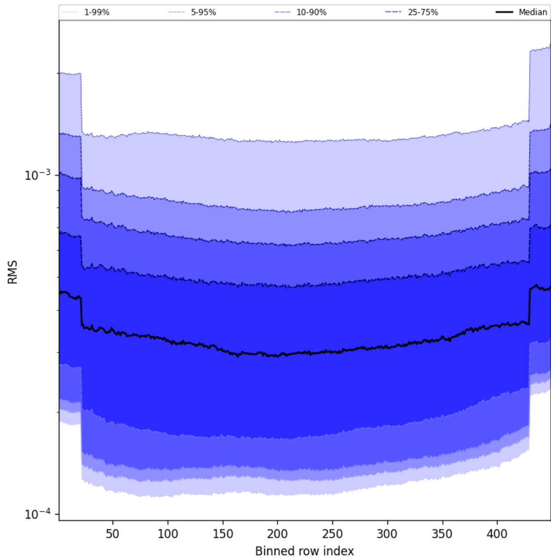
Figure 60: Along track statistics of “RMS” for 2025-04-13 to 2025-04-14
