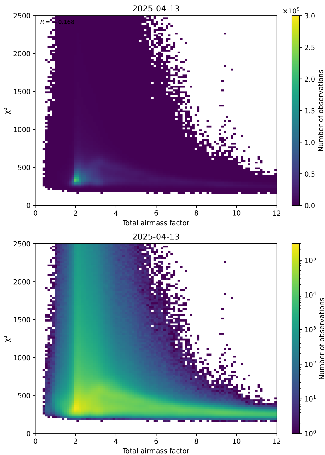
Figure 63: Scatter density plot of “Total airmass factor” against “ \chi^2 ” for 2025-04-13 to 2025-04-14.
