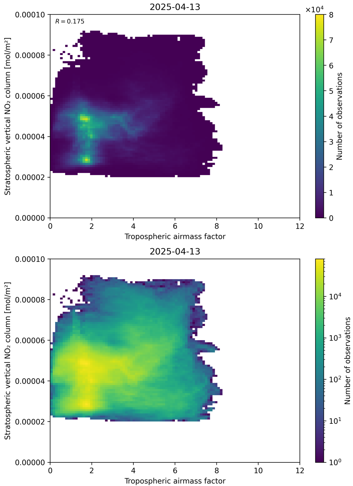
Figure 74: Scatter density plot of “Tropospheric air mass factor” against “Stratospheric vertical NO 2 column” for 2025-04-13 to 2025-04-14.
