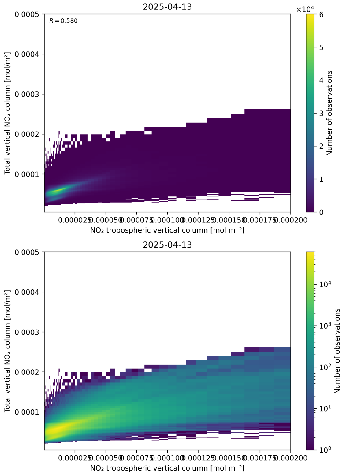
Figure 128: Scatter density plot of “NO 2 tropospheric vertical column” against “Total vertical NO 2 column” for 2025-04-13 to 2025-04-14.
