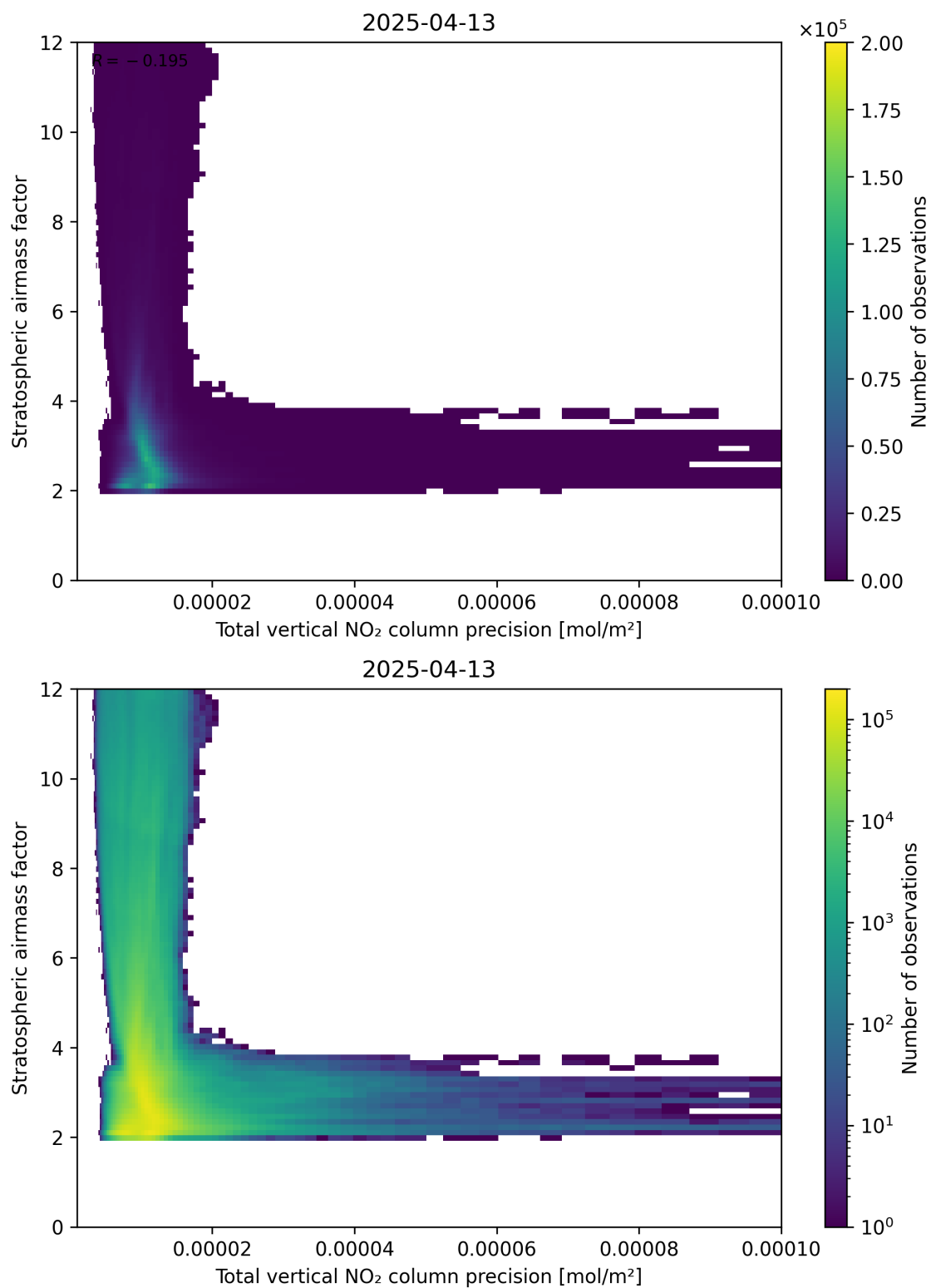
Figure 115: Scatter density plot of “Total vertical NO 2 column precision” against “Stratospheric air mass factor” for 2025-04-13 to 2025-04-14.
