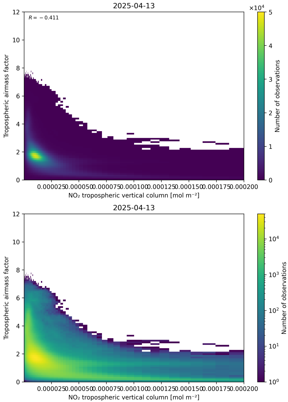
Figure 123: Scatter density plot of “NO 2 tropospheric vertical column” against “Tropospheric airmass factor” for 2025-04-13 to 2025-04-14.
