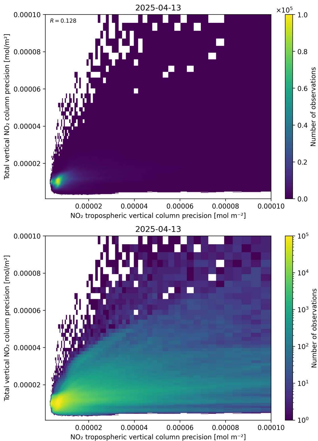
Figure 139: Scatter density plot of “NO 2 tropospheric vertical column precision” against “Total vertical NO 2 column precision” for 2025-04-13 to 2025-04-14.
