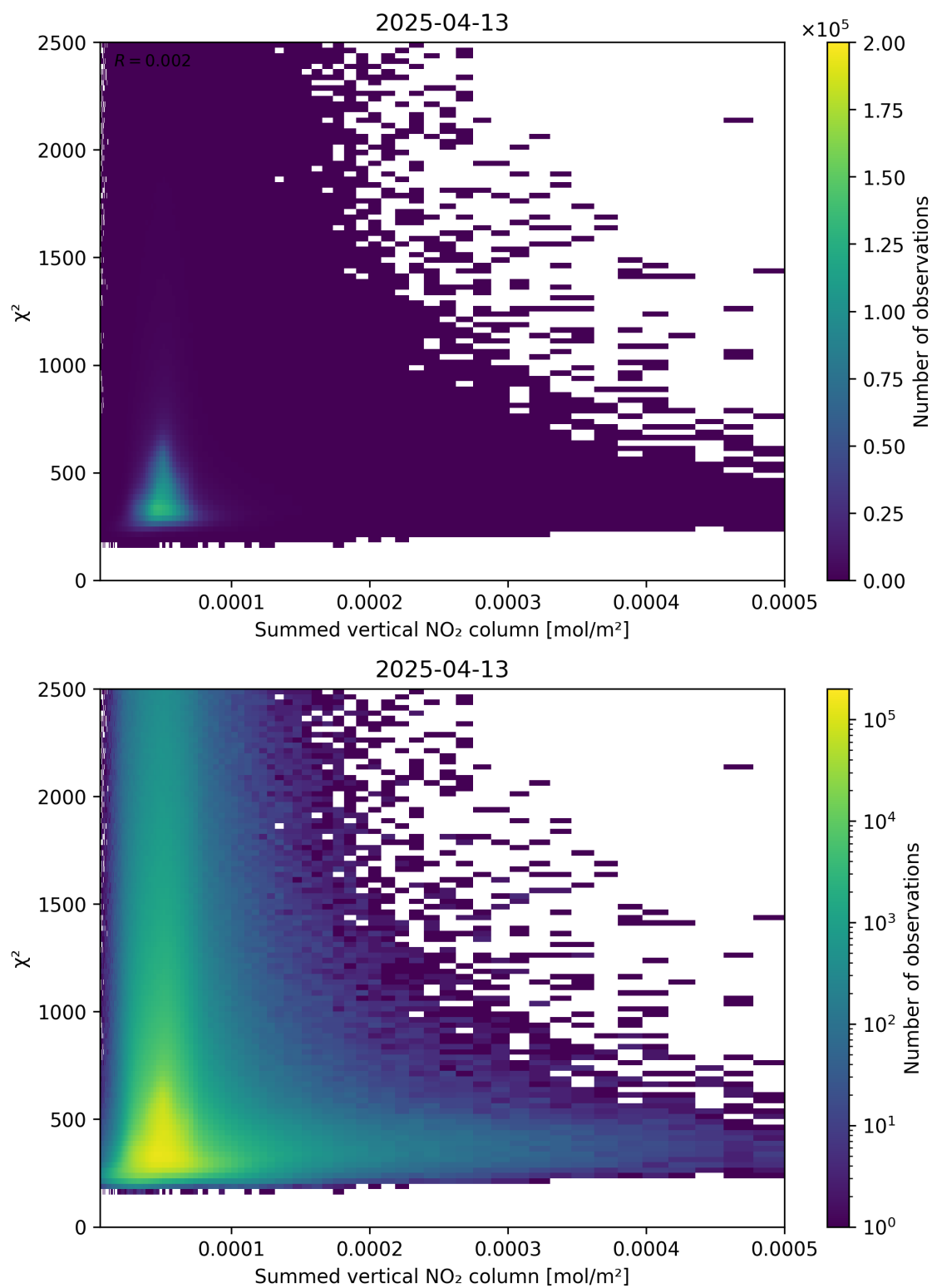
Figure 104: Scatter density plot of “Summed vertical NO 2 column” against “ \chi^2 ” for 2025-04-13 to 2025-04-14.
