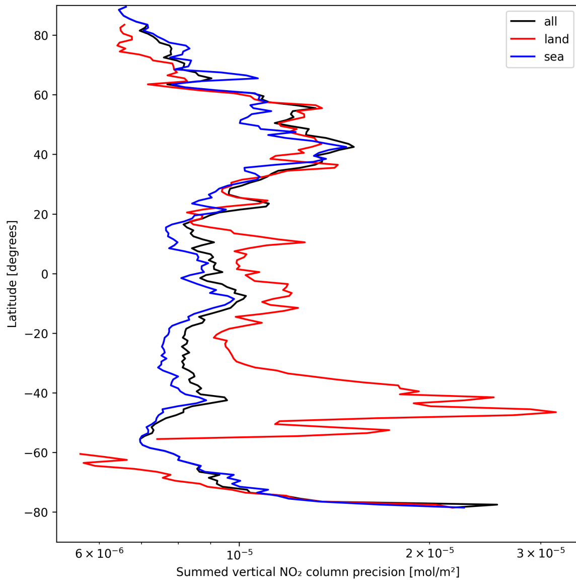
Figure 24: Zonal average of “Summed vertical NO 2 column precision” for 2025-04-13 to 2025-04-14.
