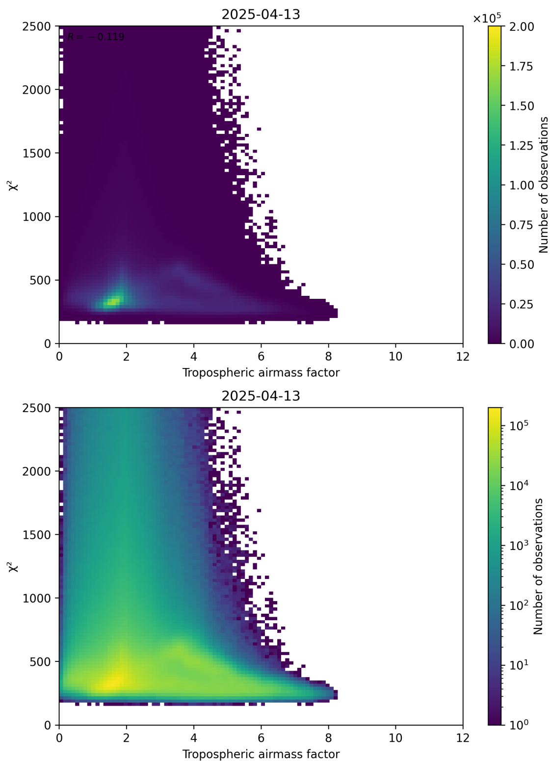
Figure 73: Scatter density plot of “Tropospheric airmass factor” against “ \chi^2 ” for 2025-04-13 to 2025-04-14.
