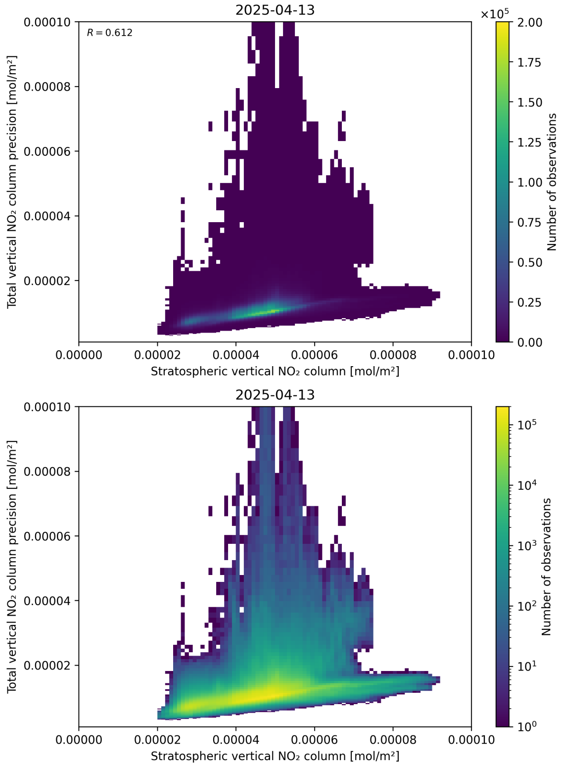
Figure 101: Scatter density plot of “Stratospheric vertical NO 2 column” against “Total vertical NO 2 column precision” for 2025-04-13 to 2025-04-14.
