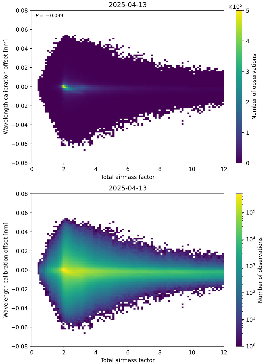
Figure 70: Scatter density plot of “Total airmass factor” against “Wavelength calibration offset” for 2025-04-13 to 2025-04-14.
