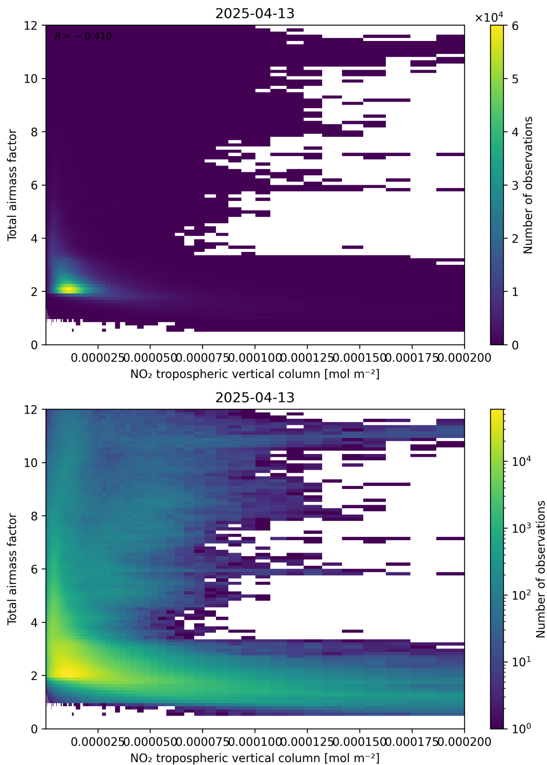
Figure 122: Scatter density plot of “NO 2 tropospheric vertical column” against “Total air mass factor” for 2025-04-13 to 2025-04-14.
