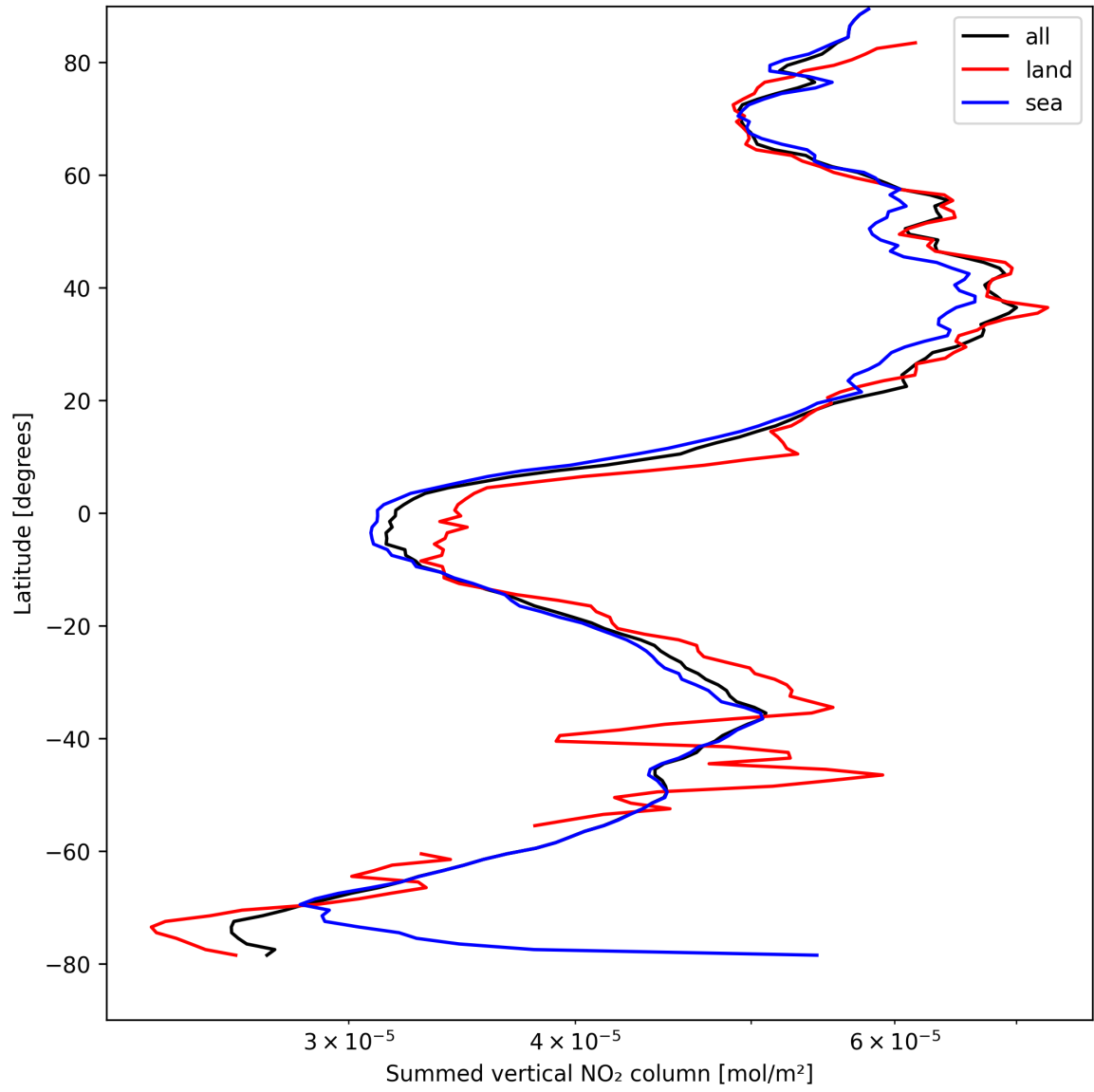
Figure 23: Zonal average of “Summed vertical NO 2 column” for 2025-04-13 to 2025-04-14.
