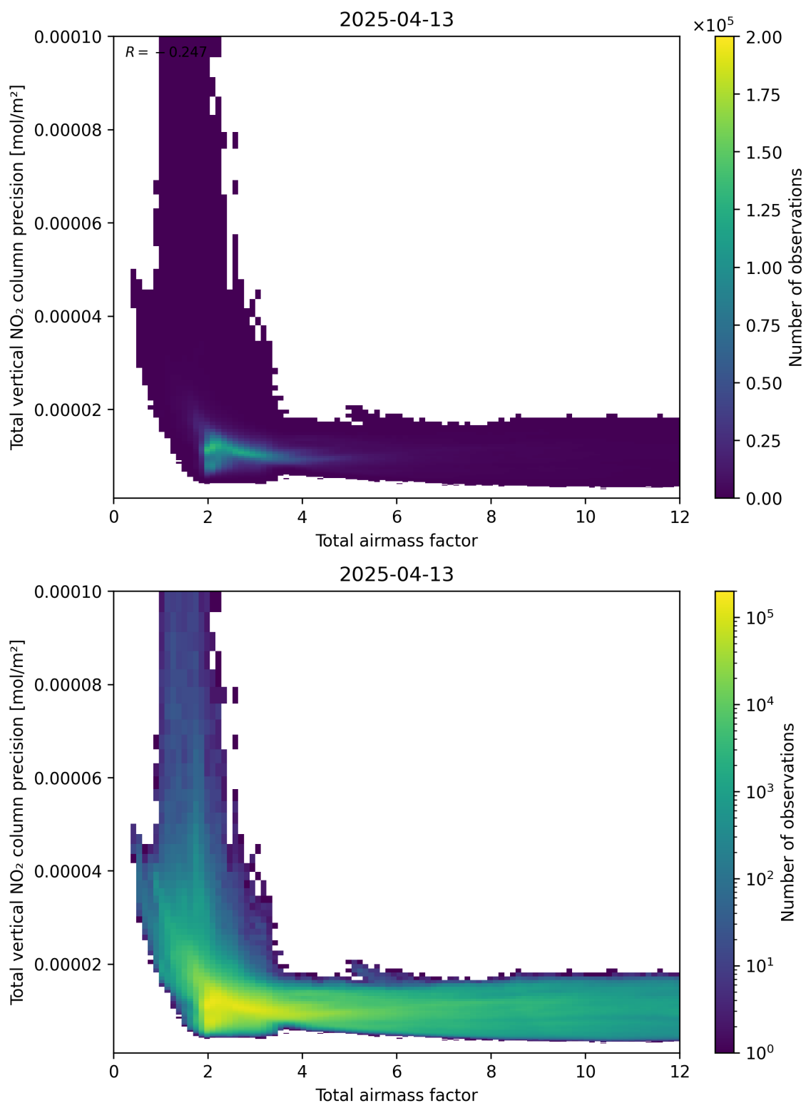
Figure 68: Scatter density plot of “Total airmass factor” against “Total vertical NO 2 column precision” for 2025-04-13 to 2025-04-14.
