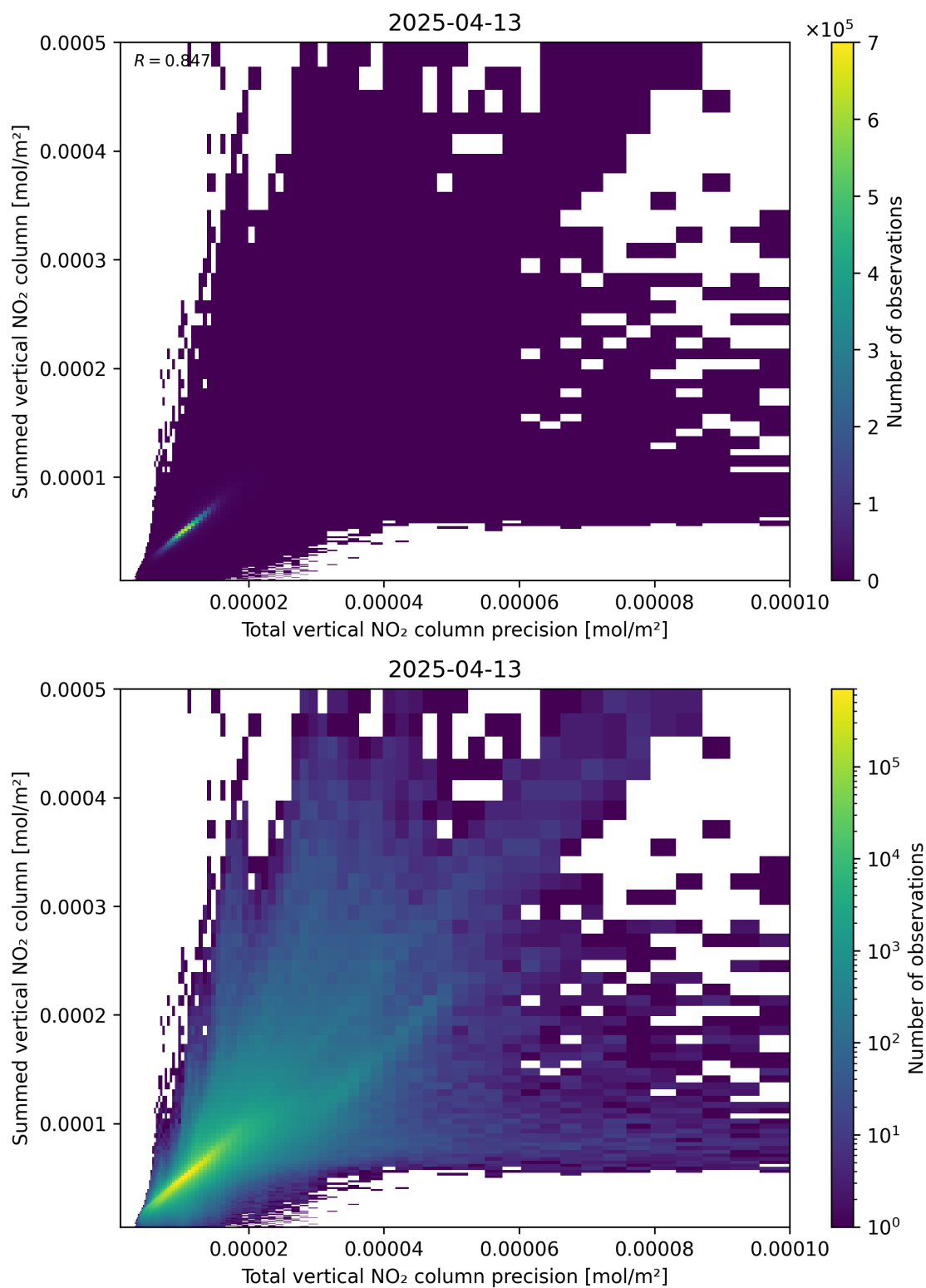
Figure 117: Scatter density plot of “Total vertical NO 2 column precision” against “Summed vertical NO 2 column” for 2025-04-13 to 2025-04-14.
