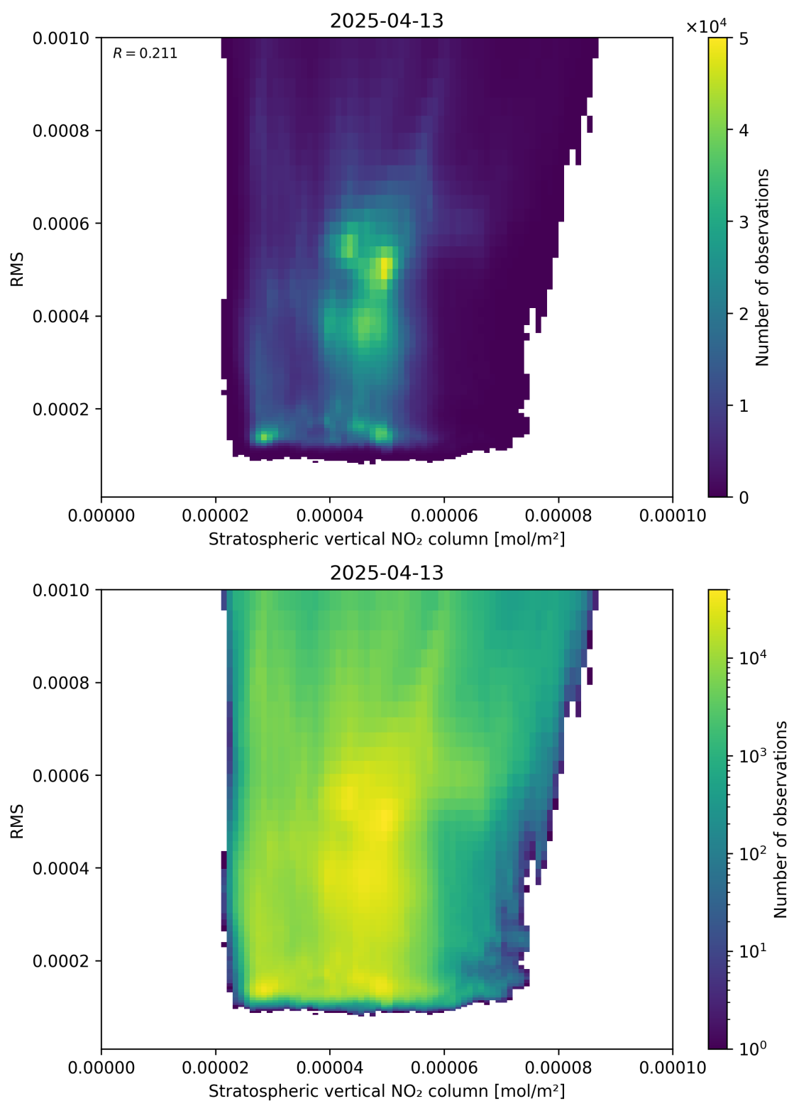
Figure 102: Scatter density plot of “Stratospheric vertical NO 2 column” against “RMS” for 2025-04-13 to 2025-04-14.
