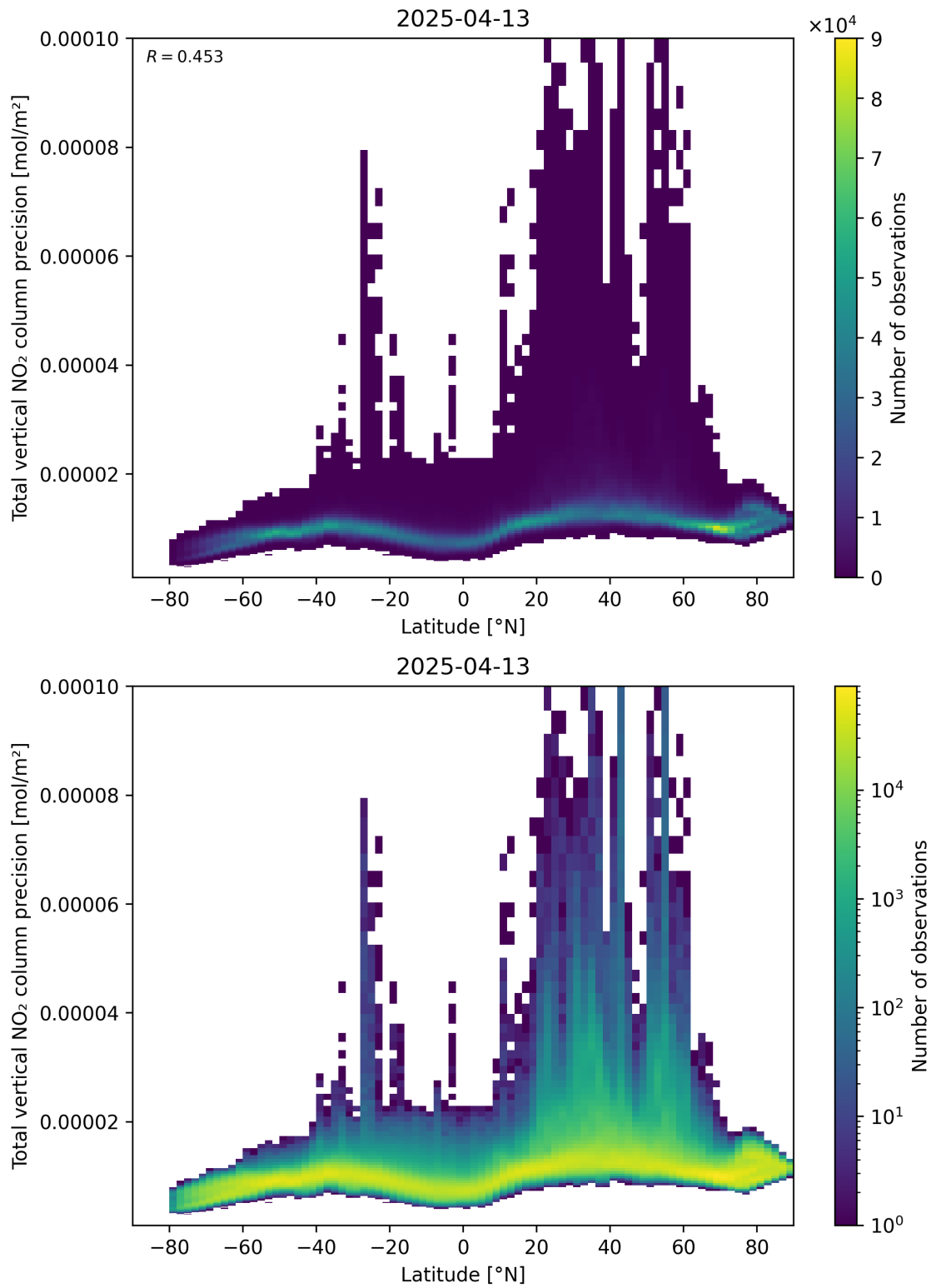
Figure 91: Scatter density plot of “Latitude” against “Total vertical NO 2 column precision” for 2025-04-13 to 2025-04-14.
