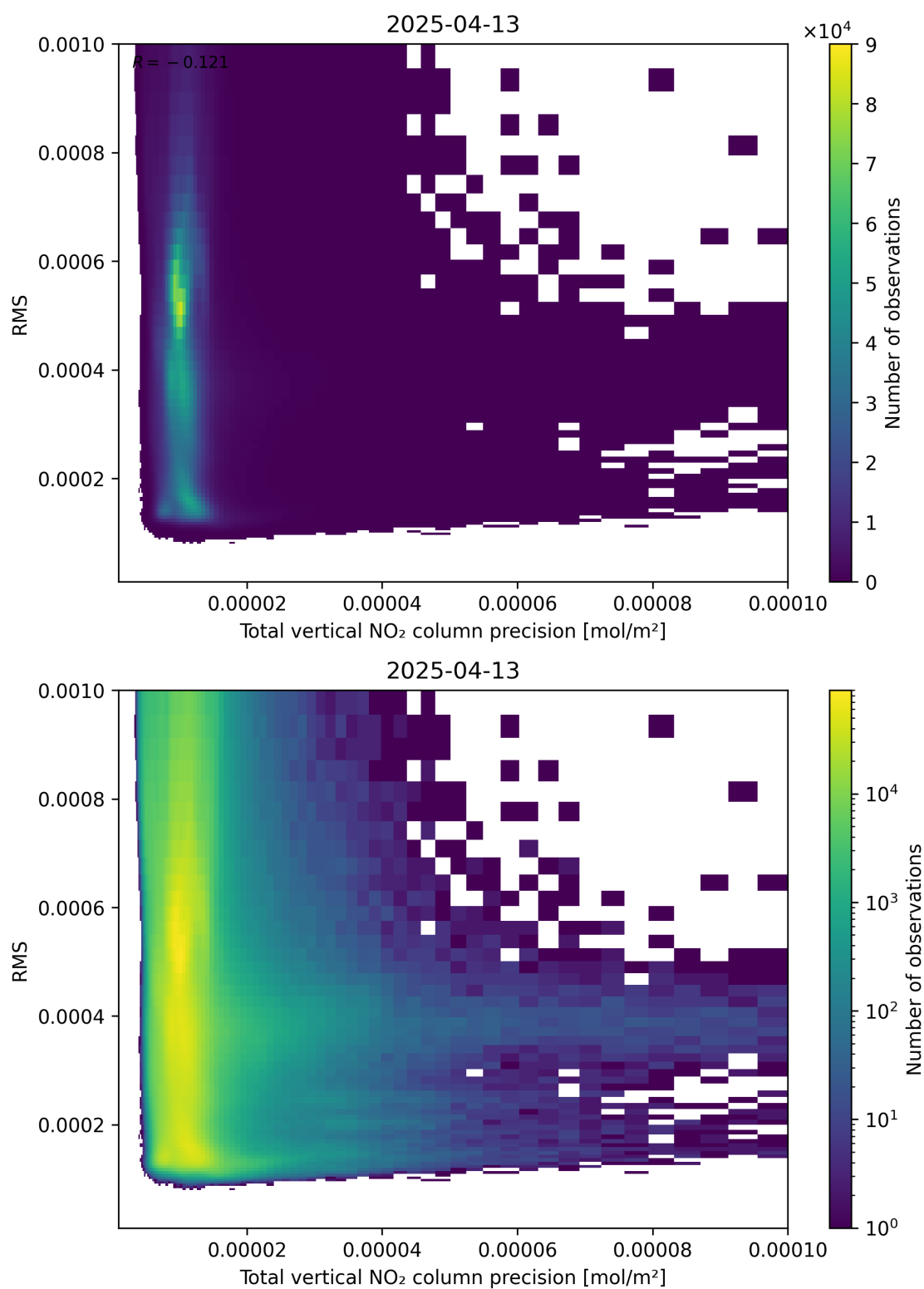
Figure 119: Scatter density plot of “Total vertical NO 2 column precision” against “RMS” for 2025-04-13 to 2025-04-14.
