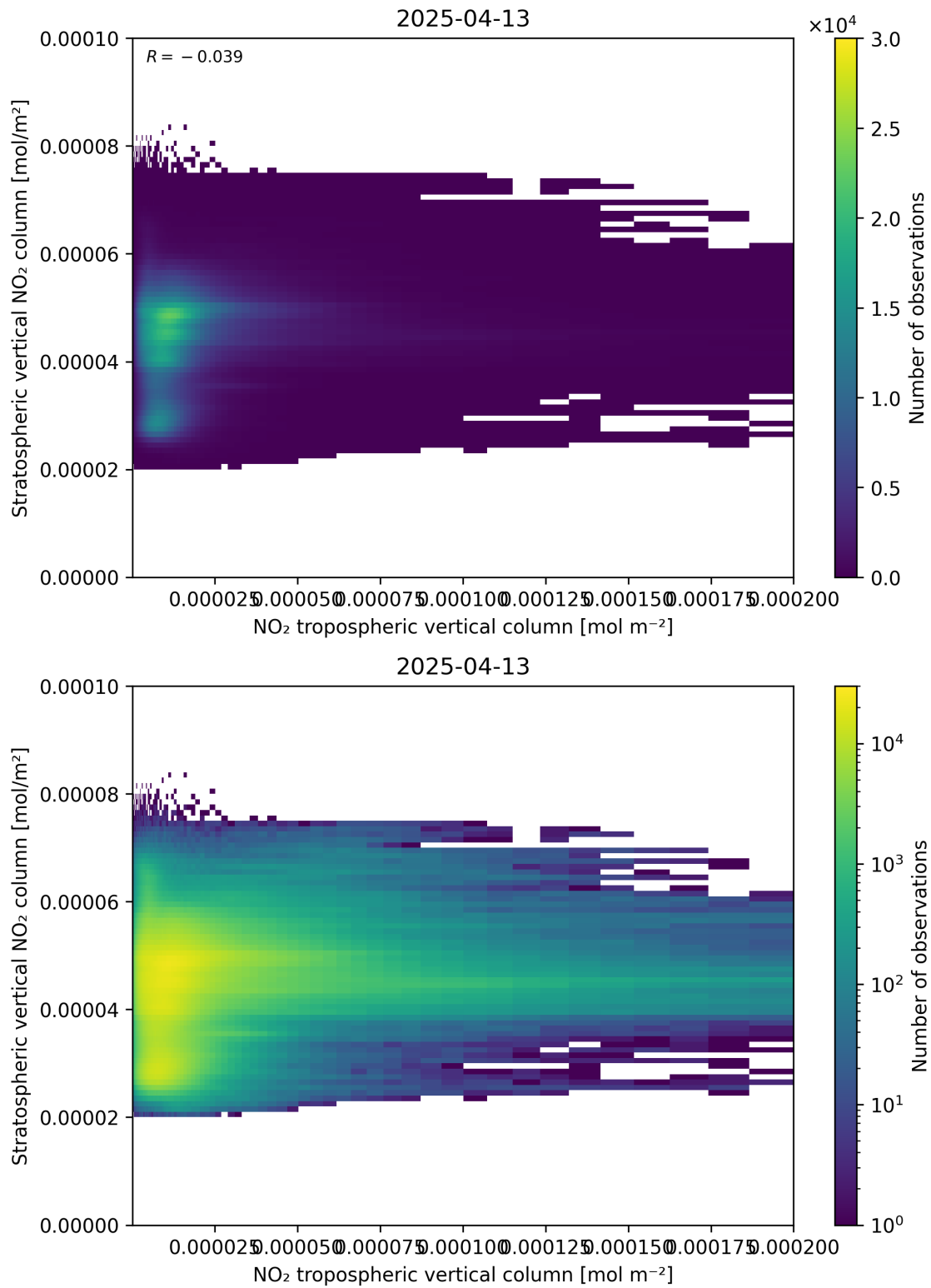
Figure 125: Scatter density plot of “NO 2 tropospheric vertical column” against “Stratospheric vertical NO 2 column” for 2025-04-13 to 2025-04-14.
