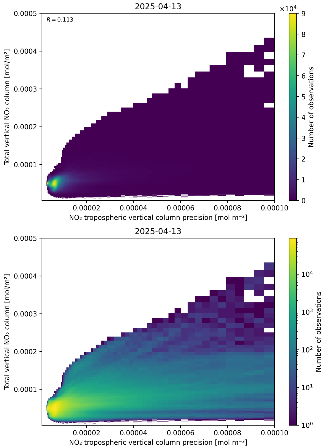
Figure 138: Scatter density plot of “NO 2 tropospheric vertical column precision” against “Total vertical NO 2 column” for 2025-04-13 to 2025-04-14.
