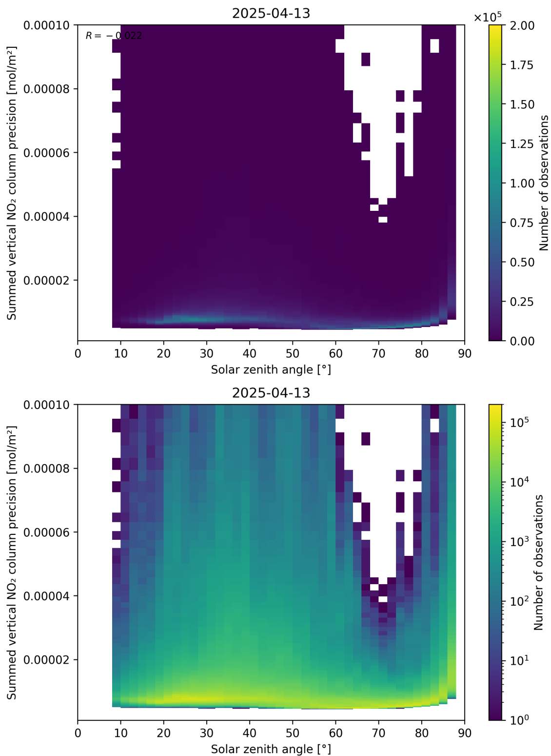
Figure 152: Scatter density plot of “Solar zenith angle” against “Summed vertical NO 2 column precision” for 2025-04-13 to 2025-04-14.
