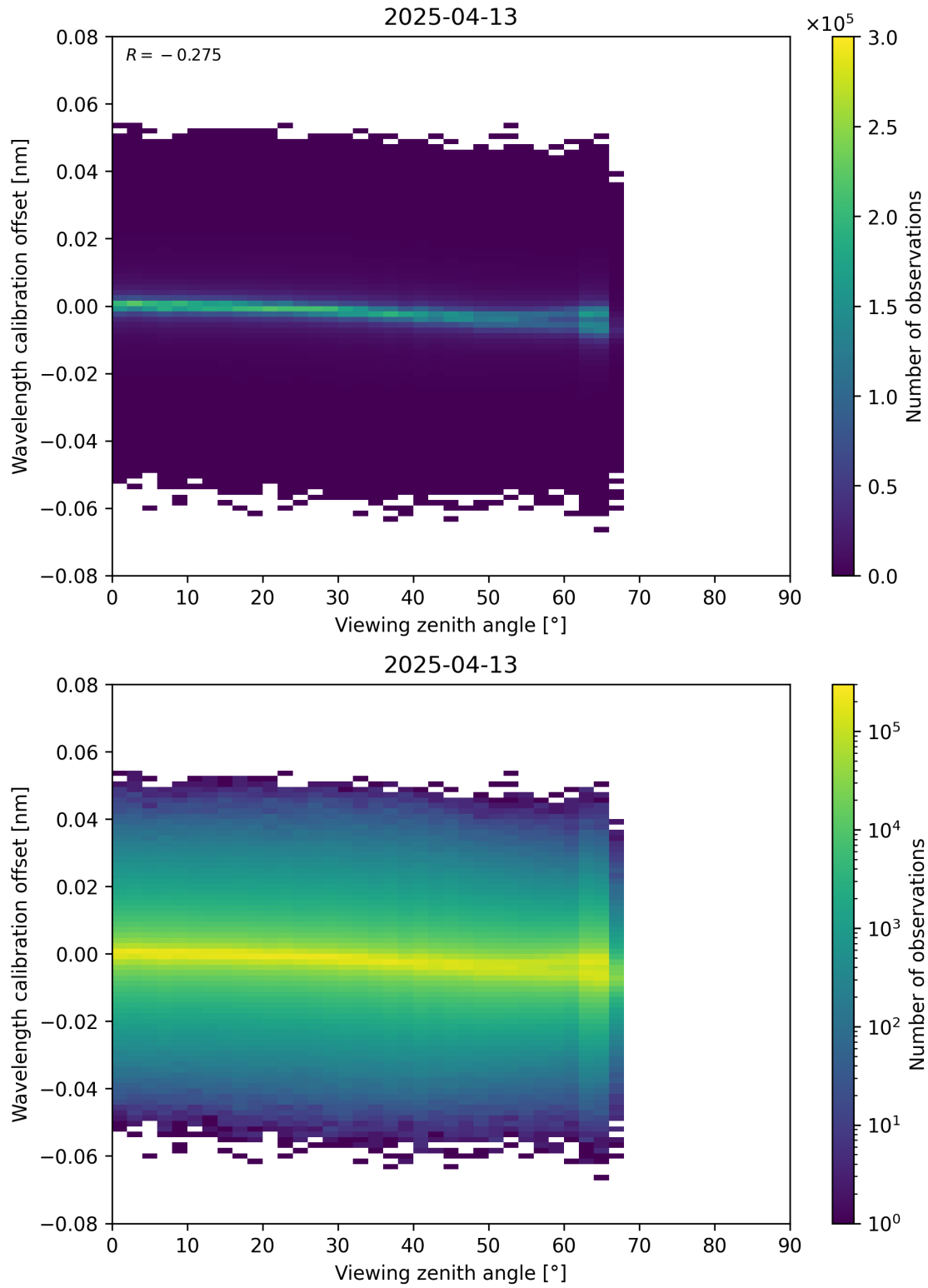
Figure 173: Scatter density plot of “Viewing zenith angle” against “Wavelength calibration offset” for 2025-04-13 to 2025-04-14.
