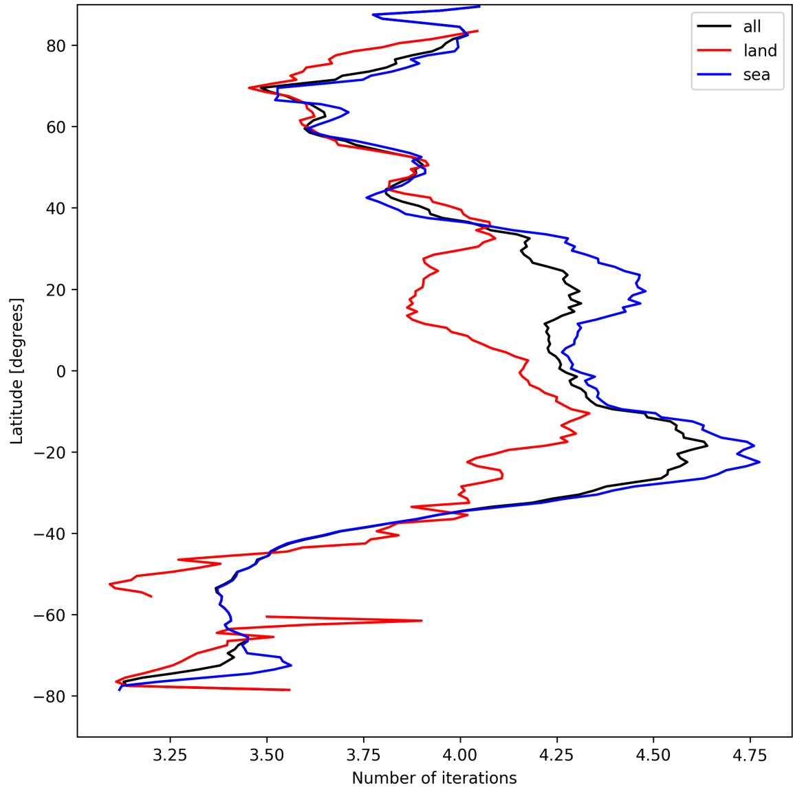
Figure 17: Zonal average of “Number of iterations” for 2025-04-13 to 2025-04-14.
