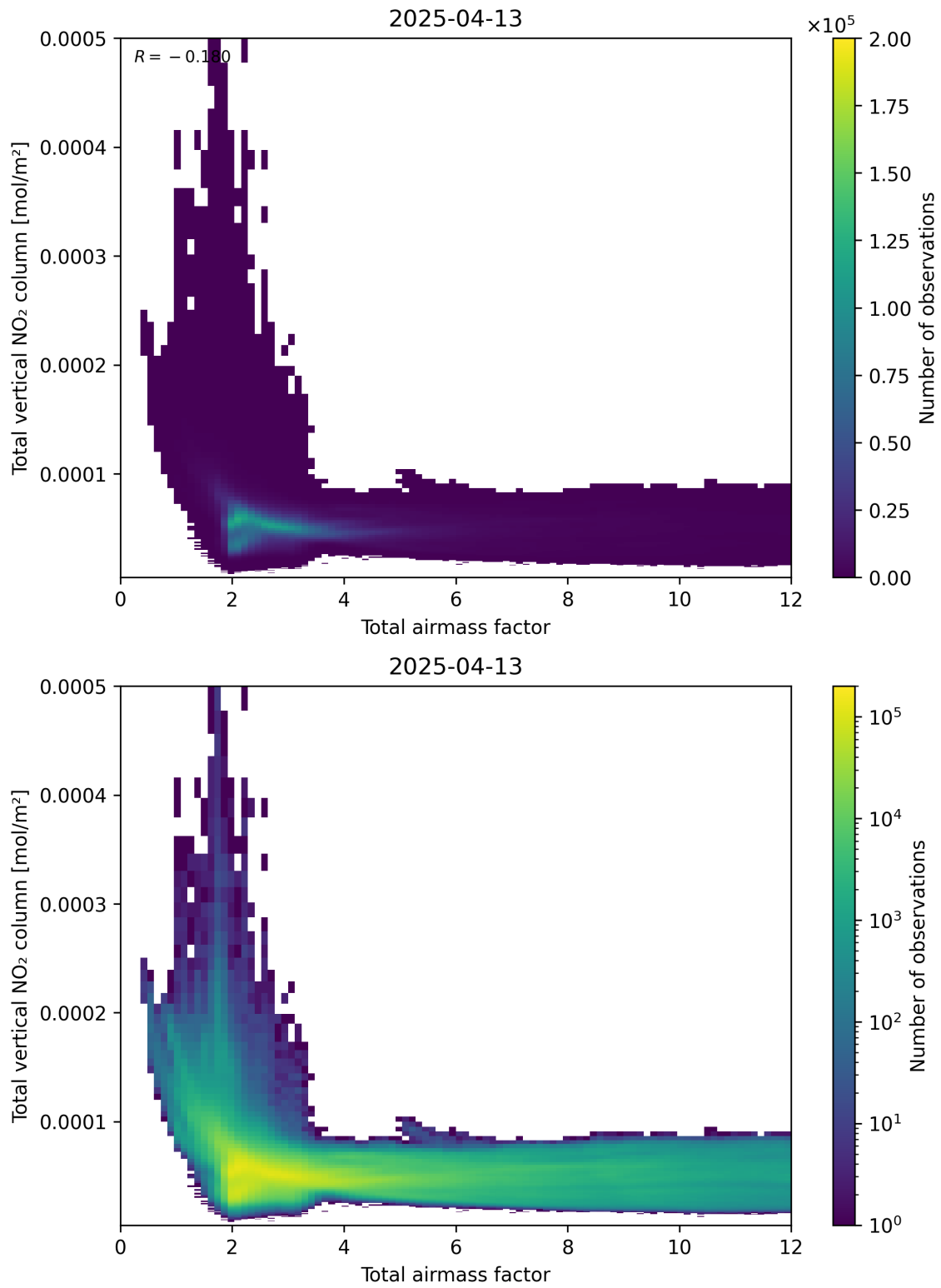
Figure 67: Scatter density plot of “Total airmass factor” against “Total vertical NO 2 column” for 2025-04-13 to 2025-04-14.
