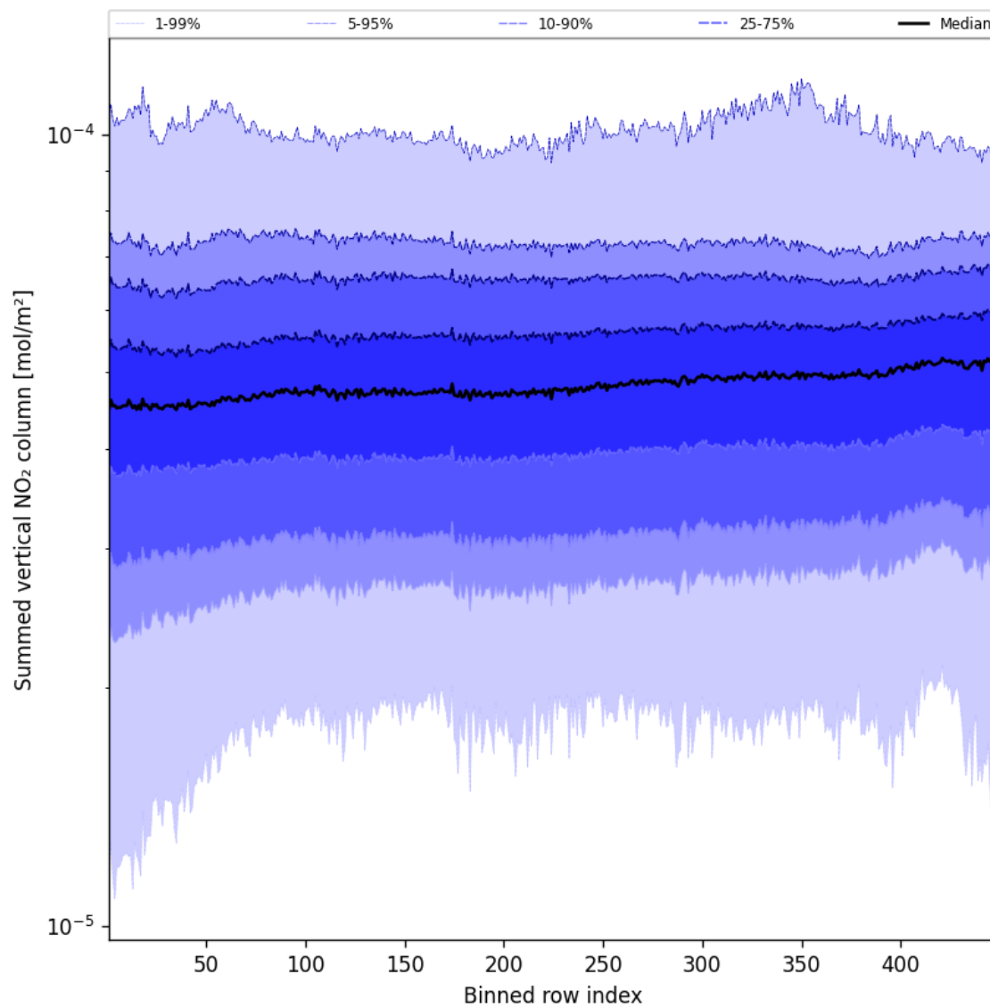
Figure 57: Along track statistics of “Summed vertical NO 2 column” for 2025-04-13 to 2025-04-14
