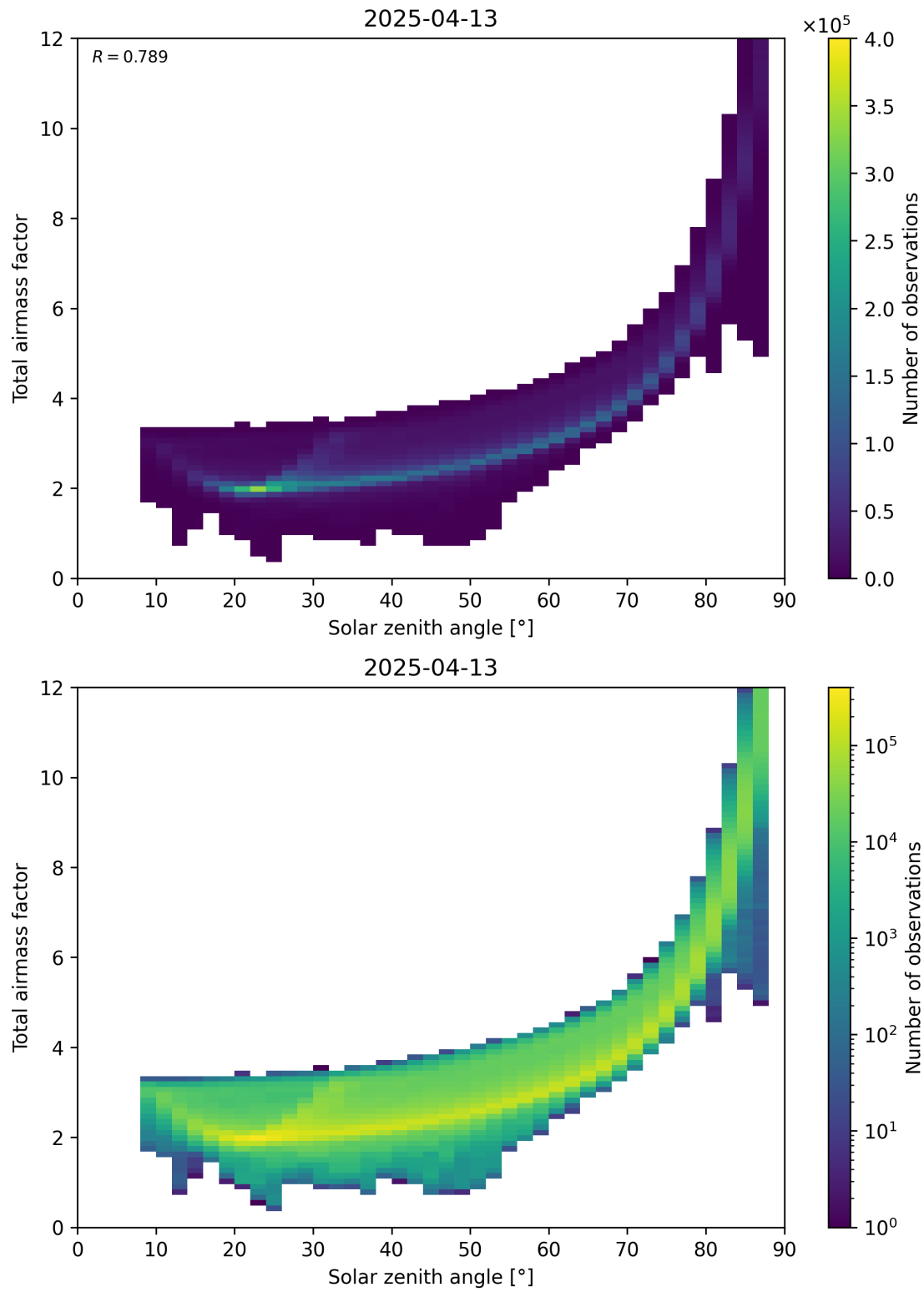
Figure 146: Scatter density plot of “Solar zenith angle” against “Total airmass factor” for 2025-04-13 to 2025-04-14.
