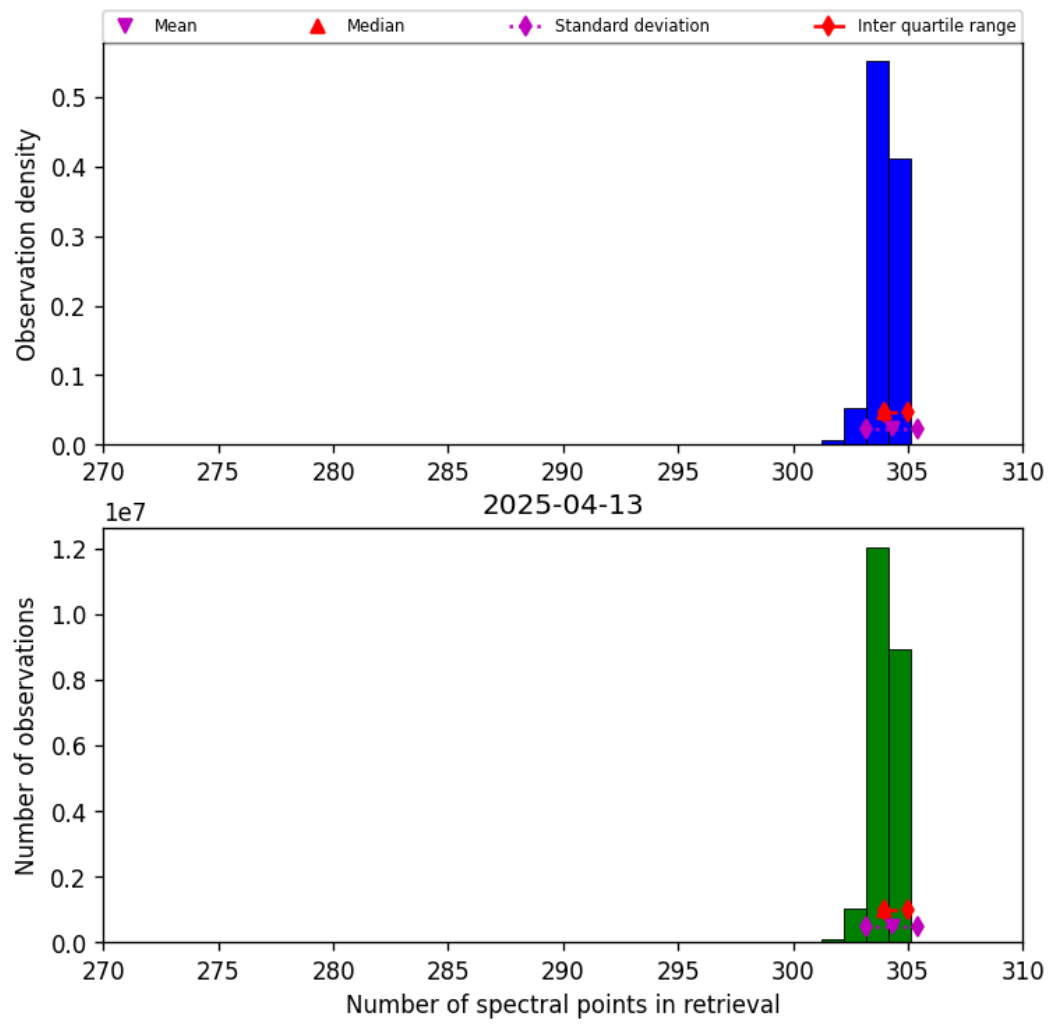
Figure 33: Histogram of “Number of spectral points in retrieval” for 2025-04-13 to 2025-04-14
