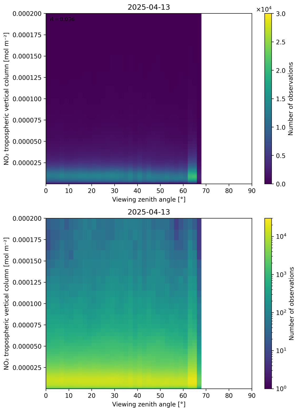
Figure 169: Scatter density plot of “Viewing zenith angle” against “NO 2 tropospheric vertical column” for 2025-04-13 to 2025-04-14.
