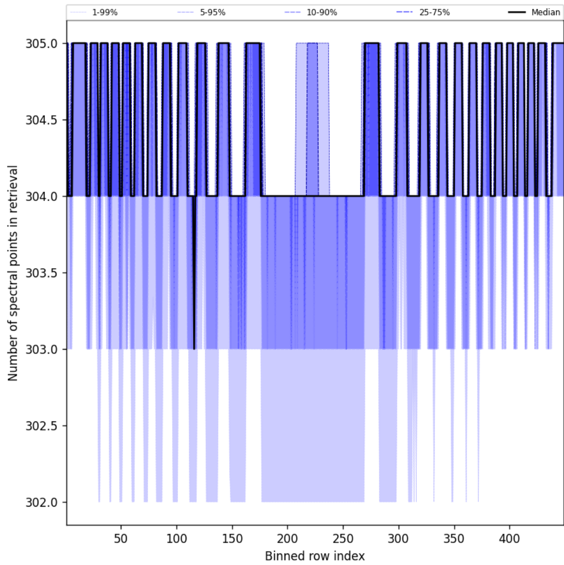
Figure 50: Along track statistics of “Number of spectral points in retrieval” for 2025-04-13 to 2025-04-14
