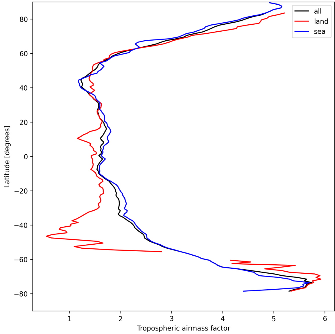
Figure 14: Zonal average of “Tropospheric airmass factor” for 2025-04-13 to 2025-04-14.
