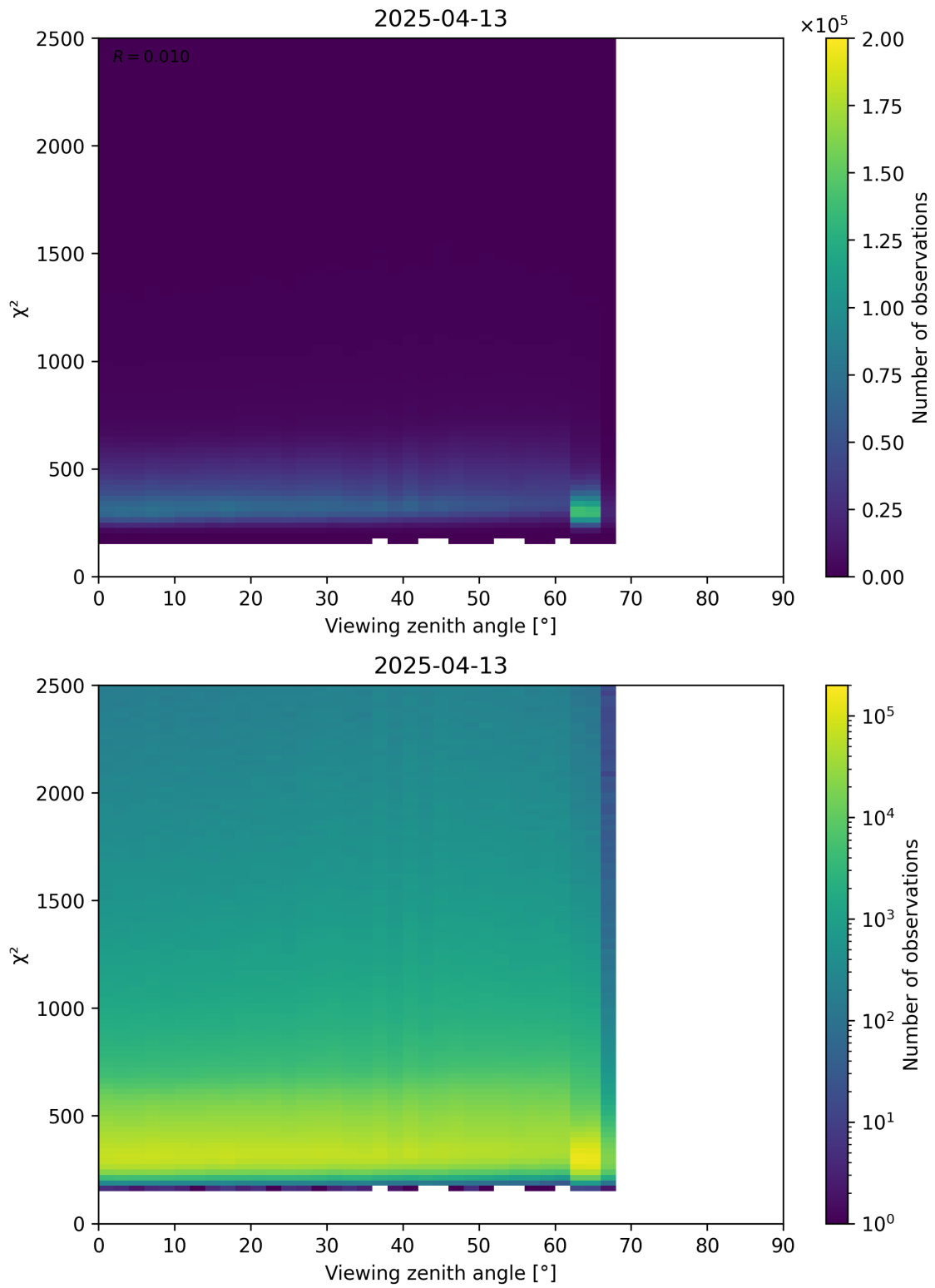
Figure 162: Scatter density plot of “Viewing zenith angle” against “ \chi^2 ” for 2025-04-13 to 2025-04-14.
