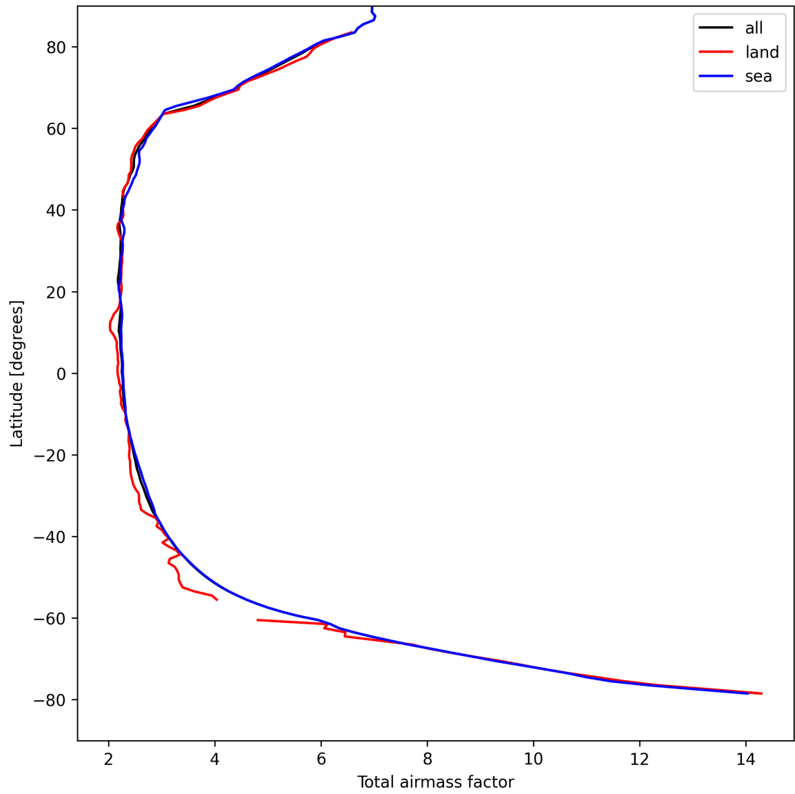
Figure 15: Zonal average of “Total airmass factor” for 2025-04-13 to 2025-04-14.
