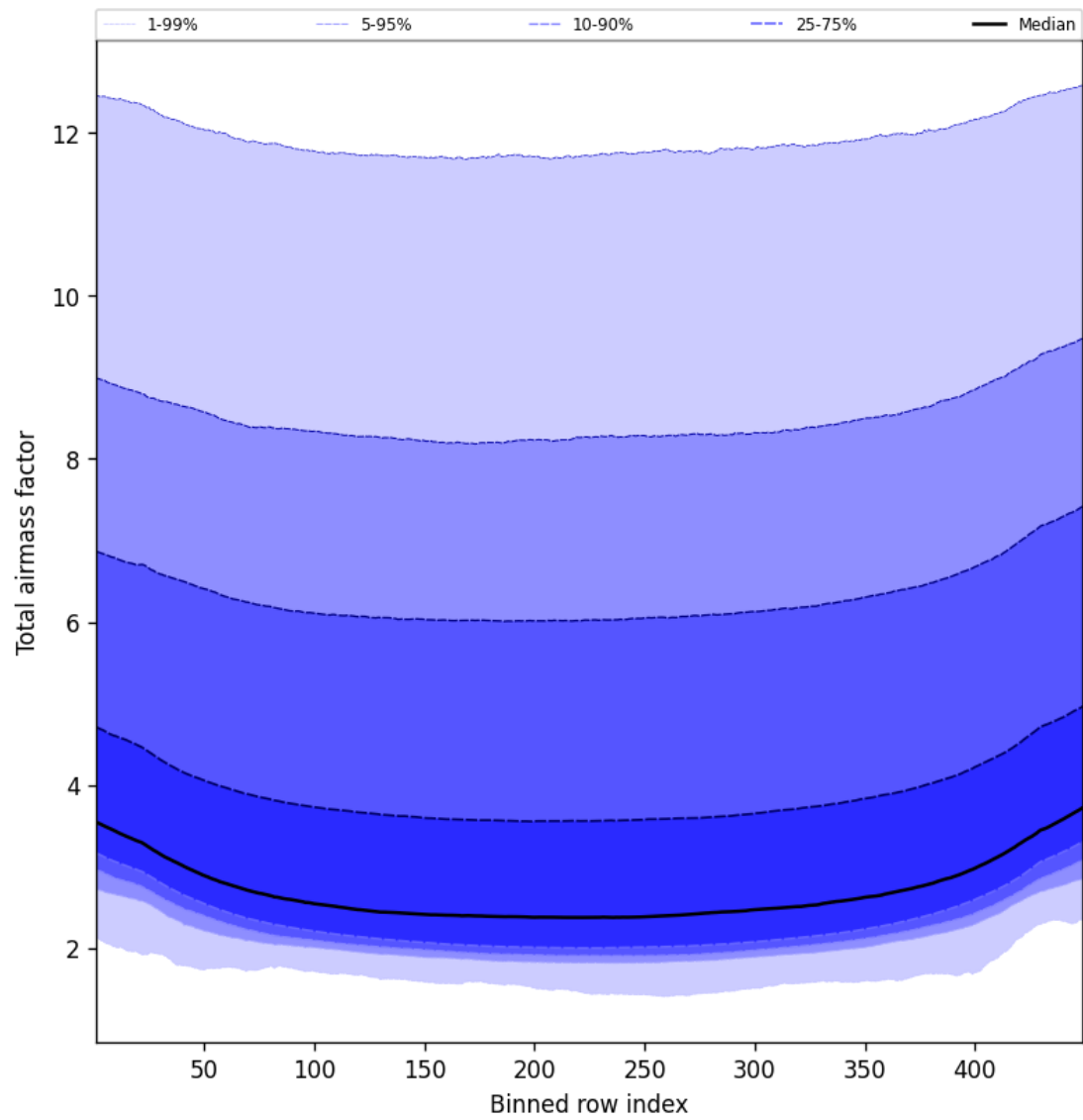
Figure 49: Along track statistics of “Total airmass factor” for 2025-04-13 to 2025-04-14
