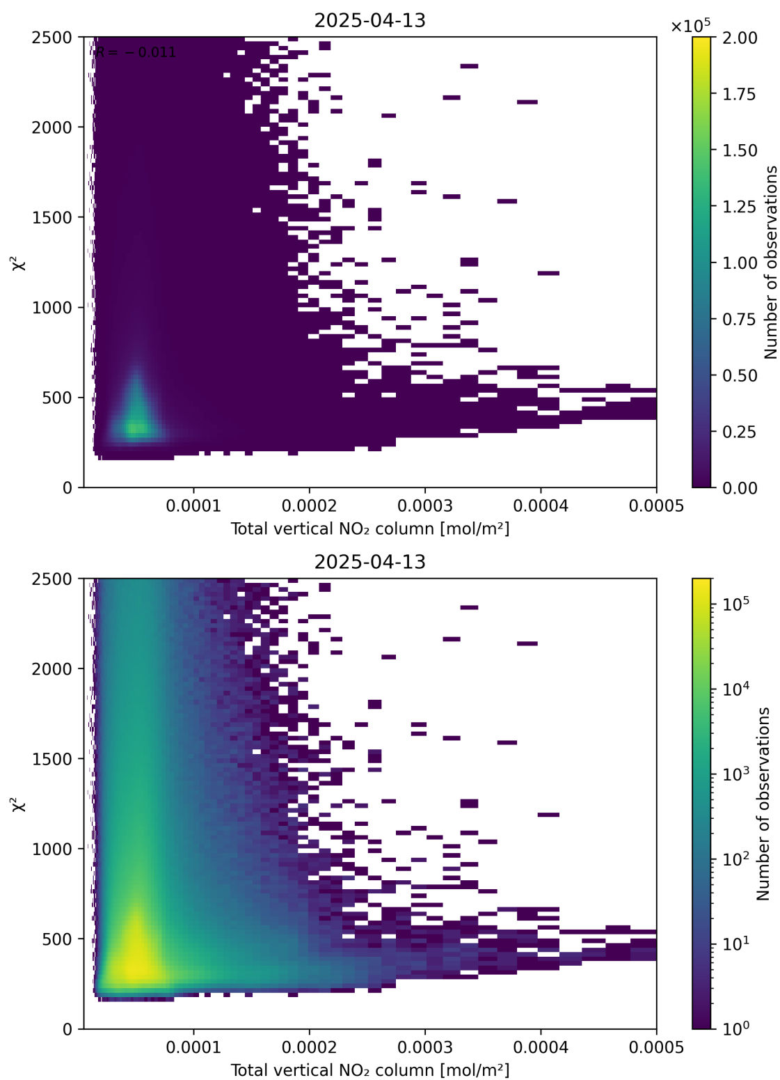
Figure 111: Scatter density plot of “Total vertical NO 2 column” against “ \chi^2 ” for 2025-04-13 to 2025-04-14.
