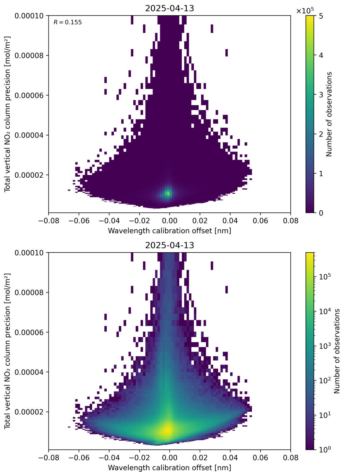
Figure 180: Scatter density plot of “Wavelength calibration offset” against “Total vertical NO 2 column precision” for 2025-04-13 to 2025-04-14.
