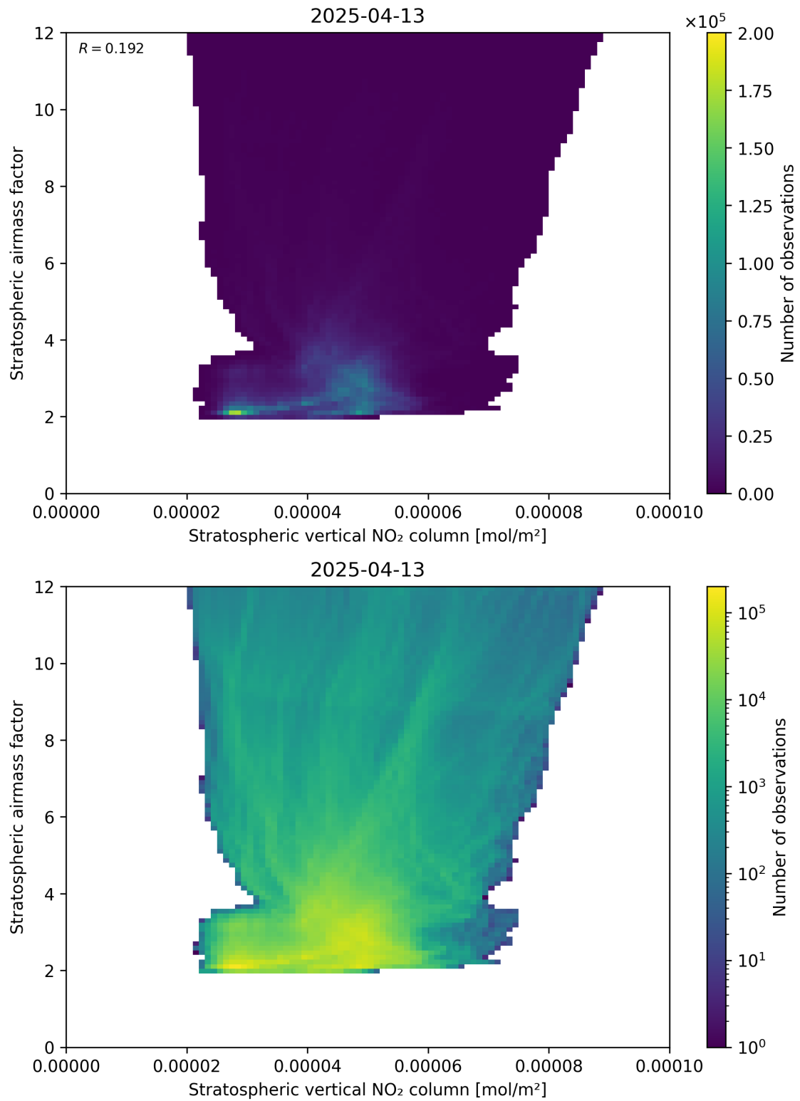
Figure 96: Scatter density plot of “Stratospheric vertical NO 2 column” against “Stratospheric airmass factor” for 2025-04-13 to 2025-04-14.
