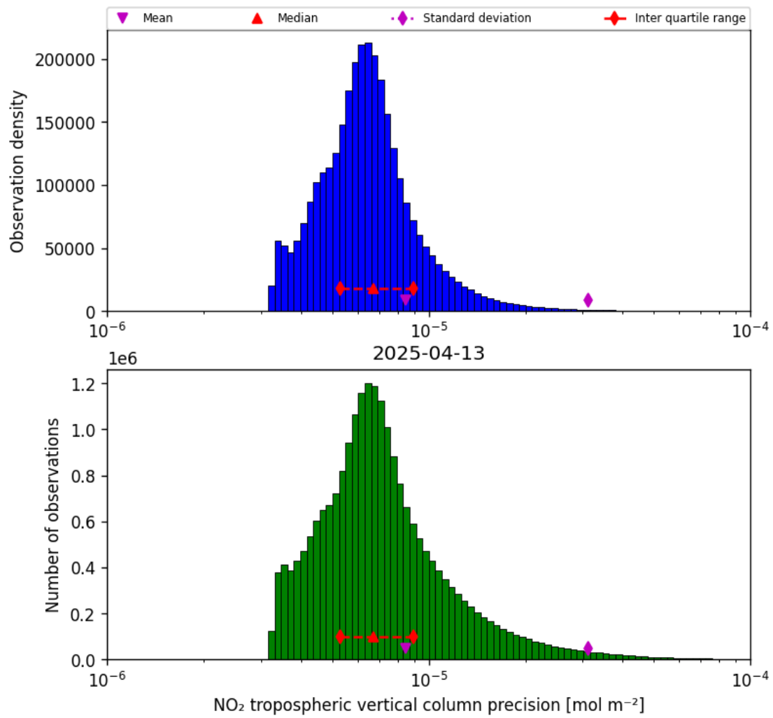
Figure 30: Histogram of “NO 2 tropospheric vertical column precision” for 2025-04-13 to 2025-04-14
