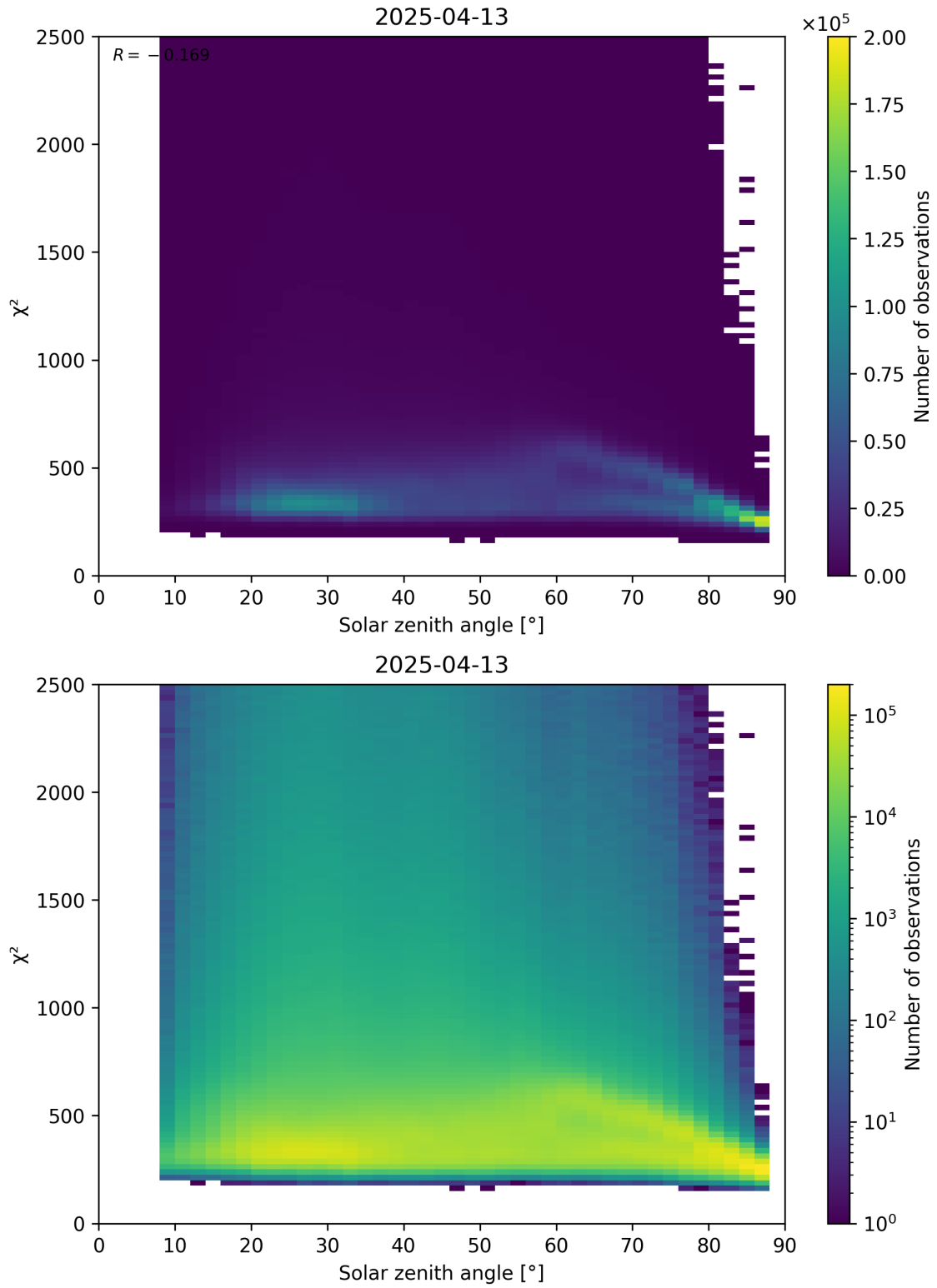
Figure 148: Scatter density plot of “Solar zenith angle” against “ \chi^2 ” for 2025-04-13 to 2025-04-14.
