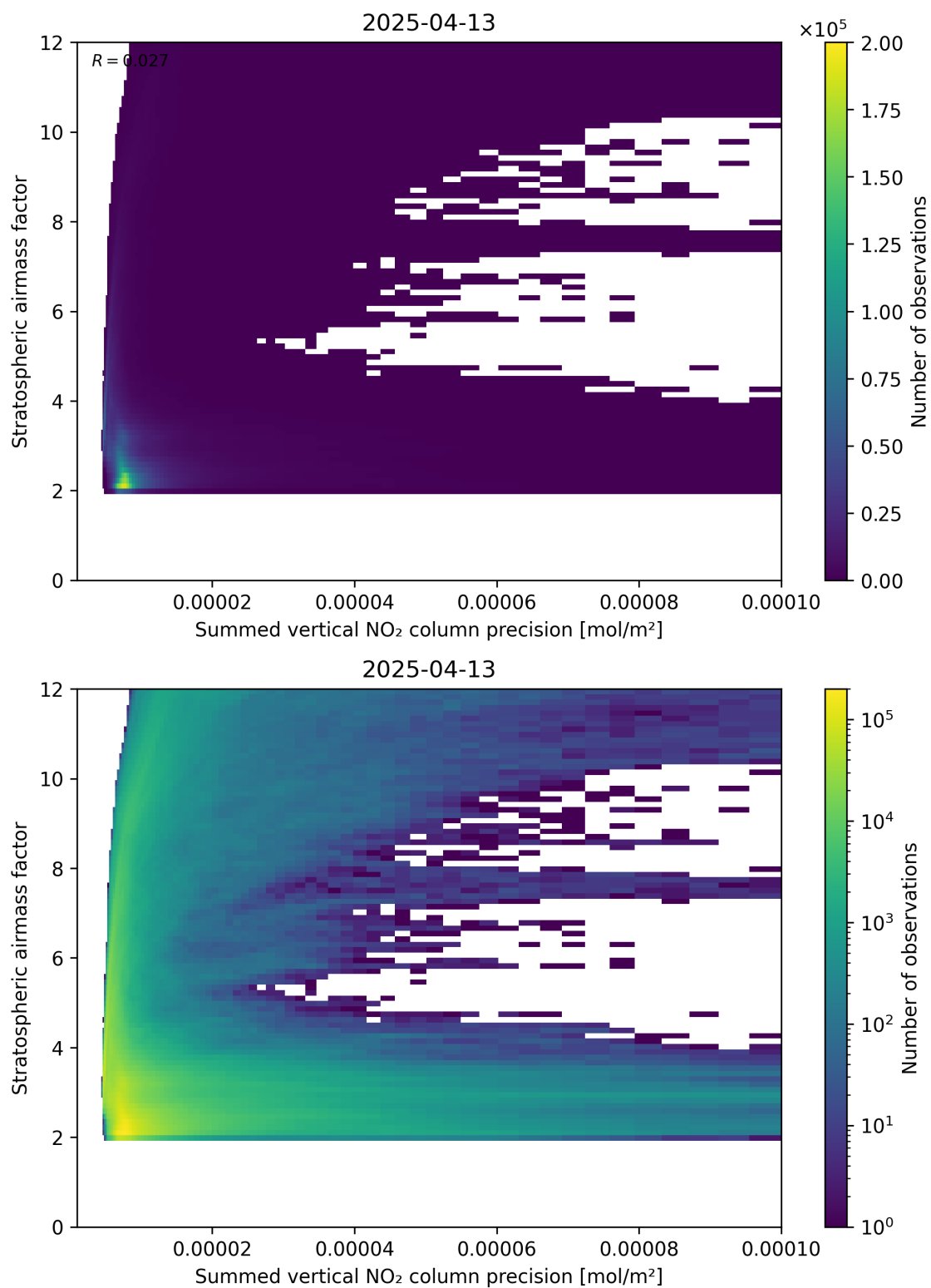
Figure 106: Scatter density plot of “Summed vertical NO 2 column precision” against “Stratospheric airmass factor” for 2025-04-13 to 2025-04-14.
