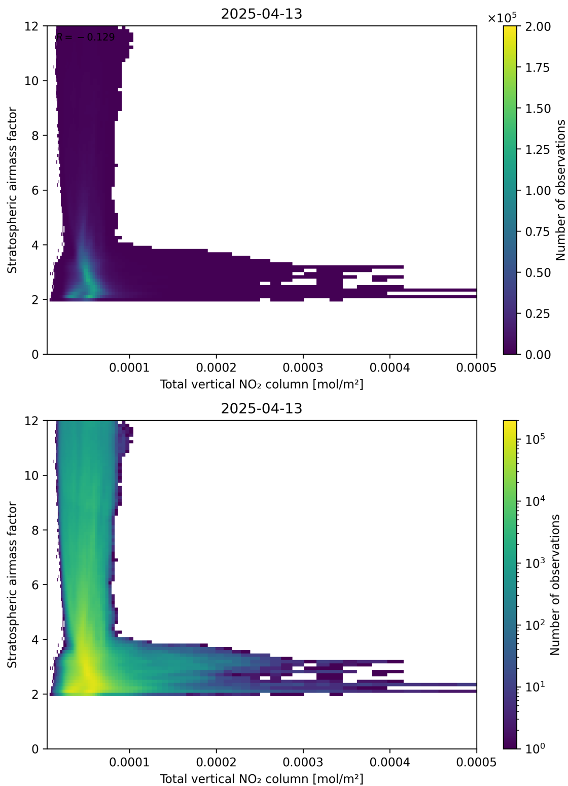
Figure 110: Scatter density plot of “Total vertical NO 2 column” against “Stratospheric airmass factor” for 2025-04-13 to 2025-04-14.
