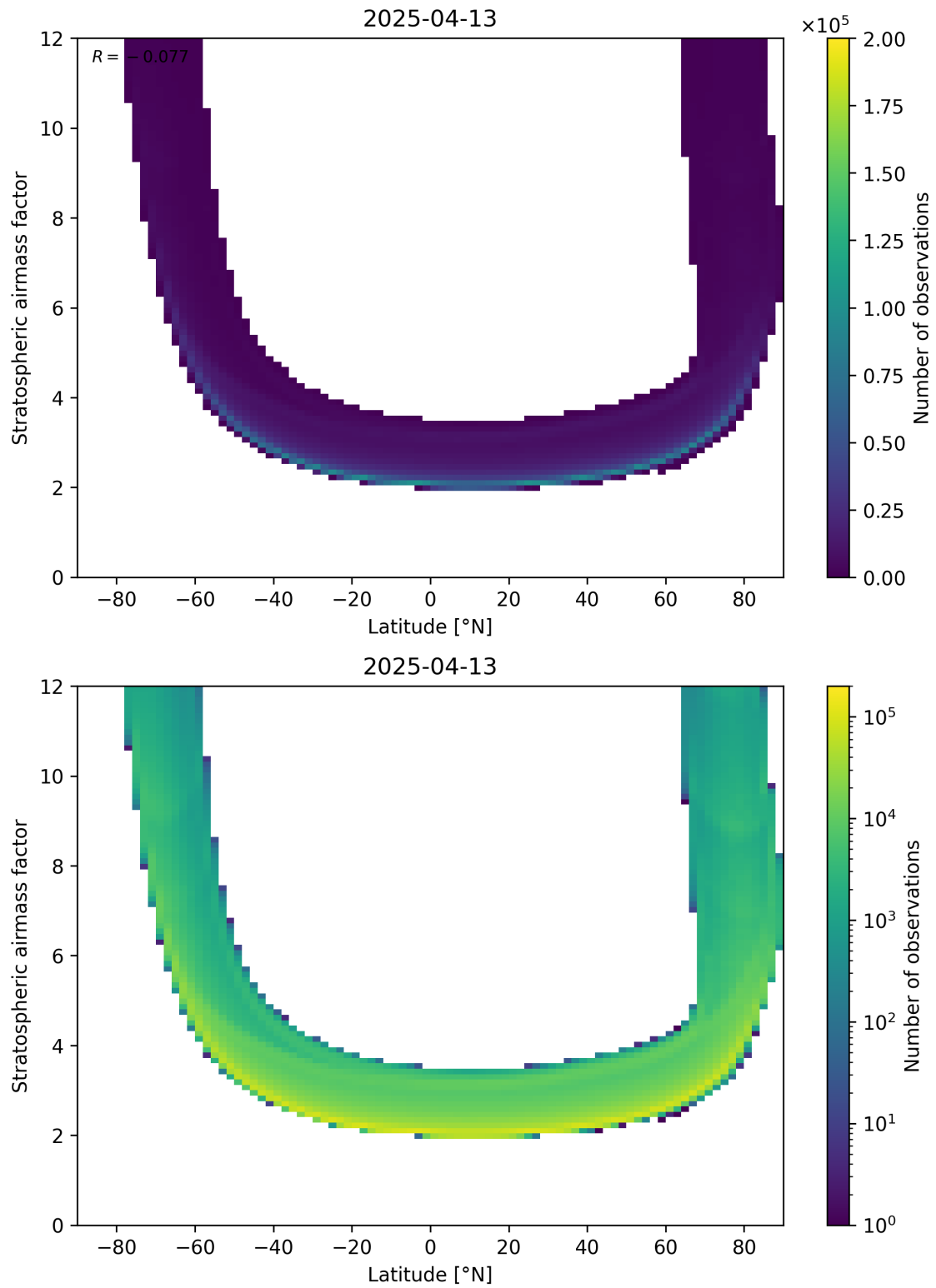
Figure 83: Scatter density plot of “Latitude” against “Stratospheric air mass factor” for 2025-04-13 to 2025-04-14.
