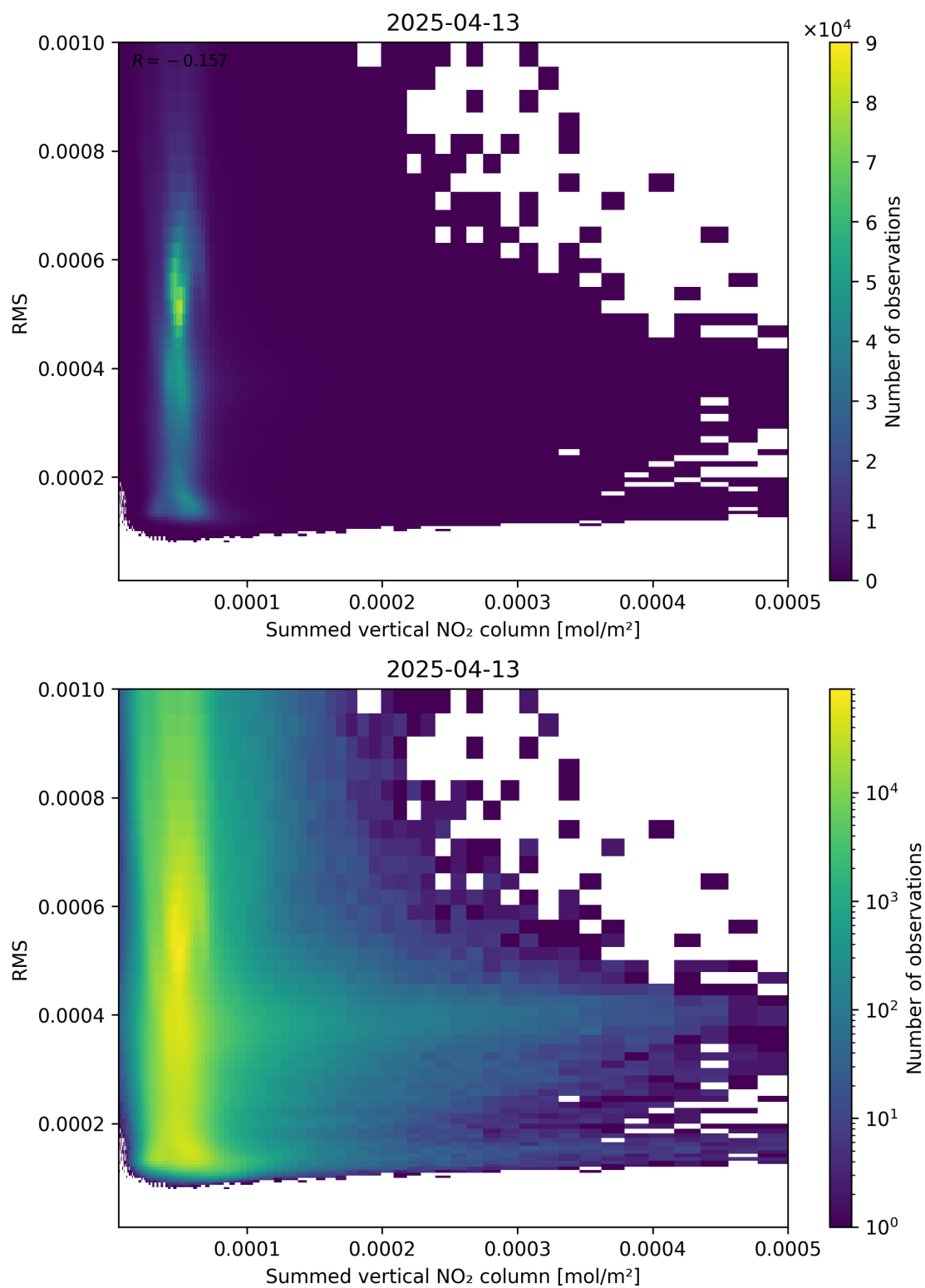
Figure 109: Scatter density plot of “Summed vertical NO 2 column” against “RMS” for 2025-04-13 to 2025-04-14.
