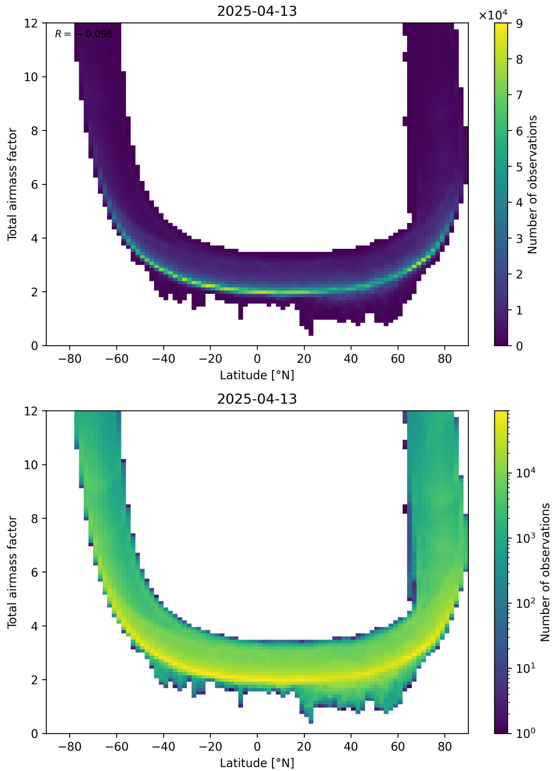
Figure 84: Scatter density plot of “Latitude” against “Total airmass factor” for 2025-04-13 to 2025-04-14.
