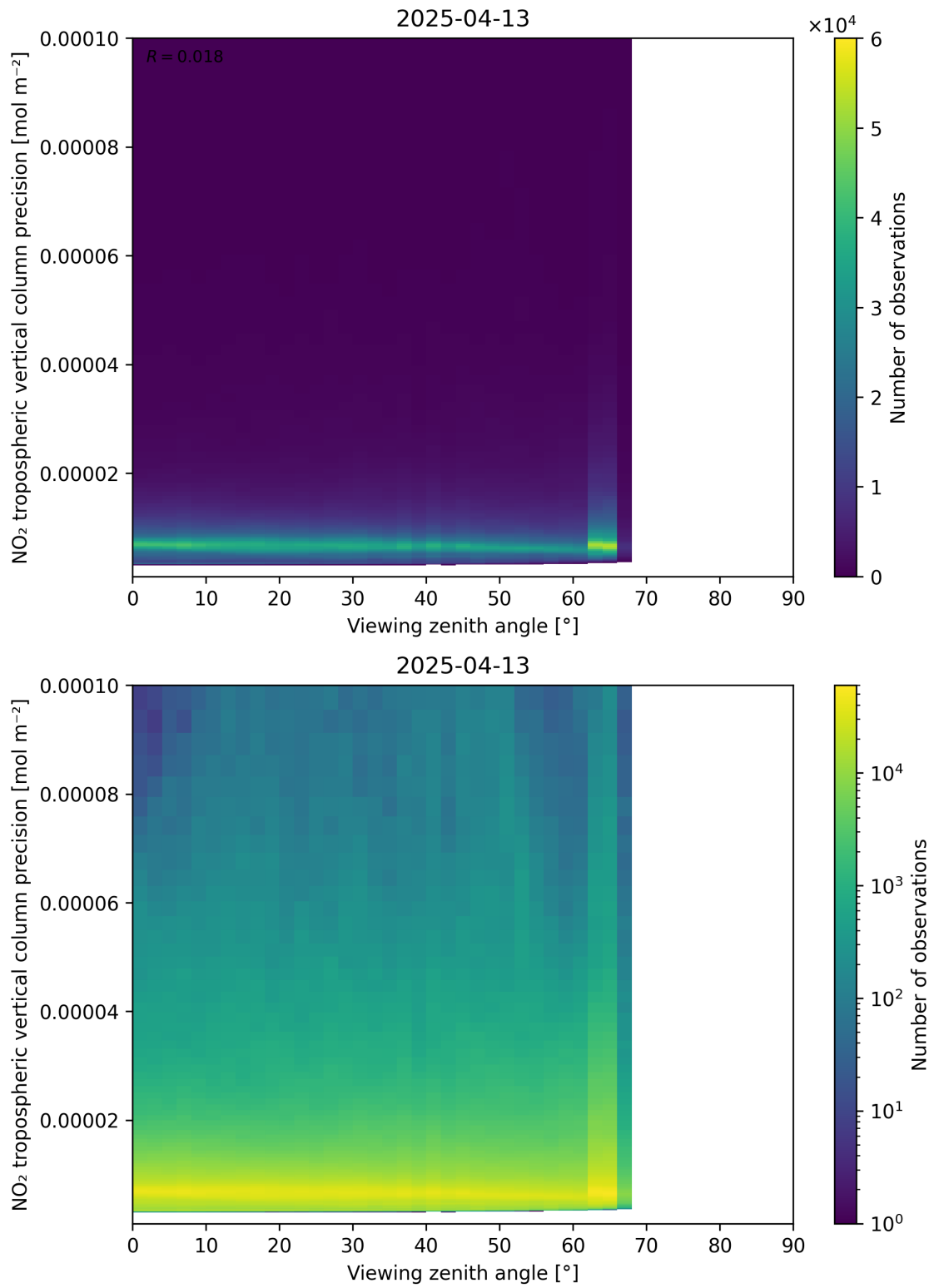
Figure 170: Scatter density plot of “Viewing zenith angle” against “NO 2 tropospheric vertical column precision” for 2025-04-13 to 2025-04-14.
