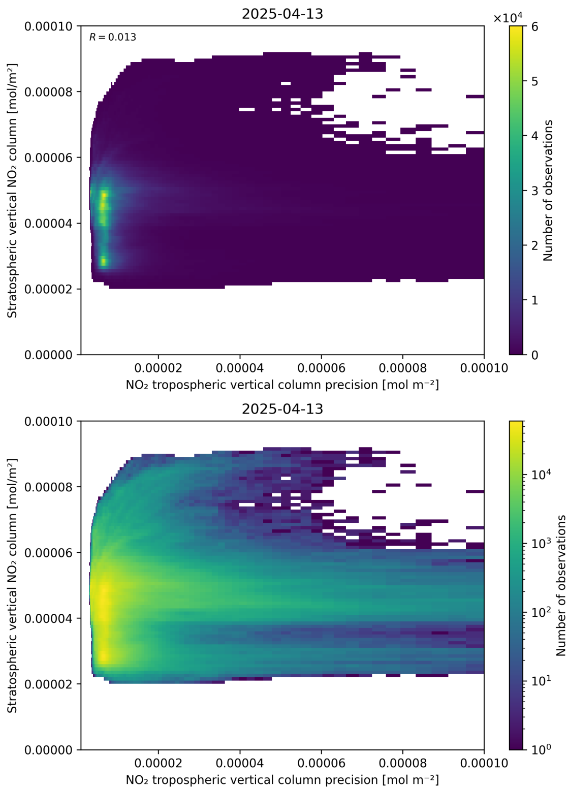
Figure 135: Scatter density plot of “NO 2 tropospheric vertical column precision” against “Stratospheric vertical NO 2 column” for 2025-04-13 to 2025-04-14.
