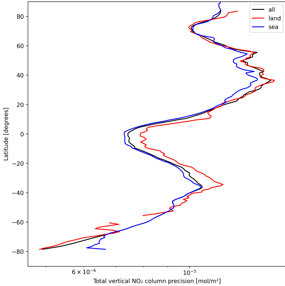
Figure 22: Zonal average of “Total vertical NO 2 column precision” for 2025-04-13 to 2025-04-14.
