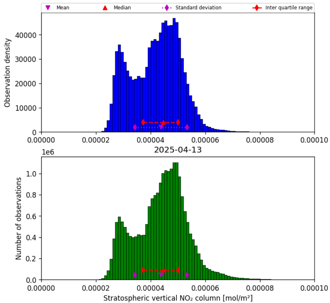
Figure 36: Histogram of “Stratospheric vertical NO 2 column” for 2025-04-13 to 2025-04-14
