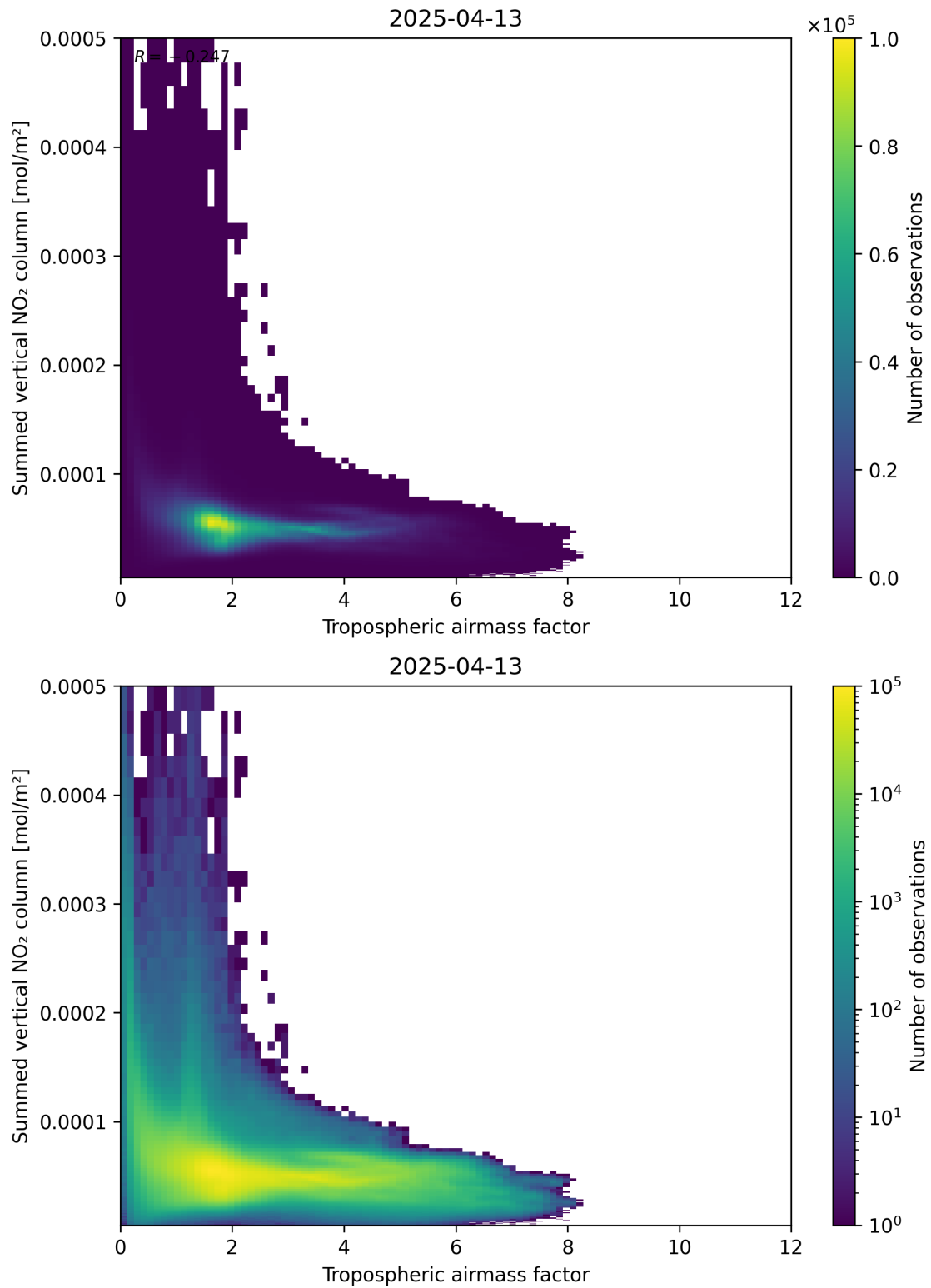
Figure 75: Scatter density plot of “Tropospheric air mass factor” against “Summed vertical NO 2 column” for 2025-04-13 to 2025-04-14.
