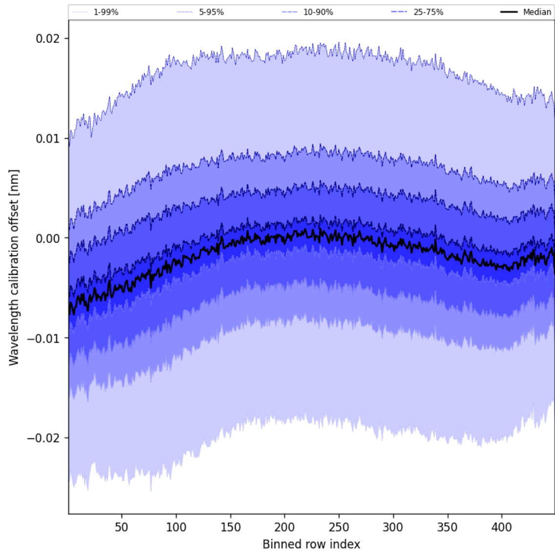
Figure 52: Along track statistics of “Wavelength calibration offset” for 2025-04-13 to 2025-04-14
