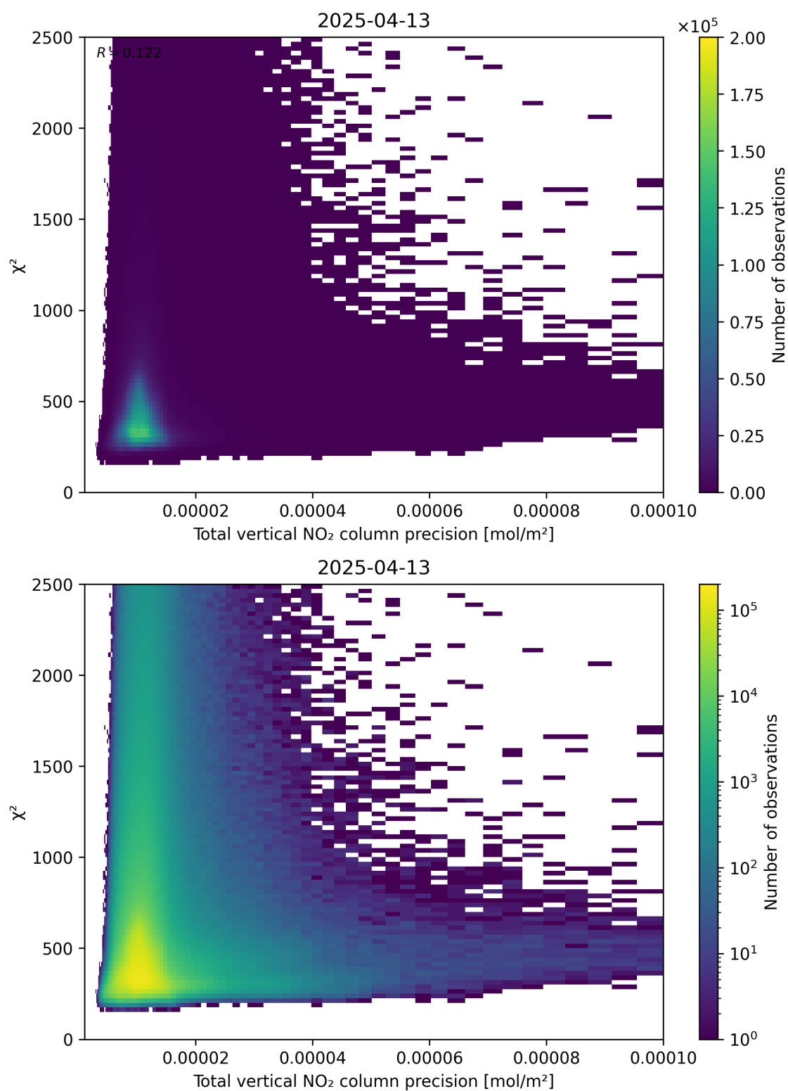
Figure 116: Scatter density plot of “Total vertical NO 2 column precision” against “ \chi^2 ” for 2025-04-13 to 2025-04-14.
