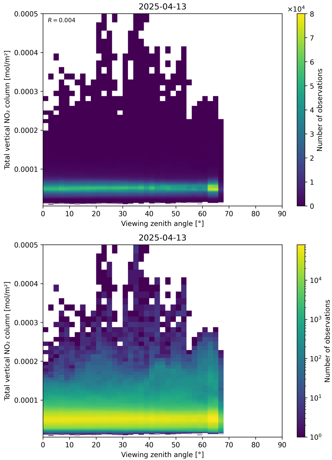
Figure 167: Scatter density plot of “Viewing zenith angle” against “Total vertical NO 2 column” for 2025-04-13 to 2025-04-14.
