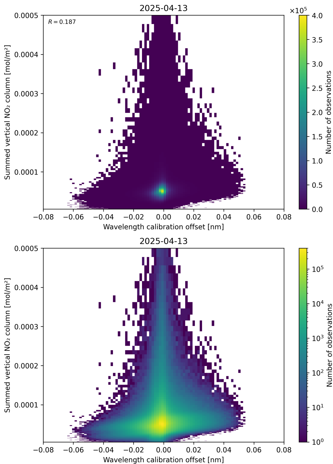
Figure 177: Scatter density plot of “Wavelength calibration offset” against “Summed vertical NO 2 column” for 2025-04-13 to 2025-04-14.
