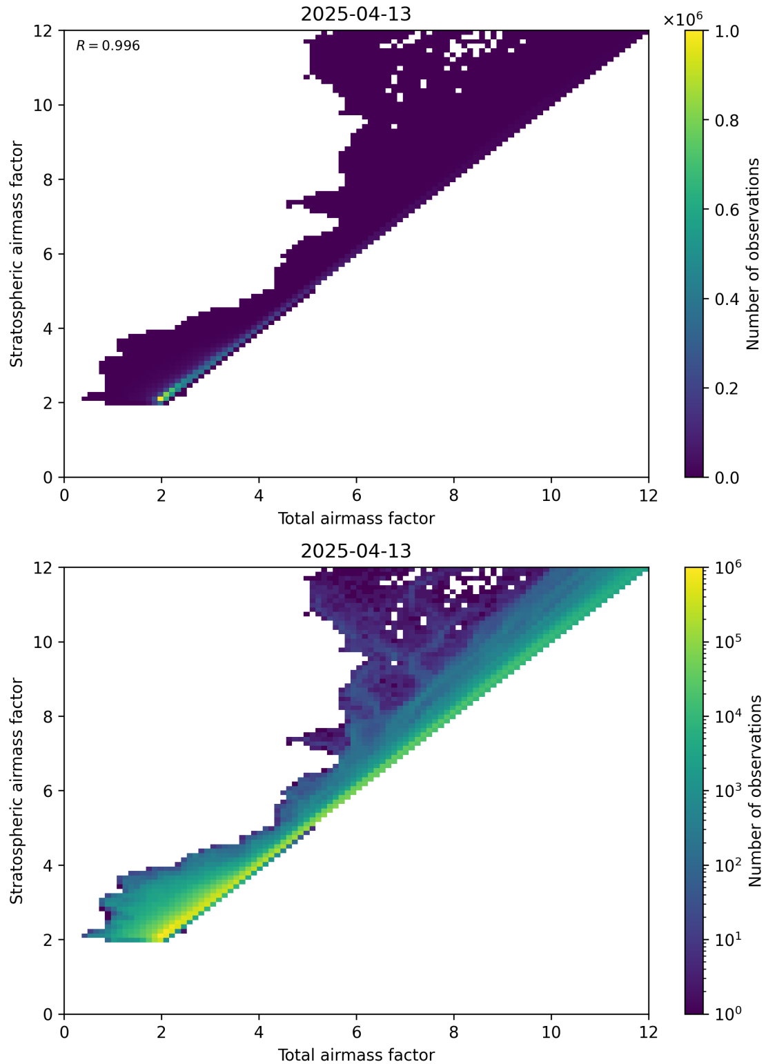
Figure 62: Scatter density plot of “Total airmass factor” against “Stratospheric airmass factor” for 2025-04-13 to 2025-04-14.
