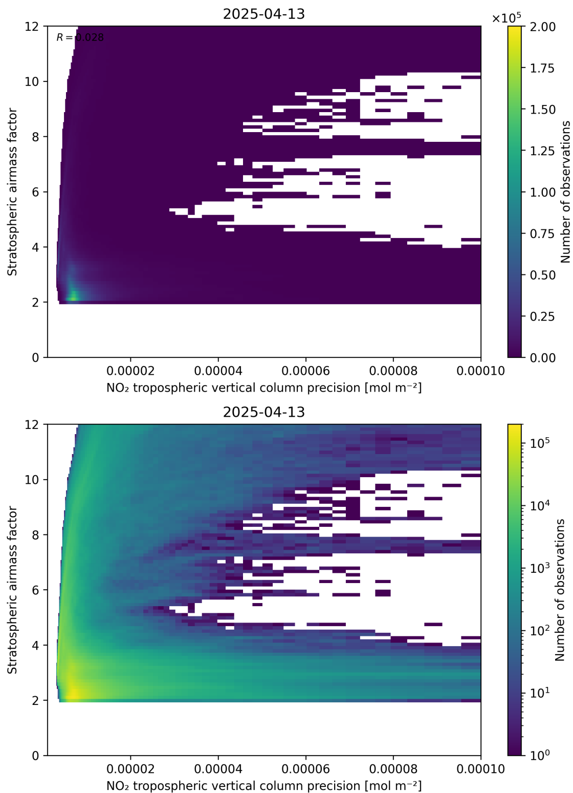
Figure 131: Scatter density plot of “NO 2 tropospheric vertical column precision” against “Stratospheric airmass factor” for 2025-04-13 to 2025-04-14.
