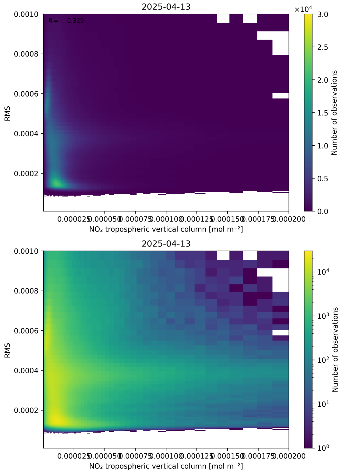
Figure 142: Scatter density plot of “NO 2 tropospheric vertical column” against “RMS” for 2025-04-13 to 2025-04-14.
