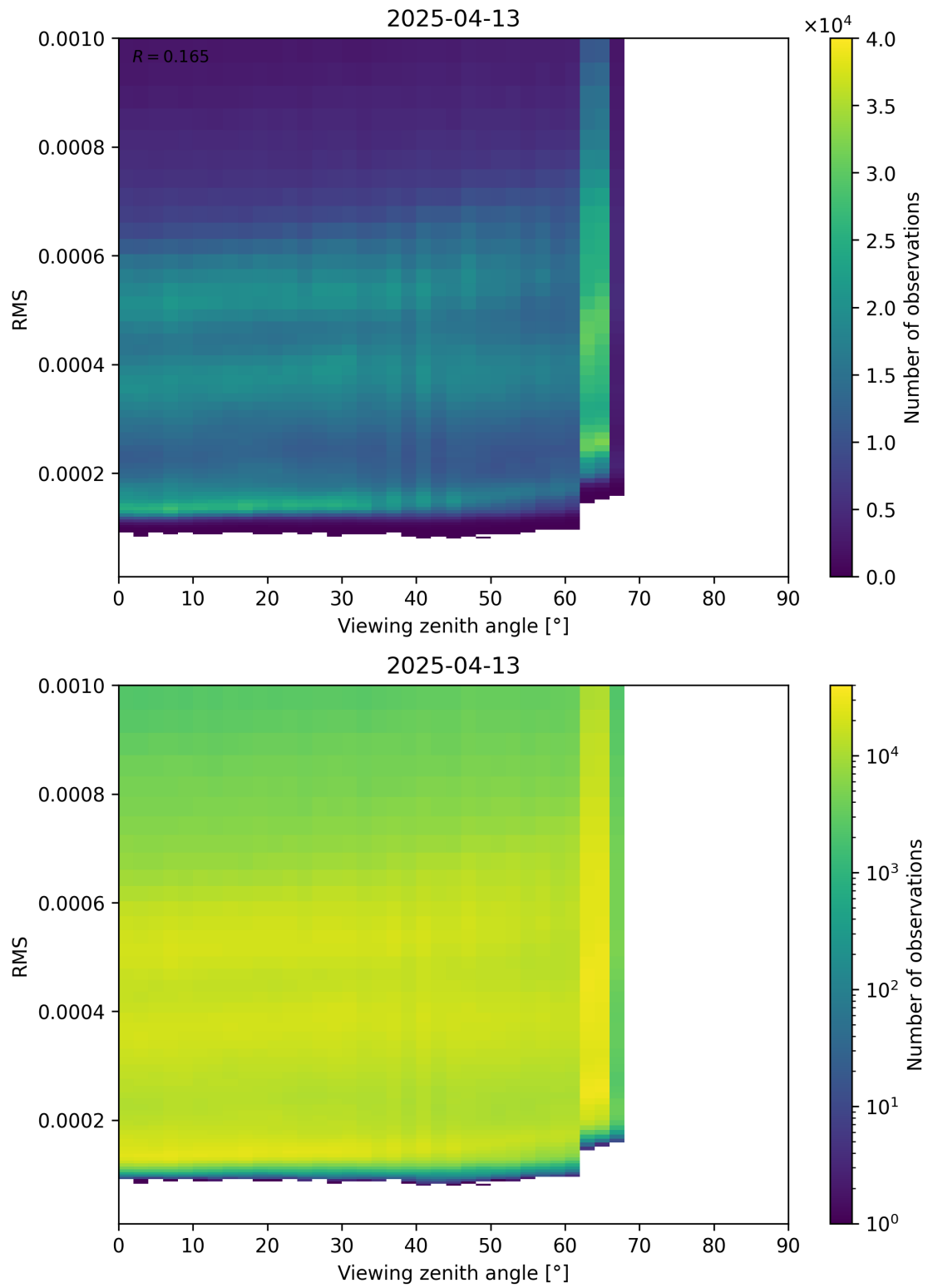
Figure 171: Scatter density plot of “Viewing zenith angle” against “RMS” for 2025-04-13 to 2025-04-14.
