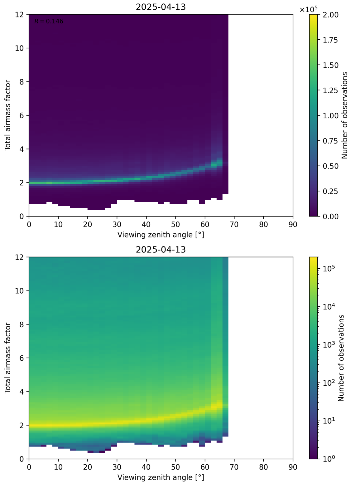
Figure 160: Scatter density plot of “Viewing zenith angle” against “Total airmass factor” for 2025-04-13 to 2025-04-14.
