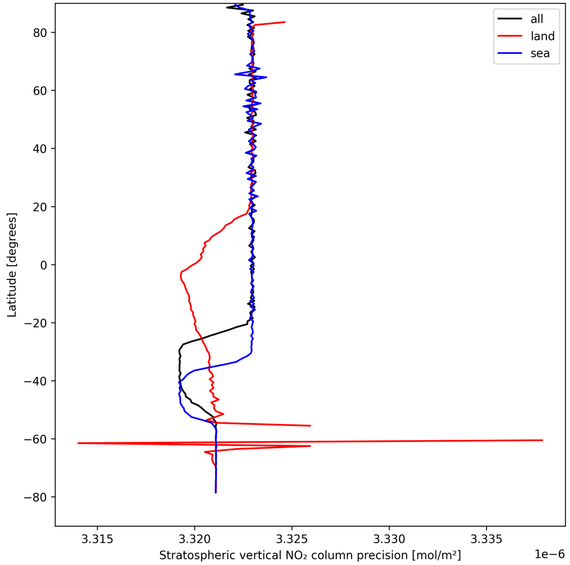
Figure 20: Zonal average of “Stratospheric vertical NO 2 column precision” for 2025-04-13 to 2025-04-14.
