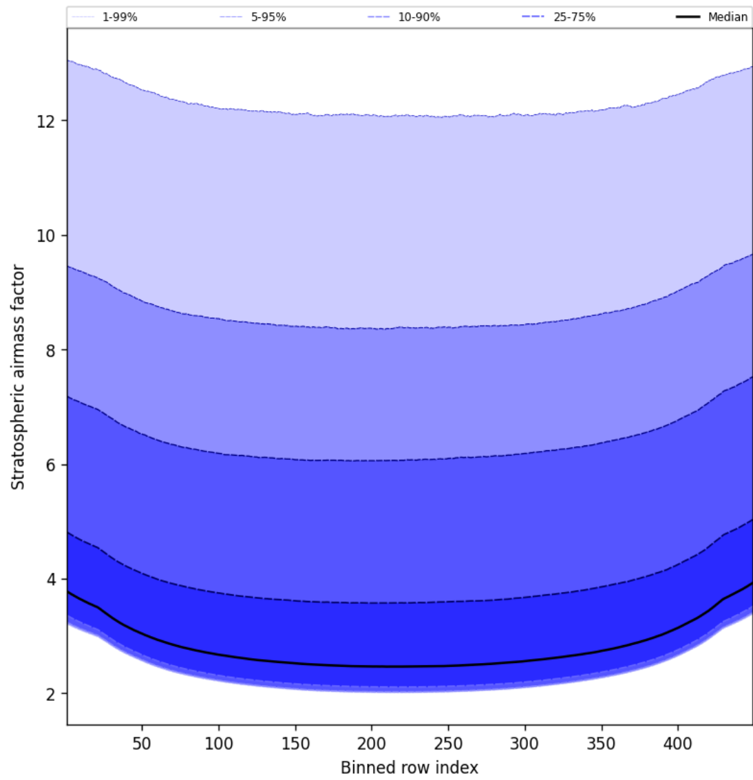
Figure 61: Along track statistics of “Stratospheric airmass factor” for 2025-04-13 to 2025-04-14
