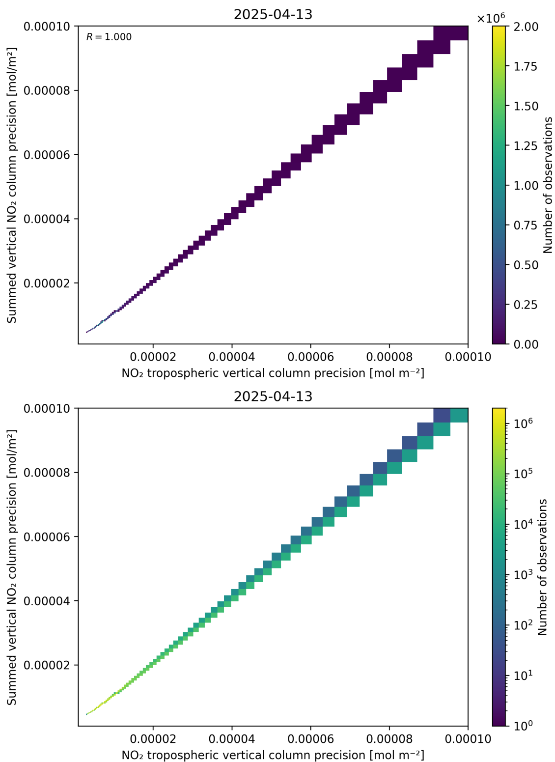
Figure 137: Scatter density plot of “NO 2 tropospheric vertical column precision” against “Summed vertical NO 2 column precision” for 2025-04-13 to 2025-04-14.
