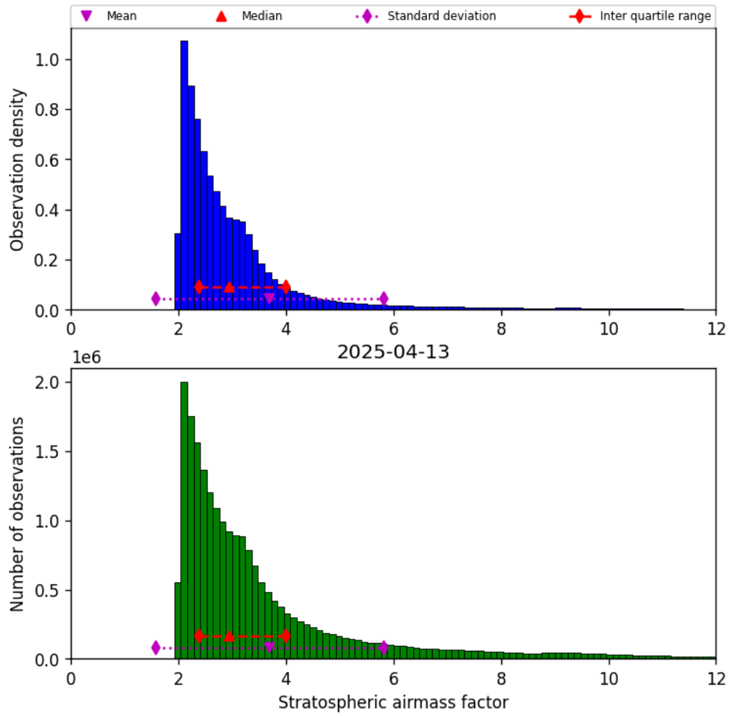
Figure 44: Histogram of “Stratospheric airmass factor” for 2025-04-13 to 2025-04-14
