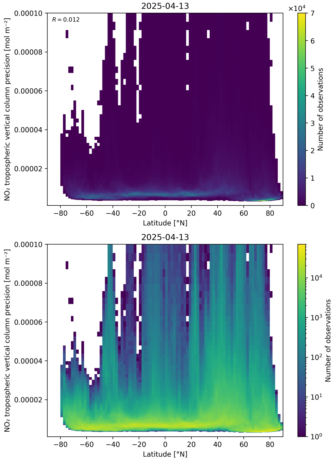
Figure 93: Scatter density plot of “Latitude” against “NO 2 tropospheric vertical column precision” for 2025-04-13 to 2025-04-14.
