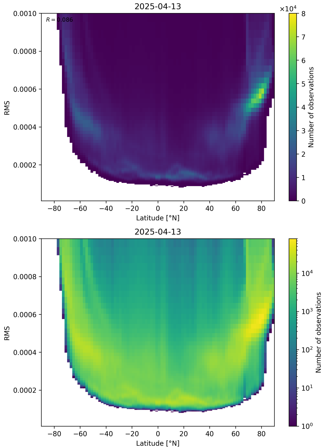
Figure 94: Scatter density plot of “Latitude” against “RMS” for 2025-04-13 to 2025-04-14.
