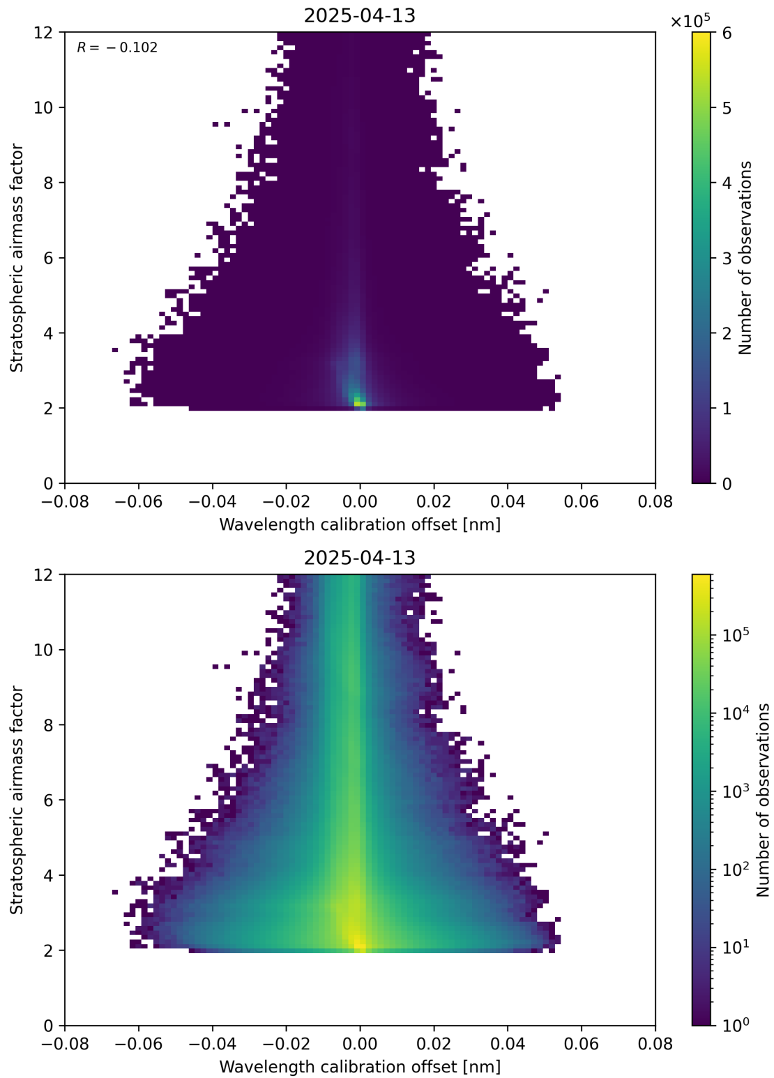
Figure 174: Scatter density plot of “Wavelength calibration offset” against “Stratospheric airmass factor” for 2025-04-13 to 2025-04-14.
