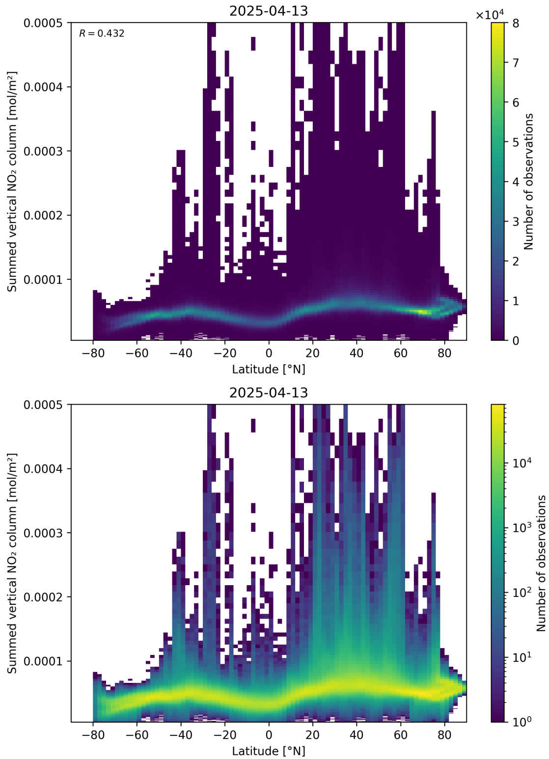
Figure 88: Scatter density plot of “Latitude” against “Summed vertical NO 2 column” for 2025-04-13 to 2025-04-14.
