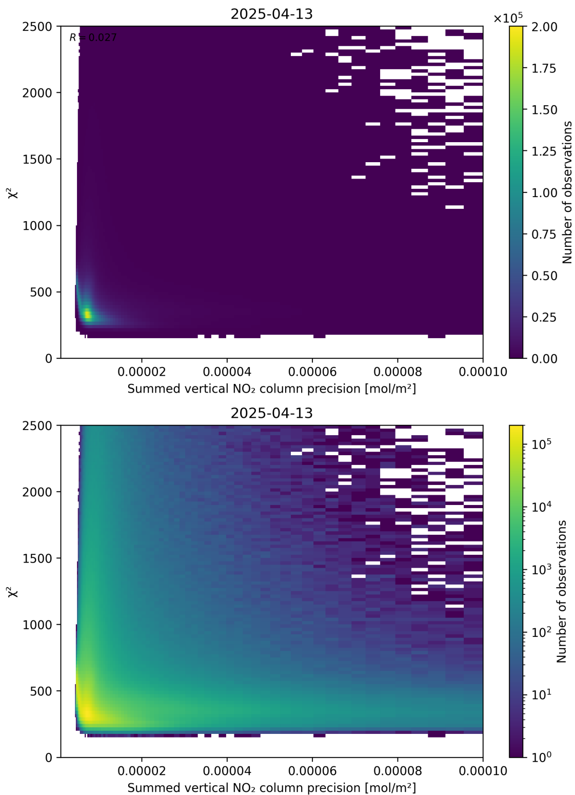
Figure 107: Scatter density plot of “Summed vertical NO 2 column precision” against “ \chi^2 ” for 2025-04-13 to 2025-04-14.
