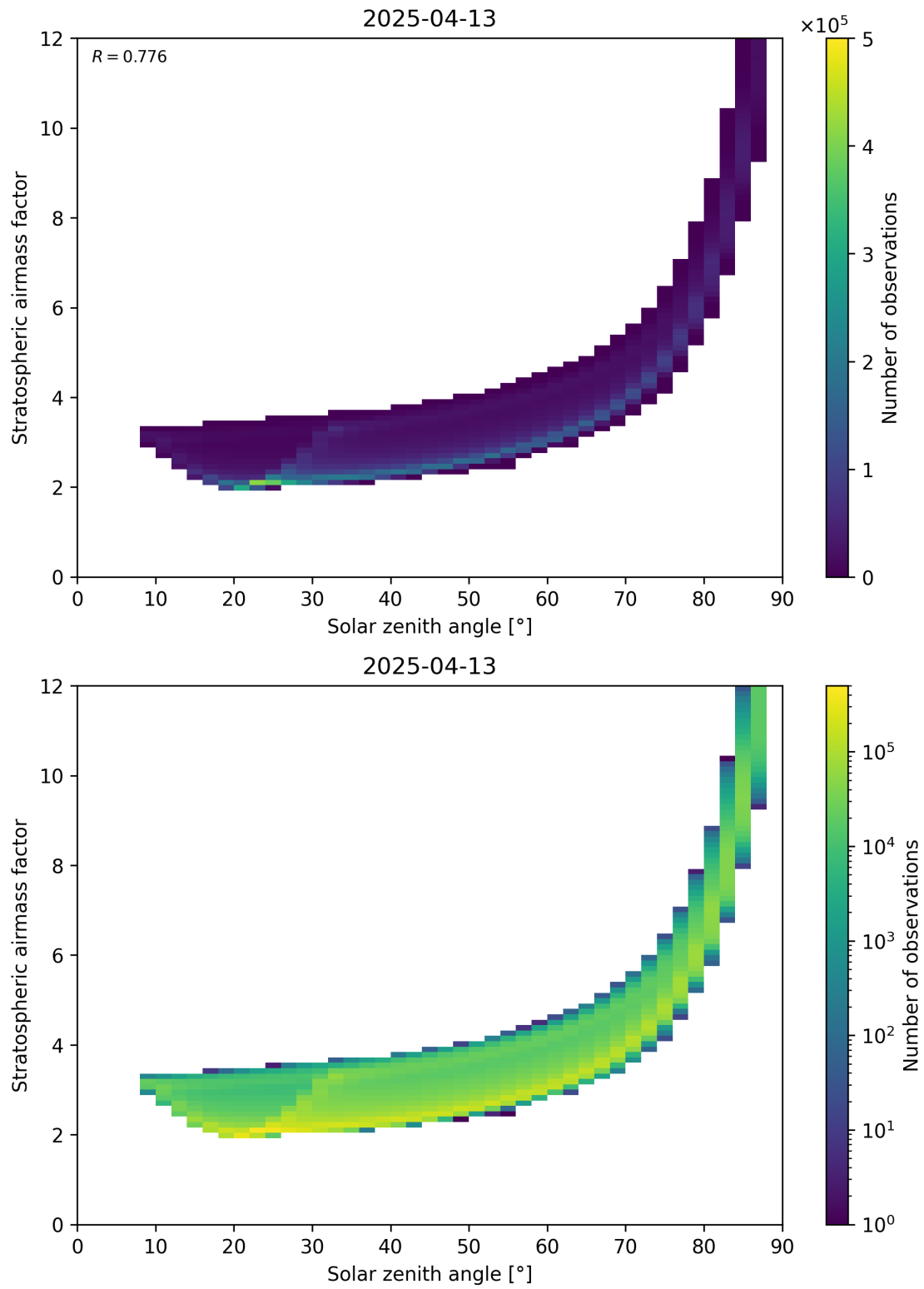
Figure 145: Scatter density plot of “Solar zenith angle” against “Stratospheric airmass factor” for 2025-04-13 to 2025-04-14.
