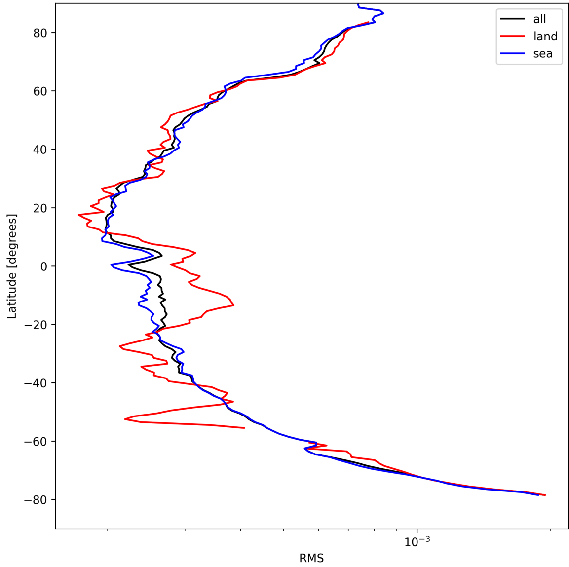
Figure 26: Zonal average of “RMS” for 2025-04-13 to 2025-04-14.
