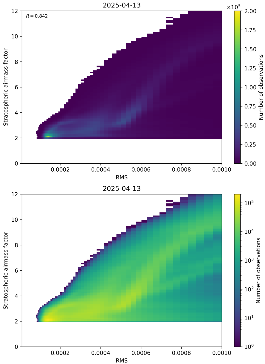
Figure 144: Scatter density plot of “RMS” against “Stratospheric airmass factor” for 2025-04-13 to 2025-04-14.
