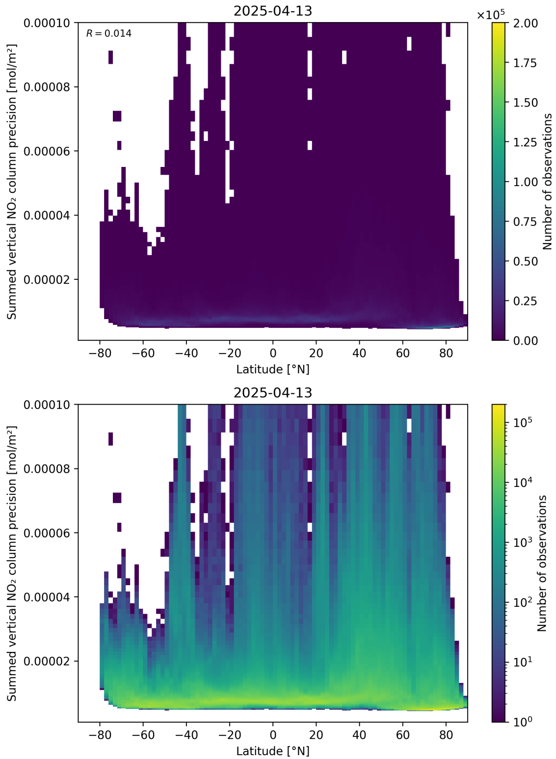
Figure 89: Scatter density plot of “Latitude” against “Summed vertical NO 2 column precision” for 2025-04-13 to 2025-04-14.
