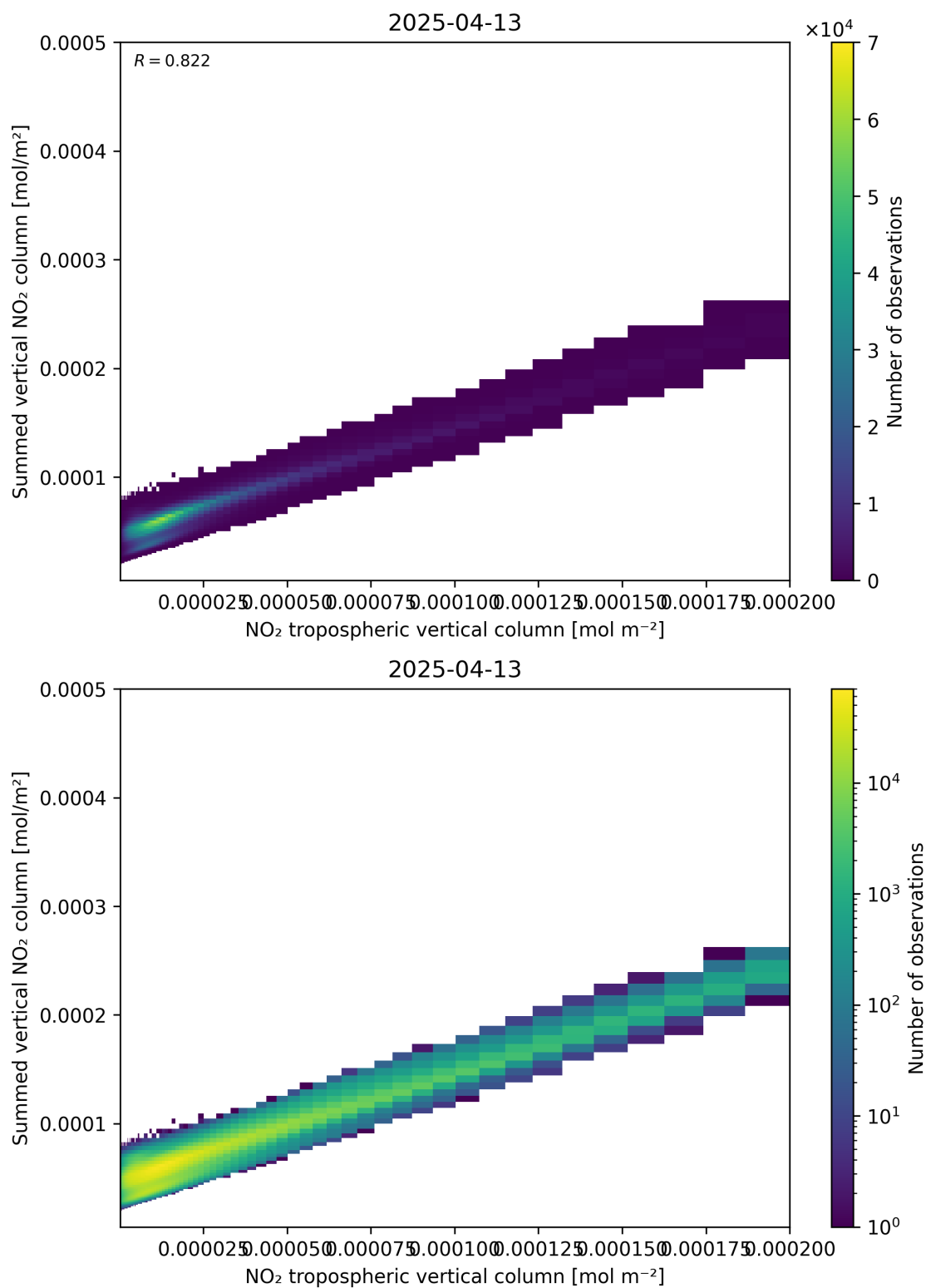
Figure 126: Scatter density plot of “NO 2 tropospheric vertical column” against “Summed vertical NO 2 column” for 2025-04-13 to 2025-04-14.
