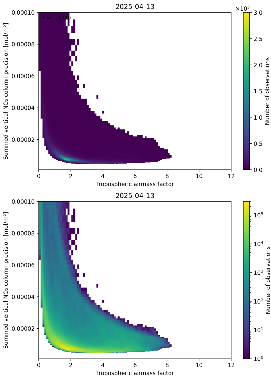
Figure 76: Scatter density plot of “Tropospheric air mass factor” against “Summed vertical NO 2 column precision” for 2025-04-13 to 2025-04-14.
