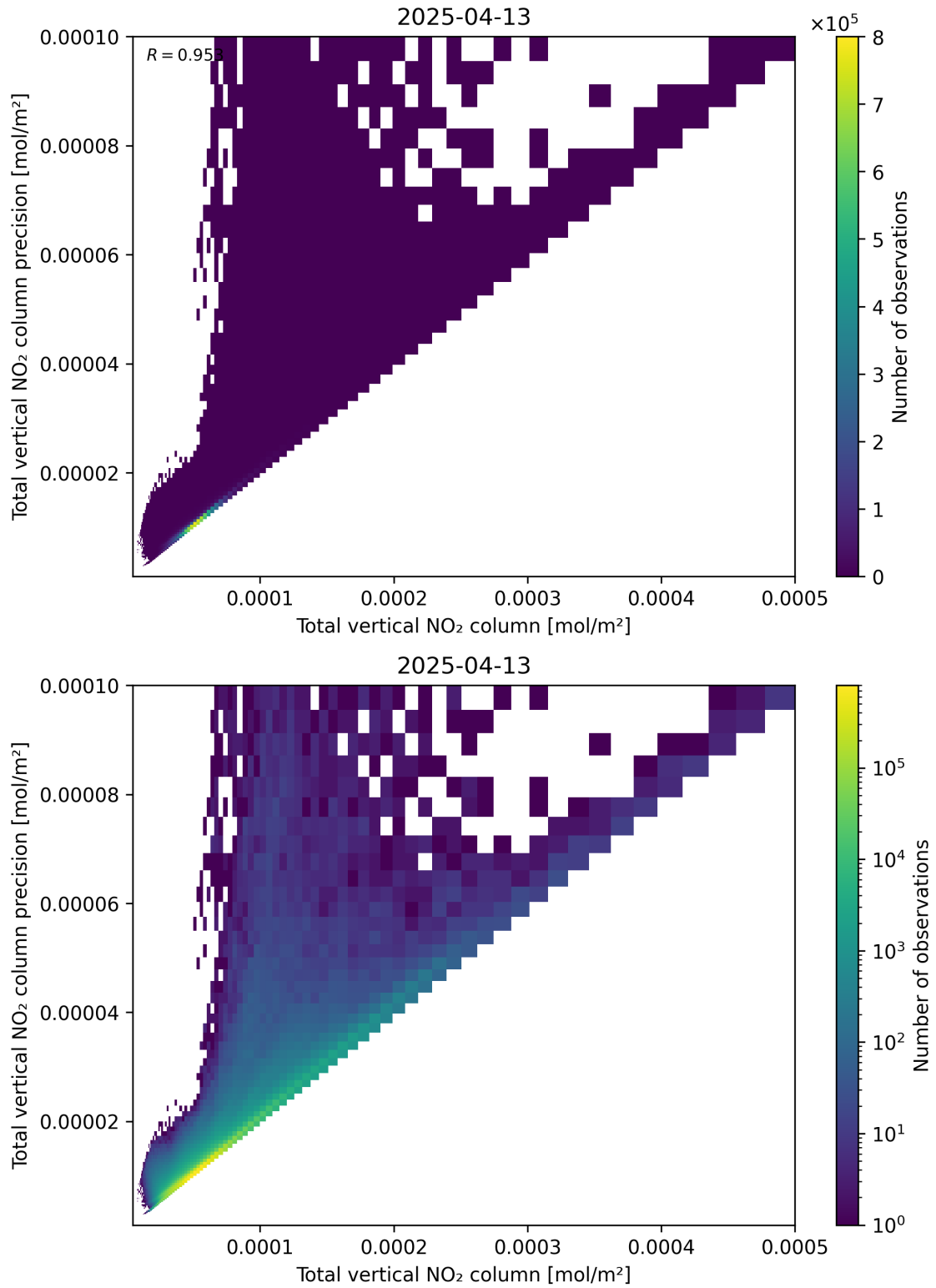
Figure 114: Scatter density plot of “Total vertical NO 2 column” against “Total vertical NO 2 column precision” for 2025-04-13 to 2025-04-14.
