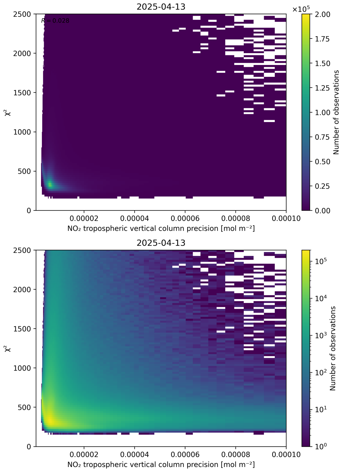
Figure 134: Scatter density plot of “NO 2 tropospheric vertical column precision” against “ \chi^2 ” for 2025-04-13 to 2025-04-14.
