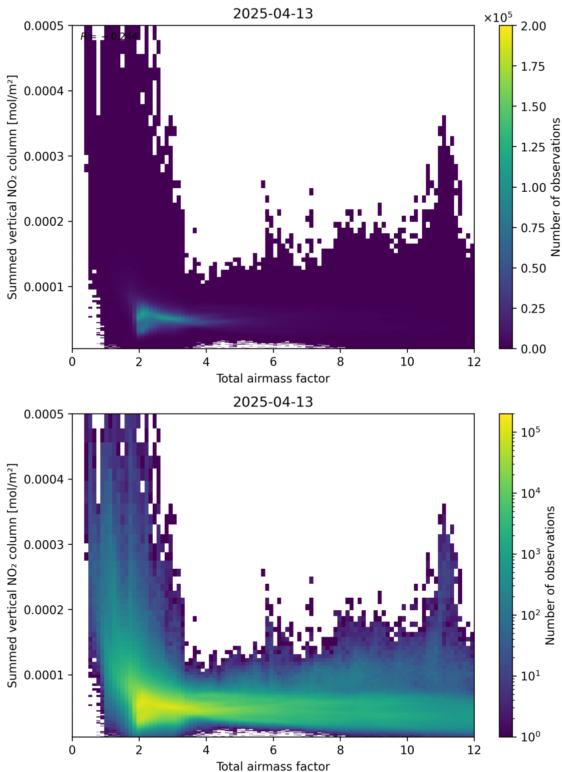
Figure 65: Scatter density plot of “Total airmass factor” against “Summed vertical NO 2 column” for 2025-04-13 to 2025-04-14.
