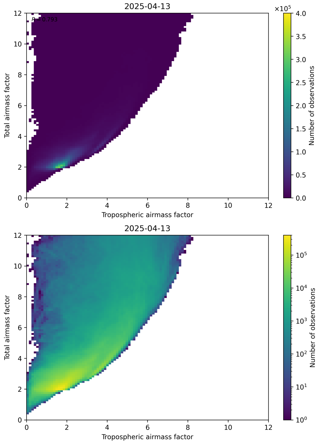
Figure 72: Scatter density plot of “Tropospheric airmass factor” against “Total airmass factor” for 2025-04-13 to 2025-04-14.
