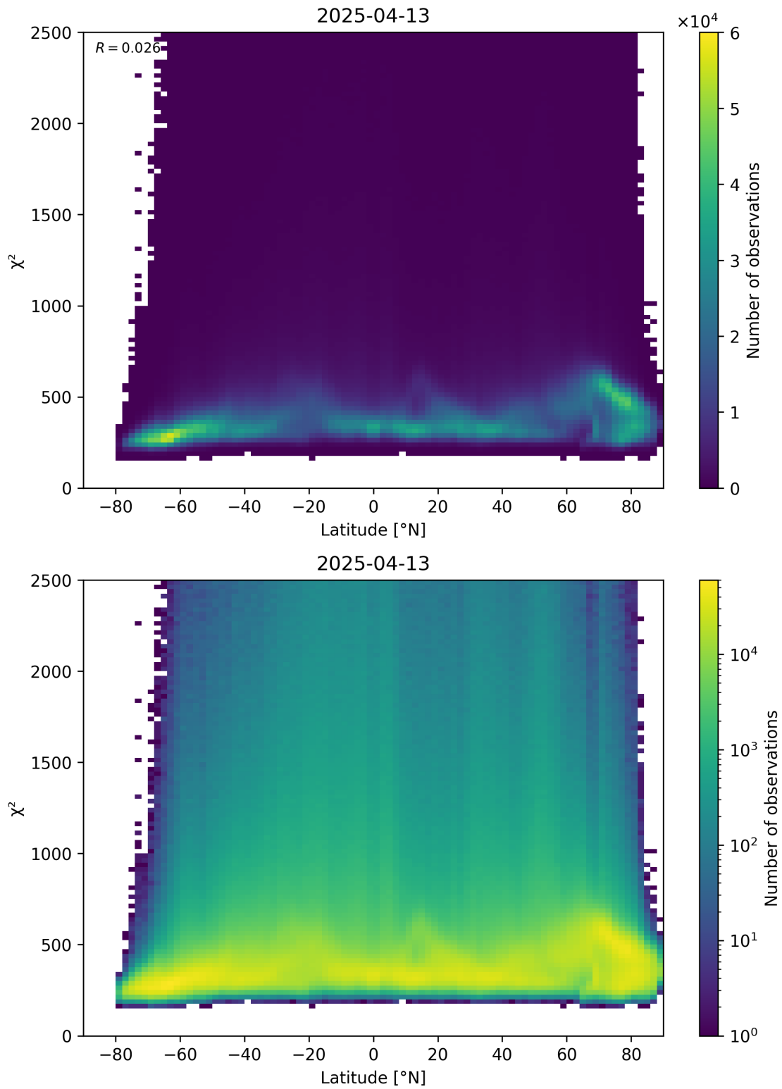
Figure 86: Scatter density plot of “Latitude” against “ \chi^2 ” for 2025-04-13 to 2025-04-14.
