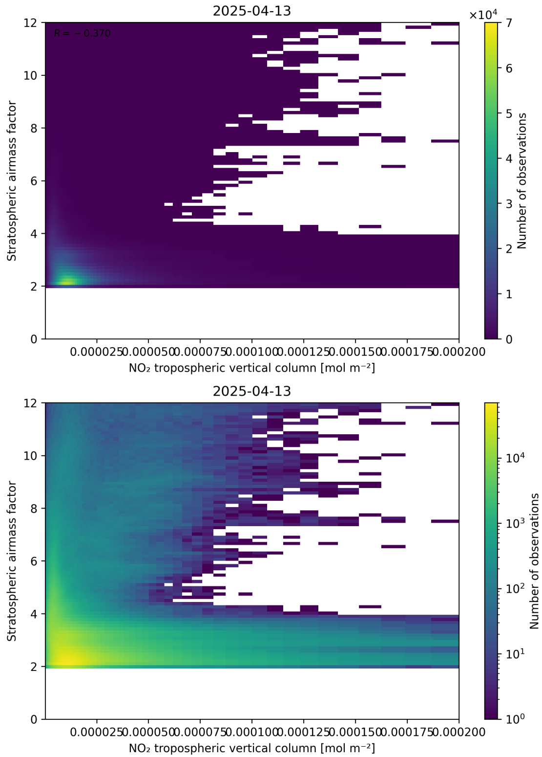
Figure 121: Scatter density plot of “NO 2 tropospheric vertical column” against “Stratospheric air mass factor” for 2025-04-13 to 2025-04-14.
