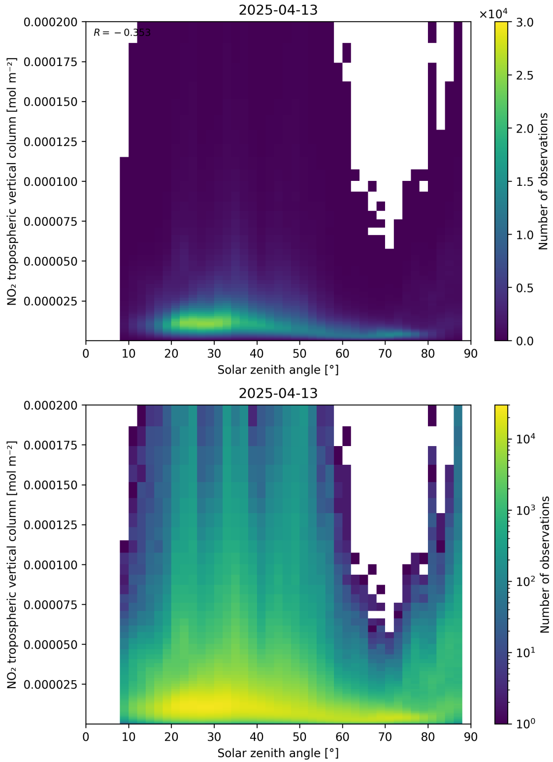
Figure 155: Scatter density plot of “Solar zenith angle” against “NO 2 tropospheric vertical column” for 2025-04-13 to 2025-04-14.
