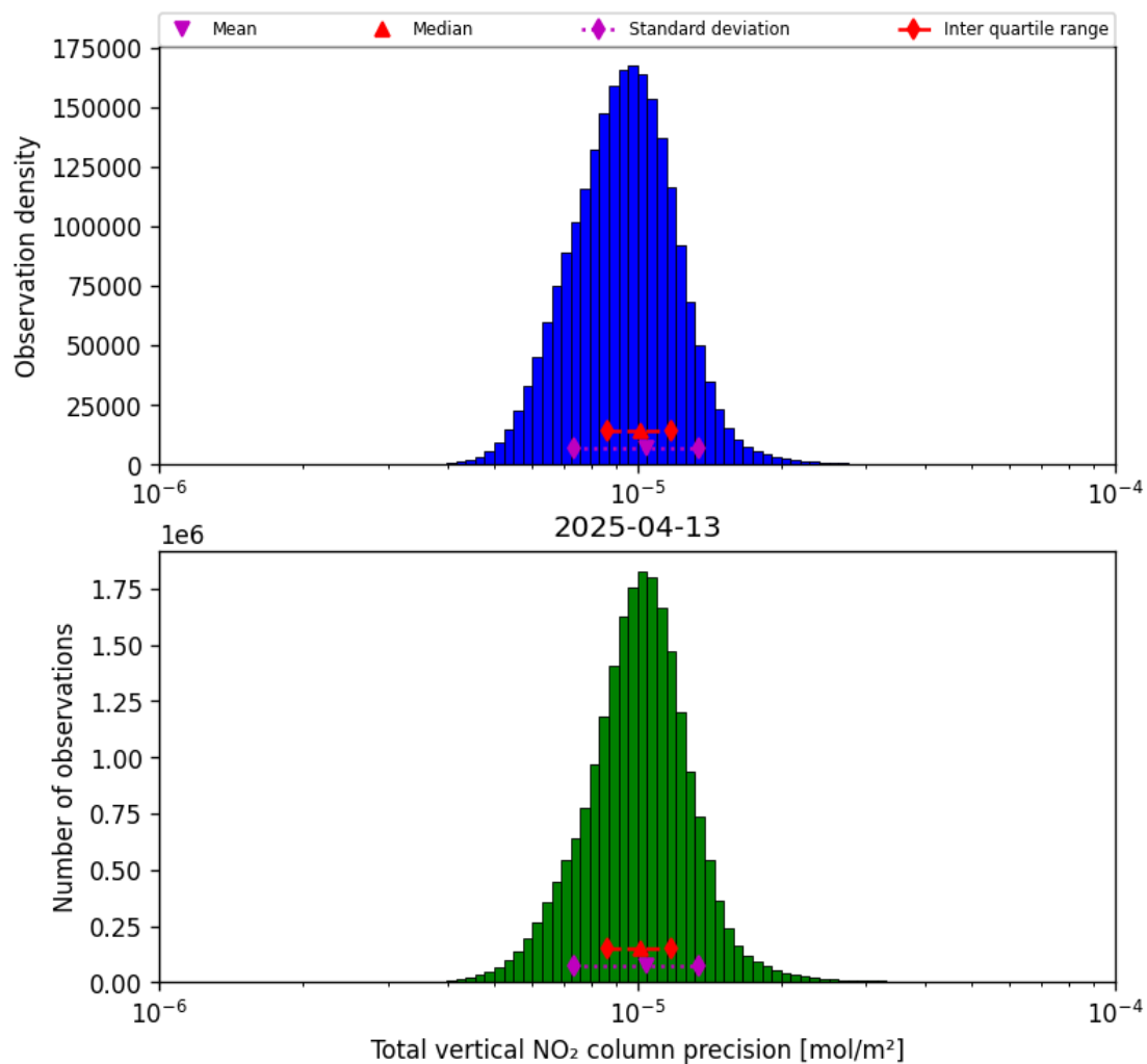
Figure 39: Histogram of “Total vertical NO 2 column precision” for 2025-04-13 to 2025-04-14
