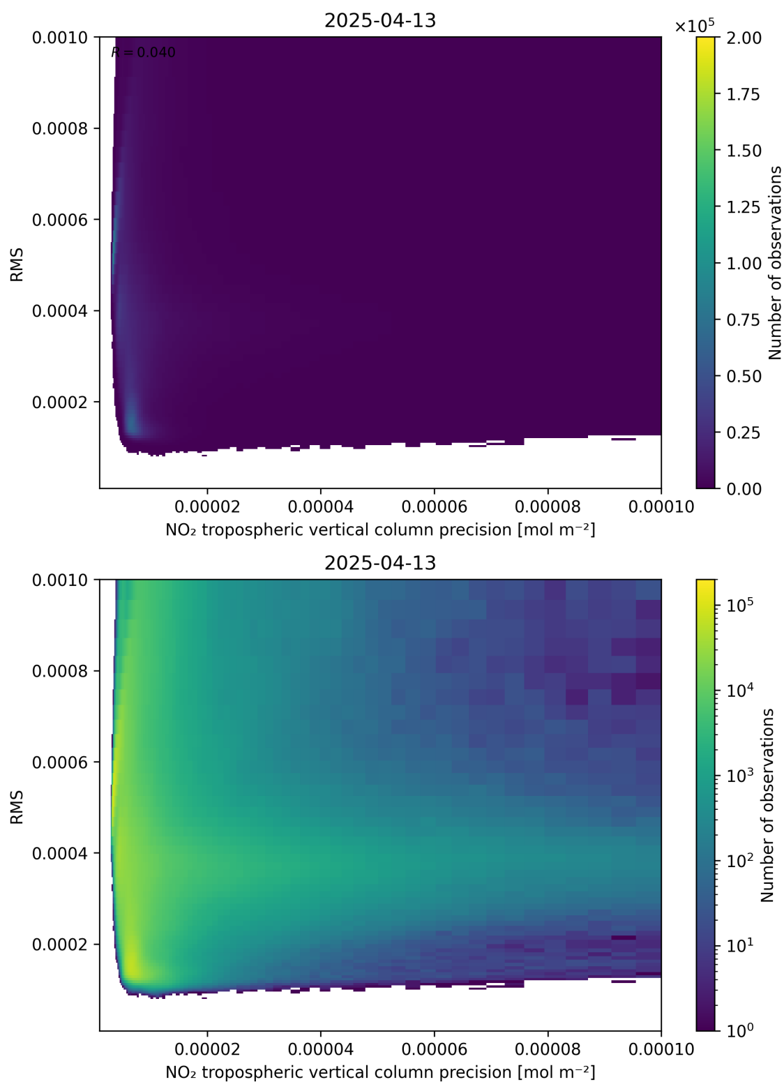
Figure 140: Scatter density plot of “NO 2 tropospheric vertical column precision” against “RMS” for 2025-04-13 to 2025-04-14.
