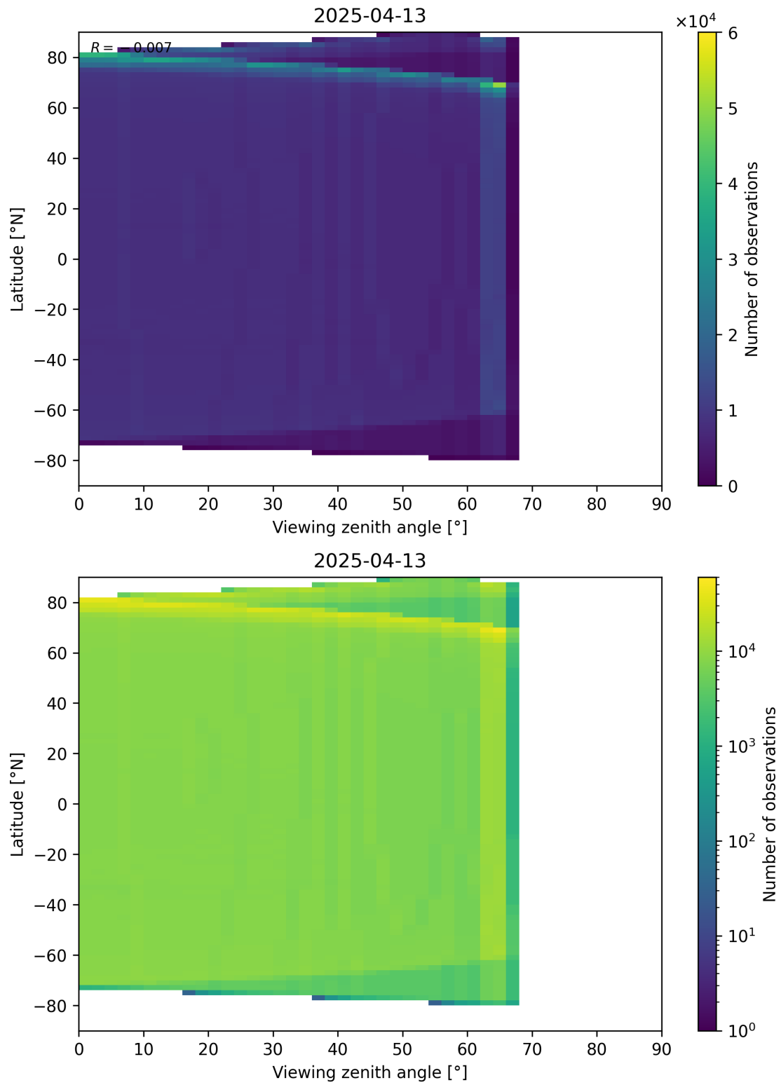
Figure 163: Scatter density plot of “Viewing zenith angle” against “Latitude” for 2025-04-13 to 2025-04-14.
