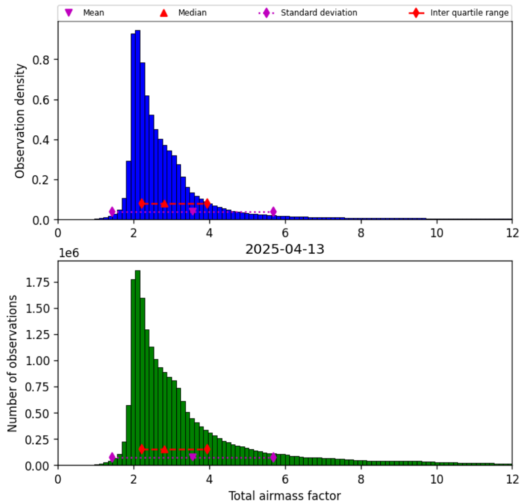
Figure 32: Histogram of “Total airmass factor” for 2025-04-13 to 2025-04-14
