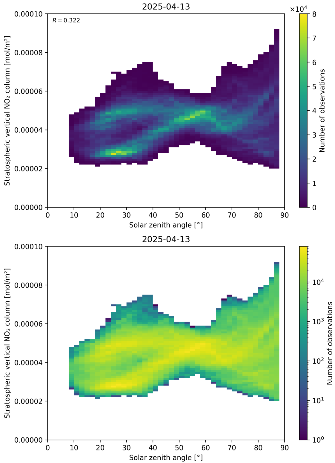
Figure 150: Scatter density plot of “Solar zenith angle” against “Stratospheric vertical NO 2 column” for 2025-04-13 to 2025-04-14.
