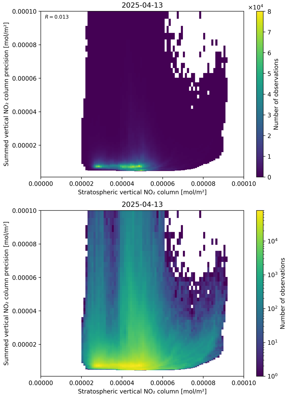
Figure 99: Scatter density plot of “Stratospheric vertical NO 2 column” against “Summed vertical NO 2 column precision” for 2025-04-13 to 2025-04-14.
