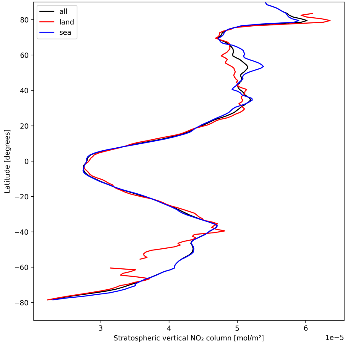
Figure 19: Zonal average of “Stratospheric vertical NO 2 column” for 2025-04-13 to 2025-04-14.
