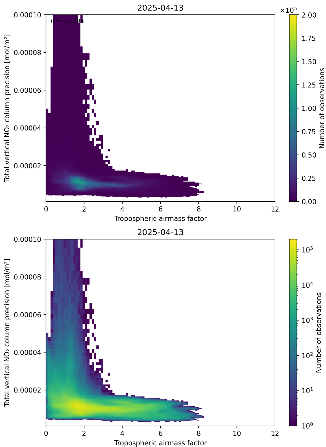
Figure 78: Scatter density plot of “Tropospheric air mass factor” against “Total vertical NO 2 column precision” for 2025-04-13 to 2025-04-14.
