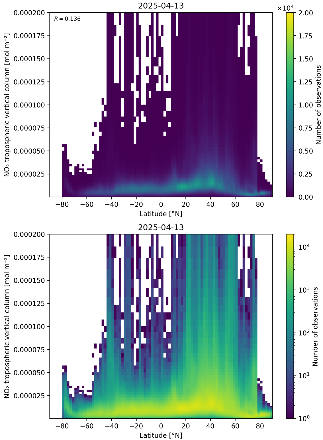
Figure 92: Scatter density plot of “Latitude” against “NO 2 tropospheric vertical column” for 2025-04-13 to 2025-04-14.
