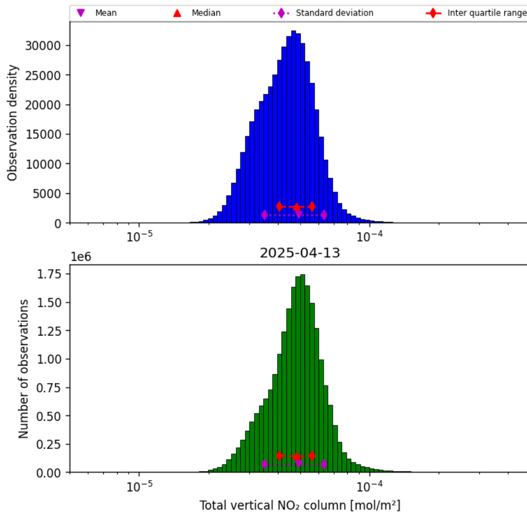
Figure 38: Histogram of “Total vertical NO 2 column” for 2025-04-13 to 2025-04-14
