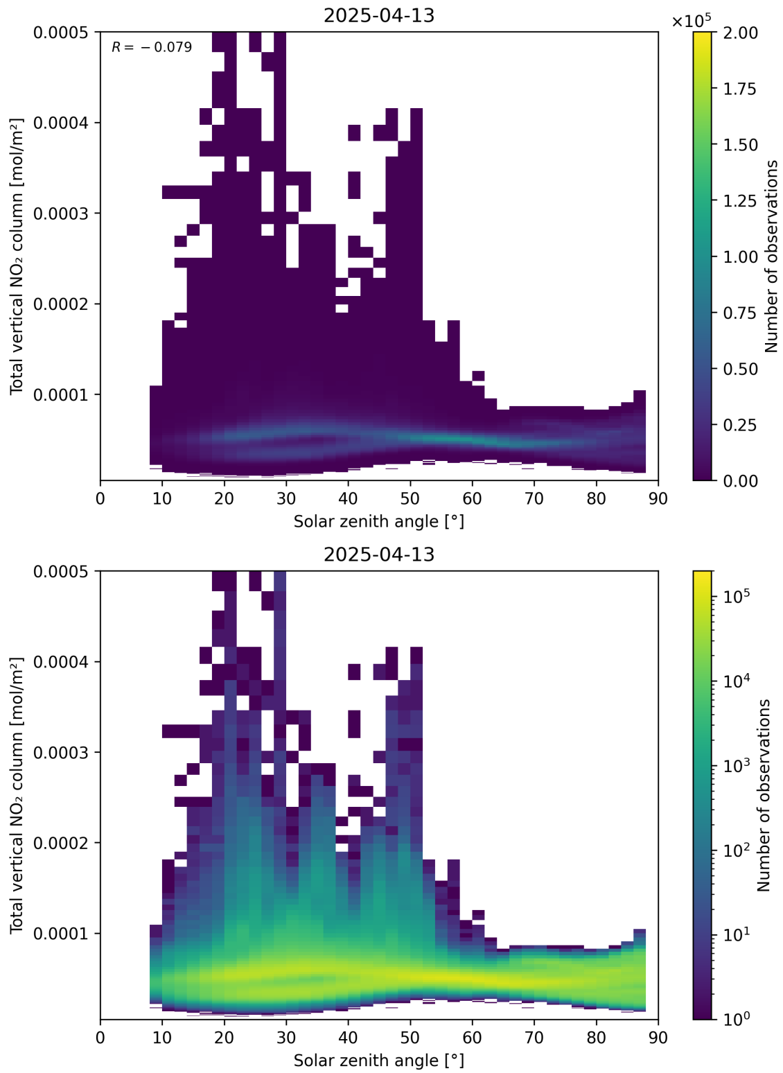
Figure 153: Scatter density plot of “Solar zenith angle” against “Total vertical NO 2 column” for 2025-04-13 to 2025-04-14.
