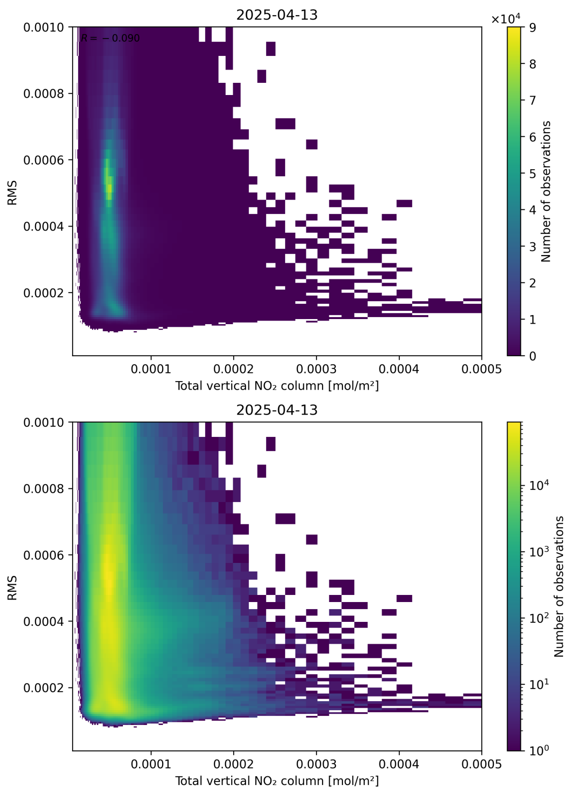
Figure 120: Scatter density plot of “Total vertical NO 2 column” against “RMS” for 2025-04-13 to 2025-04-14.
