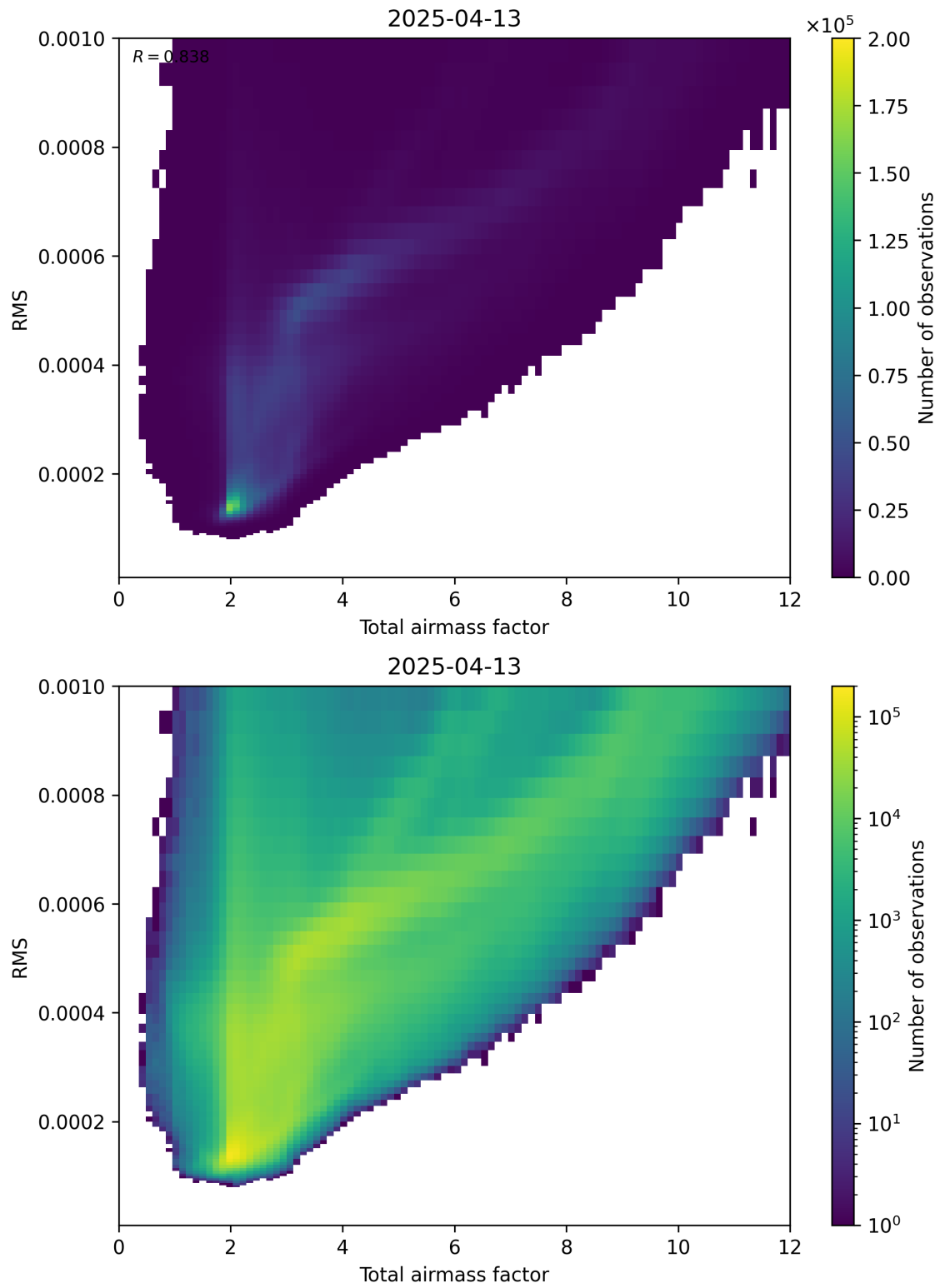
Figure 69: Scatter density plot of “Total airmass factor” against “RMS” for 2025-04-13 to 2025-04-14.
