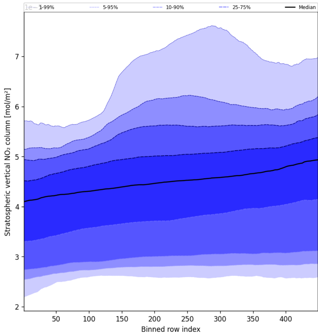
Figure 53: Along track statistics of “Stratospheric vertical NO 2 column” for 2025-04-13 to 2025-04-14
