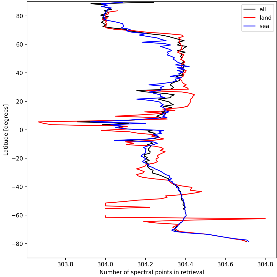
Figure 16: Zonal average of “Number of spectral points in retrieval” for 2025-04-13 to 2025-04-14.
