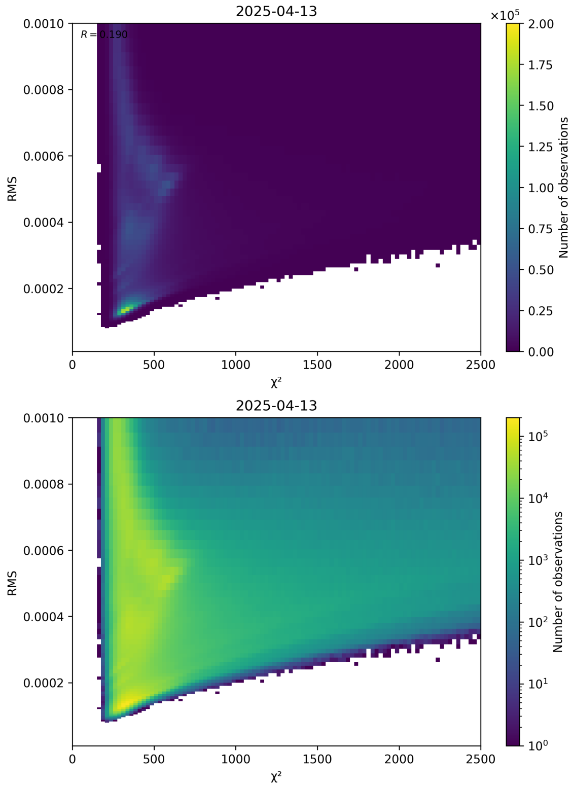
Figure 82: Scatter density plot of “ \chi^2 ” against “RMS” for 2025-04-13 to 2025-04-14.
