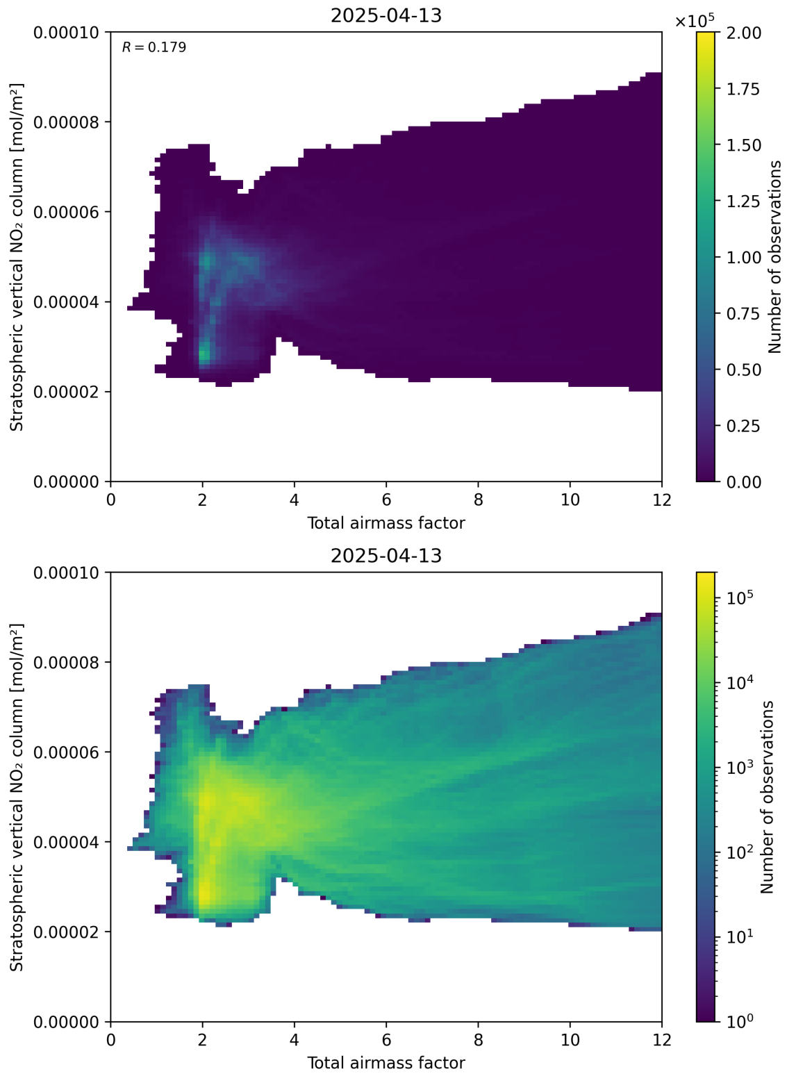
Figure 64: Scatter density plot of “Total airmass factor” against “Stratospheric vertical \text{NO}_2 column” for 2025-04-13 to 2025-04-14.
