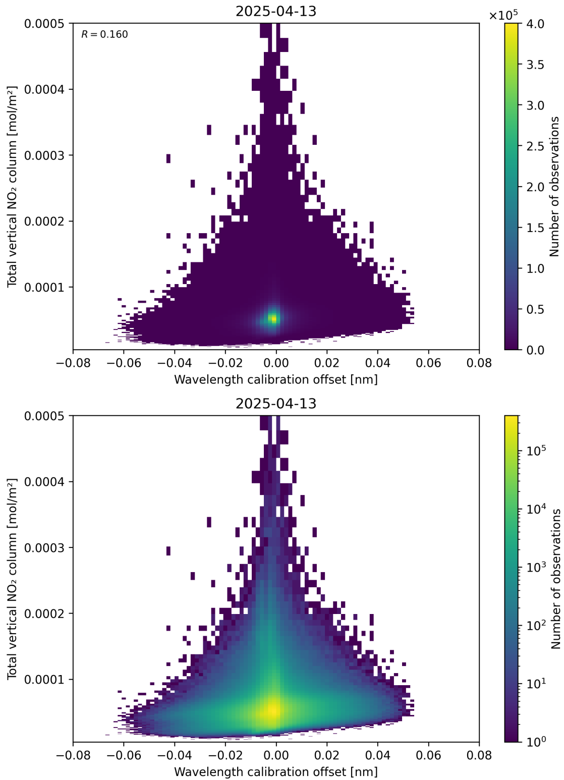
Figure 179: Scatter density plot of “Wavelength calibration offset” against “Total vertical NO 2 column” for 2025-04-13 to 2025-04-14.
