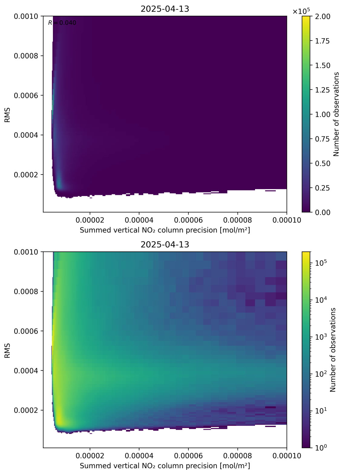
Figure 108: Scatter density plot of “Summed vertical NO 2 column precision” against “RMS” for 2025-04-13 to 2025-04-14.
