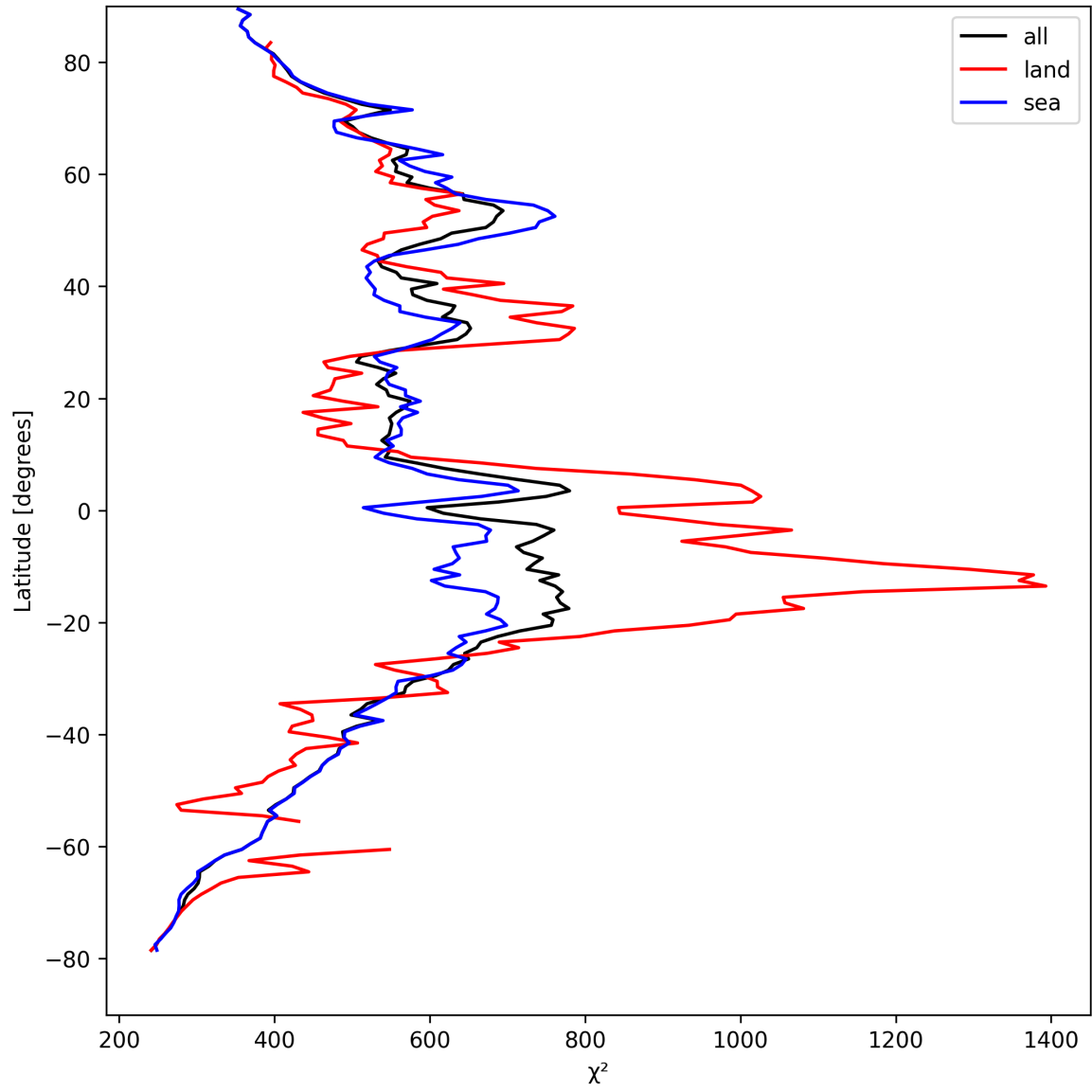
Figure 25: Zonal average of “ \chi^2 ” for 2025-04-13 to 2025-04-14.
