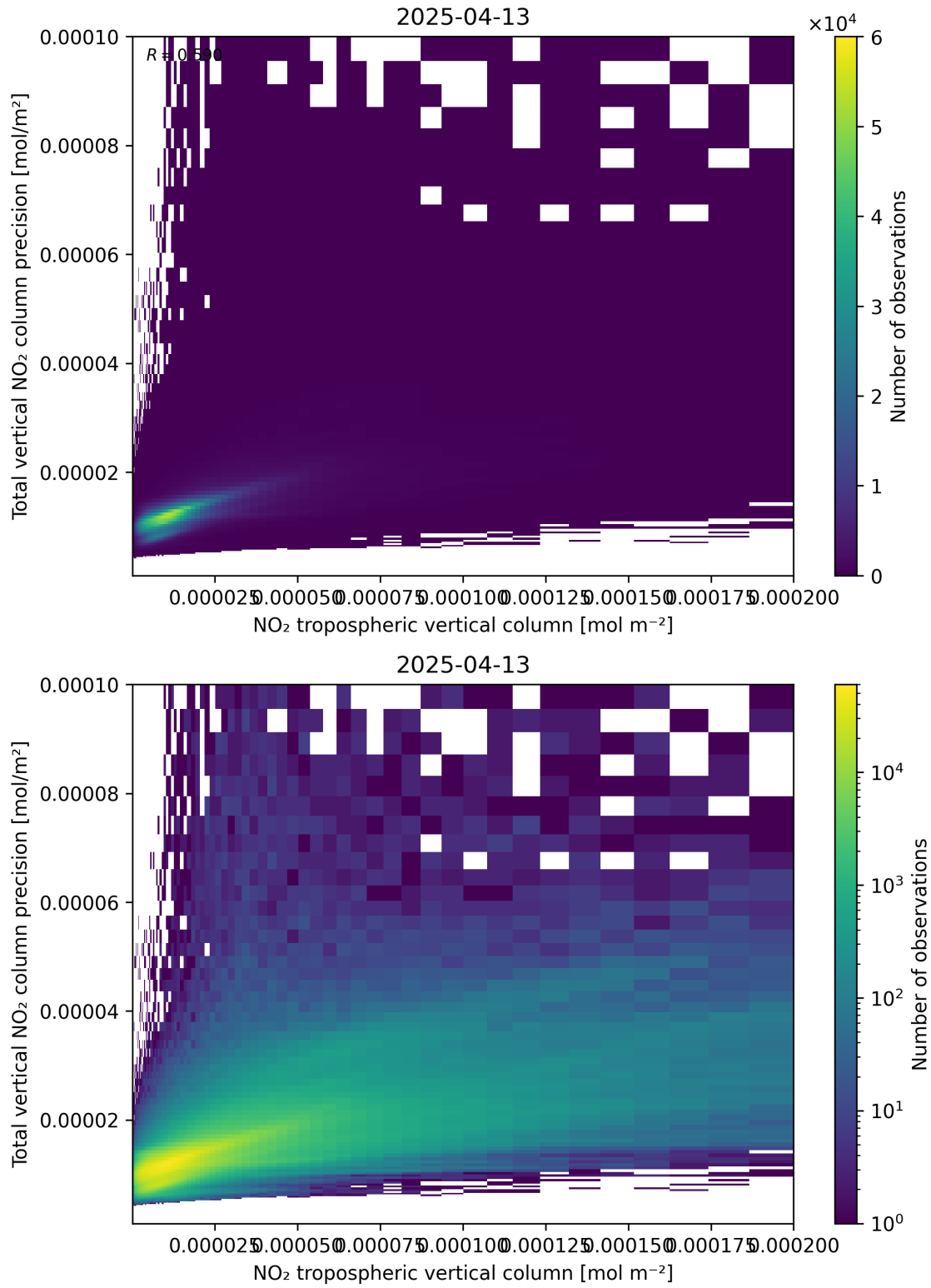
Figure 129: Scatter density plot of “NO 2 tropospheric vertical column” against “Total vertical NO 2 column precision” for 2025-04-13 to 2025-04-14.
