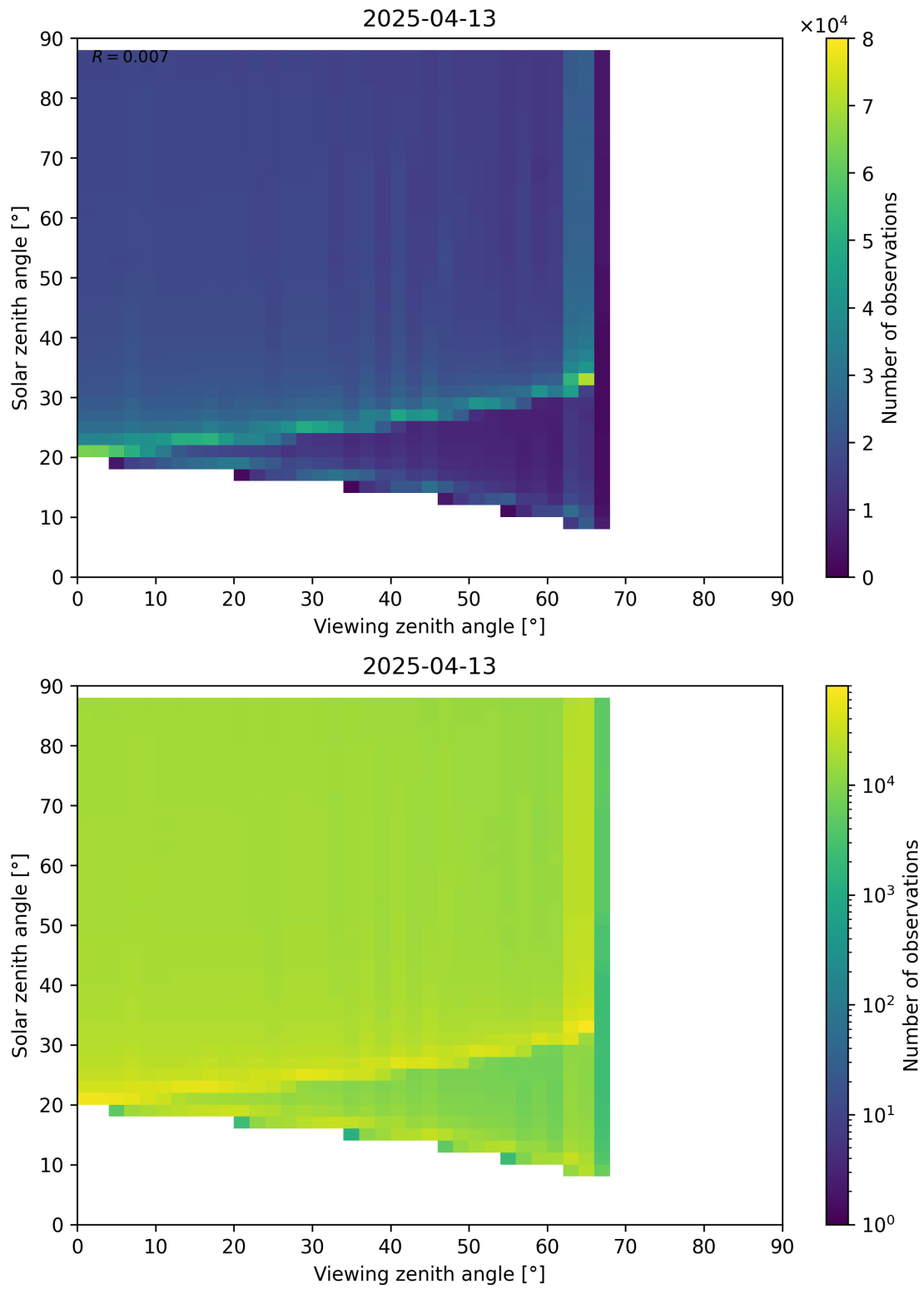
Figure 172: Scatter density plot of “Viewing zenith angle” against “Solar zenith angle” for 2025-04-13 to 2025-04-14.
