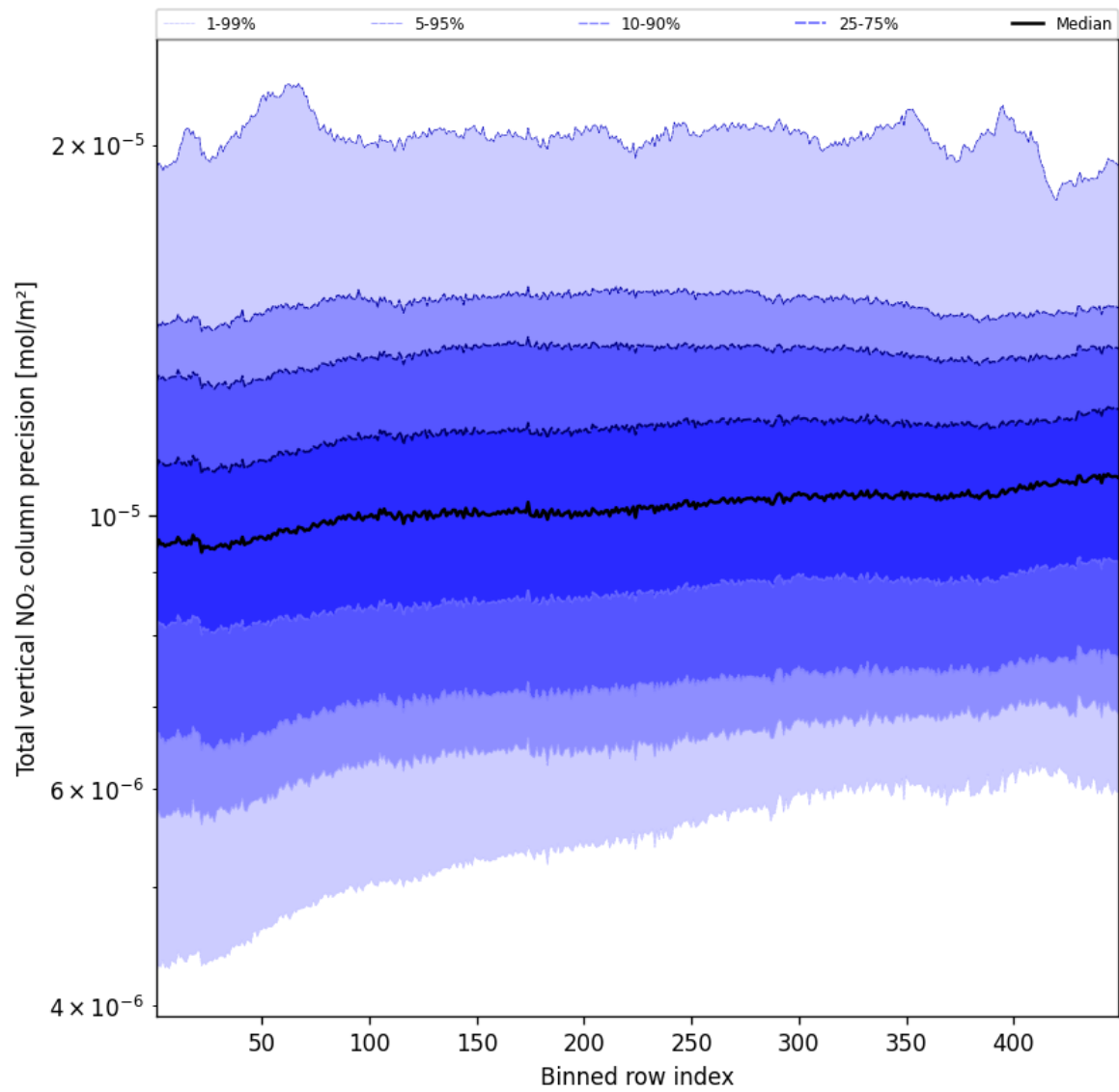
Figure 56: Along track statistics of “Total vertical NO 2 column precision” for 2025-04-13 to 2025-04-14
