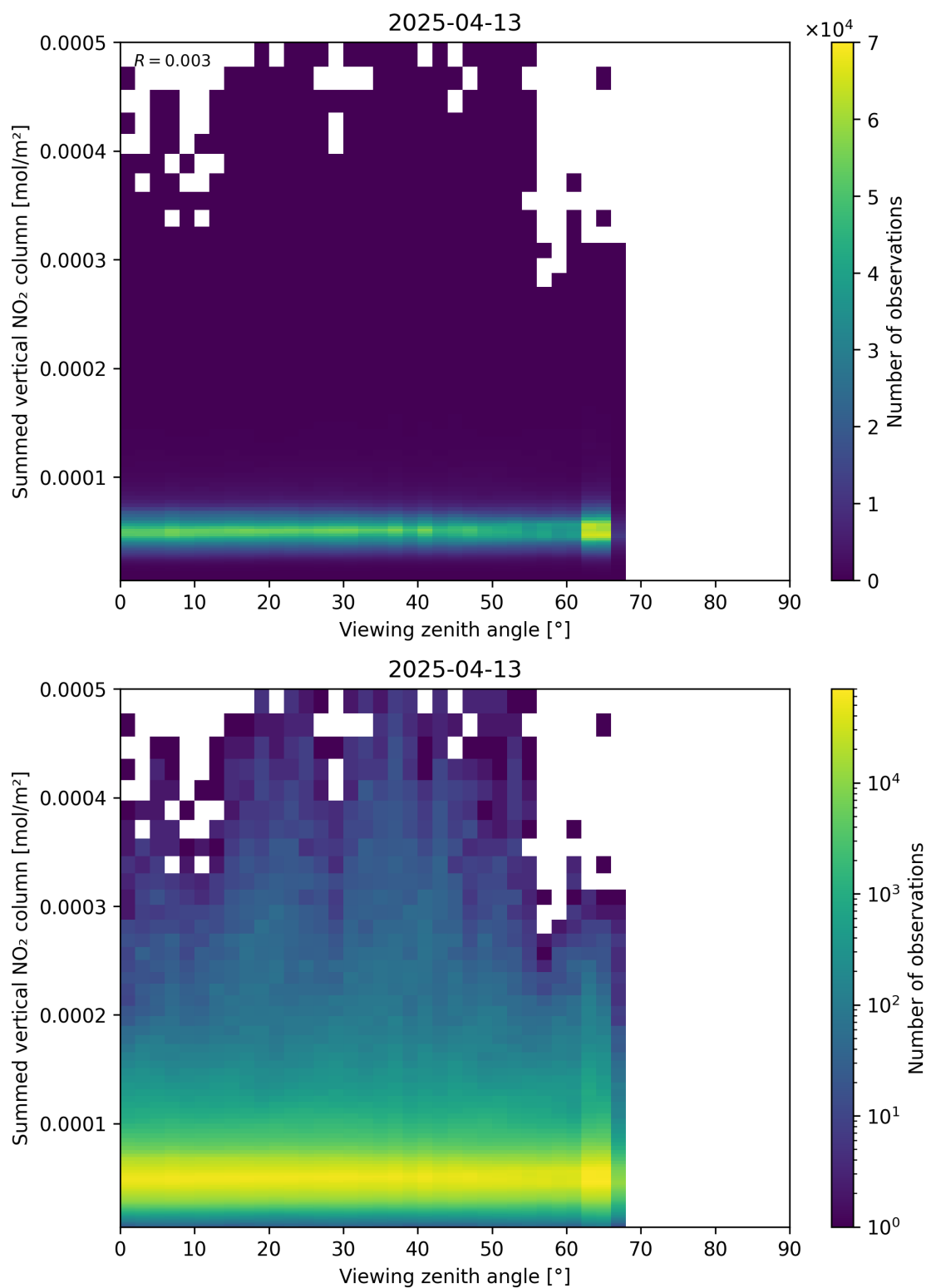
Figure 165: Scatter density plot of “Viewing zenith angle” against “Summed vertical NO 2 column” for 2025-04-13 to 2025-04-14.
