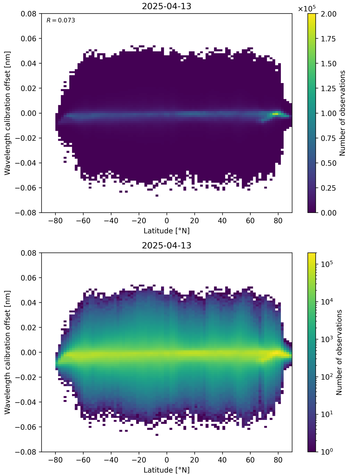
Figure 95: Scatter density plot of “Latitude” against “Wavelength calibration offset” for 2025-04-13 to 2025-04-14.
