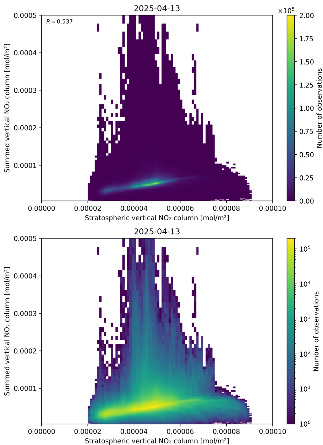
Figure 98: Scatter density plot of “Stratospheric vertical NO 2 column” against “Summed vertical NO 2 column” for 2025-04-13 to 2025-04-14.
