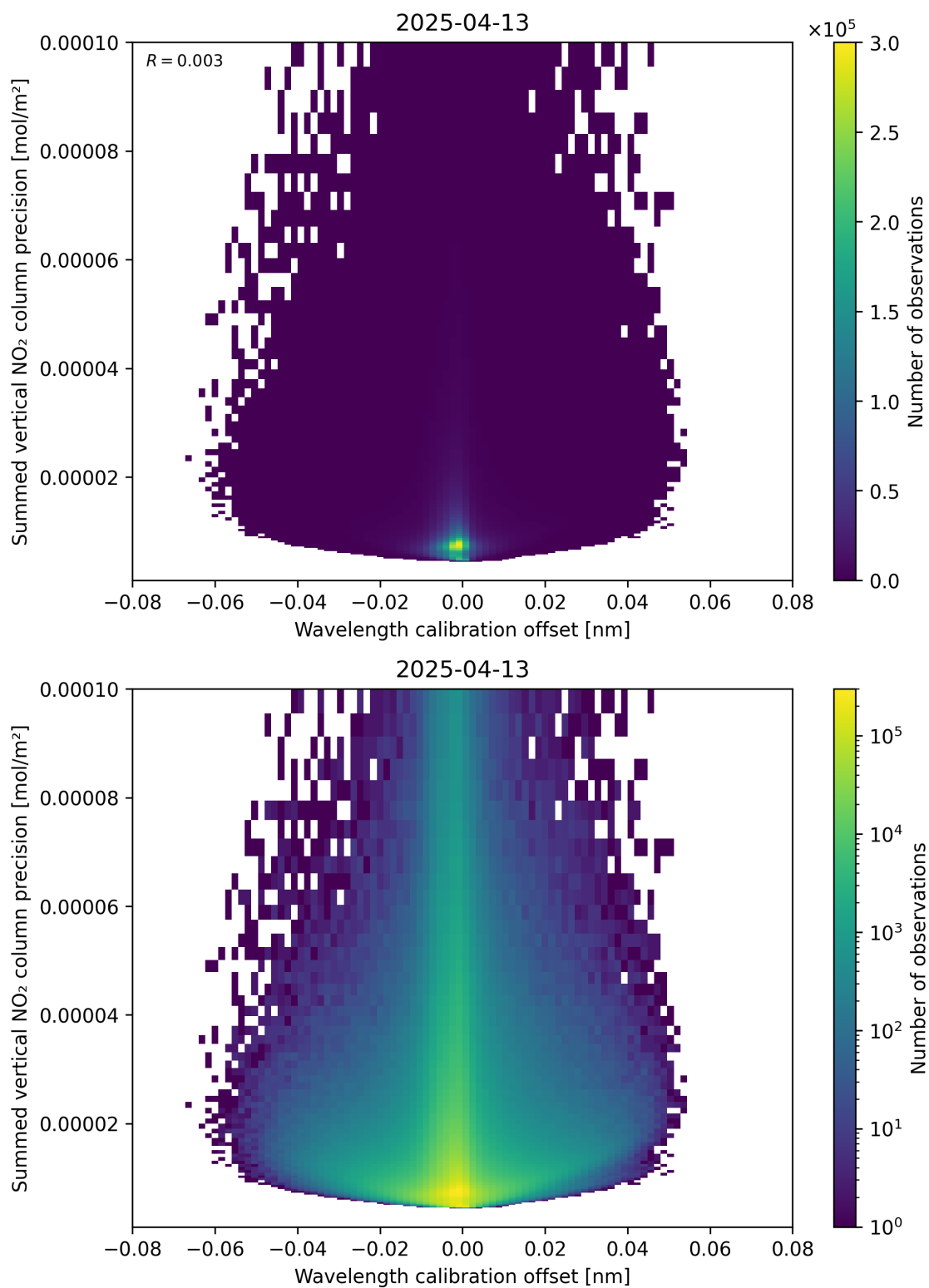
Figure 178: Scatter density plot of “Wavelength calibration offset” against “Summed vertical NO 2 column precision” for 2025-04-13 to 2025-04-14.
