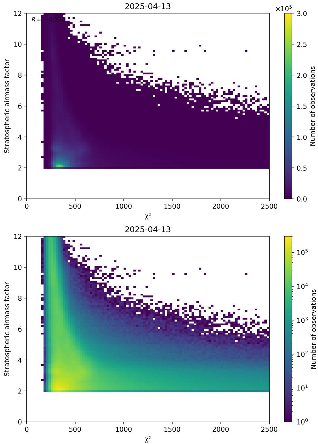
Figure 81: Scatter density plot of “ \chi^2 ” against “Stratospheric airmass factor” for 2025-04-13 to 2025-04-14.
