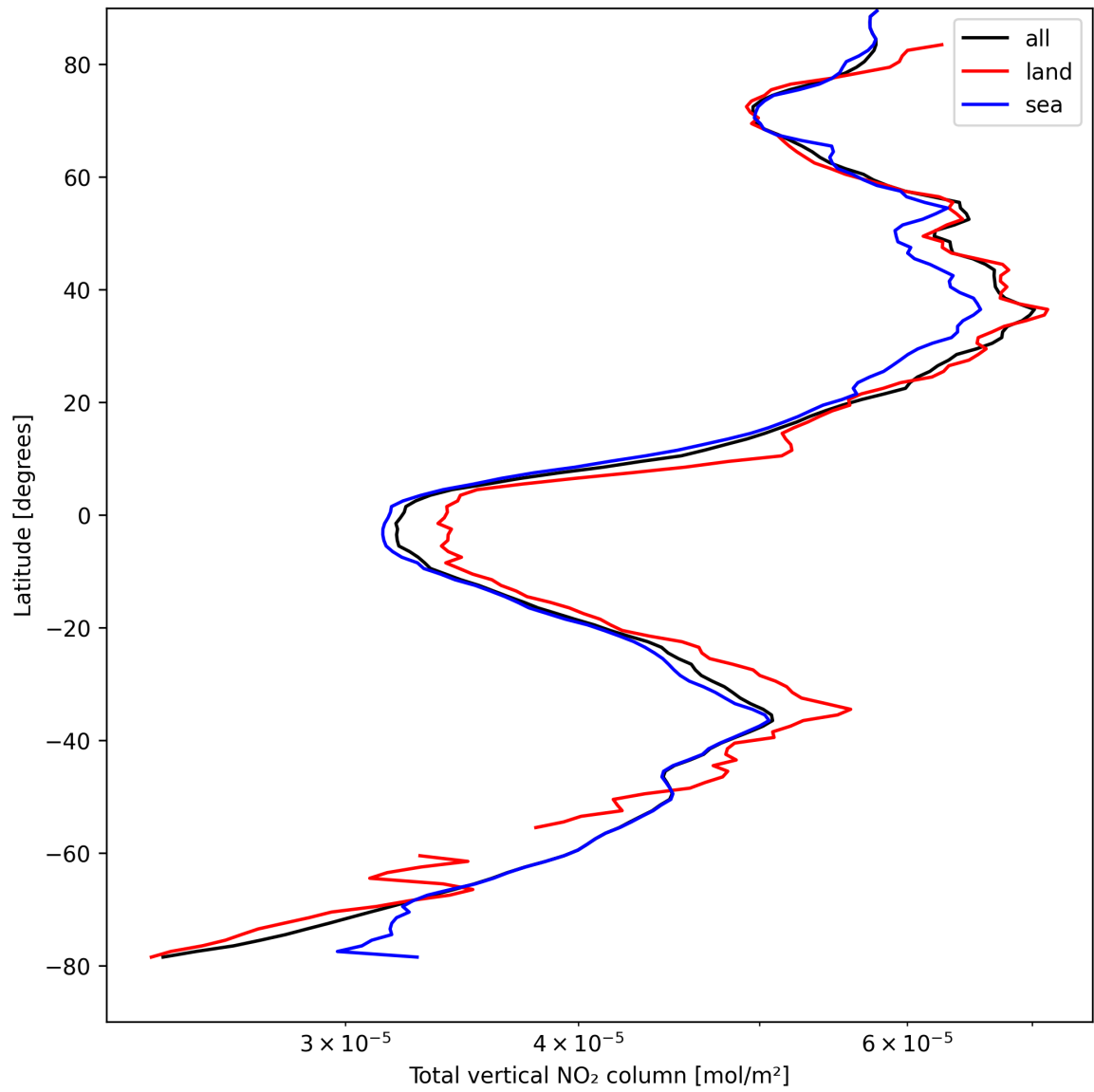
Figure 21: Zonal average of “Total vertical NO 2 column” for 2025-04-13 to 2025-04-14.
