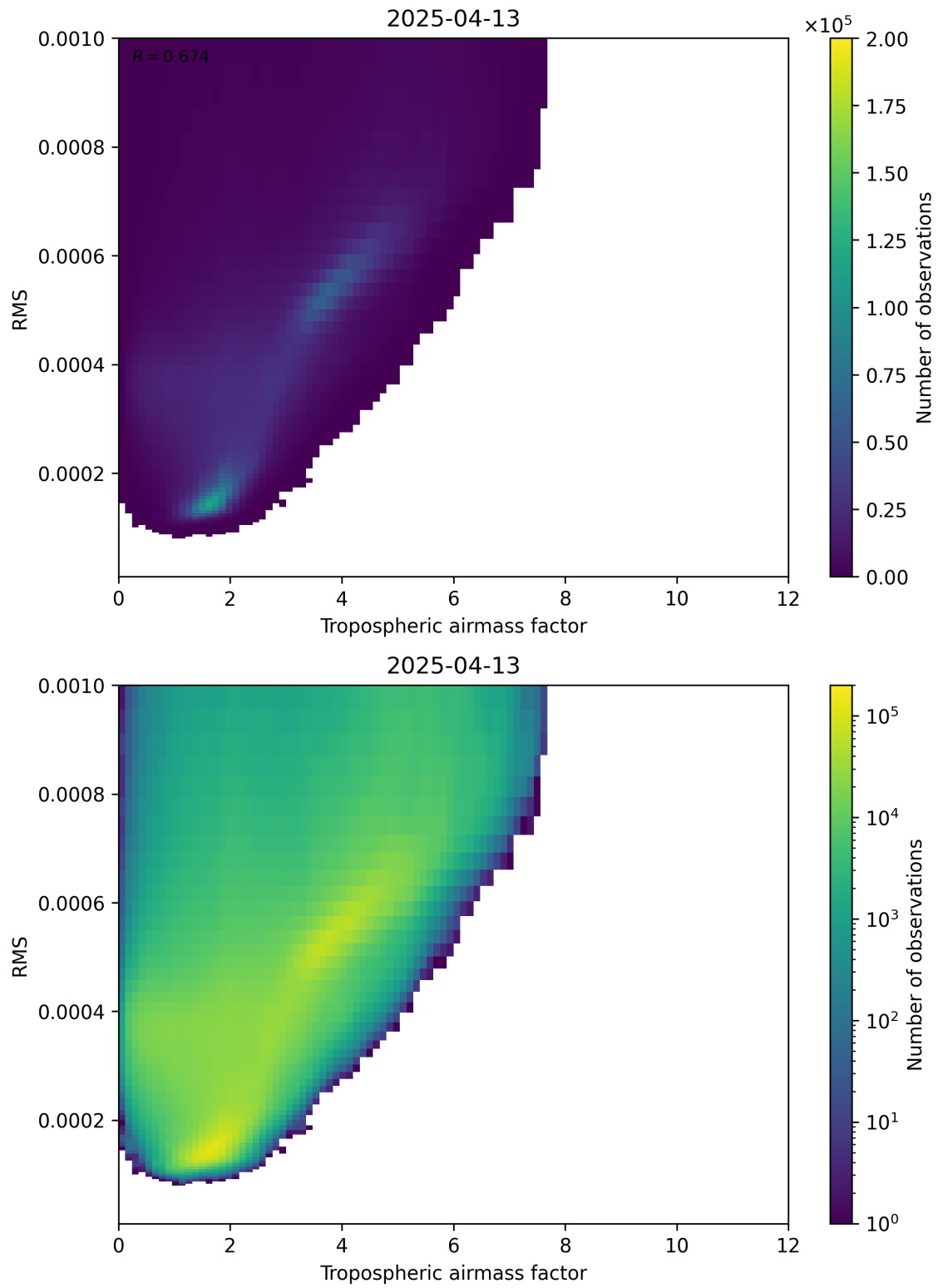
Figure 79: Scatter density plot of “Tropospheric airmass factor” against “RMS” for 2025-04-13 to 2025-04-14.
