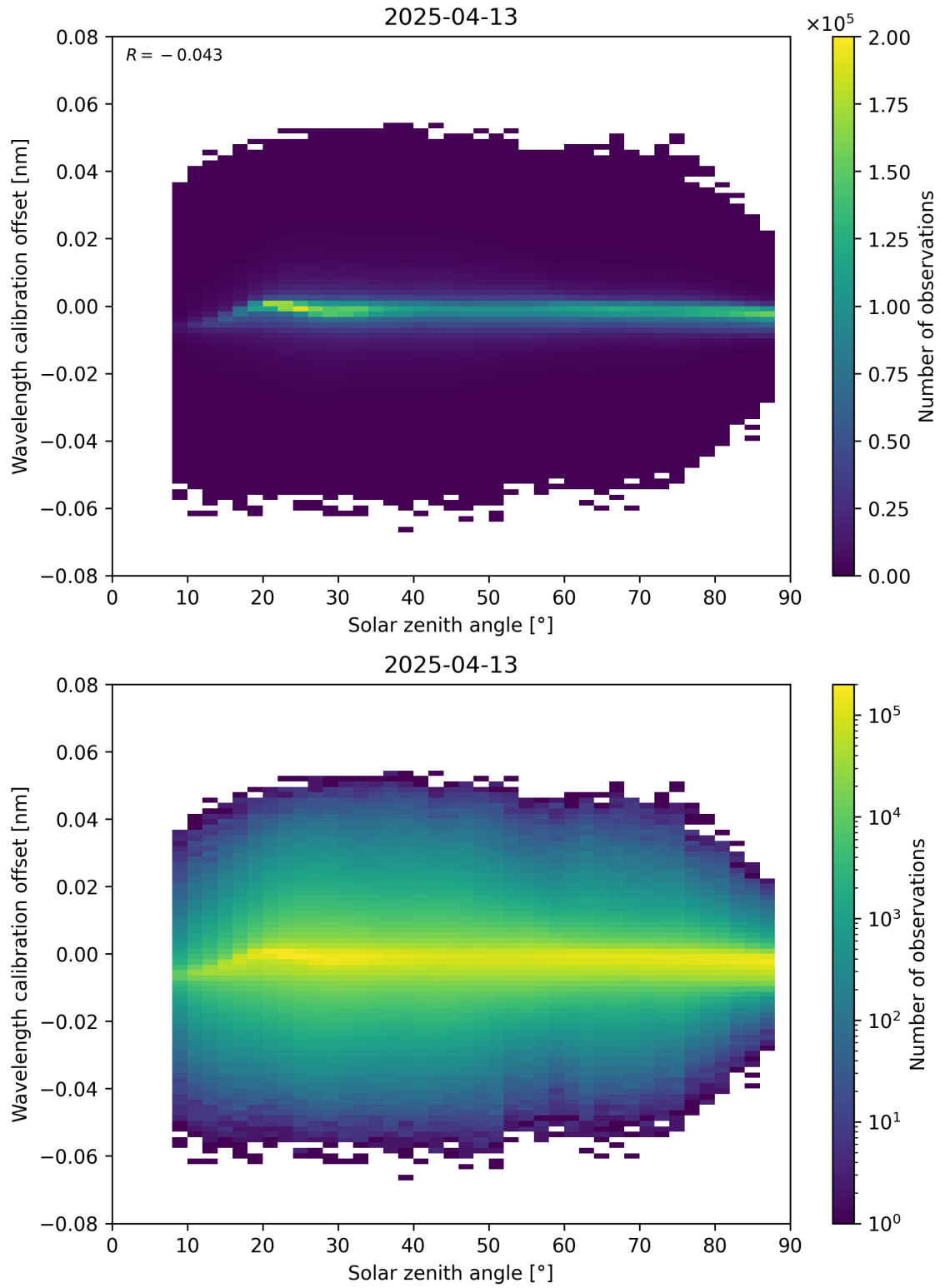
Figure 158: Scatter density plot of “Solar zenith angle” against “Wavelength calibration offset” for 2025-04-13 to 2025-04-14.
