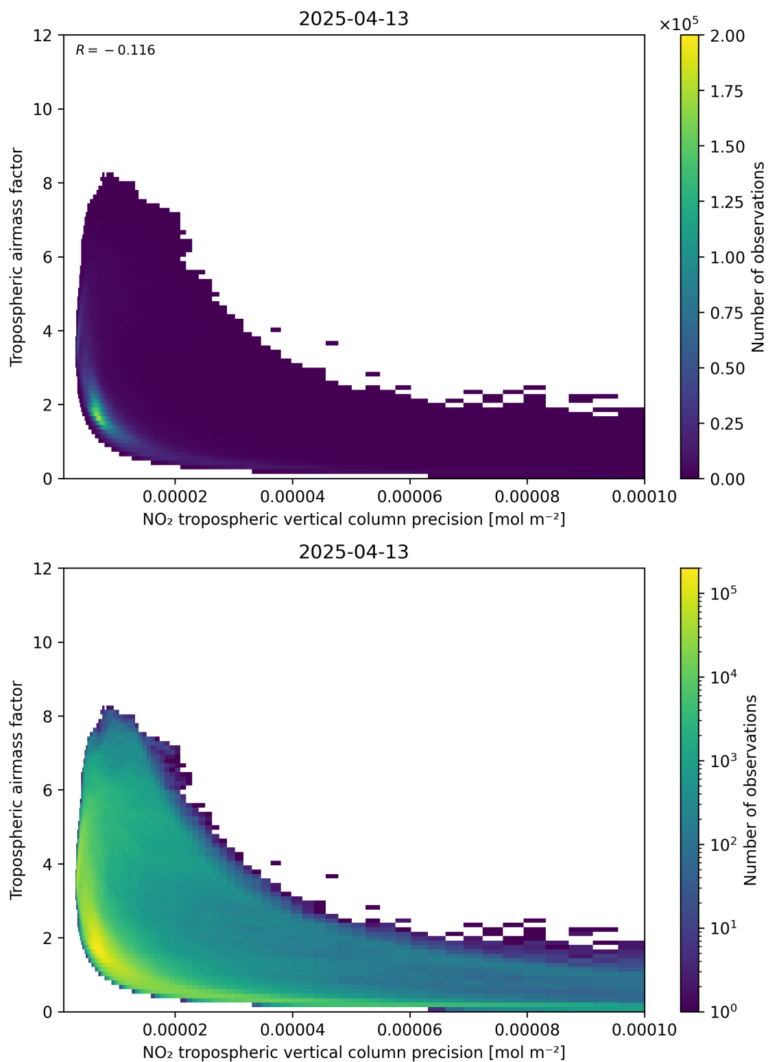
Figure 133: Scatter density plot of “NO 2 tropospheric vertical column precision” against “Tropospheric air mass factor” for 2025-04-13 to 2025-04-14.
