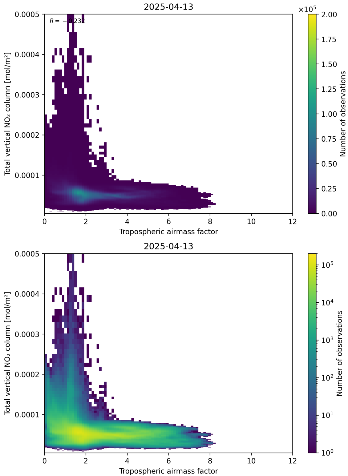
Figure 77: Scatter density plot of “Tropospheric airmass factor” against “Total vertical NO 2 column” for 2025-04-13 to 2025-04-14.
