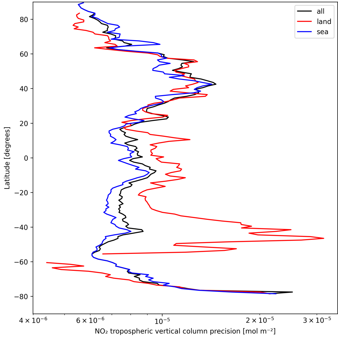
Figure 13: Zonal average of “NO 2 tropospheric vertical column precision” for 2025-04-13 to 2025-04-14.
