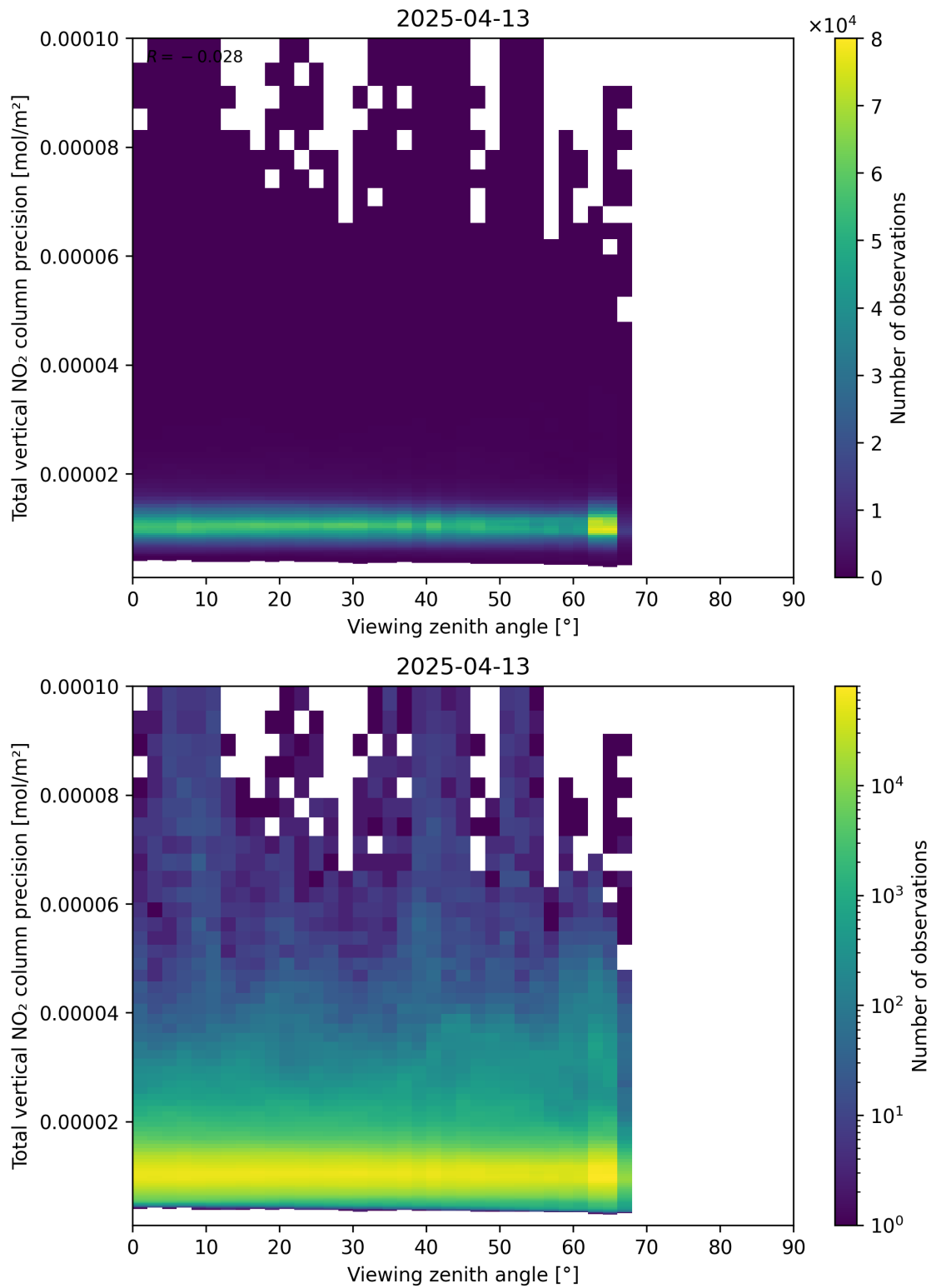
Figure 168: Scatter density plot of “Viewing zenith angle” against “Total vertical NO 2 column precision” for 2025-04-13 to 2025-04-14.
