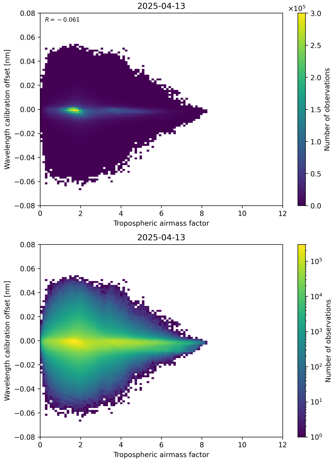
Figure 80: Scatter density plot of “Tropospheric airmass factor” against “Wavelength calibration offset” for 2025-04-13 to 2025-04-14.
