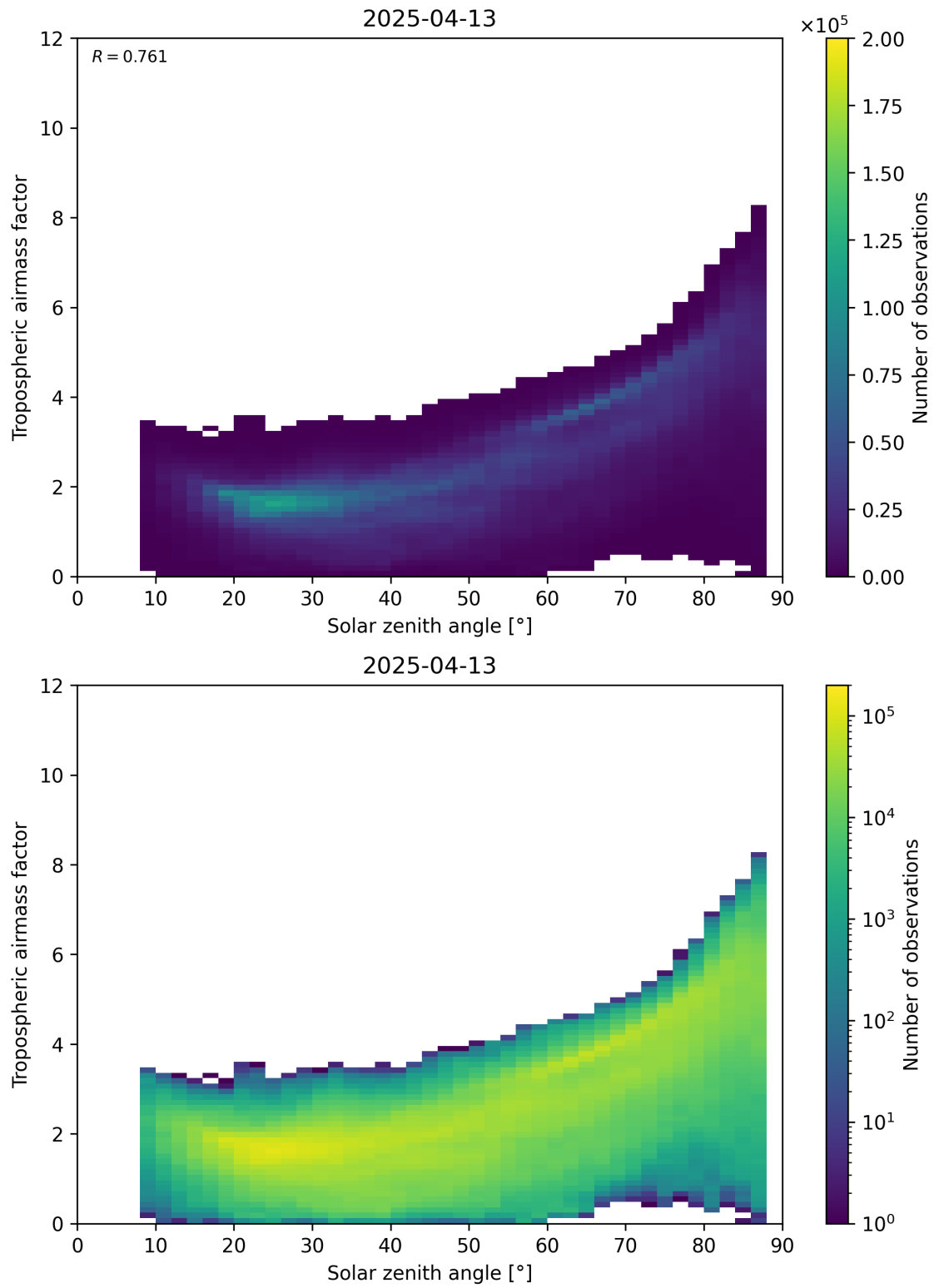
Figure 147: Scatter density plot of “Solar zenith angle” against “Tropospheric airmass factor” for 2025-04-13 to 2025-04-14.
