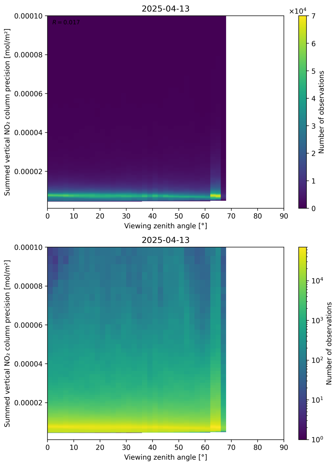
Figure 166: Scatter density plot of “Viewing zenith angle” against “Summed vertical NO 2 column precision” for 2025-04-13 to 2025-04-14.
