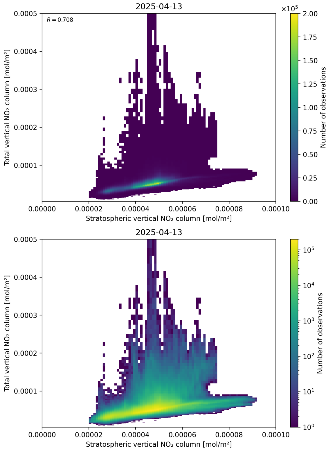
Figure 100: Scatter density plot of “Stratospheric vertical NO 2 column” against “Total vertical NO 2 column” for 2025-04-13 to 2025-04-14.
