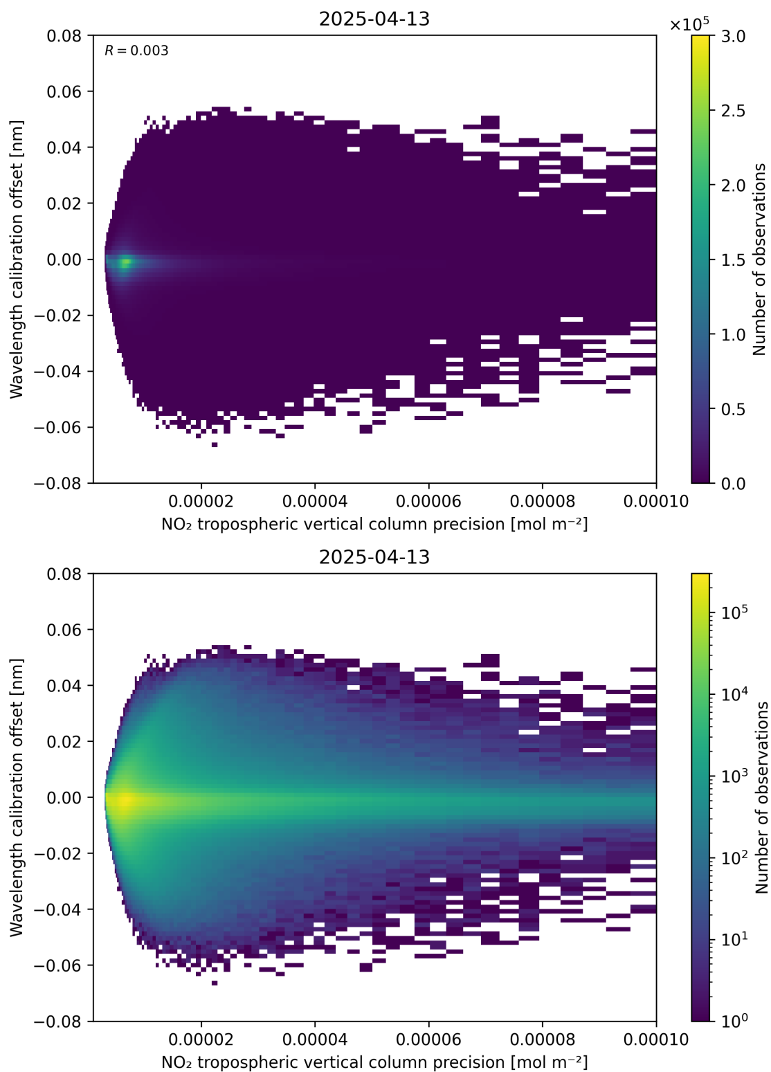
Figure 141: Scatter density plot of “NO 2 tropospheric vertical column precision” against “Wavelength calibration offset” for 2025-04-13 to 2025-04-14.
