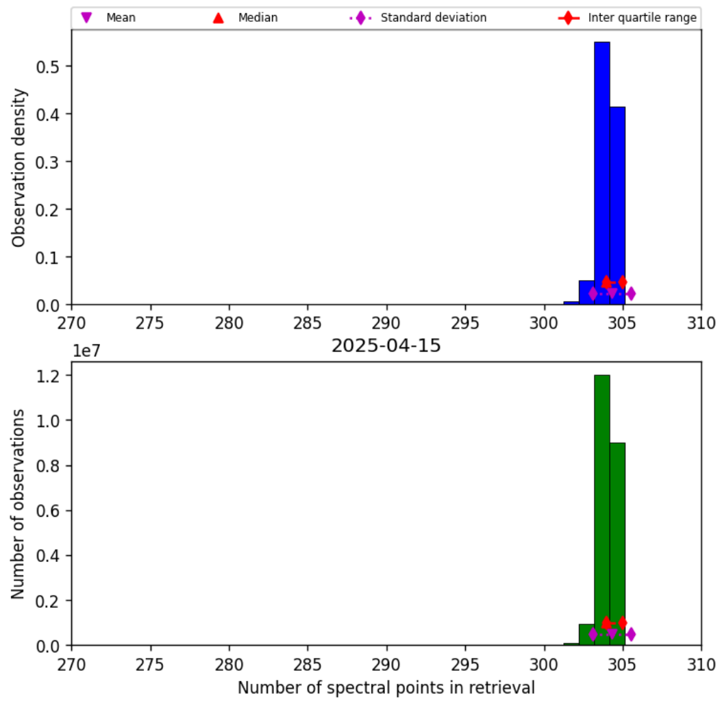
Figure 33: Histogram of “Number of spectral points in retrieval” for 2025-04-15 to 2025-04-16
