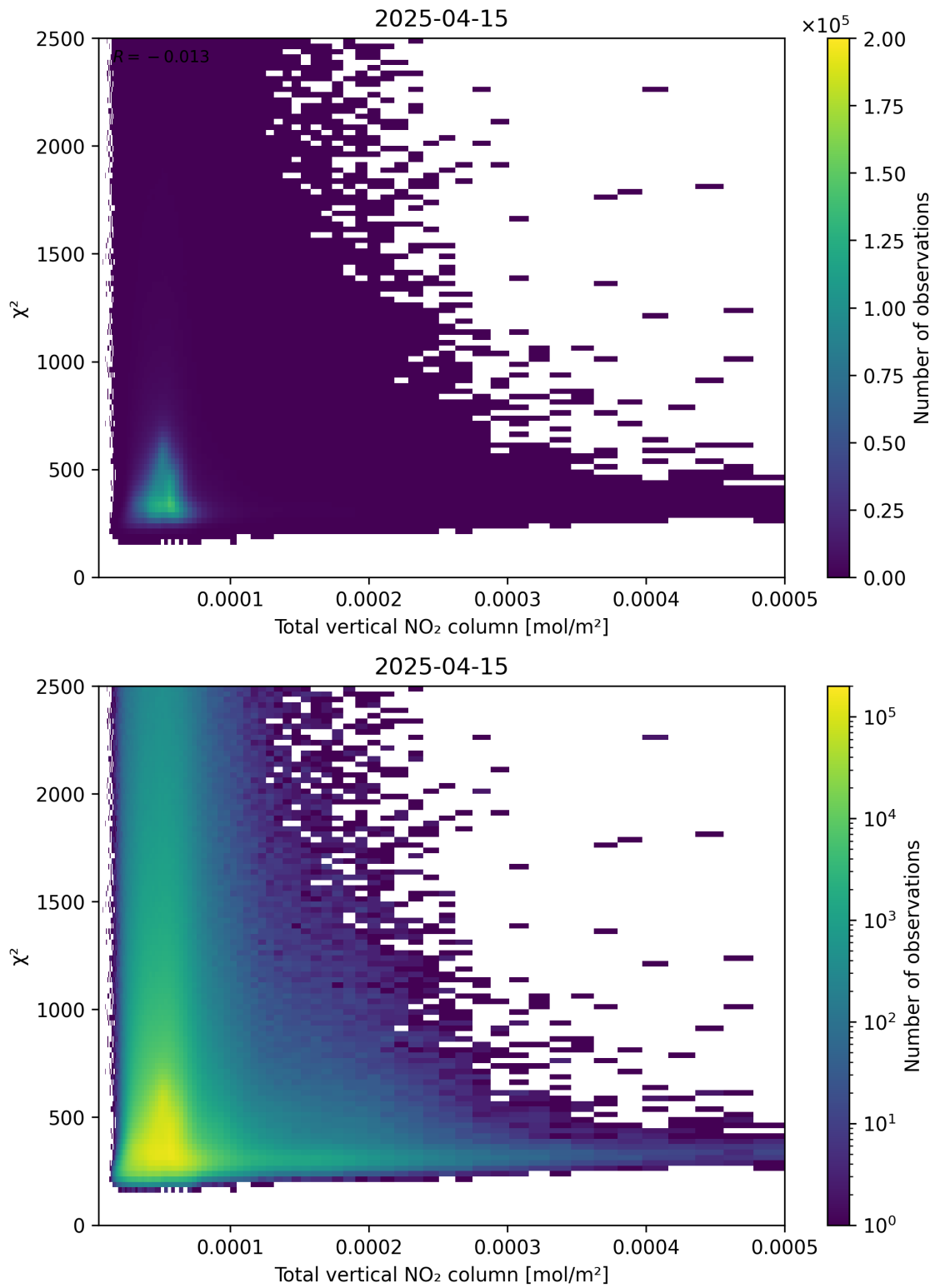
Figure 111: Scatter density plot of “Total vertical NO 2 column” against “ \chi^2 ” for 2025-04-15 to 2025-04-16.
