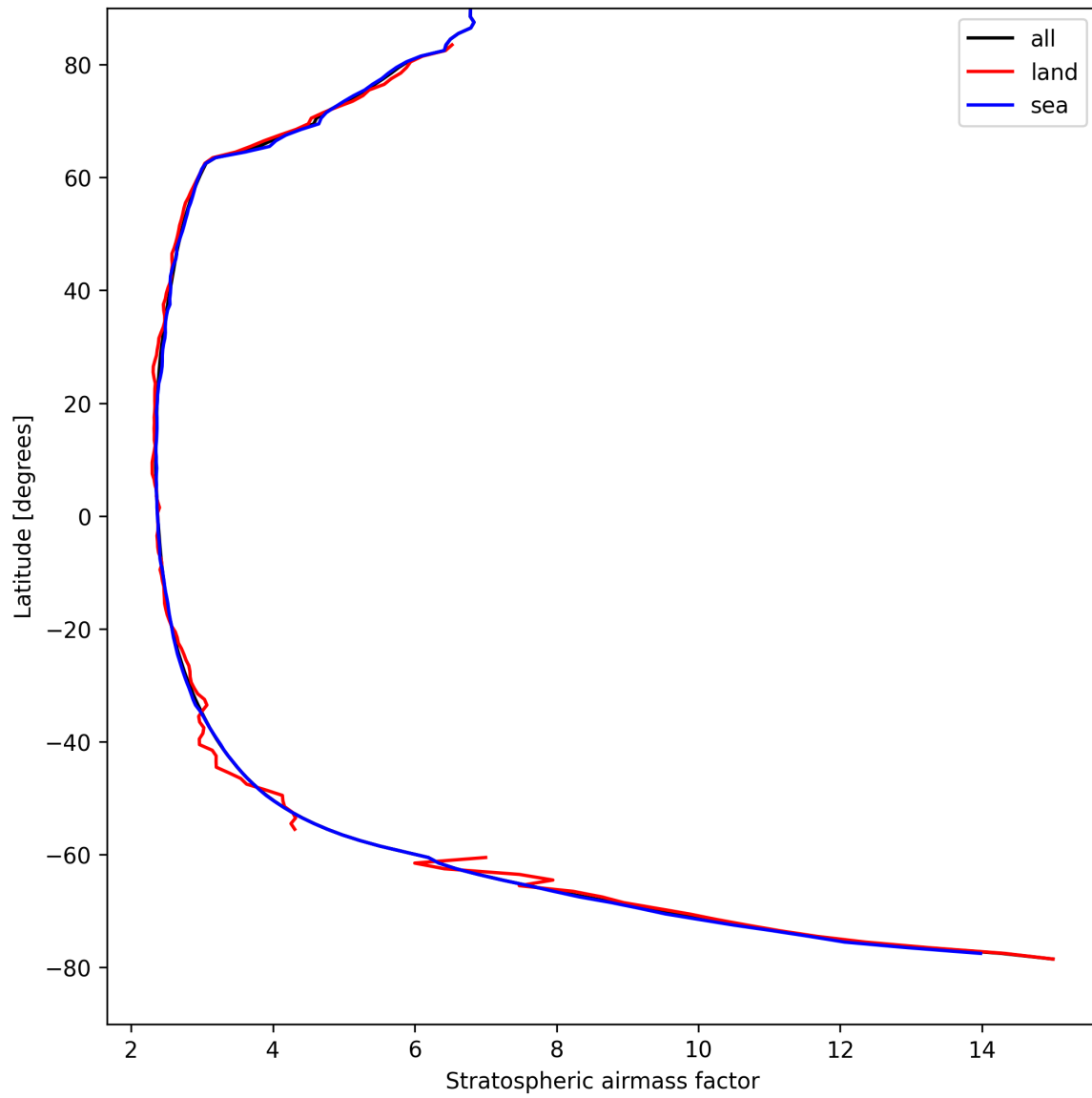
Figure 27: Zonal average of “Stratospheric airmass factor” for 2025-04-15 to 2025-04-16.
