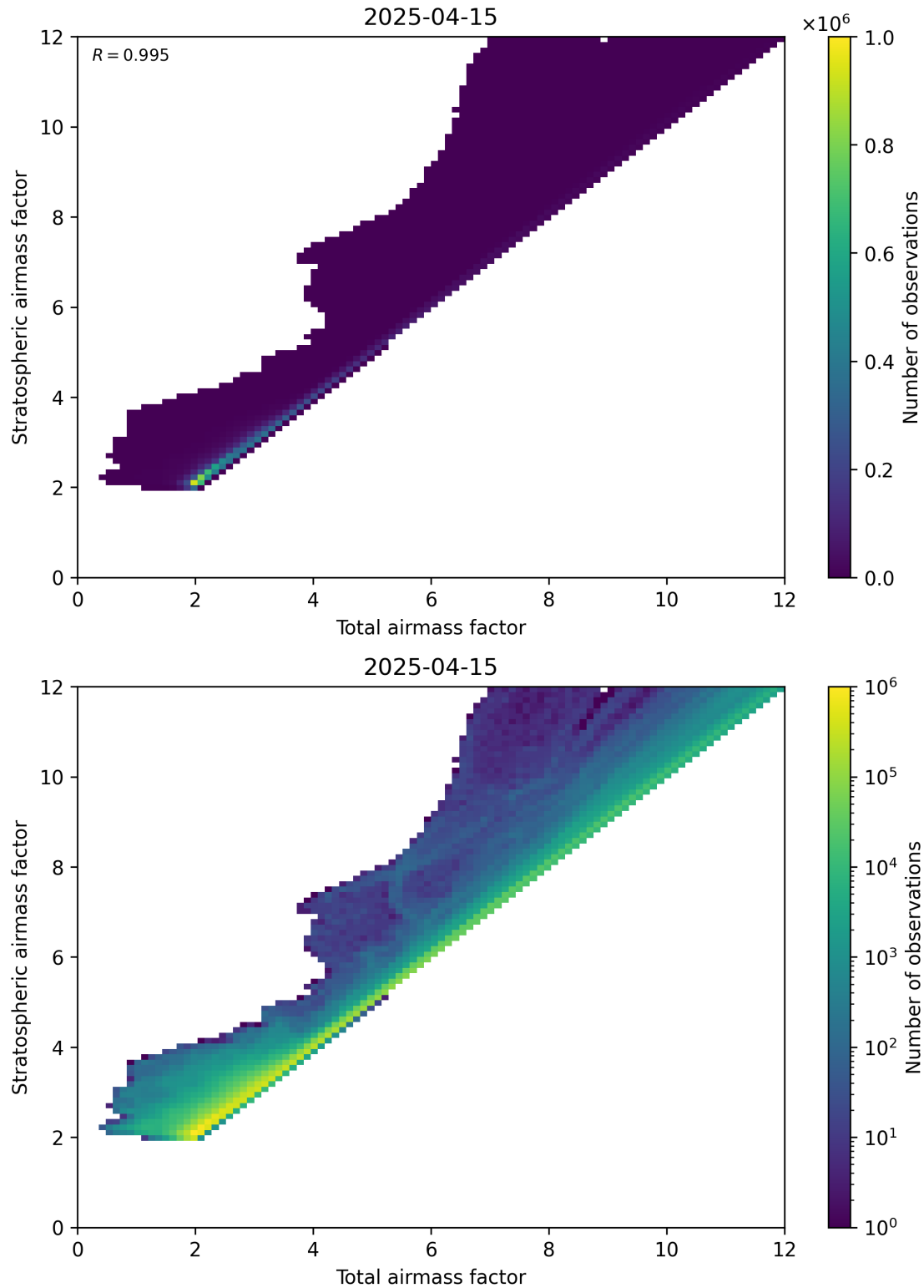
Figure 62: Scatter density plot of “Total airmass factor” against “Stratospheric airmass factor” for 2025-04-15 to 2025-04-16.
