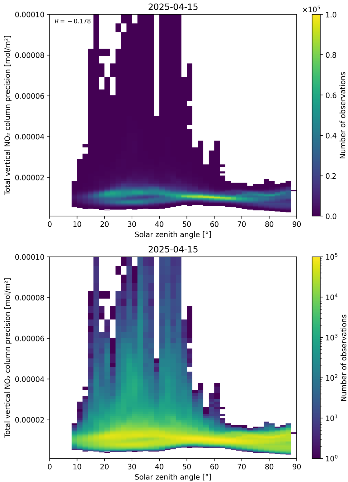
Figure 154: Scatter density plot of “Solar zenith angle” against “Total vertical NO 2 column precision” for 2025-04-15 to 2025-04-16.
