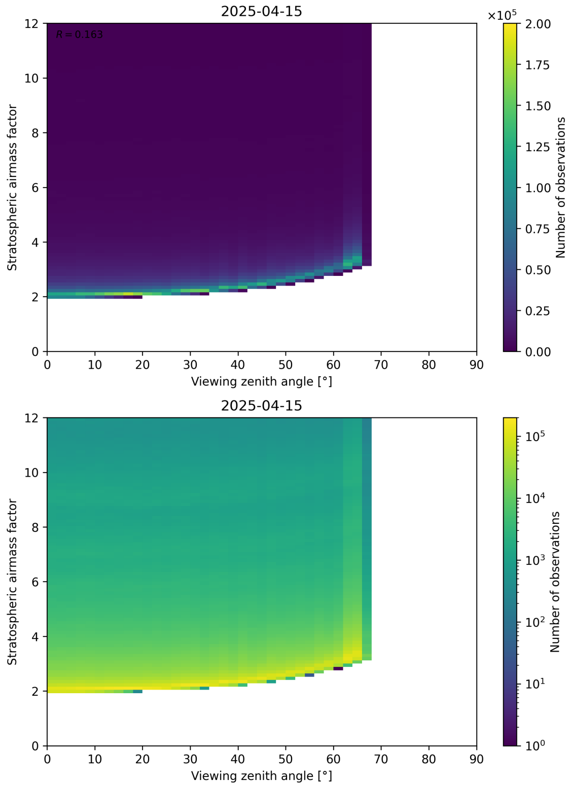
Figure 159: Scatter density plot of “Viewing zenith angle” against “Stratospheric airmass factor” for 2025-04-15 to 2025-04-16.
