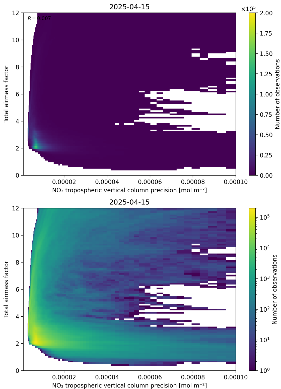
Figure 132: Scatter density plot of “NO 2 tropospheric vertical column precision” against “Total air mass factor” for 2025-04-15 to 2025-04-16.
