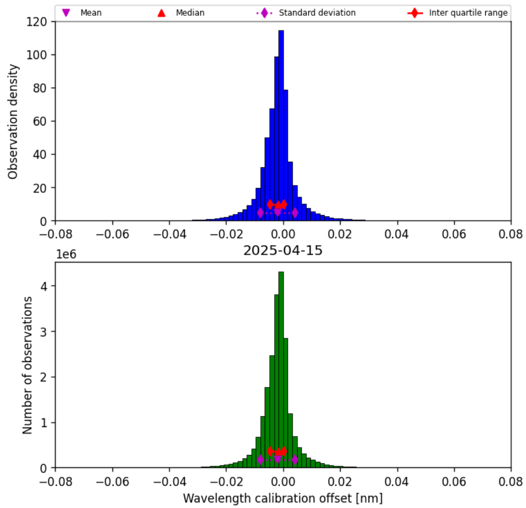
Figure 35: Histogram of “Wavelength calibration offset” for 2025-04-15 to 2025-04-16
