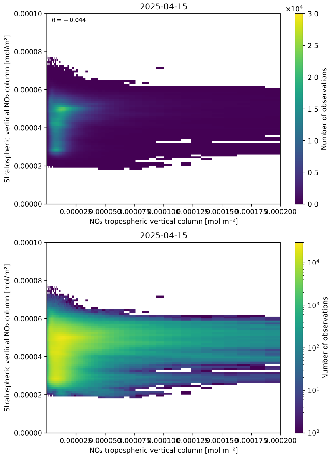
Figure 125: Scatter density plot of “NO 2 tropospheric vertical column” against “Stratospheric vertical NO 2 column” for 2025-04-15 to 2025-04-16.
