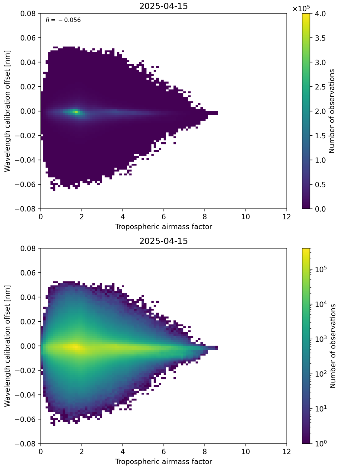
Figure 80: Scatter density plot of “Tropospheric airmass factor” against “Wavelength calibration offset” for 2025-04-15 to 2025-04-16.
