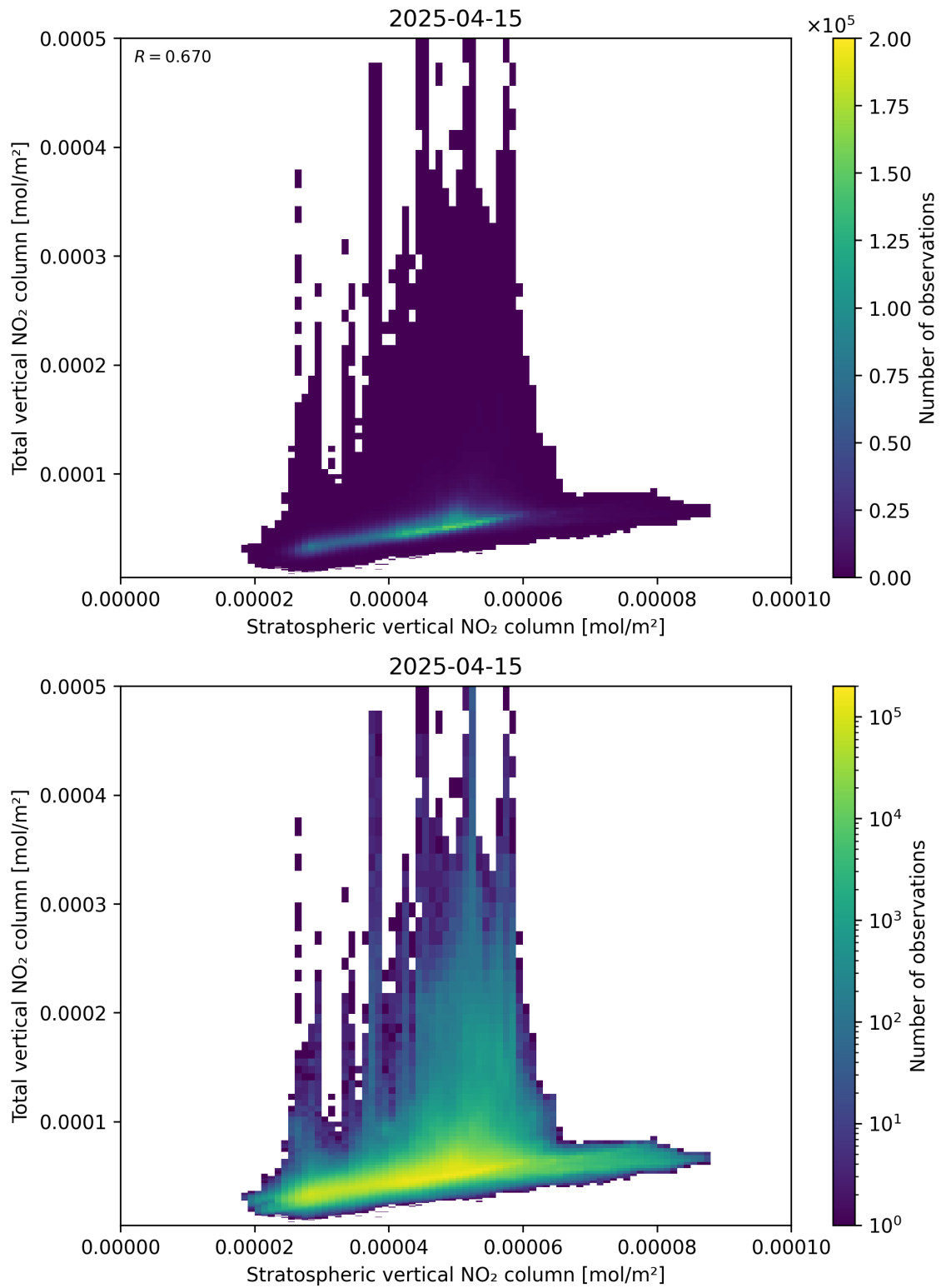
Figure 100: Scatter density plot of “Stratospheric vertical NO 2 column” against “Total vertical NO 2 column” for 2025-04-15 to 2025-04-16.
