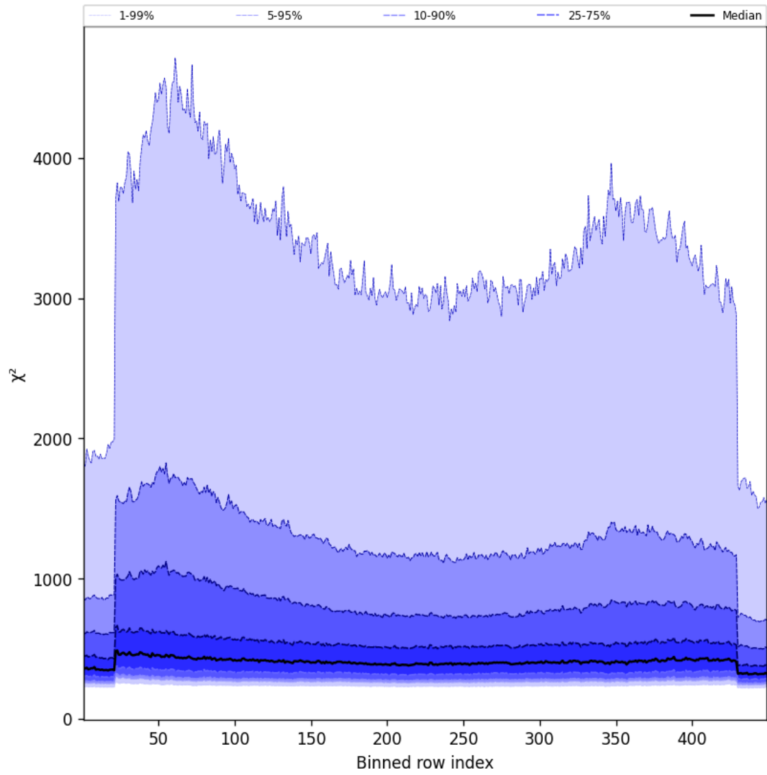
Figure 59: Along track statistics of “ \chi^2 ” for 2025-04-15 to 2025-04-16
