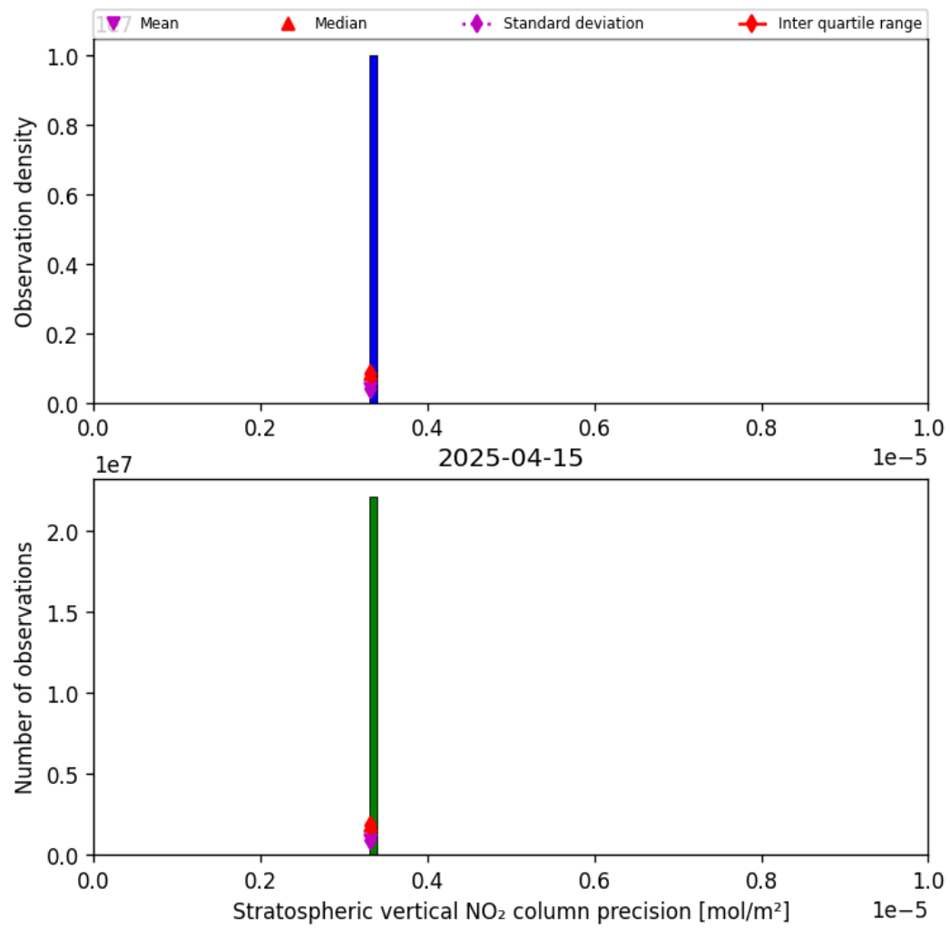
Figure 37: Histogram of “Stratospheric vertical NO 2 column precision” for 2025-04-15 to 2025-04-16
