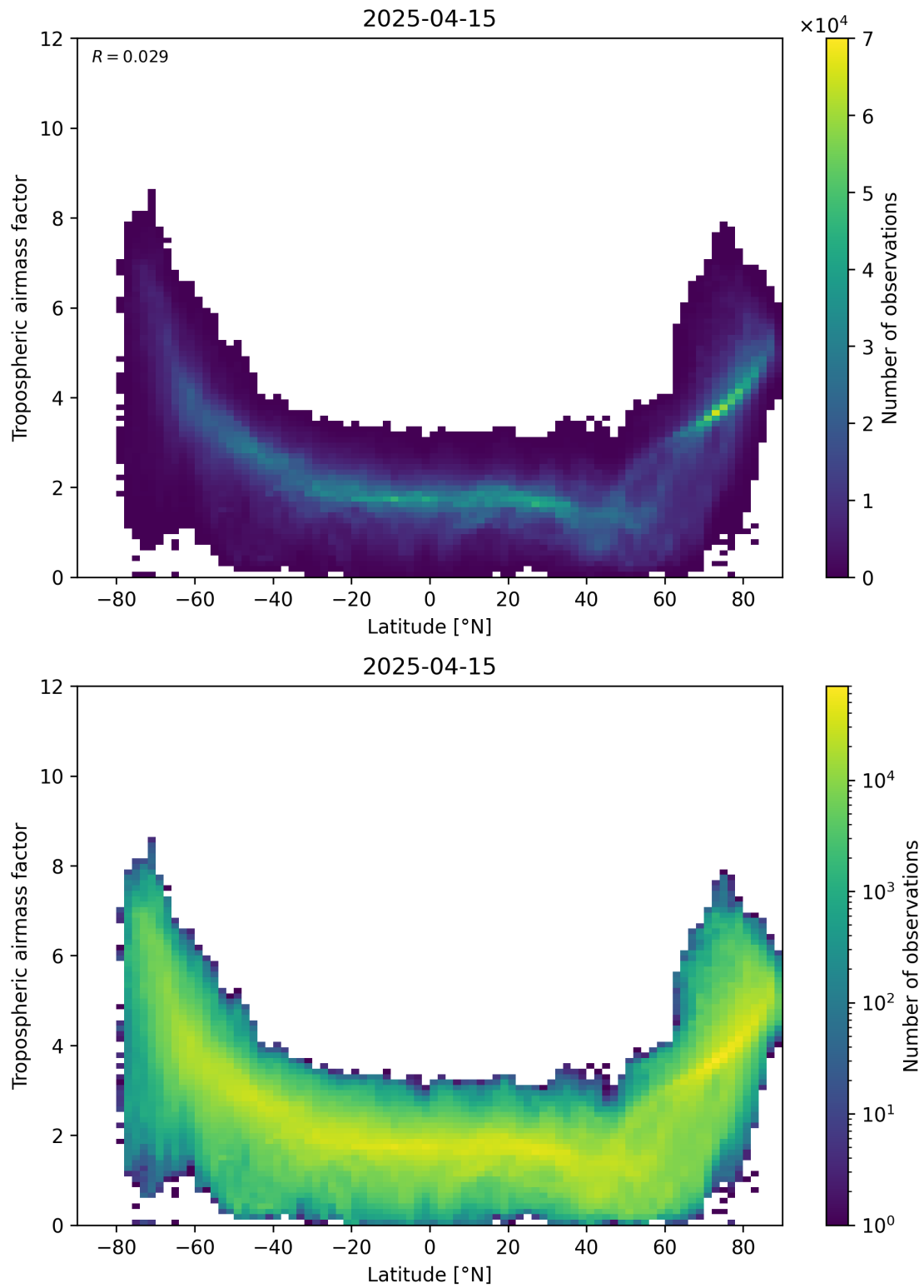
Figure 85: Scatter density plot of “Latitude” against “Tropospheric airmass factor” for 2025-04-15 to 2025-04-16.
