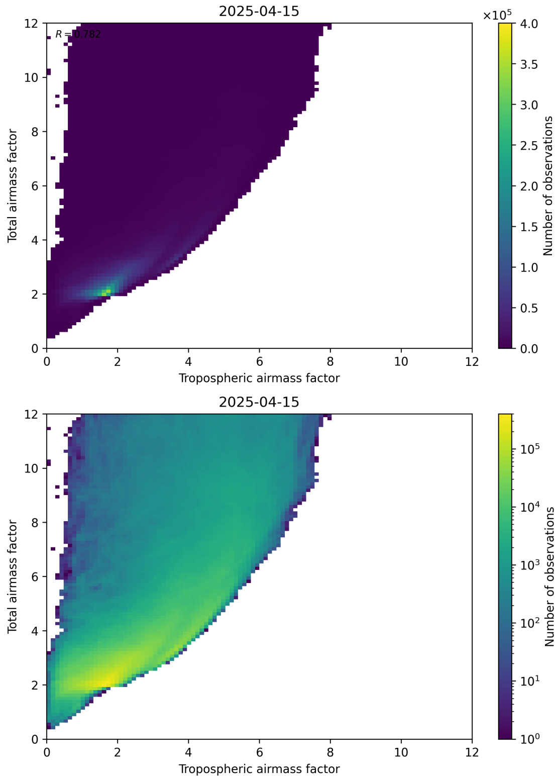
Figure 72: Scatter density plot of “Tropospheric airmass factor” against “Total airmass factor” for 2025-04-15 to 2025-04-16.
