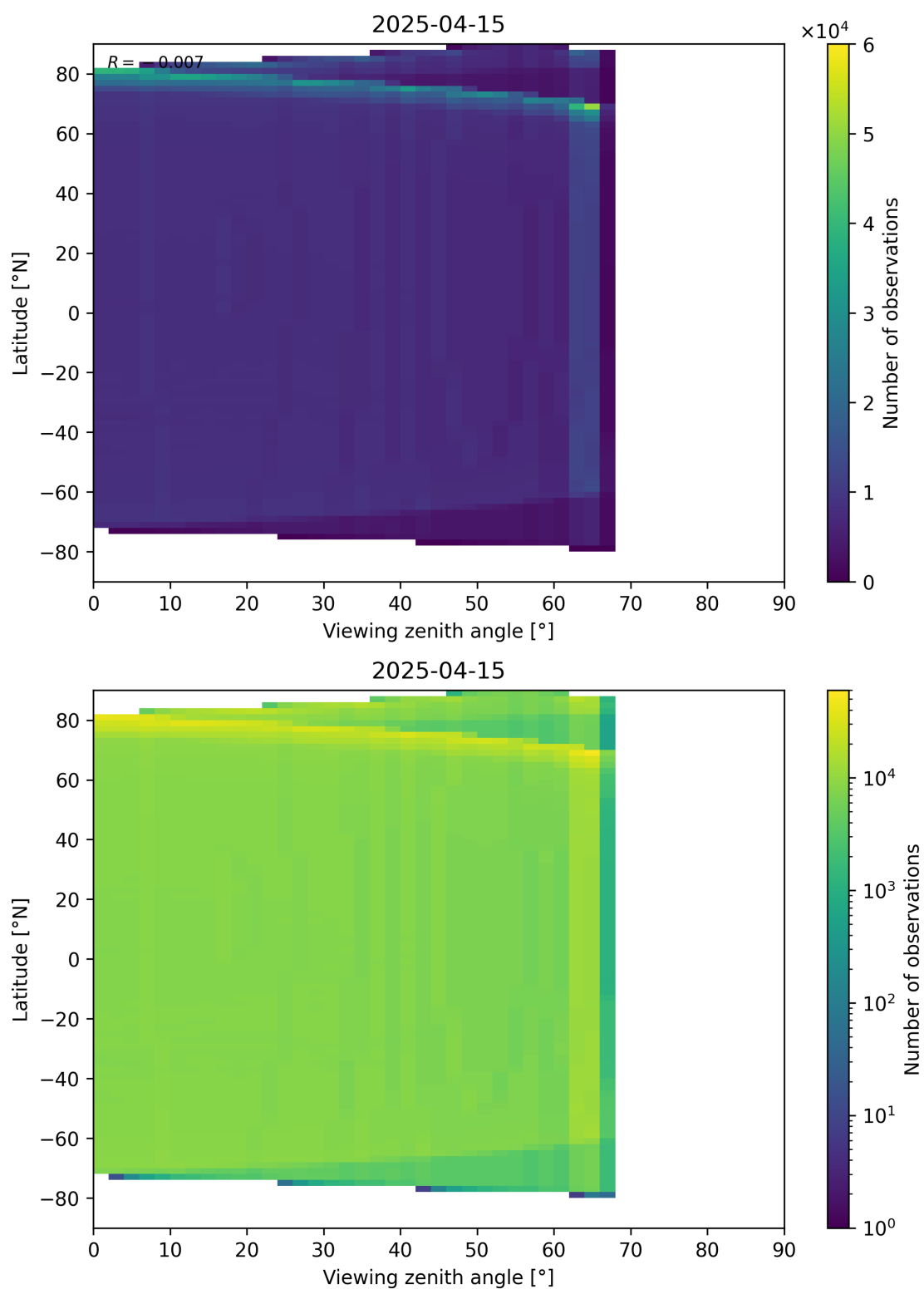
Figure 163: Scatter density plot of “Viewing zenith angle” against “Latitude” for 2025-04-15 to 2025-04-16.
