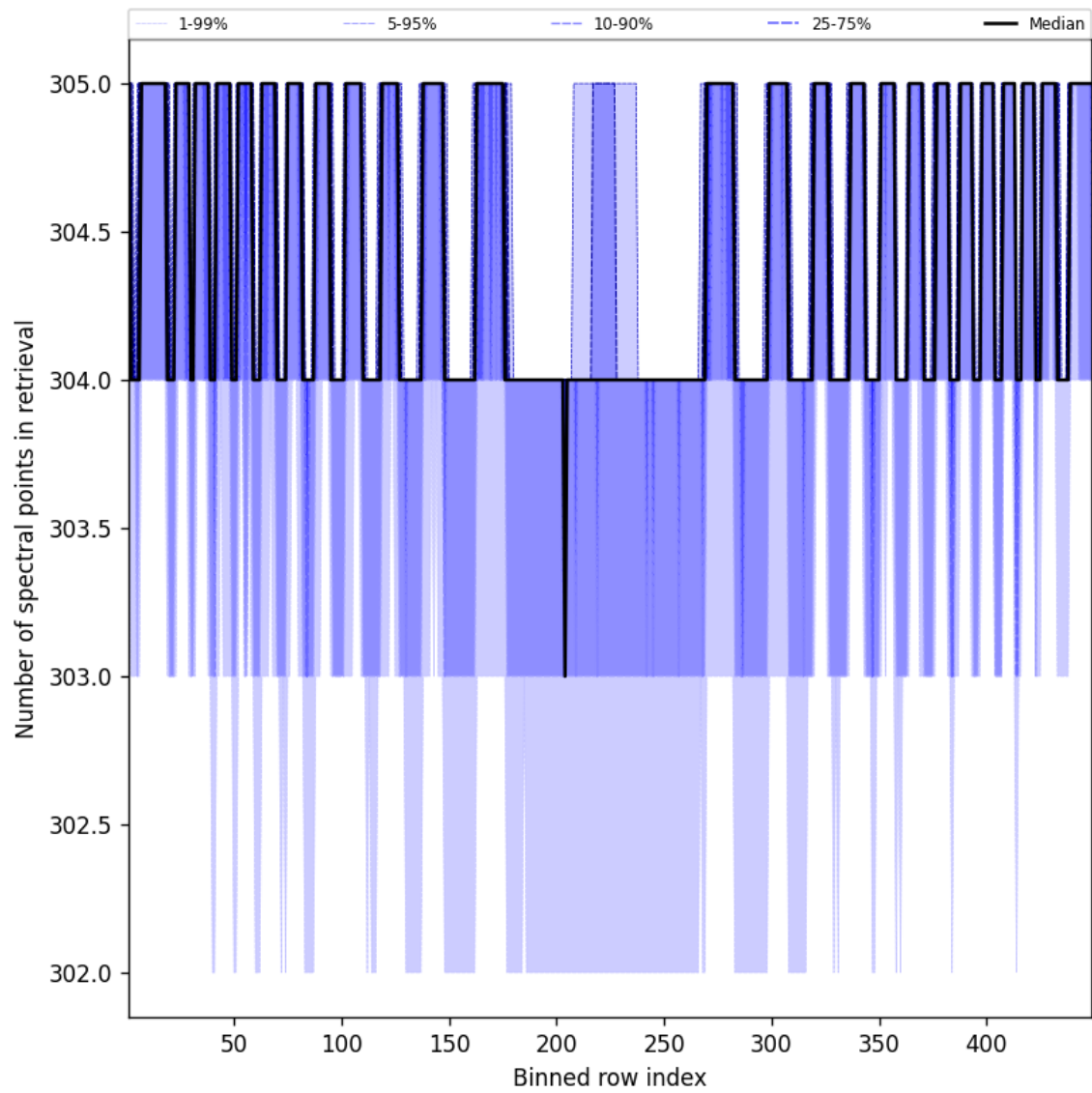
Figure 50: Along track statistics of “Number of spectral points in retrieval” for 2025-04-15 to 2025-04-16
