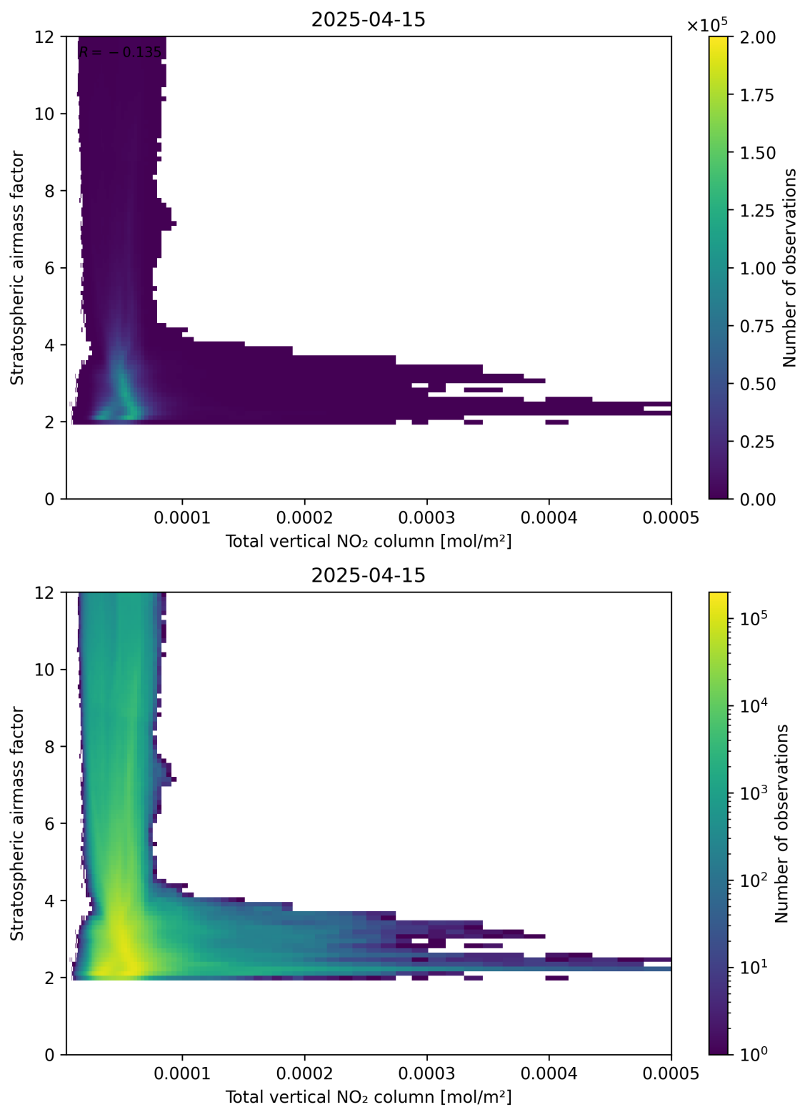
Figure 110: Scatter density plot of “Total vertical NO 2 column” against “Stratospheric airmass factor” for 2025-04-15 to 2025-04-16.
