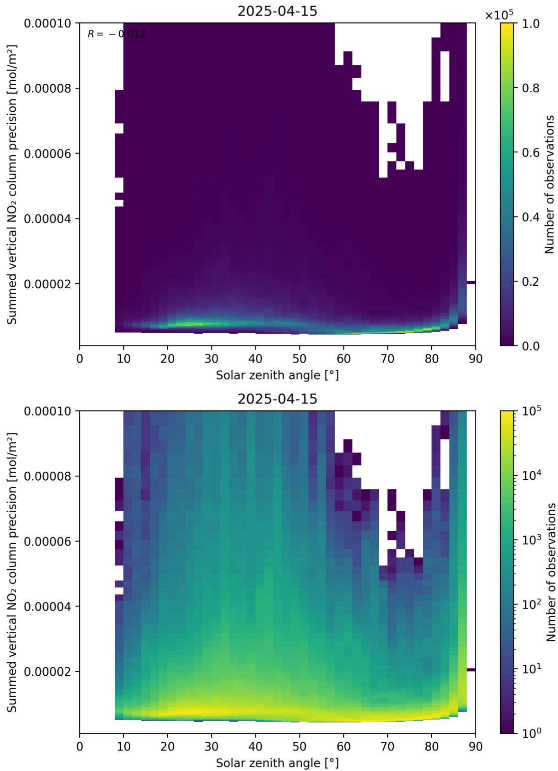
Figure 152: Scatter density plot of “Solar zenith angle” against “Summed vertical NO 2 column precision” for 2025-04-15 to 2025-04-16.
