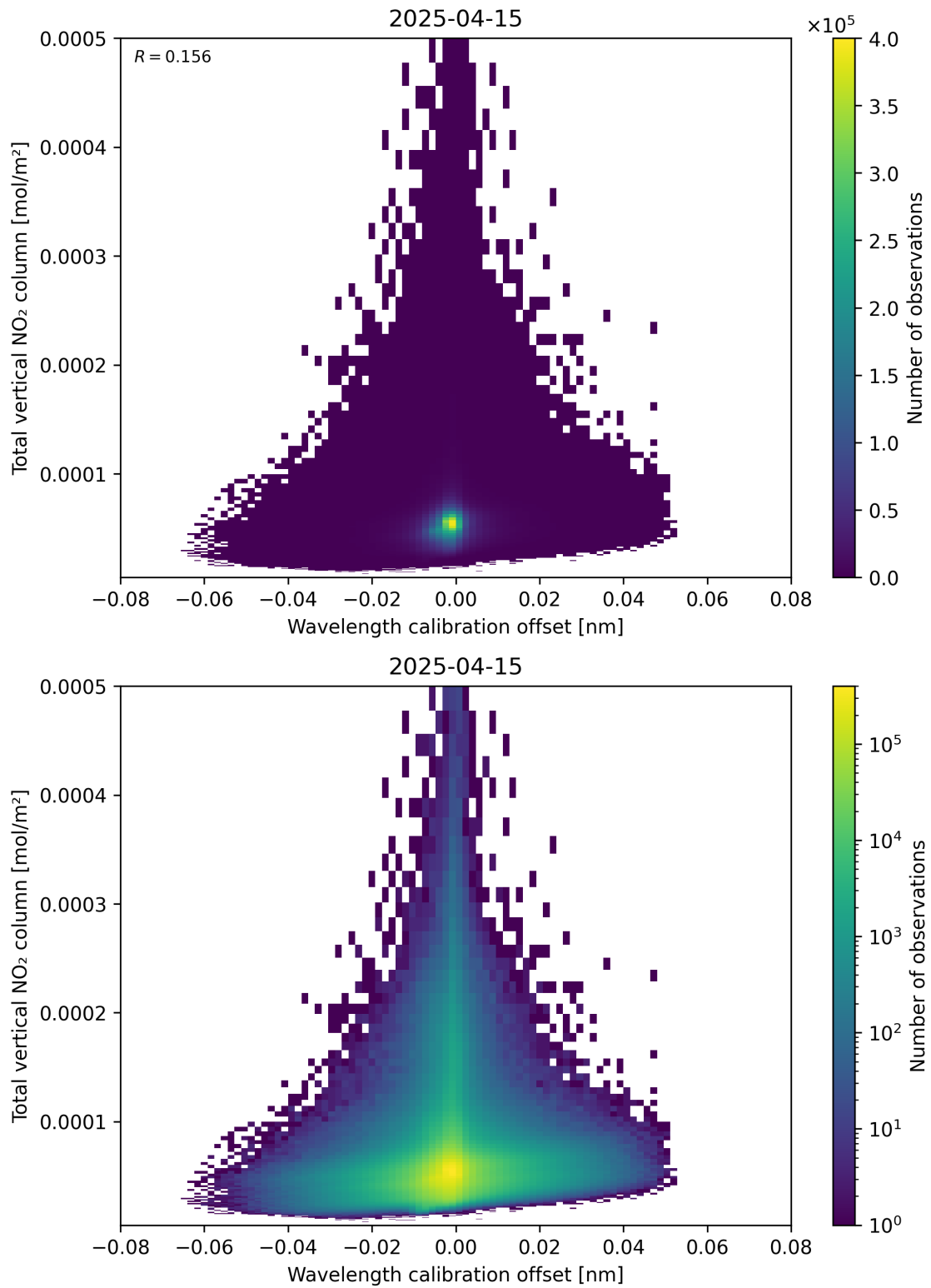
Figure 179: Scatter density plot of “Wavelength calibration offset” against “Total vertical NO 2 column” for 2025-04-15 to 2025-04-16.
