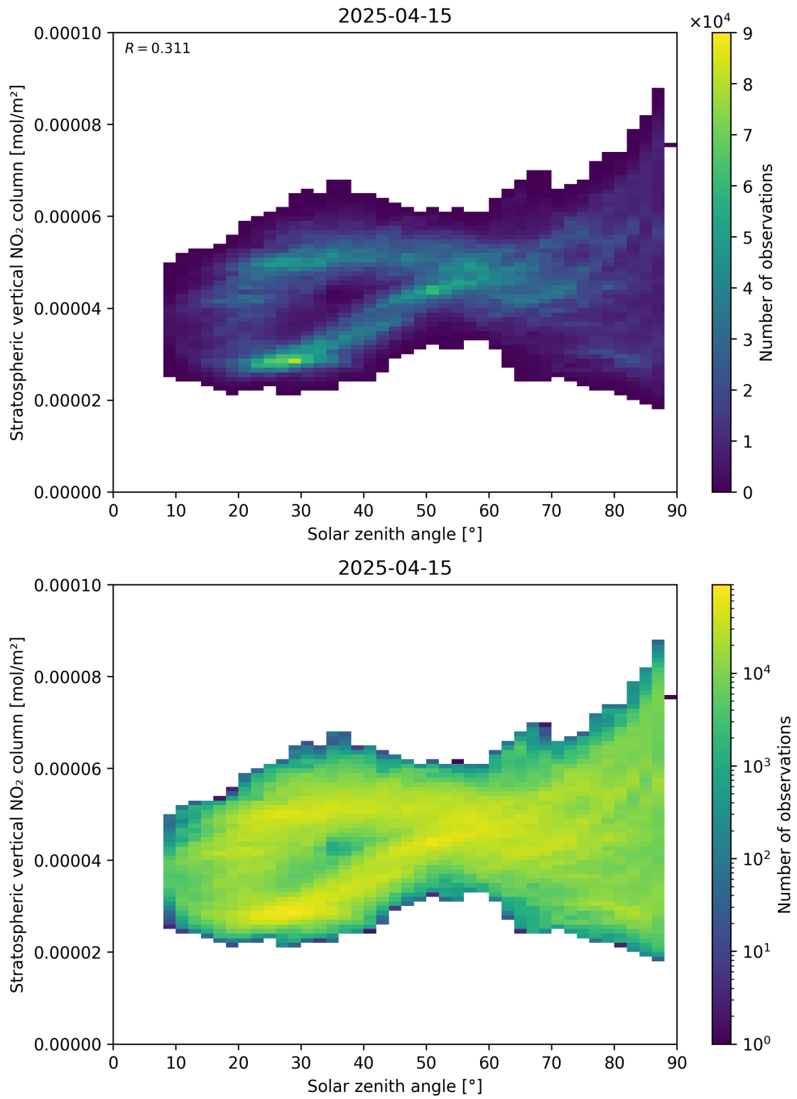
Figure 150: Scatter density plot of “Solar zenith angle” against “Stratospheric vertical NO 2 column” for 2025-04-15 to 2025-04-16.
