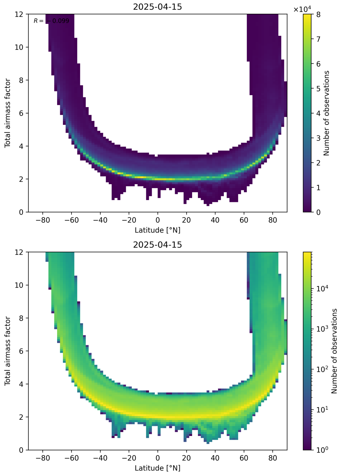
Figure 84: Scatter density plot of “Latitude” against “Total airmass factor” for 2025-04-15 to 2025-04-16.
