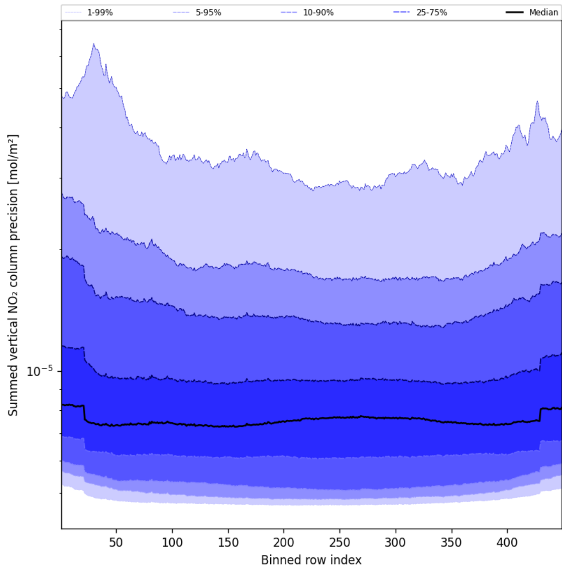
Figure 58: Along track statistics of “Summed vertical NO 2 column precision” for 2025-04-15 to 2025-04-16
