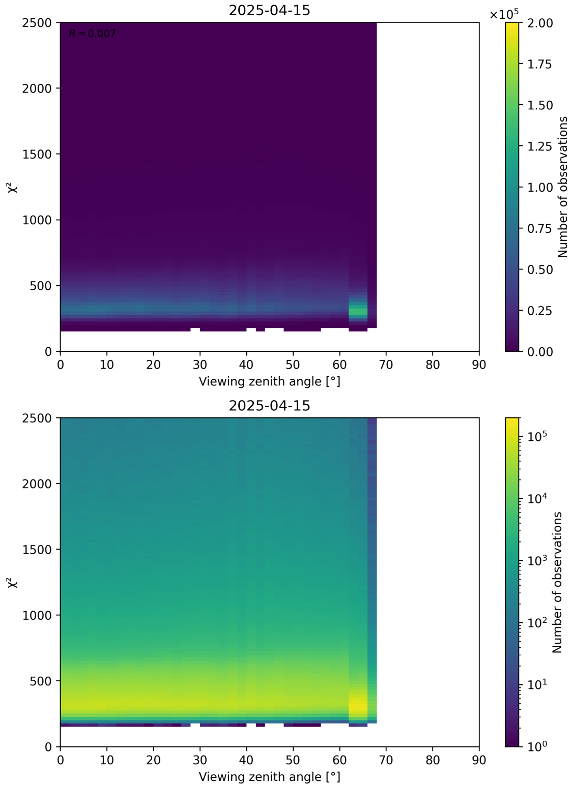
Figure 162: Scatter density plot of “Viewing zenith angle” against “ \chi^2 ” for 2025-04-15 to 2025-04-16.
