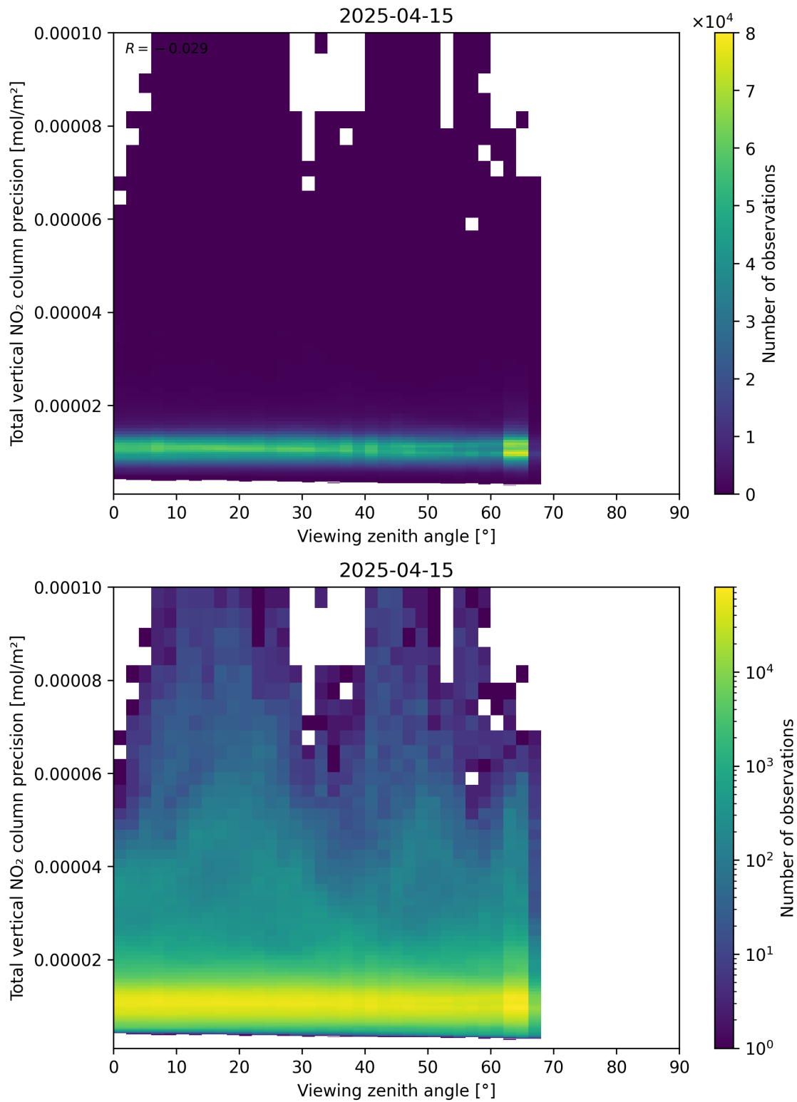
Figure 168: Scatter density plot of “Viewing zenith angle” against “Total vertical NO 2 column precision” for 2025-04-15 to 2025-04-16.
