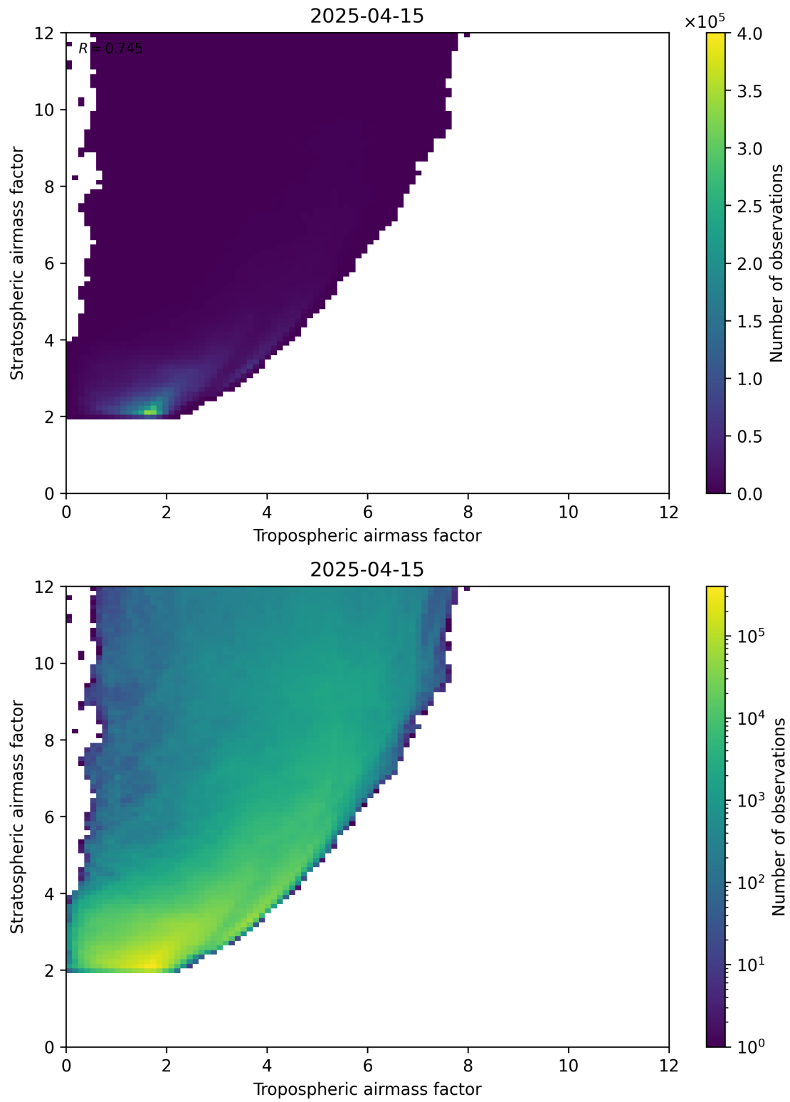
Figure 71: Scatter density plot of “Tropospheric airmass factor” against “Stratospheric airmass factor” for 2025-04-15 to 2025-04-16.
