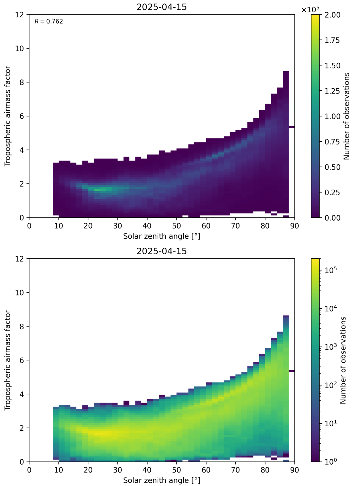
Figure 147: Scatter density plot of “Solar zenith angle” against “Tropospheric airmass factor” for 2025-04-15 to 2025-04-16.
