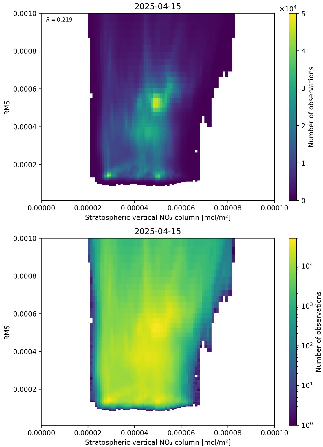
Figure 102: Scatter density plot of “Stratospheric vertical NO 2 column” against “RMS” for 2025-04-15 to 2025-04-16.
