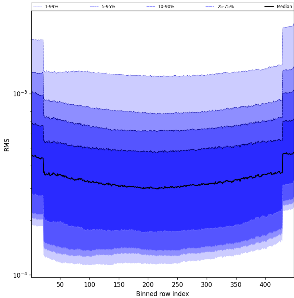
Figure 60: Along track statistics of “RMS” for 2025-04-15 to 2025-04-16
