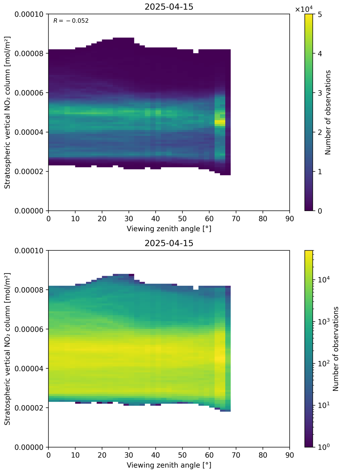
Figure 164: Scatter density plot of “Viewing zenith angle” against “Stratospheric vertical NO 2 column” for 2025-04-15 to 2025-04-16.
