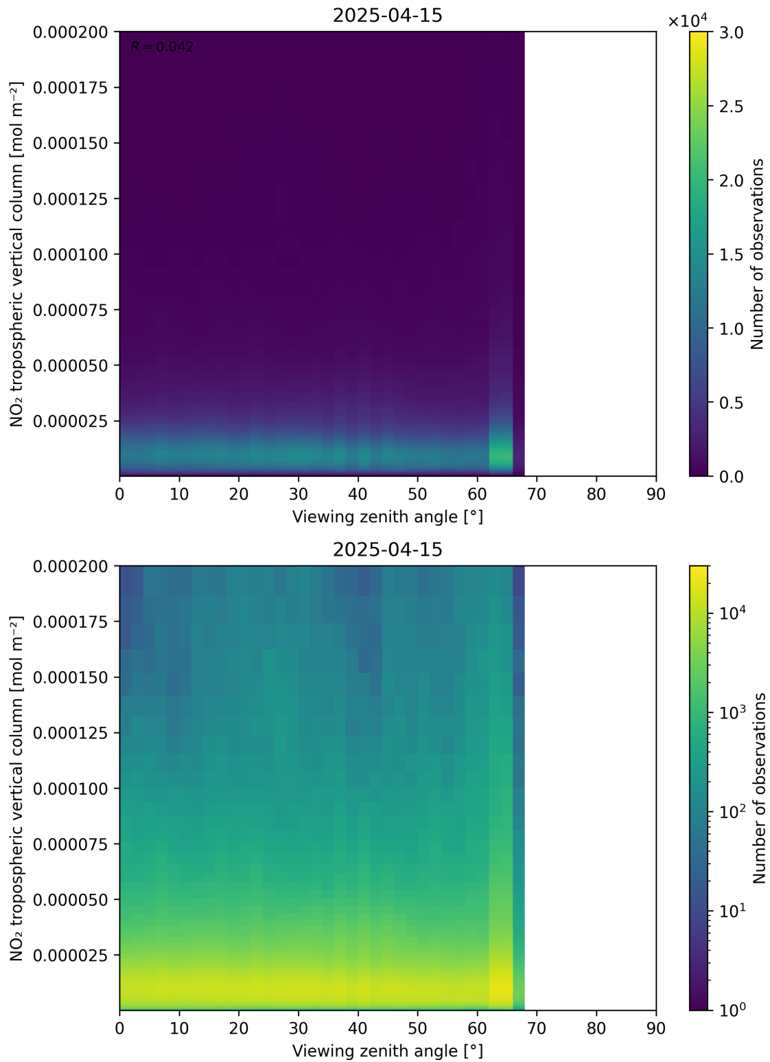
Figure 169: Scatter density plot of “Viewing zenith angle” against “NO 2 tropospheric vertical column” for 2025-04-15 to 2025-04-16.
