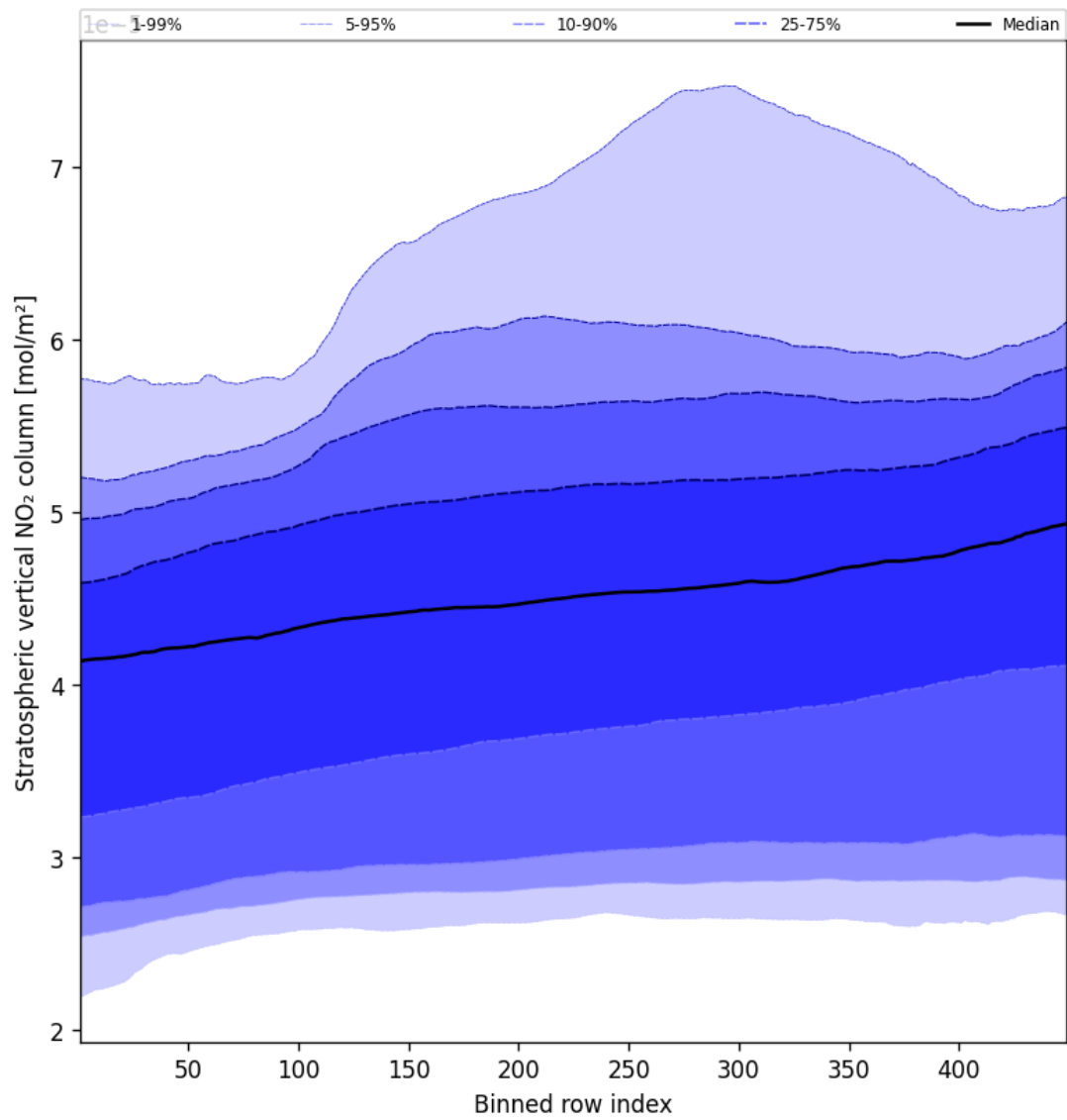
Figure 53: Along track statistics of “Stratospheric vertical NO 2 column” for 2025-04-15 to 2025-04-16
