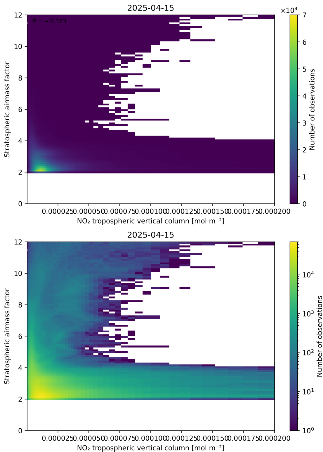
Figure 121: Scatter density plot of “NO 2 tropospheric vertical column” against “Stratospheric air mass factor” for 2025-04-15 to 2025-04-16.
