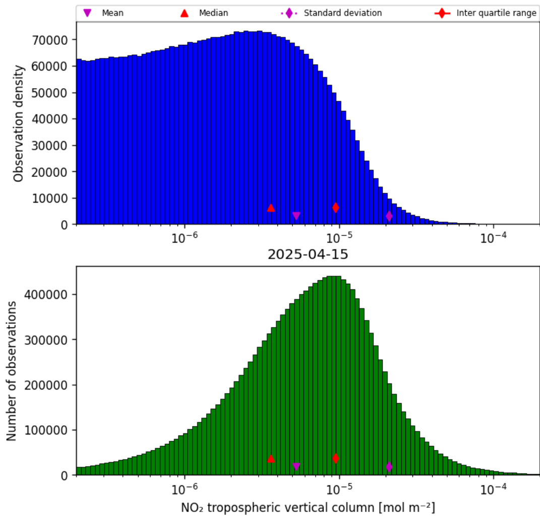
Figure 29: Histogram of “NO 2 tropospheric vertical column” for 2025-04-15 to 2025-04-16
