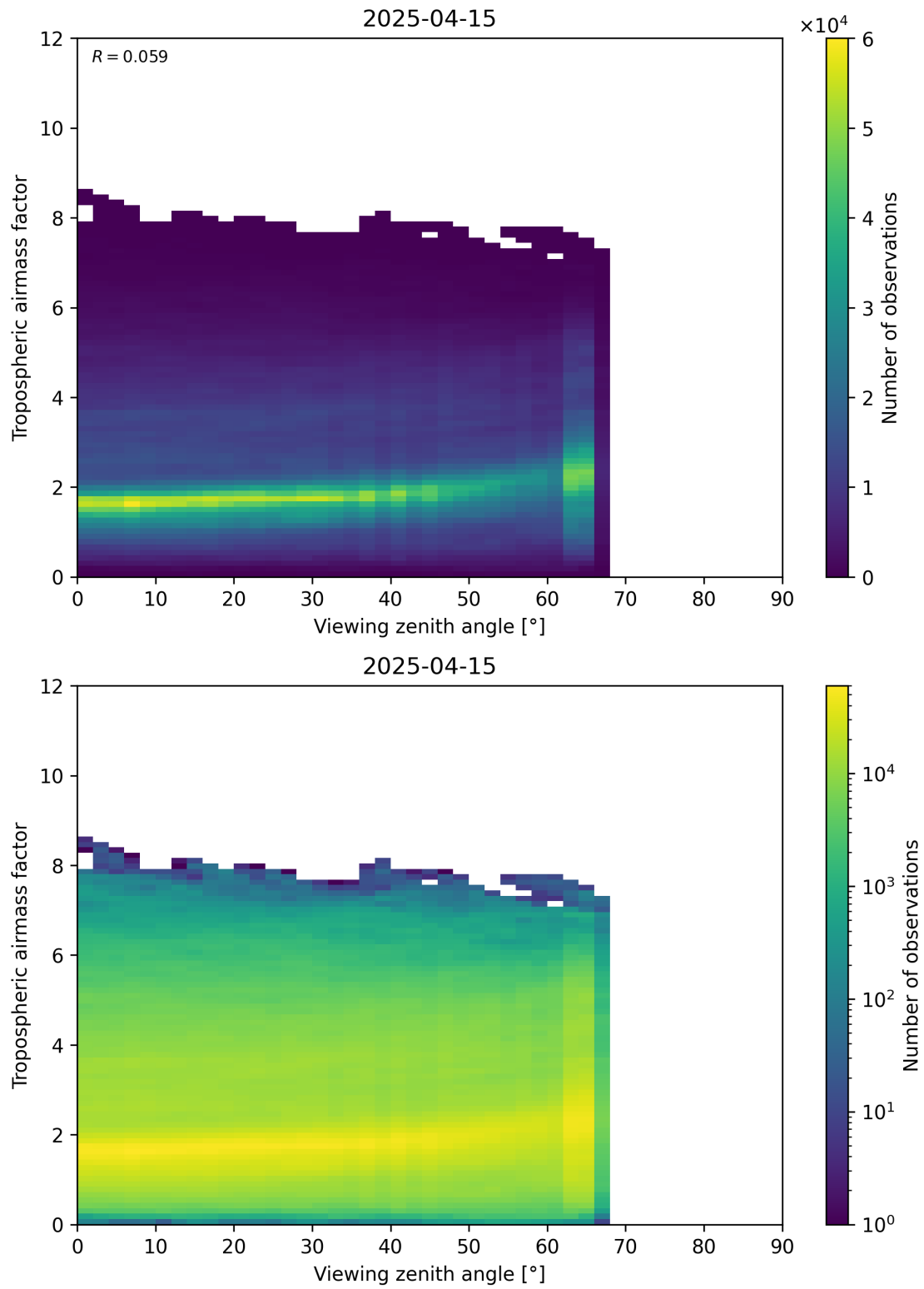
Figure 161: Scatter density plot of “Viewing zenith angle” against “Tropospheric airmass factor” for 2025-04-15 to 2025-04-16.
