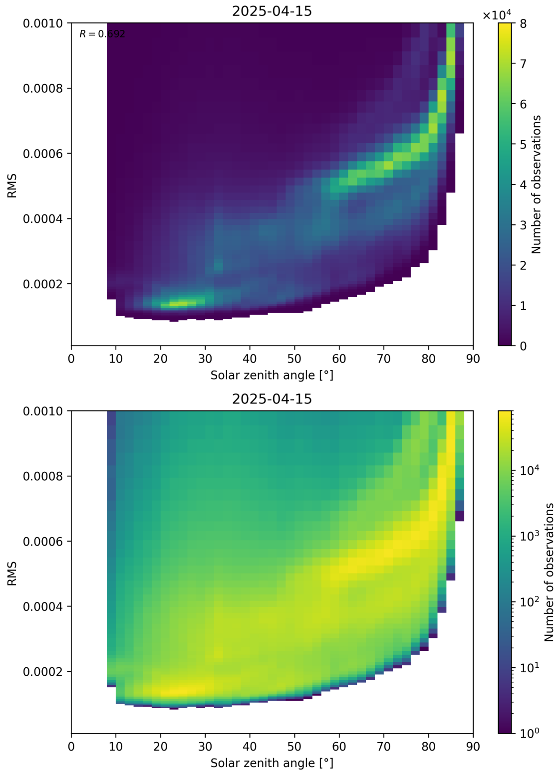
Figure 157: Scatter density plot of “Solar zenith angle” against “RMS” for 2025-04-15 to 2025-04-16.
