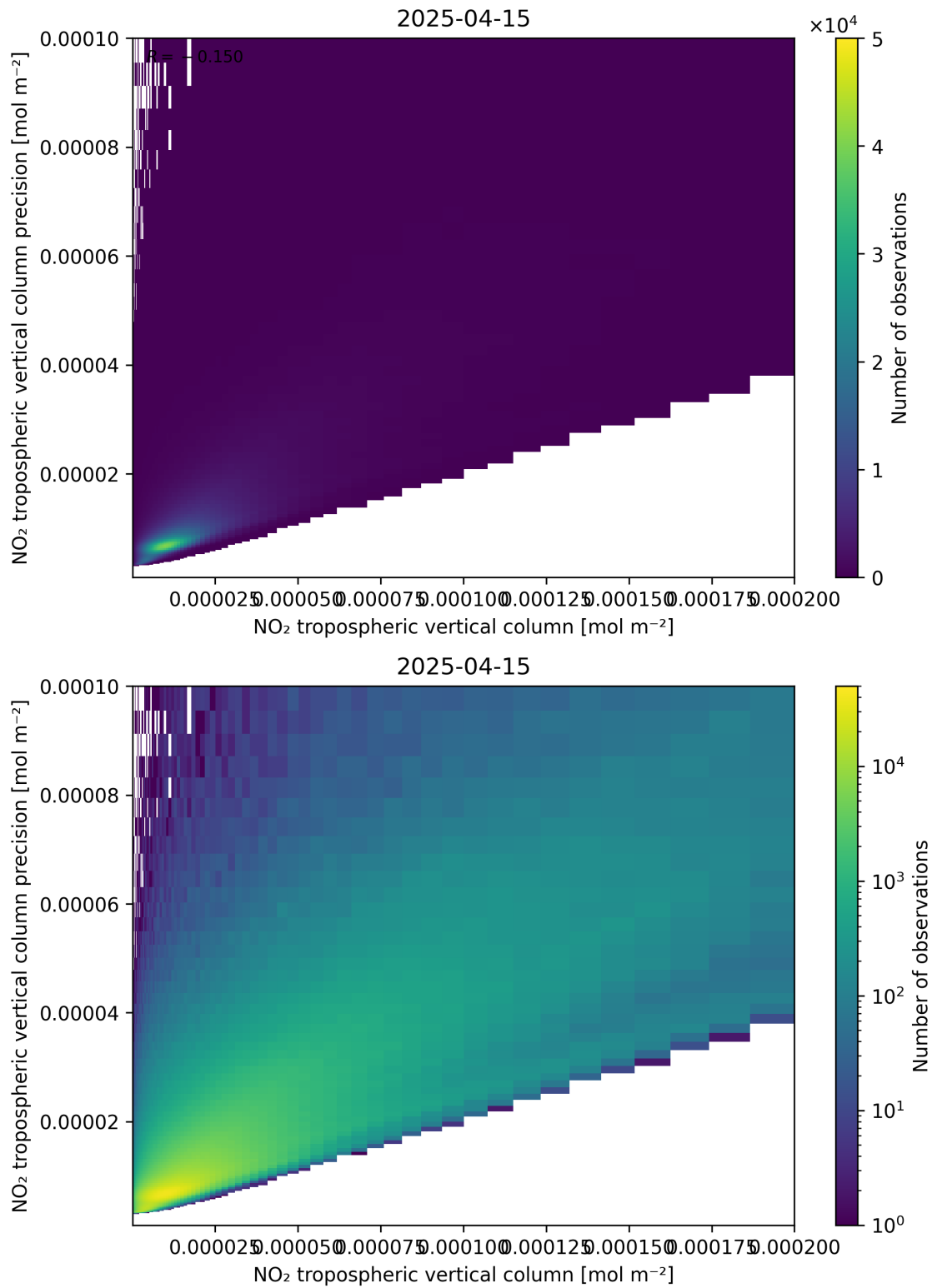
Figure 130: Scatter density plot of “NO 2 tropospheric vertical column” against “NO 2 tropospheric vertical column precision” for 2025-04-15 to 2025-04-16.
