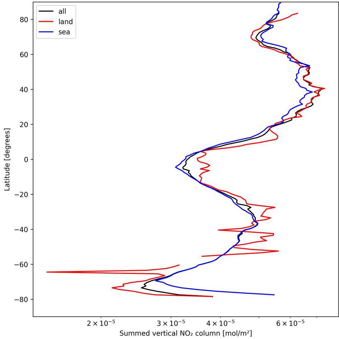
Figure 23: Zonal average of “Summed vertical NO 2 column” for 2025-04-15 to 2025-04-16.
