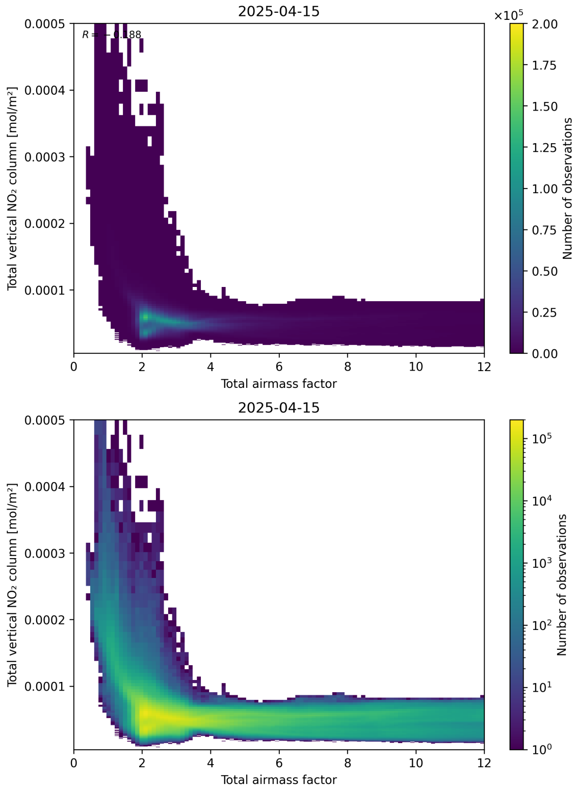
Figure 67: Scatter density plot of “Total airmass factor” against “Total vertical NO 2 column” for 2025-04-15 to 2025-04-16.
