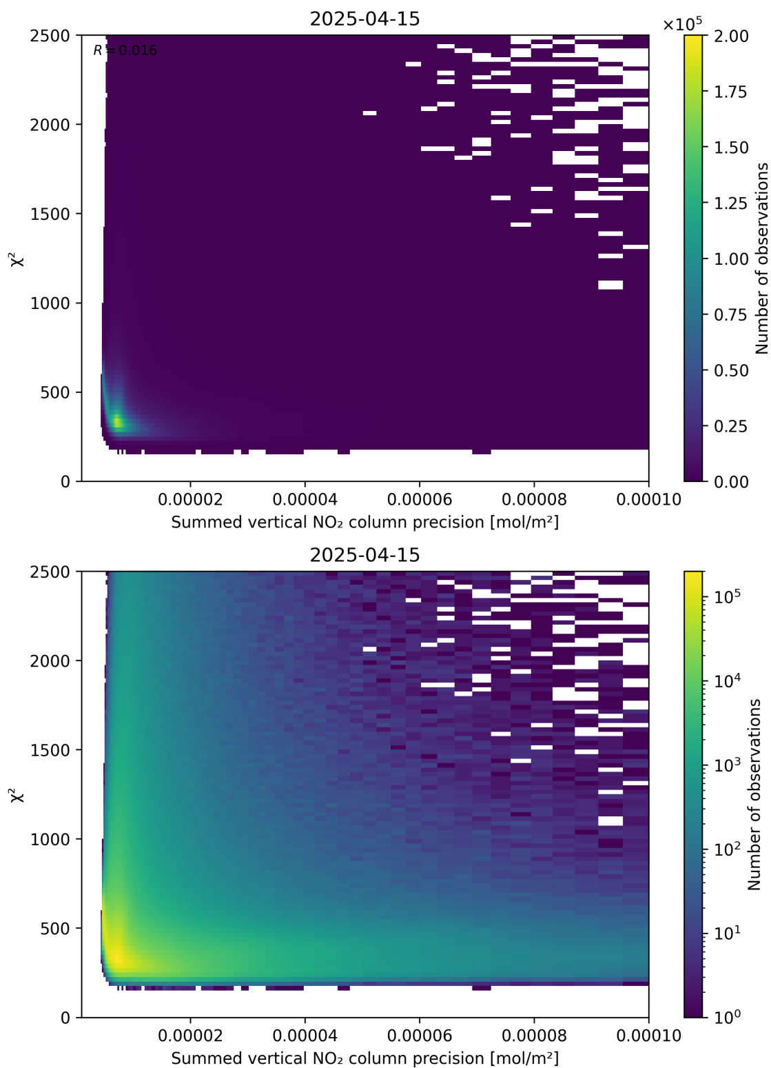
Figure 107: Scatter density plot of “Summed vertical NO 2 column precision” against “ \chi^2 ” for 2025-04-15 to 2025-04-16.
