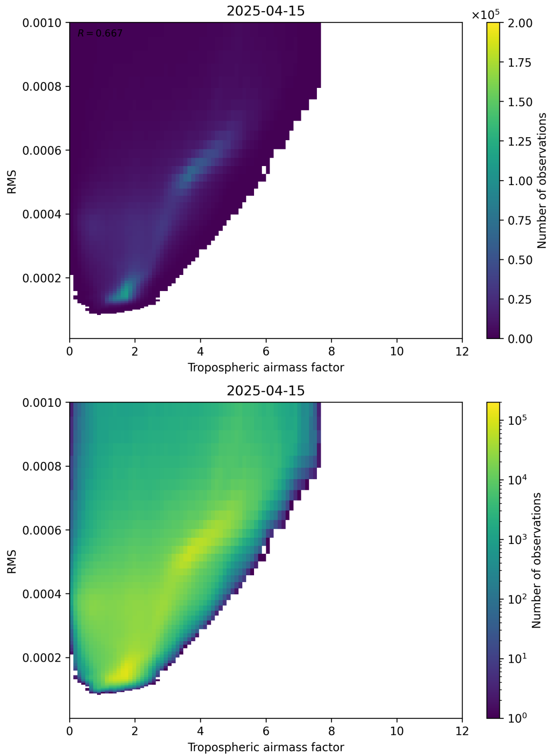
Figure 79: Scatter density plot of “Tropospheric airmass factor” against “RMS” for 2025-04-15 to 2025-04-16.
