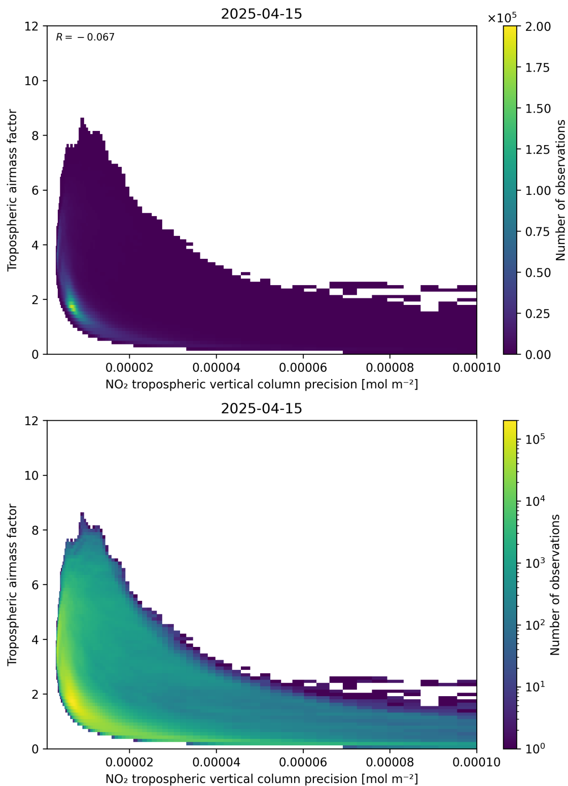
Figure 133: Scatter density plot of “NO 2 tropospheric vertical column precision” against “Tropospheric air mass factor” for 2025-04-15 to 2025-04-16.
