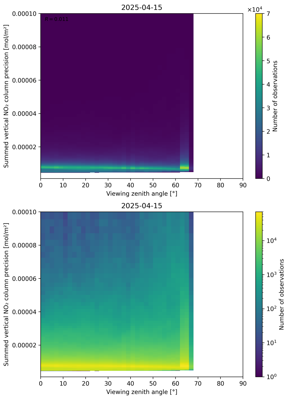
Figure 166: Scatter density plot of “Viewing zenith angle” against “Summed vertical NO 2 column precision” for 2025-04-15 to 2025-04-16.
