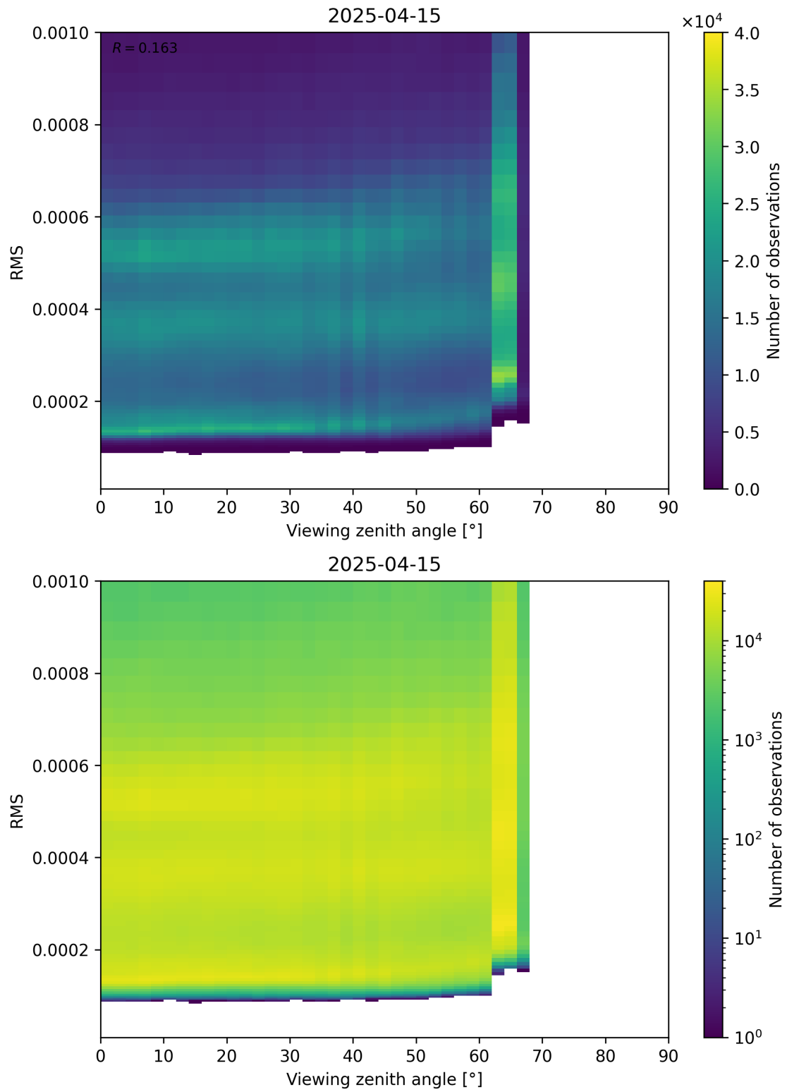
Figure 171: Scatter density plot of “Viewing zenith angle” against “RMS” for 2025-04-15 to 2025-04-16.
