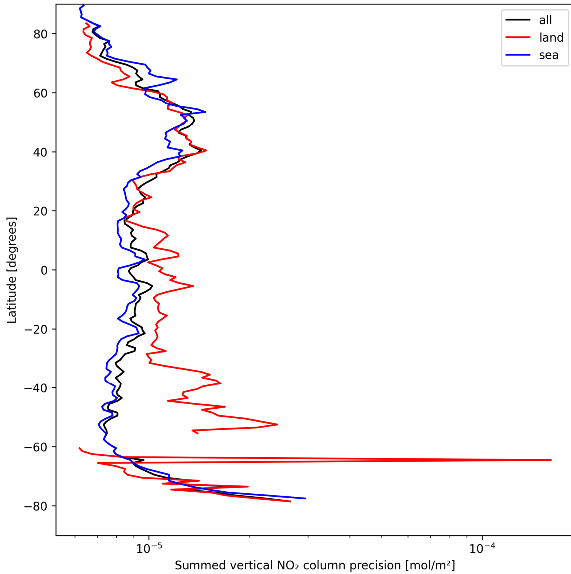
Figure 24: Zonal average of “Summed vertical NO 2 column precision” for 2025-04-15 to 2025-04-16.
