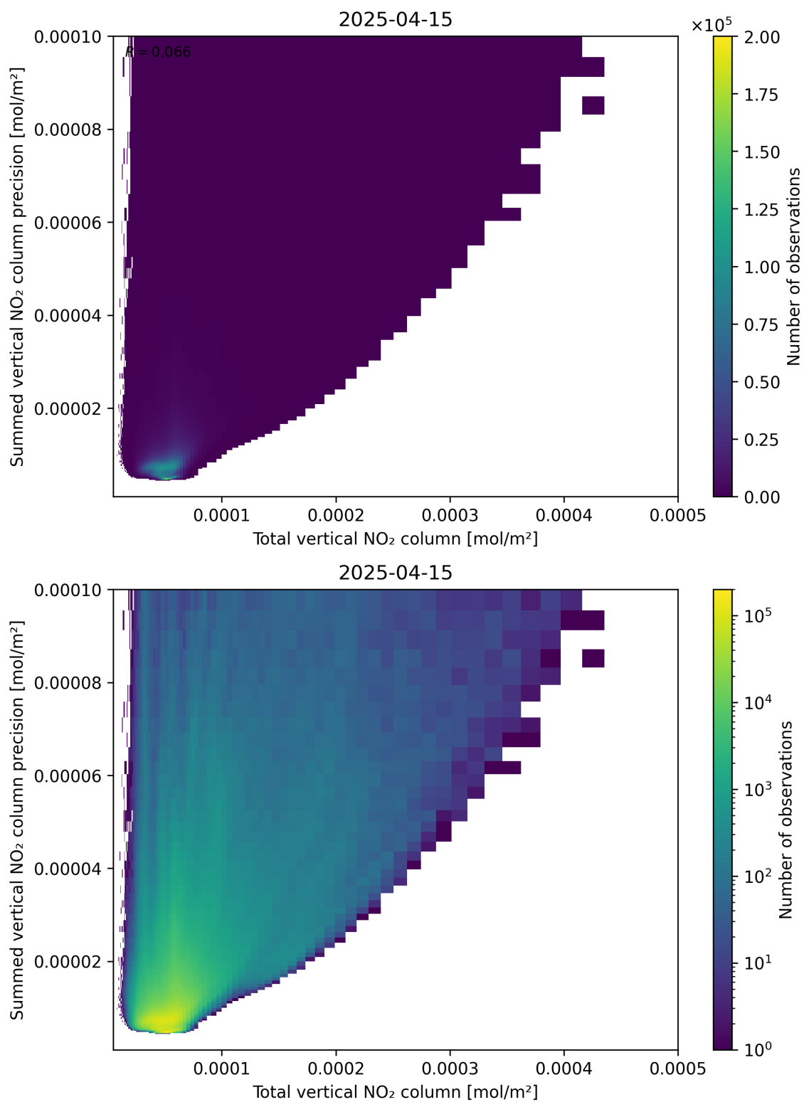
Figure 113: Scatter density plot of “Total vertical NO 2 column” against “Summed vertical NO 2 column precision” for 2025-04-15 to 2025-04-16.
