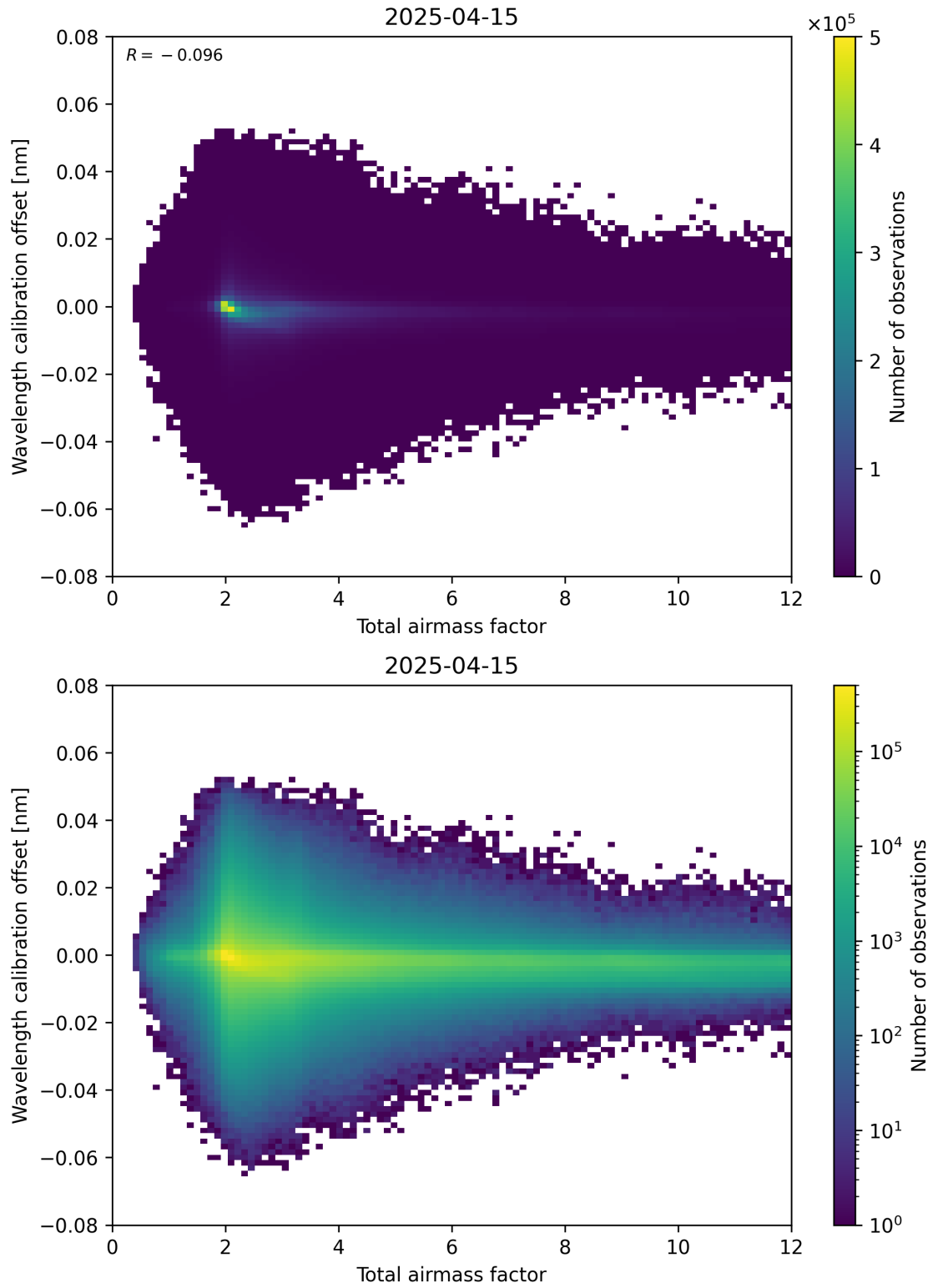
Figure 70: Scatter density plot of “Total airmass factor” against “Wavelength calibration offset” for 2025-04-15 to 2025-04-16.
