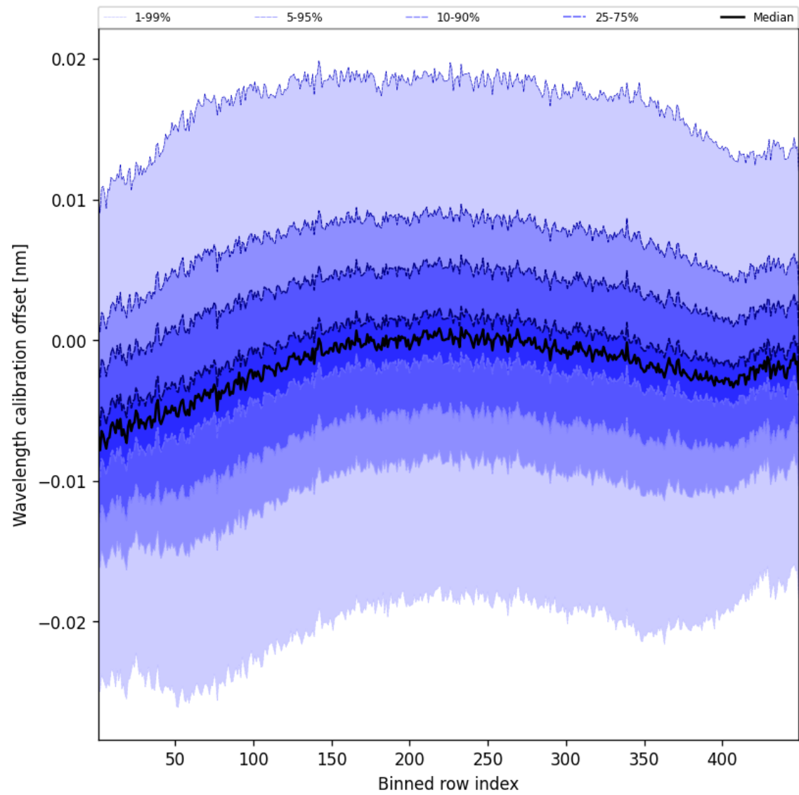
Figure 52: Along track statistics of “Wavelength calibration offset” for 2025-04-15 to 2025-04-16
