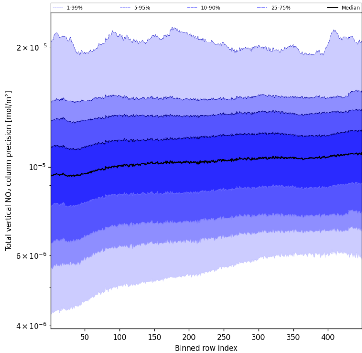
Figure 56: Along track statistics of “Total vertical NO 2 column precision” for 2025-04-15 to 2025-04-16
