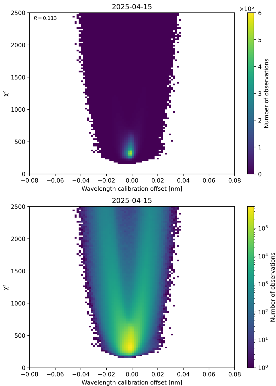
Figure 175: Scatter density plot of “Wavelength calibration offset” against “ \chi^2 ” for 2025-04-15 to 2025-04-16.
