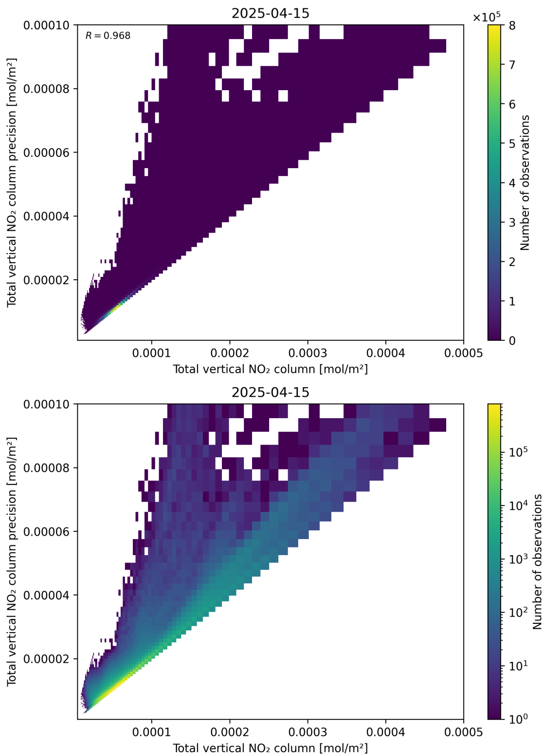
Figure 114: Scatter density plot of “Total vertical NO 2 column” against “Total vertical NO 2 column precision” for 2025-04-15 to 2025-04-16.
