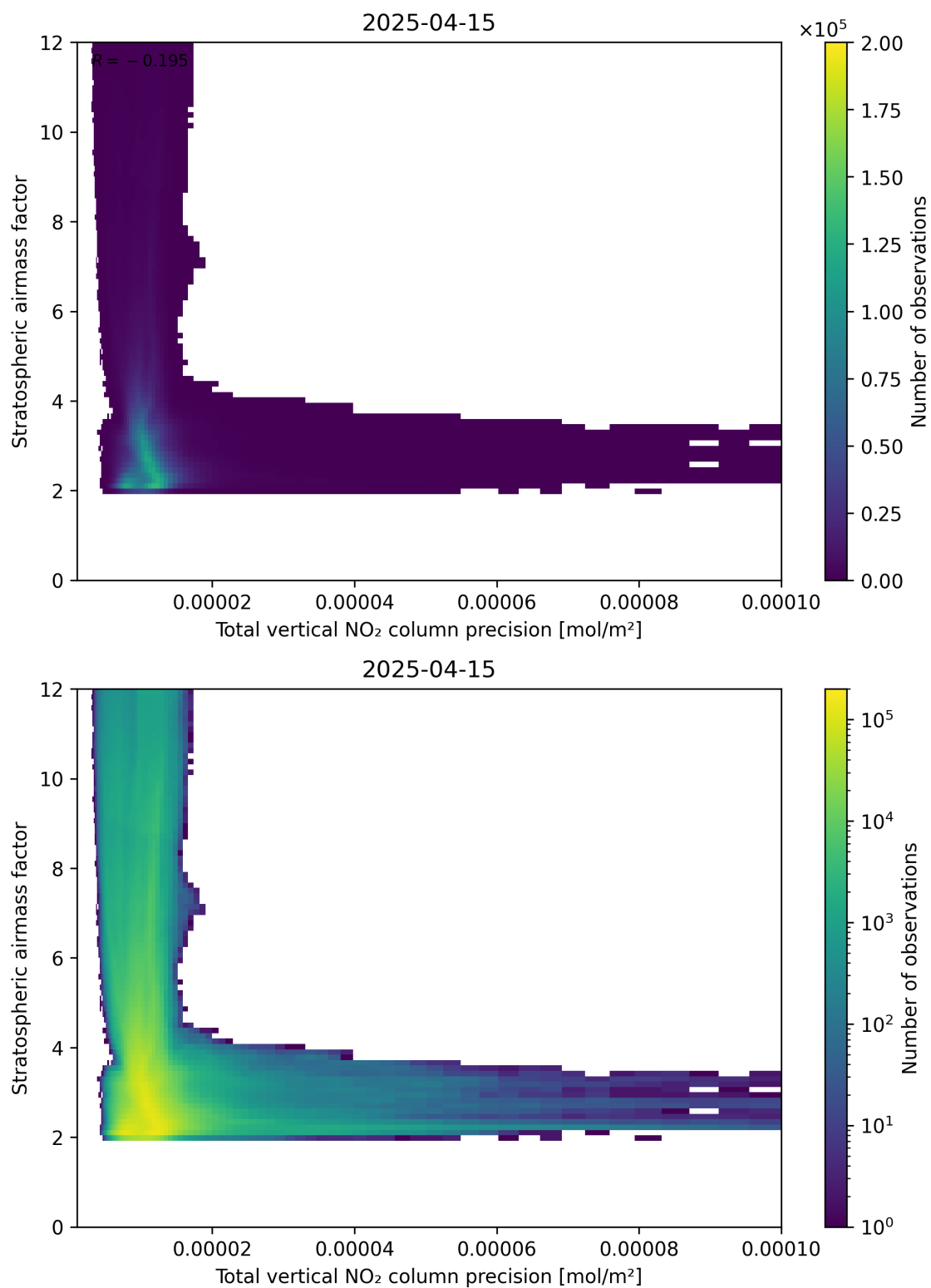
Figure 115: Scatter density plot of “Total vertical NO 2 column precision” against “Stratospheric air mass factor” for 2025-04-15 to 2025-04-16.
