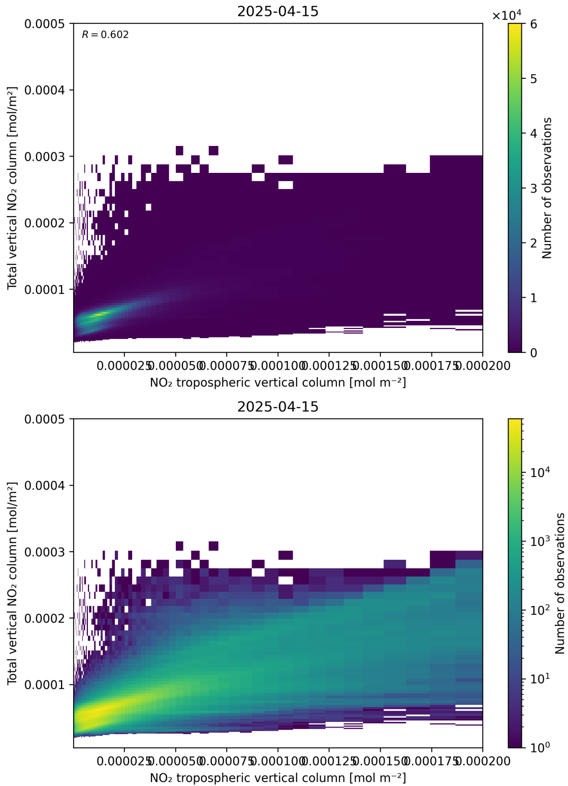
Figure 128: Scatter density plot of “NO 2 tropospheric vertical column” against “Total vertical NO 2 column” for 2025-04-15 to 2025-04-16.
