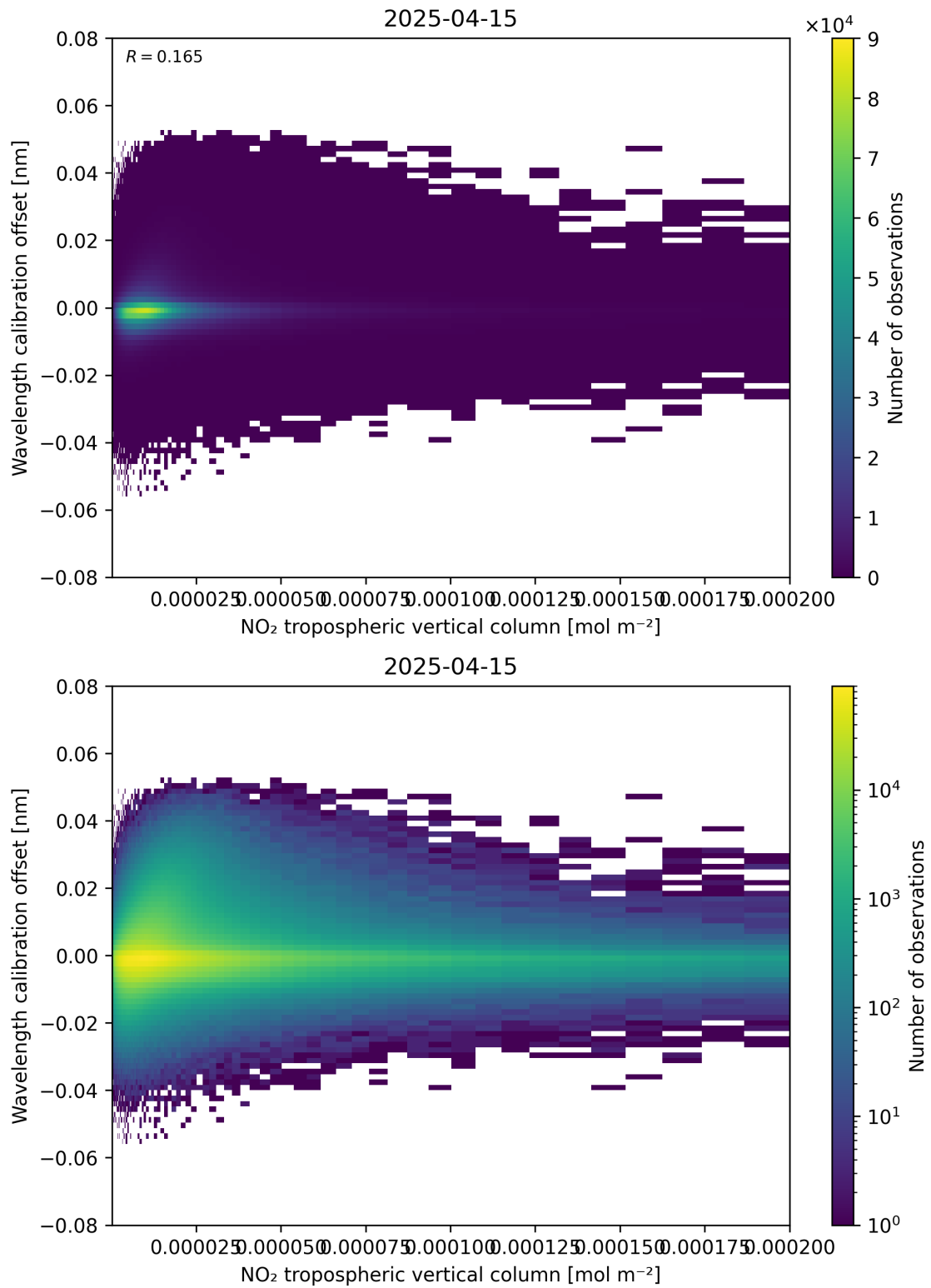
Figure 143: Scatter density plot of “NO 2 tropospheric vertical column” against “Wavelength calibration offset” for 2025-04-15 to 2025-04-16.
