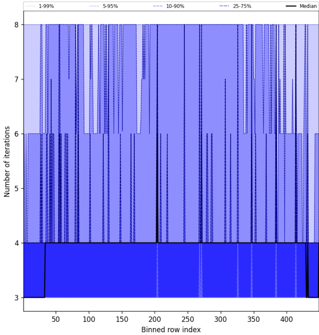
Figure 51: Along track statistics of “Number of iterations” for 2025-04-15 to 2025-04-16
