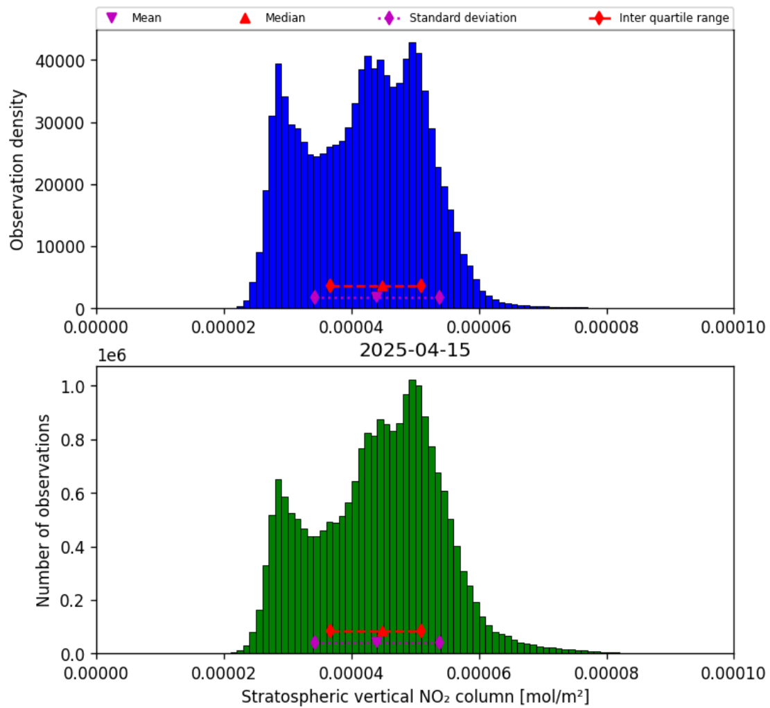
Figure 36: Histogram of “Stratospheric vertical NO 2 column” for 2025-04-15 to 2025-04-16
