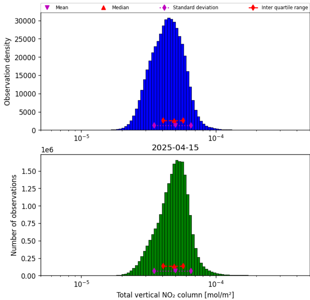
Figure 38: Histogram of “Total vertical NO 2 column” for 2025-04-15 to 2025-04-16
