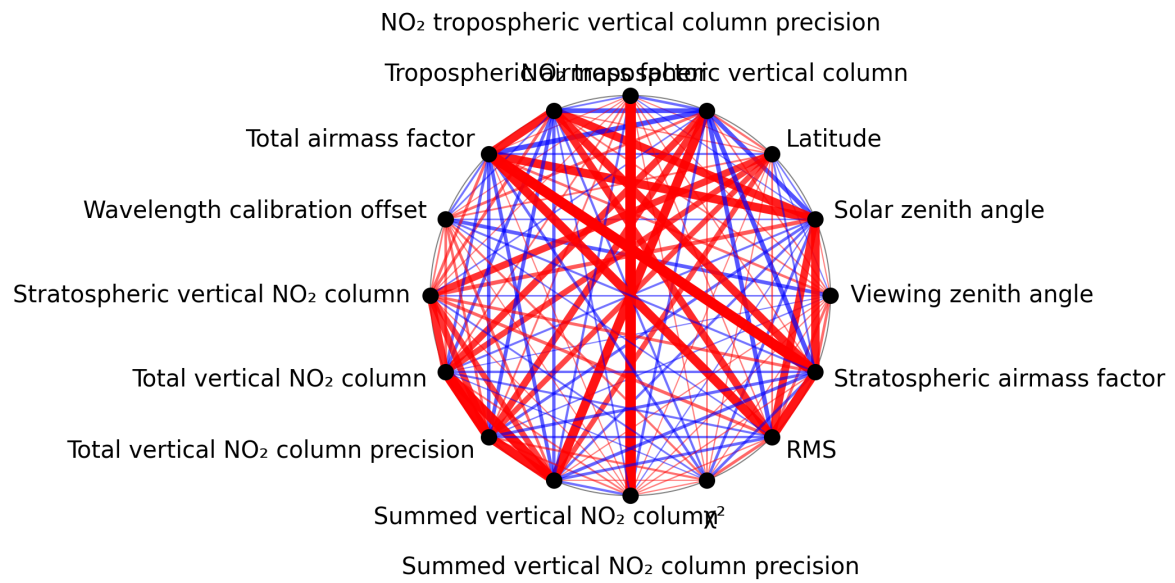
Figure 1: Map of correlation graph for 2025-04-15 to 2025-04-16.
