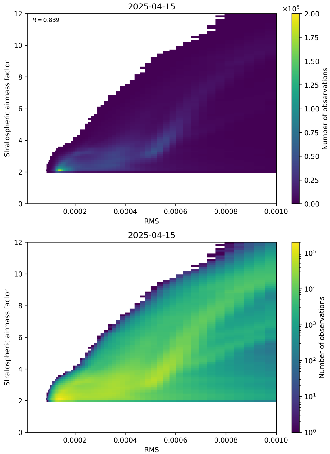
Figure 144: Scatter density plot of “RMS” against “Stratospheric airmass factor” for 2025-04-15 to 2025-04-16.
