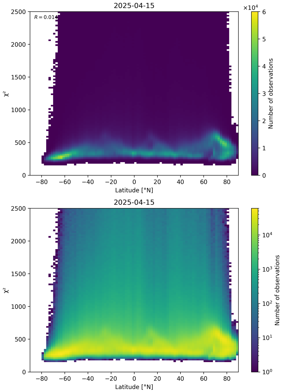
Figure 86: Scatter density plot of “Latitude” against “ \chi^2 ” for 2025-04-15 to 2025-04-16.
