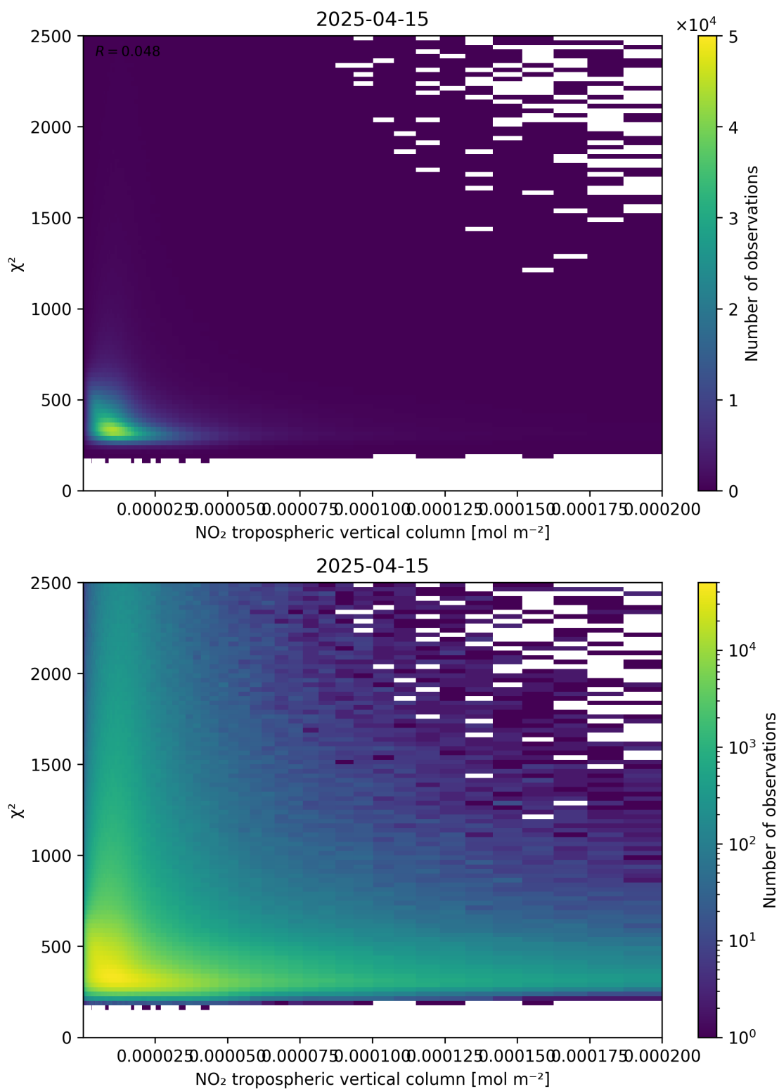
Figure 124: Scatter density plot of “NO 2 tropospheric vertical column” against “ \chi^2 ” for 2025-04-15 to 2025-04-16.
