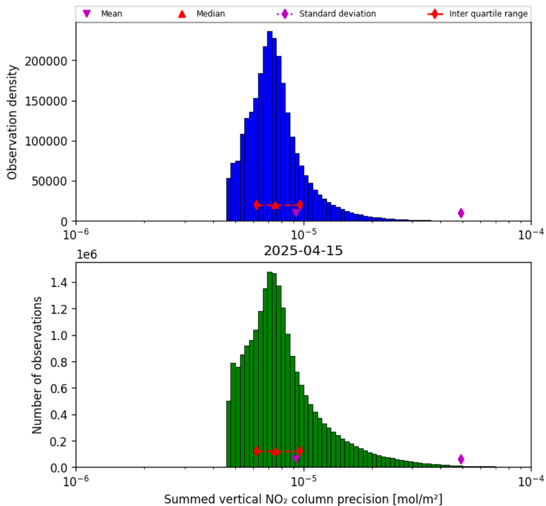
Figure 41: Histogram of "Summed vertical NO 2 column precision" for 2025-04-15 to 2025-04-16
