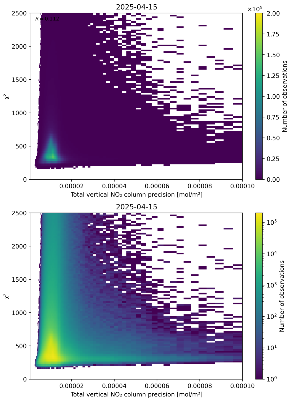
Figure 116: Scatter density plot of “Total vertical NO 2 column precision” against “ \chi^2 ” for 2025-04-15 to 2025-04-16.
