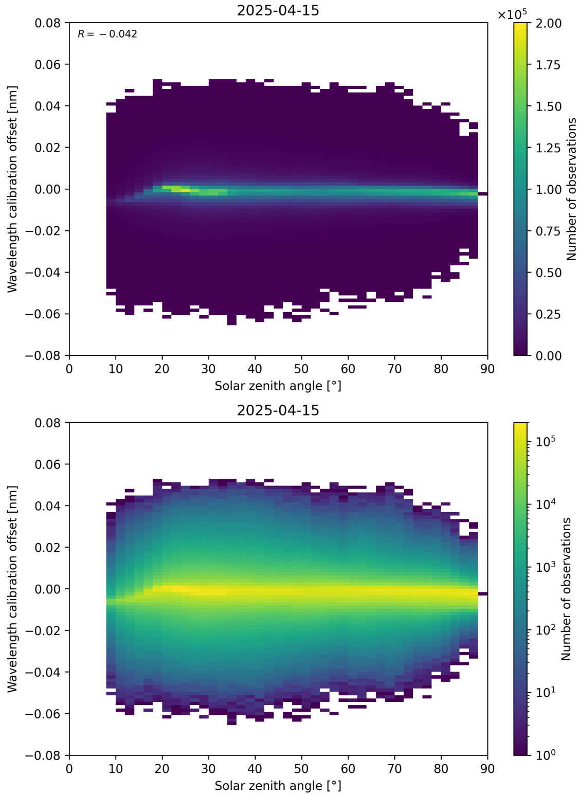
Figure 158: Scatter density plot of “Solar zenith angle” against “Wavelength calibration offset” for 2025-04-15 to 2025-04-16.
