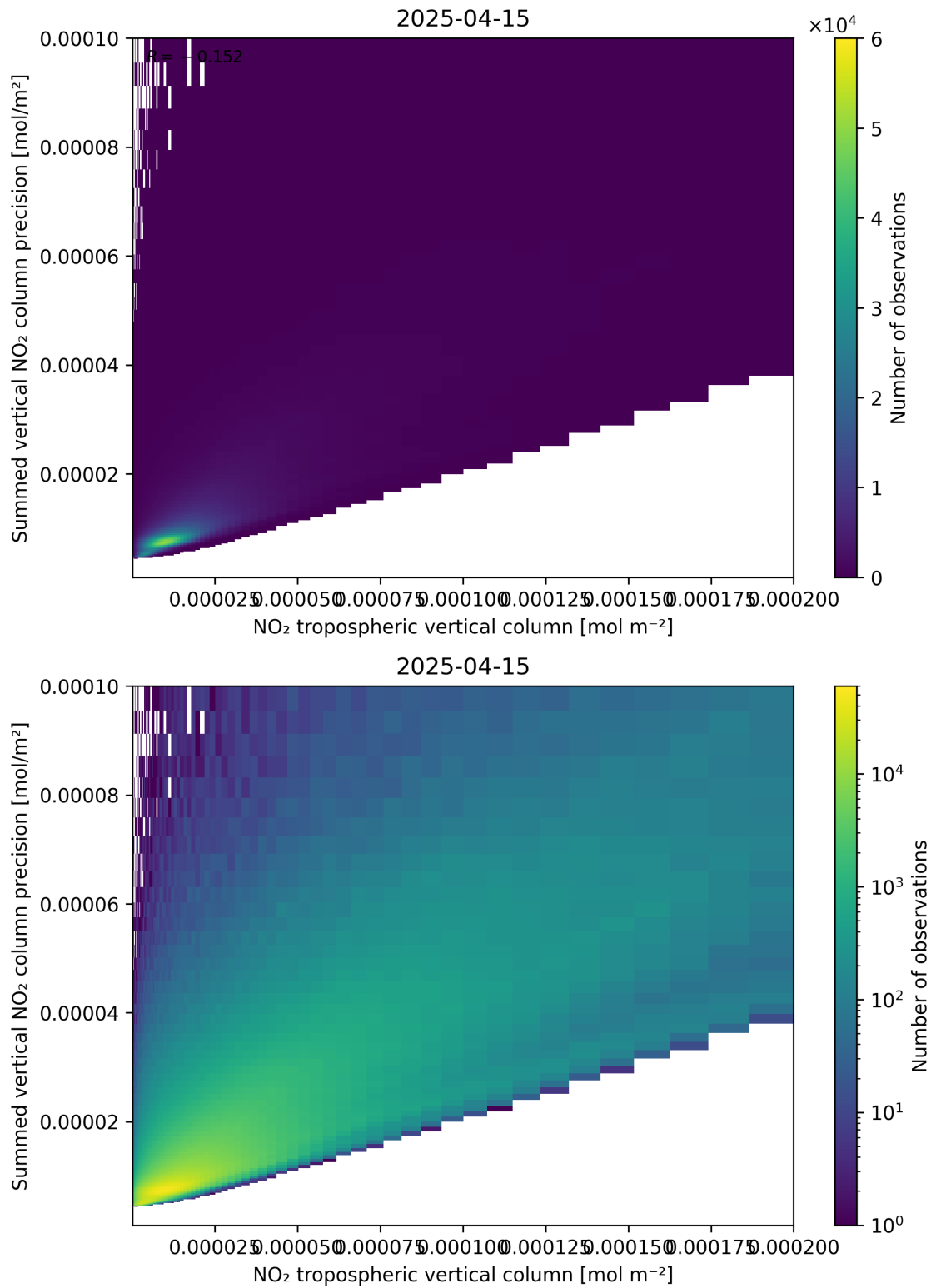
Figure 127: Scatter density plot of “NO 2 tropospheric vertical column” against “Summed vertical NO 2 column precision” for 2025-04-15 to 2025-04-16.
