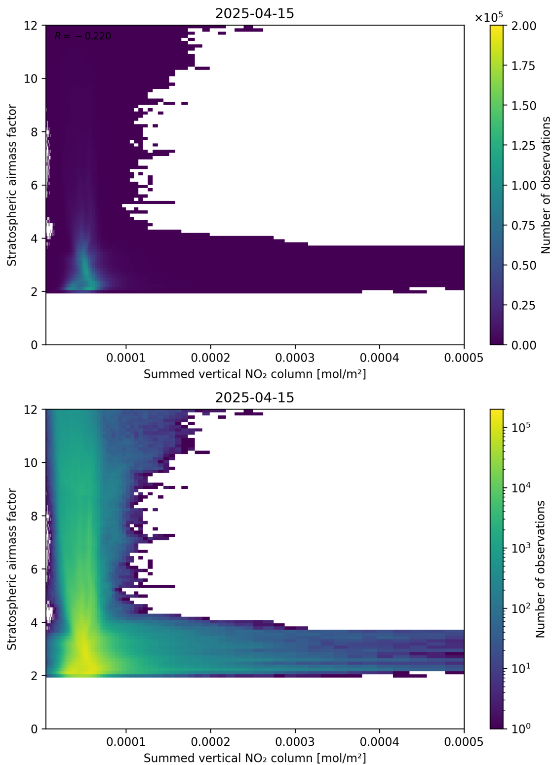
Figure 103: Scatter density plot of “Summed vertical NO 2 column” against “Stratospheric airmass factor” for 2025-04-15 to 2025-04-16.
