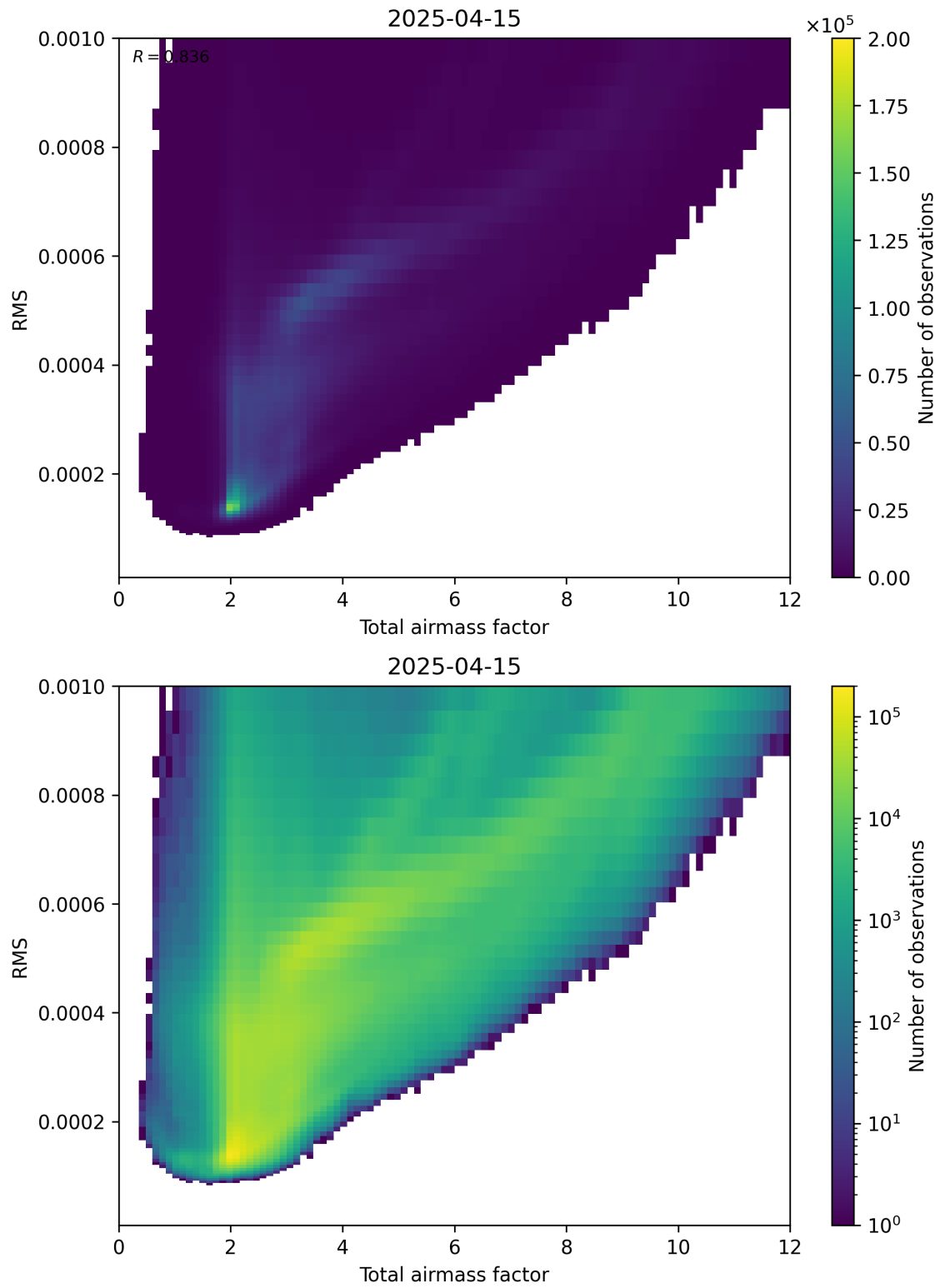
Figure 69: Scatter density plot of “Total airmass factor” against “RMS” for 2025-04-15 to 2025-04-16.
