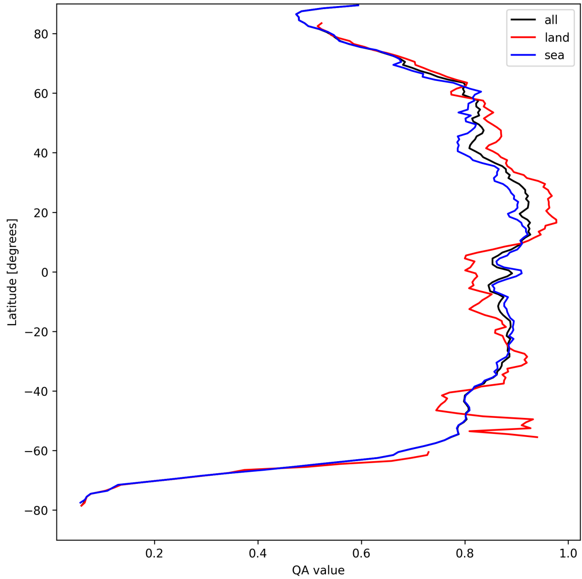
Figure 11: Zonal average of “QA value” for 2025-04-15 to 2025-04-16.
