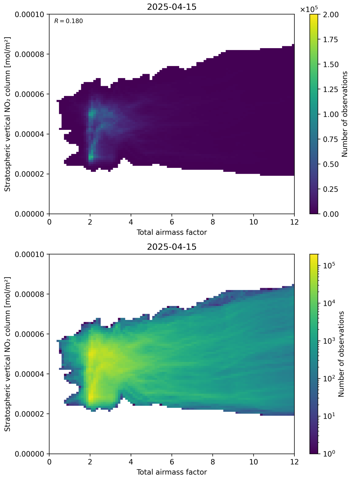
Figure 64: Scatter density plot of “Total airmass factor” against “Stratospheric vertical \text{NO}_2 column” for 2025-04-15 to 2025-04-16.
