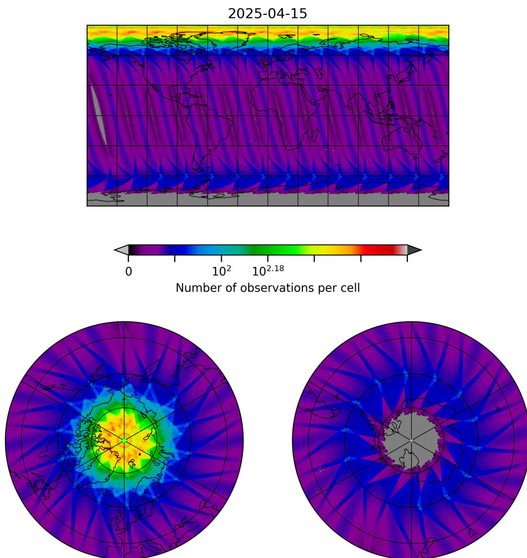
Figure 10: Map of the number of observations for 2025-04-15 to 2025-04-16
