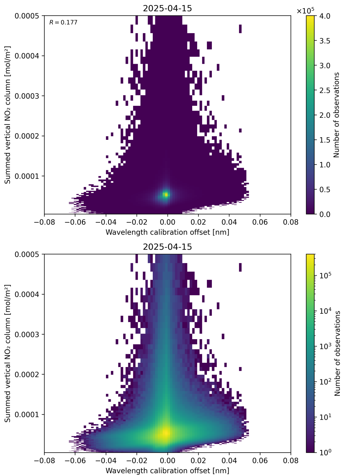
Figure 177: Scatter density plot of “Wavelength calibration offset” against “Summed vertical NO 2 column” for 2025-04-15 to 2025-04-16.
