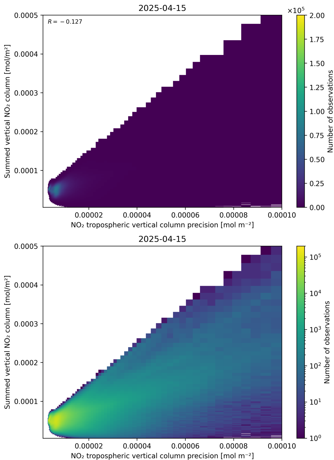
Figure 136: Scatter density plot of “NO 2 tropospheric vertical column precision” against “Summed vertical NO 2 column” for 2025-04-15 to 2025-04-16.
