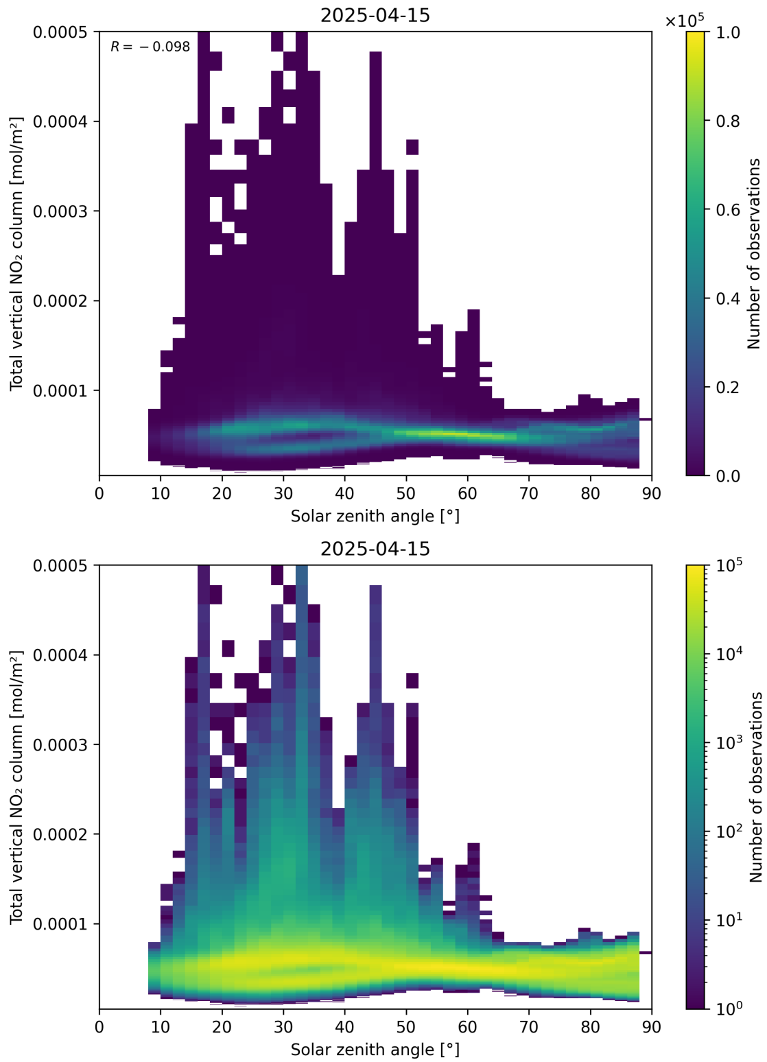
Figure 153: Scatter density plot of “Solar zenith angle” against “Total vertical NO 2 column” for 2025-04-15 to 2025-04-16.
