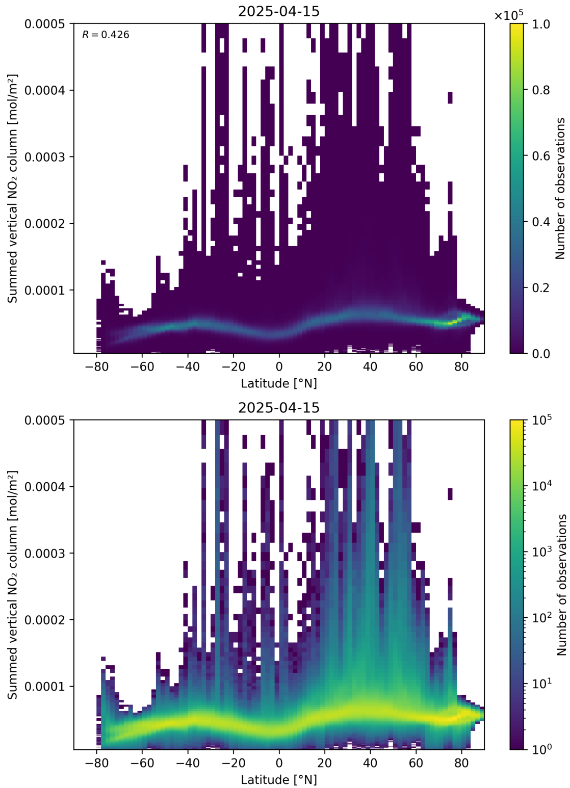
Figure 88: Scatter density plot of “Latitude” against “Summed vertical NO 2 column” for 2025-04-15 to 2025-04-16.
