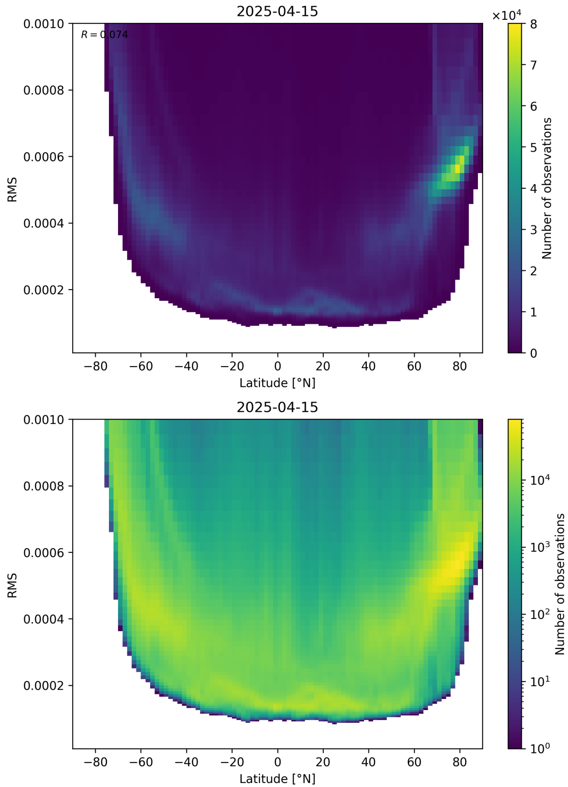
Figure 94: Scatter density plot of “Latitude” against “RMS” for 2025-04-15 to 2025-04-16.
