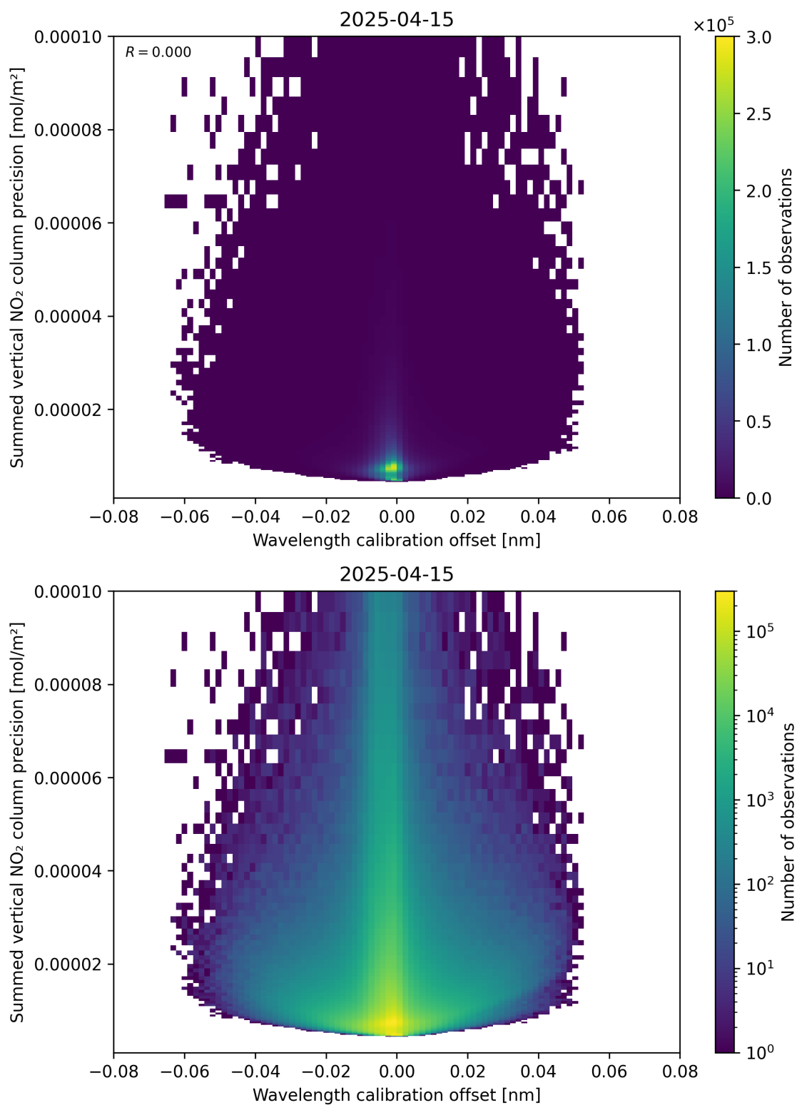
Figure 178: Scatter density plot of “Wavelength calibration offset” against “Summed vertical NO 2 column precision” for 2025-04-15 to 2025-04-16.
