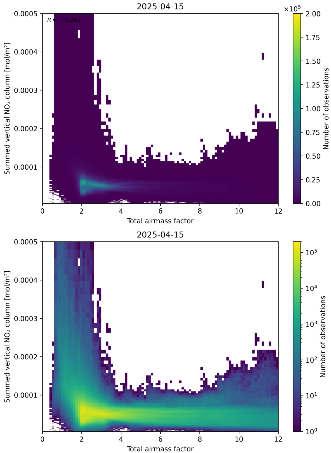
Figure 65: Scatter density plot of “Total airmass factor” against “Summed vertical NO 2 column” for 2025-04-15 to 2025-04-16.
