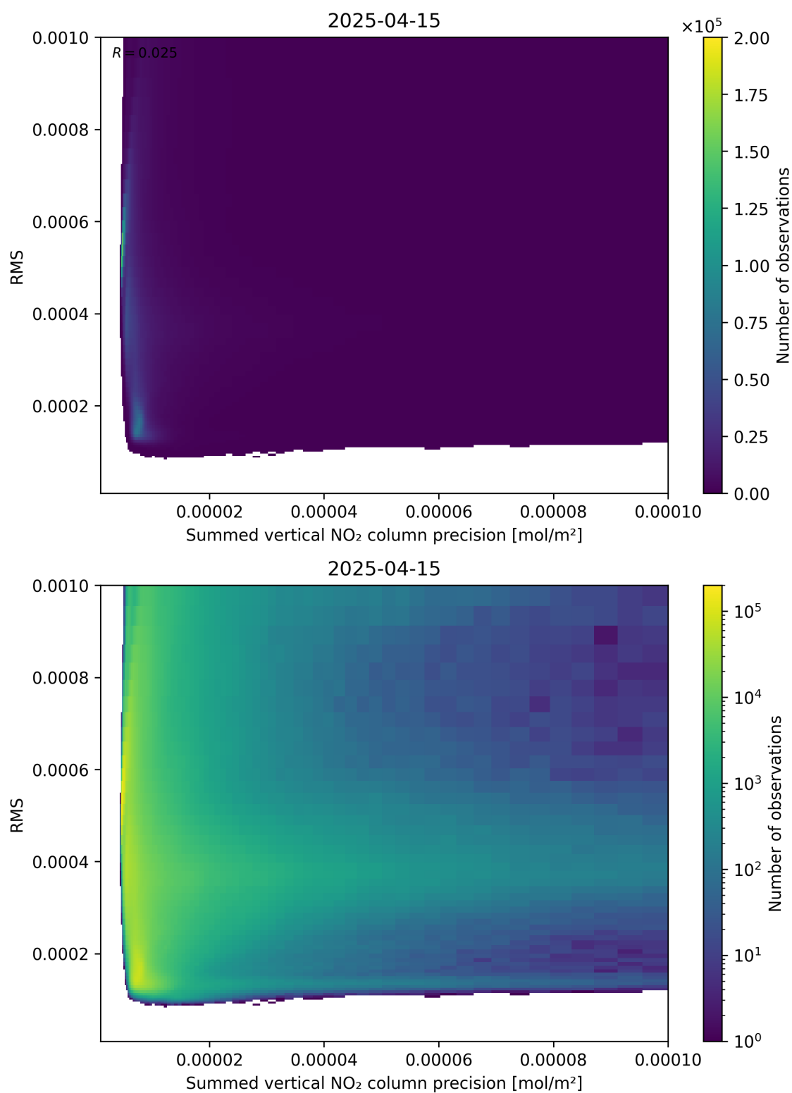
Figure 108: Scatter density plot of “Summed vertical NO 2 column precision” against “RMS” for 2025-04-15 to 2025-04-16.
