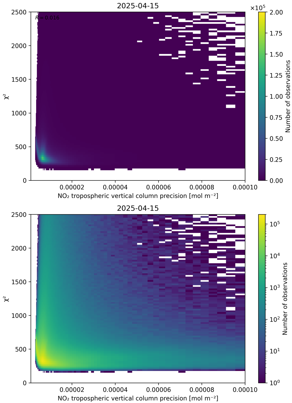
Figure 134: Scatter density plot of “NO 2 tropospheric vertical column precision” against “ \chi^2 ” for 2025-04-15 to 2025-04-16.
