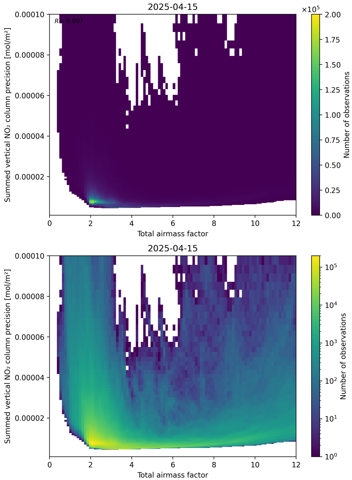
Figure 66: Scatter density plot of “Total airmass factor” against “Summed vertical NO 2 column precision” for 2025-04-15 to 2025-04-16.
