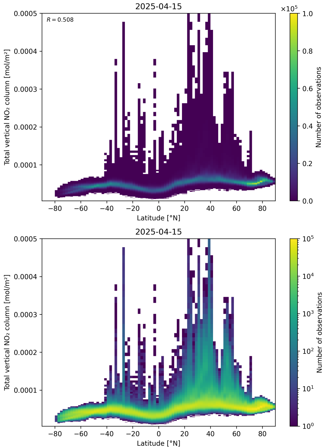
Figure 90: Scatter density plot of “Latitude” against “Total vertical NO 2 column” for 2025-04-15 to 2025-04-16.
