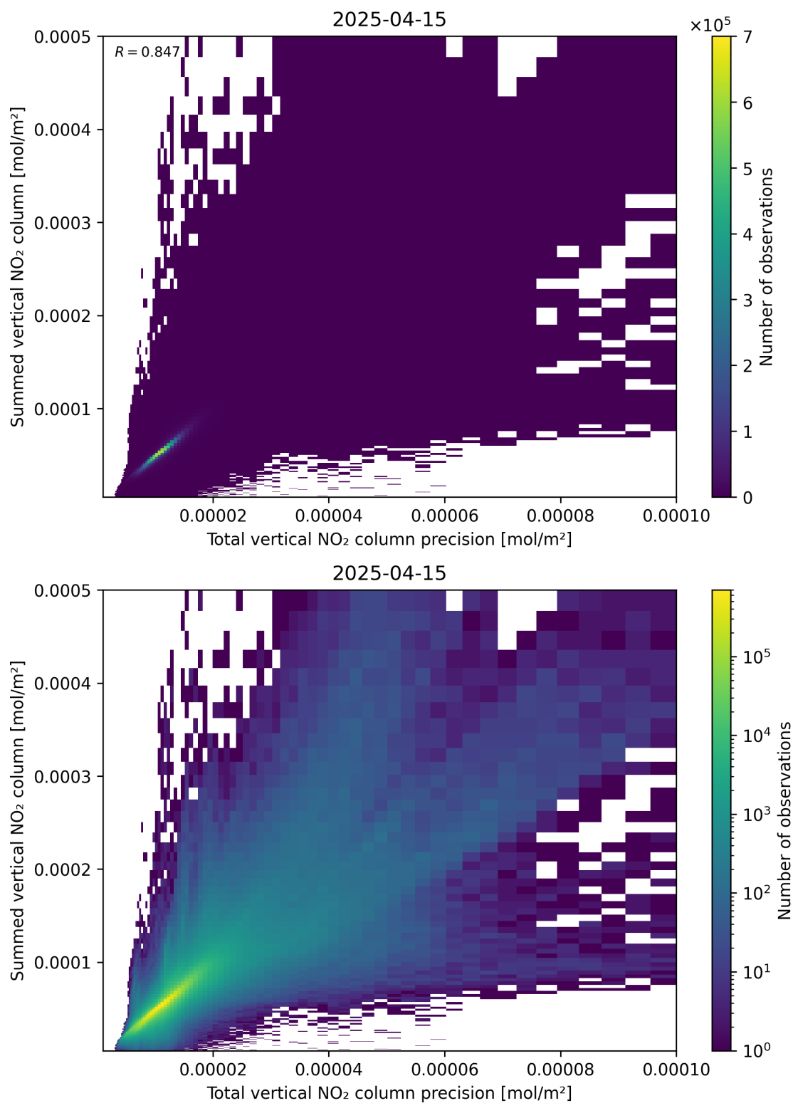
Figure 117: Scatter density plot of “Total vertical NO 2 column precision” against “Summed vertical NO 2 column” for 2025-04-15 to 2025-04-16.
