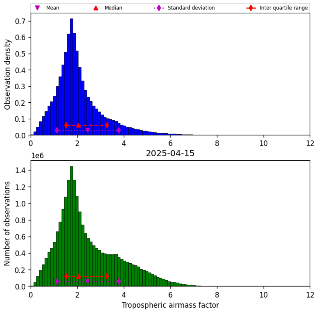
Figure 31: Histogram of “Tropospheric airmass factor” for 2025-04-15 to 2025-04-16
