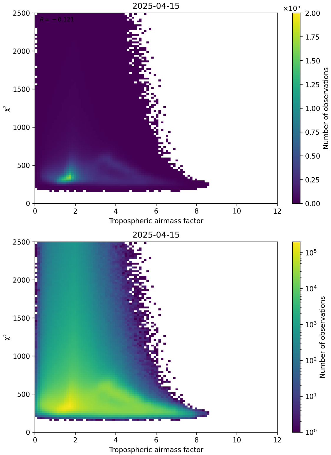
Figure 73: Scatter density plot of “Tropospheric airmass factor” against “ \chi^2 ” for 2025-04-15 to 2025-04-16.
