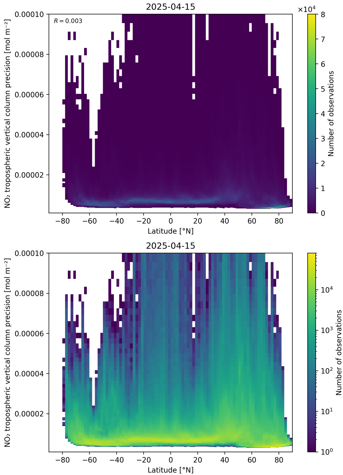
Figure 93: Scatter density plot of “Latitude” against “NO 2 tropospheric vertical column precision” for 2025-04-15 to 2025-04-16.
