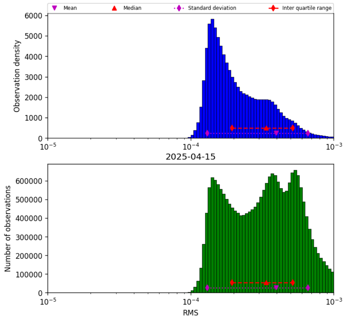
Figure 43: Histogram of “RMS” for 2025-04-15 to 2025-04-16
