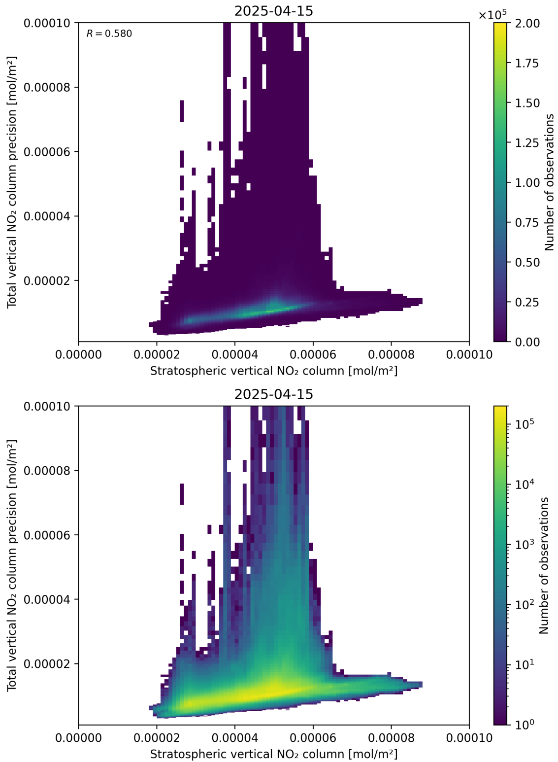
Figure 101: Scatter density plot of “Stratospheric vertical NO 2 column” against “Total vertical NO 2 column precision” for 2025-04-15 to 2025-04-16.
