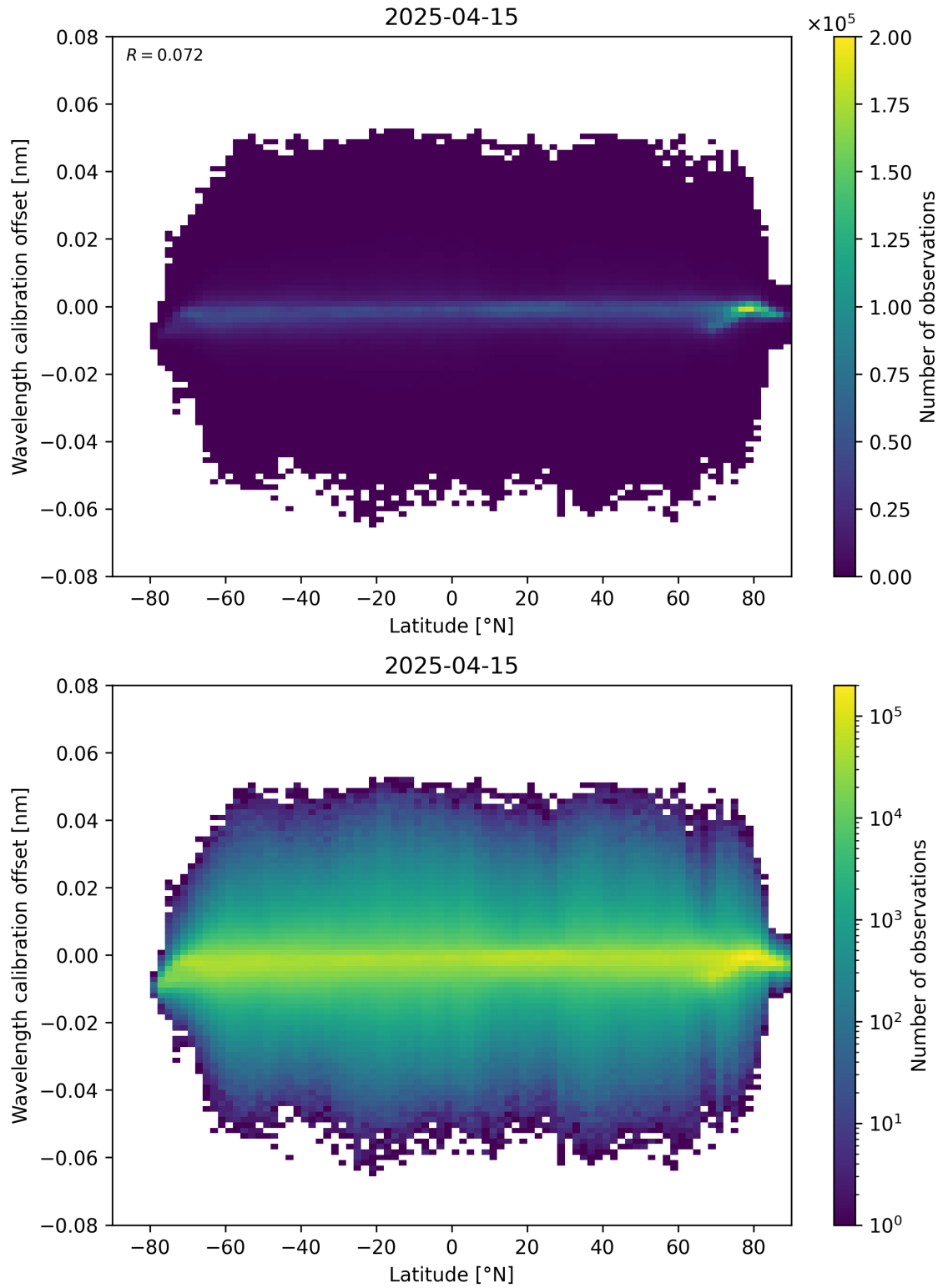
Figure 95: Scatter density plot of “Latitude” against “Wavelength calibration offset” for 2025-04-15 to 2025-04-16.
