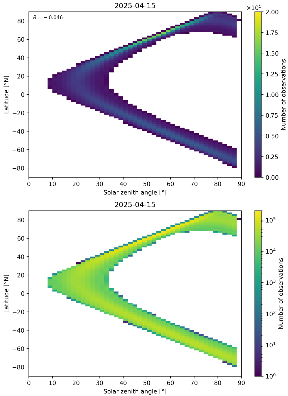
Figure 149: Scatter density plot of “Solar zenith angle” against “Latitude” for 2025-04-15 to 2025-04-16.
