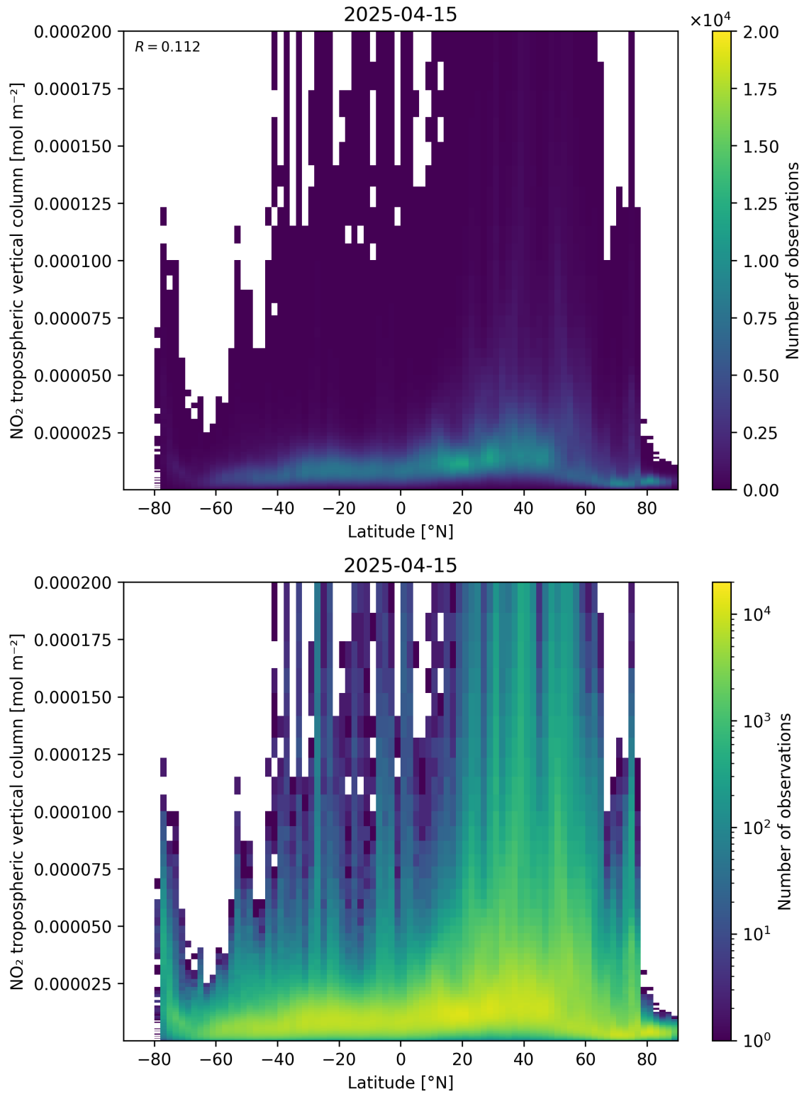
Figure 92: Scatter density plot of “Latitude” against “NO 2 tropospheric vertical column” for 2025-04-15 to 2025-04-16.
