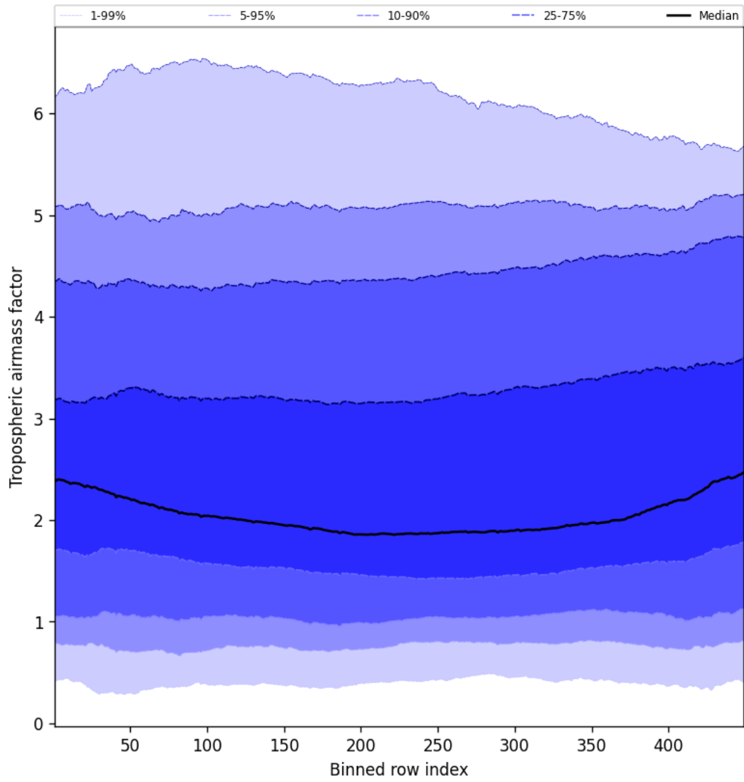
Figure 48: Along track statistics of “Tropospheric airmass factor” for 2025-04-15 to 2025-04-16
