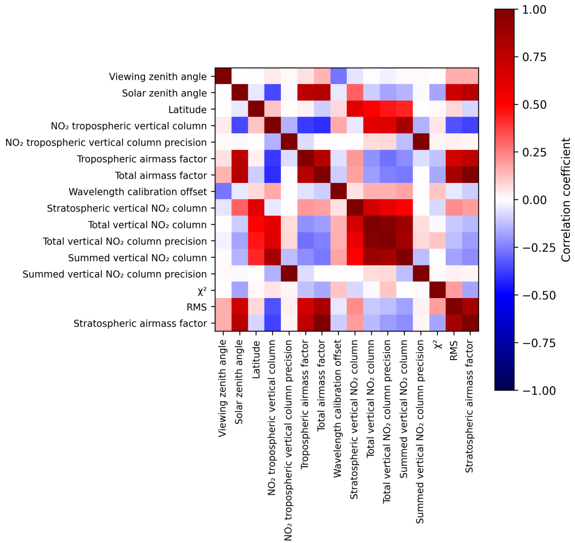
Figure 2: Map of correlation matrix for 2025-04-15 to 2025-04-16.
