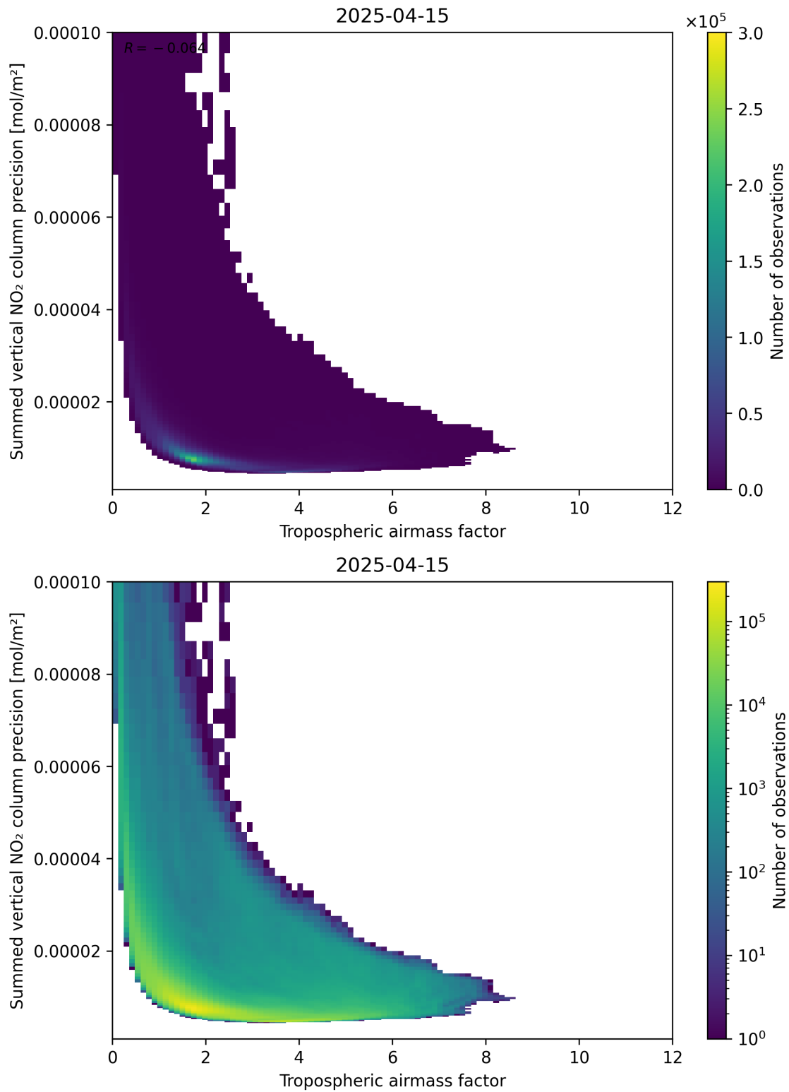
Figure 76: Scatter density plot of “Tropospheric air mass factor” against “Summed vertical NO 2 column precision” for 2025-04-15 to 2025-04-16.
