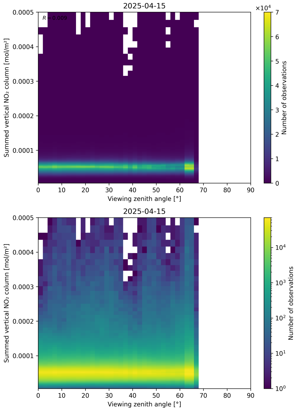
Figure 165: Scatter density plot of “Viewing zenith angle” against “Summed vertical NO 2 column” for 2025-04-15 to 2025-04-16.
