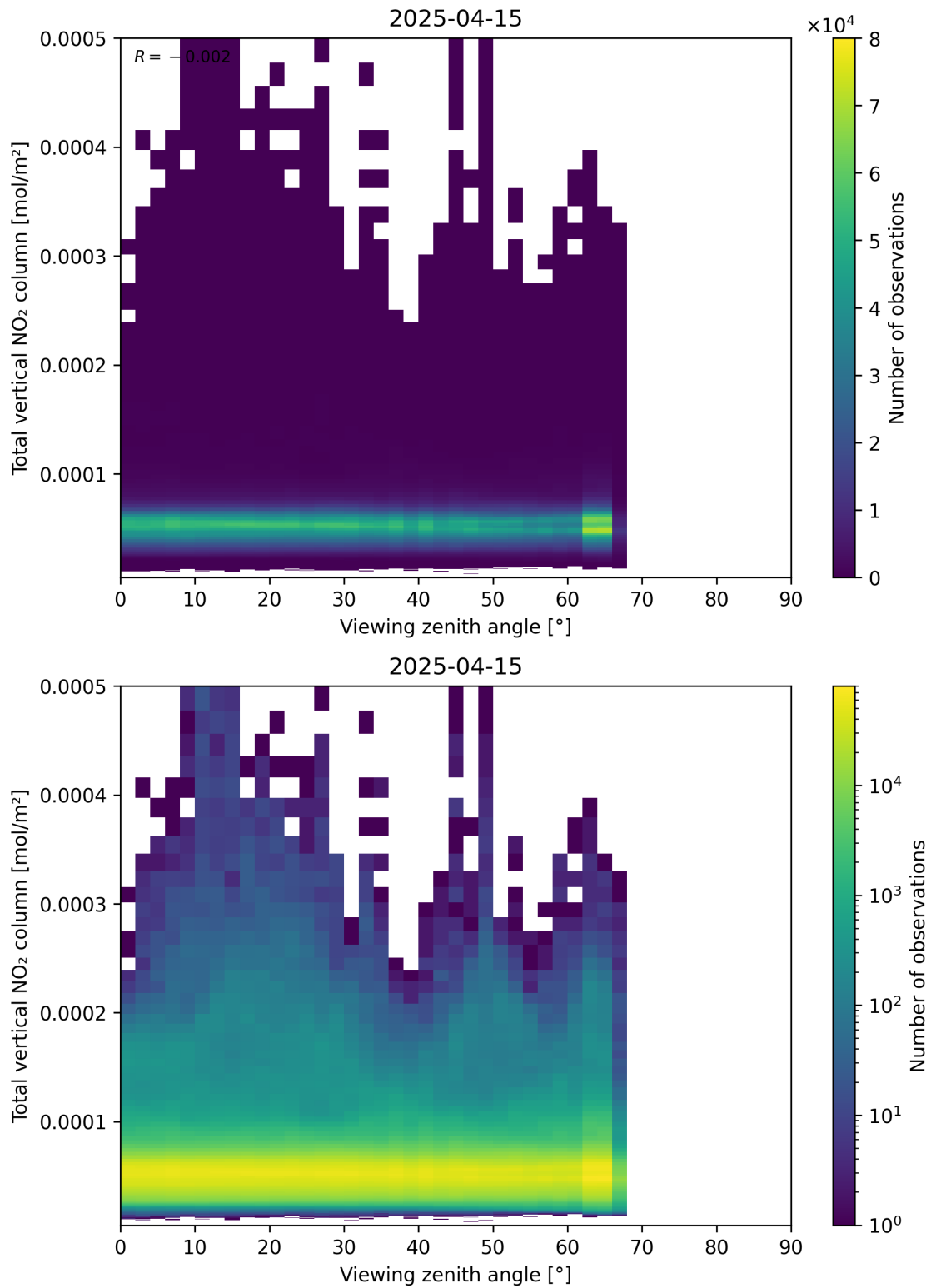
Figure 167: Scatter density plot of “Viewing zenith angle” against “Total vertical NO 2 column” for 2025-04-15 to 2025-04-16.
