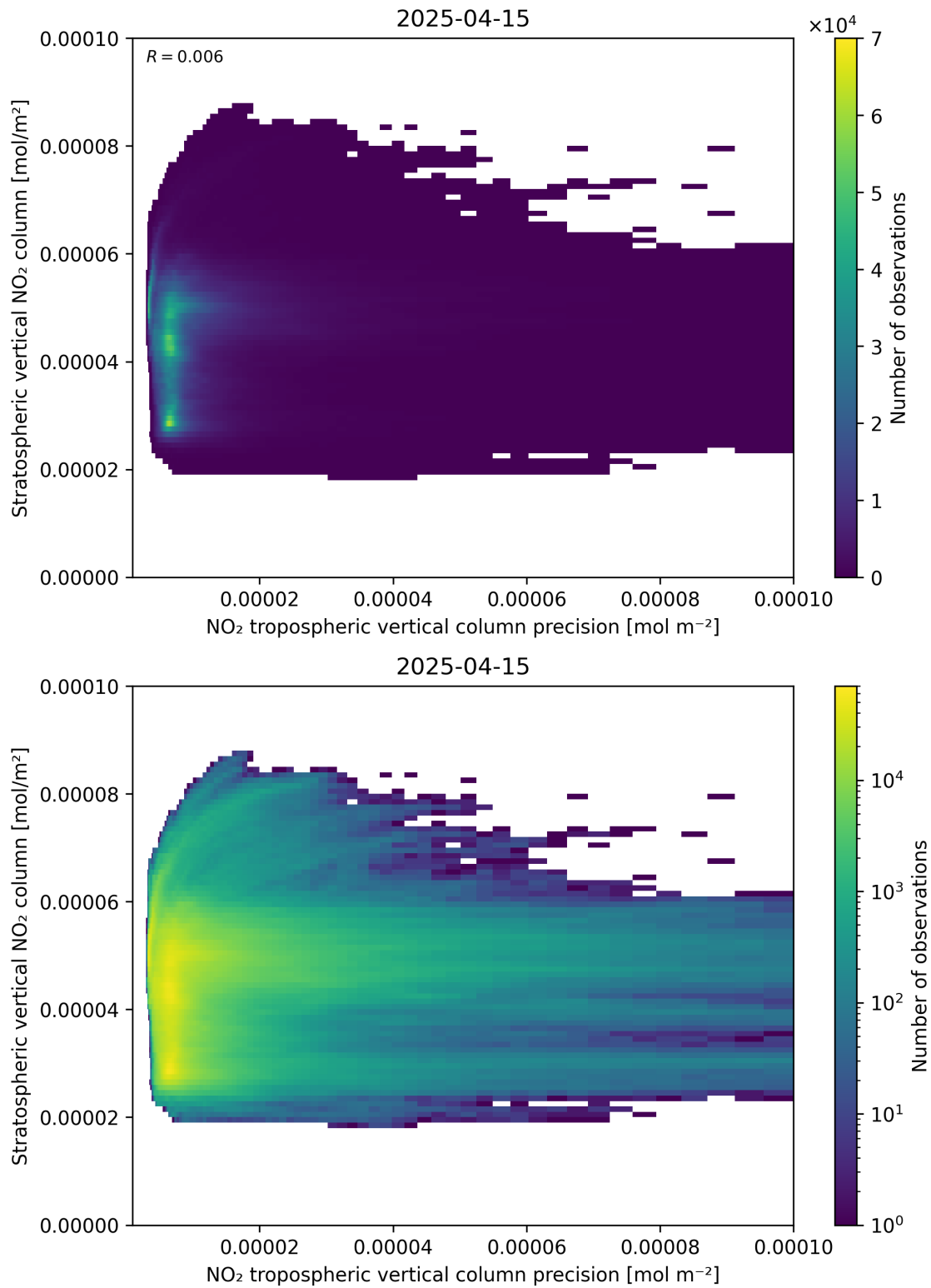
Figure 135: Scatter density plot of “NO 2 tropospheric vertical column precision” against “Stratospheric vertical NO 2 column” for 2025-04-15 to 2025-04-16.
