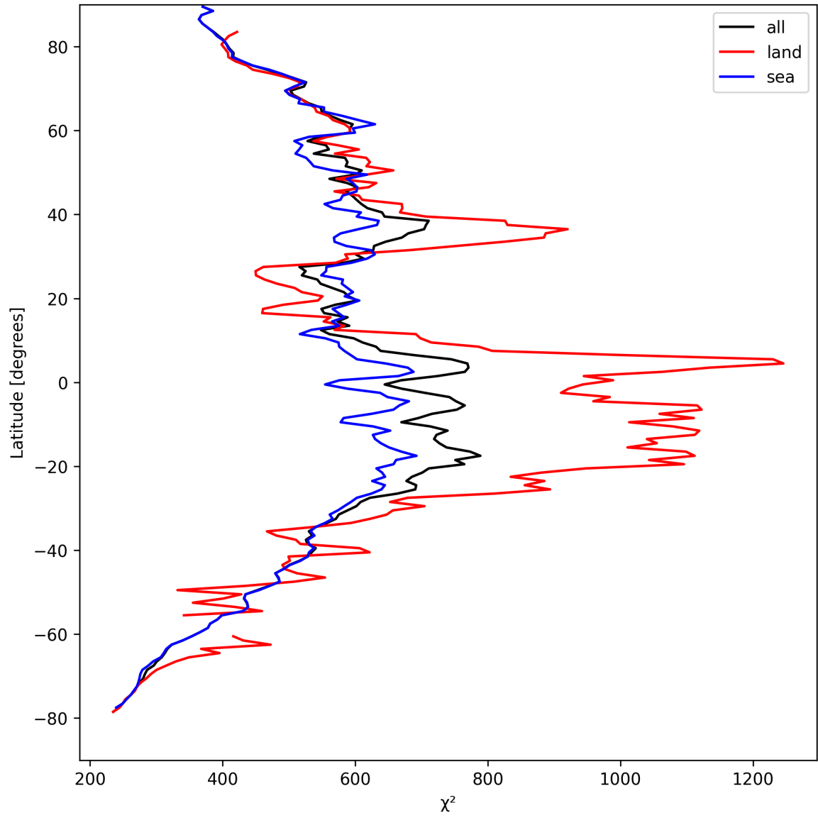
Figure 25: Zonal average of “ \chi^2 ” for 2025-04-15 to 2025-04-16.
