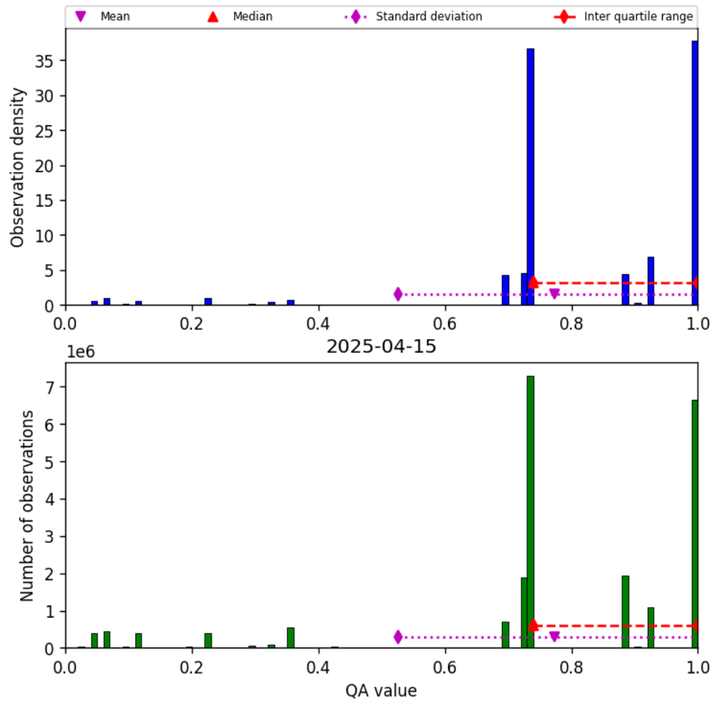
Figure 28: Histogram of “QA value” for 2025-04-15 to 2025-04-16
