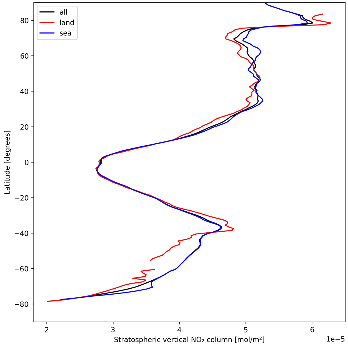
Figure 19: Zonal average of “Stratospheric vertical NO 2 column” for 2025-04-15 to 2025-04-16.
