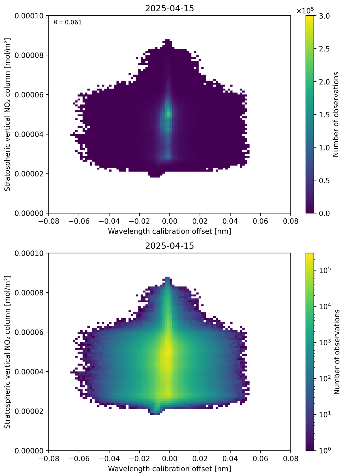
Figure 176: Scatter density plot of “Wavelength calibration offset” against “Stratospheric vertical NO 2 column” for 2025-04-15 to 2025-04-16.
