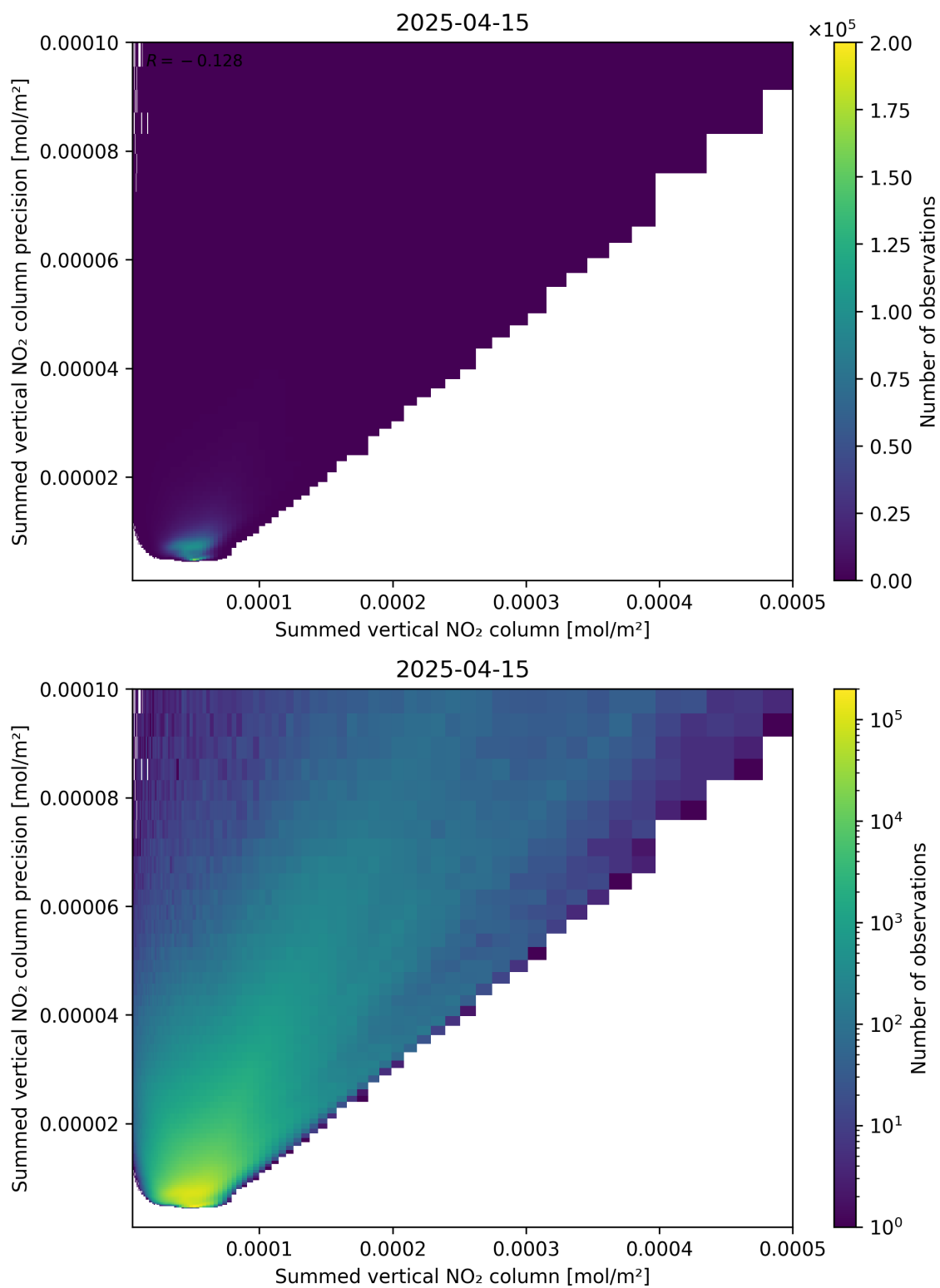
Figure 105: Scatter density plot of “Summed vertical NO 2 column” against “Summed vertical NO 2 column precision” for 2025-04-15 to 2025-04-16.
