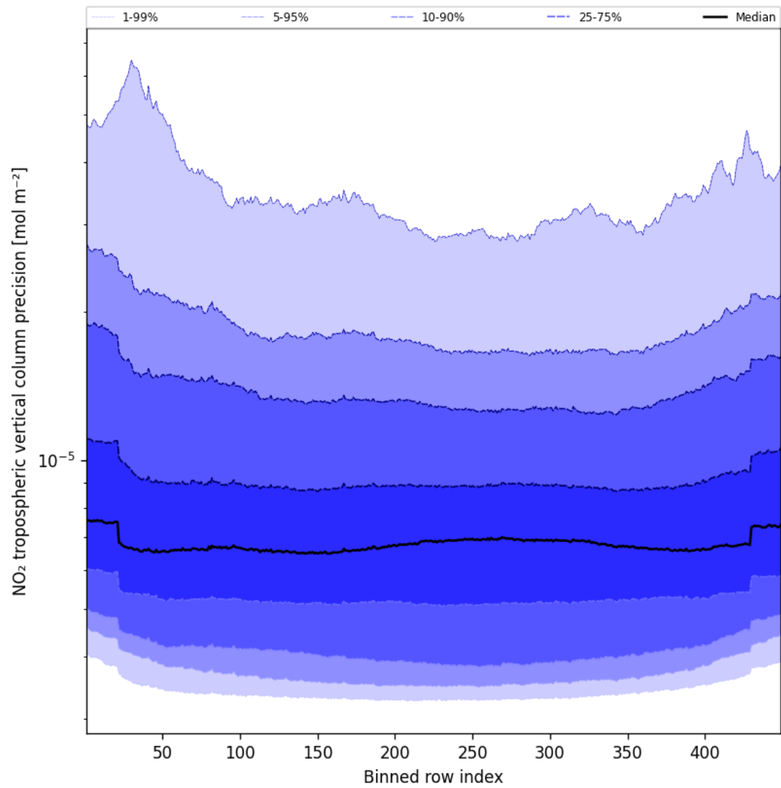
Figure 47: Along track statistics of “NO 2 tropospheric vertical column precision” for 2025-04-15 to 2025-04-16
