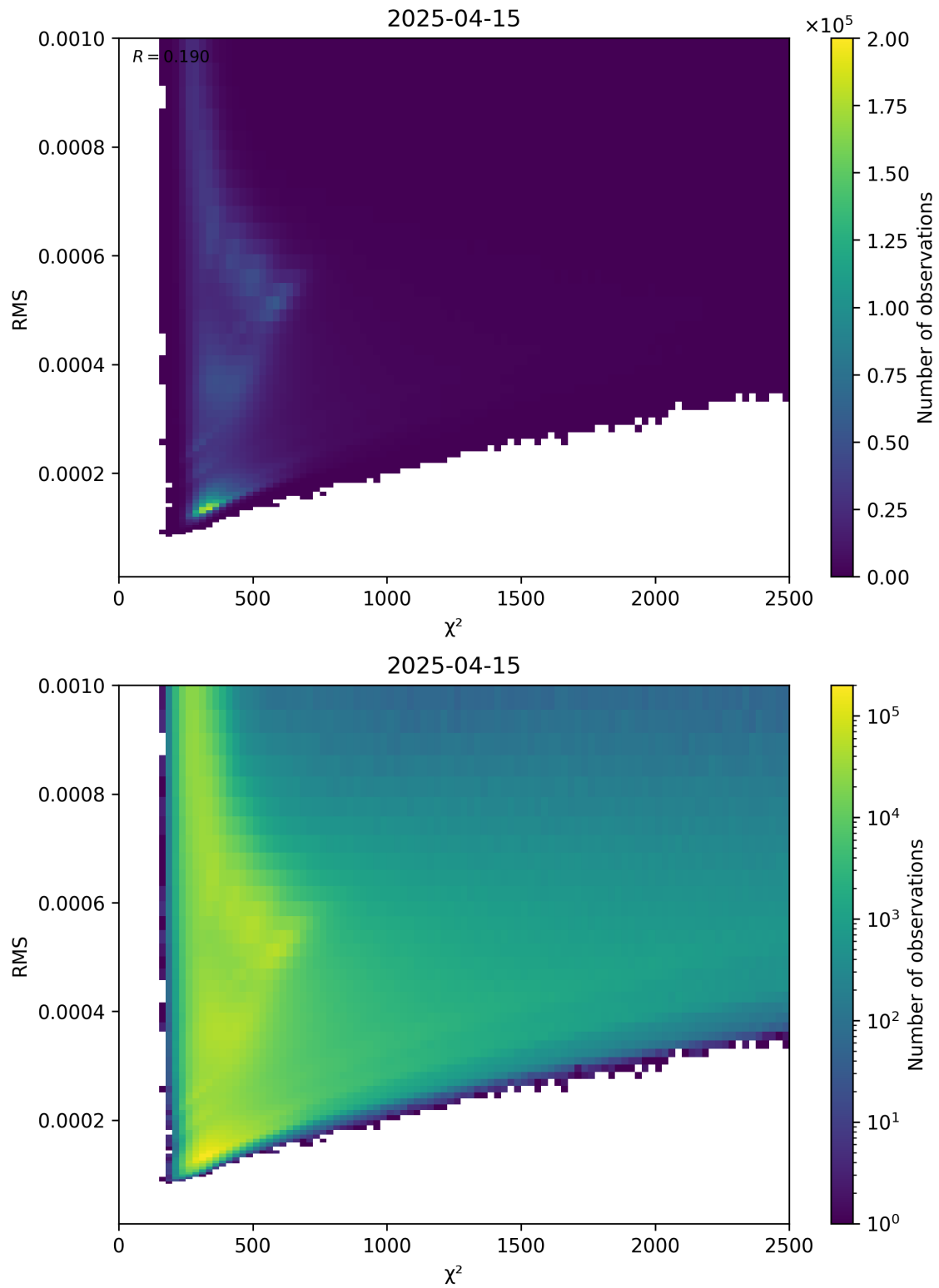
Figure 82: Scatter density plot of “ \chi^2 ” against “RMS” for 2025-04-15 to 2025-04-16.
