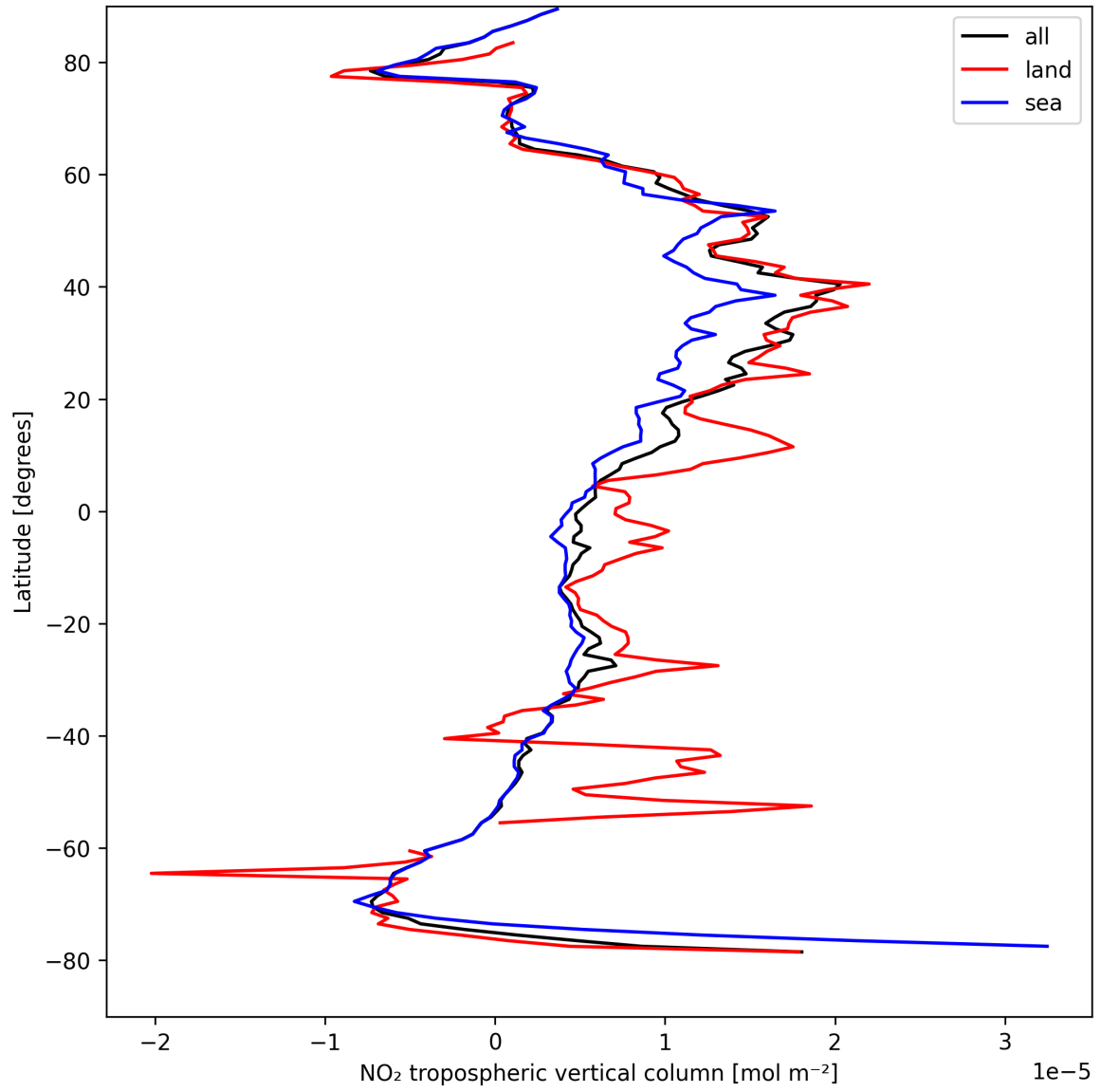
Figure 12: Zonal average of “NO 2 tropospheric vertical column” for 2025-04-15 to 2025-04-16.
