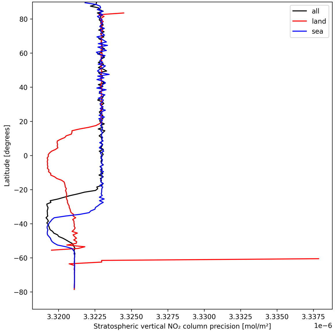
Figure 20: Zonal average of “Stratospheric vertical NO 2 column precision” for 2025-04-15 to 2025-04-16.
