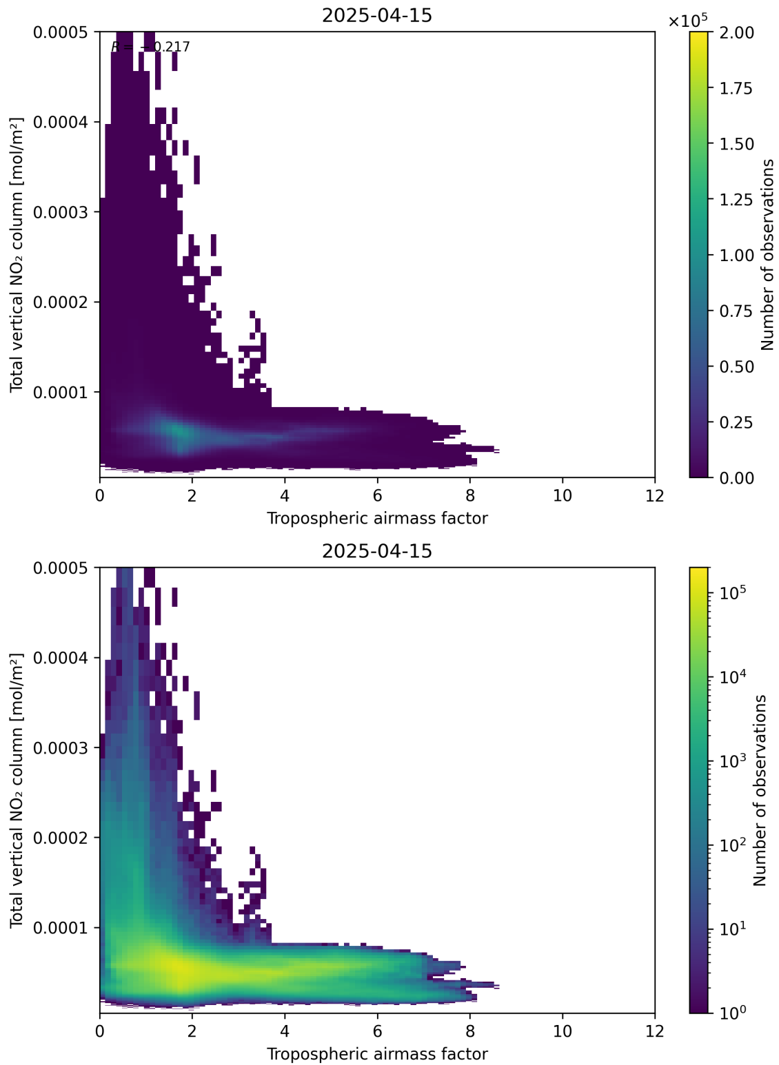
Figure 77: Scatter density plot of “Tropospheric airmass factor” against “Total vertical NO 2 column” for 2025-04-15 to 2025-04-16.
