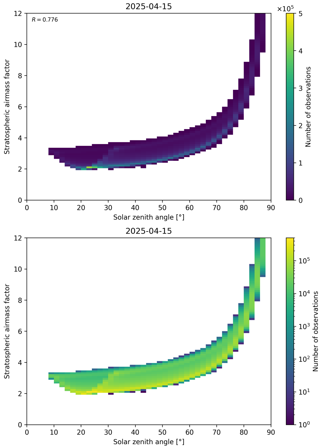
Figure 145: Scatter density plot of “Solar zenith angle” against “Stratospheric airmass factor” for 2025-04-15 to 2025-04-16.
