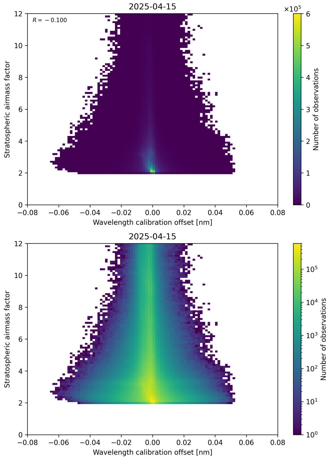
Figure 174: Scatter density plot of “Wavelength calibration offset” against “Stratospheric airmass factor” for 2025-04-15 to 2025-04-16.
