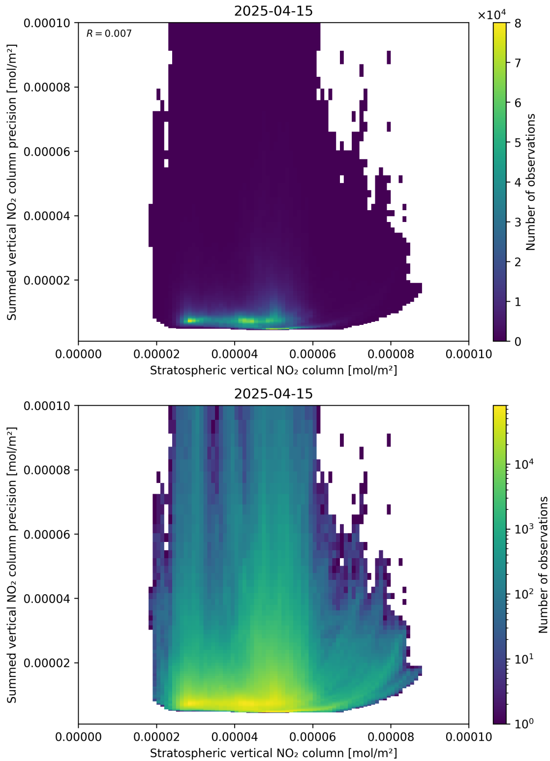
Figure 99: Scatter density plot of “Stratospheric vertical NO 2 column” against “Summed vertical NO 2 column precision” for 2025-04-15 to 2025-04-16.
