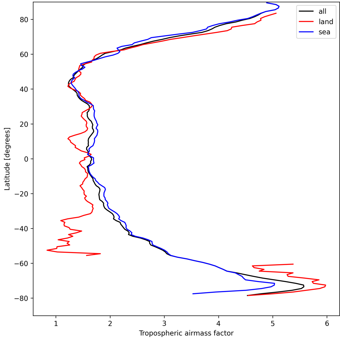
Figure 14: Zonal average of “Tropospheric airmass factor” for 2025-04-15 to 2025-04-16.
