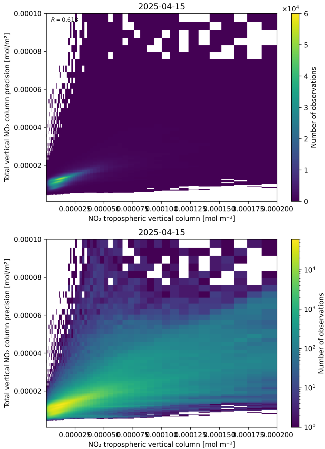
Figure 129: Scatter density plot of “NO 2 tropospheric vertical column” against “Total vertical NO 2 column precision” for 2025-04-15 to 2025-04-16.
