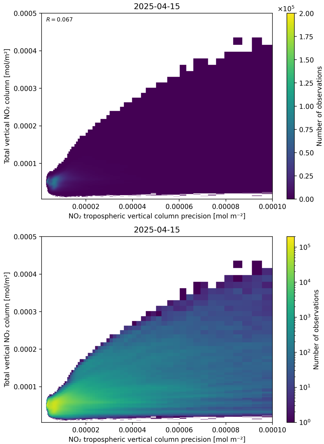
Figure 138: Scatter density plot of “NO 2 tropospheric vertical column precision” against “Total vertical NO 2 column” for 2025-04-15 to 2025-04-16.
