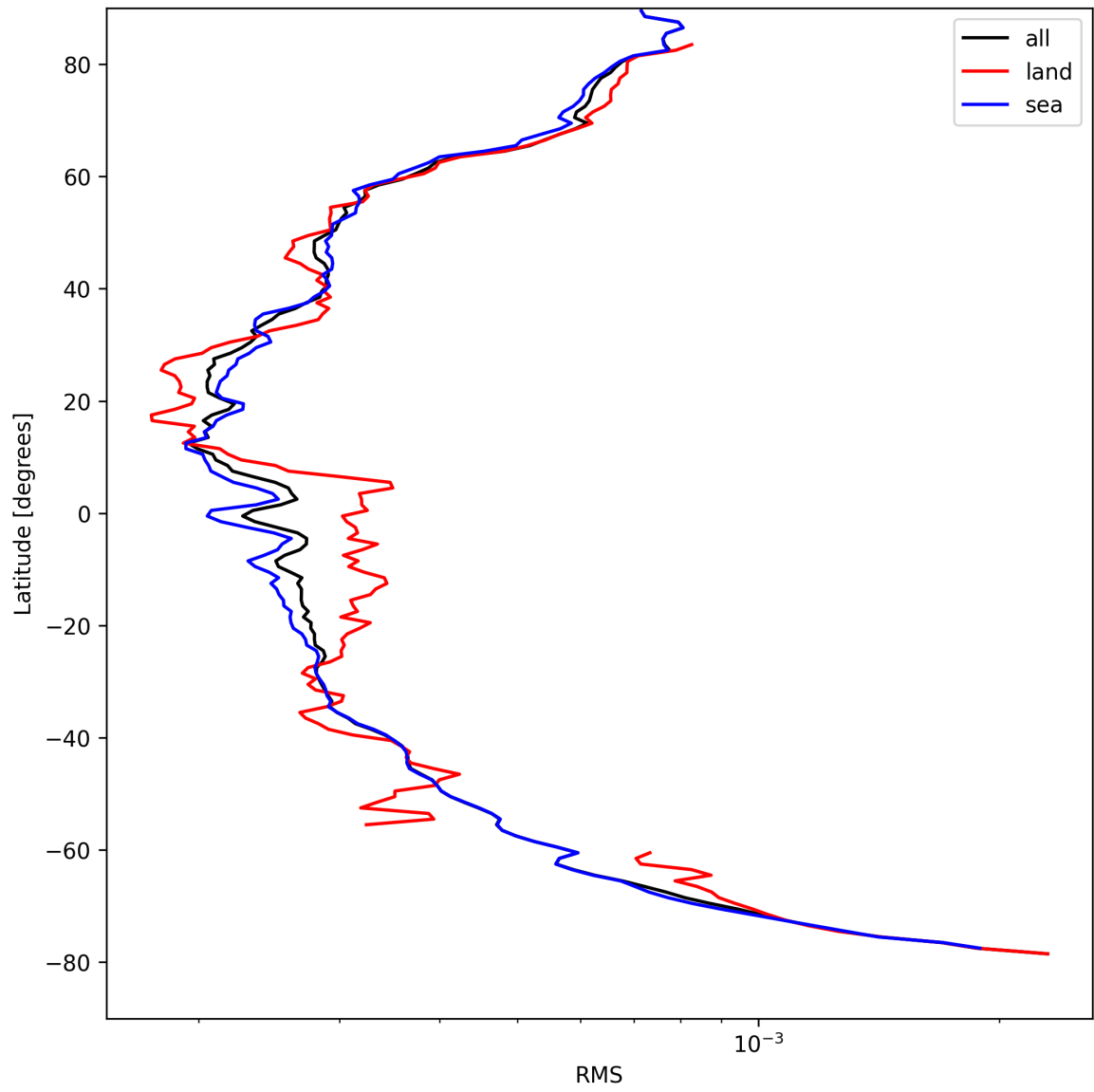
Figure 26: Zonal average of “RMS” for 2025-04-15 to 2025-04-16.
