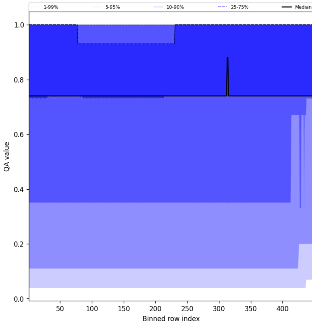
Figure 45: Along track statistics of “QA value” for 2025-04-15 to 2025-04-16
