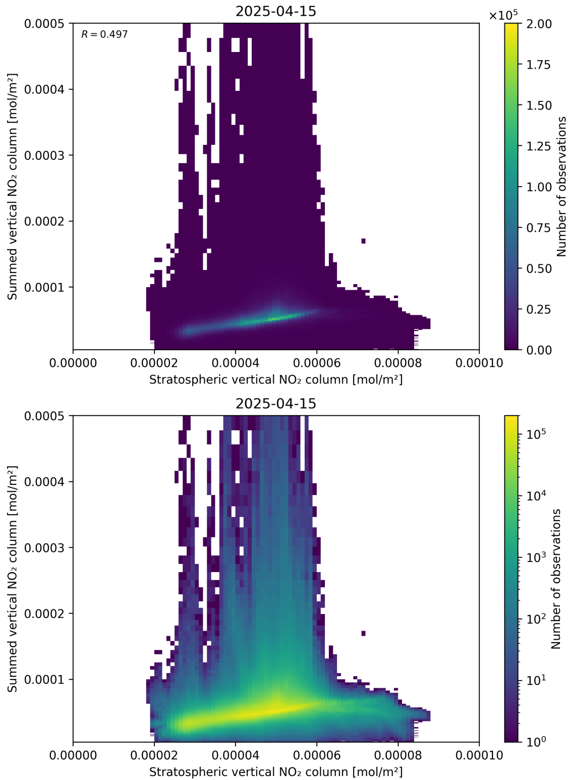
Figure 98: Scatter density plot of “Stratospheric vertical NO 2 column” against “Summed vertical NO 2 column” for 2025-04-15 to 2025-04-16.
