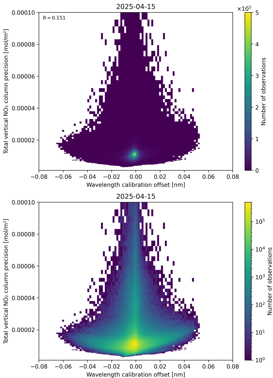
Figure 180: Scatter density plot of “Wavelength calibration offset” against “Total vertical NO 2 column precision” for 2025-04-15 to 2025-04-16.
