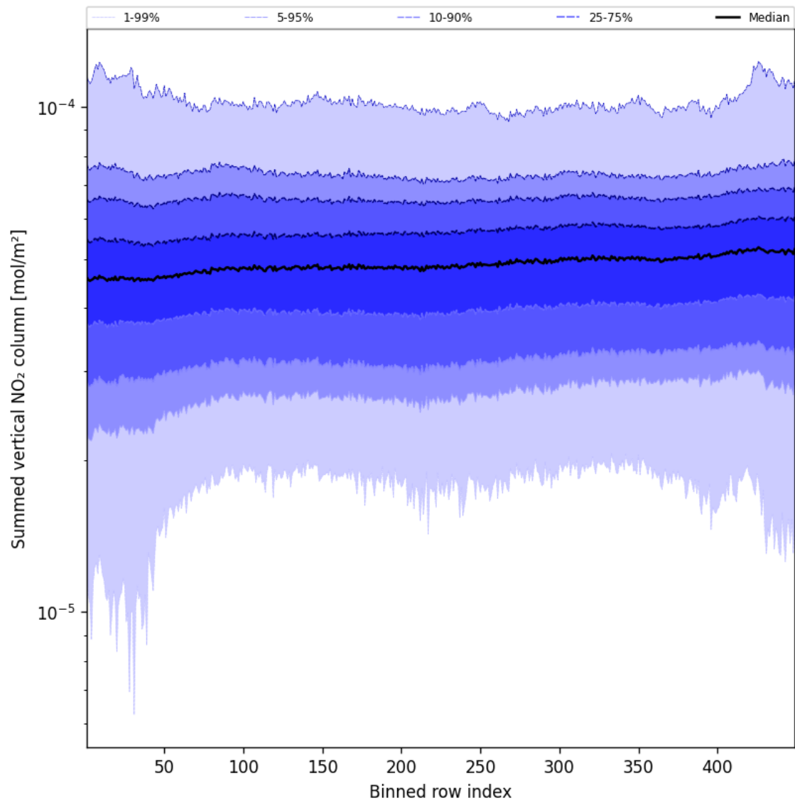
Figure 57: Along track statistics of “Summed vertical NO 2 column” for 2025-04-15 to 2025-04-16
