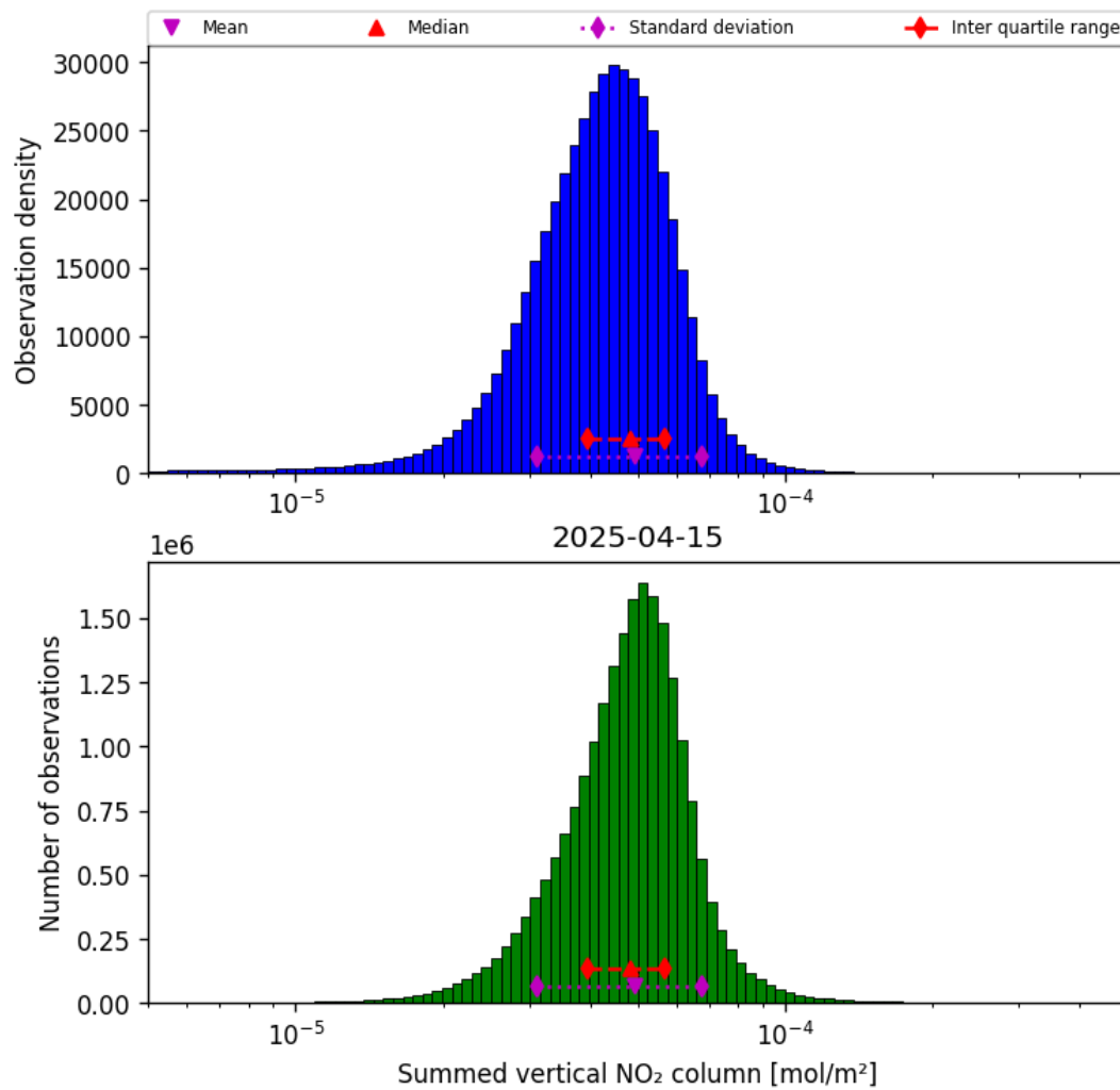
Figure 40: Histogram of “Summed vertical NO 2 column” for 2025-04-15 to 2025-04-16
