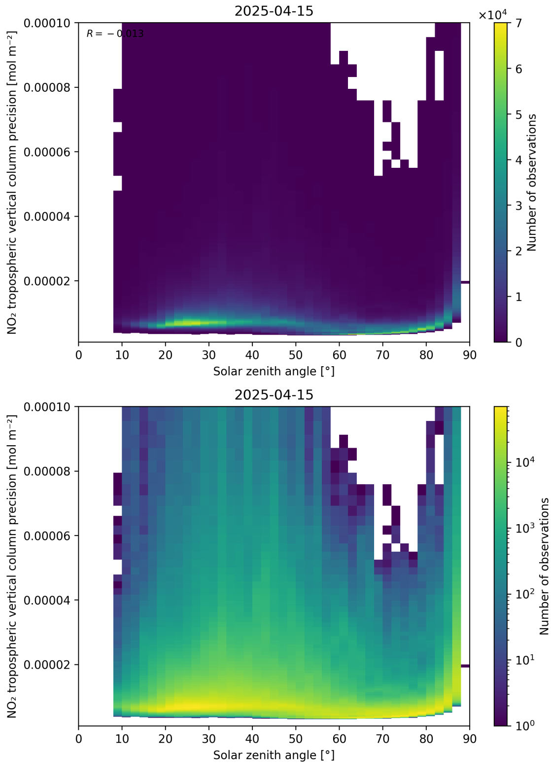
Figure 156: Scatter density plot of “Solar zenith angle” against “NO 2 tropospheric vertical column precision” for 2025-04-15 to 2025-04-16.
