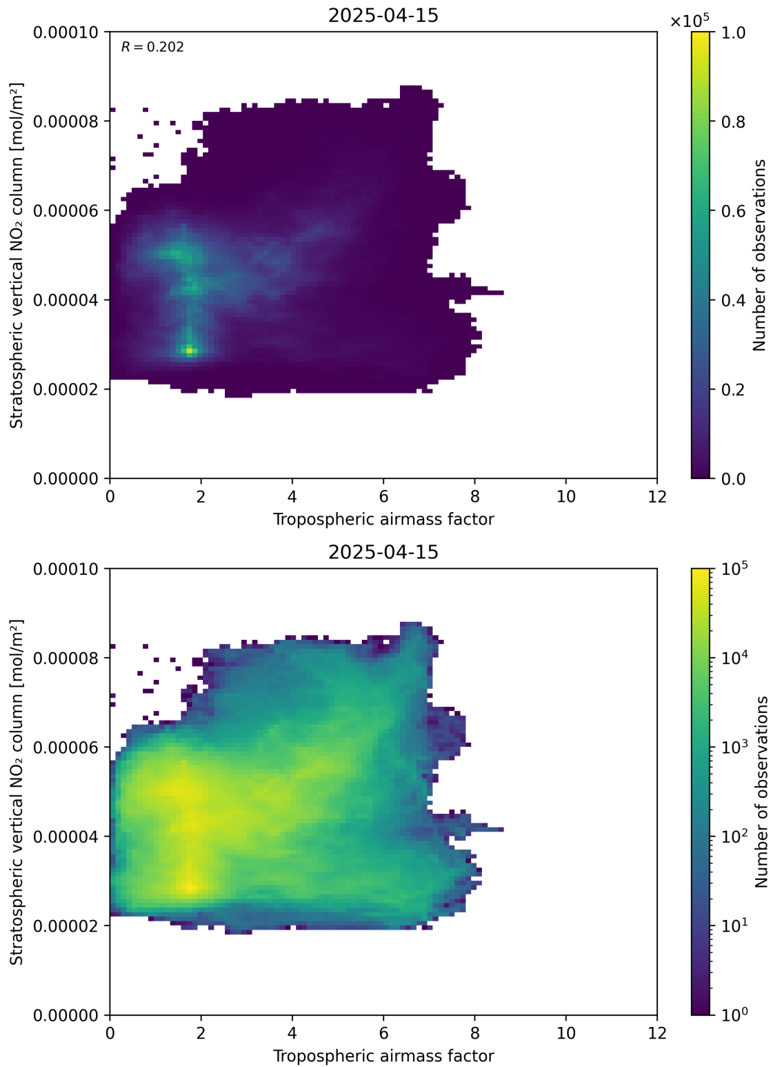
Figure 74: Scatter density plot of “Tropospheric air mass factor” against “Stratospheric vertical NO 2 column” for 2025-04-15 to 2025-04-16.
