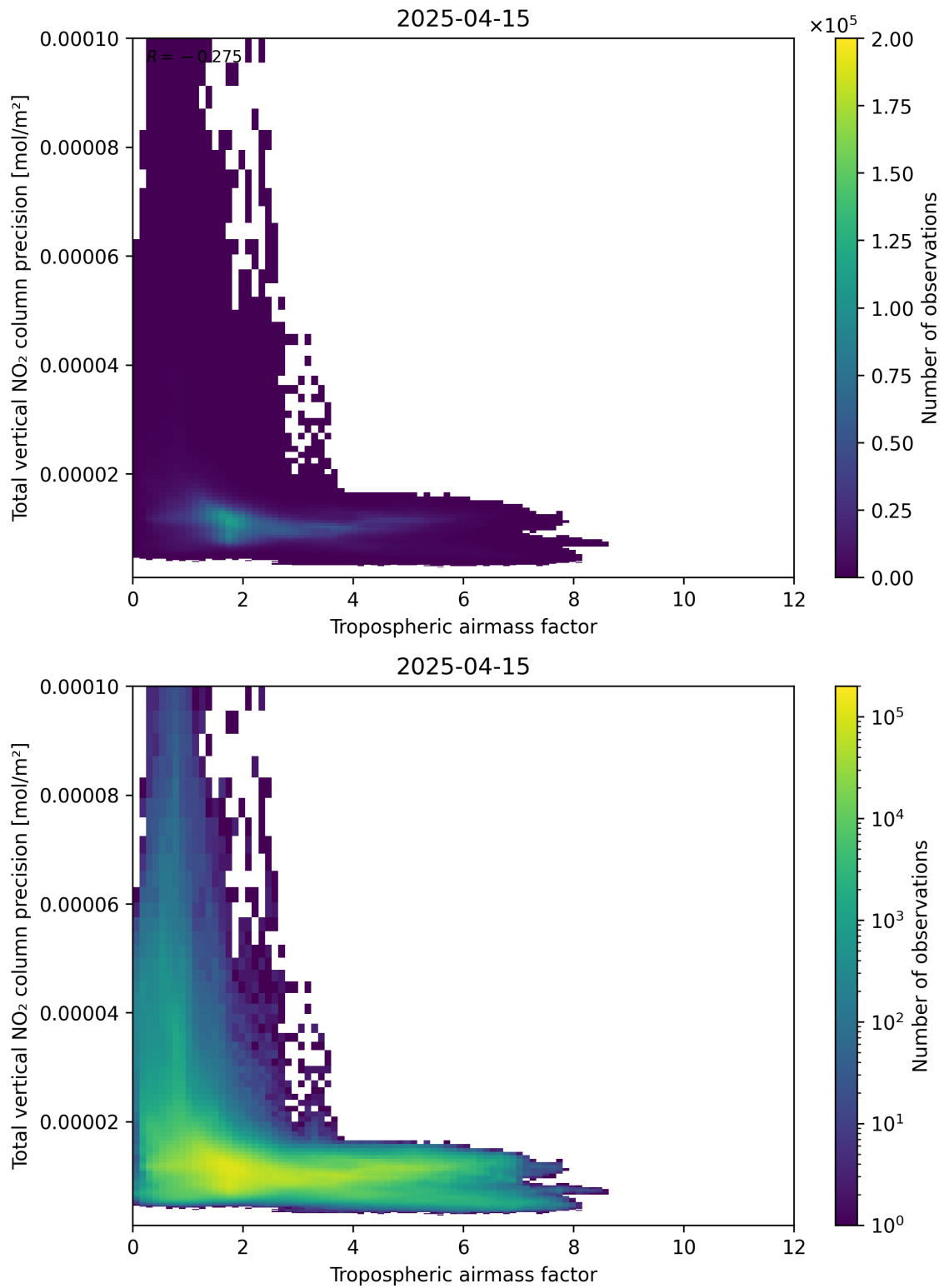
Figure 78: Scatter density plot of “Tropospheric airmass factor” against “Total vertical NO 2 column precision” for 2025-04-15 to 2025-04-16.
