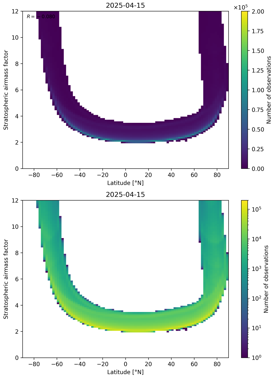
Figure 83: Scatter density plot of “Latitude” against “Stratospheric air mass factor” for 2025-04-15 to 2025-04-16.
