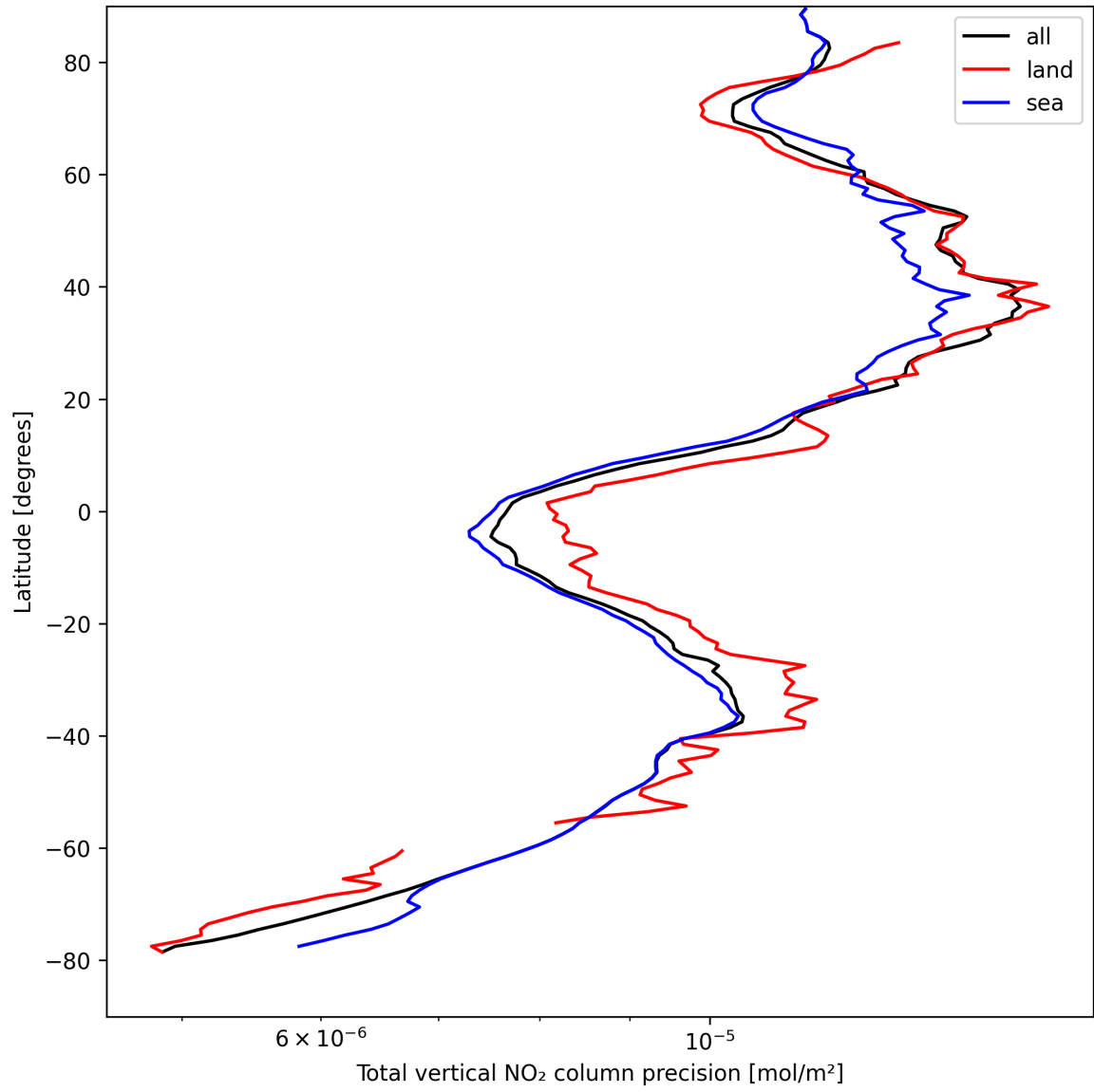
Figure 22: Zonal average of “Total vertical NO 2 column precision” for 2025-04-15 to 2025-04-16.
