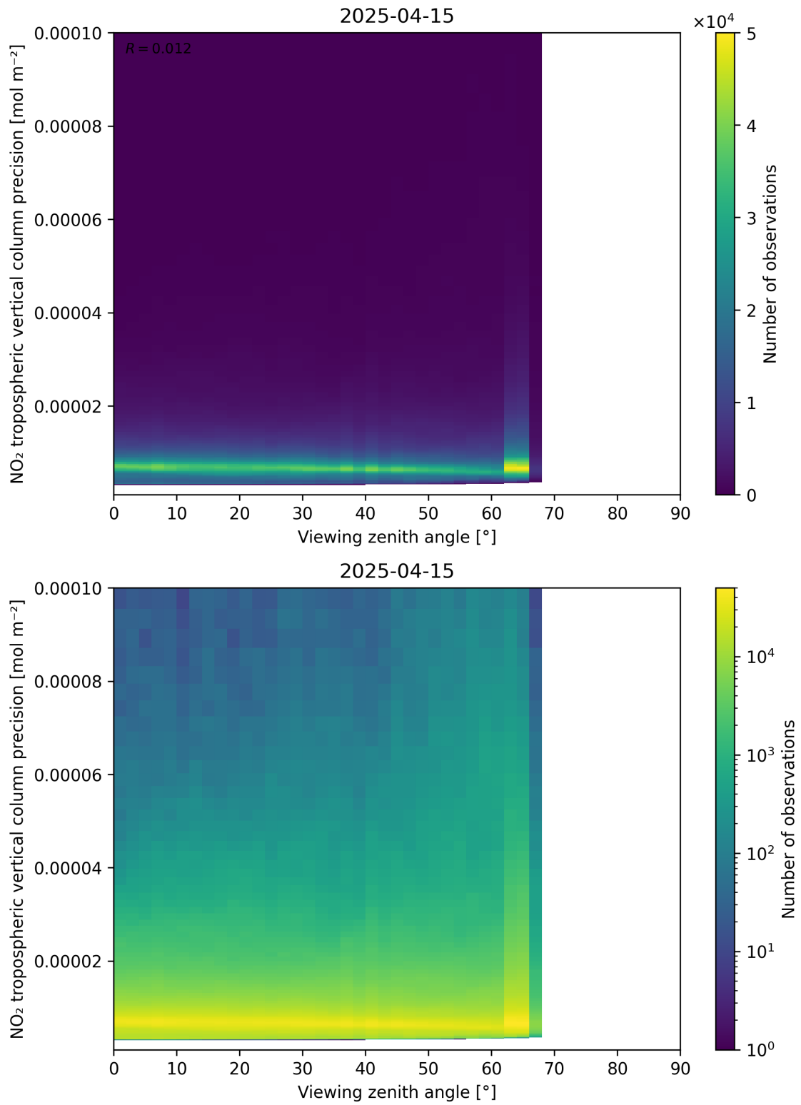
Figure 170: Scatter density plot of “Viewing zenith angle” against “NO 2 tropospheric vertical column precision” for 2025-04-15 to 2025-04-16.
