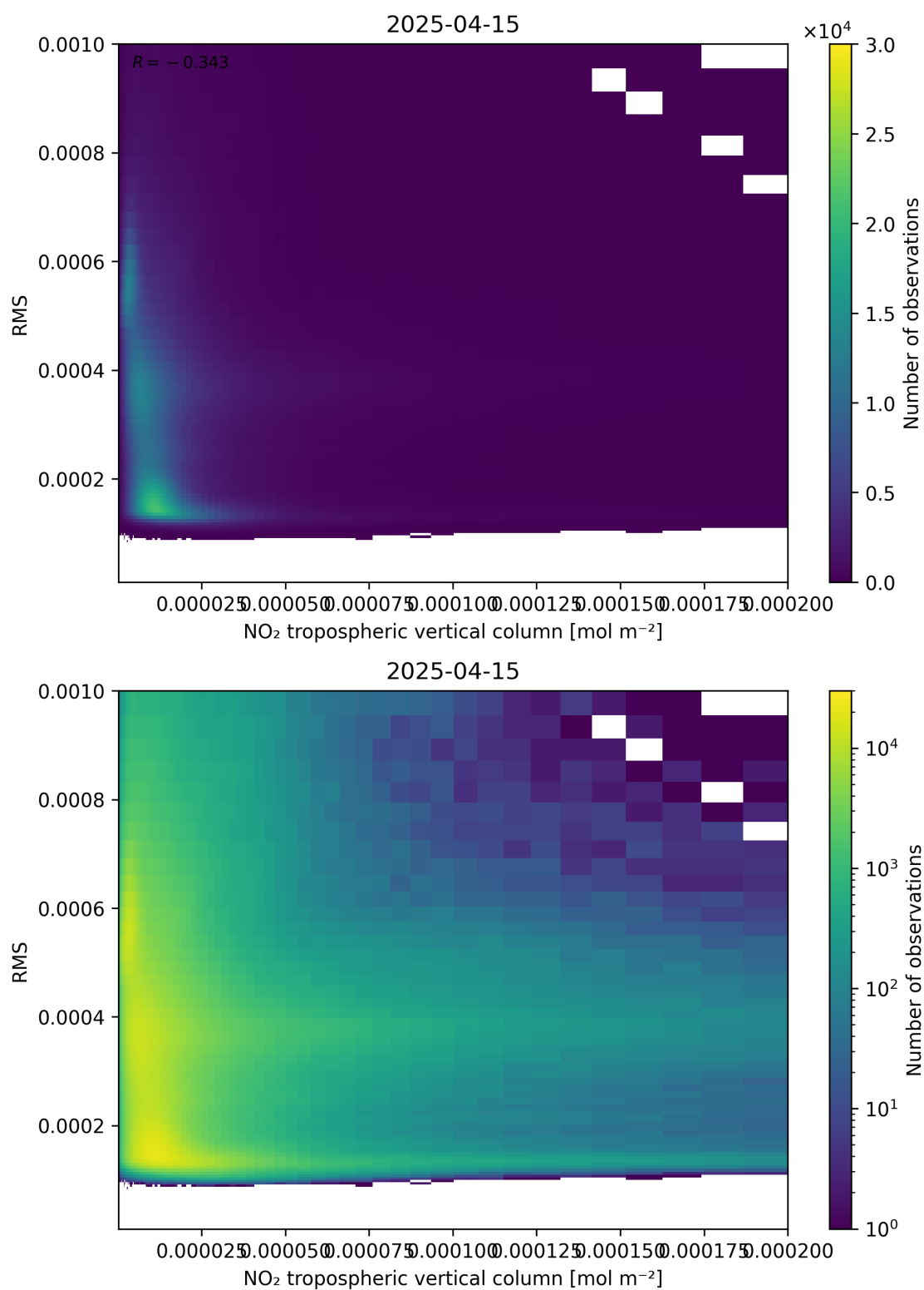
Figure 142: Scatter density plot of “NO 2 tropospheric vertical column” against “RMS” for 2025-04-15 to 2025-04-16.
