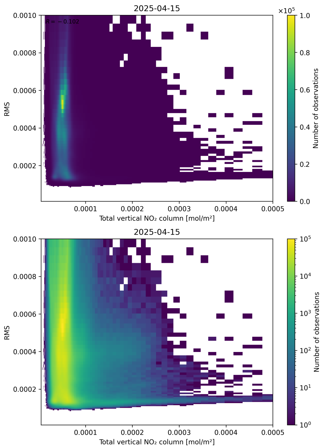
Figure 120: Scatter density plot of “Total vertical NO 2 column” against “RMS” for 2025-04-15 to 2025-04-16.
