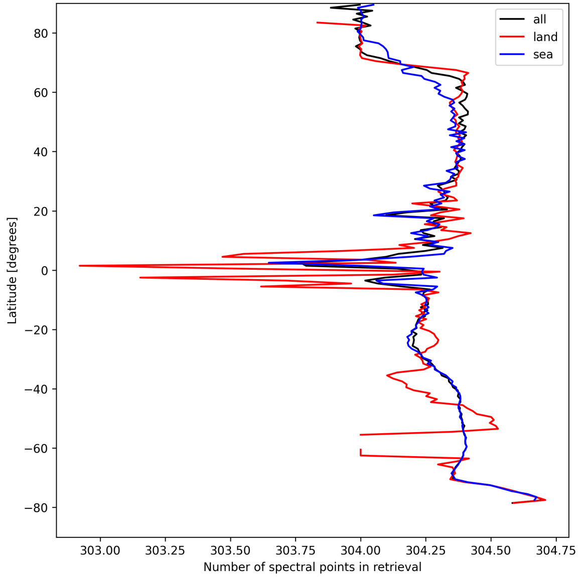
Figure 16: Zonal average of “Number of spectral points in retrieval” for 2025-04-15 to 2025-04-16.
