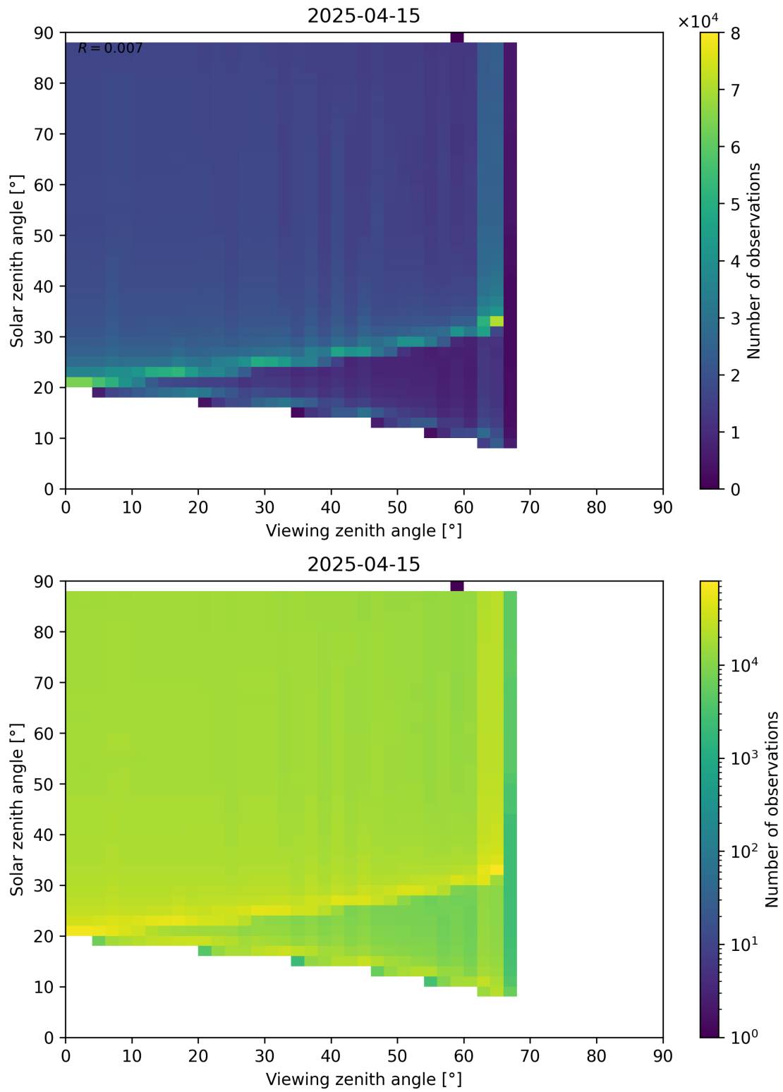
Figure 172: Scatter density plot of “Viewing zenith angle” against “Solar zenith angle” for 2025-04-15 to 2025-04-16.
