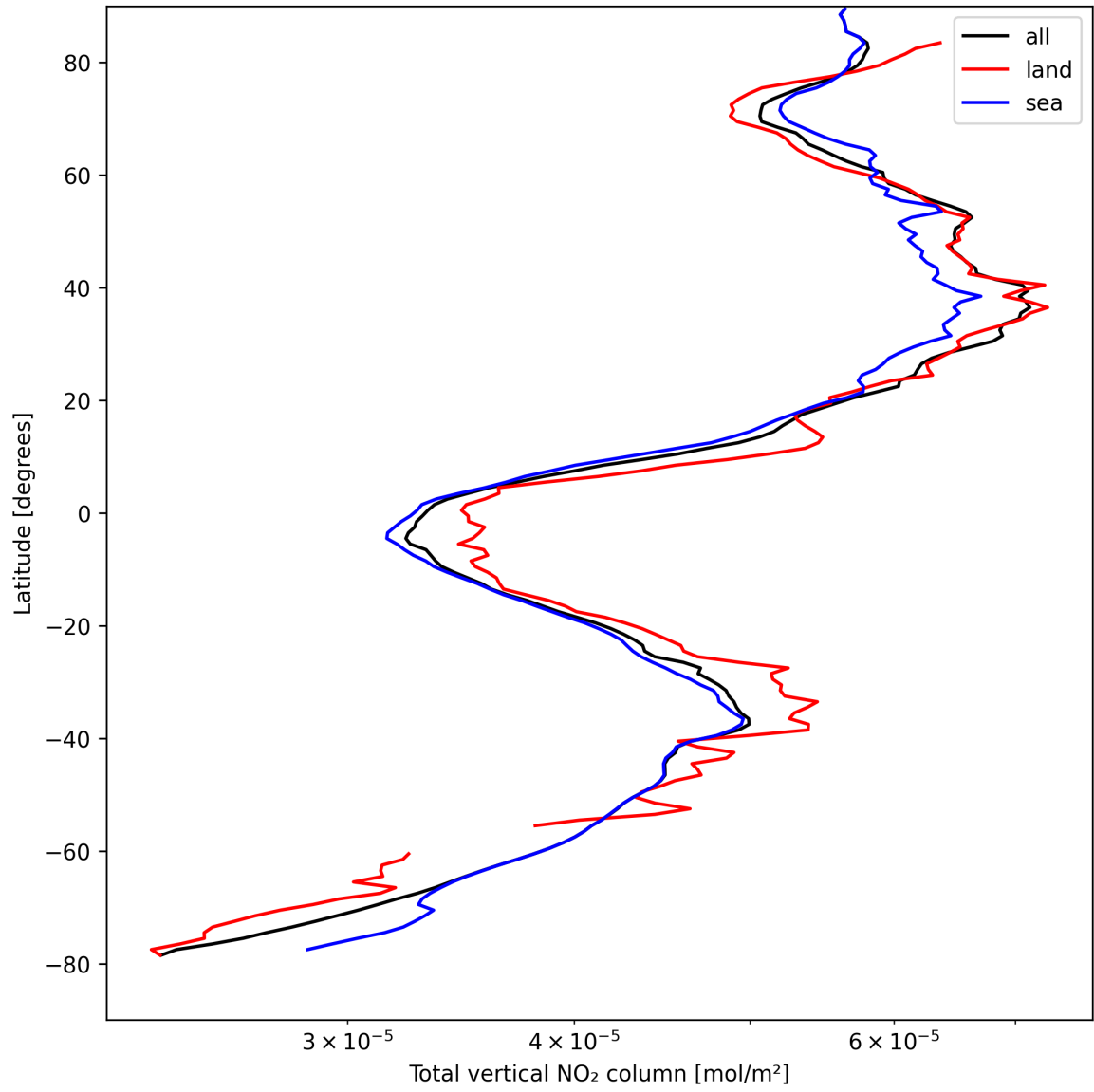
Figure 21: Zonal average of “Total vertical NO 2 column” for 2025-04-15 to 2025-04-16.
