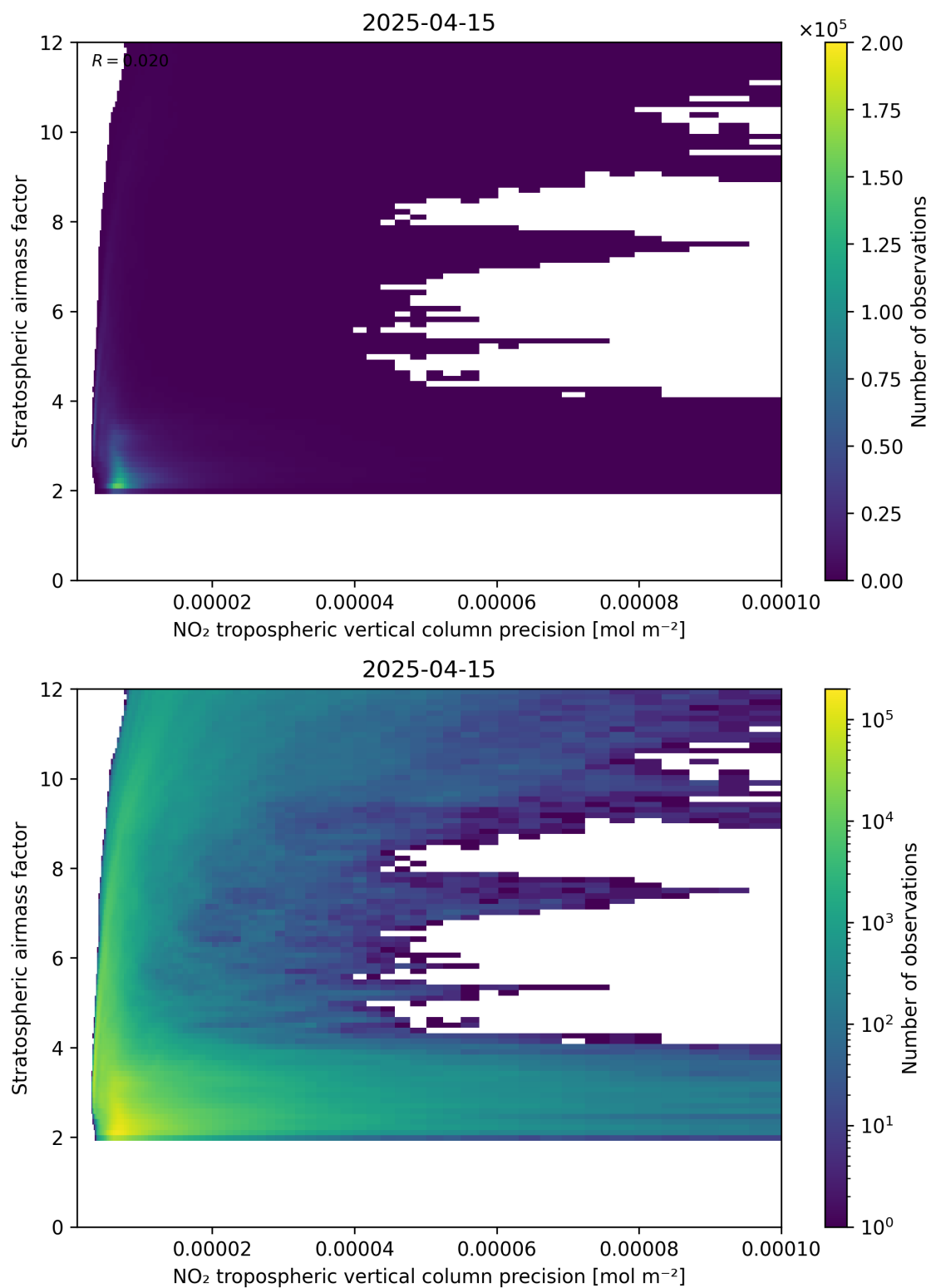
Figure 131: Scatter density plot of “NO 2 tropospheric vertical column precision” against “Stratospheric airmass factor” for 2025-04-15 to 2025-04-16.
