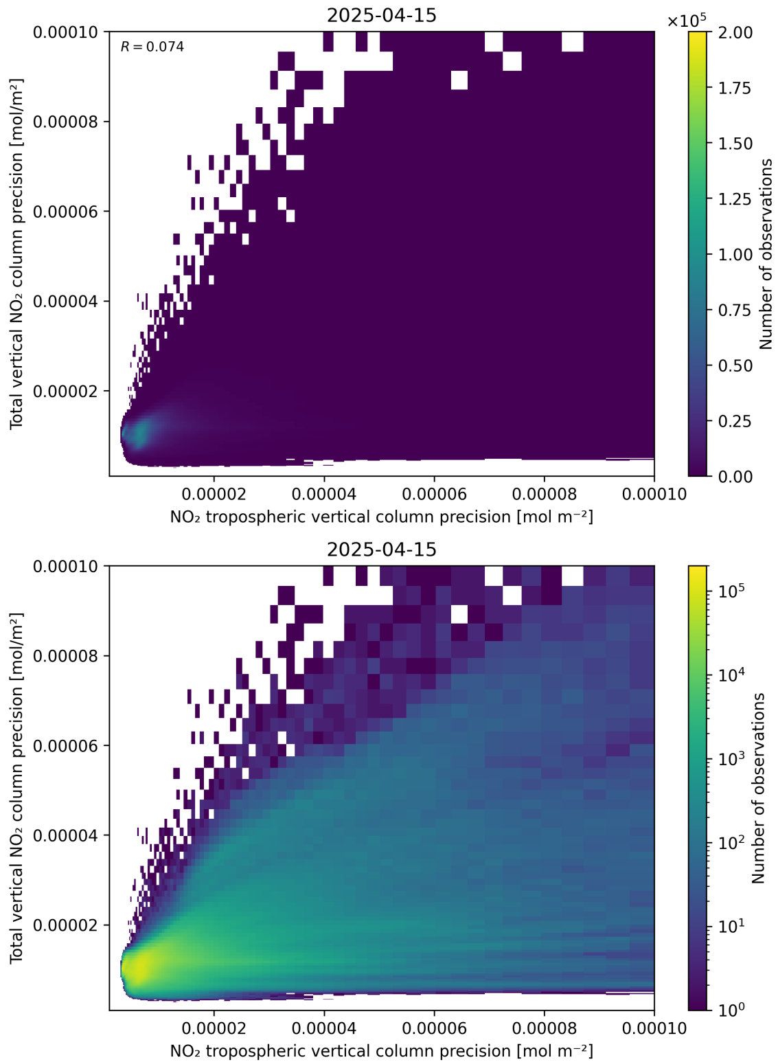
Figure 139: Scatter density plot of “NO 2 tropospheric vertical column precision” against “Total vertical NO 2 column precision” for 2025-04-15 to 2025-04-16.
