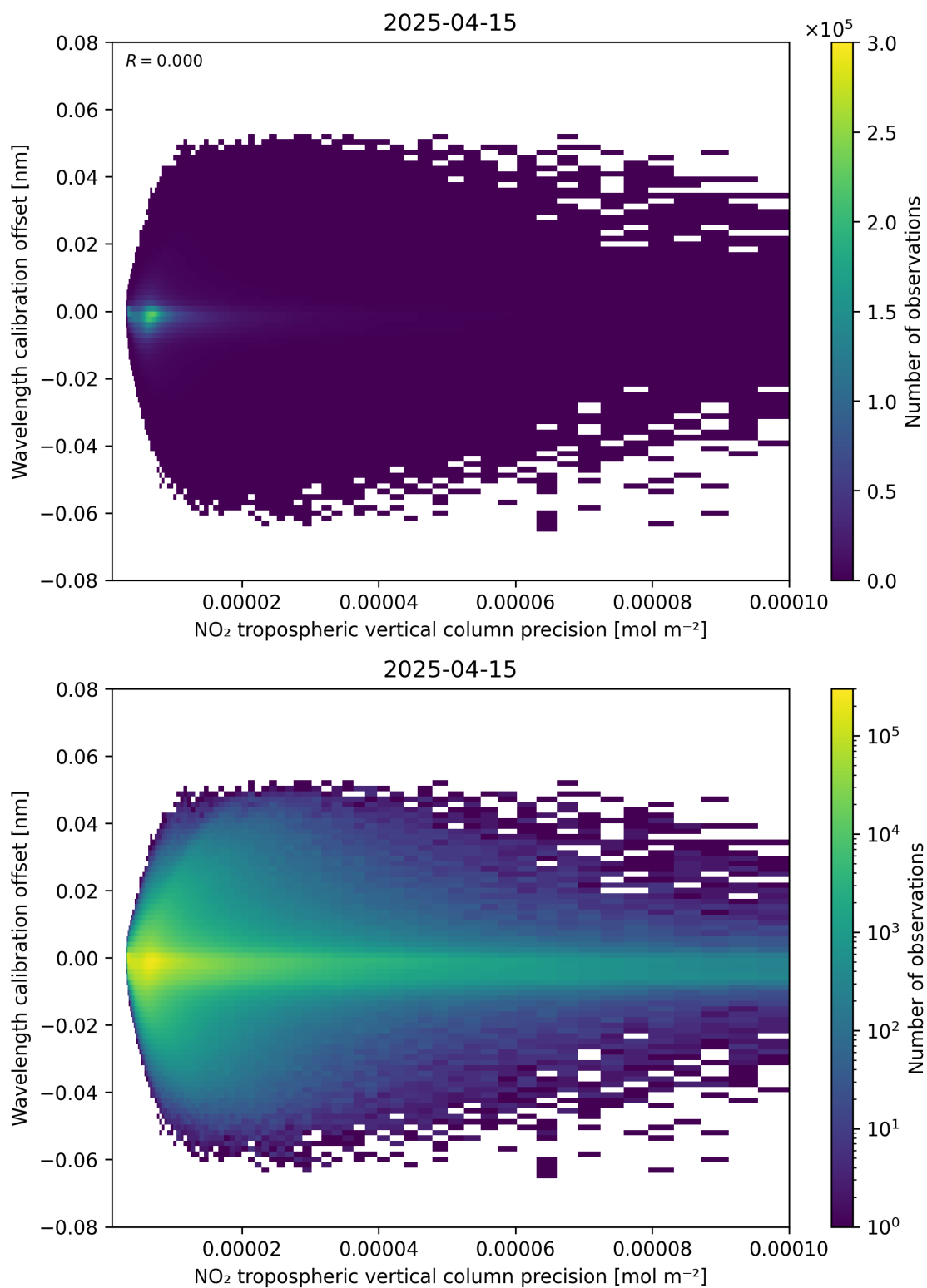
Figure 141: Scatter density plot of “NO 2 tropospheric vertical column precision” against “Wavelength calibration offset” for 2025-04-15 to 2025-04-16.
