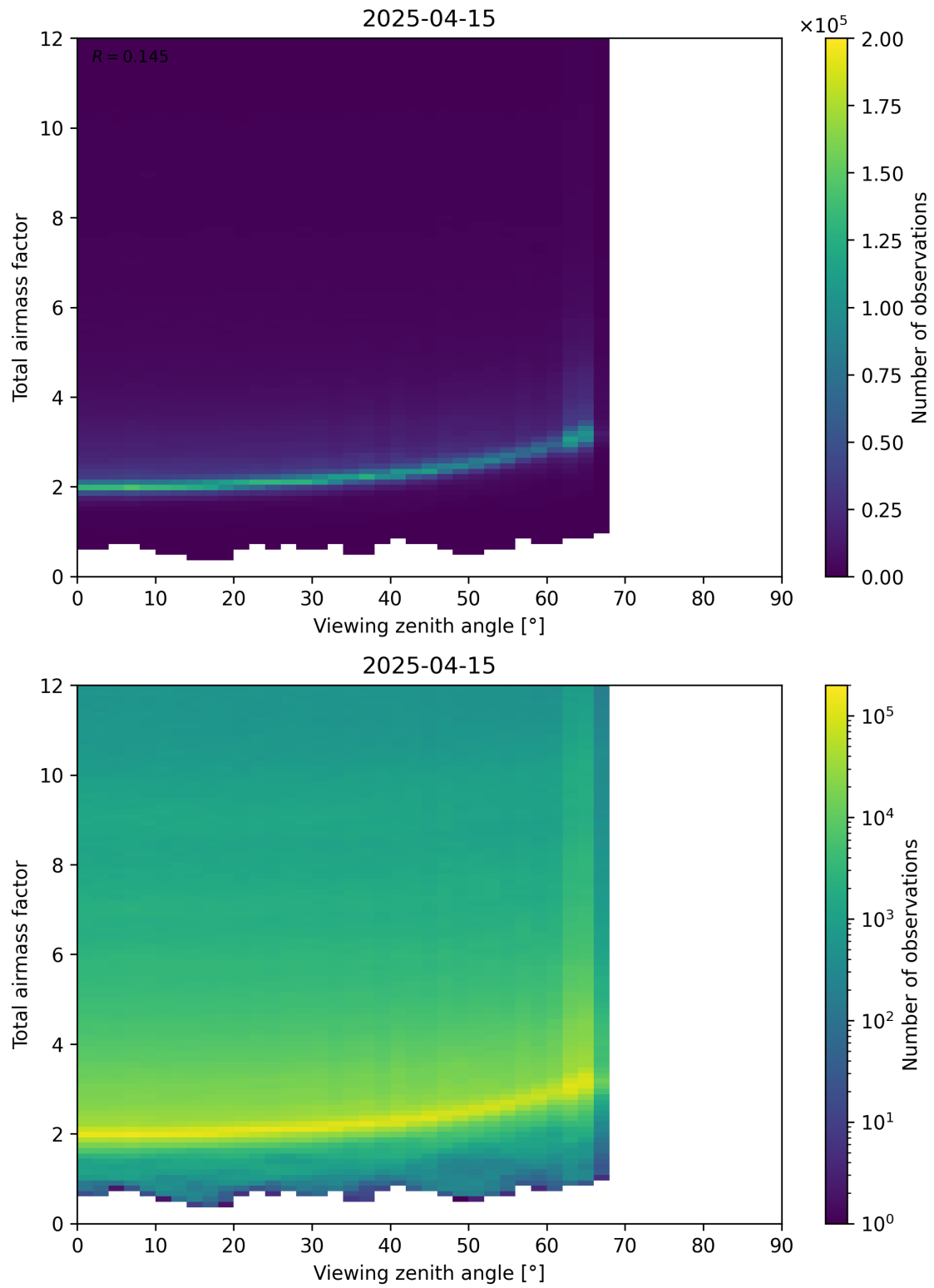
Figure 160: Scatter density plot of “Viewing zenith angle” against “Total airmass factor” for 2025-04-15 to 2025-04-16.
