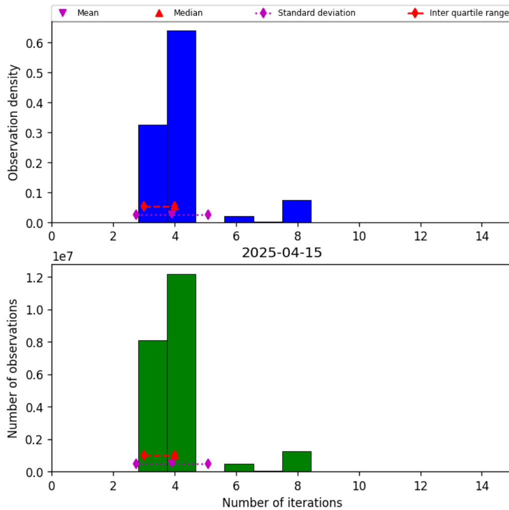
Figure 34: Histogram of “Number of iterations” for 2025-04-15 to 2025-04-16
