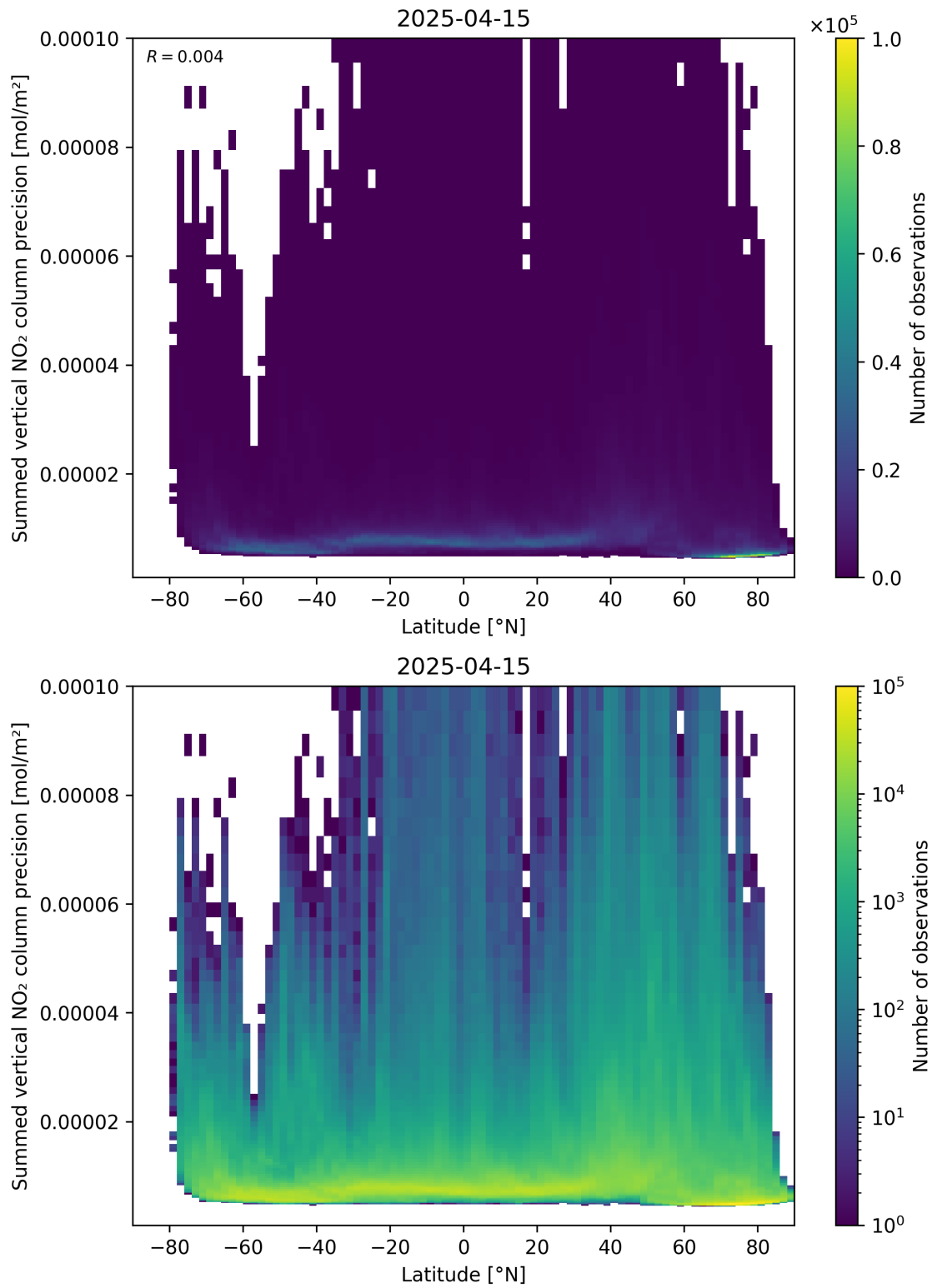
Figure 89: Scatter density plot of “Latitude” against “Summed vertical NO 2 column precision” for 2025-04-15 to 2025-04-16.
