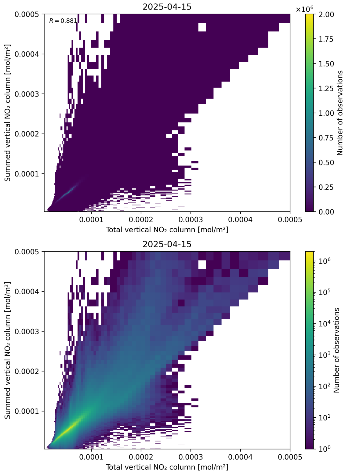
Figure 112: Scatter density plot of “Total vertical NO 2 column” against “Summed vertical NO 2 column” for 2025-04-15 to 2025-04-16.
