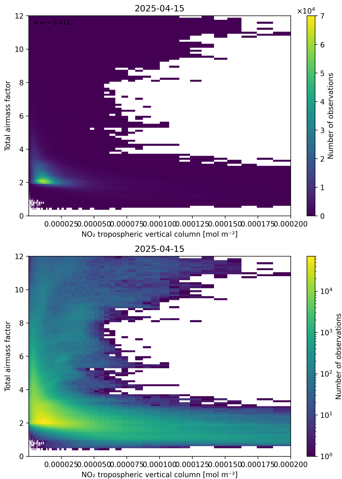
Figure 122: Scatter density plot of “NO 2 tropospheric vertical column” against “Total air mass factor” for 2025-04-15 to 2025-04-16.
