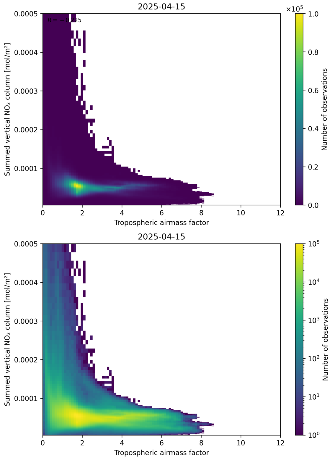
Figure 75: Scatter density plot of “Tropospheric airmass factor” against “Summed vertical NO 2 column” for 2025-04-15 to 2025-04-16.
