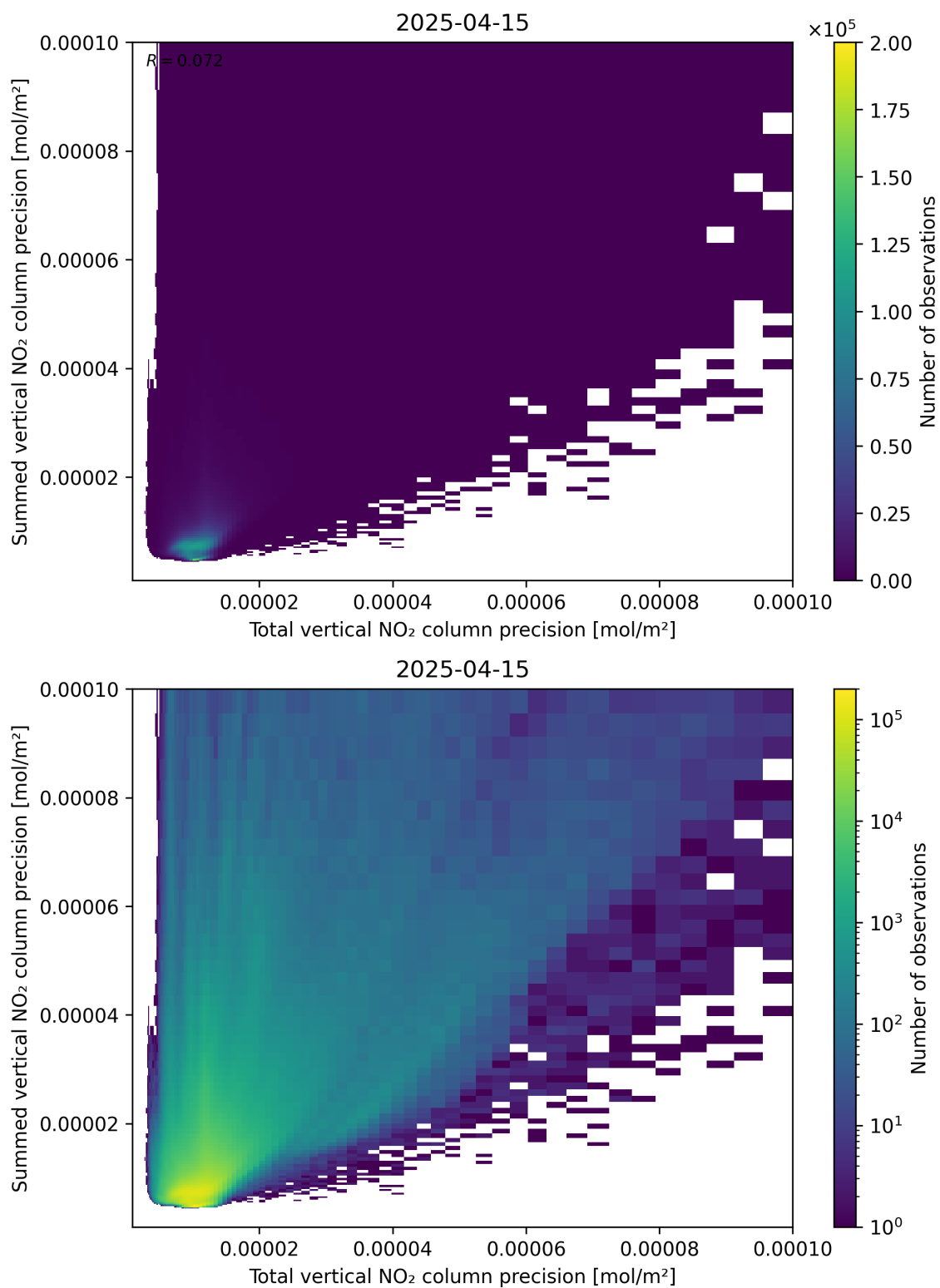
Figure 118: Scatter density plot of “Total vertical NO 2 column precision” against “Summed vertical NO 2 column precision” for 2025-04-15 to 2025-04-16.
