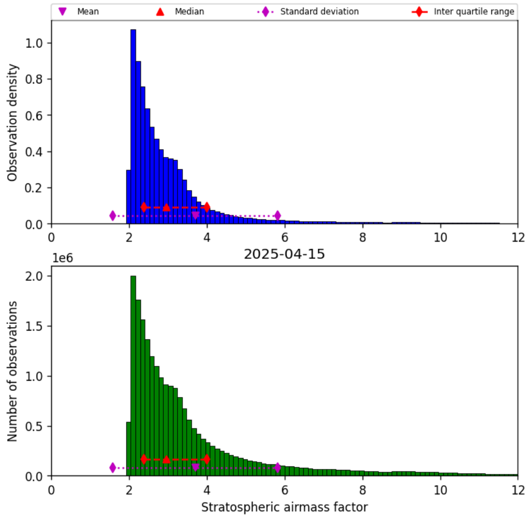
Figure 44: Histogram of “Stratospheric airmass factor” for 2025-04-15 to 2025-04-16
