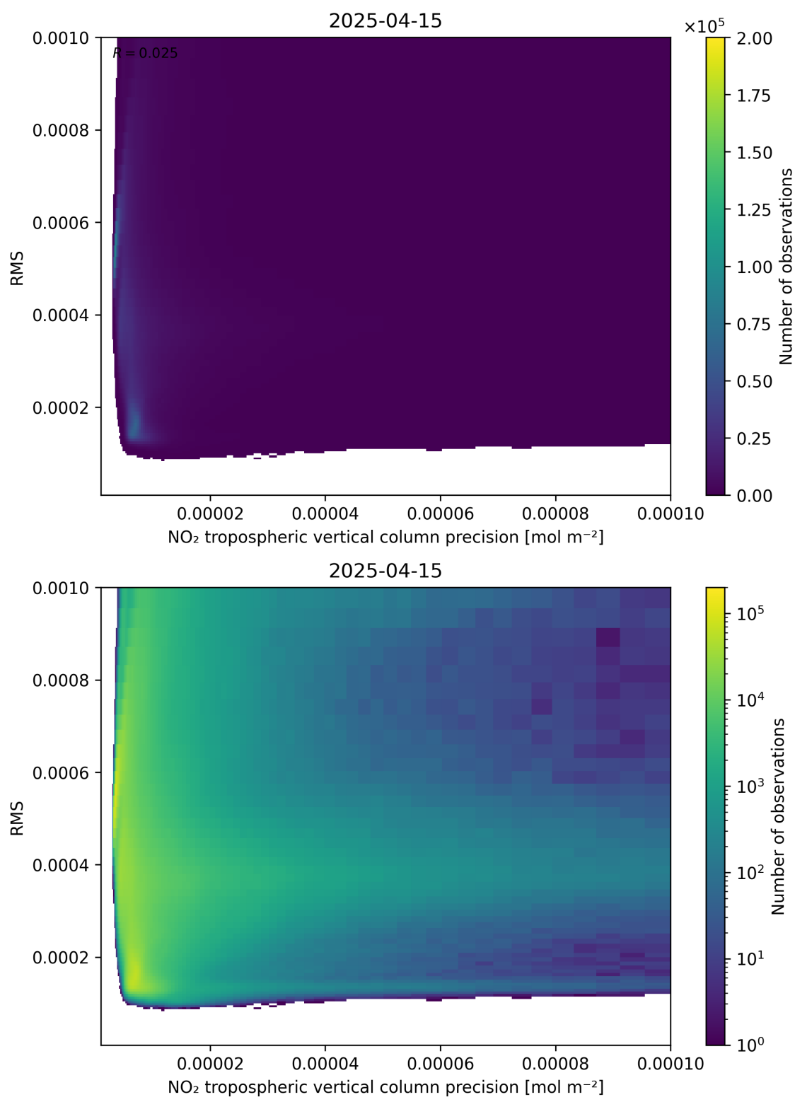
Figure 140: Scatter density plot of “NO 2 tropospheric vertical column precision” against “RMS” for 2025-04-15 to 2025-04-16.
