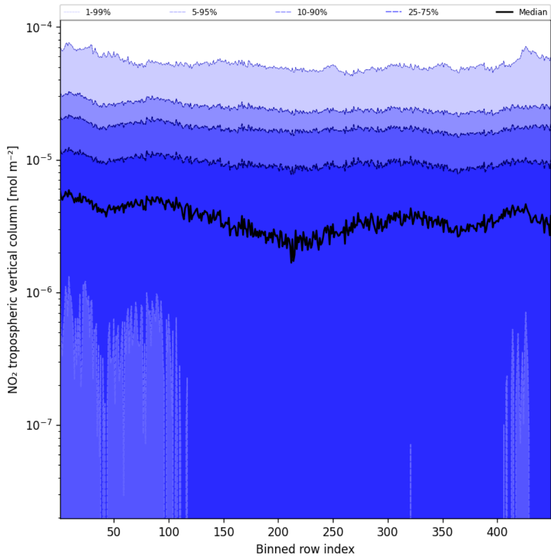
Figure 46: Along track statistics of “NO 2 tropospheric vertical column” for 2025-04-15 to 2025-04-16
