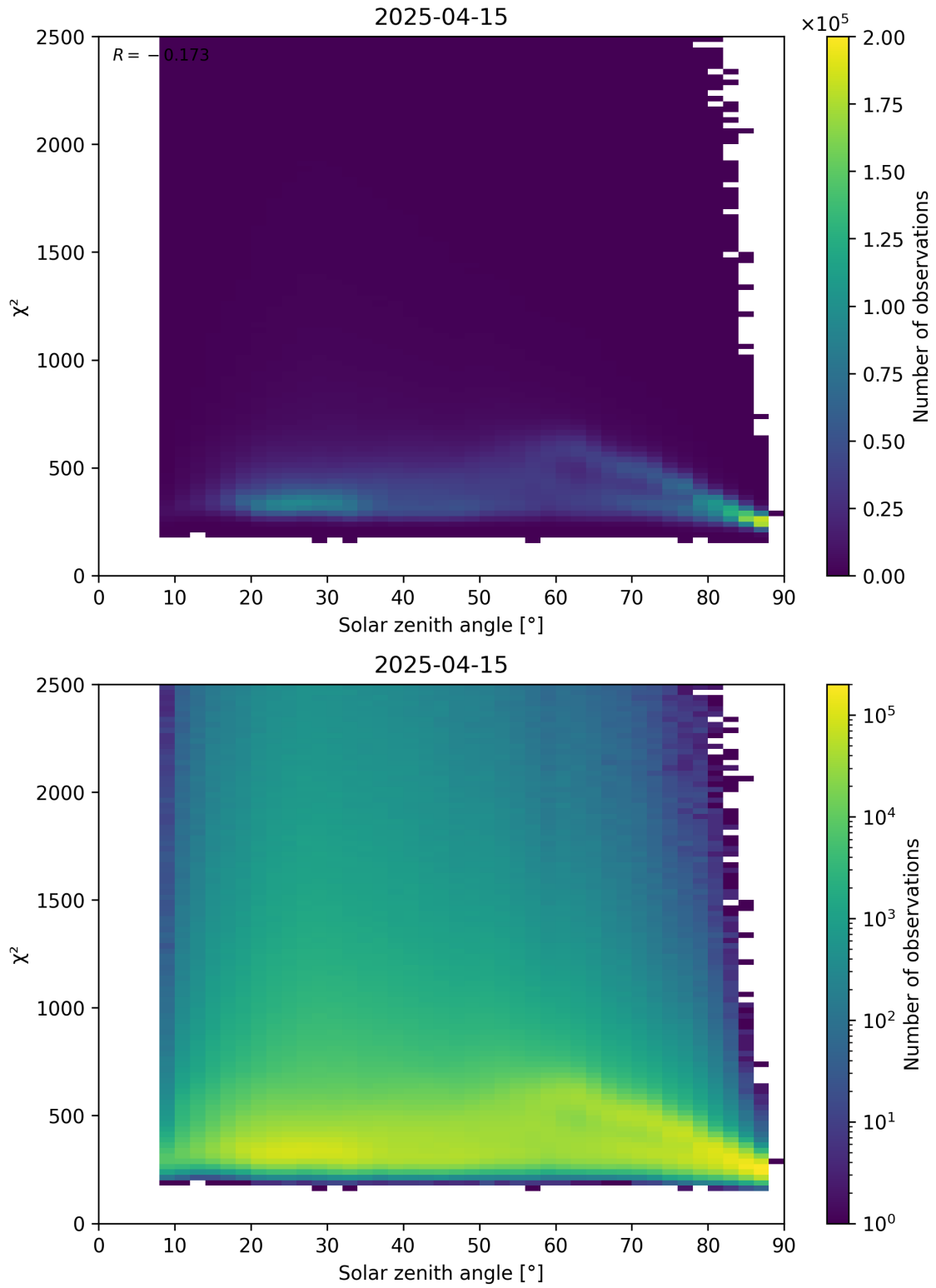
Figure 148: Scatter density plot of “Solar zenith angle” against “ \chi^2 ” for 2025-04-15 to 2025-04-16.
