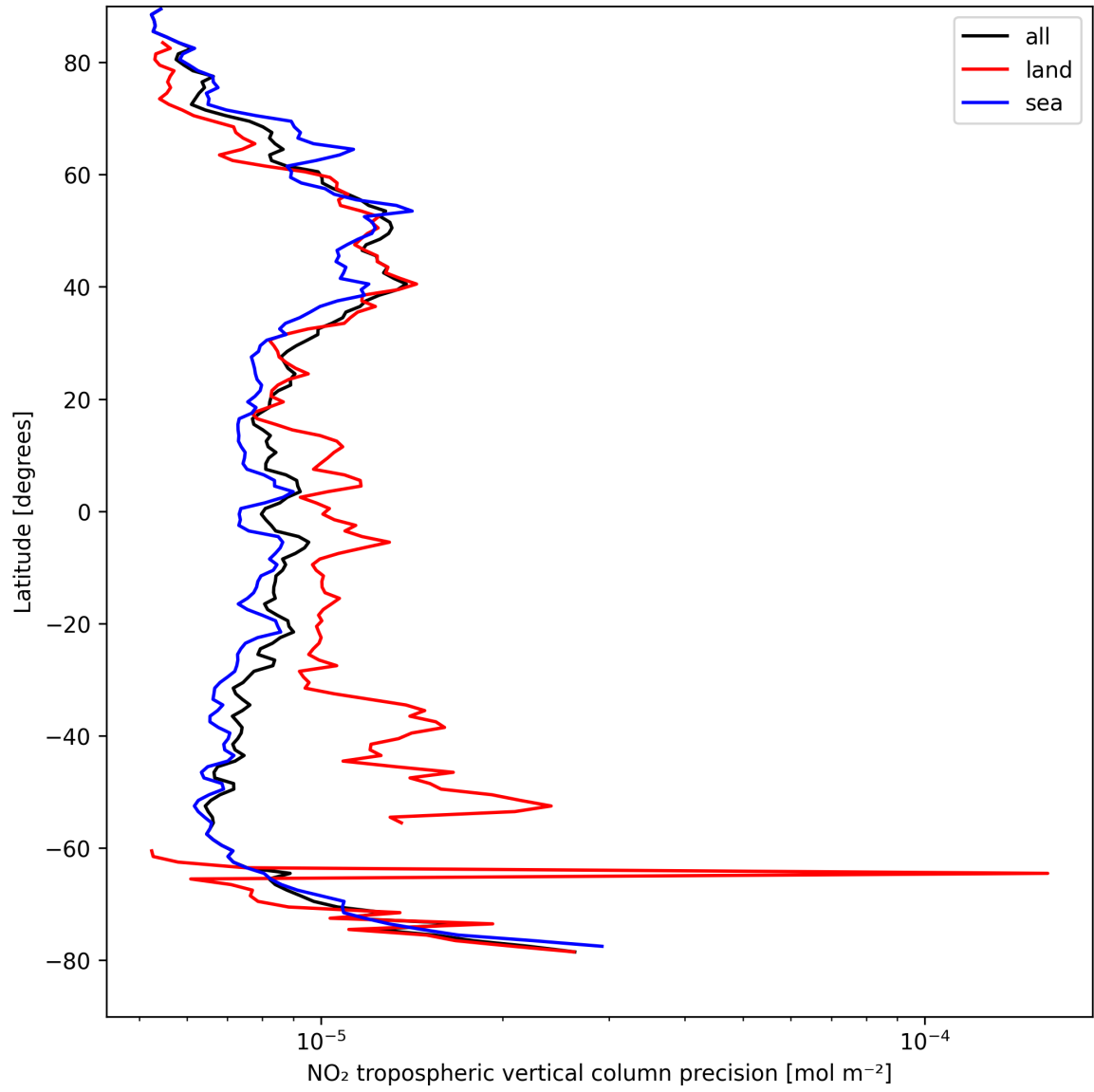
Figure 13: Zonal average of “NO 2 tropospheric vertical column precision” for 2025-04-15 to 2025-04-16.
