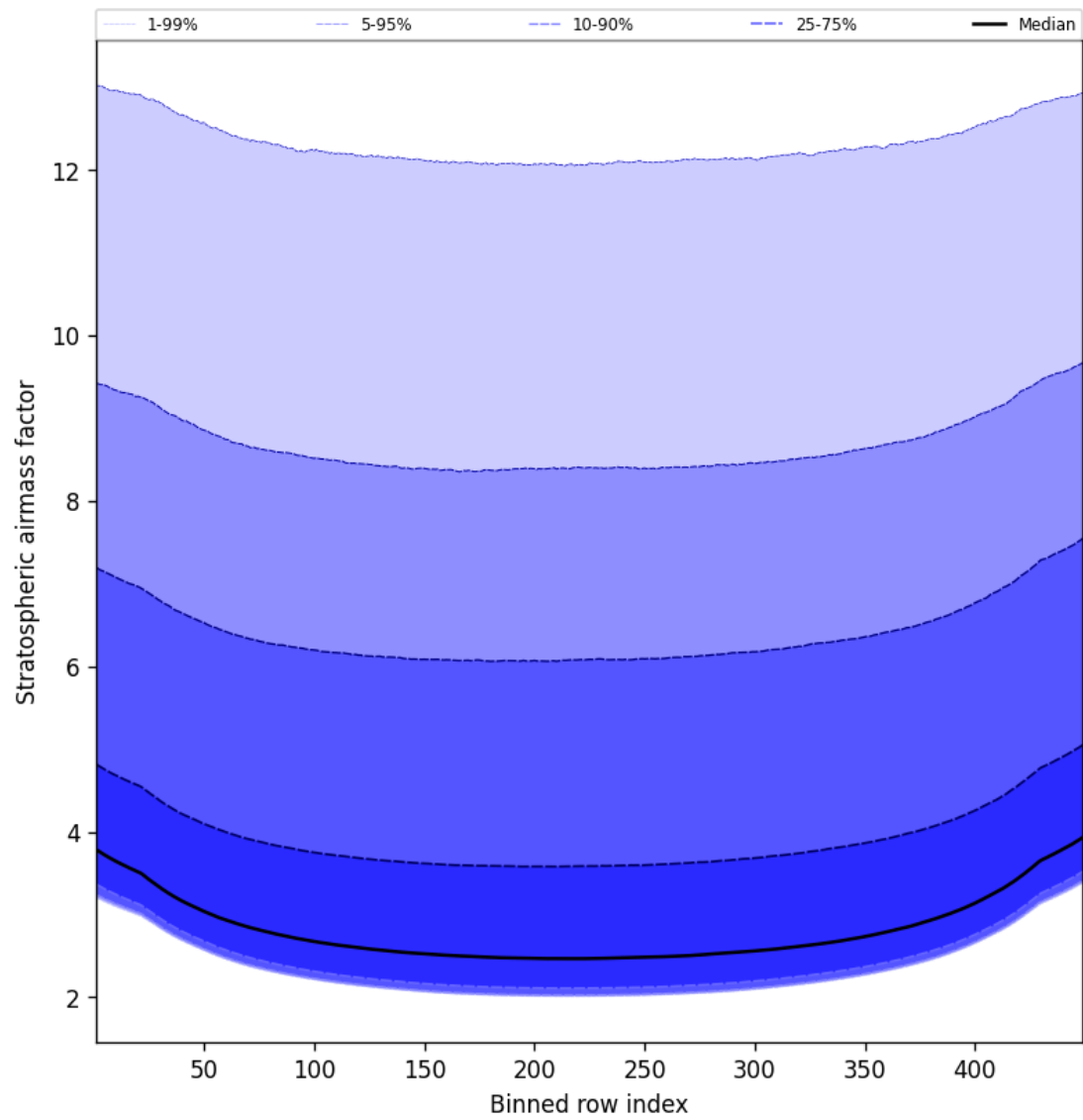
Figure 61: Along track statistics of “Stratospheric air mass factor” for 2025-04-15 to 2025-04-16
