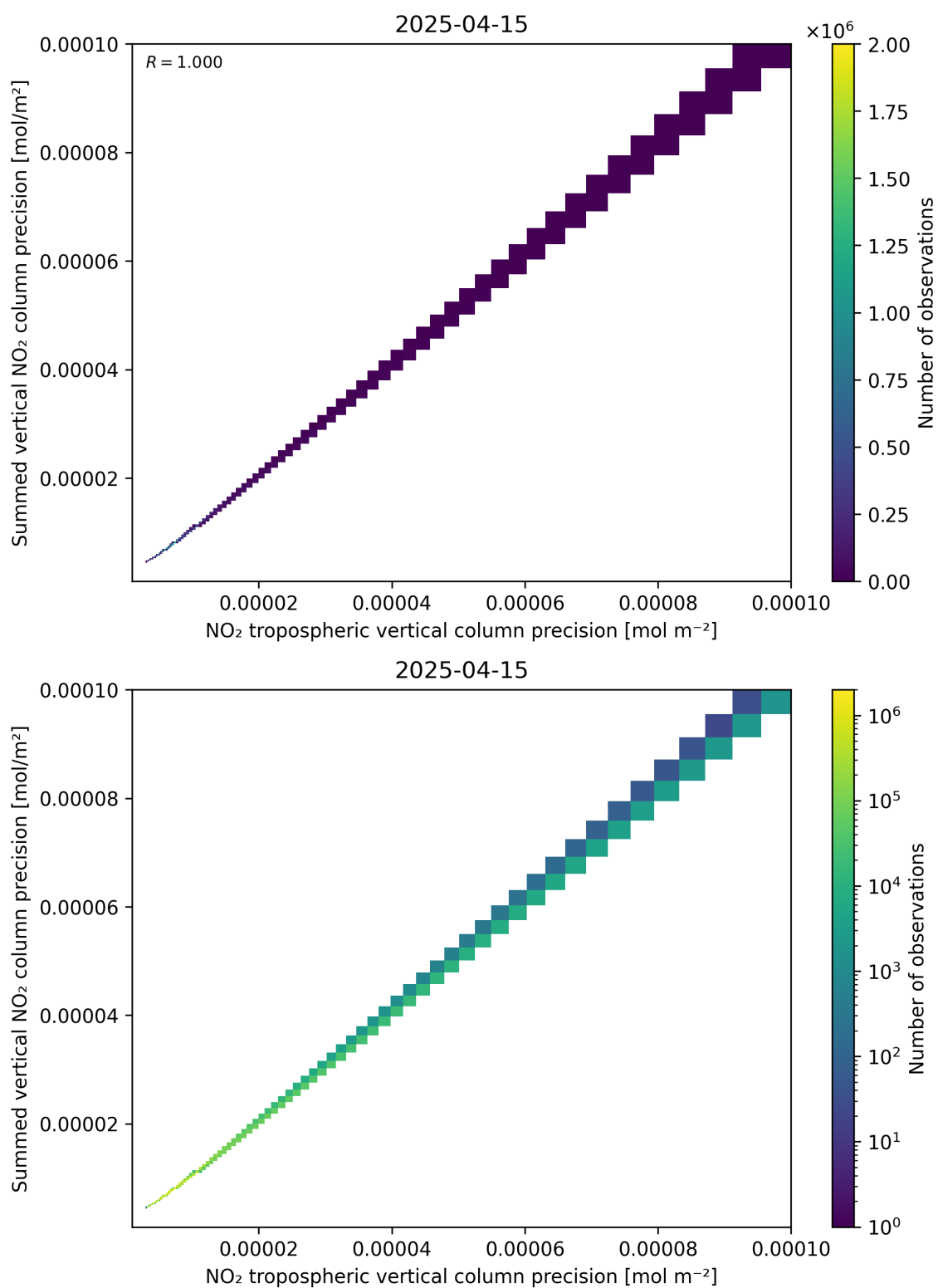
Figure 137: Scatter density plot of “NO 2 tropospheric vertical column precision” against “Summed vertical NO 2 column precision” for 2025-04-15 to 2025-04-16.
