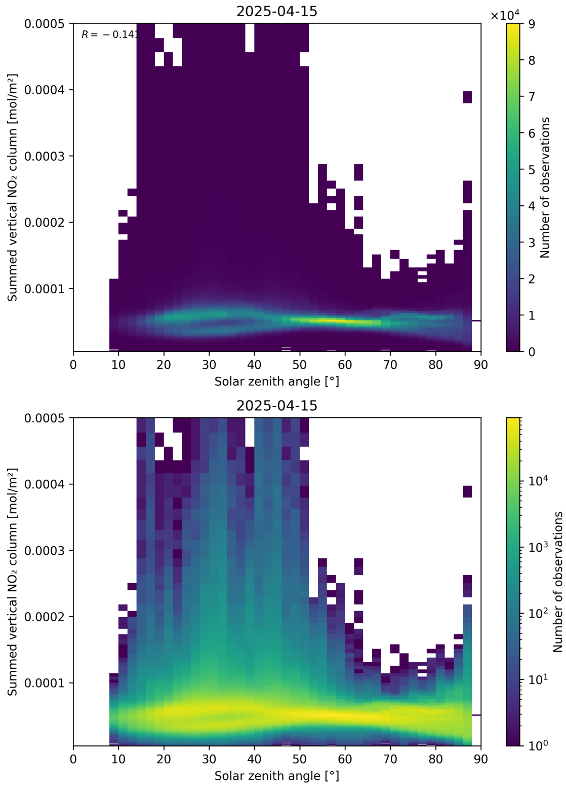
Figure 151: Scatter density plot of “Solar zenith angle” against “Summed vertical NO 2 column” for 2025-04-15 to 2025-04-16.
