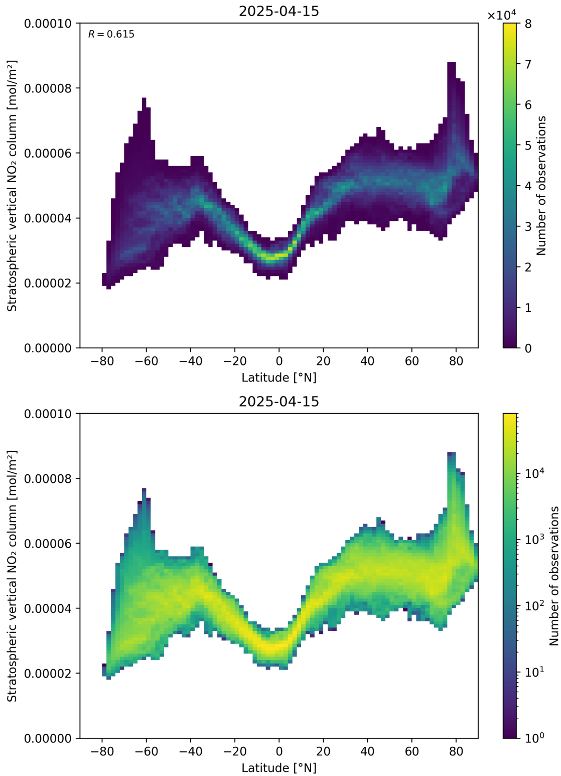
Figure 87: Scatter density plot of “Latitude” against “Stratospheric vertical NO 2 column” for 2025-04-15 to 2025-04-16.
