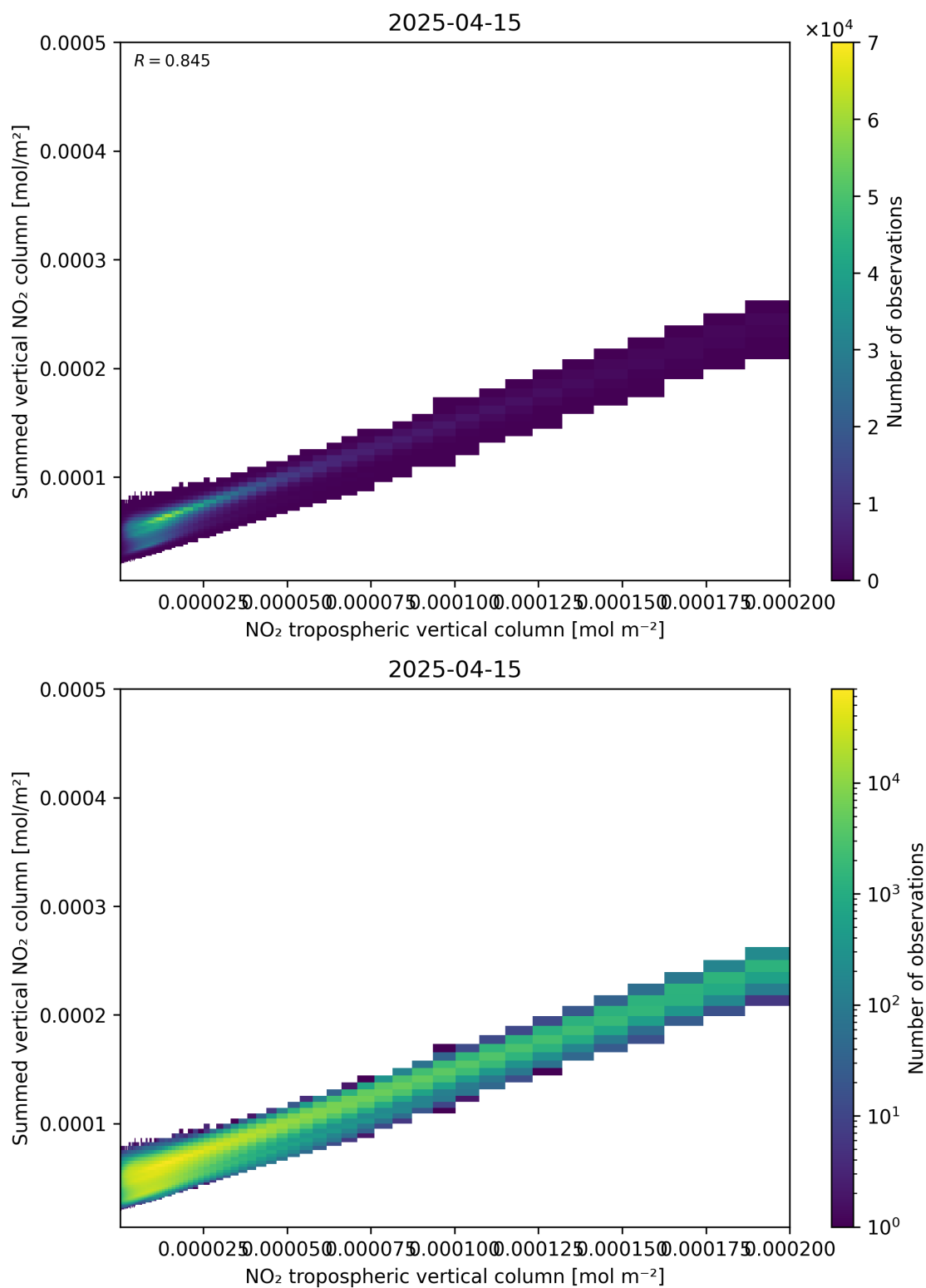
Figure 126: Scatter density plot of “NO 2 tropospheric vertical column” against “Summed vertical NO 2 column” for 2025-04-15 to 2025-04-16.
