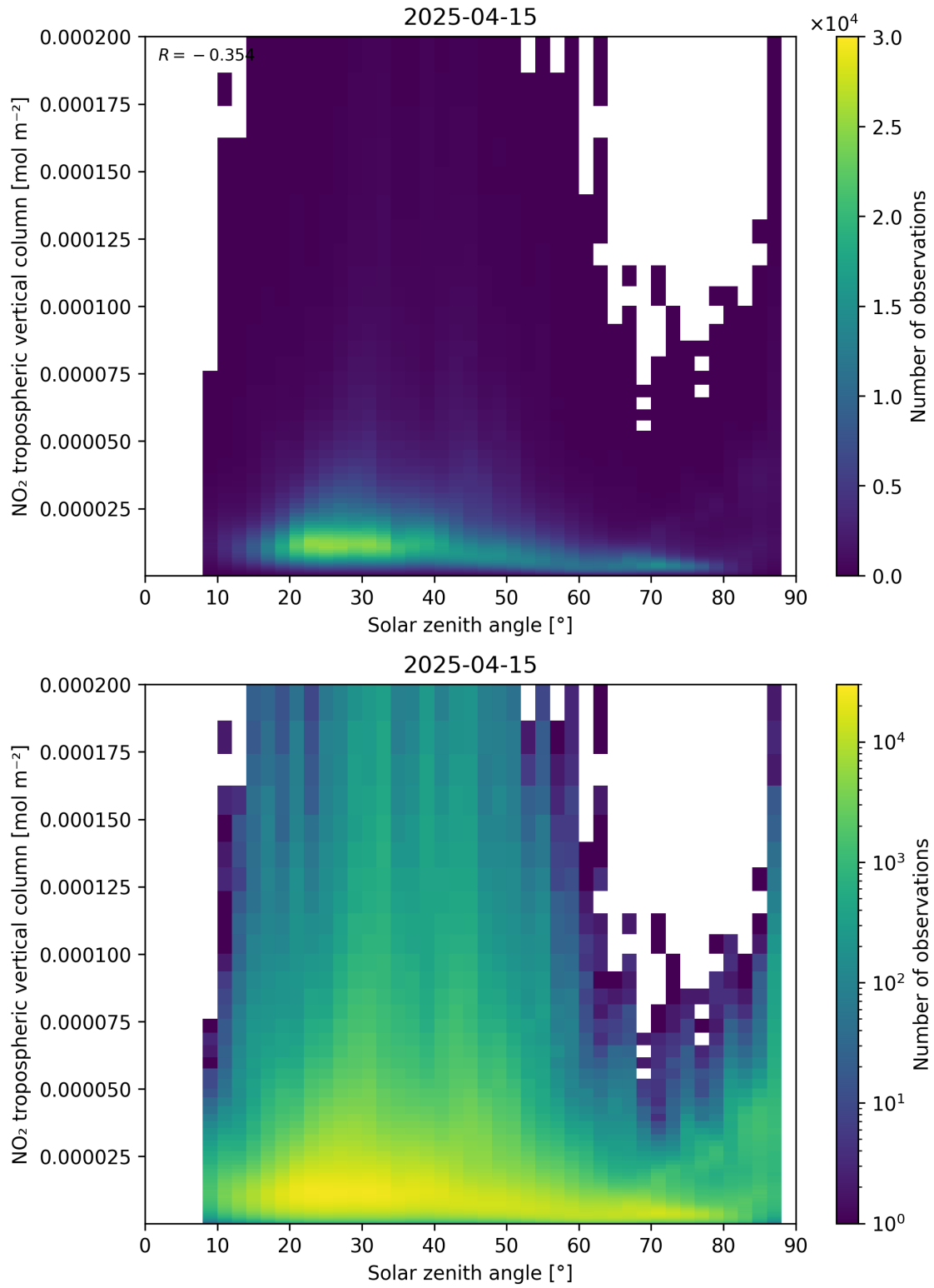
Figure 155: Scatter density plot of “Solar zenith angle” against “NO 2 tropospheric vertical column” for 2025-04-15 to 2025-04-16.
