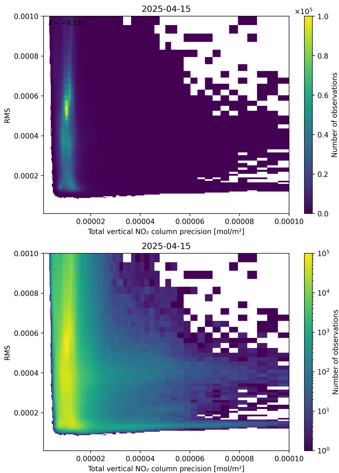
Figure 119: Scatter density plot of “Total vertical NO 2 column precision” against “RMS” for 2025-04-15 to 2025-04-16.
