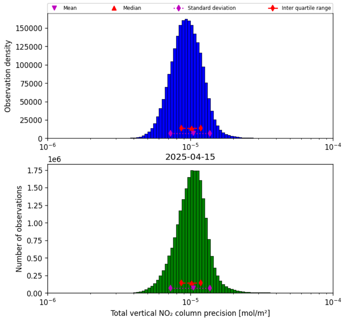
Figure 39: Histogram of “Total vertical NO 2 column precision” for 2025-04-15 to 2025-04-16
