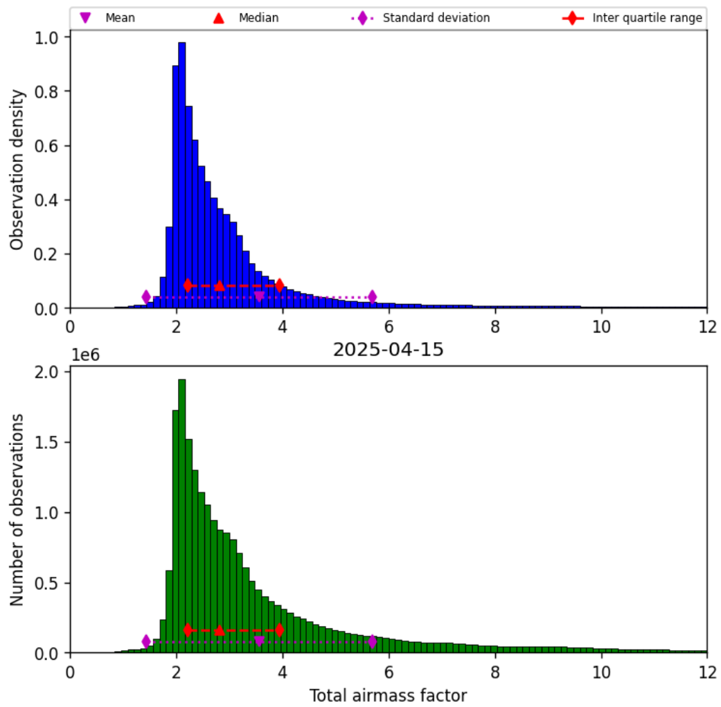
Figure 32: Histogram of “Total airmass factor” for 2025-04-15 to 2025-04-16
