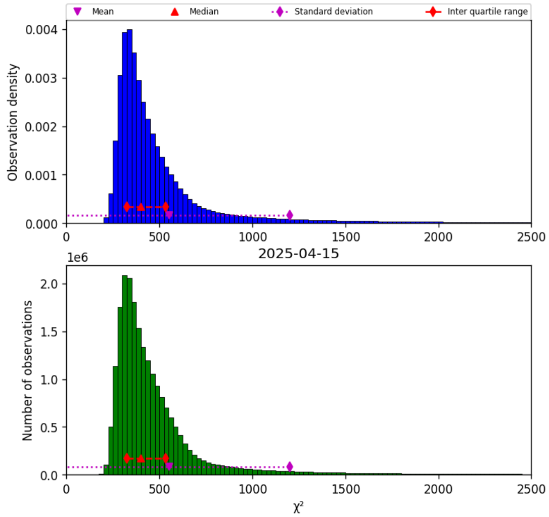
Figure 42: Histogram of “ \chi^2 ” for 2025-04-15 to 2025-04-16
