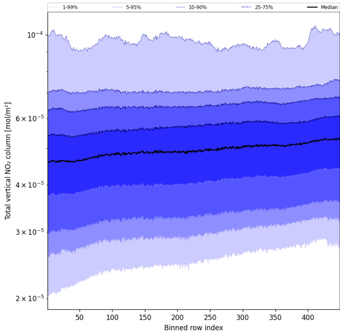
Figure 55: Along track statistics of “Total vertical NO 2 column” for 2025-04-15 to 2025-04-16
