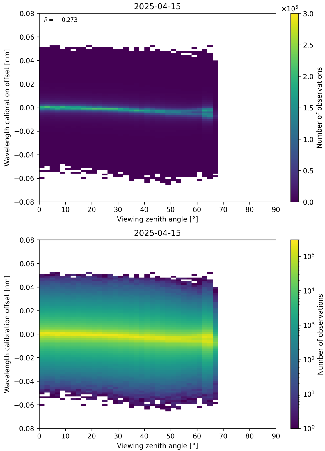
Figure 173: Scatter density plot of “Viewing zenith angle” against “Wavelength calibration offset” for 2025-04-15 to 2025-04-16.
