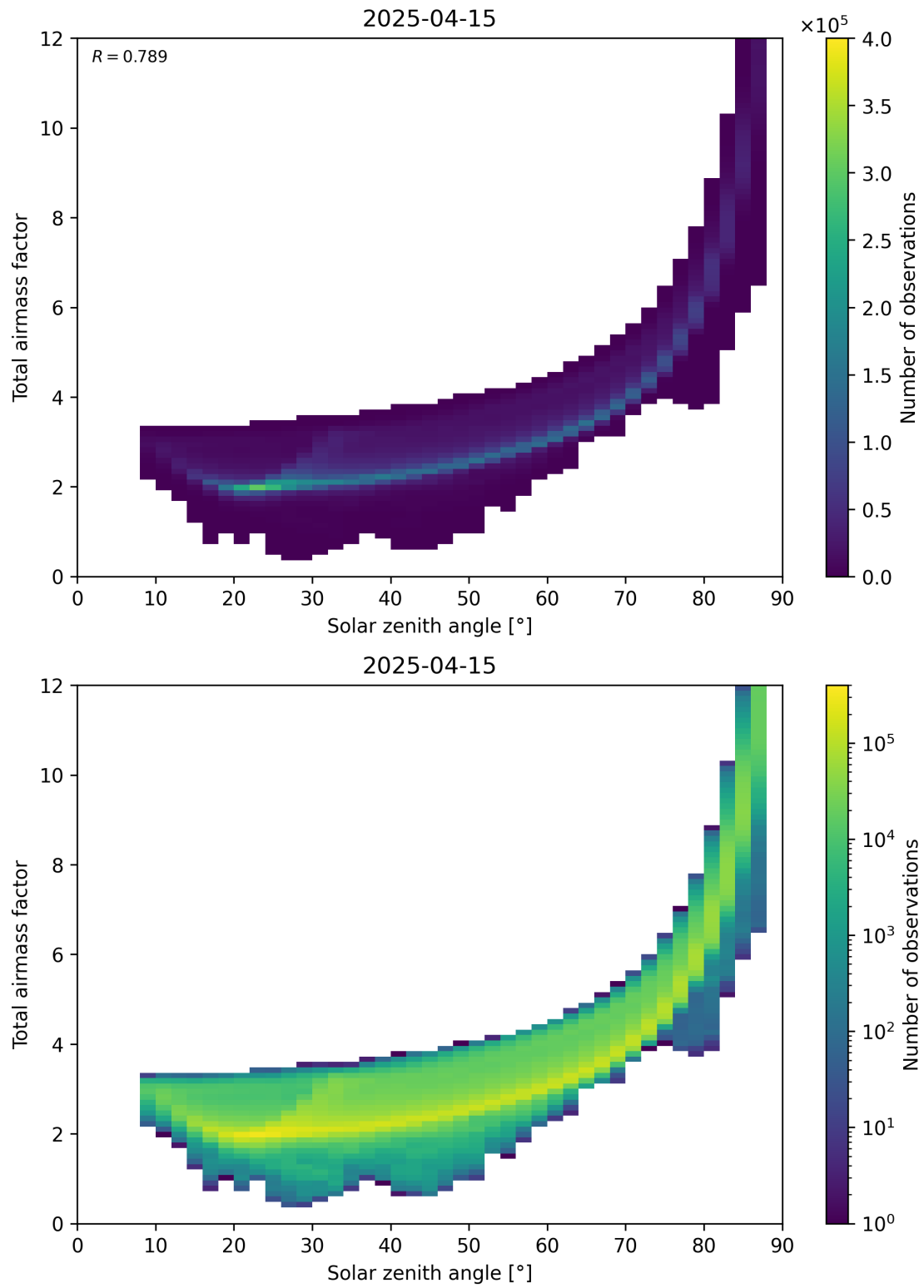
Figure 146: Scatter density plot of “Solar zenith angle” against “Total air mass factor” for 2025-04-15 to 2025-04-16.
