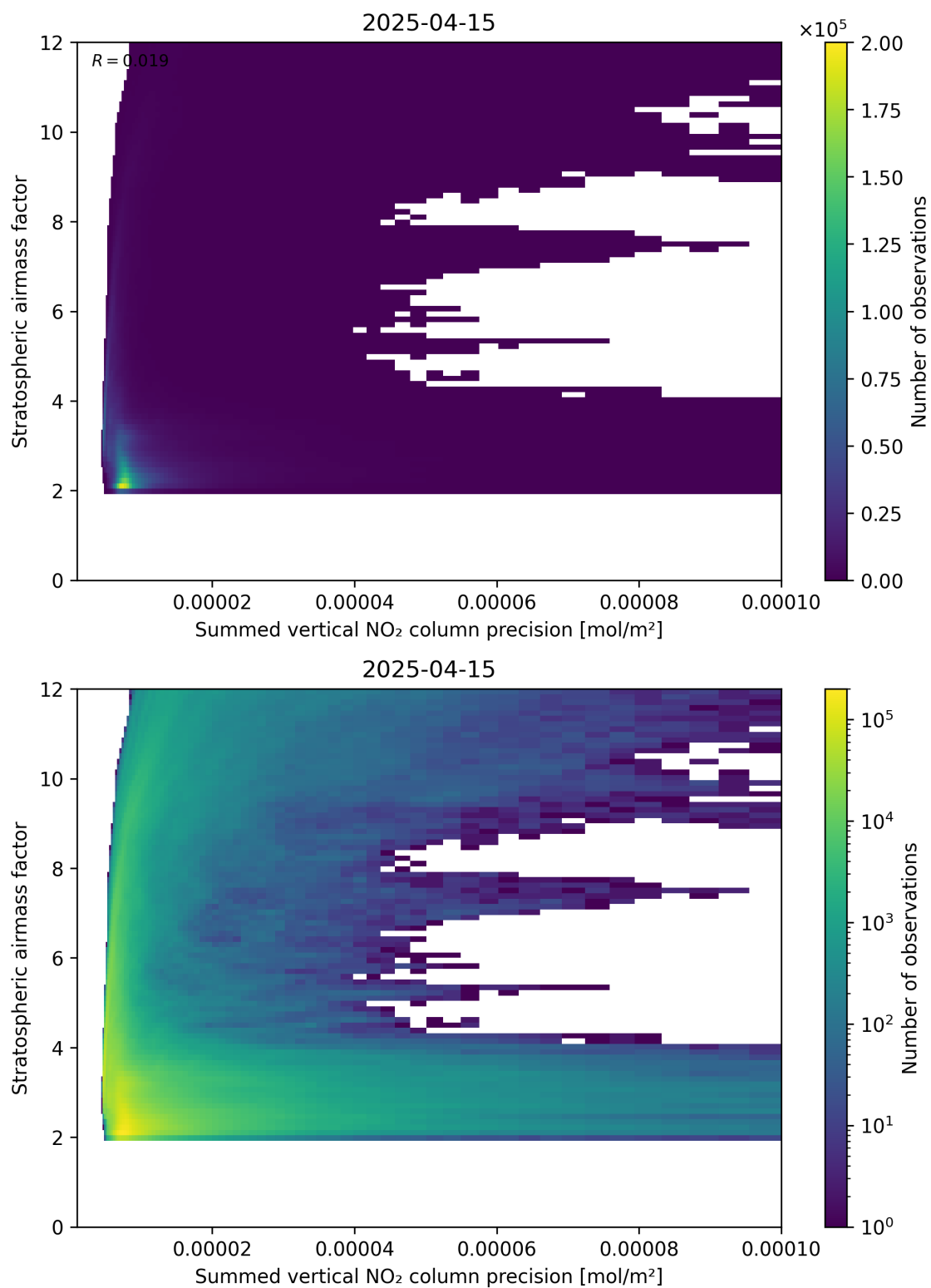
Figure 106: Scatter density plot of “Summed vertical NO 2 column precision” against “Stratospheric airmass factor” for 2025-04-15 to 2025-04-16.
