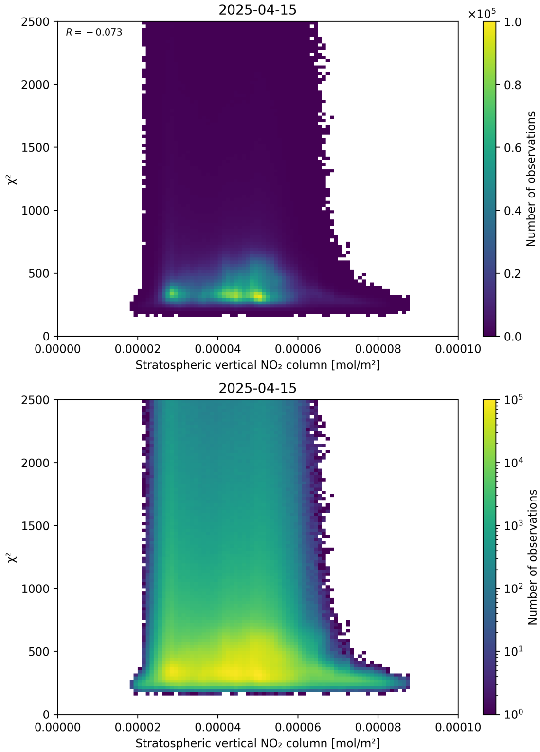
Figure 97: Scatter density plot of “Stratospheric vertical NO 2 column” against “ \chi^2 ” for 2025-04-15 to 2025-04-16.
