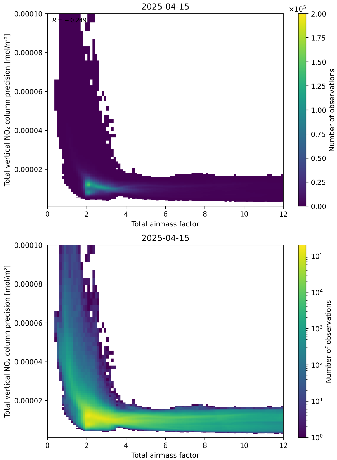
Figure 68: Scatter density plot of “Total airmass factor” against “Total vertical NO 2 column precision” for 2025-04-15 to 2025-04-16.
