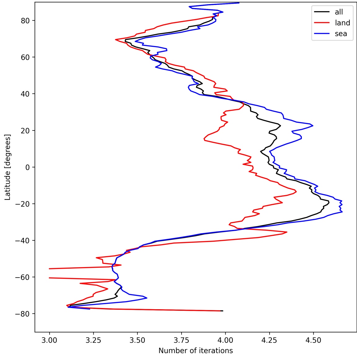
Figure 17: Zonal average of “Number of iterations” for 2025-04-15 to 2025-04-16.
