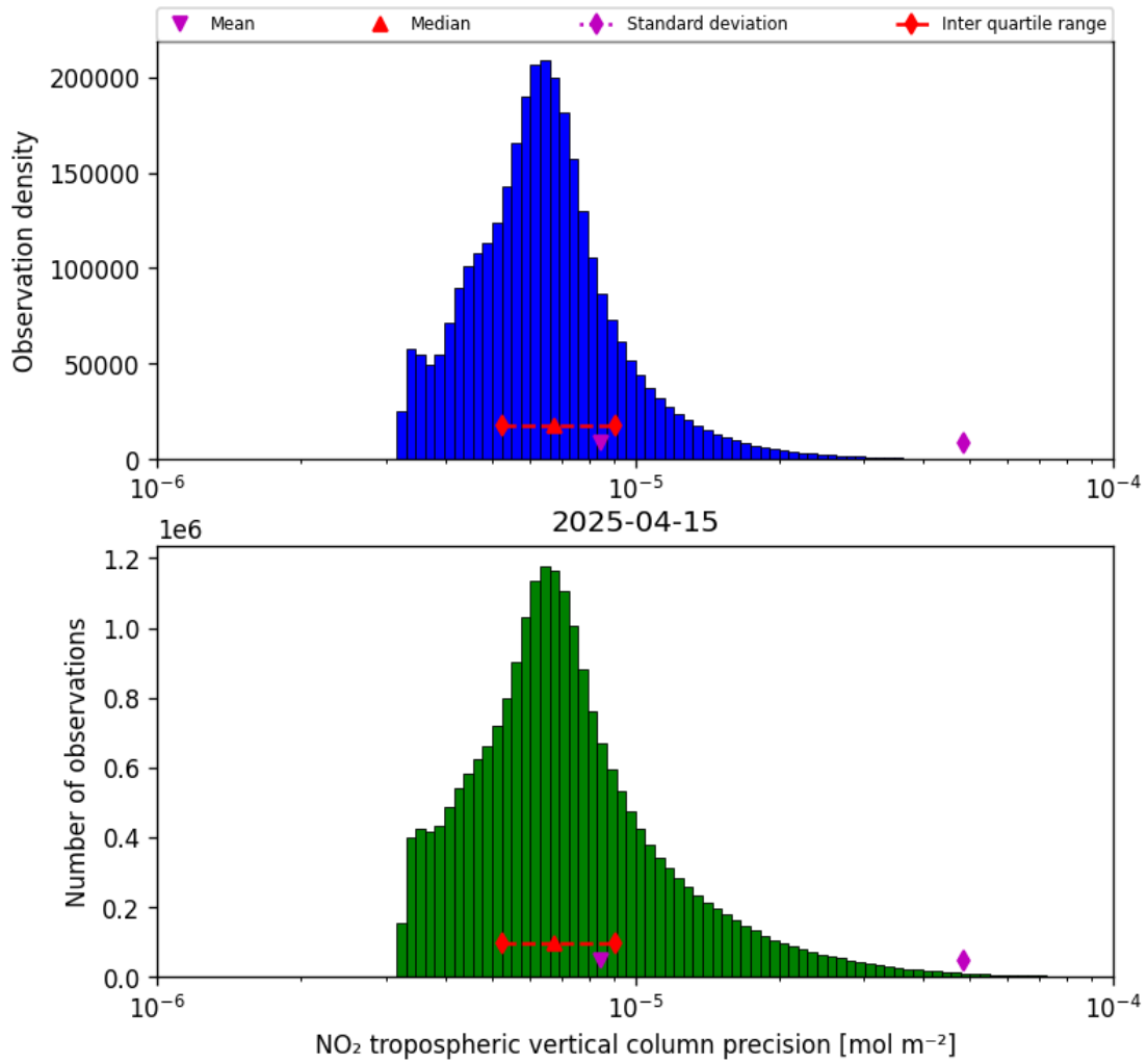
Figure 30: Histogram of “NO 2 tropospheric vertical column precision” for 2025-04-15 to 2025-04-16
