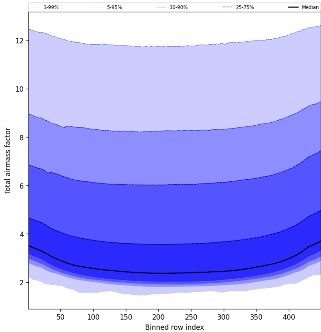
Figure 49: Along track statistics of “Total airmass factor” for 2025-04-15 to 2025-04-16
