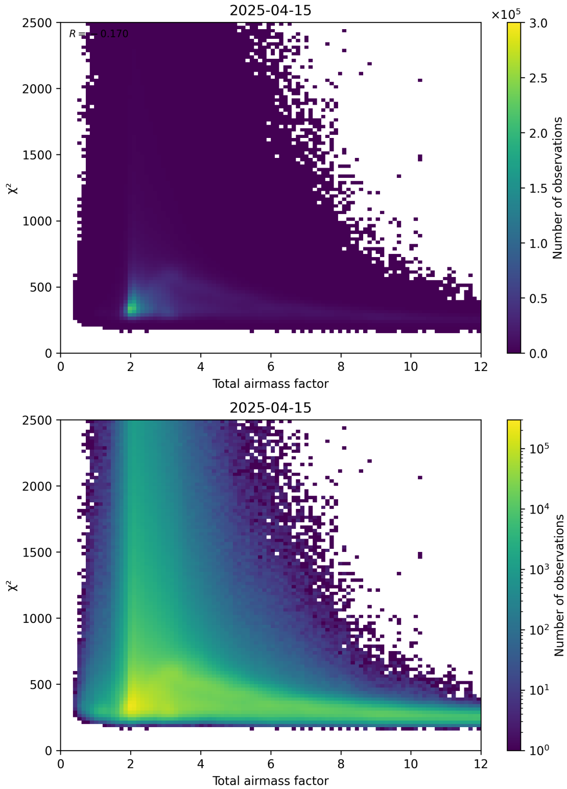
Figure 63: Scatter density plot of “Total airmass factor” against “ \chi^2 ” for 2025-04-15 to 2025-04-16.
