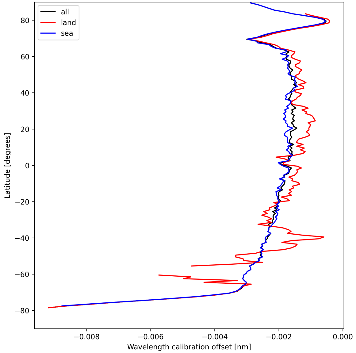
Figure 18: Zonal average of “Wavelength calibration offset” for 2025-04-15 to 2025-04-16.
