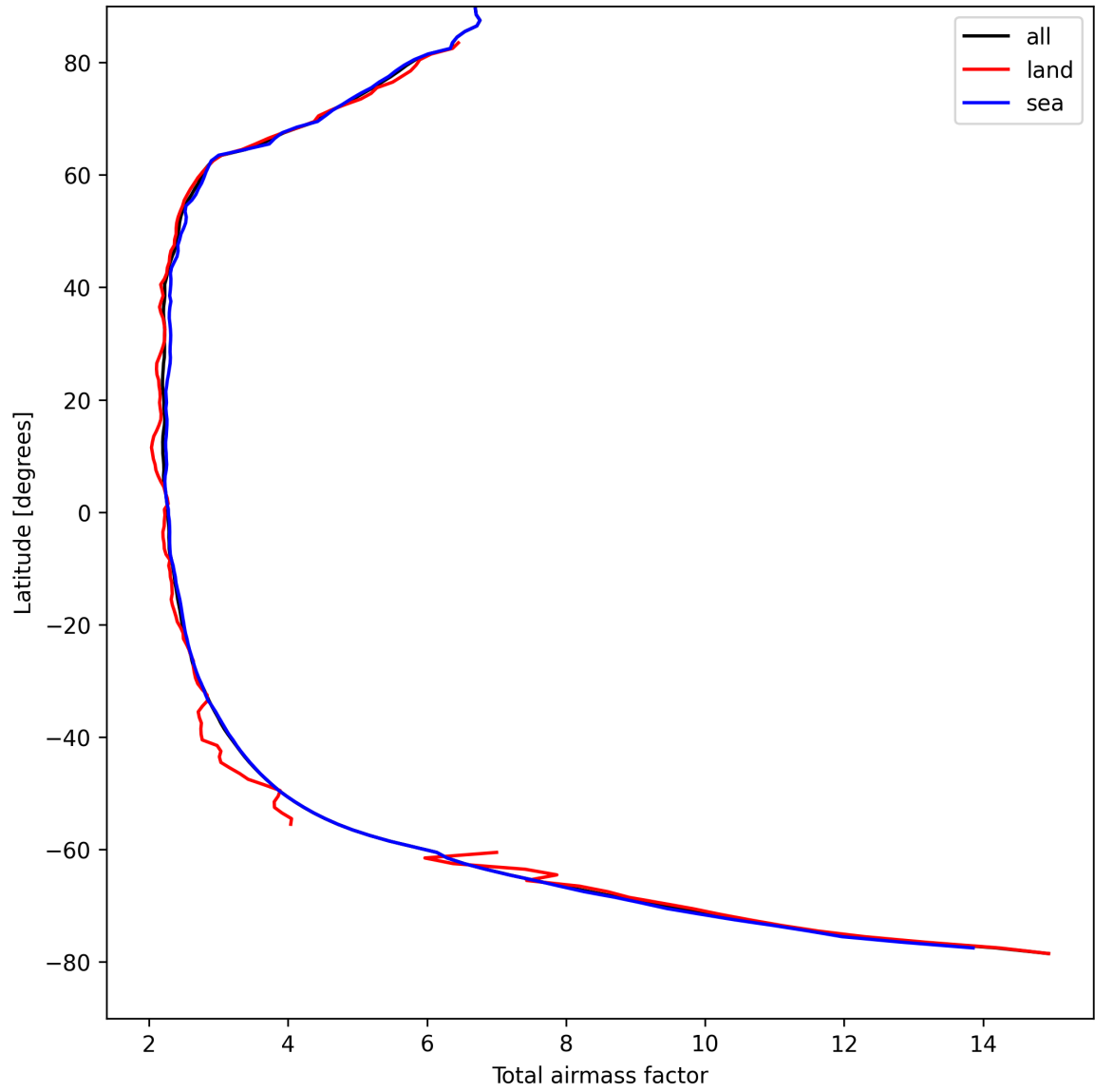
Figure 15: Zonal average of “Total airmass factor” for 2025-04-15 to 2025-04-16.
