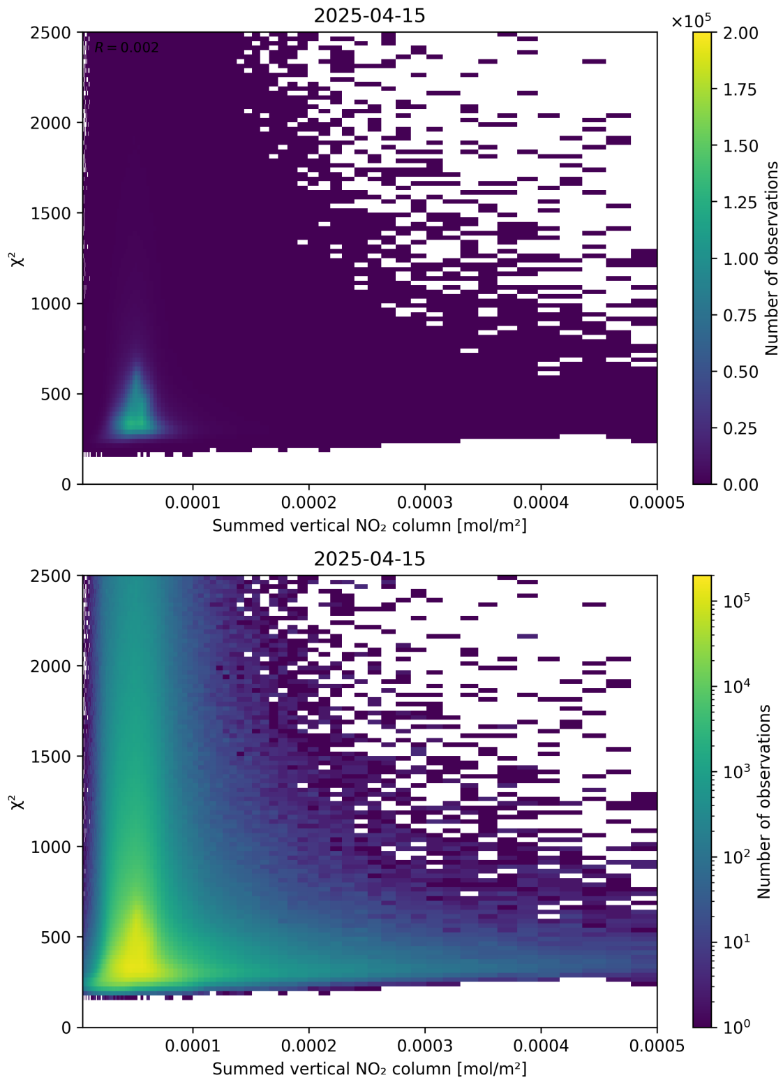
Figure 104: Scatter density plot of “Summed vertical NO 2 column” against “ \chi^2 ” for 2025-04-15 to 2025-04-16.
