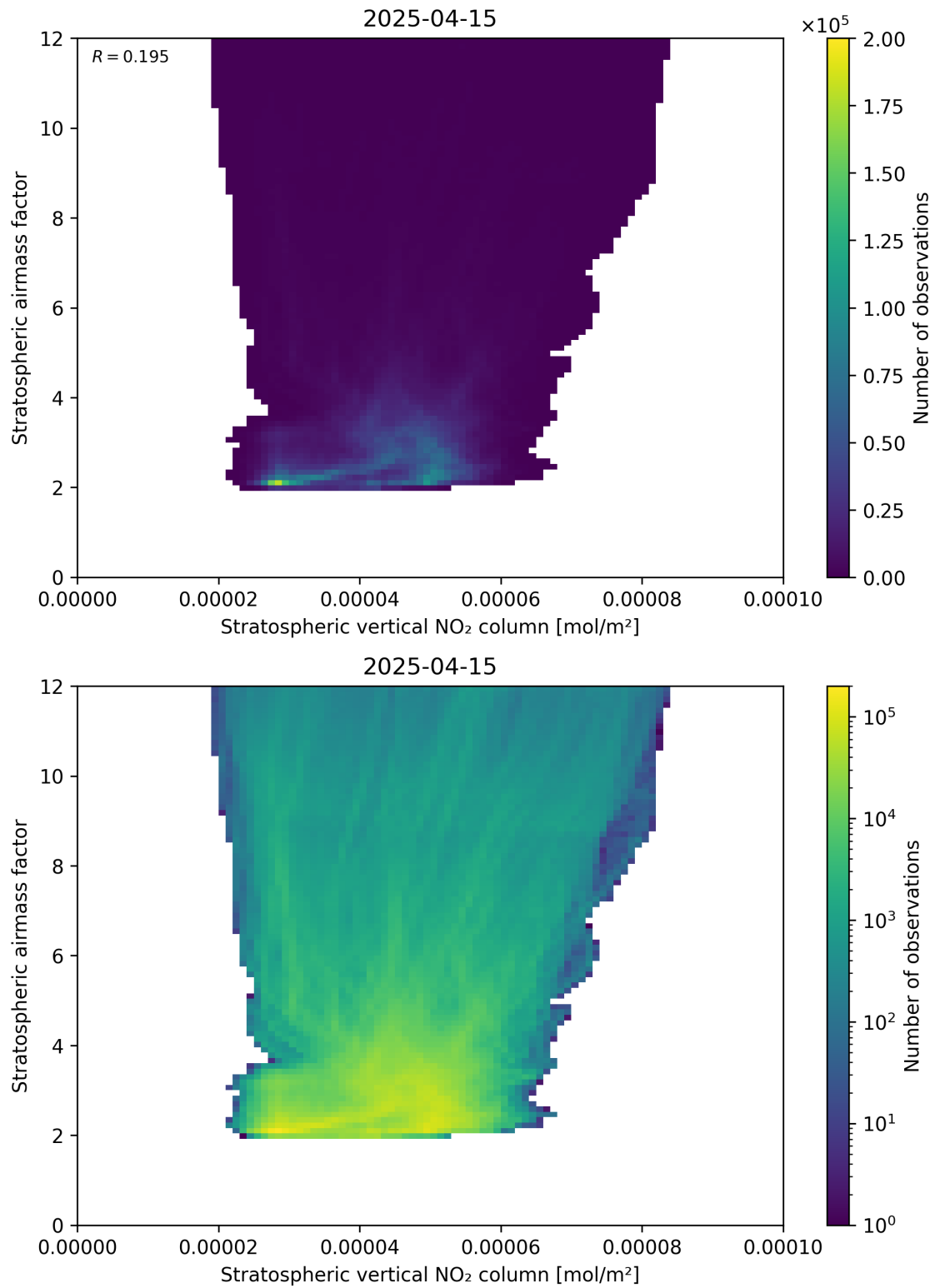
Figure 96: Scatter density plot of “Stratospheric vertical NO 2 column” against “Stratospheric airmass factor” for 2025-04-15 to 2025-04-16.
