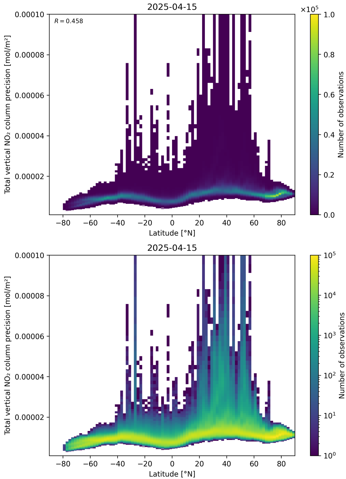
Figure 91: Scatter density plot of “Latitude” against “Total vertical NO 2 column precision” for 2025-04-15 to 2025-04-16.
