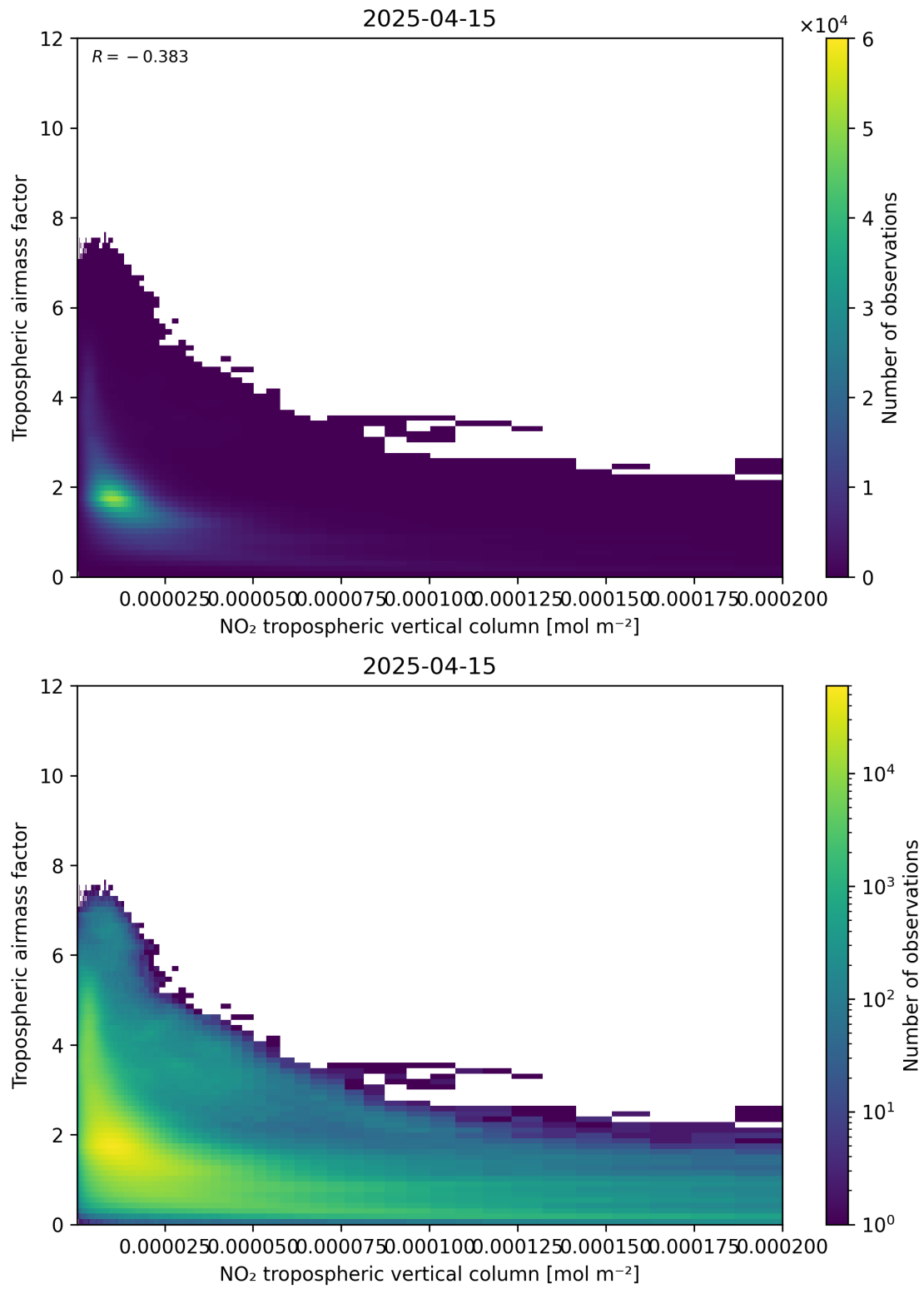
Figure 123: Scatter density plot of “NO 2 tropospheric vertical column” against “Tropospheric air mass factor” for 2025-04-15 to 2025-04-16.
