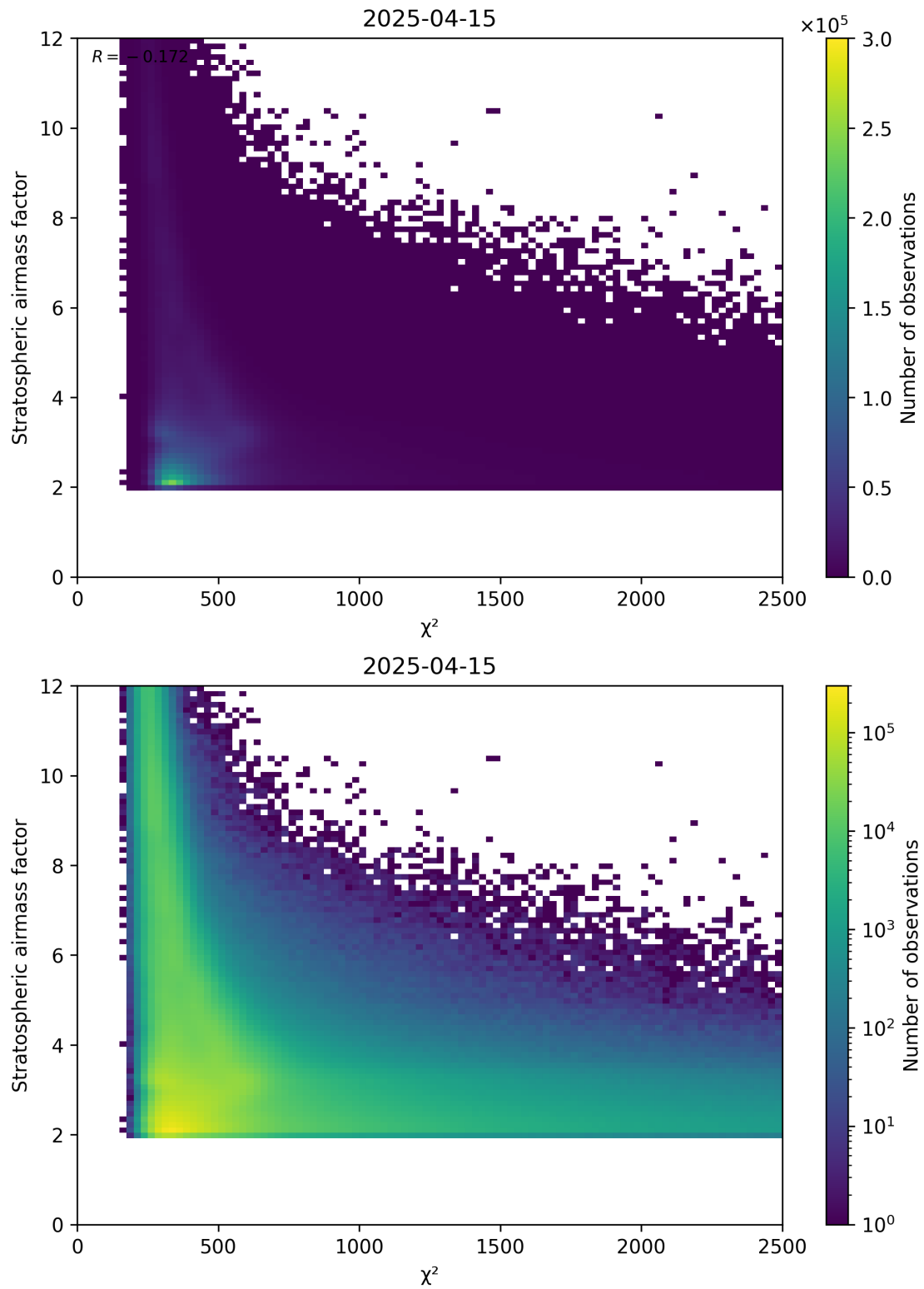
Figure 81: Scatter density plot of “ \chi^2 ” against “Stratospheric airmass factor” for 2025-04-15 to 2025-04-16.
