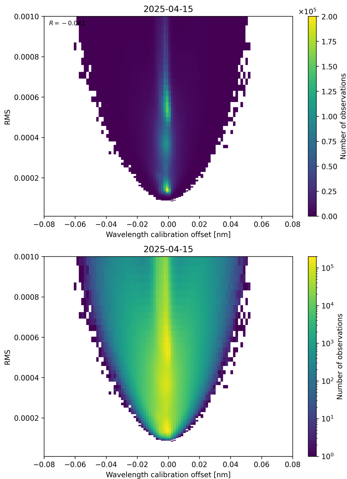
Figure 181: Scatter density plot of “Wavelength calibration offset” against “RMS” for 2025-04-15 to 2025-04-16.
