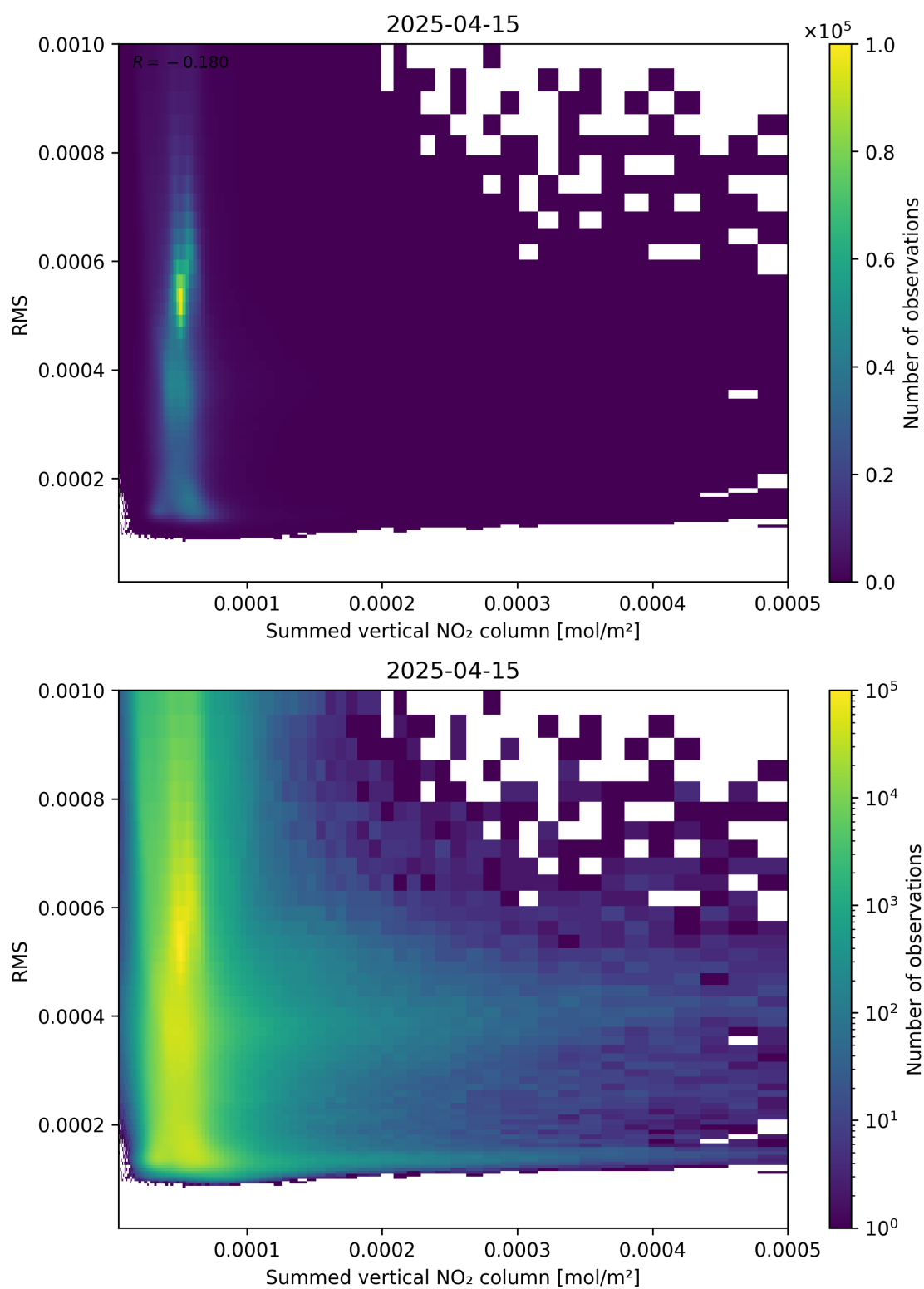
Figure 109: Scatter density plot of “Summed vertical NO 2 column” against “RMS” for 2025-04-15 to 2025-04-16.
