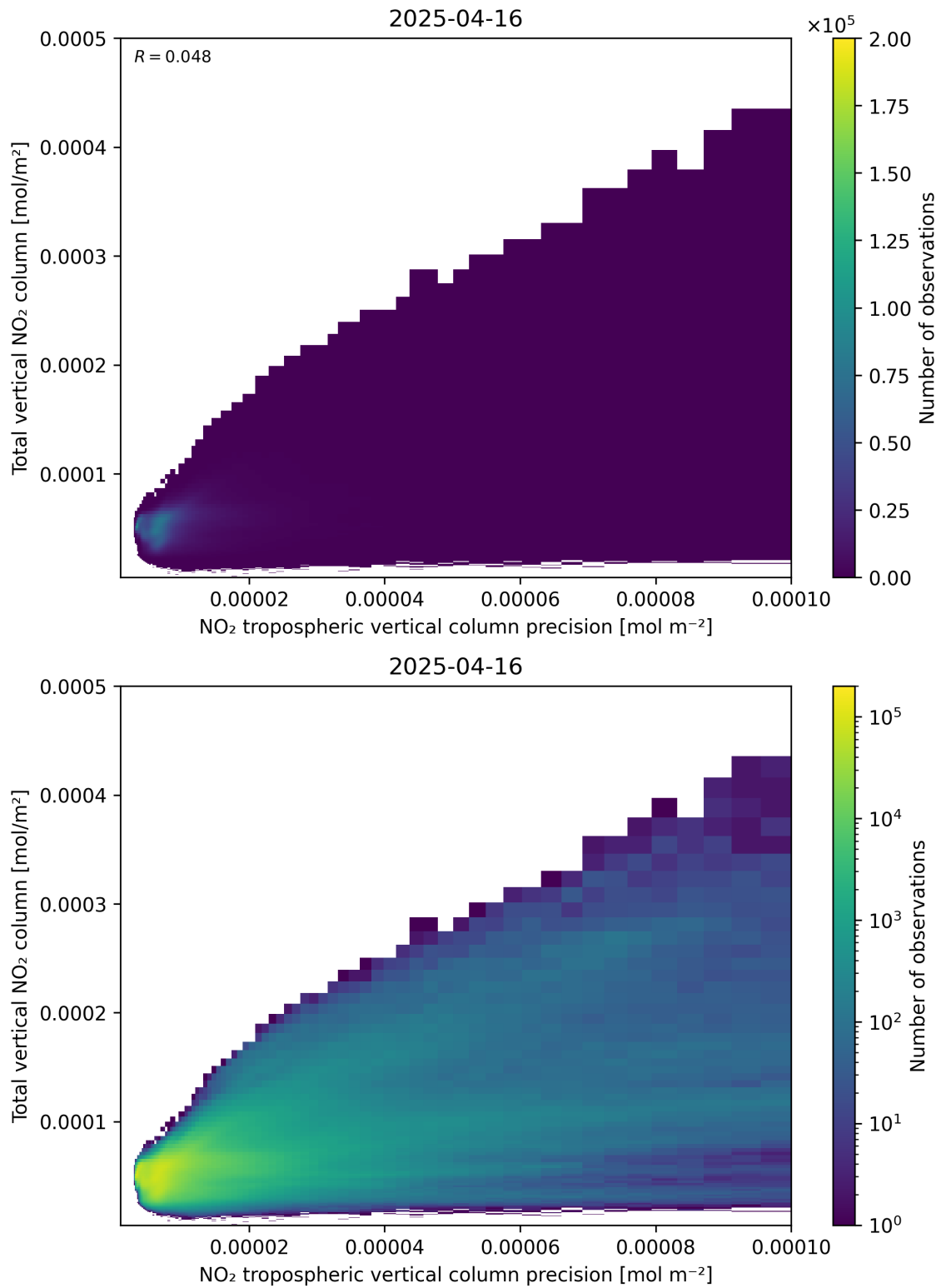
Figure 138: Scatter density plot of “NO 2 tropospheric vertical column precision” against “Total vertical NO 2 column” for 2025-04-16 to 2025-04-16.
