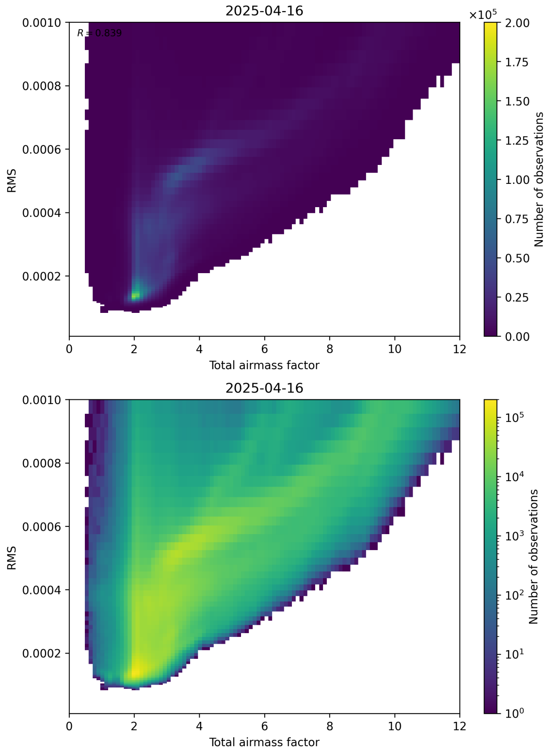
Figure 69: Scatter density plot of “Total airmass factor” against “RMS” for 2025-04-16 to 2025-04-16.
