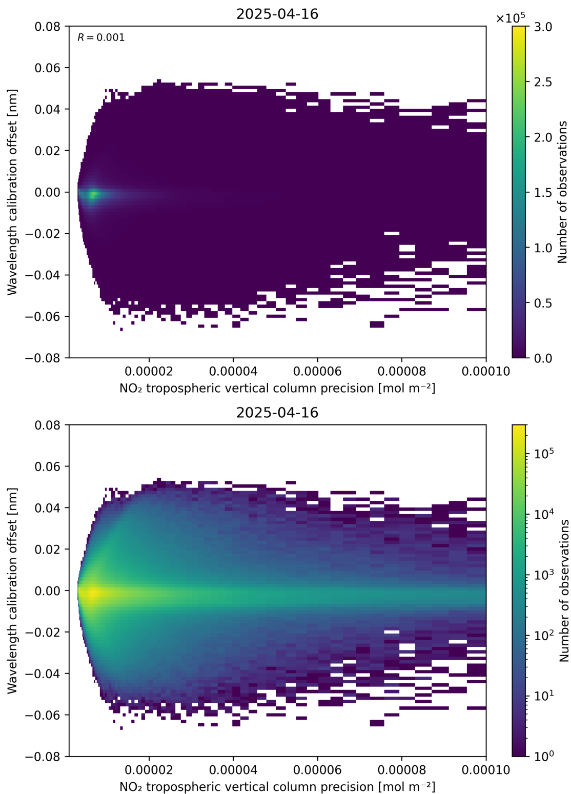
Figure 141: Scatter density plot of “NO 2 tropospheric vertical column precision” against “Wavelength calibration offset” for 2025-04-16 to 2025-04-16.
