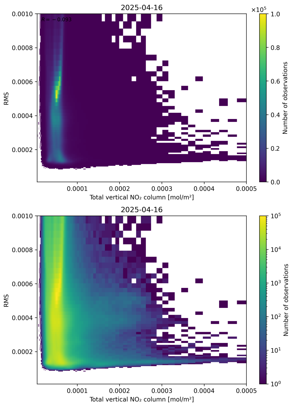
Figure 120: Scatter density plot of “Total vertical NO 2 column” against “RMS” for 2025-04-16 to 2025-04-16.
