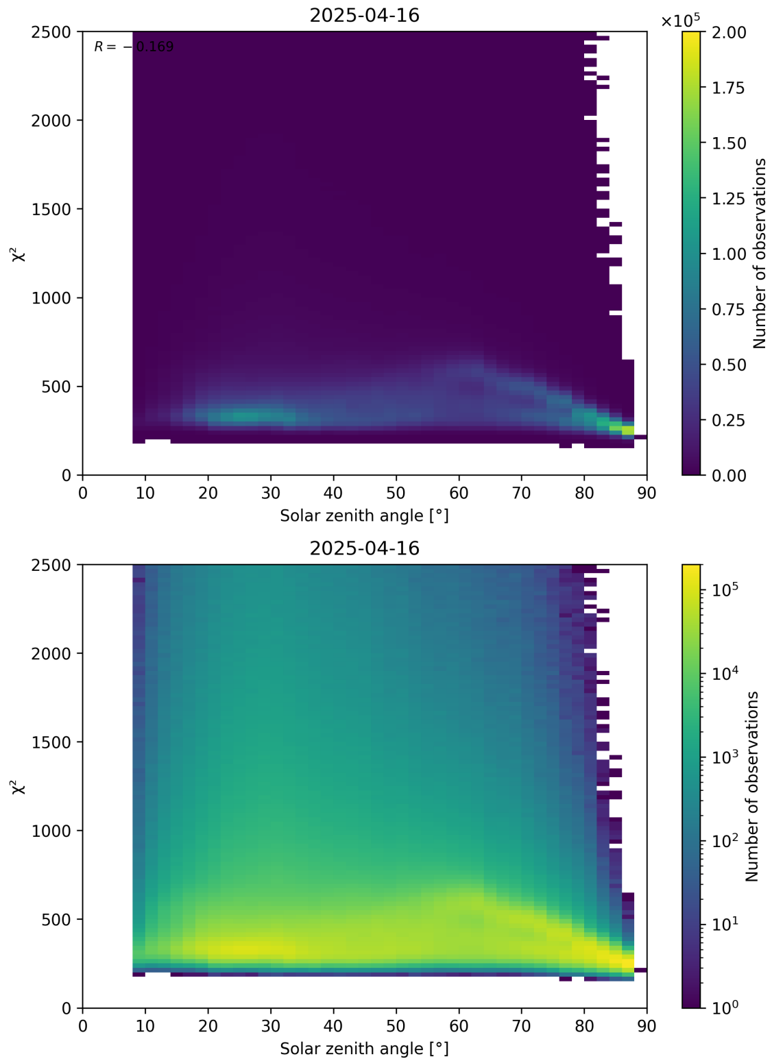
Figure 148: Scatter density plot of “Solar zenith angle” against “ \chi^2 ” for 2025-04-16 to 2025-04-16.
