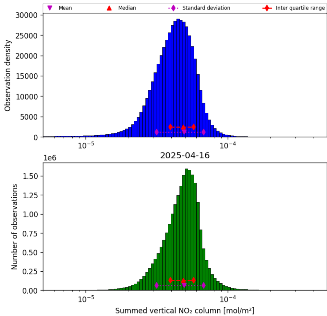
Figure 40: Histogram of “Summed vertical NO 2 column” for 2025-04-16 to 2025-04-16
