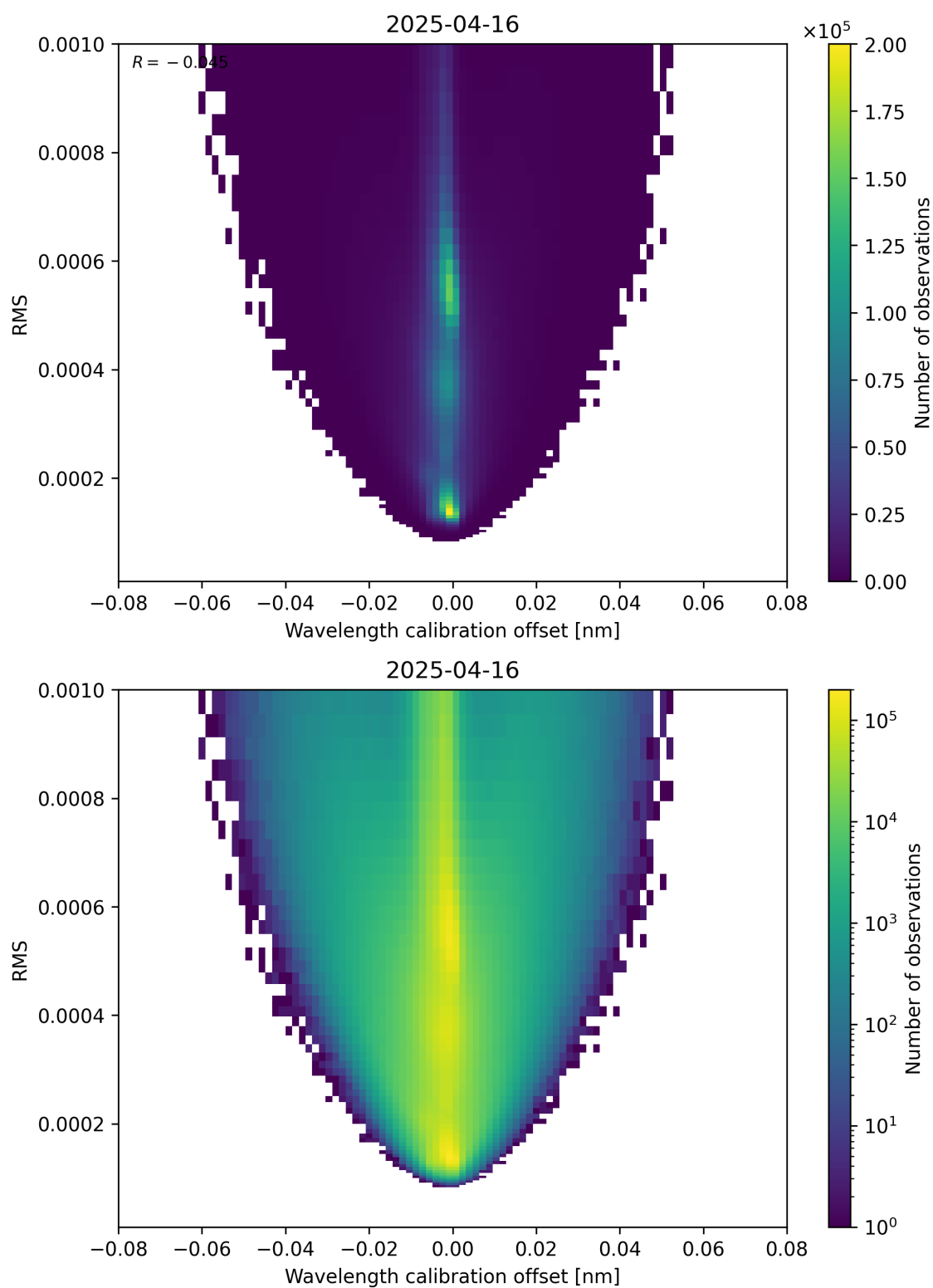
Figure 181: Scatter density plot of “Wavelength calibration offset” against “RMS” for 2025-04-16 to 2025-04-16.
