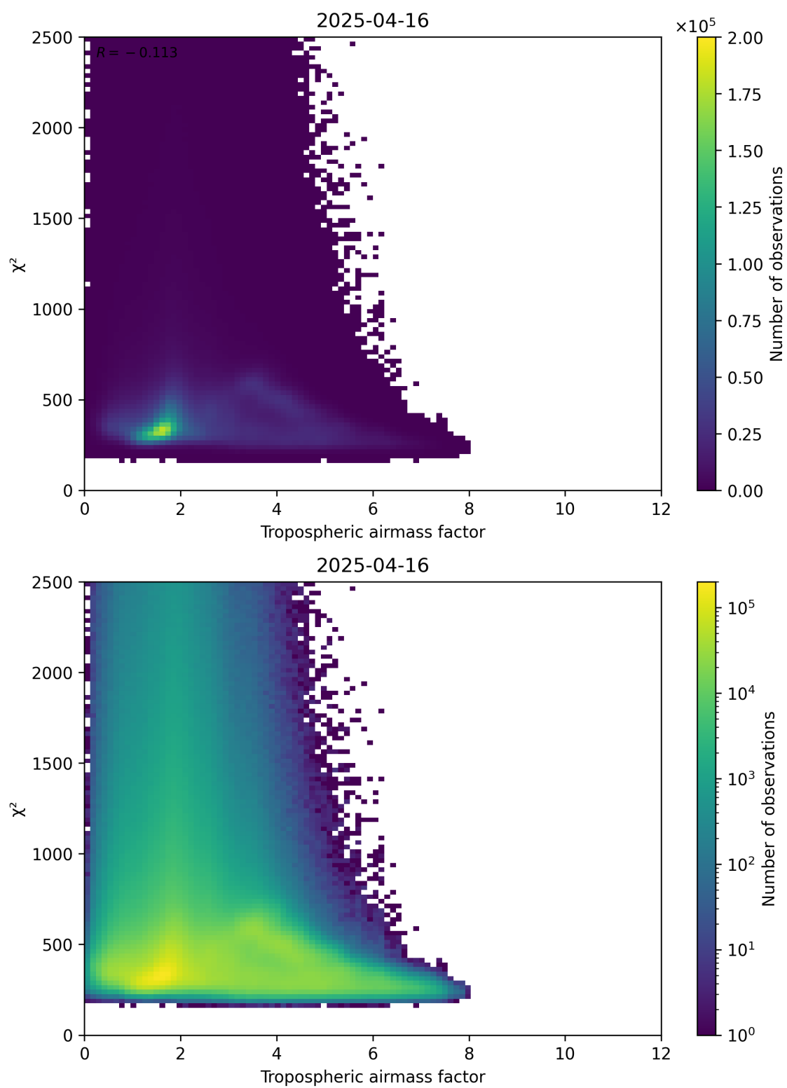
Figure 73: Scatter density plot of “Tropospheric airmass factor” against “ \chi^2 ” for 2025-04-16 to 2025-04-16.
