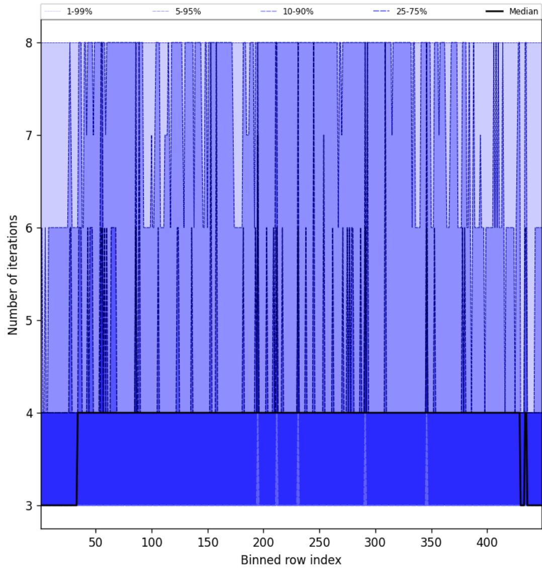
Figure 51: Along track statistics of “Number of iterations” for 2025-04-16 to 2025-04-16
