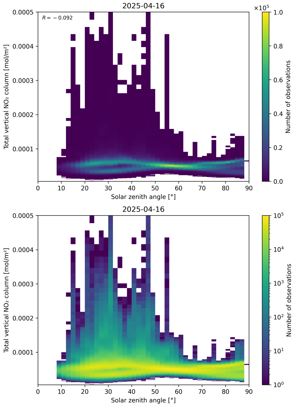
Figure 153: Scatter density plot of “Solar zenith angle” against “Total vertical NO 2 column” for 2025-04-16 to 2025-04-16.
