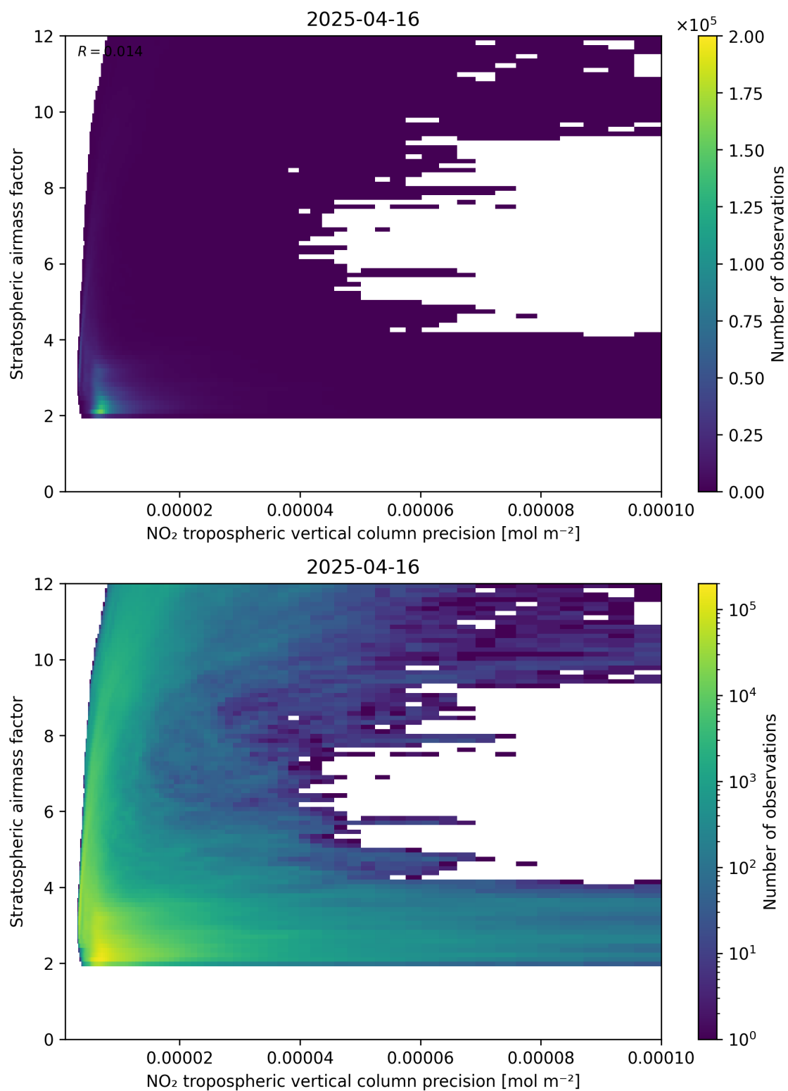
Figure 131: Scatter density plot of “NO 2 tropospheric vertical column precision” against “Stratospheric airmass factor” for 2025-04-16 to 2025-04-16.
