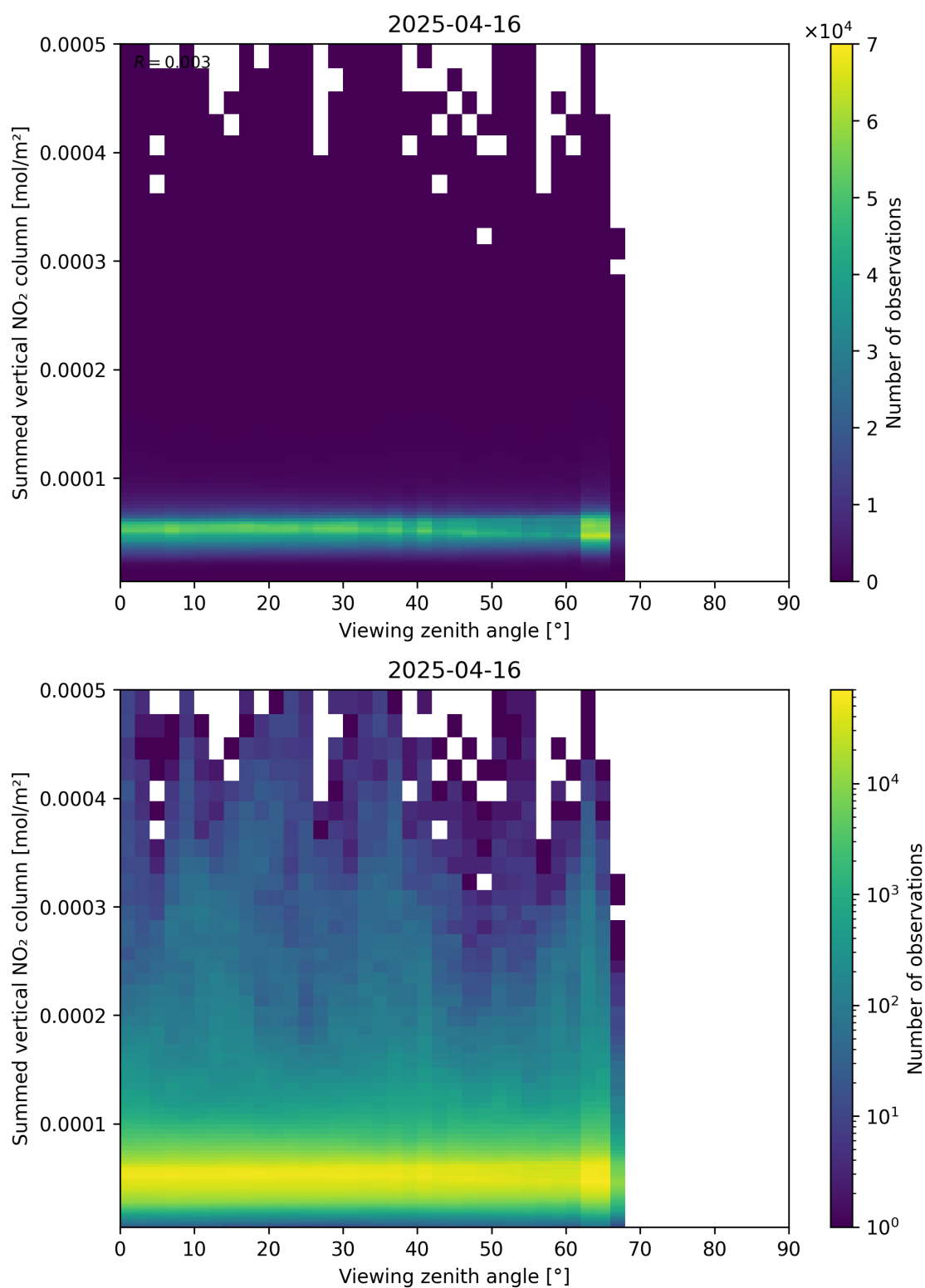
Figure 165: Scatter density plot of “Viewing zenith angle” against “Summed vertical NO 2 column” for 2025-04-16 to 2025-04-16.
