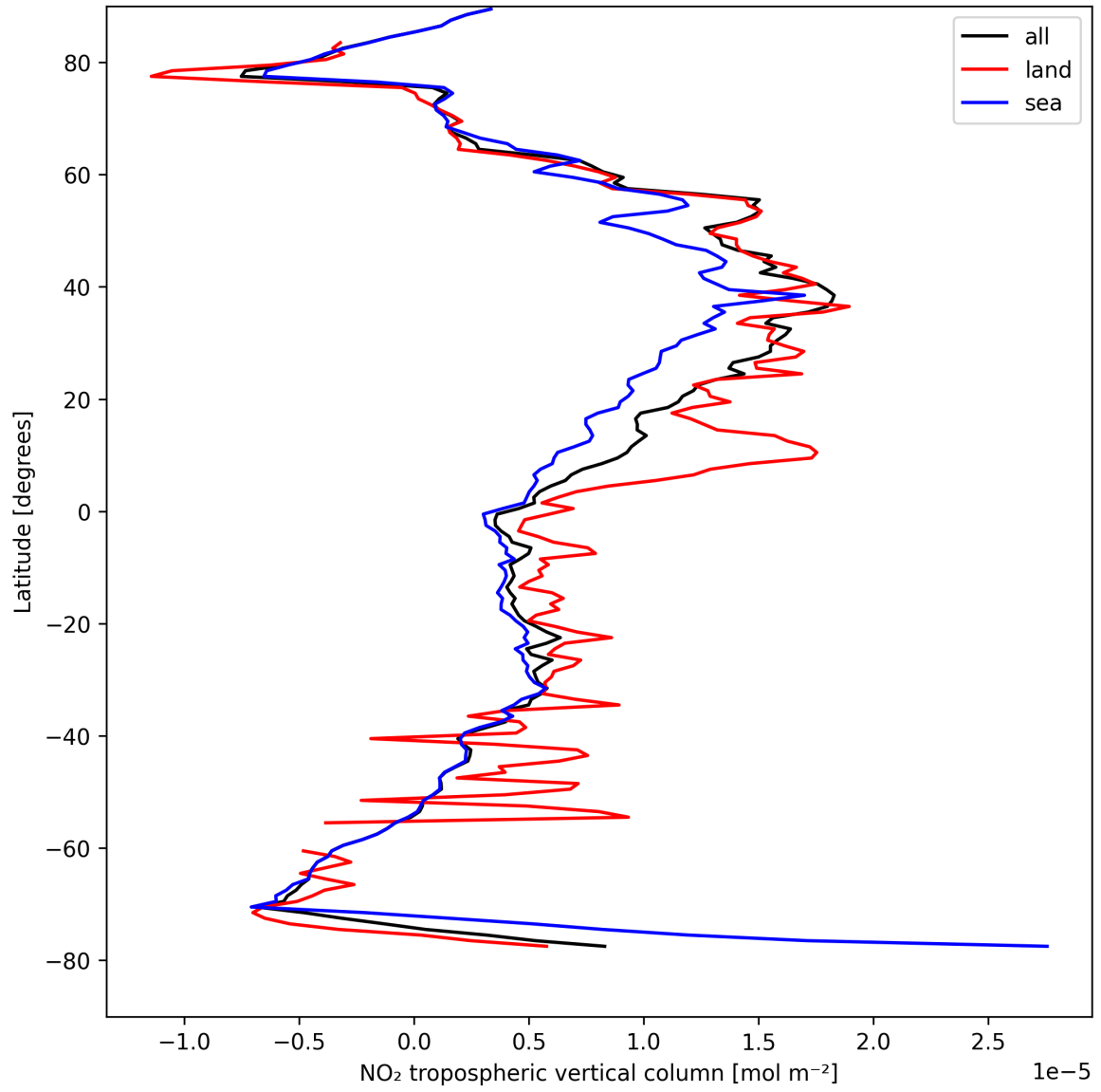
Figure 12: Zonal average of “NO 2 tropospheric vertical column” for 2025-04-16 to 2025-04-16.
