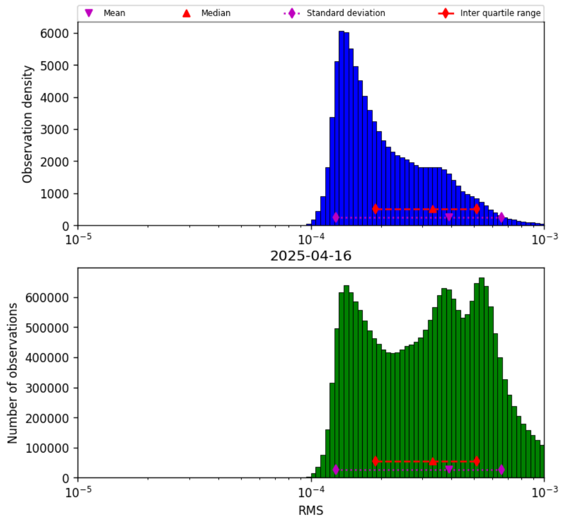
Figure 43: Histogram of “RMS” for 2025-04-16 to 2025-04-16
