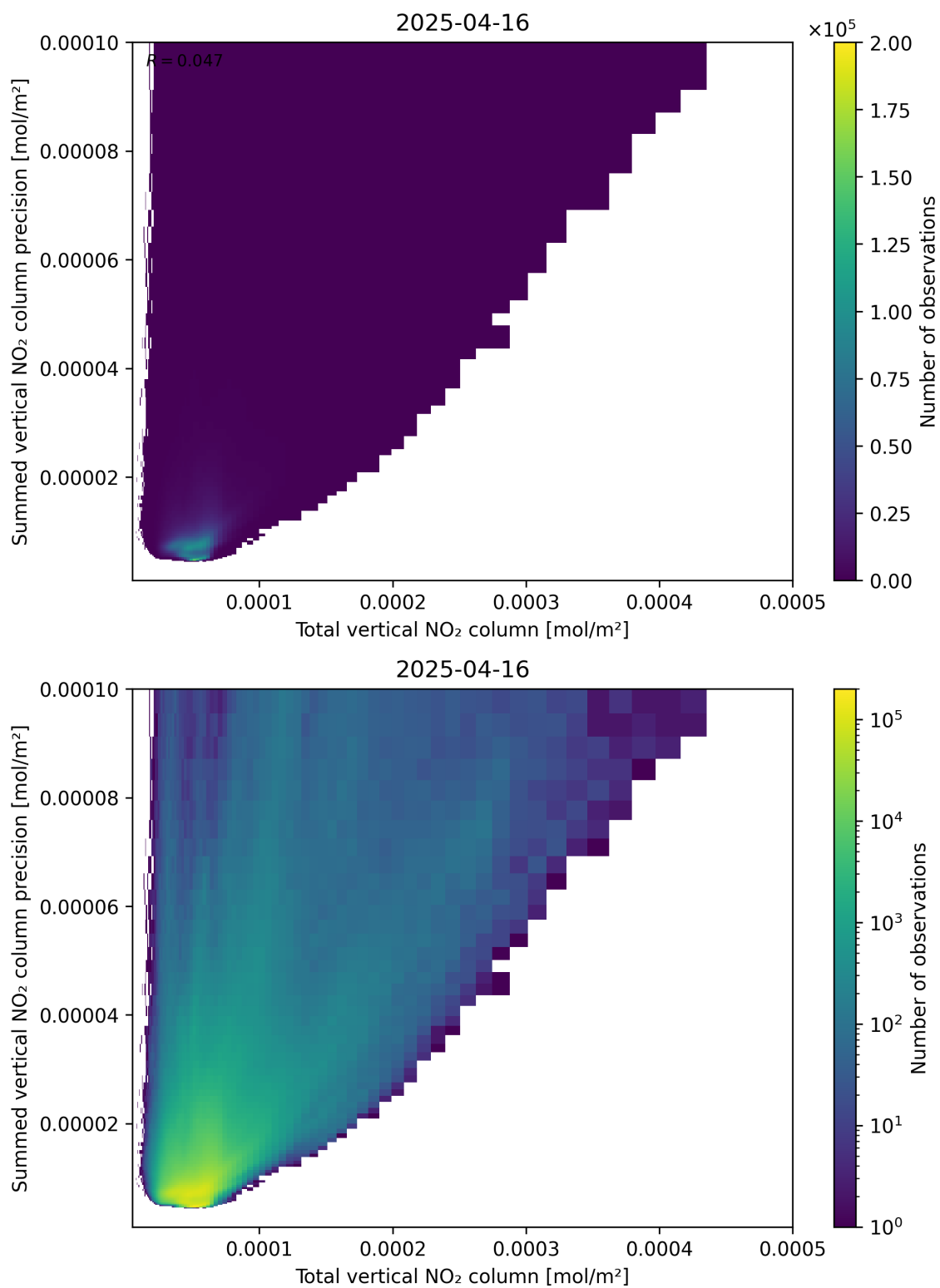
Figure 113: Scatter density plot of “Total vertical NO 2 column” against “Summed vertical NO 2 column precision” for 2025-04-16 to 2025-04-16.
