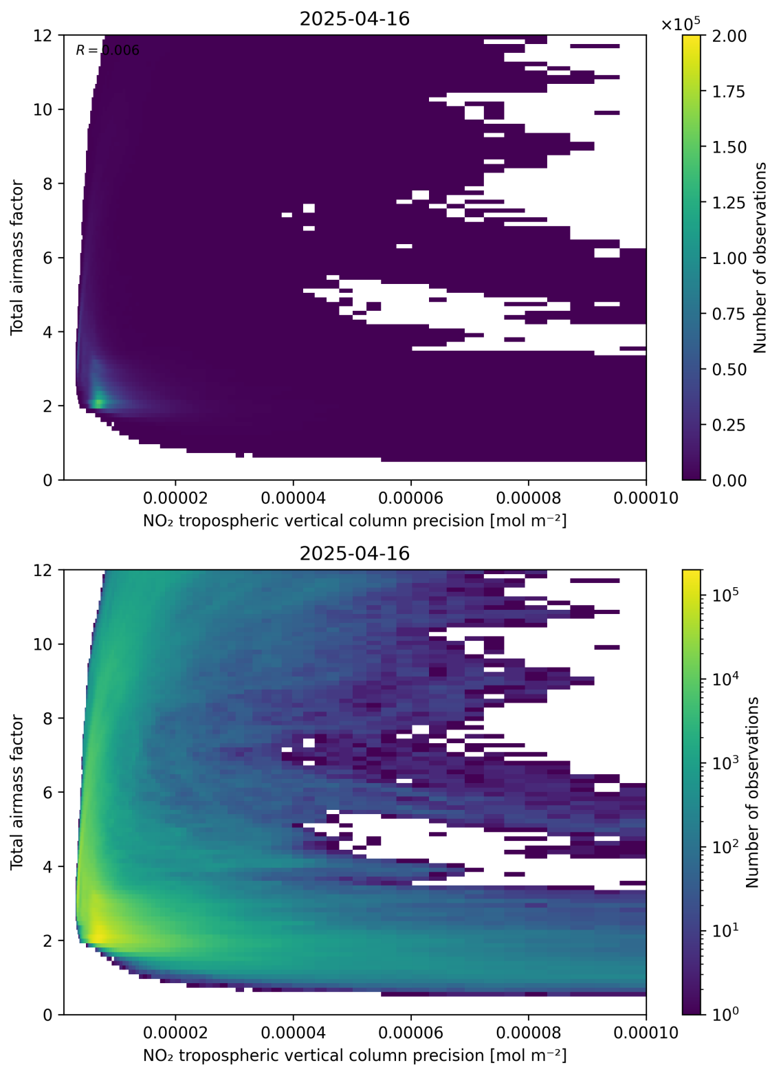
Figure 132: Scatter density plot of “NO 2 tropospheric vertical column precision” against “Total airmass factor” for 2025-04-16 to 2025-04-16.
