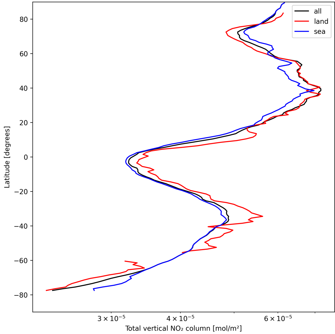
Figure 21: Zonal average of “Total vertical NO 2 column” for 2025-04-16 to 2025-04-16.
