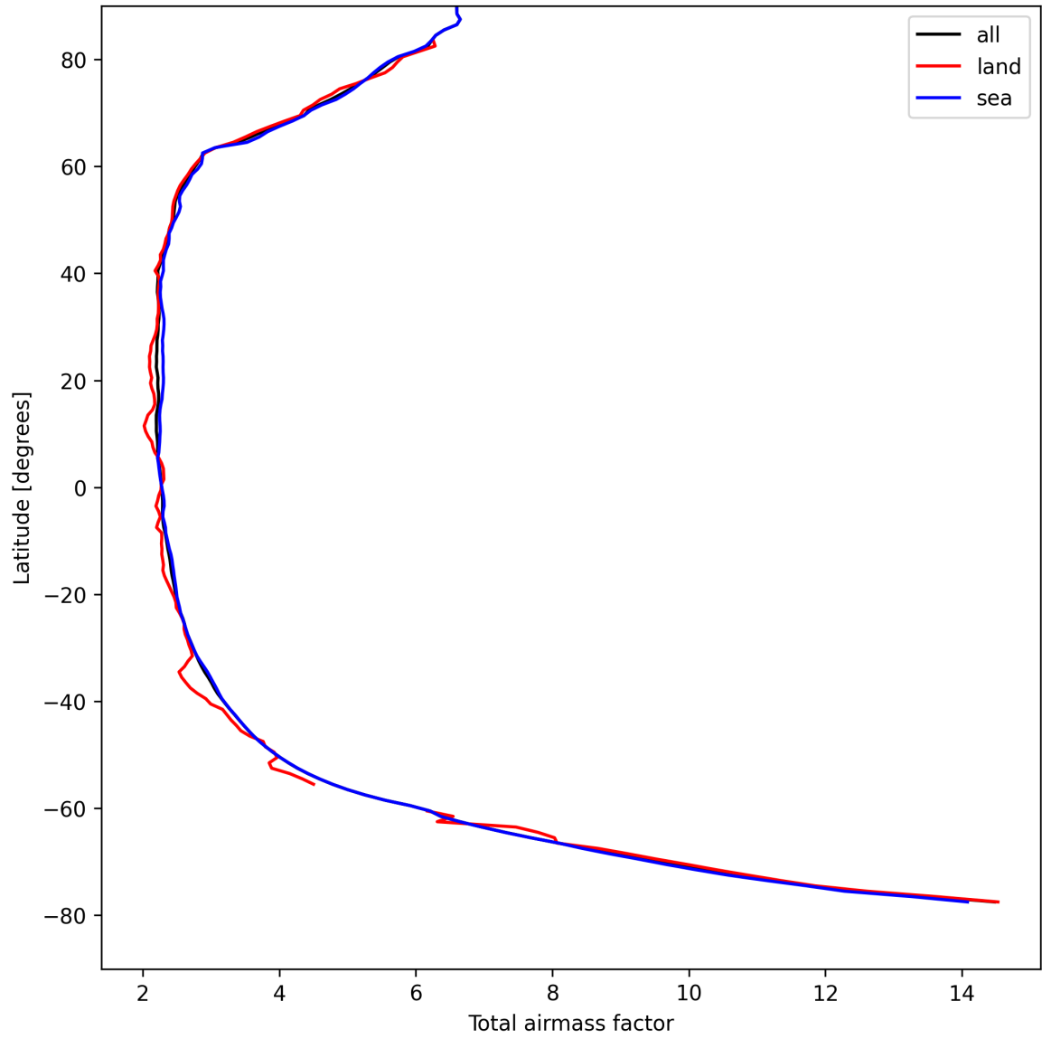
Figure 15: Zonal average of “Total airmass factor” for 2025-04-16 to 2025-04-16.
