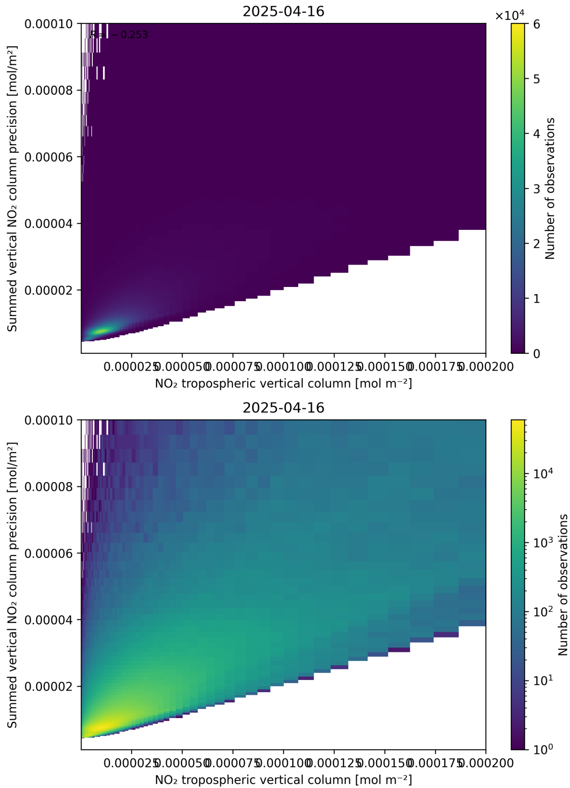
Figure 127: Scatter density plot of “NO 2 tropospheric vertical column” against “Summed vertical NO 2 column precision” for 2025-04-16 to 2025-04-16.
