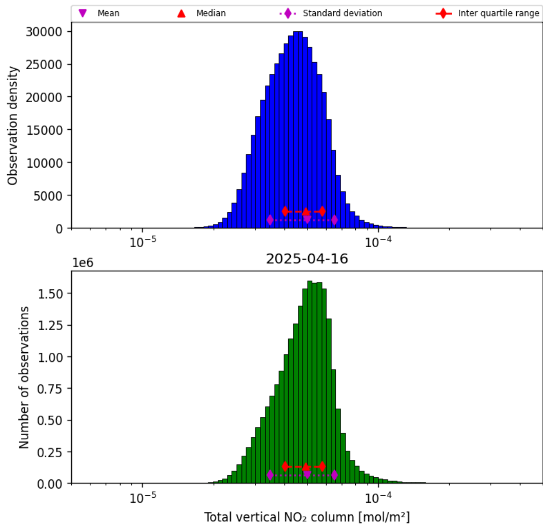
Figure 38: Histogram of "Total vertical NO 2 column" for 2025-04-16 to 2025-04-16
