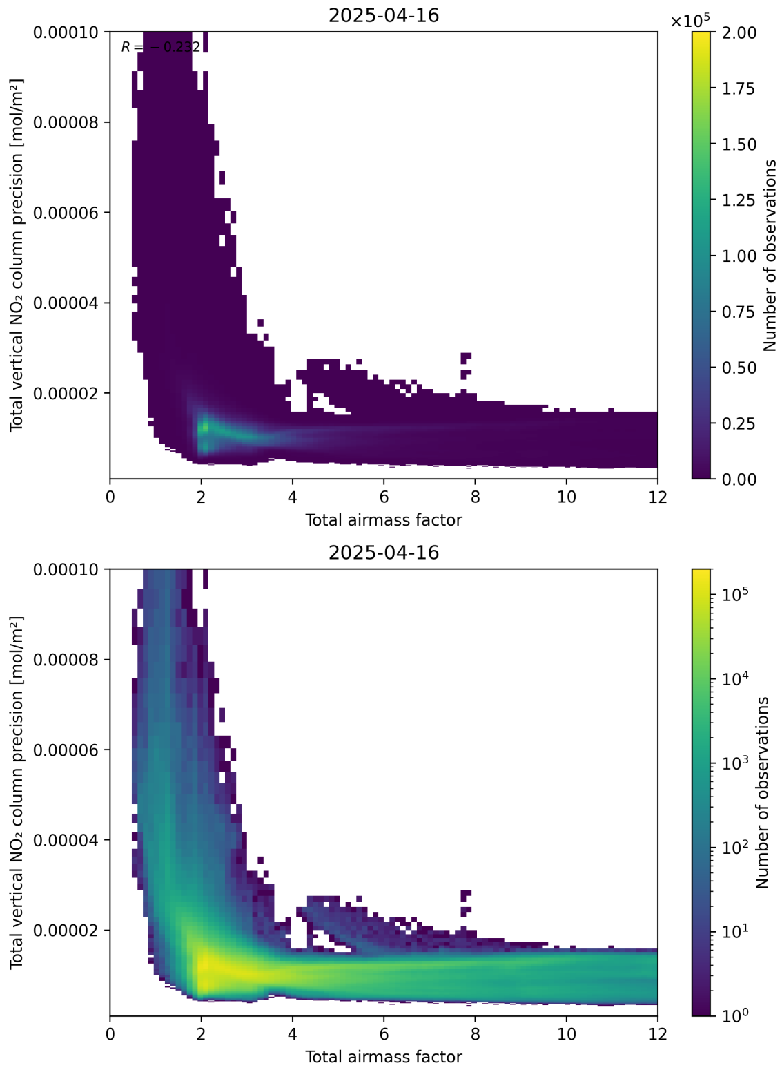
Figure 68: Scatter density plot of “Total airmass factor” against “Total vertical NO 2 column precision” for 2025-04-16 to 2025-04-16.
