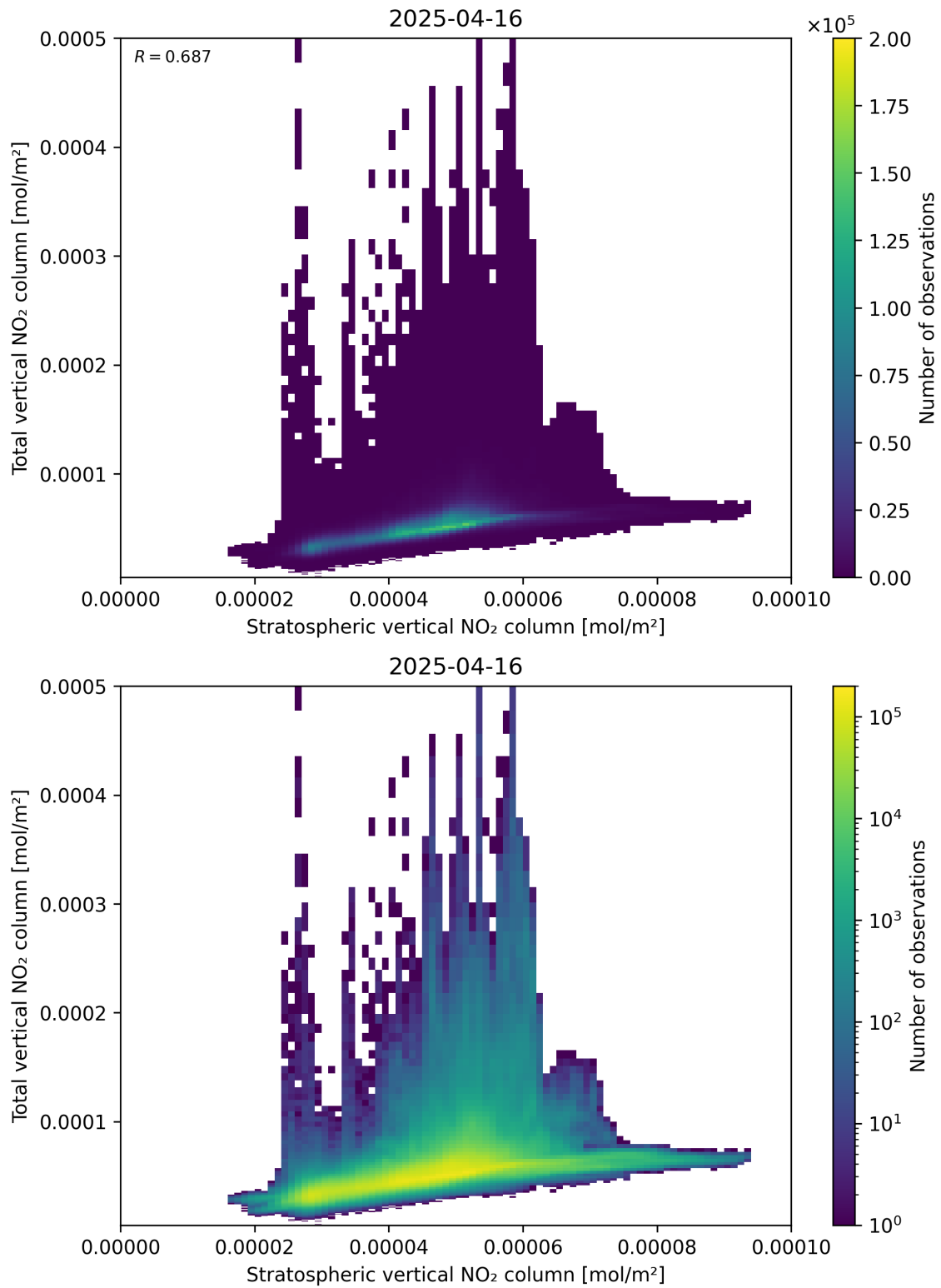
Figure 100: Scatter density plot of “Stratospheric vertical NO 2 column” against “Total vertical NO 2 column” for 2025-04-16 to 2025-04-16.
