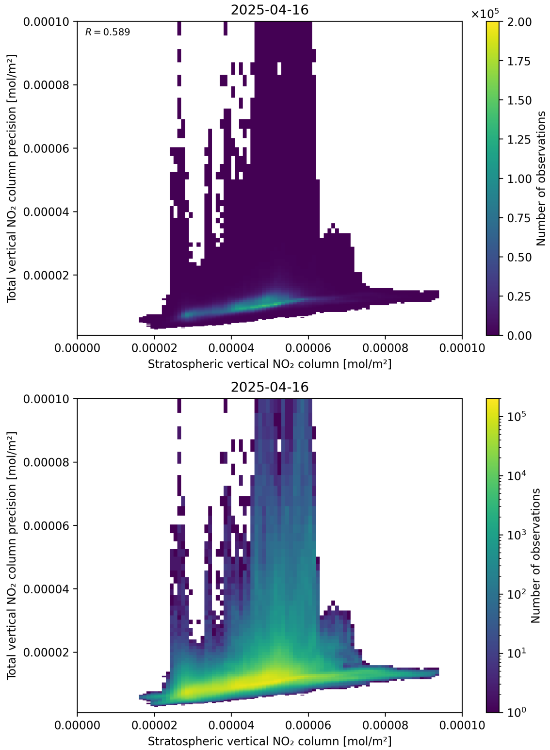
Figure 101: Scatter density plot of “Stratospheric vertical NO 2 column” against “Total vertical NO 2 column precision” for 2025-04-16 to 2025-04-16.
