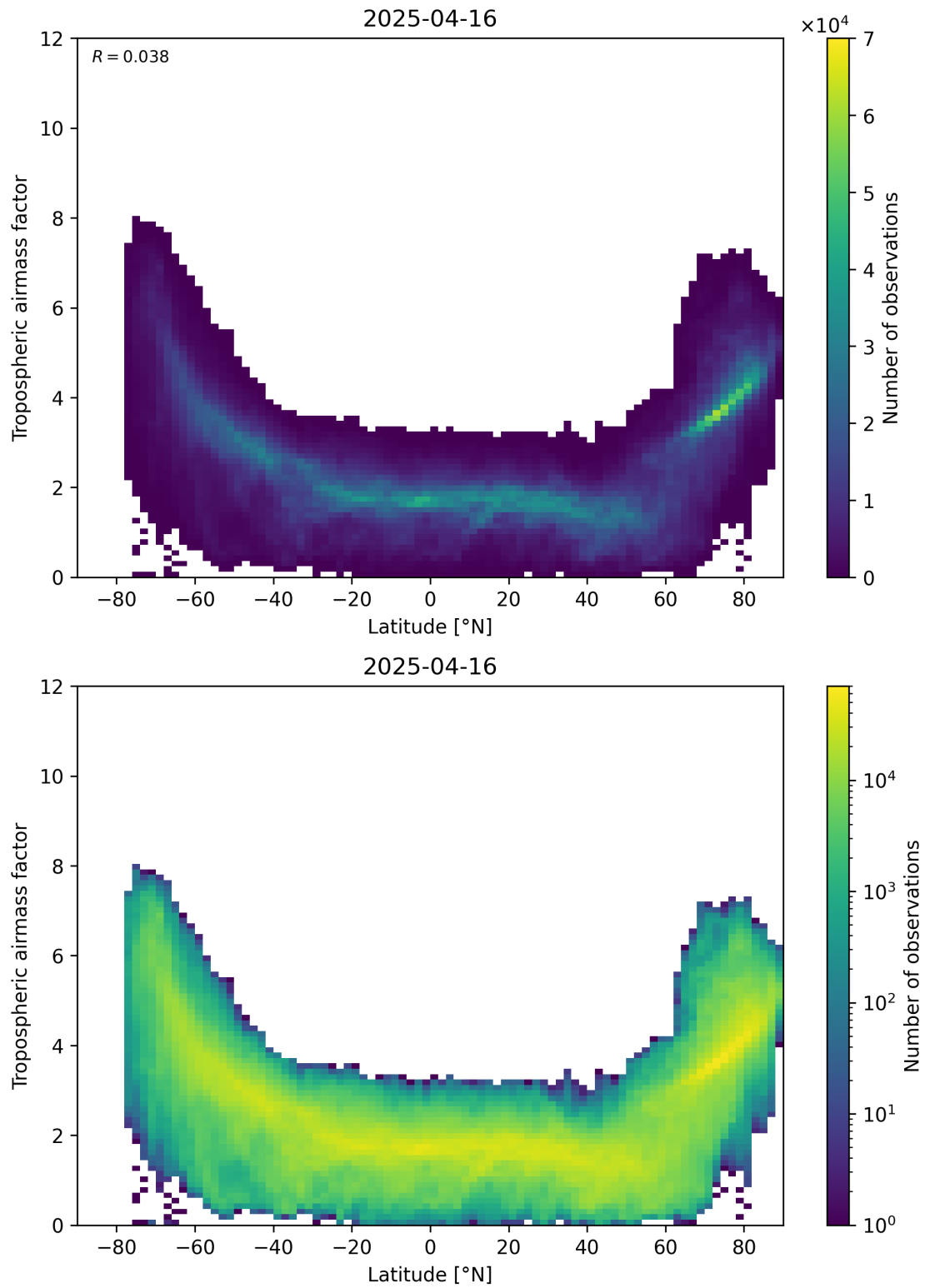
Figure 85: Scatter density plot of “Latitude” against “Tropospheric air mass factor” for 2025-04-16 to 2025-04-16.
