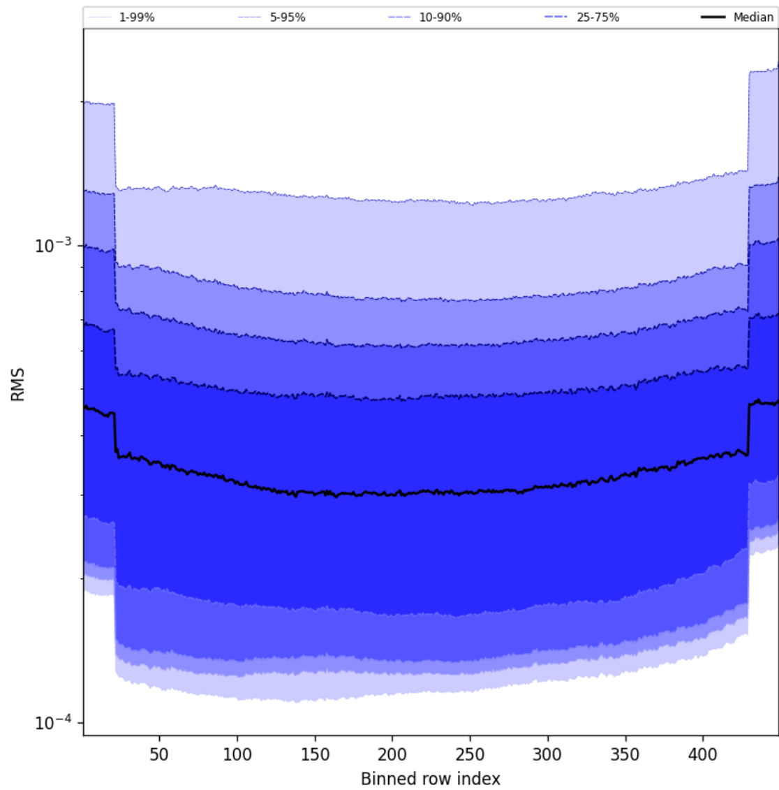
Figure 60: Along track statistics of “RMS” for 2025-04-16 to 2025-04-16
