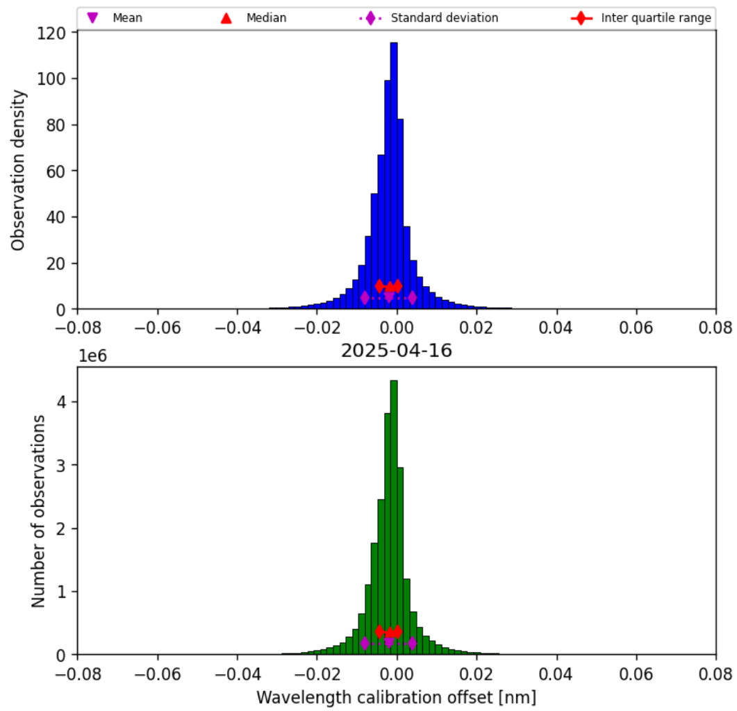
Figure 35: Histogram of “Wavelength calibration offset” for 2025-04-16 to 2025-04-16
