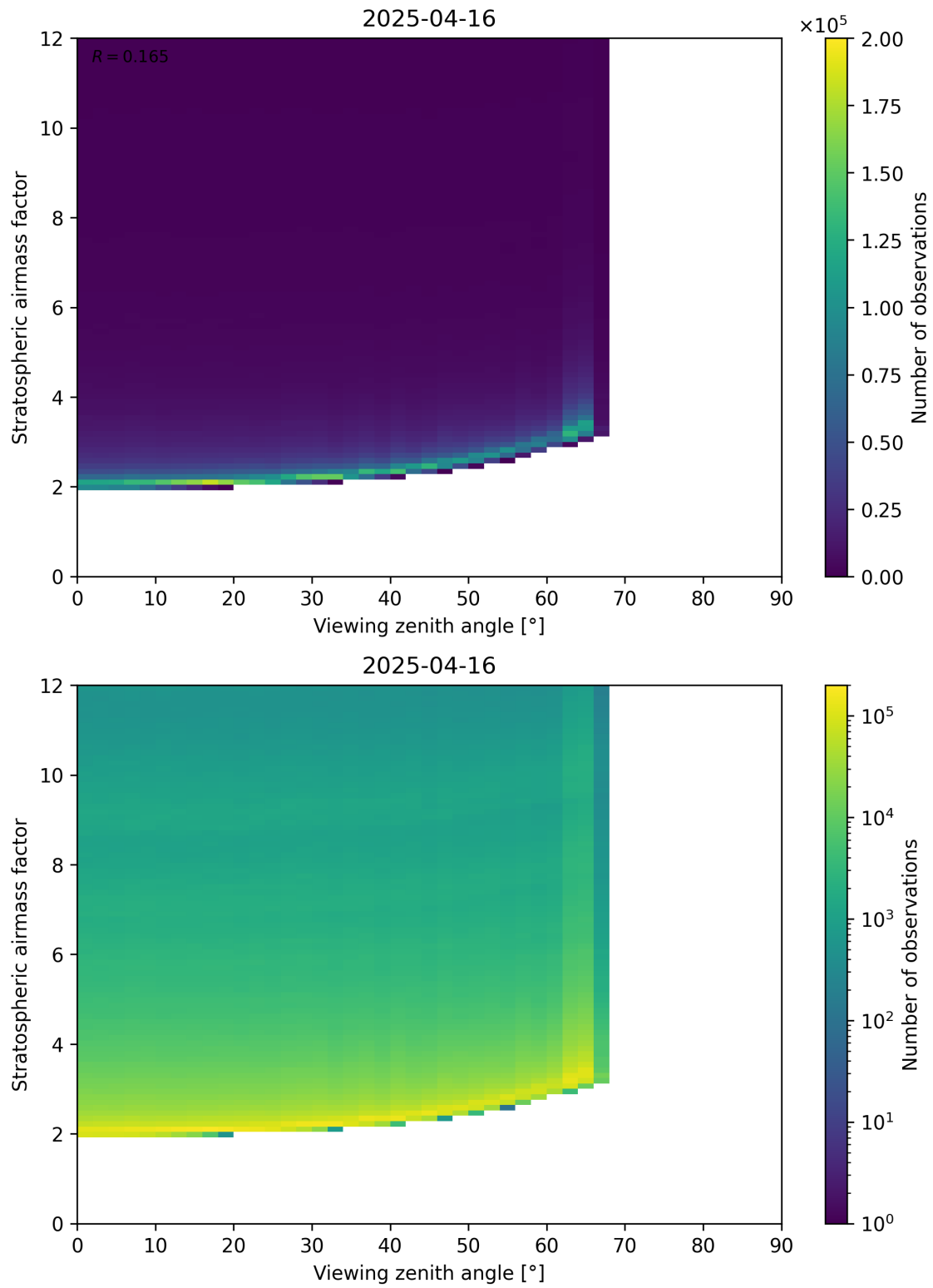
Figure 159: Scatter density plot of “Viewing zenith angle” against “Stratospheric airmass factor” for 2025-04-16 to 2025-04-16.
