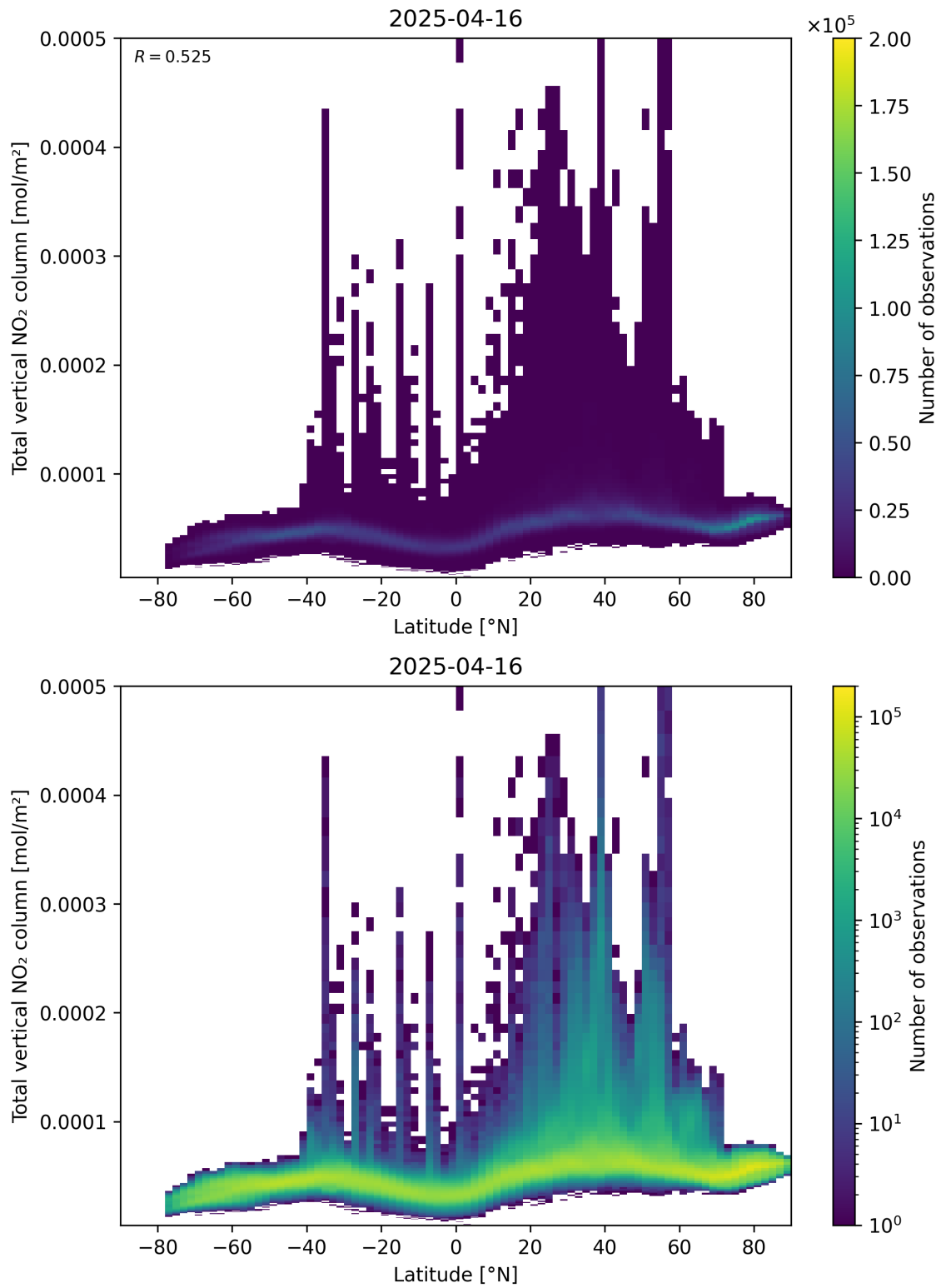
Figure 90: Scatter density plot of “Latitude” against “Total vertical NO 2 column” for 2025-04-16 to 2025-04-16.
