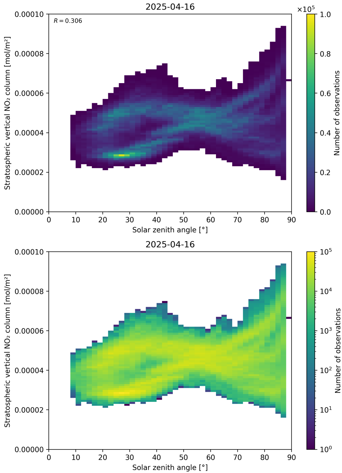
Figure 150: Scatter density plot of “Solar zenith angle” against “Stratospheric vertical NO 2 column” for 2025-04-16 to 2025-04-16.
