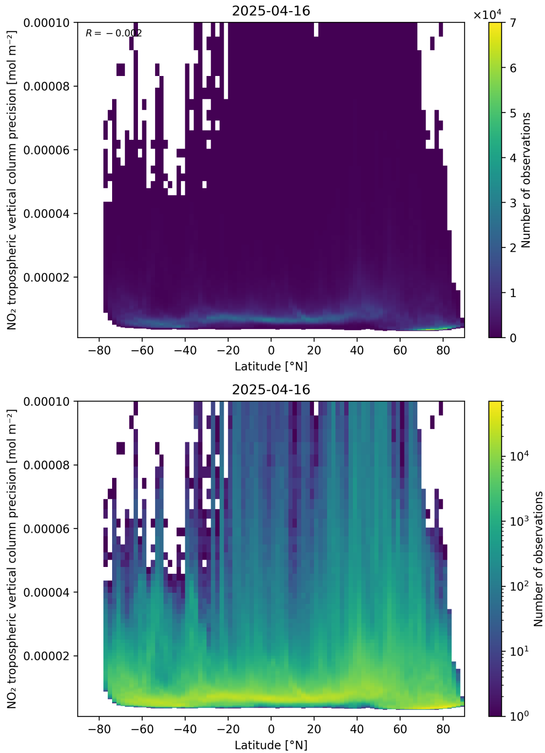
Figure 93: Scatter density plot of “Latitude” against “NO 2 tropospheric vertical column precision” for 2025-04-16 to 2025-04-16.
