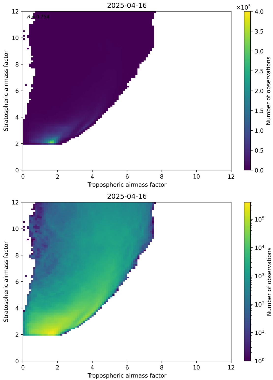
Figure 71: Scatter density plot of “Tropospheric airmass factor” against “Stratospheric airmass factor” for 2025-04-16 to 2025-04-16.
