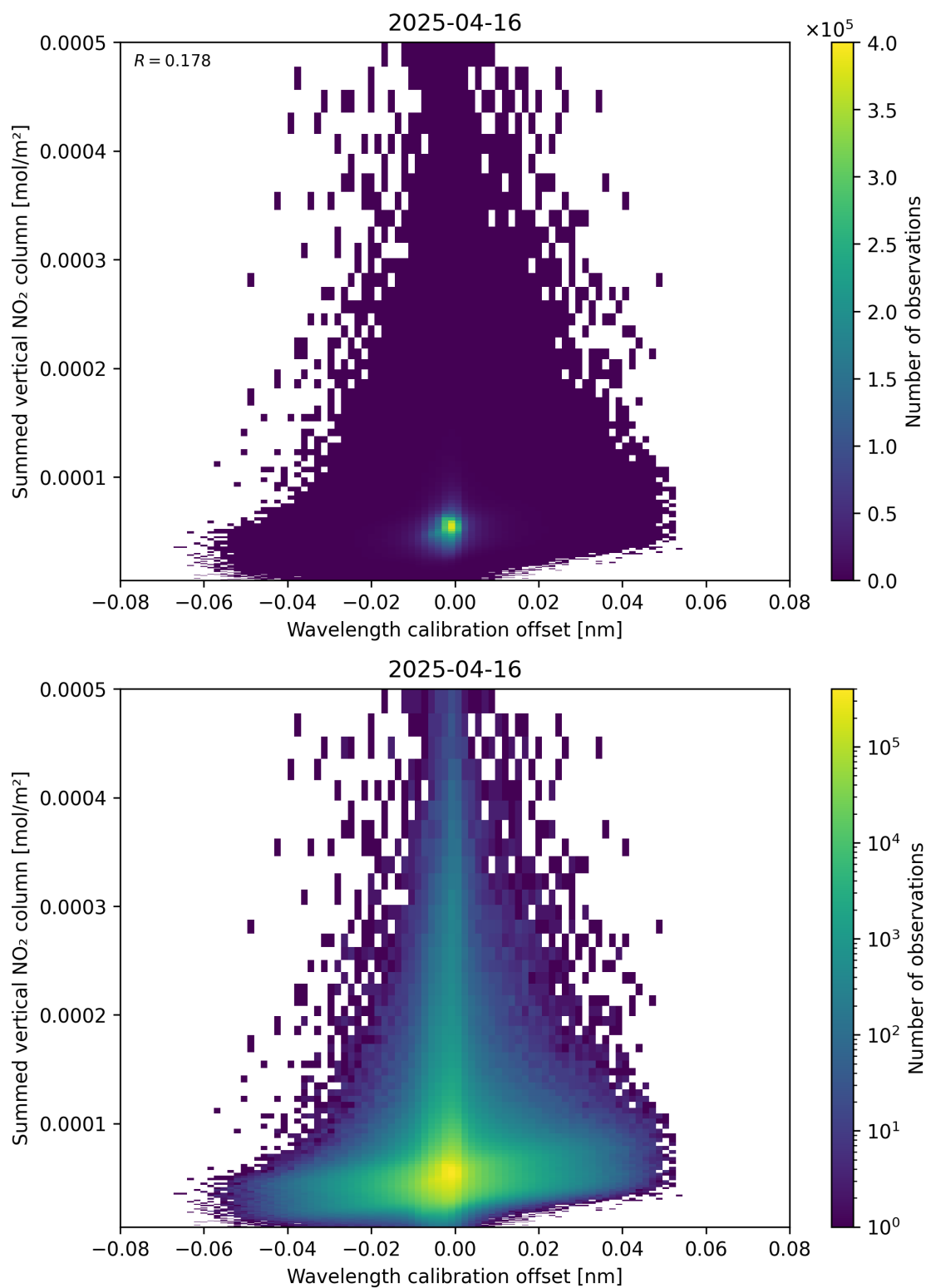
Figure 177: Scatter density plot of “Wavelength calibration offset” against “Summed vertical NO 2 column” for 2025-04-16 to 2025-04-16.
