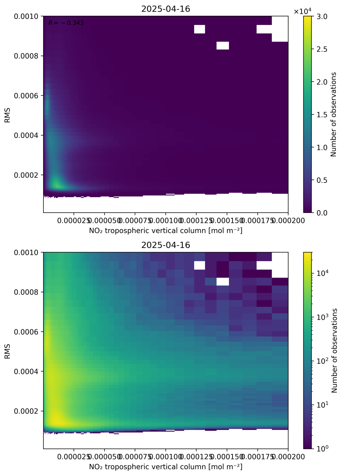
Figure 142: Scatter density plot of “NO 2 tropospheric vertical column” against “RMS” for 2025-04-16 to 2025-04-16.
