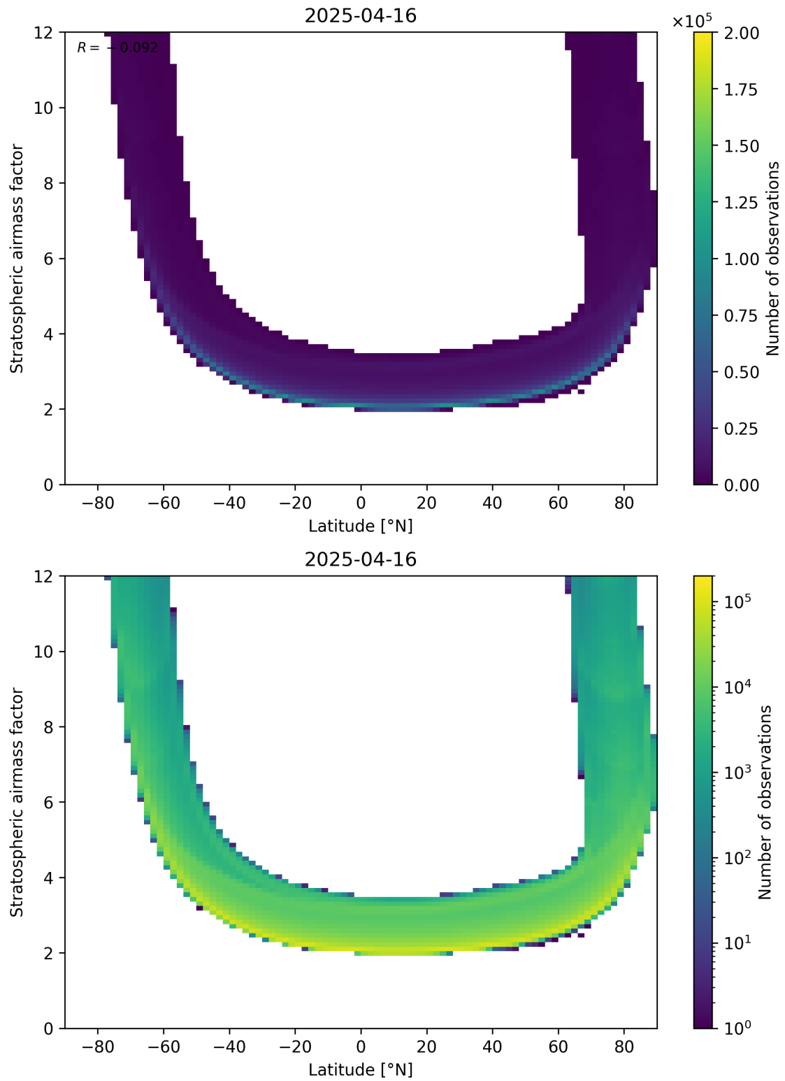
Figure 83: Scatter density plot of “Latitude” against “Stratospheric air mass factor” for 2025-04-16 to 2025-04-16.
