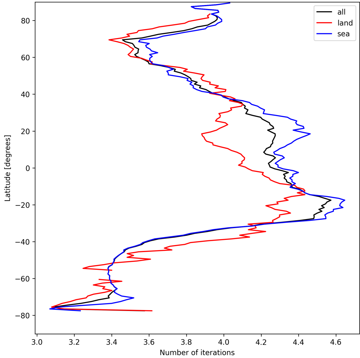
Figure 17: Zonal average of “Number of iterations” for 2025-04-16 to 2025-04-16.
