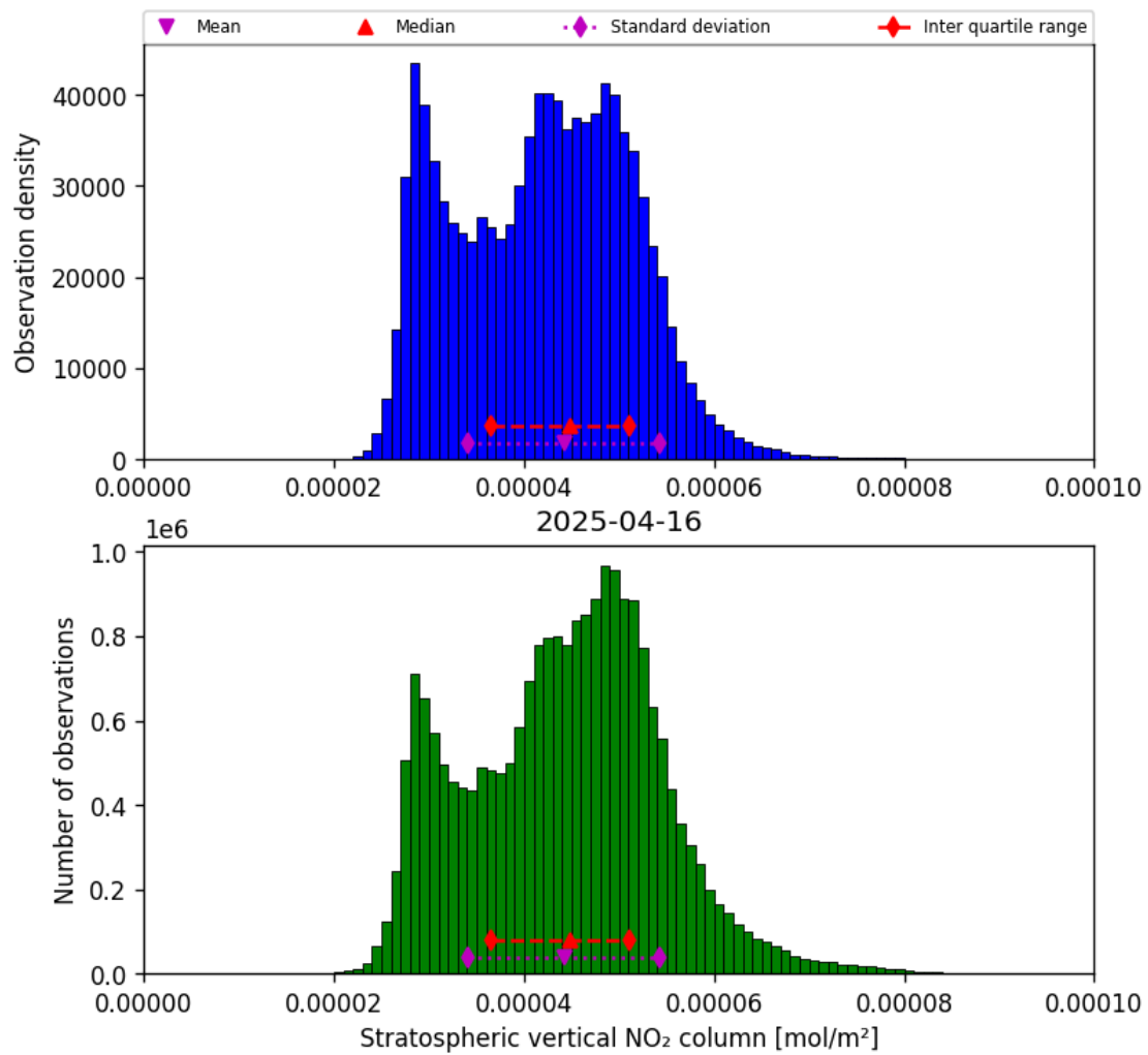
Figure 36: Histogram of “Stratospheric vertical NO 2 column” for 2025-04-16 to 2025-04-16
