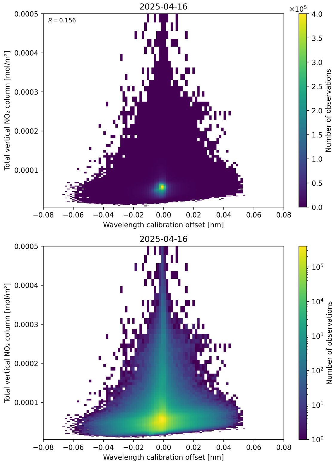
Figure 179: Scatter density plot of “Wavelength calibration offset” against “Total vertical NO 2 column” for 2025-04-16 to 2025-04-16.
