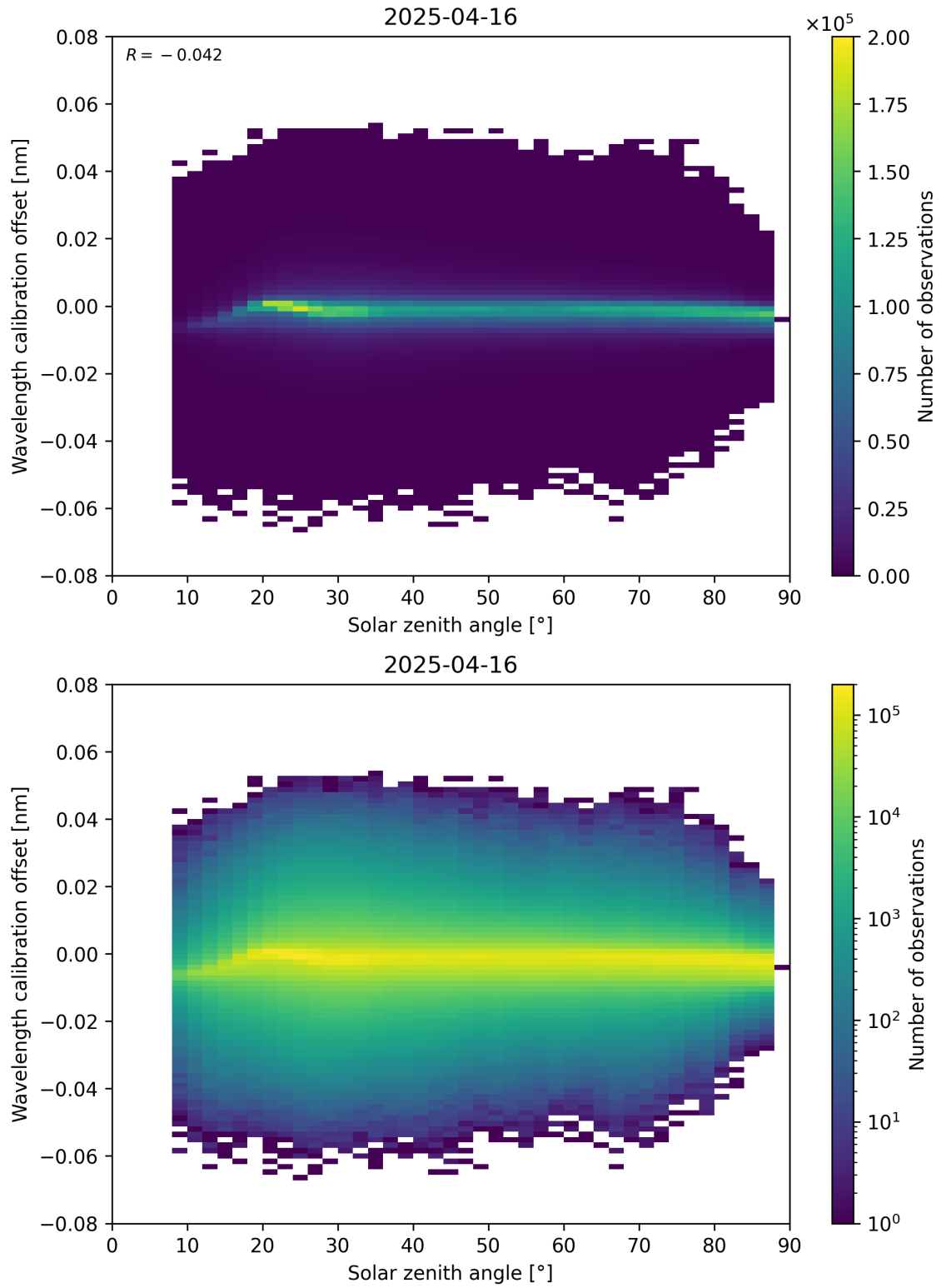
Figure 158: Scatter density plot of “Solar zenith angle” against “Wavelength calibration offset” for 2025-04-16 to 2025-04-16.
