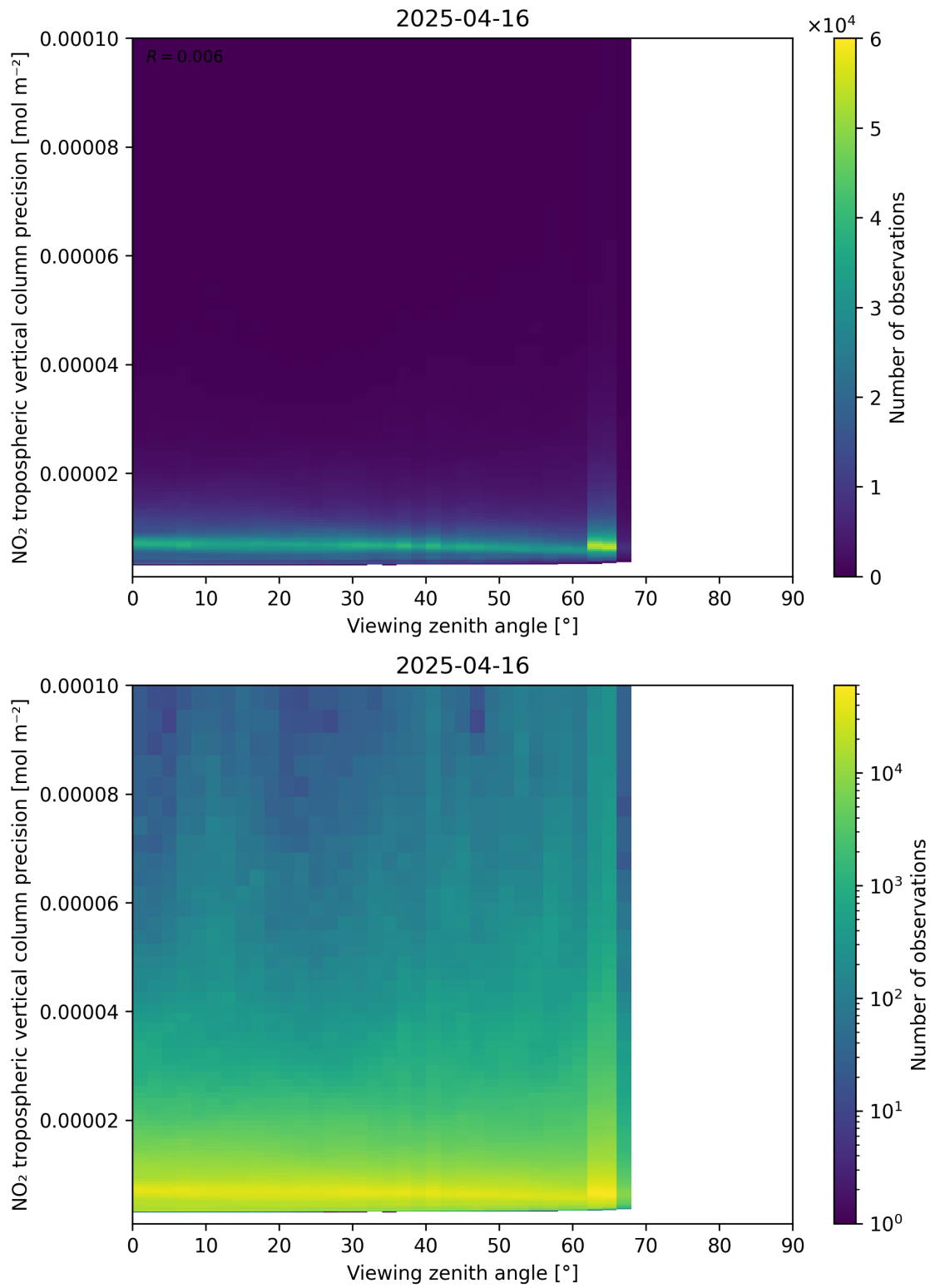
Figure 170: Scatter density plot of “Viewing zenith angle” against “NO 2 tropospheric vertical column precision” for 2025-04-16 to 2025-04-16.
