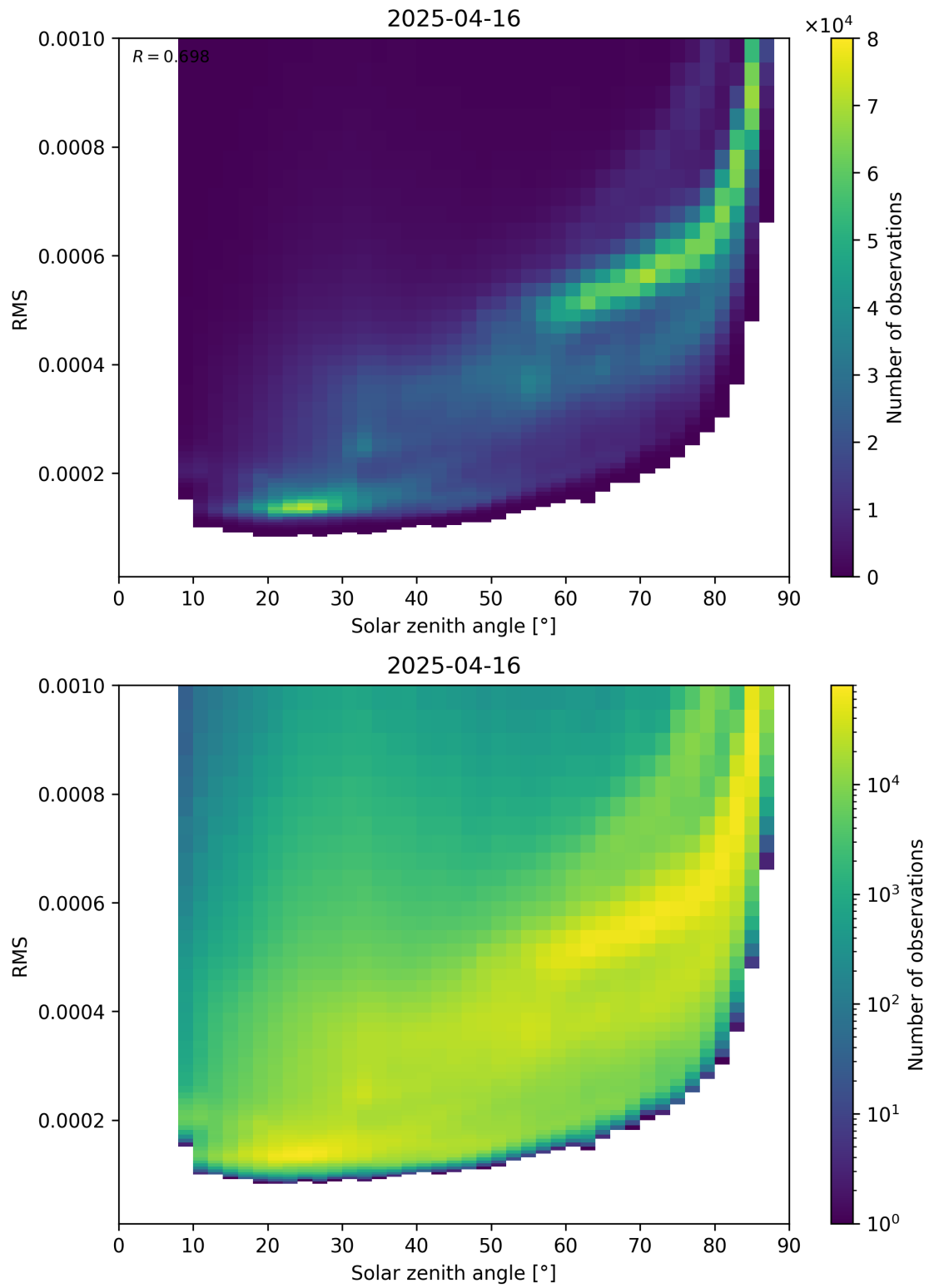
Figure 157: Scatter density plot of “Solar zenith angle” against “RMS” for 2025-04-16 to 2025-04-16.
