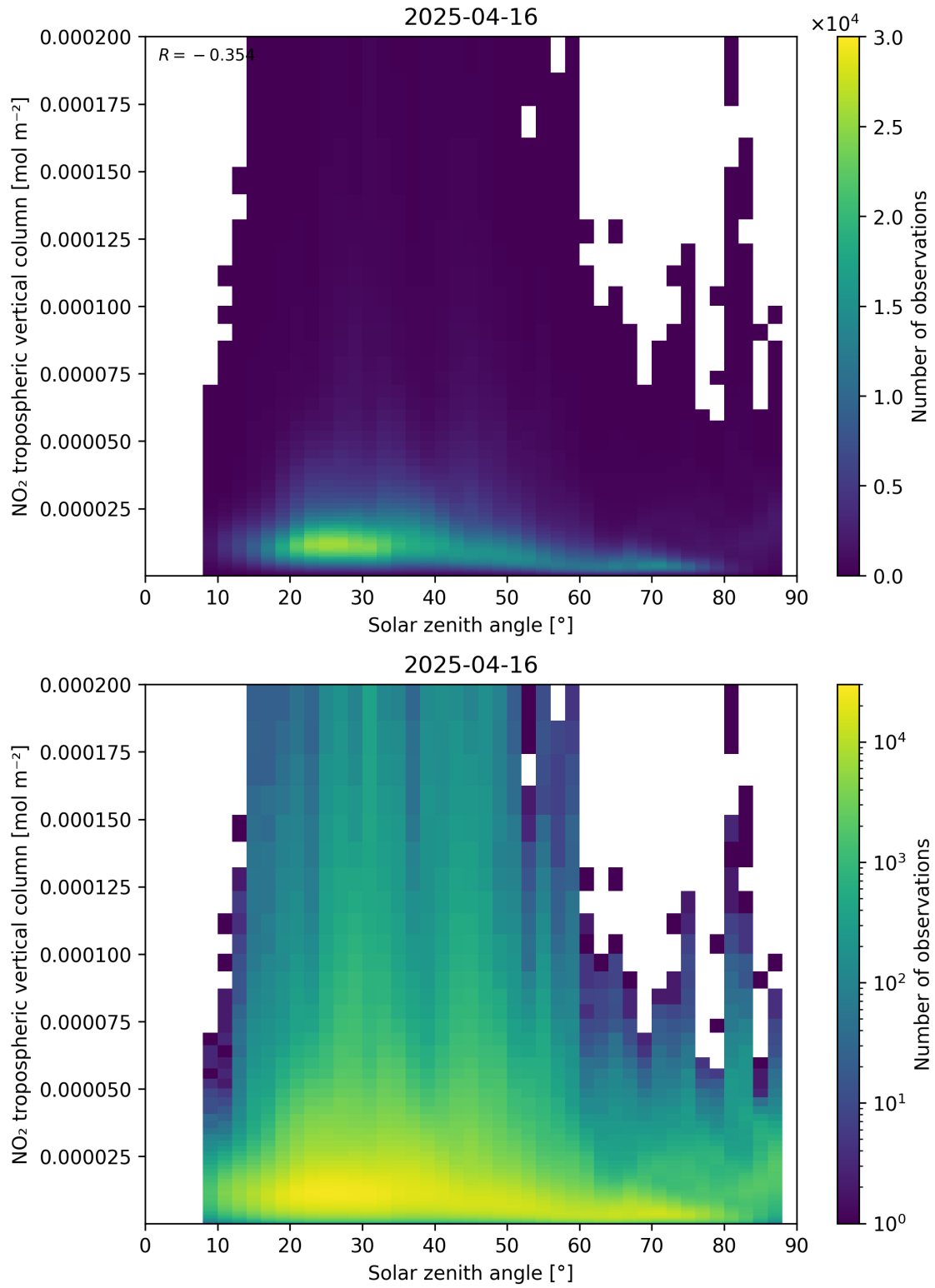
Figure 155: Scatter density plot of “Solar zenith angle” against “NO 2 tropospheric vertical column” for 2025-04-16 to 2025-04-16.
