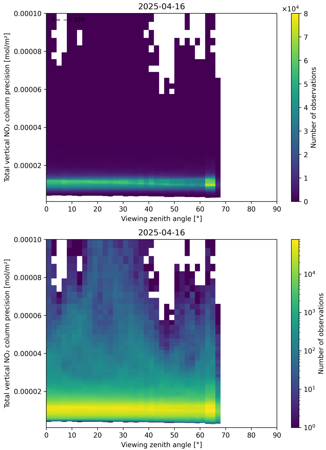
Figure 168: Scatter density plot of “Viewing zenith angle” against “Total vertical NO 2 column precision” for 2025-04-16 to 2025-04-16.
