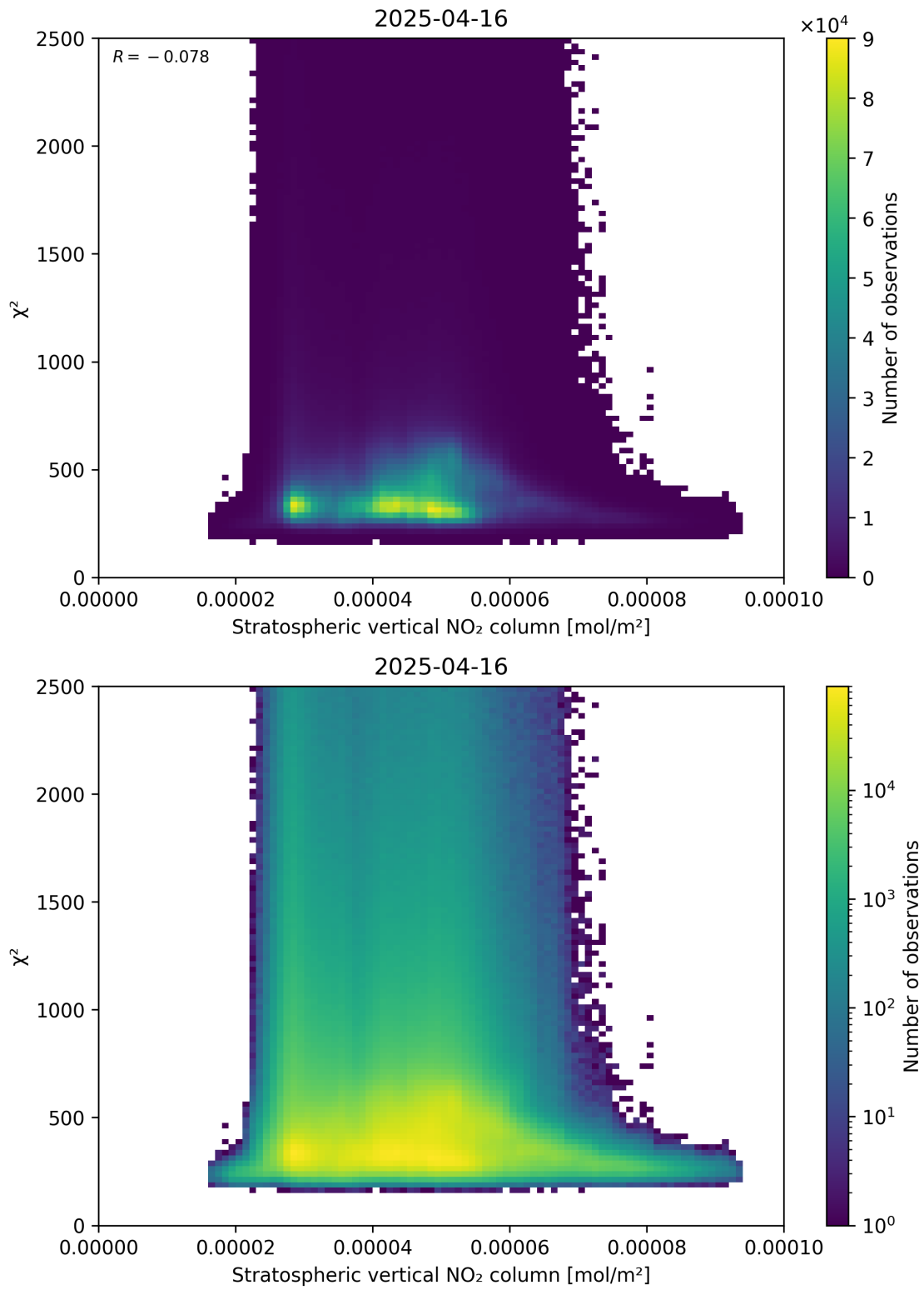
Figure 97: Scatter density plot of “Stratospheric vertical NO 2 column” against “ \chi^2 ” for 2025-04-16 to 2025-04-16.
