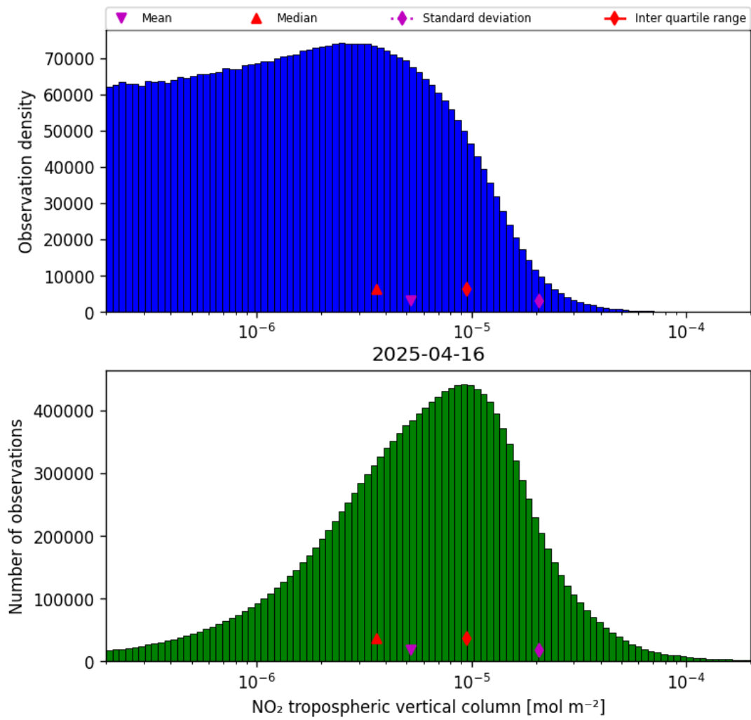
Figure 29: Histogram of “ \text{NO}_2 tropospheric vertical column” for 2025-04-16 to 2025-04-16
