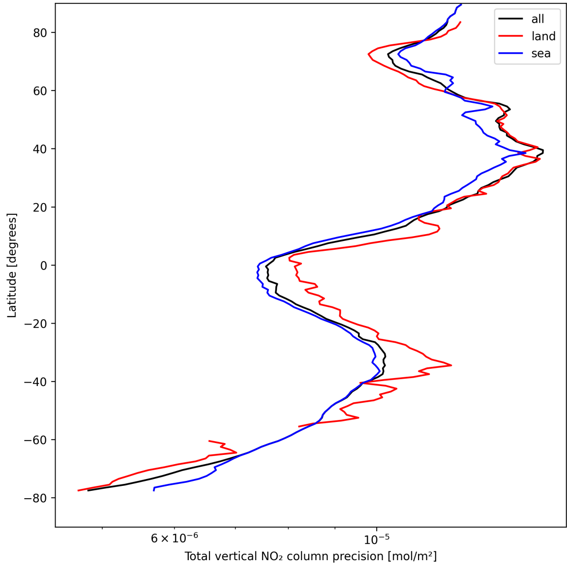
Figure 22: Zonal average of “Total vertical NO 2 column precision” for 2025-04-16 to 2025-04-16.
