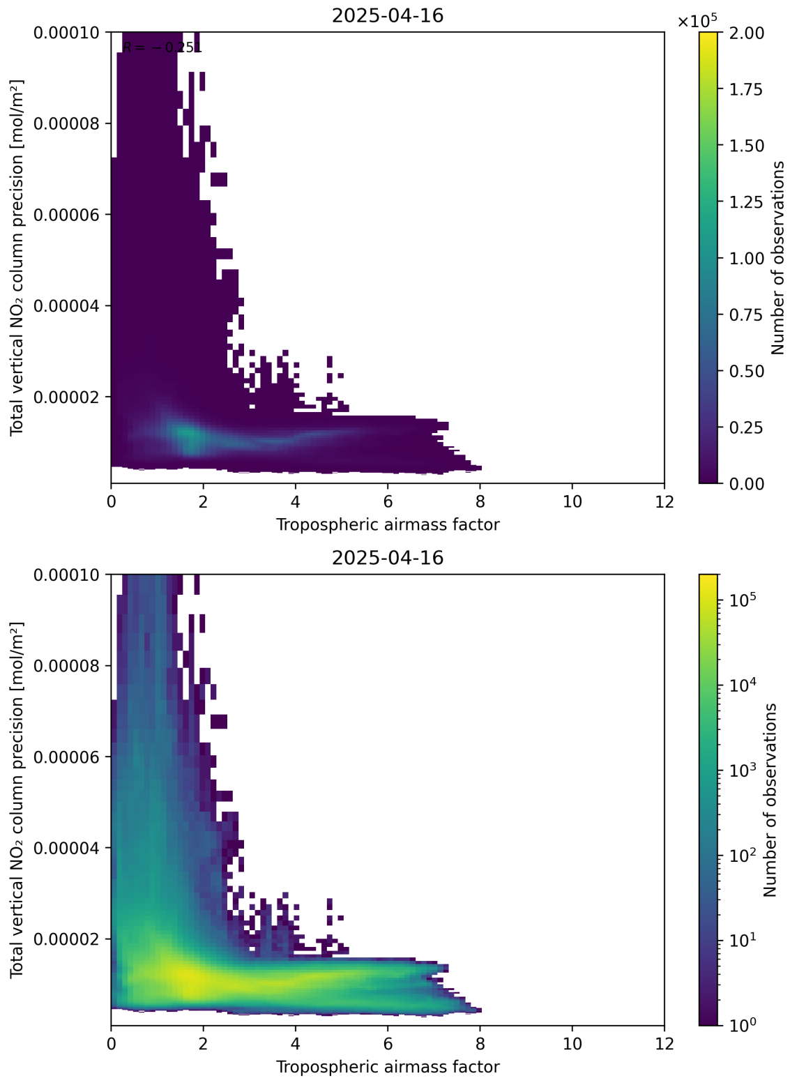
Figure 78: Scatter density plot of “Tropospheric air mass factor” against “Total vertical NO 2 column precision” for 2025-04-16 to 2025-04-16.
