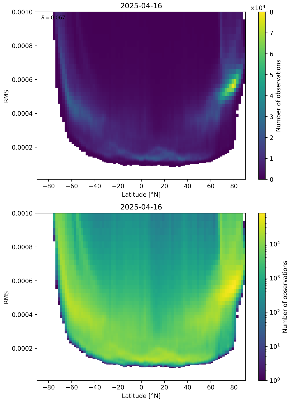
Figure 94: Scatter density plot of “Latitude” against “RMS” for 2025-04-16 to 2025-04-16.
