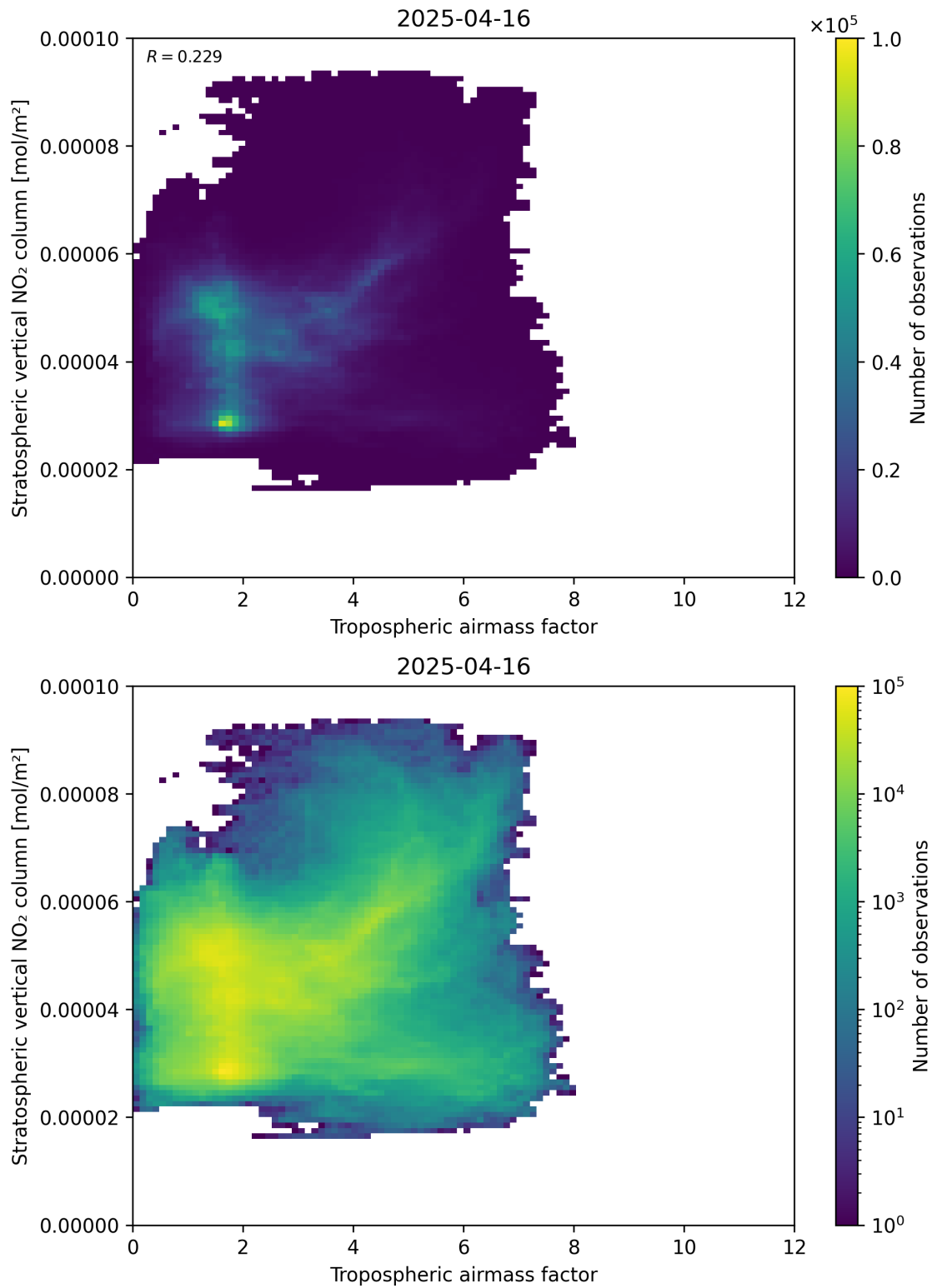
Figure 74: Scatter density plot of “Tropospheric air mass factor” against “Stratospheric vertical \text{NO}_2 column” for 2025-04-16 to 2025-04-16.
