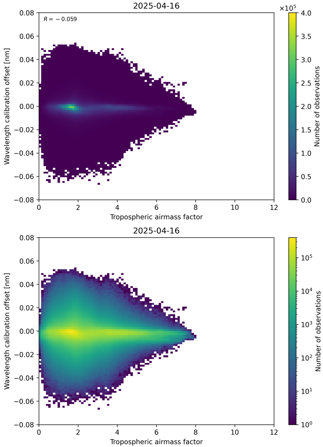
Figure 80: Scatter density plot of “Tropospheric airmass factor” against “Wavelength calibration offset” for 2025-04-16 to 2025-04-16.
