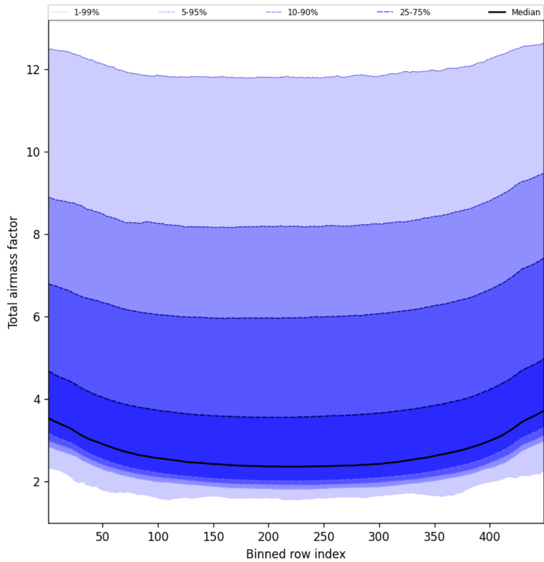
Figure 49: Along track statistics of “Total airmass factor” for 2025-04-16 to 2025-04-16
