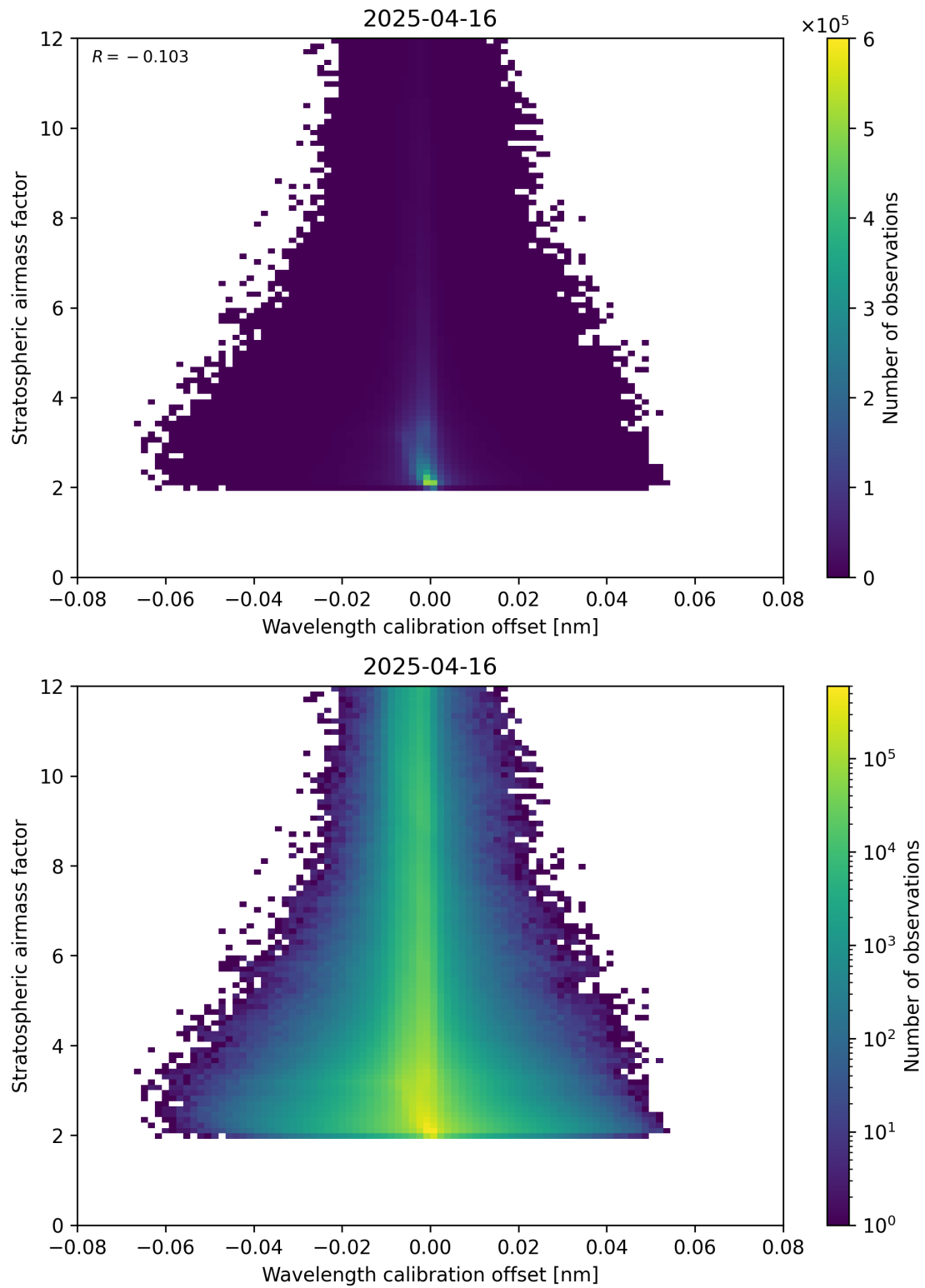
Figure 174: Scatter density plot of “Wavelength calibration offset” against “Stratospheric airmass factor” for 2025-04-16 to 2025-04-16.
