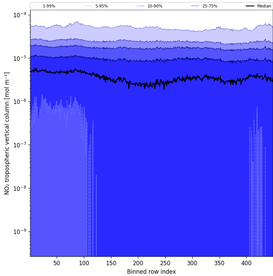
Figure 46: Along track statistics of “NO 2 tropospheric vertical column” for 2025-04-16 to 2025-04-16
