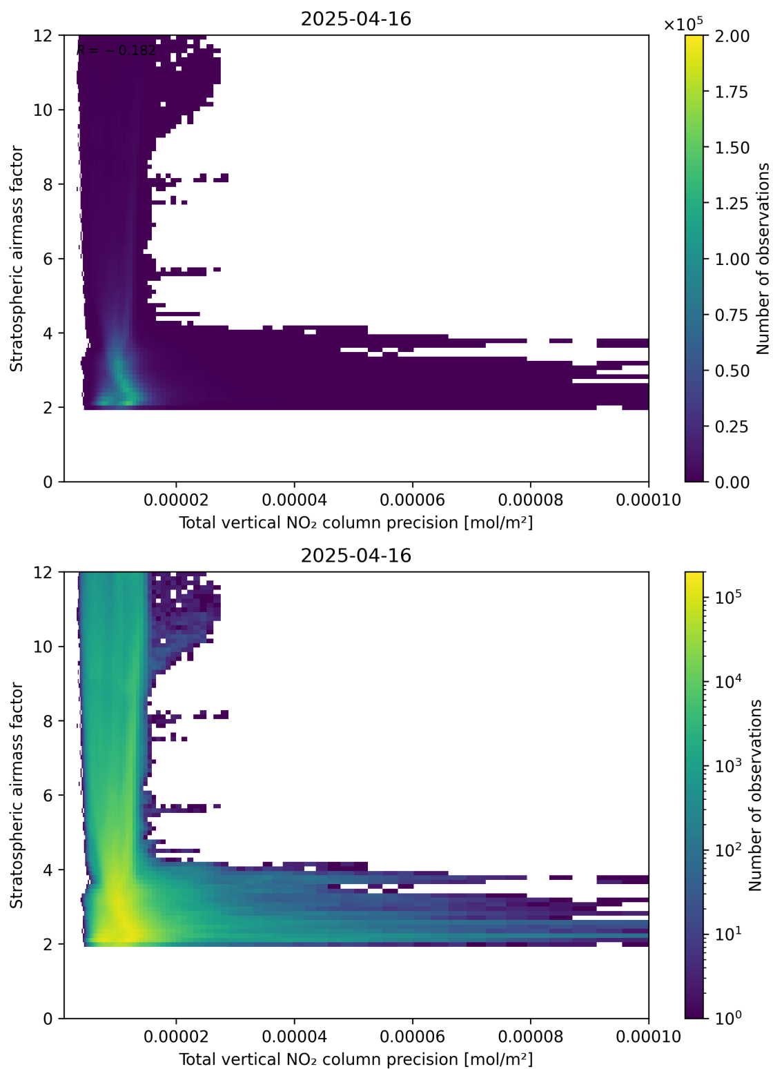
Figure 115: Scatter density plot of “Total vertical NO 2 column precision” against “Stratospheric air mass factor” for 2025-04-16 to 2025-04-16.
