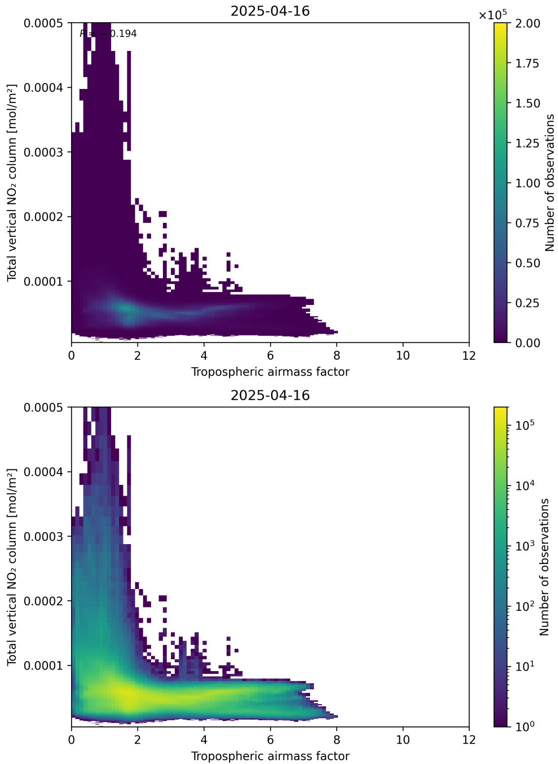
Figure 77: Scatter density plot of “Tropospheric airmass factor” against “Total vertical NO 2 column” for 2025-04-16 to 2025-04-16.
