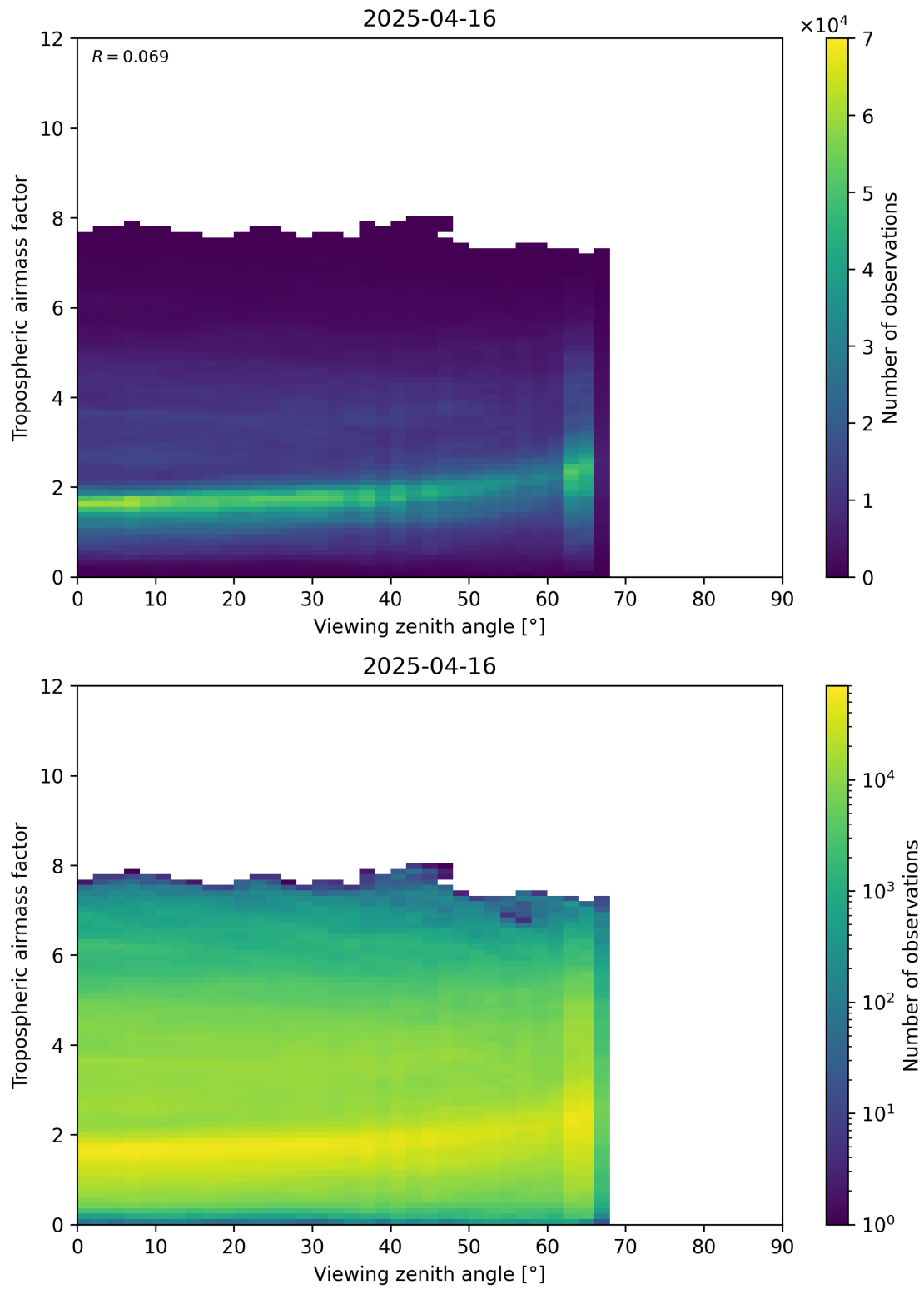
Figure 161: Scatter density plot of “Viewing zenith angle” against “Tropospheric airmass factor” for 2025-04-16 to 2025-04-16.
