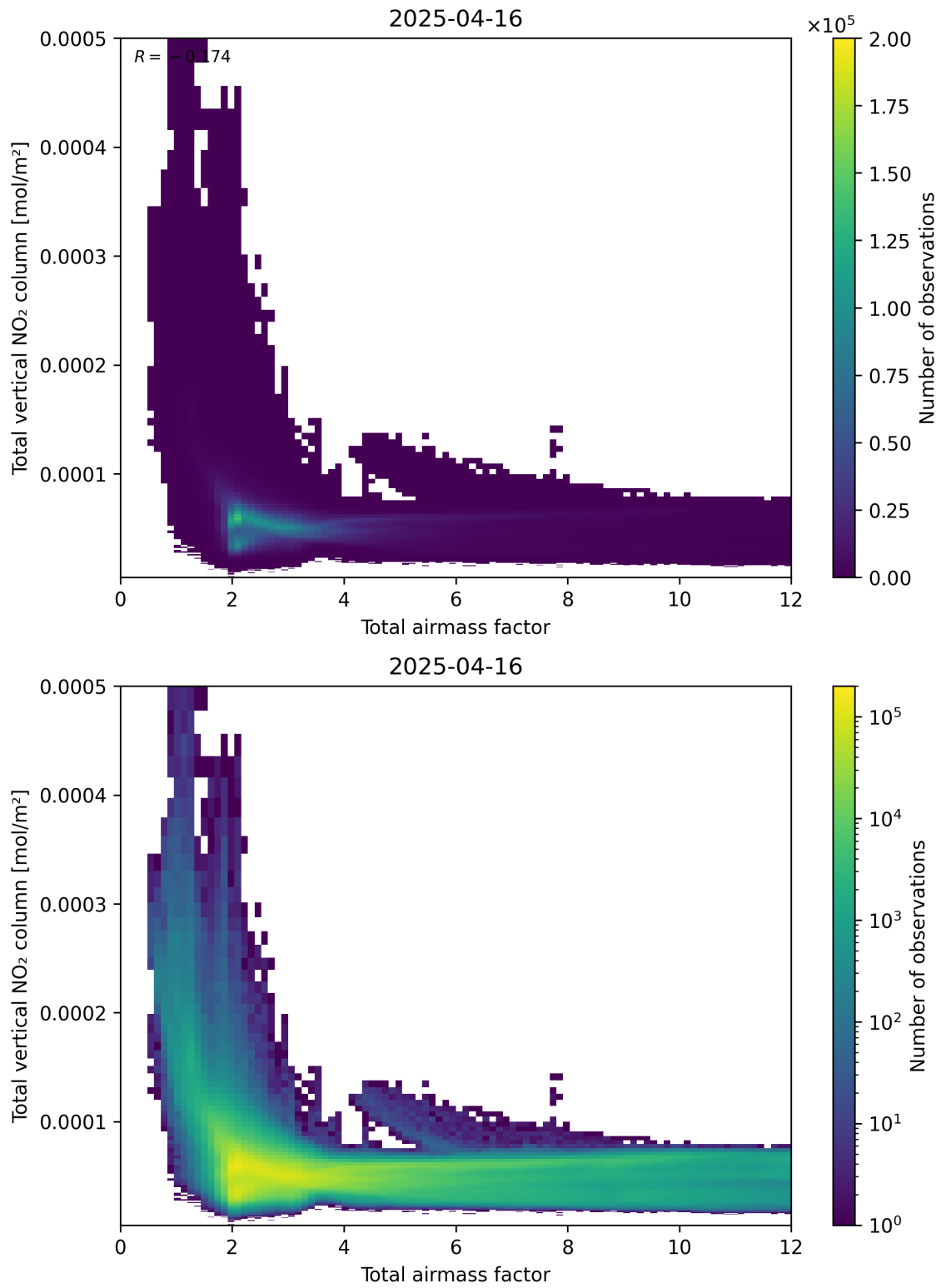
Figure 67: Scatter density plot of “Total airmass factor” against “Total vertical NO 2 column” for 2025-04-16 to 2025-04-16.
