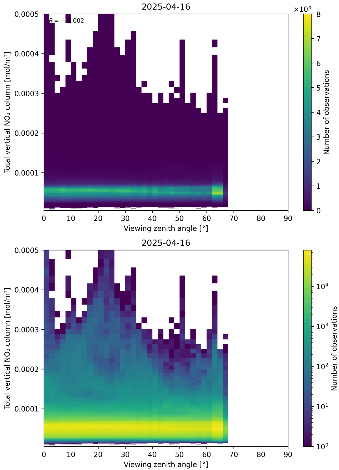
Figure 167: Scatter density plot of “Viewing zenith angle” against “Total vertical NO 2 column” for 2025-04-16 to 2025-04-16.
