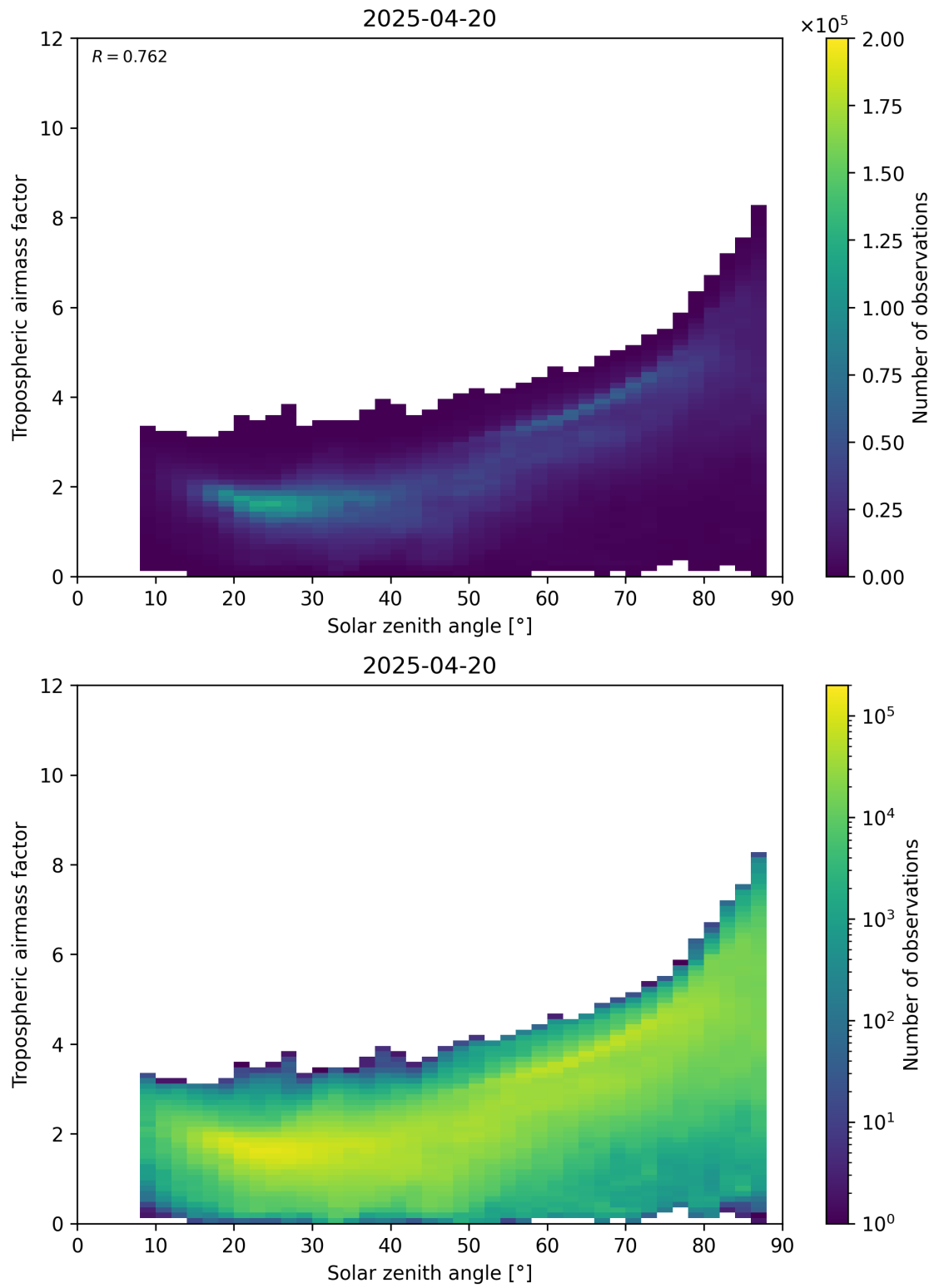
Figure 147: Scatter density plot of “Solar zenith angle” against “Tropospheric airmass factor” for 2025-04-20 to 2025-04-21.
