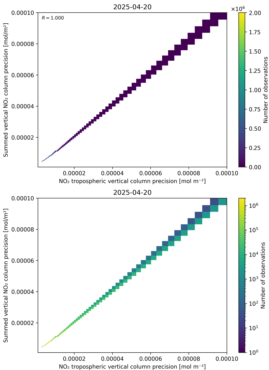
Figure 137: Scatter density plot of “NO 2 tropospheric vertical column precision” against “Summed vertical NO 2 column precision” for 2025-04-20 to 2025-04-21.
