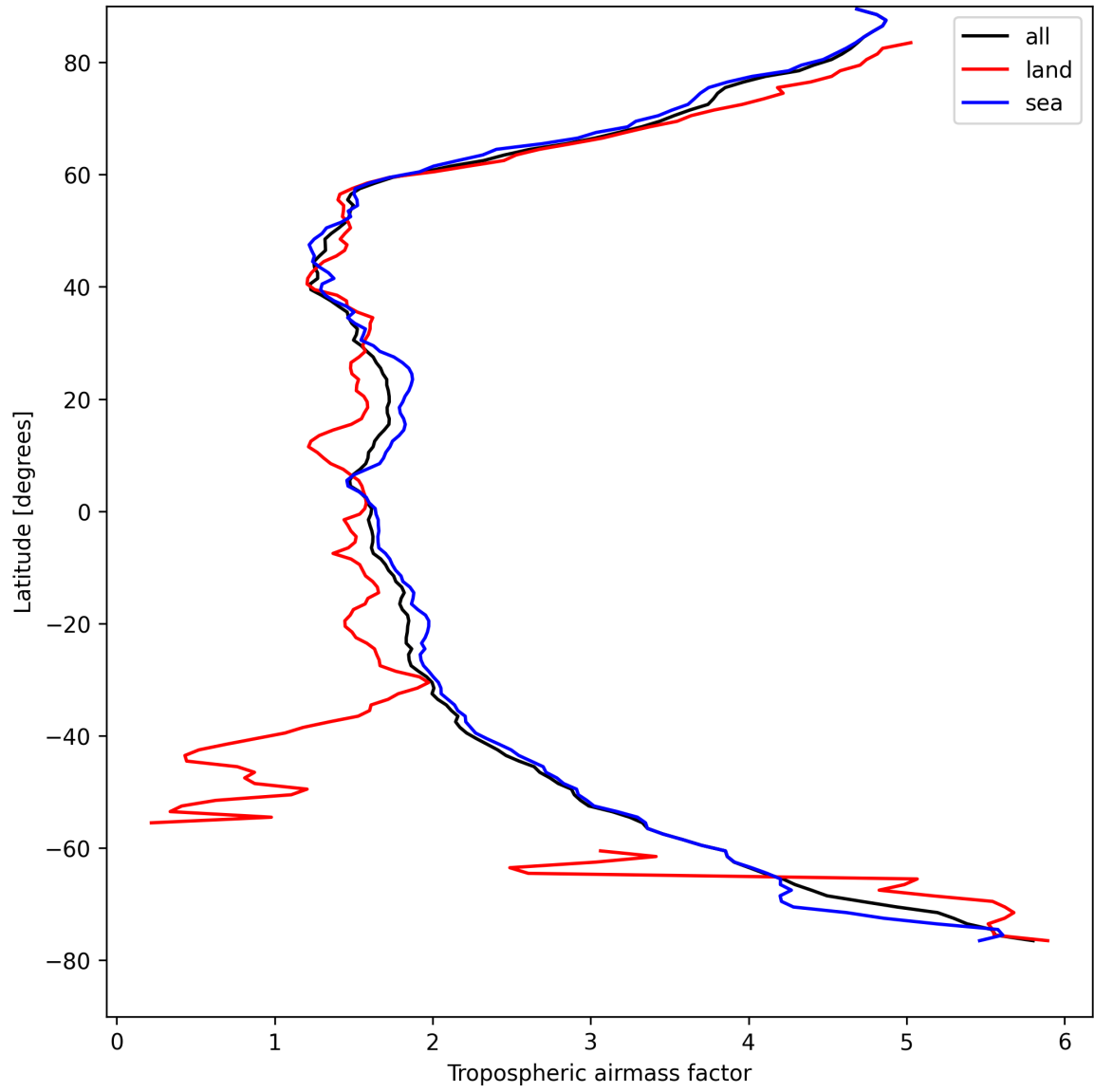
Figure 14: Zonal average of “Tropospheric airmass factor” for 2025-04-20 to 2025-04-21.
