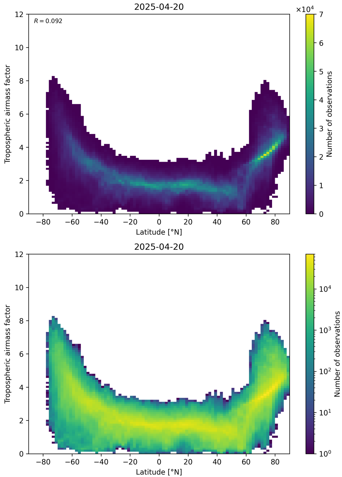
Figure 85: Scatter density plot of “Latitude” against “Tropospheric air mass factor” for 2025-04-20 to 2025-04-21.
