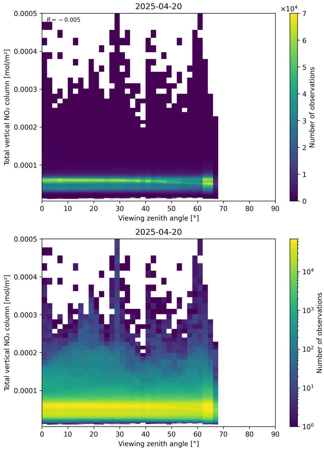
Figure 167: Scatter density plot of “Viewing zenith angle” against “Total vertical NO 2 column” for 2025-04-20 to 2025-04-21.
