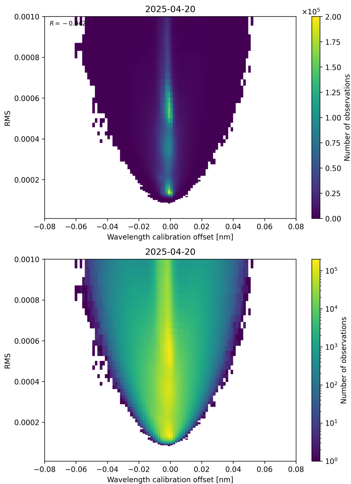
Figure 181: Scatter density plot of “Wavelength calibration offset” against “RMS” for 2025-04-20 to 2025-04-21.
