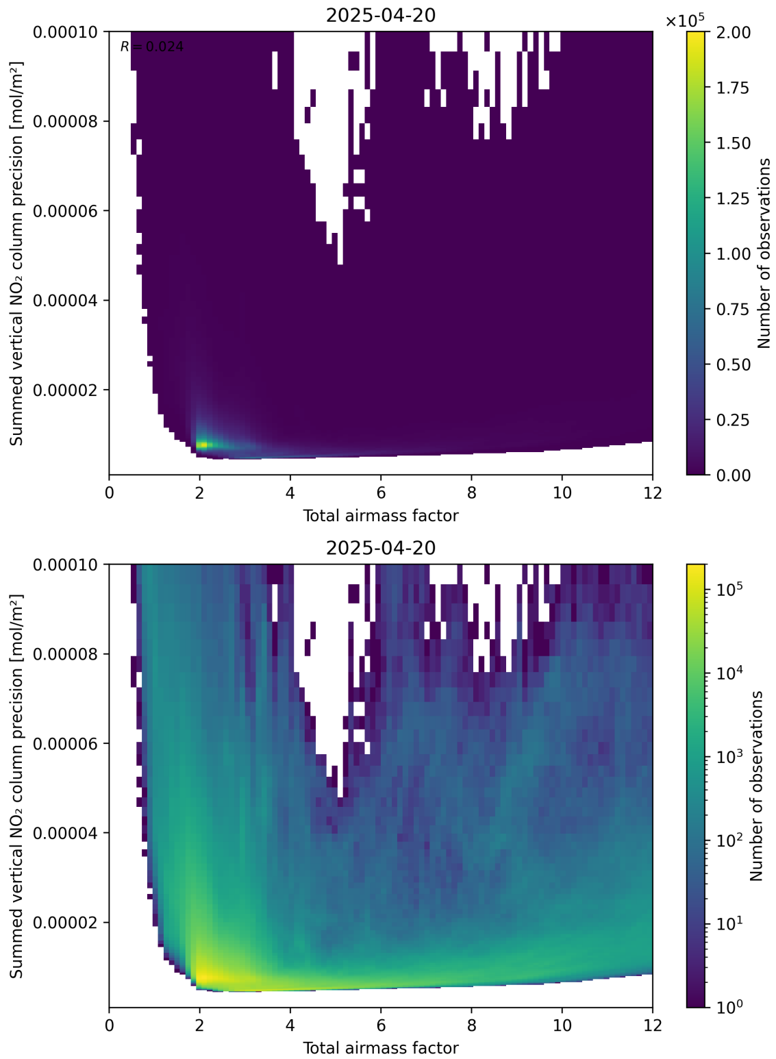
Figure 66: Scatter density plot of “Total airmass factor” against “Summed vertical NO 2 column precision” for 2025-04-20 to 2025-04-21.
