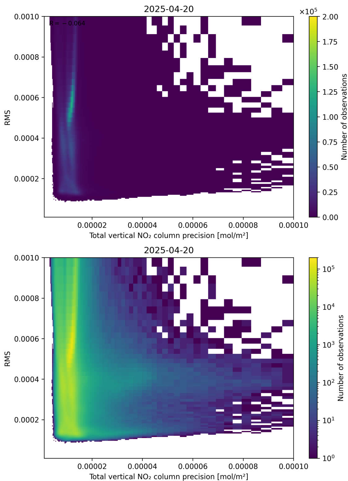
Figure 119: Scatter density plot of “Total vertical NO 2 column precision” against “RMS” for 2025-04-20 to 2025-04-21.
