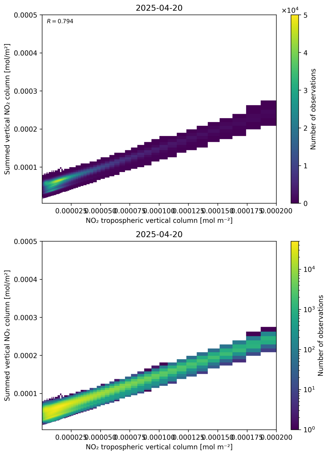
Figure 126: Scatter density plot of “NO 2 tropospheric vertical column” against “Summed vertical NO 2 column” for 2025-04-20 to 2025-04-21.
