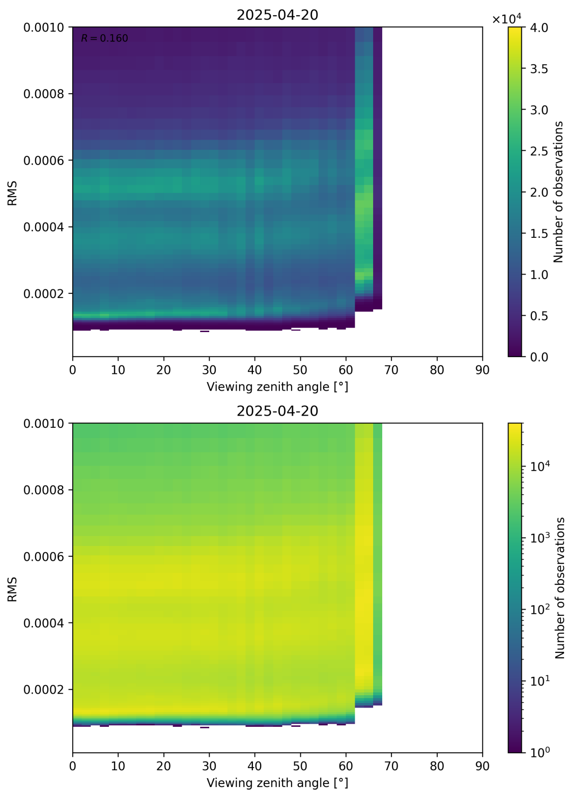
Figure 171: Scatter density plot of “Viewing zenith angle” against “RMS” for 2025-04-20 to 2025-04-21.
