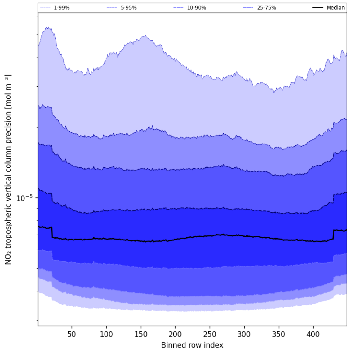
Figure 47: Along track statistics of “NO 2 tropospheric vertical column precision” for 2025-04-20 to 2025-04-21
