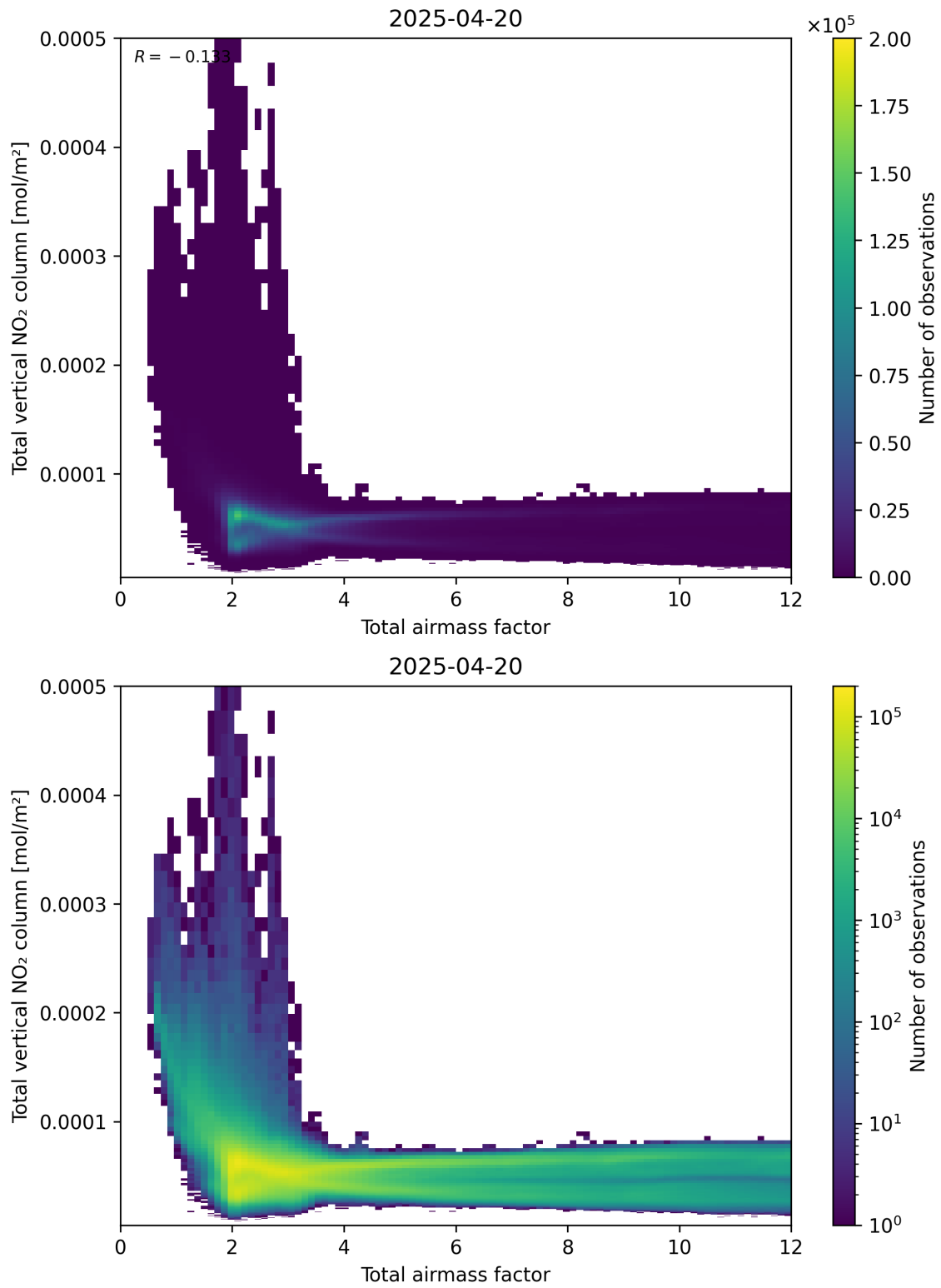
Figure 67: Scatter density plot of “Total airmass factor” against “Total vertical NO 2 column” for 2025-04-20 to 2025-04-21.
