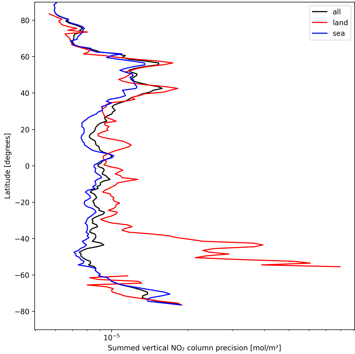
Figure 24: Zonal average of “Summed vertical NO 2 column precision” for 2025-04-20 to 2025-04-21.
