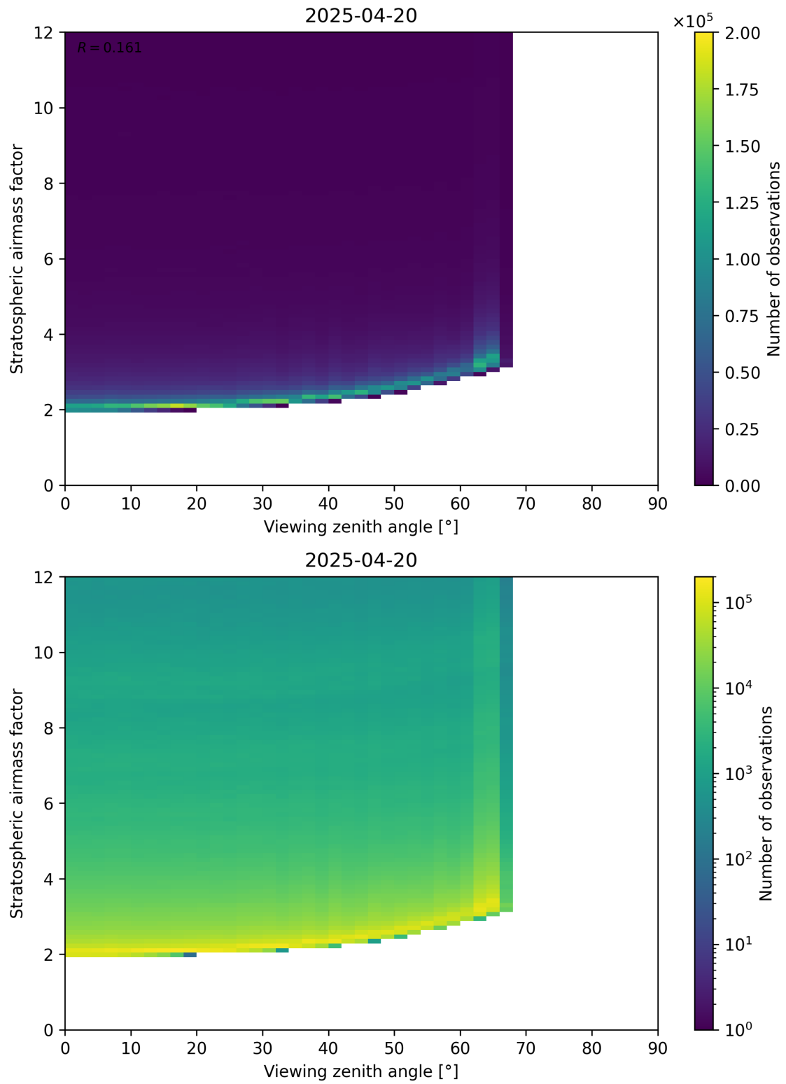
Figure 159: Scatter density plot of “Viewing zenith angle” against “Stratospheric airmass factor” for 2025-04-20 to 2025-04-21.
