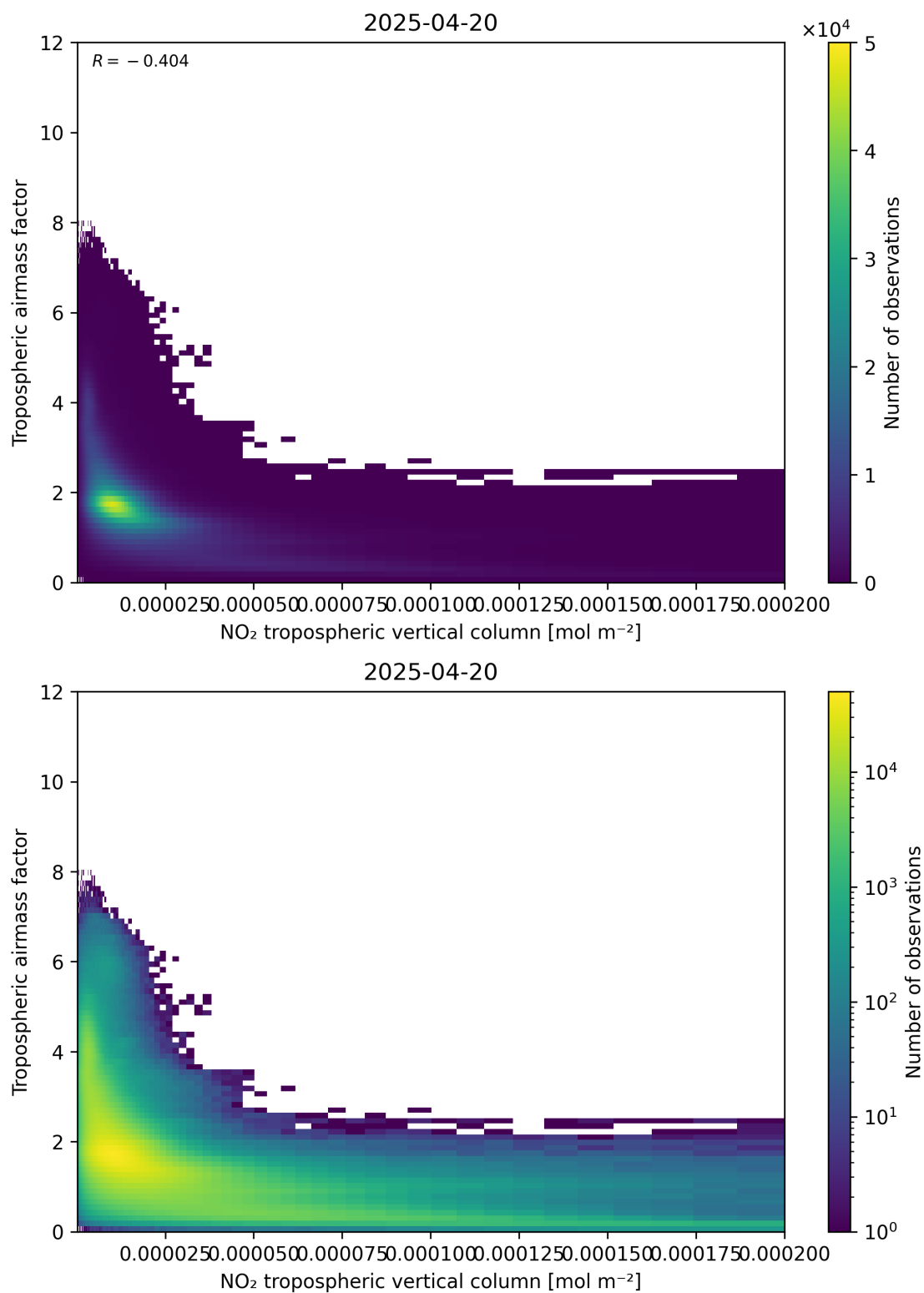
Figure 123: Scatter density plot of “NO 2 tropospheric vertical column” against “Tropospheric air mass factor” for 2025-04-20 to 2025-04-21.
