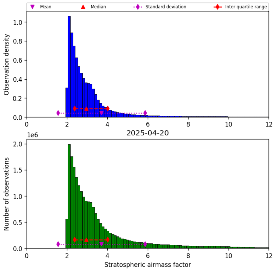
Figure 44: Histogram of “Stratospheric airmass factor” for 2025-04-20 to 2025-04-21
