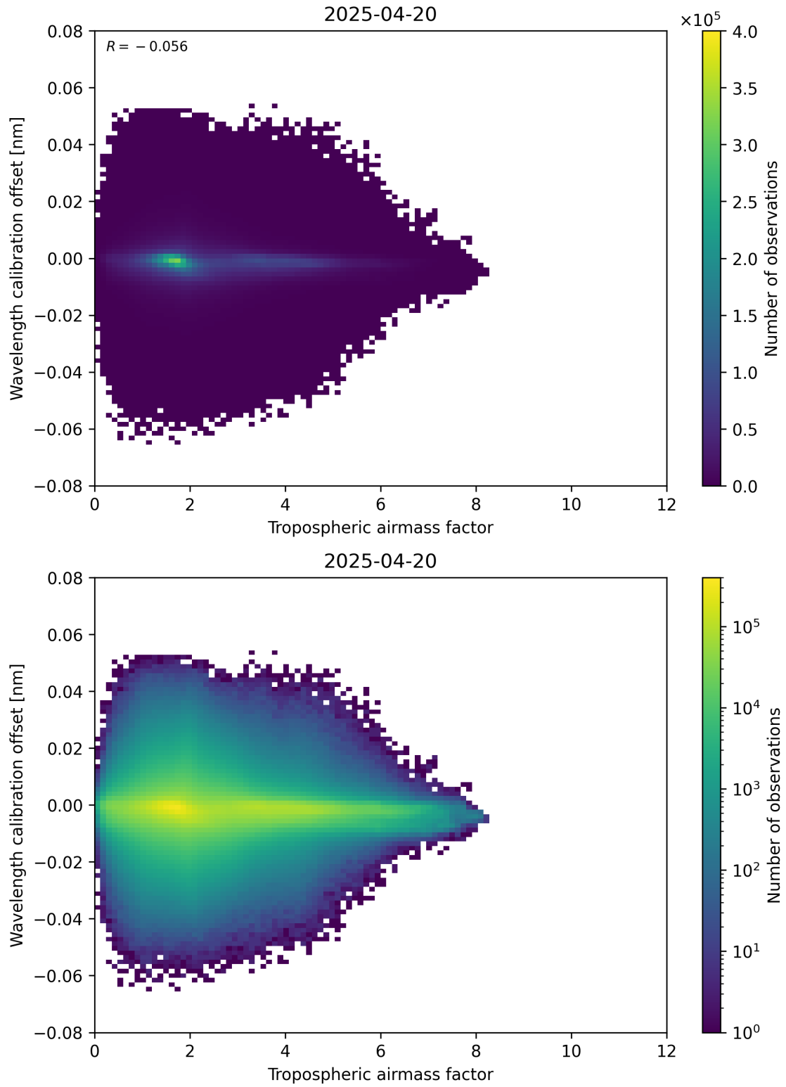
Figure 80: Scatter density plot of “Tropospheric airmass factor” against “Wavelength calibration offset” for 2025-04-20 to 2025-04-21.
