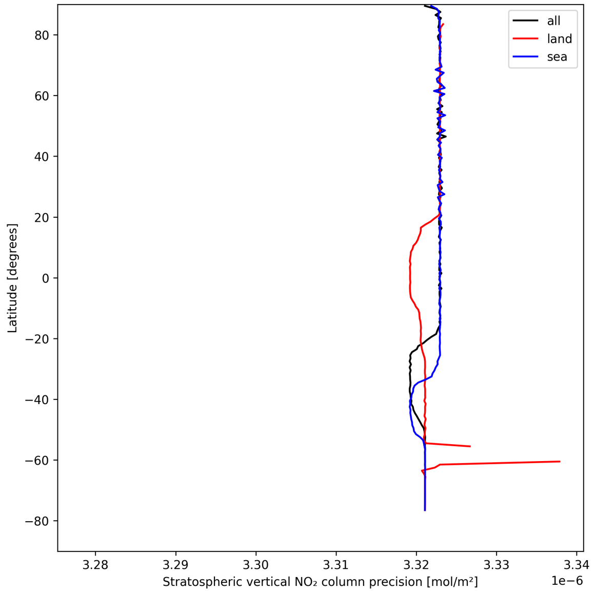
Figure 20: Zonal average of “Stratospheric vertical NO 2 column precision” for 2025-04-20 to 2025-04-21.
