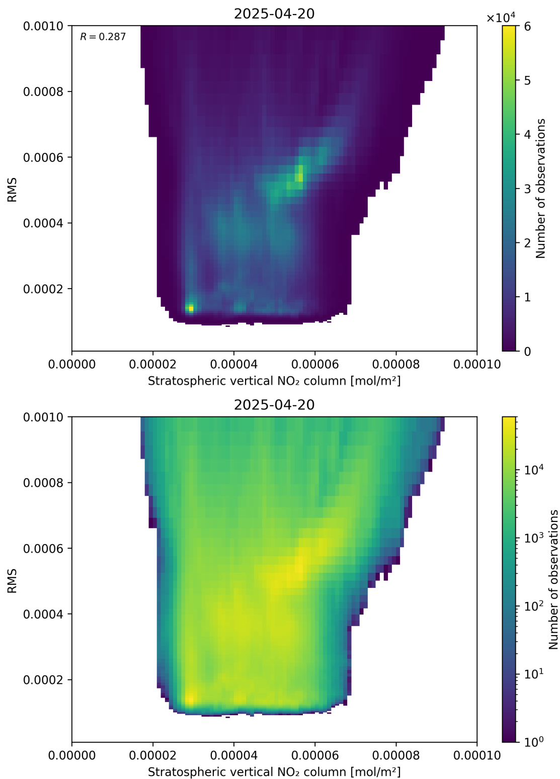
Figure 102: Scatter density plot of “Stratospheric vertical NO 2 column” against “RMS” for 2025-04-20 to 2025-04-21.
