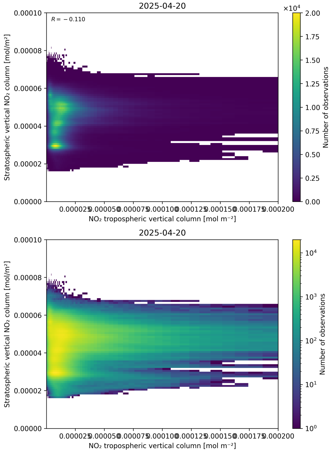
Figure 125: Scatter density plot of “NO 2 tropospheric vertical column” against “Stratospheric vertical NO 2 column” for 2025-04-20 to 2025-04-21.
