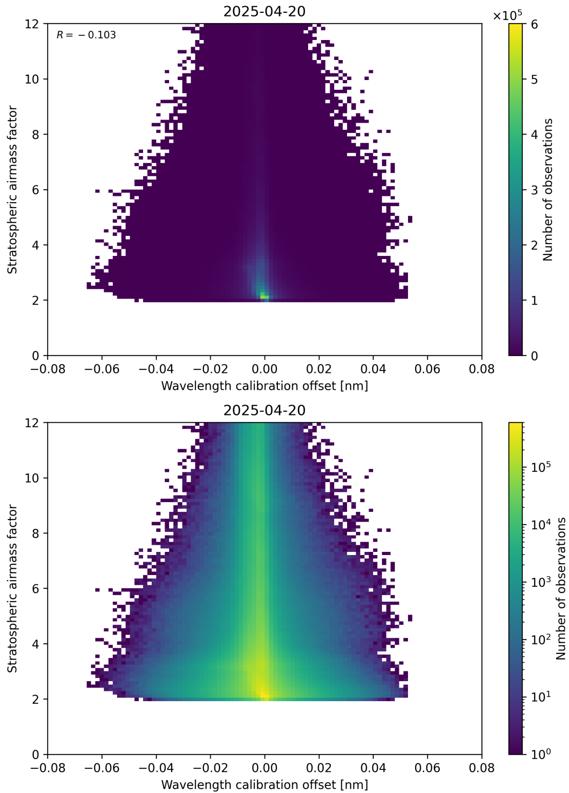
Figure 174: Scatter density plot of “Wavelength calibration offset” against “Stratospheric airmass factor” for 2025-04-20 to 2025-04-21.
