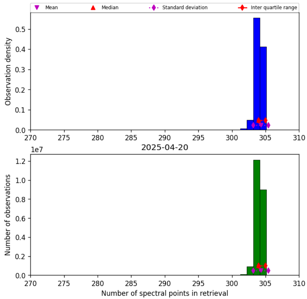
Figure 33: Histogram of “Number of spectral points in retrieval” for 2025-04-20 to 2025-04-21
