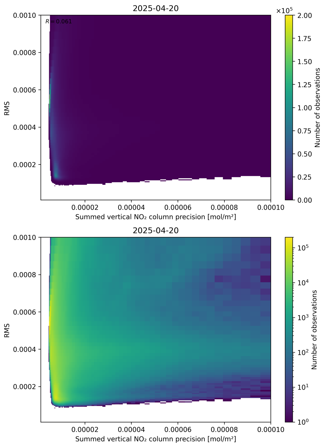
Figure 108: Scatter density plot of “Summed vertical NO 2 column precision” against “RMS” for 2025-04-20 to 2025-04-21.
