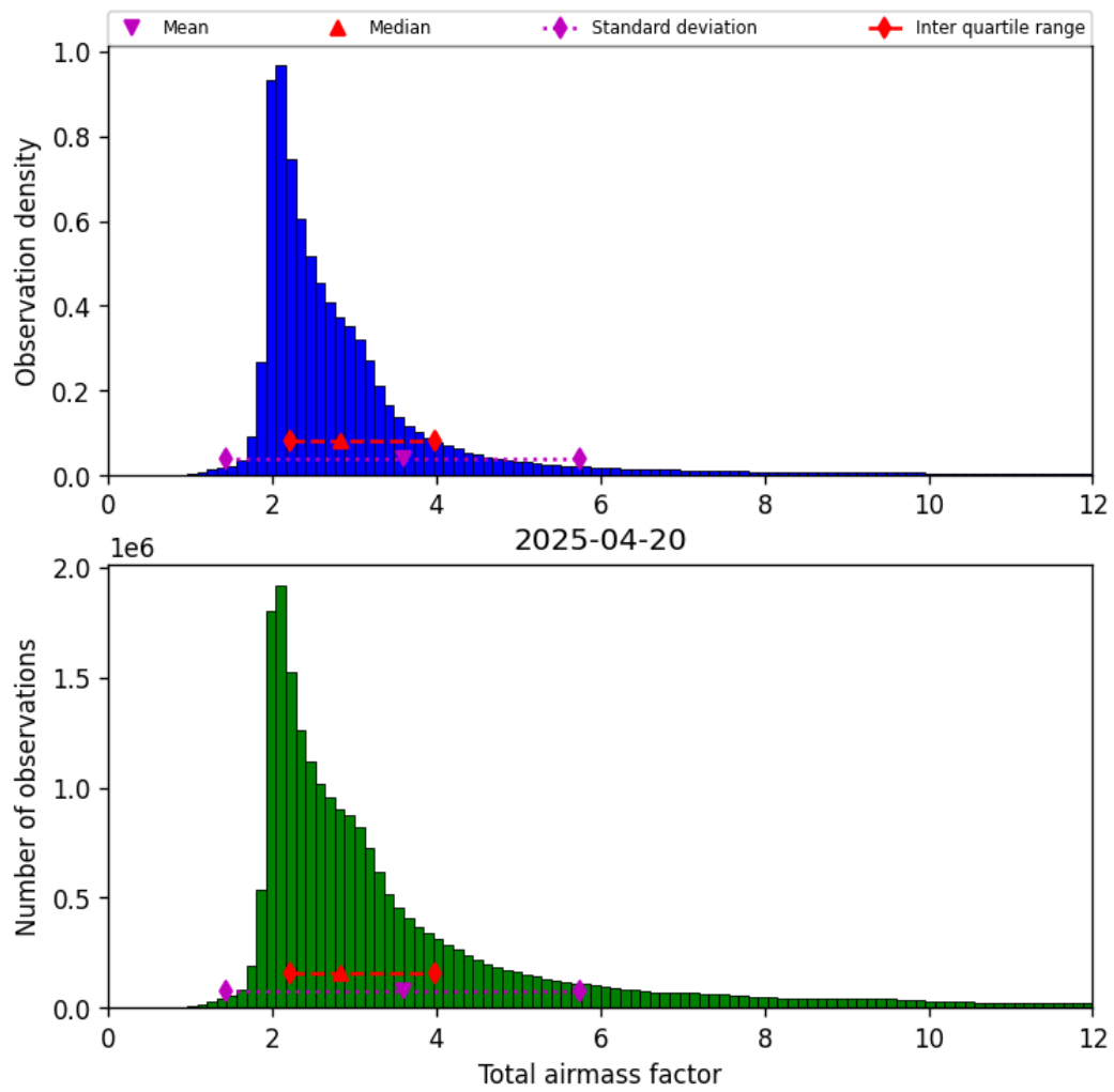
Figure 32: Histogram of “Total airmass factor” for 2025-04-20 to 2025-04-21
