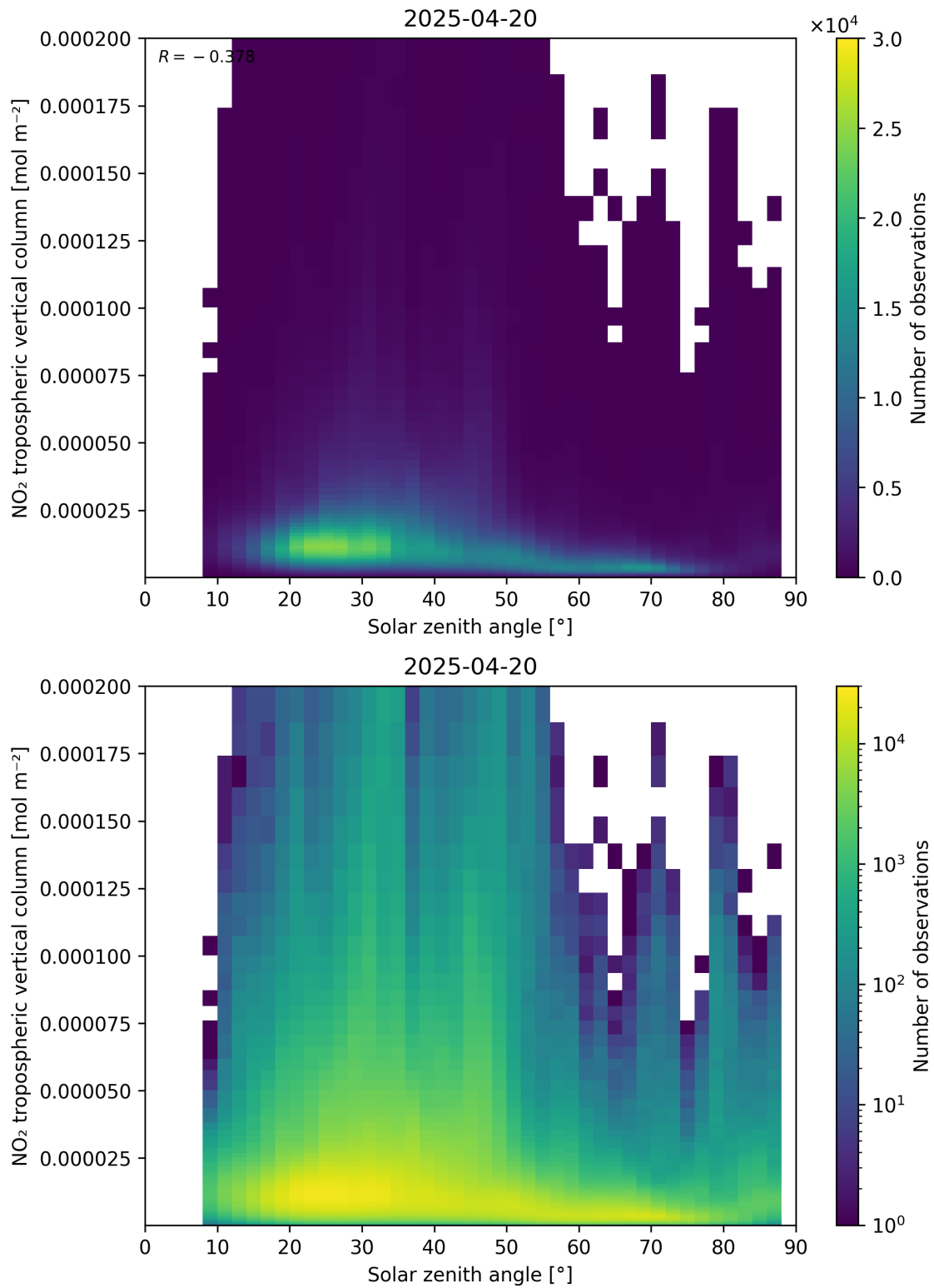
Figure 155: Scatter density plot of “Solar zenith angle” against “NO 2 tropospheric vertical column” for 2025-04-20 to 2025-04-21.
