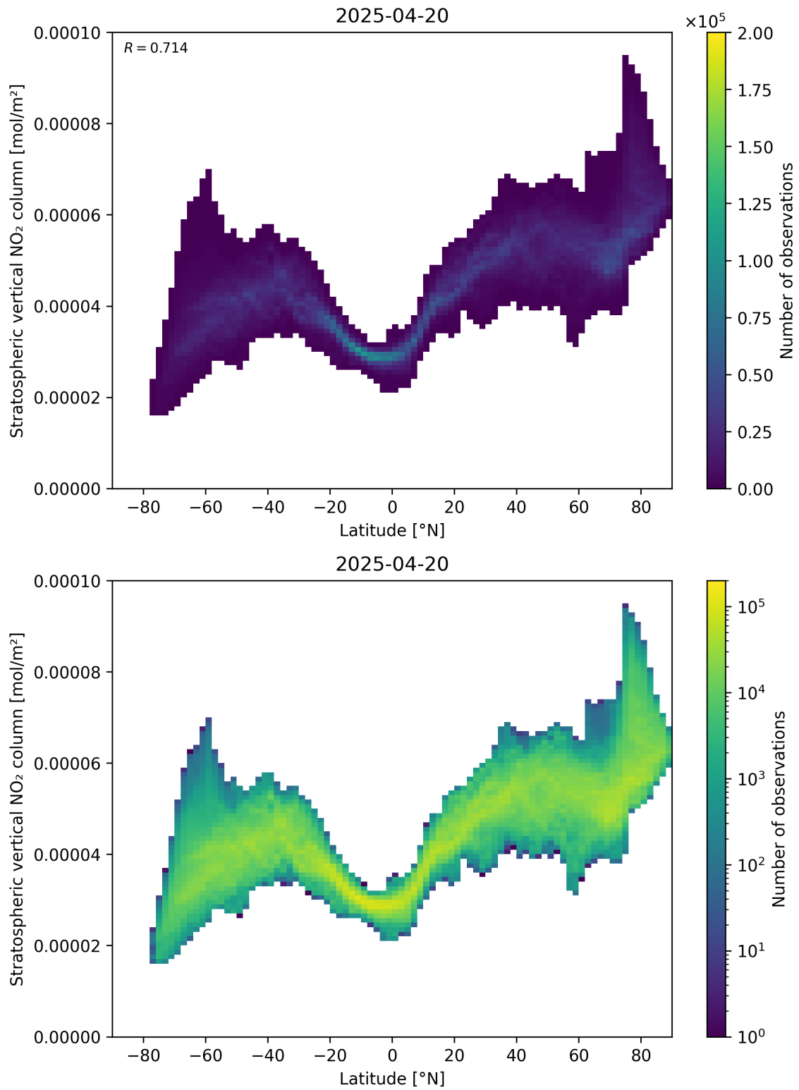
Figure 87: Scatter density plot of “Latitude” against “Stratospheric vertical NO 2 column” for 2025-04-20 to 2025-04-21.
