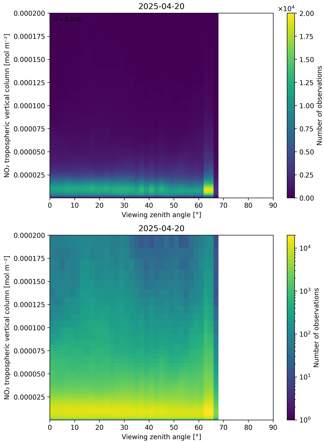
Figure 169: Scatter density plot of “Viewing zenith angle” against “NO 2 tropospheric vertical column” for 2025-04-20 to 2025-04-21.
