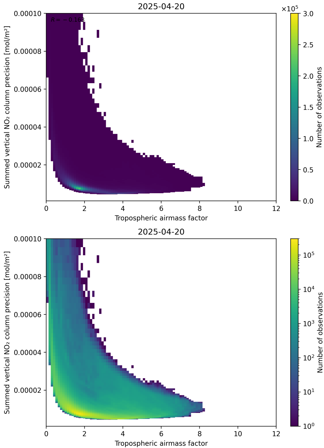
Figure 76: Scatter density plot of “Tropospheric air mass factor” against “Summed vertical NO 2 column precision” for 2025-04-20 to 2025-04-21.
