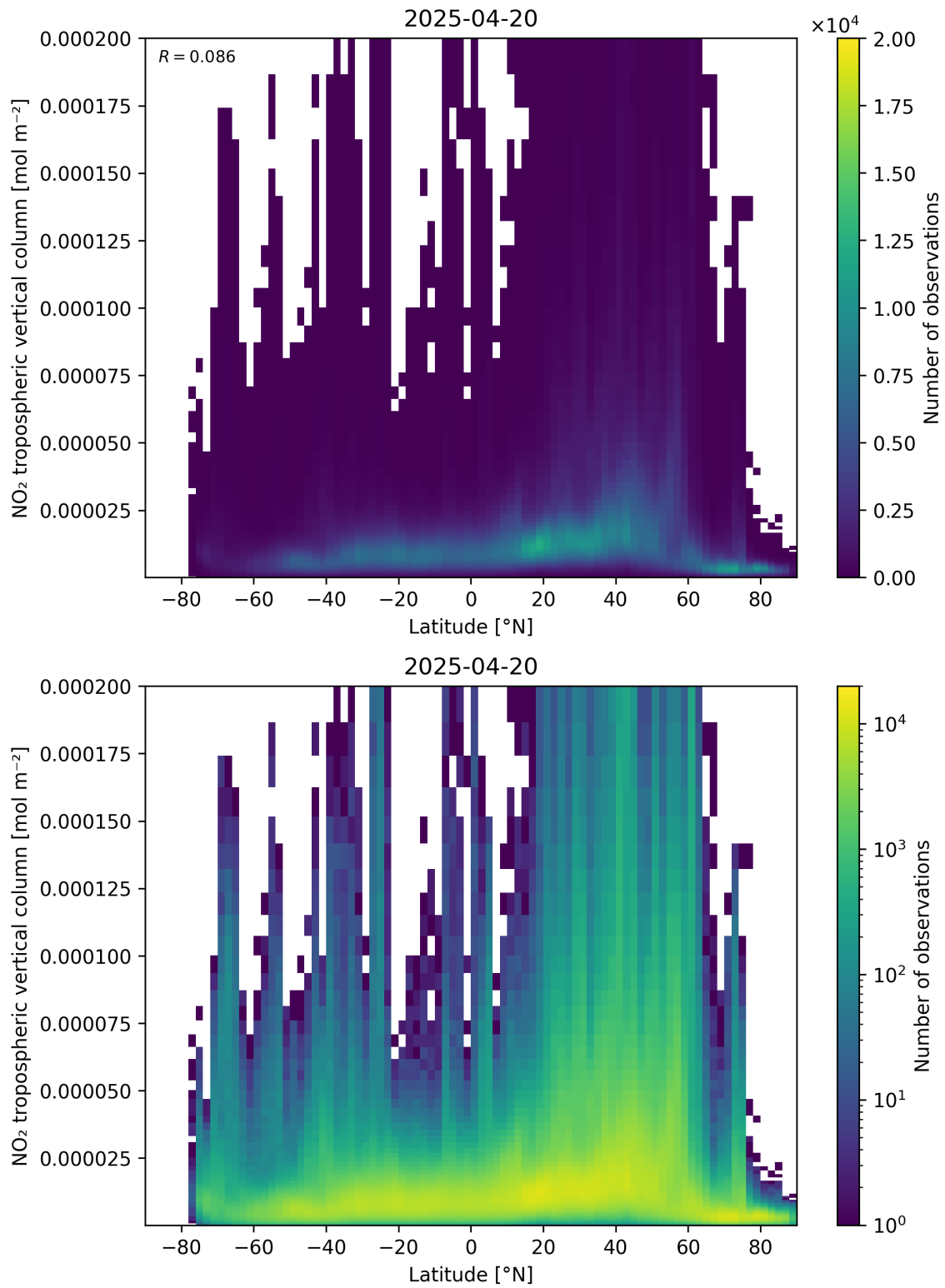
Figure 92: Scatter density plot of “Latitude” against “NO 2 tropospheric vertical column” for 2025-04-20 to 2025-04-21.
