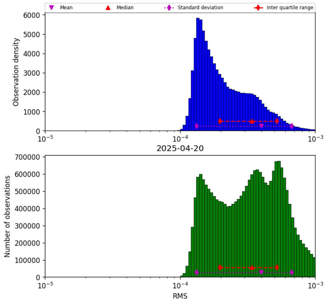
Figure 43: Histogram of “RMS” for 2025-04-20 to 2025-04-21
