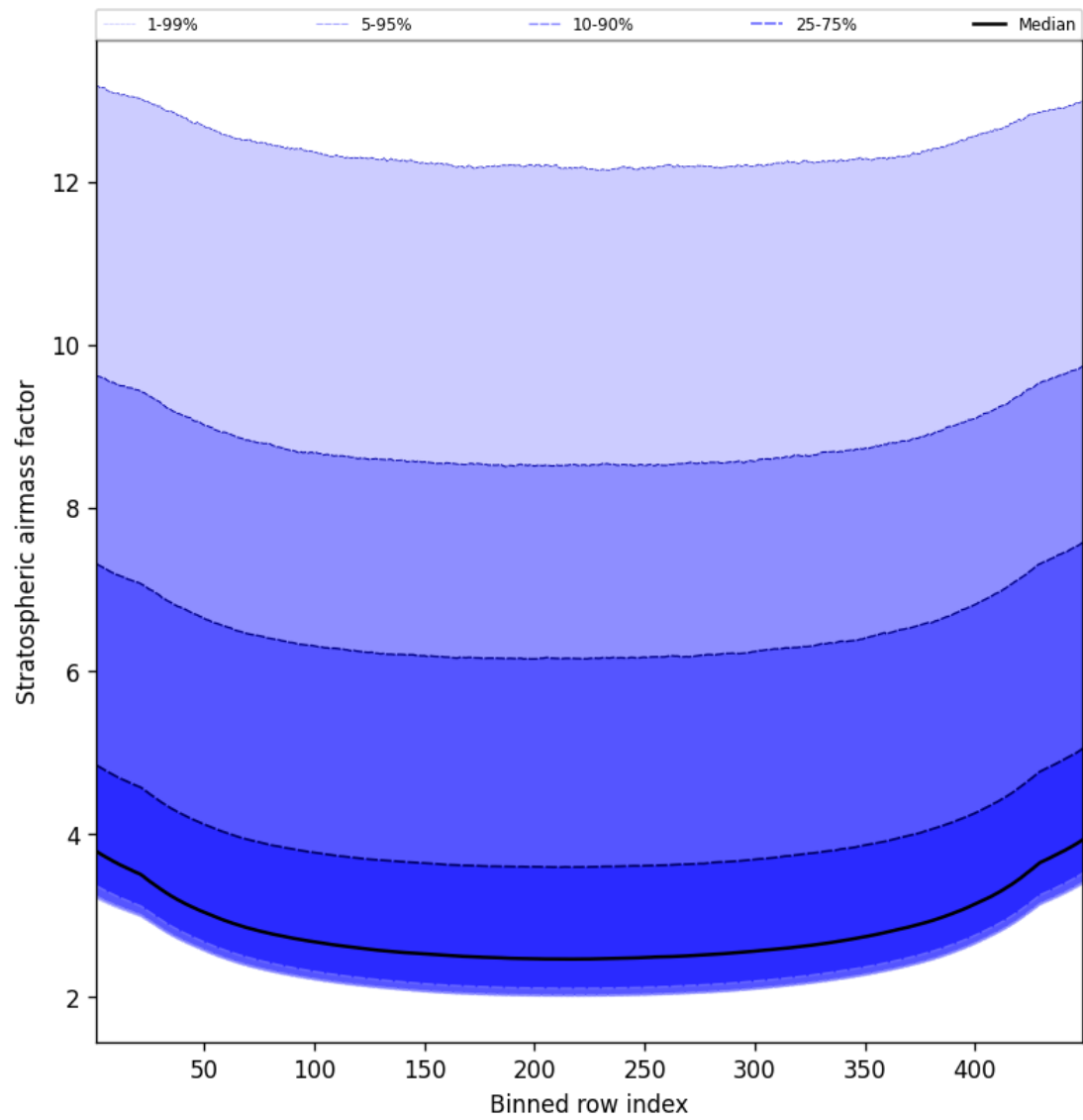
Figure 61: Along track statistics of “Stratospheric air mass factor” for 2025-04-20 to 2025-04-21
