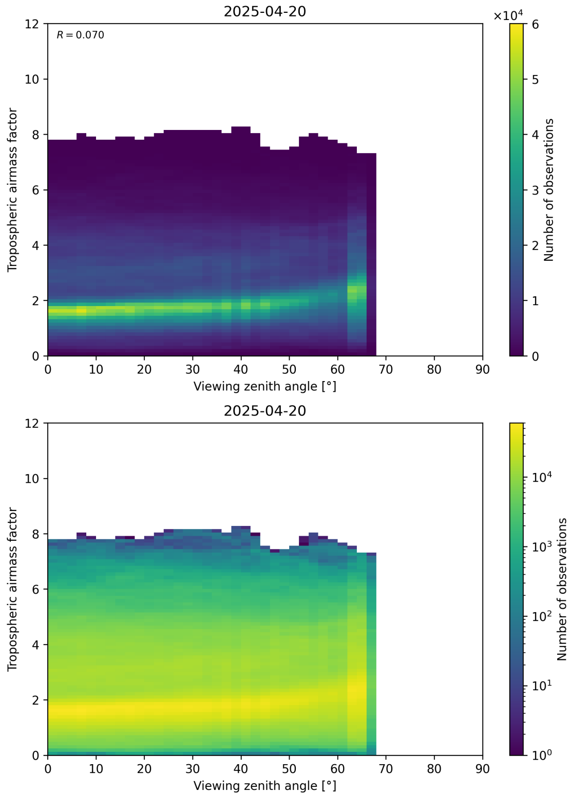
Figure 161: Scatter density plot of “Viewing zenith angle” against “Tropospheric airmass factor” for 2025-04-20 to 2025-04-21.
