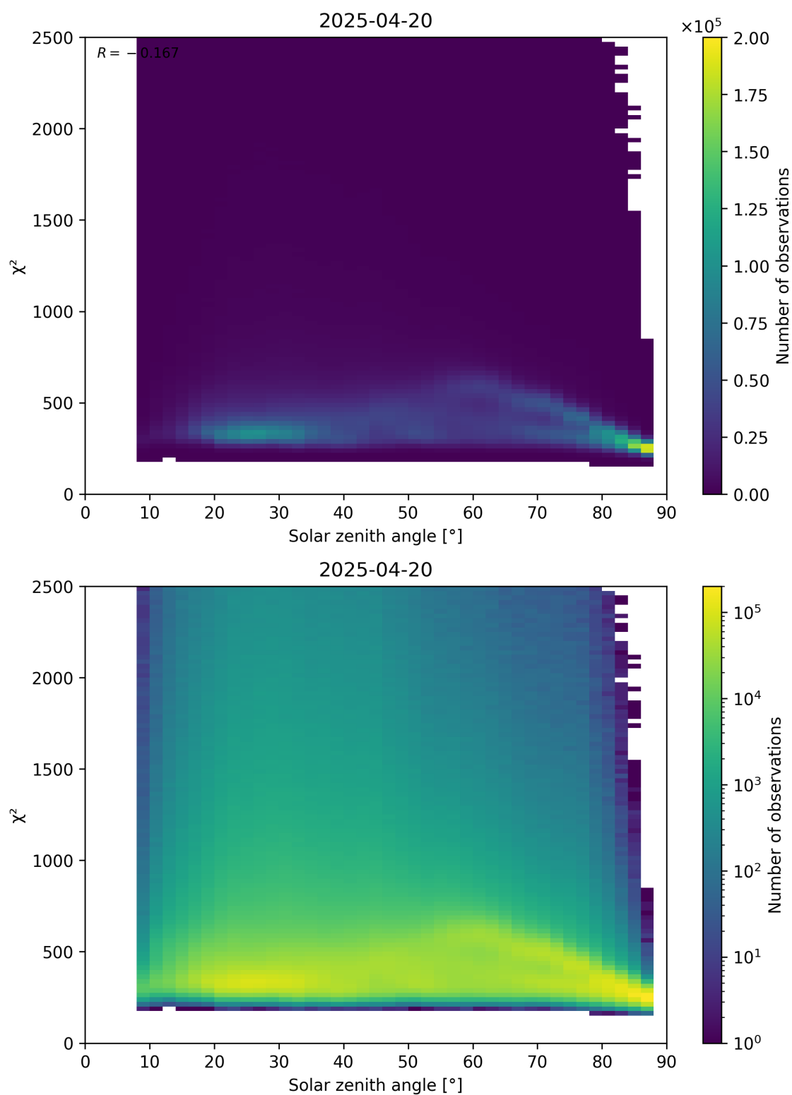
Figure 148: Scatter density plot of “Solar zenith angle” against “ \chi^2 ” for 2025-04-20 to 2025-04-21.
