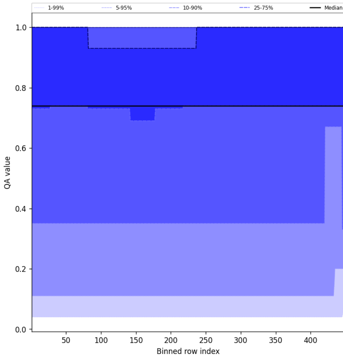
Figure 45: Along track statistics of “QA value” for 2025-04-20 to 2025-04-21
