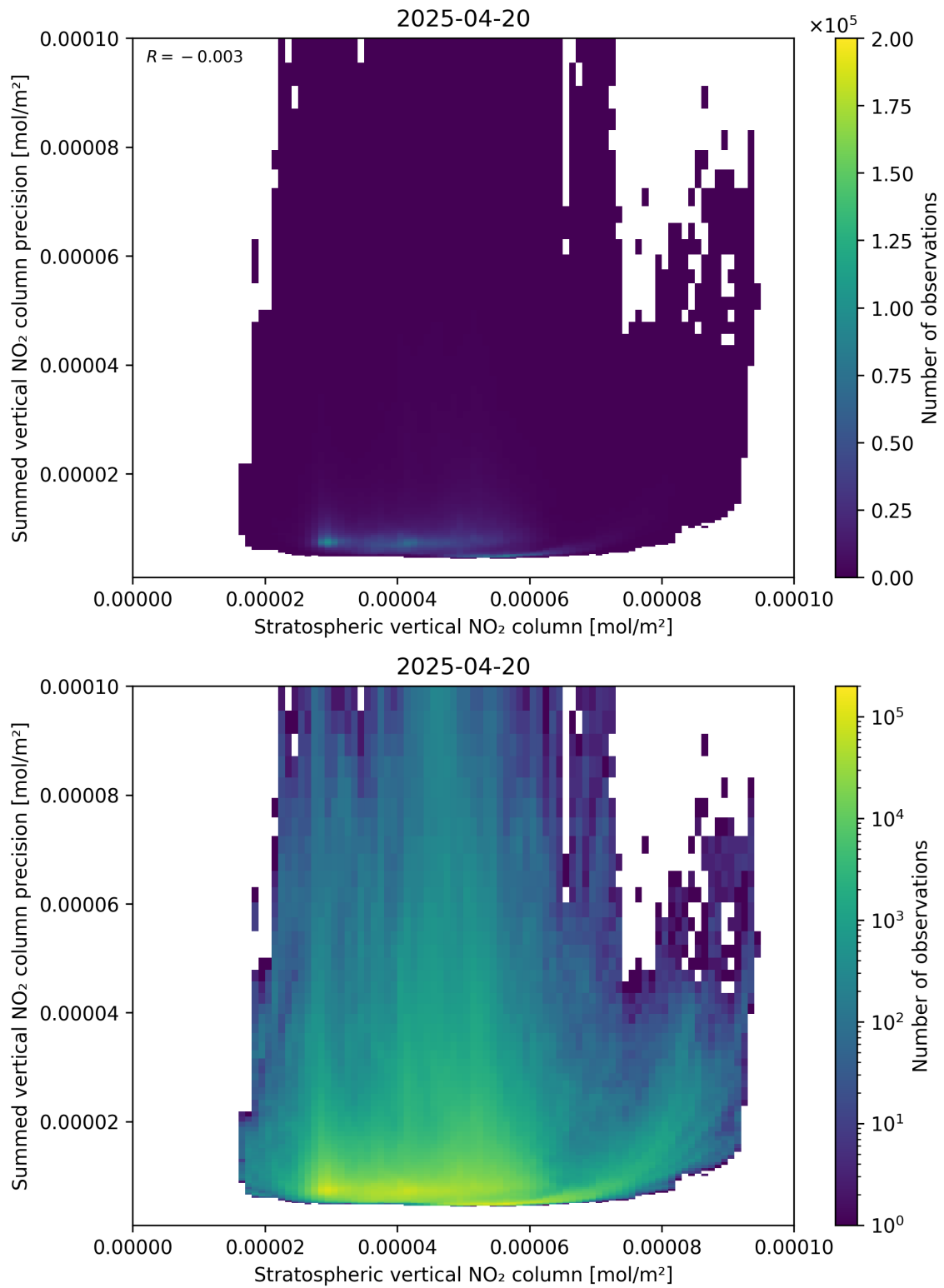
Figure 99: Scatter density plot of “Stratospheric vertical NO 2 column” against “Summed vertical NO 2 column precision” for 2025-04-20 to 2025-04-21.
