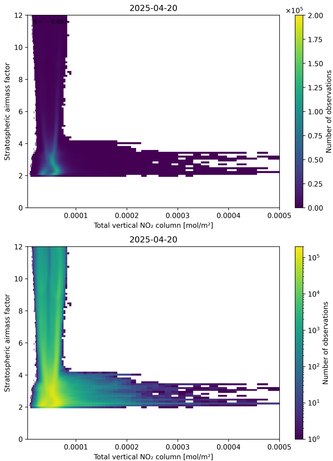
Figure 110: Scatter density plot of “Total vertical NO 2 column” against “Stratospheric airmass factor” for 2025-04-20 to 2025-04-21.
