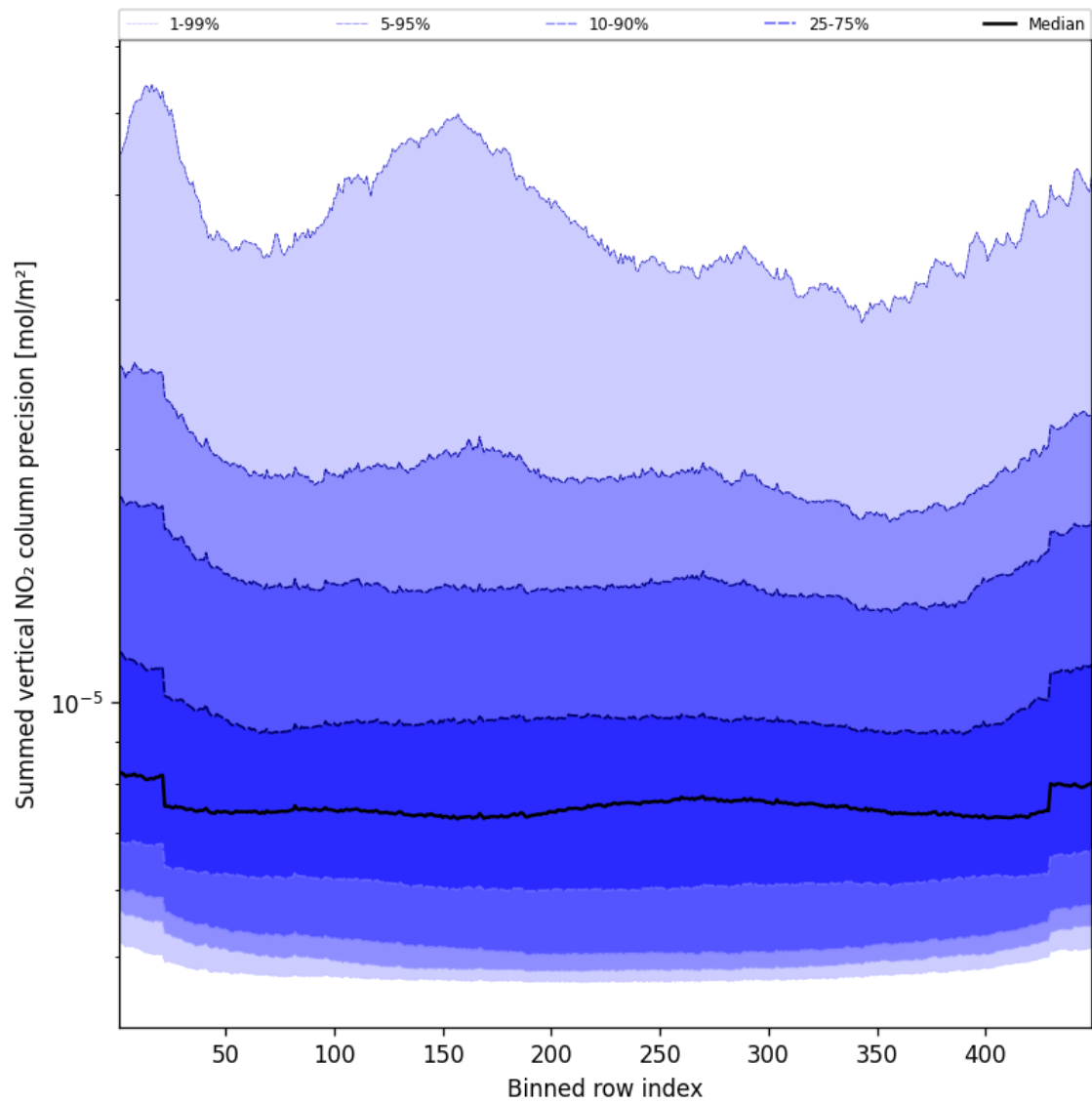
Figure 58: Along track statistics of “Summed vertical NO 2 column precision” for 2025-04-20 to 2025-04-21
