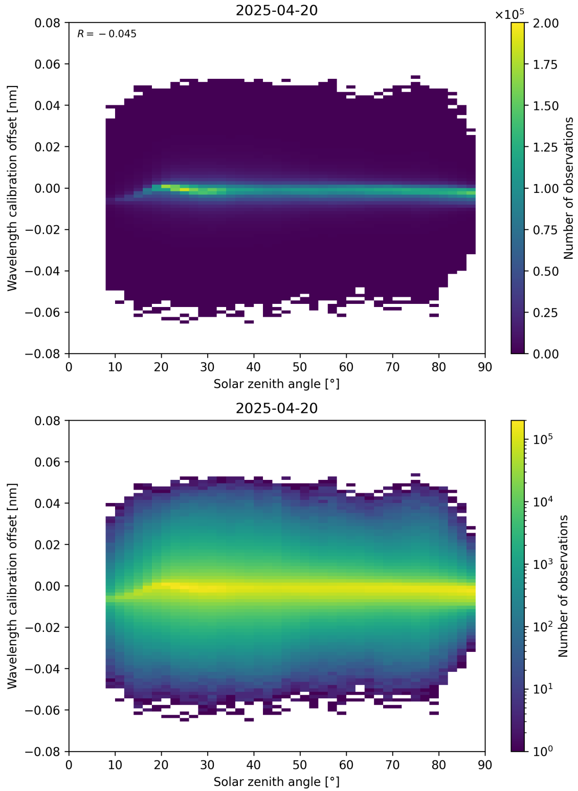
Figure 158: Scatter density plot of “Solar zenith angle” against “Wavelength calibration offset” for 2025-04-20 to 2025-04-21.
