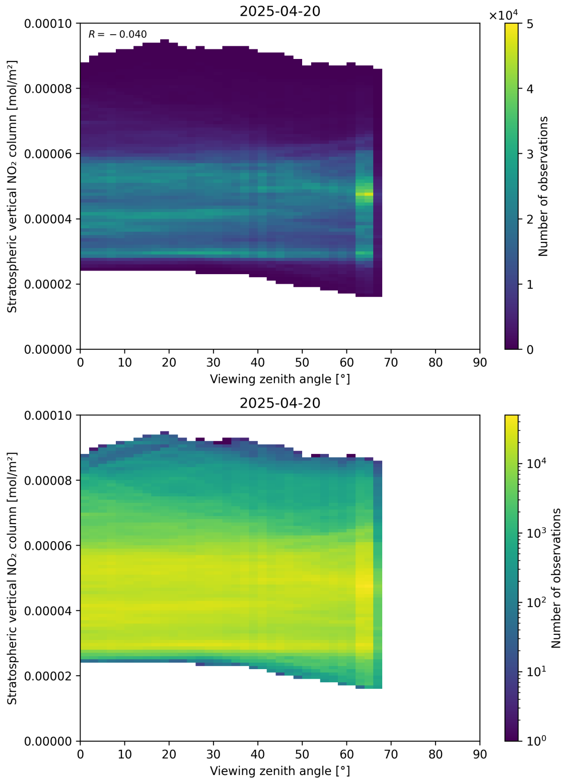
Figure 164: Scatter density plot of “Viewing zenith angle” against “Stratospheric vertical NO 2 column” for 2025-04-20 to 2025-04-21.
