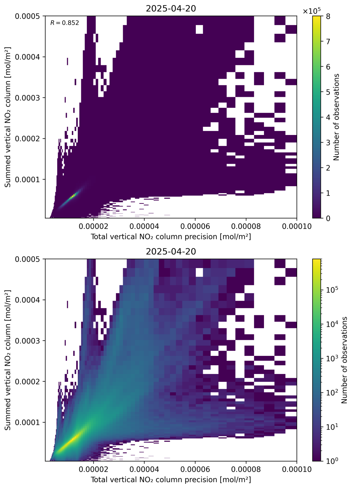
Figure 117: Scatter density plot of “Total vertical NO 2 column precision” against “Summed vertical NO 2 column” for 2025-04-20 to 2025-04-21.
