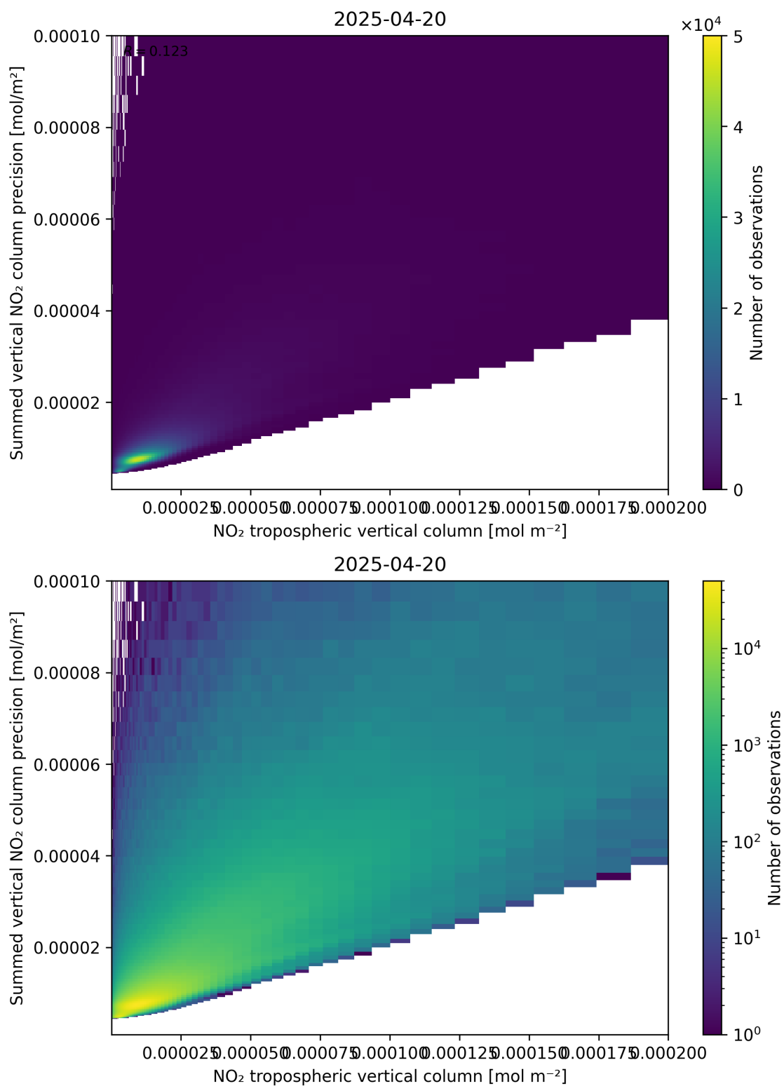
Figure 127: Scatter density plot of “NO 2 tropospheric vertical column” against “Summed vertical NO 2 column precision” for 2025-04-20 to 2025-04-21.
