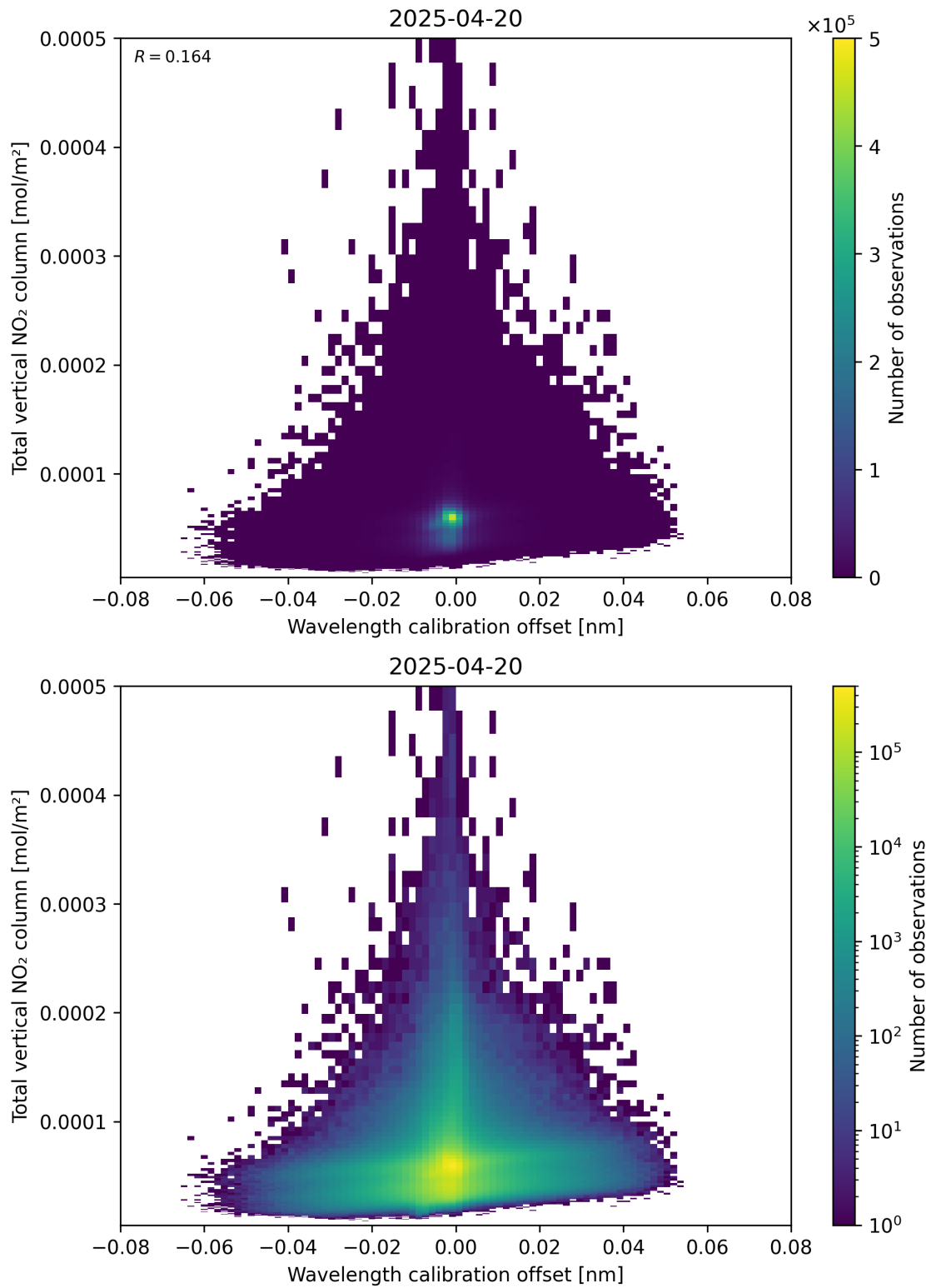
Figure 179: Scatter density plot of “Wavelength calibration offset” against “Total vertical NO 2 column” for 2025-04-20 to 2025-04-21.
