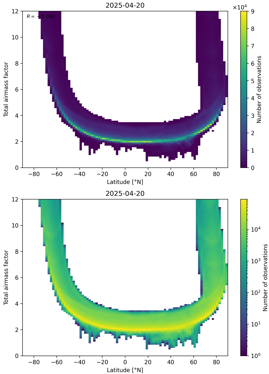
Figure 84: Scatter density plot of “Latitude” against “Total airmass factor” for 2025-04-20 to 2025-04-21.
