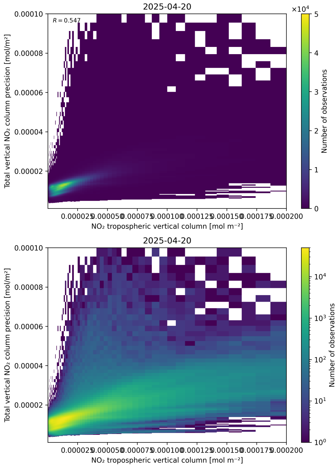
Figure 129: Scatter density plot of “NO 2 tropospheric vertical column” against “Total vertical NO 2 column precision” for 2025-04-20 to 2025-04-21.
