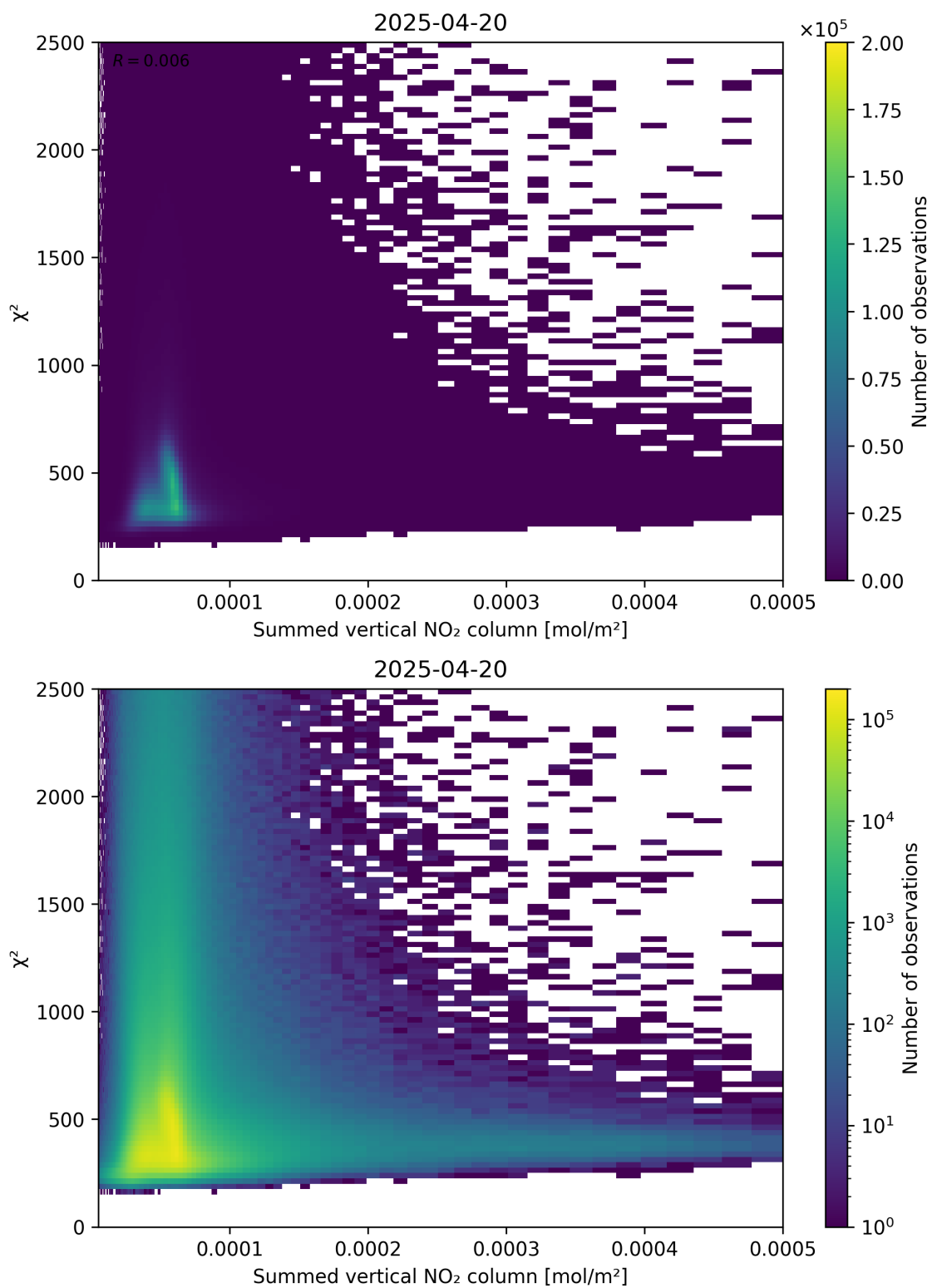
Figure 104: Scatter density plot of “Summed vertical NO 2 column” against “ \chi^2 ” for 2025-04-20 to 2025-04-21.
