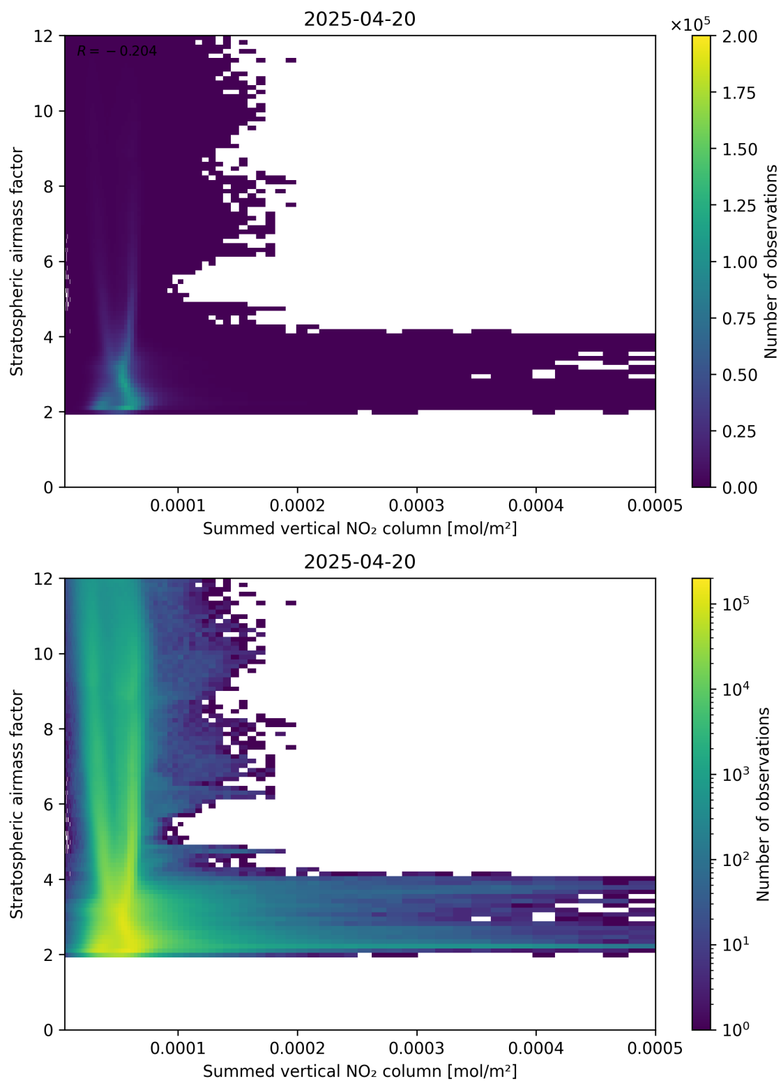
Figure 103: Scatter density plot of “Summed vertical NO 2 column” against “Stratospheric airmass factor” for 2025-04-20 to 2025-04-21.
