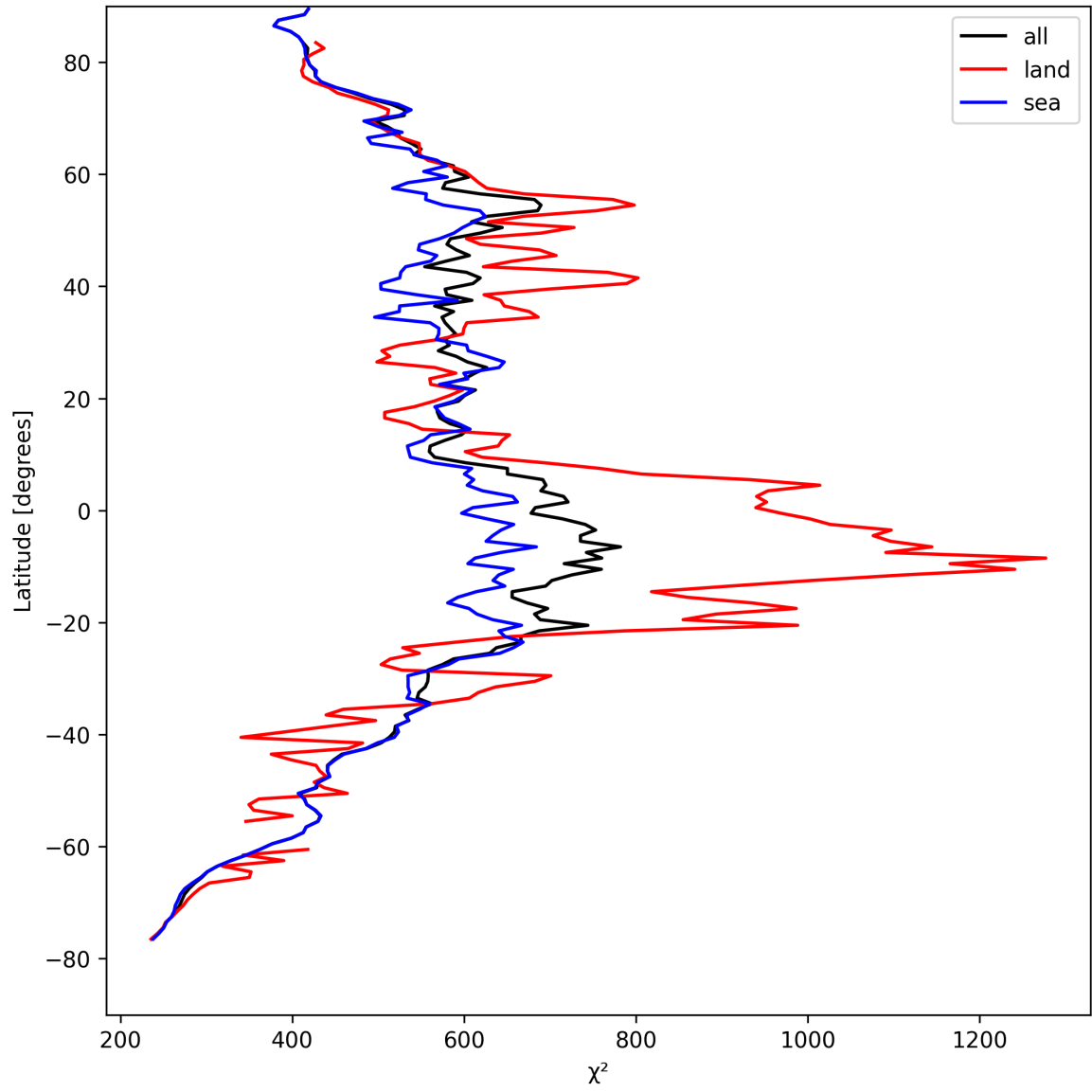
Figure 25: Zonal average of “ \chi^2 ” for 2025-04-20 to 2025-04-21.
