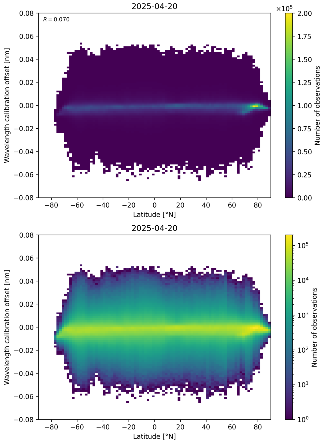
Figure 95: Scatter density plot of “Latitude” against “Wavelength calibration offset” for 2025-04-20 to 2025-04-21.
