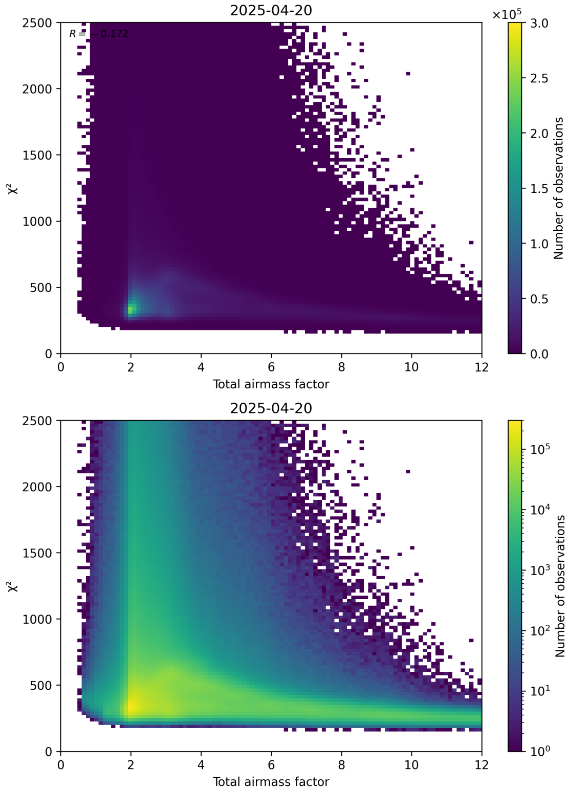
Figure 63: Scatter density plot of “Total airmass factor” against “ \chi^2 ” for 2025-04-20 to 2025-04-21.
