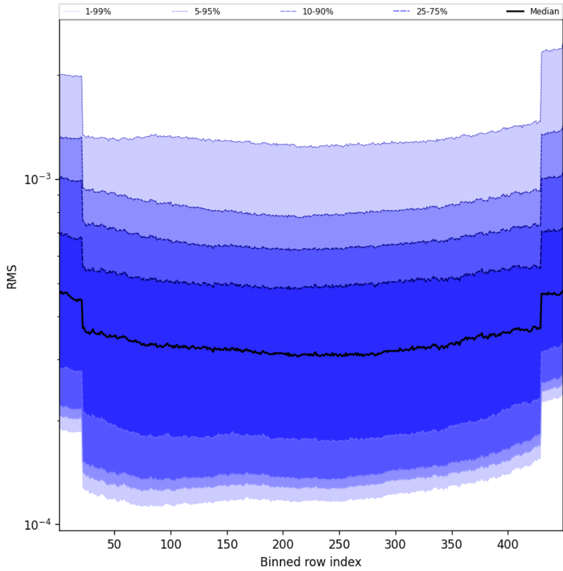
Figure 60: Along track statistics of “RMS” for 2025-04-20 to 2025-04-21
