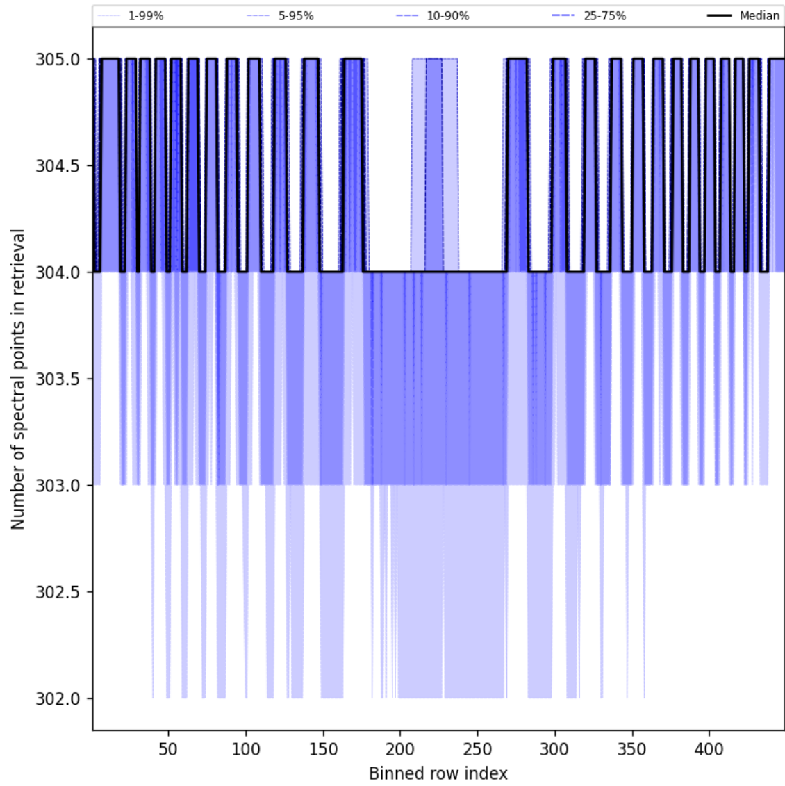
Figure 50: Along track statistics of “Number of spectral points in retrieval” for 2025-04-20 to 2025-04-21
