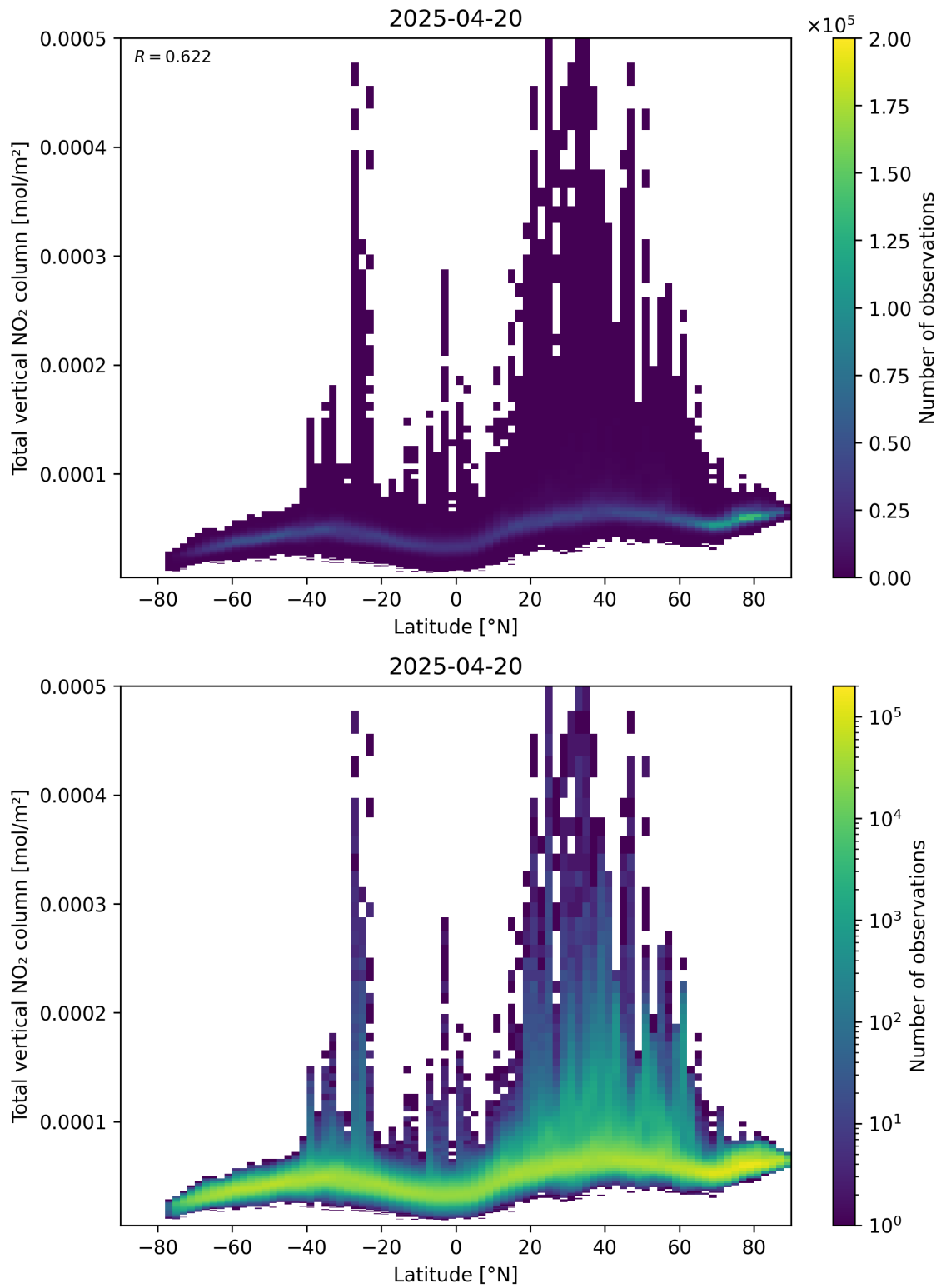
Figure 90: Scatter density plot of “Latitude” against “Total vertical NO 2 column” for 2025-04-20 to 2025-04-21.
