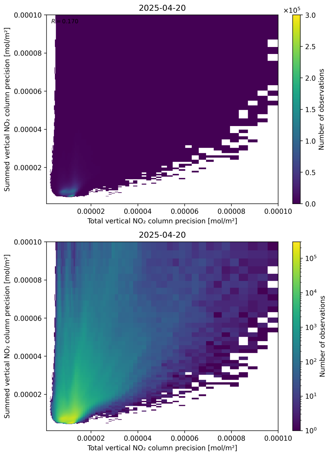
Figure 118: Scatter density plot of “Total vertical NO 2 column precision” against “Summed vertical NO 2 column precision” for 2025-04-20 to 2025-04-21.
