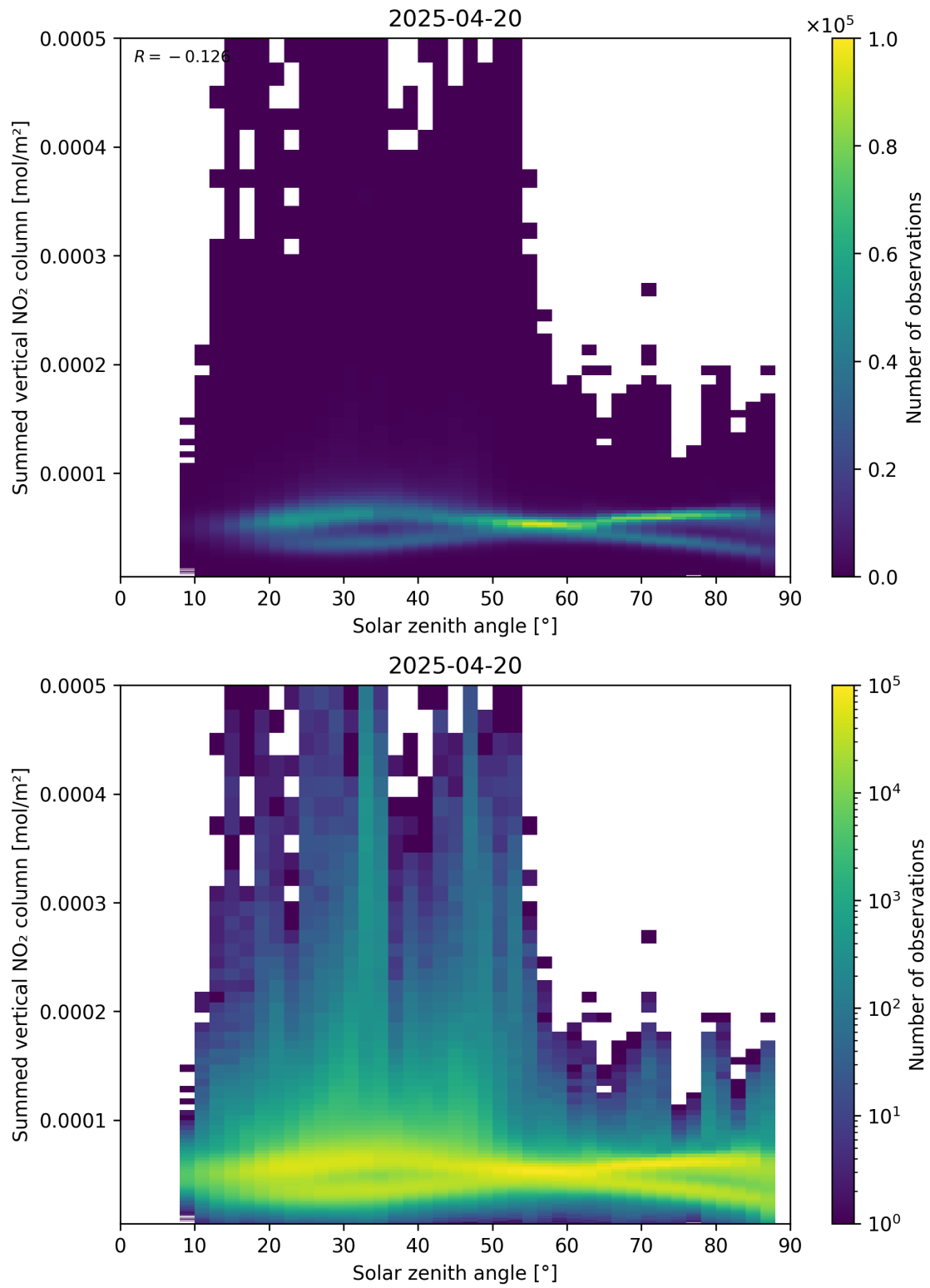
Figure 151: Scatter density plot of “Solar zenith angle” against “Summed vertical NO 2 column” for 2025-04-20 to 2025-04-21.
