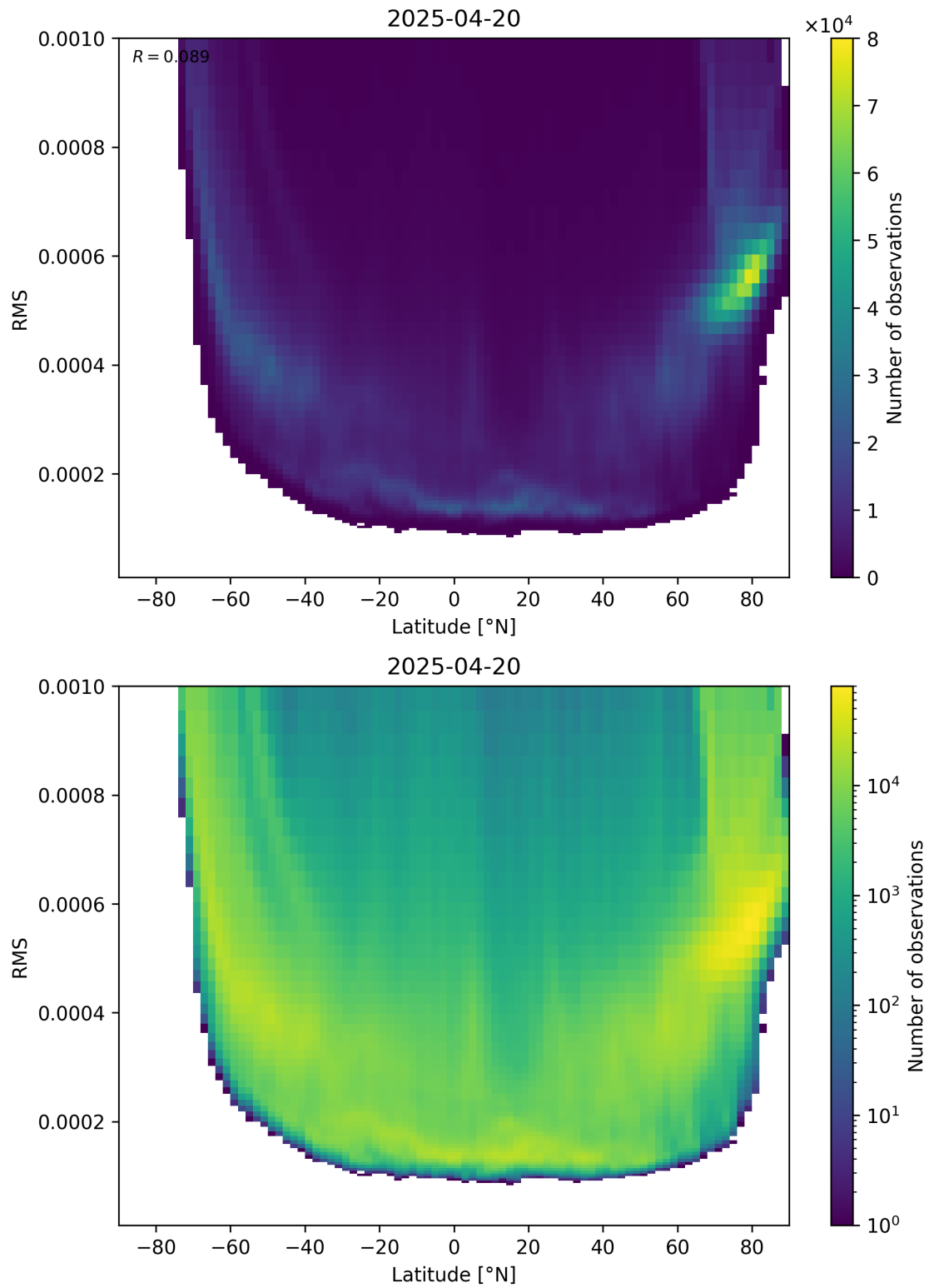
Figure 94: Scatter density plot of “Latitude” against “RMS” for 2025-04-20 to 2025-04-21.
