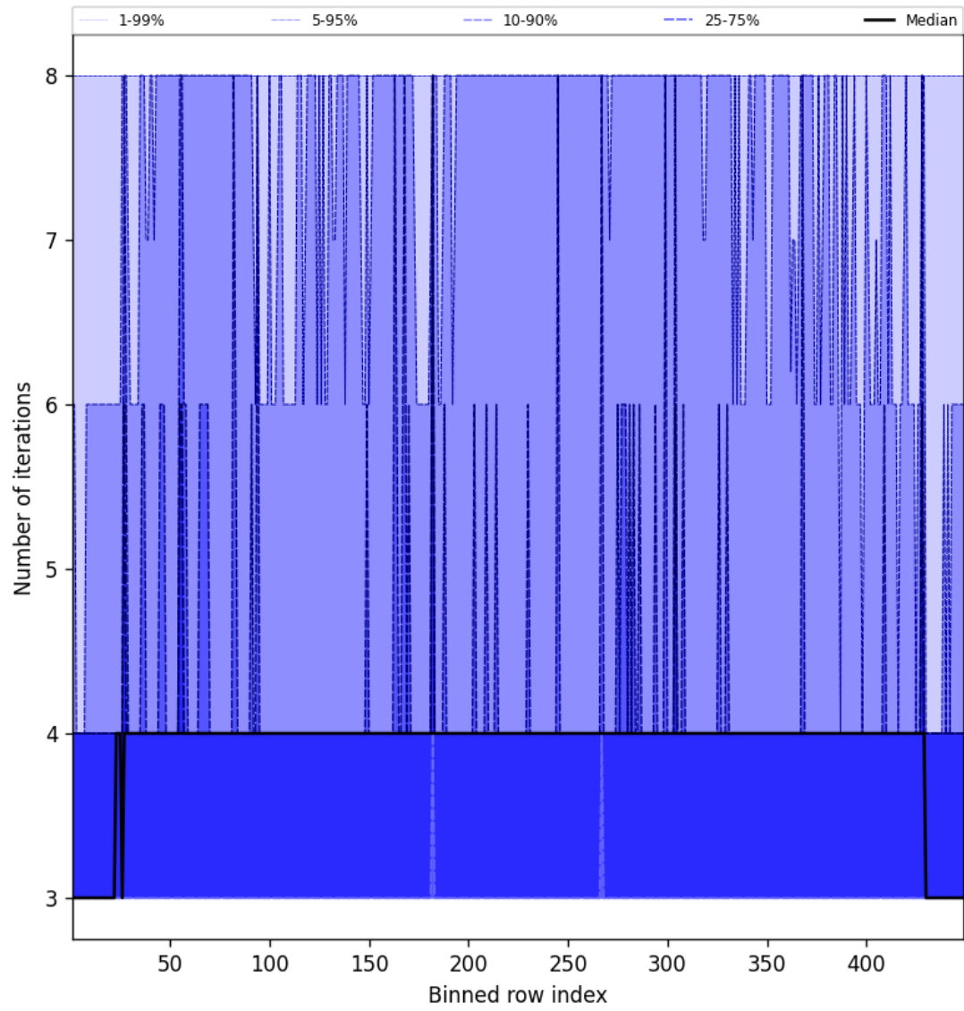
Figure 51: Along track statistics of “Number of iterations” for 2025-04-20 to 2025-04-21
