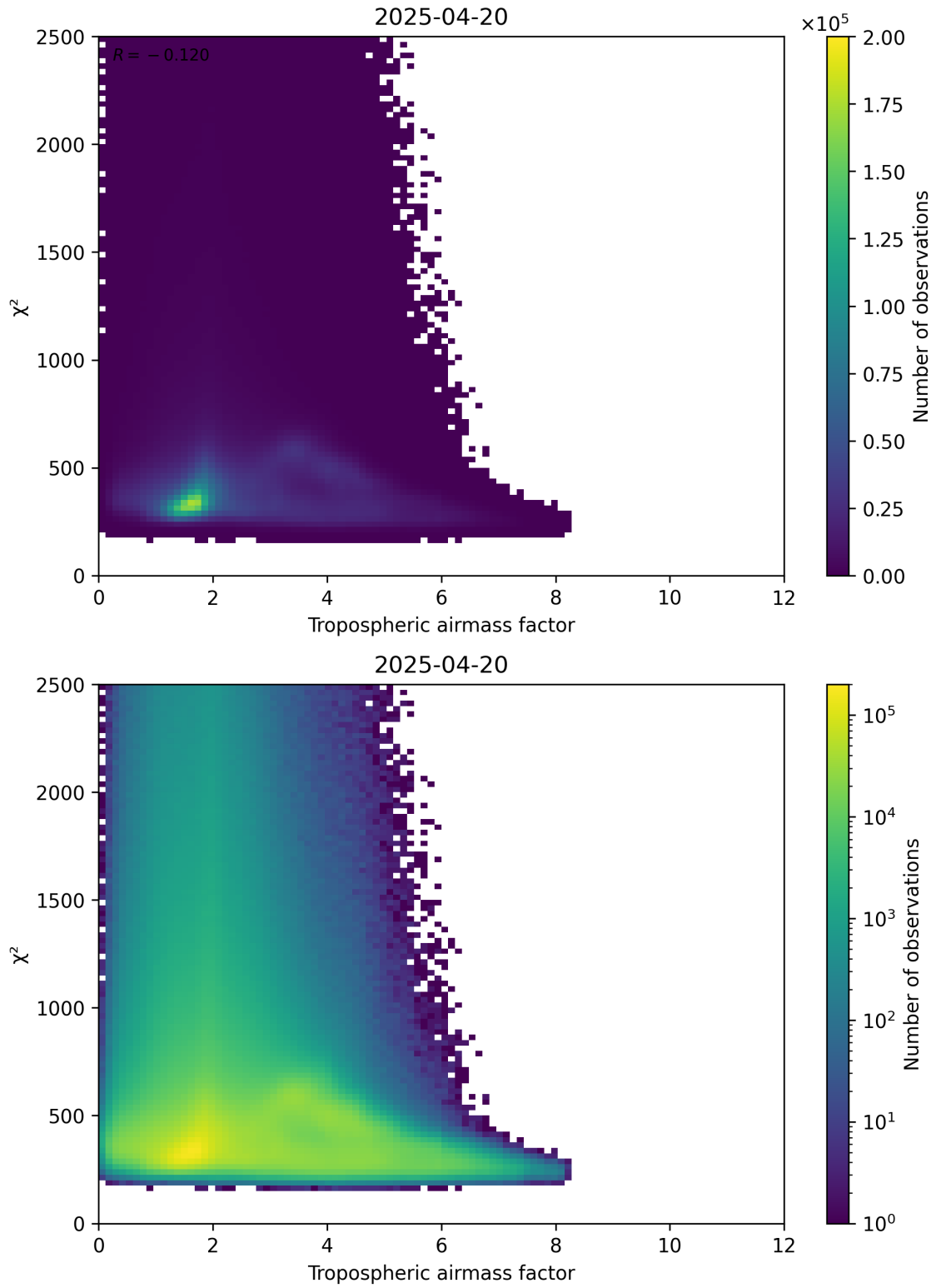
Figure 73: Scatter density plot of “Tropospheric airmass factor” against “ \chi^2 ” for 2025-04-20 to 2025-04-21.
