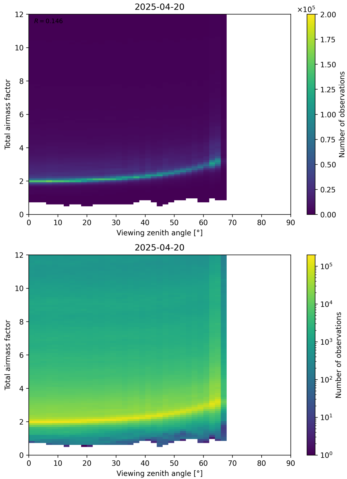
Figure 160: Scatter density plot of “Viewing zenith angle” against “Total airmass factor” for 2025-04-20 to 2025-04-21.
