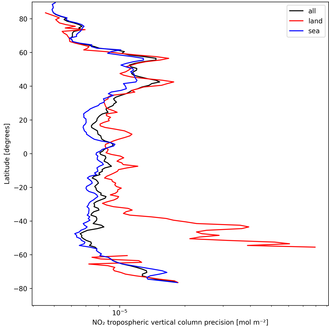
Figure 13: Zonal average of “NO 2 tropospheric vertical column precision” for 2025-04-20 to 2025-04-21.
