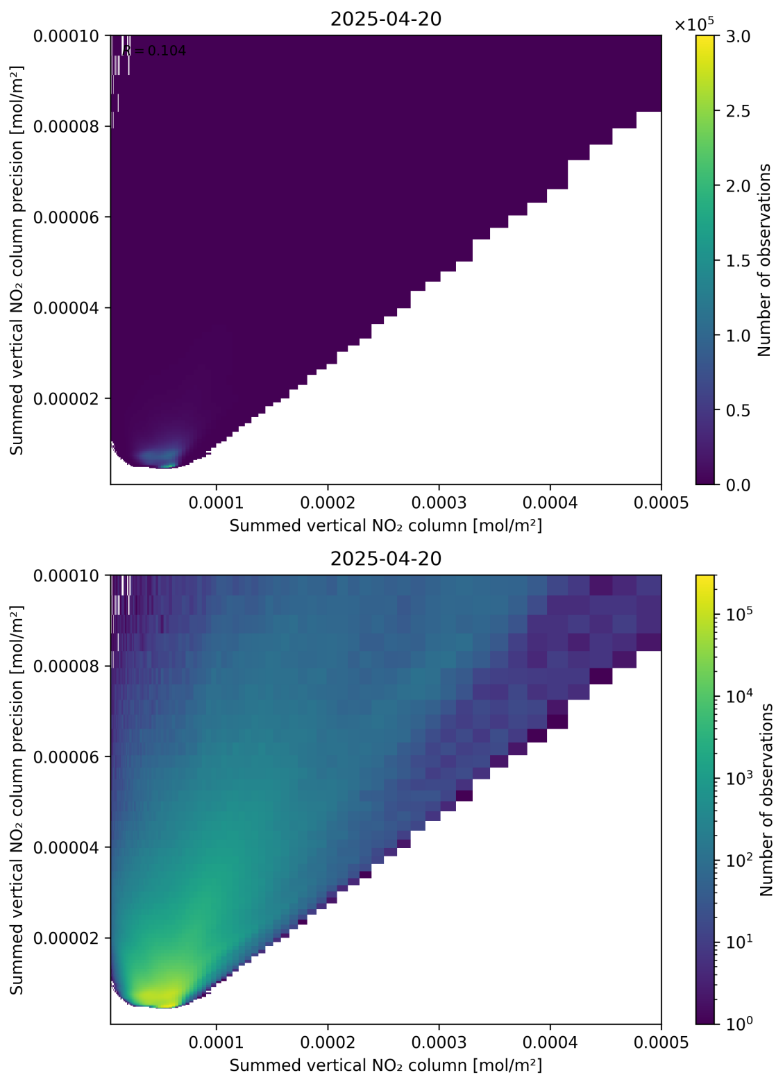
Figure 105: Scatter density plot of “Summed vertical NO 2 column” against “Summed vertical NO 2 column precision” for 2025-04-20 to 2025-04-21.
