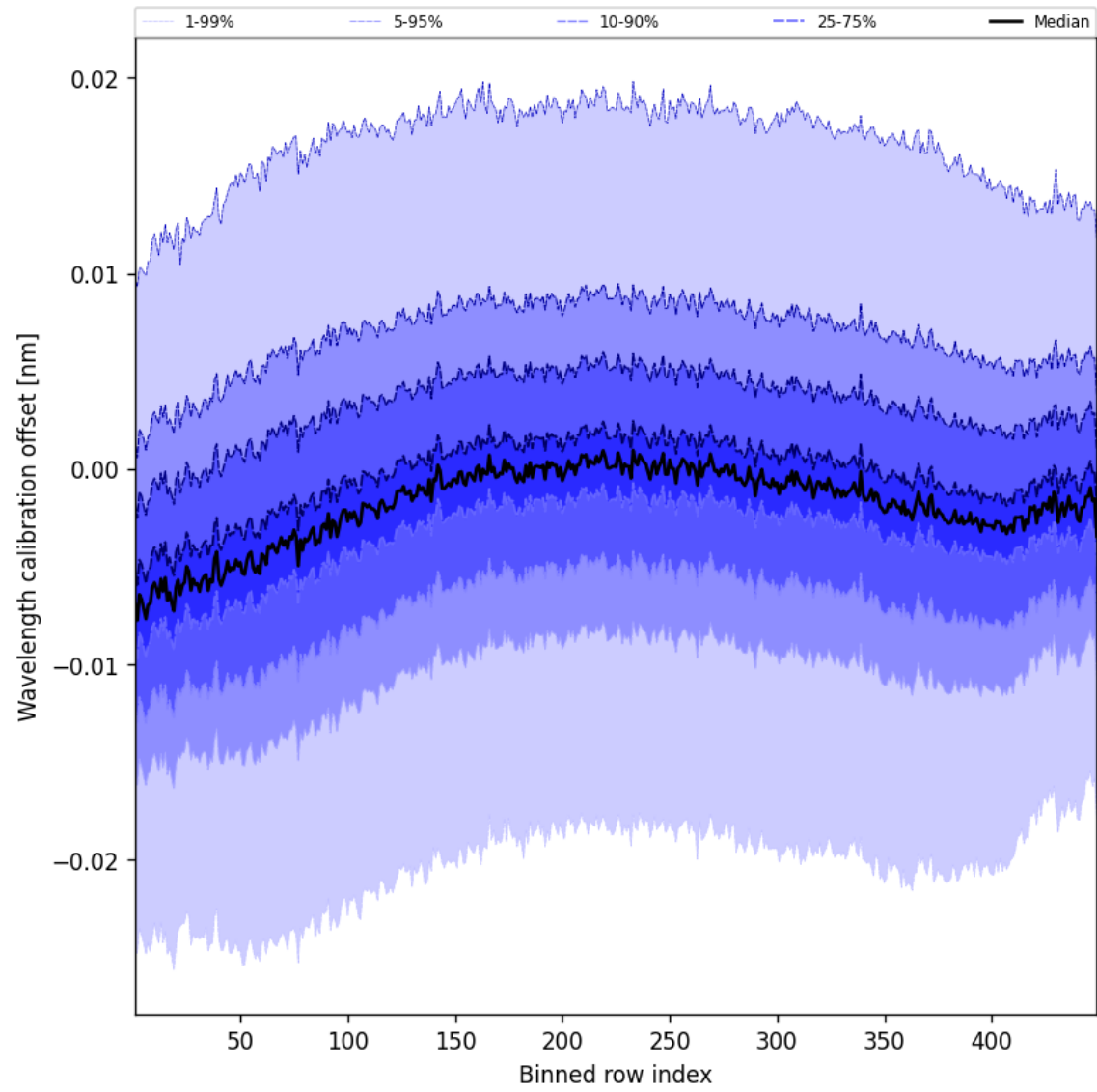
Figure 52: Along track statistics of “Wavelength calibration offset” for 2025-04-20 to 2025-04-21
