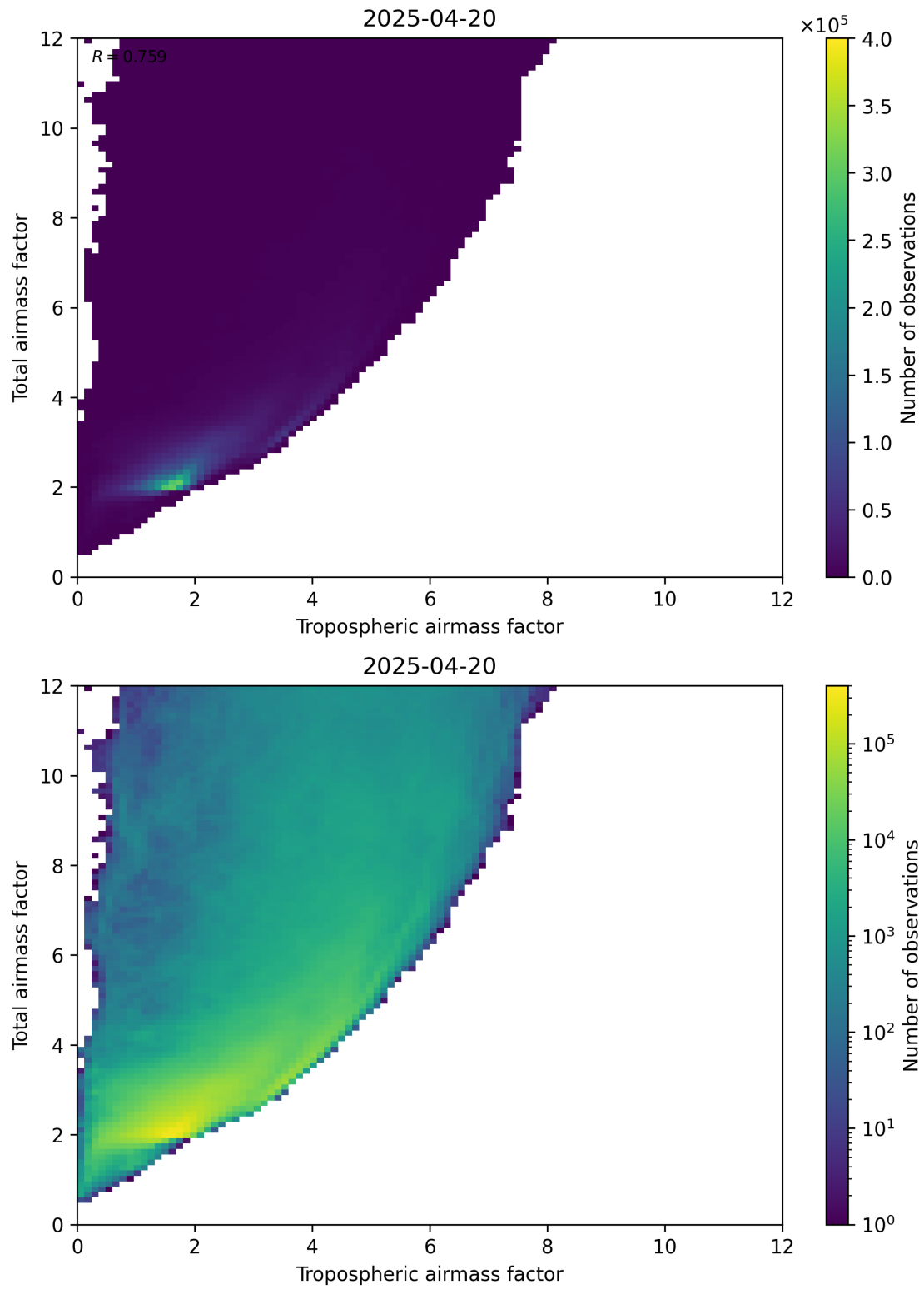
Figure 72: Scatter density plot of “Tropospheric airmass factor” against “Total airmass factor” for 2025-04-20 to 2025-04-21.
