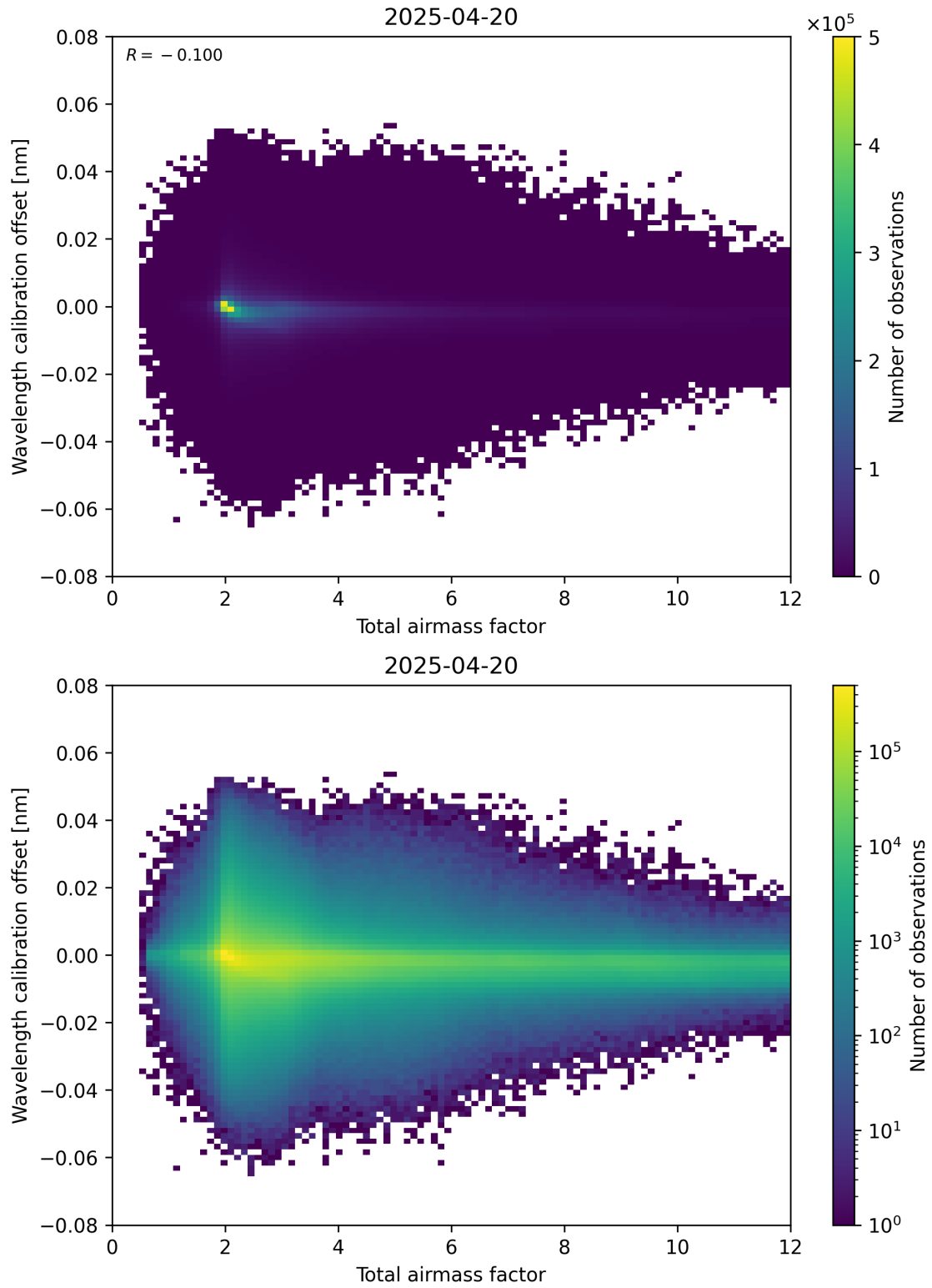
Figure 70: Scatter density plot of “Total airmass factor” against “Wavelength calibration offset” for 2025-04-20 to 2025-04-21.
