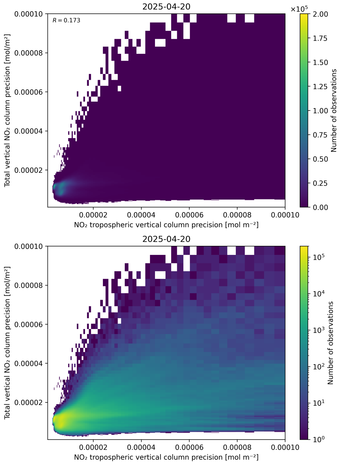
Figure 139: Scatter density plot of “NO 2 tropospheric vertical column precision” against “Total vertical NO 2 column precision” for 2025-04-20 to 2025-04-21.
