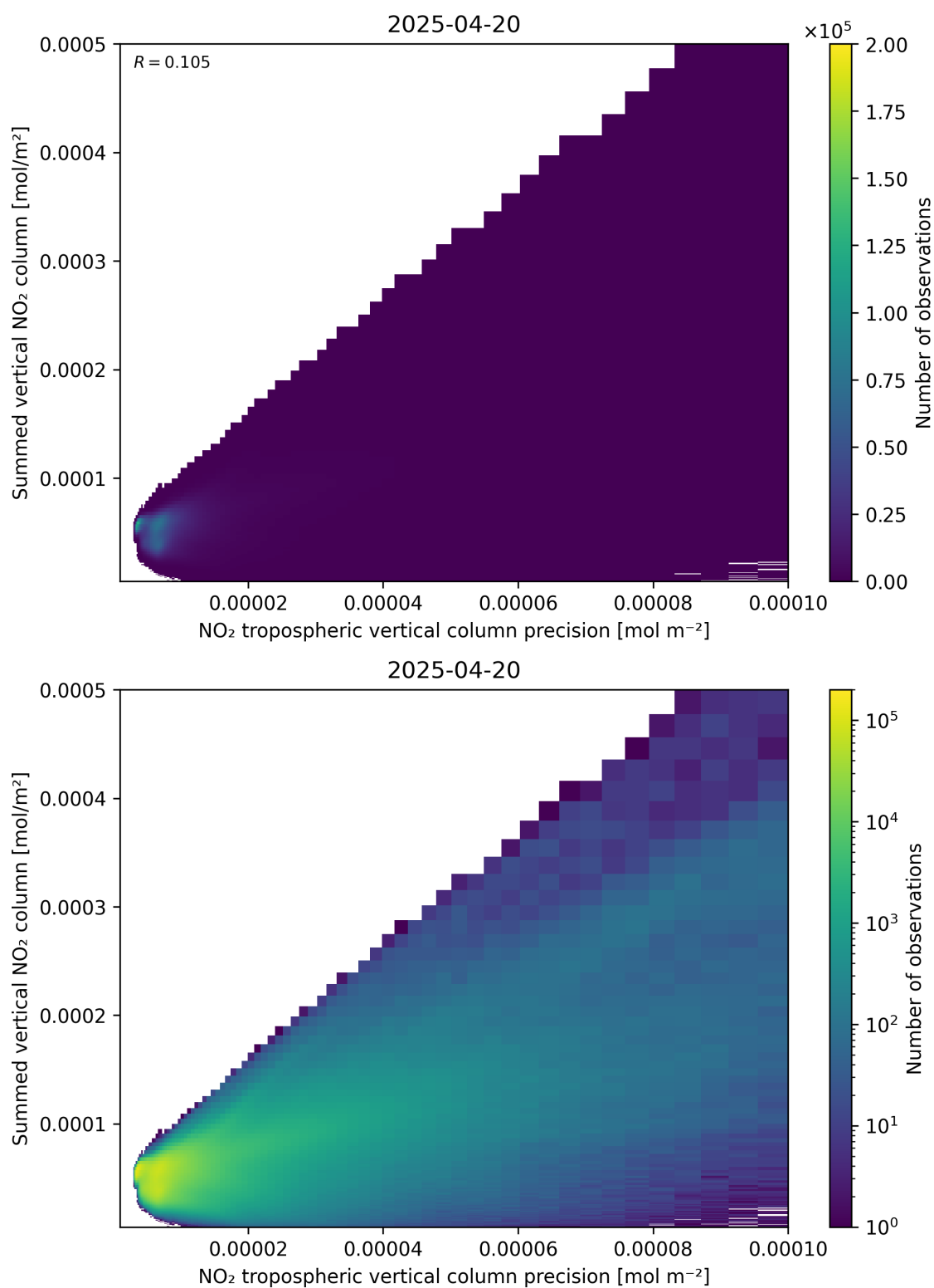
Figure 136: Scatter density plot of “NO 2 tropospheric vertical column precision” against “Summed vertical NO 2 column” for 2025-04-20 to 2025-04-21.
