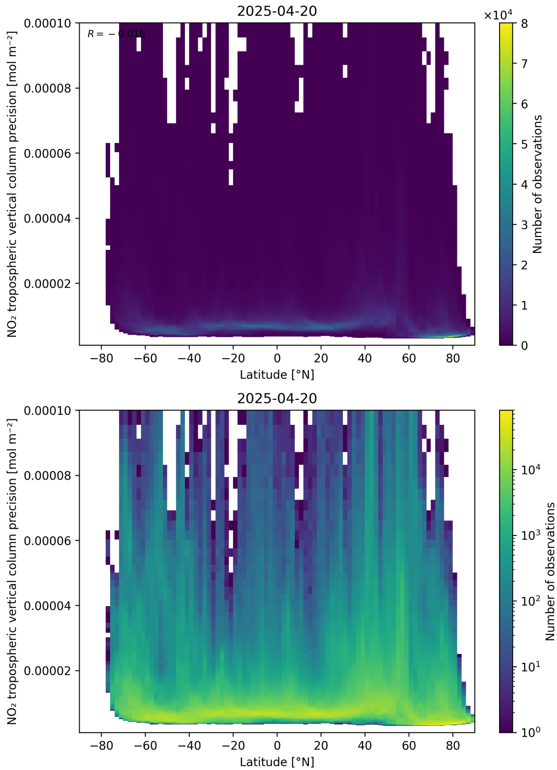
Figure 93: Scatter density plot of “Latitude” against “NO 2 tropospheric vertical column precision” for 2025-04-20 to 2025-04-21.
