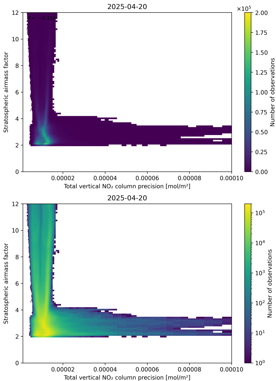
Figure 115: Scatter density plot of “Total vertical NO 2 column precision” against “Stratospheric air mass factor” for 2025-04-20 to 2025-04-21.
