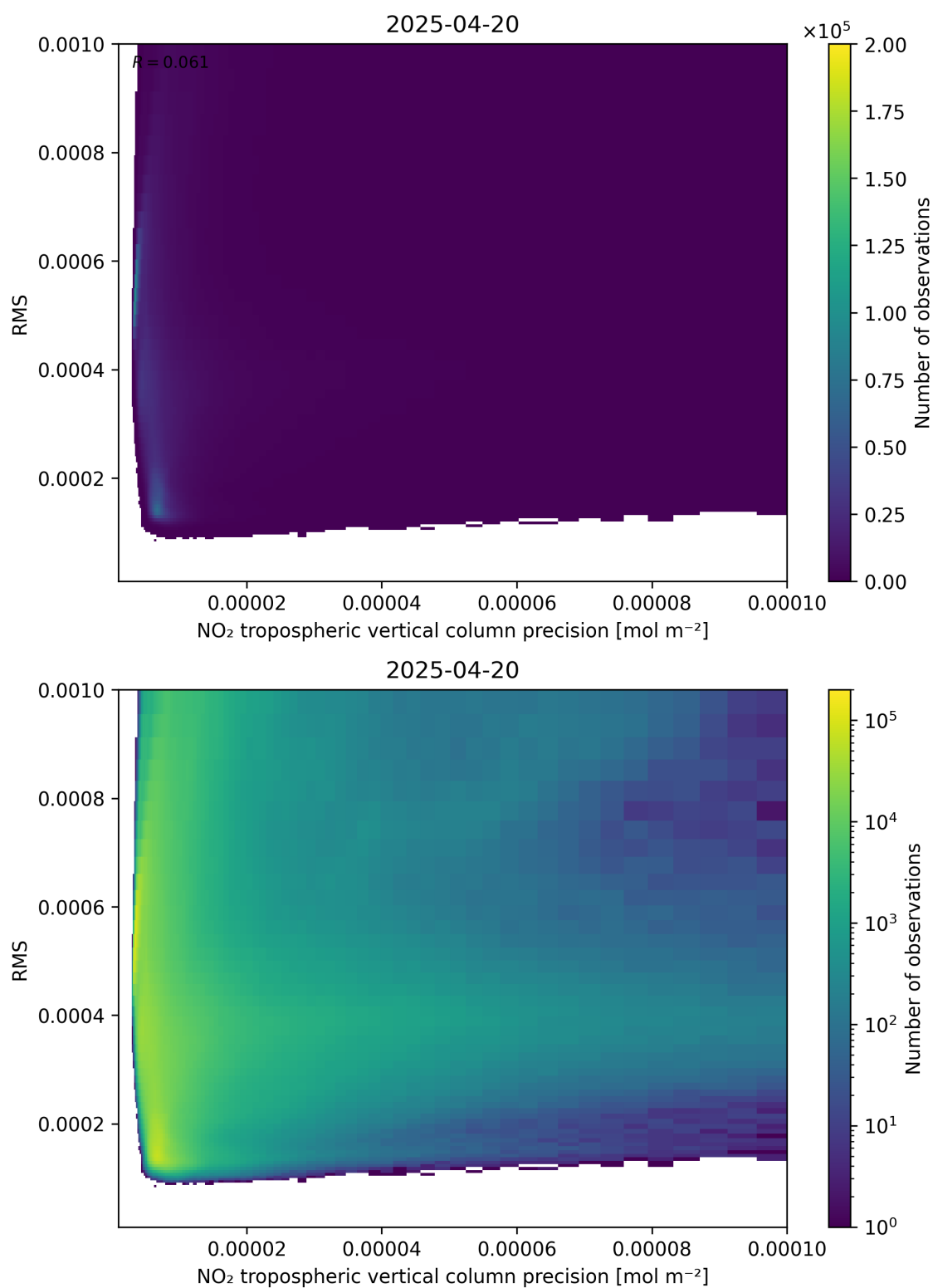
Figure 140: Scatter density plot of “NO 2 tropospheric vertical column precision” against “RMS” for 2025-04-20 to 2025-04-21.
