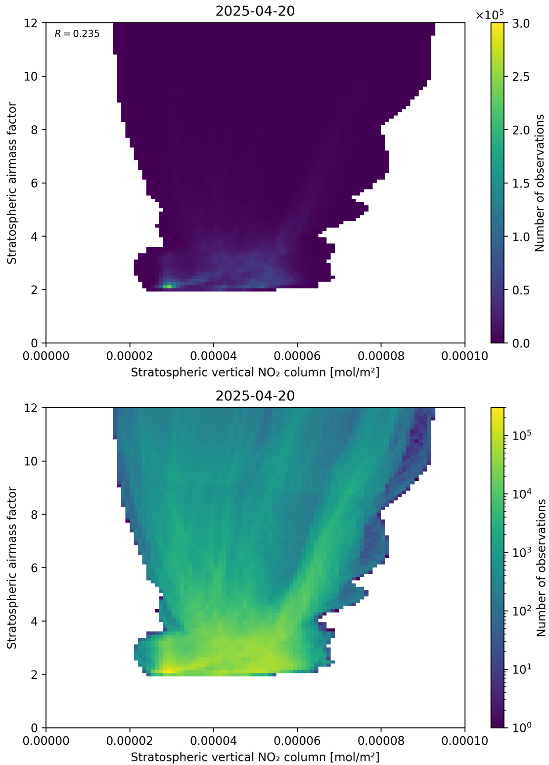
Figure 96: Scatter density plot of “Stratospheric vertical NO 2 column” against “Stratospheric airmass factor” for 2025-04-20 to 2025-04-21.
