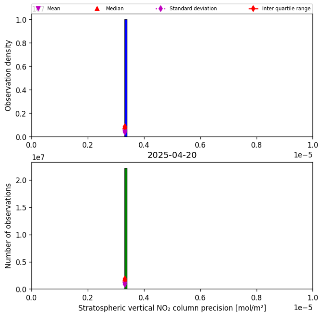
Figure 37: Histogram of “Stratospheric vertical NO 2 column precision” for 2025-04-20 to 2025-04-21
