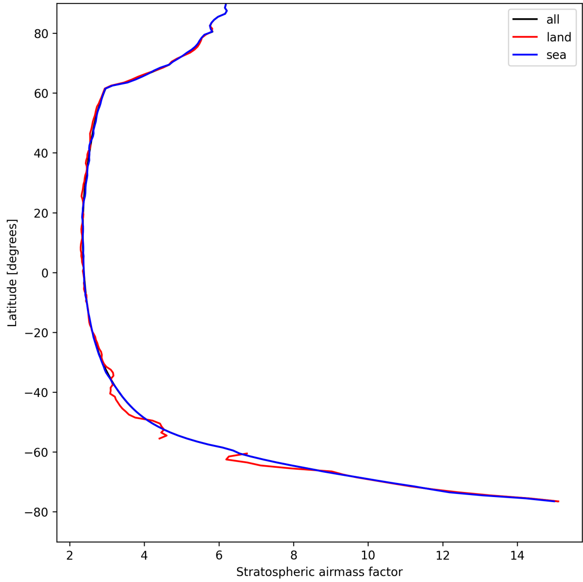
Figure 27: Zonal average of “Stratospheric airmass factor” for 2025-04-20 to 2025-04-21.
