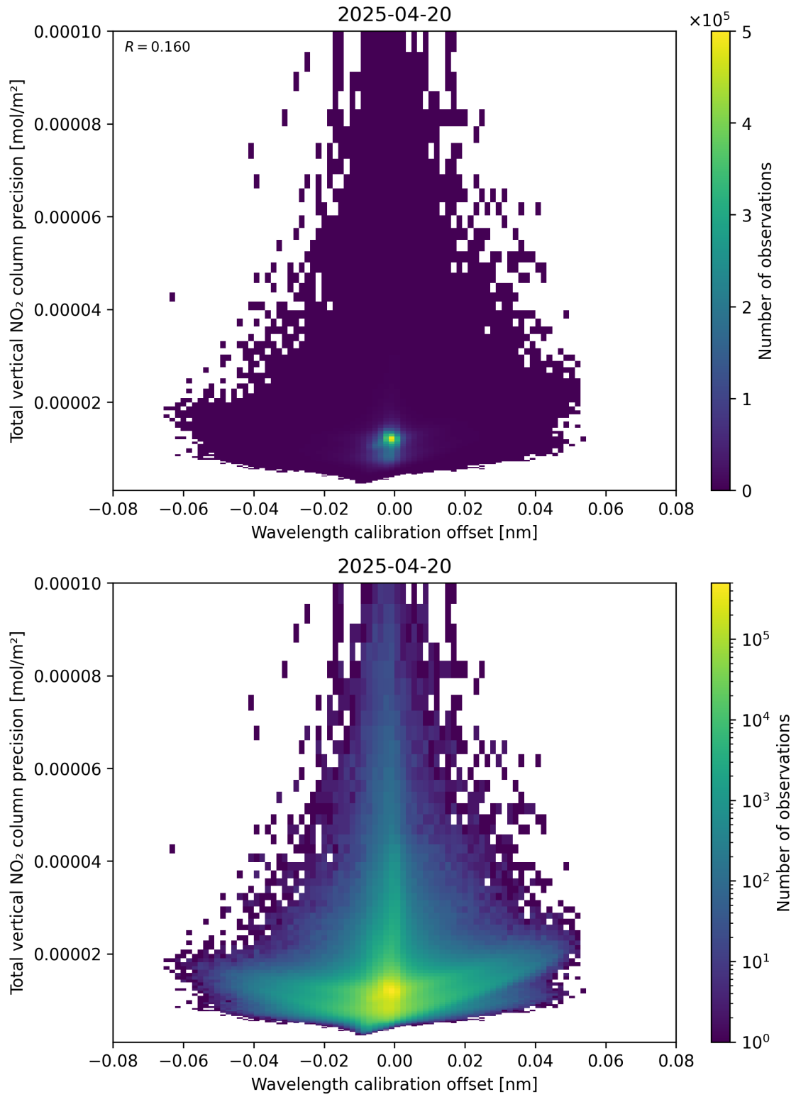
Figure 180: Scatter density plot of “Wavelength calibration offset” against “Total vertical NO 2 column precision” for 2025-04-20 to 2025-04-21.
