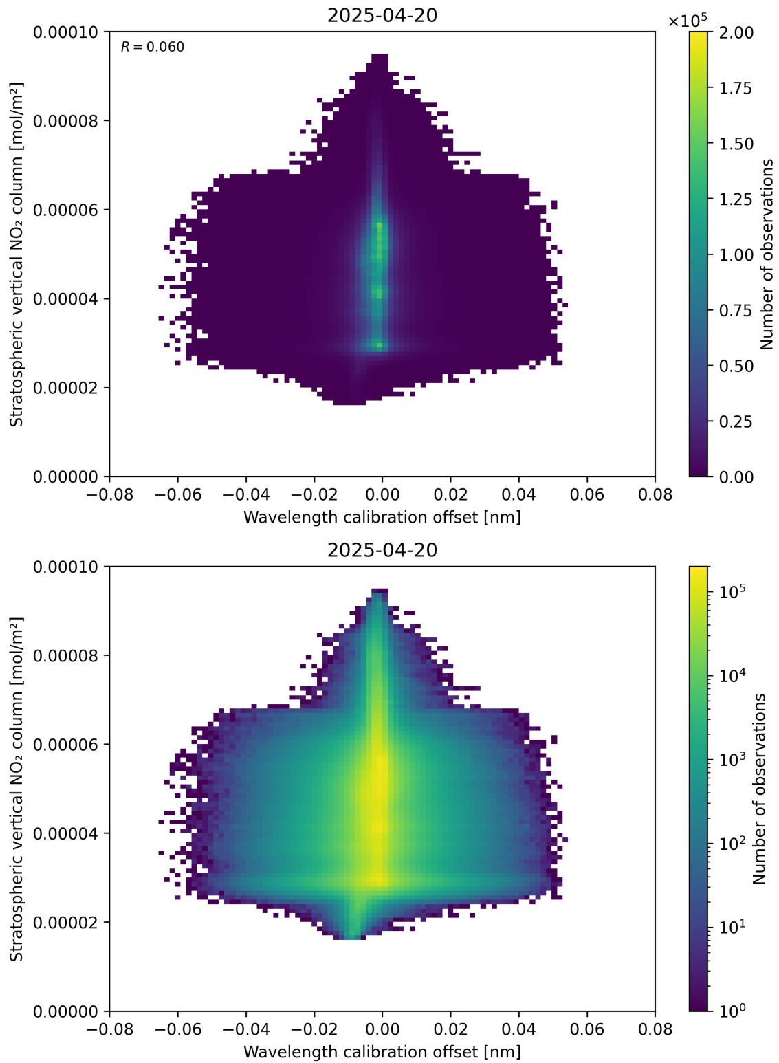
Figure 176: Scatter density plot of “Wavelength calibration offset” against “Stratospheric vertical NO 2 column” for 2025-04-20 to 2025-04-21.
