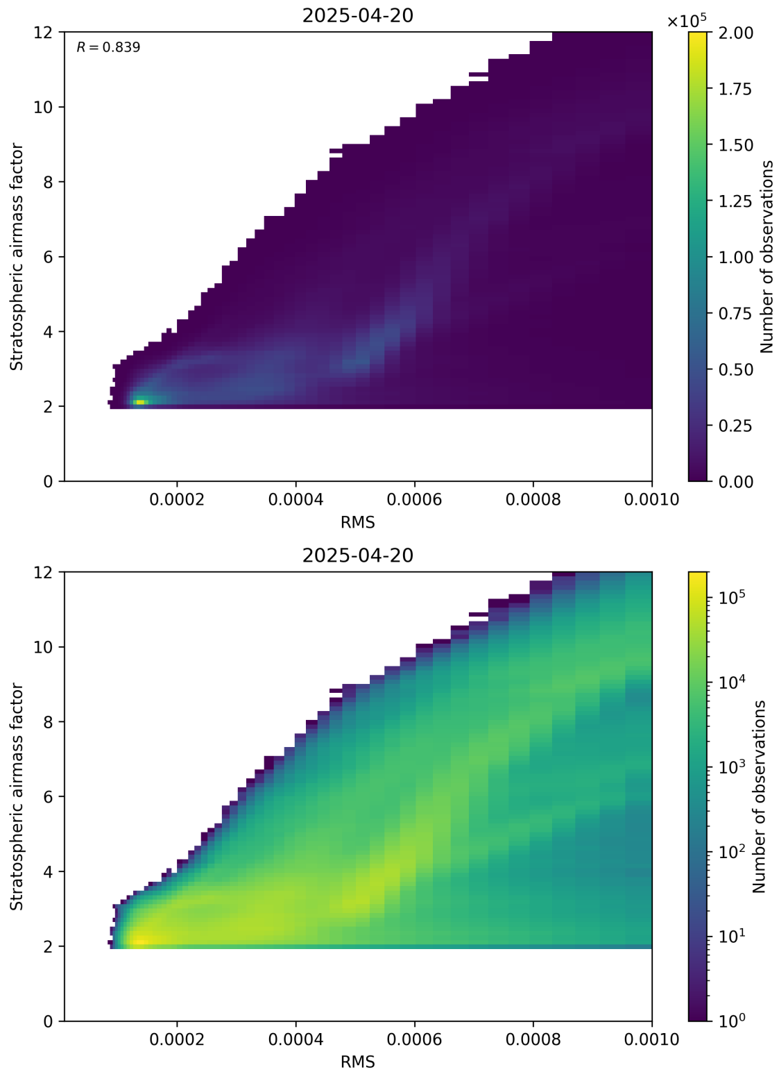
Figure 144: Scatter density plot of “RMS” against “Stratospheric airmass factor” for 2025-04-20 to 2025-04-21.
