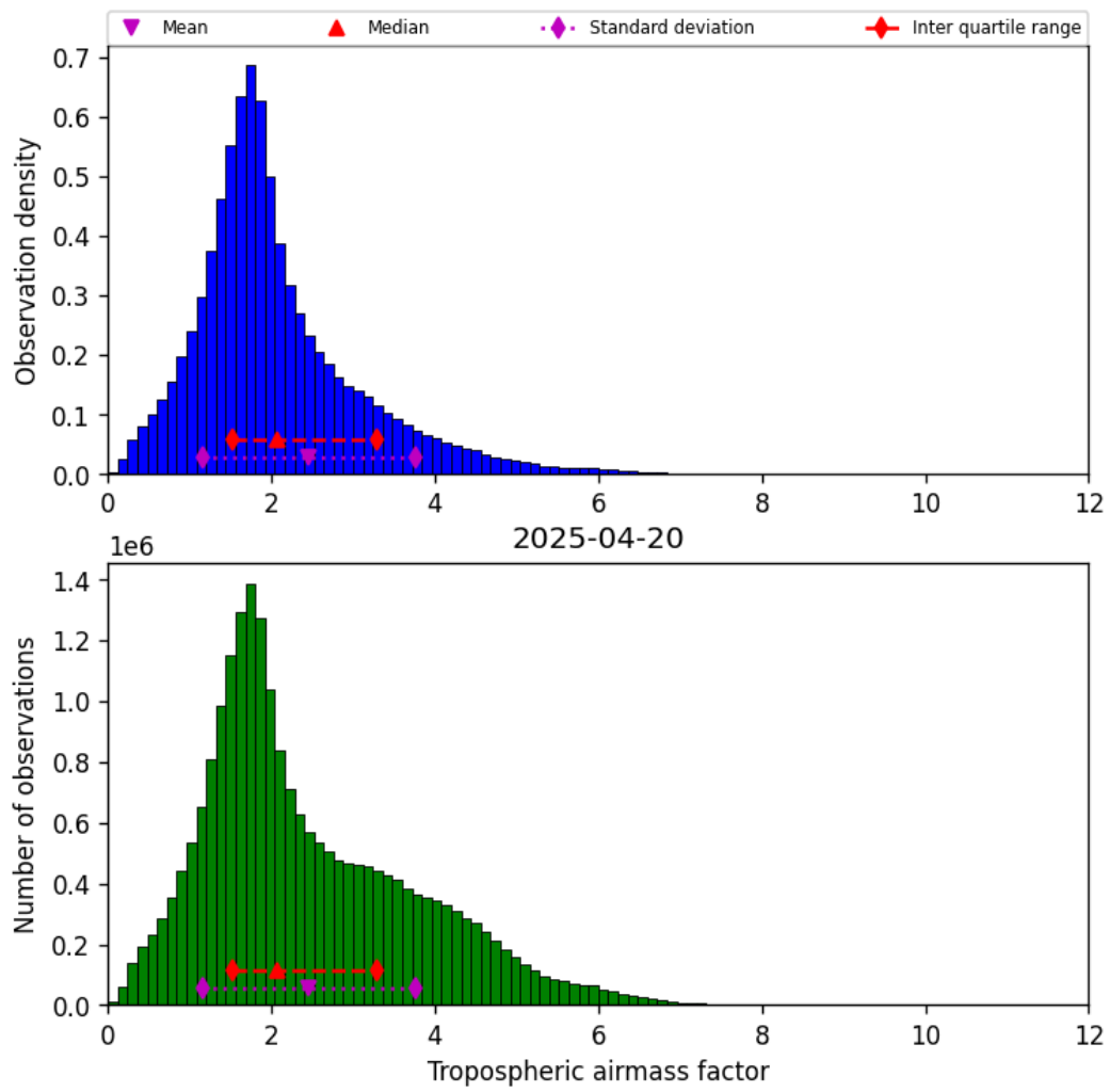
Figure 31: Histogram of “Tropospheric airmass factor” for 2025-04-20 to 2025-04-21
