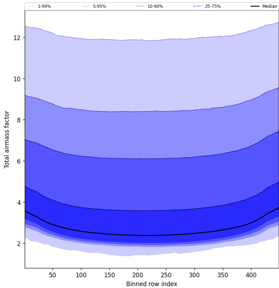
Figure 49: Along track statistics of “Total airmass factor” for 2025-04-20 to 2025-04-21
