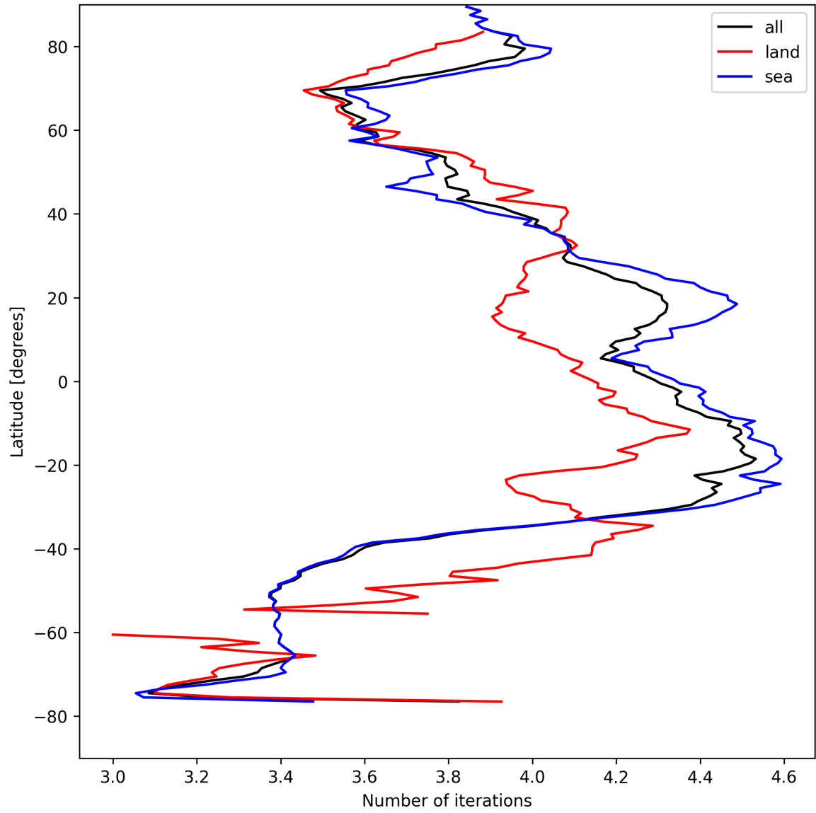
Figure 17: Zonal average of “Number of iterations” for 2025-04-20 to 2025-04-21.
