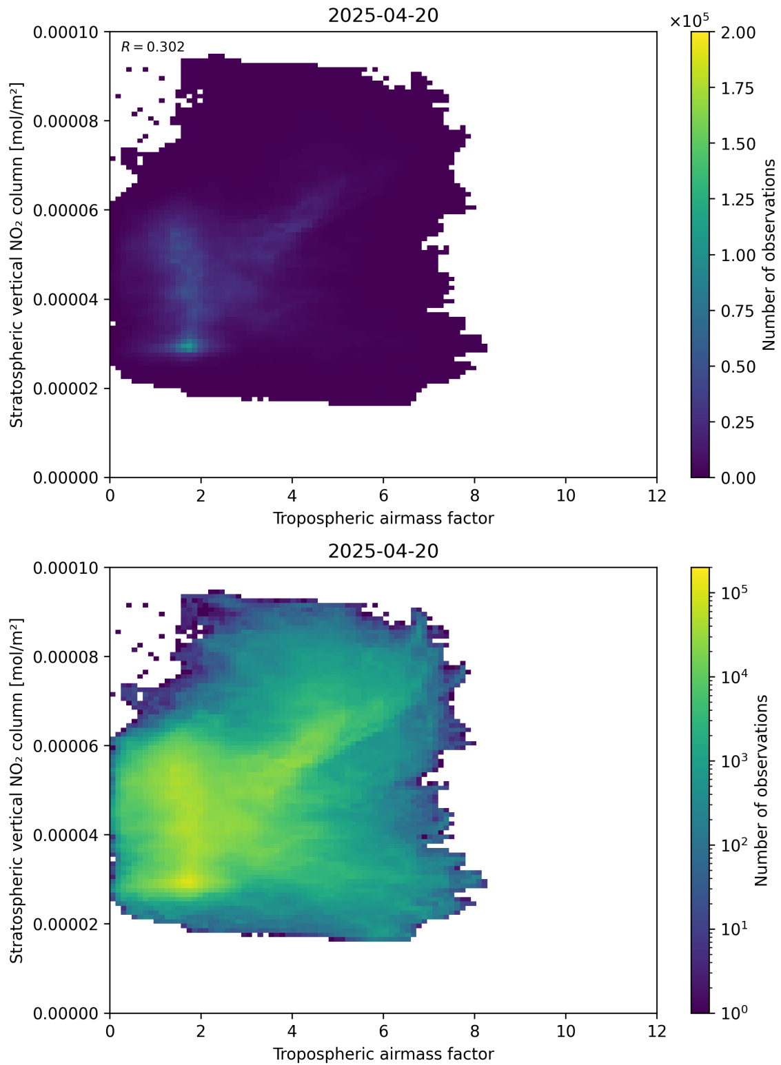
Figure 74: Scatter density plot of “Tropospheric air mass factor” against “Stratospheric vertical NO 2 column” for 2025-04-20 to 2025-04-21.
