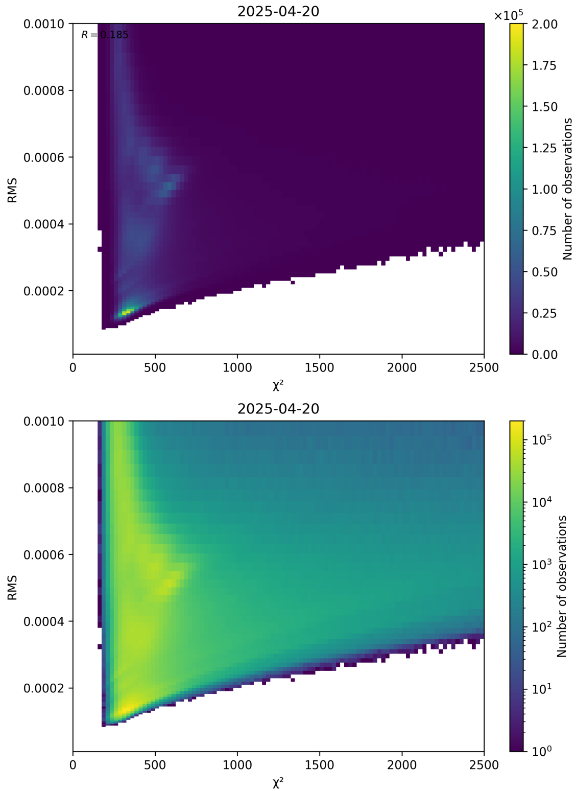
Figure 82: Scatter density plot of “ \chi^2 ” against “RMS” for 2025-04-20 to 2025-04-21.
