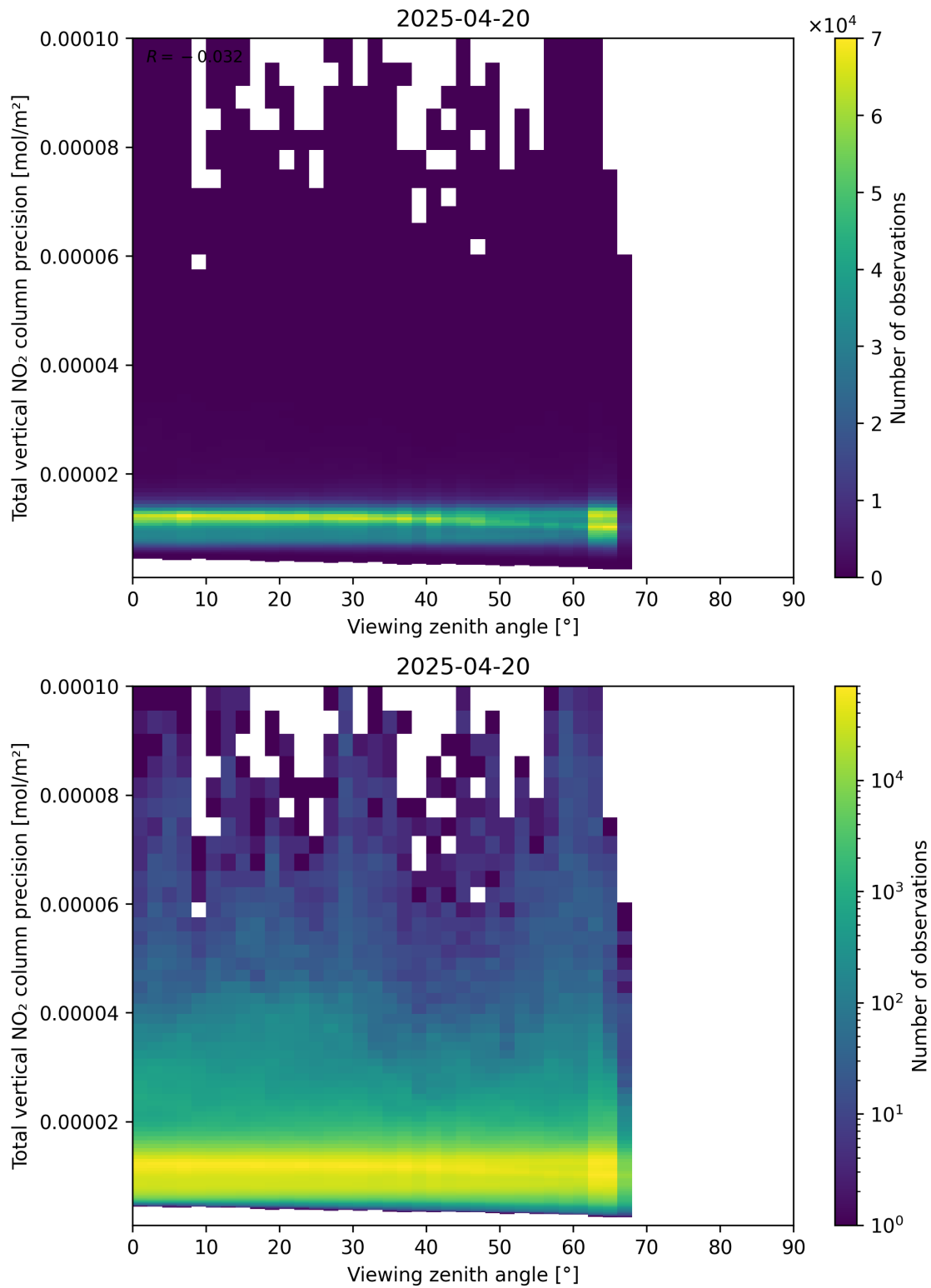
Figure 168: Scatter density plot of “Viewing zenith angle” against “Total vertical NO 2 column precision” for 2025-04-20 to 2025-04-21.
