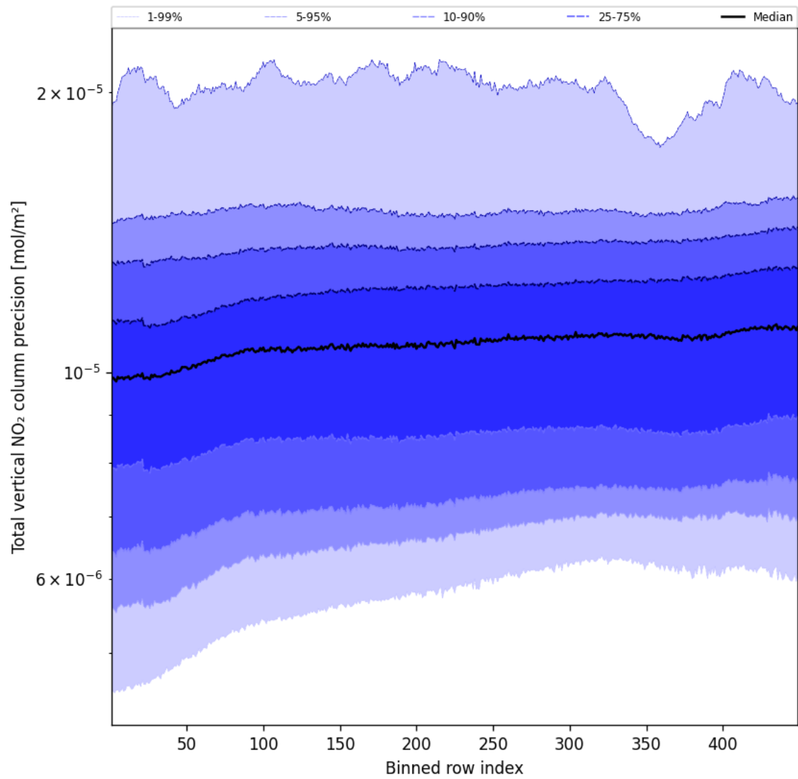
Figure 56: Along track statistics of “Total vertical NO 2 column precision” for 2025-04-20 to 2025-04-21
