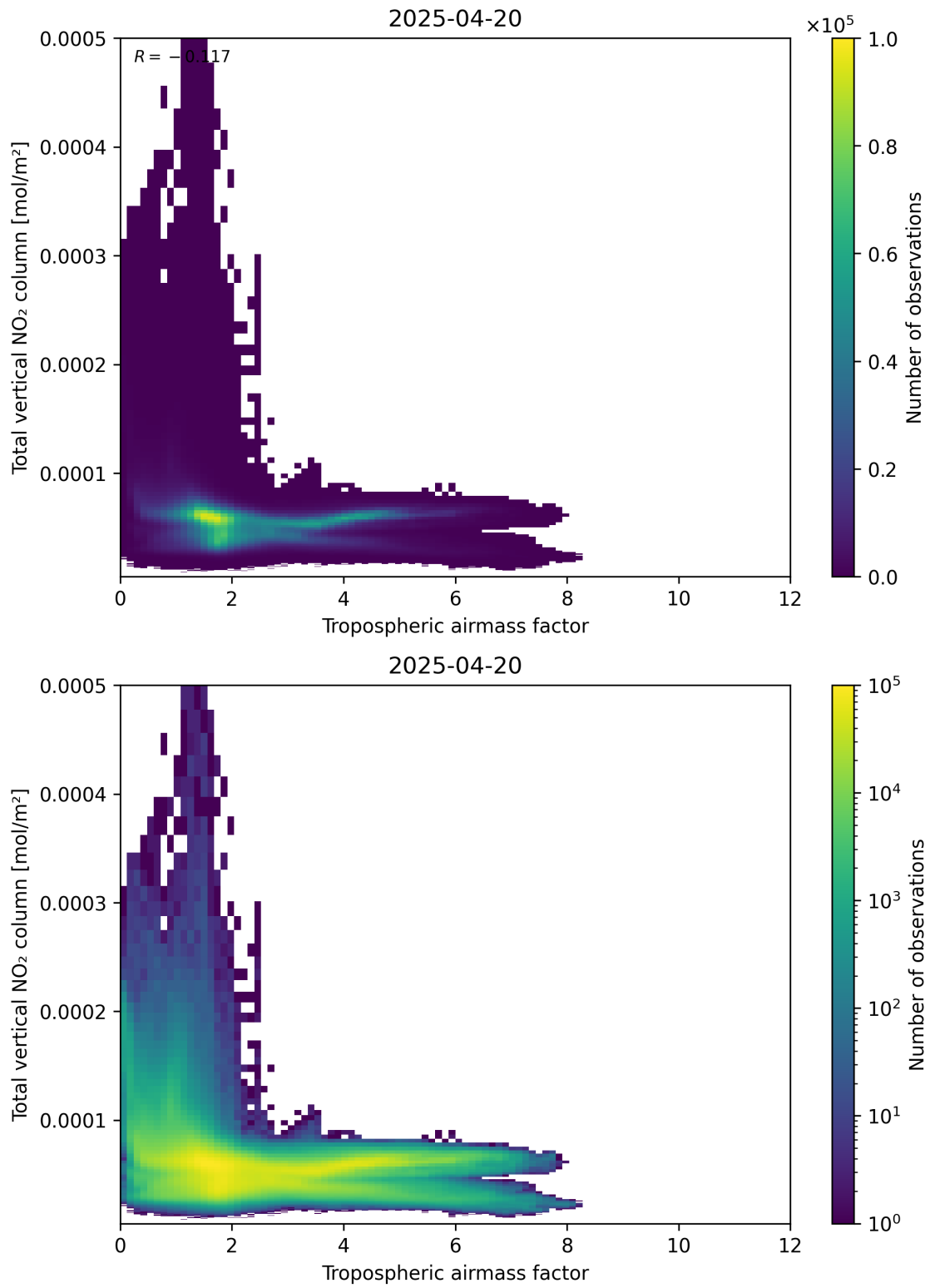
Figure 77: Scatter density plot of “Tropospheric airmass factor” against “Total vertical NO 2 column” for 2025-04-20 to 2025-04-21.
