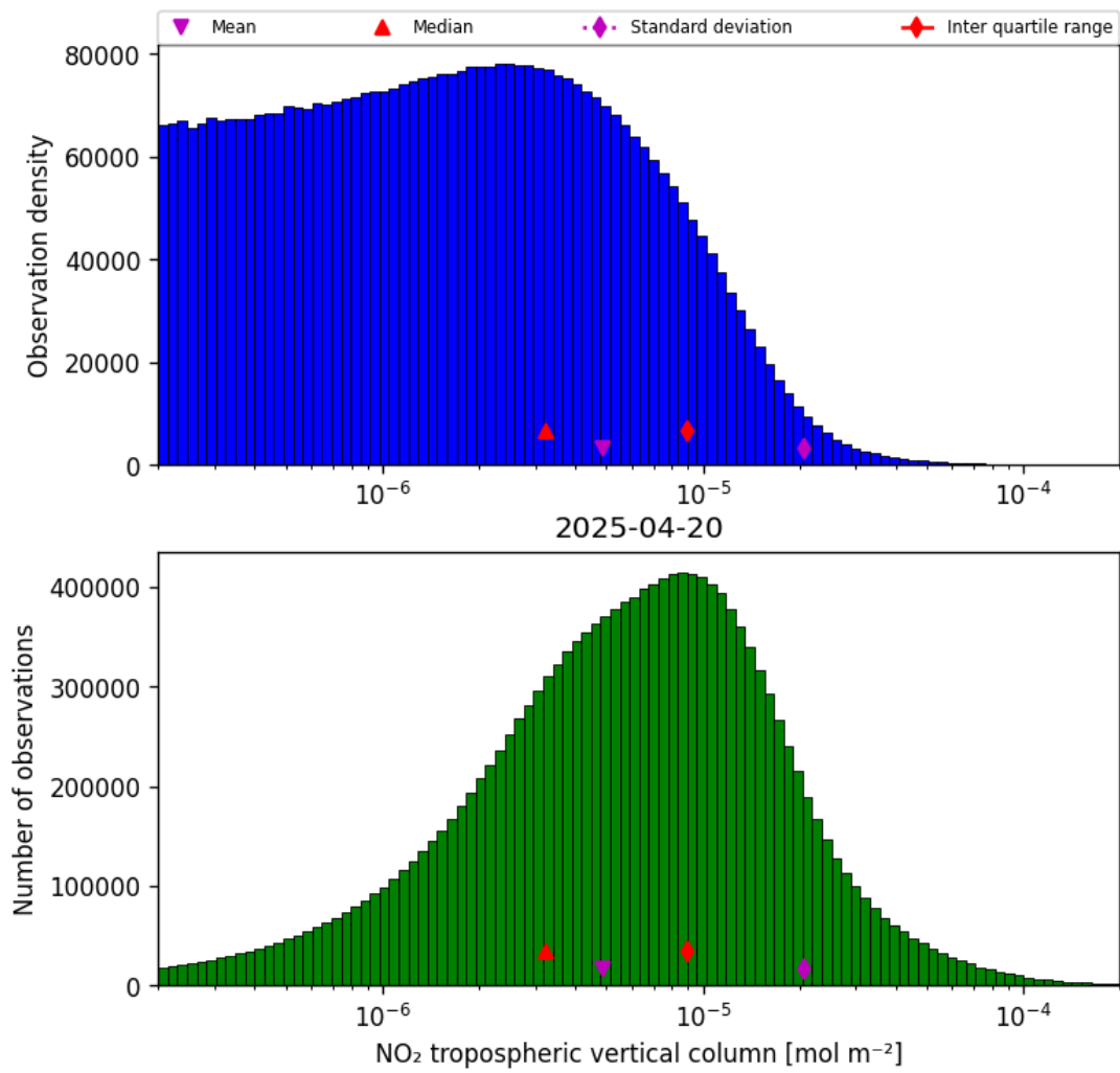
Figure 29: Histogram of “NO 2 tropospheric vertical column” for 2025-04-20 to 2025-04-21
