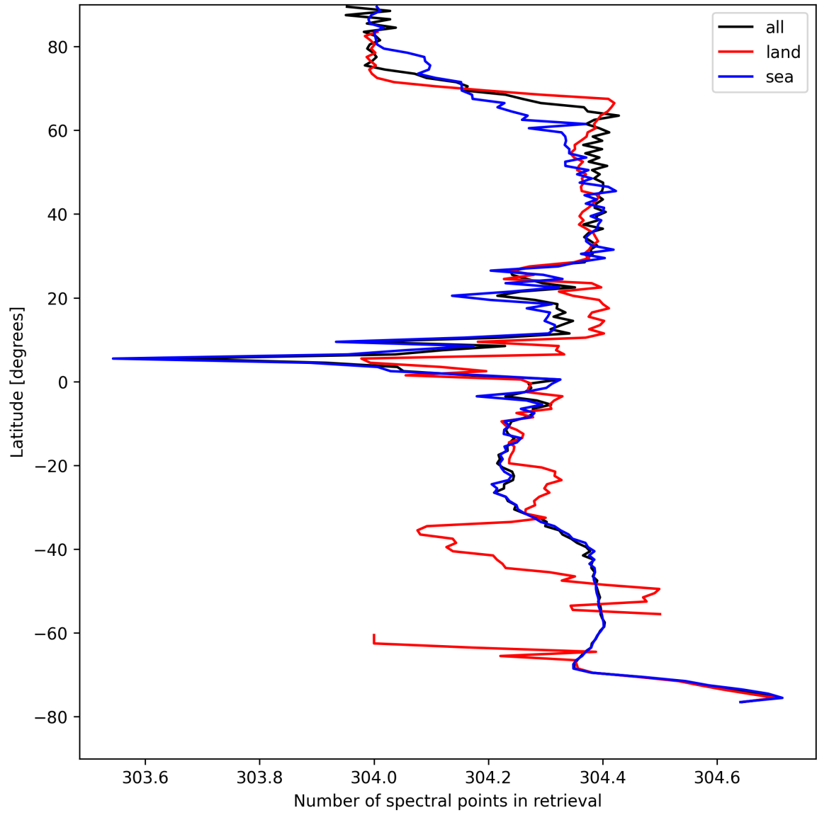
Figure 16: Zonal average of “Number of spectral points in retrieval” for 2025-04-20 to 2025-04-21.
