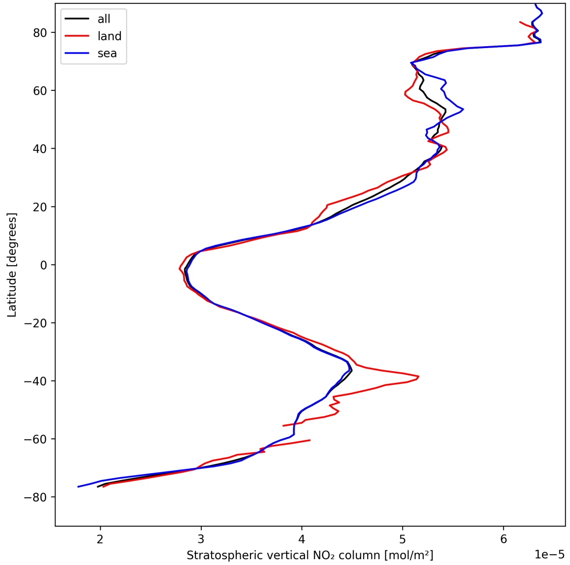
Figure 19: Zonal average of “Stratospheric vertical NO 2 column” for 2025-04-20 to 2025-04-21.
