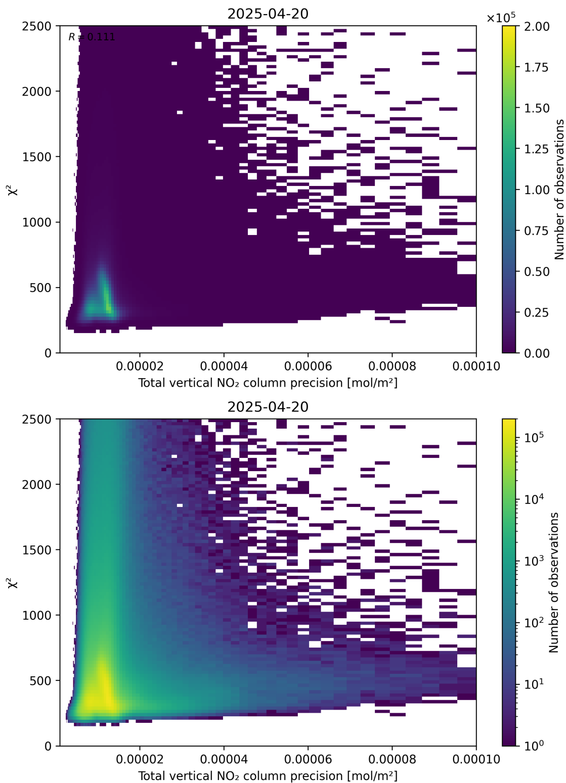
Figure 116: Scatter density plot of “Total vertical NO 2 column precision” against “ \chi^2 ” for 2025-04-20 to 2025-04-21.
