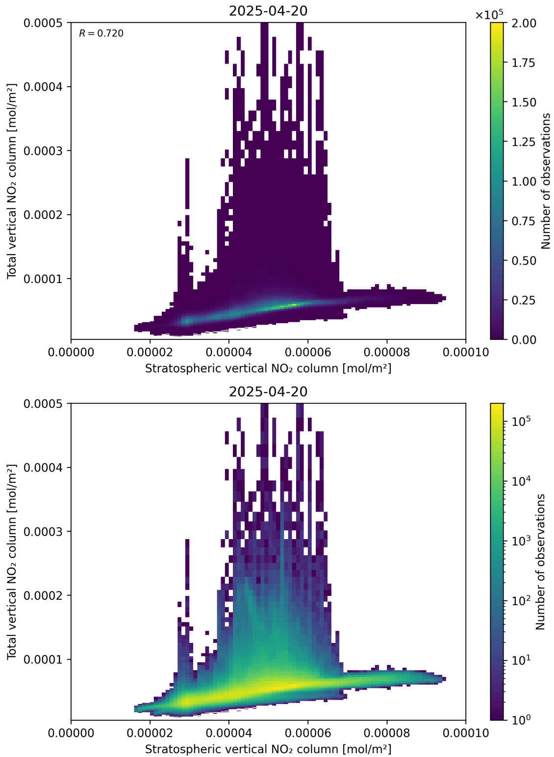
Figure 100: Scatter density plot of “Stratospheric vertical NO 2 column” against “Total vertical NO 2 column” for 2025-04-20 to 2025-04-21.
