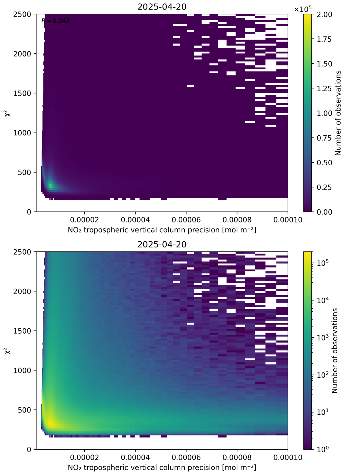
Figure 134: Scatter density plot of “NO 2 tropospheric vertical column precision” against “ \chi^2 ” for 2025-04-20 to 2025-04-21.
