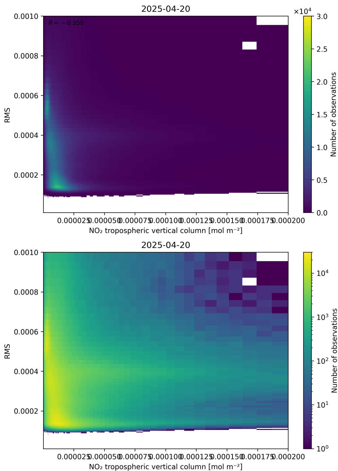
Figure 142: Scatter density plot of “NO 2 tropospheric vertical column” against “RMS” for 2025-04-20 to 2025-04-21.
