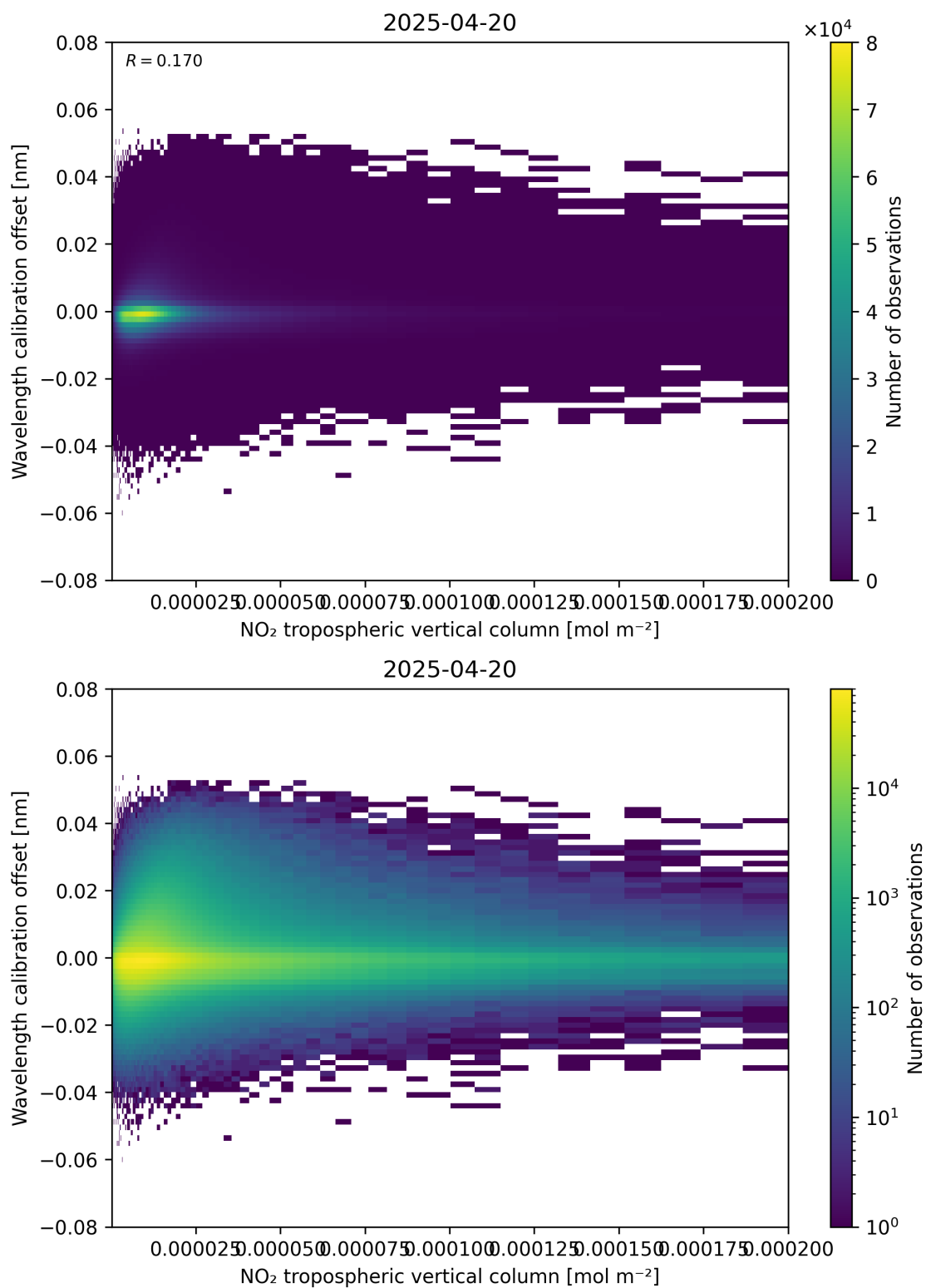
Figure 143: Scatter density plot of “NO 2 tropospheric vertical column” against “Wavelength calibration offset” for 2025-04-20 to 2025-04-21.
