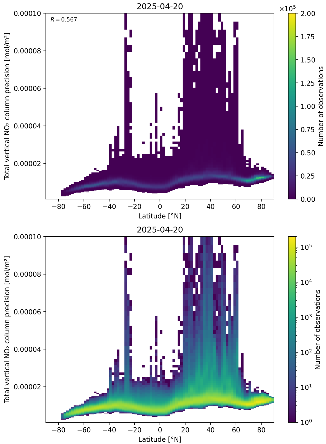
Figure 91: Scatter density plot of “Latitude” against “Total vertical NO 2 column precision” for 2025-04-20 to 2025-04-21.
