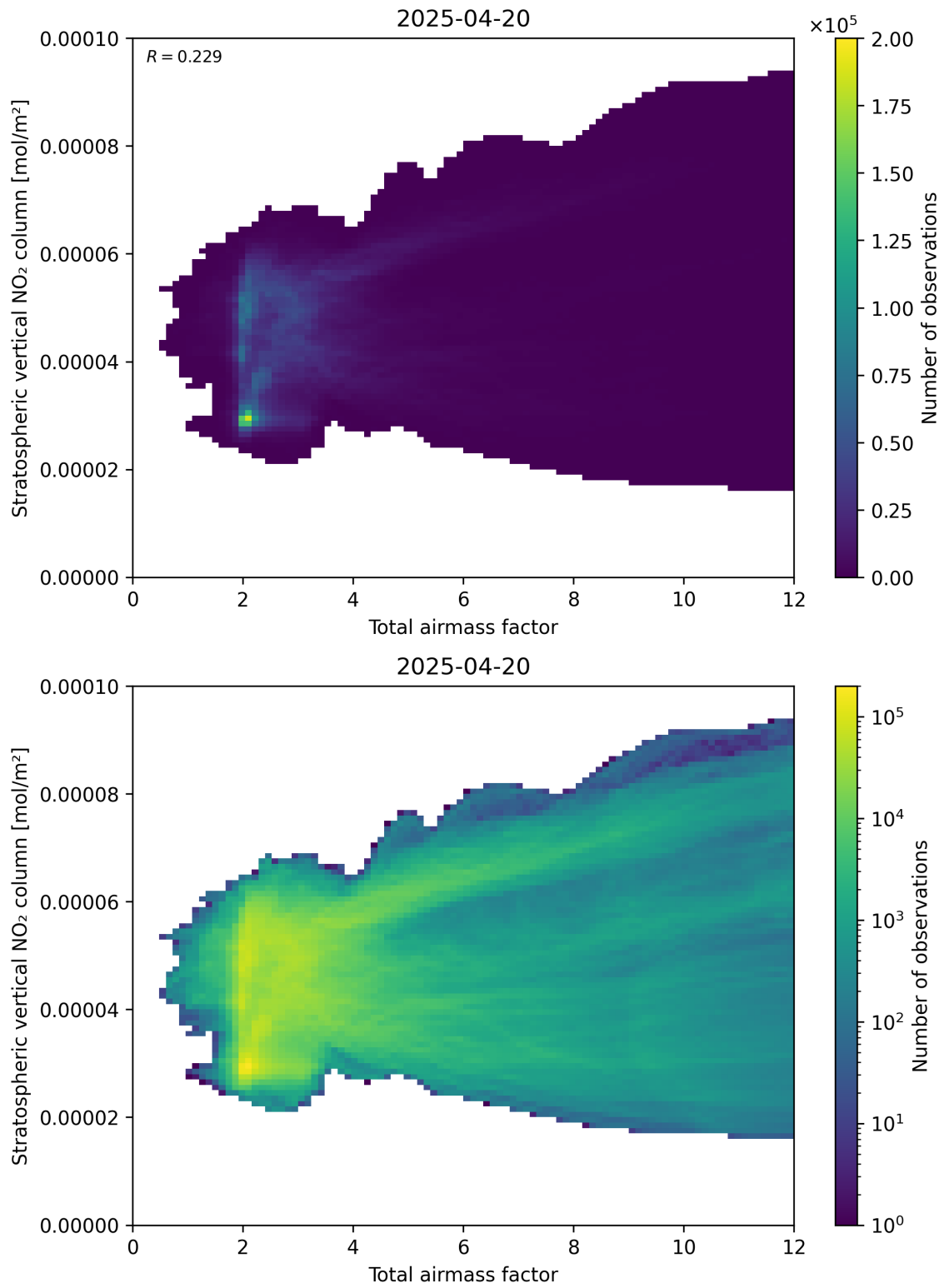
Figure 64: Scatter density plot of “Total airmass factor” against “Stratospheric vertical \text{NO}_2 column” for 2025-04-20 to 2025-04-21.
