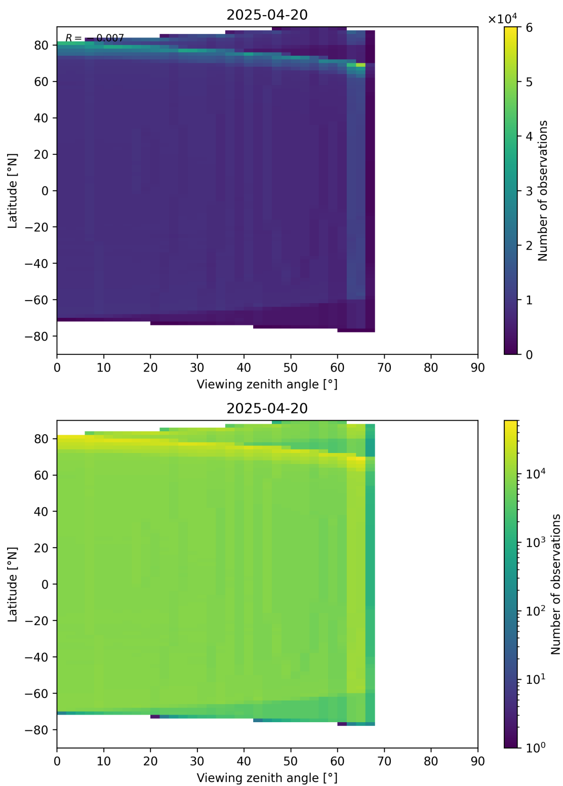
Figure 163: Scatter density plot of “Viewing zenith angle” against “Latitude” for 2025-04-20 to 2025-04-21.
