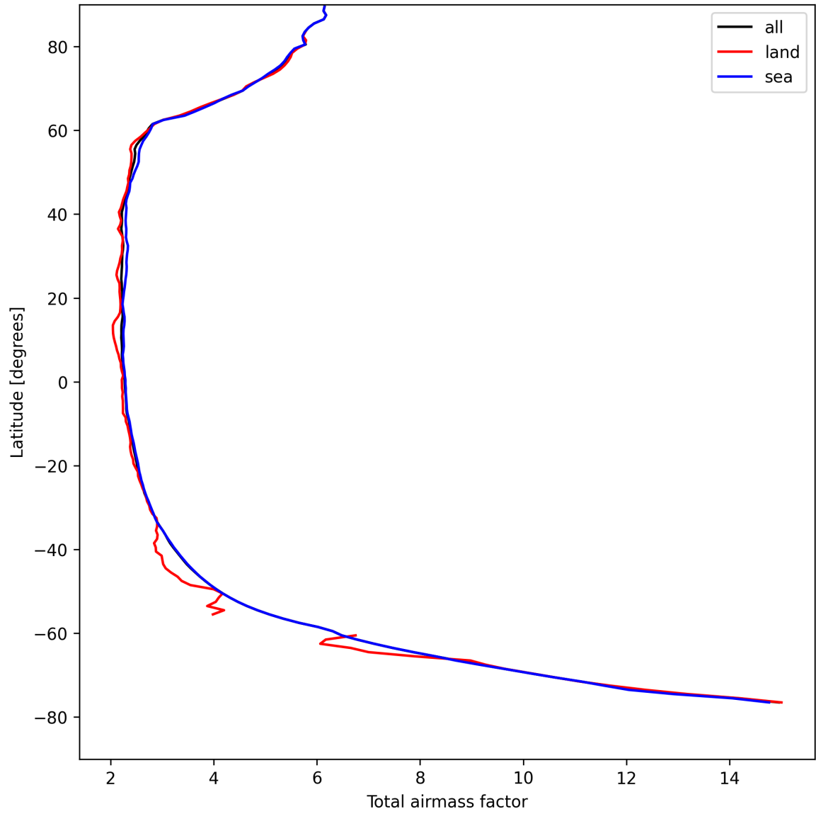
Figure 15: Zonal average of “Total airmass factor” for 2025-04-20 to 2025-04-21.
