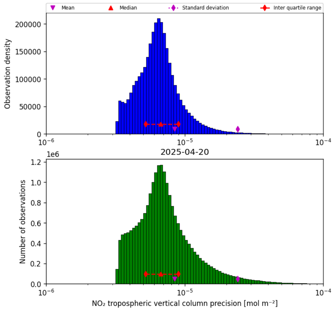
Figure 30: Histogram of “NO 2 tropospheric vertical column precision” for 2025-04-20 to 2025-04-21
