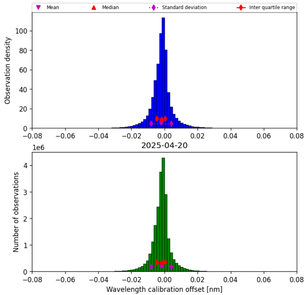
Figure 35: Histogram of “Wavelength calibration offset” for 2025-04-20 to 2025-04-21
