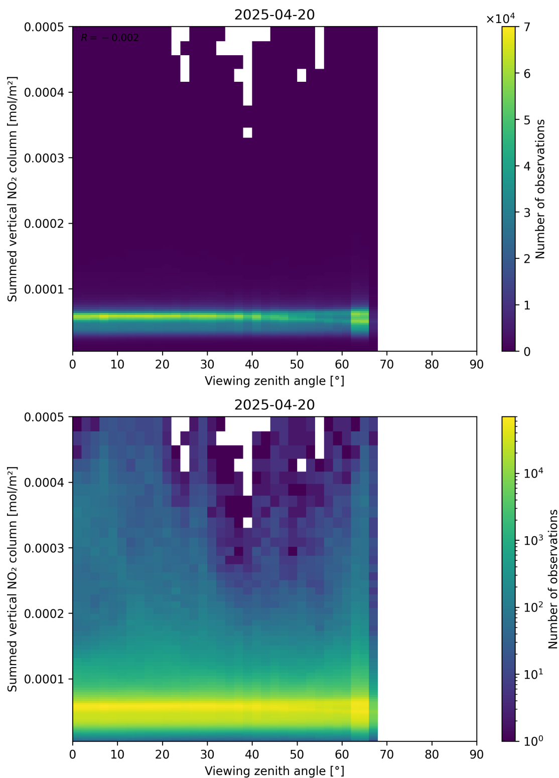
Figure 165: Scatter density plot of “Viewing zenith angle” against “Summed vertical NO 2 column” for 2025-04-20 to 2025-04-21.
