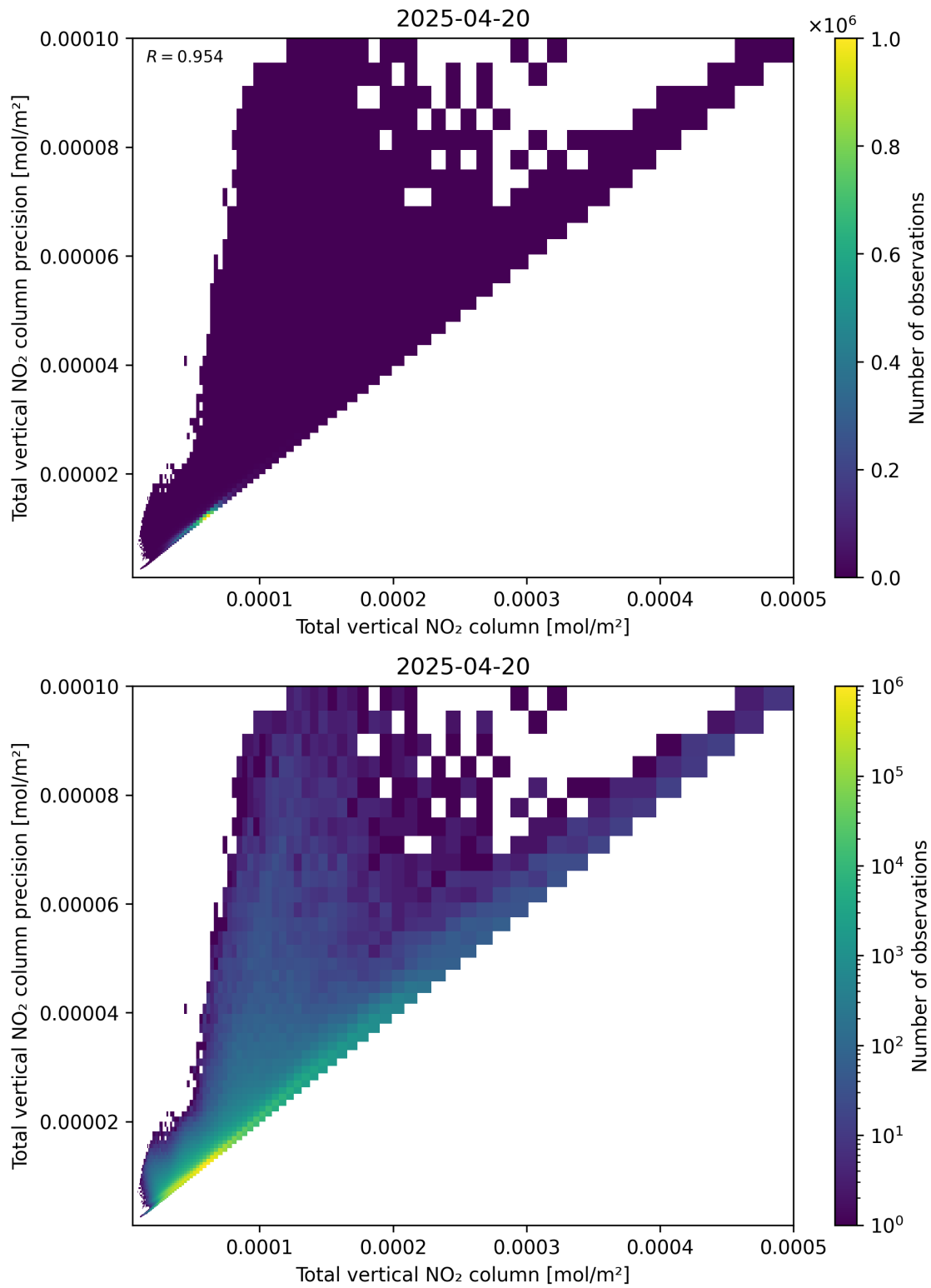
Figure 114: Scatter density plot of “Total vertical NO 2 column” against “Total vertical NO 2 column precision” for 2025-04-20 to 2025-04-21.
