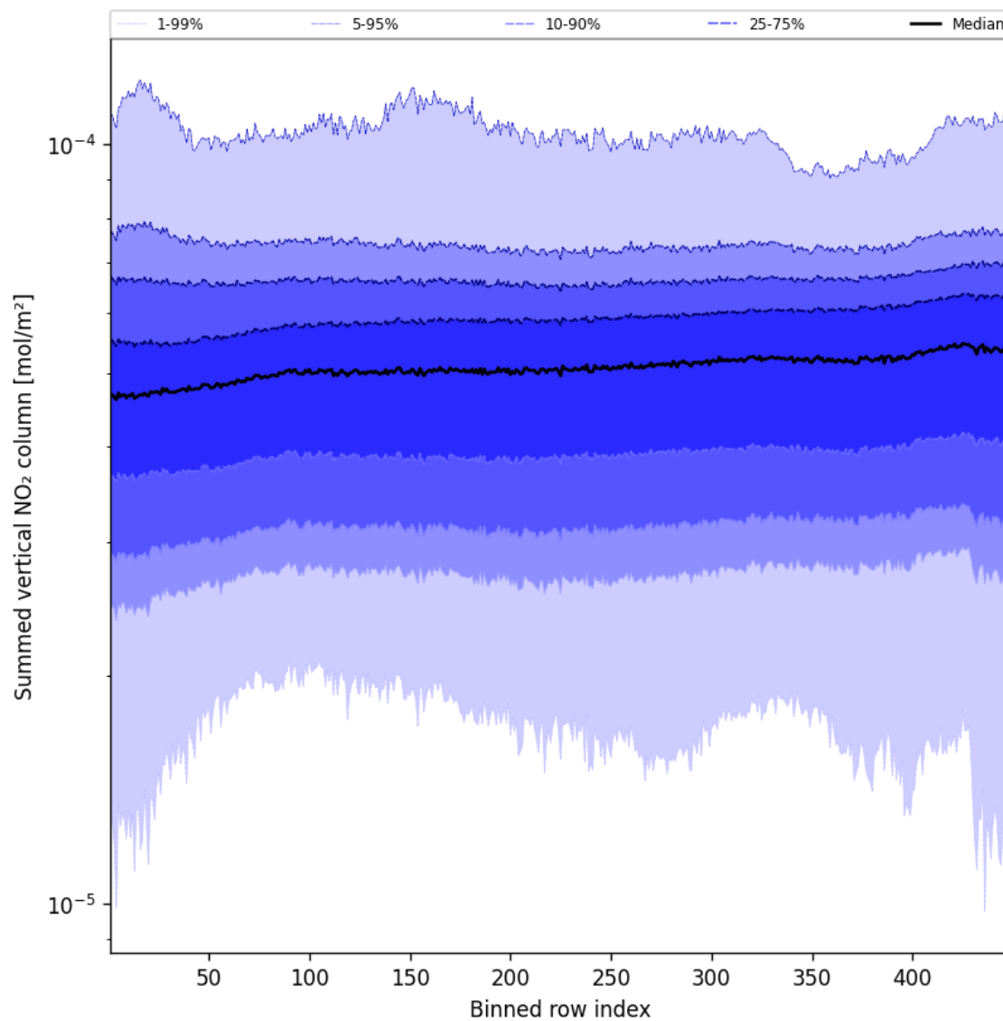
Figure 57: Along track statistics of “Summed vertical NO 2 column” for 2025-04-20 to 2025-04-21
