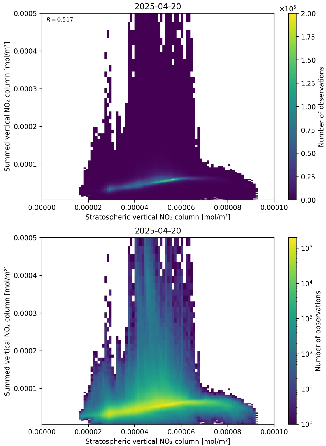
Figure 98: Scatter density plot of “Stratospheric vertical NO 2 column” against “Summed vertical NO 2 column” for 2025-04-20 to 2025-04-21.
