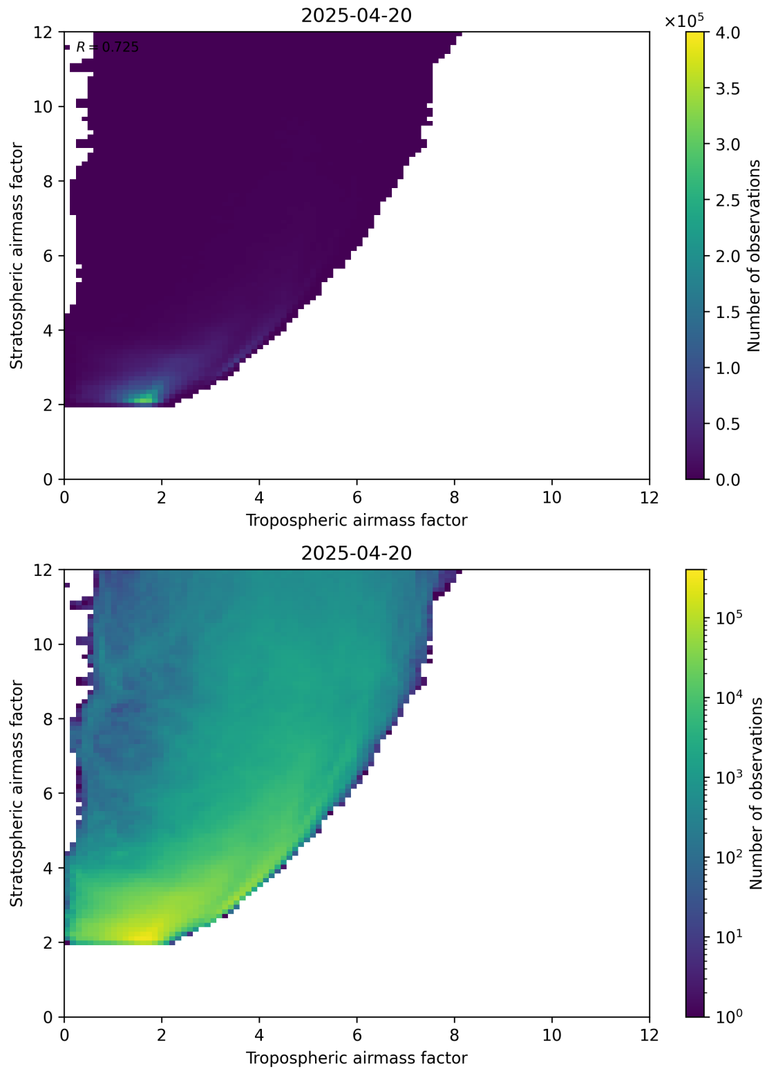
Figure 71: Scatter density plot of “Tropospheric airmass factor” against “Stratospheric airmass factor” for 2025-04-20 to 2025-04-21.
