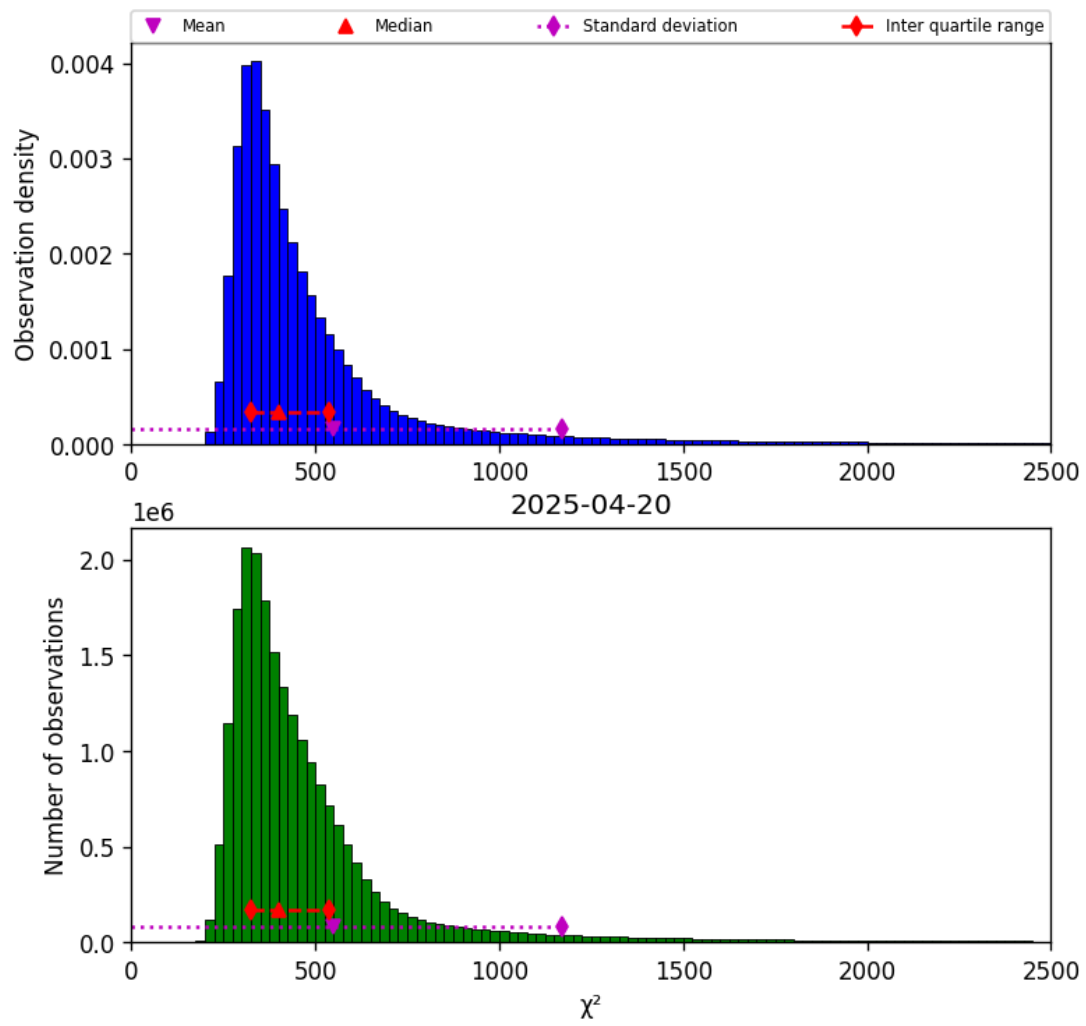
Figure 42: Histogram of “ \chi^2 ” for 2025-04-20 to 2025-04-21
