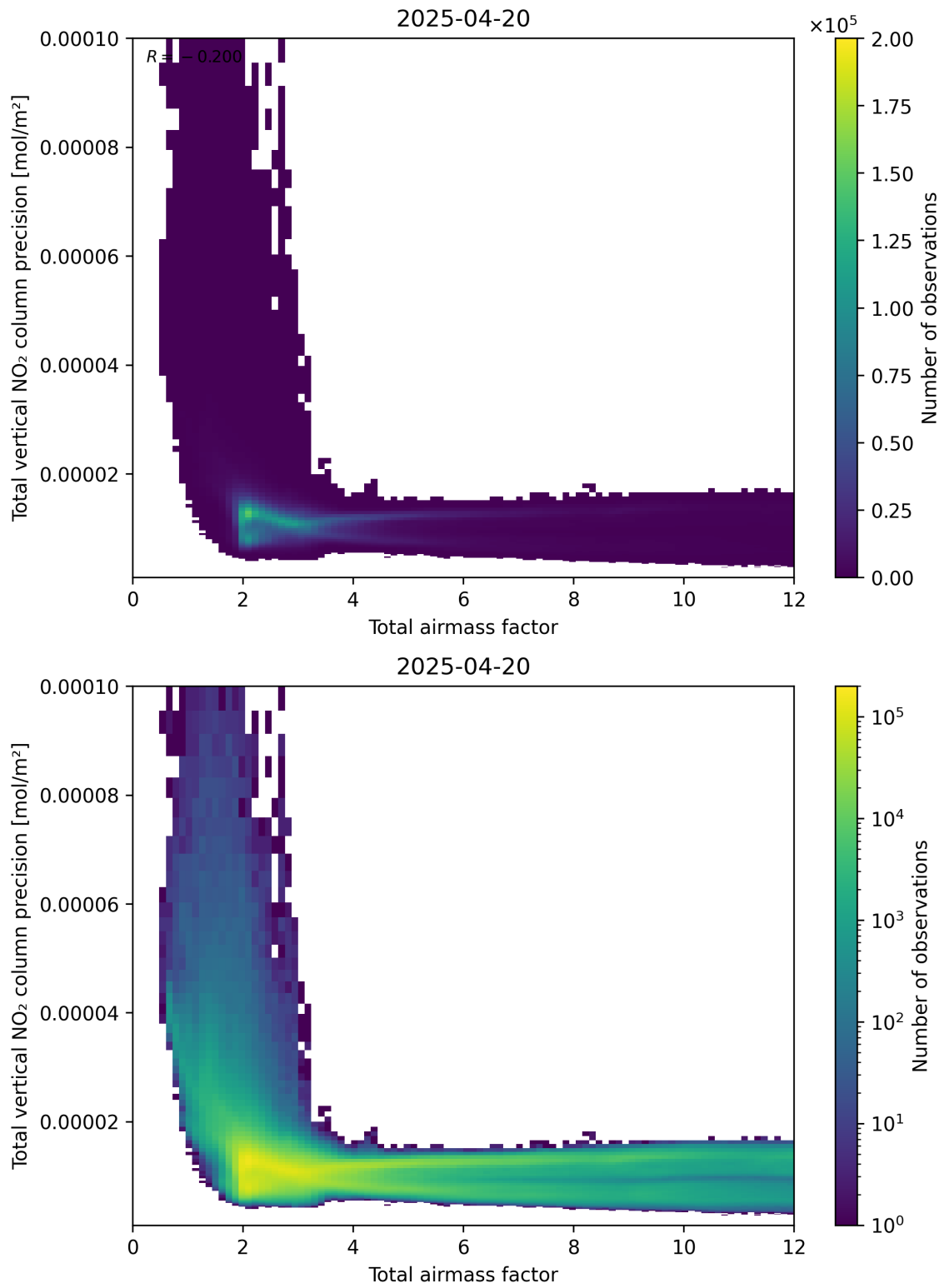
Figure 68: Scatter density plot of “Total airmass factor” against “Total vertical NO 2 column precision” for 2025-04-20 to 2025-04-21.
