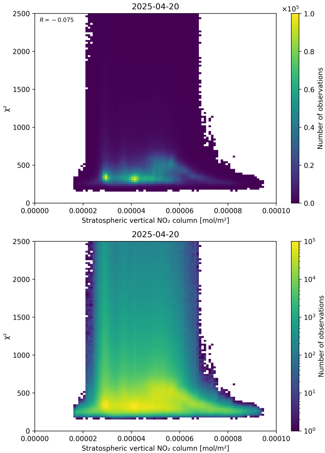
Figure 97: Scatter density plot of “Stratospheric vertical NO 2 column” against “ \chi^2 ” for 2025-04-20 to 2025-04-21.
