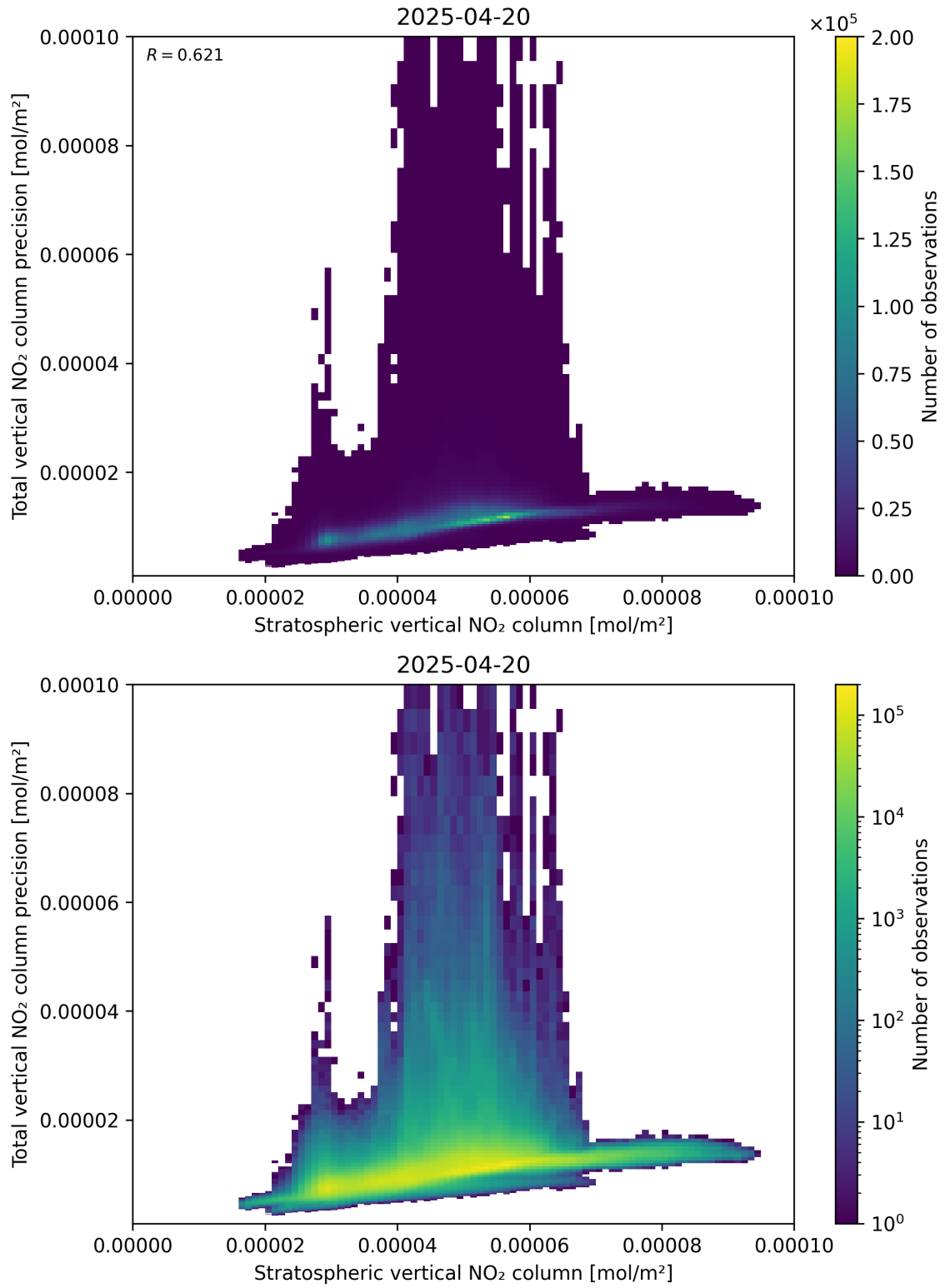
Figure 101: Scatter density plot of “Stratospheric vertical NO 2 column” against “Total vertical NO 2 column precision” for 2025-04-20 to 2025-04-21.
