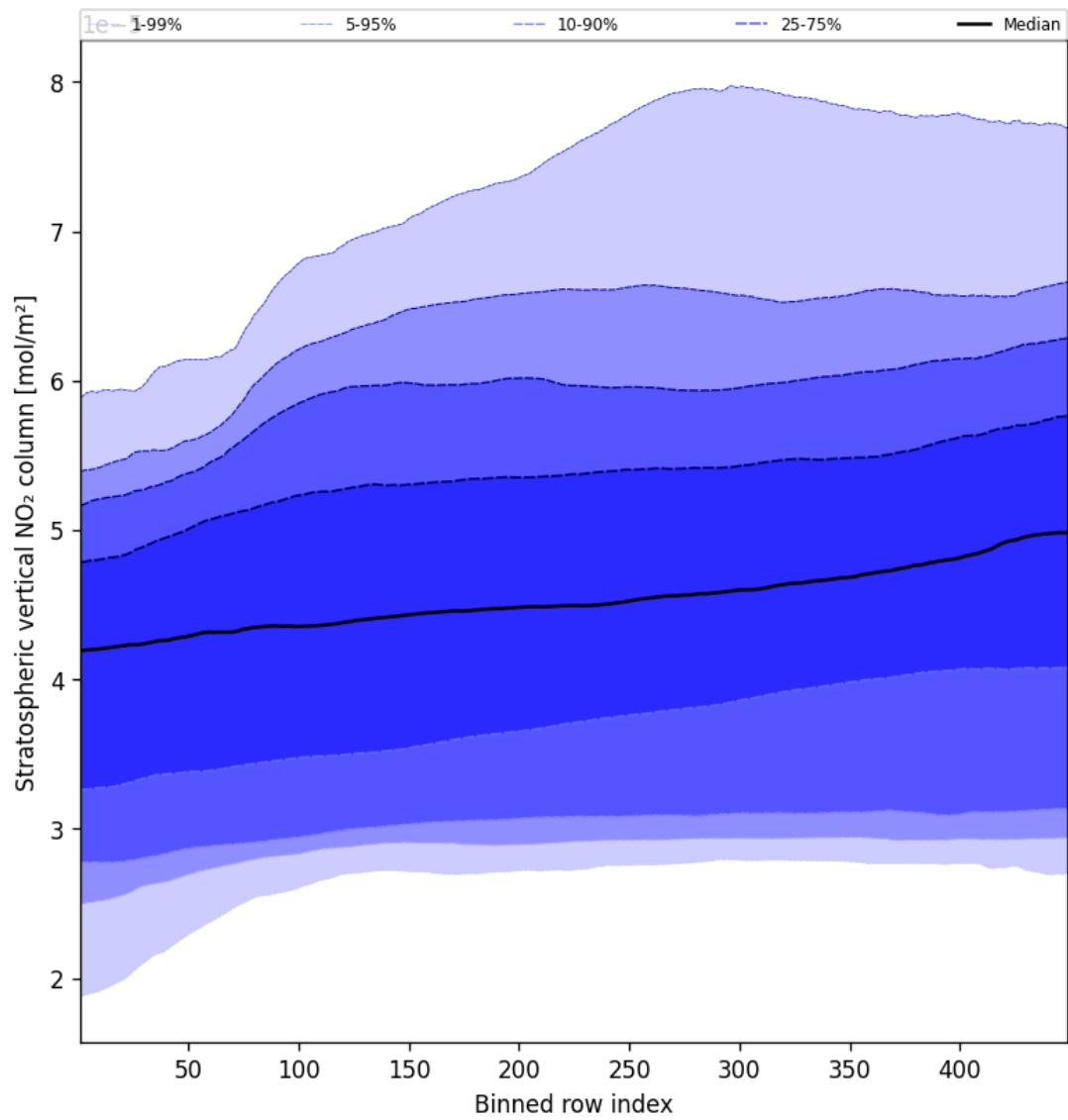
Figure 53: Along track statistics of “Stratospheric vertical NO 2 column” for 2025-04-20 to 2025-04-21
