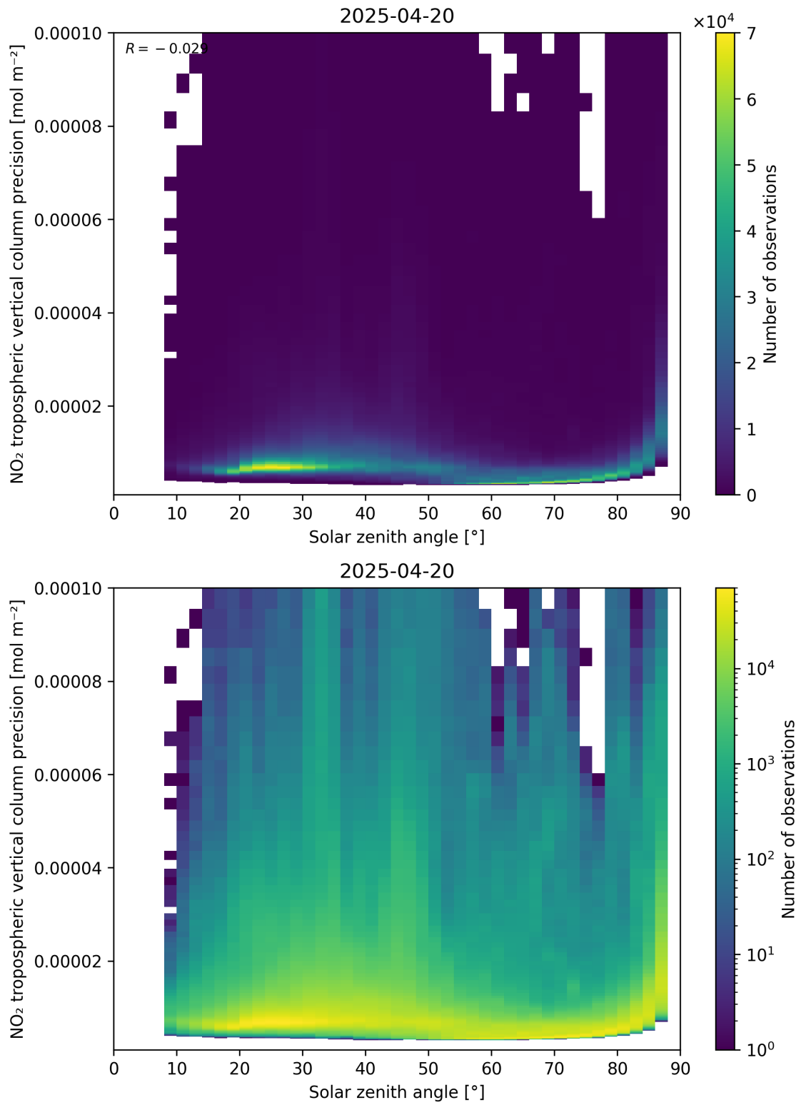
Figure 156: Scatter density plot of “Solar zenith angle” against “NO 2 tropospheric vertical column precision” for 2025-04-20 to 2025-04-21.
