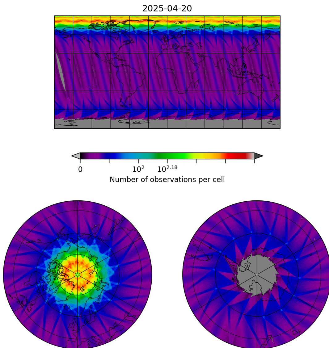
Figure 10: Map of the number of observations for 2025-04-20 to 2025-04-21
