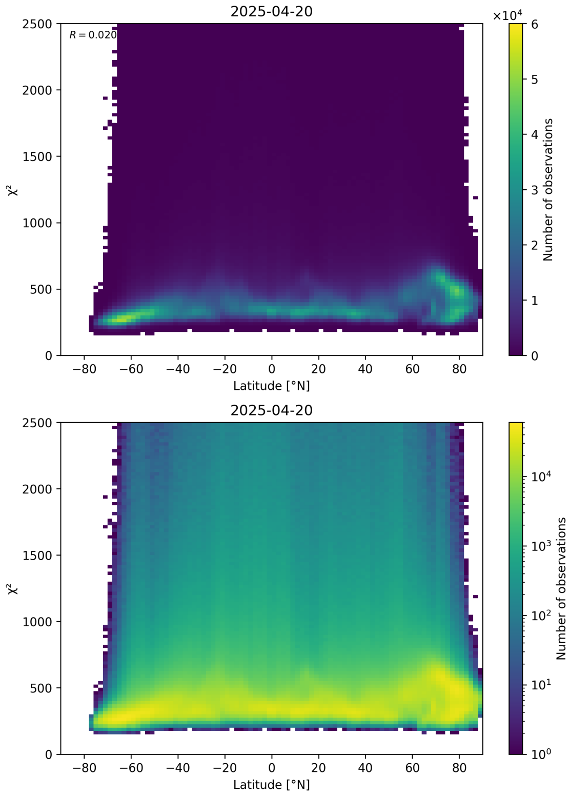
Figure 86: Scatter density plot of “Latitude” against “ \chi^2 ” for 2025-04-20 to 2025-04-21.
