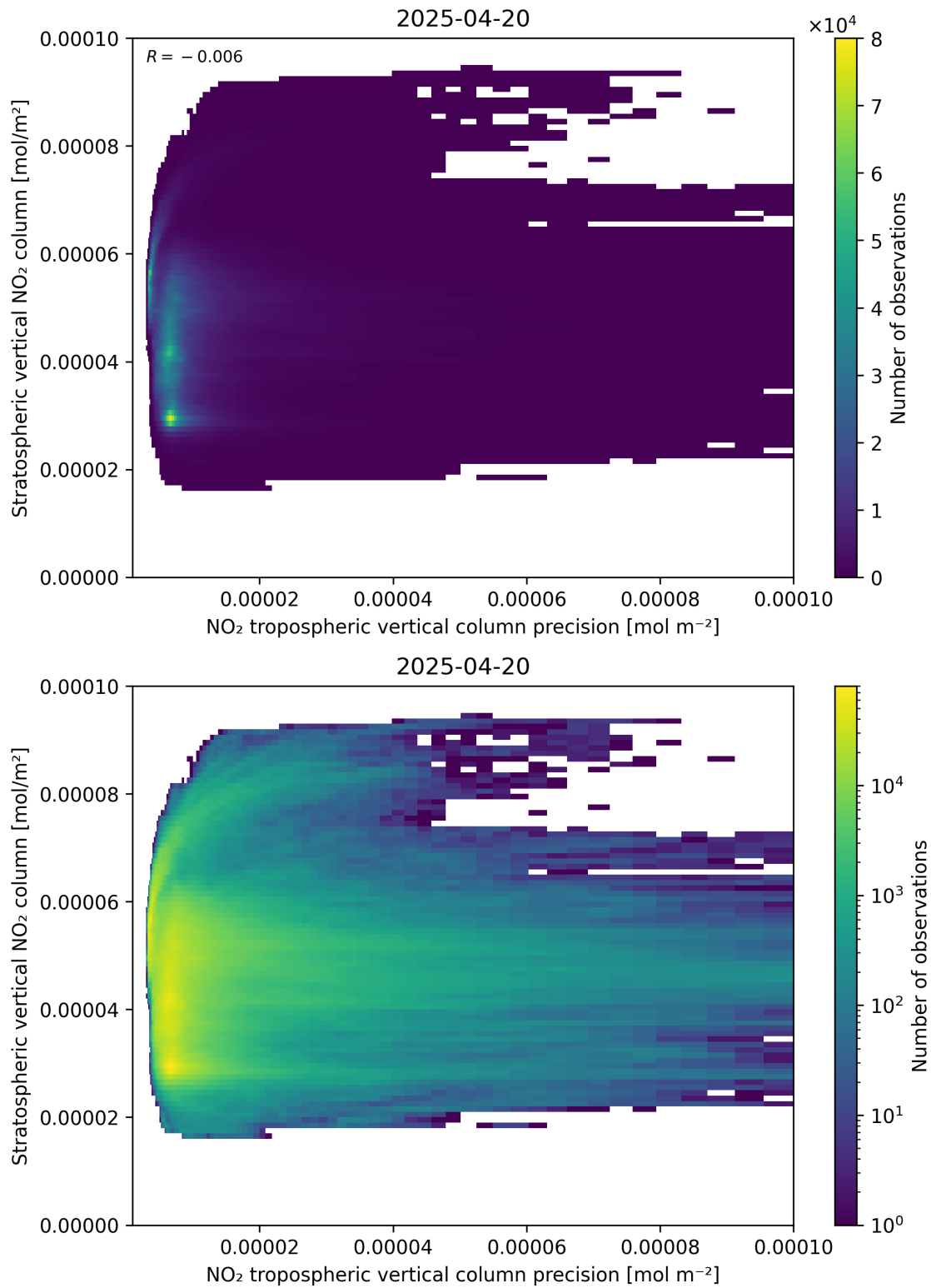
Figure 135: Scatter density plot of “NO 2 tropospheric vertical column precision” against “Stratospheric vertical NO 2 column” for 2025-04-20 to 2025-04-21.
