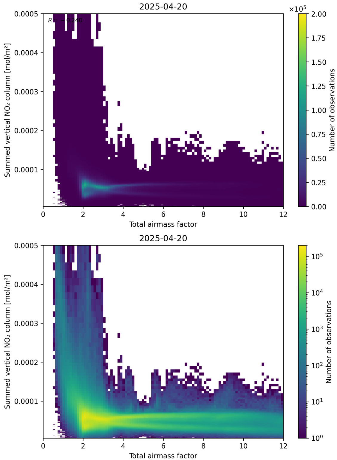
Figure 65: Scatter density plot of “Total airmass factor” against “Summed vertical NO 2 column” for 2025-04-20 to 2025-04-21.
