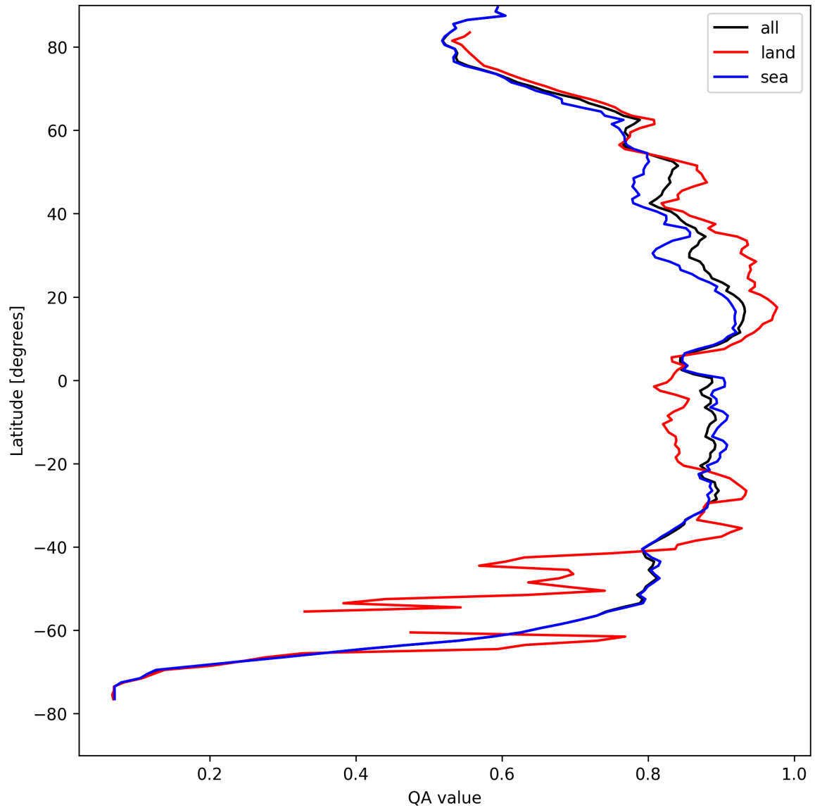
Figure 11: Zonal average of “QA value” for 2025-04-20 to 2025-04-21.
