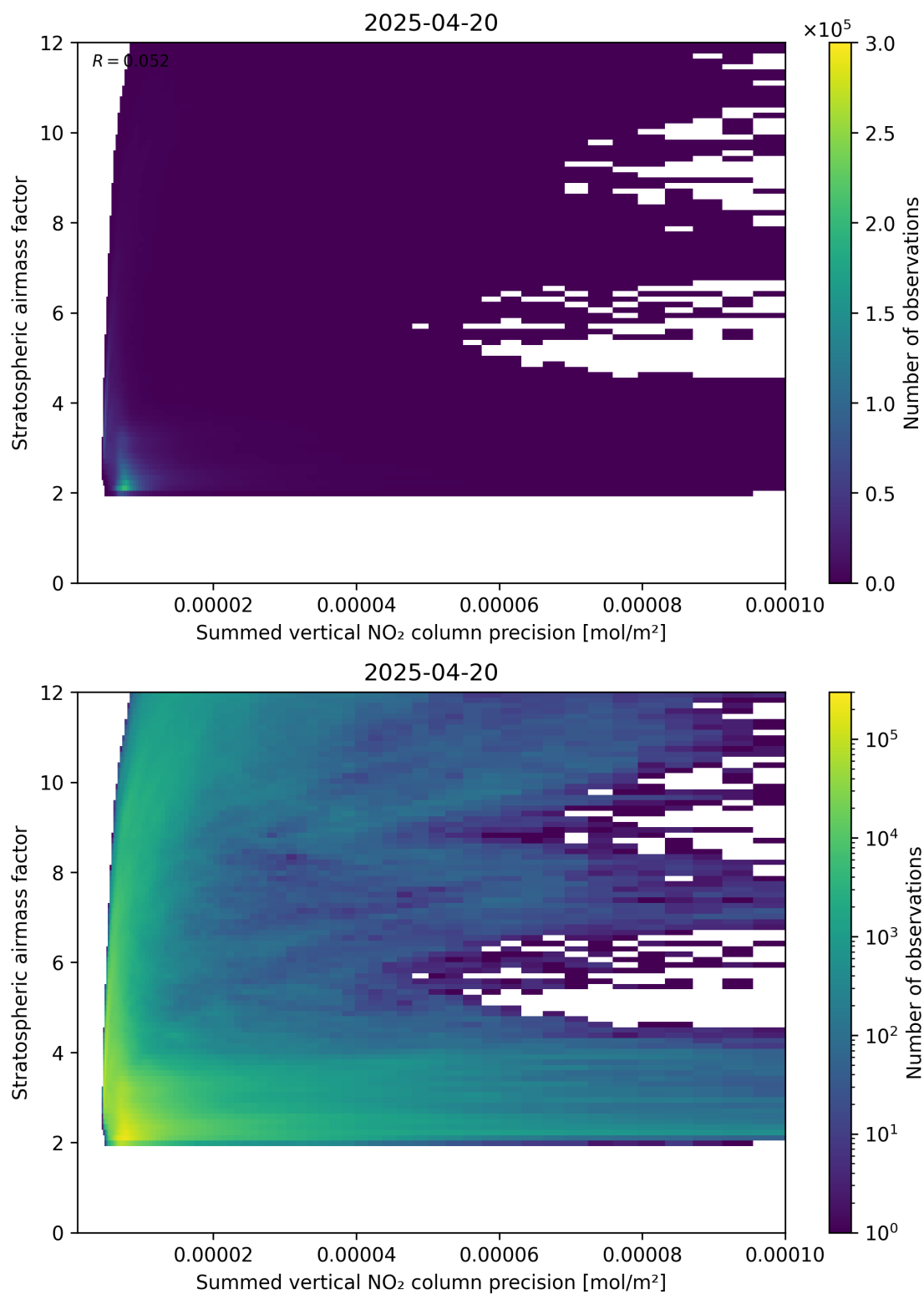
Figure 106: Scatter density plot of “Summed vertical NO 2 column precision” against “Stratospheric airmass factor” for 2025-04-20 to 2025-04-21.
