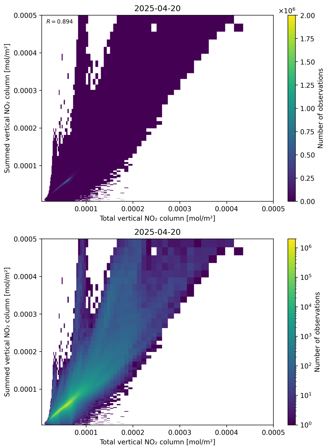
Figure 112: Scatter density plot of “Total vertical NO 2 column” against “Summed vertical NO 2 column” for 2025-04-20 to 2025-04-21.
