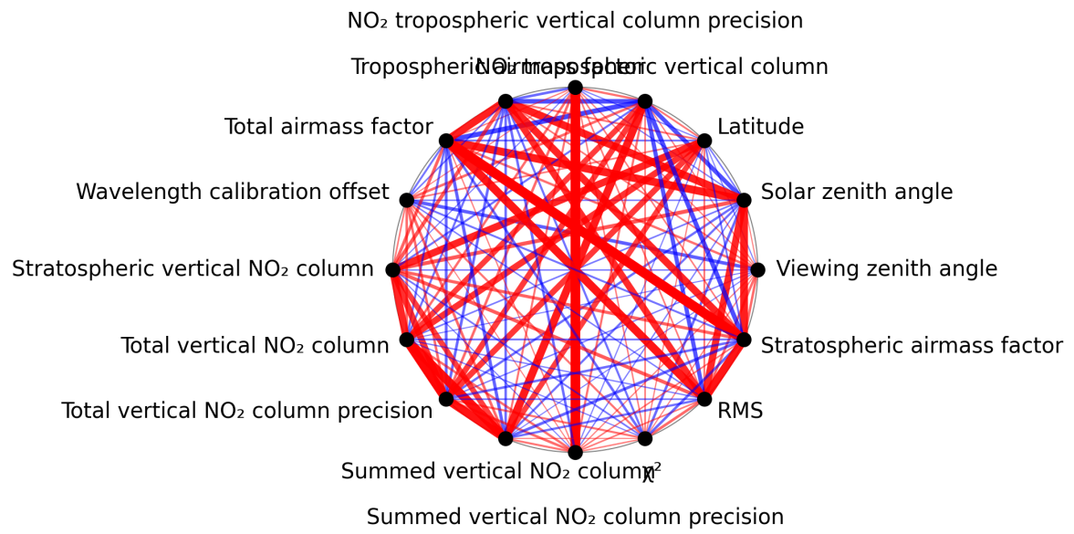
Figure 1: Map of correlation graph for 2025-04-20 to 2025-04-21.
