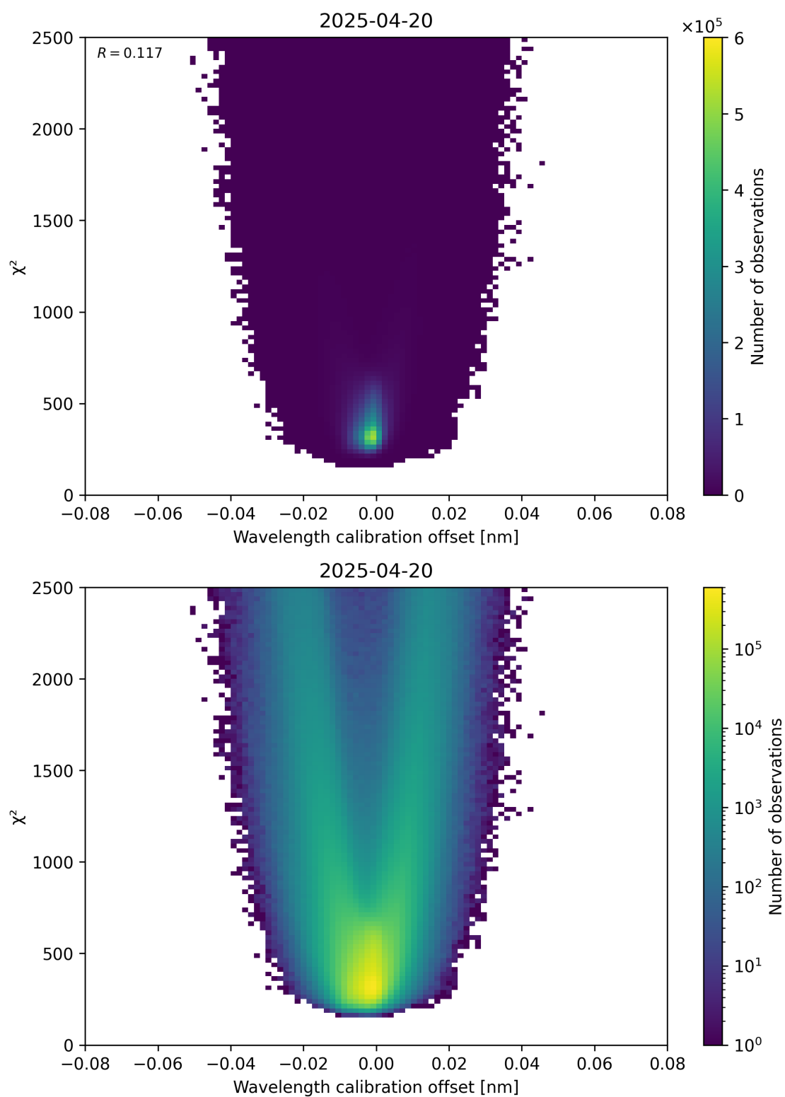
Figure 175: Scatter density plot of “Wavelength calibration offset” against “ \chi^2 ” for 2025-04-20 to 2025-04-21.
