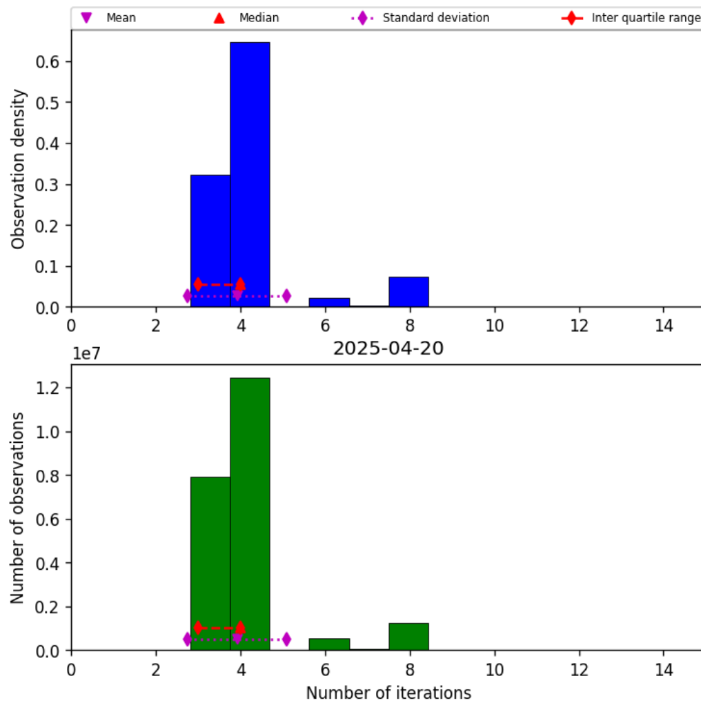
Figure 34: Histogram of “Number of iterations” for 2025-04-20 to 2025-04-21
