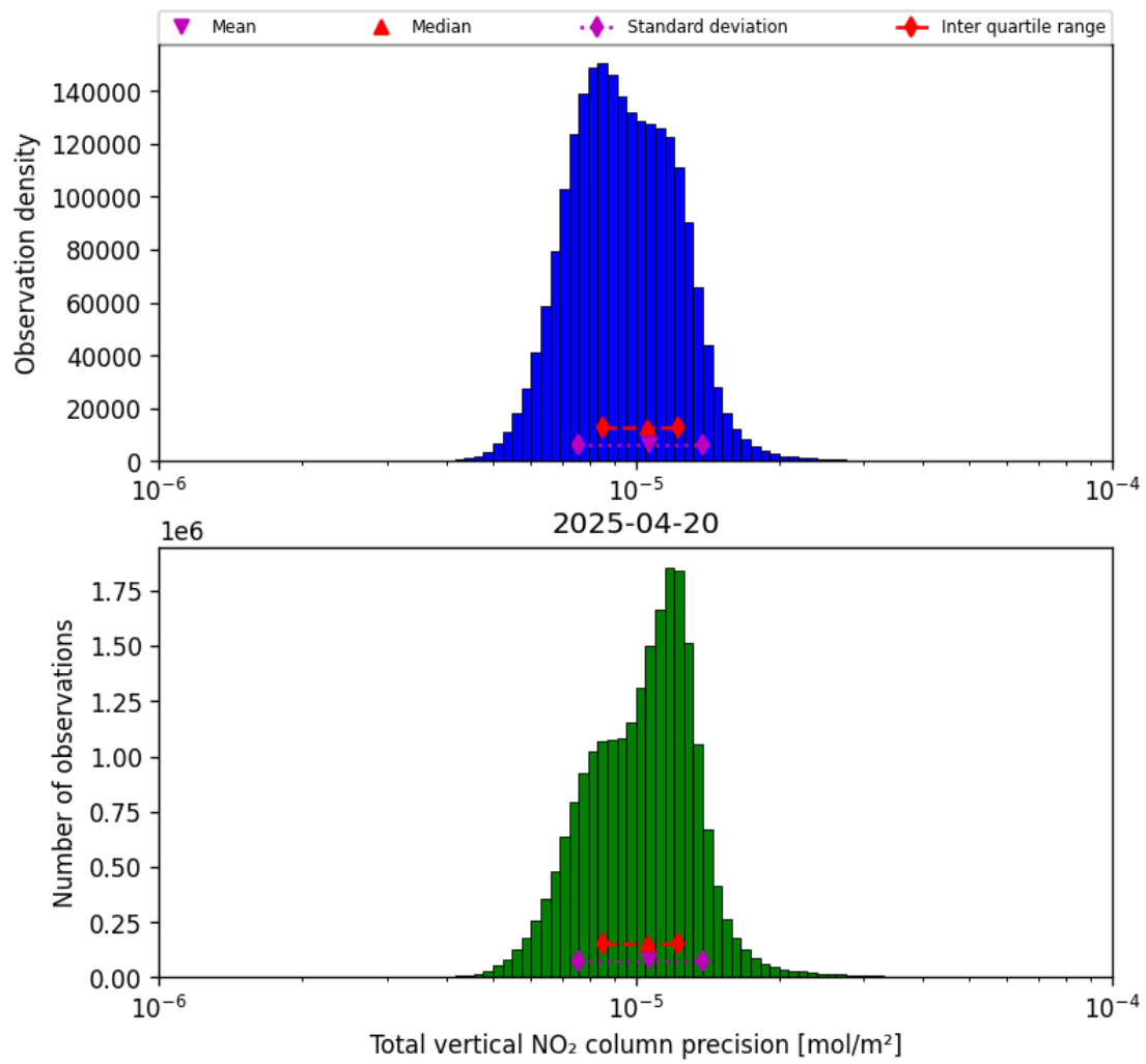
Figure 39: Histogram of “Total vertical NO 2 column precision” for 2025-04-20 to 2025-04-21
