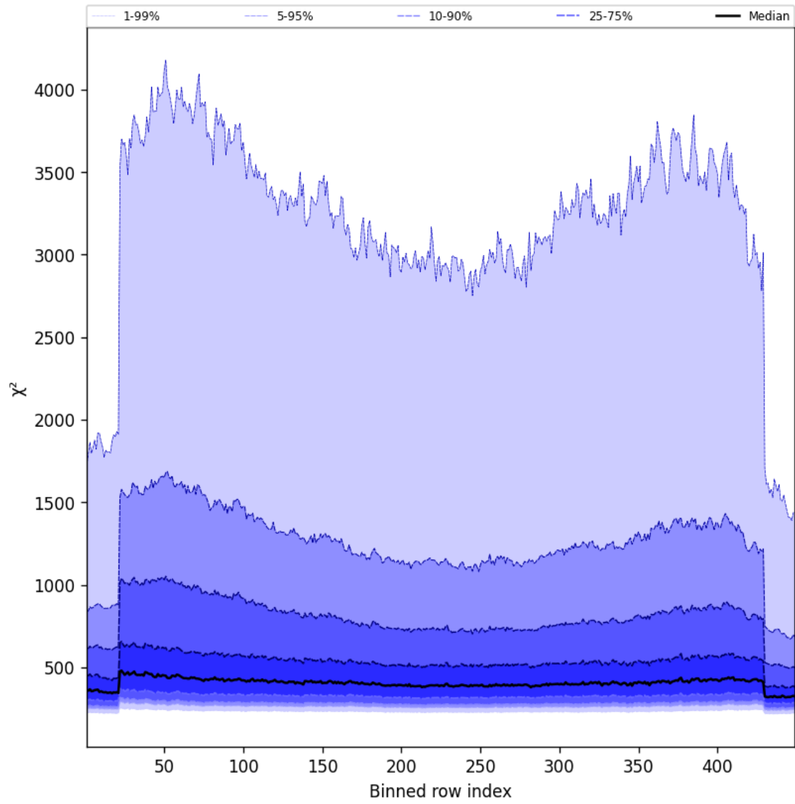
Figure 59: Along track statistics of “ \chi^2 ” for 2025-04-20 to 2025-04-21
