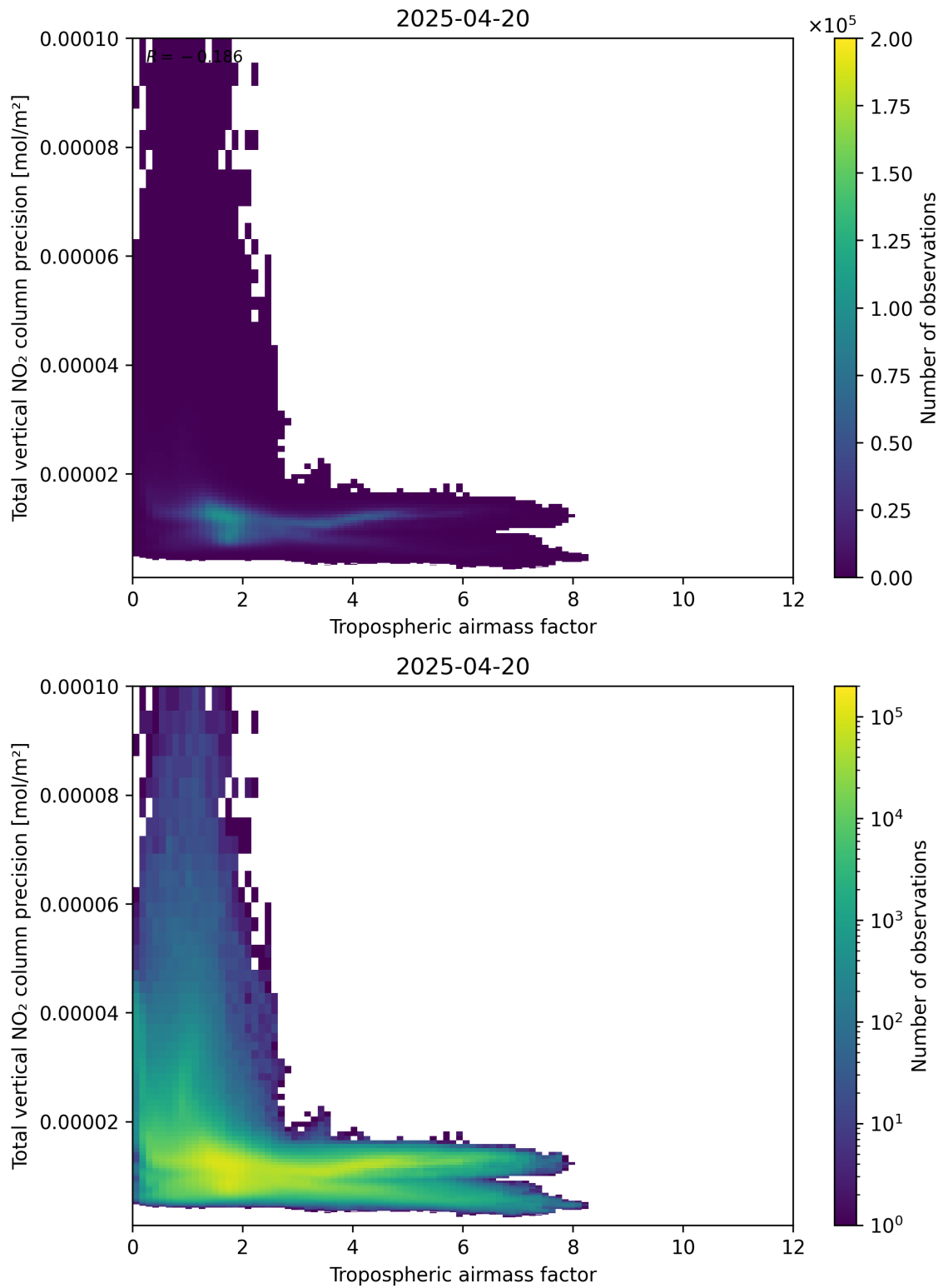
Figure 78: Scatter density plot of “Tropospheric air mass factor” against “Total vertical NO 2 column precision” for 2025-04-20 to 2025-04-21.
