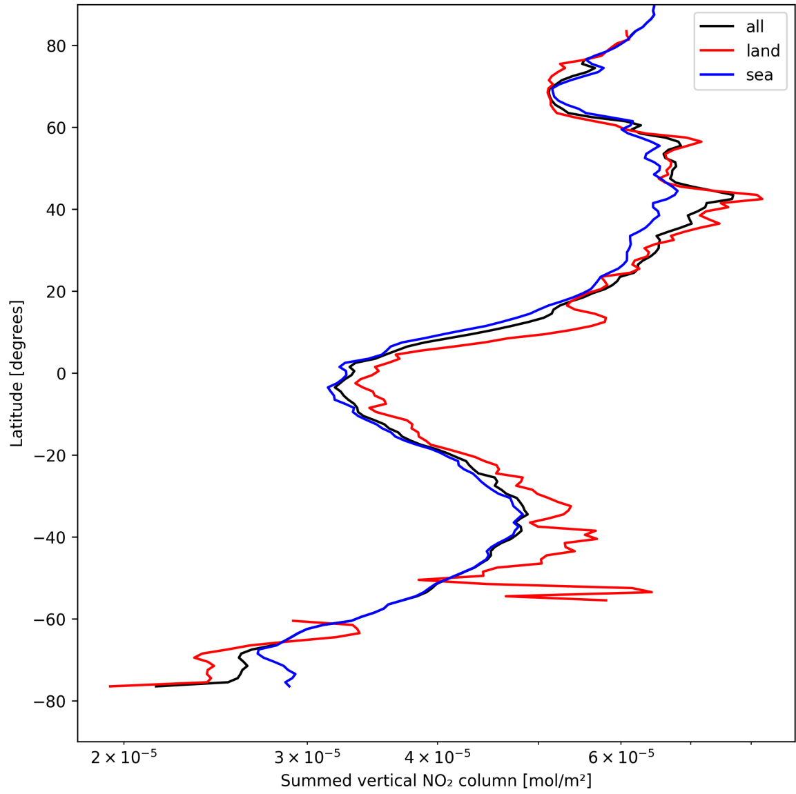
Figure 23: Zonal average of “Summed vertical NO 2 column” for 2025-04-20 to 2025-04-21.
