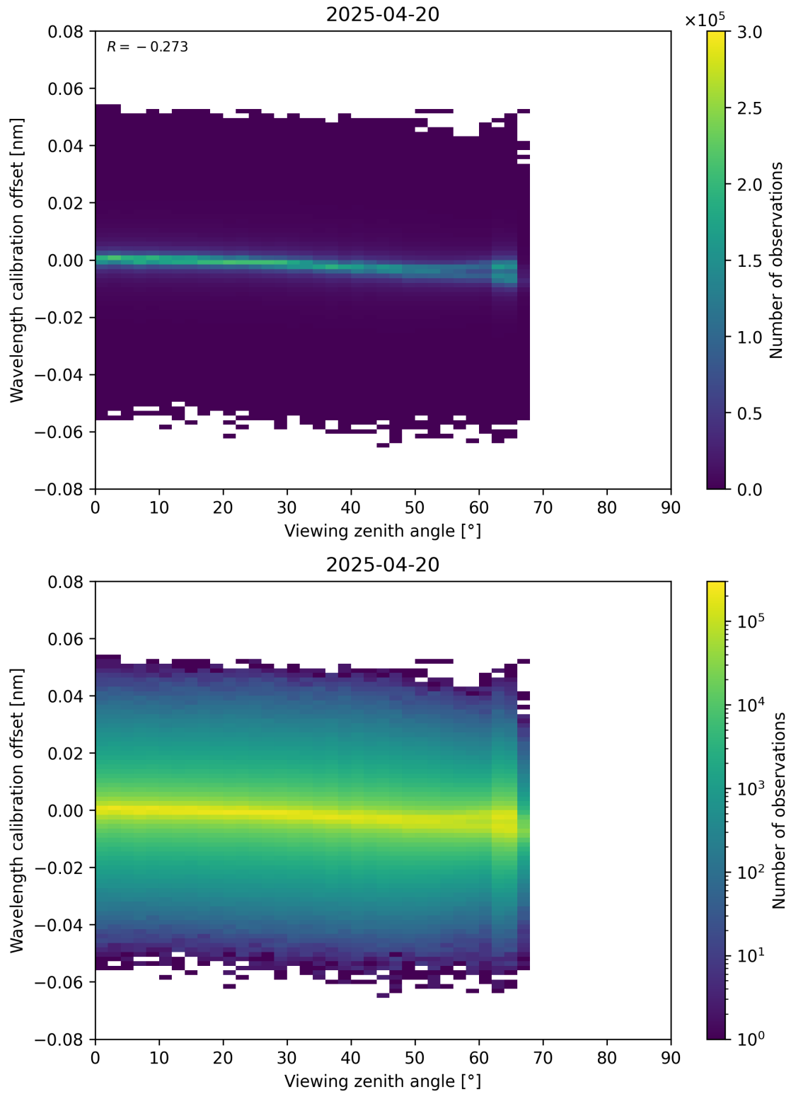
Figure 173: Scatter density plot of “Viewing zenith angle” against “Wavelength calibration offset” for 2025-04-20 to 2025-04-21.
