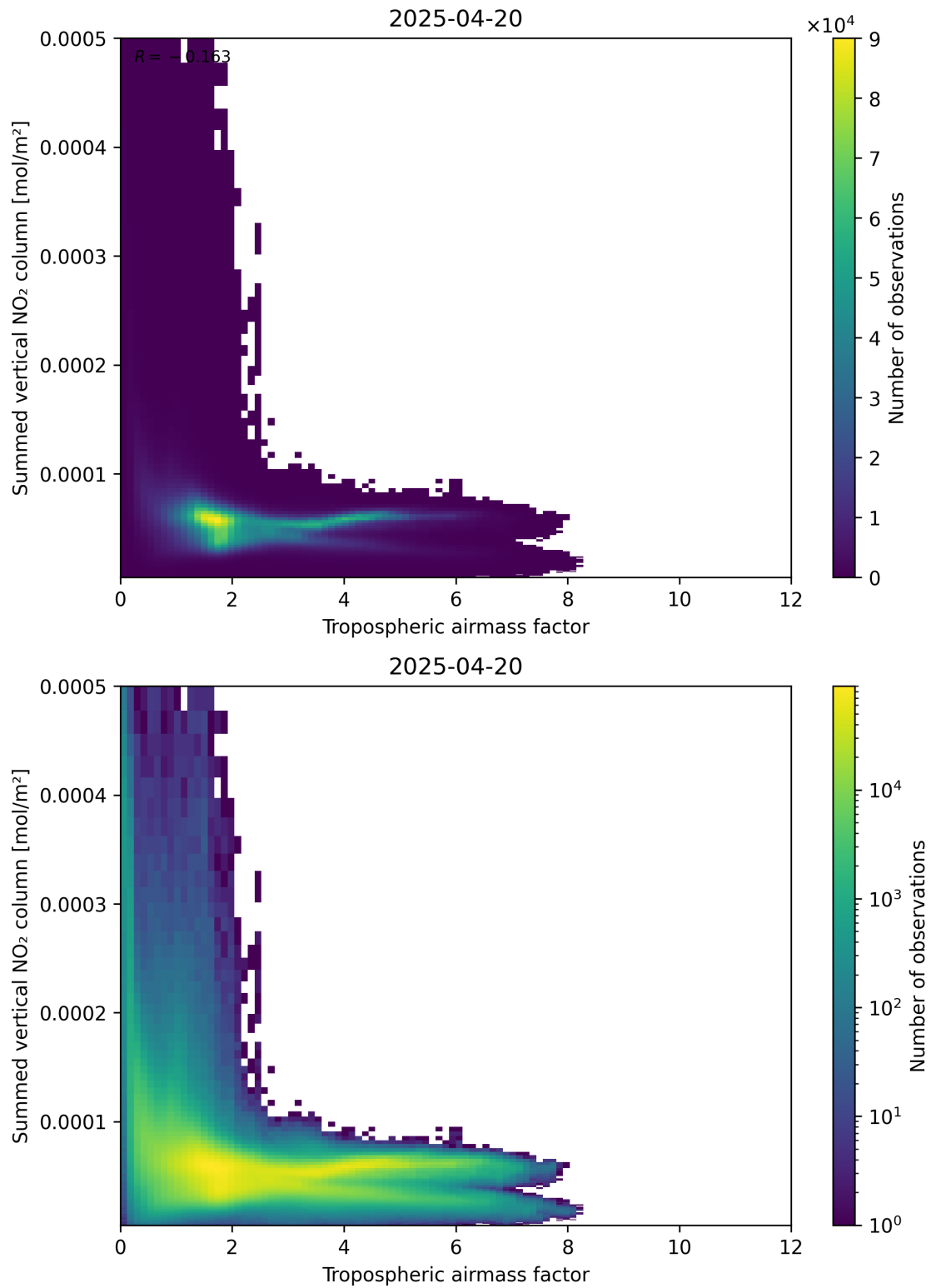
Figure 75: Scatter density plot of “Tropospheric air mass factor” against “Summed vertical NO 2 column” for 2025-04-20 to 2025-04-21.
