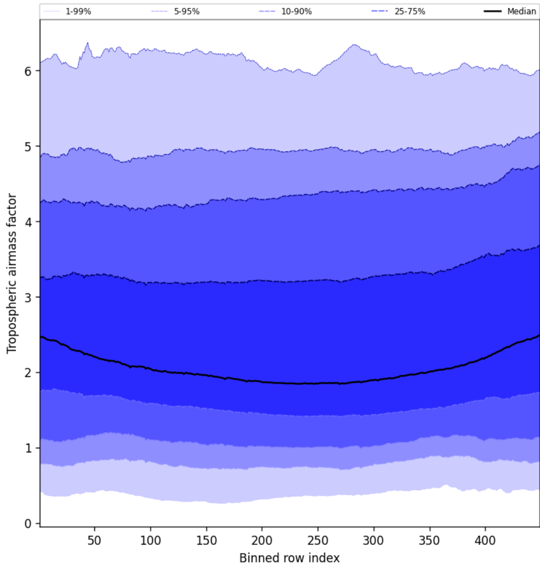
Figure 48: Along track statistics of “Tropospheric airmass factor” for 2025-04-20 to 2025-04-21
