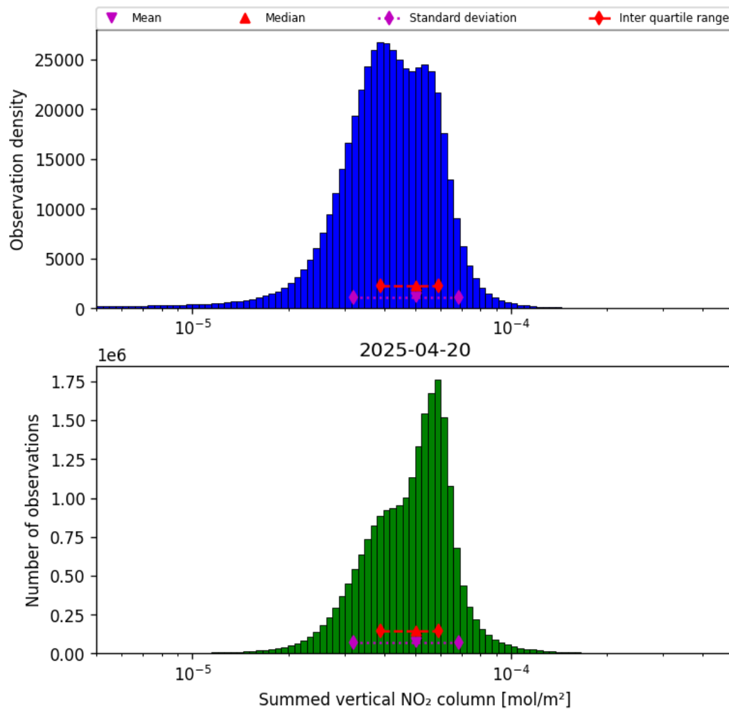
Figure 40: Histogram of “Summed vertical NO 2 column” for 2025-04-20 to 2025-04-21
