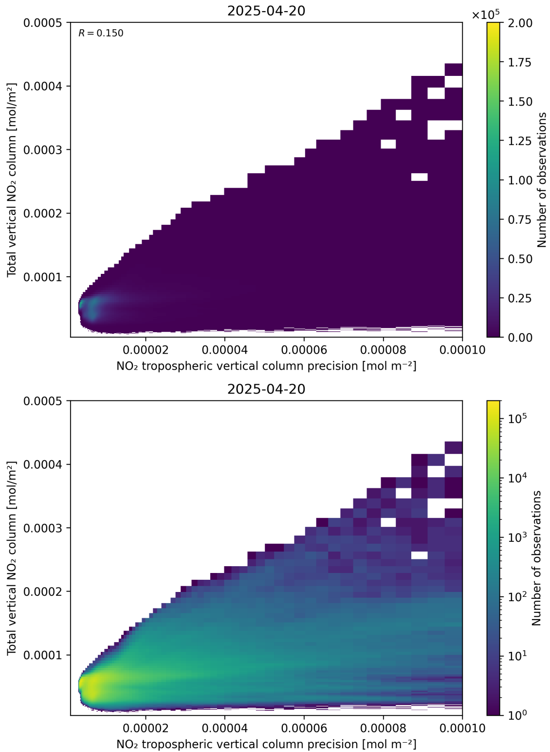
Figure 138: Scatter density plot of “NO 2 tropospheric vertical column precision” against “Total vertical NO 2 column” for 2025-04-20 to 2025-04-21.
