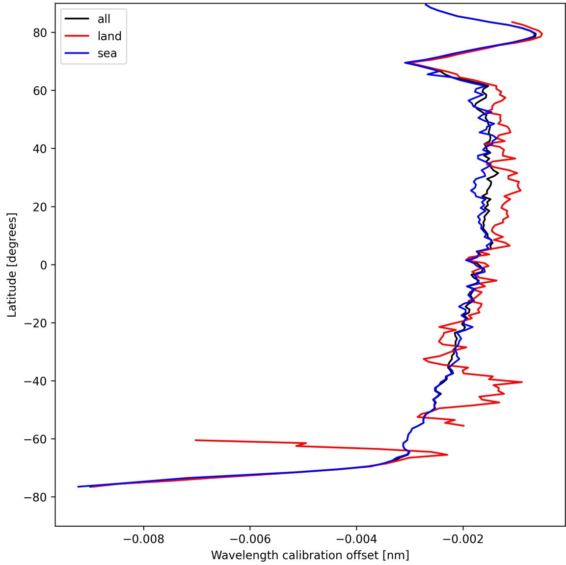
Figure 18: Zonal average of “Wavelength calibration offset” for 2025-04-20 to 2025-04-21.
