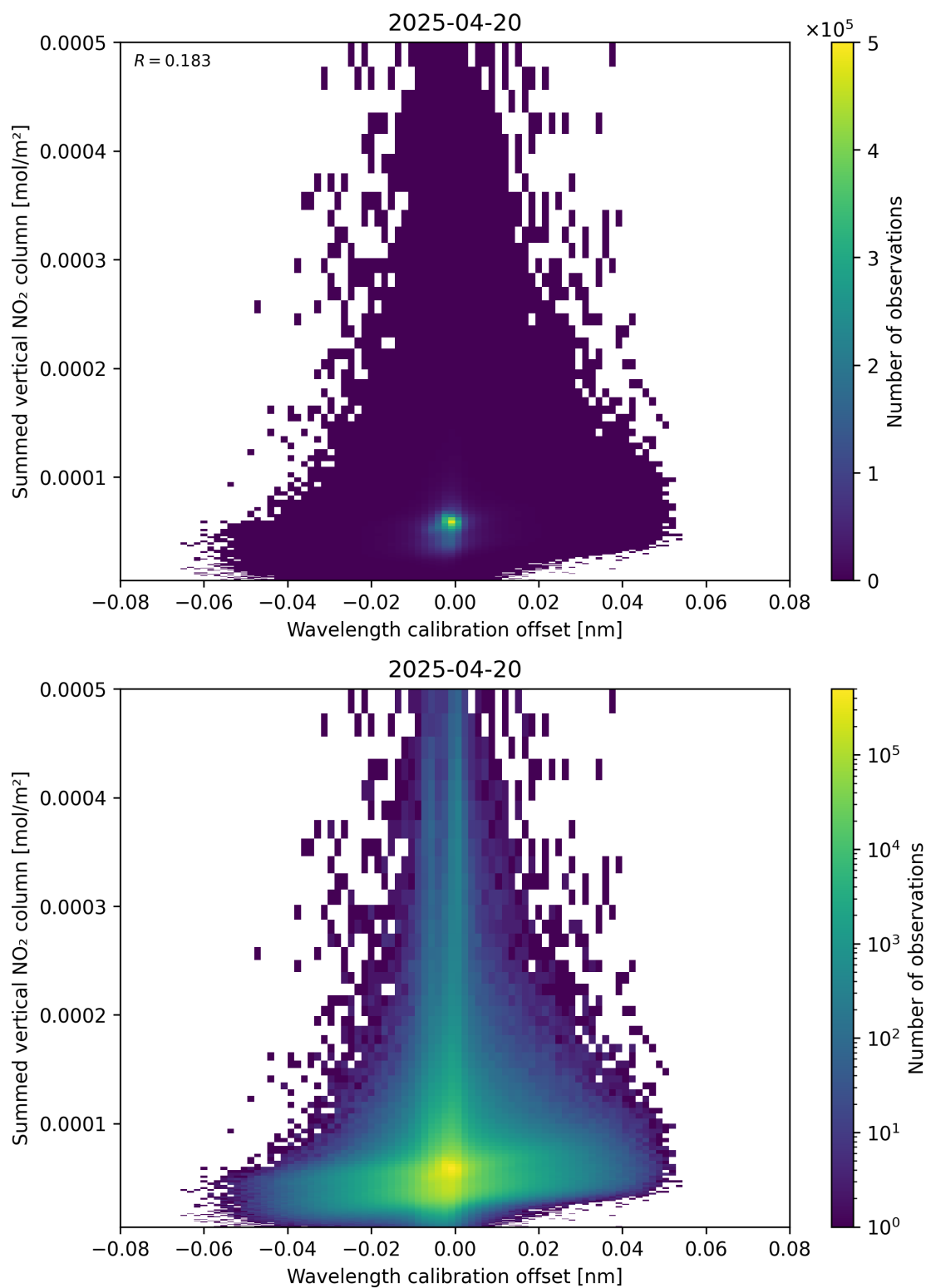
Figure 177: Scatter density plot of “Wavelength calibration offset” against “Summed vertical NO 2 column” for 2025-04-20 to 2025-04-21.
