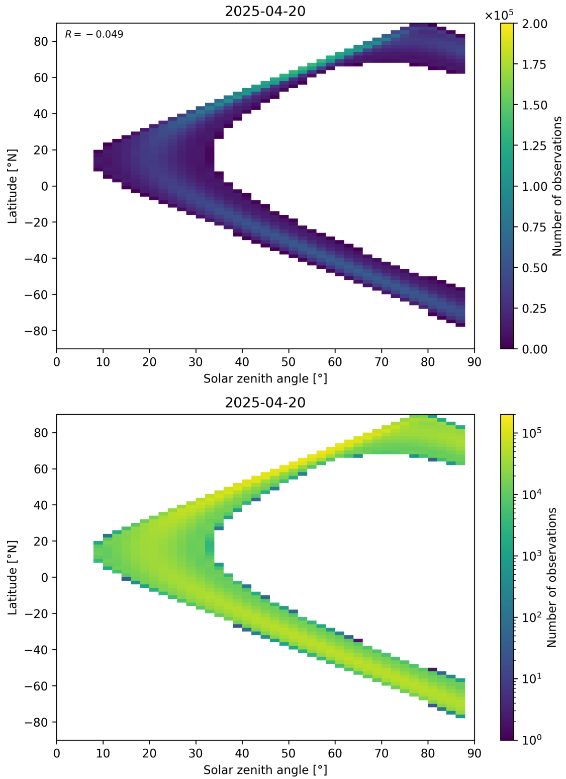
Figure 149: Scatter density plot of “Solar zenith angle” against “Latitude” for 2025-04-20 to 2025-04-21.
