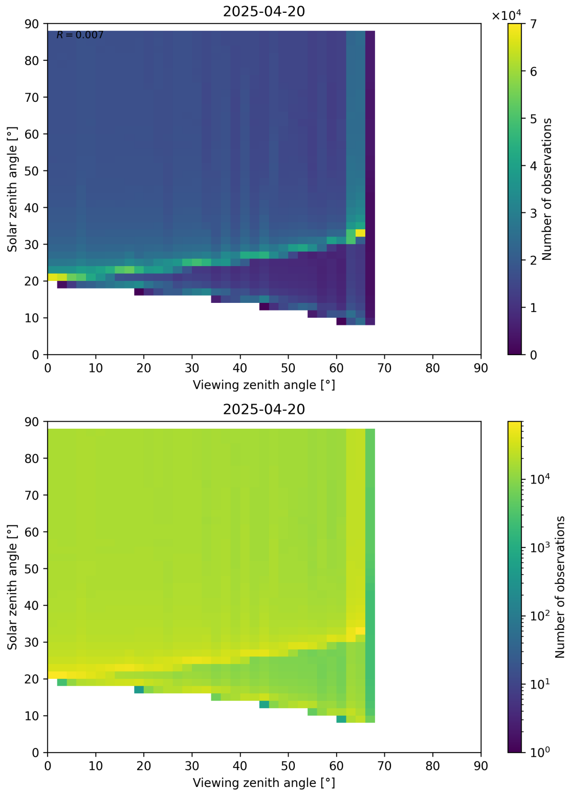
Figure 172: Scatter density plot of “Viewing zenith angle” against “Solar zenith angle” for 2025-04-20 to 2025-04-21.
