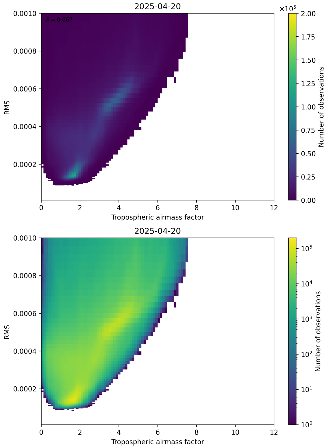
Figure 79: Scatter density plot of “Tropospheric airmass factor” against “RMS” for 2025-04-20 to 2025-04-21.
