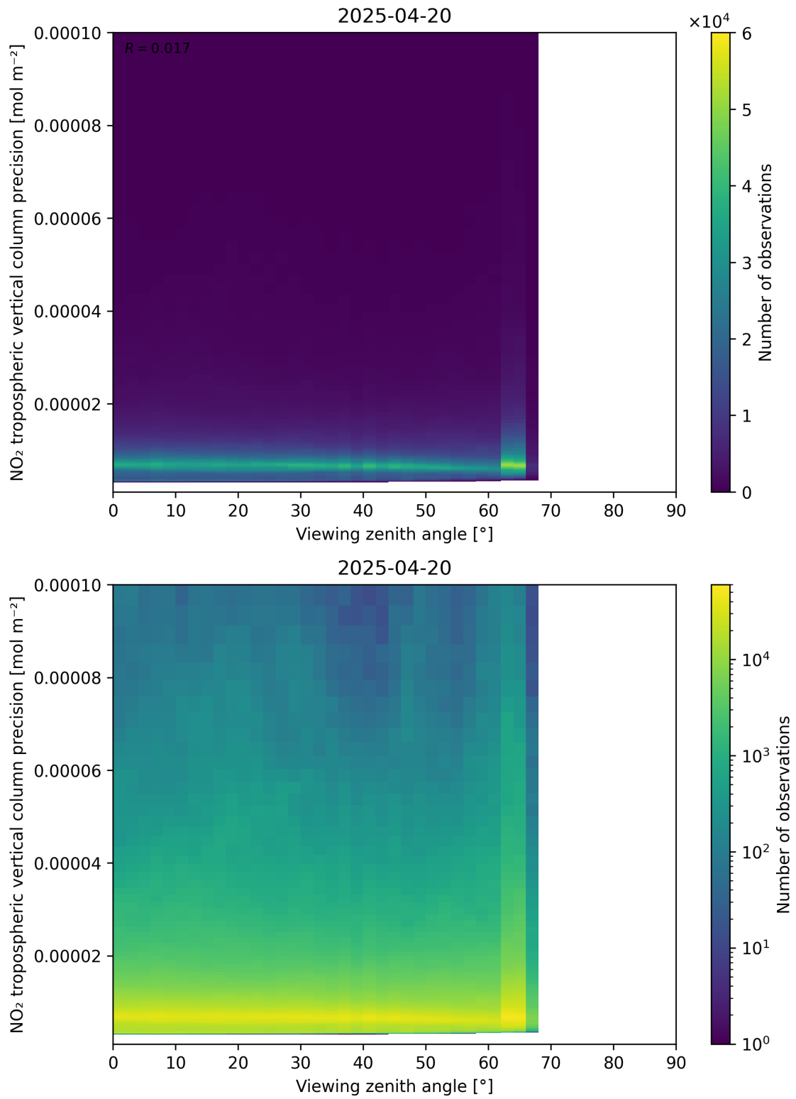
Figure 170: Scatter density plot of “Viewing zenith angle” against “NO 2 tropospheric vertical column precision” for 2025-04-20 to 2025-04-21.
