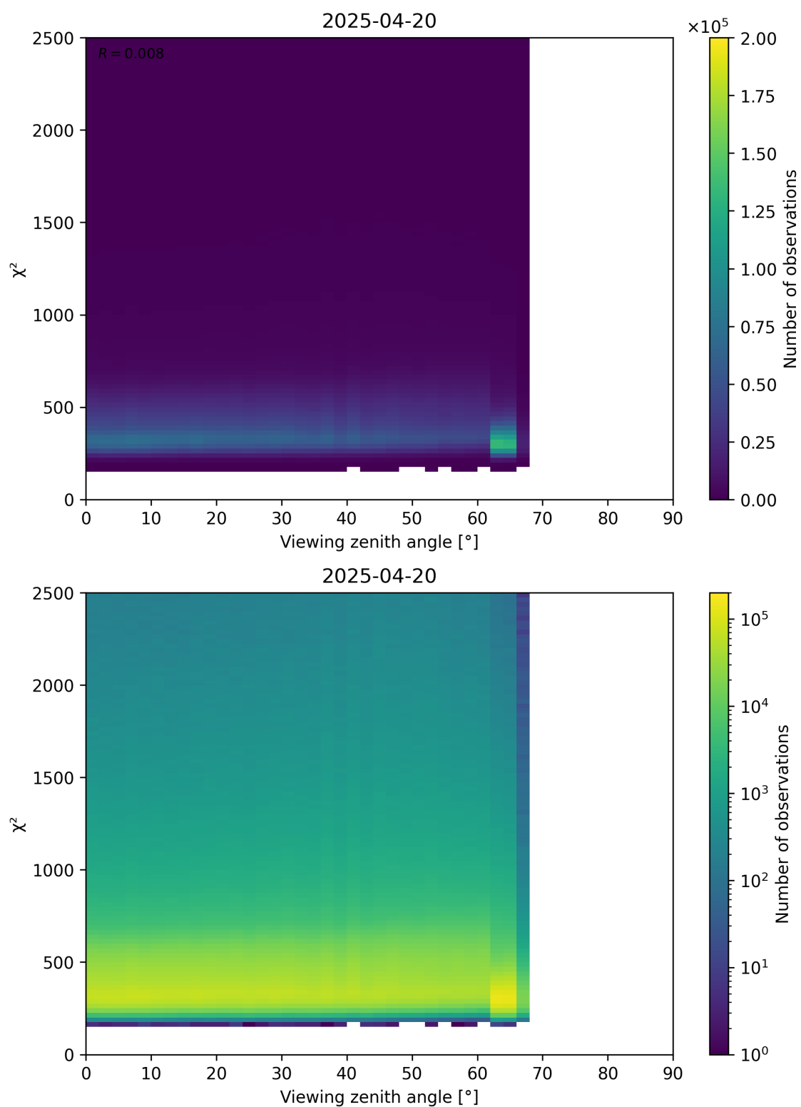
Figure 162: Scatter density plot of “Viewing zenith angle” against “ \chi^2 ” for 2025-04-20 to 2025-04-21.
