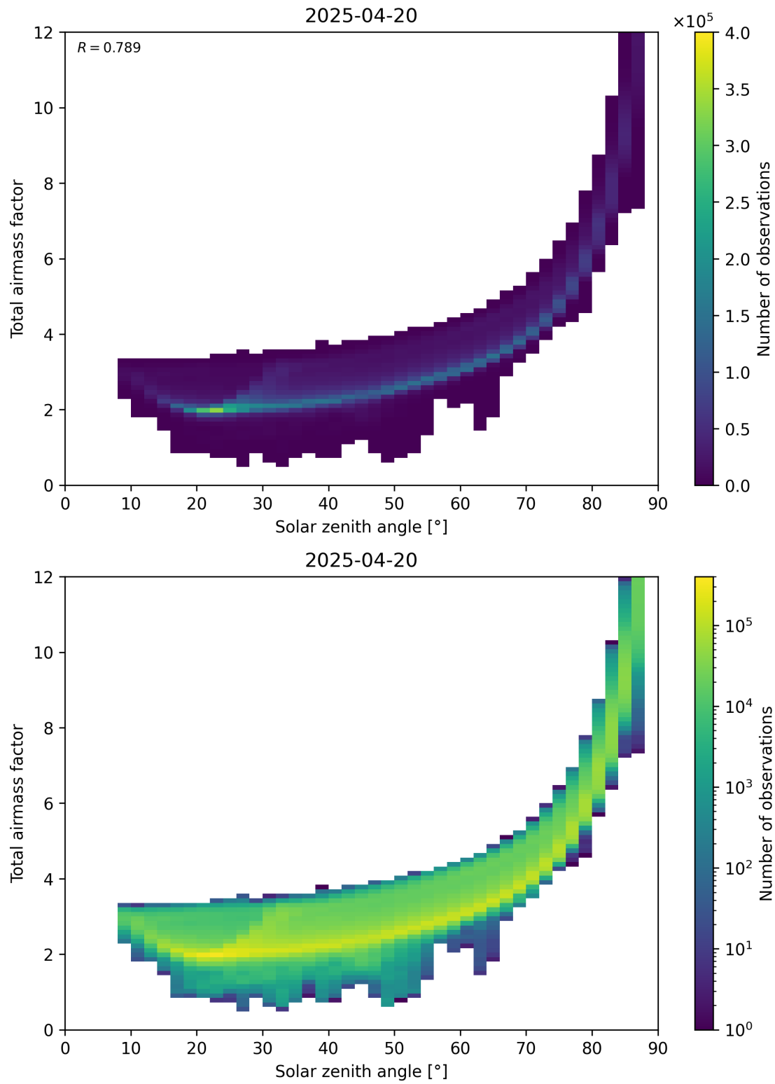
Figure 146: Scatter density plot of “Solar zenith angle” against “Total air mass factor” for 2025-04-20 to 2025-04-21.
