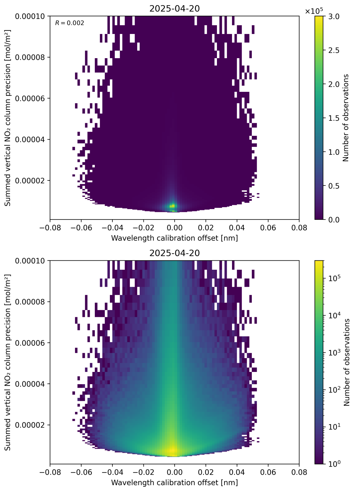
Figure 178: Scatter density plot of “Wavelength calibration offset” against “Summed vertical NO 2 column precision” for 2025-04-20 to 2025-04-21.
