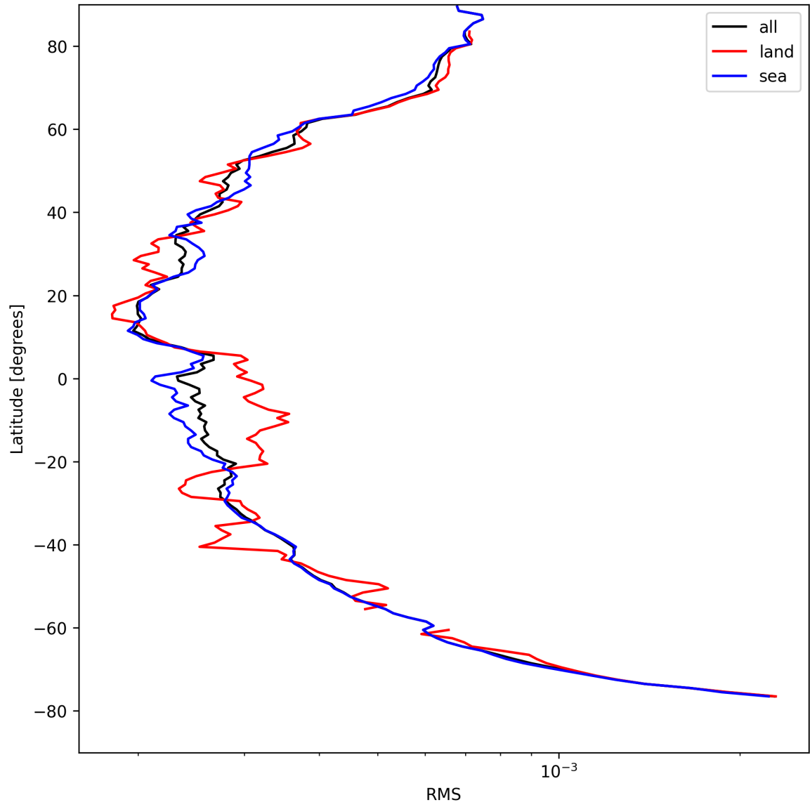
Figure 26: Zonal average of “RMS” for 2025-04-20 to 2025-04-21.
