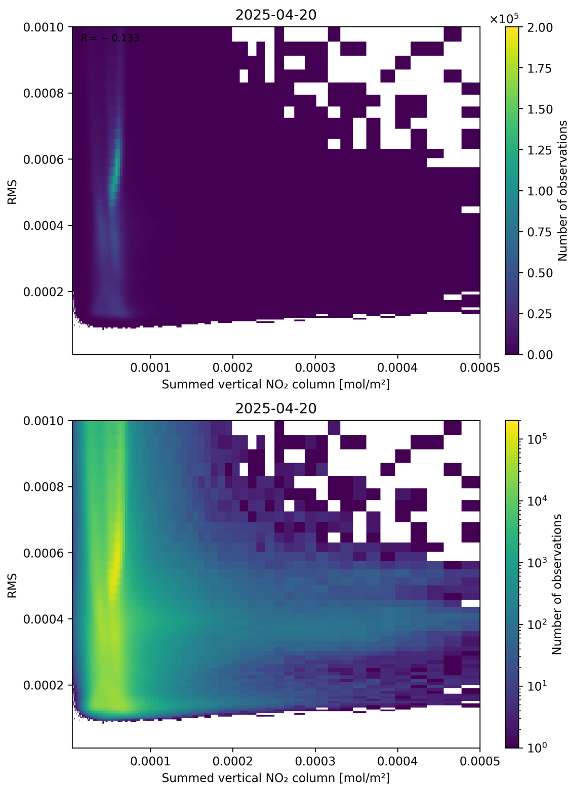
Figure 109: Scatter density plot of “Summed vertical NO 2 column” against “RMS” for 2025-04-20 to 2025-04-21.
