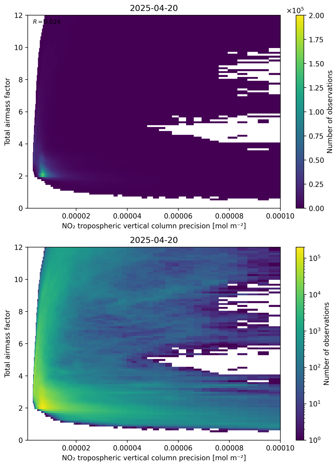
Figure 132: Scatter density plot of “NO 2 tropospheric vertical column precision” against “Total air mass factor” for 2025-04-20 to 2025-04-21.
