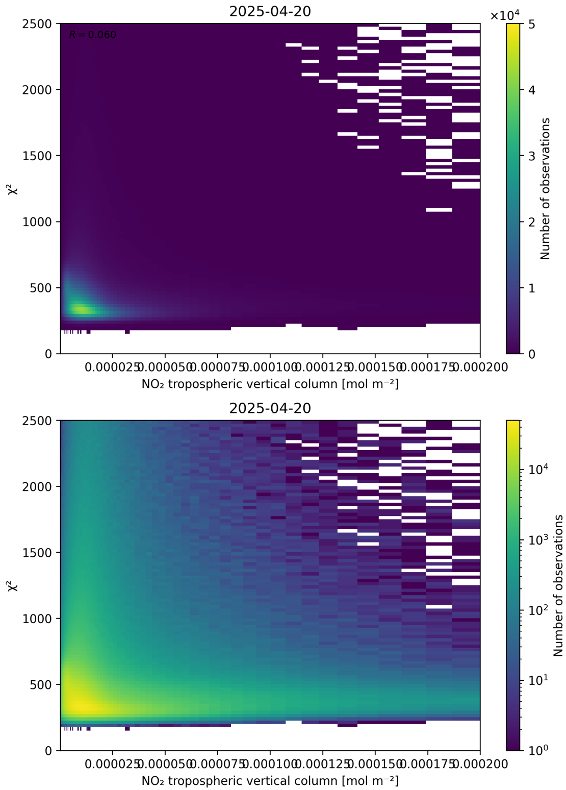
Figure 124: Scatter density plot of “NO 2 tropospheric vertical column” against “ \chi^2 ” for 2025-04-20 to 2025-04-21.
