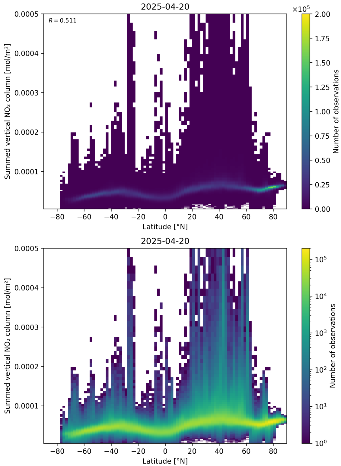
Figure 88: Scatter density plot of “Latitude” against “Summed vertical NO 2 column” for 2025-04-20 to 2025-04-21.
