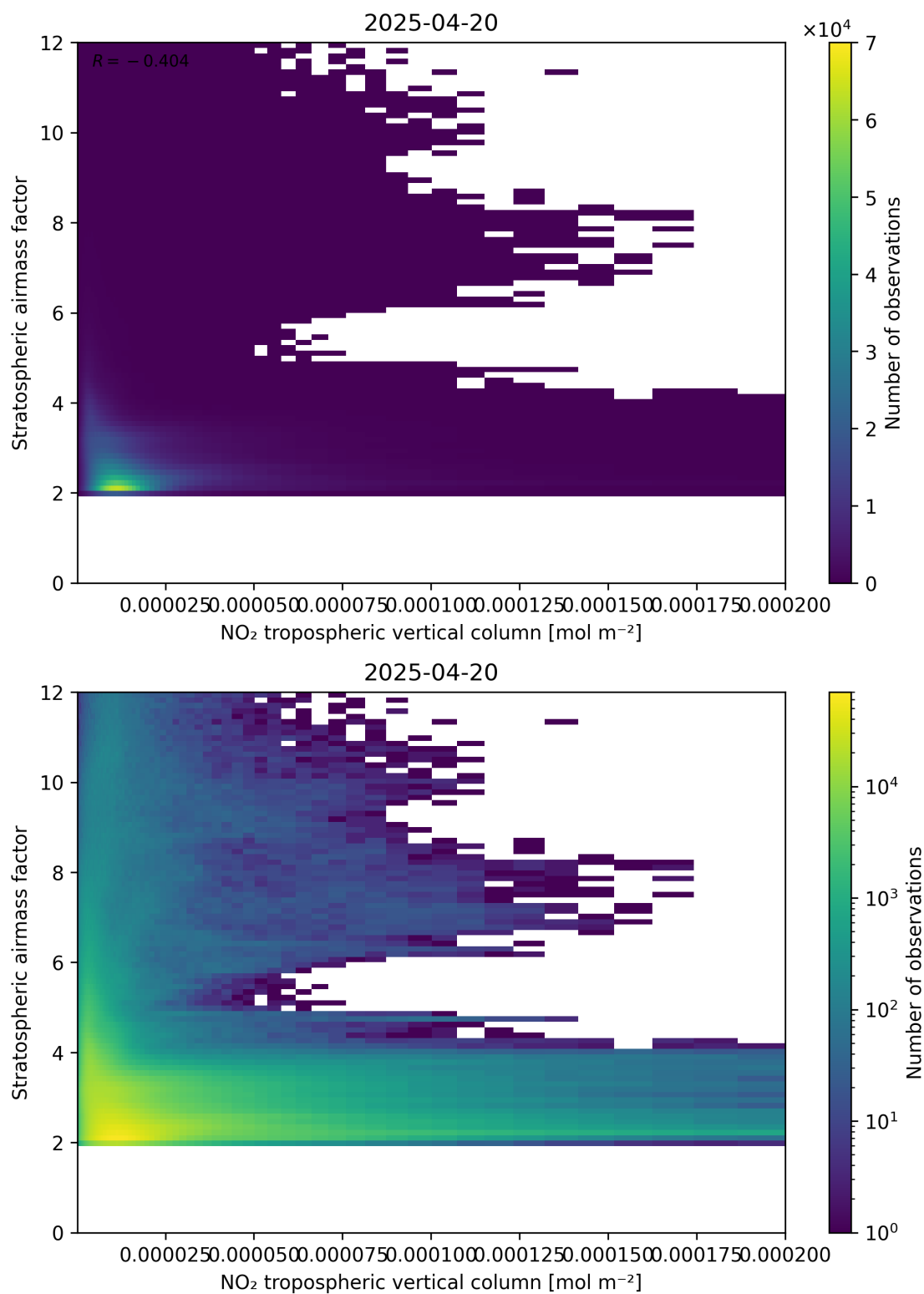
Figure 121: Scatter density plot of “NO 2 tropospheric vertical column” against “Stratospheric air mass factor” for 2025-04-20 to 2025-04-21.
