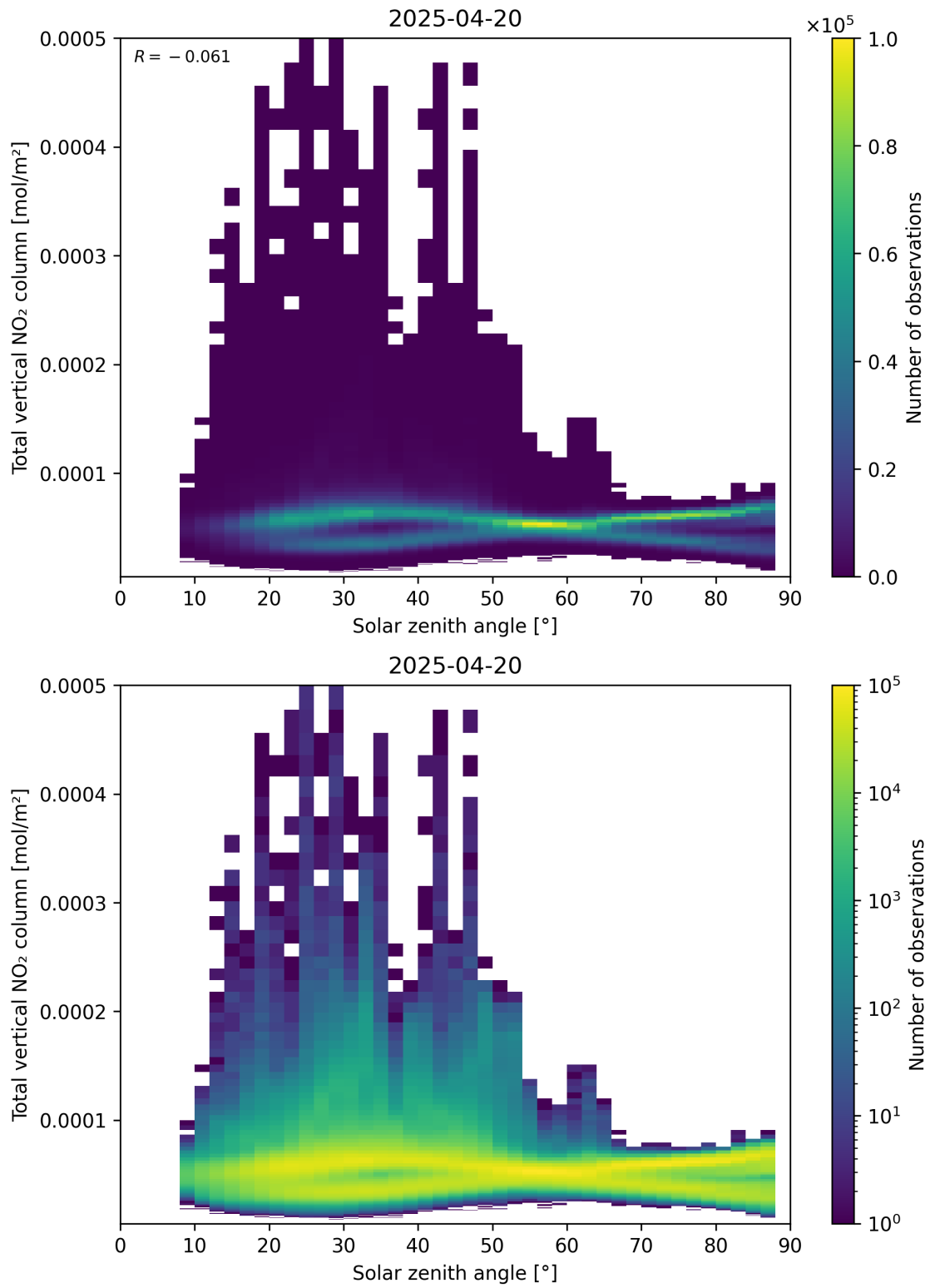
Figure 153: Scatter density plot of “Solar zenith angle” against “Total vertical NO 2 column” for 2025-04-20 to 2025-04-21.
