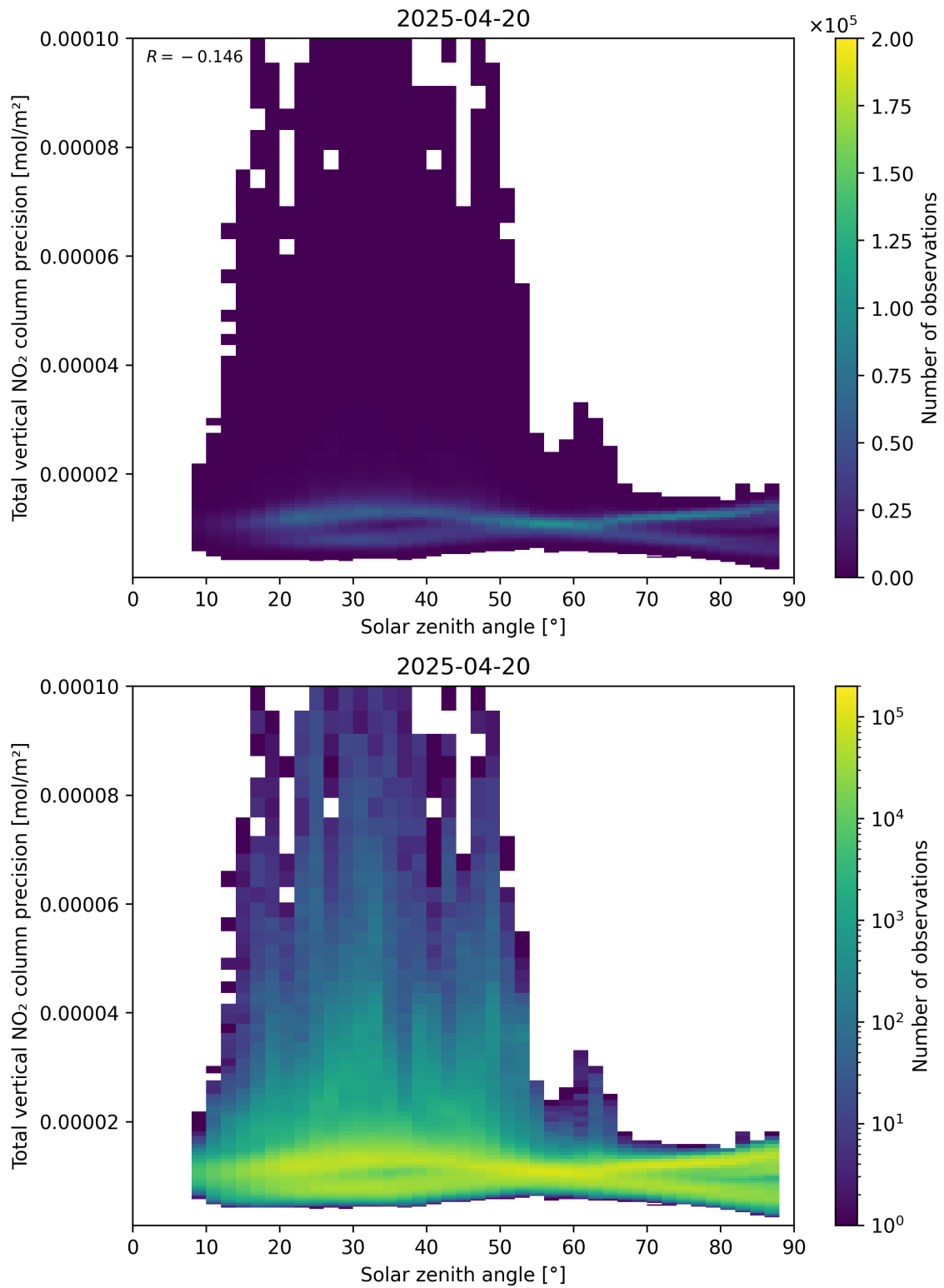
Figure 154: Scatter density plot of “Solar zenith angle” against “Total vertical NO 2 column precision” for 2025-04-20 to 2025-04-21.
