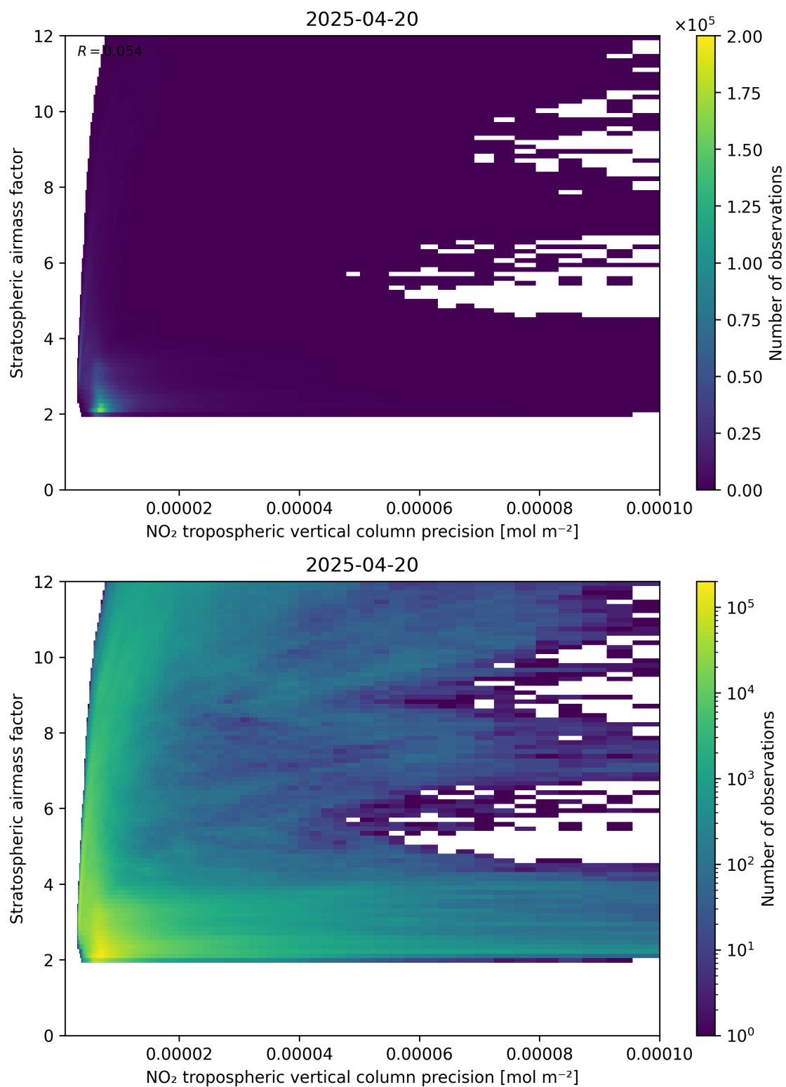
Figure 131: Scatter density plot of “NO 2 tropospheric vertical column precision” against “Stratospheric airmass factor” for 2025-04-20 to 2025-04-21.
