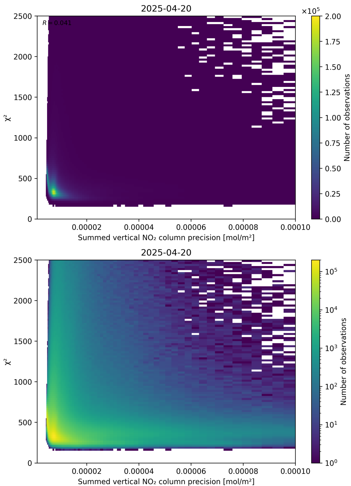
Figure 107: Scatter density plot of “Summed vertical NO 2 column precision” against “ \chi^2 ” for 2025-04-20 to 2025-04-21.
