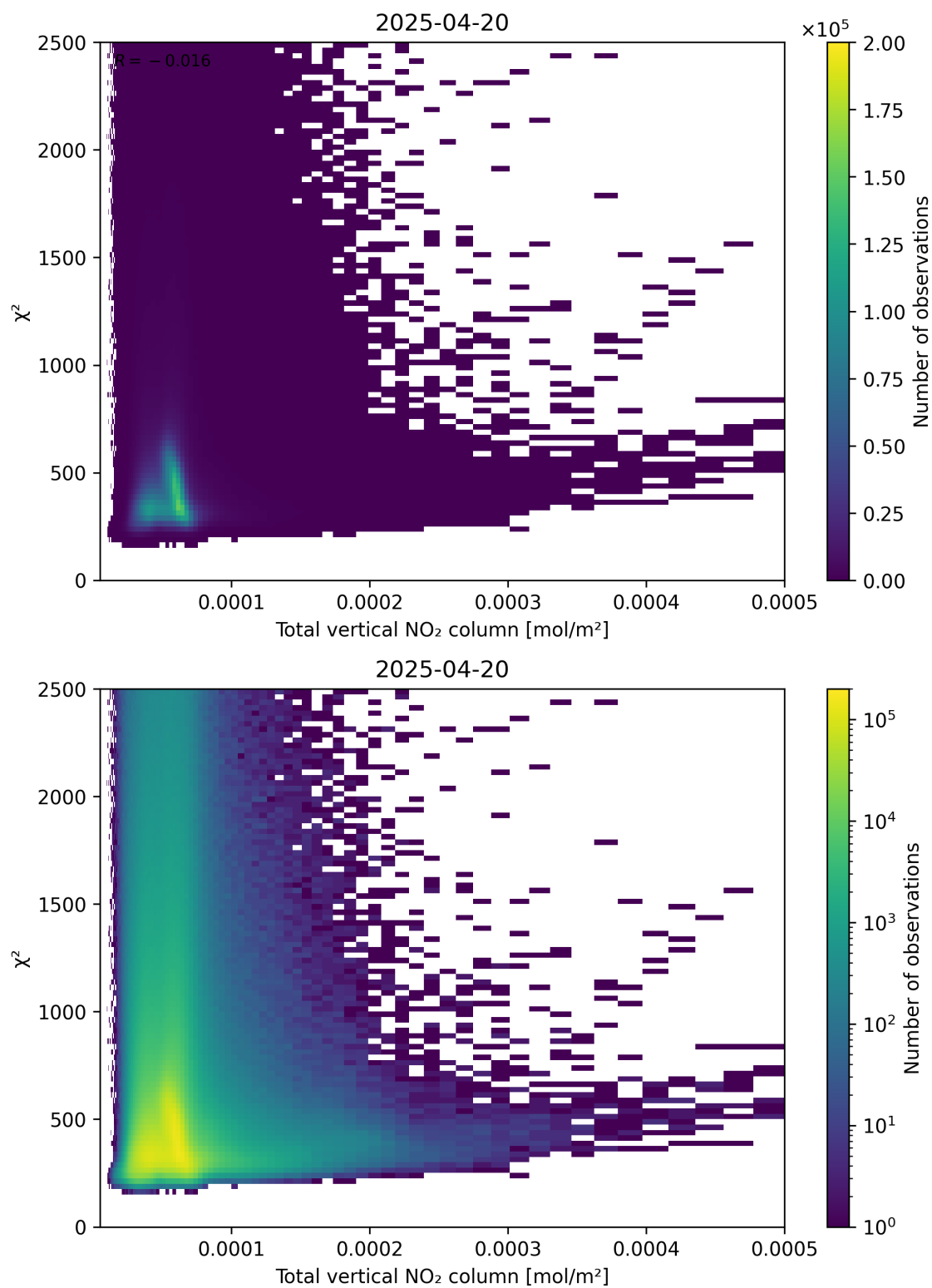
Figure 111: Scatter density plot of “Total vertical NO 2 column” against “ \chi^2 ” for 2025-04-20 to 2025-04-21.
