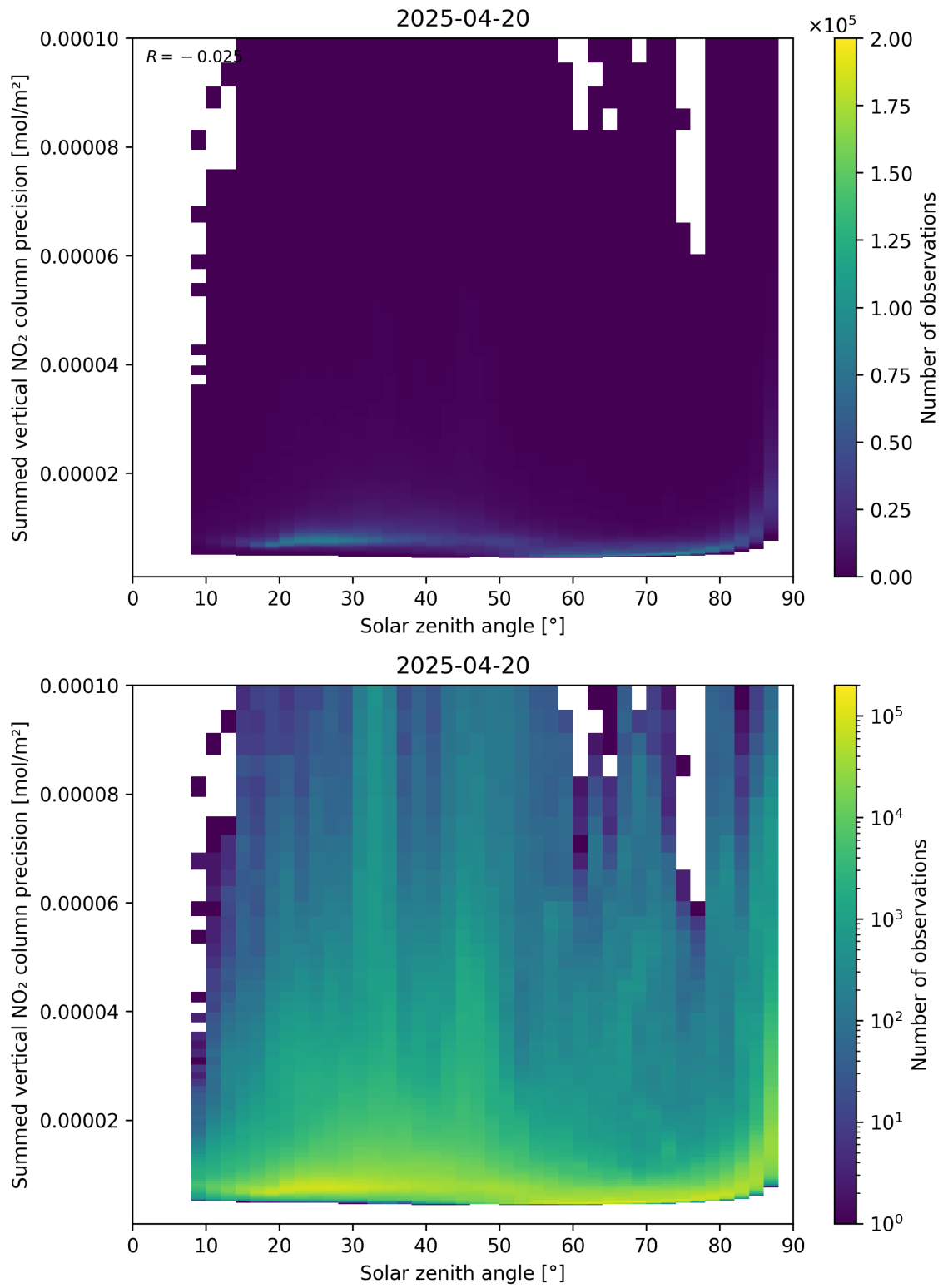
Figure 152: Scatter density plot of “Solar zenith angle” against “Summed vertical NO 2 column precision” for 2025-04-20 to 2025-04-21.
