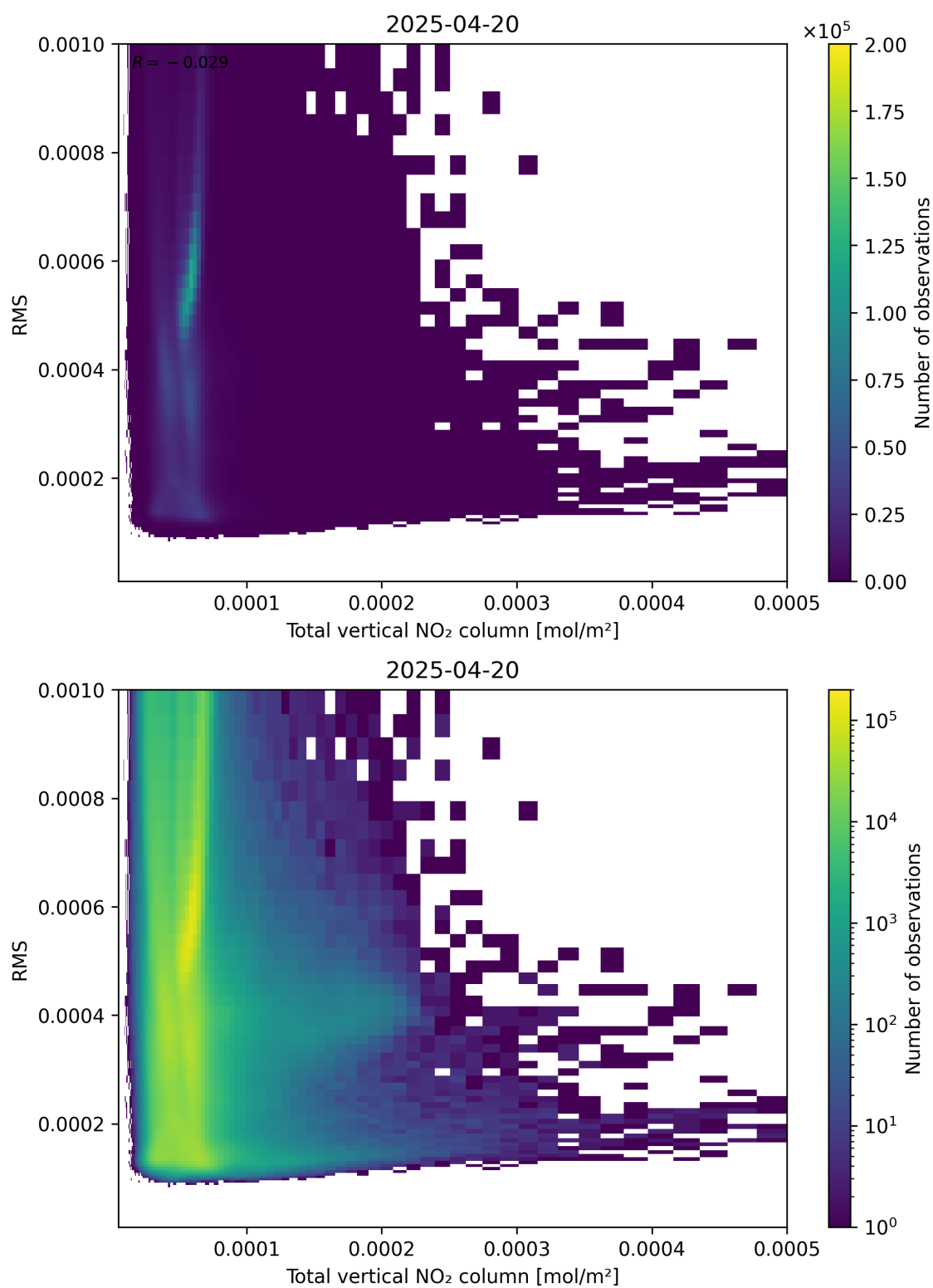
Figure 120: Scatter density plot of “Total vertical NO 2 column” against “RMS” for 2025-04-20 to 2025-04-21.
