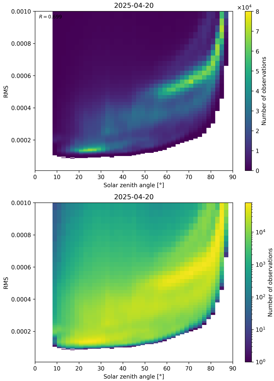
Figure 157: Scatter density plot of “Solar zenith angle” against “RMS” for 2025-04-20 to 2025-04-21.
