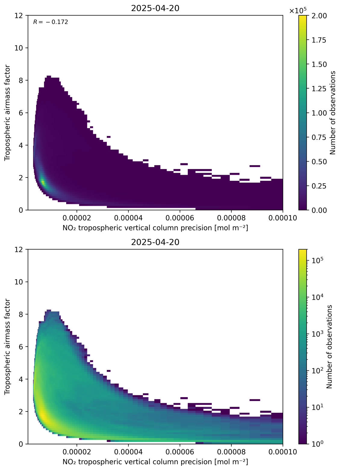
Figure 133: Scatter density plot of “NO 2 tropospheric vertical column precision” against “Tropospheric air mass factor” for 2025-04-20 to 2025-04-21.
