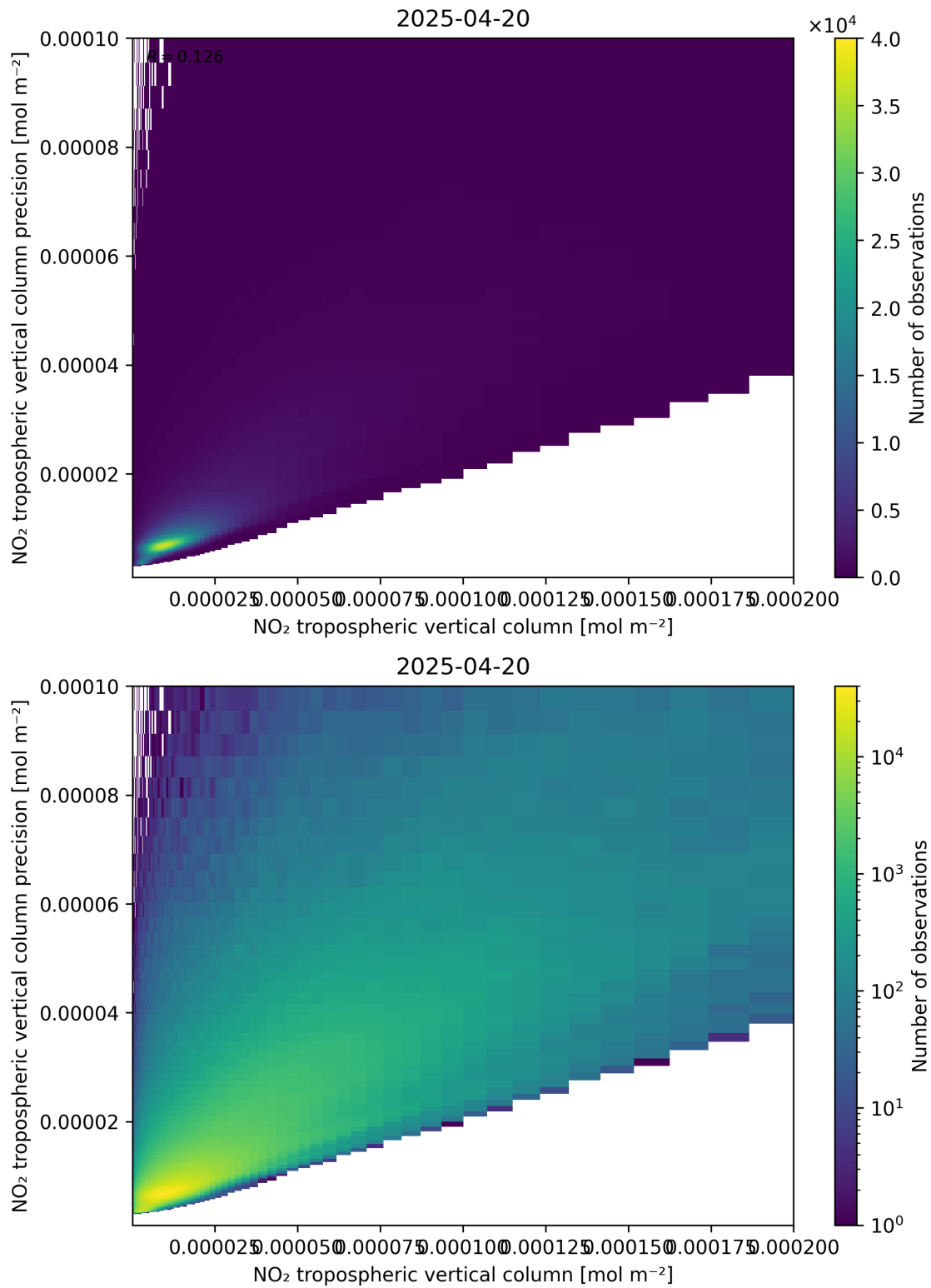
Figure 130: Scatter density plot of “NO 2 tropospheric vertical column” against “NO 2 tropospheric vertical column precision” for 2025-04-20 to 2025-04-21.
