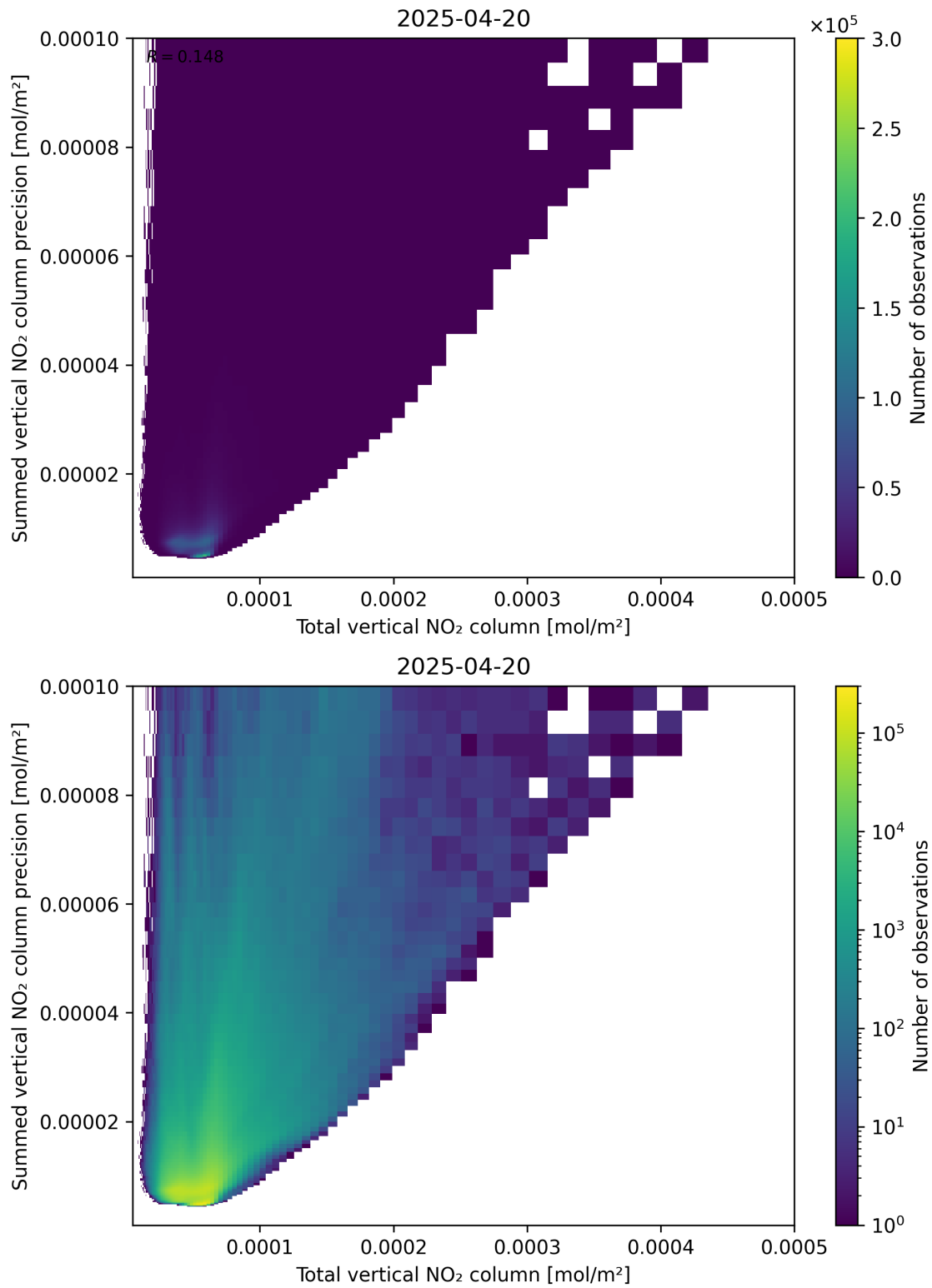
Figure 113: Scatter density plot of “Total vertical NO 2 column” against “Summed vertical NO 2 column precision” for 2025-04-20 to 2025-04-21.
