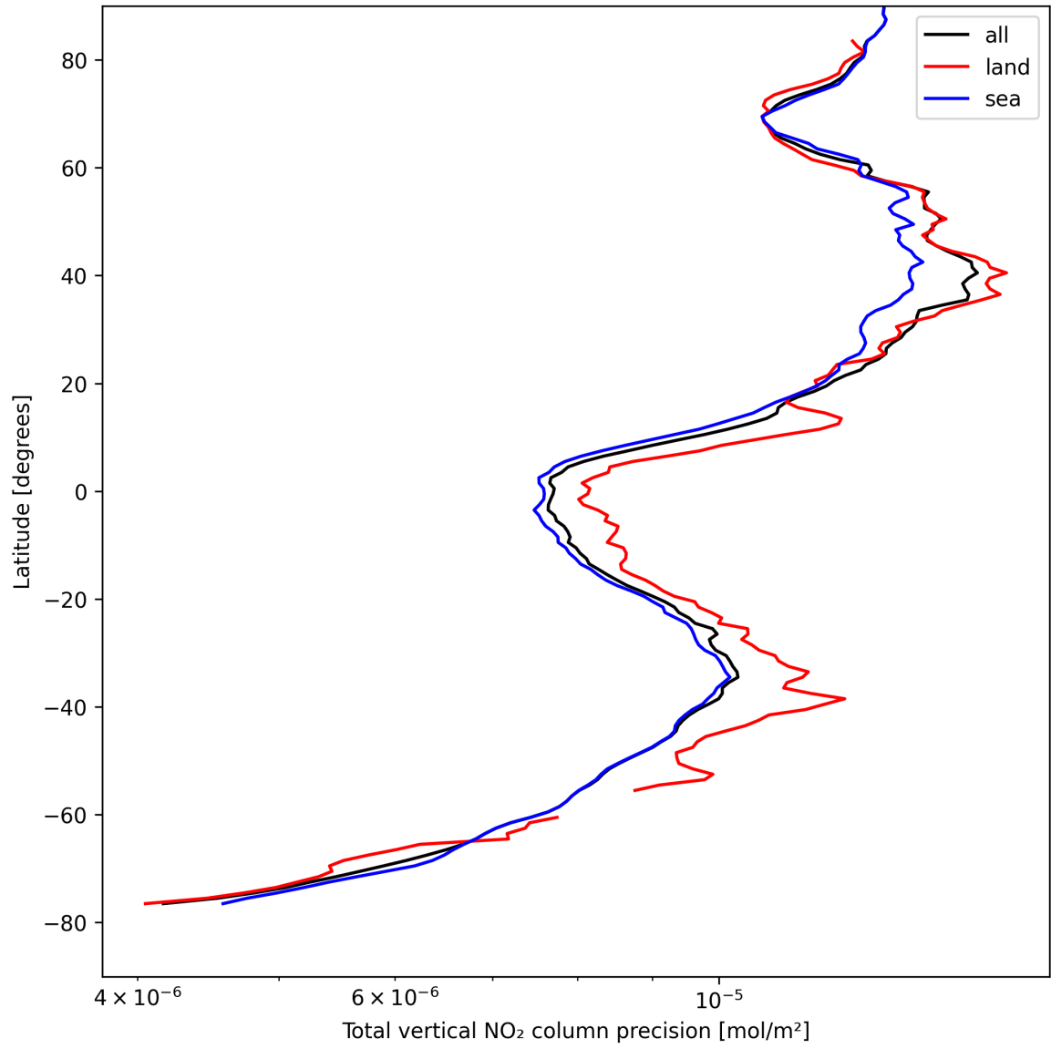
Figure 22: Zonal average of “Total vertical NO 2 column precision” for 2025-04-20 to 2025-04-21.
