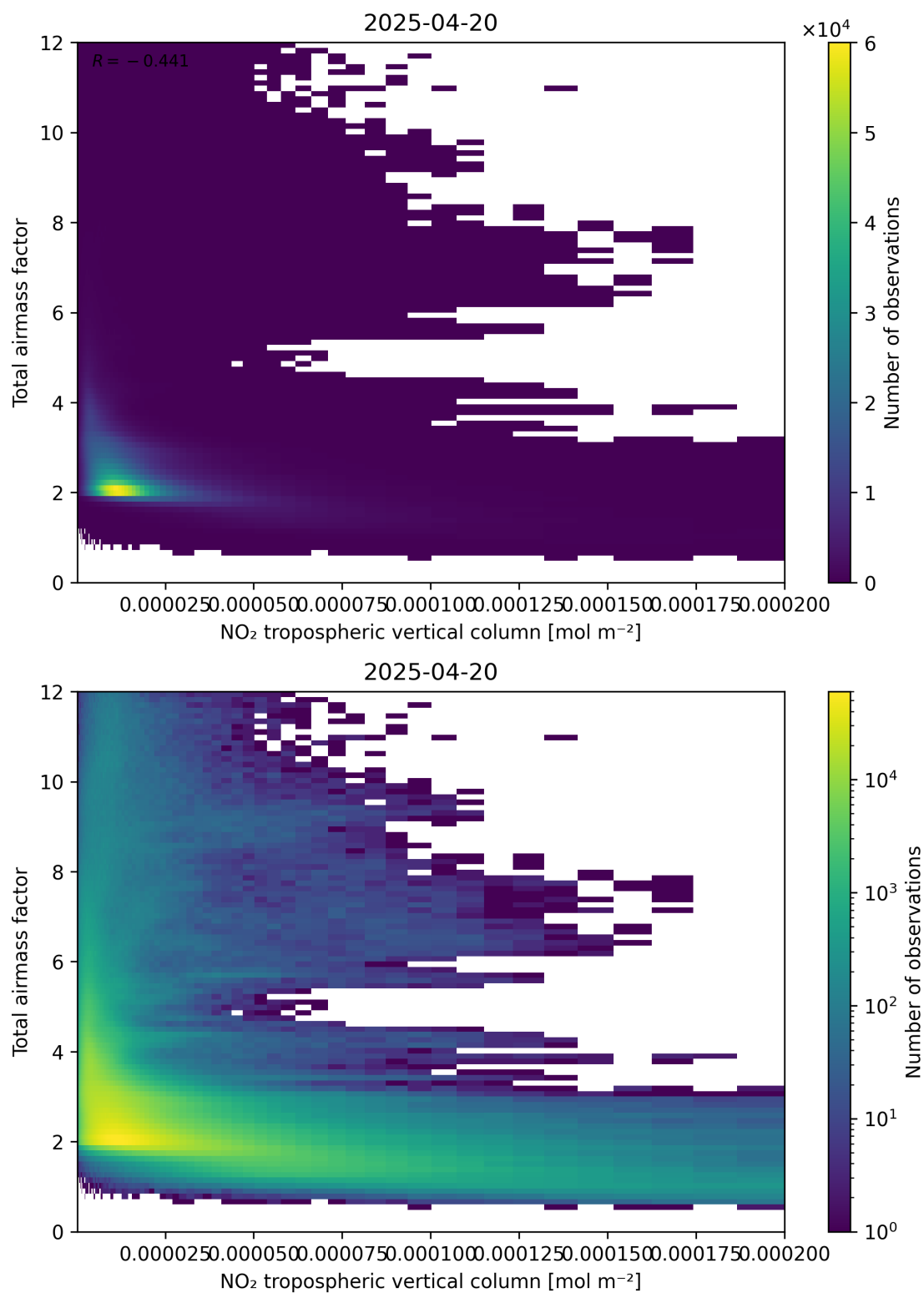
Figure 122: Scatter density plot of “NO 2 tropospheric vertical column” against “Total air mass factor” for 2025-04-20 to 2025-04-21.
