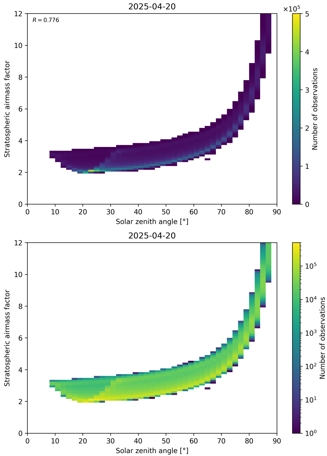
Figure 145: Scatter density plot of “Solar zenith angle” against “Stratospheric airmass factor” for 2025-04-20 to 2025-04-21.
