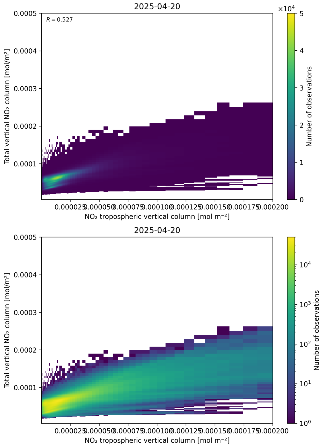
Figure 128: Scatter density plot of “NO 2 tropospheric vertical column” against “Total vertical NO 2 column” for 2025-04-20 to 2025-04-21.
