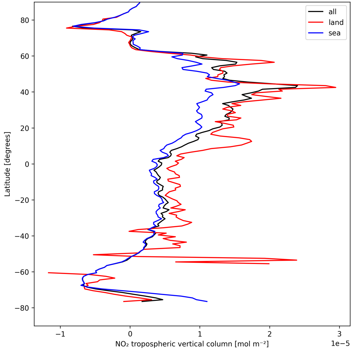
Figure 12: Zonal average of “NO 2 tropospheric vertical column” for 2025-04-20 to 2025-04-21.
