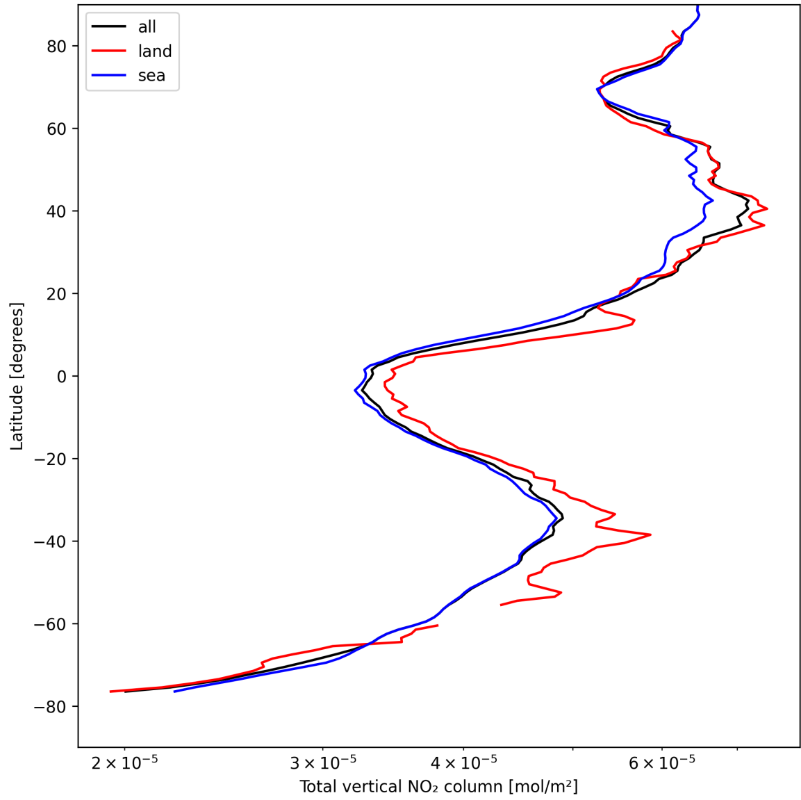
Figure 21: Zonal average of “Total vertical NO 2 column” for 2025-04-20 to 2025-04-21.
