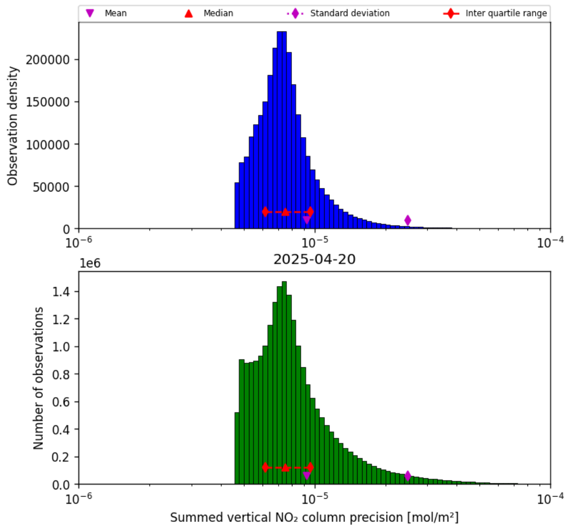
Figure 41: Histogram of "Summed vertical NO 2 column precision" for 2025-04-20 to 2025-04-21
