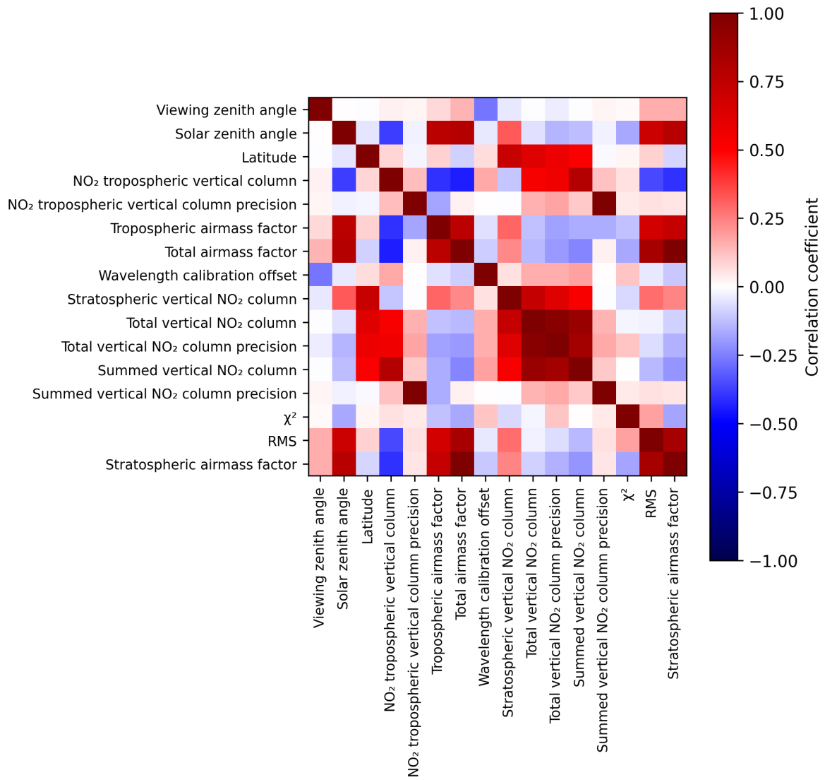
Figure 2: Map of correlation matrix for 2025-04-20 to 2025-04-21.
