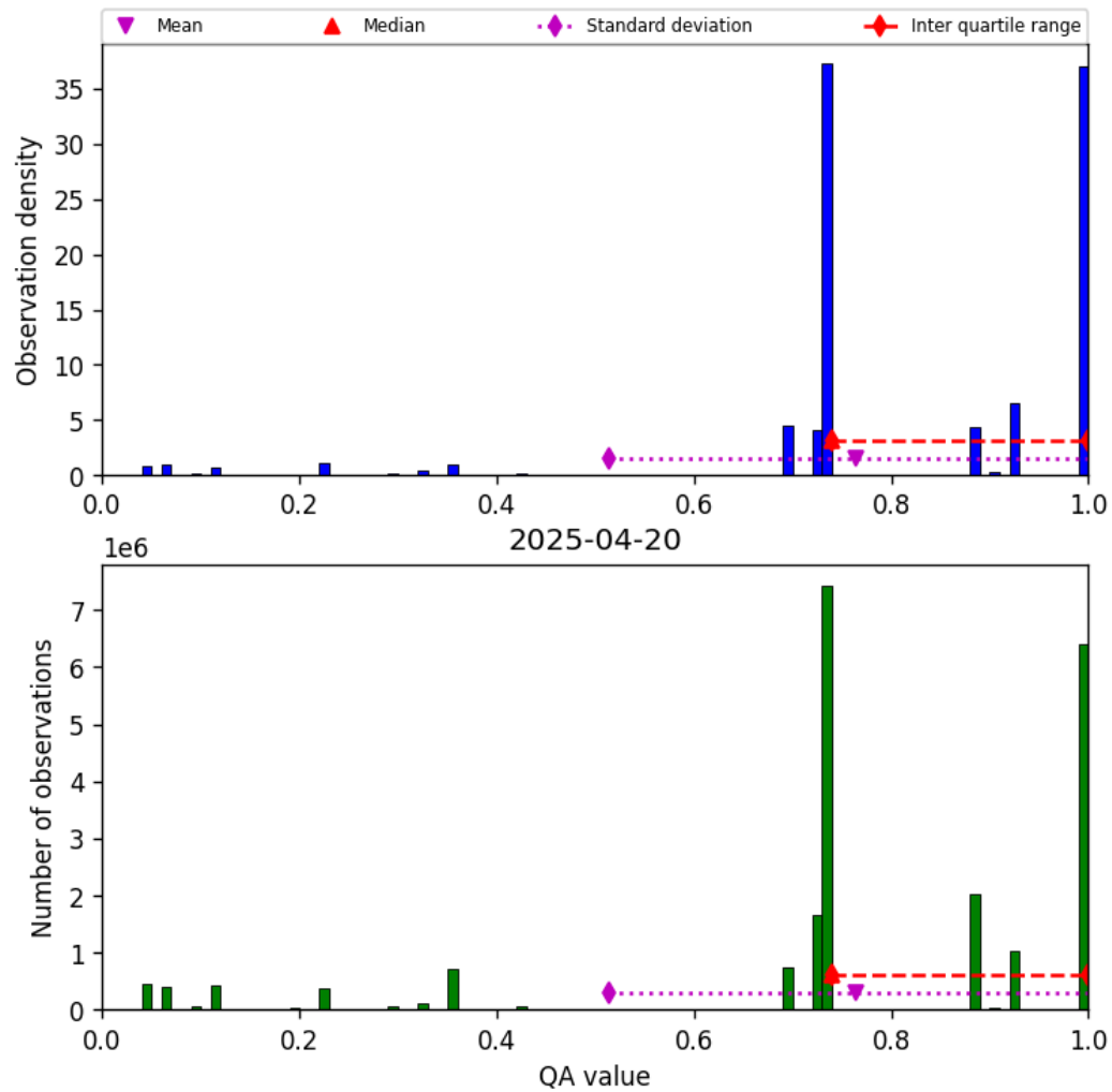
Figure 28: Histogram of “QA value” for 2025-04-20 to 2025-04-21
