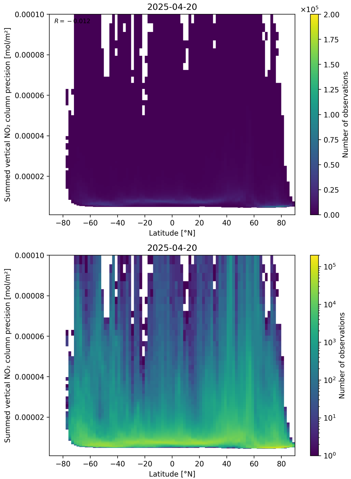
Figure 89: Scatter density plot of “Latitude” against “Summed vertical NO 2 column precision” for 2025-04-20 to 2025-04-21.
