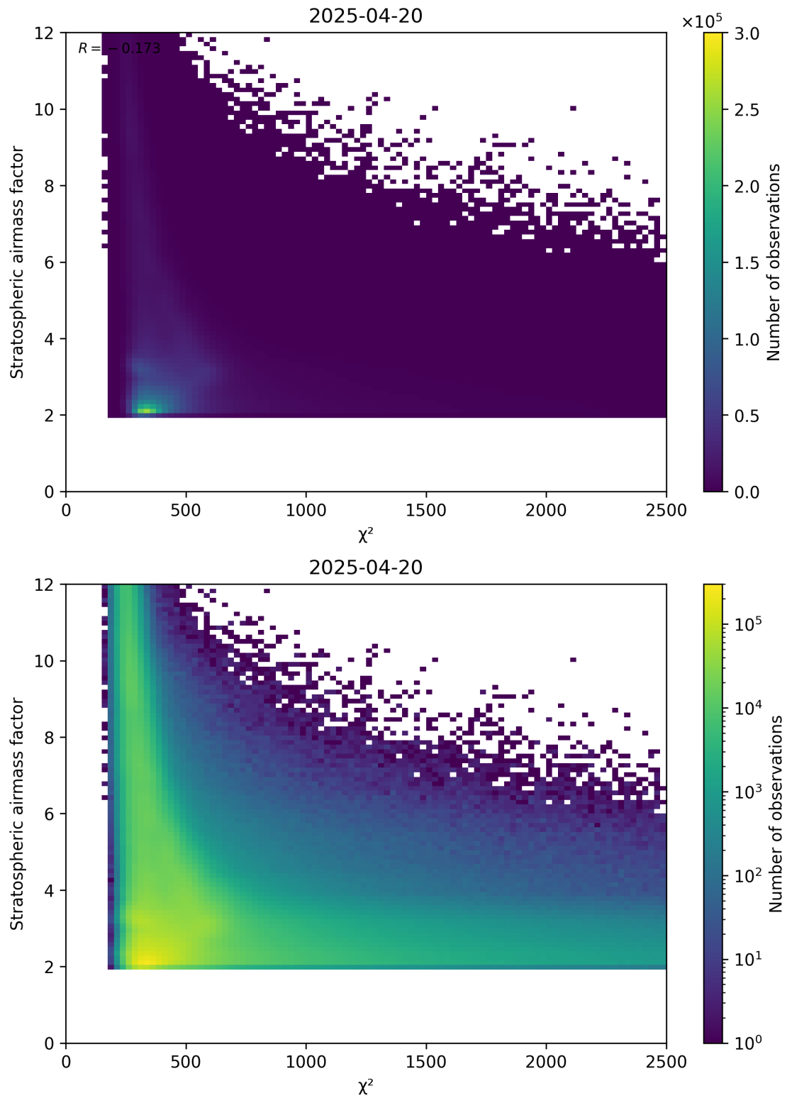
Figure 81: Scatter density plot of “ \chi^2 ” against “Stratospheric airmass factor” for 2025-04-20 to 2025-04-21.
