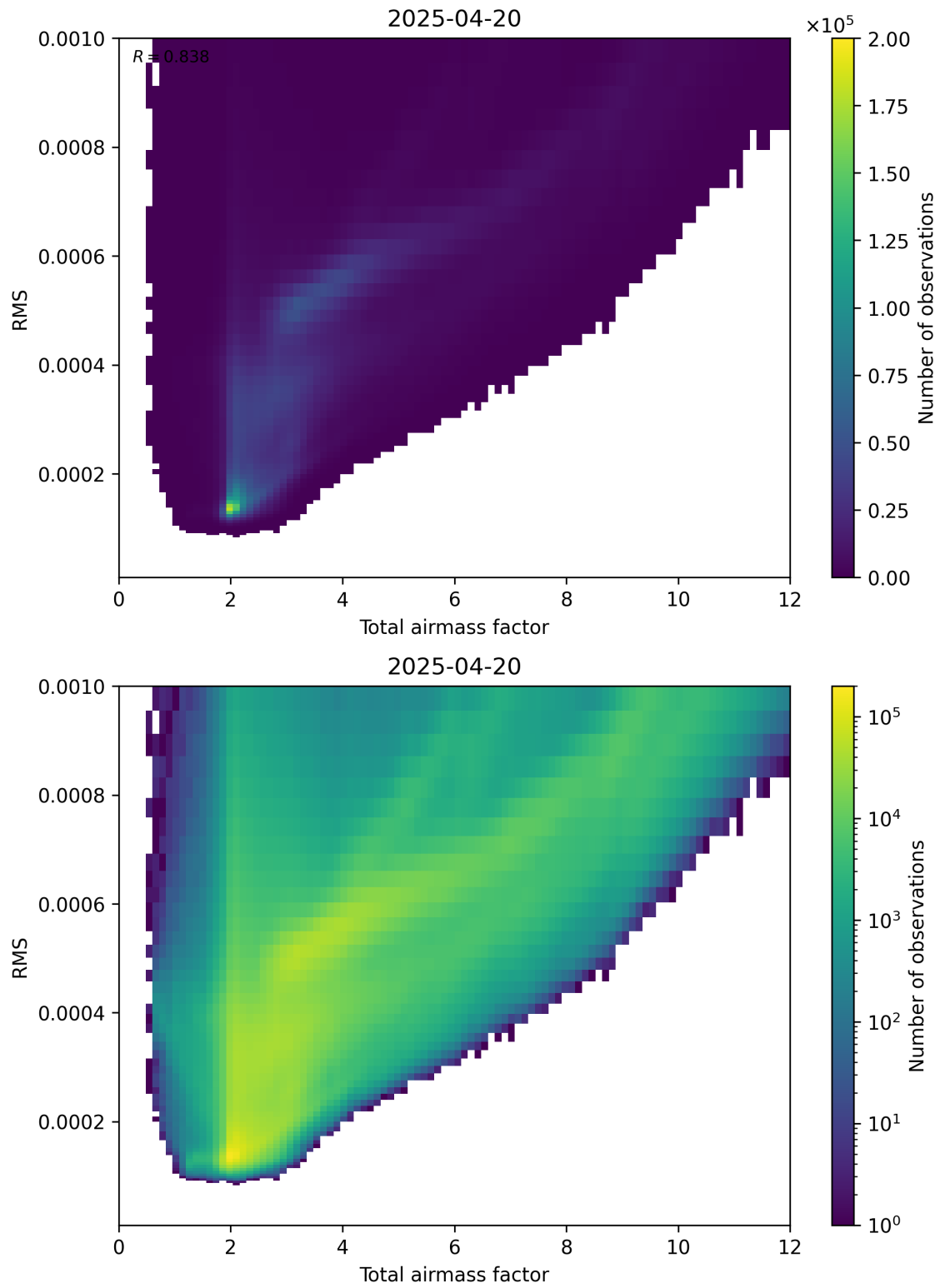
Figure 69: Scatter density plot of “Total airmass factor” against “RMS” for 2025-04-20 to 2025-04-21.
