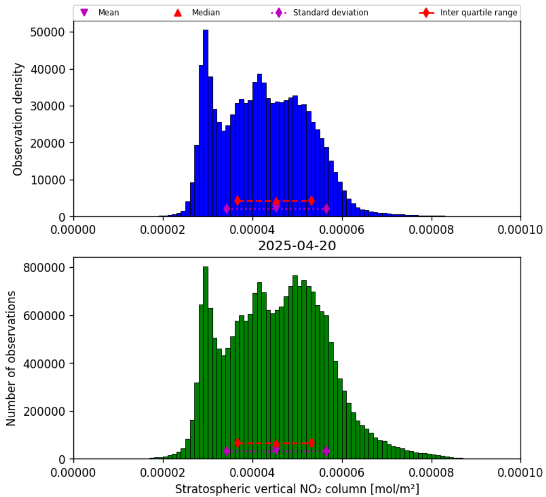
Figure 36: Histogram of “Stratospheric vertical NO 2 column” for 2025-04-20 to 2025-04-21
