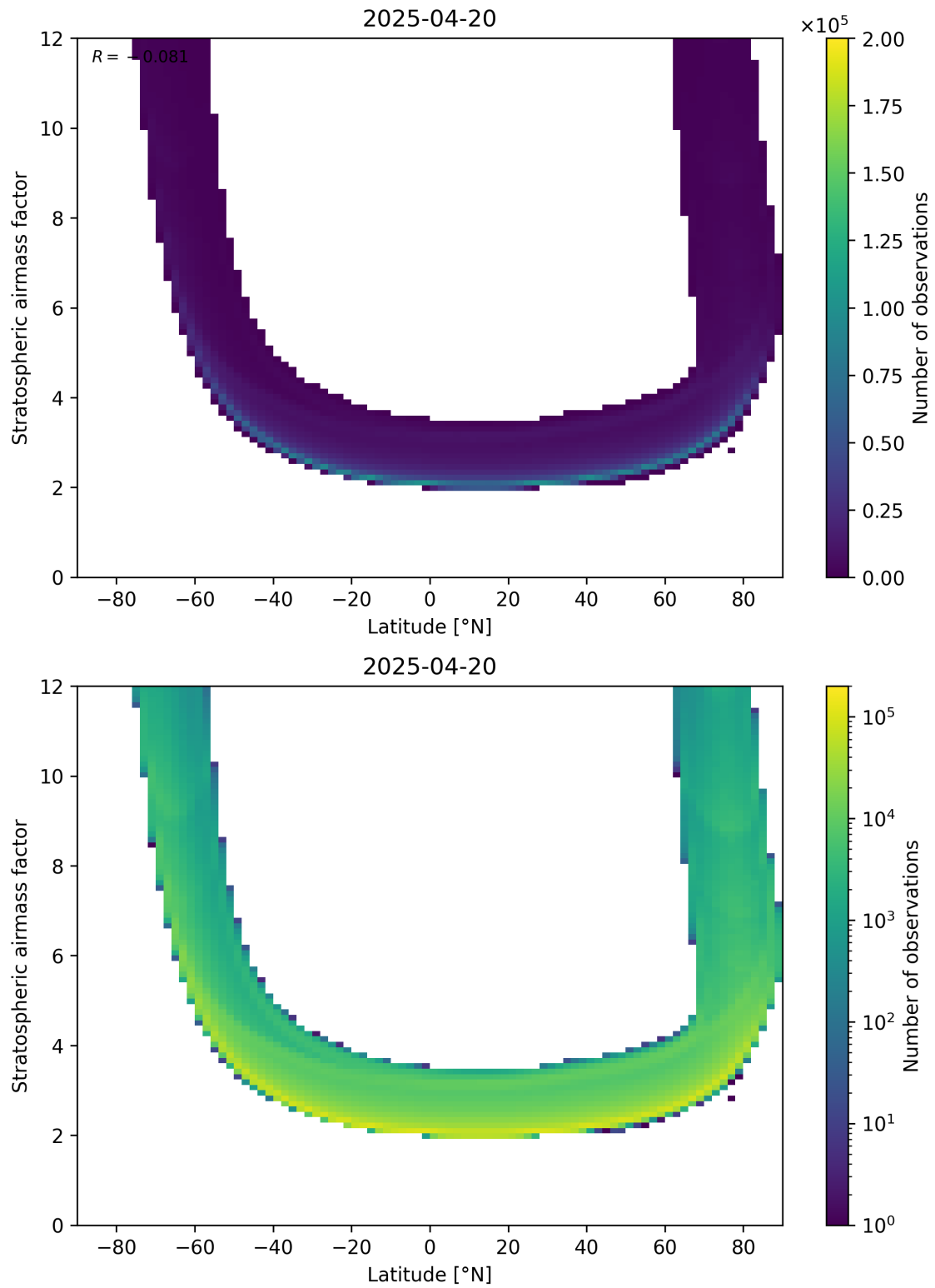
Figure 83: Scatter density plot of “Latitude” against “Stratospheric air mass factor” for 2025-04-20 to 2025-04-21.
