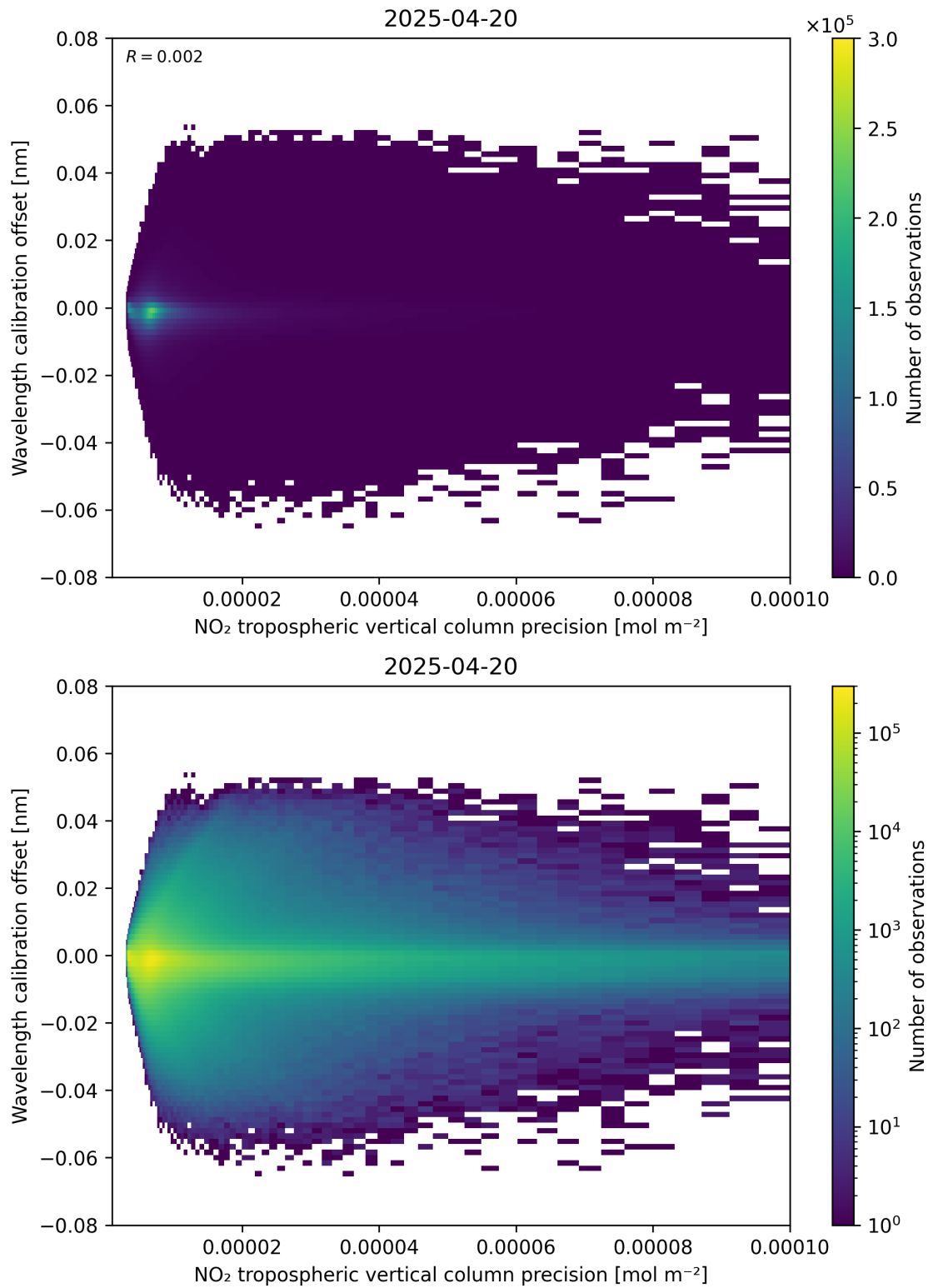
Figure 141: Scatter density plot of “NO 2 tropospheric vertical column precision” against “Wavelength calibration offset” for 2025-04-20 to 2025-04-21.
