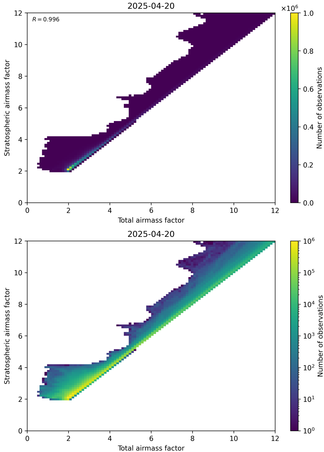
Figure 62: Scatter density plot of “Total air mass factor” against “Stratospheric air mass factor” for 2025-04-20 to 2025-04-21.
