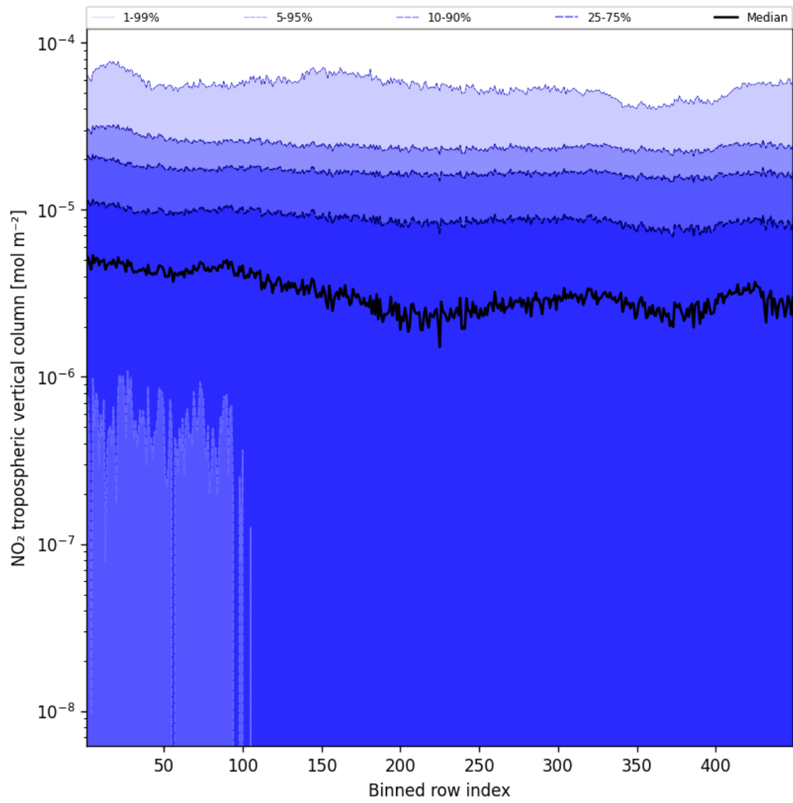
Figure 46: Along track statistics of “NO 2 tropospheric vertical column” for 2025-04-20 to 2025-04-21
