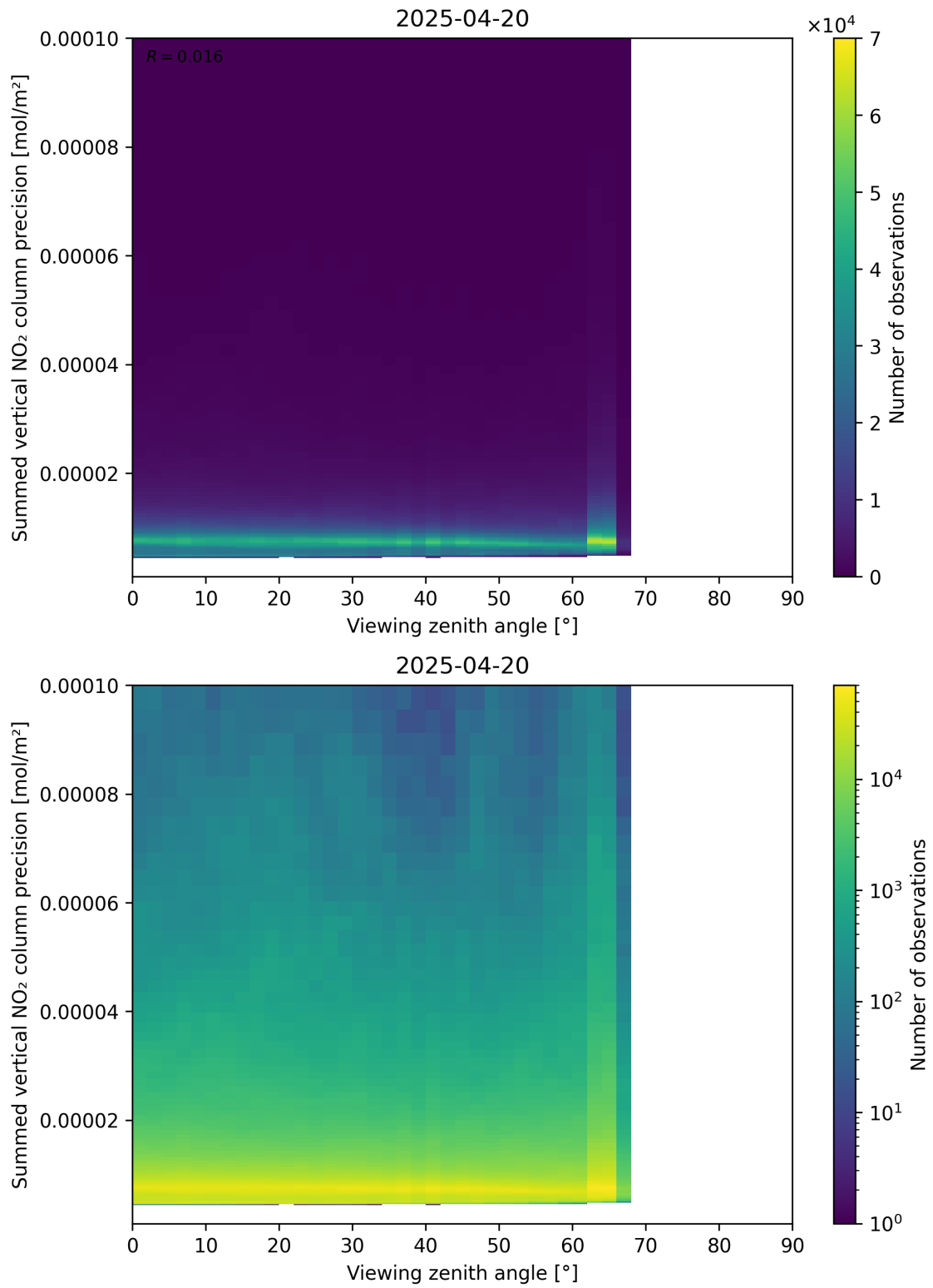
Figure 166: Scatter density plot of “Viewing zenith angle” against “Summed vertical NO 2 column precision” for 2025-04-20 to 2025-04-21.
