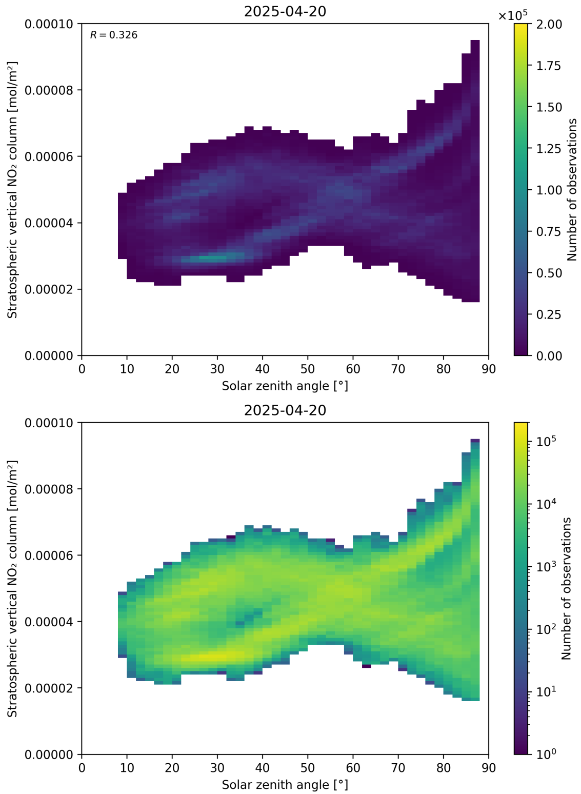
Figure 150: Scatter density plot of “Solar zenith angle” against “Stratospheric vertical NO 2 column” for 2025-04-20 to 2025-04-21.
