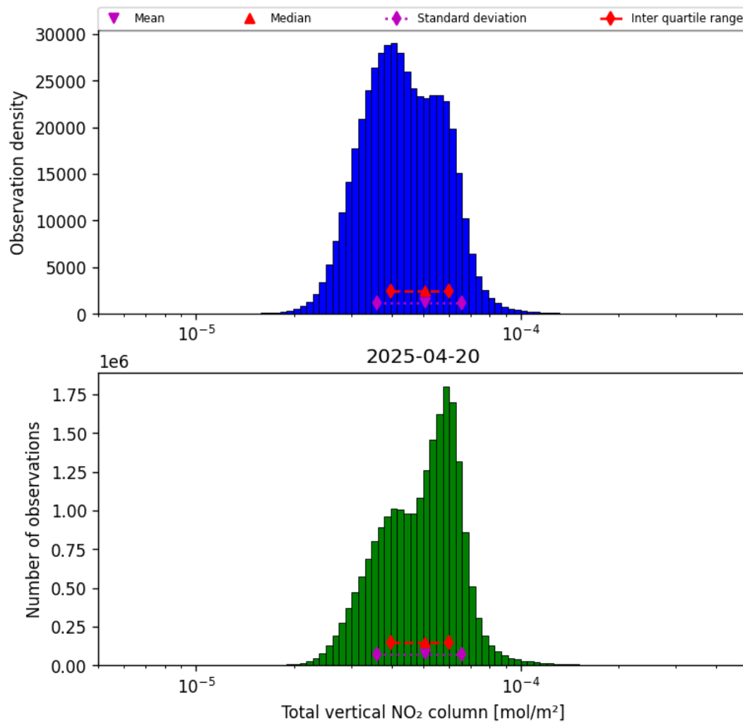
Figure 38: Histogram of “Total vertical NO 2 column” for 2025-04-20 to 2025-04-21
