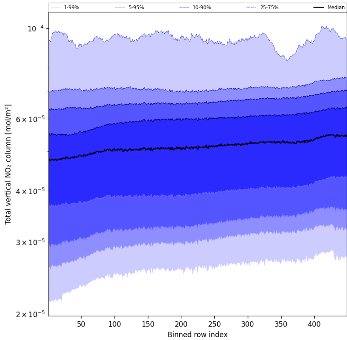
Figure 55: Along track statistics of “Total vertical NO 2 column” for 2025-04-20 to 2025-04-21
