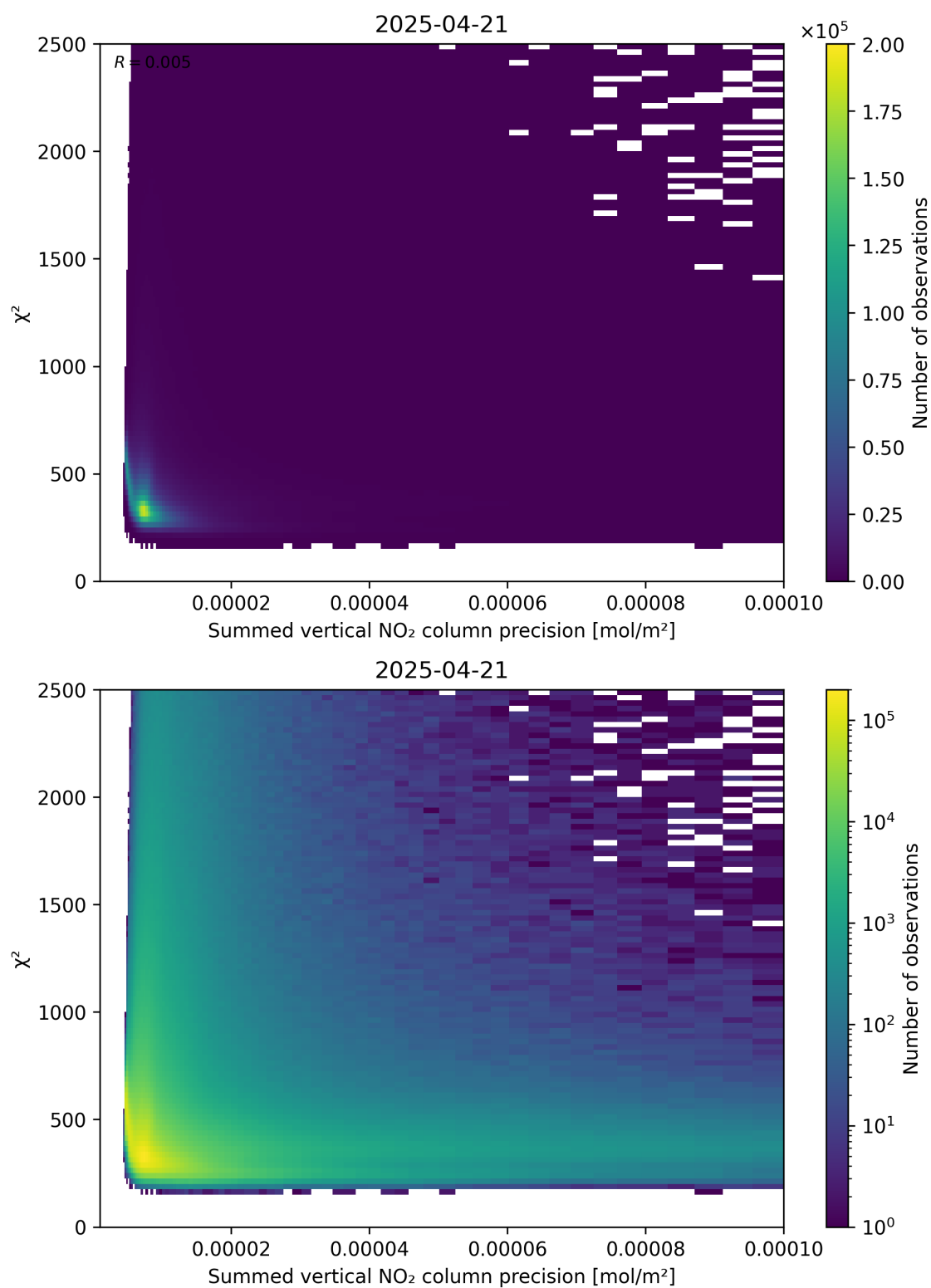
Figure 107: Scatter density plot of “Summed vertical NO 2 column precision” against “ \chi^2 ” for 2025-04-21 to 2025-04-22.
