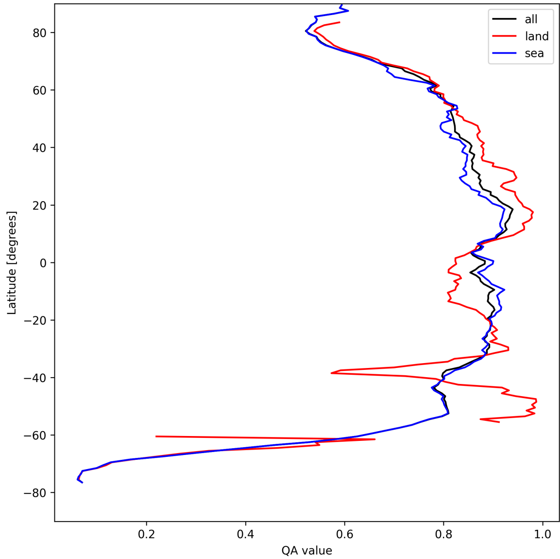
Figure 11: Zonal average of “QA value” for 2025-04-21 to 2025-04-22.
