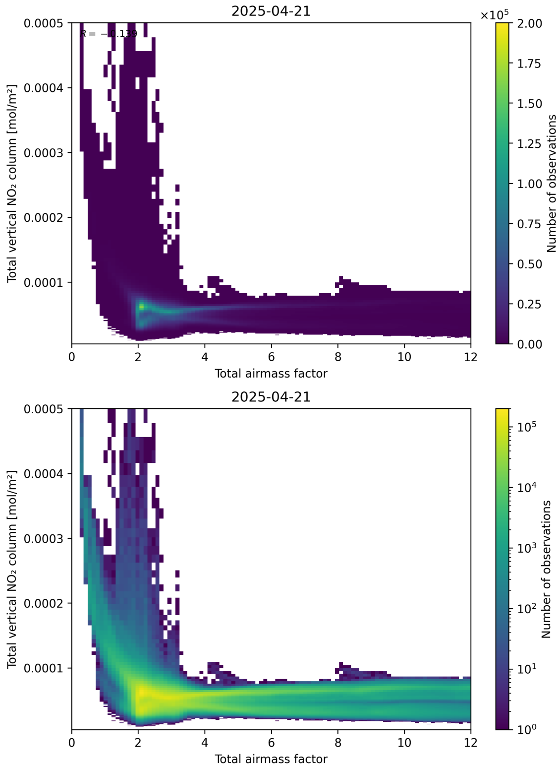
Figure 67: Scatter density plot of “Total airmass factor” against “Total vertical NO 2 column” for 2025-04-21 to 2025-04-22.
