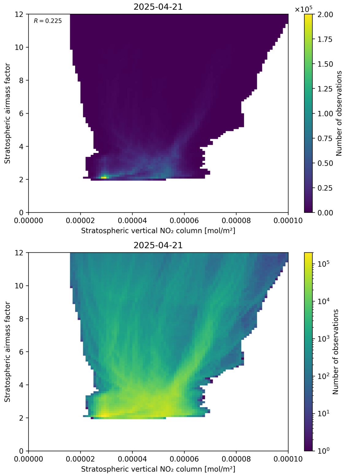
Figure 96: Scatter density plot of “Stratospheric vertical NO 2 column” against “Stratospheric airmass factor” for 2025-04-21 to 2025-04-22.
