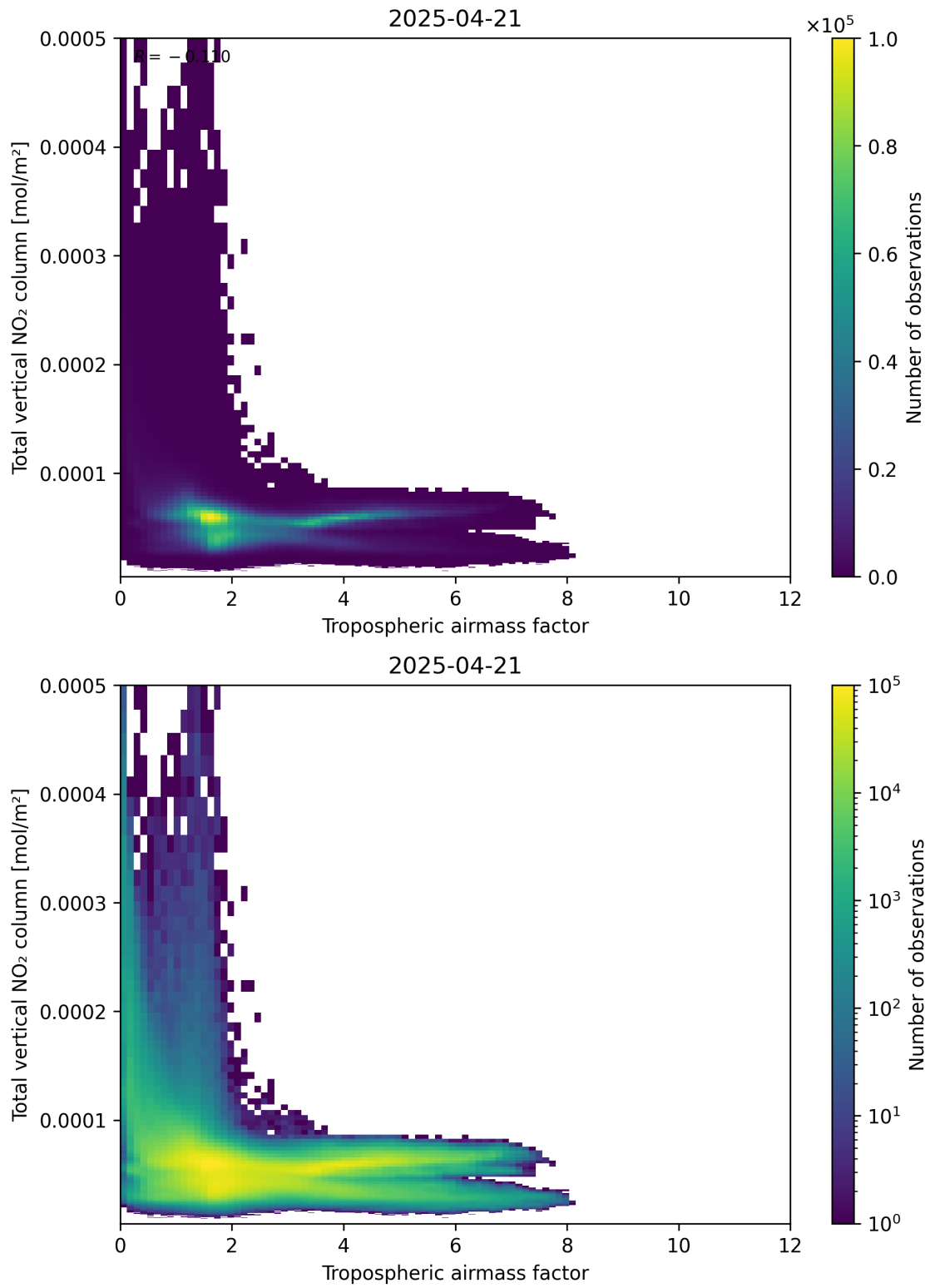
Figure 77: Scatter density plot of “Tropospheric airmass factor” against “Total vertical NO 2 column” for 2025-04-21 to 2025-04-22.
