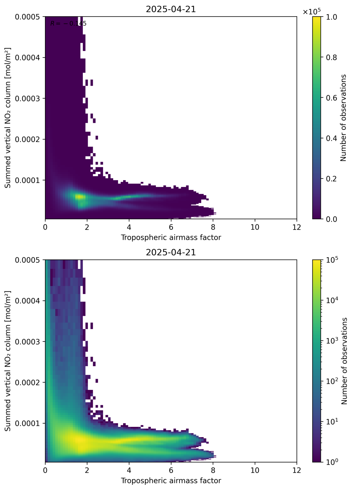
Figure 75: Scatter density plot of “Tropospheric air mass factor” against “Summed vertical NO 2 column” for 2025-04-21 to 2025-04-22.
