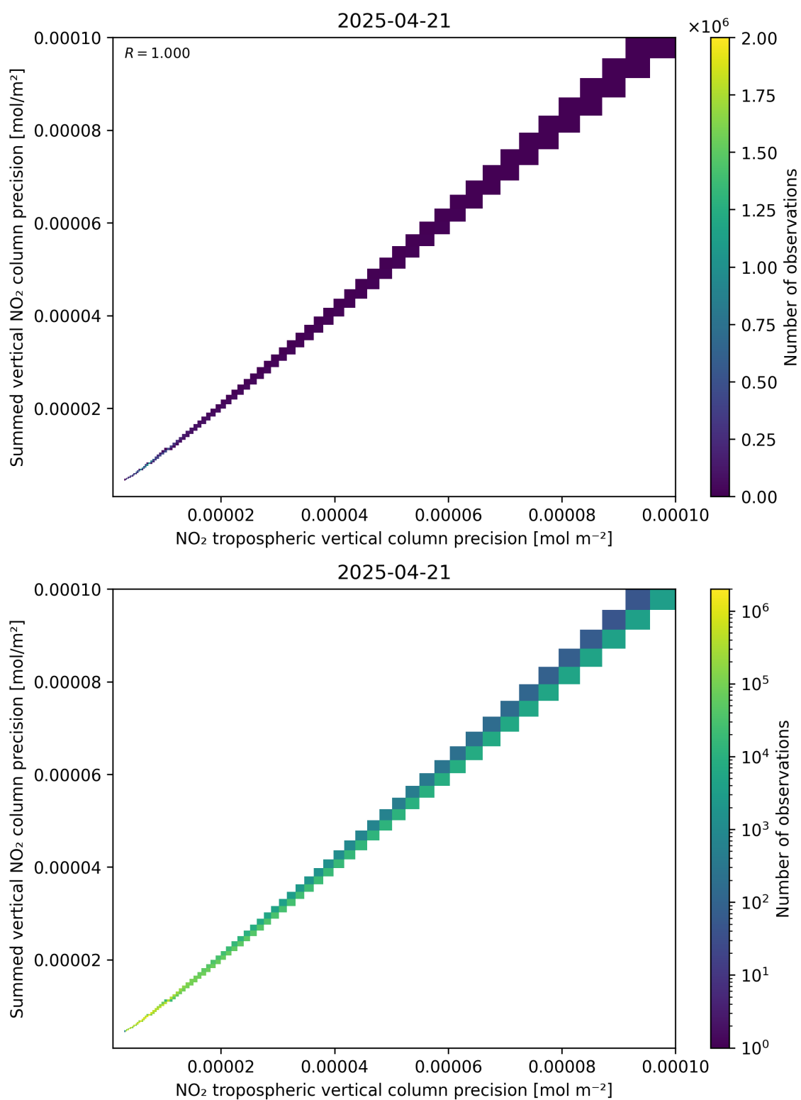
Figure 137: Scatter density plot of “NO 2 tropospheric vertical column precision” against “Summed vertical NO 2 column precision” for 2025-04-21 to 2025-04-22.
