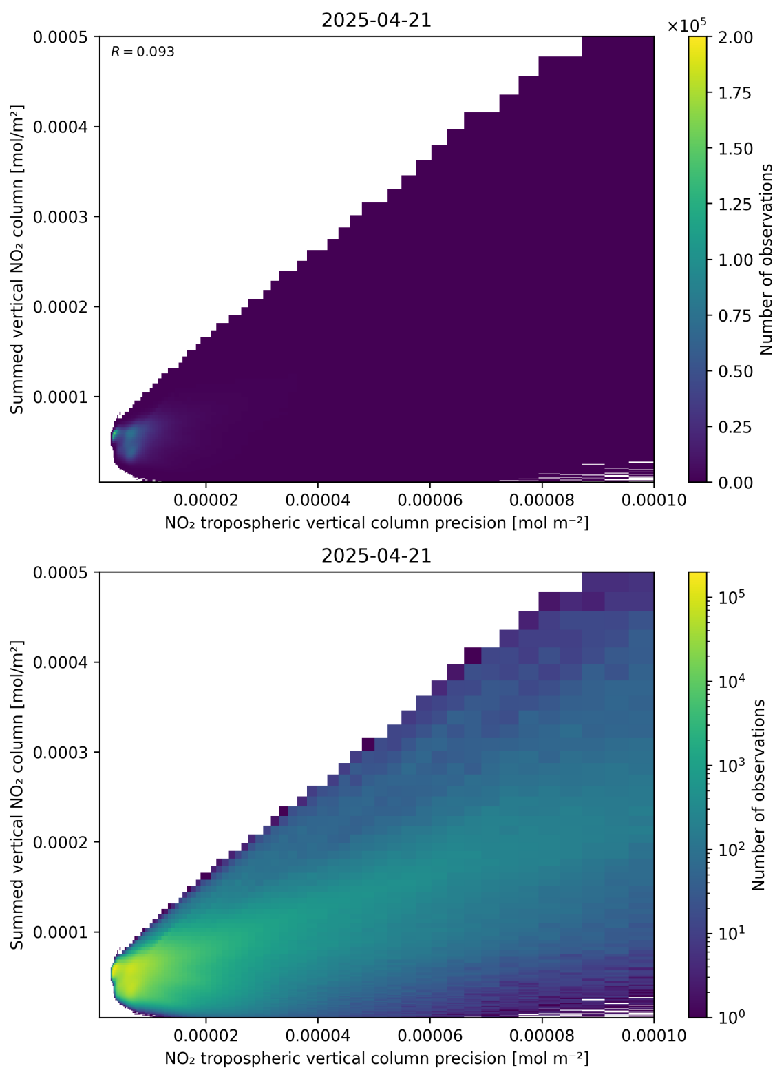
Figure 136: Scatter density plot of “NO 2 tropospheric vertical column precision” against “Summed vertical NO 2 column” for 2025-04-21 to 2025-04-22.
