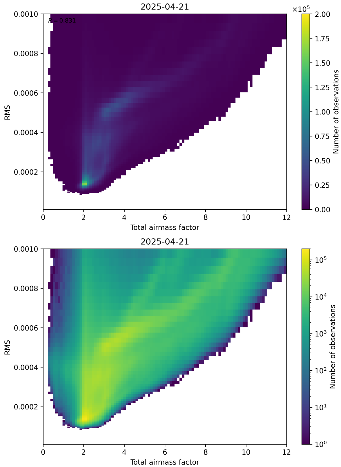
Figure 69: Scatter density plot of “Total airmass factor” against “RMS” for 2025-04-21 to 2025-04-22.
