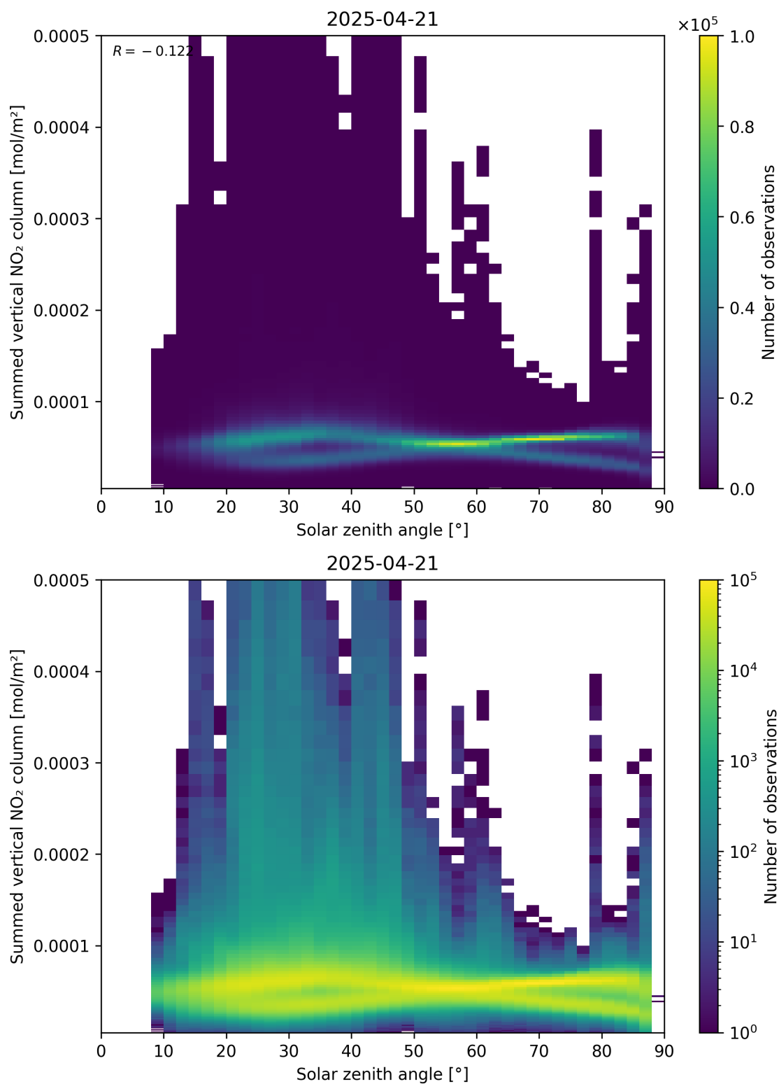
Figure 151: Scatter density plot of “Solar zenith angle” against “Summed vertical NO 2 column” for 2025-04-21 to 2025-04-22.
