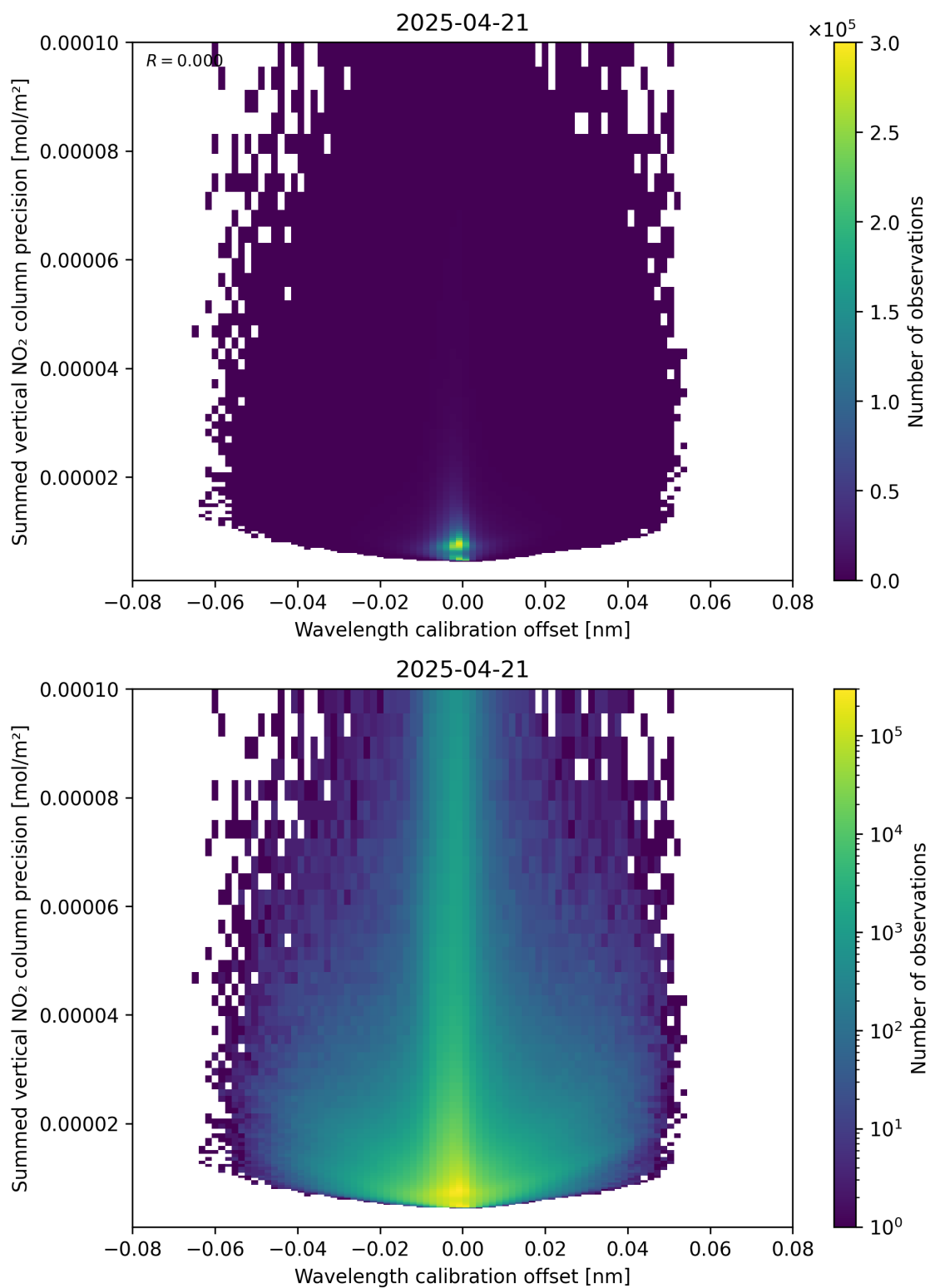
Figure 178: Scatter density plot of “Wavelength calibration offset” against “Summed vertical NO 2 column precision” for 2025-04-21 to 2025-04-22.
