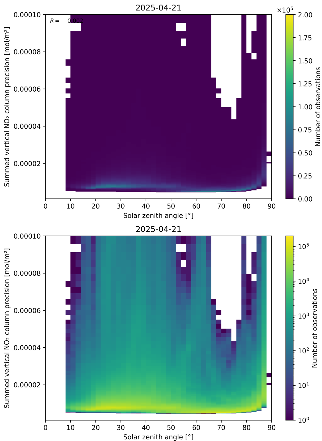
Figure 152: Scatter density plot of “Solar zenith angle” against “Summed vertical NO 2 column precision” for 2025-04-21 to 2025-04-22.
