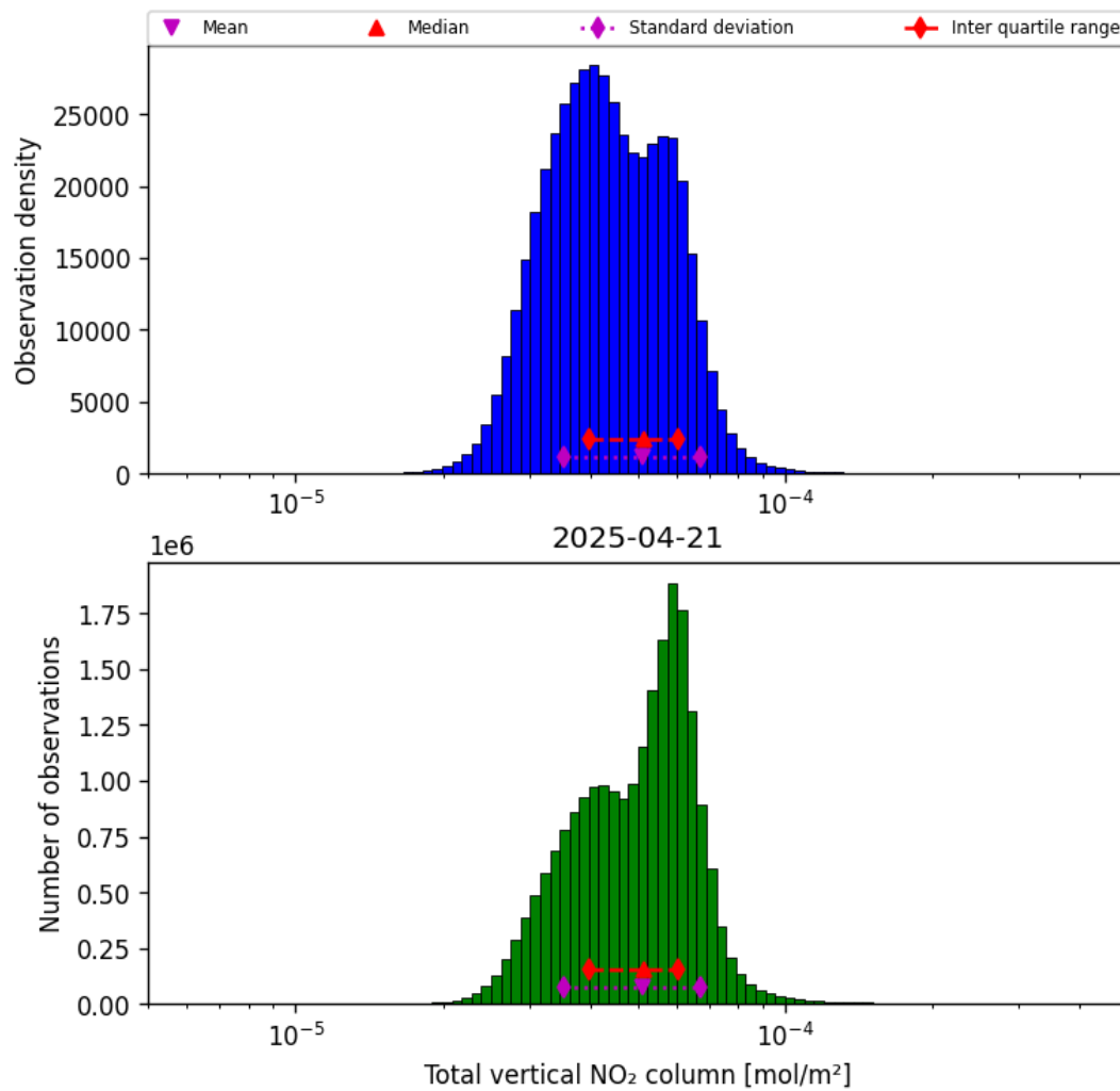
Figure 38: Histogram of “Total vertical NO 2 column” for 2025-04-21 to 2025-04-22
