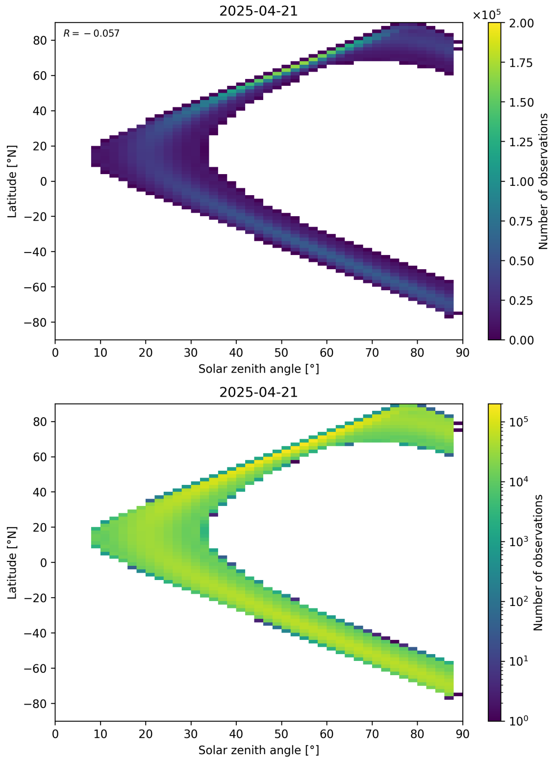
Figure 149: Scatter density plot of “Solar zenith angle” against “Latitude” for 2025-04-21 to 2025-04-22.
