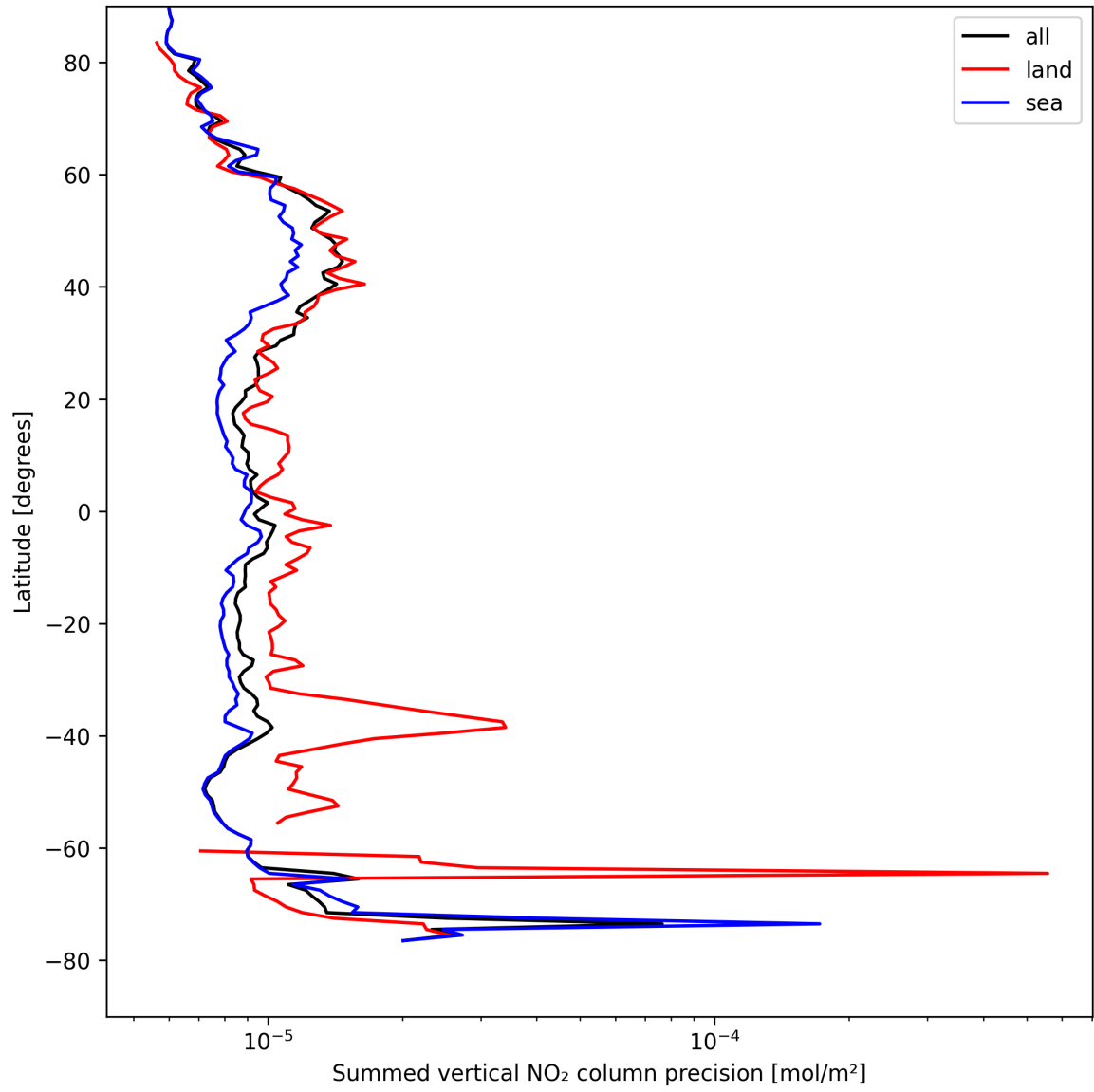
Figure 24: Zonal average of “Summed vertical NO 2 column precision” for 2025-04-21 to 2025-04-22.
