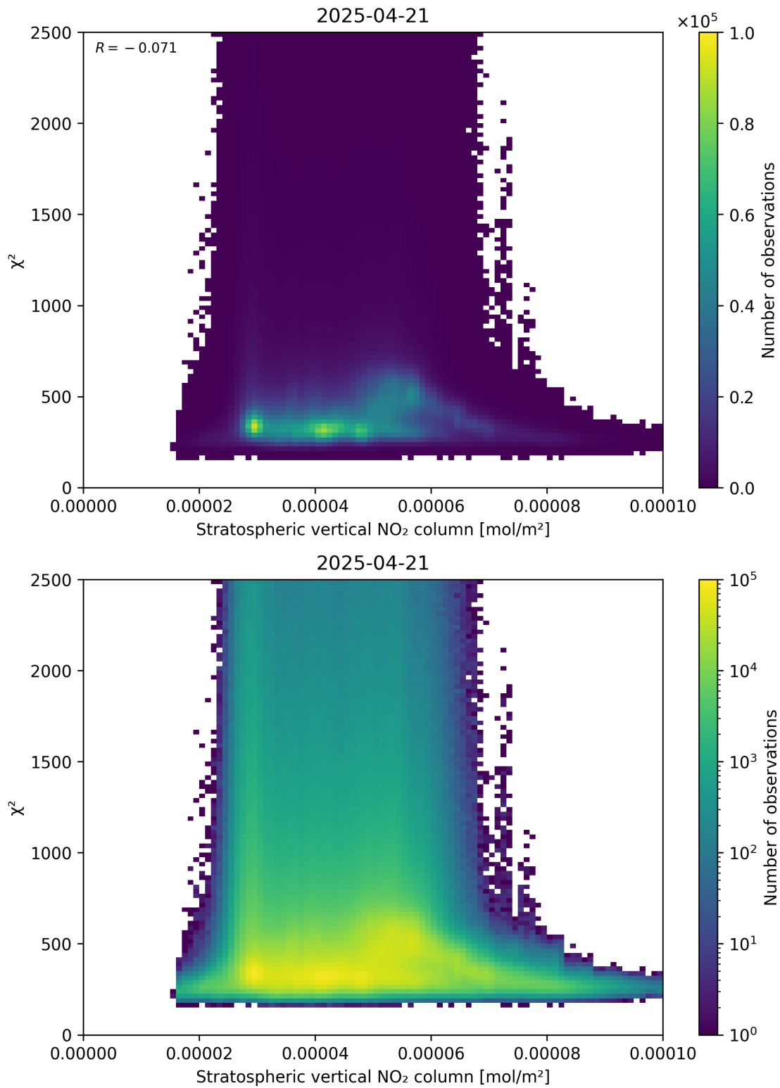
Figure 97: Scatter density plot of “Stratospheric vertical NO 2 column” against “ \chi^2 ” for 2025-04-21 to 2025-04-22.
