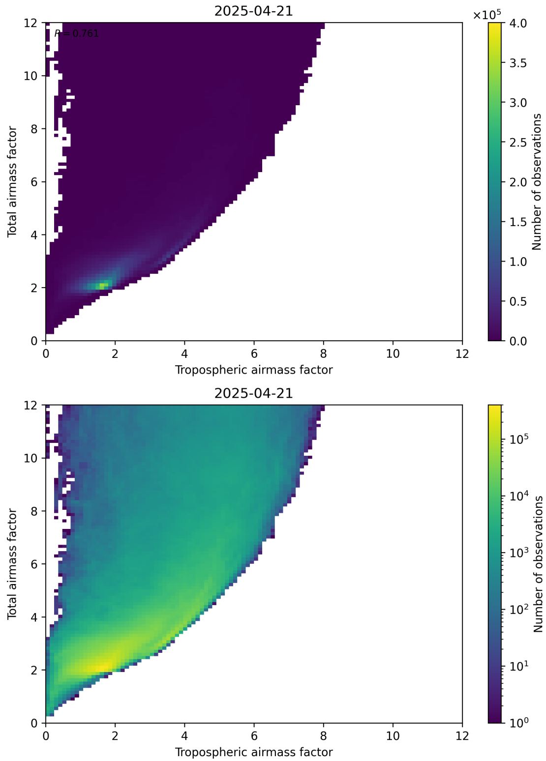
Figure 72: Scatter density plot of “Tropospheric airmass factor” against “Total airmass factor” for 2025-04-21 to 2025-04-22.
