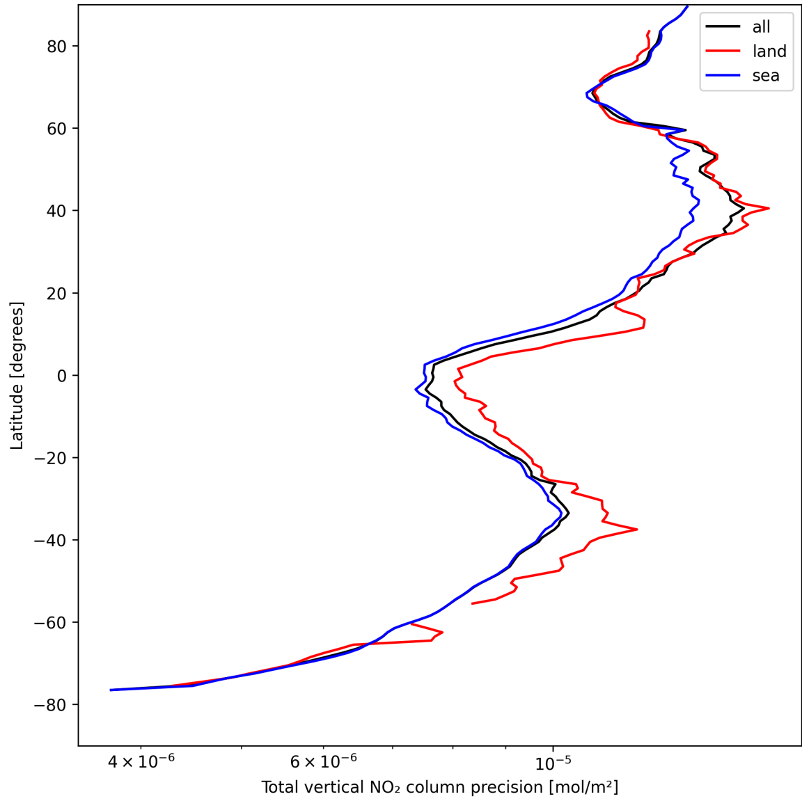
Figure 22: Zonal average of “Total vertical NO 2 column precision” for 2025-04-21 to 2025-04-22.
