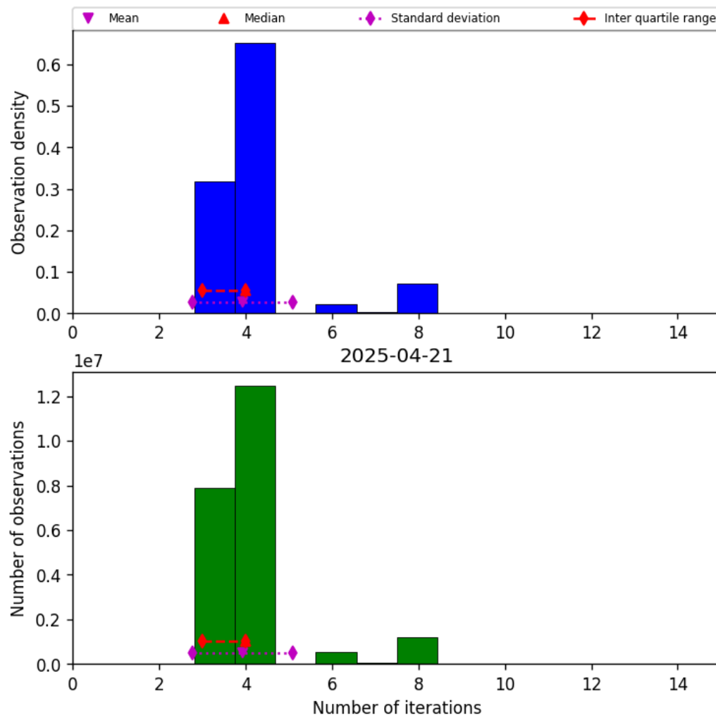
Figure 34: Histogram of “Number of iterations” for 2025-04-21 to 2025-04-22
