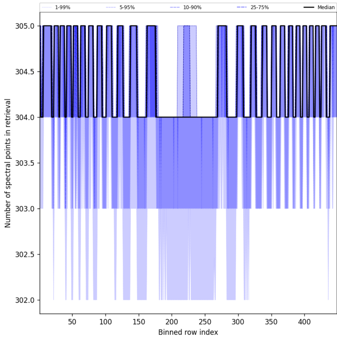
Figure 50: Along track statistics of “Number of spectral points in retrieval” for 2025-04-21 to 2025-04-22
