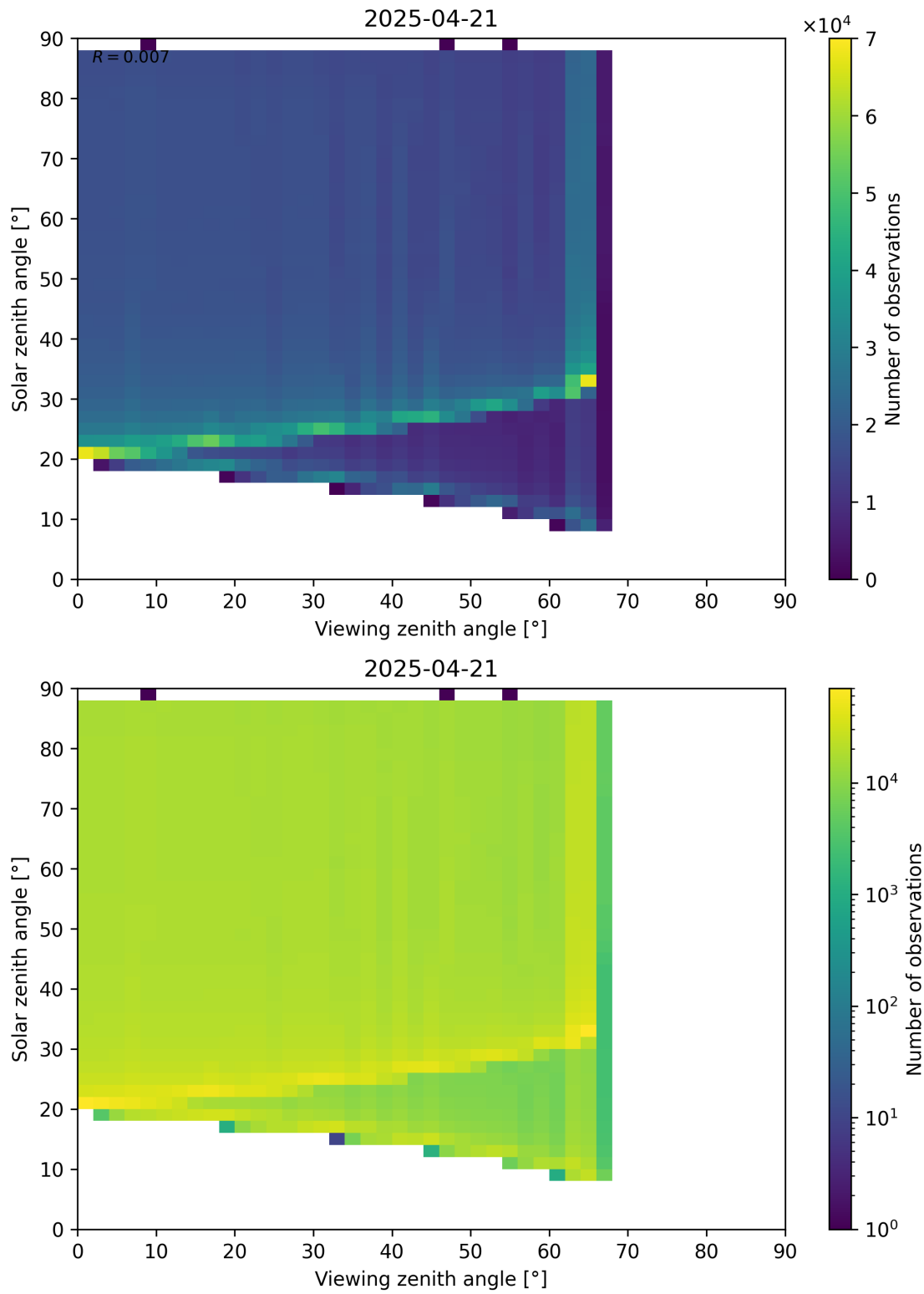
Figure 172: Scatter density plot of “Viewing zenith angle” against “Solar zenith angle” for 2025-04-21 to 2025-04-22.
