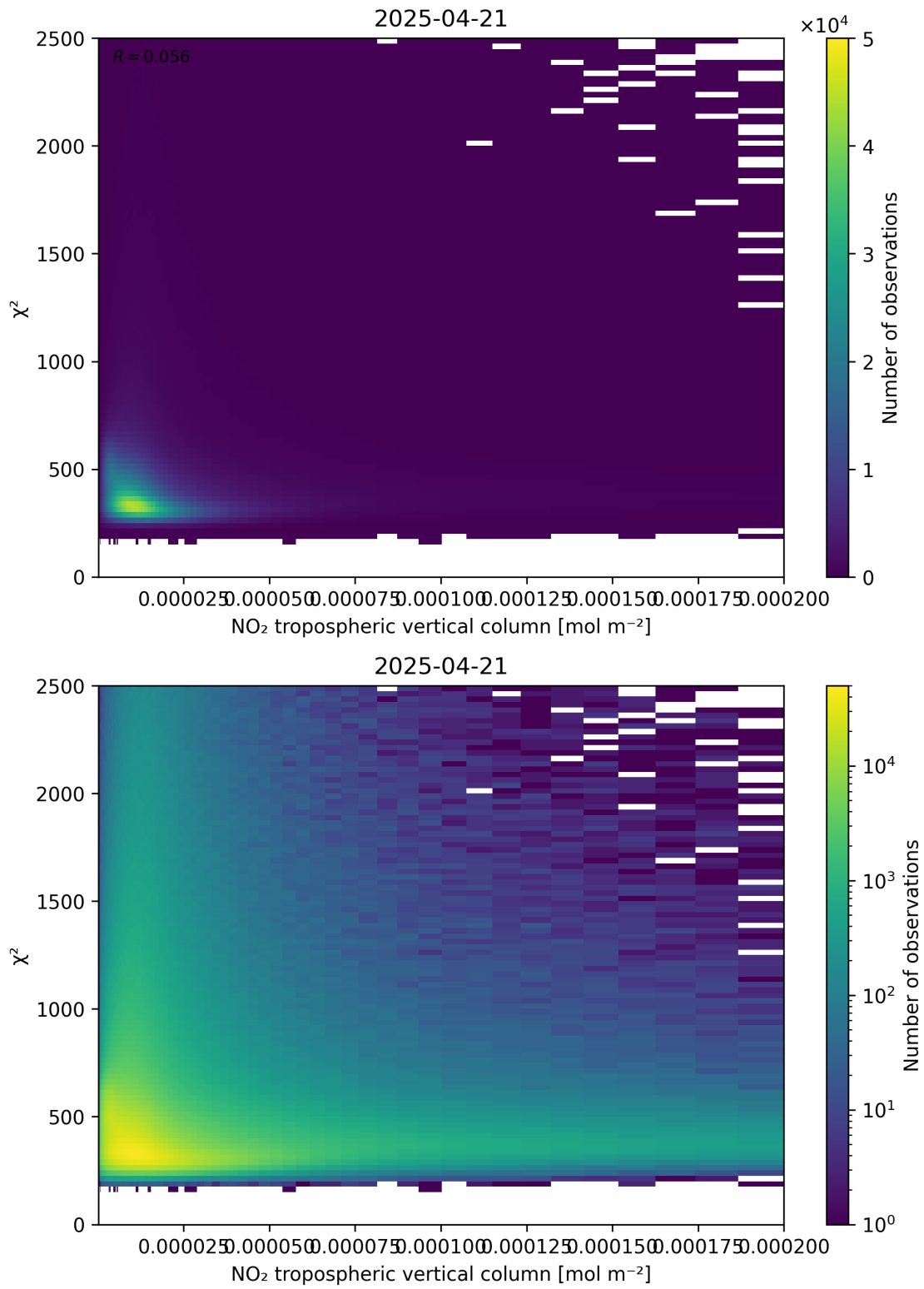
Figure 124: Scatter density plot of “NO 2 tropospheric vertical column” against “ \chi^2 ” for 2025-04-21 to 2025-04-22.
