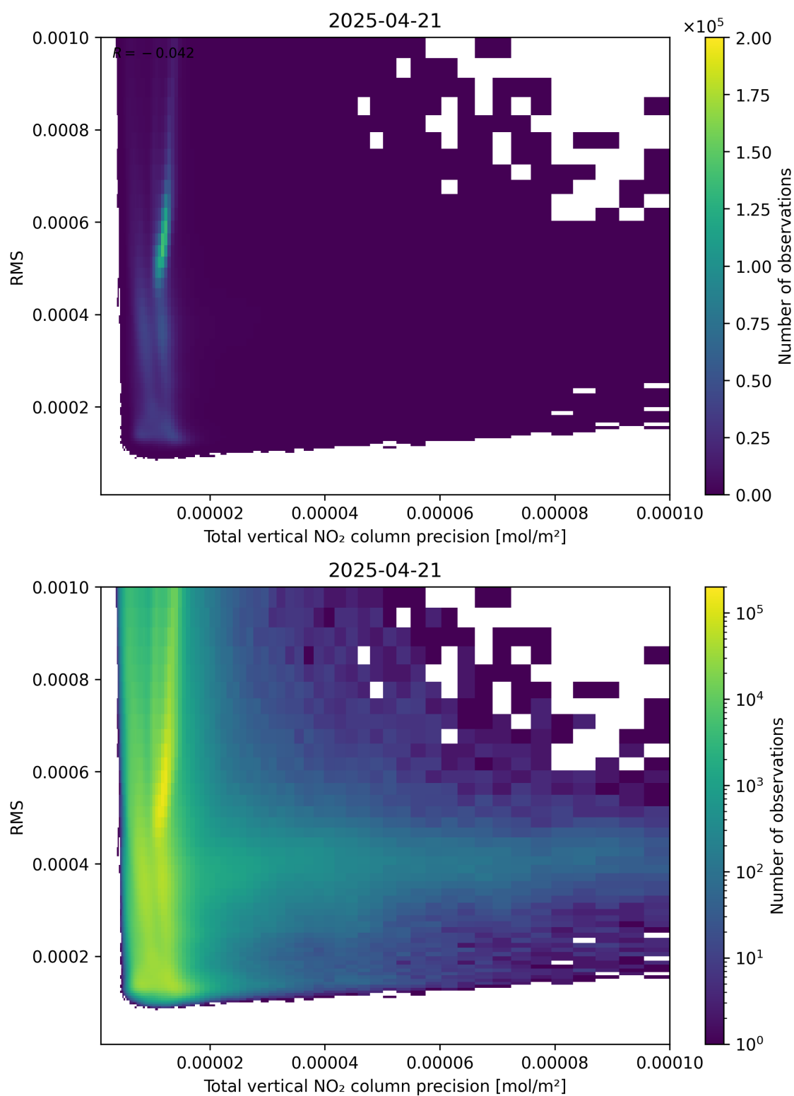
Figure 119: Scatter density plot of “Total vertical NO 2 column precision” against “RMS” for 2025-04-21 to 2025-04-22.
