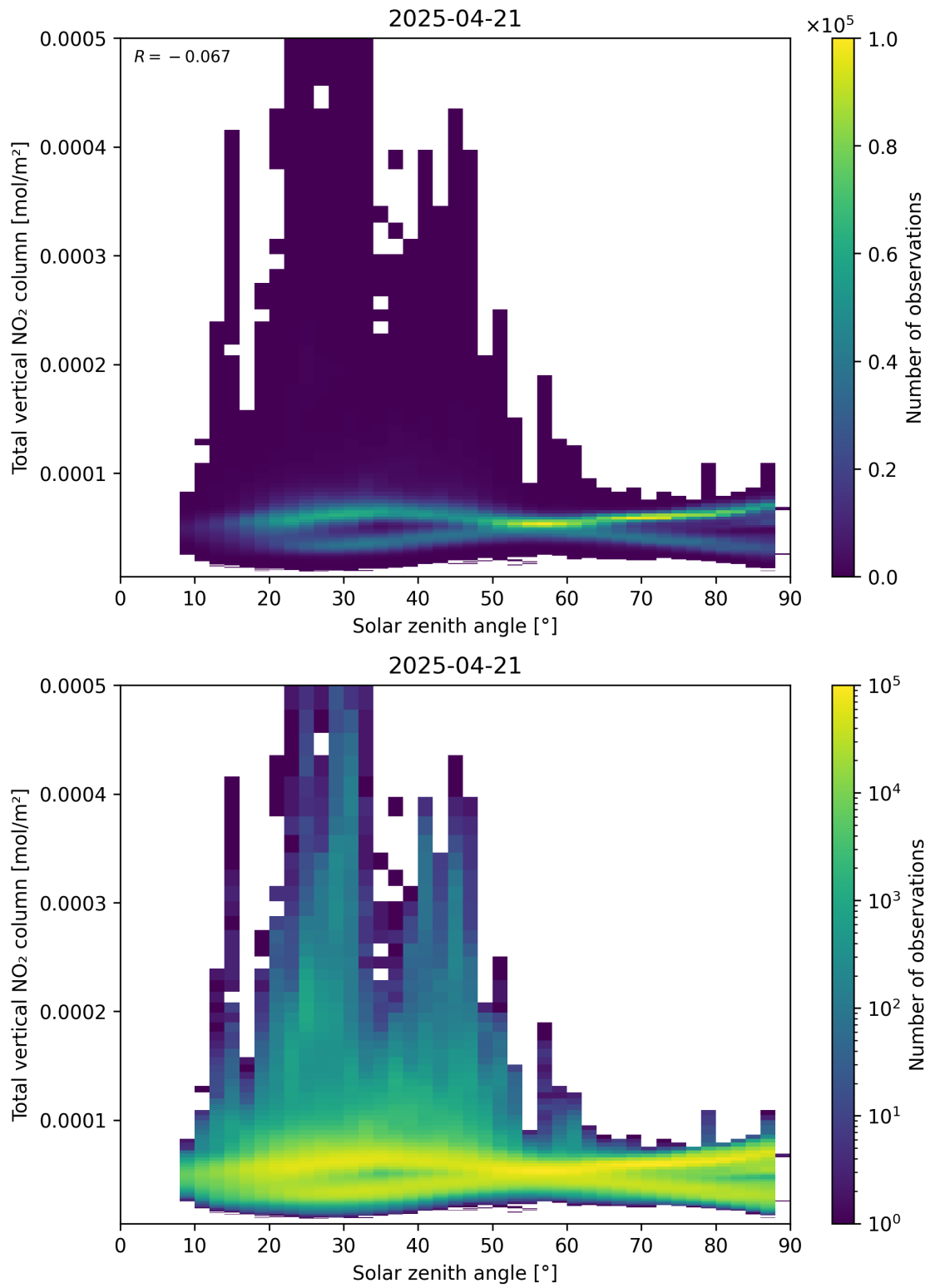
Figure 153: Scatter density plot of “Solar zenith angle” against “Total vertical NO 2 column” for 2025-04-21 to 2025-04-22.
