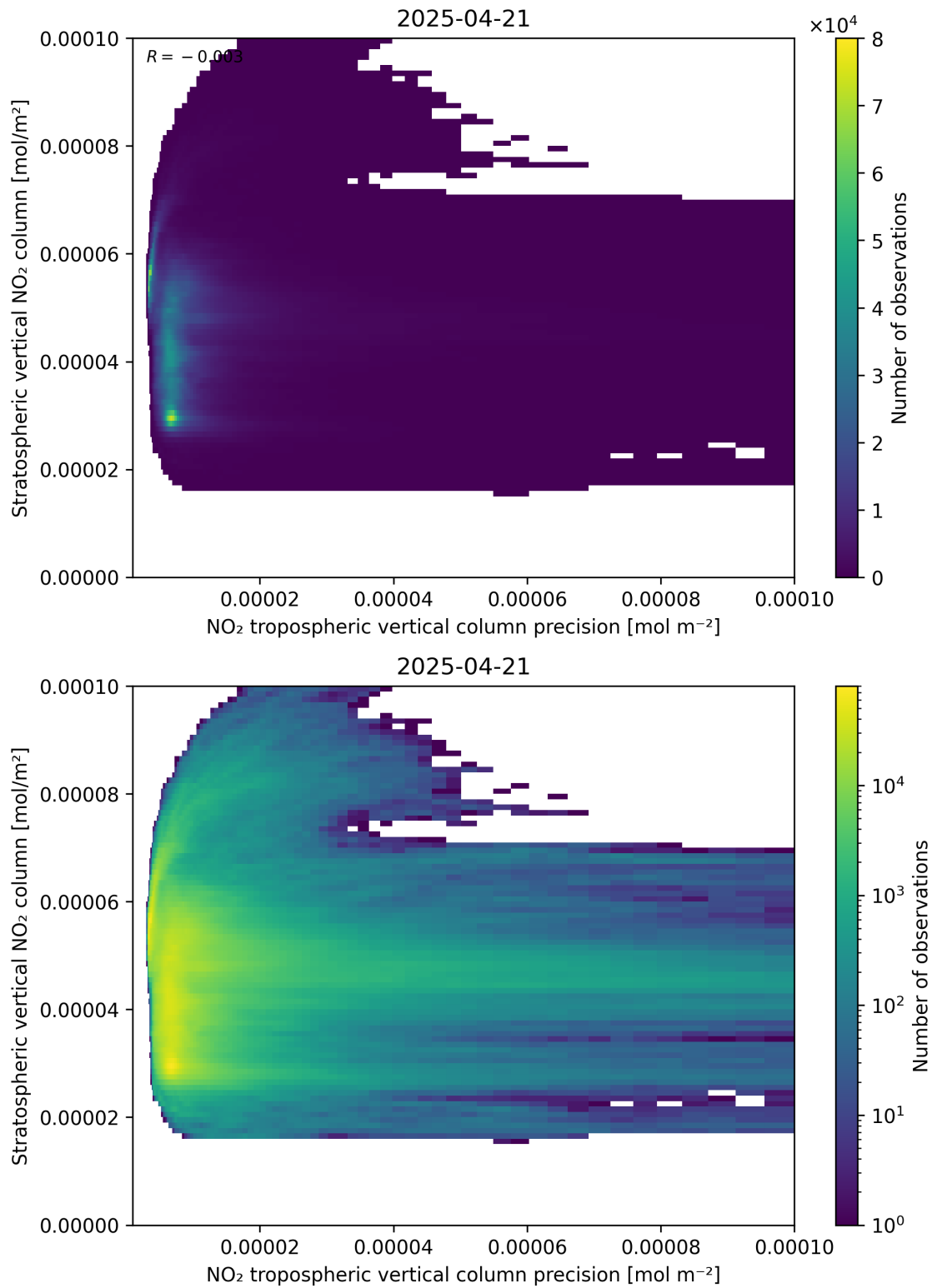
Figure 135: Scatter density plot of “NO 2 tropospheric vertical column precision” against “Stratospheric vertical NO 2 column” for 2025-04-21 to 2025-04-22.
