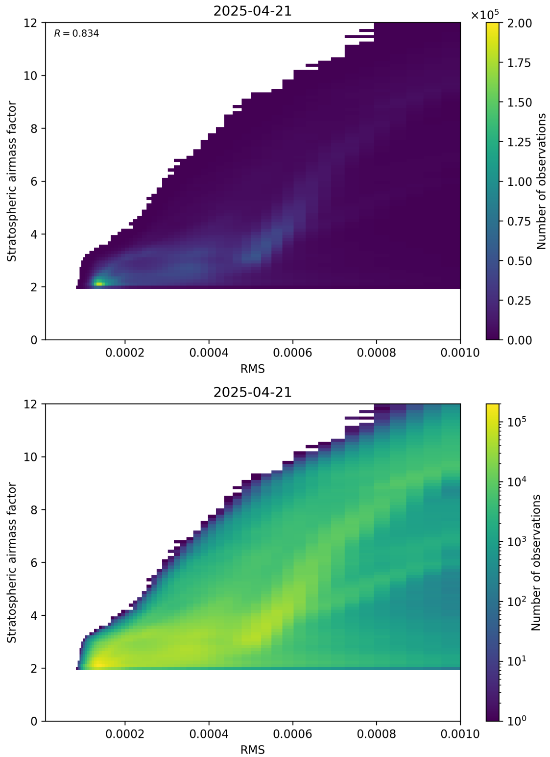
Figure 144: Scatter density plot of “RMS” against “Stratospheric airmass factor” for 2025-04-21 to 2025-04-22.
