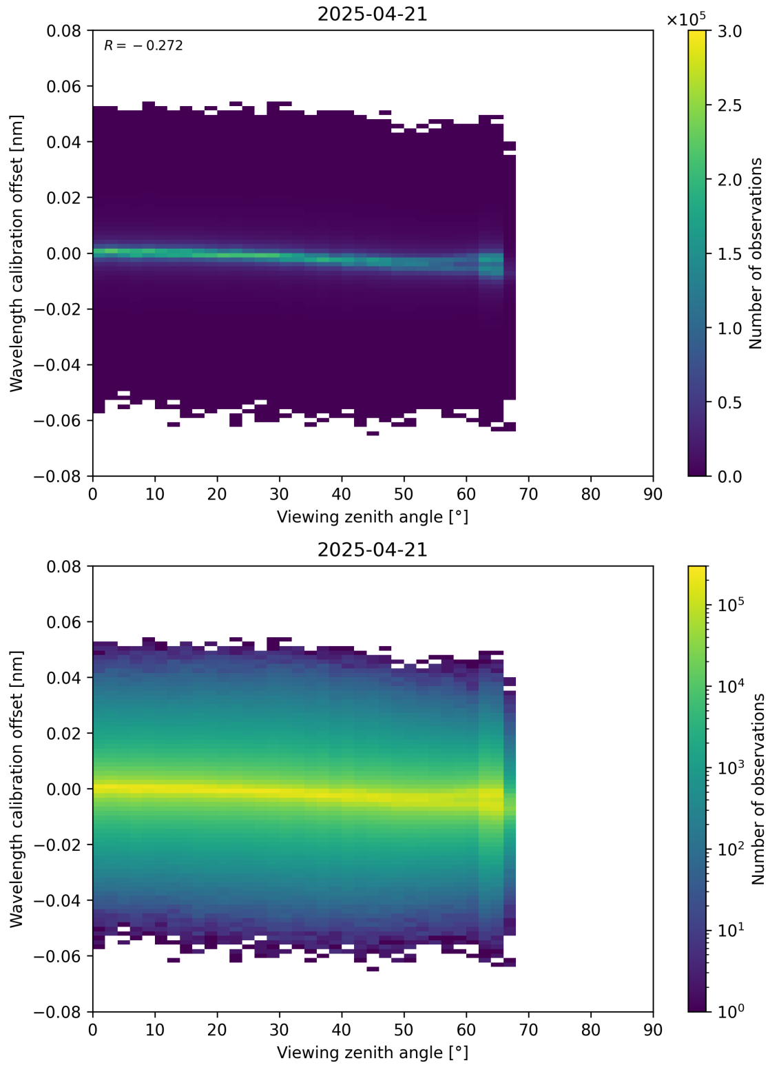
Figure 173: Scatter density plot of “Viewing zenith angle” against “Wavelength calibration offset” for 2025-04-21 to 2025-04-22.
