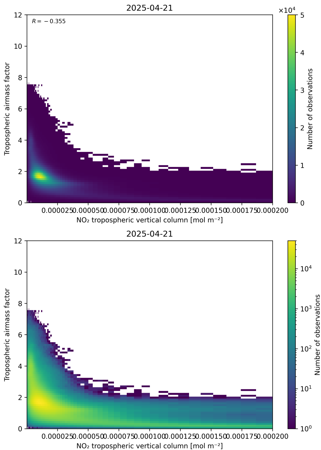
Figure 123: Scatter density plot of “NO 2 tropospheric vertical column” against “Tropospheric air mass factor” for 2025-04-21 to 2025-04-22.
