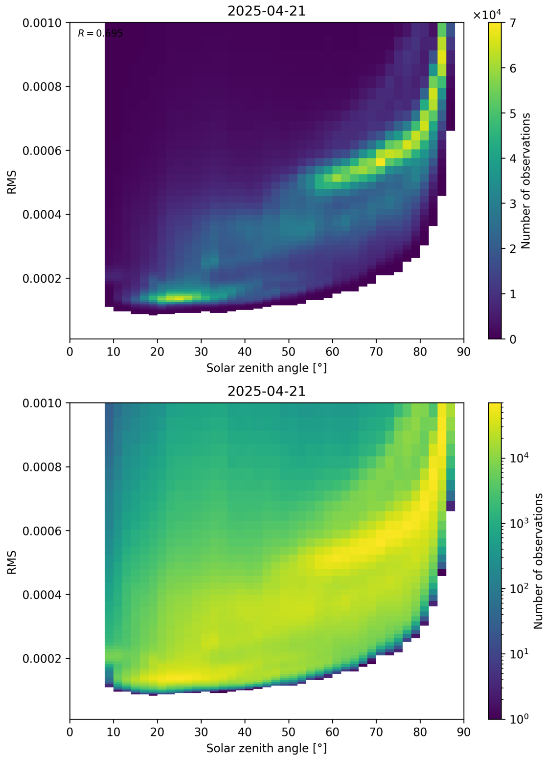
Figure 157: Scatter density plot of “Solar zenith angle” against “RMS” for 2025-04-21 to 2025-04-22.
