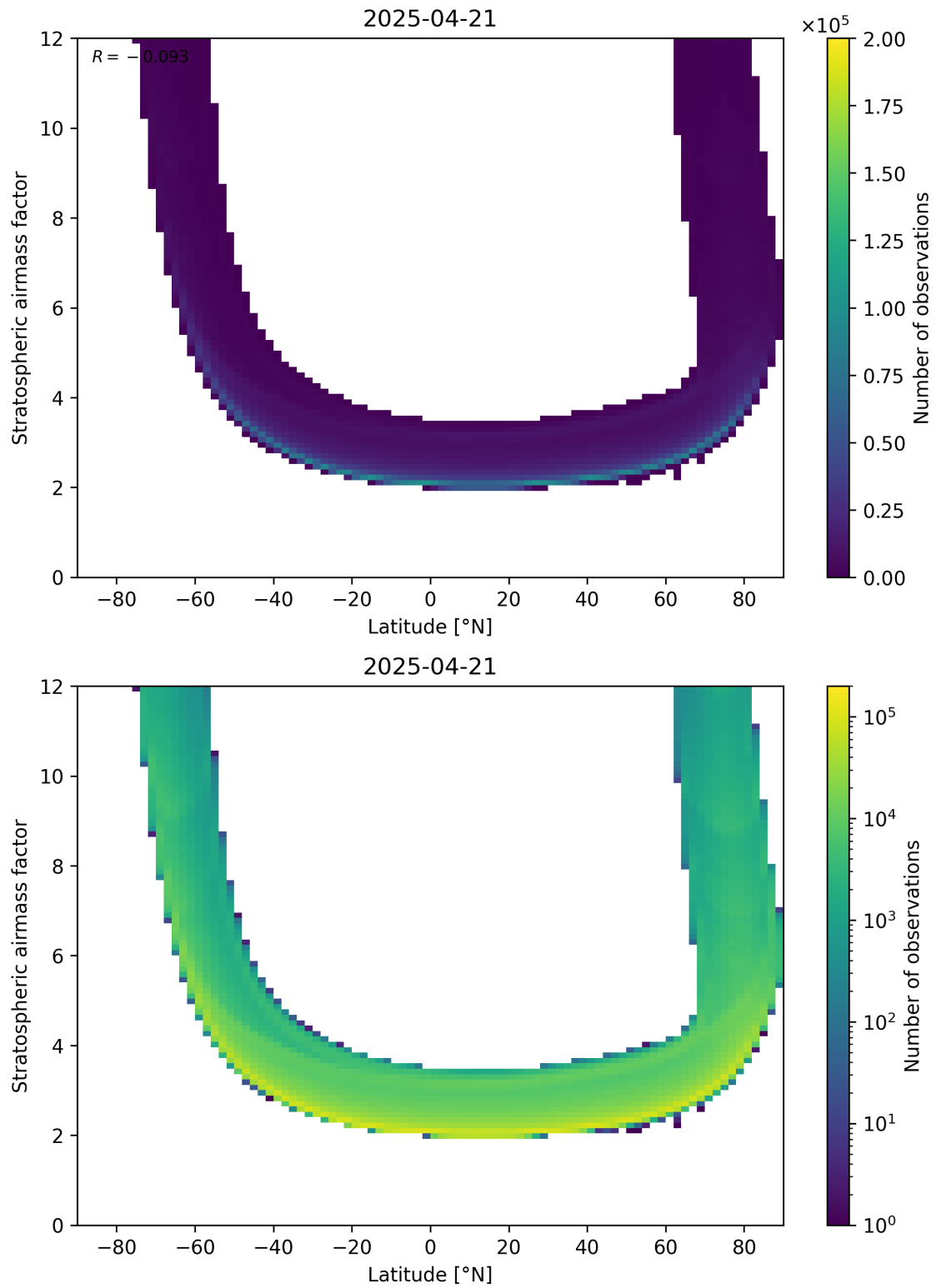
Figure 83: Scatter density plot of “Latitude” against “Stratospheric air mass factor” for 2025-04-21 to 2025-04-22.
