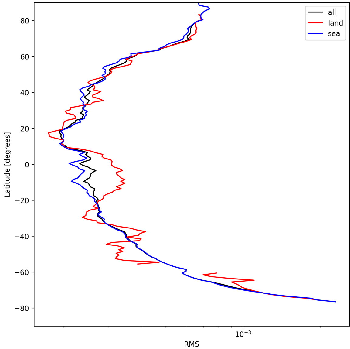
Figure 26: Zonal average of “RMS” for 2025-04-21 to 2025-04-22.
