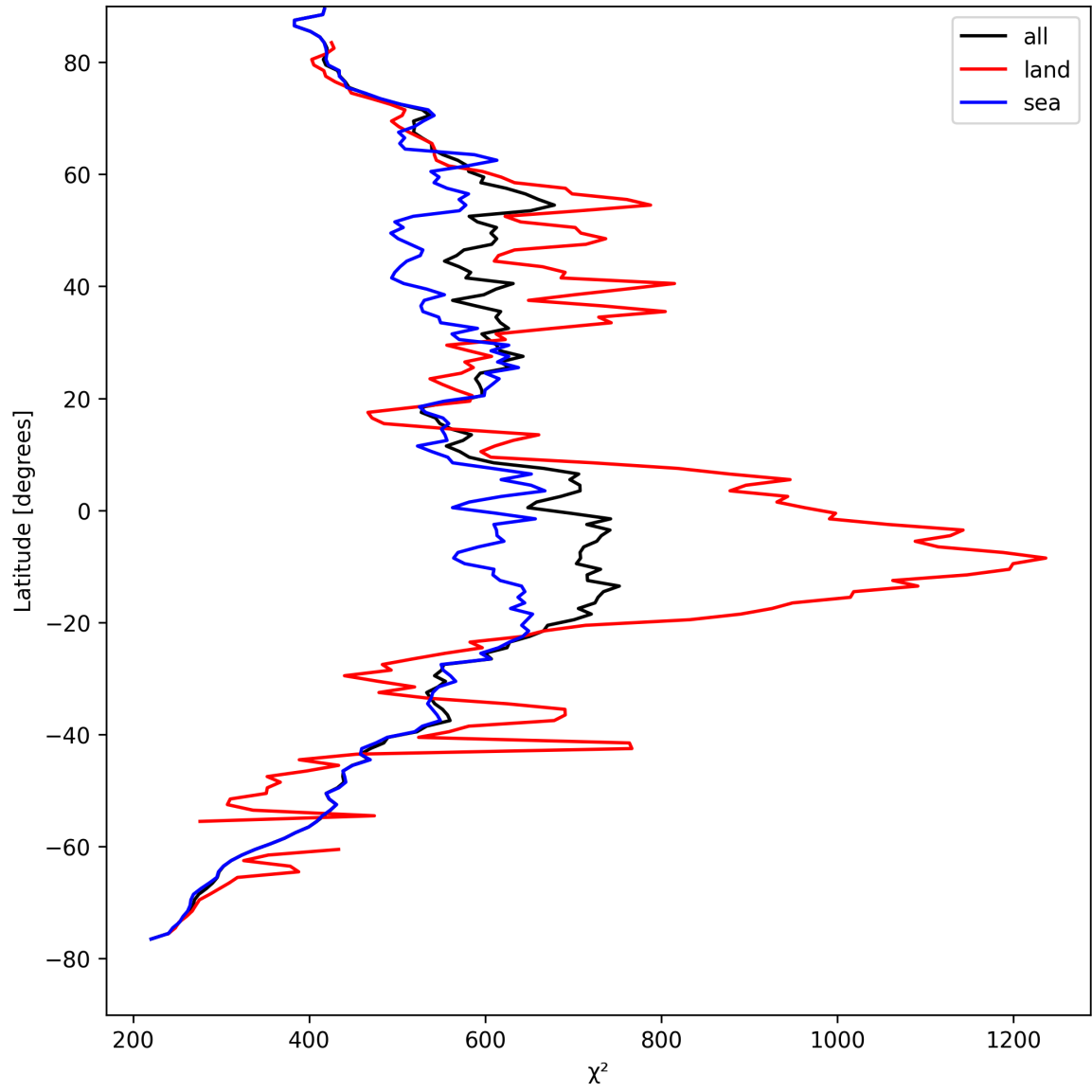
Figure 25: Zonal average of “ \chi^2 ” for 2025-04-21 to 2025-04-22.
