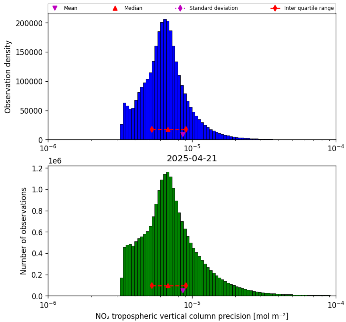
Figure 30: Histogram of “NO 2 tropospheric vertical column precision” for 2025-04-21 to 2025-04-22
