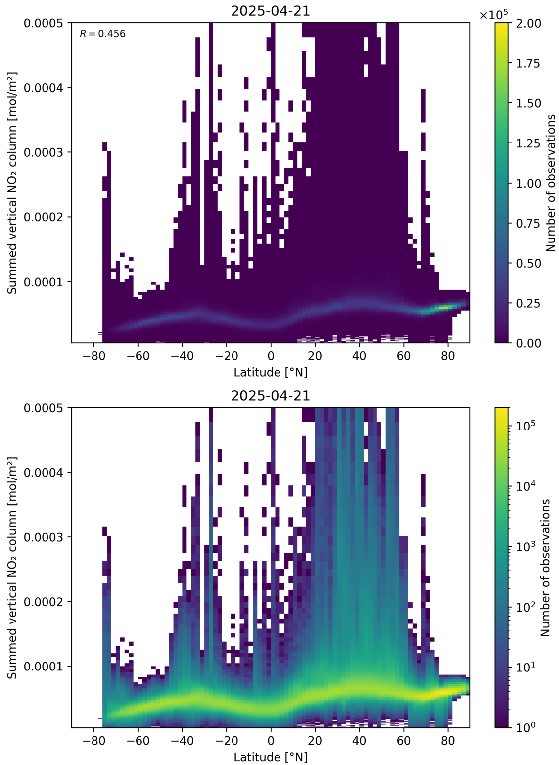
Figure 88: Scatter density plot of “Latitude” against “Summed vertical NO 2 column” for 2025-04-21 to 2025-04-22.
