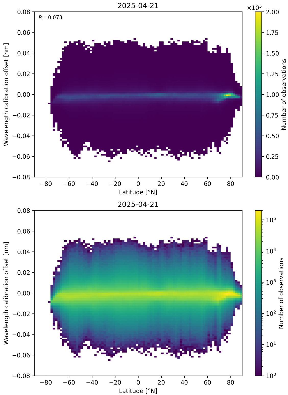
Figure 95: Scatter density plot of “Latitude” against “Wavelength calibration offset” for 2025-04-21 to 2025-04-22.
