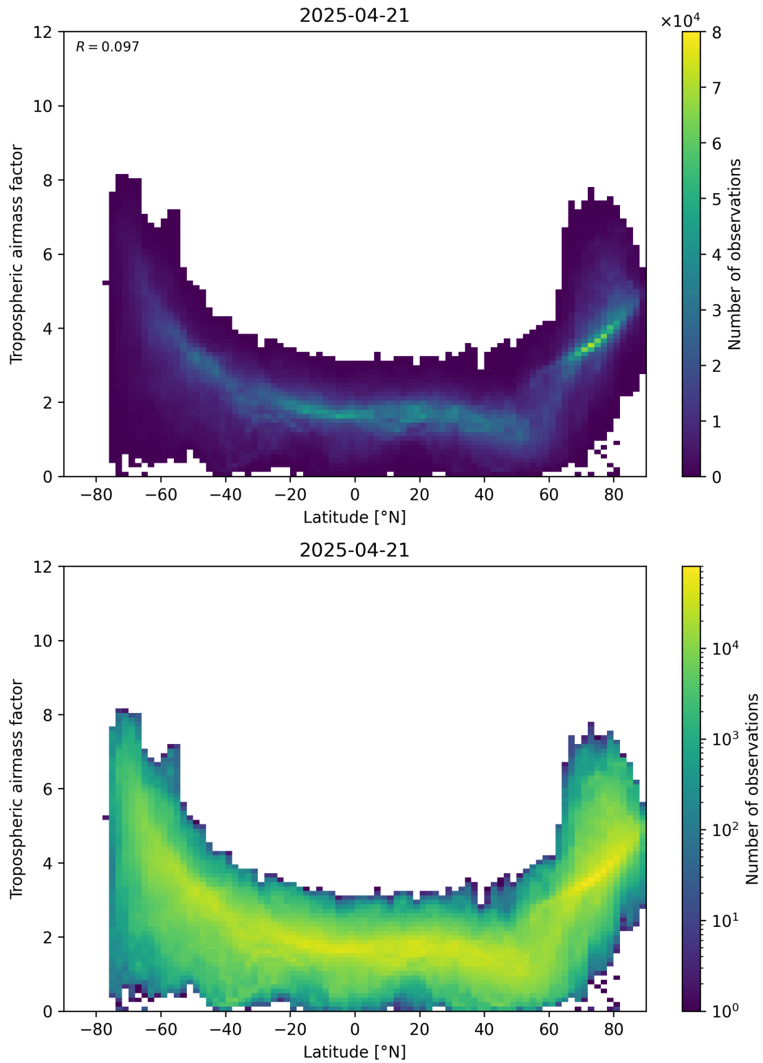
Figure 85: Scatter density plot of “Latitude” against “Tropospheric airmass factor” for 2025-04-21 to 2025-04-22.
