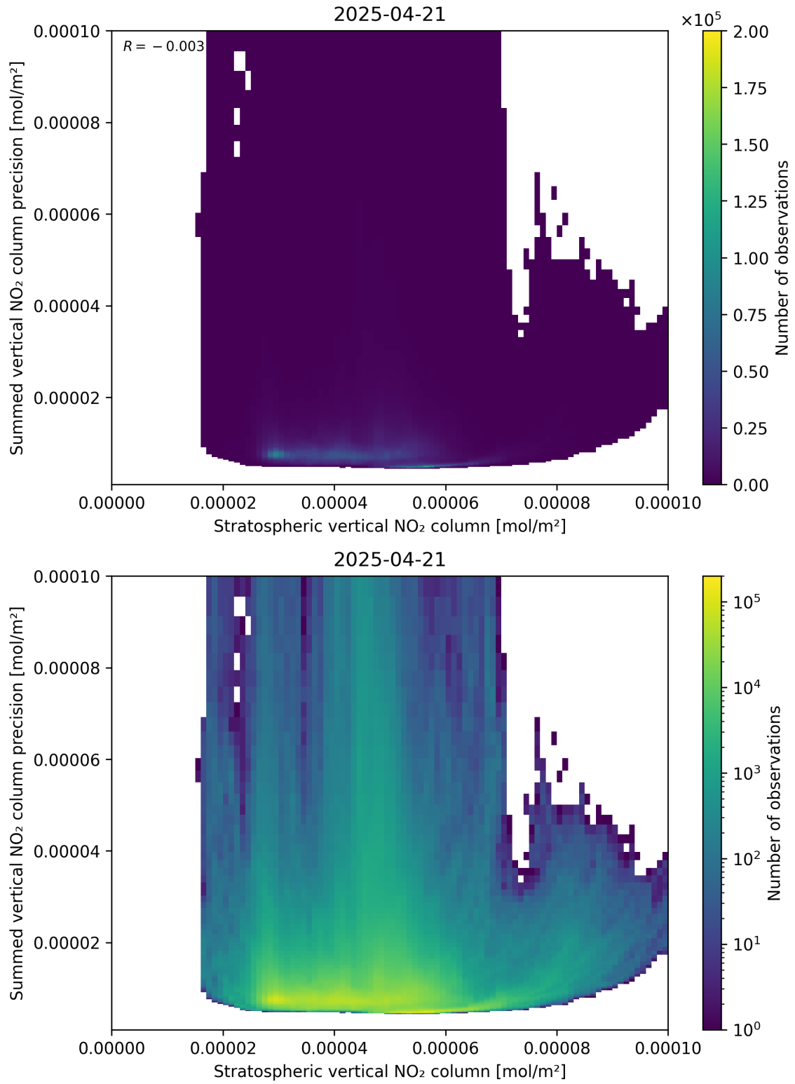
Figure 99: Scatter density plot of “Stratospheric vertical NO 2 column” against “Summed vertical NO 2 column precision” for 2025-04-21 to 2025-04-22.
