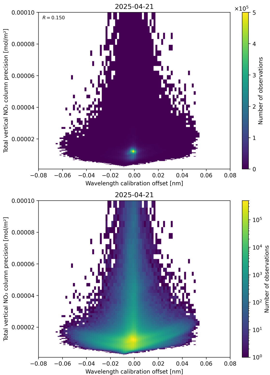
Figure 180: Scatter density plot of “Wavelength calibration offset” against “Total vertical NO 2 column precision” for 2025-04-21 to 2025-04-22.
