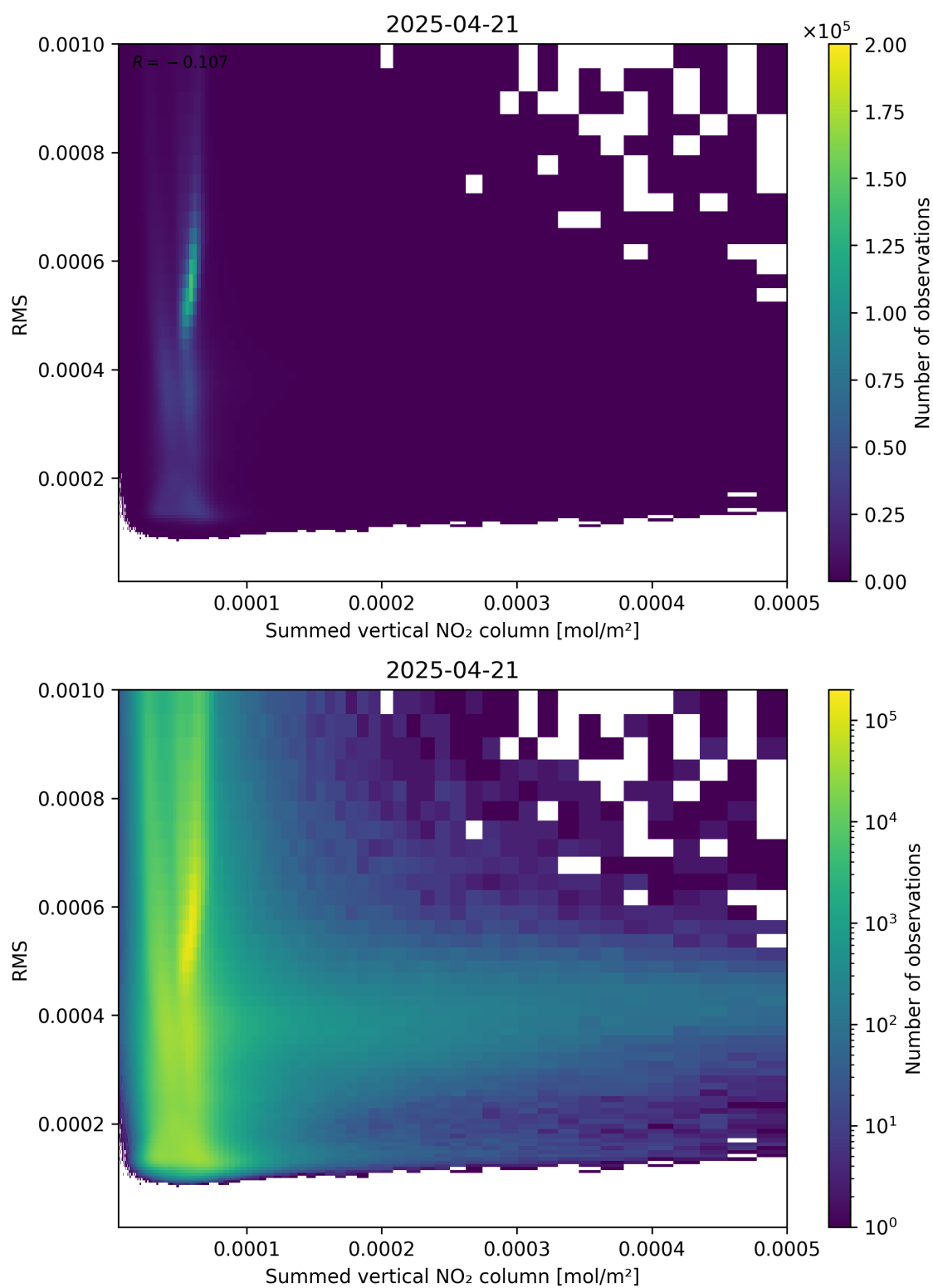
Figure 109: Scatter density plot of “Summed vertical NO 2 column” against “RMS” for 2025-04-21 to 2025-04-22.
