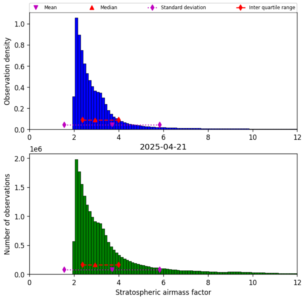
Figure 44: Histogram of “Stratospheric airmass factor” for 2025-04-21 to 2025-04-22
