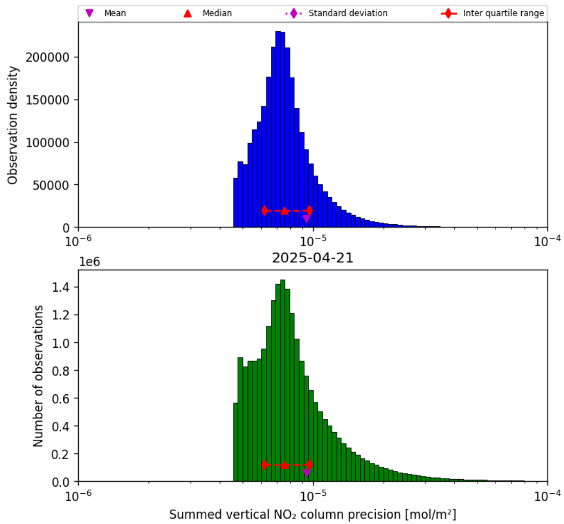
Figure 41: Histogram of "Summed vertical NO 2 column precision" for 2025-04-21 to 2025-04-22
