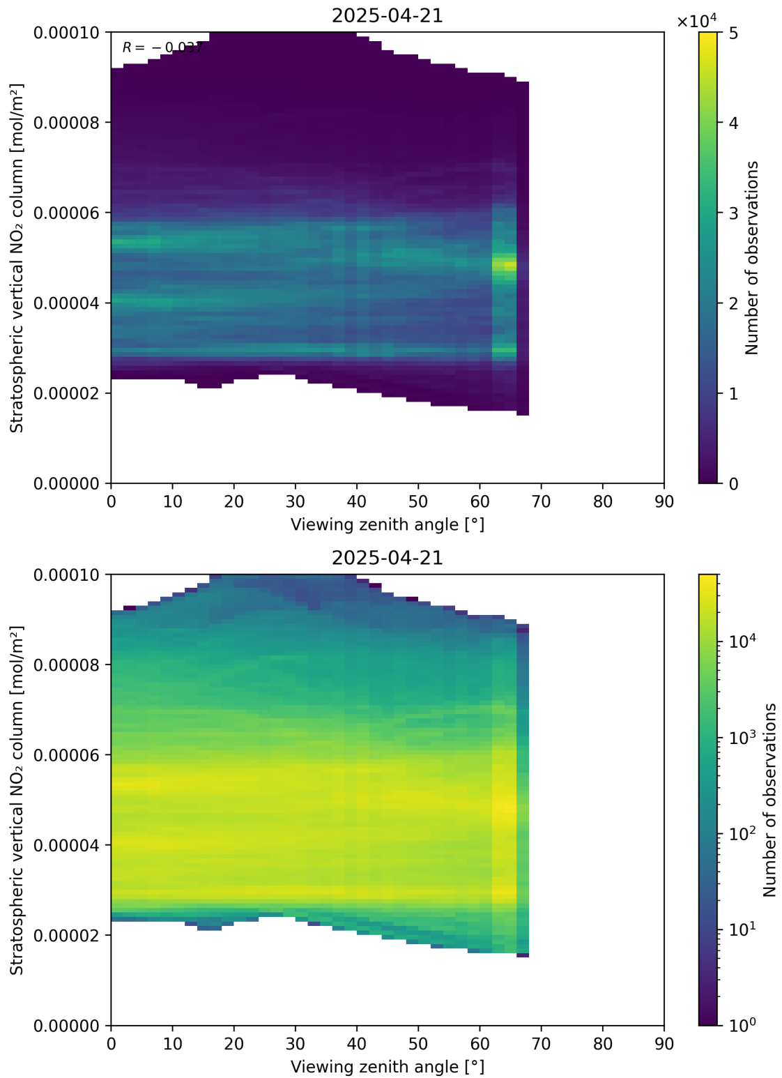
Figure 164: Scatter density plot of “Viewing zenith angle” against “Stratospheric vertical NO 2 column” for 2025-04-21 to 2025-04-22.
