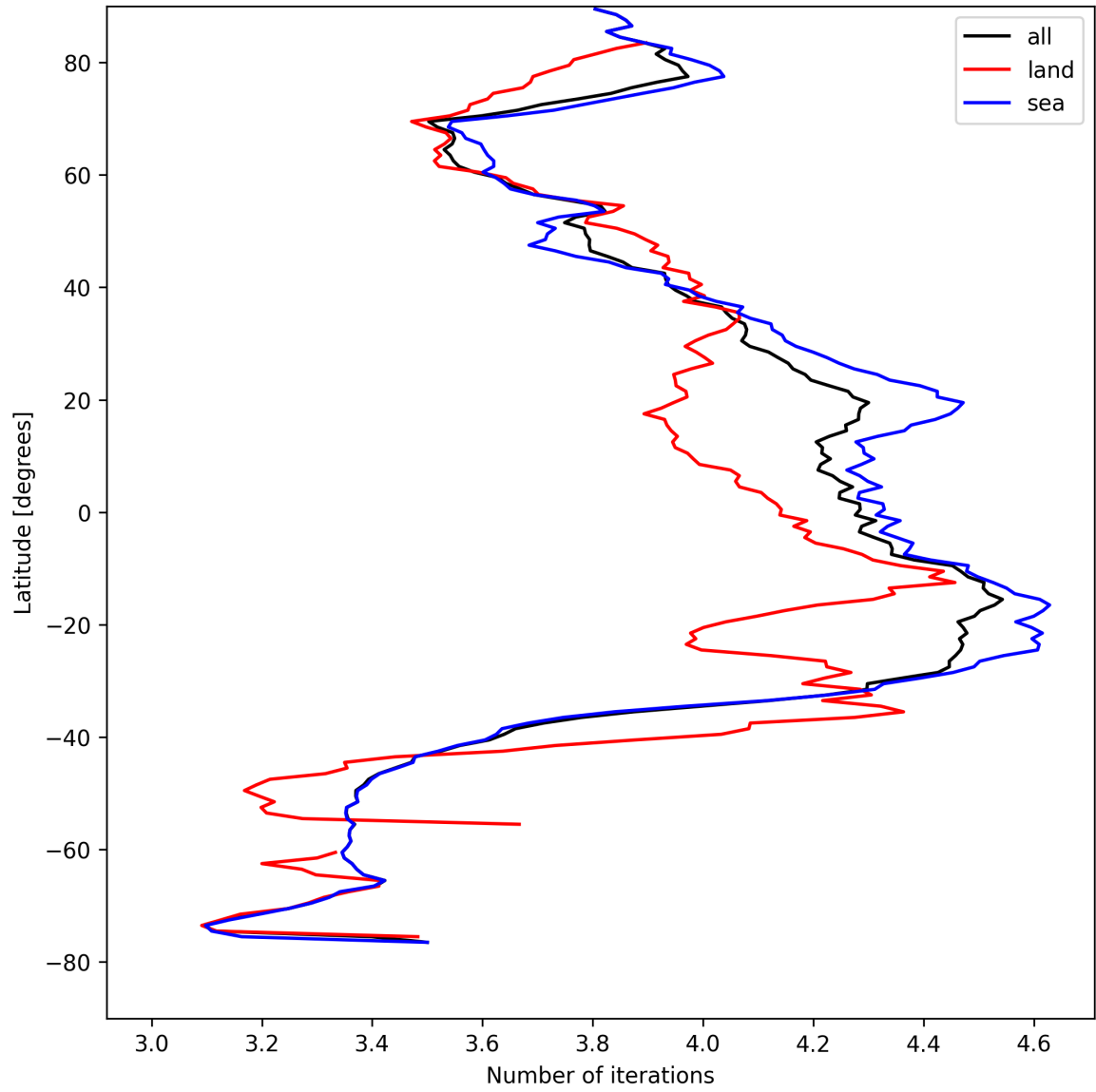
Figure 17: Zonal average of “Number of iterations” for 2025-04-21 to 2025-04-22.
