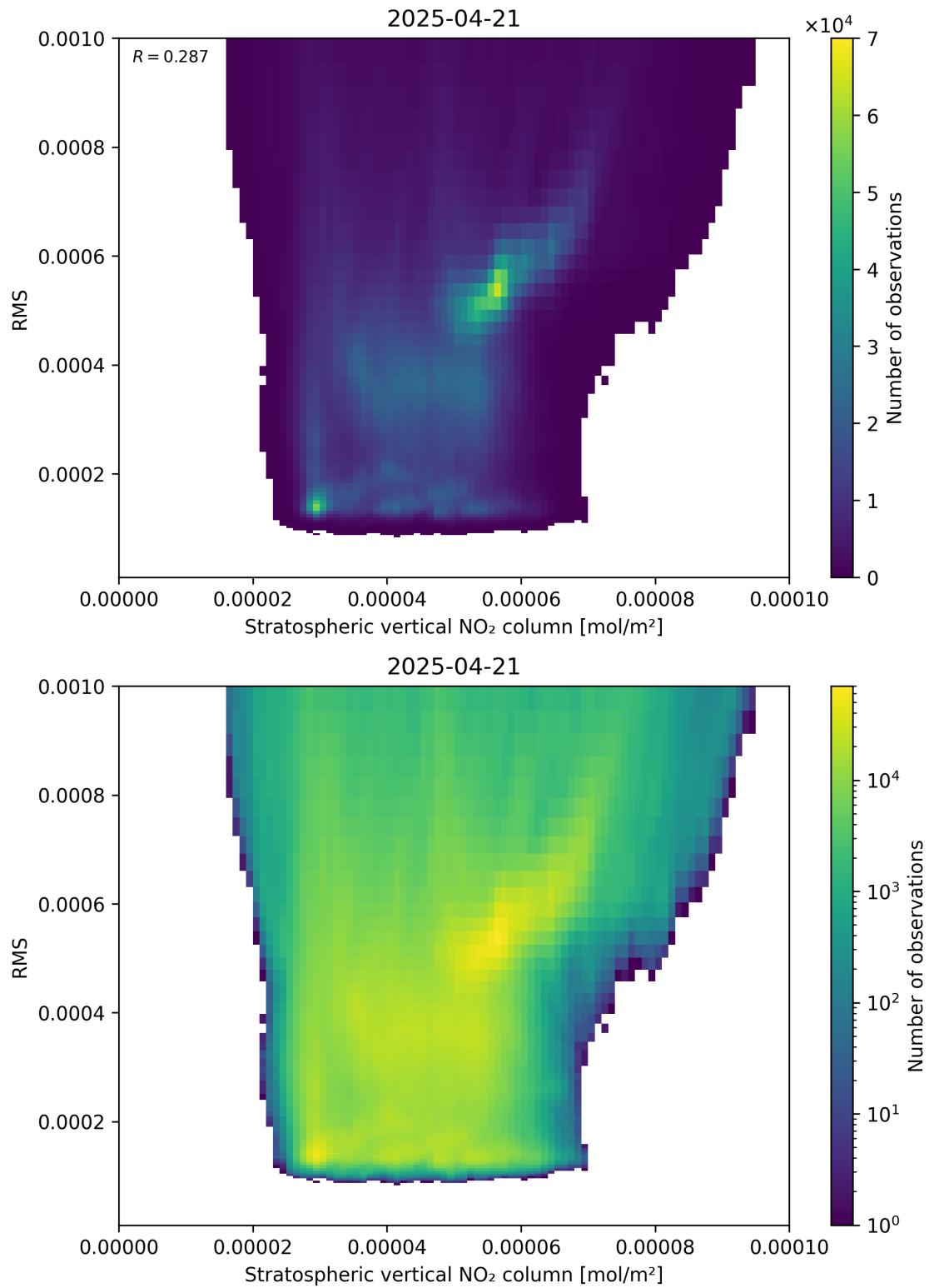
Figure 102: Scatter density plot of “Stratospheric vertical NO 2 column” against “RMS” for 2025-04-21 to 2025-04-22.
