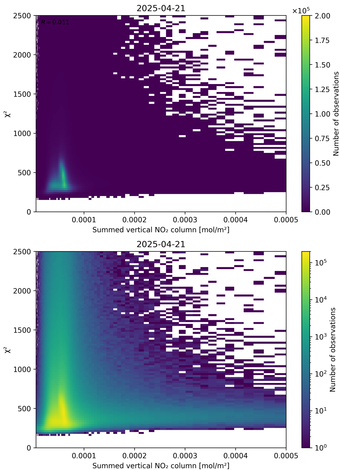
Figure 104: Scatter density plot of “Summed vertical NO 2 column” against “ \chi^2 ” for 2025-04-21 to 2025-04-22.
