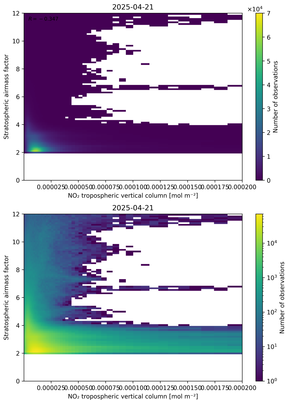
Figure 121: Scatter density plot of “NO 2 tropospheric vertical column” against “Stratospheric air mass factor” for 2025-04-21 to 2025-04-22.
