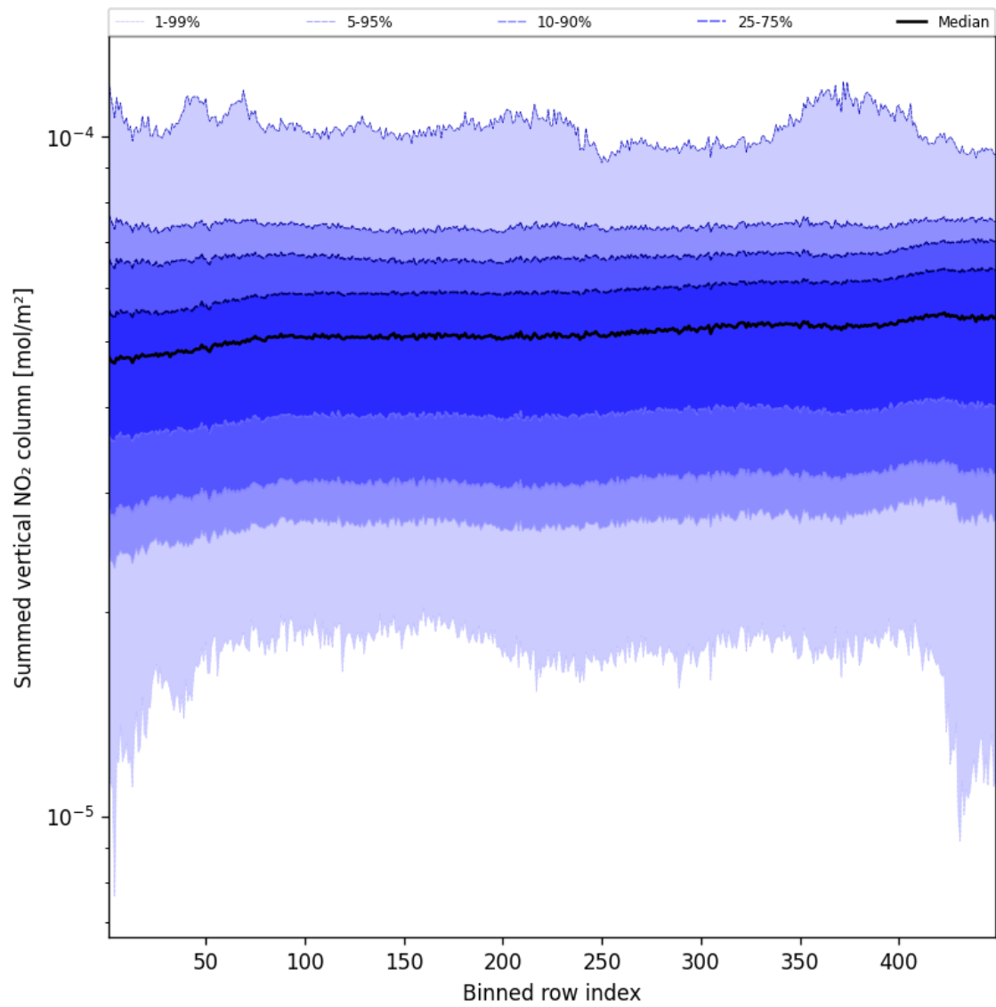
Figure 57: Along track statistics of “Summed vertical NO 2 column” for 2025-04-21 to 2025-04-22
