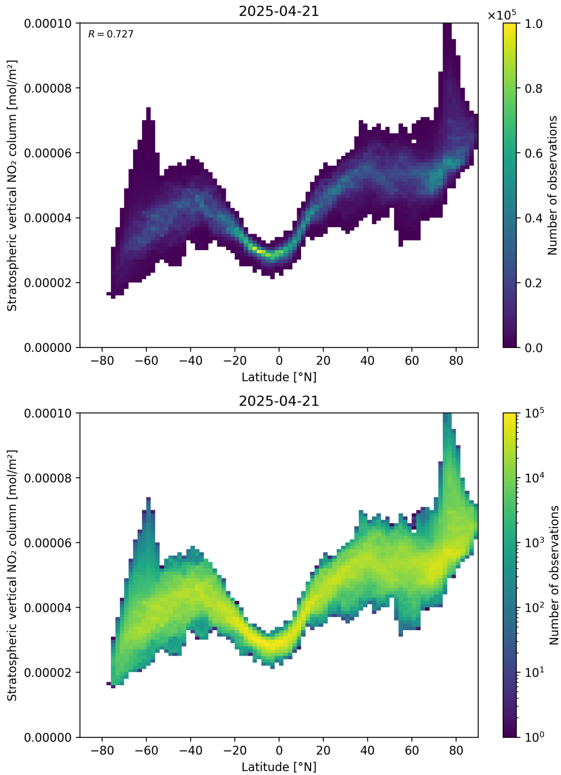
Figure 87: Scatter density plot of “Latitude” against “Stratospheric vertical NO 2 column” for 2025-04-21 to 2025-04-22.
