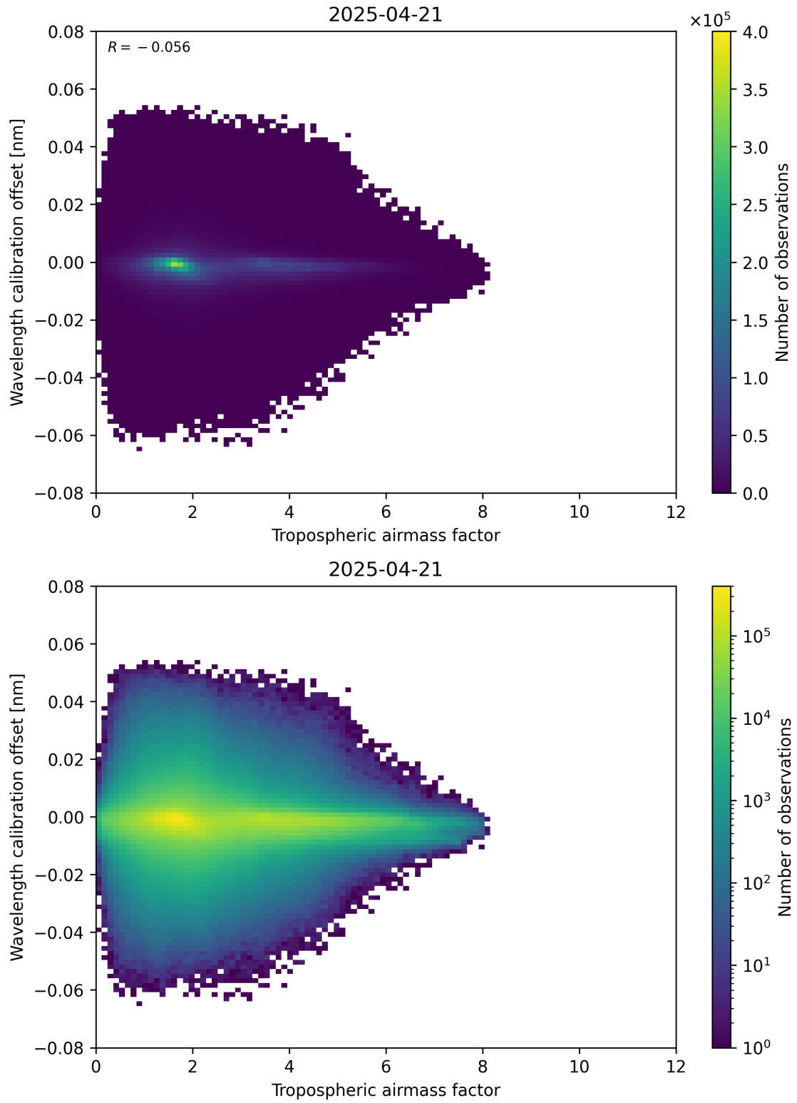
Figure 80: Scatter density plot of “Tropospheric airmass factor” against “Wavelength calibration offset” for 2025-04-21 to 2025-04-22.
