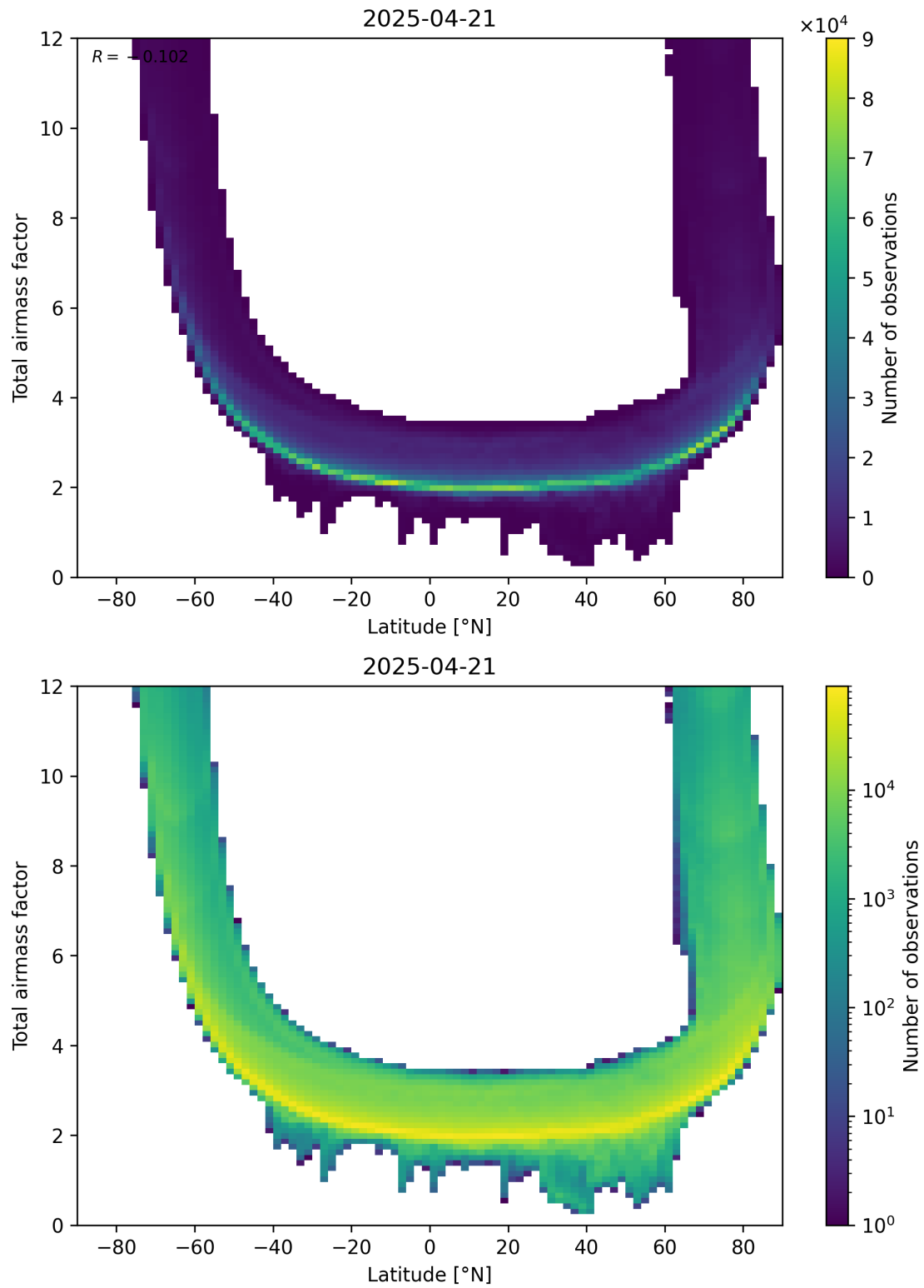
Figure 84: Scatter density plot of “Latitude” against “Total airmass factor” for 2025-04-21 to 2025-04-22.
