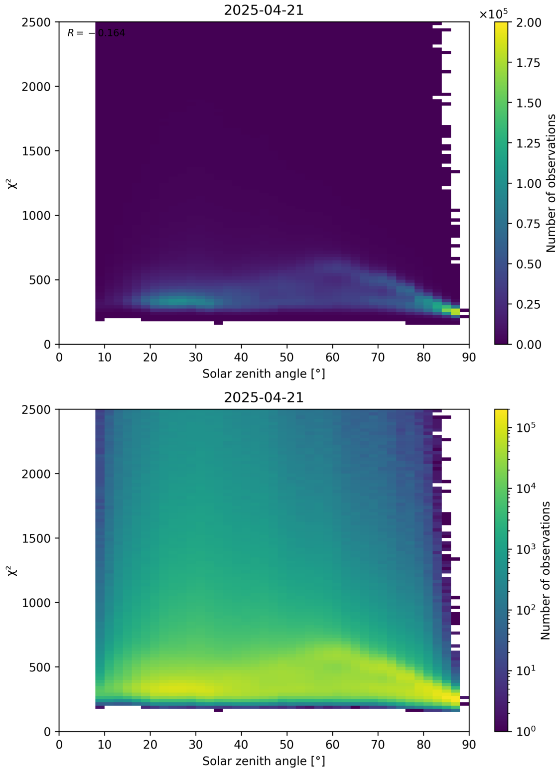
Figure 148: Scatter density plot of “Solar zenith angle” against “ \chi^2 ” for 2025-04-21 to 2025-04-22.
