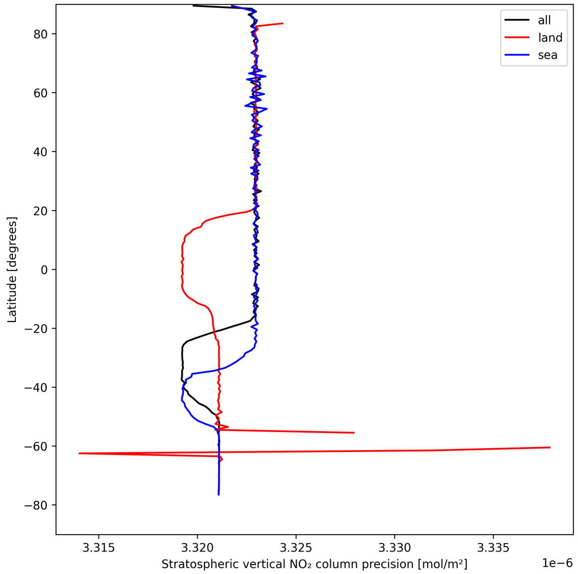
Figure 20: Zonal average of “Stratospheric vertical NO 2 column precision” for 2025-04-21 to 2025-04-22.
