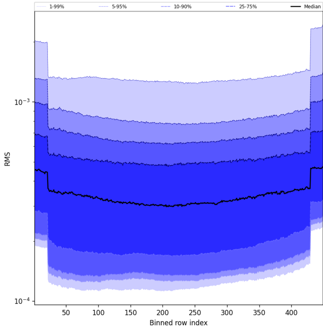
Figure 60: Along track statistics of “RMS” for 2025-04-21 to 2025-04-22
