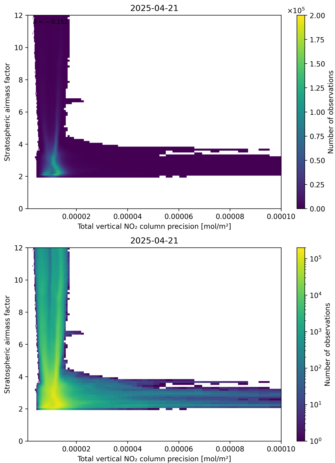
Figure 115: Scatter density plot of “Total vertical NO 2 column precision” against “Stratospheric air mass factor” for 2025-04-21 to 2025-04-22.
