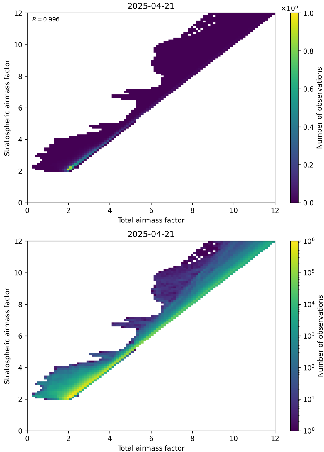
Figure 62: Scatter density plot of “Total airmass factor” against “Stratospheric airmass factor” for 2025-04-21 to 2025-04-22.
