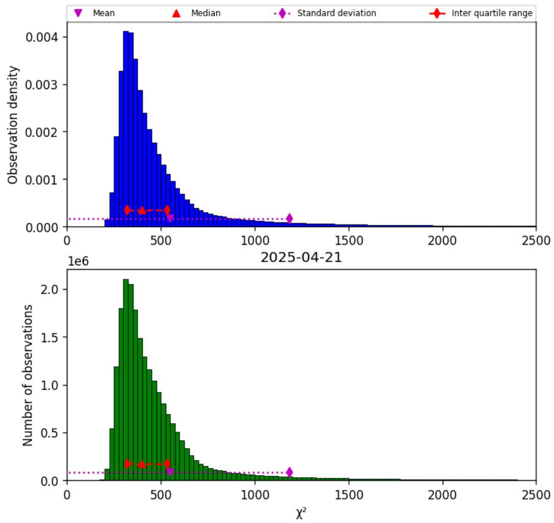
Figure 42: Histogram of “ \chi^2 ” for 2025-04-21 to 2025-04-22
