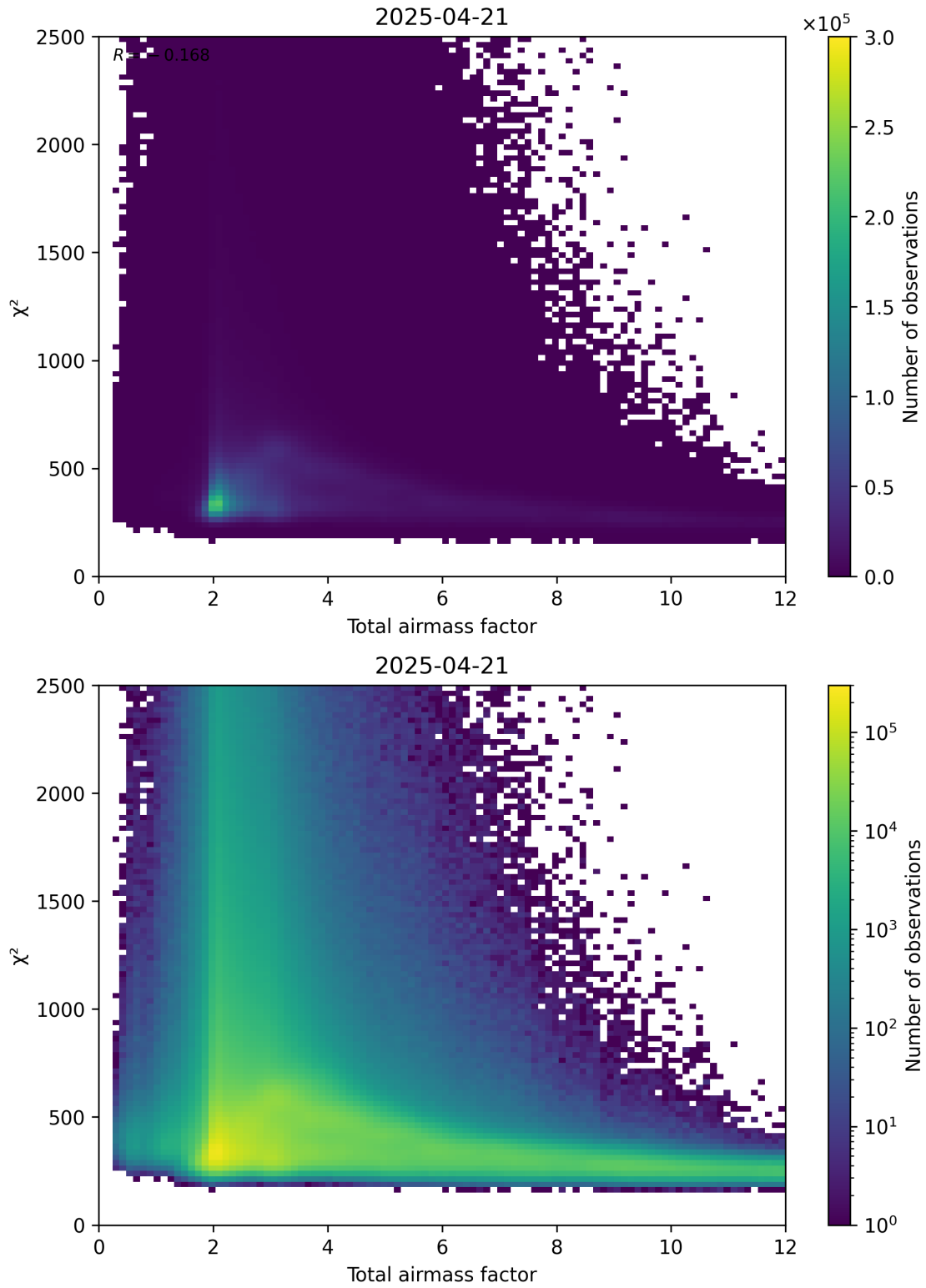
Figure 63: Scatter density plot of “Total airmass factor” against “ \chi^2 ” for 2025-04-21 to 2025-04-22.
