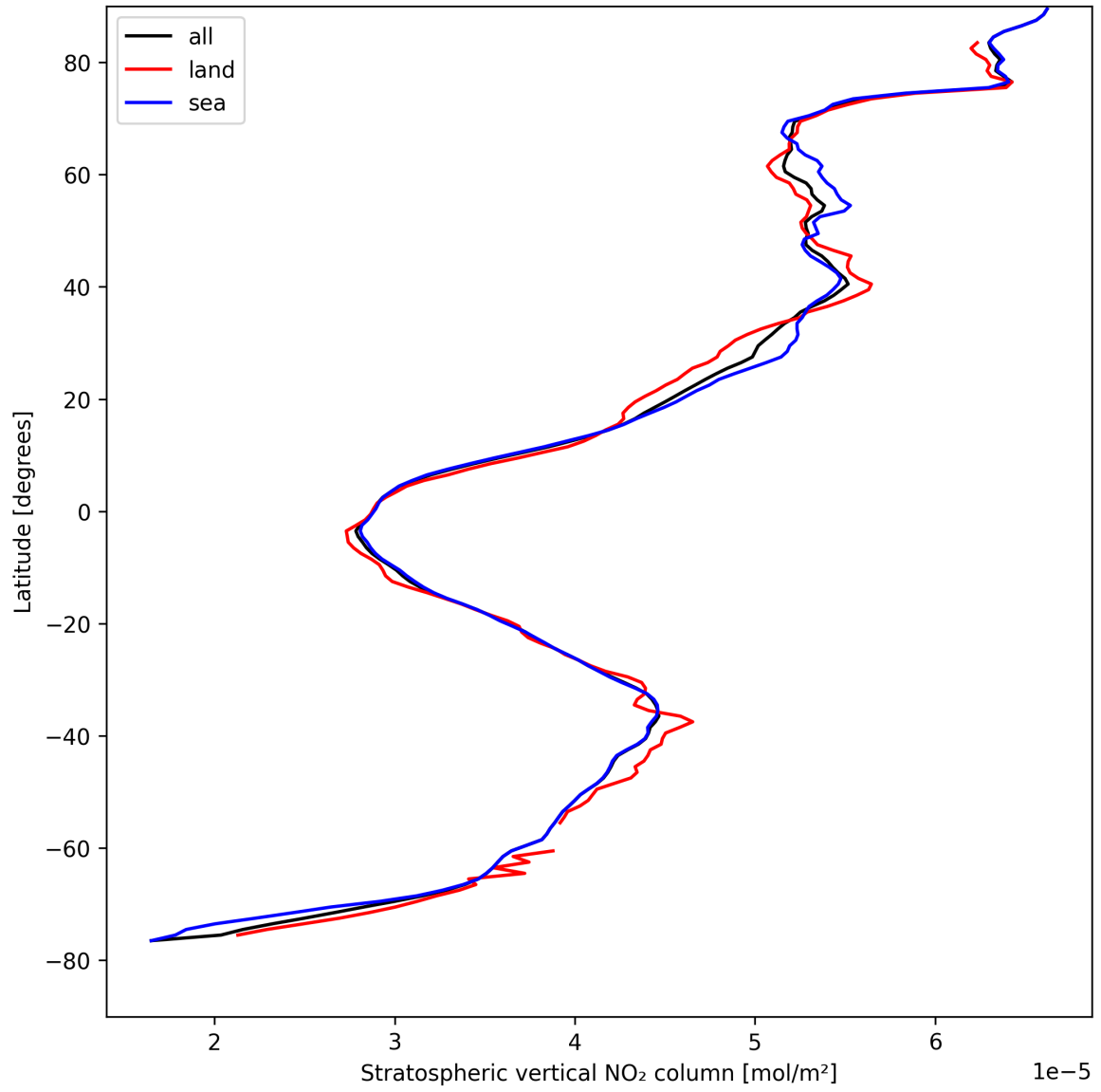
Figure 19: Zonal average of “Stratospheric vertical NO 2 column” for 2025-04-21 to 2025-04-22.
