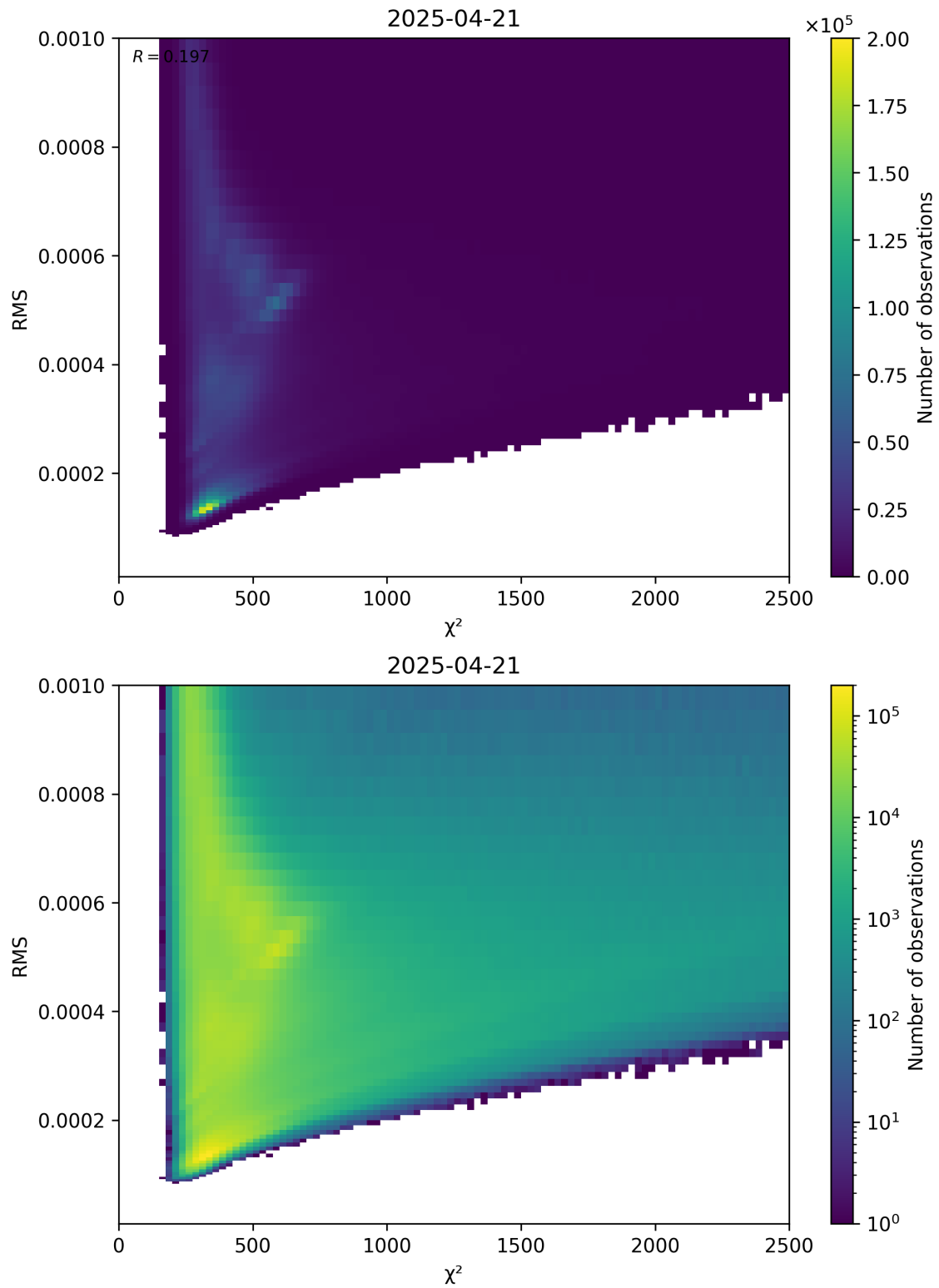
Figure 82: Scatter density plot of “ \chi^2 ” against “RMS” for 2025-04-21 to 2025-04-22.
