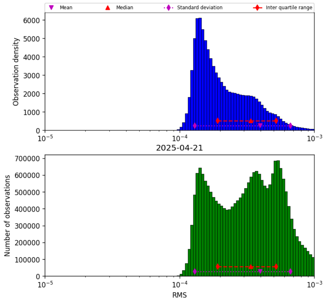
Figure 43: Histogram of “RMS” for 2025-04-21 to 2025-04-22
