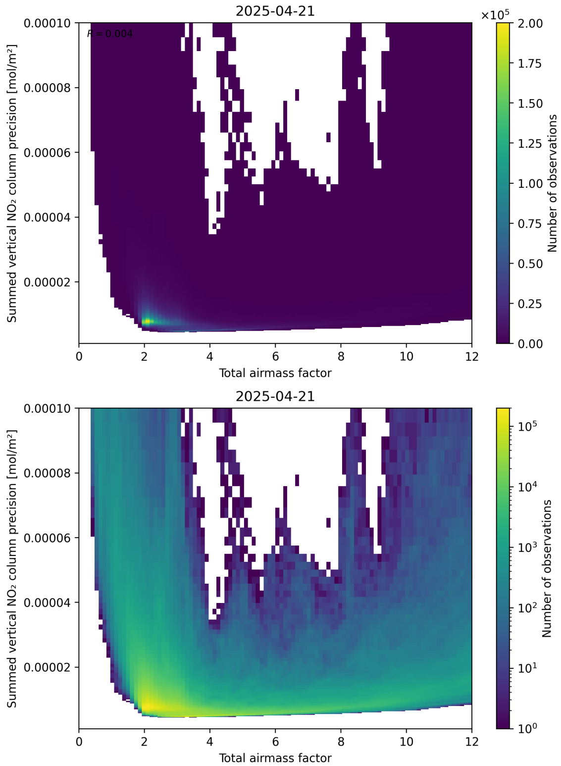
Figure 66: Scatter density plot of “Total airmass factor” against “Summed vertical NO 2 column precision” for 2025-04-21 to 2025-04-22.
