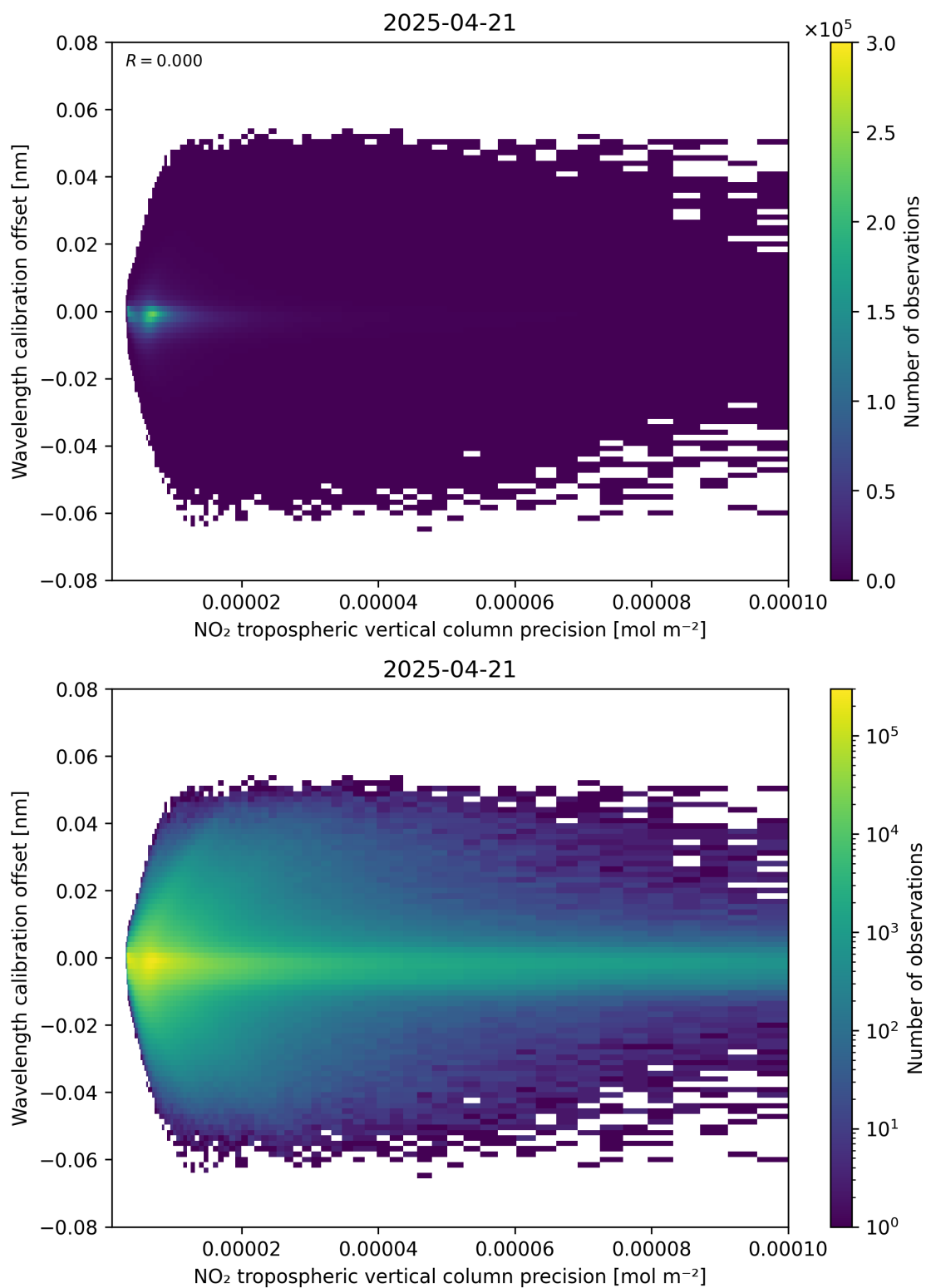
Figure 141: Scatter density plot of “NO 2 tropospheric vertical column precision” against “Wavelength calibration offset” for 2025-04-21 to 2025-04-22.
