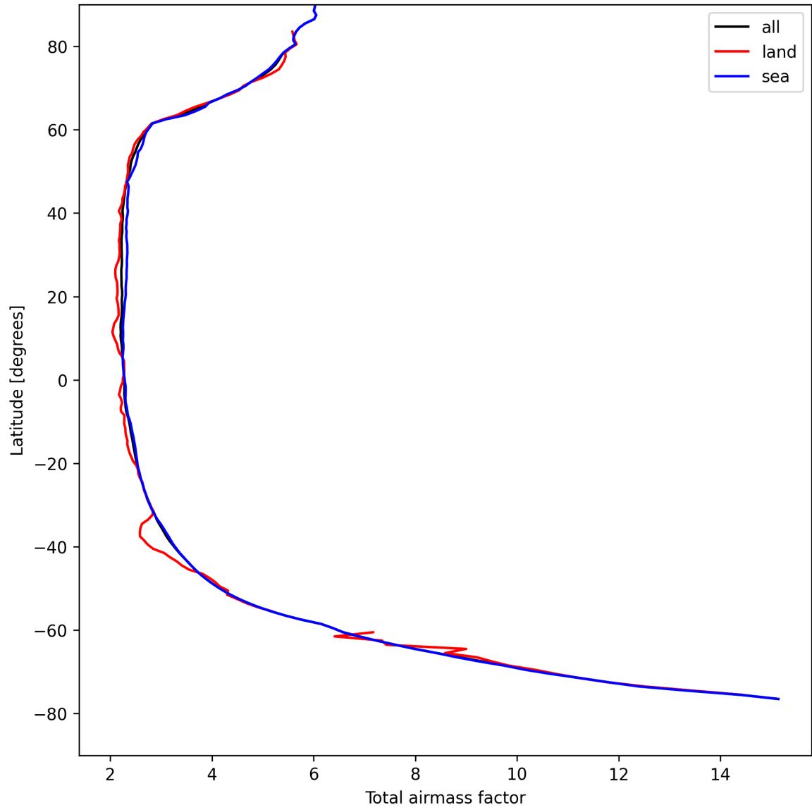
Figure 15: Zonal average of “Total airmass factor” for 2025-04-21 to 2025-04-22.
