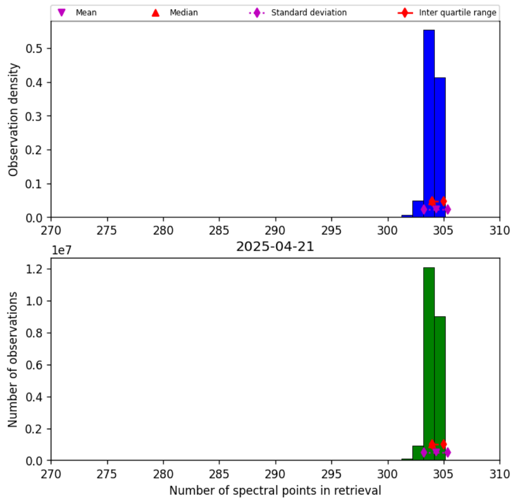
Figure 33: Histogram of “Number of spectral points in retrieval” for 2025-04-21 to 2025-04-22
