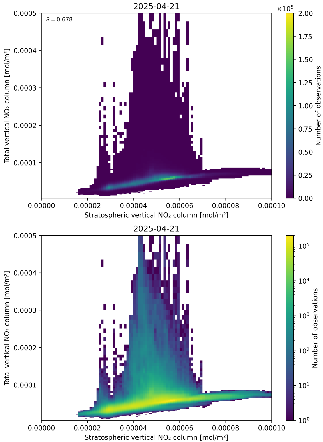
Figure 100: Scatter density plot of “Stratospheric vertical NO 2 column” against “Total vertical NO 2 column” for 2025-04-21 to 2025-04-22.
