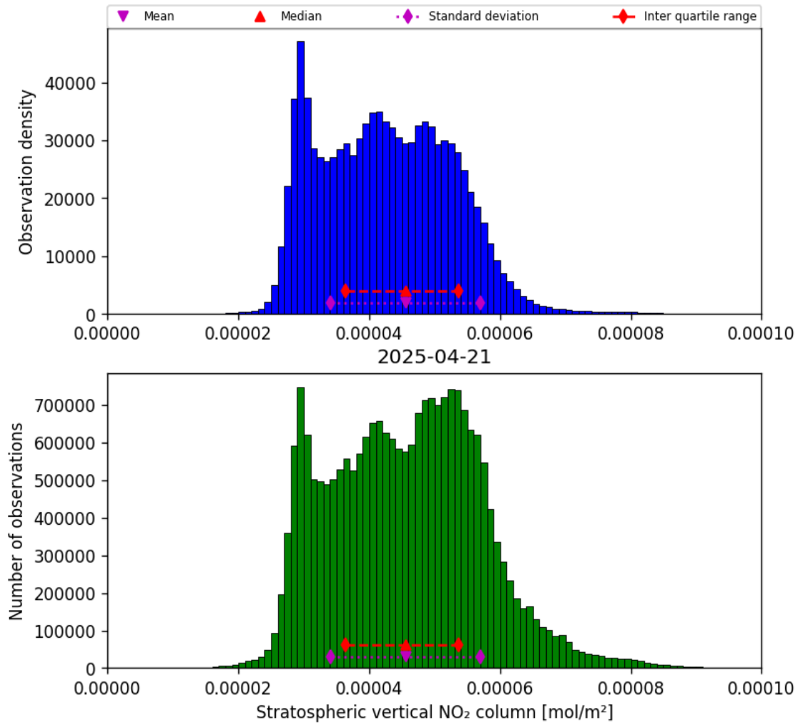
Figure 36: Histogram of “Stratospheric vertical NO 2 column” for 2025-04-21 to 2025-04-22
