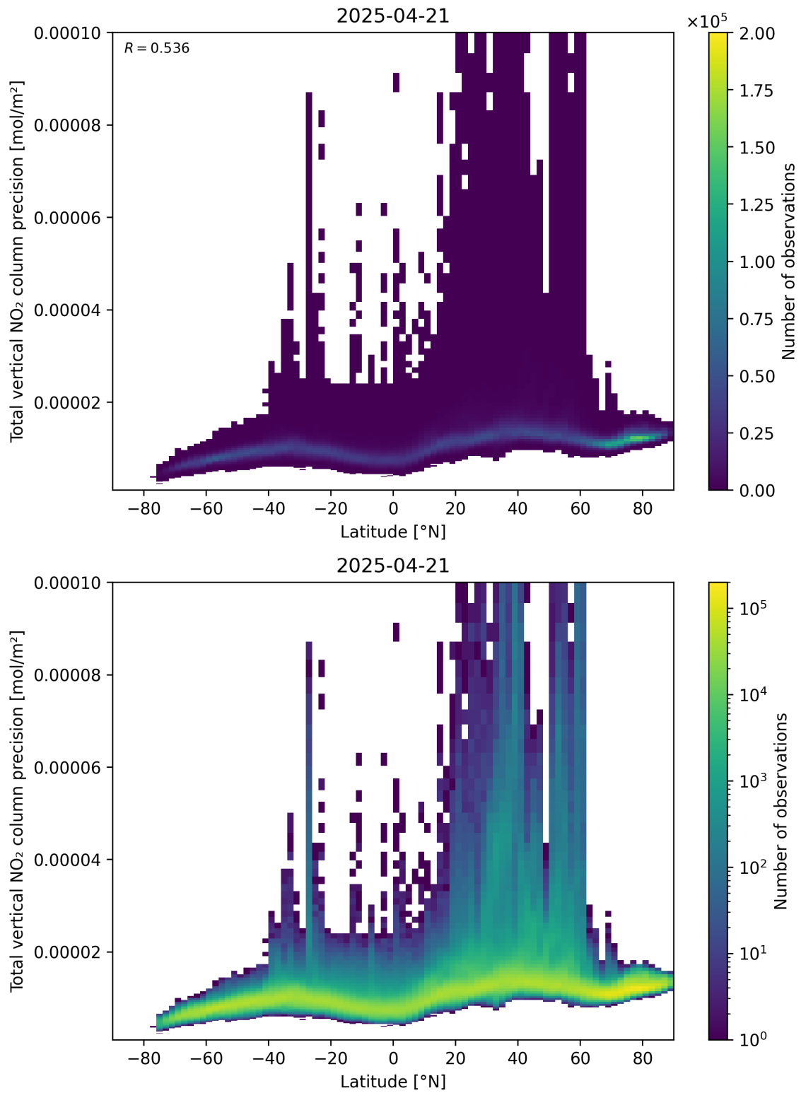
Figure 91: Scatter density plot of “Latitude” against “Total vertical NO 2 column precision” for 2025-04-21 to 2025-04-22.
