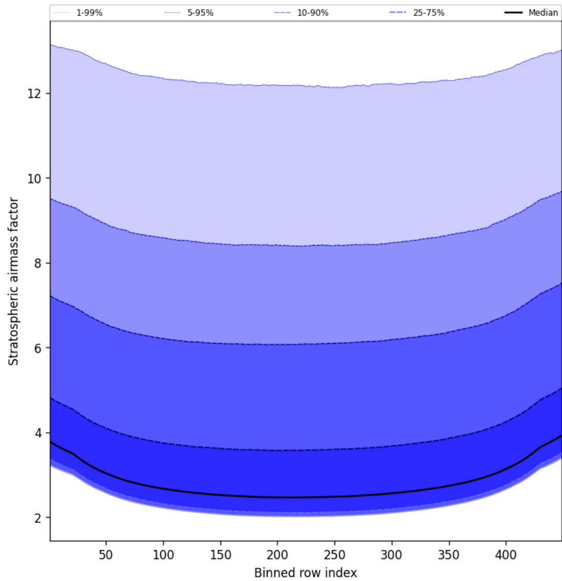
Figure 61: Along track statistics of “Stratospheric airmass factor” for 2025-04-21 to 2025-04-22
