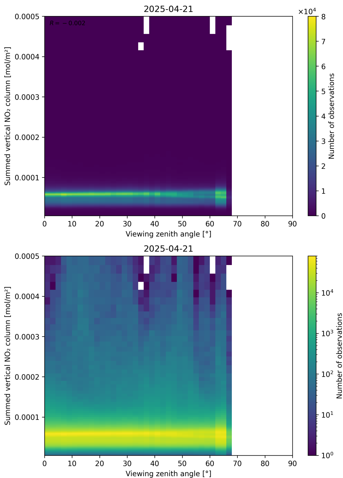
Figure 165: Scatter density plot of “Viewing zenith angle” against “Summed vertical NO 2 column” for 2025-04-21 to 2025-04-22.
