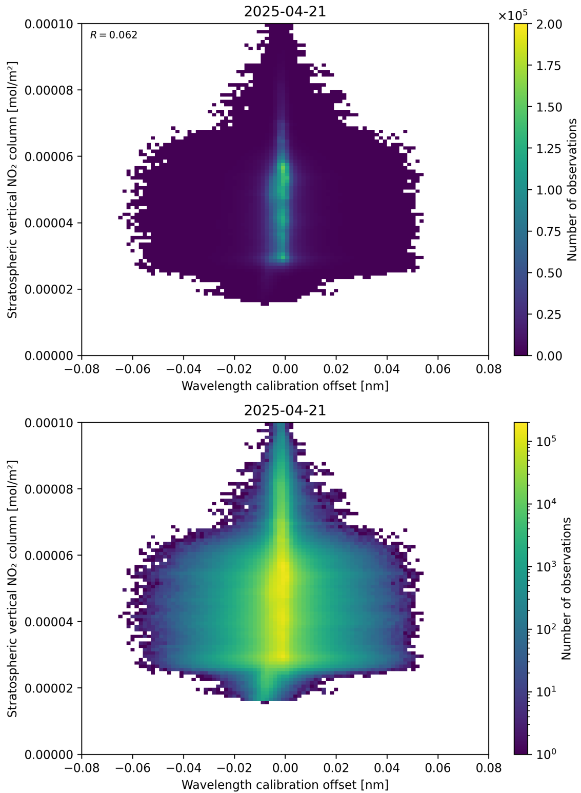
Figure 176: Scatter density plot of “Wavelength calibration offset” against “Stratospheric vertical NO 2 column” for 2025-04-21 to 2025-04-22.
