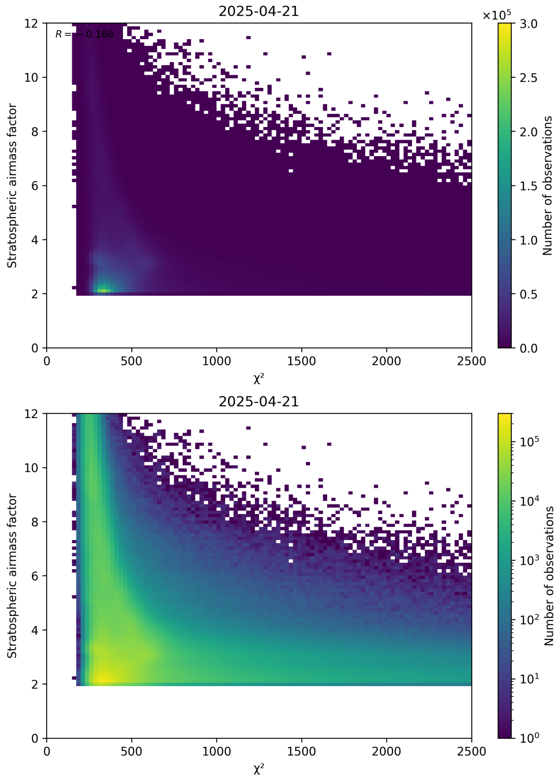
Figure 81: Scatter density plot of " \chi^2 " against "Stratospheric airmass factor" for 2025-04-21 to 2025-04-22.
