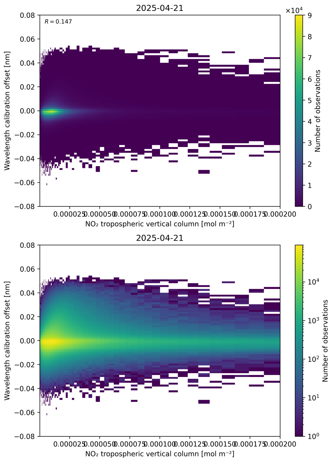
Figure 143: Scatter density plot of “NO 2 tropospheric vertical column” against “Wavelength calibration offset” for 2025-04-21 to 2025-04-22.
