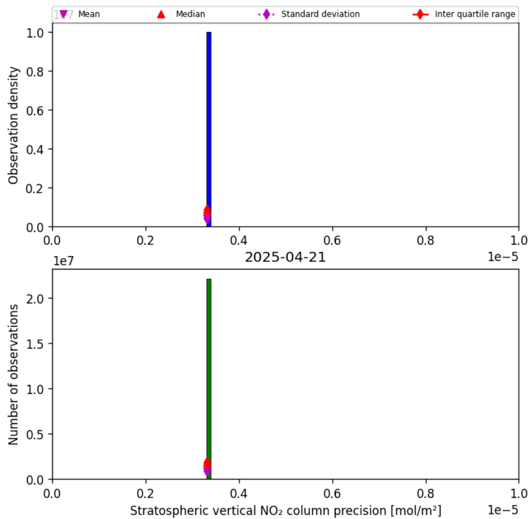
Figure 37: Histogram of “Stratospheric vertical NO 2 column precision” for 2025-04-21 to 2025-04-22
