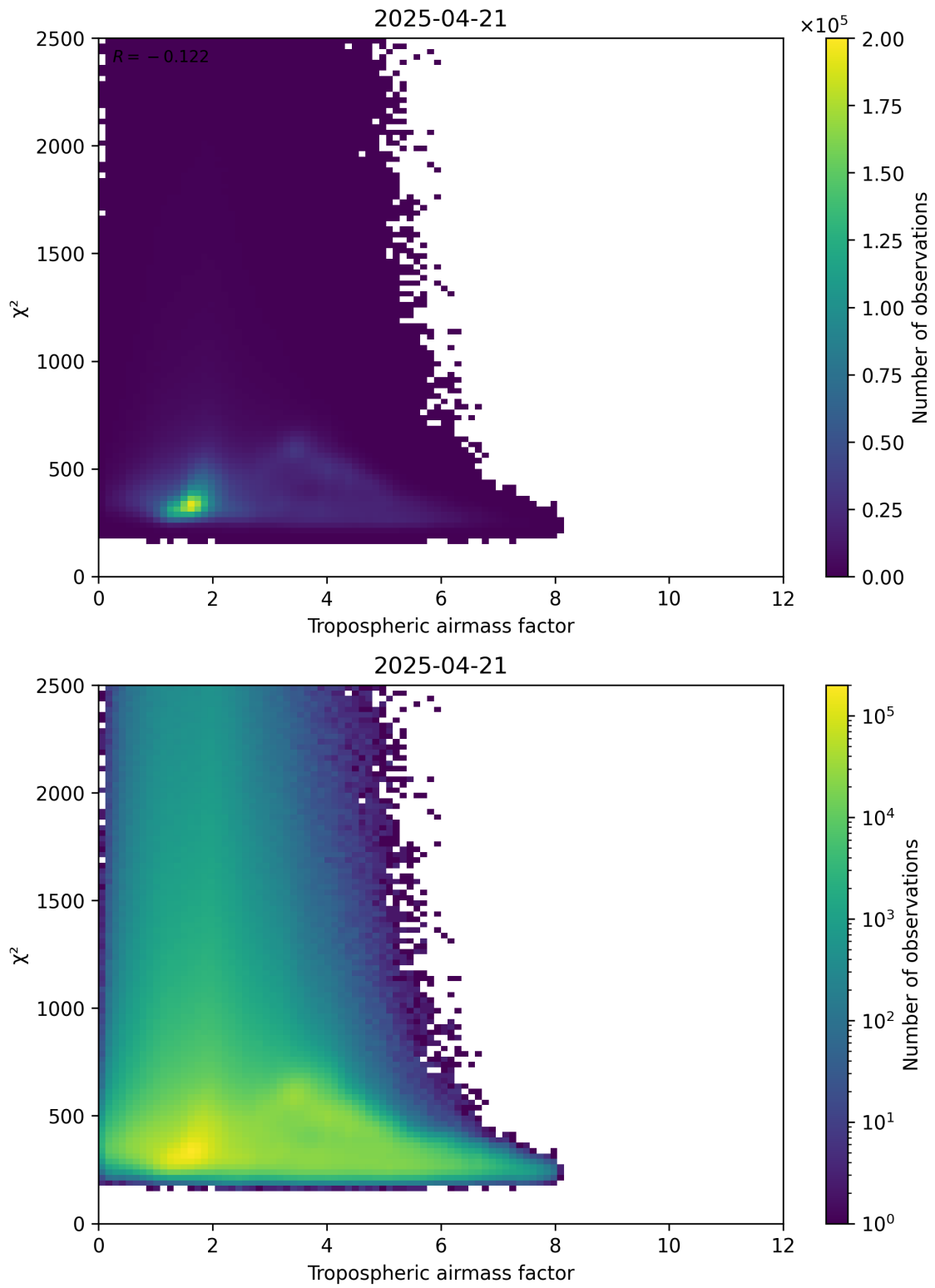
Figure 73: Scatter density plot of “Tropospheric airmass factor” against “ \chi^2 ” for 2025-04-21 to 2025-04-22.
