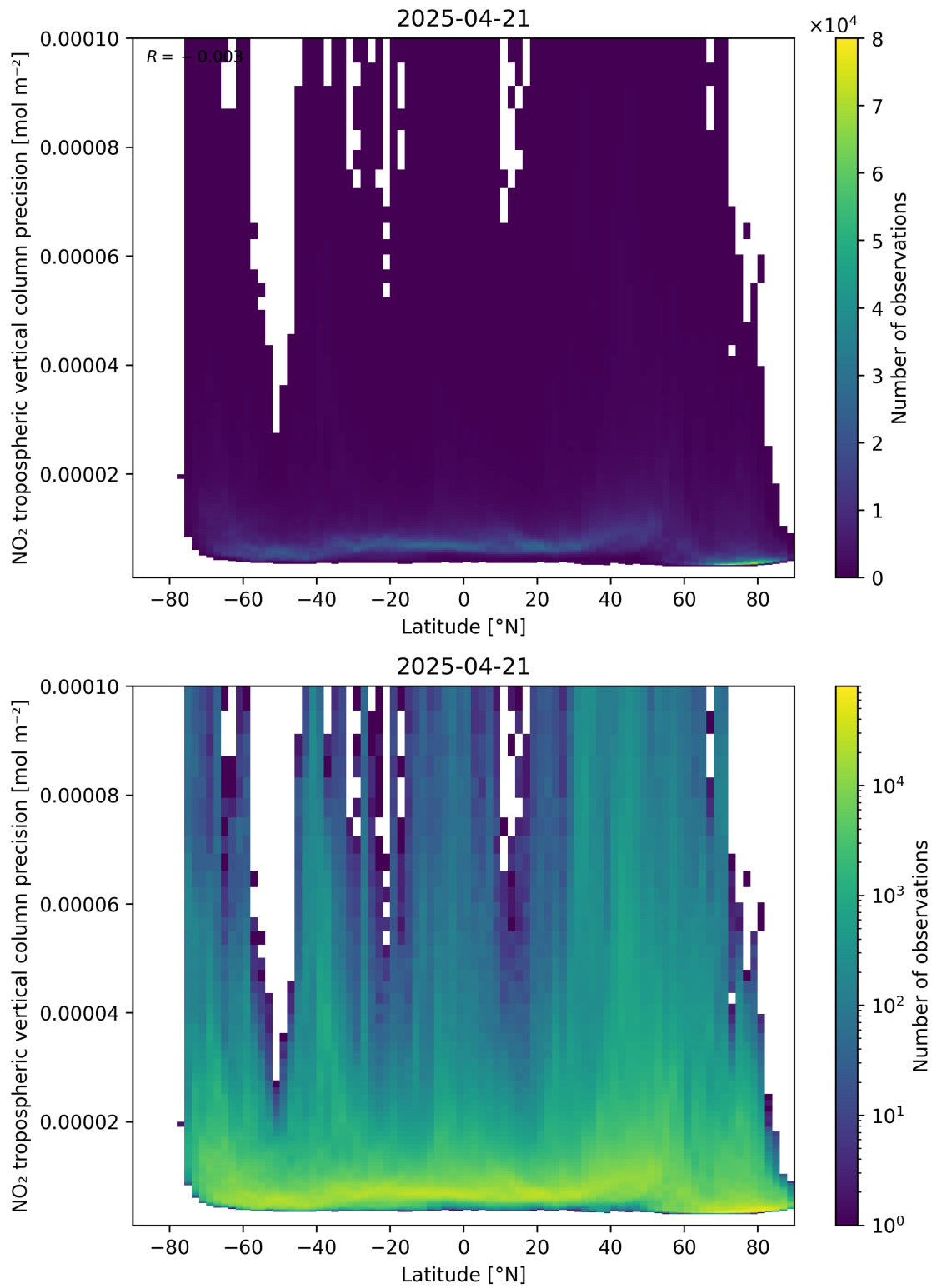
Figure 93: Scatter density plot of “Latitude” against “NO 2 tropospheric vertical column precision” for 2025-04-21 to 2025-04-22.
