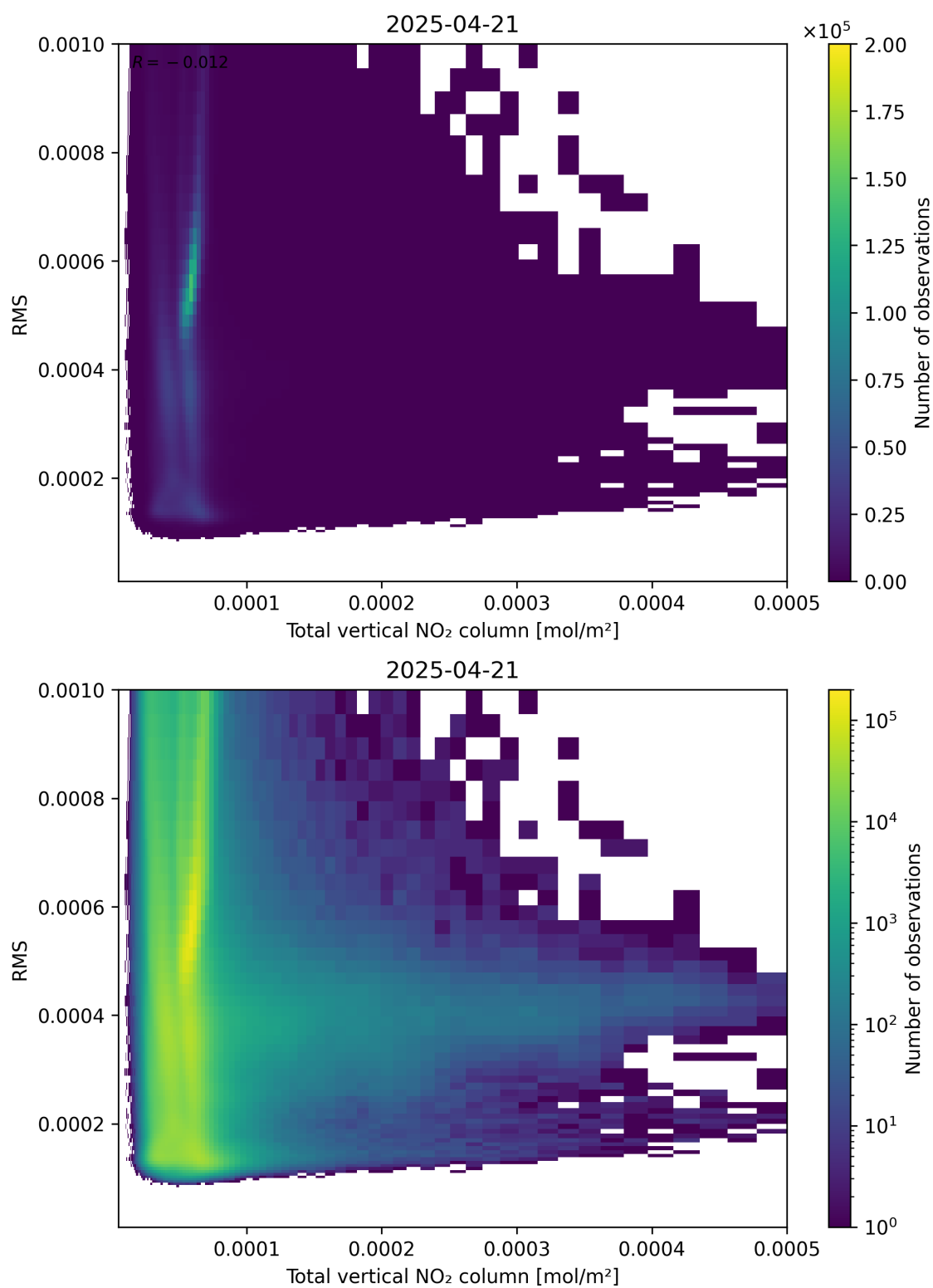
Figure 120: Scatter density plot of “Total vertical NO 2 column” against “RMS” for 2025-04-21 to 2025-04-22.
