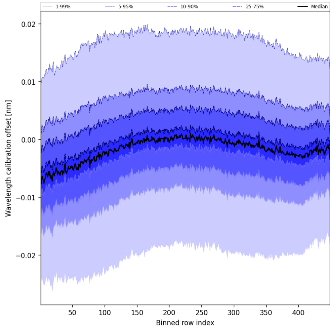
Figure 52: Along track statistics of “Wavelength calibration offset” for 2025-04-21 to 2025-04-22
