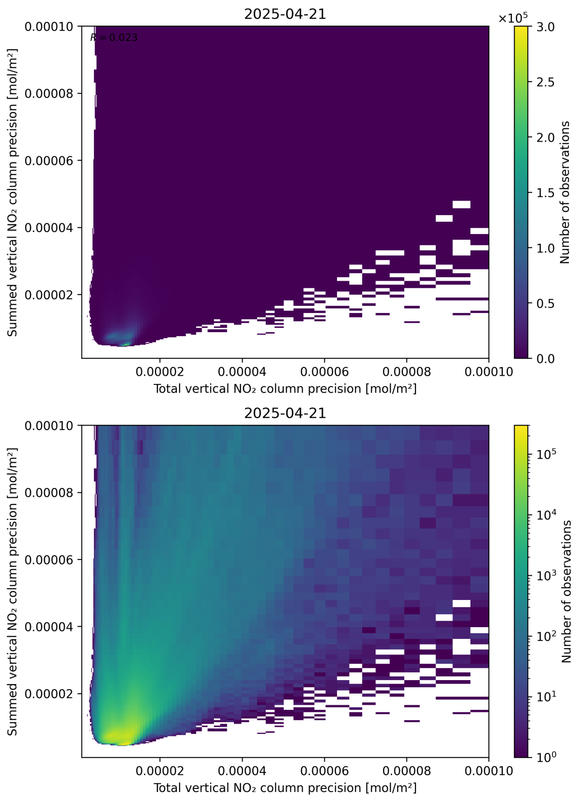
Figure 118: Scatter density plot of “Total vertical NO 2 column precision” against “Summed vertical NO 2 column precision” for 2025-04-21 to 2025-04-22.
