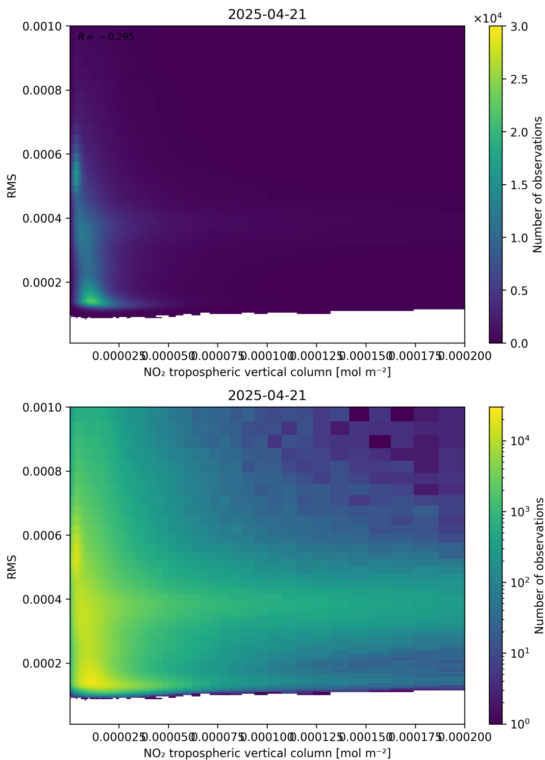
Figure 142: Scatter density plot of “NO 2 tropospheric vertical column” against “RMS” for 2025-04-21 to 2025-04-22.
