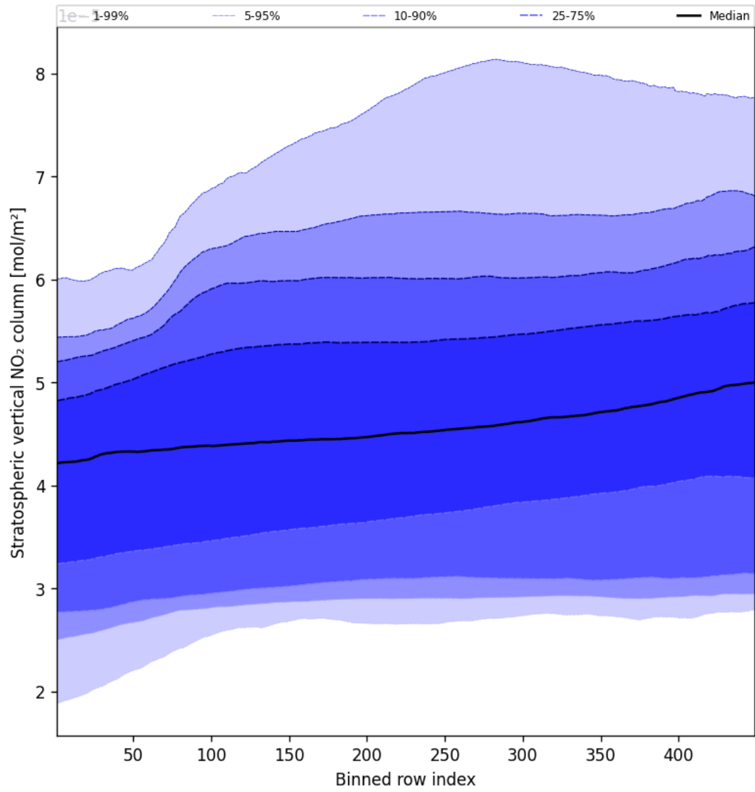
Figure 53: Along track statistics of “Stratospheric vertical NO 2 column” for 2025-04-21 to 2025-04-22
