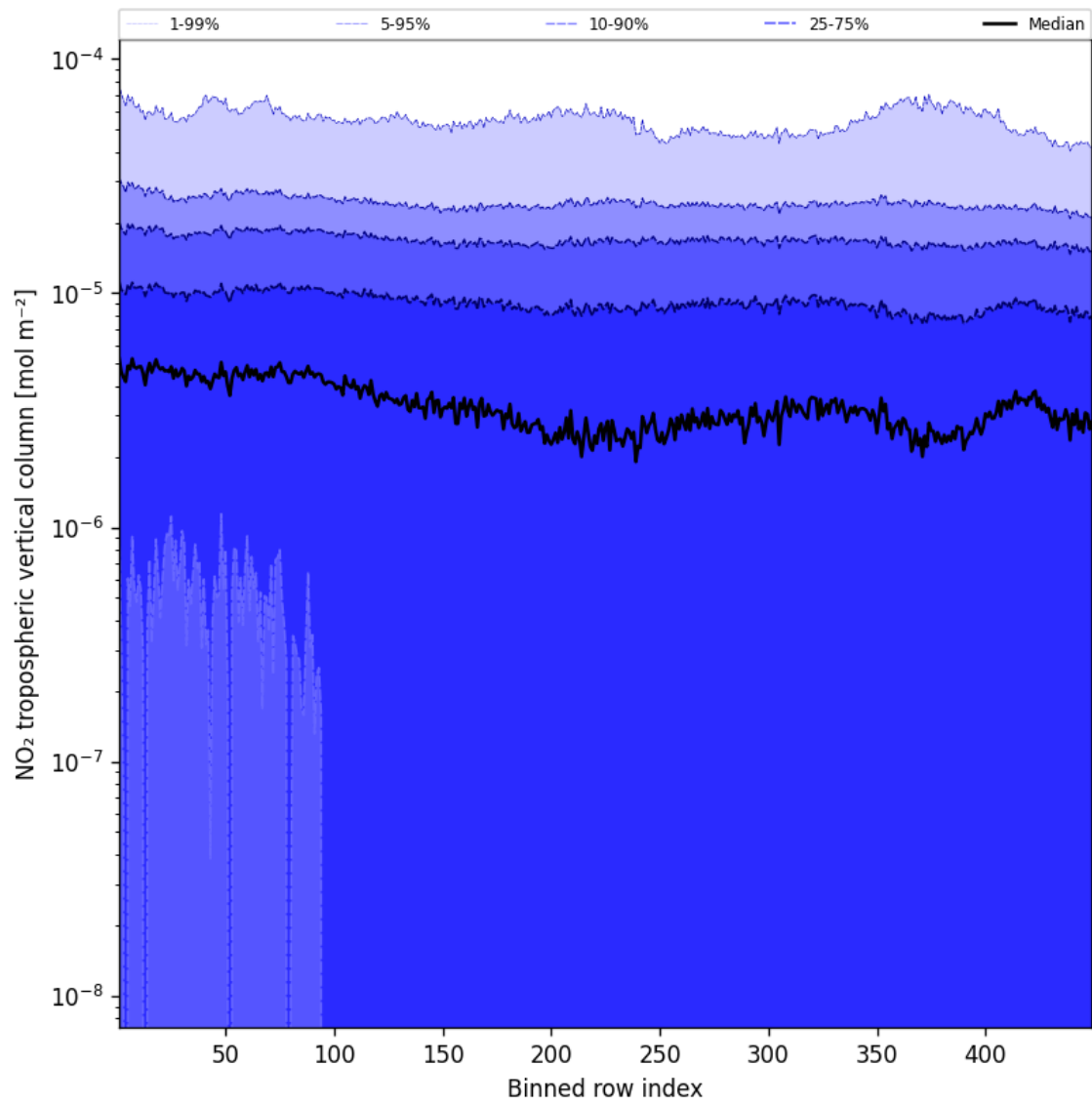
Figure 46: Along track statistics of “NO 2 tropospheric vertical column” for 2025-04-21 to 2025-04-22
