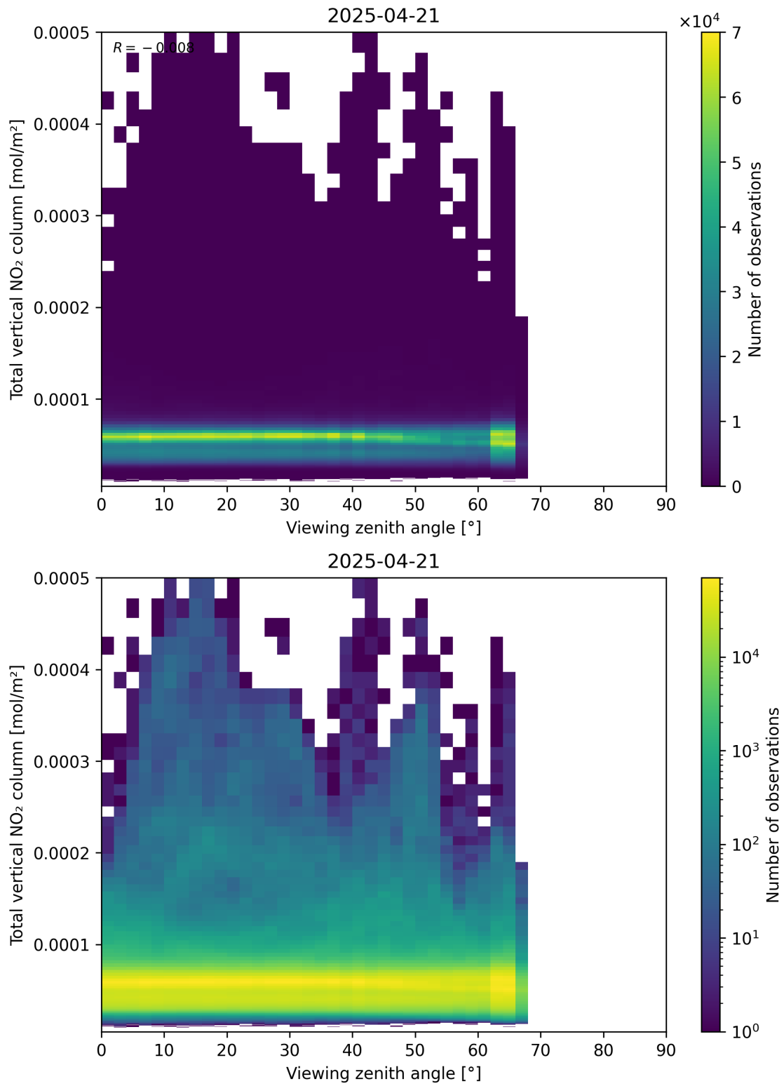
Figure 167: Scatter density plot of “Viewing zenith angle” against “Total vertical NO 2 column” for 2025-04-21 to 2025-04-22.
