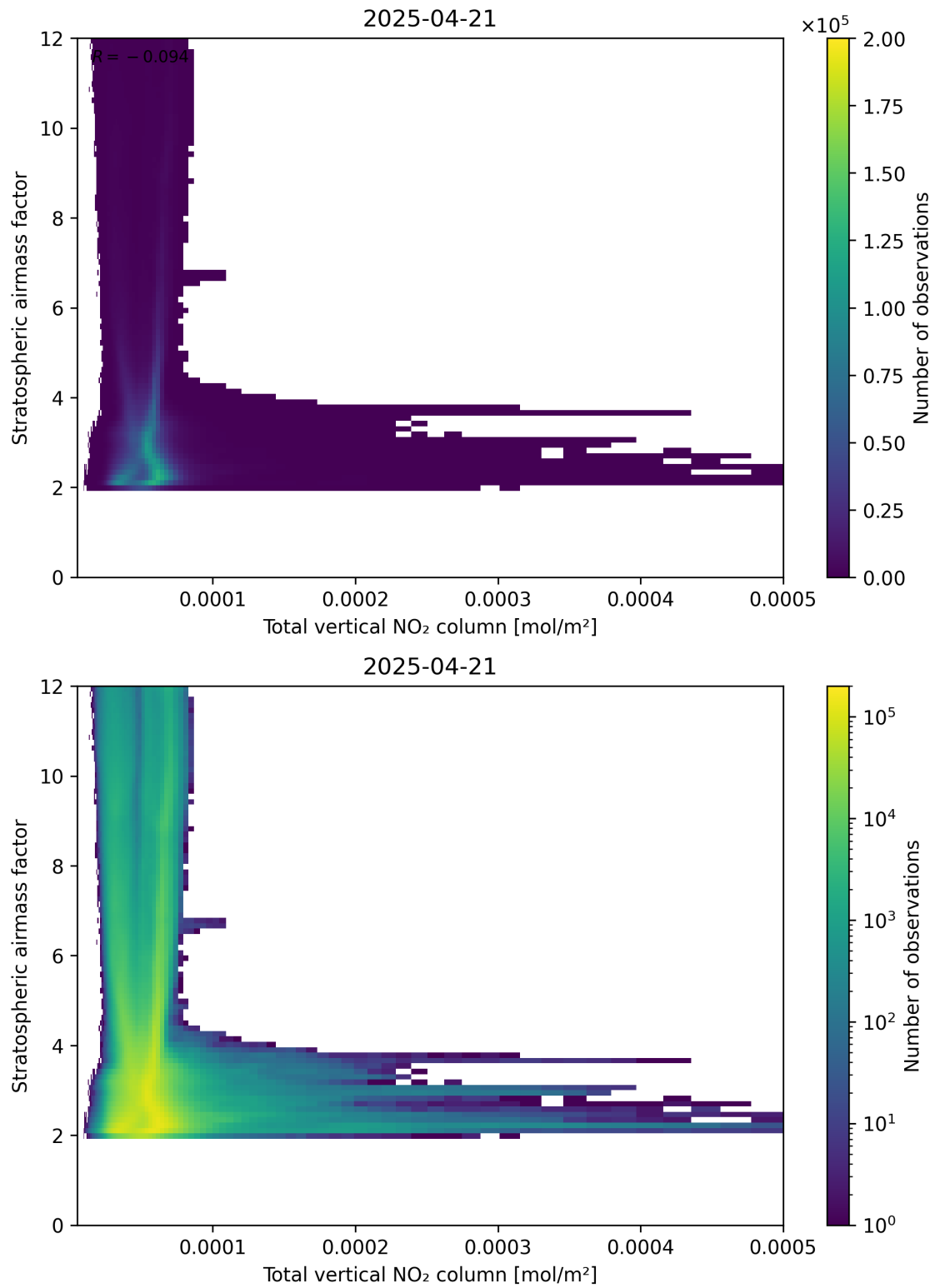
Figure 110: Scatter density plot of “Total vertical NO 2 column” against “Stratospheric airmass factor” for 2025-04-21 to 2025-04-22.
