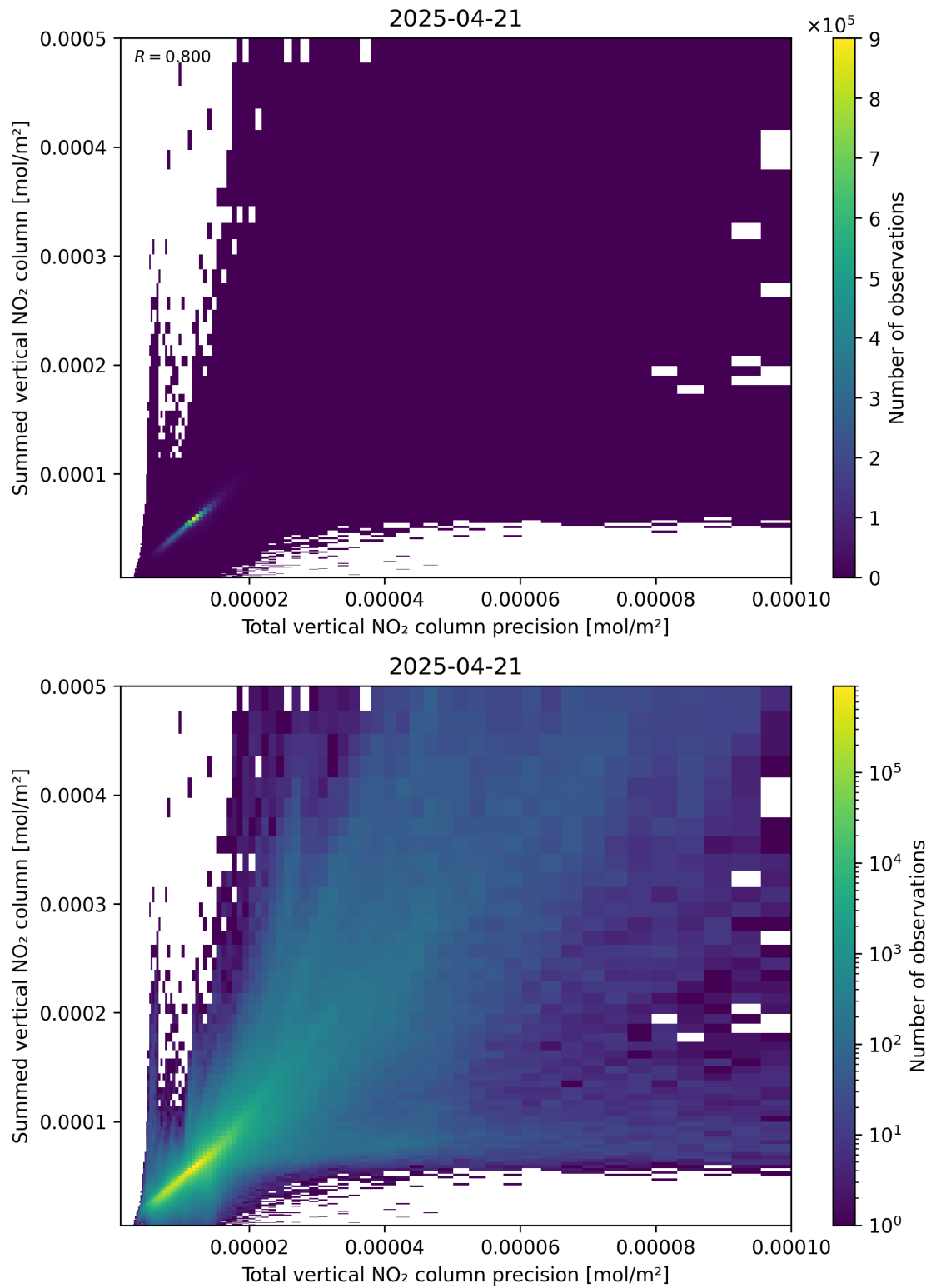
Figure 117: Scatter density plot of “Total vertical NO 2 column precision” against “Summed vertical NO 2 column” for 2025-04-21 to 2025-04-22.
