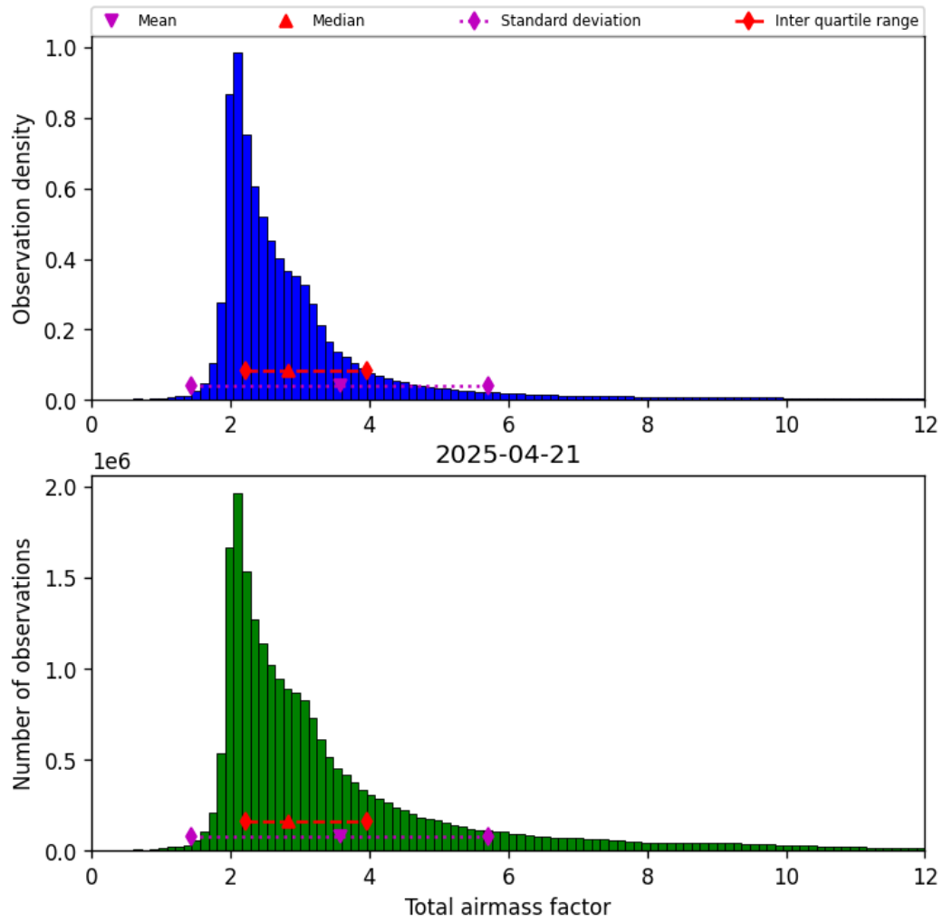
Figure 32: Histogram of “Total airmass factor” for 2025-04-21 to 2025-04-22
