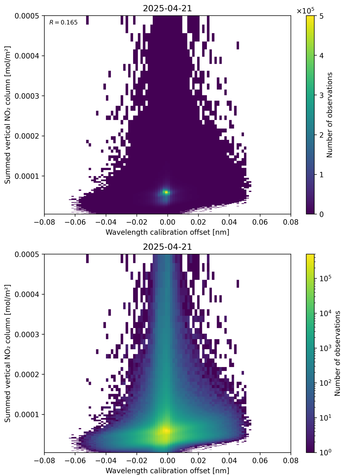
Figure 177: Scatter density plot of “Wavelength calibration offset” against “Summed vertical NO 2 column” for 2025-04-21 to 2025-04-22.
