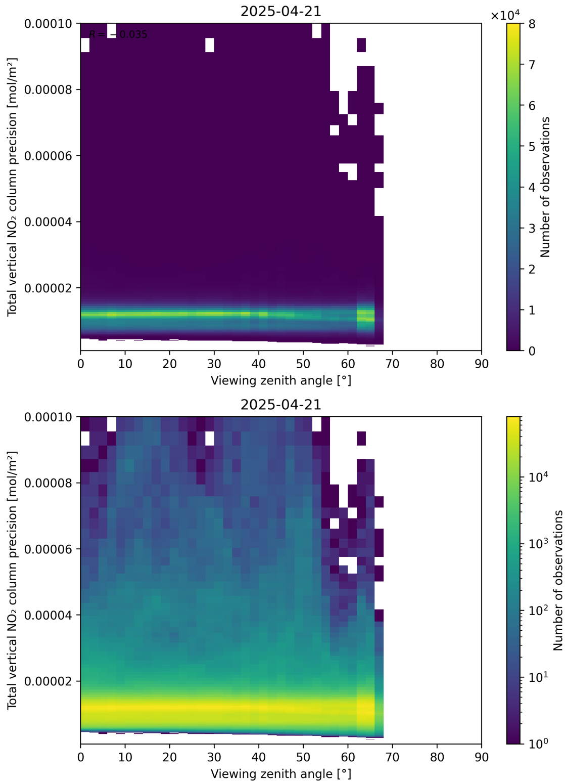
Figure 168: Scatter density plot of “Viewing zenith angle” against “Total vertical NO 2 column precision” for 2025-04-21 to 2025-04-22.
