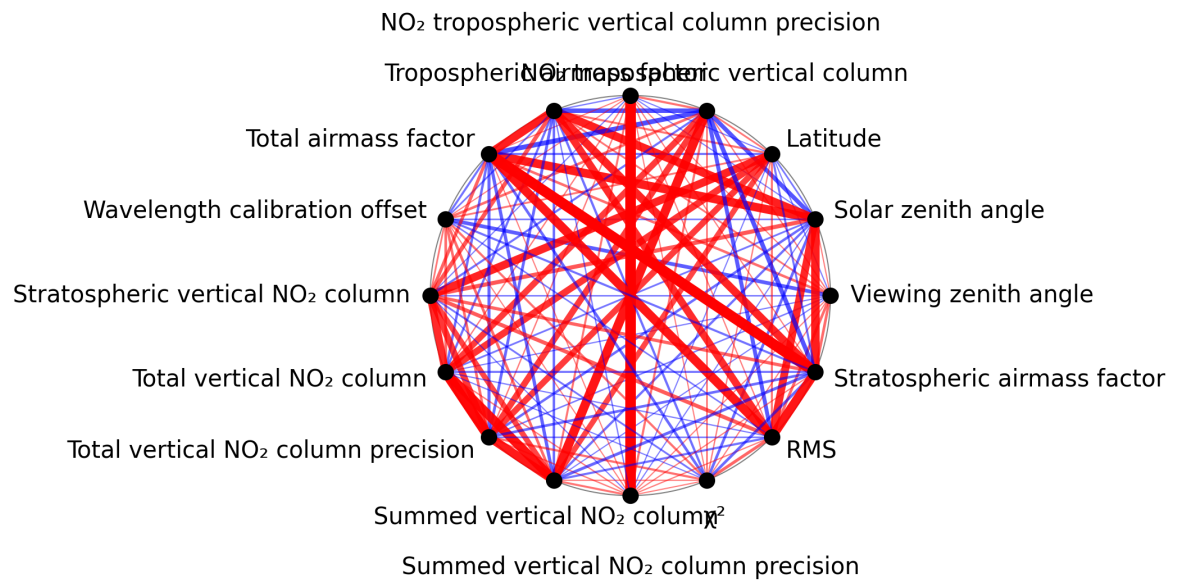
Figure 1: Map of correlation graph for 2025-04-21 to 2025-04-22.
