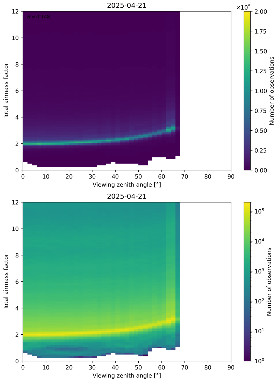
Figure 160: Scatter density plot of “Viewing zenith angle” against “Total airmass factor” for 2025-04-21 to 2025-04-22.
