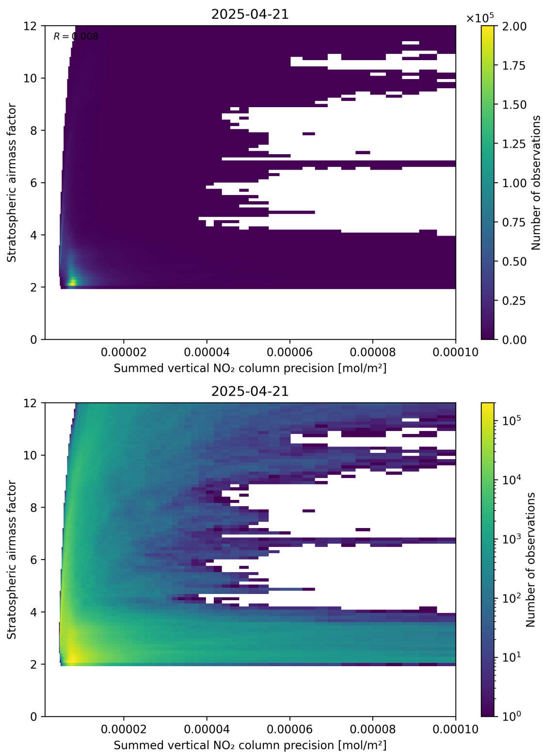
Figure 106: Scatter density plot of “Summed vertical NO 2 column precision” against “Stratospheric airmass factor” for 2025-04-21 to 2025-04-22.
