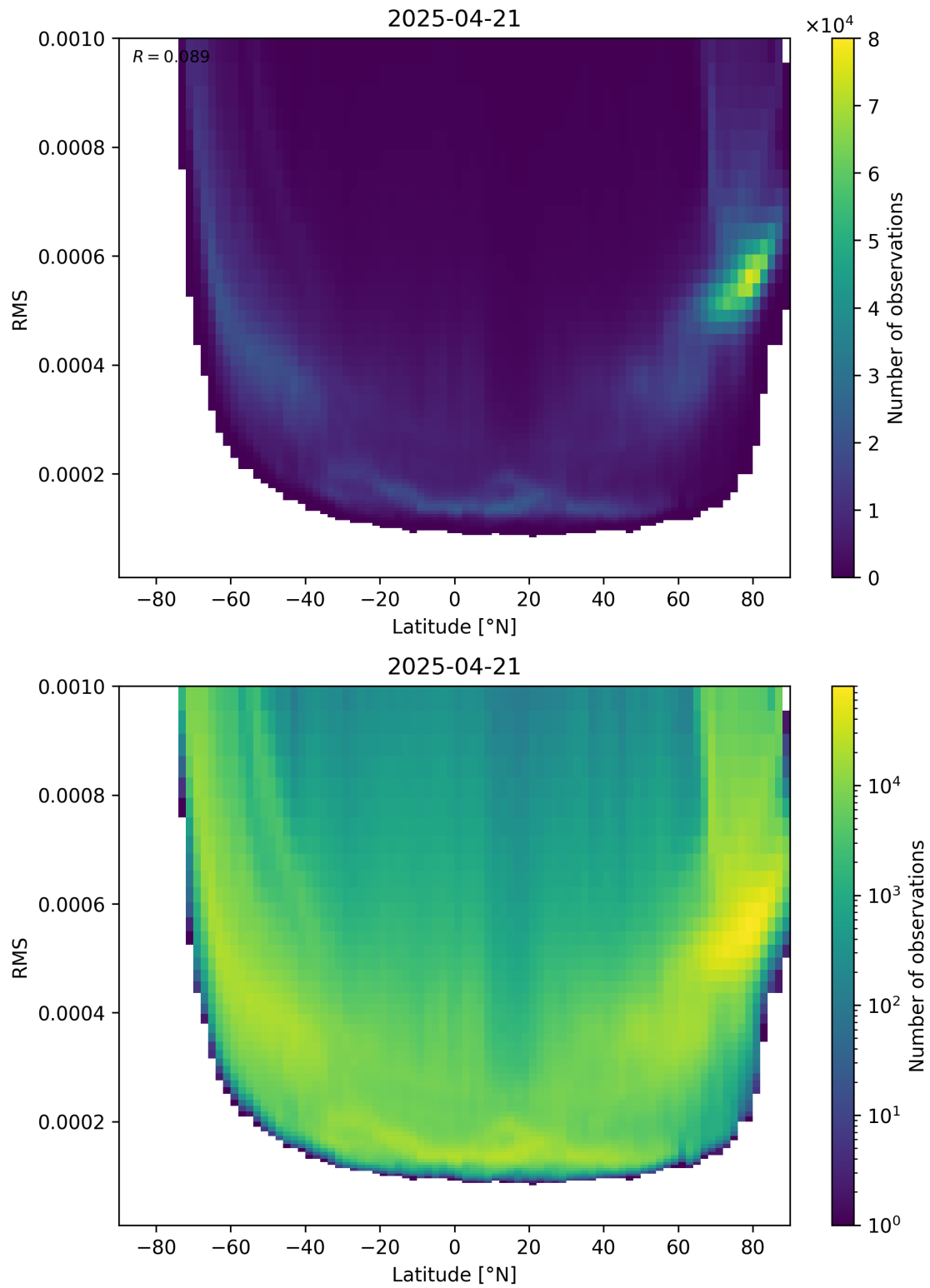
Figure 94: Scatter density plot of “Latitude” against “RMS” for 2025-04-21 to 2025-04-22.
