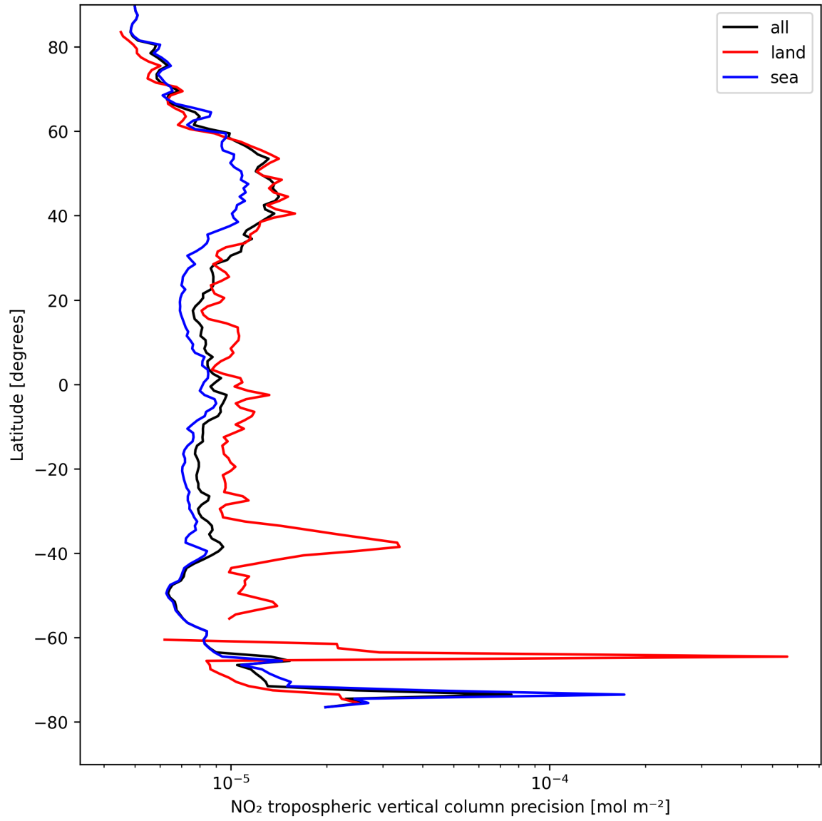
Figure 13: Zonal average of “NO 2 tropospheric vertical column precision” for 2025-04-21 to 2025-04-22.
