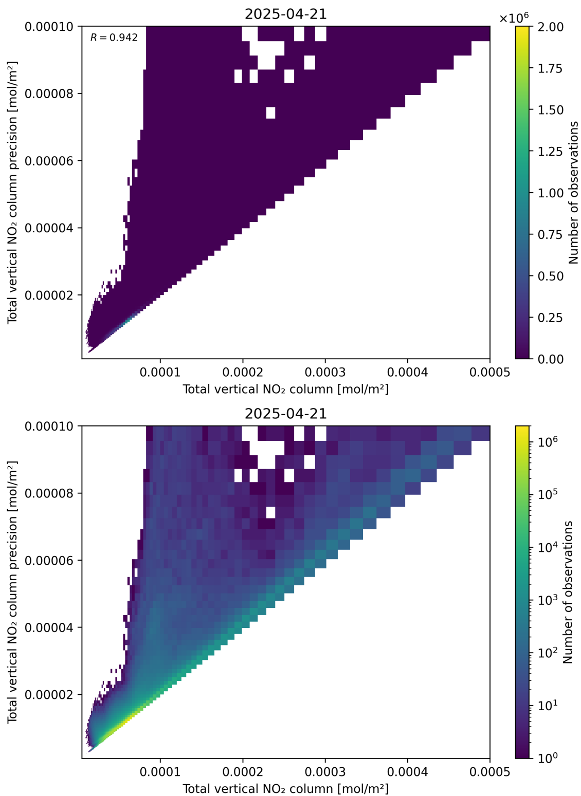
Figure 114: Scatter density plot of “Total vertical NO 2 column” against “Total vertical NO 2 column precision” for 2025-04-21 to 2025-04-22.
