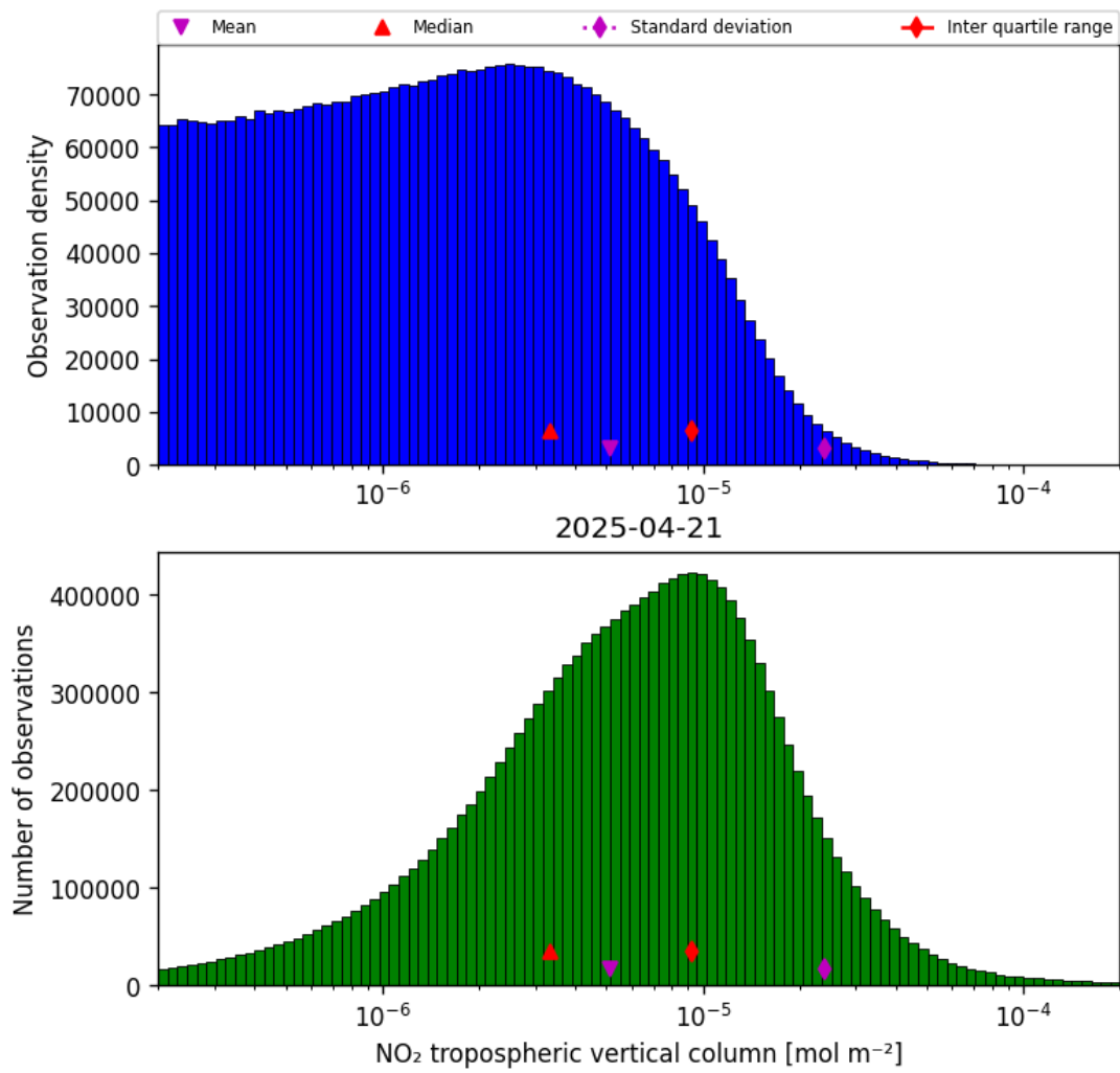
Figure 29: Histogram of “NO 2 tropospheric vertical column” for 2025-04-21 to 2025-04-22
