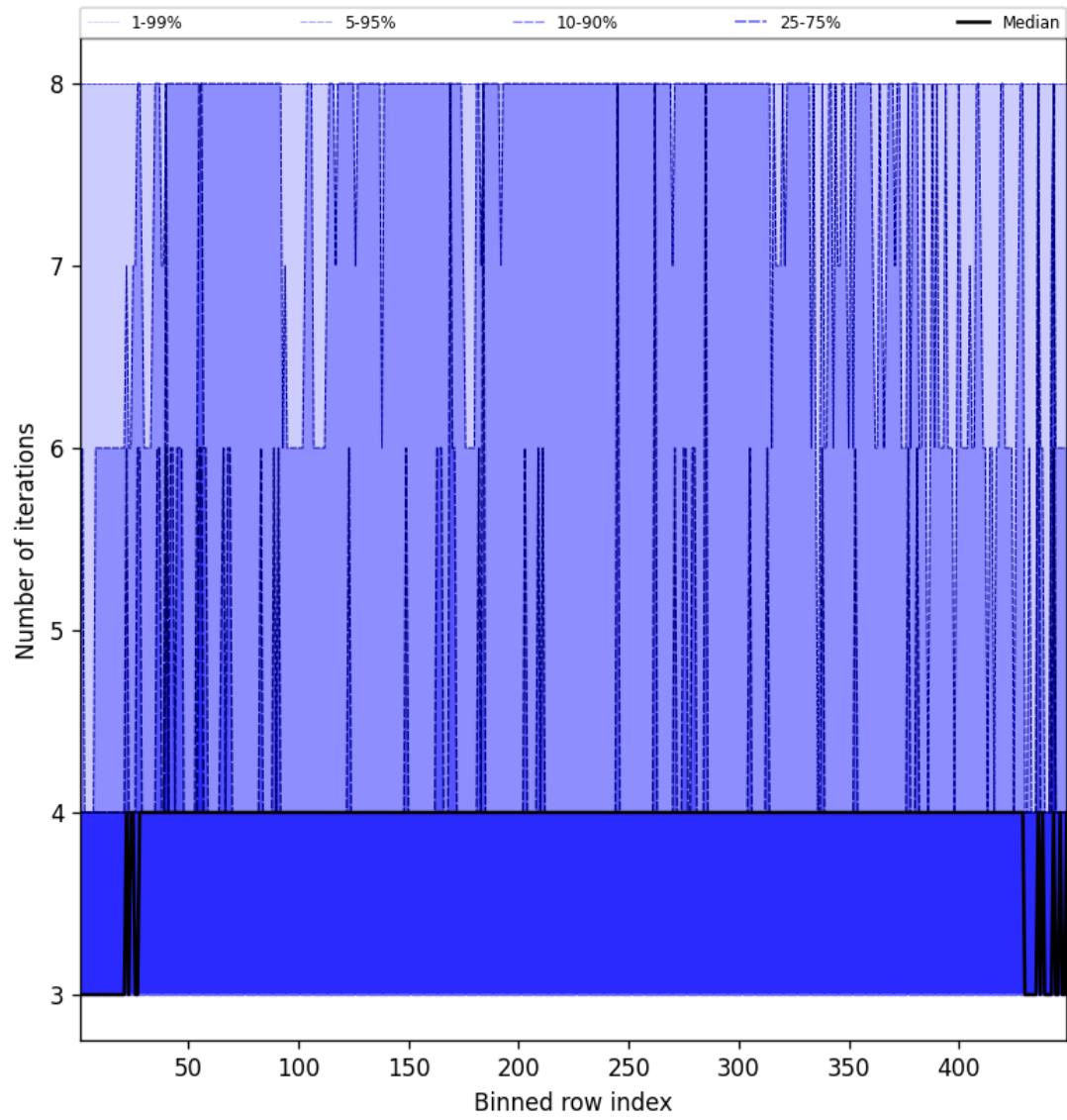
Figure 51: Along track statistics of “Number of iterations” for 2025-04-21 to 2025-04-22
