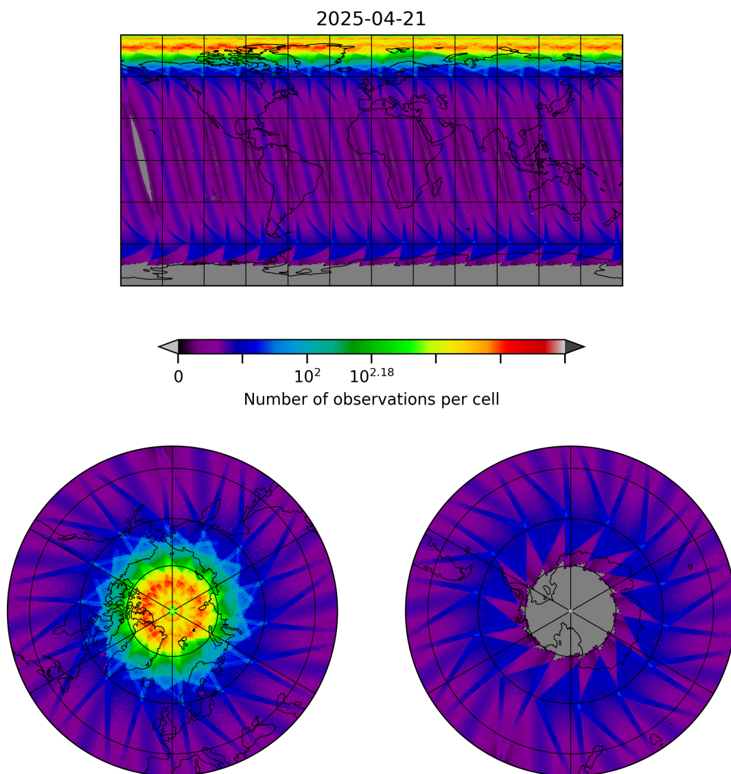
Figure 10: Map of the number of observations for 2025-04-21 to 2025-04-22
