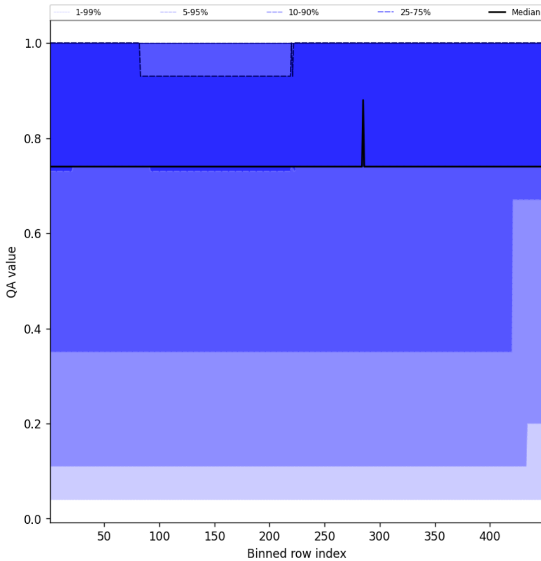
Figure 45: Along track statistics of "QA value" for 2025-04-21 to 2025-04-22
