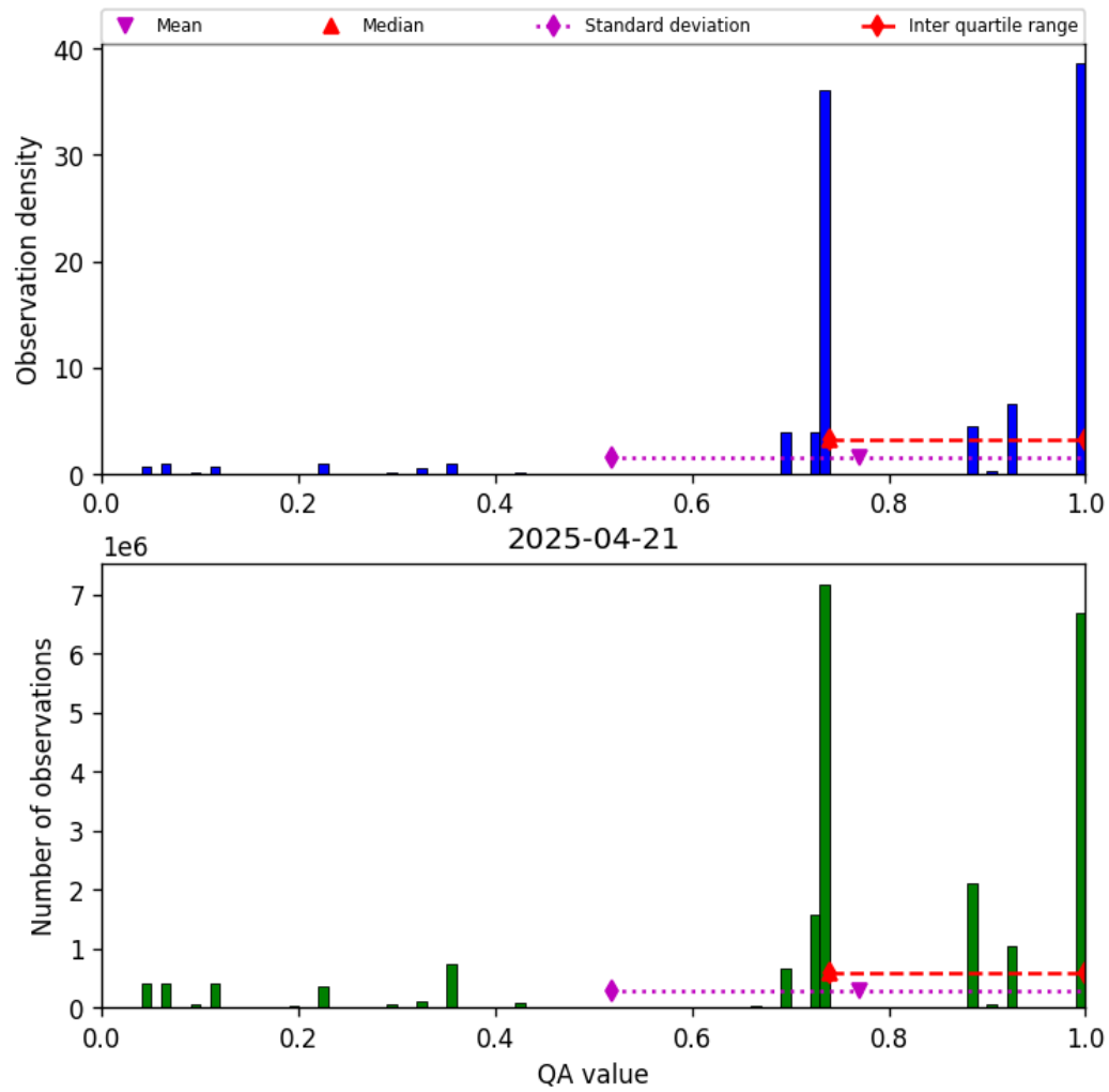
Figure 28: Histogram of “QA value” for 2025-04-21 to 2025-04-22
