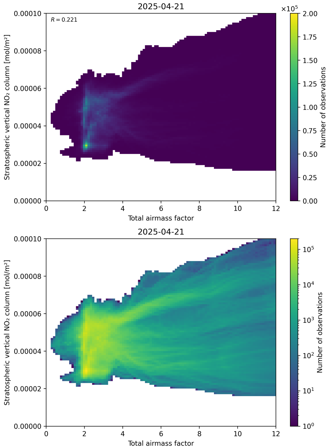
Figure 64: Scatter density plot of “Total airmass factor” against “Stratospheric vertical \text{NO}_2 column” for 2025-04-21 to 2025-04-22.
