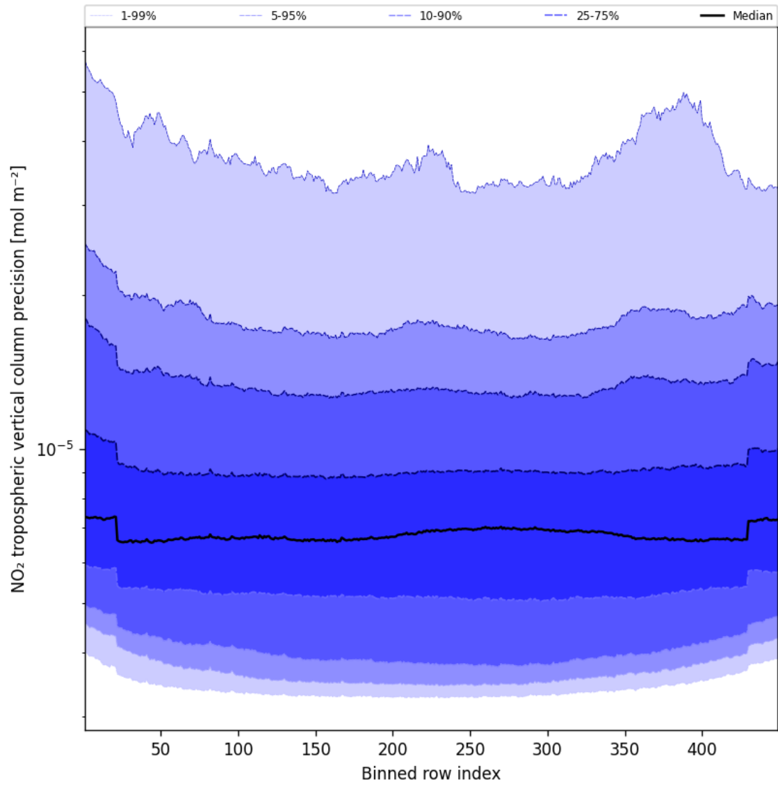
Figure 47: Along track statistics of “NO 2 tropospheric vertical column precision” for 2025-04-21 to 2025-04-22
