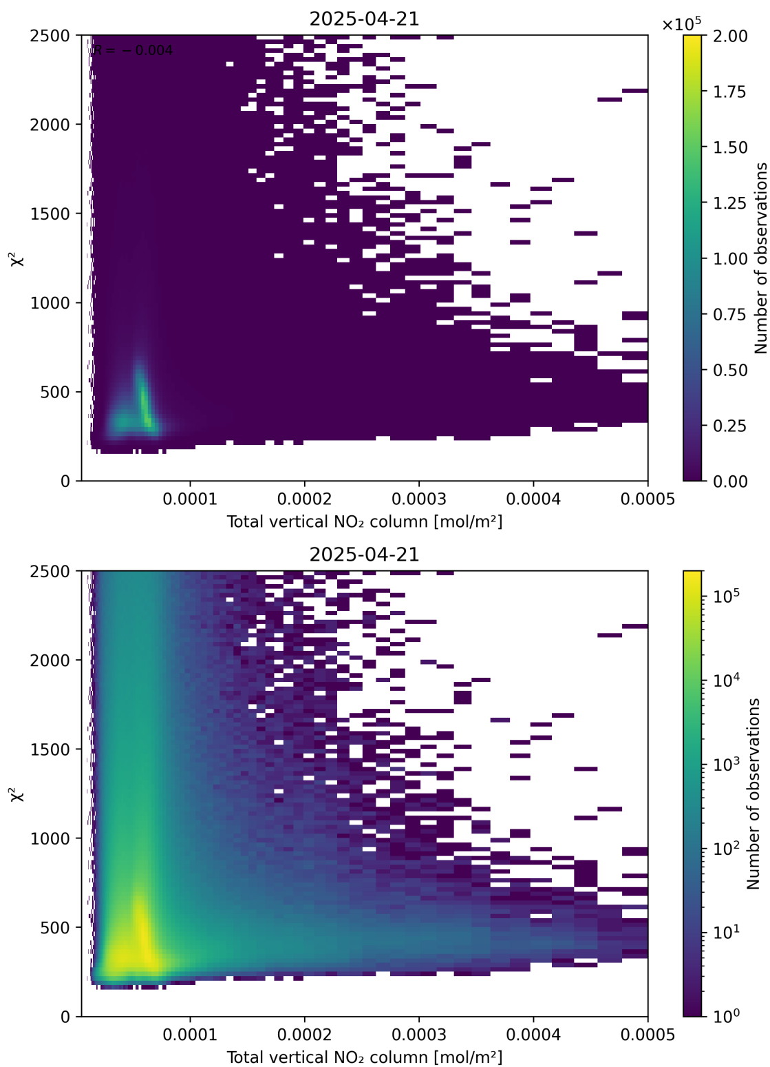
Figure 111: Scatter density plot of “Total vertical NO 2 column” against “ \chi^2 ” for 2025-04-21 to 2025-04-22.
