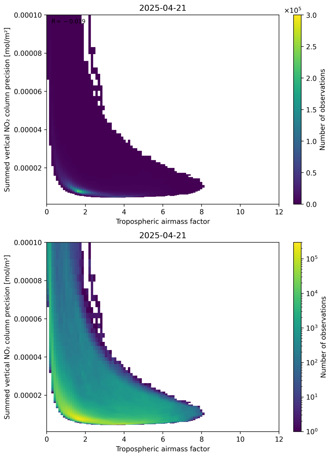
Figure 76: Scatter density plot of “Tropospheric air mass factor” against “Summed vertical NO 2 column precision” for 2025-04-21 to 2025-04-22.
