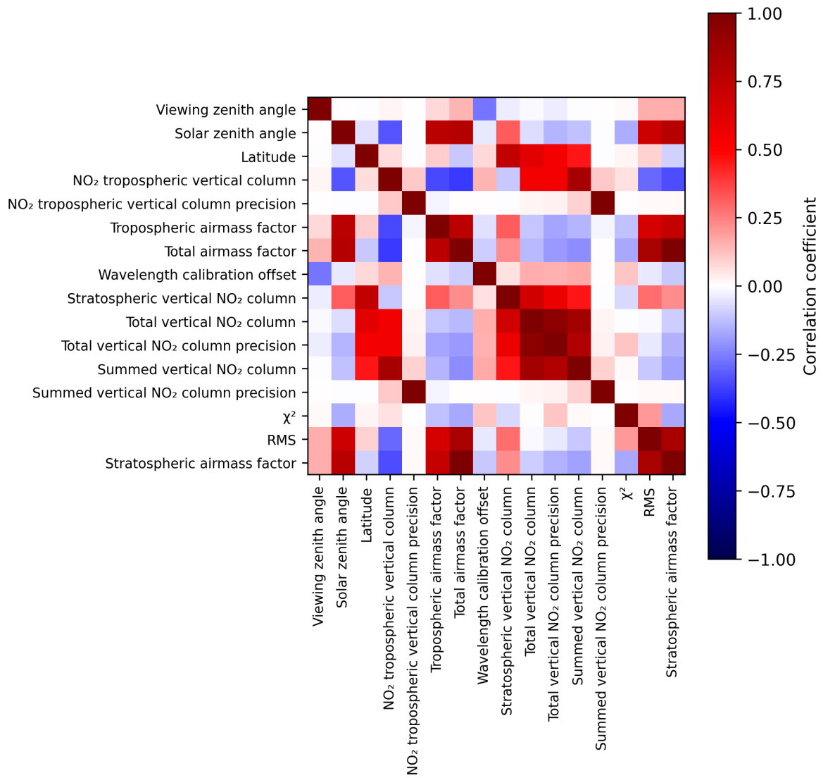
Figure 2: Map of correlation matrix for 2025-04-21 to 2025-04-22.
