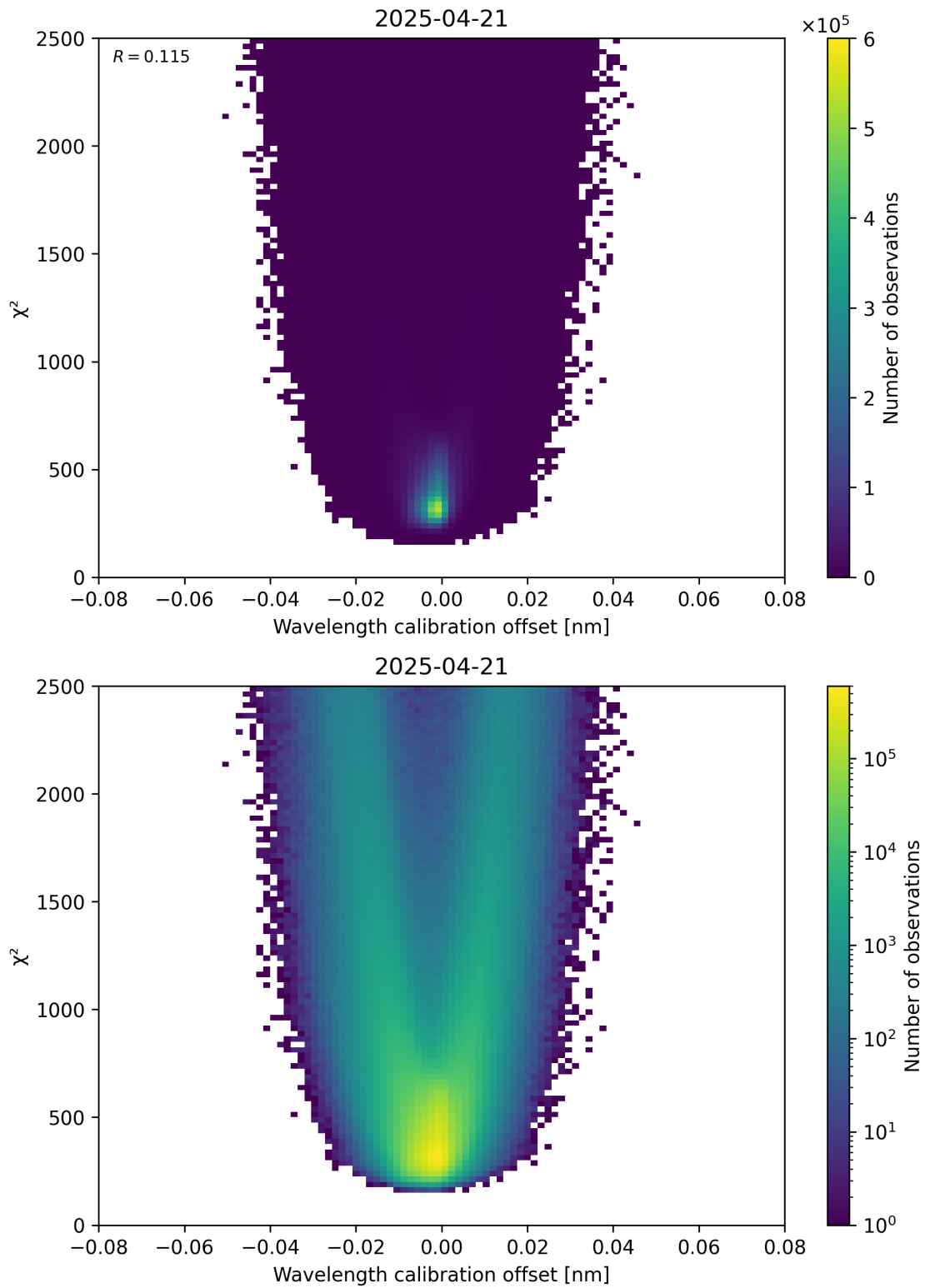
Figure 175: Scatter density plot of “Wavelength calibration offset” against “ \chi^2 ” for 2025-04-21 to 2025-04-22.
