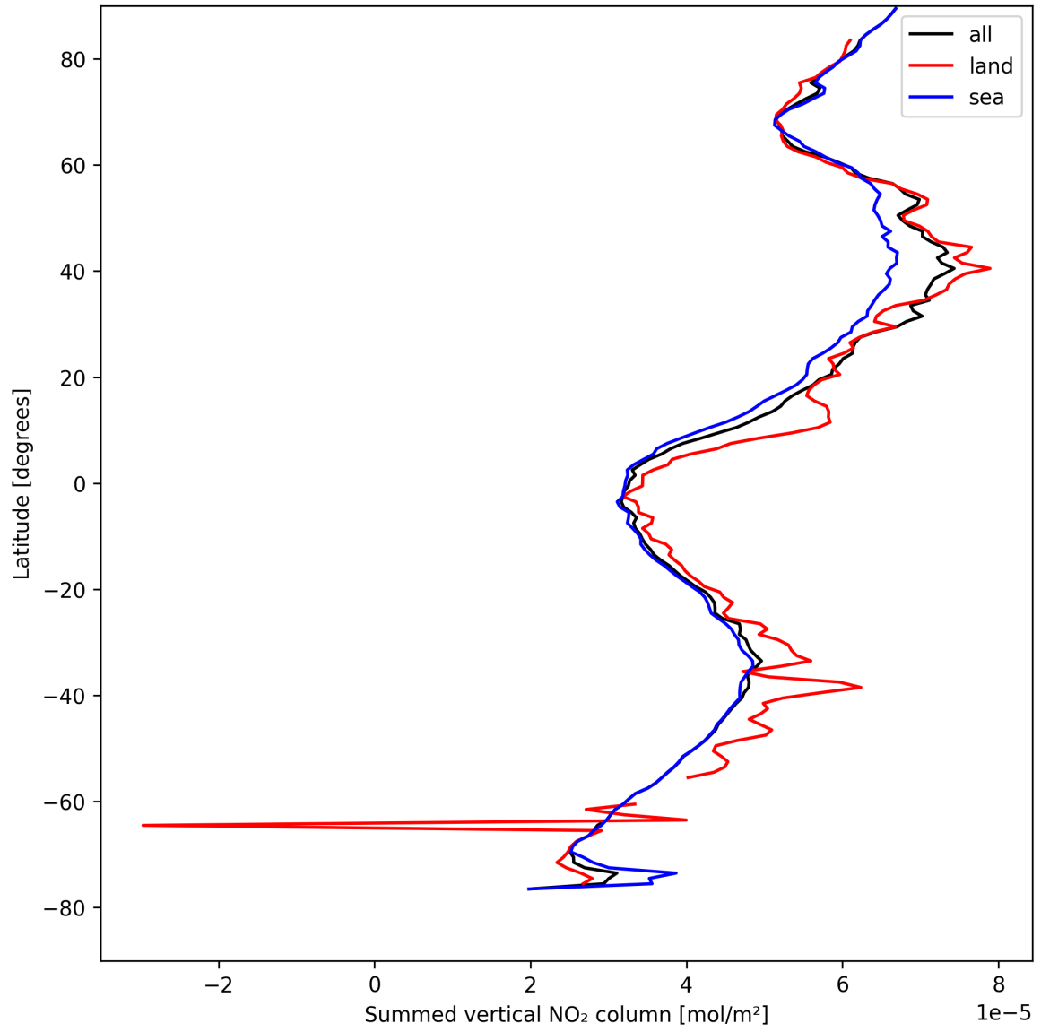
Figure 23: Zonal average of “Summed vertical NO 2 column” for 2025-04-21 to 2025-04-22.
