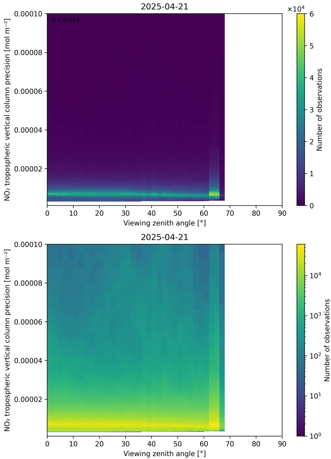
Figure 170: Scatter density plot of “Viewing zenith angle” against “NO 2 tropospheric vertical column precision” for 2025-04-21 to 2025-04-22.
