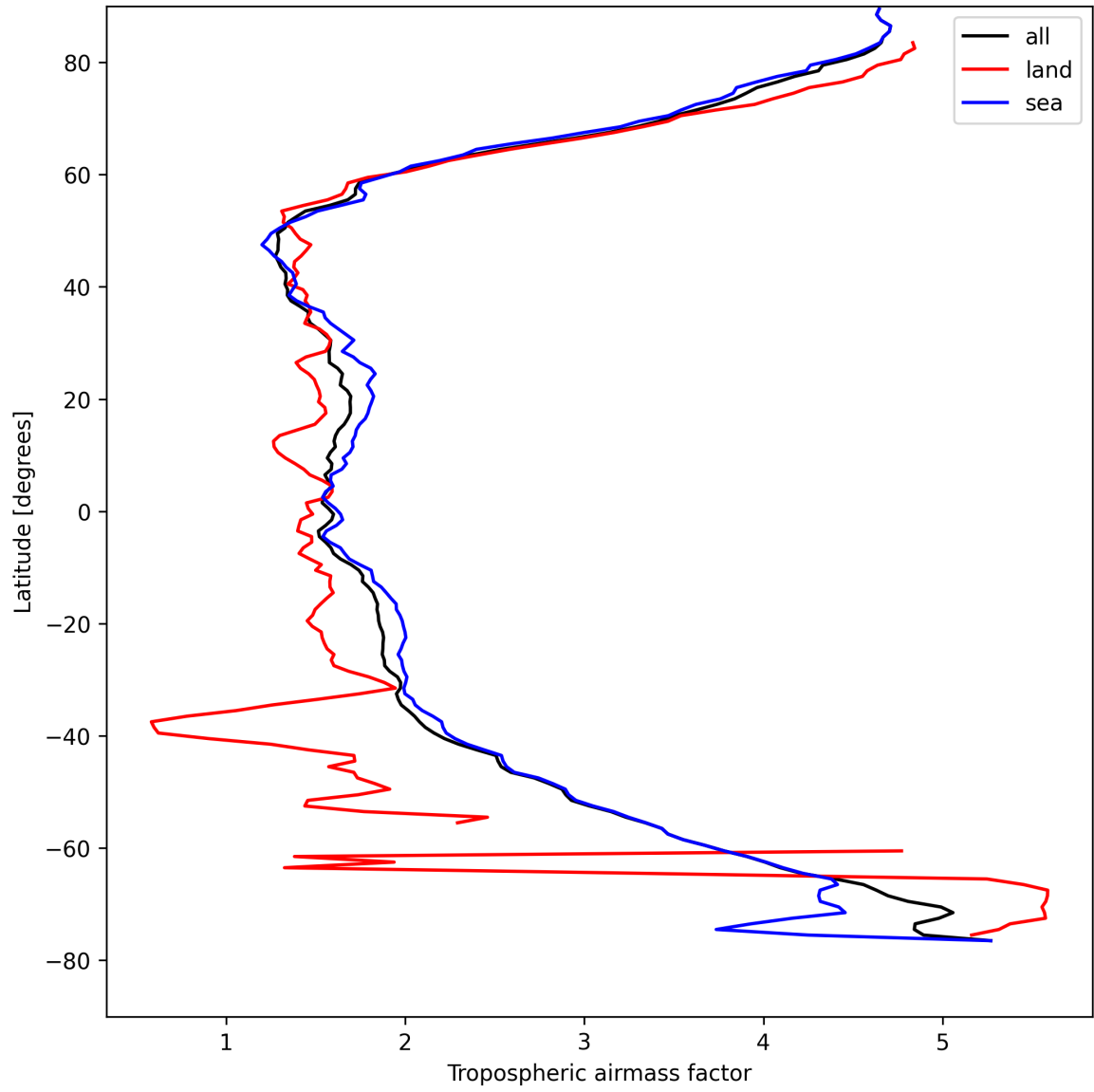
Figure 14: Zonal average of “Tropospheric airmass factor” for 2025-04-21 to 2025-04-22.
