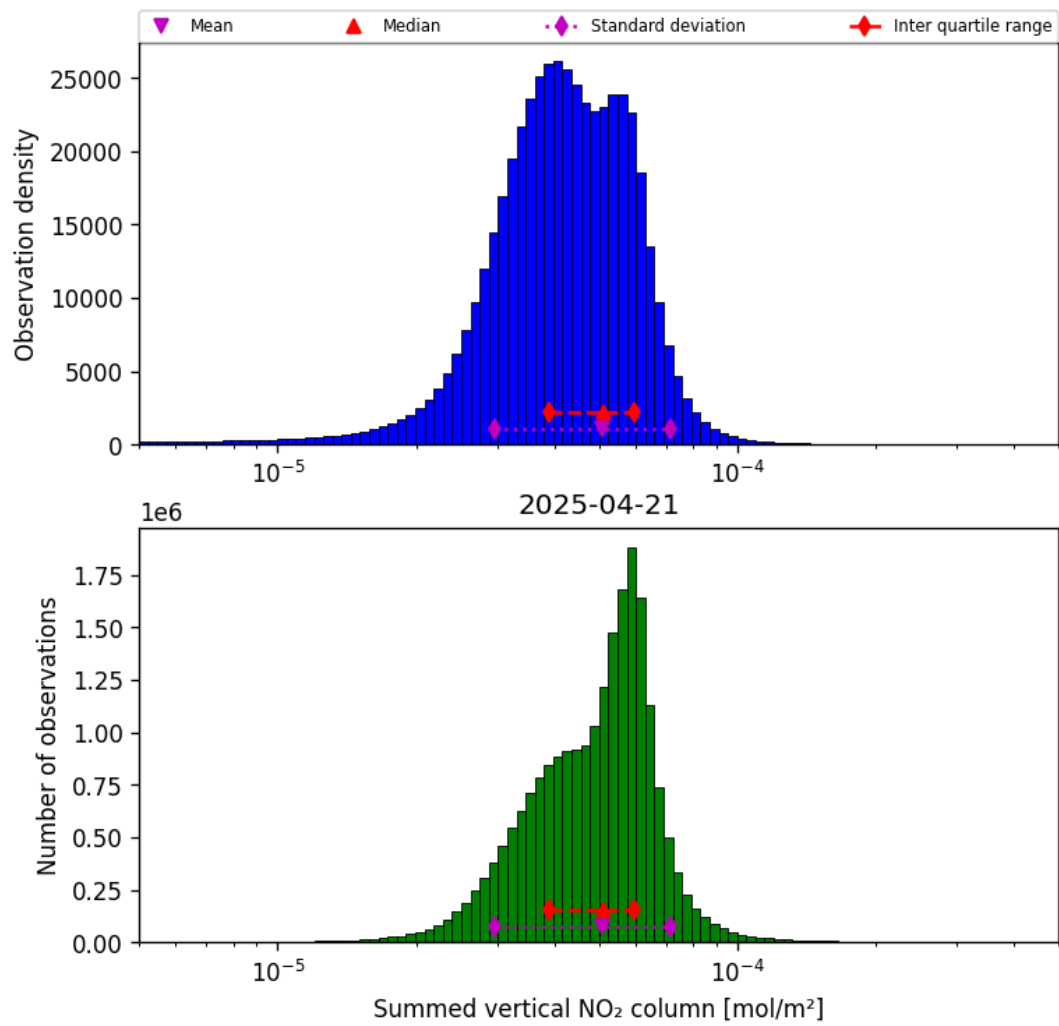
Figure 40: Histogram of “Summed vertical NO 2 column” for 2025-04-21 to 2025-04-22
