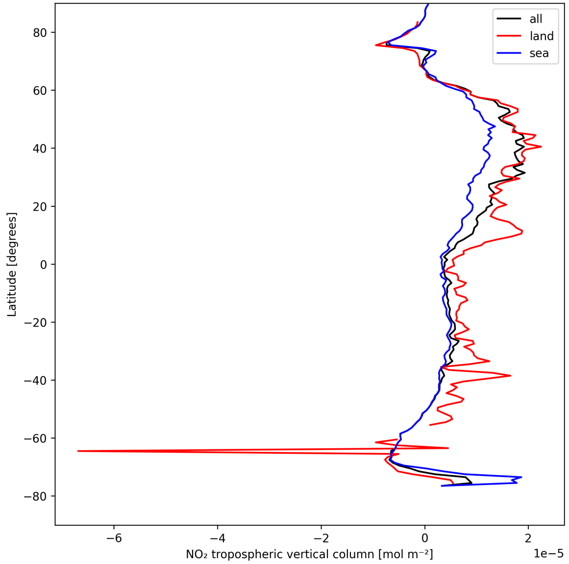
Figure 12: Zonal average of “NO 2 tropospheric vertical column” for 2025-04-21 to 2025-04-22.
