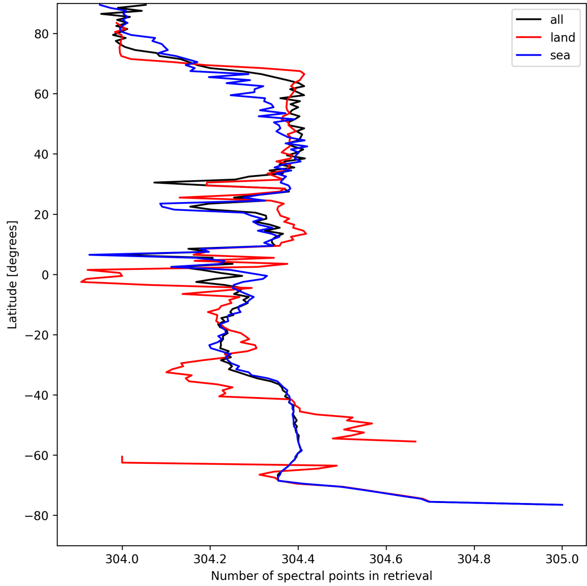
Figure 16: Zonal average of “Number of spectral points in retrieval” for 2025-04-21 to 2025-04-22.
