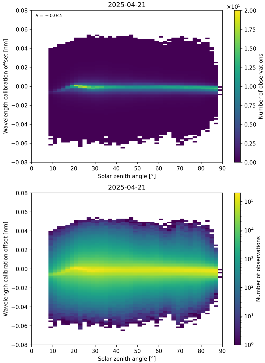
Figure 158: Scatter density plot of “Solar zenith angle” against “Wavelength calibration offset” for 2025-04-21 to 2025-04-22.
