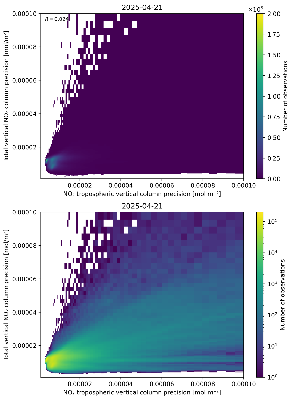
Figure 139: Scatter density plot of “NO 2 tropospheric vertical column precision” against “Total vertical NO 2 column precision” for 2025-04-21 to 2025-04-22.
