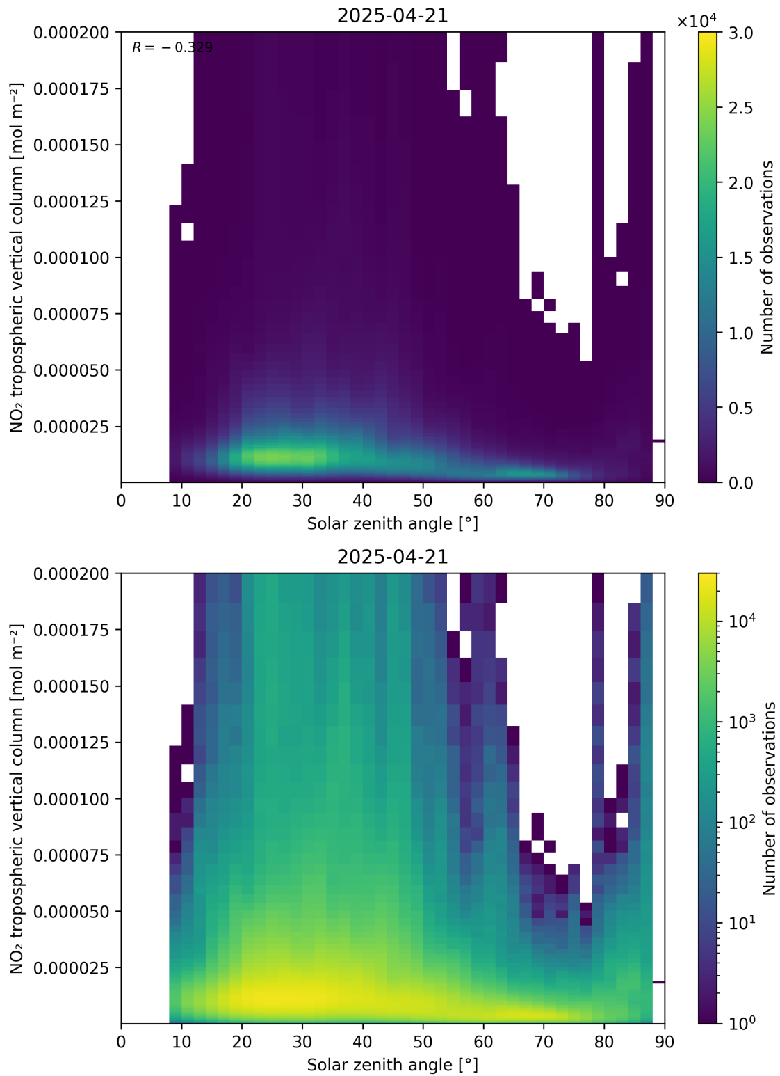
Figure 155: Scatter density plot of “Solar zenith angle” against “NO 2 tropospheric vertical column” for 2025-04-21 to 2025-04-22.
