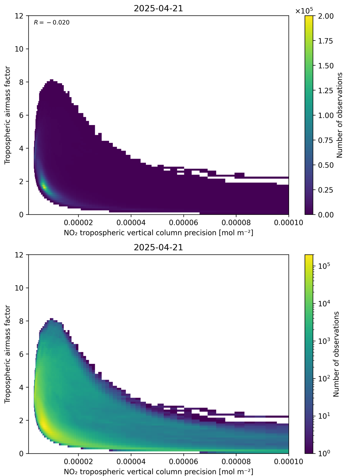
Figure 133: Scatter density plot of “NO 2 tropospheric vertical column precision” against “Tropospheric airmass factor” for 2025-04-21 to 2025-04-22.
