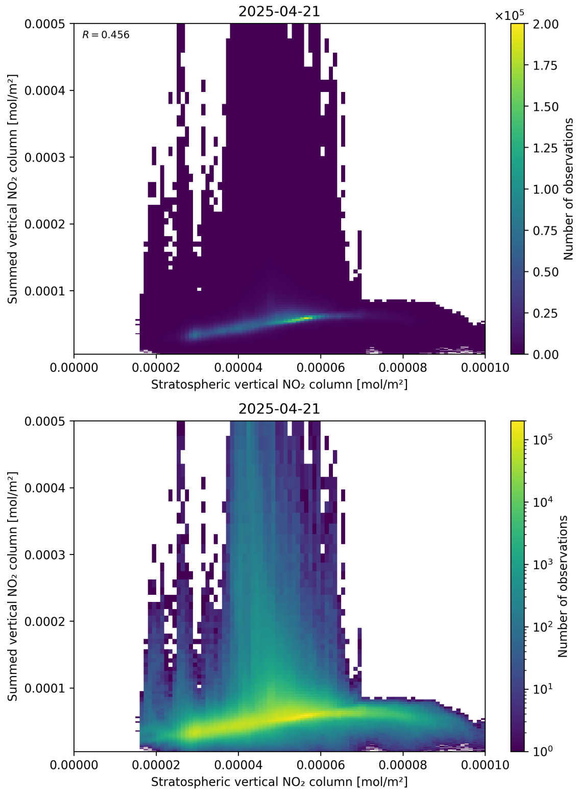
Figure 98: Scatter density plot of “Stratospheric vertical NO 2 column” against “Summed vertical NO 2 column” for 2025-04-21 to 2025-04-22.
