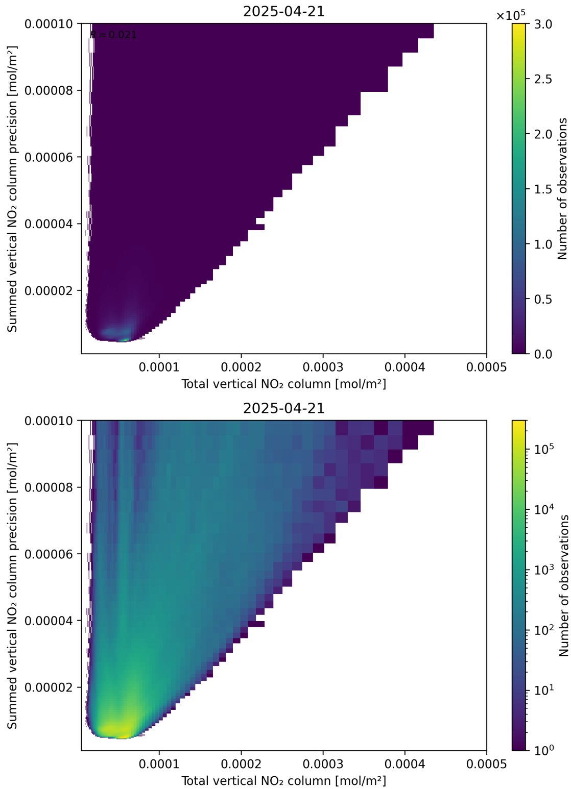
Figure 113: Scatter density plot of “Total vertical NO 2 column” against “Summed vertical NO 2 column precision” for 2025-04-21 to 2025-04-22.
