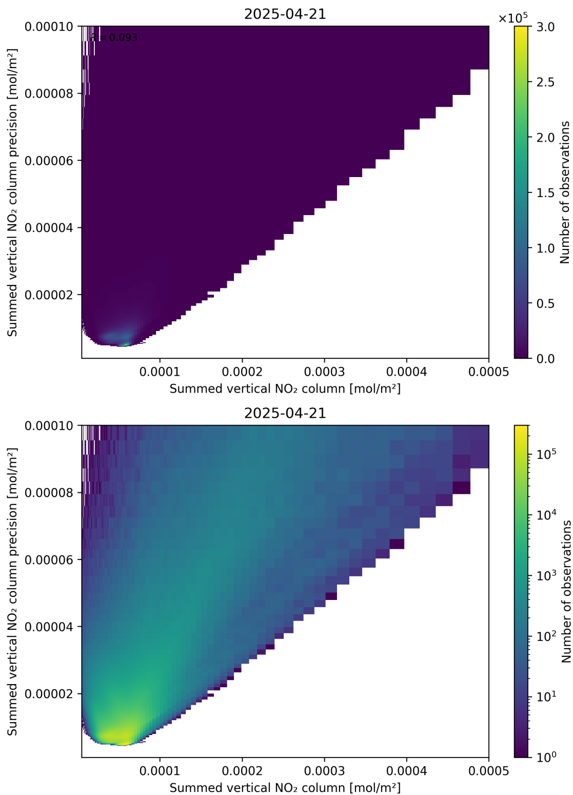
Figure 105: Scatter density plot of “Summed vertical NO 2 column” against “Summed vertical NO 2 column precision” for 2025-04-21 to 2025-04-22.
