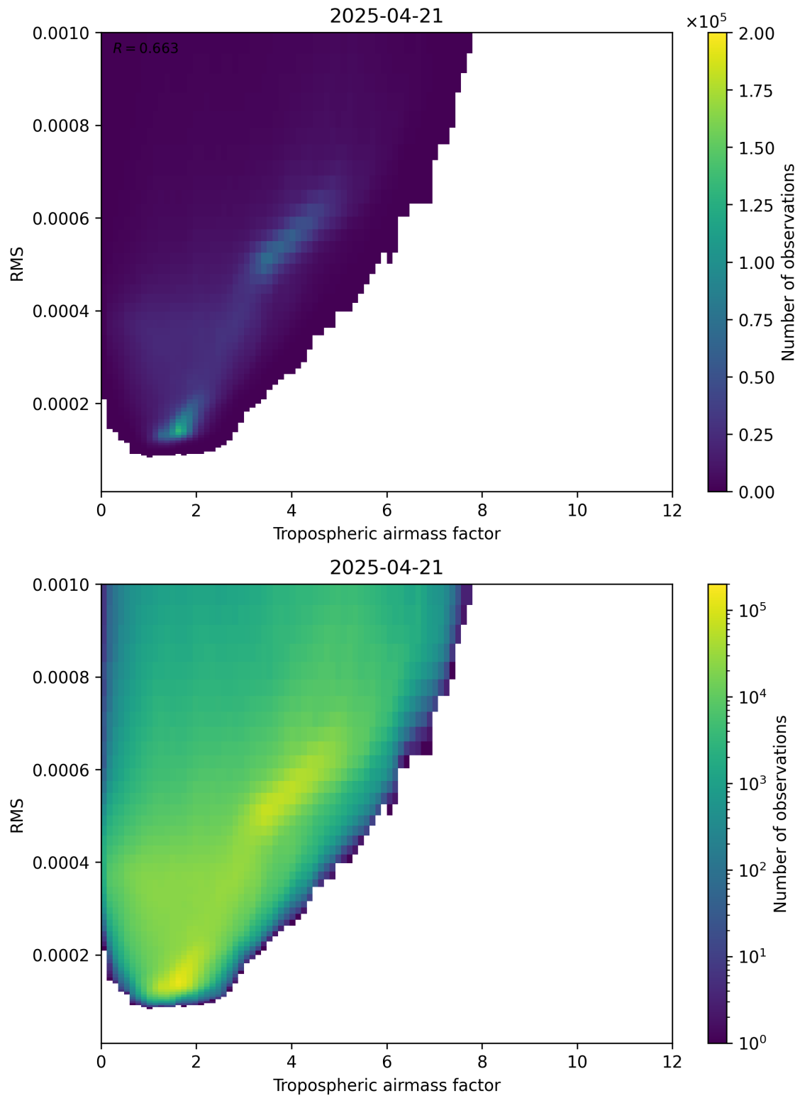
Figure 79: Scatter density plot of “Tropospheric airmass factor” against “RMS” for 2025-04-21 to 2025-04-22.
