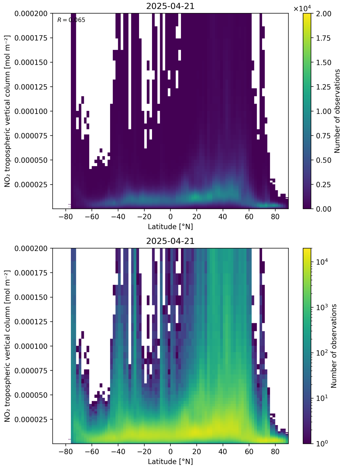
Figure 92: Scatter density plot of “Latitude” against “NO 2 tropospheric vertical column” for 2025-04-21 to 2025-04-22.
