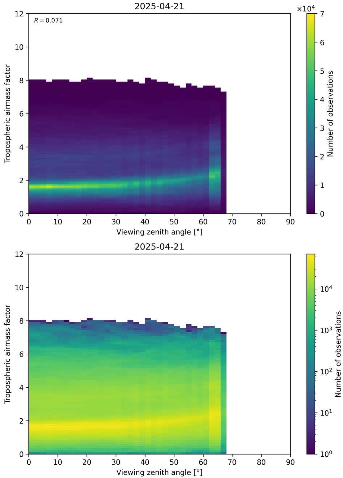
Figure 161: Scatter density plot of “Viewing zenith angle” against “Tropospheric airmass factor” for 2025-04-21 to 2025-04-22.
