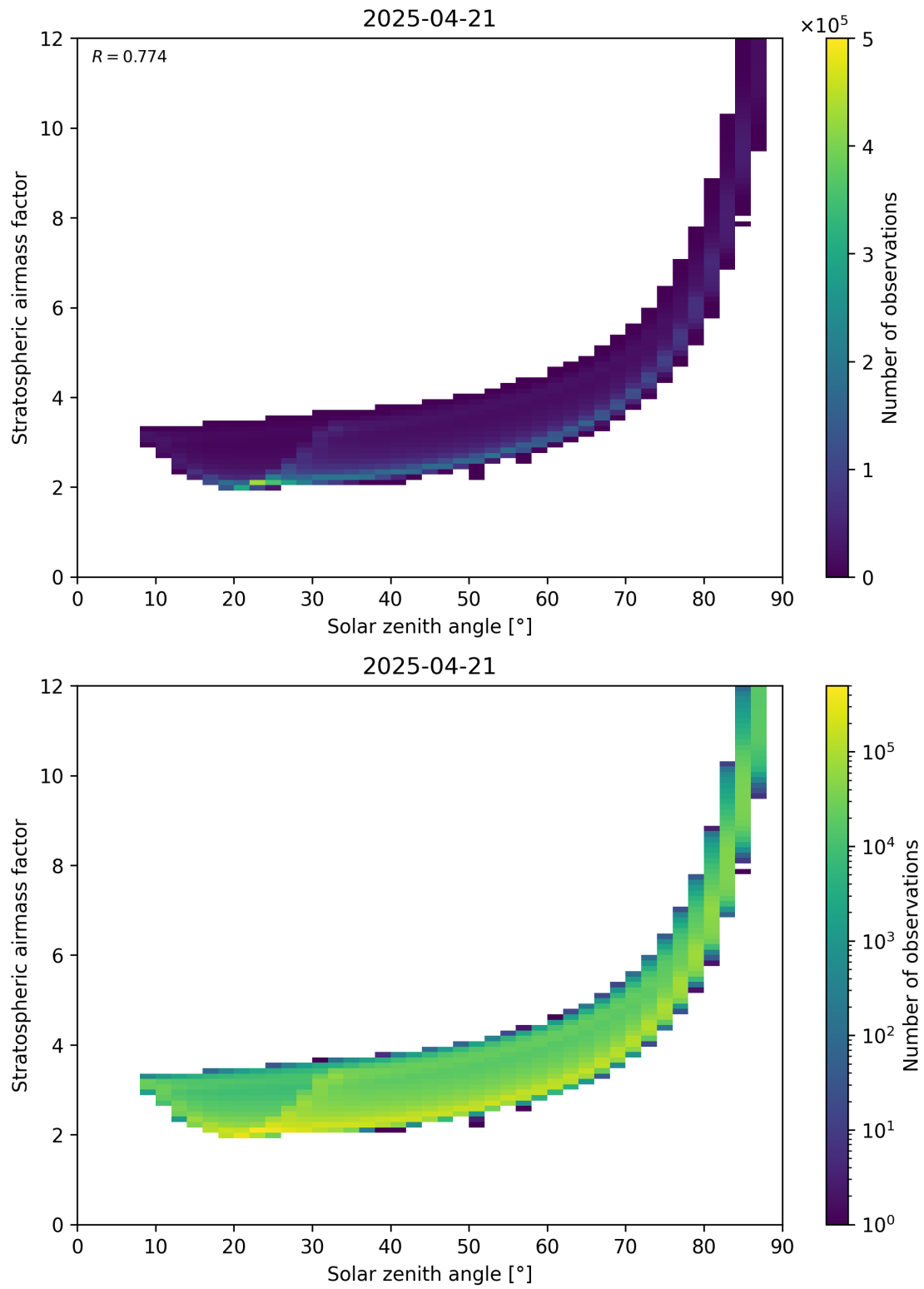
Figure 145: Scatter density plot of “Solar zenith angle” against “Stratospheric airmass factor” for 2025-04-21 to 2025-04-22.
