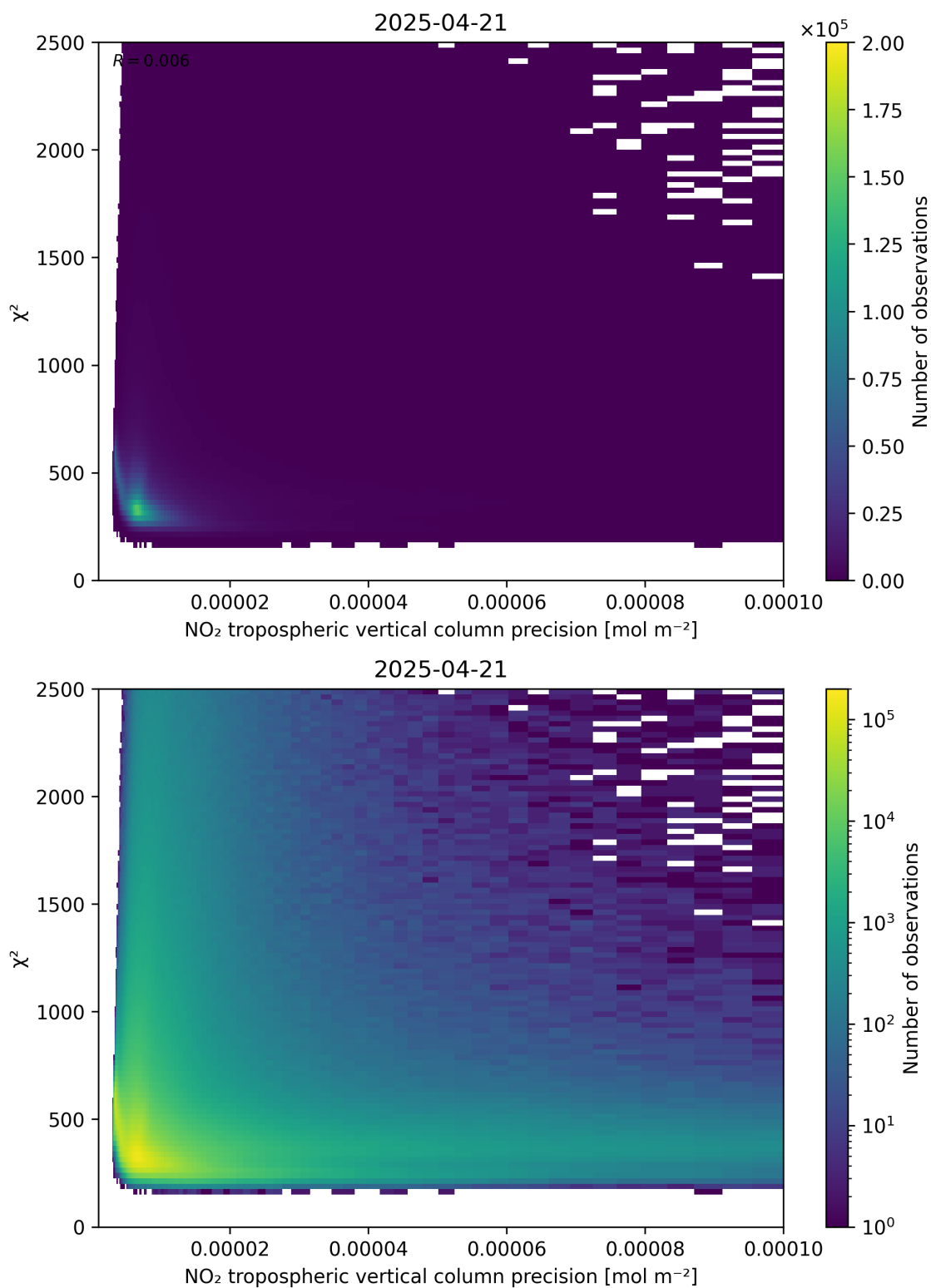
Figure 134: Scatter density plot of “NO 2 tropospheric vertical column precision” against “ \chi^2 ” for 2025-04-21 to 2025-04-22.
