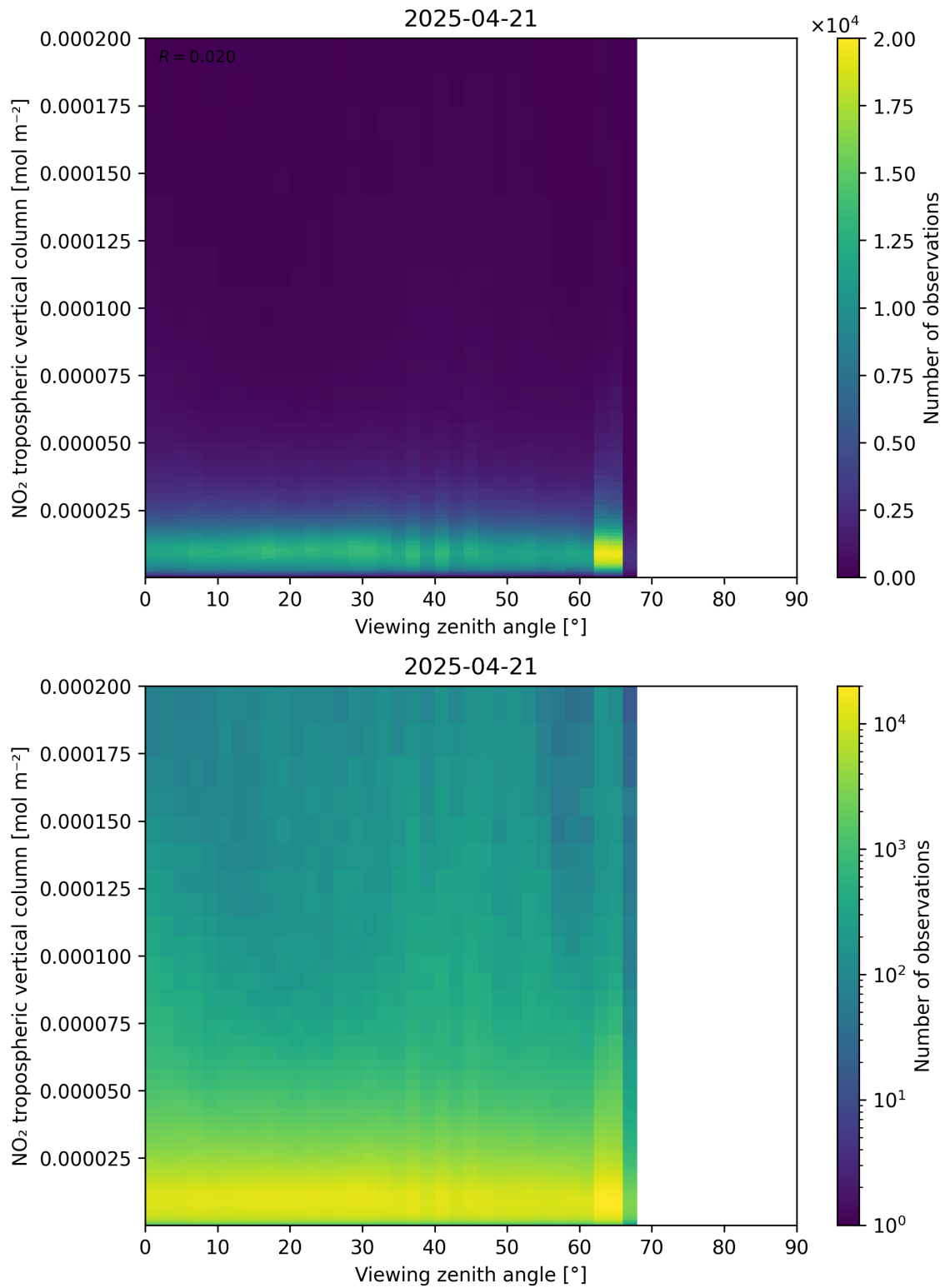
Figure 169: Scatter density plot of “Viewing zenith angle” against “NO 2 tropospheric vertical column” for 2025-04-21 to 2025-04-22.
