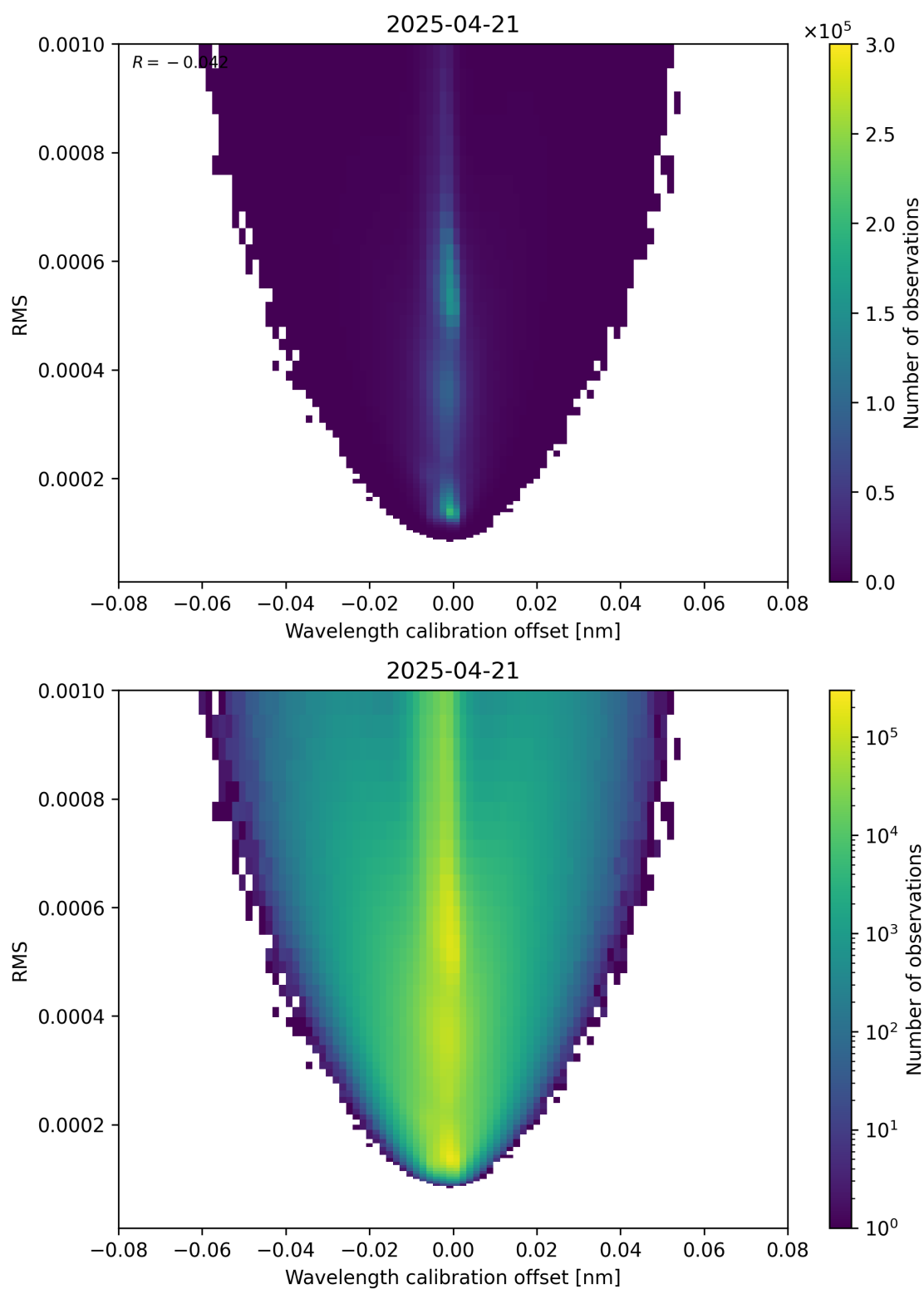
Figure 181: Scatter density plot of “Wavelength calibration offset” against “RMS” for 2025-04-21 to 2025-04-22.
