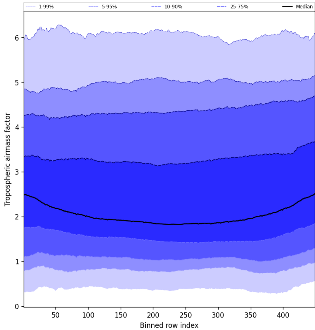
Figure 48: Along track statistics of “Tropospheric air mass factor” for 2025-04-21 to 2025-04-22
