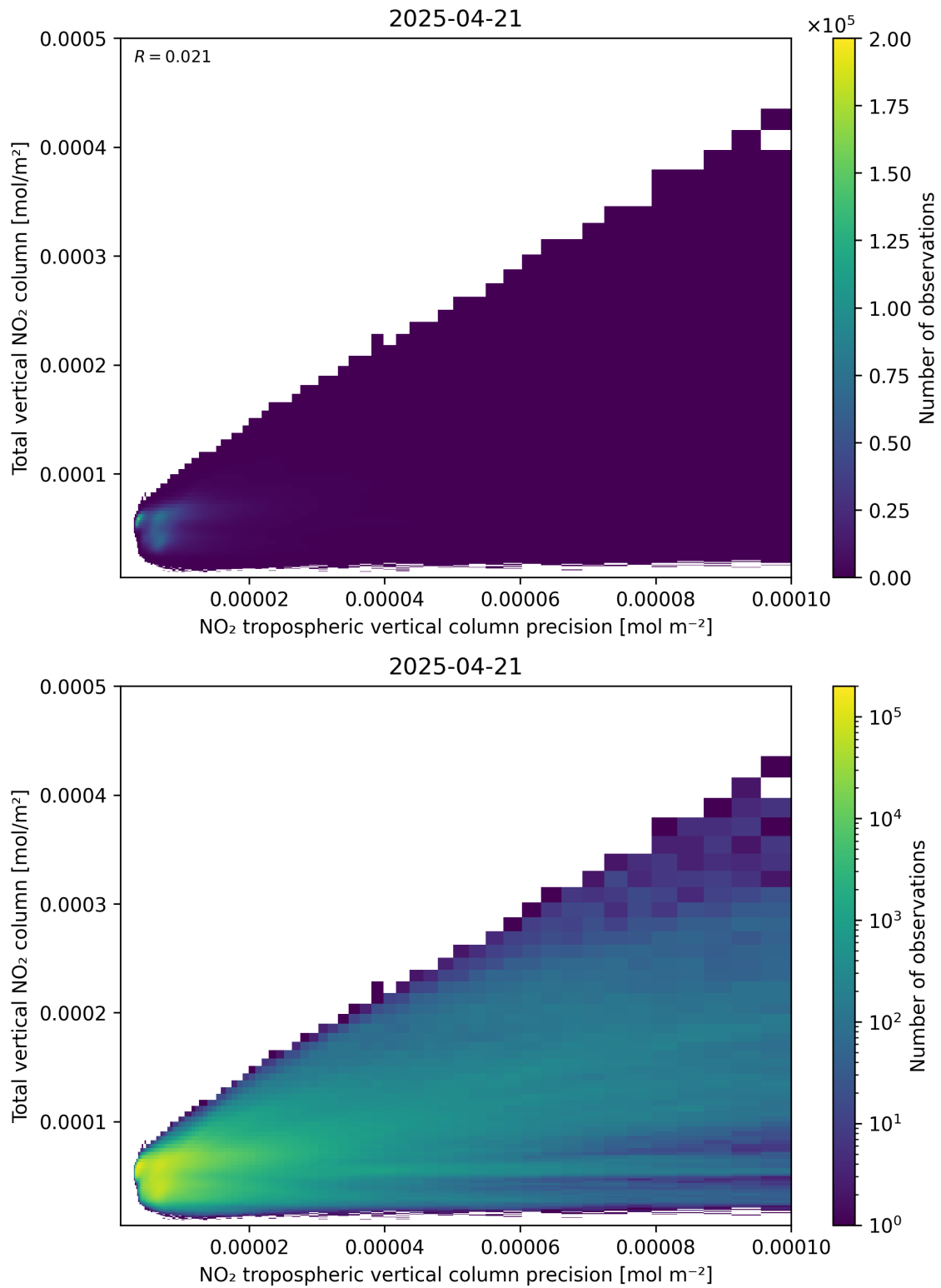
Figure 138: Scatter density plot of “NO 2 tropospheric vertical column precision” against “Total vertical NO 2 column” for 2025-04-21 to 2025-04-22.
