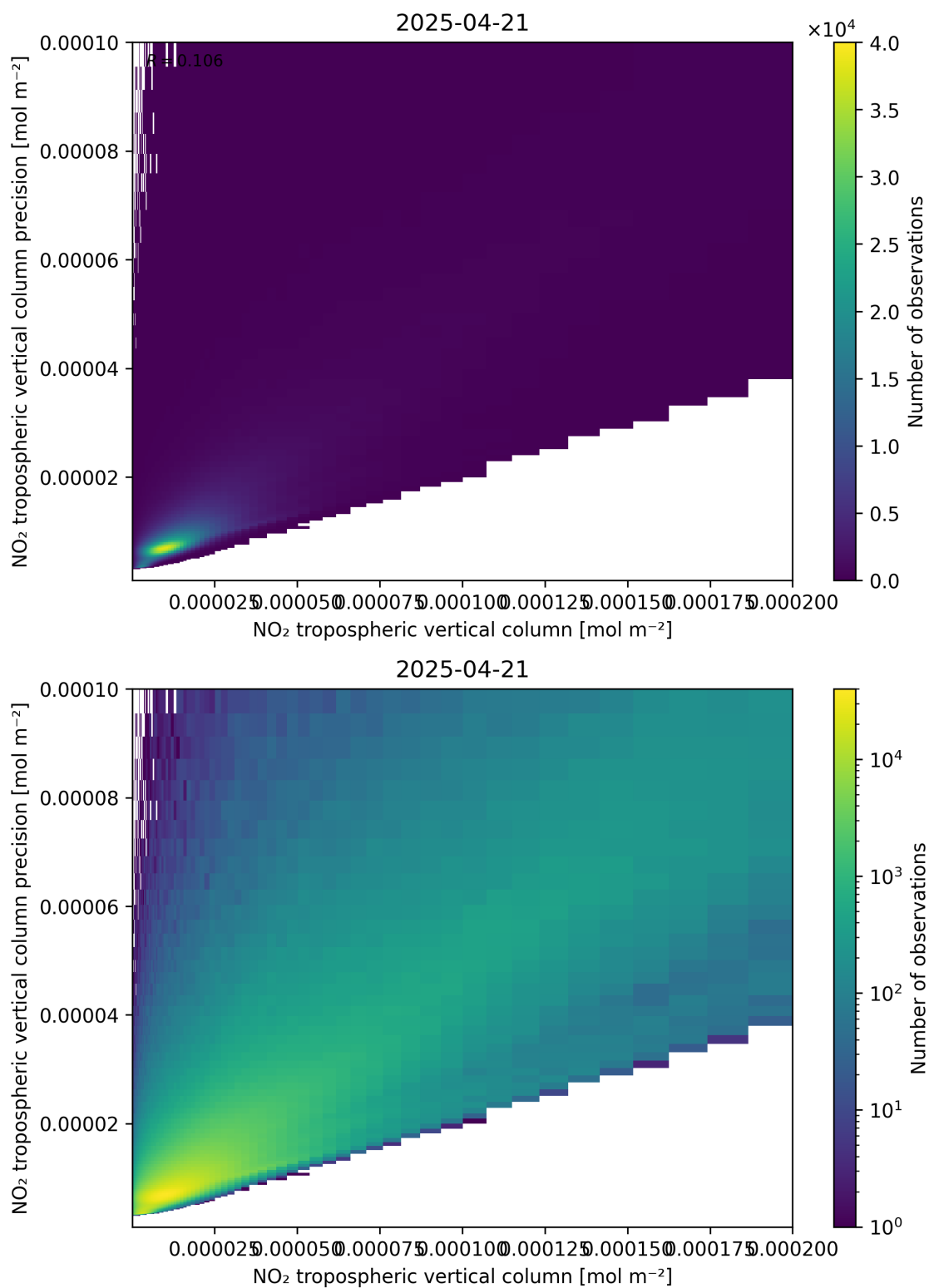
Figure 130: Scatter density plot of “NO 2 tropospheric vertical column” against “NO 2 tropospheric vertical column precision” for 2025-04-21 to 2025-04-22.
