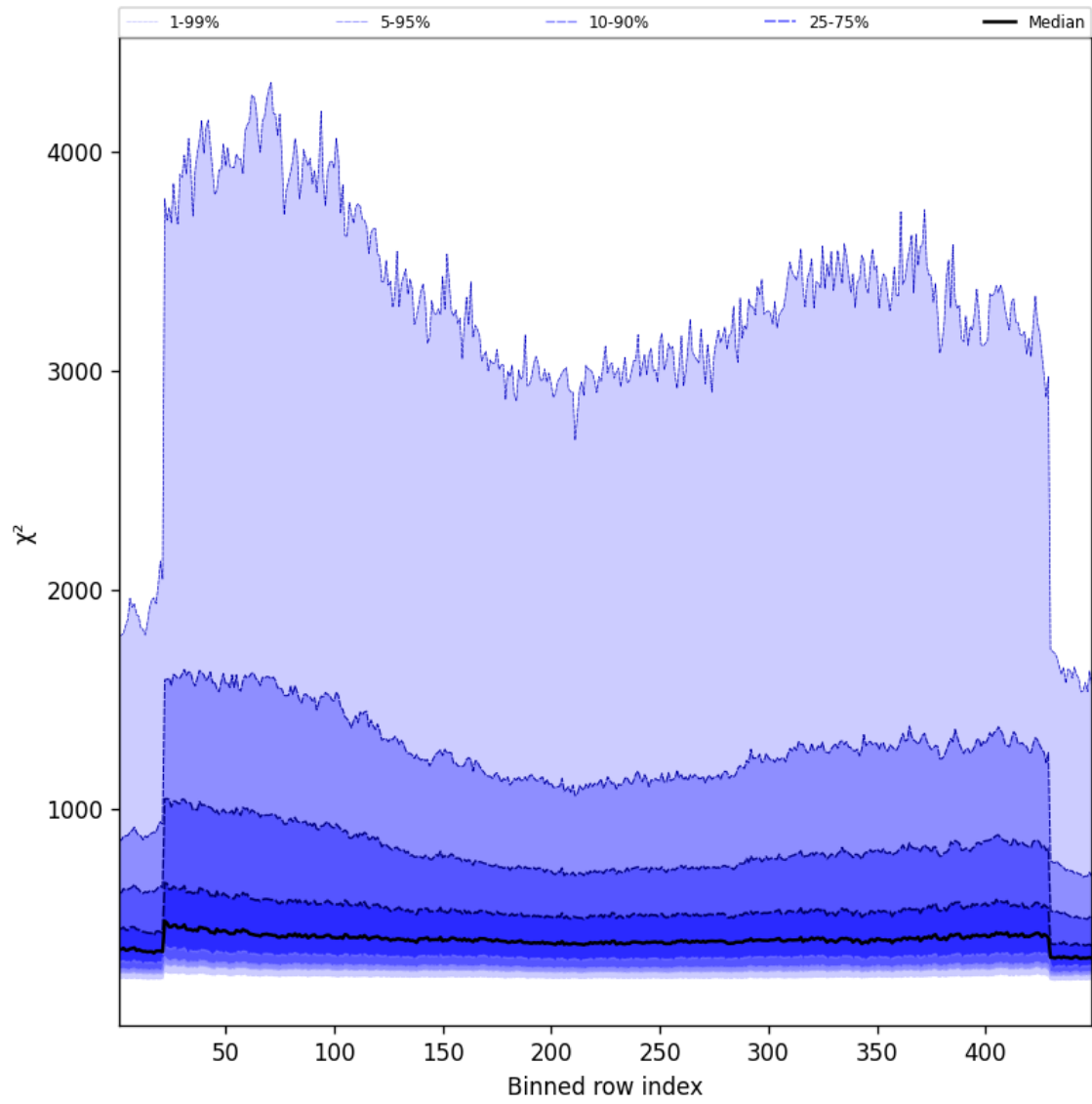
Figure 59: Along track statistics of “ \chi^2 ” for 2025-04-21 to 2025-04-22
