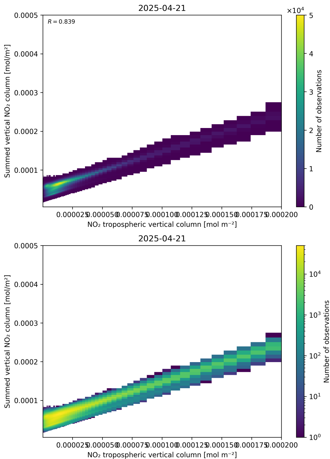
Figure 126: Scatter density plot of “NO 2 tropospheric vertical column” against “Summed vertical NO 2 column” for 2025-04-21 to 2025-04-22.
