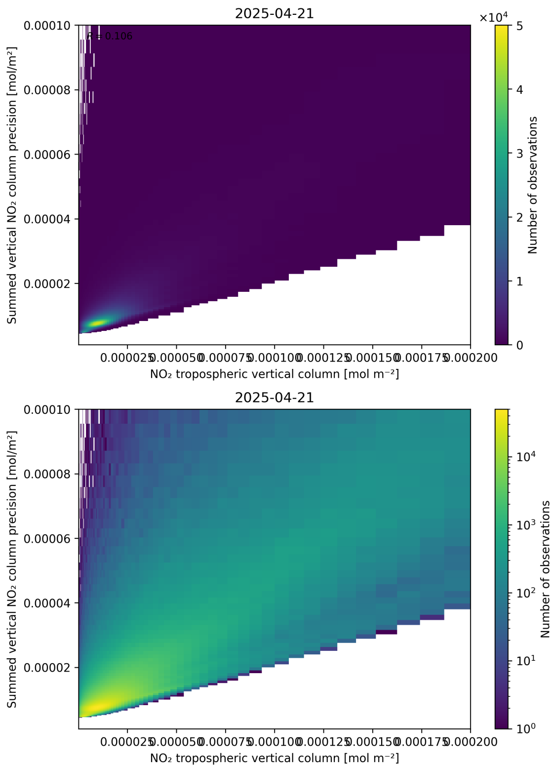
Figure 127: Scatter density plot of “NO 2 tropospheric vertical column” against “Summed vertical NO 2 column precision” for 2025-04-21 to 2025-04-22.
