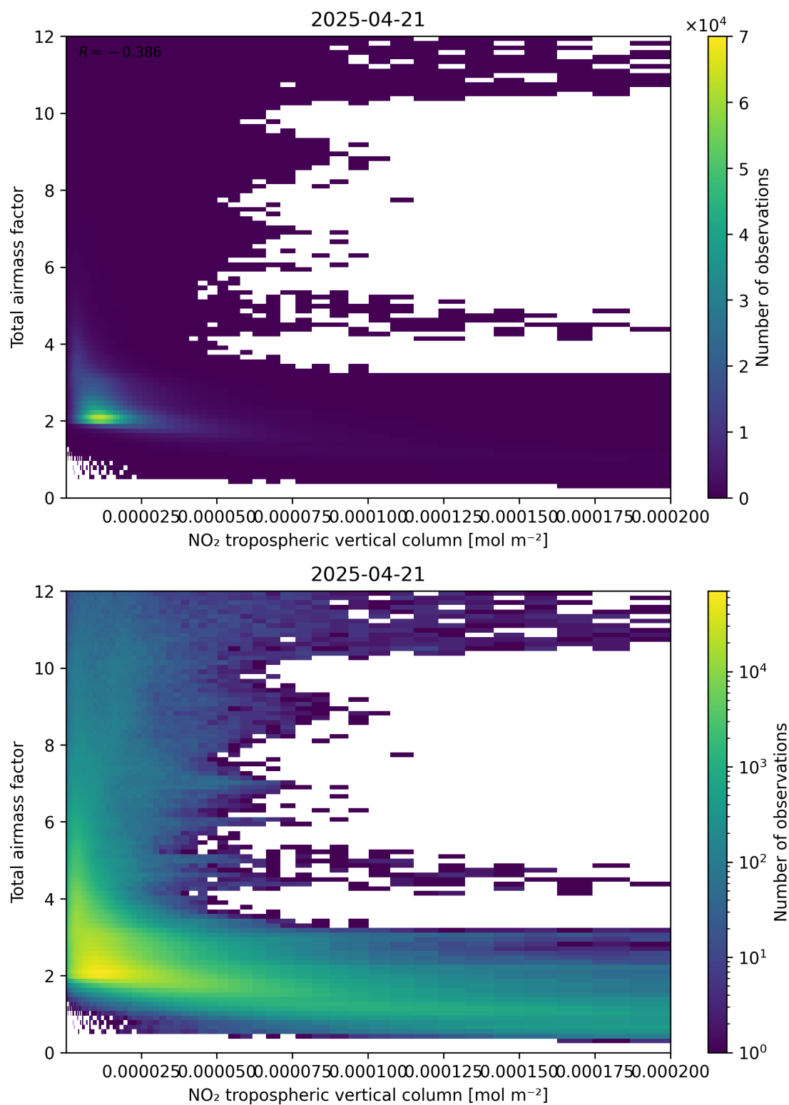
Figure 122: Scatter density plot of “NO 2 tropospheric vertical column” against “Total air mass factor” for 2025-04-21 to 2025-04-22.
