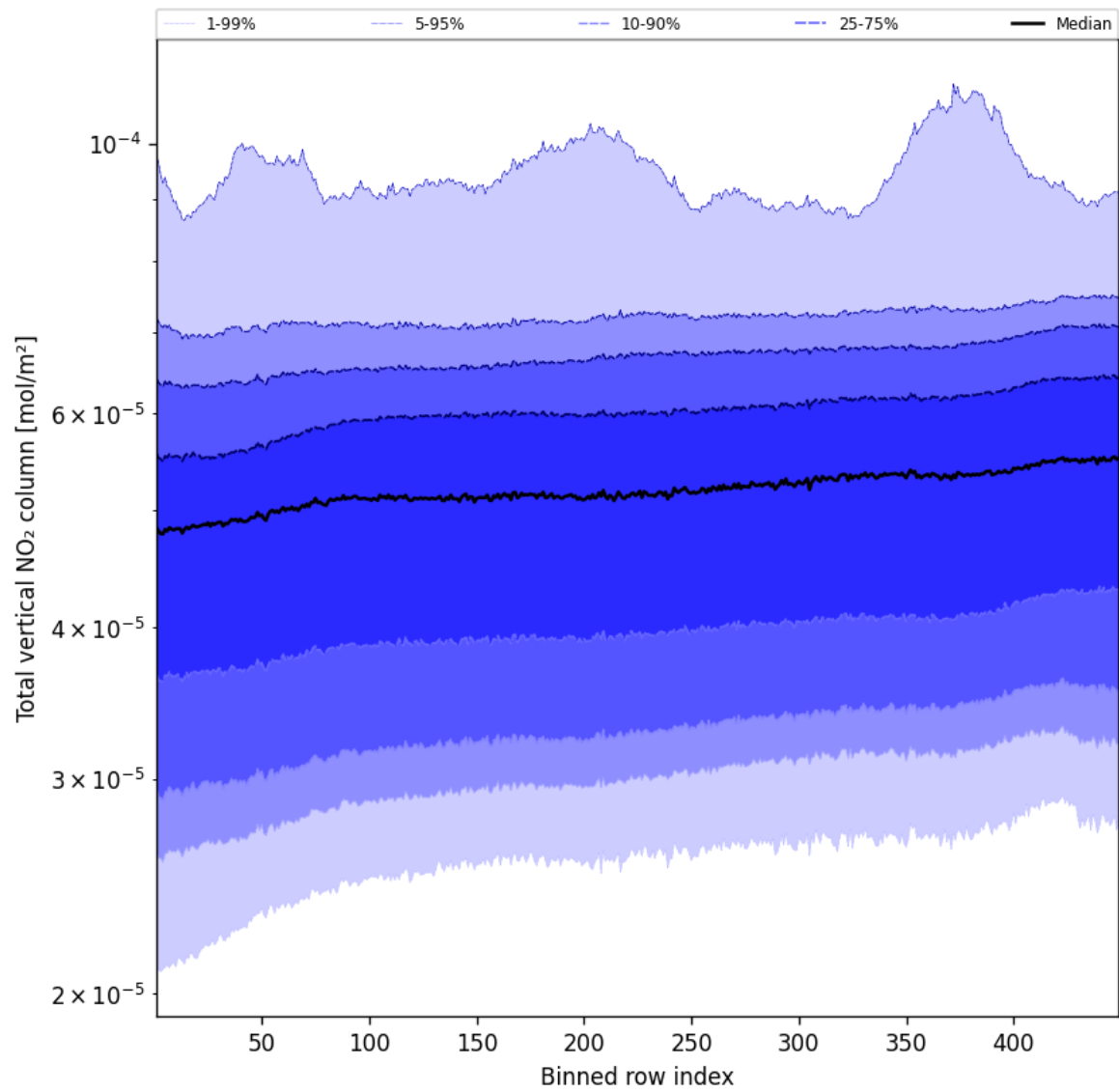
Figure 55: Along track statistics of “Total vertical NO 2 column” for 2025-04-21 to 2025-04-22
