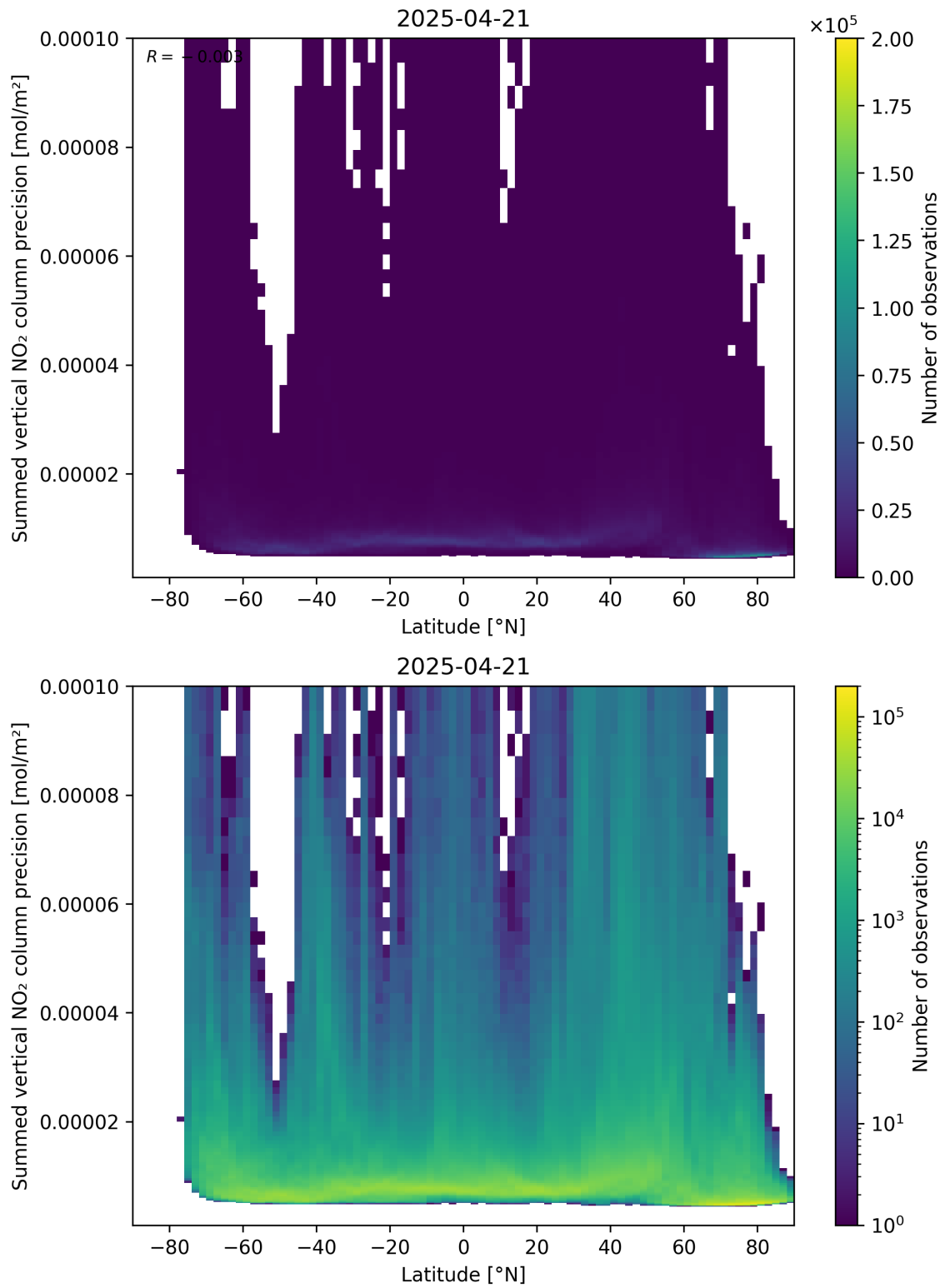
Figure 89: Scatter density plot of “Latitude” against “Summed vertical NO 2 column precision” for 2025-04-21 to 2025-04-22.
