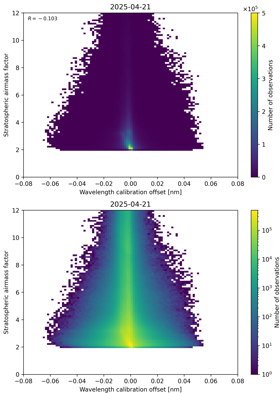
Figure 174: Scatter density plot of “Wavelength calibration offset” against “Stratospheric airmass factor” for 2025-04-21 to 2025-04-22.
