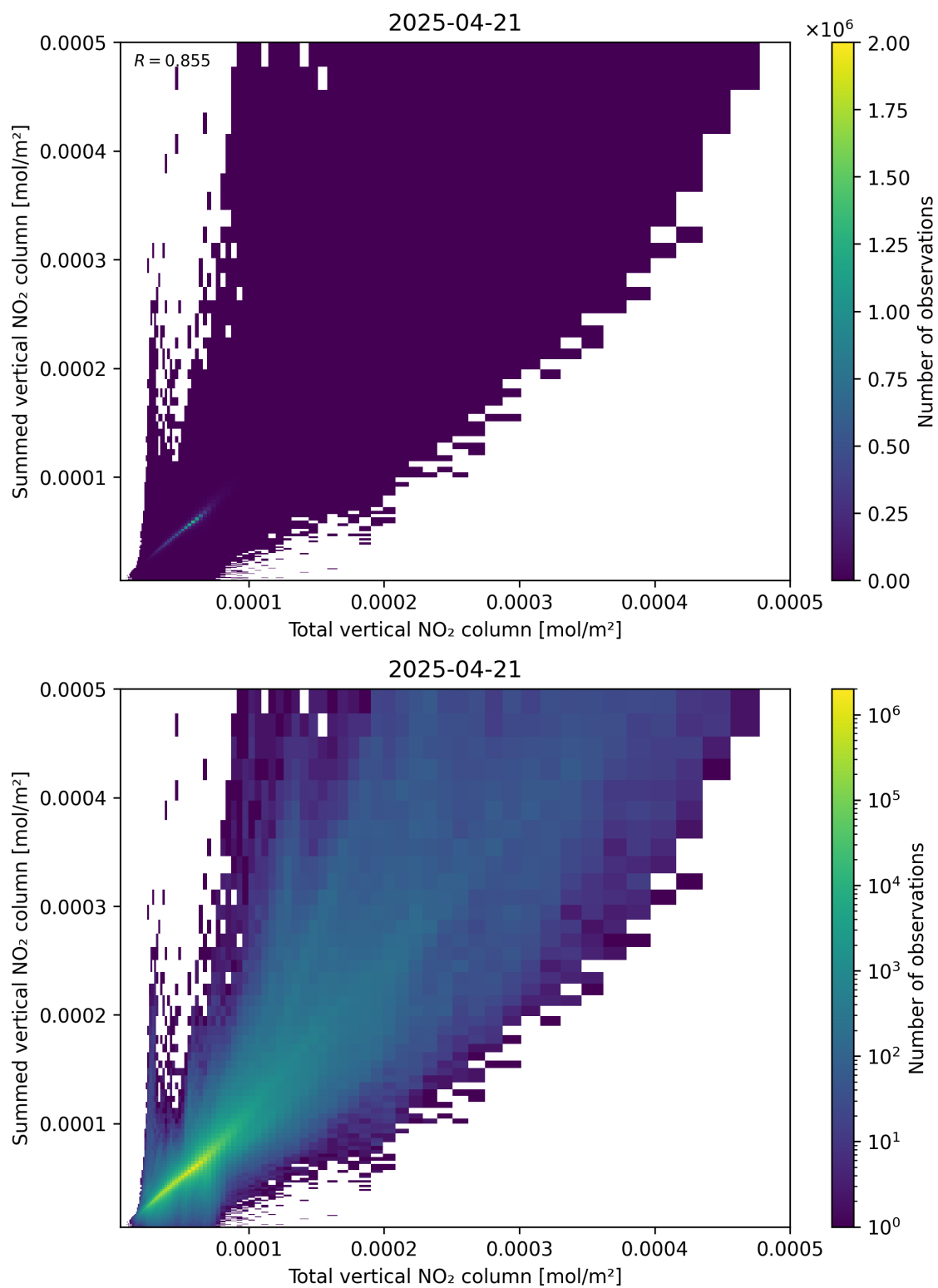
Figure 112: Scatter density plot of “Total vertical NO 2 column” against “Summed vertical NO 2 column” for 2025-04-21 to 2025-04-22.
