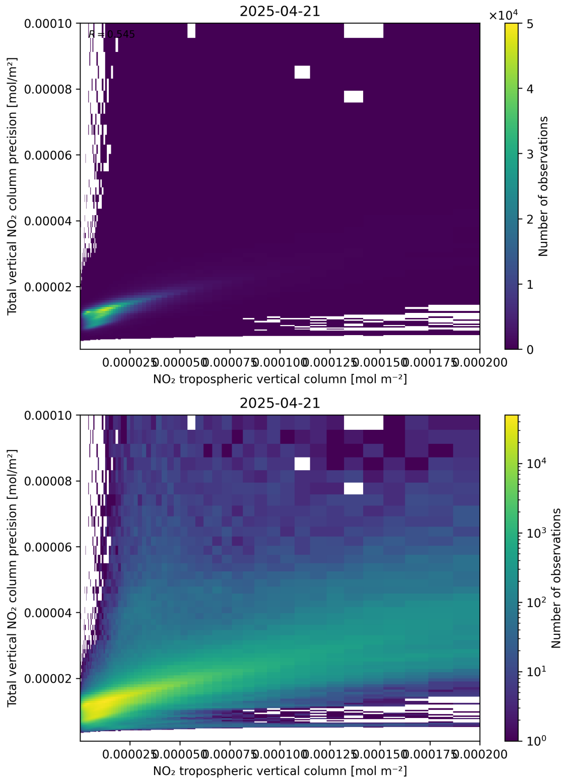
Figure 129: Scatter density plot of “NO 2 tropospheric vertical column” against “Total vertical NO 2 column precision” for 2025-04-21 to 2025-04-22.
