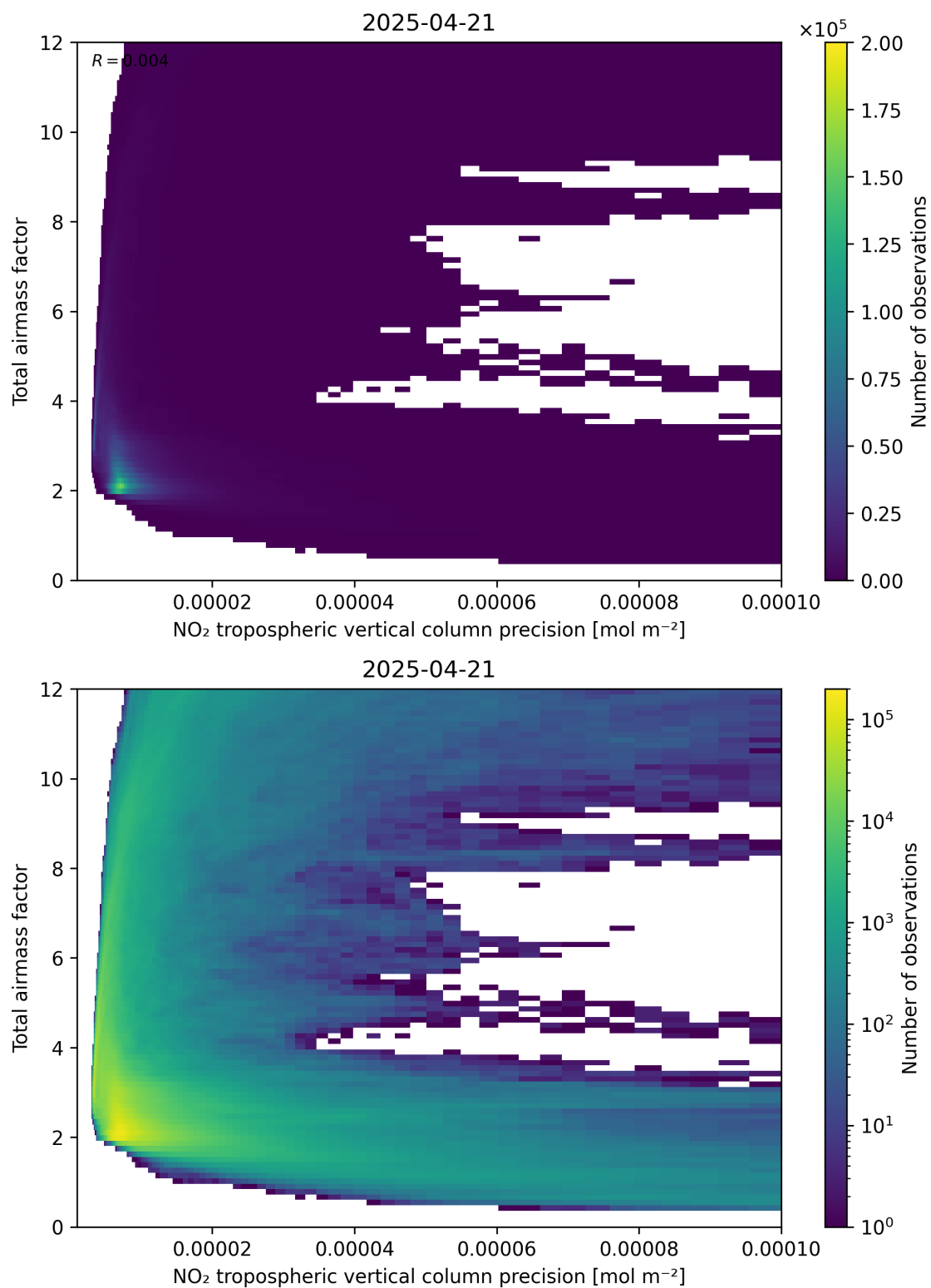
Figure 132: Scatter density plot of “NO 2 tropospheric vertical column precision” against “Total air mass factor” for 2025-04-21 to 2025-04-22.
