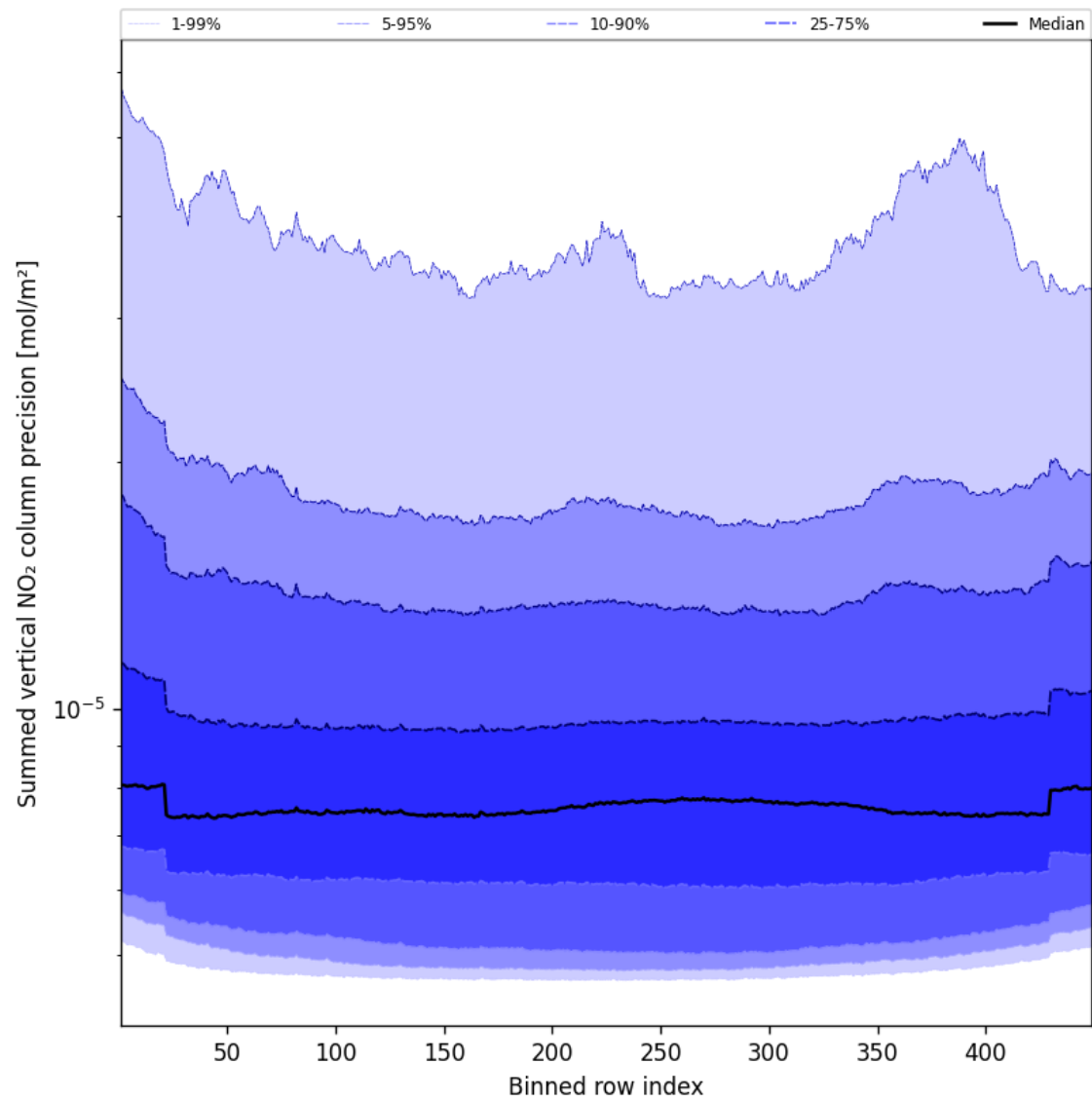
Figure 58: Along track statistics of “Summed vertical NO 2 column precision” for 2025-04-21 to 2025-04-22
