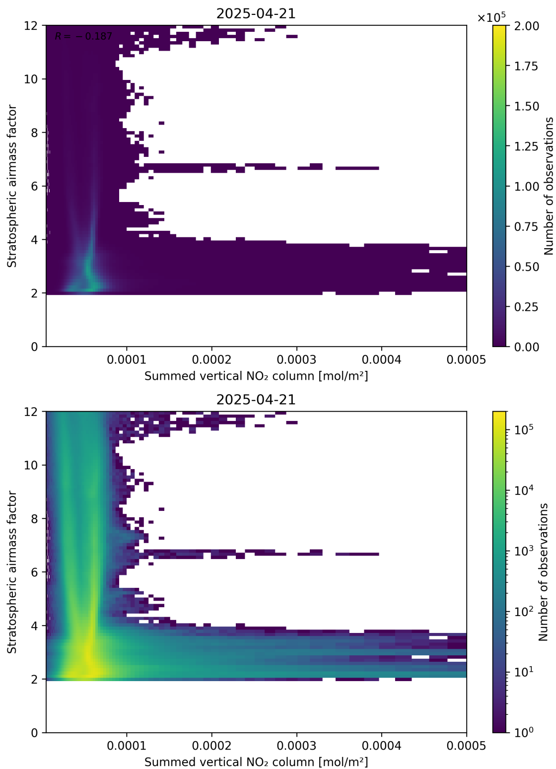
Figure 103: Scatter density plot of “Summed vertical NO 2 column” against “Stratospheric air mass factor” for 2025-04-21 to 2025-04-22.
