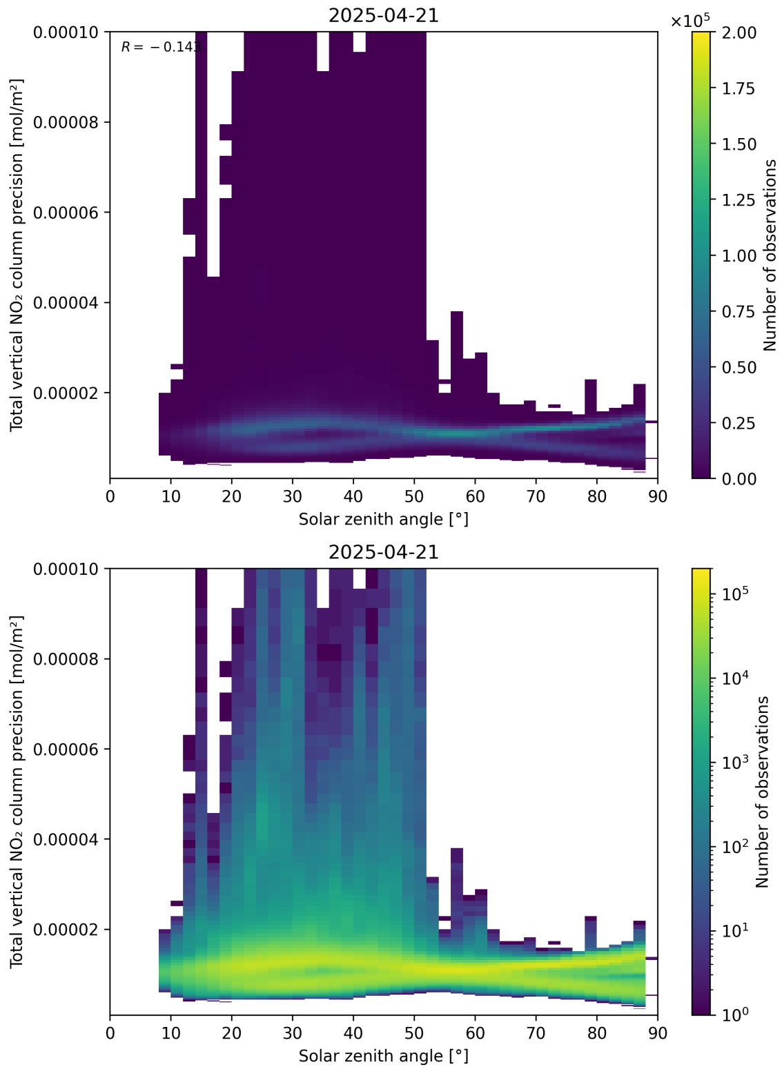
Figure 154: Scatter density plot of “Solar zenith angle” against “Total vertical NO 2 column precision” for 2025-04-21 to 2025-04-22.
