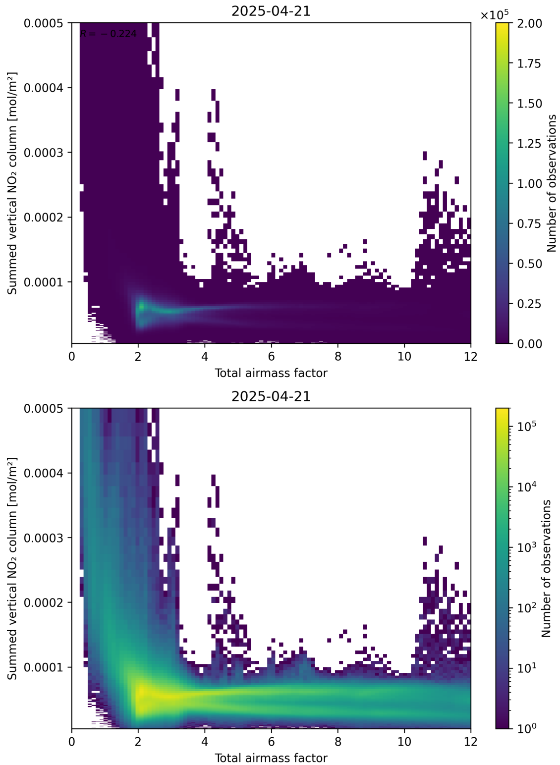
Figure 65: Scatter density plot of “Total airmass factor” against “Summed vertical NO 2 column” for 2025-04-21 to 2025-04-22.
