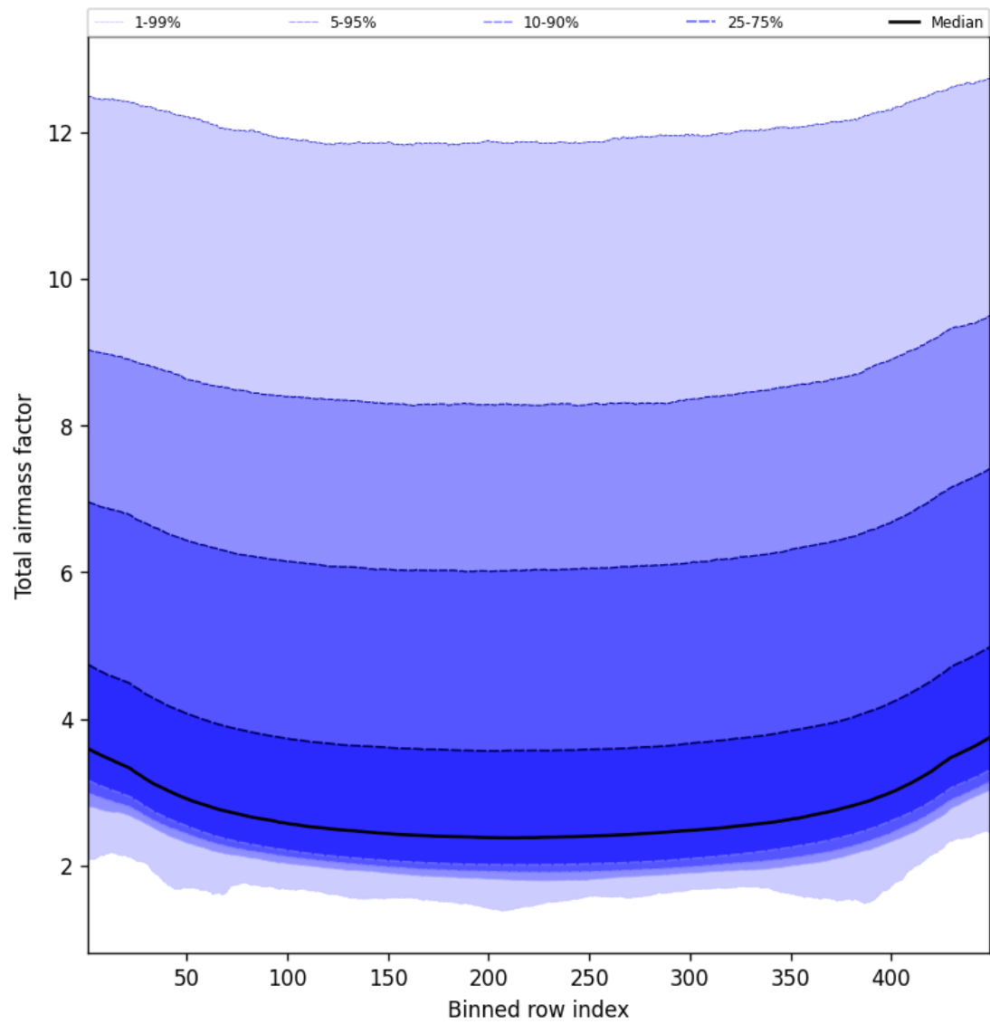
Figure 49: Along track statistics of “Total airmass factor” for 2025-04-21 to 2025-04-22
