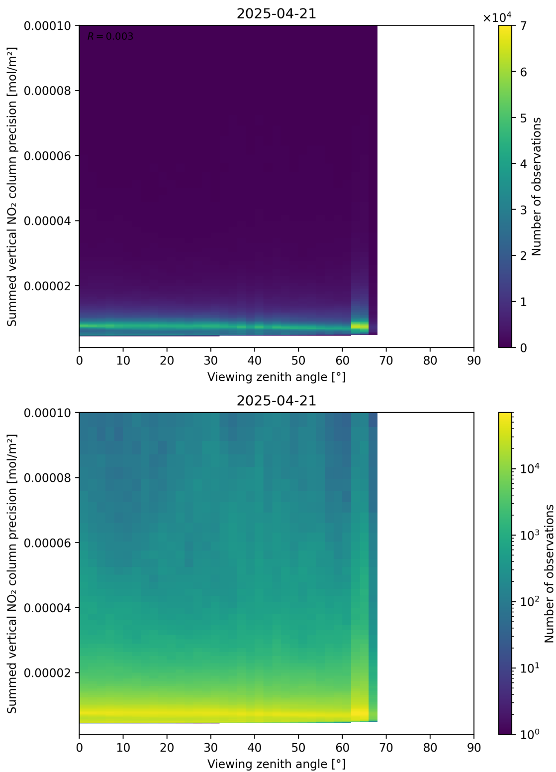
Figure 166: Scatter density plot of “Viewing zenith angle” against “Summed vertical NO 2 column precision” for 2025-04-21 to 2025-04-22.
