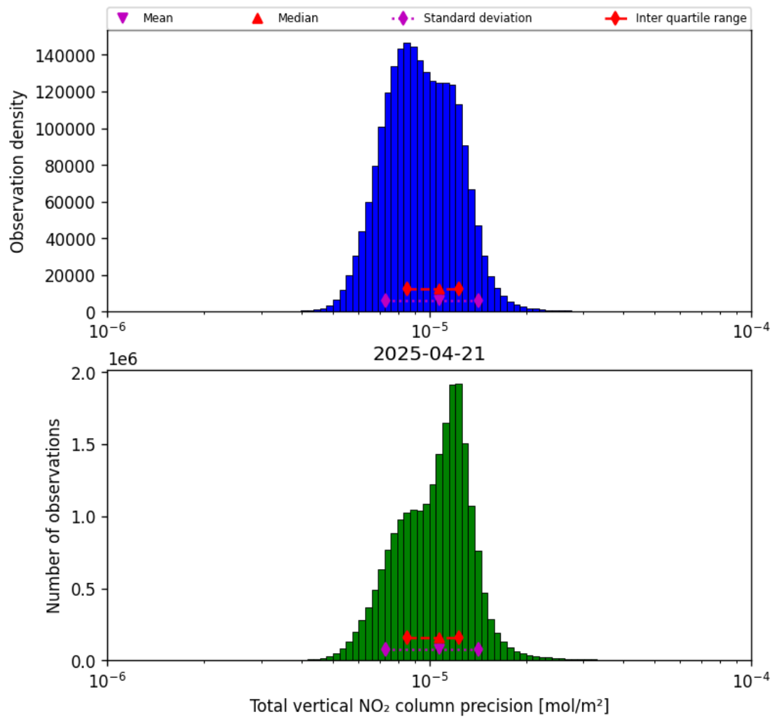
Figure 39: Histogram of “Total vertical NO 2 column precision” for 2025-04-21 to 2025-04-22
