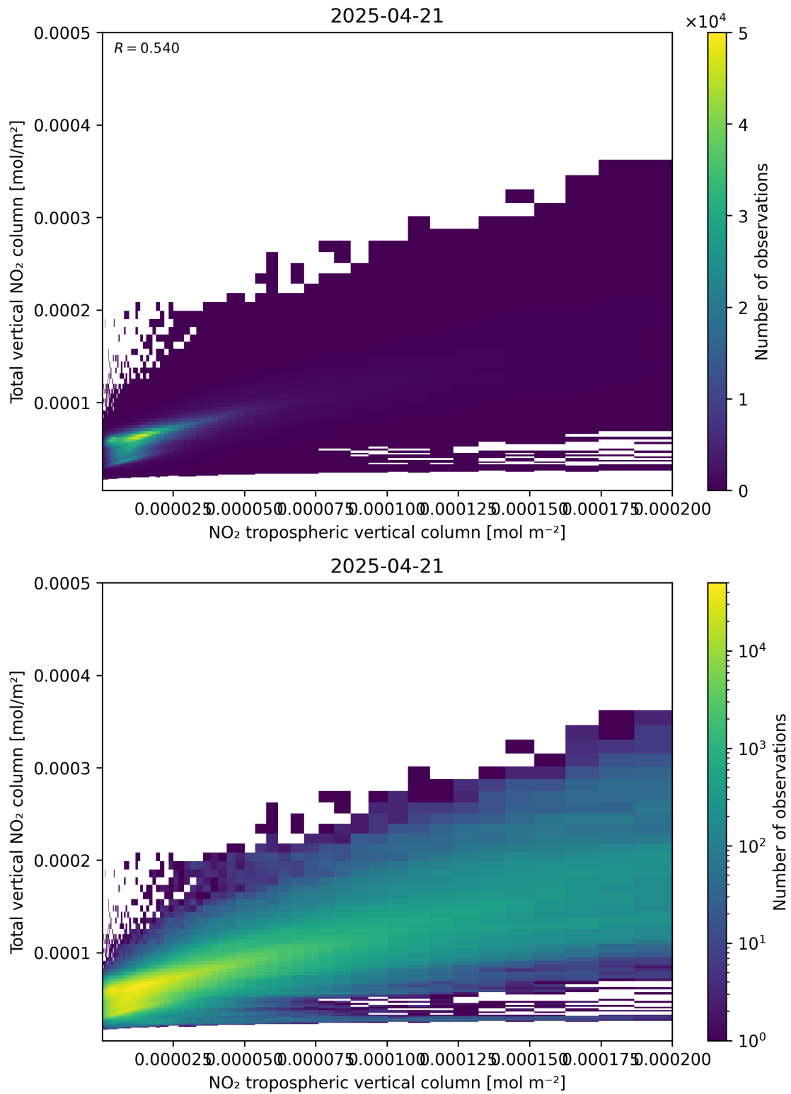
Figure 128: Scatter density plot of “NO 2 tropospheric vertical column” against “Total vertical NO 2 column” for 2025-04-21 to 2025-04-22.
