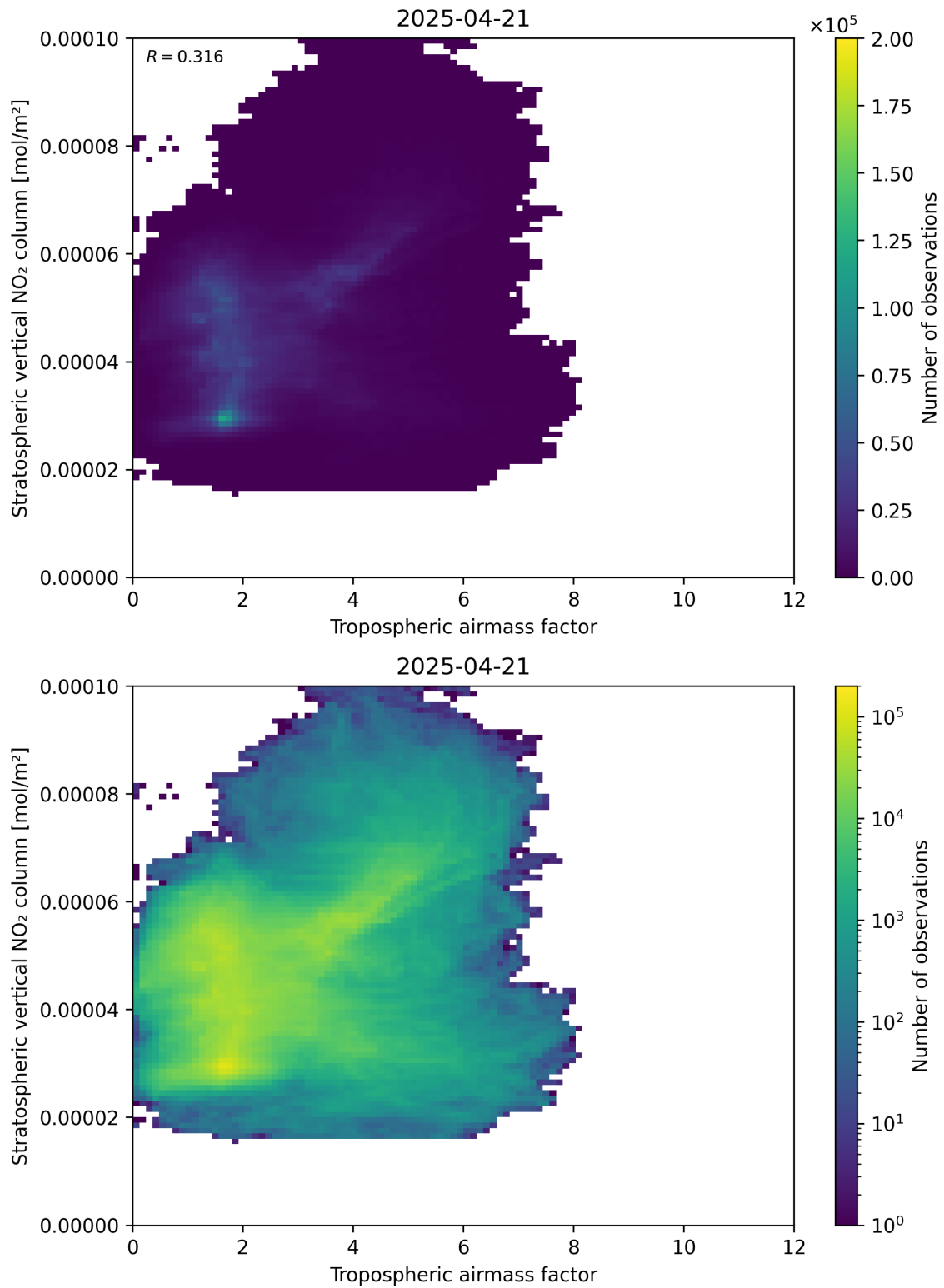
Figure 74: Scatter density plot of “Tropospheric air mass factor” against “Stratospheric vertical NO 2 column” for 2025-04-21 to 2025-04-22.
