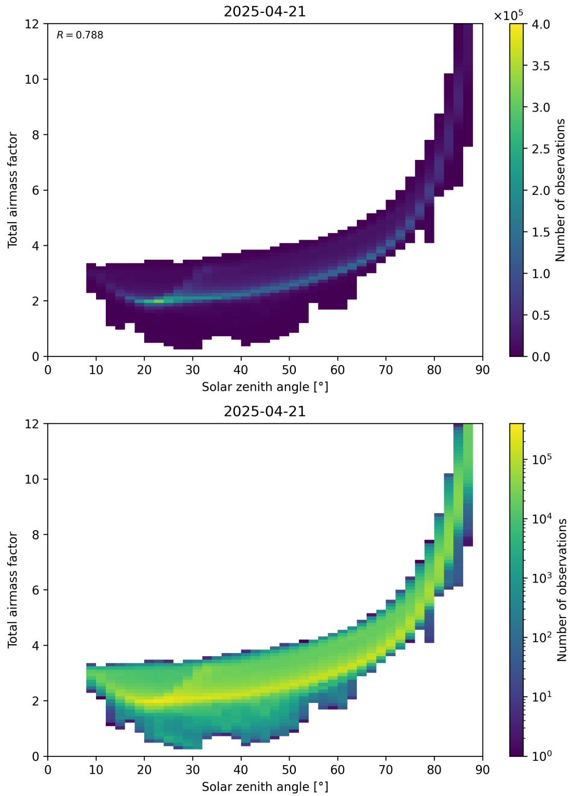
Figure 146: Scatter density plot of “Solar zenith angle” against “Total air mass factor” for 2025-04-21 to 2025-04-22.
