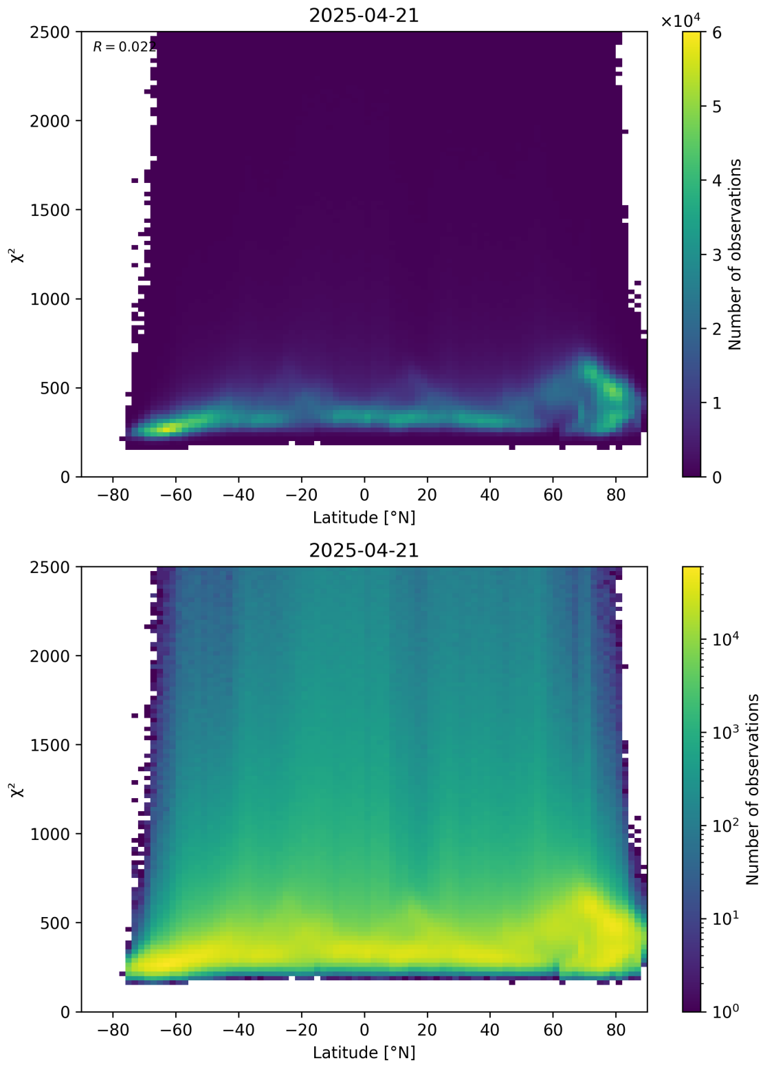
Figure 86: Scatter density plot of “Latitude” against “ \chi^2 ” for 2025-04-21 to 2025-04-22.
