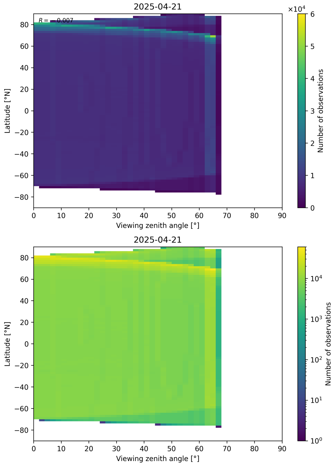
Figure 163: Scatter density plot of “Viewing zenith angle” against “Latitude” for 2025-04-21 to 2025-04-22.
