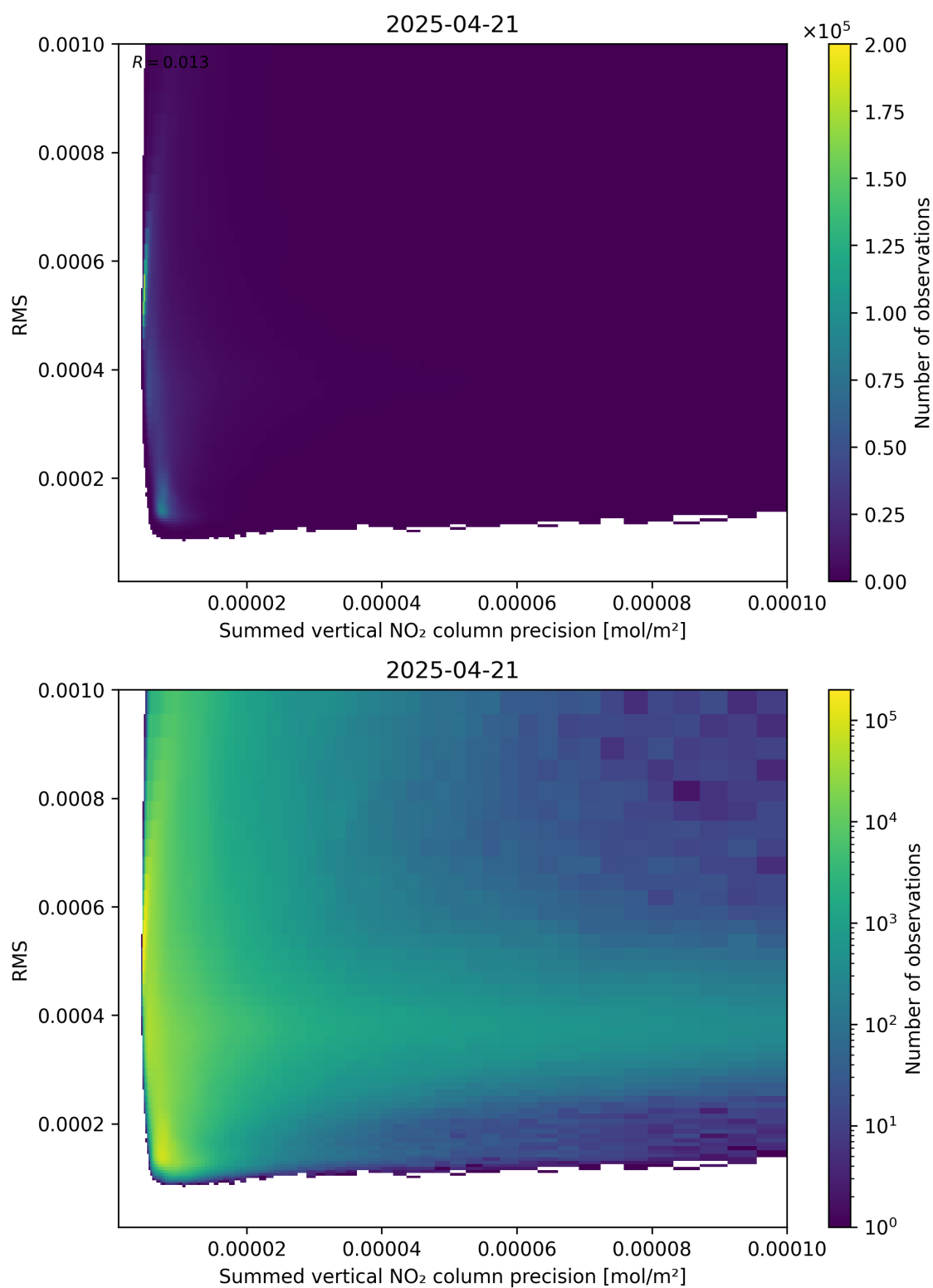
Figure 108: Scatter density plot of “Summed vertical NO 2 column precision” against “RMS” for 2025-04-21 to 2025-04-22.
