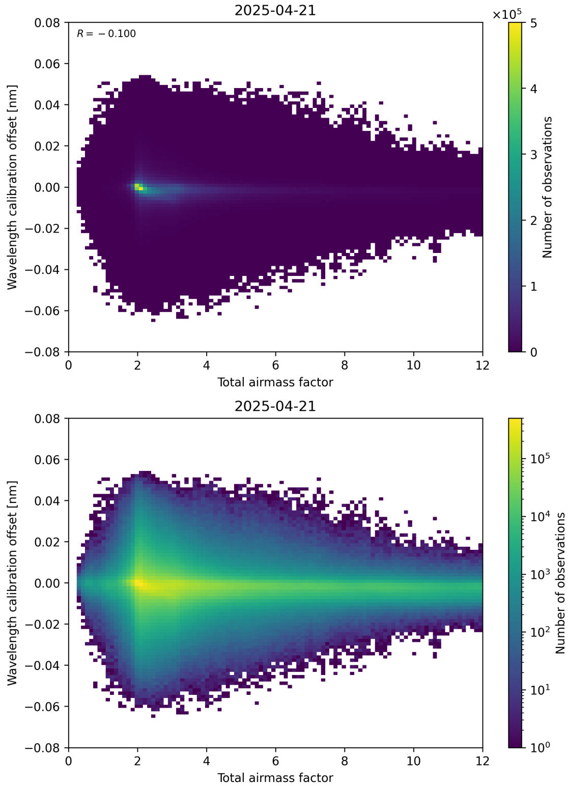
Figure 70: Scatter density plot of “Total airmass factor” against “Wavelength calibration offset” for 2025-04-21 to 2025-04-22.
