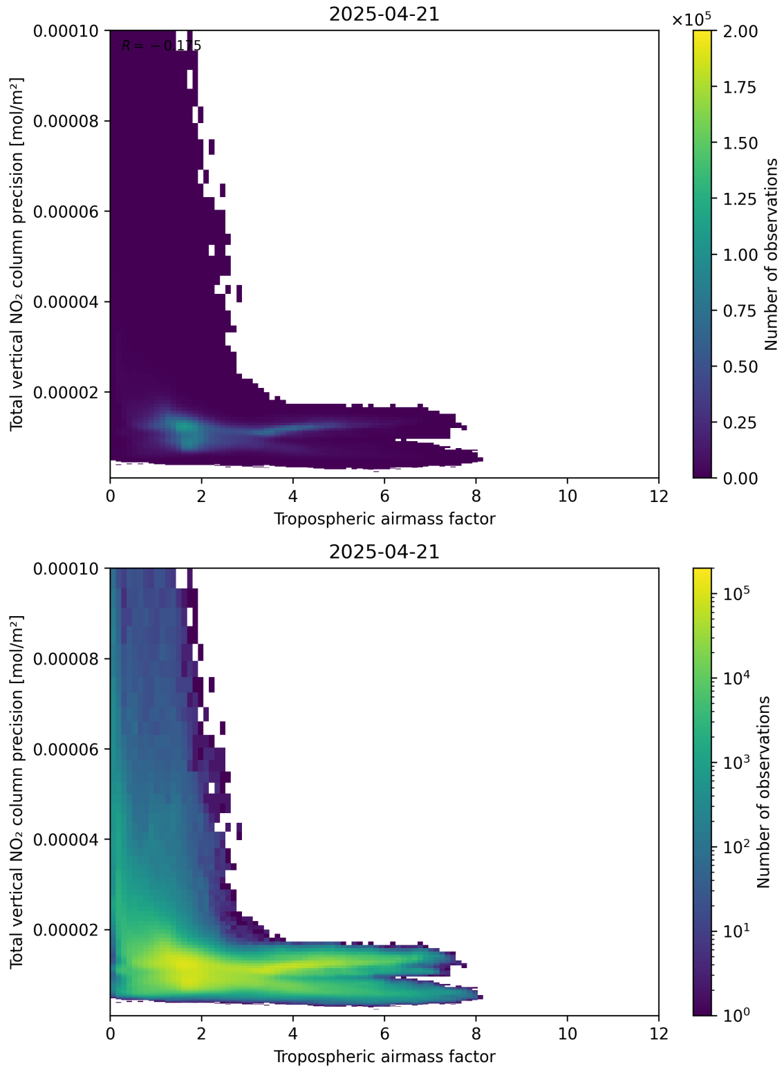
Figure 78: Scatter density plot of “Tropospheric air mass factor” against “Total vertical NO 2 column precision” for 2025-04-21 to 2025-04-22.
