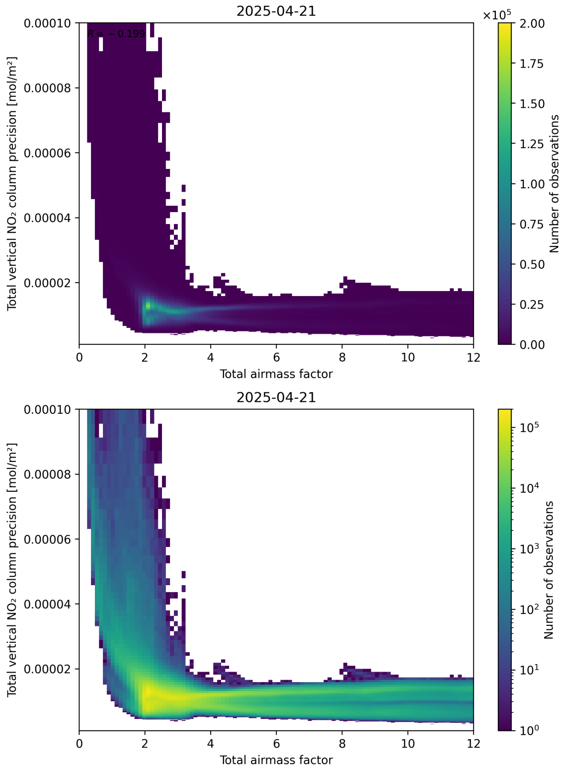
Figure 68: Scatter density plot of “Total airmass factor” against “Total vertical NO 2 column precision” for 2025-04-21 to 2025-04-22.
