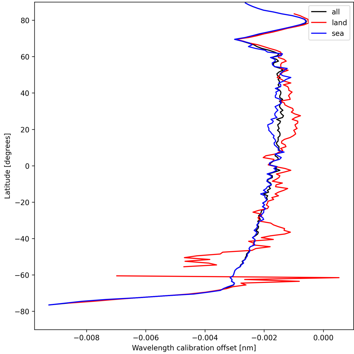
Figure 18: Zonal average of “Wavelength calibration offset” for 2025-04-21 to 2025-04-22.
