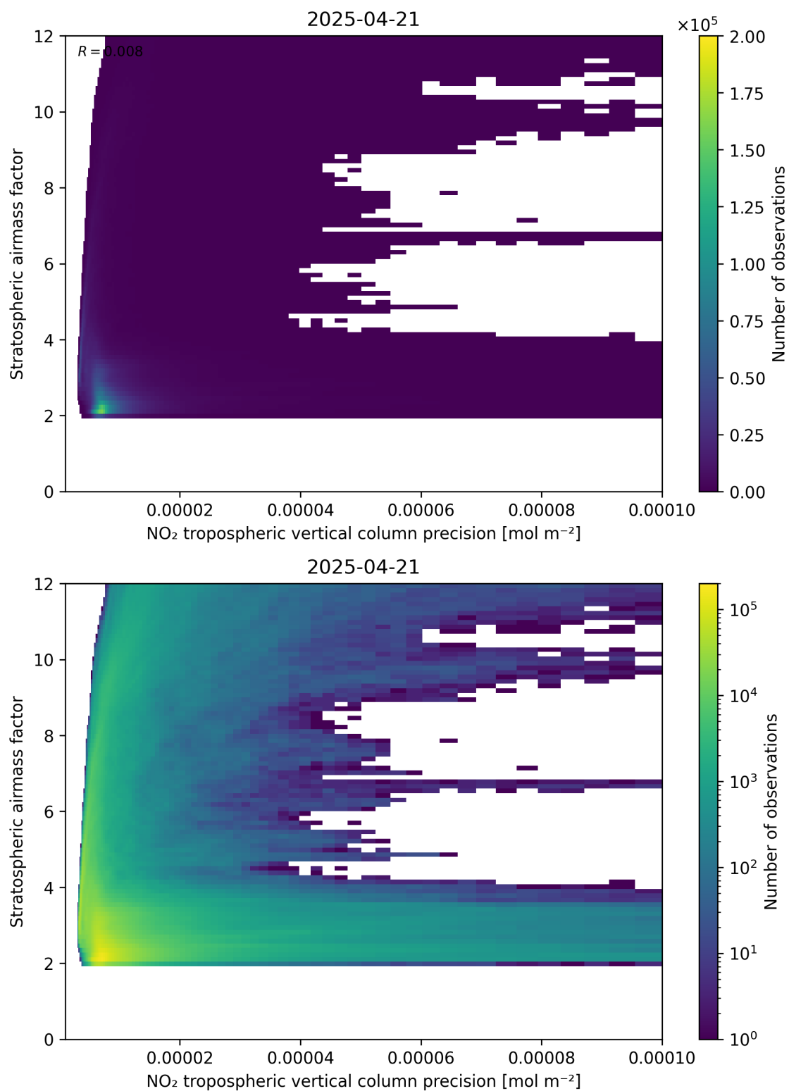
Figure 131: Scatter density plot of “NO 2 tropospheric vertical column precision” against “Stratospheric airmass factor” for 2025-04-21 to 2025-04-22.
