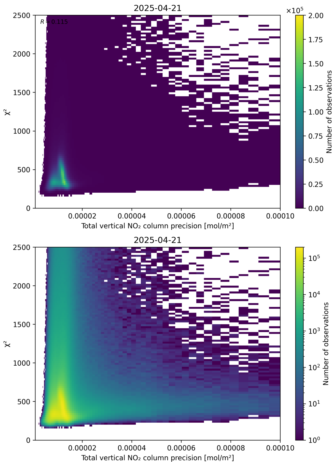
Figure 116: Scatter density plot of “Total vertical NO 2 column precision” against “ \chi^2 ” for 2025-04-21 to 2025-04-22.
