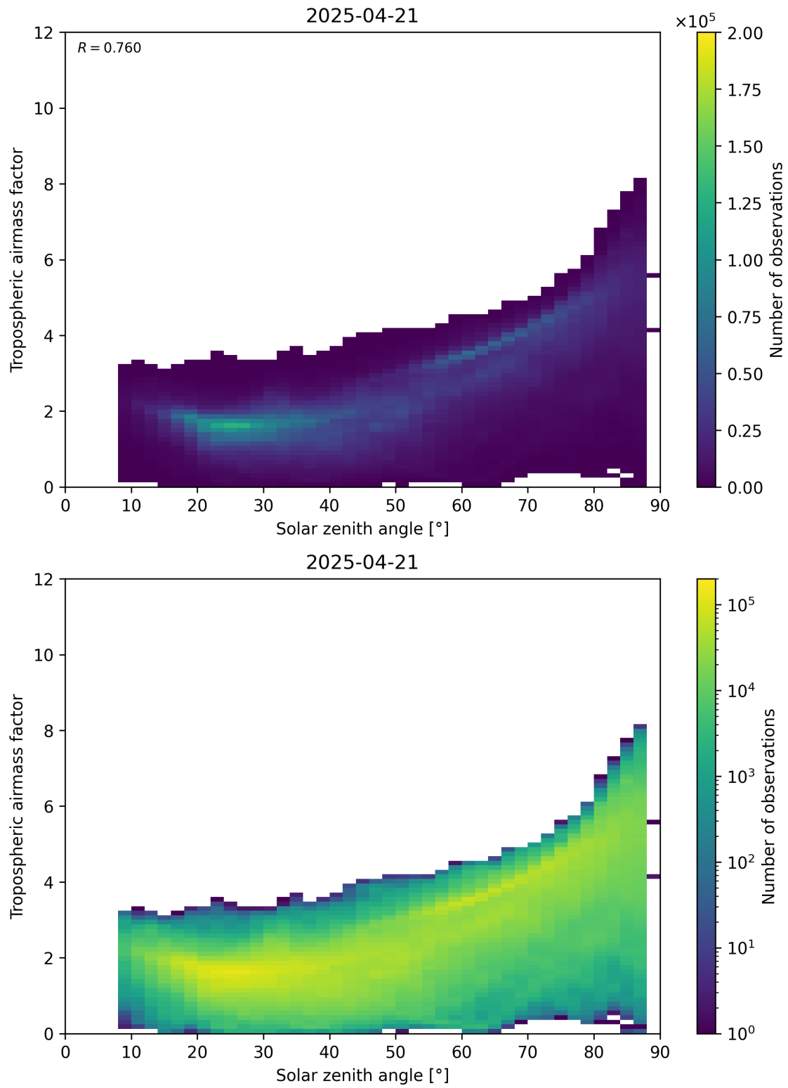
Figure 147: Scatter density plot of “Solar zenith angle” against “Tropospheric airmass factor” for 2025-04-21 to 2025-04-22.
