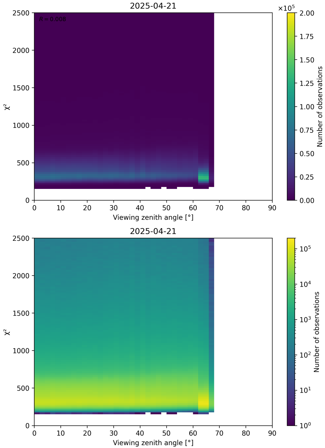
Figure 162: Scatter density plot of “Viewing zenith angle” against “ \chi^2 ” for 2025-04-21 to 2025-04-22.
