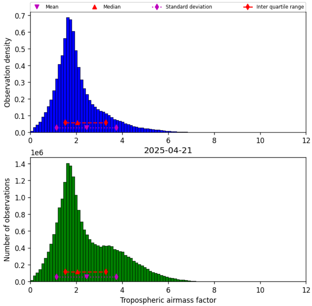
Figure 31: Histogram of “Tropospheric airmass factor” for 2025-04-21 to 2025-04-22
