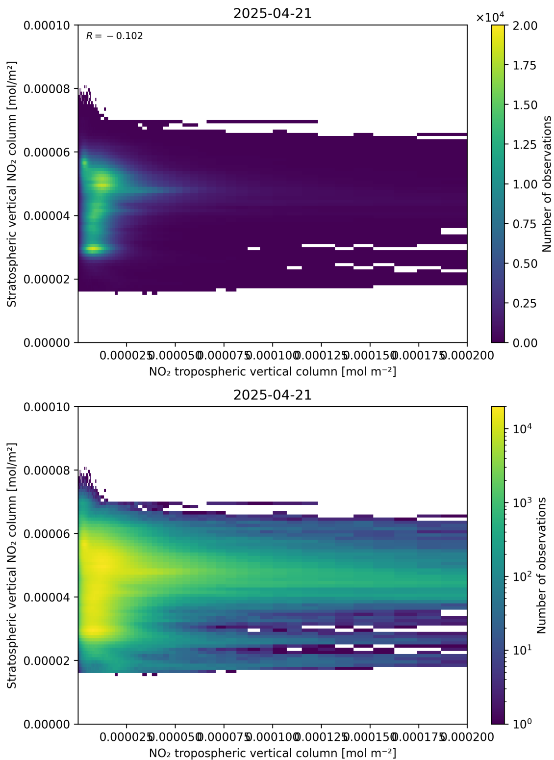
Figure 125: Scatter density plot of “NO 2 tropospheric vertical column” against “Stratospheric vertical NO 2 column” for 2025-04-21 to 2025-04-22.
