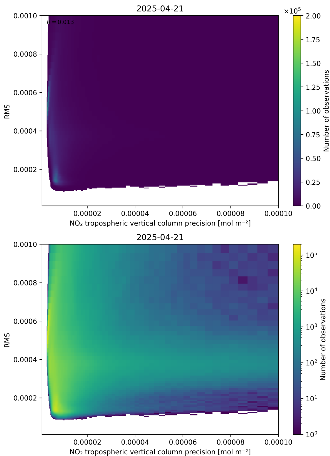
Figure 140: Scatter density plot of “NO 2 tropospheric vertical column precision” against “RMS” for 2025-04-21 to 2025-04-22.
