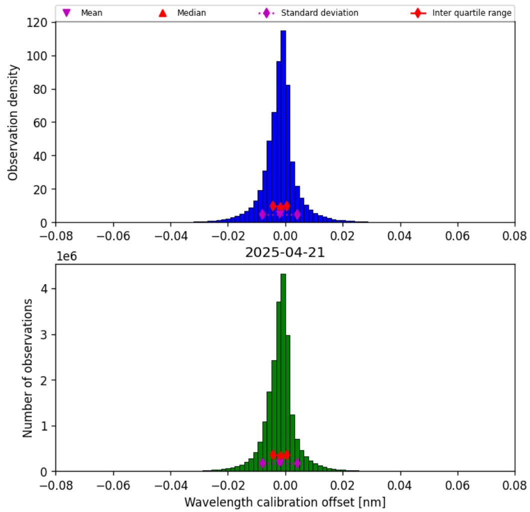
Figure 35: Histogram of “Wavelength calibration offset” for 2025-04-21 to 2025-04-22
