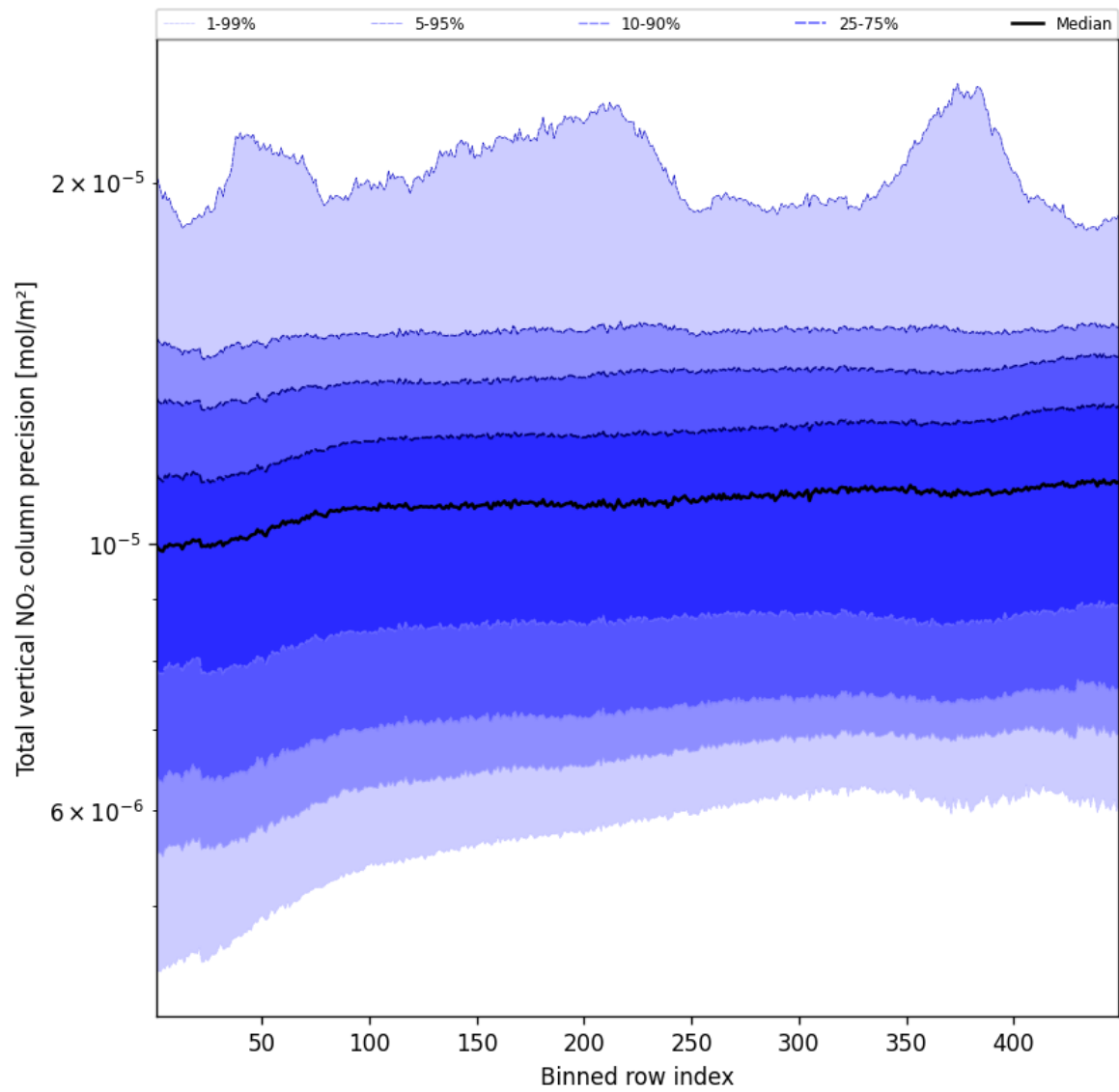
Figure 56: Along track statistics of “Total vertical NO 2 column precision” for 2025-04-21 to 2025-04-22
