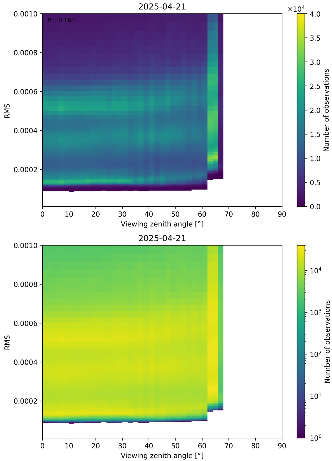
Figure 171: Scatter density plot of “Viewing zenith angle” against “RMS” for 2025-04-21 to 2025-04-22.
