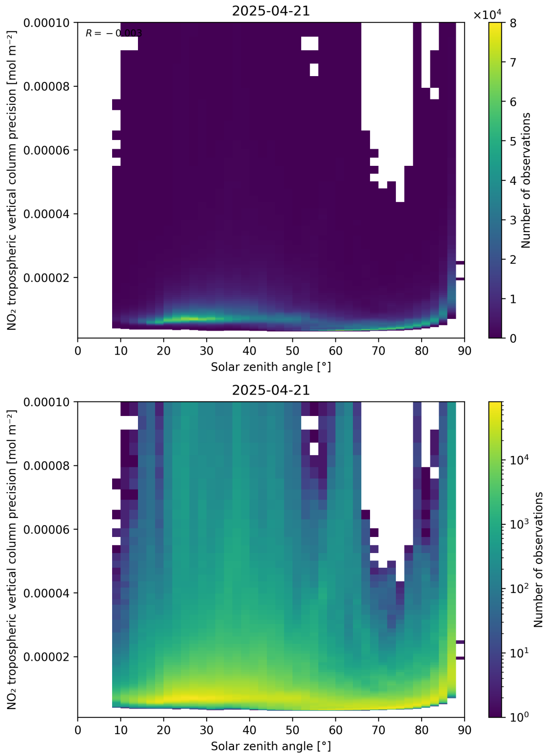
Figure 156: Scatter density plot of “Solar zenith angle” against “NO 2 tropospheric vertical column precision” for 2025-04-21 to 2025-04-22.
