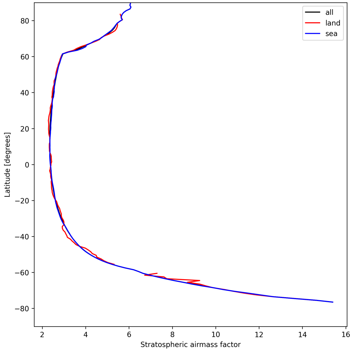
Figure 27: Zonal average of “Stratospheric airmass factor” for 2025-04-21 to 2025-04-22.
