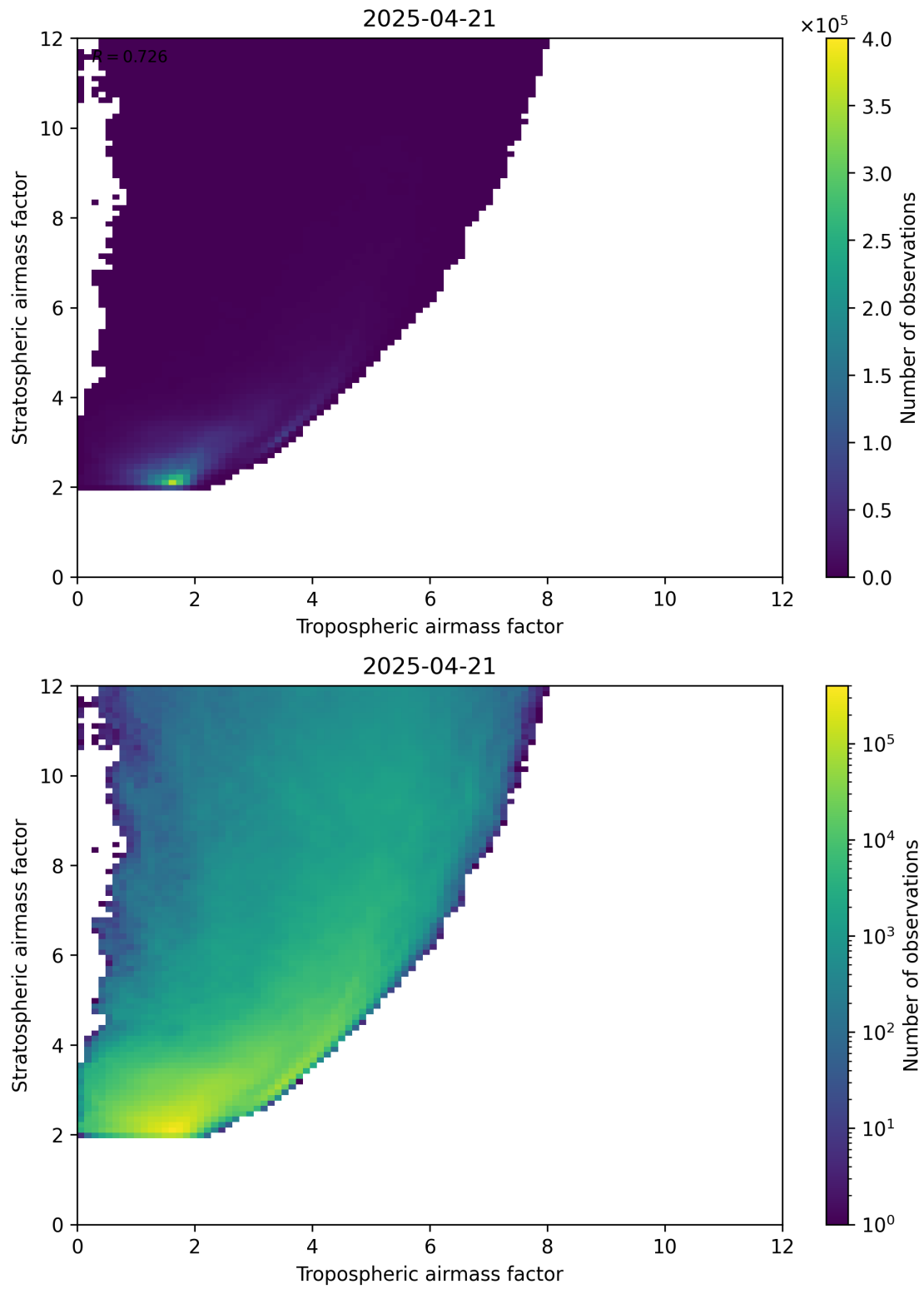
Figure 71: Scatter density plot of “Tropospheric airmass factor” against “Stratospheric airmass factor” for 2025-04-21 to 2025-04-22.
