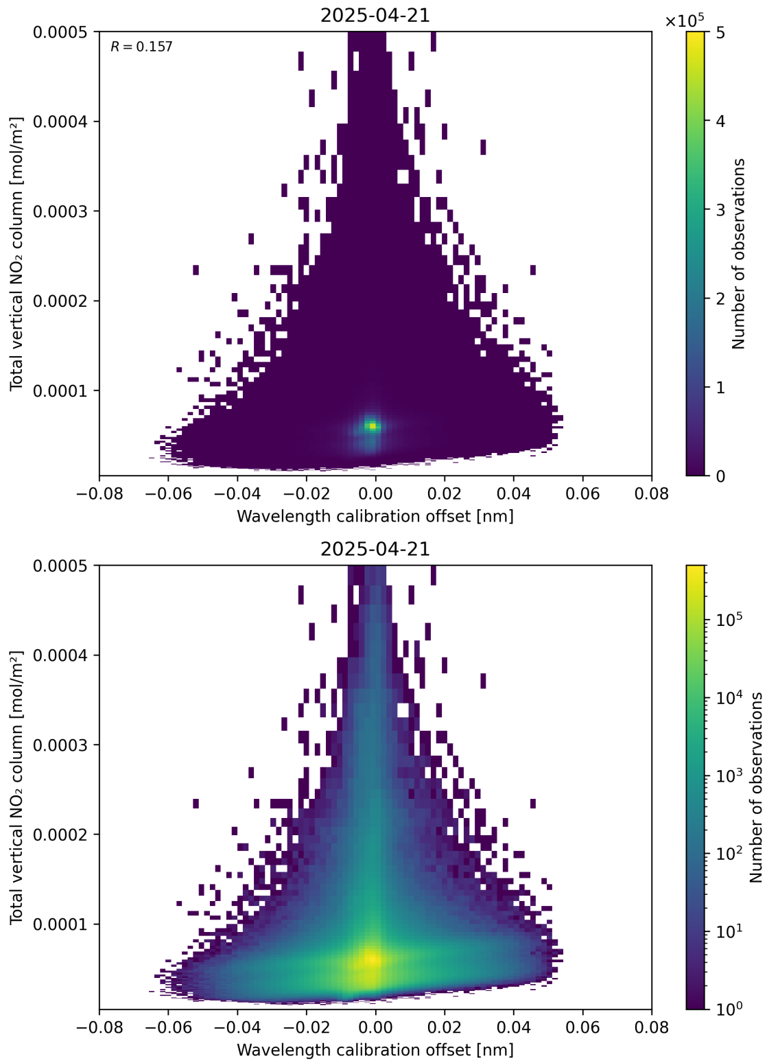
Figure 179: Scatter density plot of “Wavelength calibration offset” against “Total vertical NO 2 column” for 2025-04-21 to 2025-04-22.
