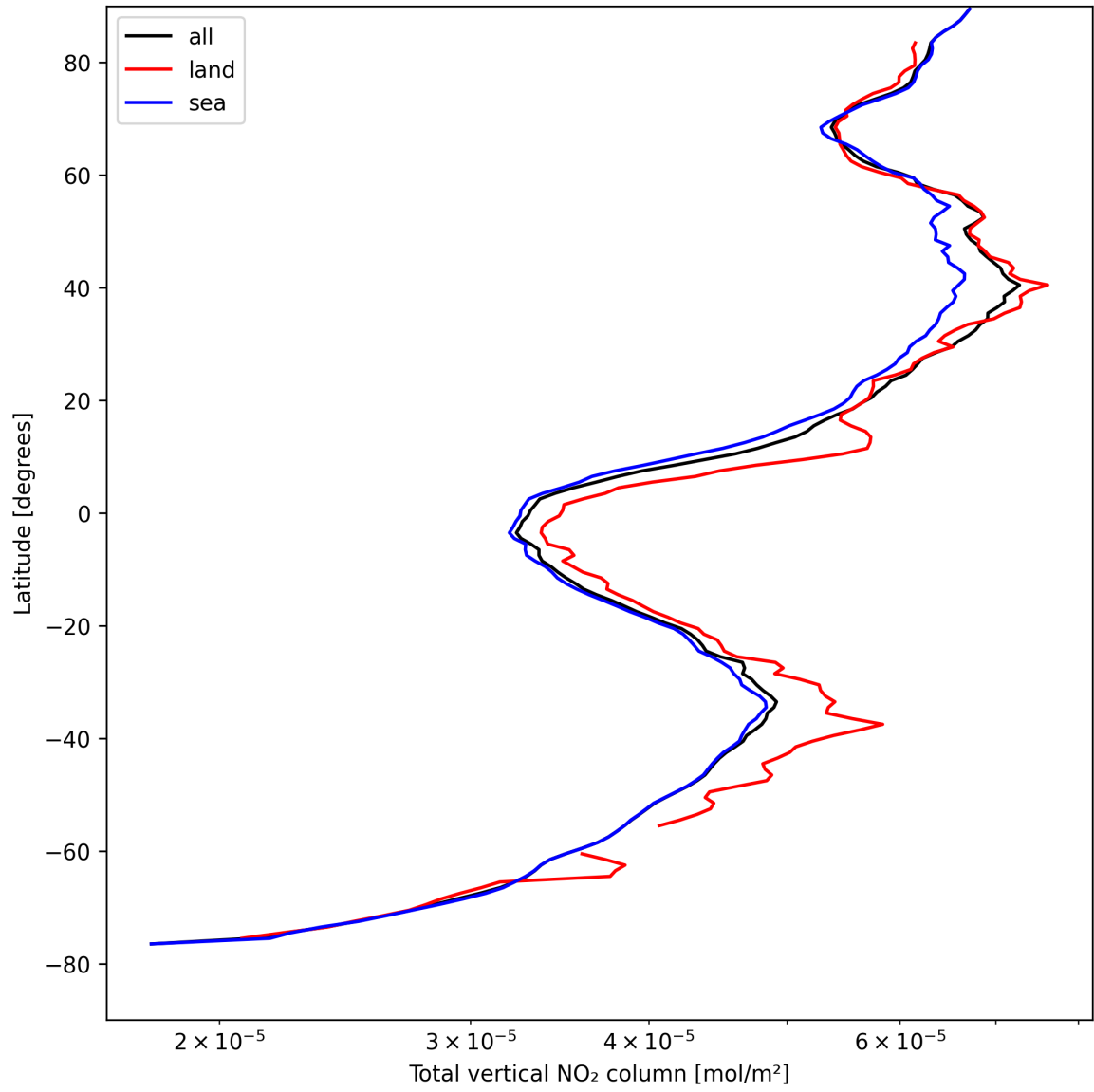
Figure 21: Zonal average of “Total vertical NO 2 column” for 2025-04-21 to 2025-04-22.
