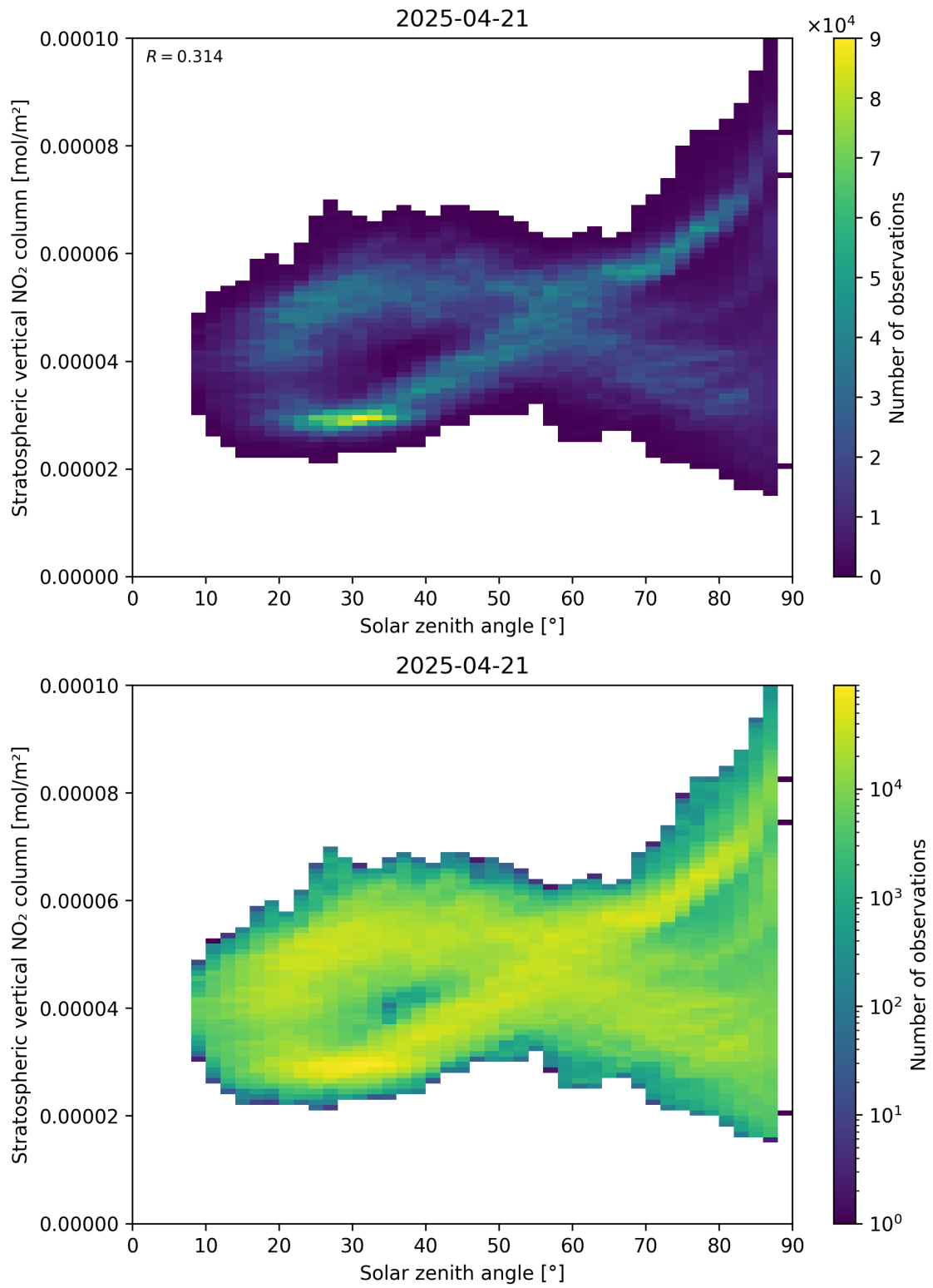
Figure 150: Scatter density plot of “Solar zenith angle” against “Stratospheric vertical NO 2 column” for 2025-04-21 to 2025-04-22.
