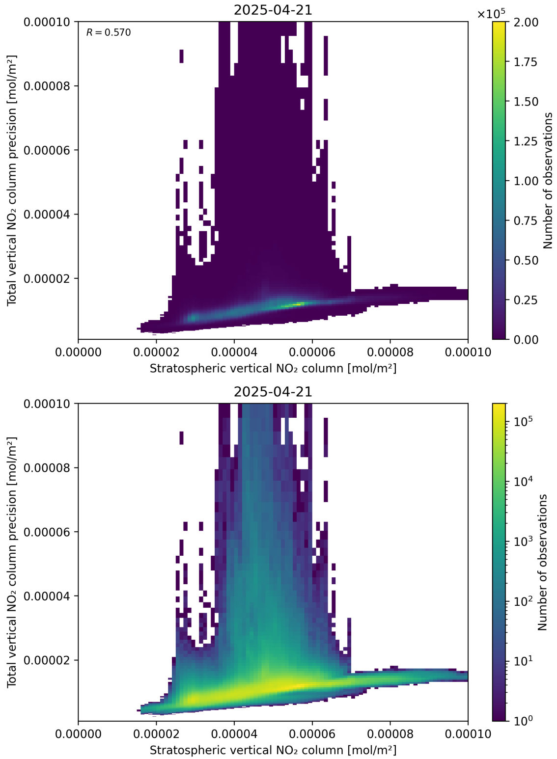
Figure 101: Scatter density plot of “Stratospheric vertical NO 2 column” against “Total vertical NO 2 column precision” for 2025-04-21 to 2025-04-22.
