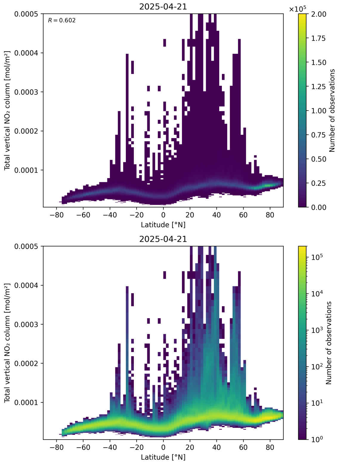
Figure 90: Scatter density plot of “Latitude” against “Total vertical NO 2 column” for 2025-04-21 to 2025-04-22.
