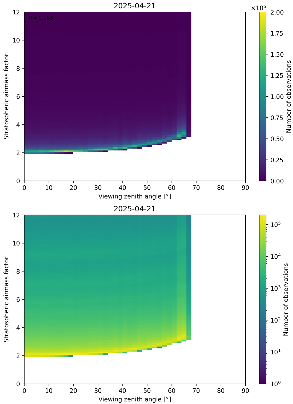
Figure 159: Scatter density plot of “Viewing zenith angle” against “Stratospheric airmass factor” for 2025-04-21 to 2025-04-22.
