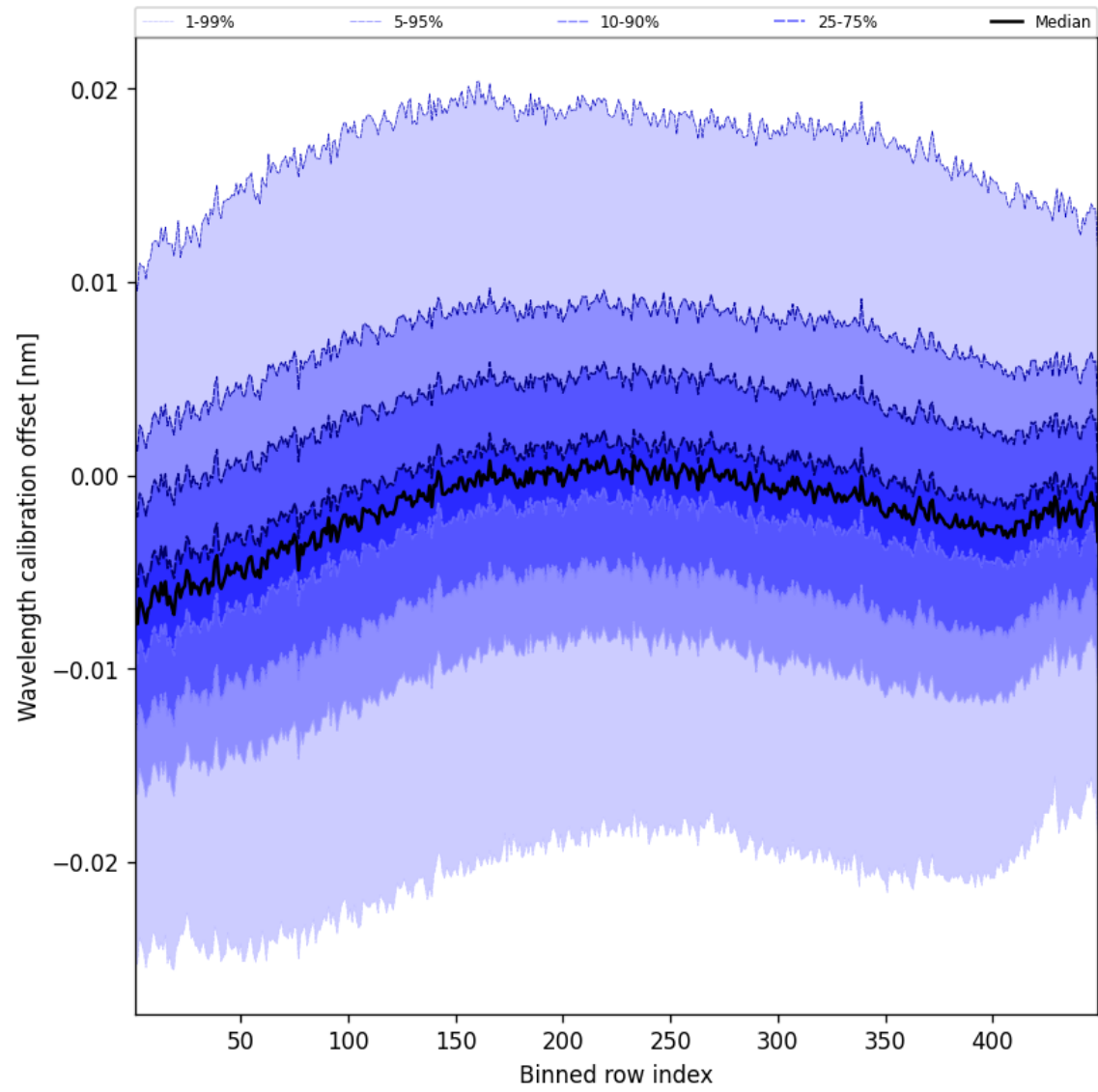
Figure 52: Along track statistics of “Wavelength calibration offset” for 2025-04-22 to 2025-04-22
