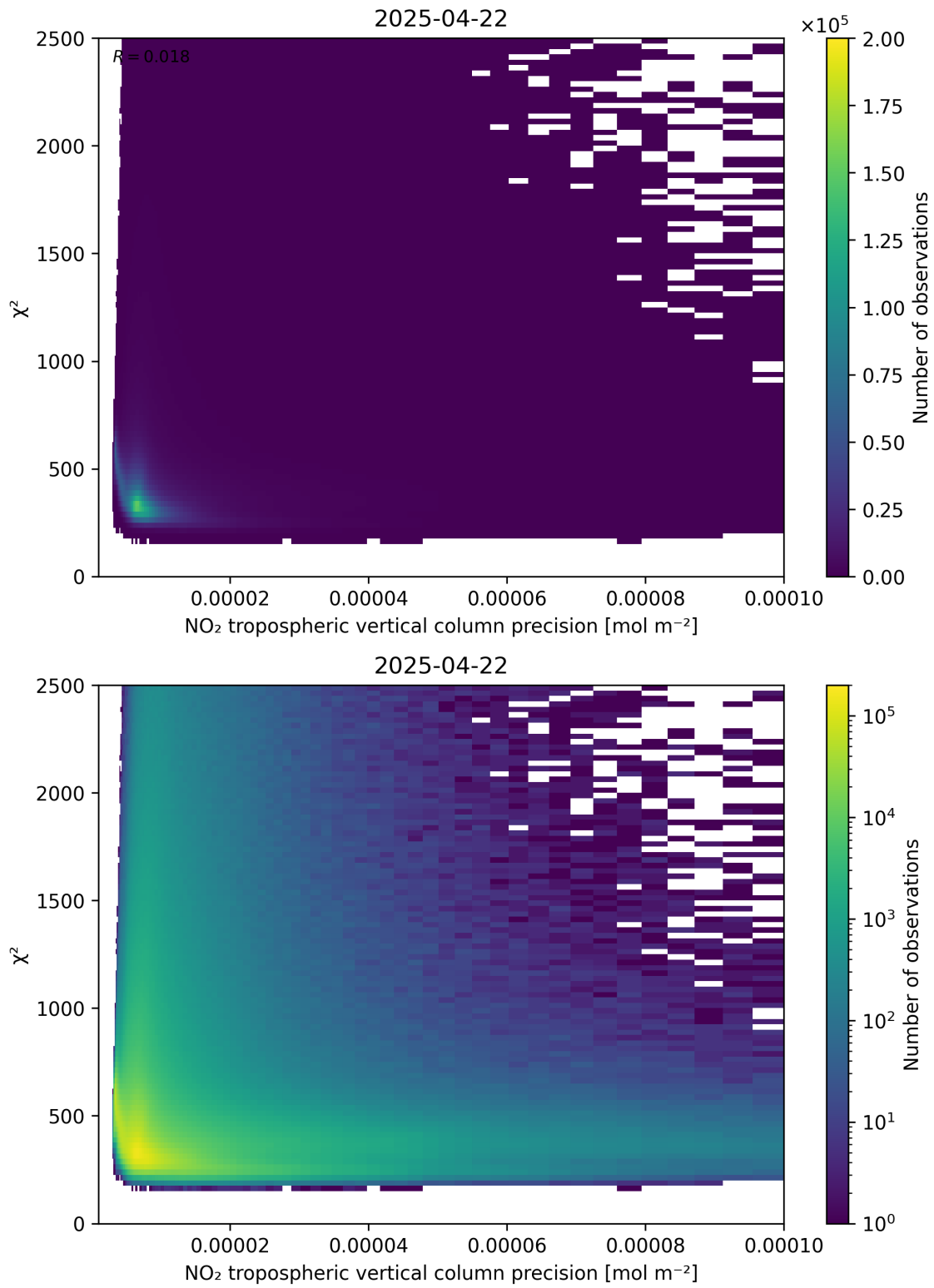
Figure 134: Scatter density plot of “NO 2 tropospheric vertical column precision” against “ \chi^2 ” for 2025-04-22 to 2025-04-22.
