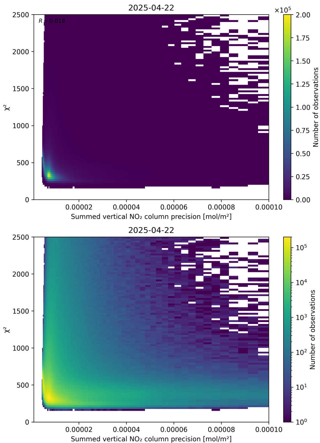
Figure 107: Scatter density plot of “Summed vertical NO 2 column precision” against “ \chi^2 ” for 2025-04-22 to 2025-04-22.
