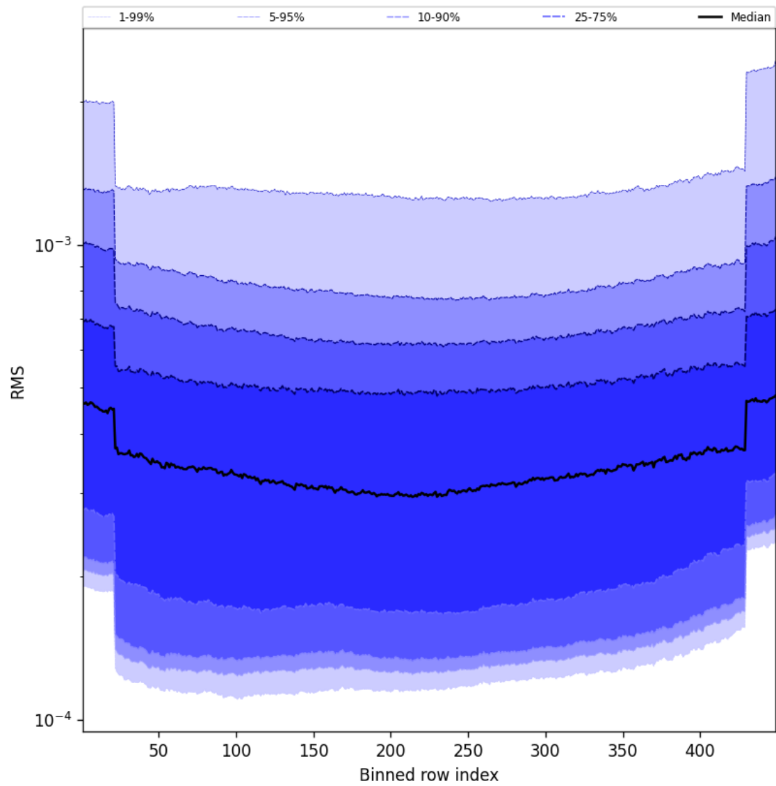
Figure 60: Along track statistics of “RMS” for 2025-04-22 to 2025-04-22
