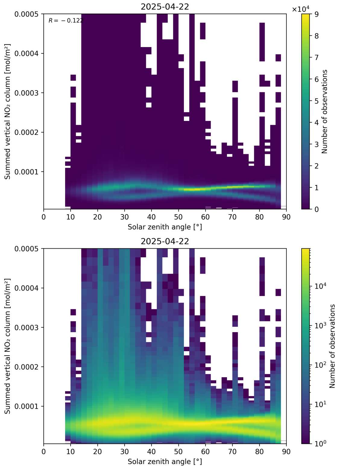
Figure 151: Scatter density plot of “Solar zenith angle” against “Summed vertical NO 2 column” for 2025-04-22 to 2025-04-22.
