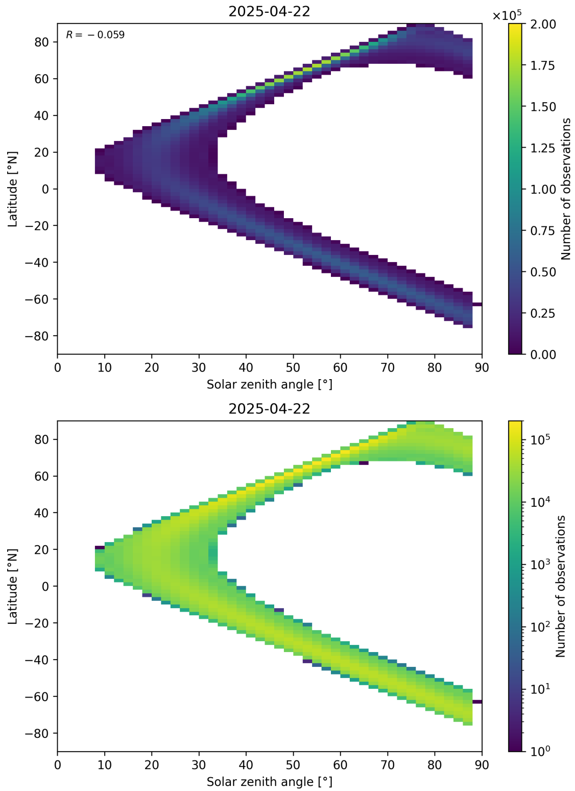
Figure 149: Scatter density plot of “Solar zenith angle” against “Latitude” for 2025-04-22 to 2025-04-22.
