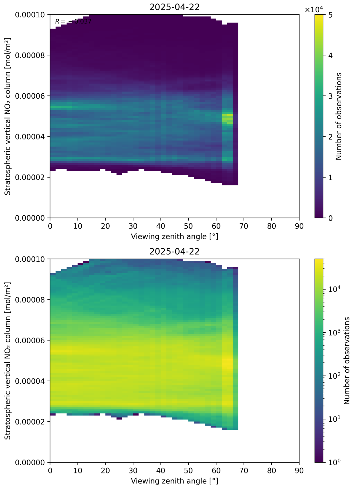
Figure 164: Scatter density plot of “Viewing zenith angle” against “Stratospheric vertical NO 2 column” for 2025-04-22 to 2025-04-22.
