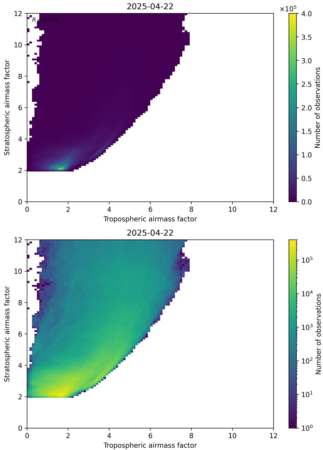
Figure 71: Scatter density plot of “Tropospheric airmass factor” against “Stratospheric airmass factor” for 2025-04-22 to 2025-04-22.
