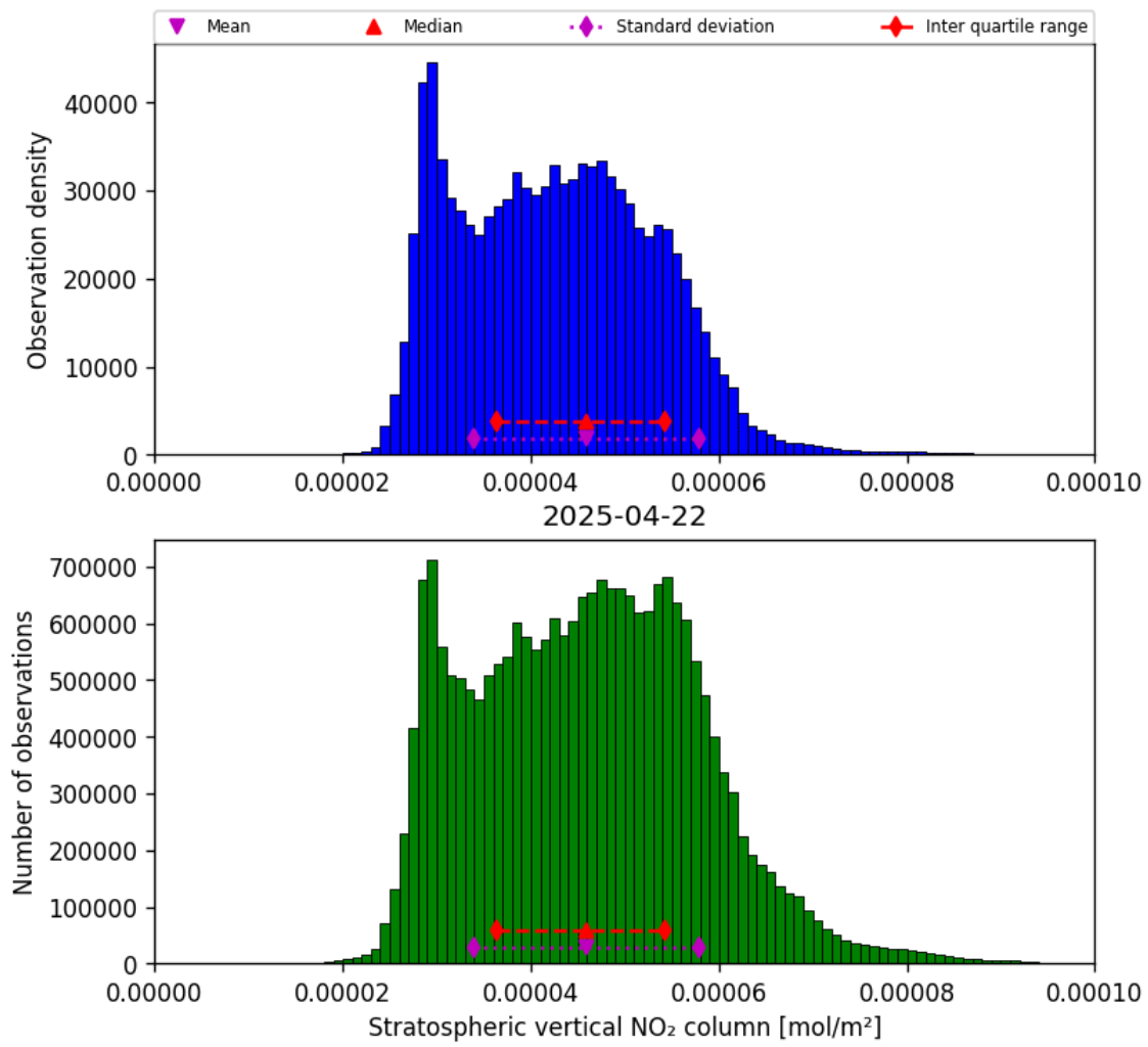
Figure 36: Histogram of “Stratospheric vertical NO 2 column” for 2025-04-22 to 2025-04-22
