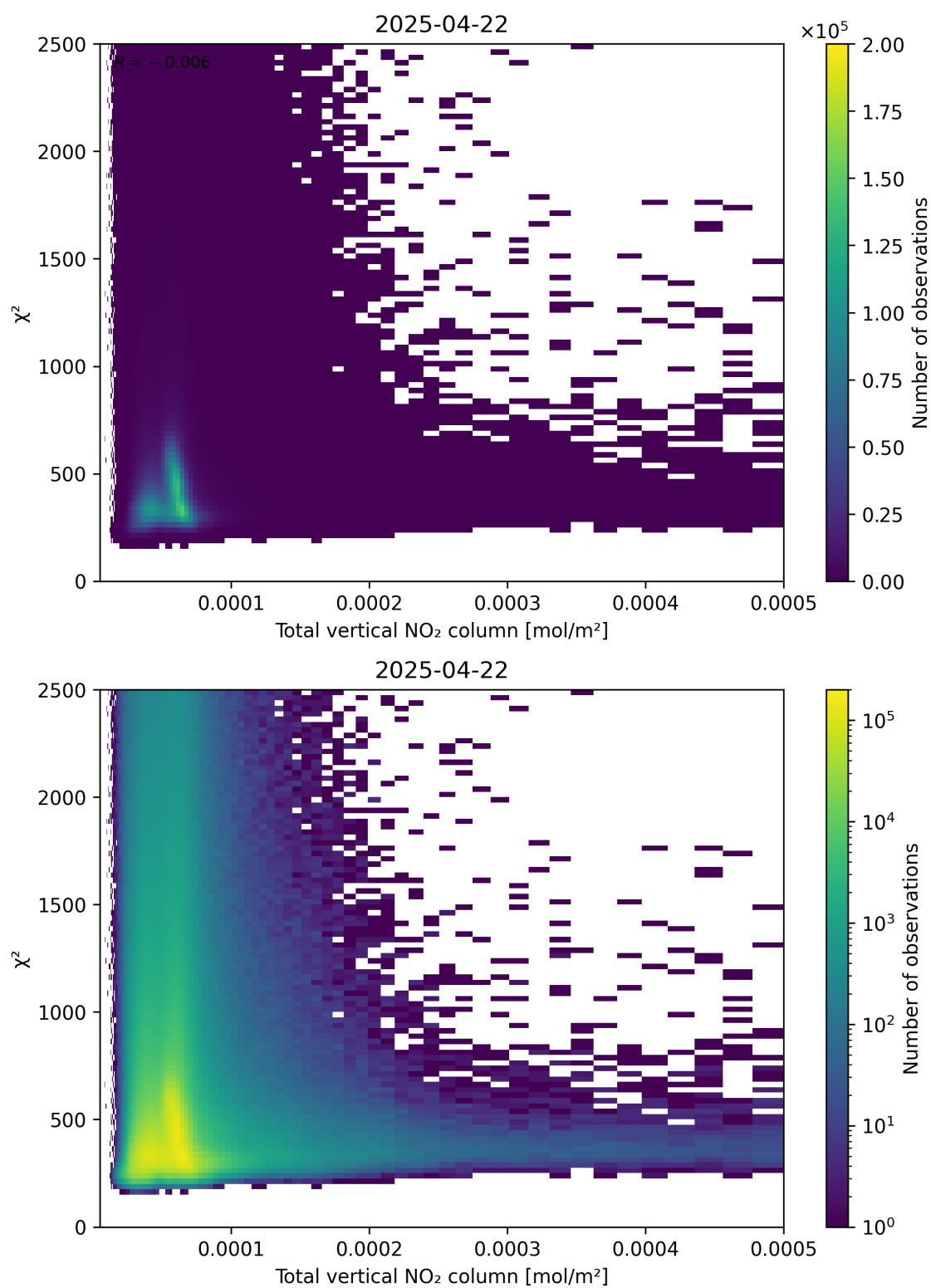
Figure 111: Scatter density plot of “Total vertical NO 2 column” against “ \chi^2 ” for 2025-04-22 to 2025-04-22.
