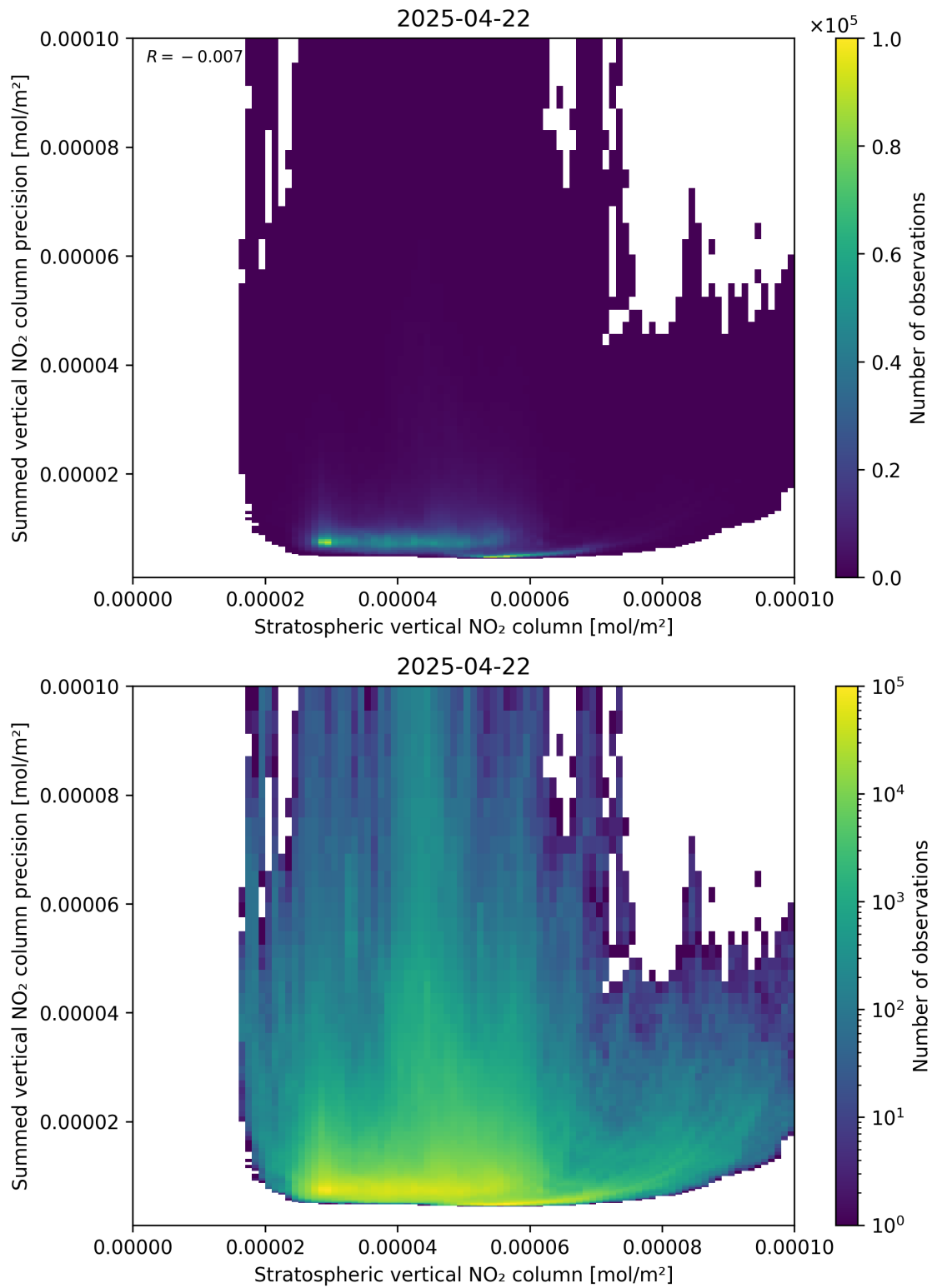
Figure 99: Scatter density plot of “Stratospheric vertical NO 2 column” against “Summed vertical NO 2 column precision” for 2025-04-22 to 2025-04-22.
