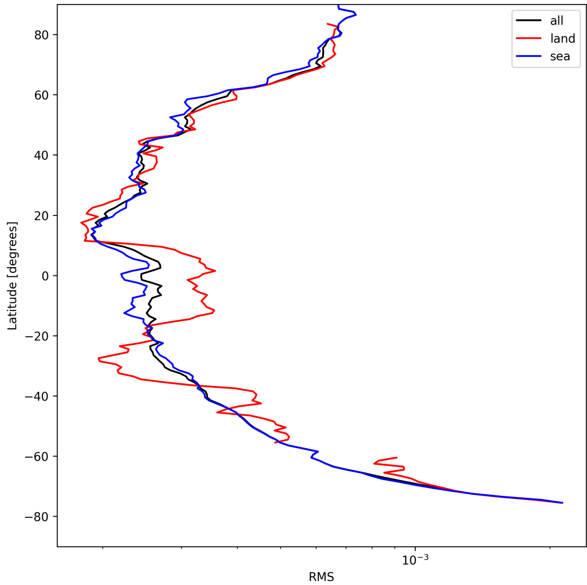
Figure 26: Zonal average of “RMS” for 2025-04-22 to 2025-04-22.
