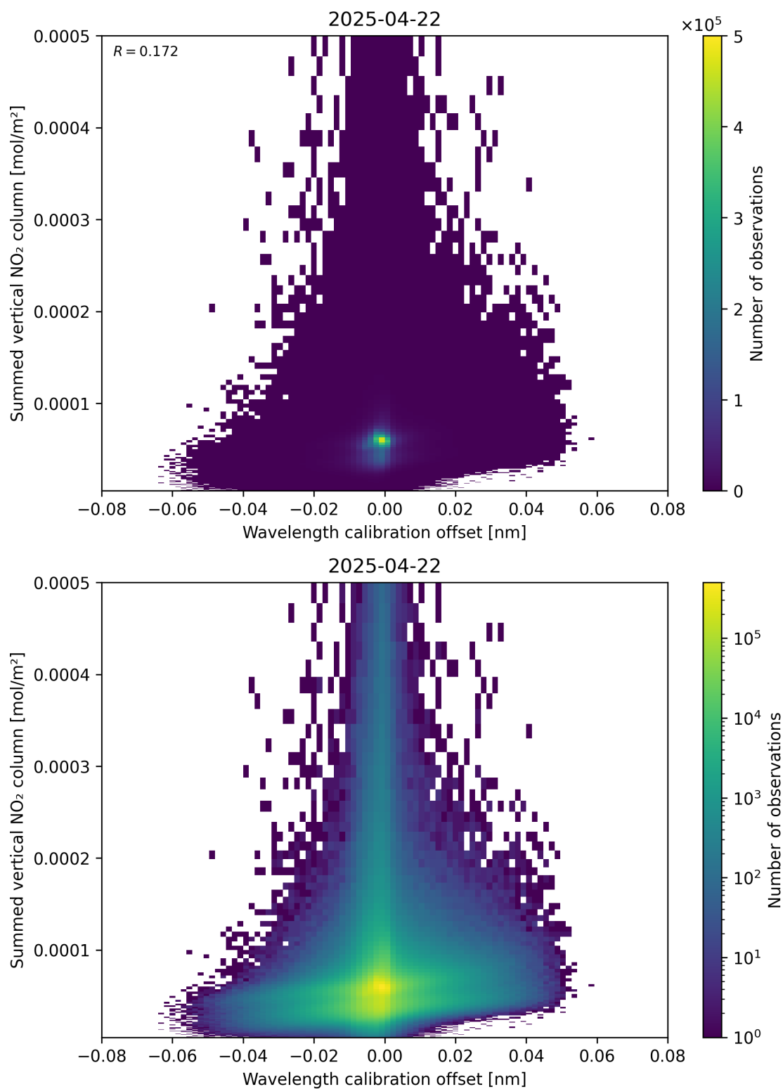
Figure 177: Scatter density plot of “Wavelength calibration offset” against “Summed vertical NO 2 column” for 2025-04-22 to 2025-04-22.
