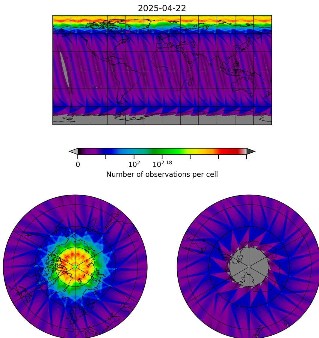
Figure 10: Map of the number of observations for 2025-04-22 to 2025-04-22
