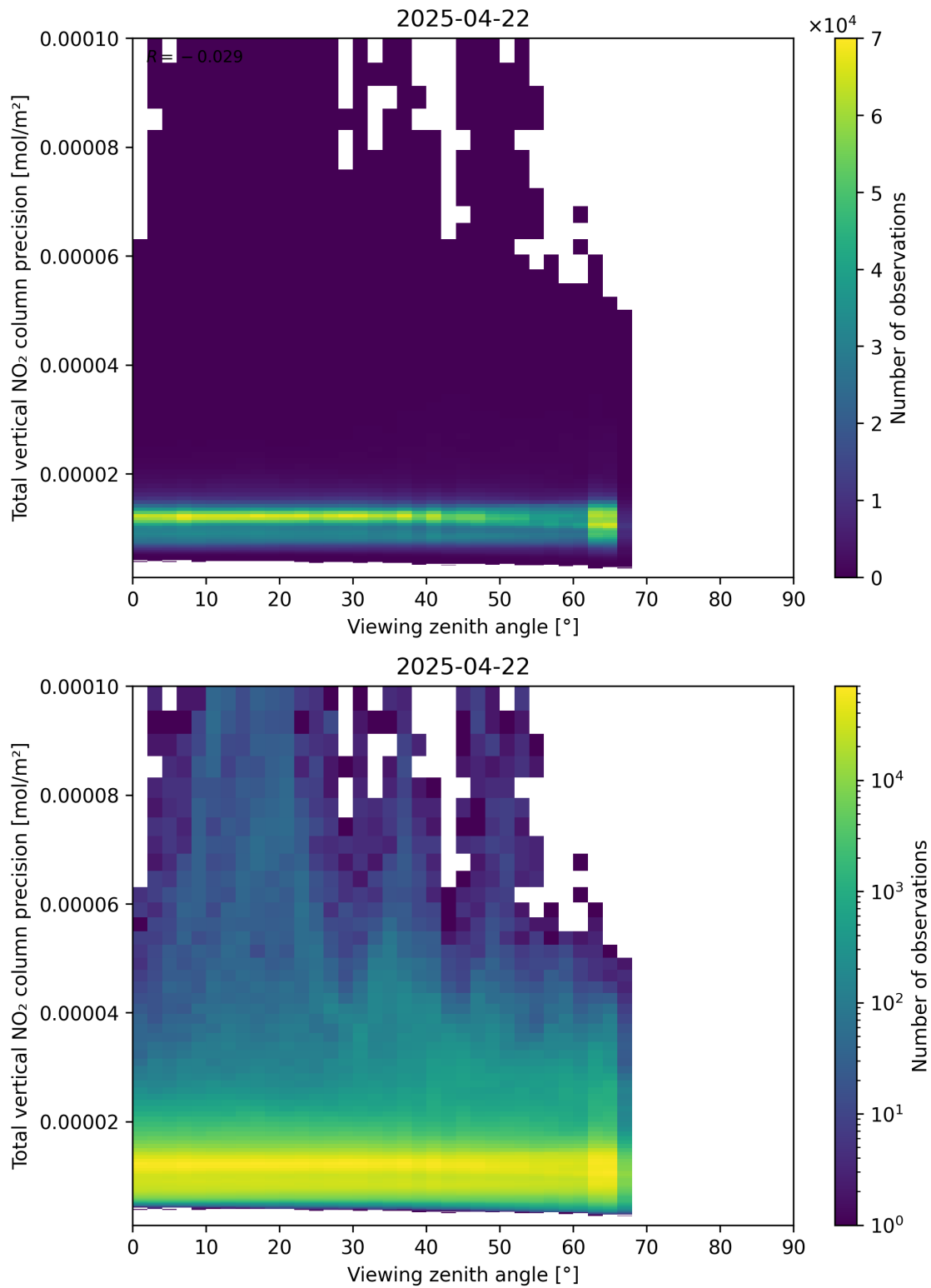
Figure 168: Scatter density plot of “Viewing zenith angle” against “Total vertical NO 2 column precision” for 2025-04-22 to 2025-04-22.
