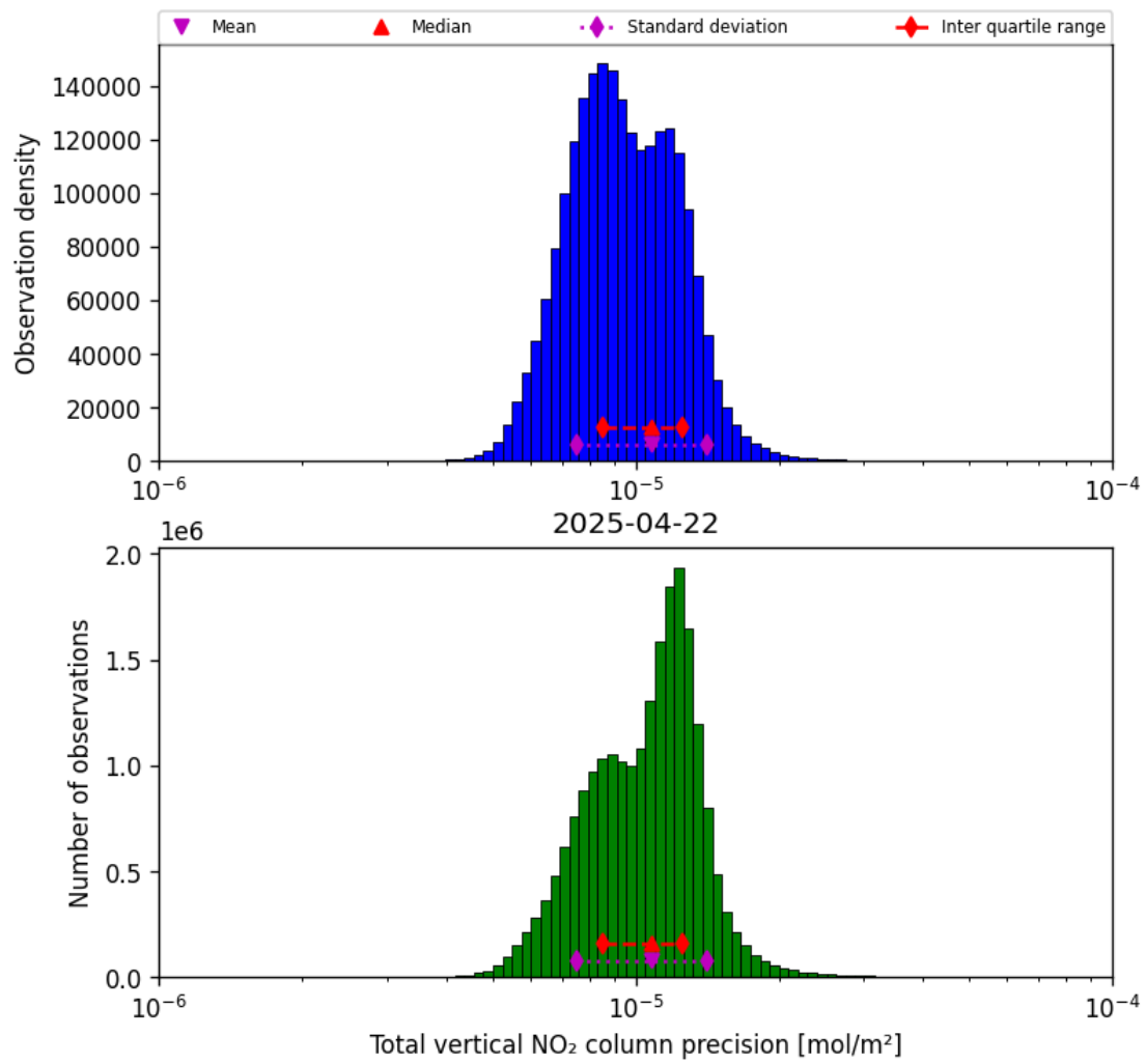
Figure 39: Histogram of "Total vertical NO 2 column precision" for 2025-04-22 to 2025-04-22
