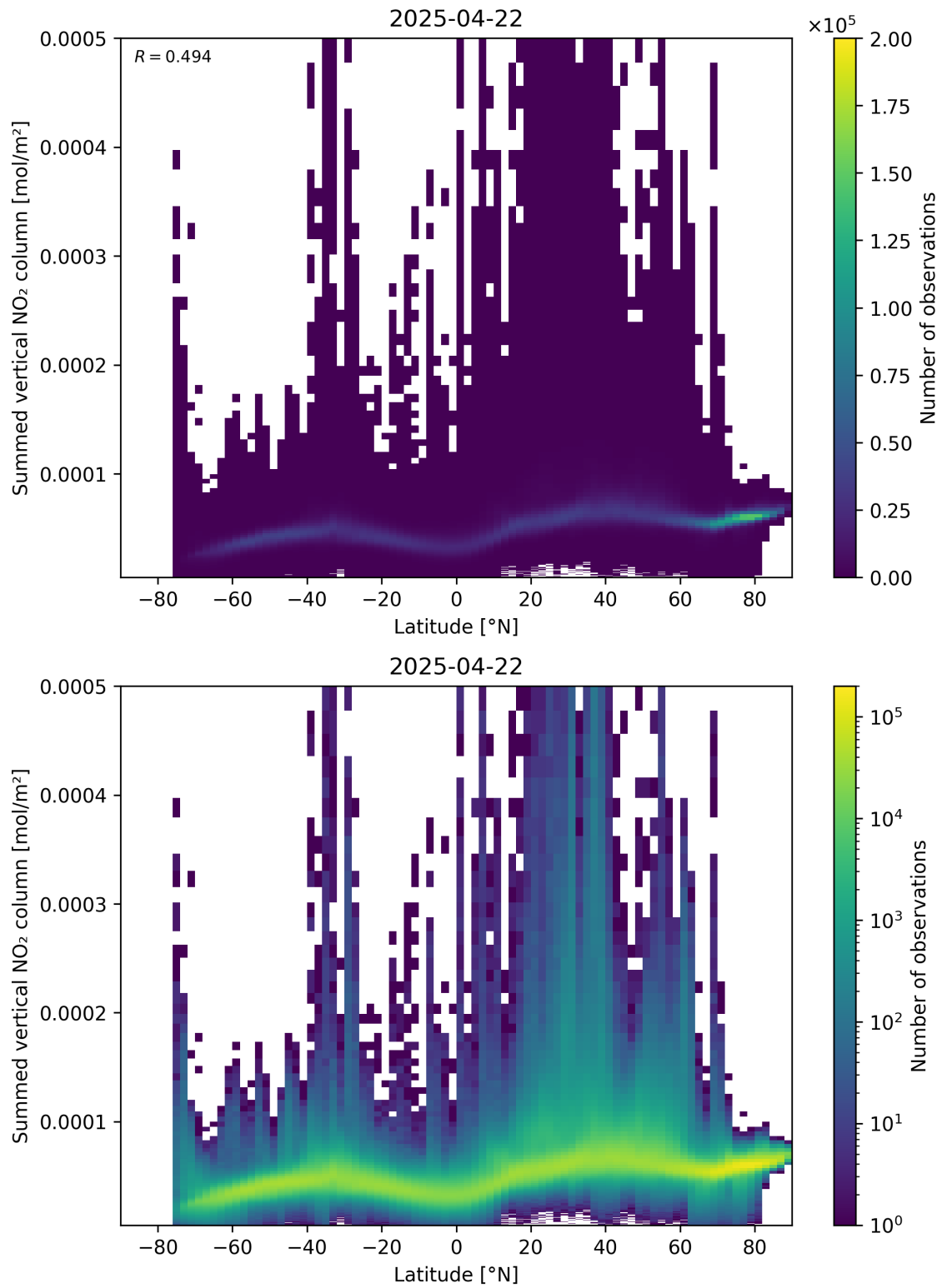
Figure 88: Scatter density plot of “Latitude” against “Summed vertical NO 2 column” for 2025-04-22 to 2025-04-22.
