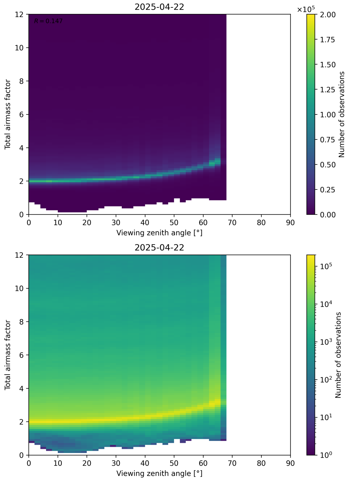
Figure 160: Scatter density plot of “Viewing zenith angle” against “Total airmass factor” for 2025-04-22 to 2025-04-22.
