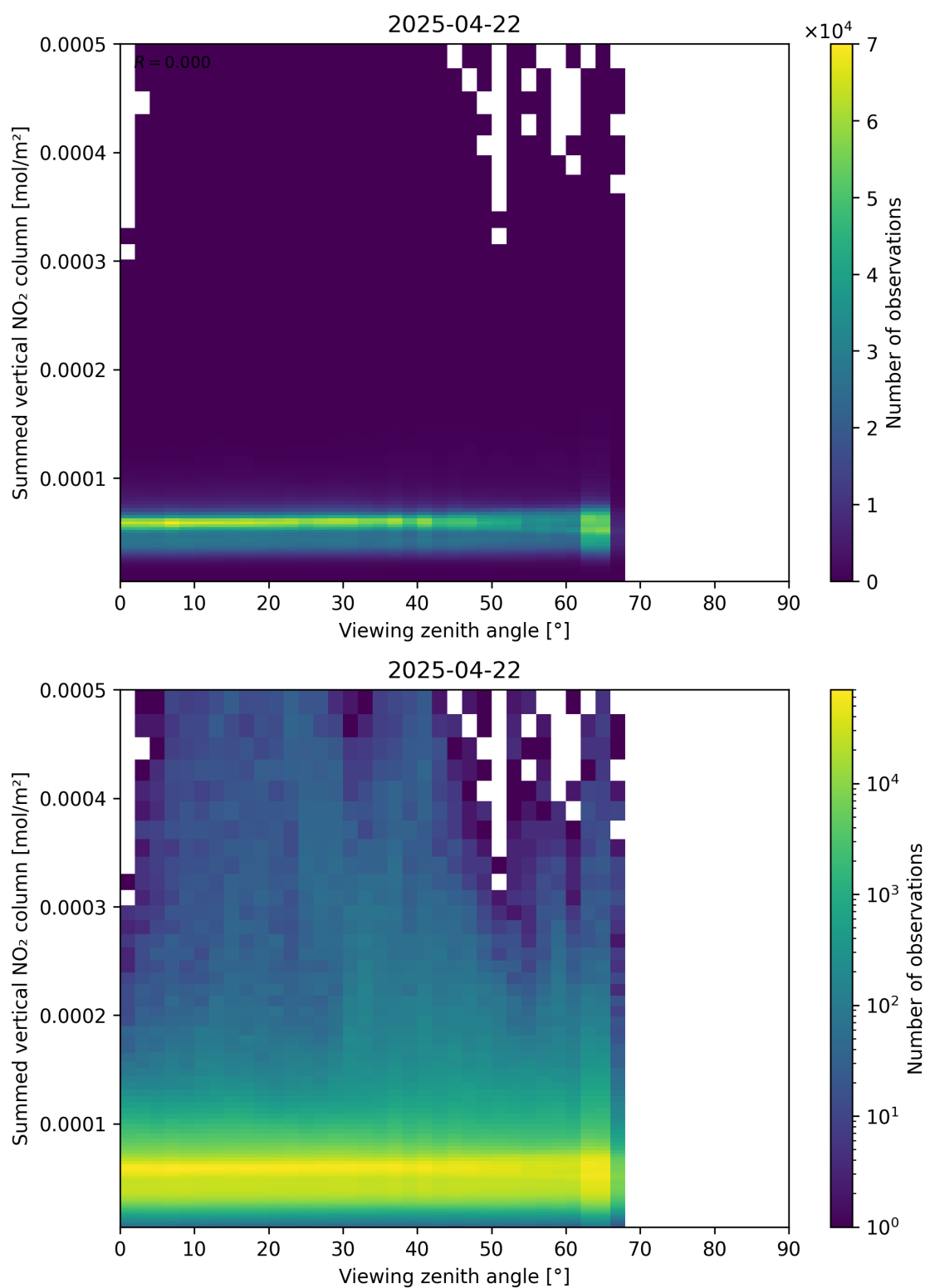
Figure 165: Scatter density plot of “Viewing zenith angle” against “Summed vertical NO 2 column” for 2025-04-22 to 2025-04-22.
