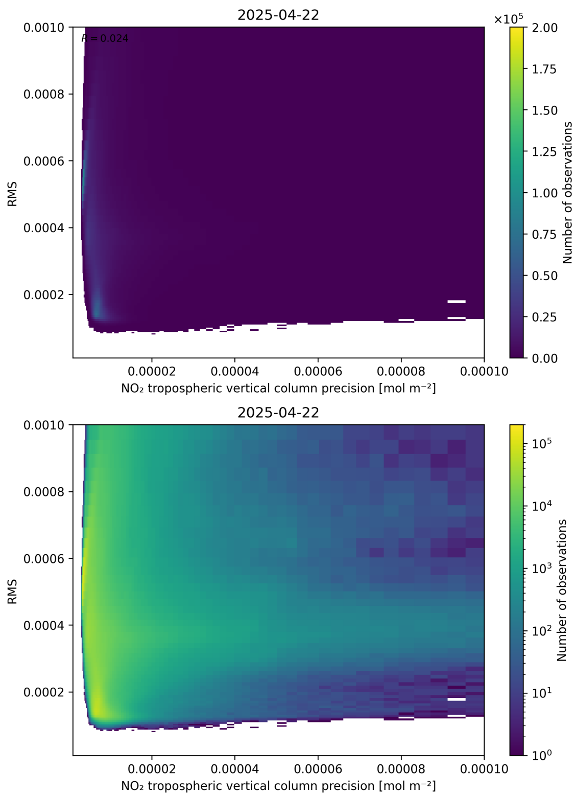
Figure 140: Scatter density plot of “NO 2 tropospheric vertical column precision” against “RMS” for 2025-04-22 to 2025-04-22.
