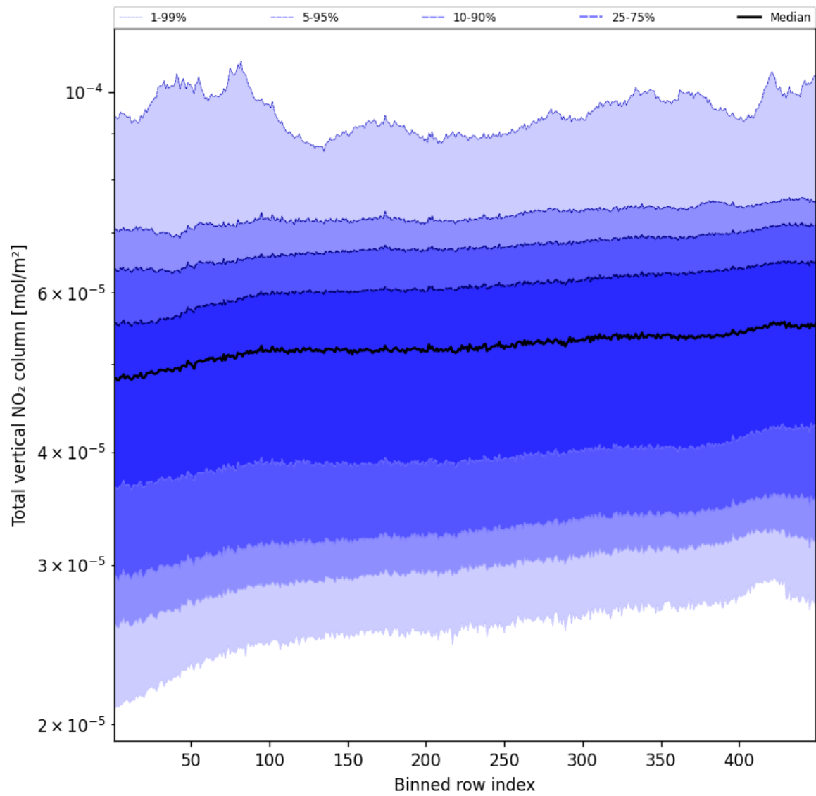
Figure 55: Along track statistics of “Total vertical NO 2 column” for 2025-04-22 to 2025-04-22
