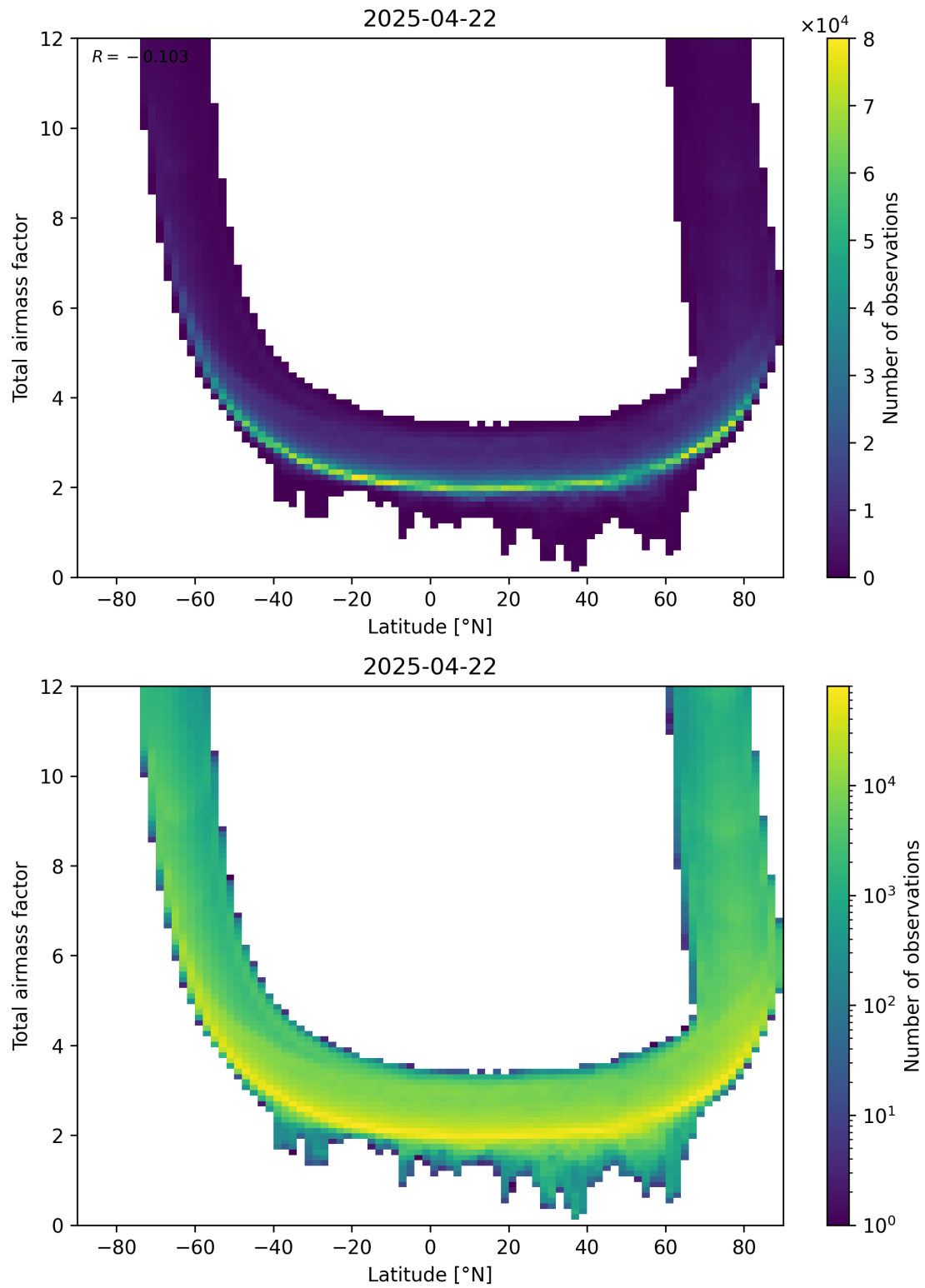
Figure 84: Scatter density plot of “Latitude” against “Total airmass factor” for 2025-04-22 to 2025-04-22.
