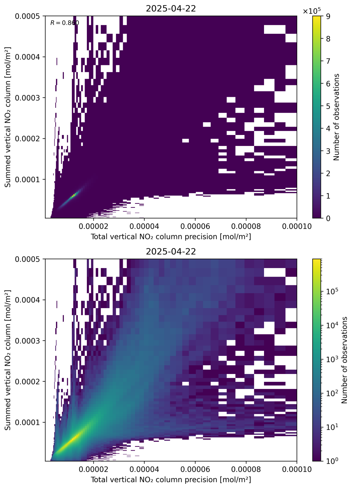
Figure 117: Scatter density plot of “Total vertical NO 2 column precision” against “Summed vertical NO 2 column” for 2025-04-22 to 2025-04-22.
