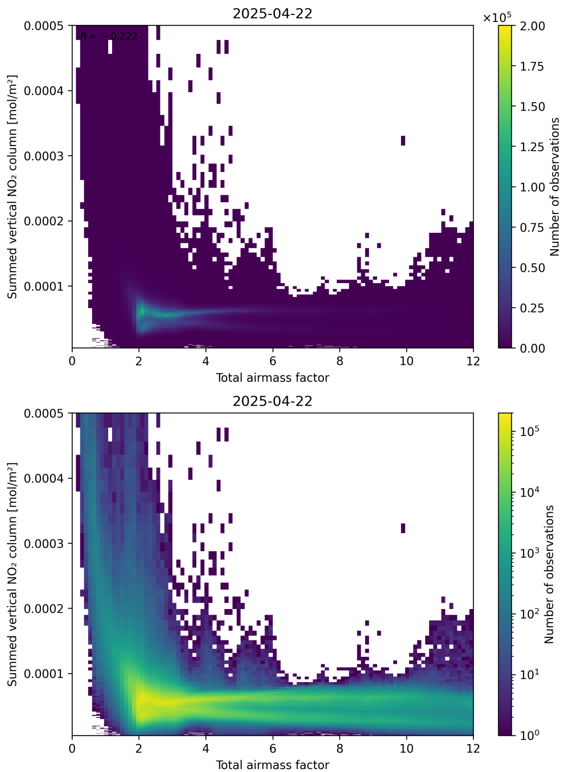
Figure 65: Scatter density plot of “Total airmass factor” against “Summed vertical NO 2 column” for 2025-04-22 to 2025-04-22.
