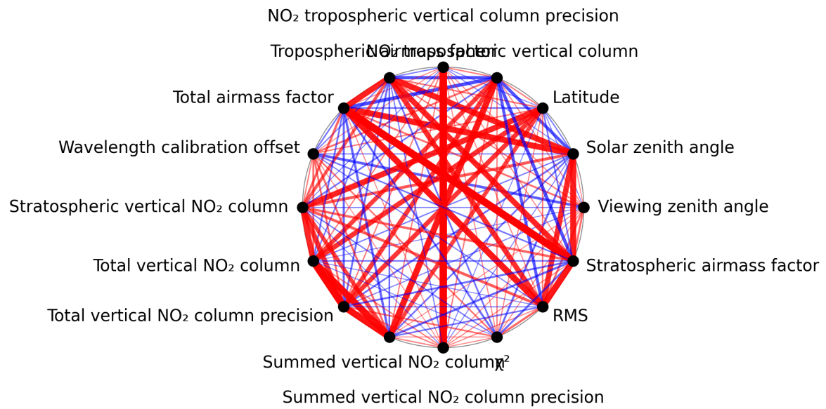
Figure 1: Map of correlation graph for 2025-04-22 to 2025-04-22.
