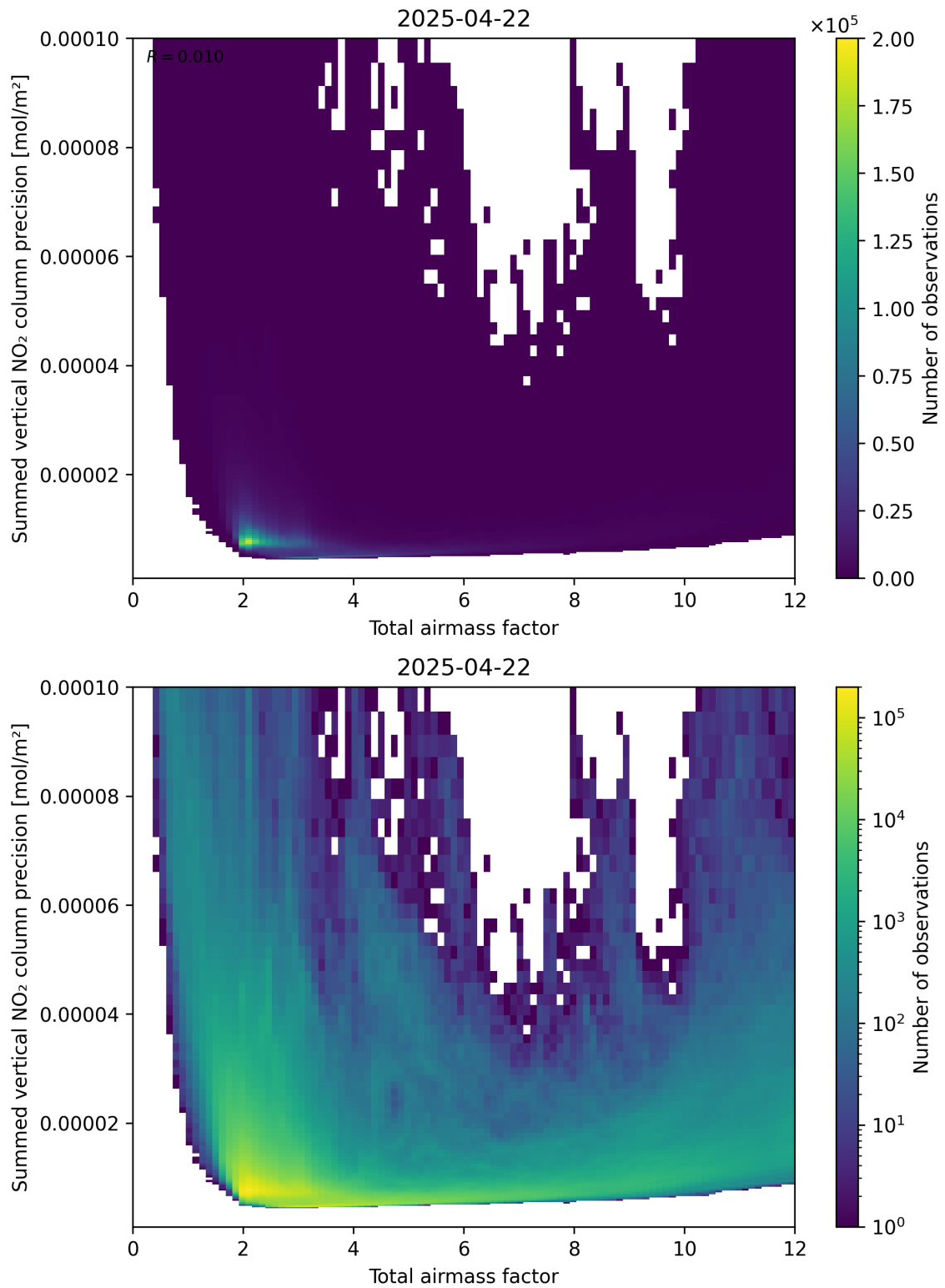
Figure 66: Scatter density plot of “Total airmass factor” against “Summed vertical NO 2 column precision” for 2025-04-22 to 2025-04-22.
