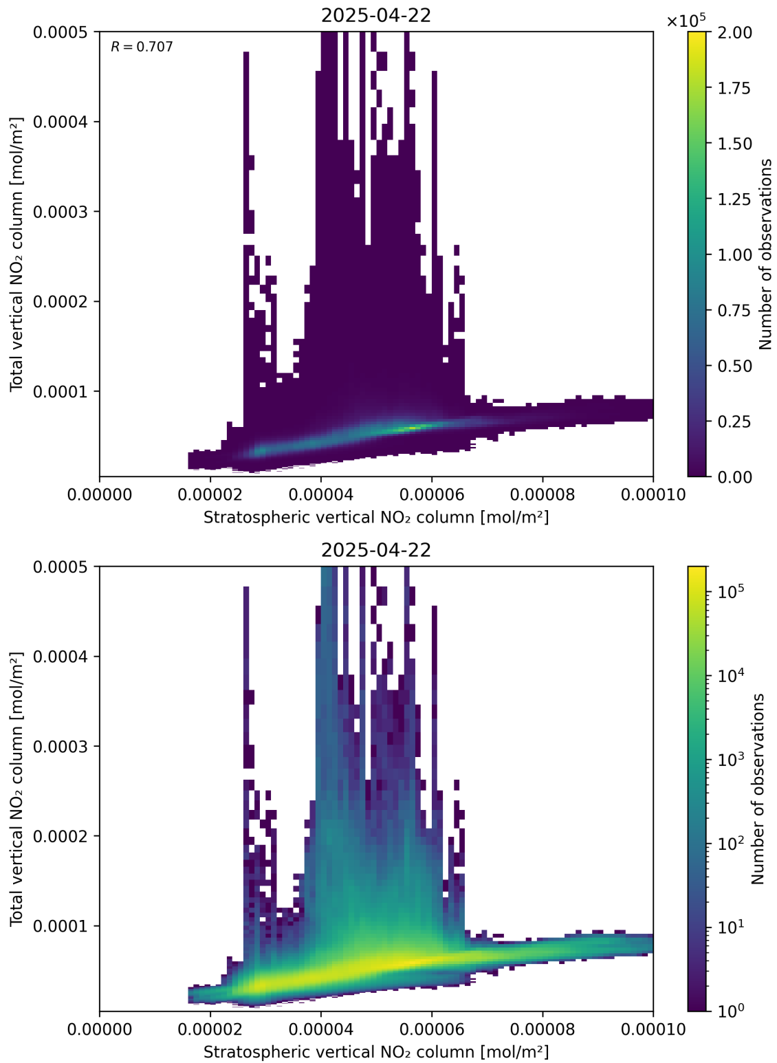
Figure 100: Scatter density plot of “Stratospheric vertical NO 2 column” against “Total vertical NO 2 column” for 2025-04-22 to 2025-04-22.
