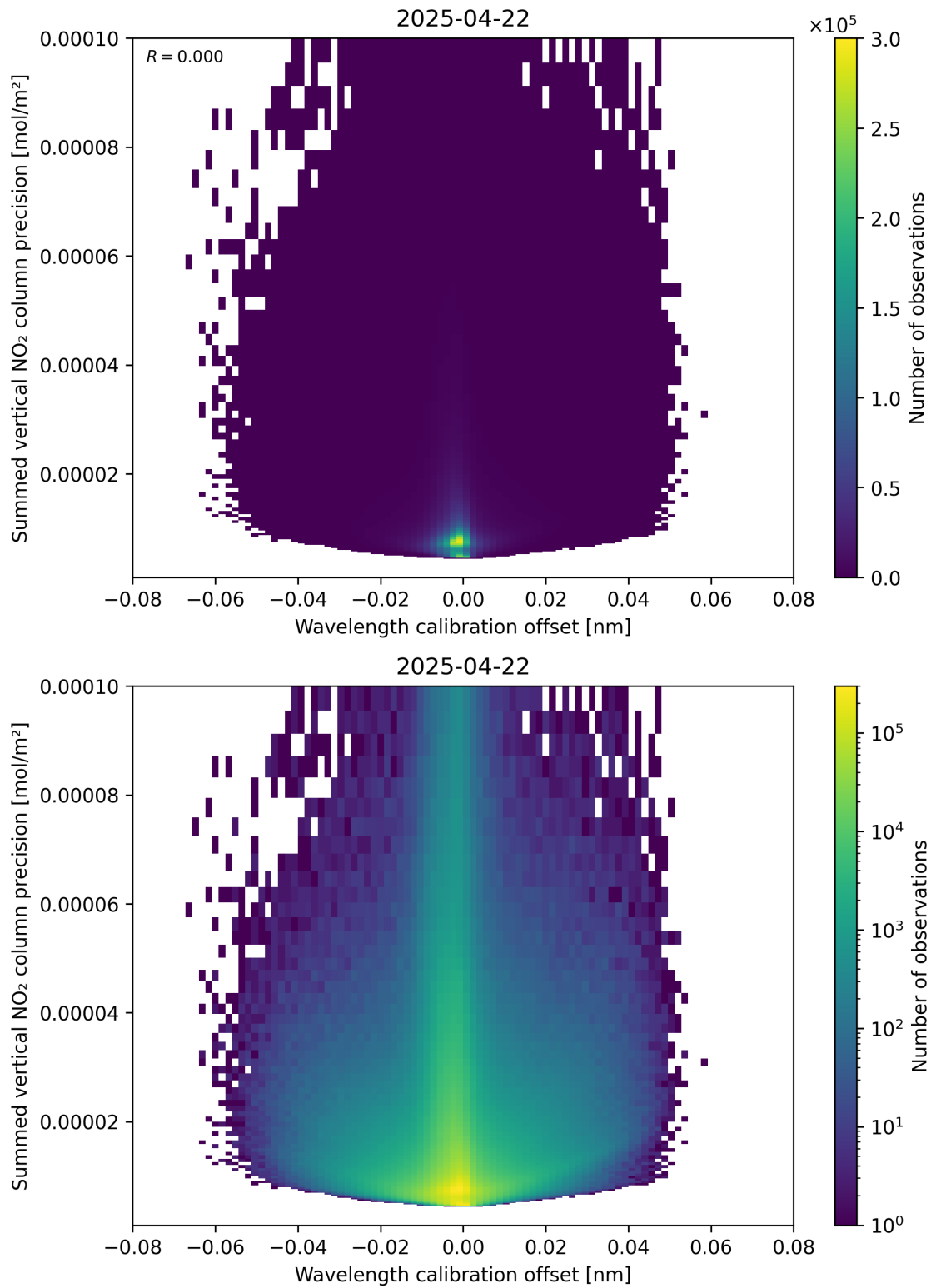
Figure 178: Scatter density plot of “Wavelength calibration offset” against “Summed vertical NO 2 column precision” for 2025-04-22 to 2025-04-22.
