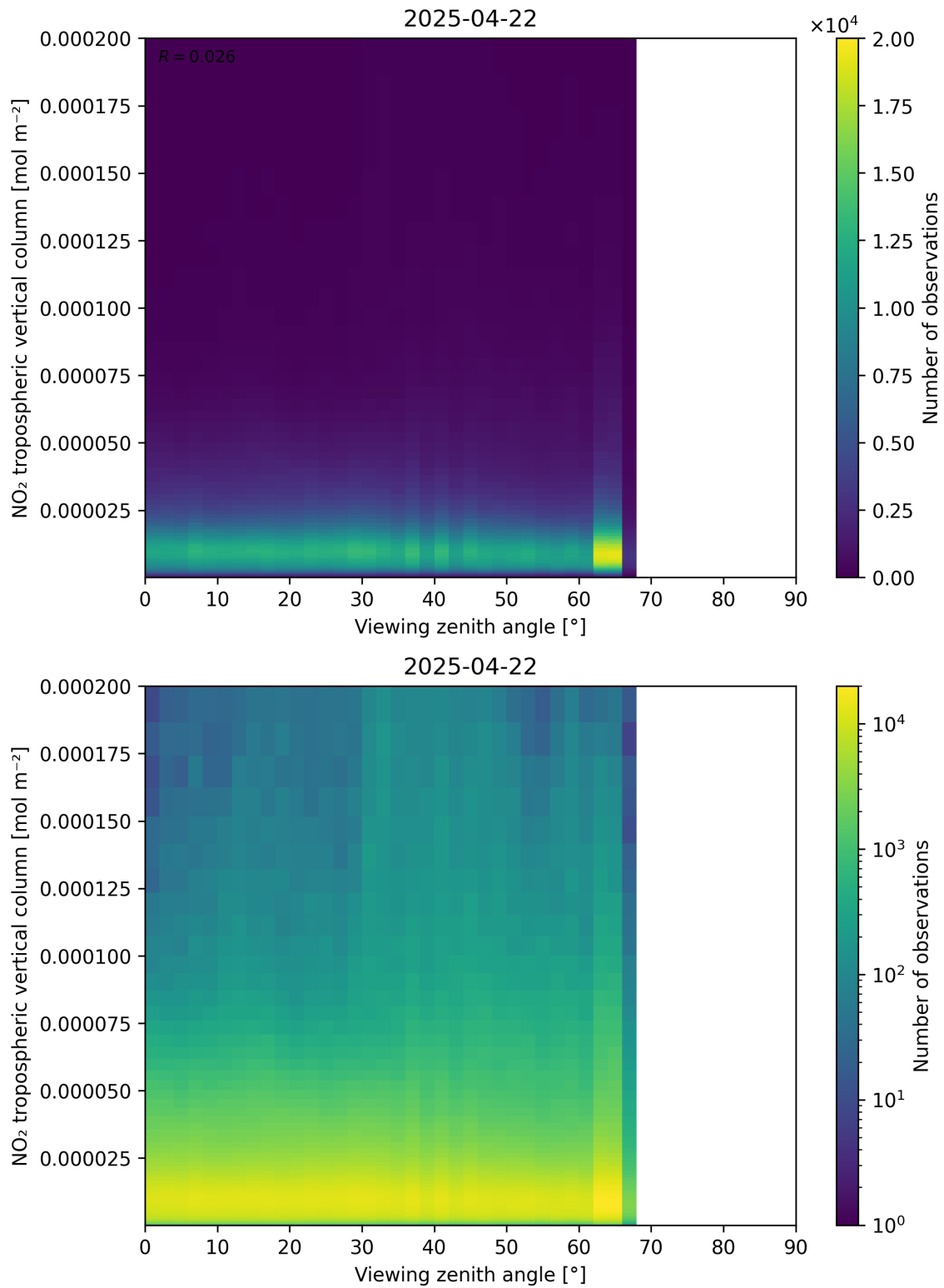
Figure 169: Scatter density plot of “Viewing zenith angle” against “NO 2 tropospheric vertical column” for 2025-04-22 to 2025-04-22.
