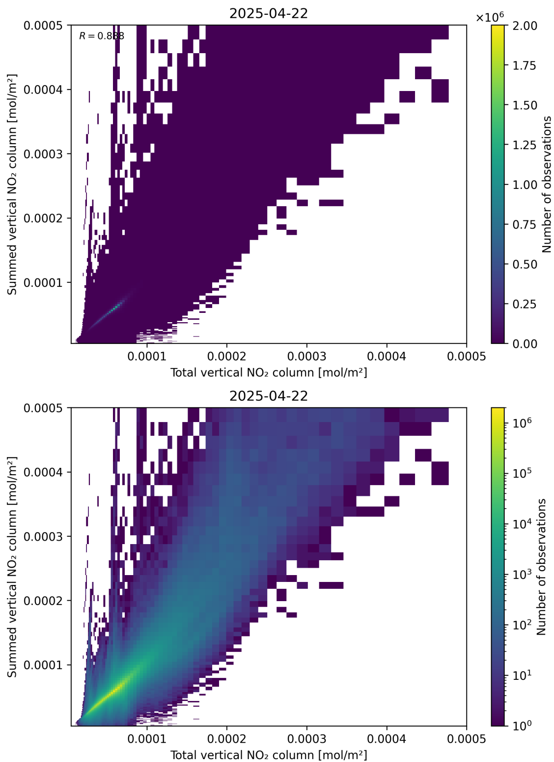
Figure 112: Scatter density plot of “Total vertical NO 2 column” against “Summed vertical NO 2 column” for 2025-04-22 to 2025-04-22.
