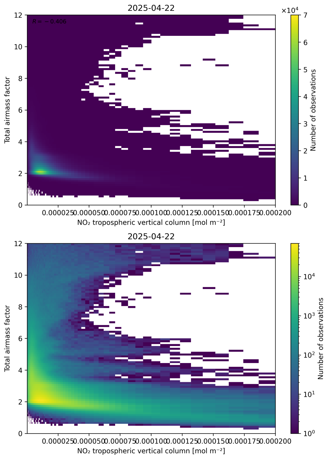
Figure 122: Scatter density plot of “NO 2 tropospheric vertical column” against “Total air mass factor” for 2025-04-22 to 2025-04-22.
