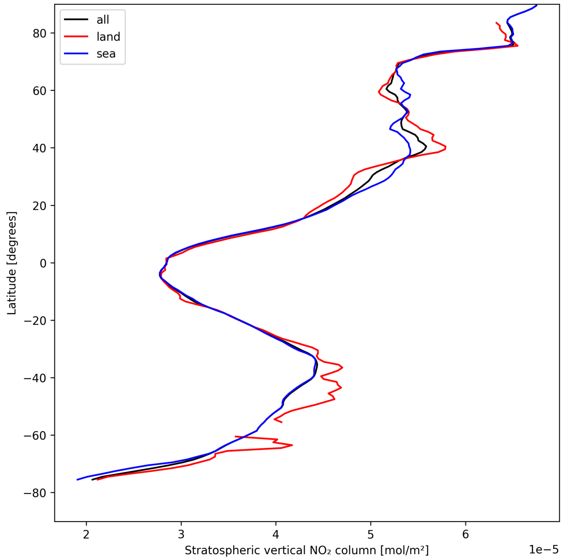
Figure 19: Zonal average of “Stratospheric vertical NO 2 column” for 2025-04-22 to 2025-04-22.
