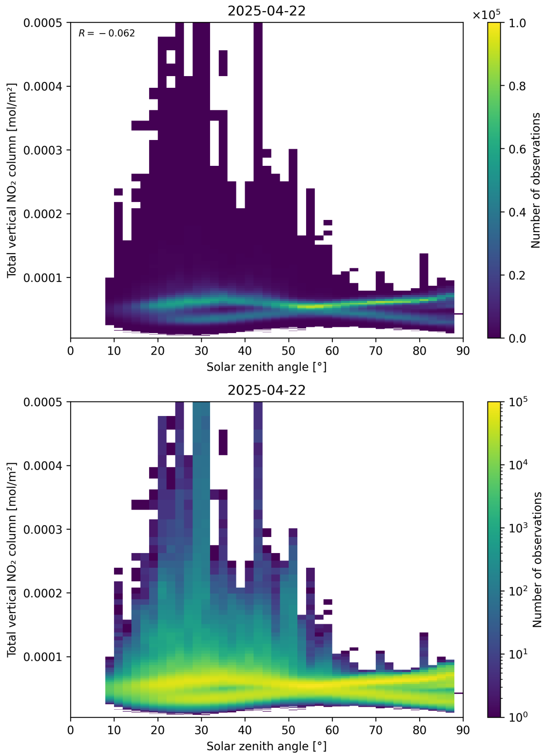
Figure 153: Scatter density plot of “Solar zenith angle” against “Total vertical NO 2 column” for 2025-04-22 to 2025-04-22.
