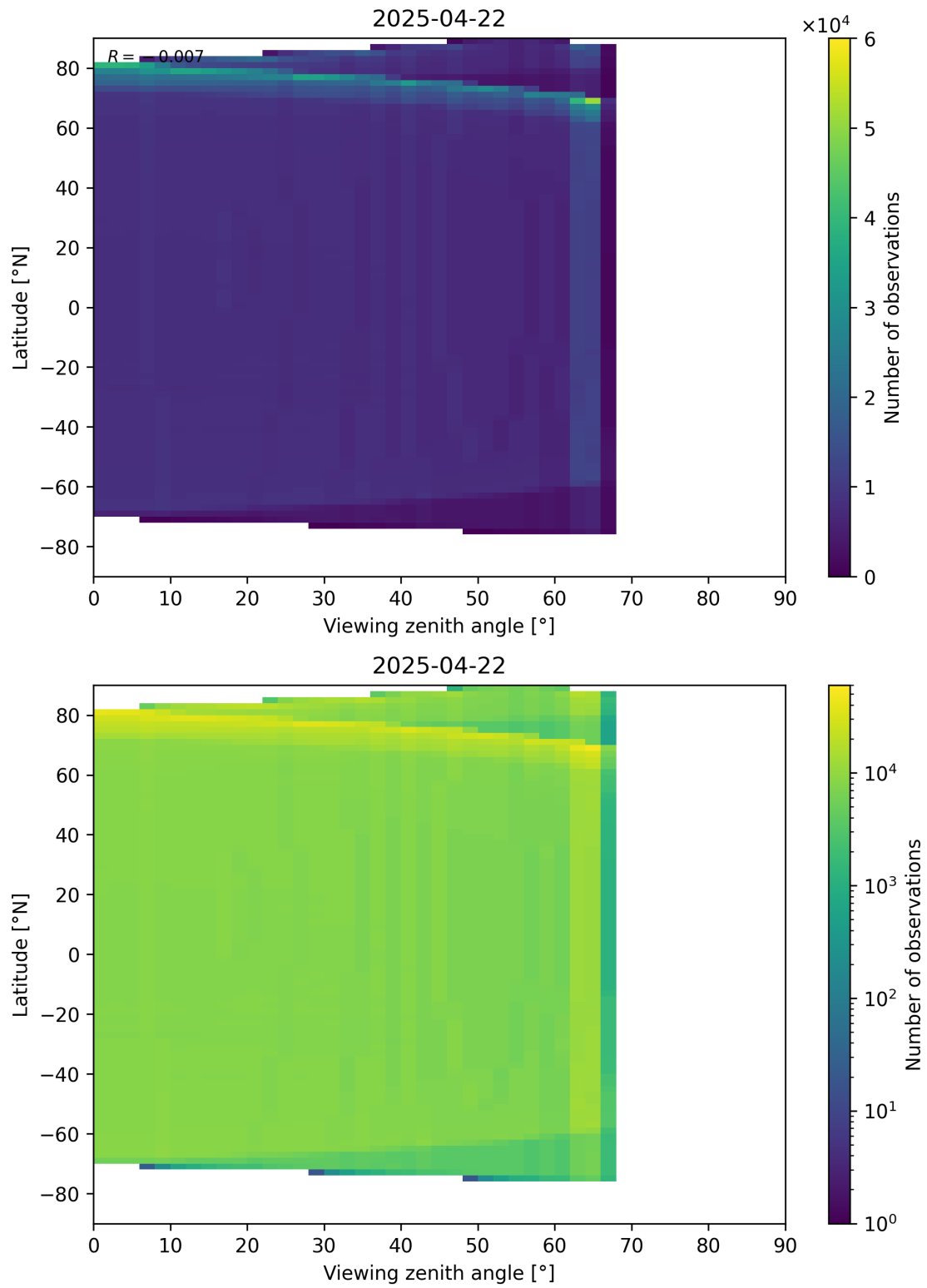
Figure 163: Scatter density plot of “Viewing zenith angle” against “Latitude” for 2025-04-22 to 2025-04-22.
