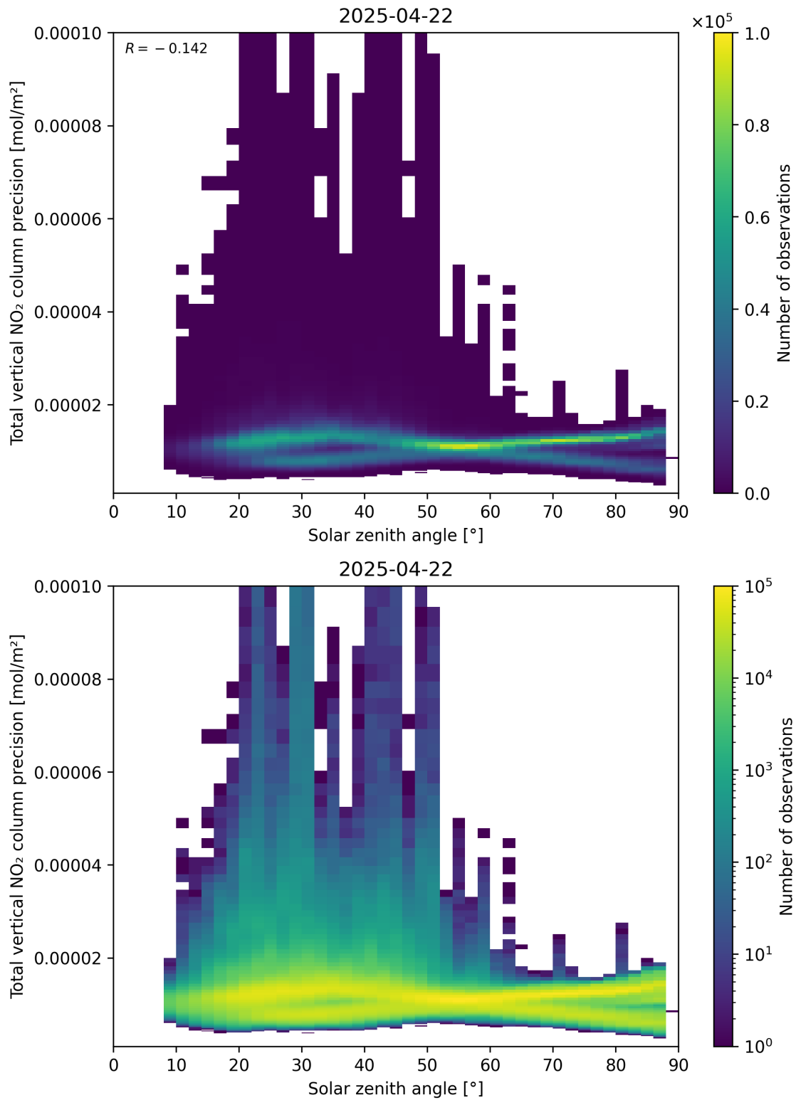
Figure 154: Scatter density plot of “Solar zenith angle” against “Total vertical NO 2 column precision” for 2025-04-22 to 2025-04-22.
