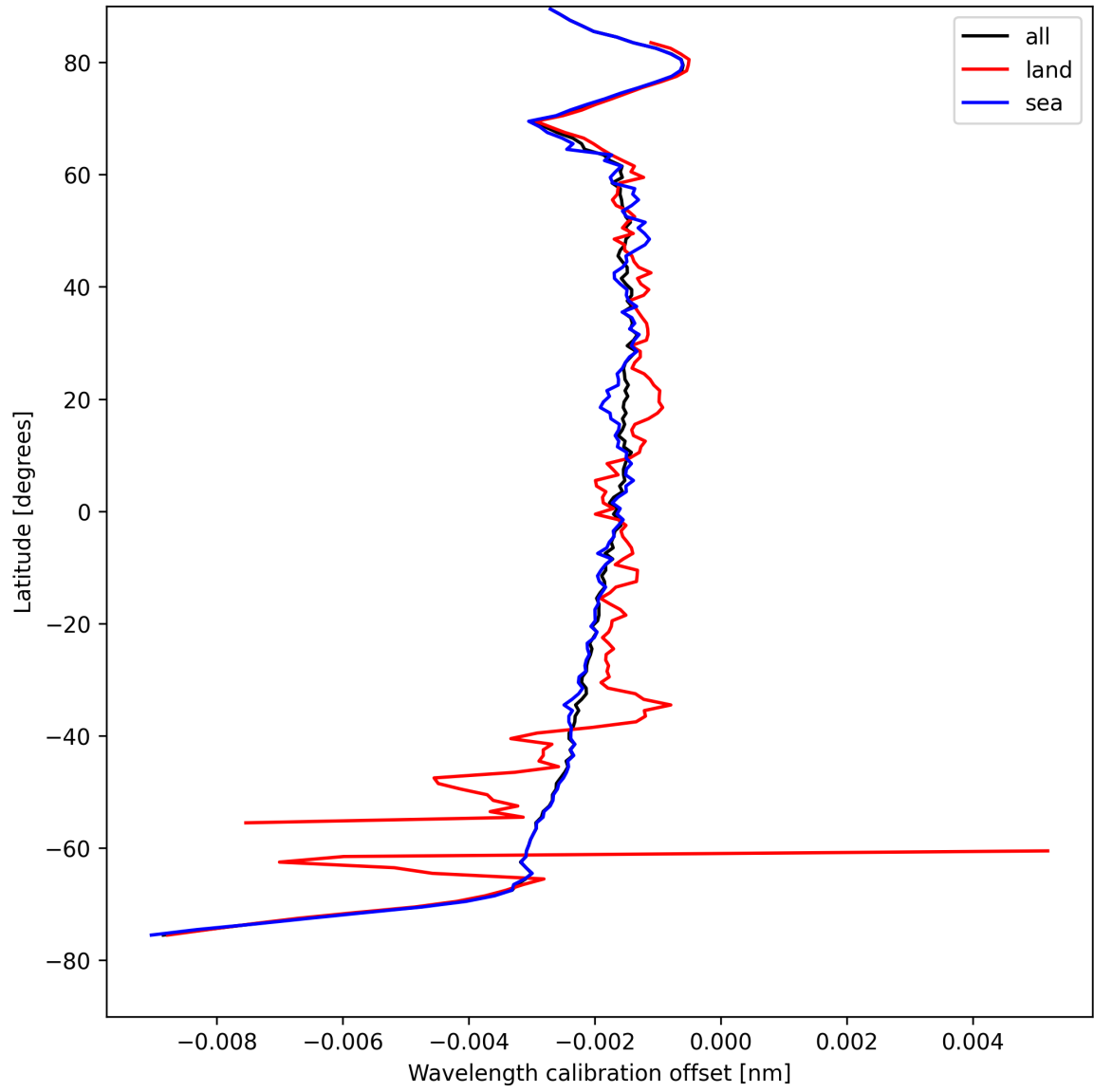
Figure 18: Zonal average of “Wavelength calibration offset” for 2025-04-22 to 2025-04-22.
