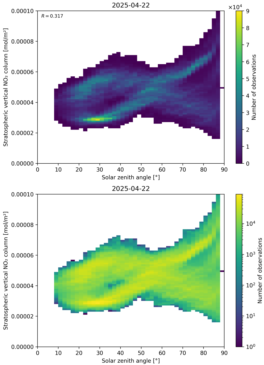
Figure 150: Scatter density plot of “Solar zenith angle” against “Stratospheric vertical NO 2 column” for 2025-04-22 to 2025-04-22.
