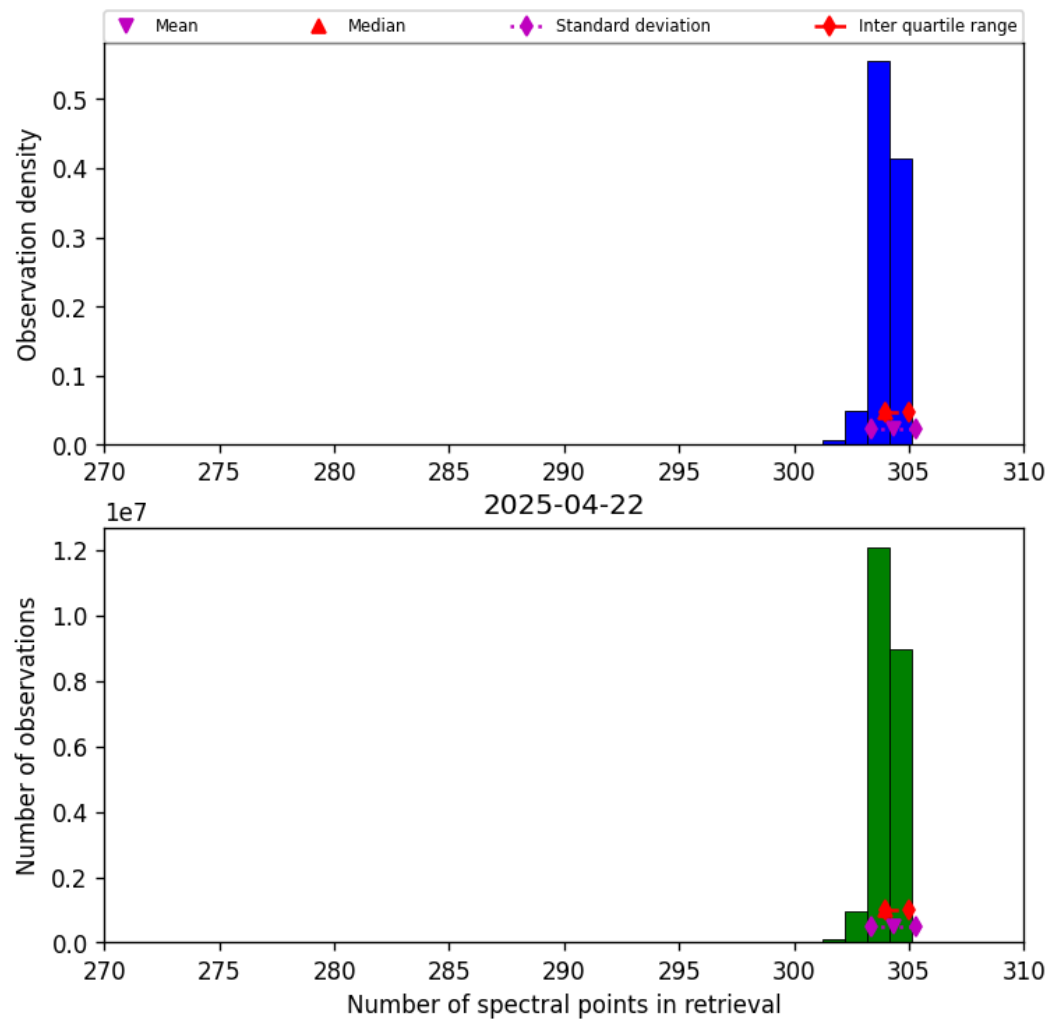
Figure 33: Histogram of “Number of spectral points in retrieval” for 2025-04-22 to 2025-04-22
