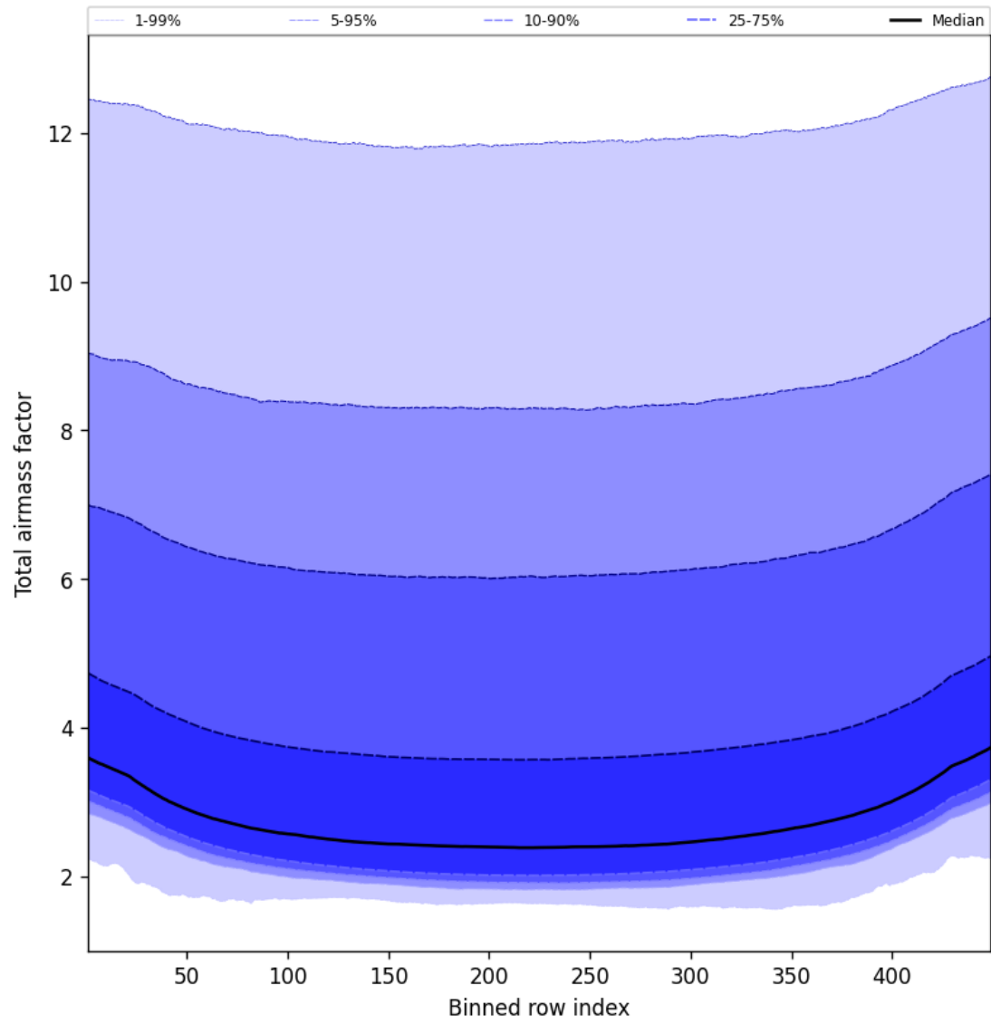
Figure 49: Along track statistics of “Total airmass factor” for 2025-04-22 to 2025-04-22
