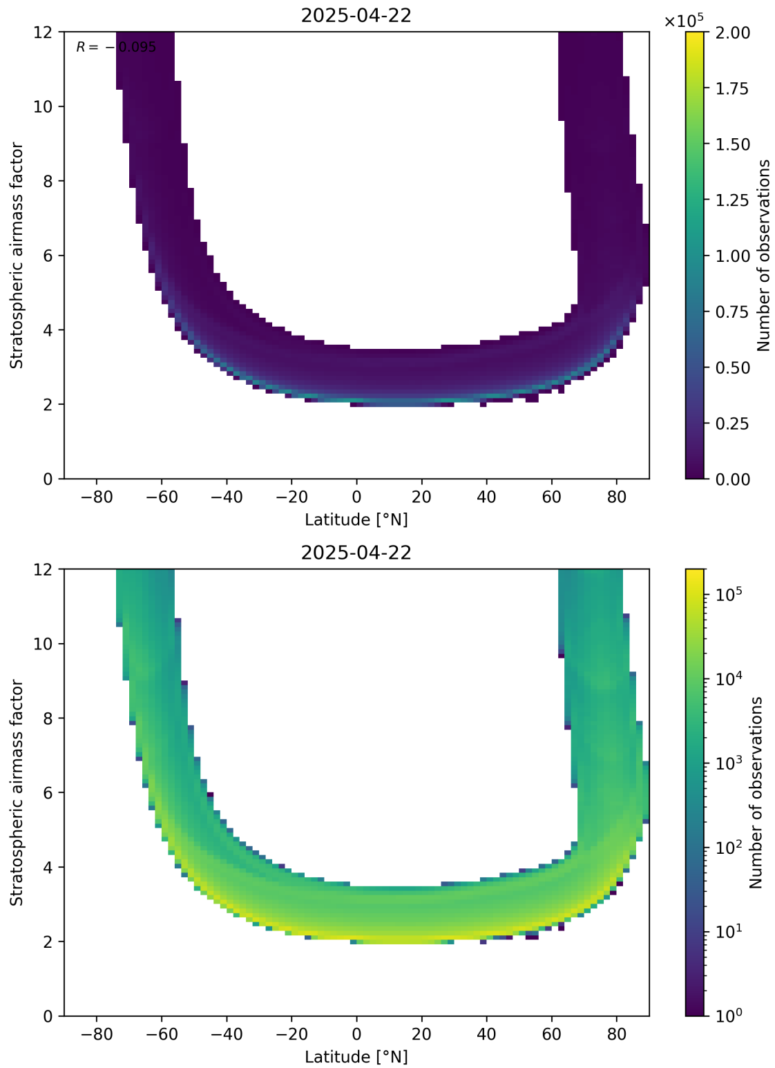
Figure 83: Scatter density plot of “Latitude” against “Stratospheric air mass factor” for 2025-04-22 to 2025-04-22.
