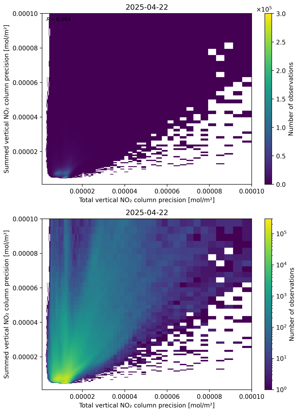
Figure 118: Scatter density plot of “Total vertical NO 2 column precision” against “Summed vertical NO 2 column precision” for 2025-04-22 to 2025-04-22.
