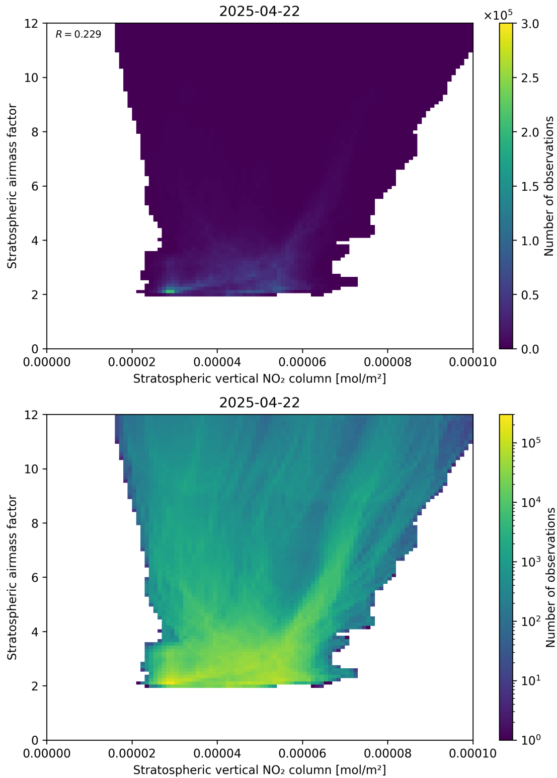
Figure 96: Scatter density plot of “Stratospheric vertical NO 2 column” against “Stratospheric airmass factor” for 2025-04-22 to 2025-04-22.
