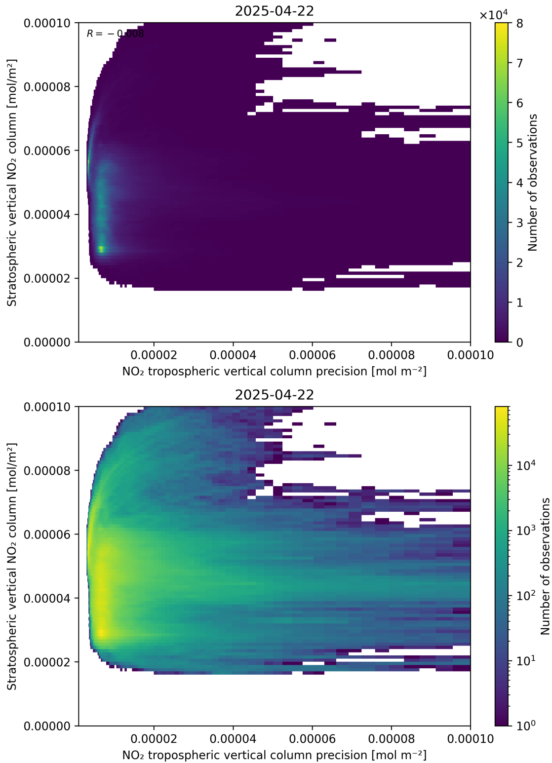
Figure 135: Scatter density plot of “NO 2 tropospheric vertical column precision” against “Stratospheric vertical NO 2 column” for 2025-04-22 to 2025-04-22.
