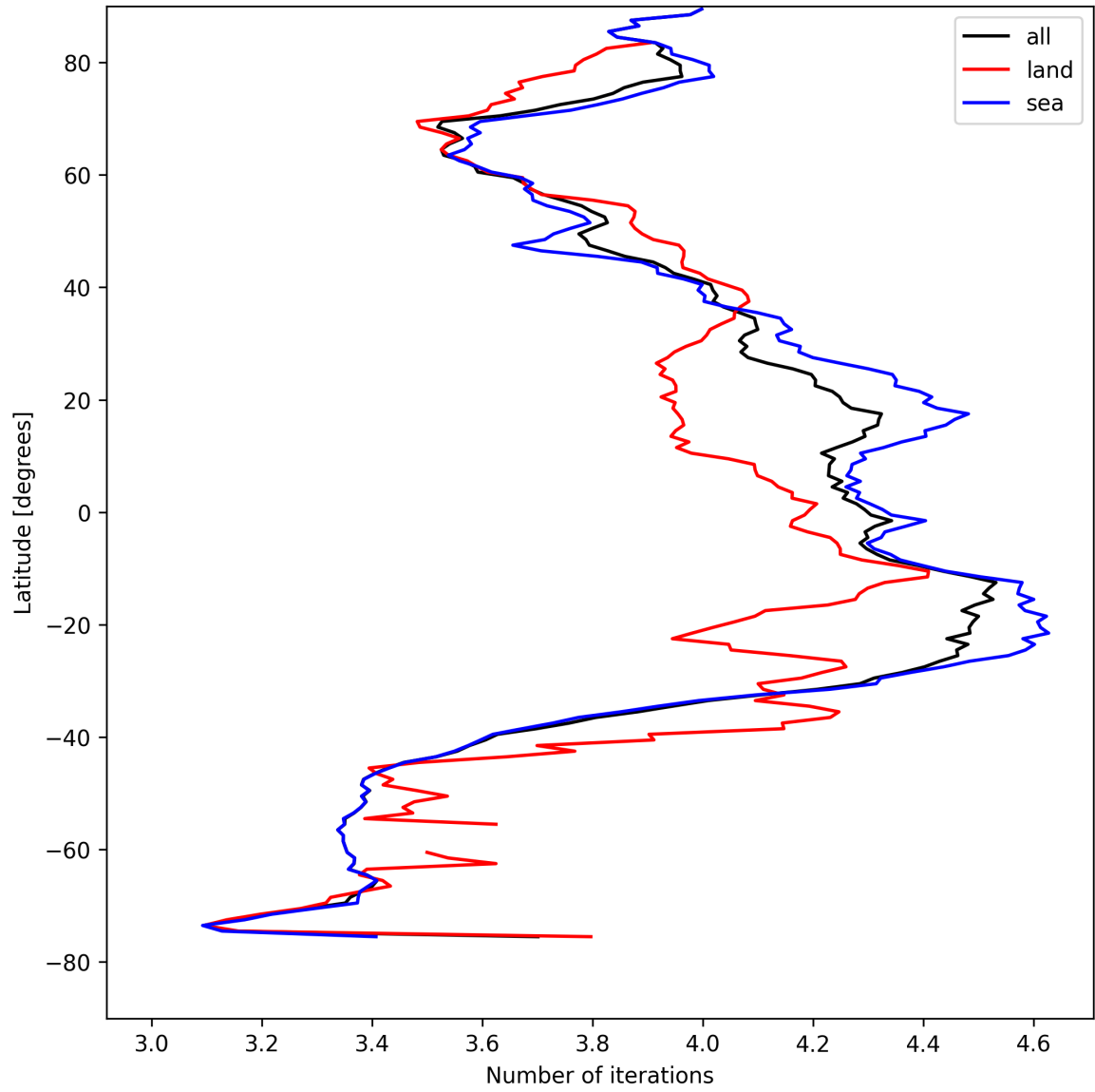
Figure 17: Zonal average of “Number of iterations” for 2025-04-22 to 2025-04-22.
