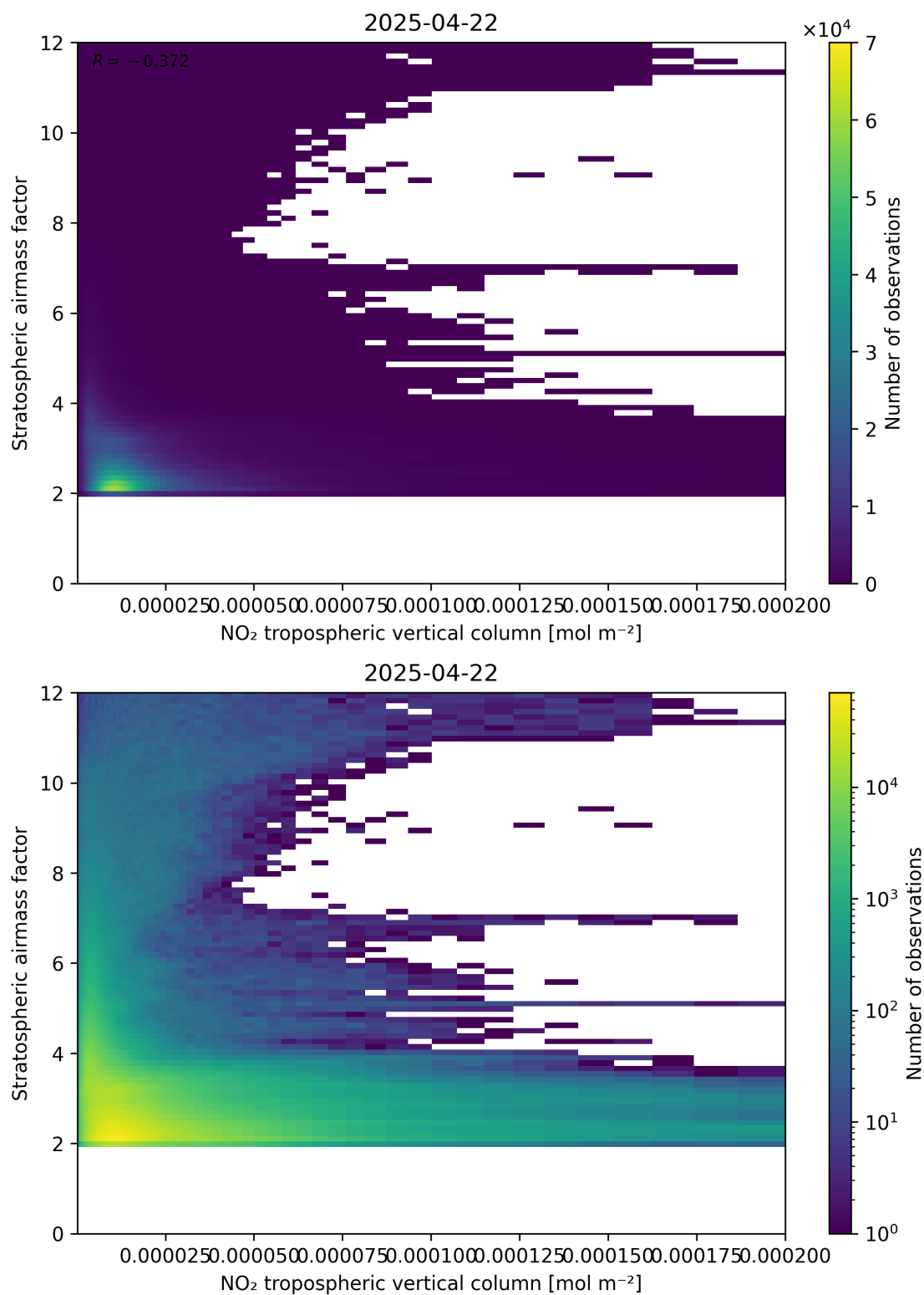
Figure 121: Scatter density plot of “NO 2 tropospheric vertical column” against “Stratospheric air mass factor” for 2025-04-22 to 2025-04-22.
