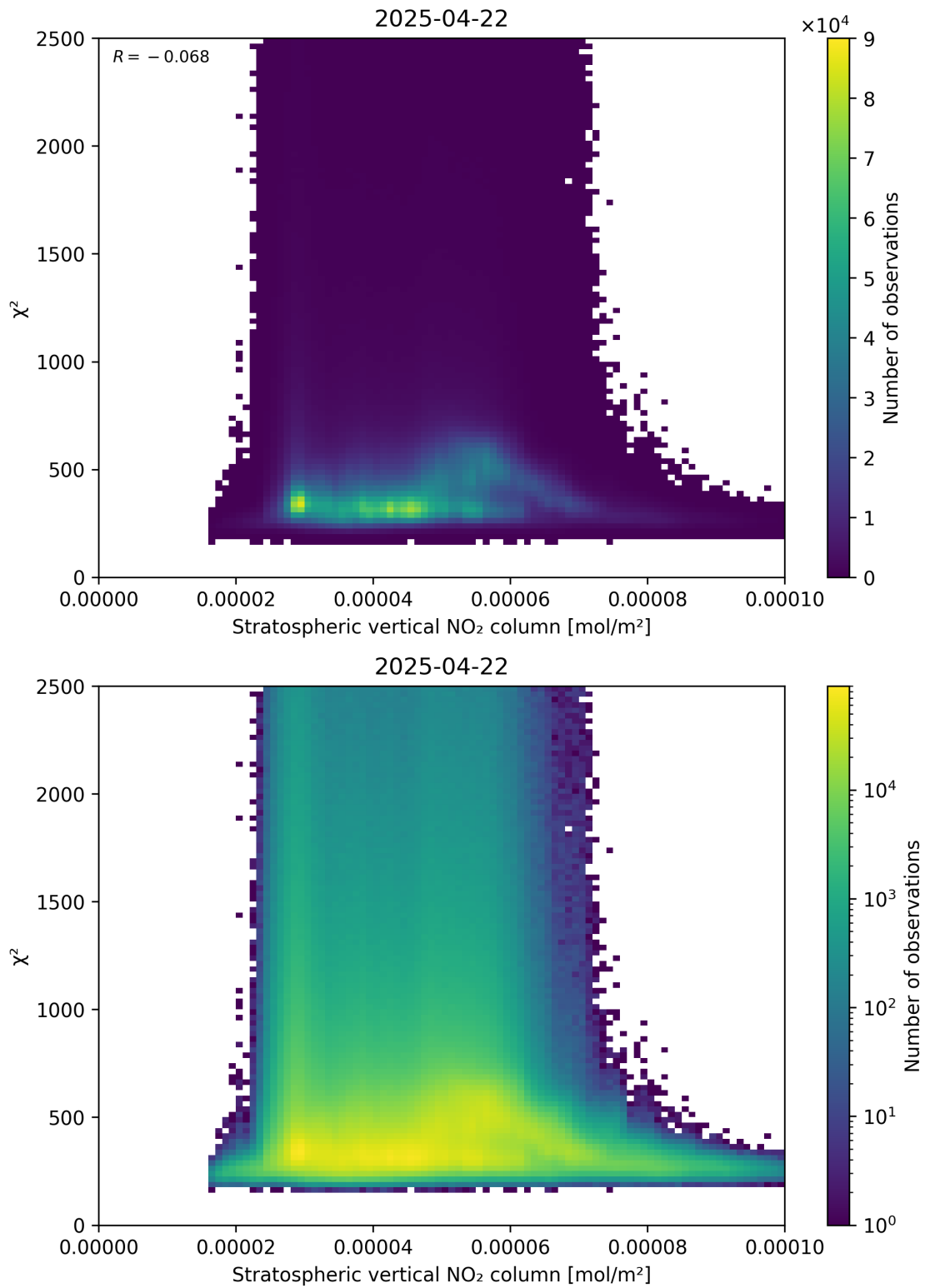
Figure 97: Scatter density plot of “Stratospheric vertical NO 2 column” against “ \chi^2 ” for 2025-04-22 to 2025-04-22.
