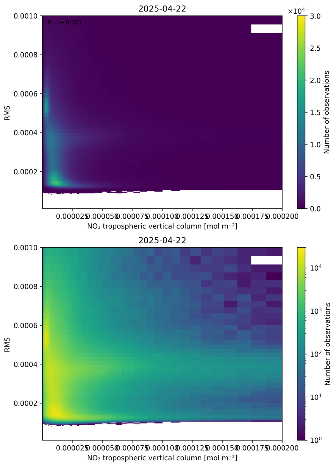
Figure 142: Scatter density plot of “NO 2 tropospheric vertical column” against “RMS” for 2025-04-22 to 2025-04-22.
