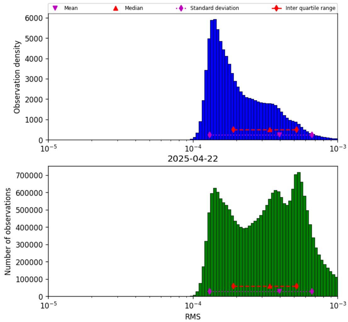
Figure 43: Histogram of “RMS” for 2025-04-22 to 2025-04-22
