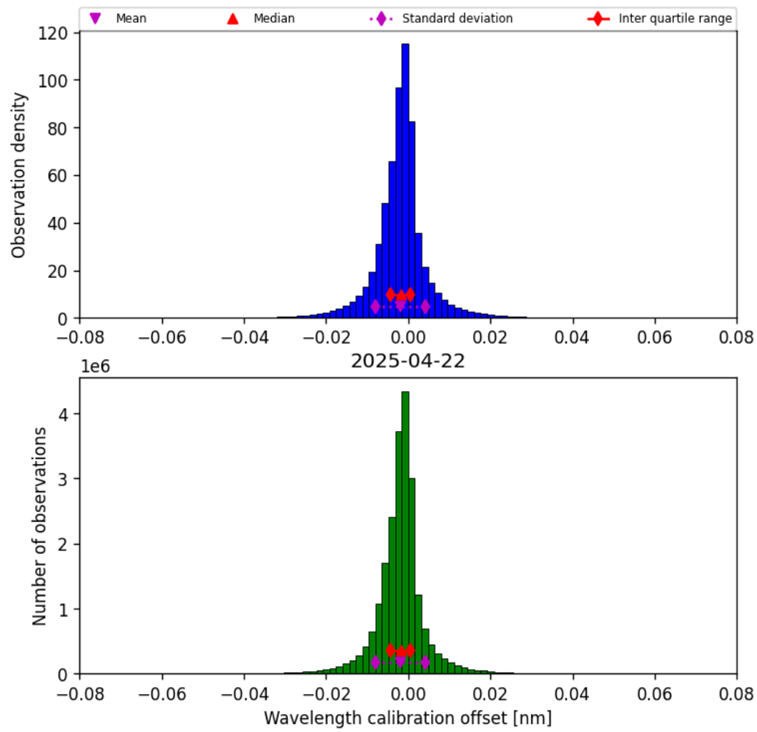
Figure 35: Histogram of “Wavelength calibration offset” for 2025-04-22 to 2025-04-22
