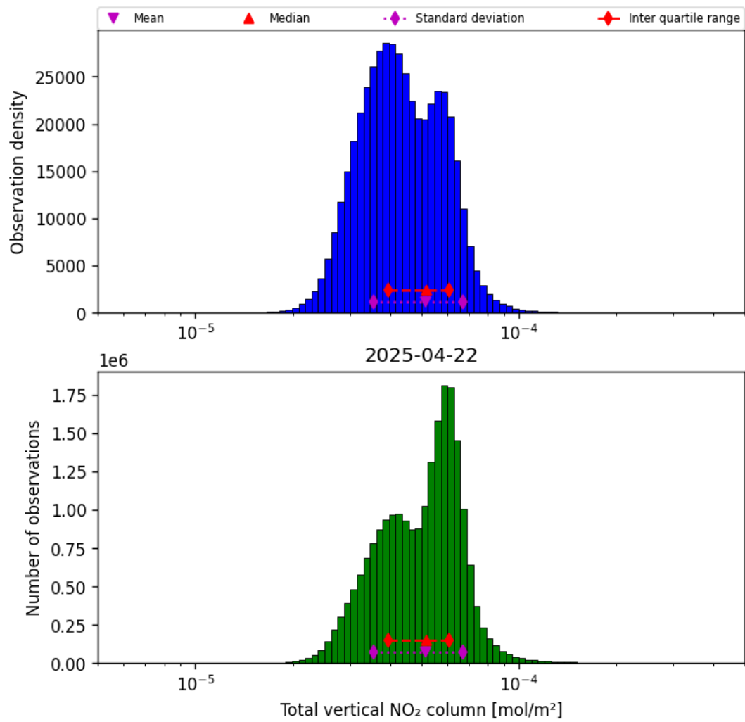
Figure 38: Histogram of “Total vertical NO 2 column” for 2025-04-22 to 2025-04-22
