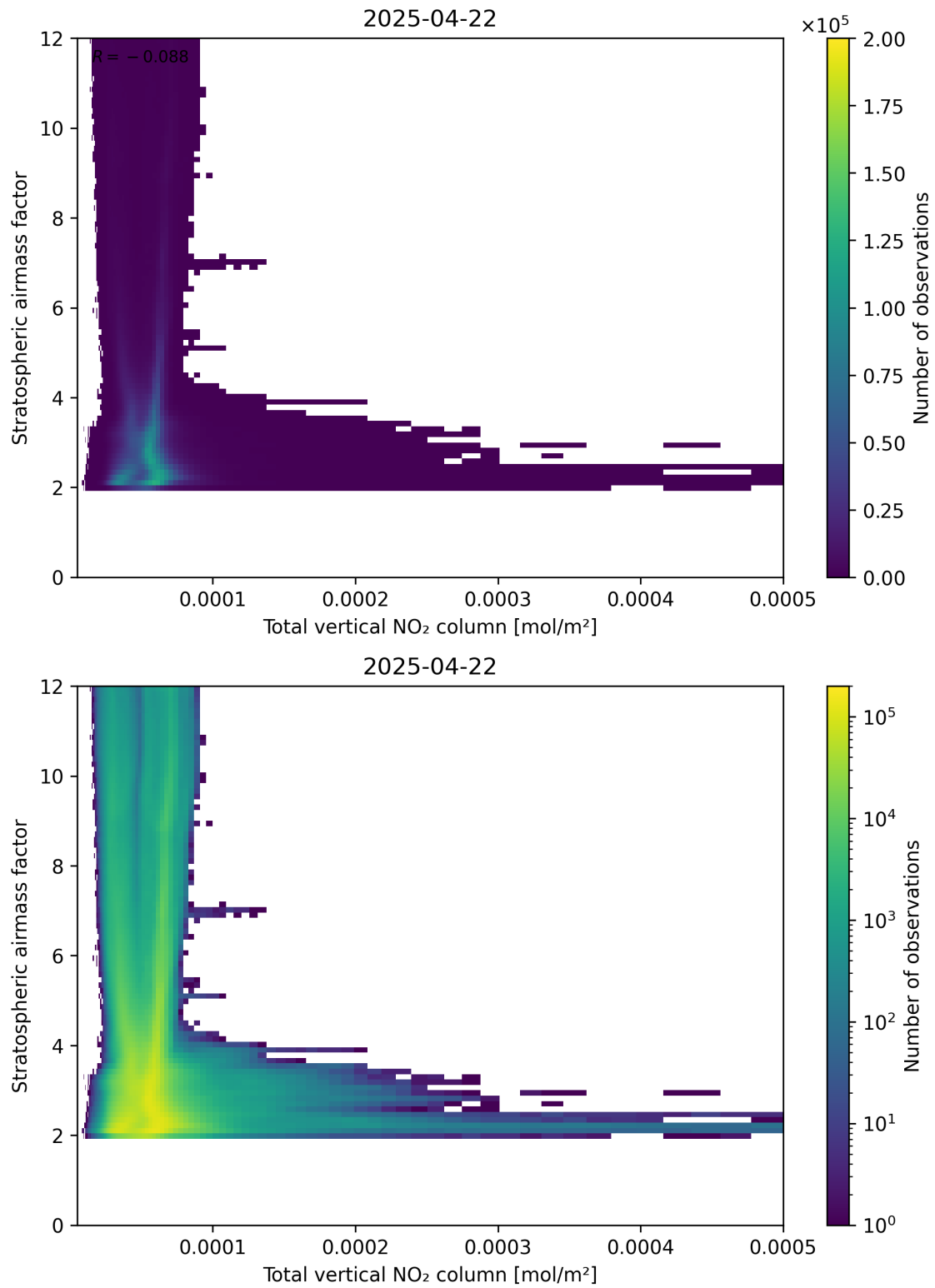
Figure 110: Scatter density plot of “Total vertical NO 2 column” against “Stratospheric airmass factor” for 2025-04-22 to 2025-04-22.
