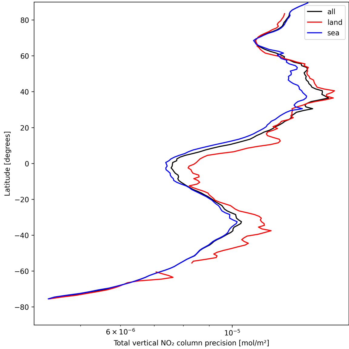
Figure 22: Zonal average of “Total vertical NO 2 column precision” for 2025-04-22 to 2025-04-22.
