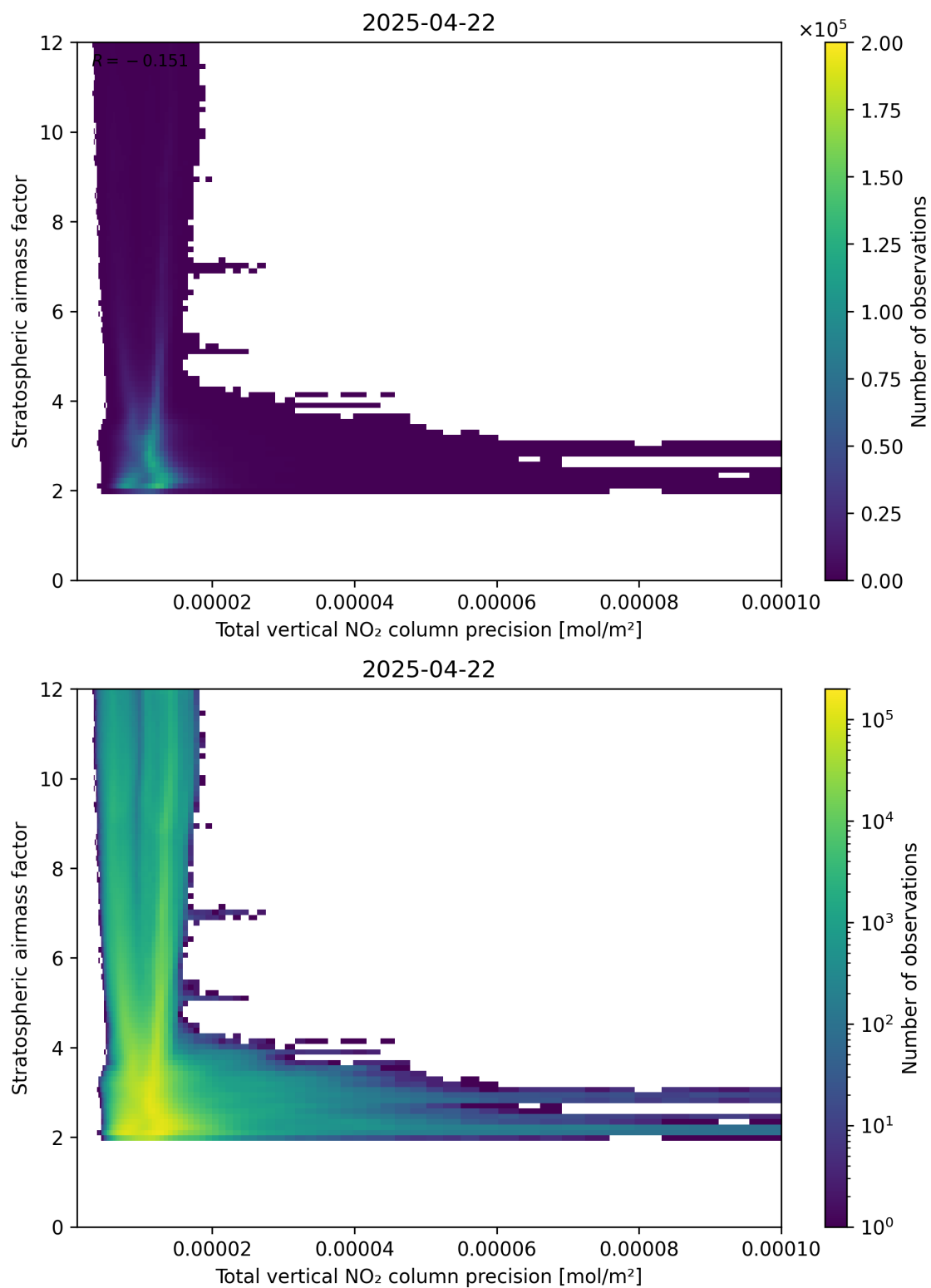
Figure 115: Scatter density plot of “Total vertical NO 2 column precision” against “Stratospheric air mass factor” for 2025-04-22 to 2025-04-22.
