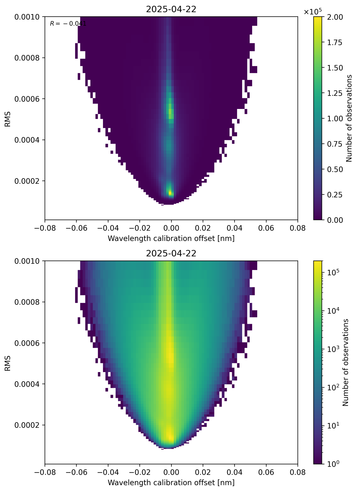
Figure 181: Scatter density plot of “Wavelength calibration offset” against “RMS” for 2025-04-22 to 2025-04-22.
