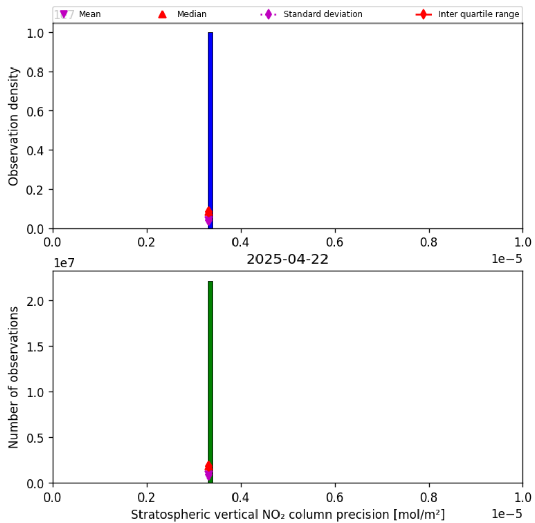
Figure 37: Histogram of “Stratospheric vertical NO 2 column precision” for 2025-04-22 to 2025-04-22
