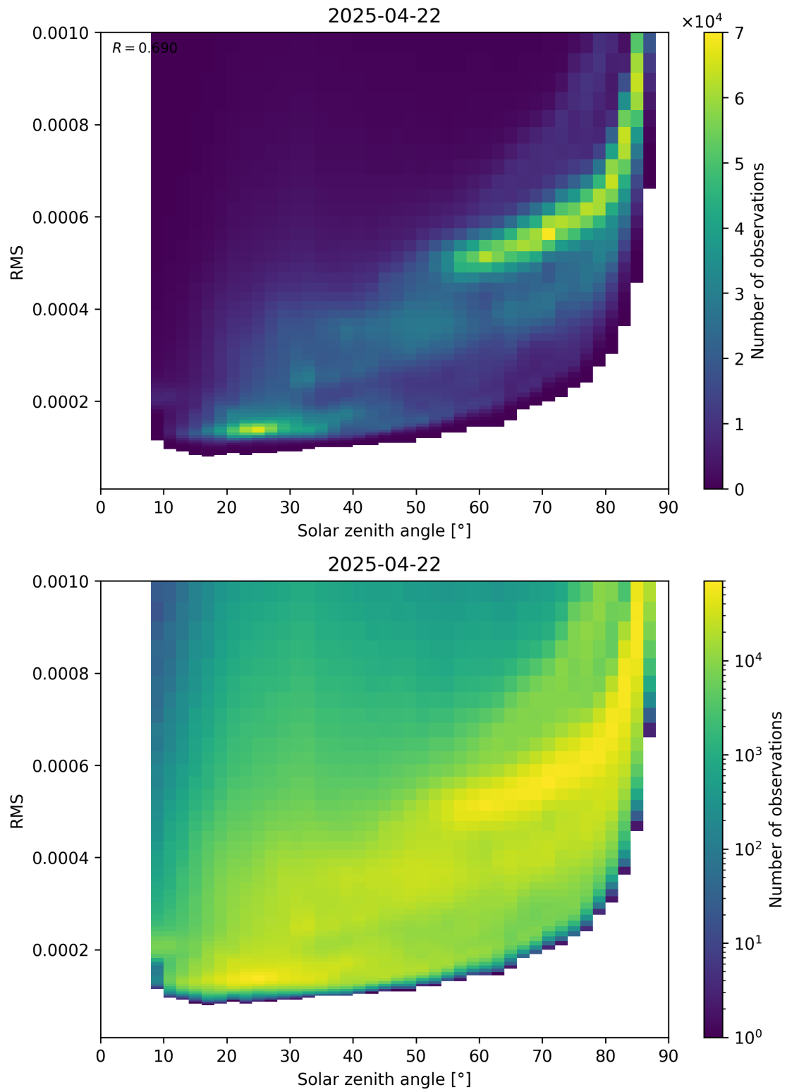
Figure 157: Scatter density plot of “Solar zenith angle” against “RMS” for 2025-04-22 to 2025-04-22.
