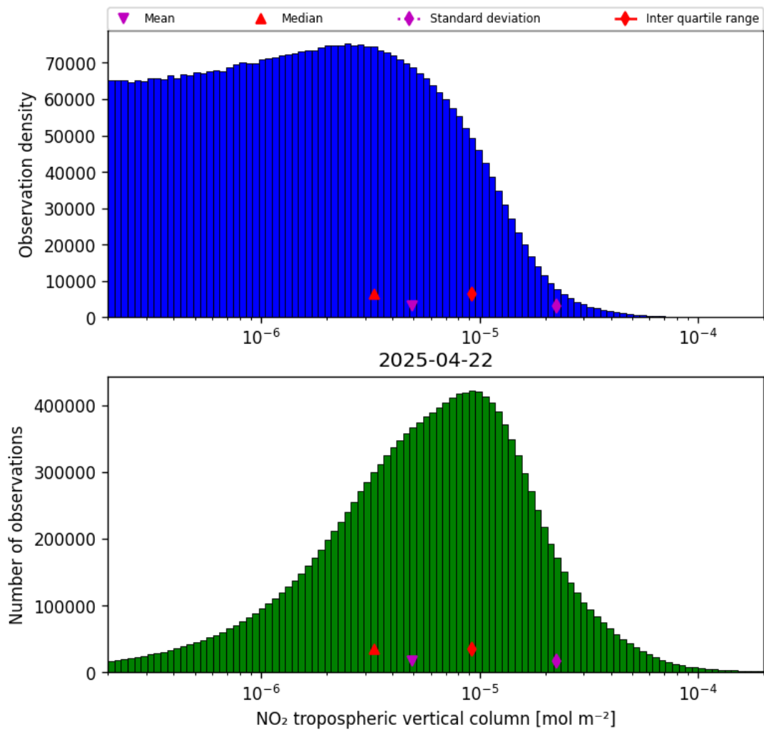
Figure 29: Histogram of “NO 2 tropospheric vertical column” for 2025-04-22 to 2025-04-22
