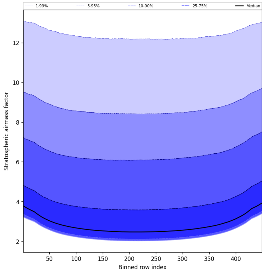
Figure 61: Along track statistics of “Stratospheric airmass factor” for 2025-04-22 to 2025-04-22
