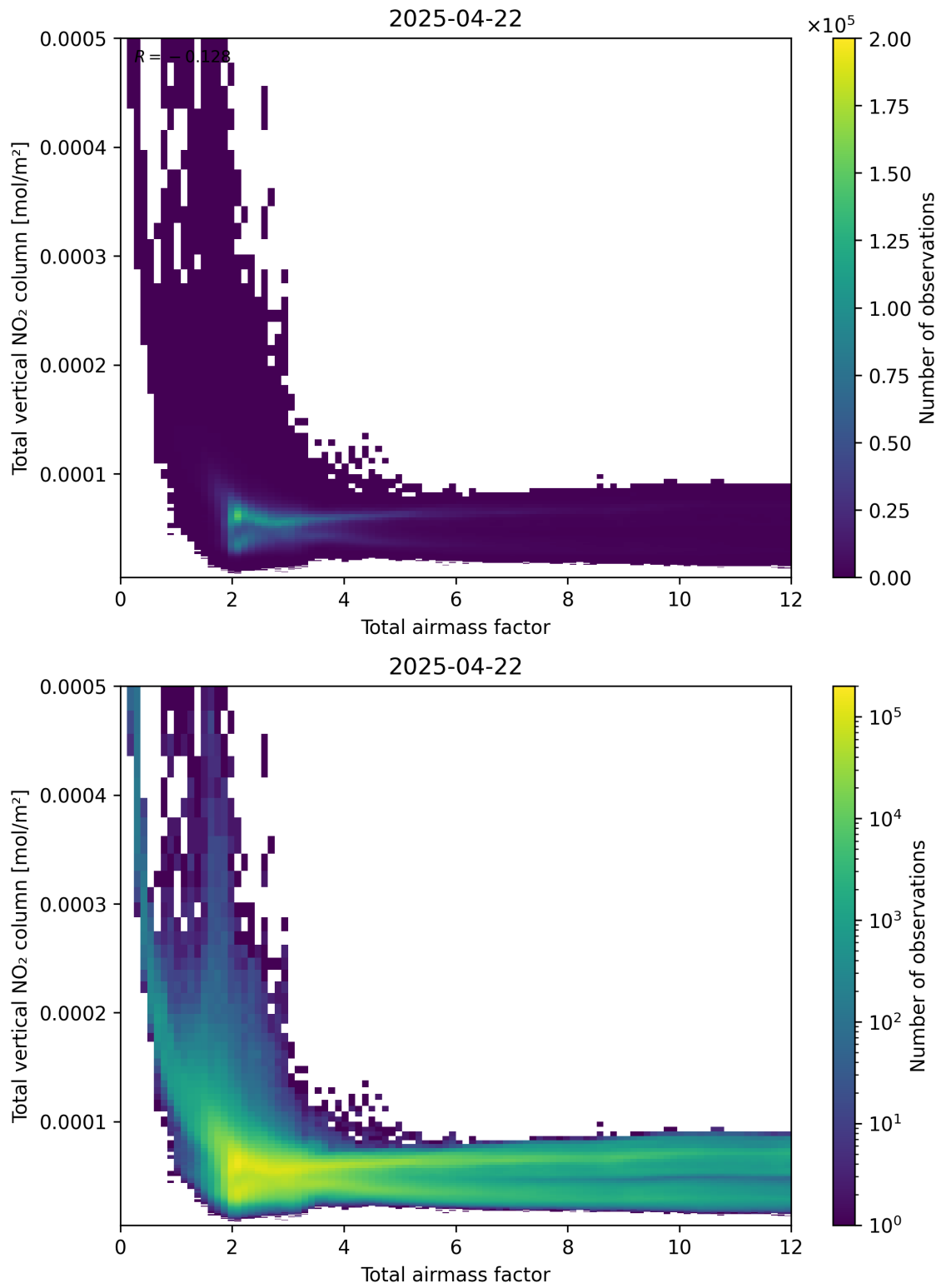
Figure 67: Scatter density plot of “Total airmass factor” against “Total vertical NO 2 column” for 2025-04-22 to 2025-04-22.
