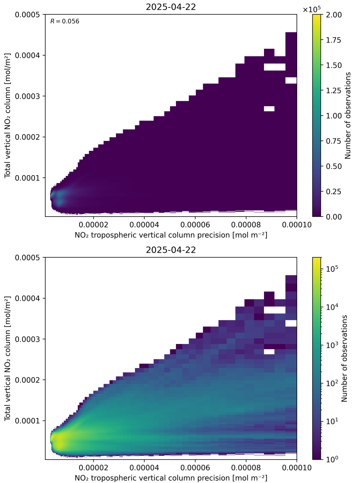
Figure 138: Scatter density plot of “NO 2 tropospheric vertical column precision” against “Total vertical NO 2 column” for 2025-04-22 to 2025-04-22.
