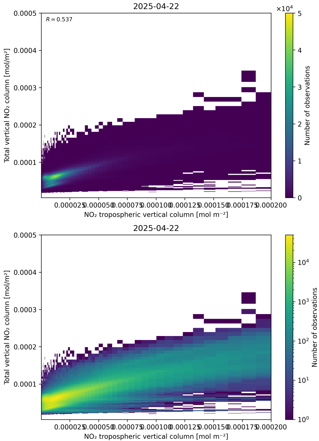
Figure 128: Scatter density plot of “NO 2 tropospheric vertical column” against “Total vertical NO 2 column” for 2025-04-22 to 2025-04-22.
