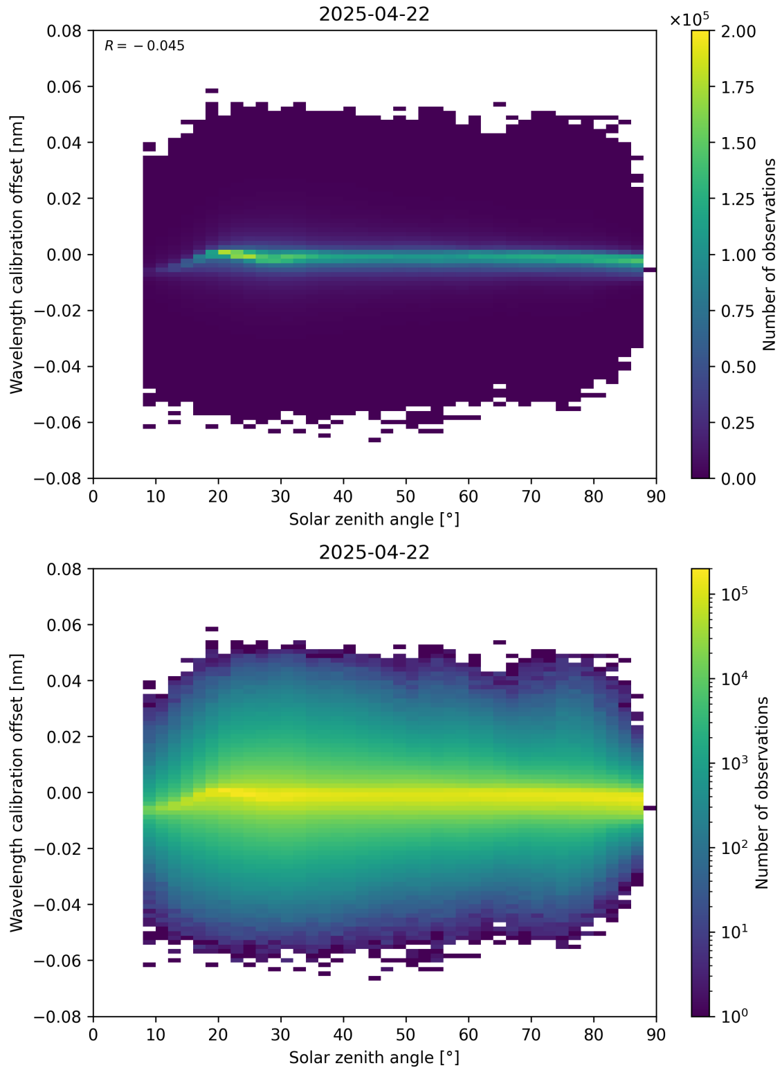
Figure 158: Scatter density plot of “Solar zenith angle” against “Wavelength calibration offset” for 2025-04-22 to 2025-04-22.
