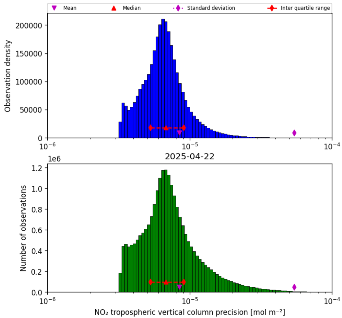
Figure 30: Histogram of “NO 2 tropospheric vertical column precision” for 2025-04-22 to 2025-04-22
