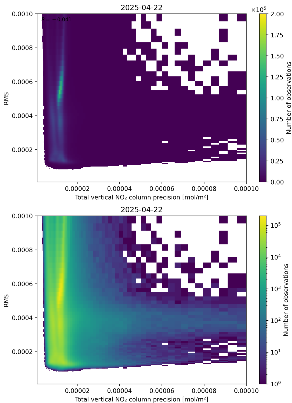
Figure 119: Scatter density plot of “Total vertical NO 2 column precision” against “RMS” for 2025-04-22 to 2025-04-22.
