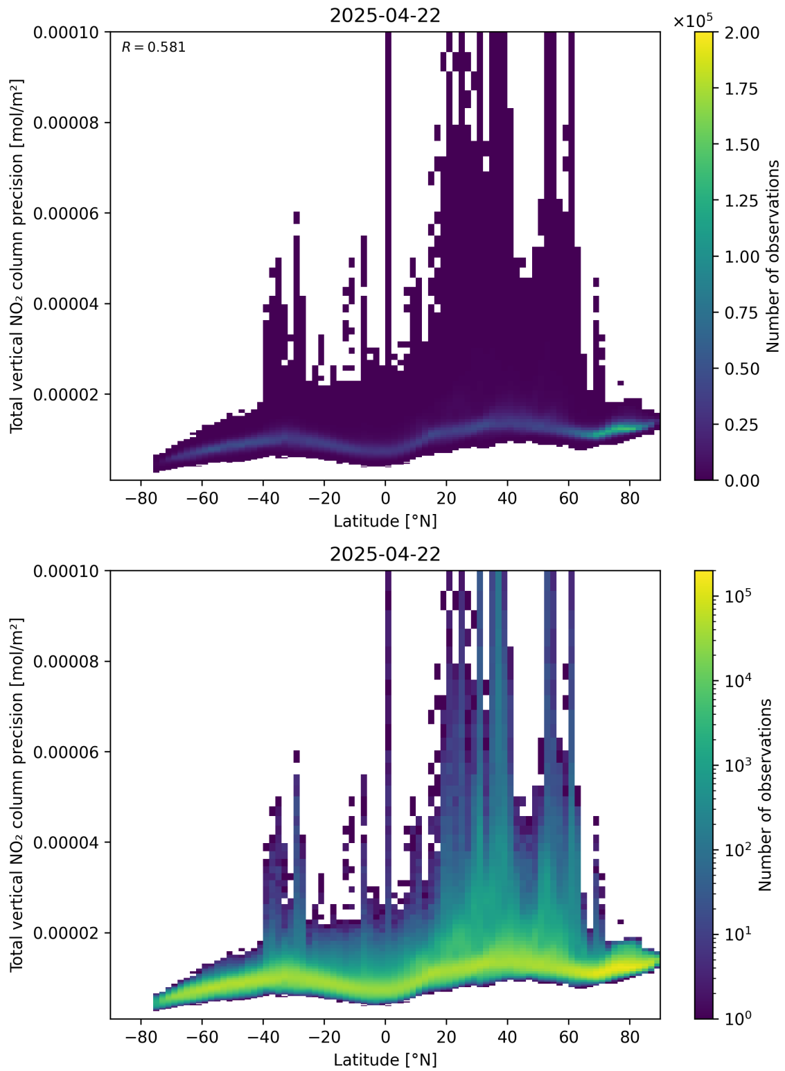
Figure 91: Scatter density plot of “Latitude” against “Total vertical NO 2 column precision” for 2025-04-22 to 2025-04-22.
