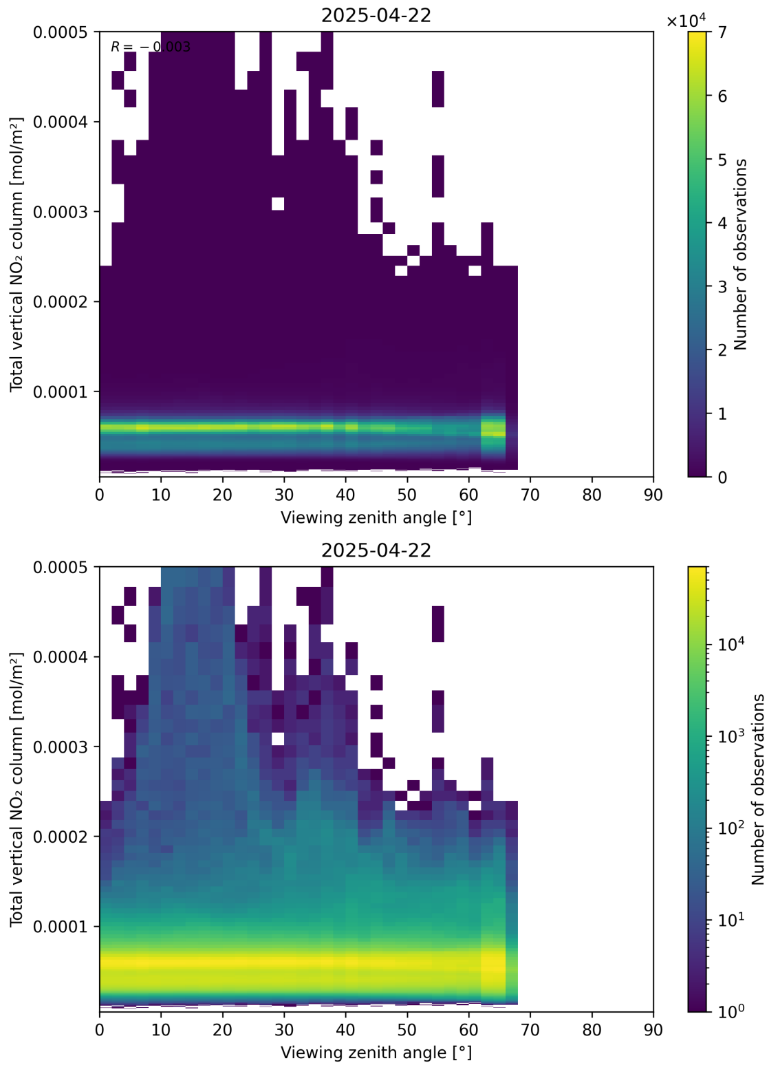
Figure 167: Scatter density plot of “Viewing zenith angle” against “Total vertical NO 2 column” for 2025-04-22 to 2025-04-22.
