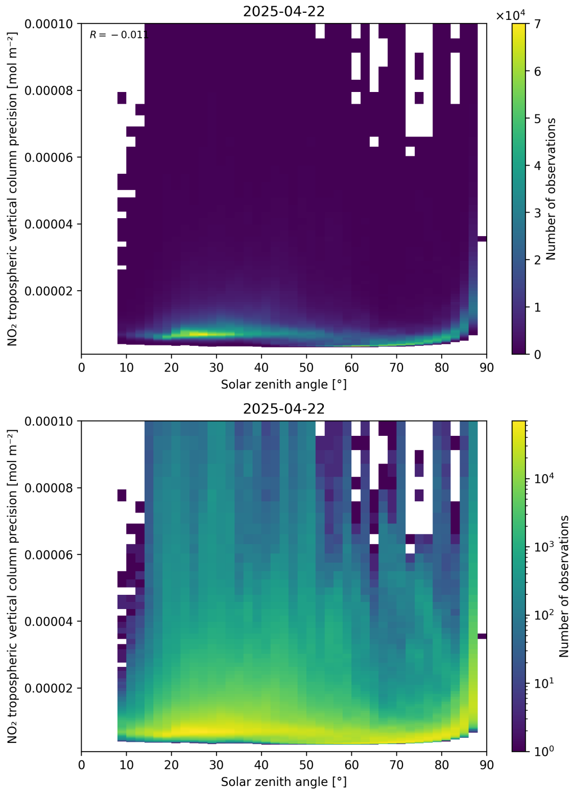
Figure 156: Scatter density plot of “Solar zenith angle” against “NO 2 tropospheric vertical column precision” for 2025-04-22 to 2025-04-22.
