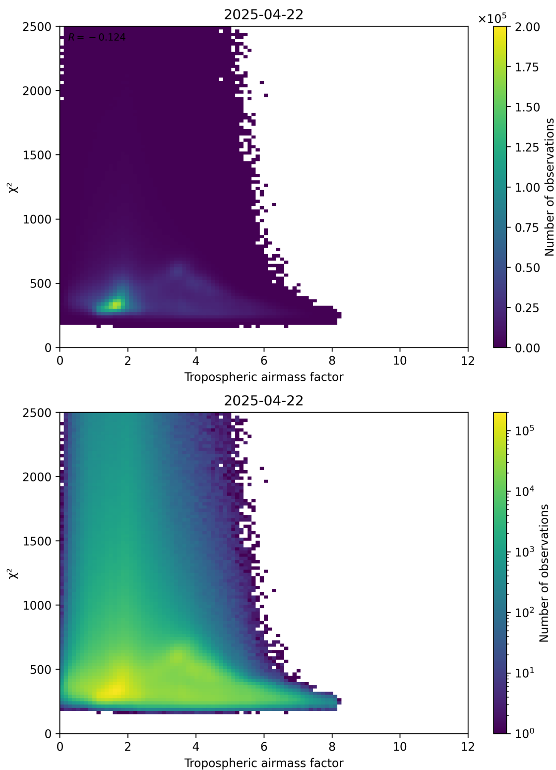
Figure 73: Scatter density plot of “Tropospheric airmass factor” against “ \chi^2 ” for 2025-04-22 to 2025-04-22.
