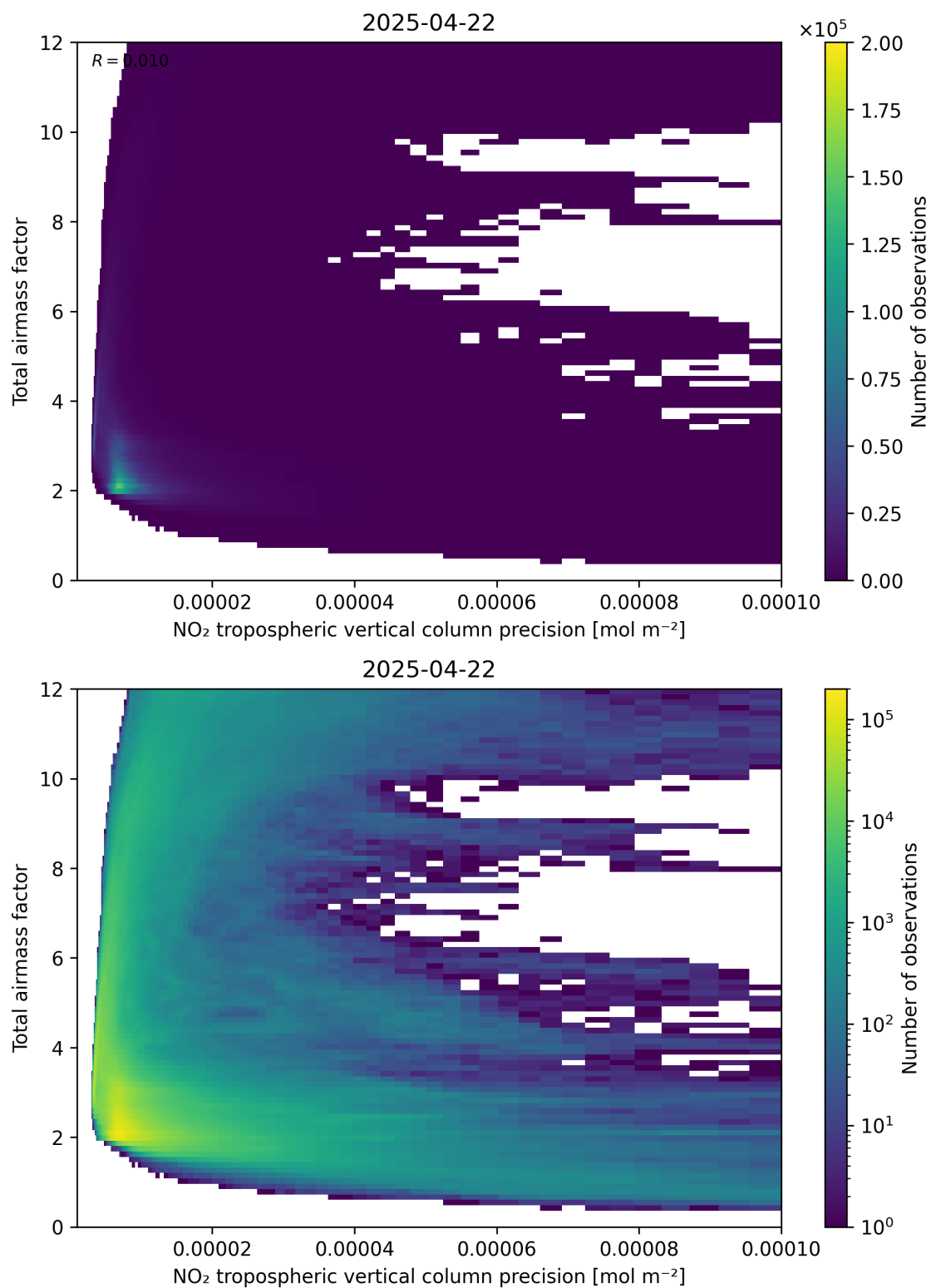
Figure 132: Scatter density plot of “NO 2 tropospheric vertical column precision” against “Total airmass factor” for 2025-04-22 to 2025-04-22.
