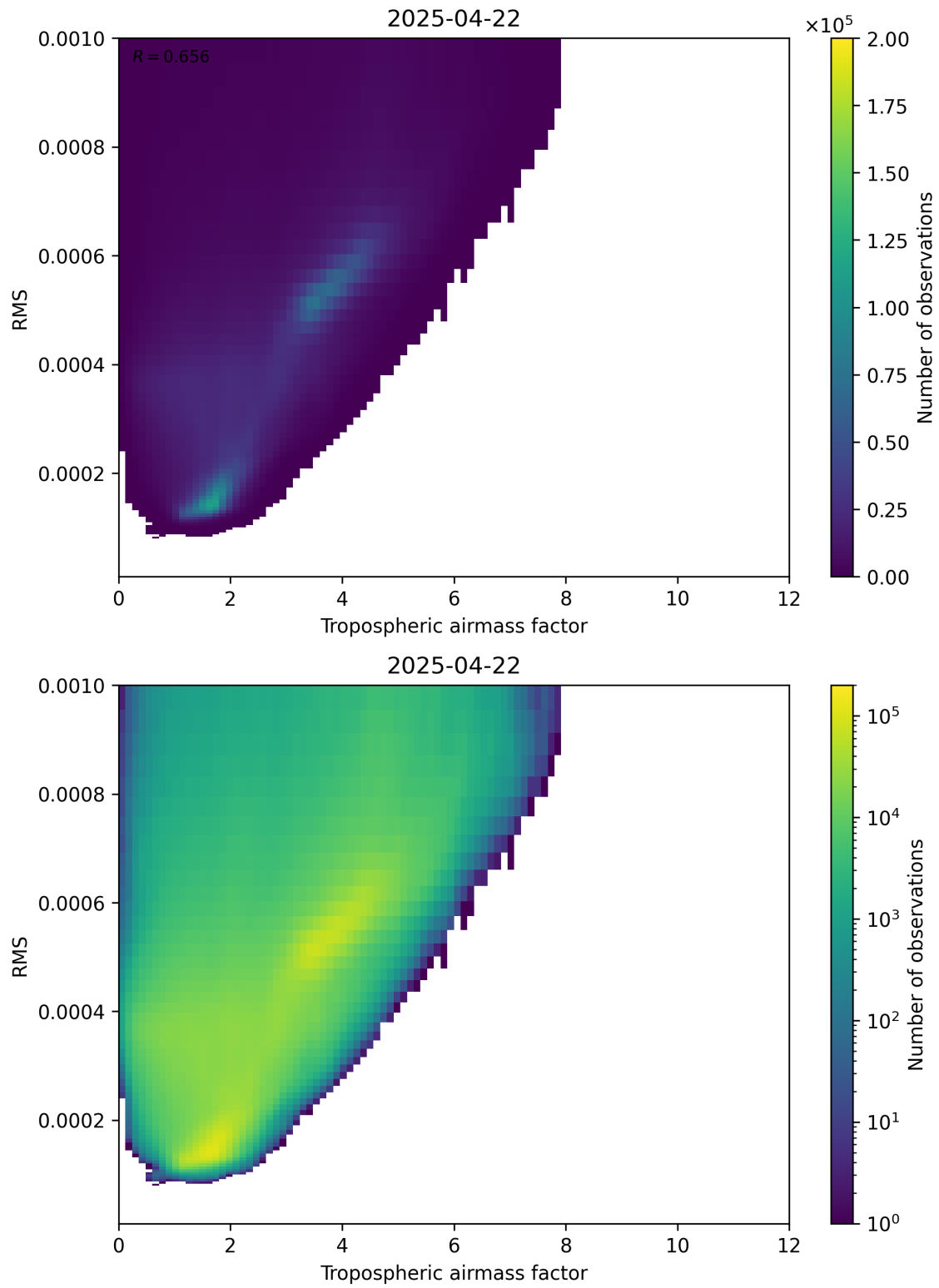
Figure 79: Scatter density plot of “Tropospheric airmass factor” against “RMS” for 2025-04-22 to 2025-04-22.
