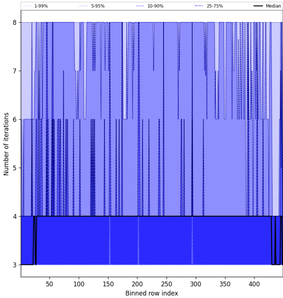
Figure 51: Along track statistics of “Number of iterations” for 2025-04-22 to 2025-04-22
