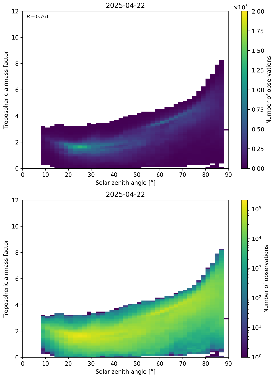
Figure 147: Scatter density plot of “Solar zenith angle” against “Tropospheric airmass factor” for 2025-04-22 to 2025-04-22.
