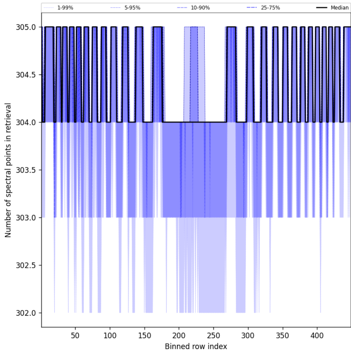
Figure 50: Along track statistics of “Number of spectral points in retrieval” for 2025-04-22 to 2025-04-22
