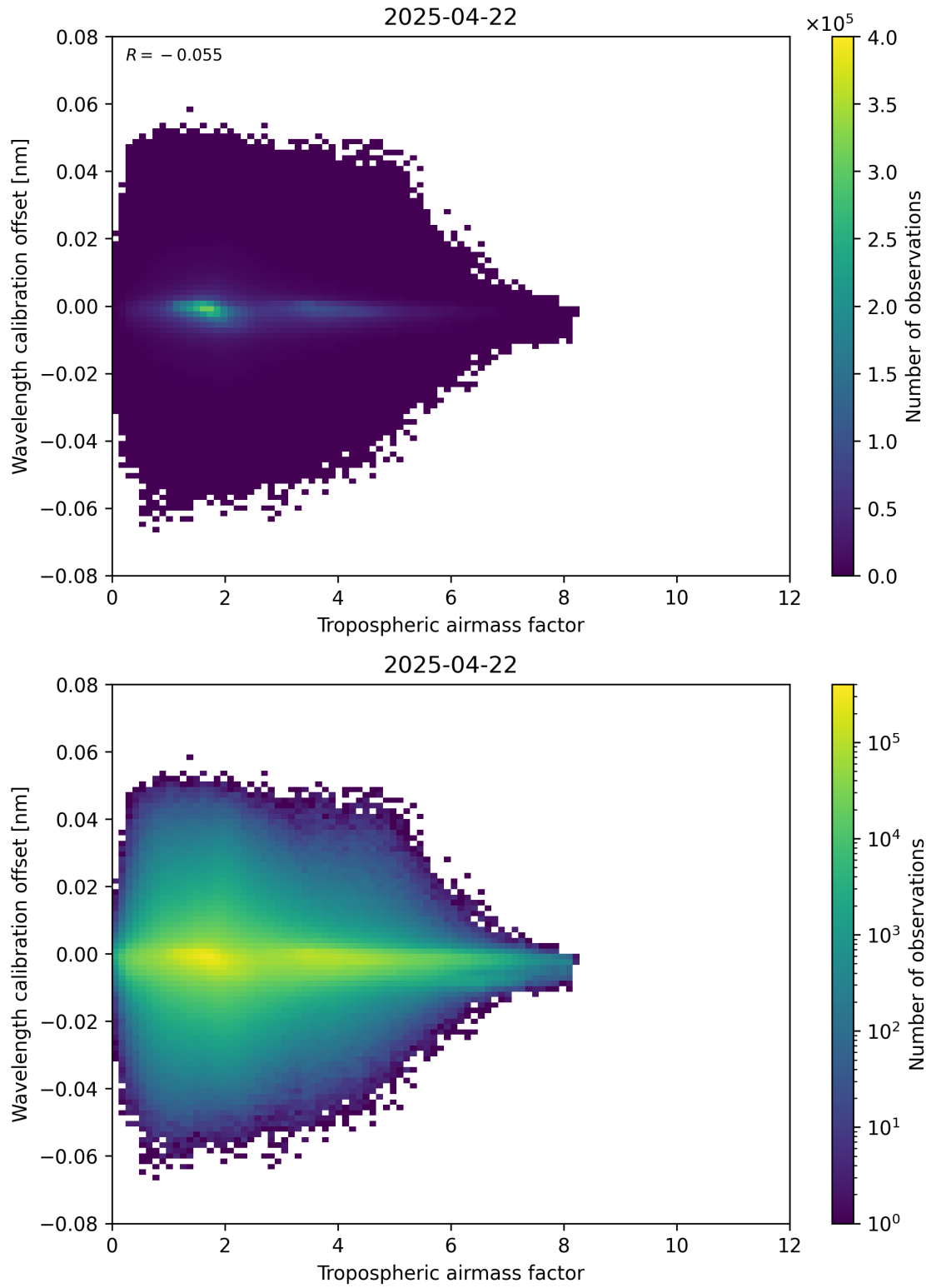
Figure 80: Scatter density plot of “Tropospheric airmass factor” against “Wavelength calibration offset” for 2025-04-22 to 2025-04-22.
