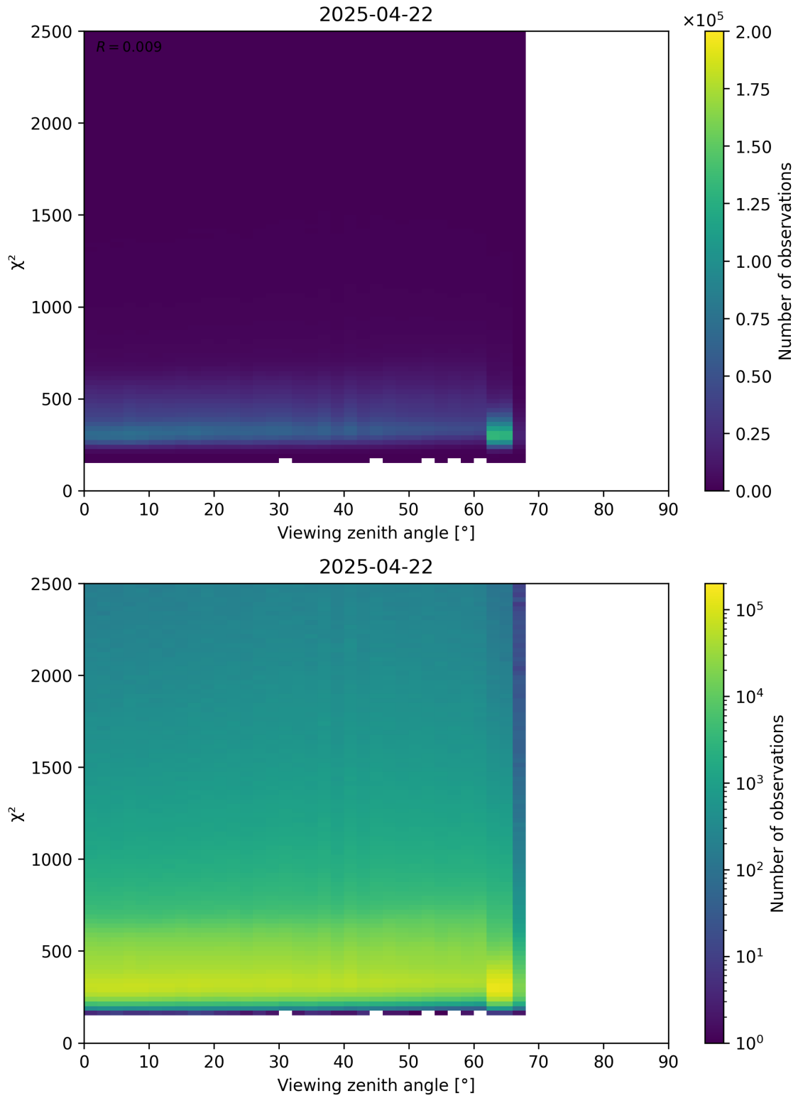
Figure 162: Scatter density plot of “Viewing zenith angle” against “ \chi^2 ” for 2025-04-22 to 2025-04-22.
