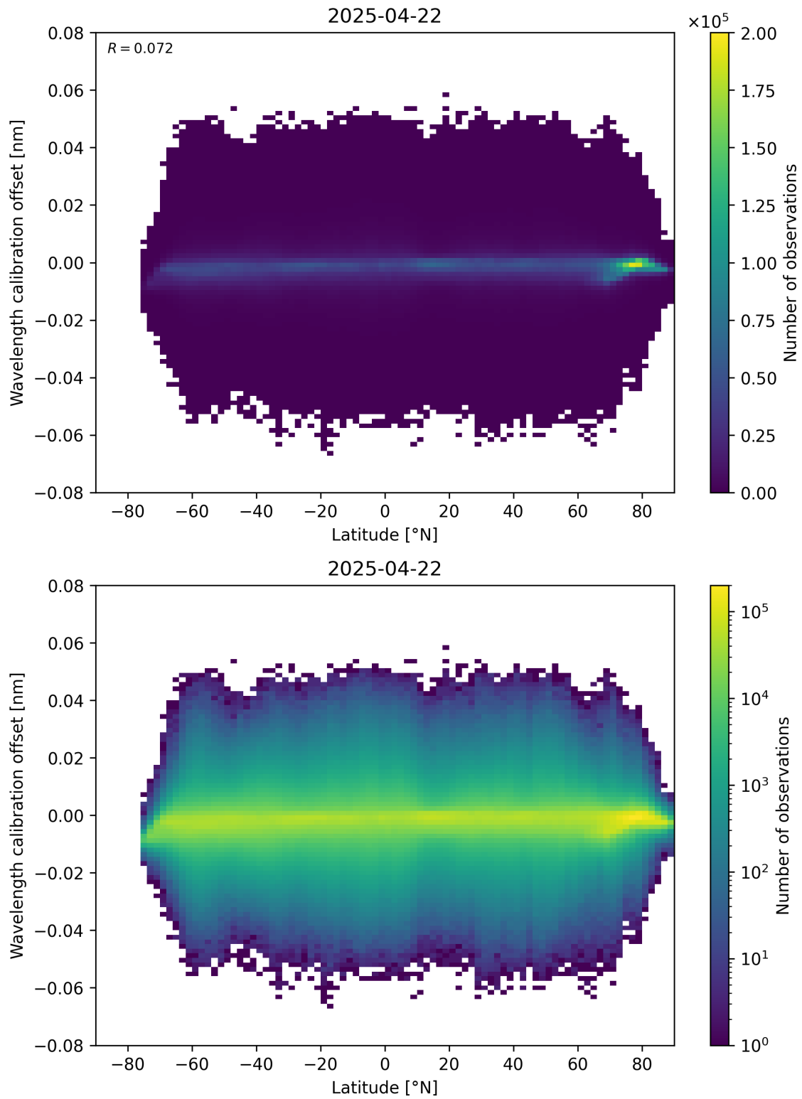
Figure 95: Scatter density plot of “Latitude” against “Wavelength calibration offset” for 2025-04-22 to 2025-04-22.
