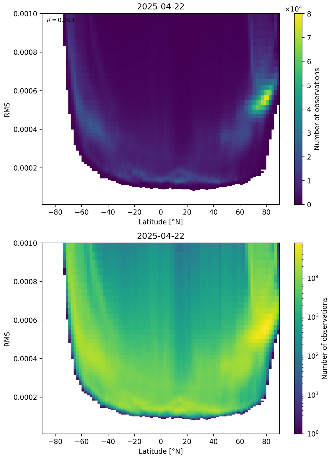
Figure 94: Scatter density plot of “Latitude” against “RMS” for 2025-04-22 to 2025-04-22.
