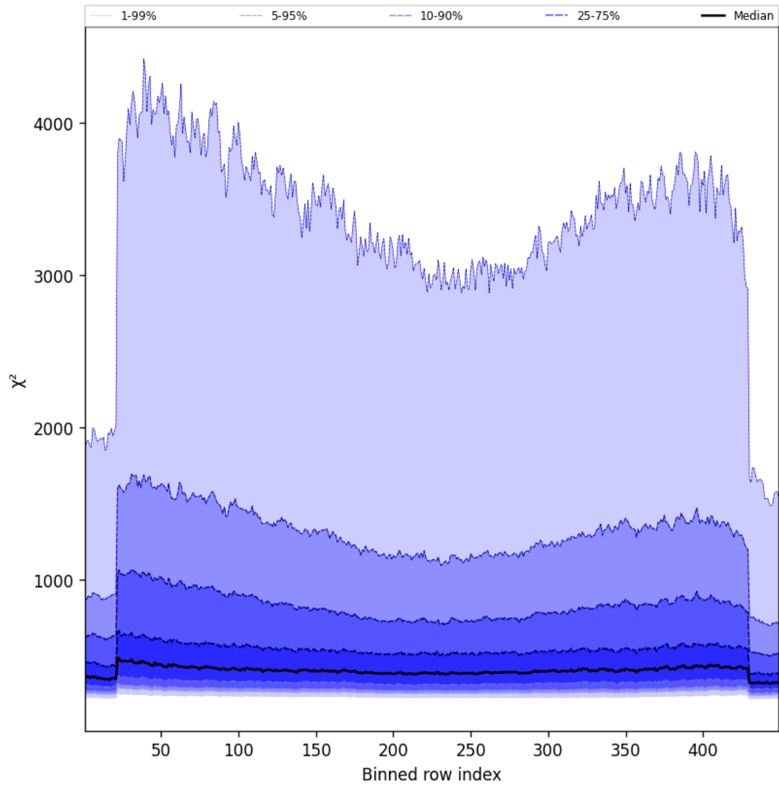
Figure 59: Along track statistics of “ \chi^2 ” for 2025-04-22 to 2025-04-22
