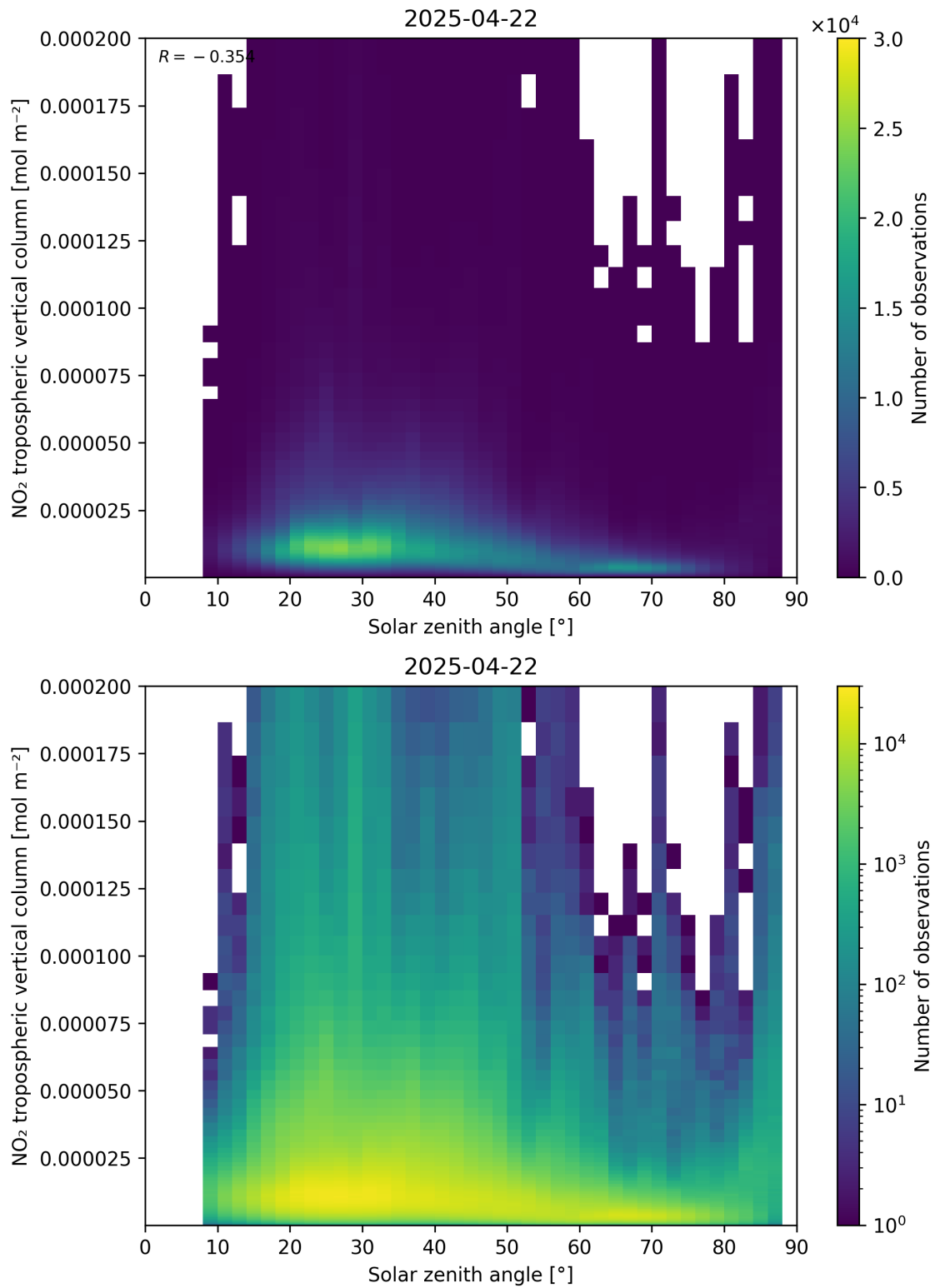
Figure 155: Scatter density plot of “Solar zenith angle” against “NO 2 tropospheric vertical column” for 2025-04-22 to 2025-04-22.
