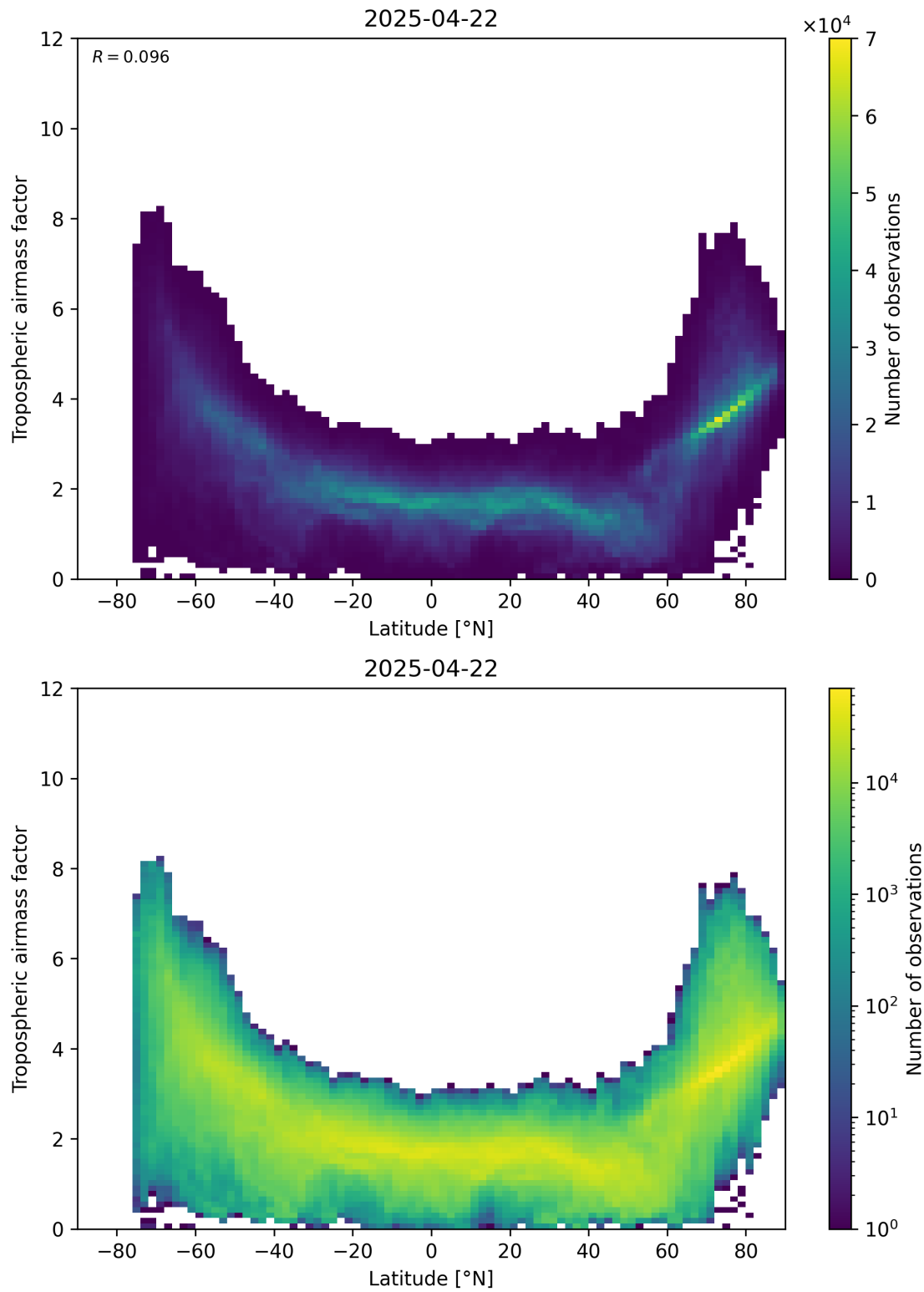
Figure 85: Scatter density plot of “Latitude” against “Tropospheric air mass factor” for 2025-04-22 to 2025-04-22.
