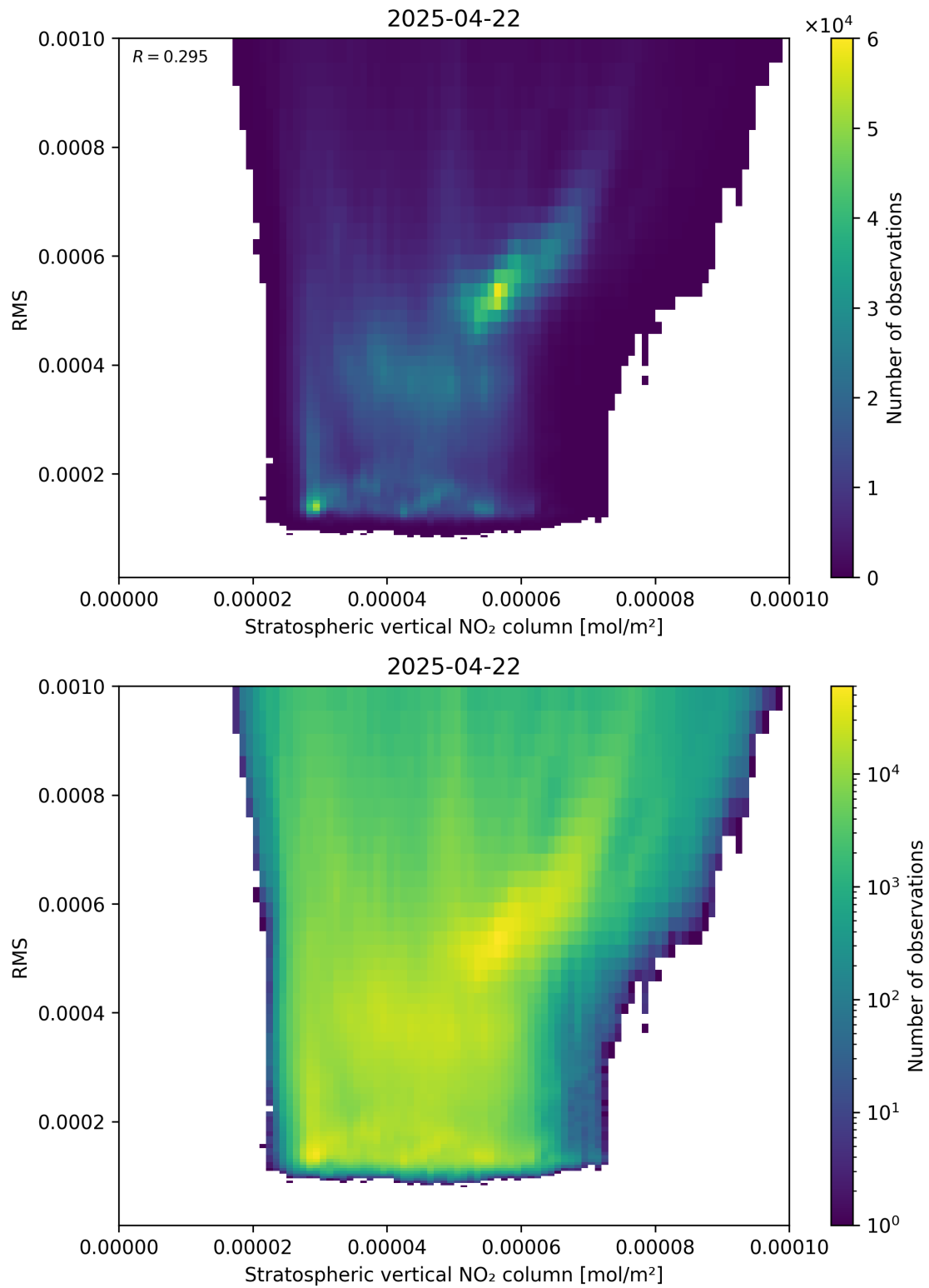
Figure 102: Scatter density plot of “Stratospheric vertical NO 2 column” against “RMS” for 2025-04-22 to 2025-04-22.
