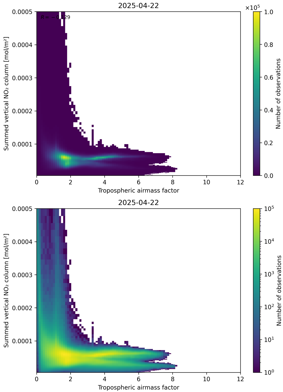
Figure 75: Scatter density plot of “Tropospheric air mass factor” against “Summed vertical NO 2 column” for 2025-04-22 to 2025-04-22.
