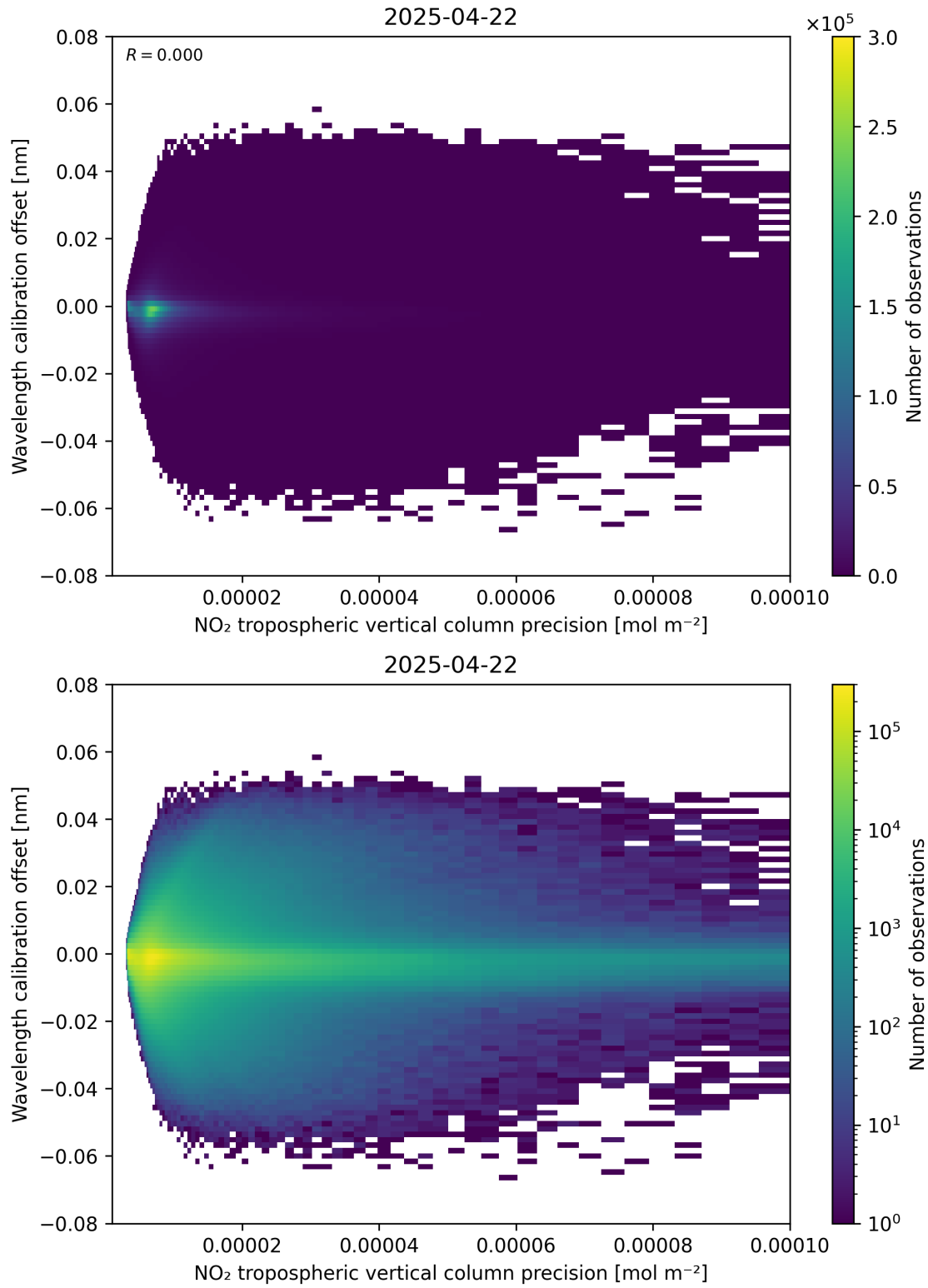
Figure 141: Scatter density plot of “NO 2 tropospheric vertical column precision” against “Wavelength calibration offset” for 2025-04-22 to 2025-04-22.
