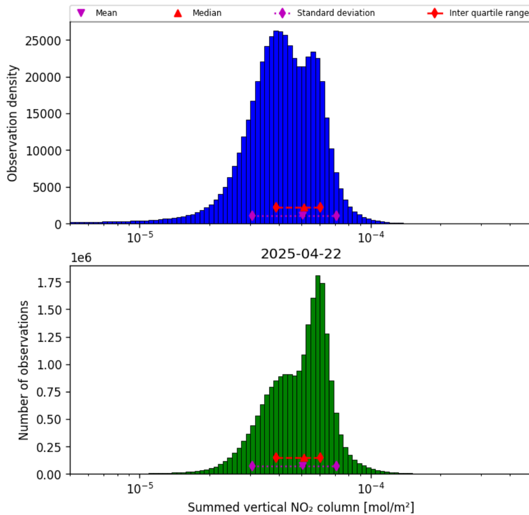
Figure 40: Histogram of “Summed vertical NO 2 column” for 2025-04-22 to 2025-04-22
