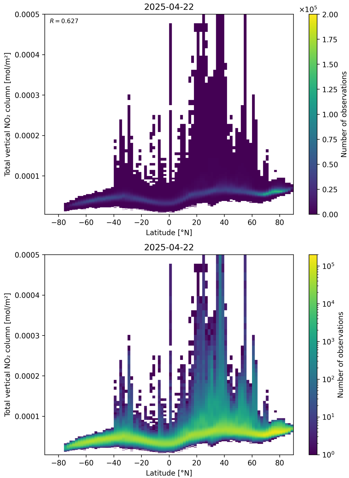
Figure 90: Scatter density plot of “Latitude” against “Total vertical NO 2 column” for 2025-04-22 to 2025-04-22.
