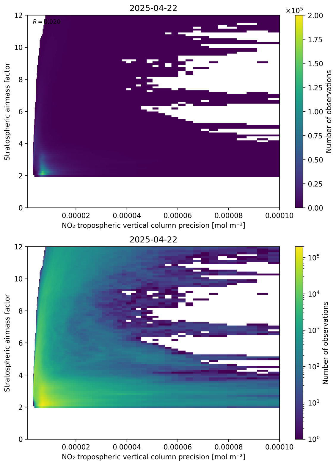
Figure 131: Scatter density plot of “NO 2 tropospheric vertical column precision” against “Stratospheric airmass factor” for 2025-04-22 to 2025-04-22.
