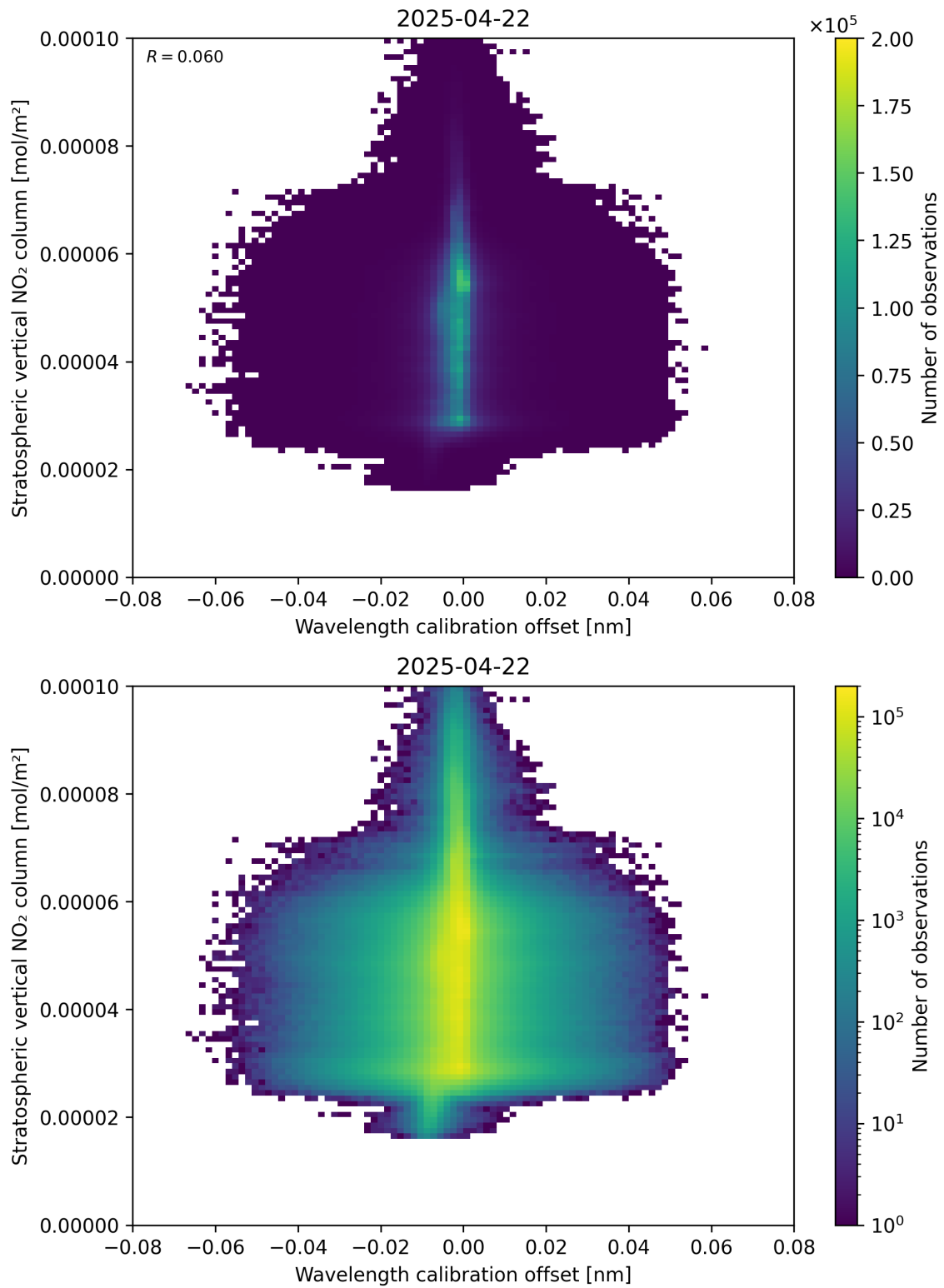
Figure 176: Scatter density plot of “Wavelength calibration offset” against “Stratospheric vertical NO 2 column” for 2025-04-22 to 2025-04-22.
