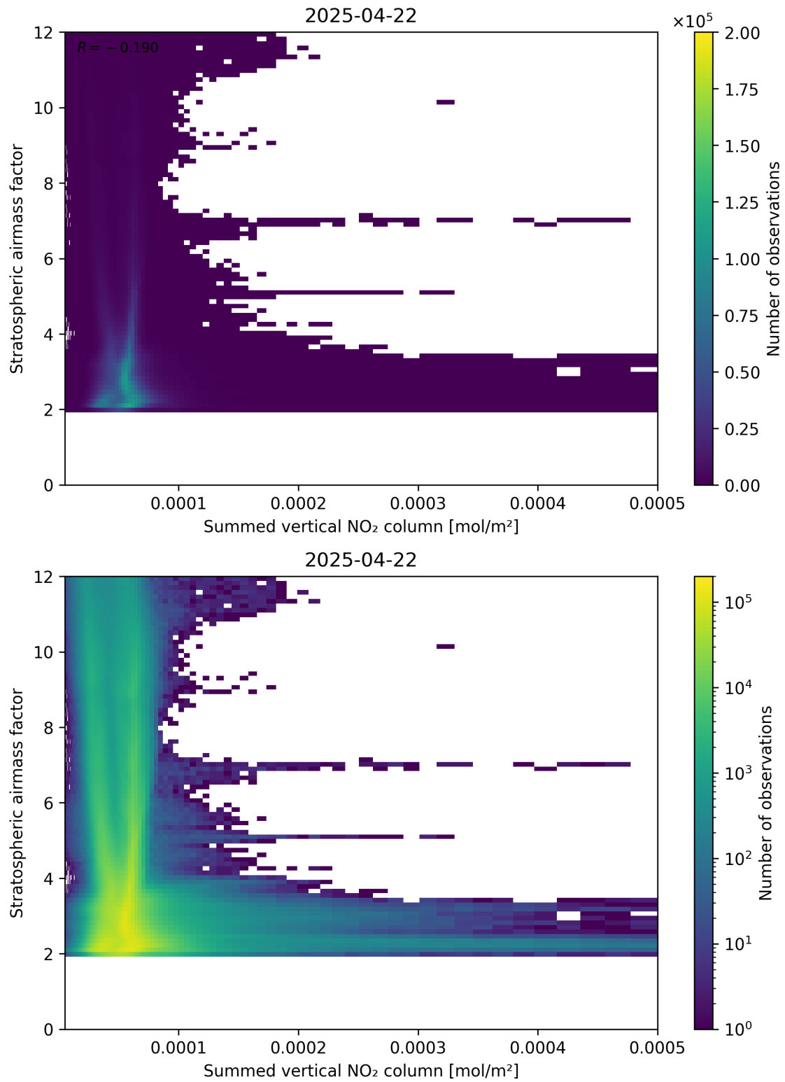
Figure 103: Scatter density plot of “Summed vertical NO 2 column” against “Stratospheric air mass factor” for 2025-04-22 to 2025-04-22.
