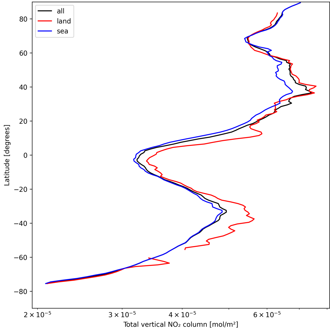
Figure 21: Zonal average of “Total vertical NO 2 column” for 2025-04-22 to 2025-04-22.
