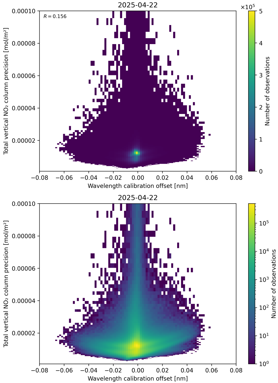
Figure 180: Scatter density plot of “Wavelength calibration offset” against “Total vertical NO 2 column precision” for 2025-04-22 to 2025-04-22.
