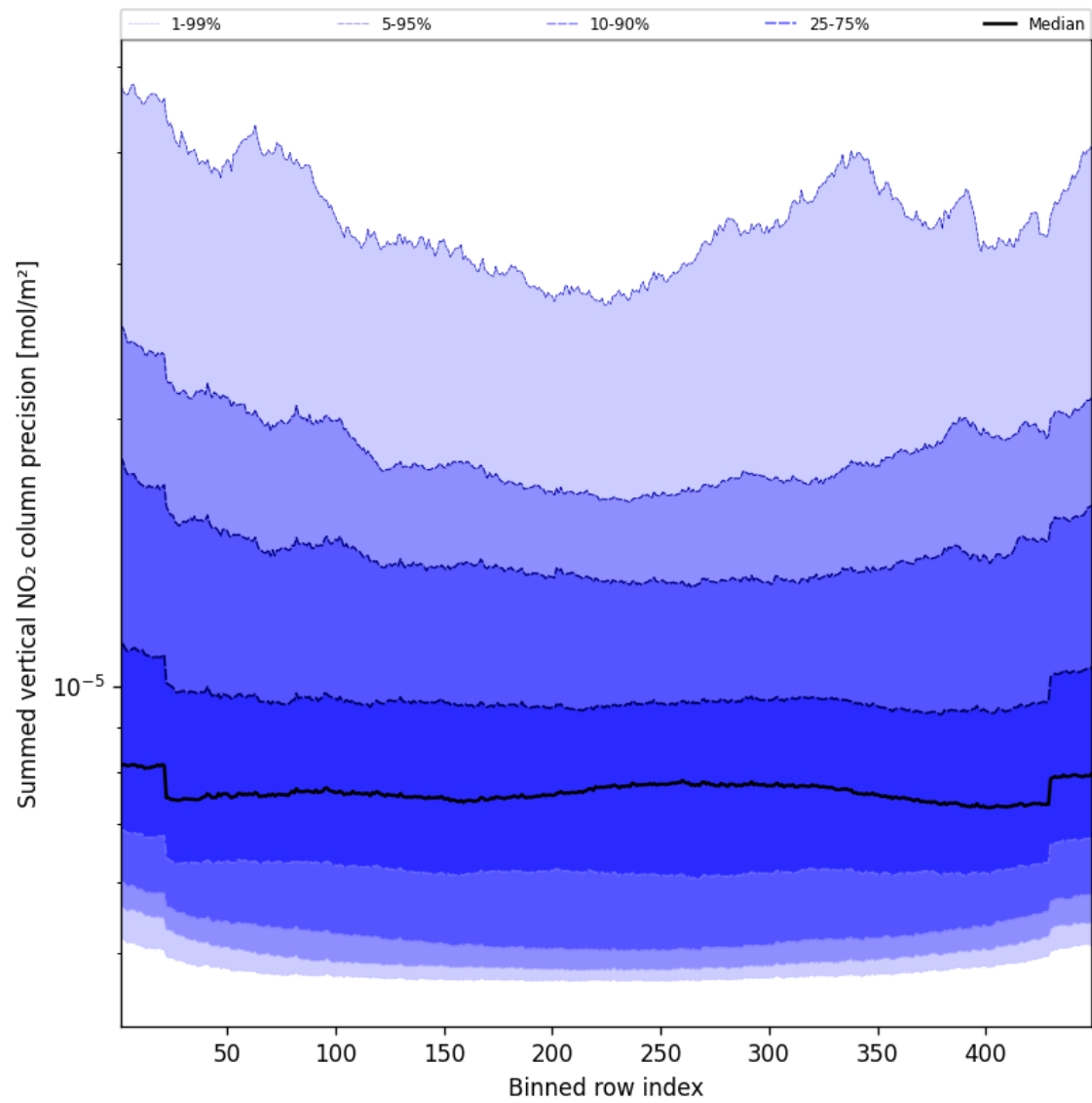
Figure 58: Along track statistics of “Summed vertical NO 2 column precision” for 2025-04-22 to 2025-04-22
