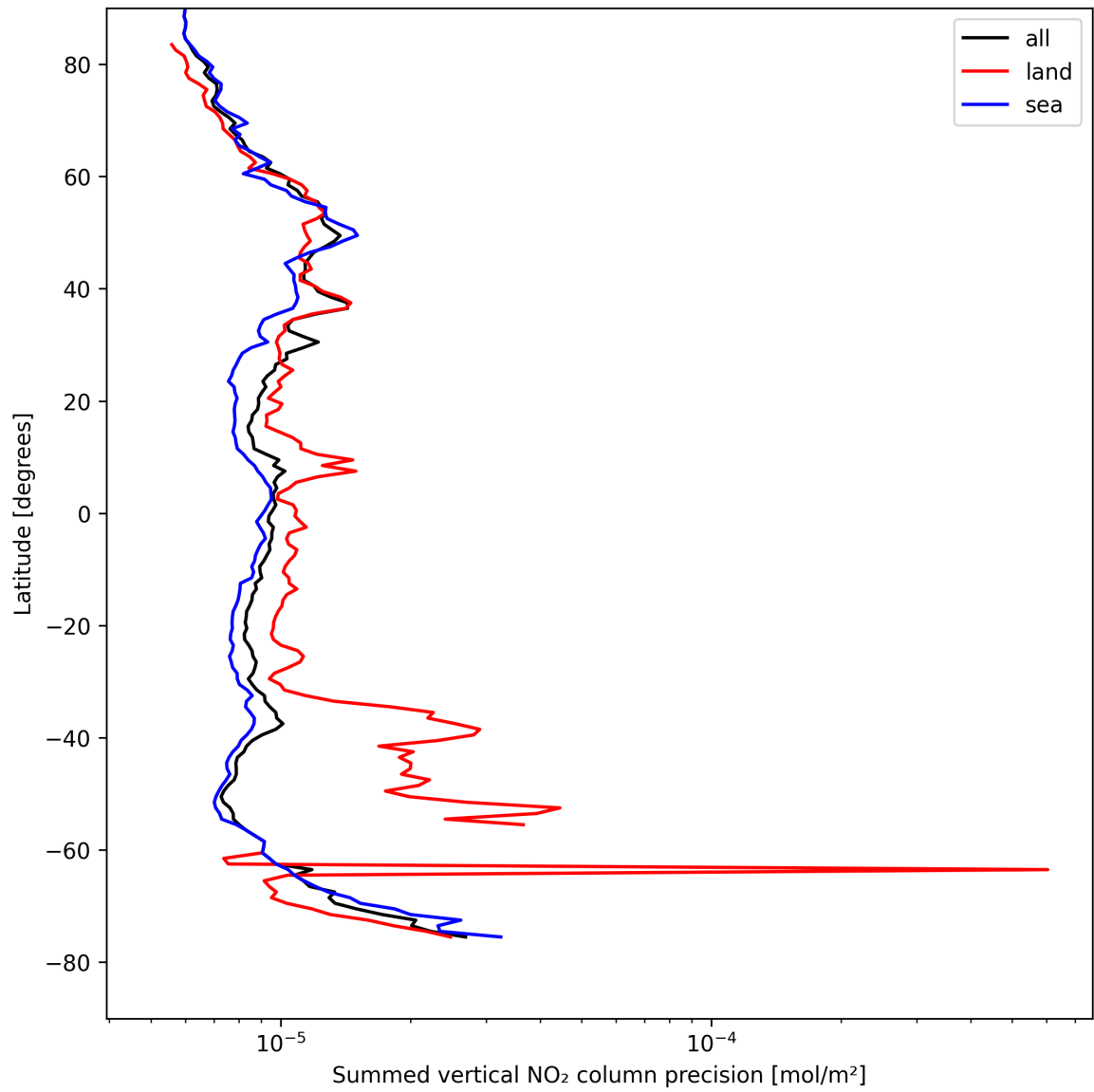
Figure 24: Zonal average of “Summed vertical NO 2 column precision” for 2025-04-22 to 2025-04-22.
