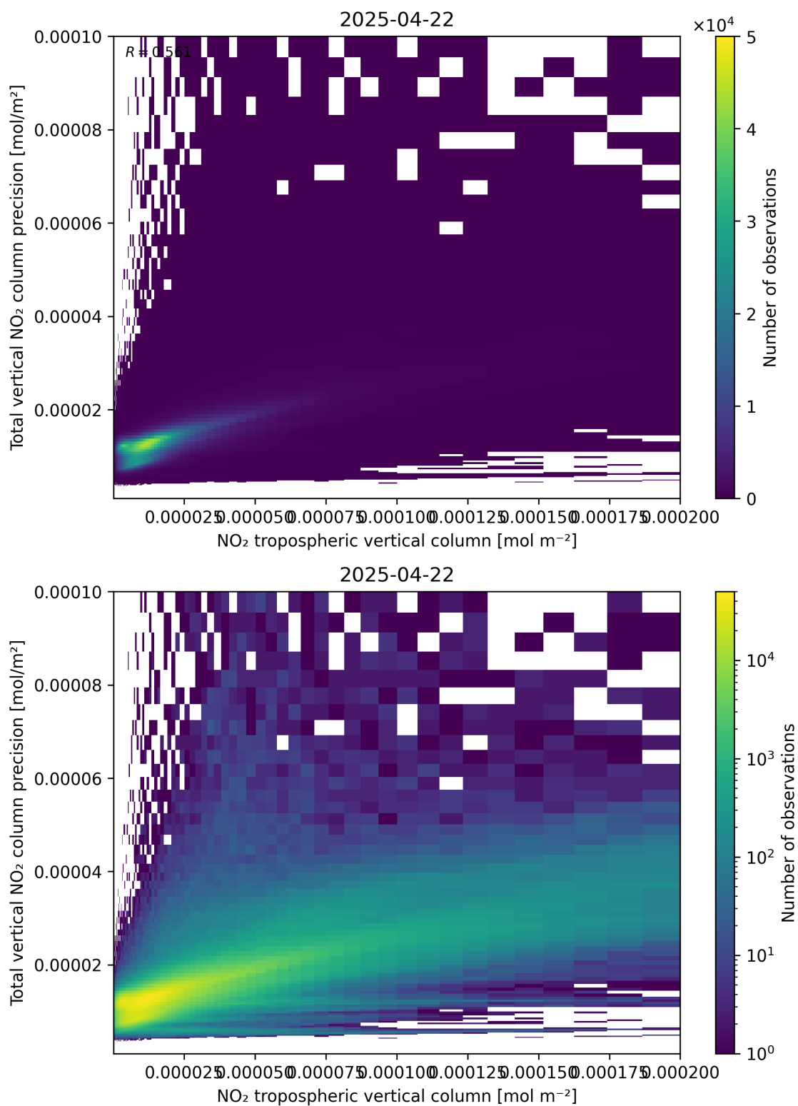
Figure 129: Scatter density plot of “NO 2 tropospheric vertical column” against “Total vertical NO 2 column precision” for 2025-04-22 to 2025-04-22.
