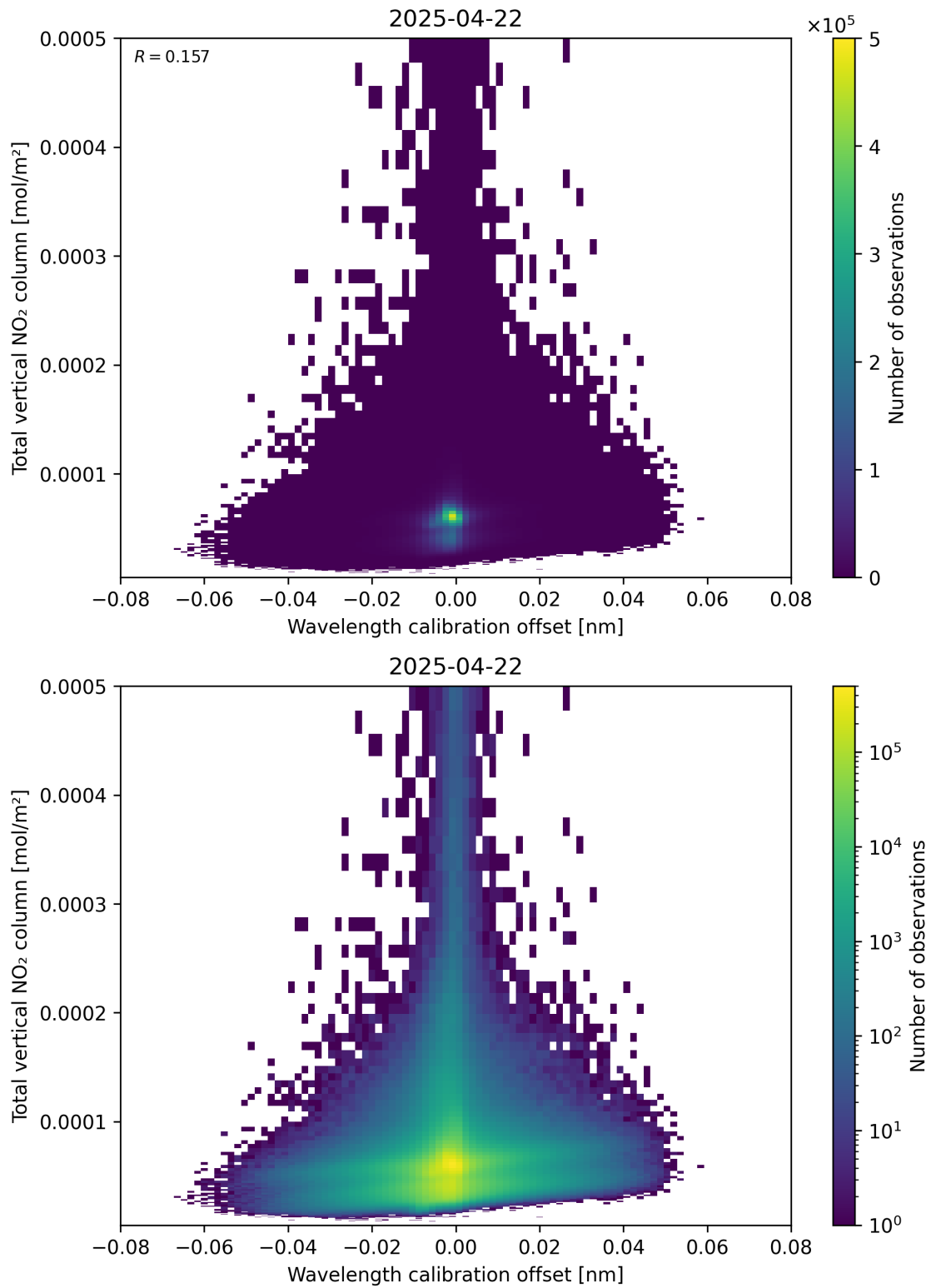
Figure 179: Scatter density plot of “Wavelength calibration offset” against “Total vertical NO 2 column” for 2025-04-22 to 2025-04-22.
