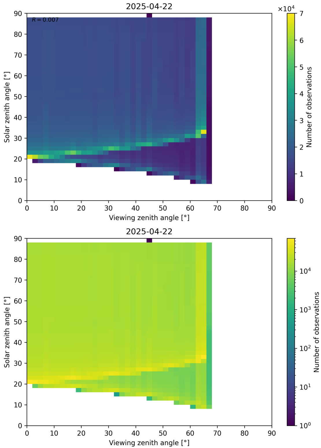
Figure 172: Scatter density plot of “Viewing zenith angle” against “Solar zenith angle” for 2025-04-22 to 2025-04-22.
