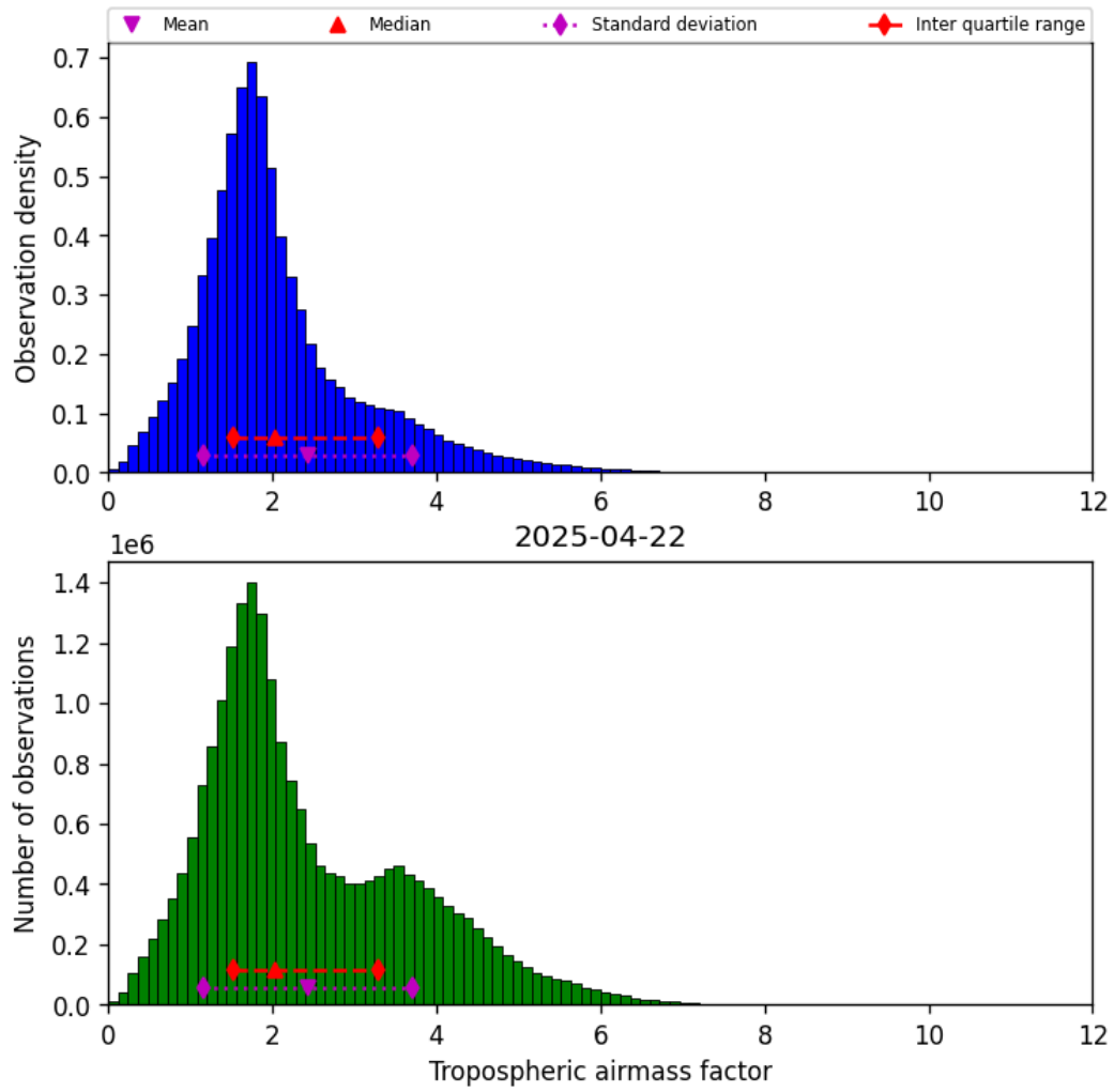
Figure 31: Histogram of “Tropospheric airmass factor” for 2025-04-22 to 2025-04-22
