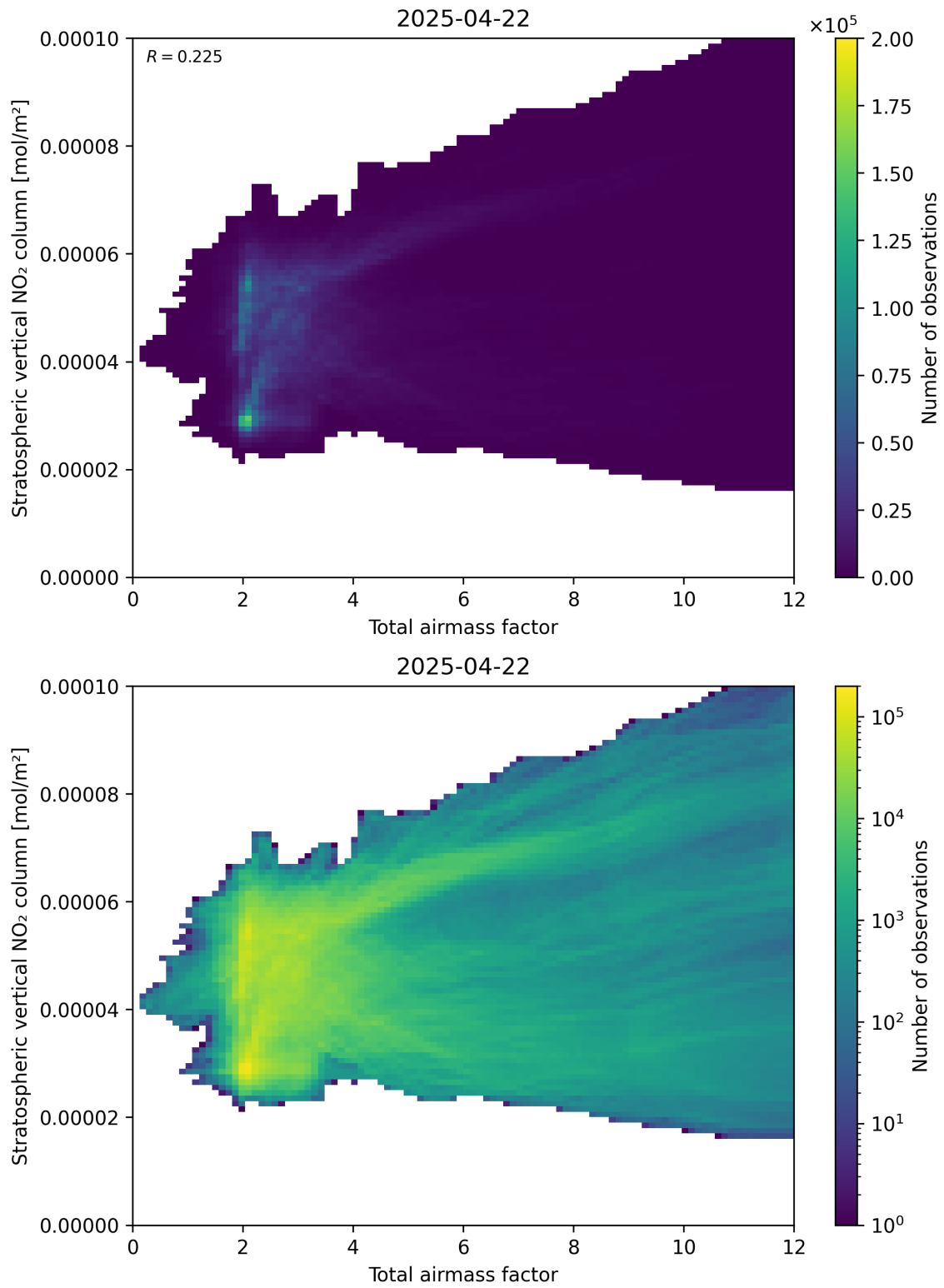
Figure 64: Scatter density plot of “Total airmass factor” against “Stratospheric vertical \text{NO}_2 column” for 2025-04-22 to 2025-04-22.
