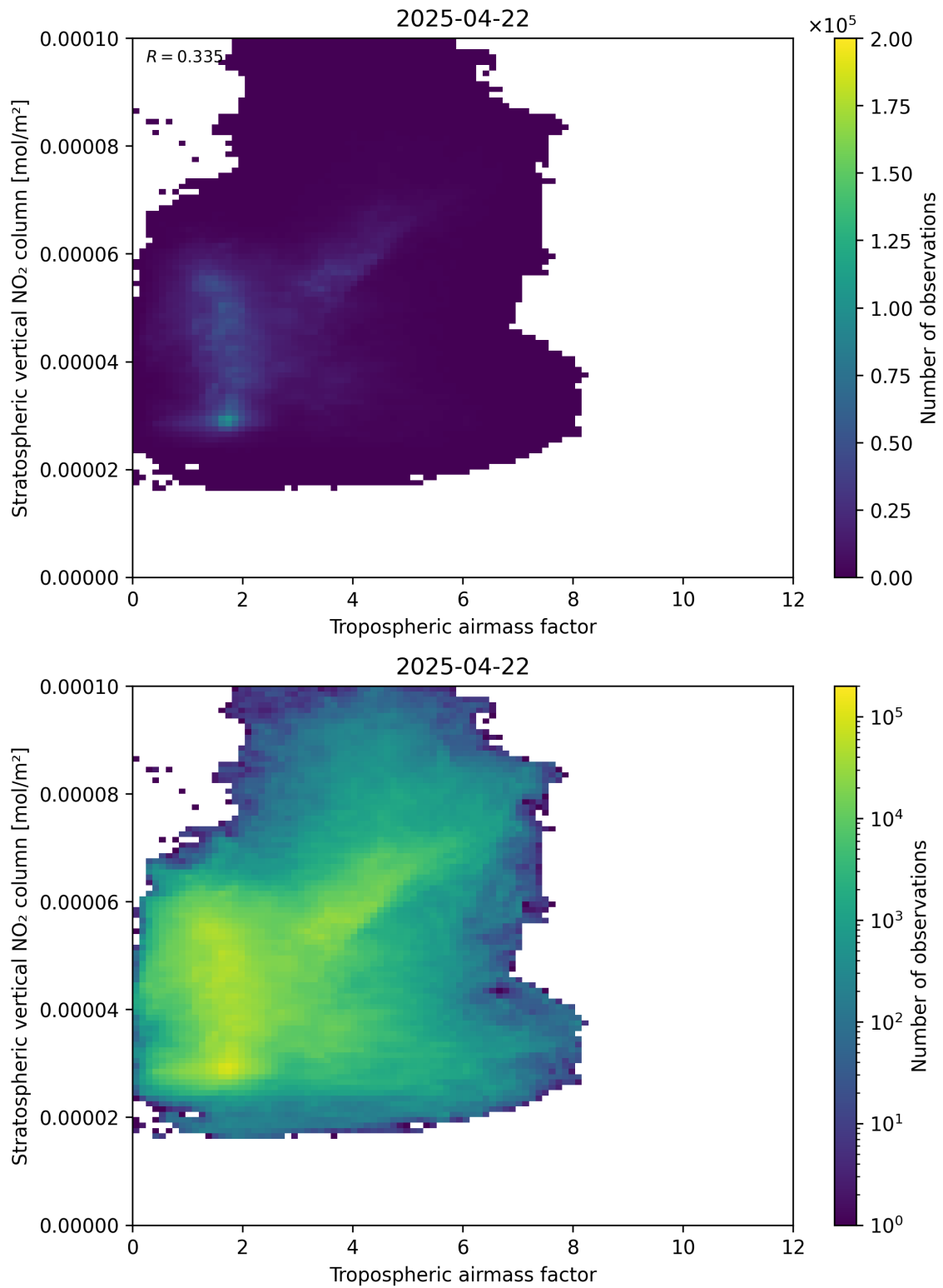
Figure 74: Scatter density plot of “Tropospheric air mass factor” against “Stratospheric vertical \text{NO}_2 column” for 2025-04-22 to 2025-04-22.
