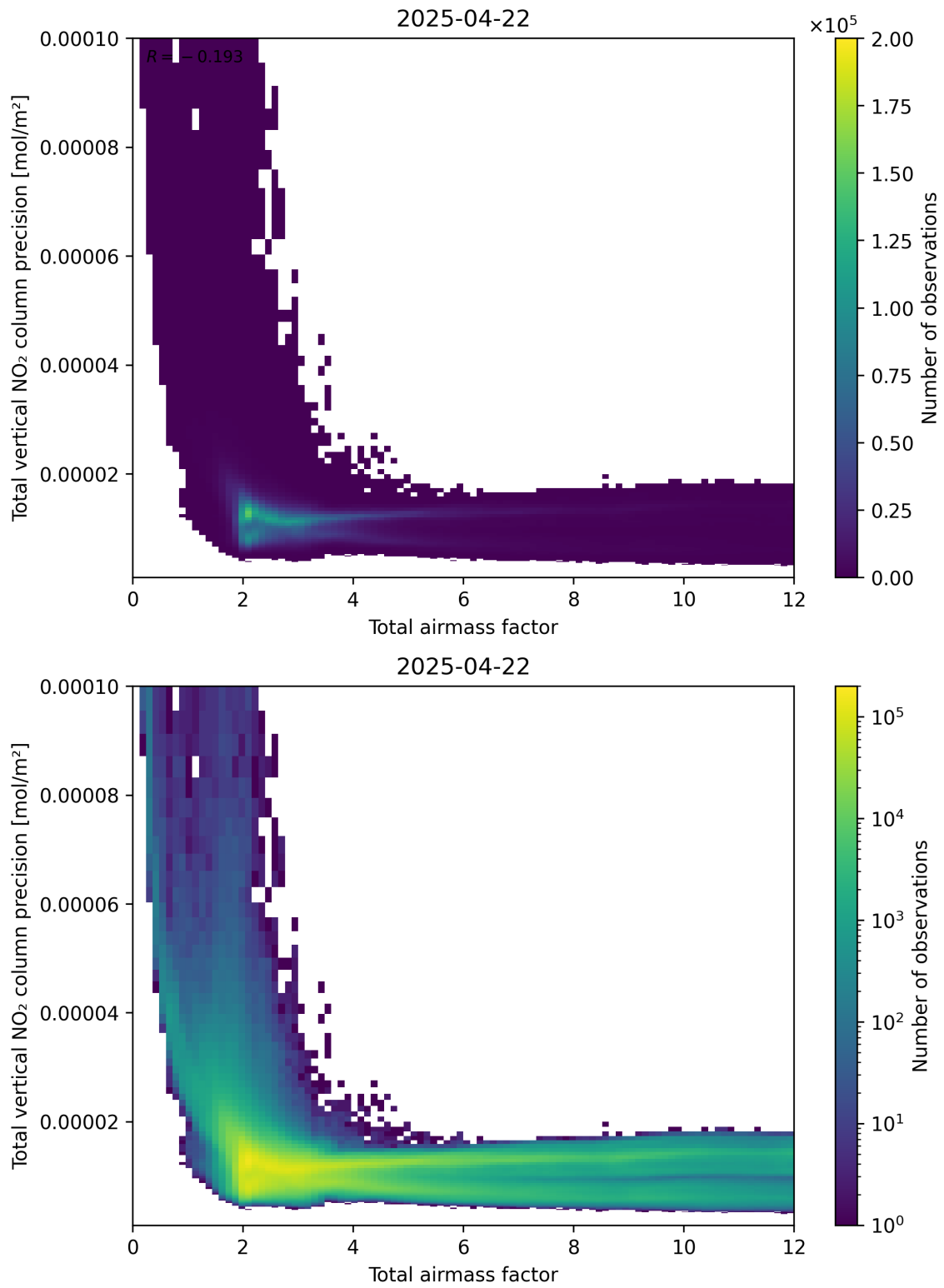
Figure 68: Scatter density plot of “Total airmass factor” against “Total vertical NO 2 column precision” for 2025-04-22 to 2025-04-22.
