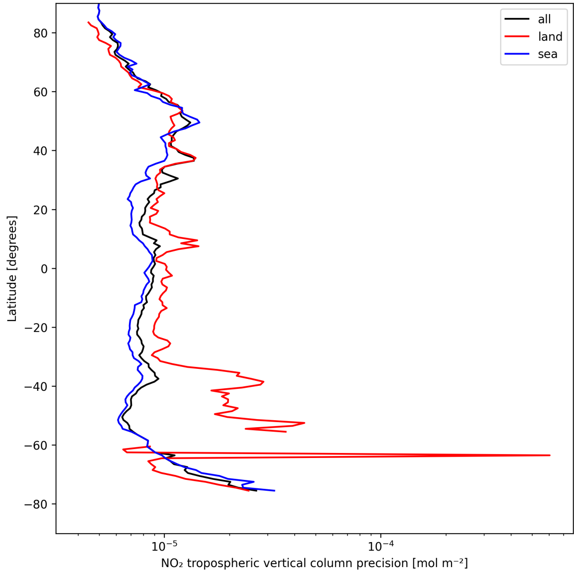
Figure 13: Zonal average of “NO 2 tropospheric vertical column precision” for 2025-04-22 to 2025-04-22.
