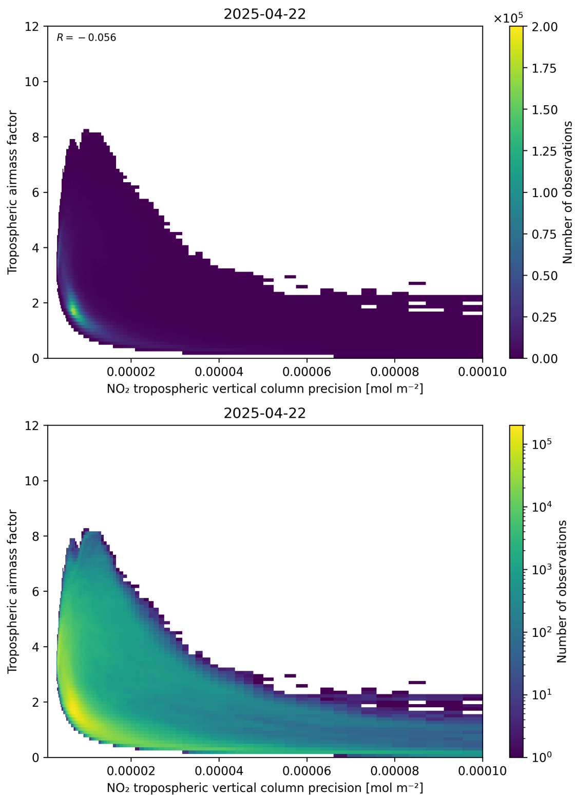
Figure 133: Scatter density plot of “NO 2 tropospheric vertical column precision” against “Tropospheric airmass factor” for 2025-04-22 to 2025-04-22.
