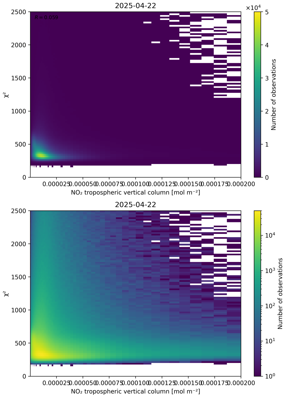
Figure 124: Scatter density plot of “NO 2 tropospheric vertical column” against “ \chi^2 ” for 2025-04-22 to 2025-04-22.
