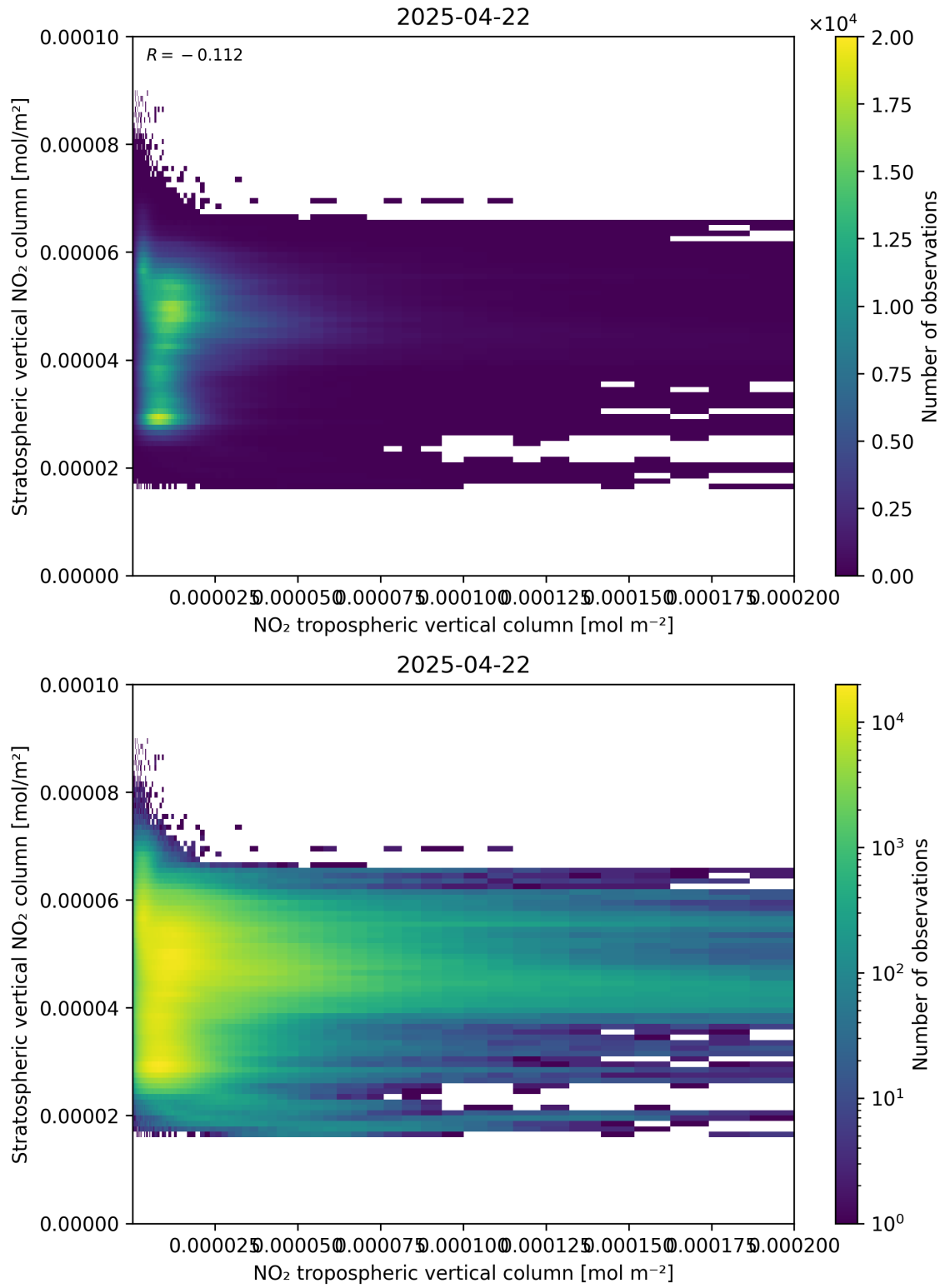
Figure 125: Scatter density plot of “NO 2 tropospheric vertical column” against “Stratospheric vertical NO 2 column” for 2025-04-22 to 2025-04-22.
