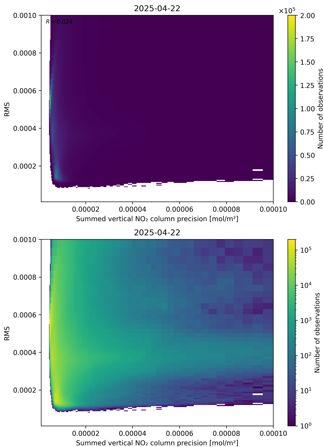
Figure 108: Scatter density plot of “Summed vertical NO 2 column precision” against “RMS” for 2025-04-22 to 2025-04-22.
