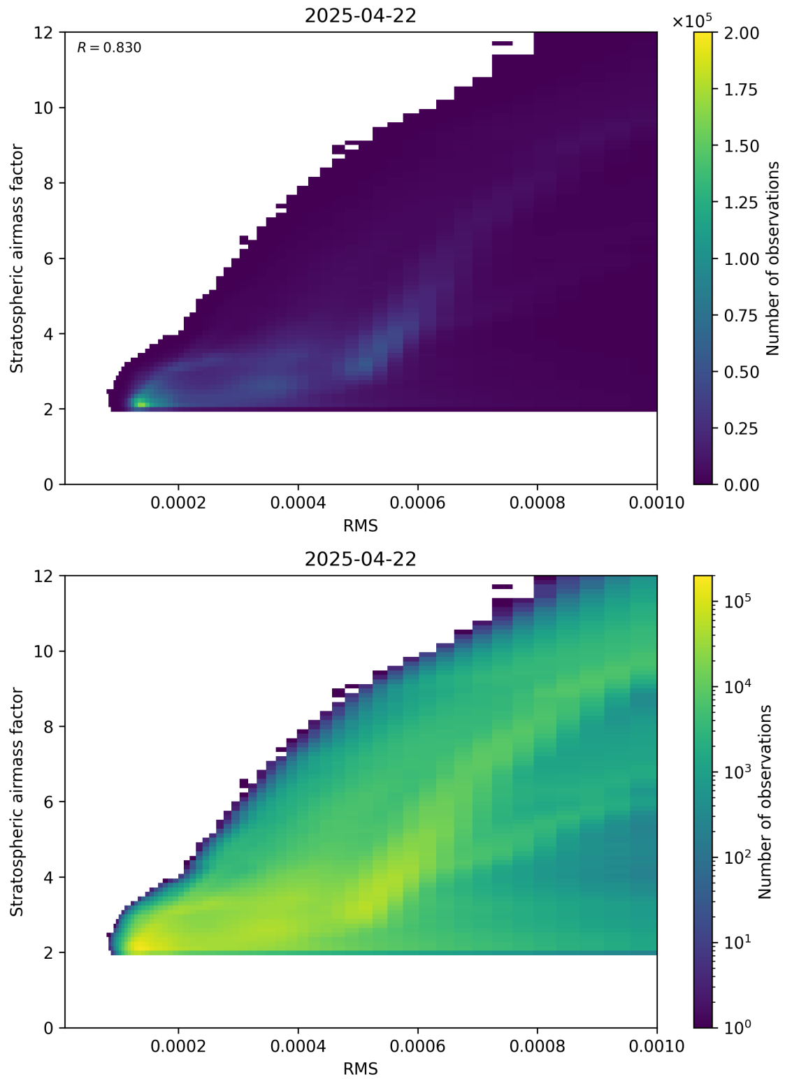
Figure 144: Scatter density plot of “RMS” against “Stratospheric airmass factor” for 2025-04-22 to 2025-04-22.
