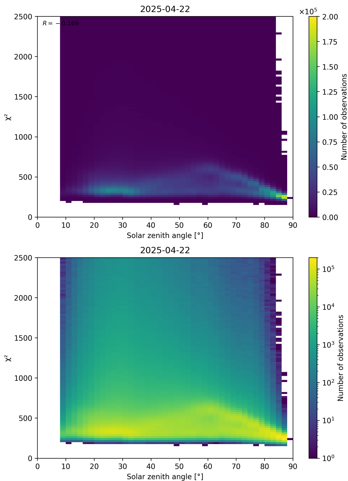
Figure 148: Scatter density plot of “Solar zenith angle” against “ \chi^2 ” for 2025-04-22 to 2025-04-22.
