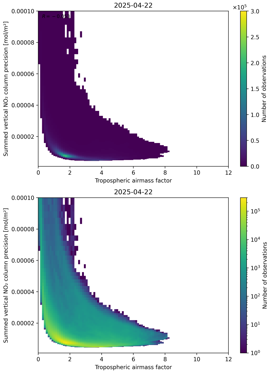
Figure 76: Scatter density plot of “Tropospheric air mass factor” against “Summed vertical NO 2 column precision” for 2025-04-22 to 2025-04-22.
