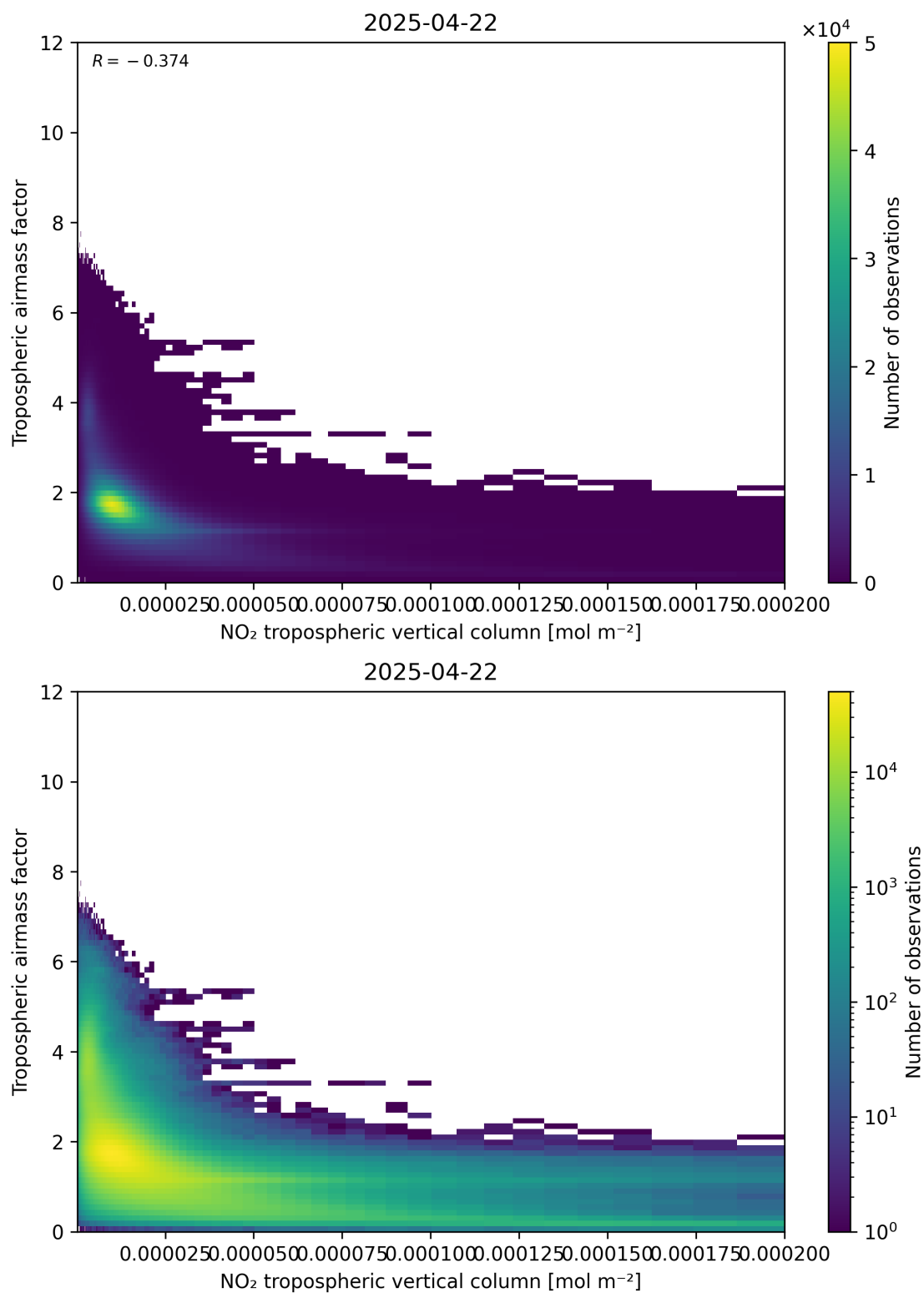
Figure 123: Scatter density plot of “NO 2 tropospheric vertical column” against “Tropospheric air mass factor” for 2025-04-22 to 2025-04-22.
