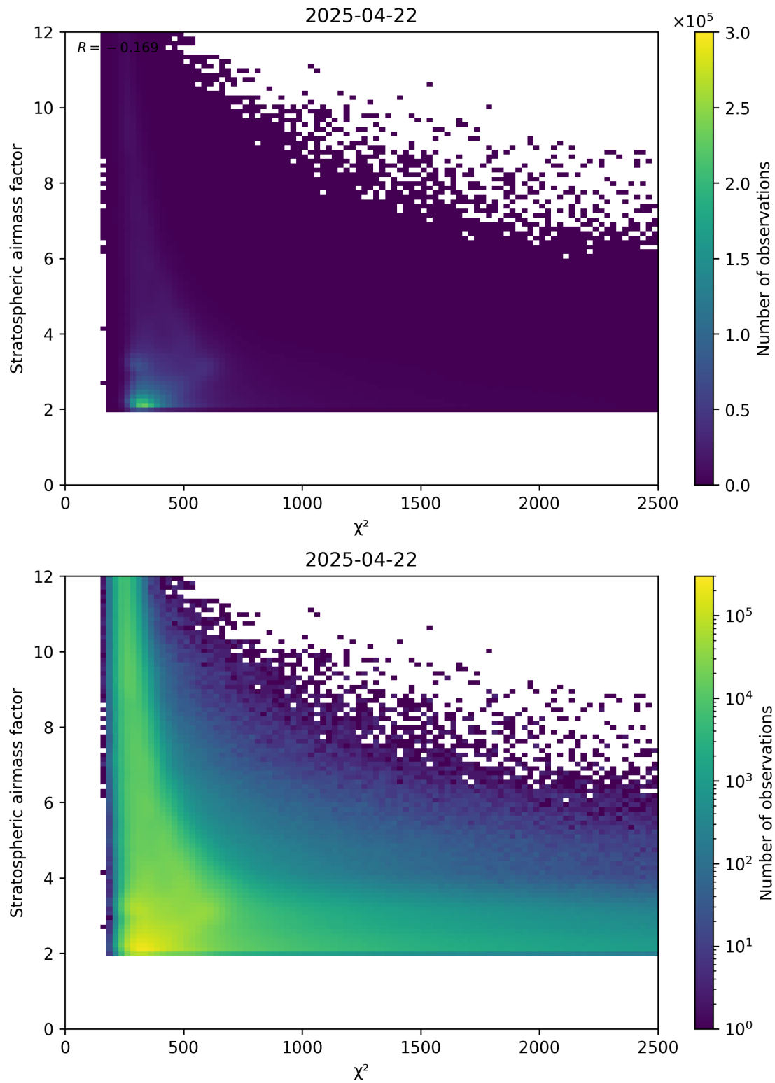
Figure 81: Scatter density plot of “ \chi^2 ” against “Stratospheric airmass factor” for 2025-04-22 to 2025-04-22.
