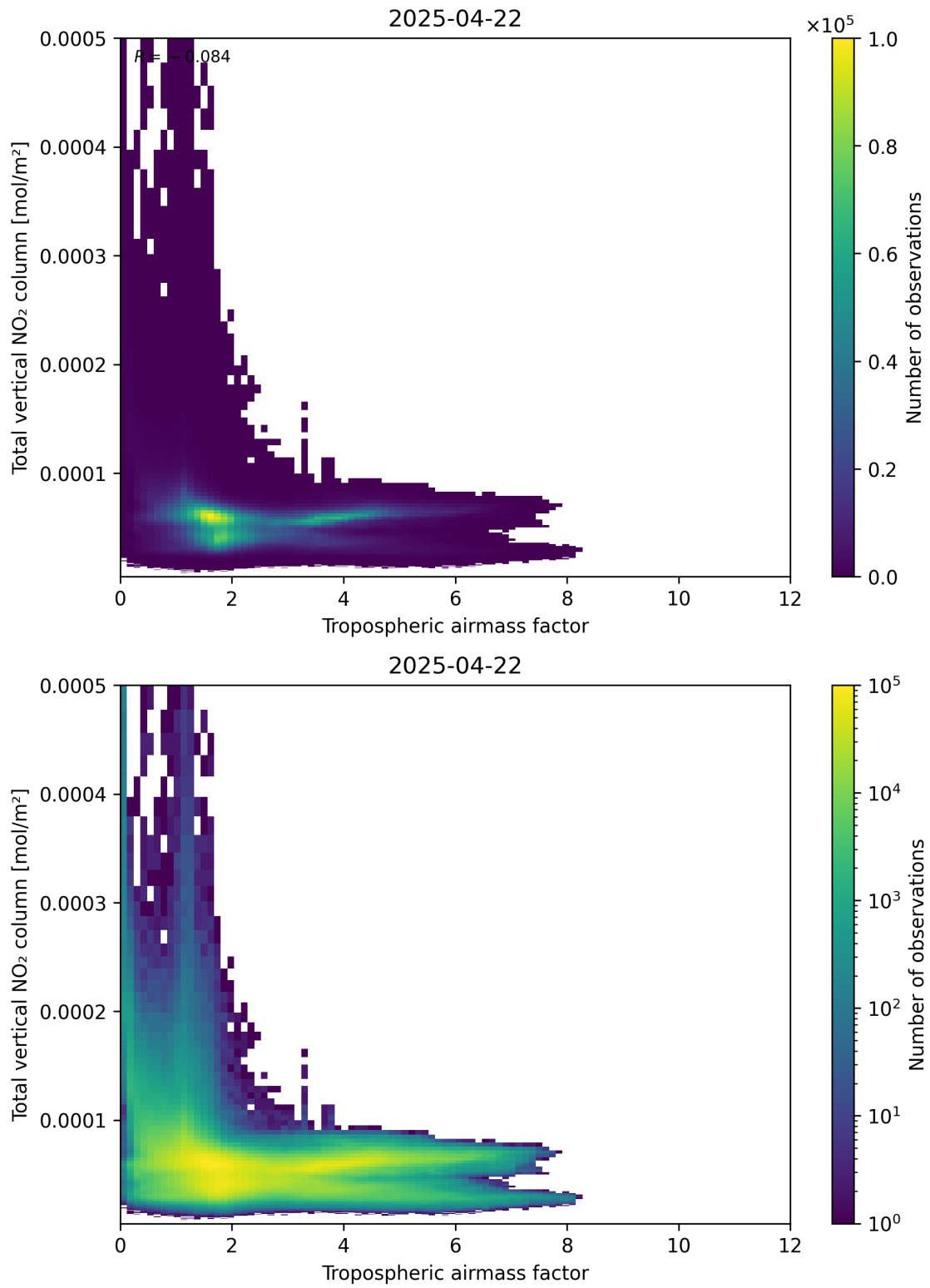
Figure 77: Scatter density plot of “Tropospheric airmass factor” against “Total vertical NO 2 column” for 2025-04-22 to 2025-04-22.
