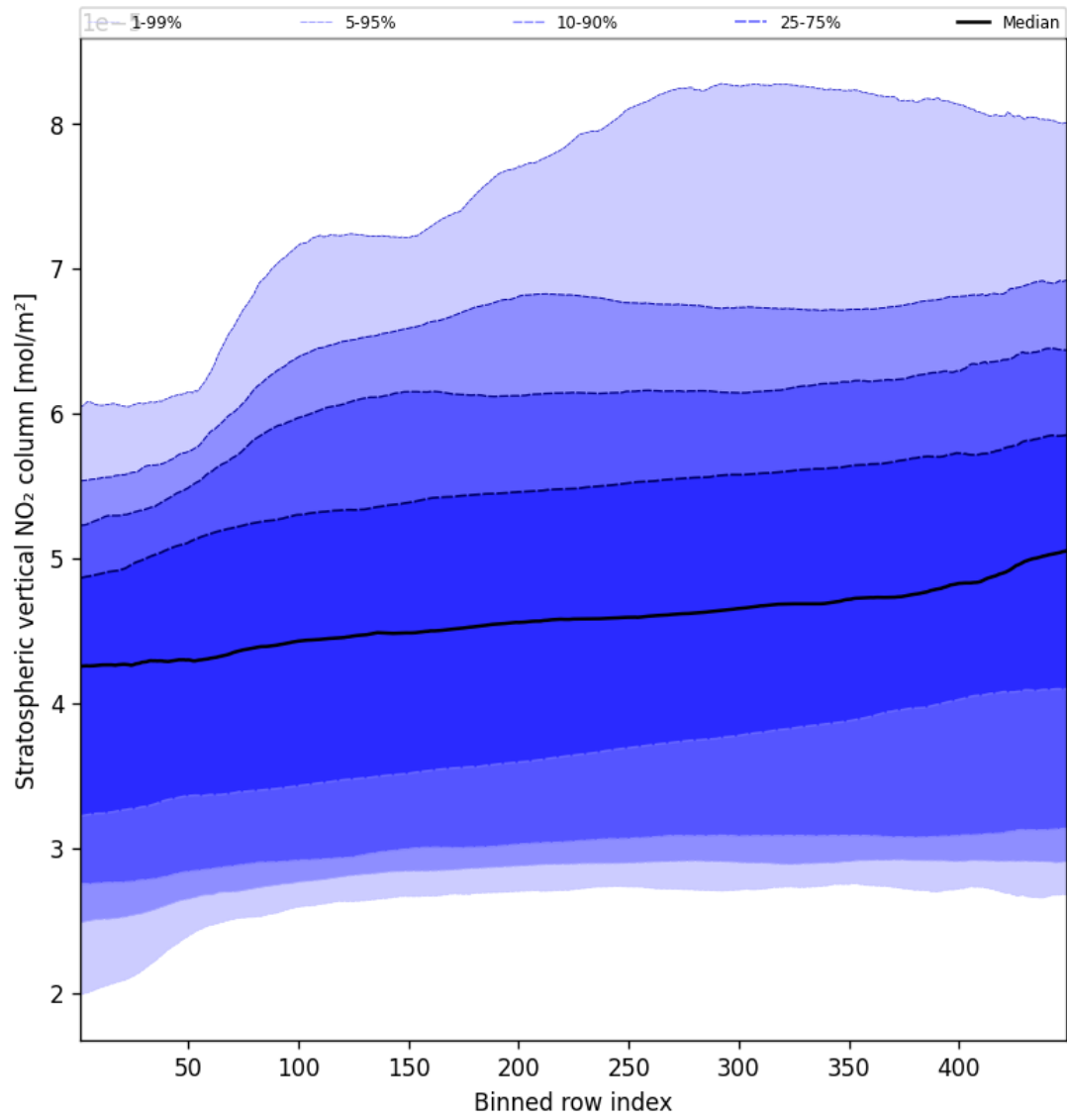
Figure 53: Along track statistics of “Stratospheric vertical NO 2 column” for 2025-04-22 to 2025-04-22
