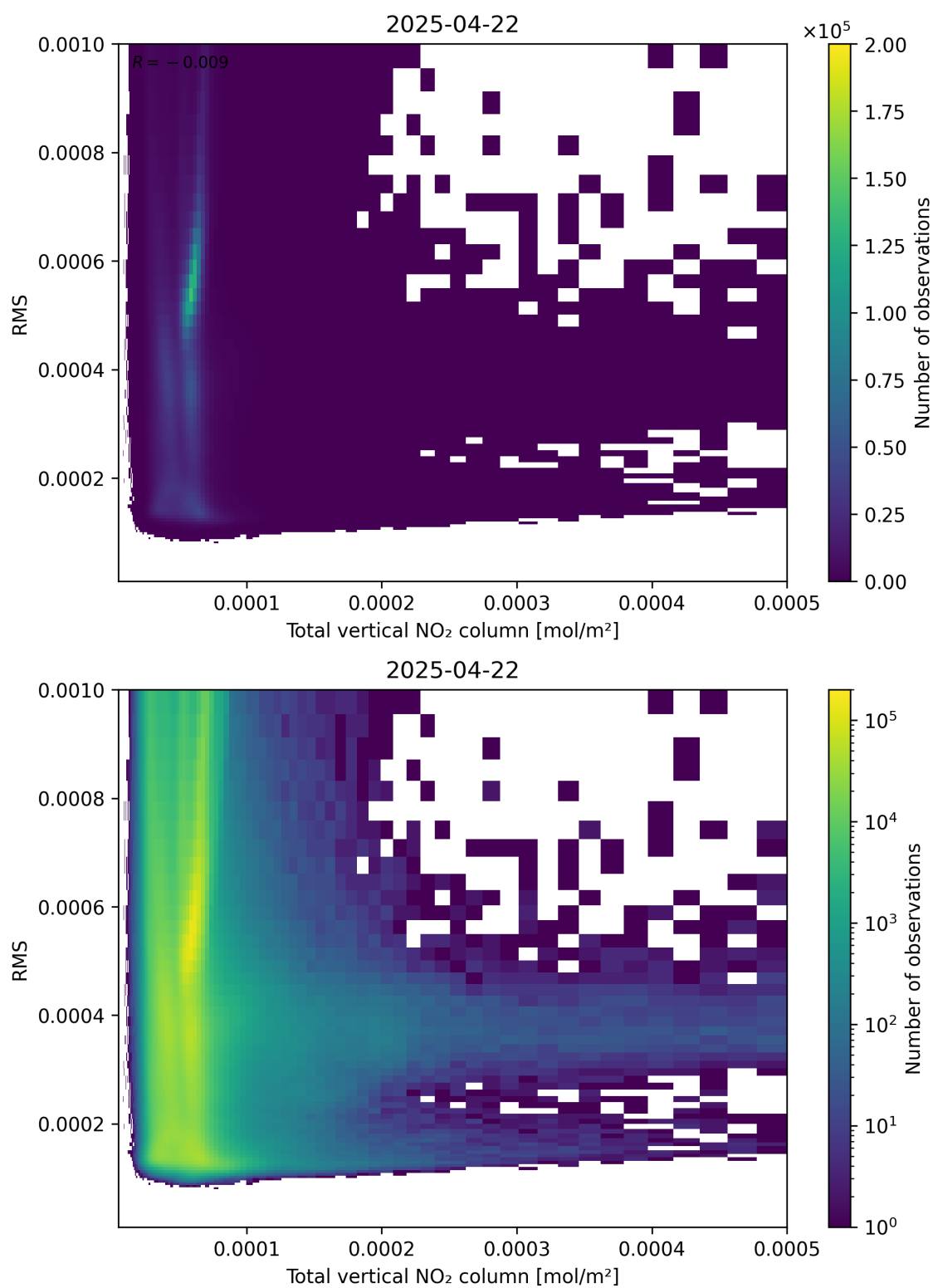
Figure 120: Scatter density plot of “Total vertical NO 2 column” against “RMS” for 2025-04-22 to 2025-04-22.
