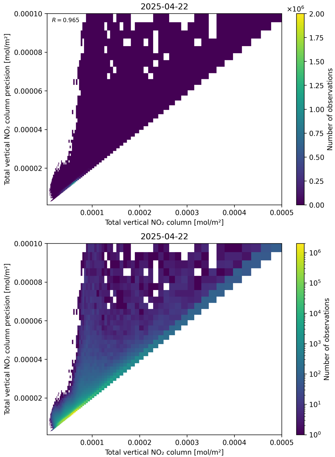
Figure 114: Scatter density plot of “Total vertical NO 2 column” against “Total vertical NO 2 column precision” for 2025-04-22 to 2025-04-22.
