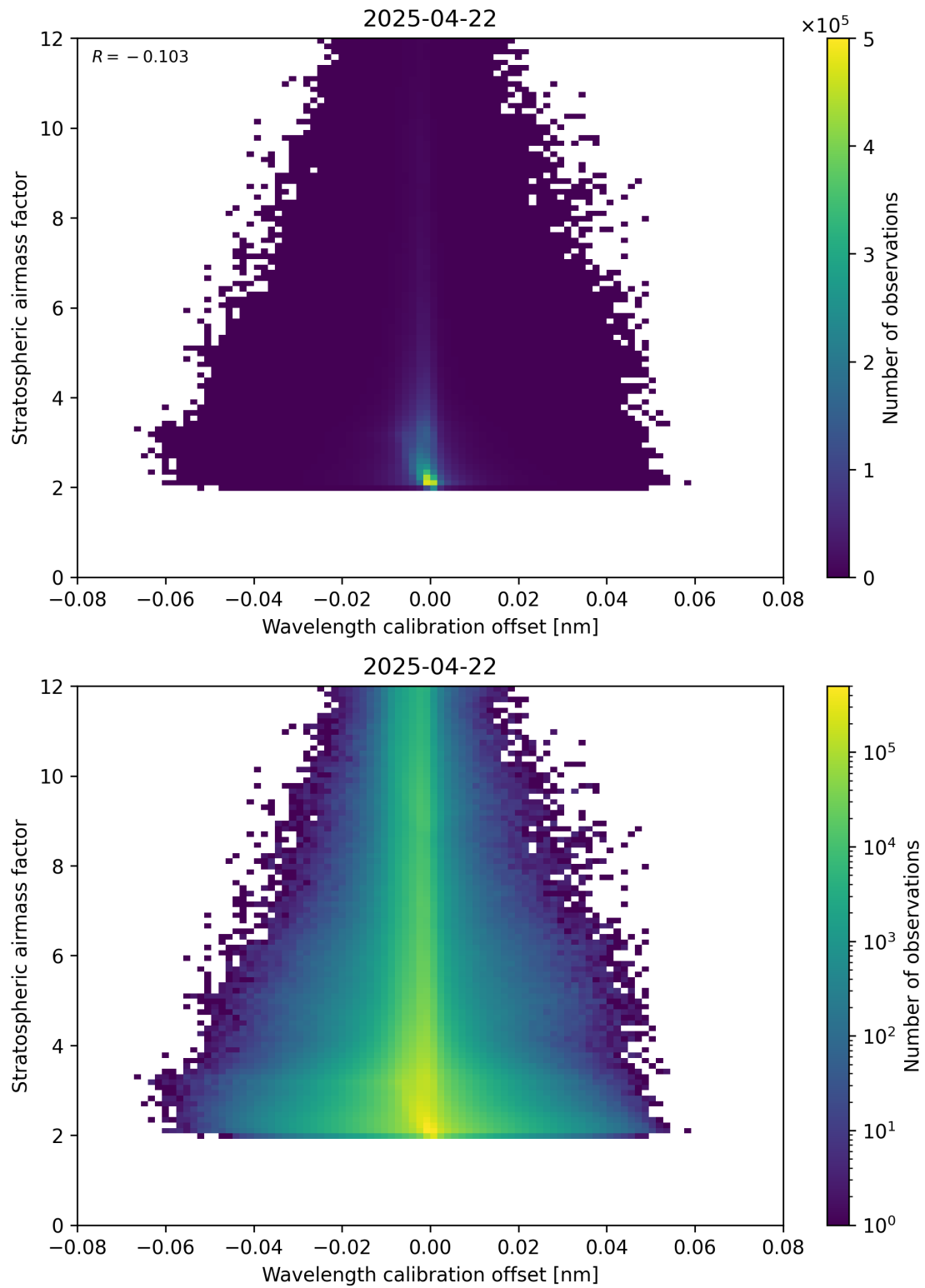
Figure 174: Scatter density plot of “Wavelength calibration offset” against “Stratospheric airmass factor” for 2025-04-22 to 2025-04-22.
