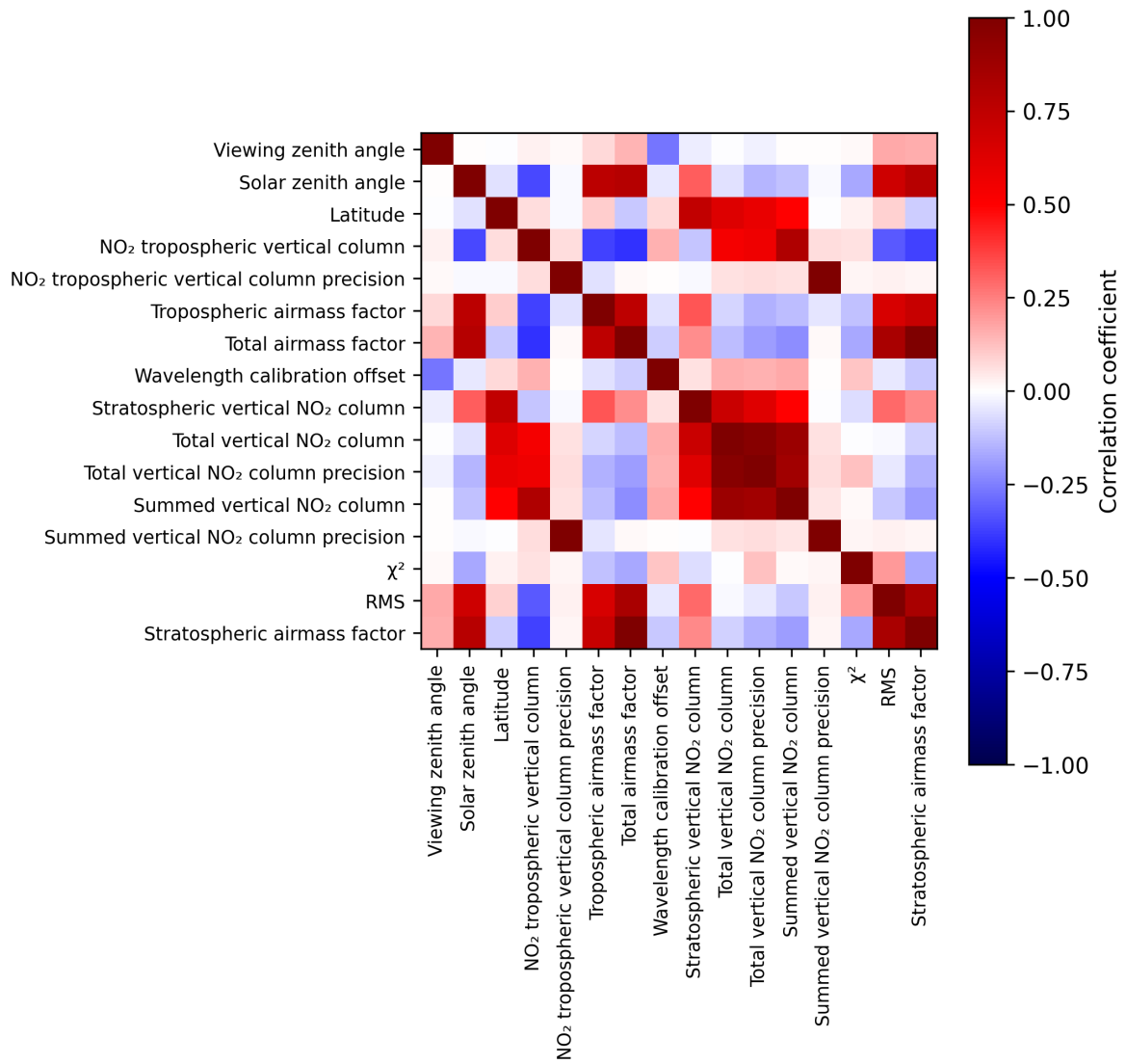
Figure 2: Map of correlation matrix for 2025-04-22 to 2025-04-22.
