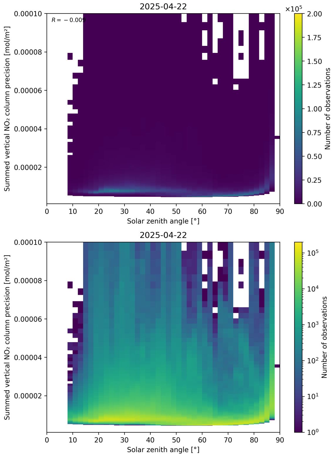
Figure 152: Scatter density plot of “Solar zenith angle” against “Summed vertical NO 2 column precision” for 2025-04-22 to 2025-04-22.
