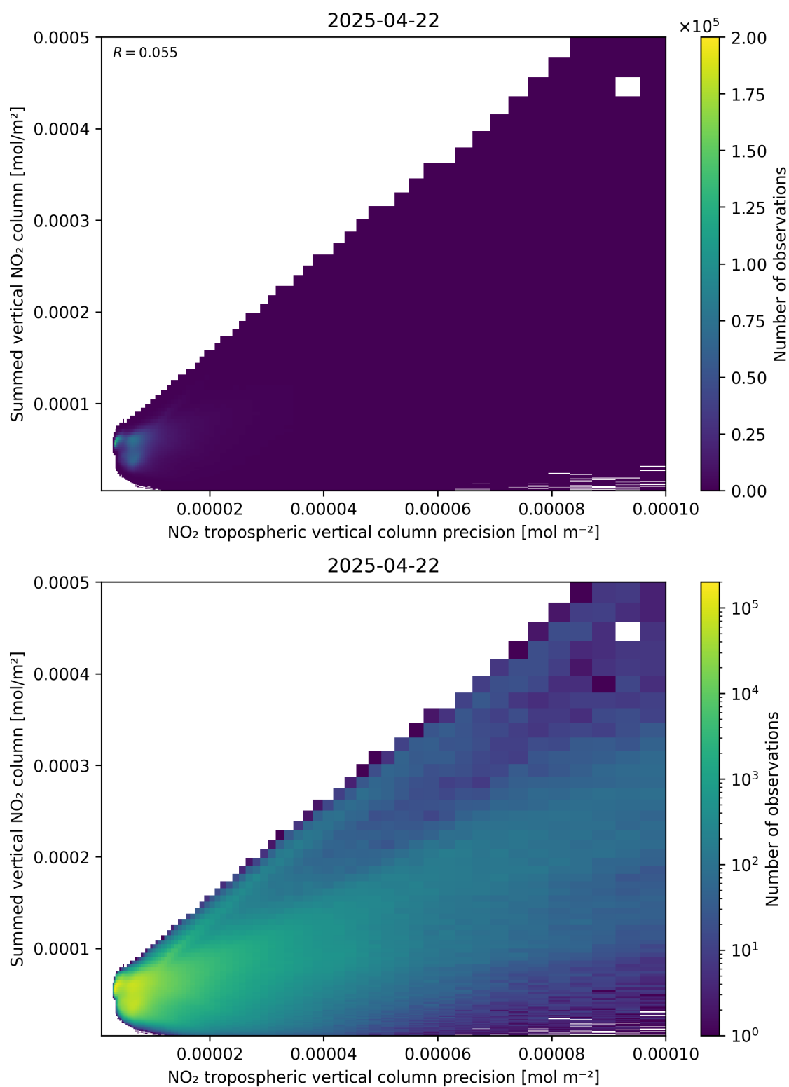
Figure 136: Scatter density plot of “NO 2 tropospheric vertical column precision” against “Summed vertical NO 2 column” for 2025-04-22 to 2025-04-22.
