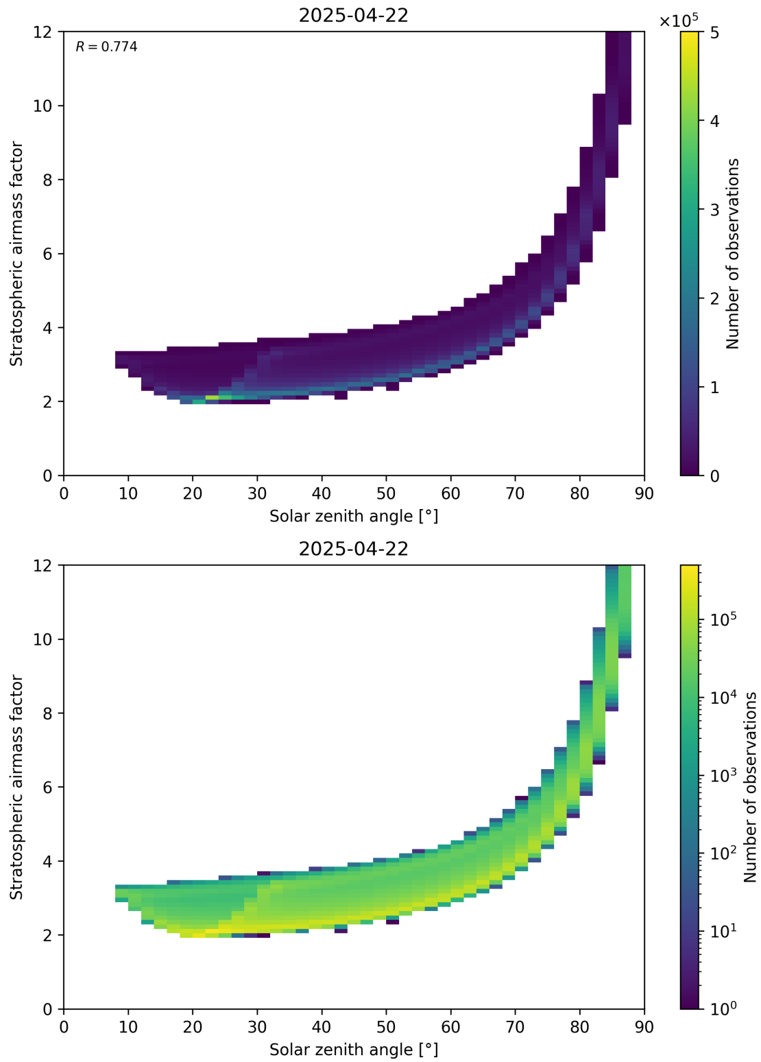
Figure 145: Scatter density plot of “Solar zenith angle” against “Stratospheric airmass factor” for 2025-04-22 to 2025-04-22.
