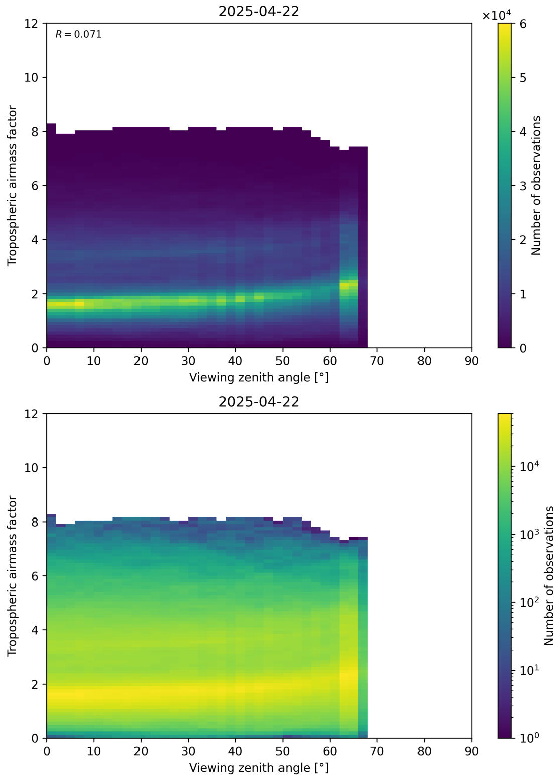
Figure 161: Scatter density plot of “Viewing zenith angle” against “Tropospheric airmass factor” for 2025-04-22 to 2025-04-22.
