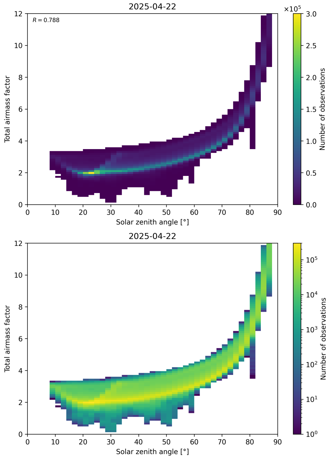
Figure 146: Scatter density plot of “Solar zenith angle” against “Total air mass factor” for 2025-04-22 to 2025-04-22.
