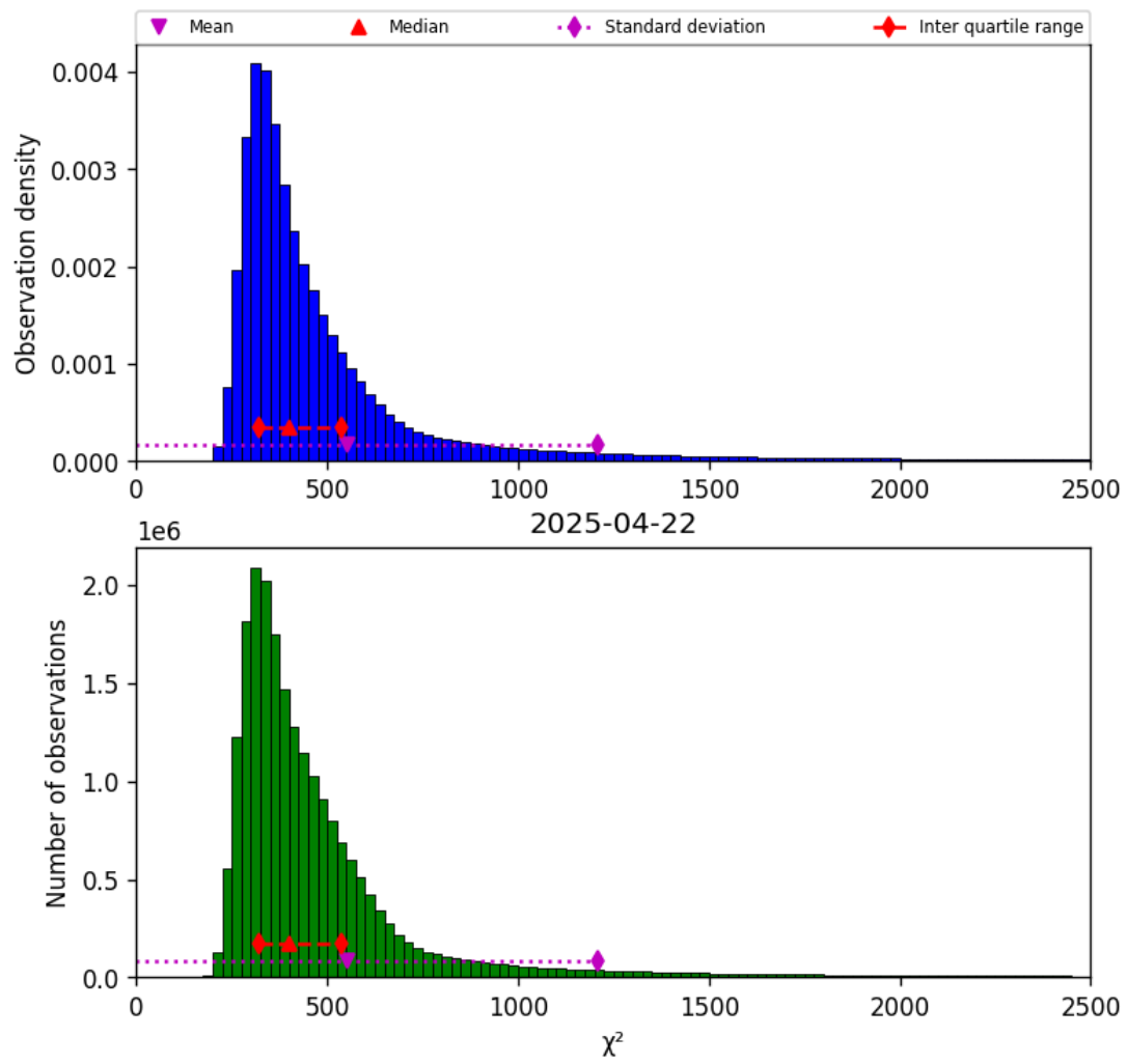
Figure 42: Histogram of “ \chi^2 ” for 2025-04-22 to 2025-04-22
