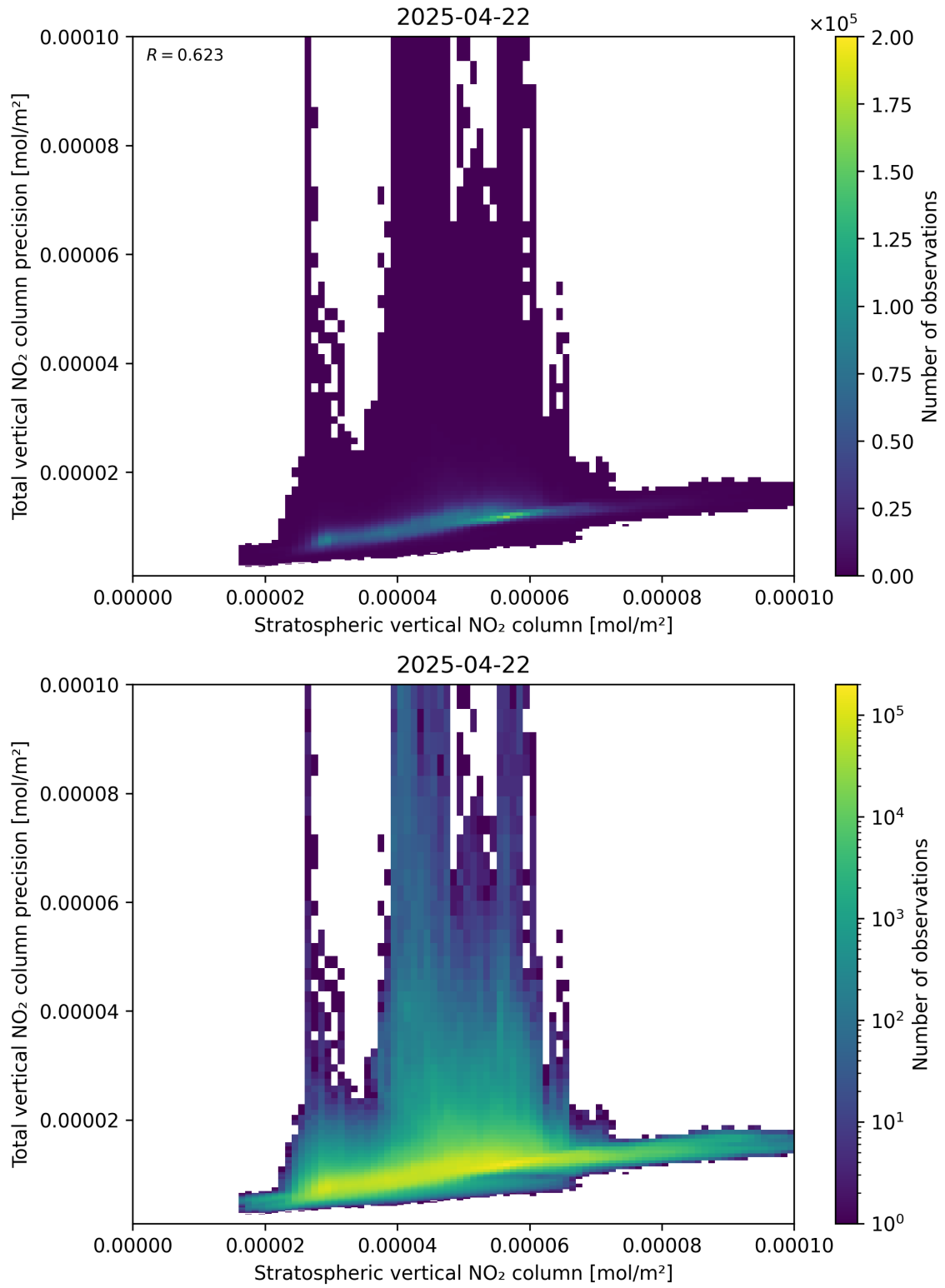
Figure 101: Scatter density plot of “Stratospheric vertical NO 2 column” against “Total vertical NO 2 column precision” for 2025-04-22 to 2025-04-22.
