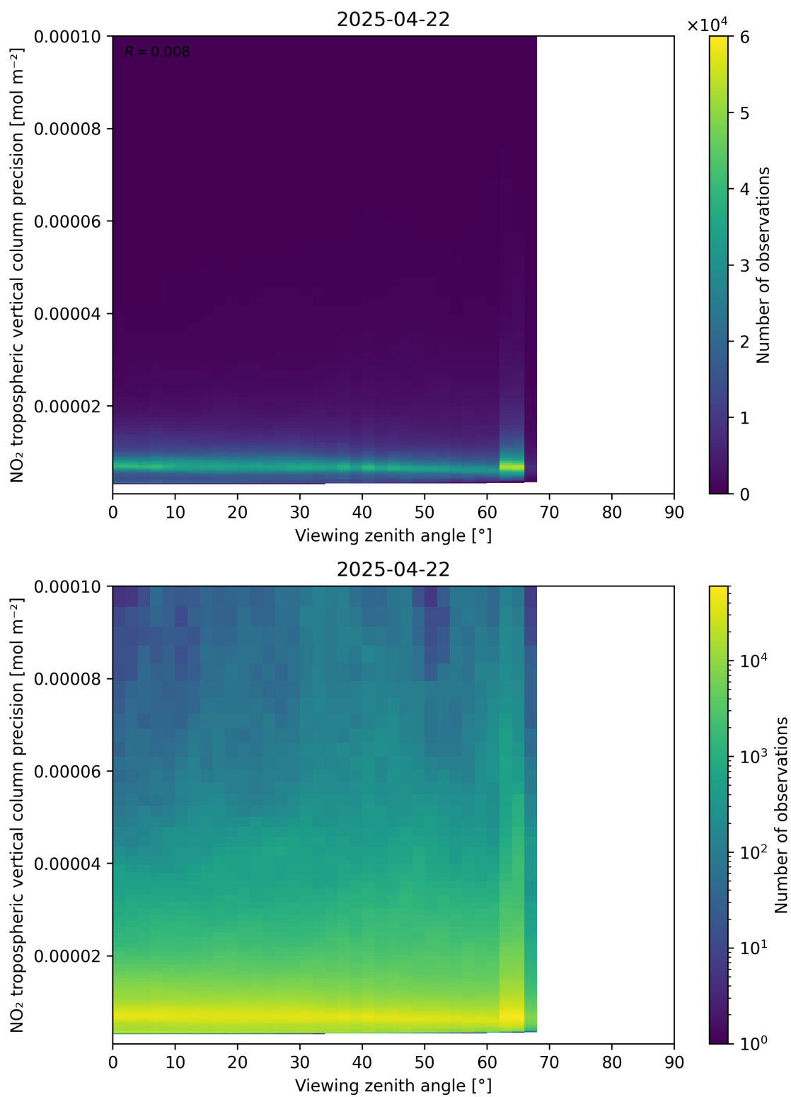
Figure 170: Scatter density plot of “Viewing zenith angle” against “NO 2 tropospheric vertical column precision” for 2025-04-22 to 2025-04-22.
