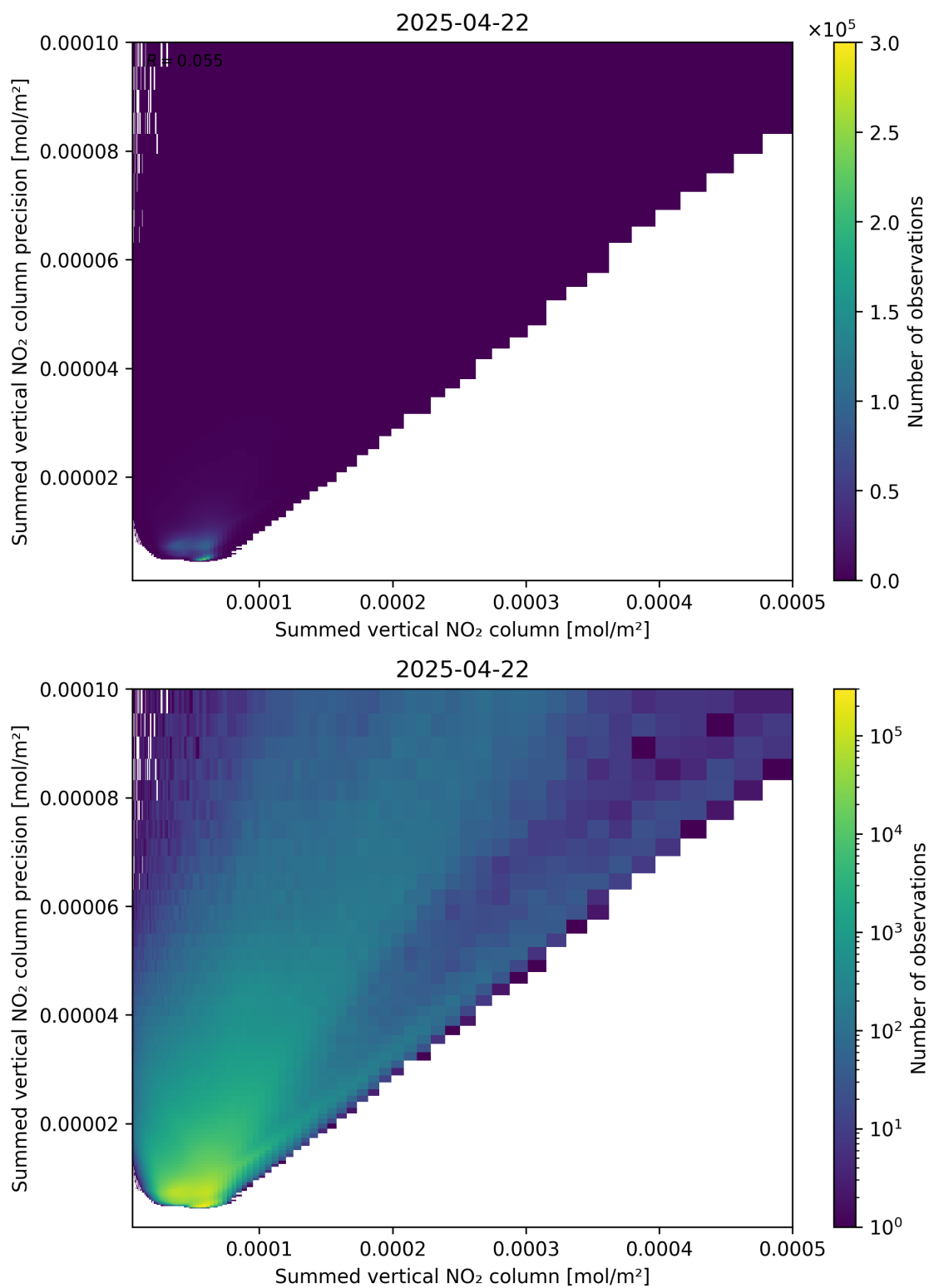
Figure 105: Scatter density plot of “Summed vertical NO 2 column” against “Summed vertical NO 2 column precision” for 2025-04-22 to 2025-04-22.
