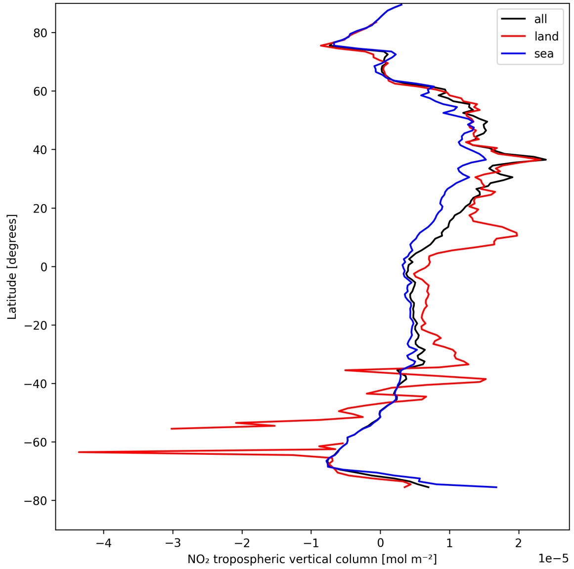
Figure 12: Zonal average of “NO 2 tropospheric vertical column” for 2025-04-22 to 2025-04-22.
