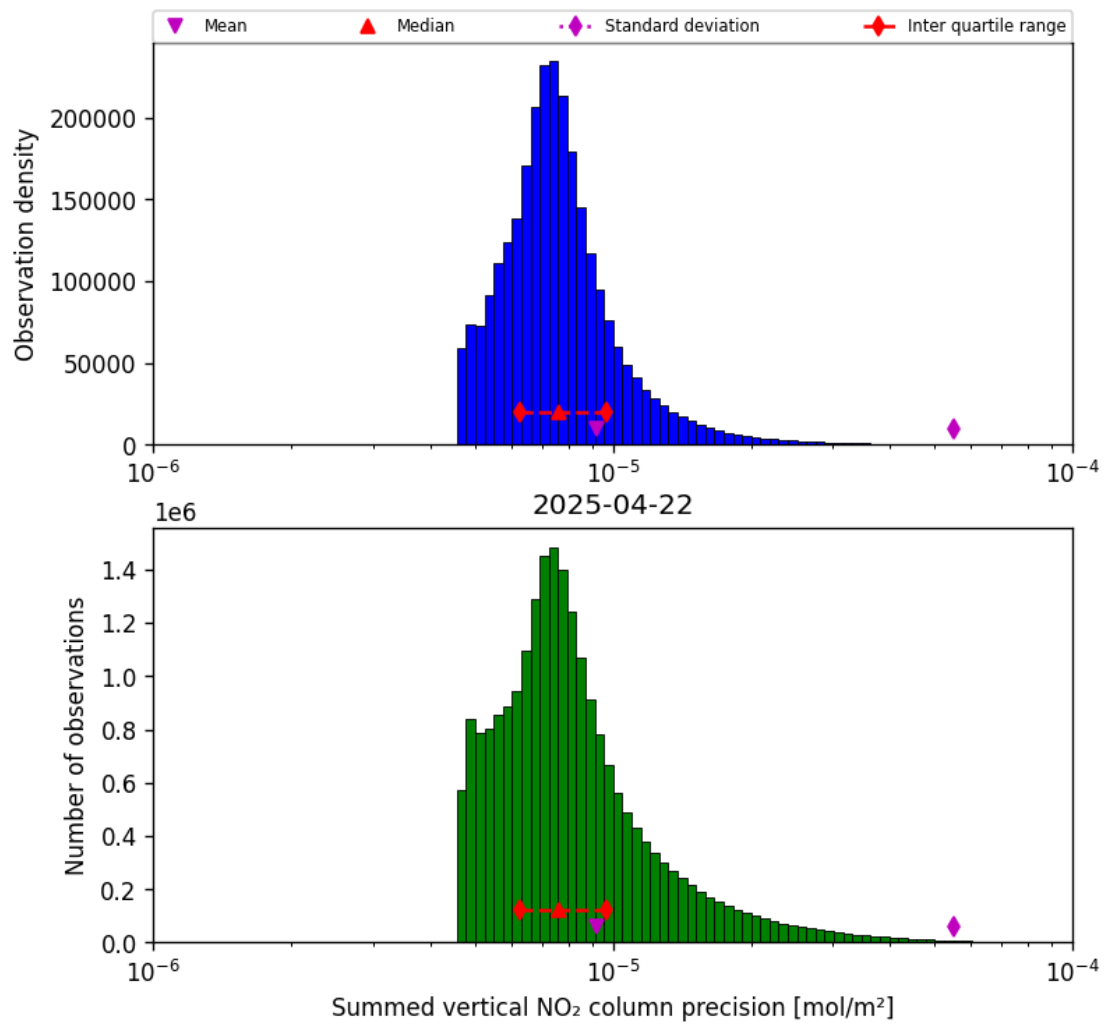
Figure 41: Histogram of "Summed vertical NO 2 column precision" for 2025-04-22 to 2025-04-22
