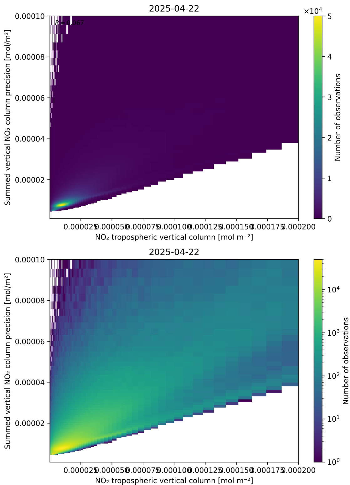
Figure 127: Scatter density plot of “NO 2 tropospheric vertical column” against “Summed vertical NO 2 column precision” for 2025-04-22 to 2025-04-22.
