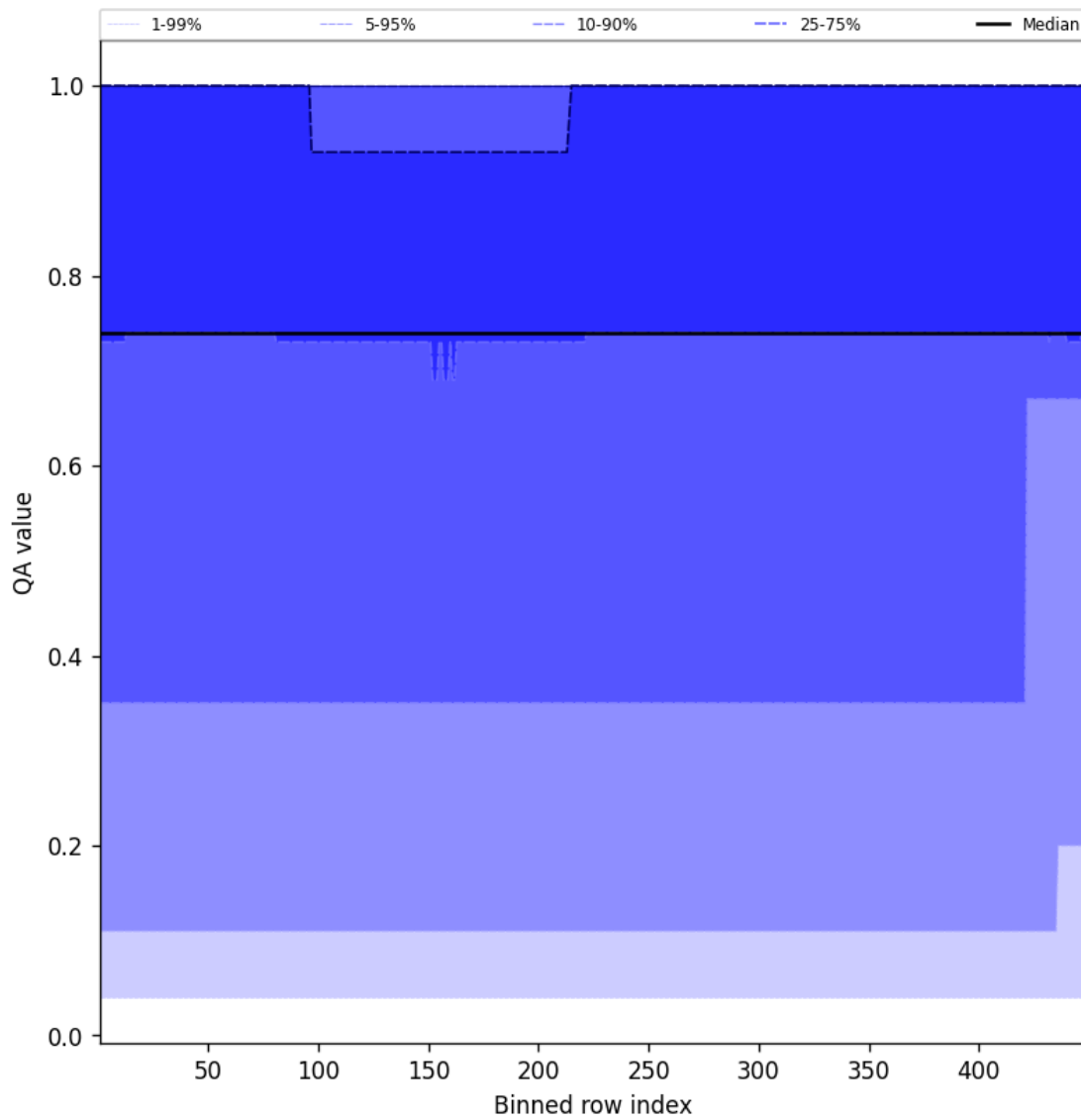
Figure 45: Along track statistics of “QA value” for 2025-04-22 to 2025-04-22
