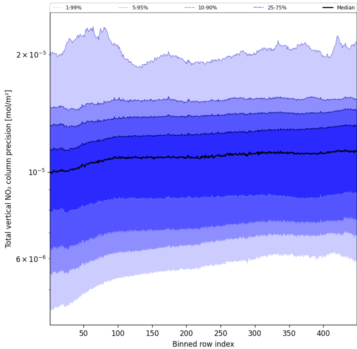
Figure 56: Along track statistics of “Total vertical NO 2 column precision” for 2025-04-22 to 2025-04-22
