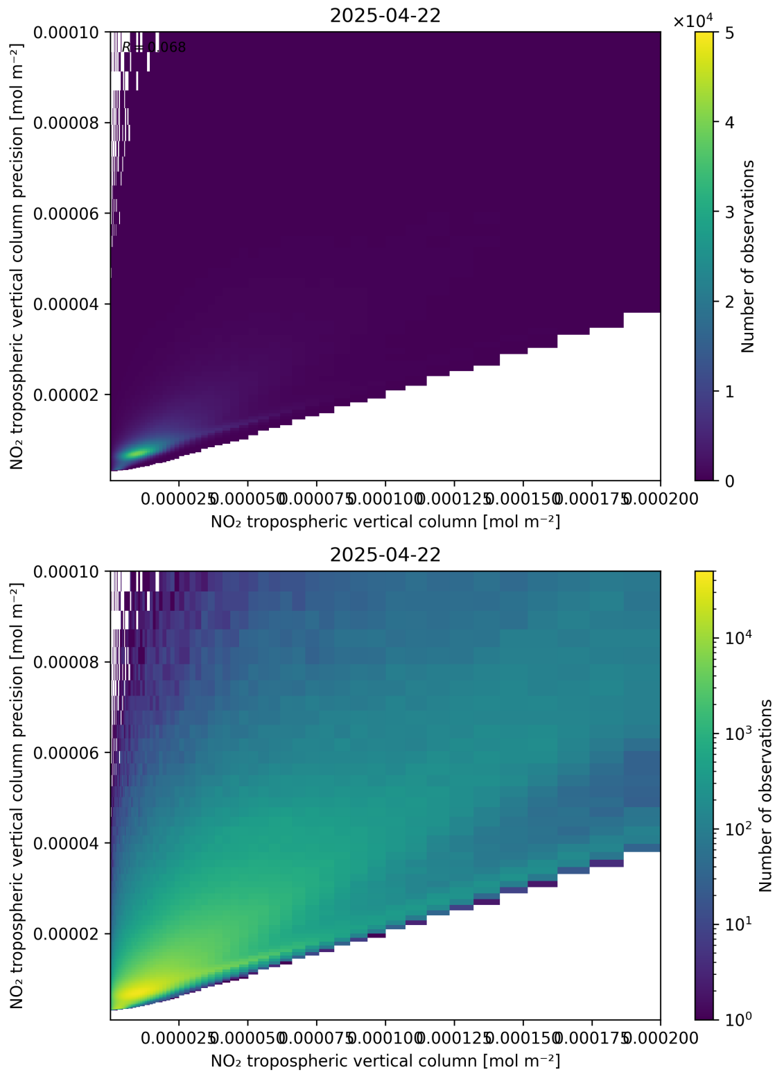
Figure 130: Scatter density plot of “NO 2 tropospheric vertical column” against “NO 2 tropospheric vertical column precision” for 2025-04-22 to 2025-04-22.
