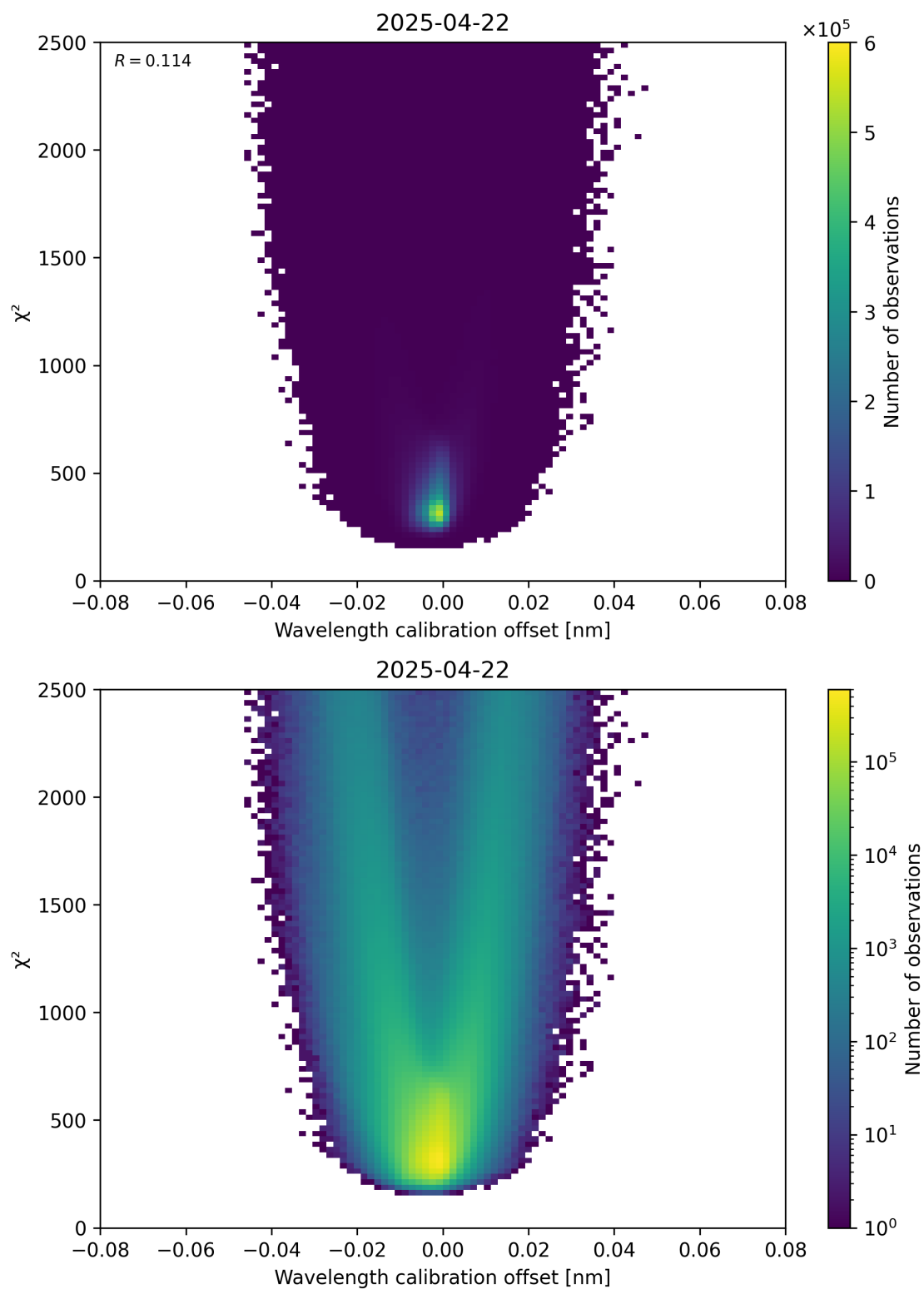
Figure 175: Scatter density plot of “Wavelength calibration offset” against “ \chi^2 ” for 2025-04-22 to 2025-04-22.
