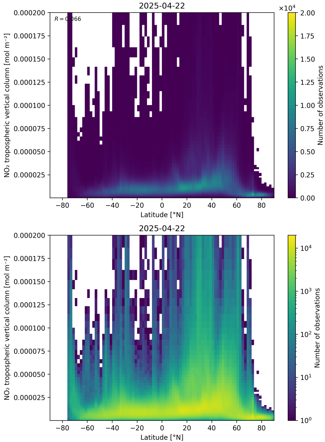
Figure 92: Scatter density plot of “Latitude” against “NO 2 tropospheric vertical column” for 2025-04-22 to 2025-04-22.
