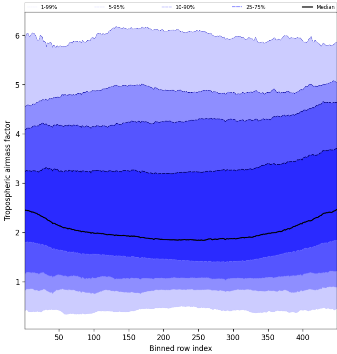
Figure 48: Along track statistics of “Tropospheric airmass factor” for 2025-04-22 to 2025-04-22
