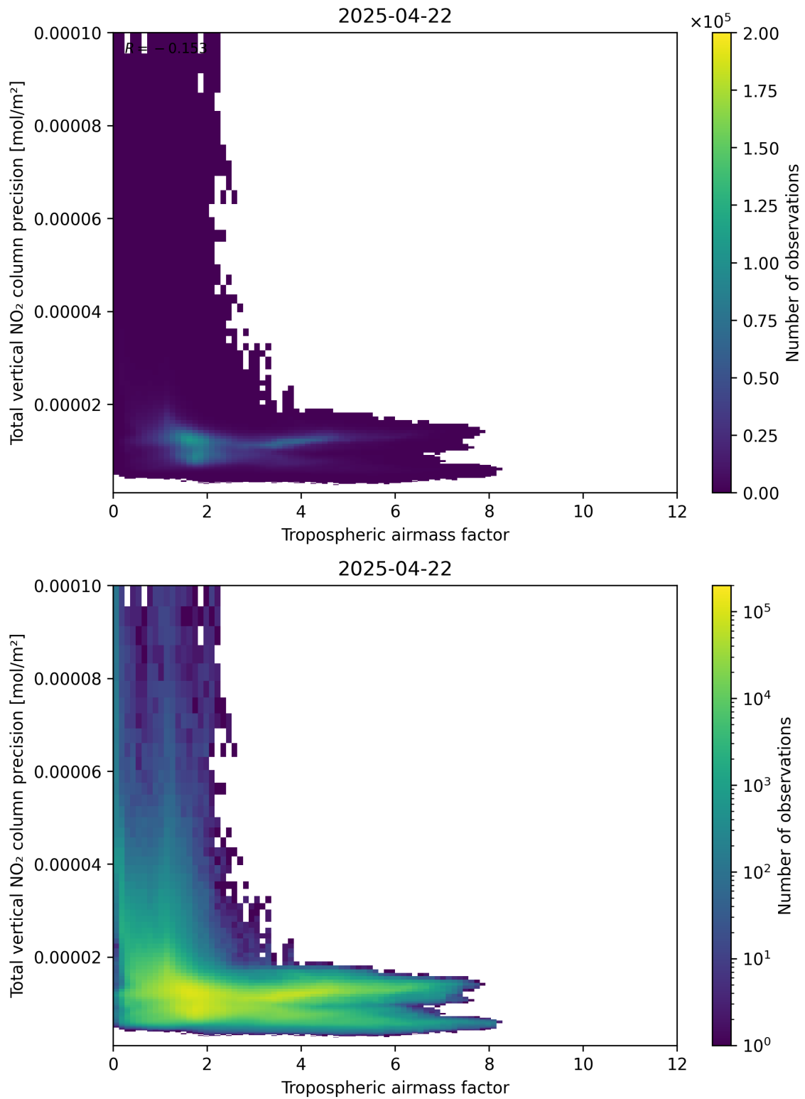
Figure 78: Scatter density plot of “Tropospheric air mass factor” against “Total vertical NO 2 column precision” for 2025-04-22 to 2025-04-22.
