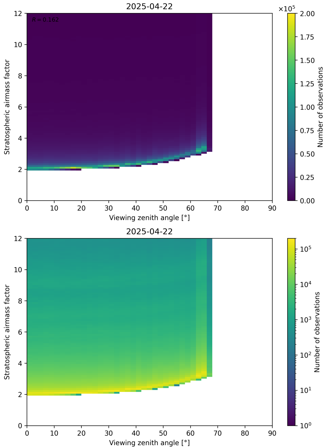
Figure 159: Scatter density plot of “Viewing zenith angle” against “Stratospheric airmass factor” for 2025-04-22 to 2025-04-22.
