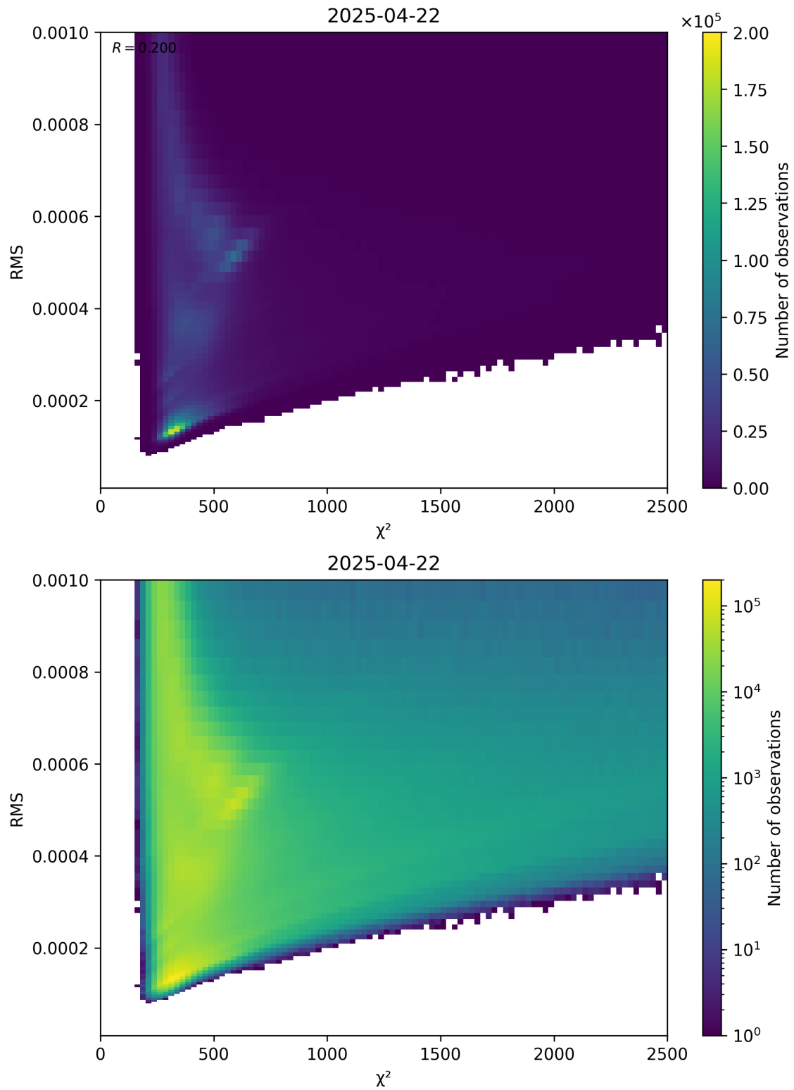
Figure 82: Scatter density plot of “ \chi^2 ” against “RMS” for 2025-04-22 to 2025-04-22.
