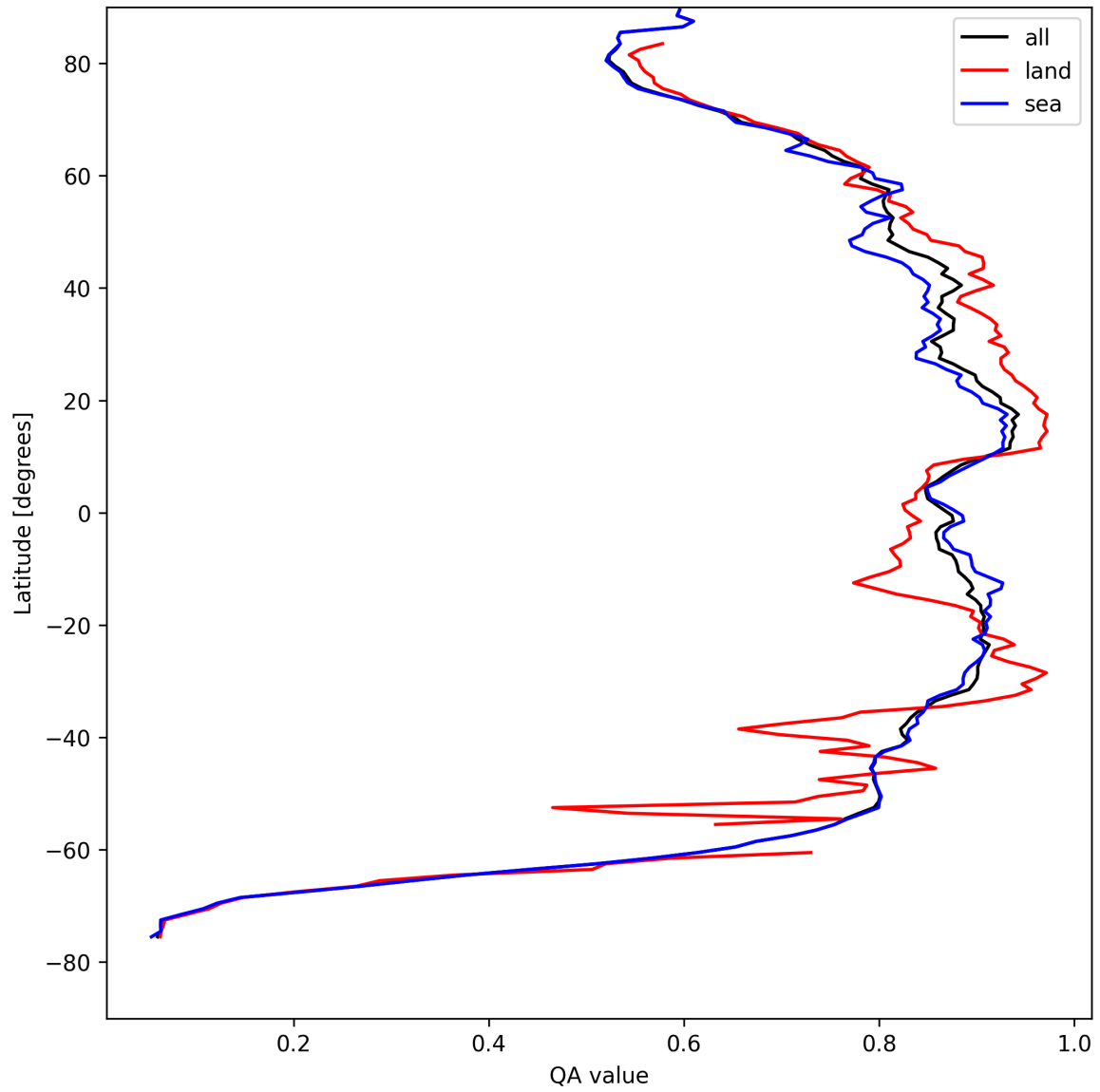
Figure 11: Zonal average of “QA value” for 2025-04-22 to 2025-04-22.
