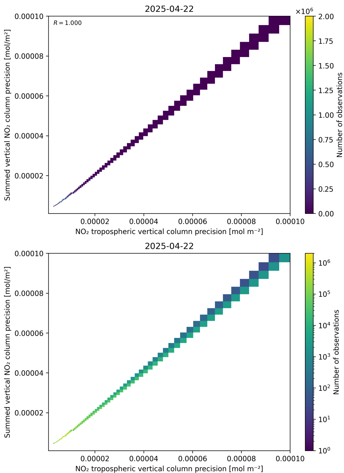
Figure 137: Scatter density plot of “NO 2 tropospheric vertical column precision” against “Summed vertical NO 2 column precision” for 2025-04-22 to 2025-04-22.
