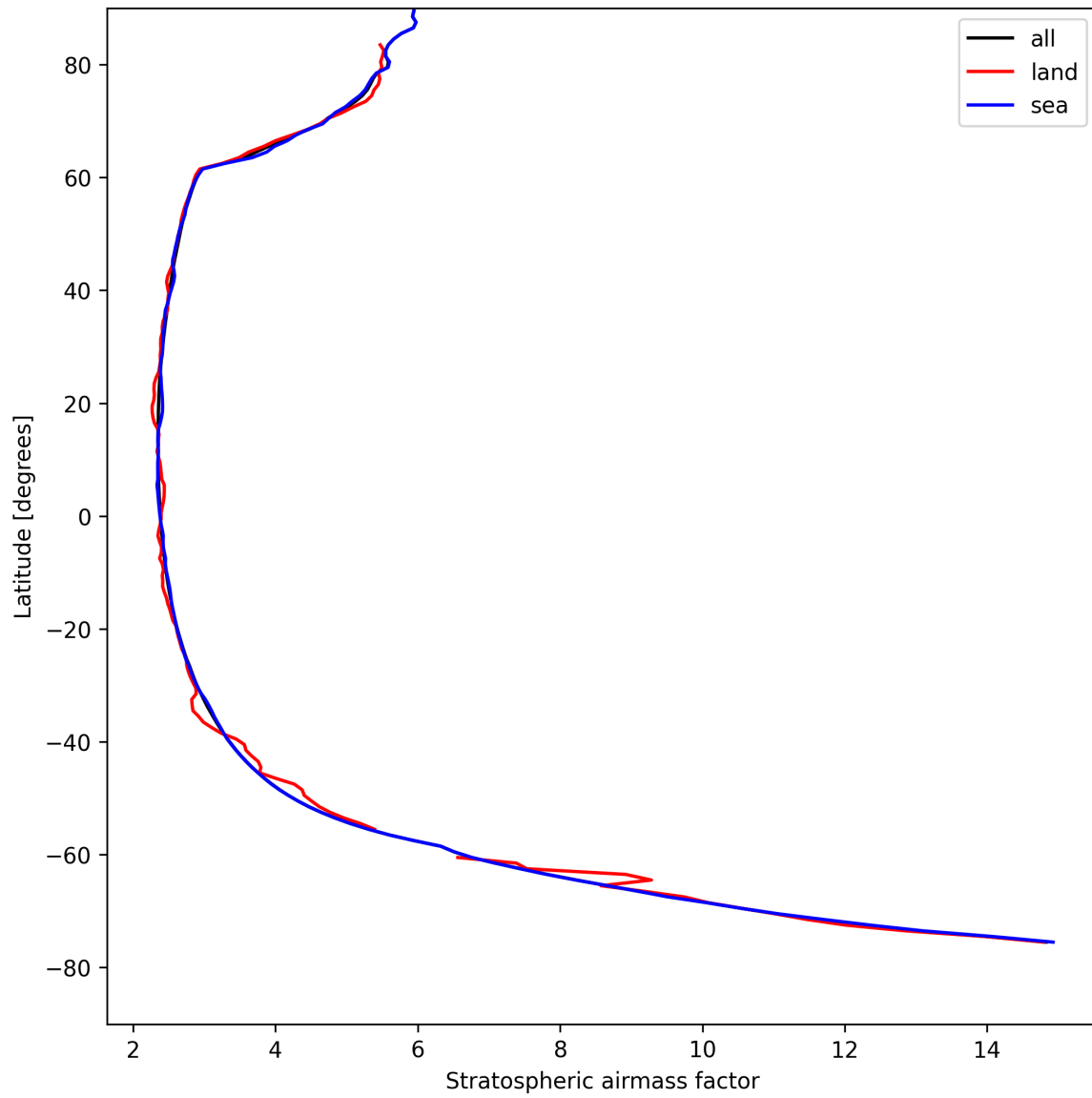
Figure 27: Zonal average of “Stratospheric airmass factor” for 2025-04-22 to 2025-04-22.
