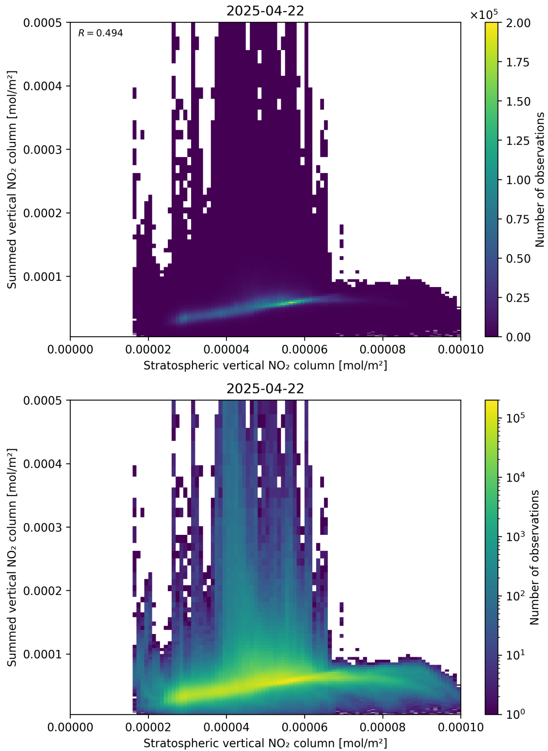
Figure 98: Scatter density plot of “Stratospheric vertical NO 2 column” against “Summed vertical NO 2 column” for 2025-04-22 to 2025-04-22.
