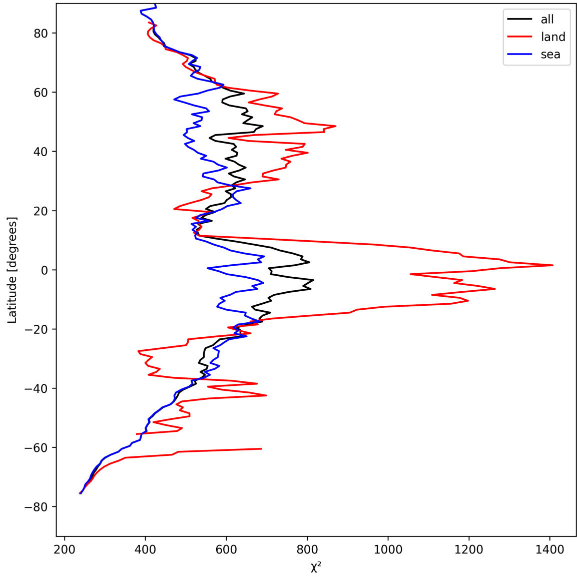
Figure 25: Zonal average of “ \chi^2 ” for 2025-04-22 to 2025-04-22.
