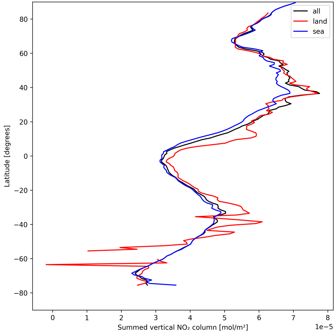
Figure 23: Zonal average of “Summed vertical NO 2 column” for 2025-04-22 to 2025-04-22.
