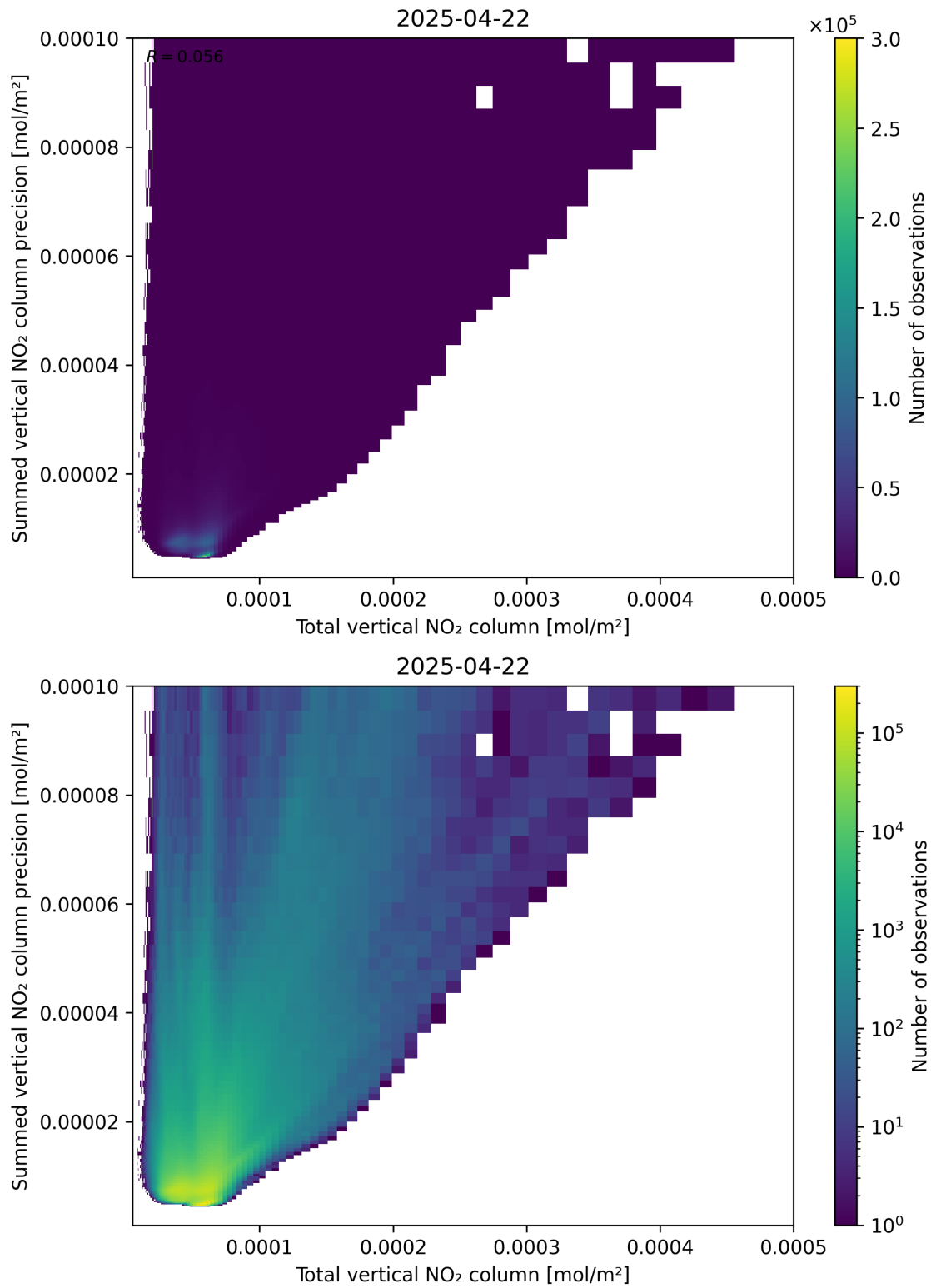
Figure 113: Scatter density plot of “Total vertical NO 2 column” against “Summed vertical NO 2 column precision” for 2025-04-22 to 2025-04-22.
