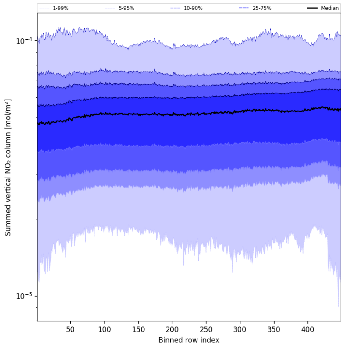
Figure 57: Along track statistics of “Summed vertical NO 2 column” for 2025-04-22 to 2025-04-22
