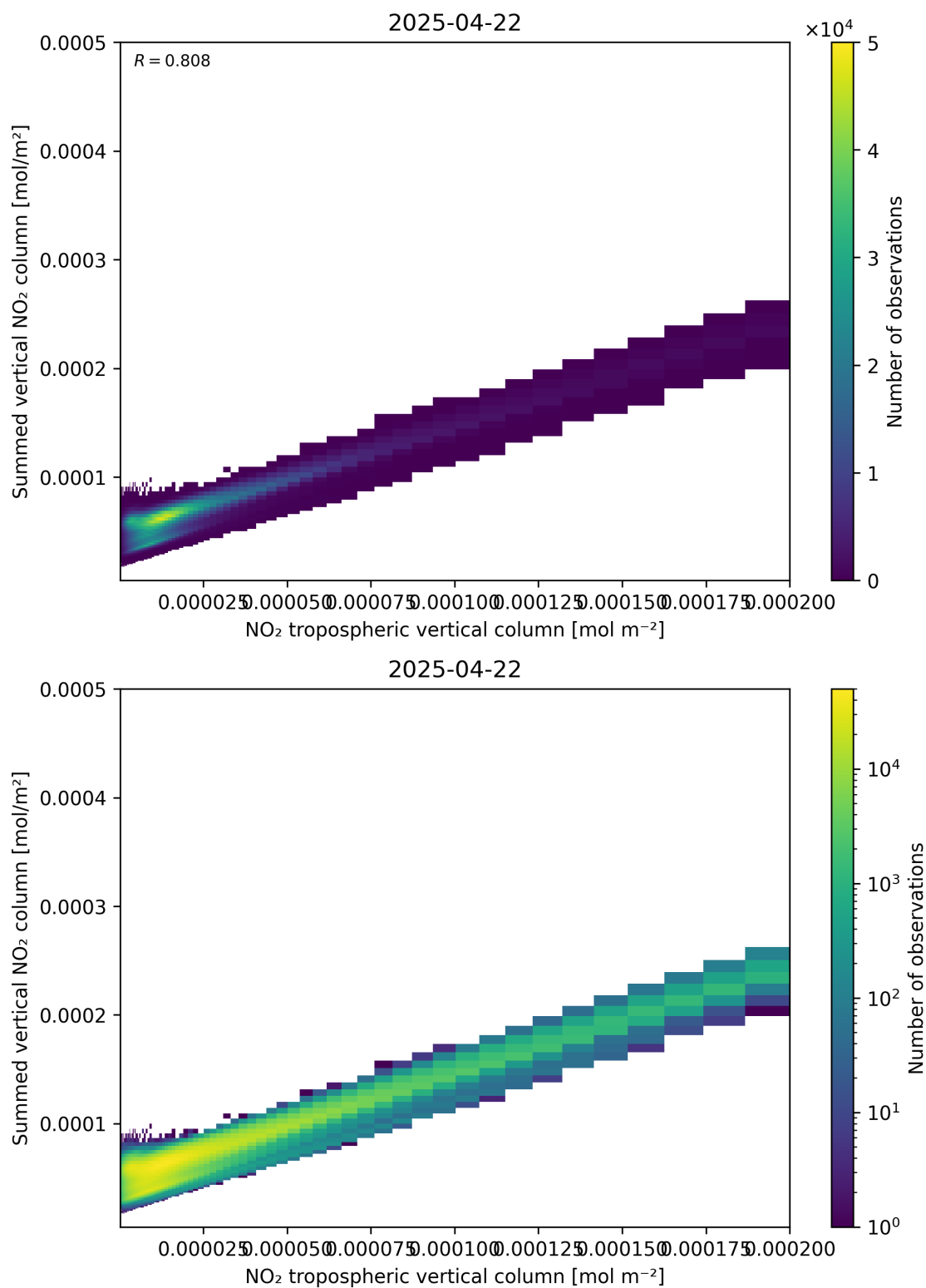
Figure 126: Scatter density plot of “NO 2 tropospheric vertical column” against “Summed vertical NO 2 column” for 2025-04-22 to 2025-04-22.
