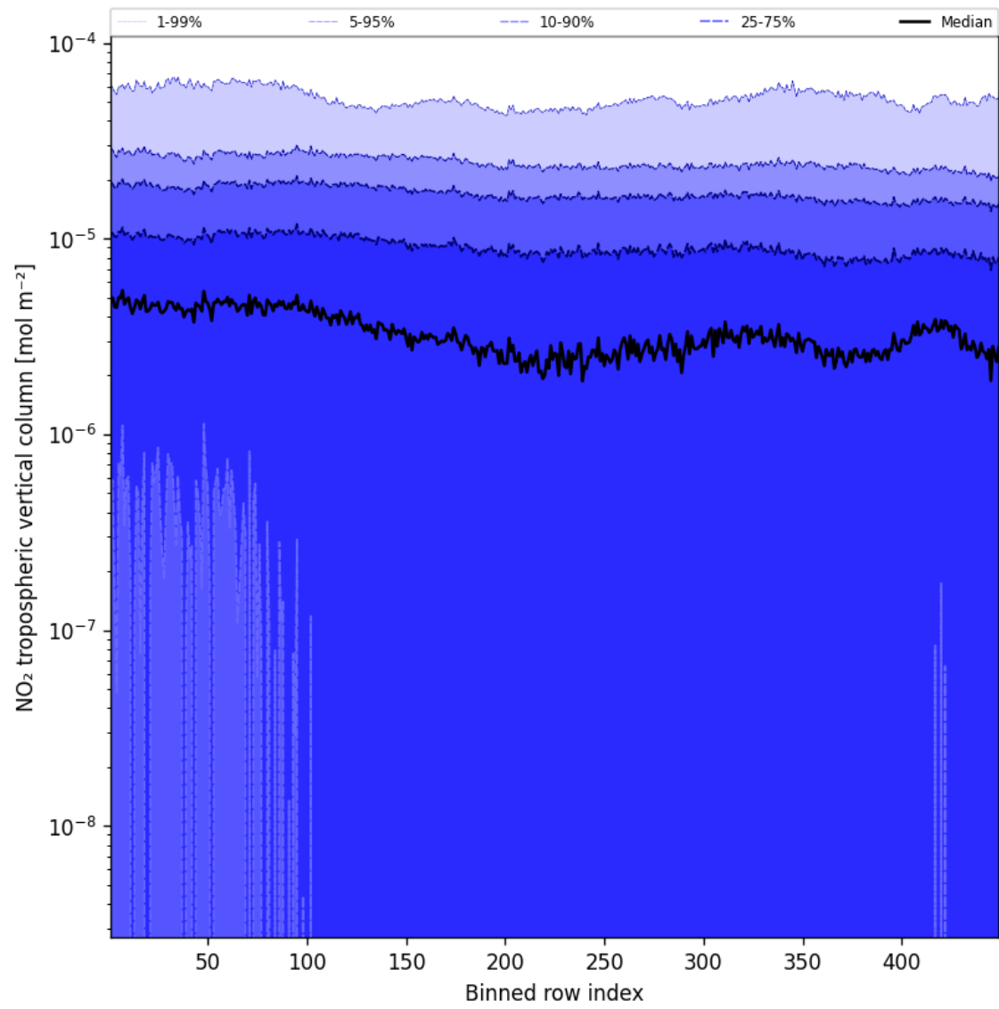
Figure 46: Along track statistics of “NO 2 tropospheric vertical column” for 2025-04-22 to 2025-04-22
