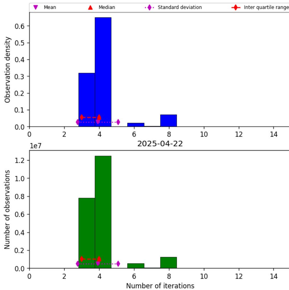
Figure 34: Histogram of “Number of iterations” for 2025-04-22 to 2025-04-22
