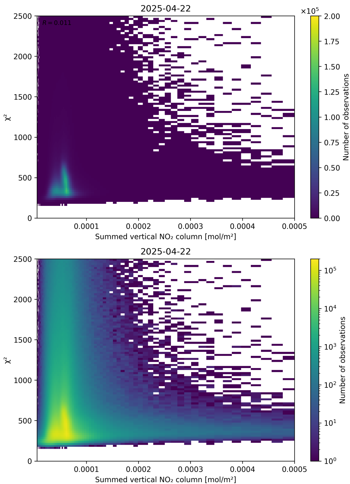
Figure 104: Scatter density plot of “Summed vertical NO 2 column” against “ \chi^2 ” for 2025-04-22 to 2025-04-22.
