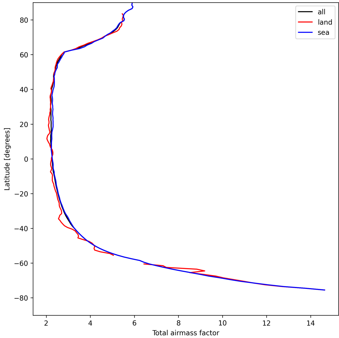
Figure 15: Zonal average of “Total airmass factor” for 2025-04-22 to 2025-04-22.
