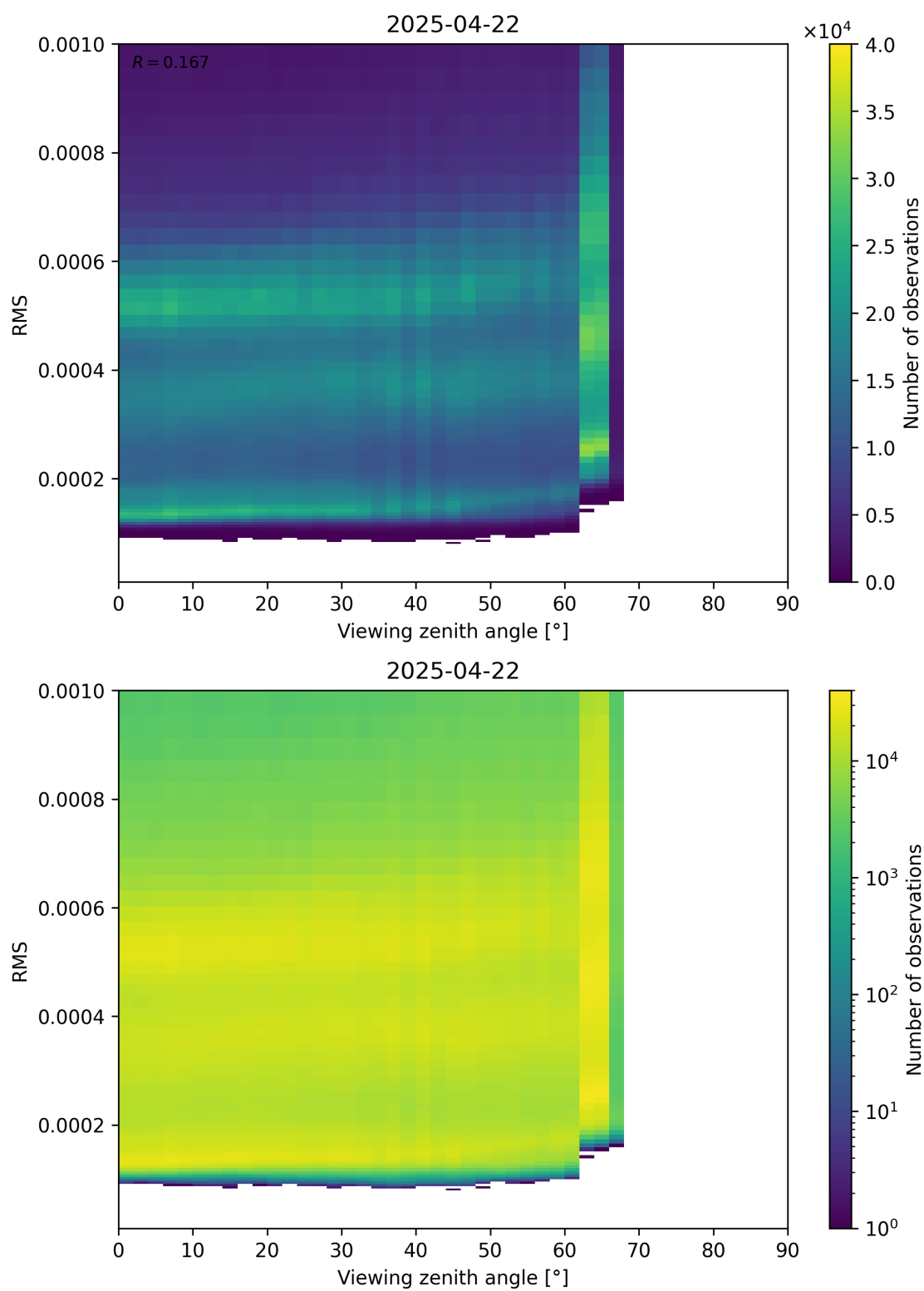
Figure 171: Scatter density plot of “Viewing zenith angle” against “RMS” for 2025-04-22 to 2025-04-22.
