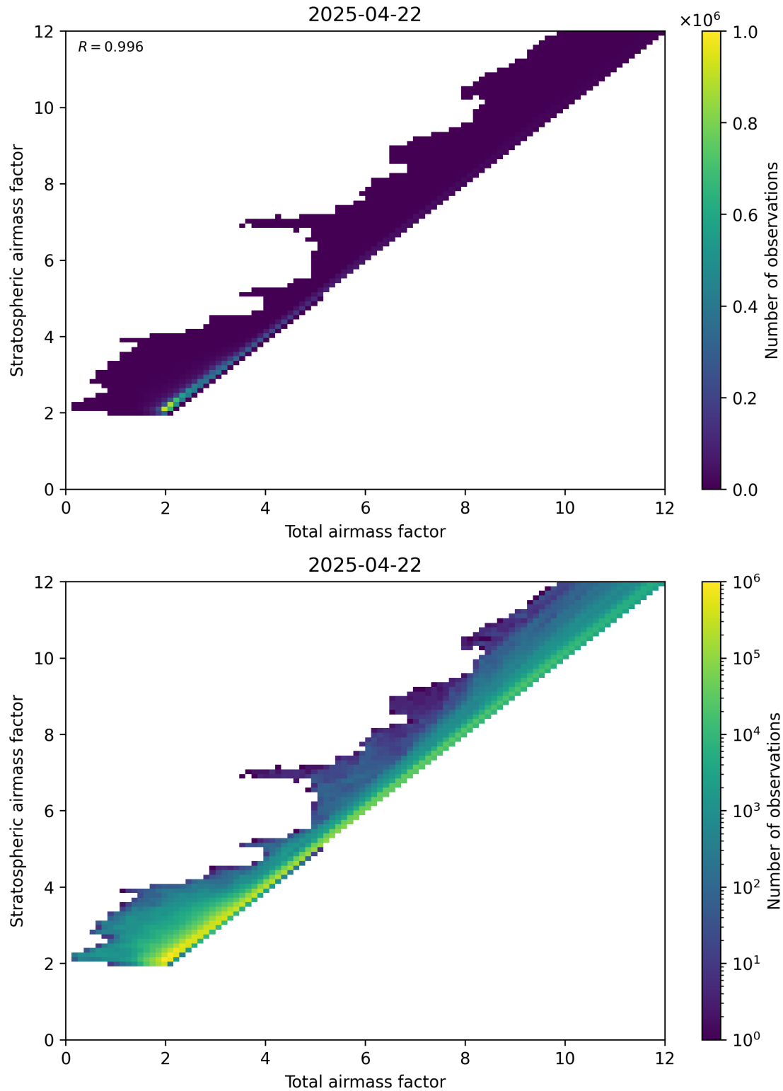
Figure 62: Scatter density plot of “Total airmass factor” against “Stratospheric airmass factor” for 2025-04-22 to 2025-04-22.
