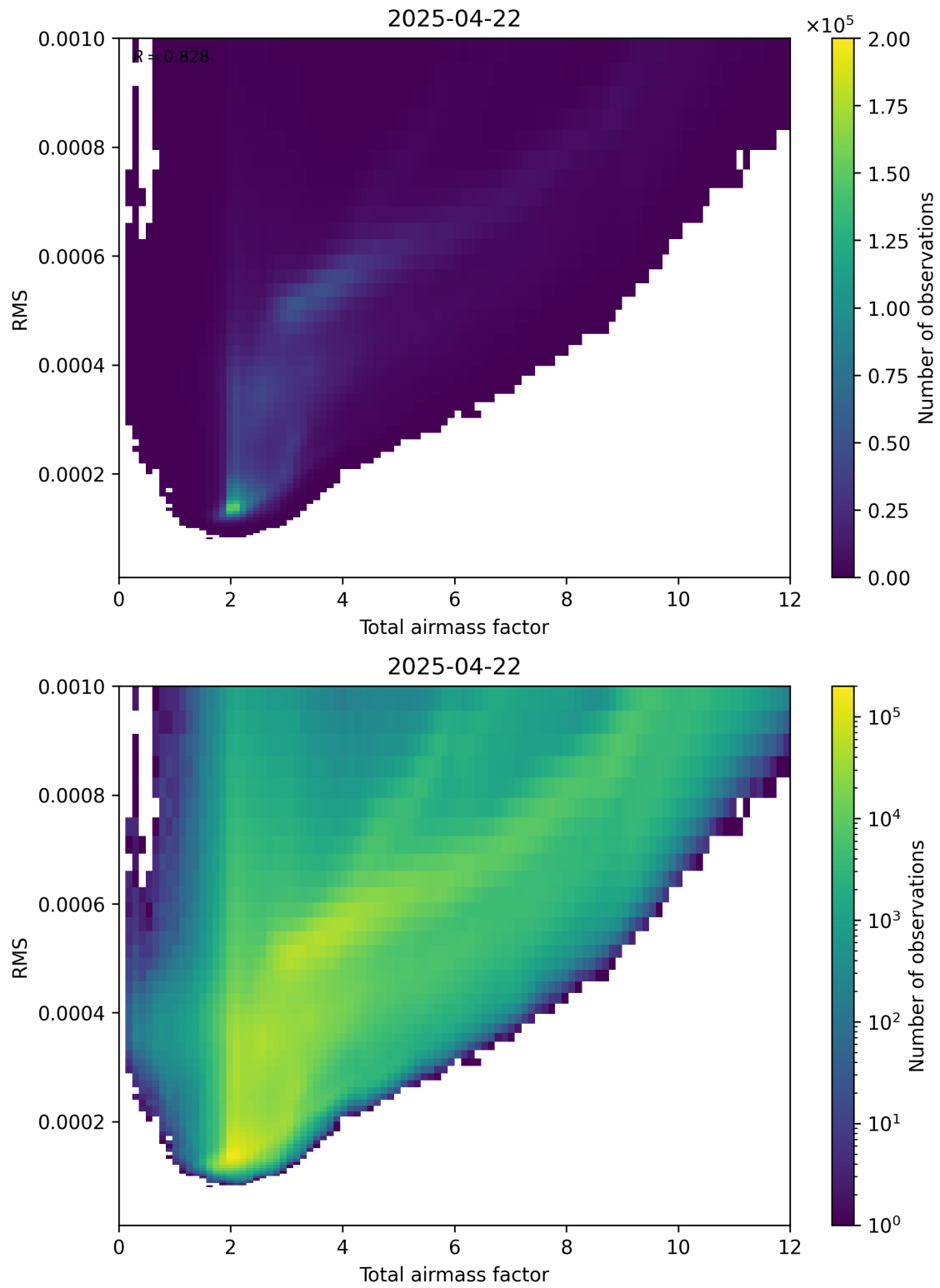
Figure 69: Scatter density plot of “Total airmass factor” against “RMS” for 2025-04-22 to 2025-04-22.
