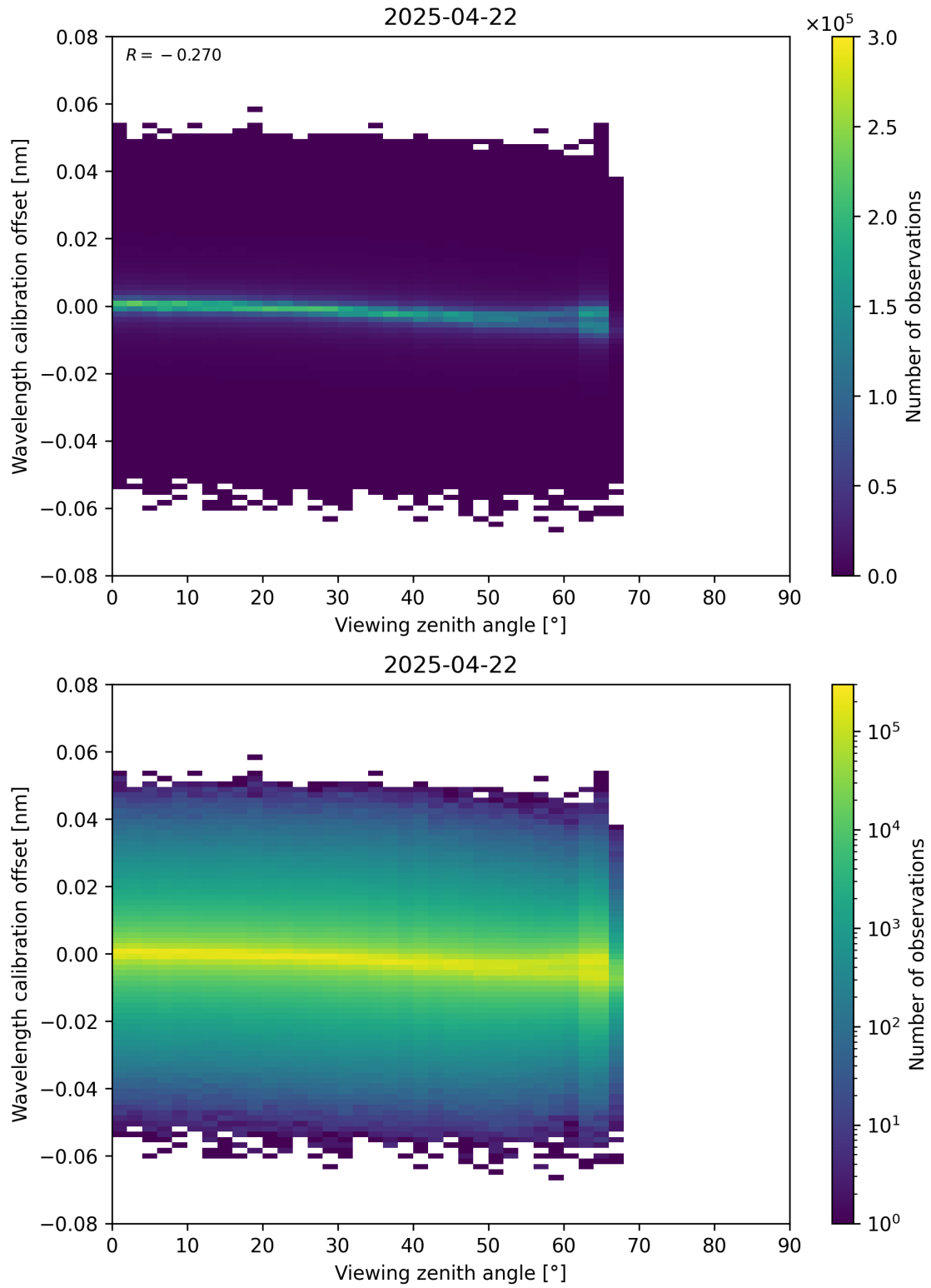
Figure 173: Scatter density plot of “Viewing zenith angle” against “Wavelength calibration offset” for 2025-04-22 to 2025-04-22.
