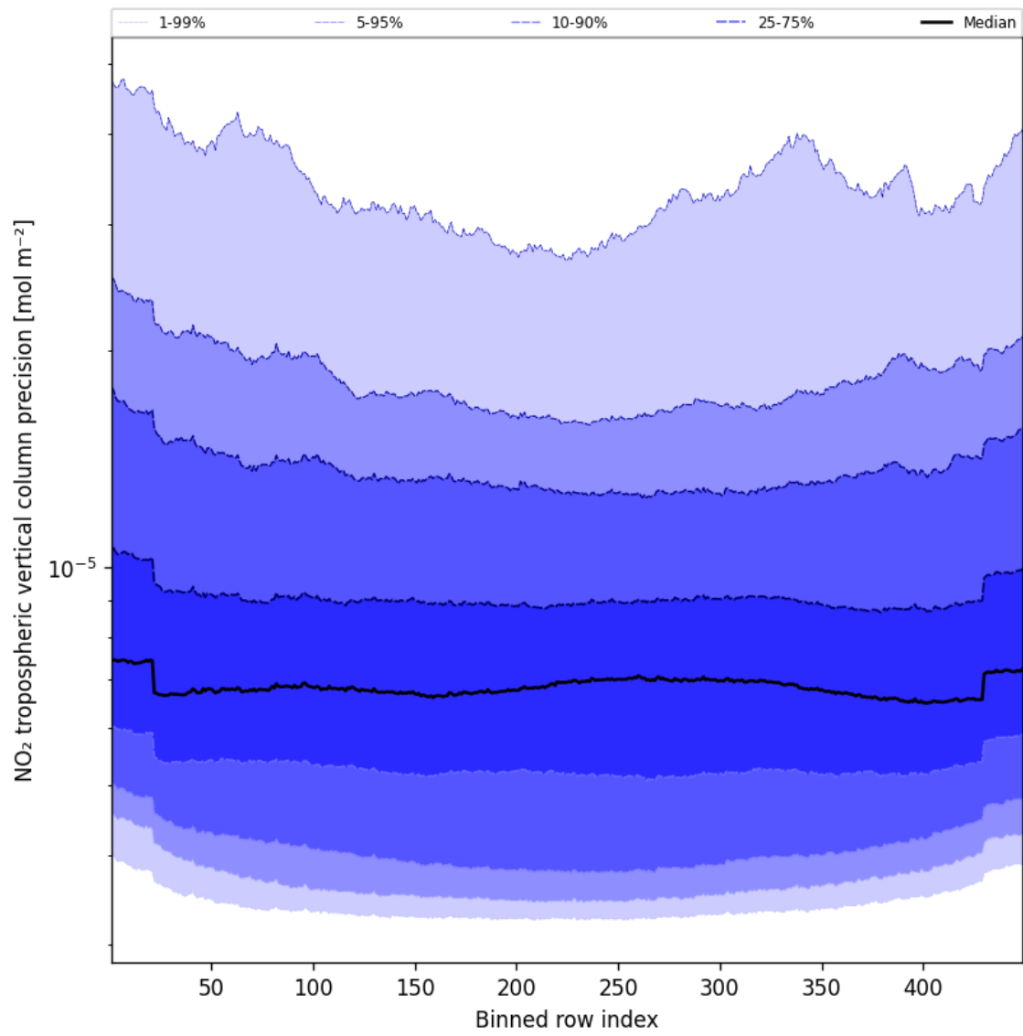
Figure 47: Along track statistics of “NO 2 tropospheric vertical column precision” for 2025-04-22 to 2025-04-22
