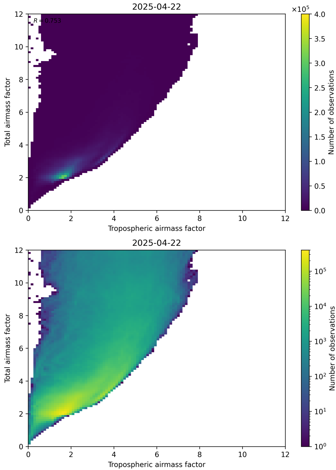
Figure 72: Scatter density plot of “Tropospheric airmass factor” against “Total airmass factor” for 2025-04-22 to 2025-04-22.
