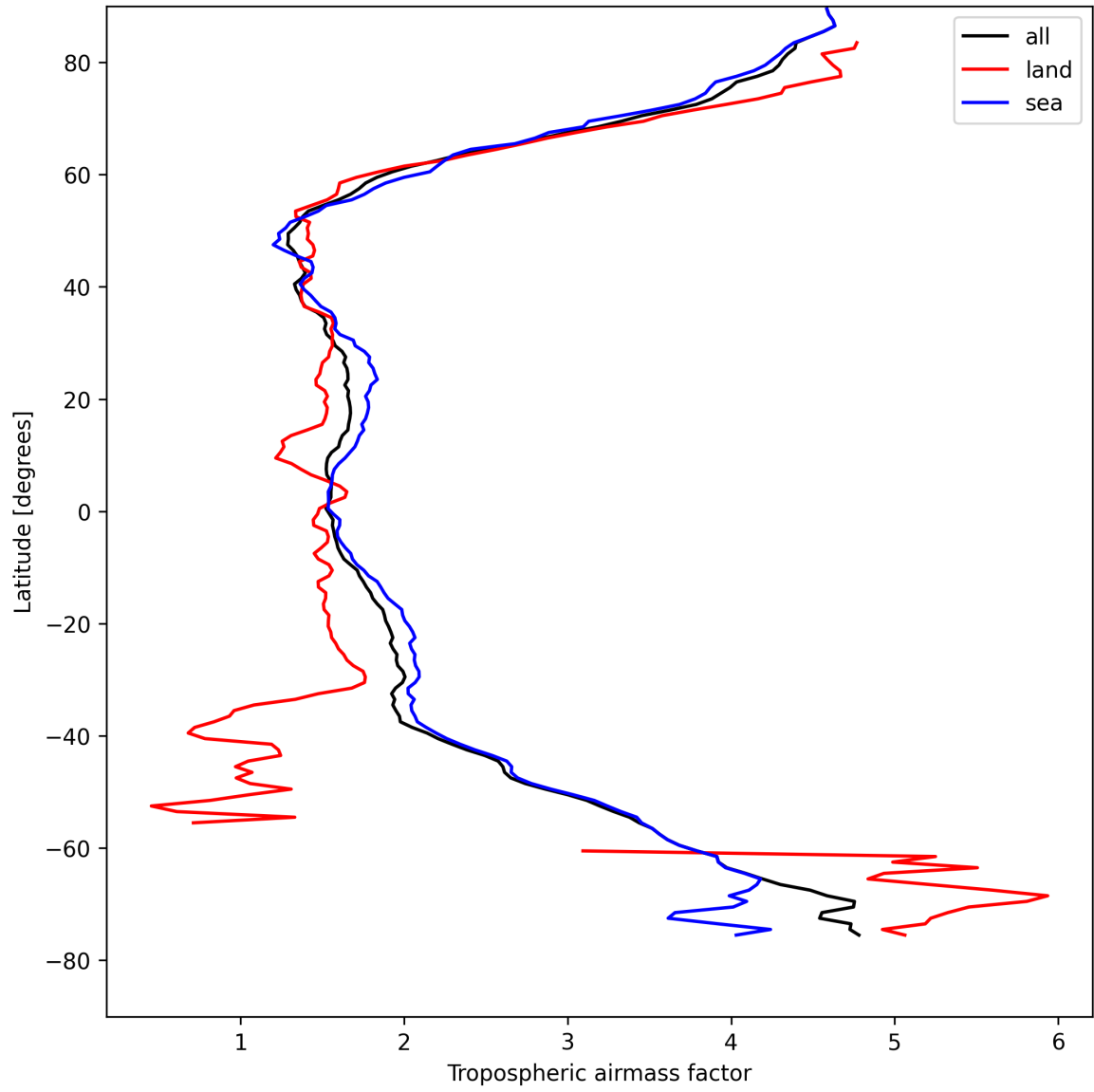
Figure 14: Zonal average of “Tropospheric airmass factor” for 2025-04-22 to 2025-04-22.
