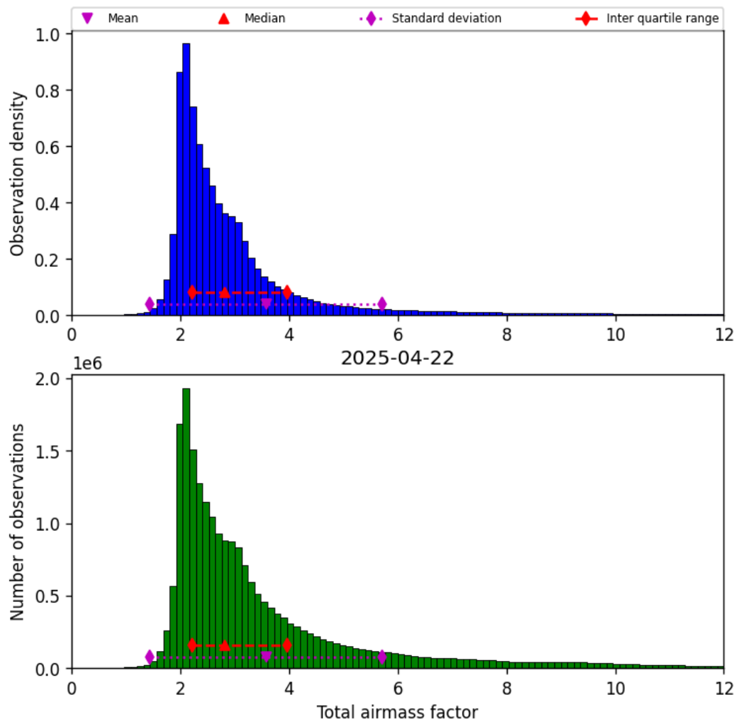
Figure 32: Histogram of “Total airmass factor” for 2025-04-22 to 2025-04-22
