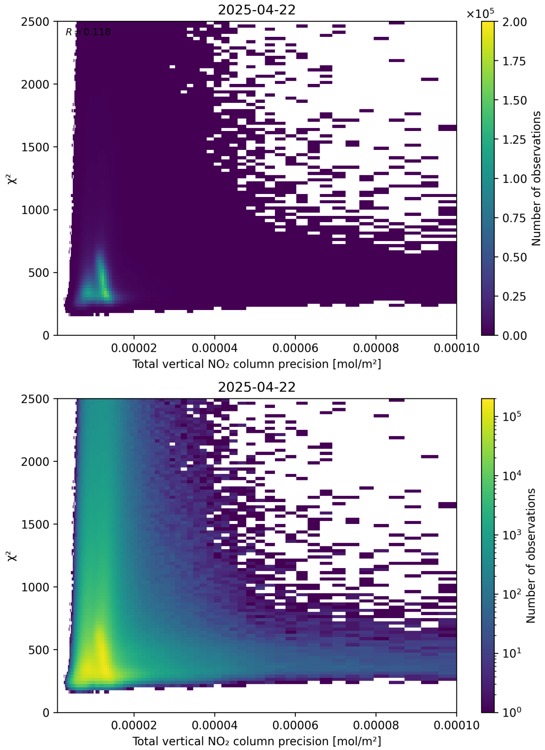
Figure 116: Scatter density plot of “Total vertical NO 2 column precision” against “ \chi^2 ” for 2025-04-22 to 2025-04-22.
