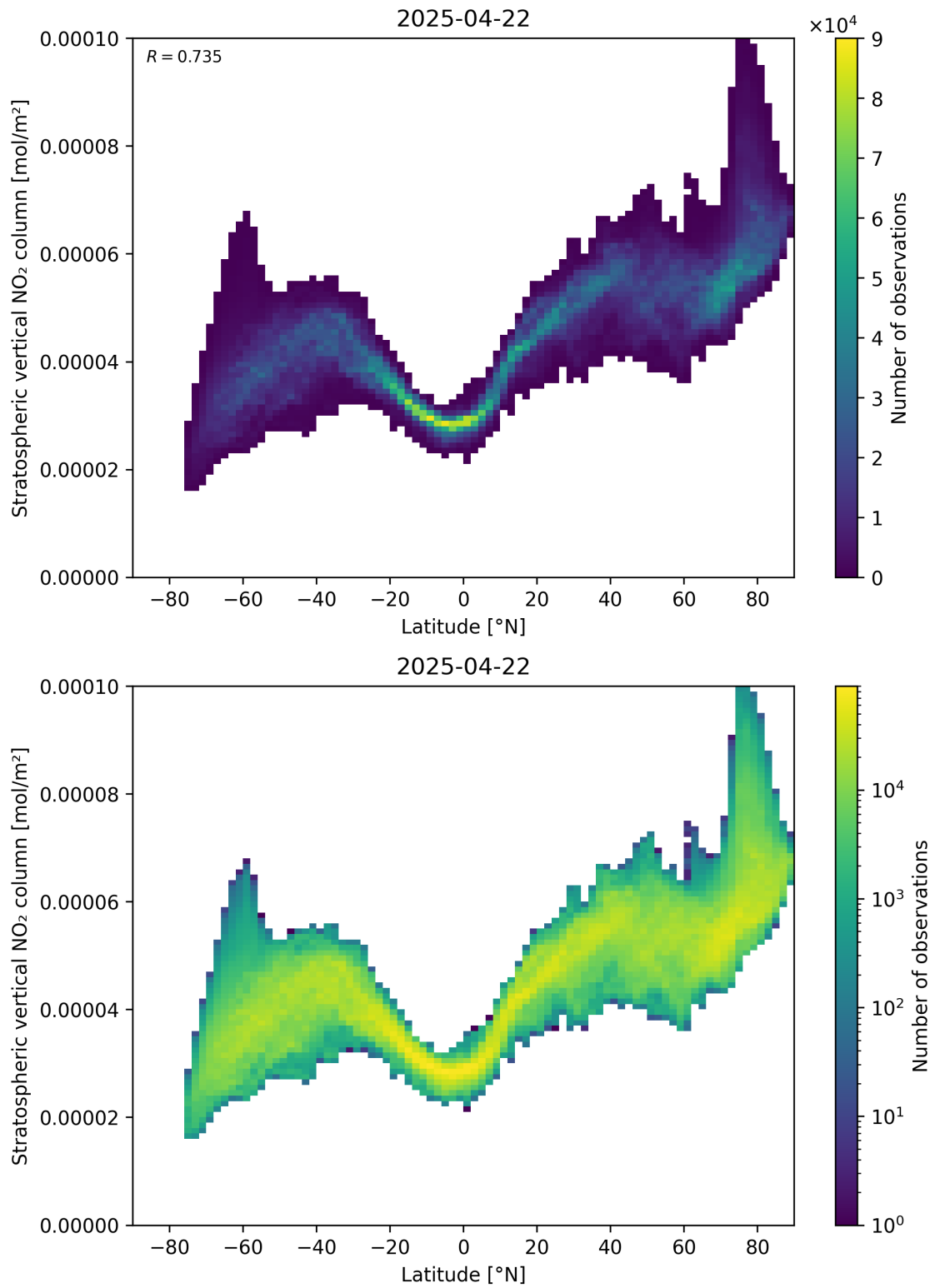
Figure 87: Scatter density plot of “Latitude” against “Stratospheric vertical NO 2 column” for 2025-04-22 to 2025-04-22.
