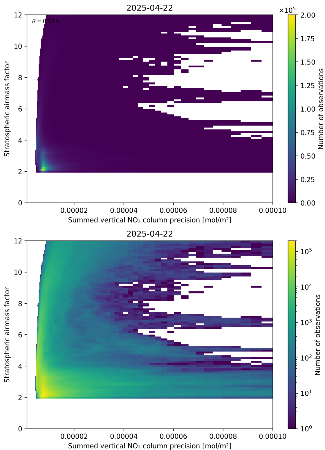
Figure 106: Scatter density plot of “Summed vertical NO 2 column precision” against “Stratospheric airmass factor” for 2025-04-22 to 2025-04-22.
