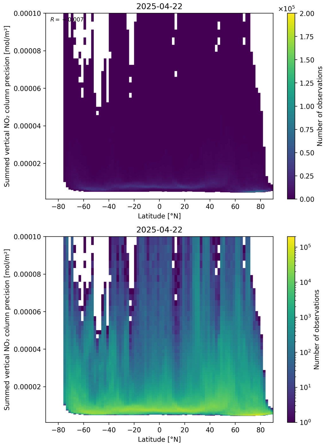
Figure 89: Scatter density plot of “Latitude” against “Summed vertical NO 2 column precision” for 2025-04-22 to 2025-04-22.
