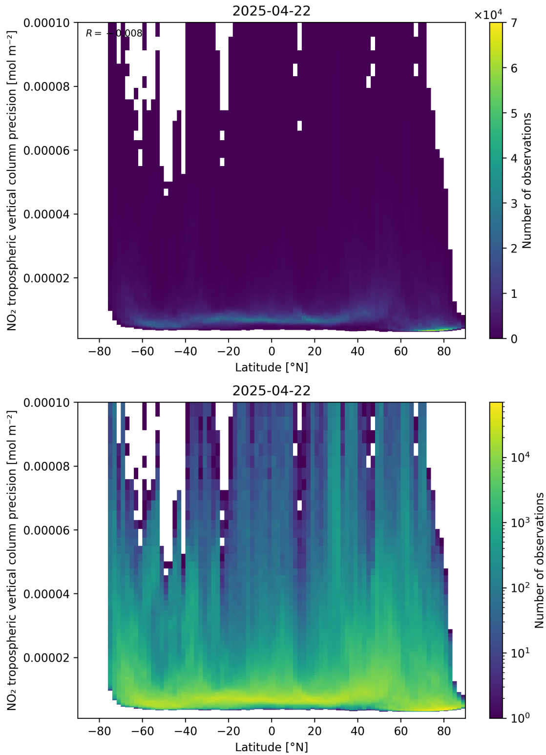
Figure 93: Scatter density plot of “Latitude” against “NO 2 tropospheric vertical column precision” for 2025-04-22 to 2025-04-22.
