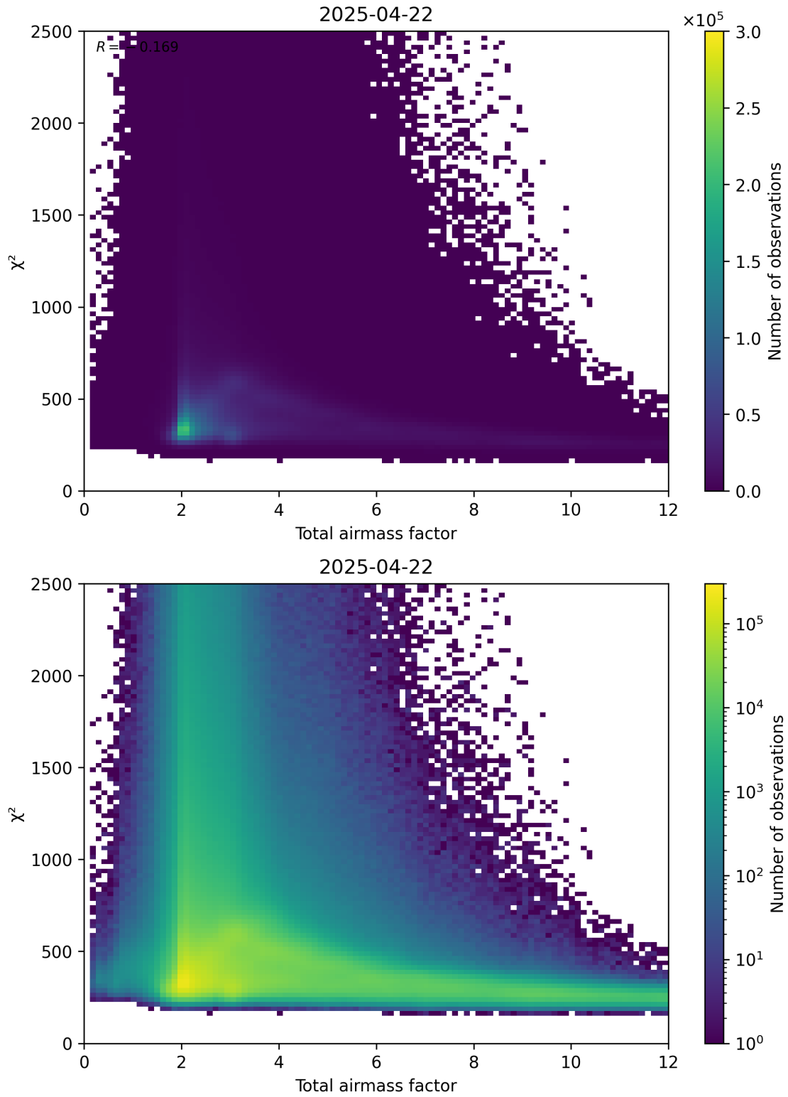
Figure 63: Scatter density plot of “Total airmass factor” against “ \chi^2 ” for 2025-04-22 to 2025-04-22.
