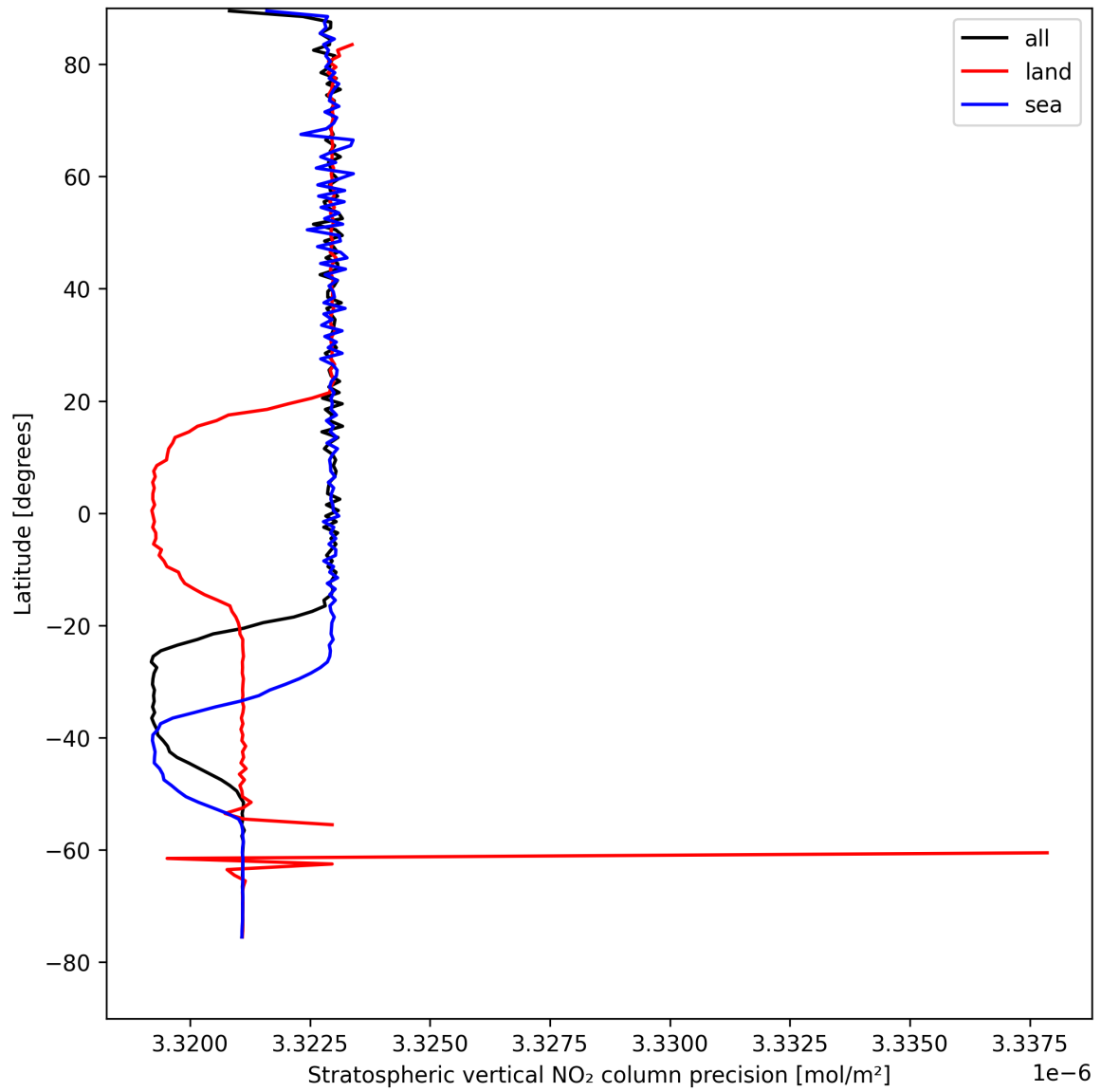
Figure 20: Zonal average of “Stratospheric vertical NO 2 column precision” for 2025-04-22 to 2025-04-22.
