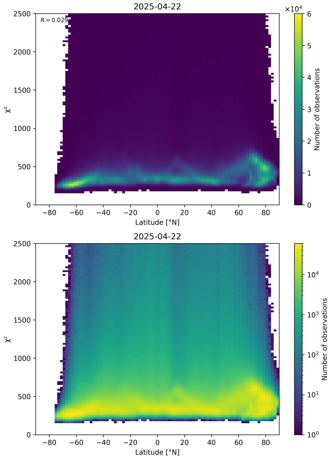
Figure 86: Scatter density plot of “Latitude” against “ \chi^2 ” for 2025-04-22 to 2025-04-22.
