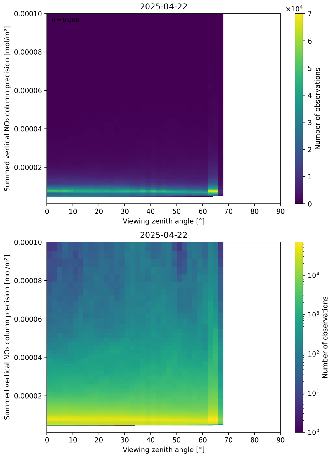
Figure 166: Scatter density plot of “Viewing zenith angle” against “Summed vertical NO 2 column precision” for 2025-04-22 to 2025-04-22.
