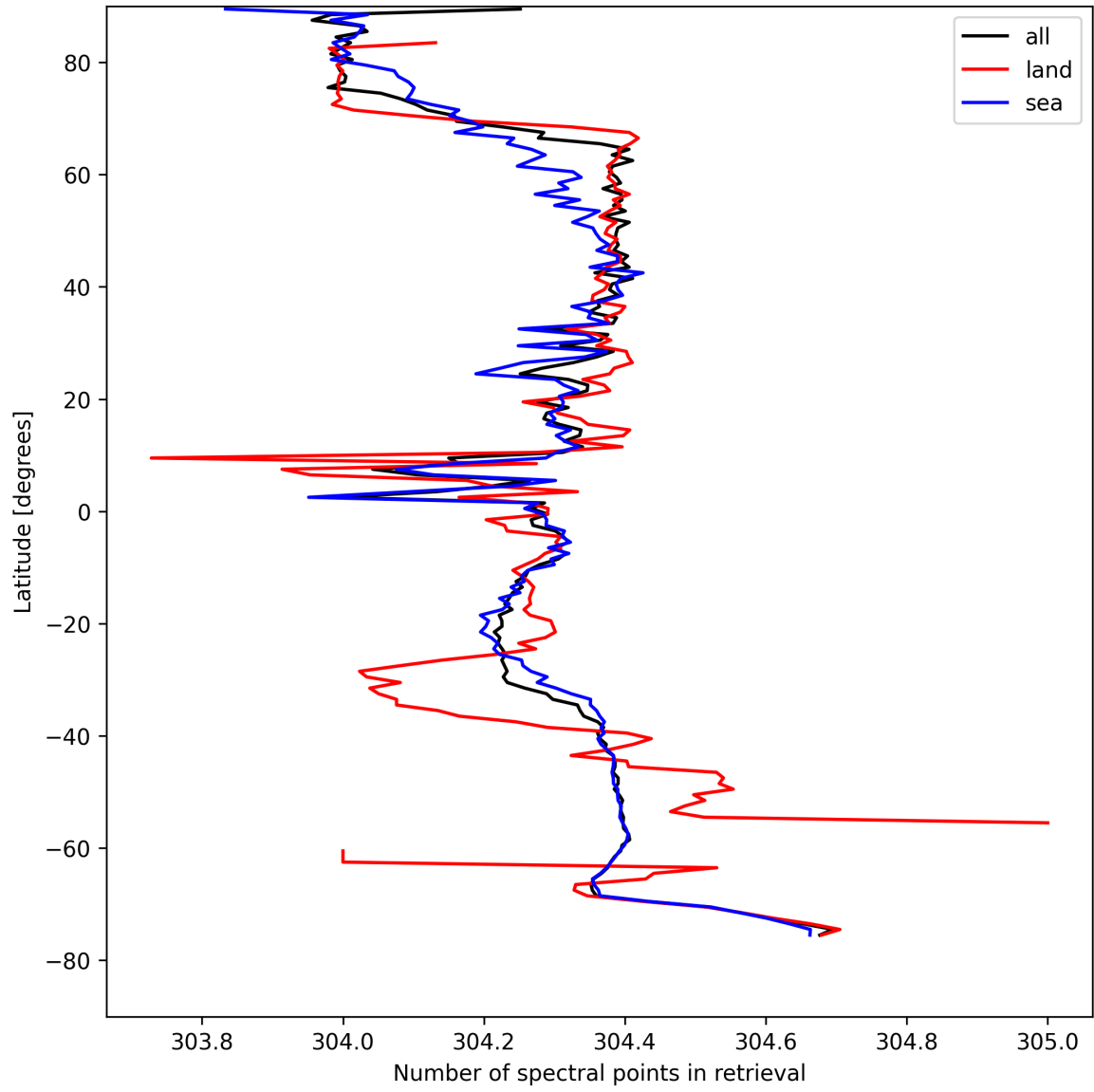
Figure 16: Zonal average of “Number of spectral points in retrieval” for 2025-04-22 to 2025-04-22.
