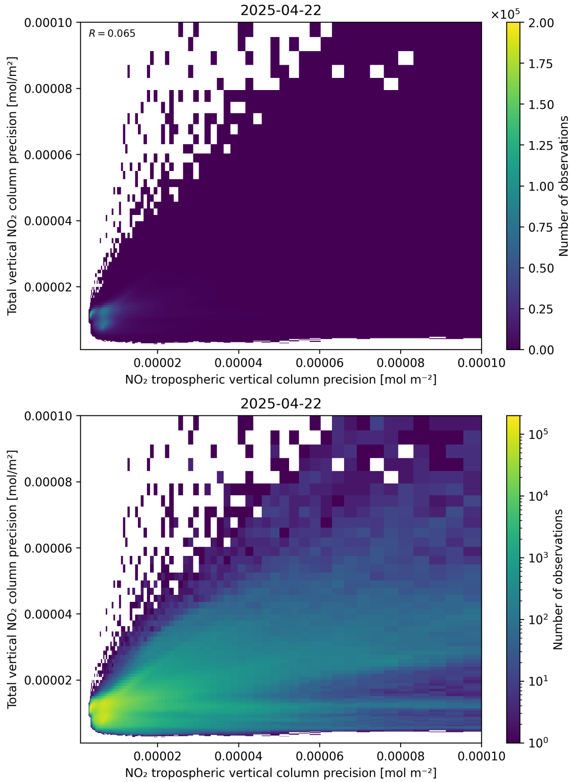
Figure 139: Scatter density plot of “NO 2 tropospheric vertical column precision” against “Total vertical NO 2 column precision” for 2025-04-22 to 2025-04-22.
