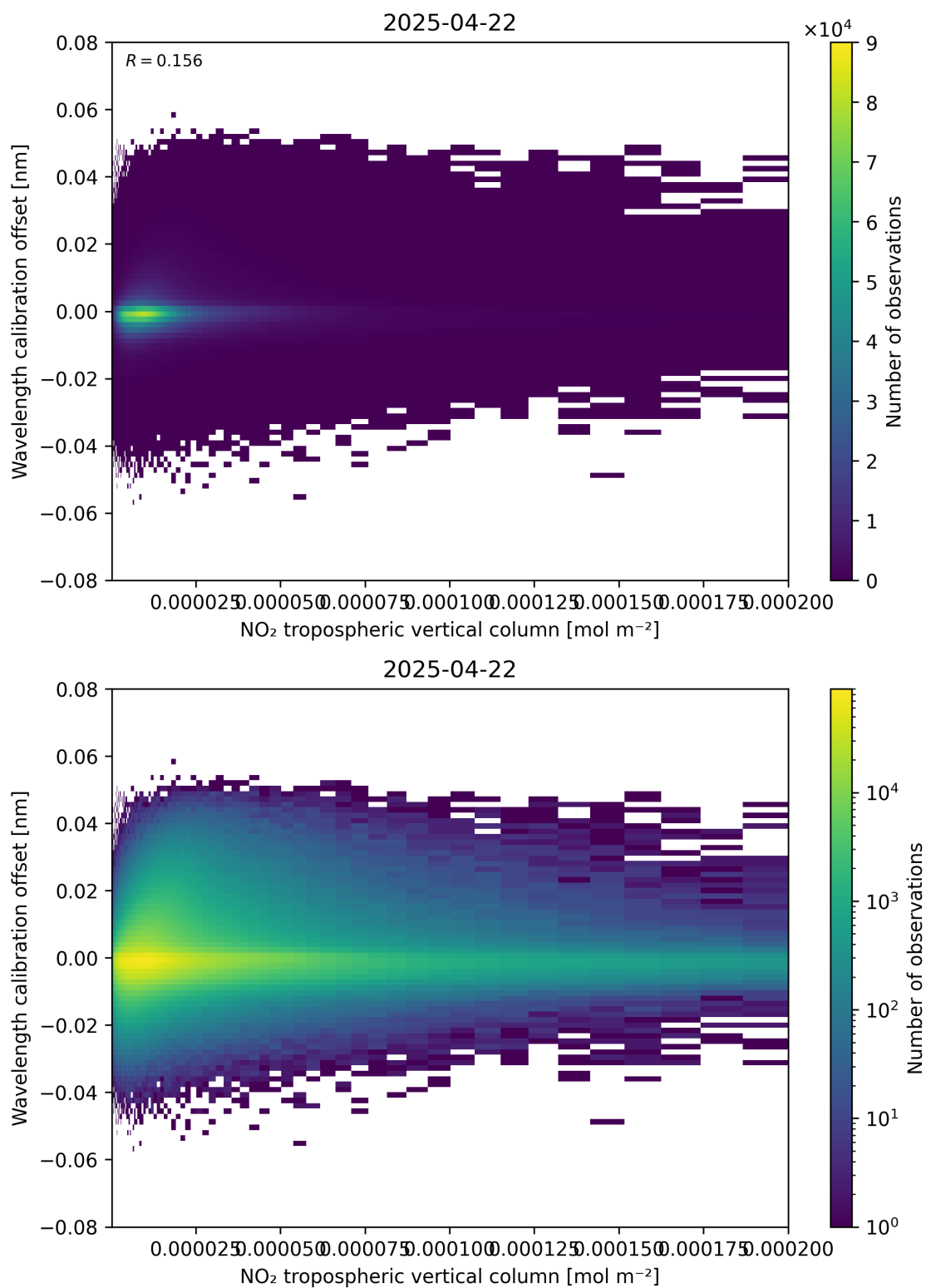
Figure 143: Scatter density plot of “NO 2 tropospheric vertical column” against “Wavelength calibration offset” for 2025-04-22 to 2025-04-22.
