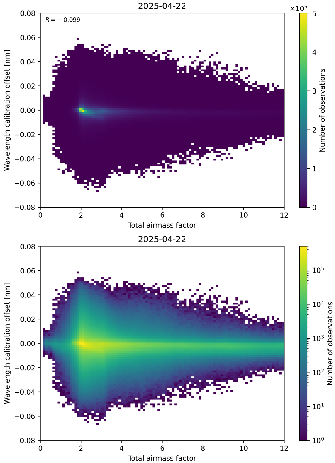
Figure 70: Scatter density plot of “Total airmass factor” against “Wavelength calibration offset” for 2025-04-22 to 2025-04-22.
