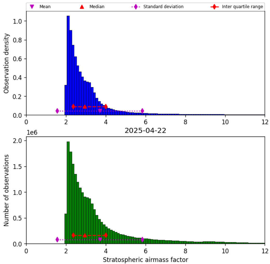
Figure 44: Histogram of “Stratospheric airmass factor” for 2025-04-22 to 2025-04-22
