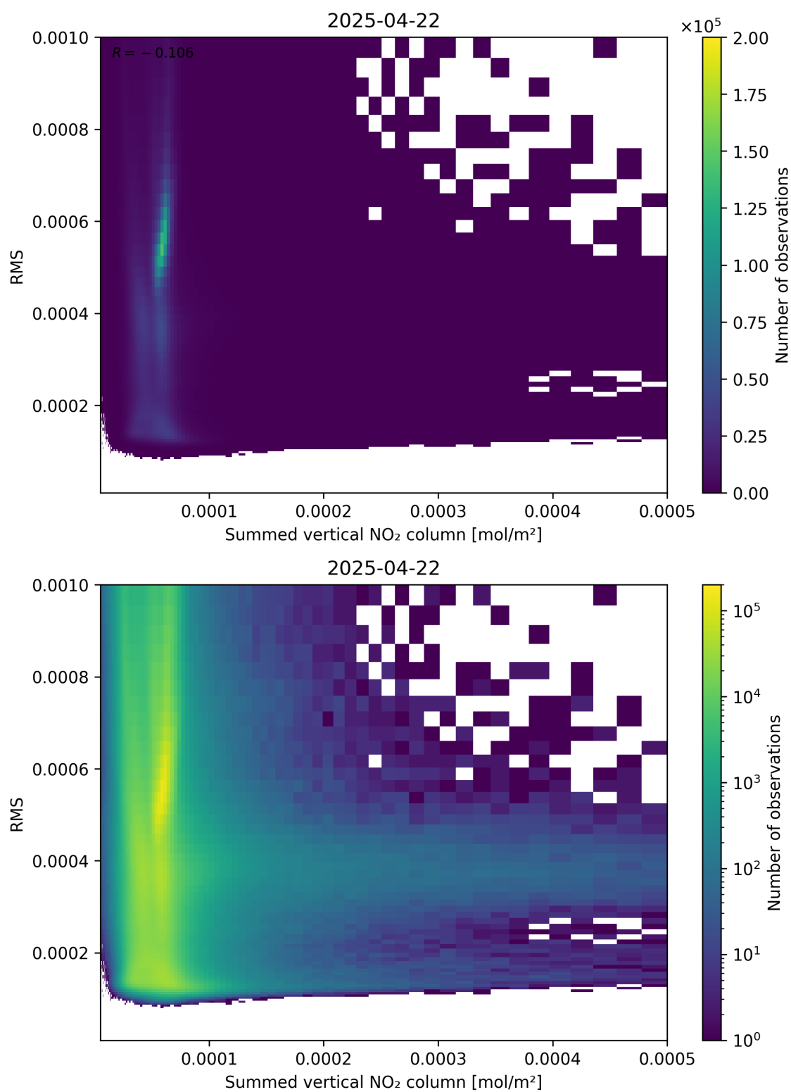
Figure 109: Scatter density plot of “Summed vertical NO 2 column” against “RMS” for 2025-04-22 to 2025-04-22.
