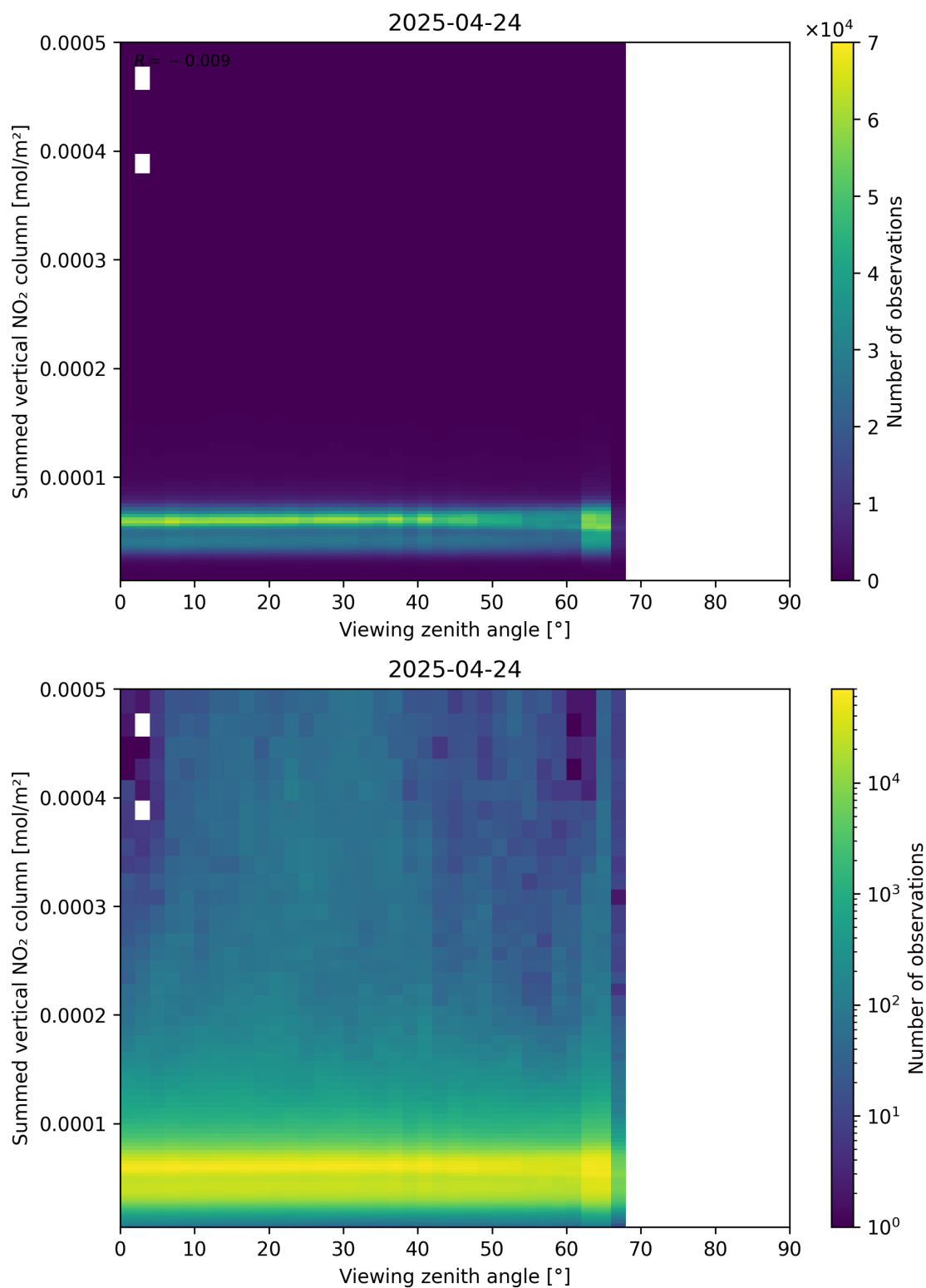
Figure 165: Scatter density plot of “Viewing zenith angle” against “Summed vertical NO 2 column” for 2025-04-24 to 2025-04-25.
