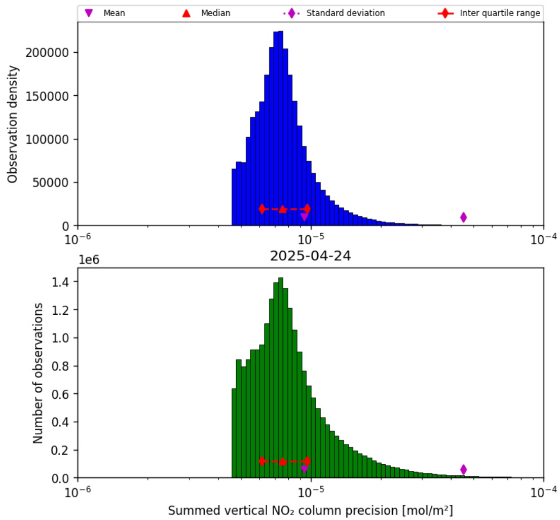
Figure 41: Histogram of “Summed vertical NO 2 column precision” for 2025-04-24 to 2025-04-25
