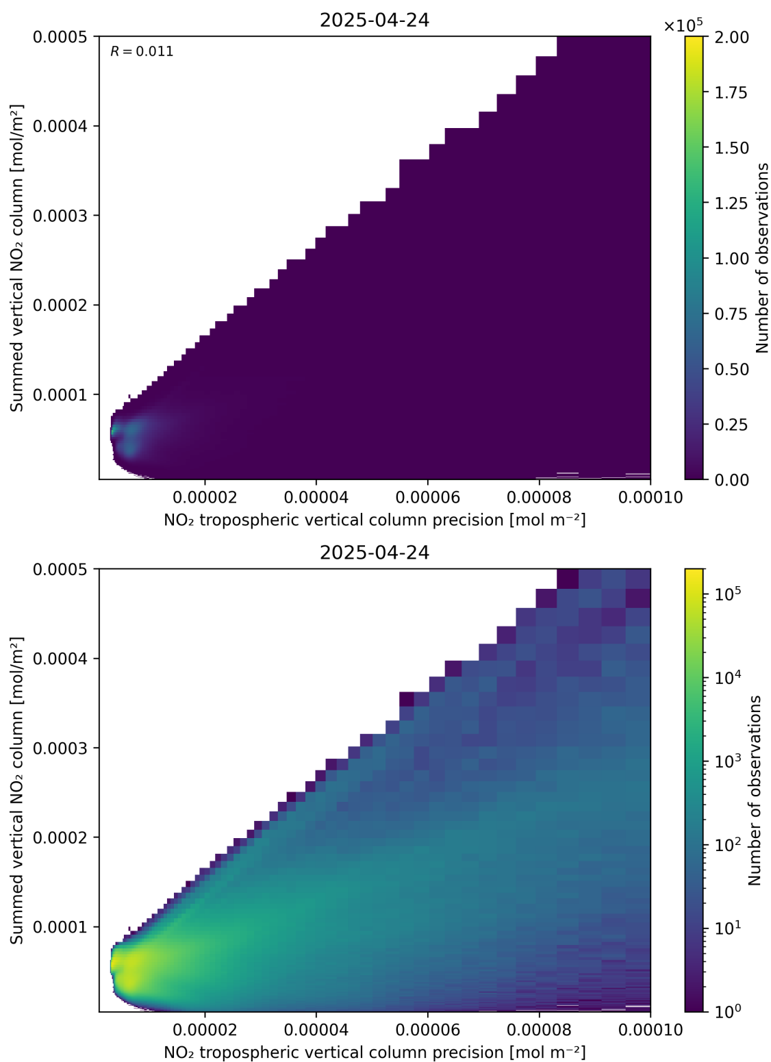
Figure 136: Scatter density plot of “NO 2 tropospheric vertical column precision” against “Summed vertical NO 2 column” for 2025-04-24 to 2025-04-25.
