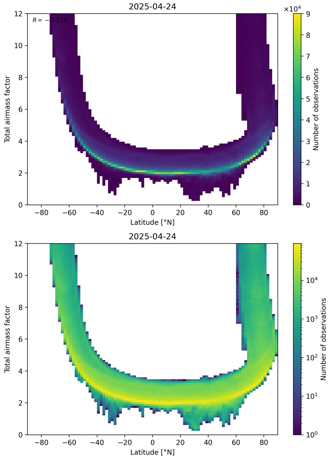
Figure 84: Scatter density plot of “Latitude” against “Total air mass factor” for 2025-04-24 to 2025-04-25.
