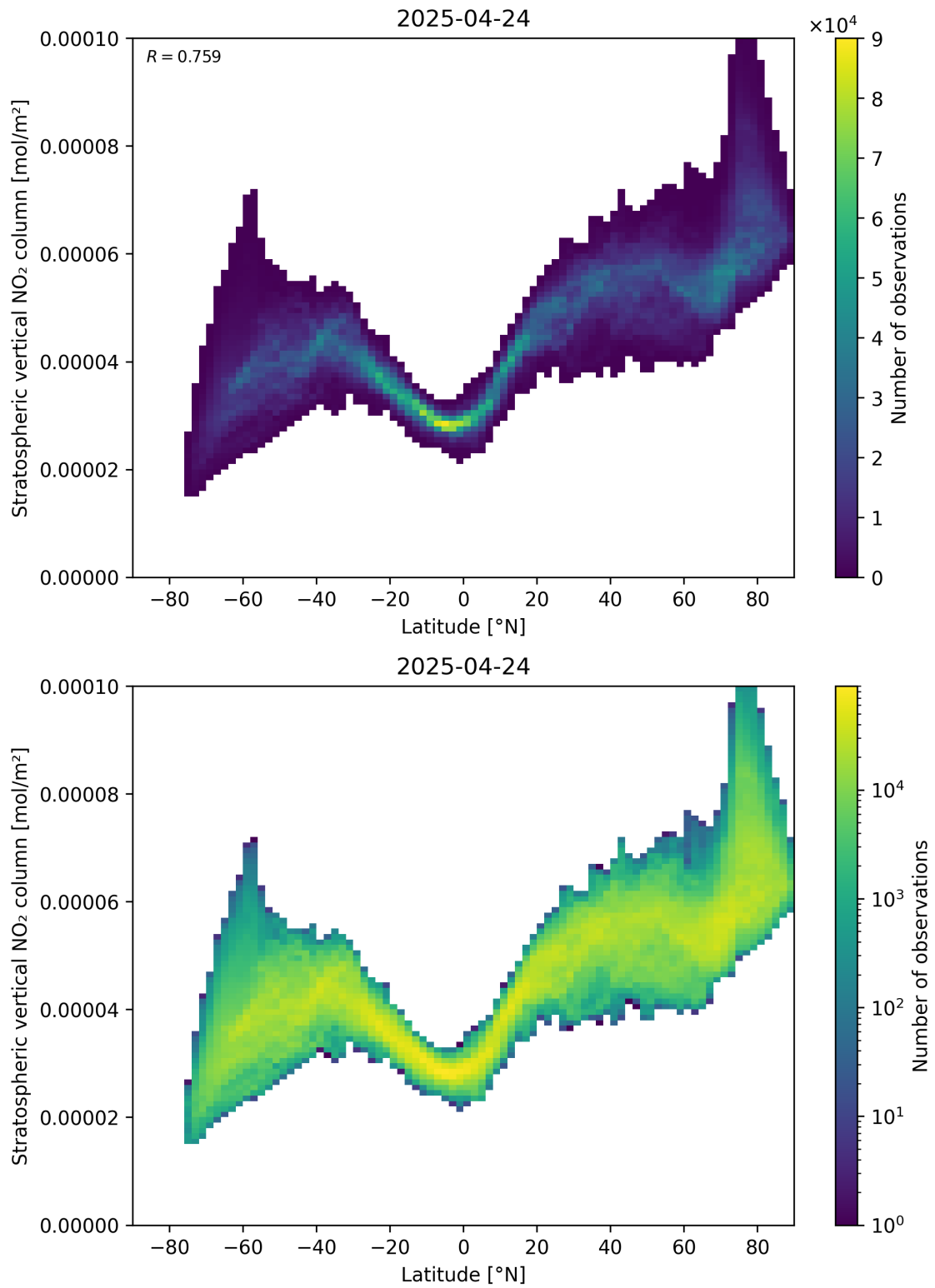
Figure 87: Scatter density plot of “Latitude” against “Stratospheric vertical NO 2 column” for 2025-04-24 to 2025-04-25.
