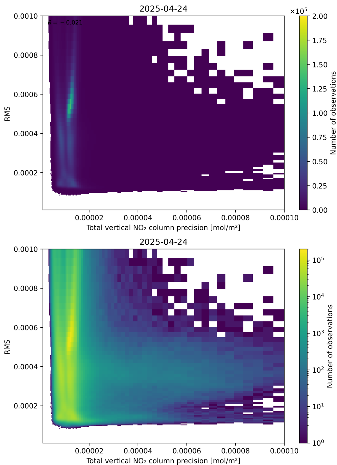
Figure 119: Scatter density plot of “Total vertical NO 2 column precision” against “RMS” for 2025-04-24 to 2025-04-25.
