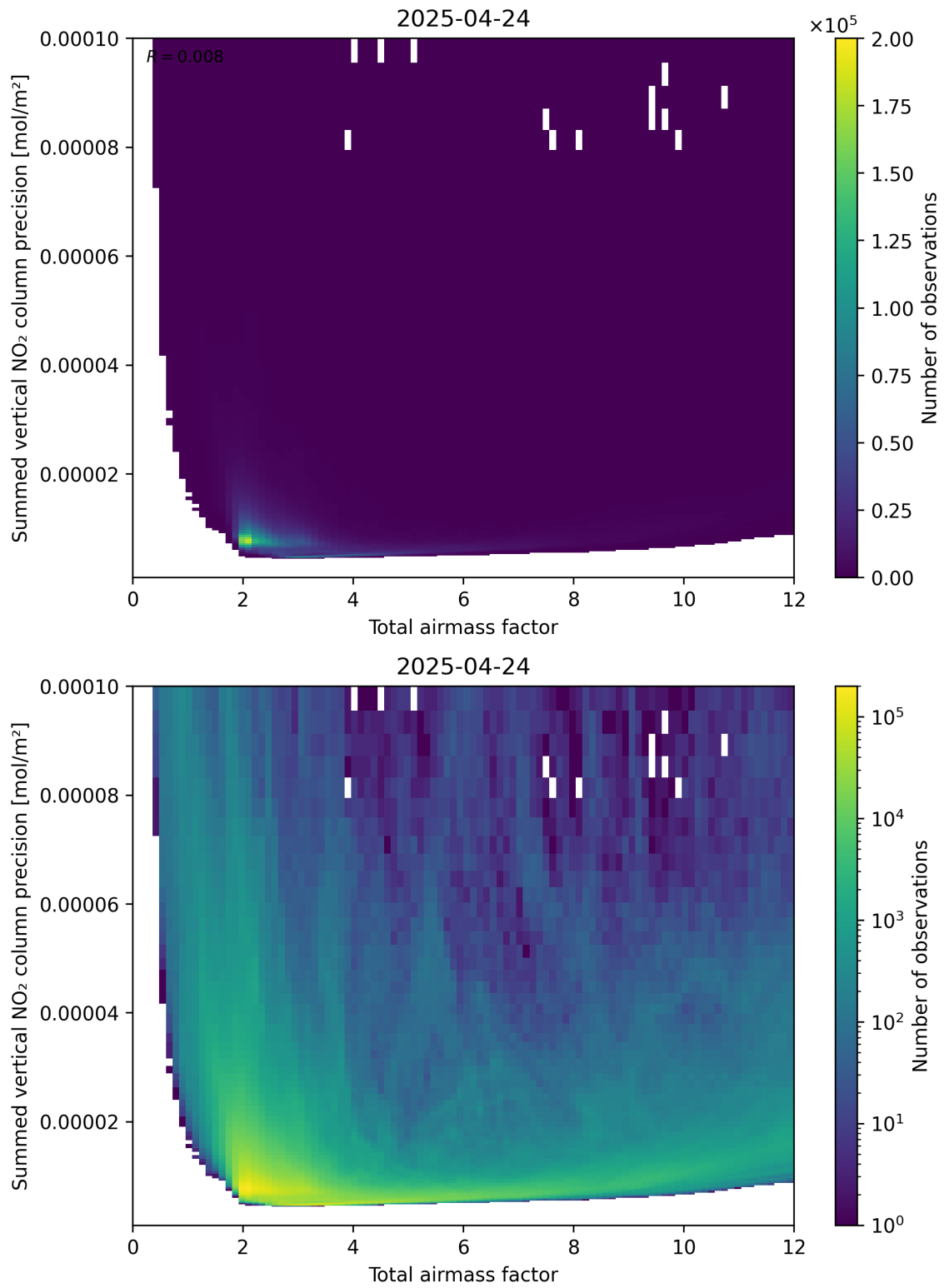
Figure 66: Scatter density plot of “Total airmass factor” against “Summed vertical NO 2 column precision” for 2025-04-24 to 2025-04-25.
