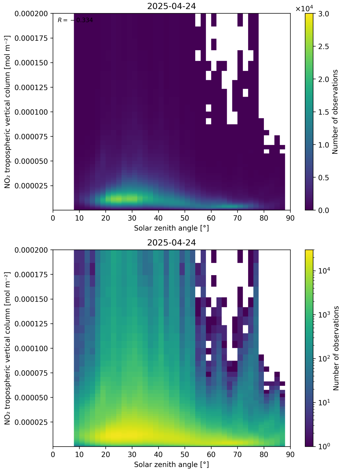
Figure 155: Scatter density plot of “Solar zenith angle” against “NO 2 tropospheric vertical column” for 2025-04-24 to 2025-04-25.
