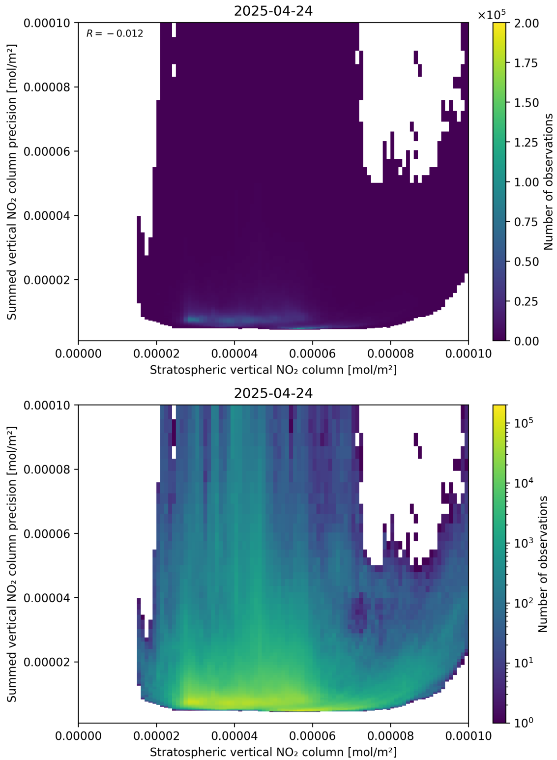
Figure 99: Scatter density plot of “Stratospheric vertical NO 2 column” against “Summed vertical NO 2 column precision” for 2025-04-24 to 2025-04-25.
