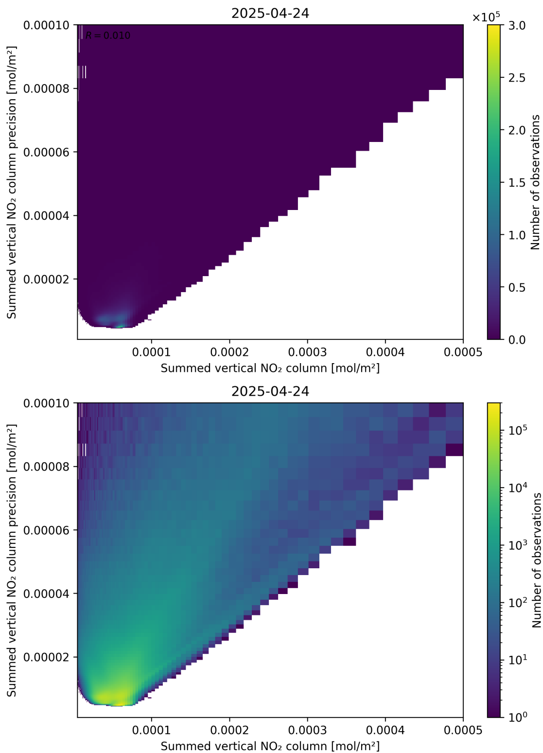
Figure 105: Scatter density plot of “Summed vertical NO 2 column” against “Summed vertical NO 2 column precision” for 2025-04-24 to 2025-04-25.
