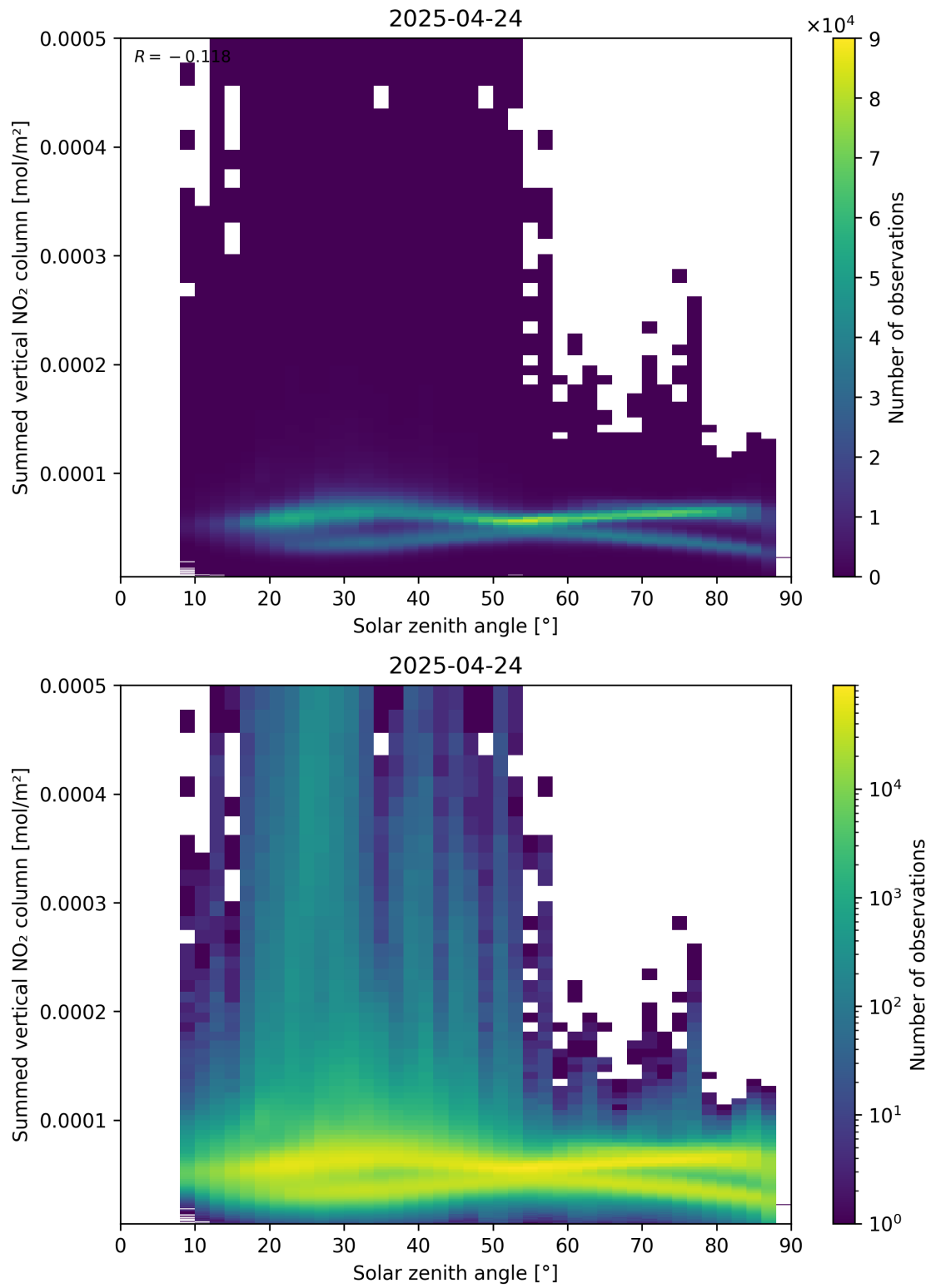
Figure 151: Scatter density plot of “Solar zenith angle” against “Summed vertical NO 2 column” for 2025-04-24 to 2025-04-25.
