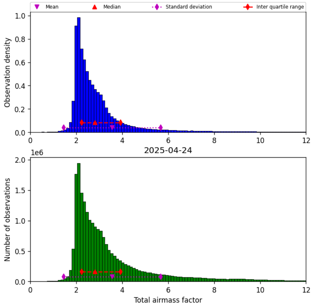
Figure 32: Histogram of “Total airmass factor” for 2025-04-24 to 2025-04-25
