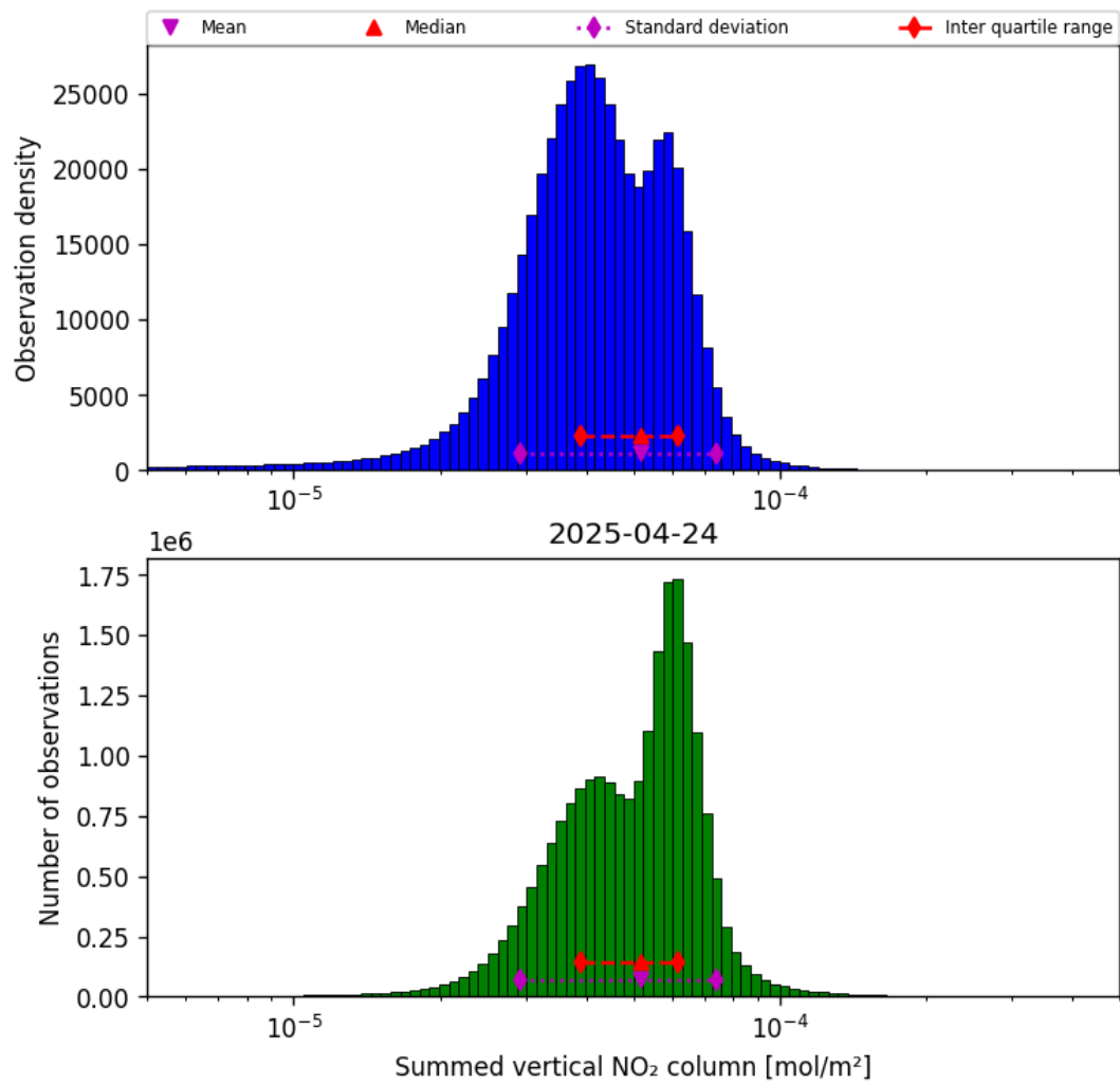
Figure 40: Histogram of “Summed vertical NO 2 column” for 2025-04-24 to 2025-04-25
