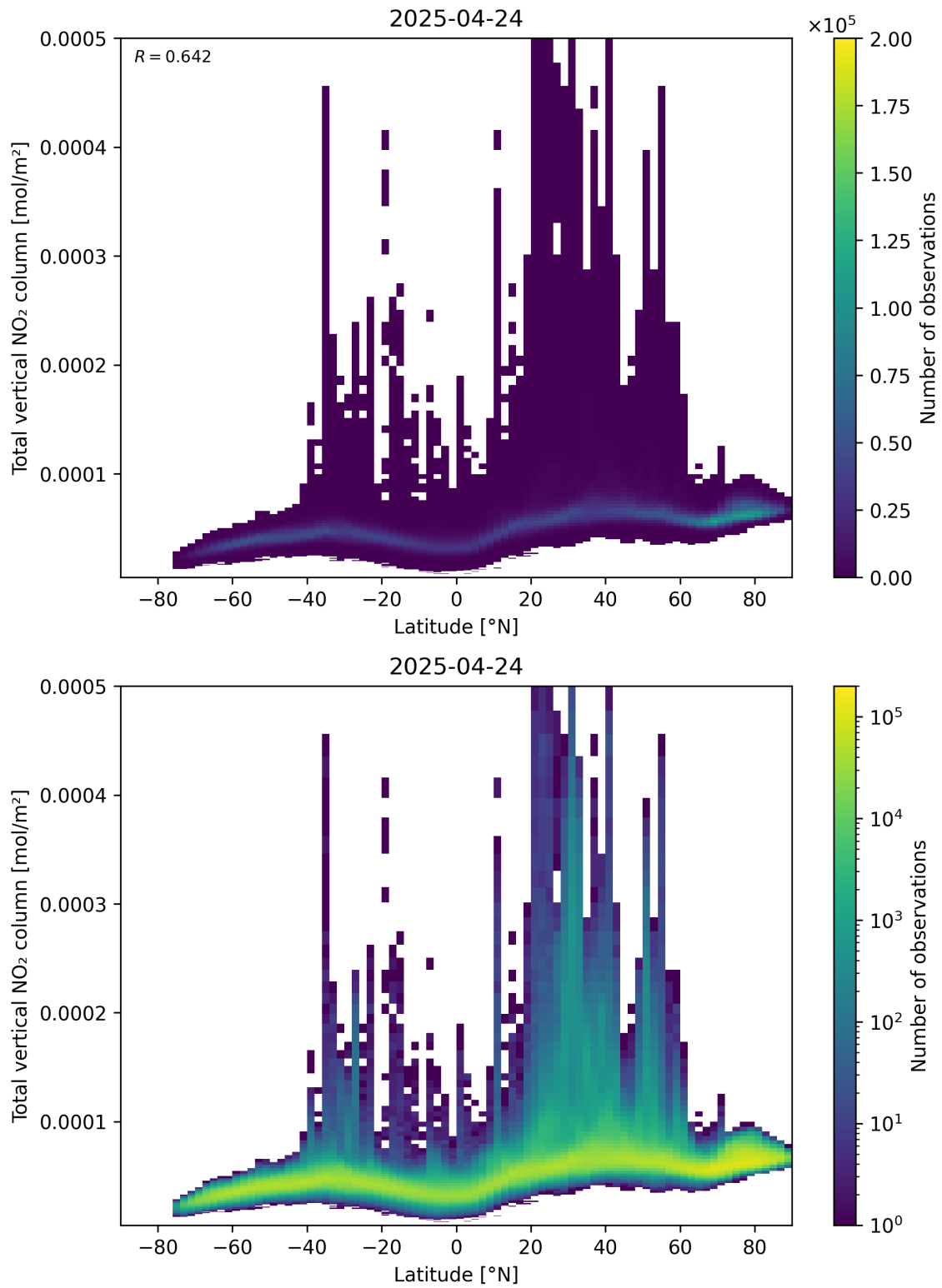
Figure 90: Scatter density plot of “Latitude” against “Total vertical NO 2 column” for 2025-04-24 to 2025-04-25.
