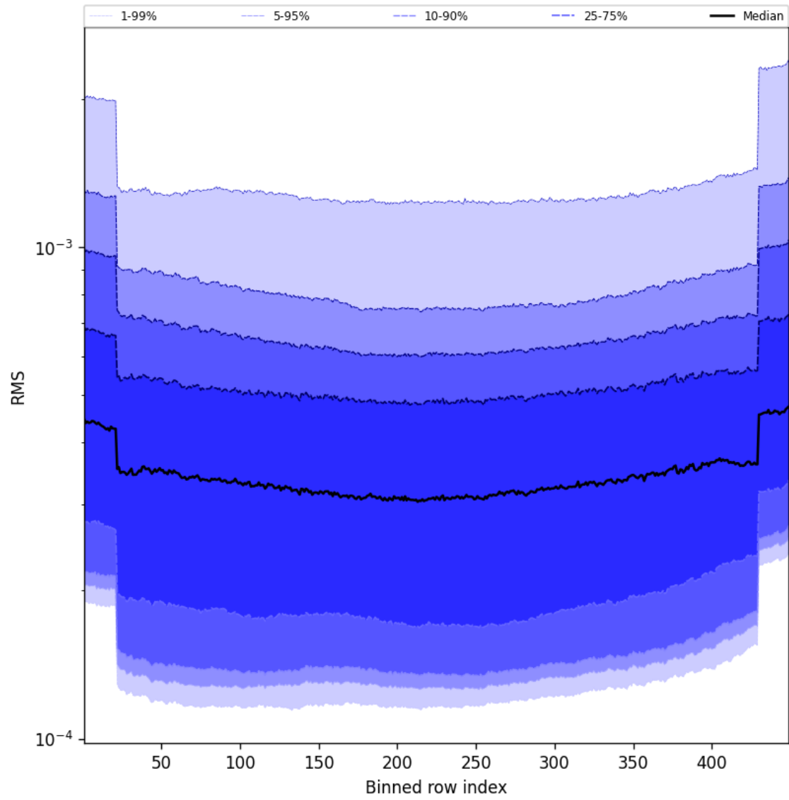
Figure 60: Along track statistics of “RMS” for 2025-04-24 to 2025-04-25
