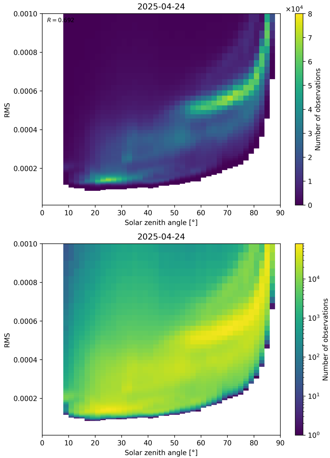
Figure 157: Scatter density plot of “Solar zenith angle” against “RMS” for 2025-04-24 to 2025-04-25.
