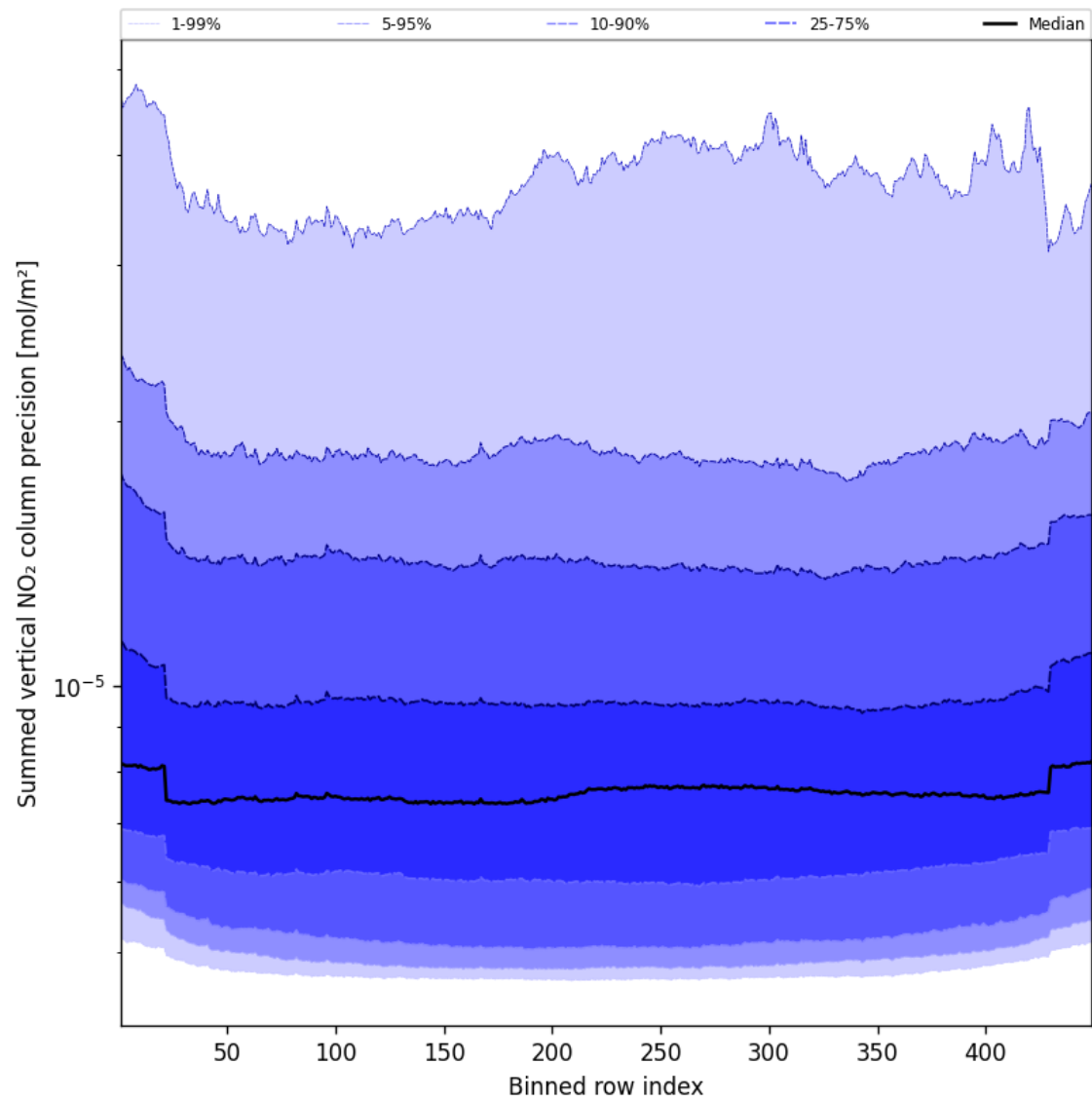
Figure 58: Along track statistics of “Summed vertical NO 2 column precision” for 2025-04-24 to 2025-04-25
