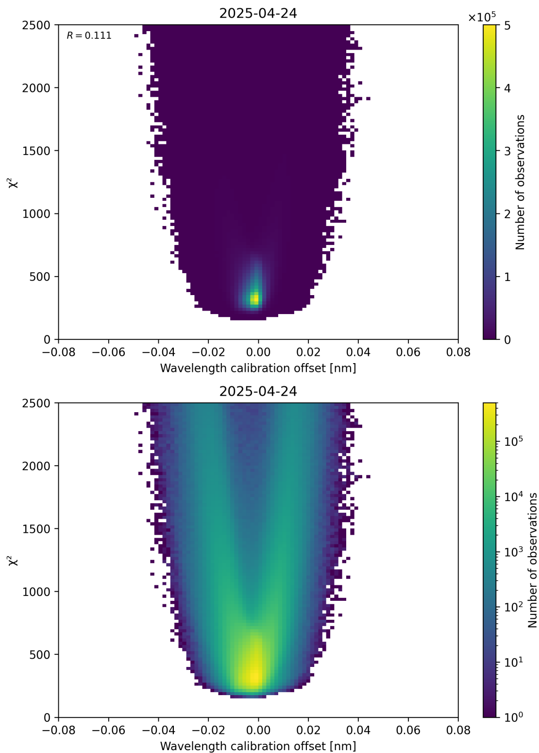
Figure 175: Scatter density plot of “Wavelength calibration offset” against “ \chi^2 ” for 2025-04-24 to 2025-04-25.
