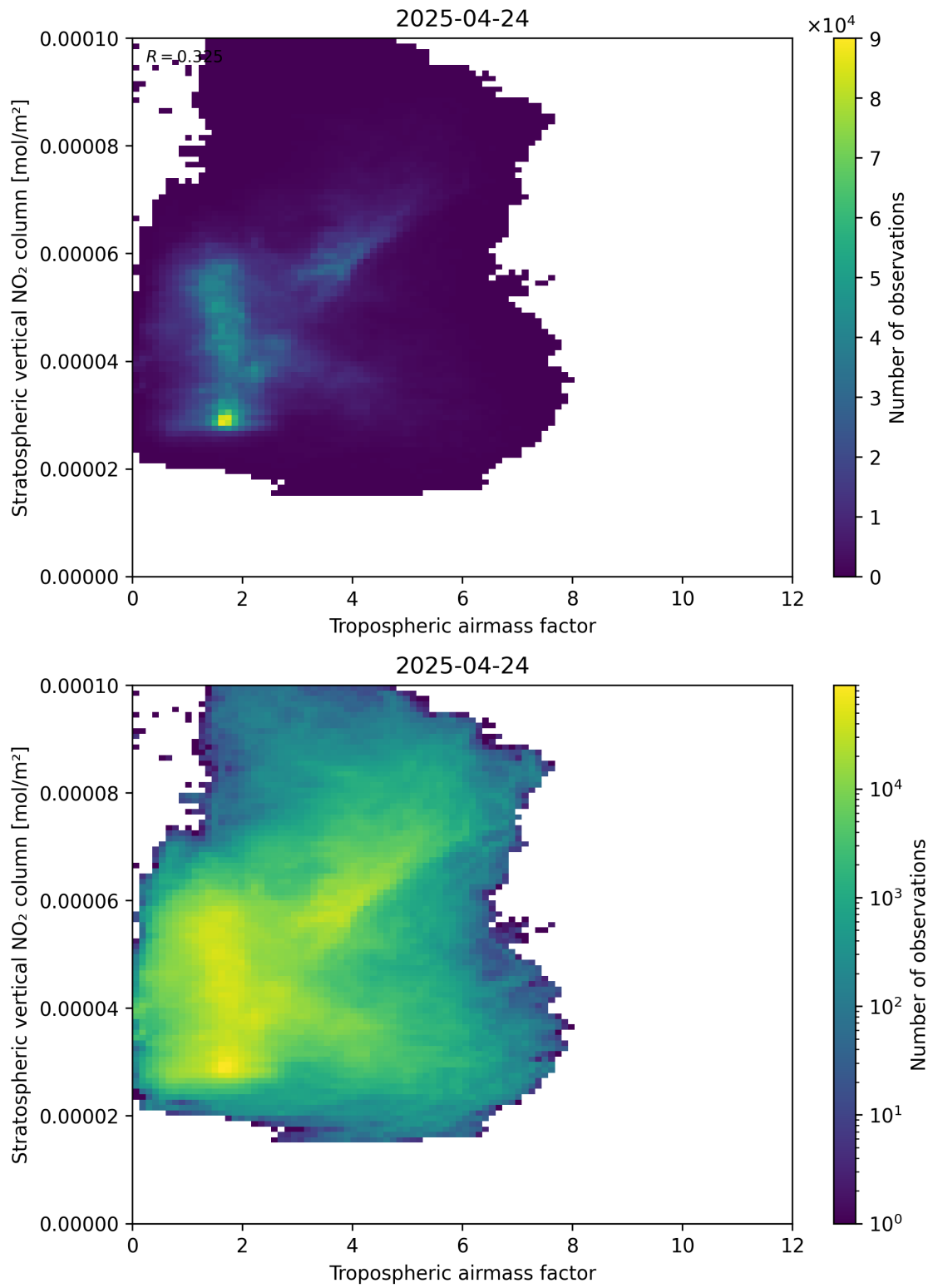
Figure 74: Scatter density plot of “Tropospheric air mass factor” against “Stratospheric vertical NO 2 column” for 2025-04-24 to 2025-04-25.
