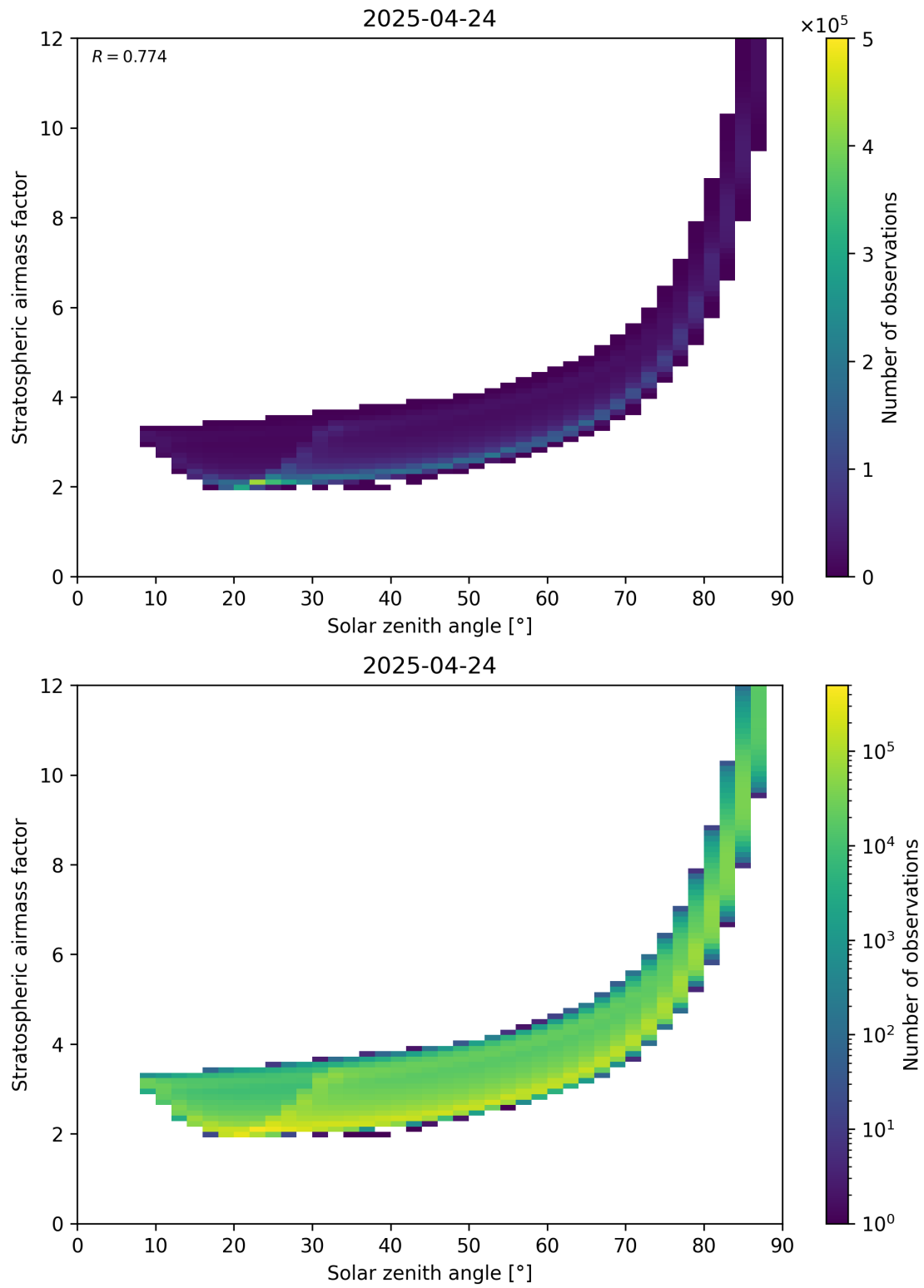
Figure 145: Scatter density plot of “Solar zenith angle” against “Stratospheric airmass factor” for 2025-04-24 to 2025-04-25.
