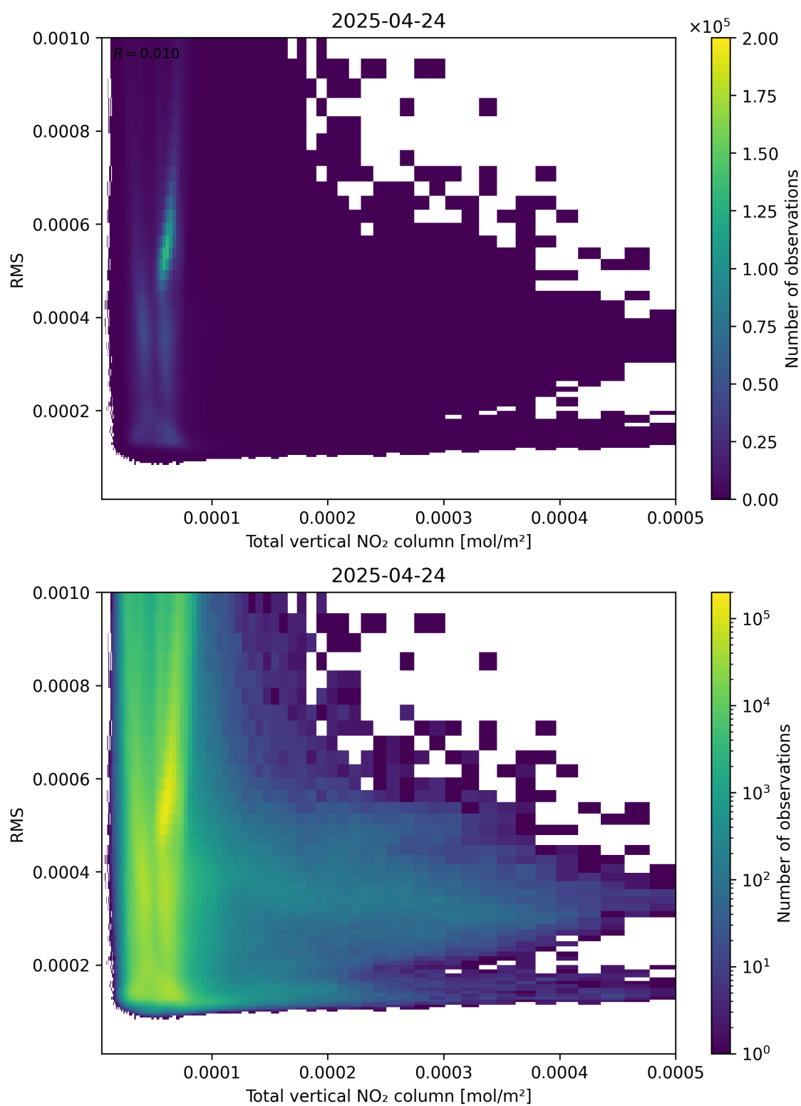
Figure 120: Scatter density plot of “Total vertical NO 2 column” against “RMS” for 2025-04-24 to 2025-04-25.
