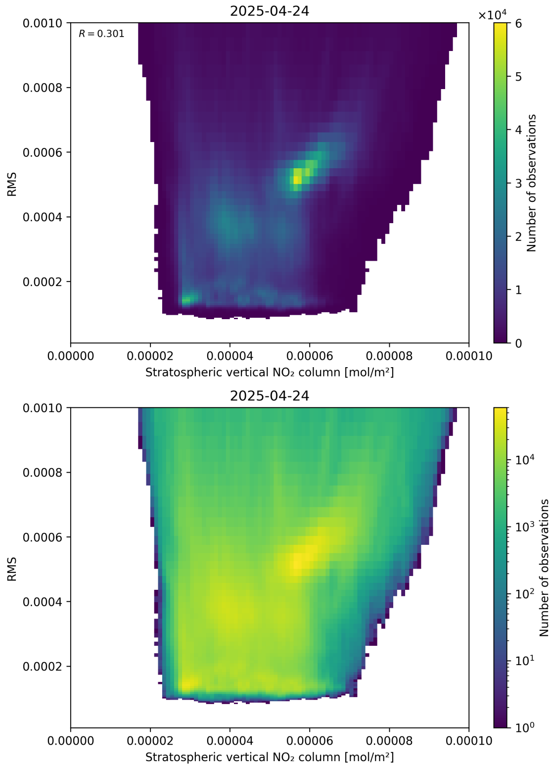
Figure 102: Scatter density plot of “Stratospheric vertical NO 2 column” against “RMS” for 2025-04-24 to 2025-04-25.
