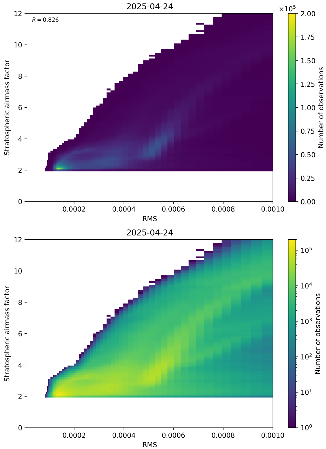
Figure 144: Scatter density plot of “RMS” against “Stratospheric airmass factor” for 2025-04-24 to 2025-04-25.
