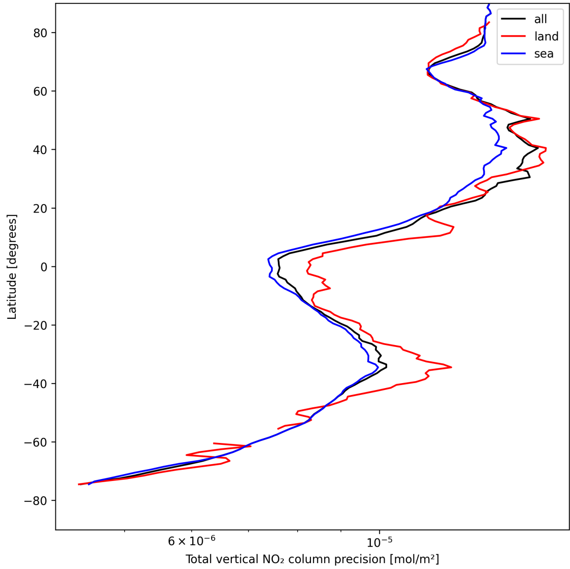
Figure 22: Zonal average of “Total vertical NO 2 column precision” for 2025-04-24 to 2025-04-25.
