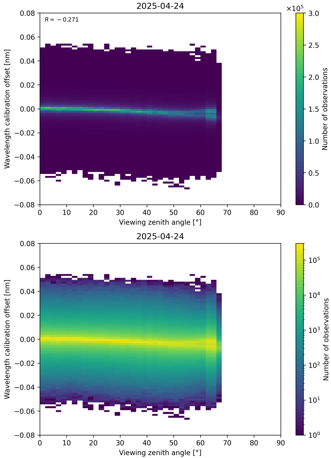
Figure 173: Scatter density plot of “Viewing zenith angle” against “Wavelength calibration offset” for 2025-04-24 to 2025-04-25.
