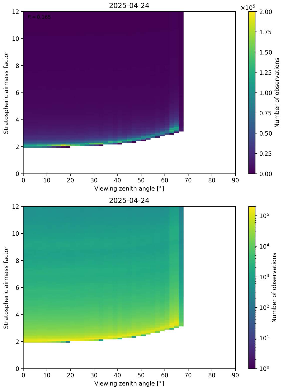
Figure 159: Scatter density plot of “Viewing zenith angle” against “Stratospheric airmass factor” for 2025-04-24 to 2025-04-25.
