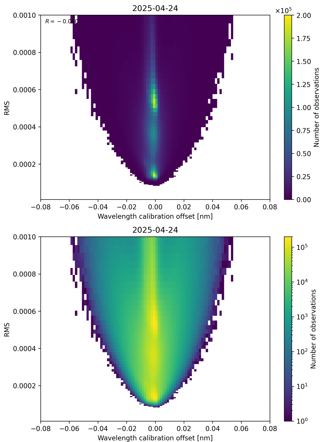
Figure 181: Scatter density plot of “Wavelength calibration offset” against “RMS” for 2025-04-24 to 2025-04-25.
