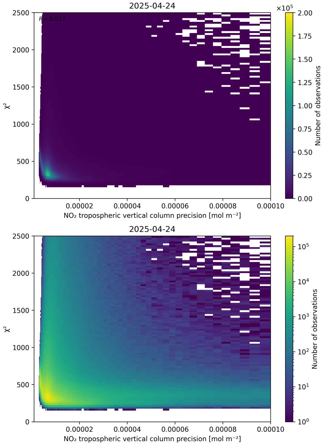
Figure 134: Scatter density plot of “NO 2 tropospheric vertical column precision” against “ \chi^2 ” for 2025-04-24 to 2025-04-25.
