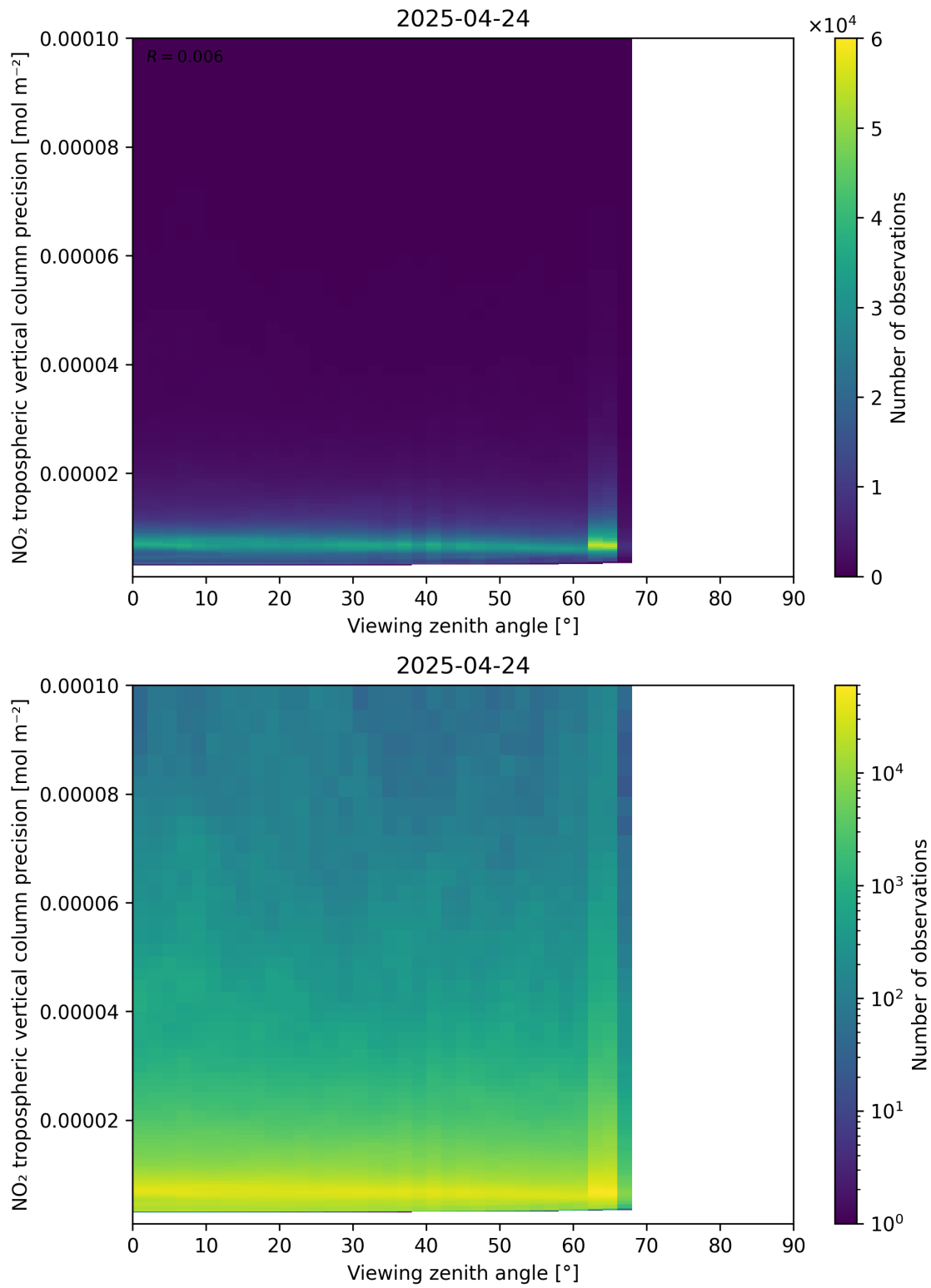
Figure 170: Scatter density plot of “Viewing zenith angle” against “NO 2 tropospheric vertical column precision” for 2025-04-24 to 2025-04-25.
