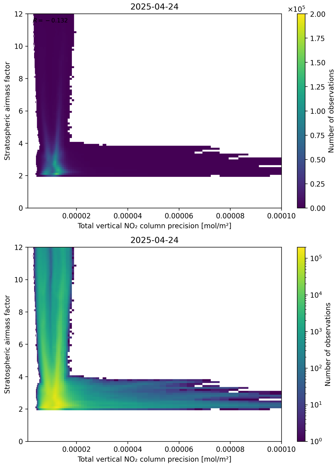
Figure 115: Scatter density plot of “Total vertical NO 2 column precision” against “Stratospheric airmass factor” for 2025-04-24 to 2025-04-25.
