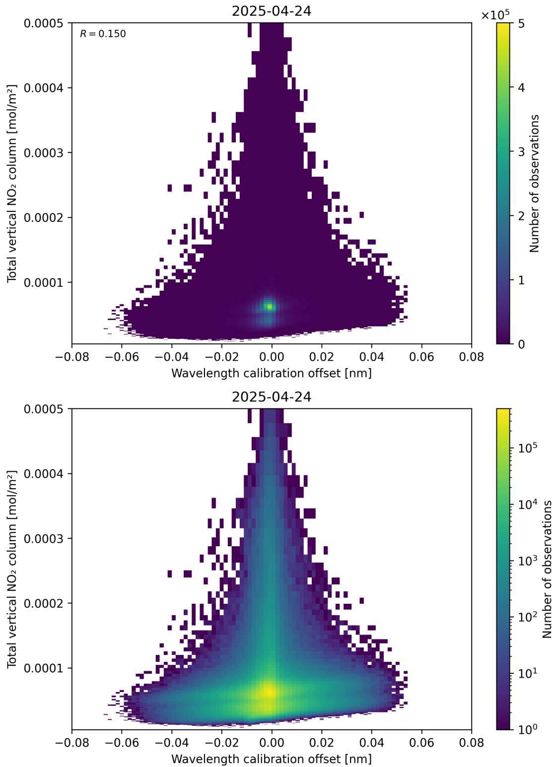
Figure 179: Scatter density plot of “Wavelength calibration offset” against “Total vertical NO 2 column” for 2025-04-24 to 2025-04-25.
