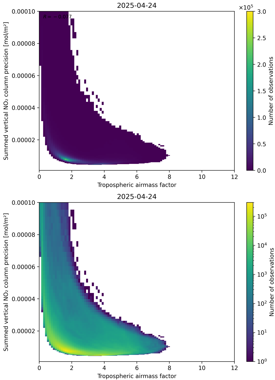
Figure 76: Scatter density plot of “Tropospheric airmass factor” against “Summed vertical NO 2 column precision” for 2025-04-24 to 2025-04-25.
