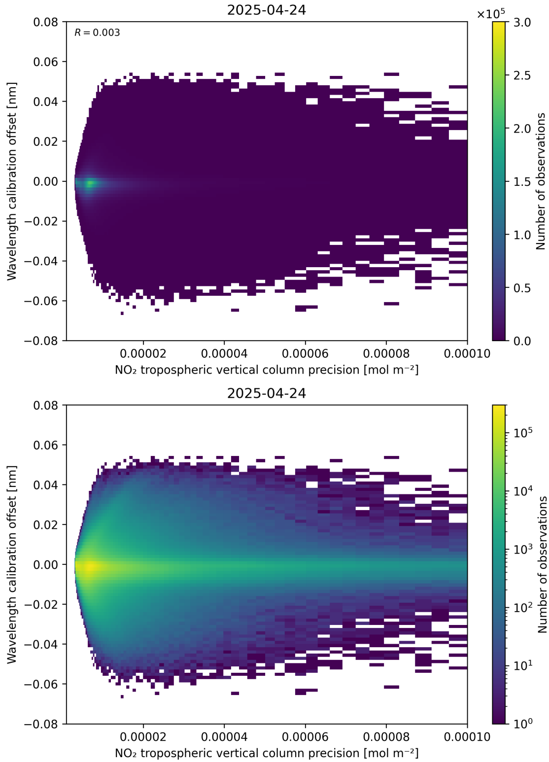
Figure 141: Scatter density plot of “NO 2 tropospheric vertical column precision” against “Wavelength calibration offset” for 2025-04-24 to 2025-04-25.
