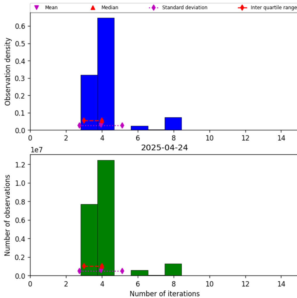
Figure 34: Histogram of “Number of iterations” for 2025-04-24 to 2025-04-25
