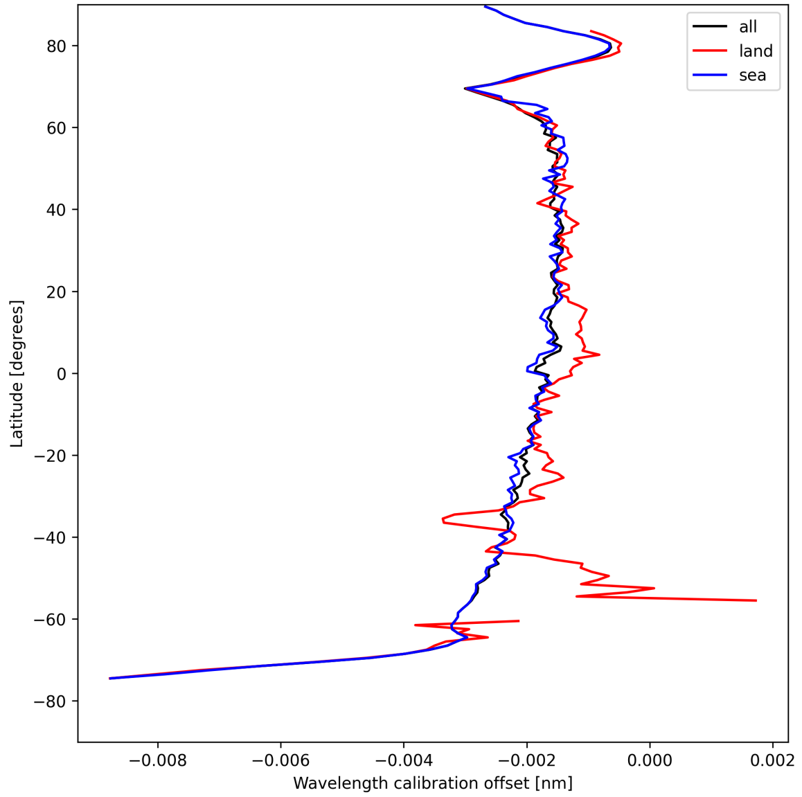
Figure 18: Zonal average of “Wavelength calibration offset” for 2025-04-24 to 2025-04-25.
