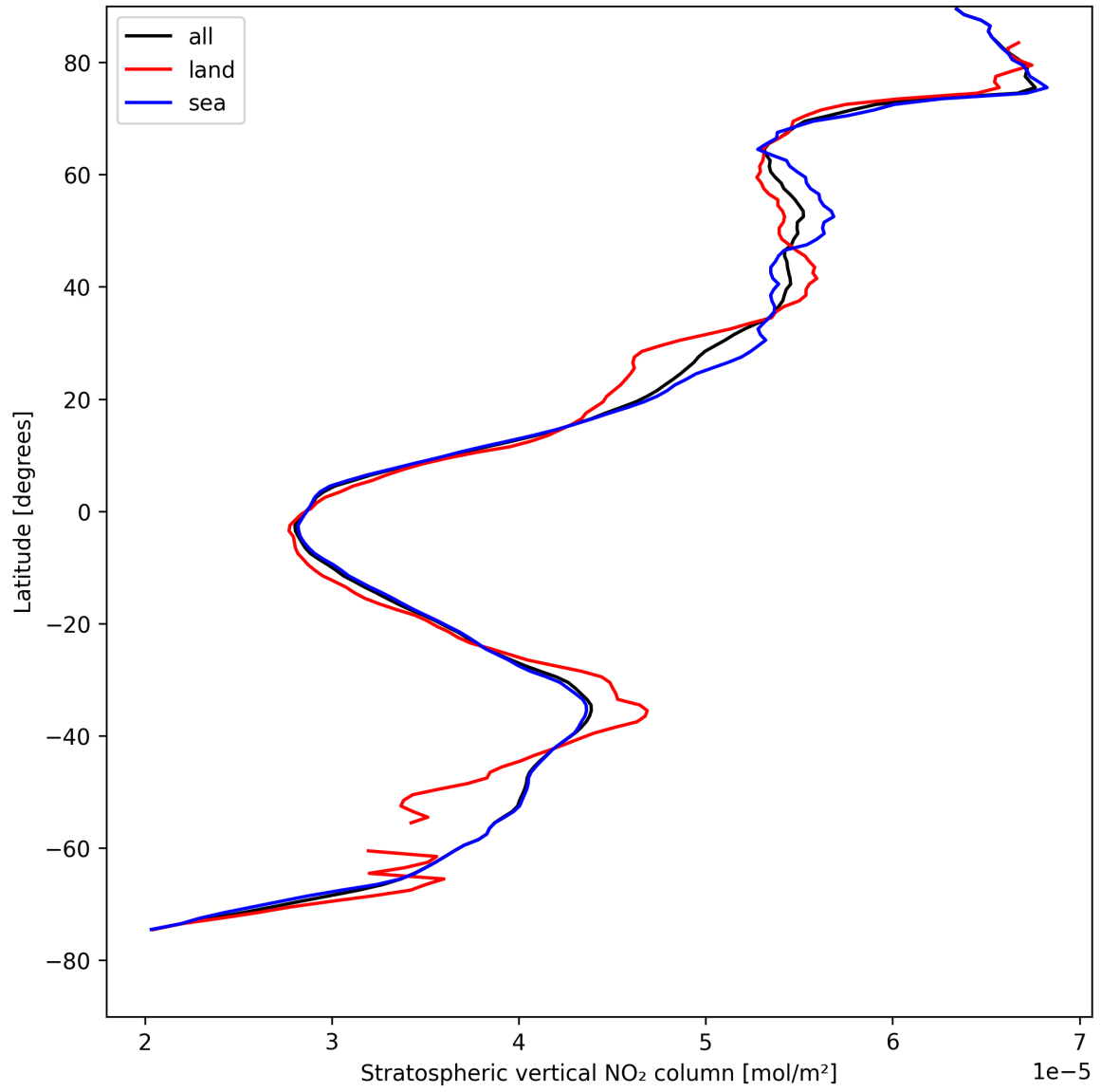
Figure 19: Zonal average of “Stratospheric vertical NO 2 column” for 2025-04-24 to 2025-04-25.
