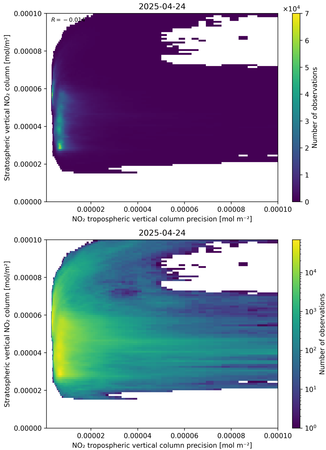
Figure 135: Scatter density plot of “NO 2 tropospheric vertical column precision” against “Stratospheric vertical NO 2 column” for 2025-04-24 to 2025-04-25.
