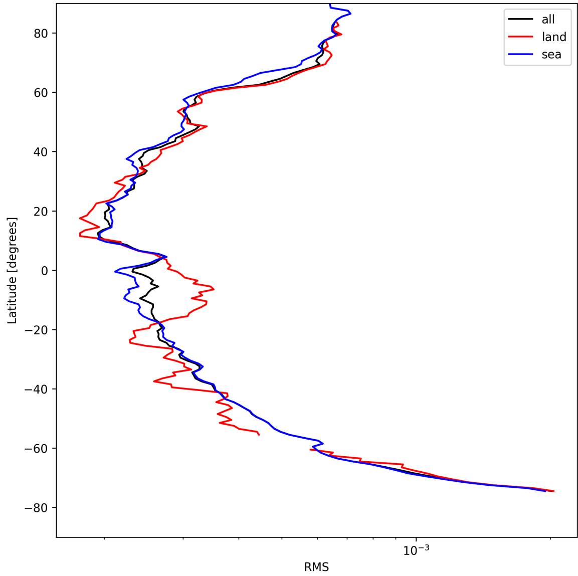
Figure 26: Zonal average of “RMS” for 2025-04-24 to 2025-04-25.
