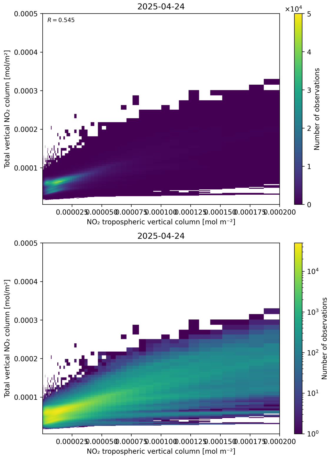
Figure 128: Scatter density plot of “NO 2 tropospheric vertical column” against “Total vertical NO 2 column” for 2025-04-24 to 2025-04-25.
