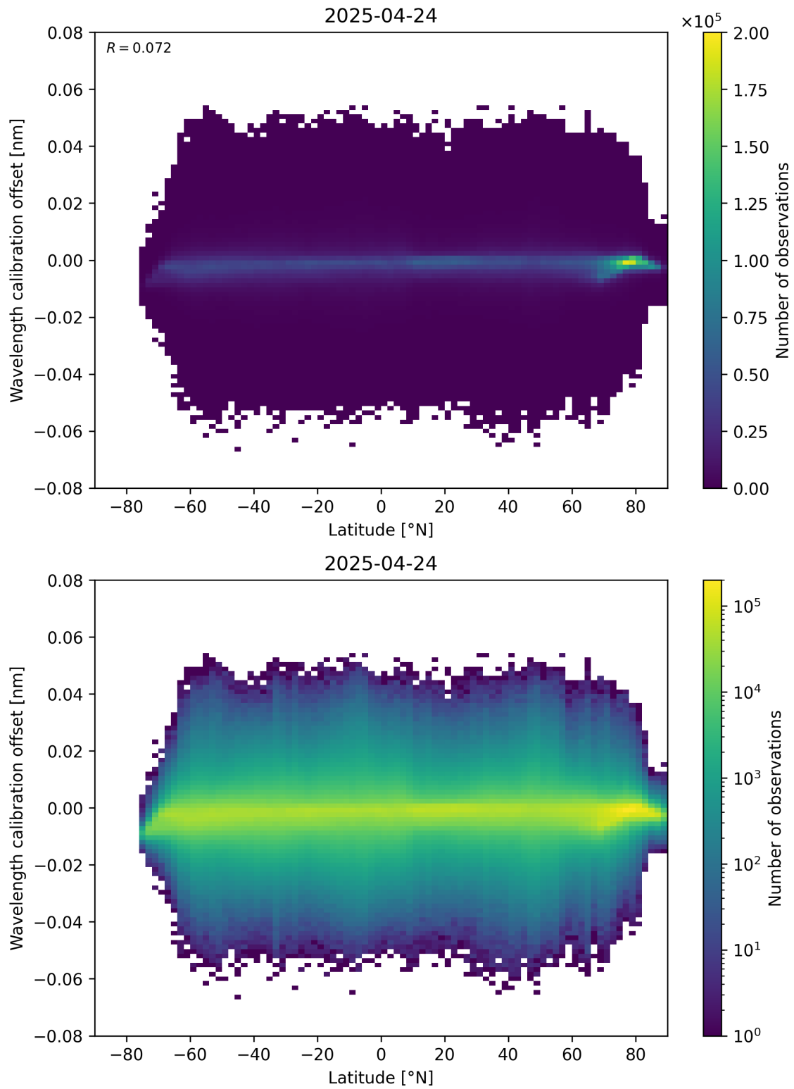
Figure 95: Scatter density plot of “Latitude” against “Wavelength calibration offset” for 2025-04-24 to 2025-04-25.
