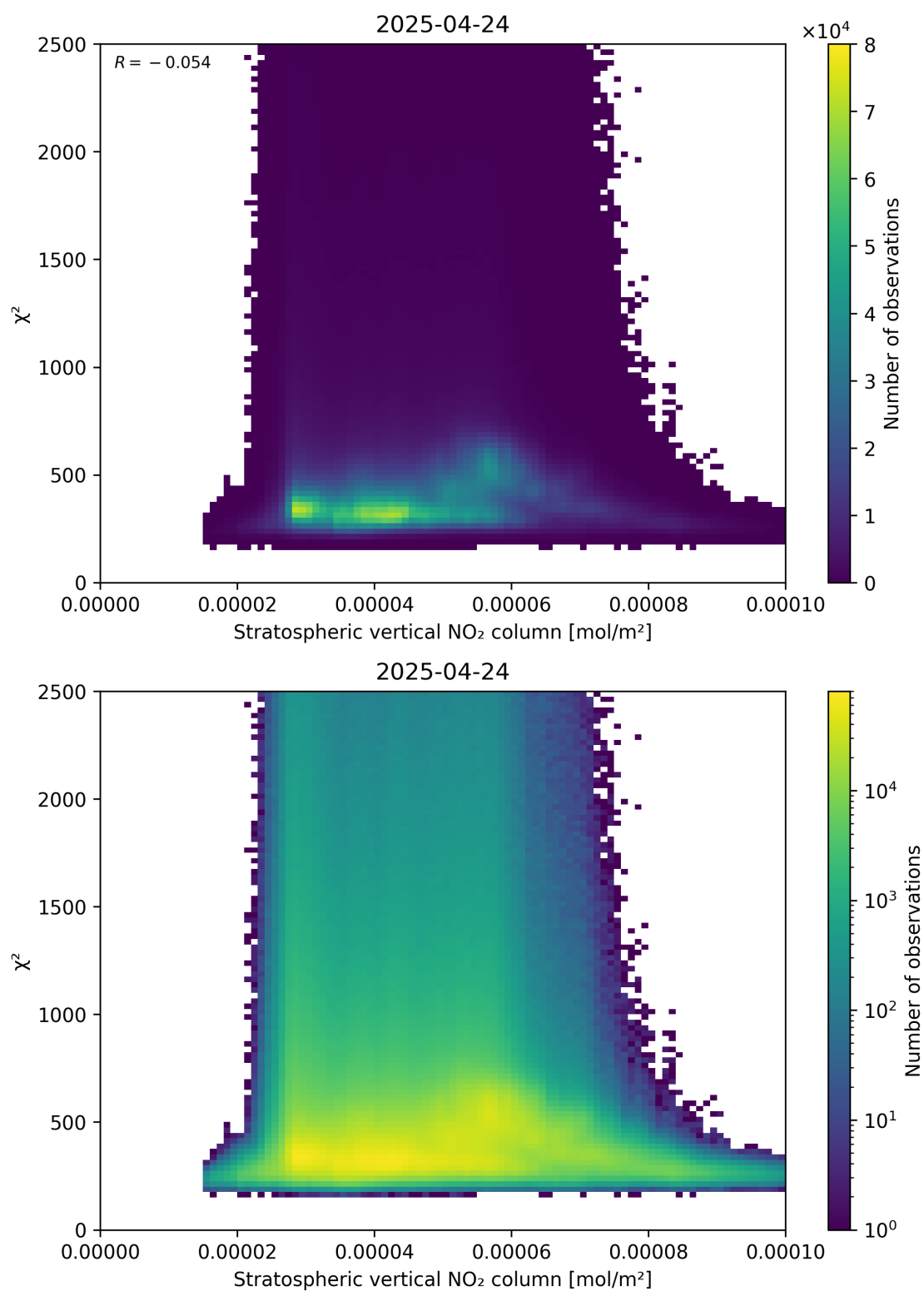
Figure 97: Scatter density plot of “Stratospheric vertical NO 2 column” against “ \chi^2 ” for 2025-04-24 to 2025-04-25.
