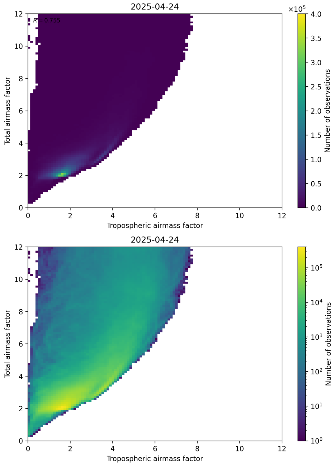
Figure 72: Scatter density plot of “Tropospheric airmass factor” against “Total airmass factor” for 2025-04-24 to 2025-04-25.
