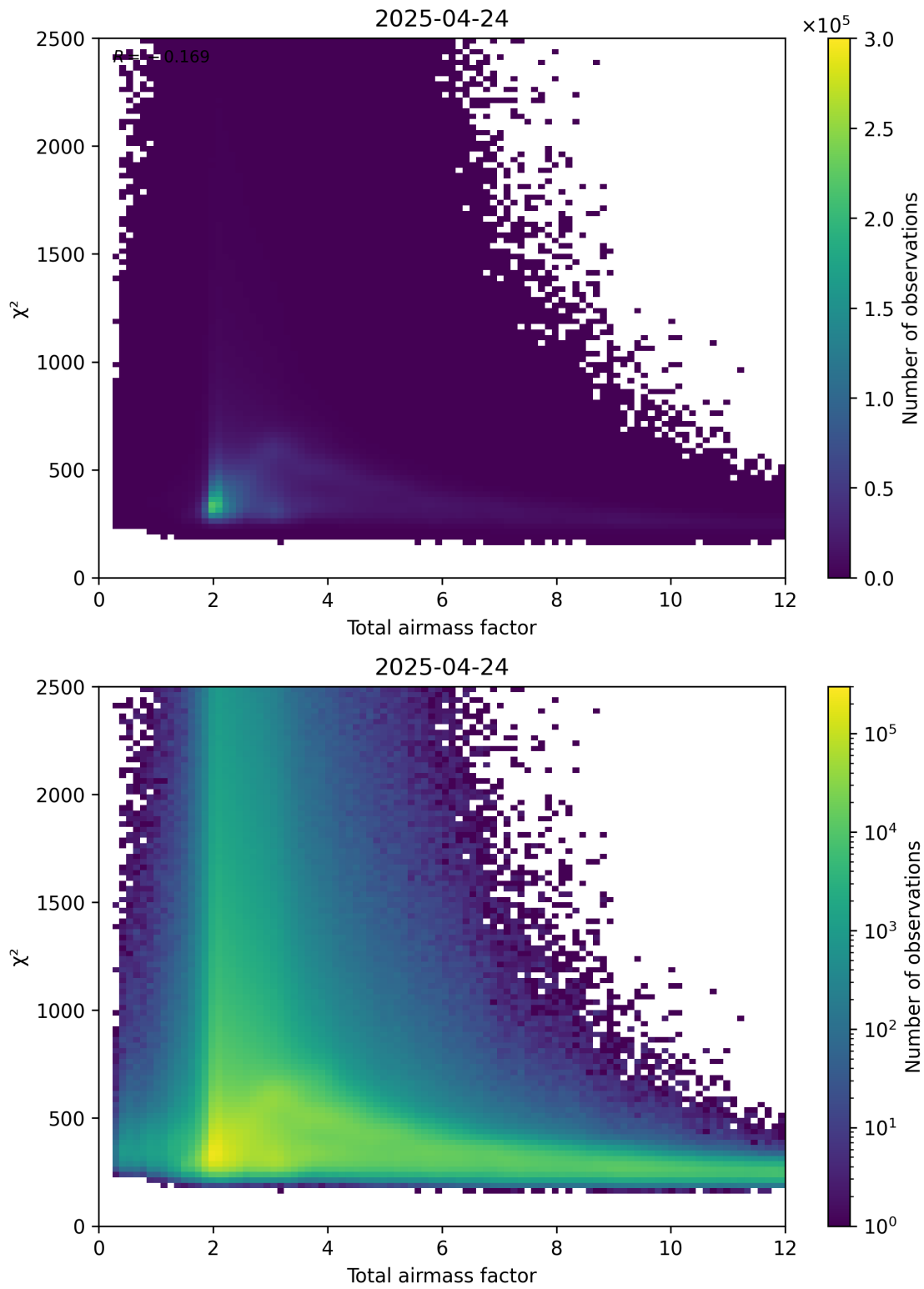
Figure 63: Scatter density plot of “Total airmass factor” against “ \chi^2 ” for 2025-04-24 to 2025-04-25.
