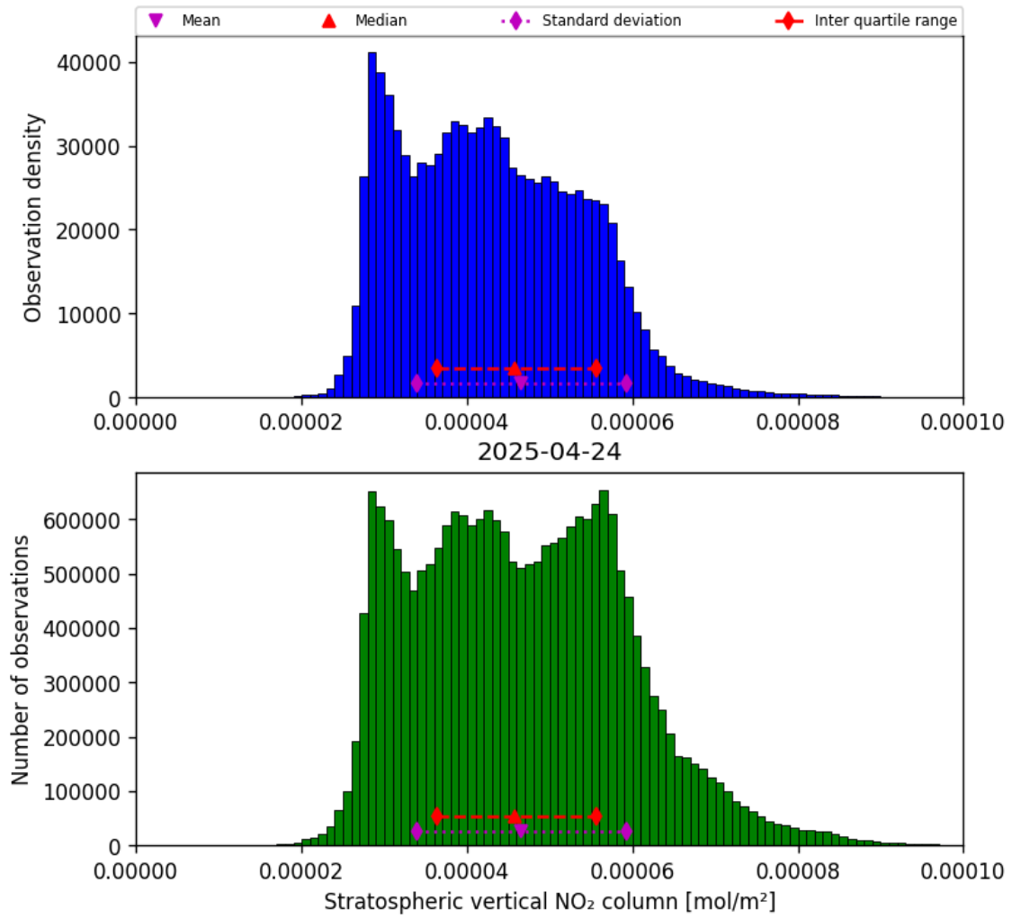
Figure 36: Histogram of “Stratospheric vertical NO 2 column” for 2025-04-24 to 2025-04-25
