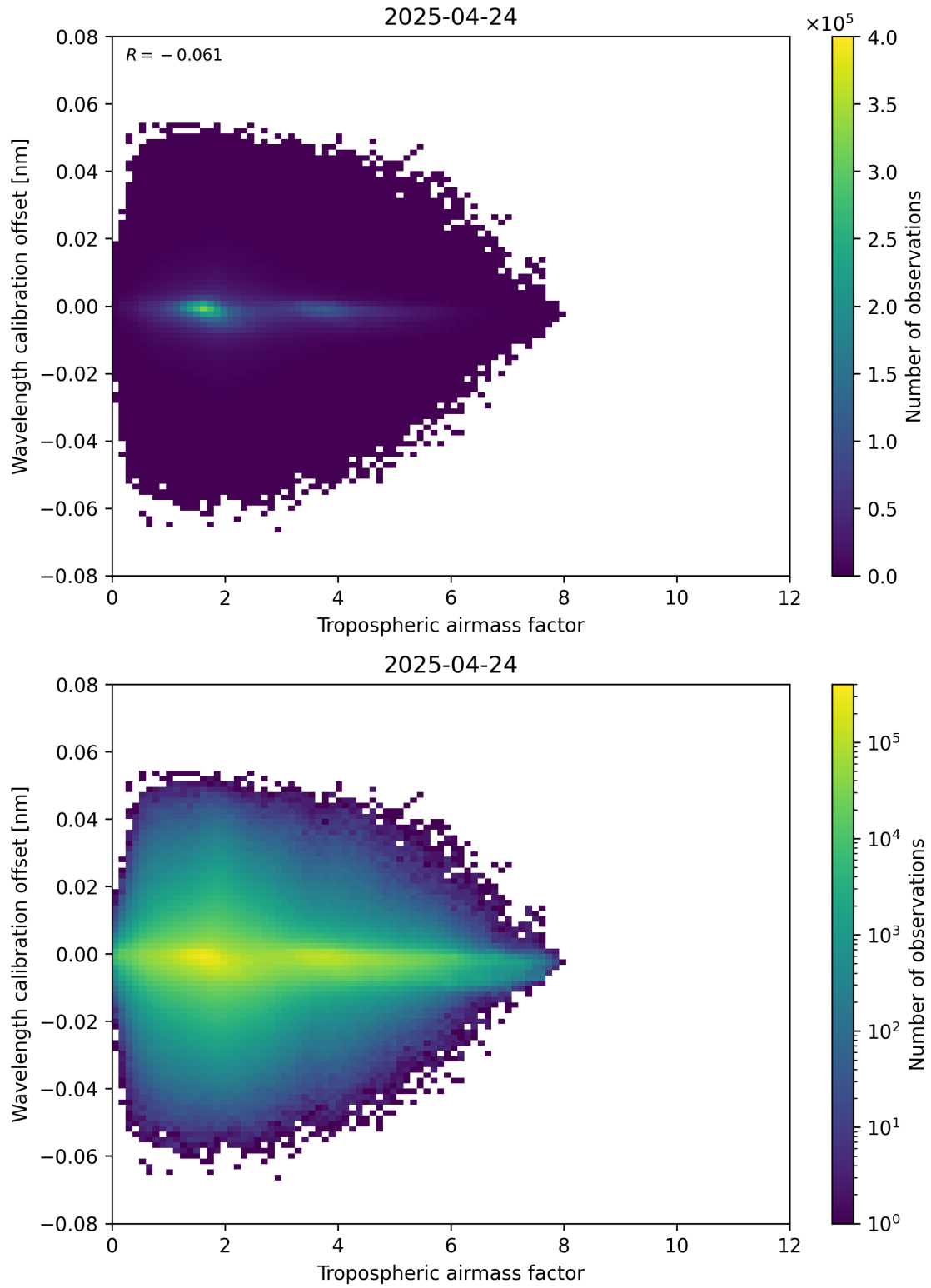
Figure 80: Scatter density plot of “Tropospheric airmass factor” against “Wavelength calibration offset” for 2025-04-24 to 2025-04-25.
