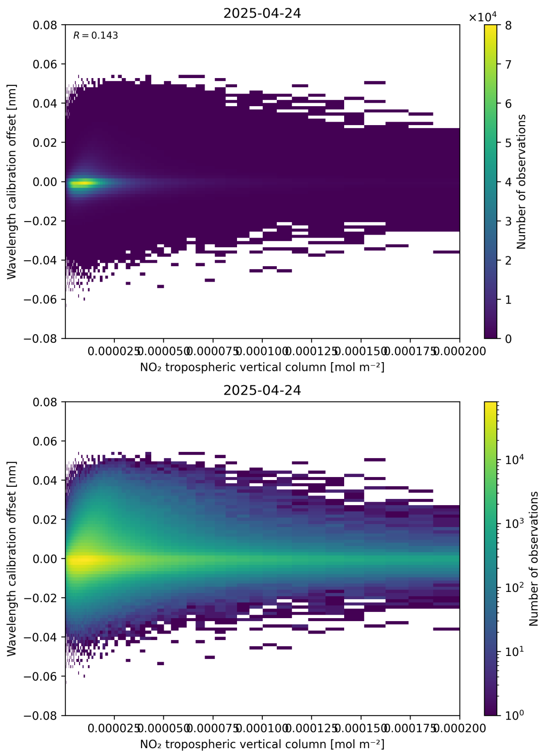
Figure 143: Scatter density plot of “NO 2 tropospheric vertical column” against “Wavelength calibration offset” for 2025-04-24 to 2025-04-25.
