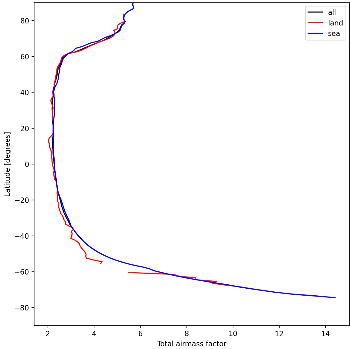
Figure 15: Zonal average of “Total airmass factor” for 2025-04-24 to 2025-04-25.
