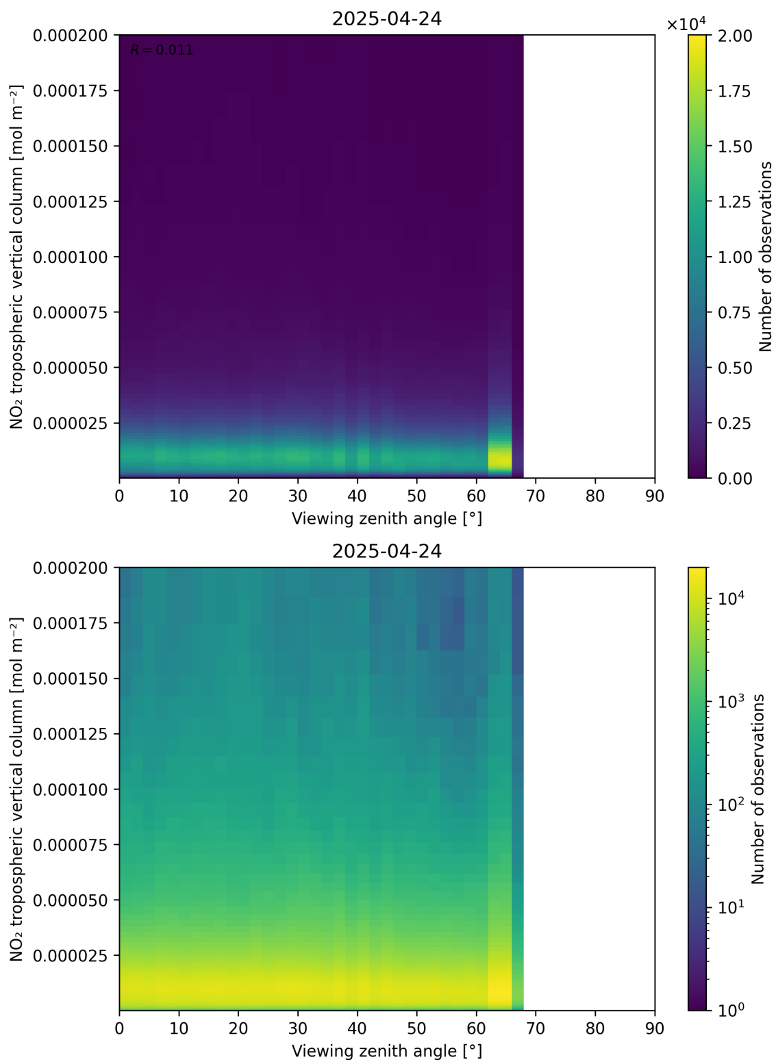
Figure 169: Scatter density plot of “Viewing zenith angle” against “NO 2 tropospheric vertical column” for 2025-04-24 to 2025-04-25.
