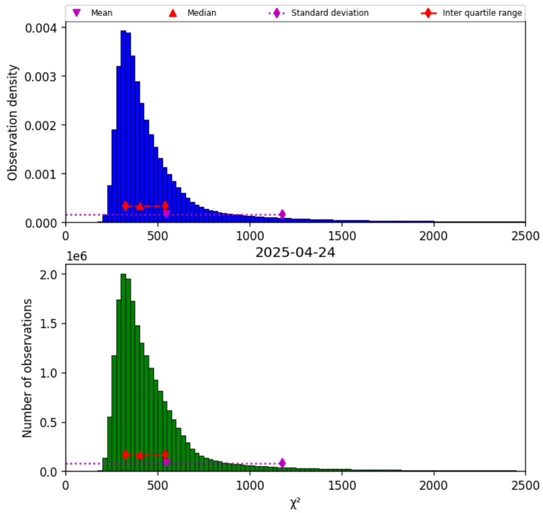
Figure 42: Histogram of " \chi^2 " for 2025-04-24 to 2025-04-25
