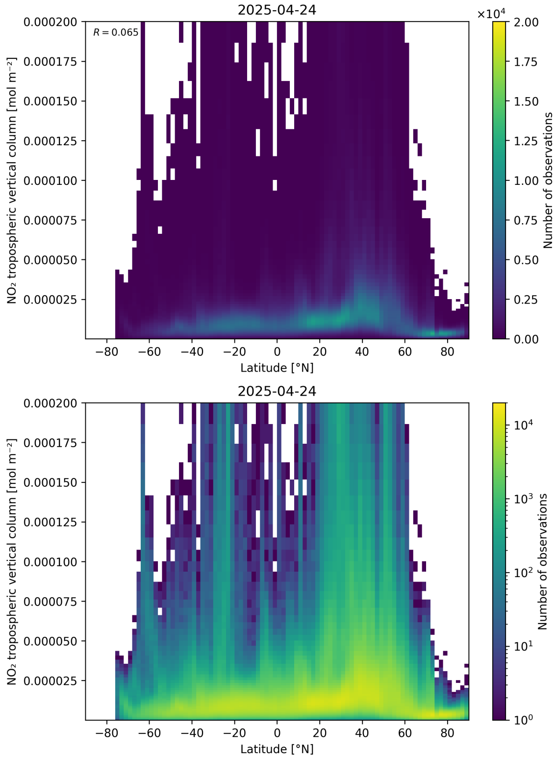
Figure 92: Scatter density plot of “Latitude” against “NO 2 tropospheric vertical column” for 2025-04-24 to 2025-04-25.
