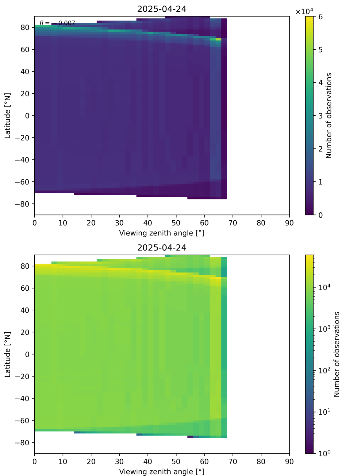
Figure 163: Scatter density plot of “Viewing zenith angle” against “Latitude” for 2025-04-24 to 2025-04-25.
