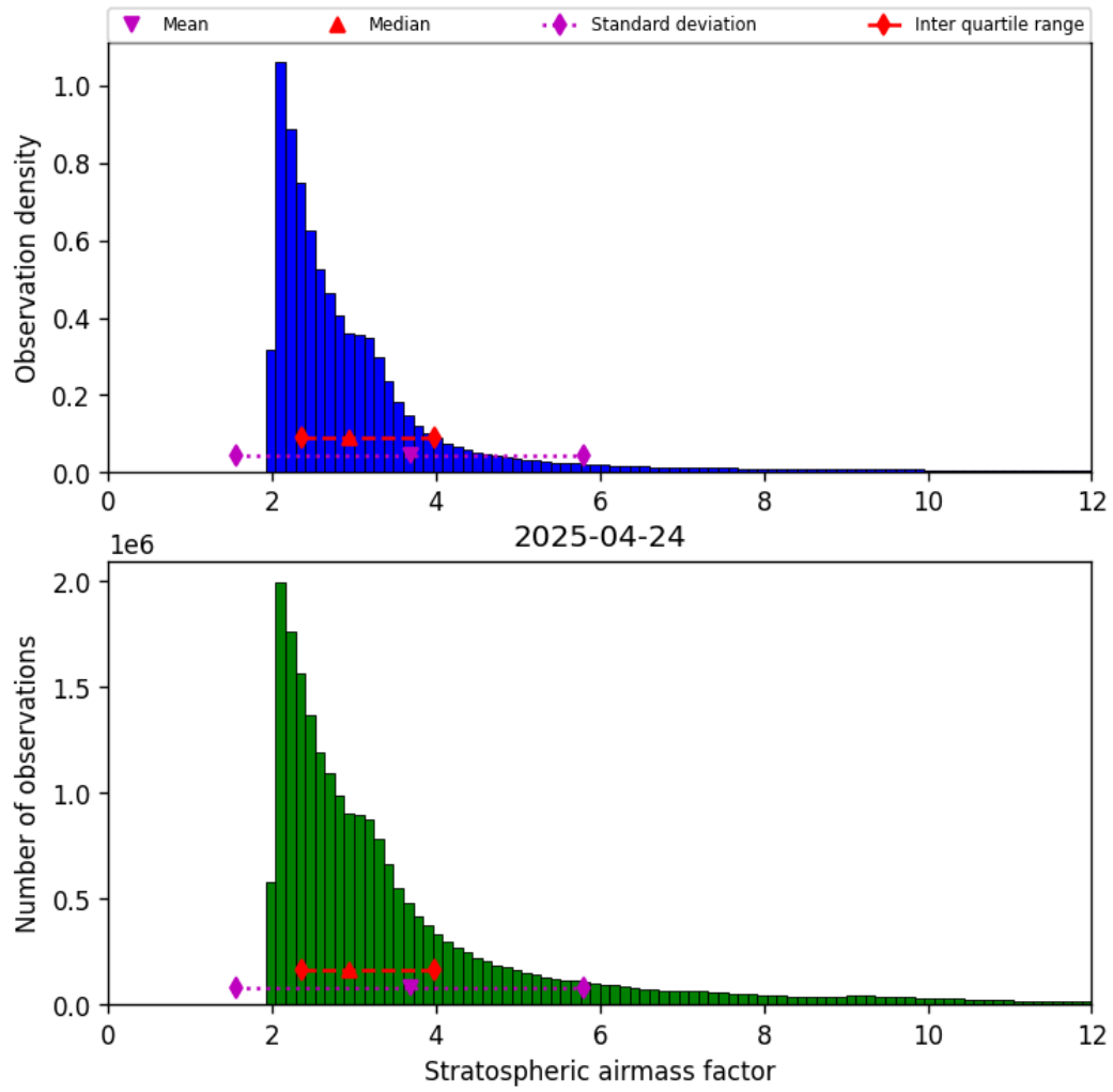
Figure 44: Histogram of “Stratospheric airmass factor” for 2025-04-24 to 2025-04-25
