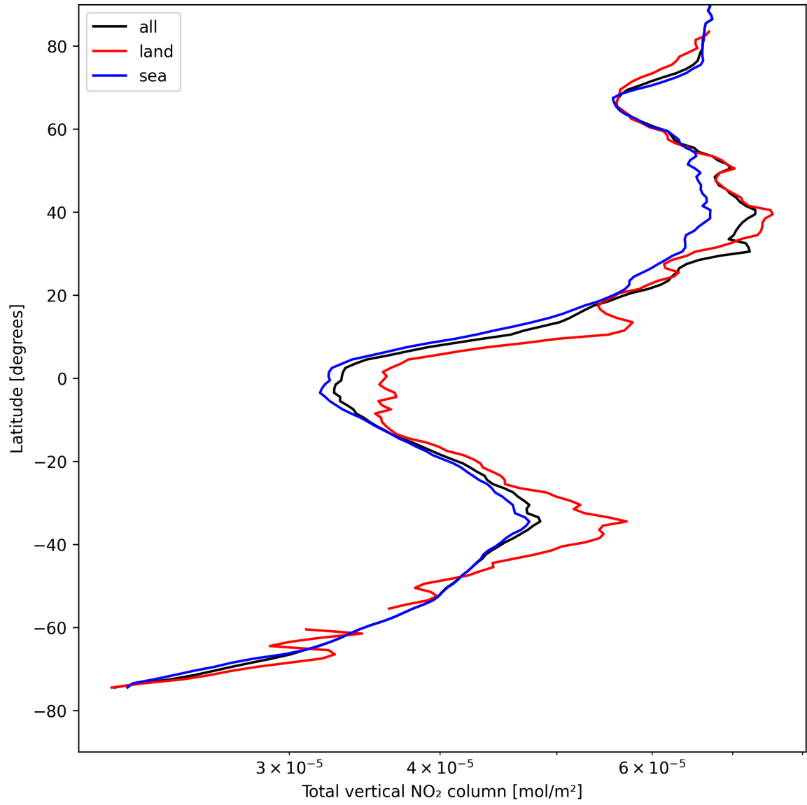
Figure 21: Zonal average of “Total vertical NO 2 column” for 2025-04-24 to 2025-04-25.
