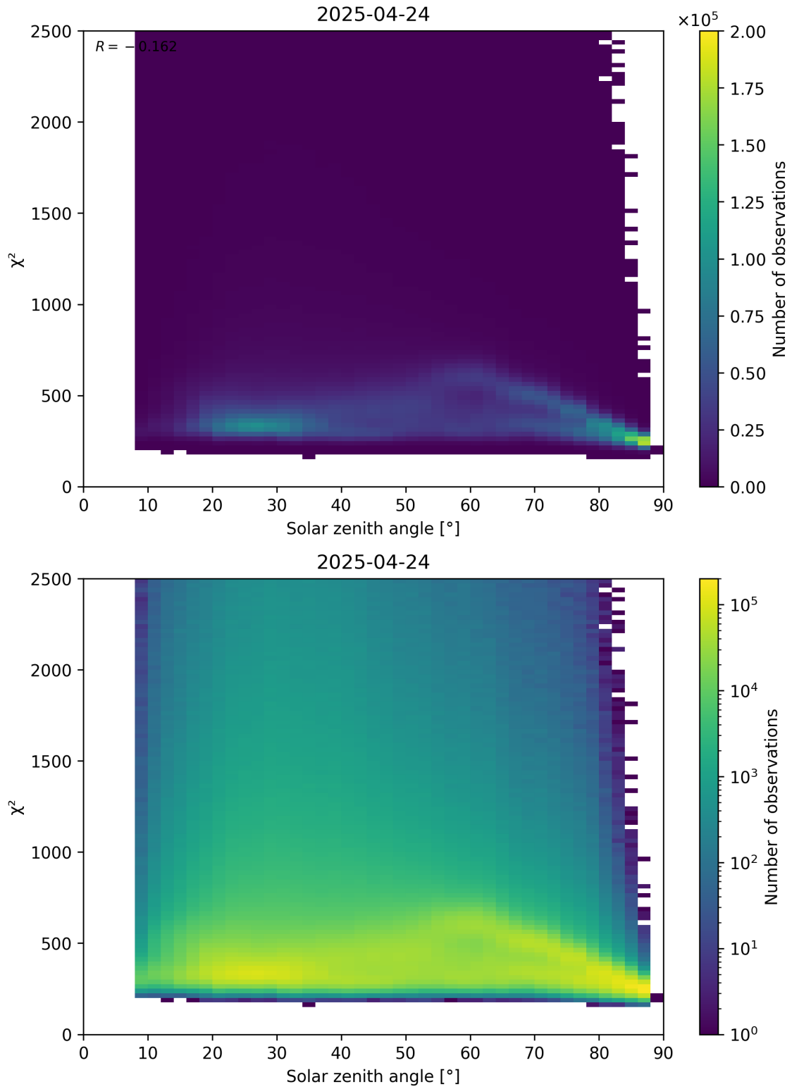
Figure 148: Scatter density plot of “Solar zenith angle” against “ \chi^2 ” for 2025-04-24 to 2025-04-25.
