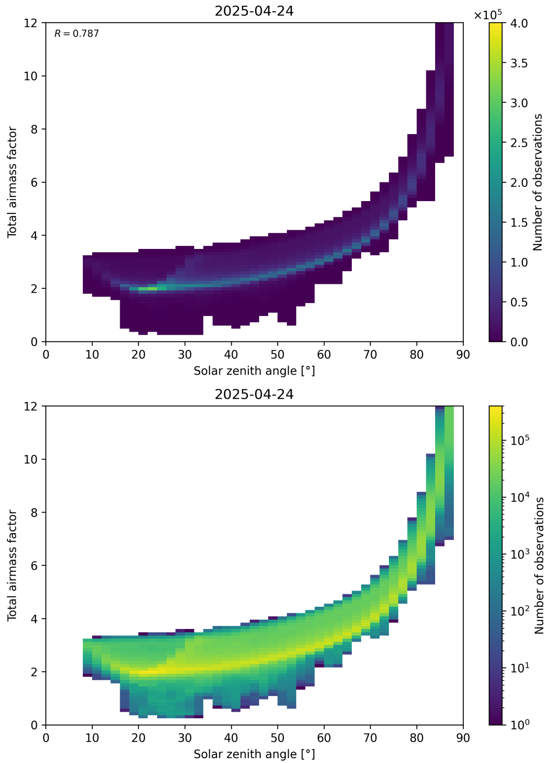
Figure 146: Scatter density plot of “Solar zenith angle” against “Total air mass factor” for 2025-04-24 to 2025-04-25.
