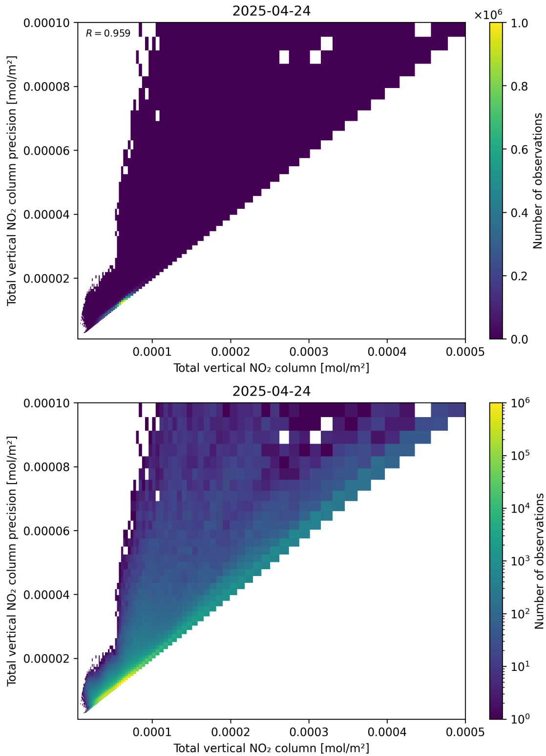
Figure 114: Scatter density plot of “Total vertical NO 2 column” against “Total vertical NO 2 column precision” for 2025-04-24 to 2025-04-25.
