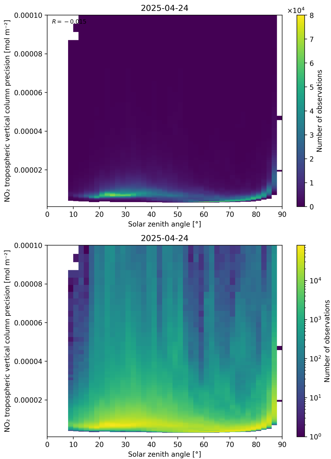
Figure 156: Scatter density plot of “Solar zenith angle” against “NO 2 tropospheric vertical column precision” for 2025-04-24 to 2025-04-25.
