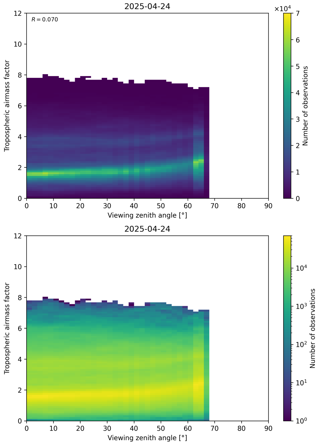
Figure 161: Scatter density plot of “Viewing zenith angle” against “Tropospheric airmass factor” for 2025-04-24 to 2025-04-25.
