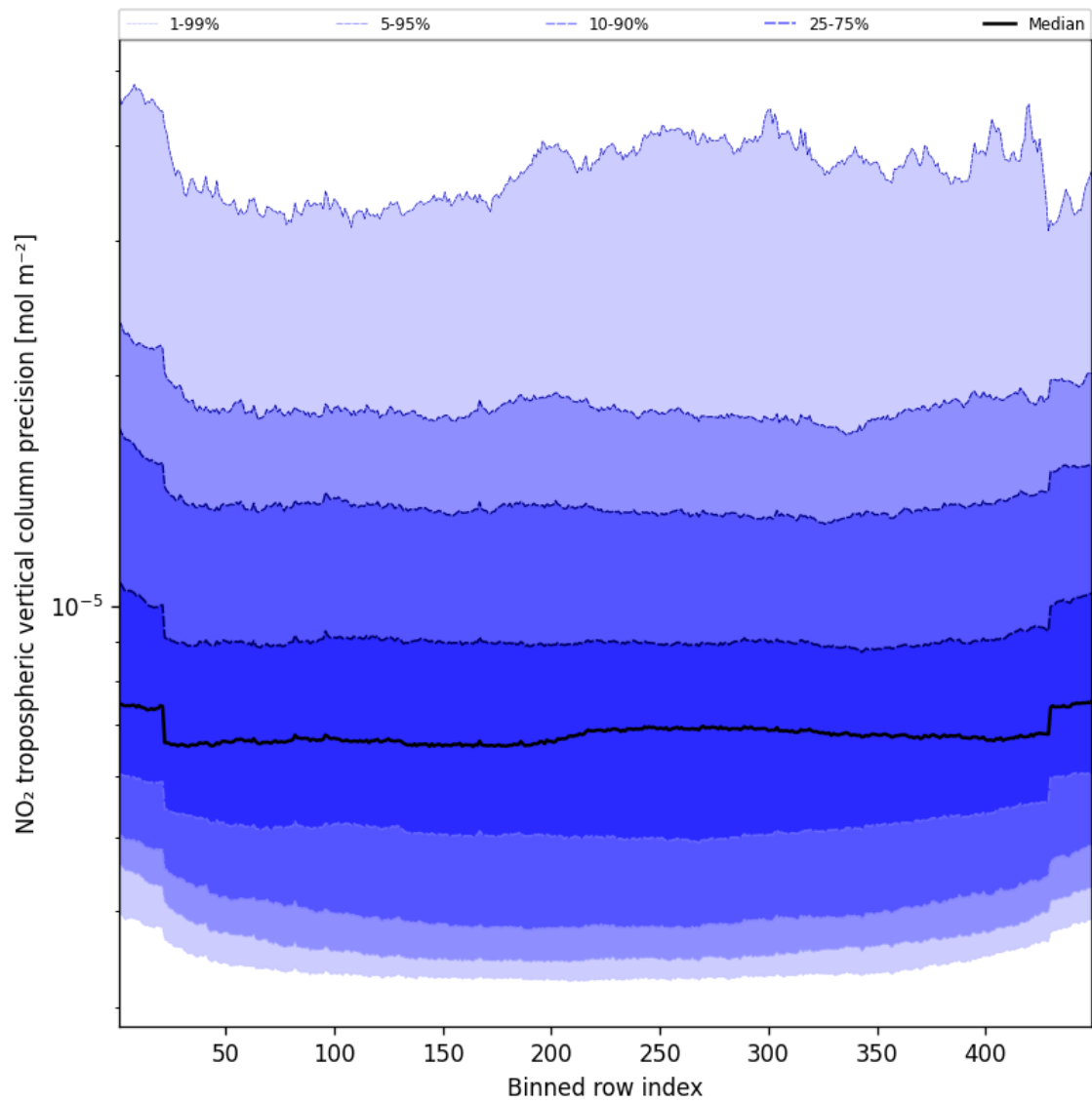
Figure 47: Along track statistics of “NO 2 tropospheric vertical column precision” for 2025-04-24 to 2025-04-25
