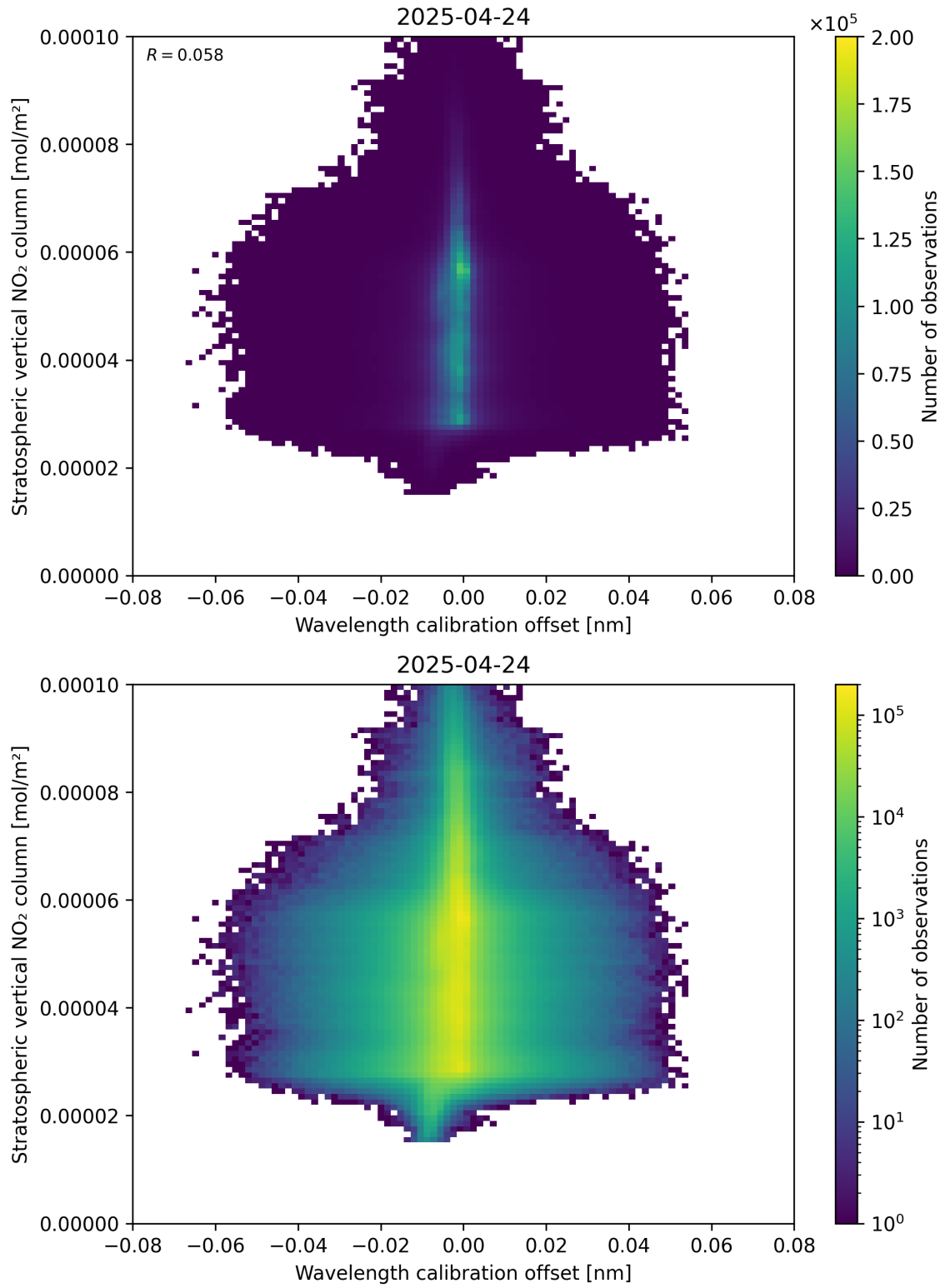
Figure 176: Scatter density plot of “Wavelength calibration offset” against “Stratospheric vertical NO 2 column” for 2025-04-24 to 2025-04-25.
