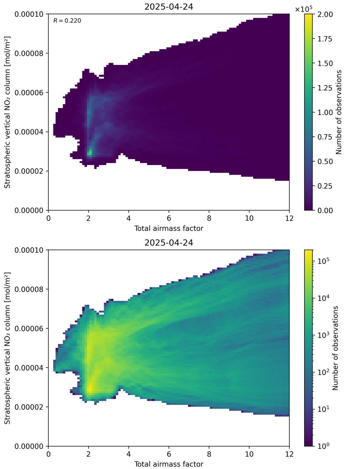
Figure 64: Scatter density plot of “Total airmass factor” against “Stratospheric vertical \text{NO}_2 column” for 2025-04-24 to 2025-04-25.
