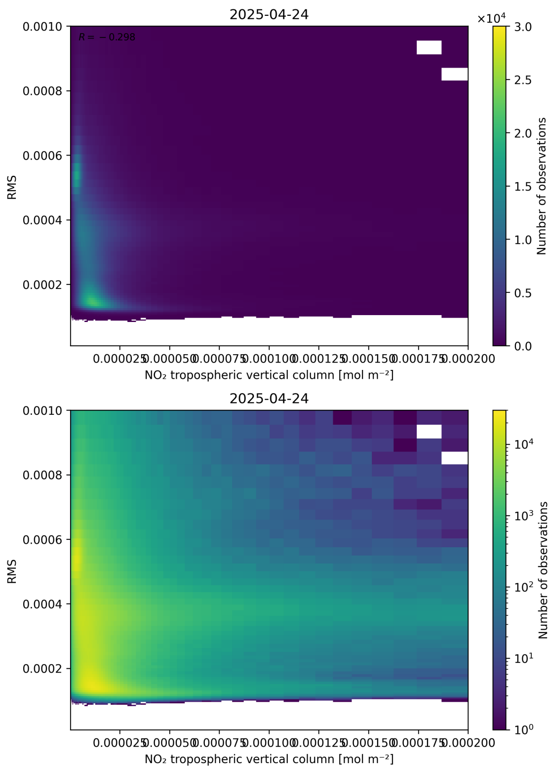
Figure 142: Scatter density plot of “NO 2 tropospheric vertical column” against “RMS” for 2025-04-24 to 2025-04-25.
