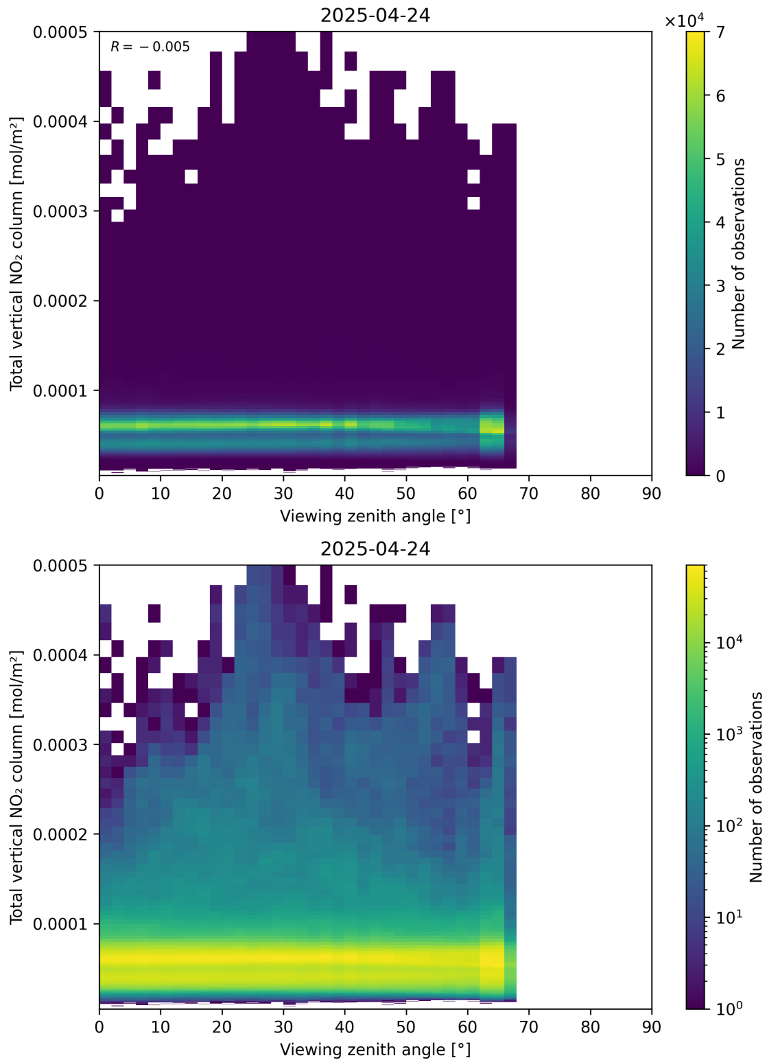
Figure 167: Scatter density plot of “Viewing zenith angle” against “Total vertical NO 2 column” for 2025-04-24 to 2025-04-25.
