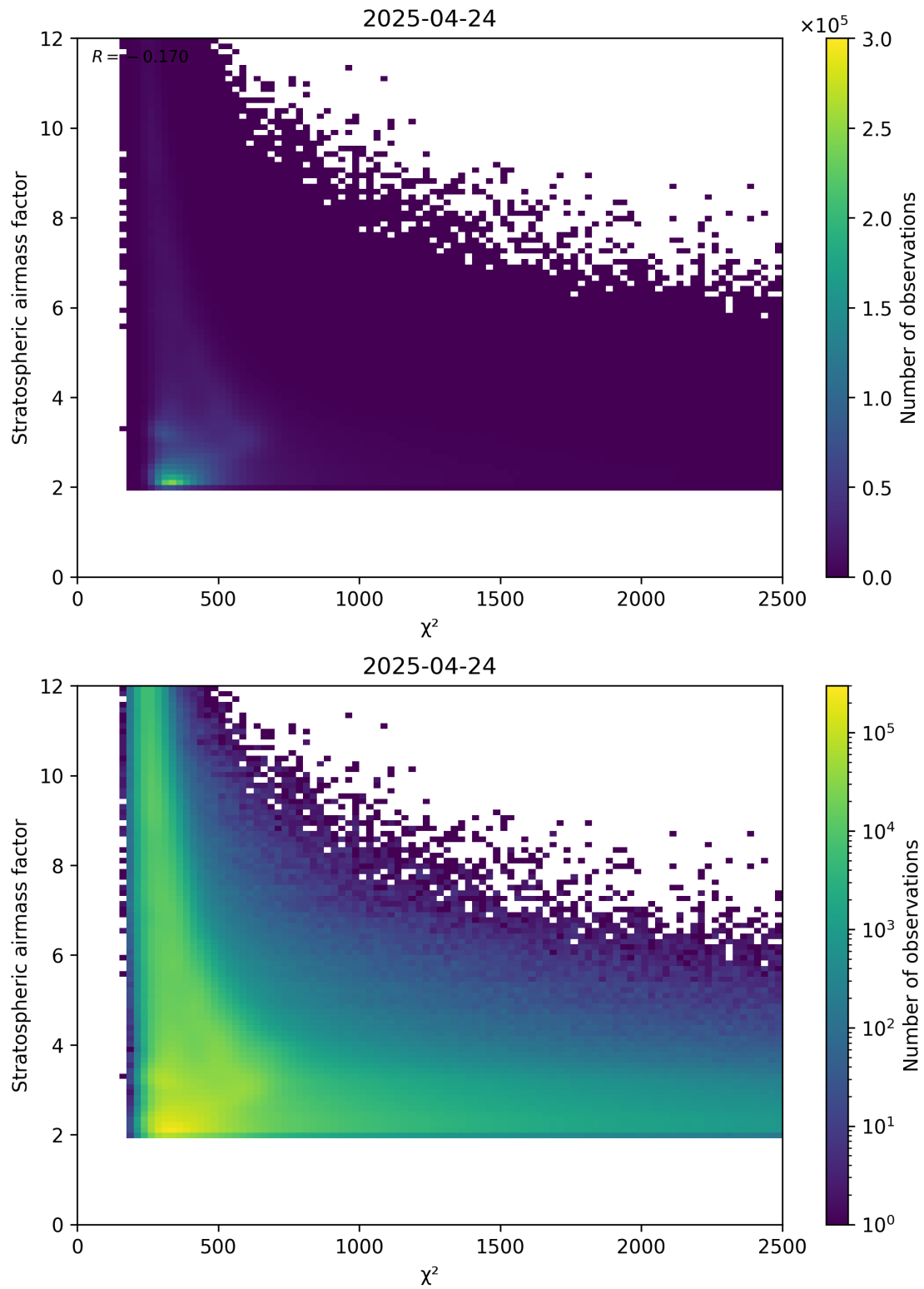
Figure 81: Scatter density plot of “ \chi^2 ” against “Stratospheric airmass factor” for 2025-04-24 to 2025-04-25.
