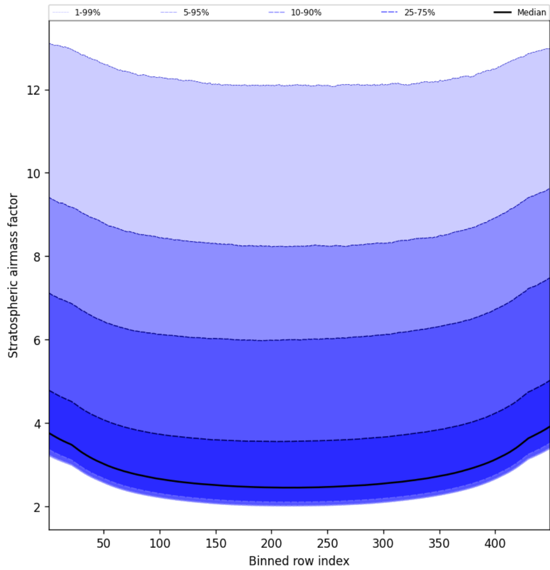
Figure 61: Along track statistics of “Stratospheric air mass factor” for 2025-04-24 to 2025-04-25
