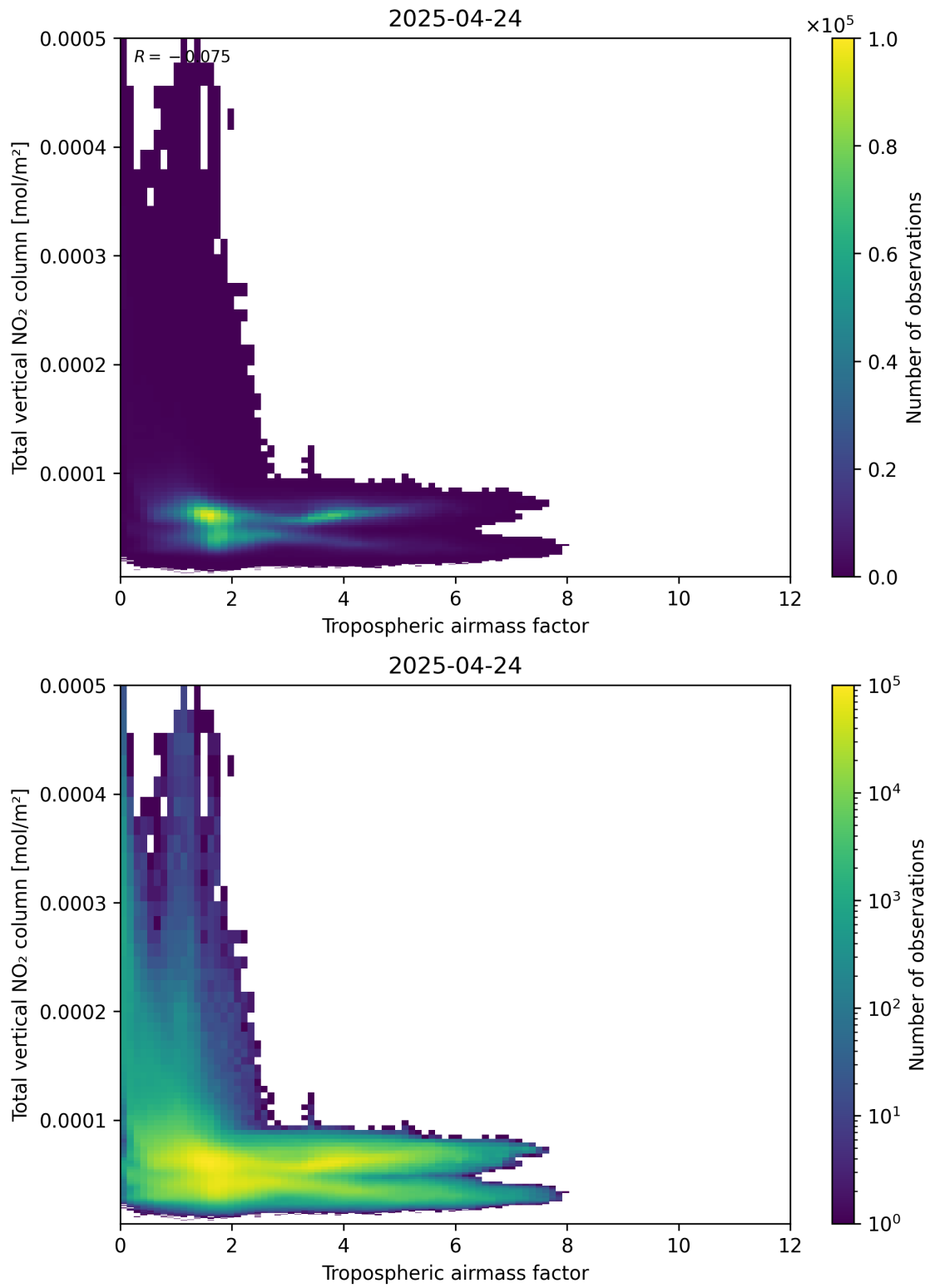
Figure 77: Scatter density plot of “Tropospheric airmass factor” against “Total vertical NO 2 column” for 2025-04-24 to 2025-04-25.
