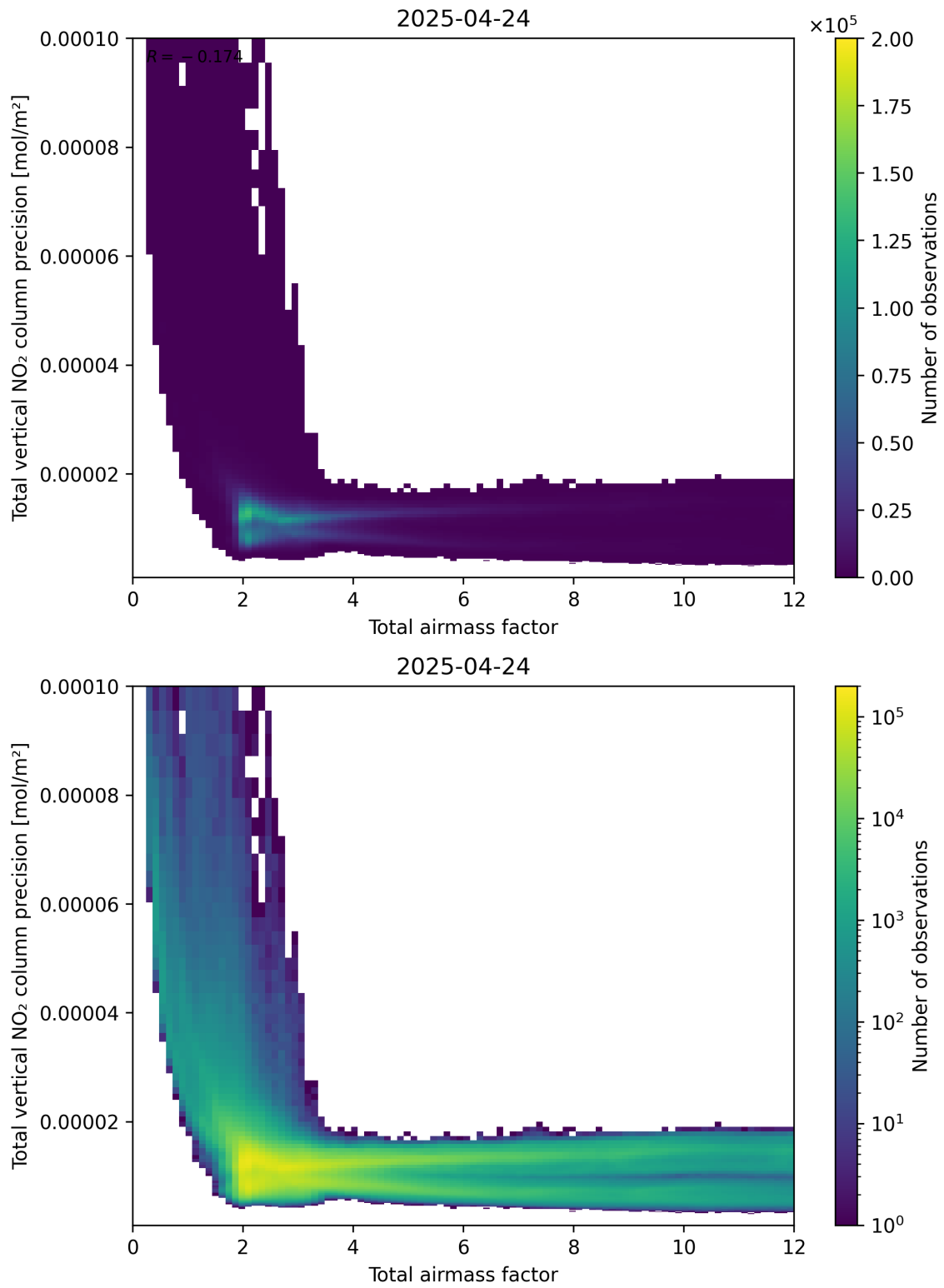
Figure 68: Scatter density plot of “Total airmass factor” against “Total vertical NO 2 column precision” for 2025-04-24 to 2025-04-25.
