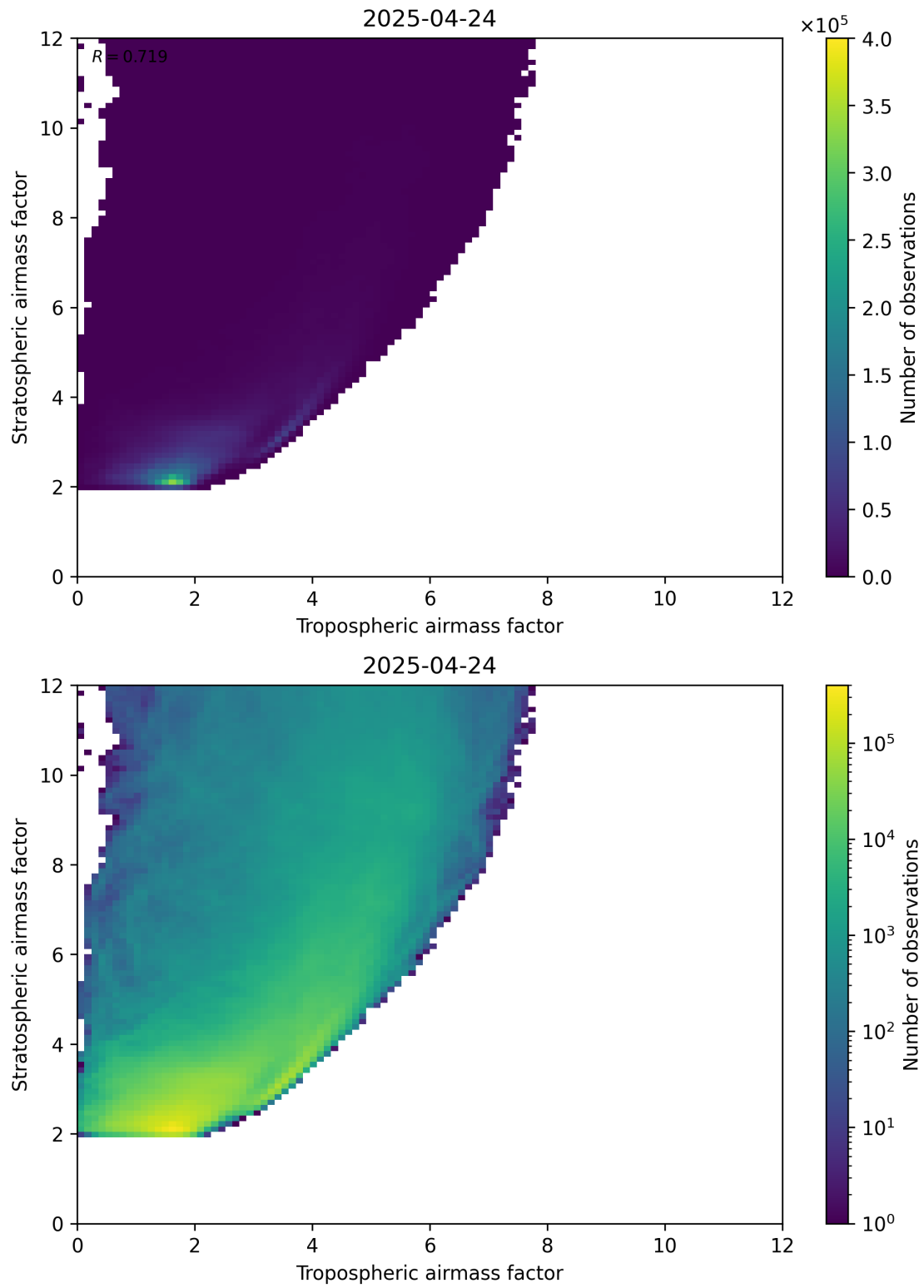
Figure 71: Scatter density plot of “Tropospheric airmass factor” against “Stratospheric airmass factor” for 2025-04-24 to 2025-04-25.
