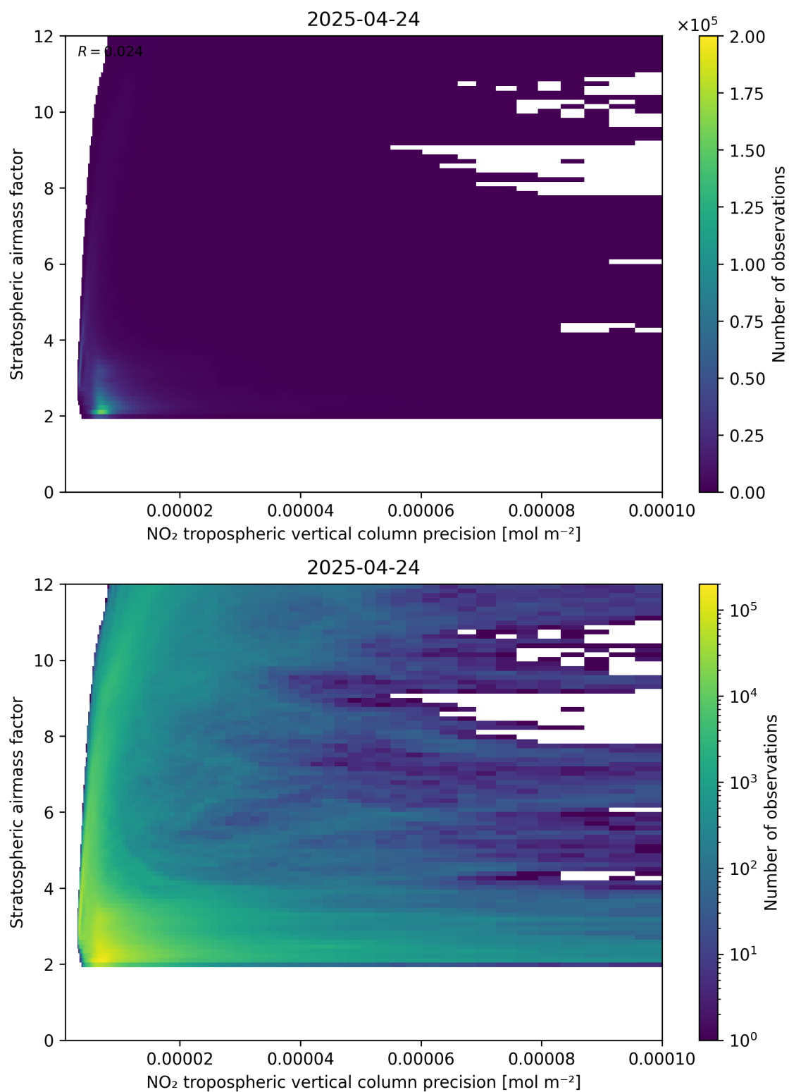
Figure 131: Scatter density plot of “NO 2 tropospheric vertical column precision” against “Stratospheric airmass factor” for 2025-04-24 to 2025-04-25.
