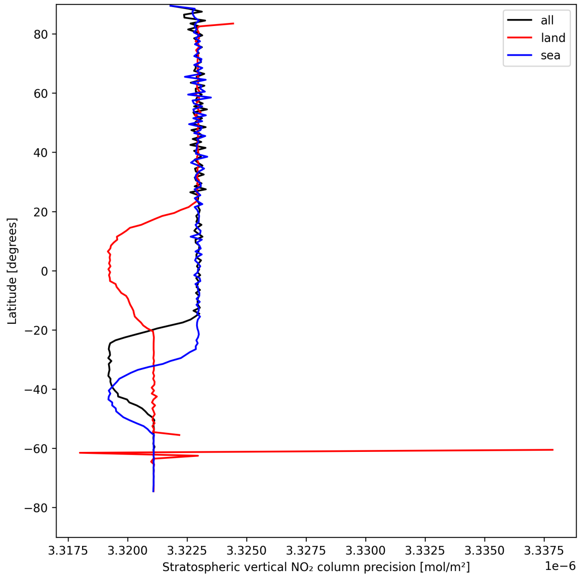
Figure 20: Zonal average of “Stratospheric vertical NO 2 column precision” for 2025-04-24 to 2025-04-25.
