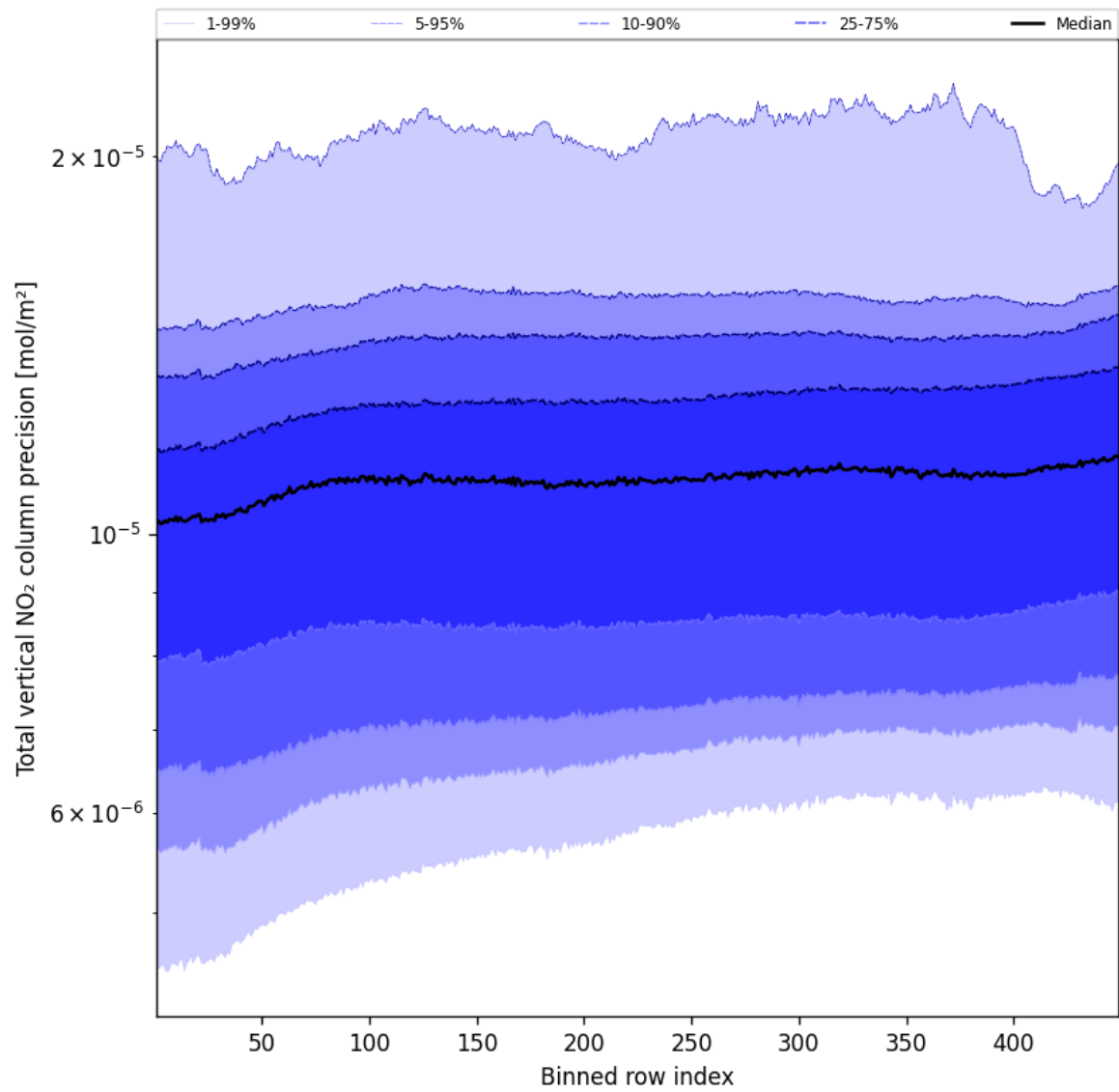
Figure 56: Along track statistics of “Total vertical NO 2 column precision” for 2025-04-24 to 2025-04-25
