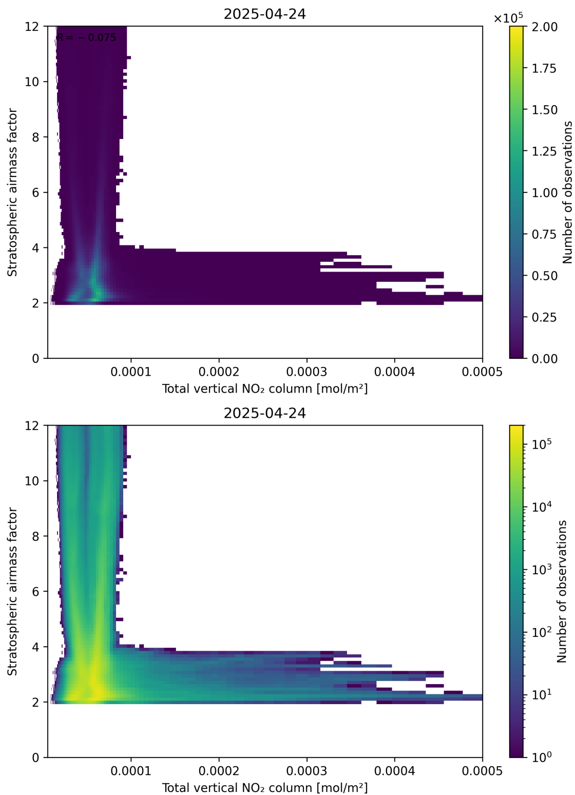
Figure 110: Scatter density plot of “Total vertical NO 2 column” against “Stratospheric airmass factor” for 2025-04-24 to 2025-04-25.
