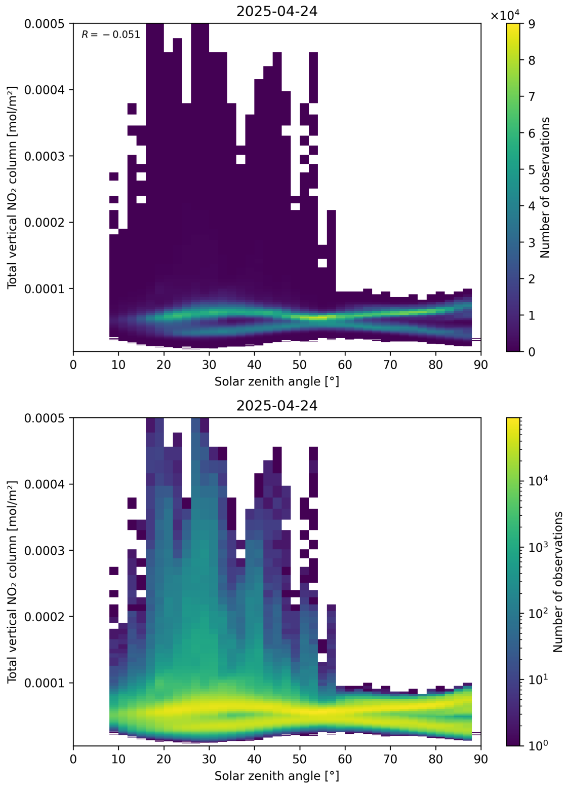
Figure 153: Scatter density plot of “Solar zenith angle” against “Total vertical NO 2 column” for 2025-04-24 to 2025-04-25.
