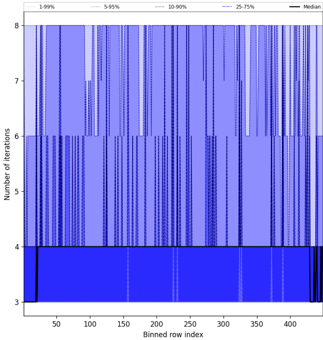
Figure 51: Along track statistics of “Number of iterations” for 2025-04-24 to 2025-04-25
