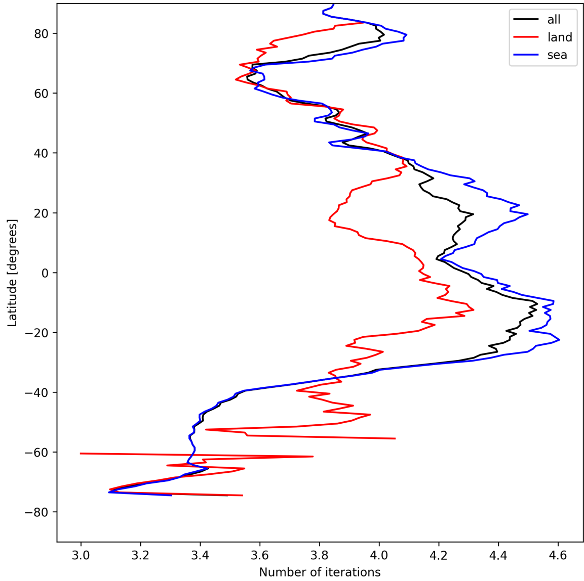
Figure 17: Zonal average of “Number of iterations” for 2025-04-24 to 2025-04-25.
