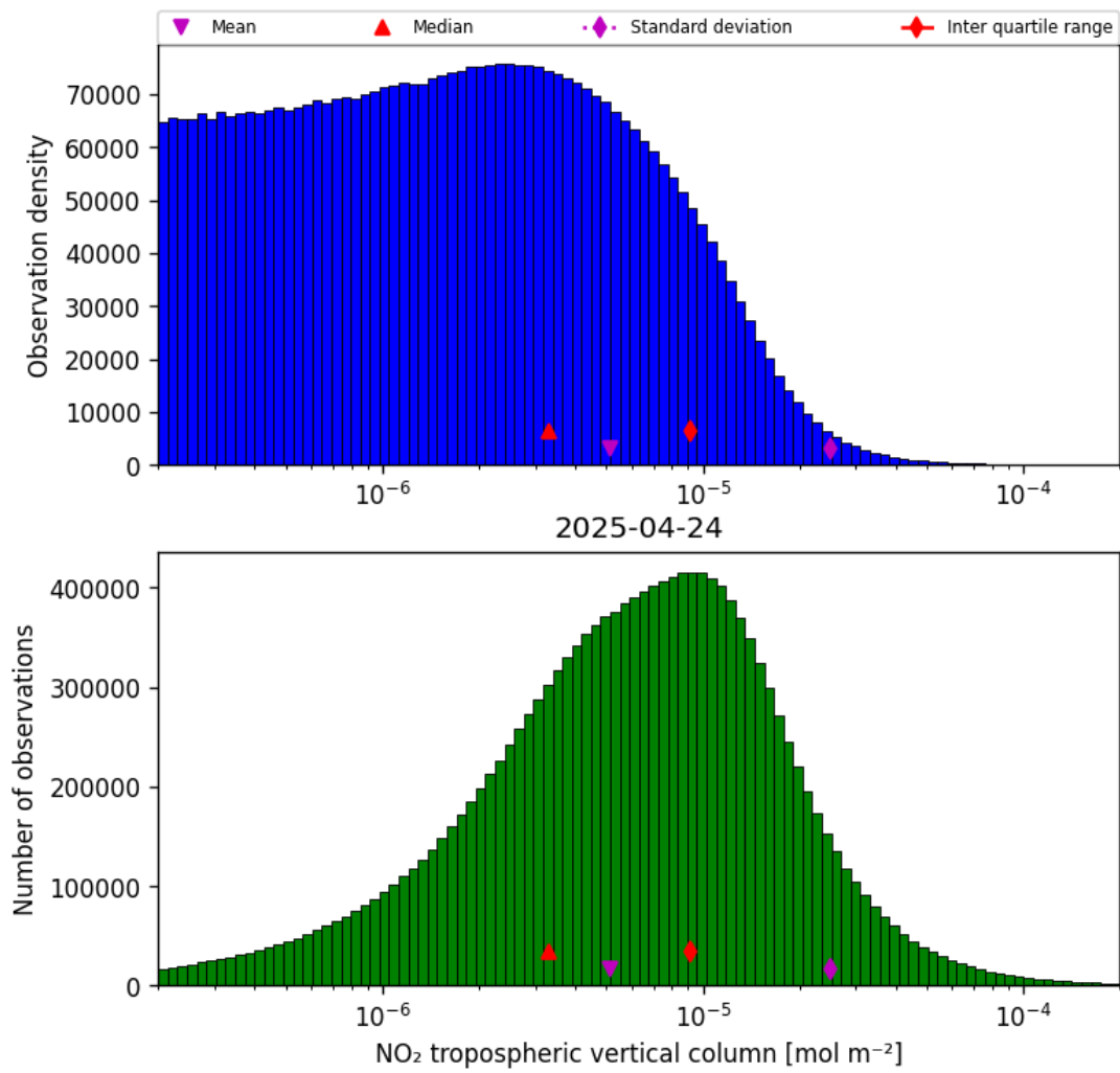
Figure 29: Histogram of “NO 2 tropospheric vertical column” for 2025-04-24 to 2025-04-25
