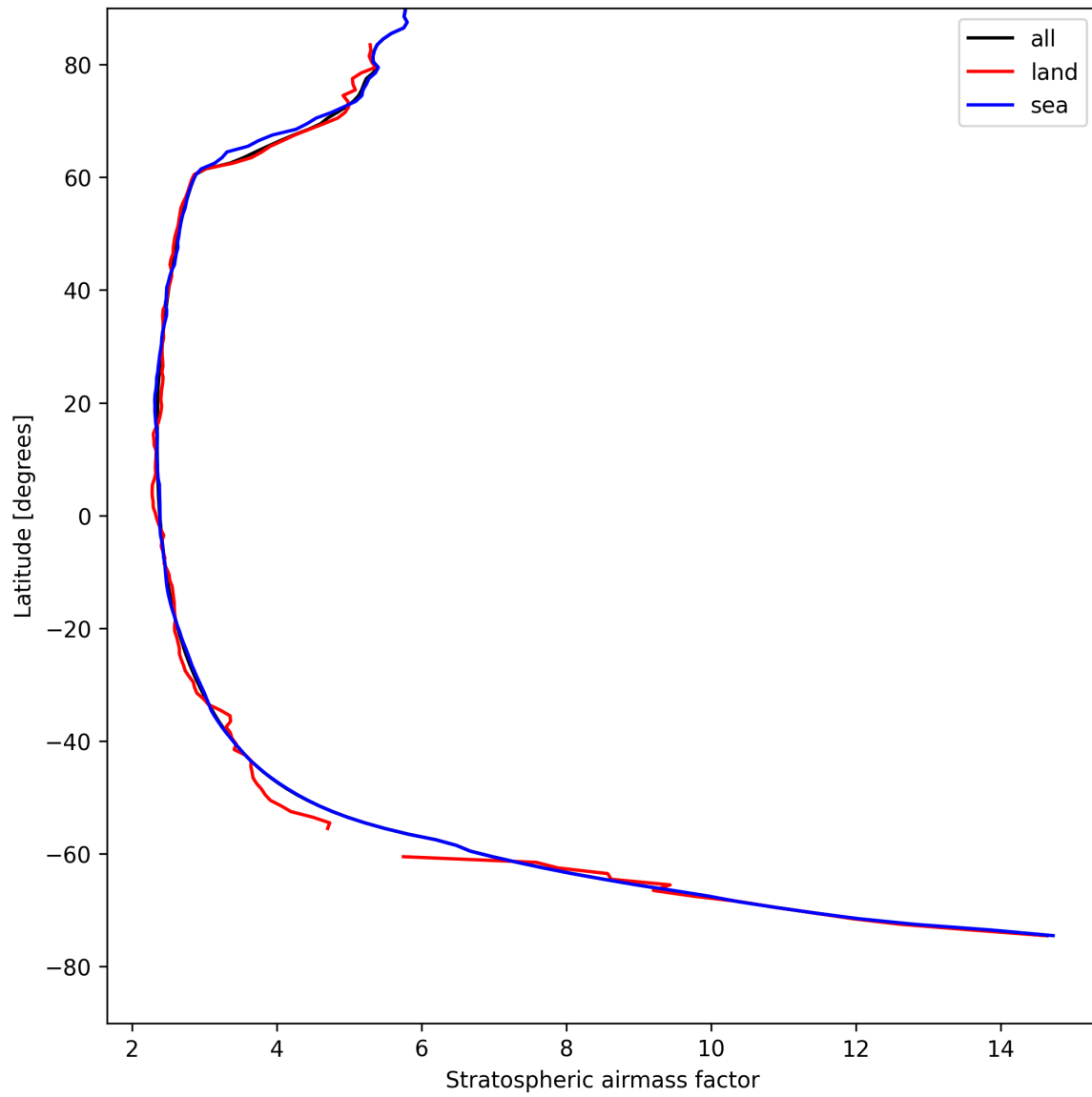
Figure 27: Zonal average of “Stratospheric airmass factor” for 2025-04-24 to 2025-04-25.
