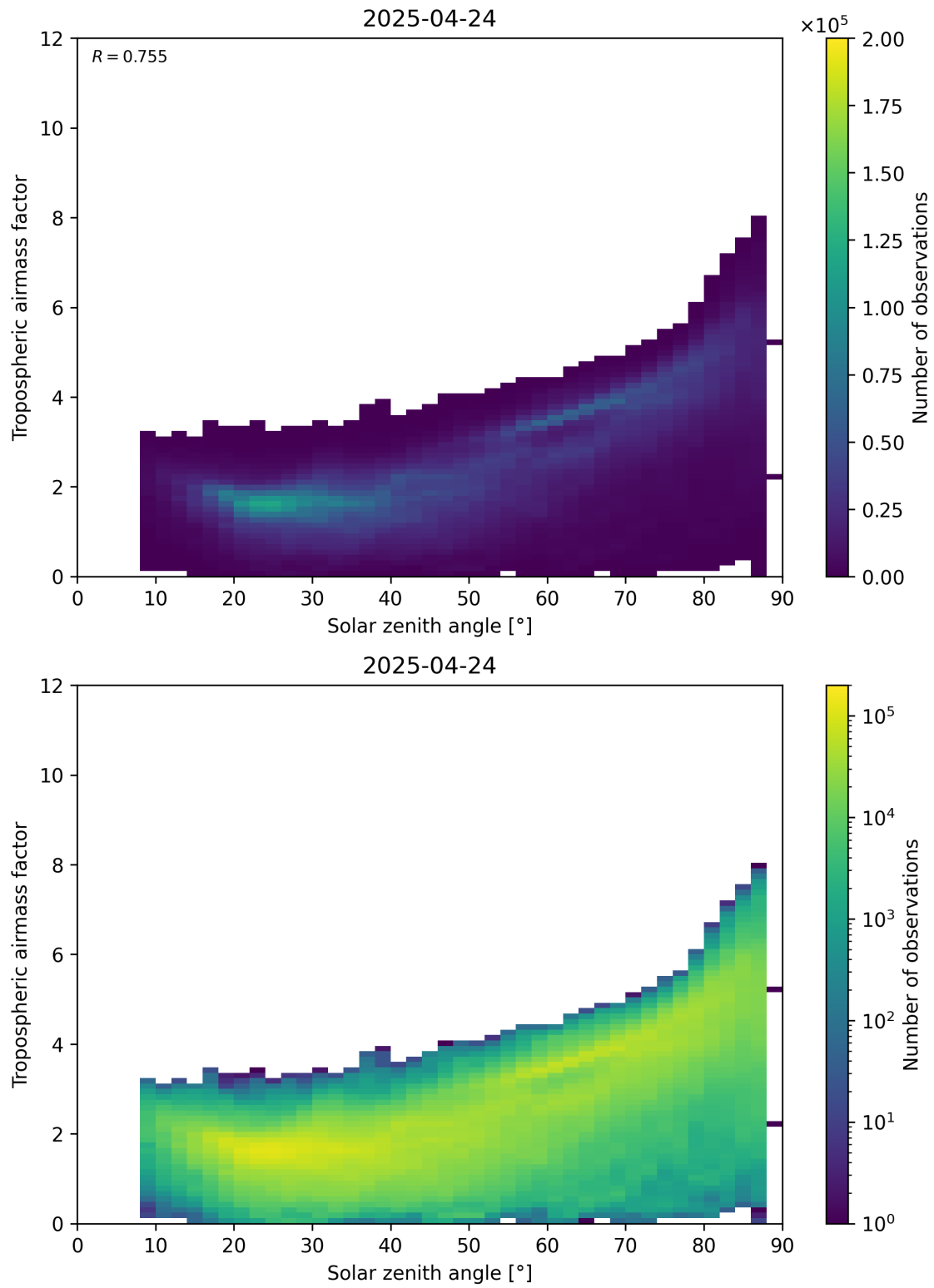
Figure 147: Scatter density plot of “Solar zenith angle” against “Tropospheric airmass factor” for 2025-04-24 to 2025-04-25.
