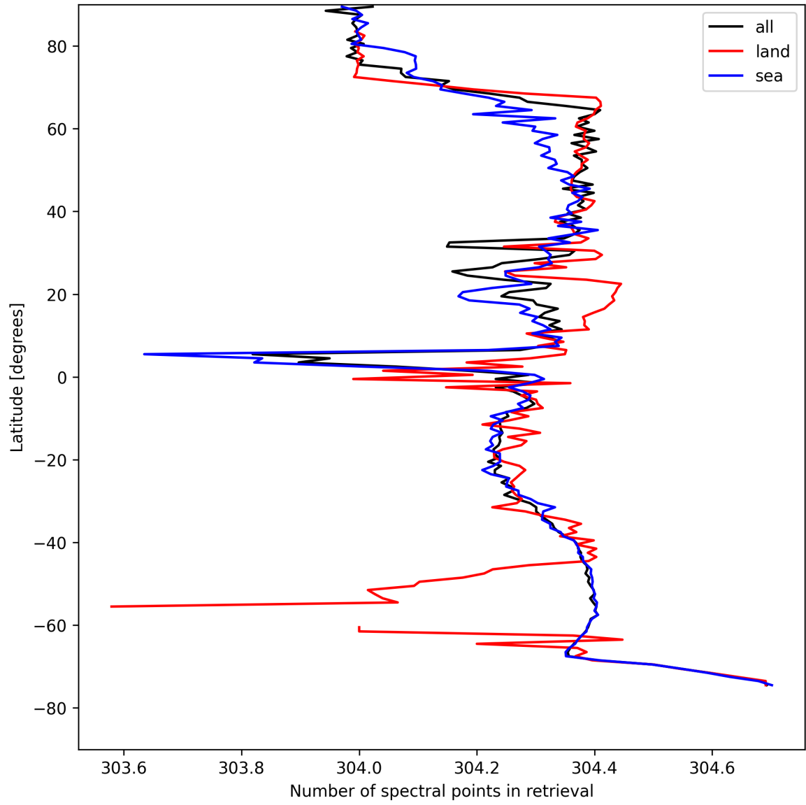
Figure 16: Zonal average of “Number of spectral points in retrieval” for 2025-04-24 to 2025-04-25.
