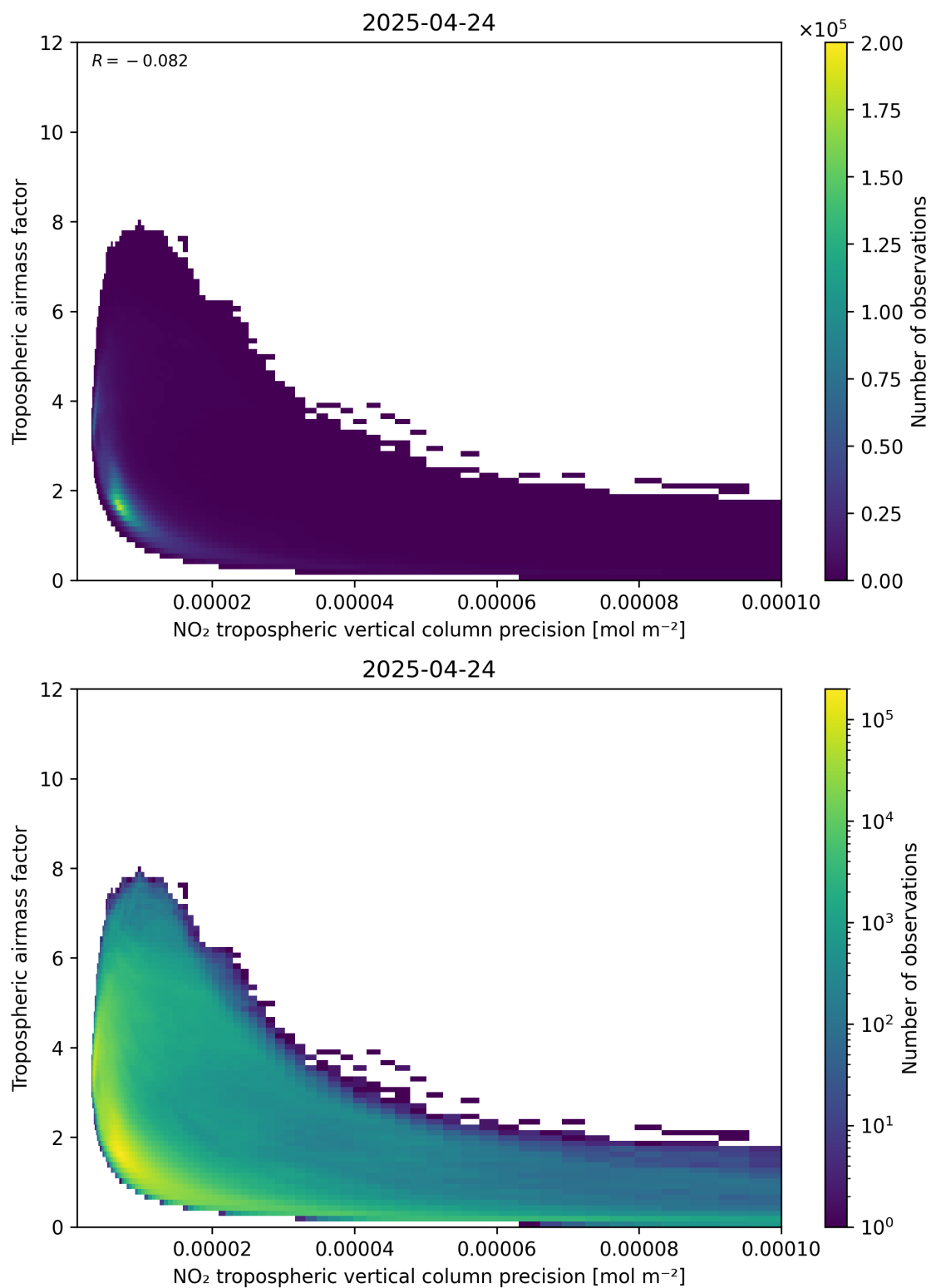
Figure 133: Scatter density plot of “NO 2 tropospheric vertical column precision” against “Tropospheric air mass factor” for 2025-04-24 to 2025-04-25.
