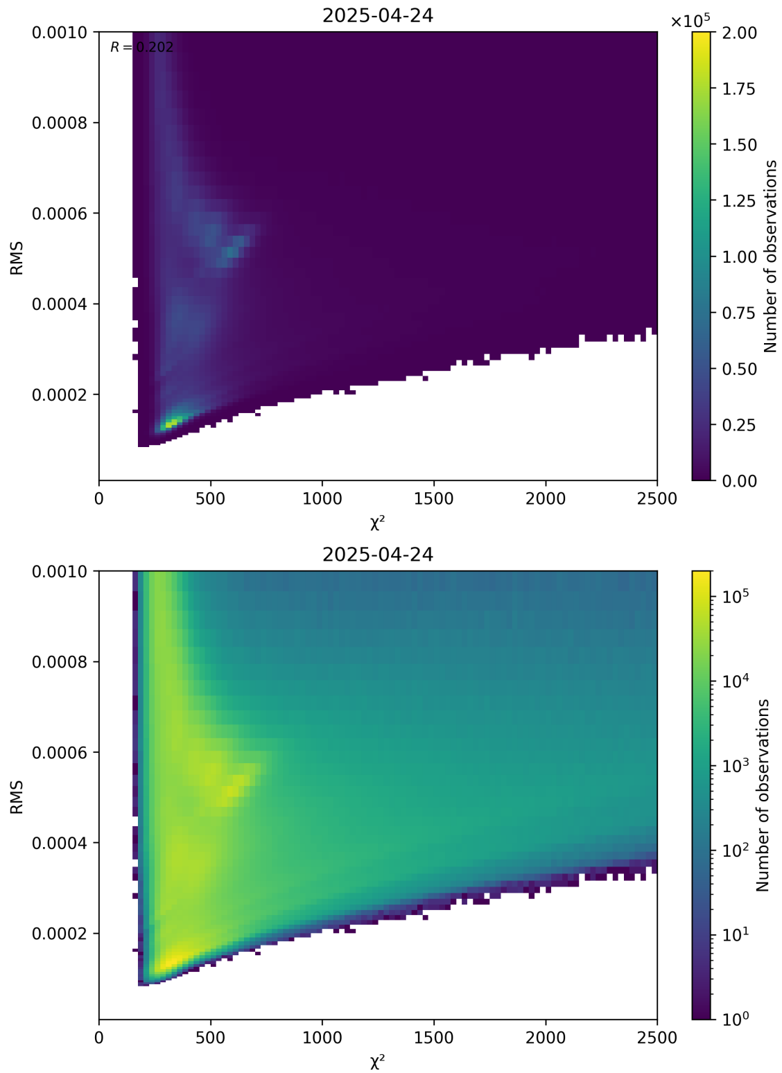
Figure 82: Scatter density plot of “ \chi^2 ” against “RMS” for 2025-04-24 to 2025-04-25.
