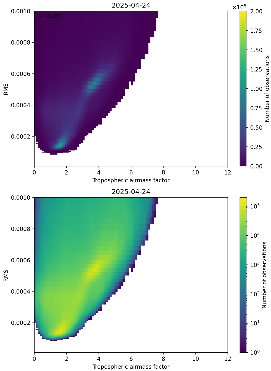
Figure 79: Scatter density plot of “Tropospheric airmass factor” against “RMS” for 2025-04-24 to 2025-04-25.
