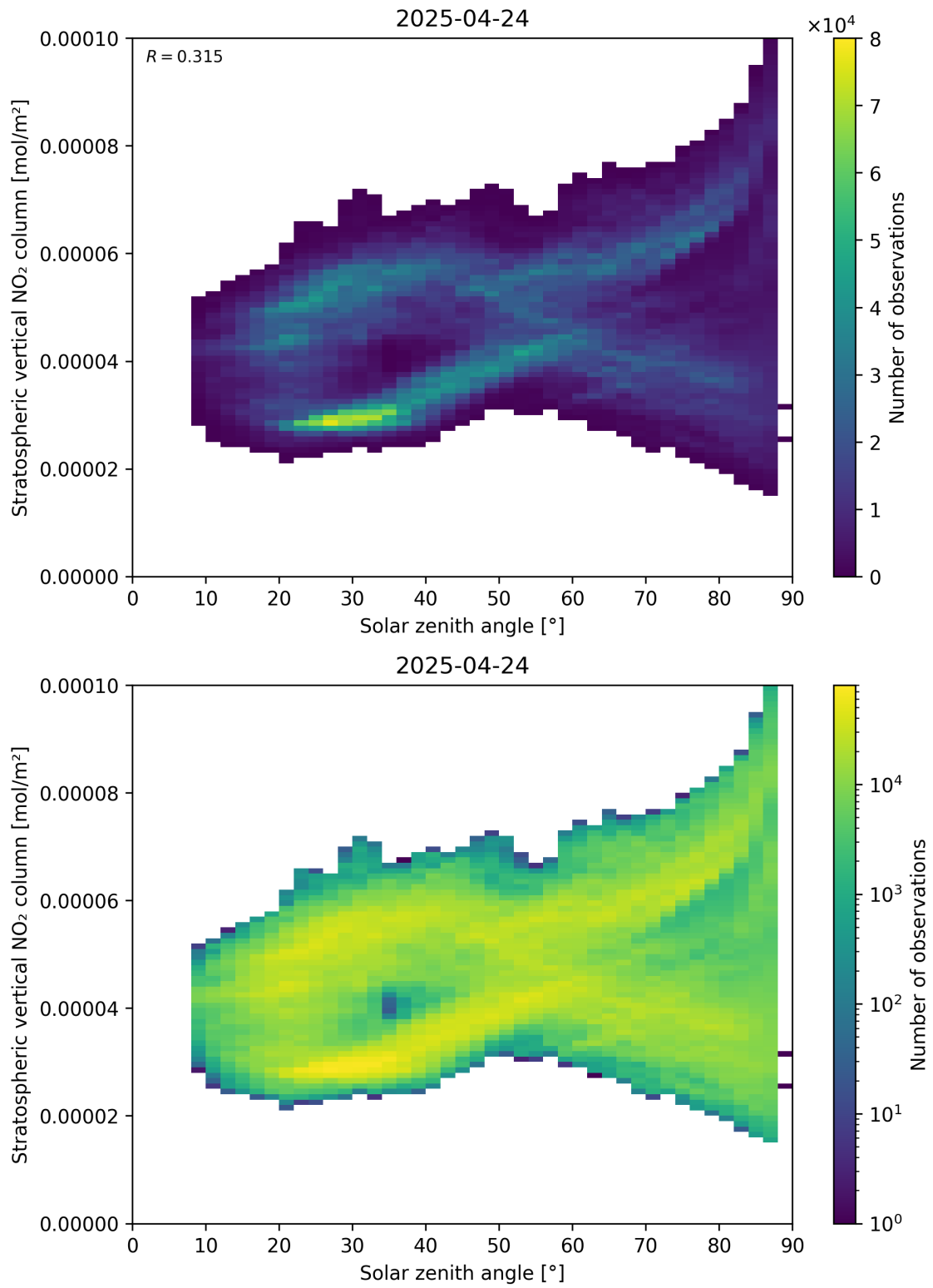
Figure 150: Scatter density plot of “Solar zenith angle” against “Stratospheric vertical NO 2 column” for 2025-04-24 to 2025-04-25.
