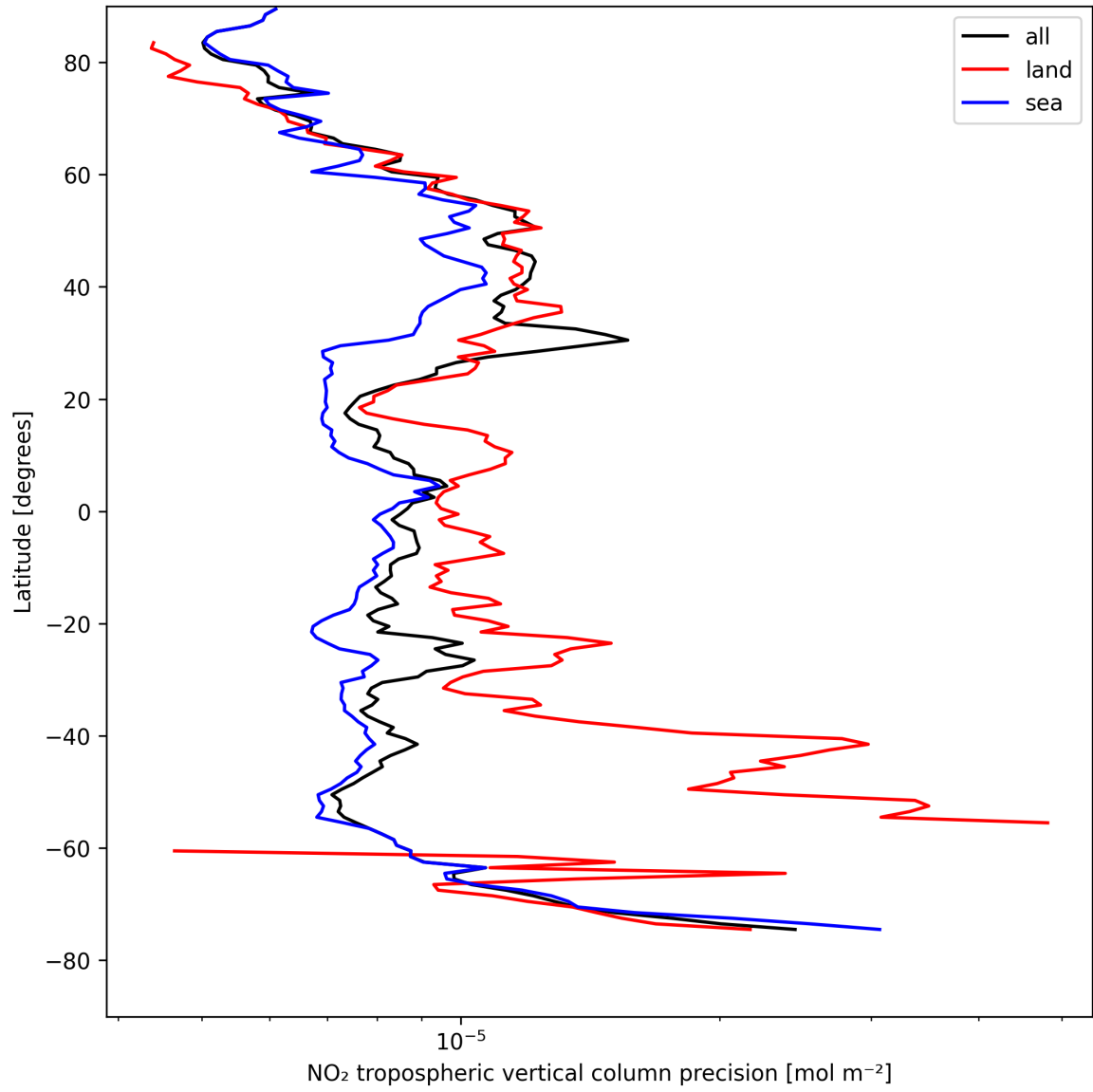
Figure 13: Zonal average of “NO 2 tropospheric vertical column precision” for 2025-04-24 to 2025-04-25.
