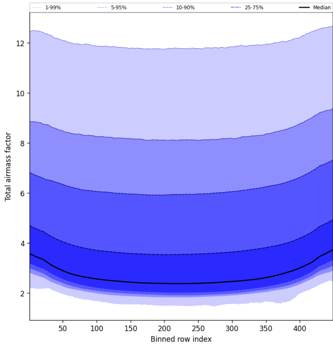
Figure 49: Along track statistics of “Total airmass factor” for 2025-04-24 to 2025-04-25
