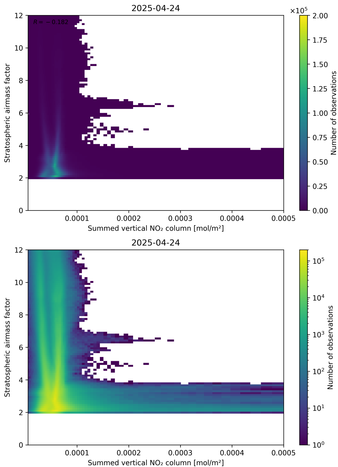
Figure 103: Scatter density plot of “Summed vertical NO 2 column” against “Stratospheric airmass factor” for 2025-04-24 to 2025-04-25.
