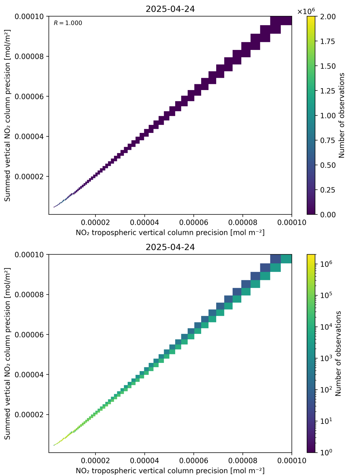
Figure 137: Scatter density plot of “NO 2 tropospheric vertical column precision” against “Summed vertical NO 2 column precision” for 2025-04-24 to 2025-04-25.
