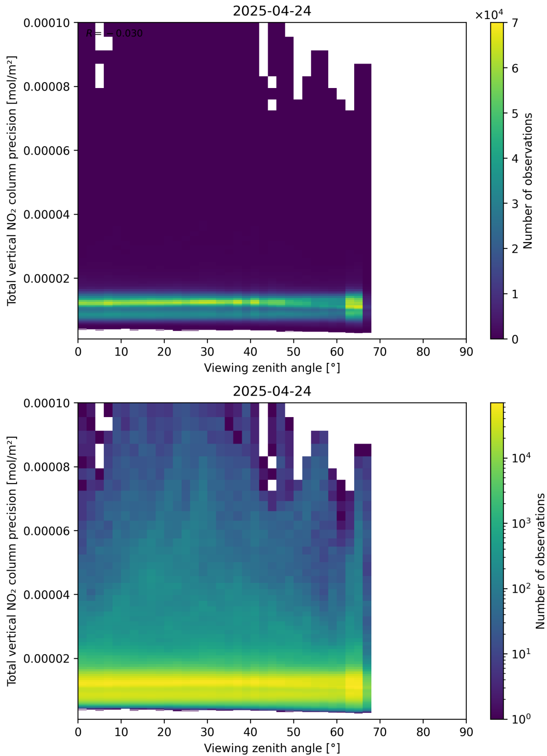
Figure 168: Scatter density plot of “Viewing zenith angle” against “Total vertical NO 2 column precision” for 2025-04-24 to 2025-04-25.
