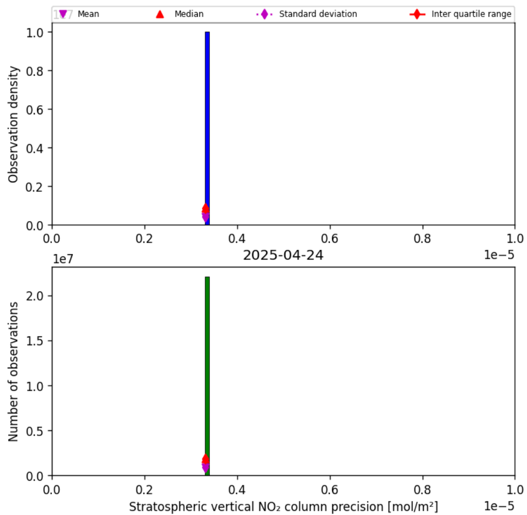
Figure 37: Histogram of “Stratospheric vertical NO 2 column precision” for 2025-04-24 to 2025-04-25
