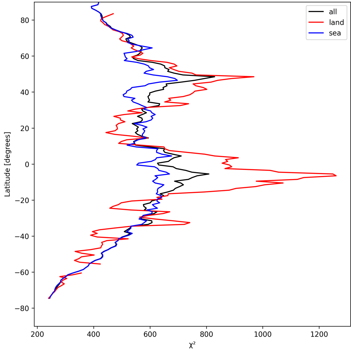
Figure 25: Zonal average of “ \chi^2 ” for 2025-04-24 to 2025-04-25.
