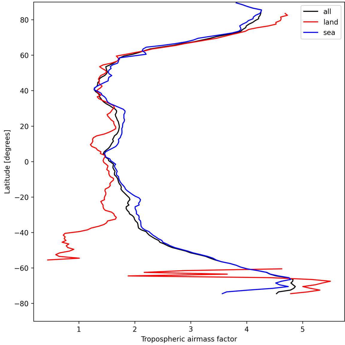
Figure 14: Zonal average of “Tropospheric airmass factor” for 2025-04-24 to 2025-04-25.
