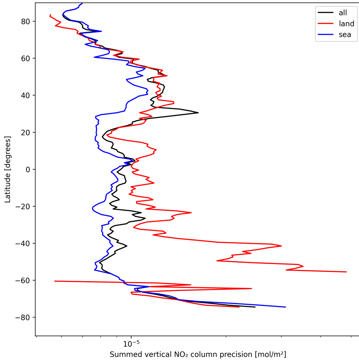
Figure 24: Zonal average of “Summed vertical NO 2 column precision” for 2025-04-24 to 2025-04-25.
