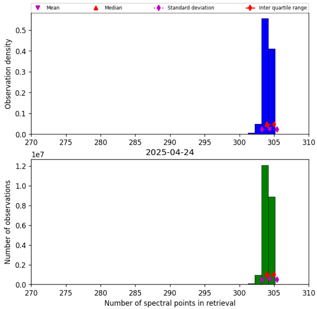
Figure 33: Histogram of “Number of spectral points in retrieval” for 2025-04-24 to 2025-04-25
