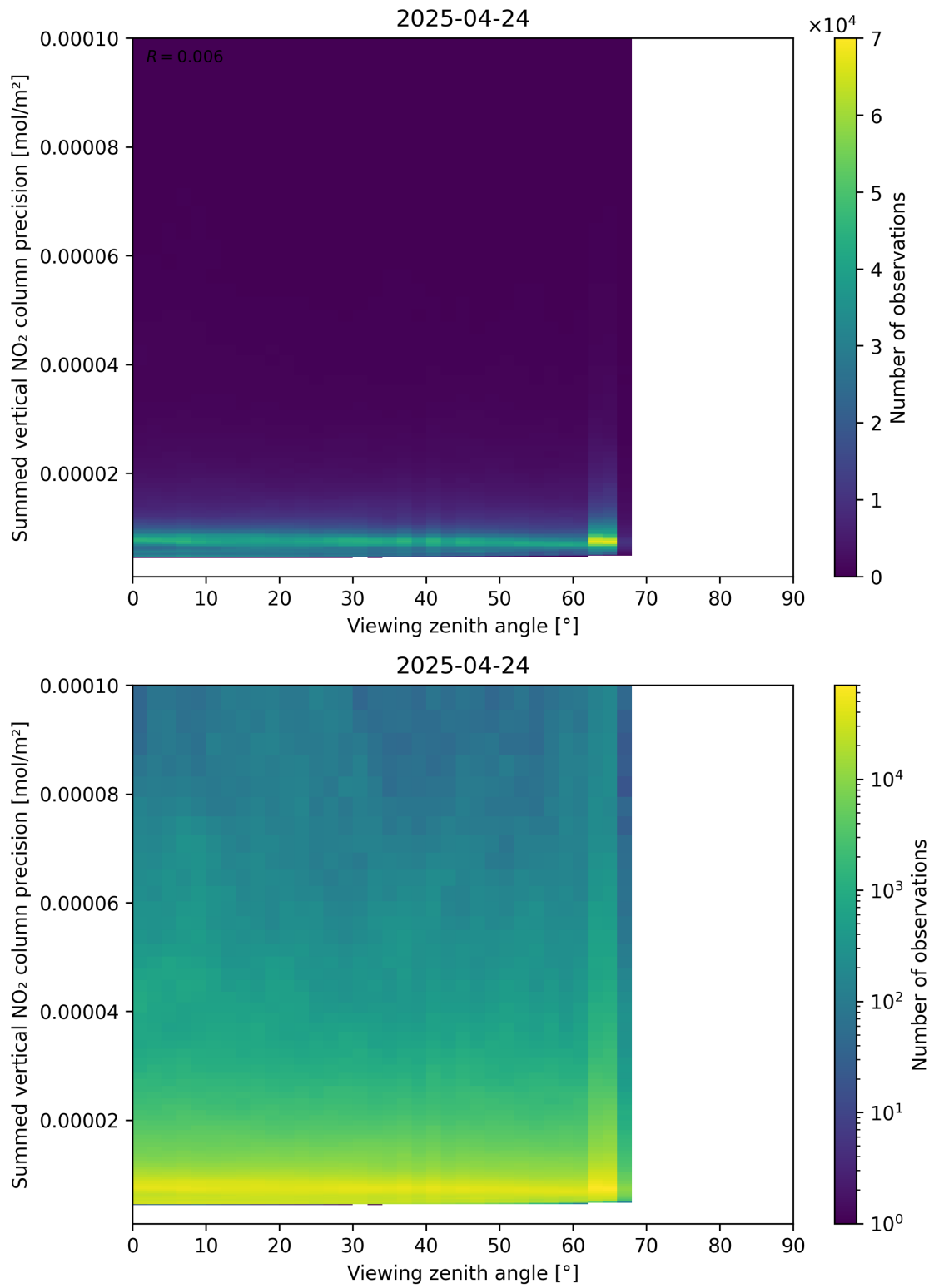
Figure 166: Scatter density plot of “Viewing zenith angle” against “Summed vertical NO 2 column precision” for 2025-04-24 to 2025-04-25.
