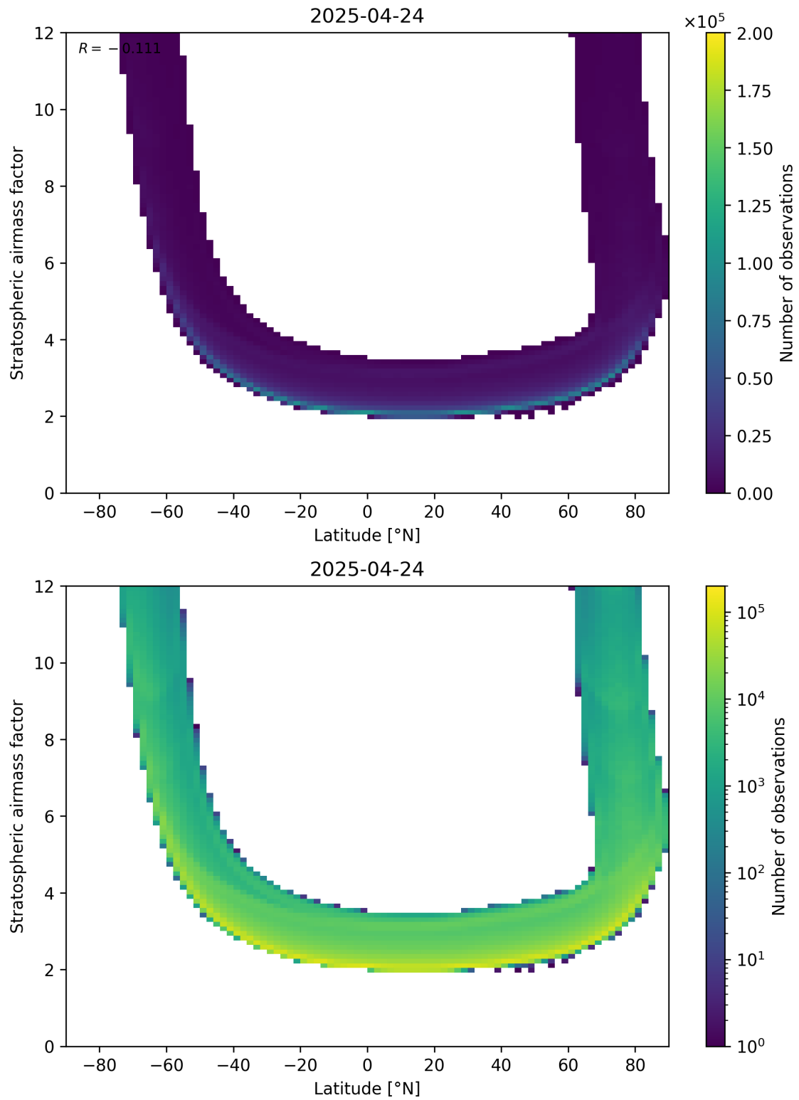
Figure 83: Scatter density plot of “Latitude” against “Stratospheric air mass factor” for 2025-04-24 to 2025-04-25.
