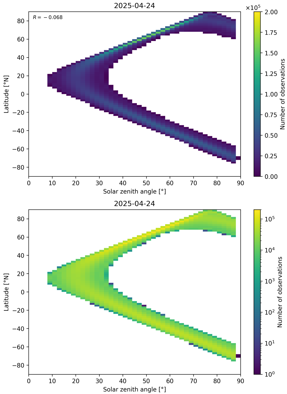
Figure 149: Scatter density plot of “Solar zenith angle” against “Latitude” for 2025-04-24 to 2025-04-25.
