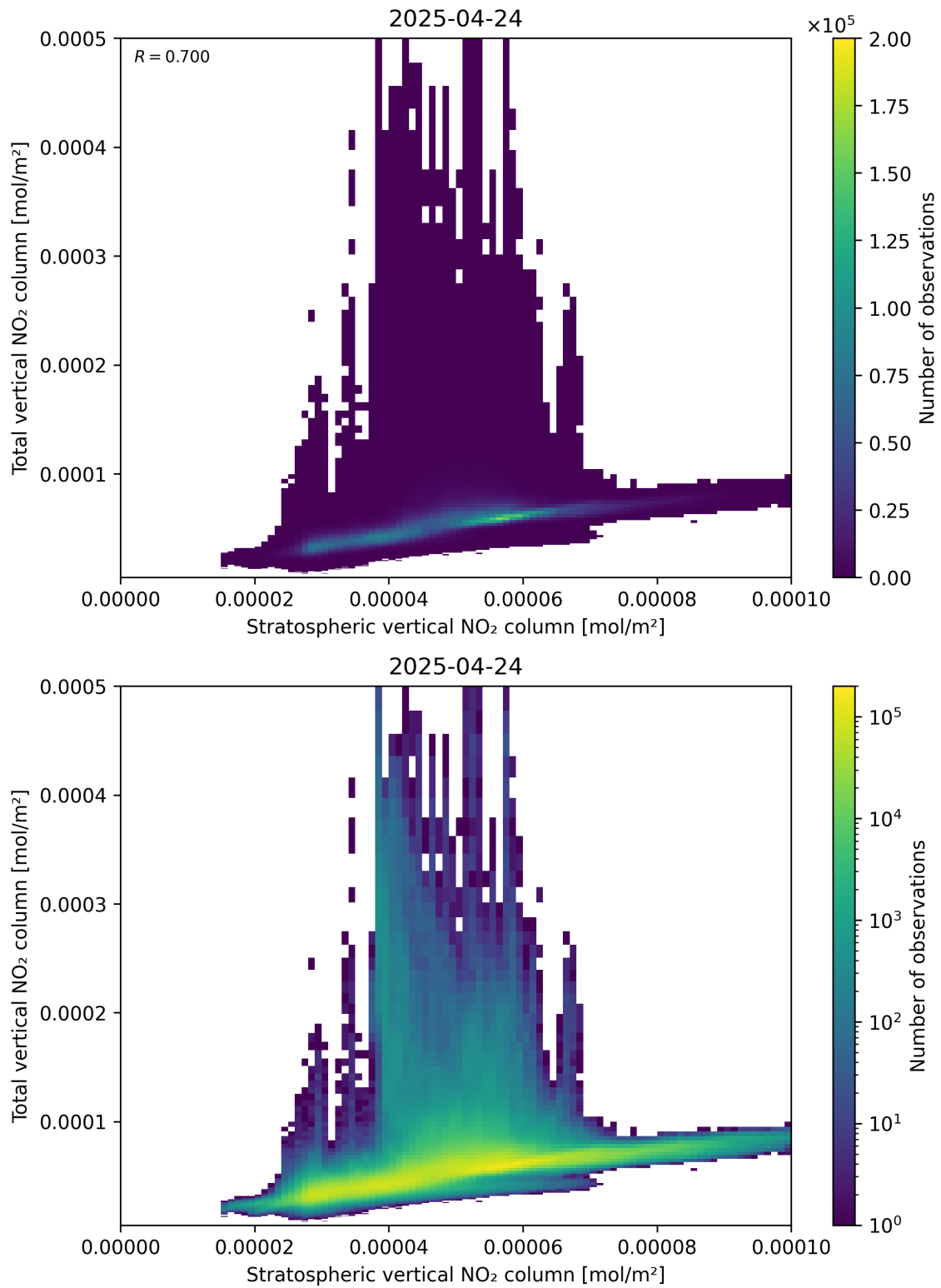
Figure 100: Scatter density plot of “Stratospheric vertical NO 2 column” against “Total vertical NO 2 column” for 2025-04-24 to 2025-04-25.
