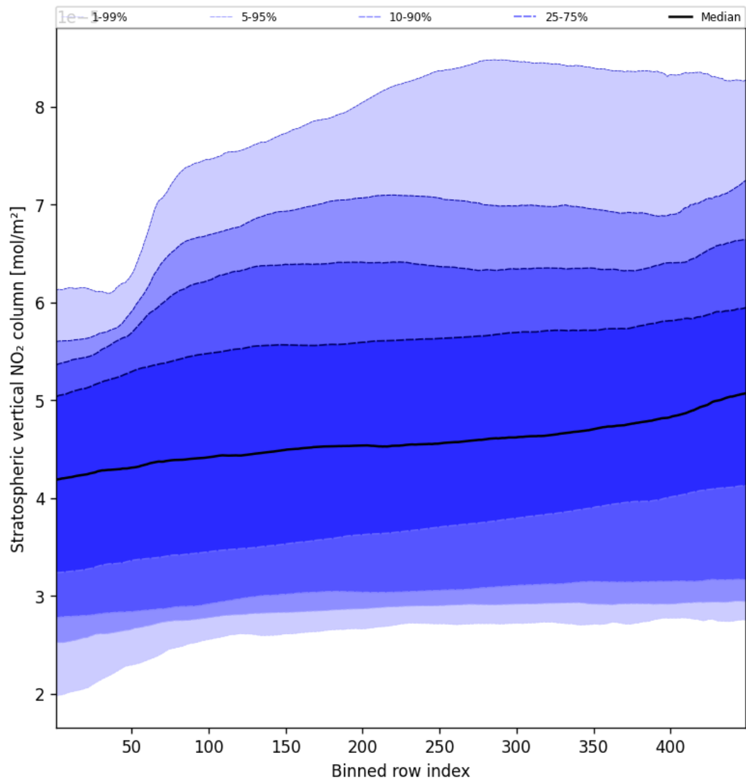
Figure 53: Along track statistics of “Stratospheric vertical NO 2 column” for 2025-04-24 to 2025-04-25
