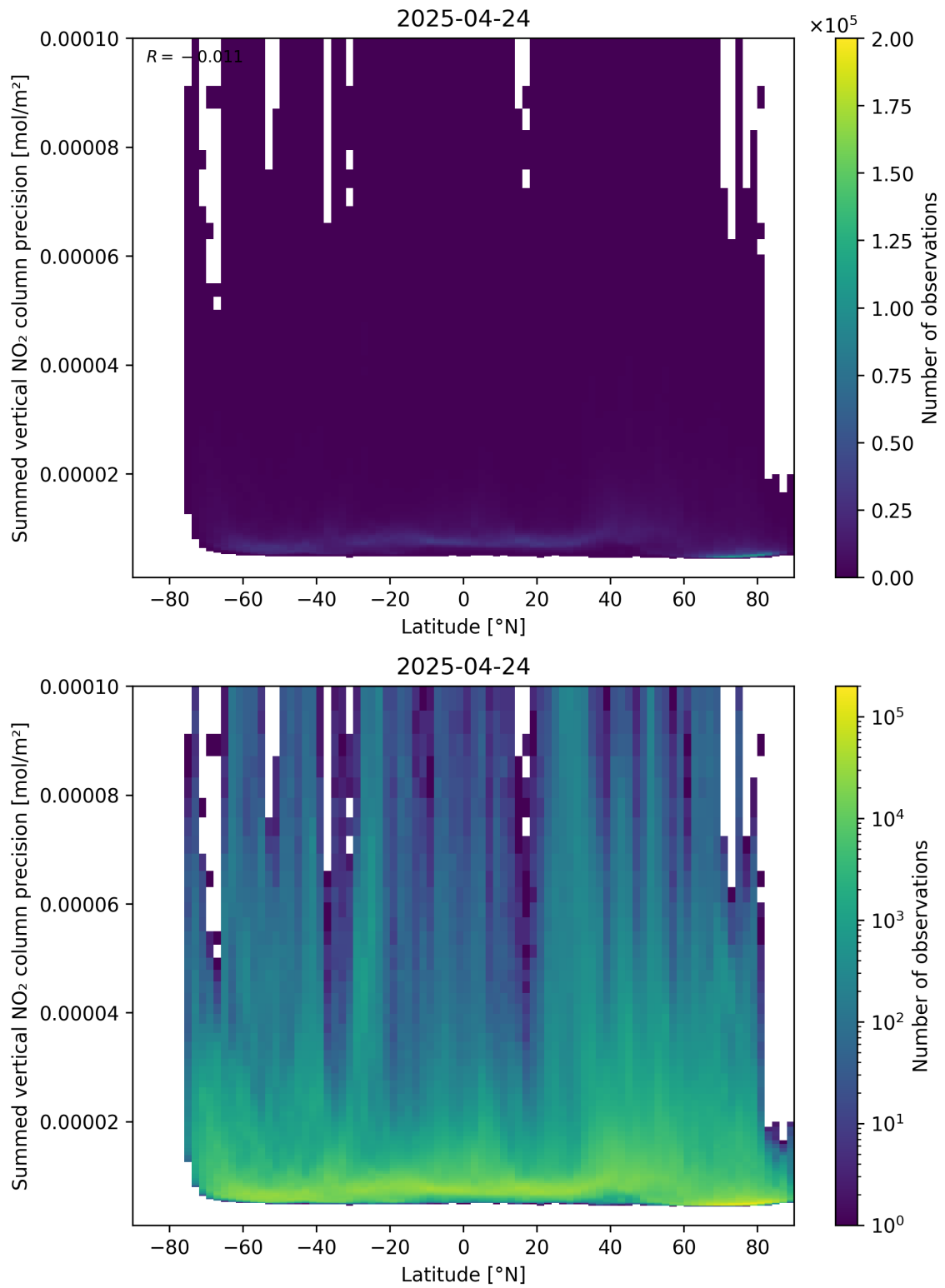
Figure 89: Scatter density plot of “Latitude” against “Summed vertical NO 2 column precision” for 2025-04-24 to 2025-04-25.
