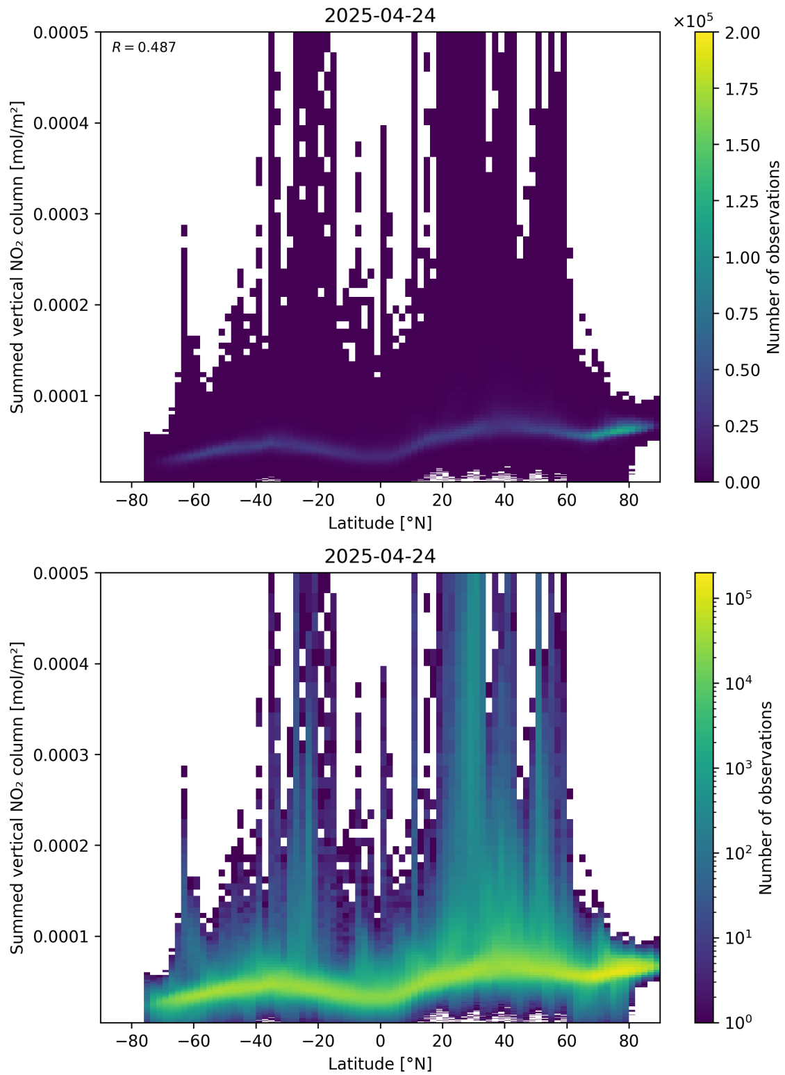
Figure 88: Scatter density plot of “Latitude” against “Summed vertical NO 2 column” for 2025-04-24 to 2025-04-25.
