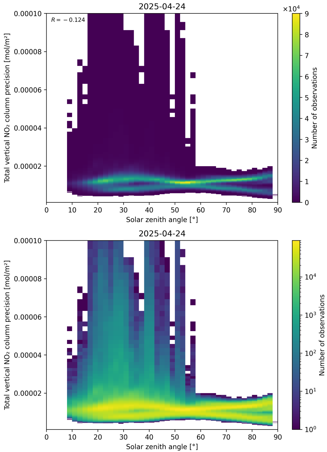
Figure 154: Scatter density plot of “Solar zenith angle” against “Total vertical NO 2 column precision” for 2025-04-24 to 2025-04-25.
