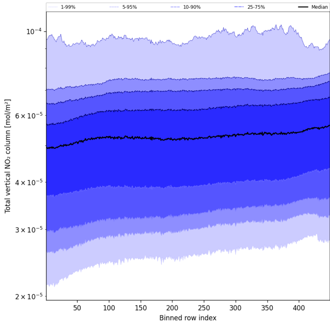
Figure 55: Along track statistics of “Total vertical NO 2 column” for 2025-04-24 to 2025-04-25
