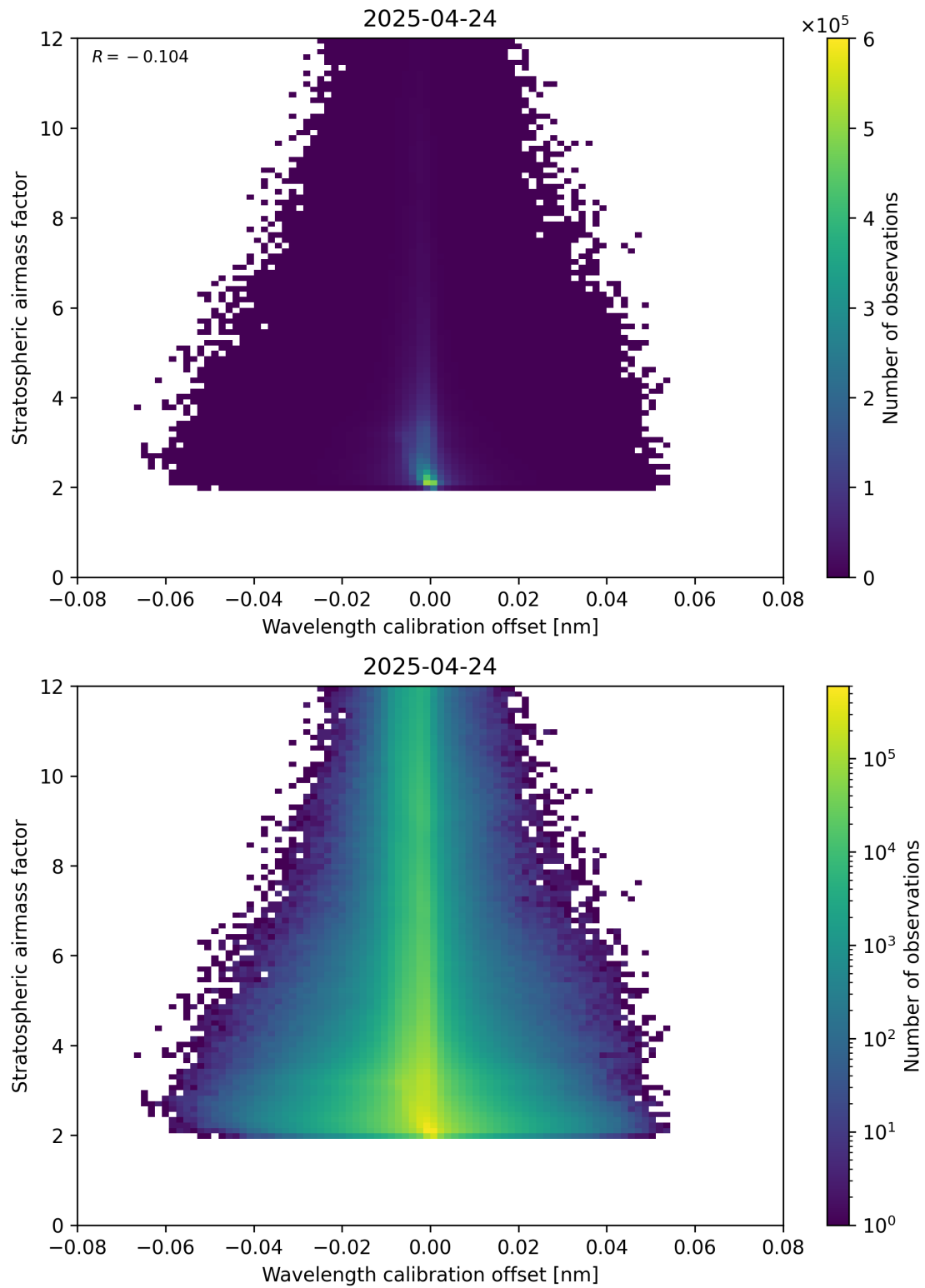
Figure 174: Scatter density plot of “Wavelength calibration offset” against “Stratospheric airmass factor” for 2025-04-24 to 2025-04-25.
