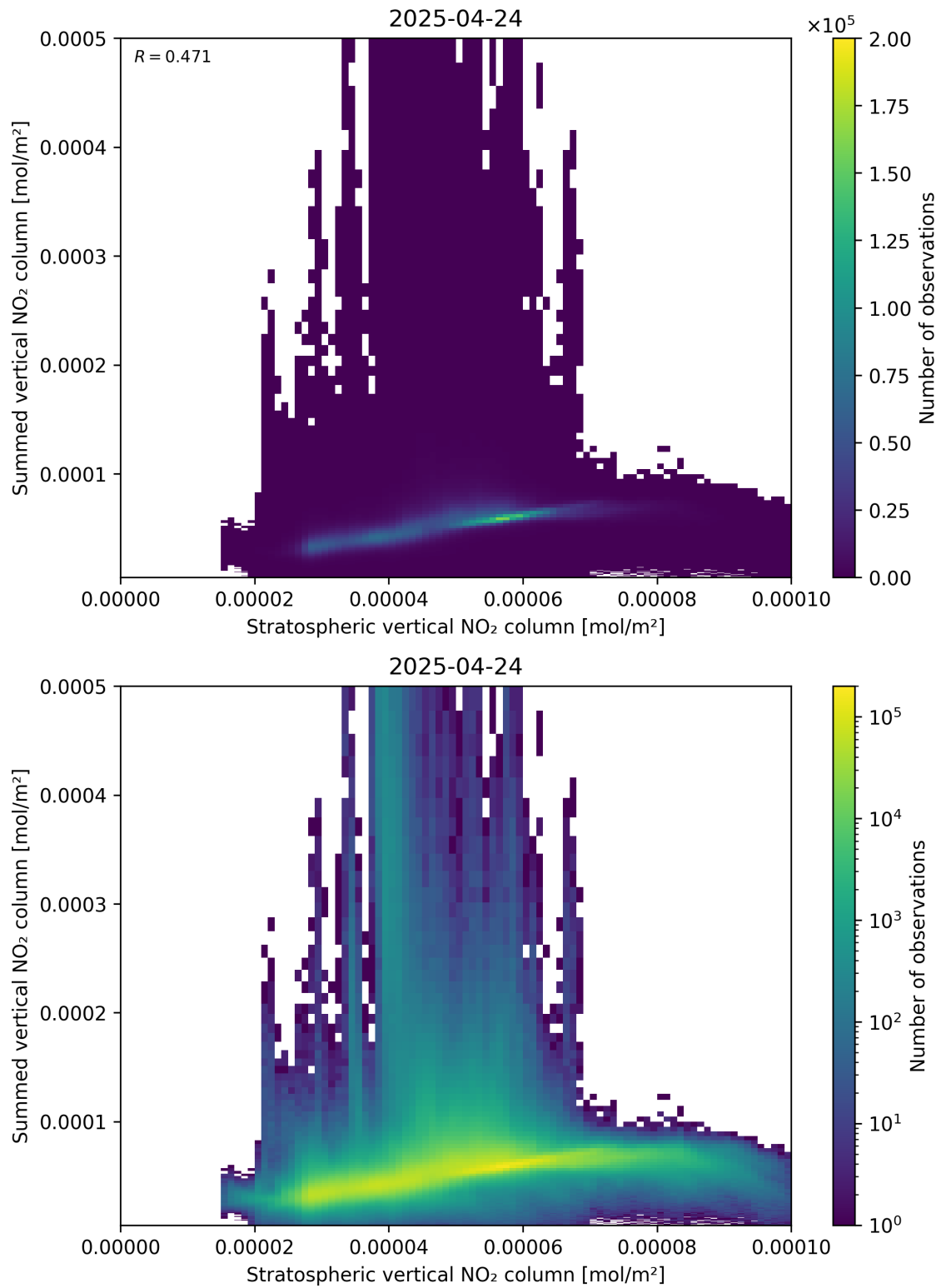
Figure 98: Scatter density plot of “Stratospheric vertical NO 2 column” against “Summed vertical NO 2 column” for 2025-04-24 to 2025-04-25.
