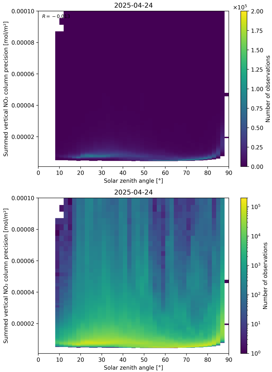
Figure 152: Scatter density plot of “Solar zenith angle” against “Summed vertical NO 2 column precision” for 2025-04-24 to 2025-04-25.
