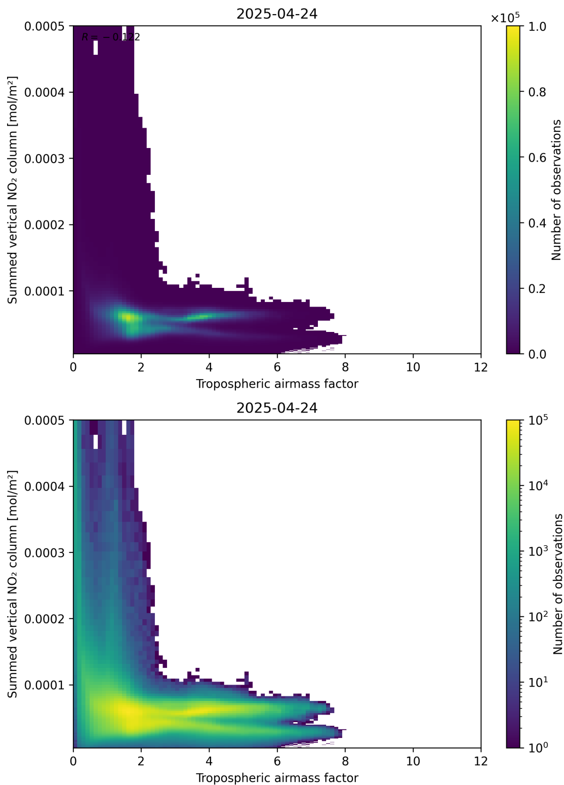
Figure 75: Scatter density plot of “Tropospheric air mass factor” against “Summed vertical NO 2 column” for 2025-04-24 to 2025-04-25.
