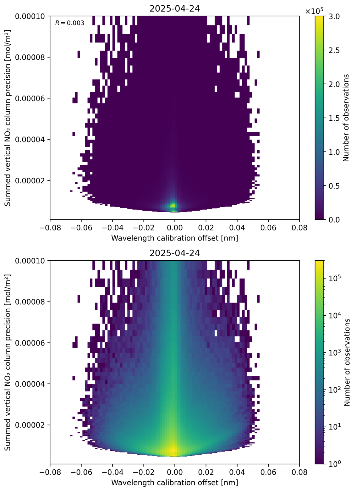
Figure 178: Scatter density plot of “Wavelength calibration offset” against “Summed vertical NO 2 column precision” for 2025-04-24 to 2025-04-25.
