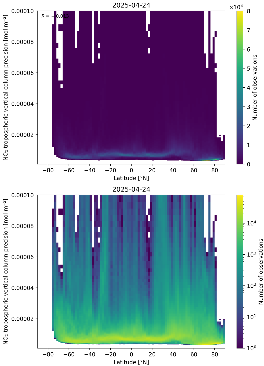
Figure 93: Scatter density plot of “Latitude” against “NO 2 tropospheric vertical column precision” for 2025-04-24 to 2025-04-25.
