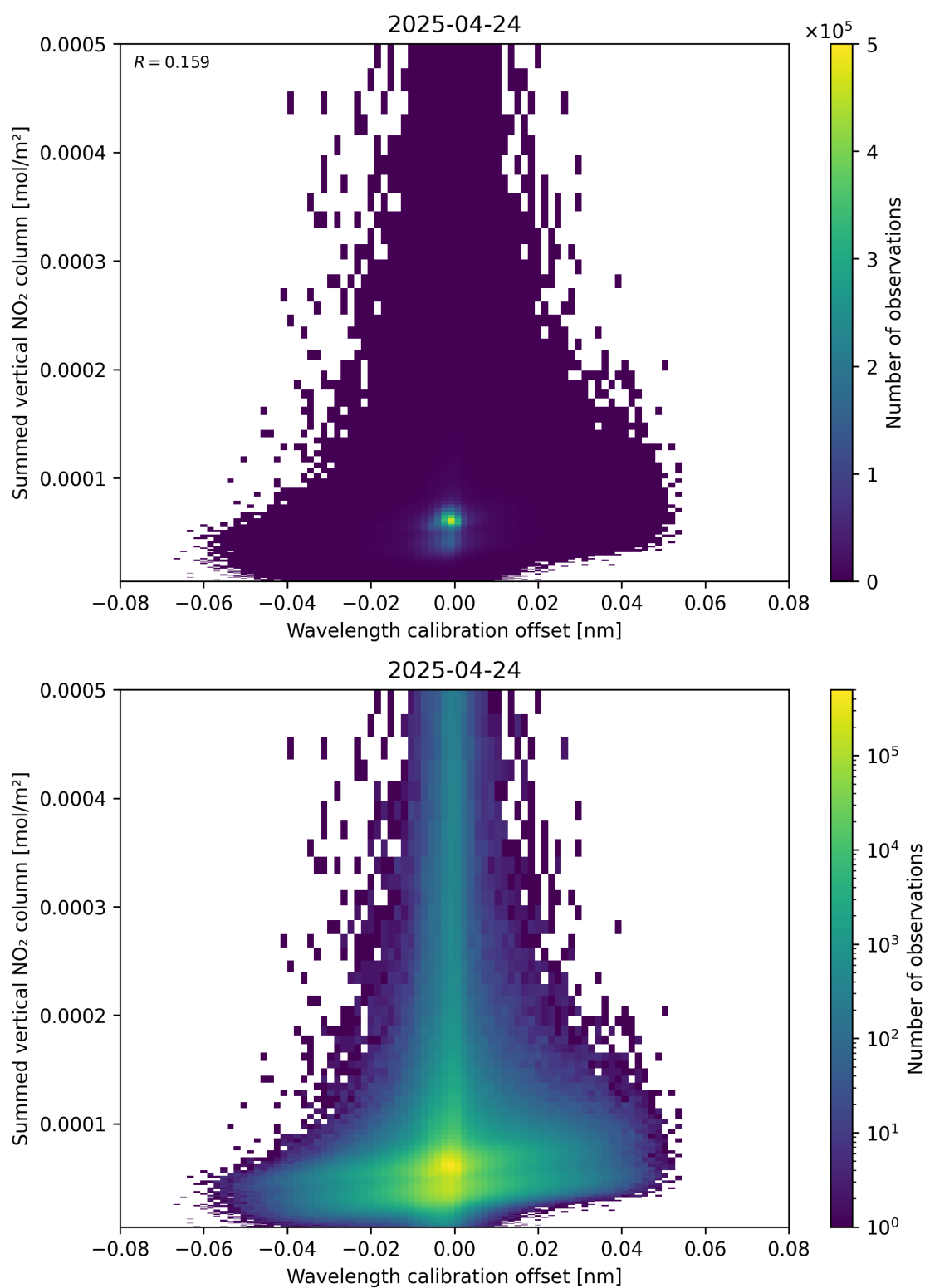
Figure 177: Scatter density plot of “Wavelength calibration offset” against “Summed vertical NO 2 column” for 2025-04-24 to 2025-04-25.
