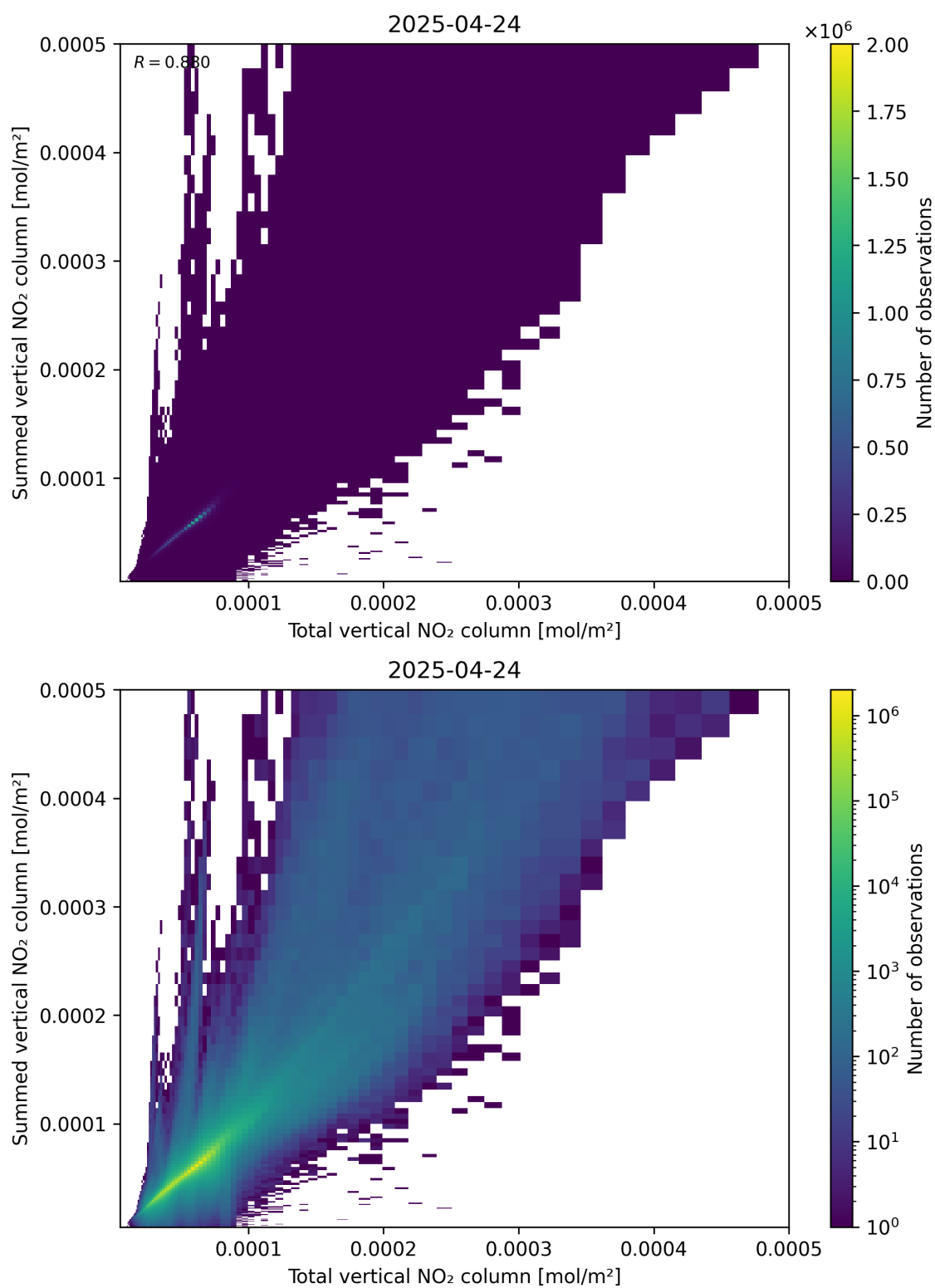
Figure 112: Scatter density plot of “Total vertical NO 2 column” against “Summed vertical NO 2 column” for 2025-04-24 to 2025-04-25.
