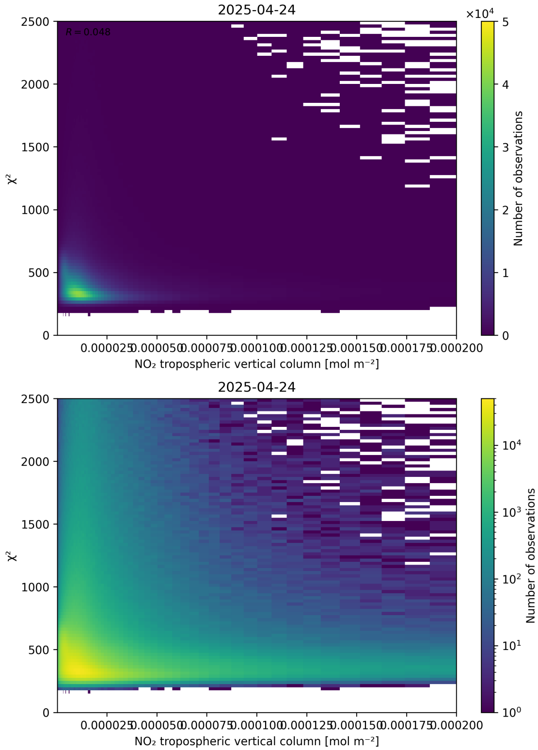
Figure 124: Scatter density plot of “NO 2 tropospheric vertical column” against “ \chi^2 ” for 2025-04-24 to 2025-04-25.
