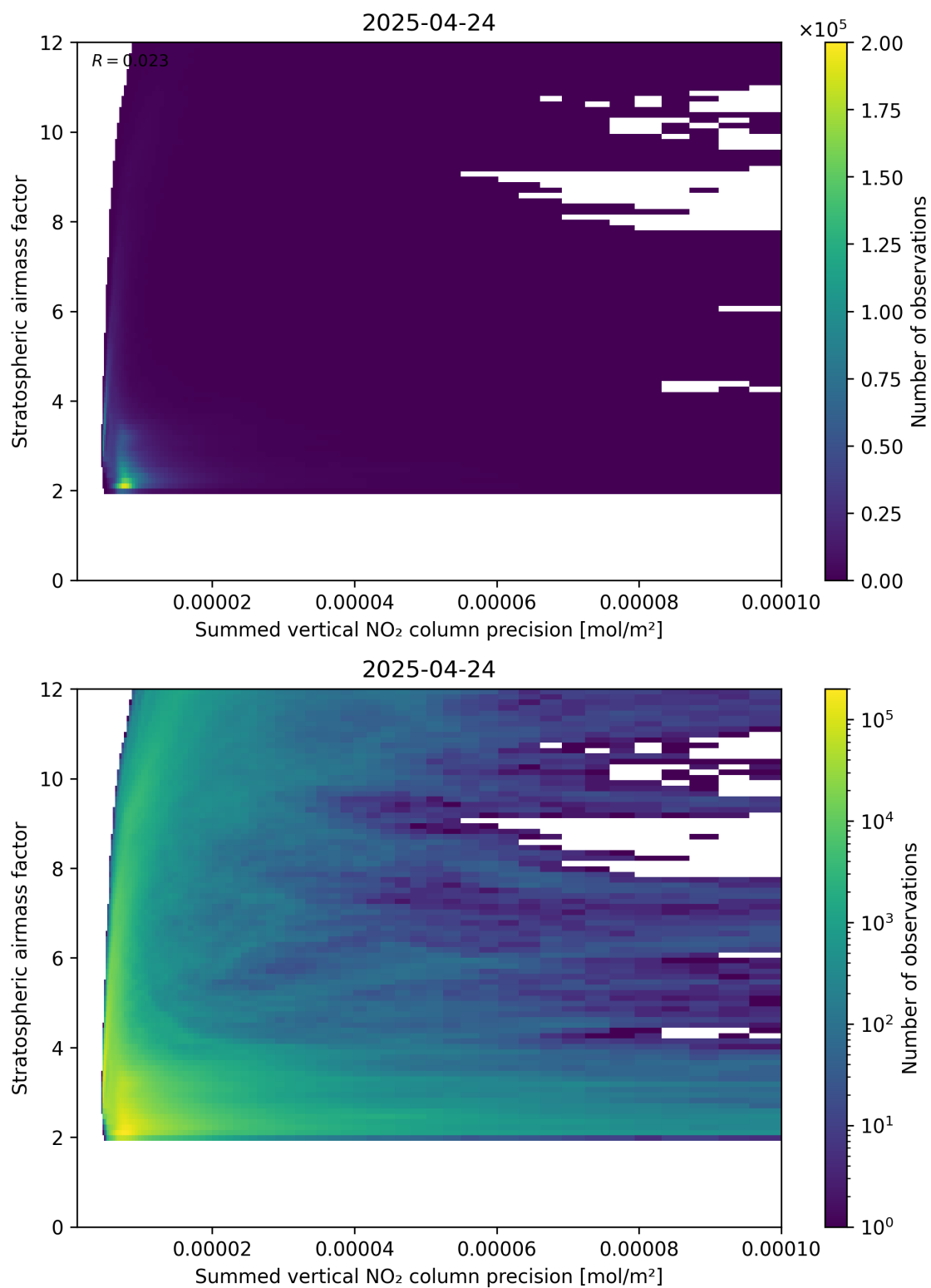
Figure 106: Scatter density plot of “Summed vertical NO 2 column precision” against “Stratospheric airmass factor” for 2025-04-24 to 2025-04-25.
