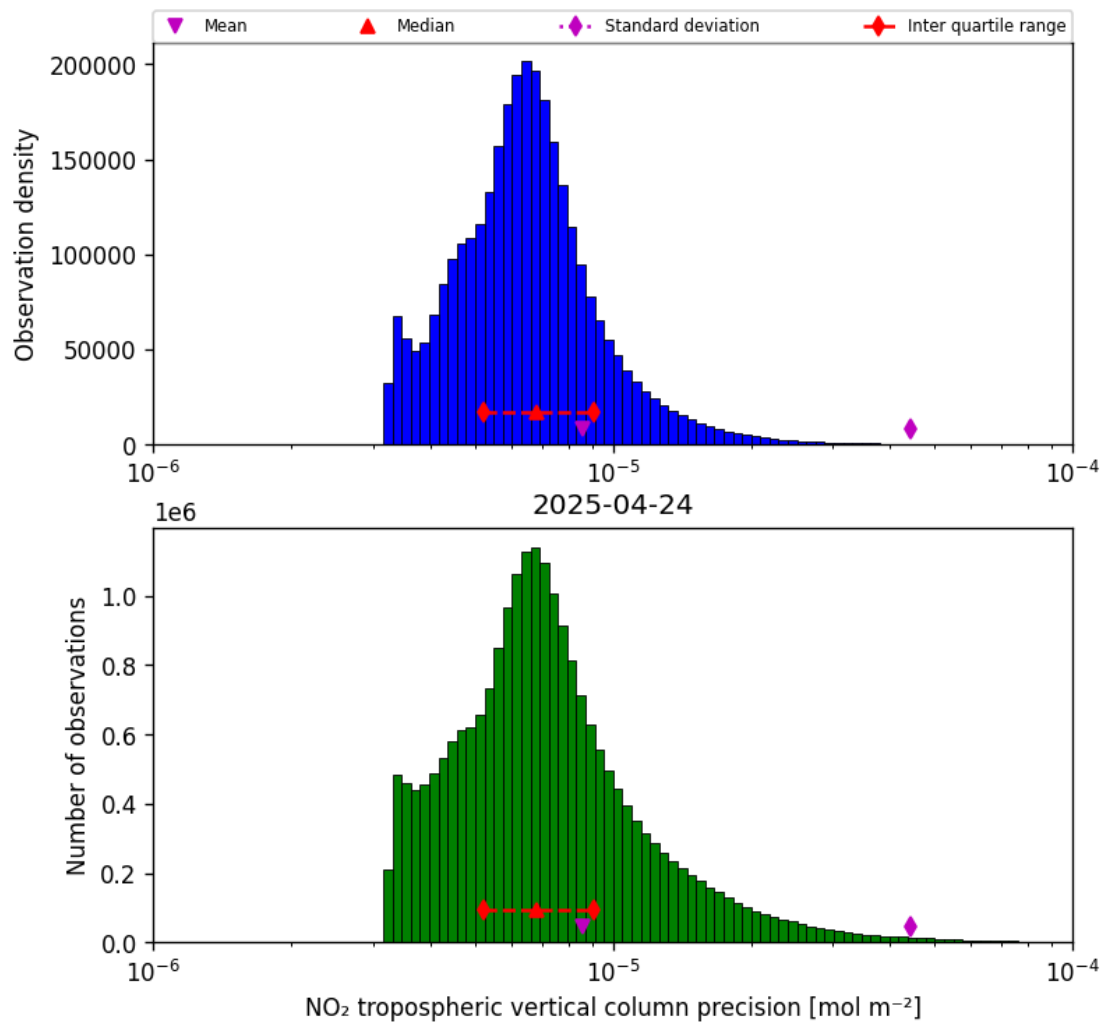
Figure 30: Histogram of “NO 2 tropospheric vertical column precision” for 2025-04-24 to 2025-04-25
