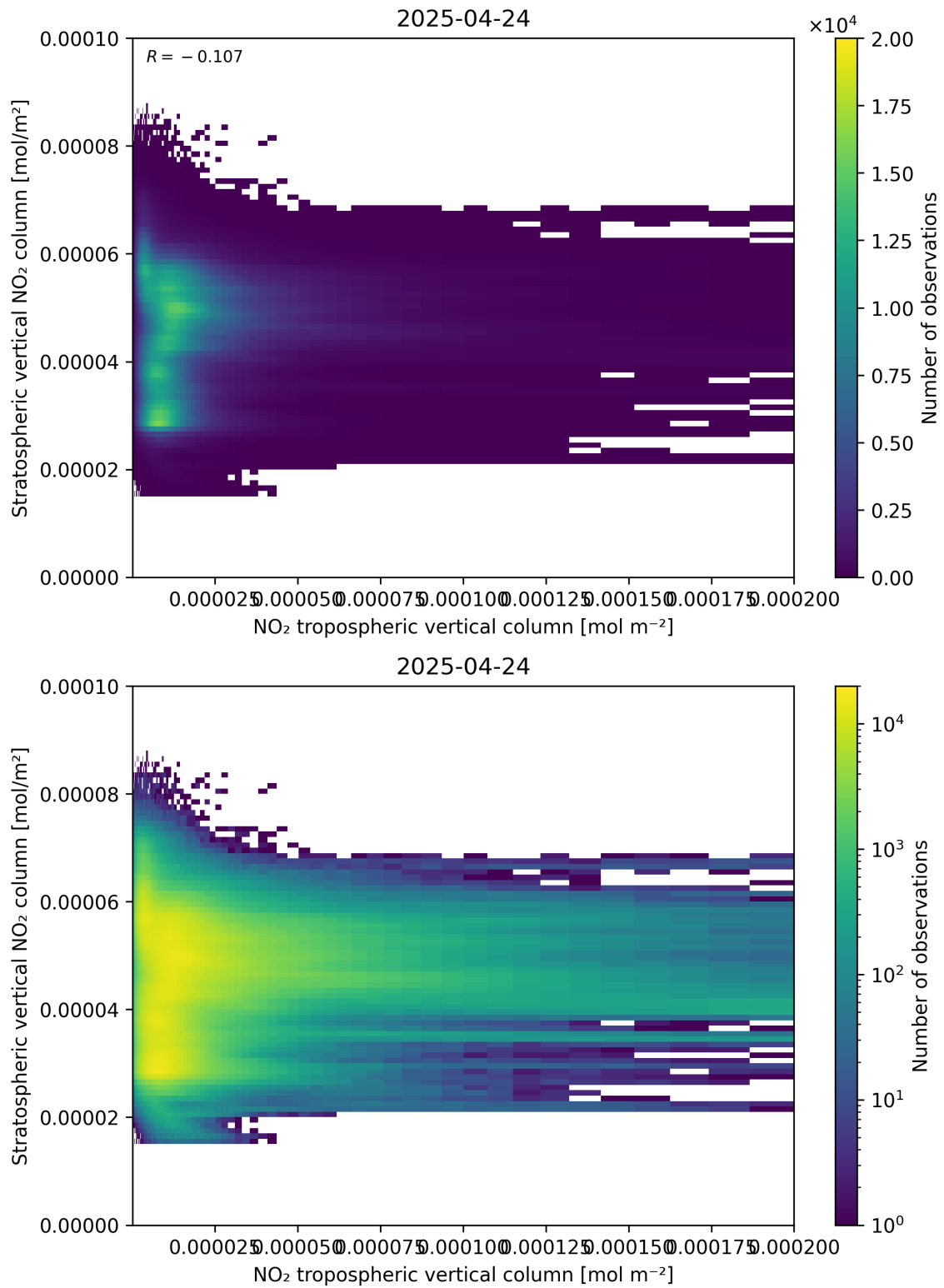
Figure 125: Scatter density plot of “NO 2 tropospheric vertical column” against “Stratospheric vertical NO 2 column” for 2025-04-24 to 2025-04-25.
