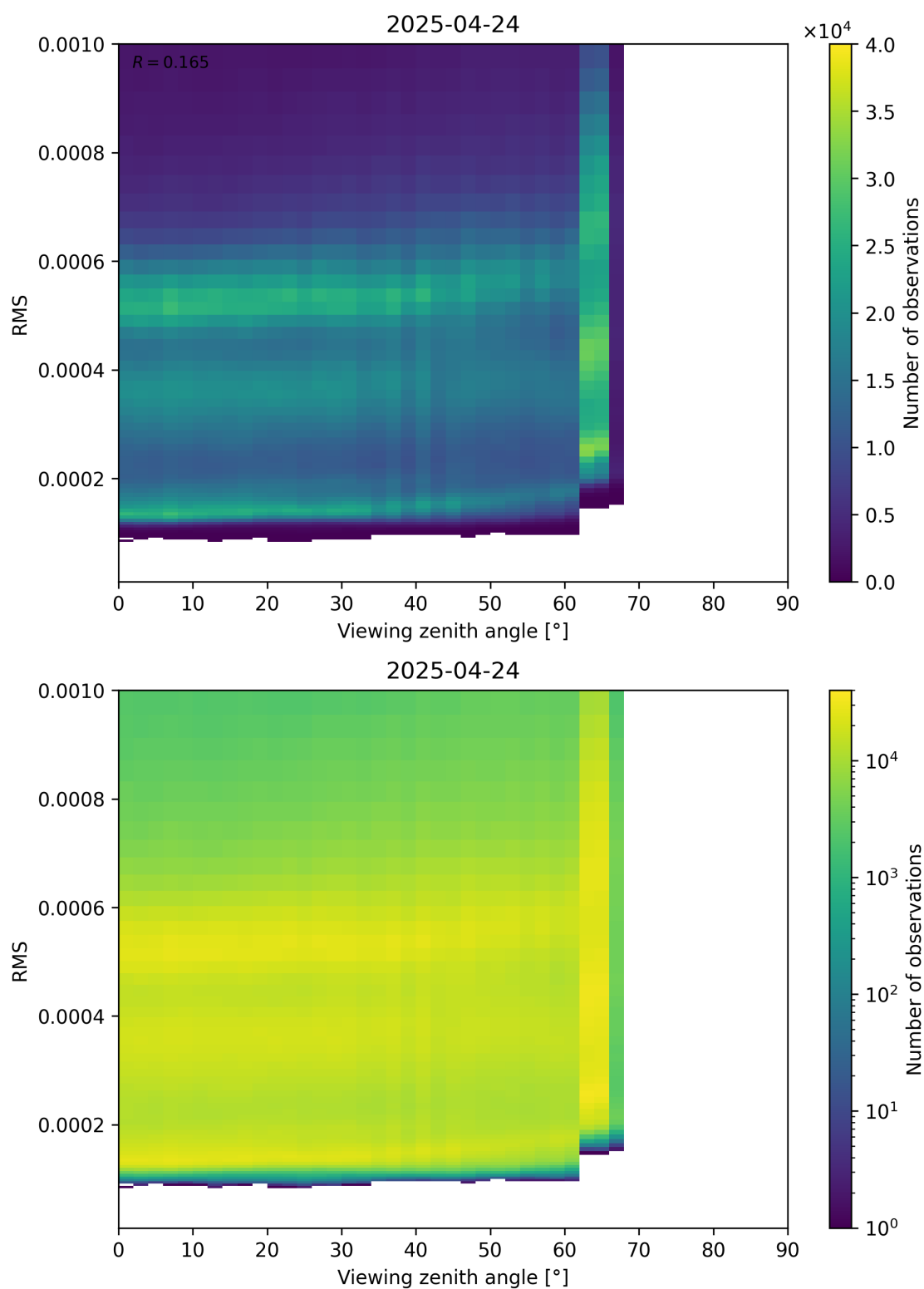
Figure 171: Scatter density plot of “Viewing zenith angle” against “RMS” for 2025-04-24 to 2025-04-25.
