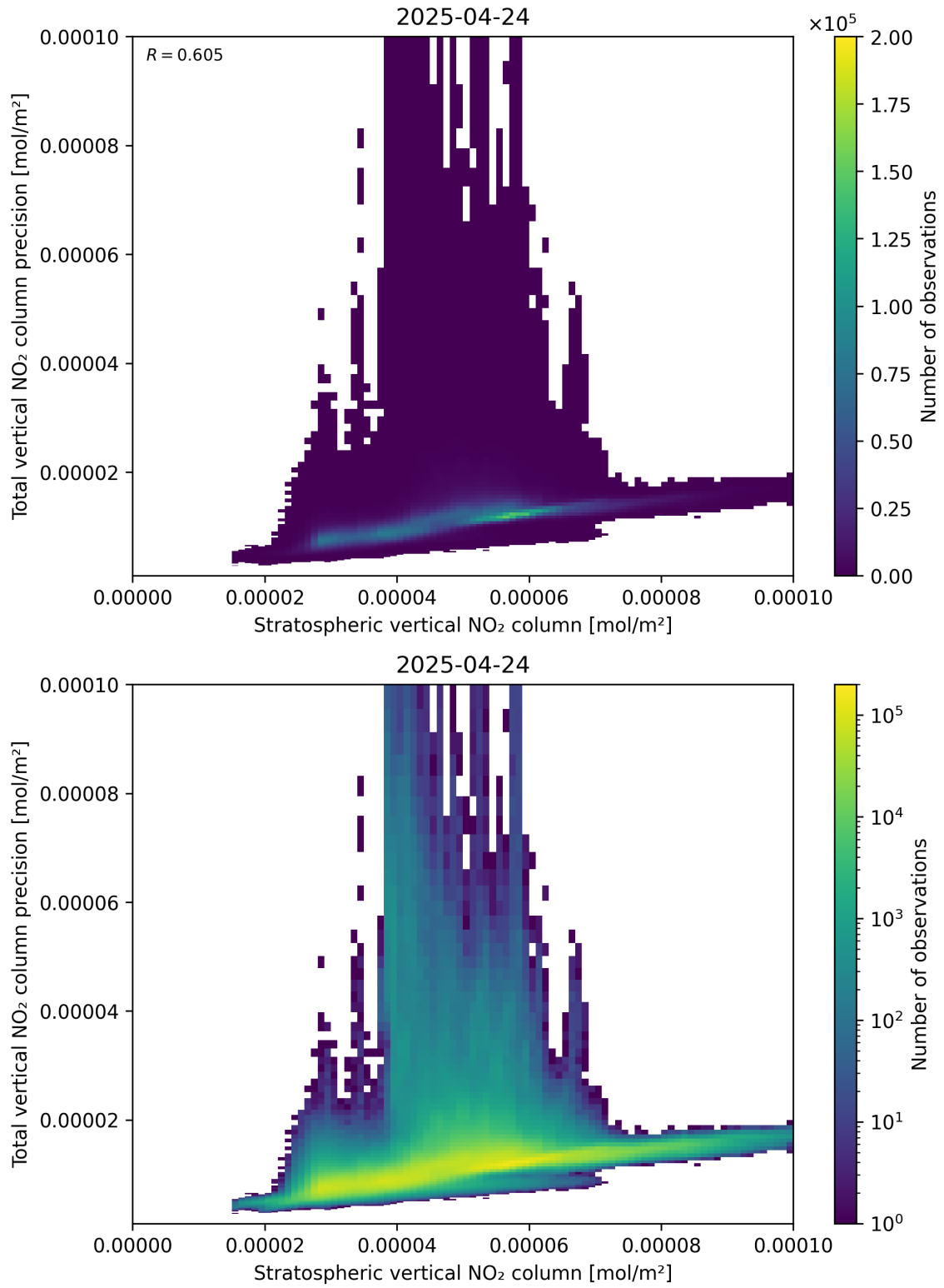
Figure 101: Scatter density plot of “Stratospheric vertical NO 2 column” against “Total vertical NO 2 column precision” for 2025-04-24 to 2025-04-25.
