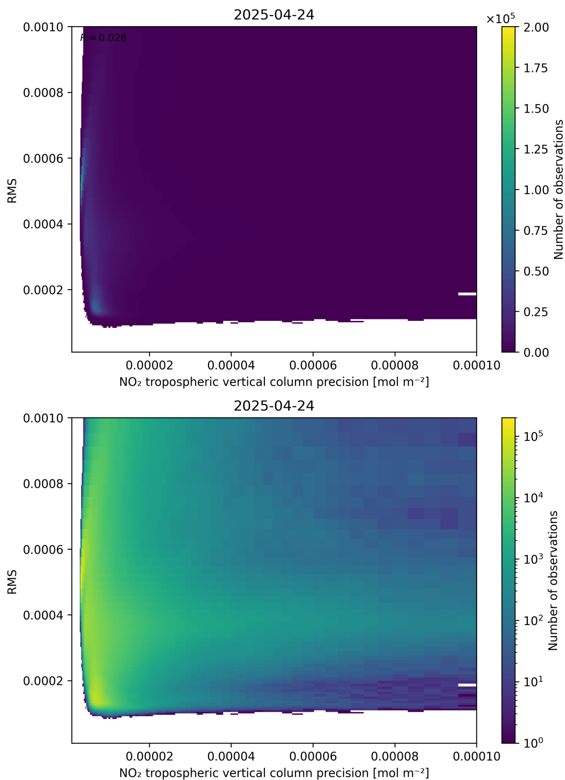
Figure 140: Scatter density plot of “NO 2 tropospheric vertical column precision” against “RMS” for 2025-04-24 to 2025-04-25.
