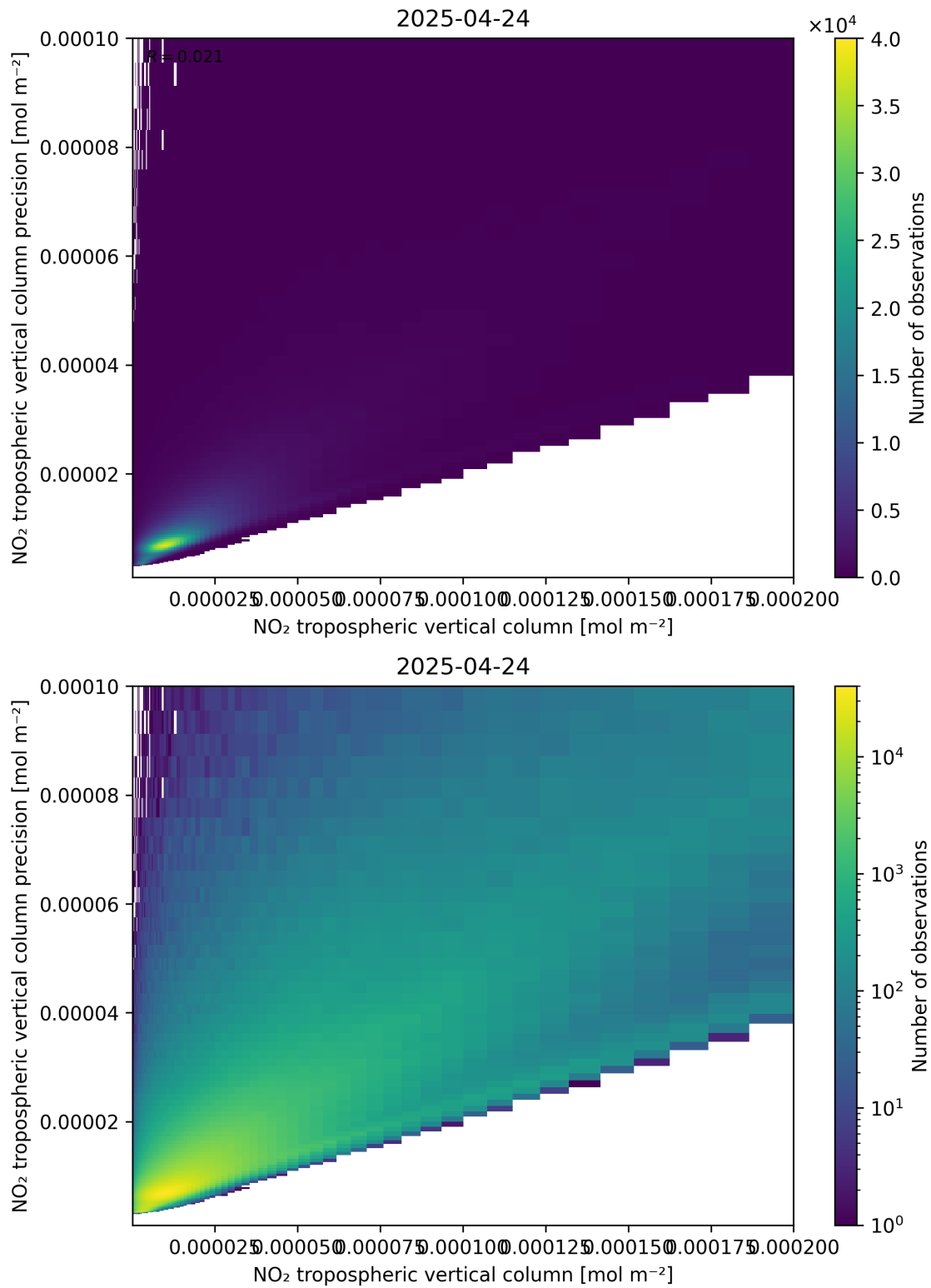
Figure 130: Scatter density plot of “NO 2 tropospheric vertical column” against “NO 2 tropospheric vertical column precision” for 2025-04-24 to 2025-04-25.
