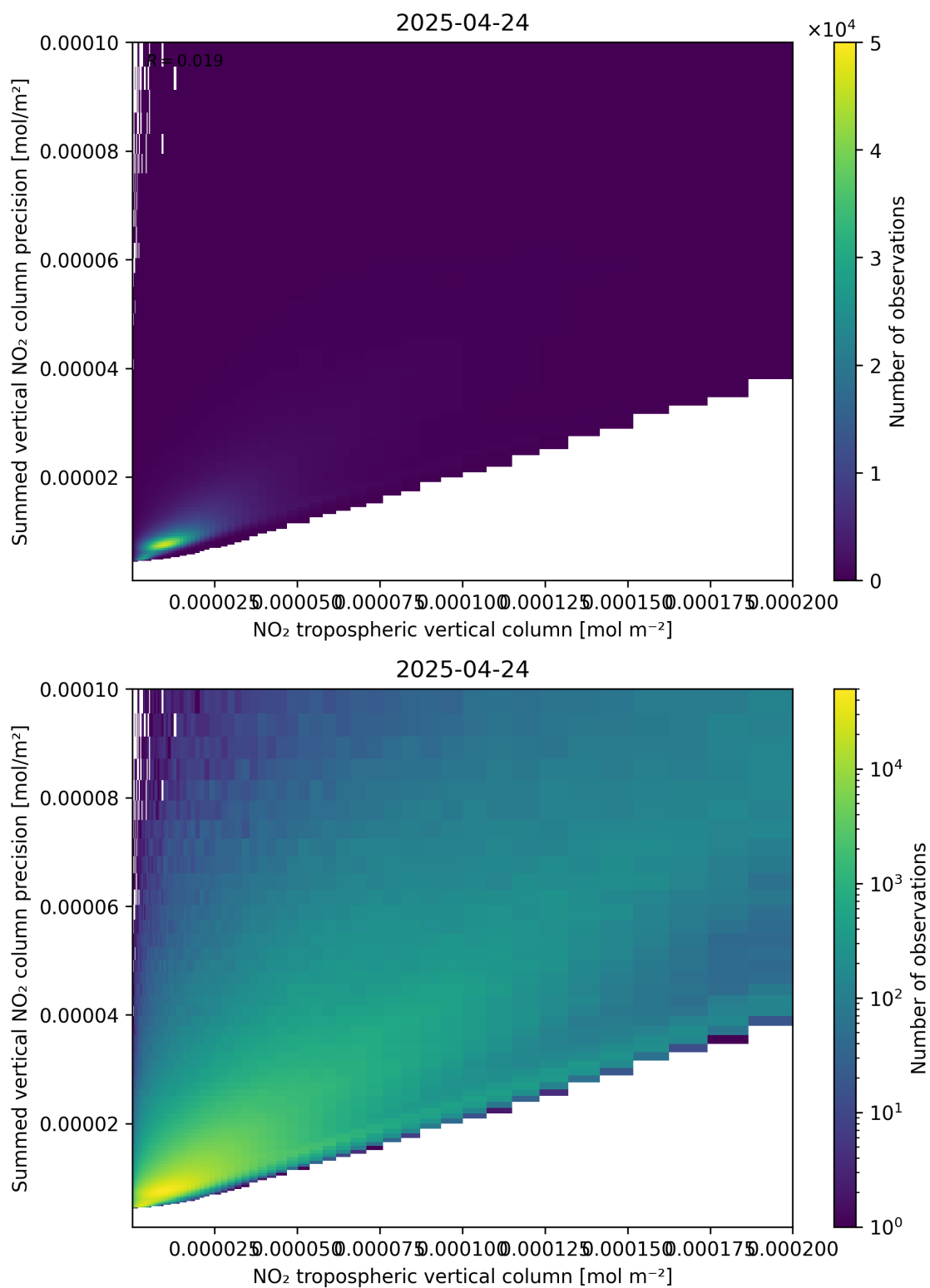
Figure 127: Scatter density plot of “NO 2 tropospheric vertical column” against “Summed vertical NO 2 column precision” for 2025-04-24 to 2025-04-25.
