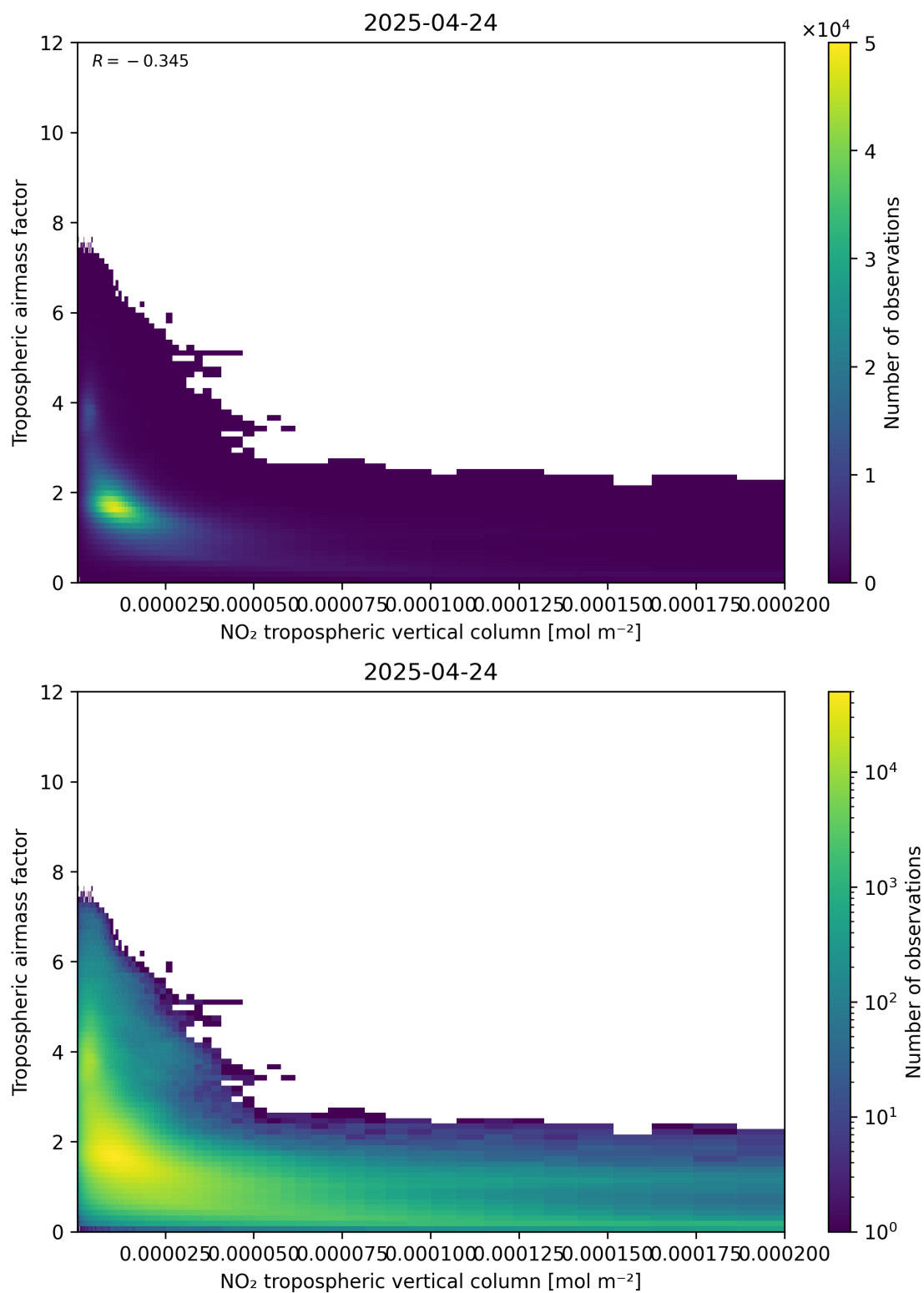
Figure 123: Scatter density plot of “NO 2 tropospheric vertical column” against “Tropospheric air mass factor” for 2025-04-24 to 2025-04-25.
