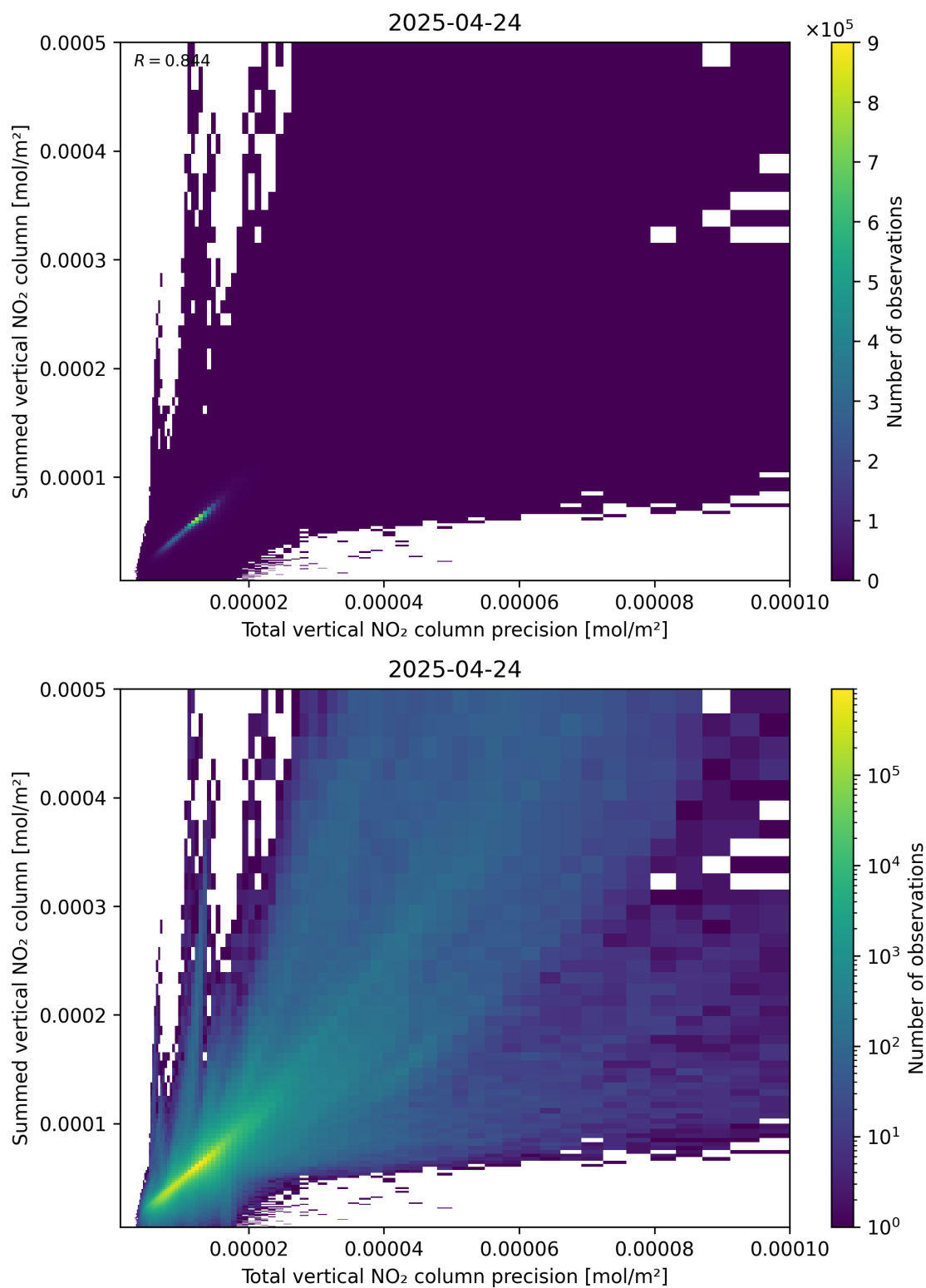
Figure 117: Scatter density plot of “Total vertical NO 2 column precision” against “Summed vertical NO 2 column” for 2025-04-24 to 2025-04-25.
