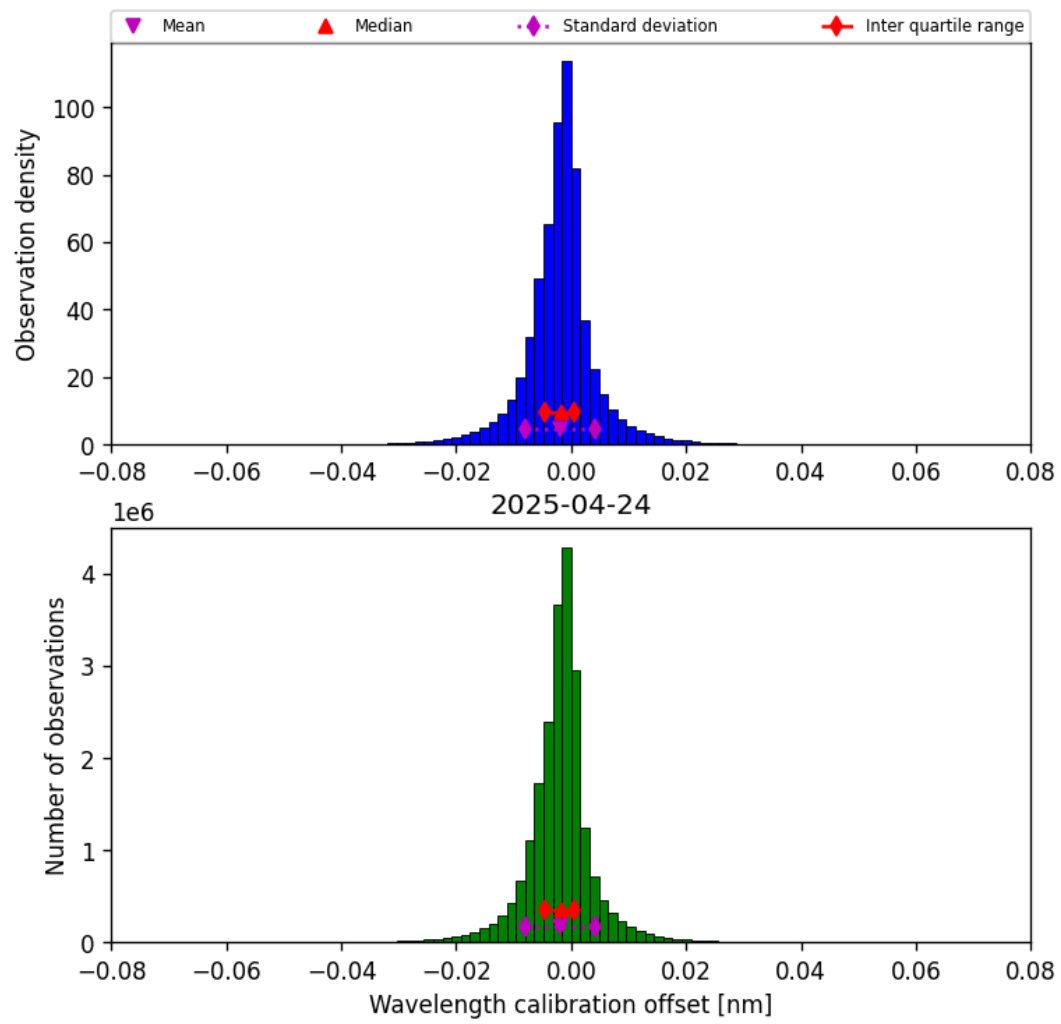
Figure 35: Histogram of “Wavelength calibration offset” for 2025-04-24 to 2025-04-25
