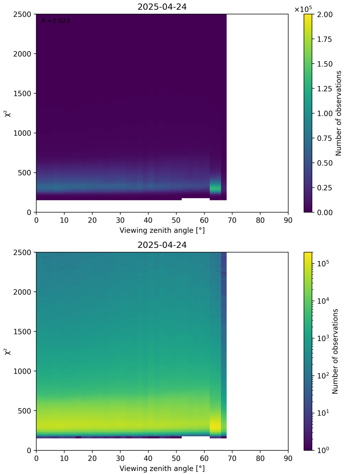
Figure 162: Scatter density plot of “Viewing zenith angle” against “ \chi^2 ” for 2025-04-24 to 2025-04-25.
