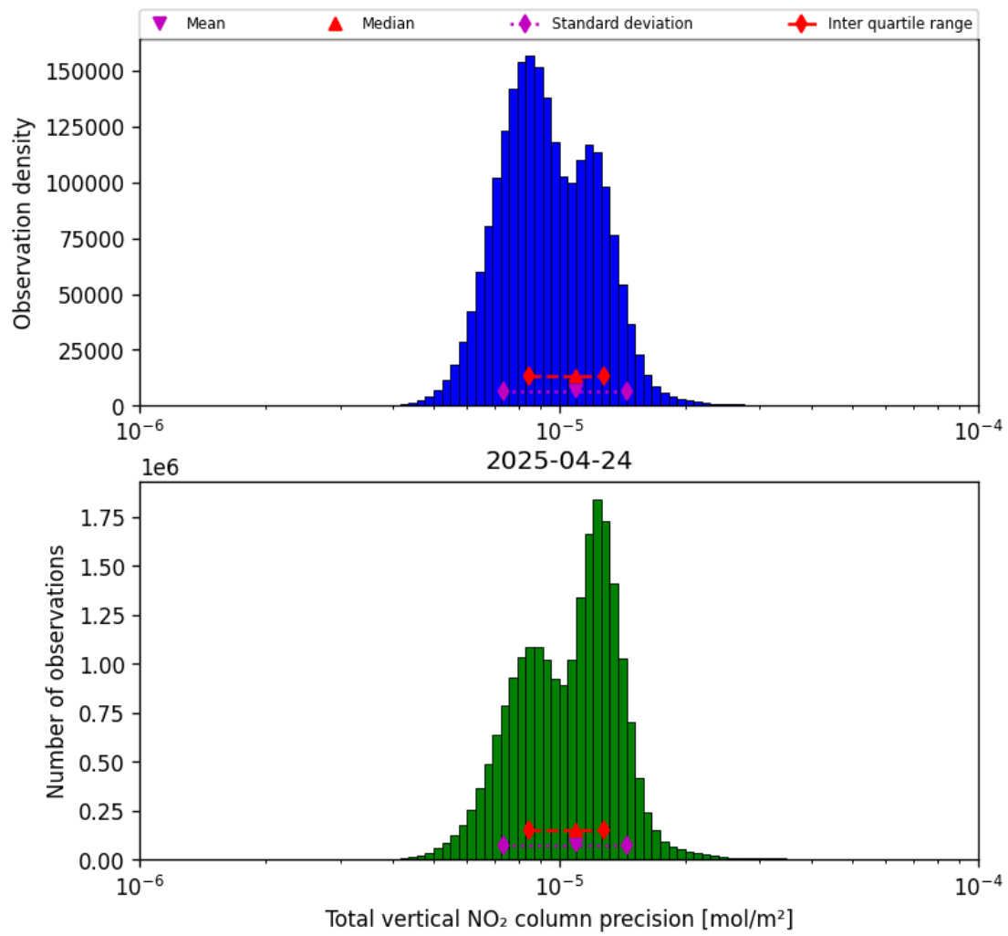
Figure 39: Histogram of “Total vertical NO 2 column precision” for 2025-04-24 to 2025-04-25
