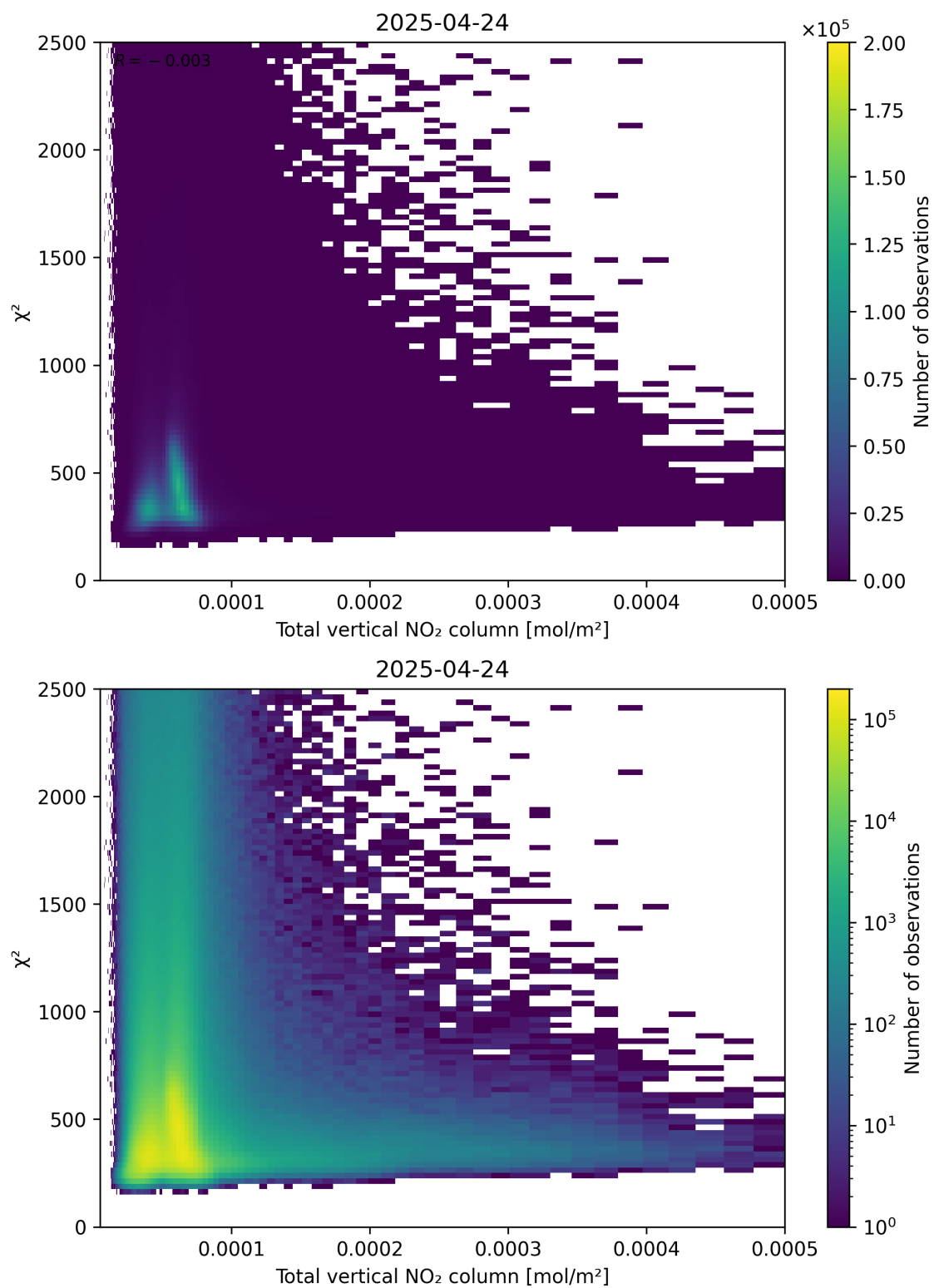
Figure 111: Scatter density plot of “Total vertical NO 2 column” against “ \chi^2 ” for 2025-04-24 to 2025-04-25.
