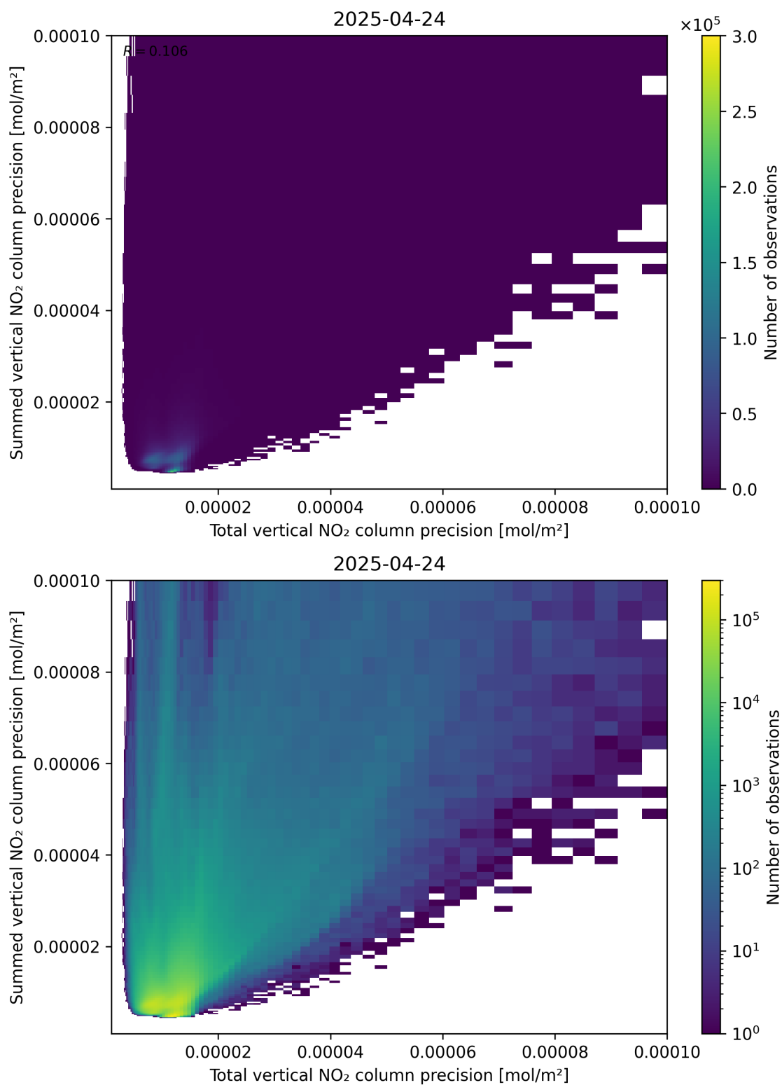
Figure 118: Scatter density plot of “Total vertical NO 2 column precision” against “Summed vertical NO 2 column precision” for 2025-04-24 to 2025-04-25.
