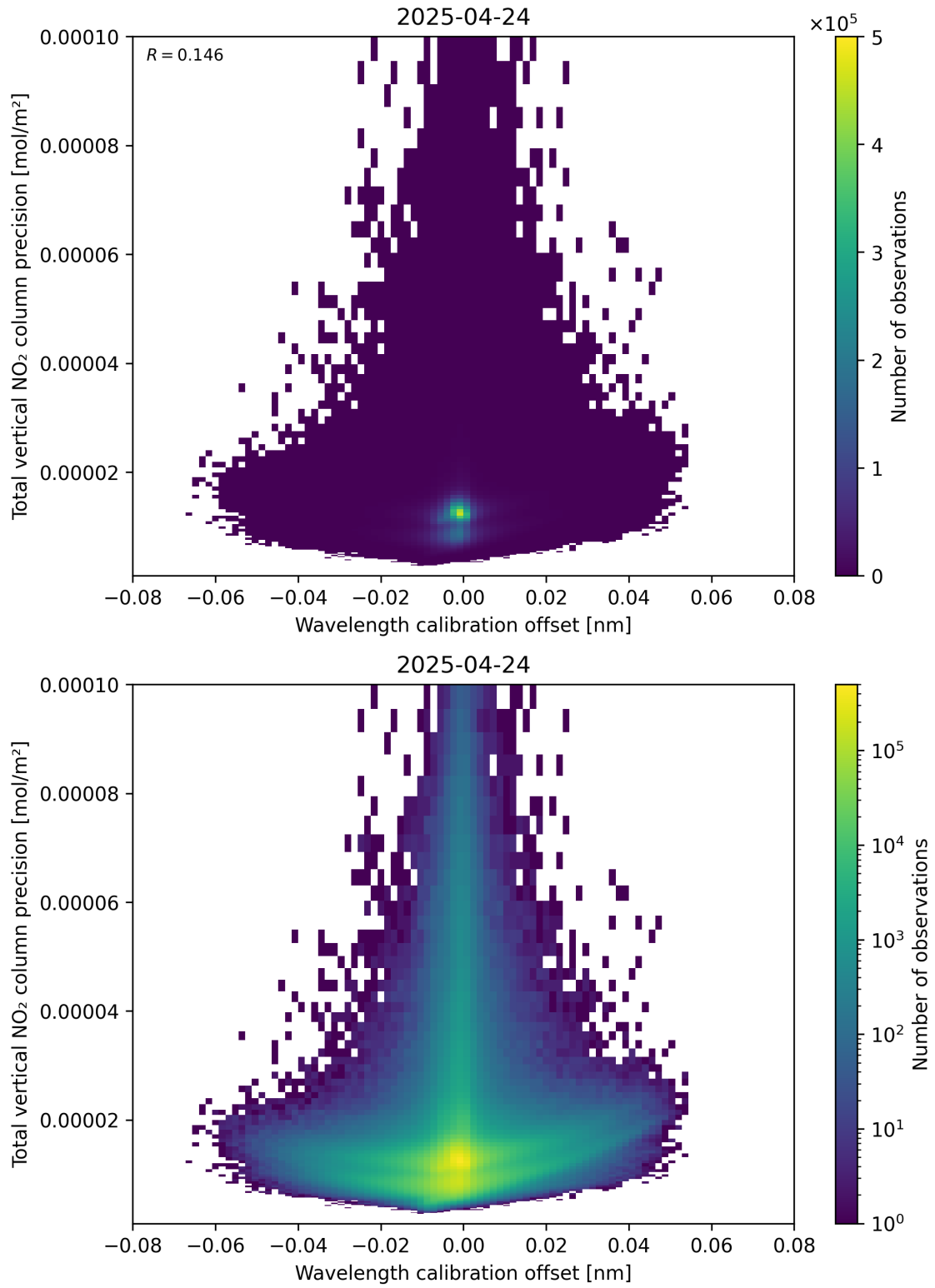
Figure 180: Scatter density plot of “Wavelength calibration offset” against “Total vertical NO 2 column precision” for 2025-04-24 to 2025-04-25.
