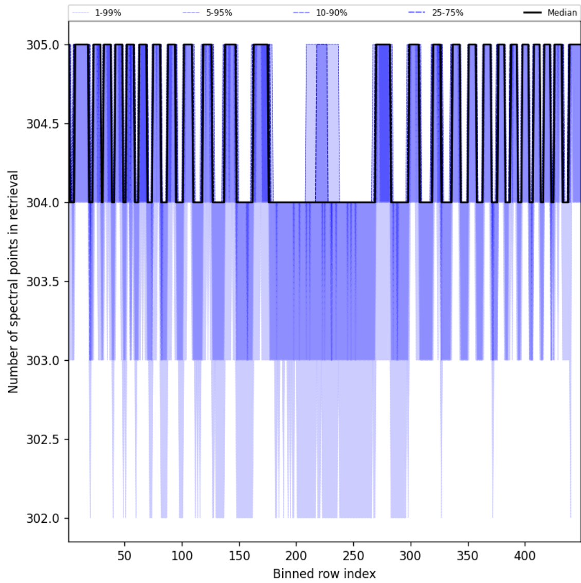
Figure 50: Along track statistics of “Number of spectral points in retrieval” for 2025-04-24 to 2025-04-25
