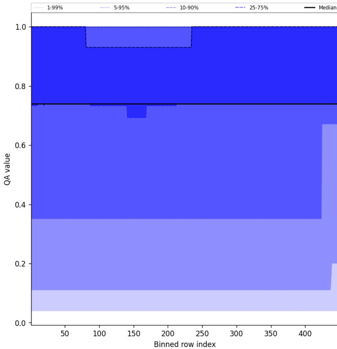
Figure 45: Along track statistics of “QA value” for 2025-04-24 to 2025-04-25
