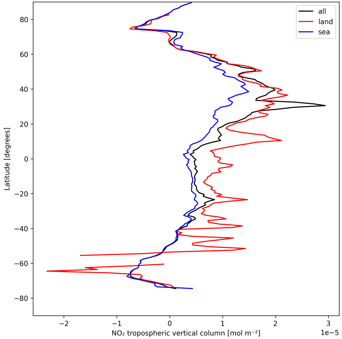
Figure 12: Zonal average of “NO 2 tropospheric vertical column” for 2025-04-24 to 2025-04-25.
