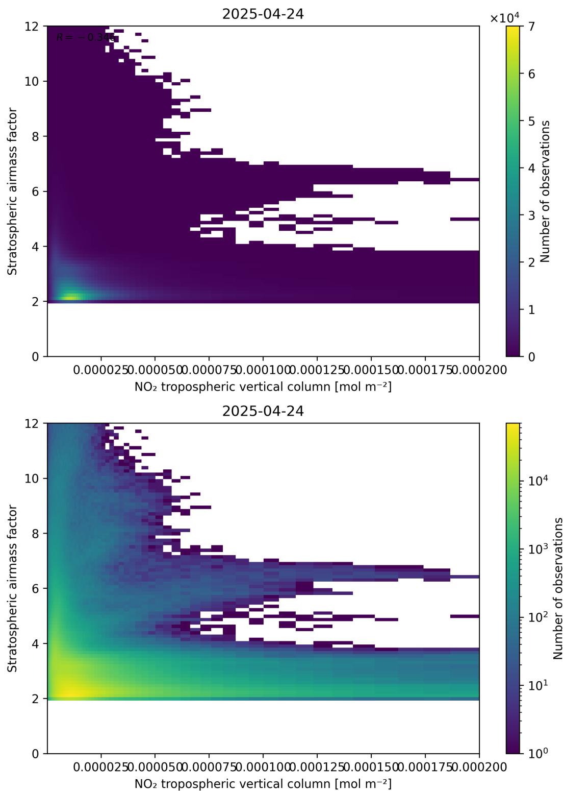
Figure 121: Scatter density plot of “NO 2 tropospheric vertical column” against “Stratospheric air mass factor” for 2025-04-24 to 2025-04-25.
