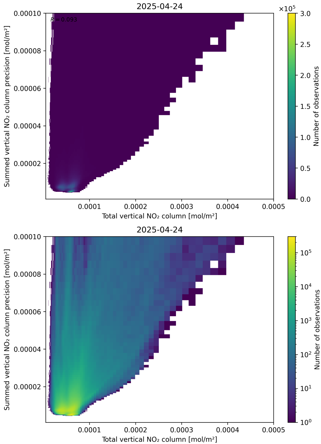
Figure 113: Scatter density plot of “Total vertical NO 2 column” against “Summed vertical NO 2 column precision” for 2025-04-24 to 2025-04-25.
