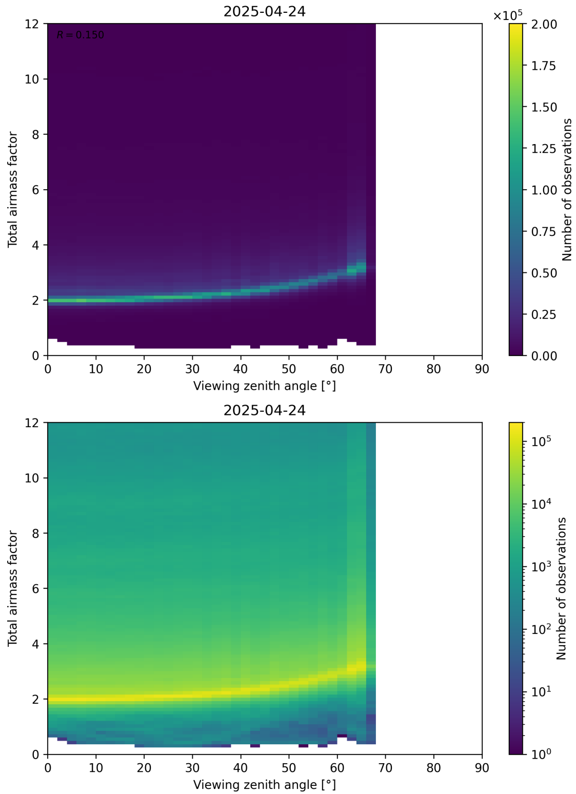
Figure 160: Scatter density plot of “Viewing zenith angle” against “Total airmass factor” for 2025-04-24 to 2025-04-25.
