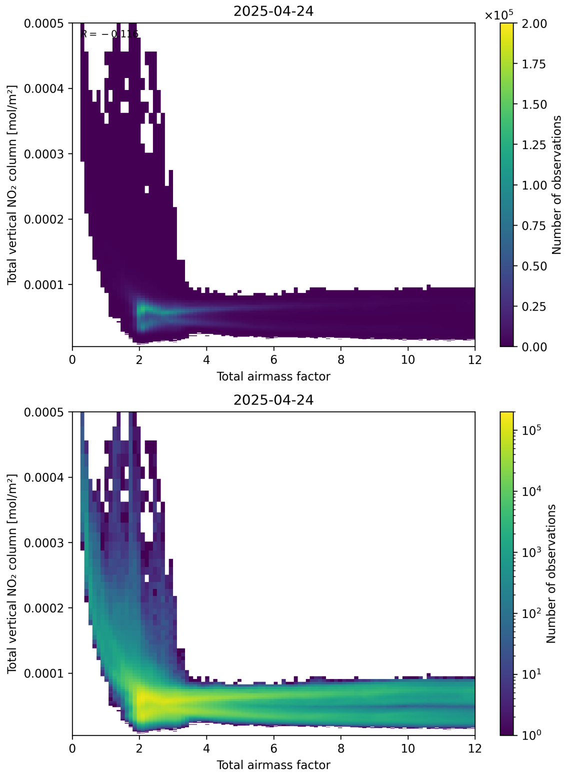
Figure 67: Scatter density plot of “Total airmass factor” against “Total vertical NO 2 column” for 2025-04-24 to 2025-04-25.
