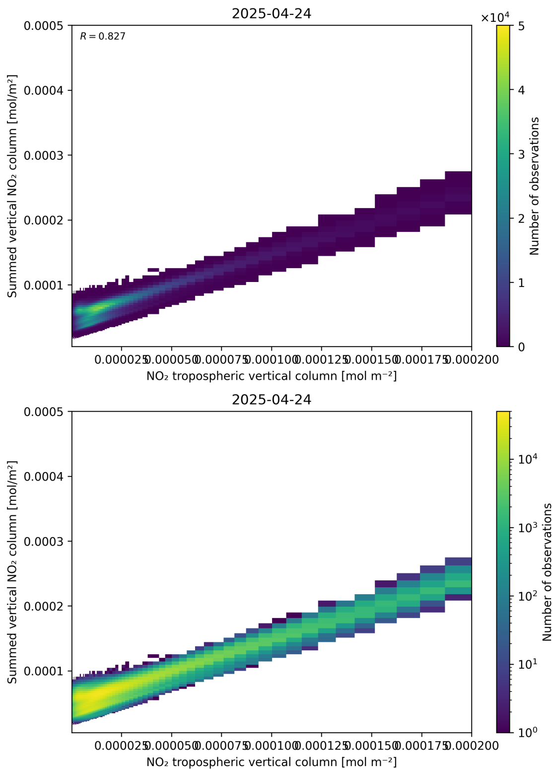
Figure 126: Scatter density plot of “NO 2 tropospheric vertical column” against “Summed vertical NO 2 column” for 2025-04-24 to 2025-04-25.
