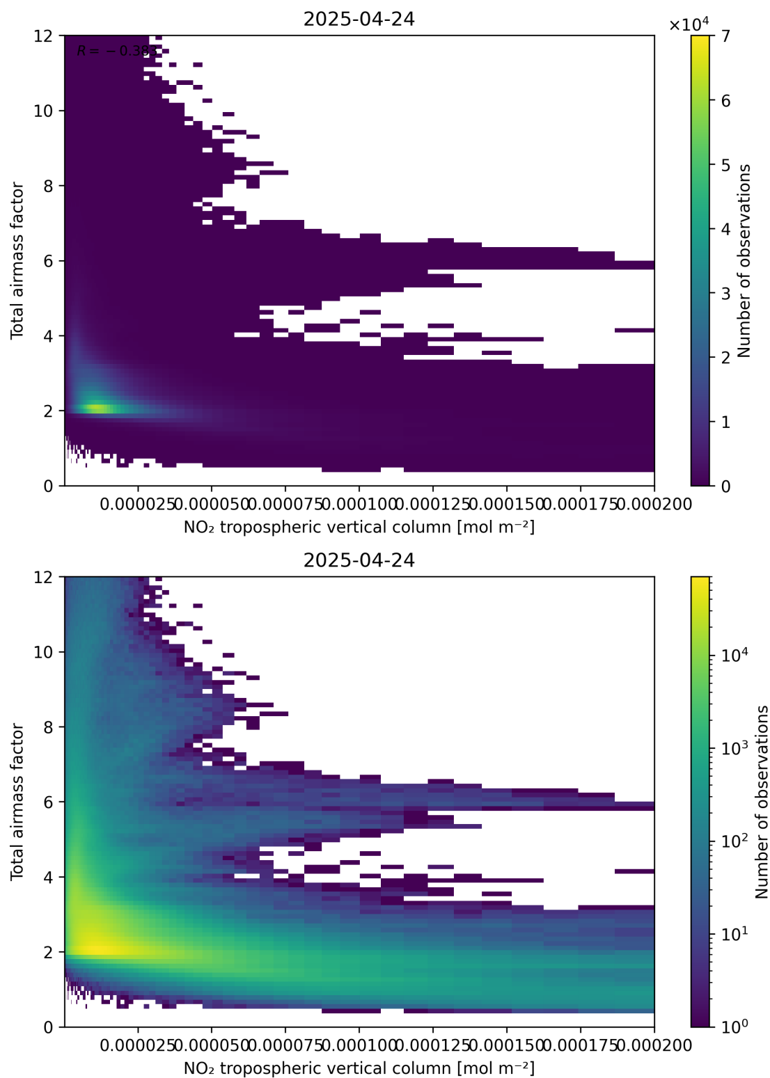
Figure 122: Scatter density plot of “NO 2 tropospheric vertical column” against “Total air mass factor” for 2025-04-24 to 2025-04-25.
