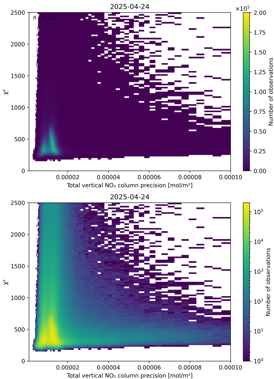
Figure 116: Scatter density plot of “Total vertical NO 2 column precision” against “ \chi^2 ” for 2025-04-24 to 2025-04-25.
