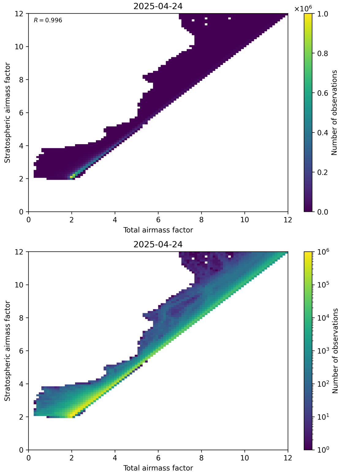
Figure 62: Scatter density plot of “Total airmass factor” against “Stratospheric airmass factor” for 2025-04-24 to 2025-04-25.
