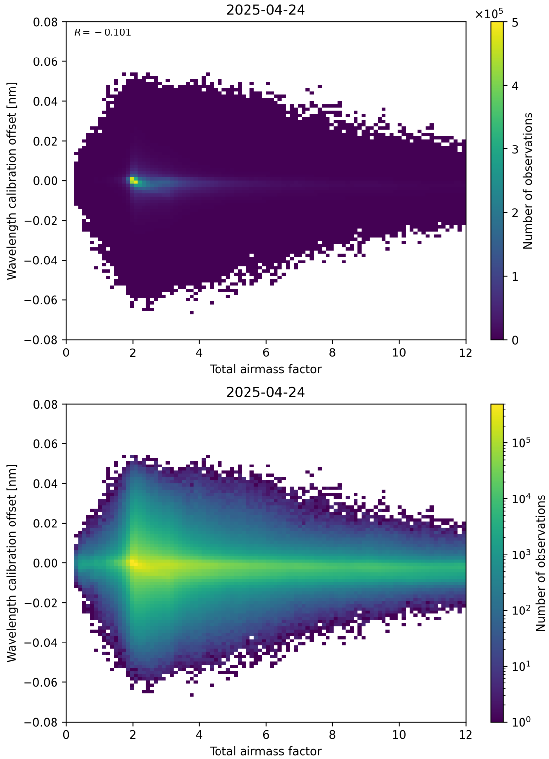
Figure 70: Scatter density plot of “Total airmass factor” against “Wavelength calibration offset” for 2025-04-24 to 2025-04-25.
