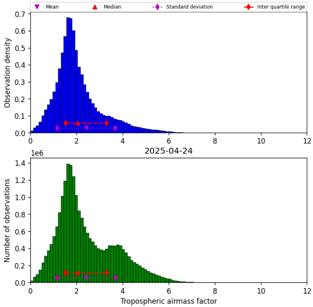
Figure 31: Histogram of “Tropospheric airmass factor” for 2025-04-24 to 2025-04-25
