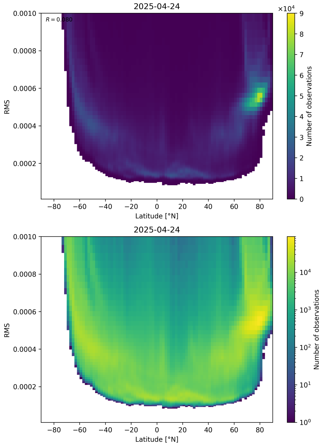
Figure 94: Scatter density plot of “Latitude” against “RMS” for 2025-04-24 to 2025-04-25.
