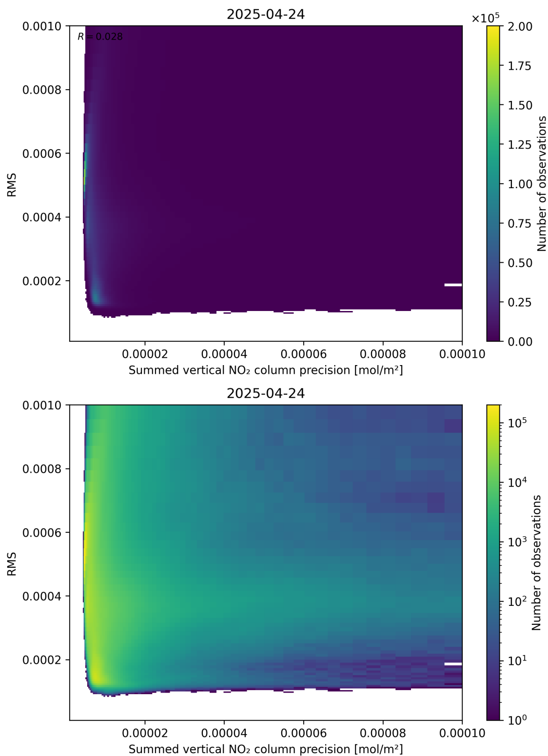
Figure 108: Scatter density plot of “Summed vertical NO 2 column precision” against “RMS” for 2025-04-24 to 2025-04-25.
