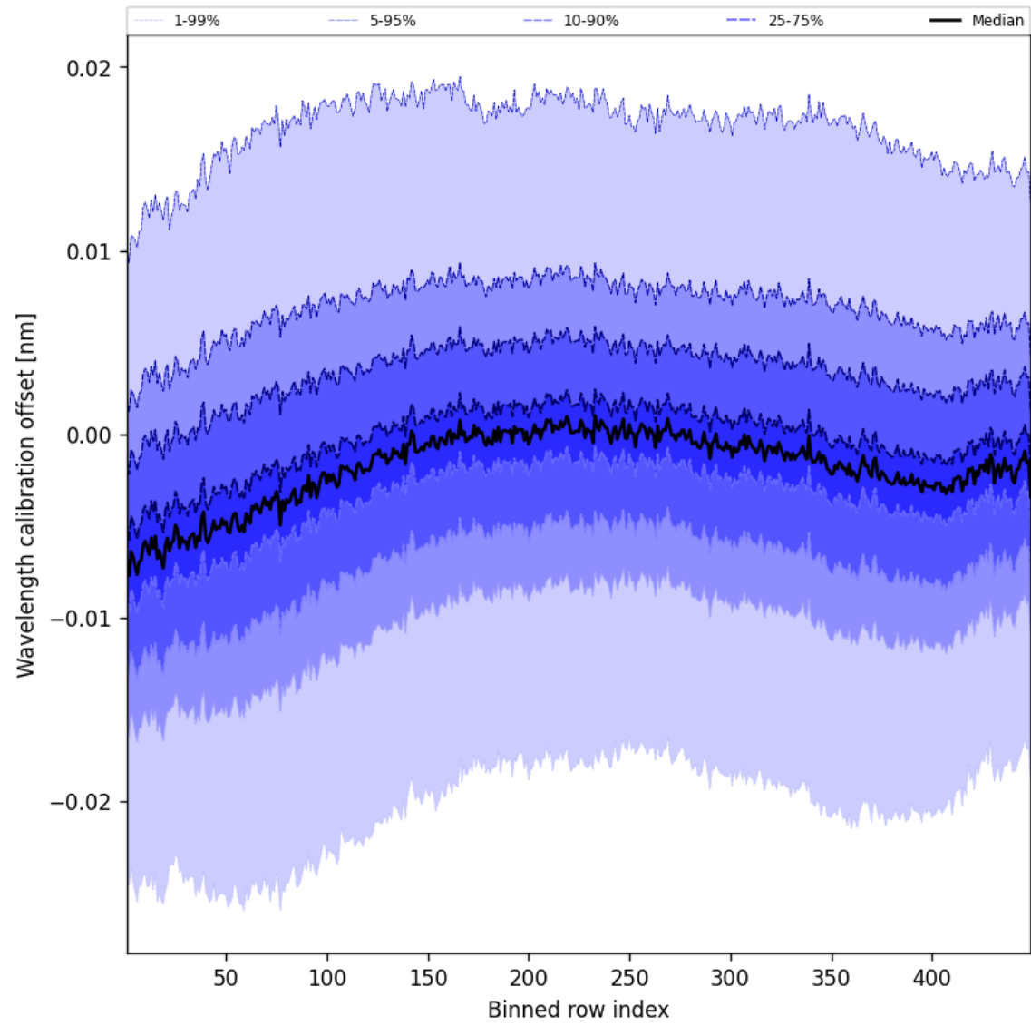
Figure 52: Along track statistics of “Wavelength calibration offset” for 2025-04-24 to 2025-04-25
