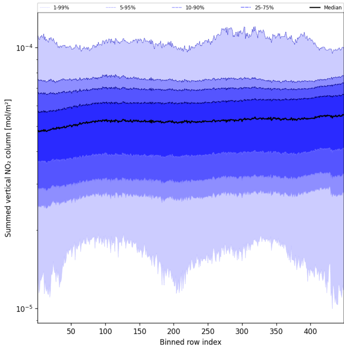
Figure 57: Along track statistics of “Summed vertical NO 2 column” for 2025-04-24 to 2025-04-25
