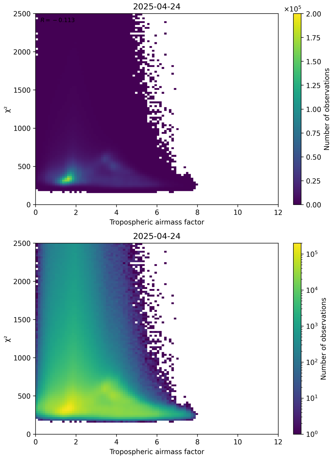
Figure 73: Scatter density plot of “Tropospheric airmass factor” against “ \chi^2 ” for 2025-04-24 to 2025-04-25.
