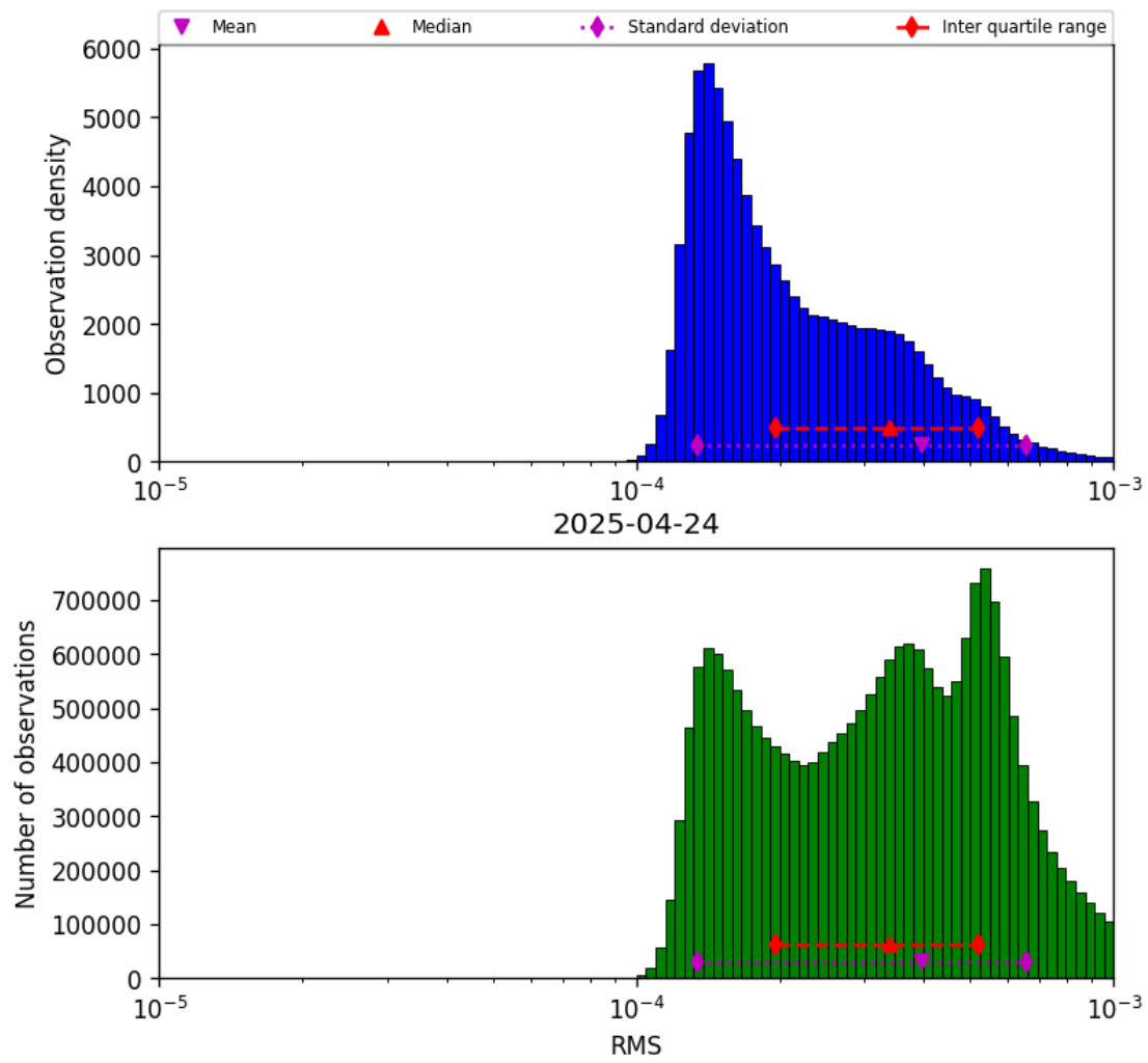
Figure 43: Histogram of “RMS” for 2025-04-24 to 2025-04-25
