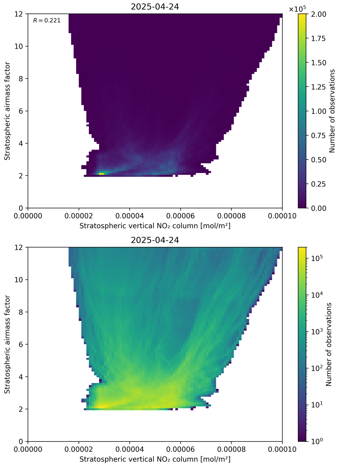
Figure 96: Scatter density plot of “Stratospheric vertical NO 2 column” against “Stratospheric airmass factor” for 2025-04-24 to 2025-04-25.
