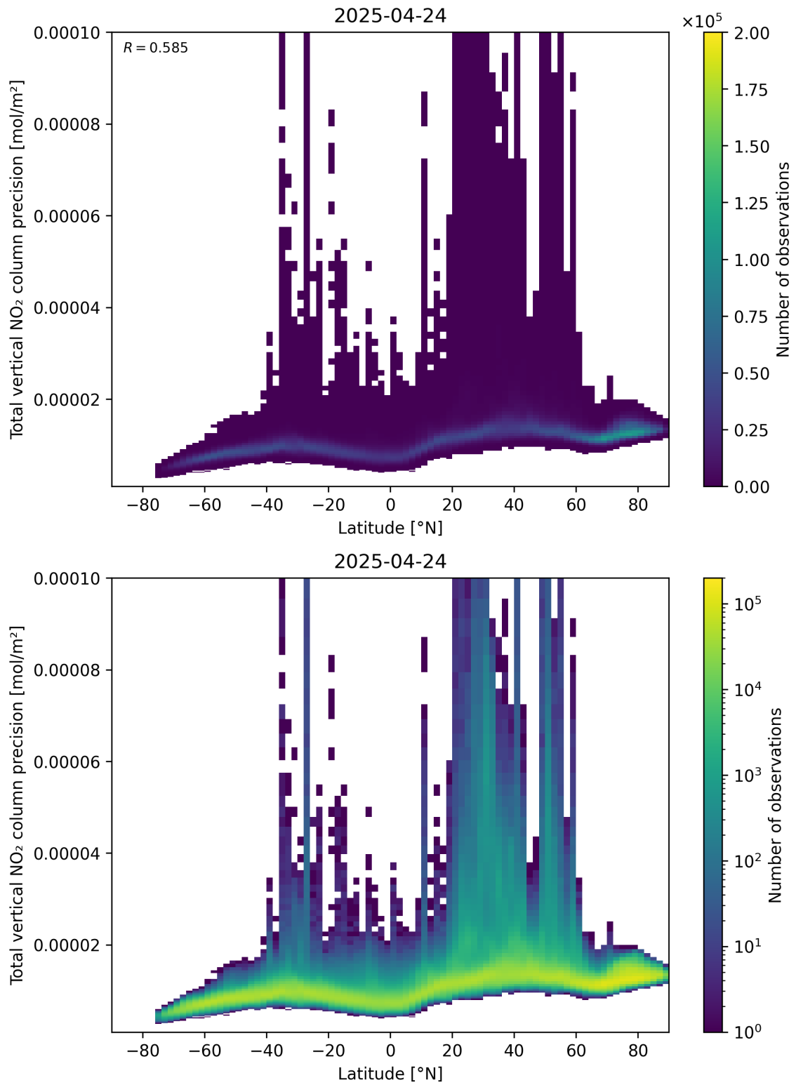
Figure 91: Scatter density plot of “Latitude” against “Total vertical NO 2 column precision” for 2025-04-24 to 2025-04-25.
