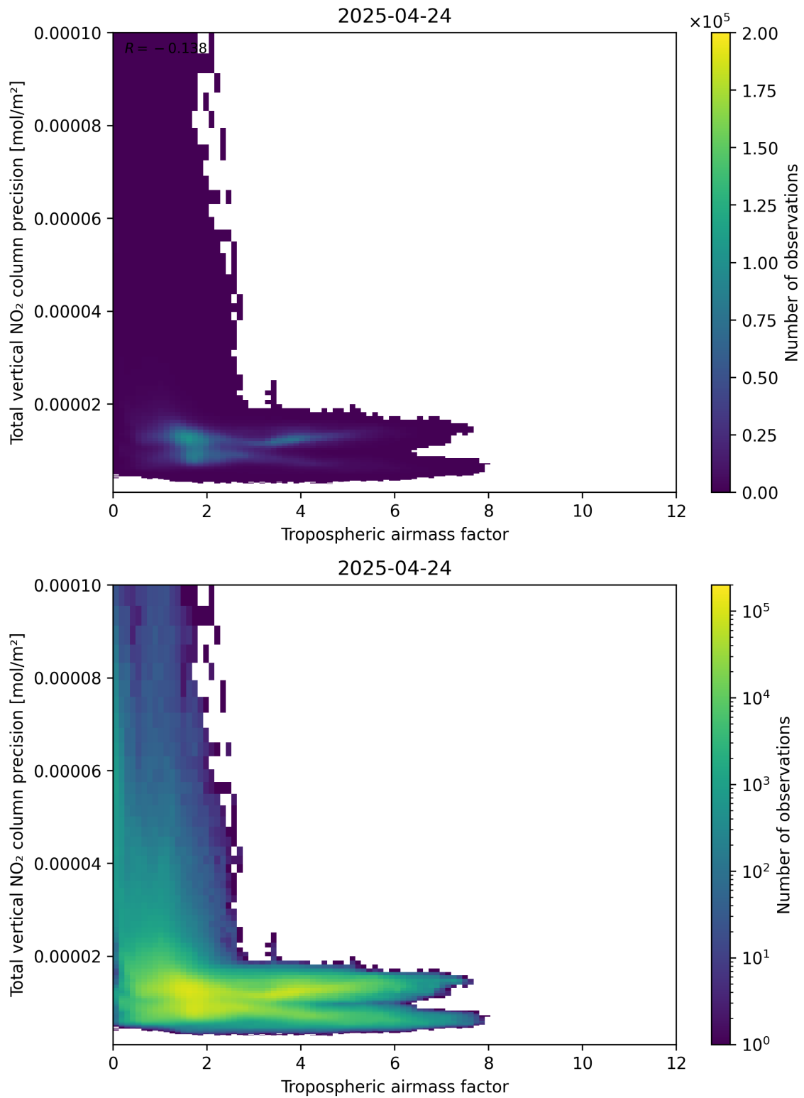
Figure 78: Scatter density plot of “Tropospheric air mass factor” against “Total vertical NO 2 column precision” for 2025-04-24 to 2025-04-25.
