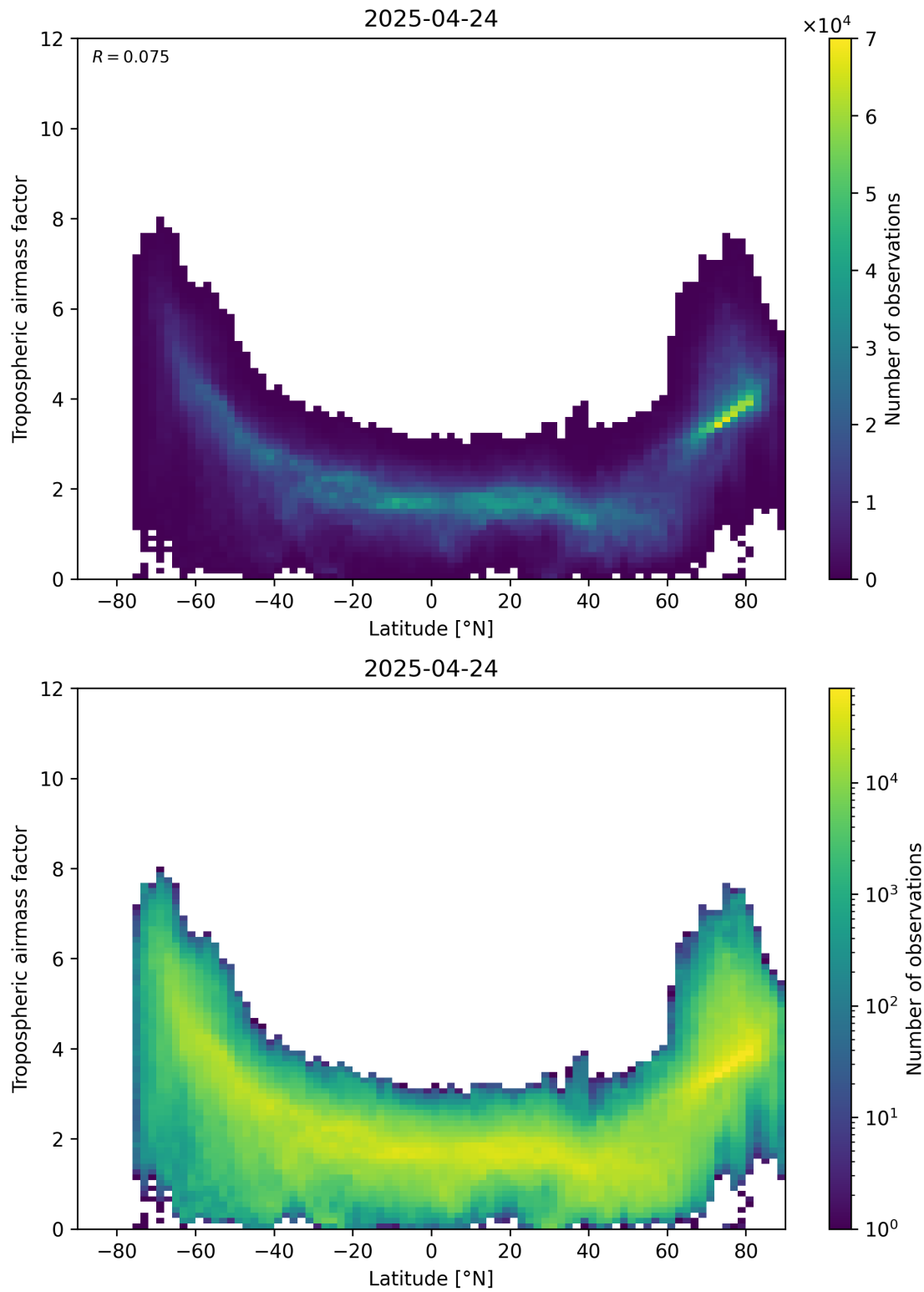
Figure 85: Scatter density plot of “Latitude” against “Tropospheric airmass factor” for 2025-04-24 to 2025-04-25.
