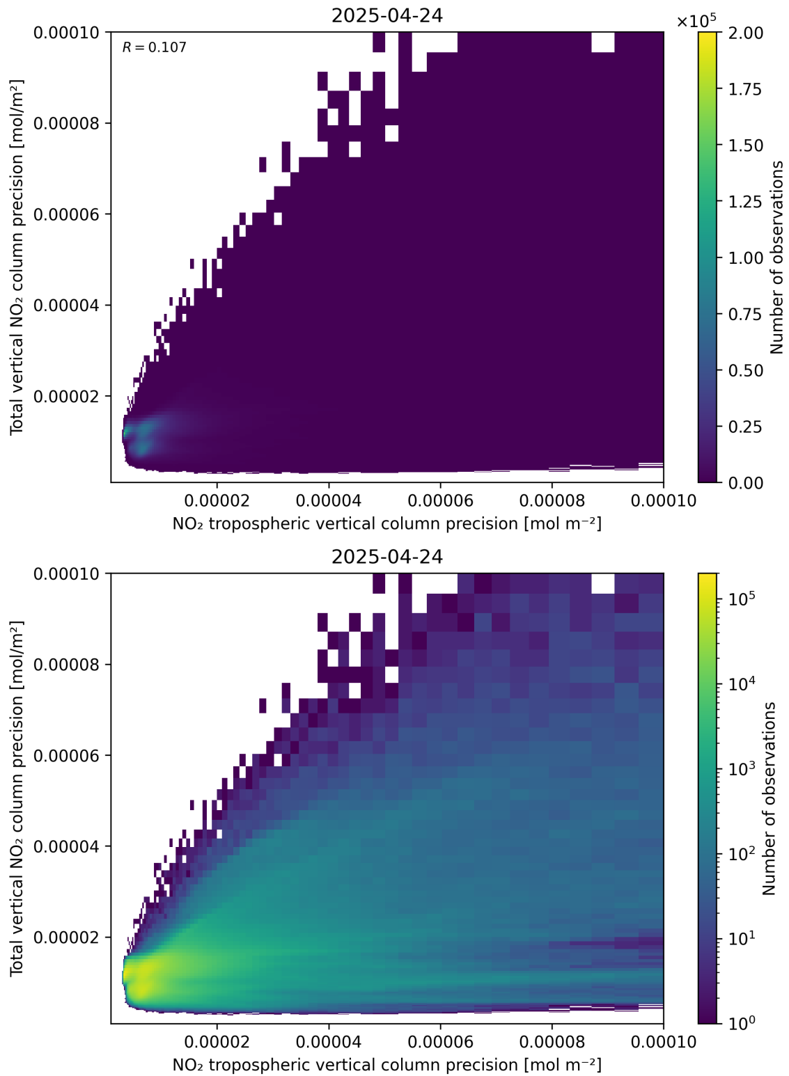
Figure 139: Scatter density plot of “NO 2 tropospheric vertical column precision” against “Total vertical NO 2 column precision” for 2025-04-24 to 2025-04-25.
