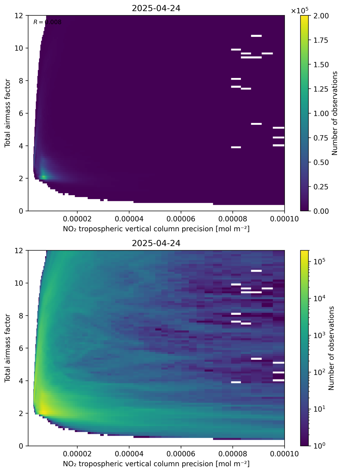
Figure 132: Scatter density plot of “NO 2 tropospheric vertical column precision” against “Total air mass factor” for 2025-04-24 to 2025-04-25.
