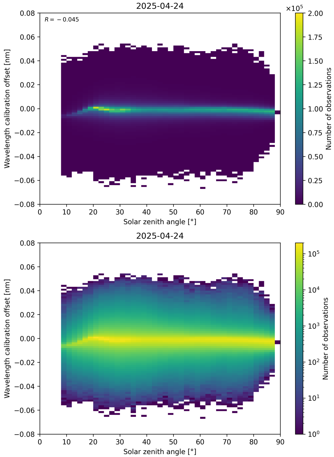
Figure 158: Scatter density plot of “Solar zenith angle” against “Wavelength calibration offset” for 2025-04-24 to 2025-04-25.
