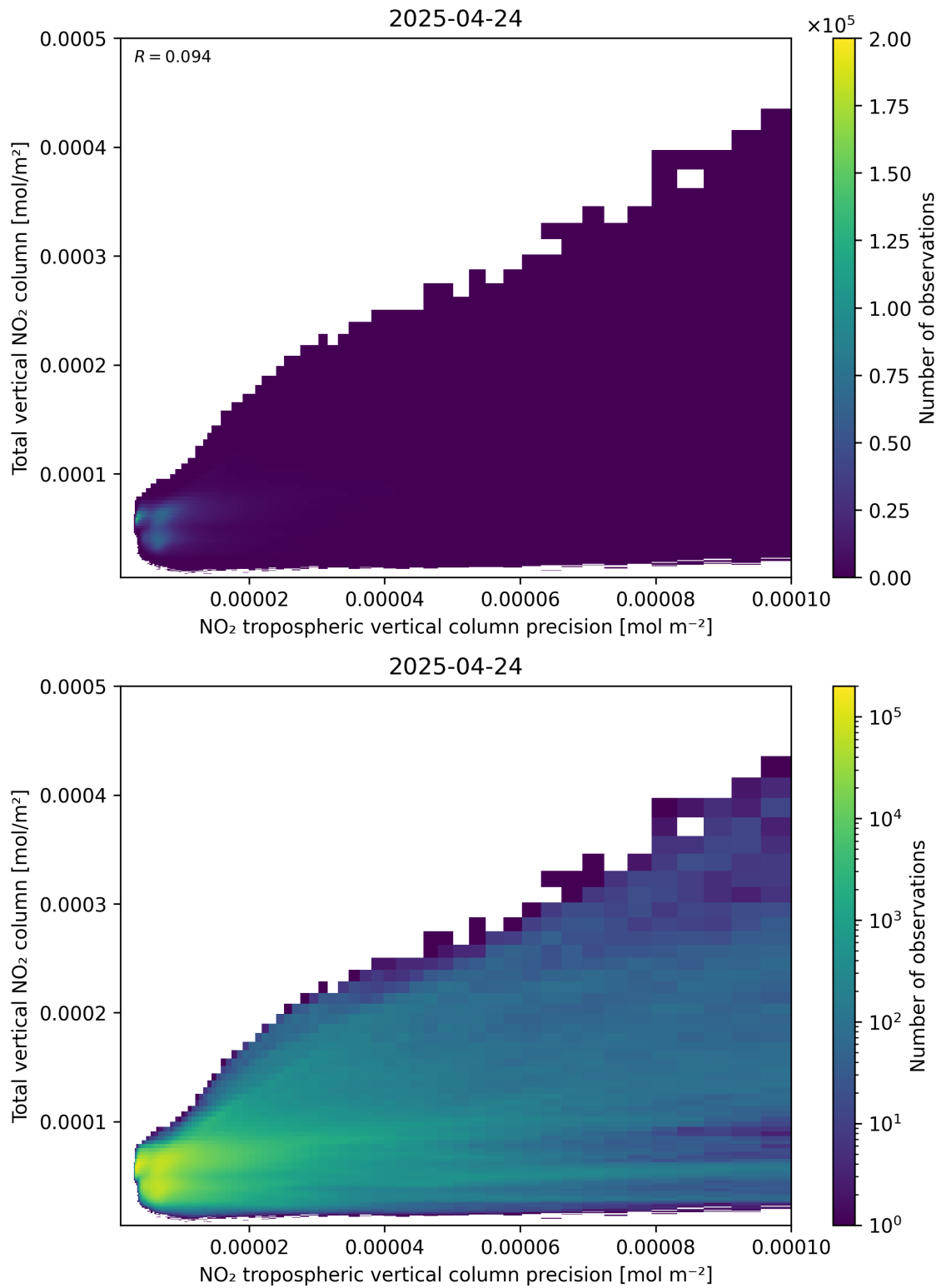
Figure 138: Scatter density plot of “NO 2 tropospheric vertical column precision” against “Total vertical NO 2 column” for 2025-04-24 to 2025-04-25.
