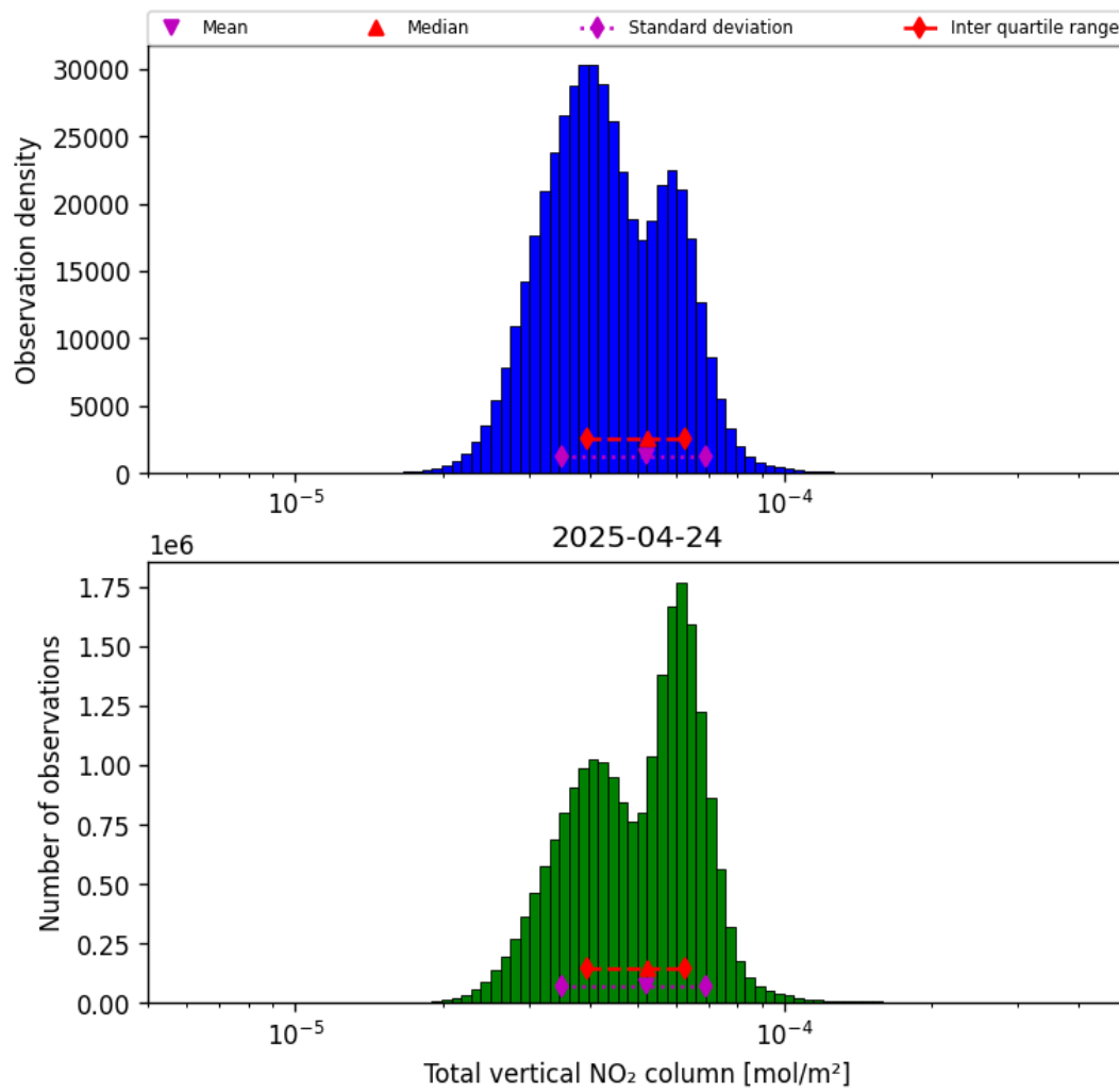
Figure 38: Histogram of "Total vertical NO 2 column" for 2025-04-24 to 2025-04-25
