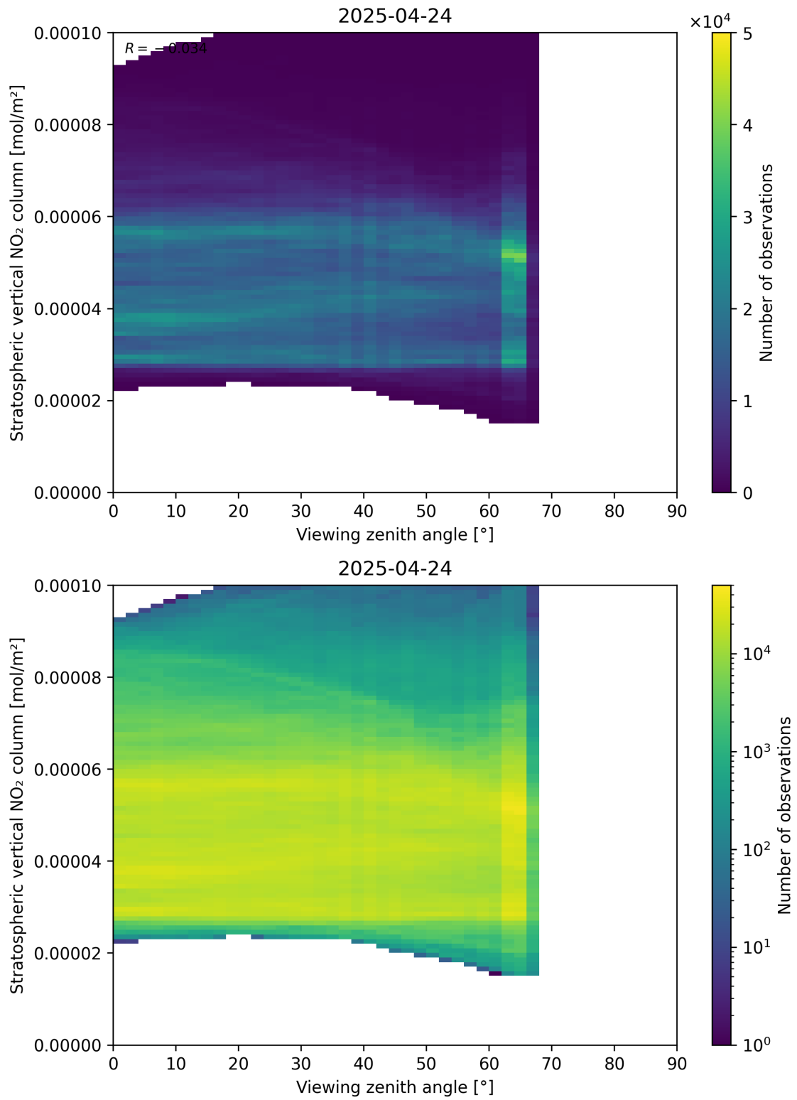
Figure 164: Scatter density plot of “Viewing zenith angle” against “Stratospheric vertical NO 2 column” for 2025-04-24 to 2025-04-25.
