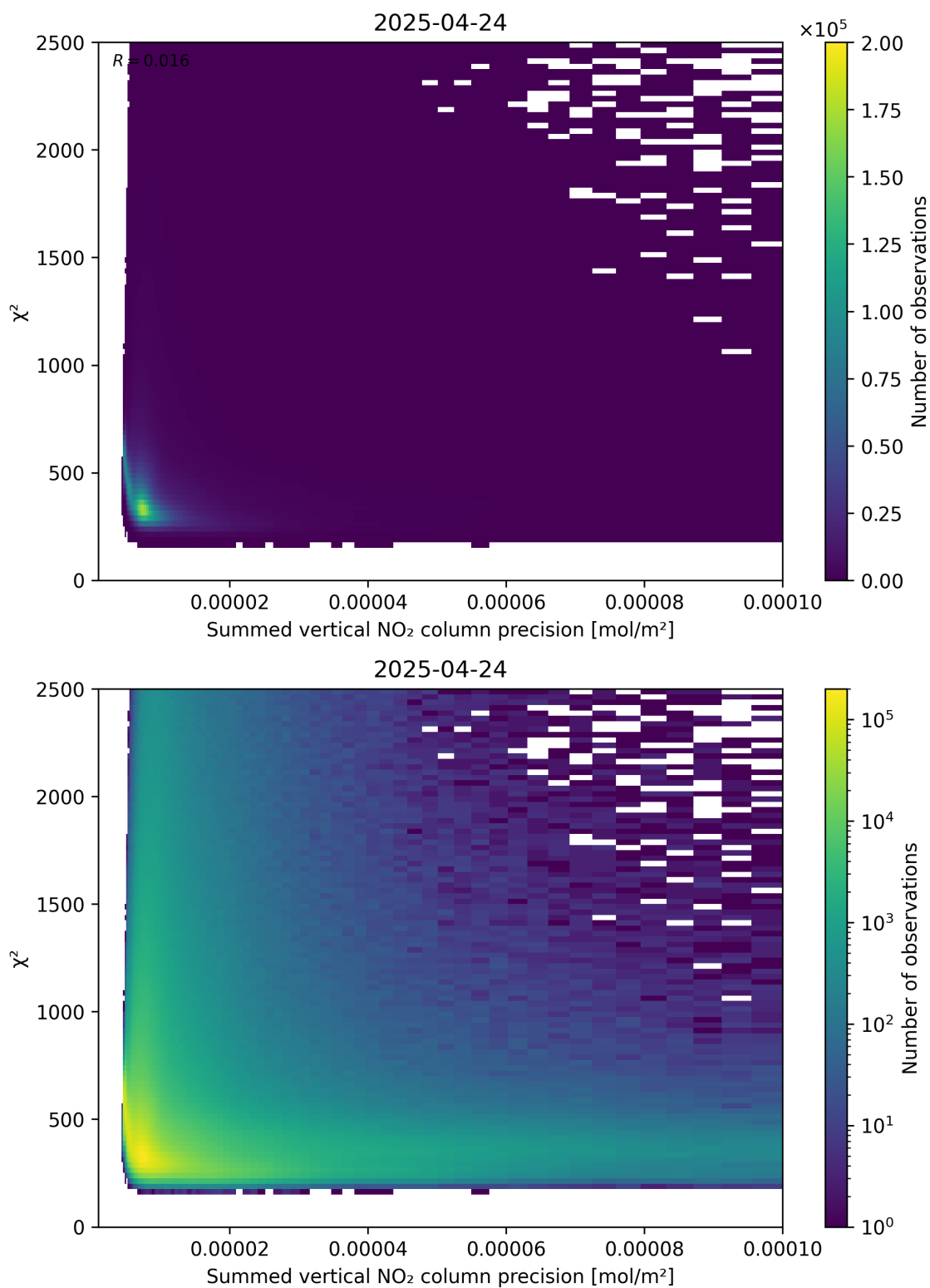
Figure 107: Scatter density plot of “Summed vertical NO 2 column precision” against “ \chi^2 ” for 2025-04-24 to 2025-04-25.
