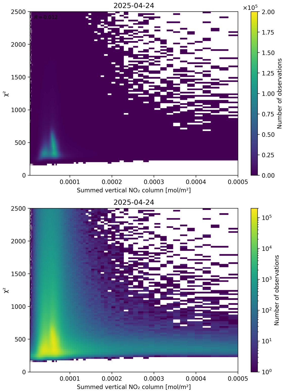
Figure 104: Scatter density plot of “Summed vertical NO 2 column” against “ \chi^2 ” for 2025-04-24 to 2025-04-25.
