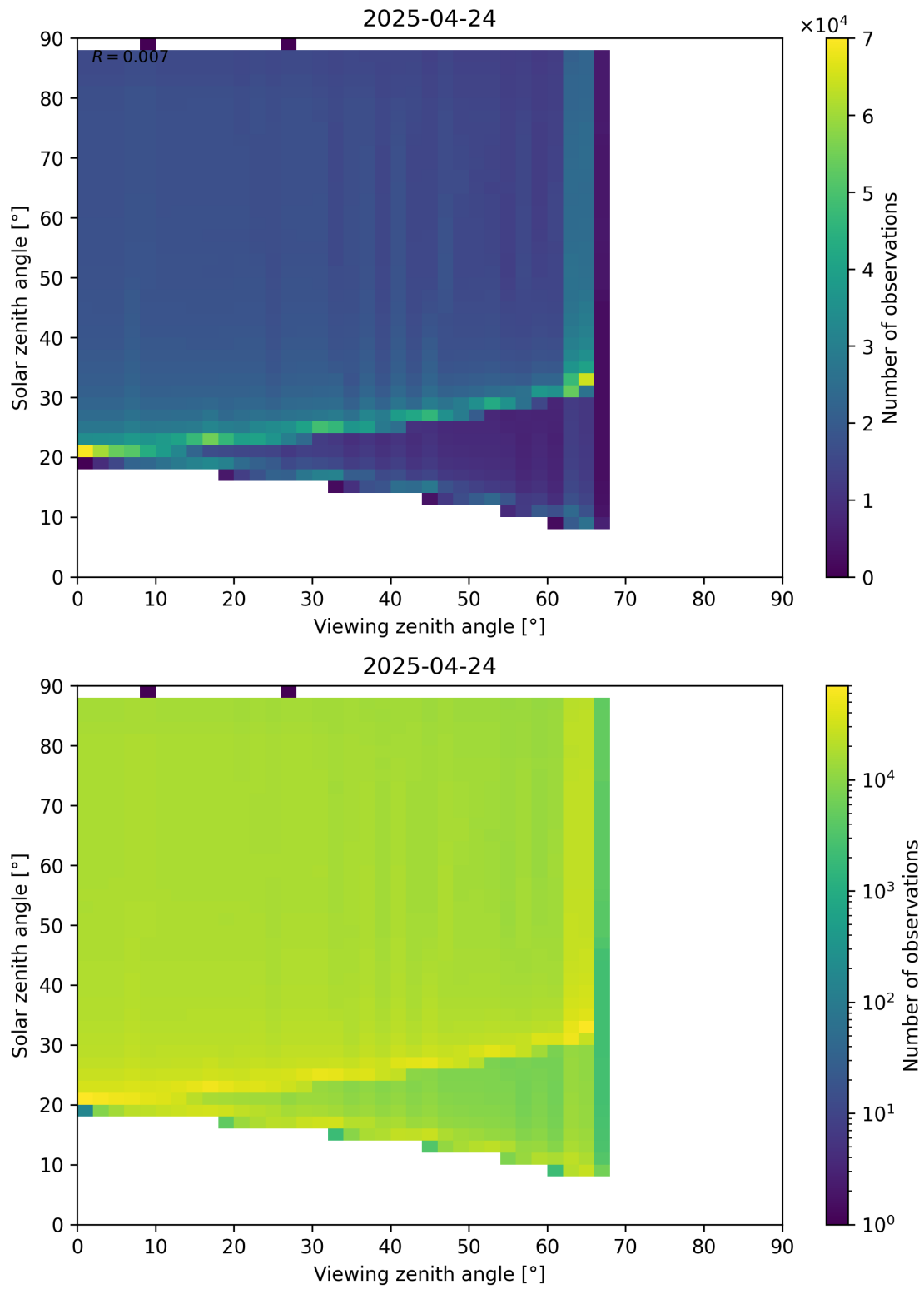
Figure 172: Scatter density plot of “Viewing zenith angle” against “Solar zenith angle” for 2025-04-24 to 2025-04-25.
