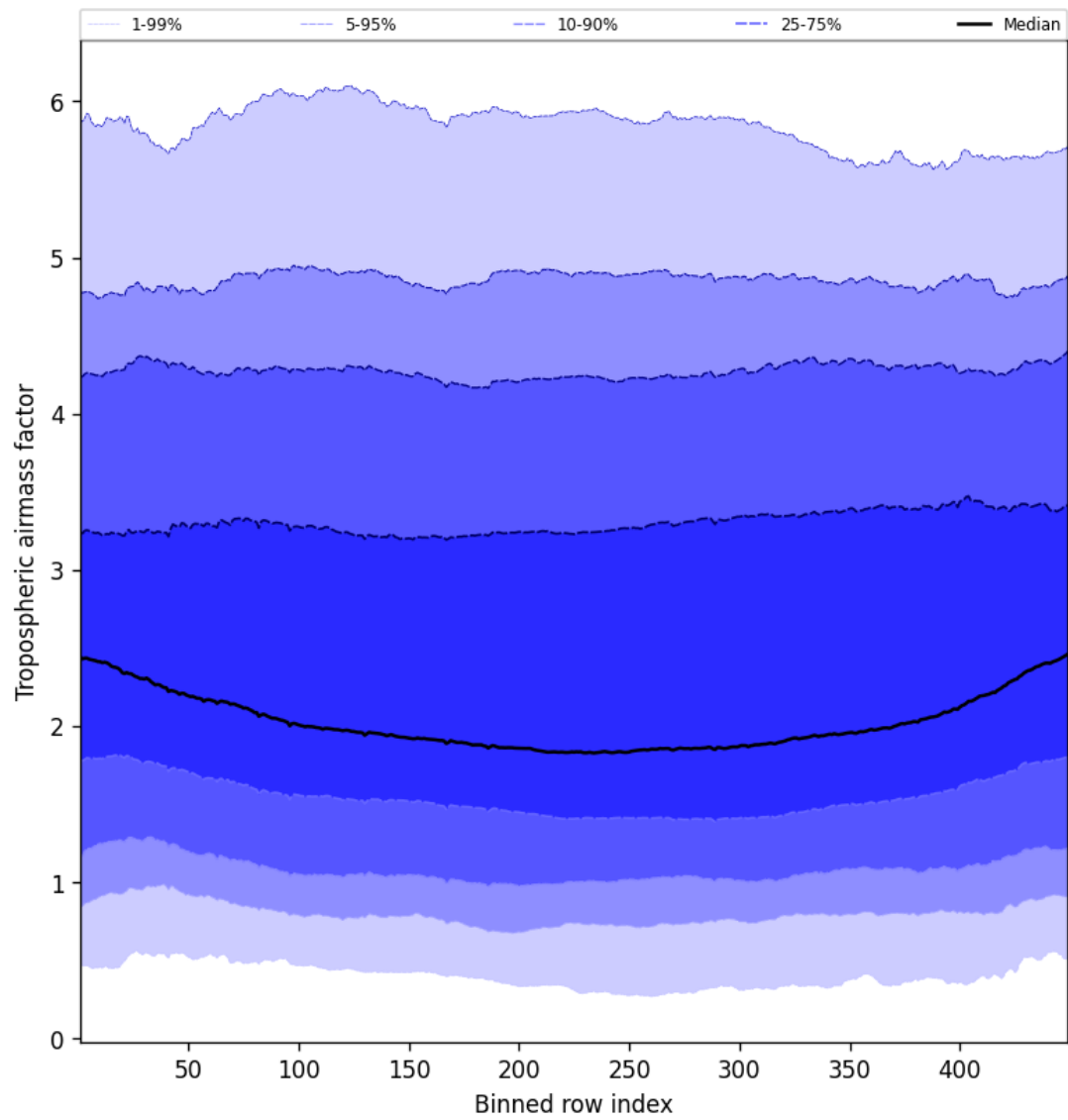
Figure 48: Along track statistics of “Tropospheric airmass factor” for 2025-04-24 to 2025-04-25
