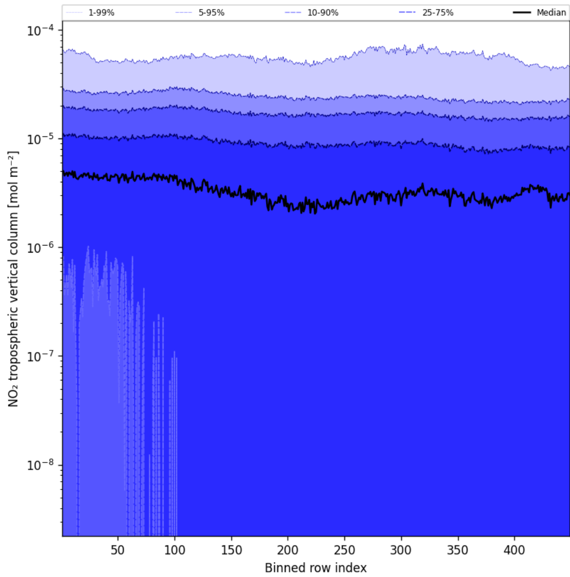
Figure 46: Along track statistics of “NO 2 tropospheric vertical column” for 2025-04-24 to 2025-04-25
