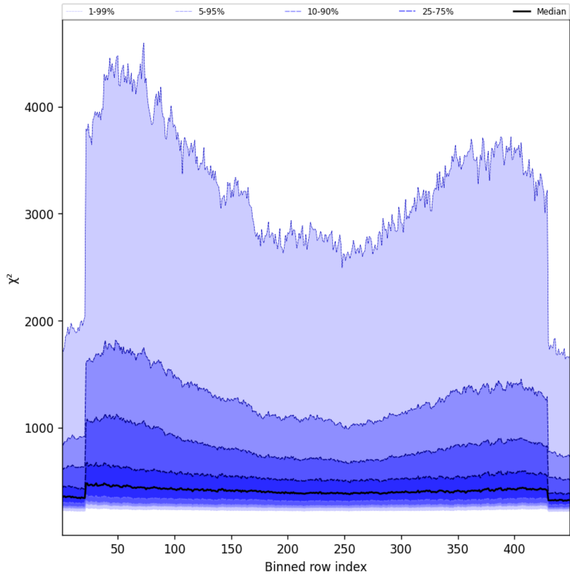
Figure 59: Along track statistics of “ \chi^2 ” for 2025-04-24 to 2025-04-25
