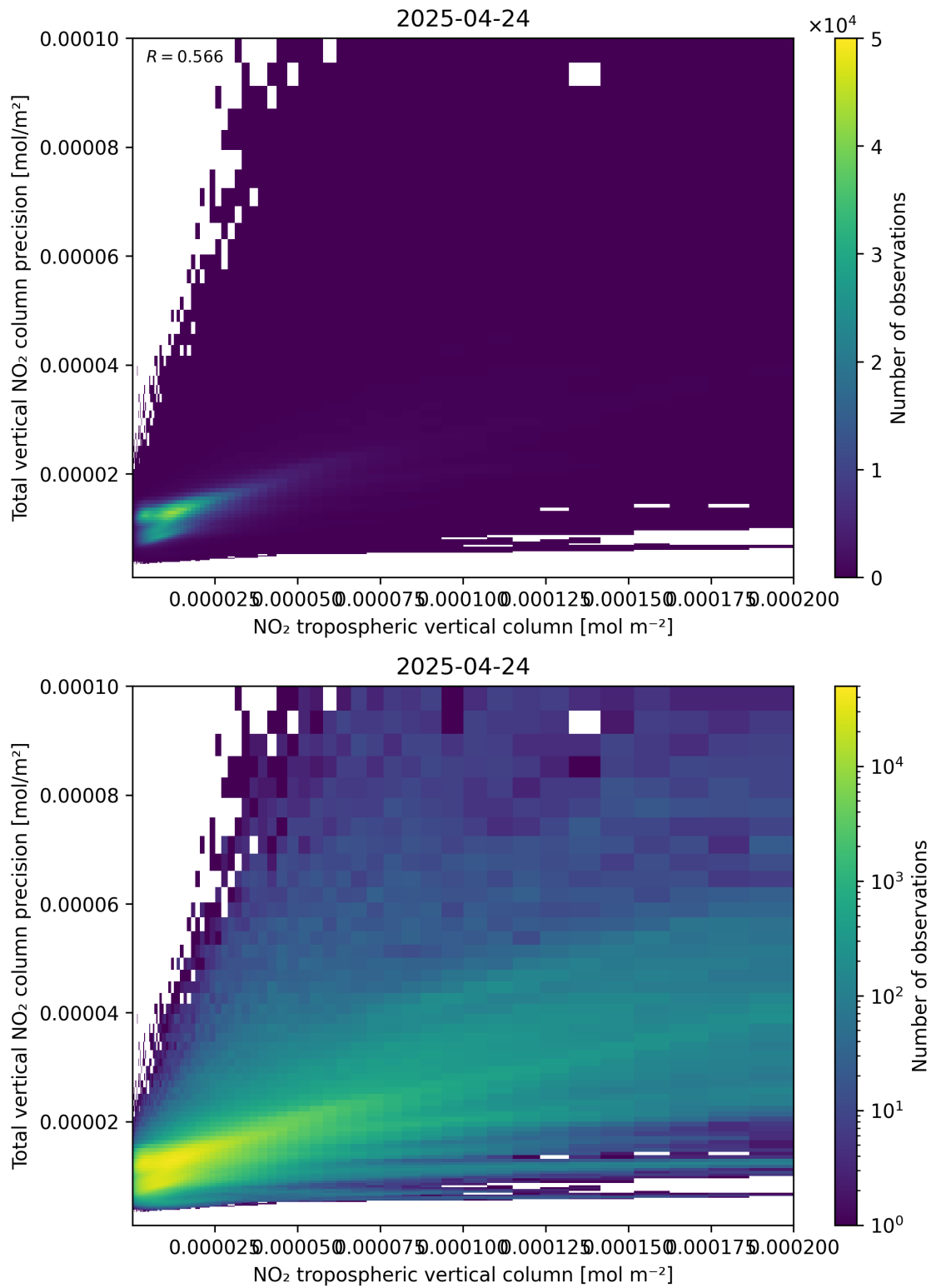
Figure 129: Scatter density plot of “NO 2 tropospheric vertical column” against “Total vertical NO 2 column precision” for 2025-04-24 to 2025-04-25.
