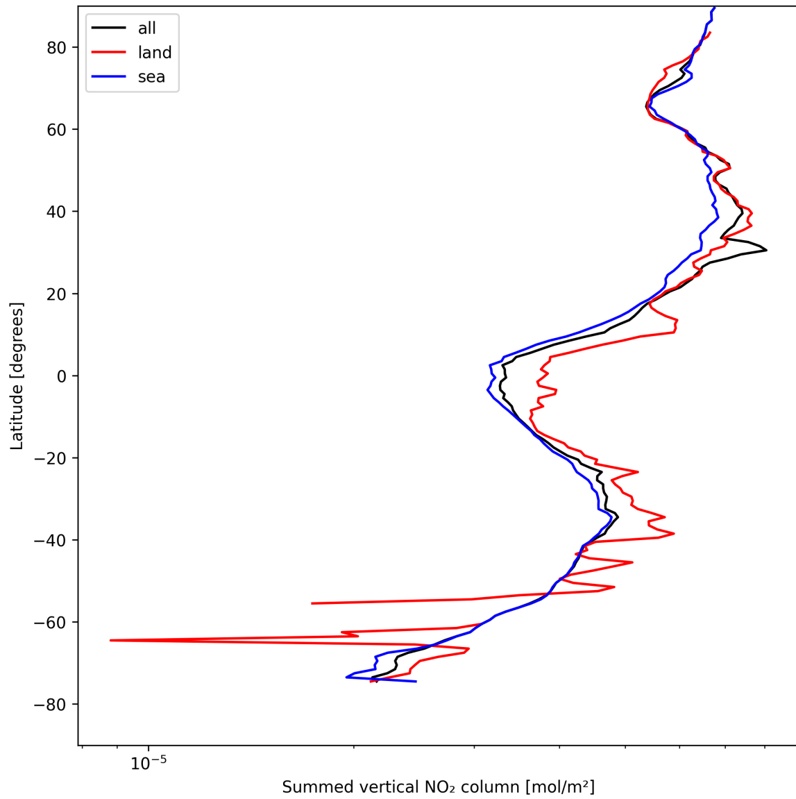
Figure 23: Zonal average of “Summed vertical NO 2 column” for 2025-04-24 to 2025-04-25.
