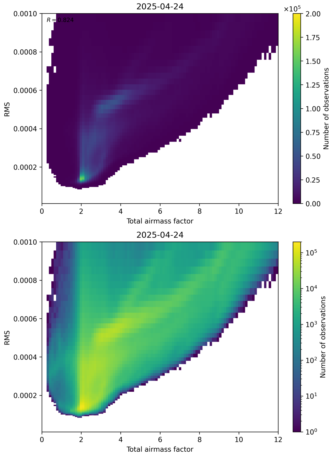
Figure 69: Scatter density plot of “Total airmass factor” against “RMS” for 2025-04-24 to 2025-04-25.
