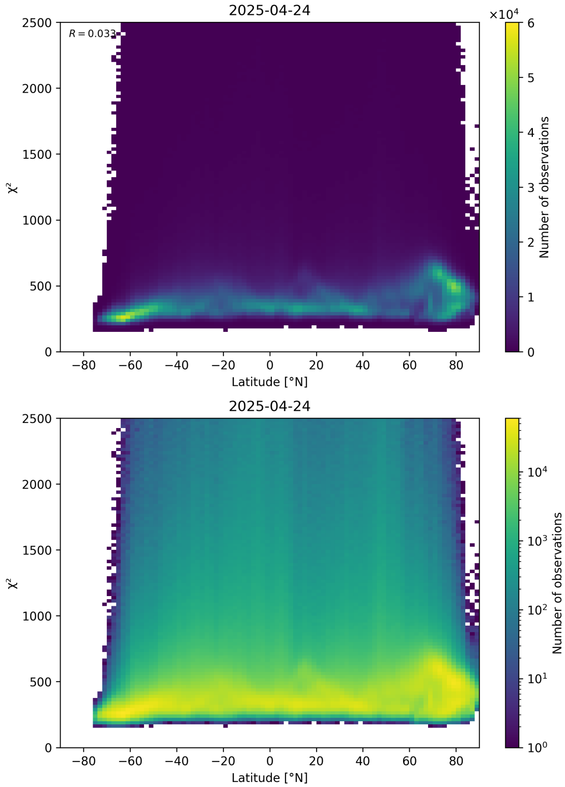
Figure 86: Scatter density plot of “Latitude” against “ \chi^2 ” for 2025-04-24 to 2025-04-25.
