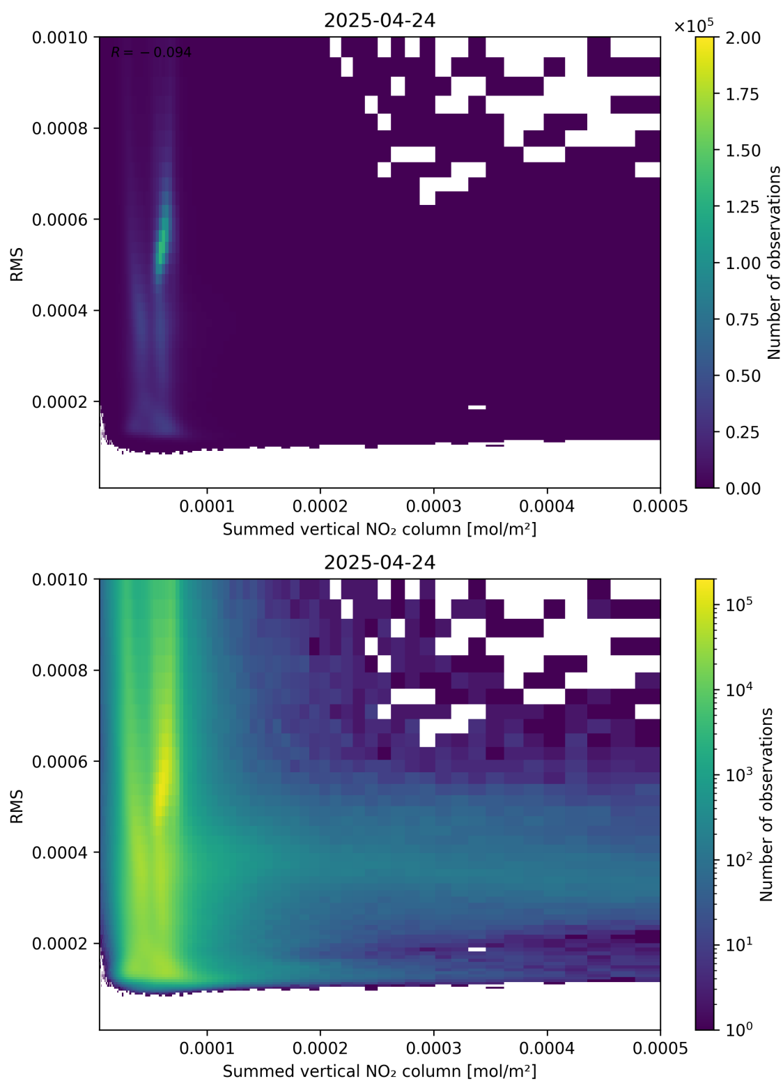
Figure 109: Scatter density plot of “Summed vertical NO 2 column” against “RMS” for 2025-04-24 to 2025-04-25.
