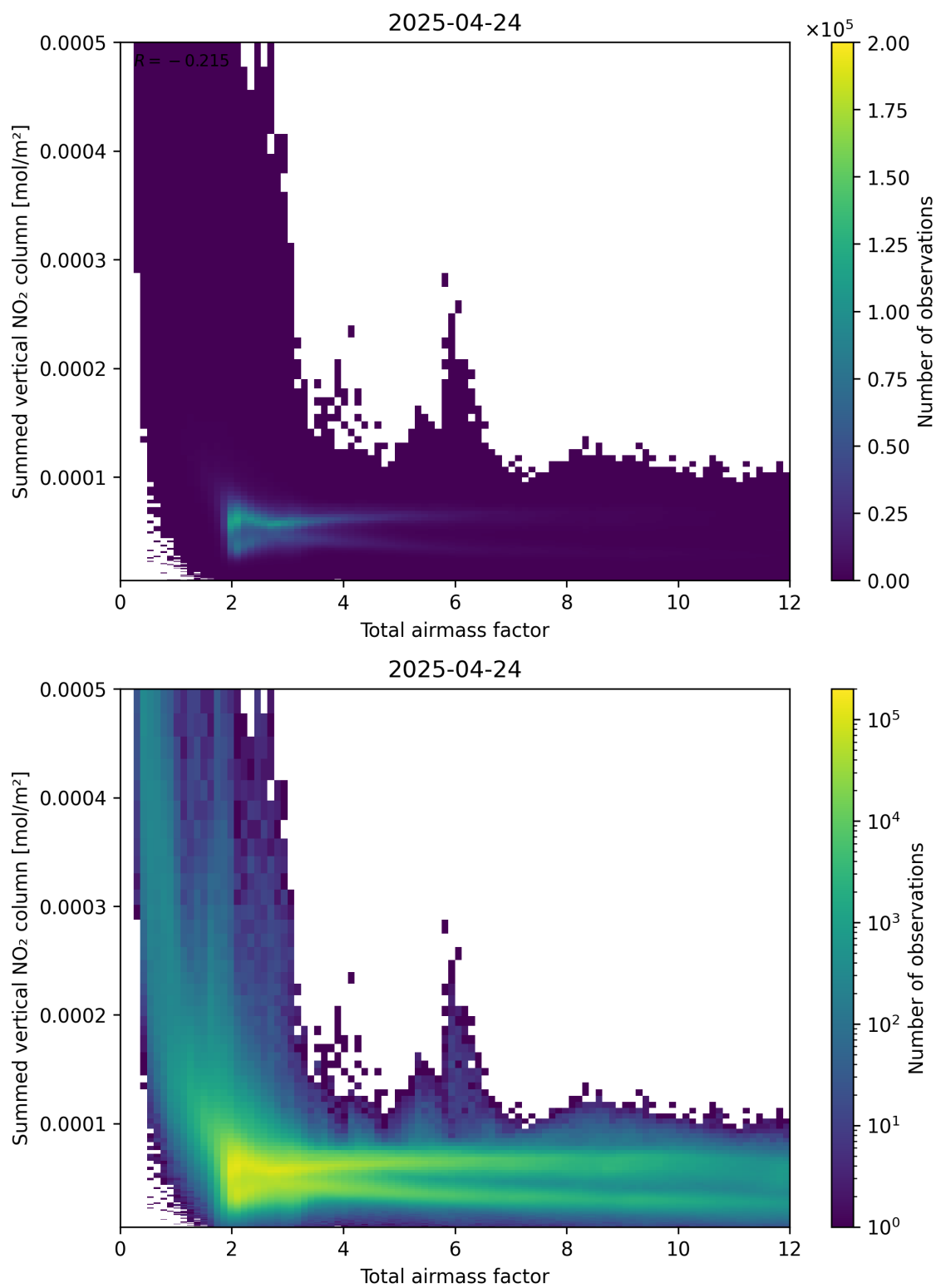
Figure 65: Scatter density plot of “Total airmass factor” against “Summed vertical NO 2 column” for 2025-04-24 to 2025-04-25.
