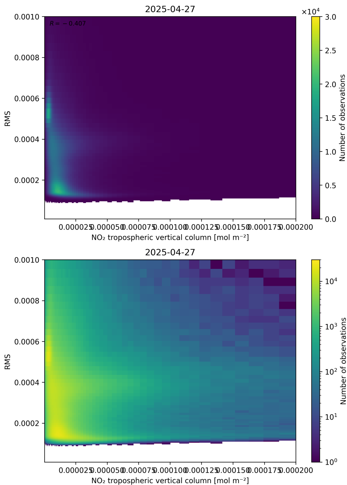
Figure 142: Scatter density plot of “NO 2 tropospheric vertical column” against “RMS” for 2025-04-27 to 2025-04-27.
