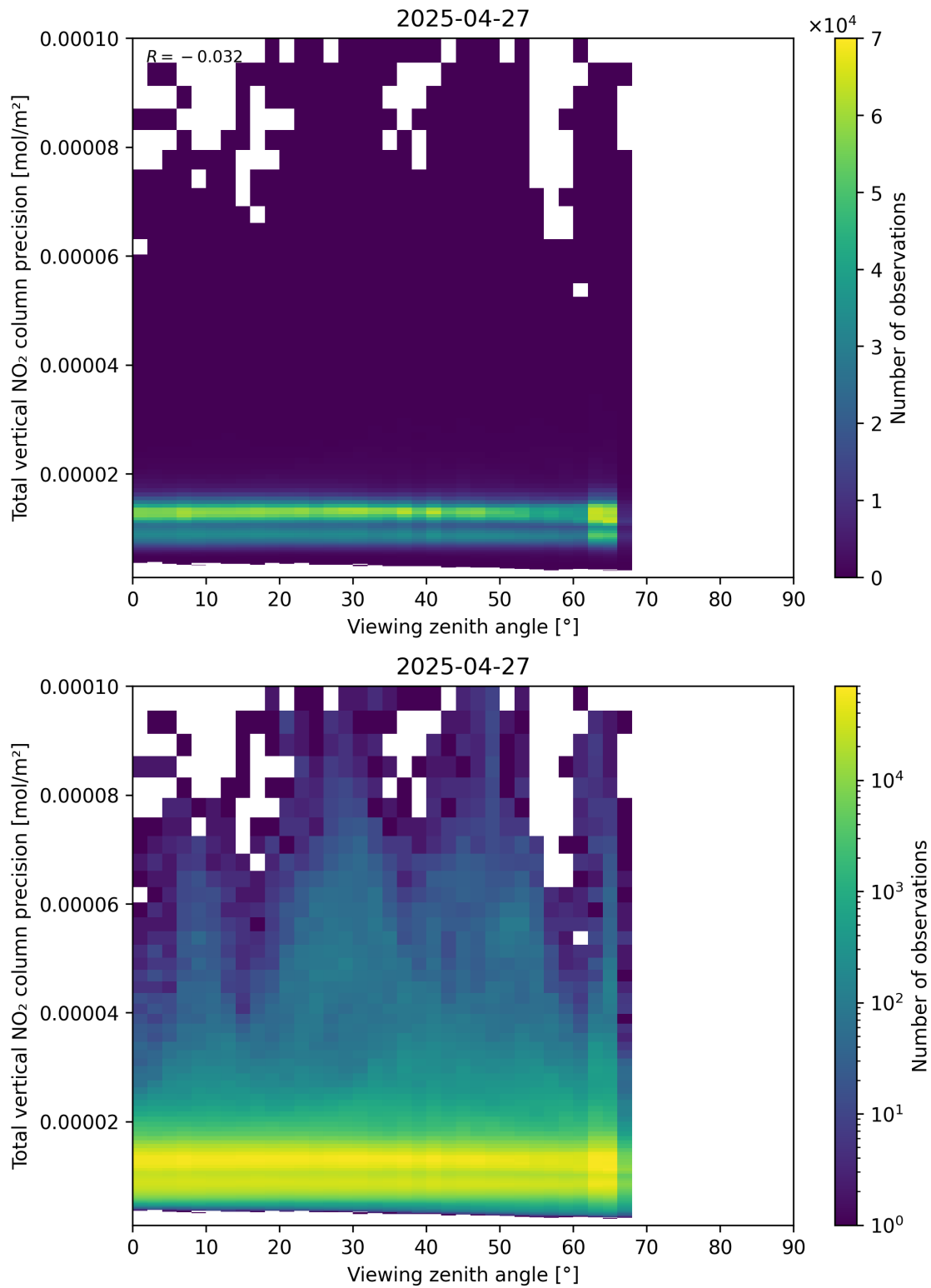
Figure 168: Scatter density plot of “Viewing zenith angle” against “Total vertical NO 2 column precision” for 2025-04-27 to 2025-04-27.
