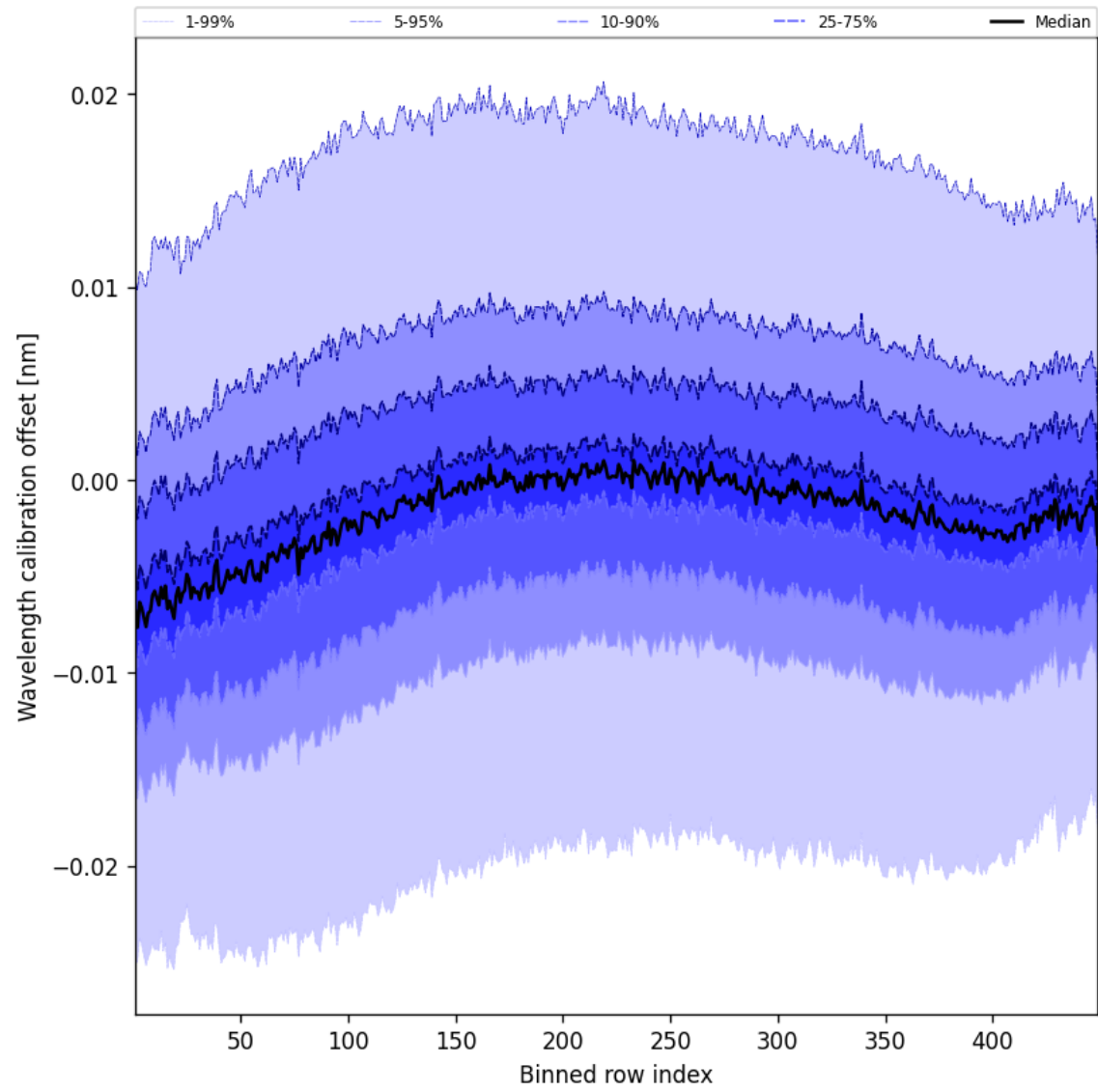
Figure 52: Along track statistics of “Wavelength calibration offset” for 2025-04-27 to 2025-04-27
