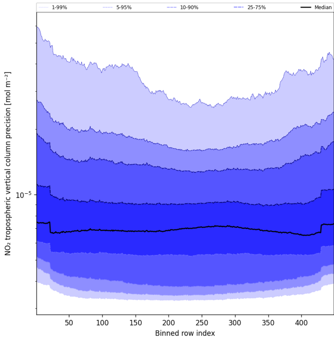
Figure 47: Along track statistics of “NO 2 tropospheric vertical column precision” for 2025-04-27 to 2025-04-27
