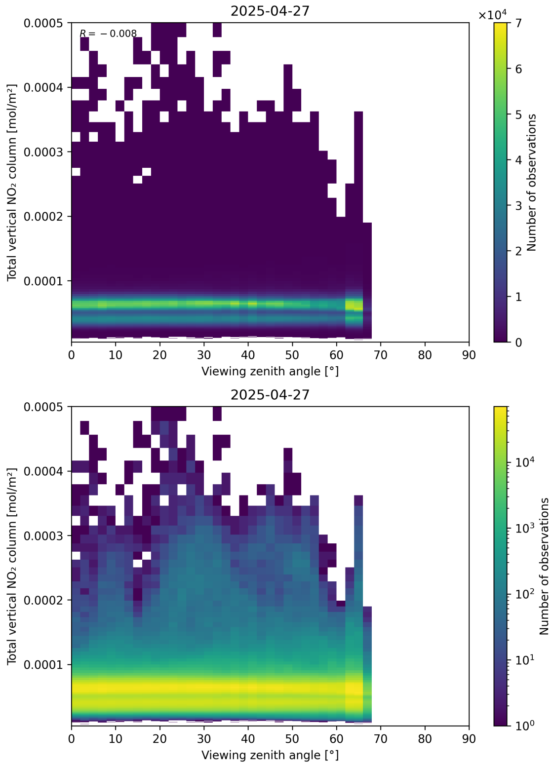
Figure 167: Scatter density plot of “Viewing zenith angle” against “Total vertical NO 2 column” for 2025-04-27 to 2025-04-27.
