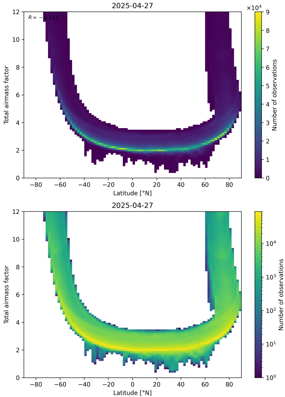
Figure 84: Scatter density plot of “Latitude” against “Total air mass factor” for 2025-04-27 to 2025-04-27.
