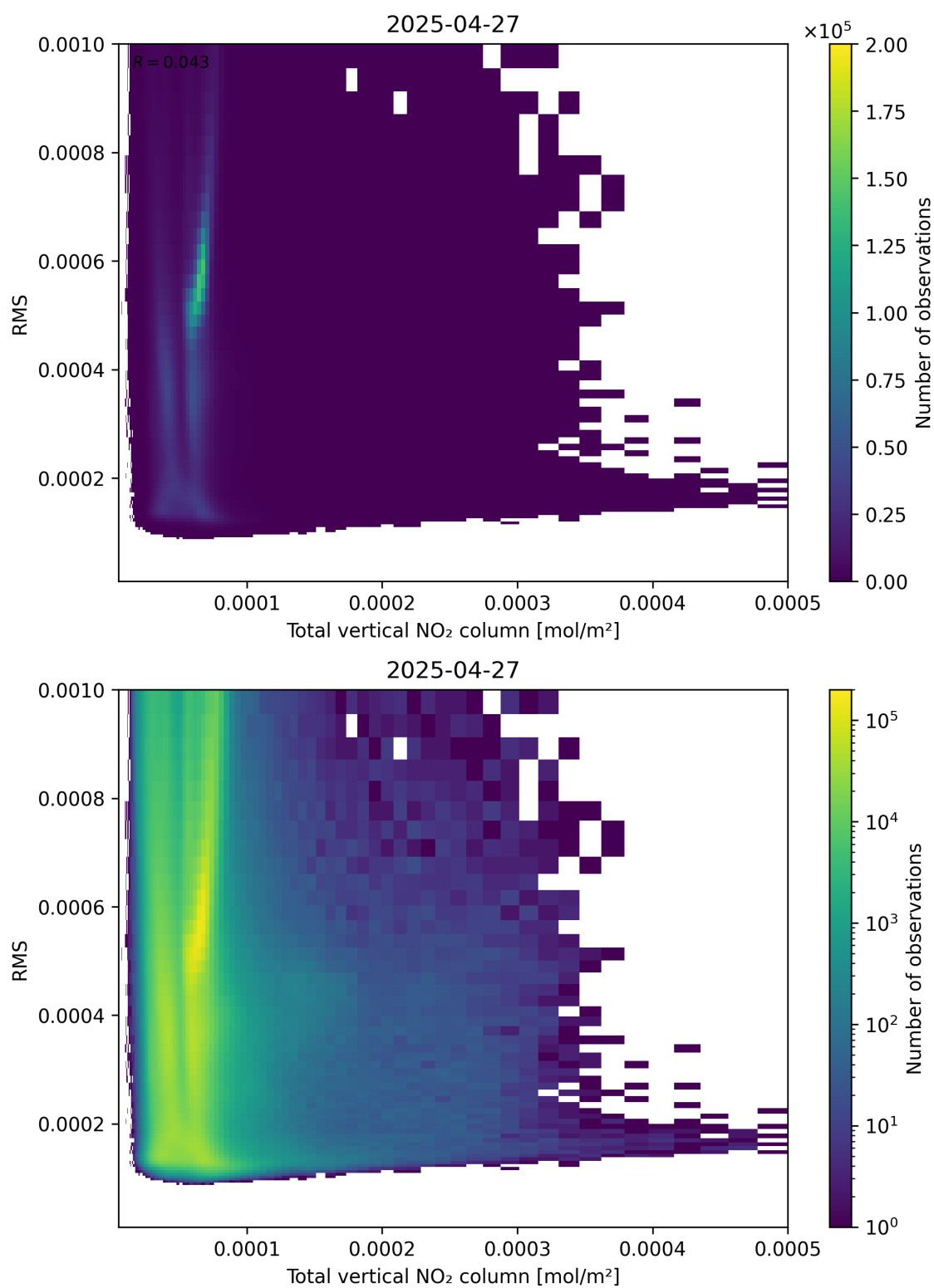
Figure 120: Scatter density plot of “Total vertical NO 2 column” against “RMS” for 2025-04-27 to 2025-04-27.
