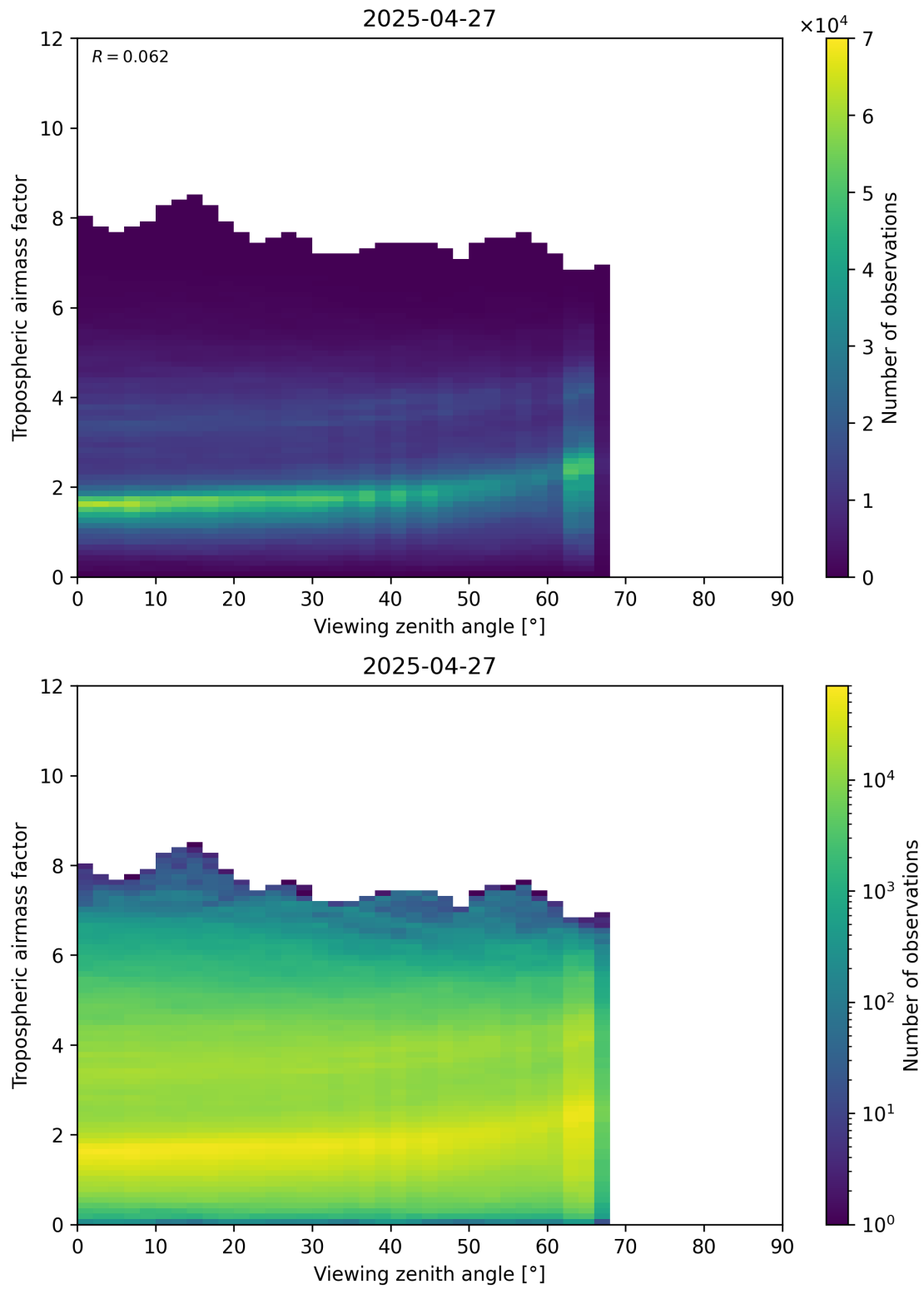
Figure 161: Scatter density plot of “Viewing zenith angle” against “Tropospheric airmass factor” for 2025-04-27 to 2025-04-27.
