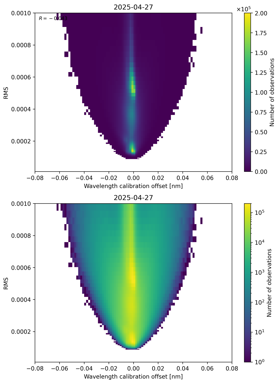
Figure 181: Scatter density plot of “Wavelength calibration offset” against “RMS” for 2025-04-27 to 2025-04-27.
