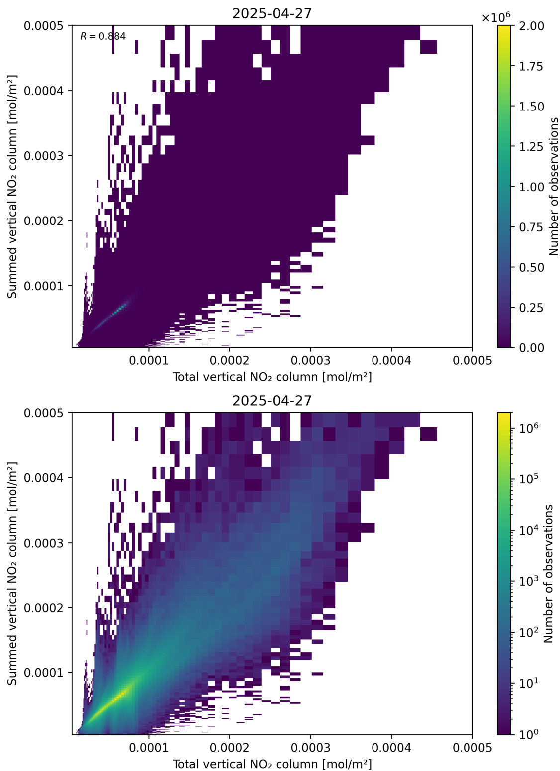
Figure 112: Scatter density plot of “Total vertical NO 2 column” against “Summed vertical NO 2 column” for 2025-04-27 to 2025-04-27.
