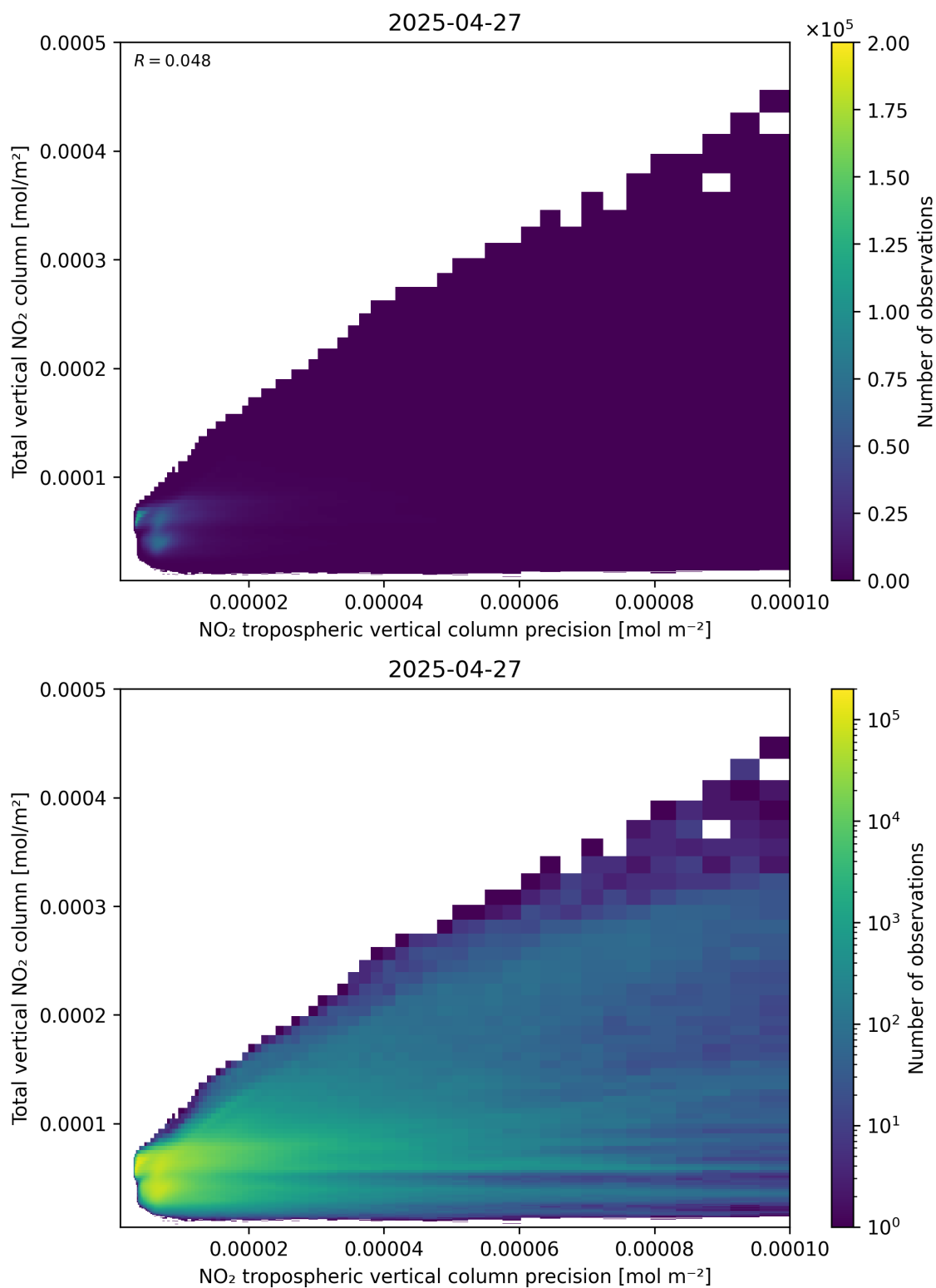
Figure 138: Scatter density plot of “NO 2 tropospheric vertical column precision” against “Total vertical NO 2 column” for 2025-04-27 to 2025-04-27.
