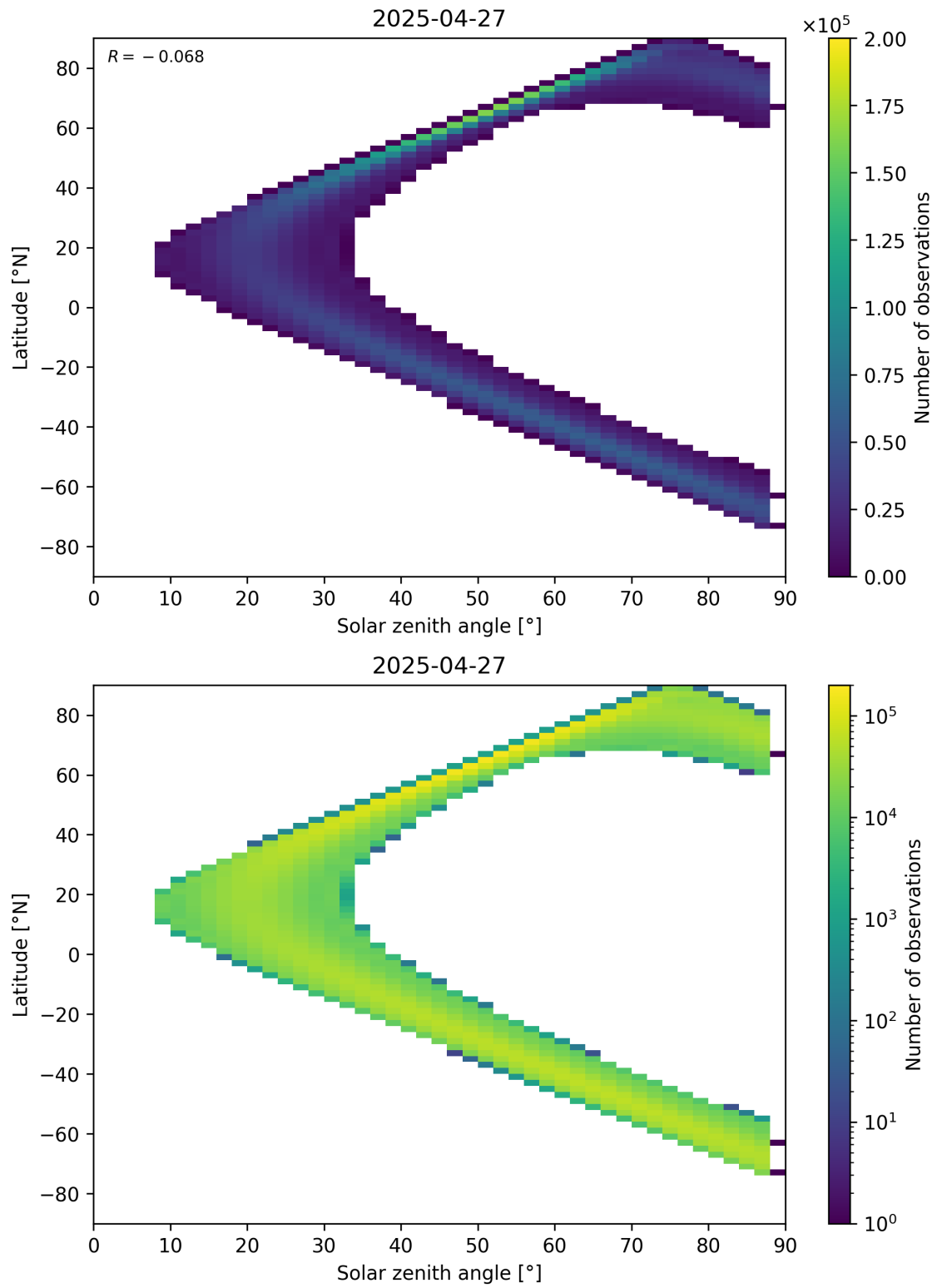
Figure 149: Scatter density plot of “Solar zenith angle” against “Latitude” for 2025-04-27 to 2025-04-27.
