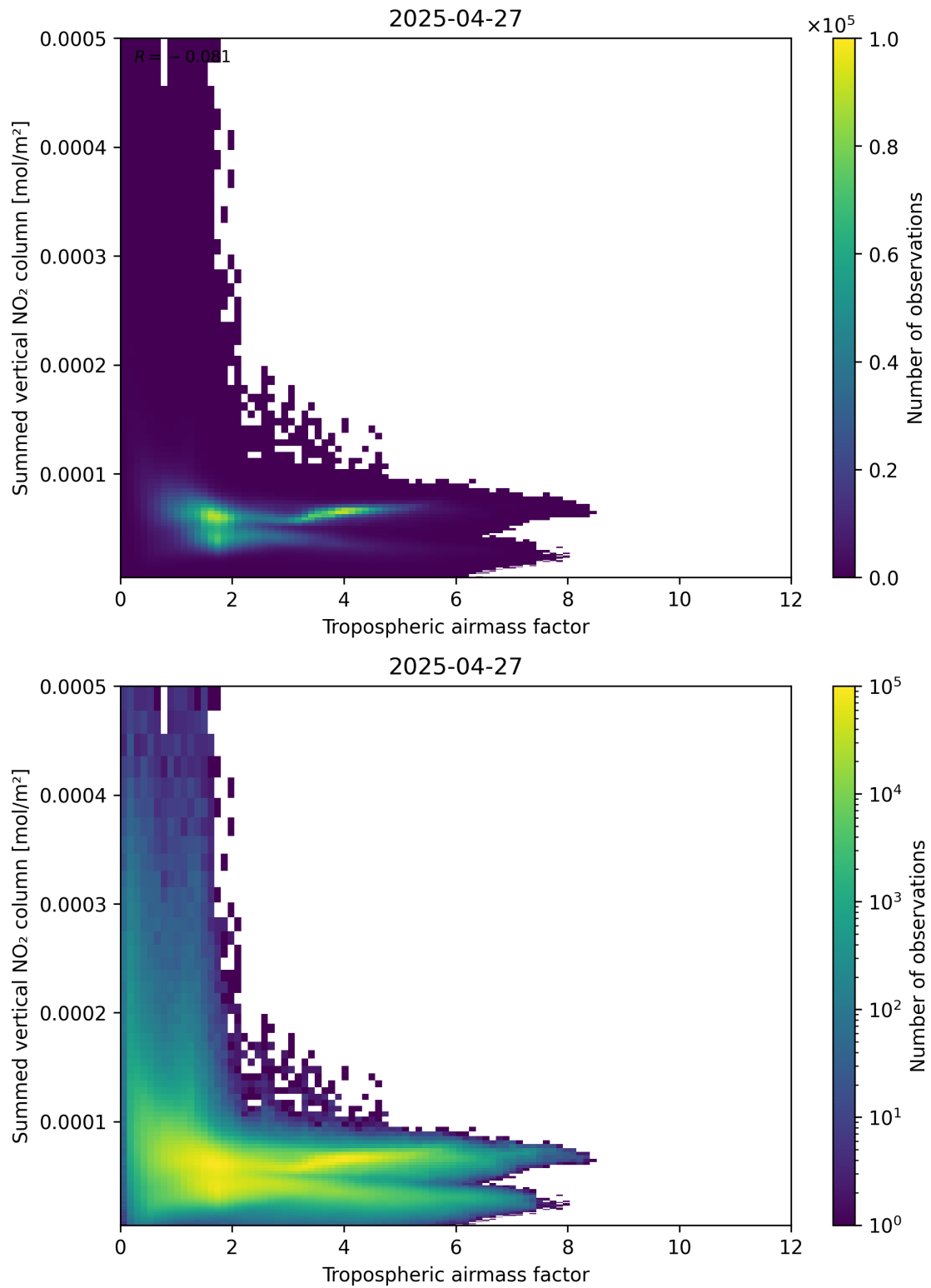
Figure 75: Scatter density plot of “Tropospheric air mass factor” against “Summed vertical NO 2 column” for 2025-04-27 to 2025-04-27.
