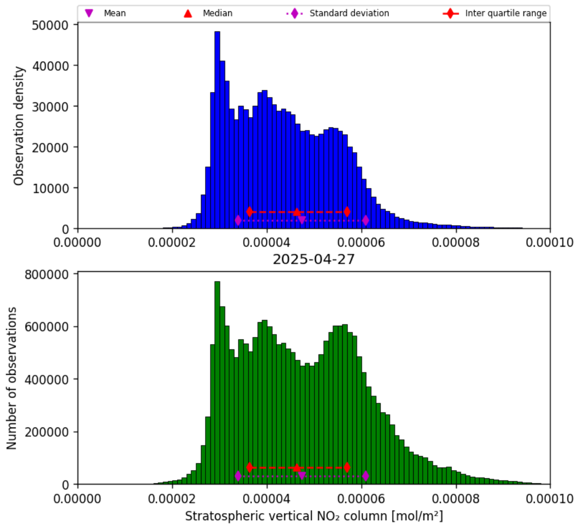
Figure 36: Histogram of “Stratospheric vertical NO 2 column” for 2025-04-27 to 2025-04-27
