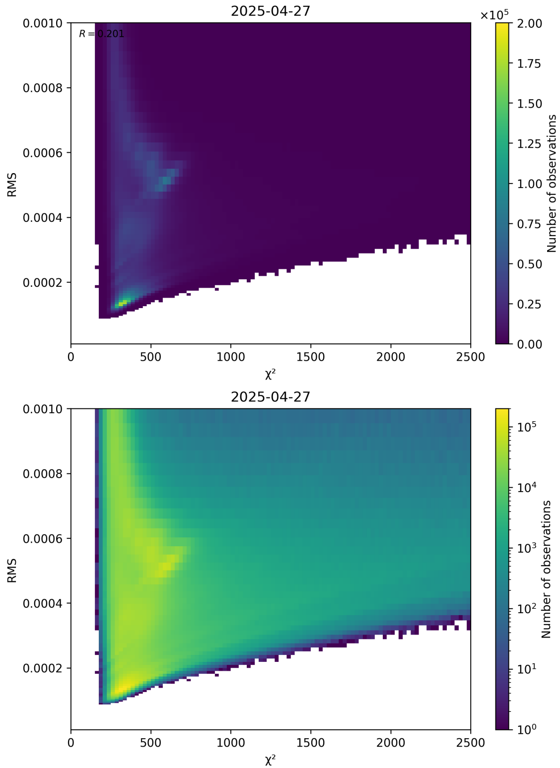
Figure 82: Scatter density plot of “ \chi^2 ” against “RMS” for 2025-04-27 to 2025-04-27.
