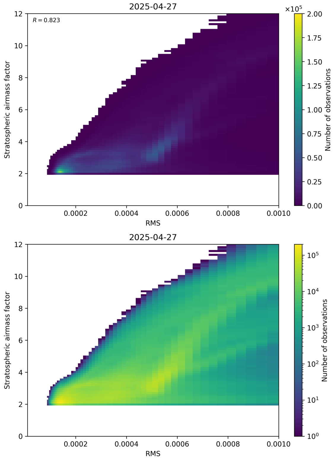
Figure 144: Scatter density plot of “RMS” against “Stratospheric airmass factor” for 2025-04-27 to 2025-04-27.
