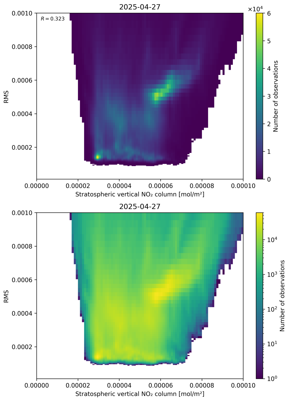
Figure 102: Scatter density plot of “Stratospheric vertical NO 2 column” against “RMS” for 2025-04-27 to 2025-04-27.
