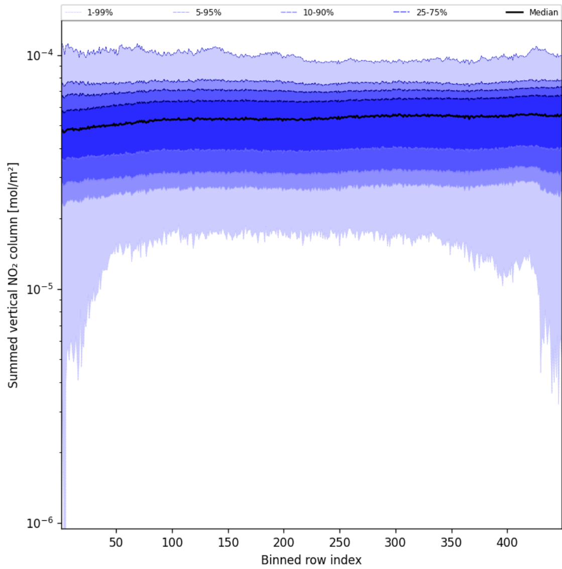
Figure 57: Along track statistics of “Summed vertical NO 2 column” for 2025-04-27 to 2025-04-27
