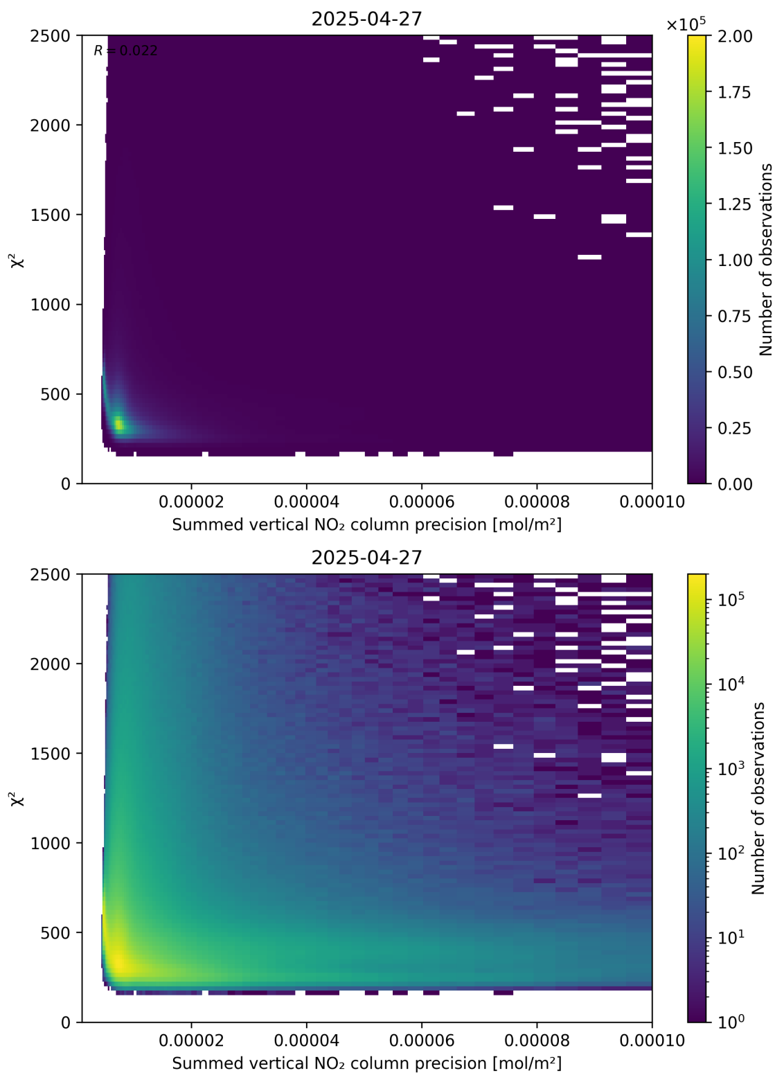
Figure 107: Scatter density plot of “Summed vertical NO 2 column precision” against “ \chi^2 ” for 2025-04-27 to 2025-04-27.
