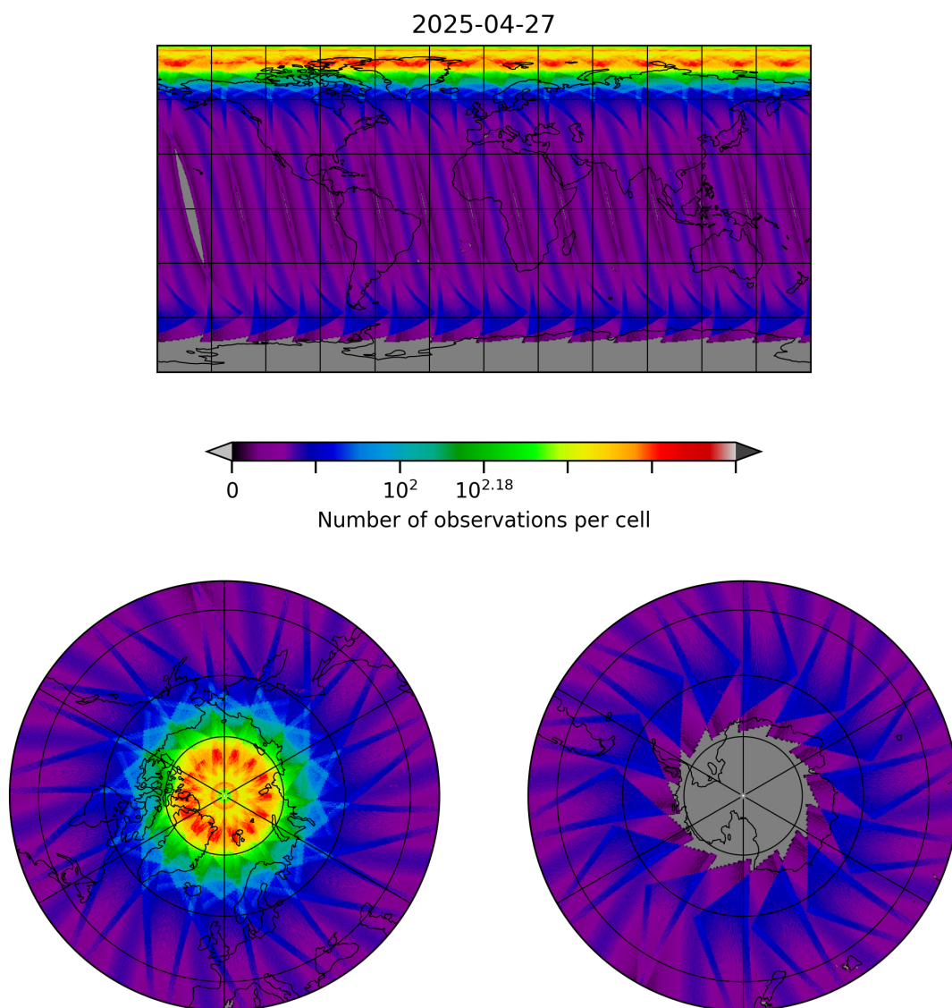
Figure 10: Map of the number of observations for 2025-04-27 to 2025-04-27
