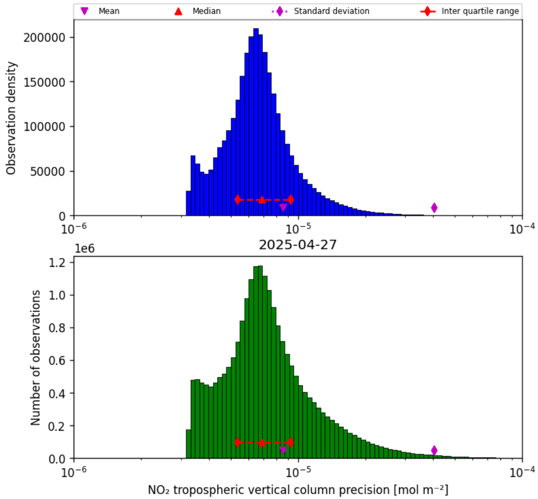
Figure 30: Histogram of “NO 2 tropospheric vertical column precision” for 2025-04-27 to 2025-04-27
