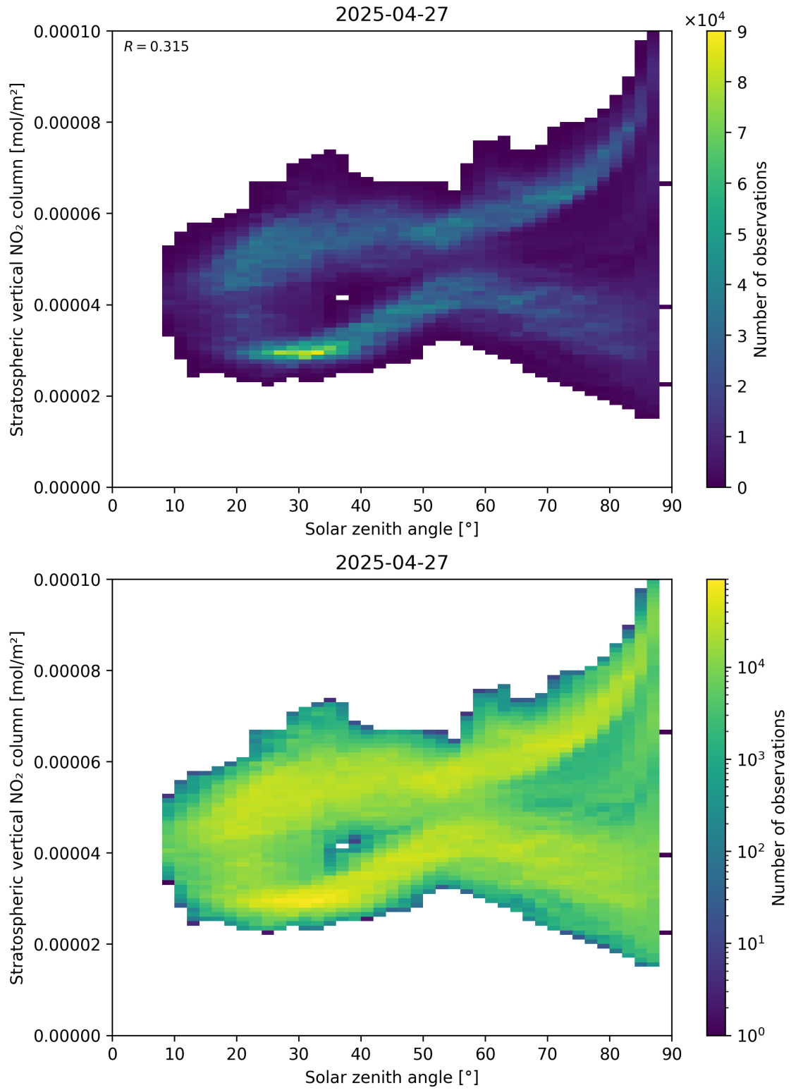
Figure 150: Scatter density plot of “Solar zenith angle” against “Stratospheric vertical NO 2 column” for 2025-04-27 to 2025-04-27.
