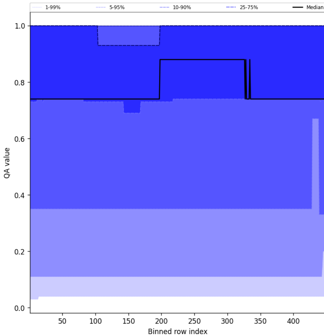
Figure 45: Along track statistics of “QA value” for 2025-04-27 to 2025-04-27
