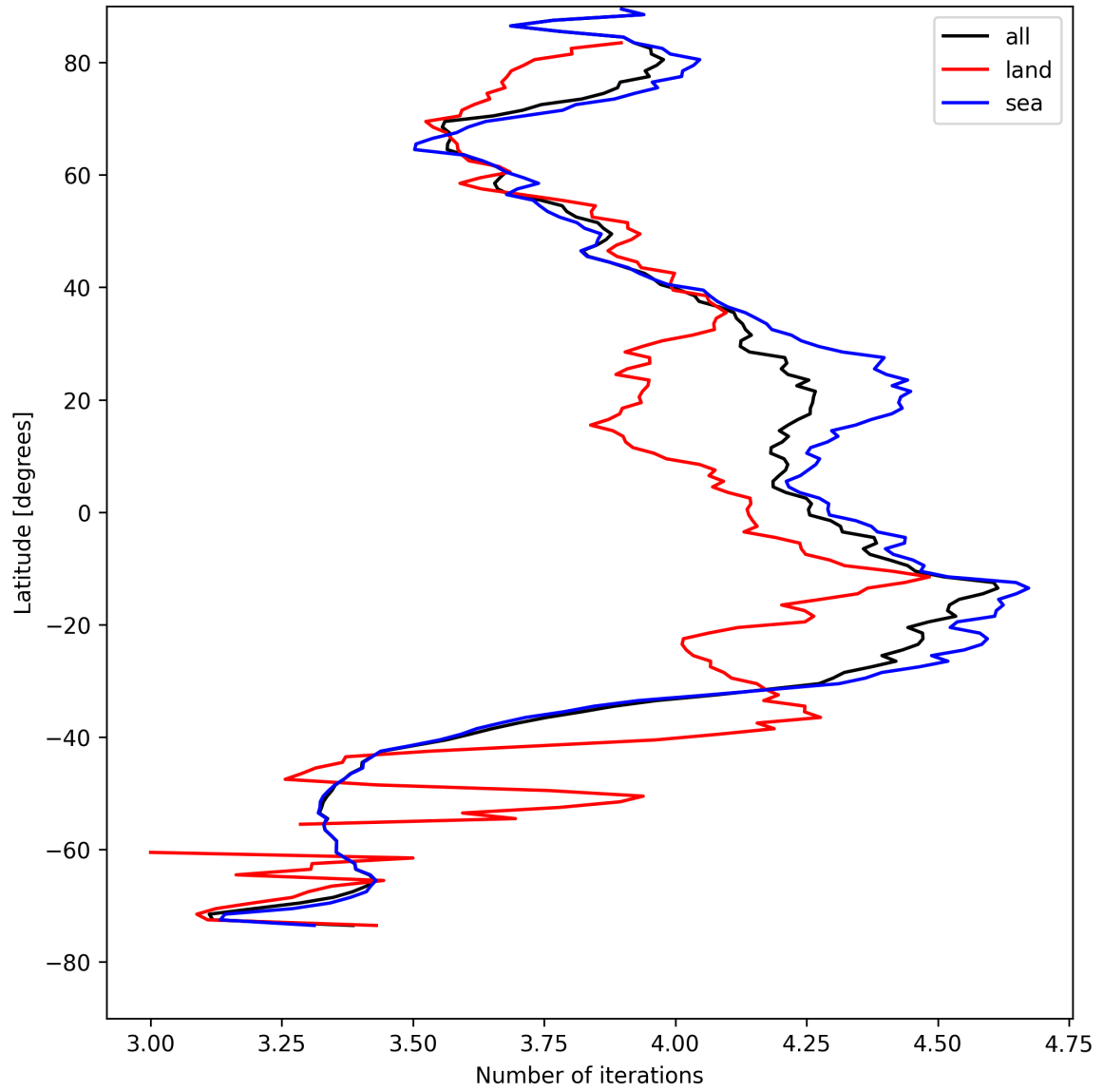
Figure 17: Zonal average of “Number of iterations” for 2025-04-27 to 2025-04-27.
