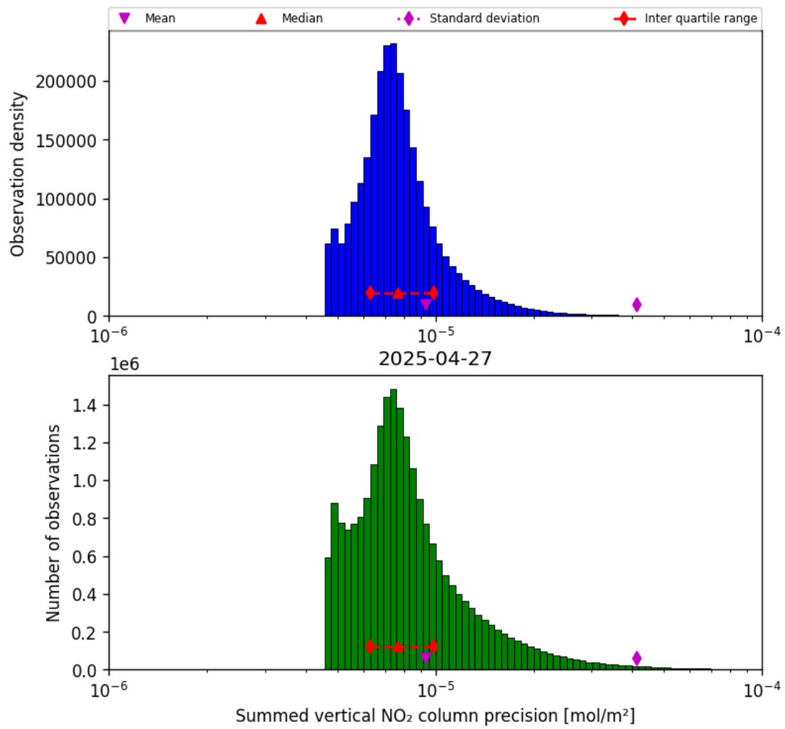
Figure 41: Histogram of "Summed vertical NO 2 column precision" for 2025-04-27 to 2025-04-27
