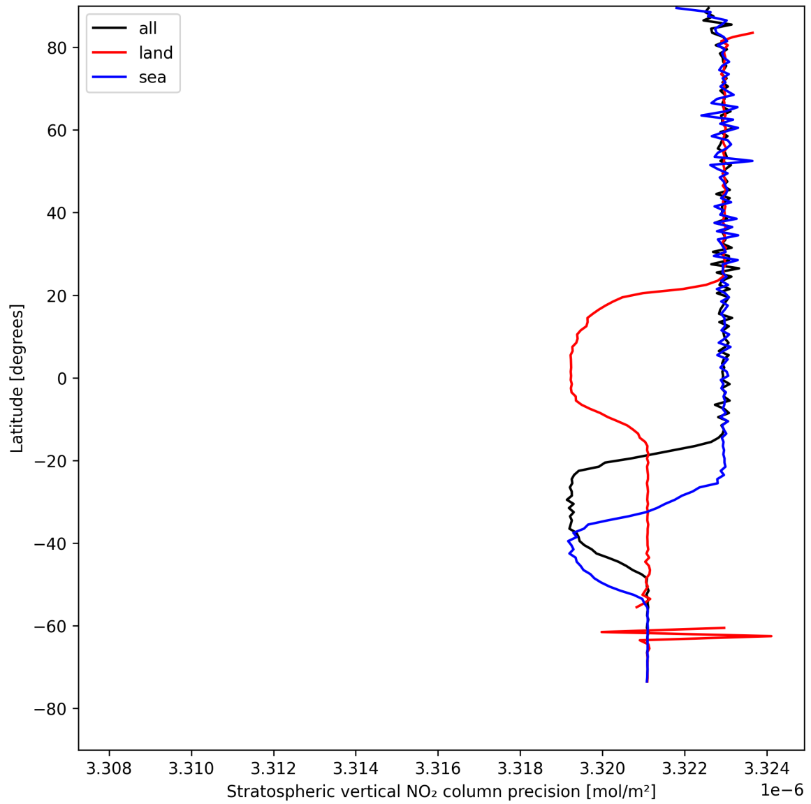
Figure 20: Zonal average of “Stratospheric vertical NO 2 column precision” for 2025-04-27 to 2025-04-27.
