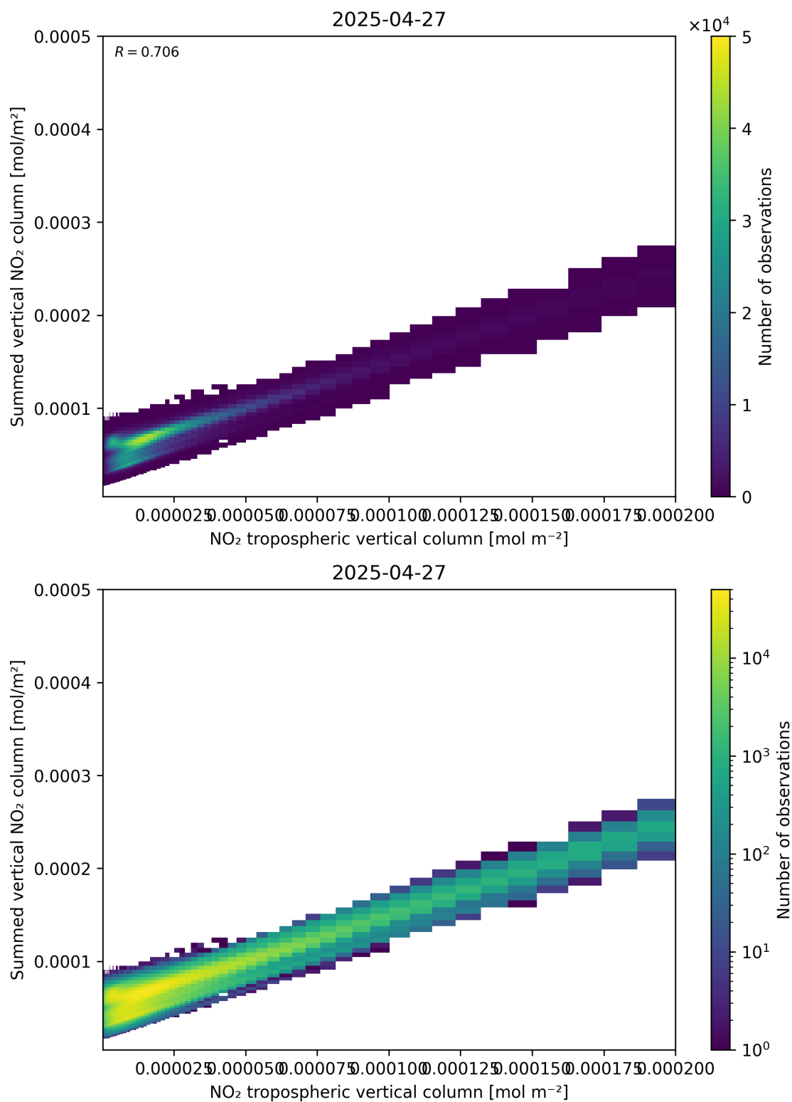
Figure 126: Scatter density plot of “NO 2 tropospheric vertical column” against “Summed vertical NO 2 column” for 2025-04-27 to 2025-04-27.
