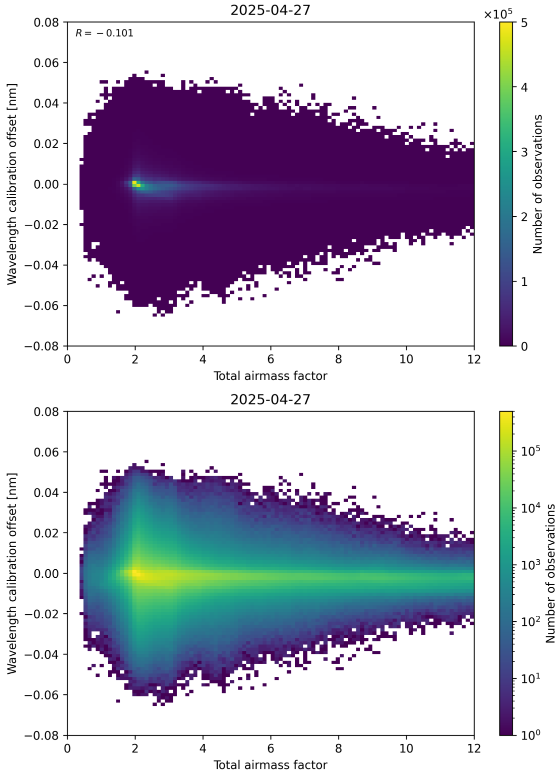
Figure 70: Scatter density plot of “Total airmass factor” against “Wavelength calibration offset” for 2025-04-27 to 2025-04-27.
