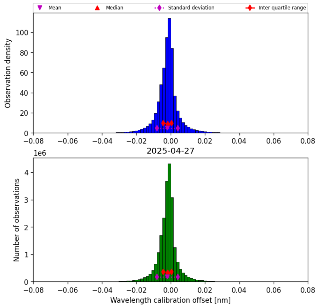
Figure 35: Histogram of “Wavelength calibration offset” for 2025-04-27 to 2025-04-27
