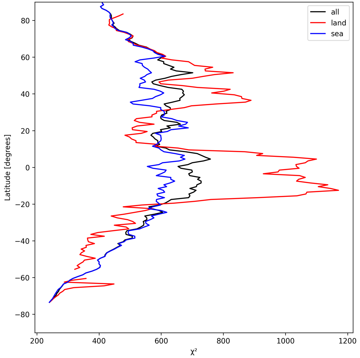
Figure 25: Zonal average of “ \chi^2 ” for 2025-04-27 to 2025-04-27.
