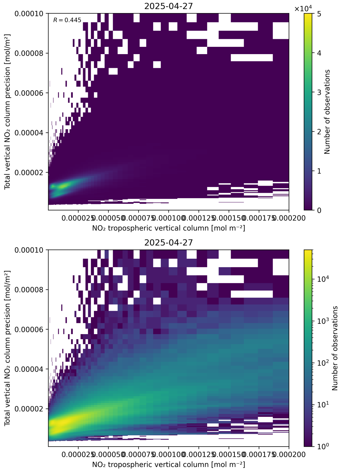
Figure 129: Scatter density plot of “NO 2 tropospheric vertical column” against “Total vertical NO 2 column precision” for 2025-04-27 to 2025-04-27.
