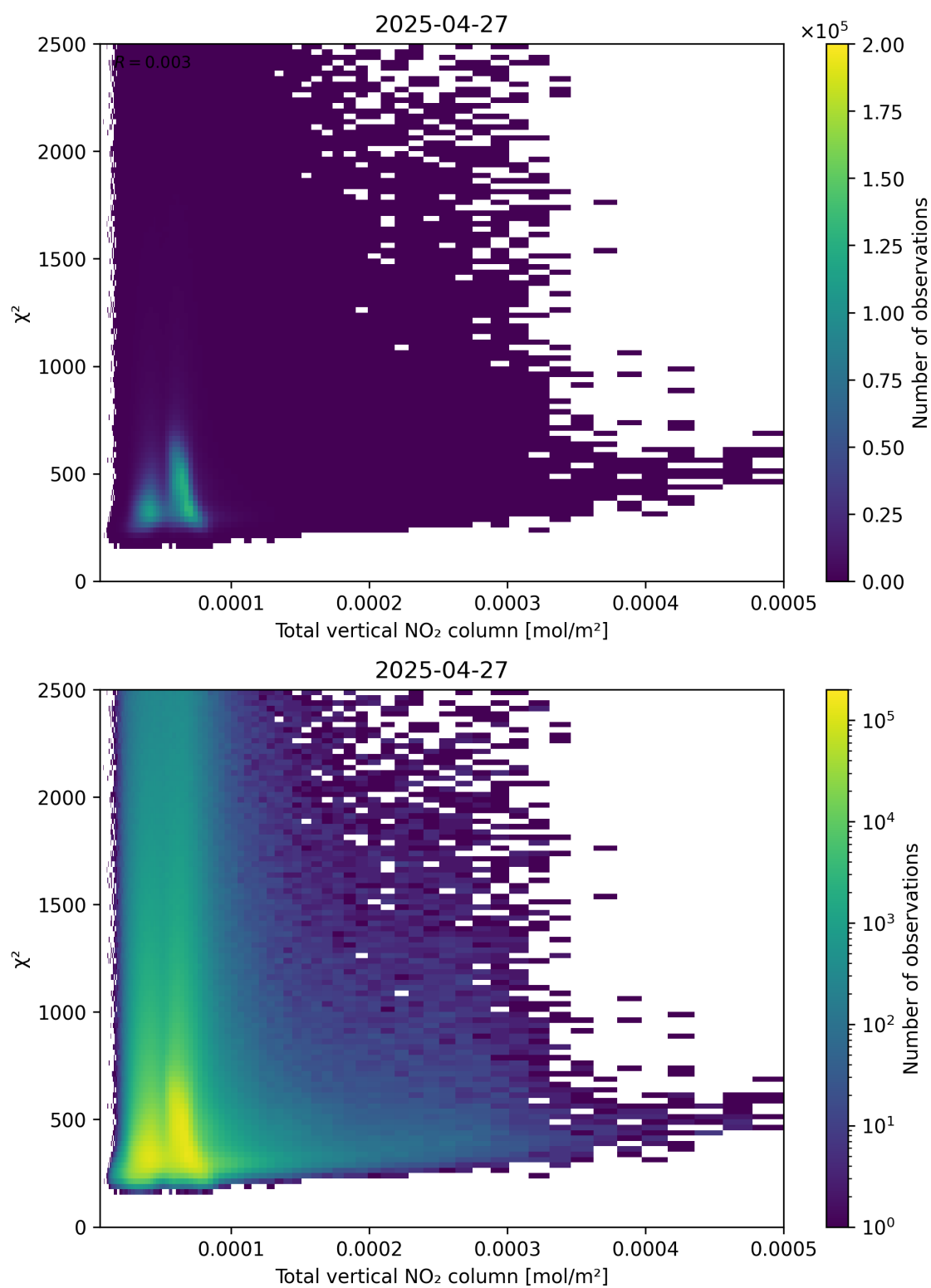
Figure 111: Scatter density plot of “Total vertical NO 2 column” against “ \chi^2 ” for 2025-04-27 to 2025-04-27.
