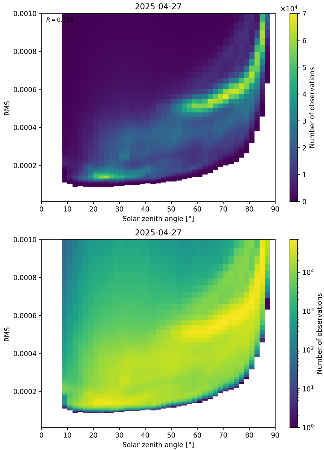
Figure 157: Scatter density plot of “Solar zenith angle” against “RMS” for 2025-04-27 to 2025-04-27.
