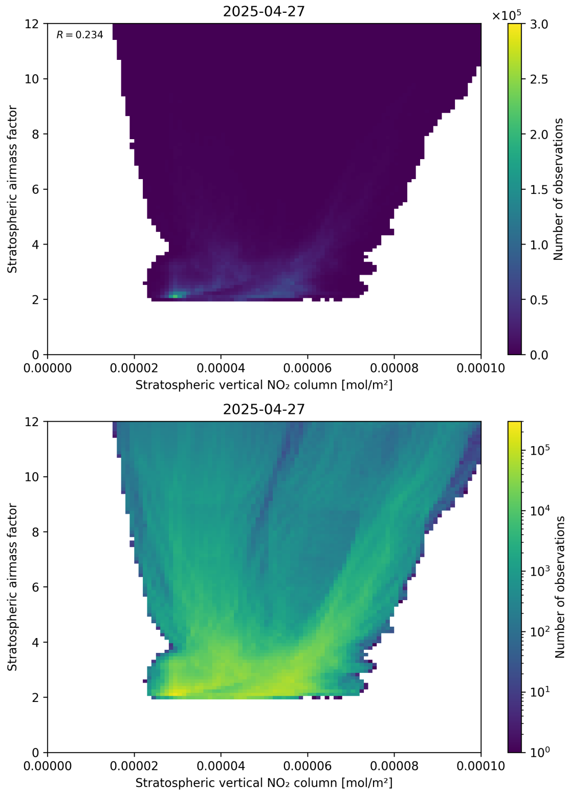
Figure 96: Scatter density plot of “Stratospheric vertical NO 2 column” against “Stratospheric airmass factor” for 2025-04-27 to 2025-04-27.
