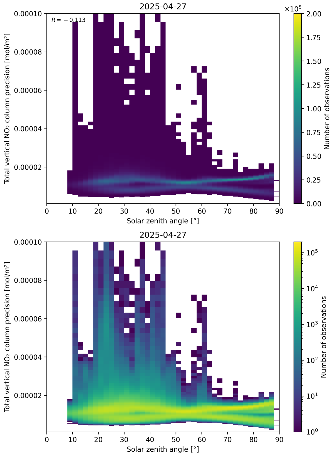
Figure 154: Scatter density plot of “Solar zenith angle” against “Total vertical NO 2 column precision” for 2025-04-27 to 2025-04-27.
