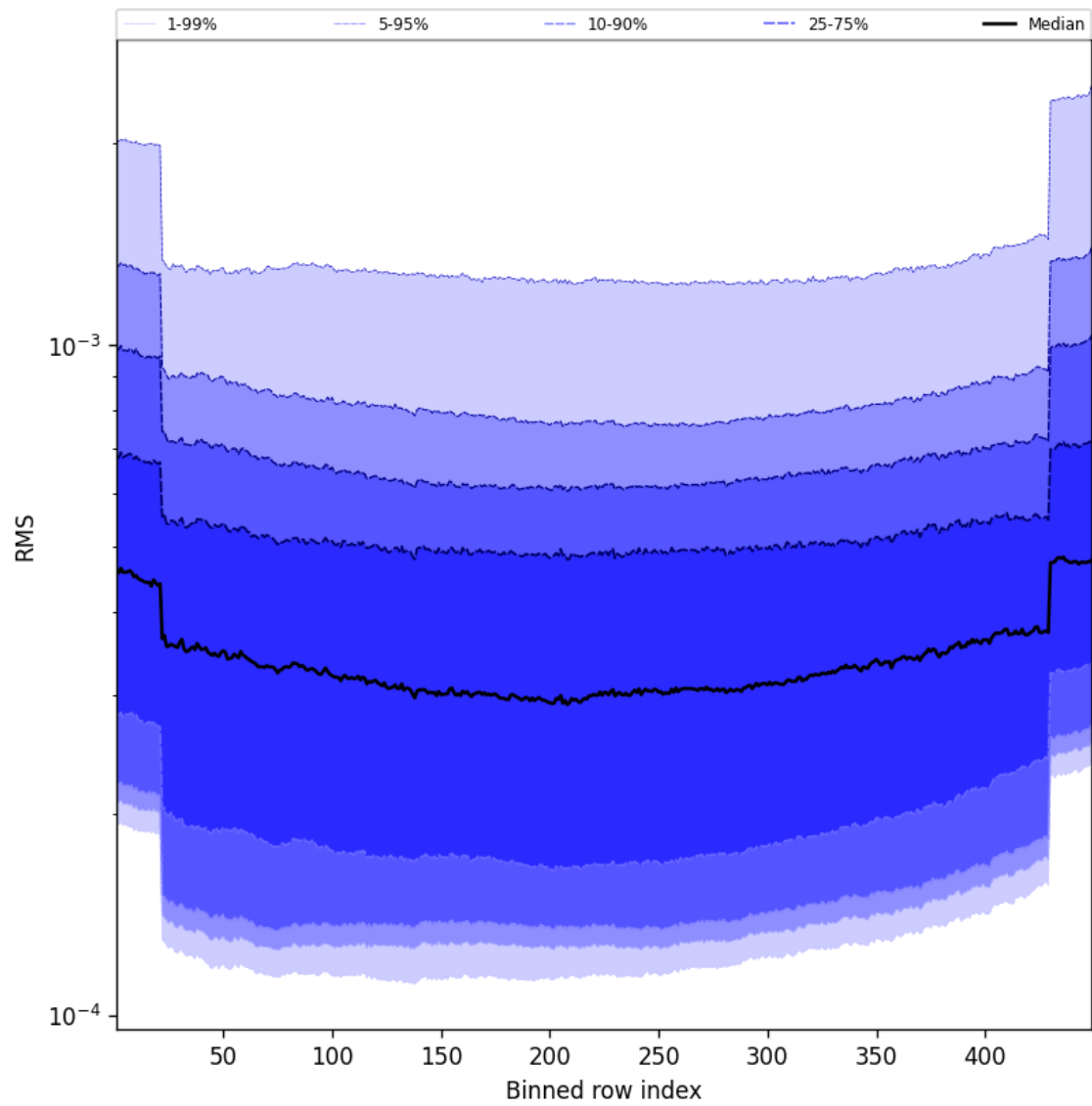
Figure 60: Along track statistics of “RMS” for 2025-04-27 to 2025-04-27
