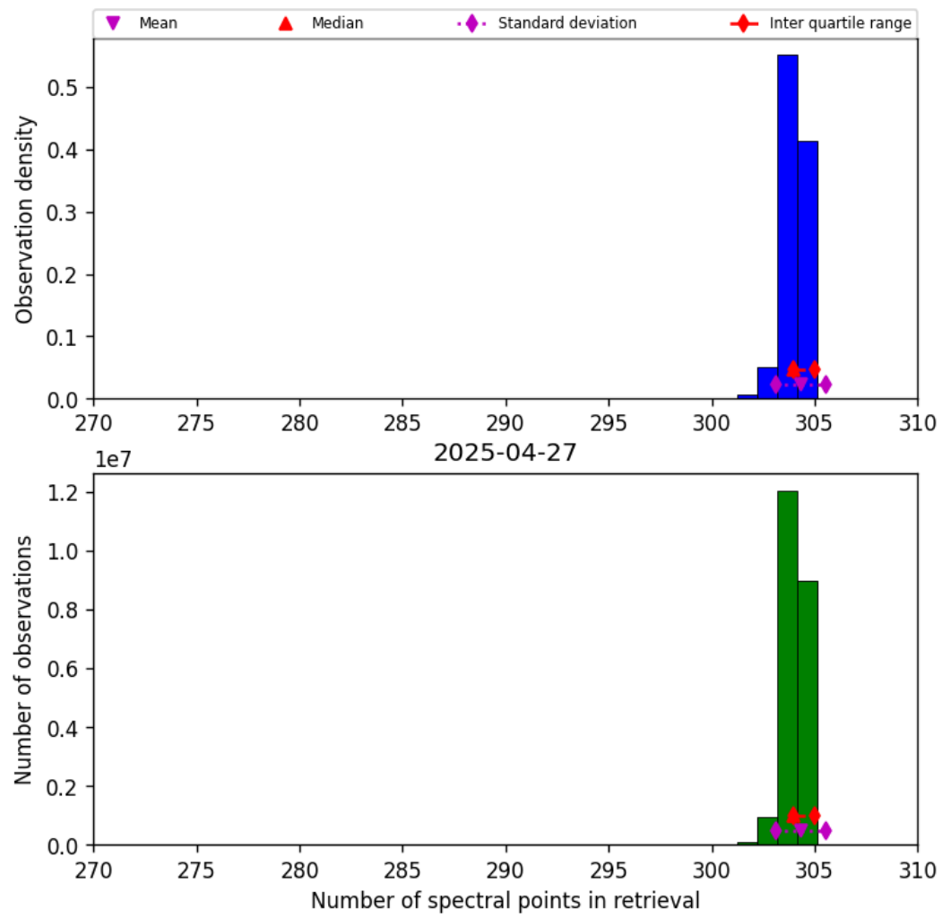
Figure 33: Histogram of “Number of spectral points in retrieval” for 2025-04-27 to 2025-04-27
