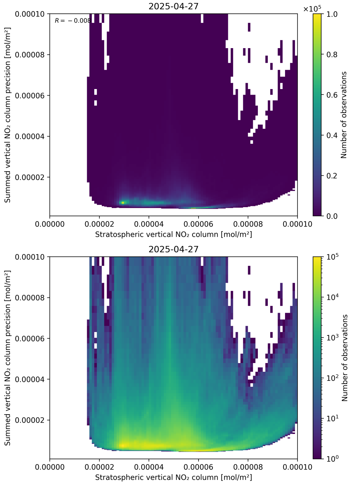
Figure 99: Scatter density plot of “Stratospheric vertical NO 2 column” against “Summed vertical NO 2 column precision” for 2025-04-27 to 2025-04-27.
