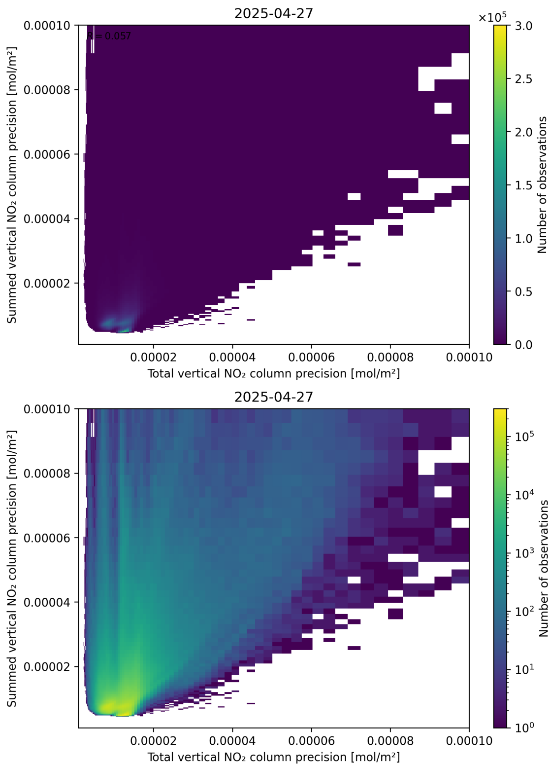
Figure 118: Scatter density plot of “Total vertical NO 2 column precision” against “Summed vertical NO 2 column precision” for 2025-04-27 to 2025-04-27.
