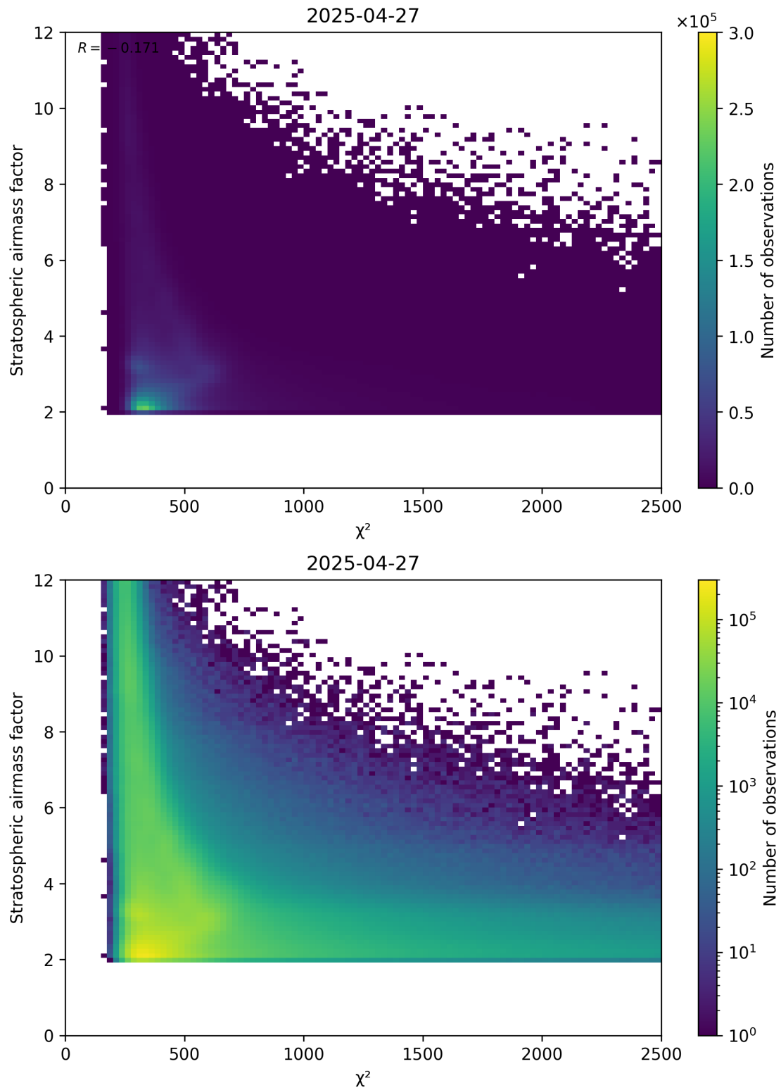
Figure 81: Scatter density plot of “ \chi^2 ” against “Stratospheric airmass factor” for 2025-04-27 to 2025-04-27.
