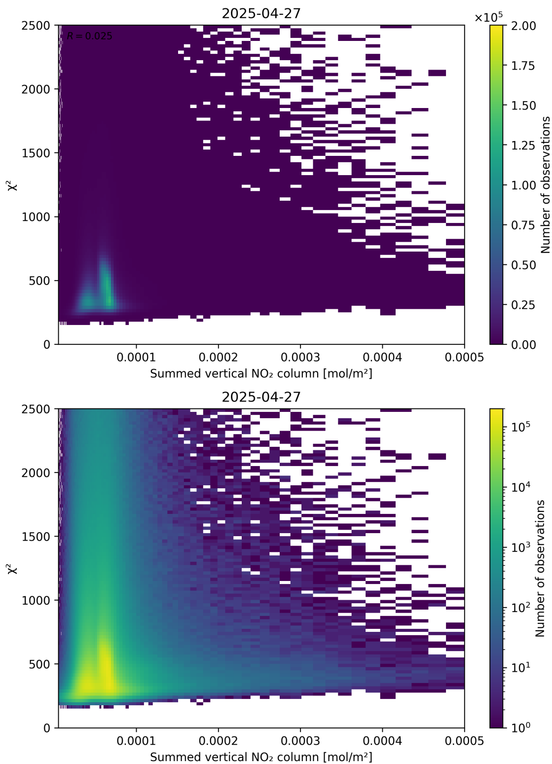
Figure 104: Scatter density plot of “Summed vertical NO 2 column” against “ \chi^2 ” for 2025-04-27 to 2025-04-27.
