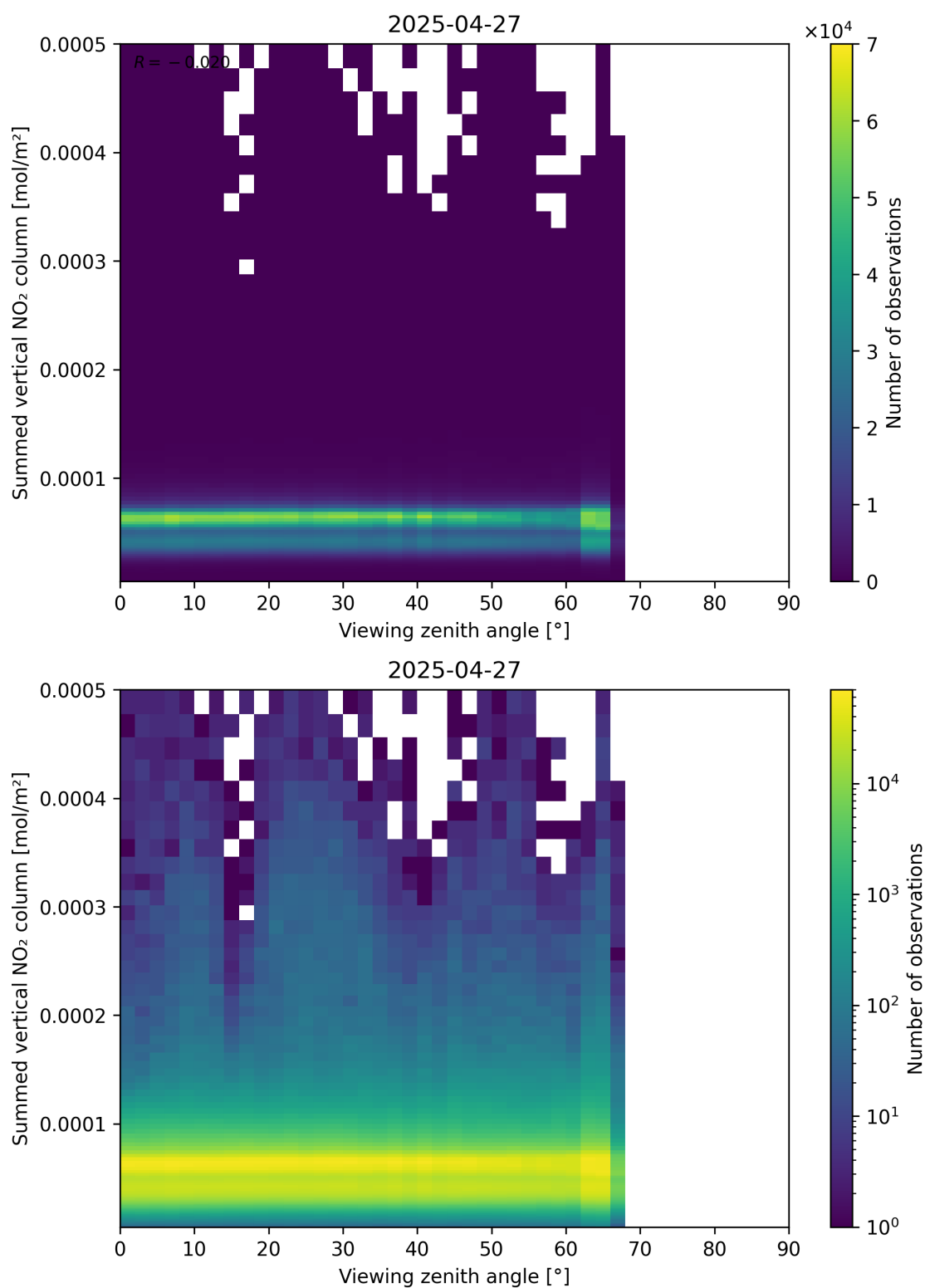
Figure 165: Scatter density plot of “Viewing zenith angle” against “Summed vertical NO 2 column” for 2025-04-27 to 2025-04-27.
