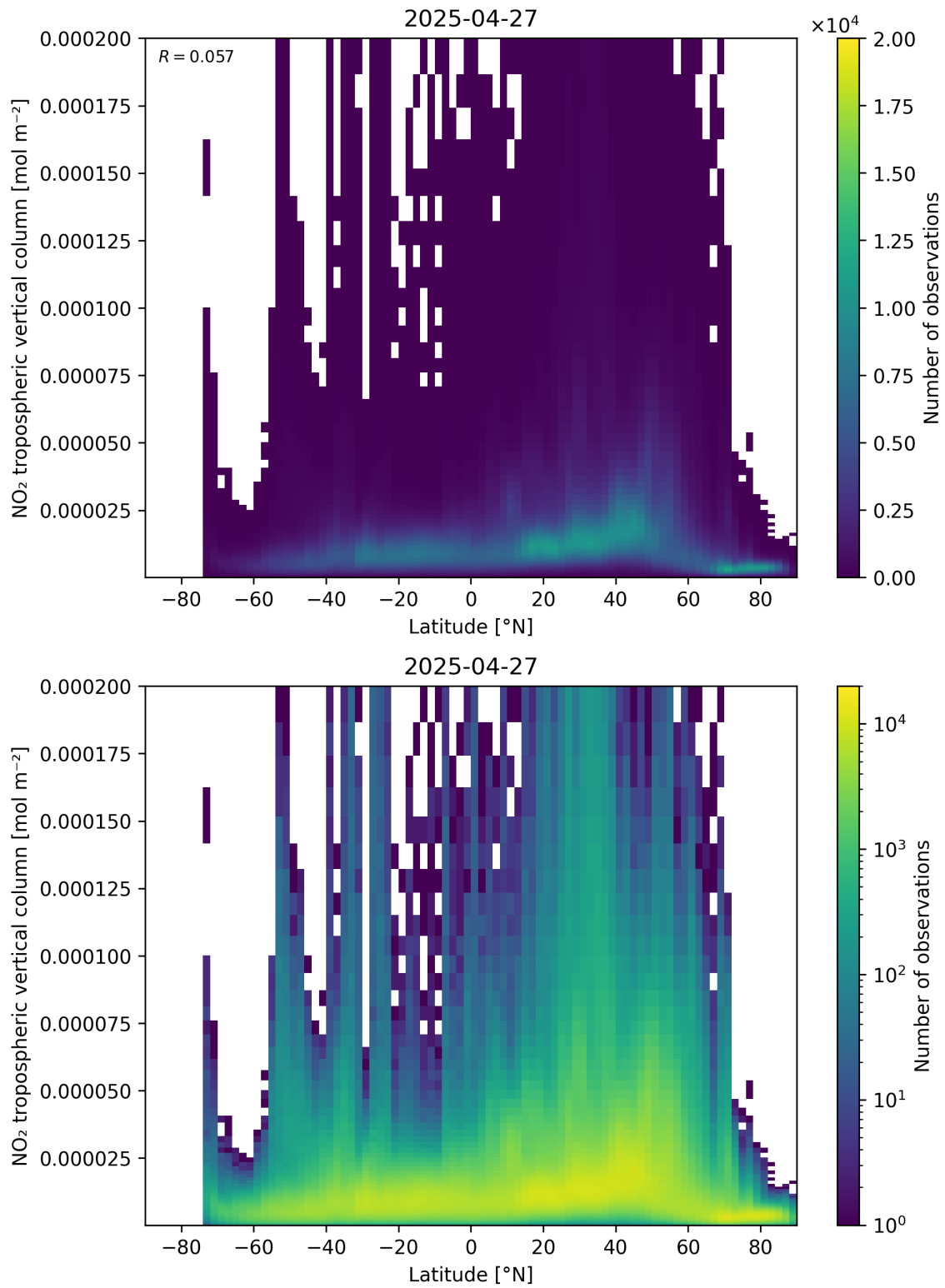
Figure 92: Scatter density plot of “Latitude” against “NO 2 tropospheric vertical column” for 2025-04-27 to 2025-04-27.
