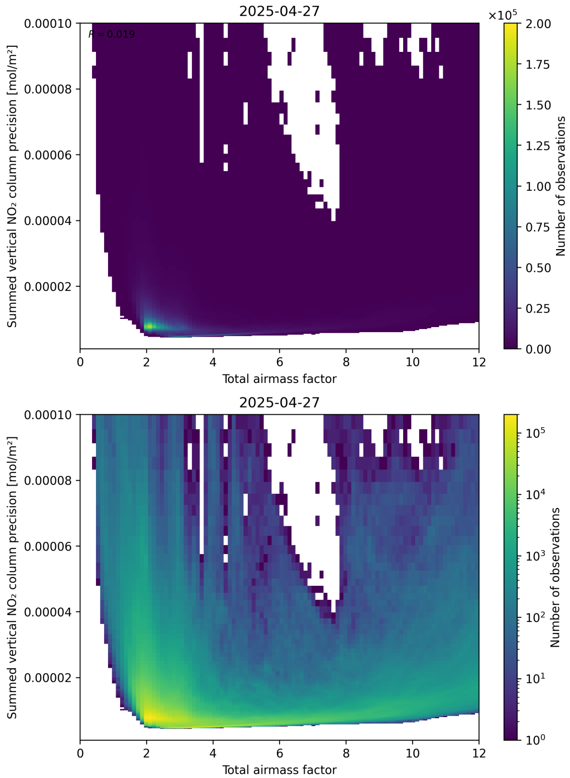
Figure 66: Scatter density plot of “Total airmass factor” against “Summed vertical NO 2 column precision” for 2025-04-27 to 2025-04-27.
