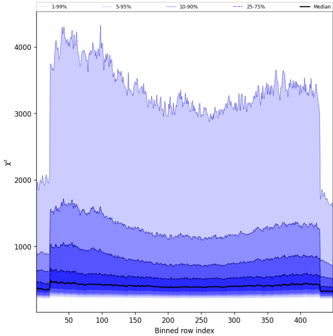
Figure 59: Along track statistics of “ \chi^2 ” for 2025-04-27 to 2025-04-27
