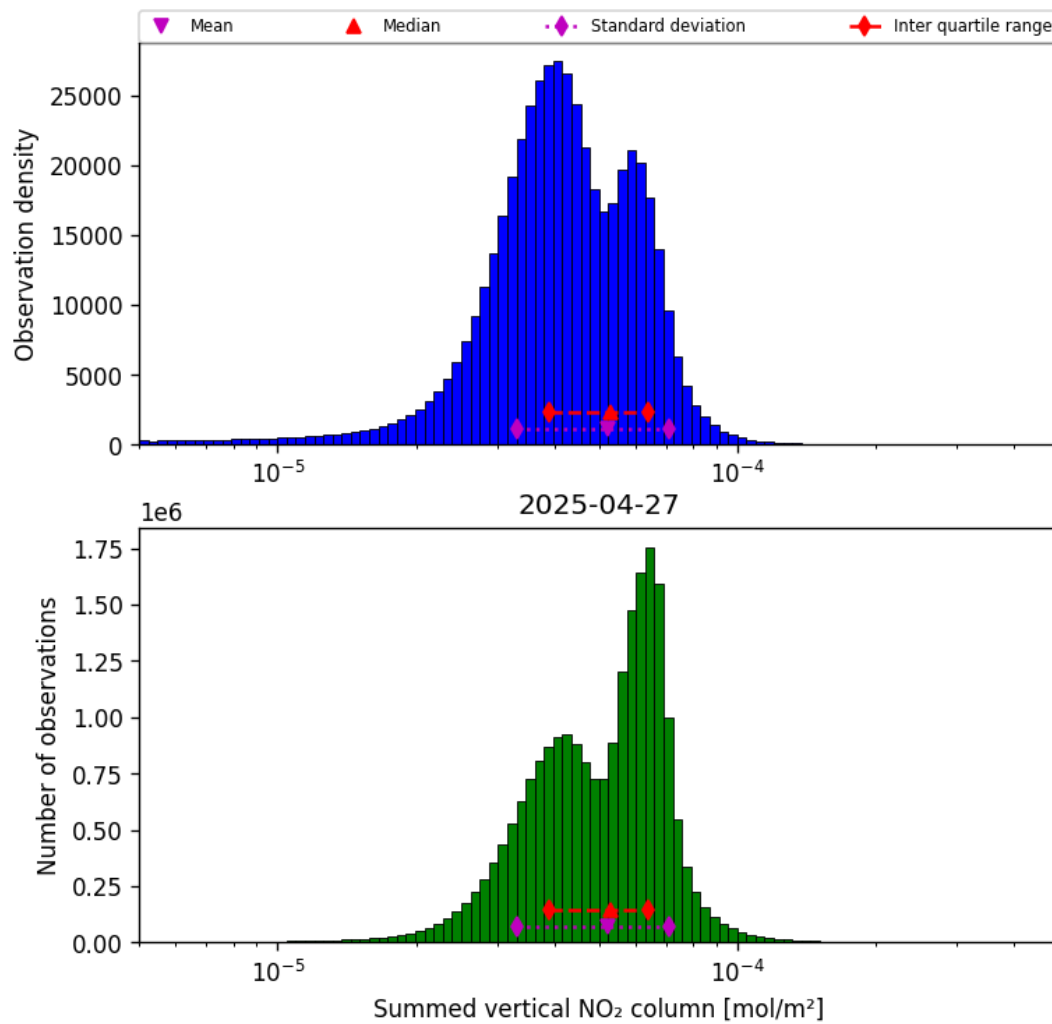
Figure 40: Histogram of “Summed vertical NO 2 column” for 2025-04-27 to 2025-04-27
