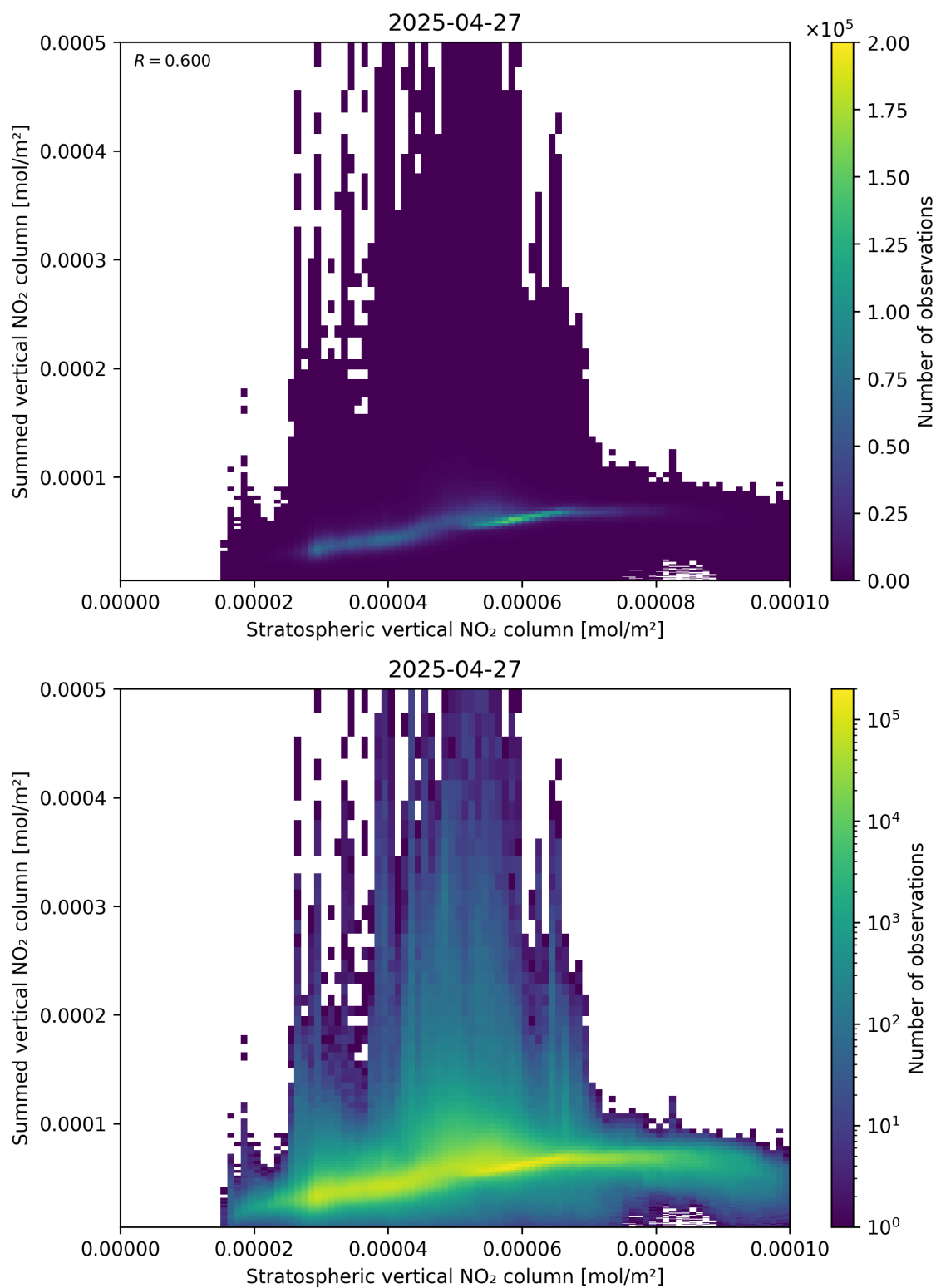
Figure 98: Scatter density plot of “Stratospheric vertical NO 2 column” against “Summed vertical NO 2 column” for 2025-04-27 to 2025-04-27.
