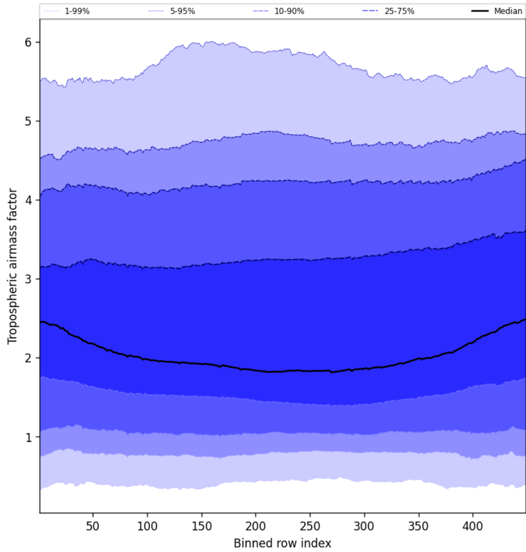
Figure 48: Along track statistics of “Tropospheric airmass factor” for 2025-04-27 to 2025-04-27
