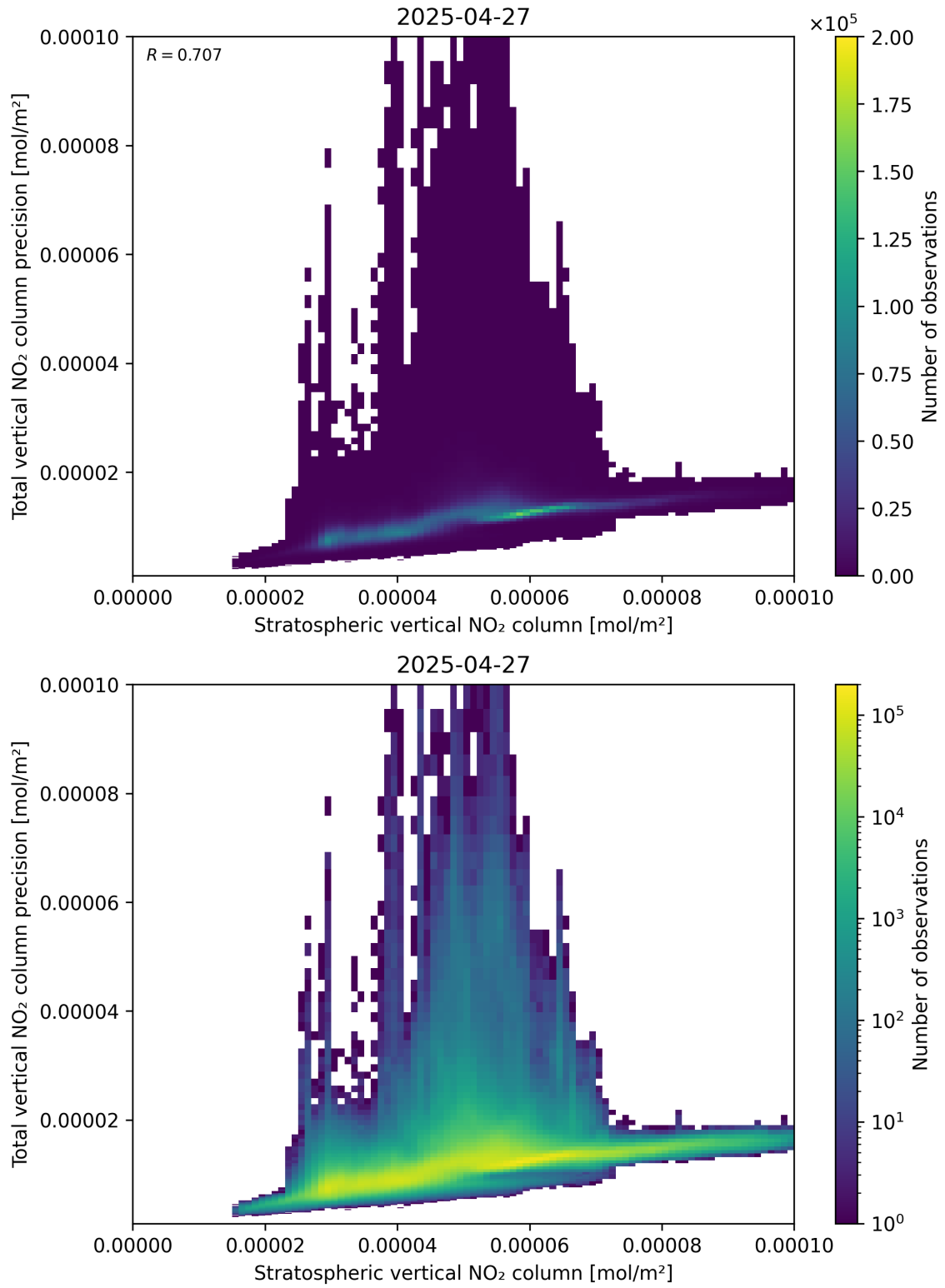
Figure 101: Scatter density plot of “Stratospheric vertical NO 2 column” against “Total vertical NO 2 column precision” for 2025-04-27 to 2025-04-27.
