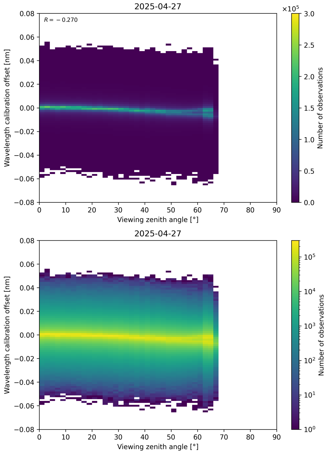
Figure 173: Scatter density plot of “Viewing zenith angle” against “Wavelength calibration offset” for 2025-04-27 to 2025-04-27.
