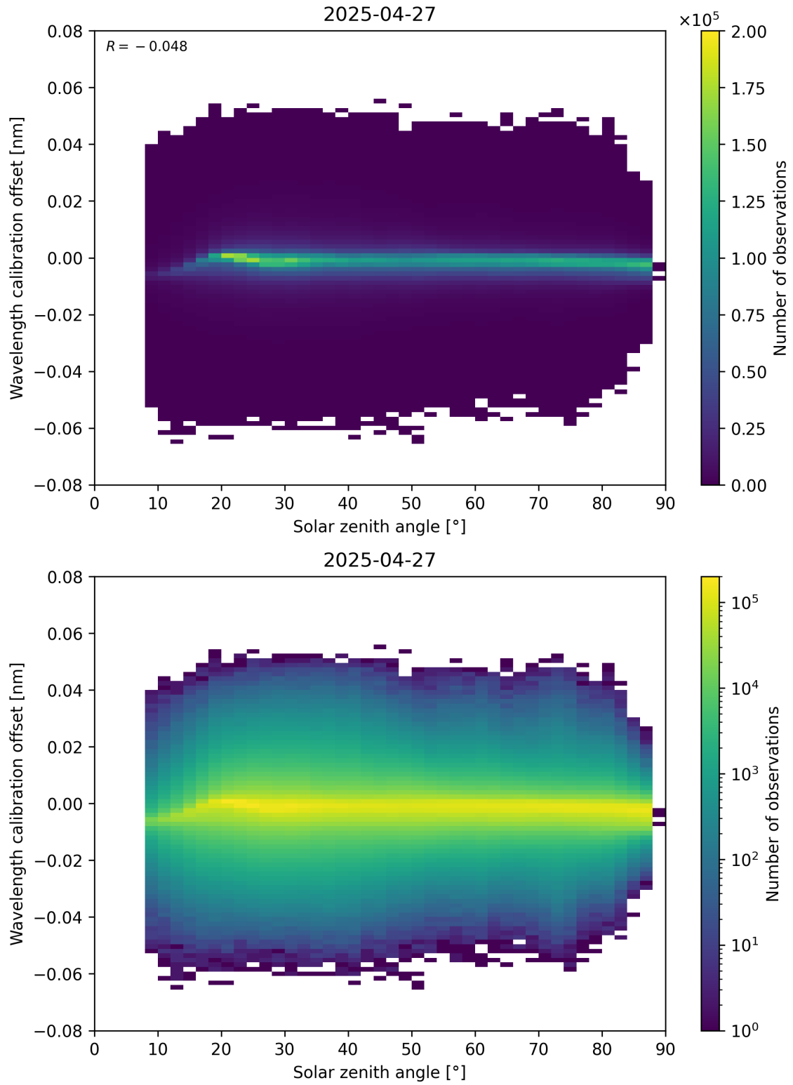
Figure 158: Scatter density plot of “Solar zenith angle” against “Wavelength calibration offset” for 2025-04-27 to 2025-04-27.
