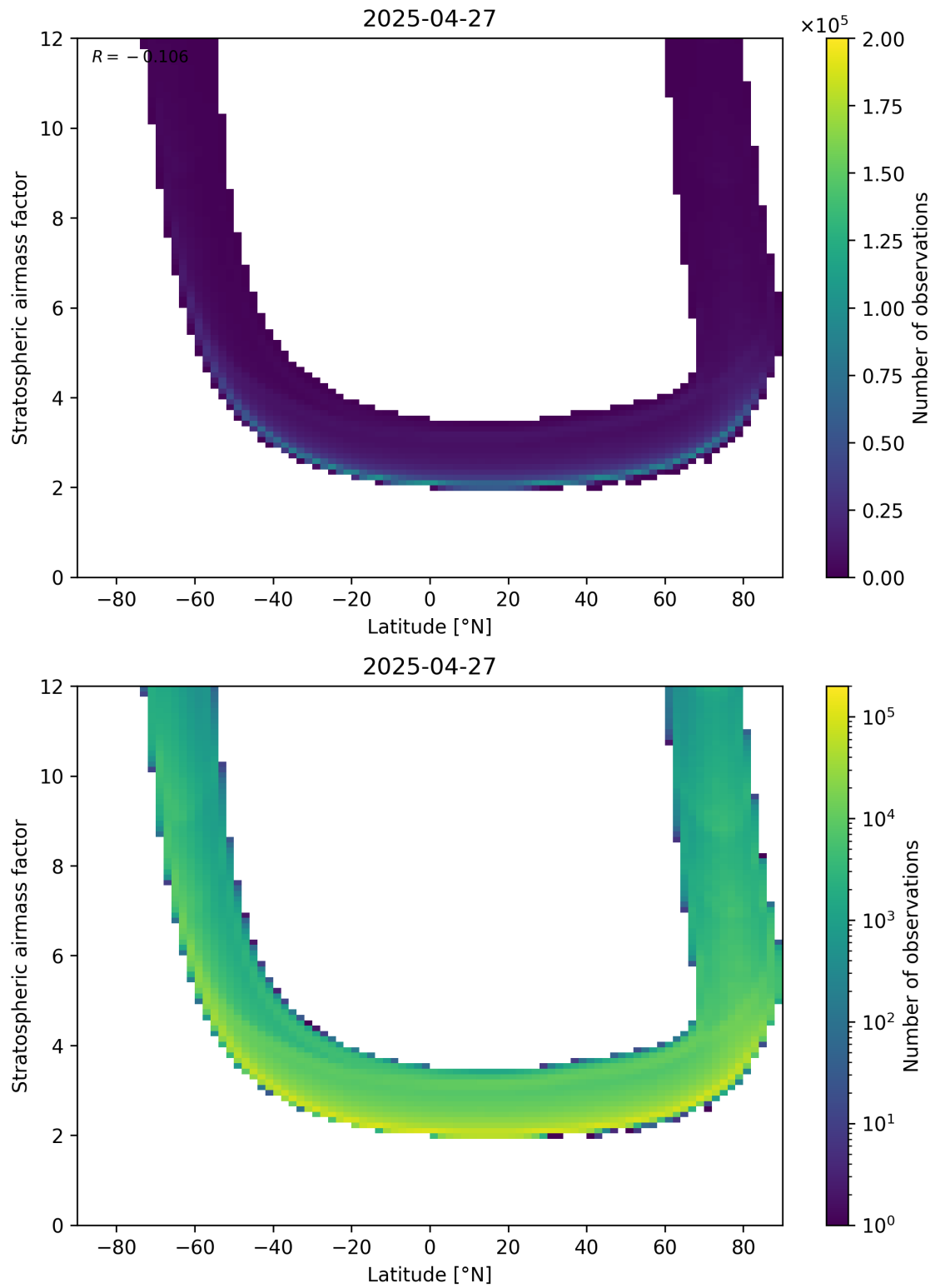
Figure 83: Scatter density plot of “Latitude” against “Stratospheric air mass factor” for 2025-04-27 to 2025-04-27.
