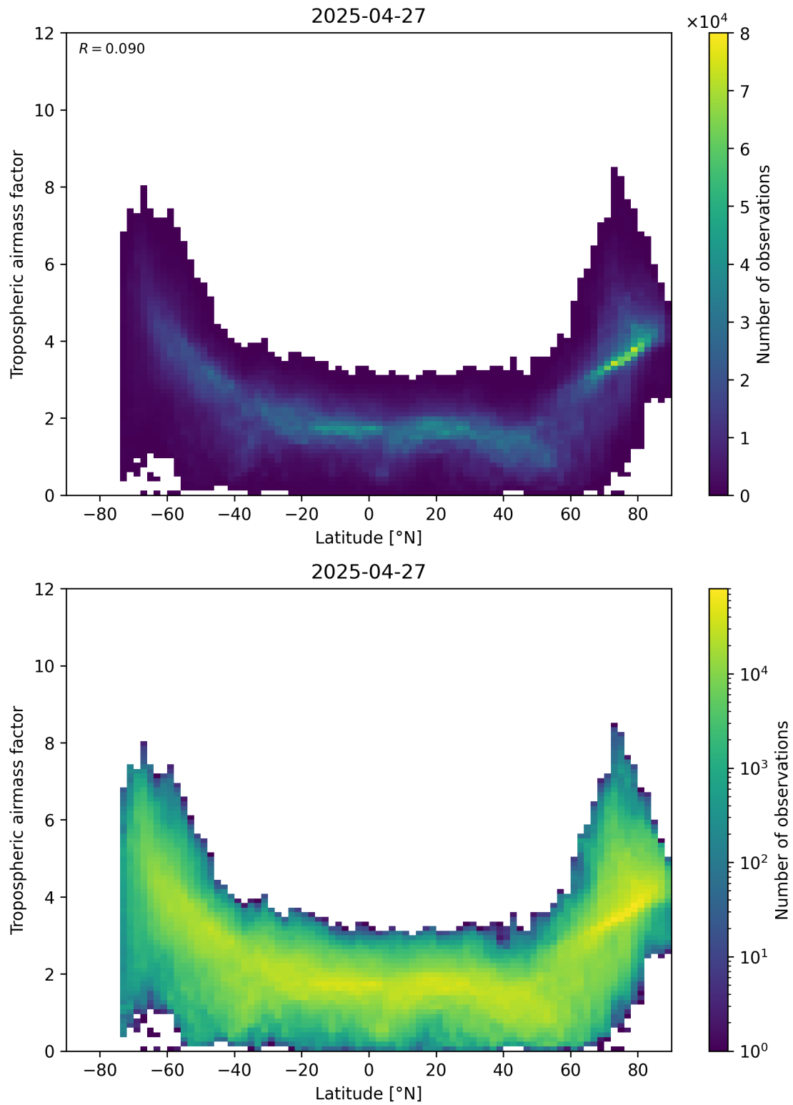
Figure 85: Scatter density plot of “Latitude” against “Tropospheric airmass factor” for 2025-04-27 to 2025-04-27.
