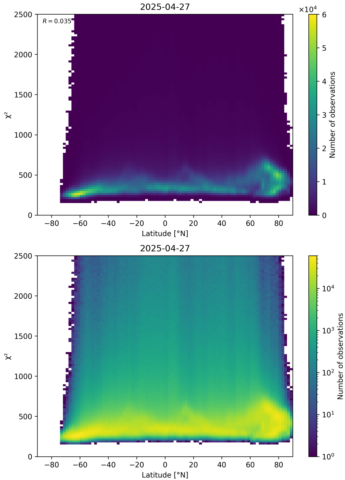
Figure 86: Scatter density plot of “Latitude” against “ \chi^2 ” for 2025-04-27 to 2025-04-27.
