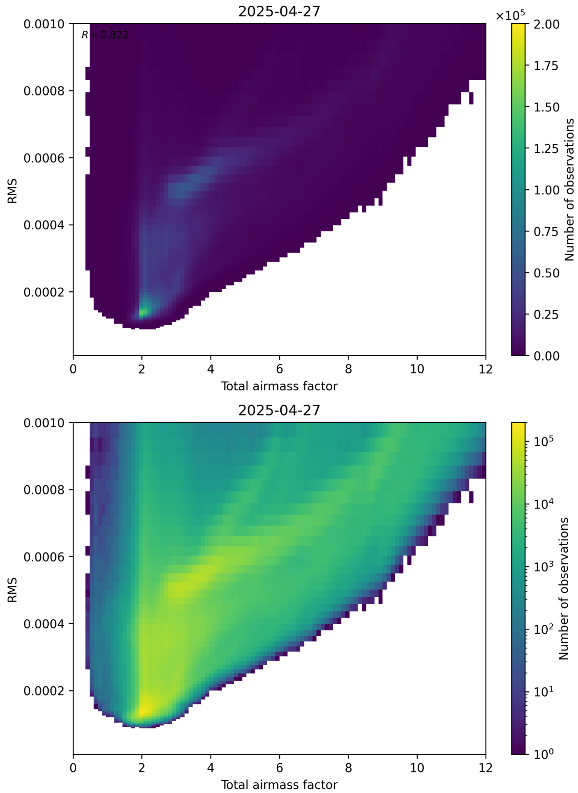
Figure 69: Scatter density plot of “Total airmass factor” against “RMS” for 2025-04-27 to 2025-04-27.
