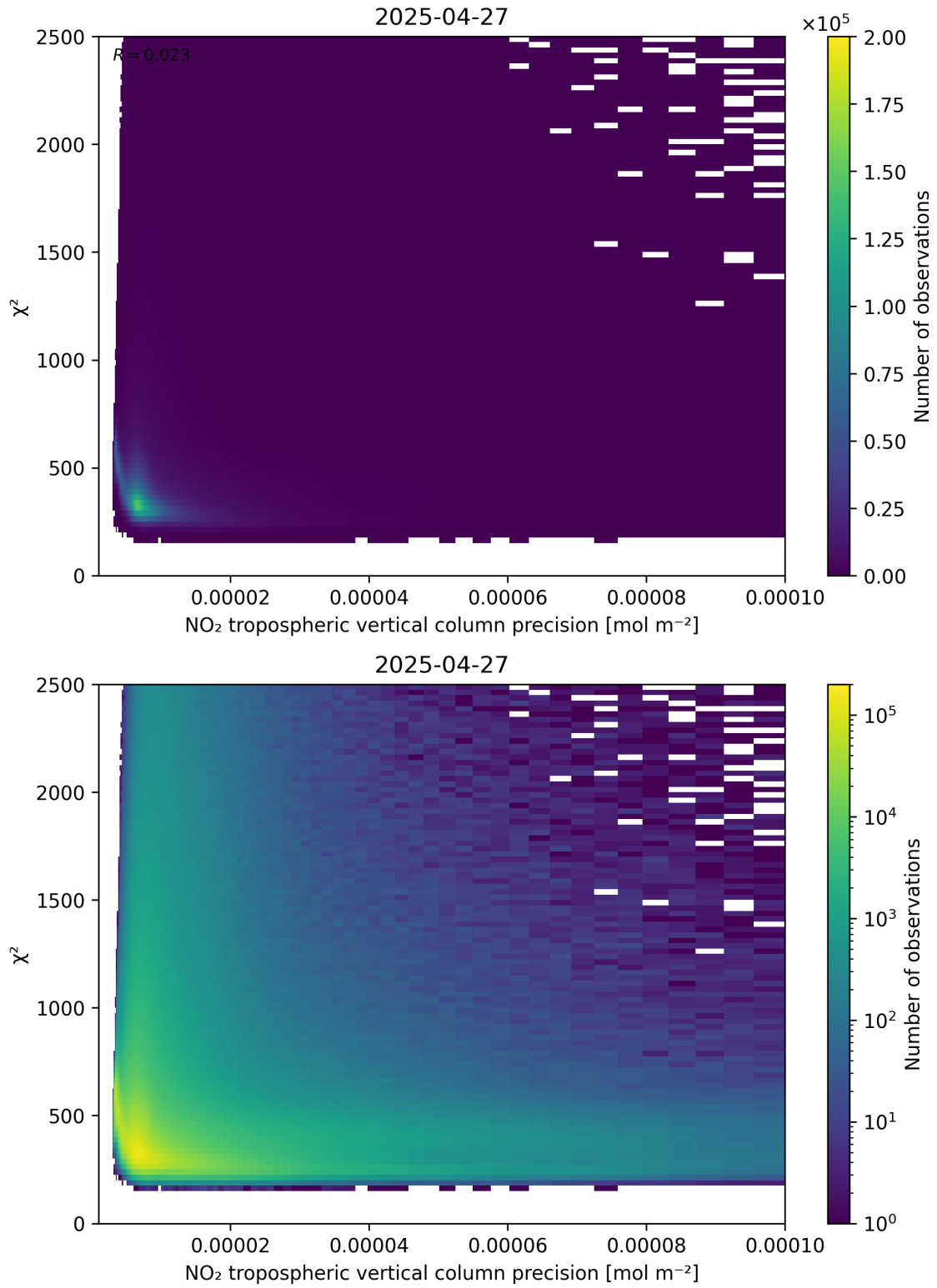
Figure 134: Scatter density plot of “NO 2 tropospheric vertical column precision” against “ \chi^2 ” for 2025-04-27 to 2025-04-27.
