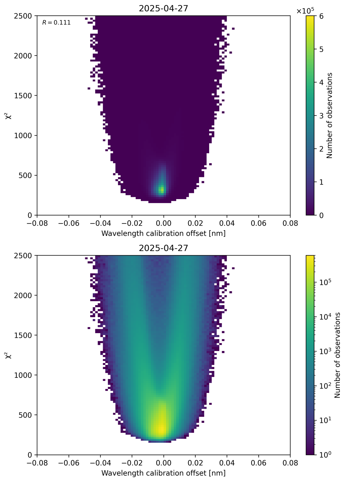
Figure 175: Scatter density plot of “Wavelength calibration offset” against “ \chi^2 ” for 2025-04-27 to 2025-04-27.
