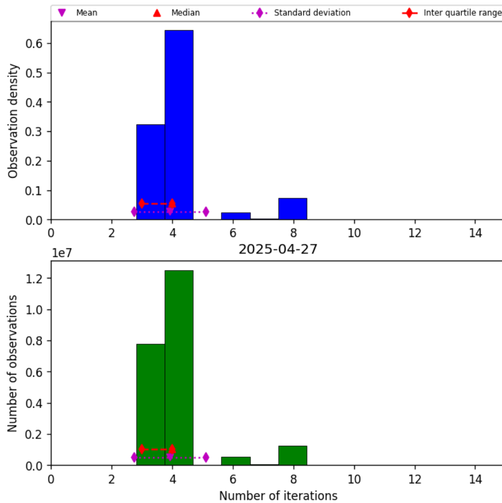
Figure 34: Histogram of “Number of iterations” for 2025-04-27 to 2025-04-27
