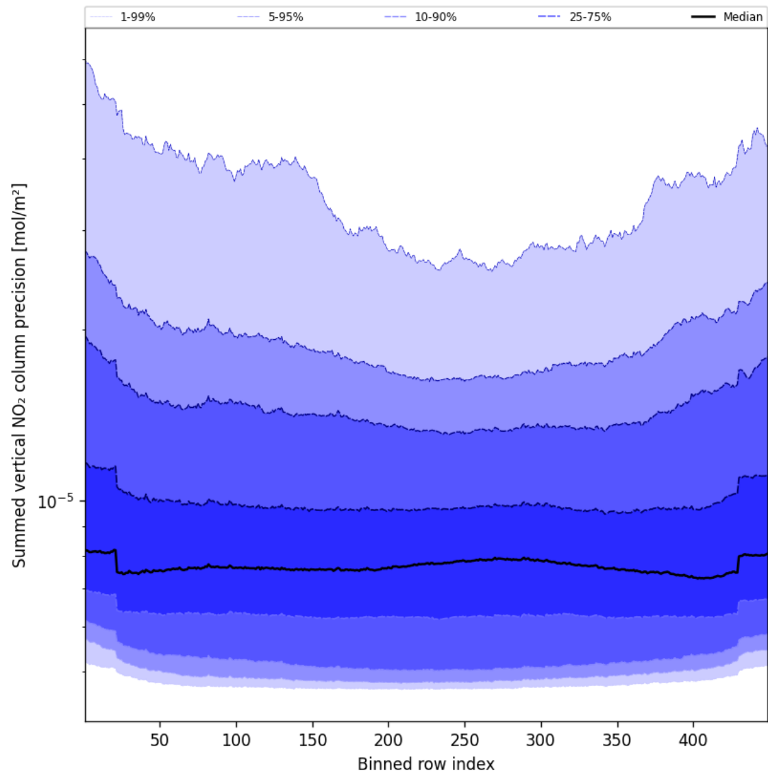
Figure 58: Along track statistics of “Summed vertical NO 2 column precision” for 2025-04-27 to 2025-04-27
