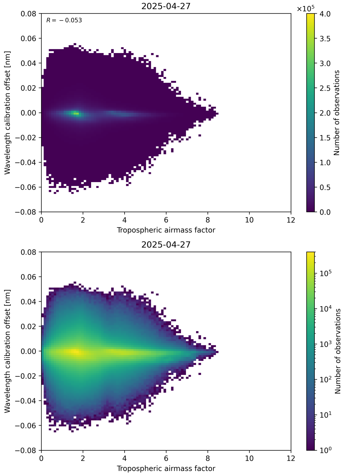
Figure 80: Scatter density plot of “Tropospheric airmass factor” against “Wavelength calibration offset” for 2025-04-27 to 2025-04-27.
