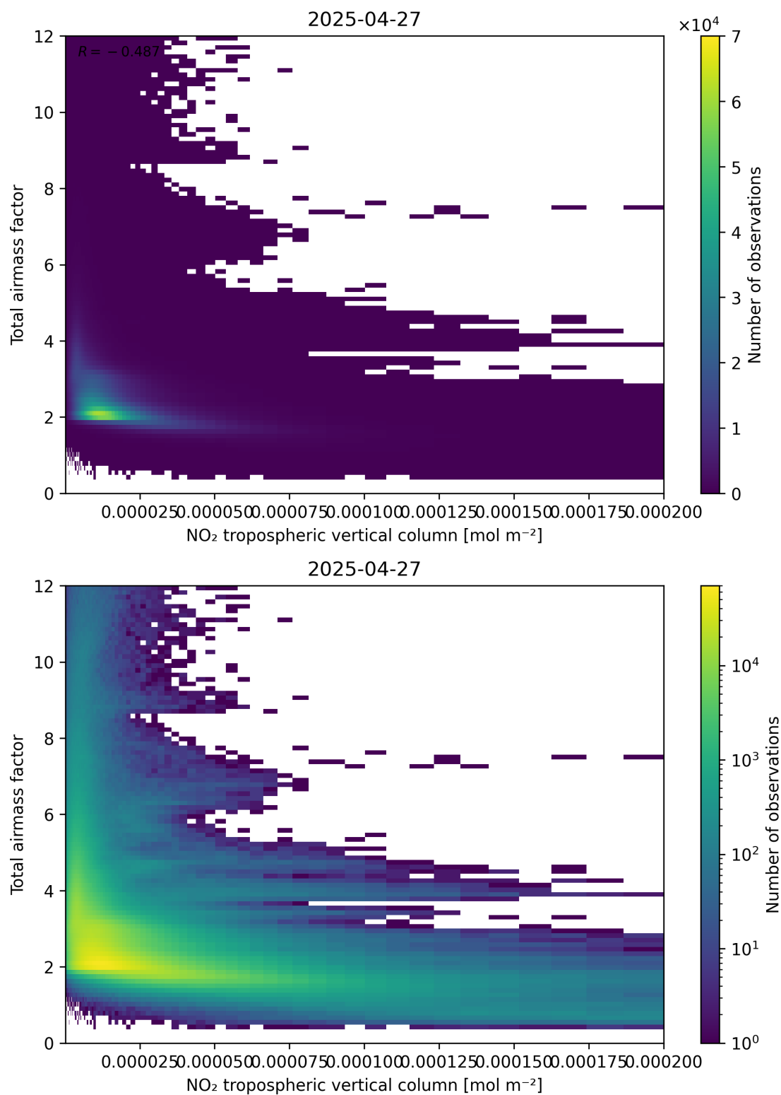
Figure 122: Scatter density plot of “NO 2 tropospheric vertical column” against “Total air mass factor” for 2025-04-27 to 2025-04-27.
