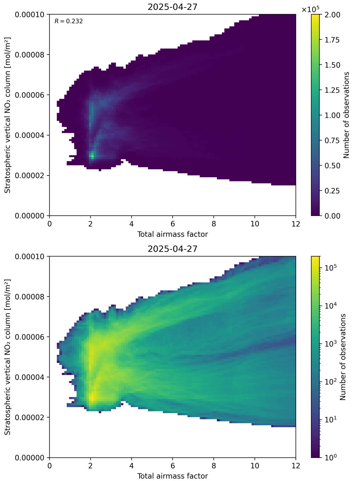
Figure 64: Scatter density plot of “Total airmass factor” against “Stratospheric vertical NO 2 column” for 2025-04-27 to 2025-04-27.
