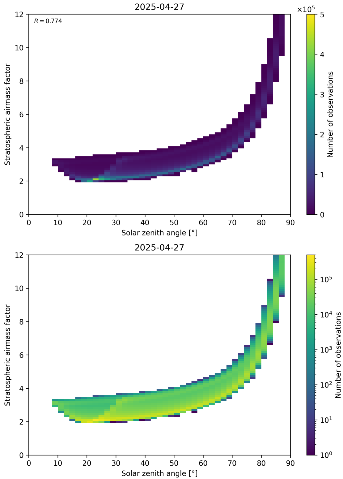
Figure 145: Scatter density plot of “Solar zenith angle” against “Stratospheric airmass factor” for 2025-04-27 to 2025-04-27.
