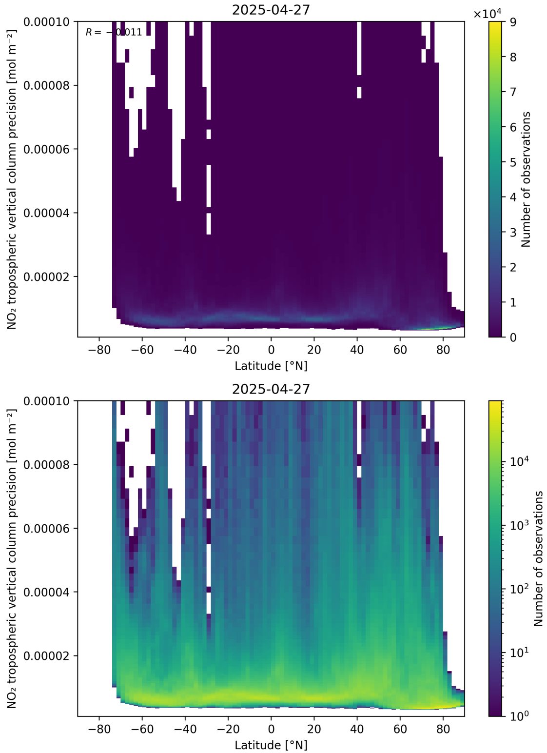
Figure 93: Scatter density plot of “Latitude” against “NO 2 tropospheric vertical column precision” for 2025-04-27 to 2025-04-27.
