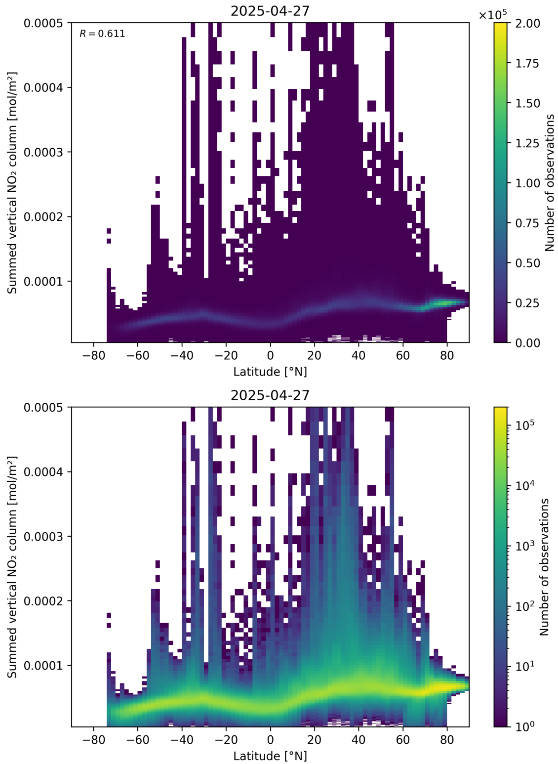
Figure 88: Scatter density plot of “Latitude” against “Summed vertical NO 2 column” for 2025-04-27 to 2025-04-27.
