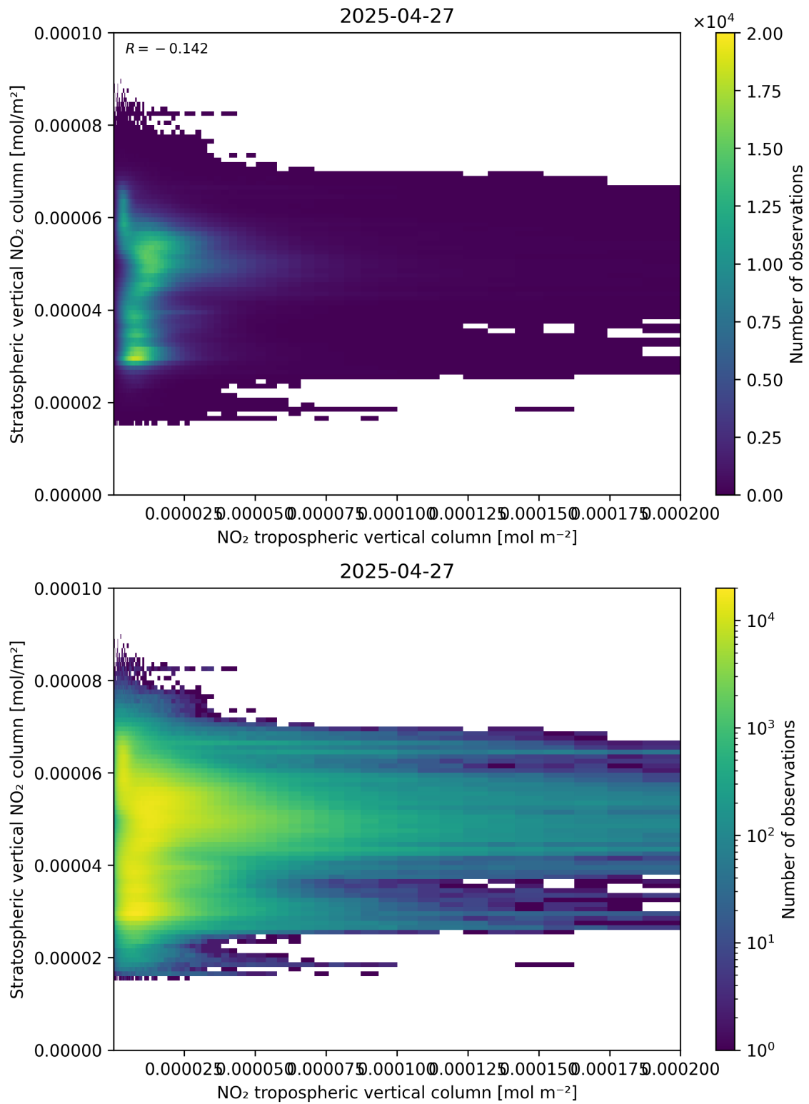
Figure 125: Scatter density plot of “NO 2 tropospheric vertical column” against “Stratospheric vertical NO 2 column” for 2025-04-27 to 2025-04-27.
