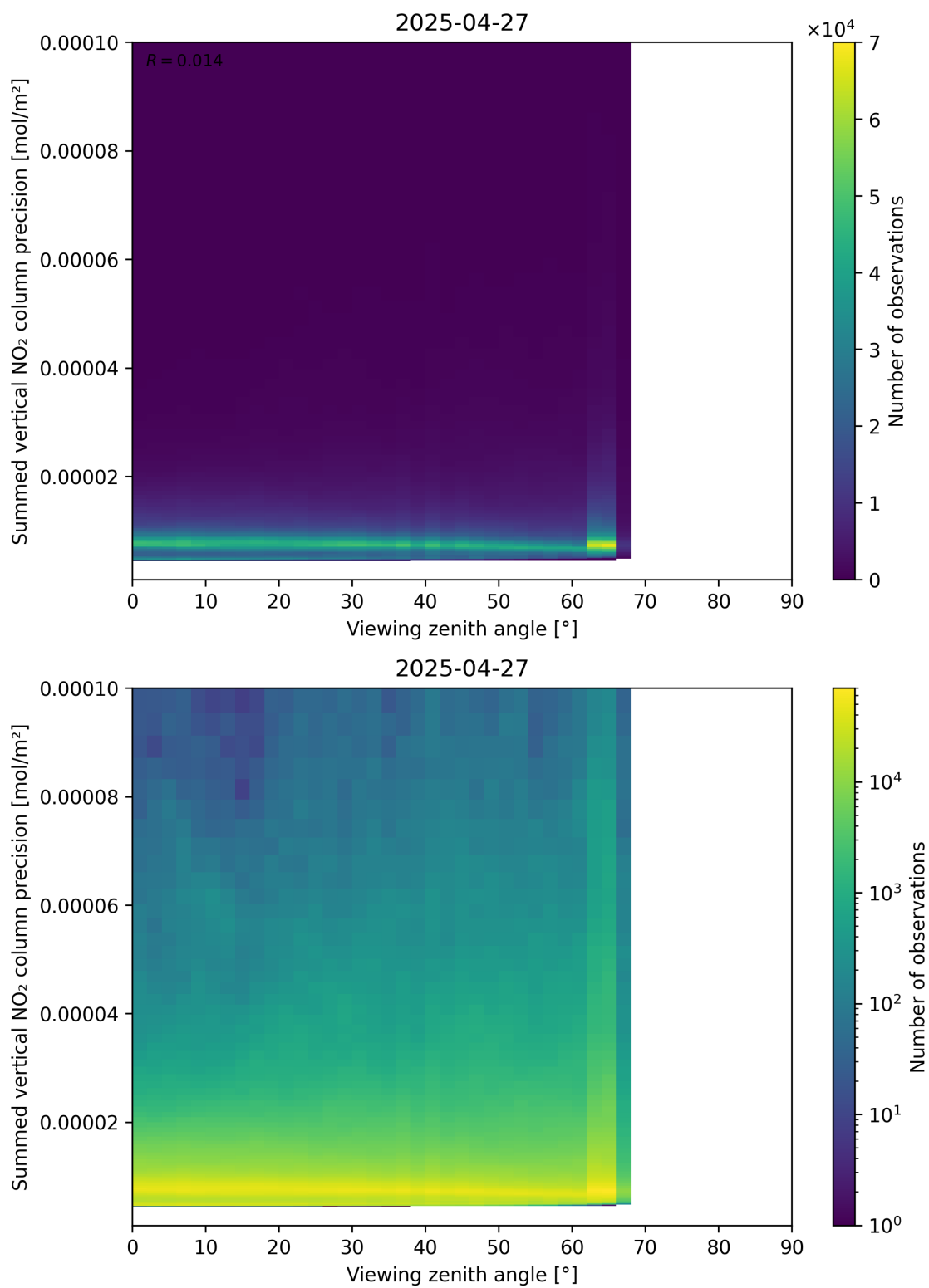
Figure 166: Scatter density plot of “Viewing zenith angle” against “Summed vertical NO 2 column precision” for 2025-04-27 to 2025-04-27.
