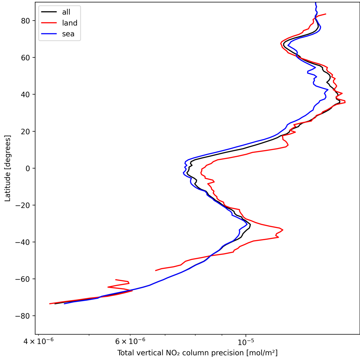
Figure 22: Zonal average of “Total vertical NO 2 column precision” for 2025-04-27 to 2025-04-27.
