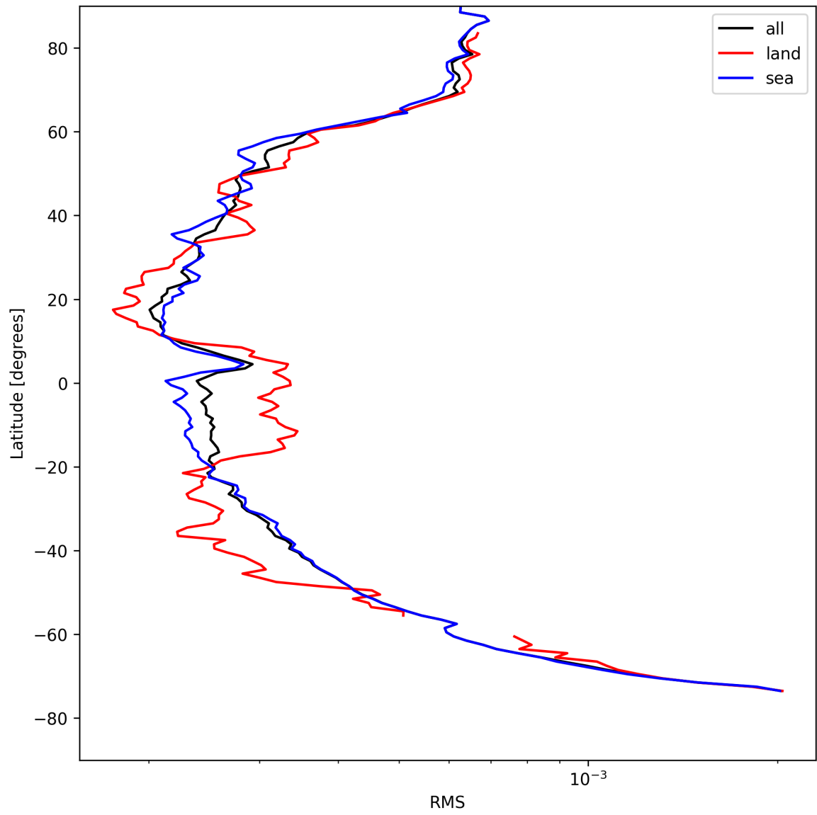
Figure 26: Zonal average of “RMS” for 2025-04-27 to 2025-04-27.
