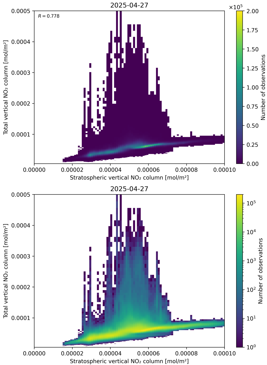
Figure 100: Scatter density plot of “Stratospheric vertical NO 2 column” against “Total vertical NO 2 column” for 2025-04-27 to 2025-04-27.
