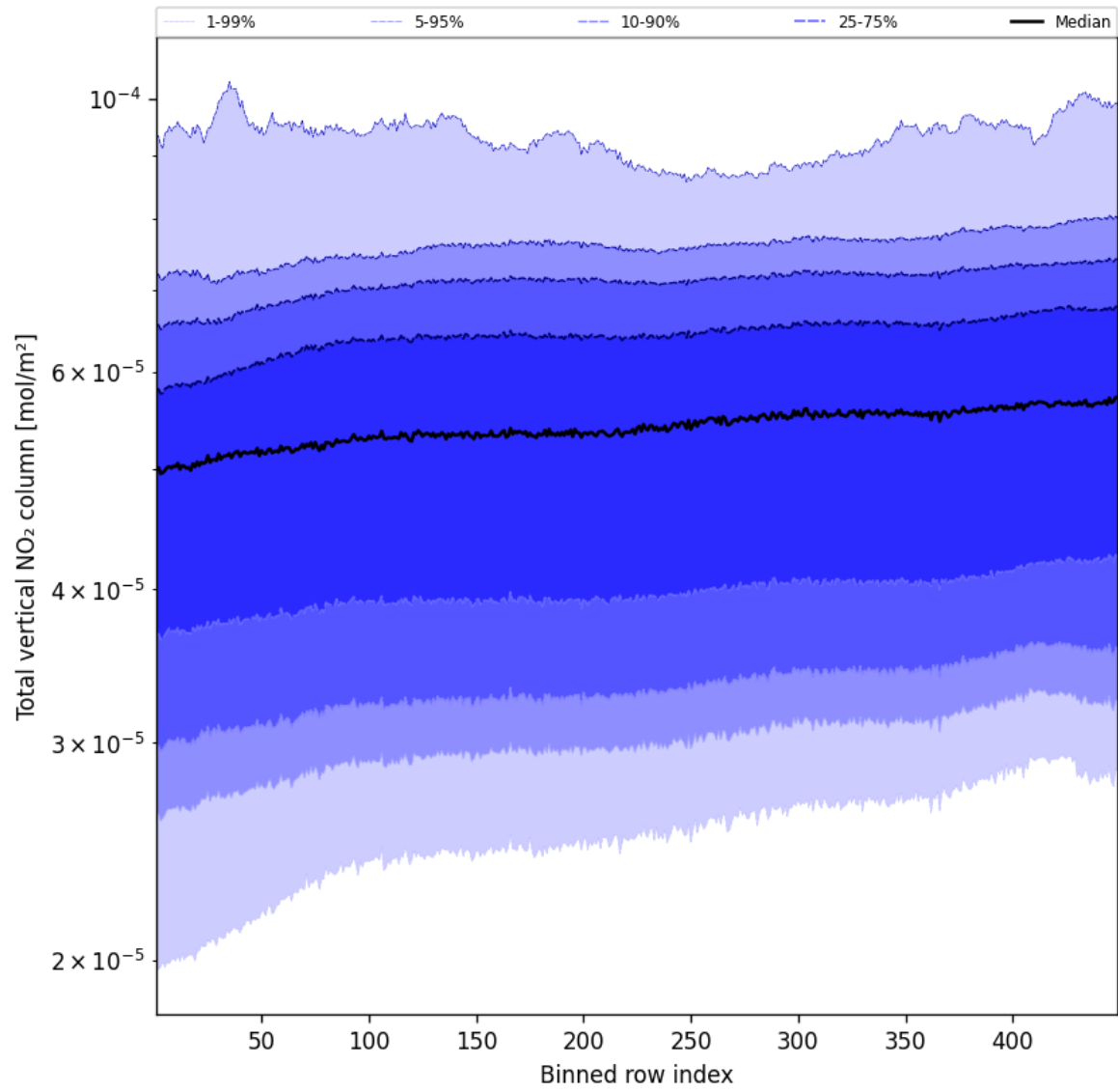
Figure 55: Along track statistics of “Total vertical NO 2 column” for 2025-04-27 to 2025-04-27
