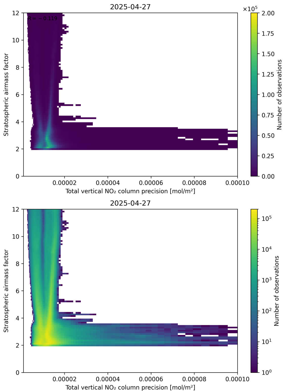
Figure 115: Scatter density plot of “Total vertical NO 2 column precision” against “Stratospheric air mass factor” for 2025-04-27 to 2025-04-27.
