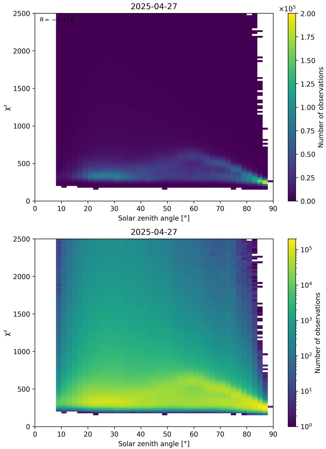
Figure 148: Scatter density plot of “Solar zenith angle” against “ \chi^2 ” for 2025-04-27 to 2025-04-27.
