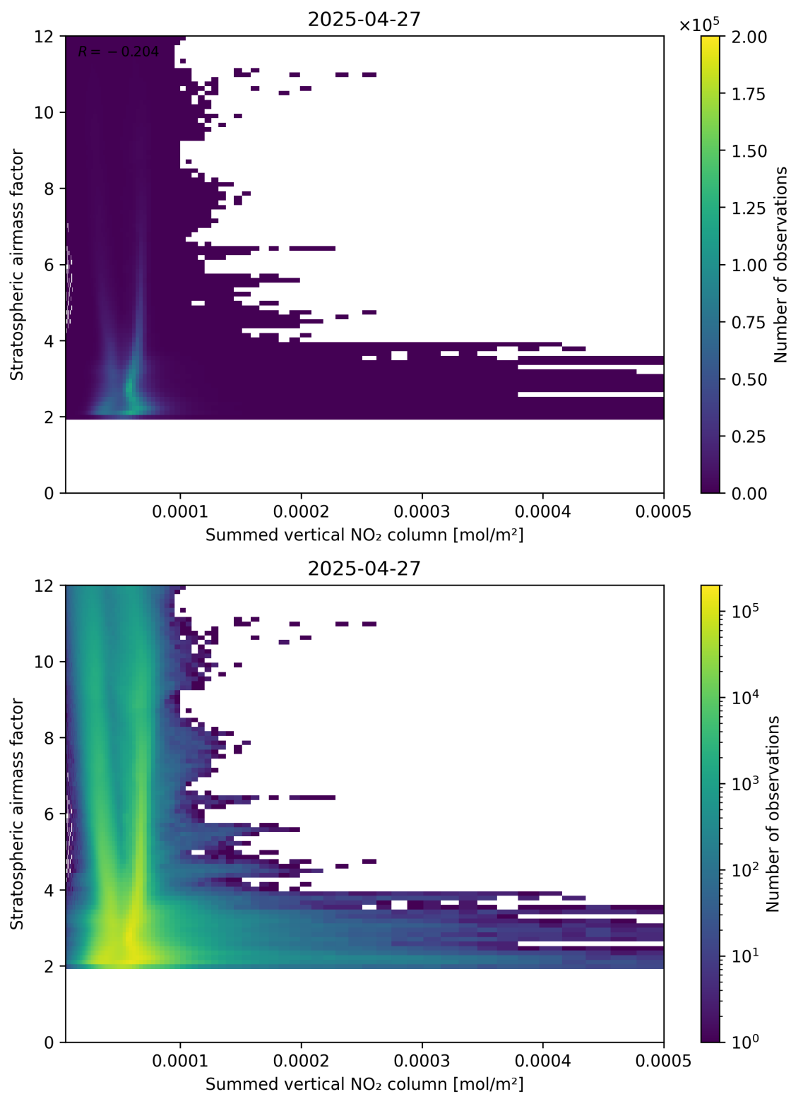
Figure 103: Scatter density plot of “Summed vertical NO 2 column” against “Stratospheric airmass factor” for 2025-04-27 to 2025-04-27.
