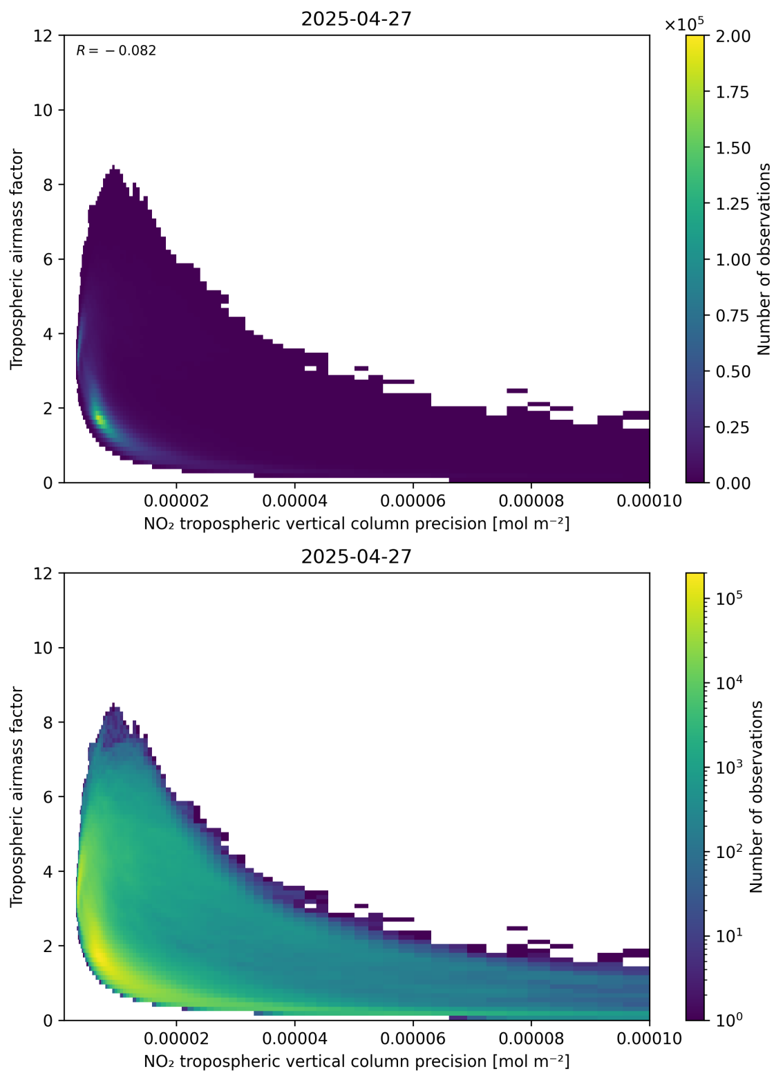
Figure 133: Scatter density plot of “NO 2 tropospheric vertical column precision” against “Tropospheric airmass factor” for 2025-04-27 to 2025-04-27.
