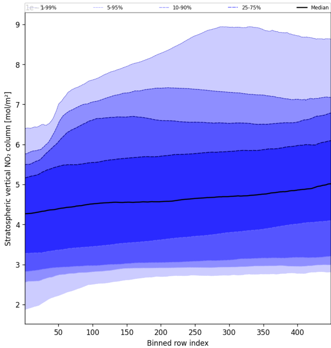
Figure 53: Along track statistics of “Stratospheric vertical NO 2 column” for 2025-04-27 to 2025-04-27
