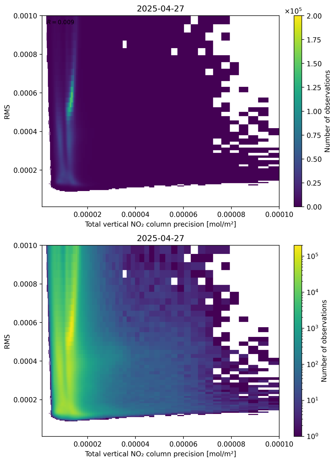
Figure 119: Scatter density plot of “Total vertical NO 2 column precision” against “RMS” for 2025-04-27 to 2025-04-27.
