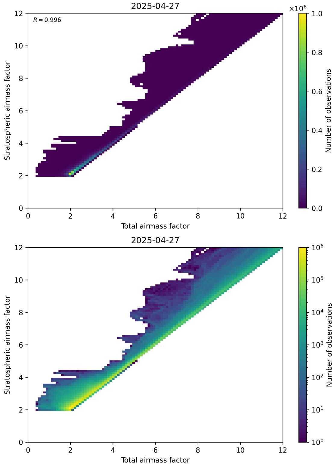
Figure 62: Scatter density plot of “Total airmass factor” against “Stratospheric airmass factor” for 2025-04-27 to 2025-04-27.
