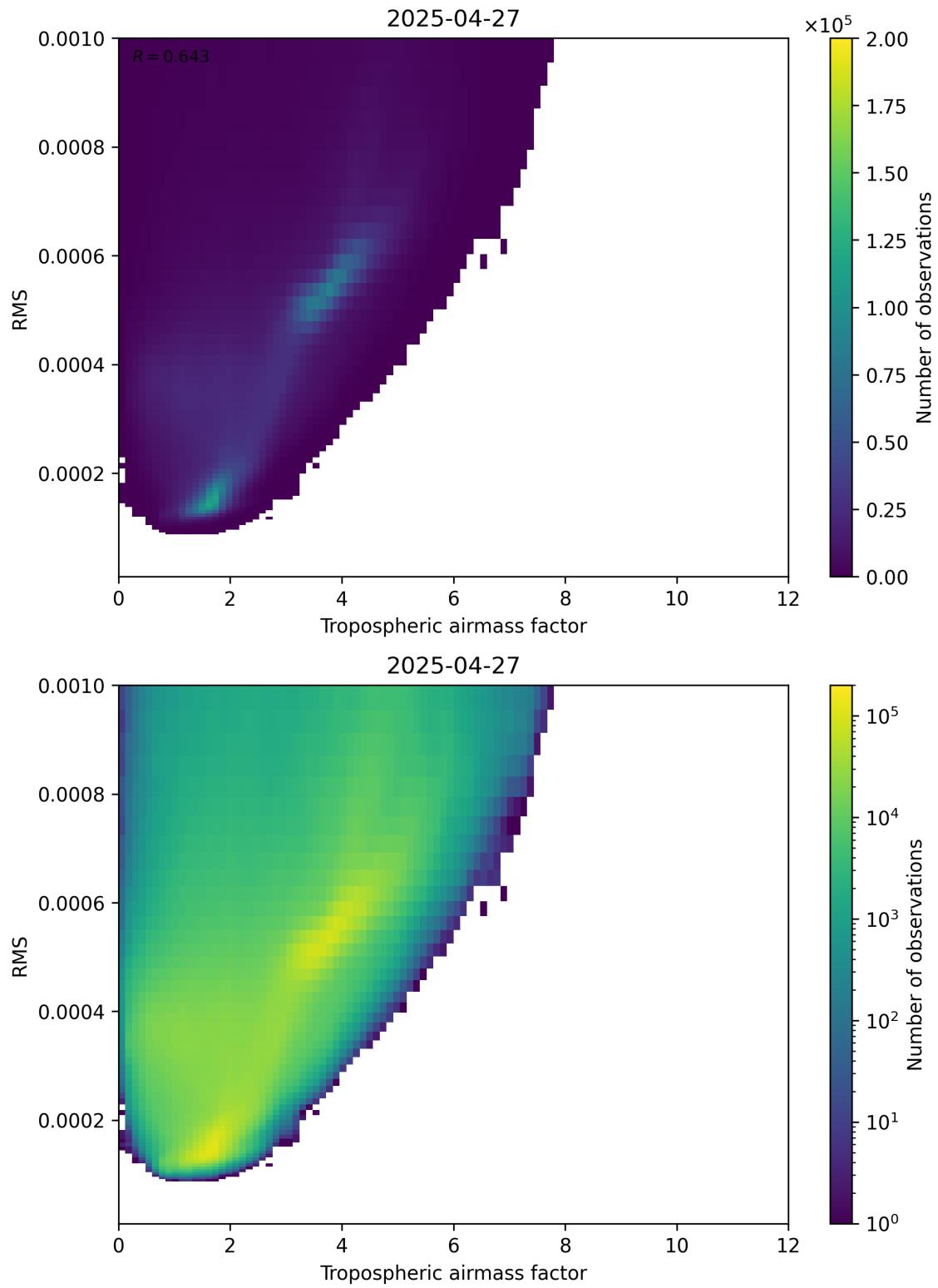
Figure 79: Scatter density plot of “Tropospheric airmass factor” against “RMS” for 2025-04-27 to 2025-04-27.
