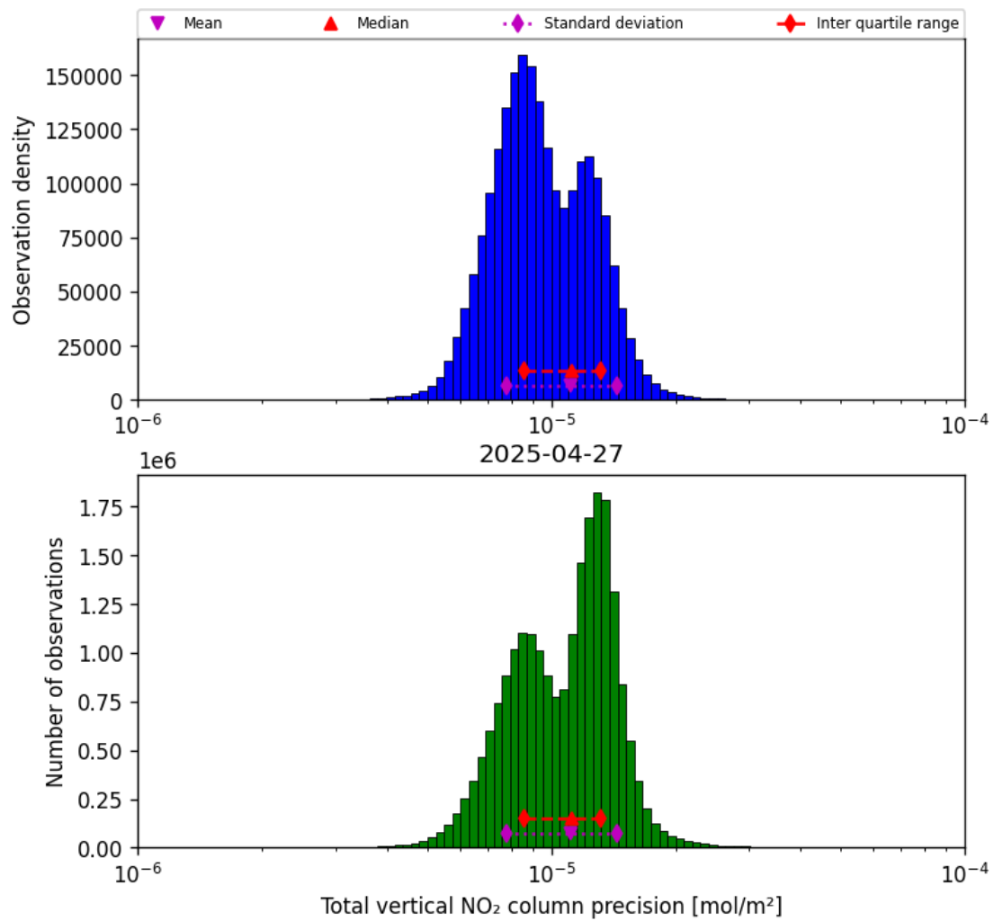
Figure 39: Histogram of “Total vertical NO 2 column precision” for 2025-04-27 to 2025-04-27
