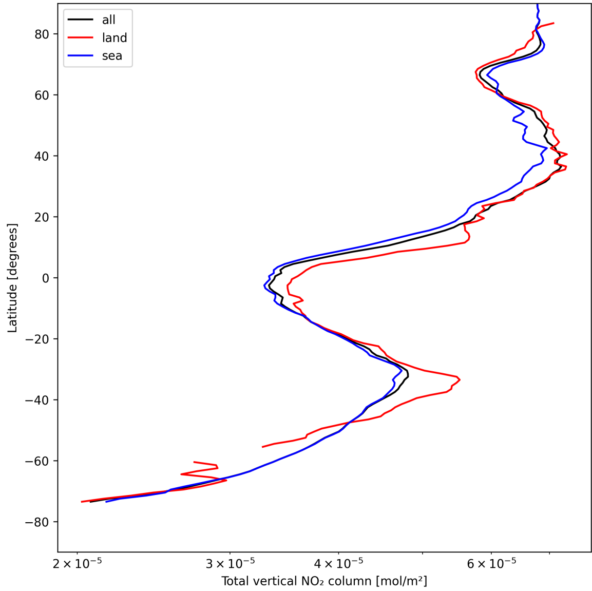
Figure 21: Zonal average of “Total vertical NO 2 column” for 2025-04-27 to 2025-04-27.
