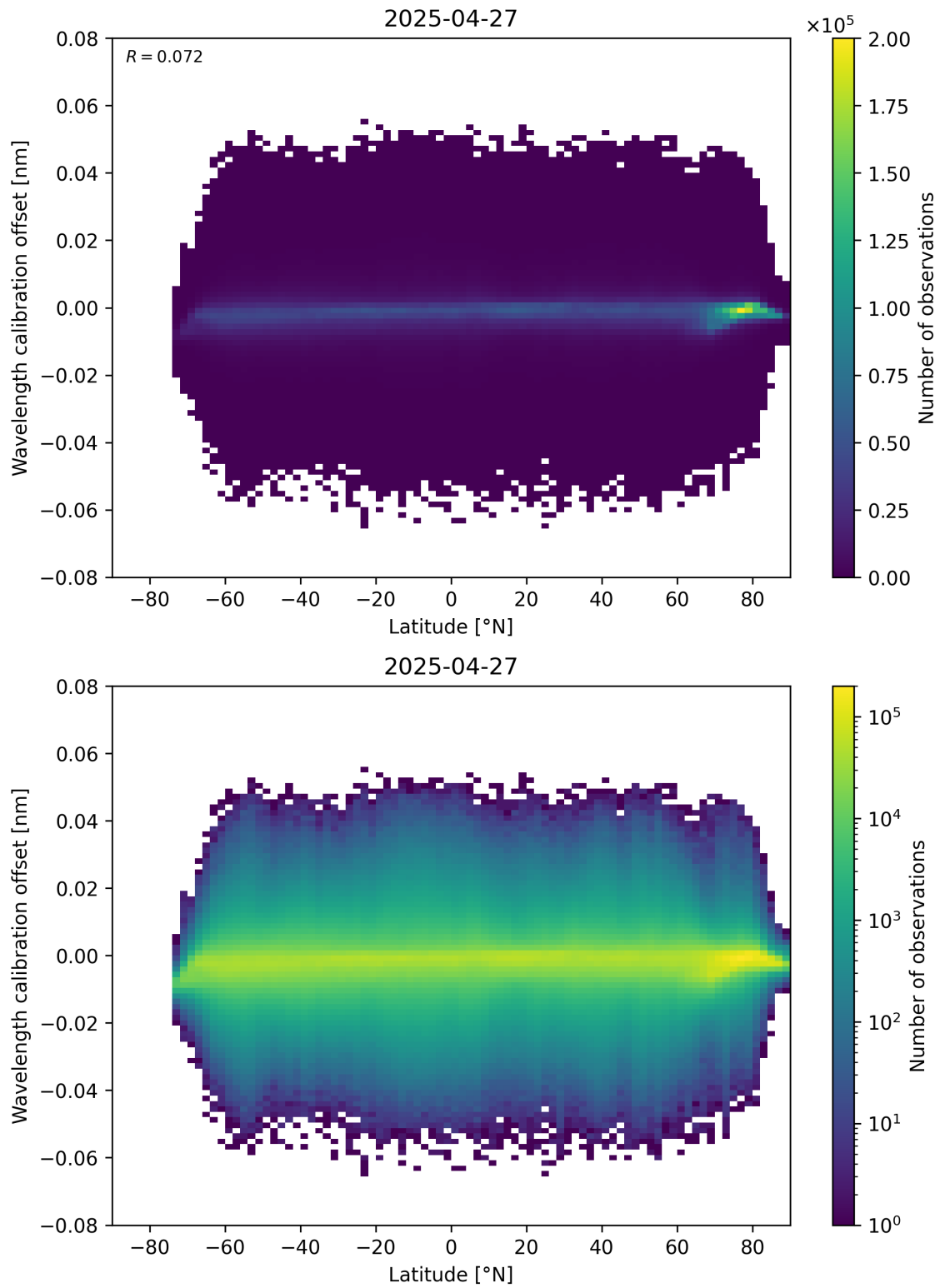
Figure 95: Scatter density plot of “Latitude” against “Wavelength calibration offset” for 2025-04-27 to 2025-04-27.
