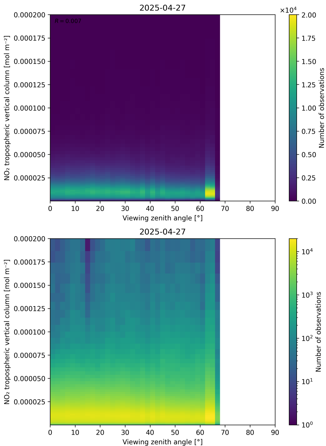
Figure 169: Scatter density plot of “Viewing zenith angle” against “NO 2 tropospheric vertical column” for 2025-04-27 to 2025-04-27.
