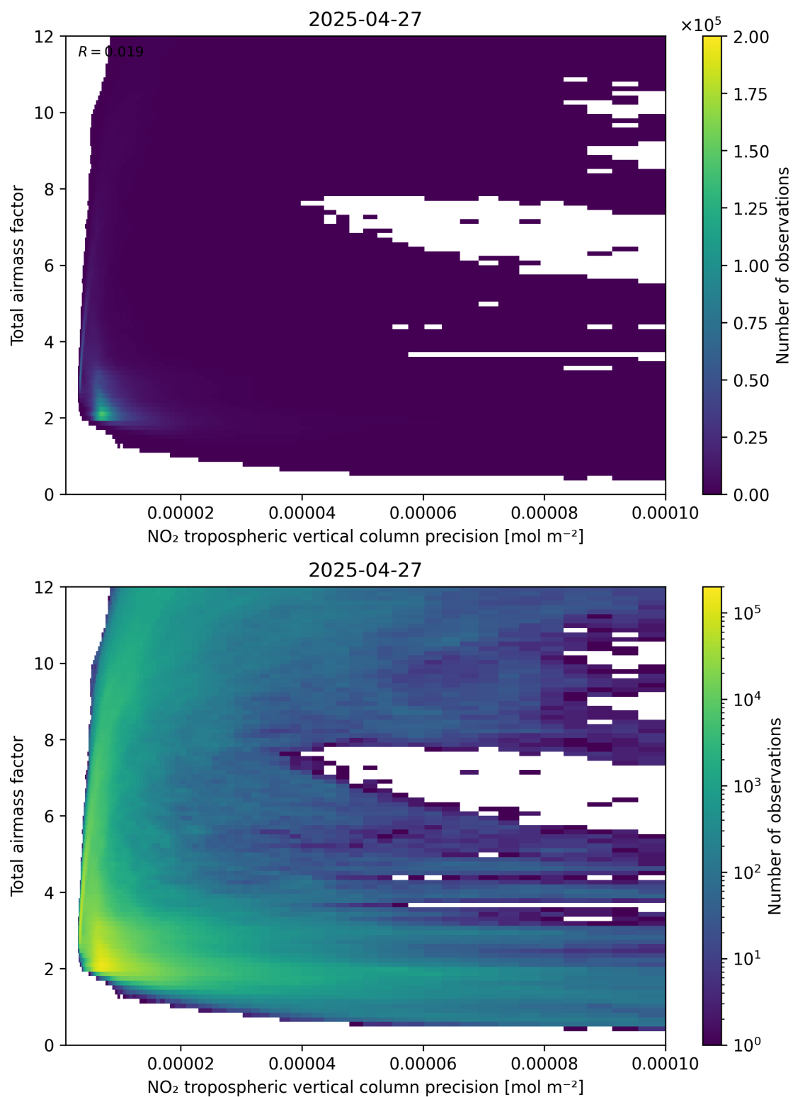
Figure 132: Scatter density plot of “NO 2 tropospheric vertical column precision” against “Total air mass factor” for 2025-04-27 to 2025-04-27.
