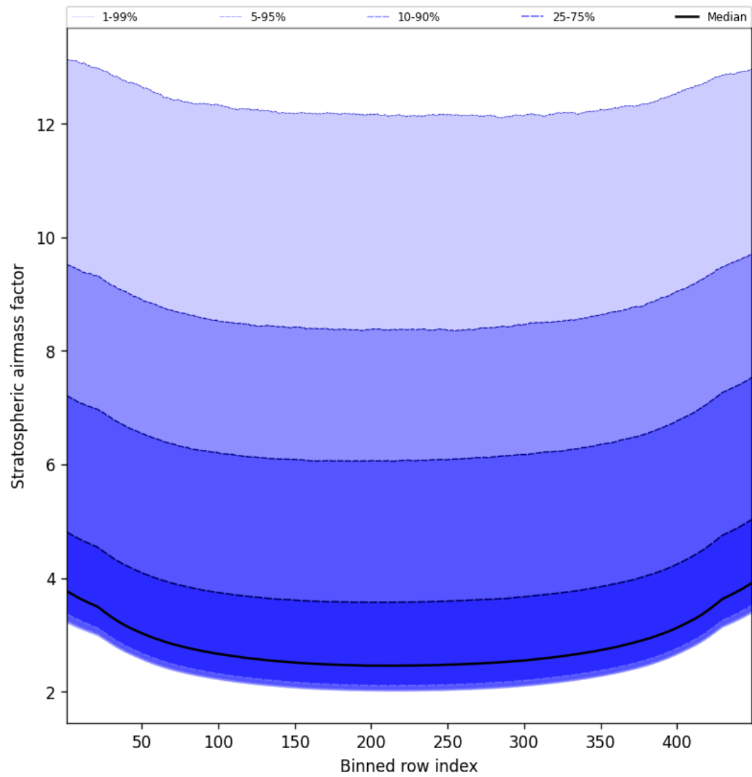
Figure 61: Along track statistics of “Stratospheric airmass factor” for 2025-04-27 to 2025-04-27
