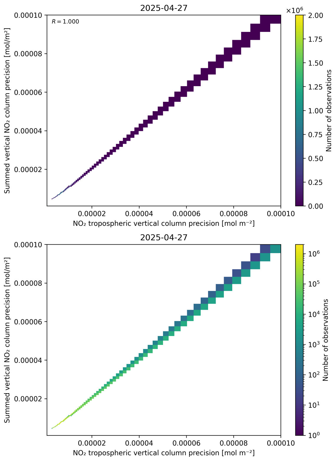
Figure 137: Scatter density plot of “NO 2 tropospheric vertical column precision” against “Summed vertical NO 2 column precision” for 2025-04-27 to 2025-04-27.
