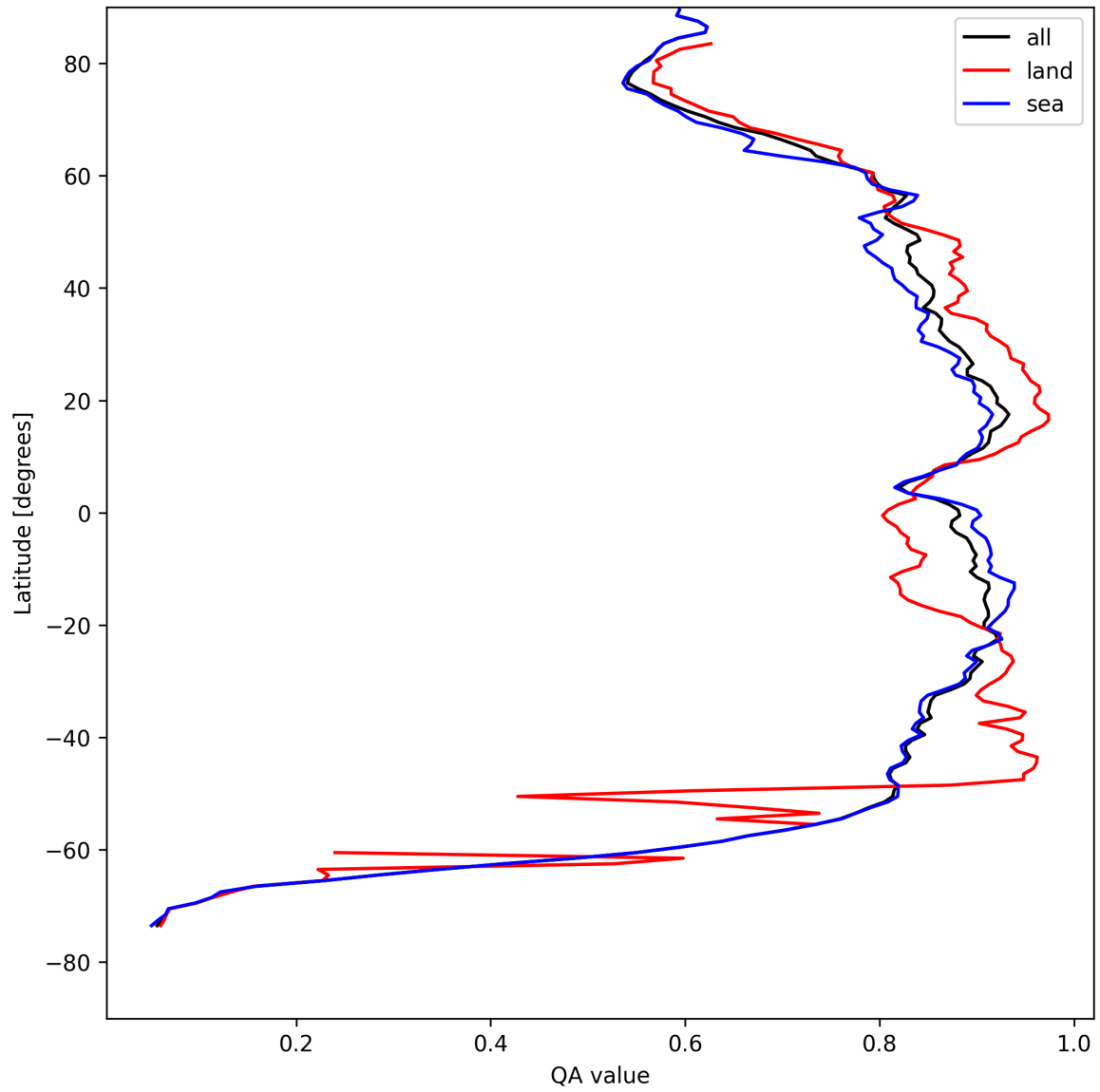
Figure 11: Zonal average of “QA value” for 2025-04-27 to 2025-04-27.
