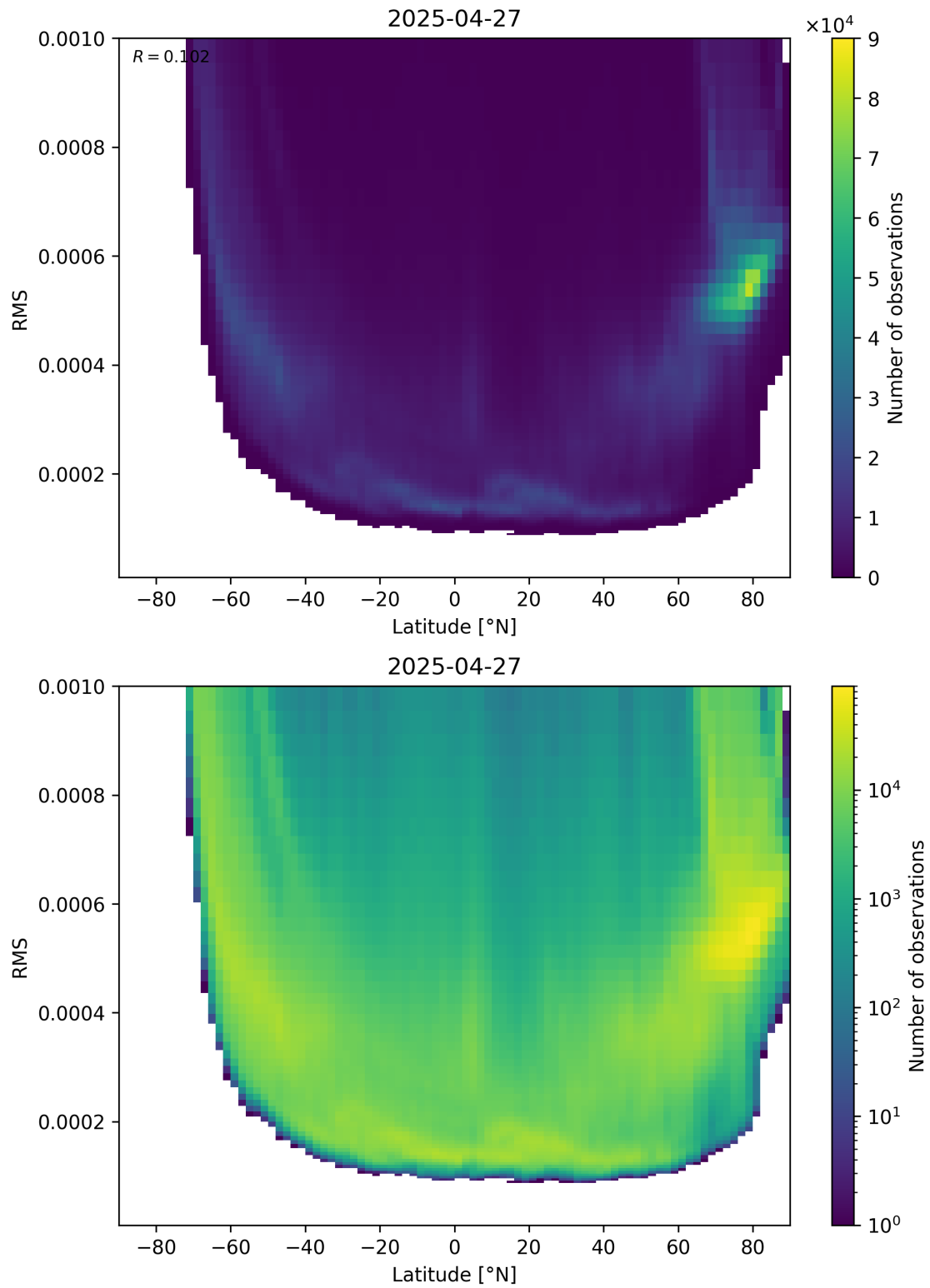
Figure 94: Scatter density plot of “Latitude” against “RMS” for 2025-04-27 to 2025-04-27.
