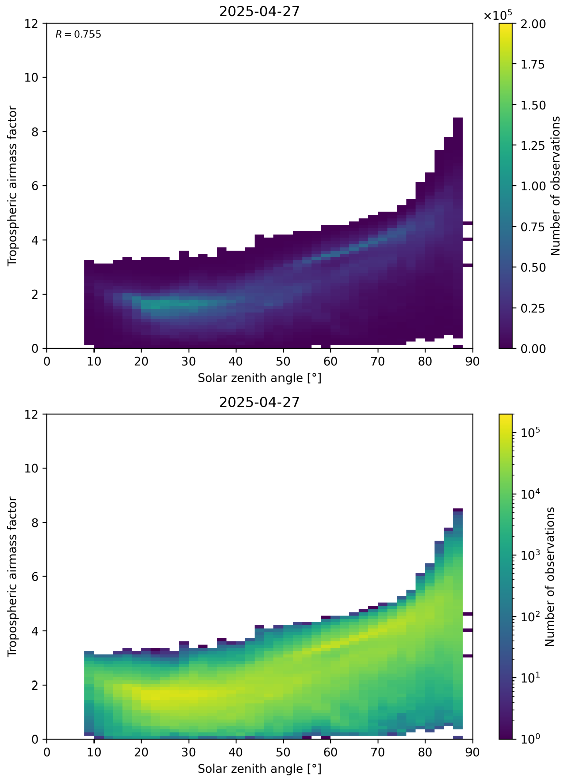
Figure 147: Scatter density plot of “Solar zenith angle” against “Tropospheric airmass factor” for 2025-04-27 to 2025-04-27.
