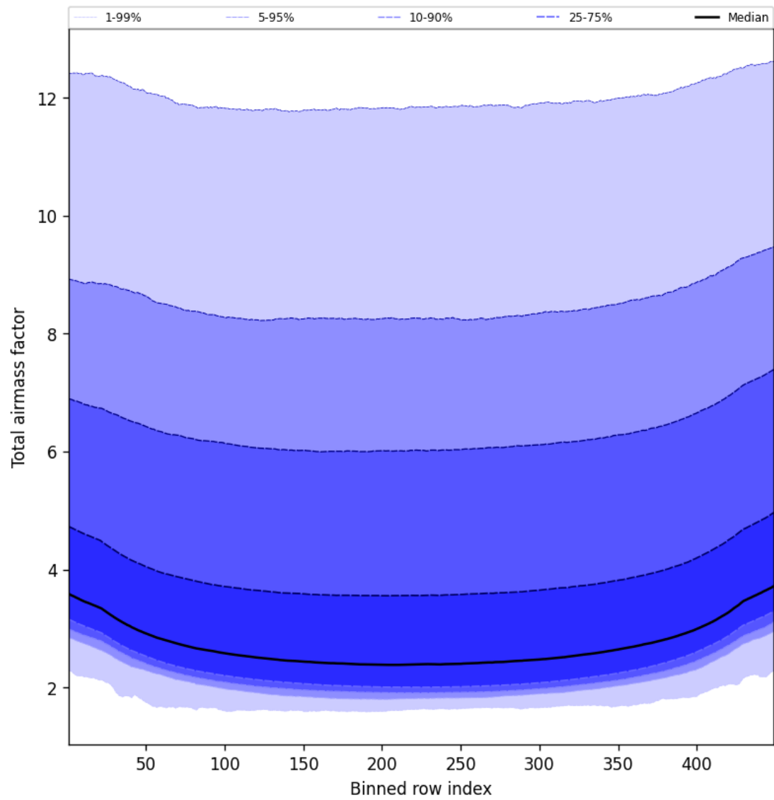
Figure 49: Along track statistics of “Total airmass factor” for 2025-04-27 to 2025-04-27
