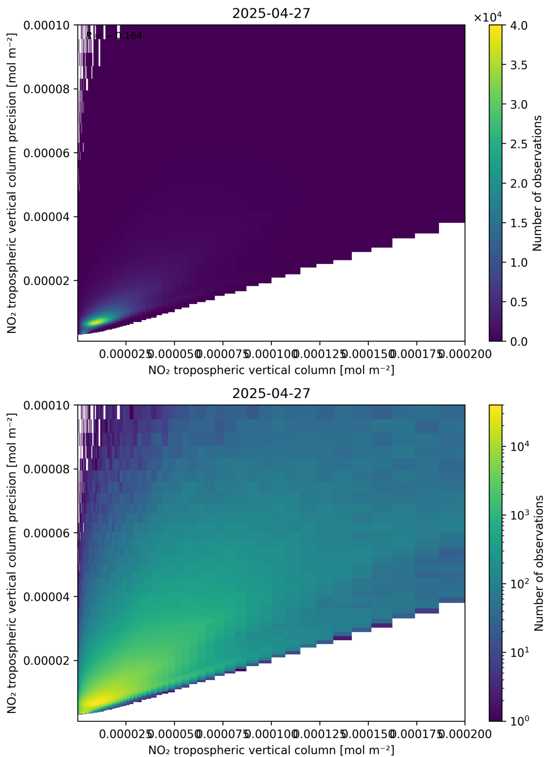
Figure 130: Scatter density plot of “NO 2 tropospheric vertical column” against “NO 2 tropospheric vertical column precision” for 2025-04-27 to 2025-04-27.
