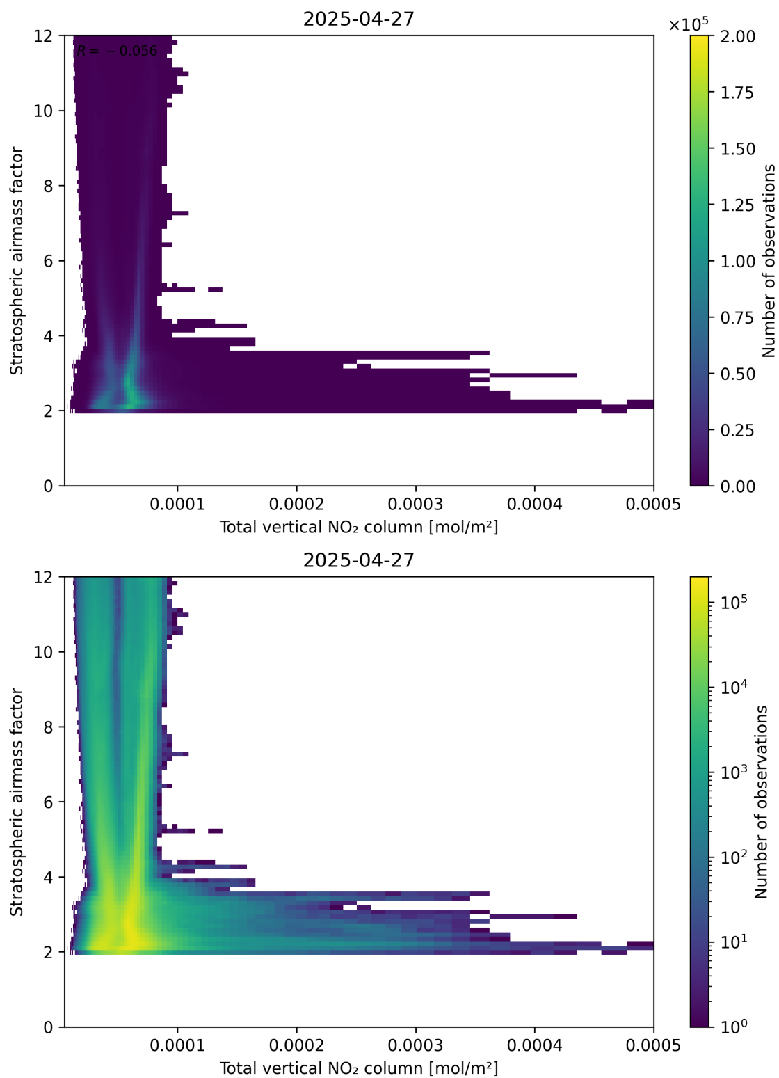
Figure 110: Scatter density plot of “Total vertical NO 2 column” against “Stratospheric airmass factor” for 2025-04-27 to 2025-04-27.
