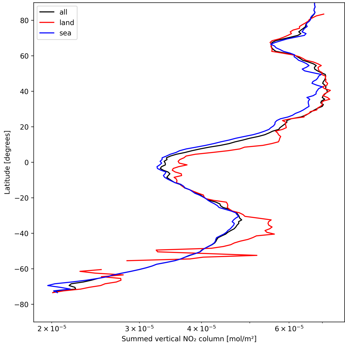
Figure 23: Zonal average of “Summed vertical NO 2 column” for 2025-04-27 to 2025-04-27.
