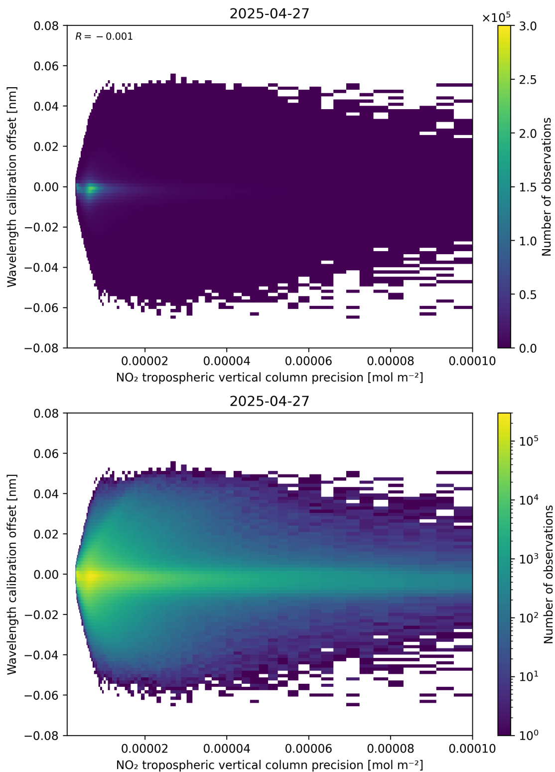
Figure 141: Scatter density plot of “NO 2 tropospheric vertical column precision” against “Wavelength calibration offset” for 2025-04-27 to 2025-04-27.
