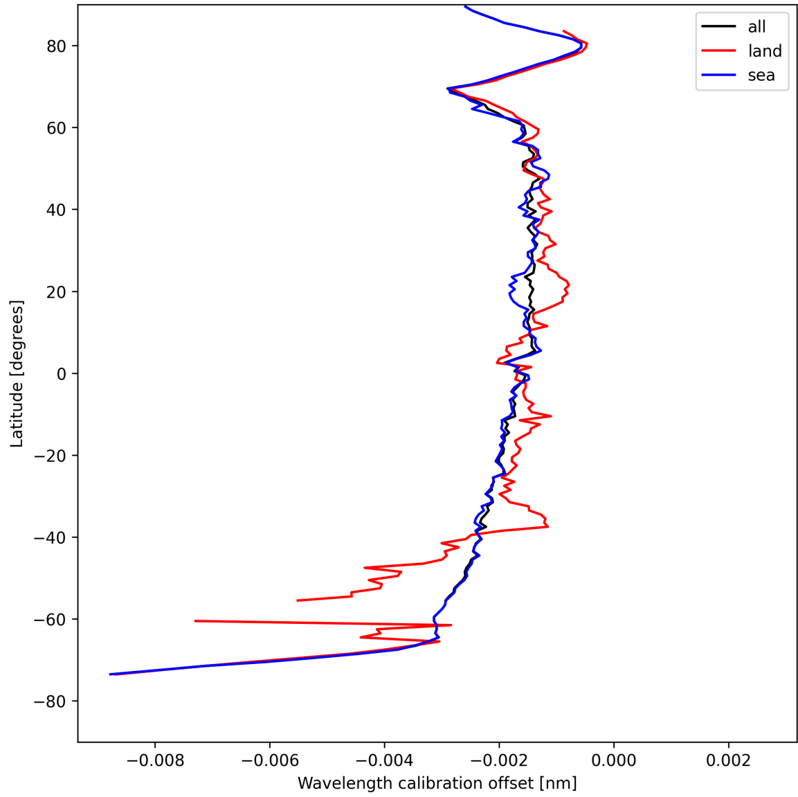
Figure 18: Zonal average of “Wavelength calibration offset” for 2025-04-27 to 2025-04-27.
