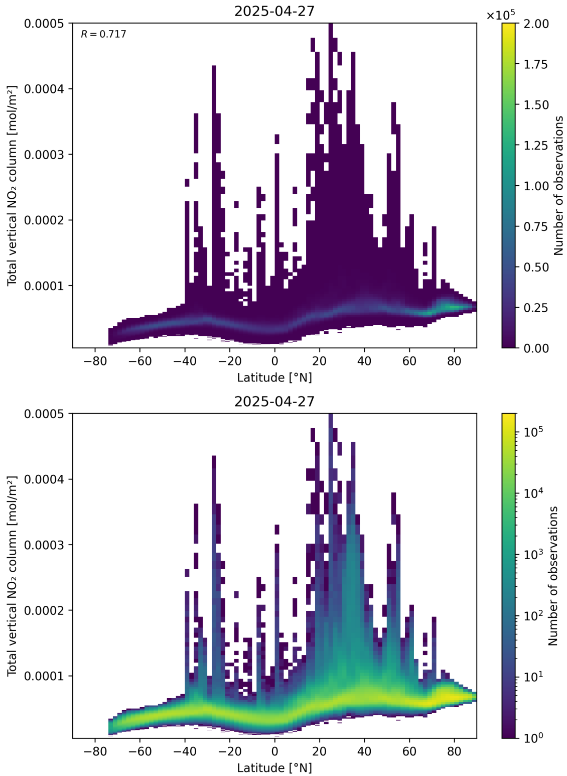
Figure 90: Scatter density plot of “Latitude” against “Total vertical NO 2 column” for 2025-04-27 to 2025-04-27.
