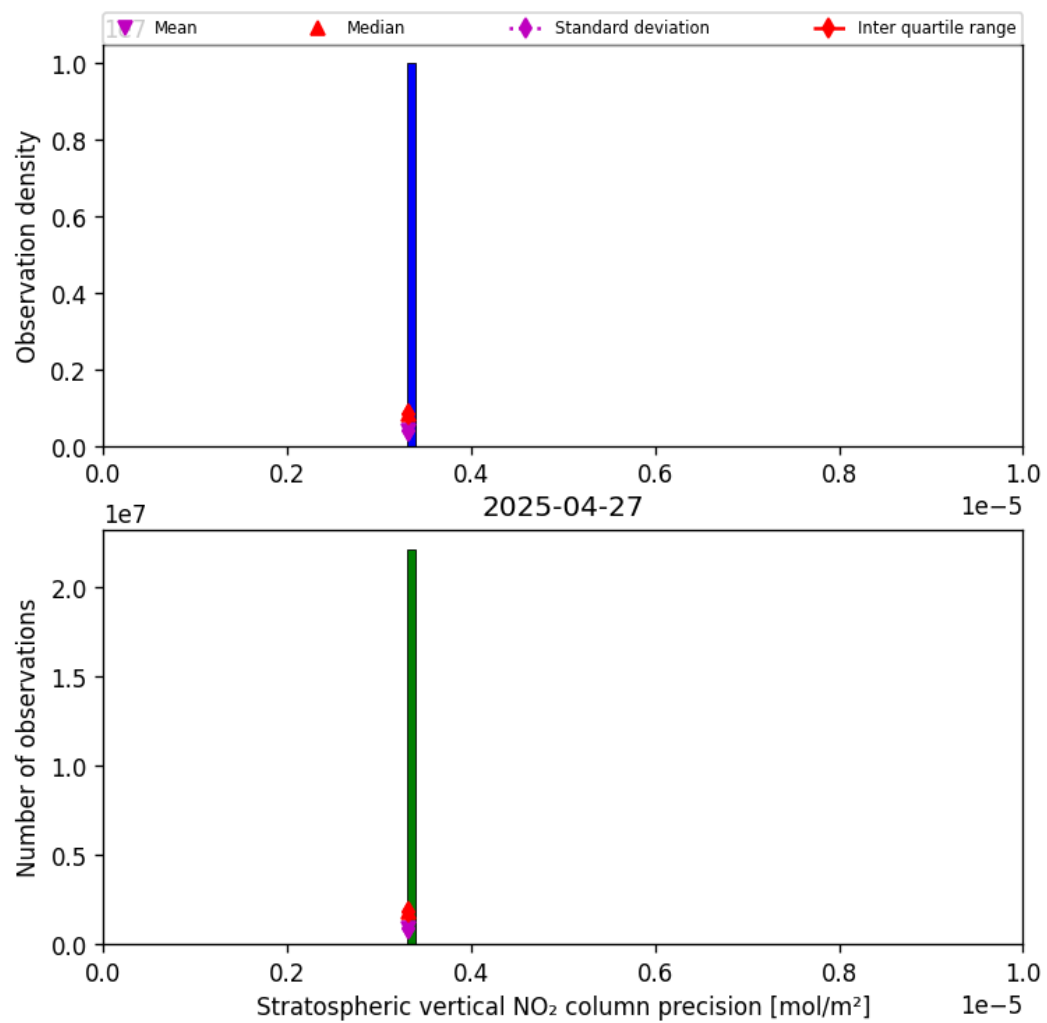
Figure 37: Histogram of “Stratospheric vertical NO 2 column precision” for 2025-04-27 to 2025-04-27
