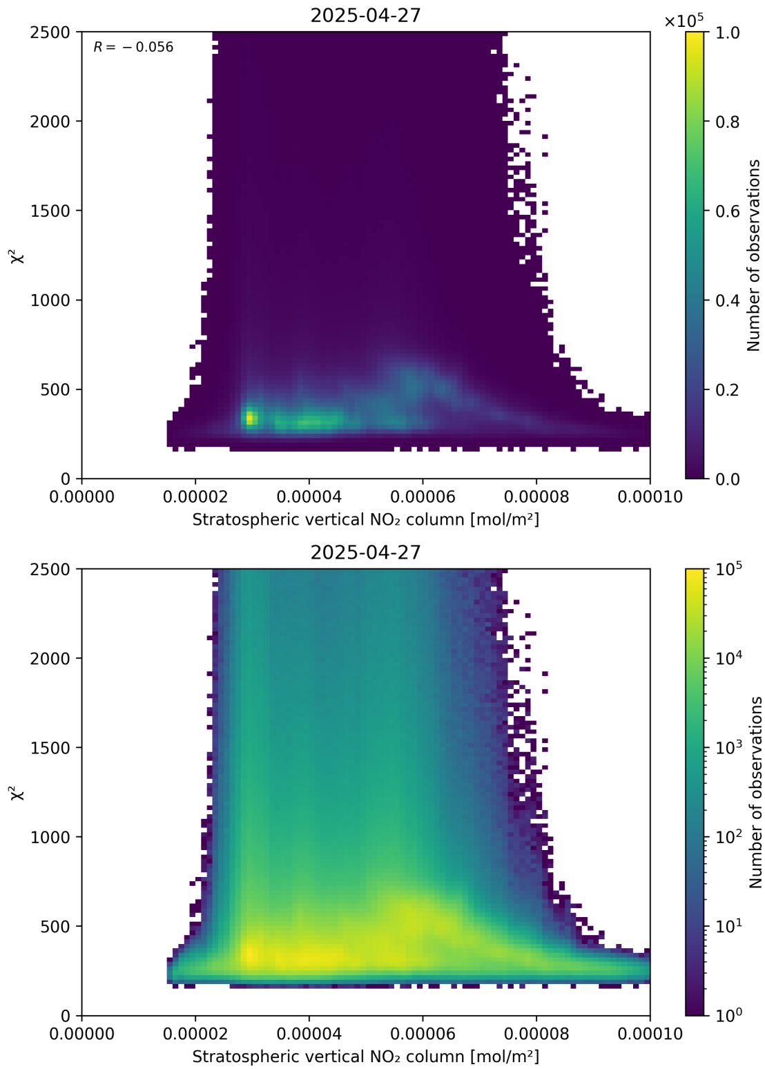
Figure 97: Scatter density plot of “Stratospheric vertical NO 2 column” against “ \chi^2 ” for 2025-04-27 to 2025-04-27.
