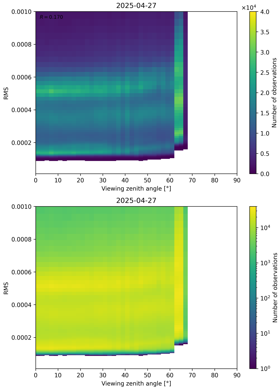
Figure 171: Scatter density plot of “Viewing zenith angle” against “RMS” for 2025-04-27 to 2025-04-27.
