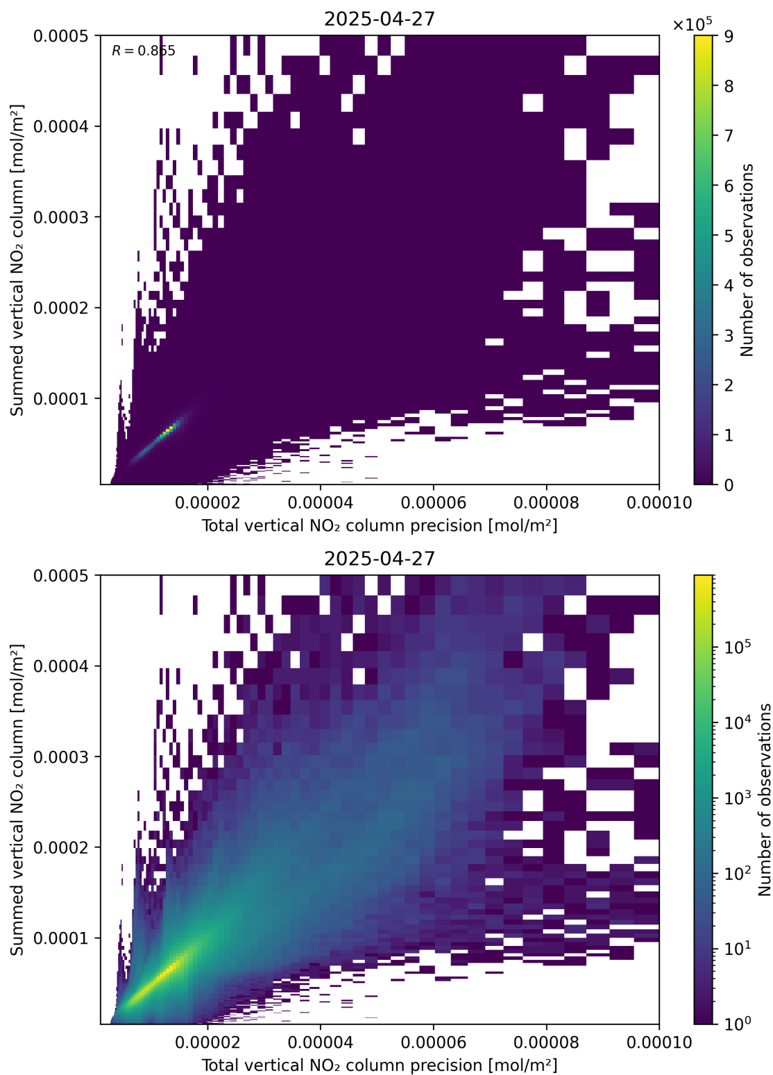
Figure 117: Scatter density plot of “Total vertical NO 2 column precision” against “Summed vertical NO 2 column” for 2025-04-27 to 2025-04-27.
