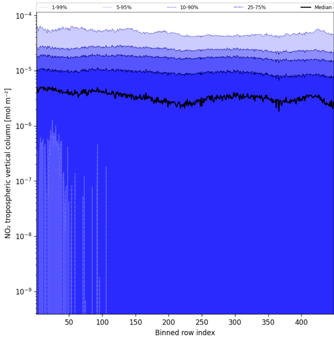
Figure 46: Along track statistics of “NO 2 tropospheric vertical column” for 2025-04-27 to 2025-04-27
