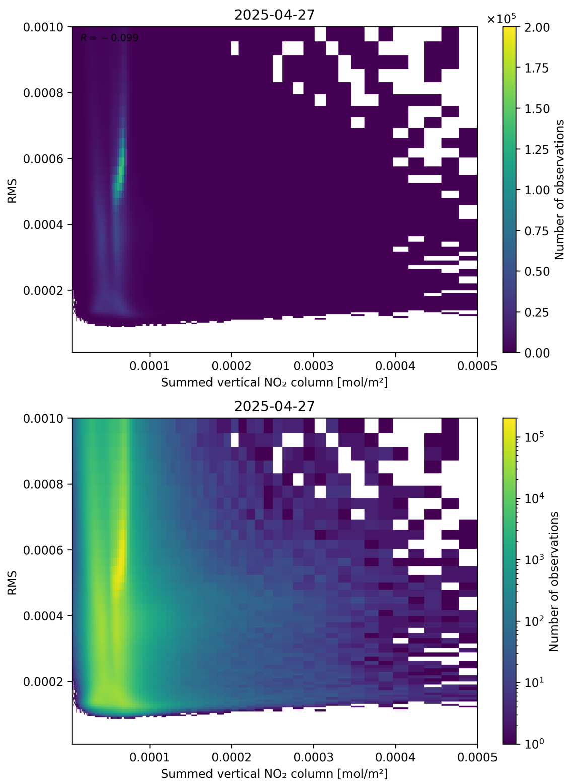
Figure 109: Scatter density plot of “Summed vertical NO 2 column” against “RMS” for 2025-04-27 to 2025-04-27.
