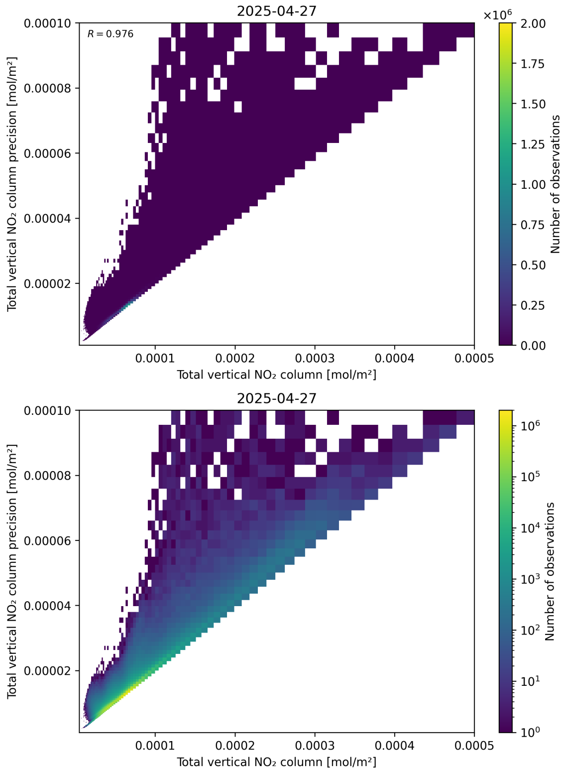
Figure 114: Scatter density plot of “Total vertical NO 2 column” against “Total vertical NO 2 column precision” for 2025-04-27 to 2025-04-27.
