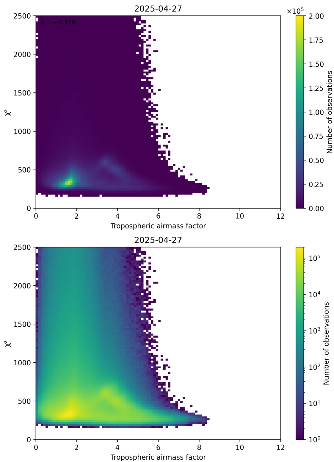
Figure 73: Scatter density plot of “Tropospheric airmass factor” against “ \chi^2 ” for 2025-04-27 to 2025-04-27.
