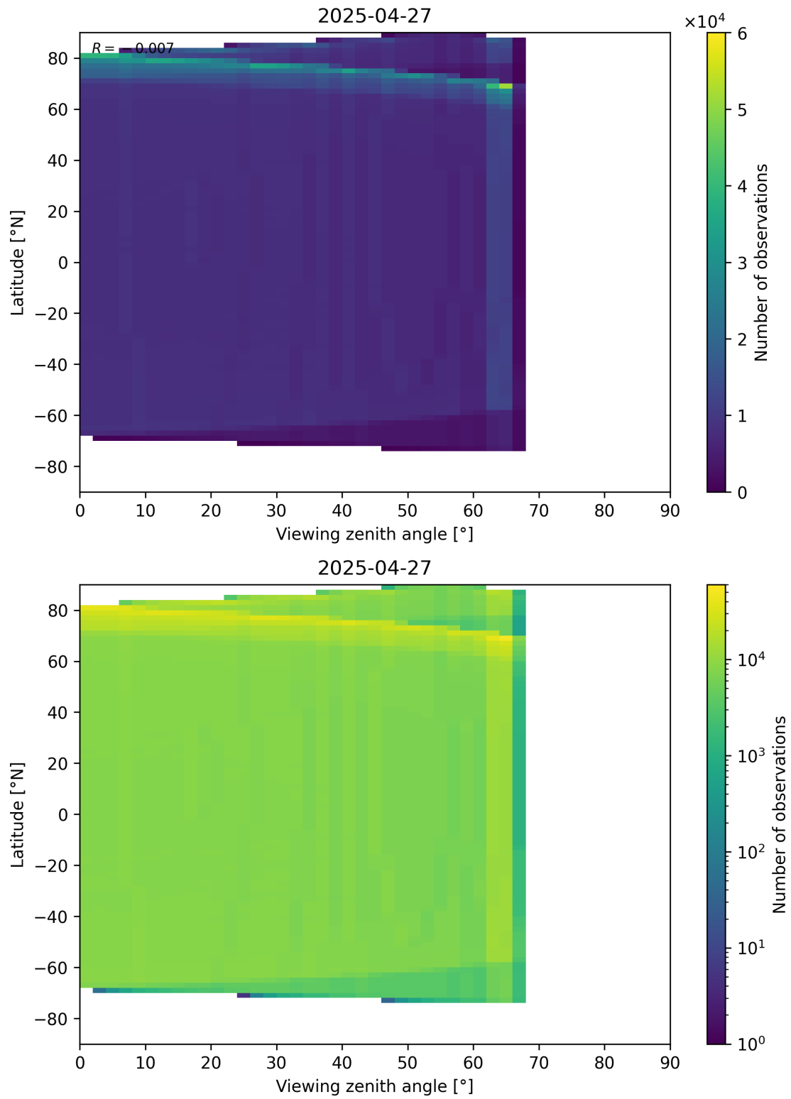
Figure 163: Scatter density plot of “Viewing zenith angle” against “Latitude” for 2025-04-27 to 2025-04-27.
