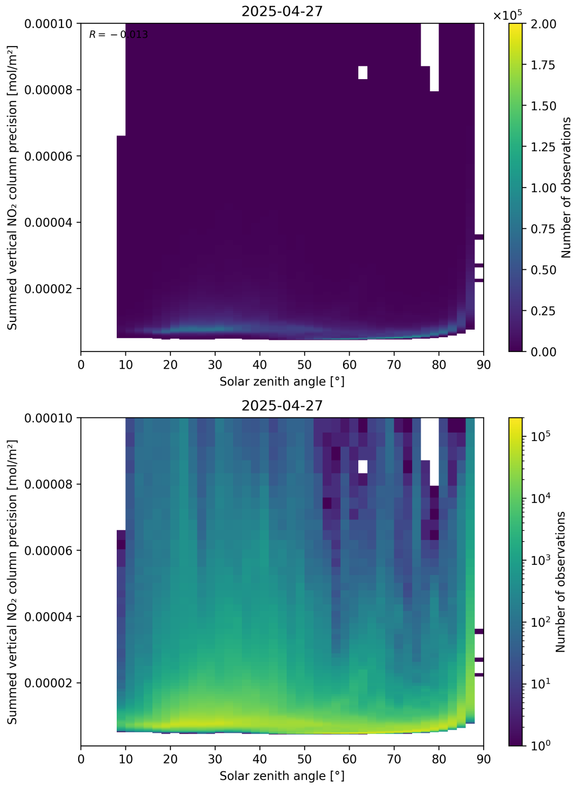
Figure 152: Scatter density plot of “Solar zenith angle” against “Summed vertical NO 2 column precision” for 2025-04-27 to 2025-04-27.
