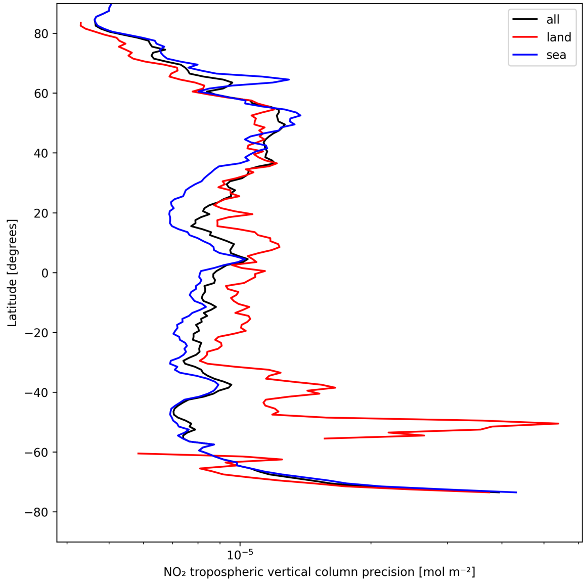
Figure 13: Zonal average of “NO 2 tropospheric vertical column precision” for 2025-04-27 to 2025-04-27.
