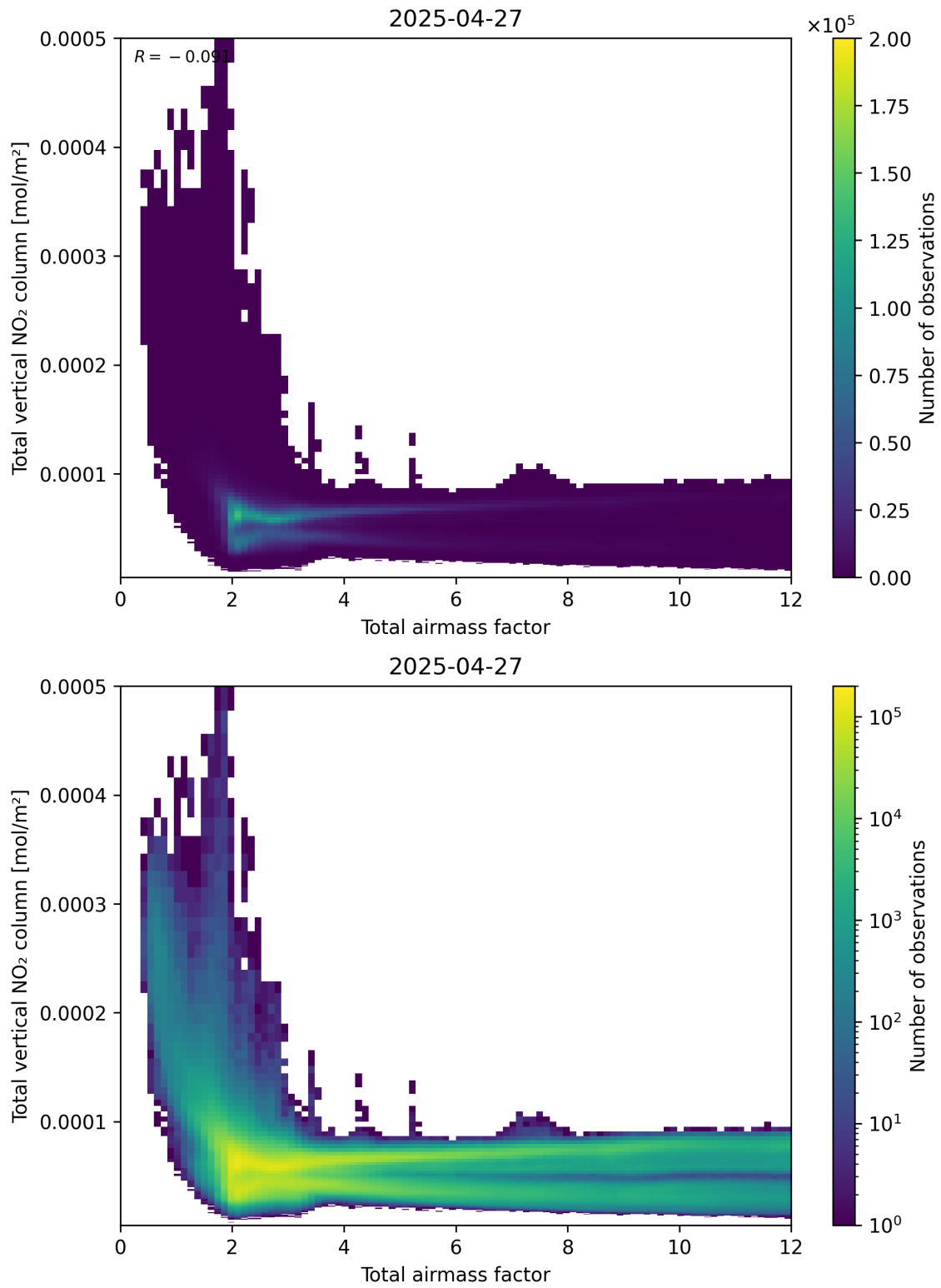
Figure 67: Scatter density plot of “Total airmass factor” against “Total vertical NO 2 column” for 2025-04-27 to 2025-04-27.
