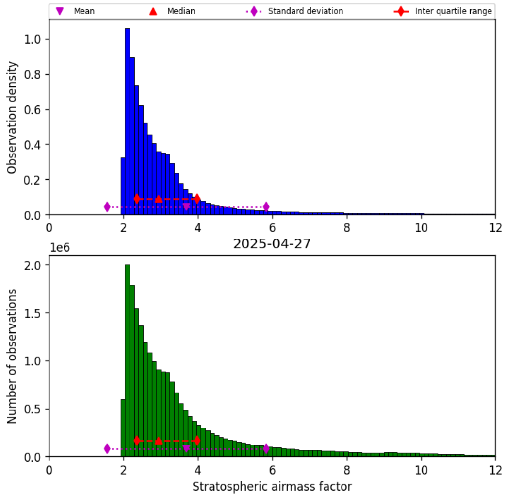
Figure 44: Histogram of “Stratospheric airmass factor” for 2025-04-27 to 2025-04-27
