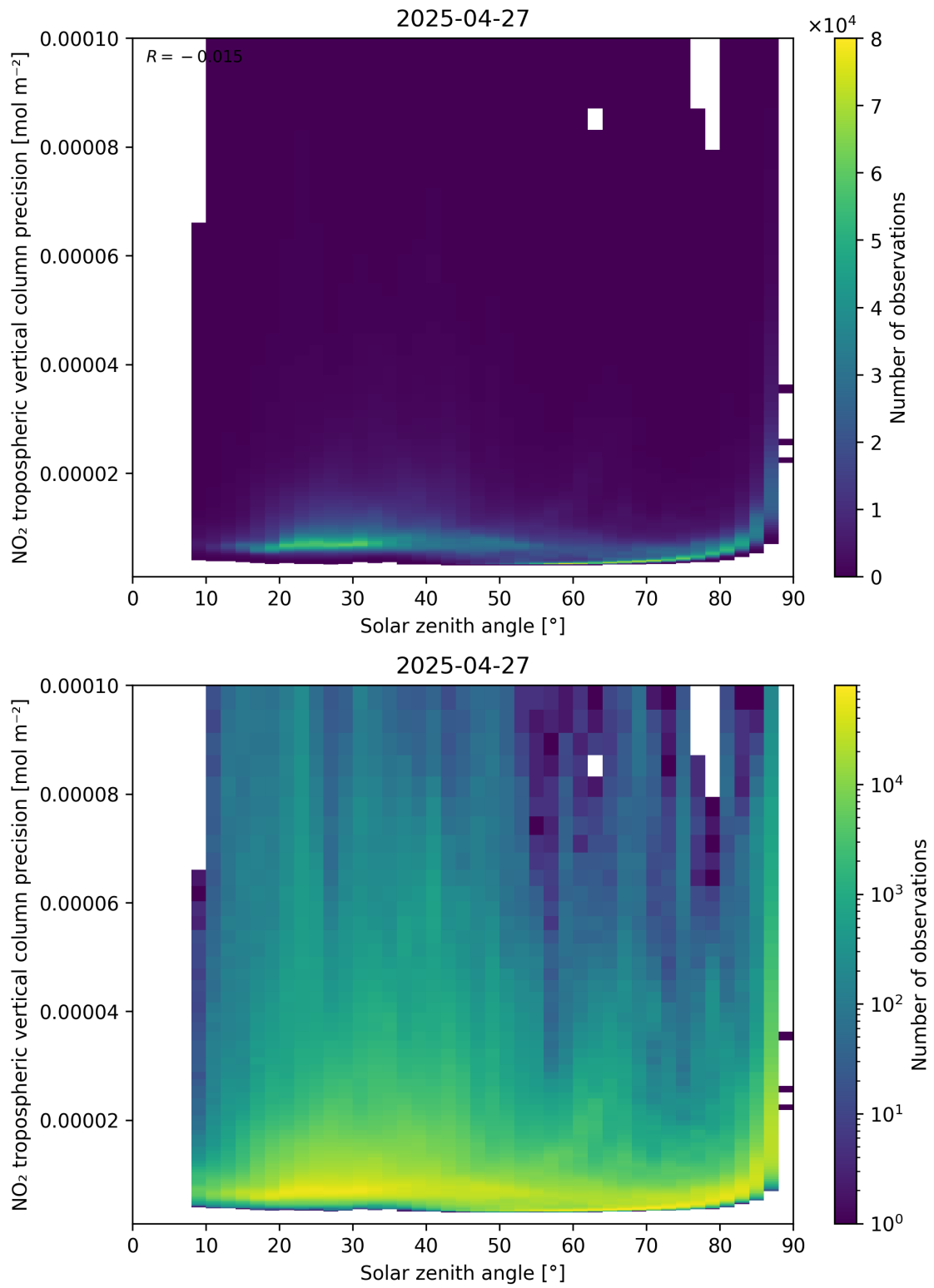
Figure 156: Scatter density plot of “Solar zenith angle” against “NO 2 tropospheric vertical column precision” for 2025-04-27 to 2025-04-27.
