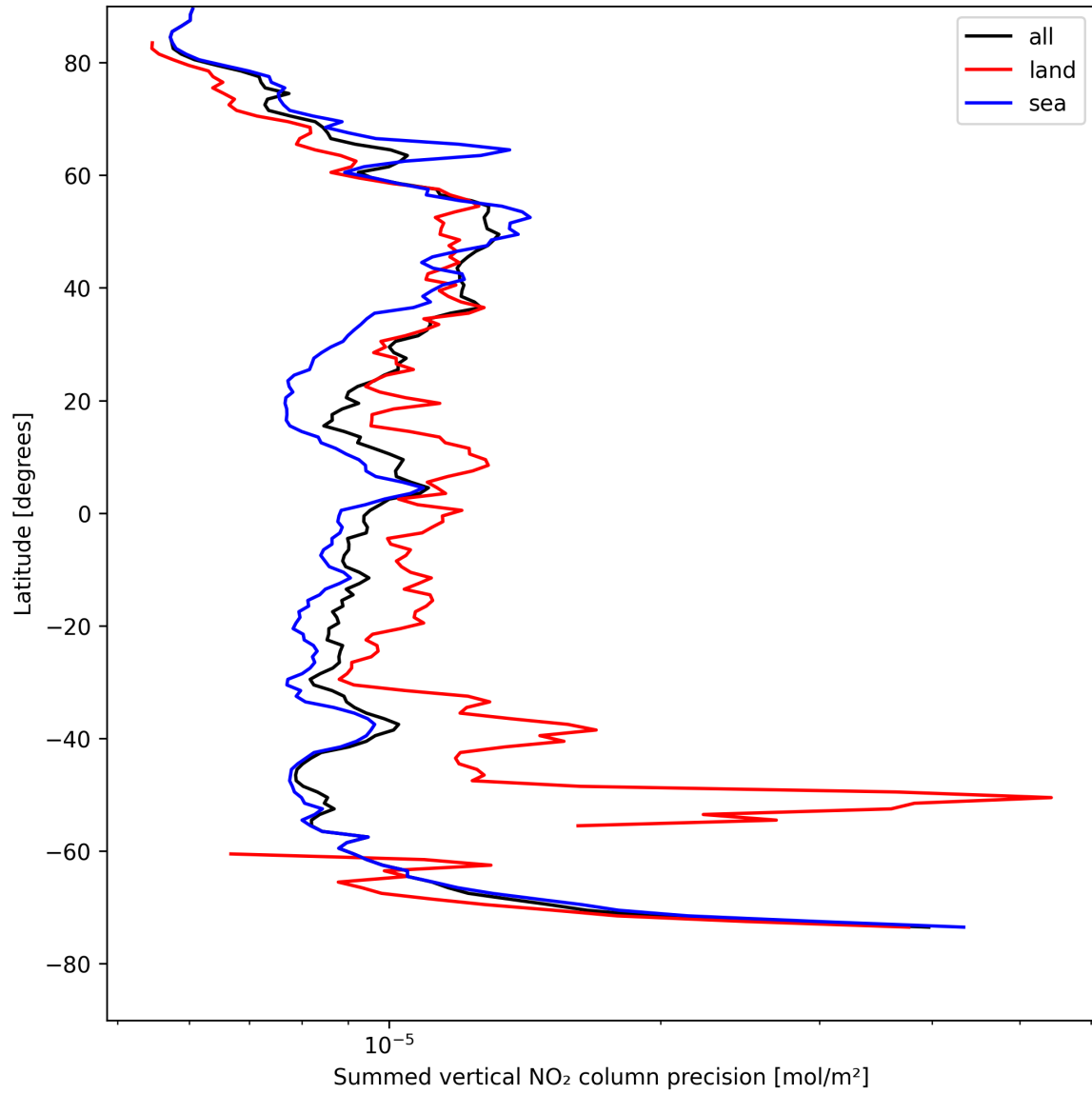
Figure 24: Zonal average of “Summed vertical NO 2 column precision” for 2025-04-27 to 2025-04-27.
