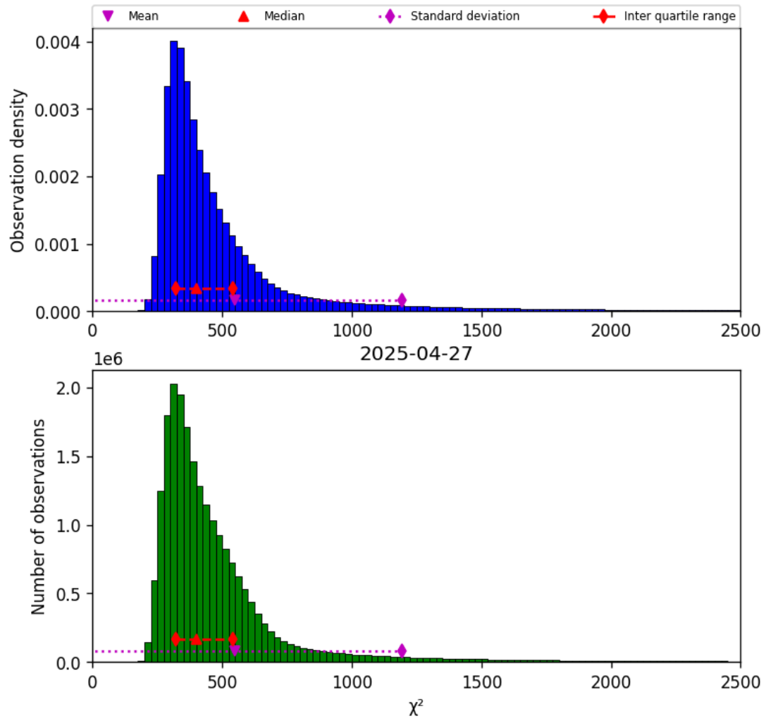
Figure 42: Histogram of " \chi^2 " for 2025-04-27 to 2025-04-27
