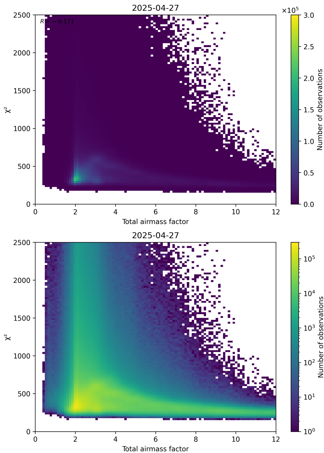
Figure 63: Scatter density plot of “Total airmass factor” against “ \chi^2 ” for 2025-04-27 to 2025-04-27.
