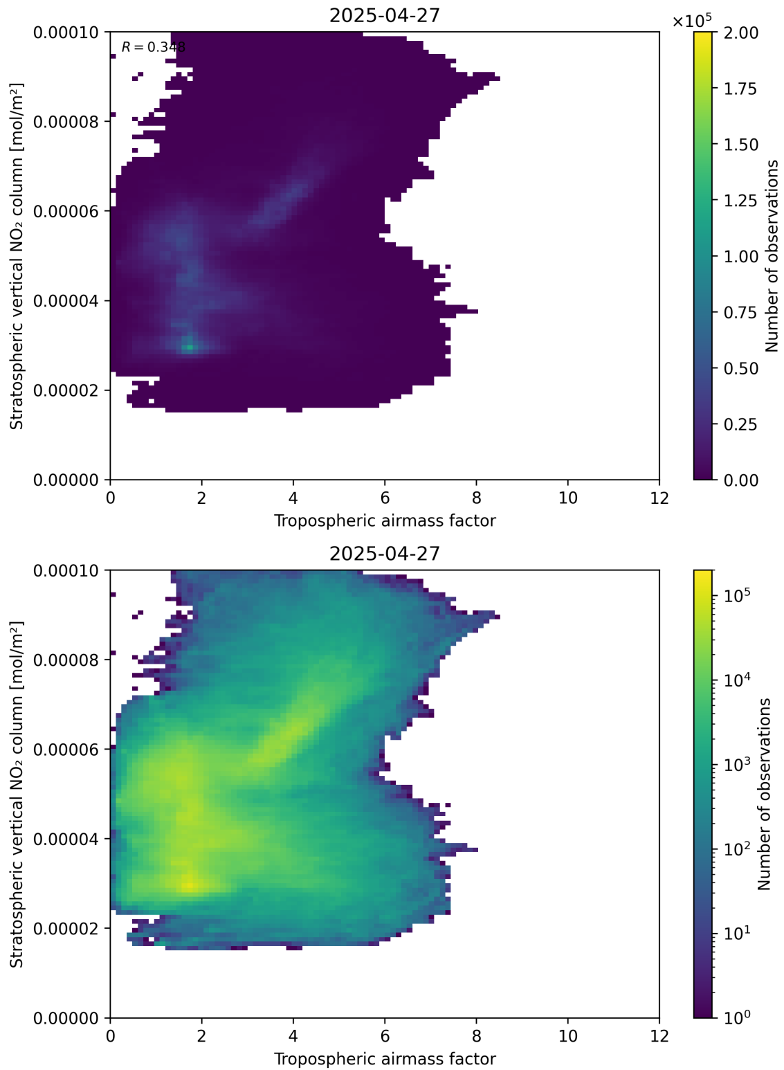
Figure 74: Scatter density plot of “Tropospheric air mass factor” against “Stratospheric vertical NO 2 column” for 2025-04-27 to 2025-04-27.
