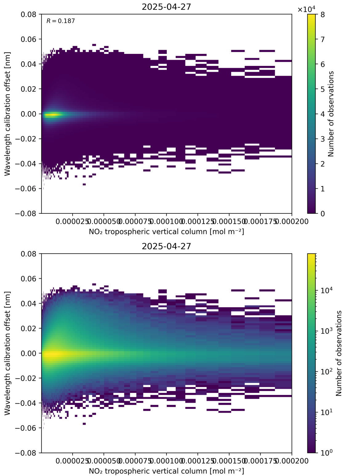
Figure 143: Scatter density plot of “NO 2 tropospheric vertical column” against “Wavelength calibration offset” for 2025-04-27 to 2025-04-27.
