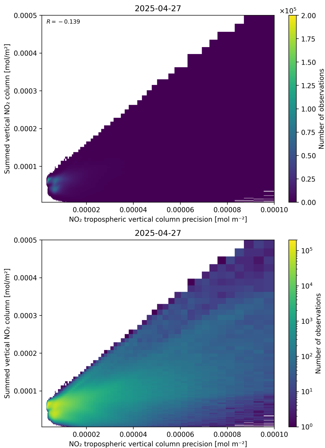
Figure 136: Scatter density plot of “NO 2 tropospheric vertical column precision” against “Summed vertical NO 2 column” for 2025-04-27 to 2025-04-27.
