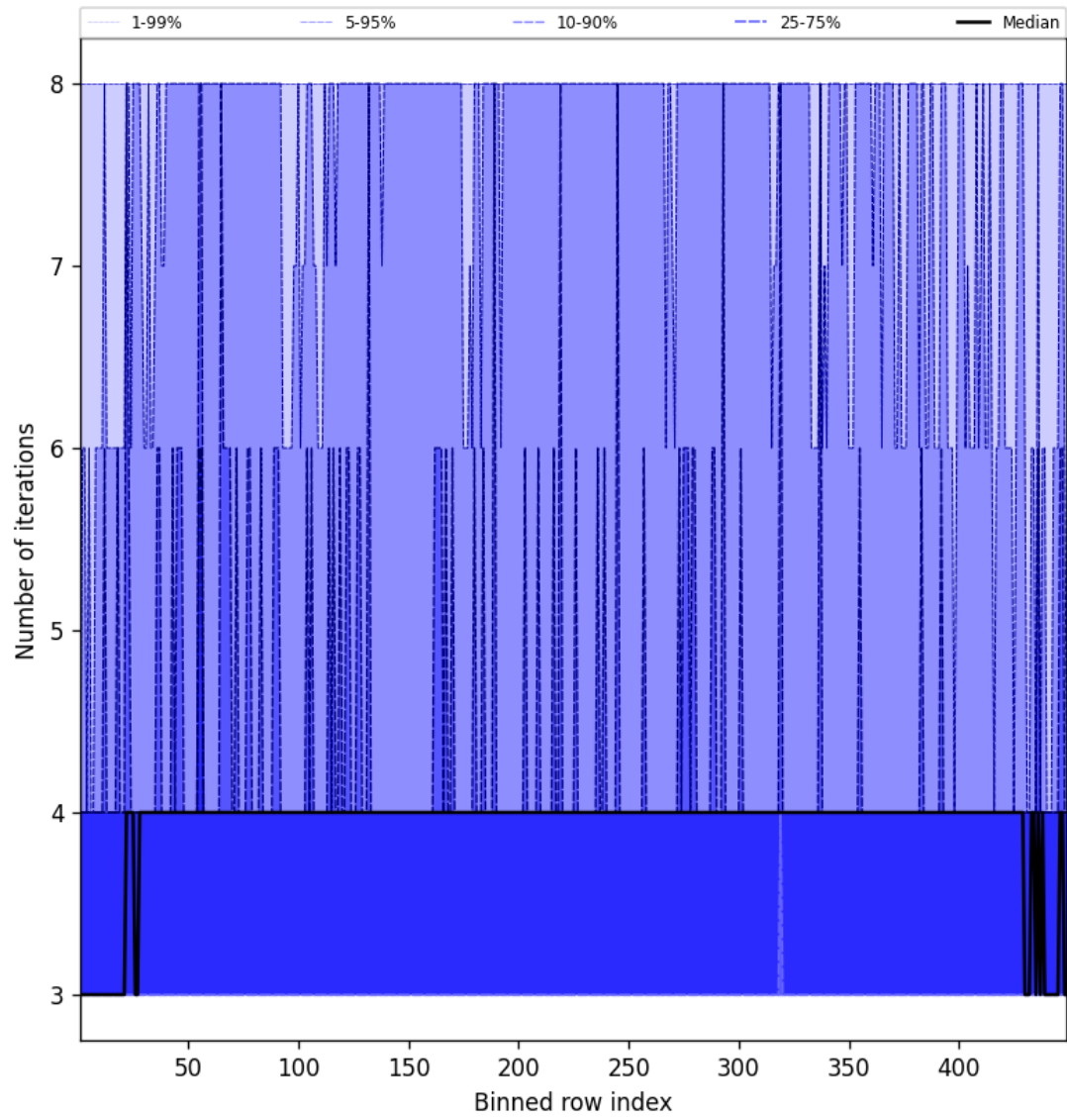
Figure 51: Along track statistics of “Number of iterations” for 2025-04-27 to 2025-04-27
