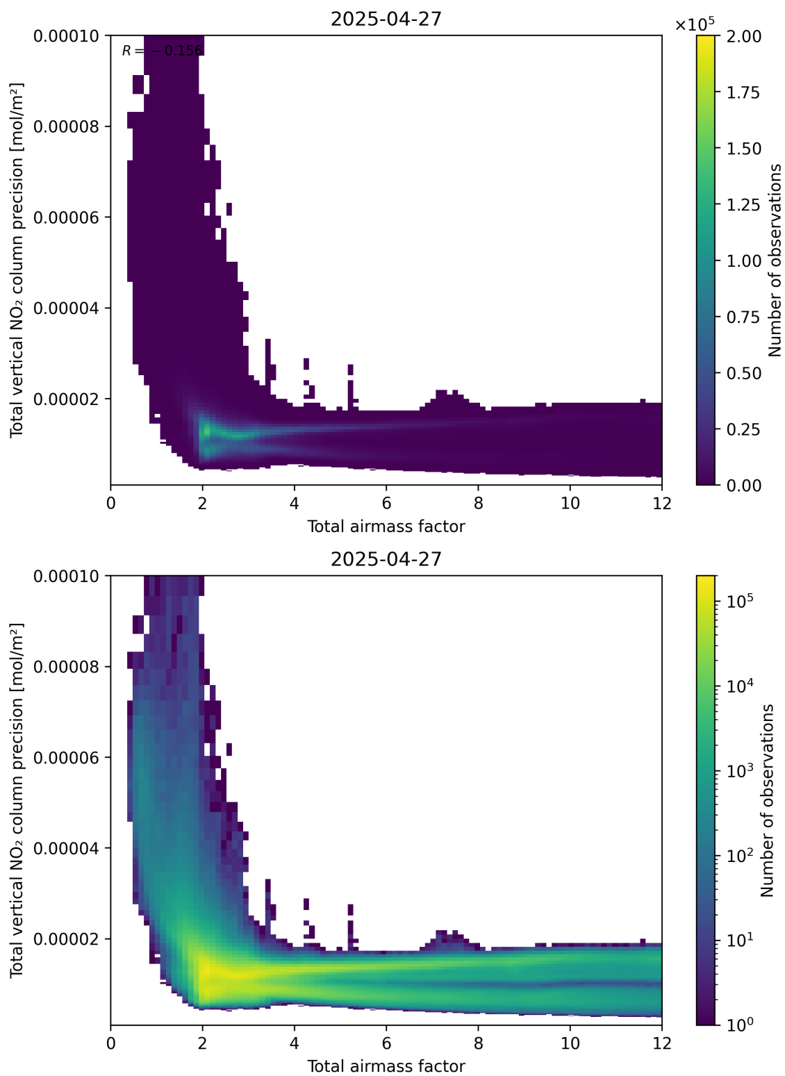
Figure 68: Scatter density plot of “Total airmass factor” against “Total vertical NO 2 column precision” for 2025-04-27 to 2025-04-27.
