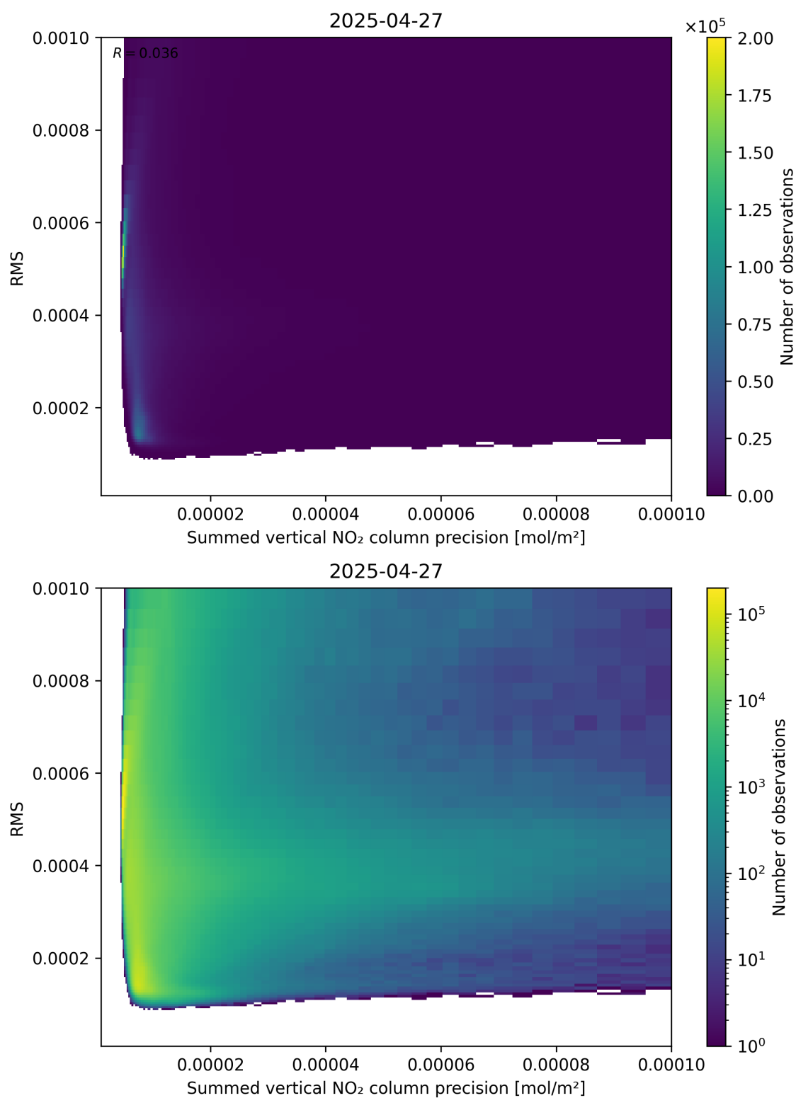
Figure 108: Scatter density plot of “Summed vertical NO 2 column precision” against “RMS” for 2025-04-27 to 2025-04-27.
