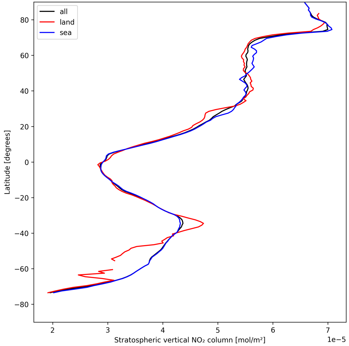
Figure 19: Zonal average of “Stratospheric vertical NO 2 column” for 2025-04-27 to 2025-04-27.
