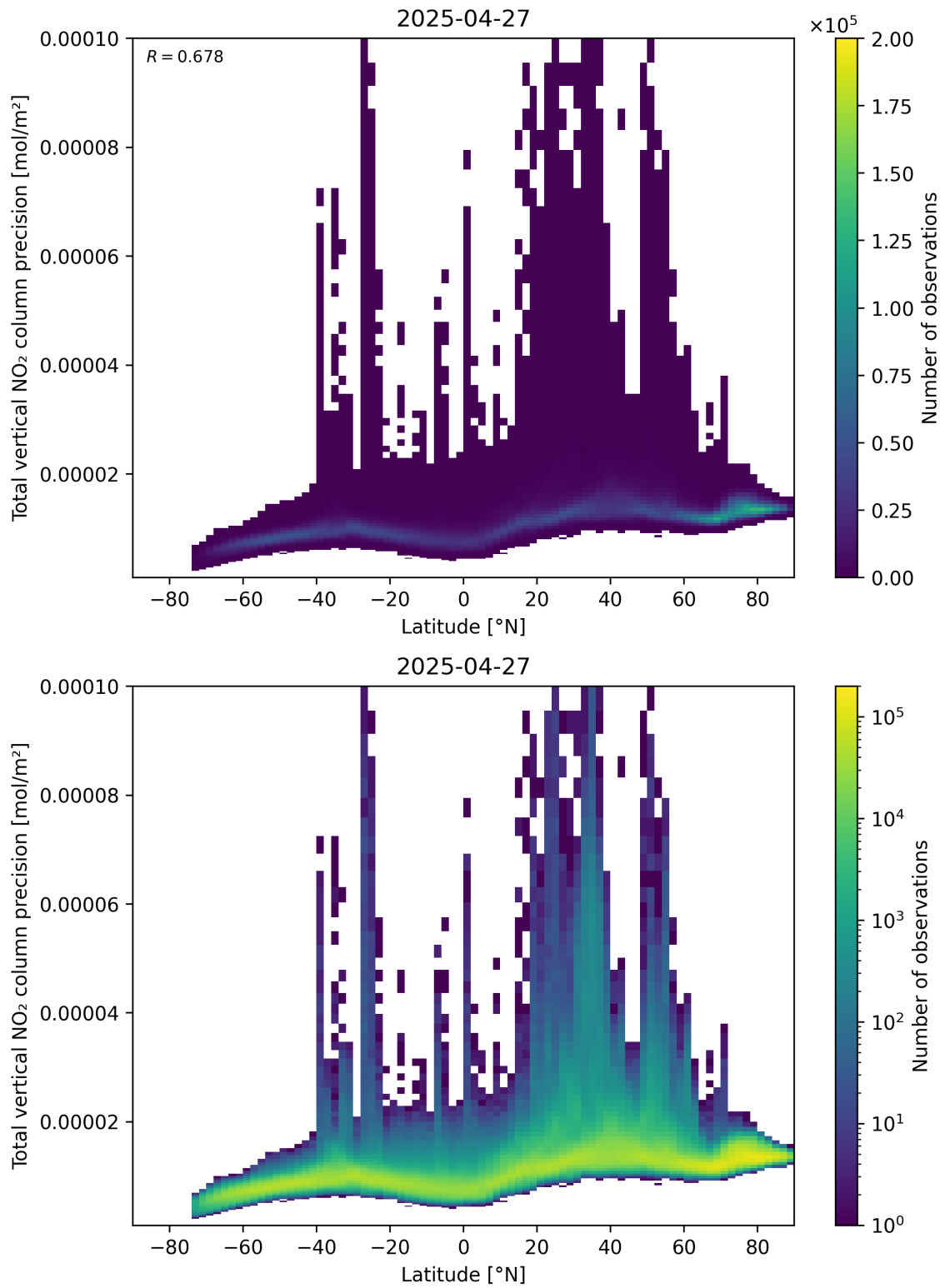
Figure 91: Scatter density plot of “Latitude” against “Total vertical NO 2 column precision” for 2025-04-27 to 2025-04-27.
