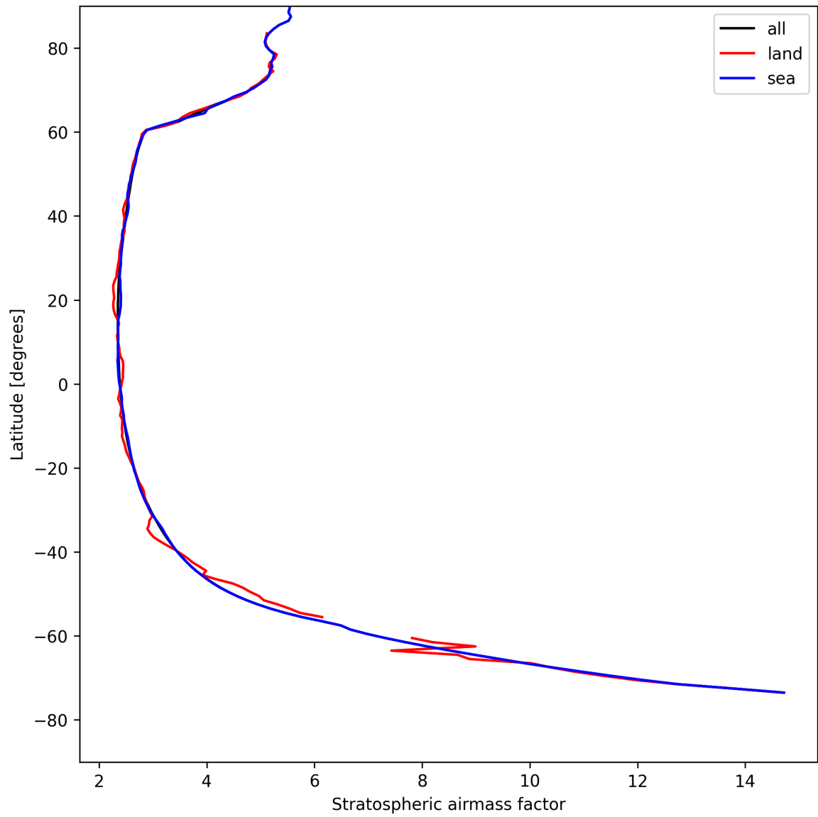
Figure 27: Zonal average of “Stratospheric air mass factor” for 2025-04-27 to 2025-04-27.
