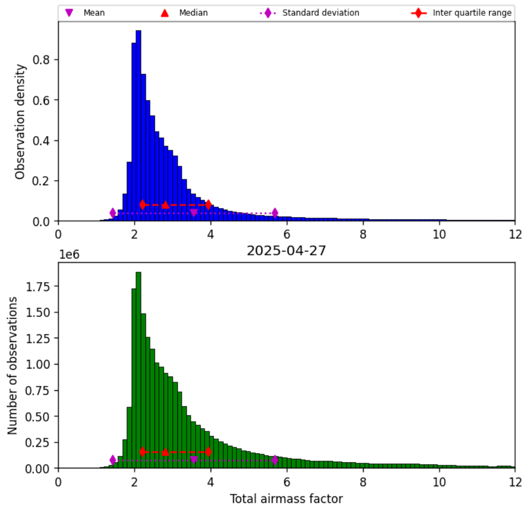
Figure 32: Histogram of “Total airmass factor” for 2025-04-27 to 2025-04-27
