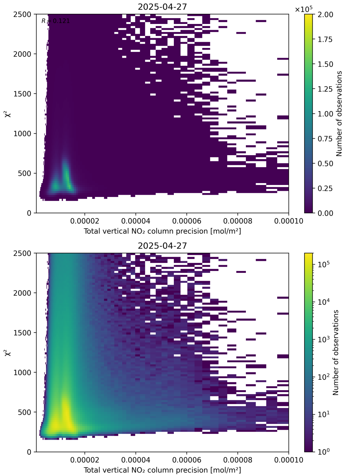
Figure 116: Scatter density plot of “Total vertical NO 2 column precision” against “ \chi^2 ” for 2025-04-27 to 2025-04-27.
