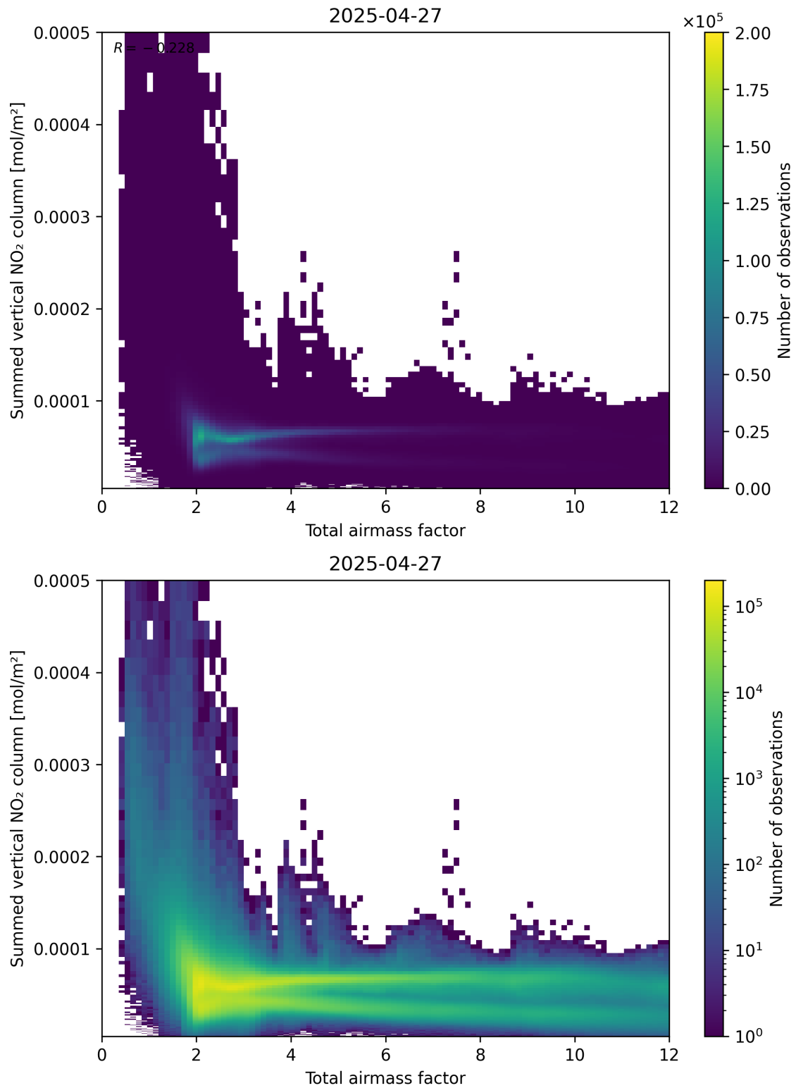
Figure 65: Scatter density plot of “Total airmass factor” against “Summed vertical NO 2 column” for 2025-04-27 to 2025-04-27.
