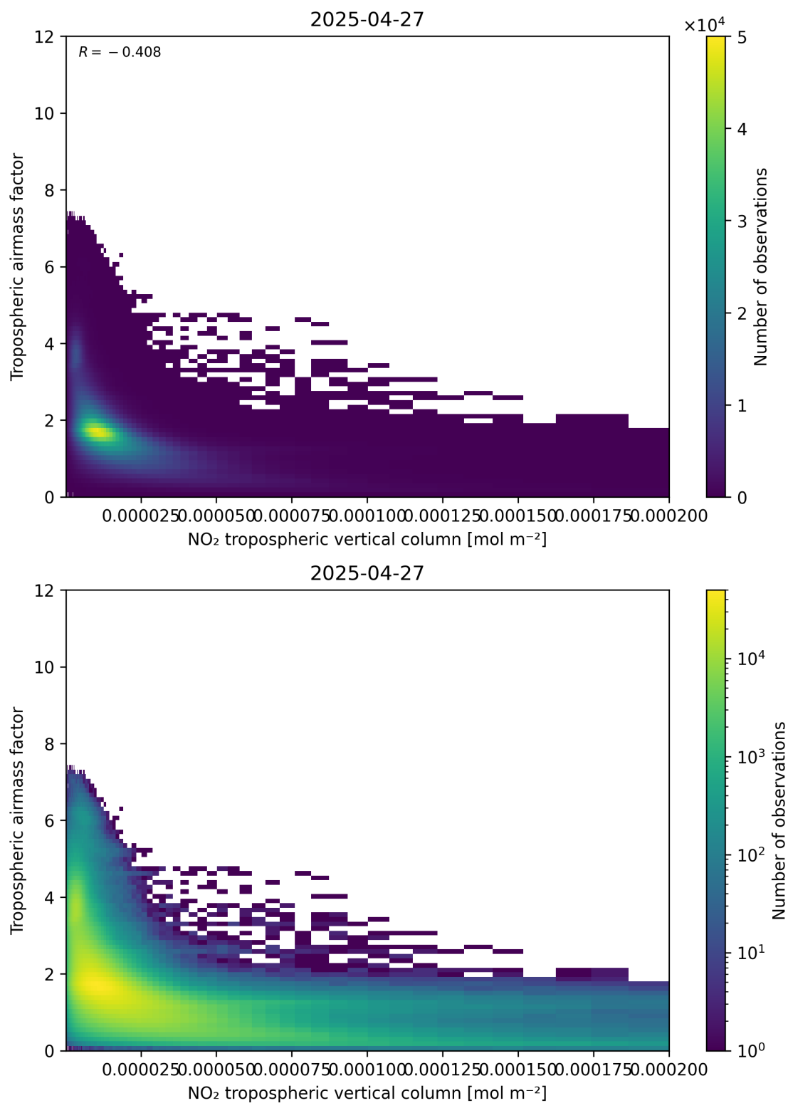
Figure 123: Scatter density plot of “NO 2 tropospheric vertical column” against “Tropospheric air mass factor” for 2025-04-27 to 2025-04-27.
