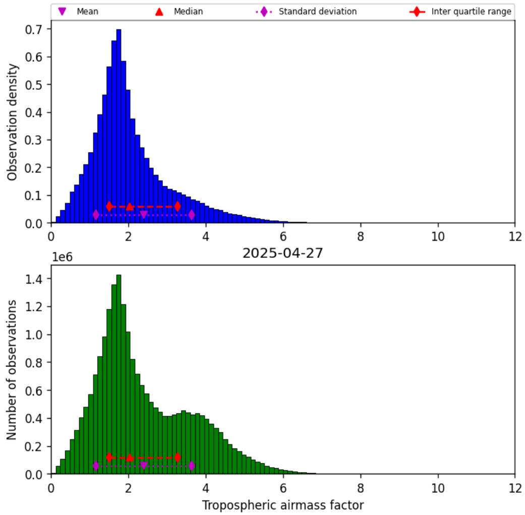
Figure 31: Histogram of “Tropospheric airmass factor” for 2025-04-27 to 2025-04-27
