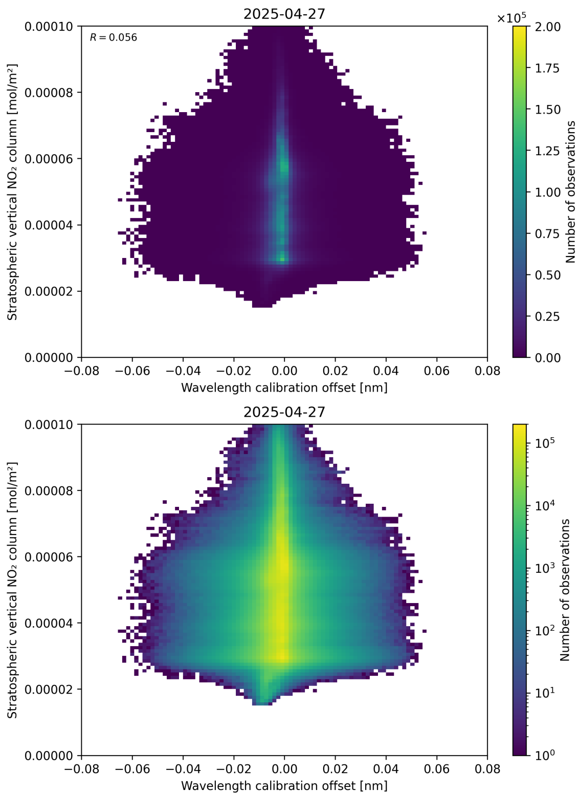
Figure 176: Scatter density plot of “Wavelength calibration offset” against “Stratospheric vertical NO 2 column” for 2025-04-27 to 2025-04-27.
