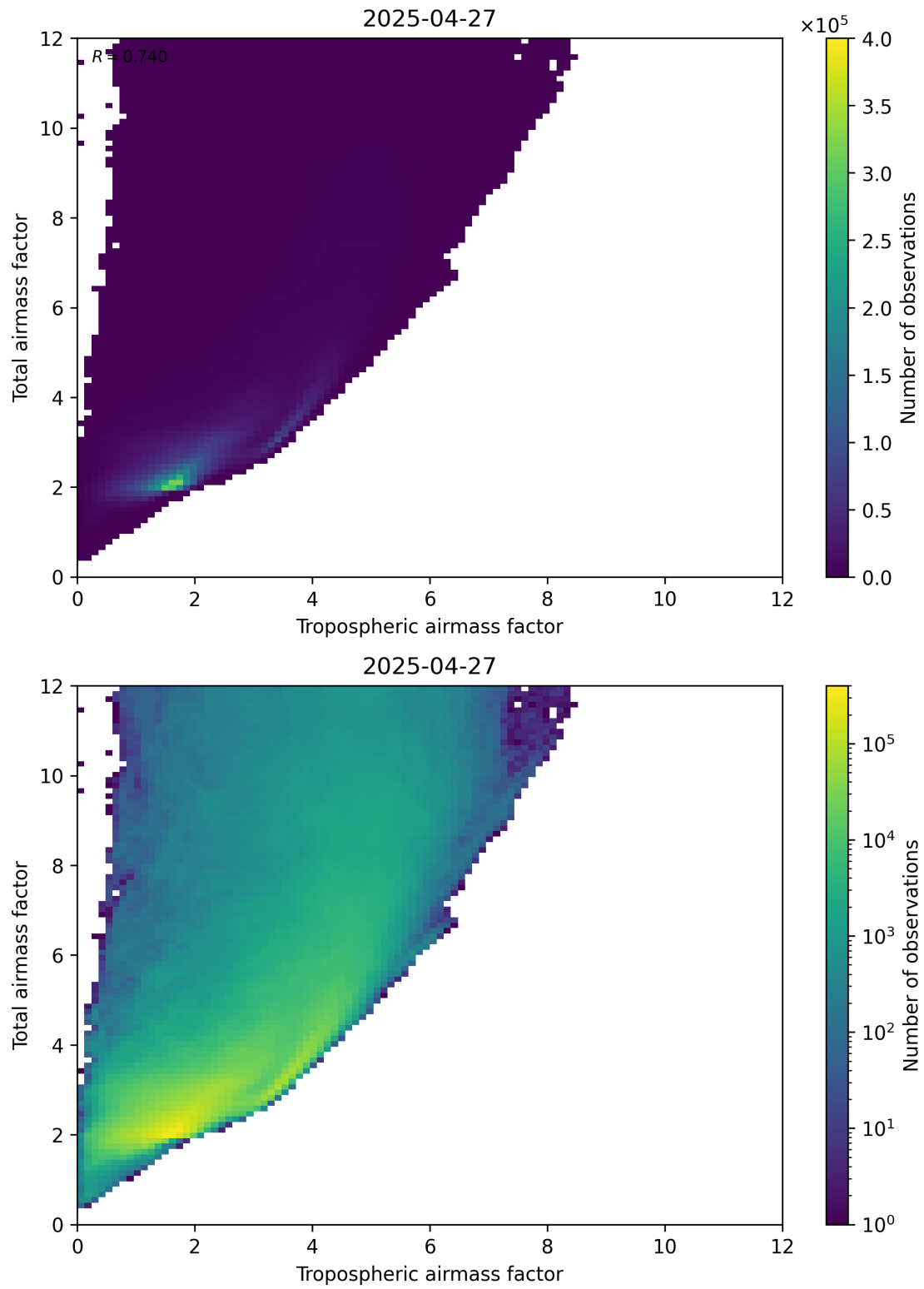
Figure 72: Scatter density plot of “Tropospheric airmass factor” against “Total airmass factor” for 2025-04-27 to 2025-04-27.
