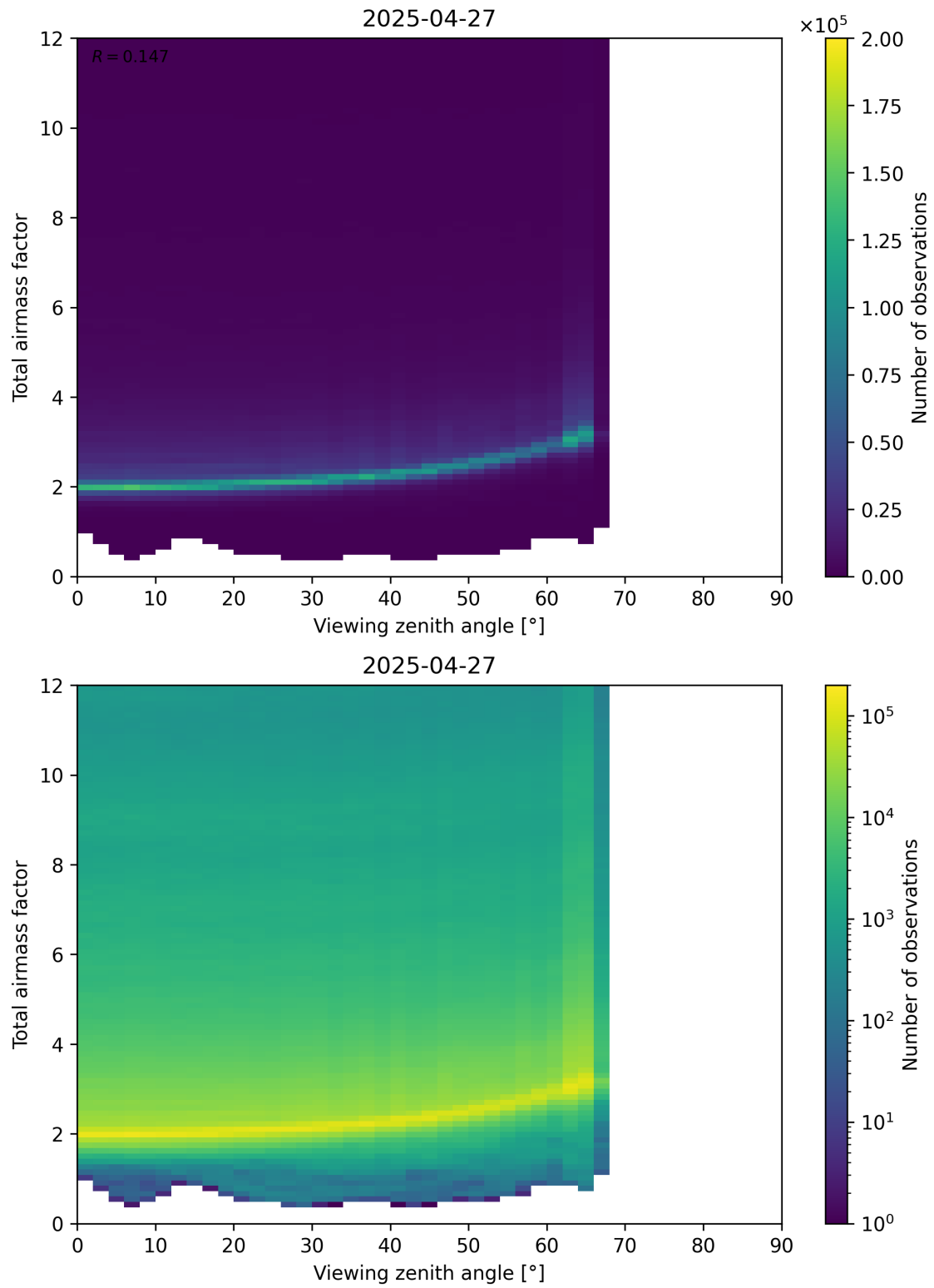
Figure 160: Scatter density plot of “Viewing zenith angle” against “Total airmass factor” for 2025-04-27 to 2025-04-27.
