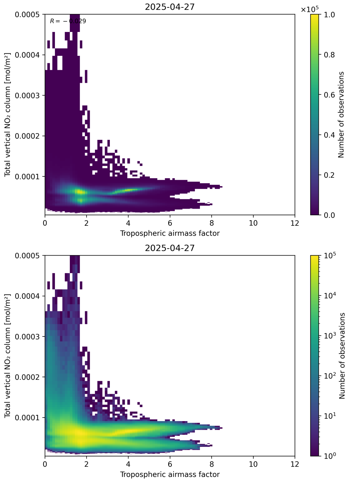
Figure 77: Scatter density plot of “Tropospheric airmass factor” against “Total vertical NO 2 column” for 2025-04-27 to 2025-04-27.
