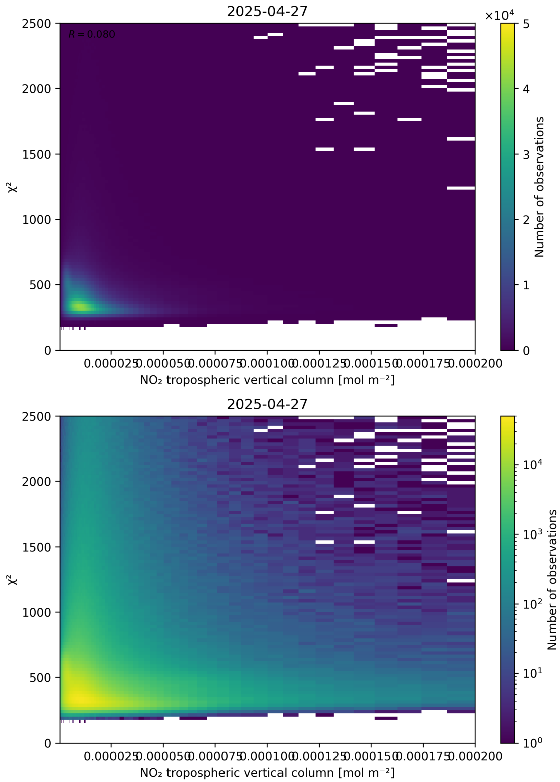
Figure 124: Scatter density plot of “NO 2 tropospheric vertical column” against “ \chi^2 ” for 2025-04-27 to 2025-04-27.
