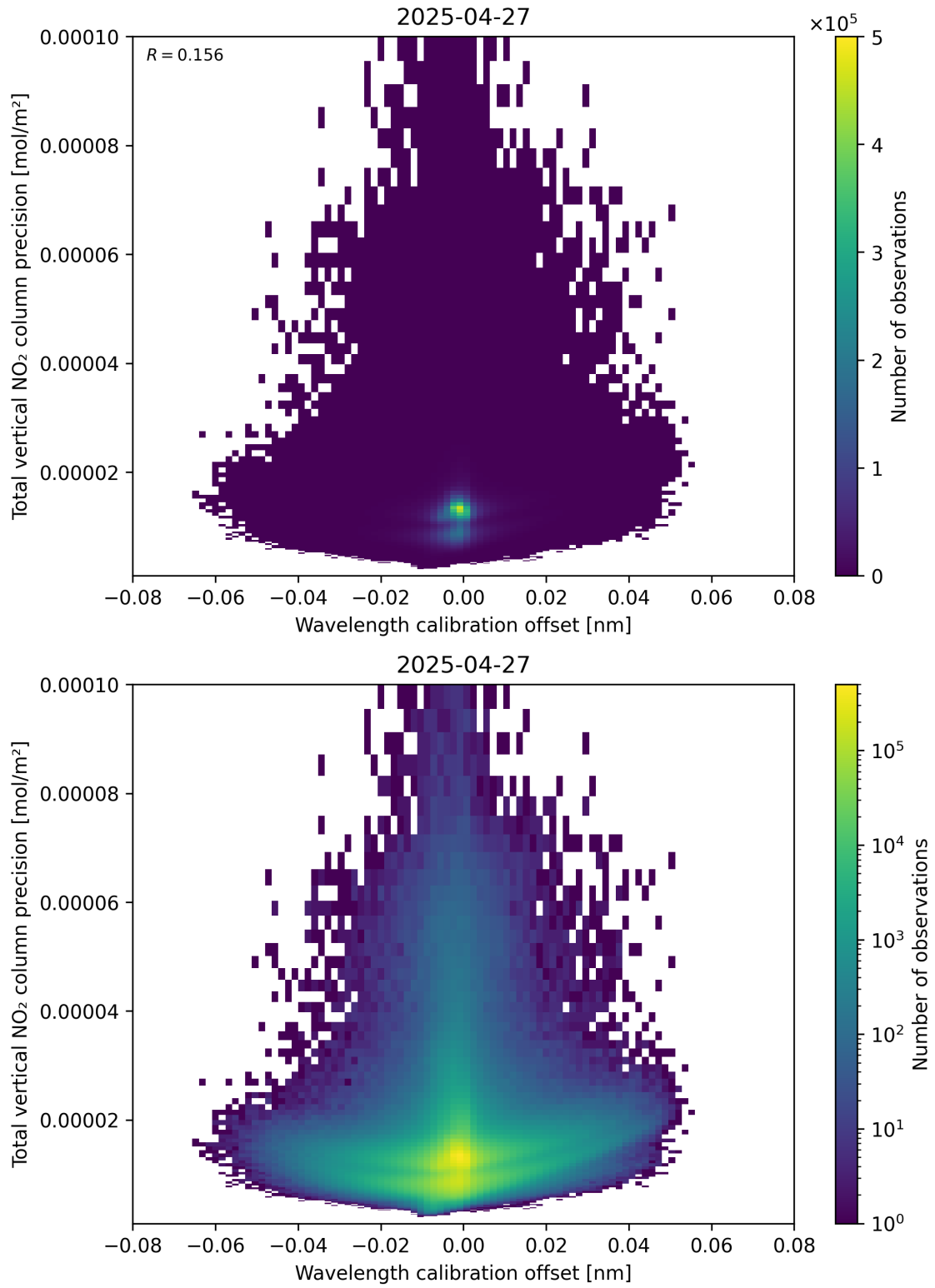
Figure 180: Scatter density plot of “Wavelength calibration offset” against “Total vertical NO 2 column precision” for 2025-04-27 to 2025-04-27.
