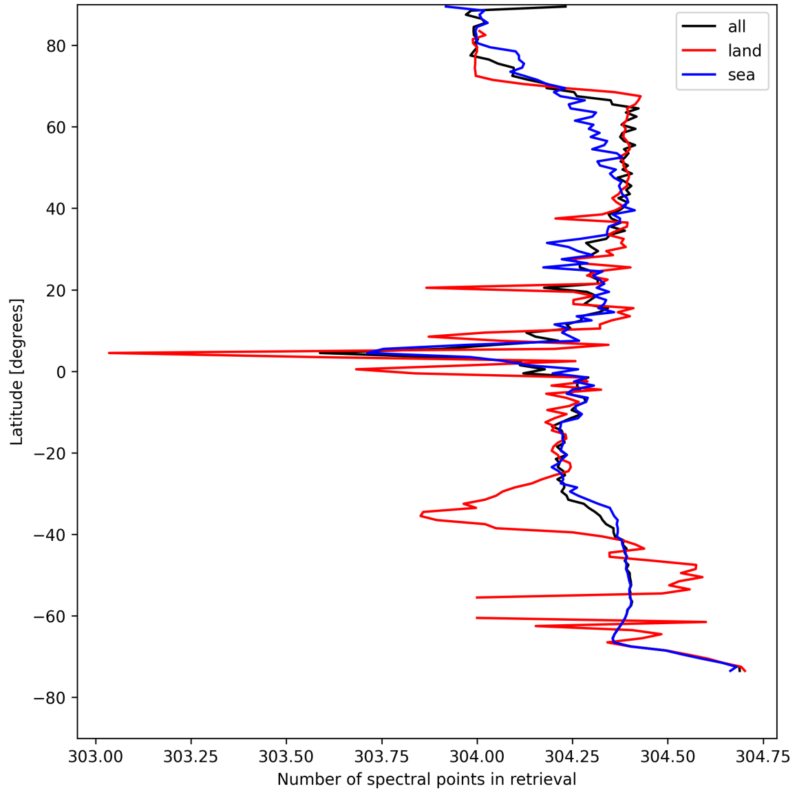
Figure 16: Zonal average of “Number of spectral points in retrieval” for 2025-04-27 to 2025-04-27.
