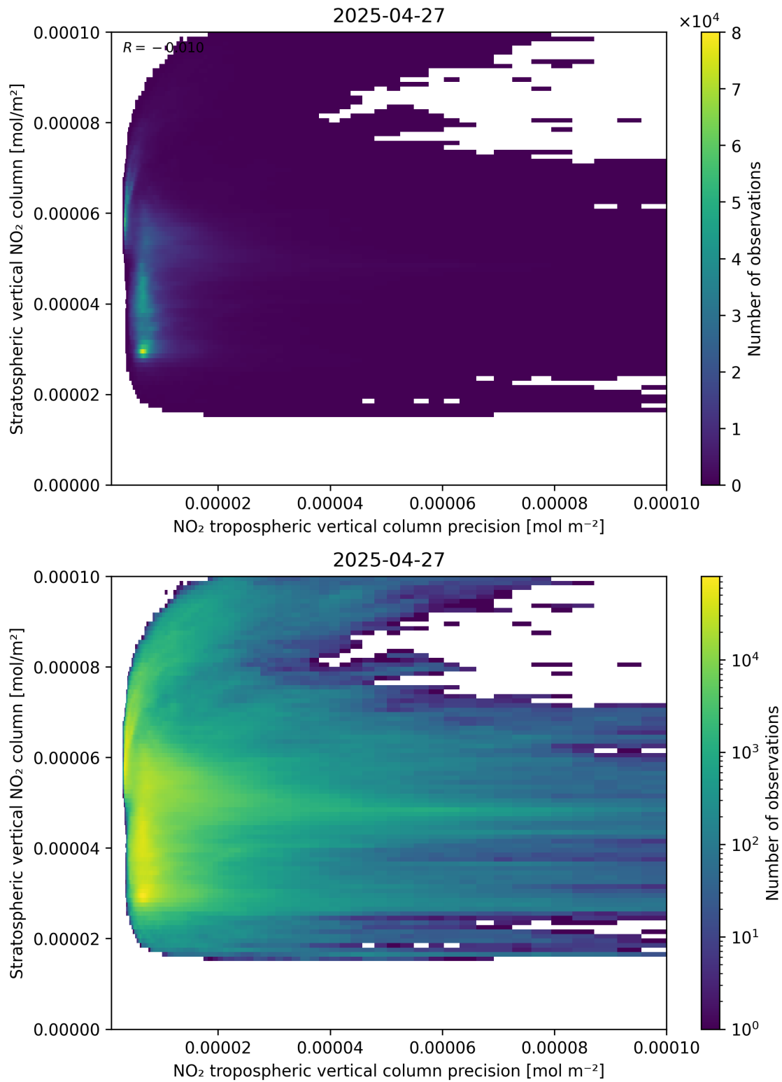
Figure 135: Scatter density plot of “NO 2 tropospheric vertical column precision” against “Stratospheric vertical NO 2 column” for 2025-04-27 to 2025-04-27.
