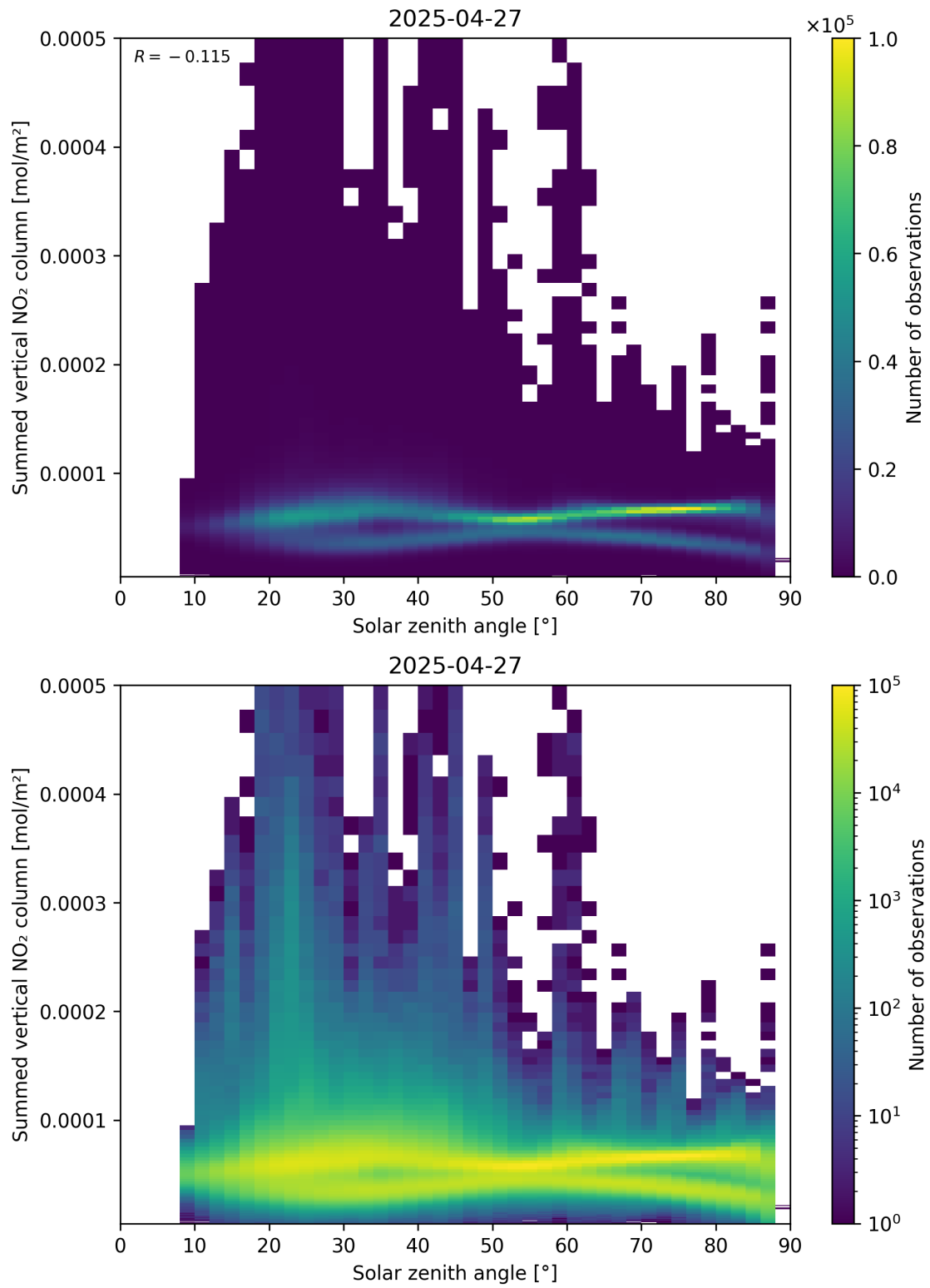
Figure 151: Scatter density plot of “Solar zenith angle” against “Summed vertical NO 2 column” for 2025-04-27 to 2025-04-27.
