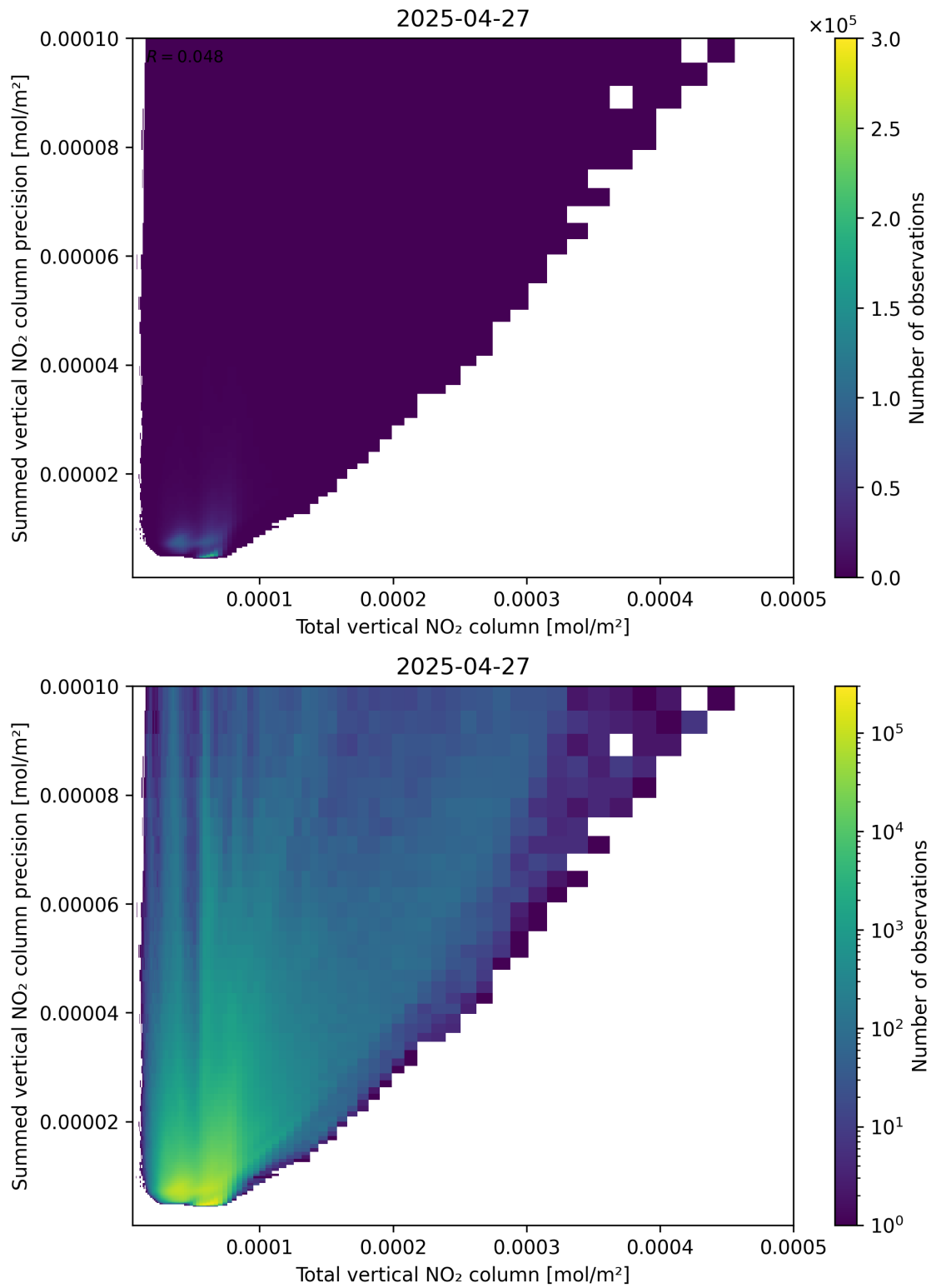
Figure 113: Scatter density plot of “Total vertical NO 2 column” against “Summed vertical NO 2 column precision” for 2025-04-27 to 2025-04-27.
