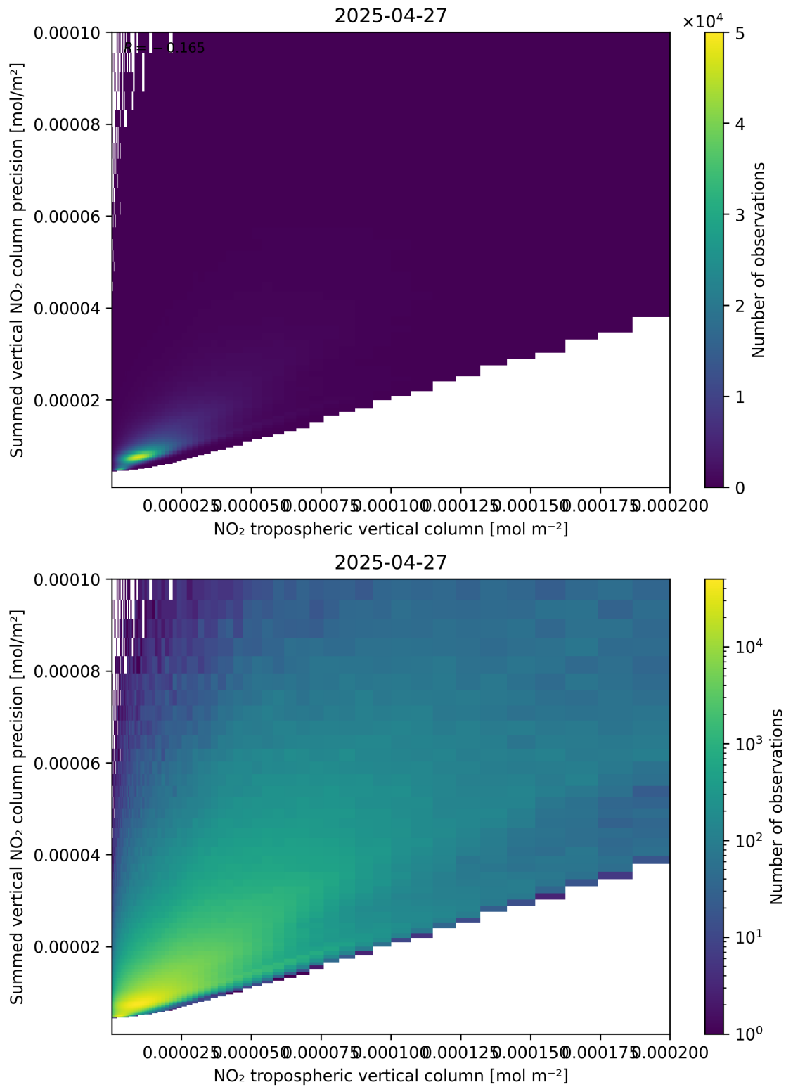
Figure 127: Scatter density plot of “NO 2 tropospheric vertical column” against “Summed vertical NO 2 column precision” for 2025-04-27 to 2025-04-27.
