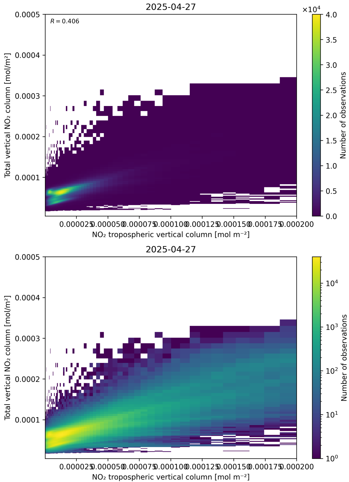
Figure 128: Scatter density plot of “NO 2 tropospheric vertical column” against “Total vertical NO 2 column” for 2025-04-27 to 2025-04-27.
