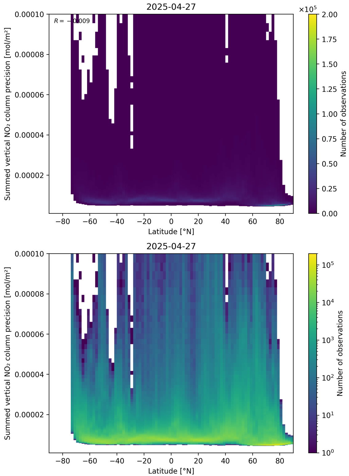
Figure 89: Scatter density plot of “Latitude” against “Summed vertical NO 2 column precision” for 2025-04-27 to 2025-04-27.
