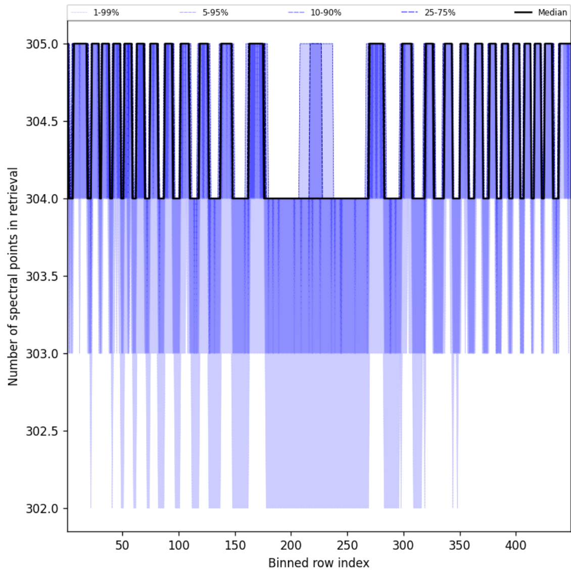
Figure 50: Along track statistics of “Number of spectral points in retrieval” for 2025-04-27 to 2025-04-27
