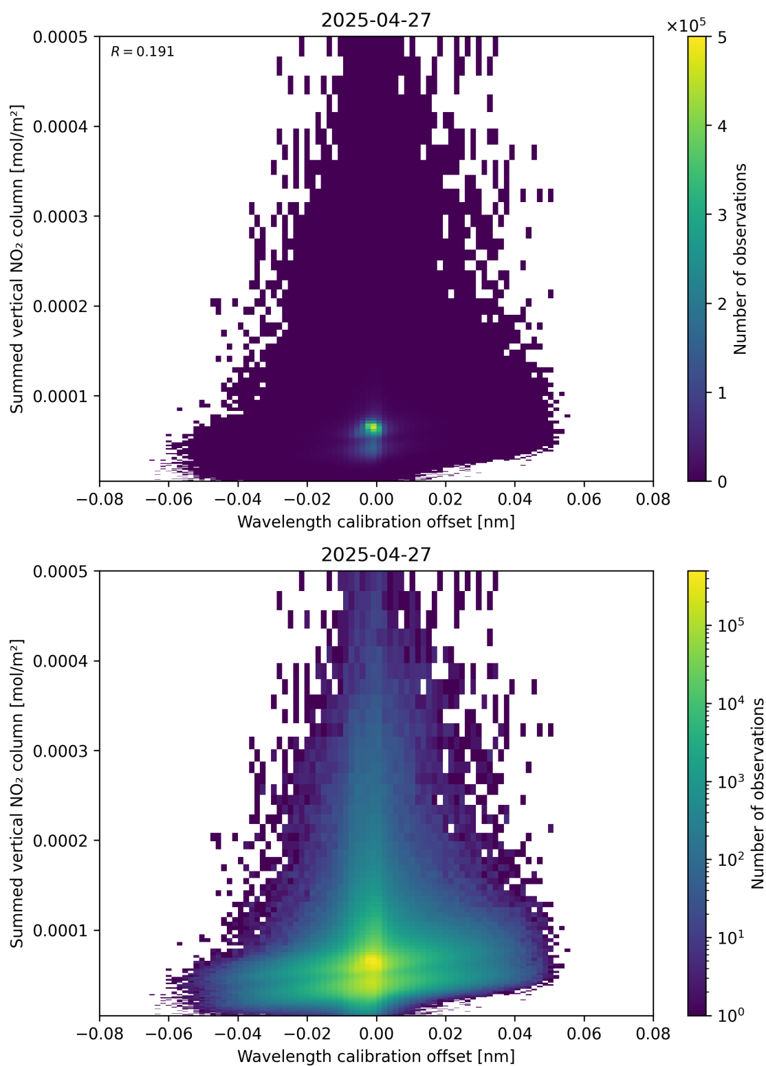
Figure 177: Scatter density plot of “Wavelength calibration offset” against “Summed vertical NO 2 column” for 2025-04-27 to 2025-04-27.
