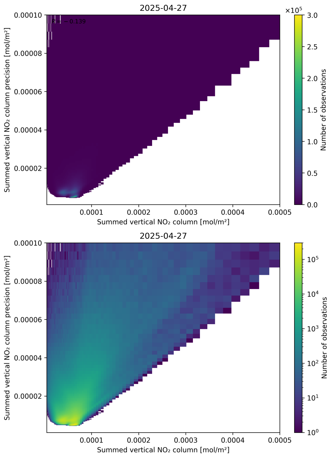
Figure 105: Scatter density plot of “Summed vertical NO 2 column” against “Summed vertical NO 2 column precision” for 2025-04-27 to 2025-04-27.
