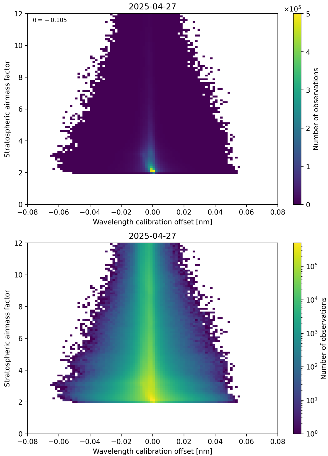
Figure 174: Scatter density plot of “Wavelength calibration offset” against “Stratospheric airmass factor” for 2025-04-27 to 2025-04-27.
