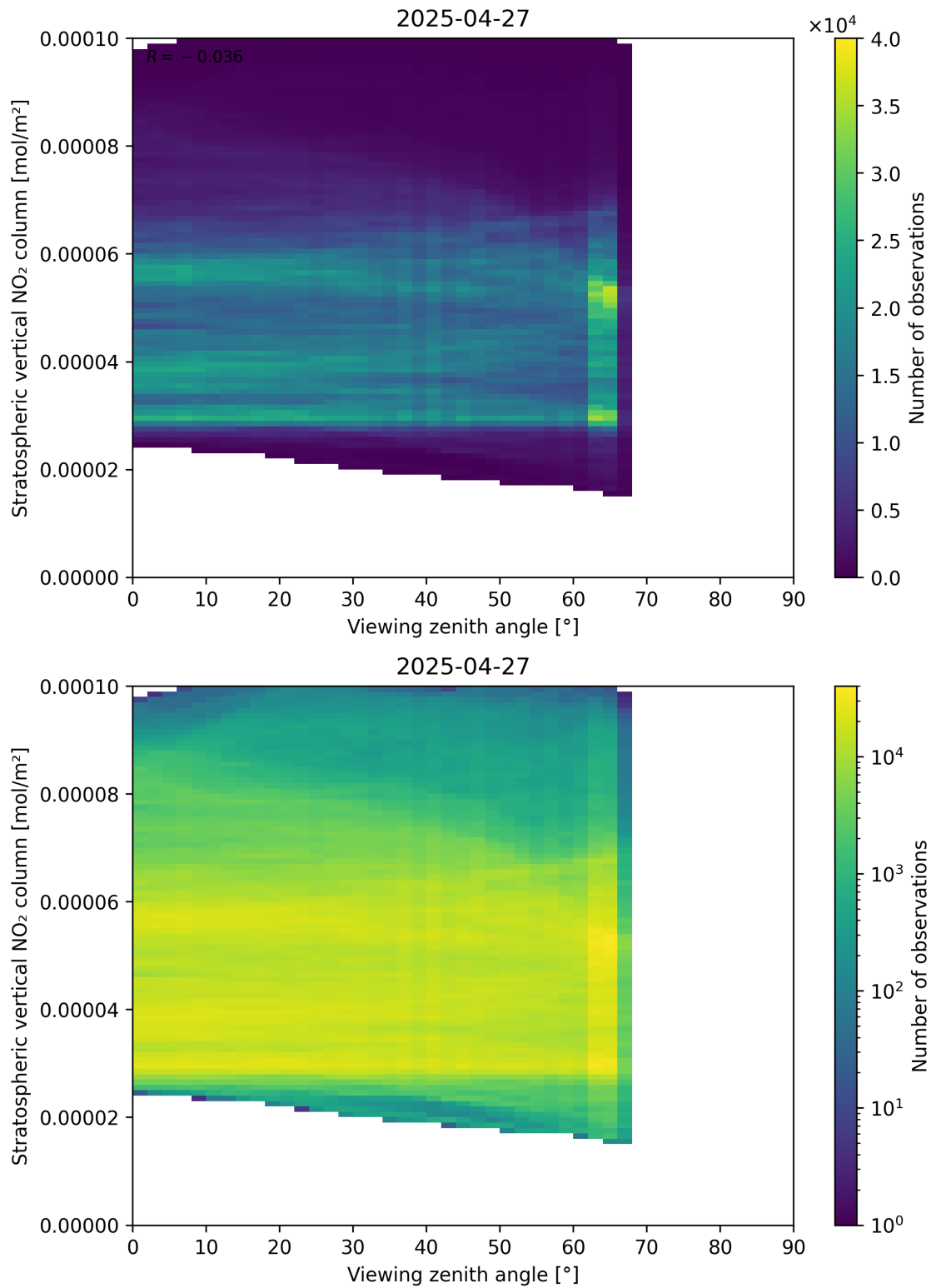
Figure 164: Scatter density plot of “Viewing zenith angle” against “Stratospheric vertical NO 2 column” for 2025-04-27 to 2025-04-27.
