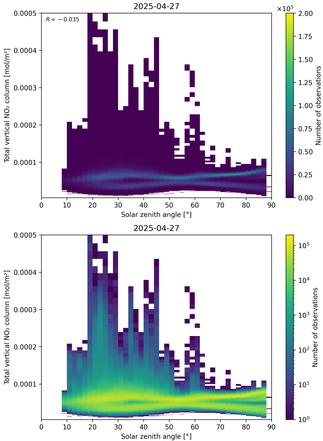
Figure 153: Scatter density plot of “Solar zenith angle” against “Total vertical NO 2 column” for 2025-04-27 to 2025-04-27.
