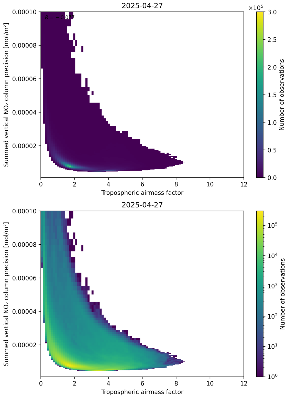
Figure 76: Scatter density plot of “Tropospheric air mass factor” against “Summed vertical NO 2 column precision” for 2025-04-27 to 2025-04-27.
