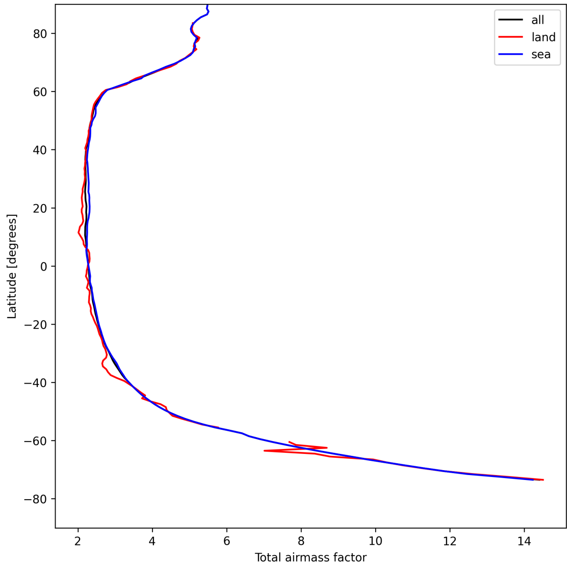
Figure 15: Zonal average of “Total airmass factor” for 2025-04-27 to 2025-04-27.
