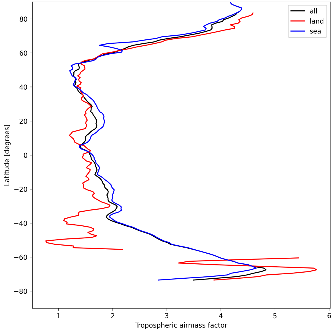
Figure 14: Zonal average of “Tropospheric airmass factor” for 2025-04-27 to 2025-04-27.
