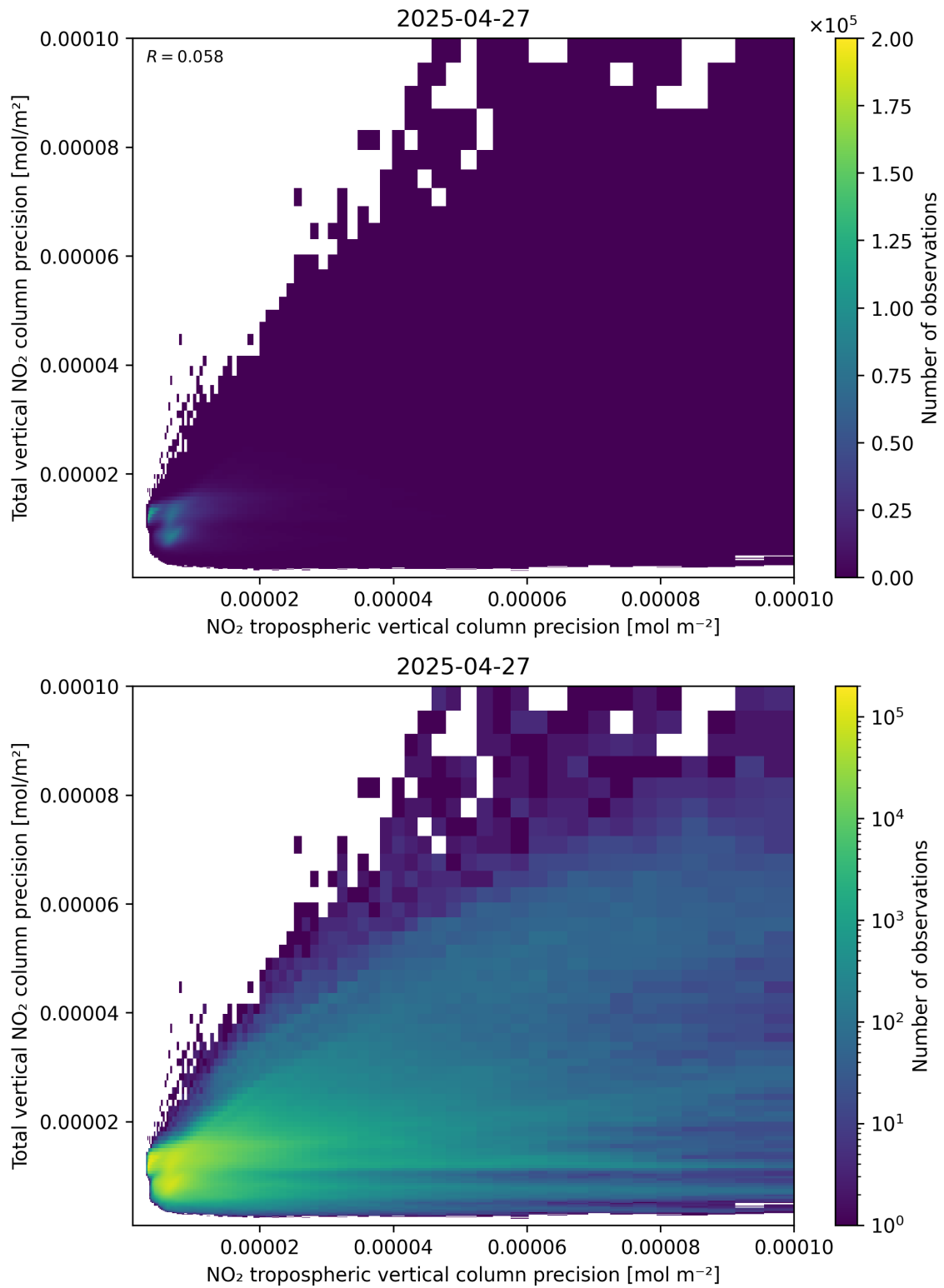
Figure 139: Scatter density plot of “NO 2 tropospheric vertical column precision” against “Total vertical NO 2 column precision” for 2025-04-27 to 2025-04-27.
