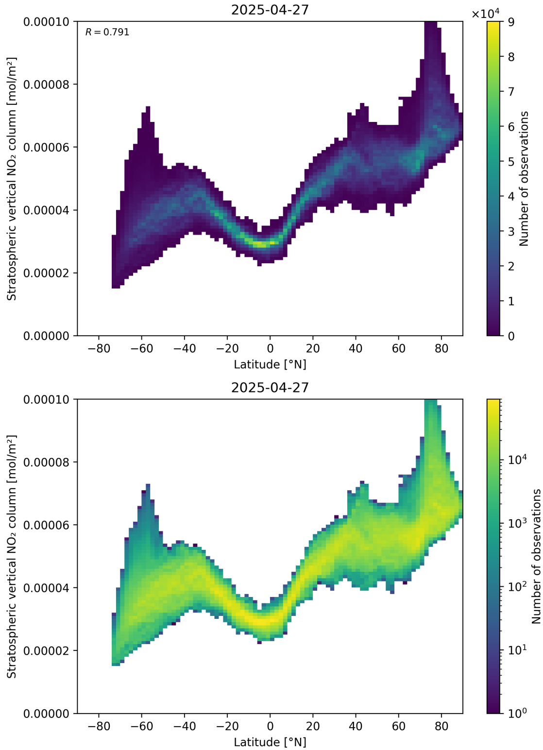
Figure 87: Scatter density plot of “Latitude” against “Stratospheric vertical \text{NO}_2 column” for 2025-04-27 to 2025-04-27.
