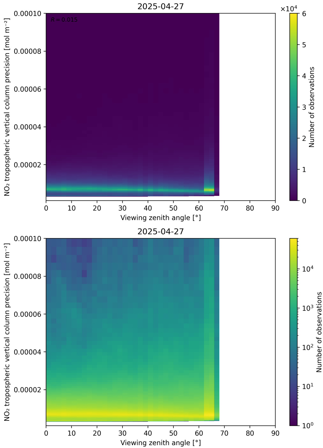
Figure 170: Scatter density plot of “Viewing zenith angle” against “NO 2 tropospheric vertical column precision” for 2025-04-27 to 2025-04-27.
