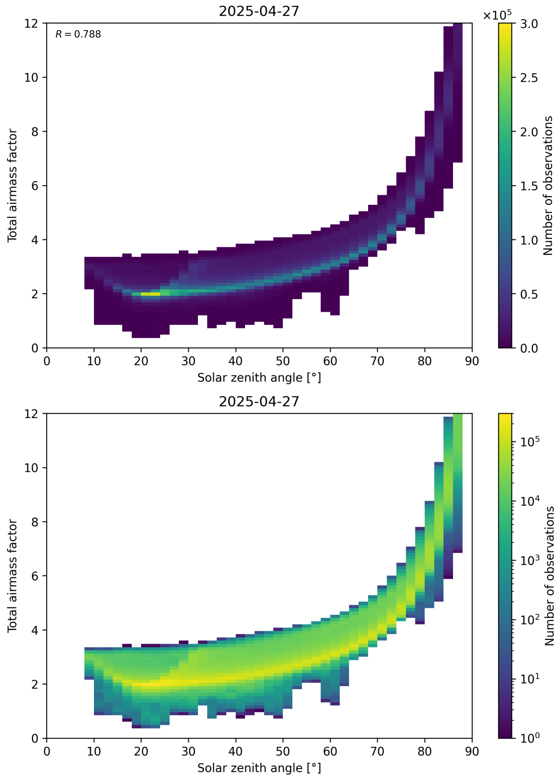
Figure 146: Scatter density plot of “Solar zenith angle” against “Total airmass factor” for 2025-04-27 to 2025-04-27.
