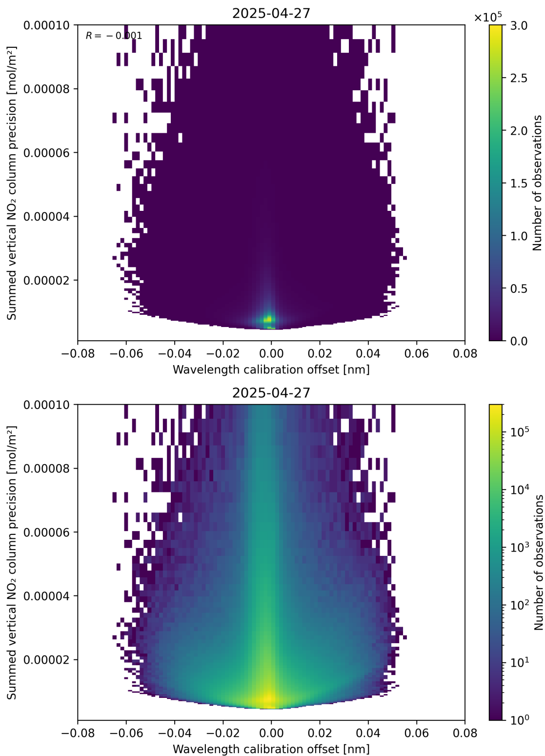
Figure 178: Scatter density plot of “Wavelength calibration offset” against “Summed vertical NO 2 column precision” for 2025-04-27 to 2025-04-27.
