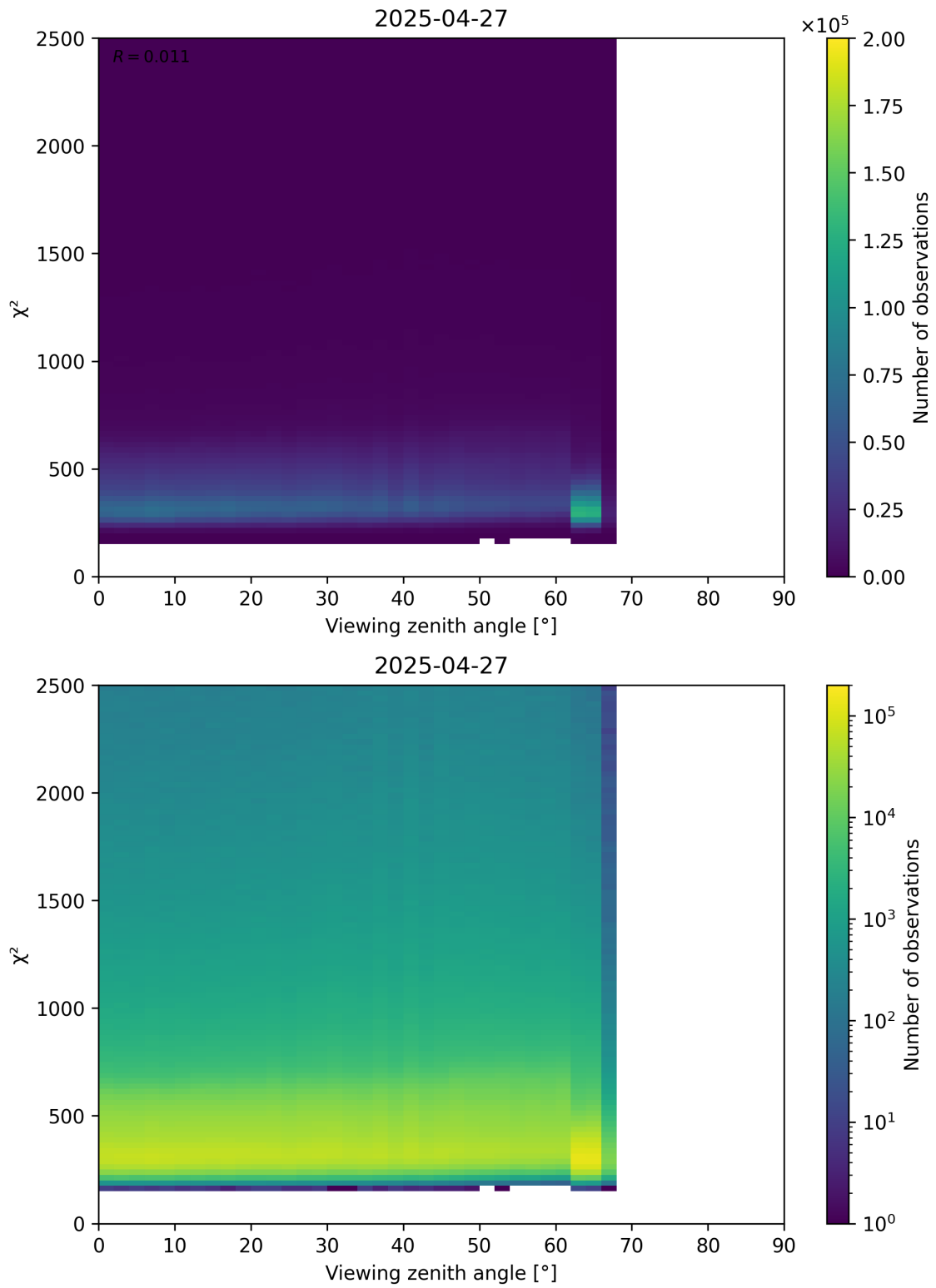
Figure 162: Scatter density plot of “Viewing zenith angle” against “ \chi^2 ” for 2025-04-27 to 2025-04-27.
