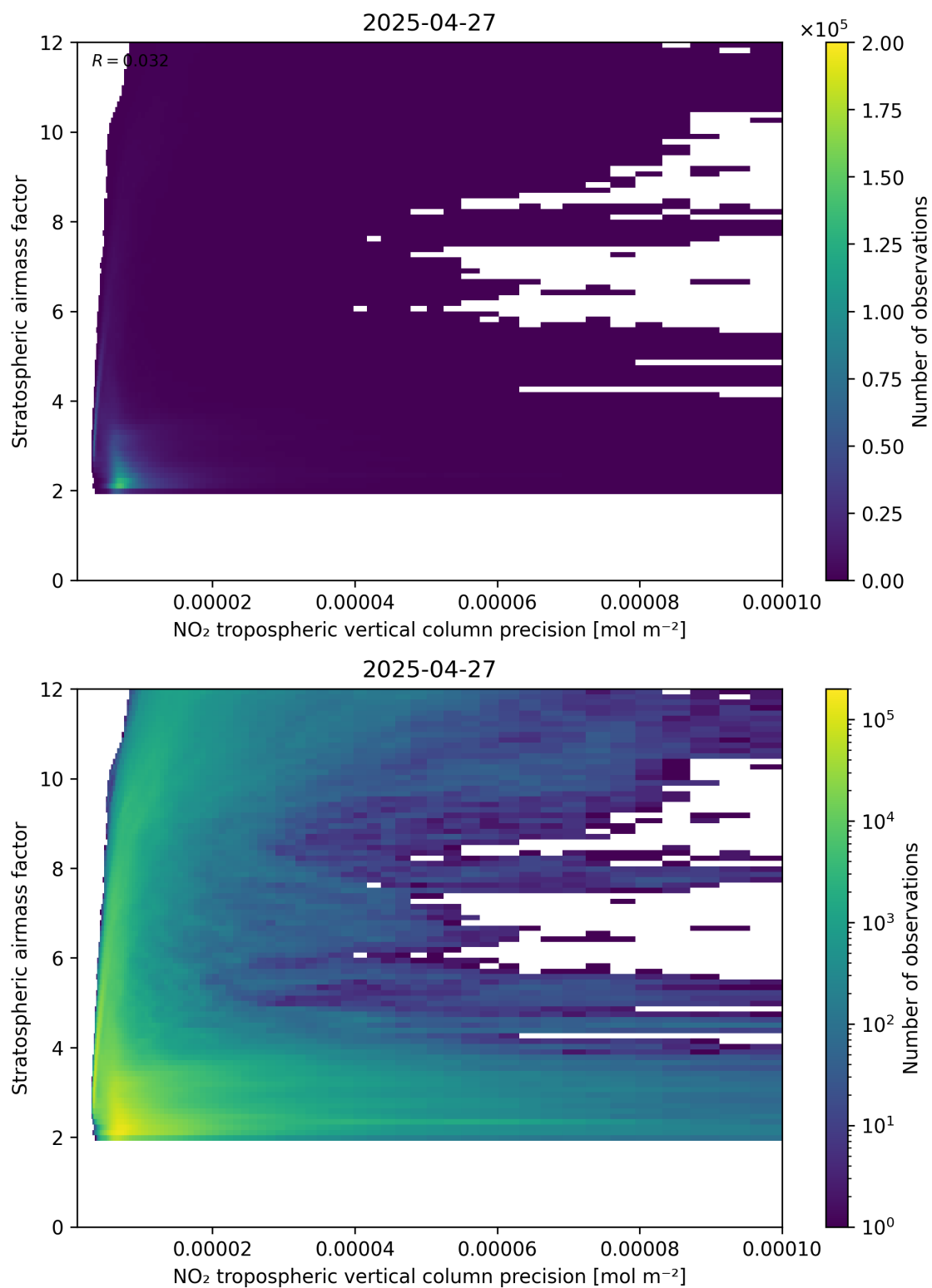
Figure 131: Scatter density plot of “NO 2 tropospheric vertical column precision” against “Stratospheric airmass factor” for 2025-04-27 to 2025-04-27.
