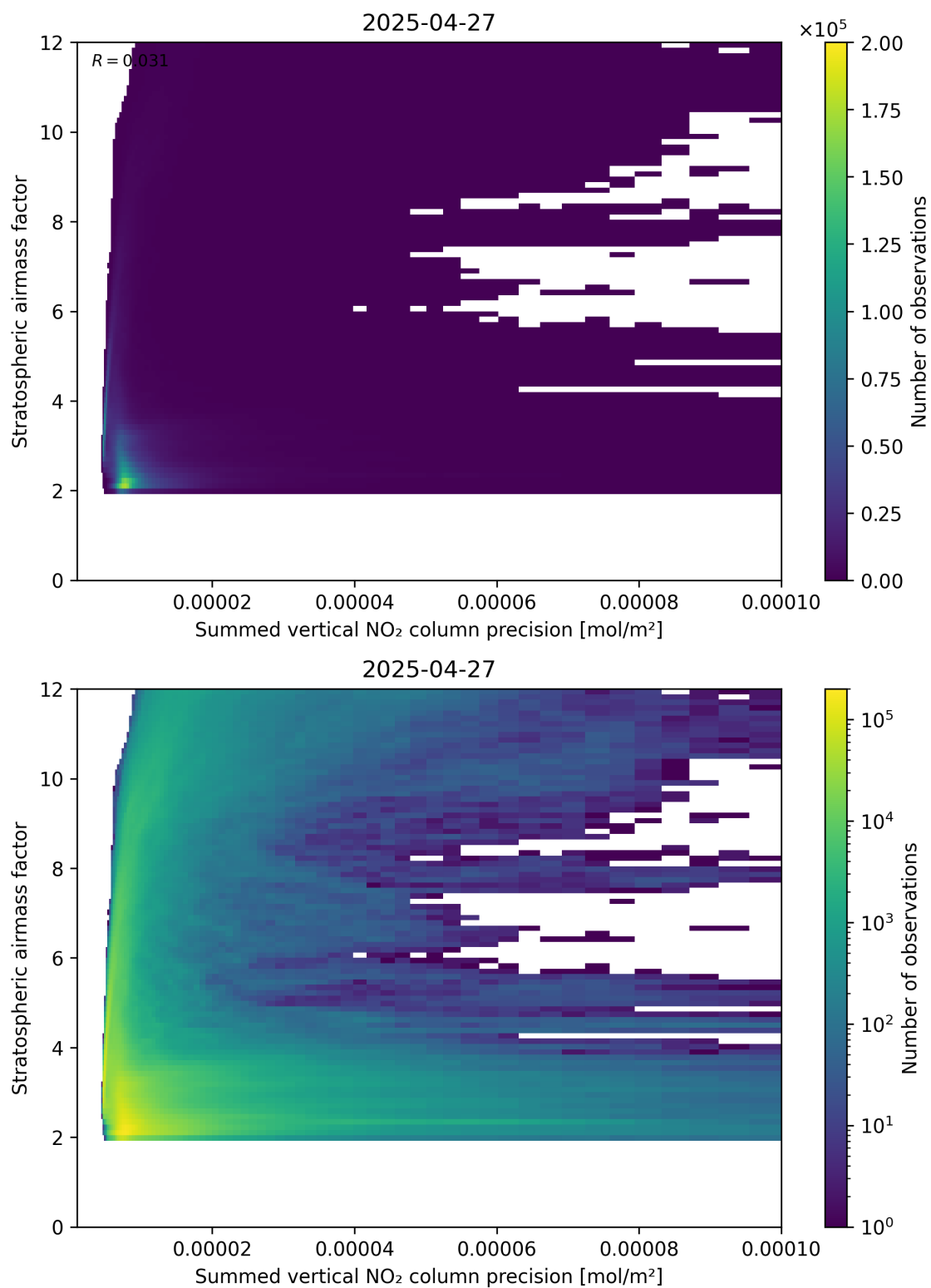
Figure 106: Scatter density plot of “Summed vertical NO 2 column precision” against “Stratospheric airmass factor” for 2025-04-27 to 2025-04-27.
