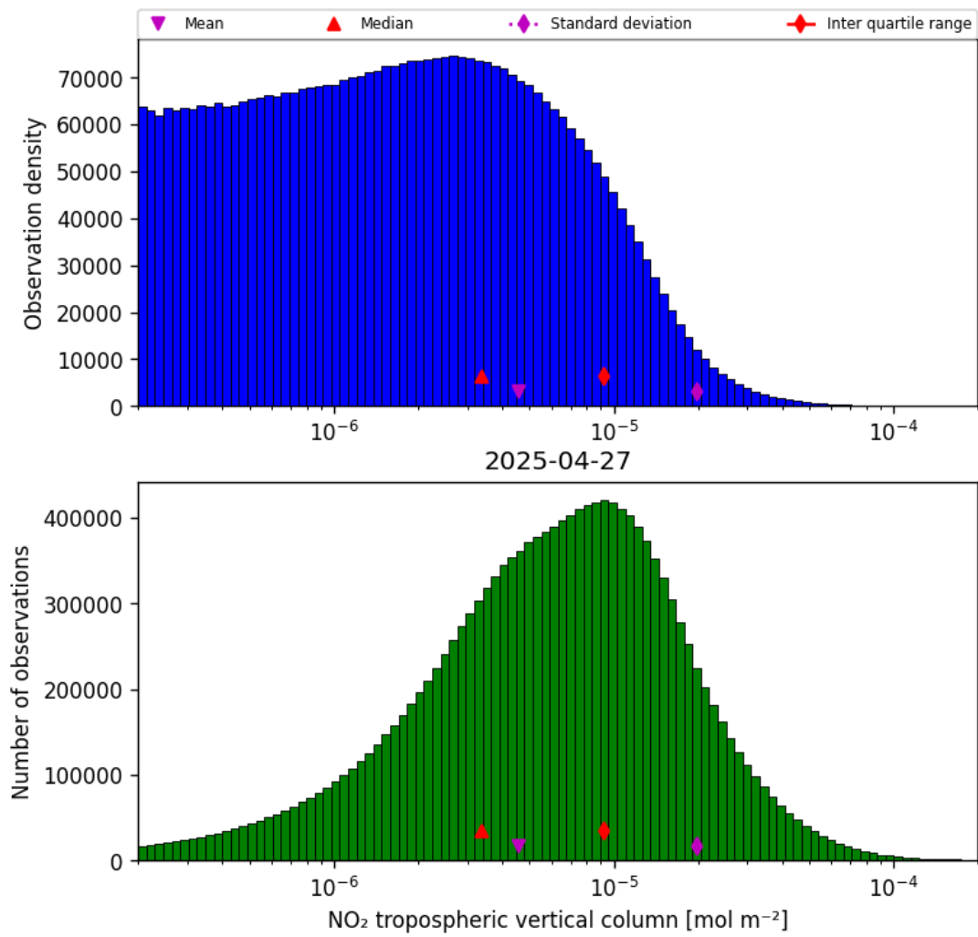
Figure 29: Histogram of “NO 2 tropospheric vertical column” for 2025-04-27 to 2025-04-27
