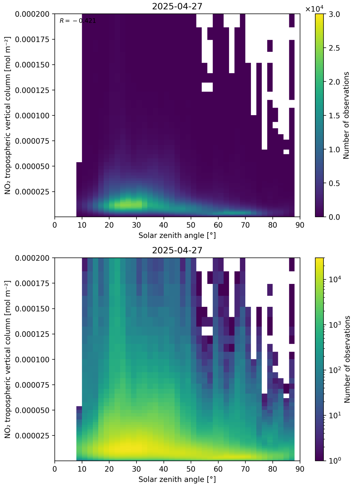
Figure 155: Scatter density plot of “Solar zenith angle” against “NO 2 tropospheric vertical column” for 2025-04-27 to 2025-04-27.
