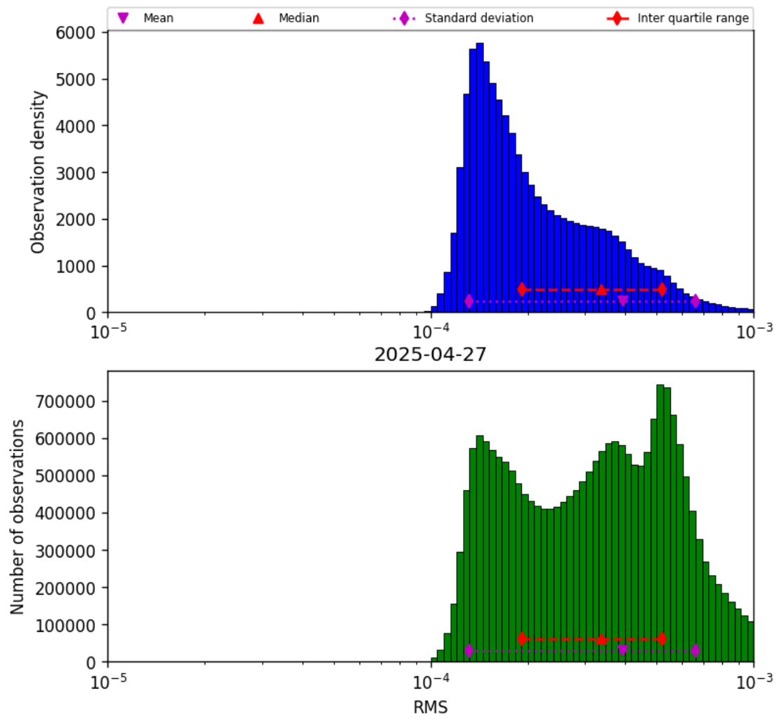
Figure 43: Histogram of “RMS” for 2025-04-27 to 2025-04-27
