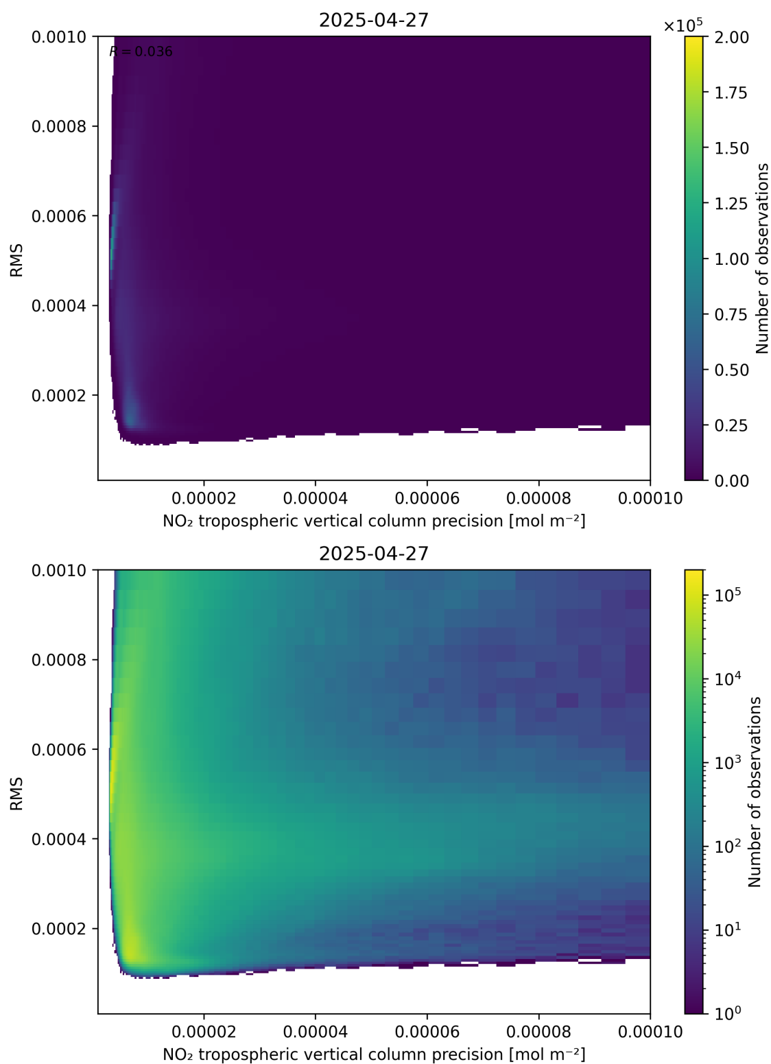
Figure 140: Scatter density plot of “NO 2 tropospheric vertical column precision” against “RMS” for 2025-04-27 to 2025-04-27.
