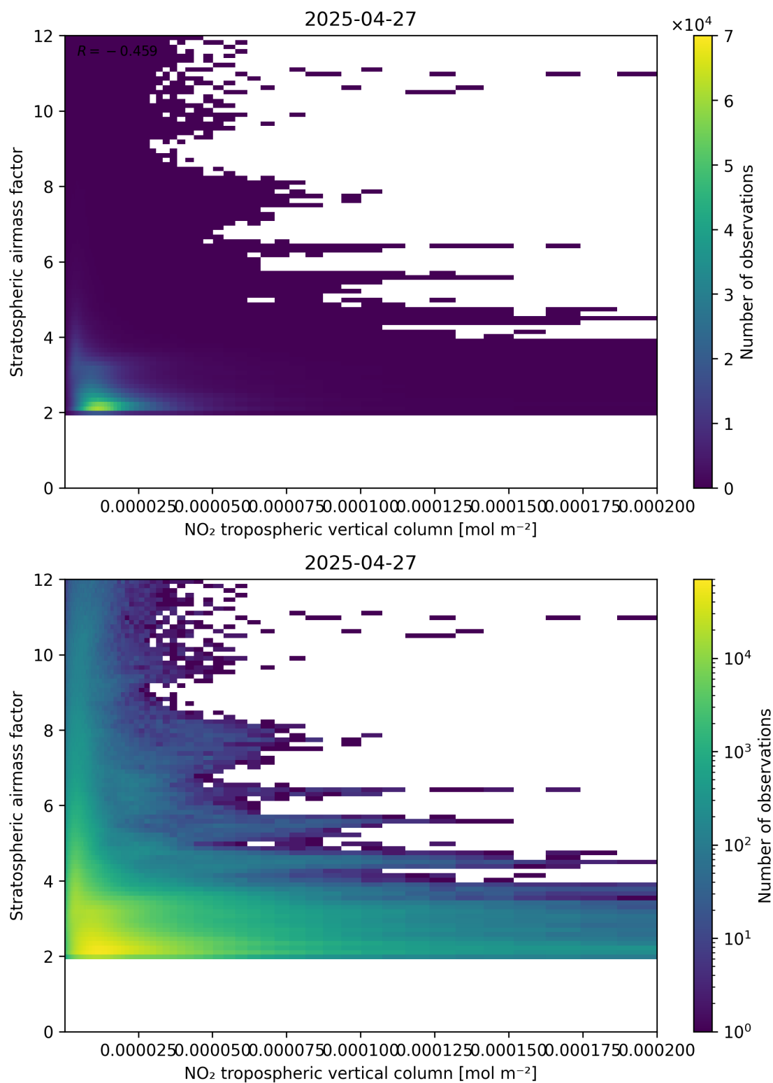
Figure 121: Scatter density plot of “NO 2 tropospheric vertical column” against “Stratospheric air mass factor” for 2025-04-27 to 2025-04-27.
