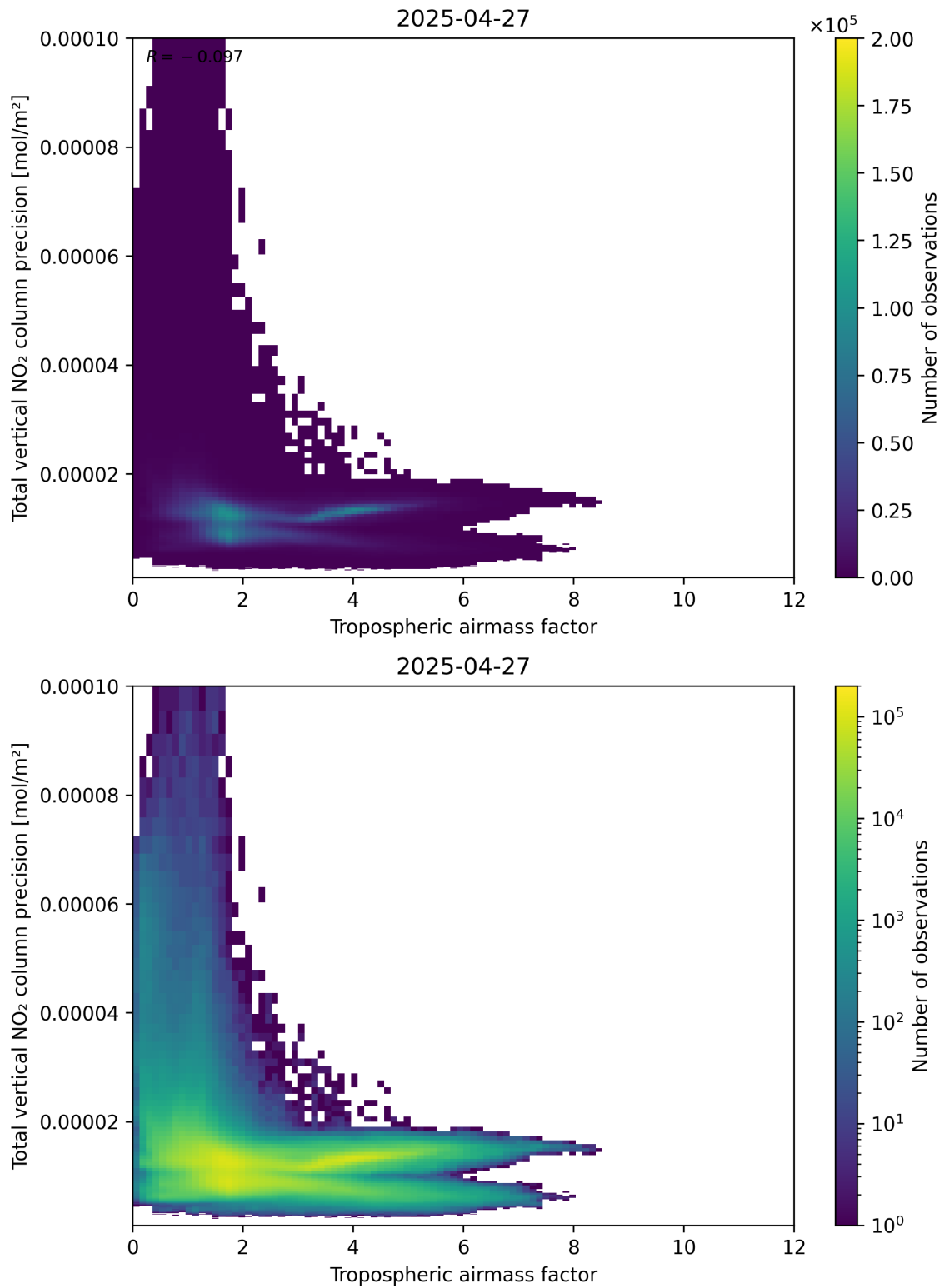
Figure 78: Scatter density plot of “Tropospheric air mass factor” against “Total vertical NO 2 column precision” for 2025-04-27 to 2025-04-27.
