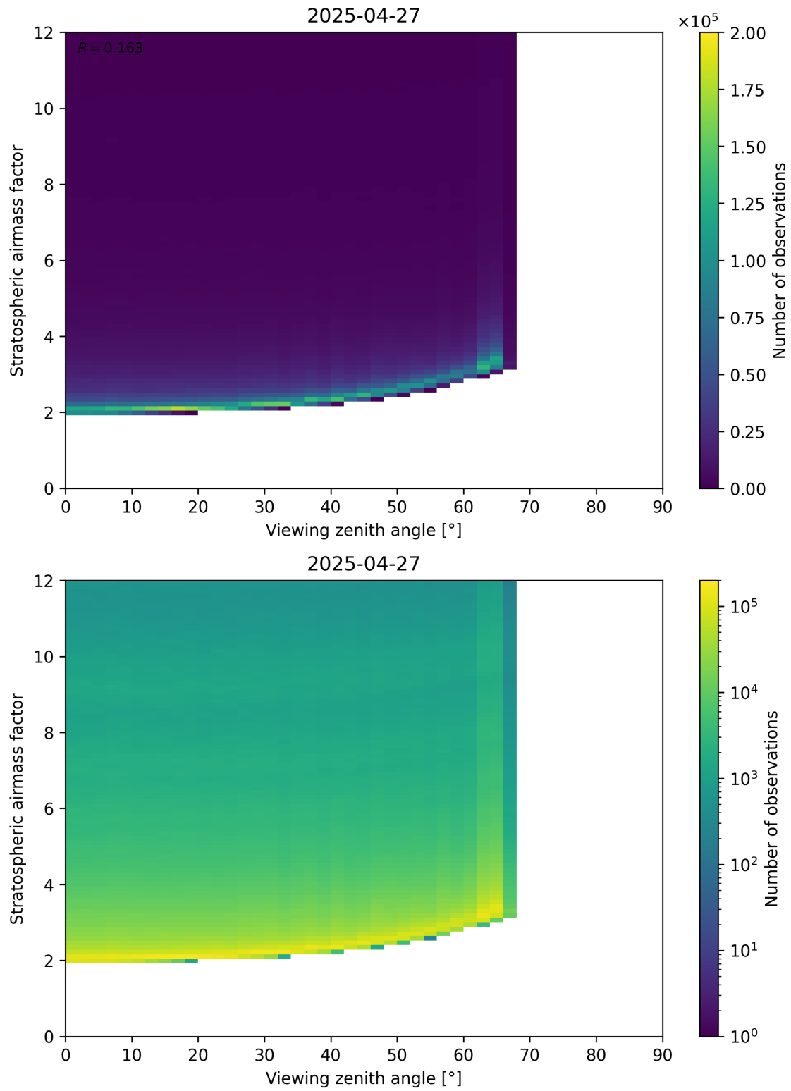
Figure 159: Scatter density plot of “Viewing zenith angle” against “Stratospheric airmass factor” for 2025-04-27 to 2025-04-27.
