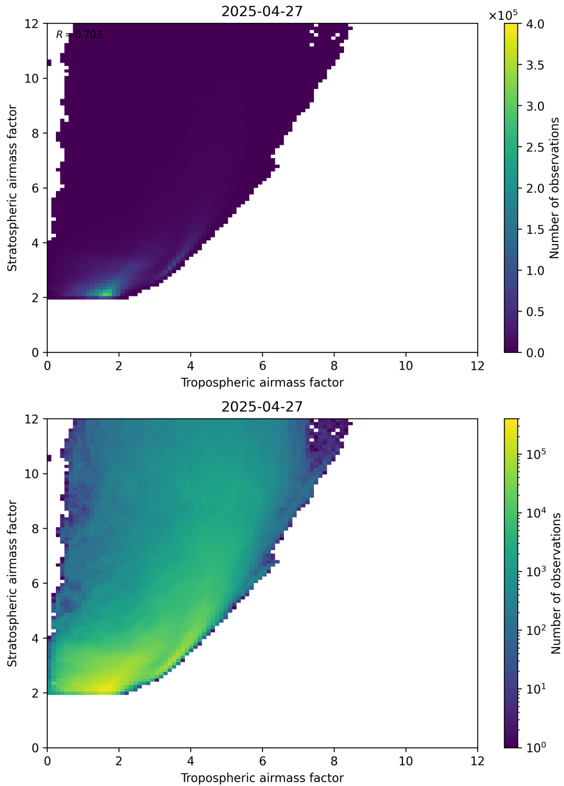
Figure 71: Scatter density plot of “Tropospheric airmass factor” against “Stratospheric airmass factor” for 2025-04-27 to 2025-04-27.
