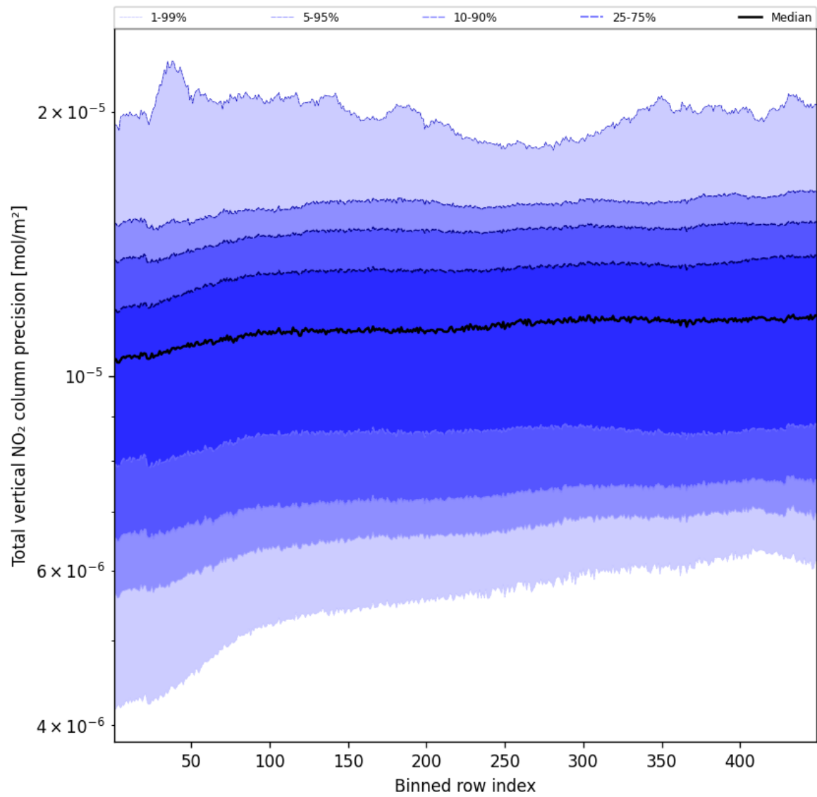
Figure 56: Along track statistics of “Total vertical NO 2 column precision” for 2025-04-27 to 2025-04-27
