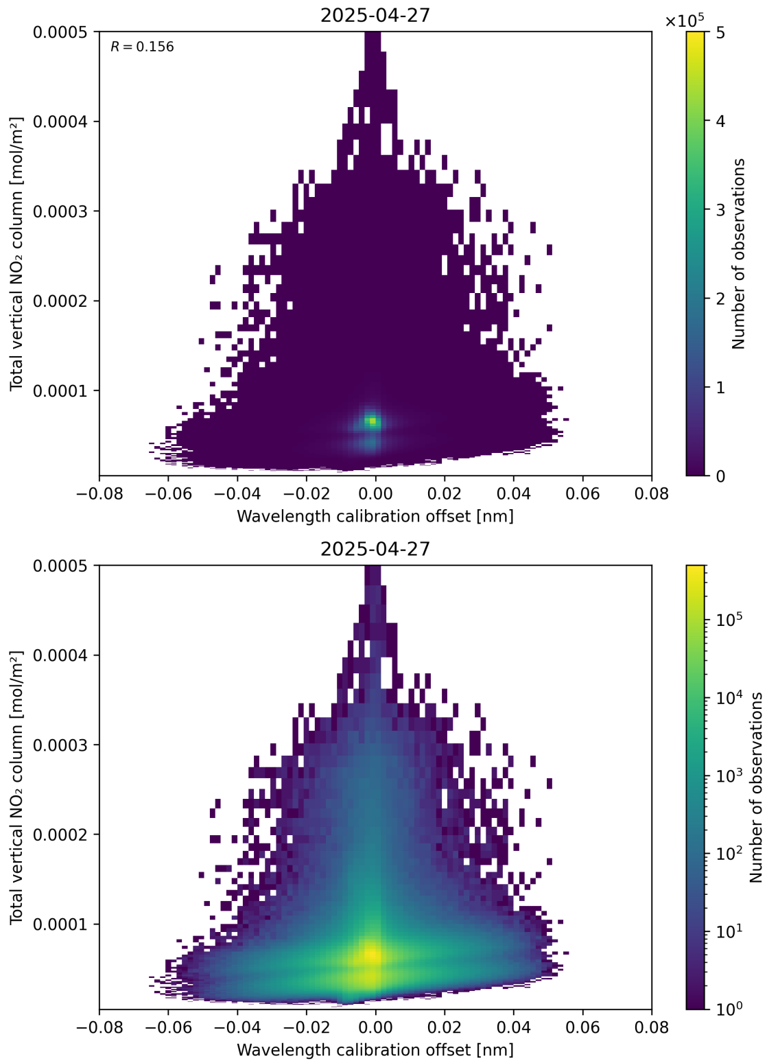
Figure 179: Scatter density plot of “Wavelength calibration offset” against “Total vertical NO 2 column” for 2025-04-27 to 2025-04-27.
