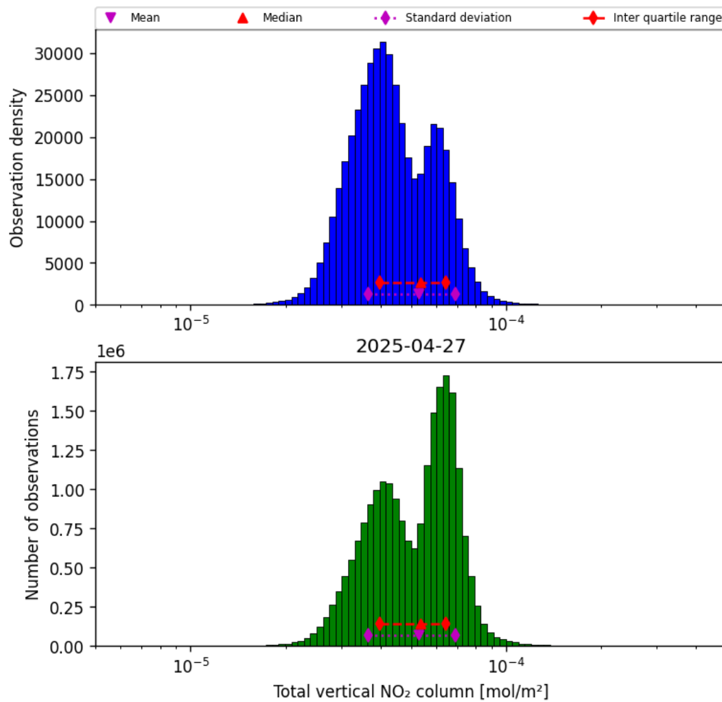
Figure 38: Histogram of “Total vertical NO 2 column” for 2025-04-27 to 2025-04-27
