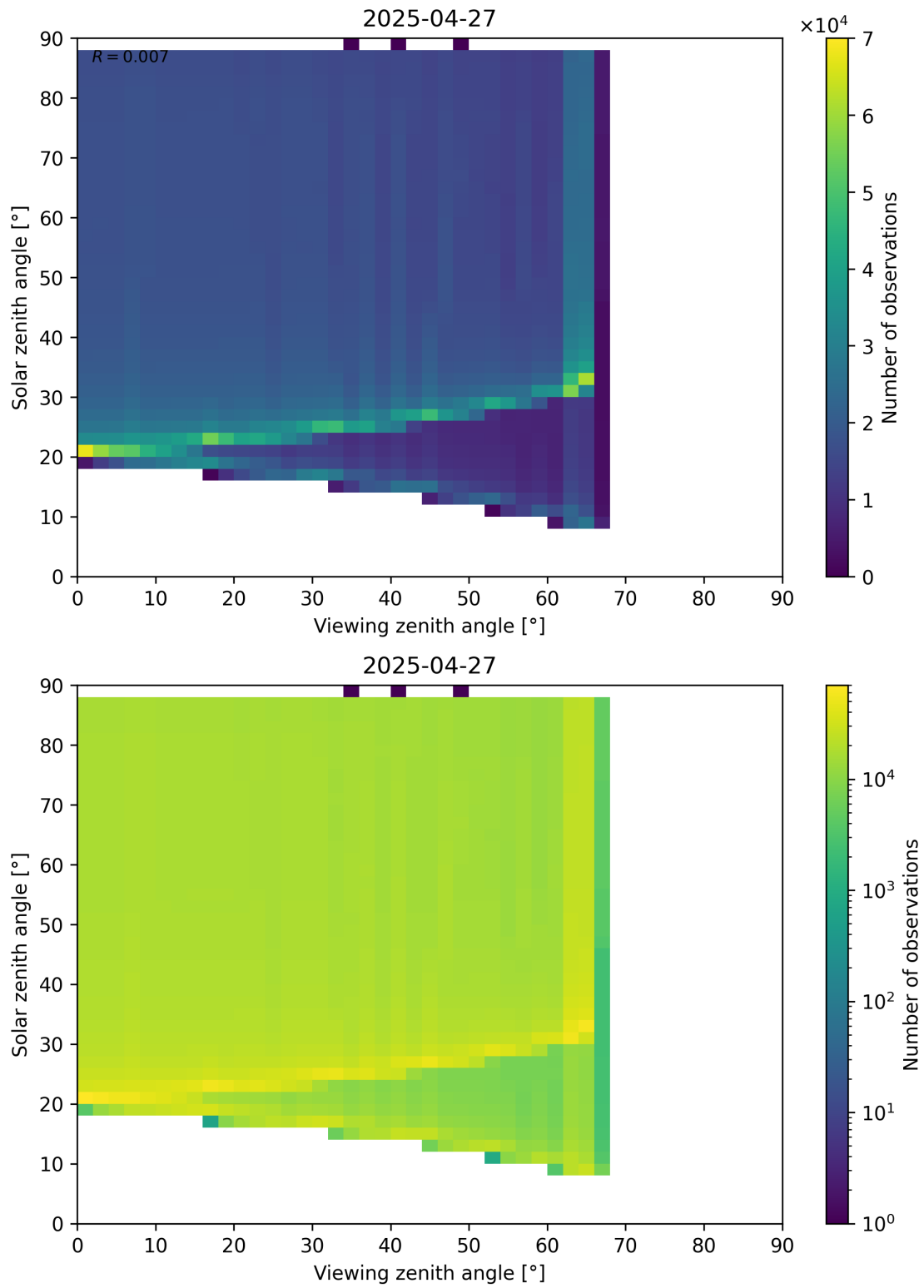
Figure 172: Scatter density plot of “Viewing zenith angle” against “Solar zenith angle” for 2025-04-27 to 2025-04-27.
