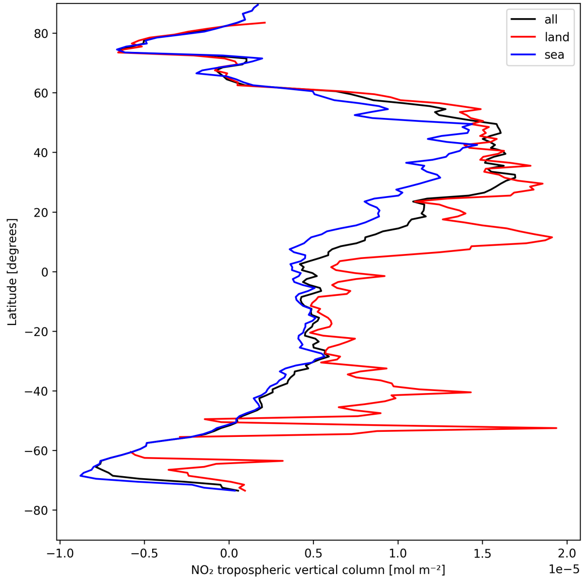
Figure 12: Zonal average of “NO 2 tropospheric vertical column” for 2025-04-27 to 2025-04-27.
