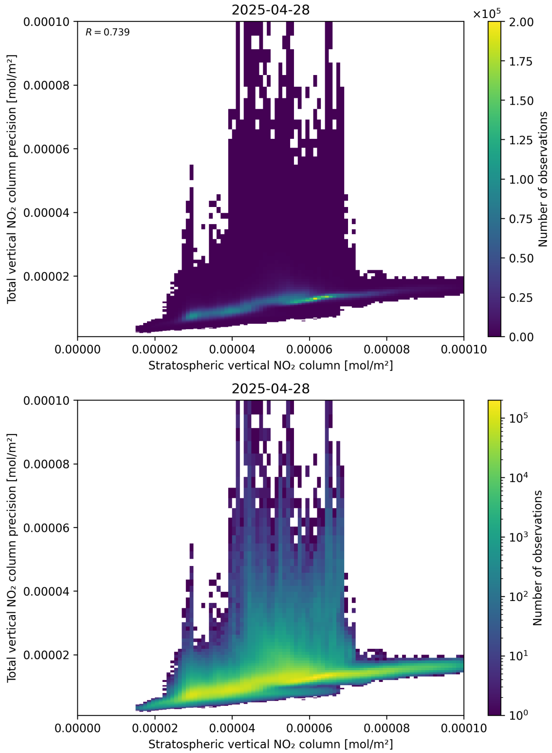
Figure 101: Scatter density plot of “Stratospheric vertical NO 2 column” against “Total vertical NO 2 column precision” for 2025-04-28 to 2025-04-29.
