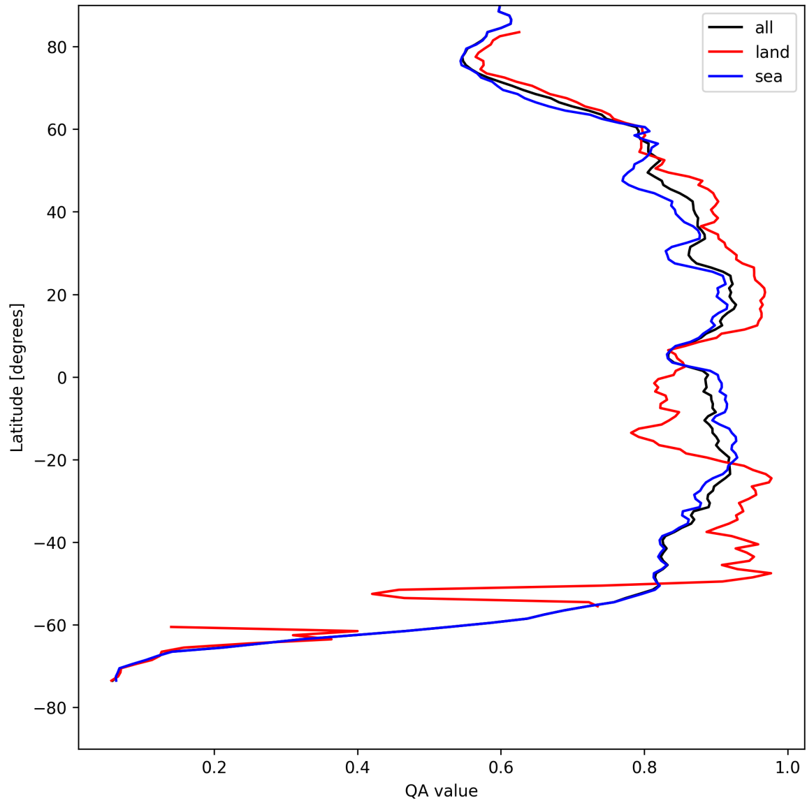
Figure 11: Zonal average of “QA value” for 2025-04-28 to 2025-04-29.
