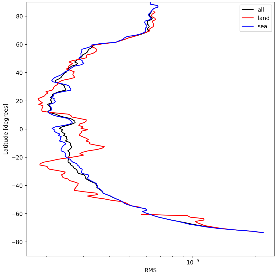
Figure 26: Zonal average of “RMS” for 2025-04-28 to 2025-04-29.
