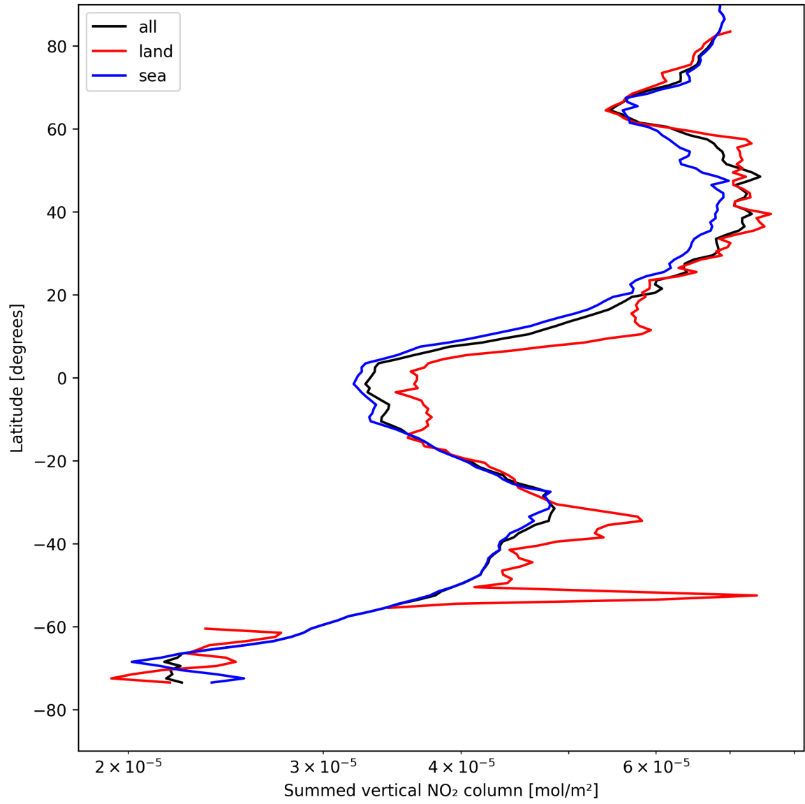
Figure 23: Zonal average of “Summed vertical NO 2 column” for 2025-04-28 to 2025-04-29.
