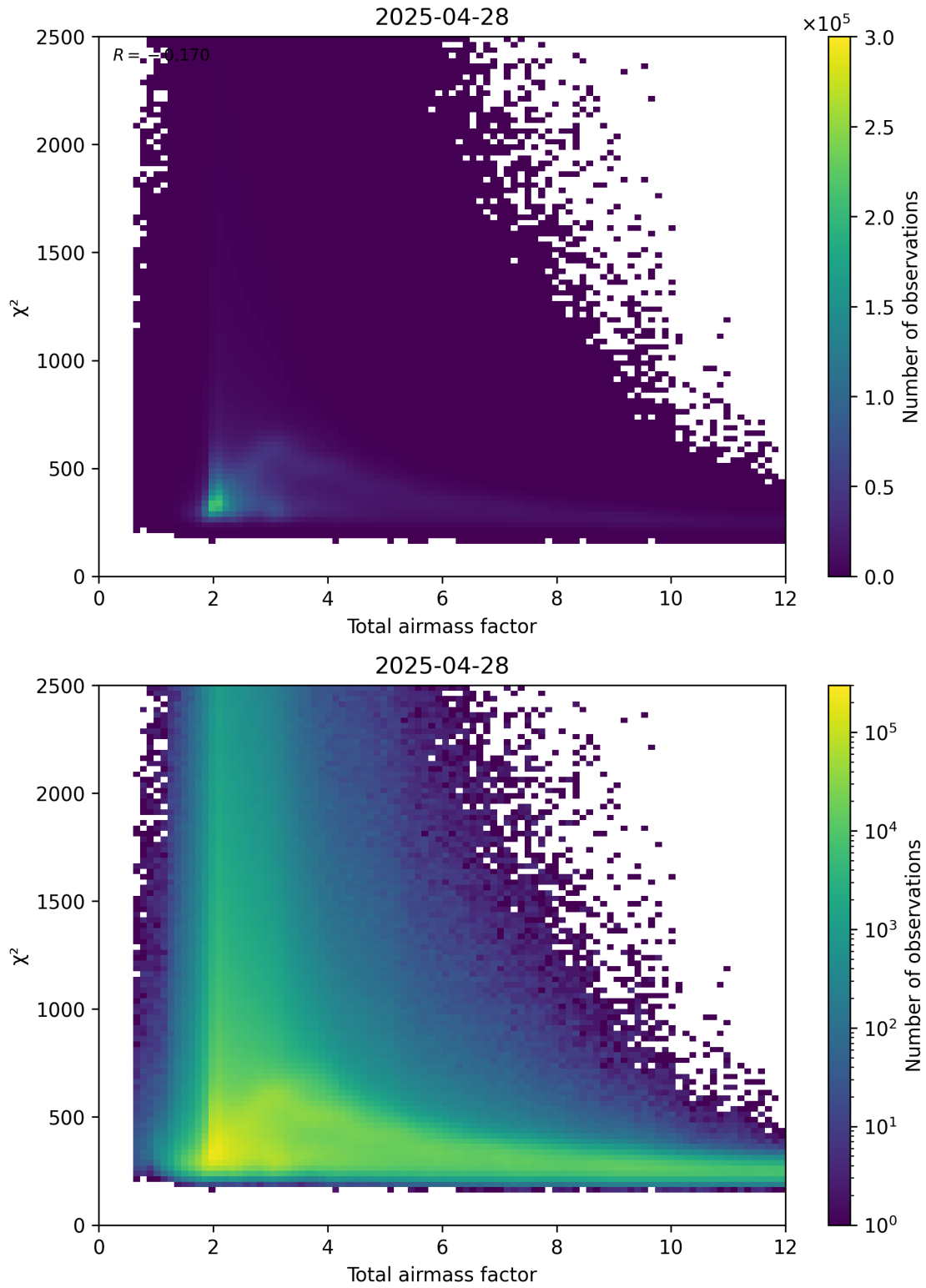
Figure 63: Scatter density plot of “Total airmass factor” against “ \chi^2 ” for 2025-04-28 to 2025-04-29.
