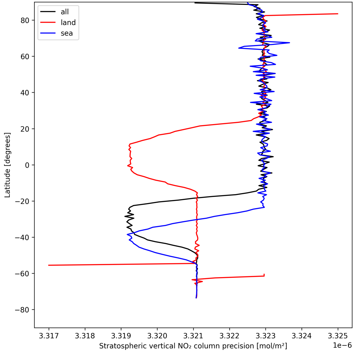
Figure 20: Zonal average of “Stratospheric vertical NO 2 column precision” for 2025-04-28 to 2025-04-29.
