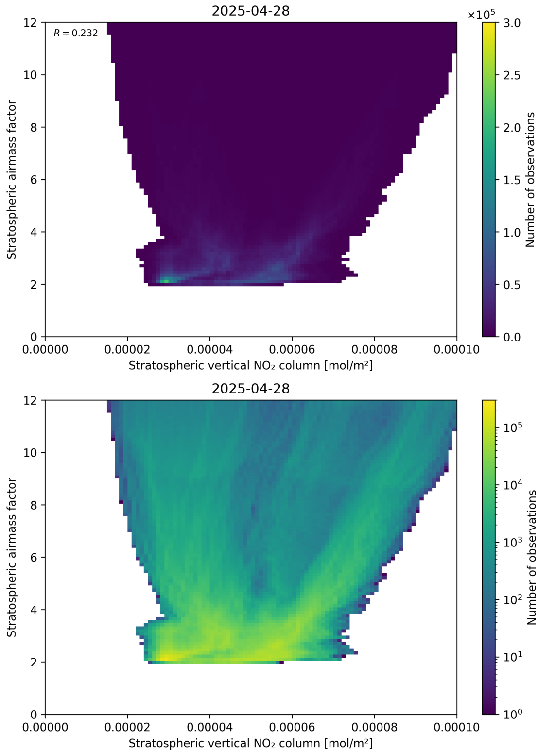
Figure 96: Scatter density plot of “Stratospheric vertical NO 2 column” against “Stratospheric airmass factor” for 2025-04-28 to 2025-04-29.
