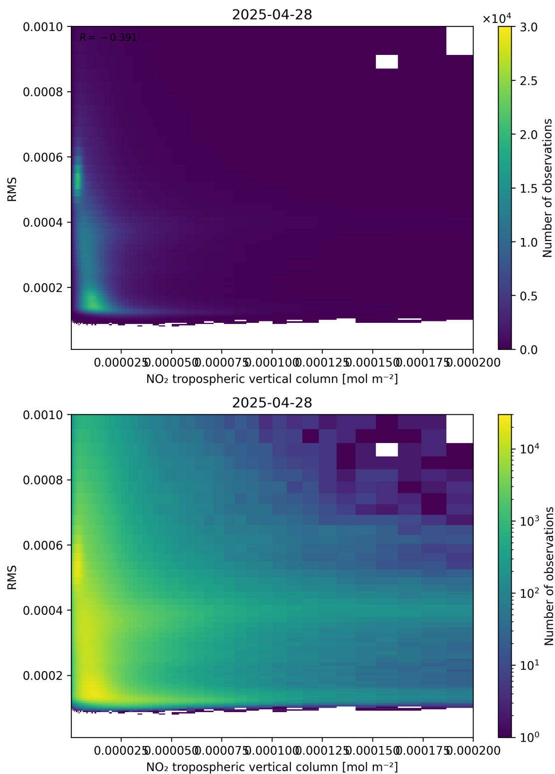
Figure 142: Scatter density plot of “NO 2 tropospheric vertical column” against “RMS” for 2025-04-28 to 2025-04-29.
