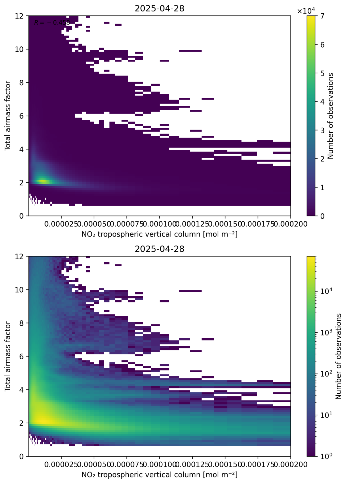
Figure 122: Scatter density plot of “NO 2 tropospheric vertical column” against “Total air mass factor” for 2025-04-28 to 2025-04-29.
