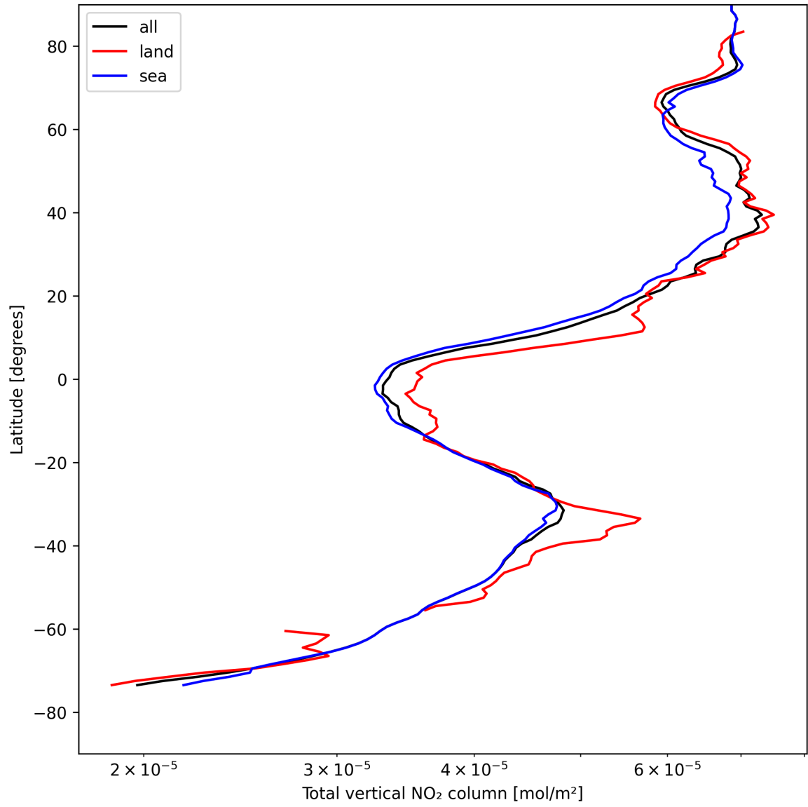
Figure 21: Zonal average of “Total vertical NO 2 column” for 2025-04-28 to 2025-04-29.
