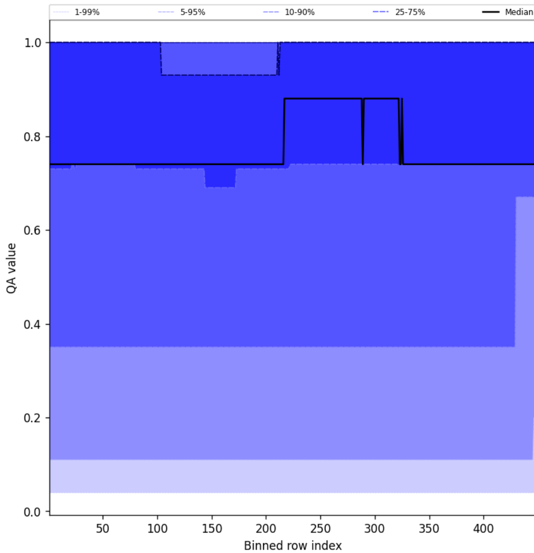
Figure 45: Along track statistics of “QA value” for 2025-04-28 to 2025-04-29
