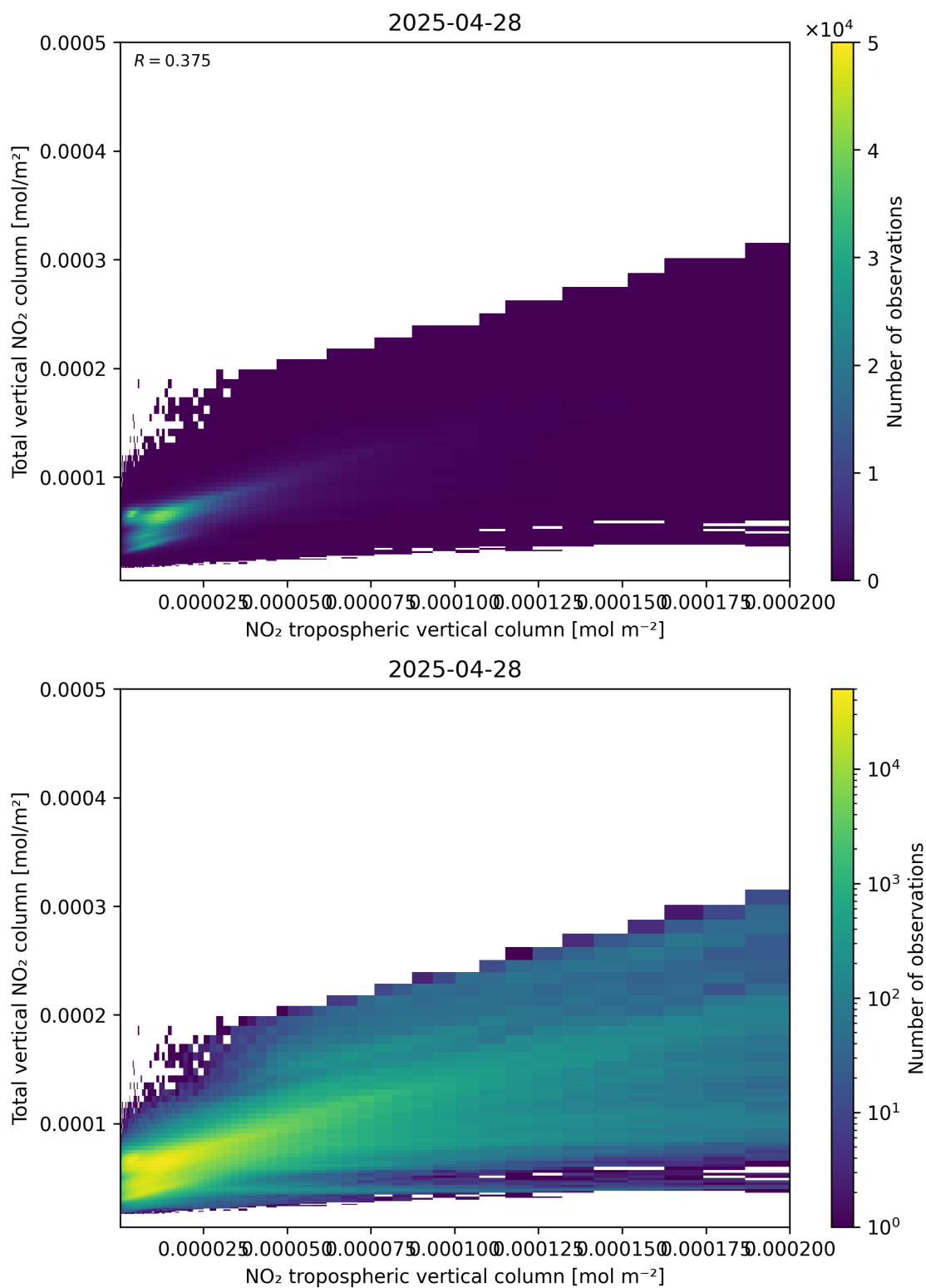
Figure 128: Scatter density plot of “NO 2 tropospheric vertical column” against “Total vertical NO 2 column” for 2025-04-28 to 2025-04-29.
