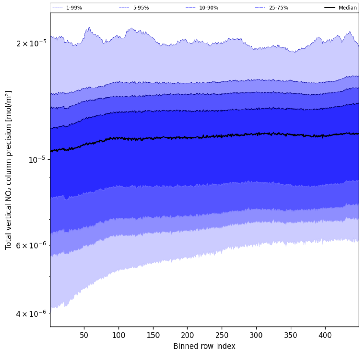
Figure 56: Along track statistics of "Total vertical NO 2 column precision" for 2025-04-28 to 2025-04-29
