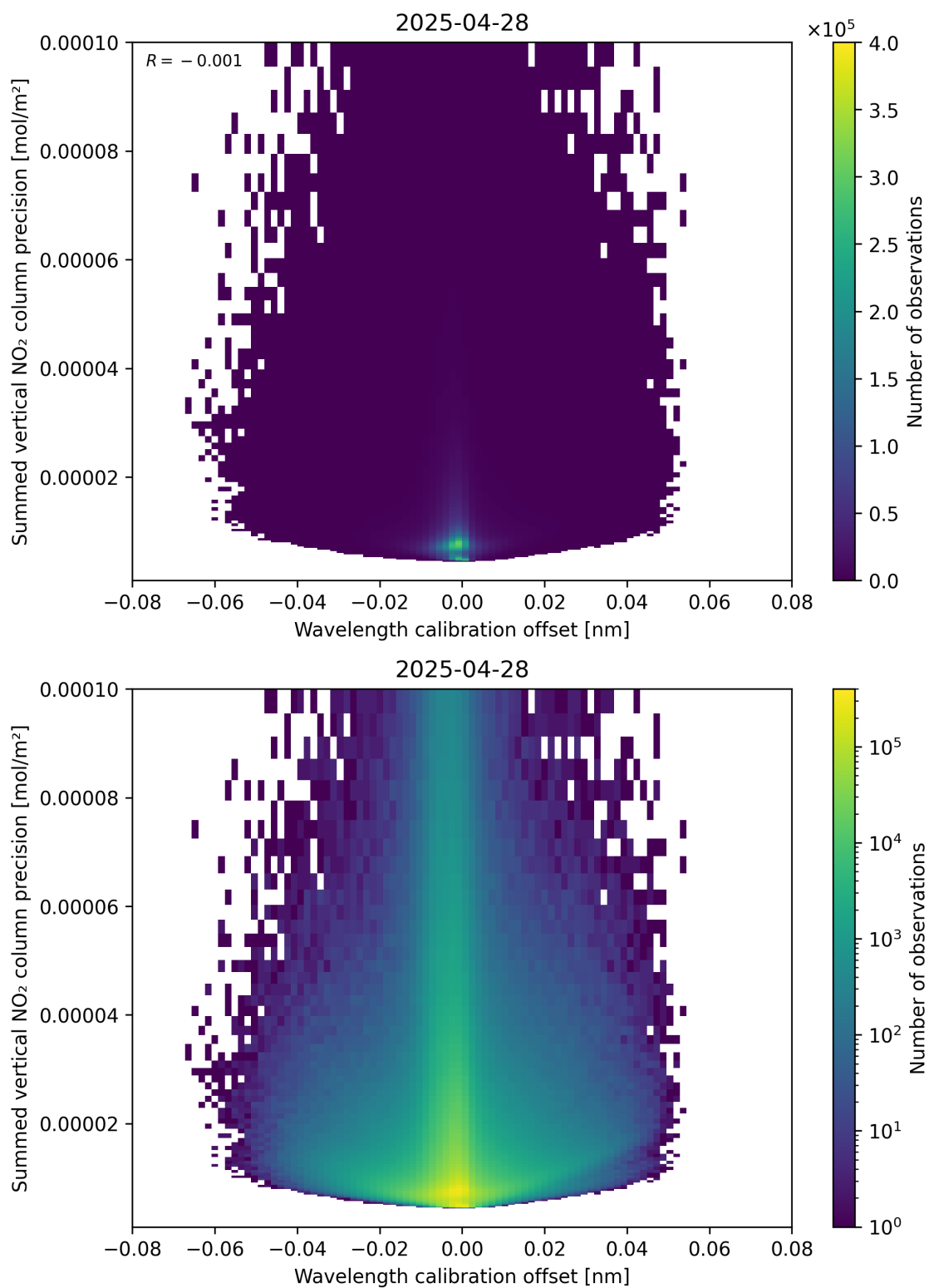
Figure 178: Scatter density plot of “Wavelength calibration offset” against “Summed vertical NO 2 column precision” for 2025-04-28 to 2025-04-29.
