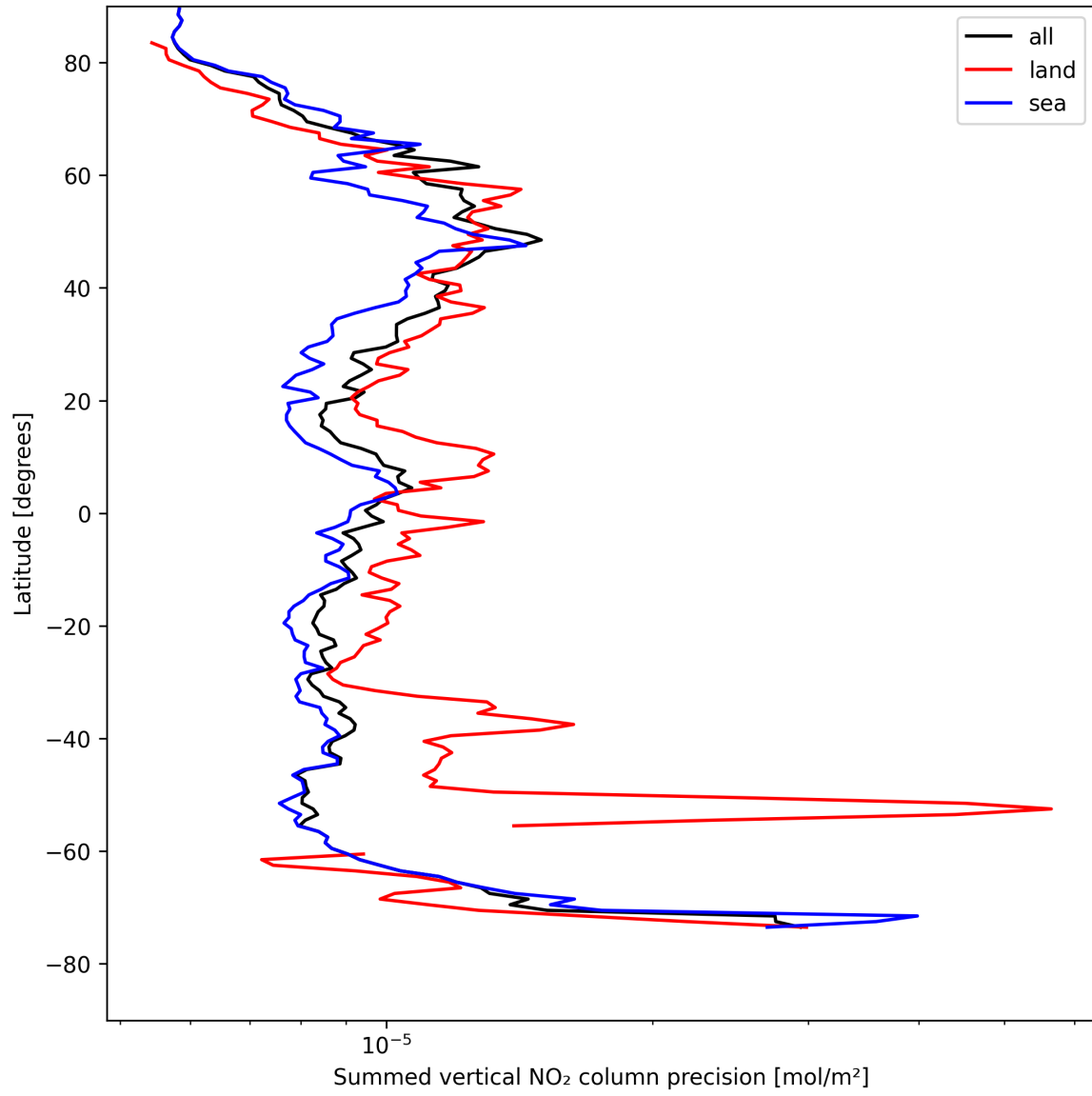
Figure 24: Zonal average of “Summed vertical NO 2 column precision” for 2025-04-28 to 2025-04-29.
