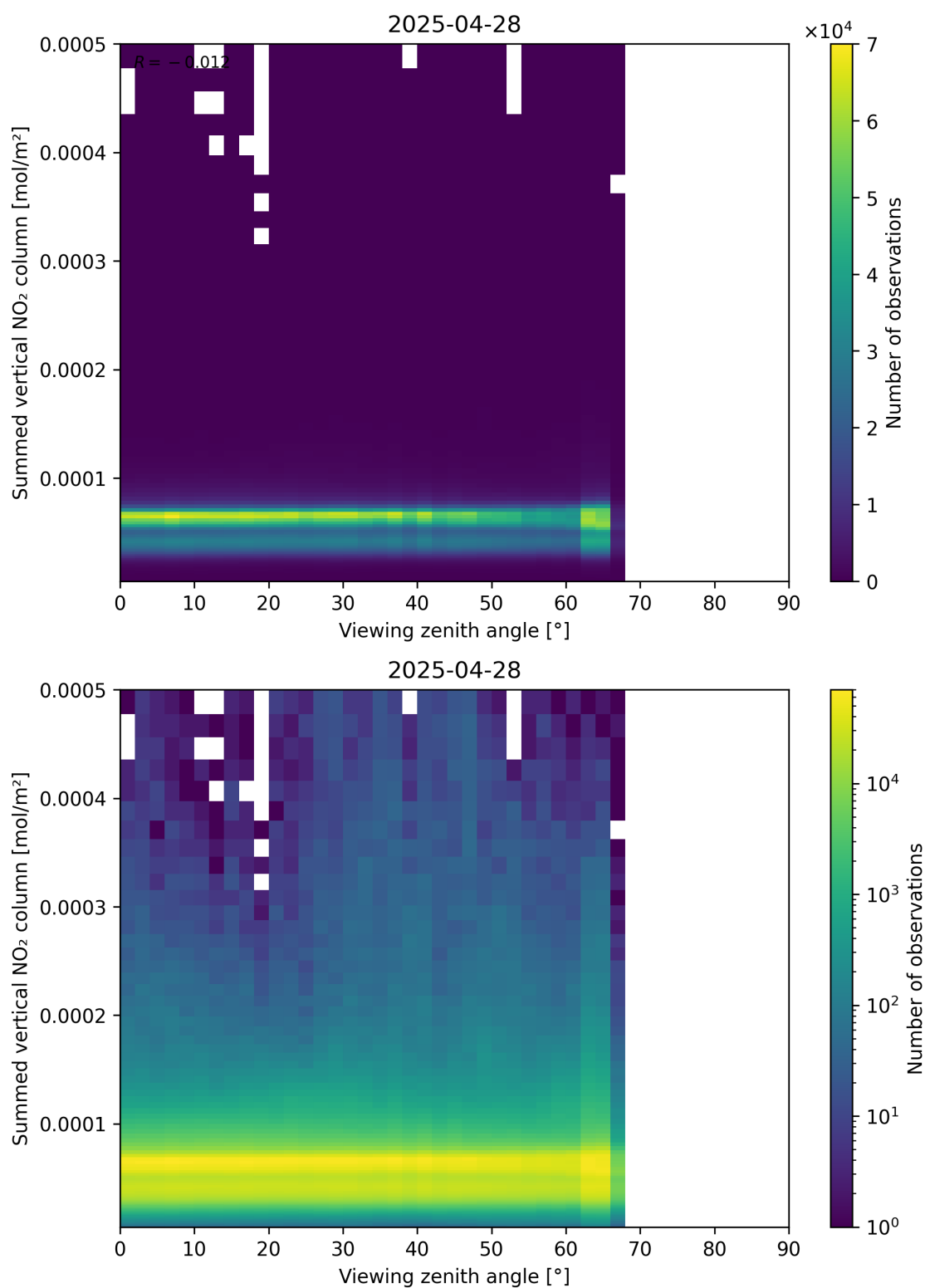
Figure 165: Scatter density plot of “Viewing zenith angle” against “Summed vertical NO 2 column” for 2025-04-28 to 2025-04-29.
