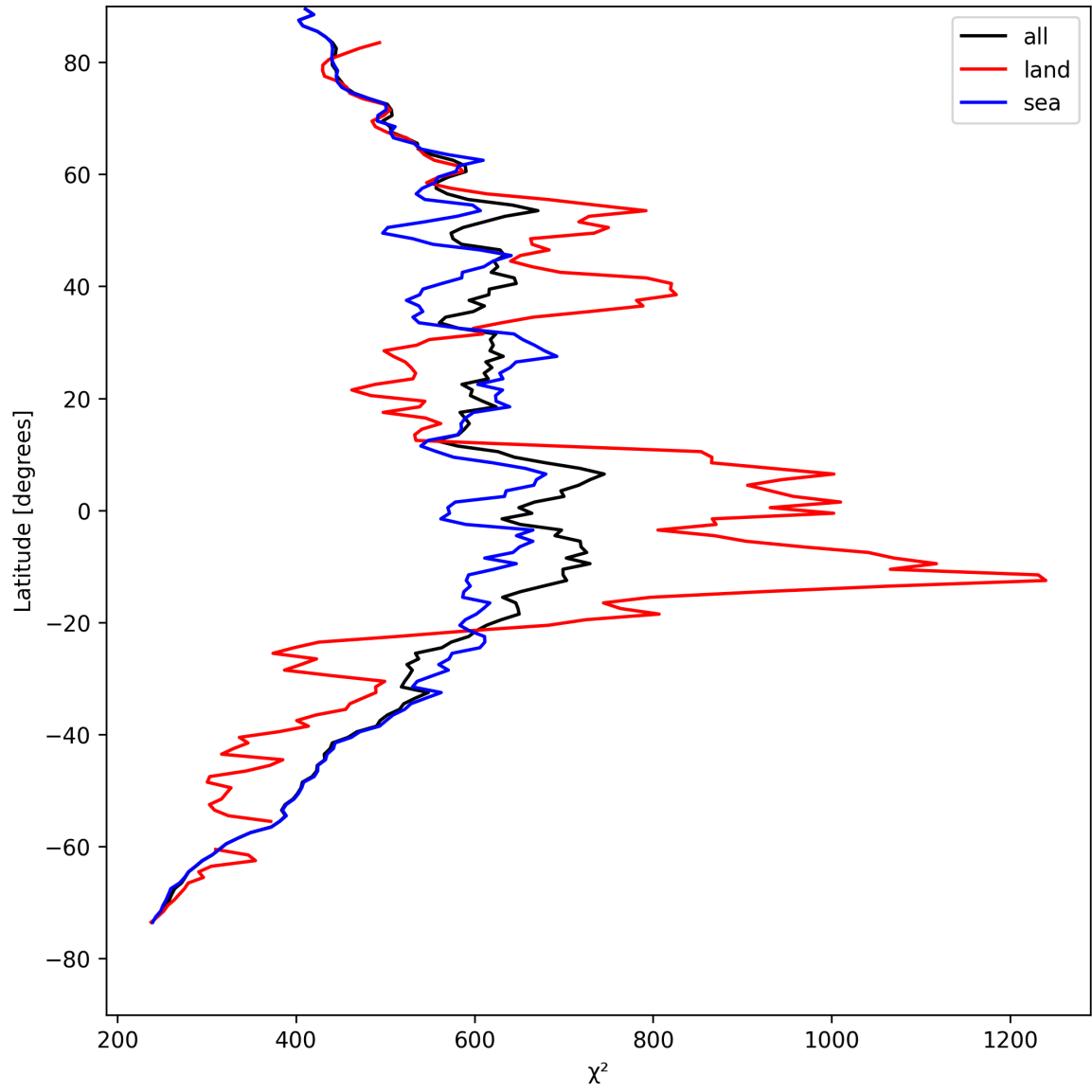
Figure 25: Zonal average of “ \chi^2 ” for 2025-04-28 to 2025-04-29.
