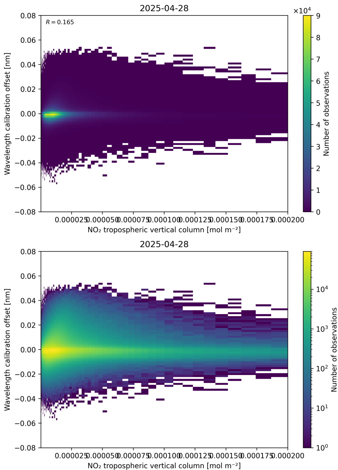
Figure 143: Scatter density plot of “NO 2 tropospheric vertical column” against “Wavelength calibration offset” for 2025-04-28 to 2025-04-29.
