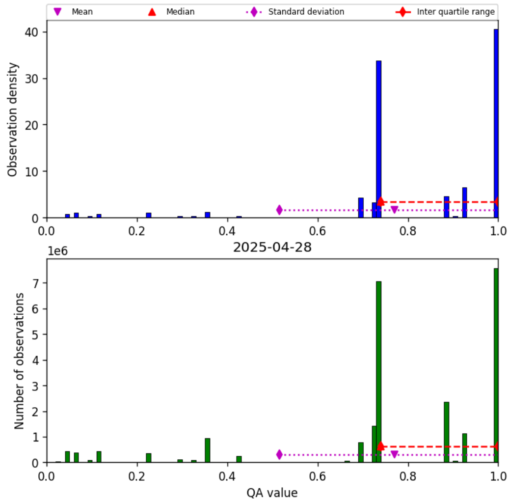
Figure 28: Histogram of “QA value” for 2025-04-28 to 2025-04-29
