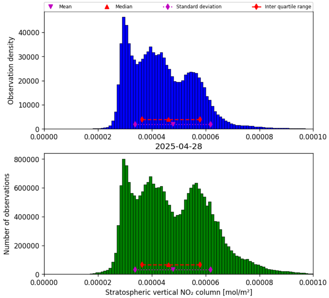
Figure 36: Histogram of “Stratospheric vertical NO 2 column” for 2025-04-28 to 2025-04-29
