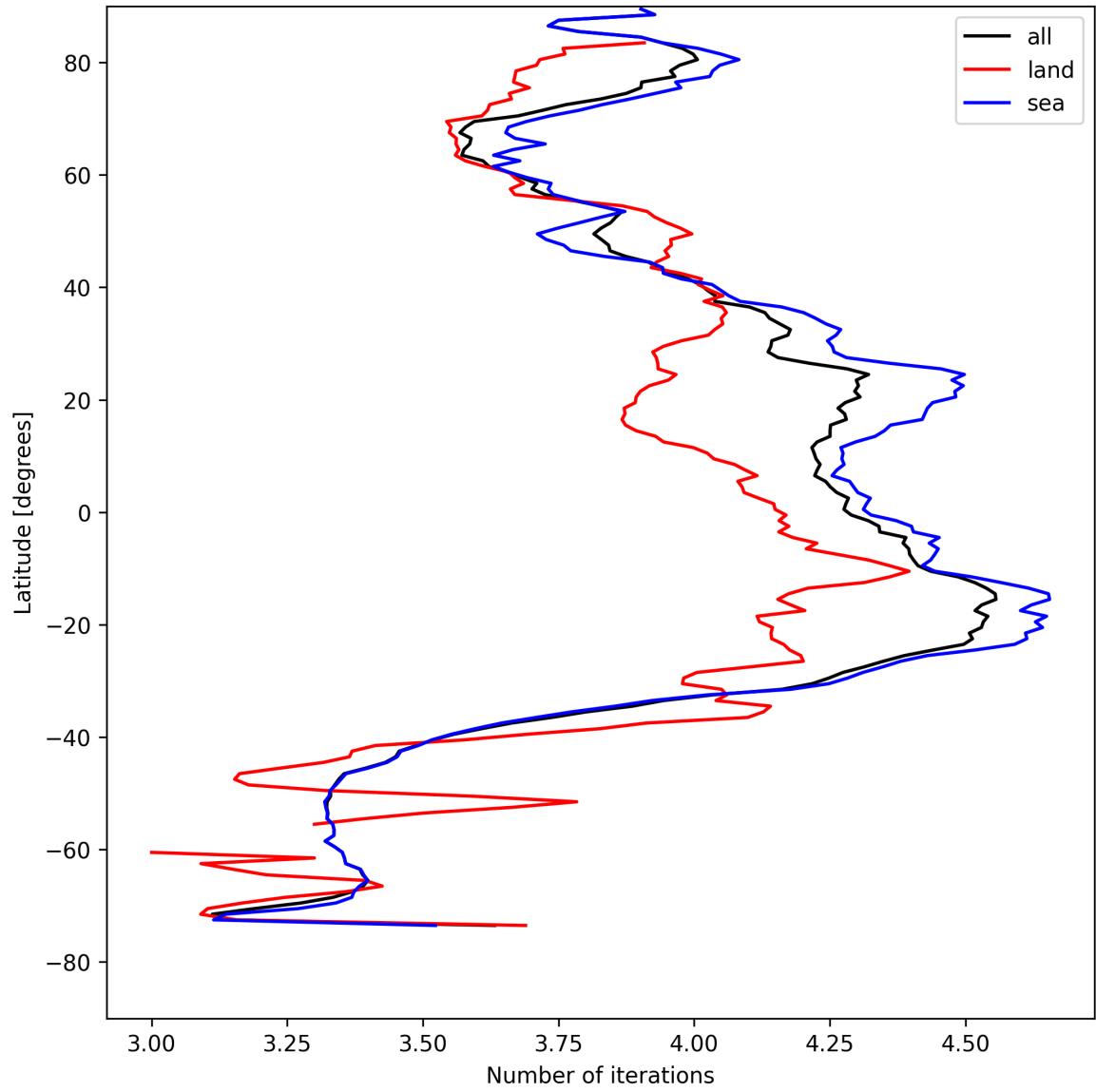
Figure 17: Zonal average of “Number of iterations” for 2025-04-28 to 2025-04-29.
