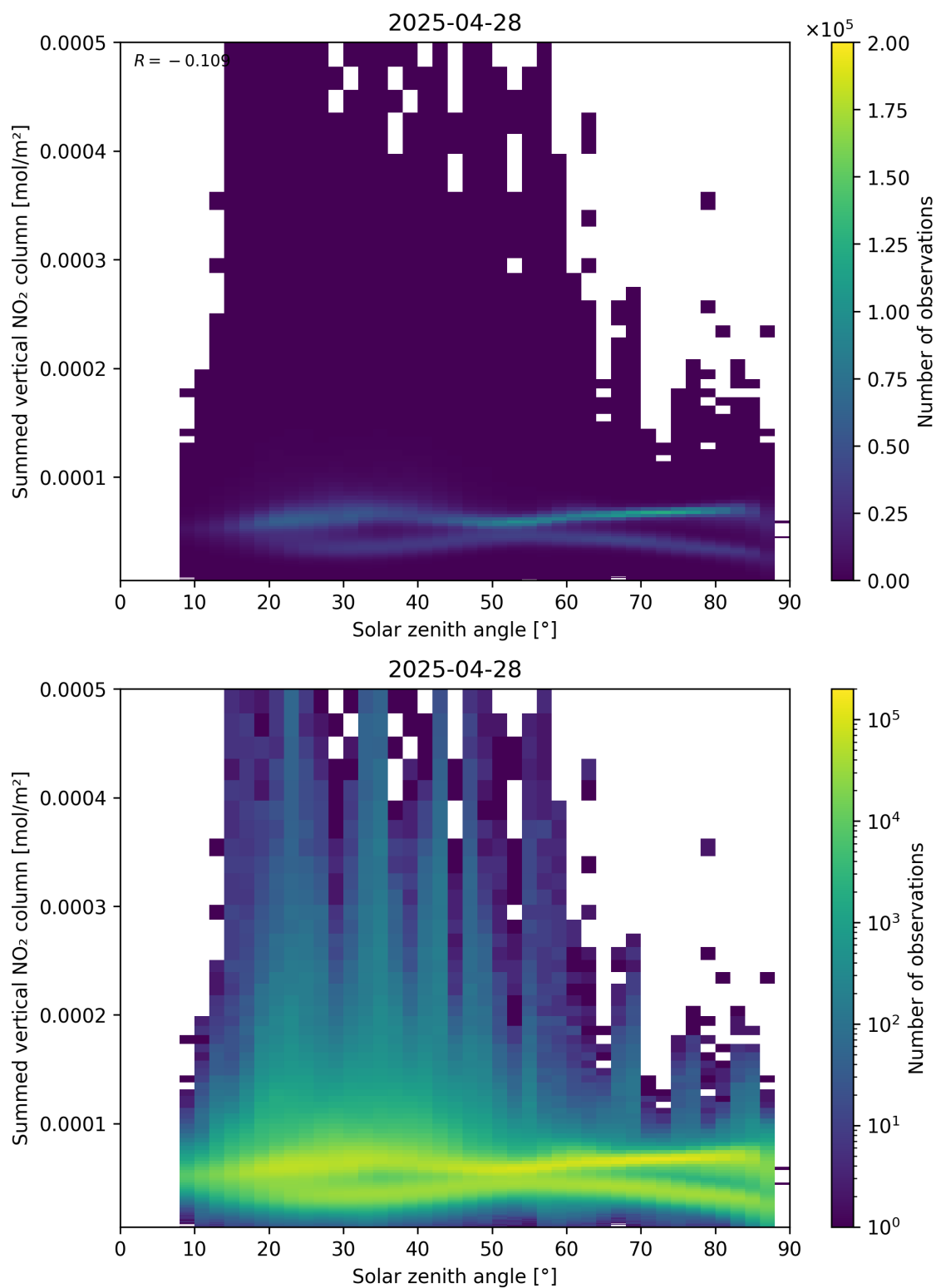
Figure 151: Scatter density plot of “Solar zenith angle” against “Summed vertical NO 2 column” for 2025-04-28 to 2025-04-29.
