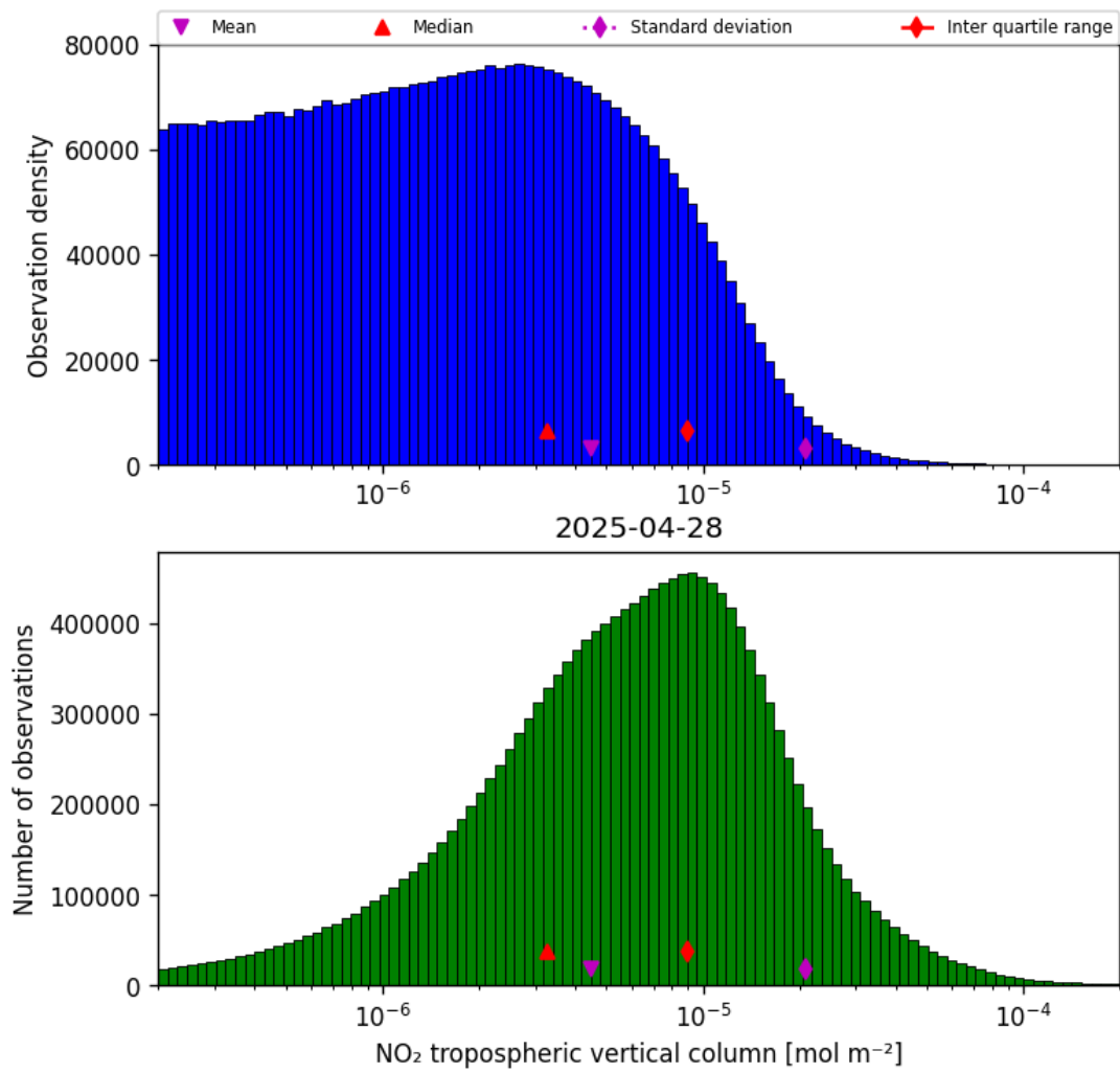
Figure 29: Histogram of “NO 2 tropospheric vertical column” for 2025-04-28 to 2025-04-29
