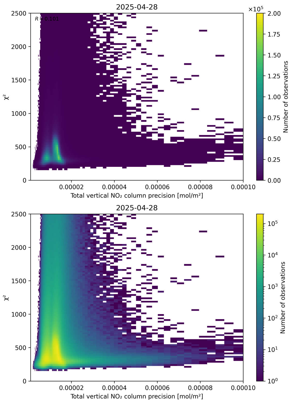
Figure 116: Scatter density plot of “Total vertical NO 2 column precision” against “ \chi^2 ” for 2025-04-28 to 2025-04-29.
