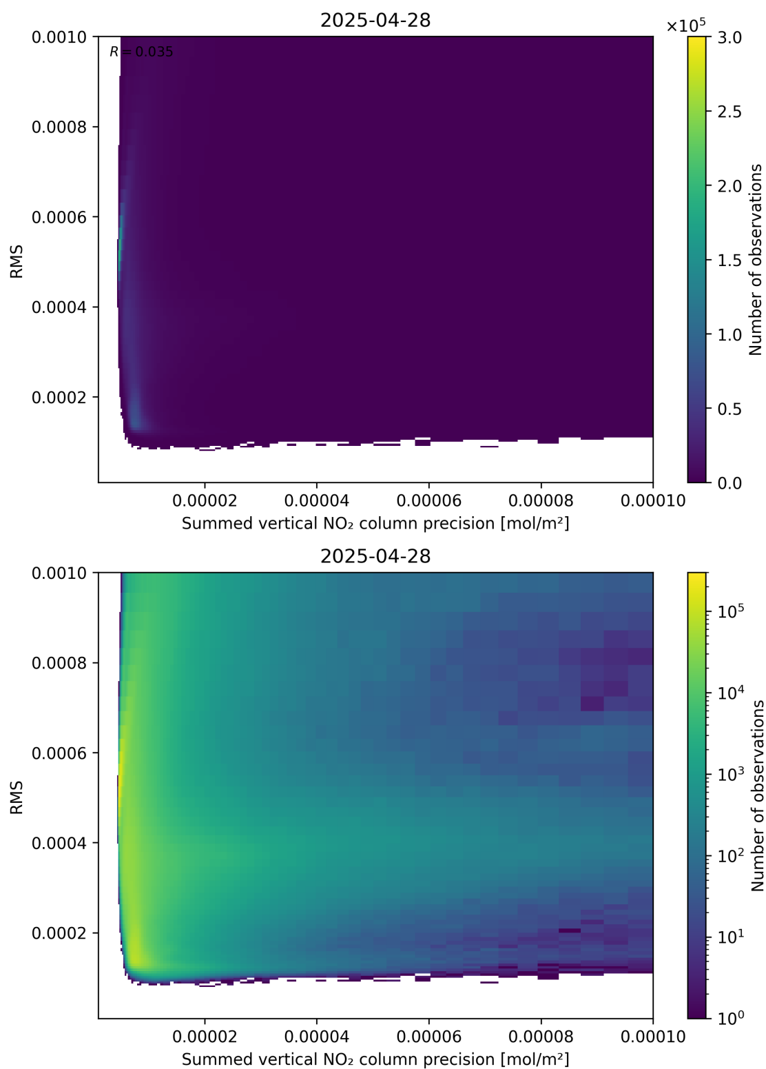
Figure 108: Scatter density plot of “Summed vertical NO 2 column precision” against “RMS” for 2025-04-28 to 2025-04-29.
