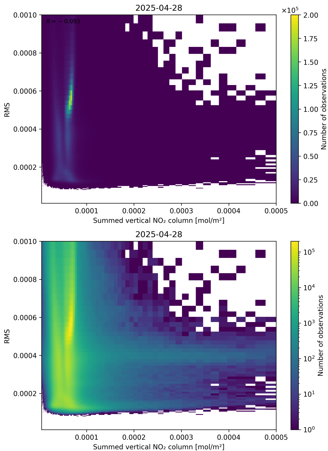
Figure 109: Scatter density plot of “Summed vertical NO 2 column” against “RMS” for 2025-04-28 to 2025-04-29.
