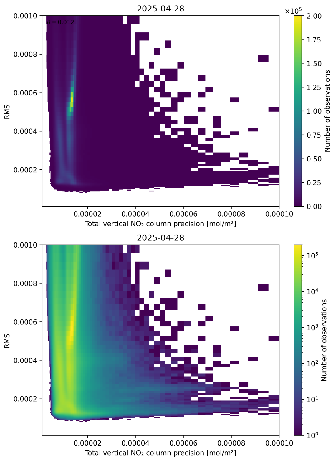
Figure 119: Scatter density plot of “Total vertical NO 2 column precision” against “RMS” for 2025-04-28 to 2025-04-29.
