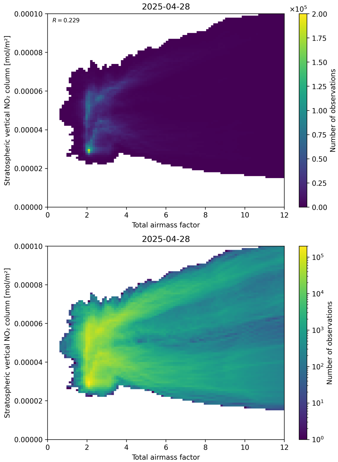
Figure 64: Scatter density plot of “Total airmass factor” against “Stratospheric vertical NO 2 column” for 2025-04-28 to 2025-04-29.
