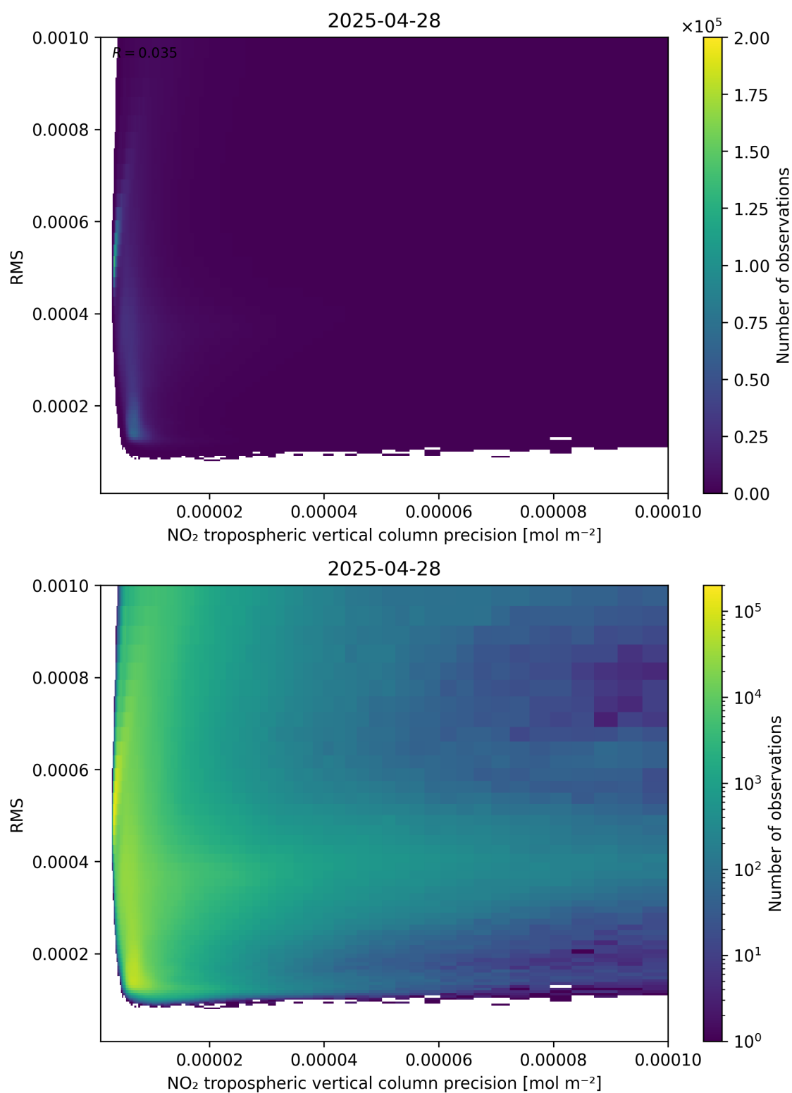
Figure 140: Scatter density plot of “NO 2 tropospheric vertical column precision” against “RMS” for 2025-04-28 to 2025-04-29.
