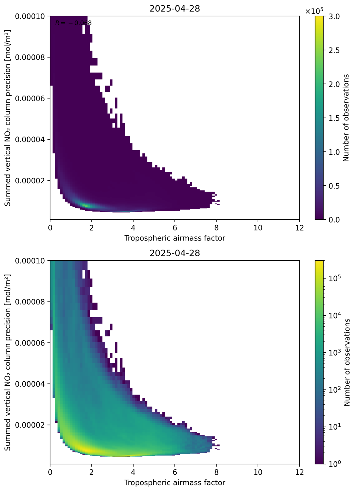
Figure 76: Scatter density plot of “Tropospheric air mass factor” against “Summed vertical NO 2 column precision” for 2025-04-28 to 2025-04-29.
