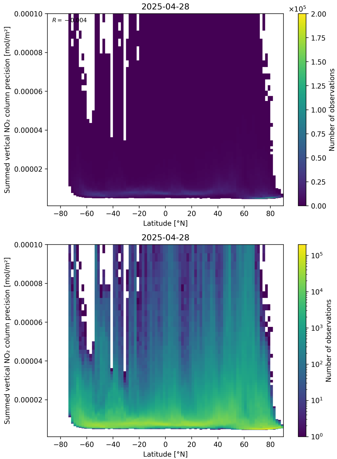
Figure 89: Scatter density plot of “Latitude” against “Summed vertical NO 2 column precision” for 2025-04-28 to 2025-04-29.
