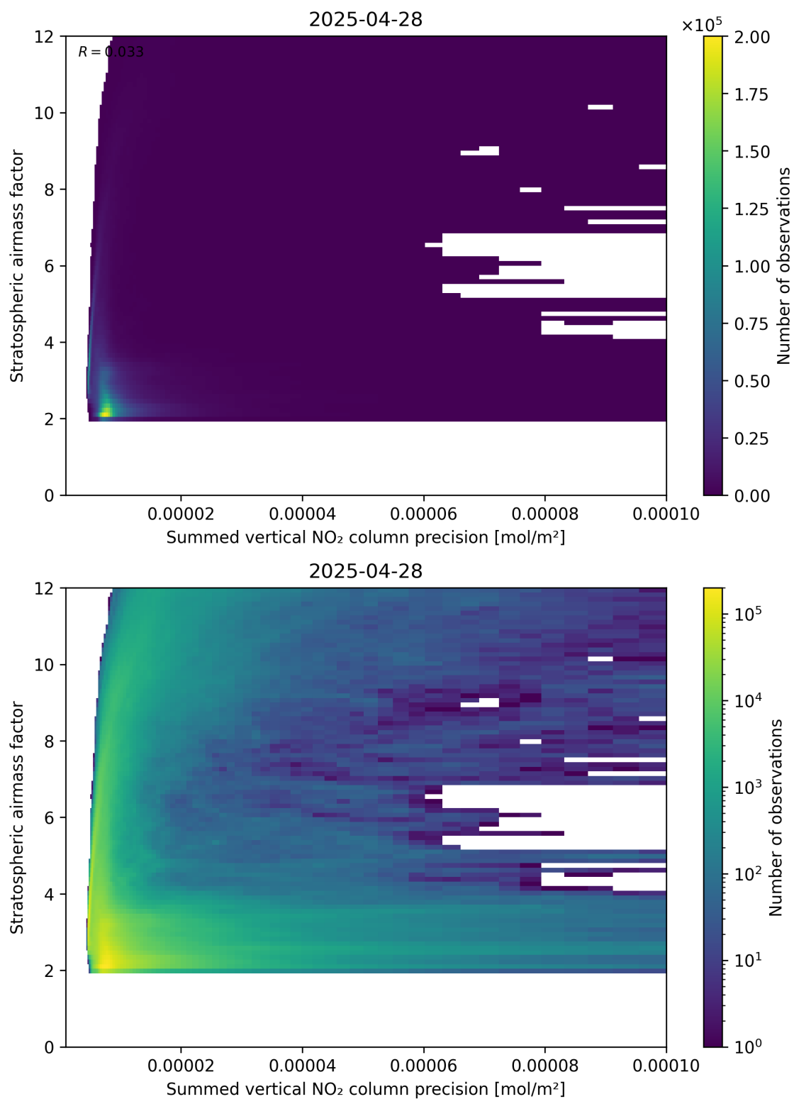
Figure 106: Scatter density plot of “Summed vertical NO 2 column precision” against “Stratospheric airmass factor” for 2025-04-28 to 2025-04-29.
