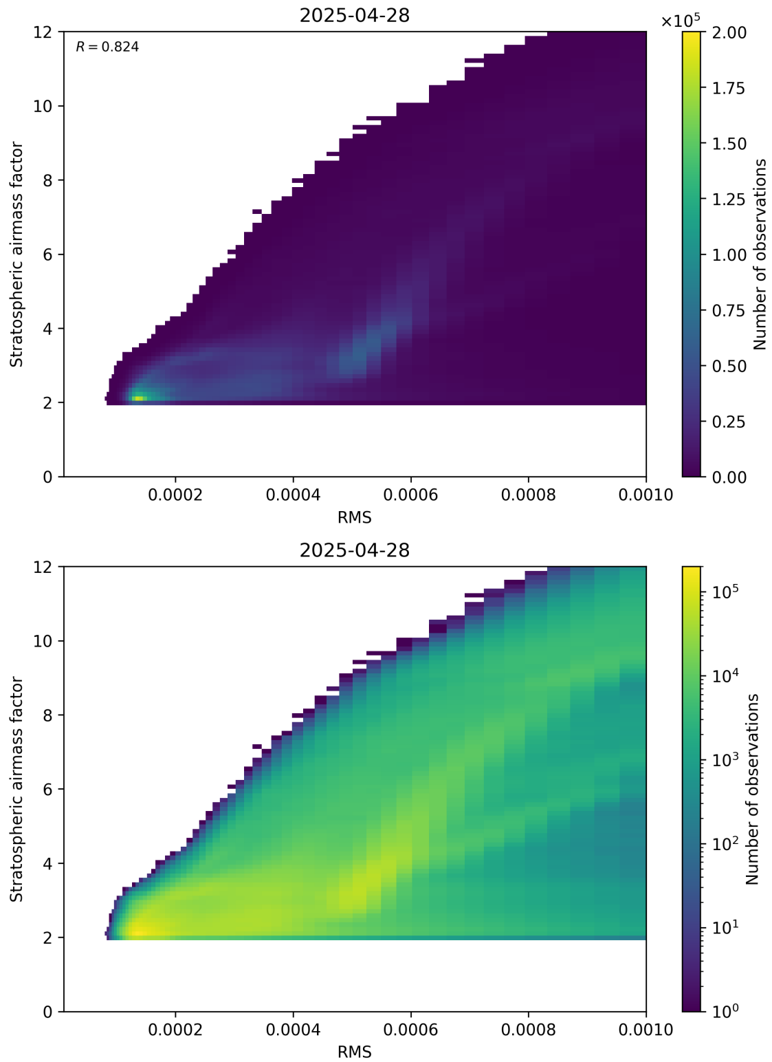
Figure 144: Scatter density plot of “RMS” against “Stratospheric airmass factor” for 2025-04-28 to 2025-04-29.
