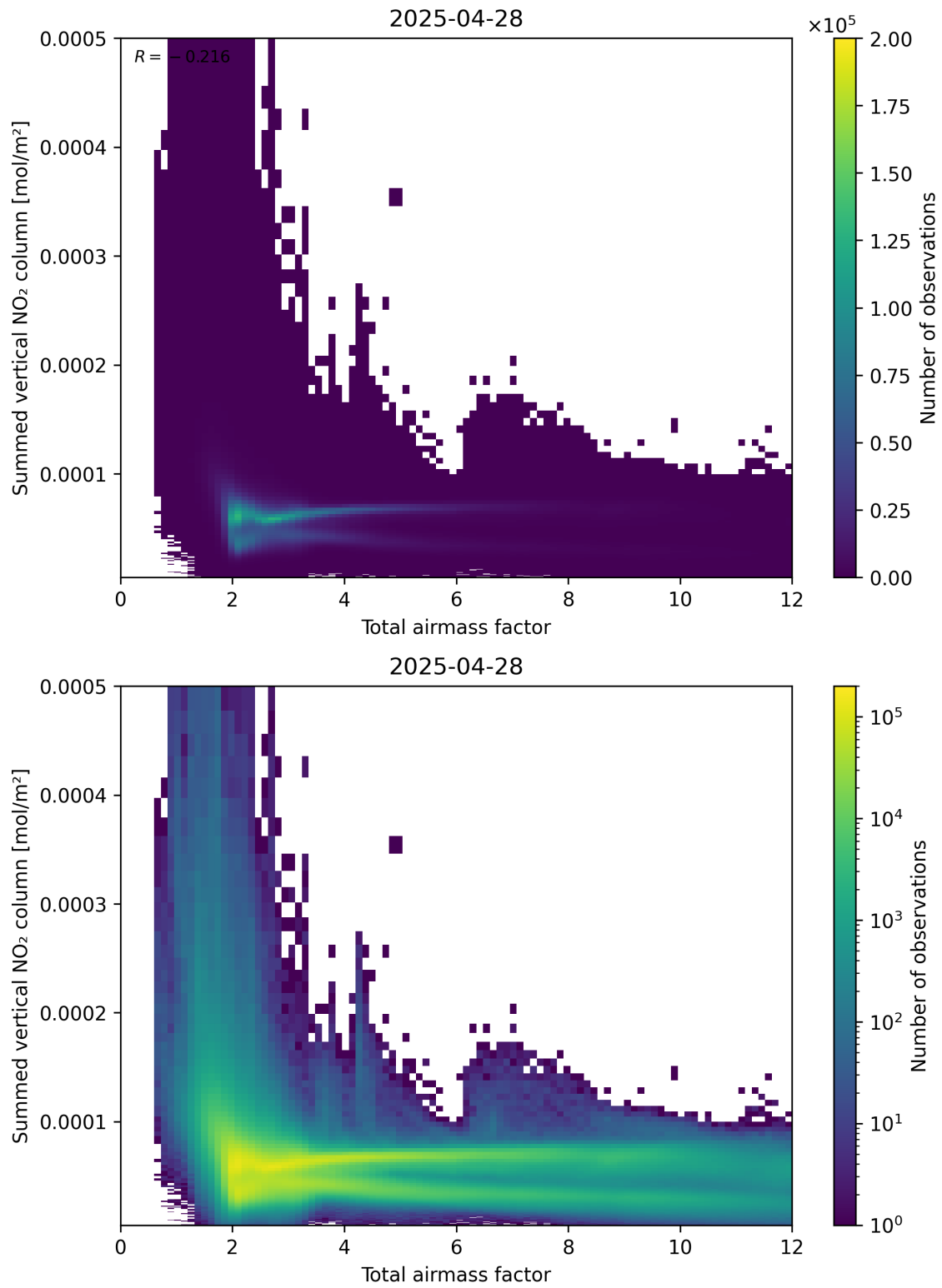
Figure 65: Scatter density plot of “Total airmass factor” against “Summed vertical NO 2 column” for 2025-04-28 to 2025-04-29.
