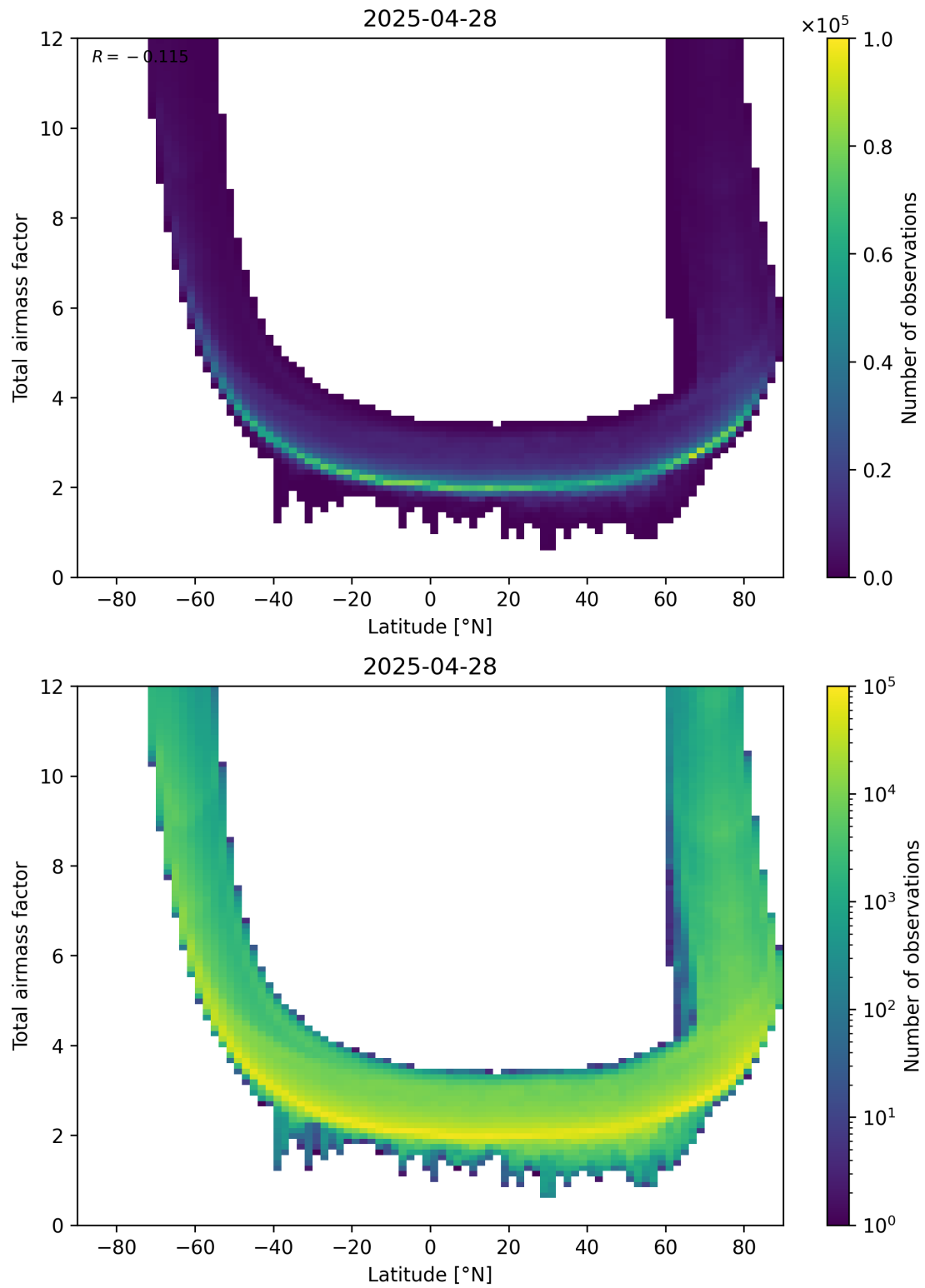
Figure 84: Scatter density plot of “Latitude” against “Total airmass factor” for 2025-04-28 to 2025-04-29.
