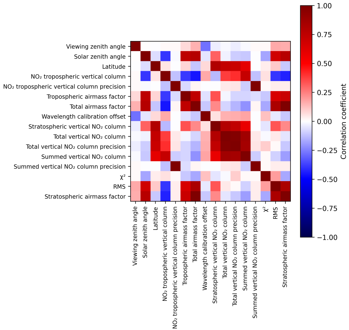
Figure 2: Map of correlation matrix for 2025-04-28 to 2025-04-29.
