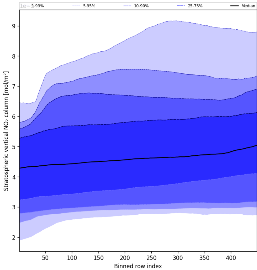
Figure 53: Along track statistics of “Stratospheric vertical NO 2 column” for 2025-04-28 to 2025-04-29
