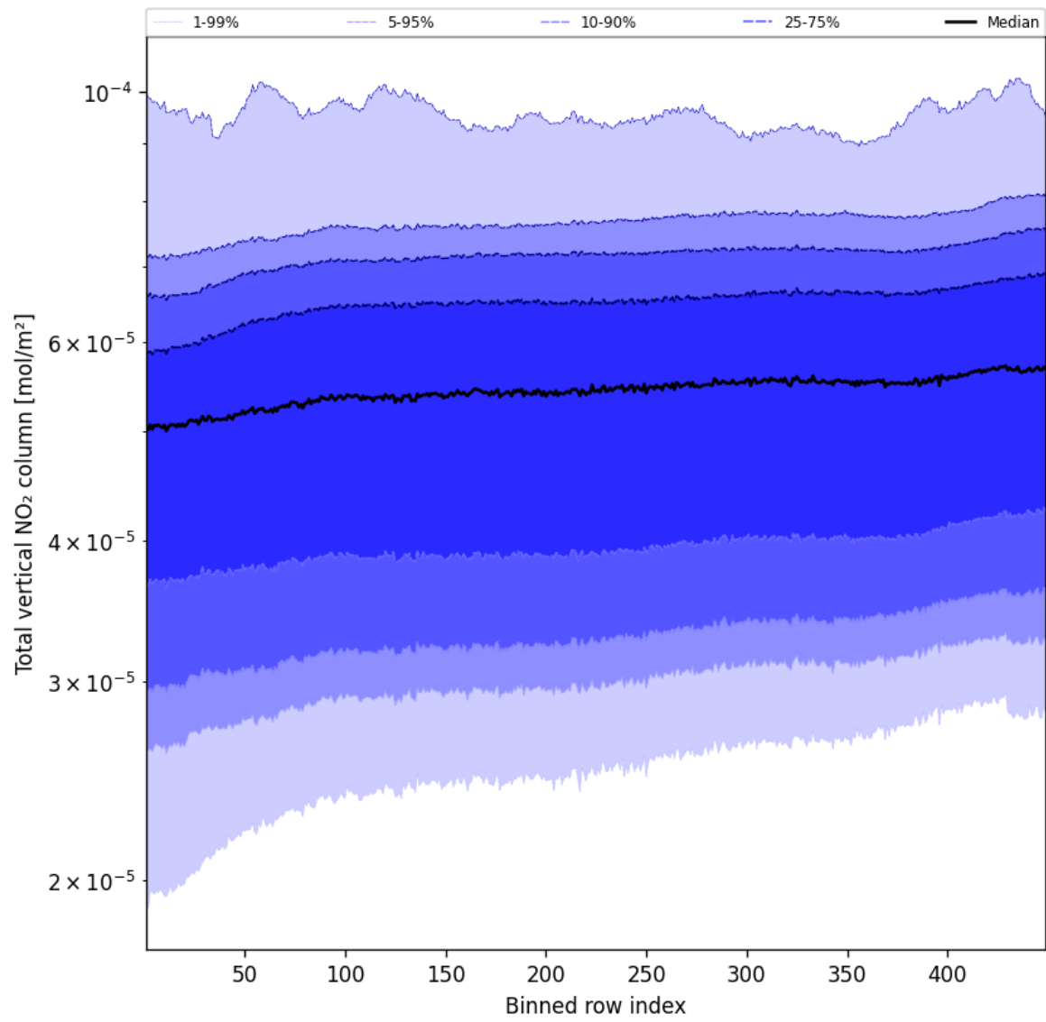
Figure 55: Along track statistics of “Total vertical NO 2 column” for 2025-04-28 to 2025-04-29
