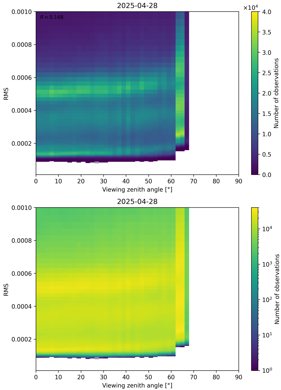
Figure 171: Scatter density plot of “Viewing zenith angle” against “RMS” for 2025-04-28 to 2025-04-29.
