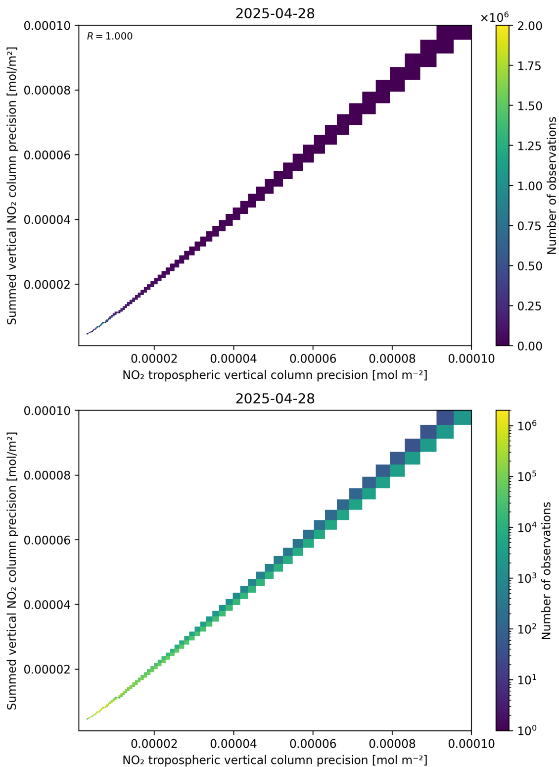
Figure 137: Scatter density plot of “NO 2 tropospheric vertical column precision” against “Summed vertical NO 2 column precision” for 2025-04-28 to 2025-04-29.
