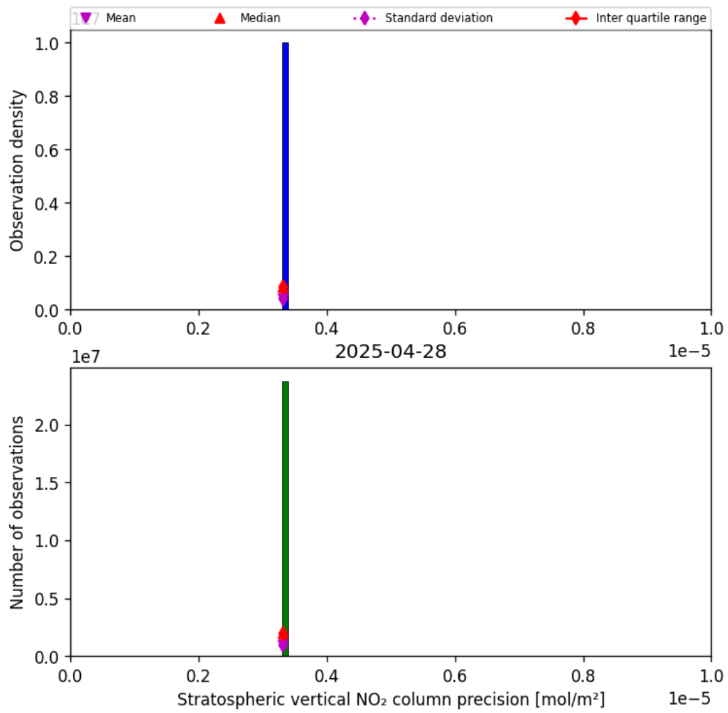
Figure 37: Histogram of “Stratospheric vertical NO 2 column precision” for 2025-04-28 to 2025-04-29
