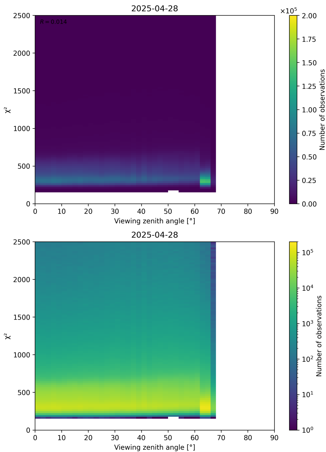
Figure 162: Scatter density plot of “Viewing zenith angle” against “ \chi^2 ” for 2025-04-28 to 2025-04-29.
