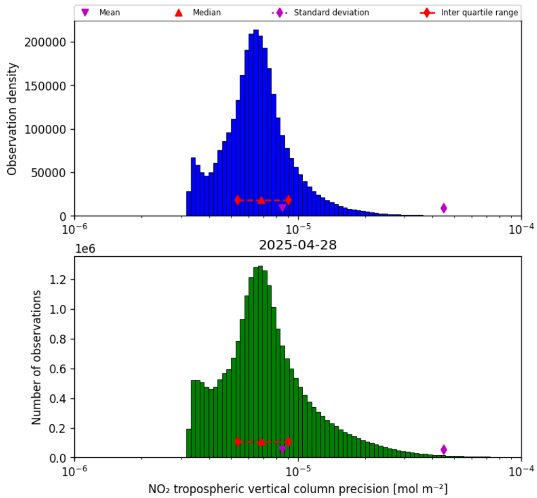
Figure 30: Histogram of “NO 2 tropospheric vertical column precision” for 2025-04-28 to 2025-04-29
