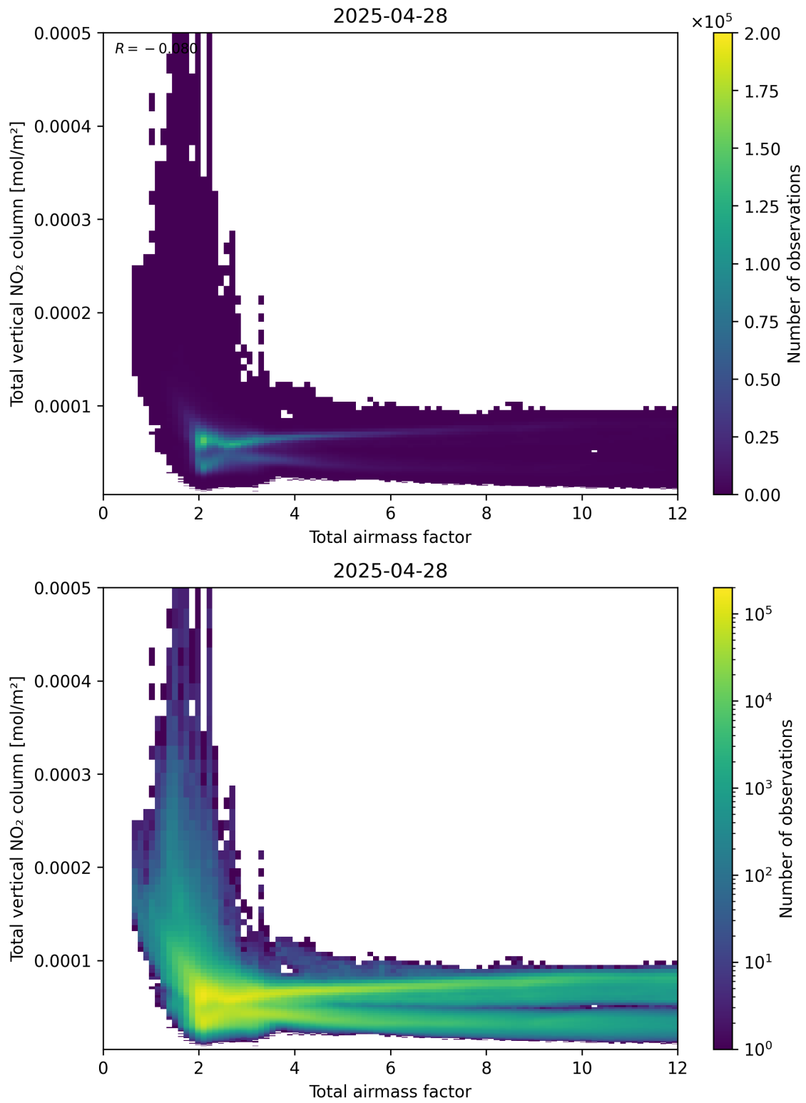
Figure 67: Scatter density plot of “Total airmass factor” against “Total vertical NO 2 column” for 2025-04-28 to 2025-04-29.
