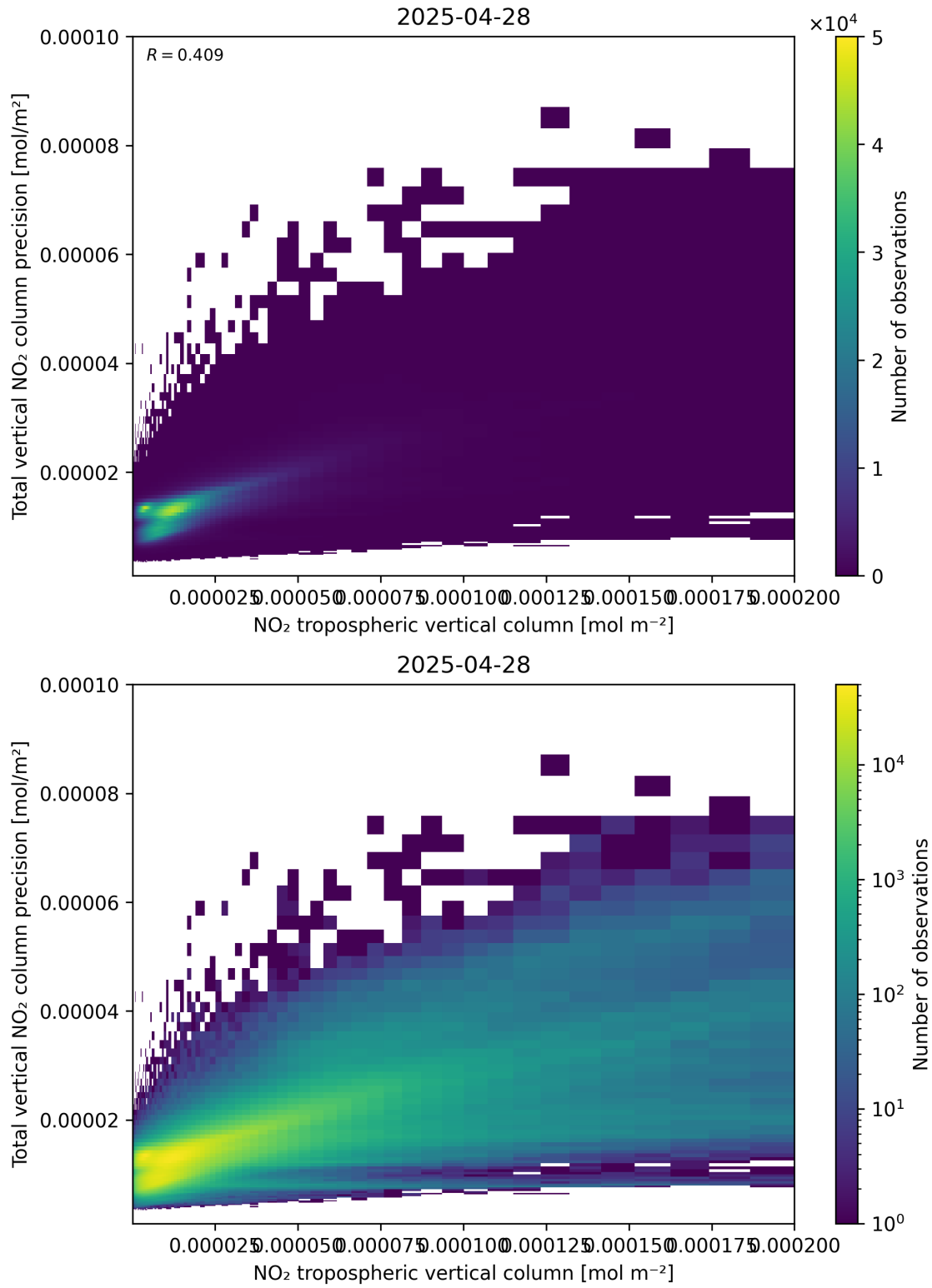
Figure 129: Scatter density plot of “NO 2 tropospheric vertical column” against “Total vertical NO 2 column precision” for 2025-04-28 to 2025-04-29.
