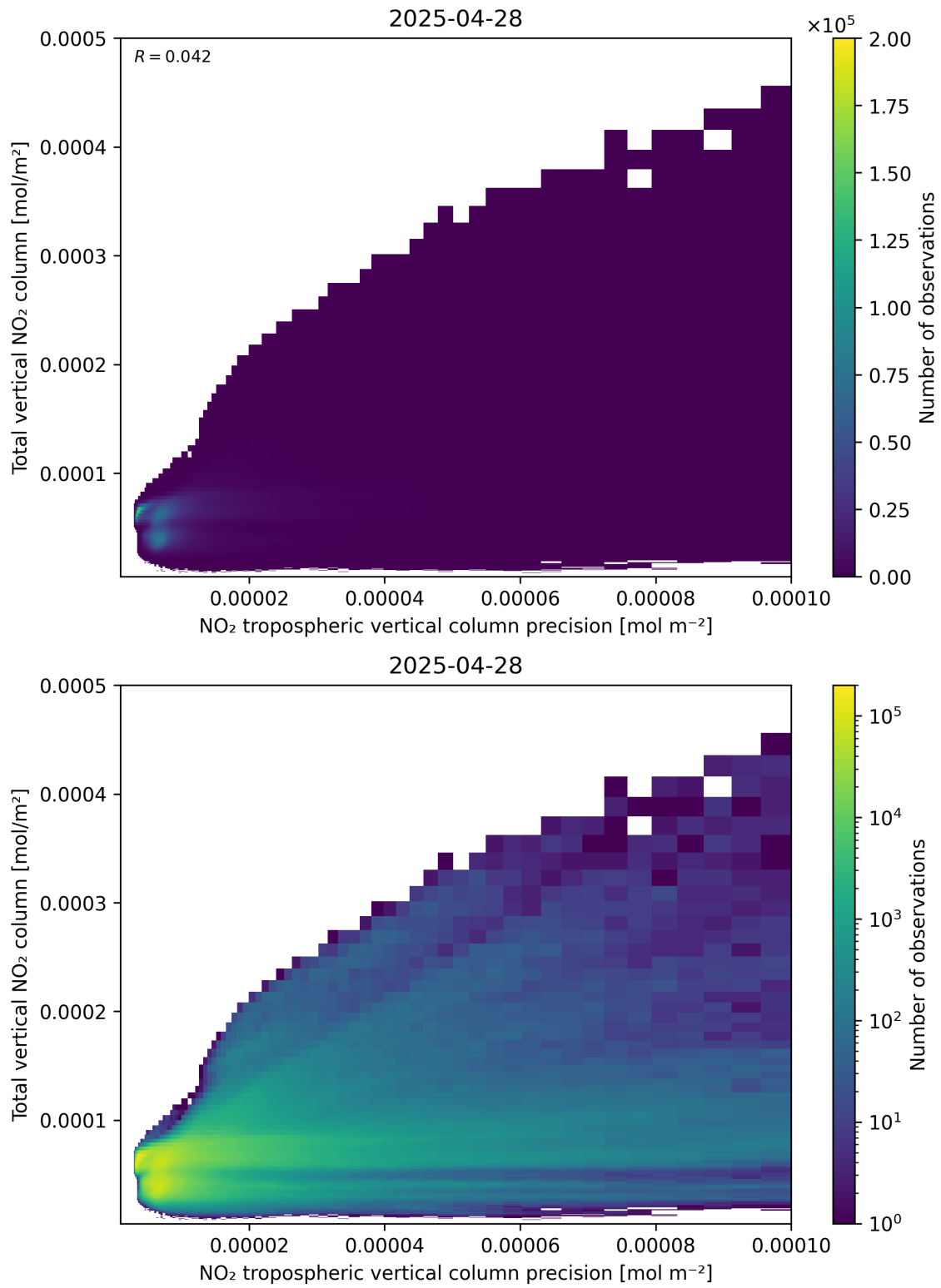
Figure 138: Scatter density plot of “NO 2 tropospheric vertical column precision” against “Total vertical NO 2 column” for 2025-04-28 to 2025-04-29.
