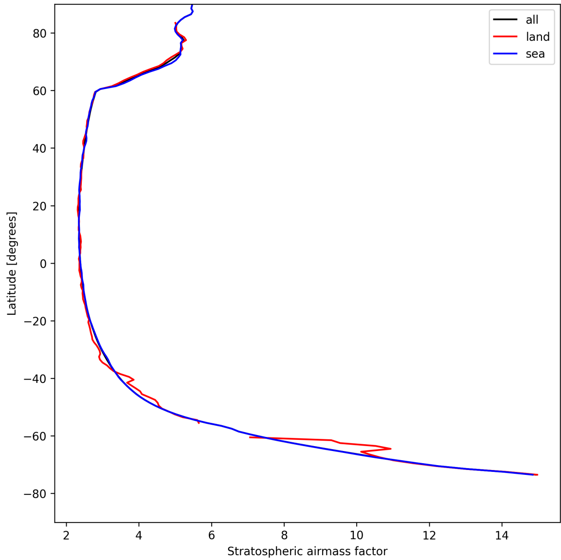
Figure 27: Zonal average of “Stratospheric airmass factor” for 2025-04-28 to 2025-04-29.
