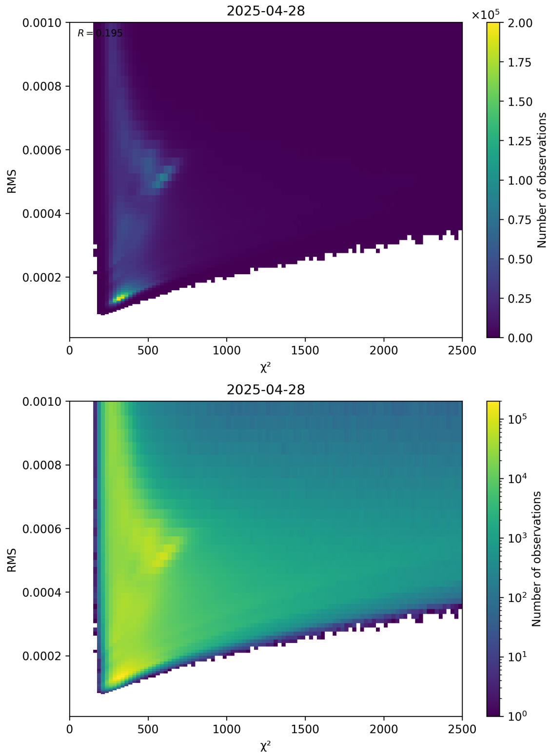
Figure 82: Scatter density plot of “ \chi^2 ” against “RMS” for 2025-04-28 to 2025-04-29.
