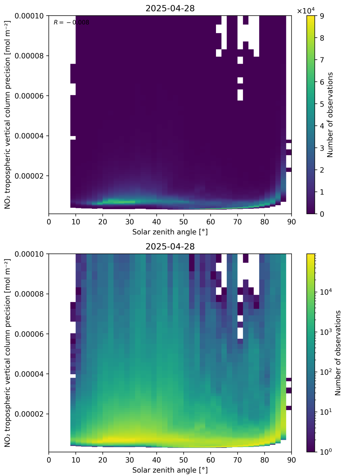
Figure 156: Scatter density plot of “Solar zenith angle” against “NO 2 tropospheric vertical column precision” for 2025-04-28 to 2025-04-29.
