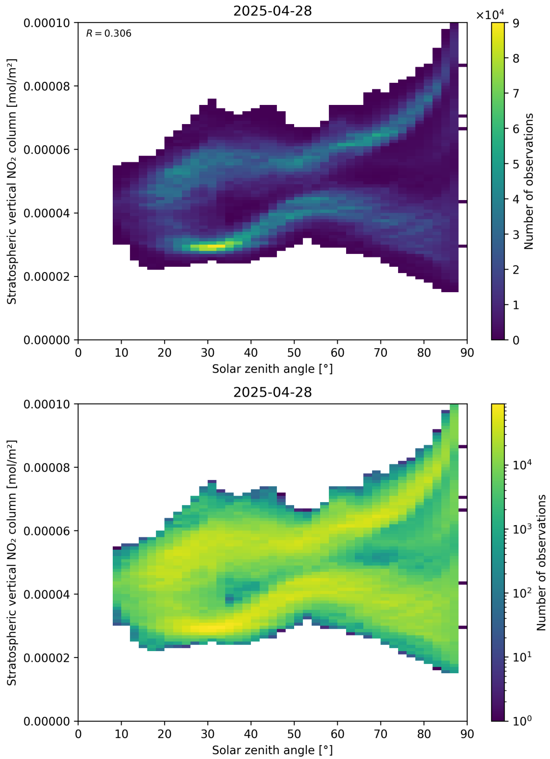
Figure 150: Scatter density plot of “Solar zenith angle” against “Stratospheric vertical NO 2 column” for 2025-04-28 to 2025-04-29.
