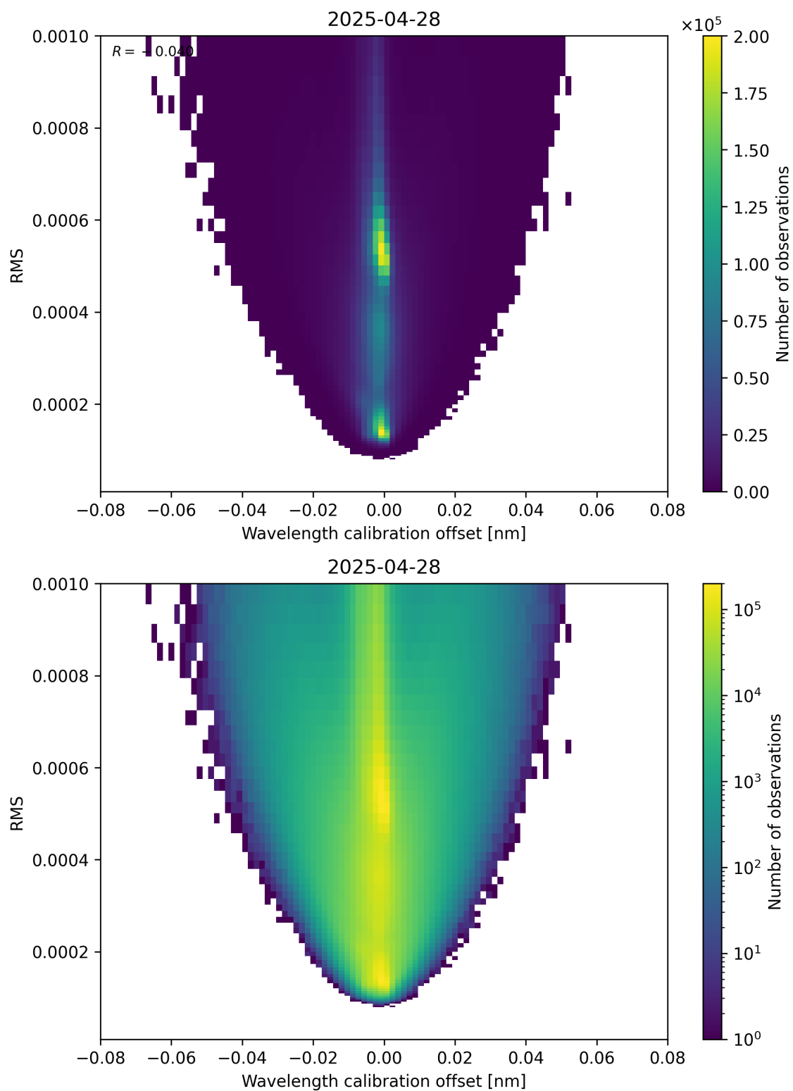
Figure 181: Scatter density plot of “Wavelength calibration offset” against “RMS” for 2025-04-28 to 2025-04-29.
