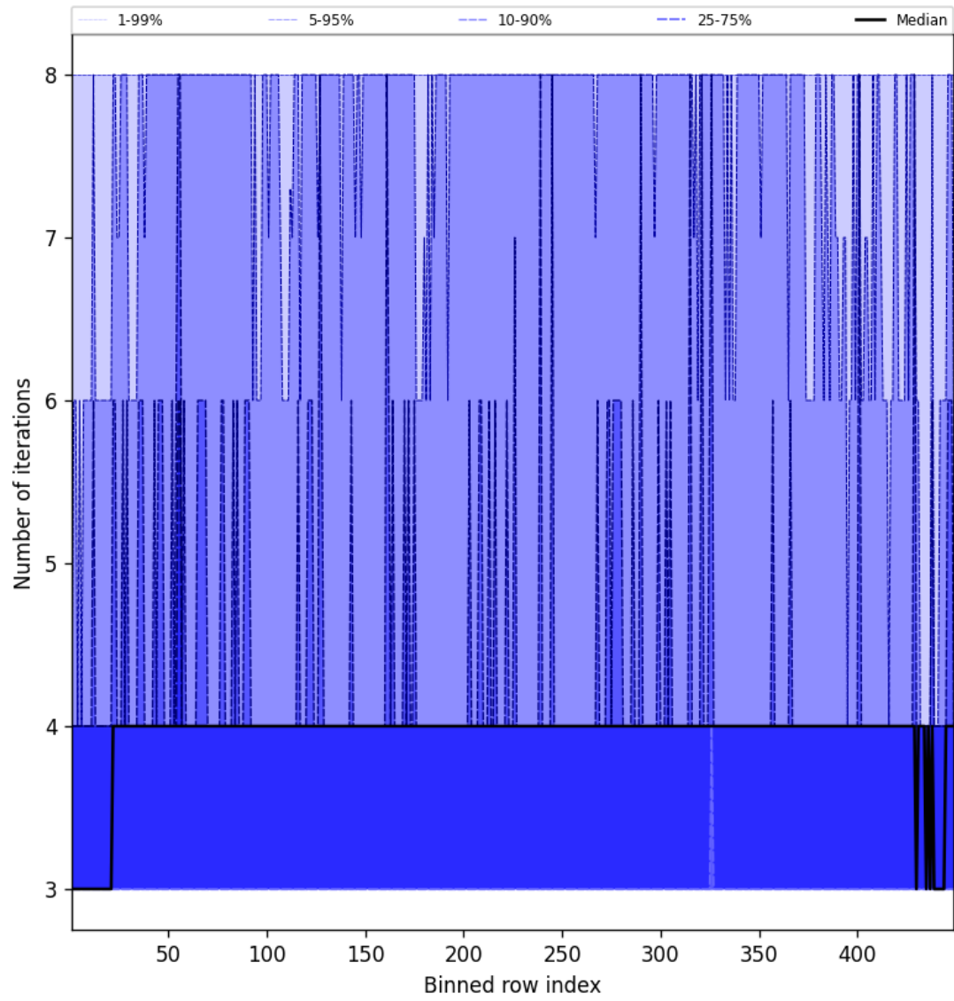
Figure 51: Along track statistics of “Number of iterations” for 2025-04-28 to 2025-04-29
