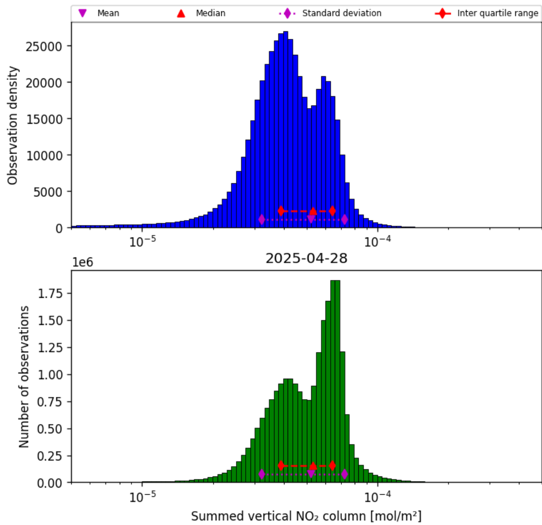
Figure 40: Histogram of “Summed vertical NO 2 column” for 2025-04-28 to 2025-04-29
