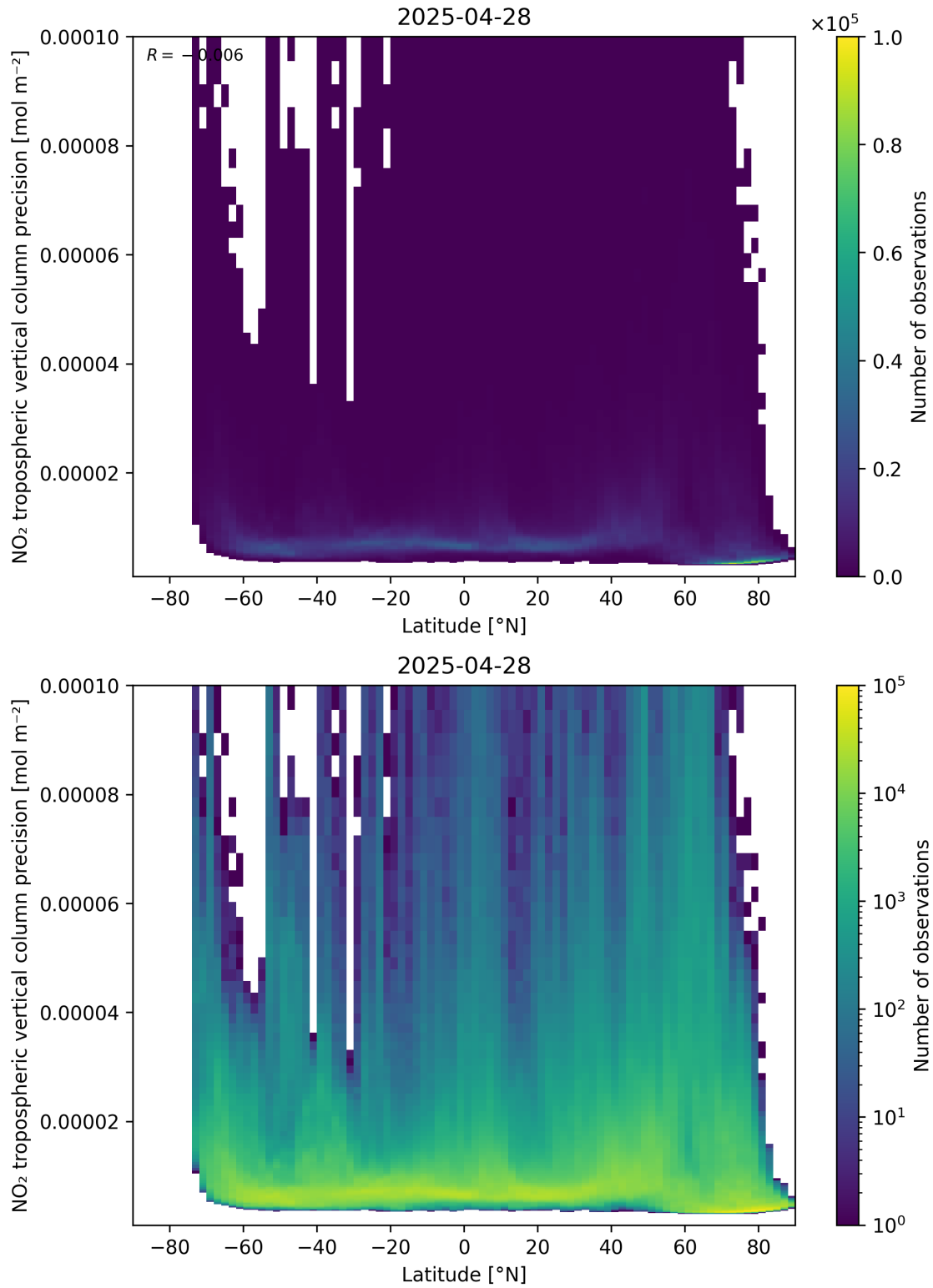
Figure 93: Scatter density plot of “Latitude” against “NO 2 tropospheric vertical column precision” for 2025-04-28 to 2025-04-29.
