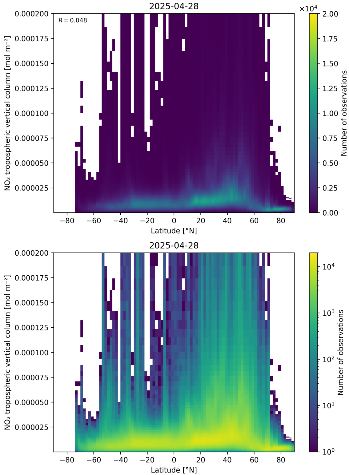
Figure 92: Scatter density plot of “Latitude” against “NO 2 tropospheric vertical column” for 2025-04-28 to 2025-04-29.
