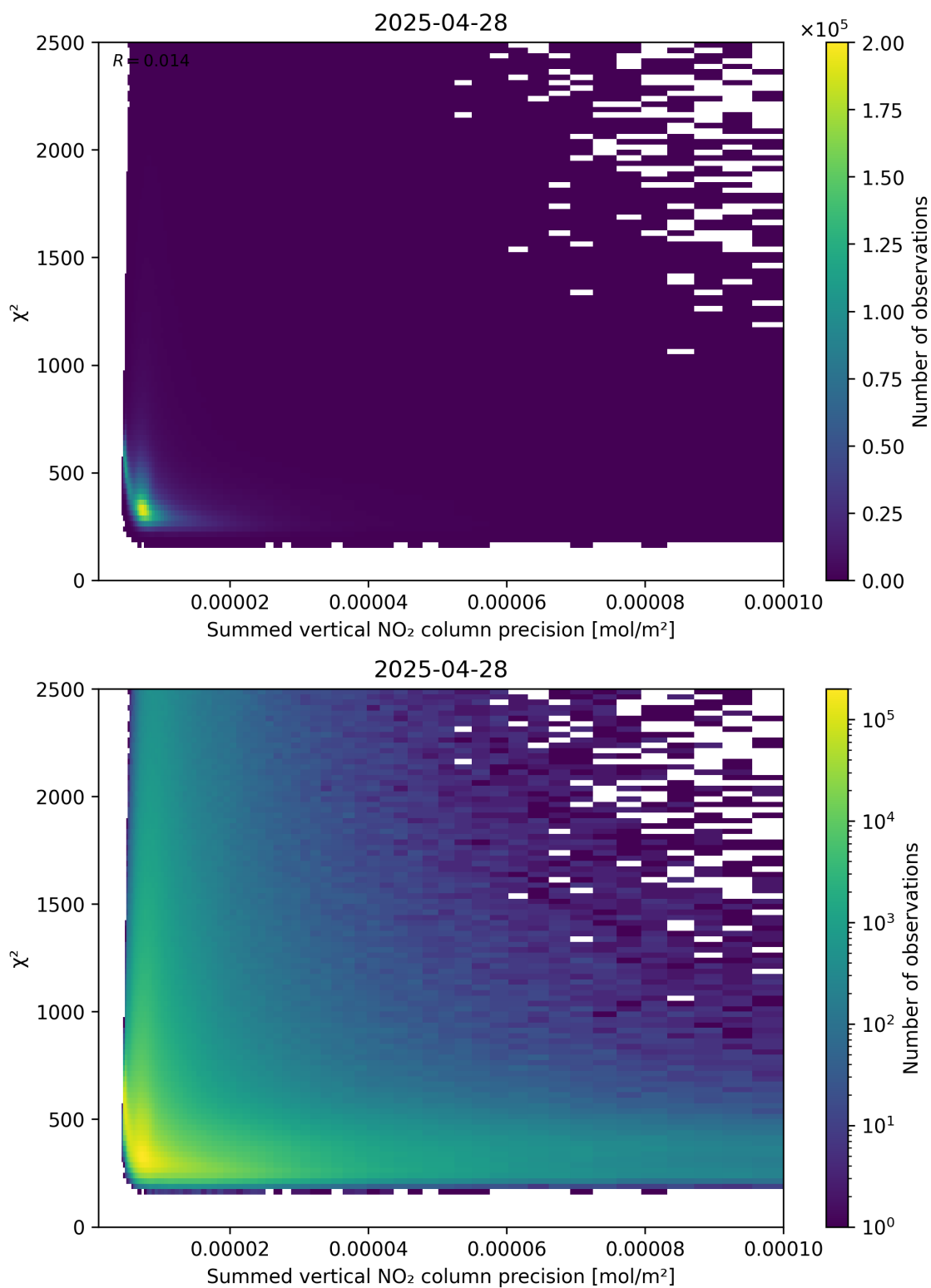
Figure 107: Scatter density plot of “Summed vertical NO 2 column precision” against “ \chi^2 ” for 2025-04-28 to 2025-04-29.
