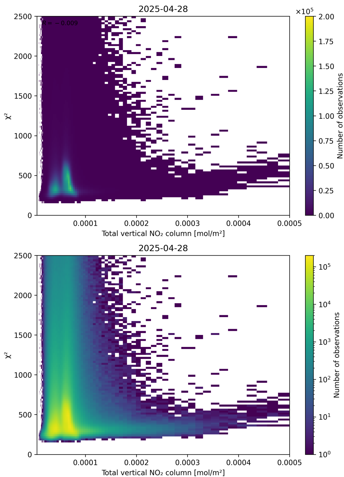
Figure 111: Scatter density plot of “Total vertical NO 2 column” against “ \chi^2 ” for 2025-04-28 to 2025-04-29.
