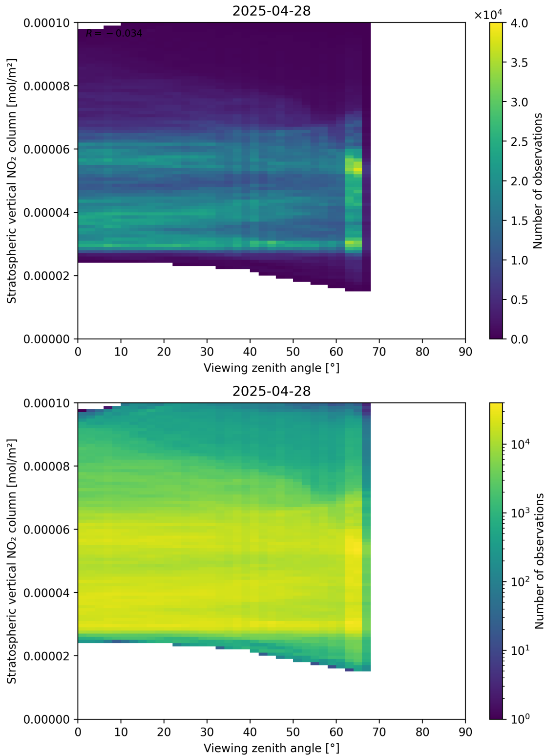
Figure 164: Scatter density plot of “Viewing zenith angle” against “Stratospheric vertical NO 2 column” for 2025-04-28 to 2025-04-29.
