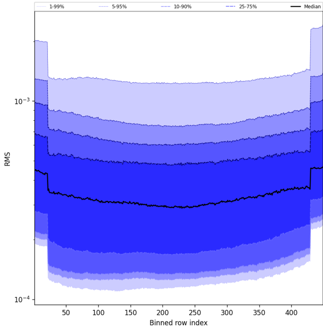
Figure 60: Along track statistics of “RMS” for 2025-04-28 to 2025-04-29
