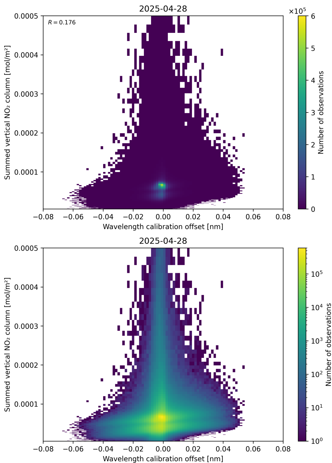
Figure 177: Scatter density plot of “Wavelength calibration offset” against “Summed vertical NO 2 column” for 2025-04-28 to 2025-04-29.
