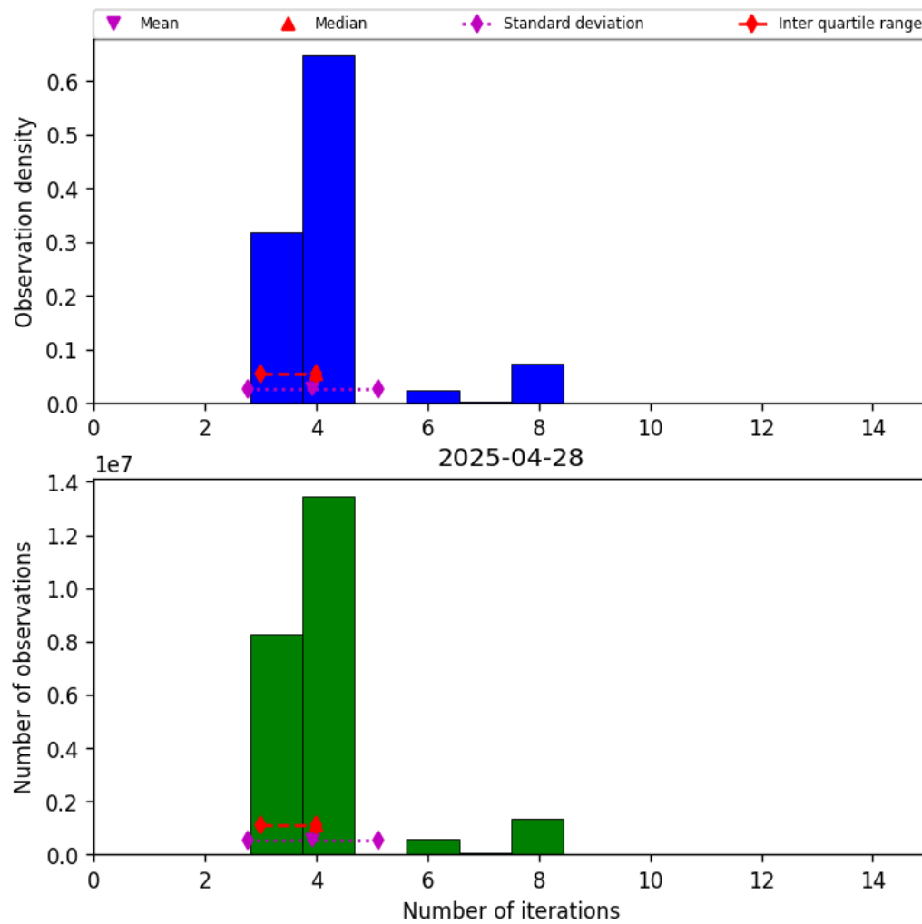
Figure 34: Histogram of “Number of iterations” for 2025-04-28 to 2025-04-29
