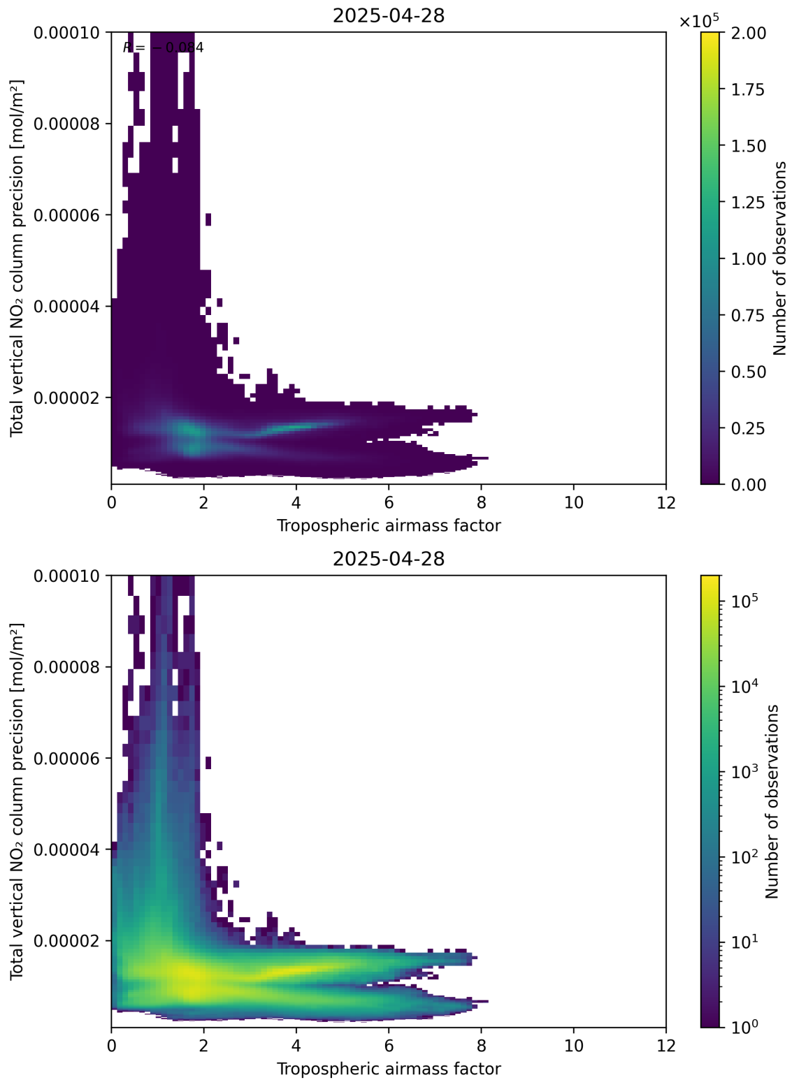
Figure 78: Scatter density plot of “Tropospheric airmass factor” against “Total vertical NO 2 column precision” for 2025-04-28 to 2025-04-29.
