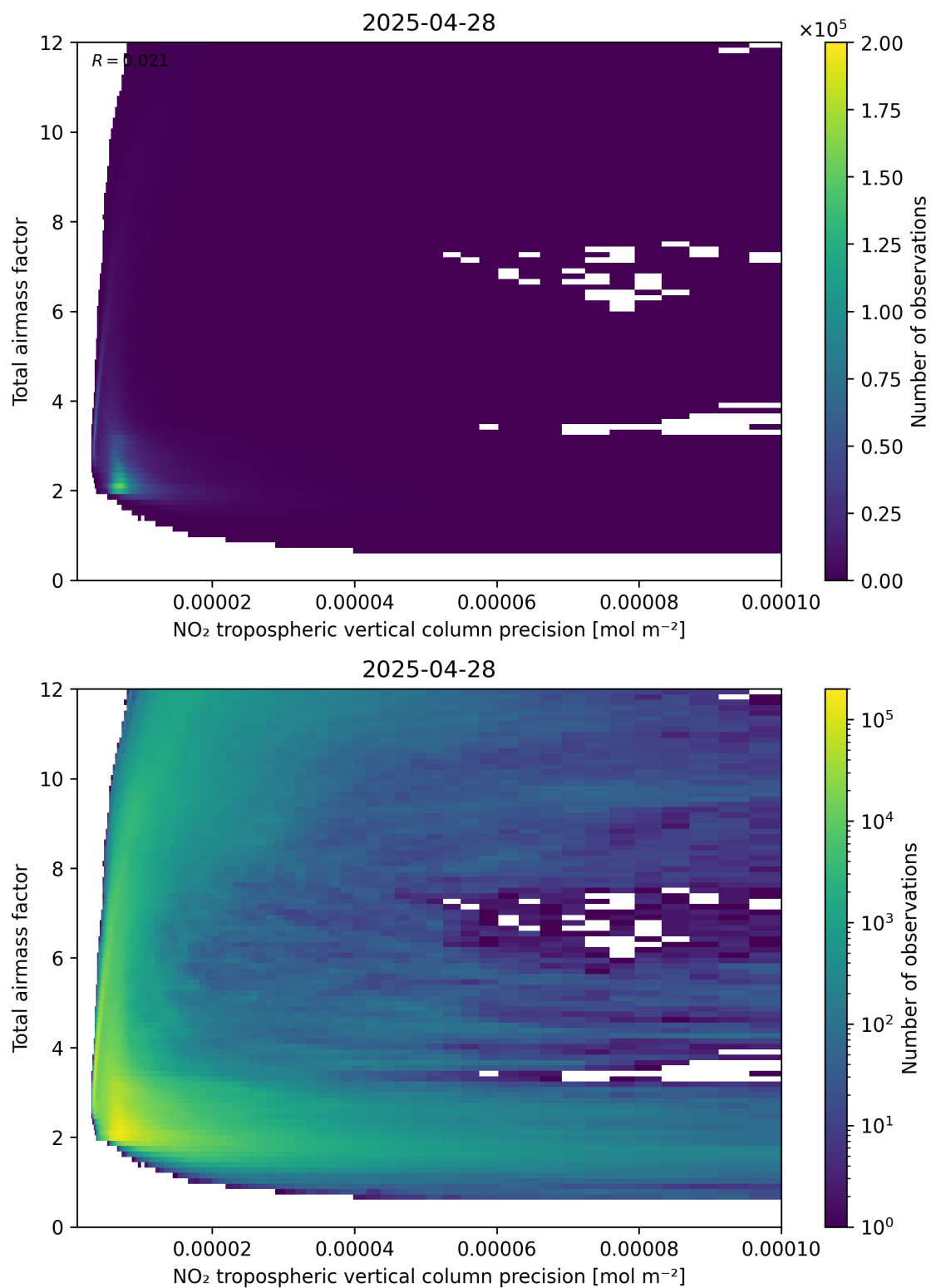
Figure 132: Scatter density plot of “NO 2 tropospheric vertical column precision” against “Total air mass factor” for 2025-04-28 to 2025-04-29.
