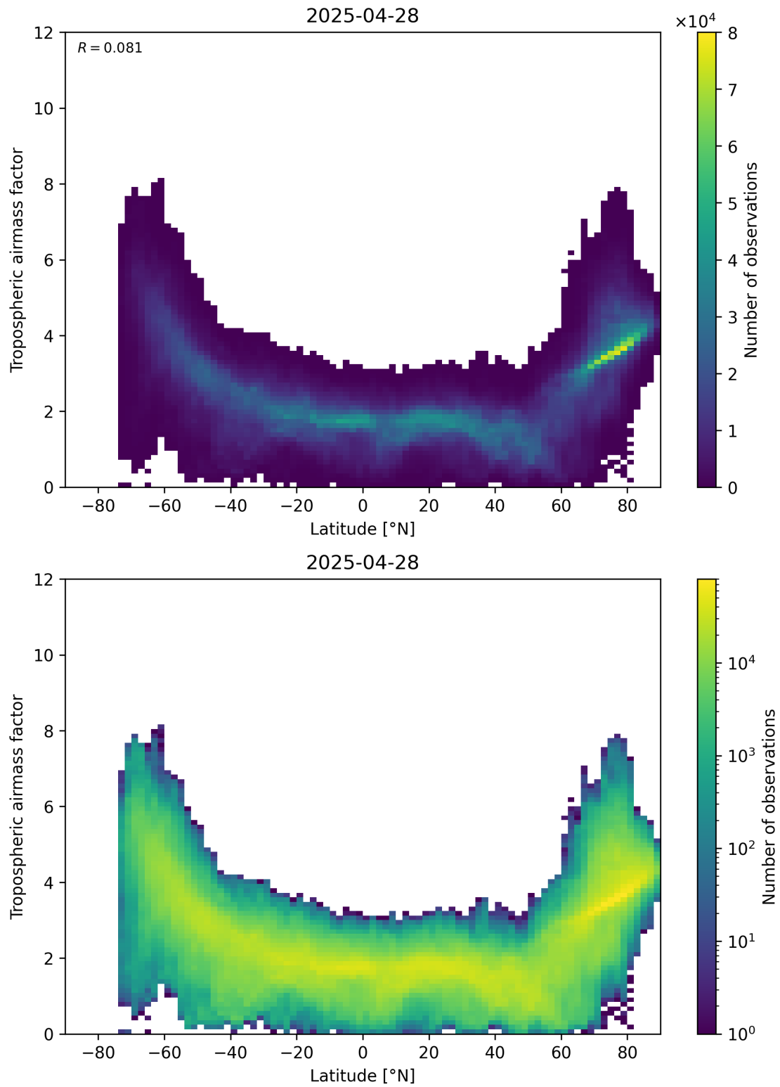
Figure 85: Scatter density plot of “Latitude” against “Tropospheric airmass factor” for 2025-04-28 to 2025-04-29.
