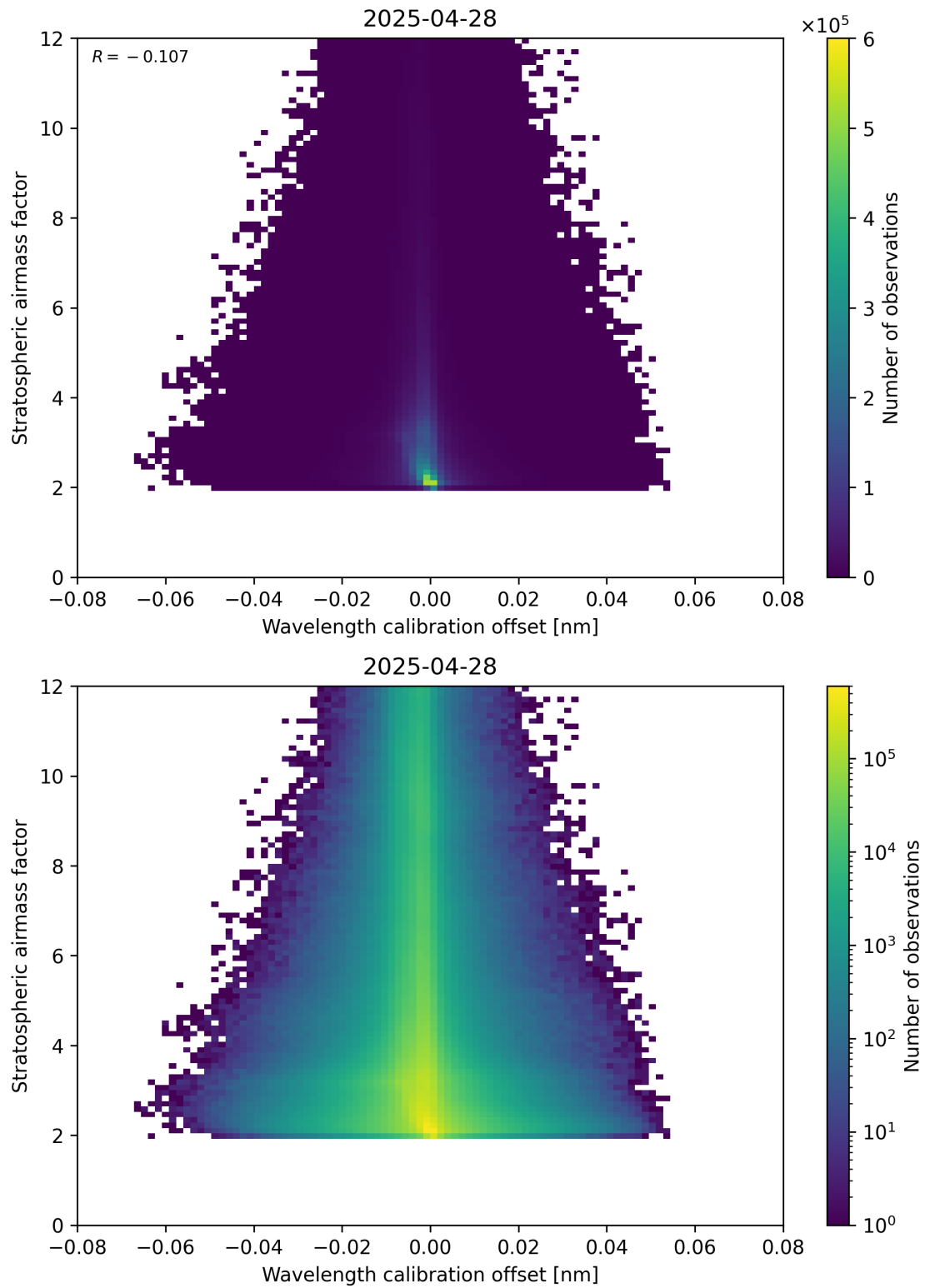
Figure 174: Scatter density plot of “Wavelength calibration offset” against “Stratospheric airmass factor” for 2025-04-28 to 2025-04-29.
