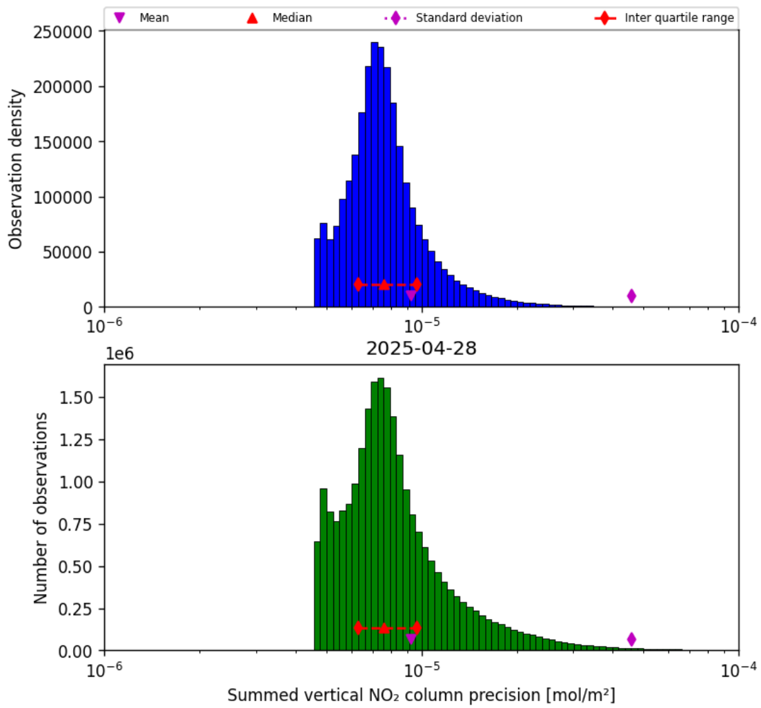
Figure 41: Histogram of “Summed vertical NO 2 column precision” for 2025-04-28 to 2025-04-29
