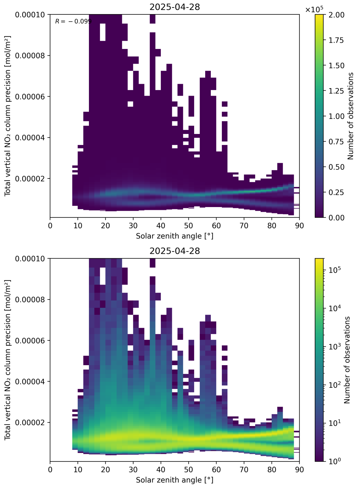
Figure 154: Scatter density plot of “Solar zenith angle” against “Total vertical NO 2 column precision” for 2025-04-28 to 2025-04-29.
