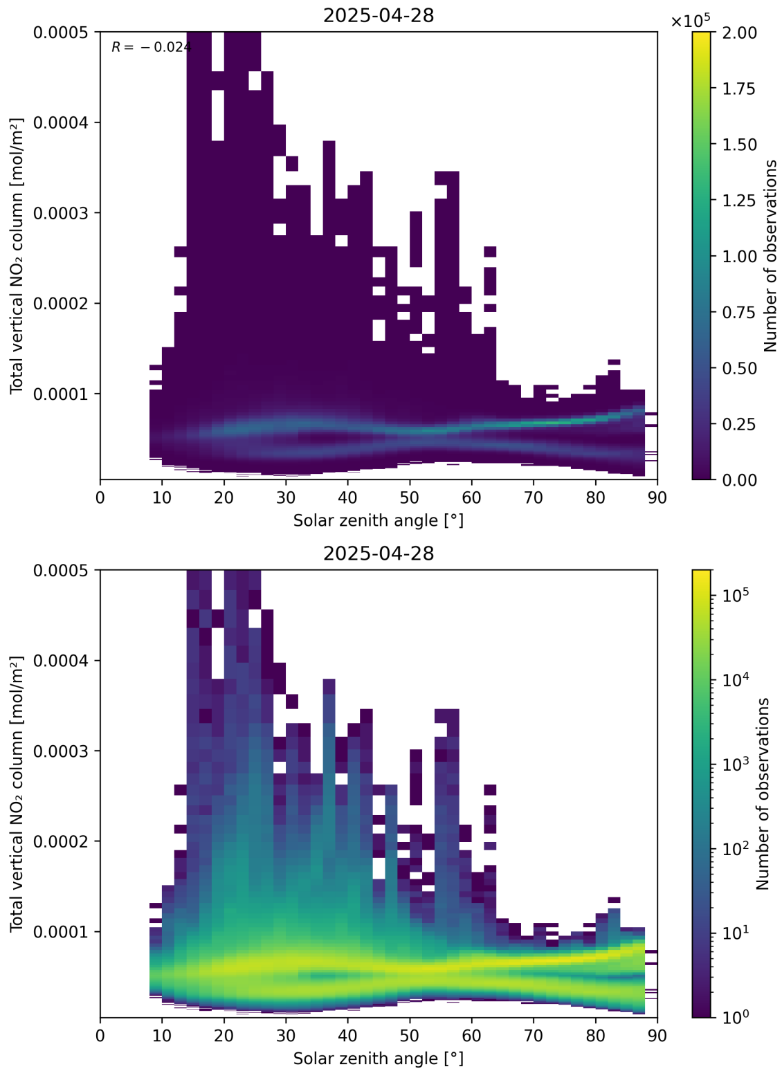
Figure 153: Scatter density plot of “Solar zenith angle” against “Total vertical NO 2 column” for 2025-04-28 to 2025-04-29.
