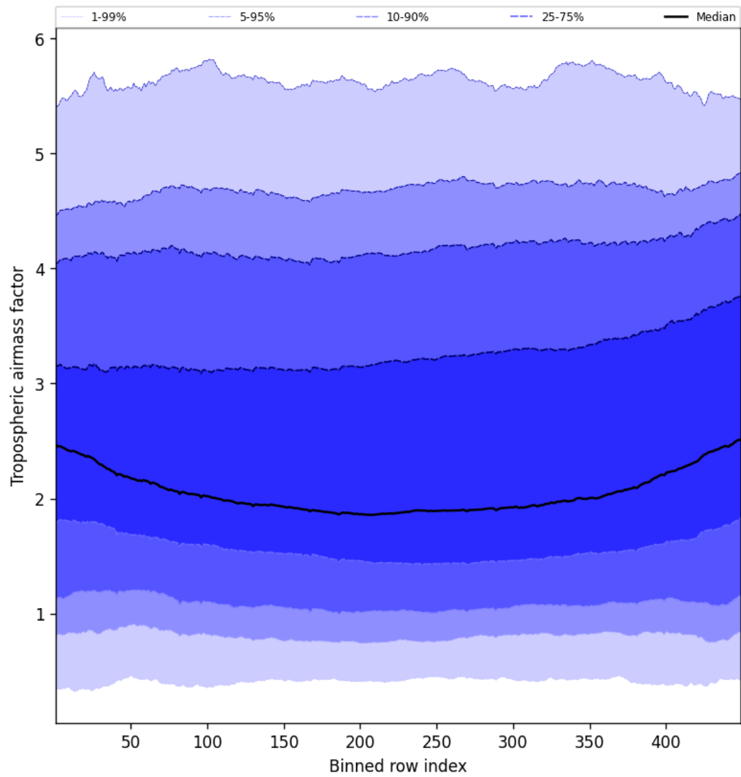
Figure 48: Along track statistics of “Tropospheric airmass factor” for 2025-04-28 to 2025-04-29
