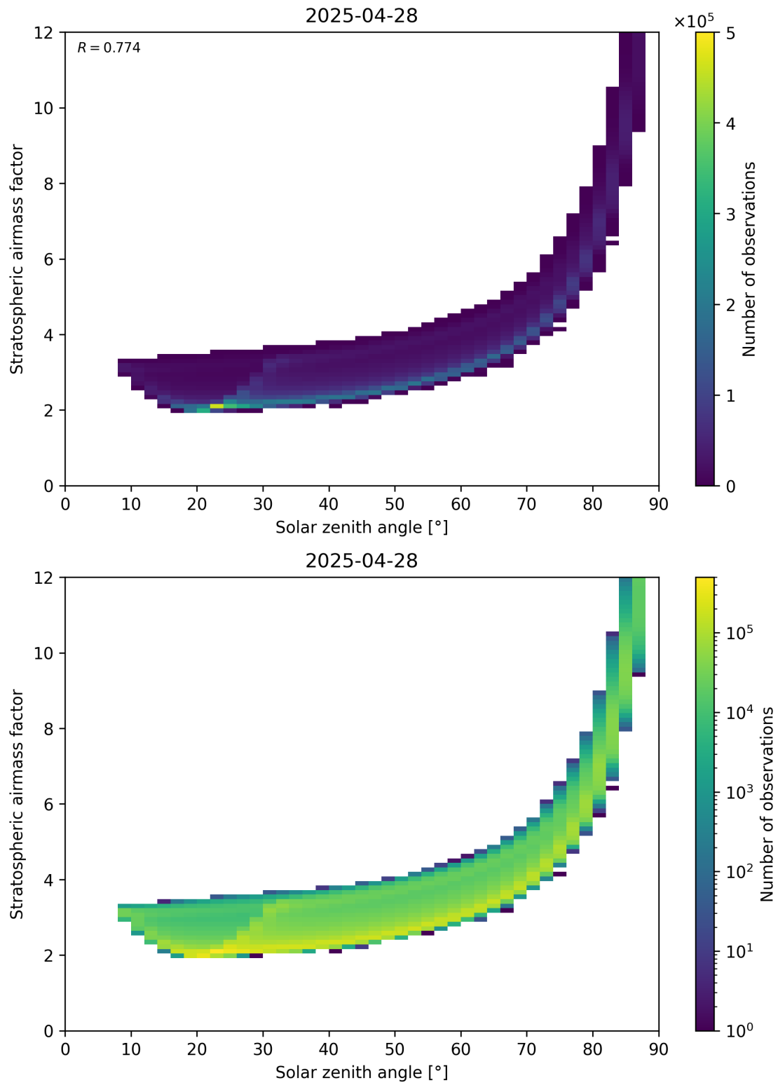
Figure 145: Scatter density plot of “Solar zenith angle” against “Stratospheric airmass factor” for 2025-04-28 to 2025-04-29.
