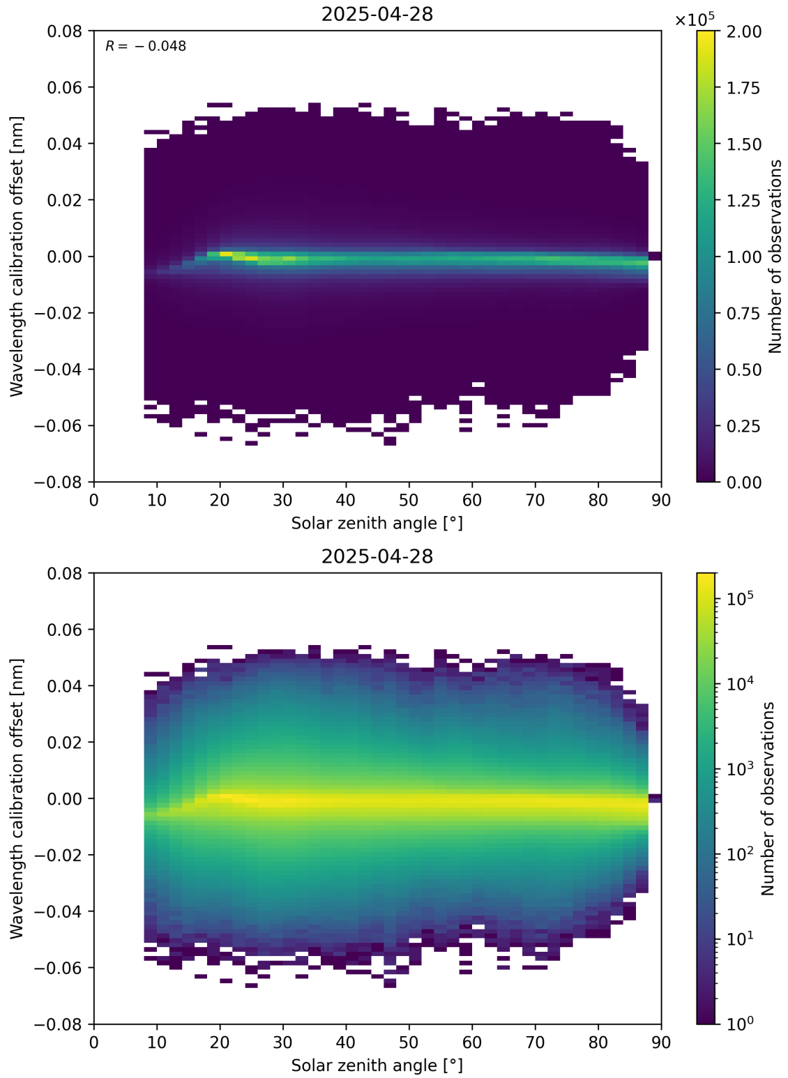
Figure 158: Scatter density plot of “Solar zenith angle” against “Wavelength calibration offset” for 2025-04-28 to 2025-04-29.
