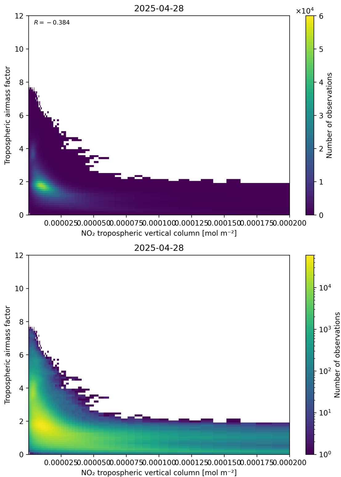
Figure 123: Scatter density plot of “NO 2 tropospheric vertical column” against “Tropospheric air mass factor” for 2025-04-28 to 2025-04-29.
