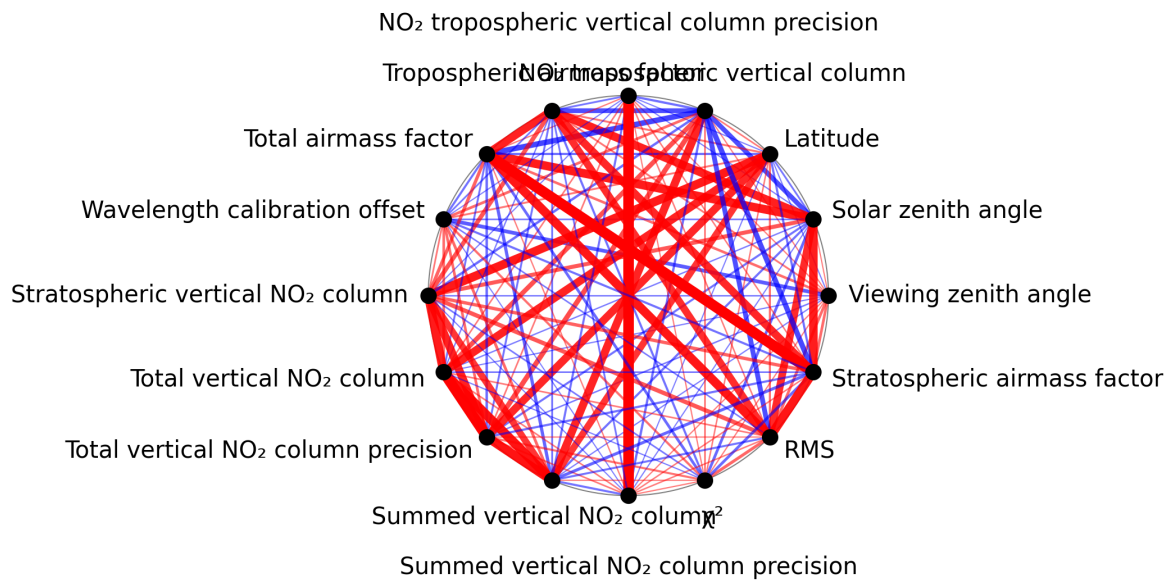
Figure 1: Map of correlation graph for 2025-04-28 to 2025-04-29.
