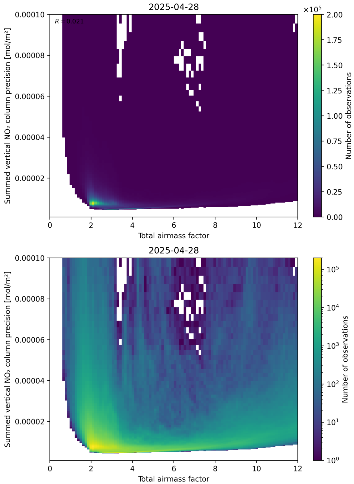
Figure 66: Scatter density plot of “Total airmass factor” against “Summed vertical NO 2 column precision” for 2025-04-28 to 2025-04-29.
