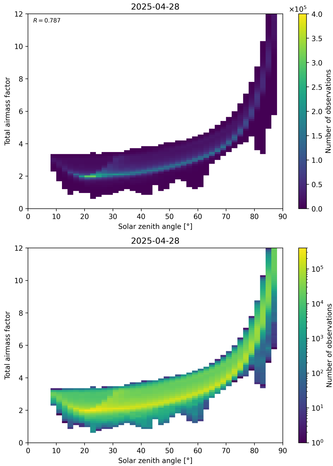
Figure 146: Scatter density plot of “Solar zenith angle” against “Total air mass factor” for 2025-04-28 to 2025-04-29.
