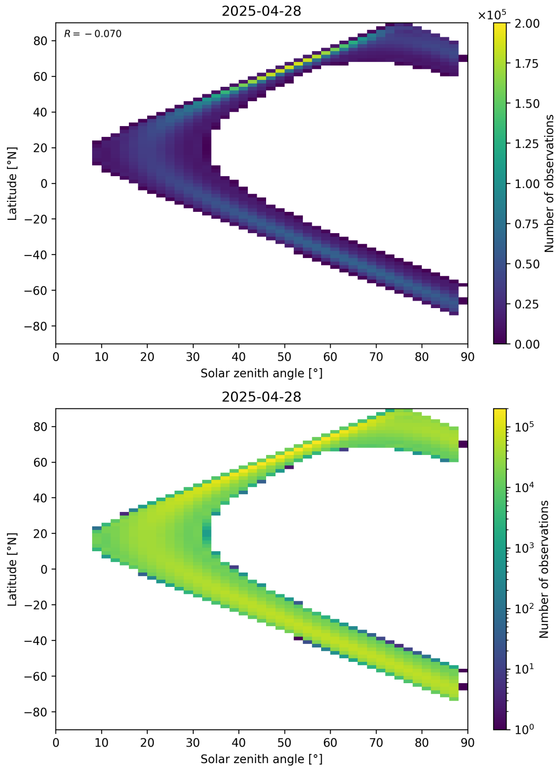
Figure 149: Scatter density plot of “Solar zenith angle” against “Latitude” for 2025-04-28 to 2025-04-29.
