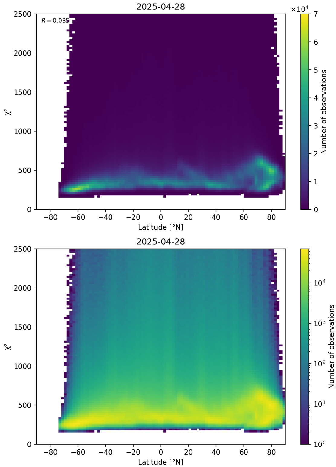
Figure 86: Scatter density plot of “Latitude” against “ \chi^2 ” for 2025-04-28 to 2025-04-29.
