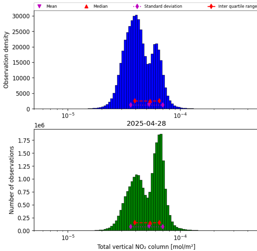
Figure 38: Histogram of “Total vertical NO 2 column” for 2025-04-28 to 2025-04-29
