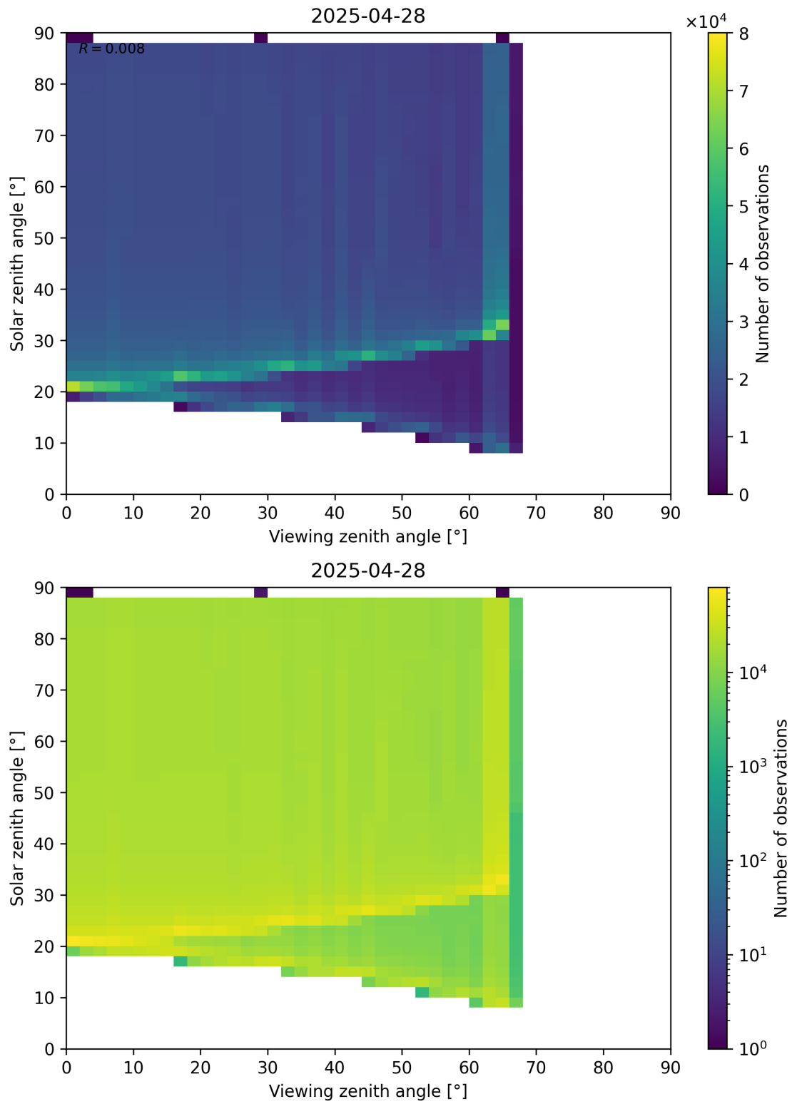
Figure 172: Scatter density plot of “Viewing zenith angle” against “Solar zenith angle” for 2025-04-28 to 2025-04-29.
