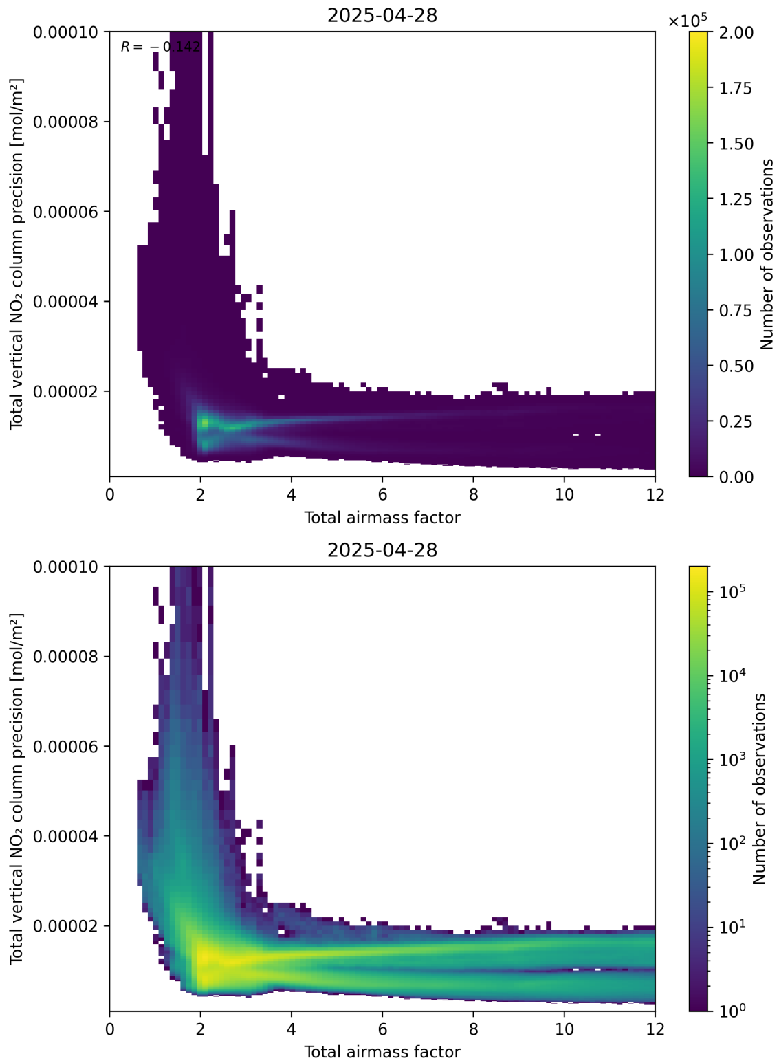
Figure 68: Scatter density plot of “Total airmass factor” against “Total vertical NO 2 column precision” for 2025-04-28 to 2025-04-29.
