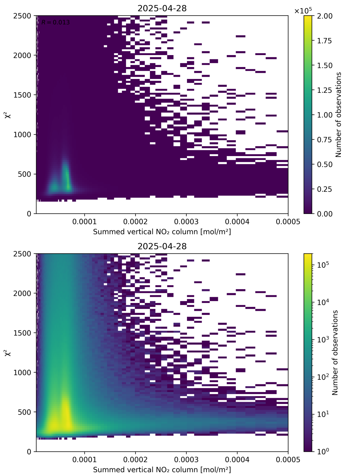
Figure 104: Scatter density plot of “Summed vertical NO 2 column” against “ \chi^2 ” for 2025-04-28 to 2025-04-29.
