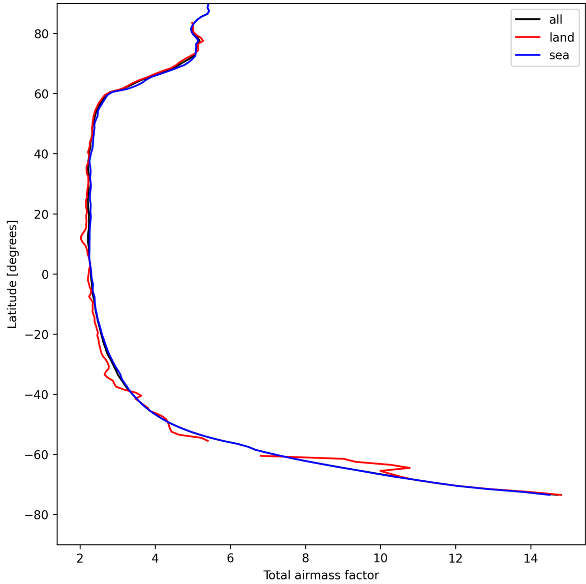
Figure 15: Zonal average of “Total airmass factor” for 2025-04-28 to 2025-04-29.
