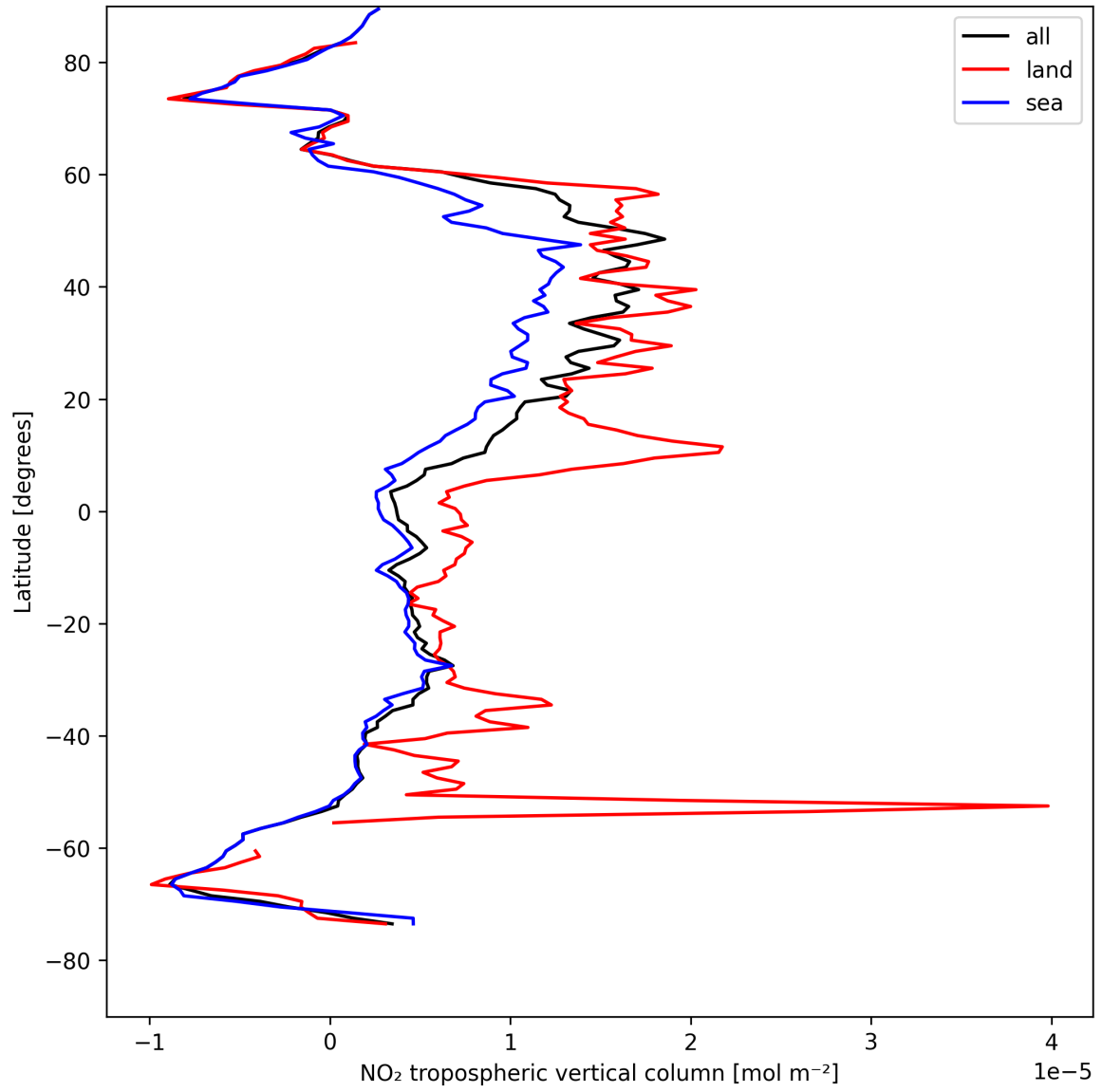
Figure 12: Zonal average of “NO 2 tropospheric vertical column” for 2025-04-28 to 2025-04-29.
