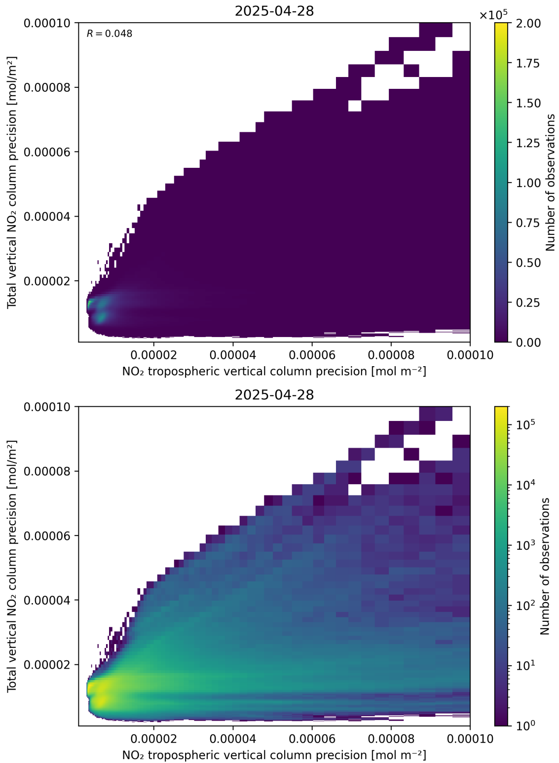
Figure 139: Scatter density plot of “NO 2 tropospheric vertical column precision” against “Total vertical NO 2 column precision” for 2025-04-28 to 2025-04-29.
