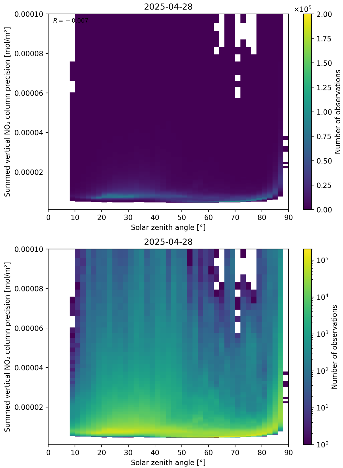
Figure 152: Scatter density plot of “Solar zenith angle” against “Summed vertical NO 2 column precision” for 2025-04-28 to 2025-04-29.
