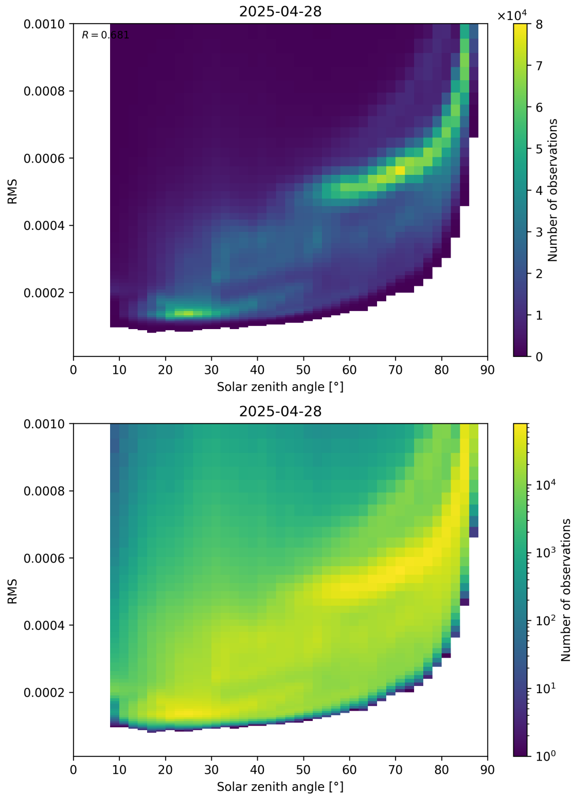
Figure 157: Scatter density plot of “Solar zenith angle” against “RMS” for 2025-04-28 to 2025-04-29.
