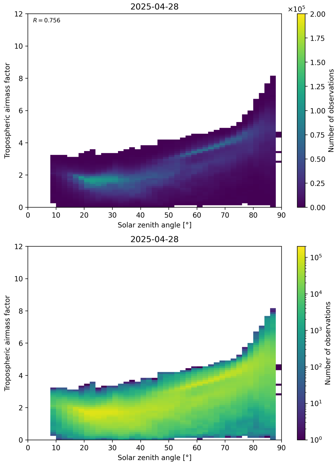
Figure 147: Scatter density plot of “Solar zenith angle” against “Tropospheric airmass factor” for 2025-04-28 to 2025-04-29.
