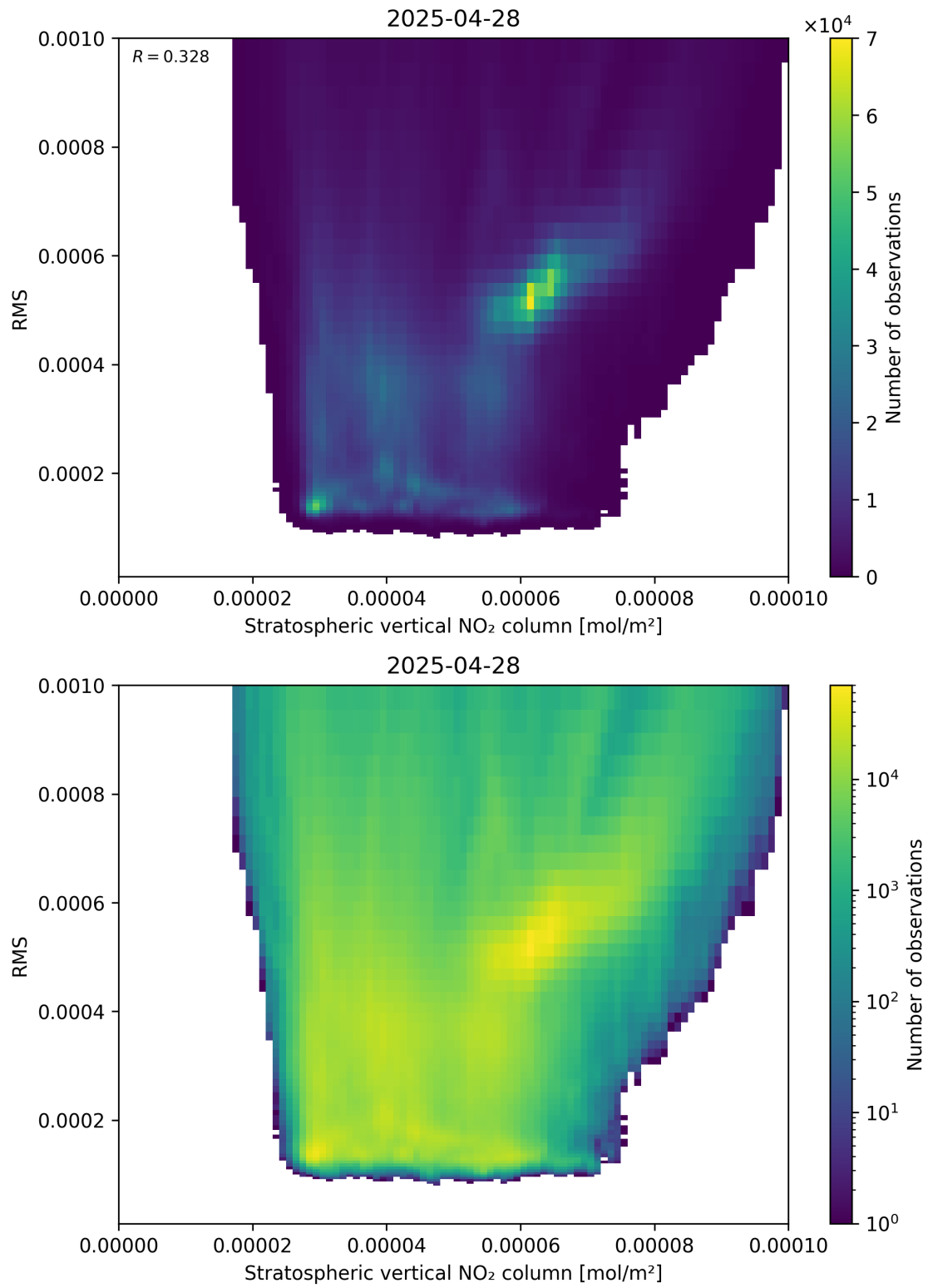
Figure 102: Scatter density plot of “Stratospheric vertical NO 2 column” against “RMS” for 2025-04-28 to 2025-04-29.
