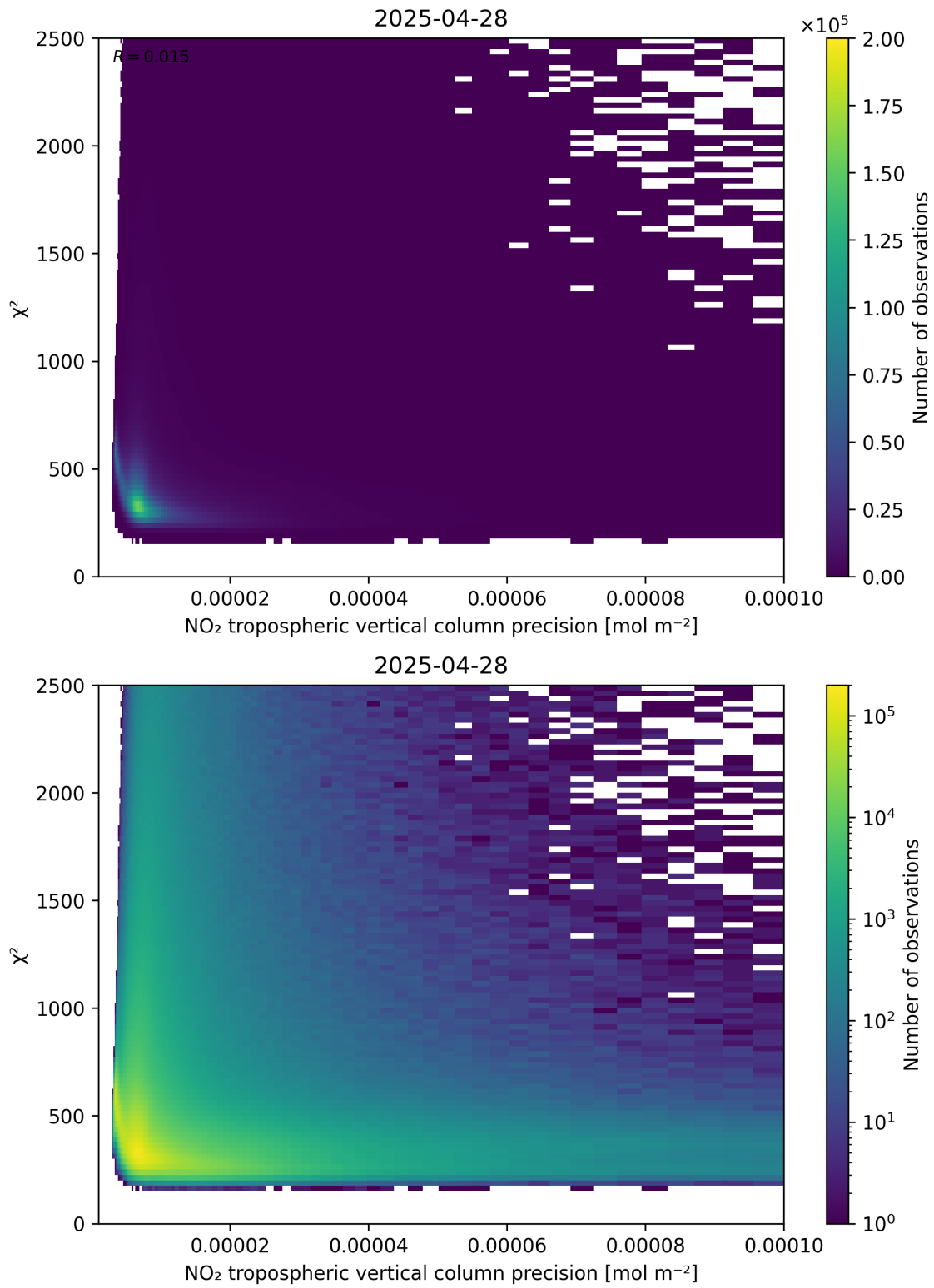
Figure 134: Scatter density plot of “NO 2 tropospheric vertical column precision” against “ \chi^2 ” for 2025-04-28 to 2025-04-29.
