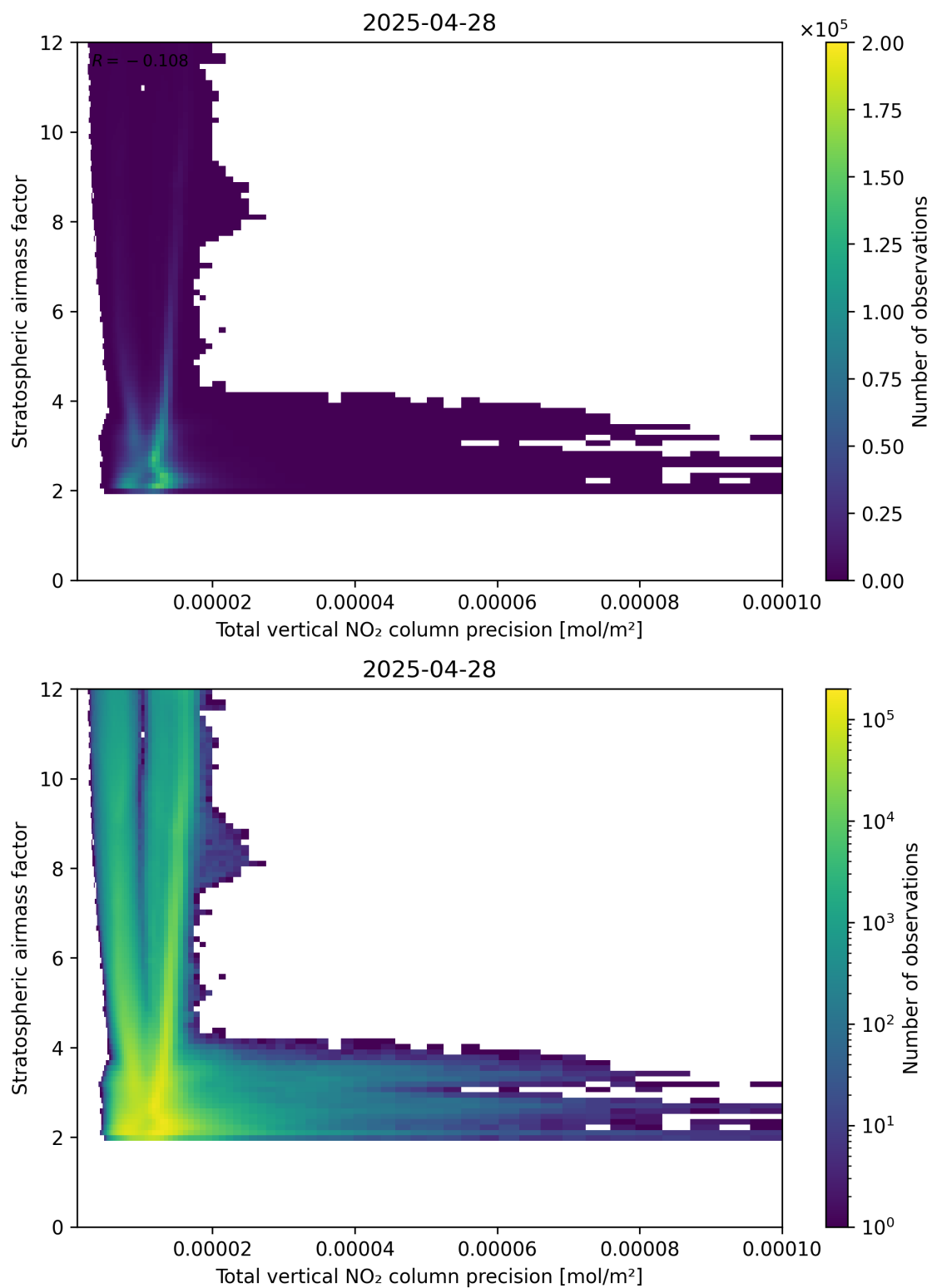
Figure 115: Scatter density plot of “Total vertical NO 2 column precision” against “Stratospheric air mass factor” for 2025-04-28 to 2025-04-29.
