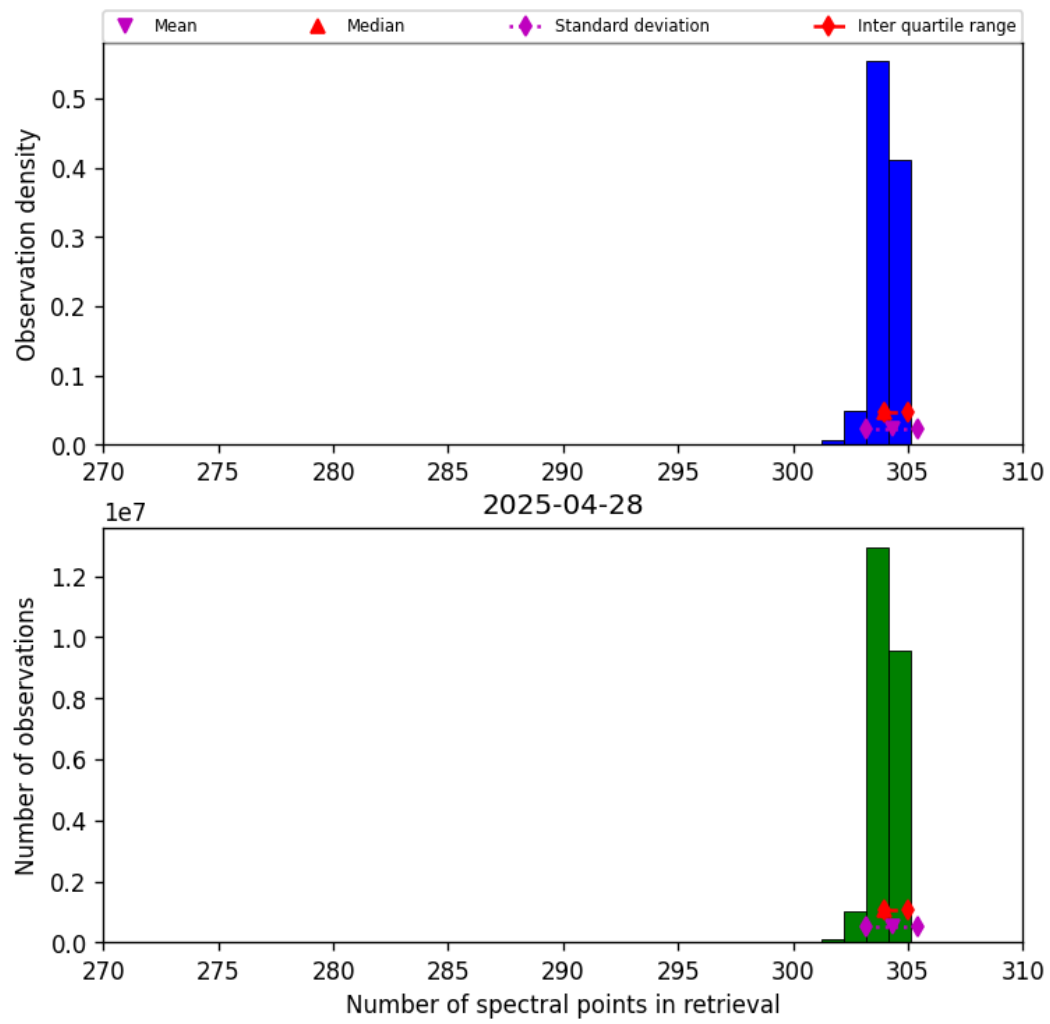
Figure 33: Histogram of “Number of spectral points in retrieval” for 2025-04-28 to 2025-04-29
