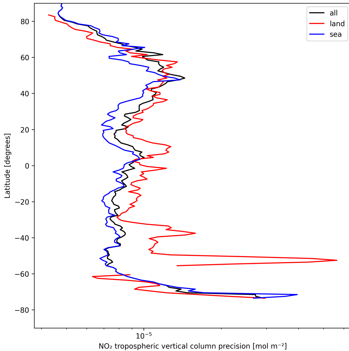
Figure 13: Zonal average of “NO 2 tropospheric vertical column precision” for 2025-04-28 to 2025-04-29.
