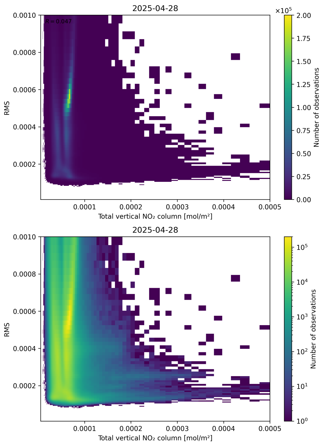
Figure 120: Scatter density plot of “Total vertical NO 2 column” against “RMS” for 2025-04-28 to 2025-04-29.
