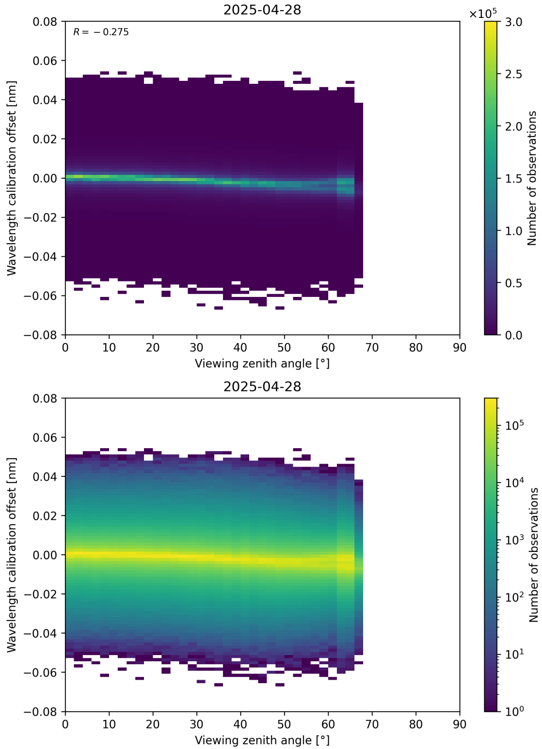
Figure 173: Scatter density plot of “Viewing zenith angle” against “Wavelength calibration offset” for 2025-04-28 to 2025-04-29.
