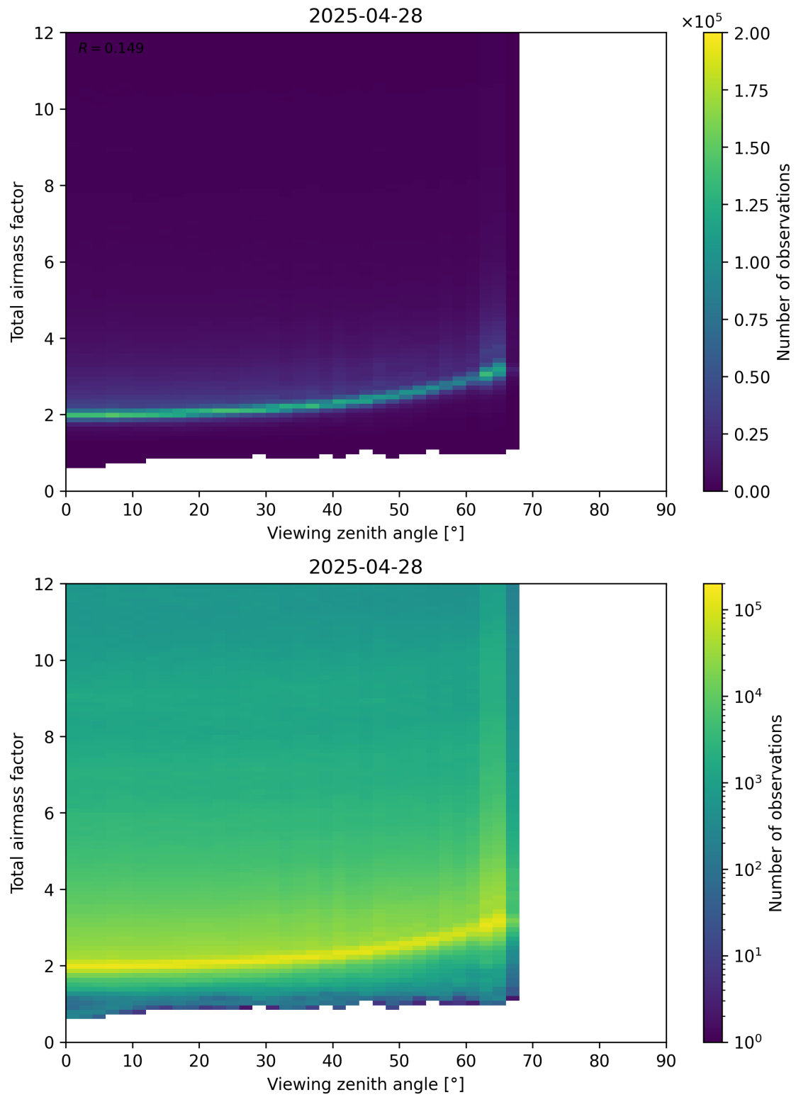
Figure 160: Scatter density plot of “Viewing zenith angle” against “Total airmass factor” for 2025-04-28 to 2025-04-29.
