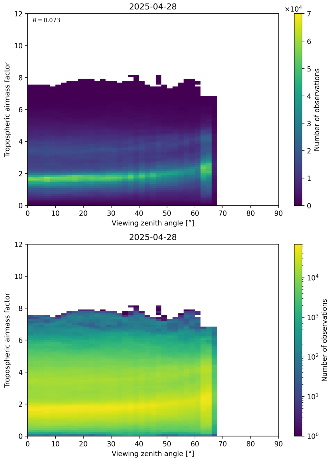
Figure 161: Scatter density plot of “Viewing zenith angle” against “Tropospheric airmass factor” for 2025-04-28 to 2025-04-29.
