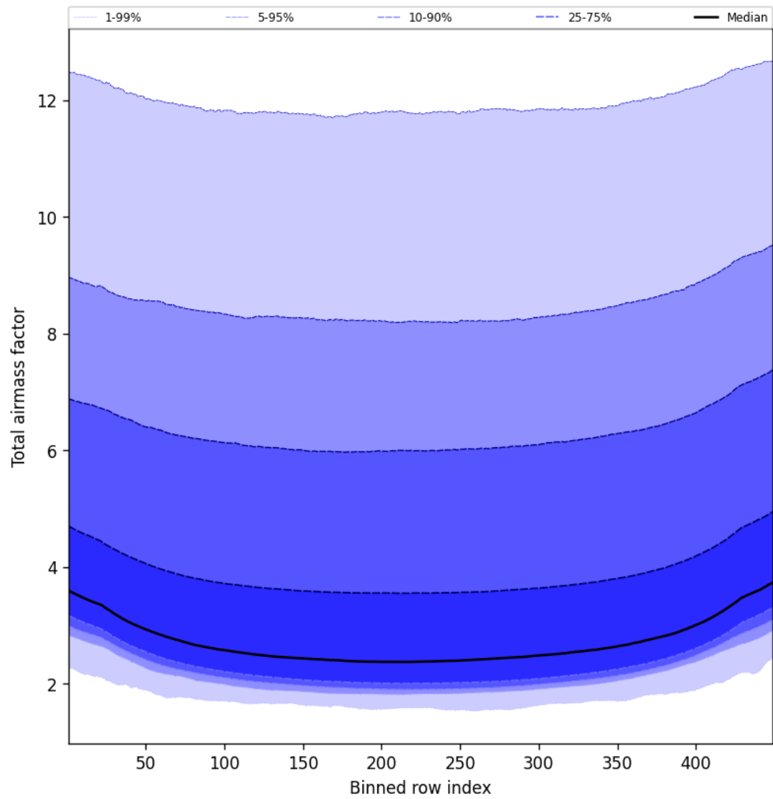
Figure 49: Along track statistics of “Total airmass factor” for 2025-04-28 to 2025-04-29
