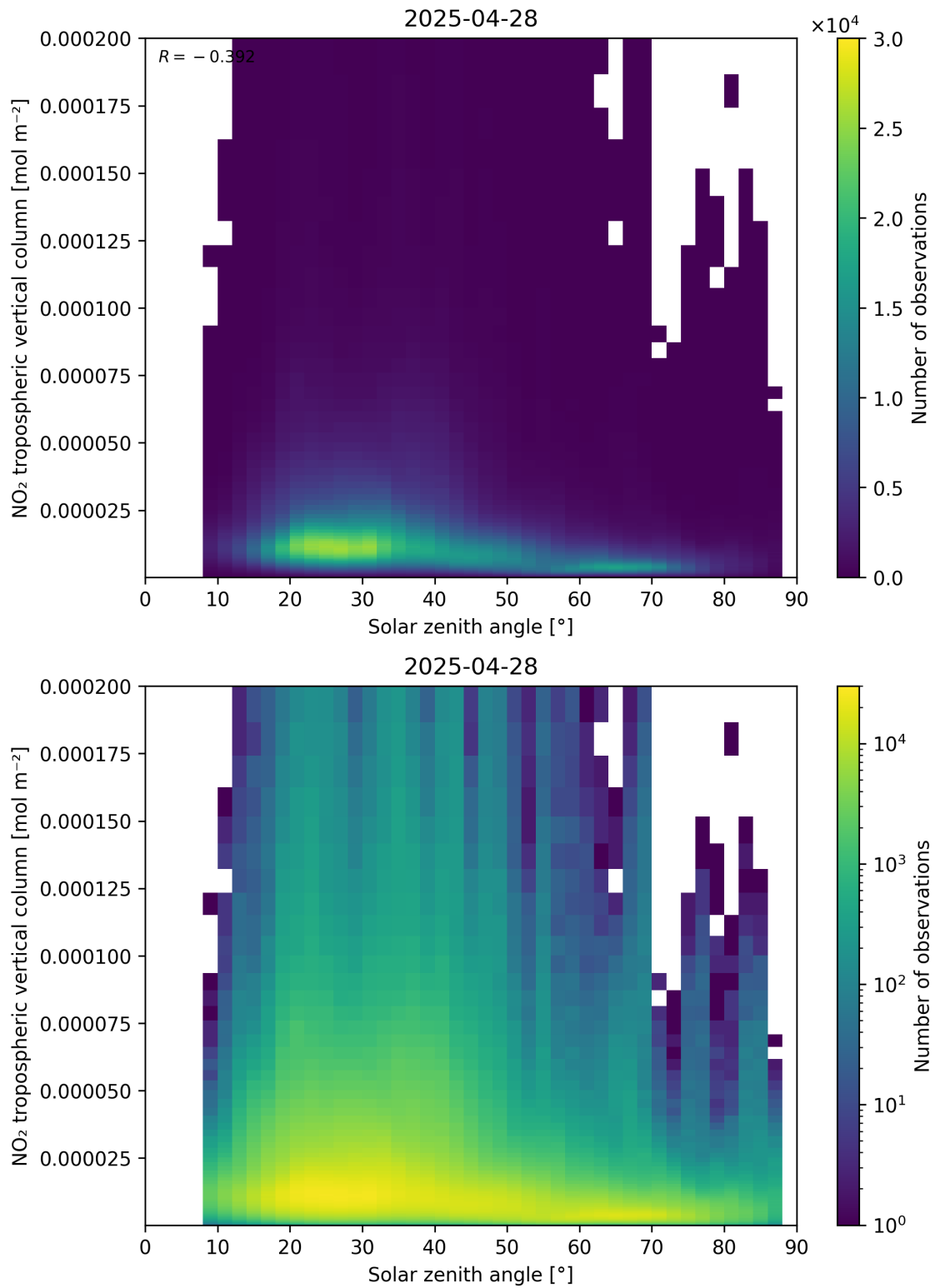
Figure 155: Scatter density plot of “Solar zenith angle” against “NO 2 tropospheric vertical column” for 2025-04-28 to 2025-04-29.
