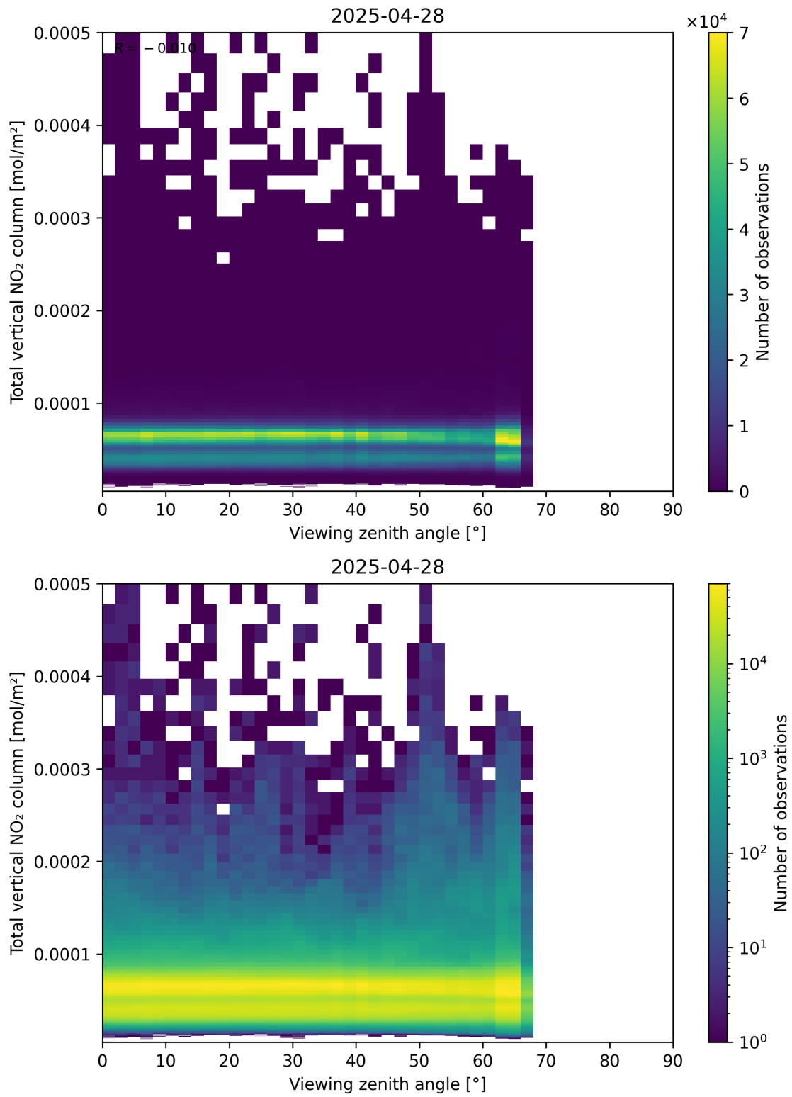
Figure 167: Scatter density plot of “Viewing zenith angle” against “Total vertical NO 2 column” for 2025-04-28 to 2025-04-29.
