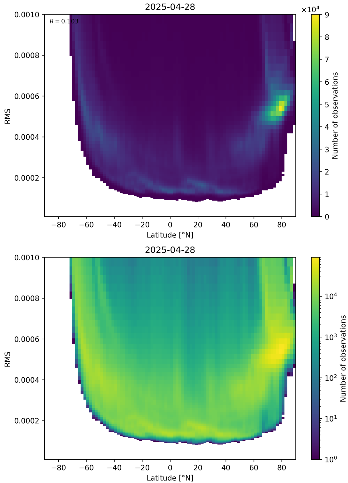
Figure 94: Scatter density plot of “Latitude” against “RMS” for 2025-04-28 to 2025-04-29.
