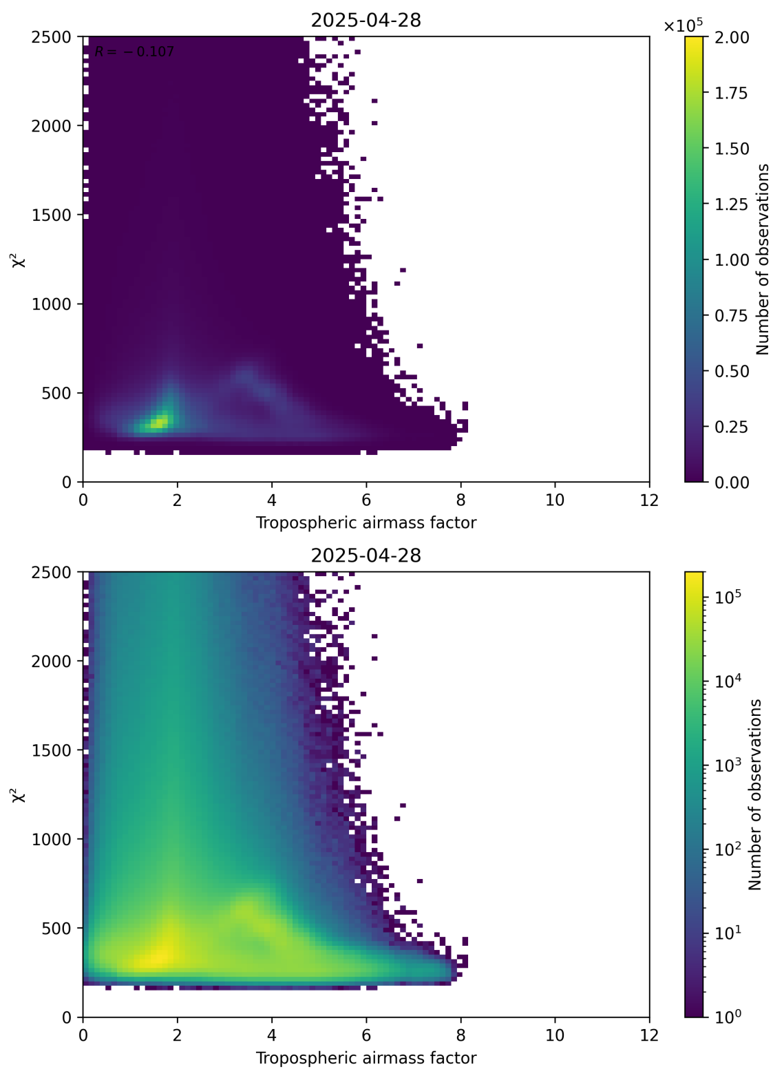
Figure 73: Scatter density plot of “Tropospheric airmass factor” against “ \chi^2 ” for 2025-04-28 to 2025-04-29.
