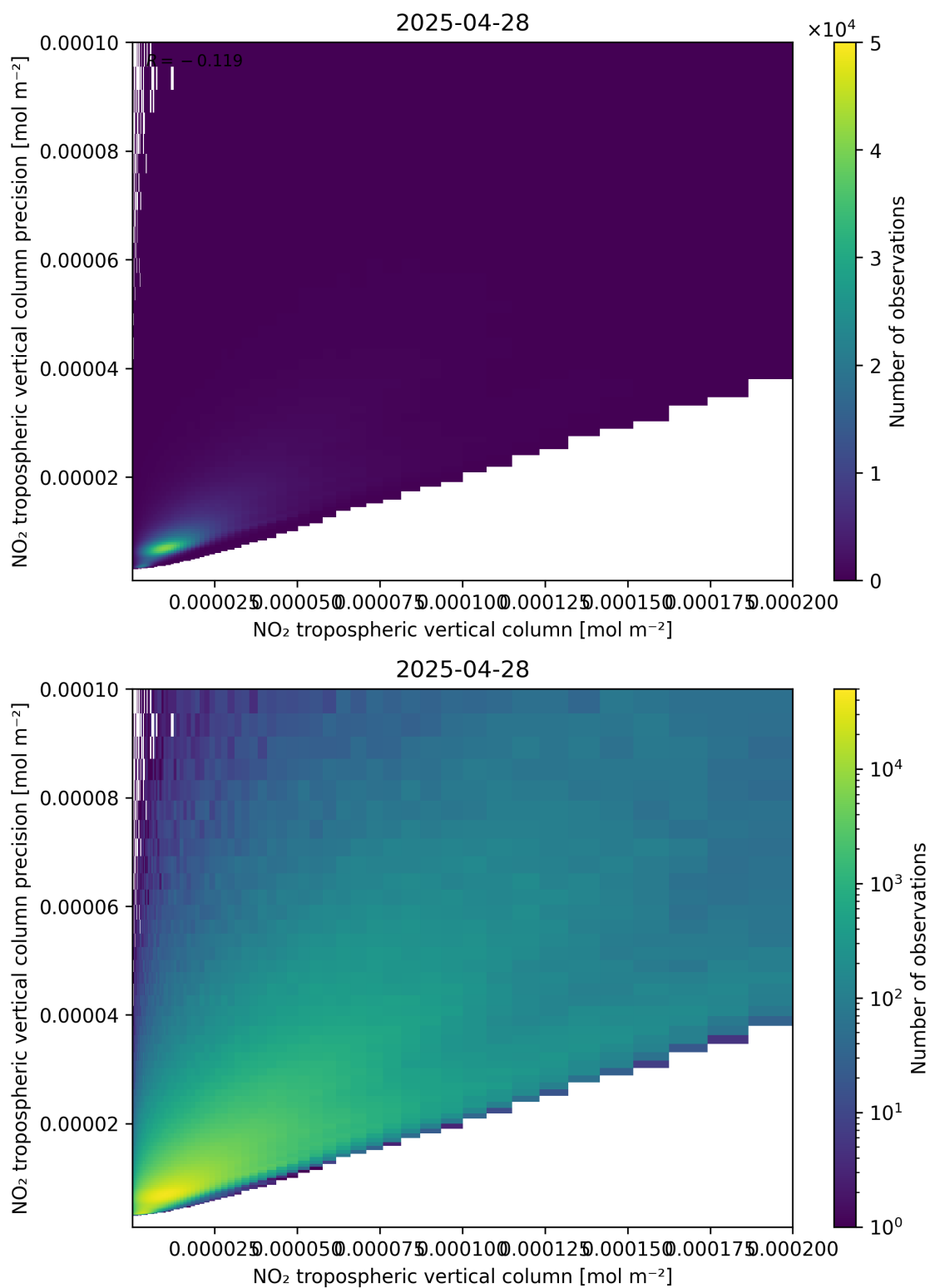
Figure 130: Scatter density plot of “NO 2 tropospheric vertical column” against “NO 2 tropospheric vertical column precision” for 2025-04-28 to 2025-04-29.
