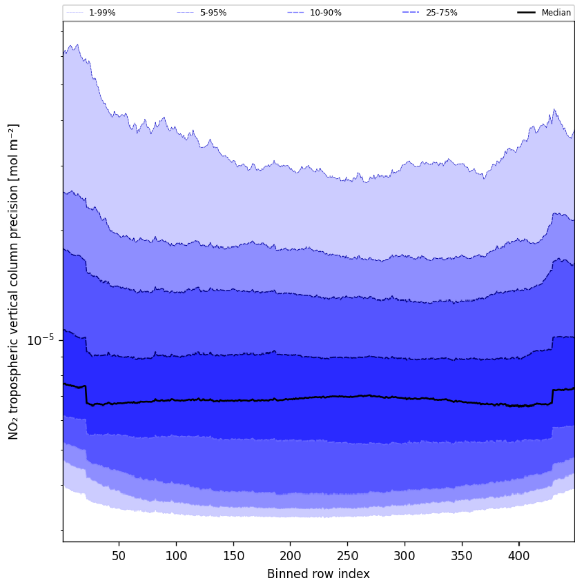
Figure 47: Along track statistics of “NO 2 tropospheric vertical column precision” for 2025-04-28 to 2025-04-29
