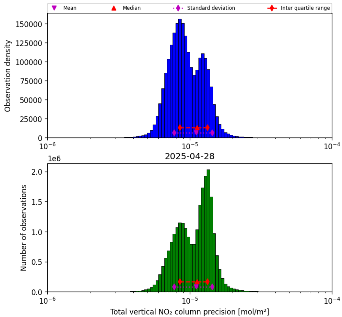
Figure 39: Histogram of “Total vertical NO 2 column precision” for 2025-04-28 to 2025-04-29
