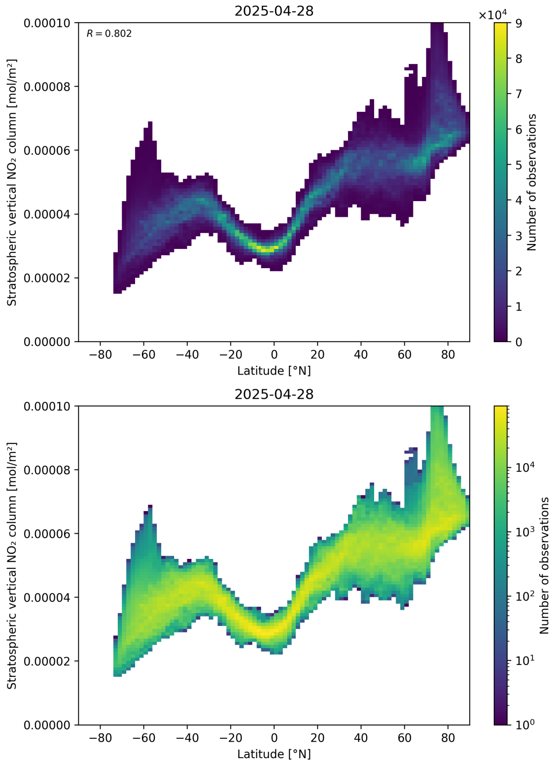
Figure 87: Scatter density plot of “Latitude” against “Stratospheric vertical NO 2 column” for 2025-04-28 to 2025-04-29.
