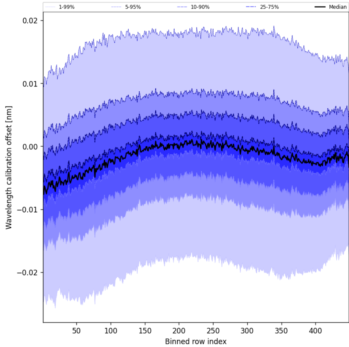
Figure 52: Along track statistics of “Wavelength calibration offset” for 2025-04-28 to 2025-04-29
