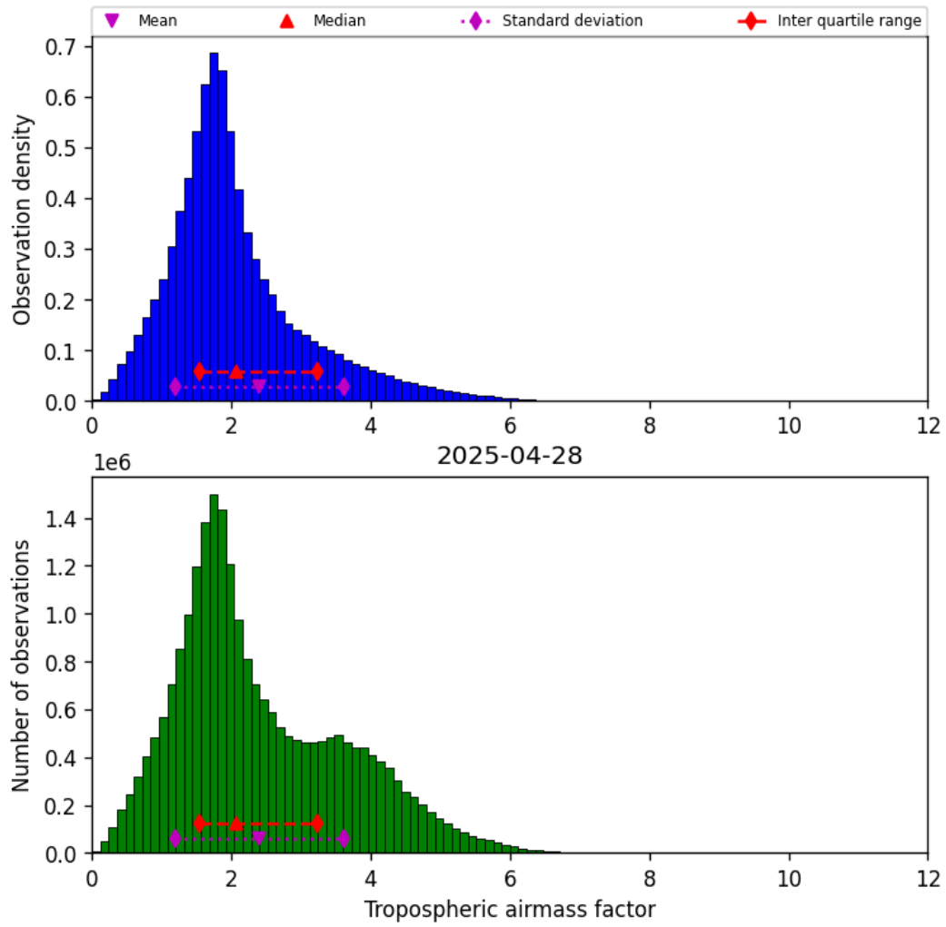
Figure 31: Histogram of “Tropospheric airmass factor” for 2025-04-28 to 2025-04-29
