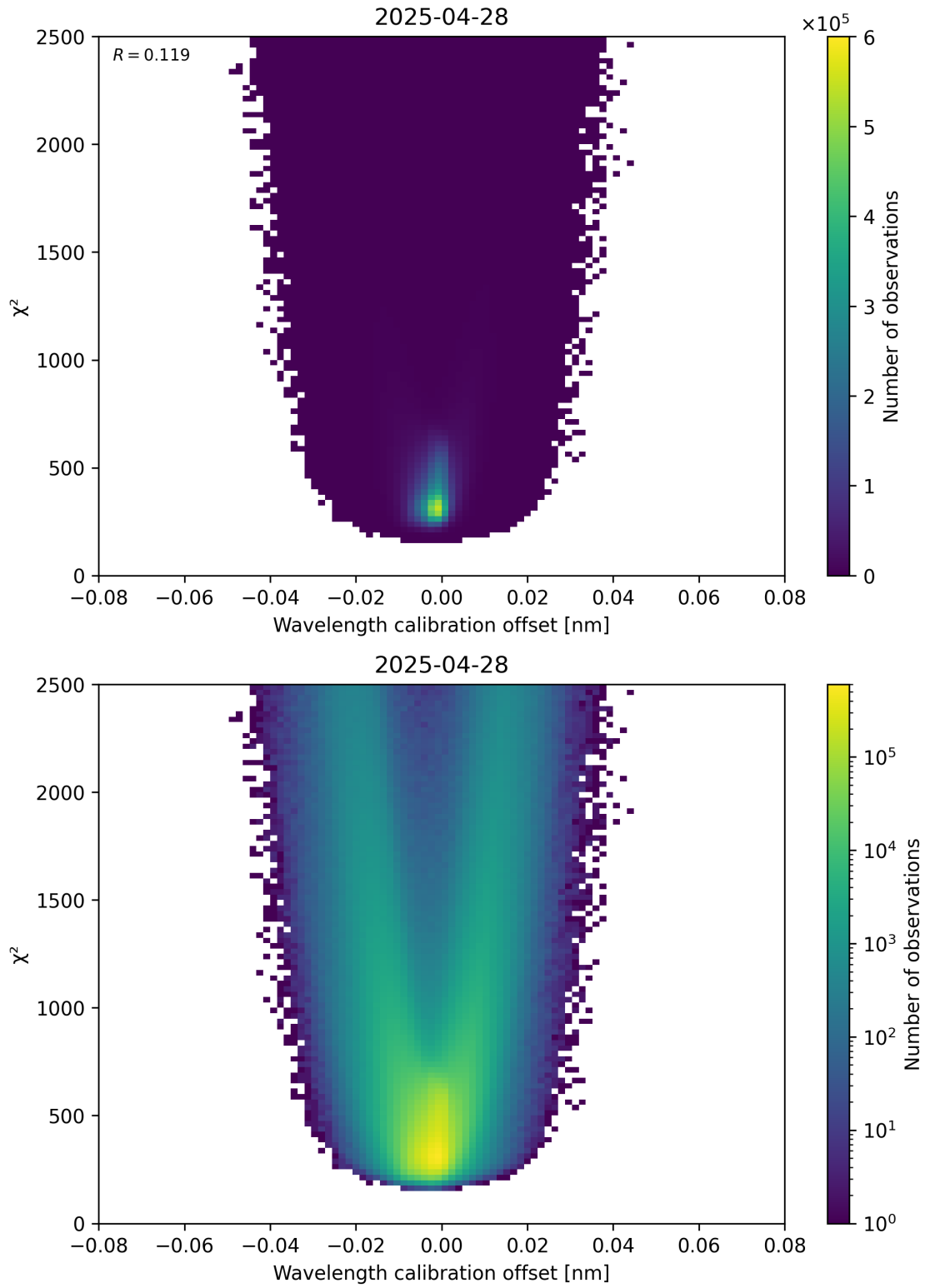
Figure 175: Scatter density plot of “Wavelength calibration offset” against “ \chi^2 ” for 2025-04-28 to 2025-04-29.
