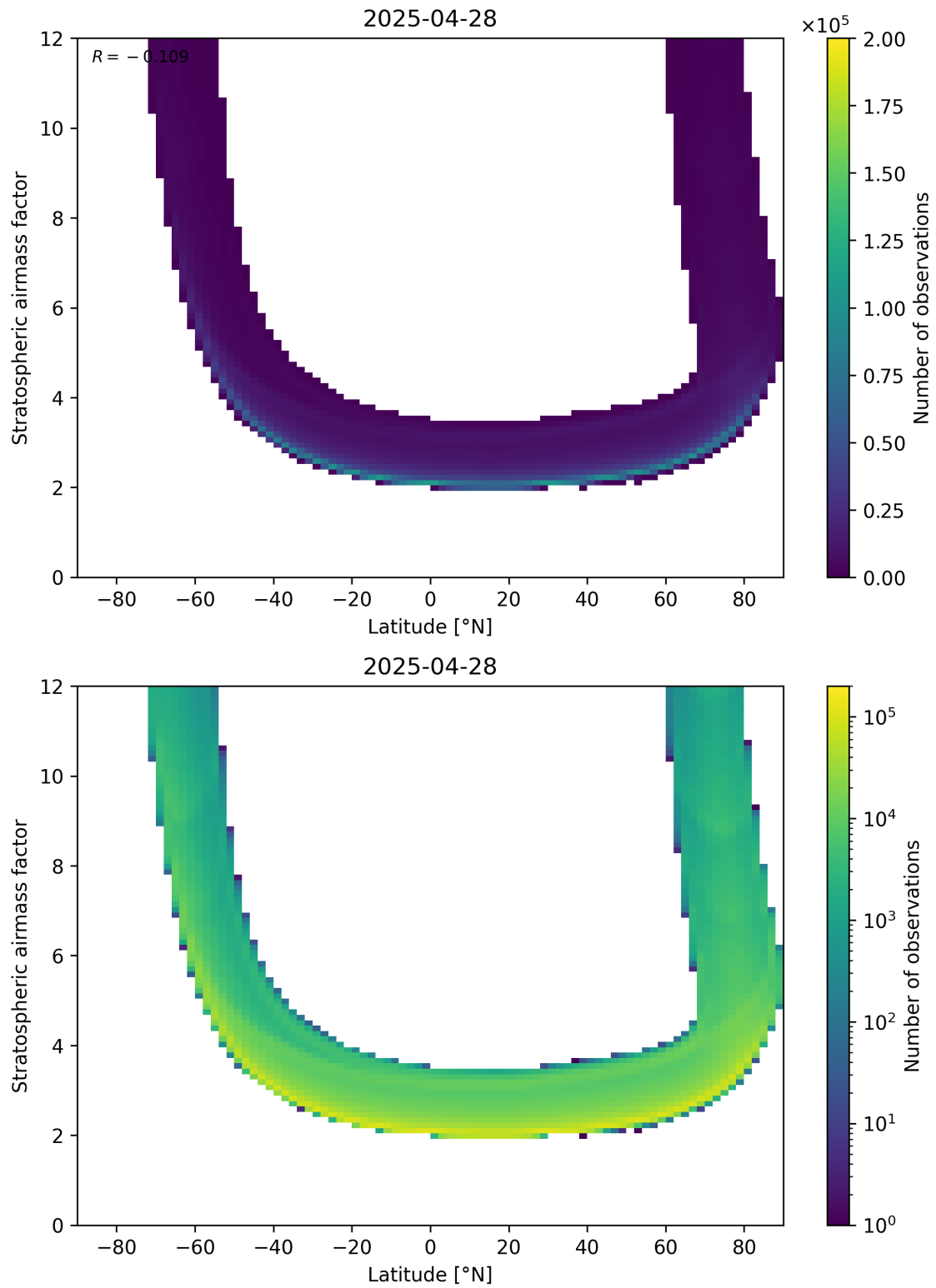
Figure 83: Scatter density plot of “Latitude” against “Stratospheric air mass factor” for 2025-04-28 to 2025-04-29.
