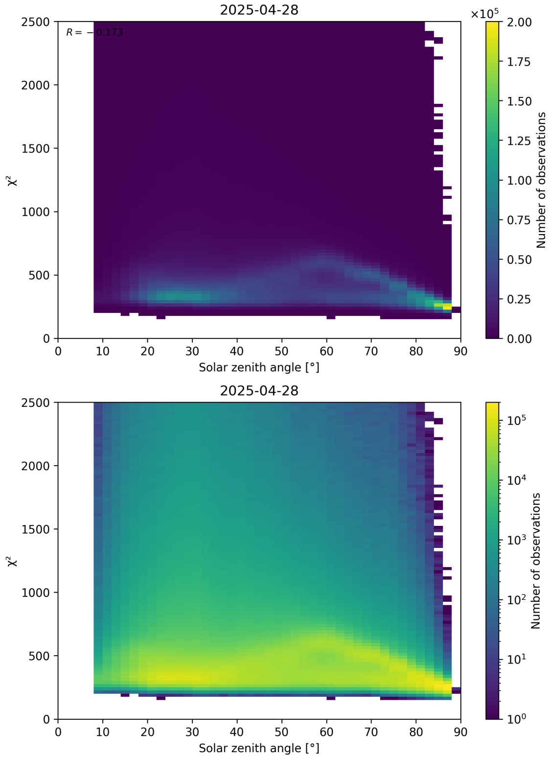
Figure 148: Scatter density plot of “Solar zenith angle” against “ \chi^2 ” for 2025-04-28 to 2025-04-29.
