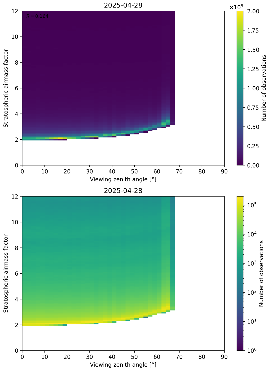
Figure 159: Scatter density plot of “Viewing zenith angle” against “Stratospheric airmass factor” for 2025-04-28 to 2025-04-29.
