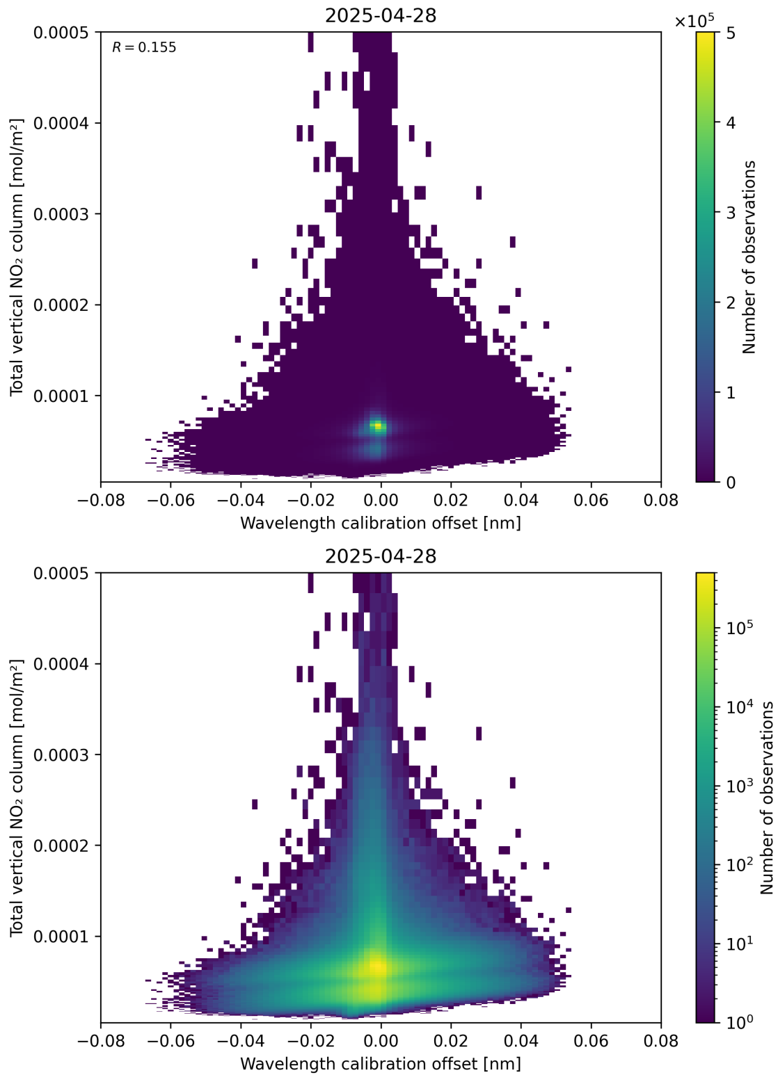
Figure 179: Scatter density plot of “Wavelength calibration offset” against “Total vertical NO 2 column” for 2025-04-28 to 2025-04-29.
