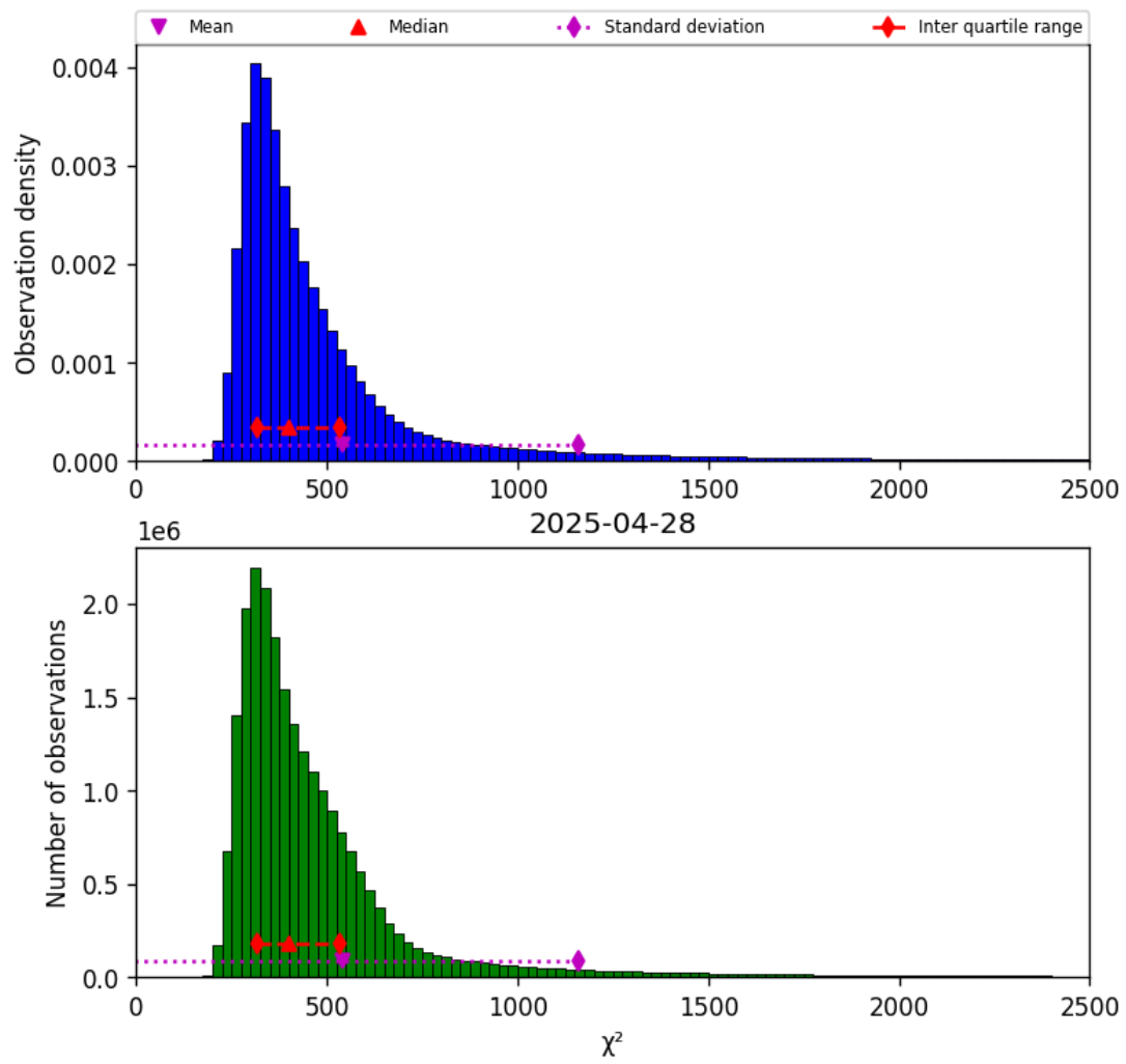
Figure 42: Histogram of “ \chi^2 ” for 2025-04-28 to 2025-04-29
