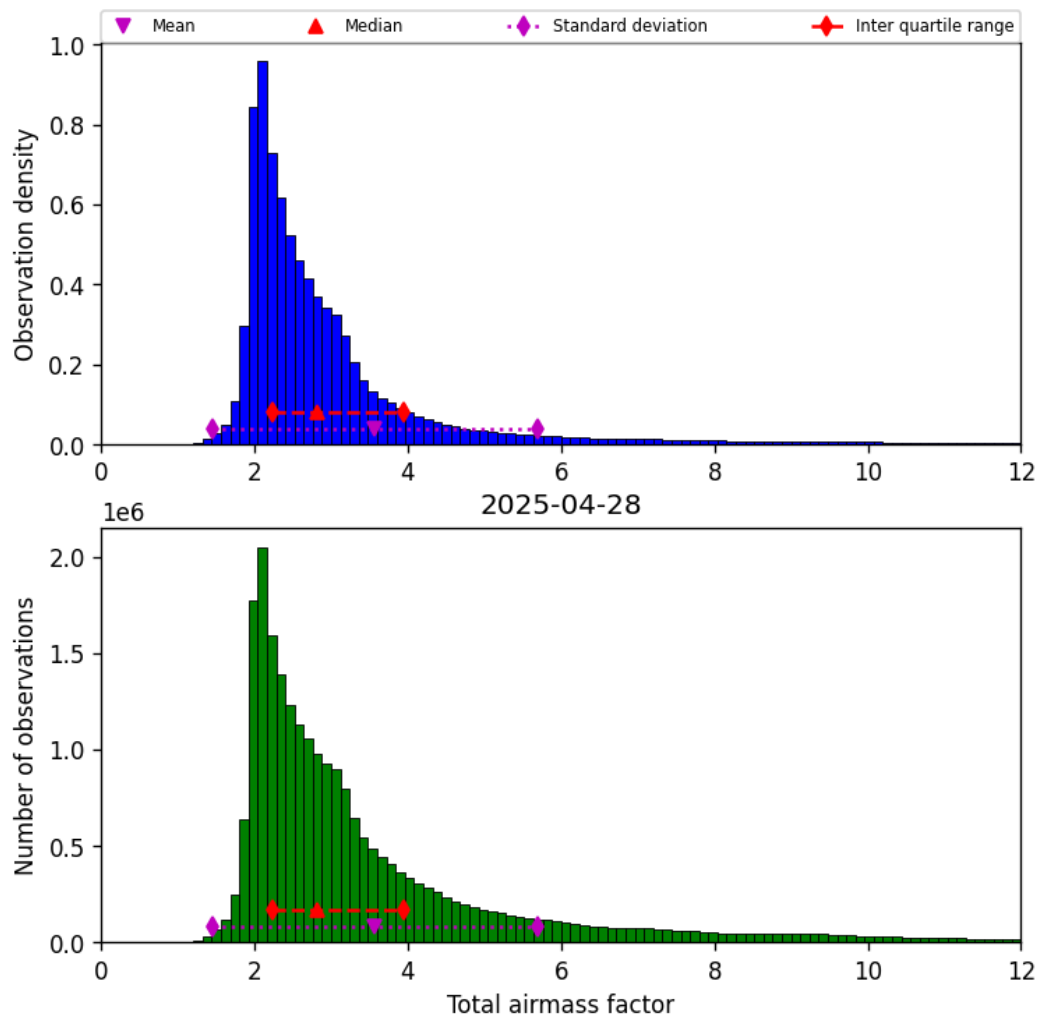
Figure 32: Histogram of “Total airmass factor” for 2025-04-28 to 2025-04-29
