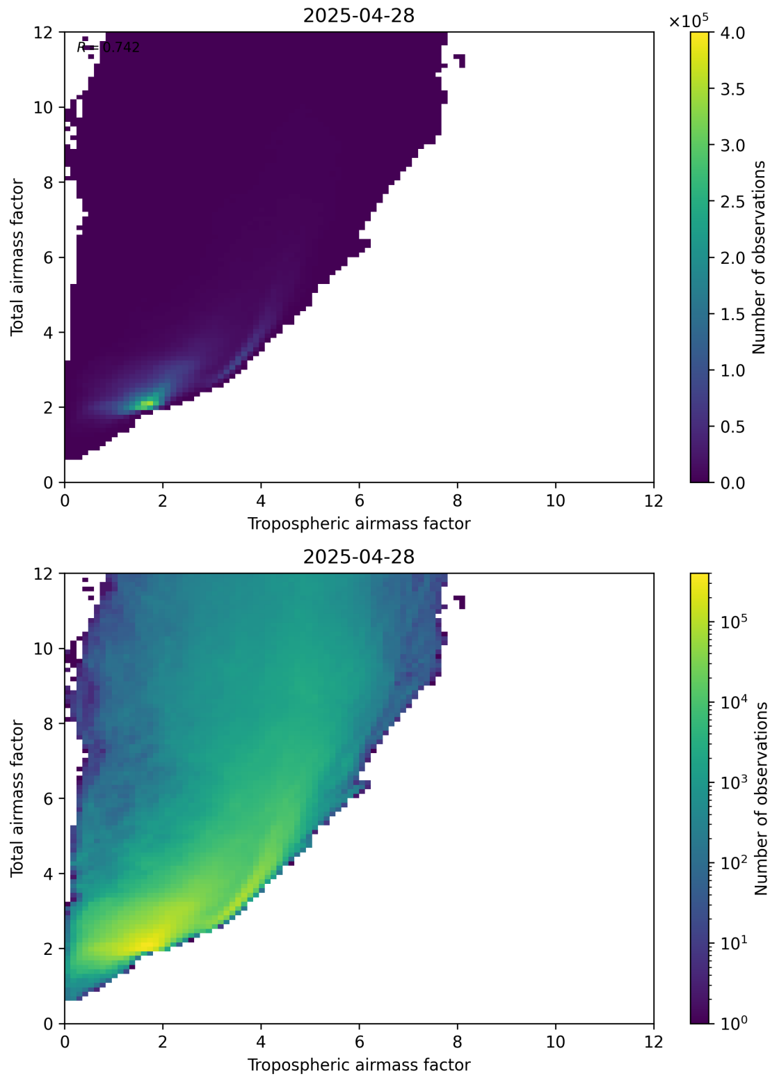
Figure 72: Scatter density plot of “Tropospheric airmass factor” against “Total airmass factor” for 2025-04-28 to 2025-04-29.
