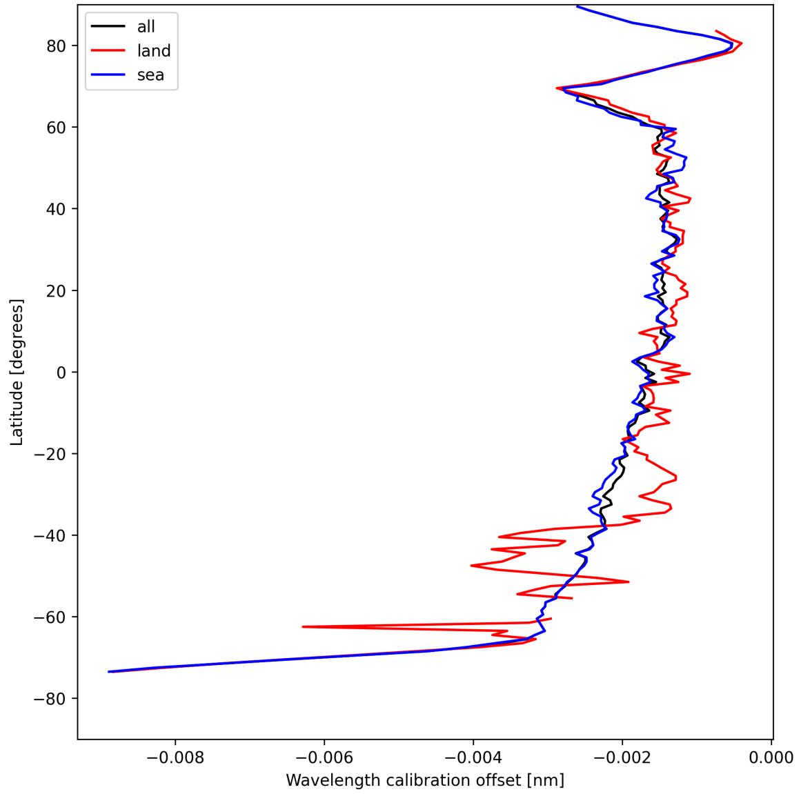
Figure 18: Zonal average of “Wavelength calibration offset” for 2025-04-28 to 2025-04-29.
