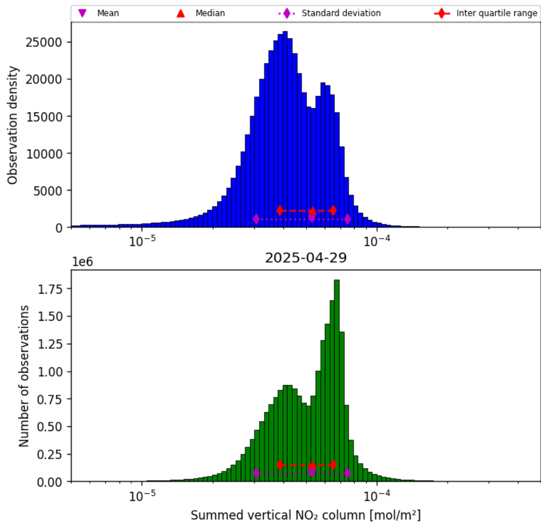
Figure 40: Histogram of “Summed vertical NO 2 column” for 2025-04-29 to 2025-04-30
