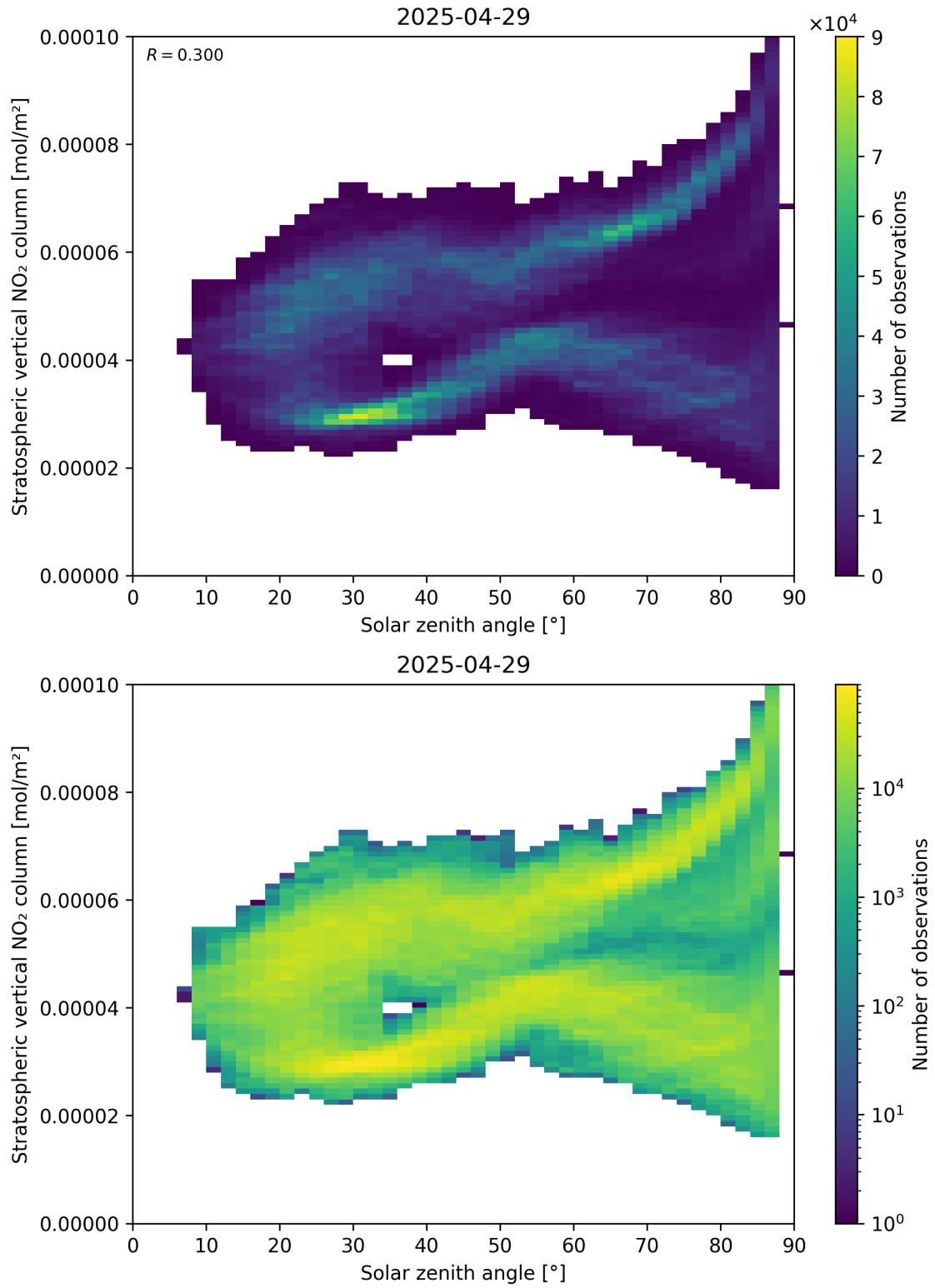
Figure 150: Scatter density plot of “Solar zenith angle” against “Stratospheric vertical NO 2 column” for 2025-04-29 to 2025-04-30.
