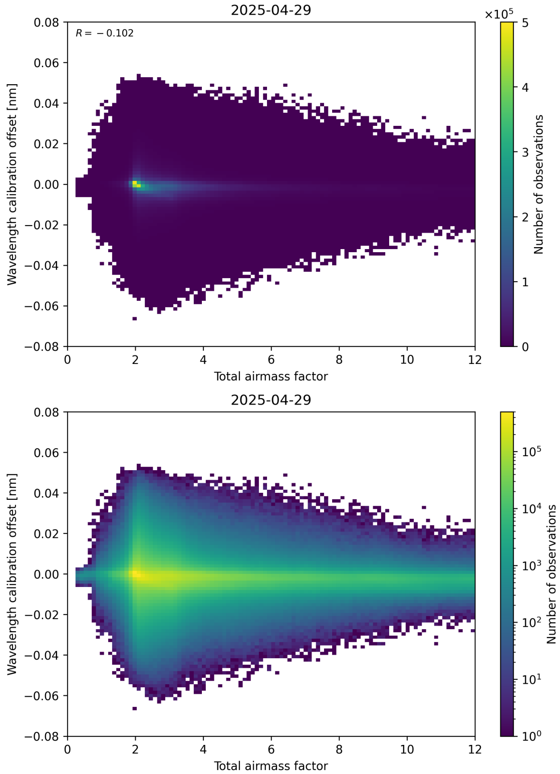
Figure 70: Scatter density plot of “Total airmass factor” against “Wavelength calibration offset” for 2025-04-29 to 2025-04-30.
