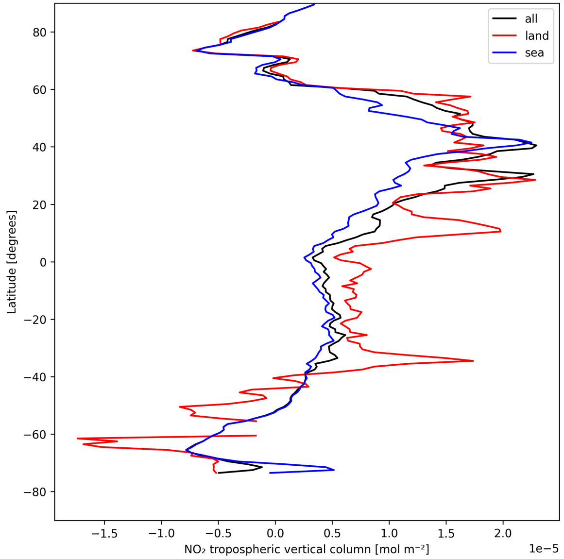
Figure 12: Zonal average of “NO 2 tropospheric vertical column” for 2025-04-29 to 2025-04-30.
