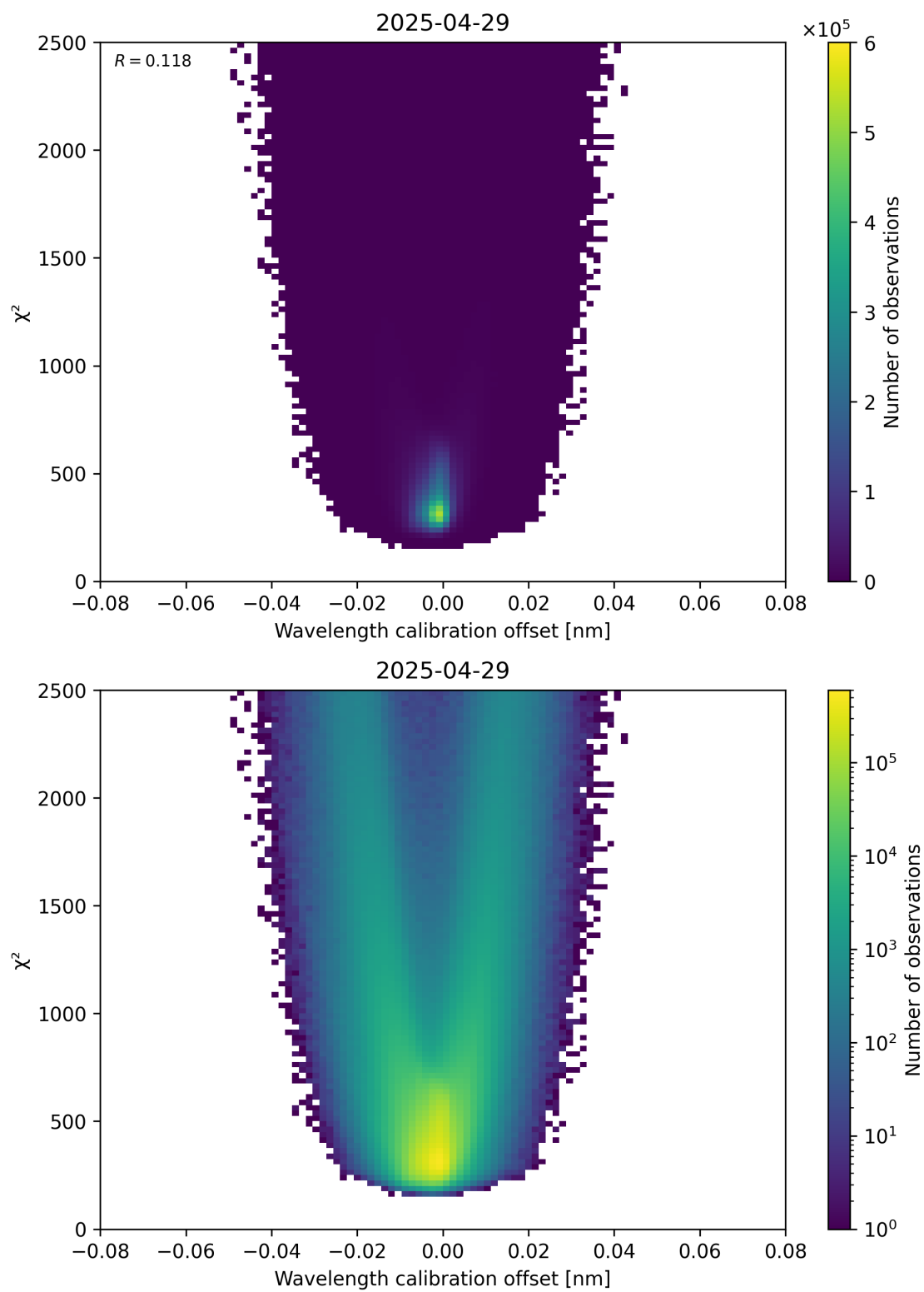
Figure 175: Scatter density plot of “Wavelength calibration offset” against “ \chi^2 ” for 2025-04-29 to 2025-04-30.
