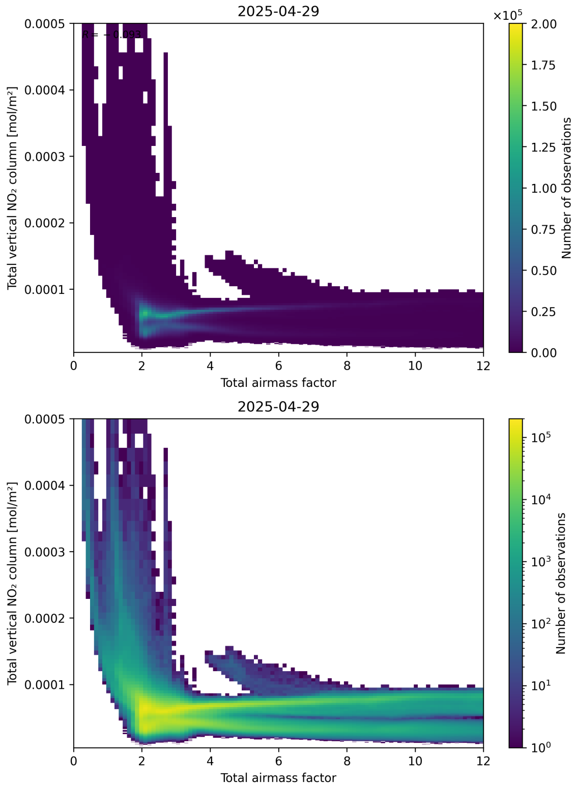
Figure 67: Scatter density plot of “Total airmass factor” against “Total vertical NO 2 column” for 2025-04-29 to 2025-04-30.
