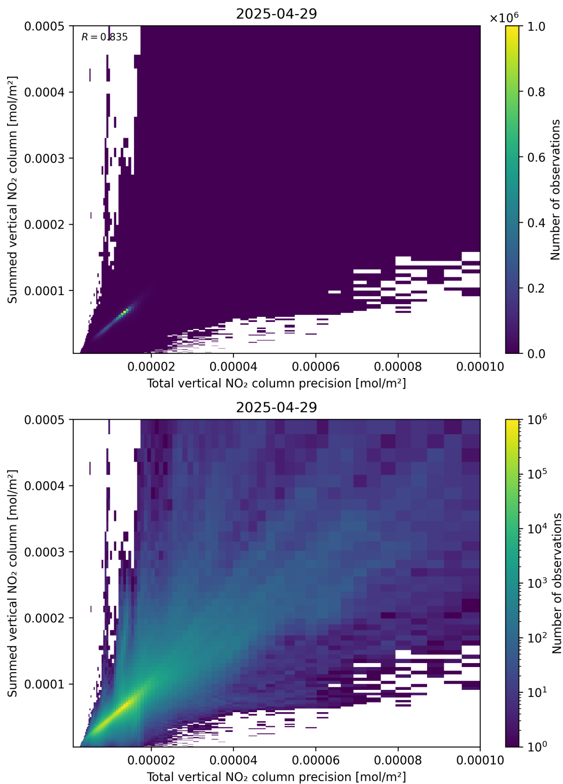
Figure 117: Scatter density plot of “Total vertical NO 2 column precision” against “Summed vertical NO 2 column” for 2025-04-29 to 2025-04-30.
