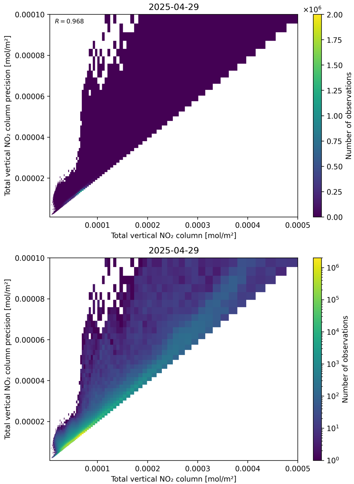
Figure 114: Scatter density plot of “Total vertical NO 2 column” against “Total vertical NO 2 column precision” for 2025-04-29 to 2025-04-30.
