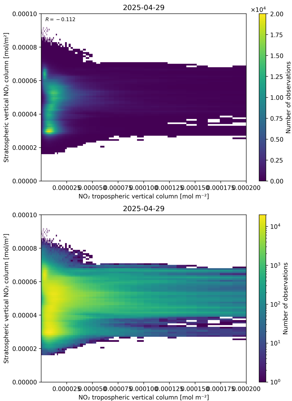
Figure 125: Scatter density plot of “NO 2 tropospheric vertical column” against “Stratospheric vertical NO 2 column” for 2025-04-29 to 2025-04-30.
