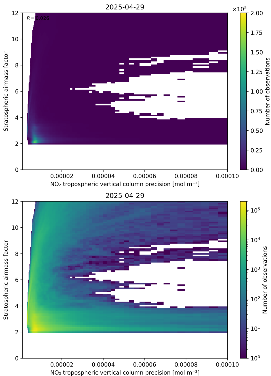
Figure 131: Scatter density plot of “NO 2 tropospheric vertical column precision” against “Stratospheric airmass factor” for 2025-04-29 to 2025-04-30.
