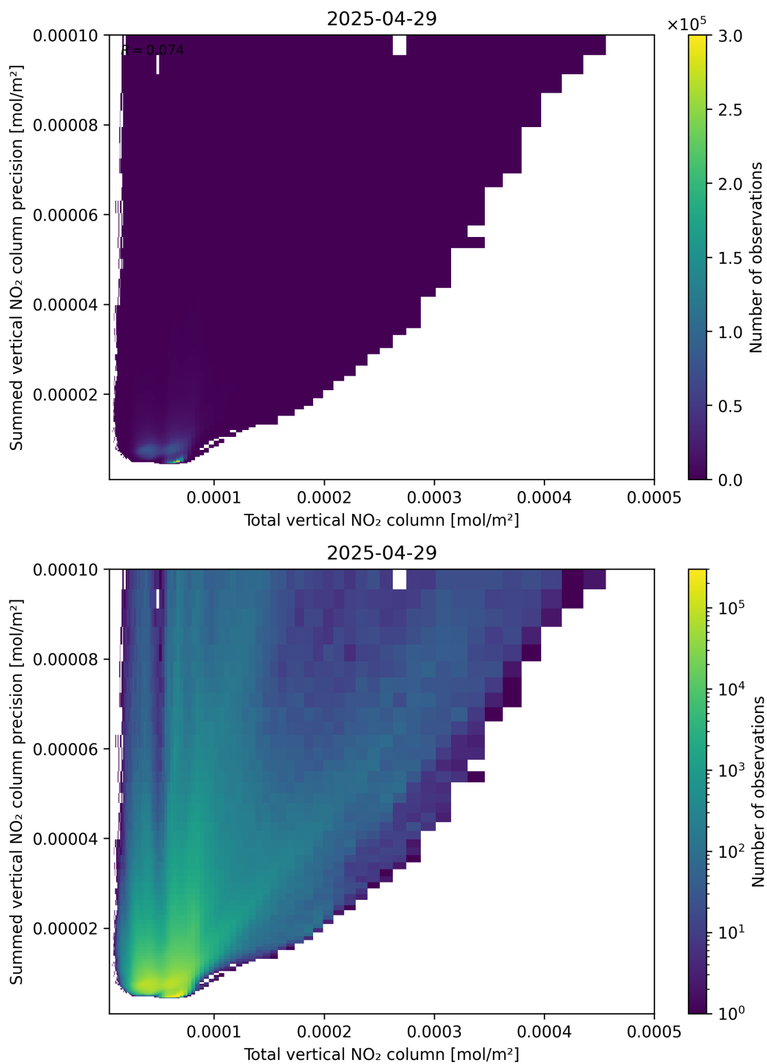
Figure 113: Scatter density plot of “Total vertical NO 2 column” against “Summed vertical NO 2 column precision” for 2025-04-29 to 2025-04-30.
