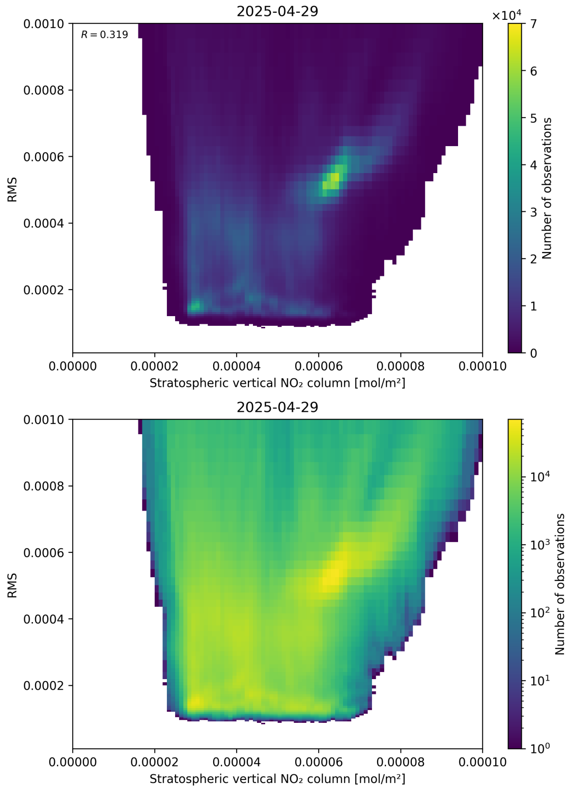
Figure 102: Scatter density plot of “Stratospheric vertical NO 2 column” against “RMS” for 2025-04-29 to 2025-04-30.
