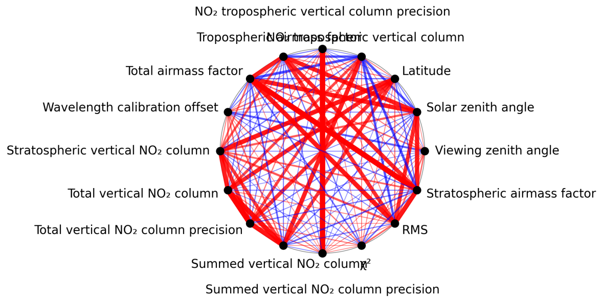
Figure 1: Map of correlation graph for 2025-04-29 to 2025-04-30.
