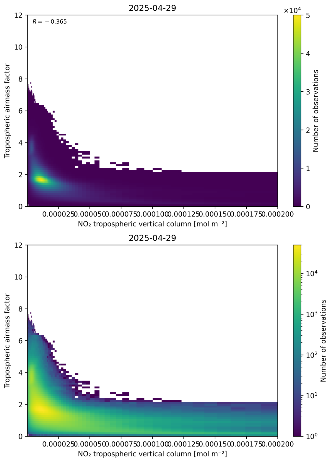
Figure 123: Scatter density plot of “NO 2 tropospheric vertical column” against “Tropospheric air mass factor” for 2025-04-29 to 2025-04-30.
