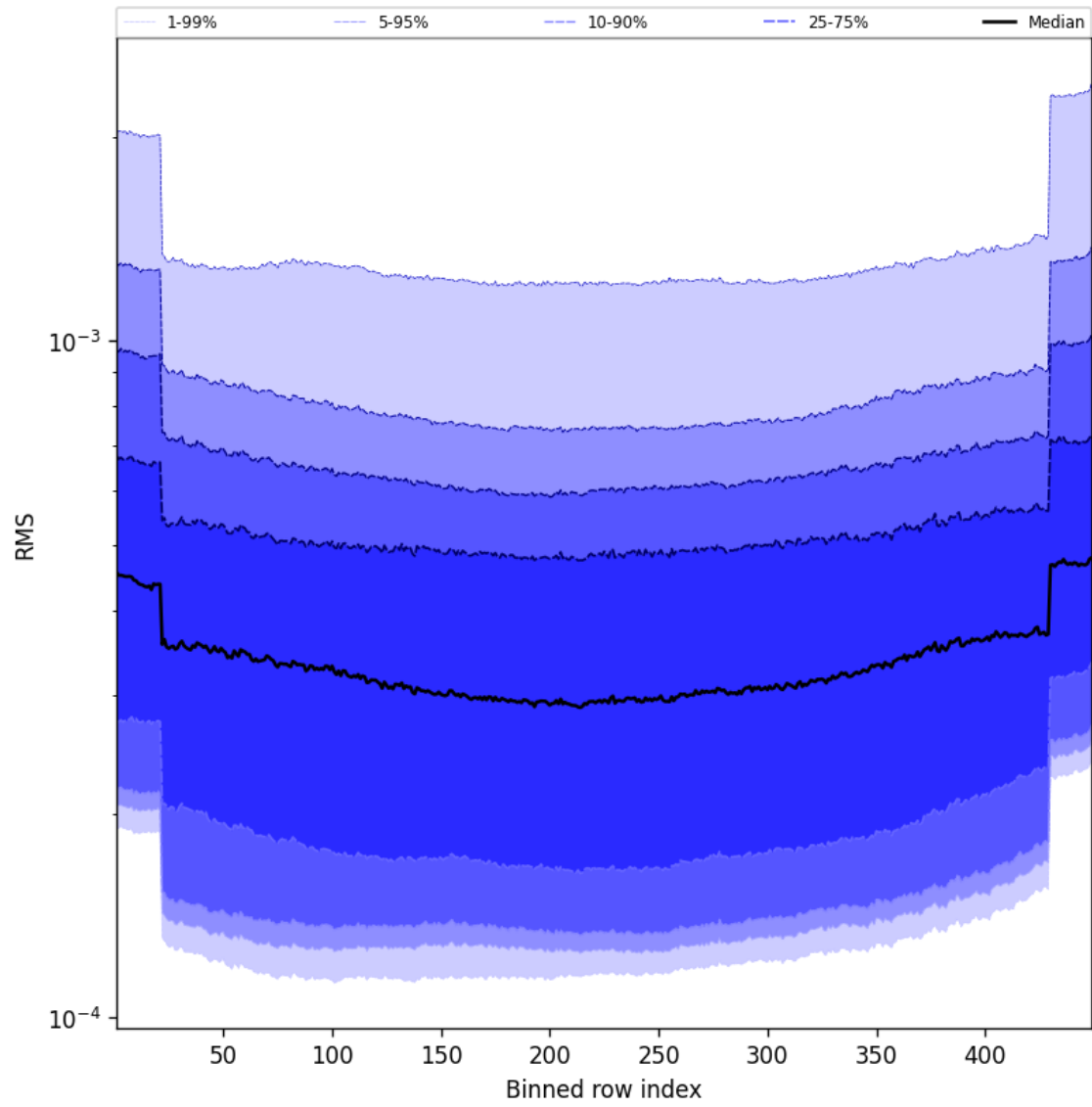
Figure 60: Along track statistics of “RMS” for 2025-04-29 to 2025-04-30
