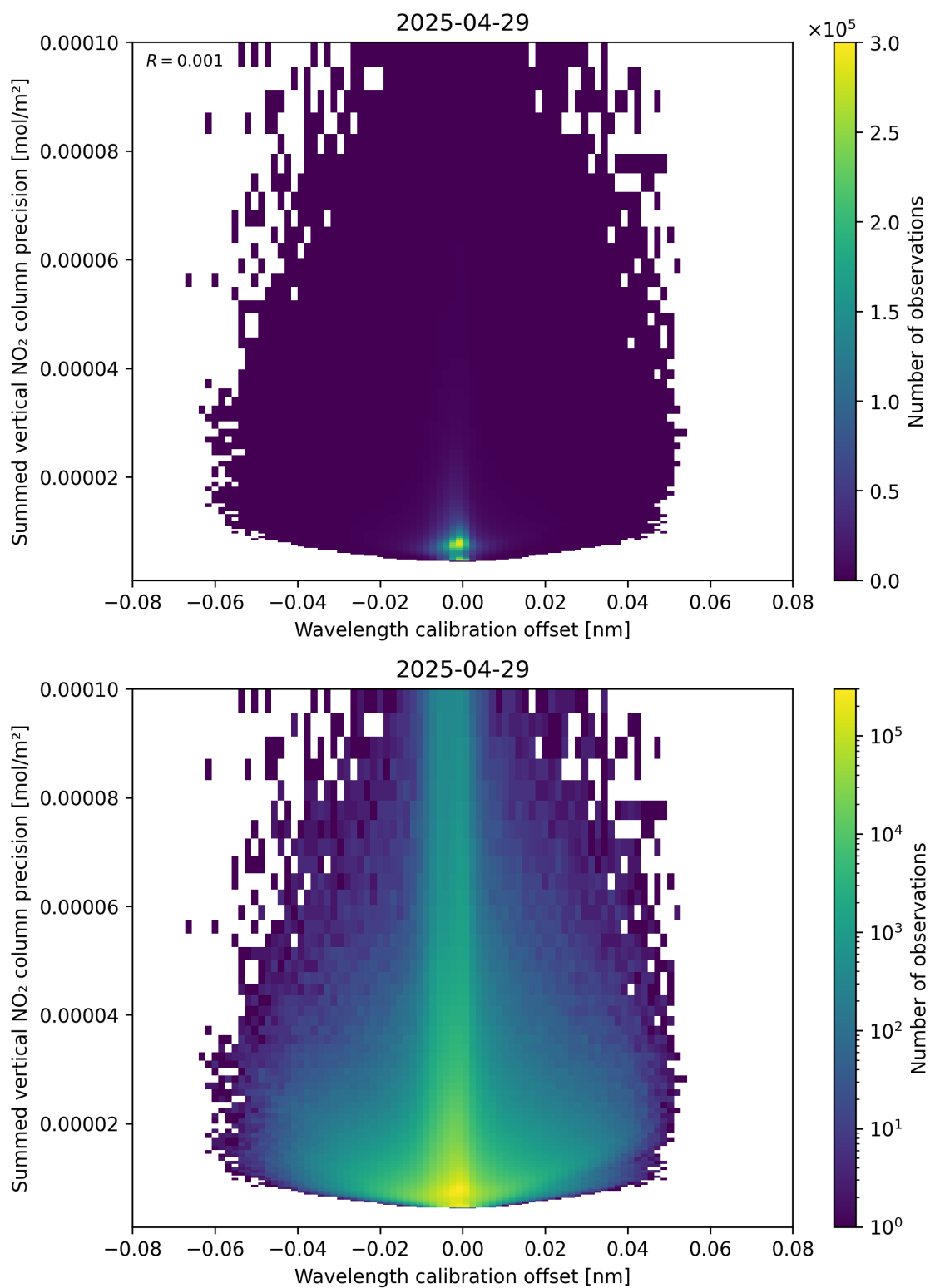
Figure 178: Scatter density plot of “Wavelength calibration offset” against “Summed vertical NO 2 column precision” for 2025-04-29 to 2025-04-30.
