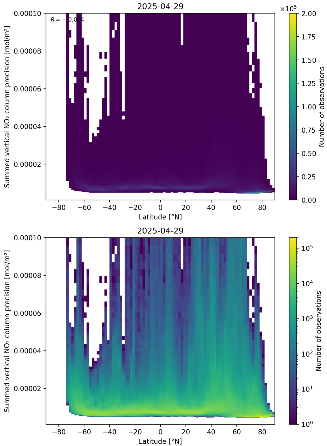
Figure 89: Scatter density plot of “Latitude” against “Summed vertical NO 2 column precision” for 2025-04-29 to 2025-04-30.
