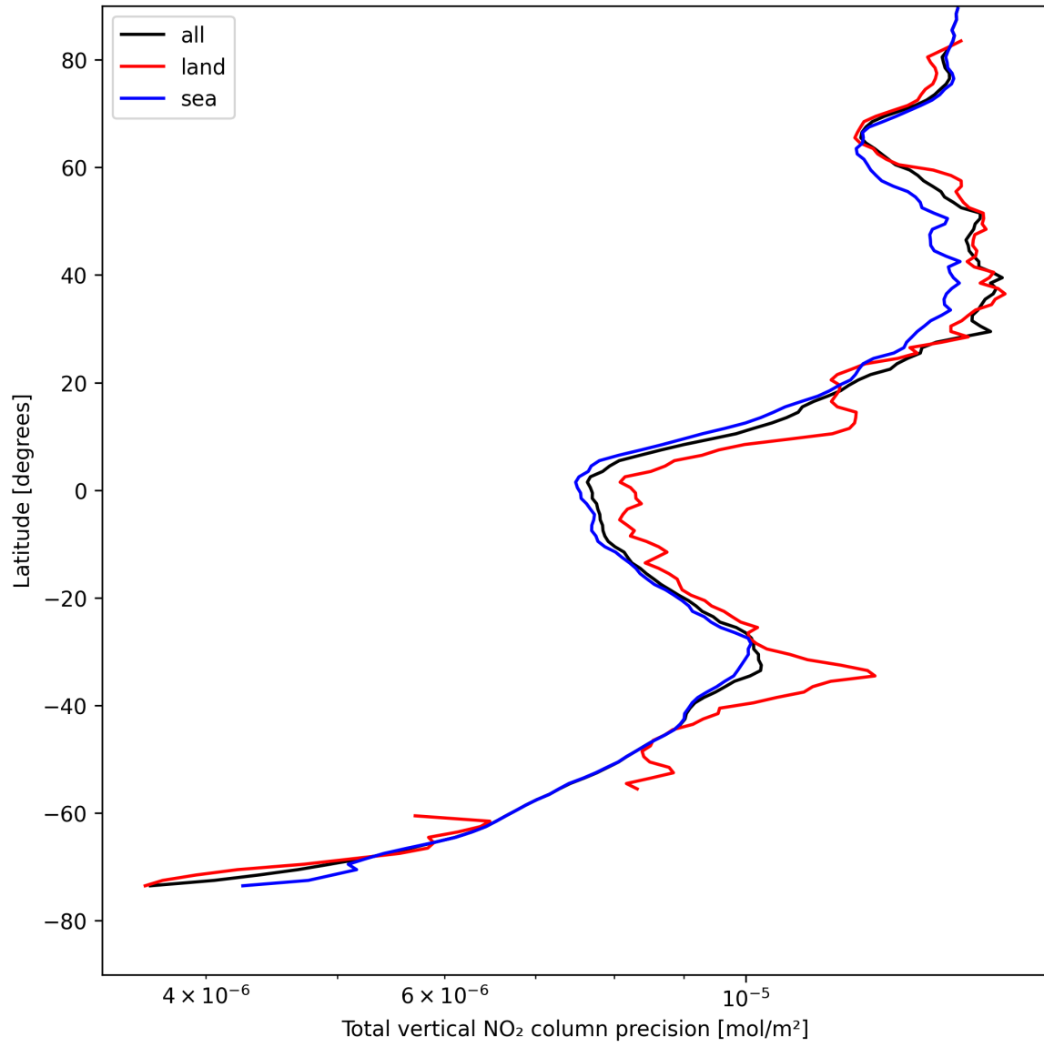
Figure 22: Zonal average of “Total vertical NO 2 column precision” for 2025-04-29 to 2025-04-30.
