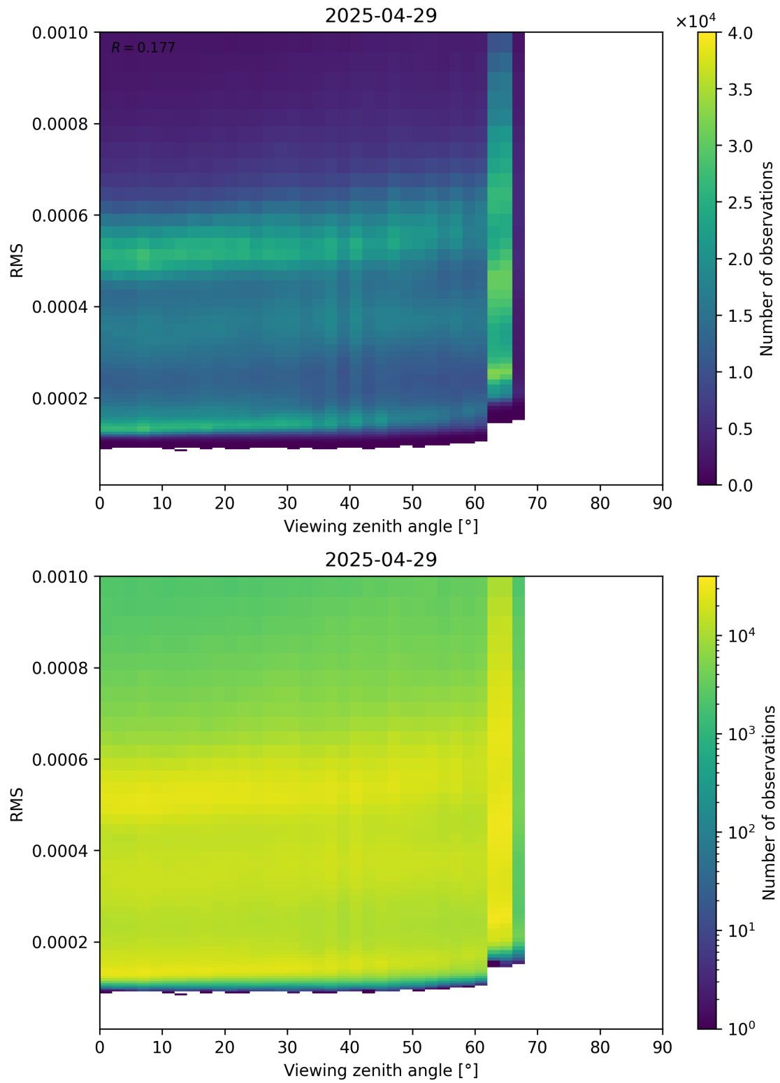
Figure 171: Scatter density plot of “Viewing zenith angle” against “RMS” for 2025-04-29 to 2025-04-30.
