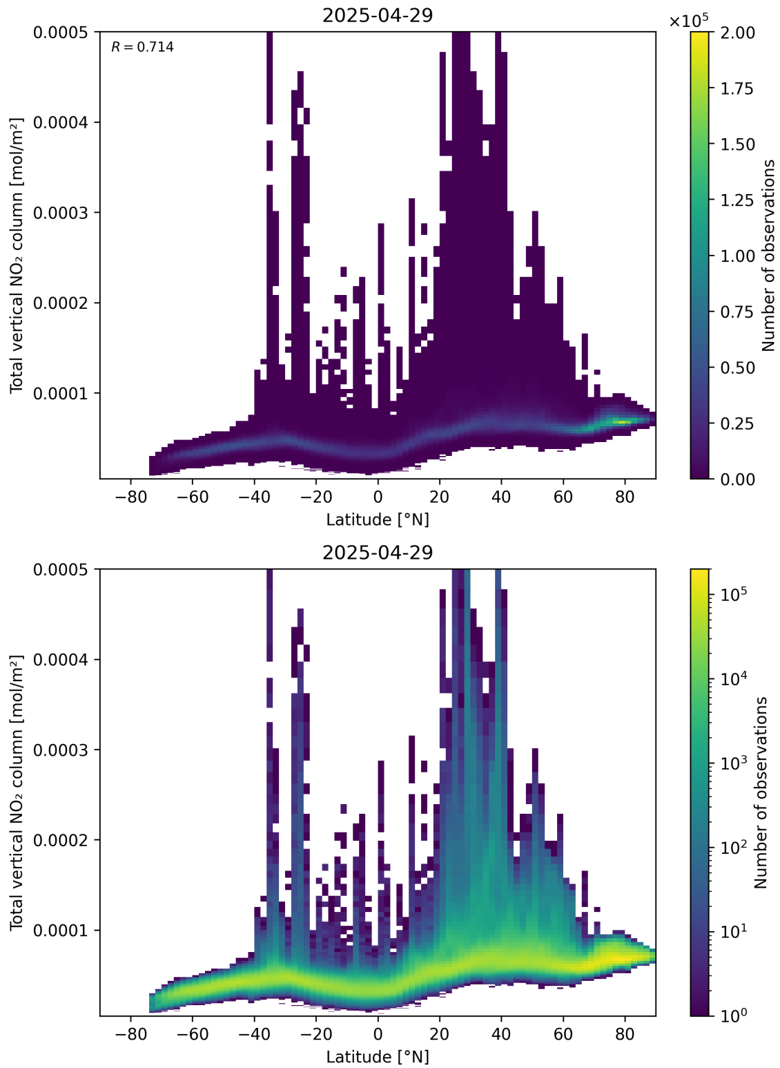
Figure 90: Scatter density plot of “Latitude” against “Total vertical NO 2 column” for 2025-04-29 to 2025-04-30.
