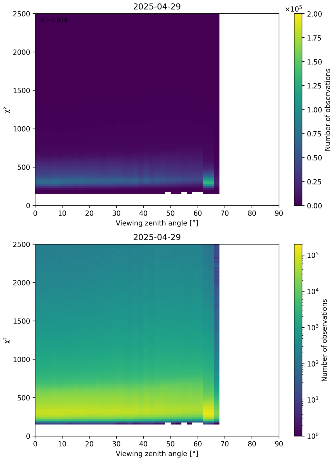
Figure 162: Scatter density plot of “Viewing zenith angle” against “ \chi^2 ” for 2025-04-29 to 2025-04-30.
