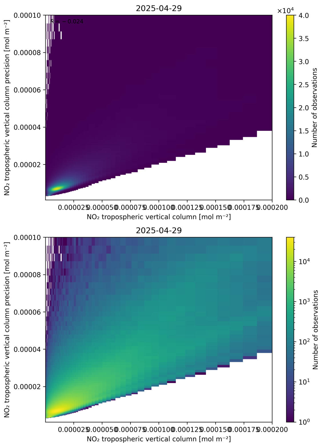
Figure 130: Scatter density plot of “NO 2 tropospheric vertical column” against “NO 2 tropospheric vertical column precision” for 2025-04-29 to 2025-04-30.
