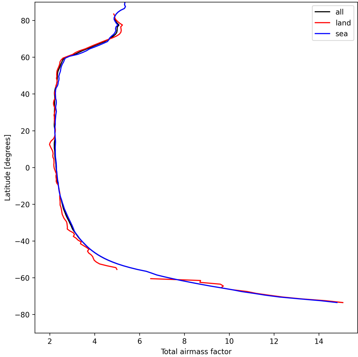
Figure 15: Zonal average of “Total airmass factor” for 2025-04-29 to 2025-04-30.
