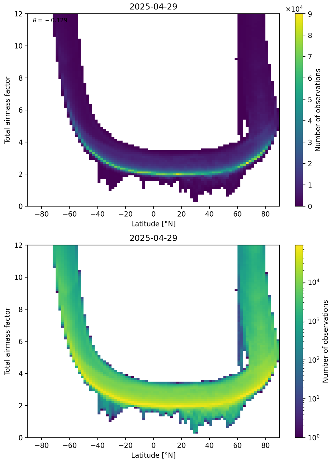
Figure 84: Scatter density plot of “Latitude” against “Total airmass factor” for 2025-04-29 to 2025-04-30.
