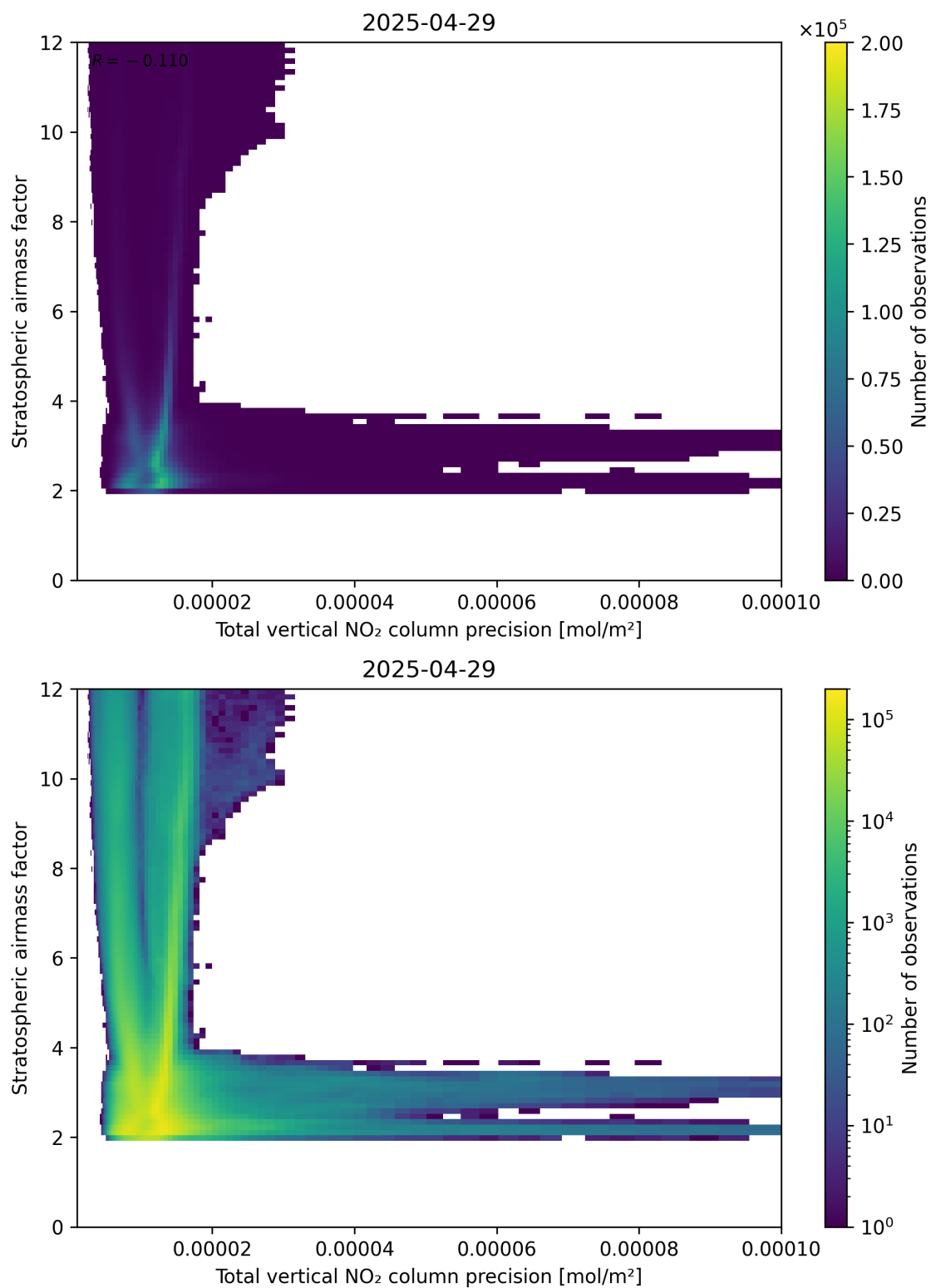
Figure 115: Scatter density plot of “Total vertical NO 2 column precision” against “Stratospheric air mass factor” for 2025-04-29 to 2025-04-30.
