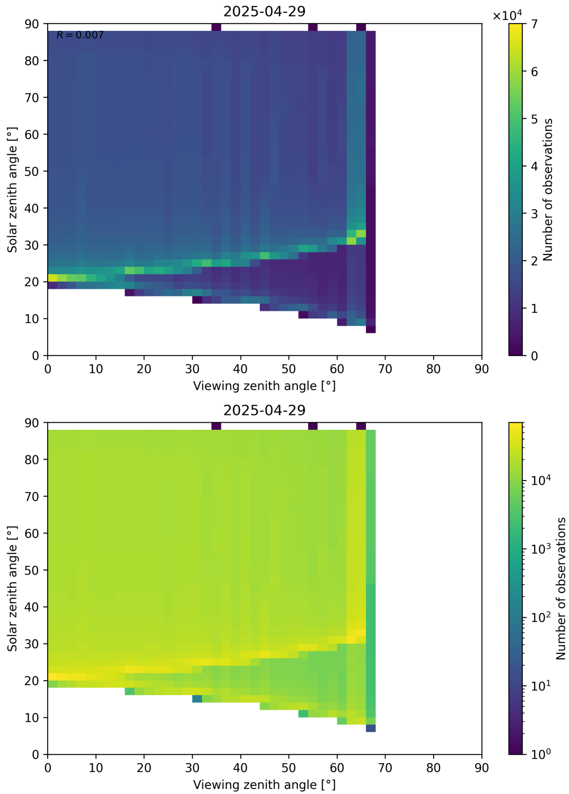
Figure 172: Scatter density plot of “Viewing zenith angle” against “Solar zenith angle” for 2025-04-29 to 2025-04-30.
