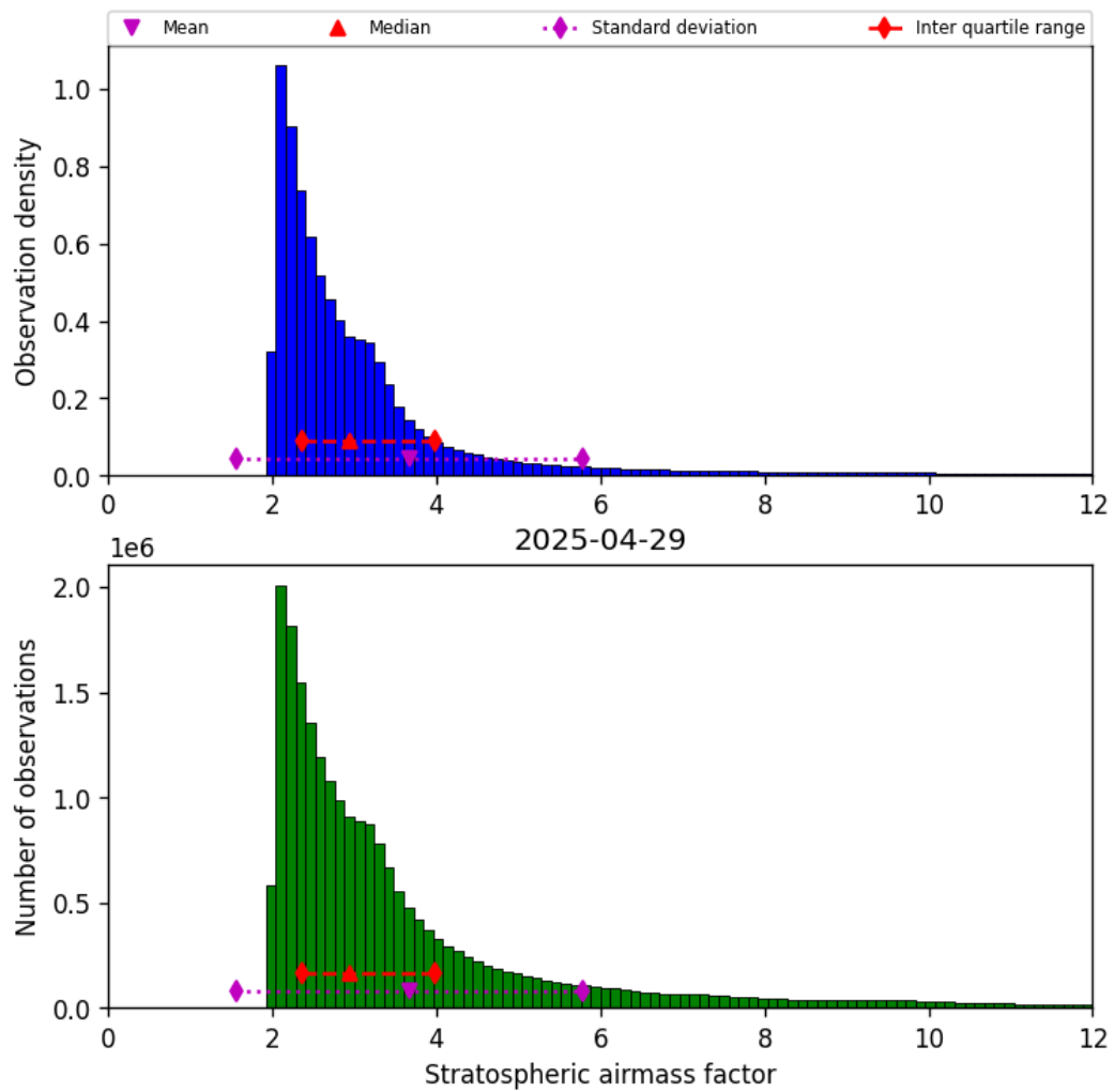
Figure 44: Histogram of “Stratospheric airmass factor” for 2025-04-29 to 2025-04-30
