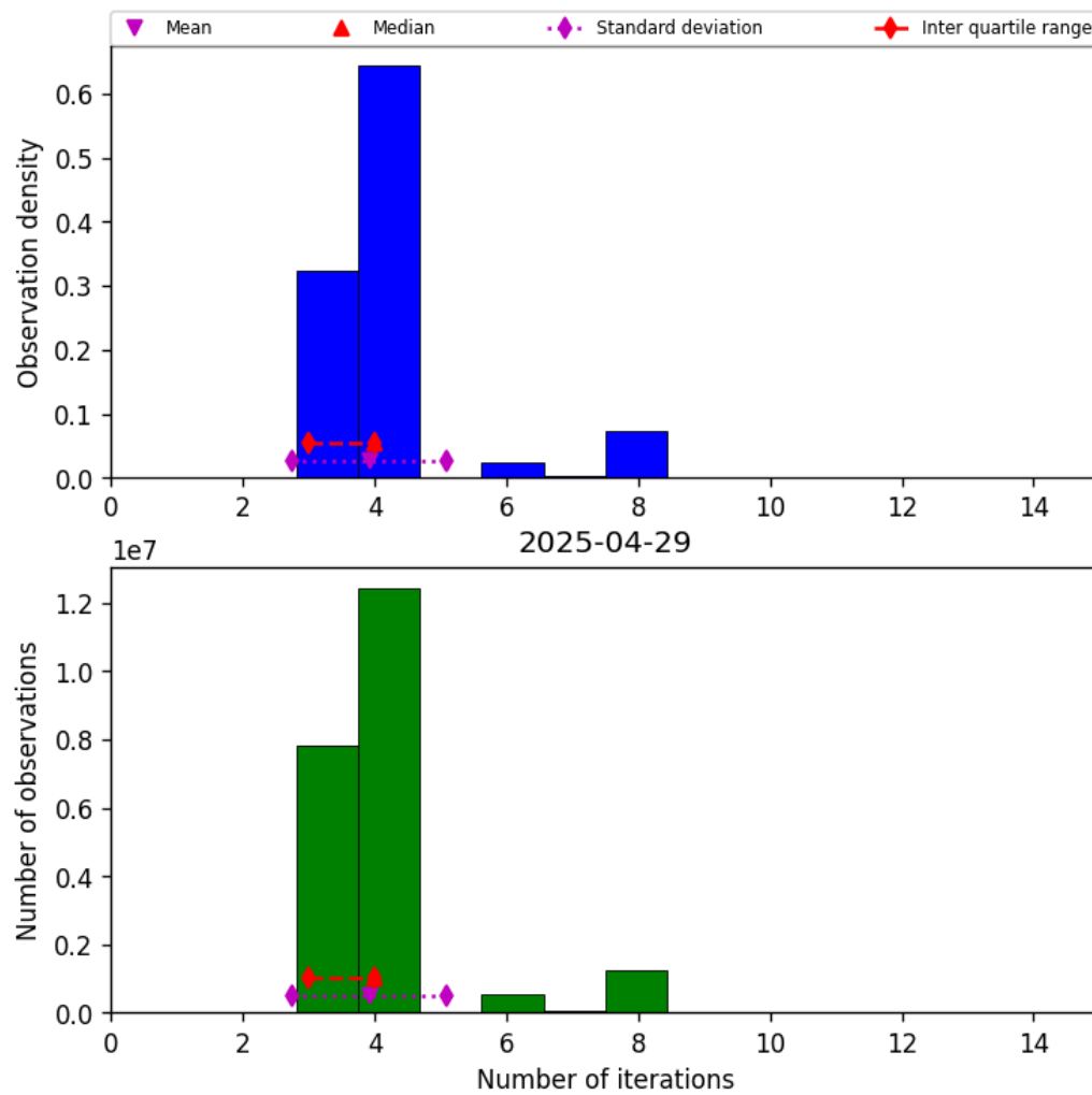
Figure 34: Histogram of “Number of iterations” for 2025-04-29 to 2025-04-30
