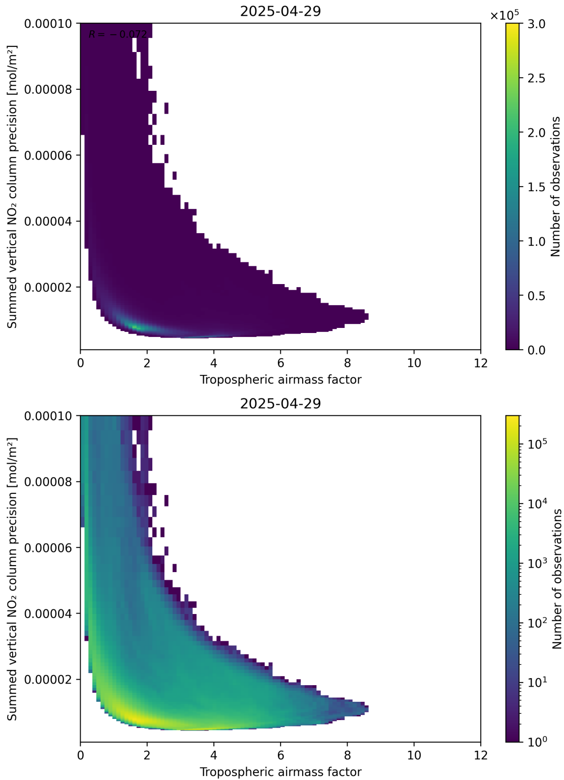
Figure 76: Scatter density plot of “Tropospheric air mass factor” against “Summed vertical NO 2 column precision” for 2025-04-29 to 2025-04-30.
