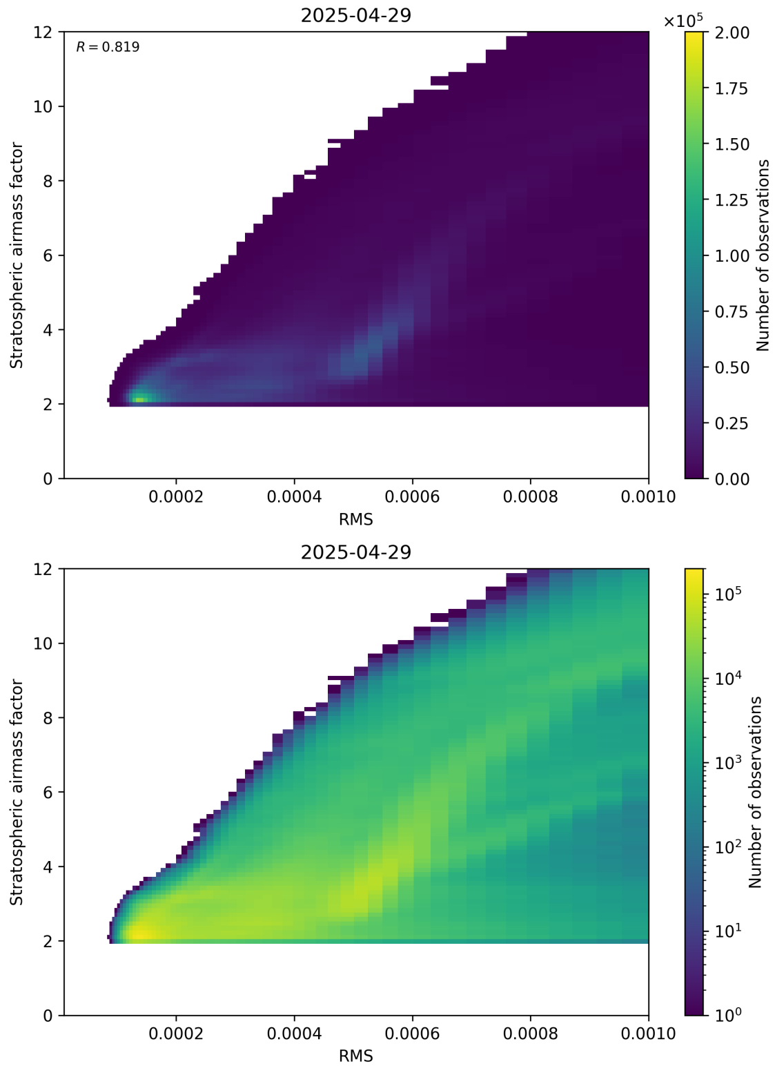
Figure 144: Scatter density plot of “RMS” against “Stratospheric airmass factor” for 2025-04-29 to 2025-04-30.
