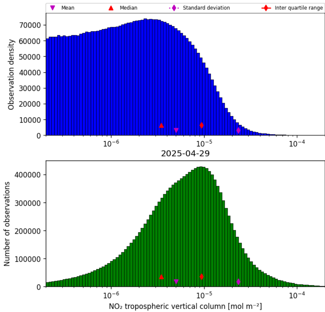
Figure 29: Histogram of “NO 2 tropospheric vertical column” for 2025-04-29 to 2025-04-30
