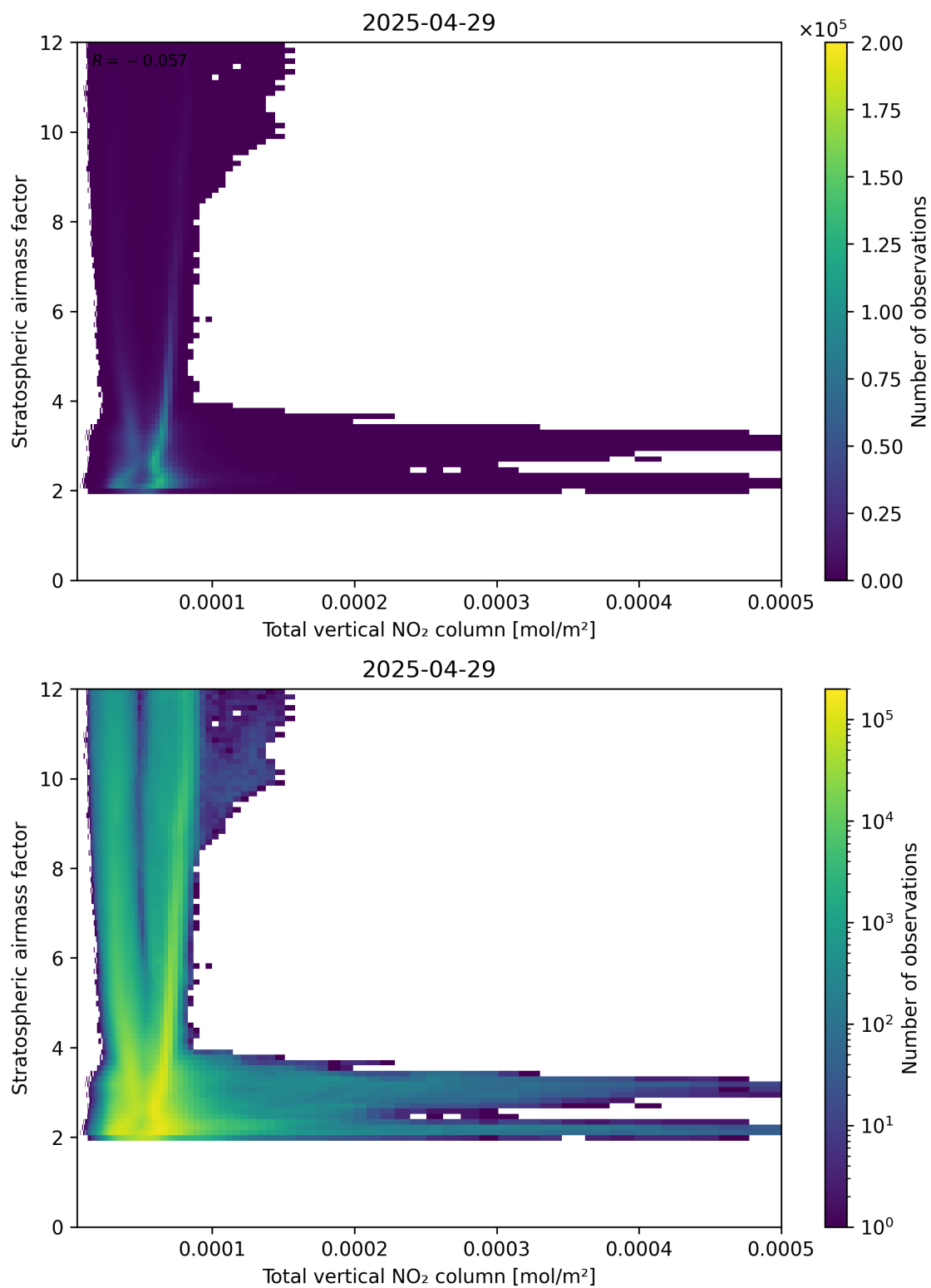
Figure 110: Scatter density plot of “Total vertical NO 2 column” against “Stratospheric airmass factor” for 2025-04-29 to 2025-04-30.
