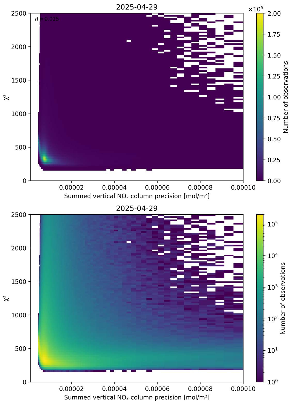
Figure 107: Scatter density plot of “Summed vertical NO 2 column precision” against “ \chi^2 ” for 2025-04-29 to 2025-04-30.
