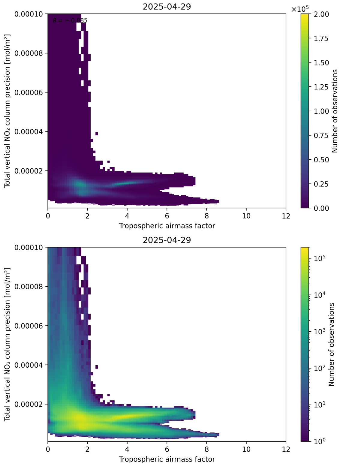
Figure 78: Scatter density plot of “Tropospheric air mass factor” against “Total vertical NO 2 column precision” for 2025-04-29 to 2025-04-30.
