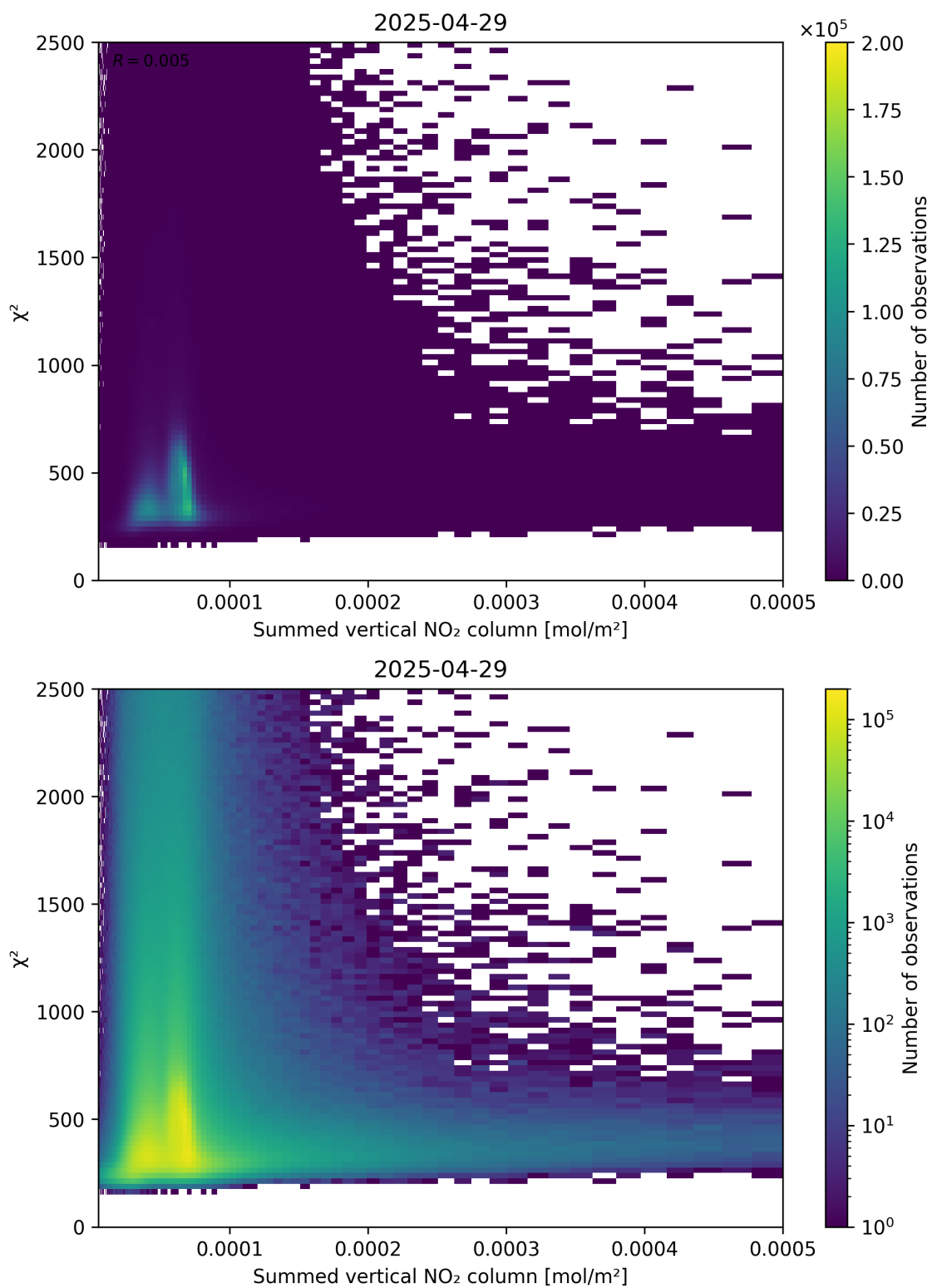
Figure 104: Scatter density plot of “Summed vertical NO 2 column” against “ \chi^2 ” for 2025-04-29 to 2025-04-30.
