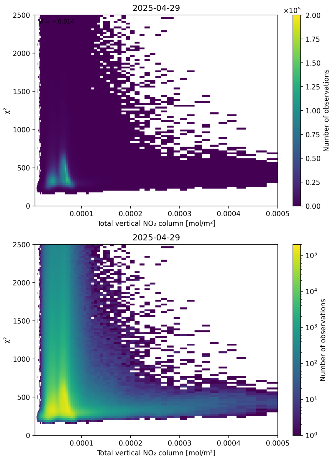
Figure 111: Scatter density plot of “Total vertical NO 2 column” against “ \chi^2 ” for 2025-04-29 to 2025-04-30.
