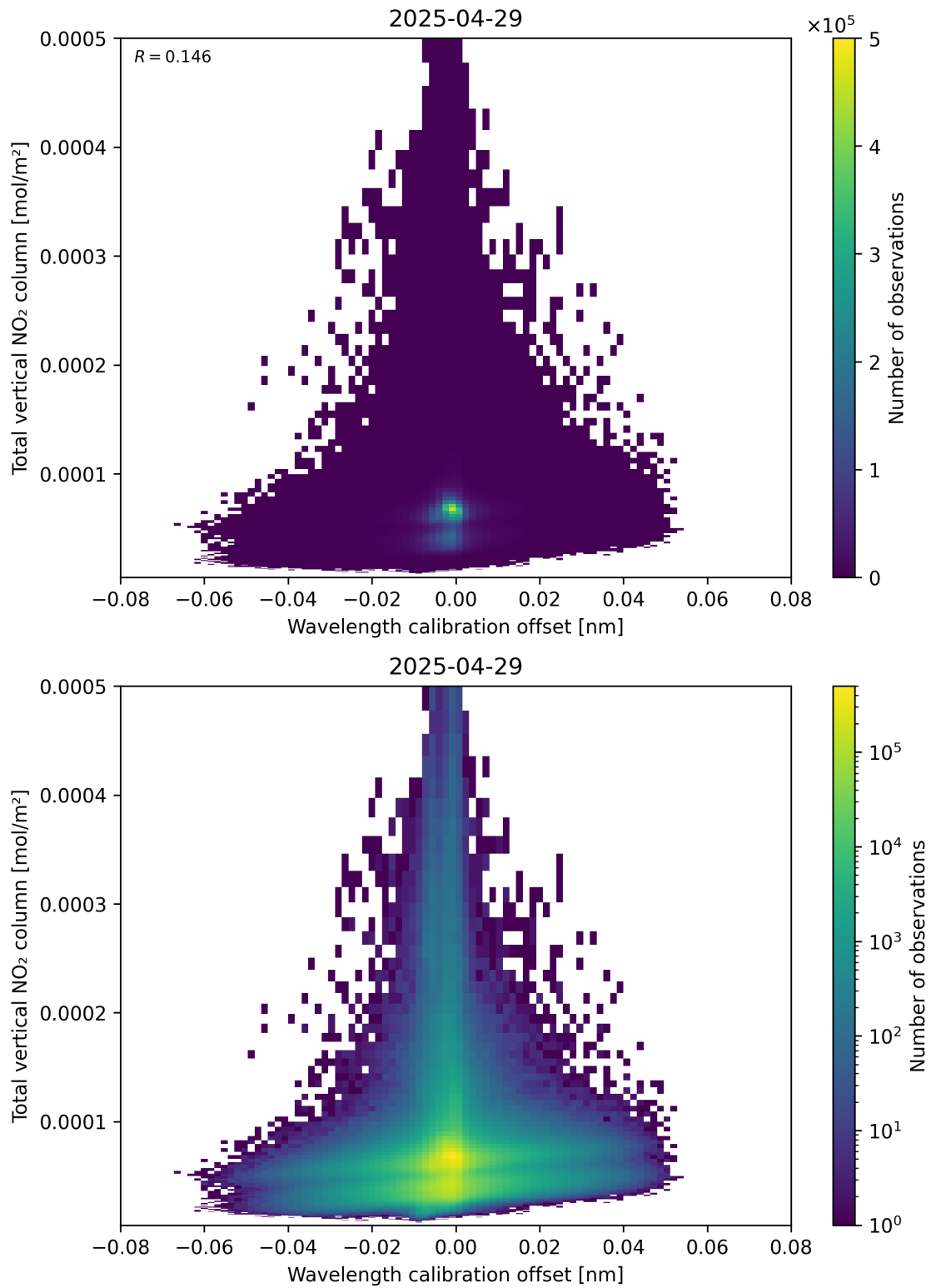
Figure 179: Scatter density plot of “Wavelength calibration offset” against “Total vertical NO 2 column” for 2025-04-29 to 2025-04-30.
