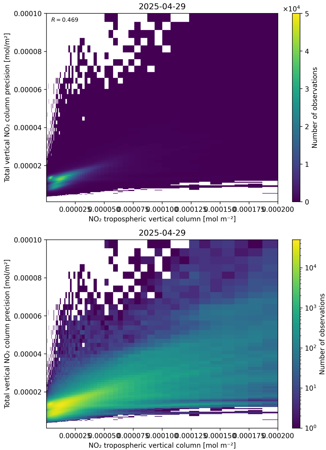
Figure 129: Scatter density plot of “NO 2 tropospheric vertical column” against “Total vertical NO 2 column precision” for 2025-04-29 to 2025-04-30.
