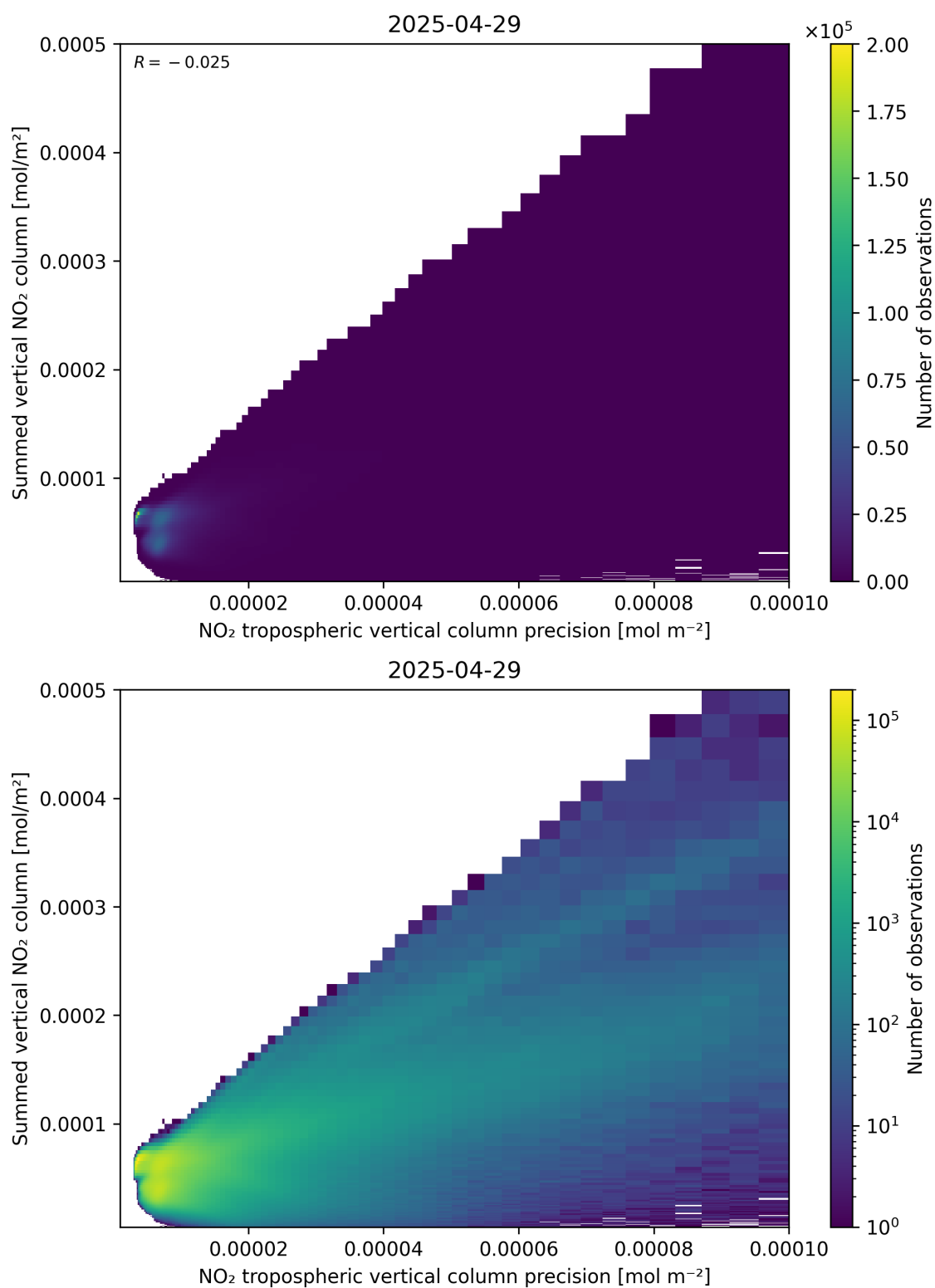
Figure 136: Scatter density plot of “NO 2 tropospheric vertical column precision” against “Summed vertical NO 2 column” for 2025-04-29 to 2025-04-30.
