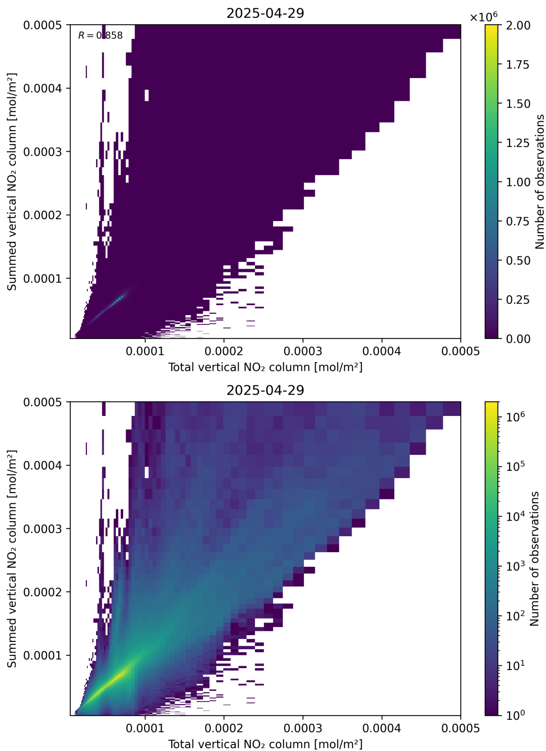
Figure 112: Scatter density plot of “Total vertical NO 2 column” against “Summed vertical NO 2 column” for 2025-04-29 to 2025-04-30.
