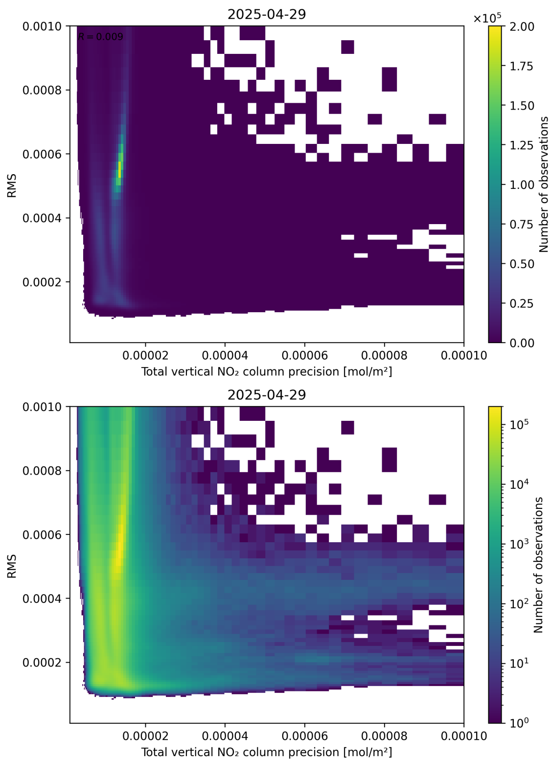
Figure 119: Scatter density plot of “Total vertical NO 2 column precision” against “RMS” for 2025-04-29 to 2025-04-30.
