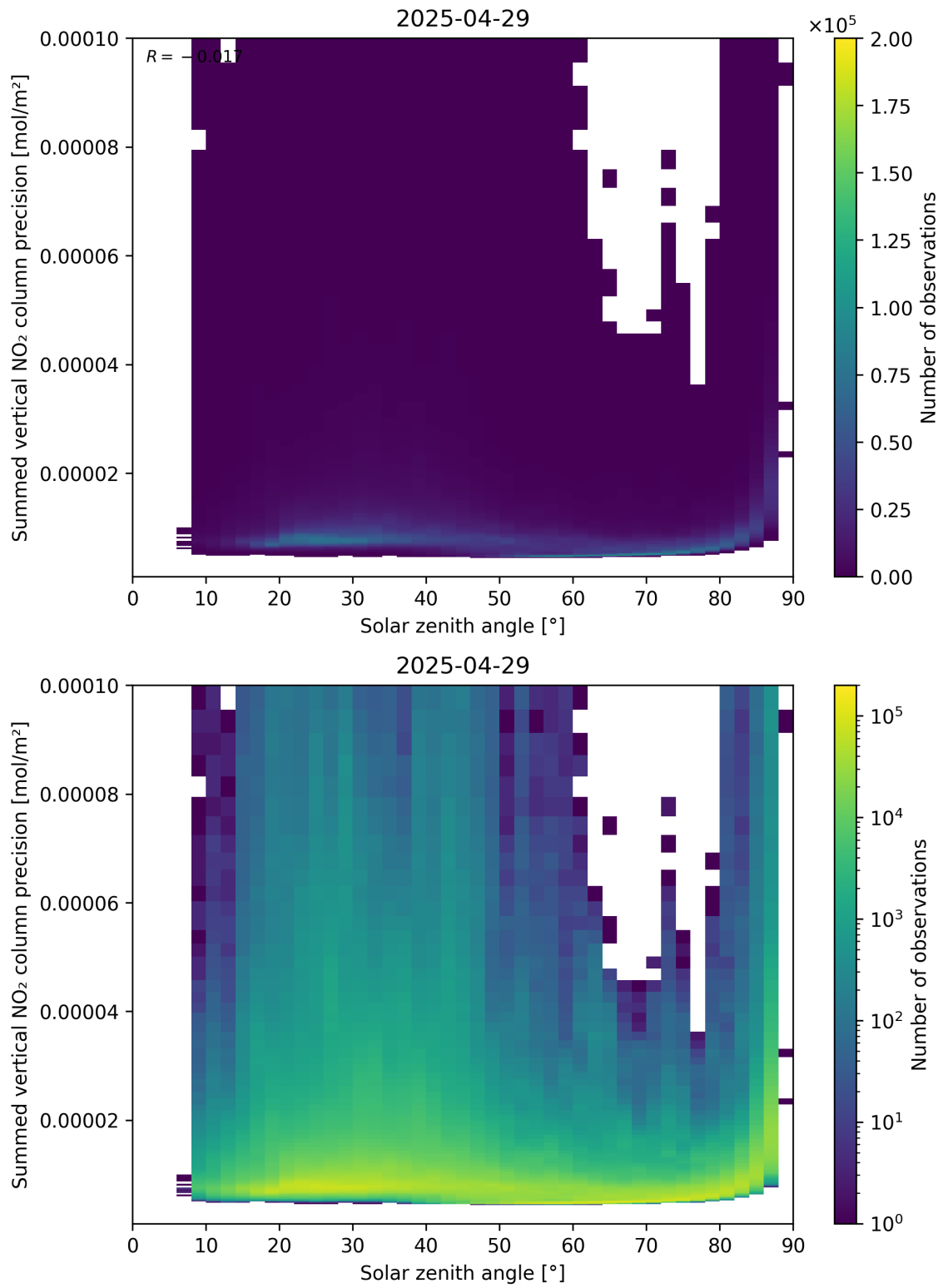
Figure 152: Scatter density plot of “Solar zenith angle” against “Summed vertical NO 2 column precision” for 2025-04-29 to 2025-04-30.
