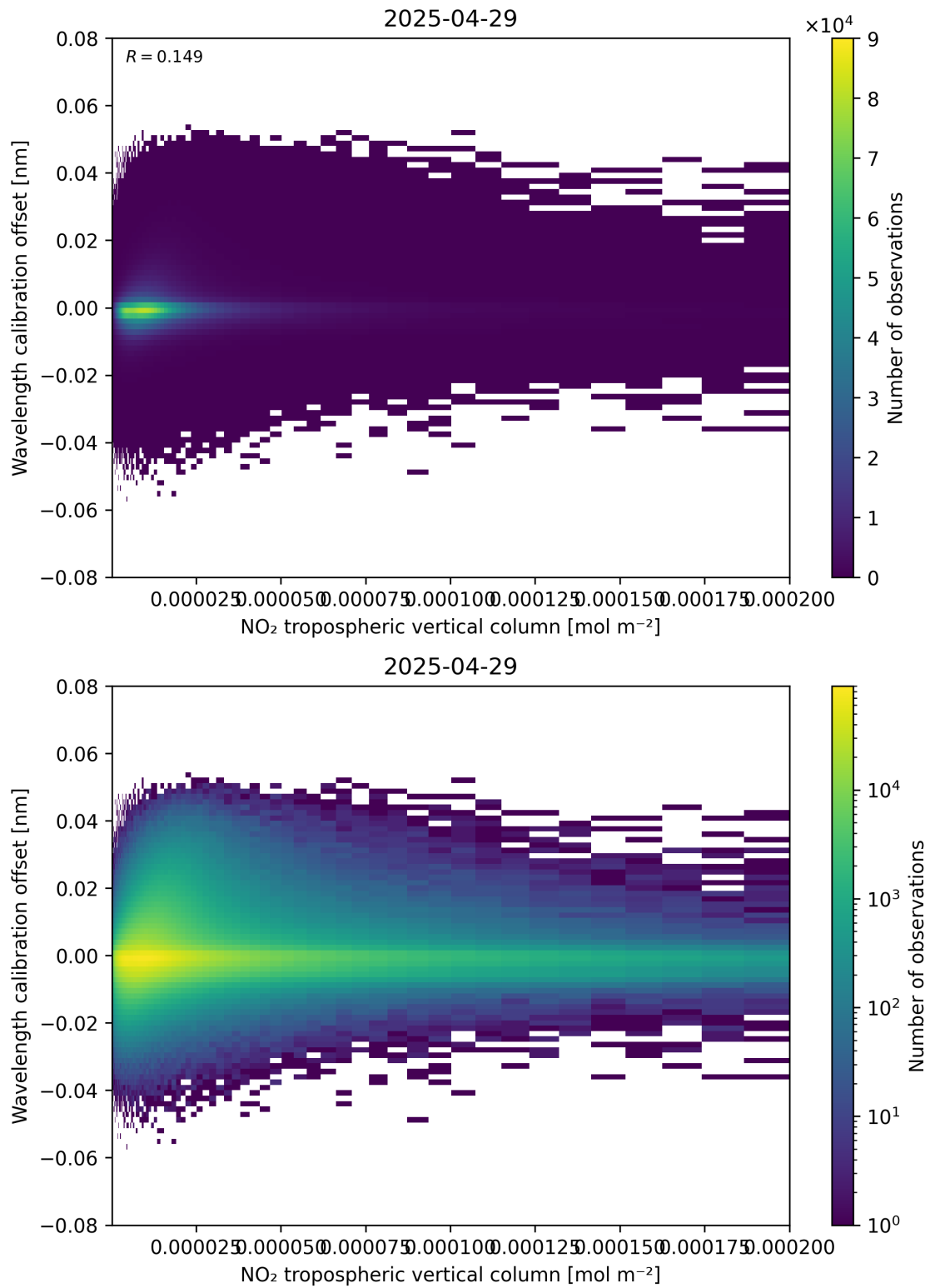
Figure 143: Scatter density plot of “NO 2 tropospheric vertical column” against “Wavelength calibration offset” for 2025-04-29 to 2025-04-30.
