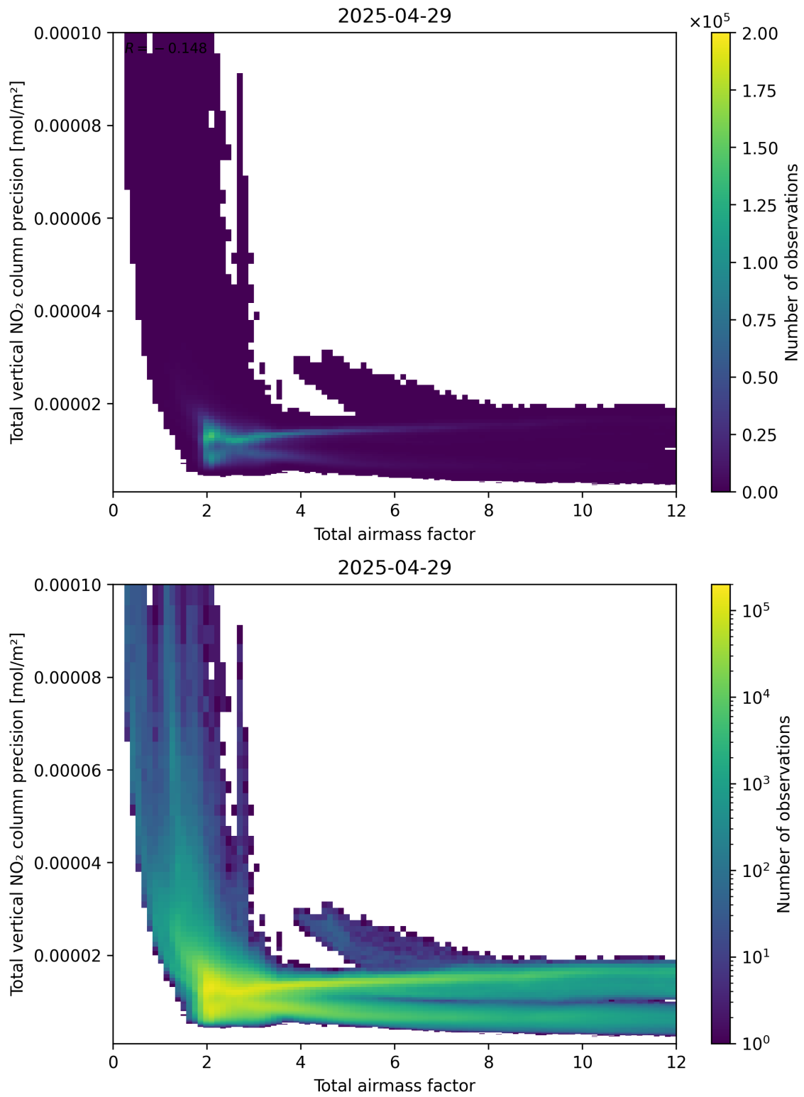
Figure 68: Scatter density plot of “Total airmass factor” against “Total vertical NO 2 column precision” for 2025-04-29 to 2025-04-30.
