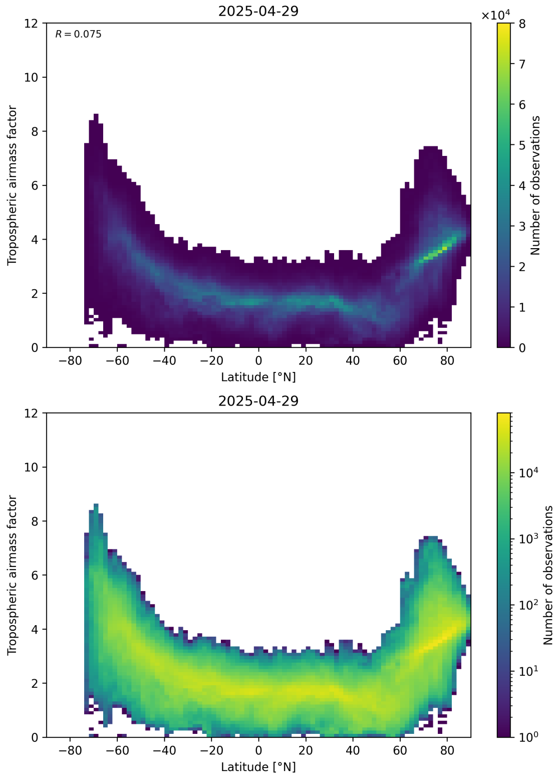
Figure 85: Scatter density plot of “Latitude” against “Tropospheric airmass factor” for 2025-04-29 to 2025-04-30.
