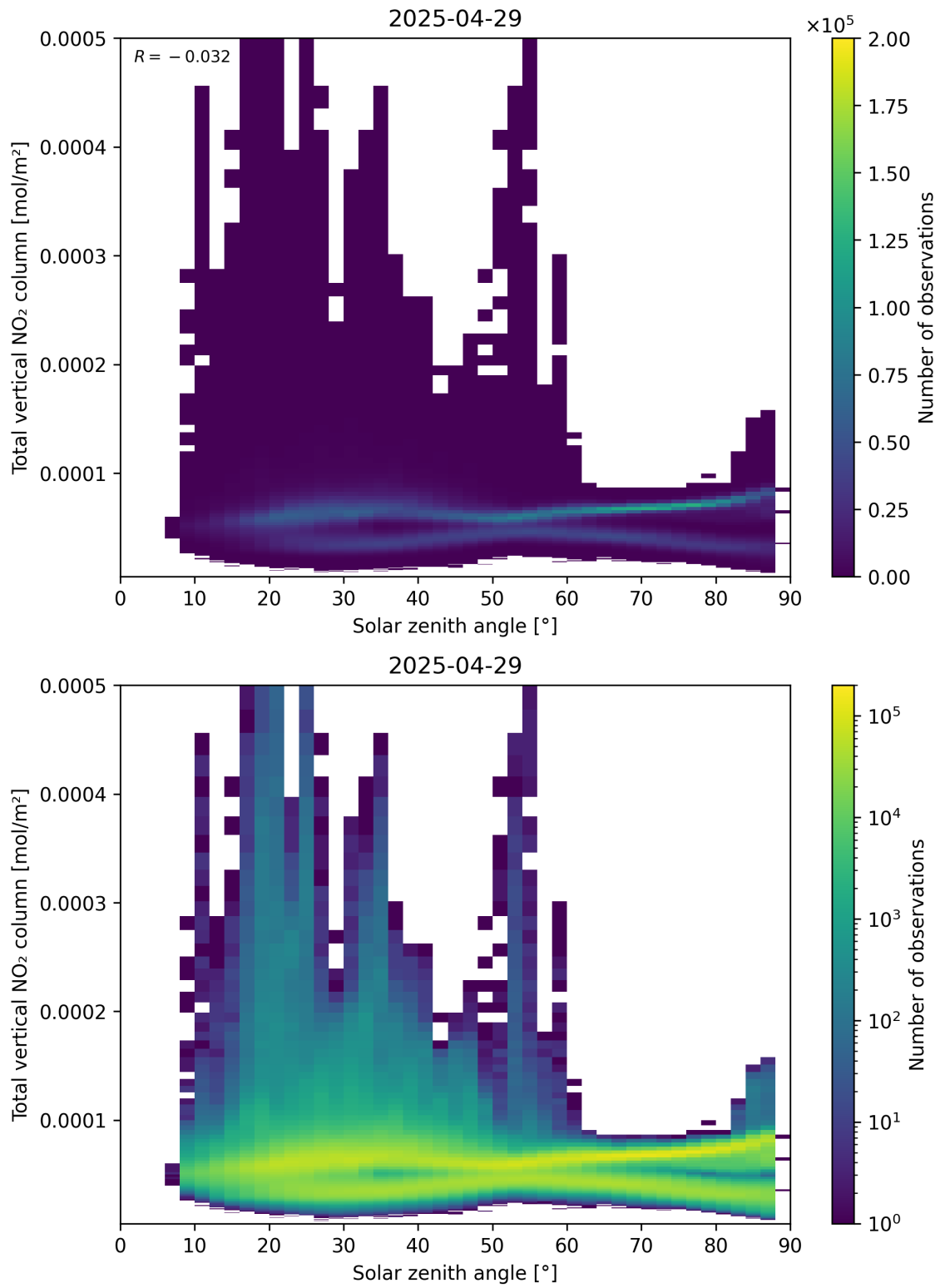
Figure 153: Scatter density plot of “Solar zenith angle” against “Total vertical NO 2 column” for 2025-04-29 to 2025-04-30.
