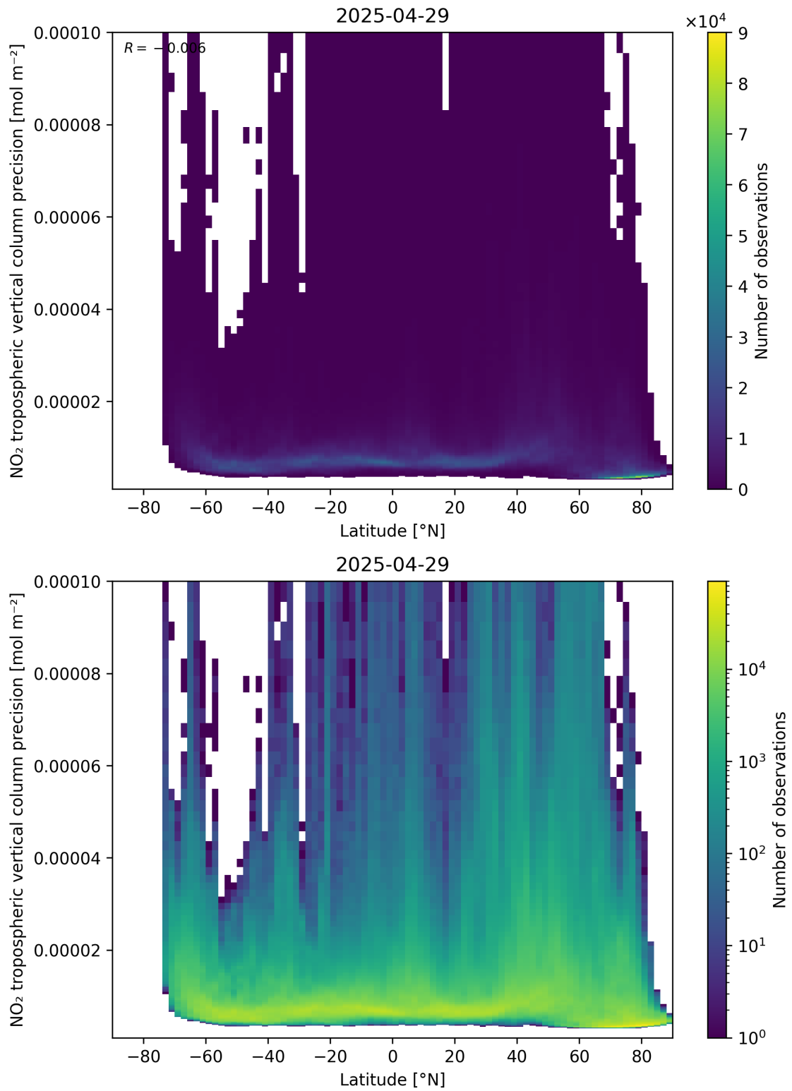
Figure 93: Scatter density plot of “Latitude” against “NO 2 tropospheric vertical column precision” for 2025-04-29 to 2025-04-30.
