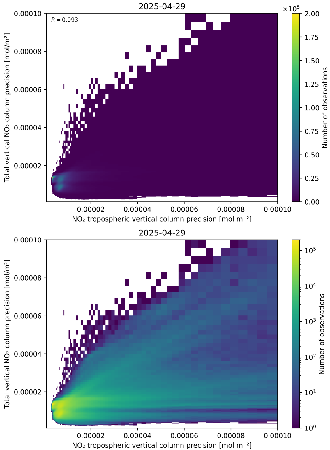
Figure 139: Scatter density plot of “NO 2 tropospheric vertical column precision” against “Total vertical NO 2 column precision” for 2025-04-29 to 2025-04-30.
