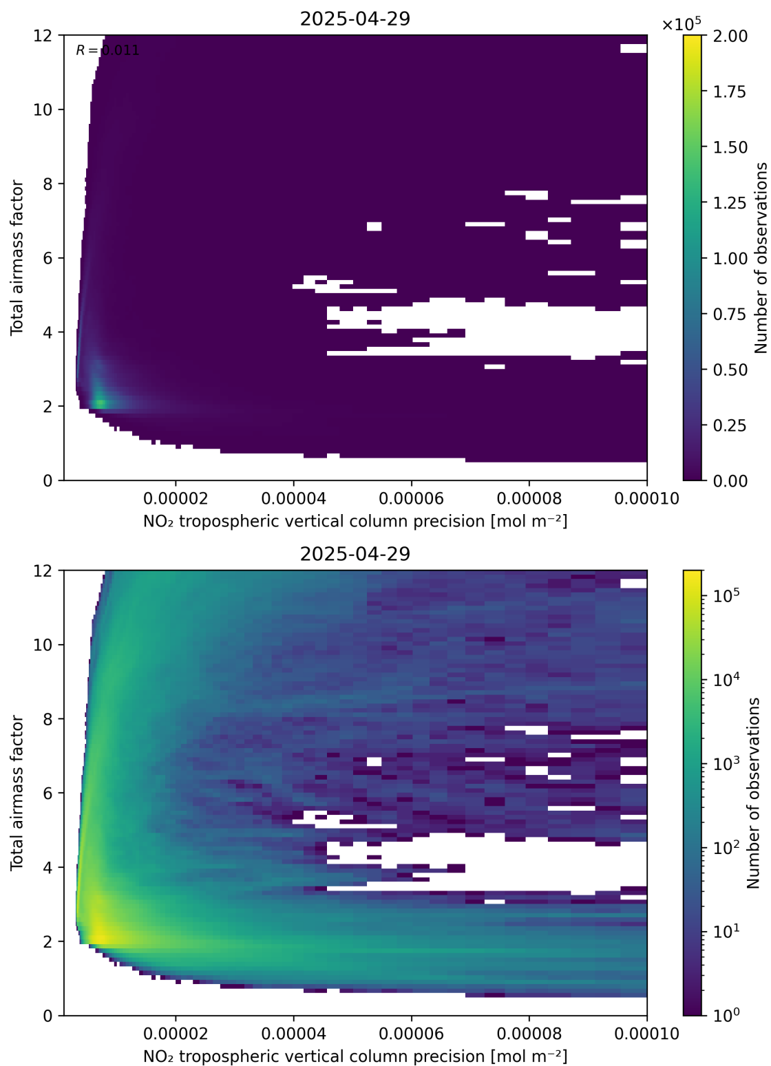
Figure 132: Scatter density plot of “NO 2 tropospheric vertical column precision” against “Total air mass factor” for 2025-04-29 to 2025-04-30.
