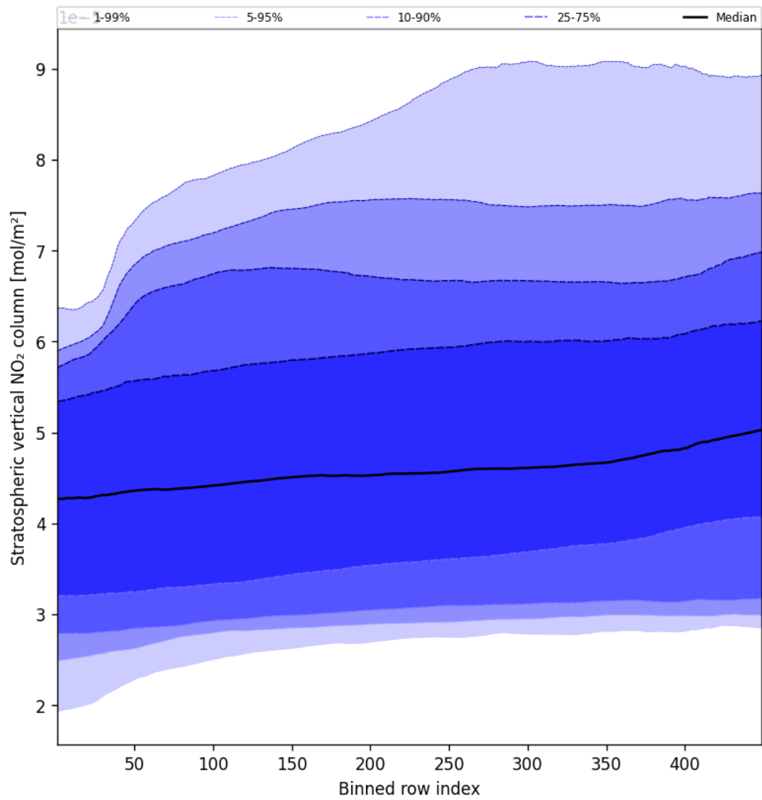
Figure 53: Along track statistics of “Stratospheric vertical NO 2 column” for 2025-04-29 to 2025-04-30
