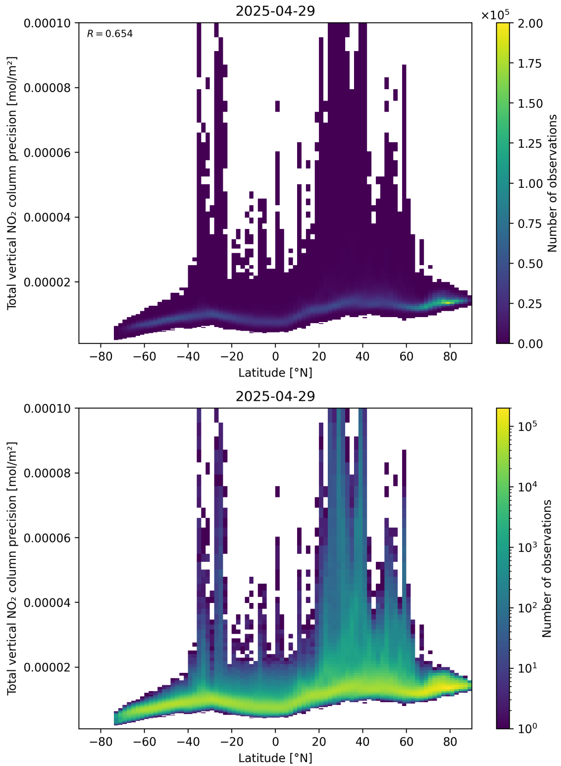
Figure 91: Scatter density plot of “Latitude” against “Total vertical NO 2 column precision” for 2025-04-29 to 2025-04-30.
