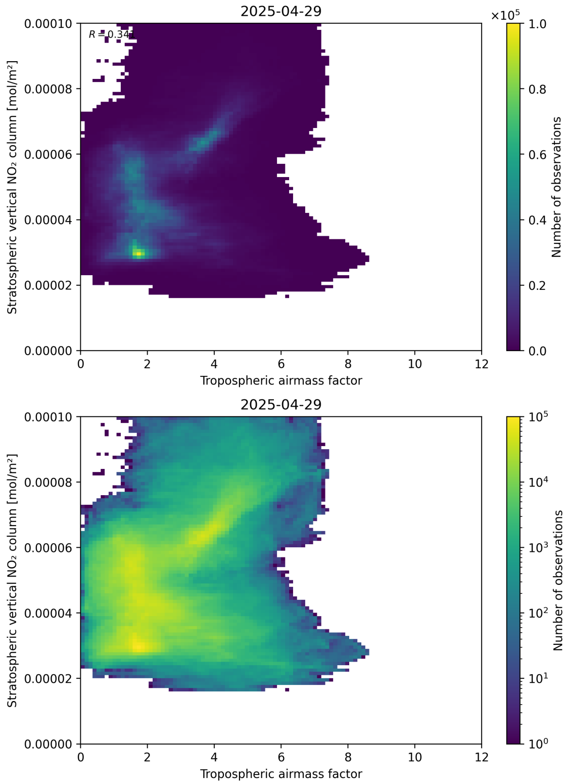
Figure 74: Scatter density plot of “Tropospheric air mass factor” against “Stratospheric vertical NO 2 column” for 2025-04-29 to 2025-04-30.
