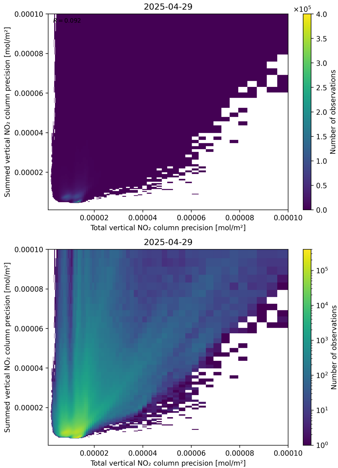
Figure 118: Scatter density plot of “Total vertical NO 2 column precision” against “Summed vertical NO 2 column precision” for 2025-04-29 to 2025-04-30.
