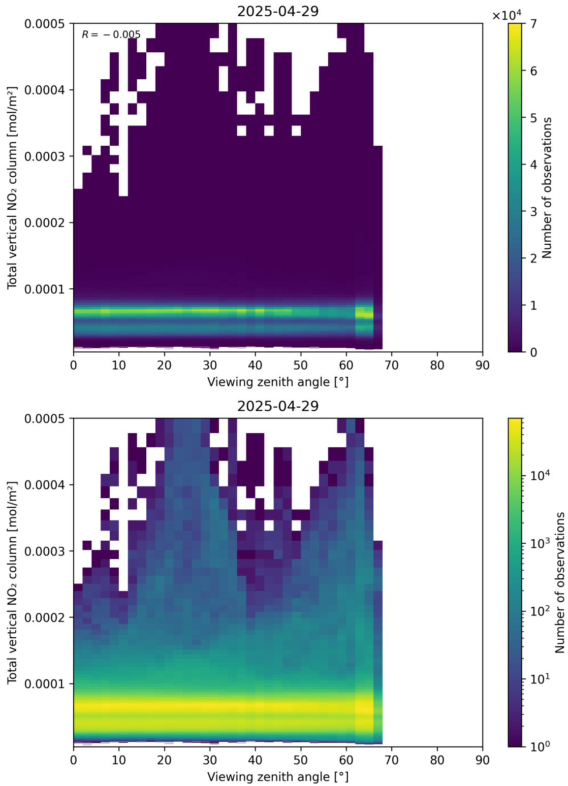
Figure 167: Scatter density plot of “Viewing zenith angle” against “Total vertical NO 2 column” for 2025-04-29 to 2025-04-30.
