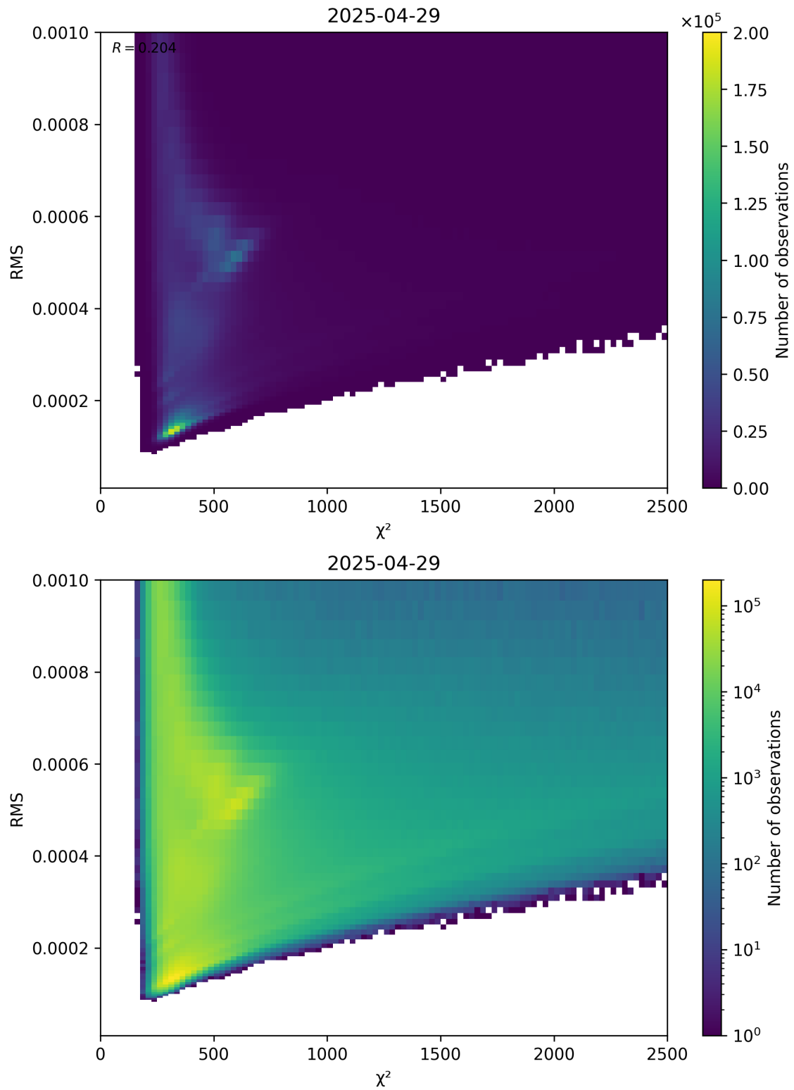
Figure 82: Scatter density plot of “ \chi^2 ” against “RMS” for 2025-04-29 to 2025-04-30.
