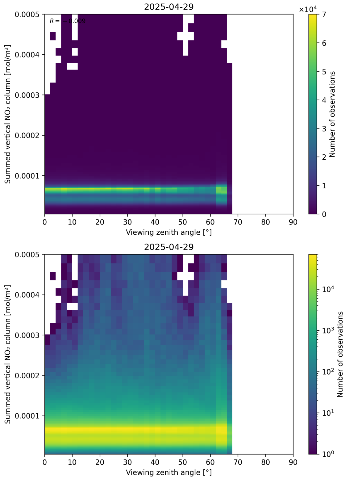
Figure 165: Scatter density plot of “Viewing zenith angle” against “Summed vertical NO 2 column” for 2025-04-29 to 2025-04-30.
