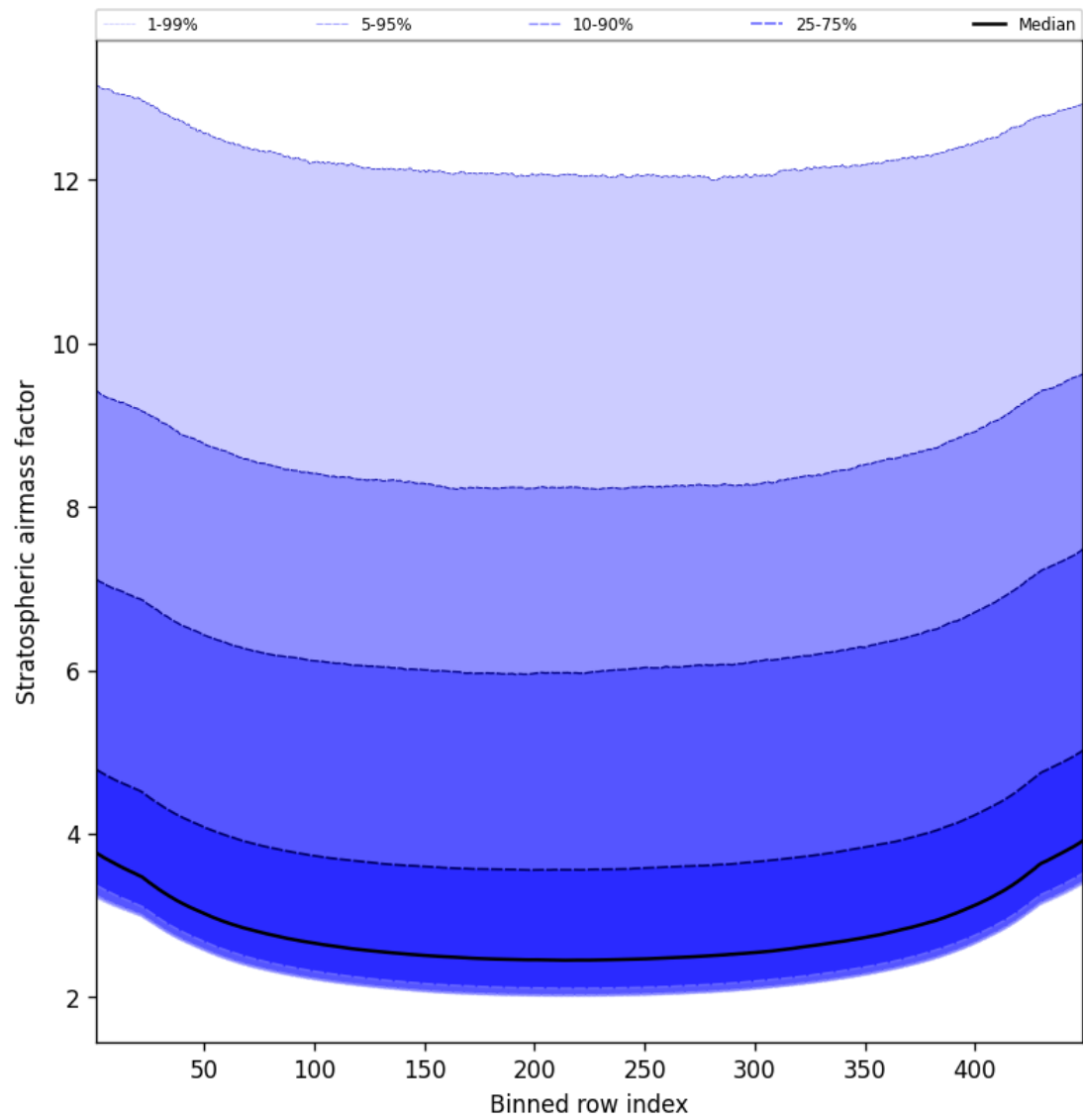
Figure 61: Along track statistics of “Stratospheric air mass factor” for 2025-04-29 to 2025-04-30
