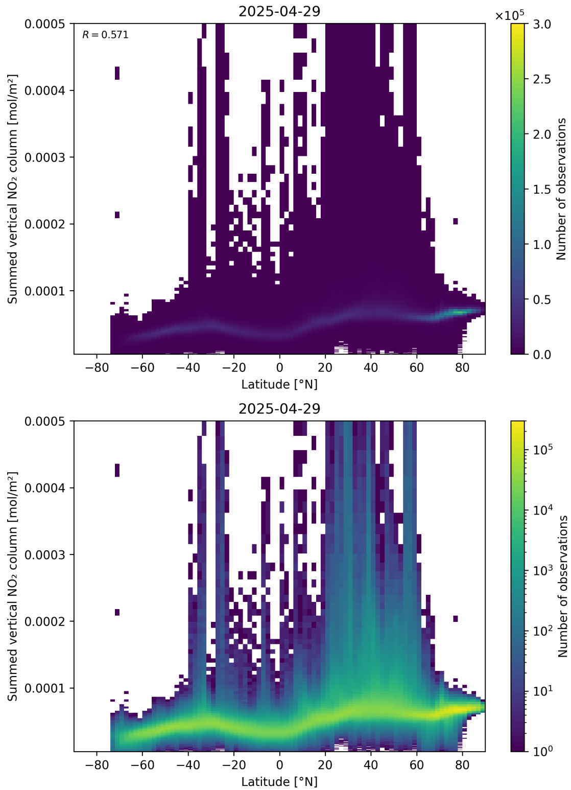
Figure 88: Scatter density plot of “Latitude” against “Summed vertical NO 2 column” for 2025-04-29 to 2025-04-30.
