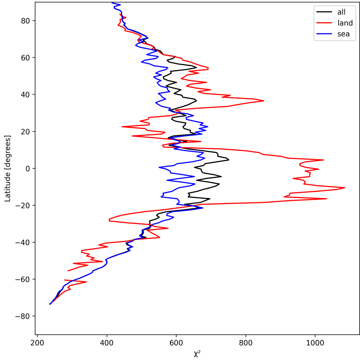
Figure 25: Zonal average of “ \chi^2 ” for 2025-04-29 to 2025-04-30.
