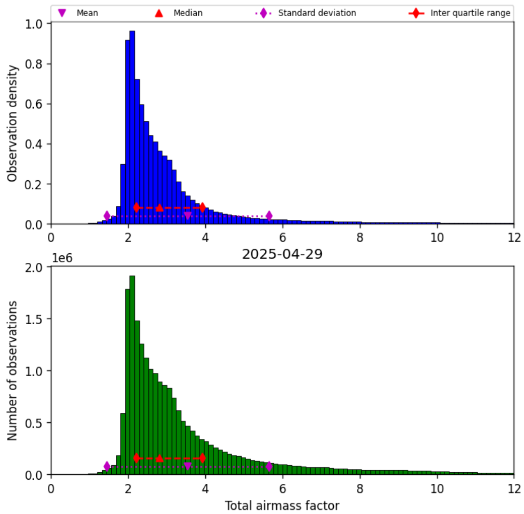
Figure 32: Histogram of “Total airmass factor” for 2025-04-29 to 2025-04-30
