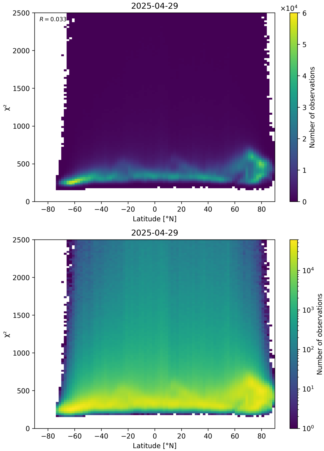
Figure 86: Scatter density plot of “Latitude” against “ \chi^2 ” for 2025-04-29 to 2025-04-30.
