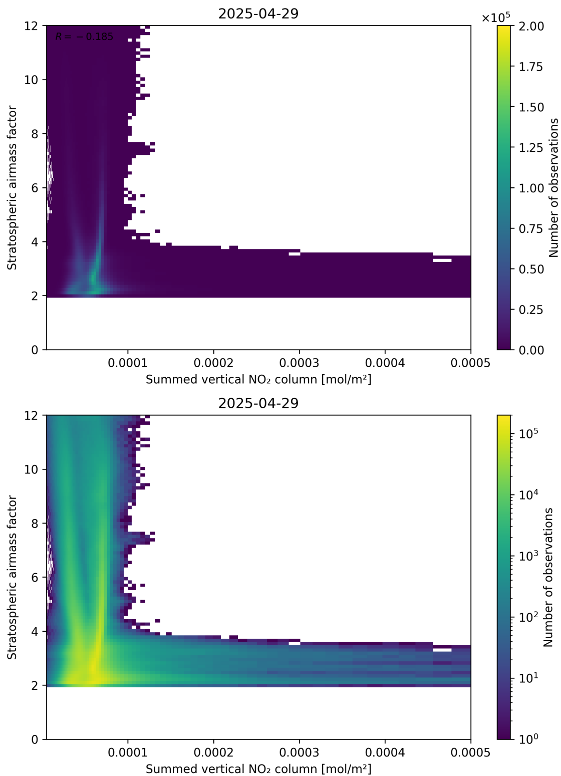
Figure 103: Scatter density plot of “Summed vertical NO 2 column” against “Stratospheric airmass factor” for 2025-04-29 to 2025-04-30.
