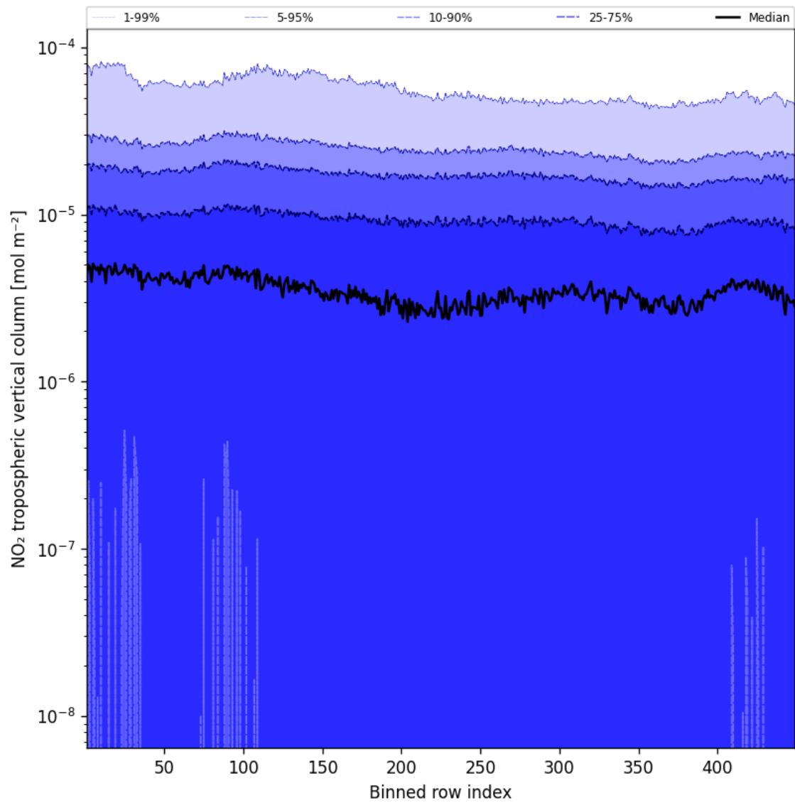
Figure 46: Along track statistics of “NO 2 tropospheric vertical column” for 2025-04-29 to 2025-04-30
