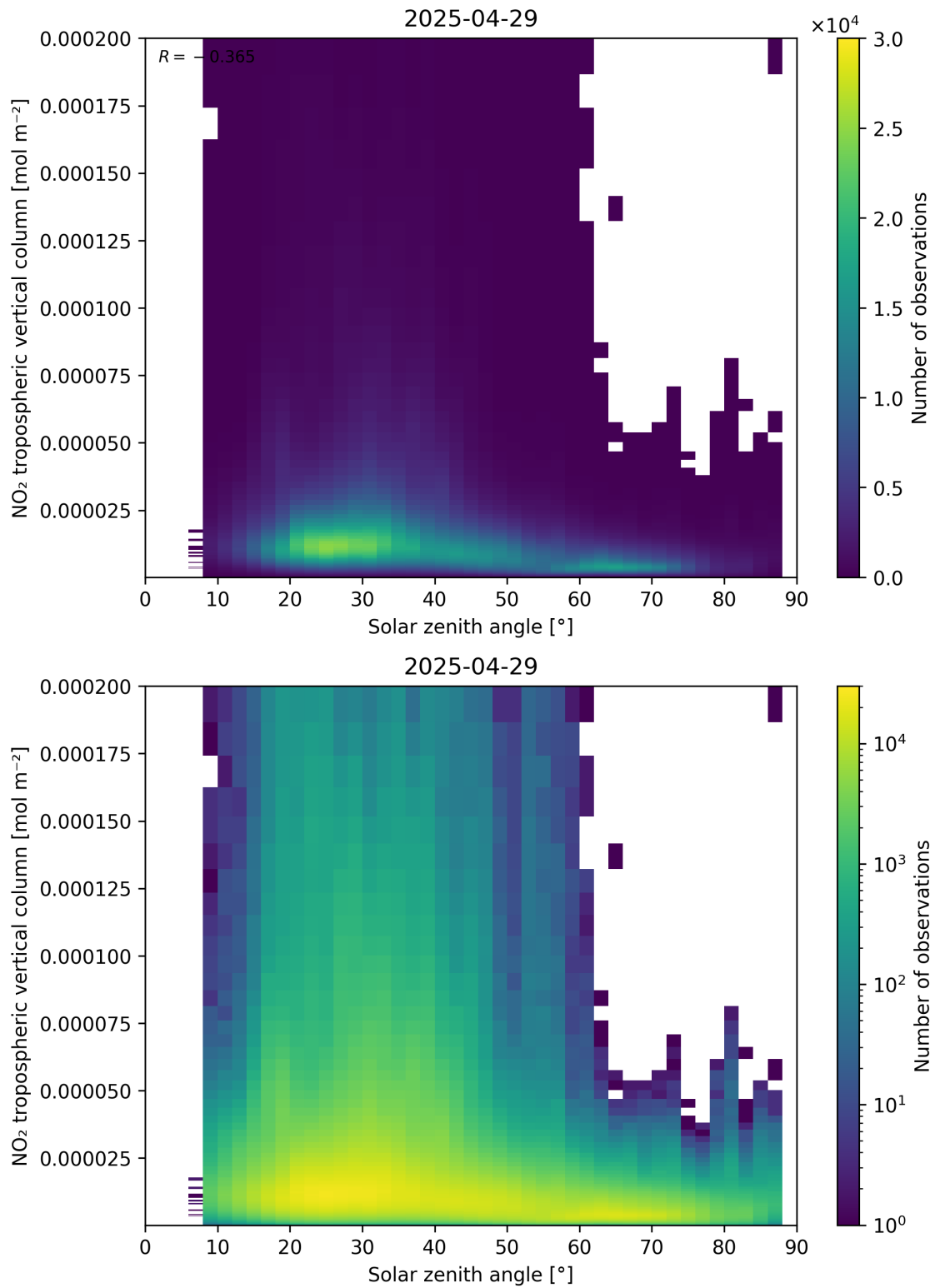
Figure 155: Scatter density plot of “Solar zenith angle” against “NO 2 tropospheric vertical column” for 2025-04-29 to 2025-04-30.
