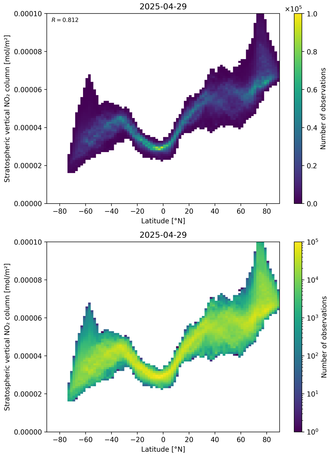
Figure 87: Scatter density plot of “Latitude” against “Stratospheric vertical NO 2 column” for 2025-04-29 to 2025-04-30.
