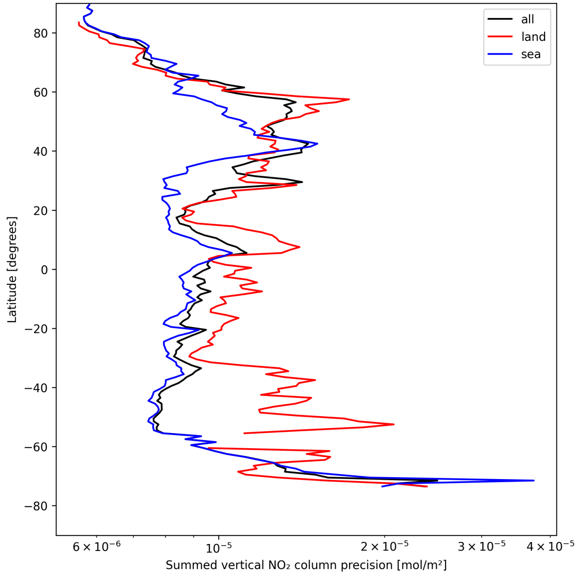
Figure 24: Zonal average of “Summed vertical NO 2 column precision” for 2025-04-29 to 2025-04-30.
