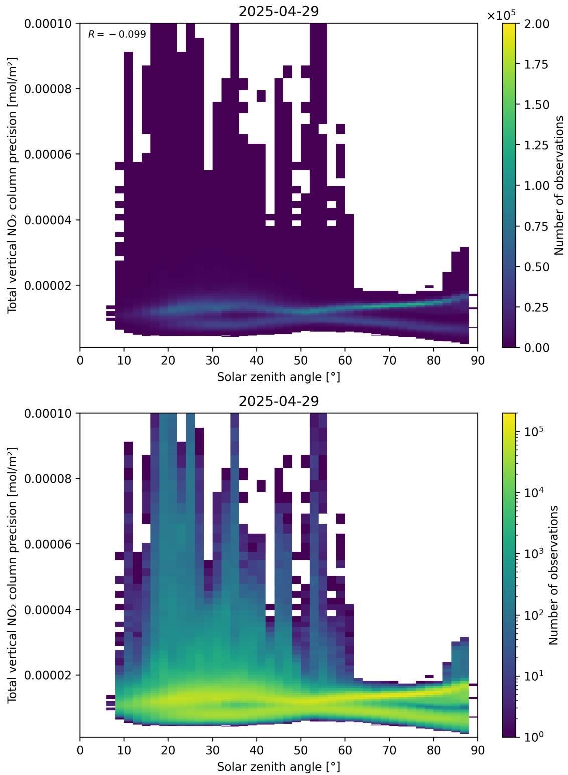
Figure 154: Scatter density plot of “Solar zenith angle” against “Total vertical NO 2 column precision” for 2025-04-29 to 2025-04-30.
