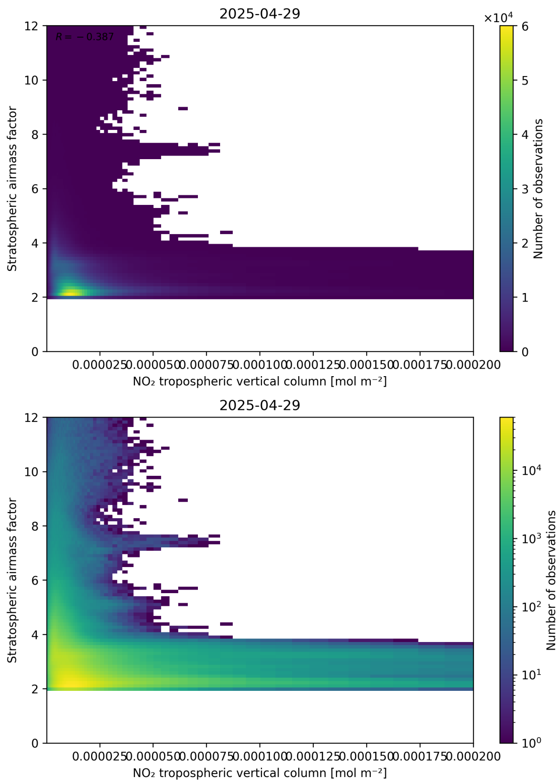
Figure 121: Scatter density plot of “NO 2 tropospheric vertical column” against “Stratospheric airmass factor” for 2025-04-29 to 2025-04-30.
