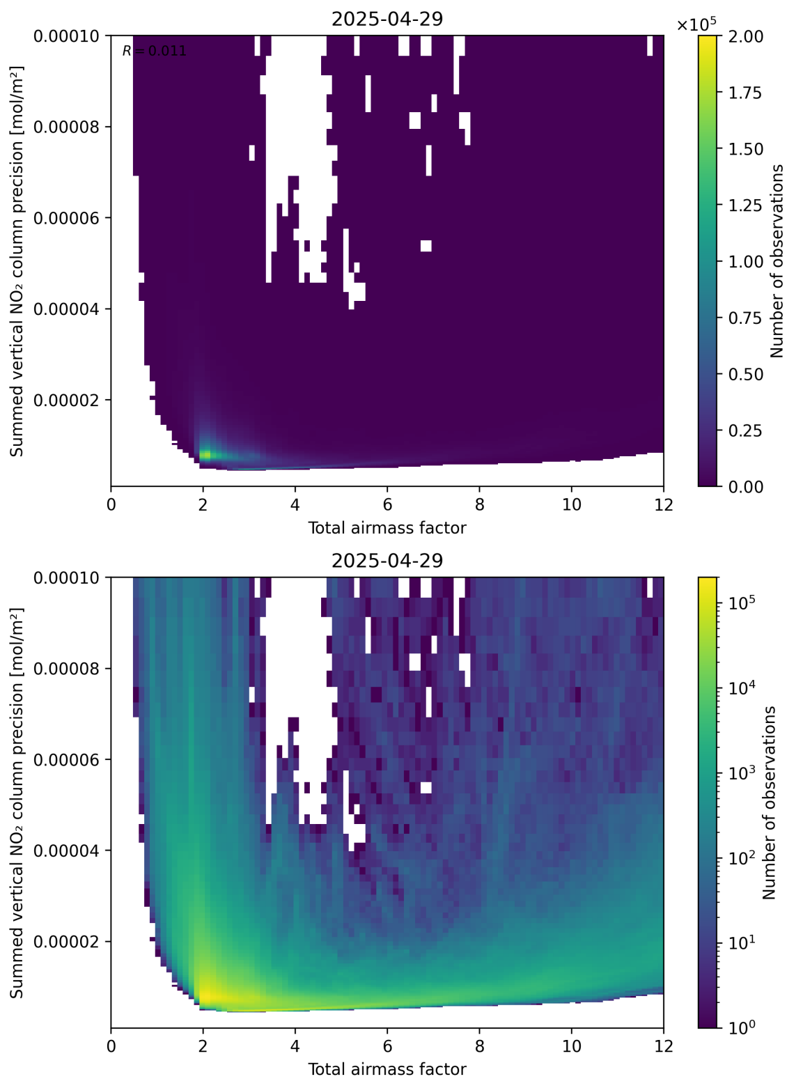
Figure 66: Scatter density plot of “Total airmass factor” against “Summed vertical NO 2 column precision” for 2025-04-29 to 2025-04-30.
