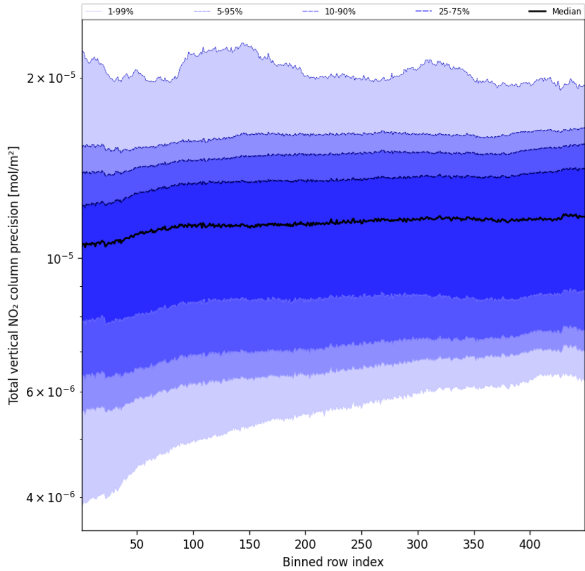
Figure 56: Along track statistics of “Total vertical NO 2 column precision” for 2025-04-29 to 2025-04-30
