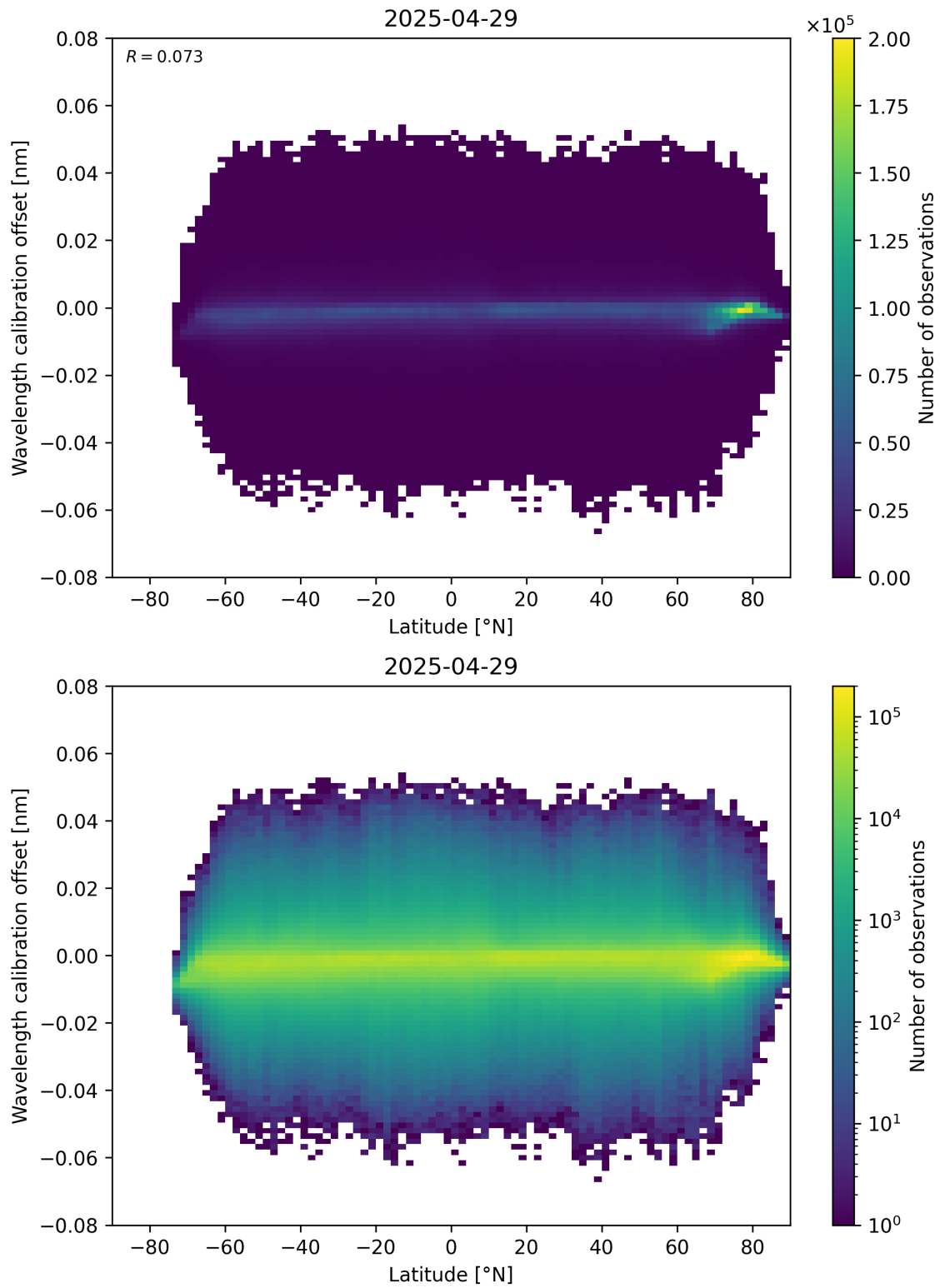
Figure 95: Scatter density plot of “Latitude” against “Wavelength calibration offset” for 2025-04-29 to 2025-04-30.
