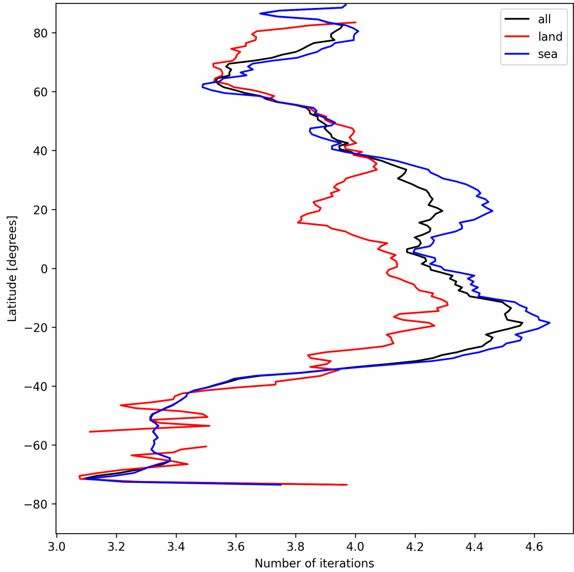
Figure 17: Zonal average of “Number of iterations” for 2025-04-29 to 2025-04-30.
