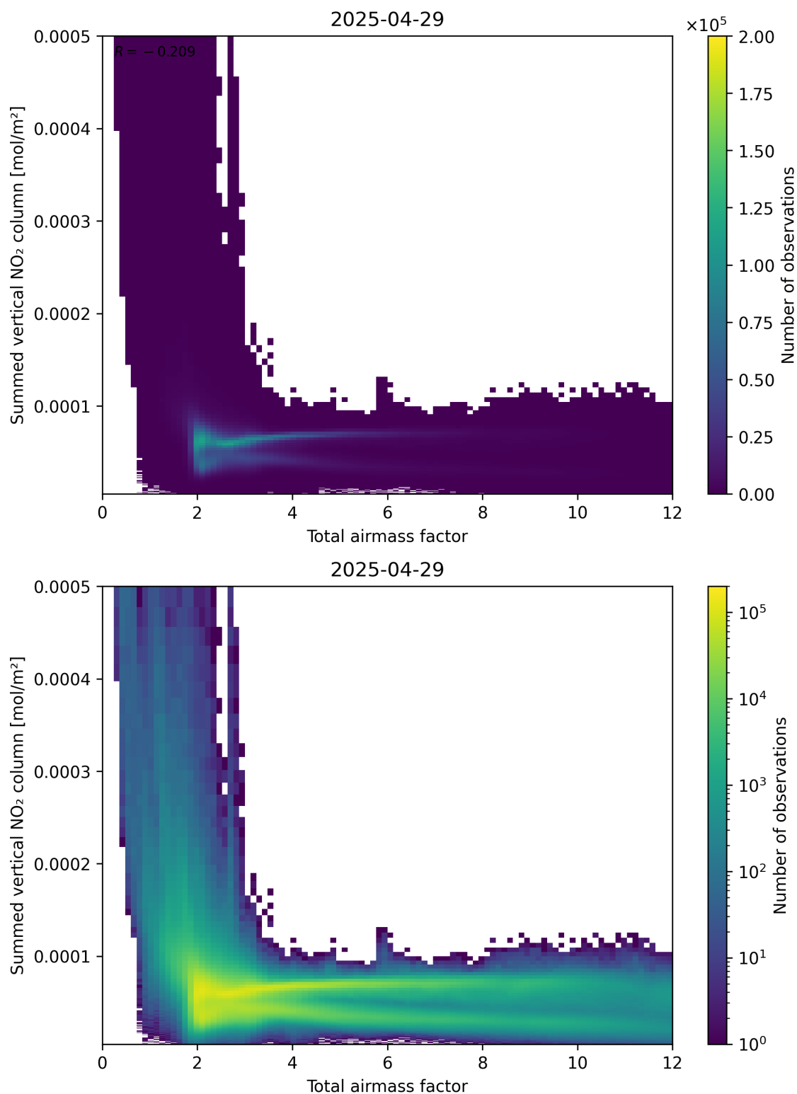
Figure 65: Scatter density plot of “Total airmass factor” against “Summed vertical NO 2 column” for 2025-04-29 to 2025-04-30.
