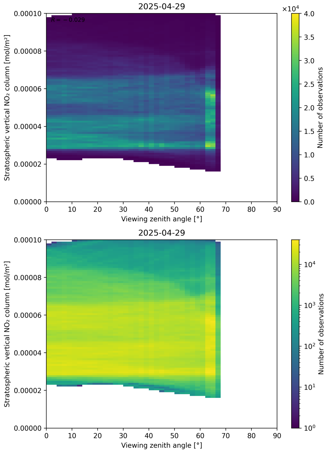
Figure 164: Scatter density plot of “Viewing zenith angle” against “Stratospheric vertical NO 2 column” for 2025-04-29 to 2025-04-30.
