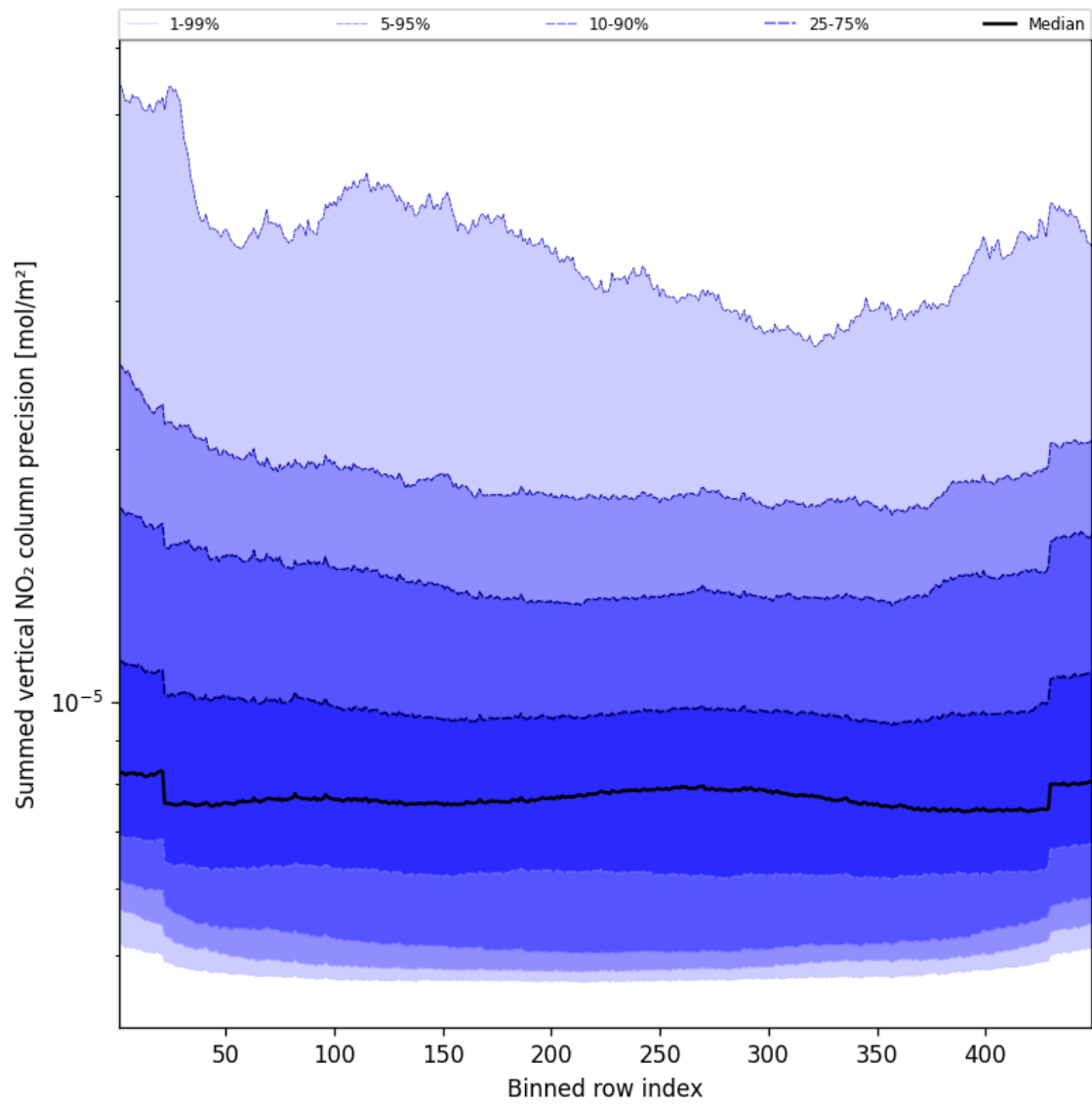
Figure 58: Along track statistics of “Summed vertical NO 2 column precision” for 2025-04-29 to 2025-04-30
