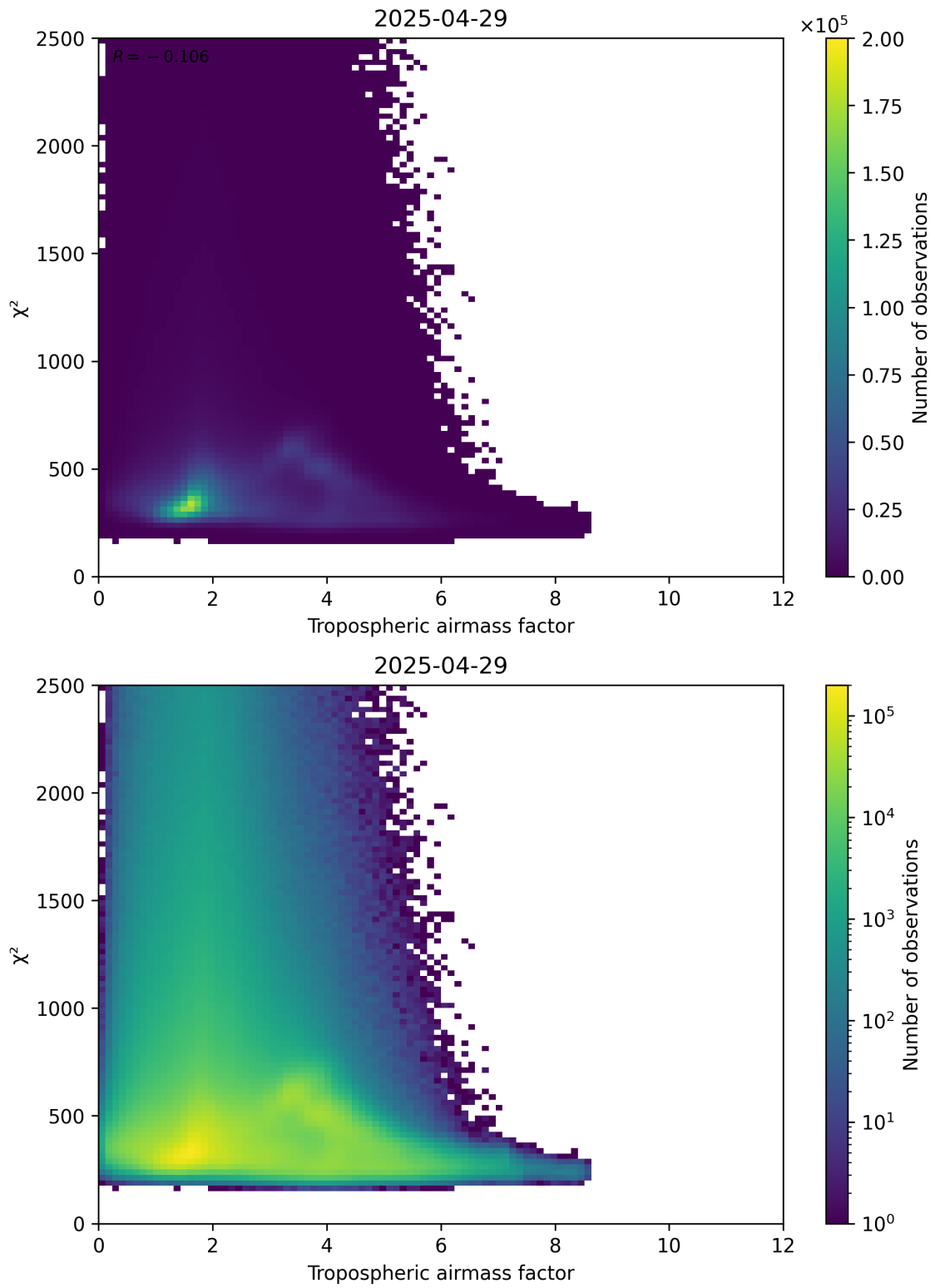
Figure 73: Scatter density plot of “Tropospheric airmass factor” against “ \chi^2 ” for 2025-04-29 to 2025-04-30.
