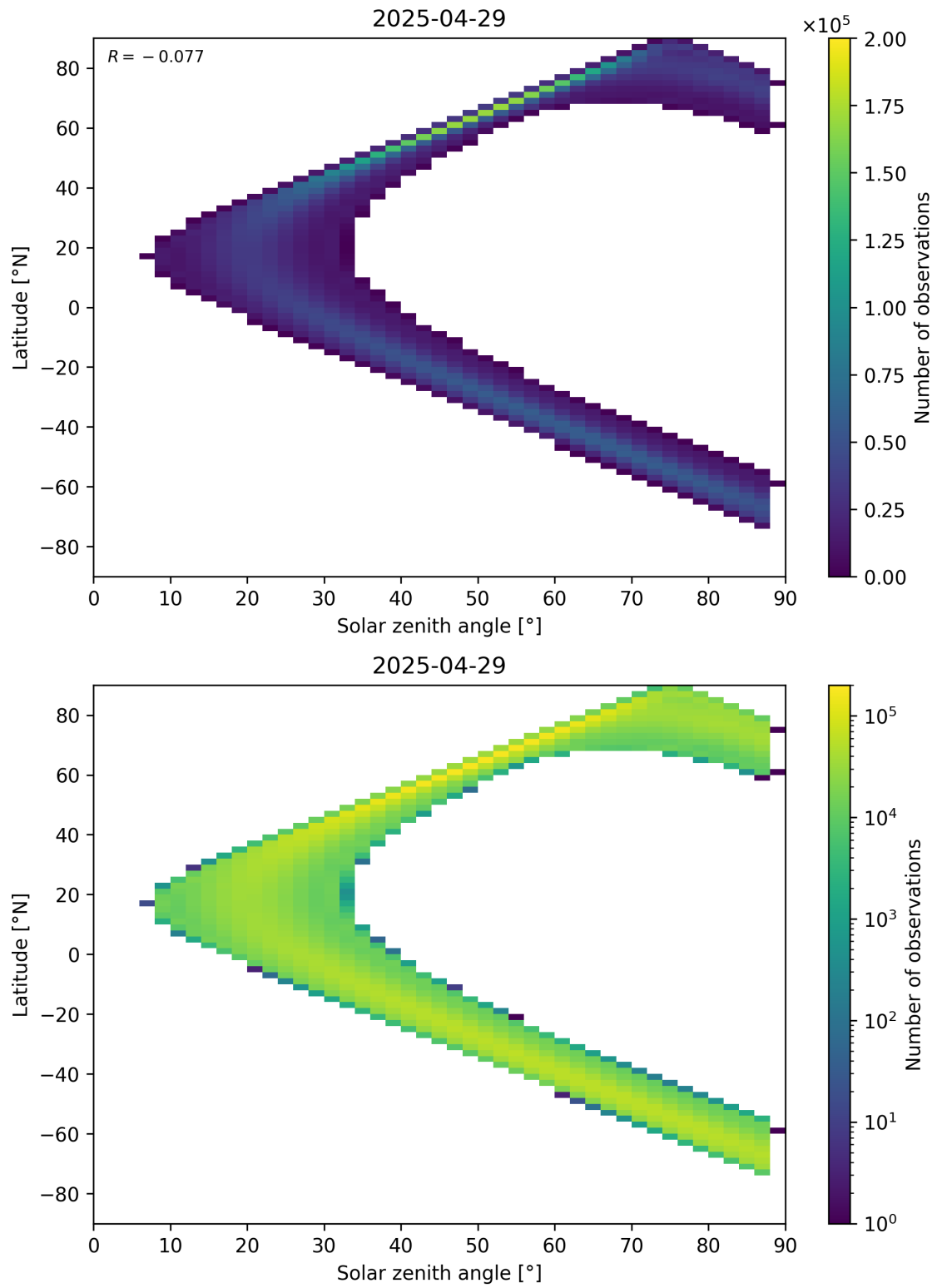
Figure 149: Scatter density plot of “Solar zenith angle” against “Latitude” for 2025-04-29 to 2025-04-30.
