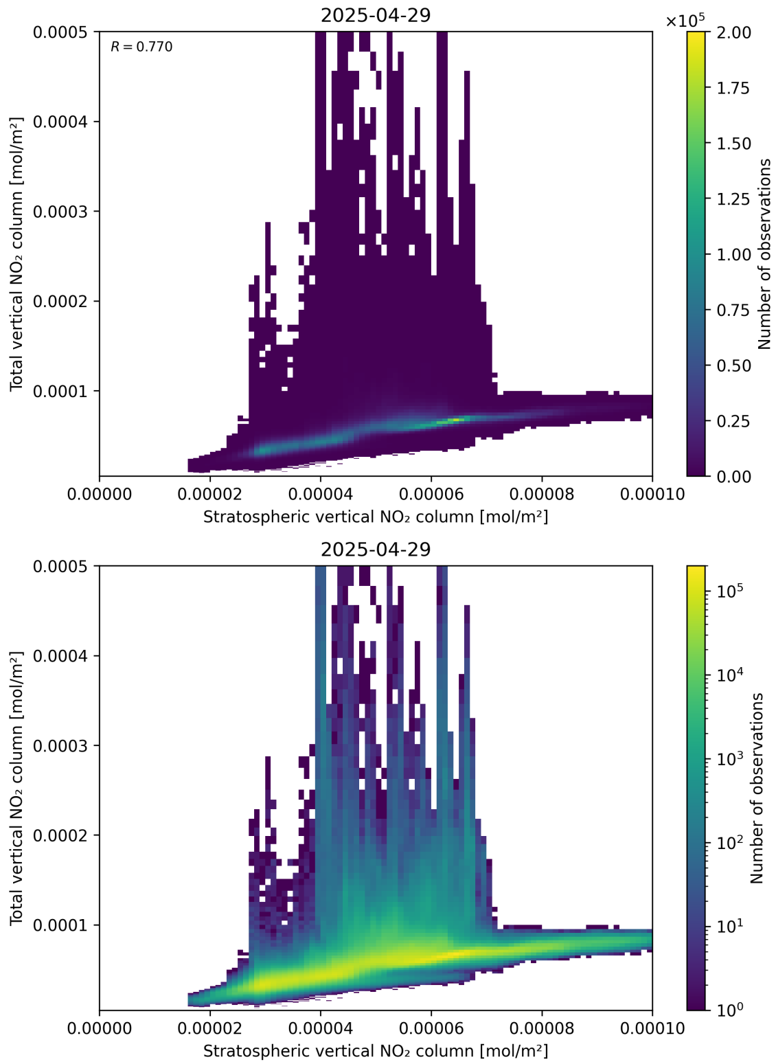
Figure 100: Scatter density plot of “Stratospheric vertical NO 2 column” against “Total vertical NO 2 column” for 2025-04-29 to 2025-04-30.
