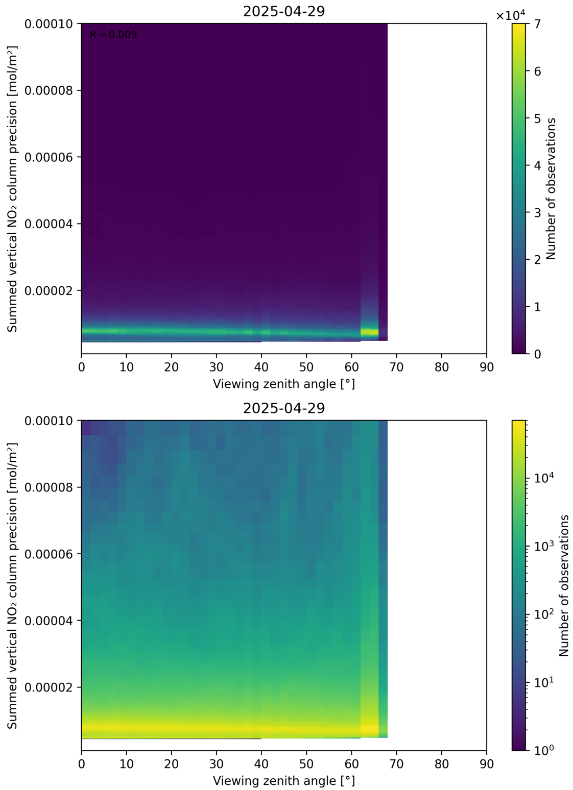
Figure 166: Scatter density plot of “Viewing zenith angle” against “Summed vertical NO 2 column precision” for 2025-04-29 to 2025-04-30.
