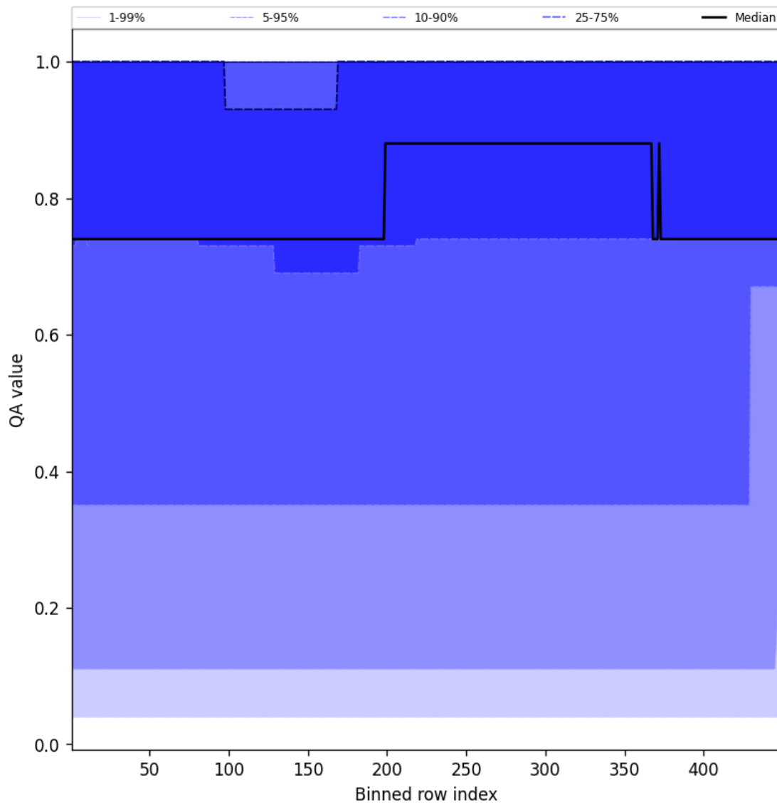
Figure 45: Along track statistics of “QA value” for 2025-04-29 to 2025-04-30
