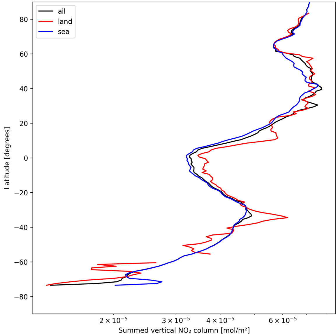
Figure 23: Zonal average of “Summed vertical NO 2 column” for 2025-04-29 to 2025-04-30.
