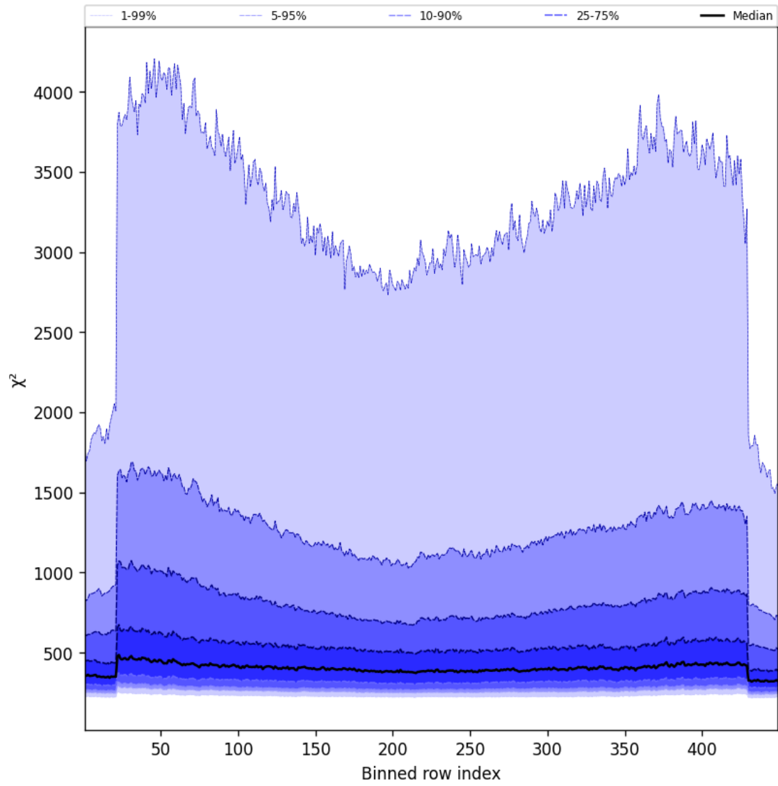
Figure 59: Along track statistics of “ \chi^2 ” for 2025-04-29 to 2025-04-30
