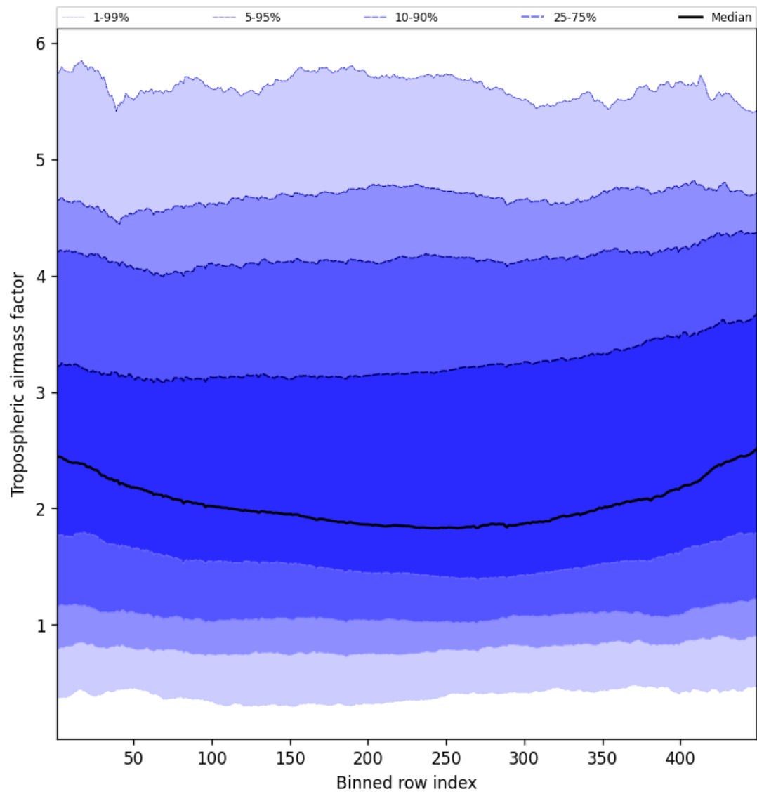
Figure 48: Along track statistics of “Tropospheric airmass factor” for 2025-04-29 to 2025-04-30
