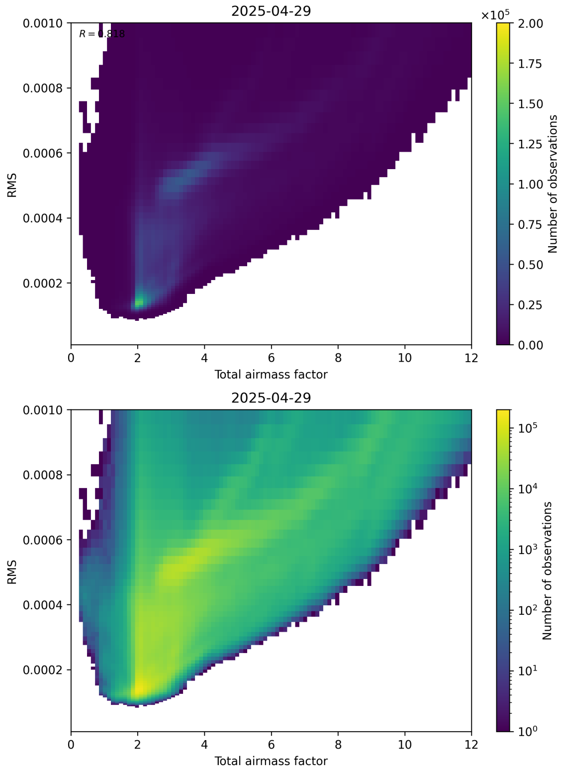
Figure 69: Scatter density plot of “Total airmass factor” against “RMS” for 2025-04-29 to 2025-04-30.
