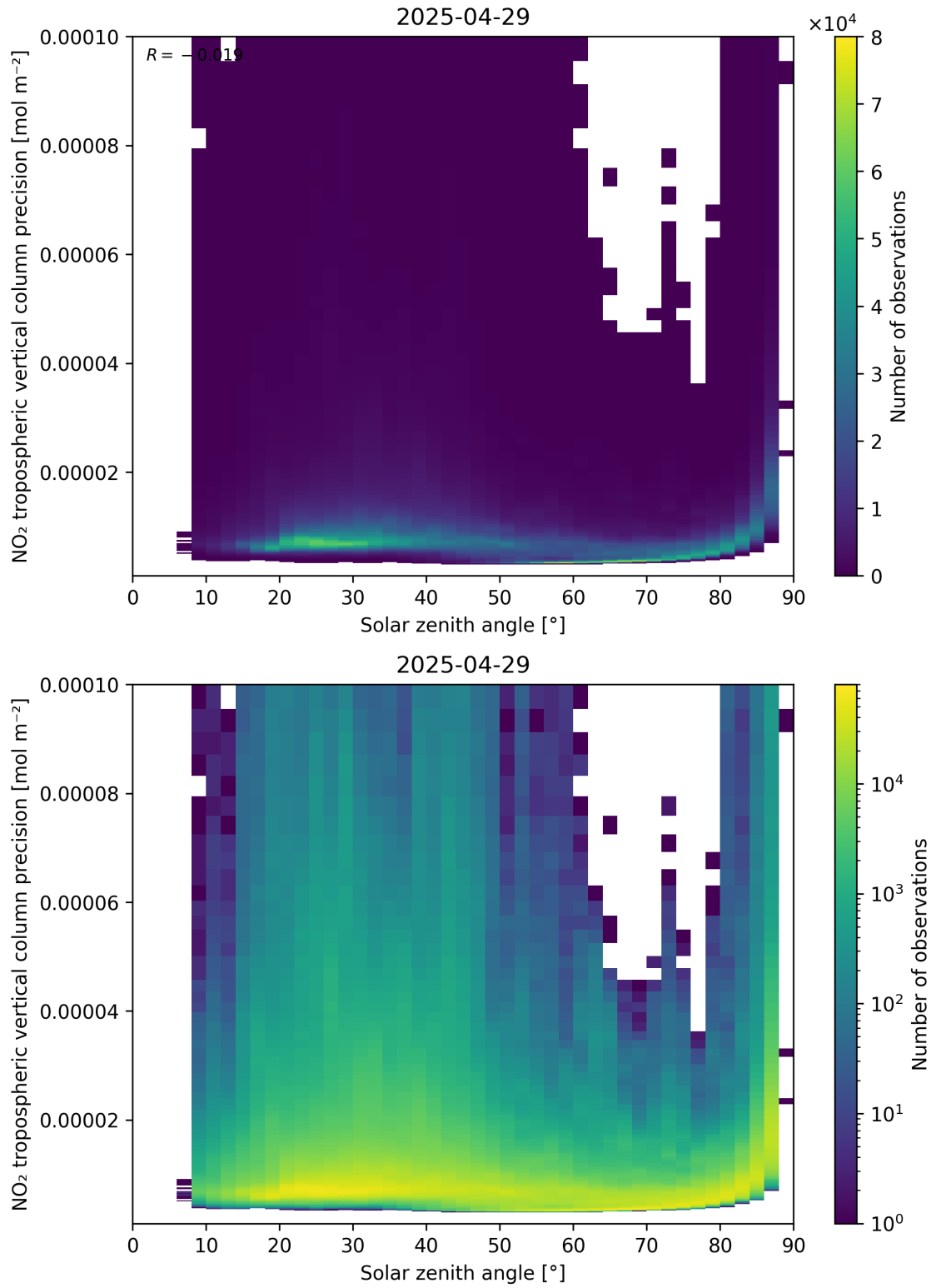
Figure 156: Scatter density plot of “Solar zenith angle” against “NO 2 tropospheric vertical column precision” for 2025-04-29 to 2025-04-30.
