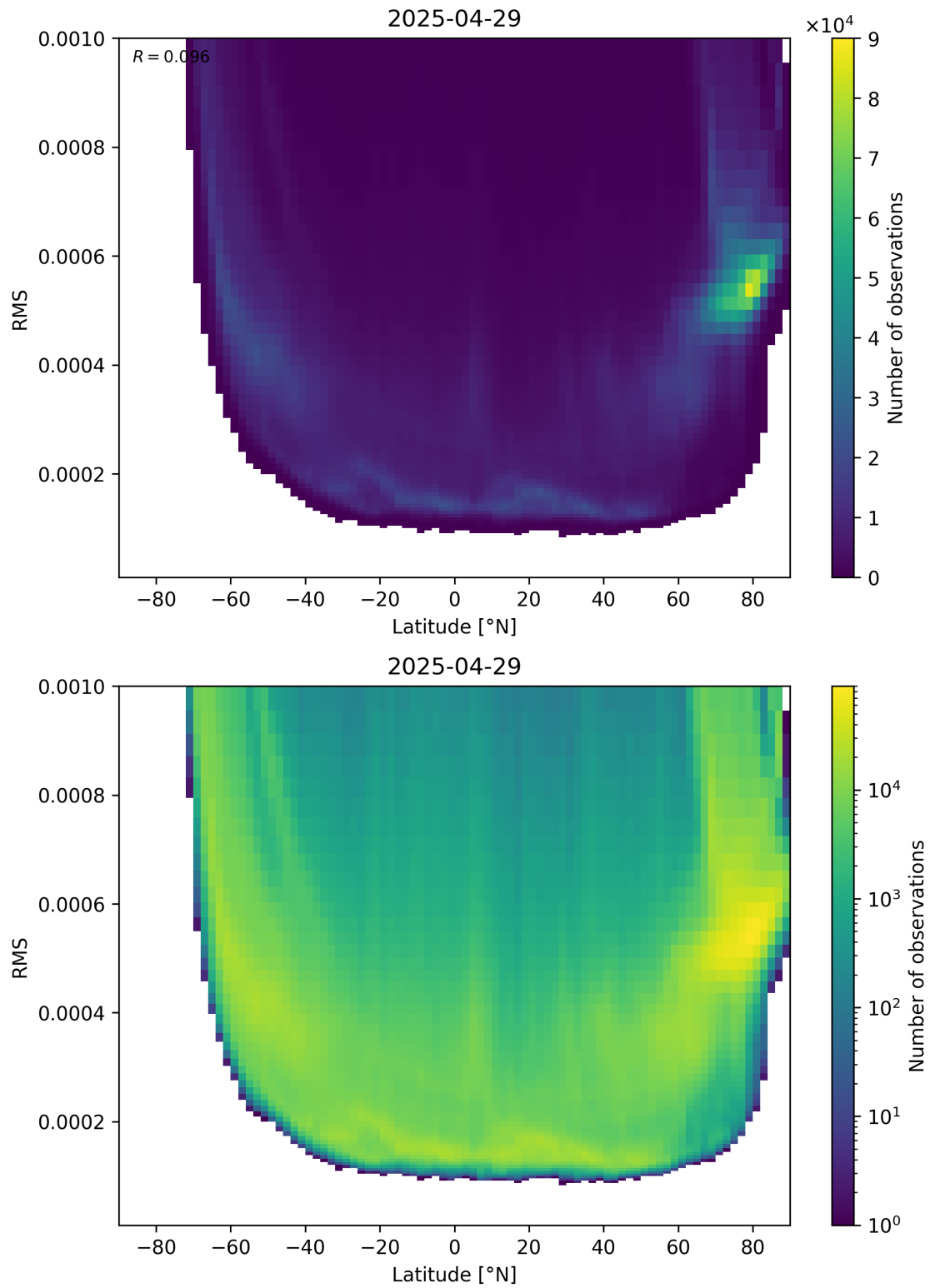
Figure 94: Scatter density plot of “Latitude” against “RMS” for 2025-04-29 to 2025-04-30.
