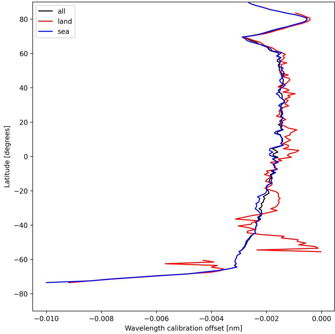
Figure 18: Zonal average of “Wavelength calibration offset” for 2025-04-29 to 2025-04-30.
