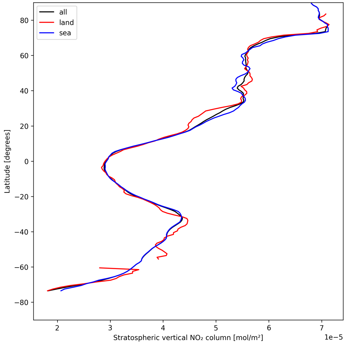
Figure 19: Zonal average of “Stratospheric vertical NO 2 column” for 2025-04-29 to 2025-04-30.
