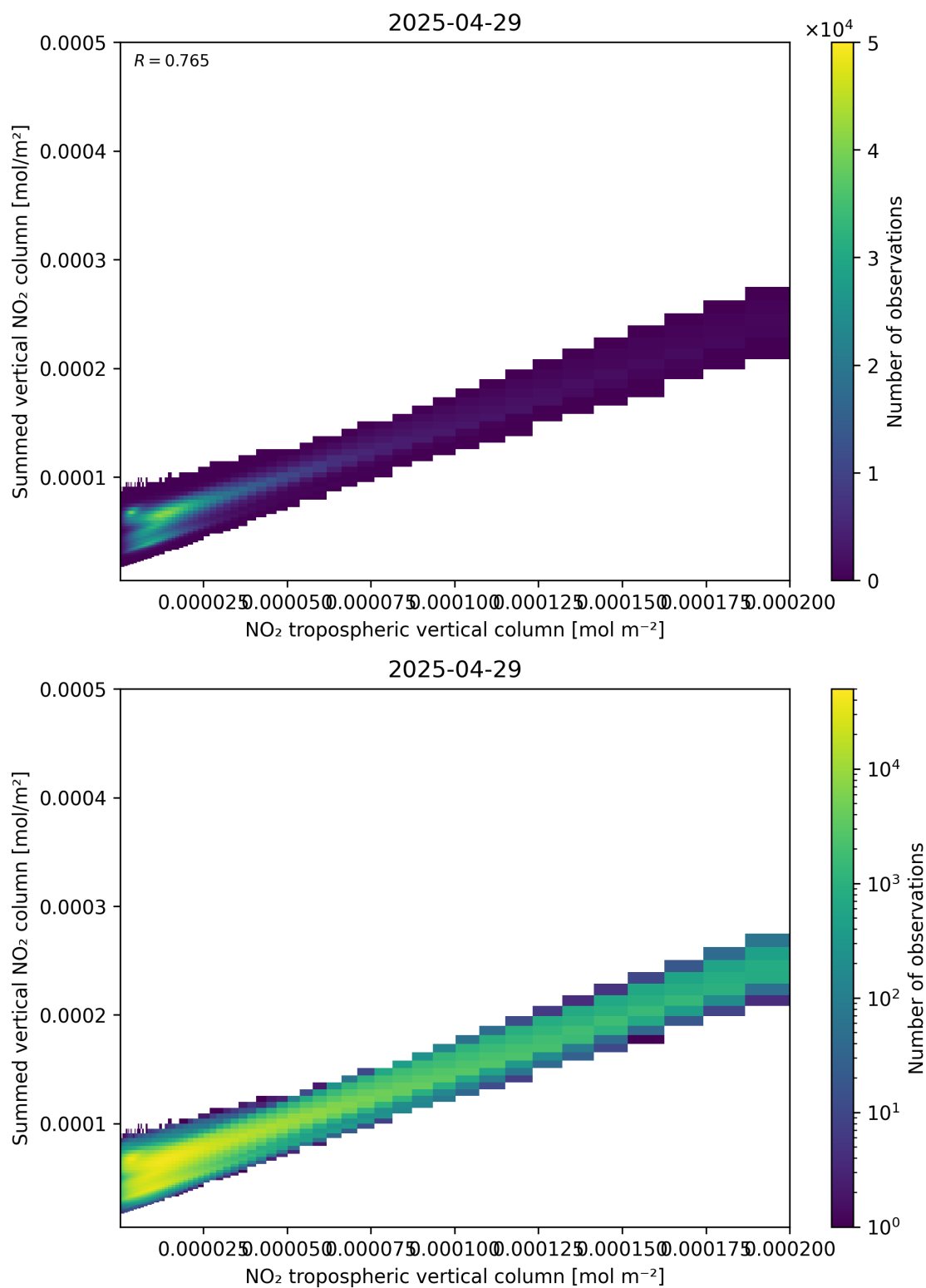
Figure 126: Scatter density plot of “NO 2 tropospheric vertical column” against “Summed vertical NO 2 column” for 2025-04-29 to 2025-04-30.
