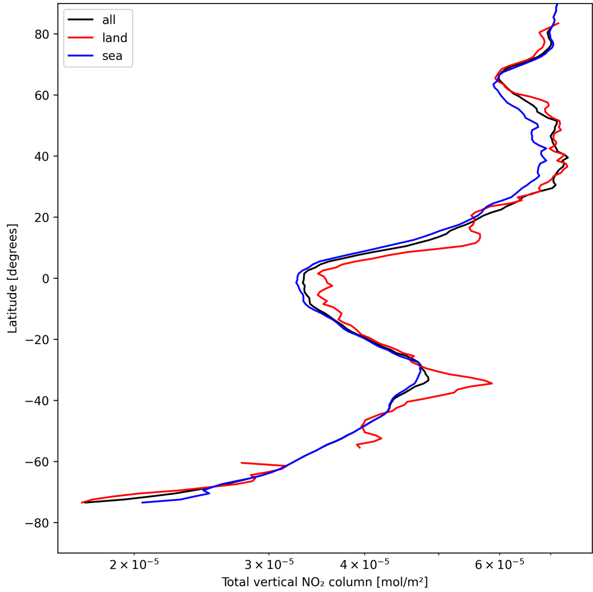
Figure 21: Zonal average of “Total vertical NO 2 column” for 2025-04-29 to 2025-04-30.
