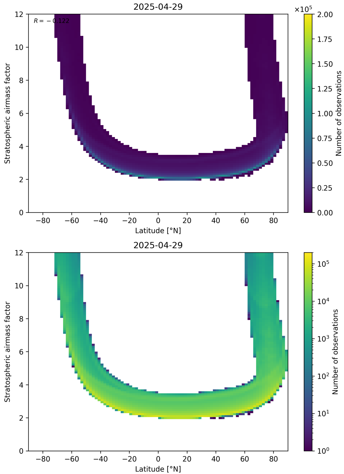
Figure 83: Scatter density plot of “Latitude” against “Stratospheric air mass factor” for 2025-04-29 to 2025-04-30.
