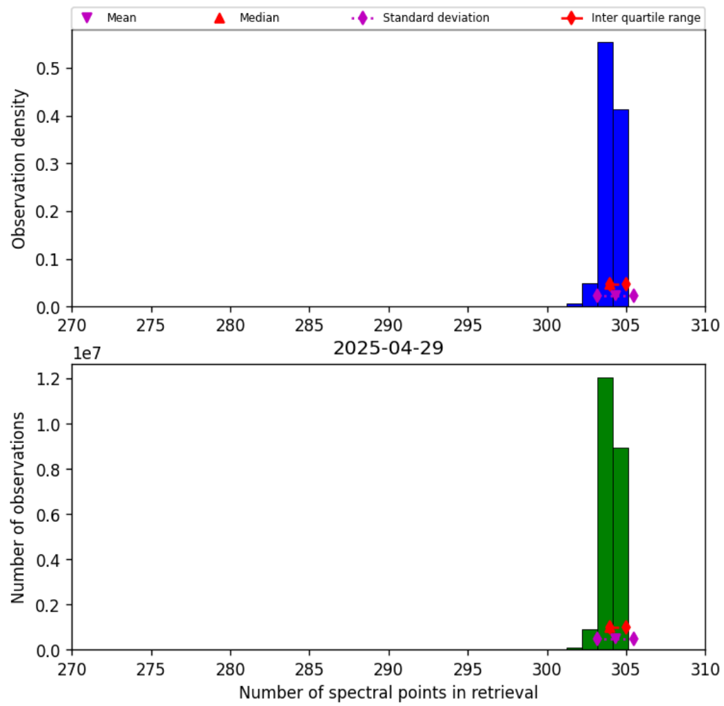
Figure 33: Histogram of “Number of spectral points in retrieval” for 2025-04-29 to 2025-04-30
