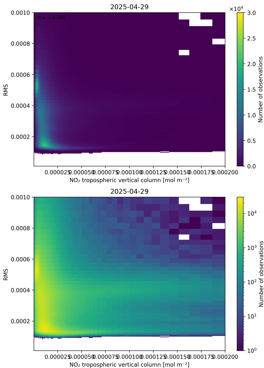
Figure 142: Scatter density plot of “NO 2 tropospheric vertical column” against “RMS” for 2025-04-29 to 2025-04-30.
