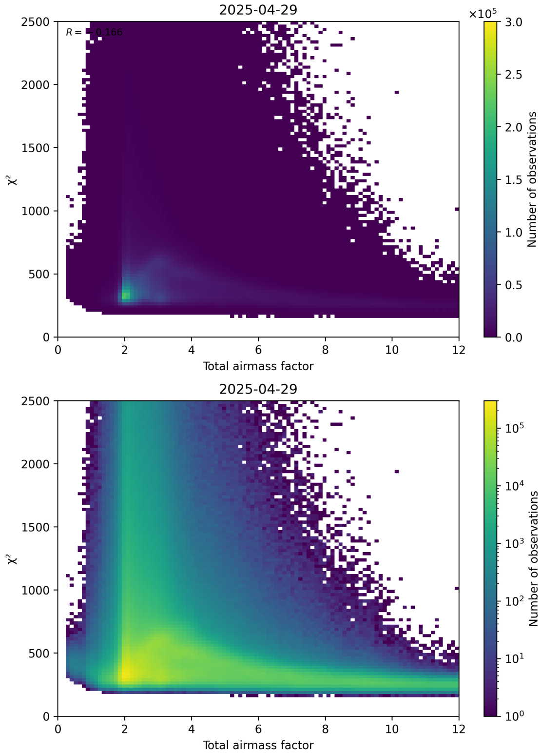
Figure 63: Scatter density plot of “Total airmass factor” against “ \chi^2 ” for 2025-04-29 to 2025-04-30.
