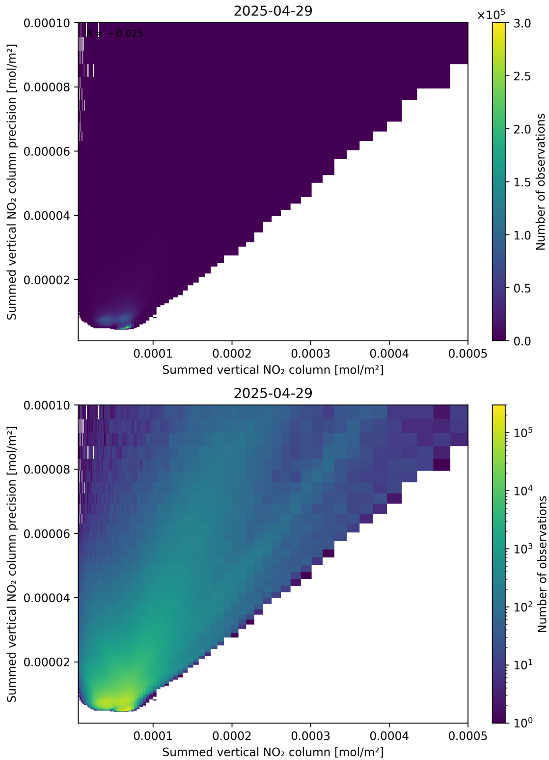
Figure 105: Scatter density plot of “Summed vertical NO 2 column” against “Summed vertical NO 2 column precision” for 2025-04-29 to 2025-04-30.
