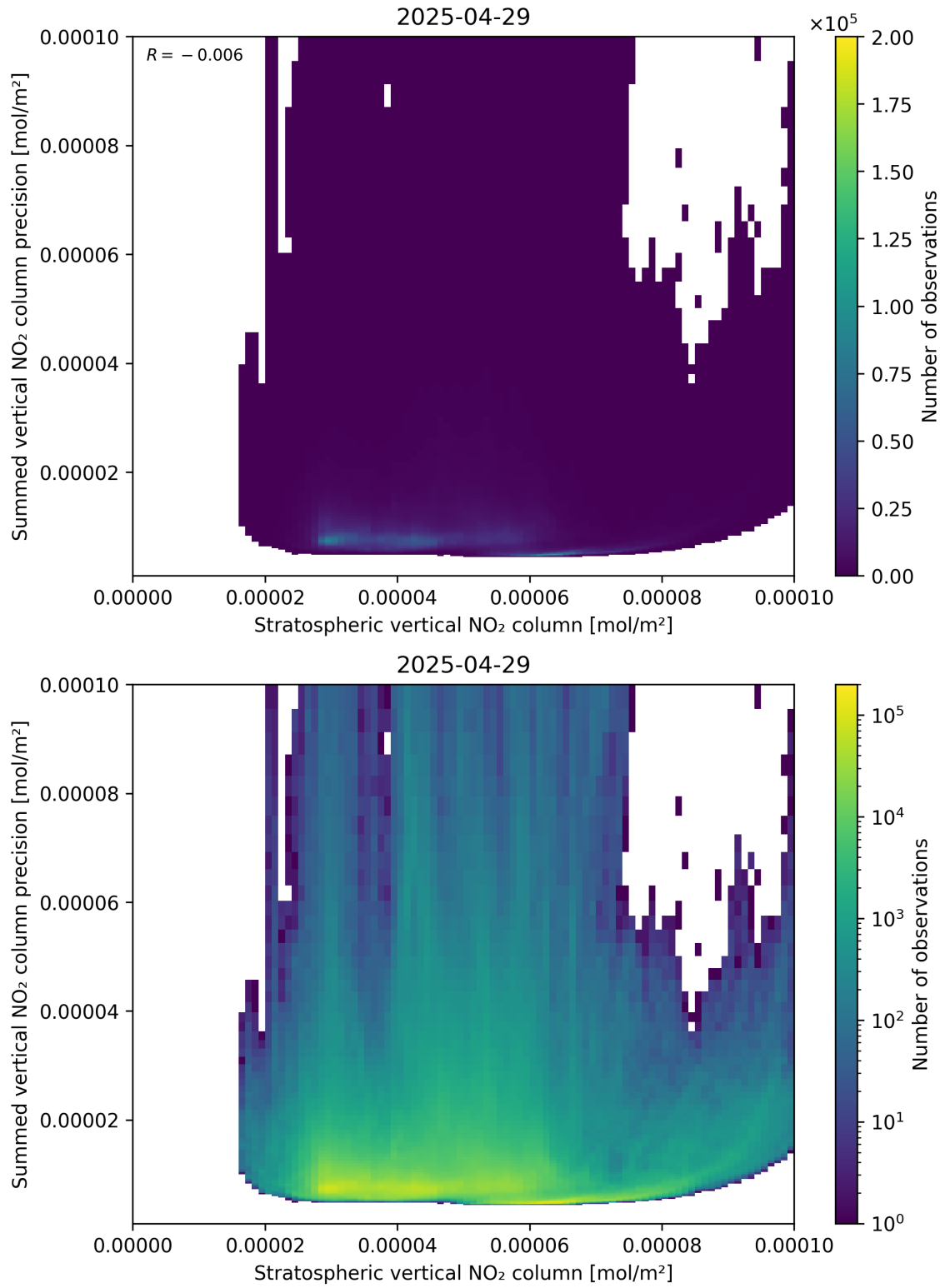
Figure 99: Scatter density plot of “Stratospheric vertical NO 2 column” against “Summed vertical NO 2 column precision” for 2025-04-29 to 2025-04-30.
