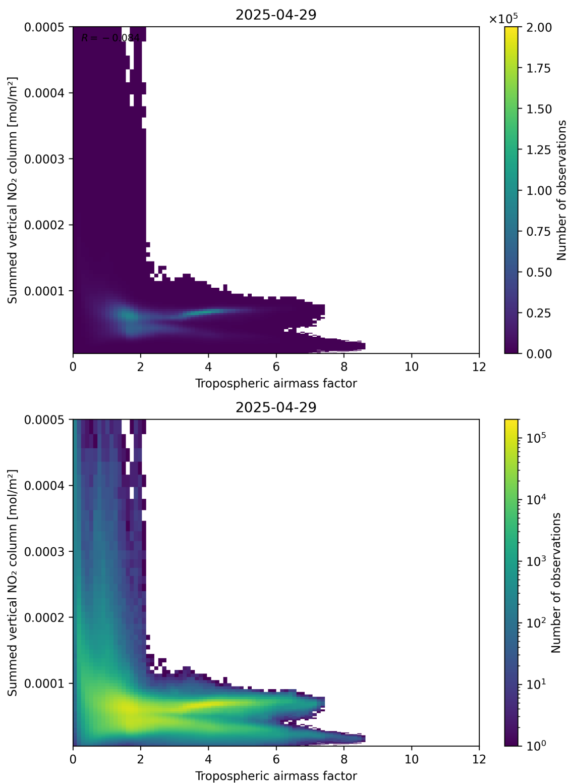
Figure 75: Scatter density plot of “Tropospheric air mass factor” against “Summed vertical NO 2 column” for 2025-04-29 to 2025-04-30.
