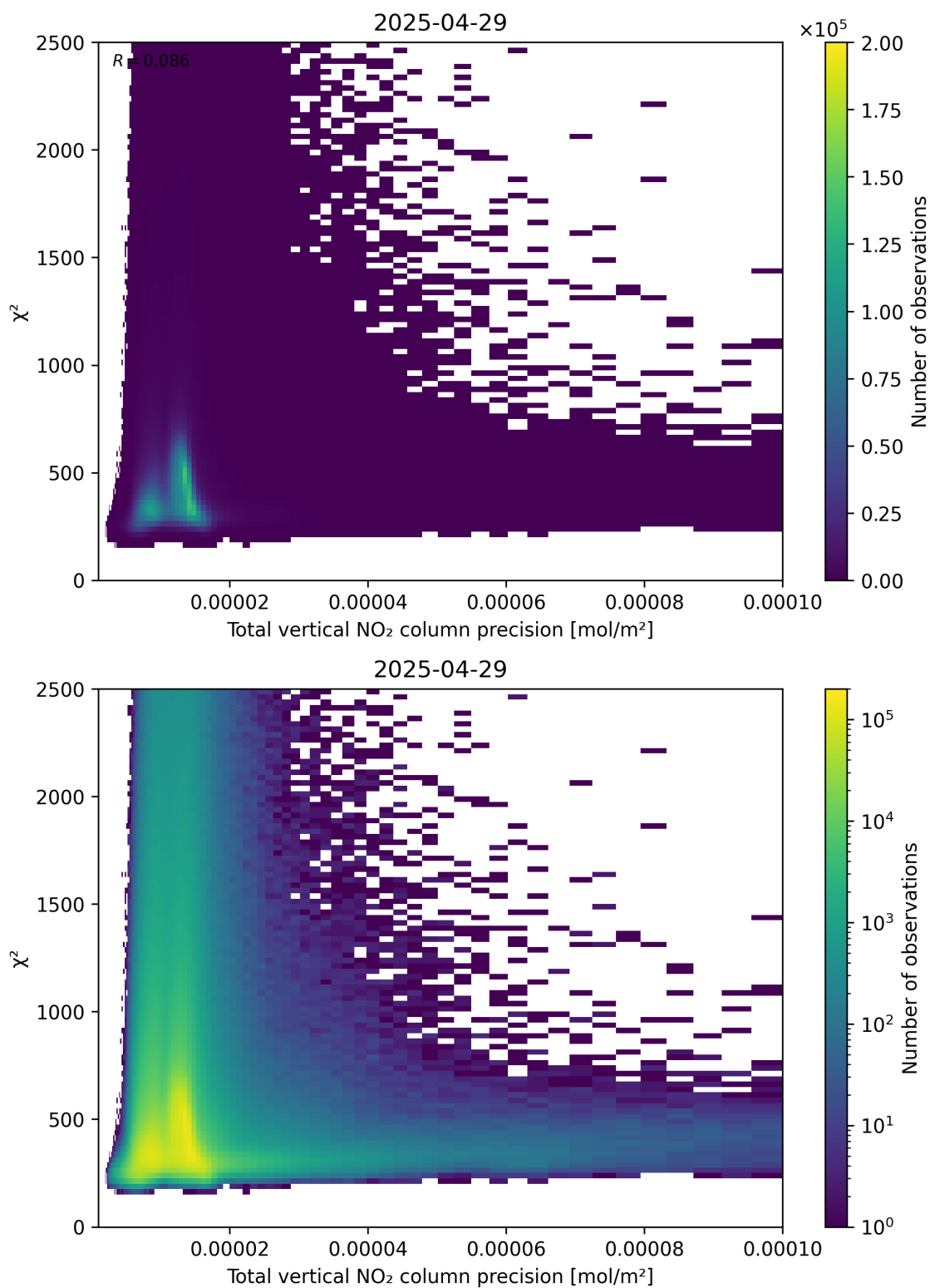
Figure 116: Scatter density plot of “Total vertical NO 2 column precision” against “ \chi^2 ” for 2025-04-29 to 2025-04-30.
