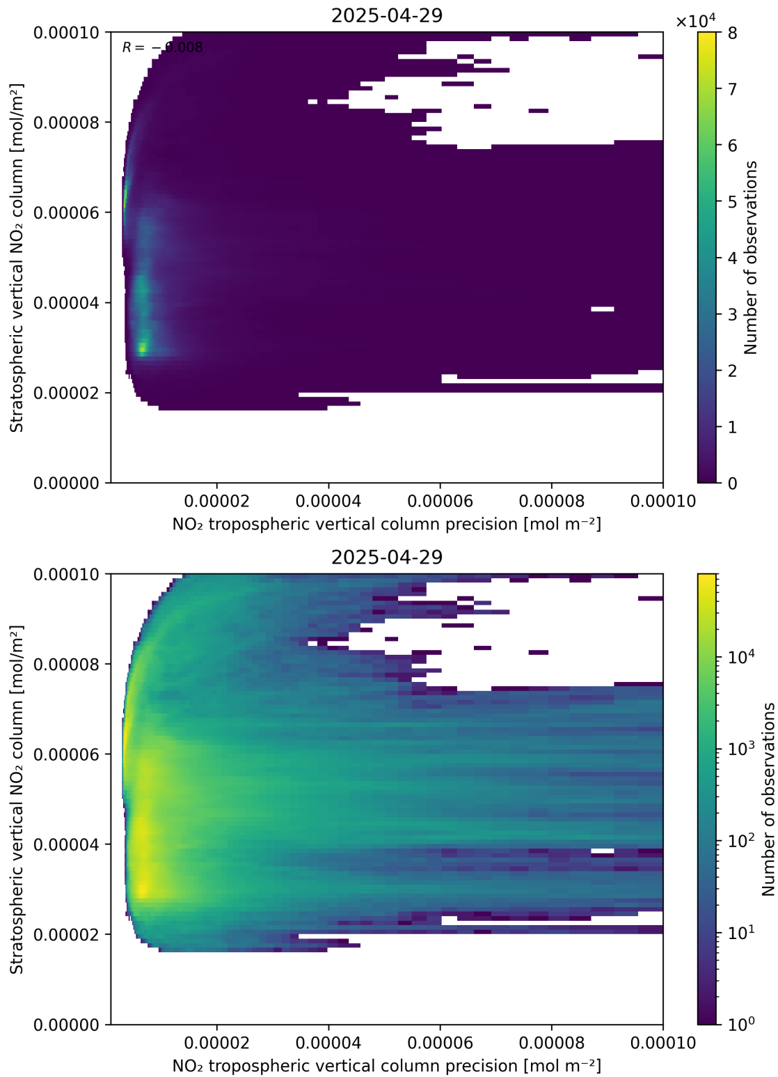
Figure 135: Scatter density plot of “NO 2 tropospheric vertical column precision” against “Stratospheric vertical NO 2 column” for 2025-04-29 to 2025-04-30.
