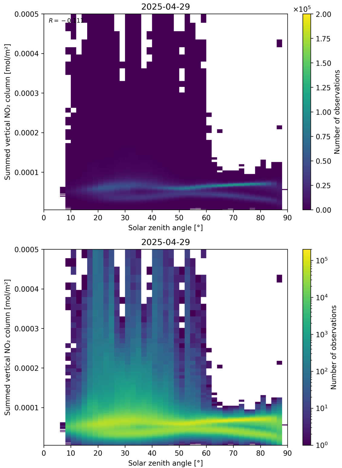
Figure 151: Scatter density plot of “Solar zenith angle” against “Summed vertical NO 2 column” for 2025-04-29 to 2025-04-30.
