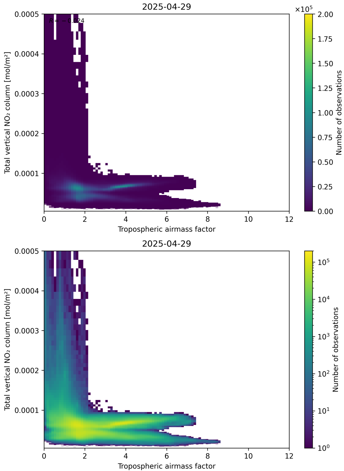
Figure 77: Scatter density plot of “Tropospheric airmass factor” against “Total vertical NO 2 column” for 2025-04-29 to 2025-04-30.
