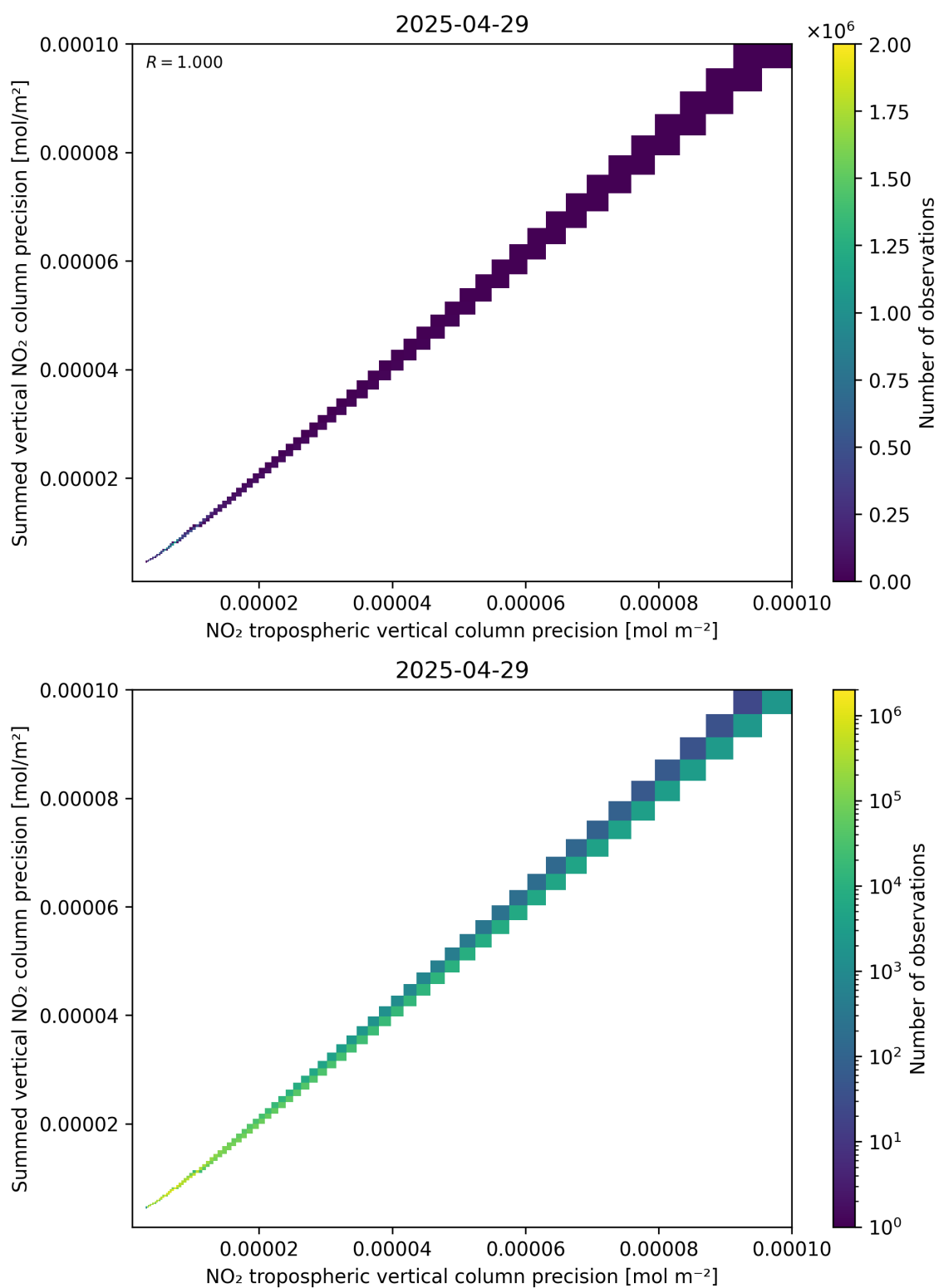
Figure 137: Scatter density plot of “NO 2 tropospheric vertical column precision” against “Summed vertical NO 2 column precision” for 2025-04-29 to 2025-04-30.
