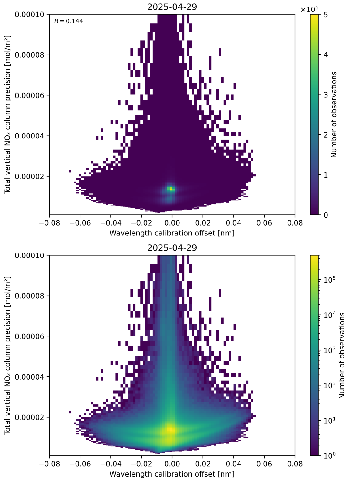
Figure 180: Scatter density plot of “Wavelength calibration offset” against “Total vertical NO 2 column precision” for 2025-04-29 to 2025-04-30.
