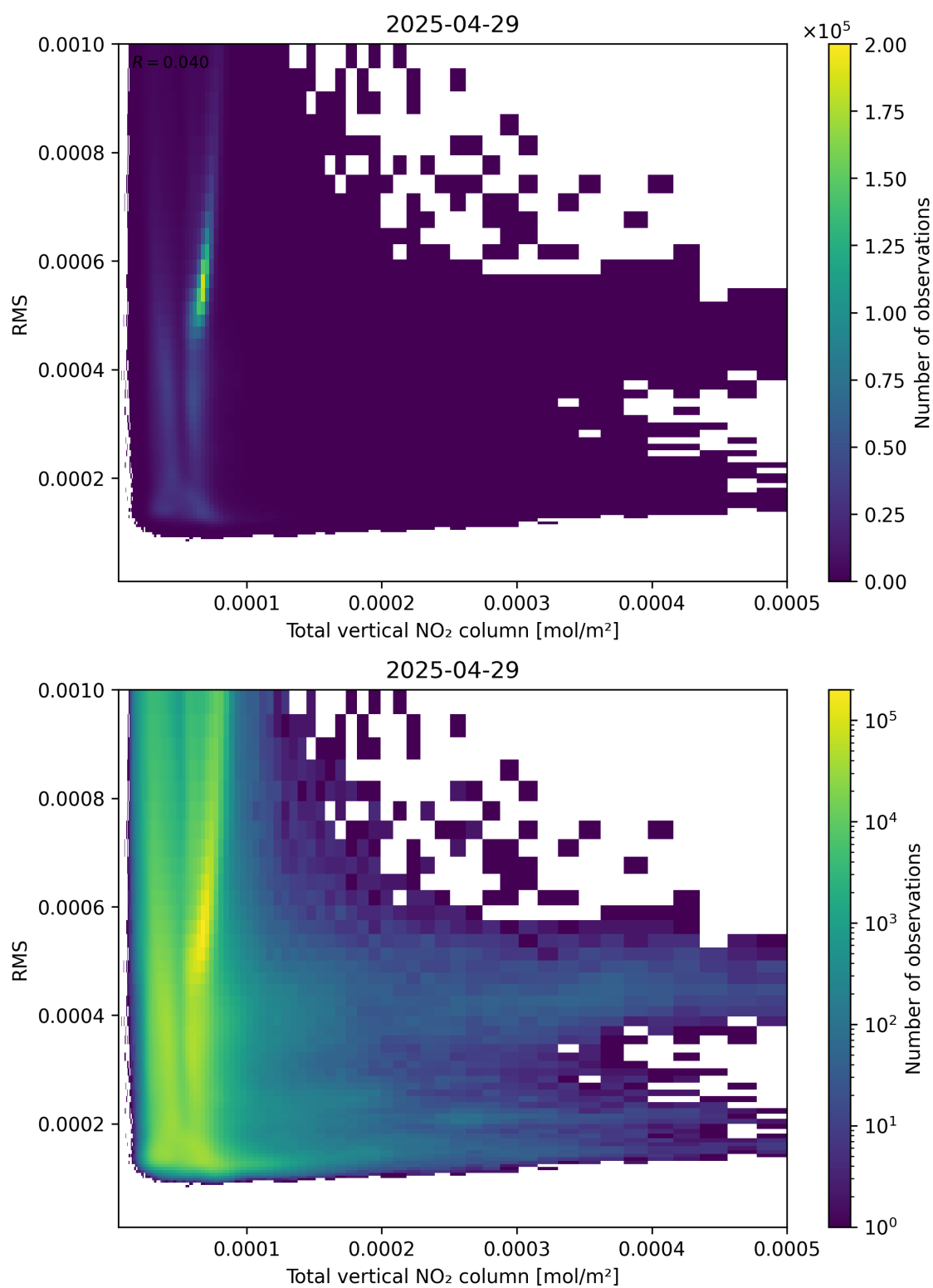
Figure 120: Scatter density plot of “Total vertical NO 2 column” against “RMS” for 2025-04-29 to 2025-04-30.
