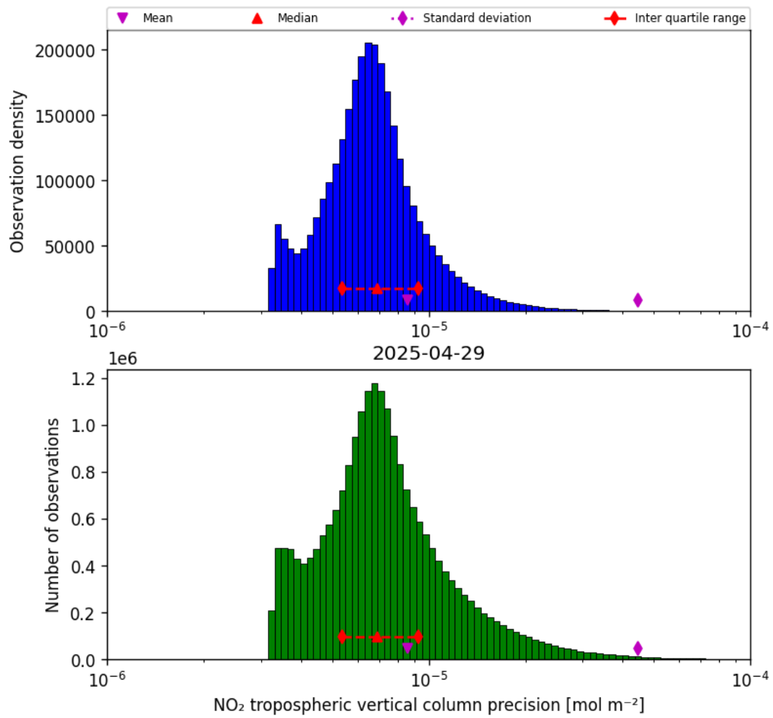
Figure 30: Histogram of “NO 2 tropospheric vertical column precision” for 2025-04-29 to 2025-04-30
