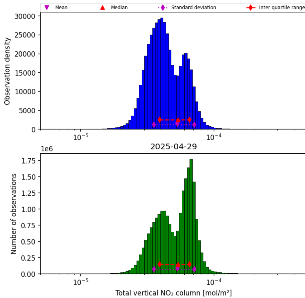
Figure 38: Histogram of “Total vertical NO 2 column” for 2025-04-29 to 2025-04-30
