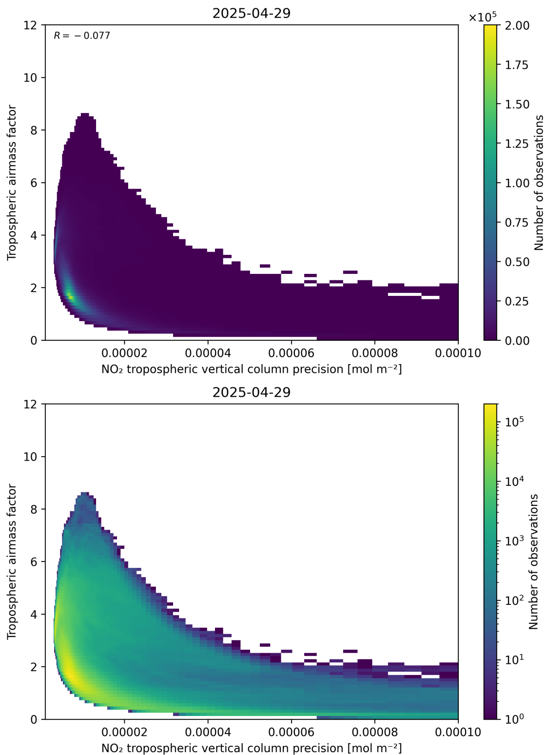
Figure 133: Scatter density plot of “NO 2 tropospheric vertical column precision” against “Tropospheric air mass factor” for 2025-04-29 to 2025-04-30.
