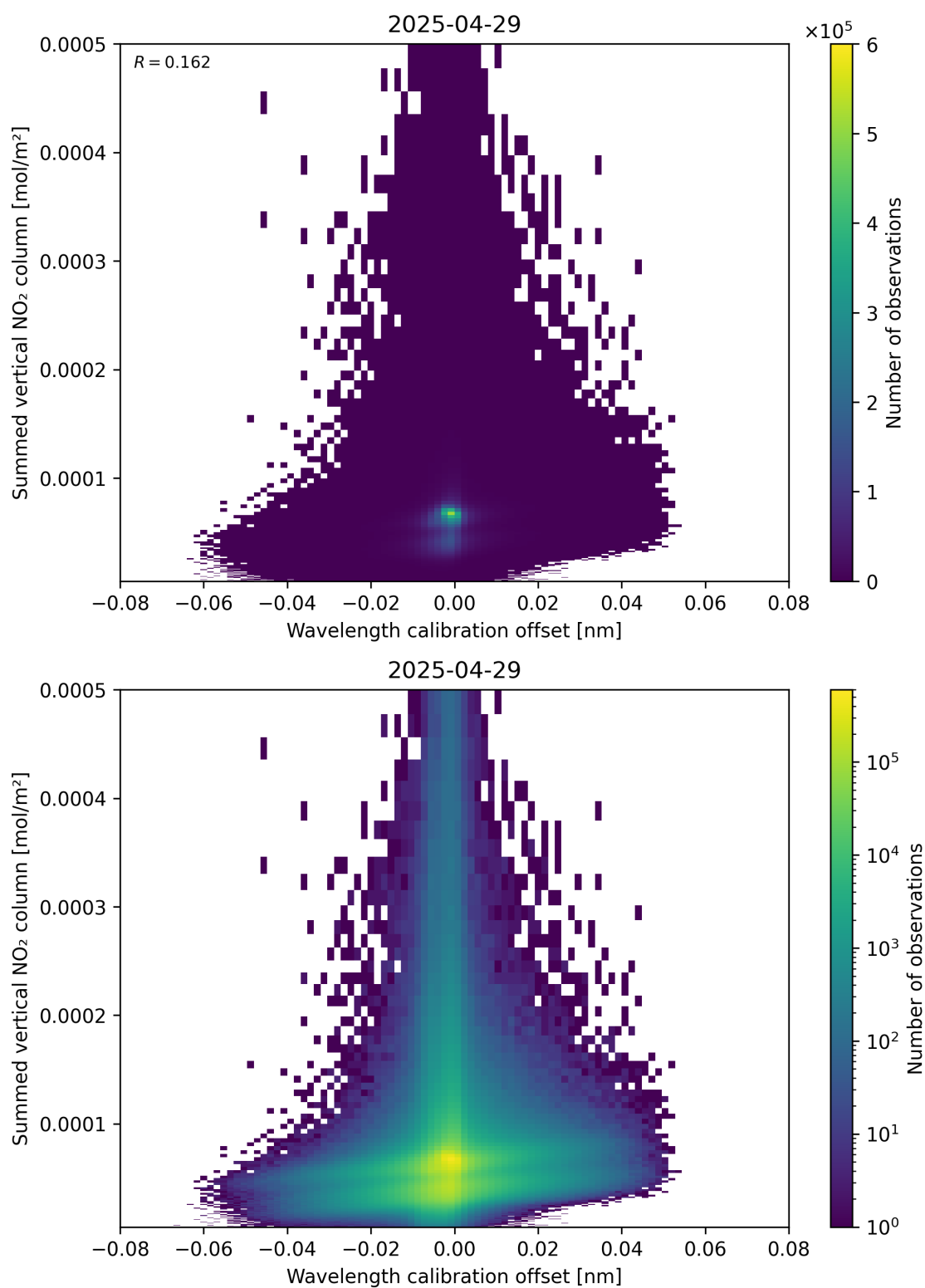
Figure 177: Scatter density plot of “Wavelength calibration offset” against “Summed vertical NO 2 column” for 2025-04-29 to 2025-04-30.
