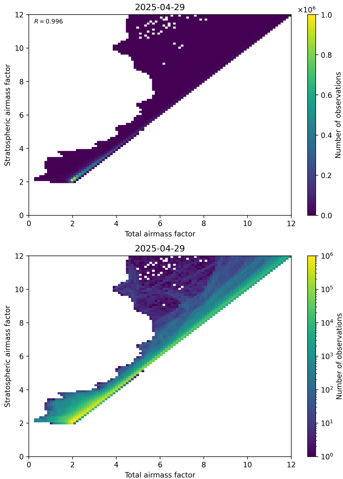
Figure 62: Scatter density plot of “Total airmass factor” against “Stratospheric airmass factor” for 2025-04-29 to 2025-04-30.
