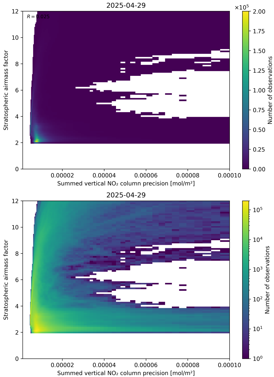
Figure 106: Scatter density plot of “Summed vertical NO 2 column precision” against “Stratospheric airmass factor” for 2025-04-29 to 2025-04-30.
