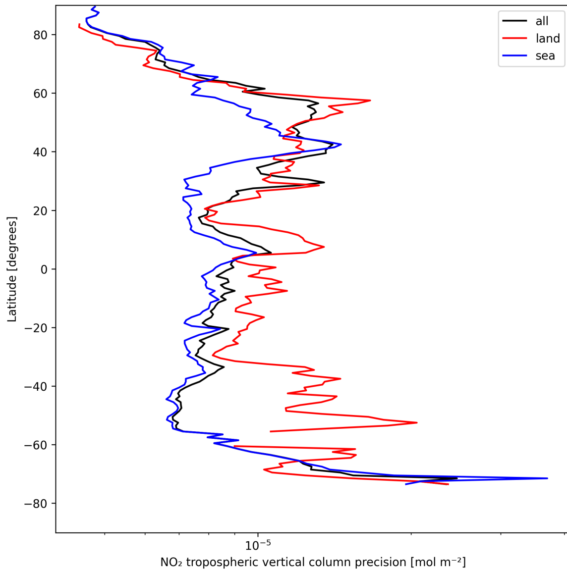
Figure 13: Zonal average of “NO 2 tropospheric vertical column precision” for 2025-04-29 to 2025-04-30.
