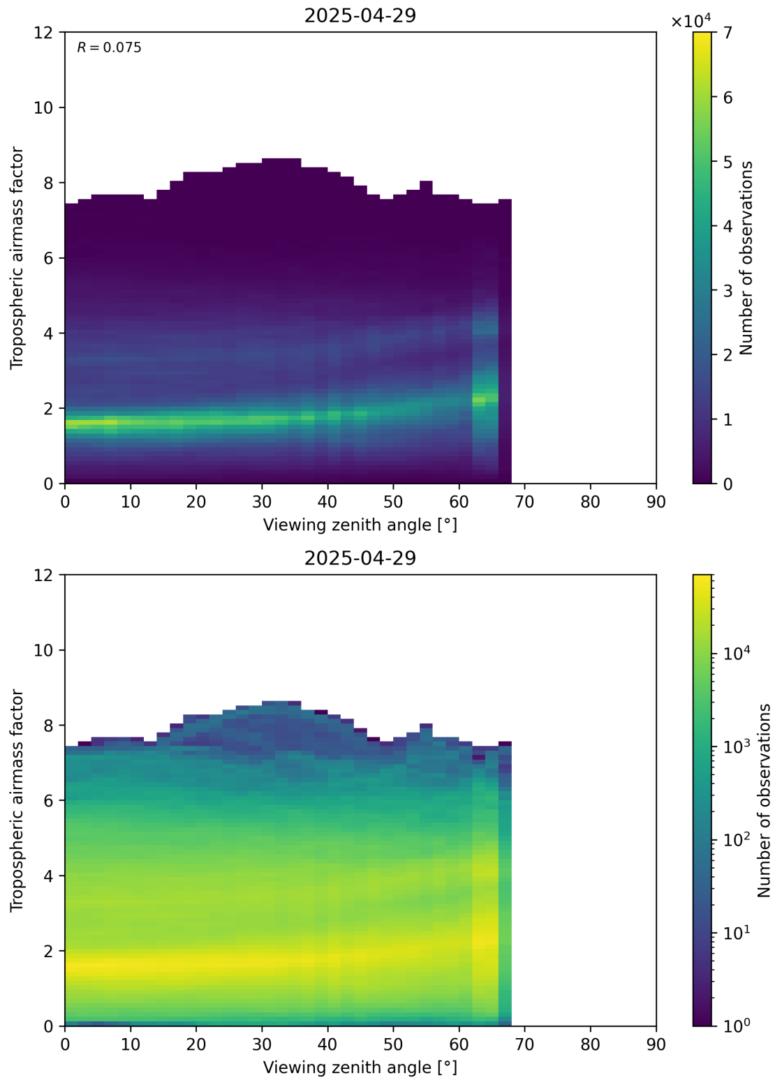
Figure 161: Scatter density plot of “Viewing zenith angle” against “Tropospheric airmass factor” for 2025-04-29 to 2025-04-30.
