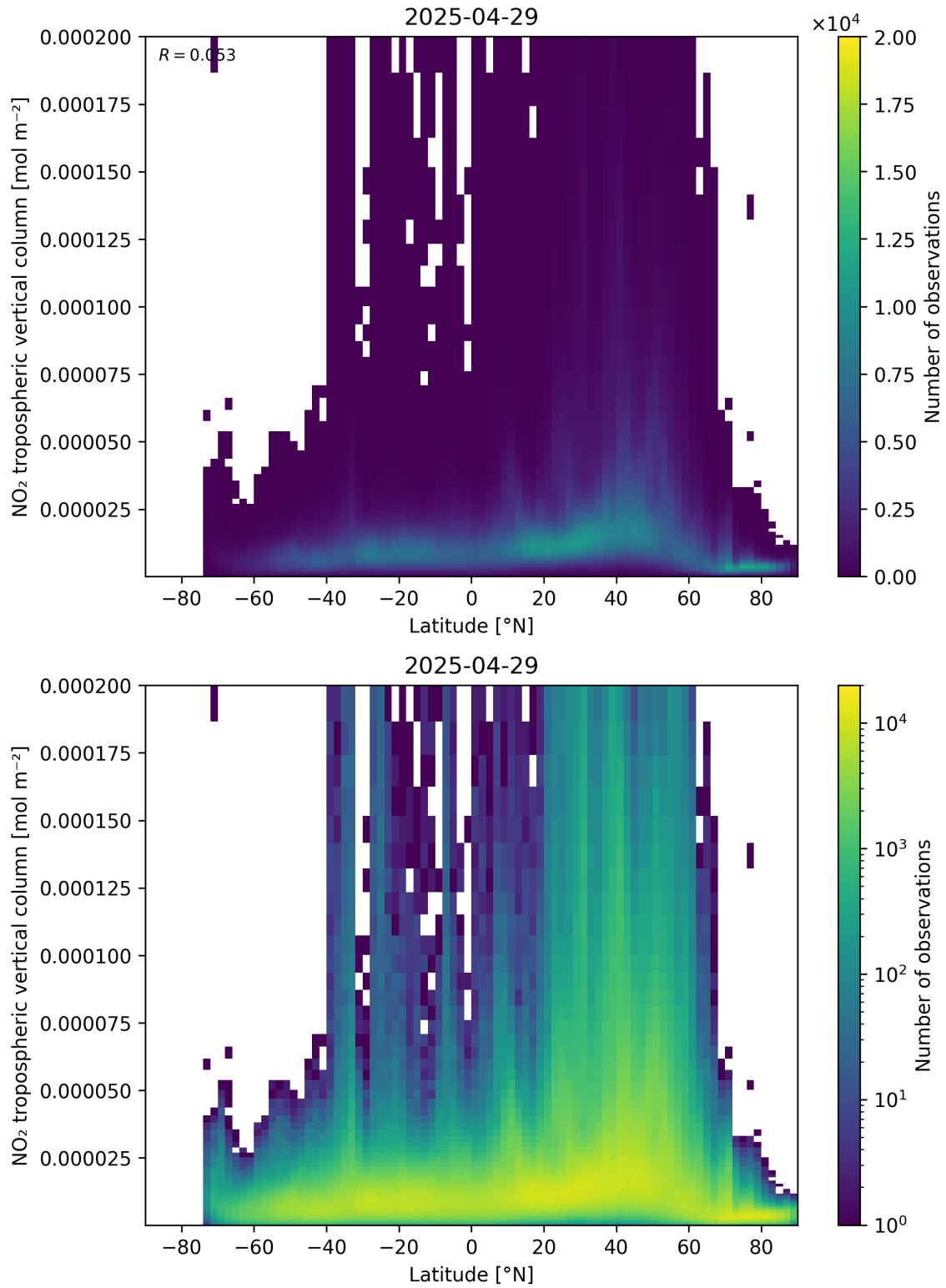
Figure 92: Scatter density plot of “Latitude” against “NO 2 tropospheric vertical column” for 2025-04-29 to 2025-04-30.
