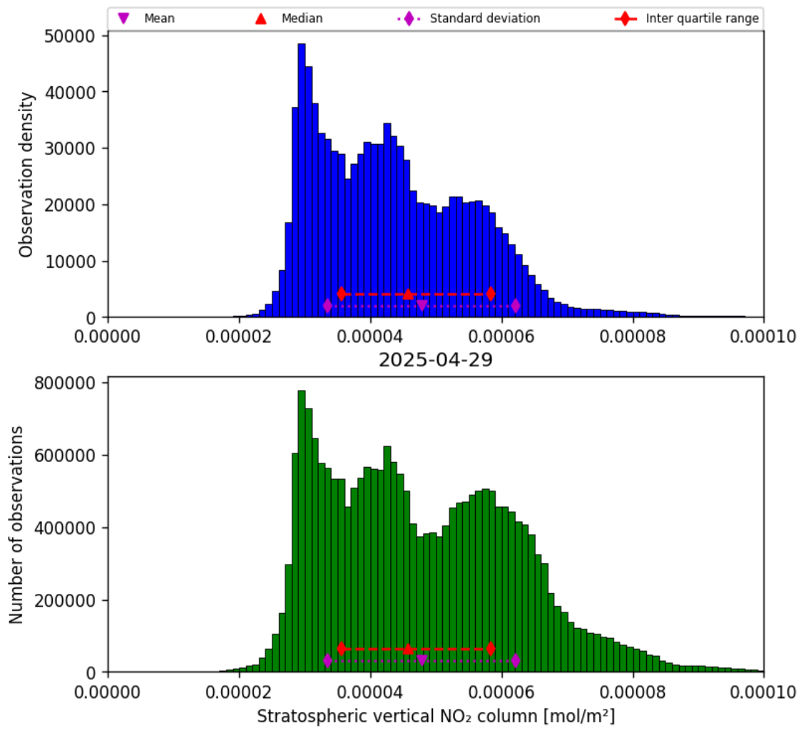
Figure 36: Histogram of “Stratospheric vertical NO 2 column” for 2025-04-29 to 2025-04-30
