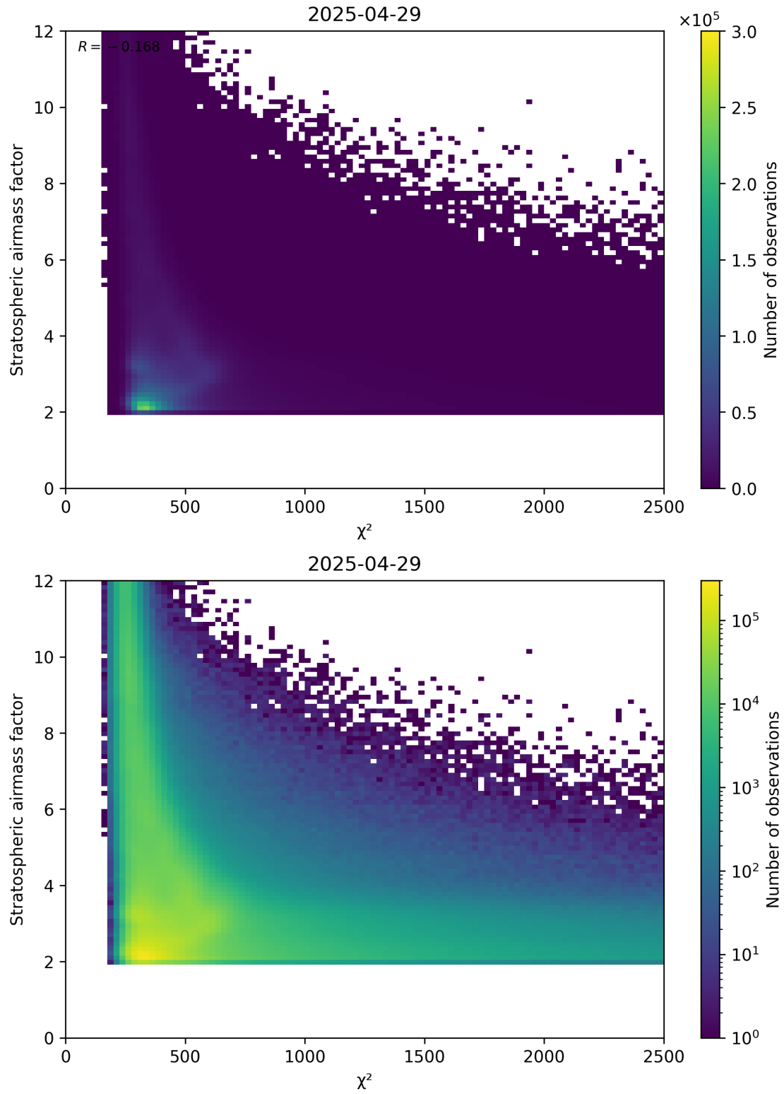
Figure 81: Scatter density plot of “ \chi^2 ” against “Stratospheric airmass factor” for 2025-04-29 to 2025-04-30.
