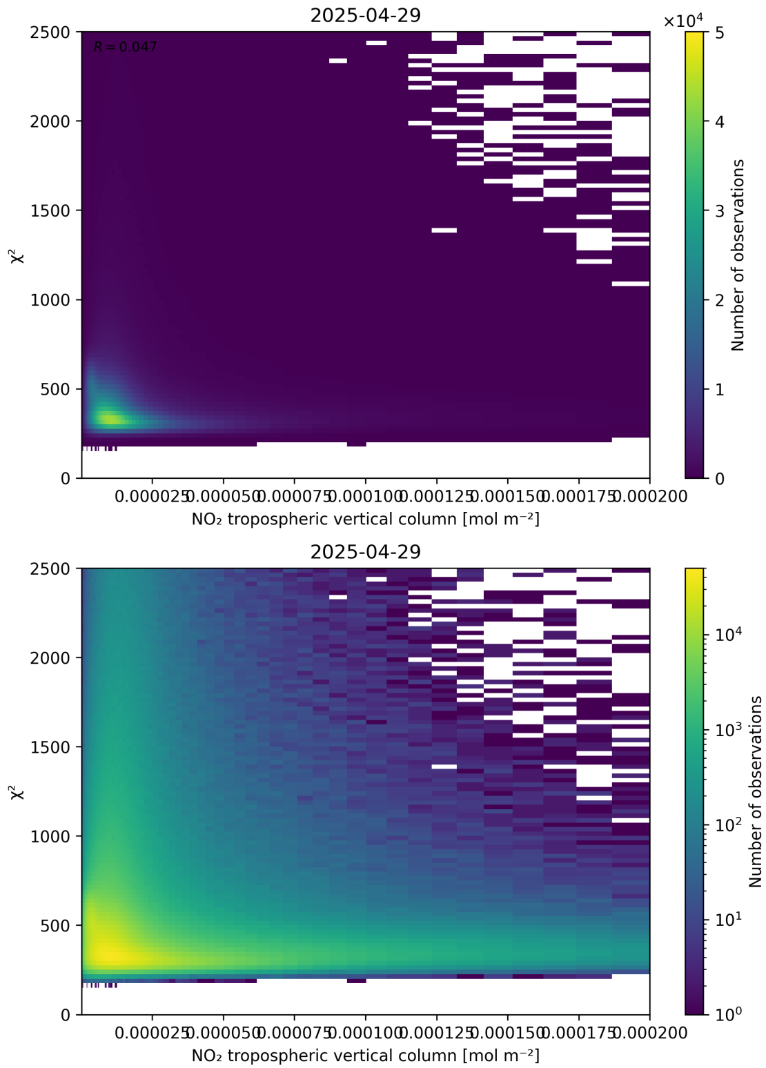
Figure 124: Scatter density plot of “NO 2 tropospheric vertical column” against “ \chi^2 ” for 2025-04-29 to 2025-04-30.
