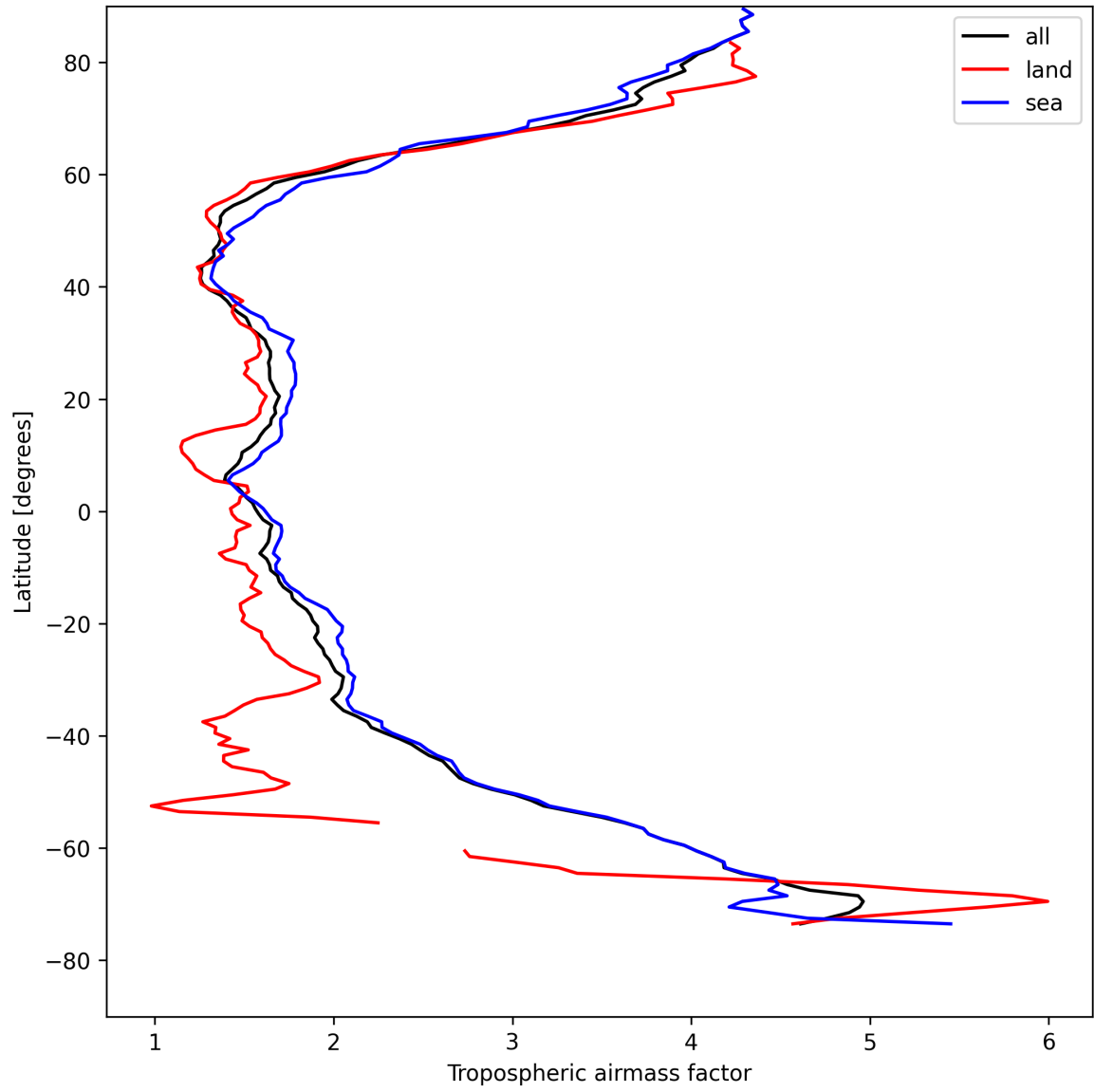
Figure 14: Zonal average of “Tropospheric airmass factor” for 2025-04-29 to 2025-04-30.
