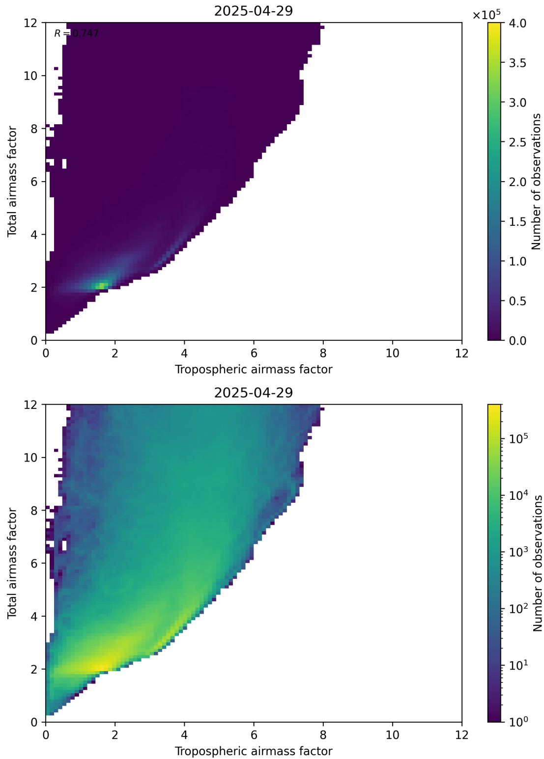
Figure 72: Scatter density plot of “Tropospheric airmass factor” against “Total airmass factor” for 2025-04-29 to 2025-04-30.
