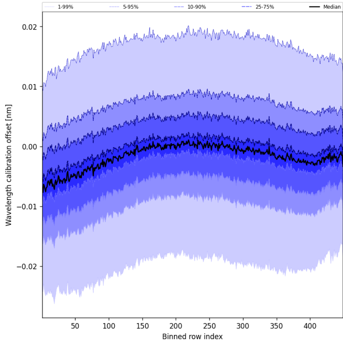
Figure 52: Along track statistics of “Wavelength calibration offset” for 2025-04-29 to 2025-04-30
