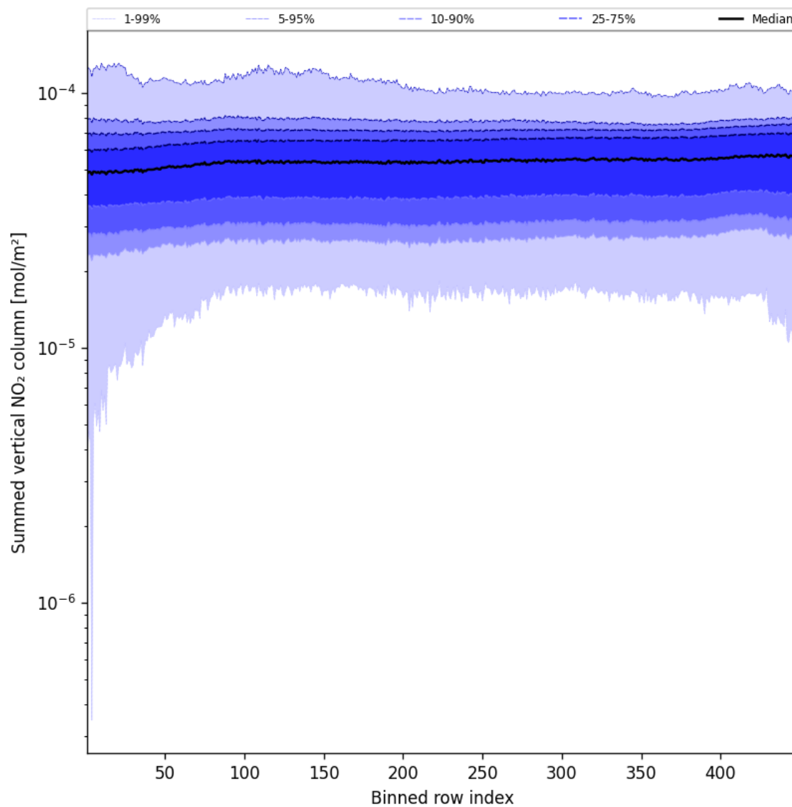
Figure 57: Along track statistics of “Summed vertical NO 2 column” for 2025-04-29 to 2025-04-30
