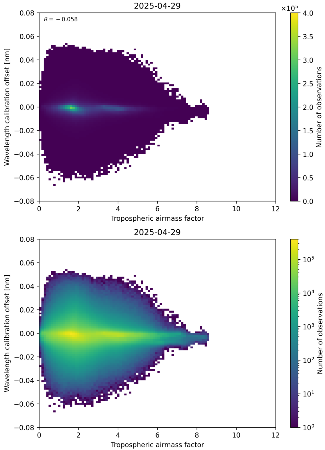
Figure 80: Scatter density plot of “Tropospheric airmass factor” against “Wavelength calibration offset” for 2025-04-29 to 2025-04-30.
