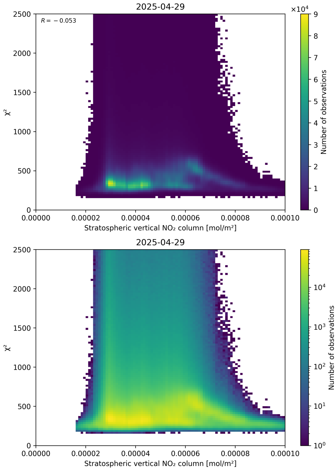
Figure 97: Scatter density plot of “Stratospheric vertical NO 2 column” against “ \chi^2 ” for 2025-04-29 to 2025-04-30.
