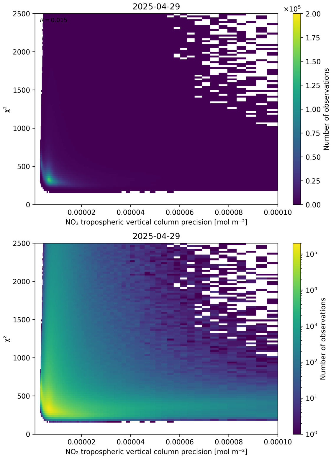
Figure 134: Scatter density plot of “NO 2 tropospheric vertical column precision” against “ \chi^2 ” for 2025-04-29 to 2025-04-30.
