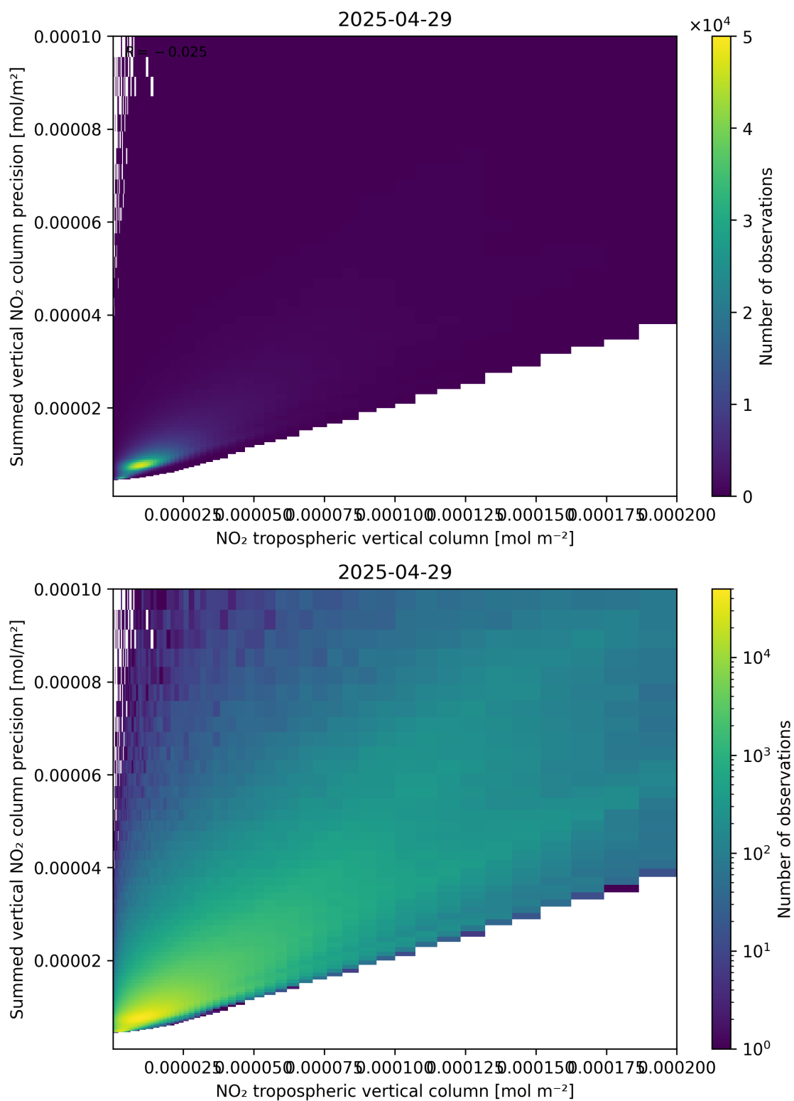
Figure 127: Scatter density plot of “NO 2 tropospheric vertical column” against “Summed vertical NO 2 column precision” for 2025-04-29 to 2025-04-30.
