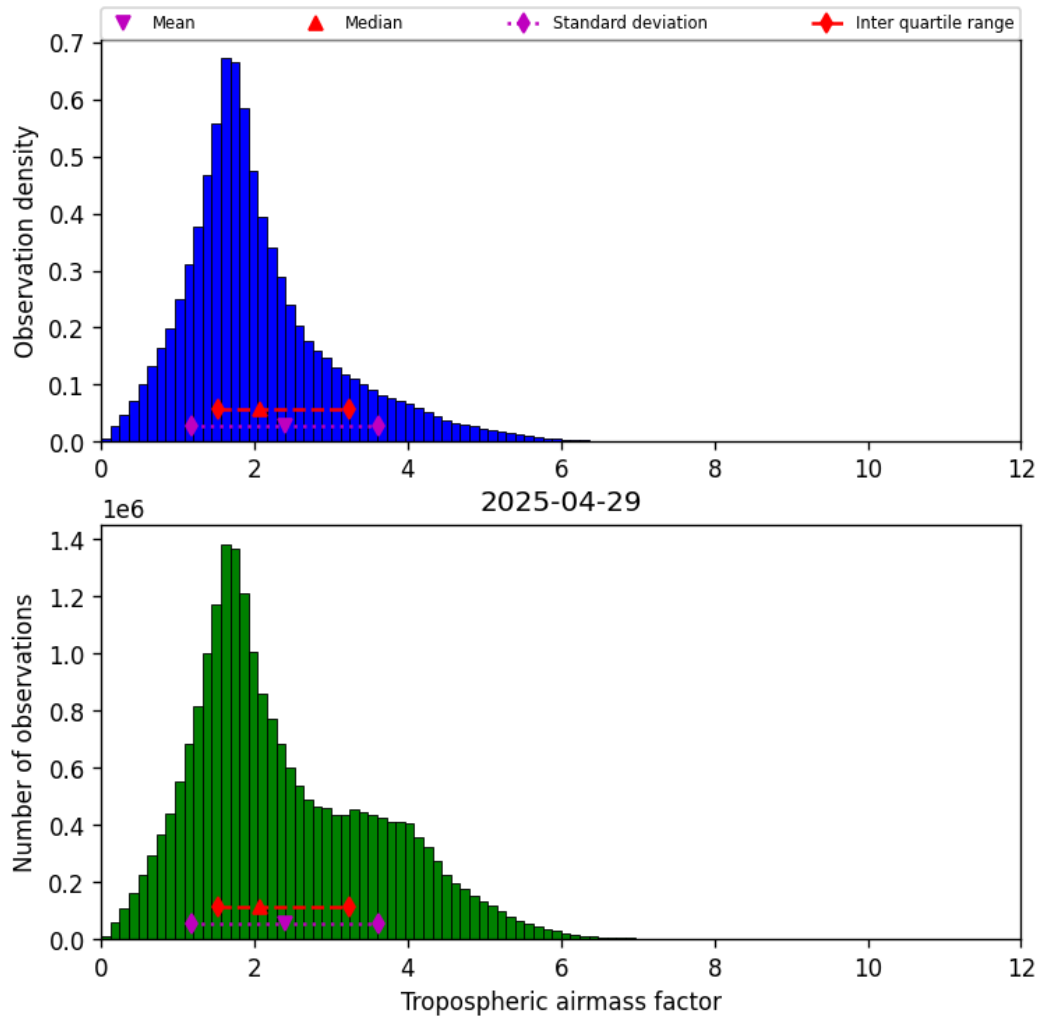
Figure 31: Histogram of “Tropospheric airmass factor” for 2025-04-29 to 2025-04-30
