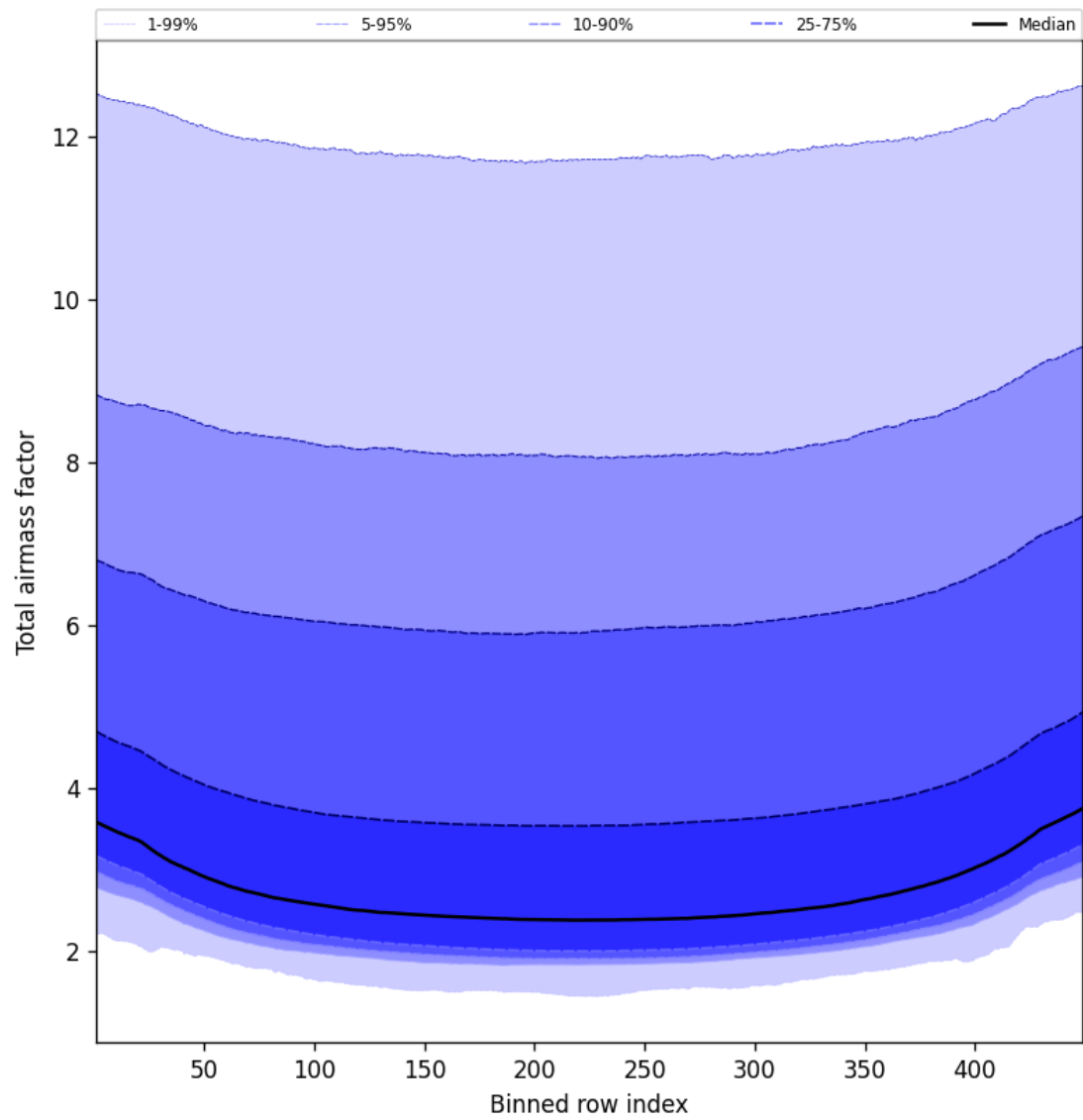
Figure 49: Along track statistics of “Total airmass factor” for 2025-04-29 to 2025-04-30
