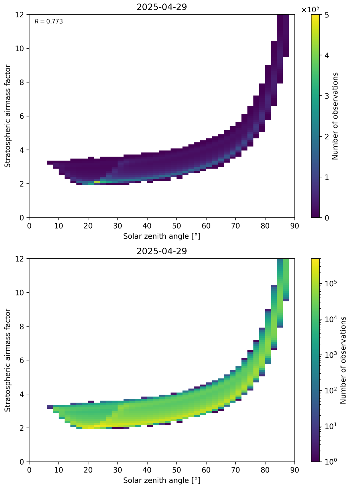
Figure 145: Scatter density plot of “Solar zenith angle” against “Stratospheric airmass factor” for 2025-04-29 to 2025-04-30.
