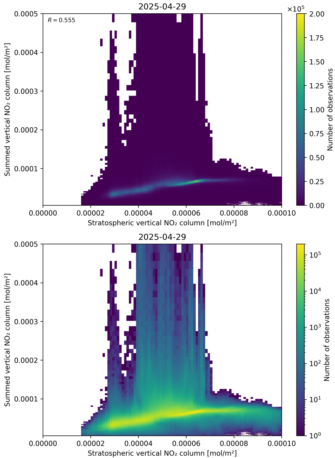
Figure 98: Scatter density plot of “Stratospheric vertical NO 2 column” against “Summed vertical NO 2 column” for 2025-04-29 to 2025-04-30.
