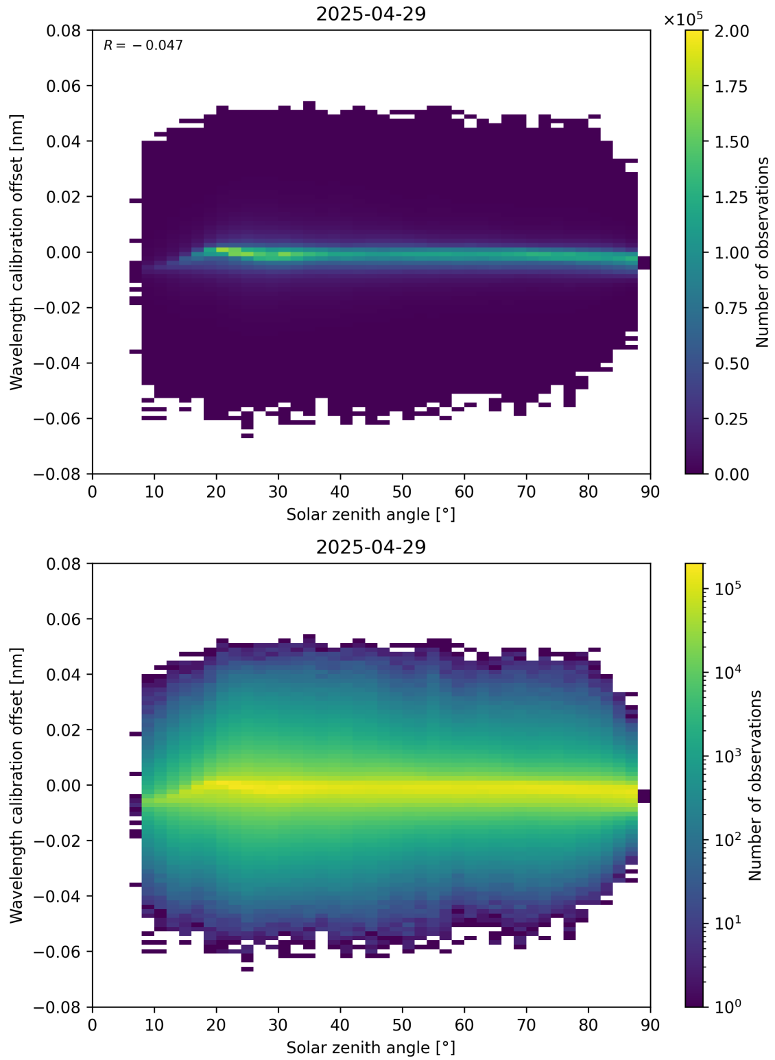
Figure 158: Scatter density plot of “Solar zenith angle” against “Wavelength calibration offset” for 2025-04-29 to 2025-04-30.
