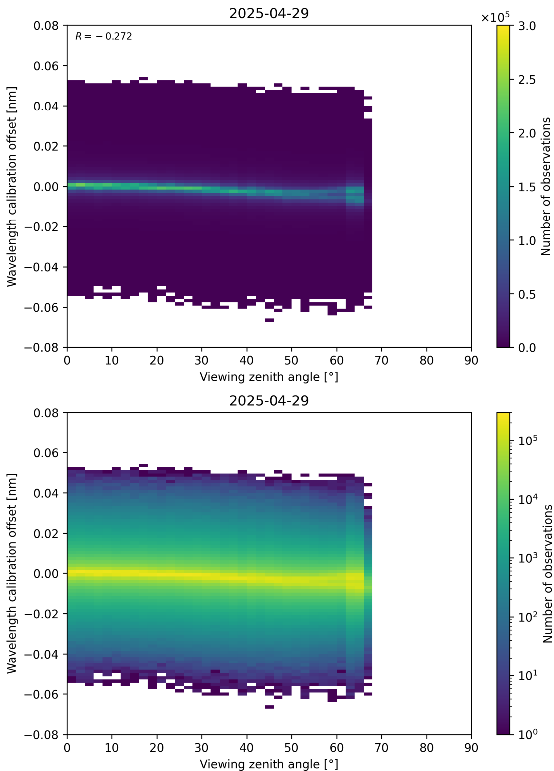
Figure 173: Scatter density plot of “Viewing zenith angle” against “Wavelength calibration offset” for 2025-04-29 to 2025-04-30.
