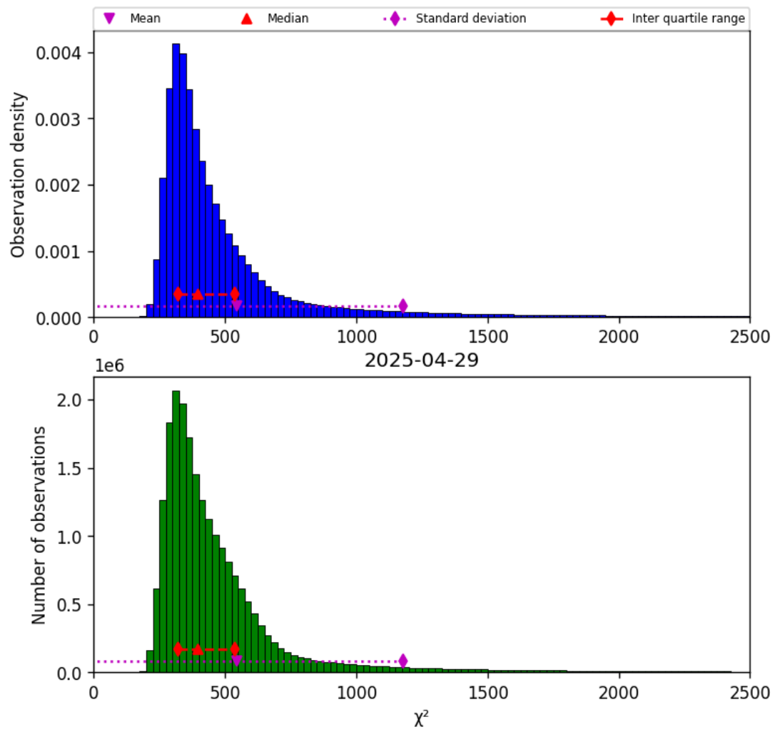
Figure 42: Histogram of “ \chi^2 ” for 2025-04-29 to 2025-04-30
