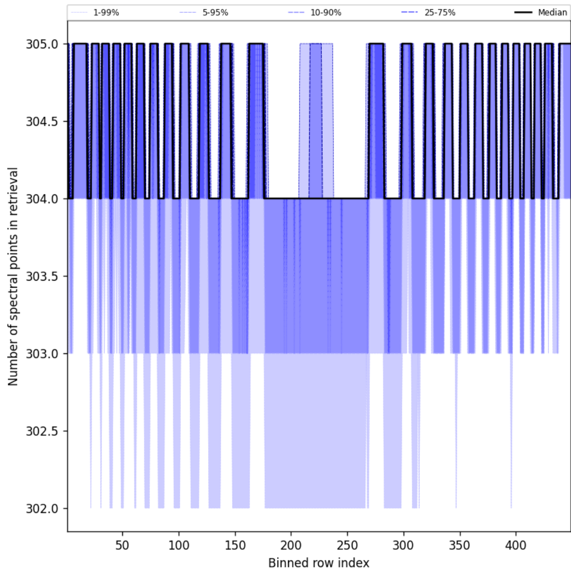
Figure 50: Along track statistics of “Number of spectral points in retrieval” for 2025-04-29 to 2025-04-30
