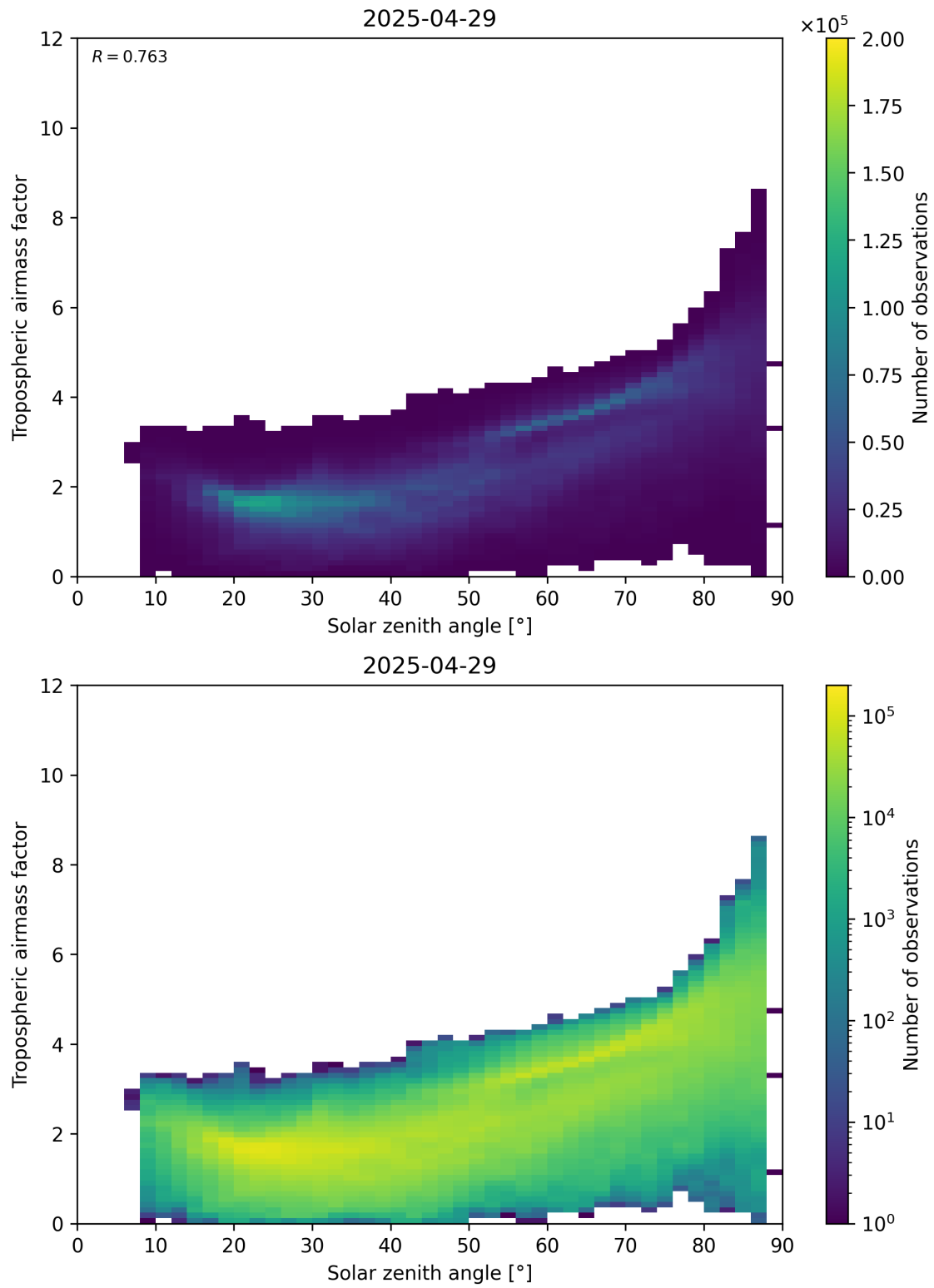
Figure 147: Scatter density plot of “Solar zenith angle” against “Tropospheric airmass factor” for 2025-04-29 to 2025-04-30.
