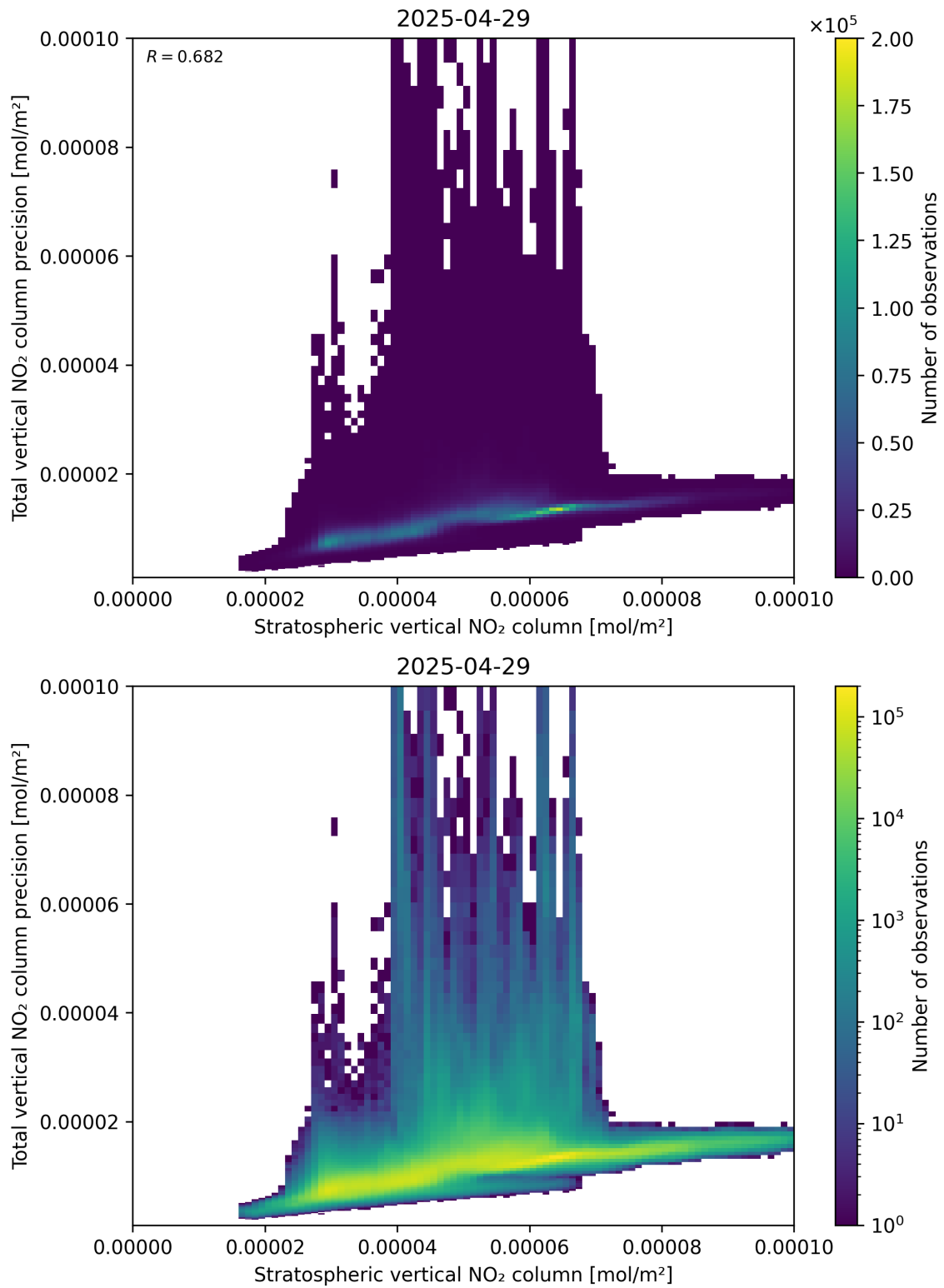
Figure 101: Scatter density plot of “Stratospheric vertical NO 2 column” against “Total vertical NO 2 column precision” for 2025-04-29 to 2025-04-30.
