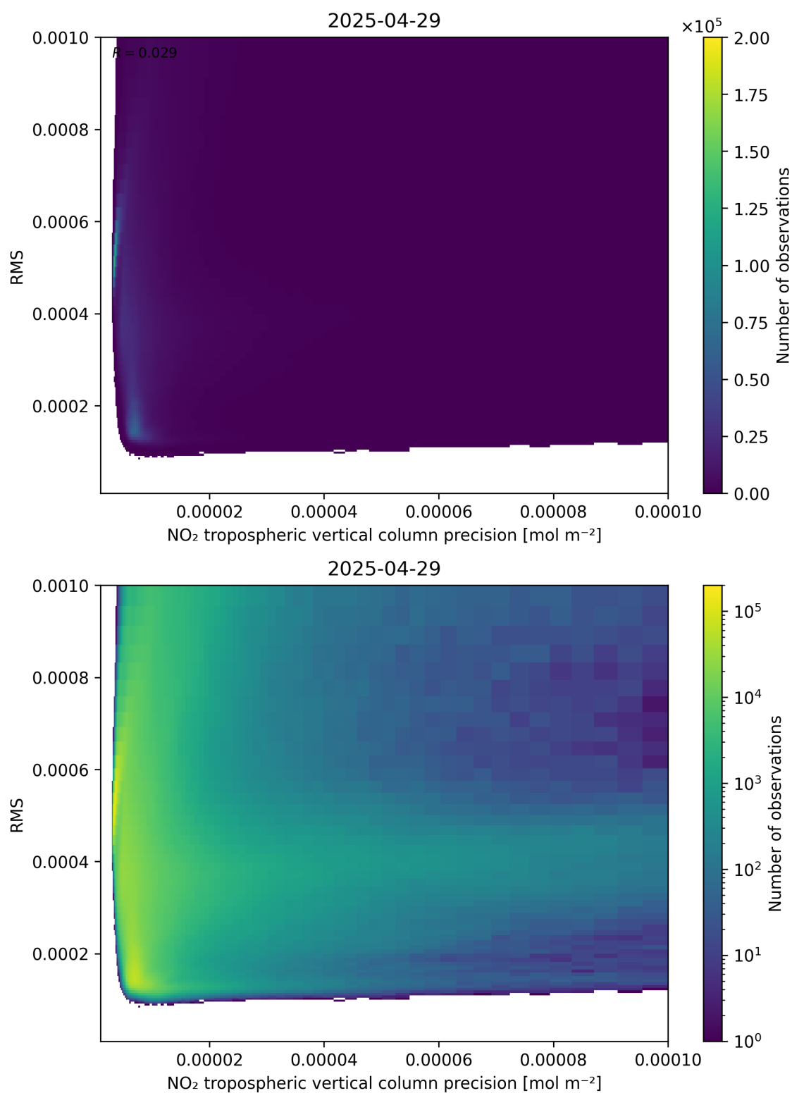
Figure 140: Scatter density plot of “NO 2 tropospheric vertical column precision” against “RMS” for 2025-04-29 to 2025-04-30.
