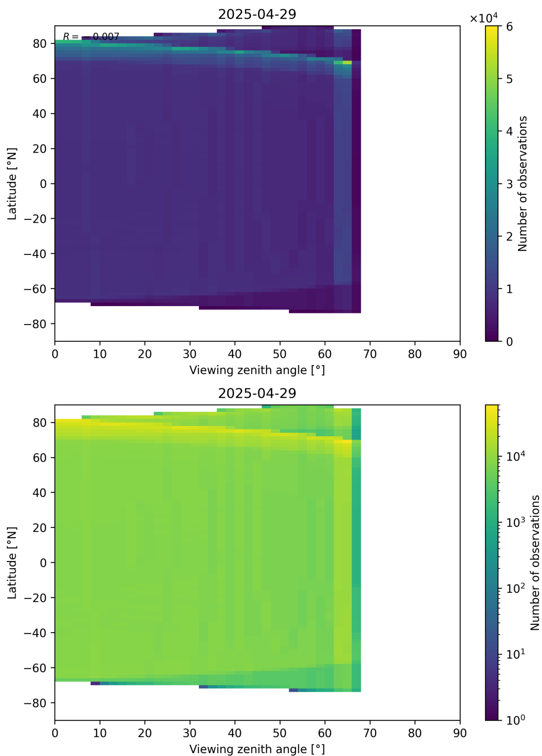
Figure 163: Scatter density plot of “Viewing zenith angle” against “Latitude” for 2025-04-29 to 2025-04-30.
