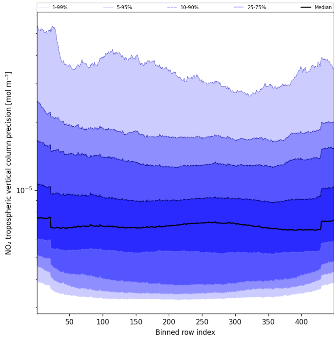
Figure 47: Along track statistics of “NO 2 tropospheric vertical column precision” for 2025-04-29 to 2025-04-30
