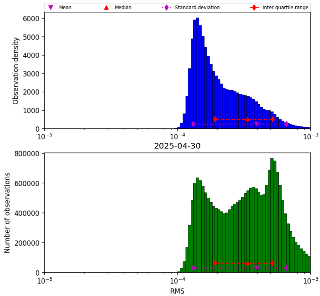
Figure 43: Histogram of “RMS” for 2025-04-30 to 2025-05-01
