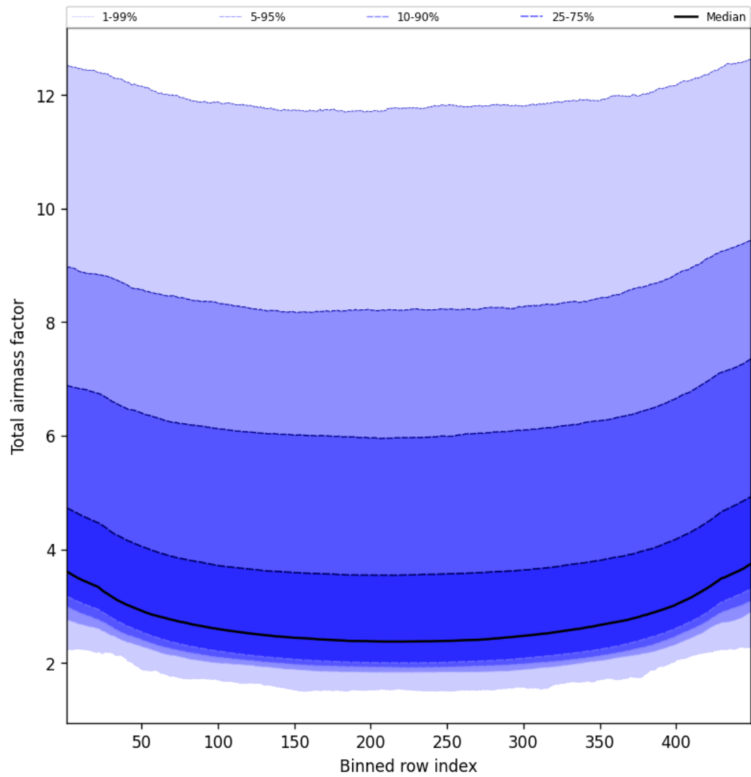
Figure 49: Along track statistics of “Total airmass factor” for 2025-04-30 to 2025-05-01
