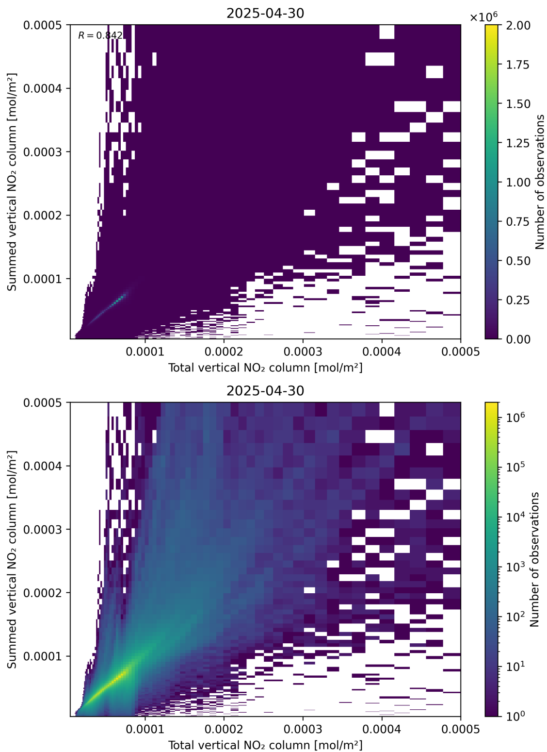
Figure 112: Scatter density plot of “Total vertical NO 2 column” against “Summed vertical NO 2 column” for 2025-04-30 to 2025-05-01.
