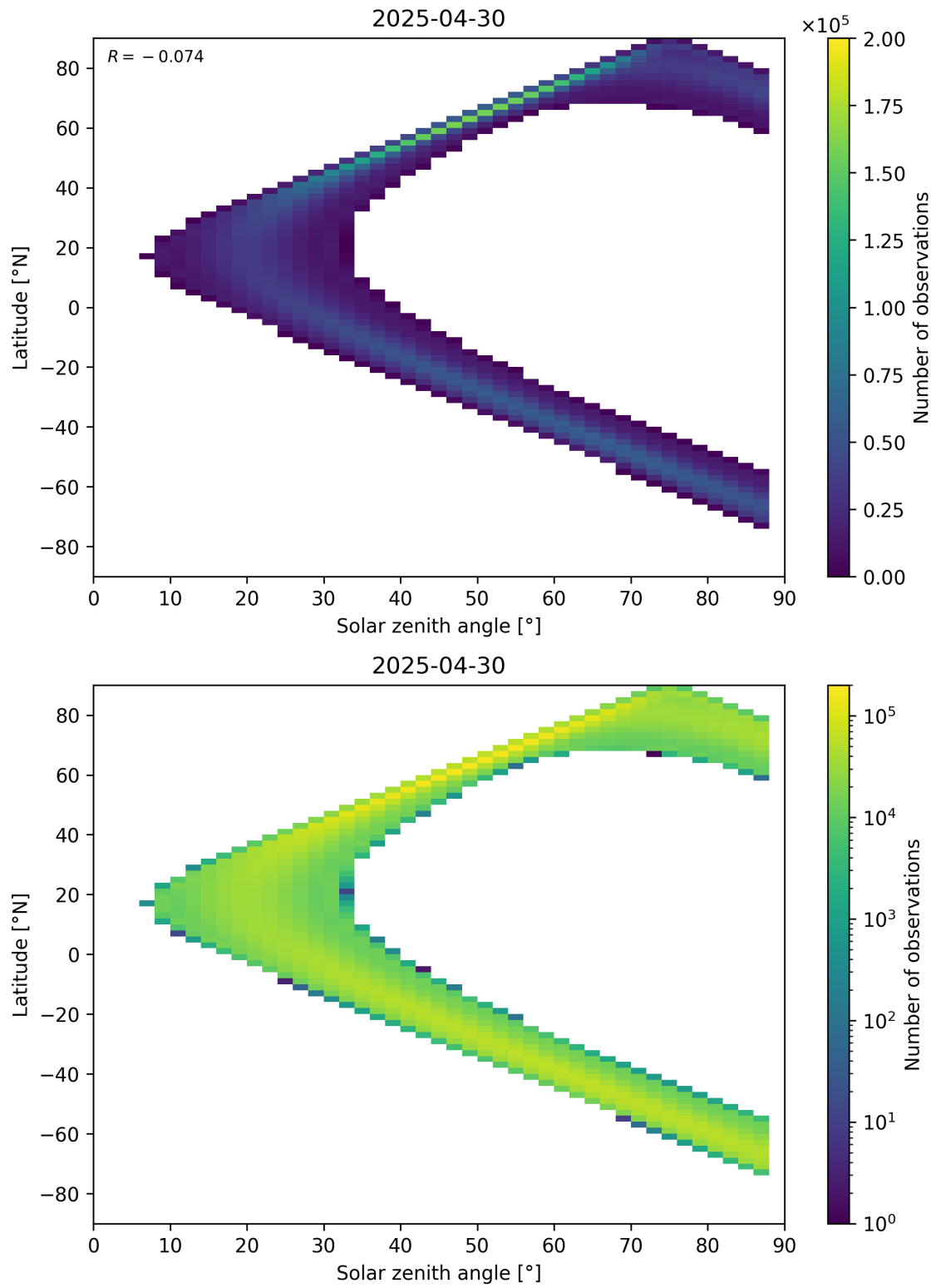
Figure 149: Scatter density plot of “Solar zenith angle” against “Latitude” for 2025-04-30 to 2025-05-01.
