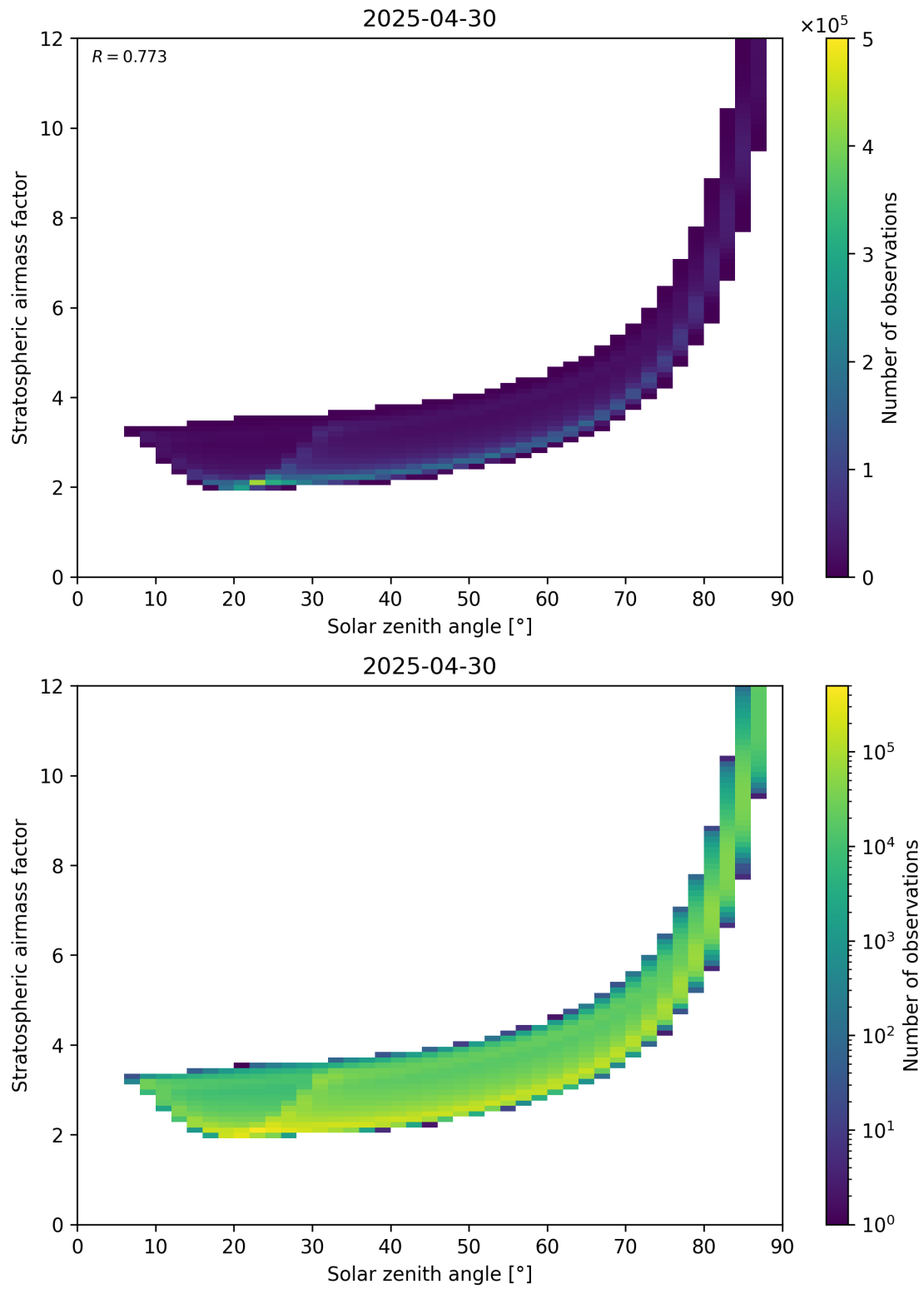
Figure 145: Scatter density plot of “Solar zenith angle” against “Stratospheric airmass factor” for 2025-04-30 to 2025-05-01.
