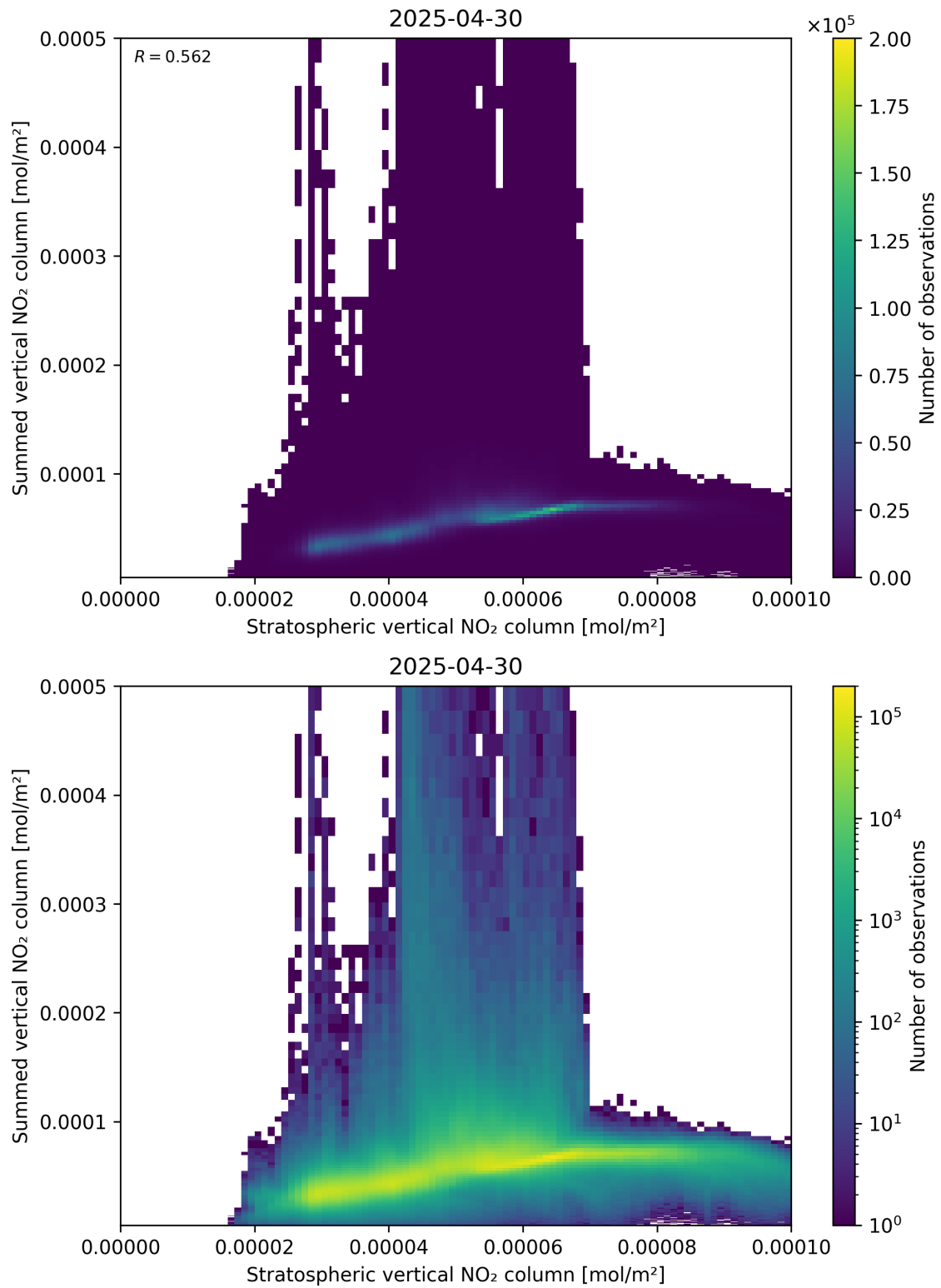
Figure 98: Scatter density plot of “Stratospheric vertical NO 2 column” against “Summed vertical NO 2 column” for 2025-04-30 to 2025-05-01.
