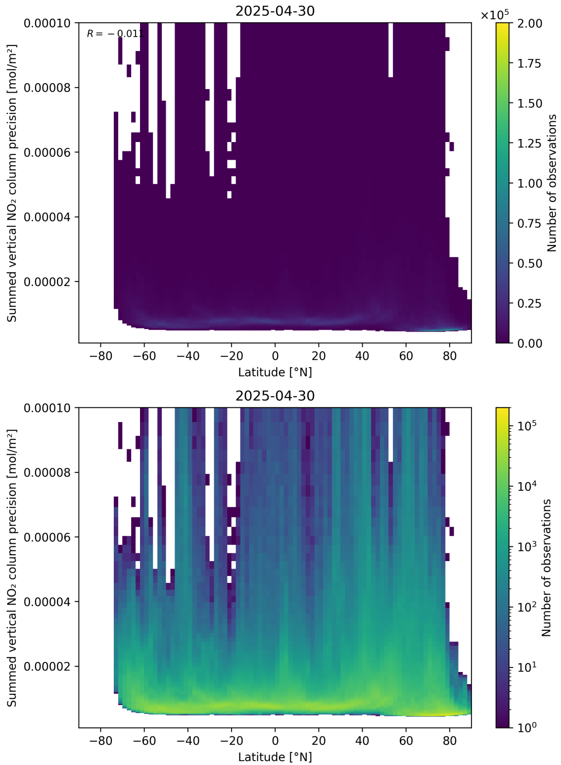
Figure 89: Scatter density plot of “Latitude” against “Summed vertical NO 2 column precision” for 2025-04-30 to 2025-05-01.
