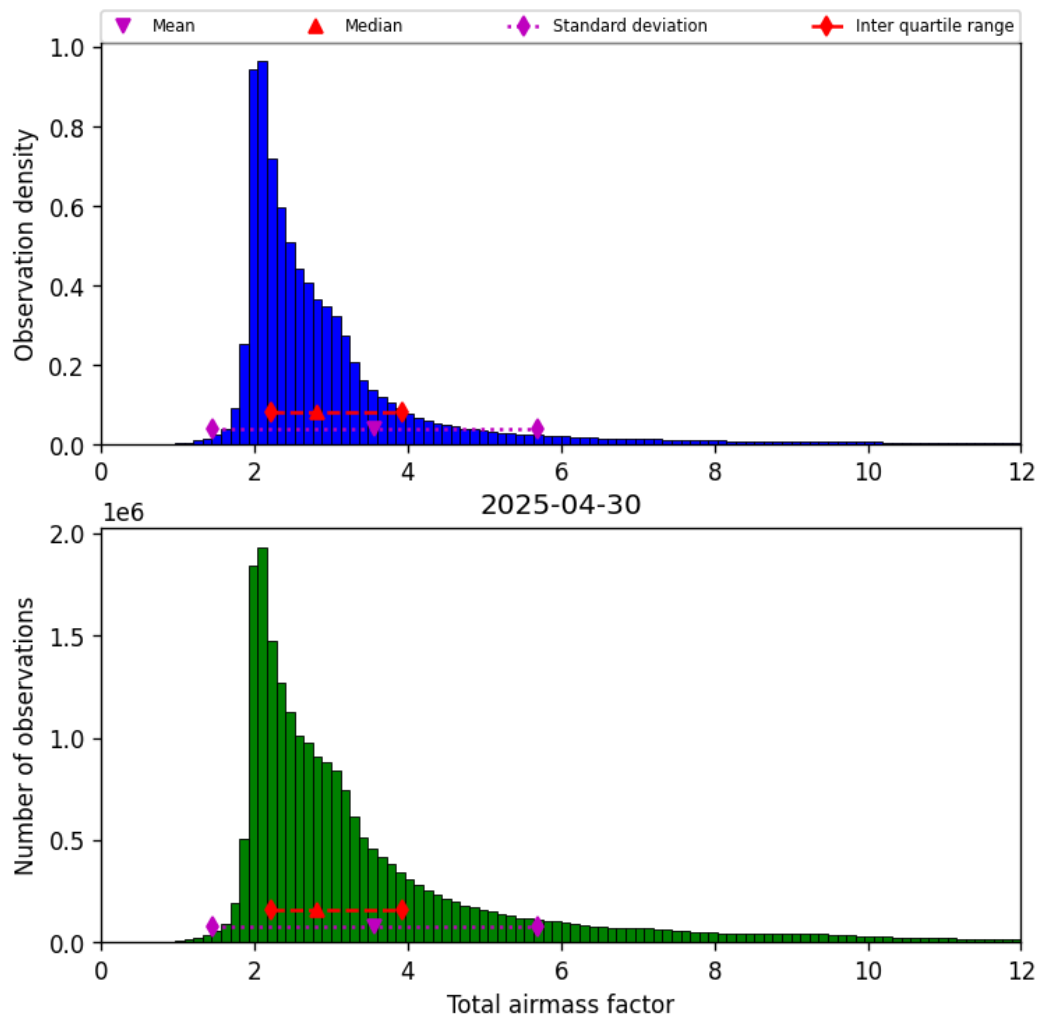
Figure 32: Histogram of “Total airmass factor” for 2025-04-30 to 2025-05-01
