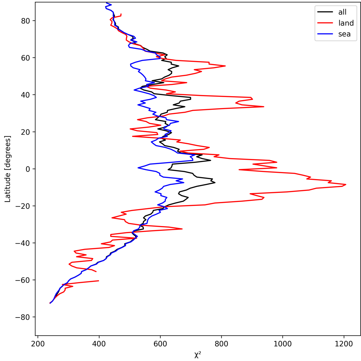
Figure 25: Zonal average of “ \chi^2 ” for 2025-04-30 to 2025-05-01.
