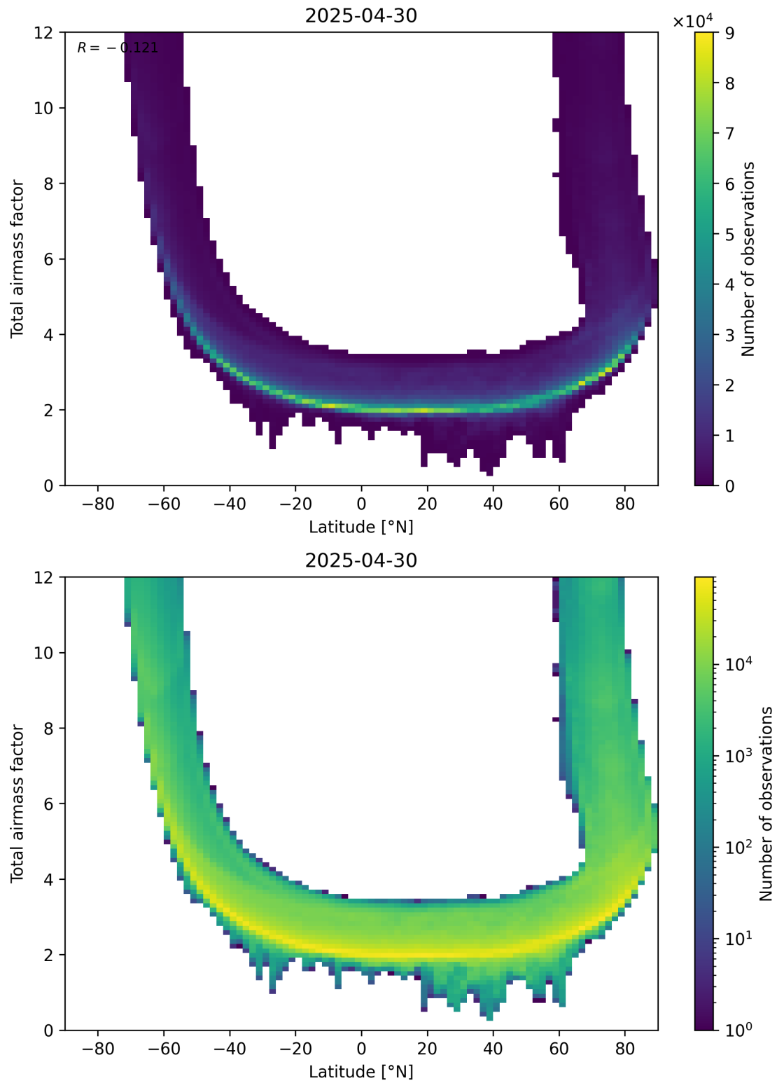
Figure 84: Scatter density plot of “Latitude” against “Total airmass factor” for 2025-04-30 to 2025-05-01.
