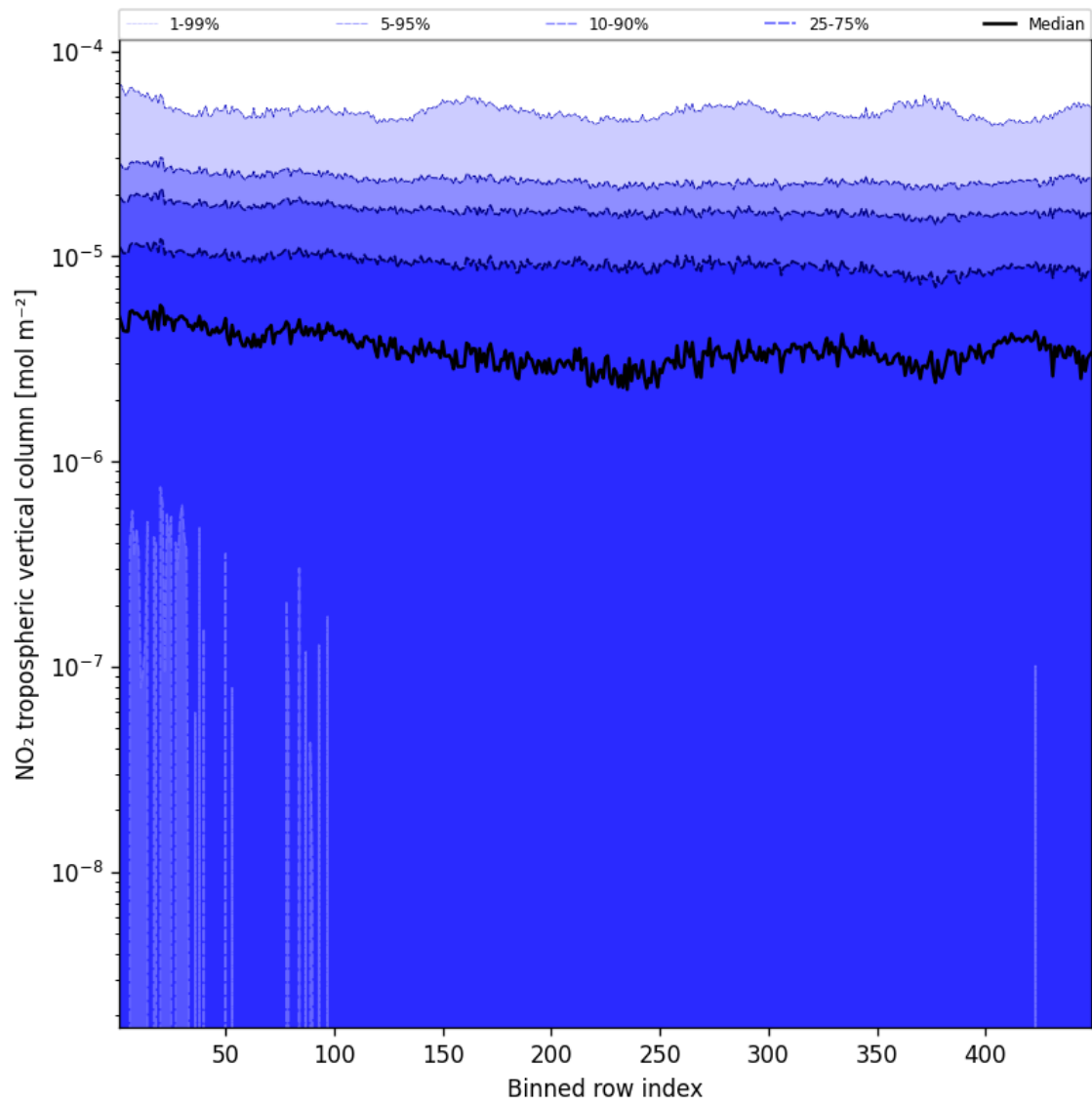
Figure 46: Along track statistics of “NO 2 tropospheric vertical column” for 2025-04-30 to 2025-05-01
