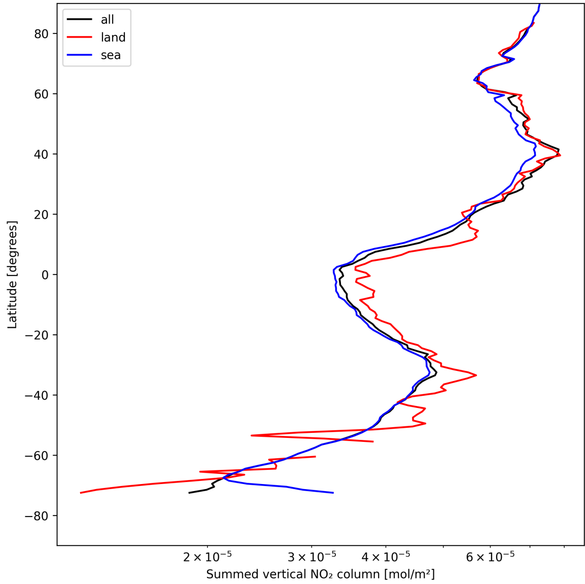
Figure 23: Zonal average of “Summed vertical NO 2 column” for 2025-04-30 to 2025-05-01.
