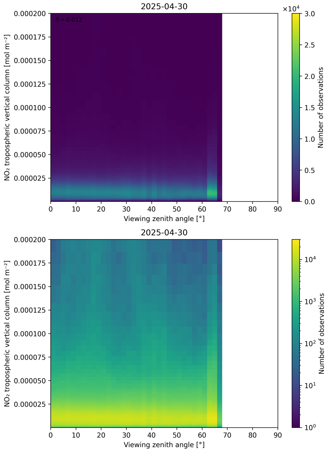
Figure 169: Scatter density plot of “Viewing zenith angle” against “NO 2 tropospheric vertical column” for 2025-04-30 to 2025-05-01.
