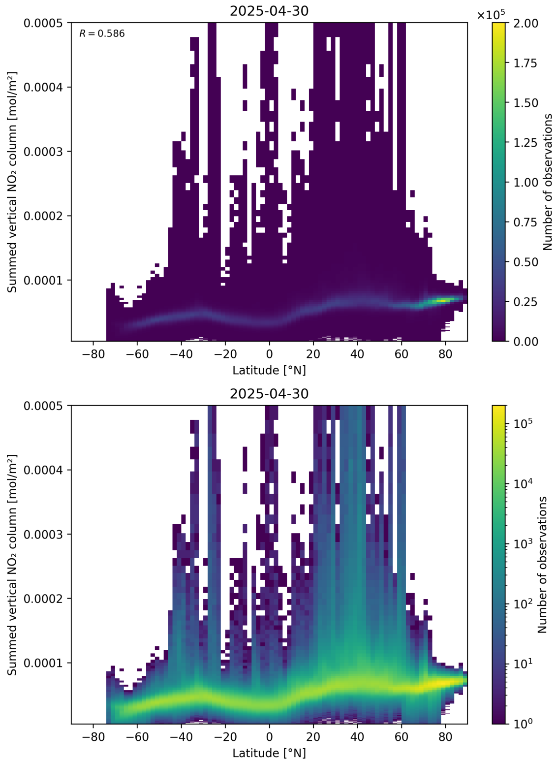
Figure 88: Scatter density plot of “Latitude” against “Summed vertical NO 2 column” for 2025-04-30 to 2025-05-01.
