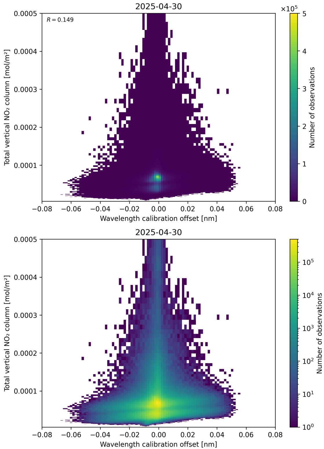
Figure 179: Scatter density plot of “Wavelength calibration offset” against “Total vertical NO 2 column” for 2025-04-30 to 2025-05-01.
