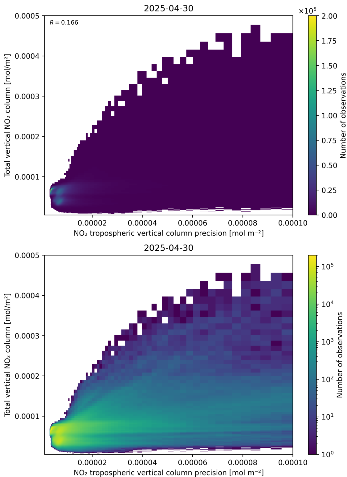
Figure 138: Scatter density plot of “NO 2 tropospheric vertical column precision” against “Total vertical NO 2 column” for 2025-04-30 to 2025-05-01.
