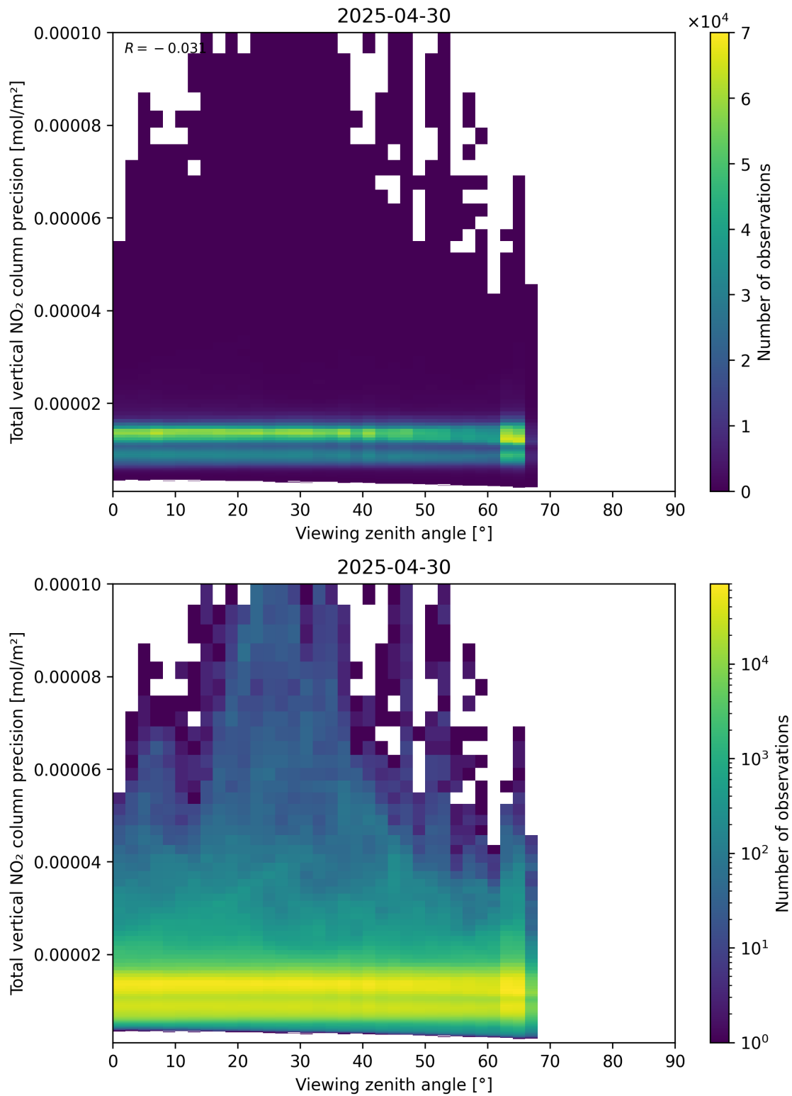
Figure 168: Scatter density plot of “Viewing zenith angle” against “Total vertical NO 2 column precision” for 2025-04-30 to 2025-05-01.
