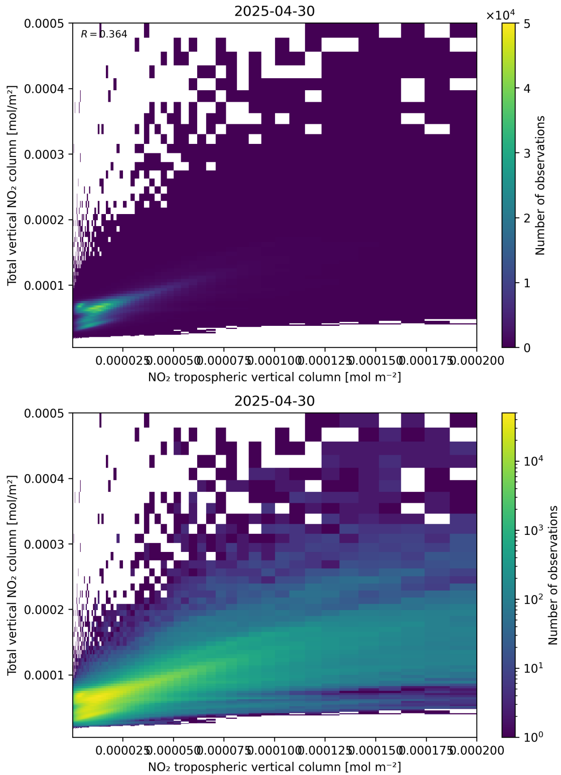
Figure 128: Scatter density plot of “NO 2 tropospheric vertical column” against “Total vertical NO 2 column” for 2025-04-30 to 2025-05-01.
