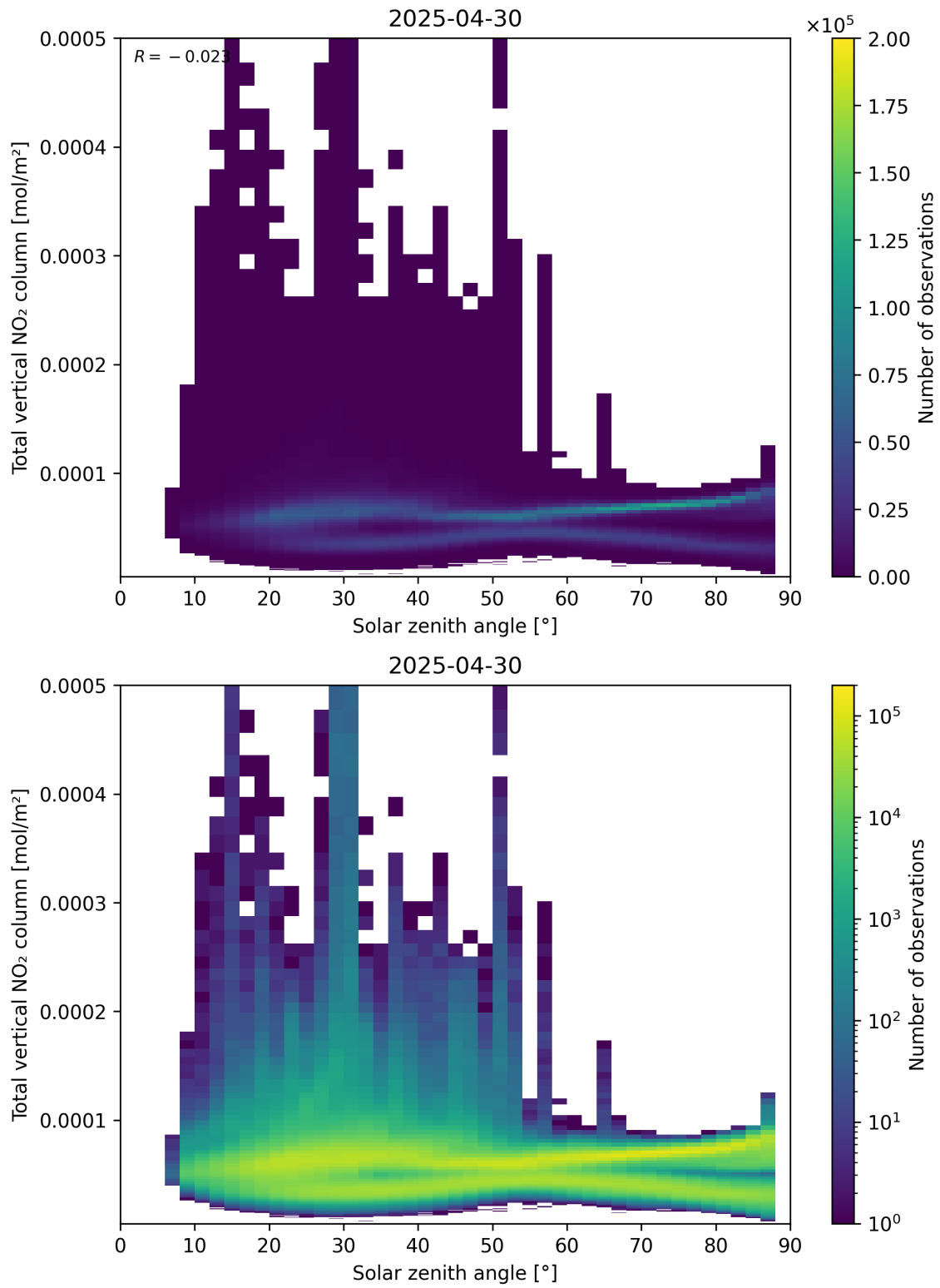
Figure 153: Scatter density plot of “Solar zenith angle” against “Total vertical NO 2 column” for 2025-04-30 to 2025-05-01.
