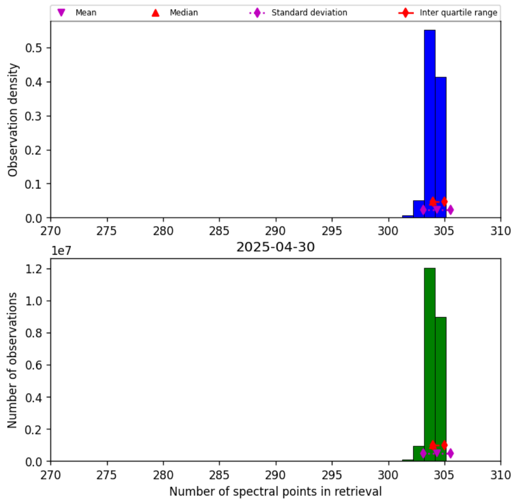
Figure 33: Histogram of “Number of spectral points in retrieval” for 2025-04-30 to 2025-05-01
