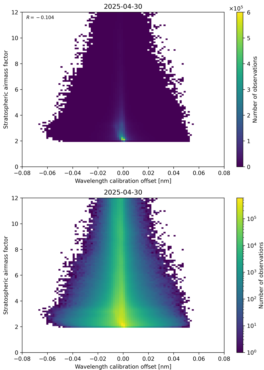
Figure 174: Scatter density plot of “Wavelength calibration offset” against “Stratospheric airmass factor” for 2025-04-30 to 2025-05-01.
