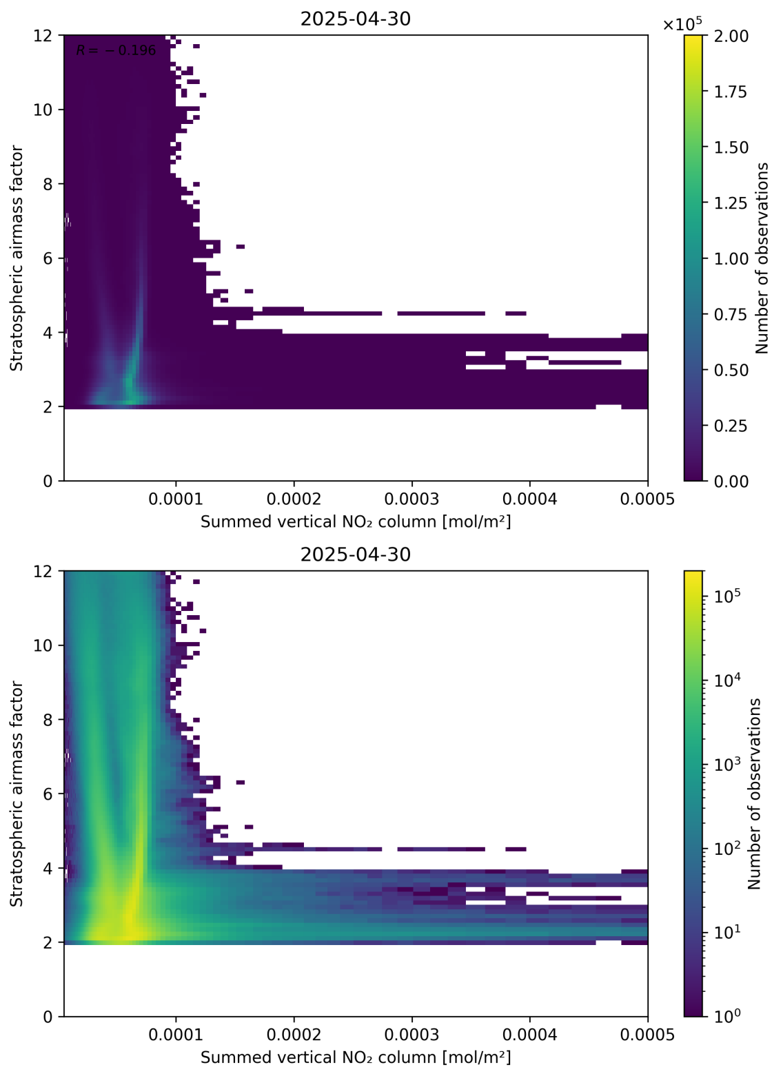
Figure 103: Scatter density plot of “Summed vertical NO 2 column” against “Stratospheric airmass factor” for 2025-04-30 to 2025-05-01.
