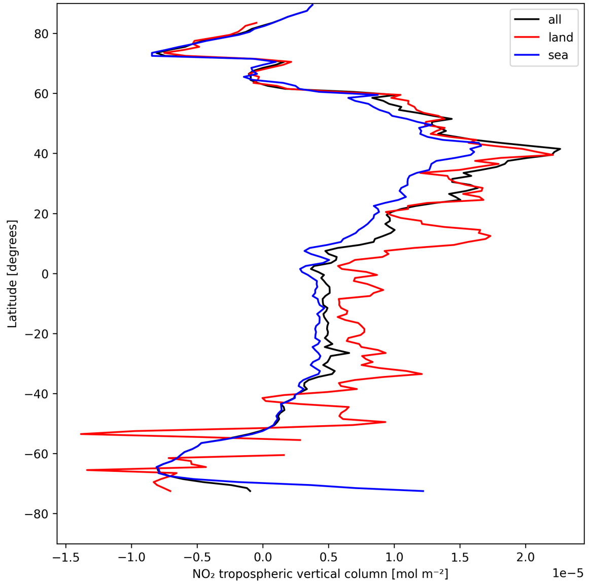
Figure 12: Zonal average of “NO 2 tropospheric vertical column” for 2025-04-30 to 2025-05-01.
