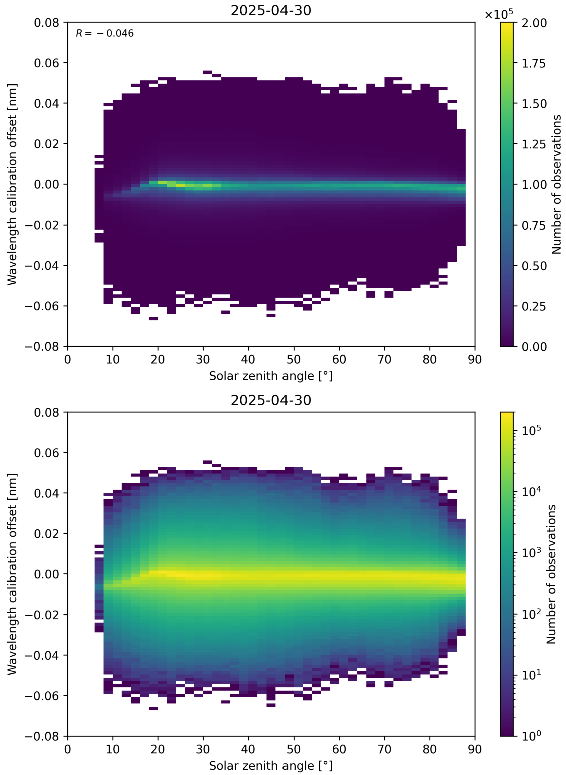
Figure 158: Scatter density plot of “Solar zenith angle” against “Wavelength calibration offset” for 2025-04-30 to 2025-05-01.
