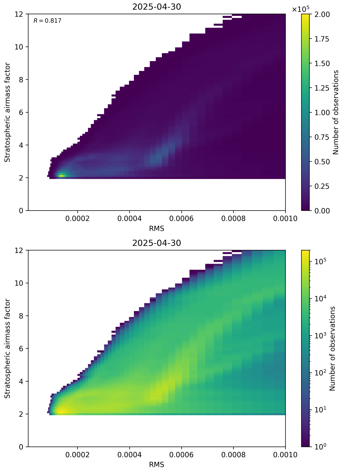
Figure 144: Scatter density plot of “RMS” against “Stratospheric airmass factor” for 2025-04-30 to 2025-05-01.
