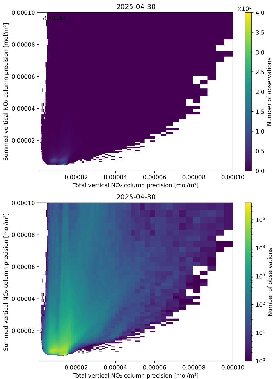
Figure 118: Scatter density plot of “Total vertical NO 2 column precision” against “Summed vertical NO 2 column precision” for 2025-04-30 to 2025-05-01.
