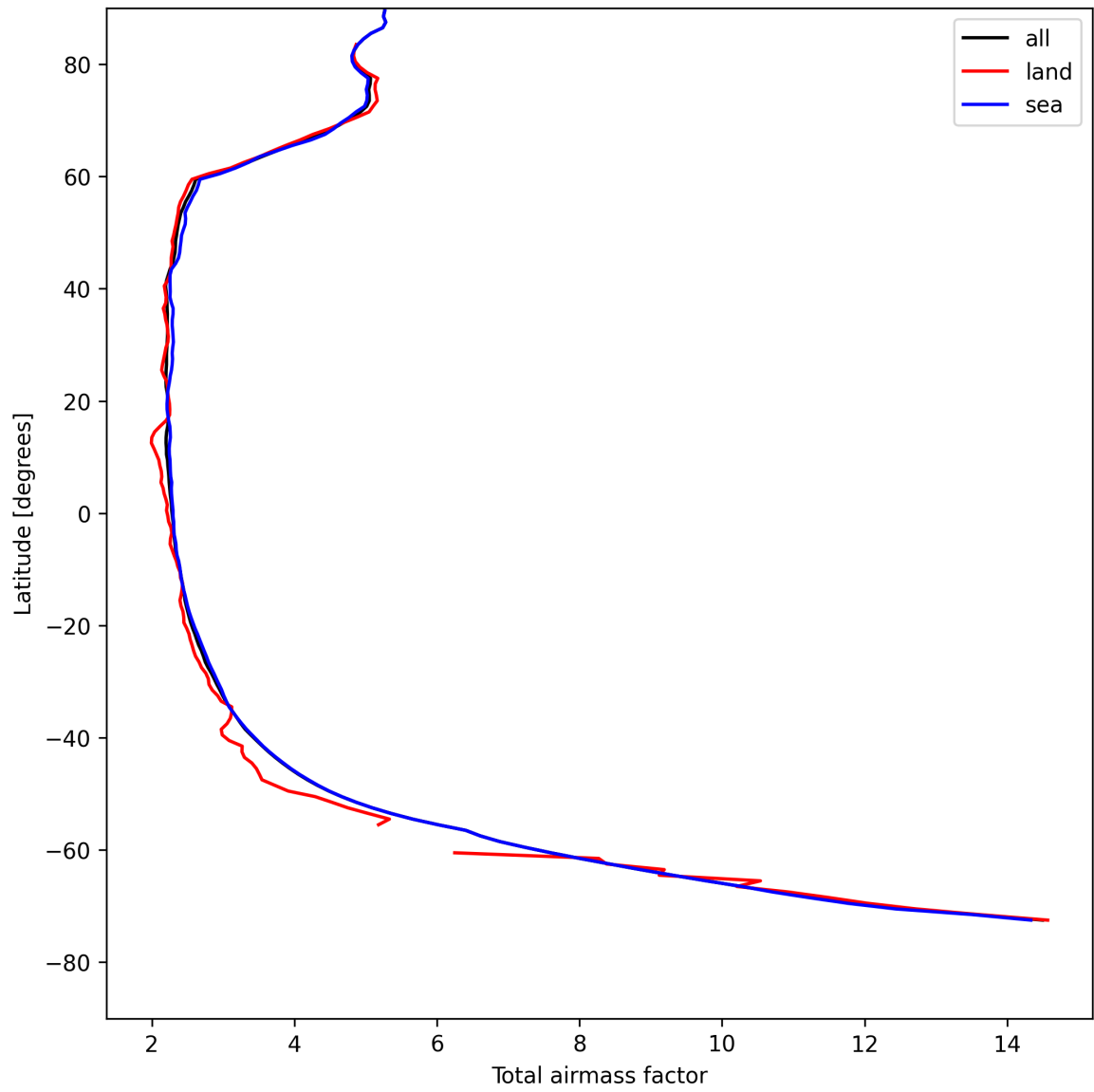
Figure 15: Zonal average of “Total airmass factor” for 2025-04-30 to 2025-05-01.
