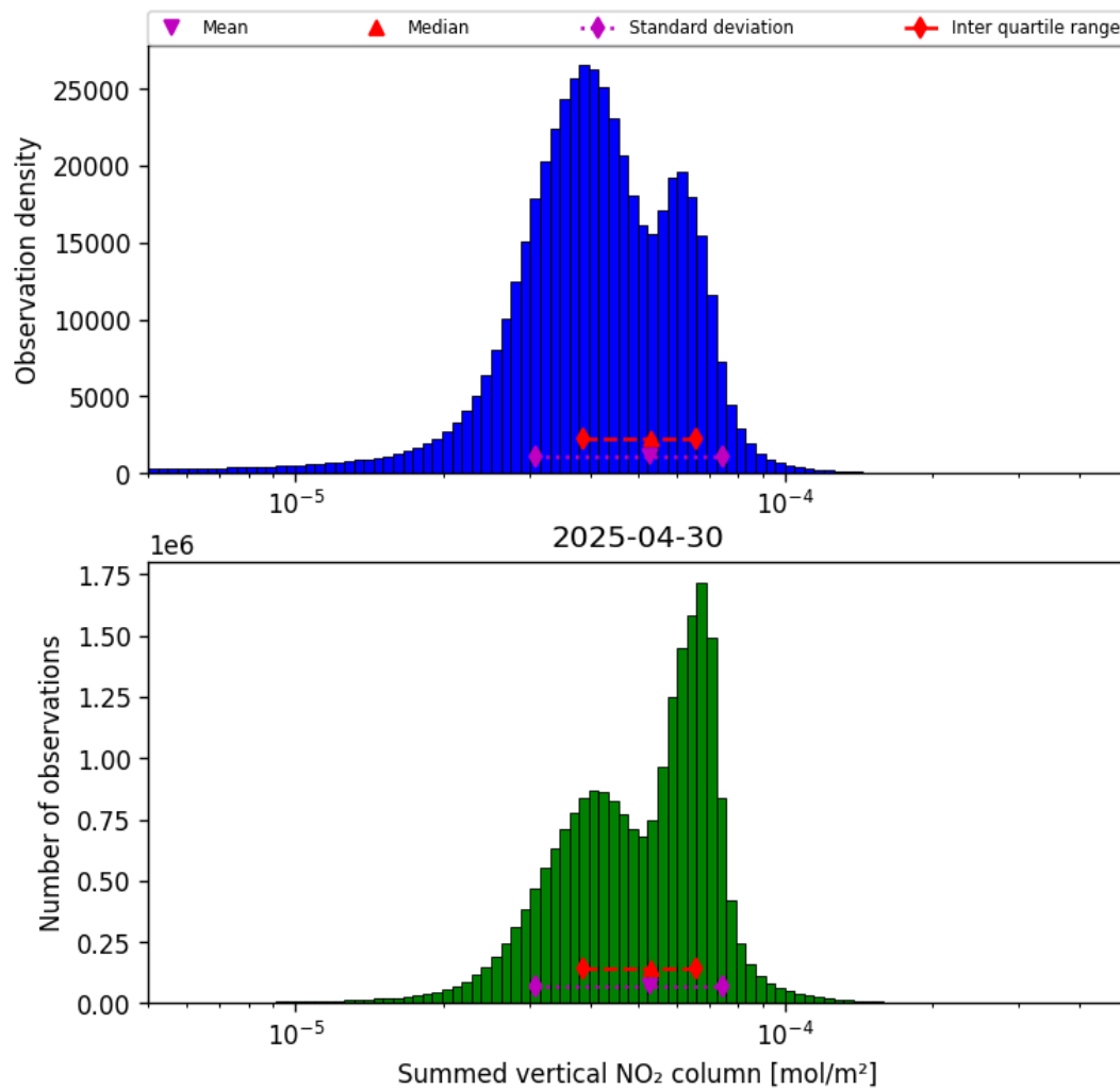
Figure 40: Histogram of “Summed vertical NO 2 column” for 2025-04-30 to 2025-05-01
