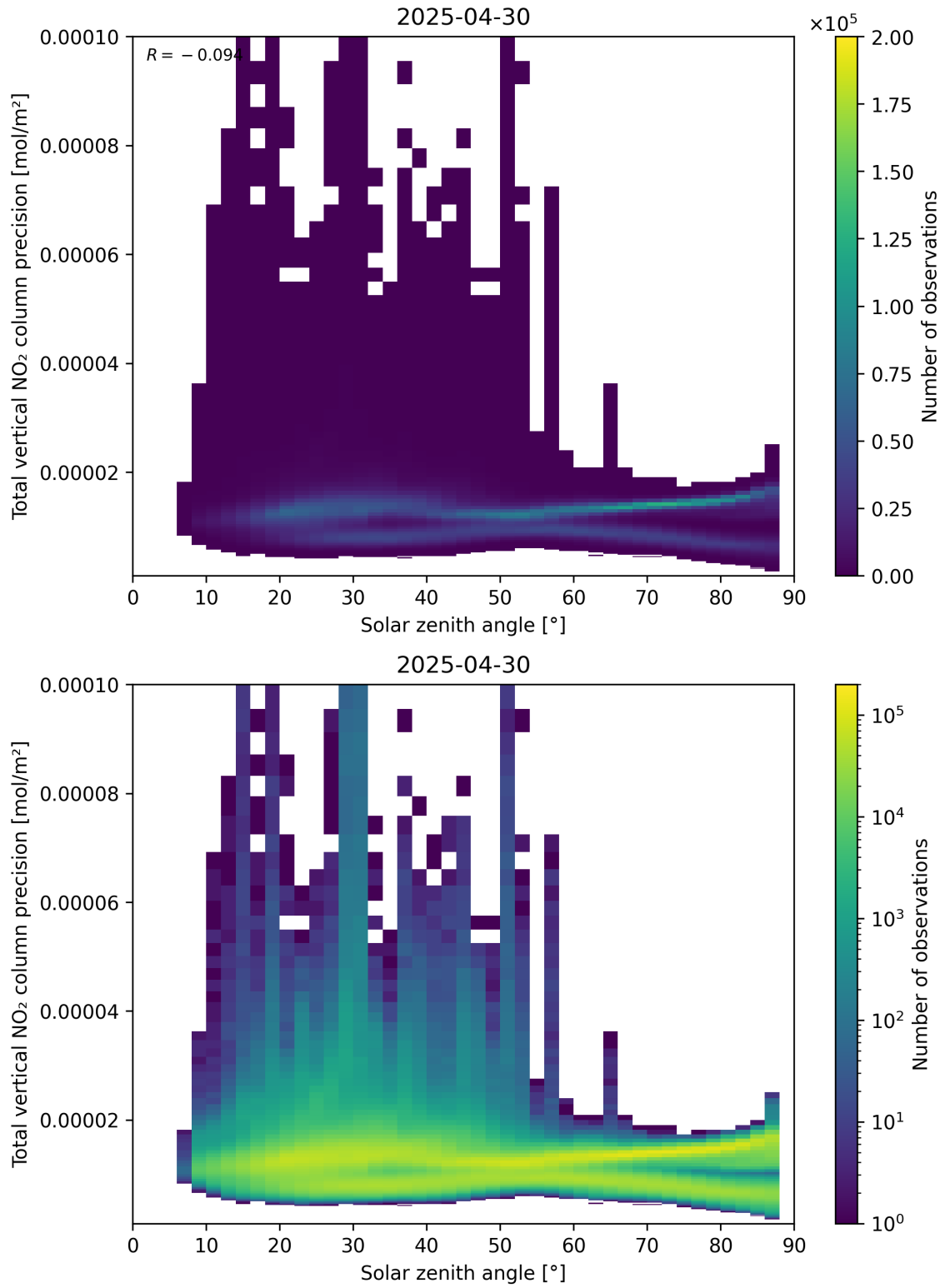
Figure 154: Scatter density plot of “Solar zenith angle” against “Total vertical NO 2 column precision” for 2025-04-30 to 2025-05-01.
