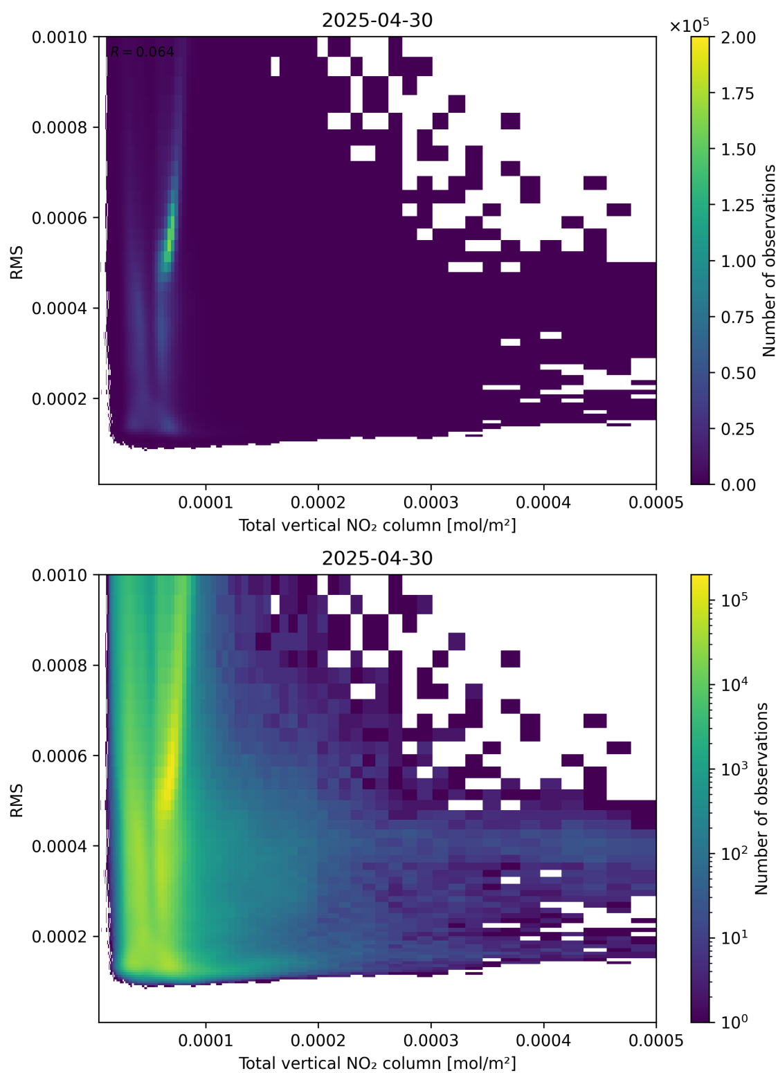
Figure 120: Scatter density plot of “Total vertical NO 2 column” against “RMS” for 2025-04-30 to 2025-05-01.
