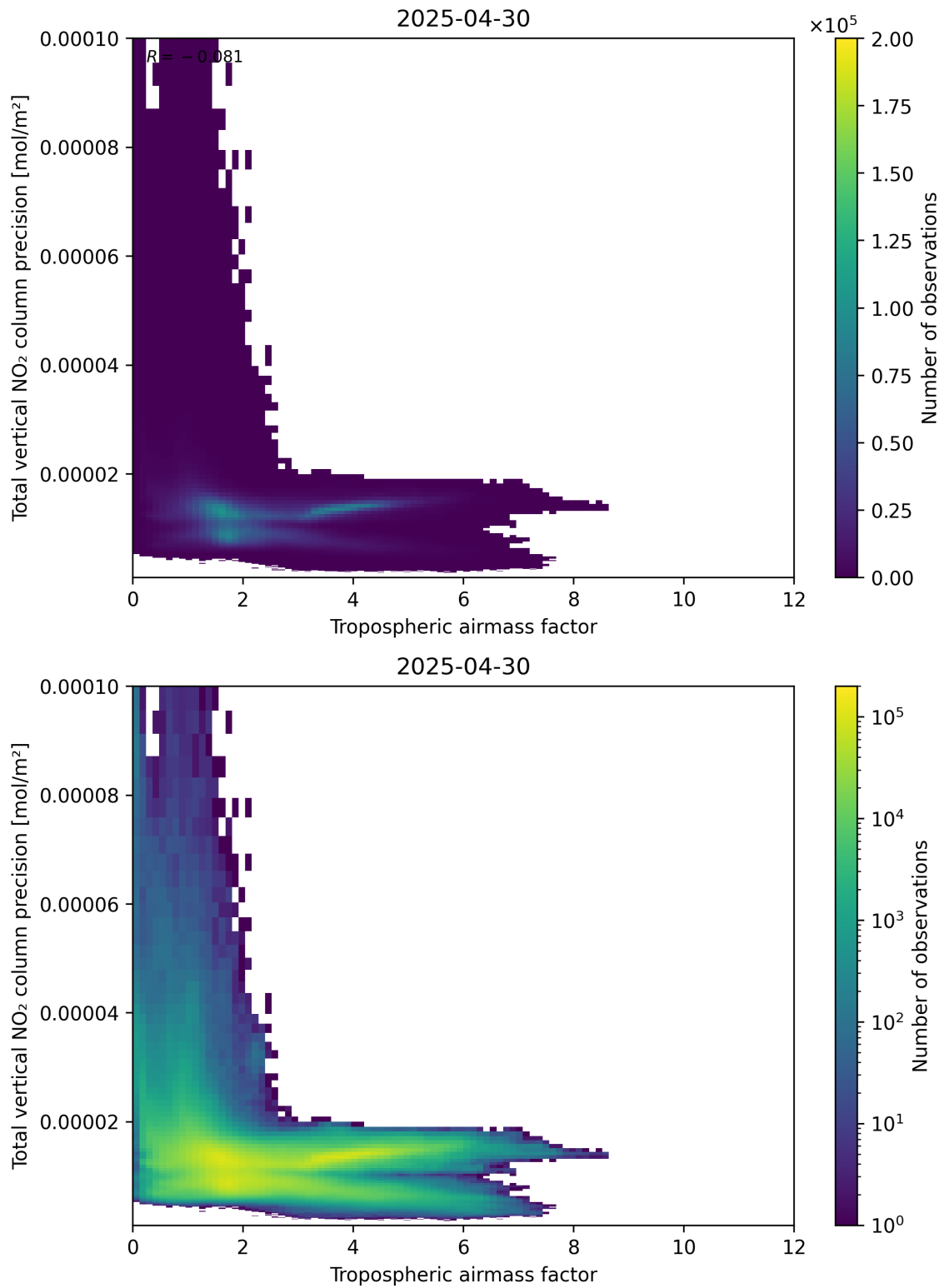
Figure 78: Scatter density plot of “Tropospheric air mass factor” against “Total vertical NO 2 column precision” for 2025-04-30 to 2025-05-01.
