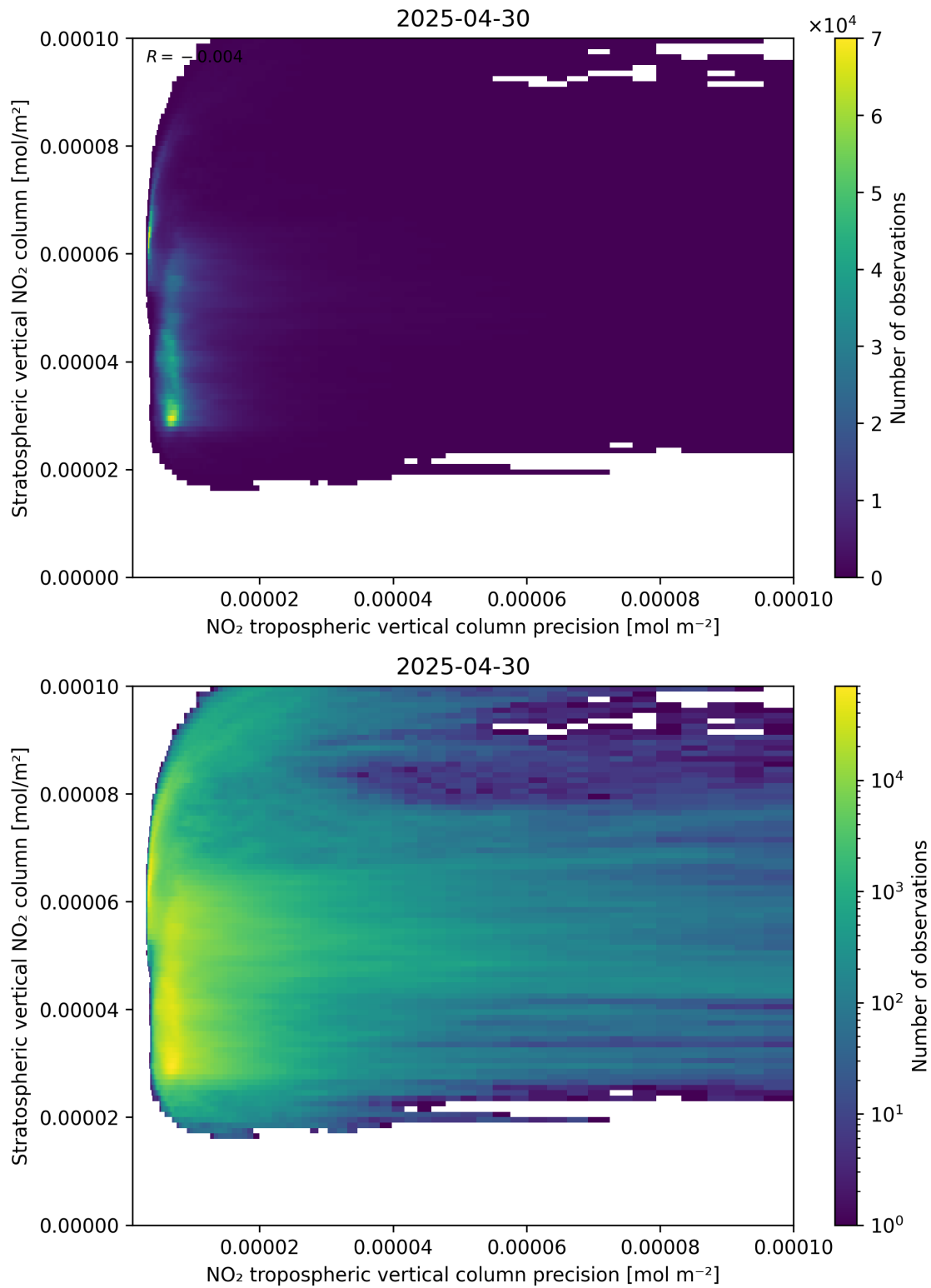
Figure 135: Scatter density plot of “NO 2 tropospheric vertical column precision” against “Stratospheric vertical NO 2 column” for 2025-04-30 to 2025-05-01.
