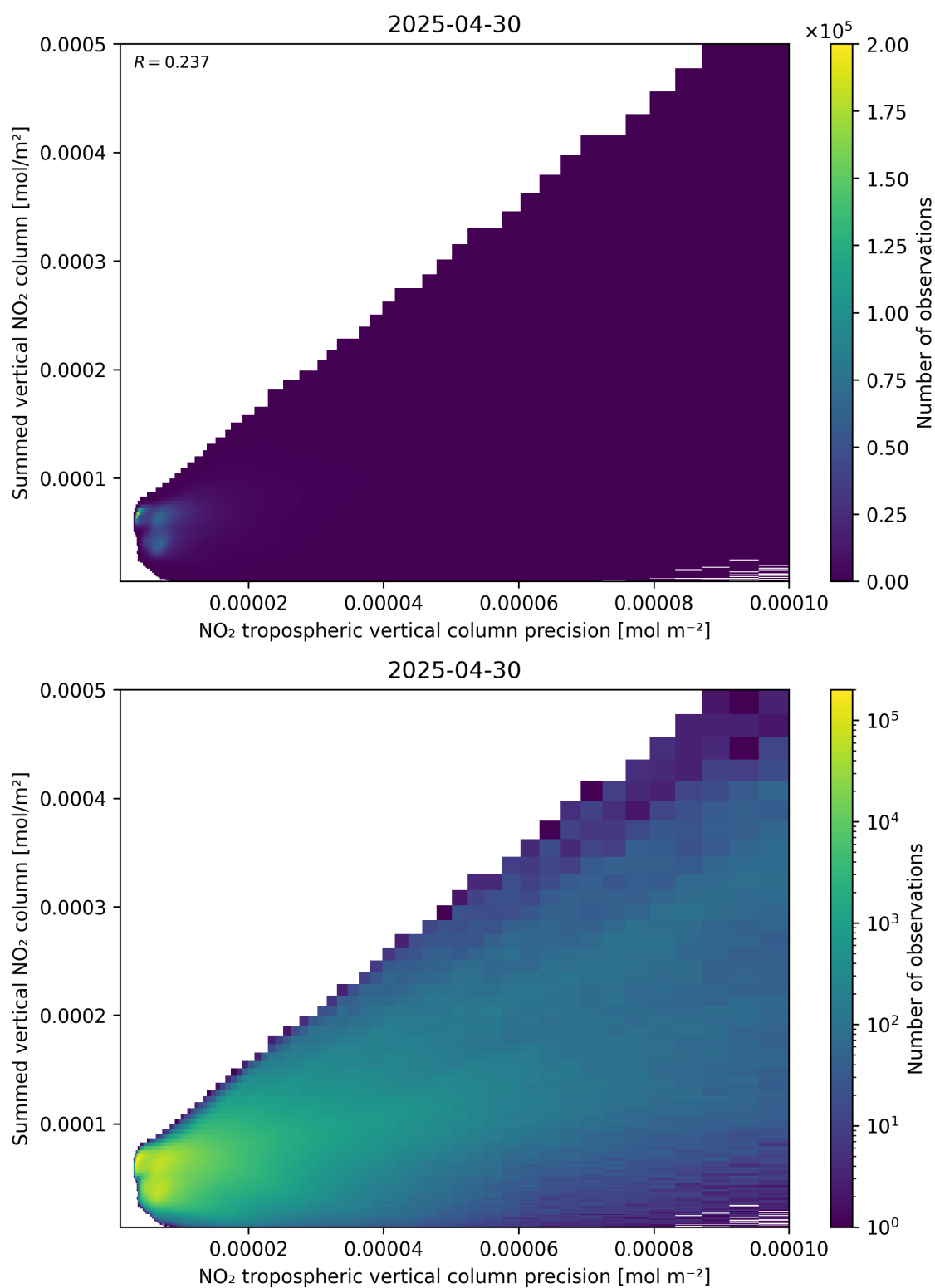
Figure 136: Scatter density plot of “NO 2 tropospheric vertical column precision” against “Summed vertical NO 2 column” for 2025-04-30 to 2025-05-01.
