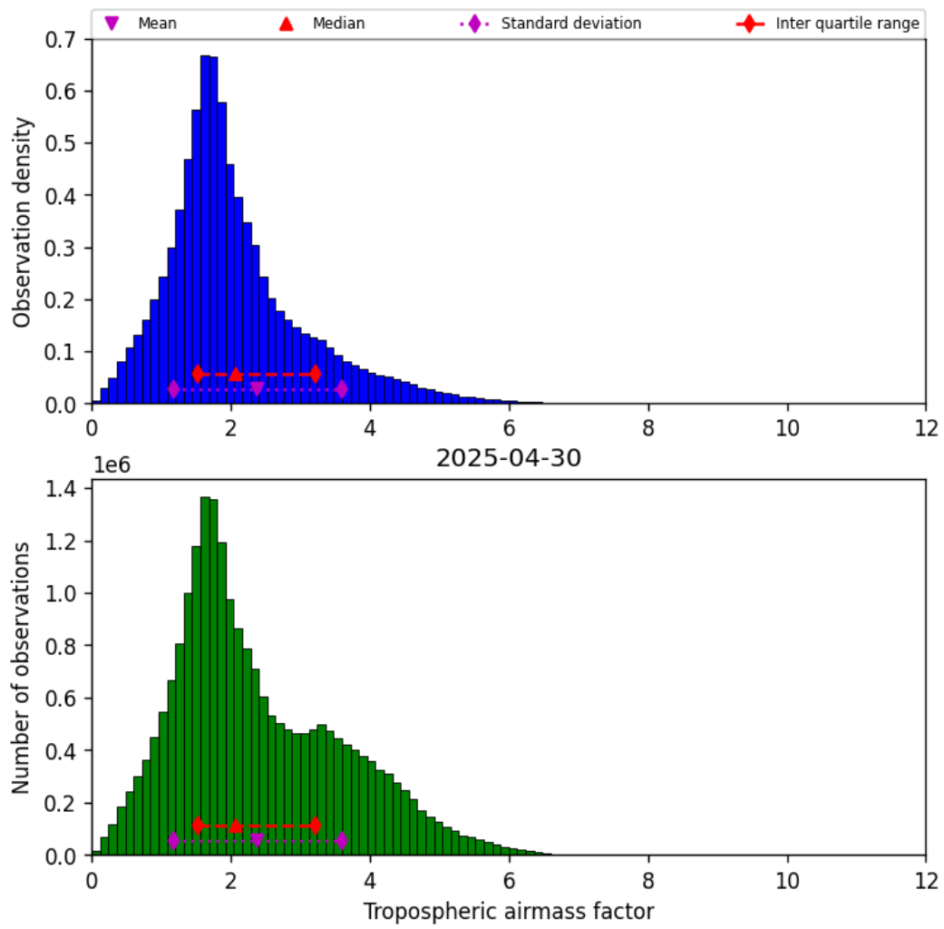
Figure 31: Histogram of “Tropospheric airmass factor” for 2025-04-30 to 2025-05-01
