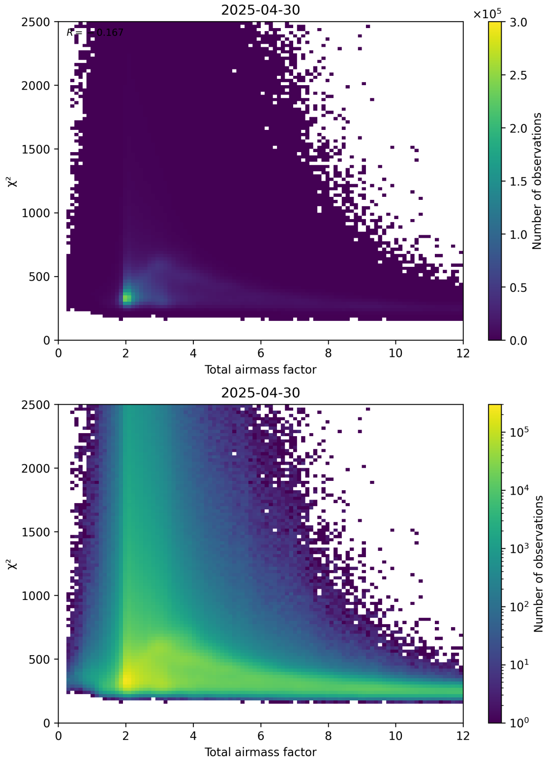
Figure 63: Scatter density plot of “Total airmass factor” against “ \chi^2 ” for 2025-04-30 to 2025-05-01.
