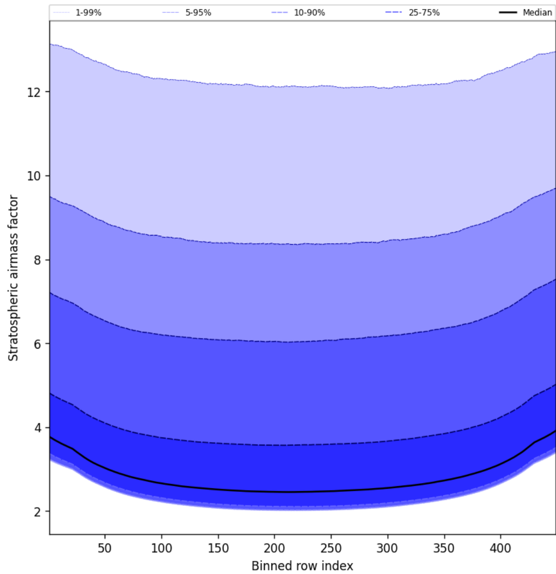
Figure 61: Along track statistics of “Stratospheric airmass factor” for 2025-04-30 to 2025-05-01
