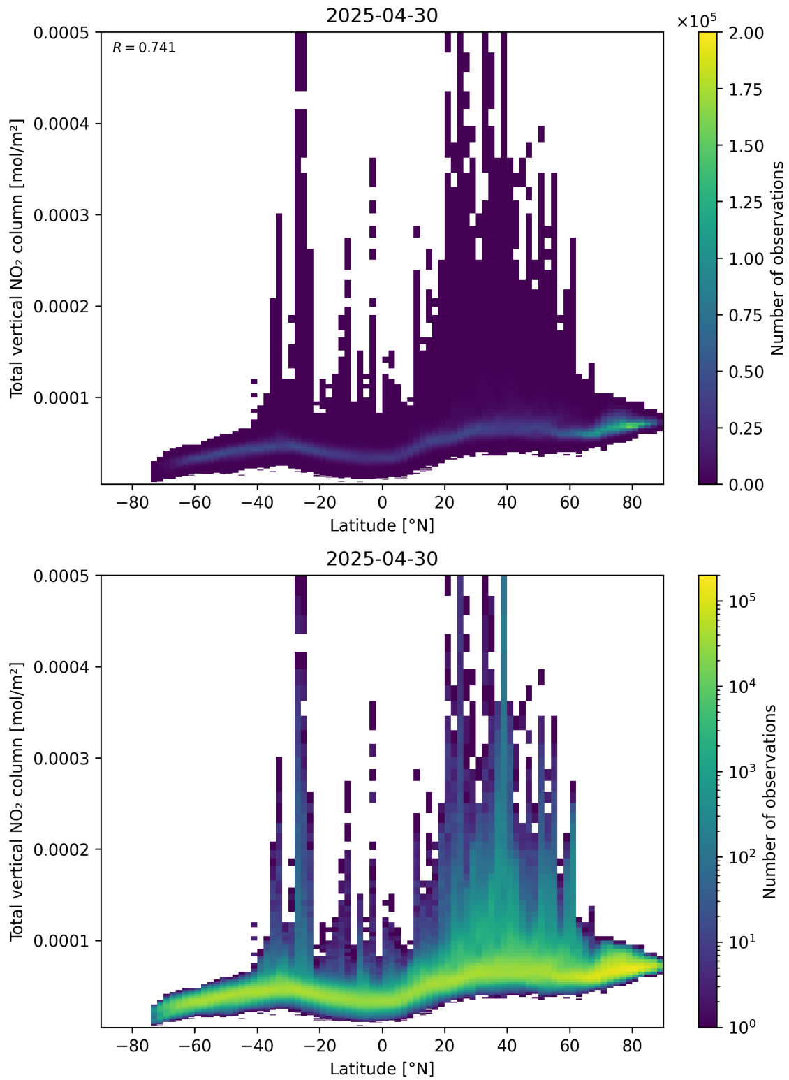
Figure 90: Scatter density plot of “Latitude” against “Total vertical NO 2 column” for 2025-04-30 to 2025-05-01.
