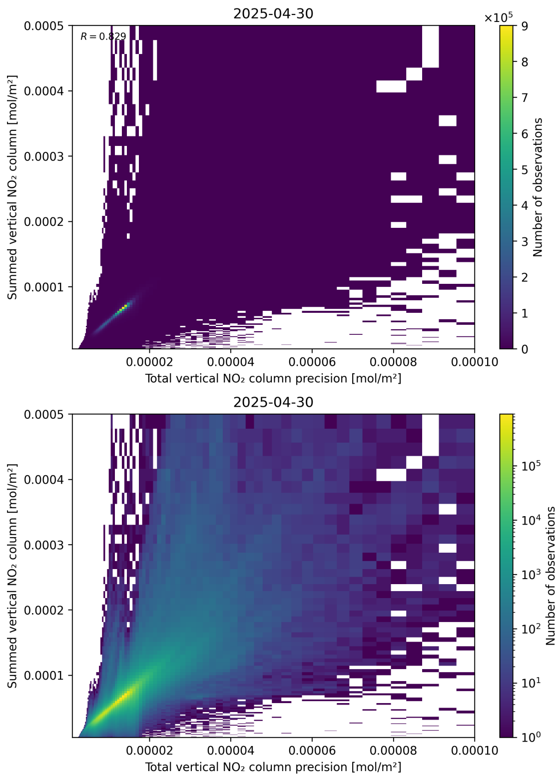
Figure 117: Scatter density plot of “Total vertical NO 2 column precision” against “Summed vertical NO 2 column” for 2025-04-30 to 2025-05-01.
