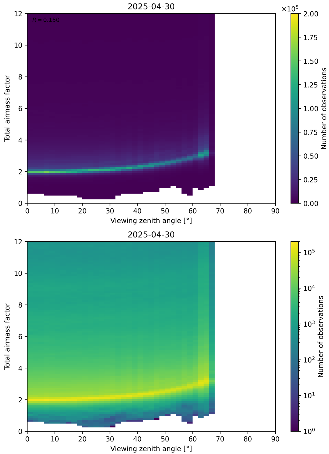
Figure 160: Scatter density plot of “Viewing zenith angle” against “Total airmass factor” for 2025-04-30 to 2025-05-01.
