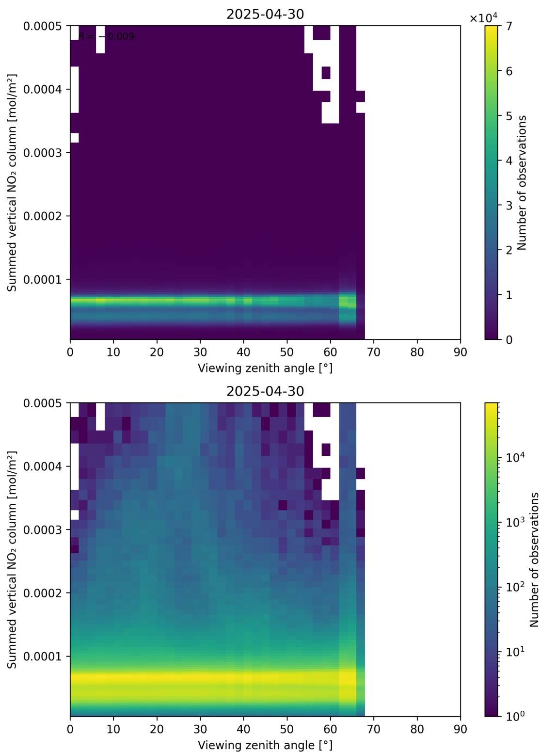
Figure 165: Scatter density plot of “Viewing zenith angle” against “Summed vertical NO 2 column” for 2025-04-30 to 2025-05-01.
