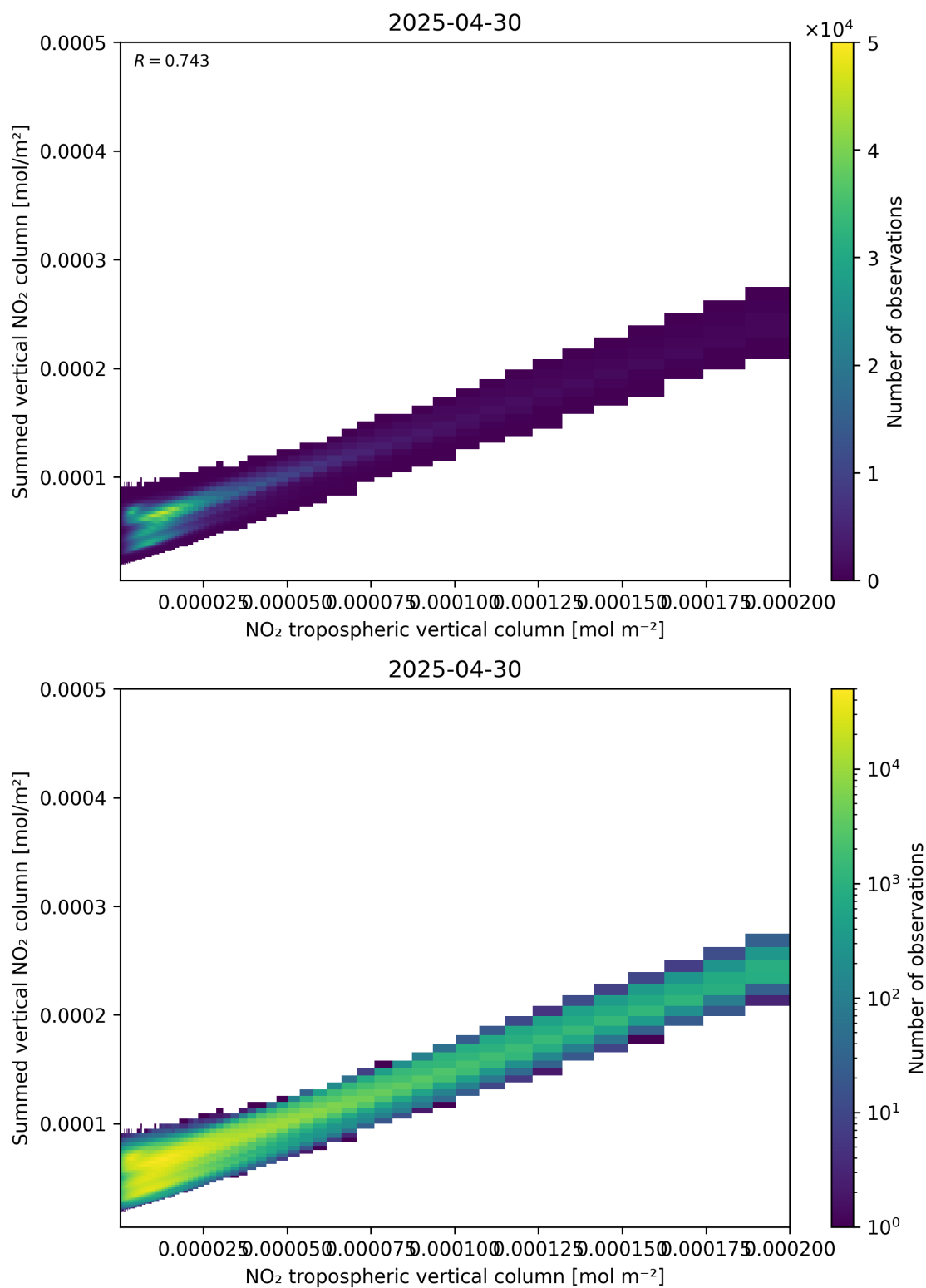
Figure 126: Scatter density plot of “NO 2 tropospheric vertical column” against “Summed vertical NO 2 column” for 2025-04-30 to 2025-05-01.
