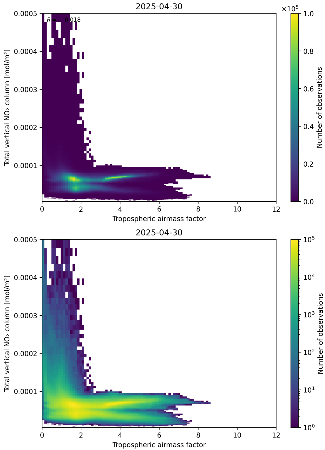
Figure 77: Scatter density plot of “Tropospheric airmass factor” against “Total vertical NO 2 column” for 2025-04-30 to 2025-05-01.
