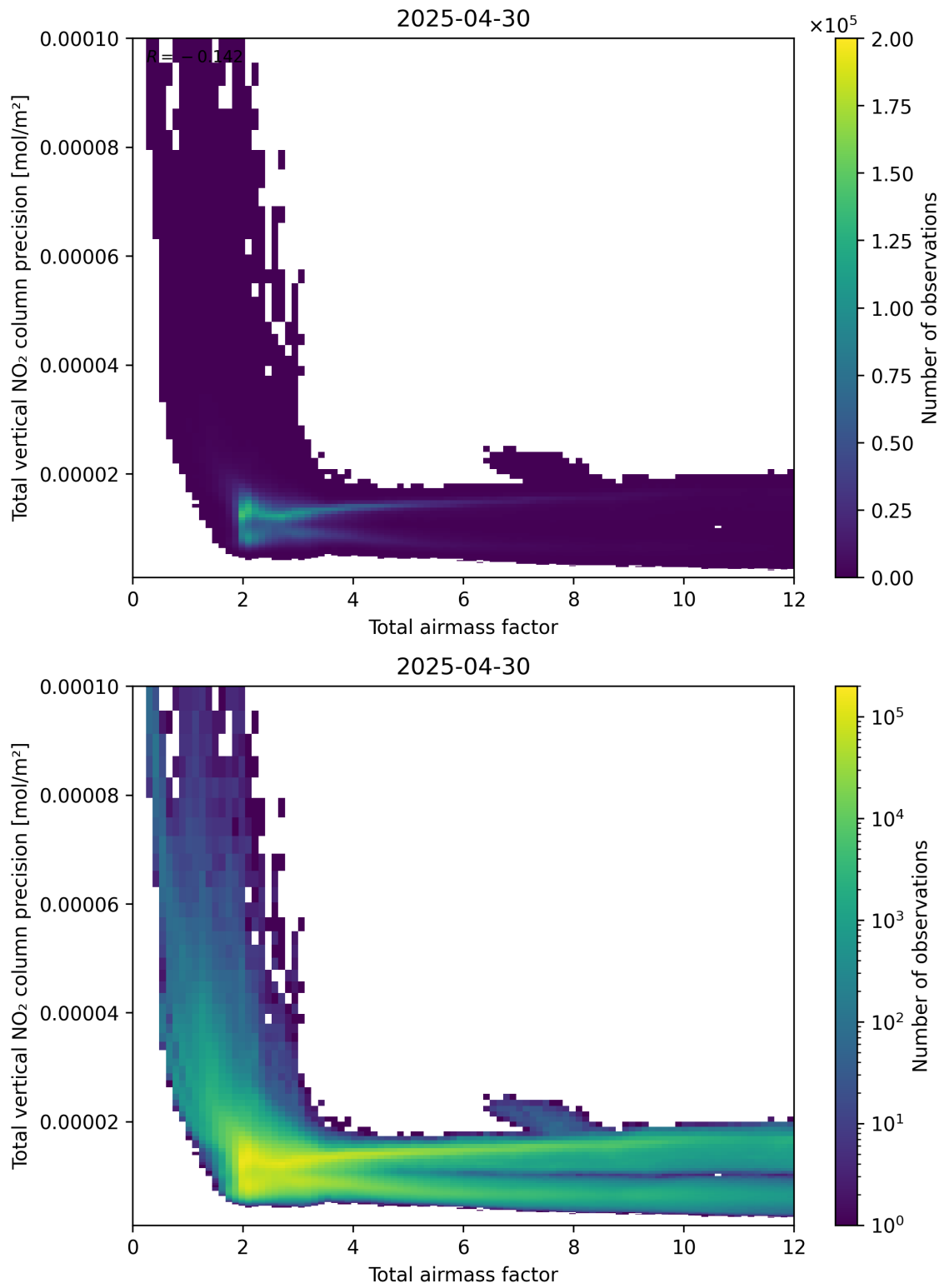
Figure 68: Scatter density plot of “Total airmass factor” against “Total vertical NO 2 column precision” for 2025-04-30 to 2025-05-01.
