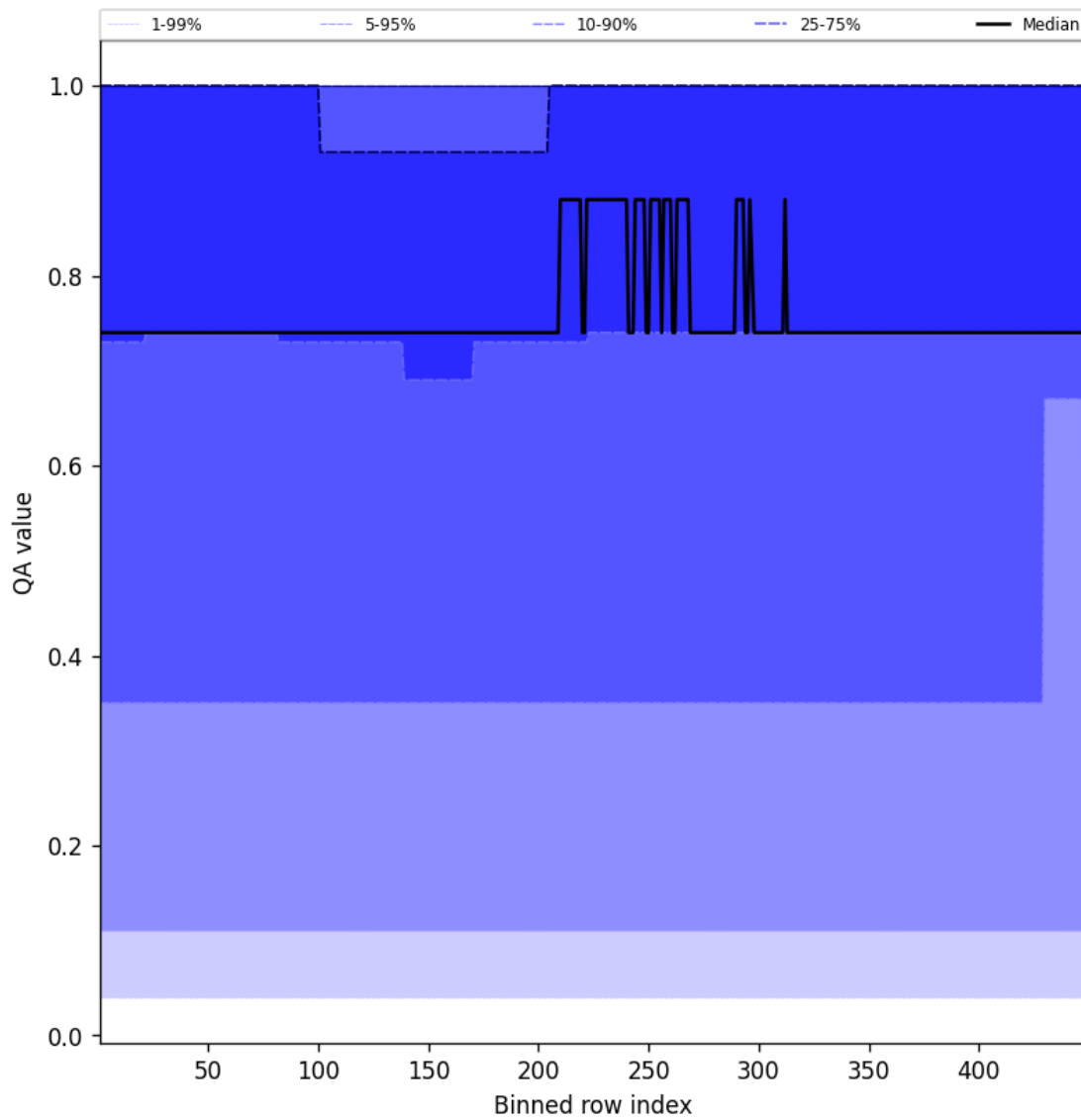
Figure 45: Along track statistics of “QA value” for 2025-04-30 to 2025-05-01
