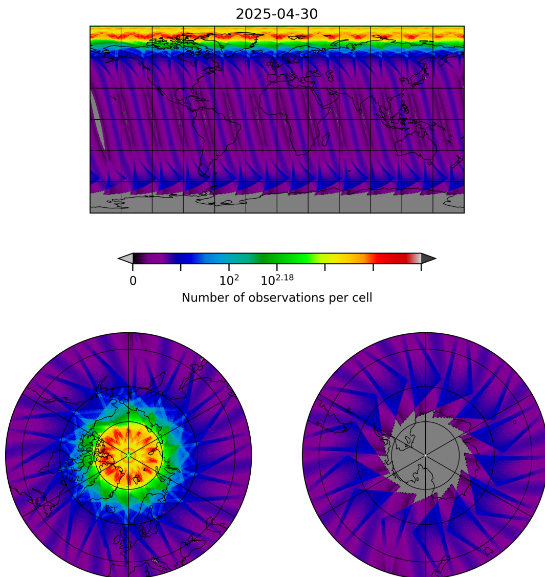
Figure 10: Map of the number of observations for 2025-04-30 to 2025-05-01
