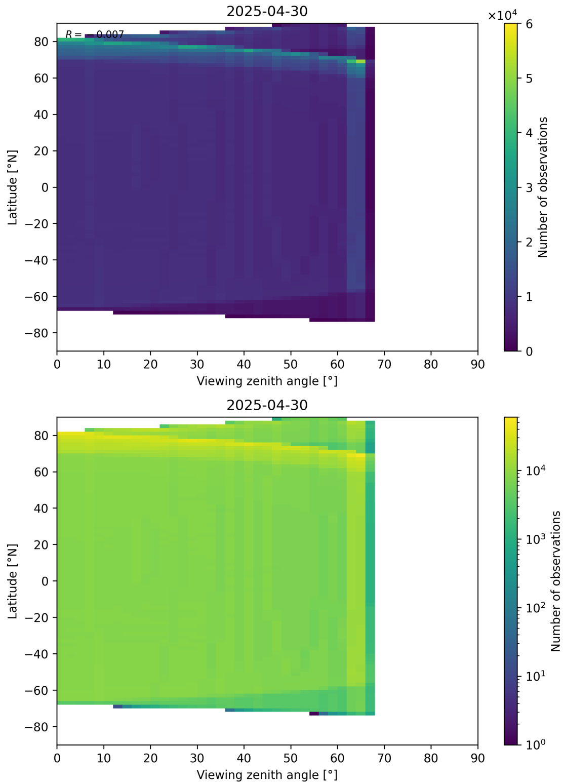
Figure 163: Scatter density plot of “Viewing zenith angle” against “Latitude” for 2025-04-30 to 2025-05-01.
