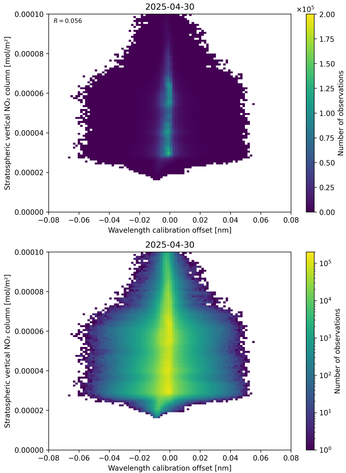
Figure 176: Scatter density plot of “Wavelength calibration offset” against “Stratospheric vertical NO 2 column” for 2025-04-30 to 2025-05-01.
