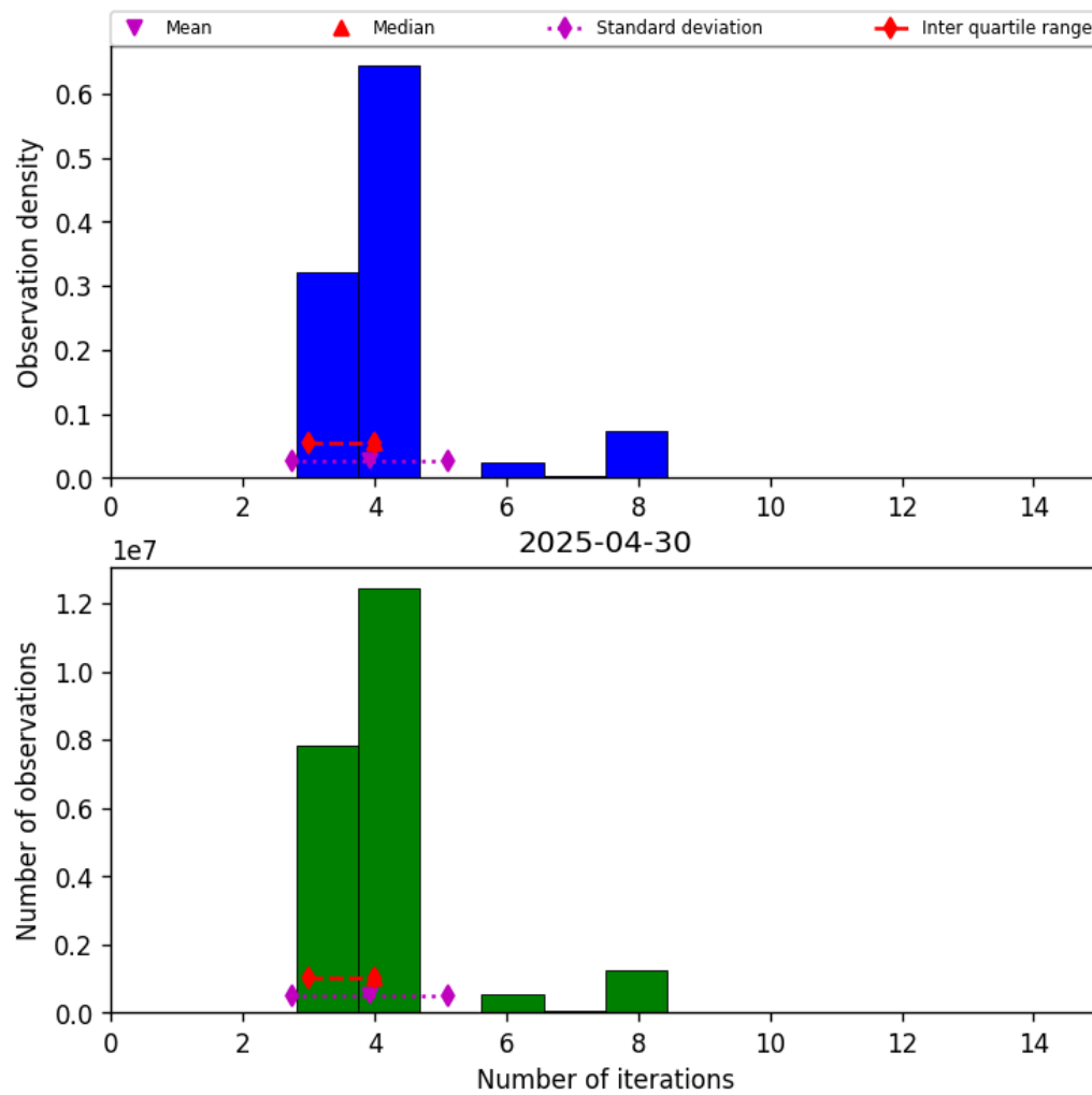
Figure 34: Histogram of “Number of iterations” for 2025-04-30 to 2025-05-01
