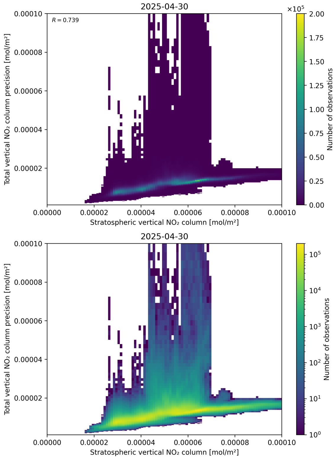
Figure 101: Scatter density plot of “Stratospheric vertical NO 2 column” against “Total vertical NO 2 column precision” for 2025-04-30 to 2025-05-01.
