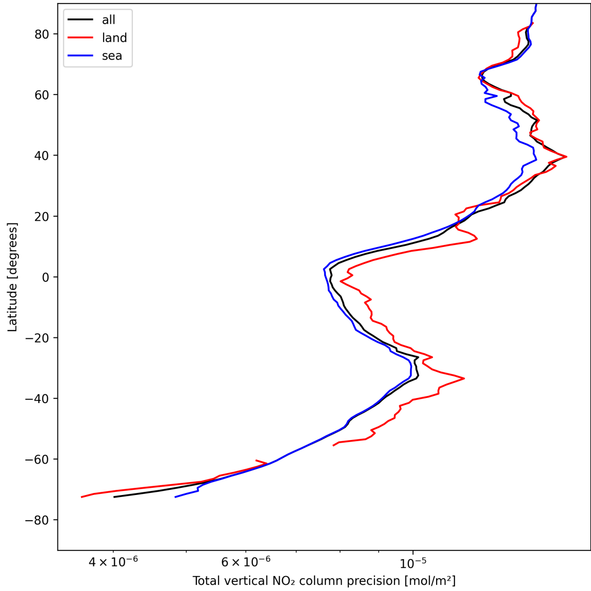
Figure 22: Zonal average of “Total vertical NO 2 column precision” for 2025-04-30 to 2025-05-01.
