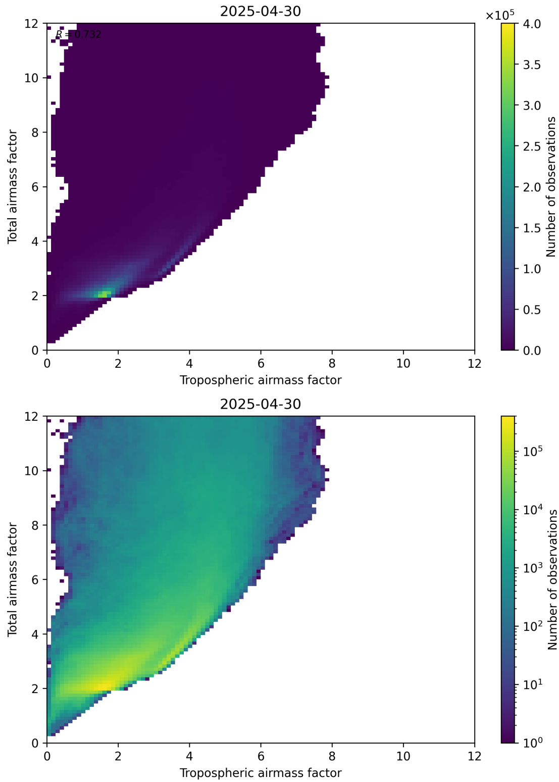
Figure 72: Scatter density plot of “Tropospheric airmass factor” against “Total airmass factor” for 2025-04-30 to 2025-05-01.
