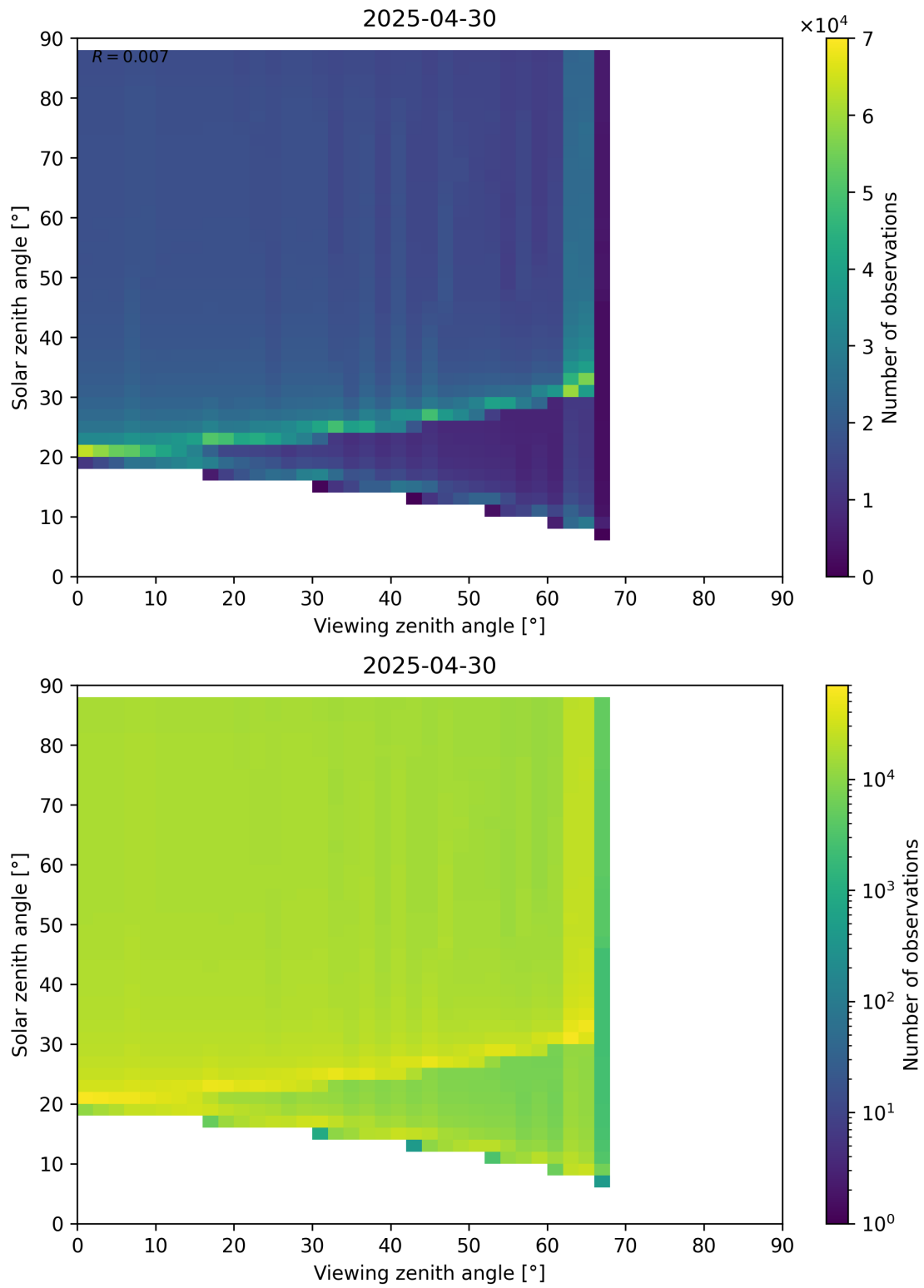
Figure 172: Scatter density plot of “Viewing zenith angle” against “Solar zenith angle” for 2025-04-30 to 2025-05-01.
