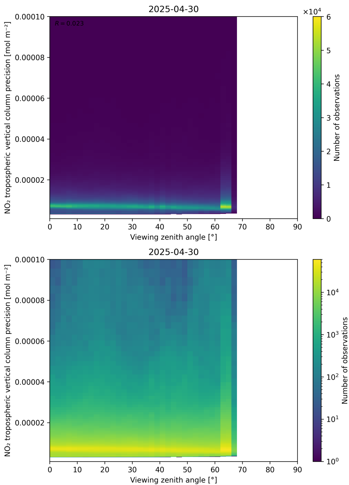
Figure 170: Scatter density plot of “Viewing zenith angle” against “NO 2 tropospheric vertical column precision” for 2025-04-30 to 2025-05-01.
