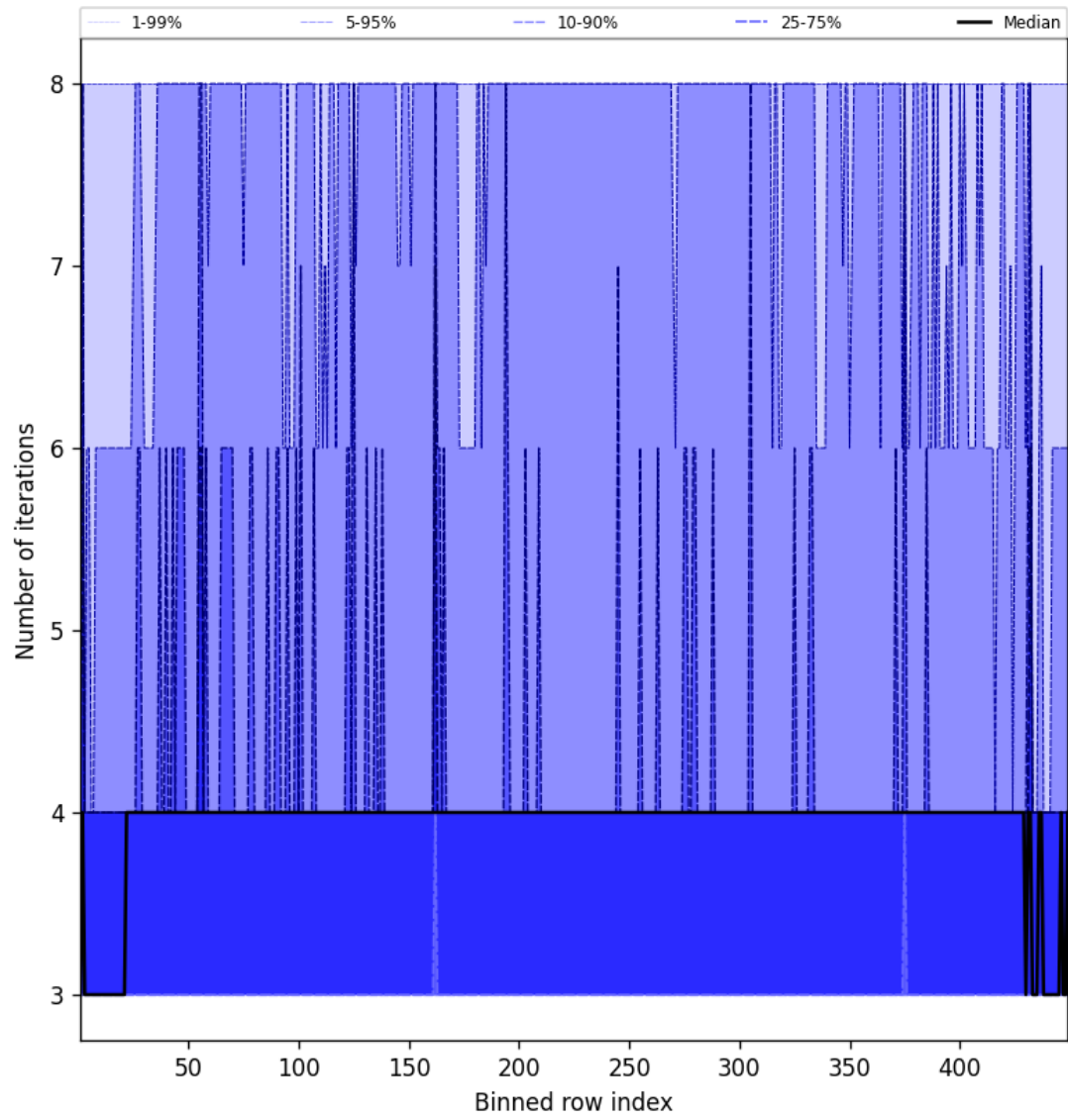
Figure 51: Along track statistics of “Number of iterations” for 2025-04-30 to 2025-05-01
