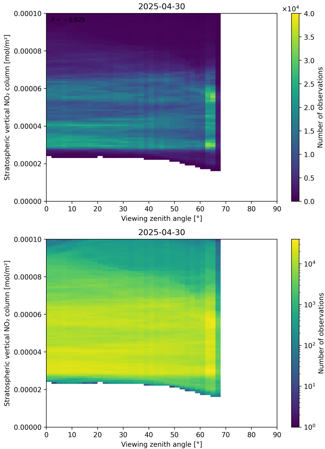
Figure 164: Scatter density plot of “Viewing zenith angle” against “Stratospheric vertical NO 2 column” for 2025-04-30 to 2025-05-01.
