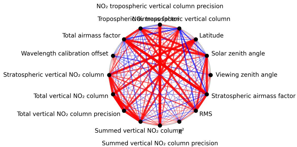
Figure 1: Map of correlation graph for 2025-04-30 to 2025-05-01.
