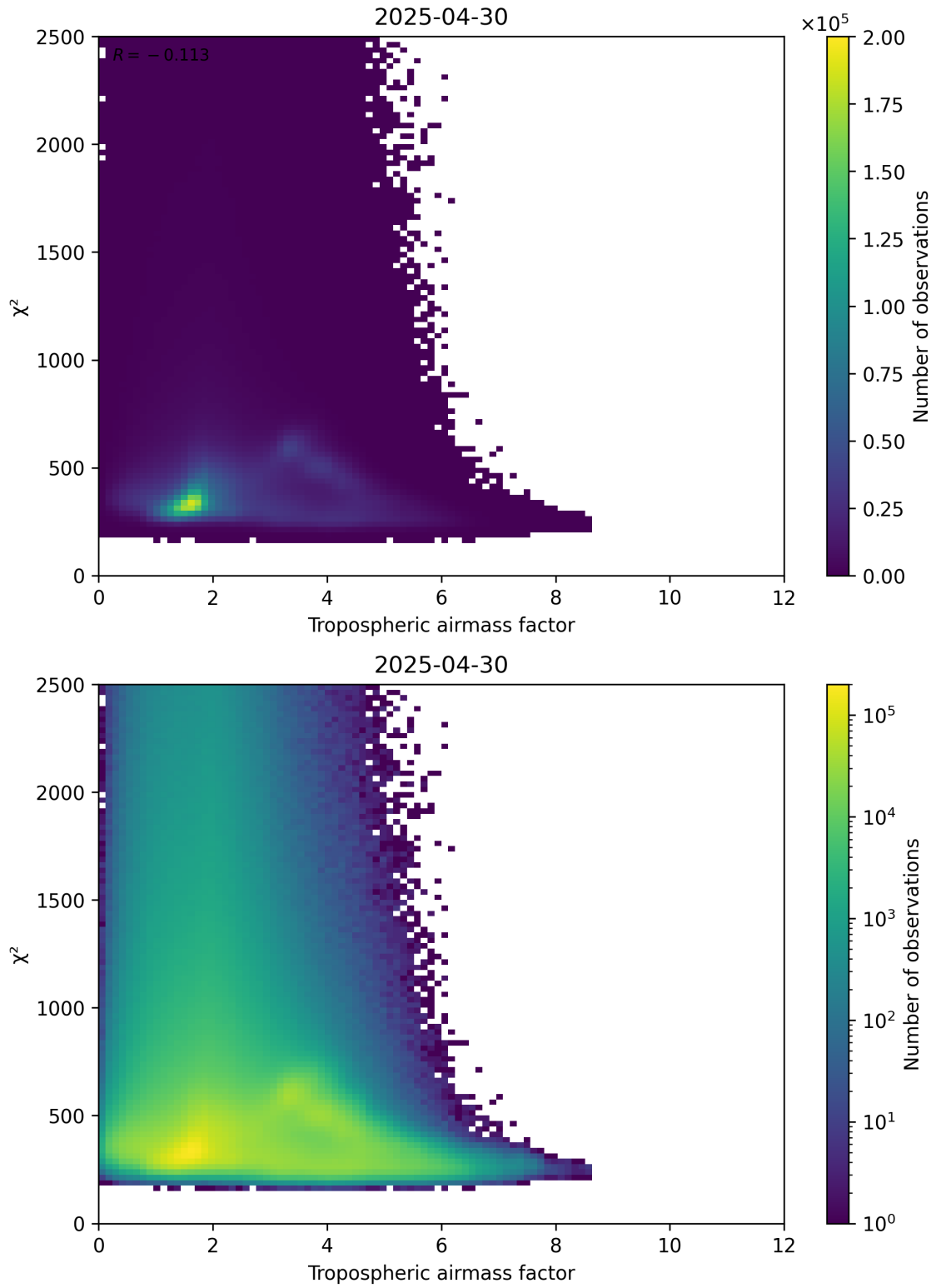
Figure 73: Scatter density plot of “Tropospheric airmass factor” against “ \chi^2 ” for 2025-04-30 to 2025-05-01.
