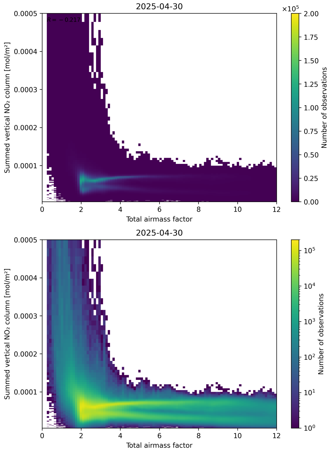
Figure 65: Scatter density plot of “Total airmass factor” against “Summed vertical NO 2 column” for 2025-04-30 to 2025-05-01.
