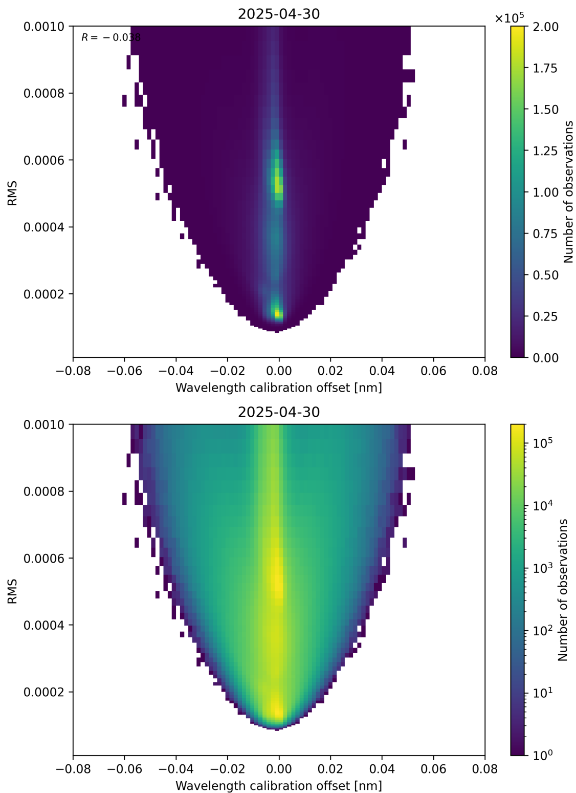
Figure 181: Scatter density plot of “Wavelength calibration offset” against “RMS” for 2025-04-30 to 2025-05-01.
