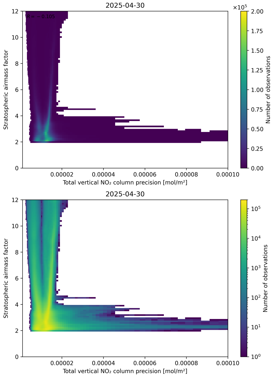
Figure 115: Scatter density plot of “Total vertical NO 2 column precision” against “Stratospheric air mass factor” for 2025-04-30 to 2025-05-01.
