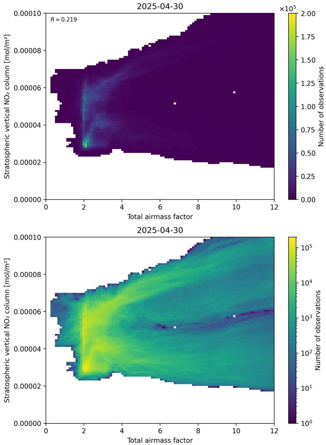
Figure 64: Scatter density plot of “Total airmass factor” against “Stratospheric vertical \text{NO}_2 column” for 2025-04-30 to 2025-05-01.
