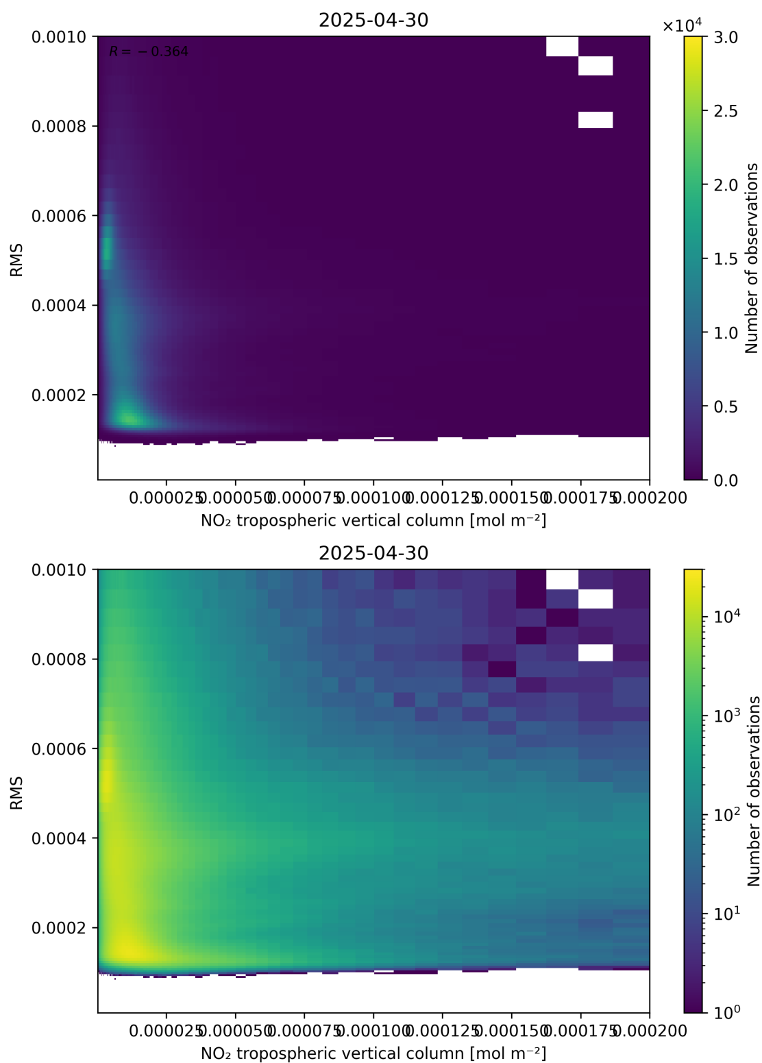
Figure 142: Scatter density plot of “NO 2 tropospheric vertical column” against “RMS” for 2025-04-30 to 2025-05-01.
