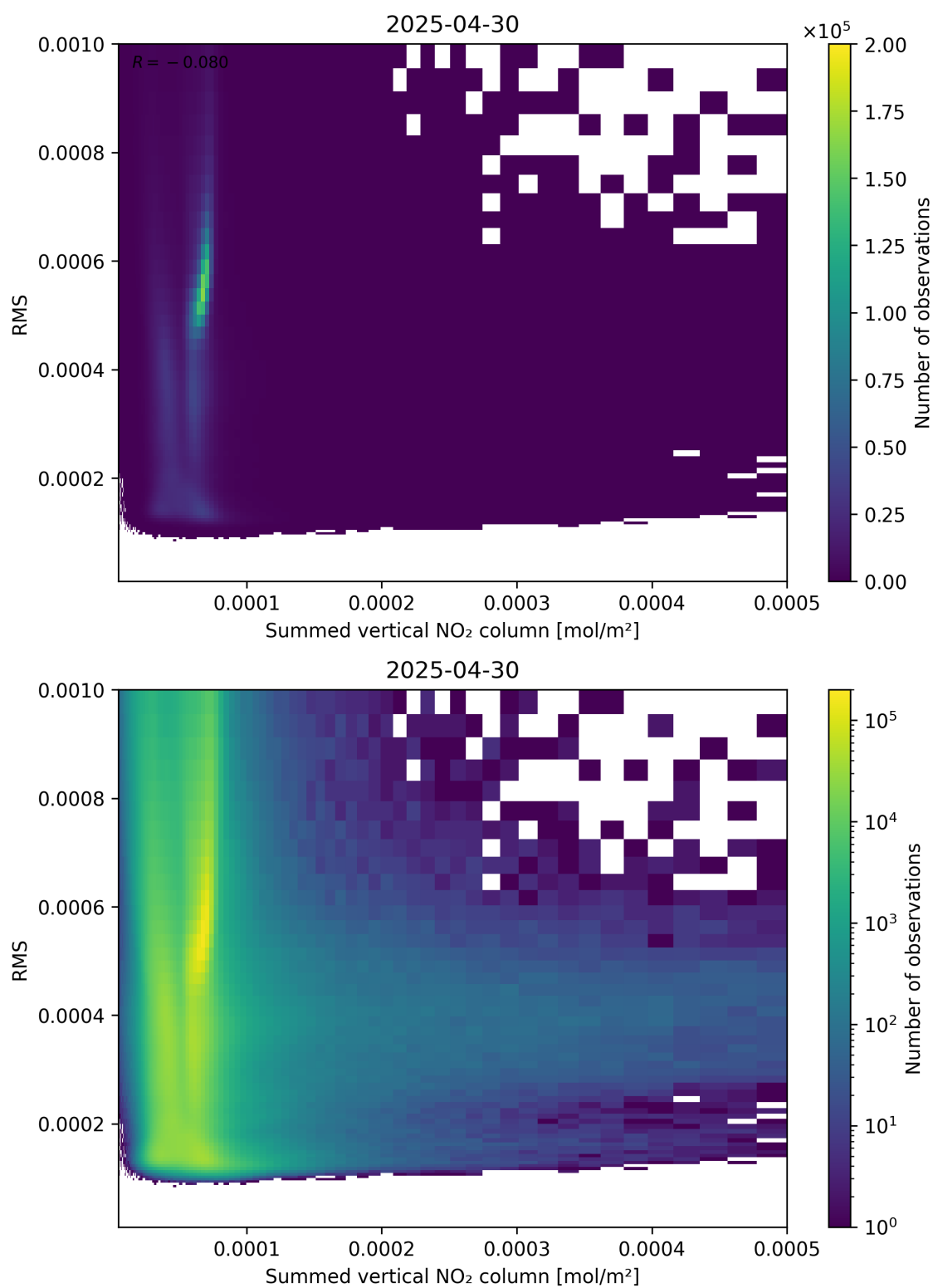
Figure 109: Scatter density plot of “Summed vertical NO 2 column” against “RMS” for 2025-04-30 to 2025-05-01.
