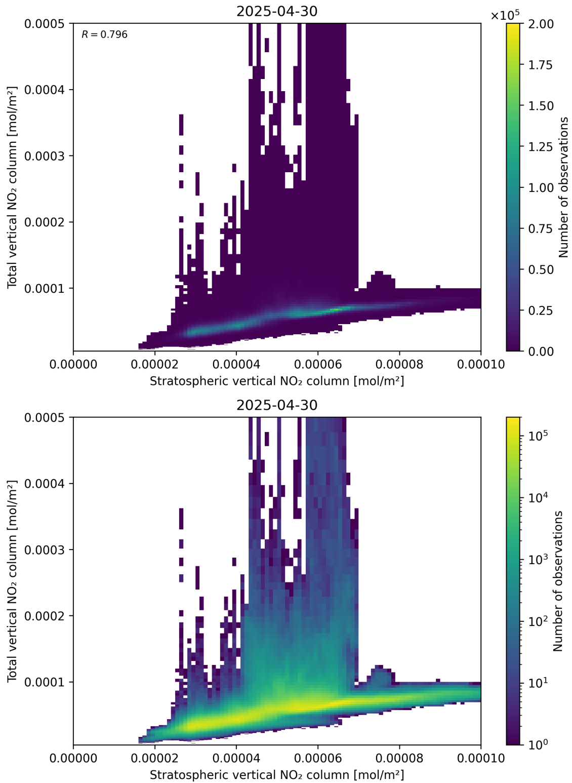
Figure 100: Scatter density plot of “Stratospheric vertical NO 2 column” against “Total vertical NO 2 column” for 2025-04-30 to 2025-05-01.
