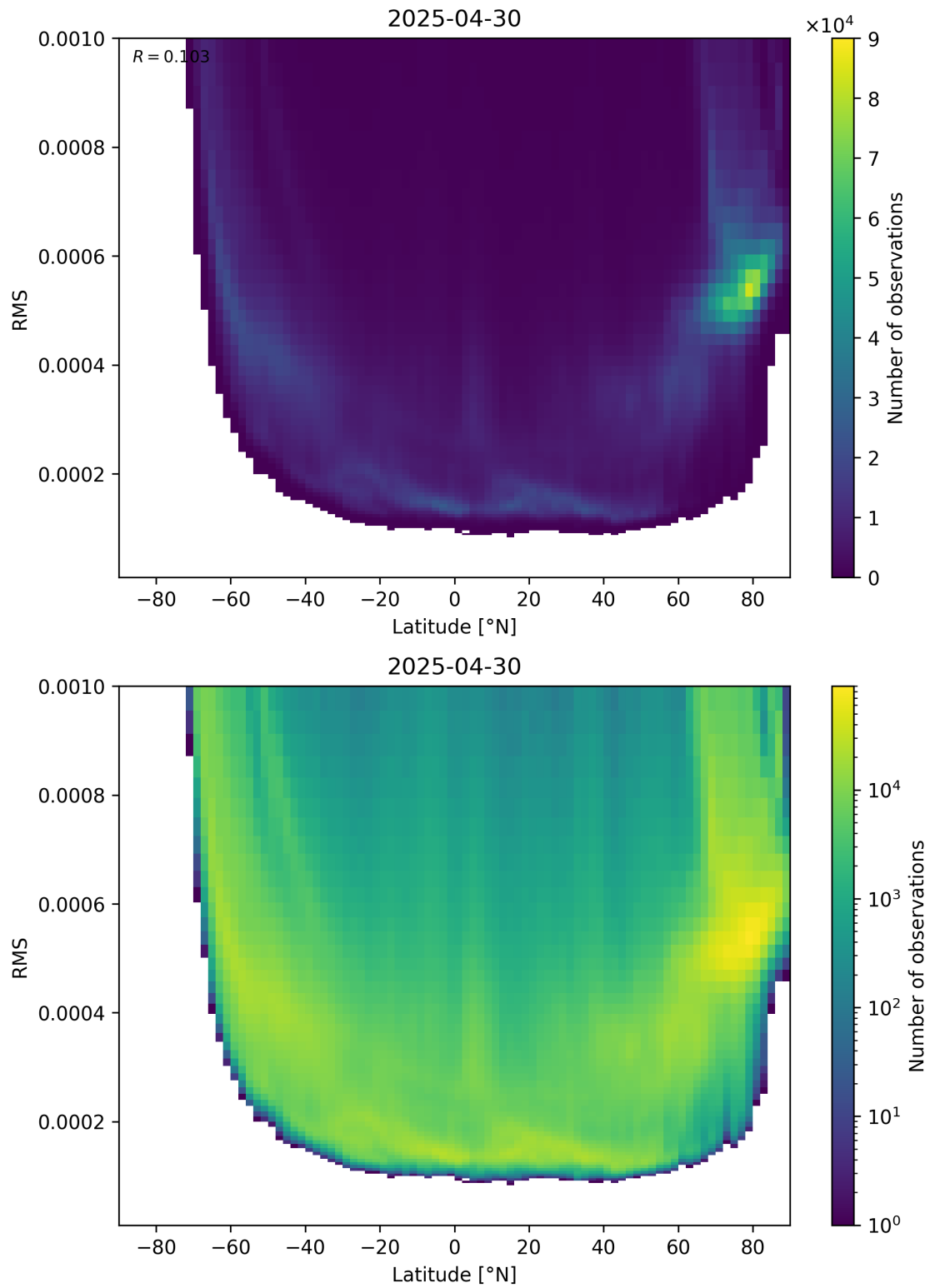
Figure 94: Scatter density plot of “Latitude” against “RMS” for 2025-04-30 to 2025-05-01.
