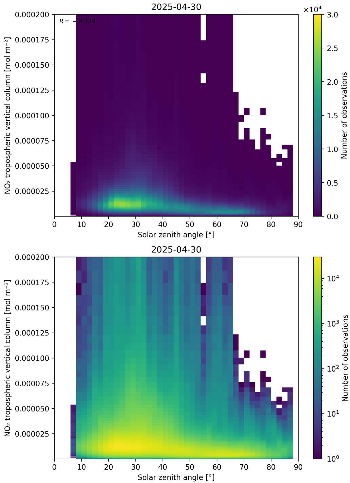
Figure 155: Scatter density plot of “Solar zenith angle” against “NO 2 tropospheric vertical column” for 2025-04-30 to 2025-05-01.
