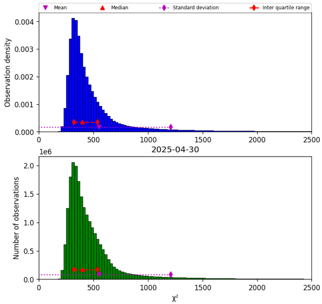
Figure 42: Histogram of “ \chi^2 ” for 2025-04-30 to 2025-05-01
