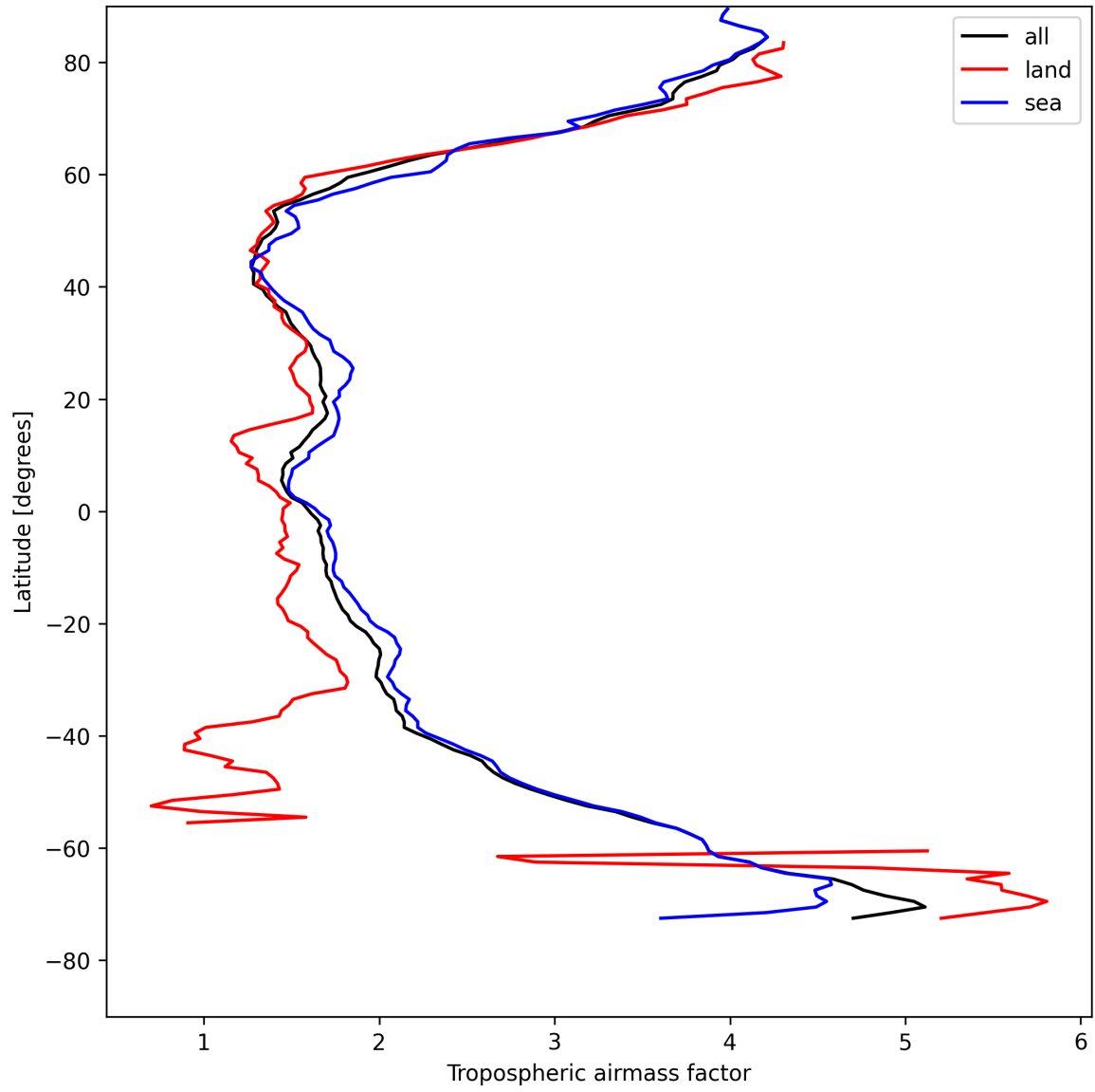
Figure 14: Zonal average of “Tropospheric air mass factor” for 2025-04-30 to 2025-05-01.
