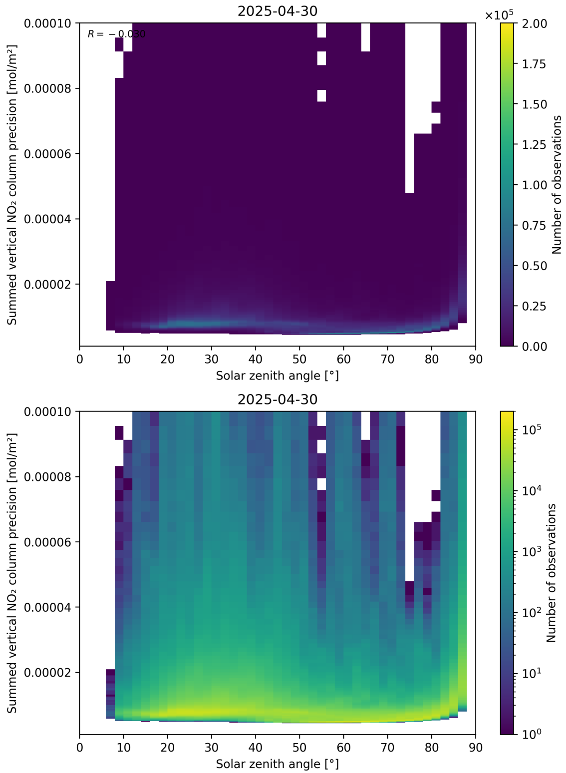
Figure 152: Scatter density plot of “Solar zenith angle” against “Summed vertical NO 2 column precision” for 2025-04-30 to 2025-05-01.
