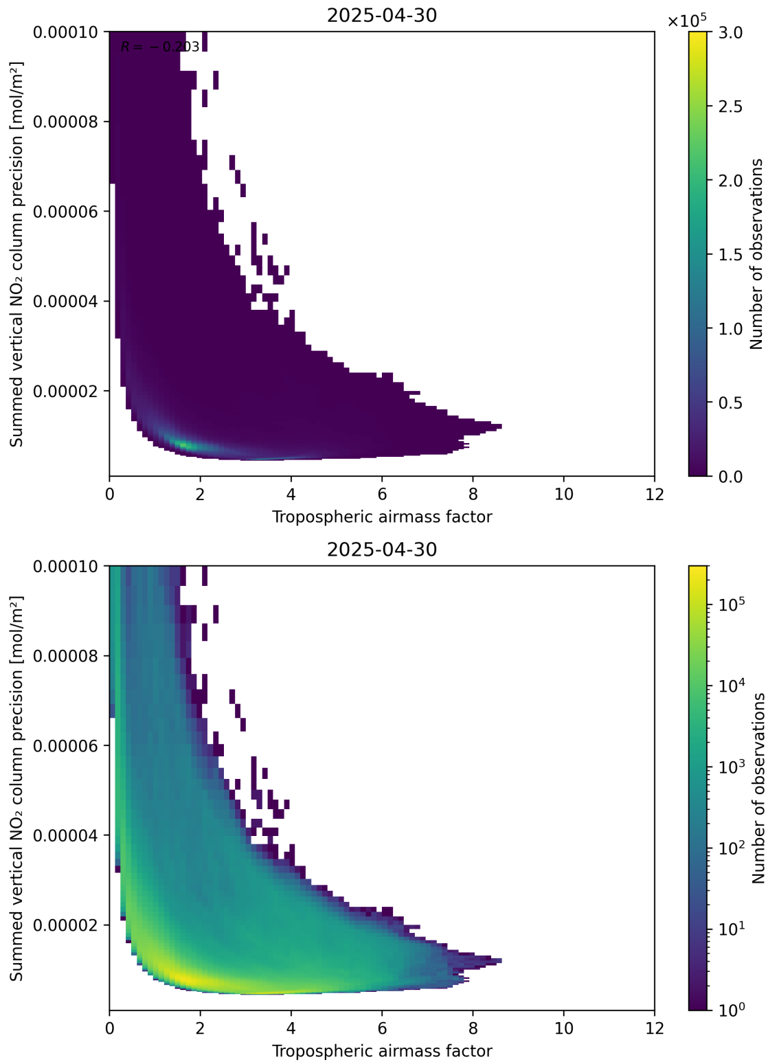
Figure 76: Scatter density plot of “Tropospheric air mass factor” against “Summed vertical NO 2 column precision” for 2025-04-30 to 2025-05-01.
