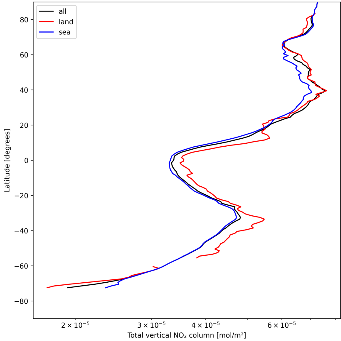
Figure 21: Zonal average of “Total vertical NO 2 column” for 2025-04-30 to 2025-05-01.
