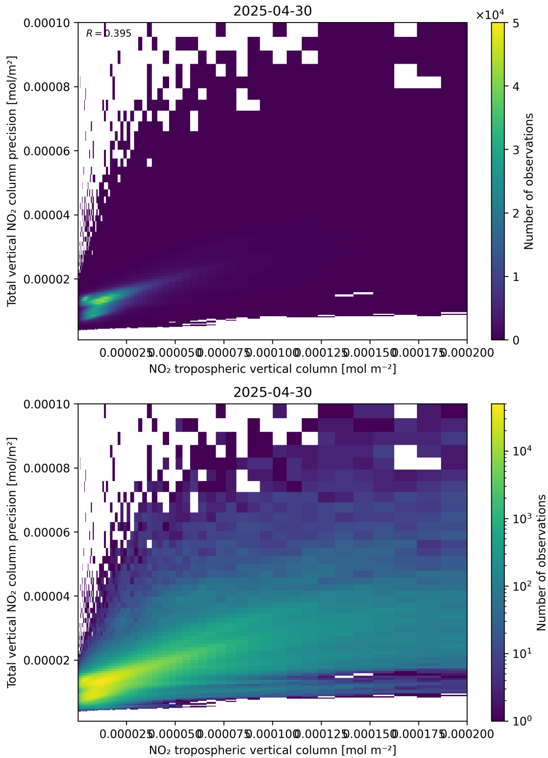
Figure 129: Scatter density plot of “NO 2 tropospheric vertical column” against “Total vertical NO 2 column precision” for 2025-04-30 to 2025-05-01.
