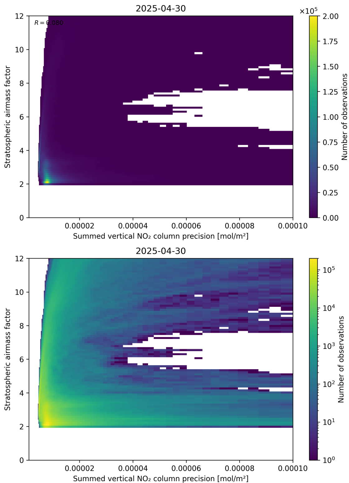
Figure 106: Scatter density plot of “Summed vertical NO 2 column precision” against “Stratospheric airmass factor” for 2025-04-30 to 2025-05-01.
