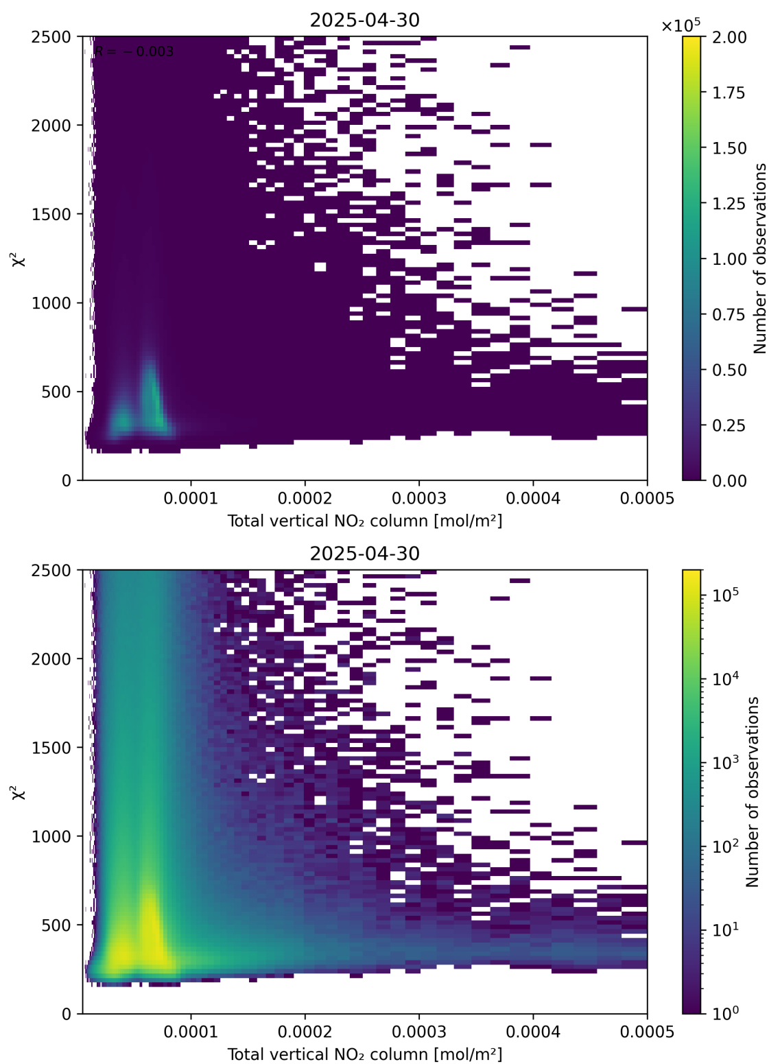
Figure 111: Scatter density plot of “Total vertical NO 2 column” against “ \chi^2 ” for 2025-04-30 to 2025-05-01.
