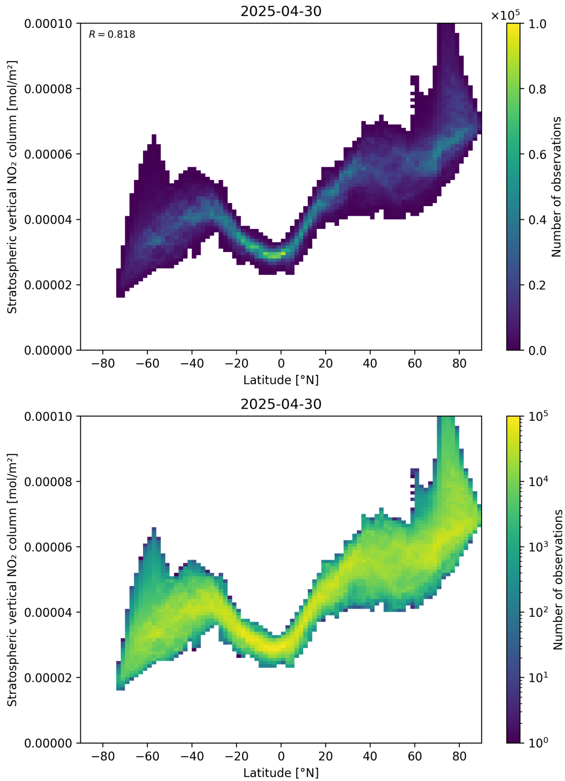
Figure 87: Scatter density plot of “Latitude” against “Stratospheric vertical \text{NO}_2 column” for 2025-04-30 to 2025-05-01.
