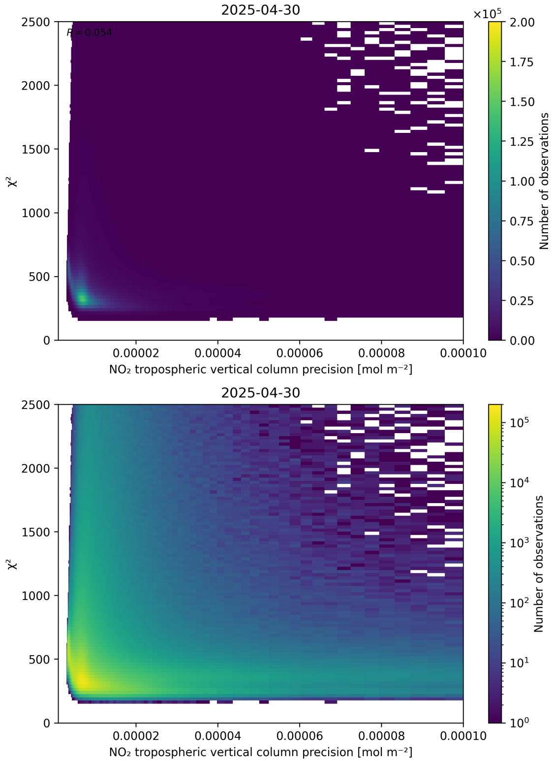
Figure 134: Scatter density plot of “NO 2 tropospheric vertical column precision” against “ \chi^2 ” for 2025-04-30 to 2025-05-01.
