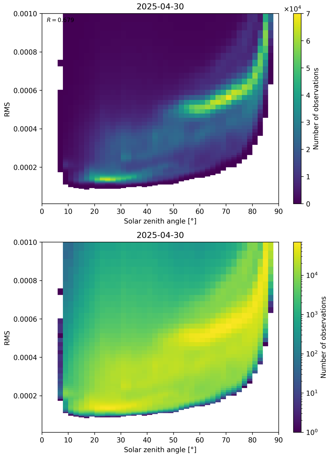
Figure 157: Scatter density plot of “Solar zenith angle” against “RMS” for 2025-04-30 to 2025-05-01.
