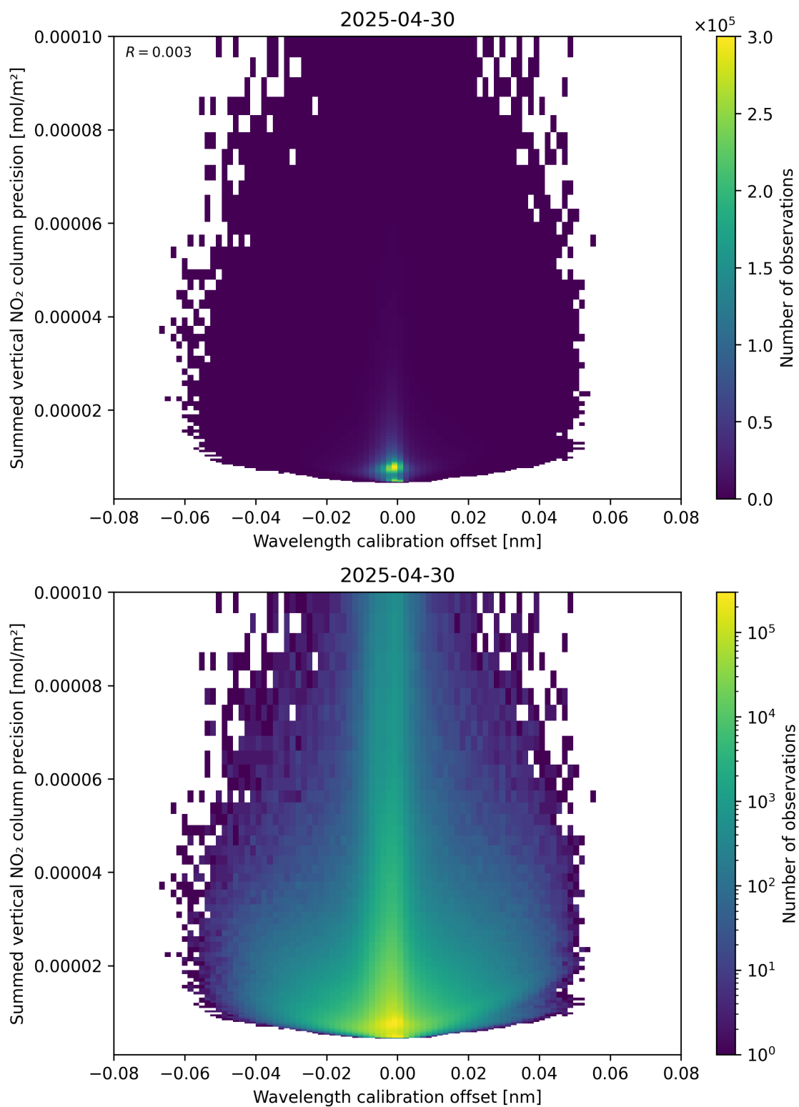
Figure 178: Scatter density plot of “Wavelength calibration offset” against “Summed vertical NO 2 column precision” for 2025-04-30 to 2025-05-01.
