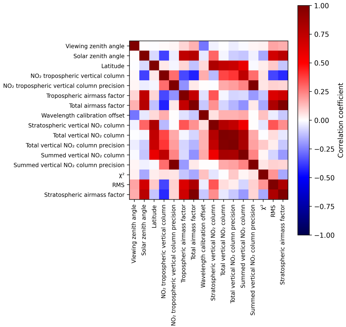
Figure 2: Map of correlation matrix for 2025-04-30 to 2025-05-01.
