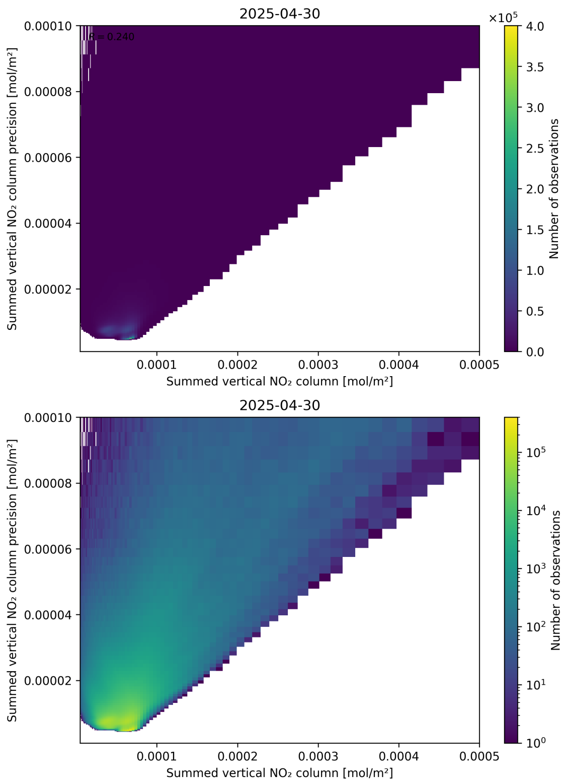
Figure 105: Scatter density plot of “Summed vertical NO 2 column” against “Summed vertical NO 2 column precision” for 2025-04-30 to 2025-05-01.
