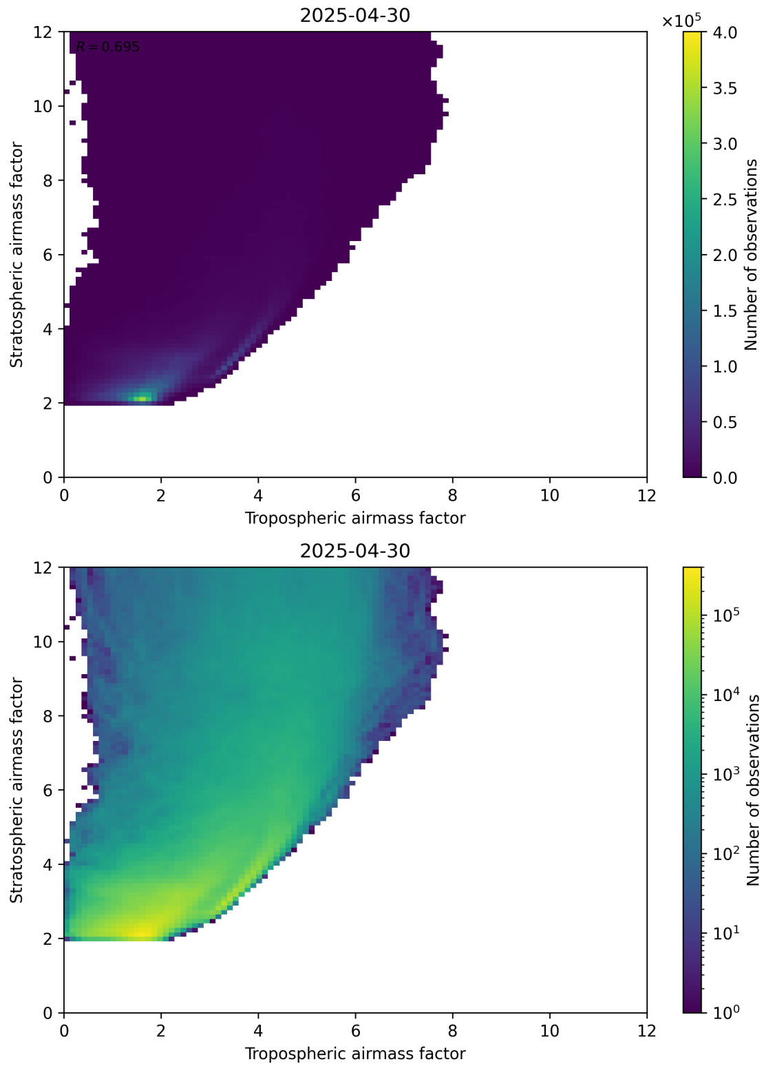
Figure 71: Scatter density plot of “Tropospheric airmass factor” against “Stratospheric airmass factor” for 2025-04-30 to 2025-05-01.
