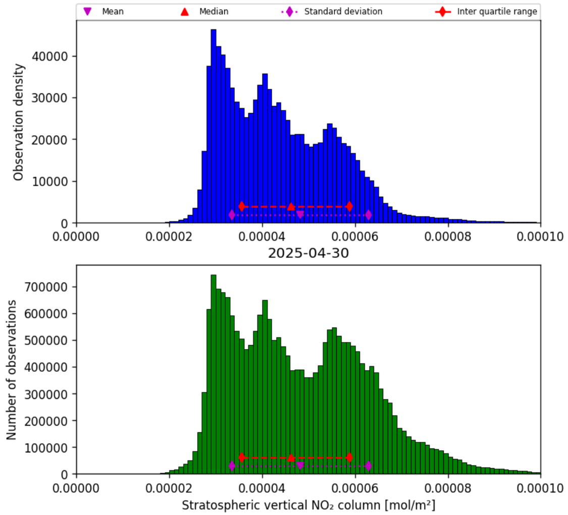
Figure 36: Histogram of “Stratospheric vertical NO 2 column” for 2025-04-30 to 2025-05-01
