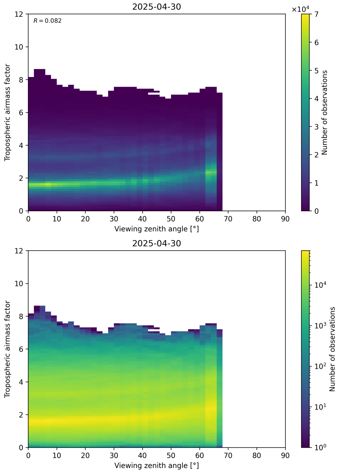
Figure 161: Scatter density plot of “Viewing zenith angle” against “Tropospheric airmass factor” for 2025-04-30 to 2025-05-01.
