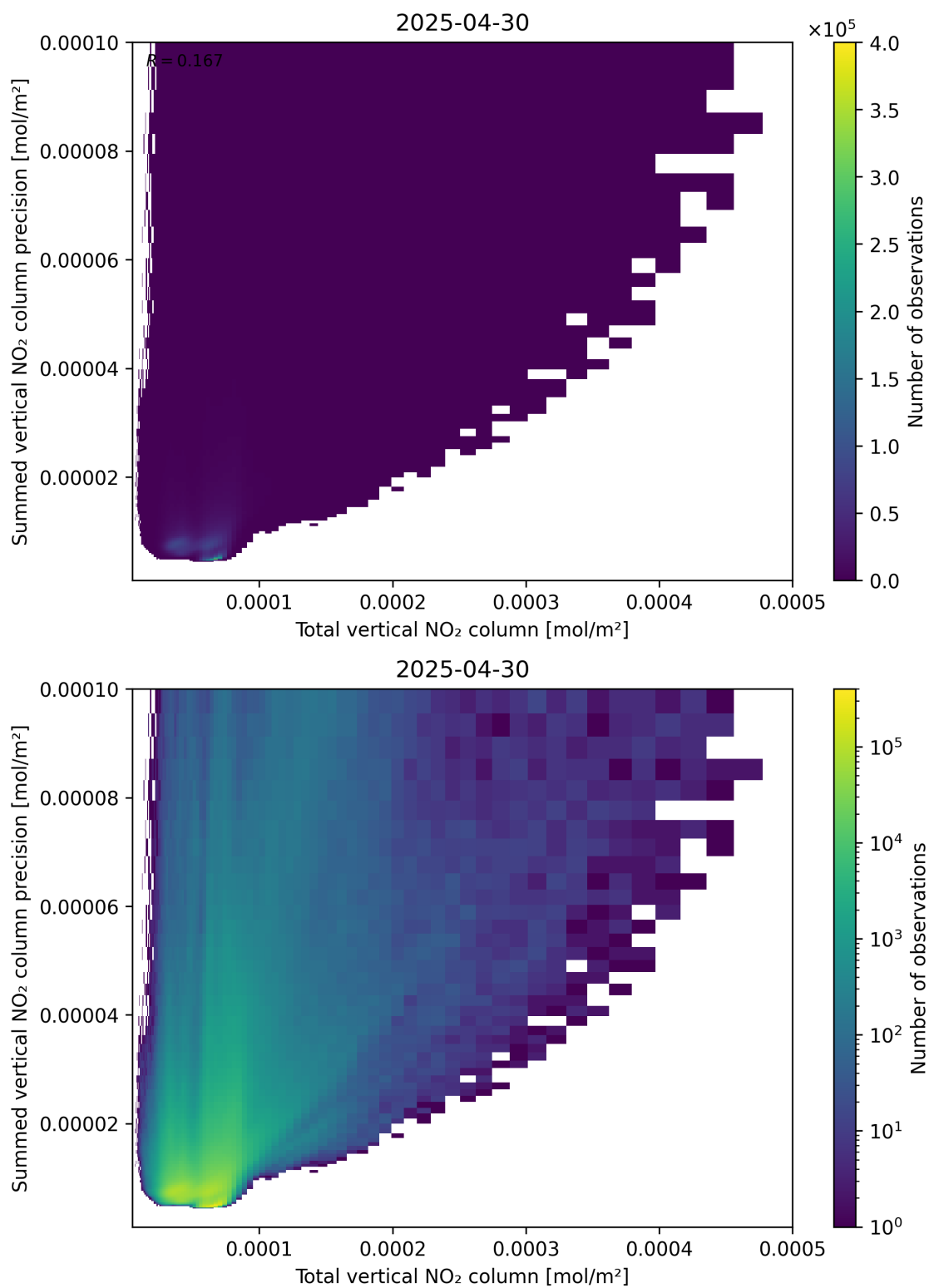
Figure 113: Scatter density plot of “Total vertical NO 2 column” against “Summed vertical NO 2 column precision” for 2025-04-30 to 2025-05-01.
