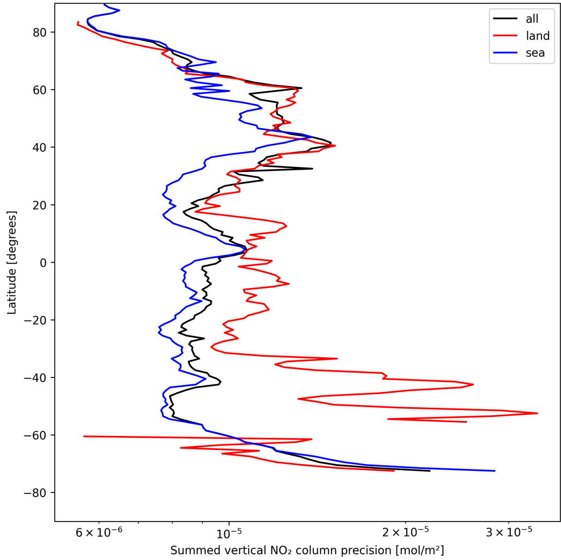
Figure 24: Zonal average of “Summed vertical NO 2 column precision” for 2025-04-30 to 2025-05-01.
