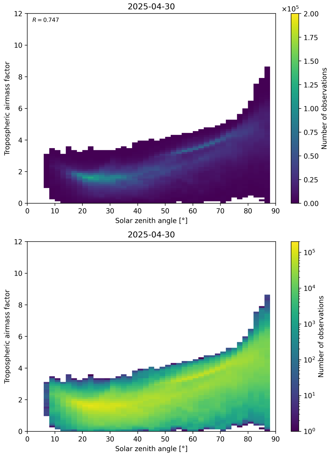
Figure 147: Scatter density plot of “Solar zenith angle” against “Tropospheric airmass factor” for 2025-04-30 to 2025-05-01.
