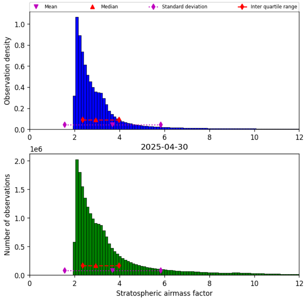
Figure 44: Histogram of “Stratospheric airmass factor” for 2025-04-30 to 2025-05-01
