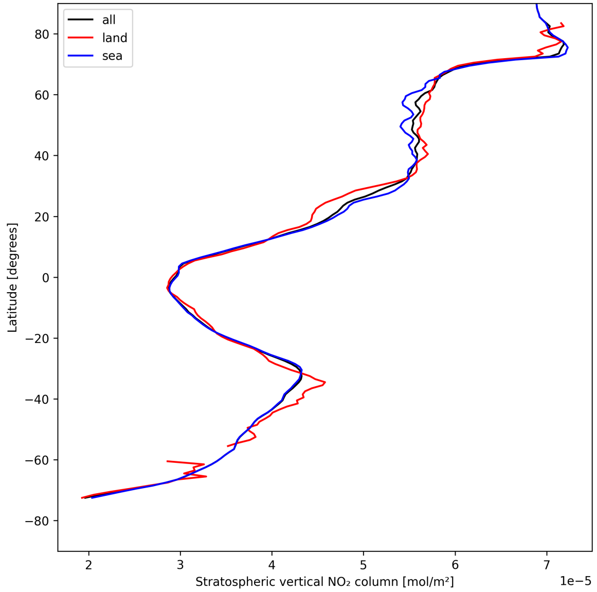
Figure 19: Zonal average of “Stratospheric vertical NO 2 column” for 2025-04-30 to 2025-05-01.
