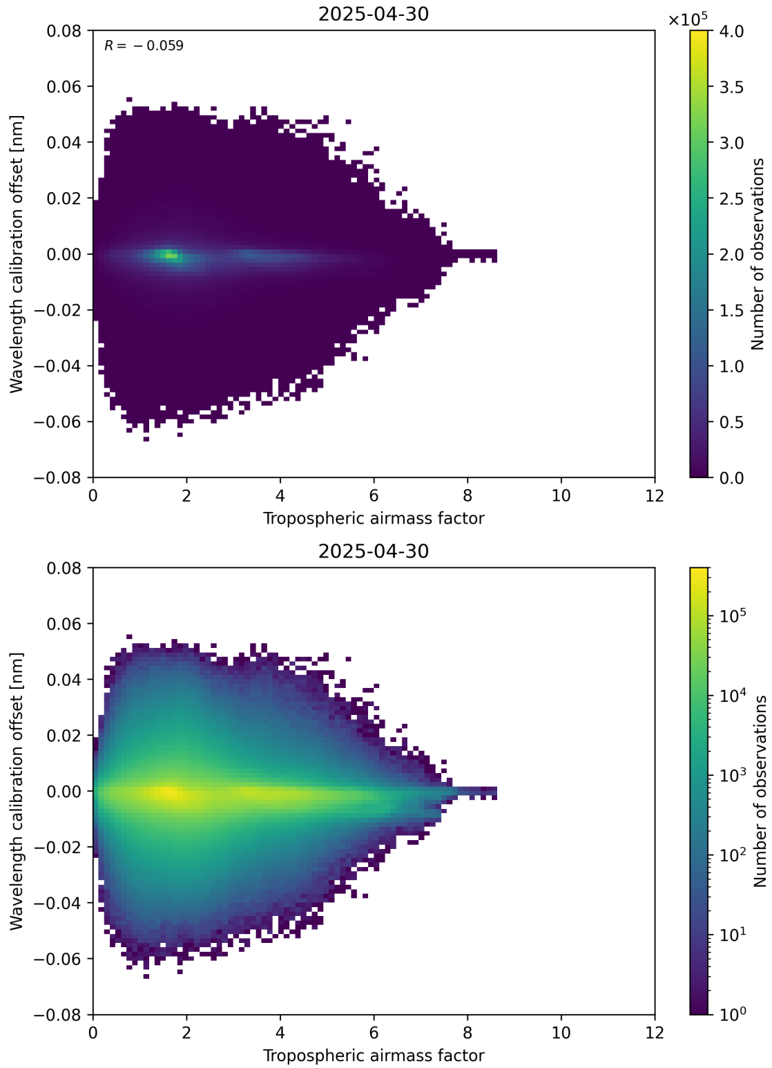
Figure 80: Scatter density plot of “Tropospheric airmass factor” against “Wavelength calibration offset” for 2025-04-30 to 2025-05-01.
