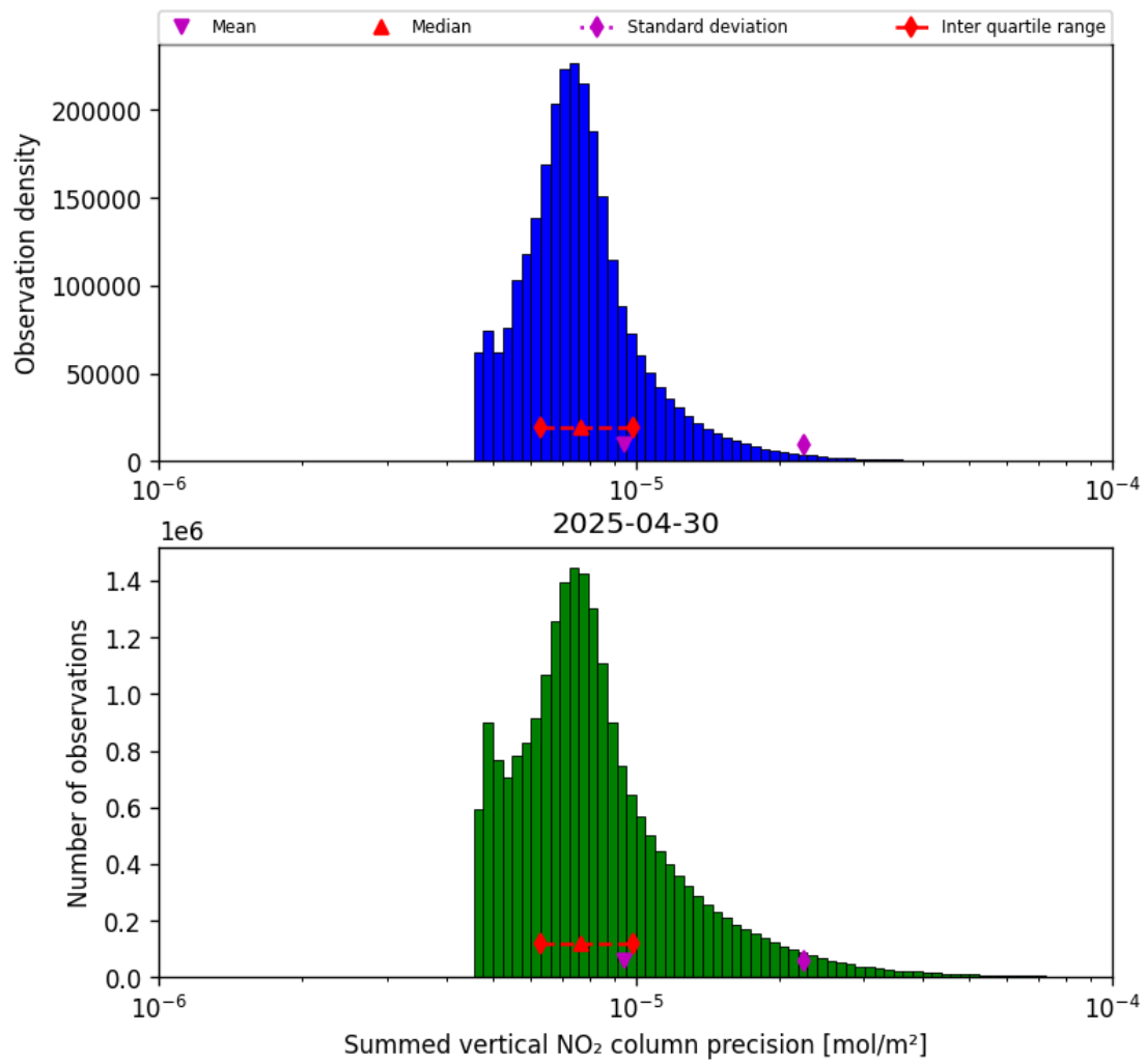
Figure 41: Histogram of "Summed vertical NO 2 column precision" for 2025-04-30 to 2025-05-01
