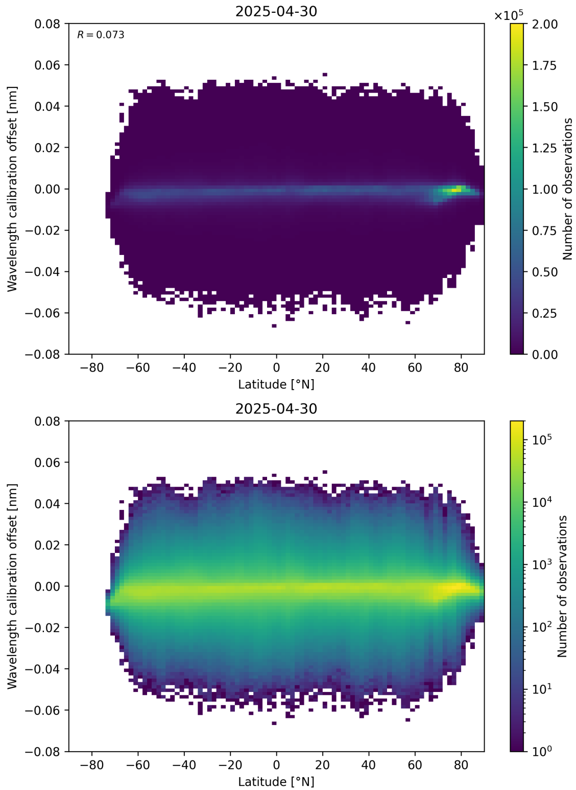
Figure 95: Scatter density plot of “Latitude” against “Wavelength calibration offset” for 2025-04-30 to 2025-05-01.
