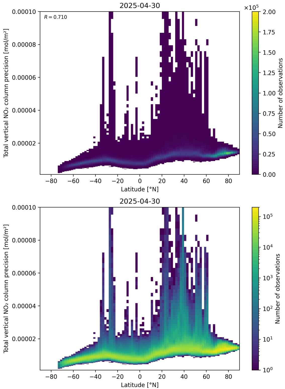
Figure 91: Scatter density plot of “Latitude” against “Total vertical NO 2 column precision” for 2025-04-30 to 2025-05-01.
