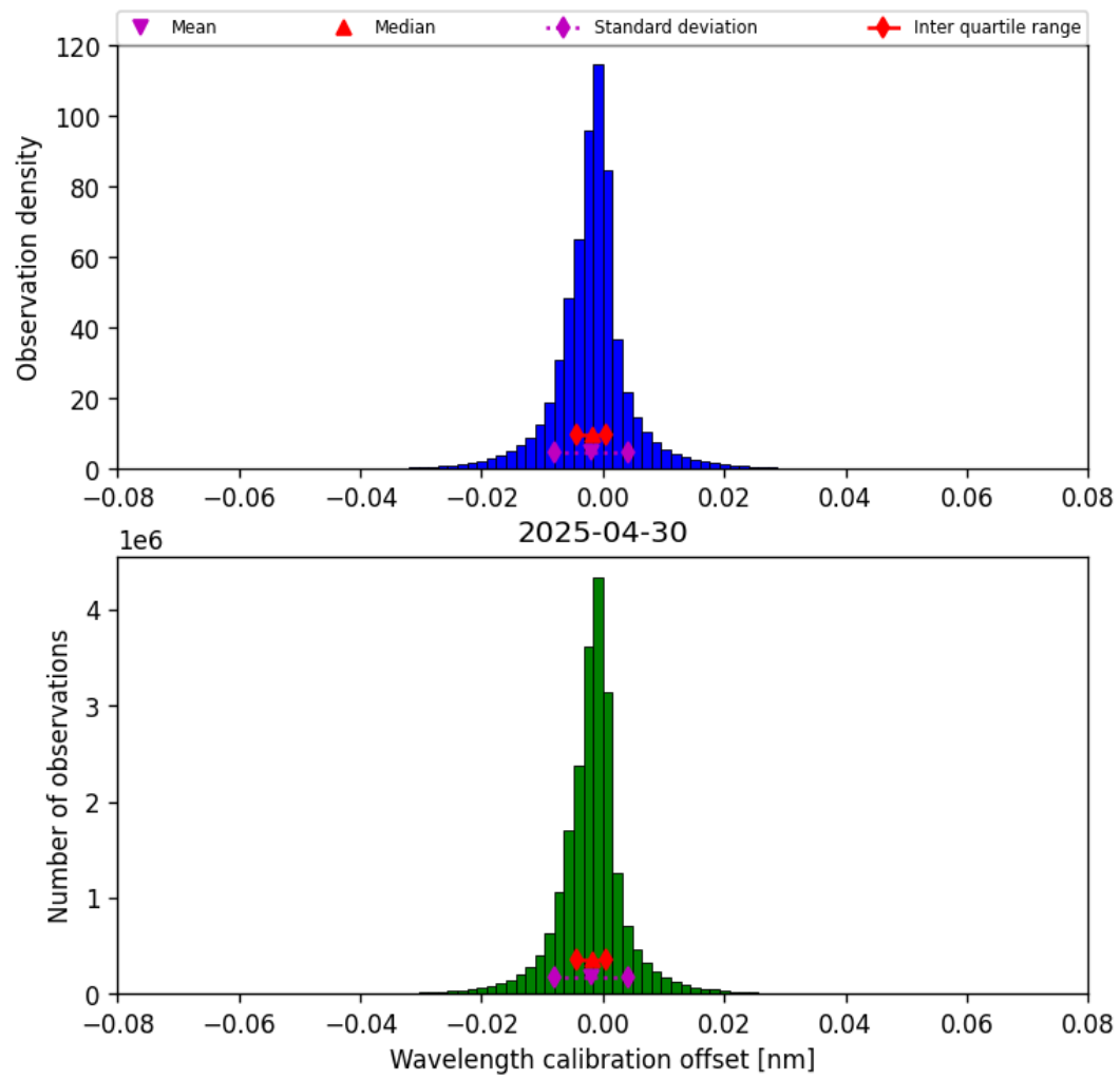
Figure 35: Histogram of “Wavelength calibration offset” for 2025-04-30 to 2025-05-01
