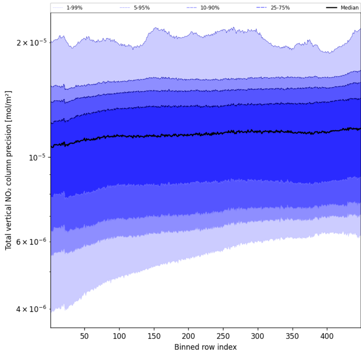
Figure 56: Along track statistics of “Total vertical NO 2 column precision” for 2025-04-30 to 2025-05-01
