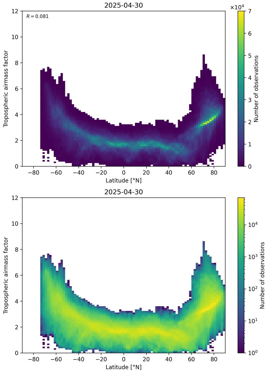
Figure 85: Scatter density plot of “Latitude” against “Tropospheric air mass factor” for 2025-04-30 to 2025-05-01.
