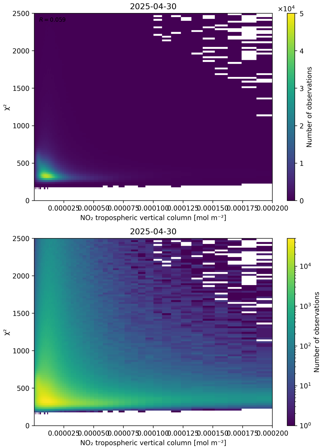
Figure 124: Scatter density plot of “NO 2 tropospheric vertical column” against “ \chi^2 ” for 2025-04-30 to 2025-05-01.
