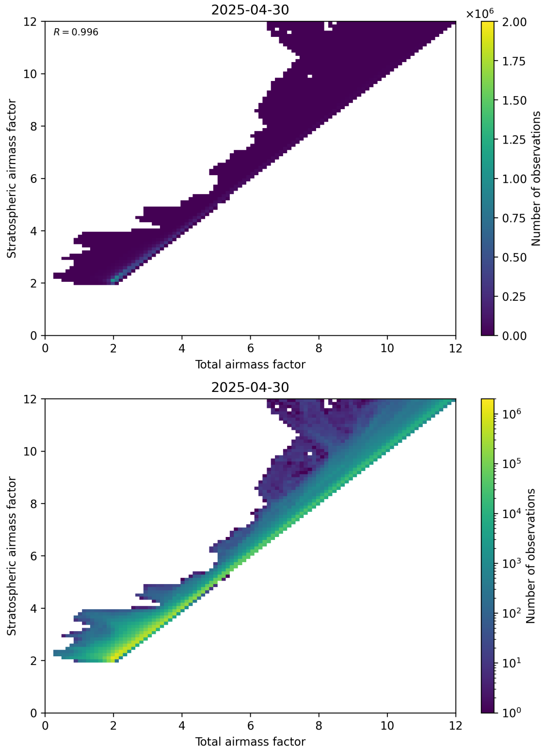
Figure 62: Scatter density plot of “Total airmass factor” against “Stratospheric airmass factor” for 2025-04-30 to 2025-05-01.
