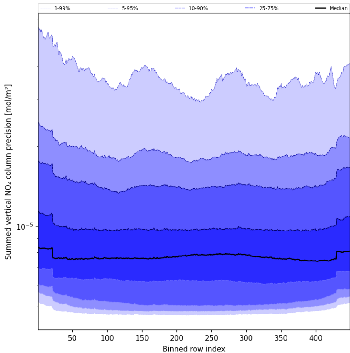
Figure 58: Along track statistics of “Summed vertical NO 2 column precision” for 2025-04-30 to 2025-05-01
