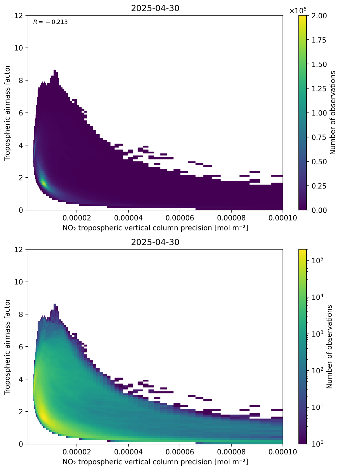
Figure 133: Scatter density plot of “NO 2 tropospheric vertical column precision” against “Tropospheric air mass factor” for 2025-04-30 to 2025-05-01.
