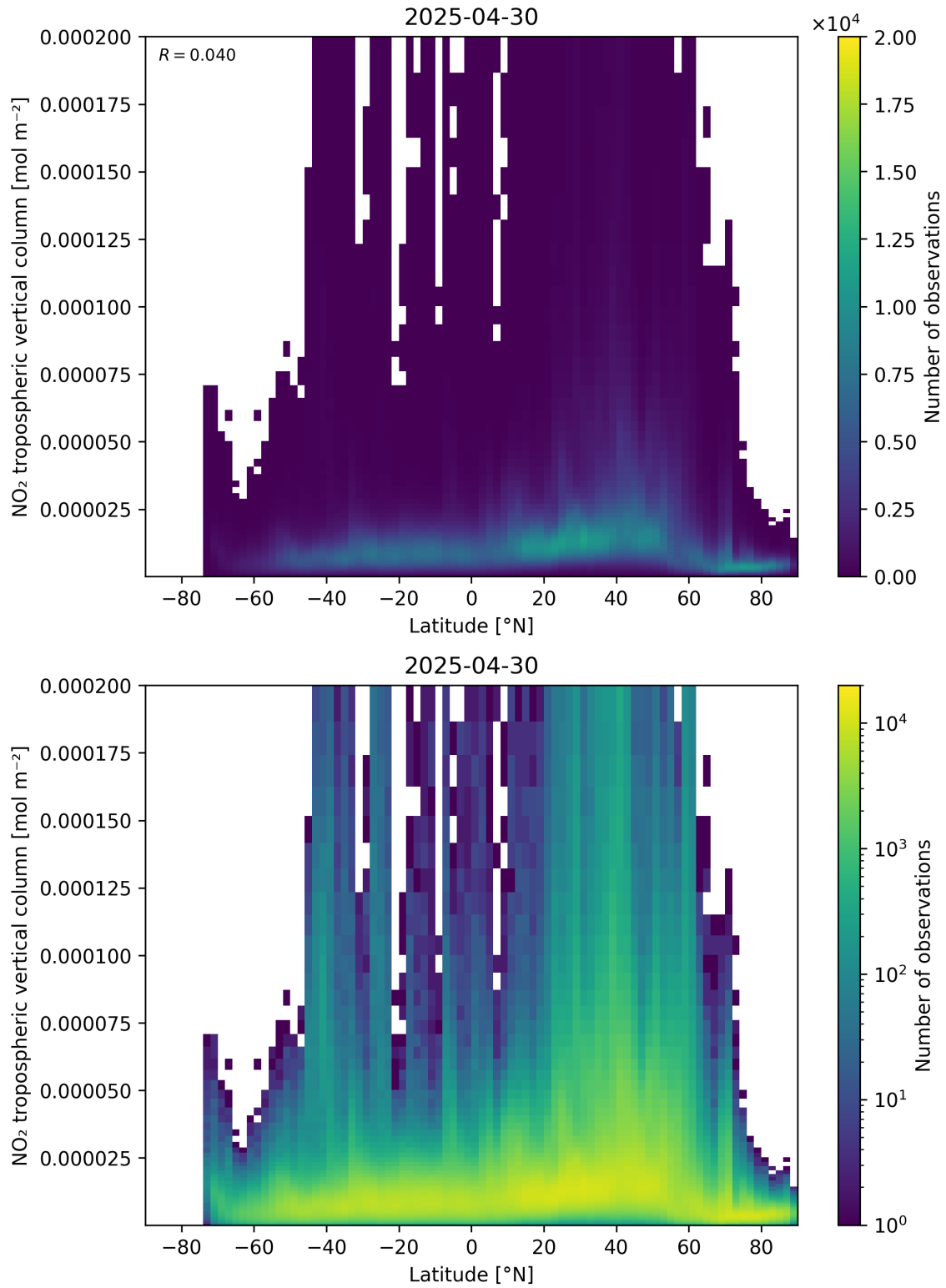
Figure 92: Scatter density plot of “Latitude” against “NO 2 tropospheric vertical column” for 2025-04-30 to 2025-05-01.
