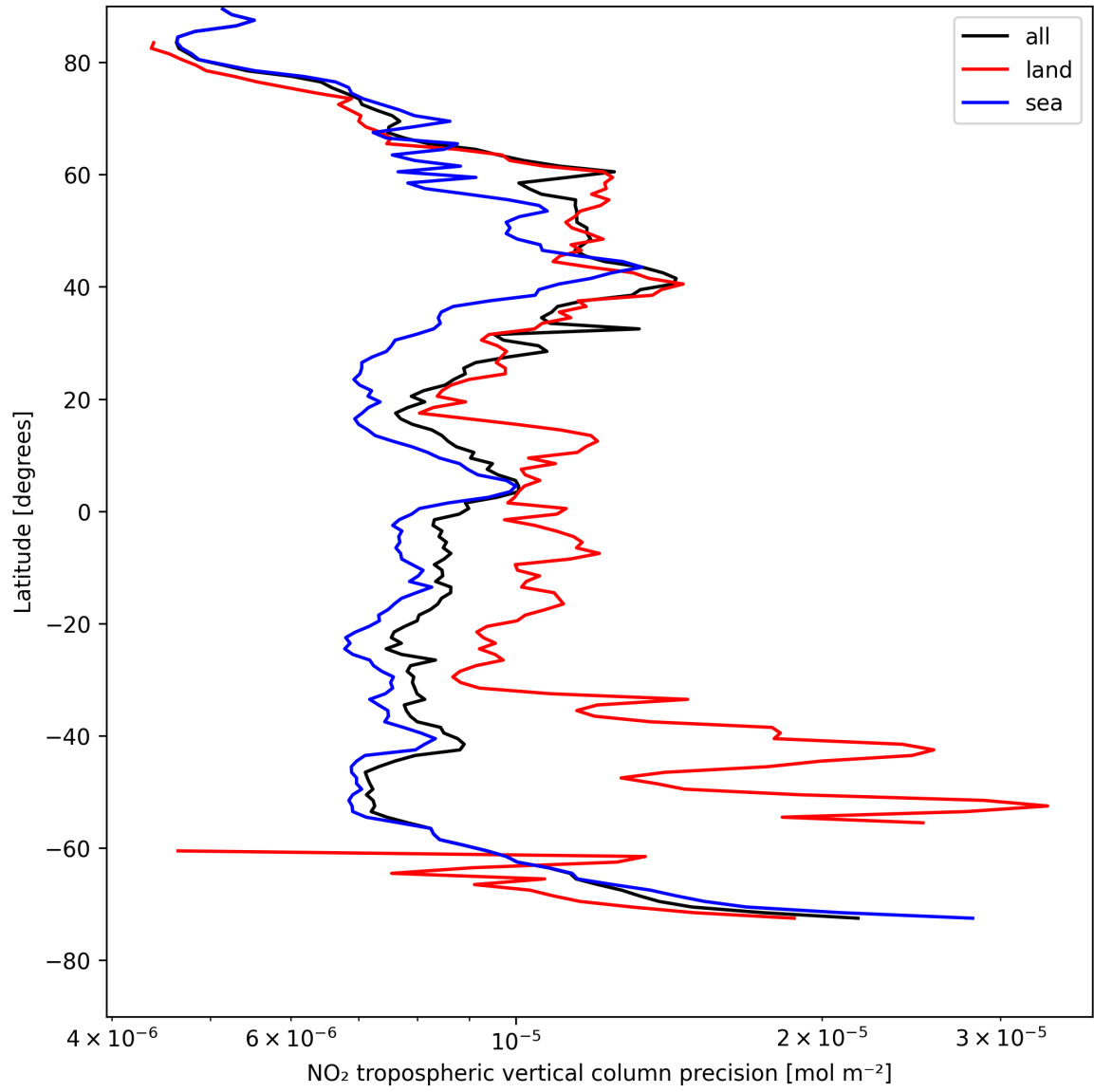
Figure 13: Zonal average of “NO 2 tropospheric vertical column precision” for 2025-04-30 to 2025-05-01.
