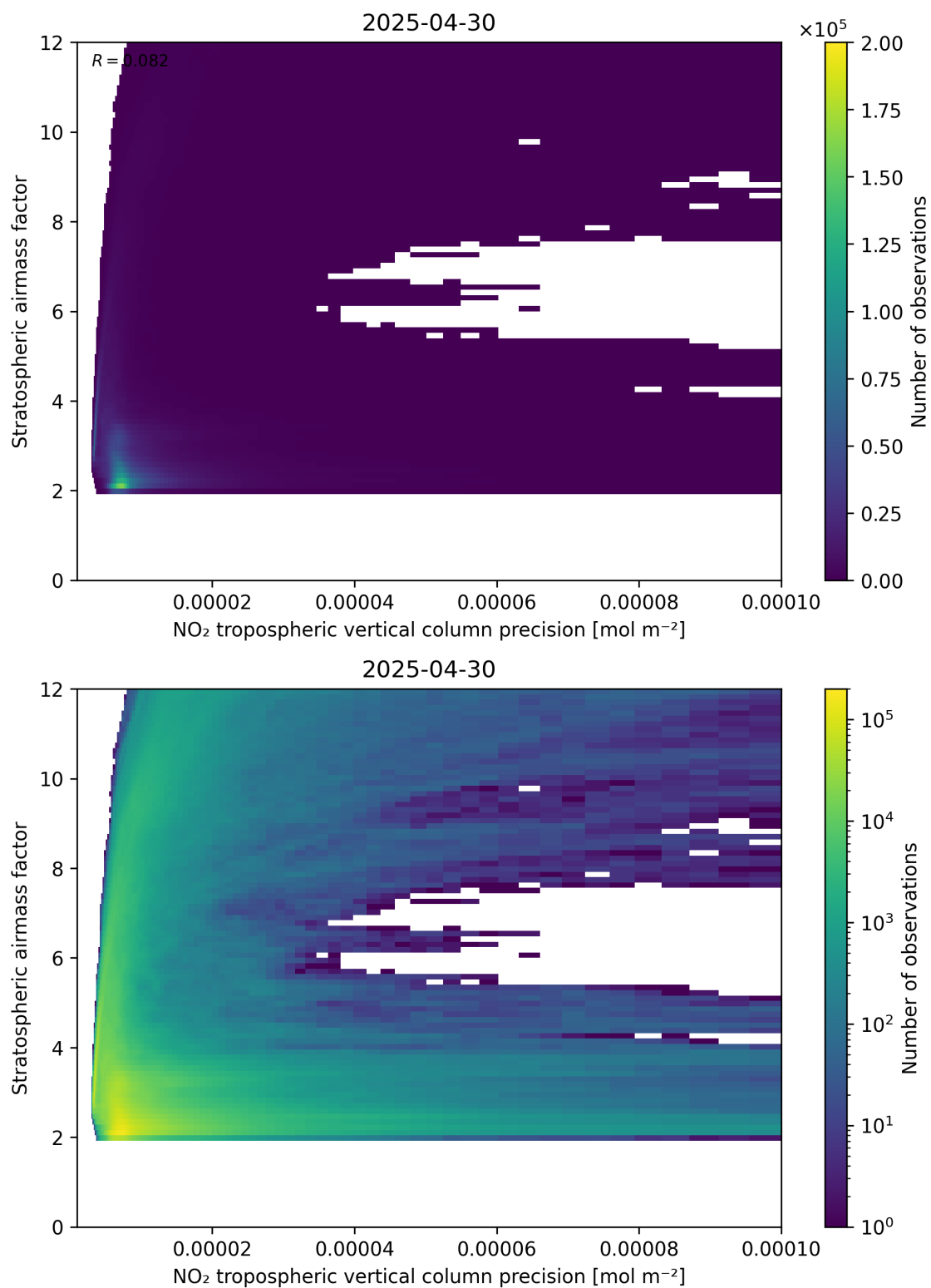
Figure 131: Scatter density plot of “NO 2 tropospheric vertical column precision” against “Stratospheric airmass factor” for 2025-04-30 to 2025-05-01.
