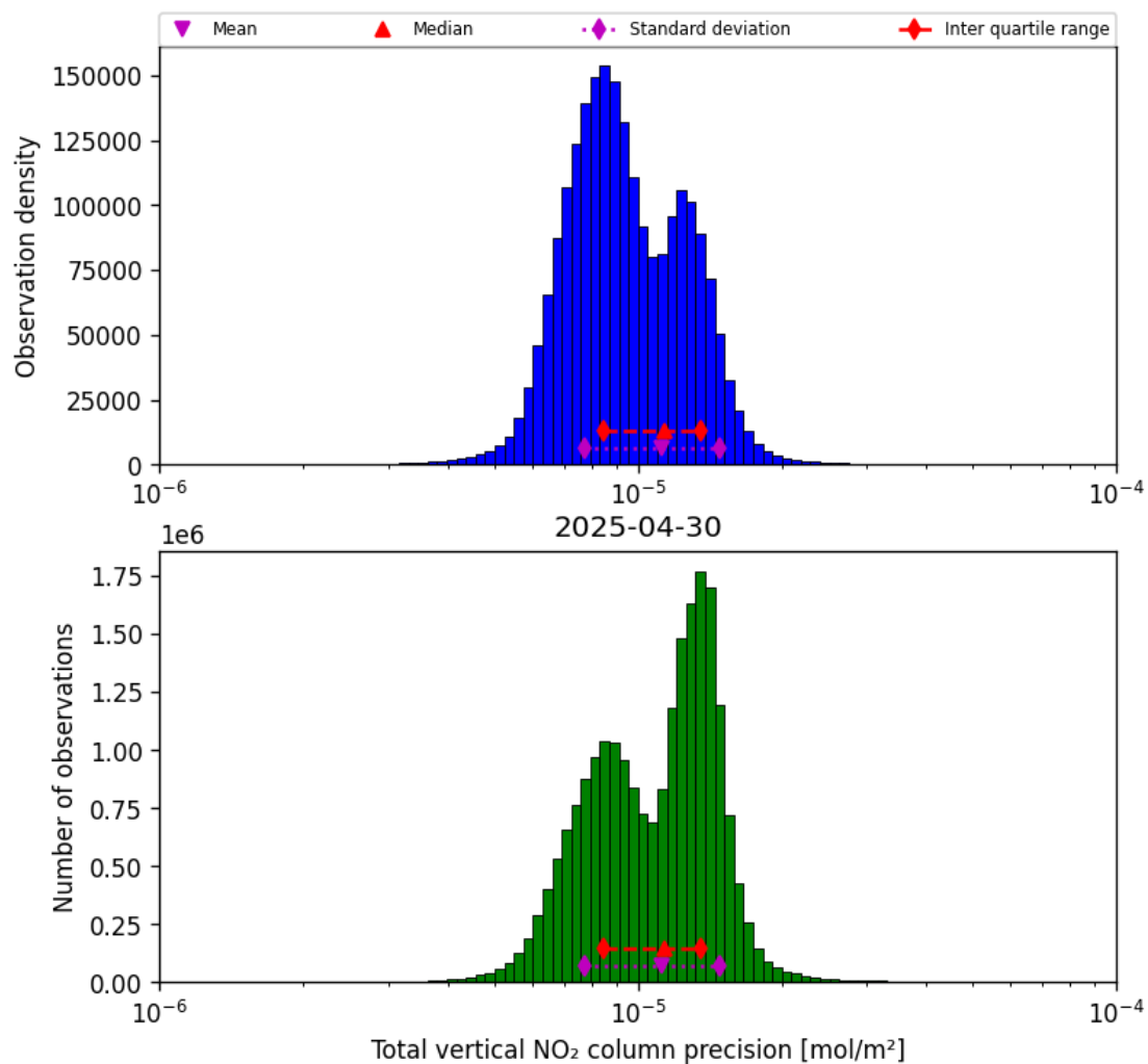
Figure 39: Histogram of “Total vertical NO 2 column precision” for 2025-04-30 to 2025-05-01
