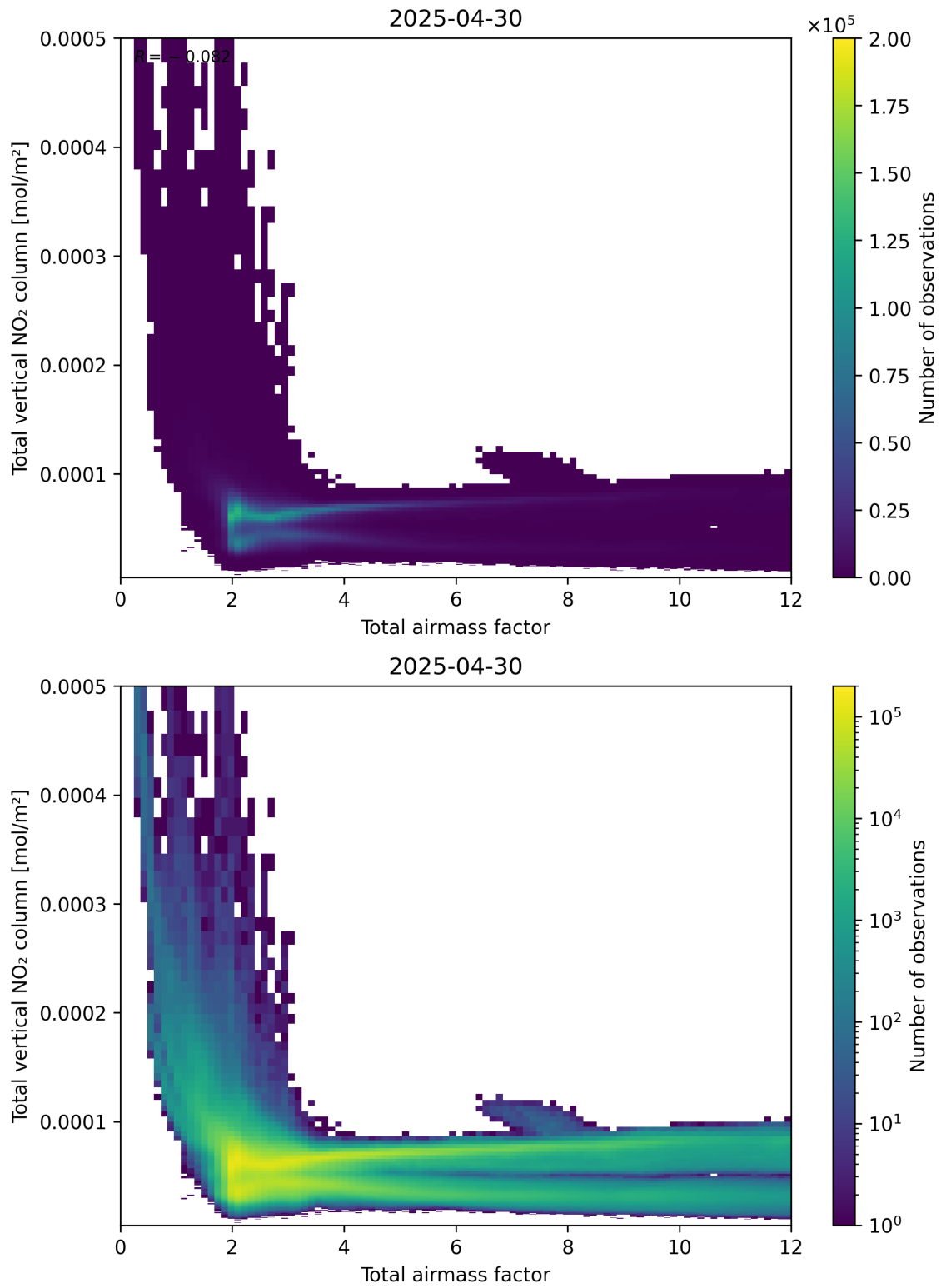
Figure 67: Scatter density plot of “Total airmass factor” against “Total vertical NO 2 column” for 2025-04-30 to 2025-05-01.
