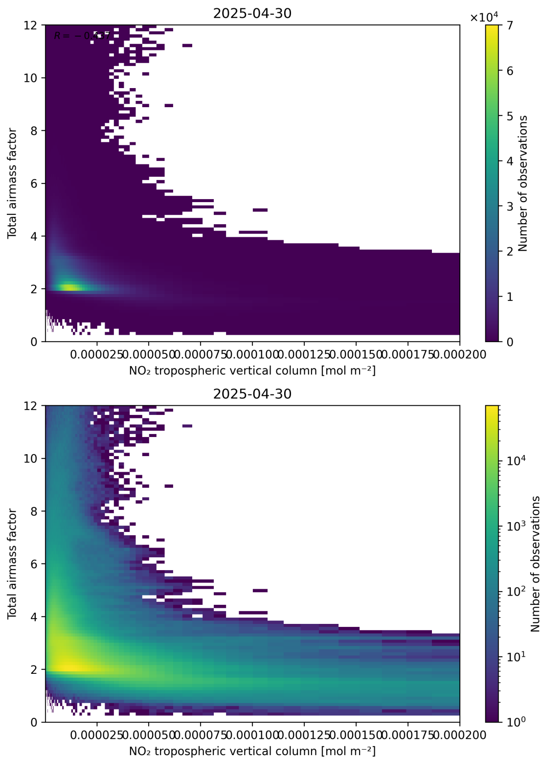
Figure 122: Scatter density plot of “NO 2 tropospheric vertical column” against “Total airmass factor” for 2025-04-30 to 2025-05-01.
