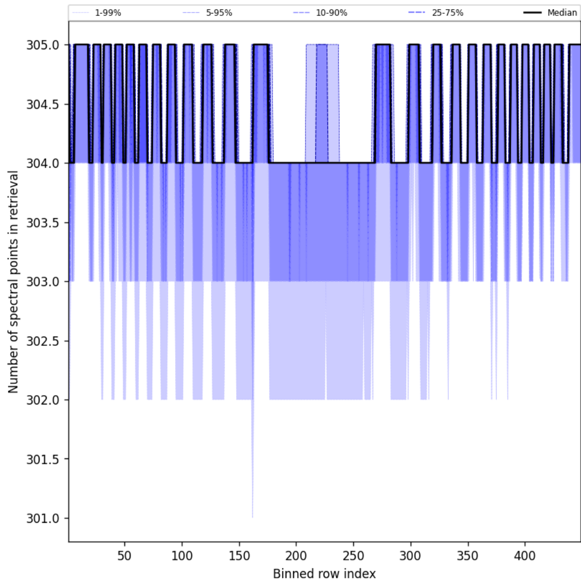
Figure 50: Along track statistics of “Number of spectral points in retrieval” for 2025-04-30 to 2025-05-01
