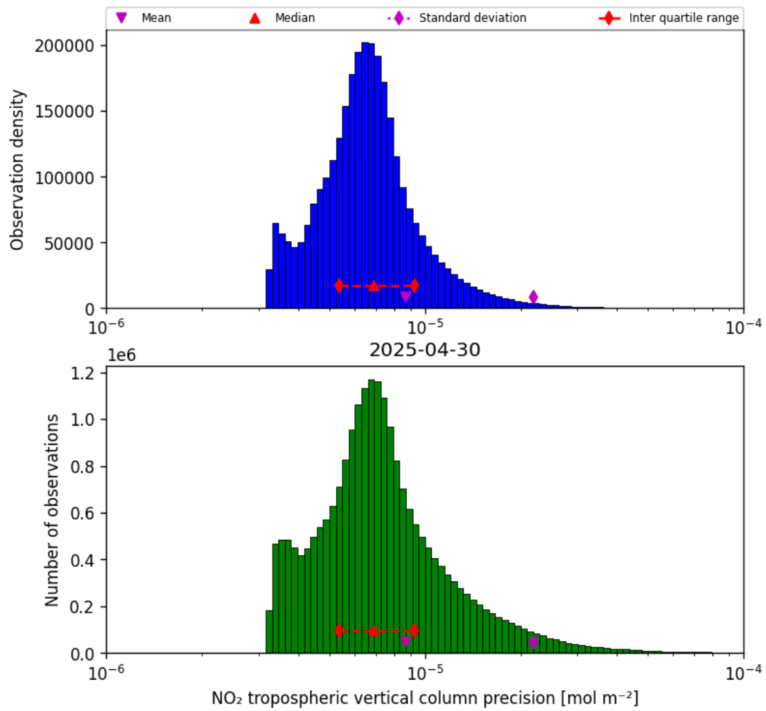
Figure 30: Histogram of “NO 2 tropospheric vertical column precision” for 2025-04-30 to 2025-05-01
