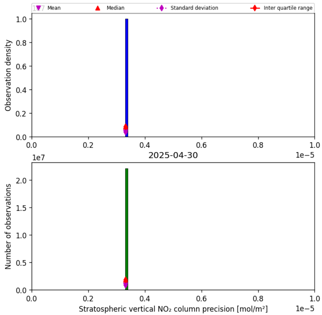
Figure 37: Histogram of “Stratospheric vertical NO 2 column precision” for 2025-04-30 to 2025-05-01
