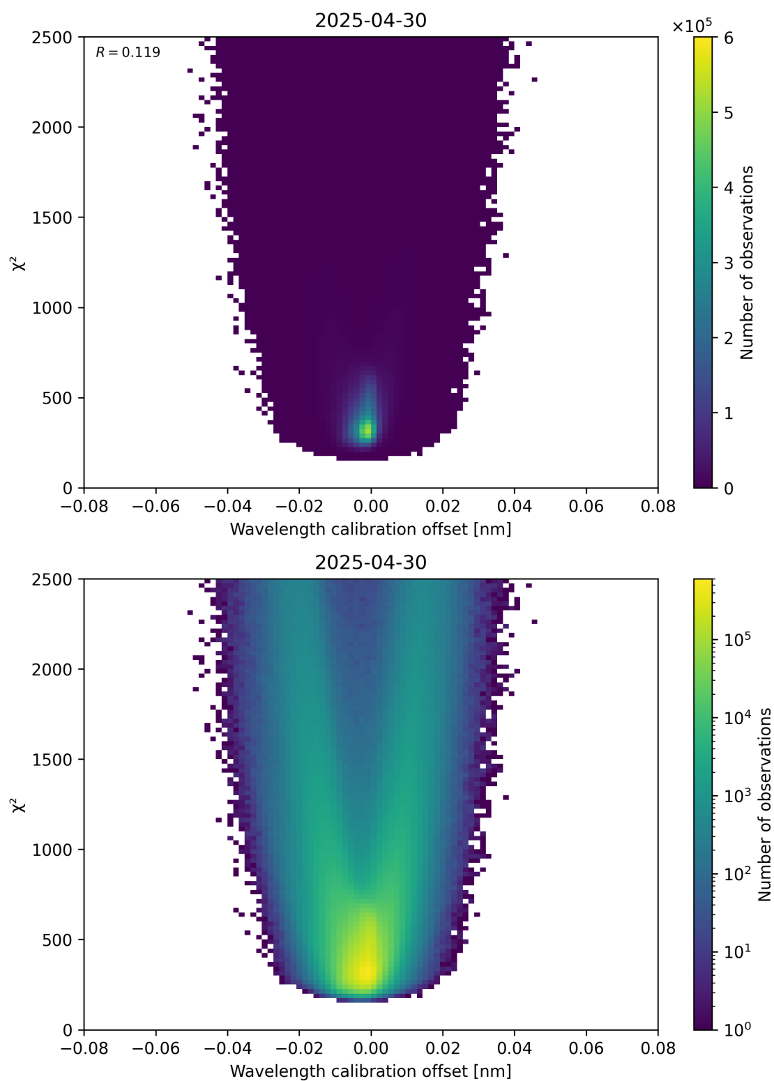
Figure 175: Scatter density plot of “Wavelength calibration offset” against “ \chi^2 ” for 2025-04-30 to 2025-05-01.
