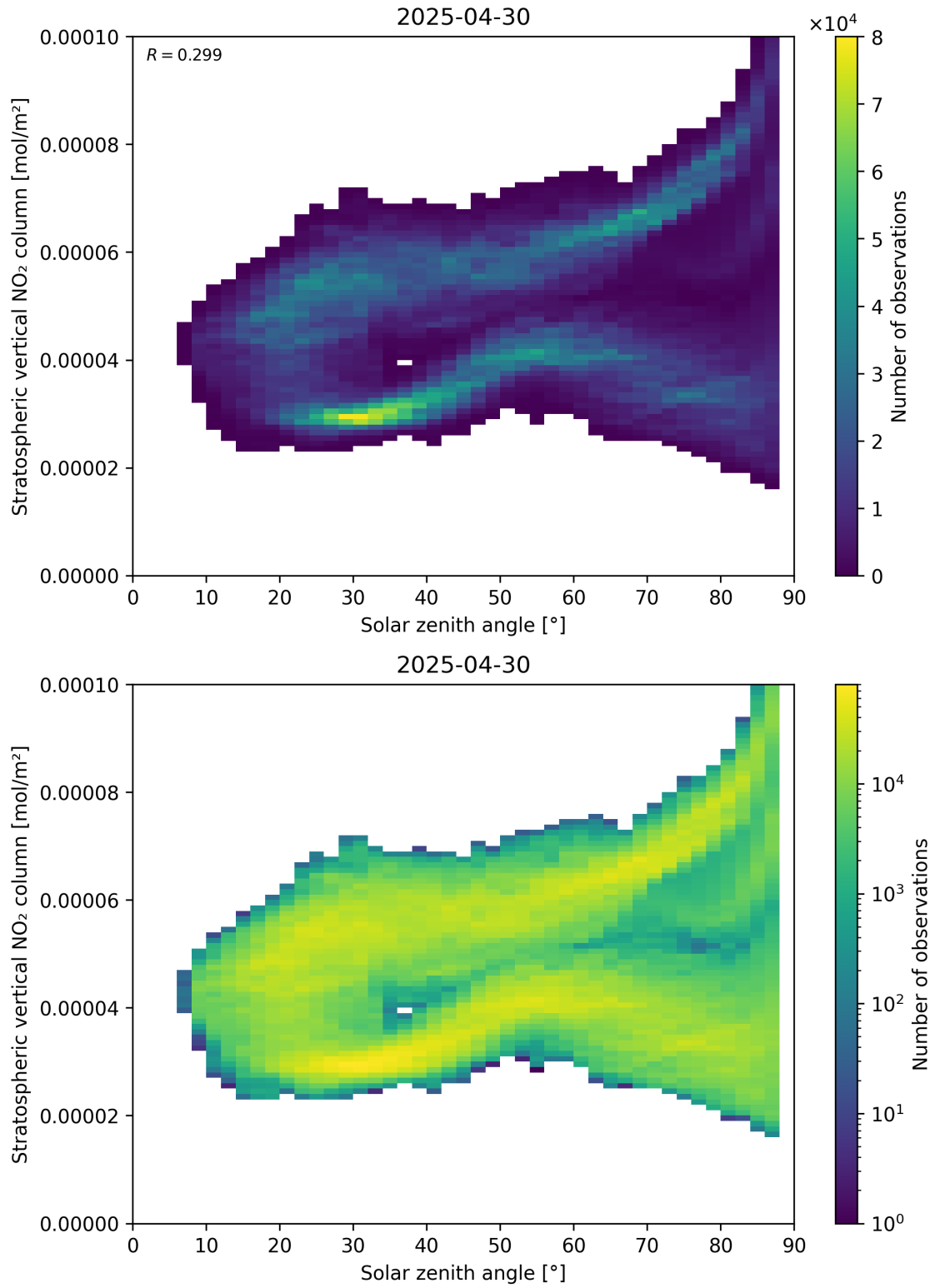
Figure 150: Scatter density plot of “Solar zenith angle” against “Stratospheric vertical NO 2 column” for 2025-04-30 to 2025-05-01.
