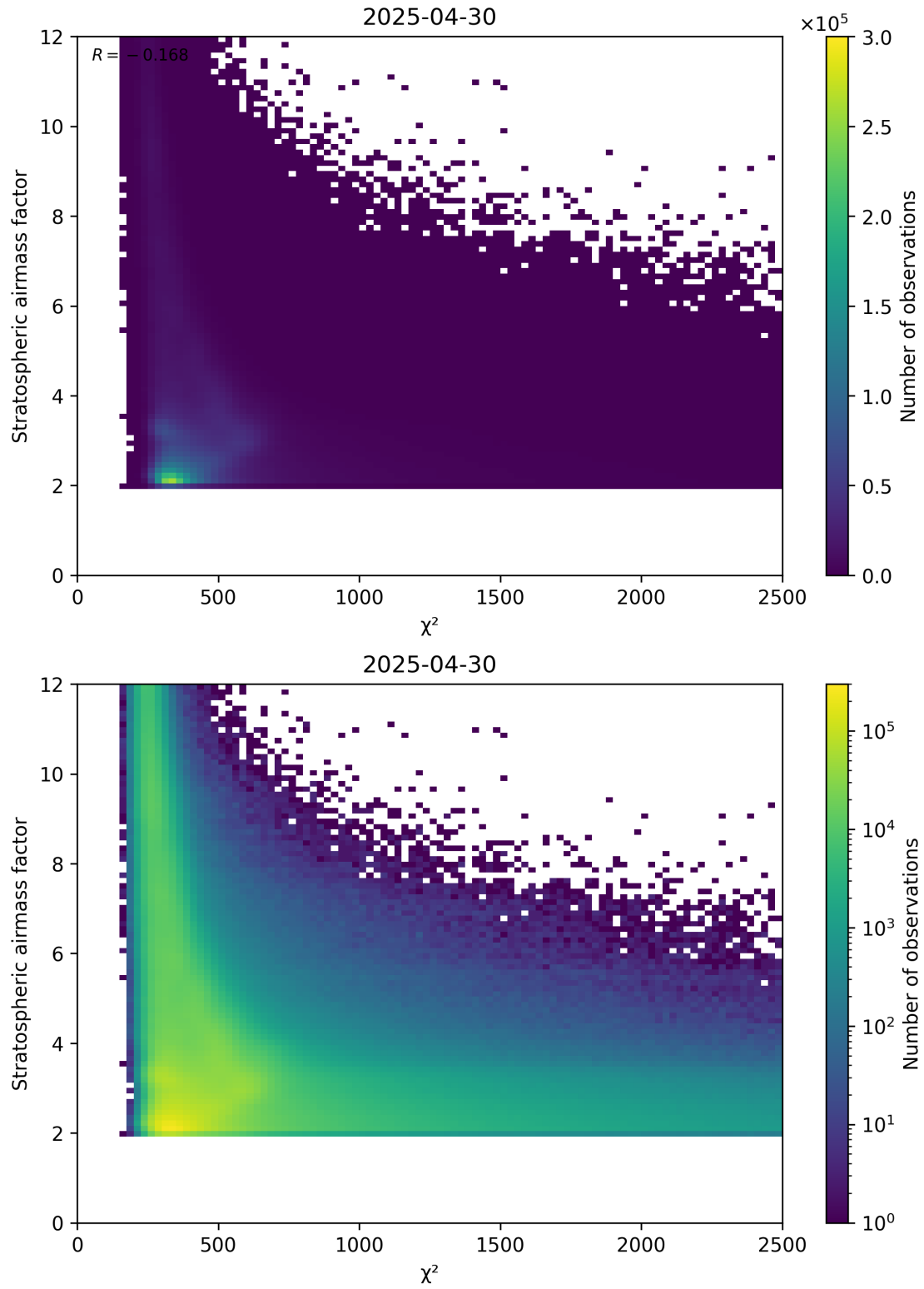
Figure 81: Scatter density plot of “ \chi^2 ” against “Stratospheric airmass factor” for 2025-04-30 to 2025-05-01.
