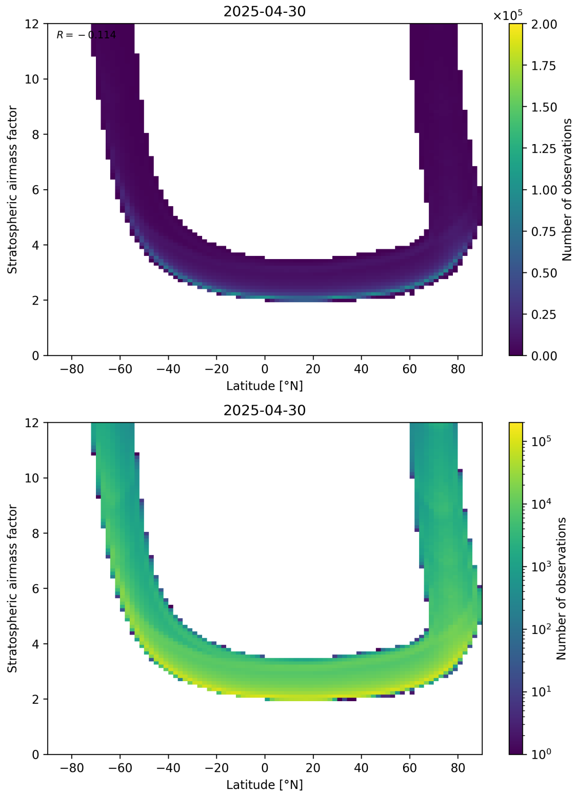
Figure 83: Scatter density plot of “Latitude” against “Stratospheric air mass factor” for 2025-04-30 to 2025-05-01.
