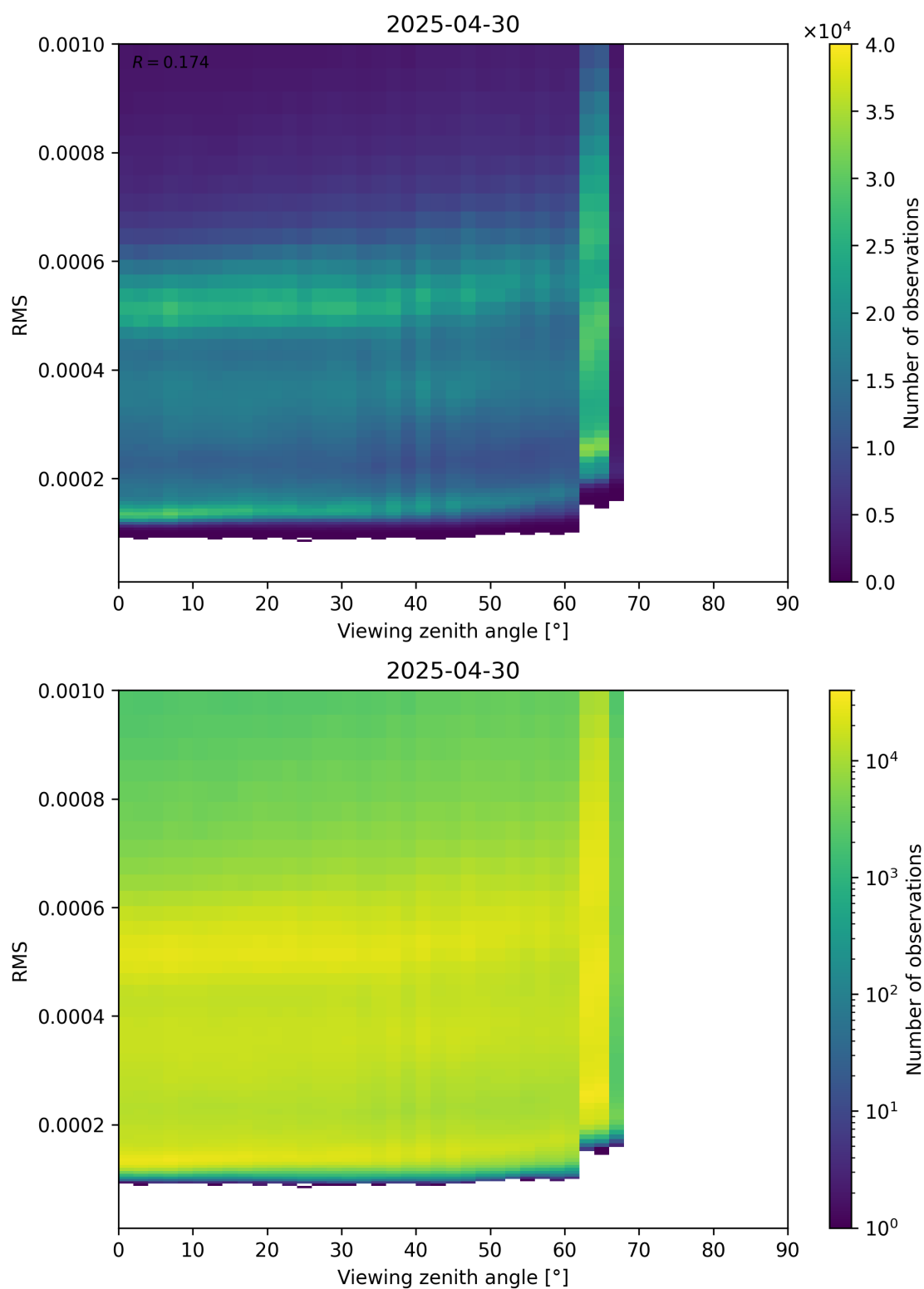
Figure 171: Scatter density plot of “Viewing zenith angle” against “RMS” for 2025-04-30 to 2025-05-01.
