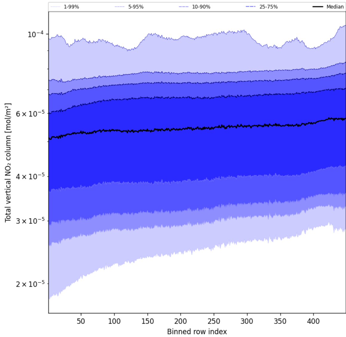
Figure 55: Along track statistics of “Total vertical NO 2 column” for 2025-04-30 to 2025-05-01
