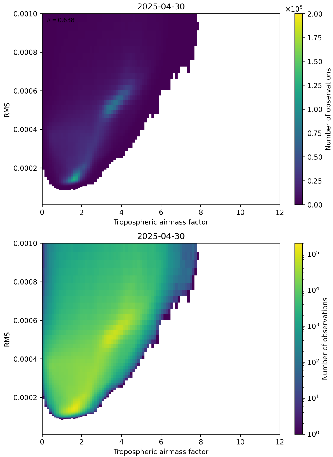
Figure 79: Scatter density plot of “Tropospheric airmass factor” against “RMS” for 2025-04-30 to 2025-05-01.
