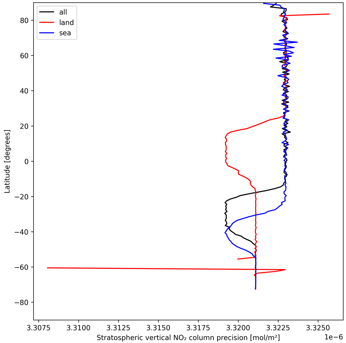
Figure 20: Zonal average of “Stratospheric vertical NO 2 column precision” for 2025-04-30 to 2025-05-01.
