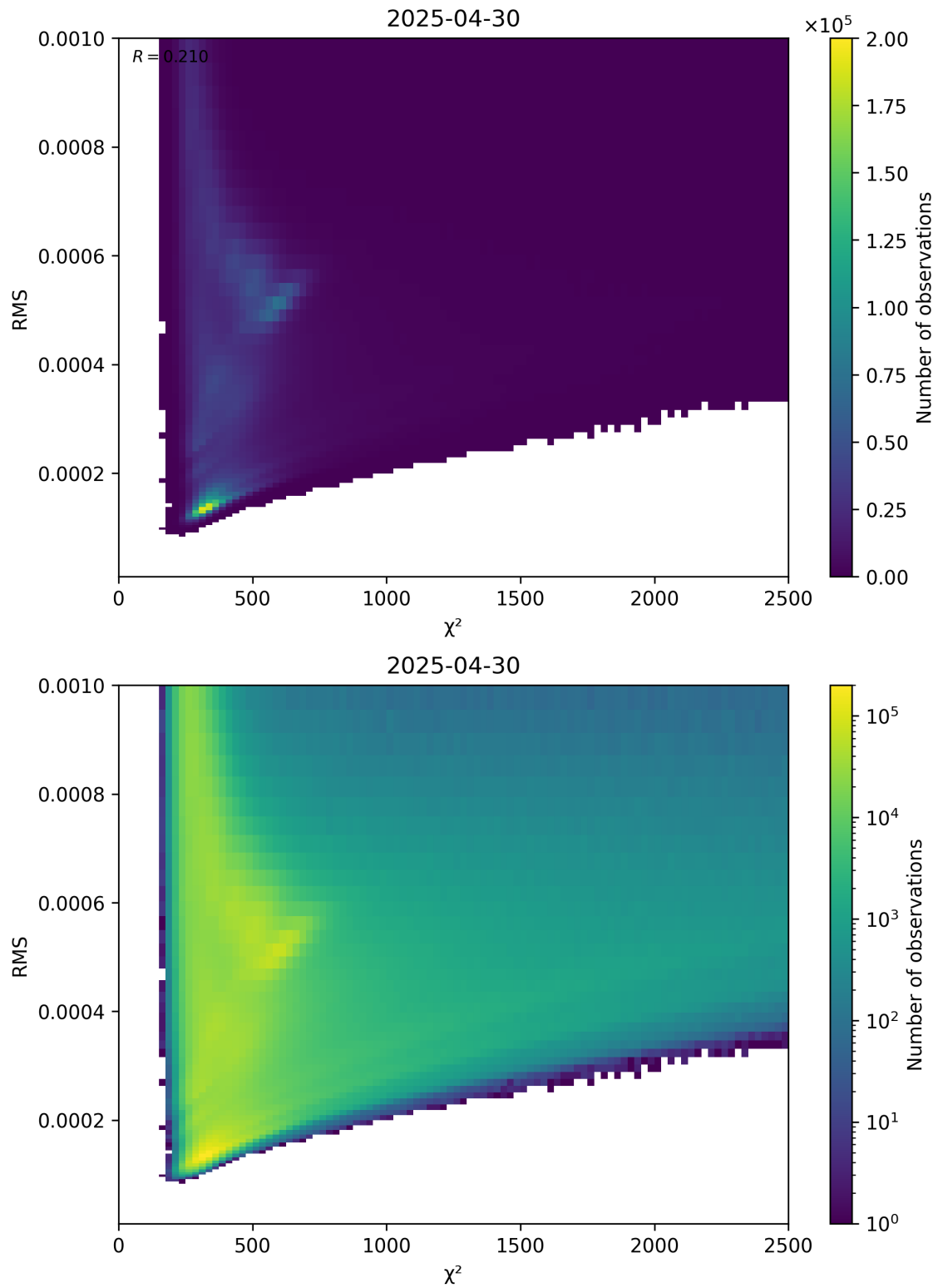
Figure 82: Scatter density plot of “ \chi^2 ” against “RMS” for 2025-04-30 to 2025-05-01.
