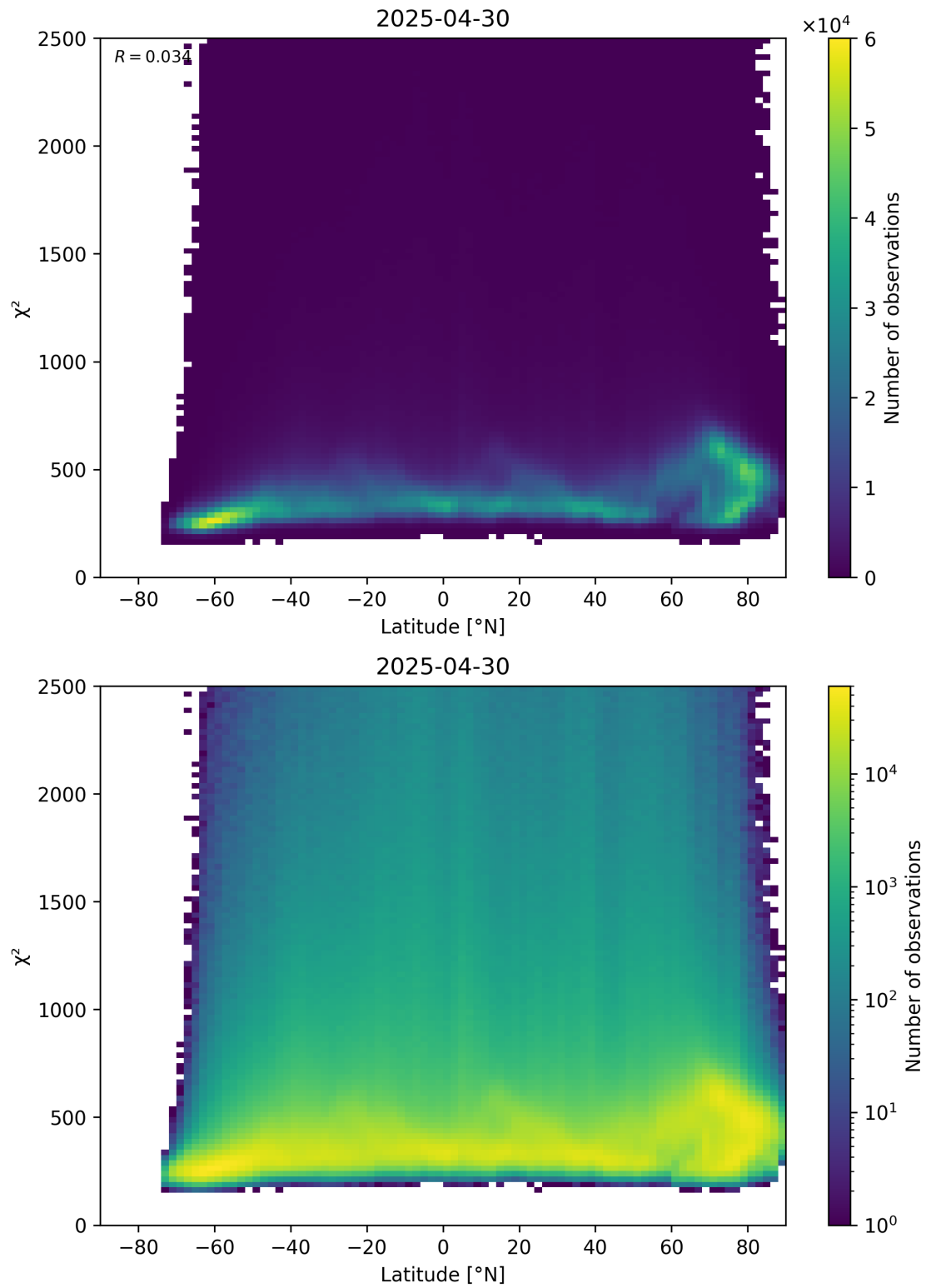
Figure 86: Scatter density plot of “Latitude” against “ \chi^2 ” for 2025-04-30 to 2025-05-01.
