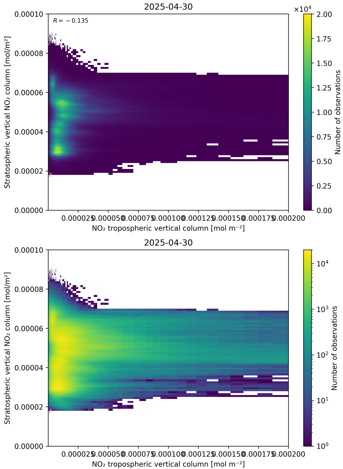
Figure 125: Scatter density plot of “NO 2 tropospheric vertical column” against “Stratospheric vertical NO 2 column” for 2025-04-30 to 2025-05-01.
