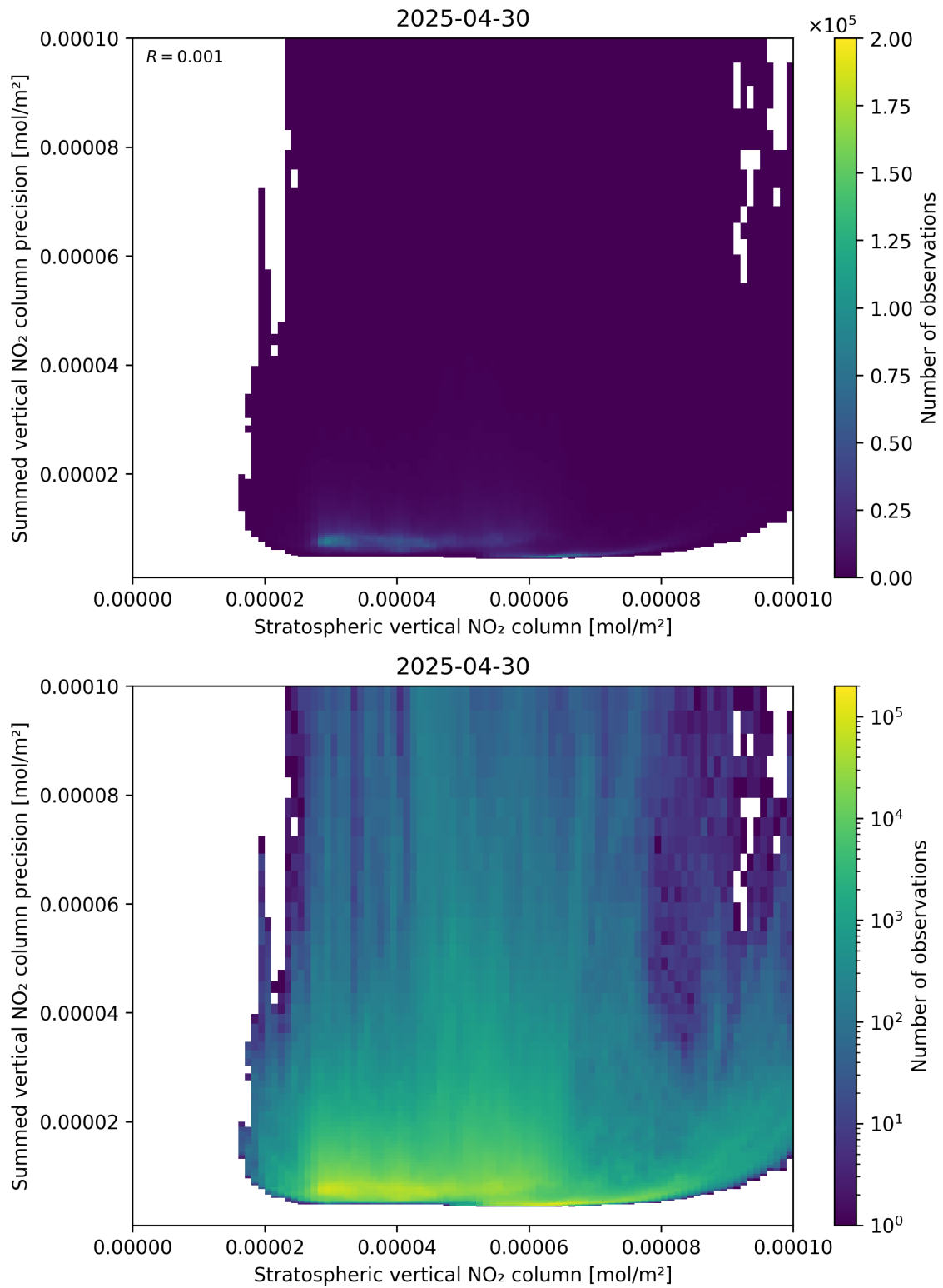
Figure 99: Scatter density plot of “Stratospheric vertical NO 2 column” against “Summed vertical NO 2 column precision” for 2025-04-30 to 2025-05-01.
