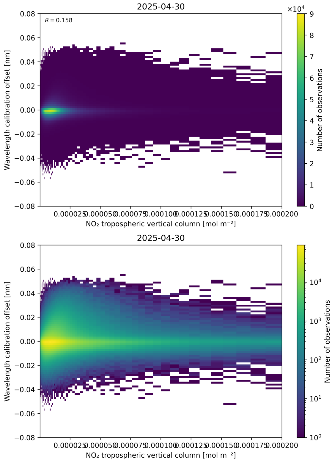
Figure 143: Scatter density plot of “NO 2 tropospheric vertical column” against “Wavelength calibration offset” for 2025-04-30 to 2025-05-01.
