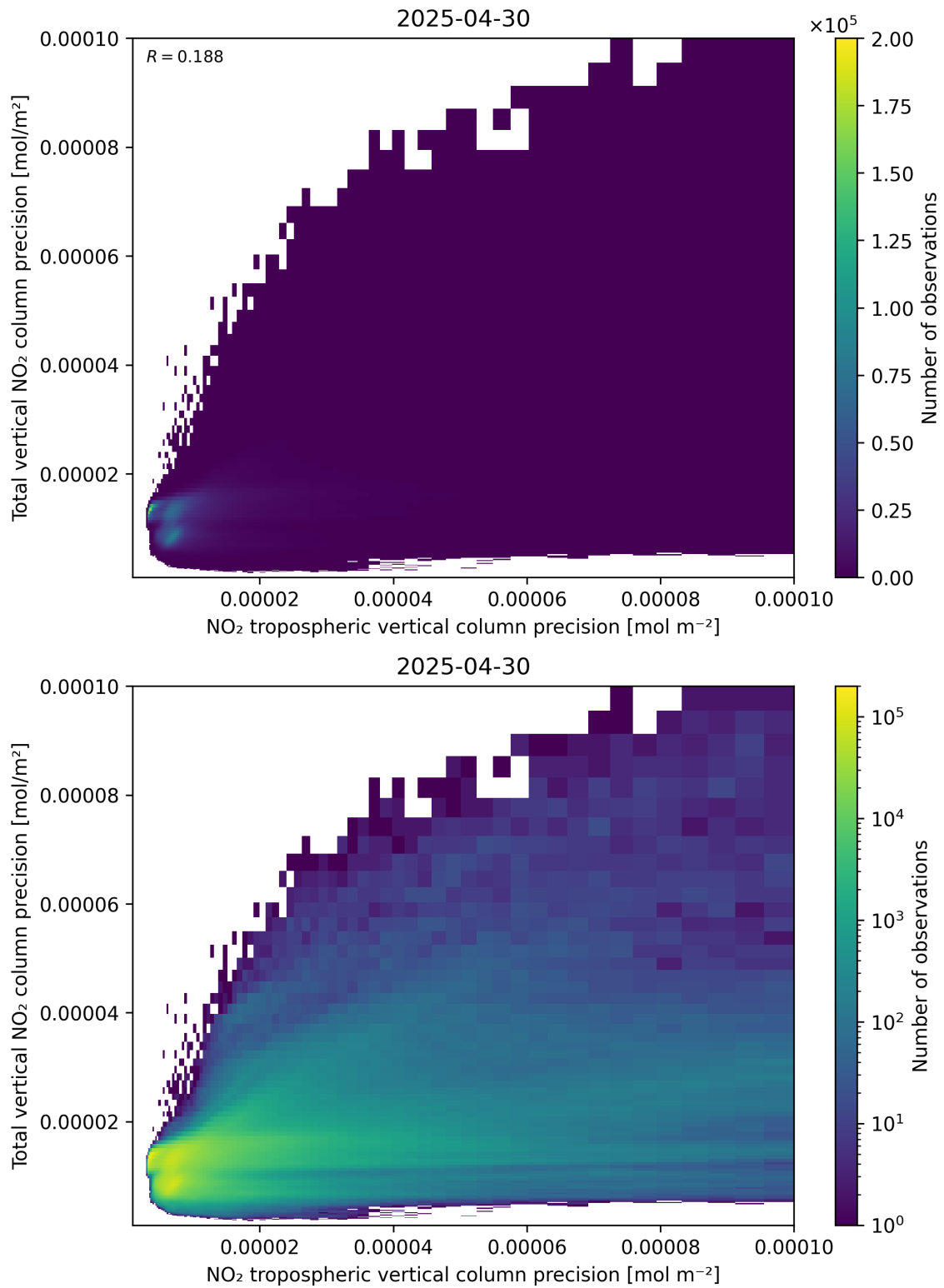
Figure 139: Scatter density plot of “NO 2 tropospheric vertical column precision” against “Total vertical NO 2 column precision” for 2025-04-30 to 2025-05-01.
