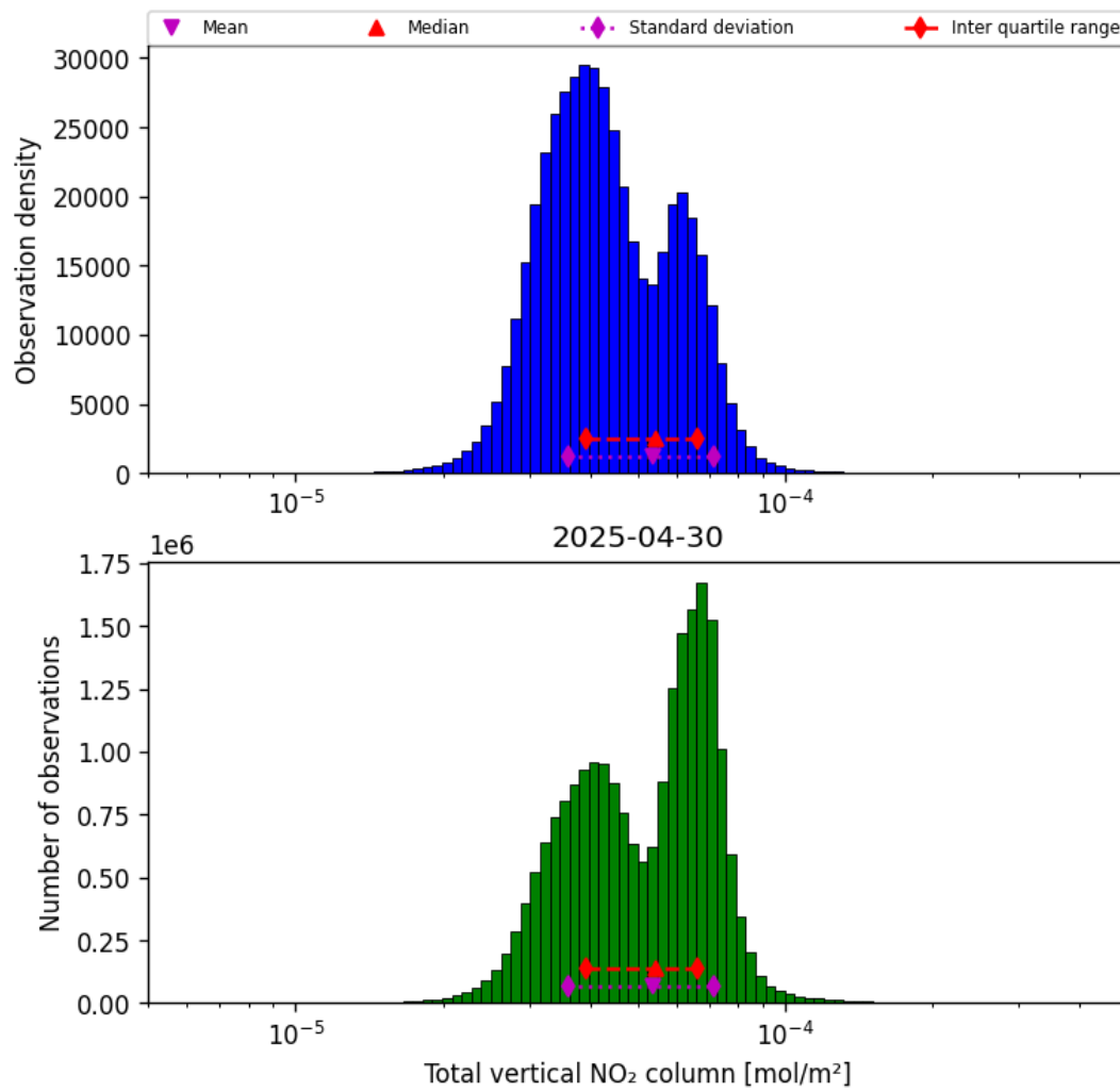
Figure 38: Histogram of “Total vertical NO 2 column” for 2025-04-30 to 2025-05-01
