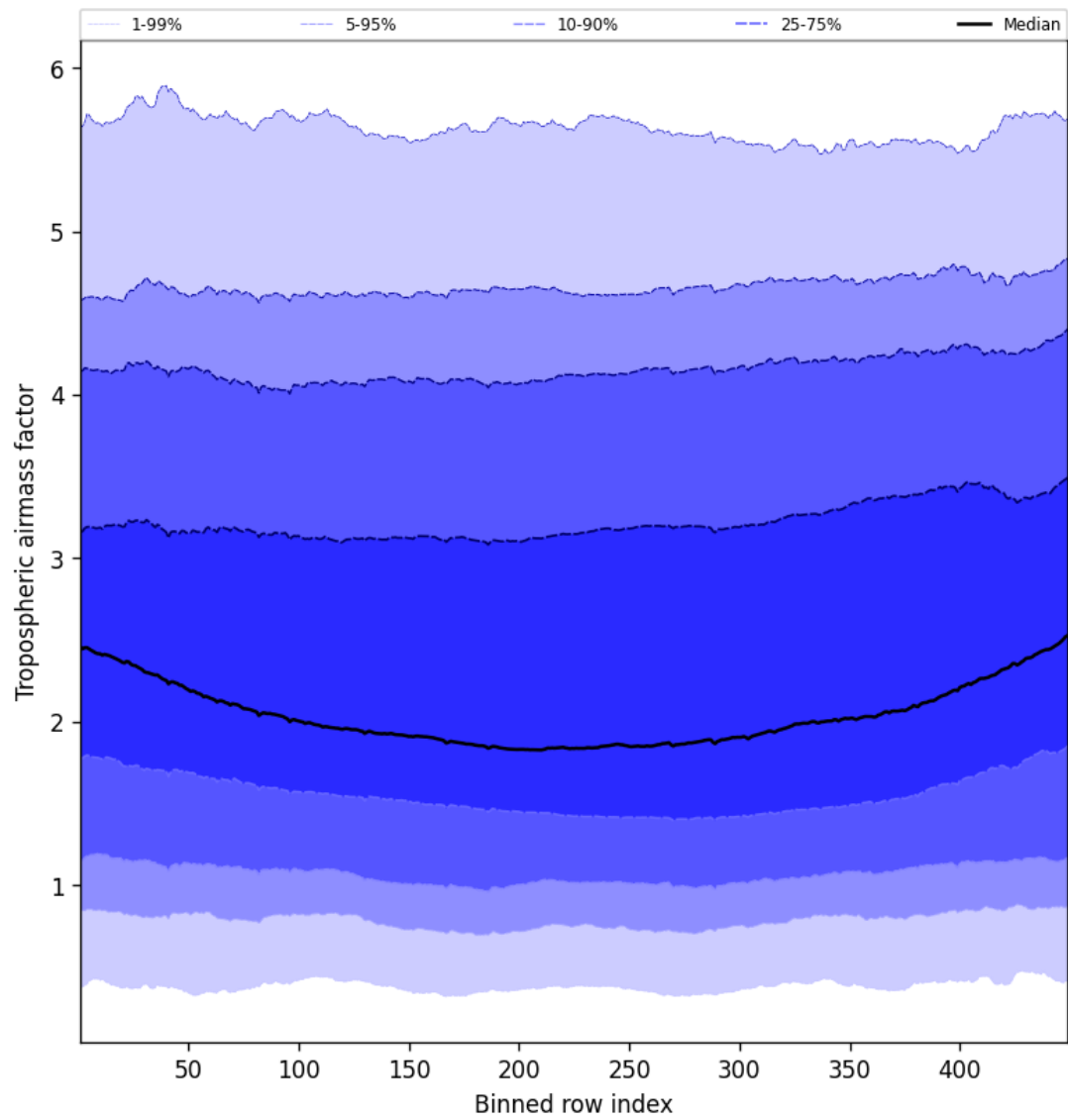
Figure 48: Along track statistics of “Tropospheric airmass factor” for 2025-04-30 to 2025-05-01
