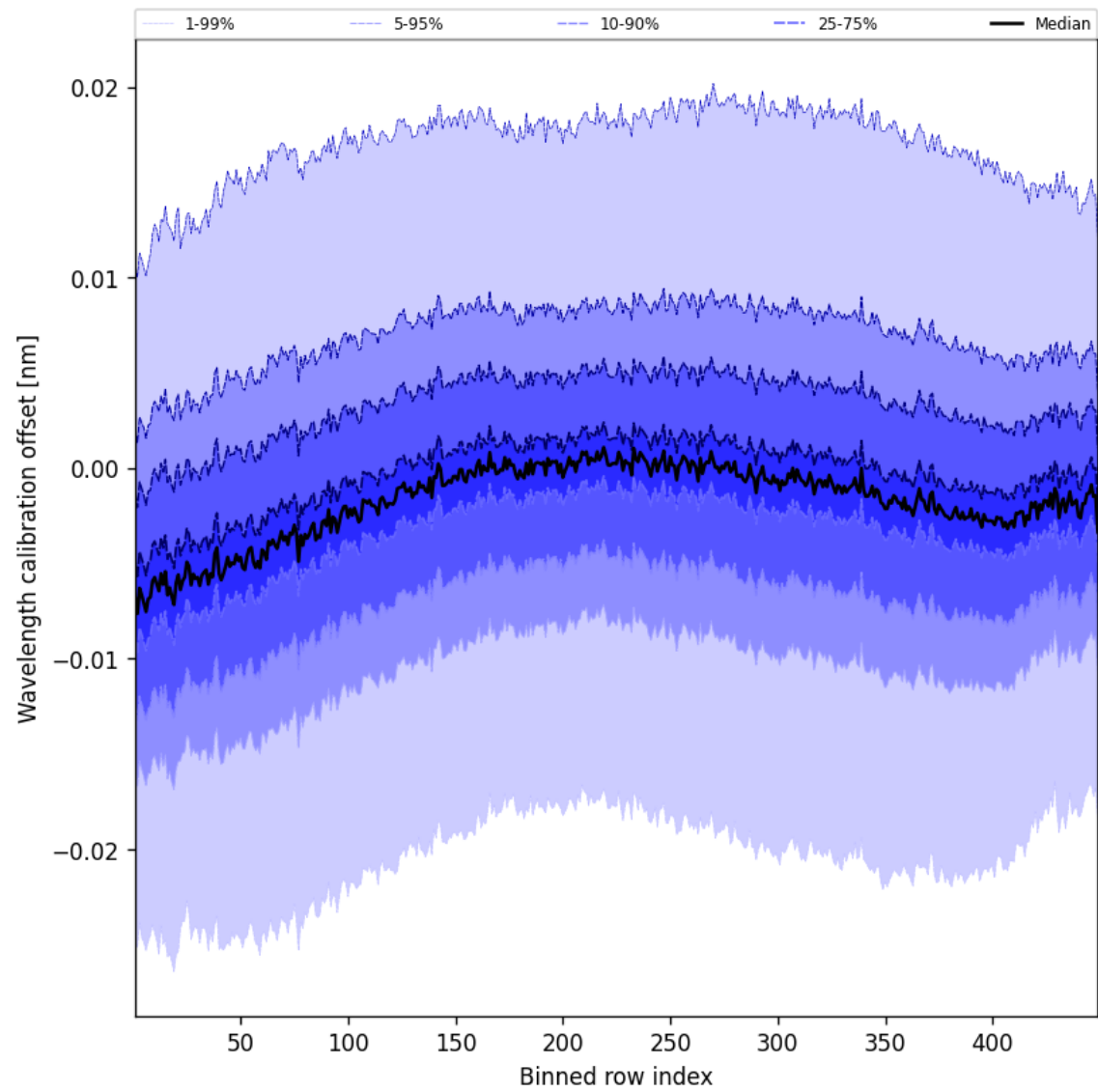
Figure 52: Along track statistics of “Wavelength calibration offset” for 2025-04-30 to 2025-05-01
