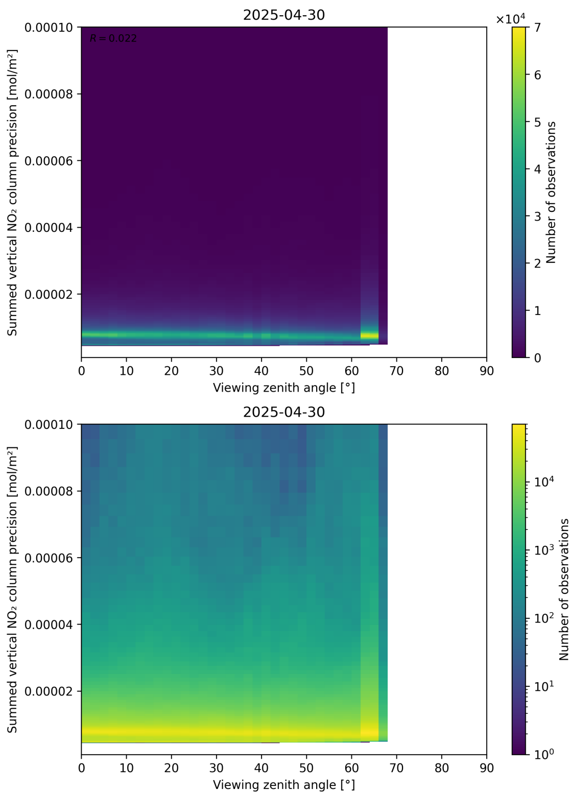
Figure 166: Scatter density plot of “Viewing zenith angle” against “Summed vertical NO 2 column precision” for 2025-04-30 to 2025-05-01.
