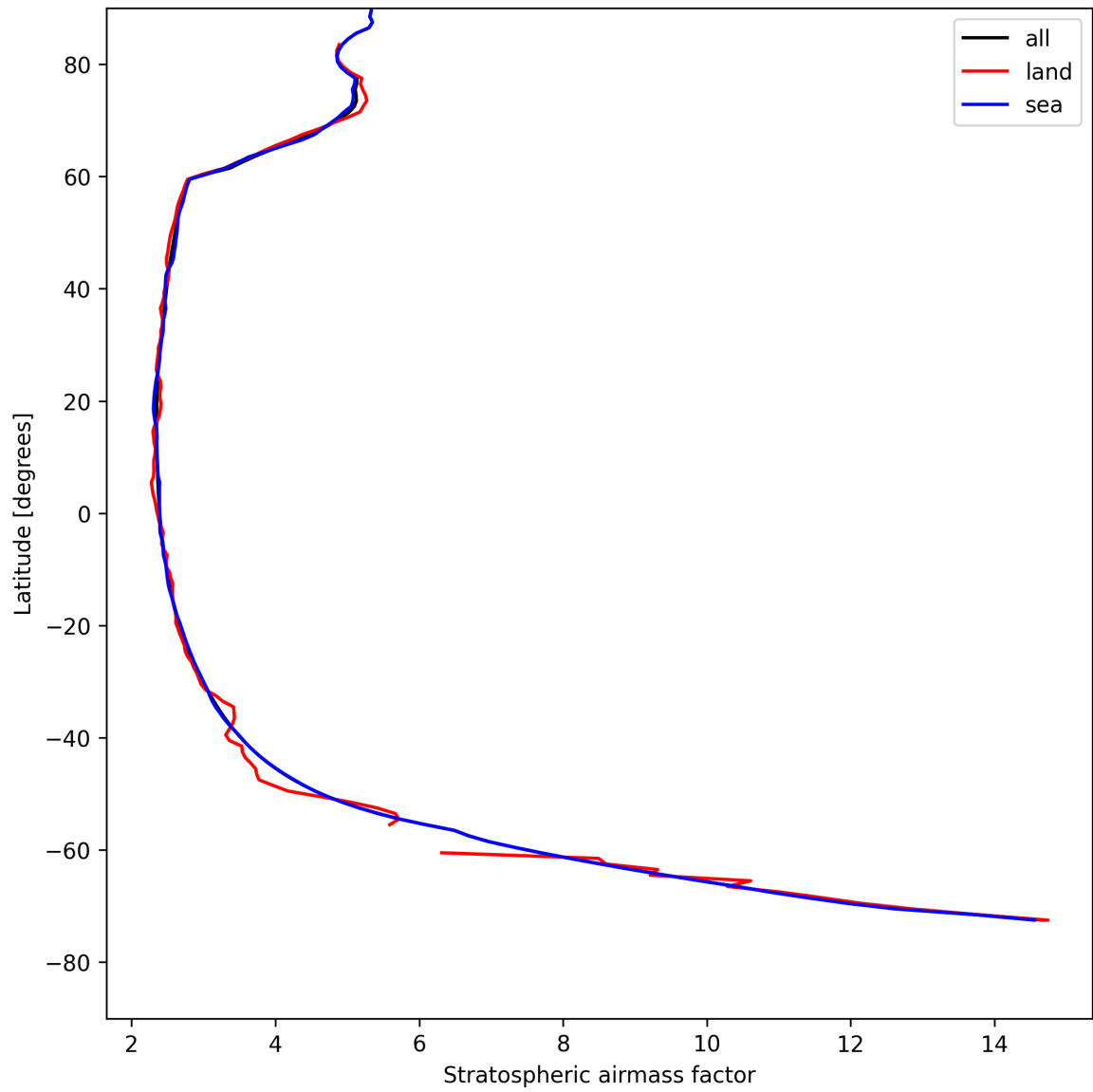
Figure 27: Zonal average of “Stratospheric air mass factor” for 2025-04-30 to 2025-05-01.
