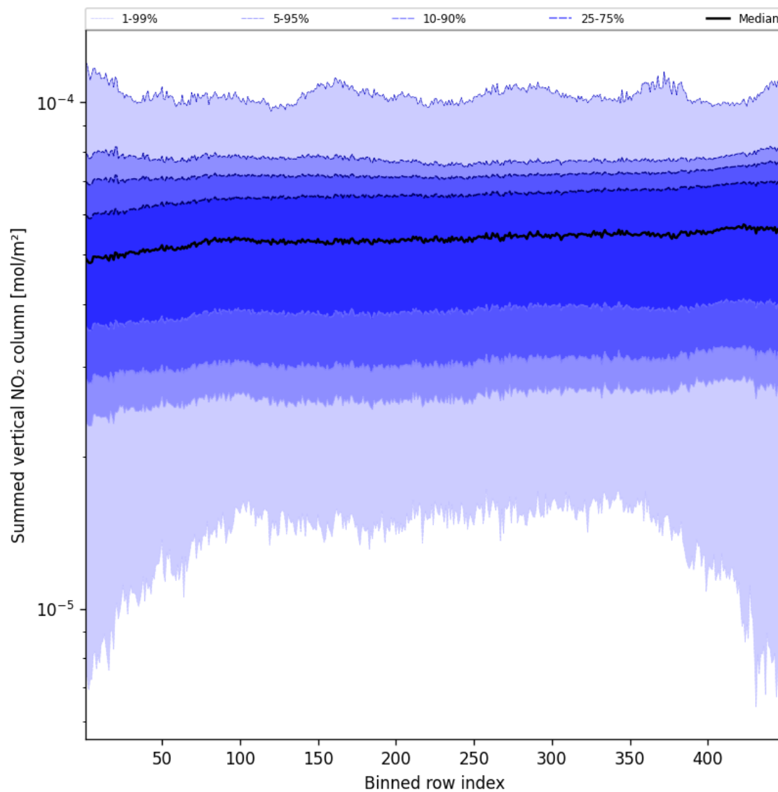
Figure 57: Along track statistics of “Summed vertical NO 2 column” for 2025-04-30 to 2025-05-01
