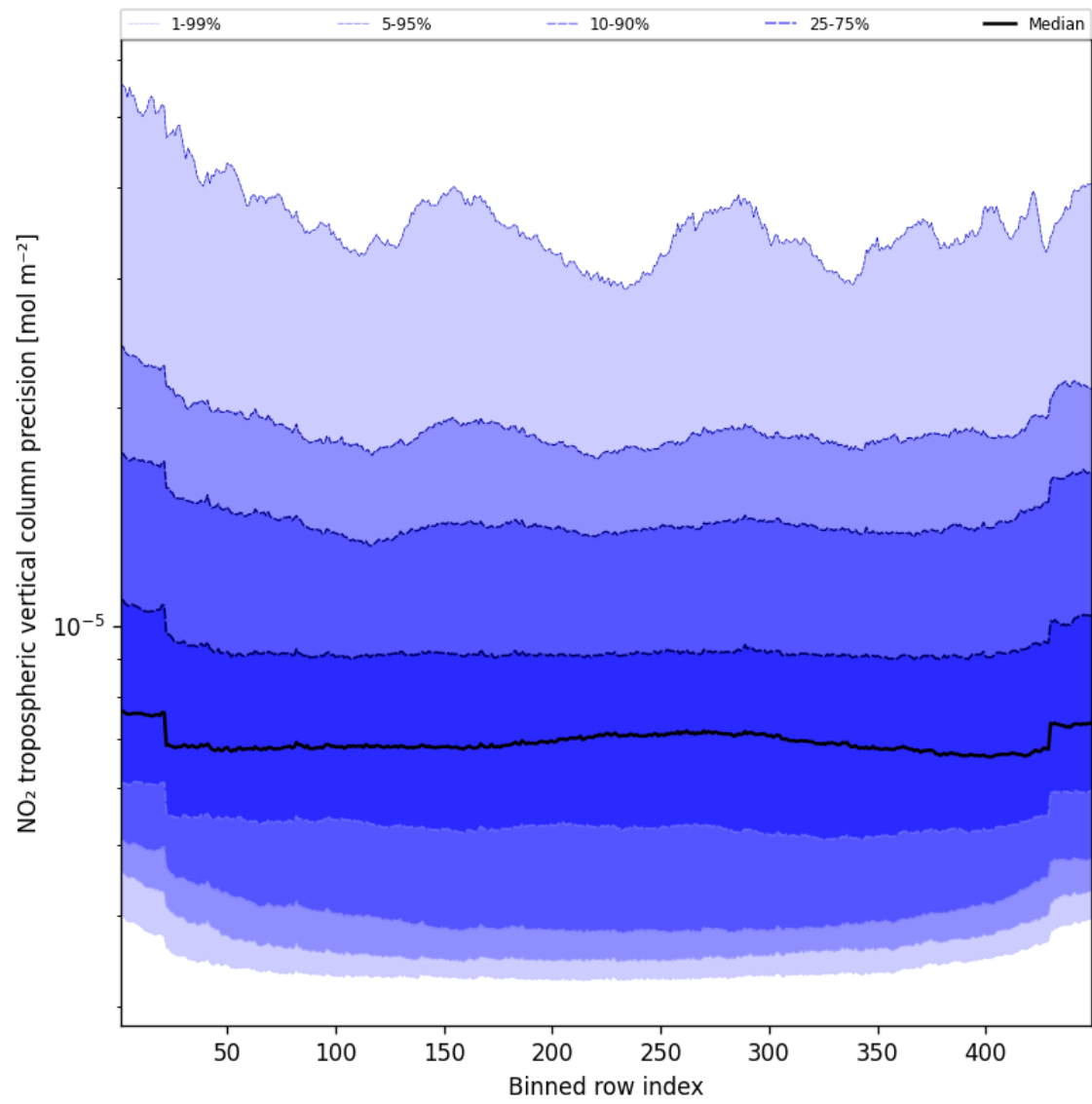
Figure 47: Along track statistics of “NO 2 tropospheric vertical column precision” for 2025-04-30 to 2025-05-01
