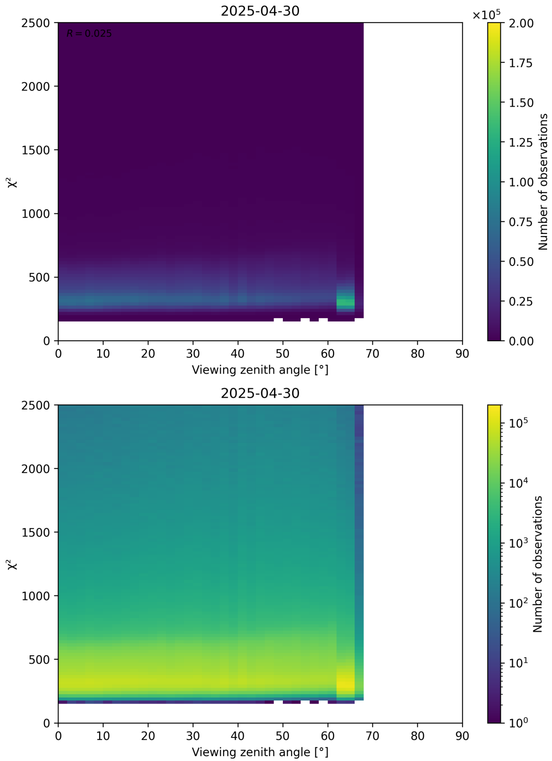
Figure 162: Scatter density plot of “Viewing zenith angle” against “ \chi^2 ” for 2025-04-30 to 2025-05-01.
