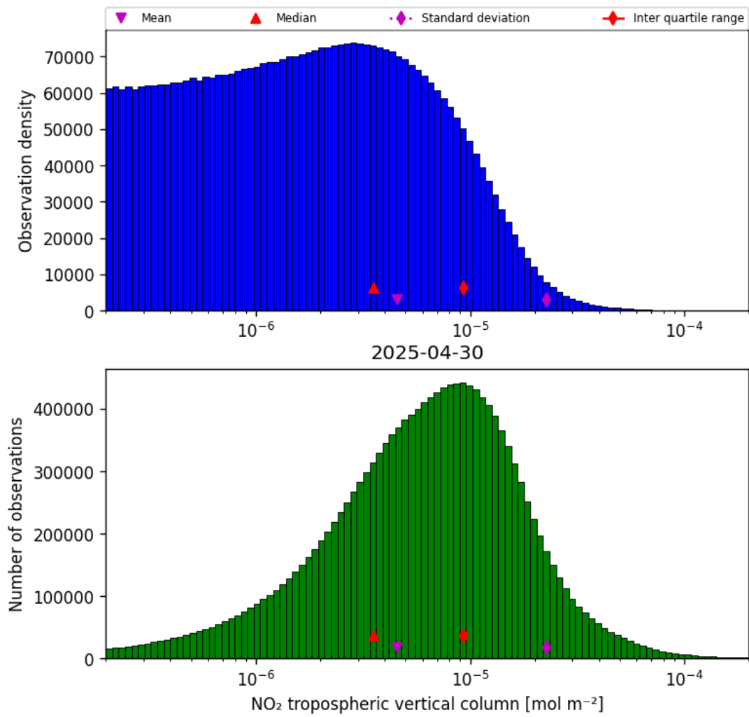
Figure 29: Histogram of “NO 2 tropospheric vertical column” for 2025-04-30 to 2025-05-01
