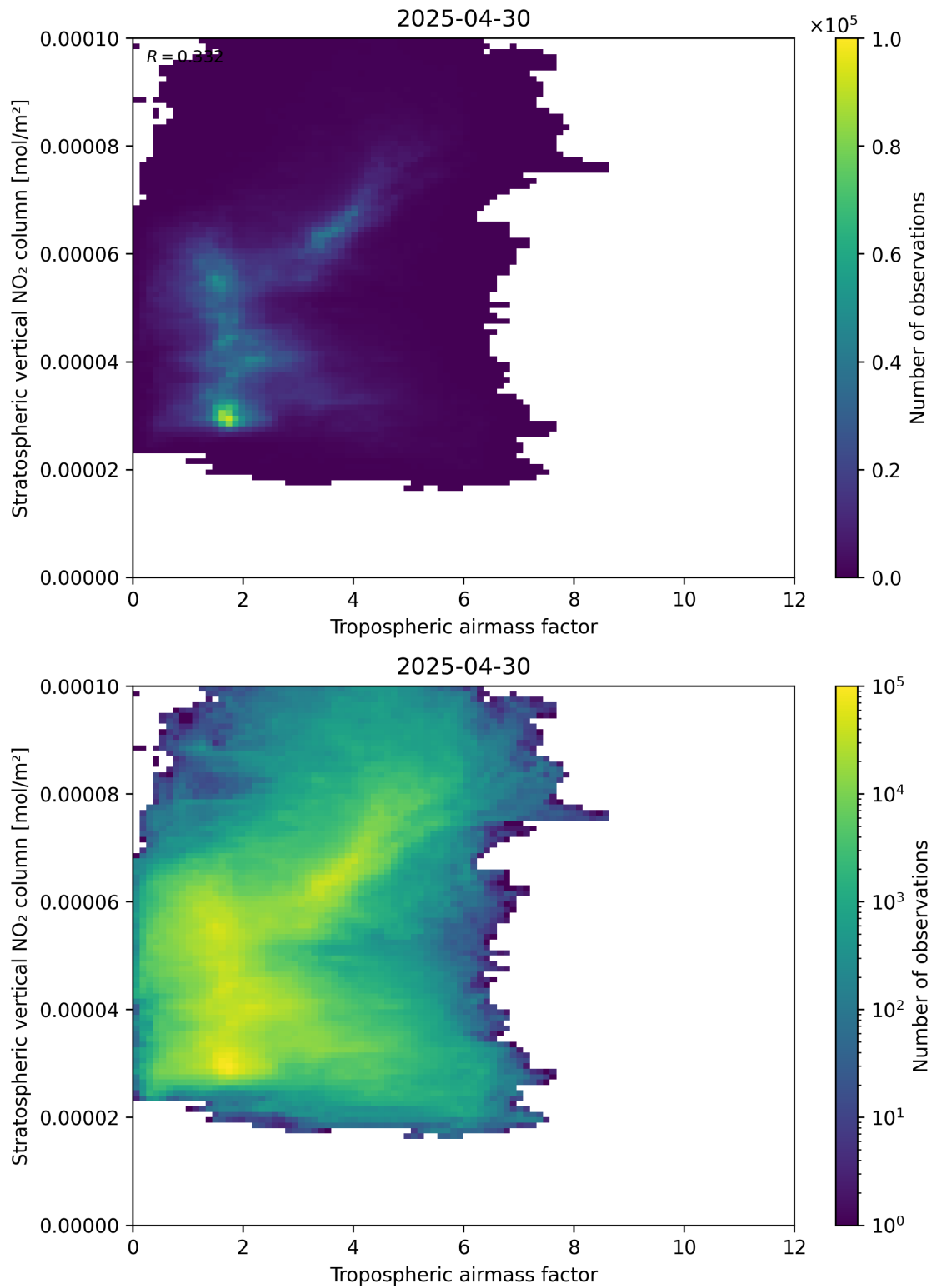
Figure 74: Scatter density plot of “Tropospheric airmass factor” against “Stratospheric vertical NO 2 column” for 2025-04-30 to 2025-05-01.
