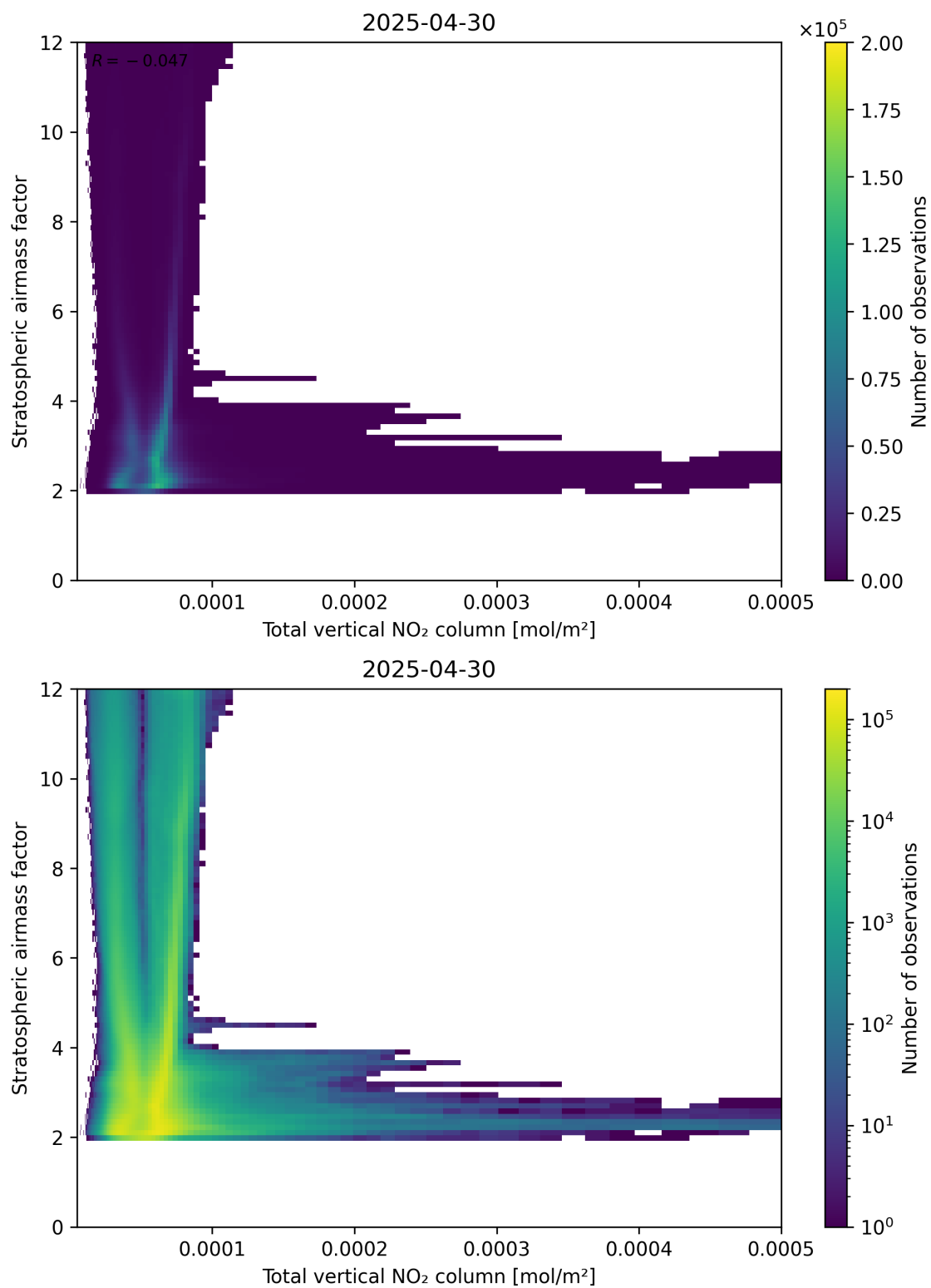
Figure 110: Scatter density plot of “Total vertical NO 2 column” against “Stratospheric airmass factor” for 2025-04-30 to 2025-05-01.
