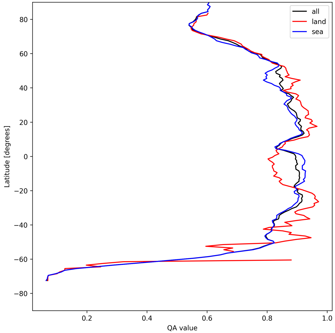
Figure 11: Zonal average of “QA value” for 2025-04-30 to 2025-05-01.
