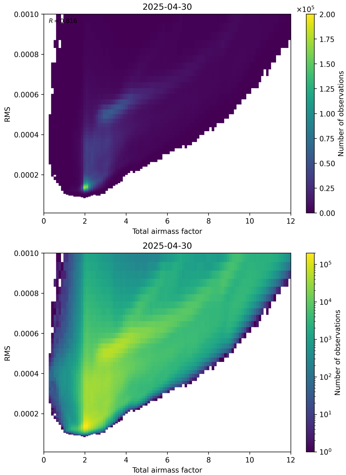
Figure 69: Scatter density plot of “Total airmass factor” against “RMS” for 2025-04-30 to 2025-05-01.
