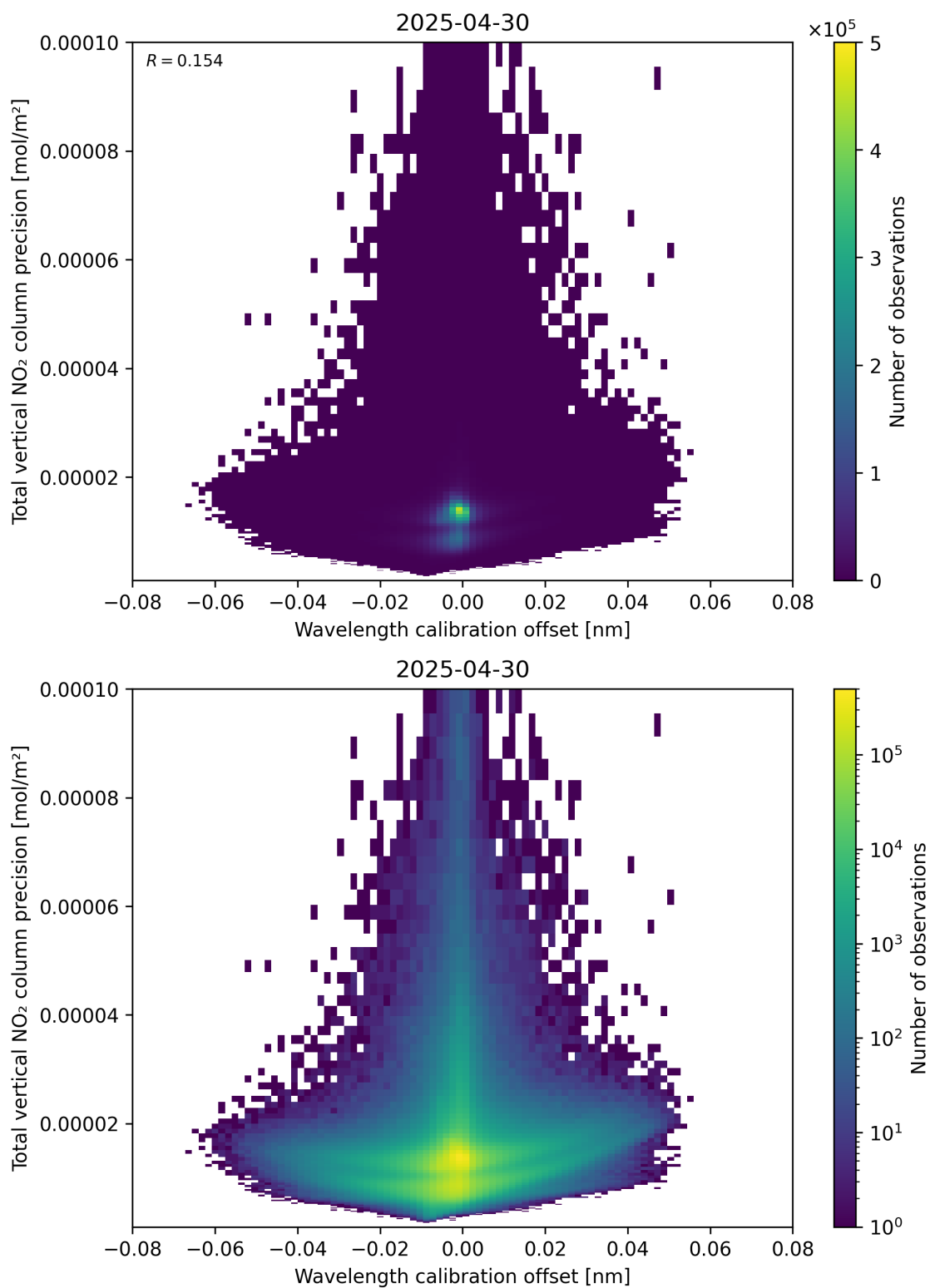
Figure 180: Scatter density plot of “Wavelength calibration offset” against “Total vertical NO 2 column precision” for 2025-04-30 to 2025-05-01.
