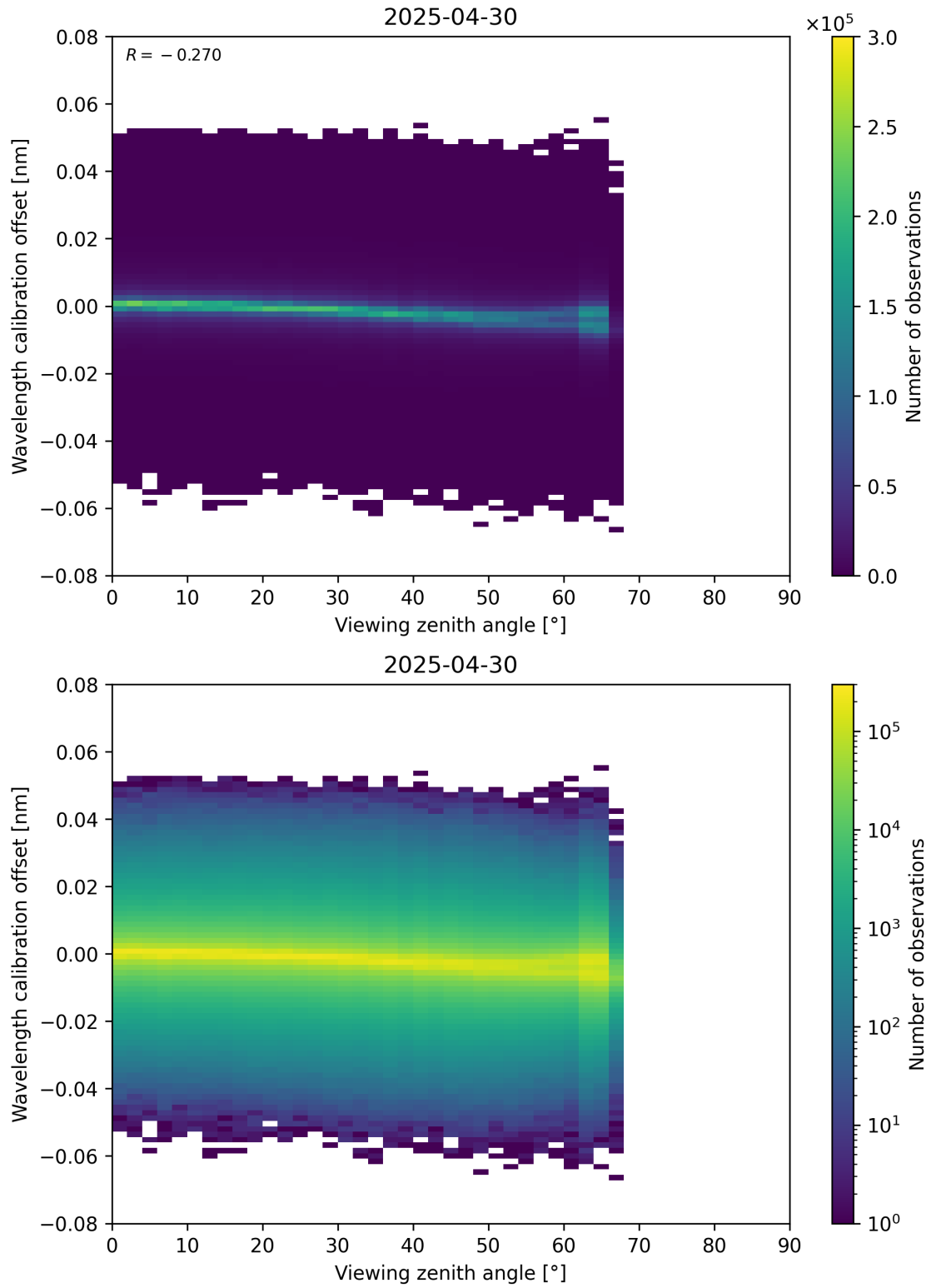
Figure 173: Scatter density plot of “Viewing zenith angle” against “Wavelength calibration offset” for 2025-04-30 to 2025-05-01.
