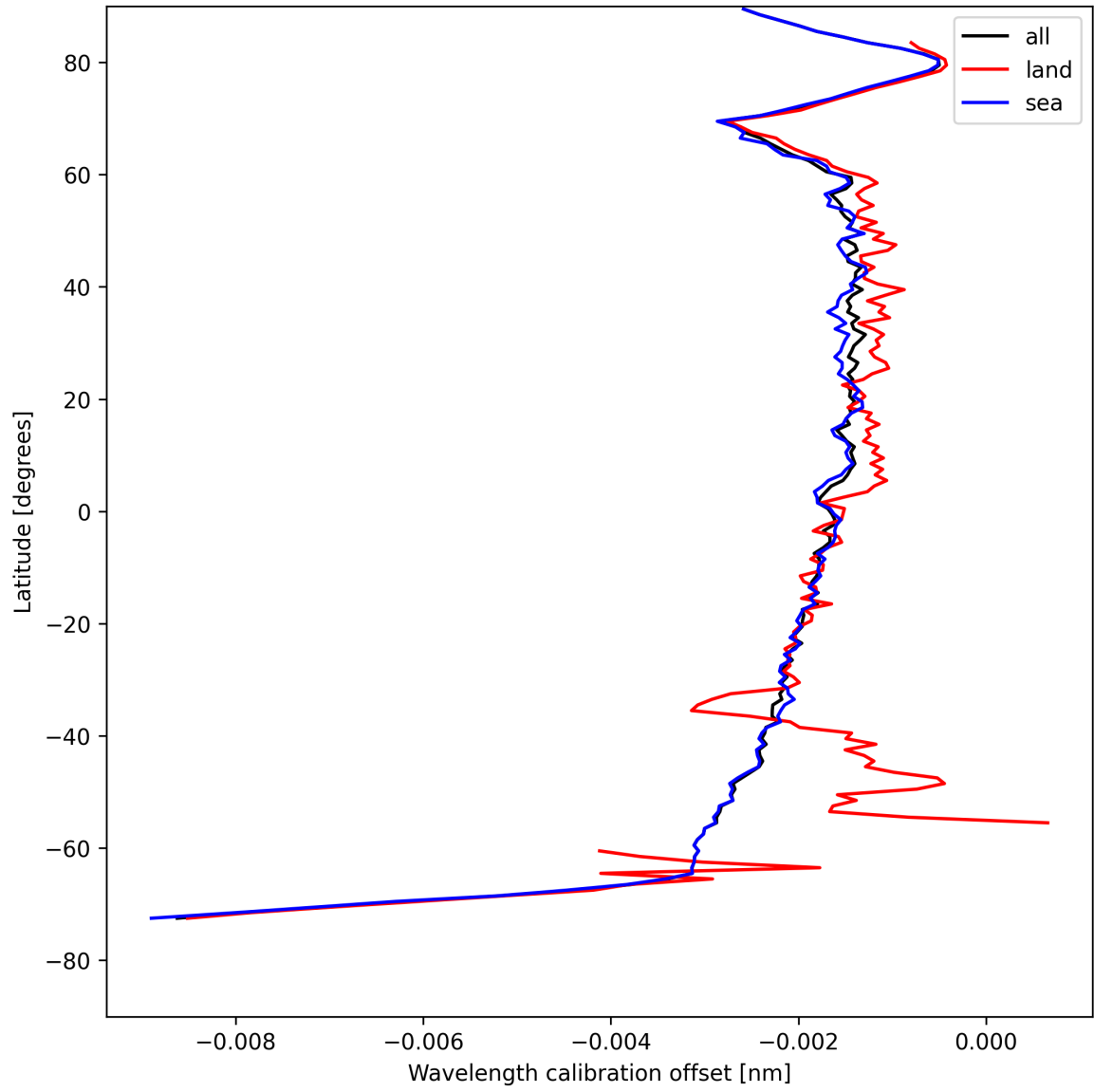
Figure 18: Zonal average of “Wavelength calibration offset” for 2025-04-30 to 2025-05-01.
