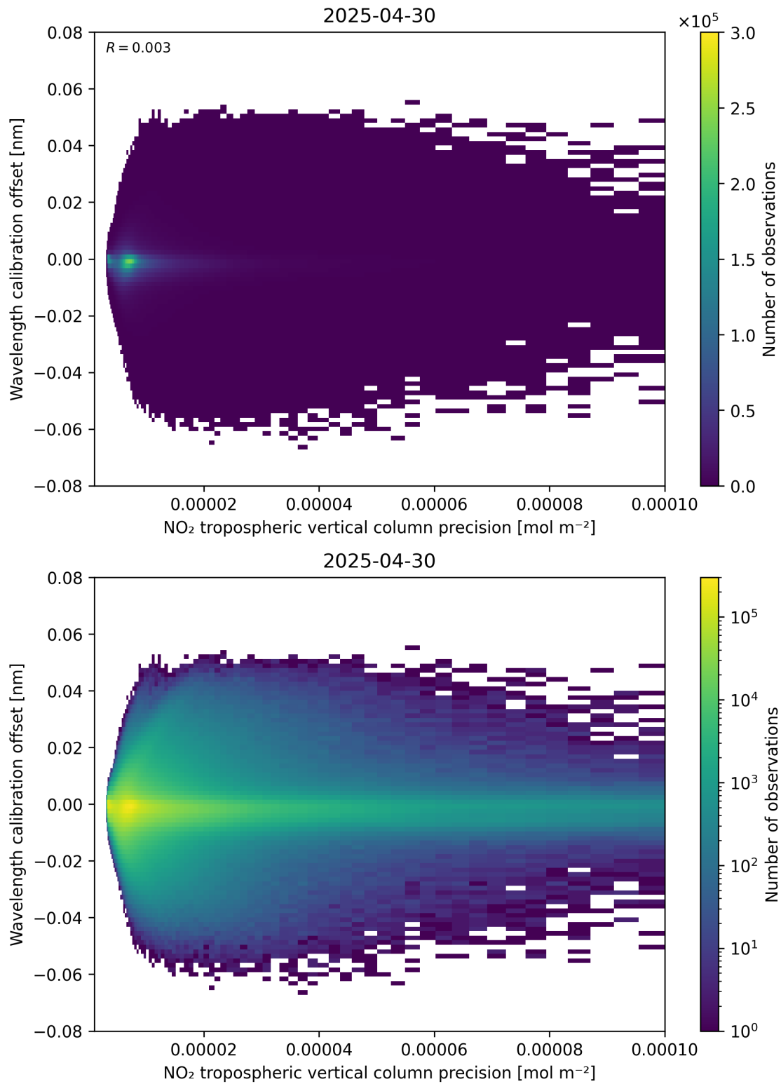
Figure 141: Scatter density plot of “NO 2 tropospheric vertical column precision” against “Wavelength calibration offset” for 2025-04-30 to 2025-05-01.
