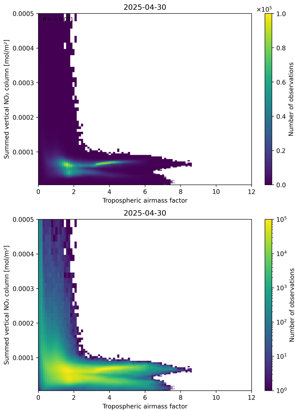
Figure 75: Scatter density plot of “Tropospheric air mass factor” against “Summed vertical NO 2 column” for 2025-04-30 to 2025-05-01.
