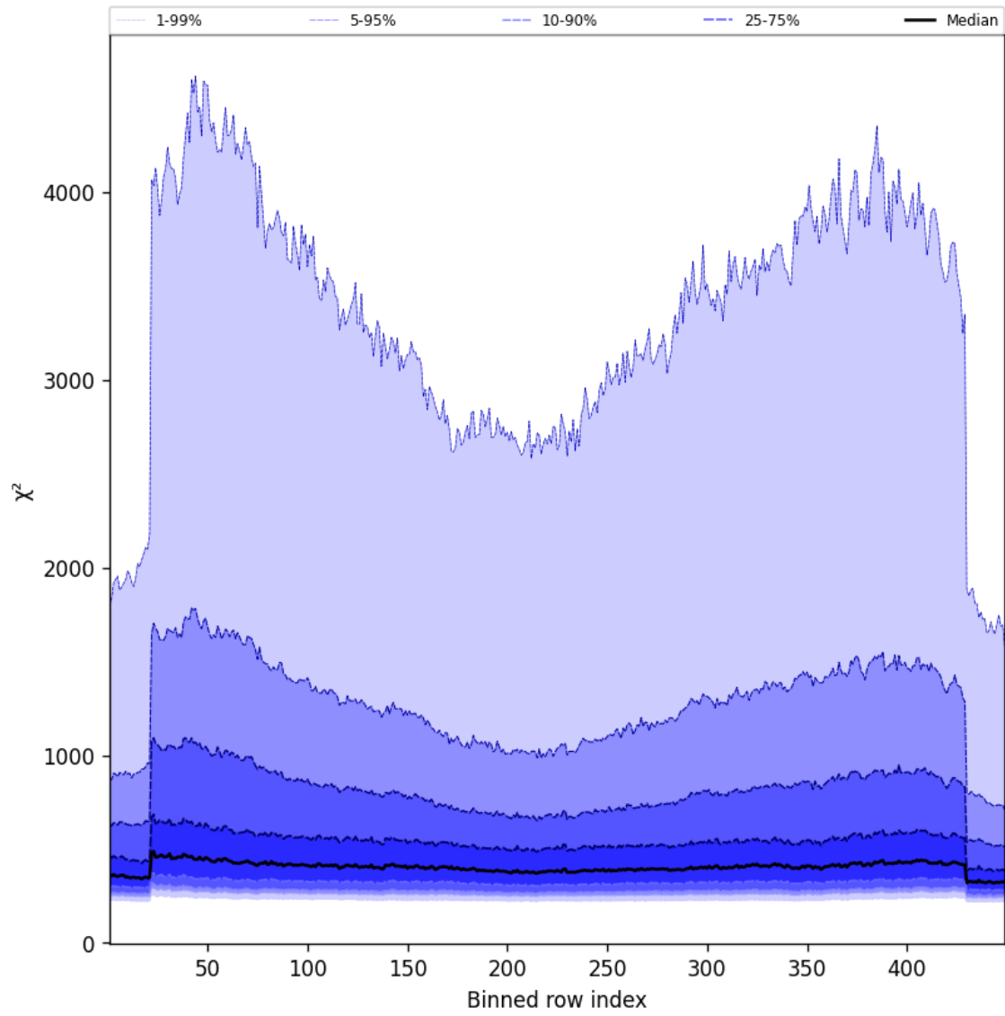
Figure 59: Along track statistics of “ \chi^2 ” for 2025-04-30 to 2025-05-01
