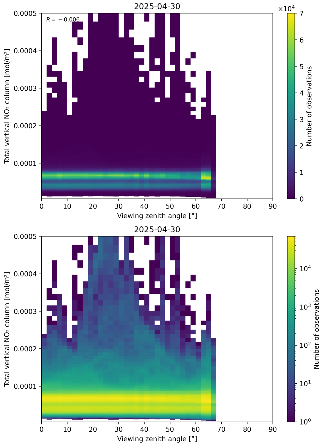
Figure 167: Scatter density plot of “Viewing zenith angle” against “Total vertical NO 2 column” for 2025-04-30 to 2025-05-01.
