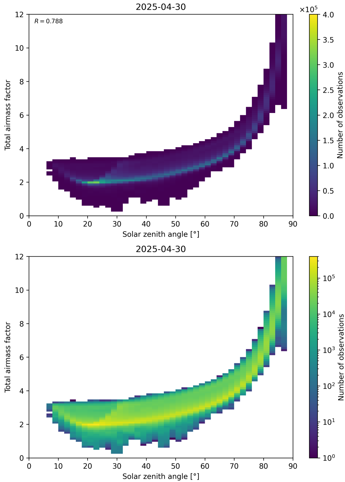
Figure 146: Scatter density plot of “Solar zenith angle” against “Total air mass factor” for 2025-04-30 to 2025-05-01.
