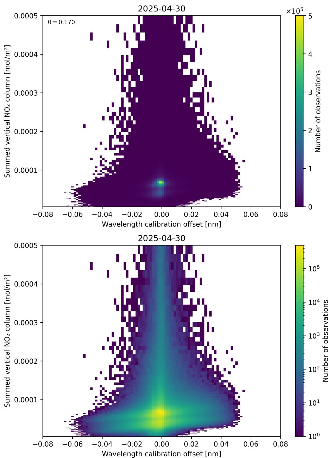
Figure 177: Scatter density plot of “Wavelength calibration offset” against “Summed vertical NO 2 column” for 2025-04-30 to 2025-05-01.
