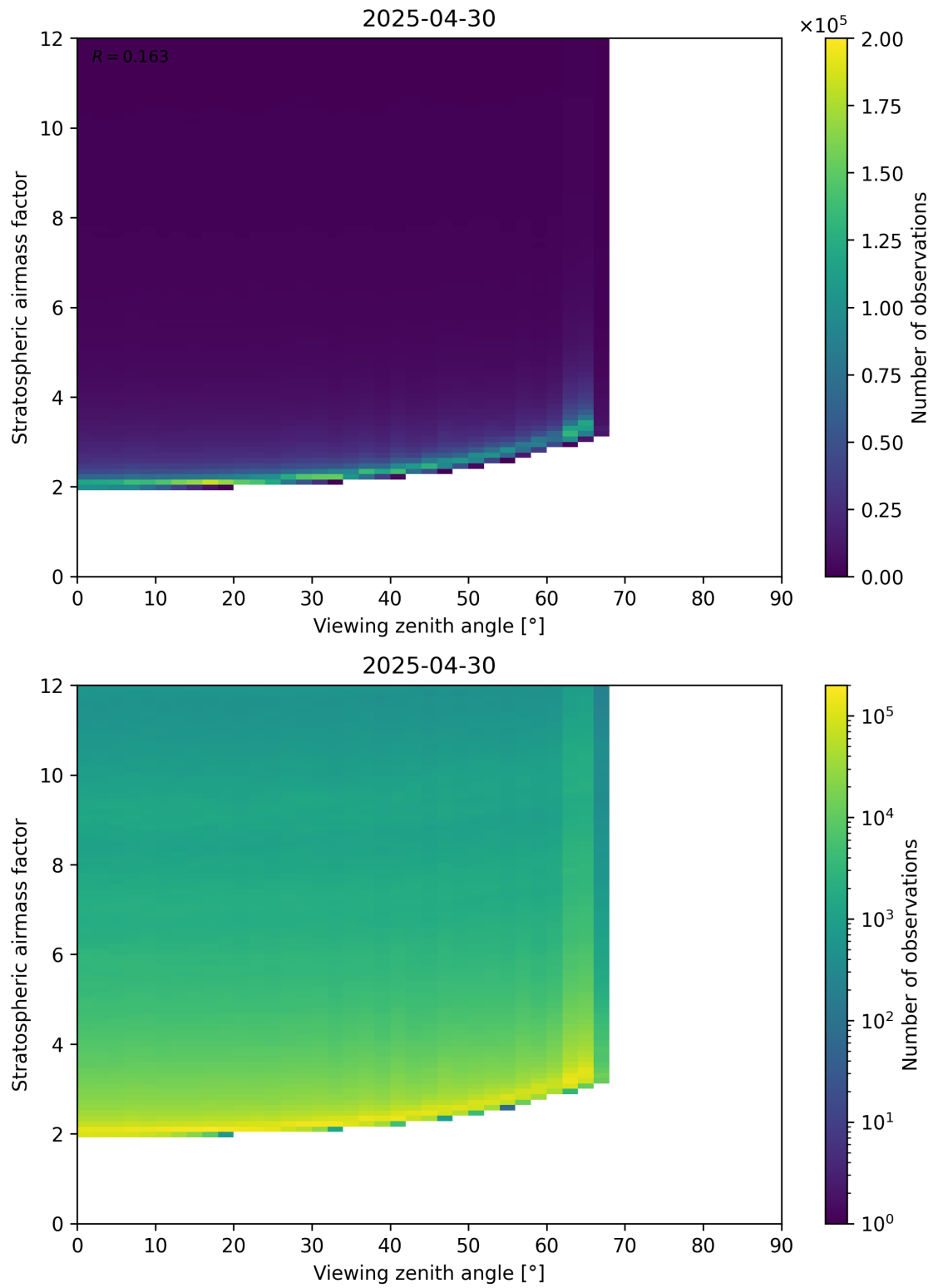
Figure 159: Scatter density plot of “Viewing zenith angle” against “Stratospheric airmass factor” for 2025-04-30 to 2025-05-01.
