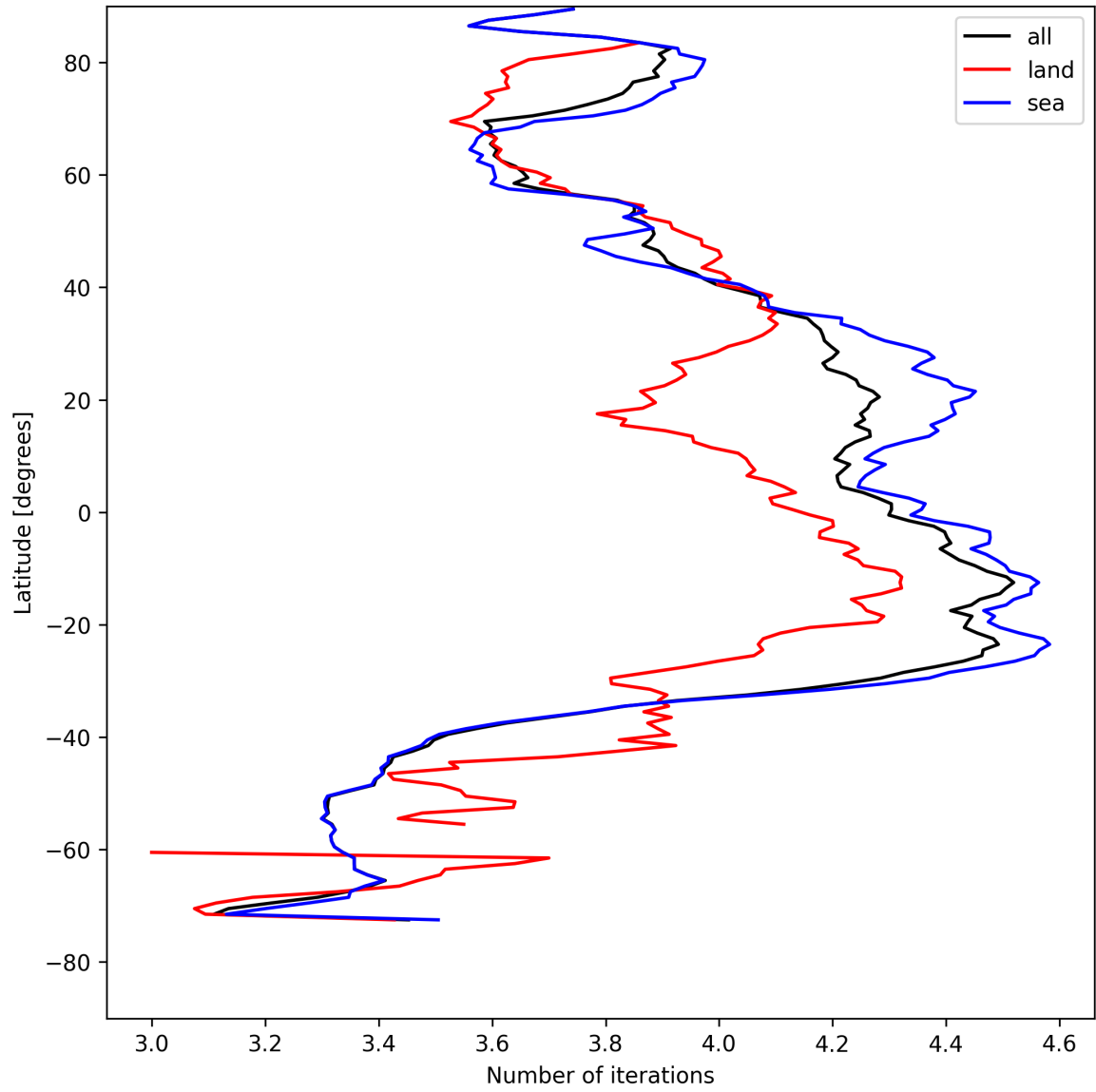
Figure 17: Zonal average of “Number of iterations” for 2025-04-30 to 2025-05-01.
