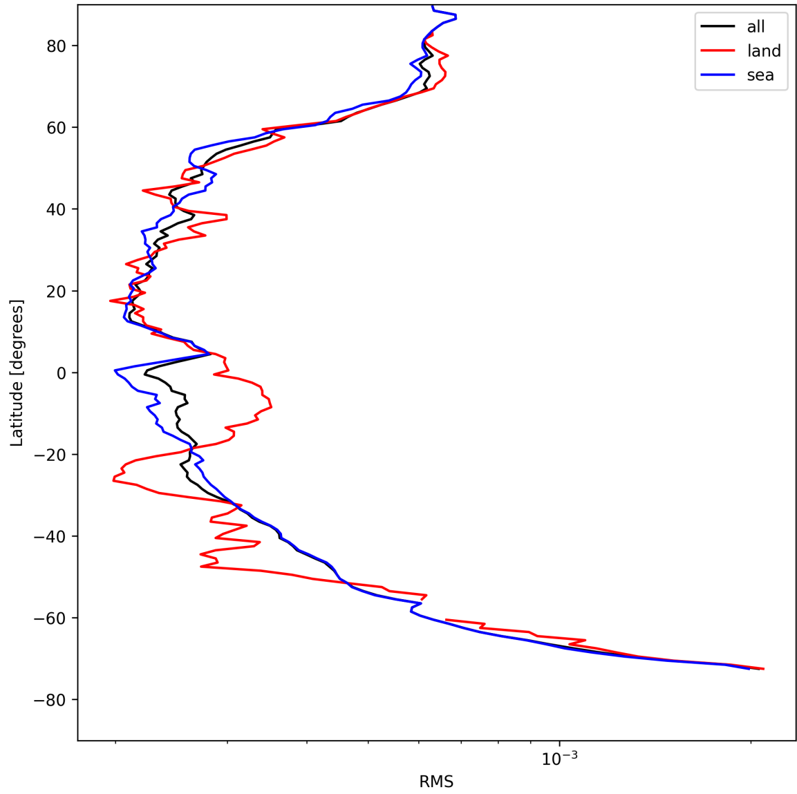
Figure 26: Zonal average of “RMS” for 2025-04-30 to 2025-05-01.
