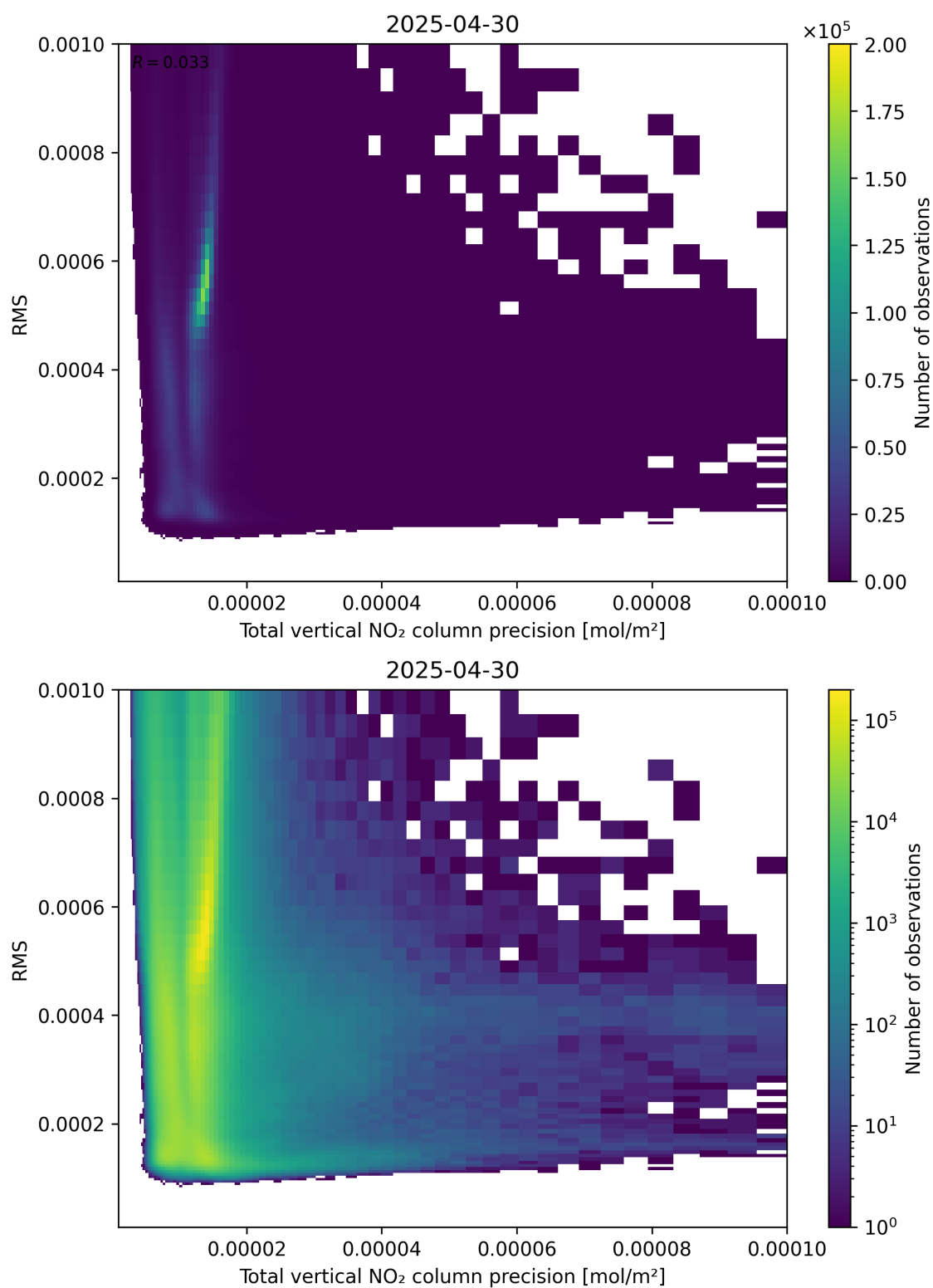
Figure 119: Scatter density plot of “Total vertical NO 2 column precision” against “RMS” for 2025-04-30 to 2025-05-01.
