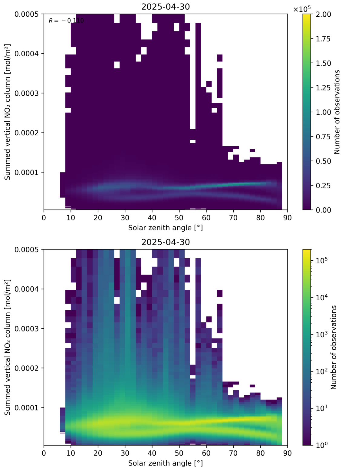
Figure 151: Scatter density plot of “Solar zenith angle” against “Summed vertical NO 2 column” for 2025-04-30 to 2025-05-01.
