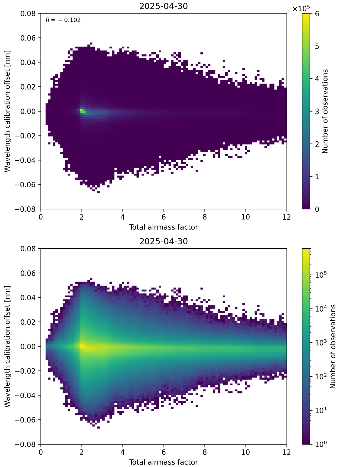
Figure 70: Scatter density plot of “Total airmass factor” against “Wavelength calibration offset” for 2025-04-30 to 2025-05-01.
