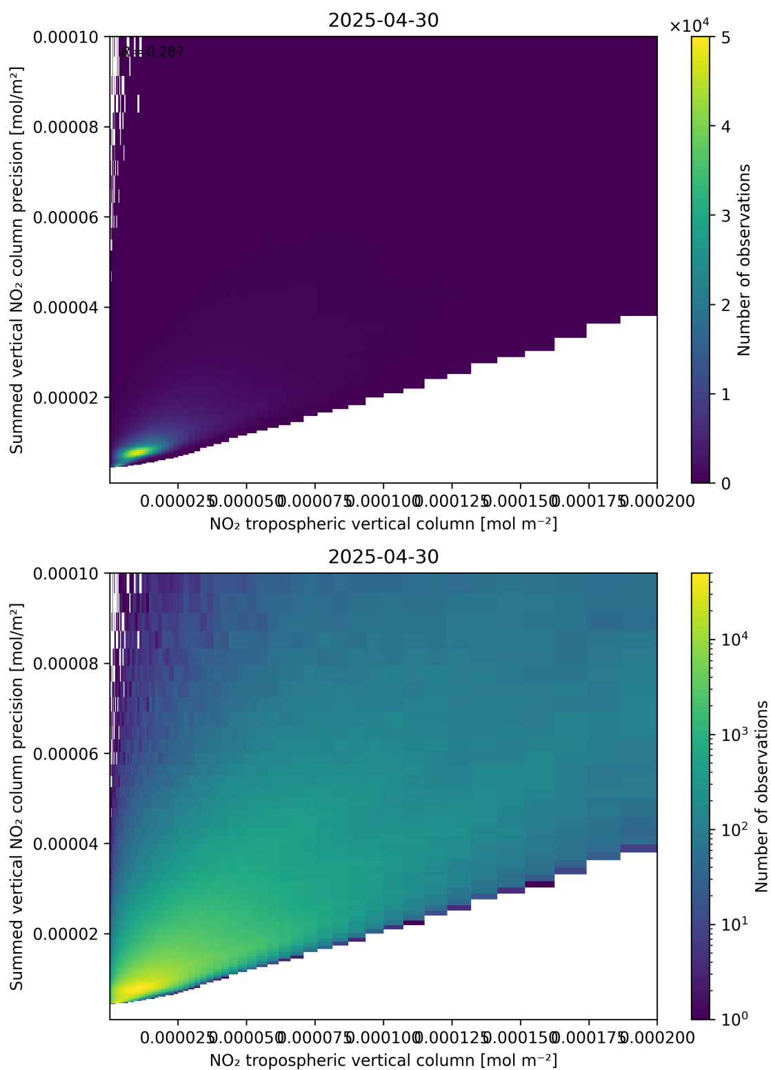
Figure 127: Scatter density plot of “NO 2 tropospheric vertical column” against “Summed vertical NO 2 column precision” for 2025-04-30 to 2025-05-01.
