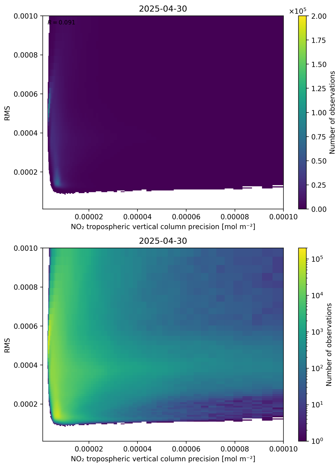
Figure 140: Scatter density plot of “NO 2 tropospheric vertical column precision” against “RMS” for 2025-04-30 to 2025-05-01.
