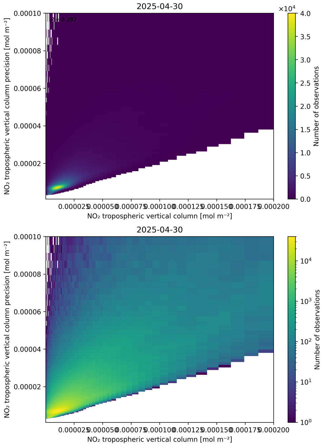
Figure 130: Scatter density plot of “NO 2 tropospheric vertical column” against “NO 2 tropospheric vertical column precision” for 2025-04-30 to 2025-05-01.
