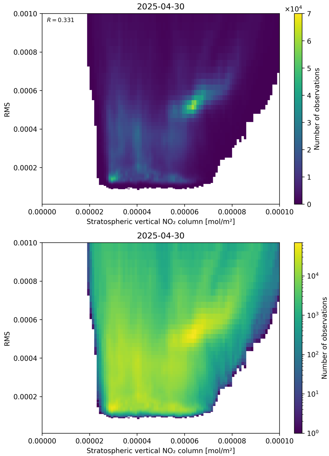
Figure 102: Scatter density plot of “Stratospheric vertical NO 2 column” against “RMS” for 2025-04-30 to 2025-05-01.
