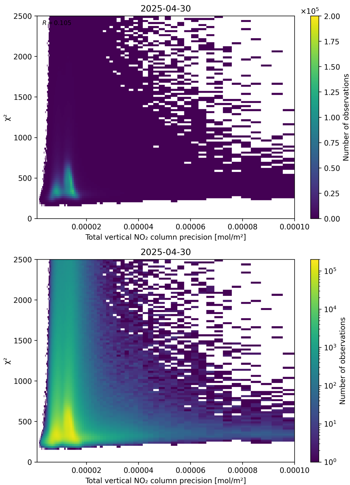
Figure 116: Scatter density plot of “Total vertical NO 2 column precision” against “ \chi^2 ” for 2025-04-30 to 2025-05-01.
