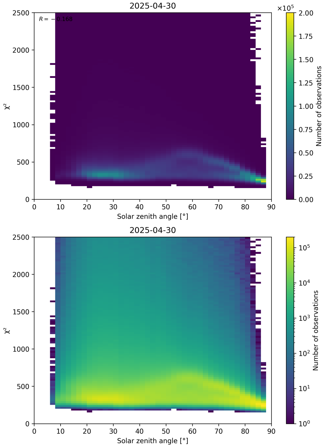
Figure 148: Scatter density plot of “Solar zenith angle” against “ \chi^2 ” for 2025-04-30 to 2025-05-01.
