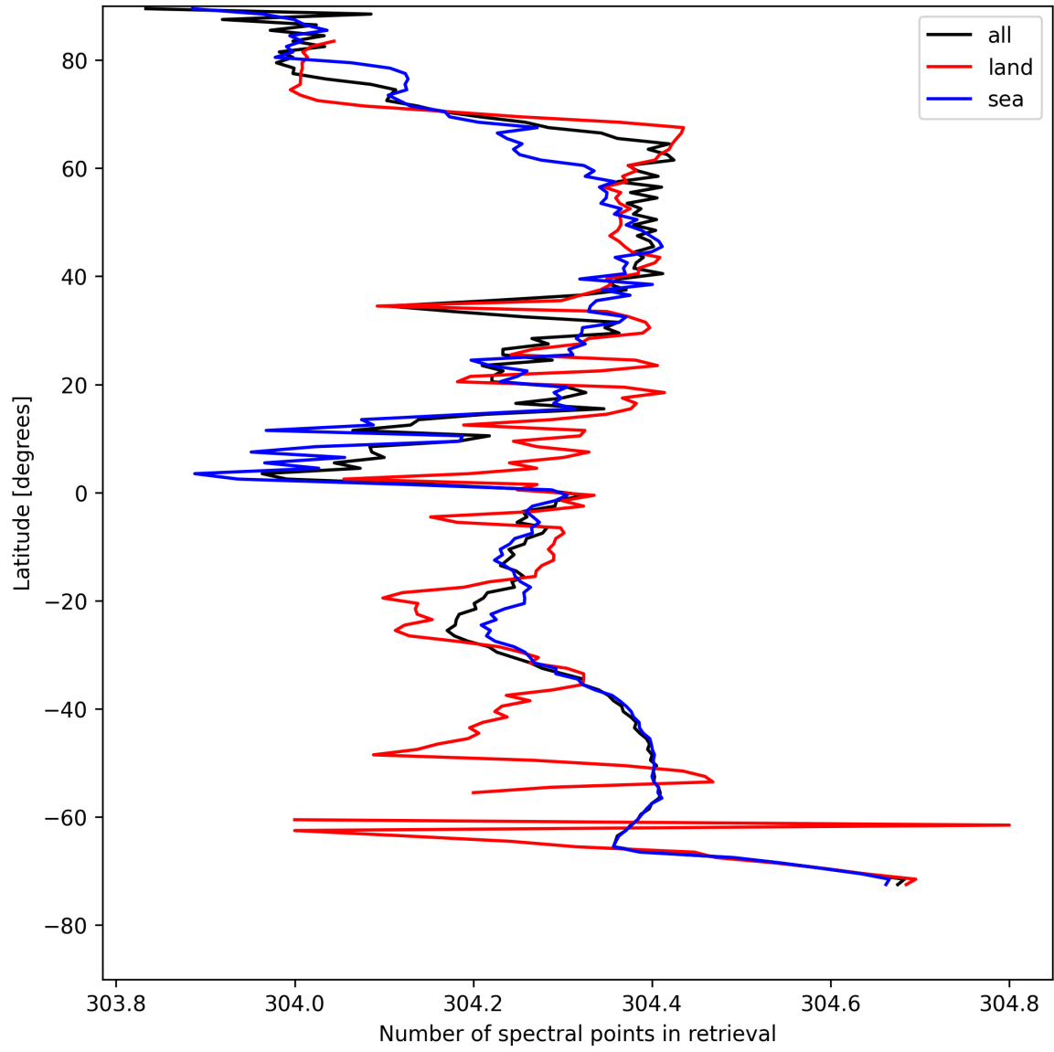
Figure 16: Zonal average of “Number of spectral points in retrieval” for 2025-04-30 to 2025-05-01.
