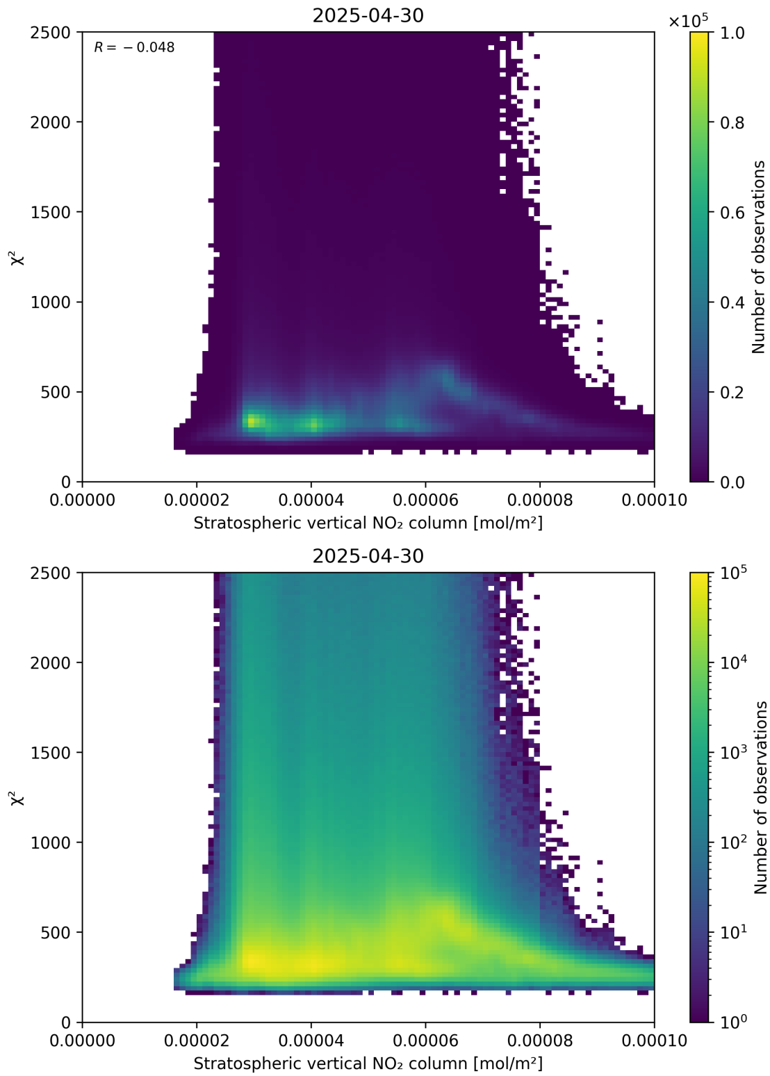
Figure 97: Scatter density plot of “Stratospheric vertical NO 2 column” against “ \chi^2 ” for 2025-04-30 to 2025-05-01.
