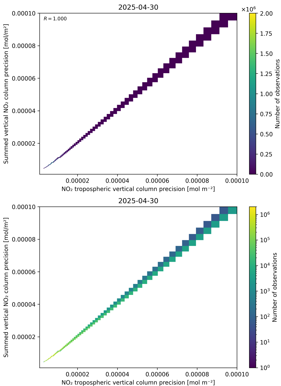
Figure 137: Scatter density plot of “NO 2 tropospheric vertical column precision” against “Summed vertical NO 2 column precision” for 2025-04-30 to 2025-05-01.
