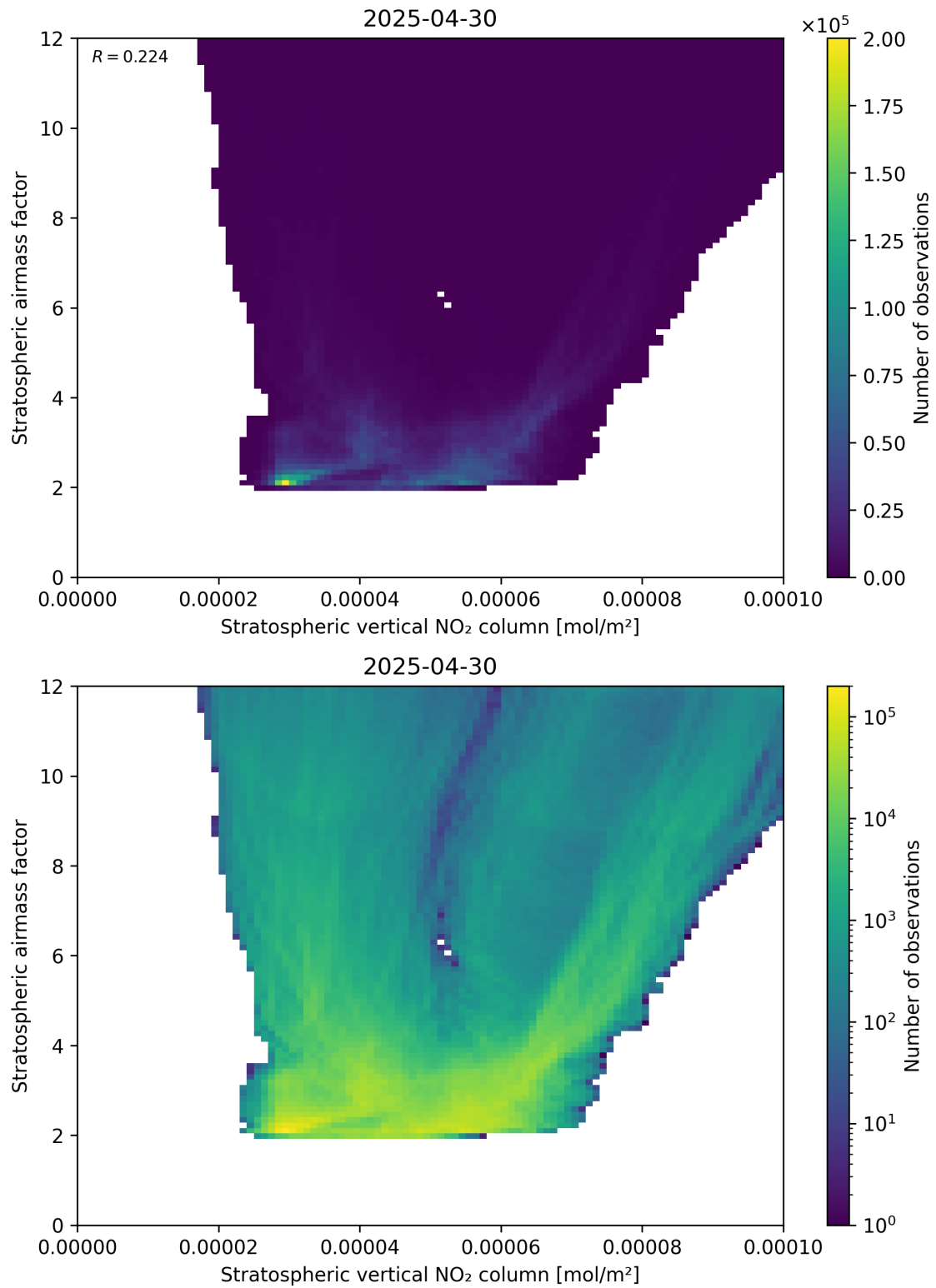
Figure 96: Scatter density plot of “Stratospheric vertical NO 2 column” against “Stratospheric airmass factor” for 2025-04-30 to 2025-05-01.
