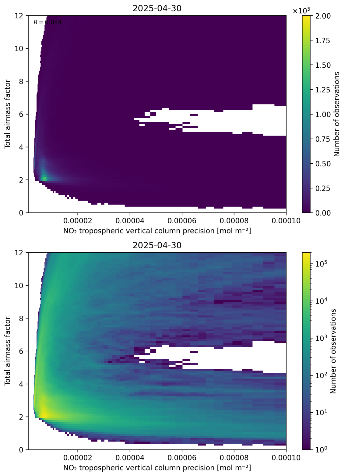
Figure 132: Scatter density plot of “NO 2 tropospheric vertical column precision” against “Total air mass factor” for 2025-04-30 to 2025-05-01.
