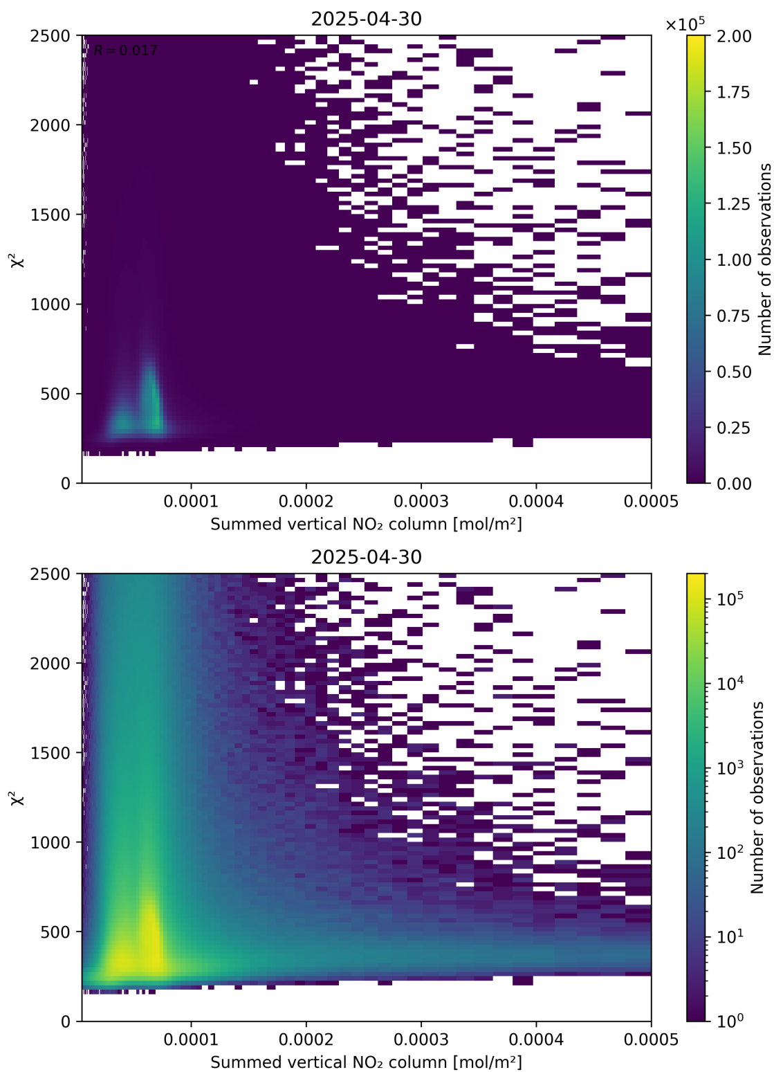
Figure 104: Scatter density plot of “Summed vertical NO 2 column” against “ \chi^2 ” for 2025-04-30 to 2025-05-01.
