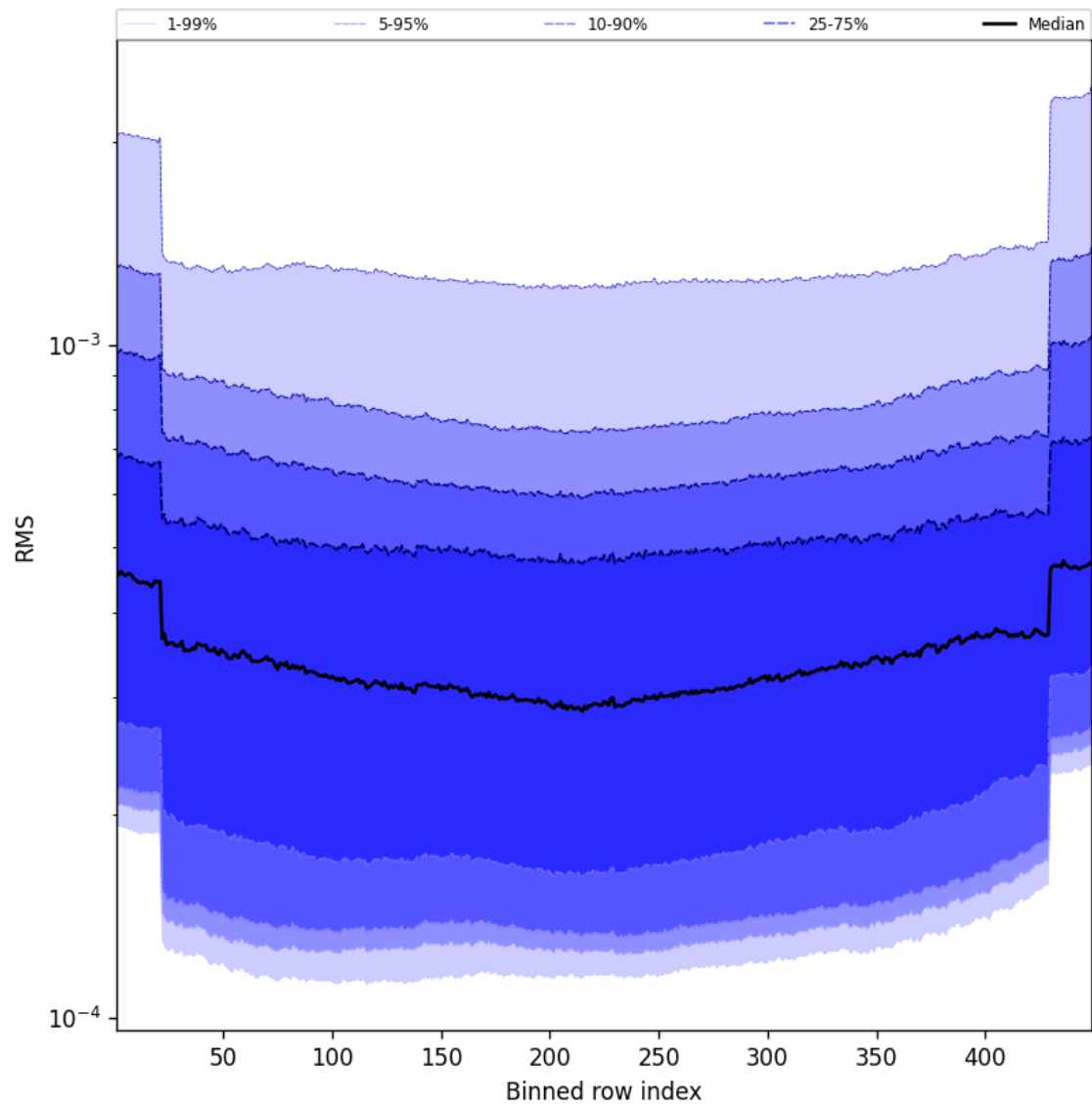
Figure 60: Along track statistics of “RMS” for 2025-04-30 to 2025-05-01
