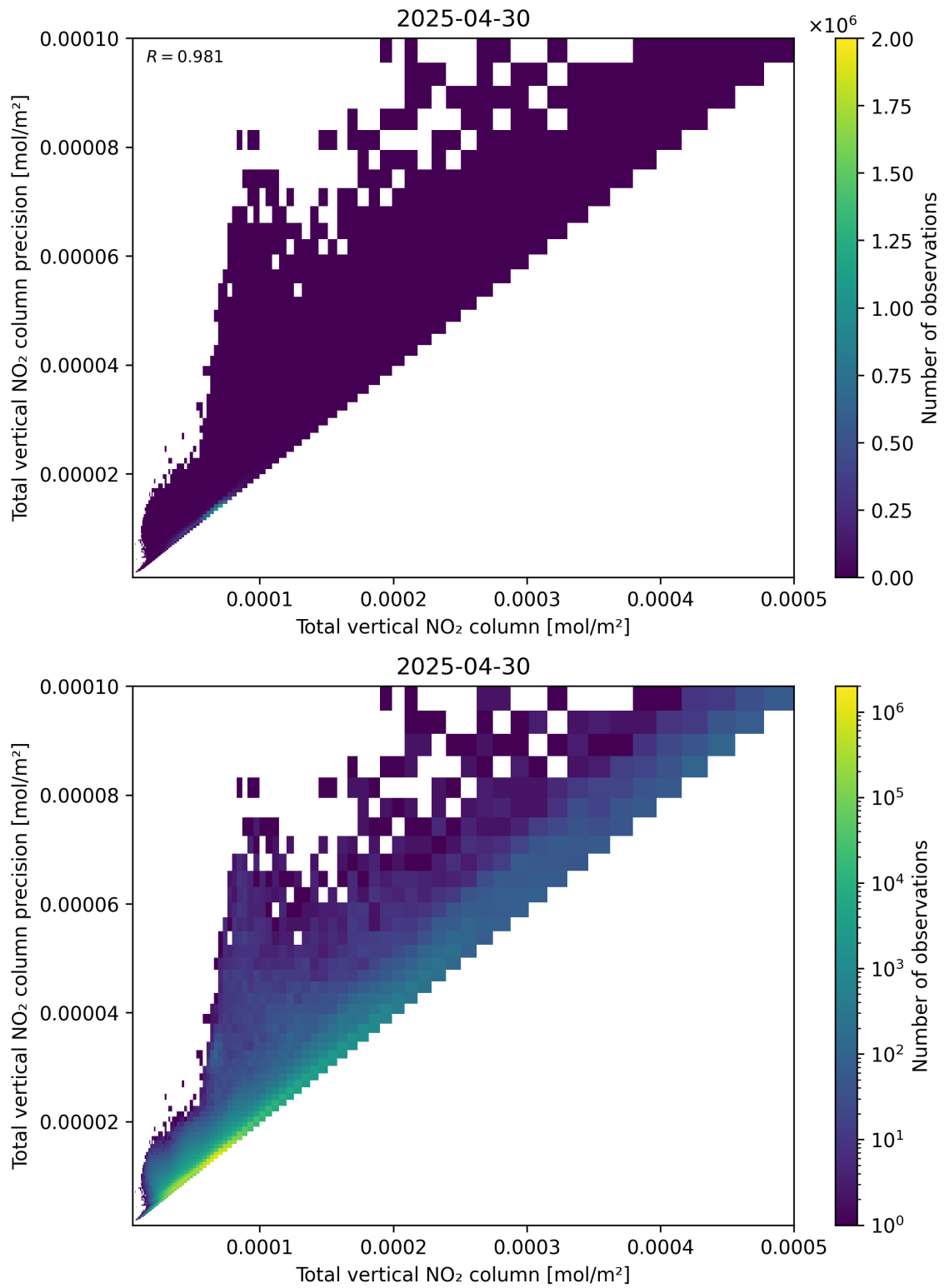
Figure 114: Scatter density plot of “Total vertical NO 2 column” against “Total vertical NO 2 column precision” for 2025-04-30 to 2025-05-01.
