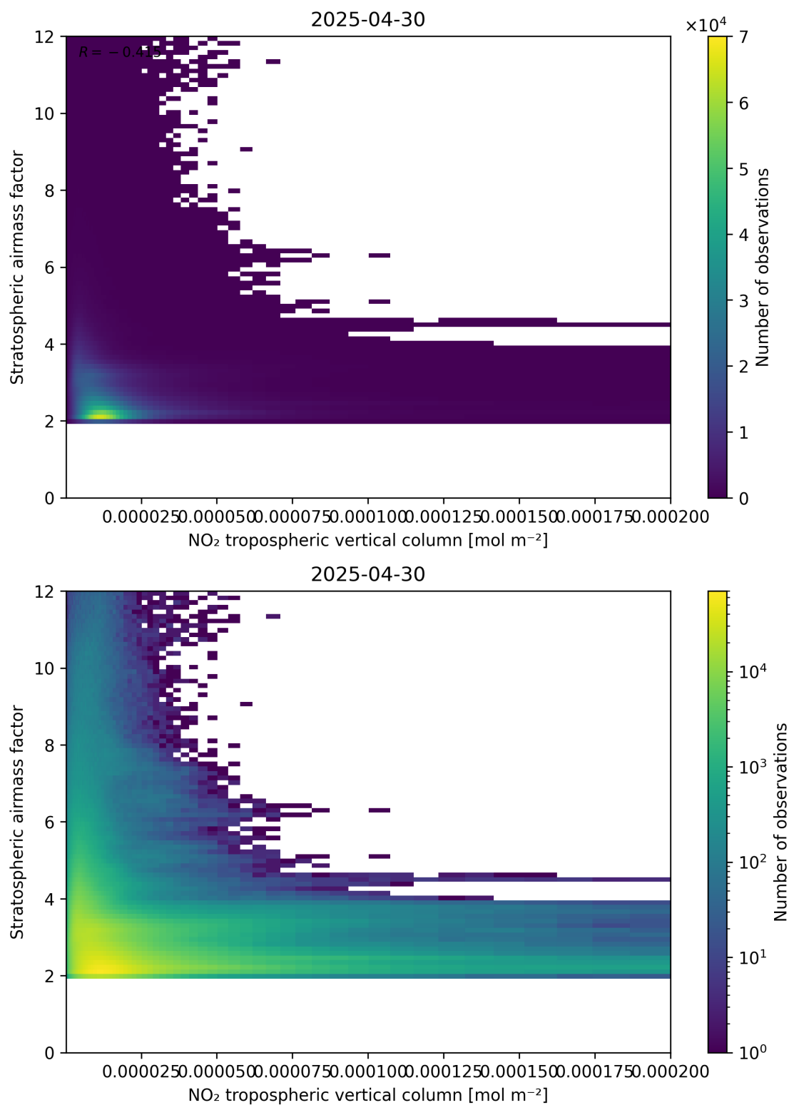
Figure 121: Scatter density plot of “NO 2 tropospheric vertical column” against “Stratospheric air mass factor” for 2025-04-30 to 2025-05-01.
