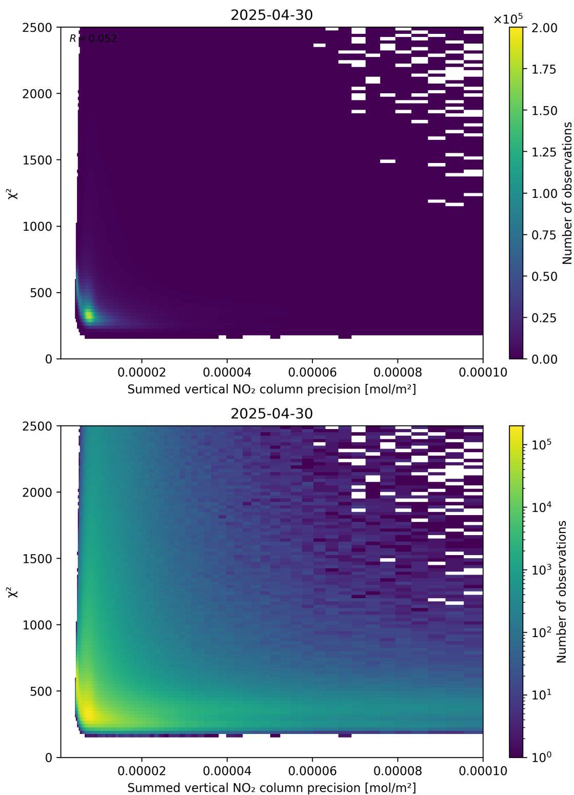
Figure 107: Scatter density plot of “Summed vertical NO 2 column precision” against “ \chi^2 ” for 2025-04-30 to 2025-05-01.
