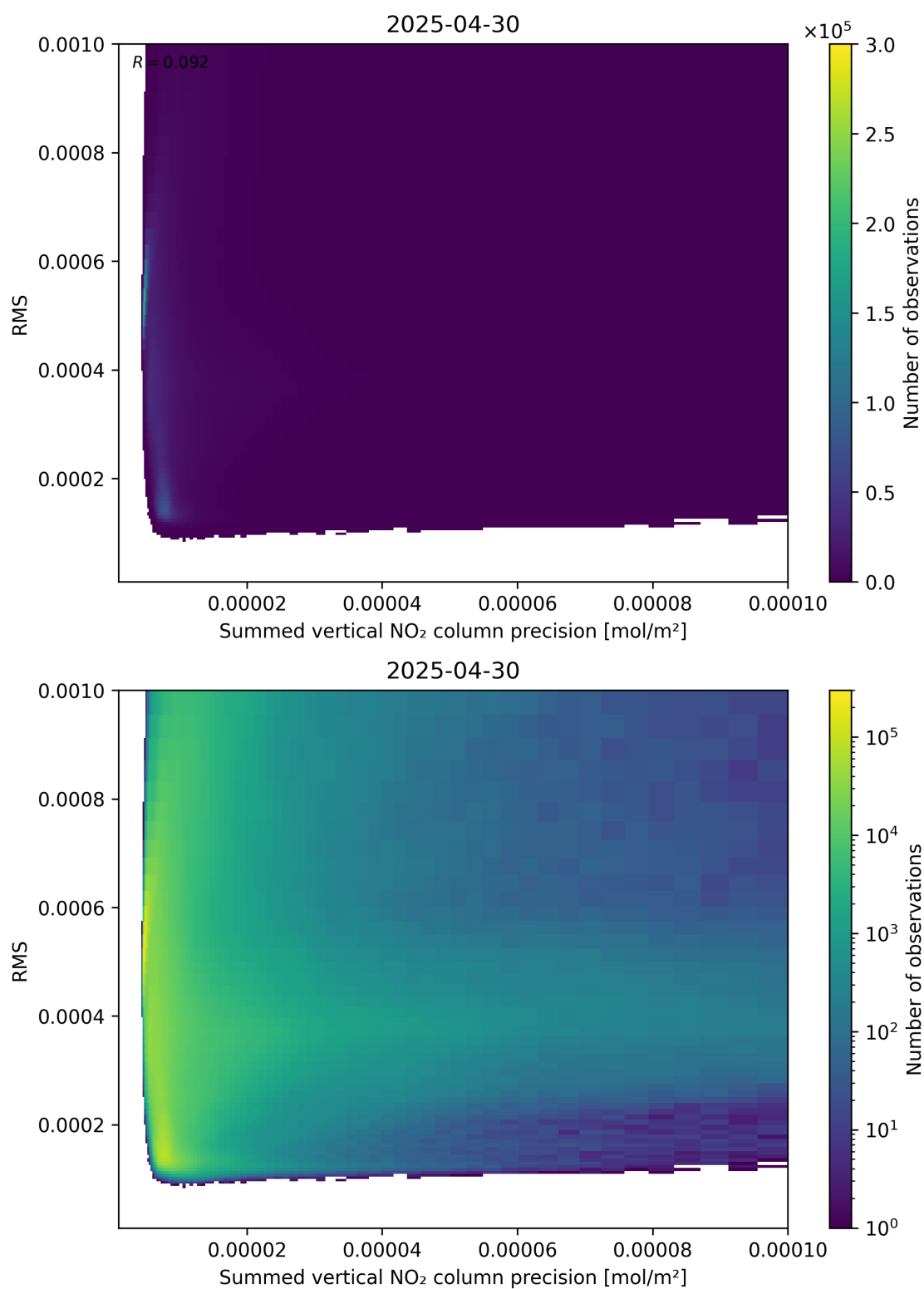
Figure 108: Scatter density plot of “Summed vertical NO 2 column precision” against “RMS” for 2025-04-30 to 2025-05-01.
