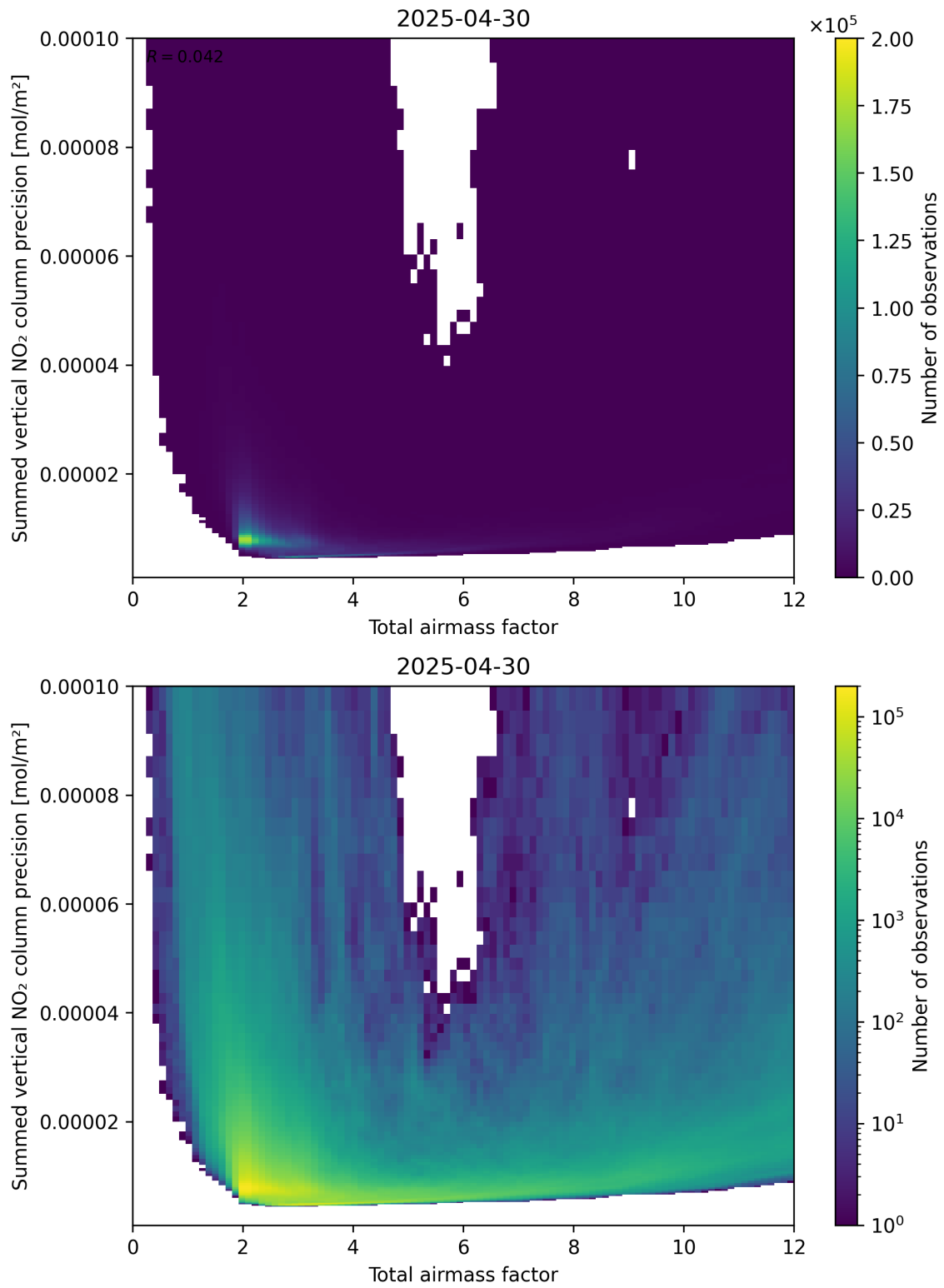
Figure 66: Scatter density plot of “Total airmass factor” against “Summed vertical NO 2 column precision” for 2025-04-30 to 2025-05-01.
