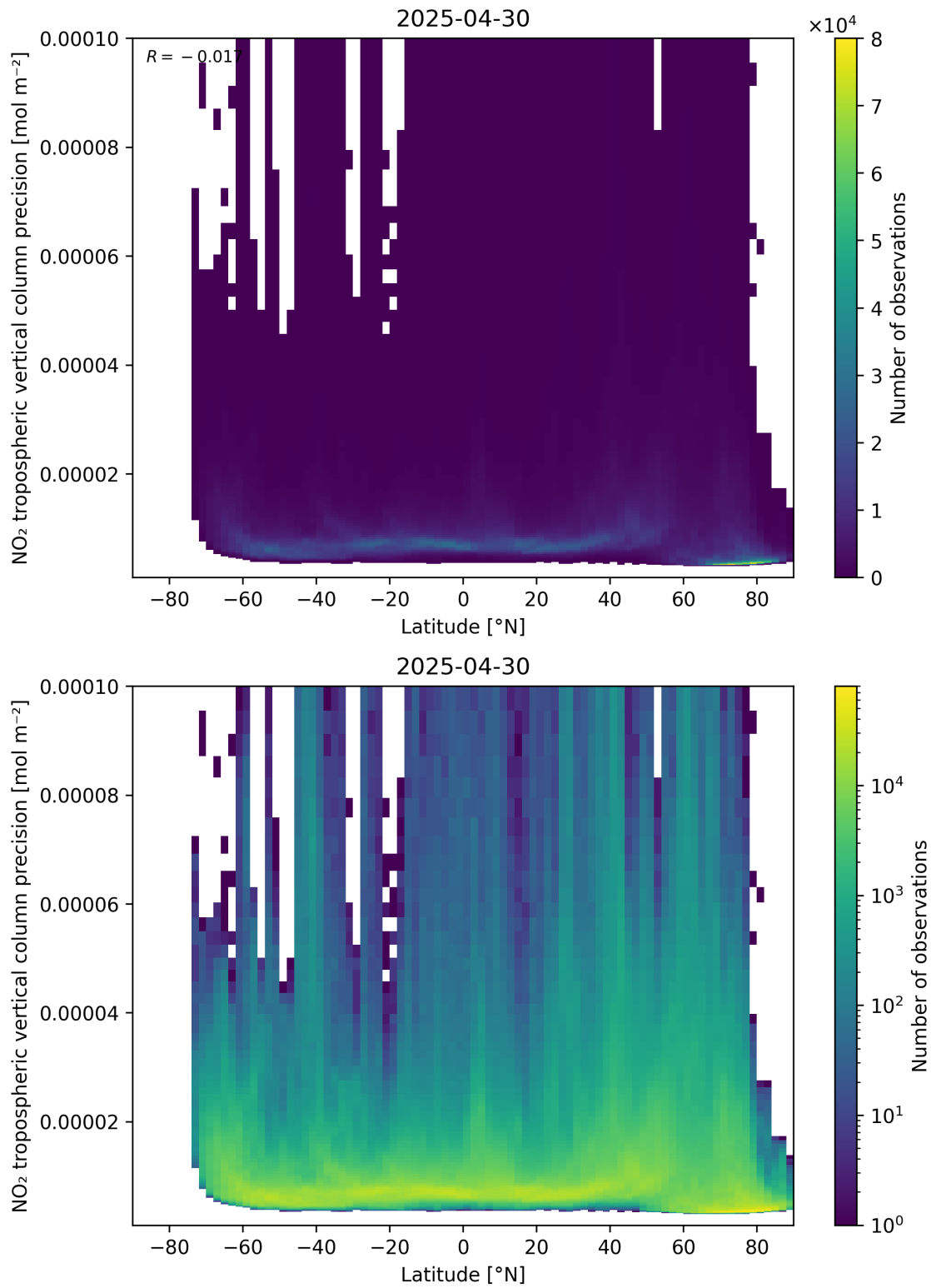
Figure 93: Scatter density plot of “Latitude” against “NO 2 tropospheric vertical column precision” for 2025-04-30 to 2025-05-01.
