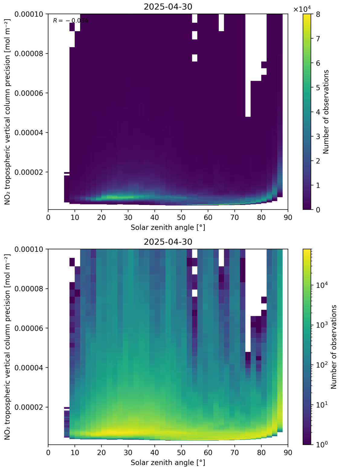
Figure 156: Scatter density plot of “Solar zenith angle” against “NO 2 tropospheric vertical column precision” for 2025-04-30 to 2025-05-01.
