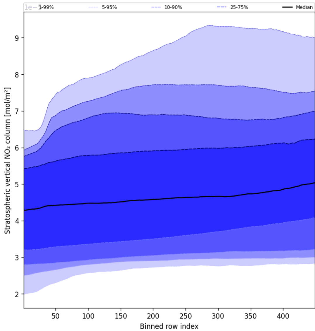
Figure 53: Along track statistics of “Stratospheric vertical NO 2 column” for 2025-04-30 to 2025-05-01
