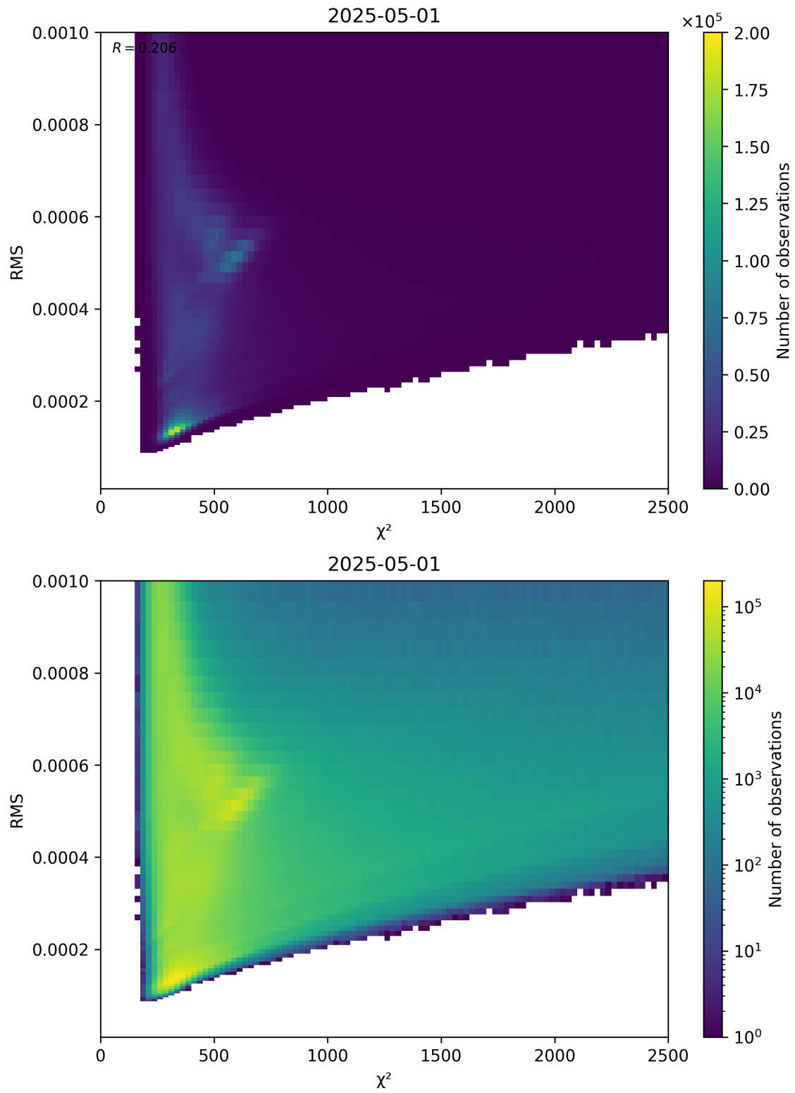
Figure 82: Scatter density plot of “ \chi^2 ” against “RMS” for 2025-05-01 to 2025-05-02.
