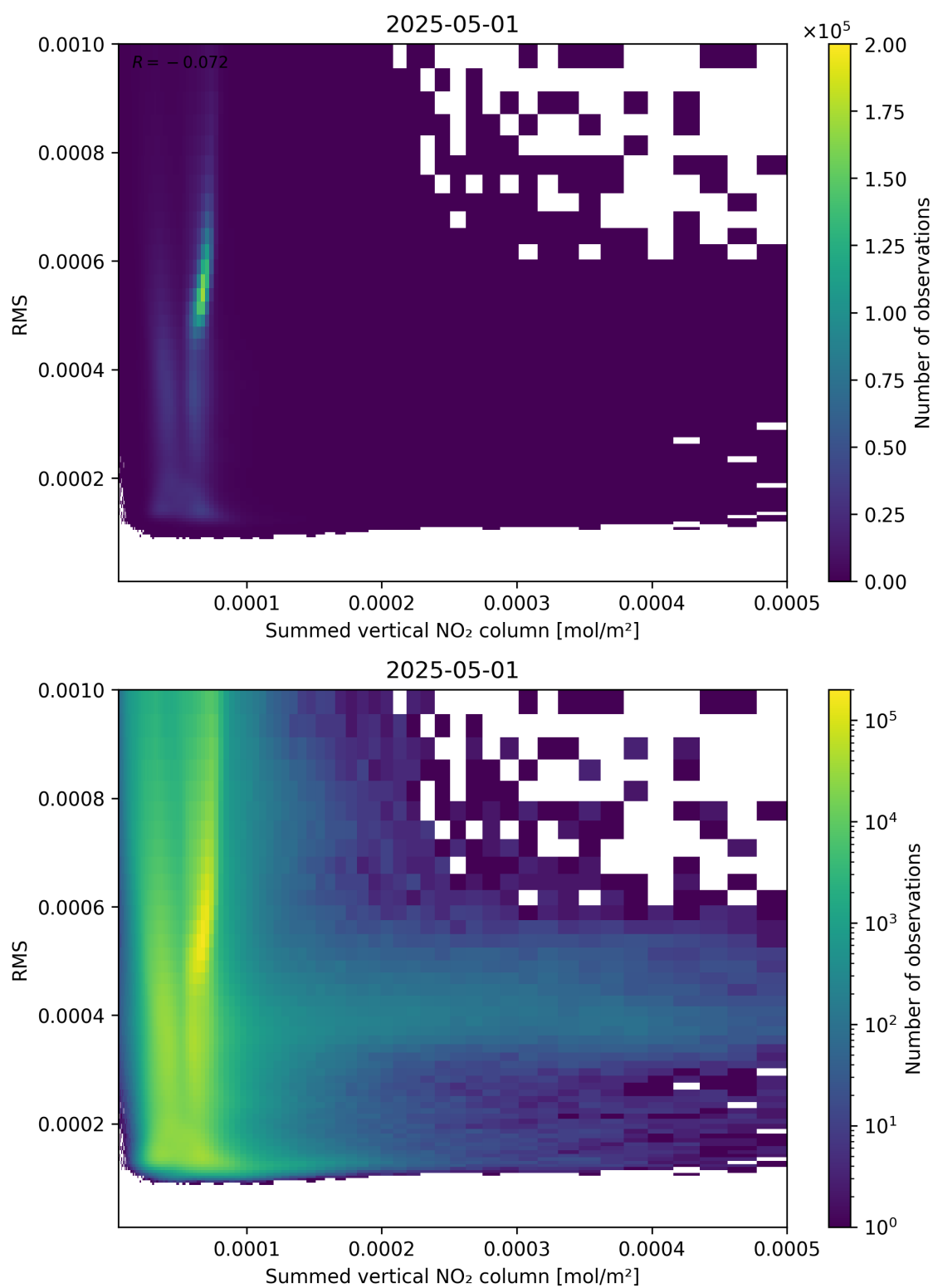
Figure 109: Scatter density plot of “Summed vertical NO 2 column” against “RMS” for 2025-05-01 to 2025-05-02.
