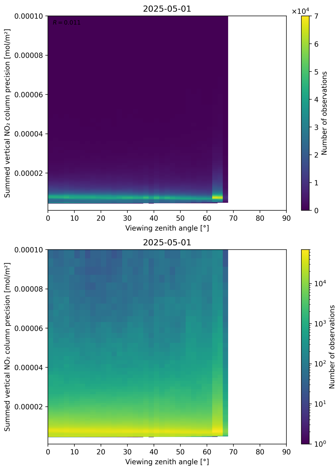
Figure 166: Scatter density plot of “Viewing zenith angle” against “Summed vertical NO 2 column precision” for 2025-05-01 to 2025-05-02.
