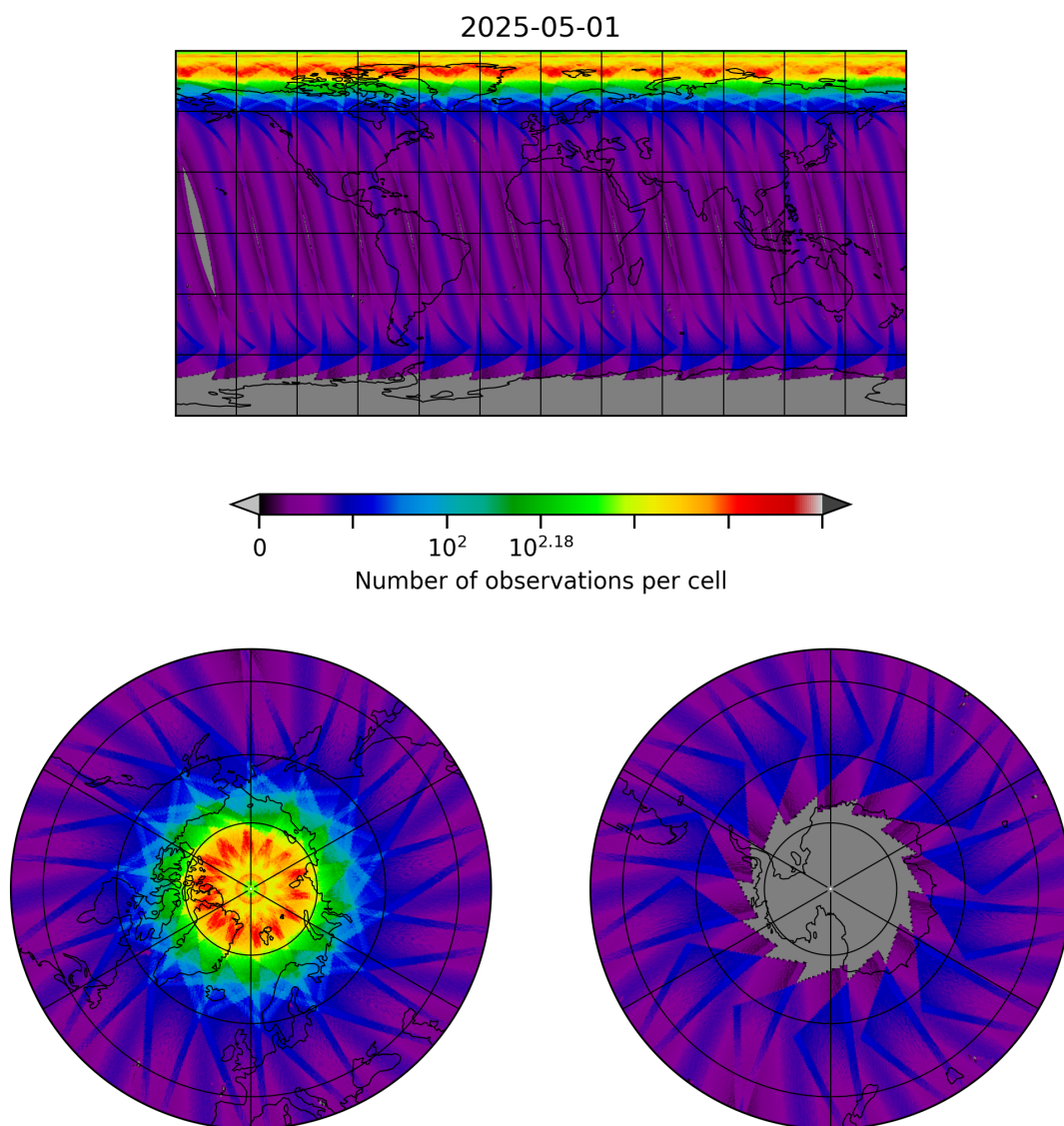
Figure 10: Map of the number of observations for 2025-05-01 to 2025-05-02
