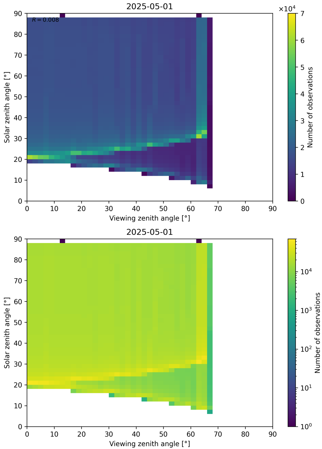
Figure 172: Scatter density plot of “Viewing zenith angle” against “Solar zenith angle” for 2025-05-01 to 2025-05-02.
