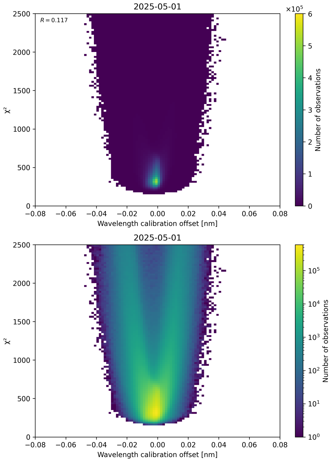
Figure 175: Scatter density plot of “Wavelength calibration offset” against “ \chi^2 ” for 2025-05-01 to 2025-05-02.
