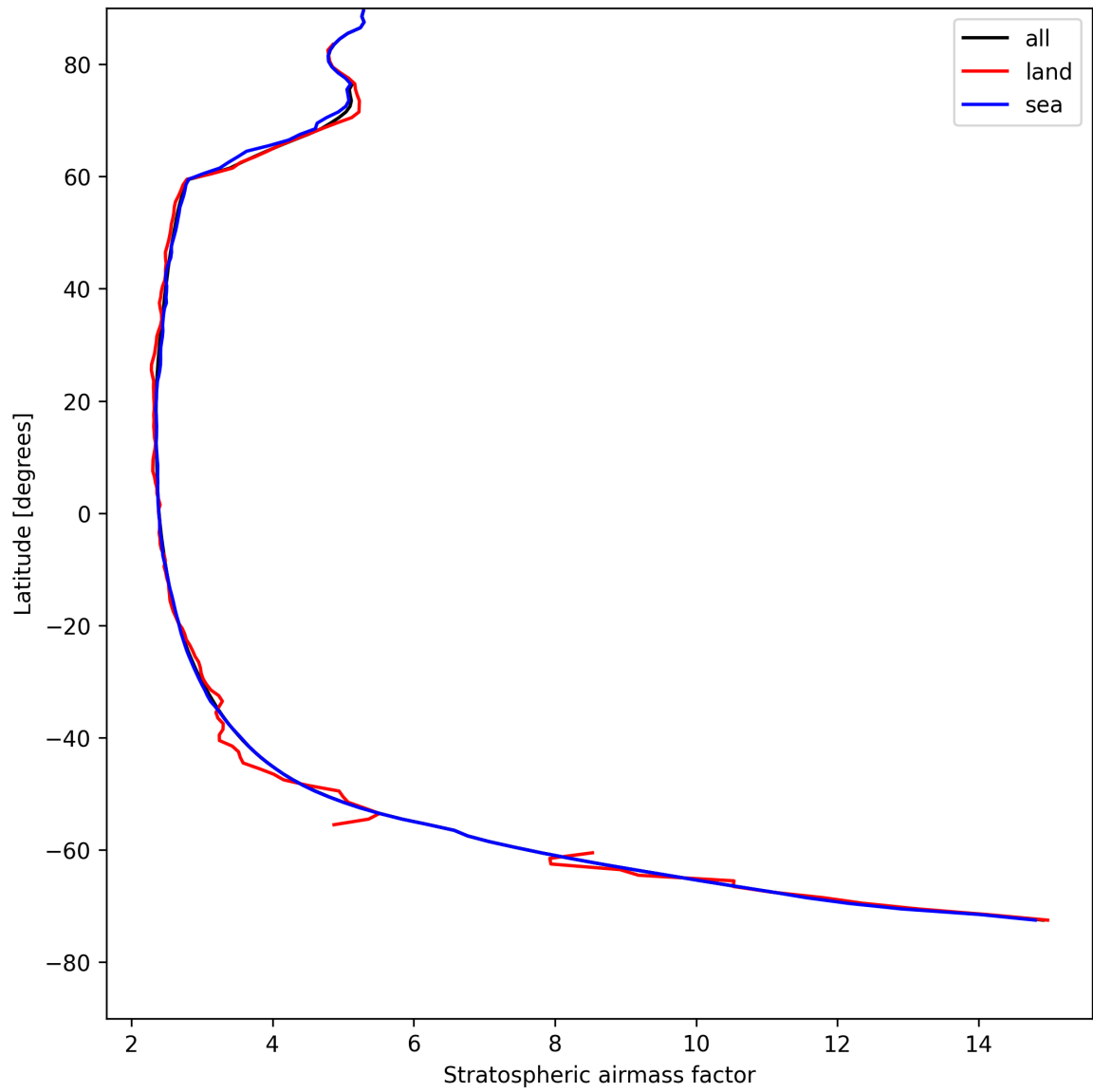
Figure 27: Zonal average of “Stratospheric air mass factor” for 2025-05-01 to 2025-05-02.
