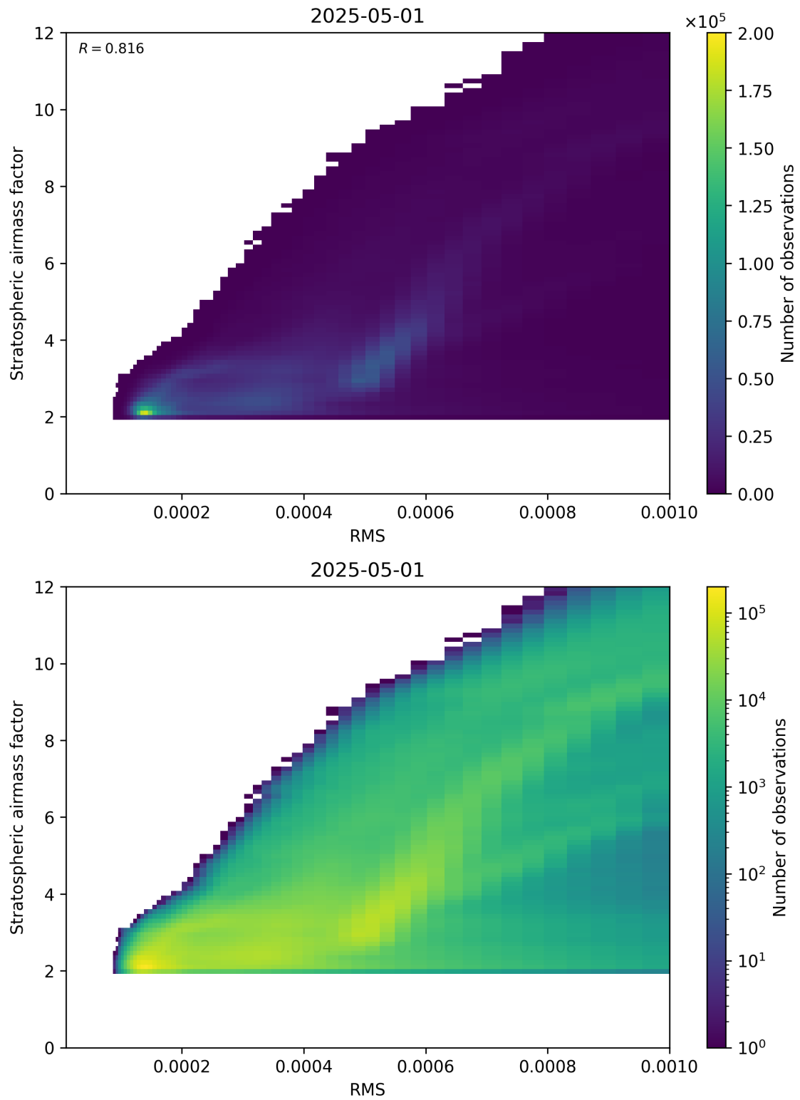
Figure 144: Scatter density plot of “RMS” against “Stratospheric airmass factor” for 2025-05-01 to 2025-05-02.
