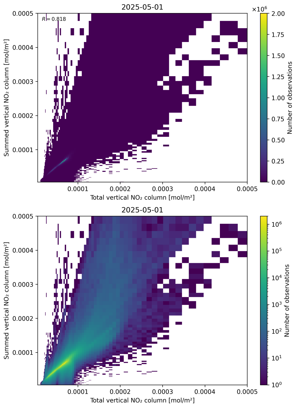
Figure 112: Scatter density plot of “Total vertical NO 2 column” against “Summed vertical NO 2 column” for 2025-05-01 to 2025-05-02.
