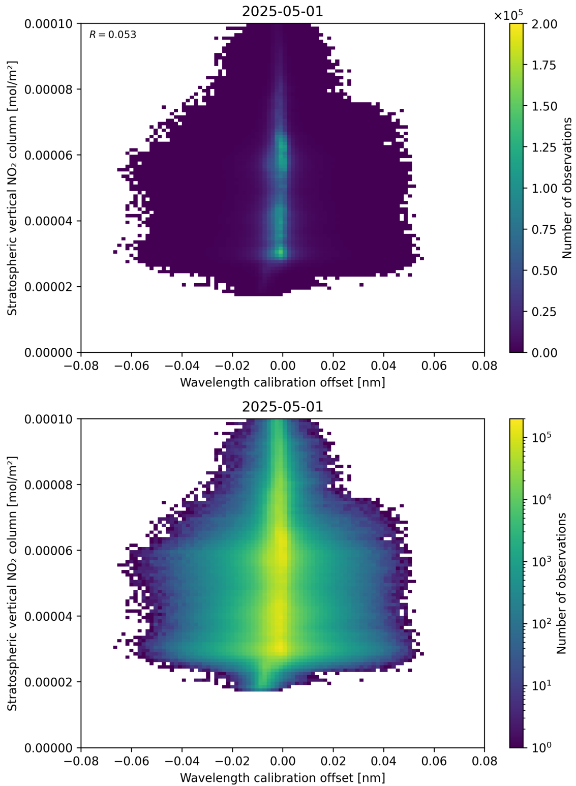
Figure 176: Scatter density plot of “Wavelength calibration offset” against “Stratospheric vertical NO 2 column” for 2025-05-01 to 2025-05-02.
