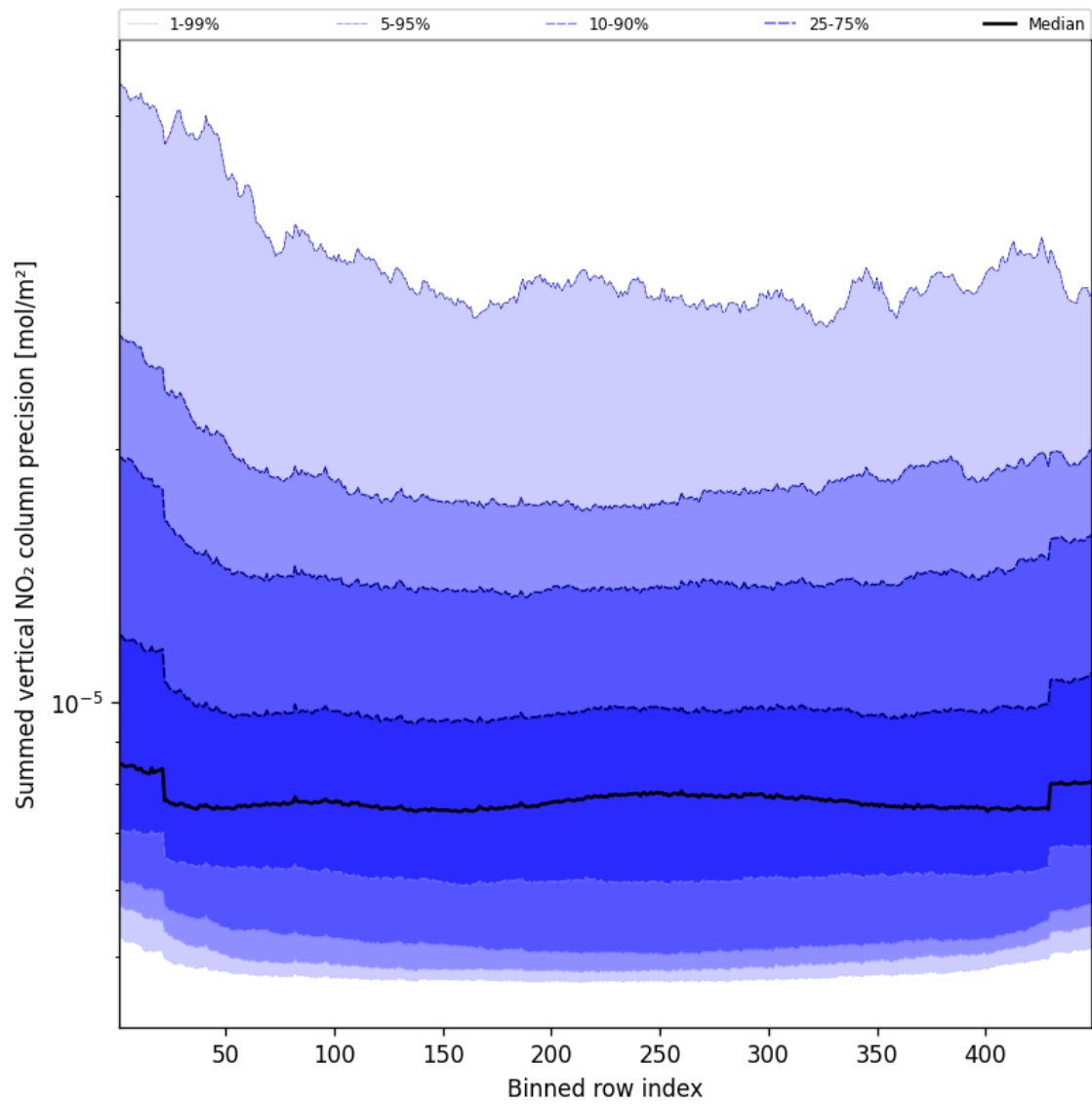
Figure 58: Along track statistics of “Summed vertical NO 2 column precision” for 2025-05-01 to 2025-05-02
