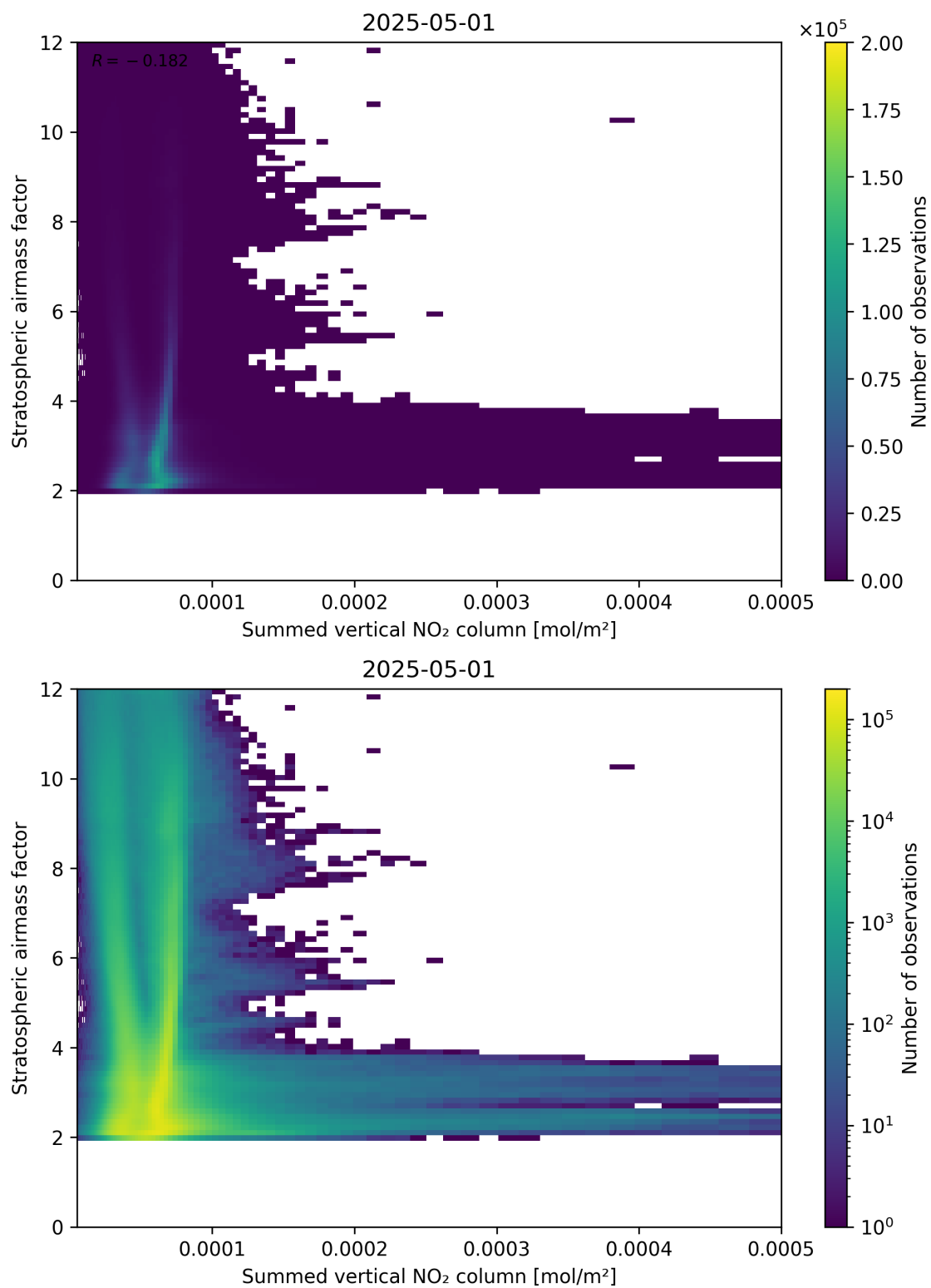
Figure 103: Scatter density plot of “Summed vertical NO 2 column” against “Stratospheric air mass factor” for 2025-05-01 to 2025-05-02.
