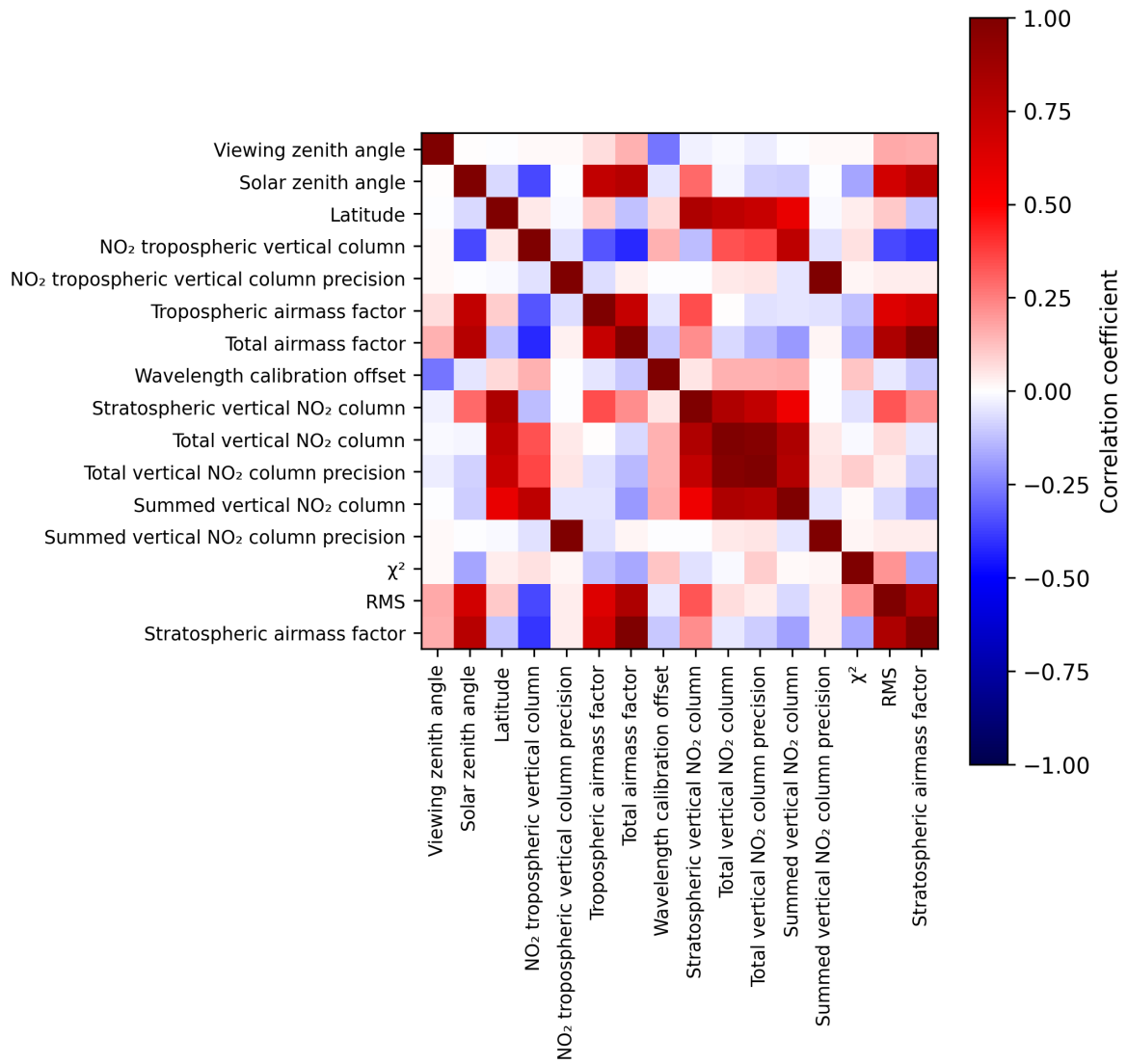
Figure 2: Map of correlation matrix for 2025-05-01 to 2025-05-02.
