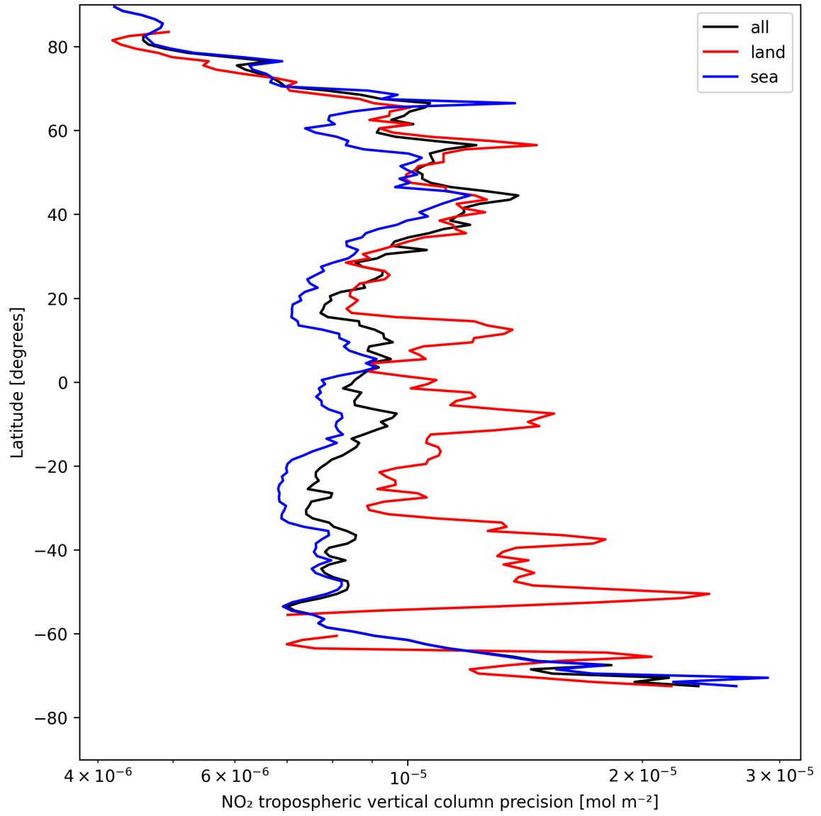
Figure 13: Zonal average of “NO 2 tropospheric vertical column precision” for 2025-05-01 to 2025-05-02.
