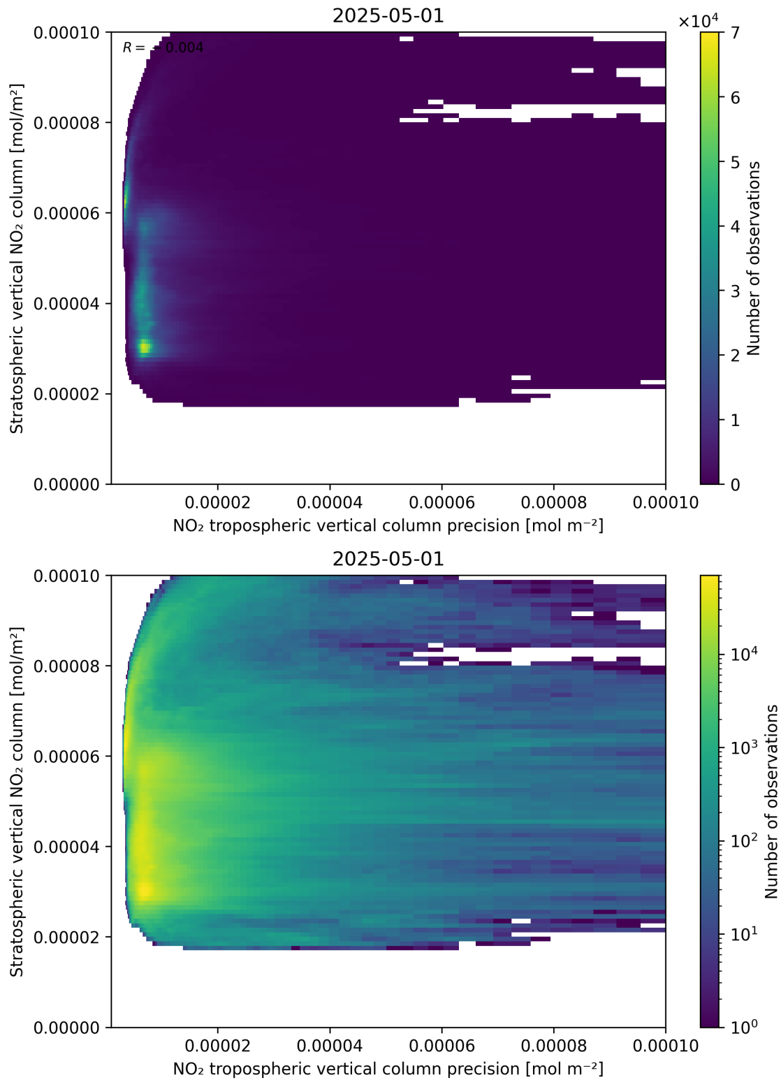
Figure 135: Scatter density plot of “NO 2 tropospheric vertical column precision” against “Stratospheric vertical NO 2 column” for 2025-05-01 to 2025-05-02.
