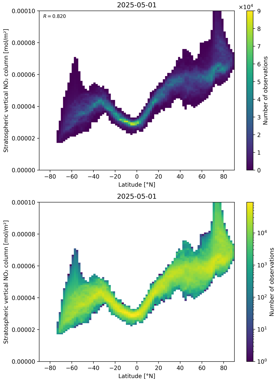
Figure 87: Scatter density plot of “Latitude” against “Stratospheric vertical \text{NO}_2 column” for 2025-05-01 to 2025-05-02.
