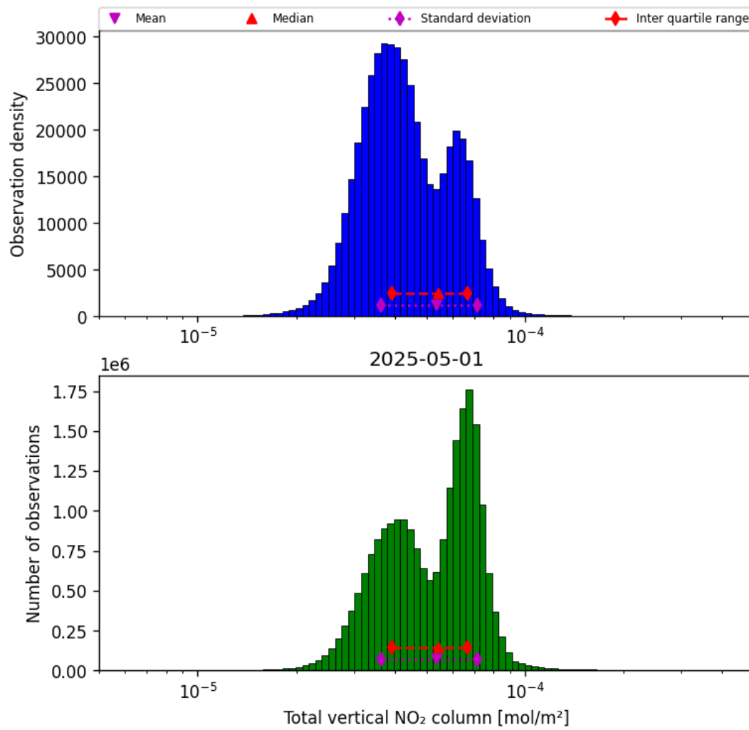
Figure 38: Histogram of "Total vertical NO 2 column" for 2025-05-01 to 2025-05-02
