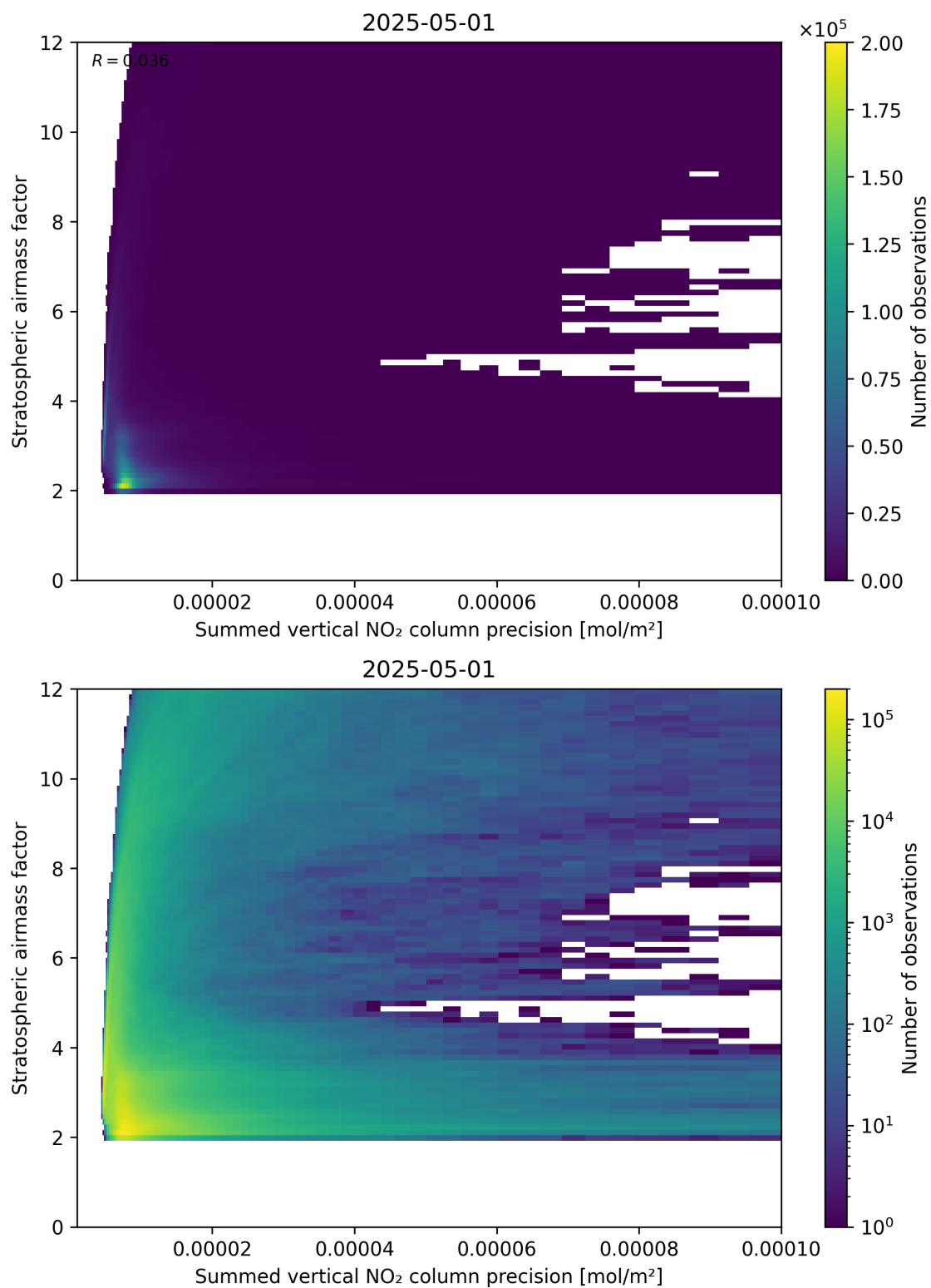
Figure 106: Scatter density plot of “Summed vertical NO 2 column precision” against “Stratospheric airmass factor” for 2025-05-01 to 2025-05-02.
