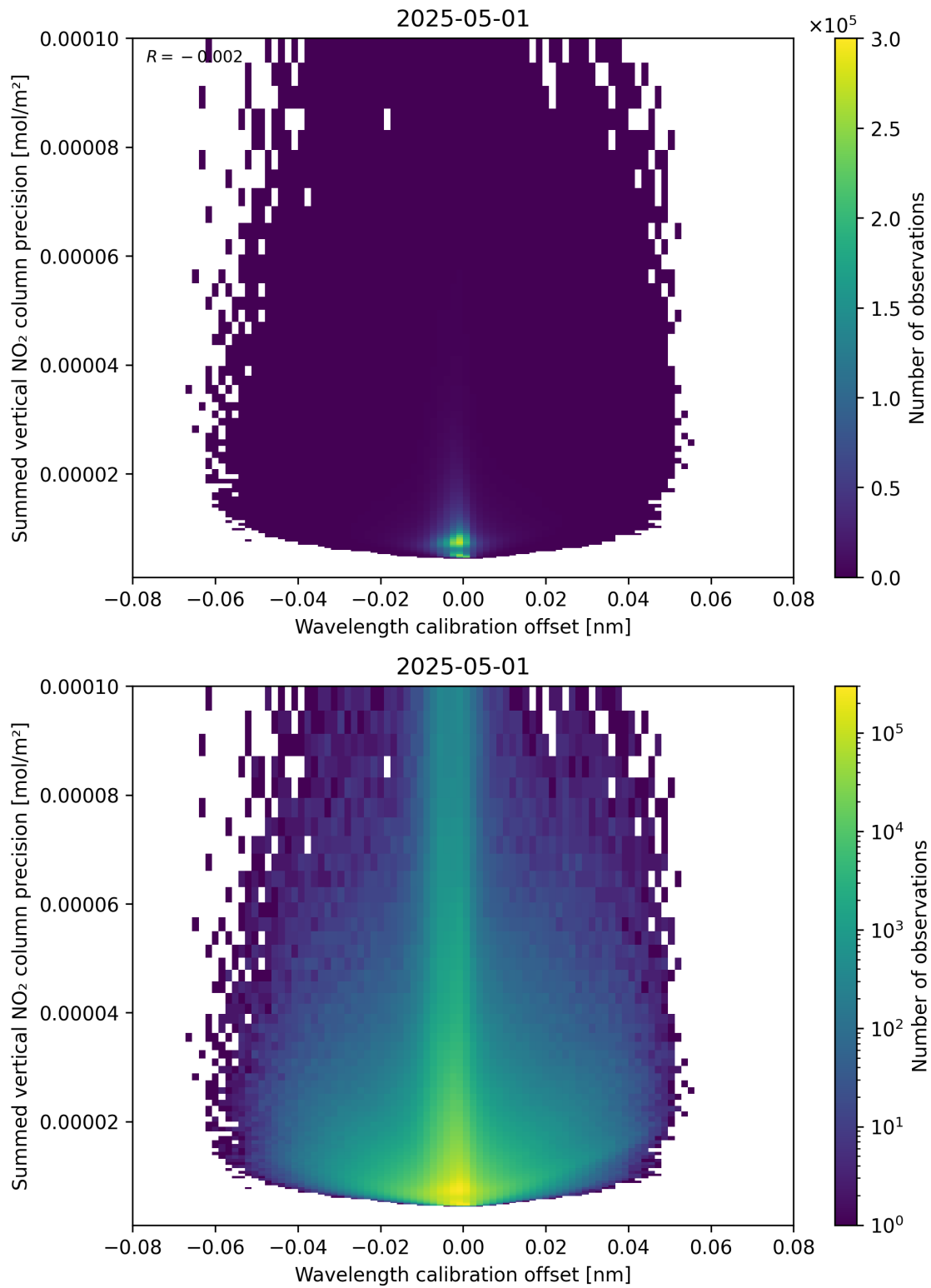
Figure 178: Scatter density plot of “Wavelength calibration offset” against “Summed vertical NO 2 column precision” for 2025-05-01 to 2025-05-02.
