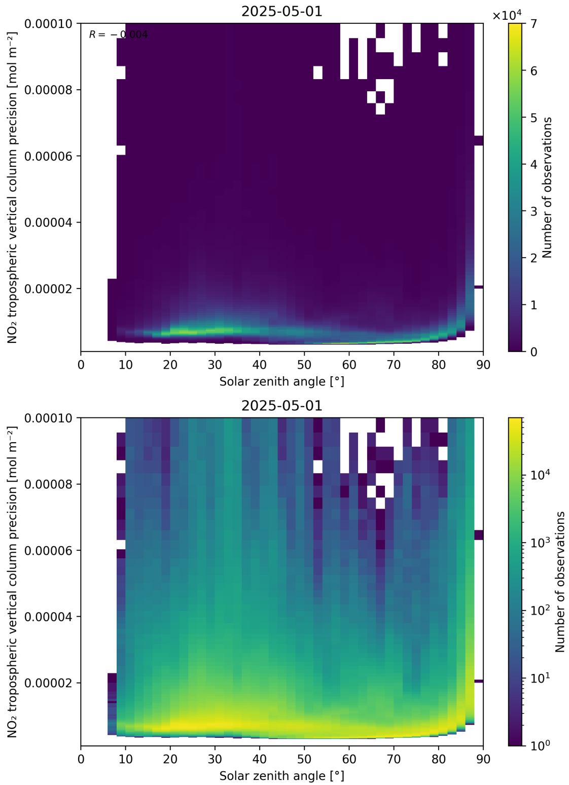
Figure 156: Scatter density plot of “Solar zenith angle” against “NO 2 tropospheric vertical column precision” for 2025-05-01 to 2025-05-02.
