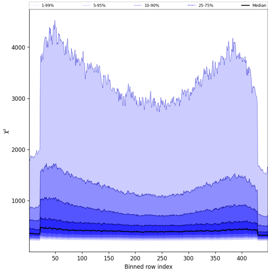
Figure 59: Along track statistics of “ \chi^2 ” for 2025-05-01 to 2025-05-02
