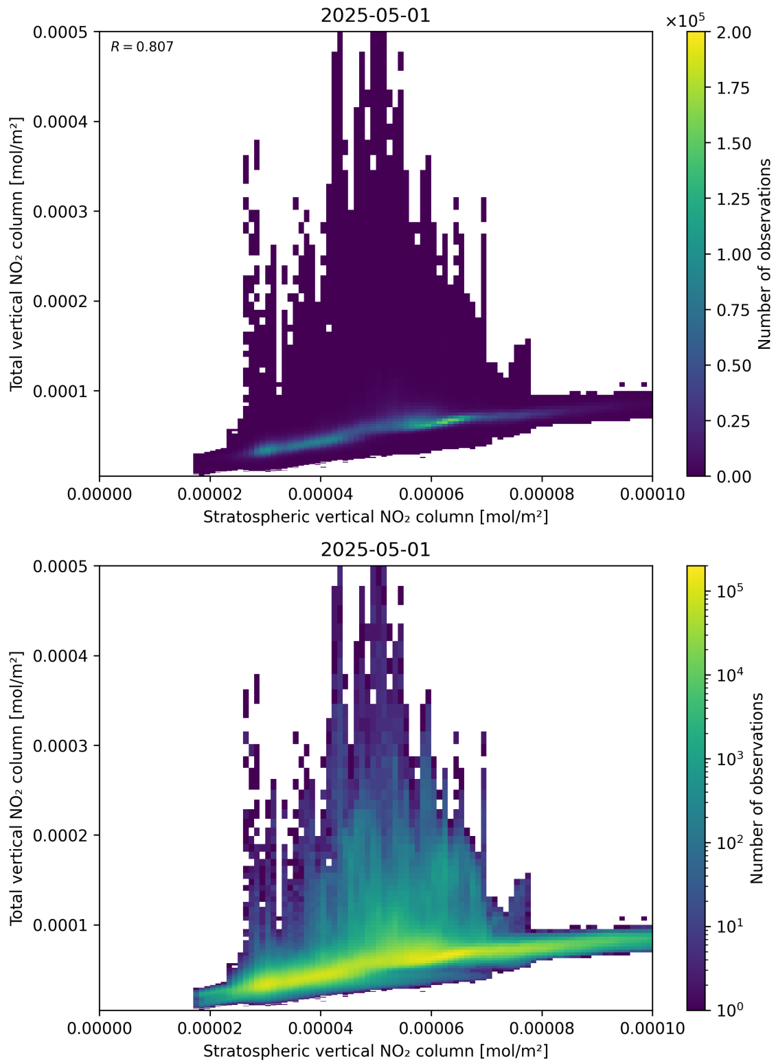
Figure 100: Scatter density plot of “Stratospheric vertical NO 2 column” against “Total vertical NO 2 column” for 2025-05-01 to 2025-05-02.
