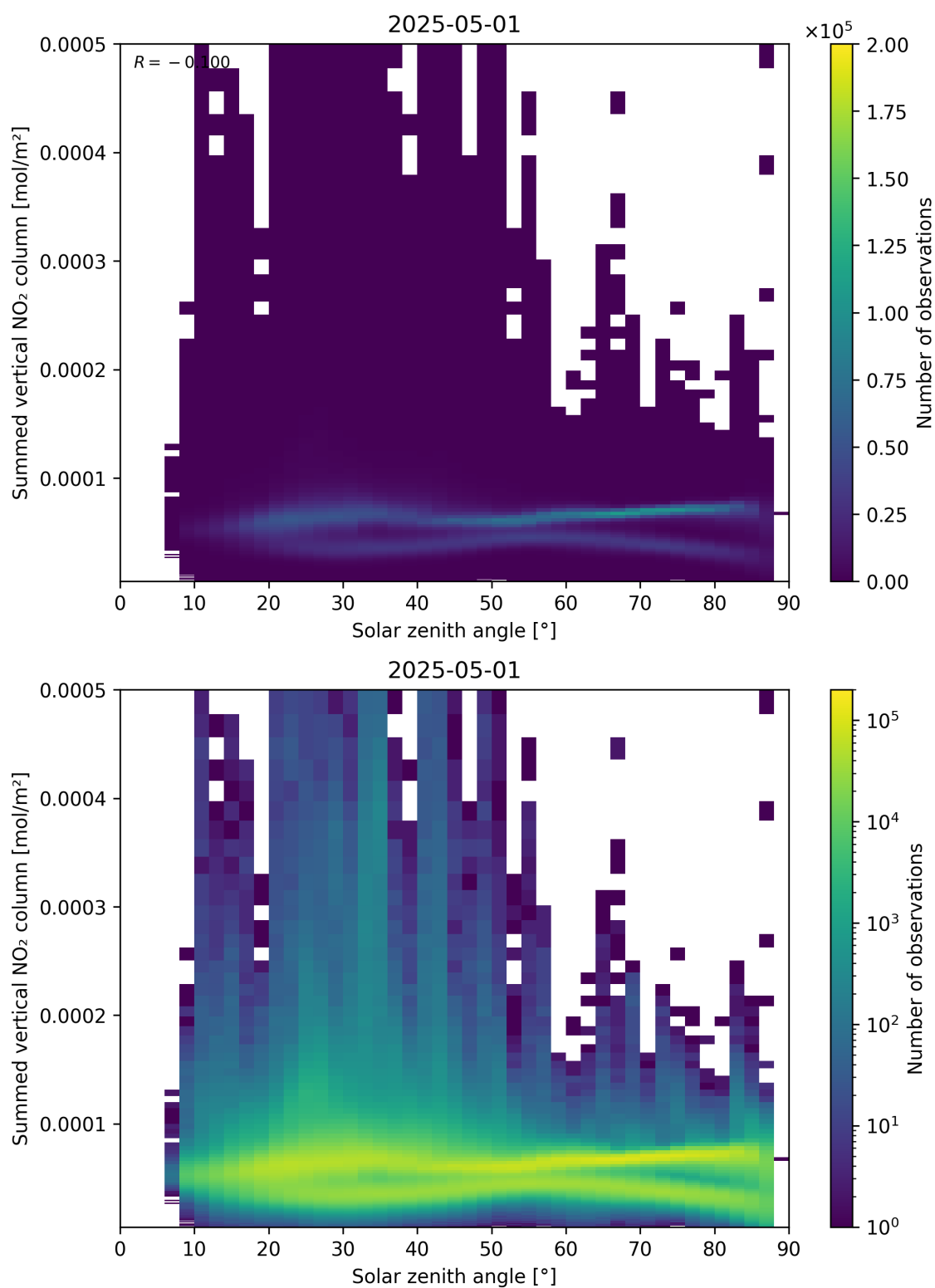
Figure 151: Scatter density plot of “Solar zenith angle” against “Summed vertical NO 2 column” for 2025-05-01 to 2025-05-02.
