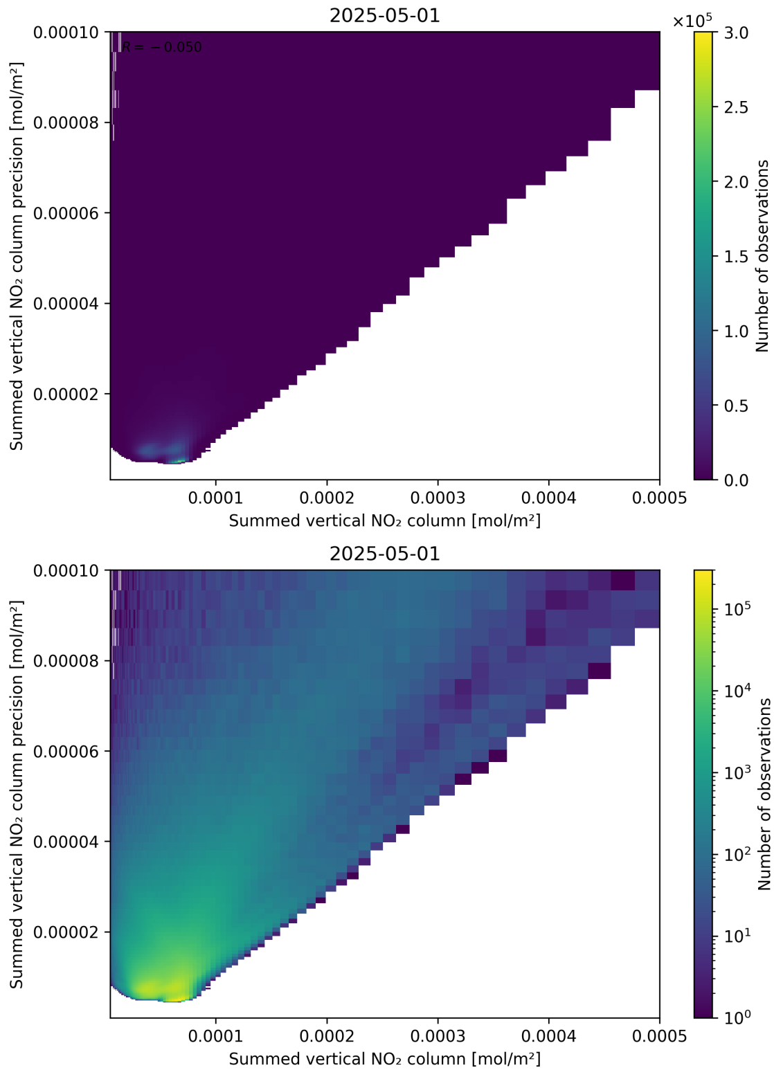
Figure 105: Scatter density plot of “Summed vertical NO 2 column” against “Summed vertical NO 2 column precision” for 2025-05-01 to 2025-05-02.
