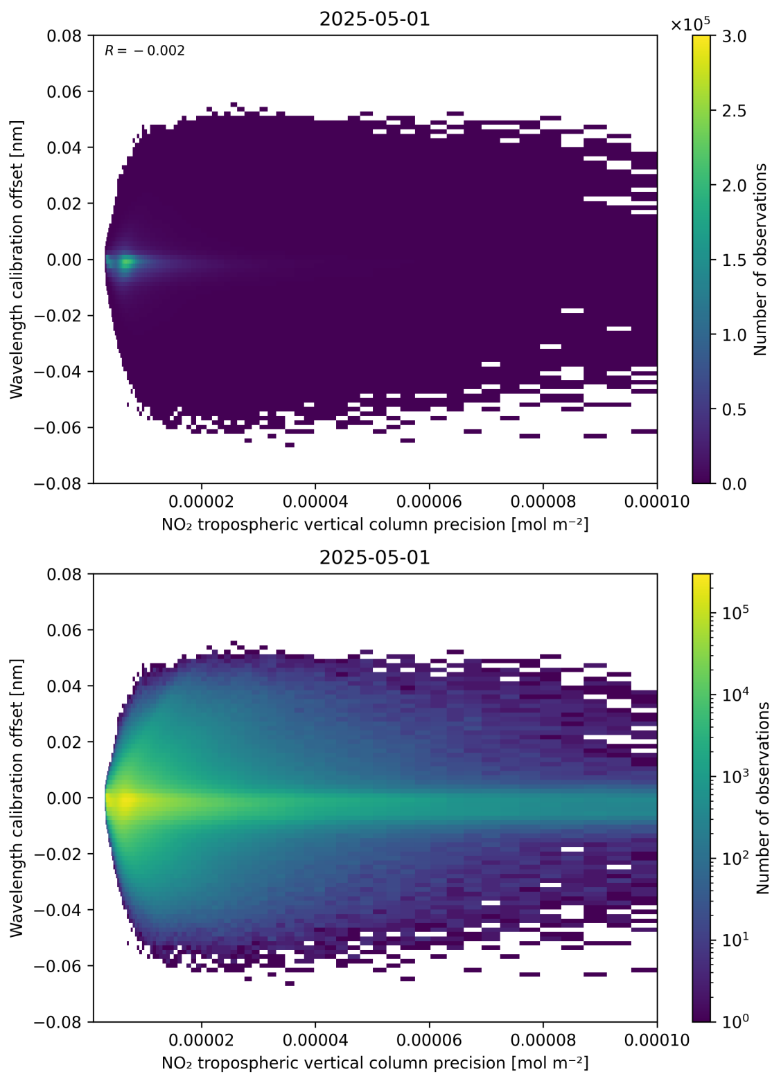
Figure 141: Scatter density plot of “NO 2 tropospheric vertical column precision” against “Wavelength calibration offset” for 2025-05-01 to 2025-05-02.
