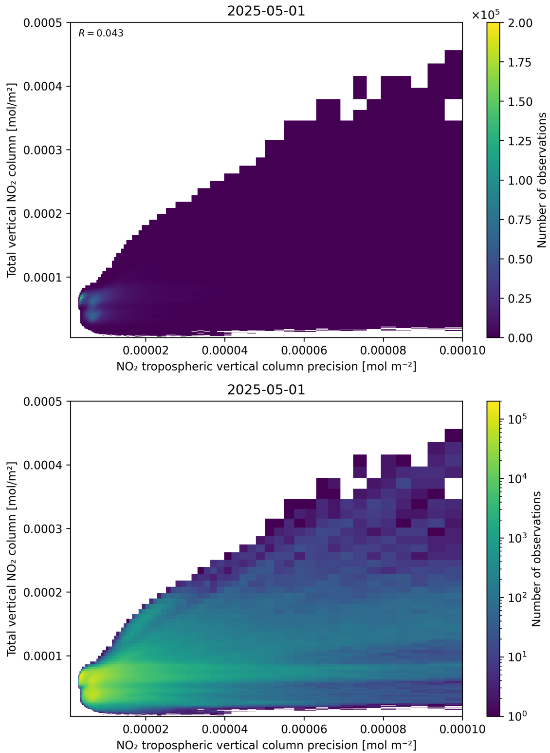
Figure 138: Scatter density plot of “NO 2 tropospheric vertical column precision” against “Total vertical NO 2 column” for 2025-05-01 to 2025-05-02.
