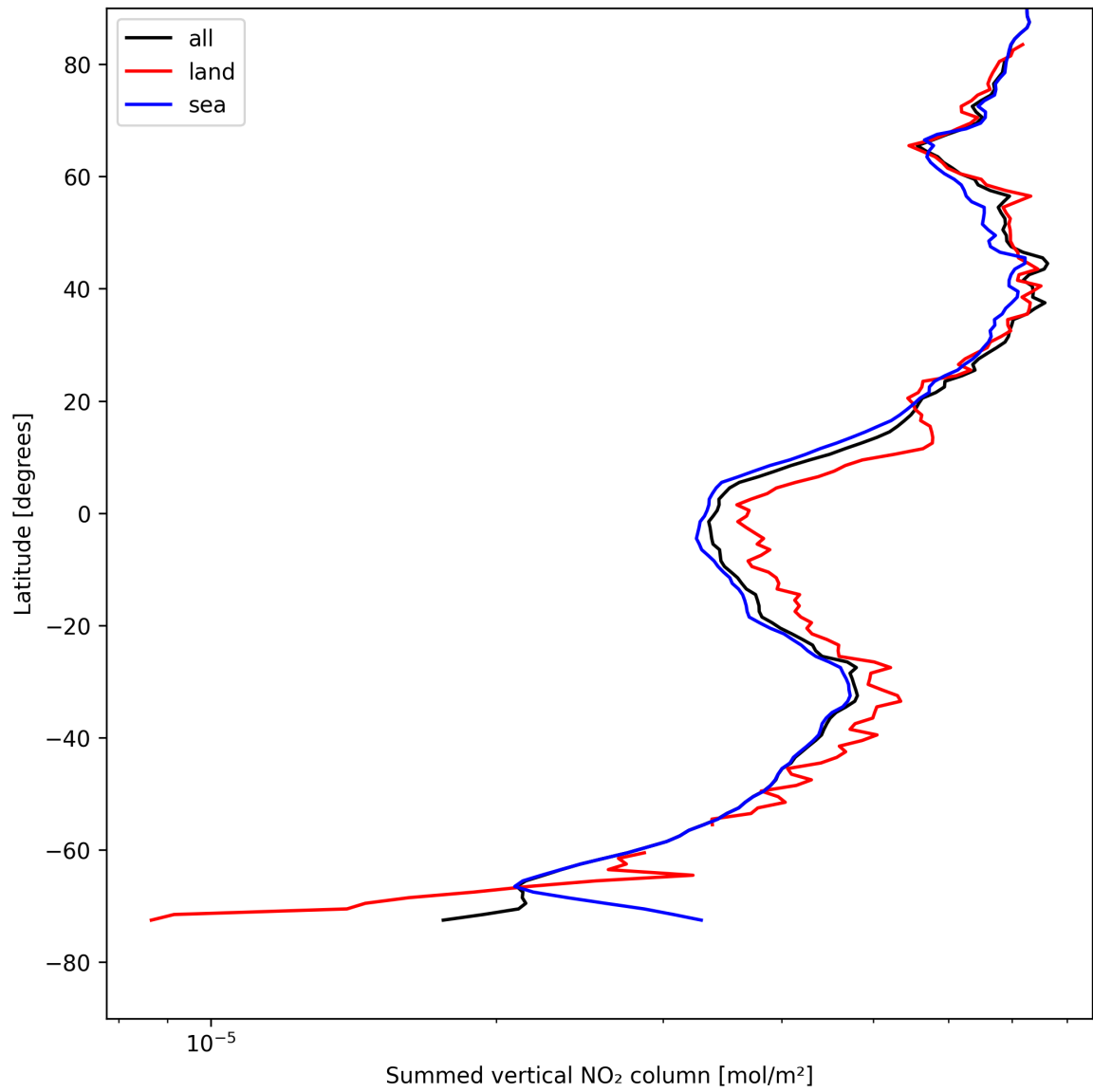
Figure 23: Zonal average of “Summed vertical NO 2 column” for 2025-05-01 to 2025-05-02.
