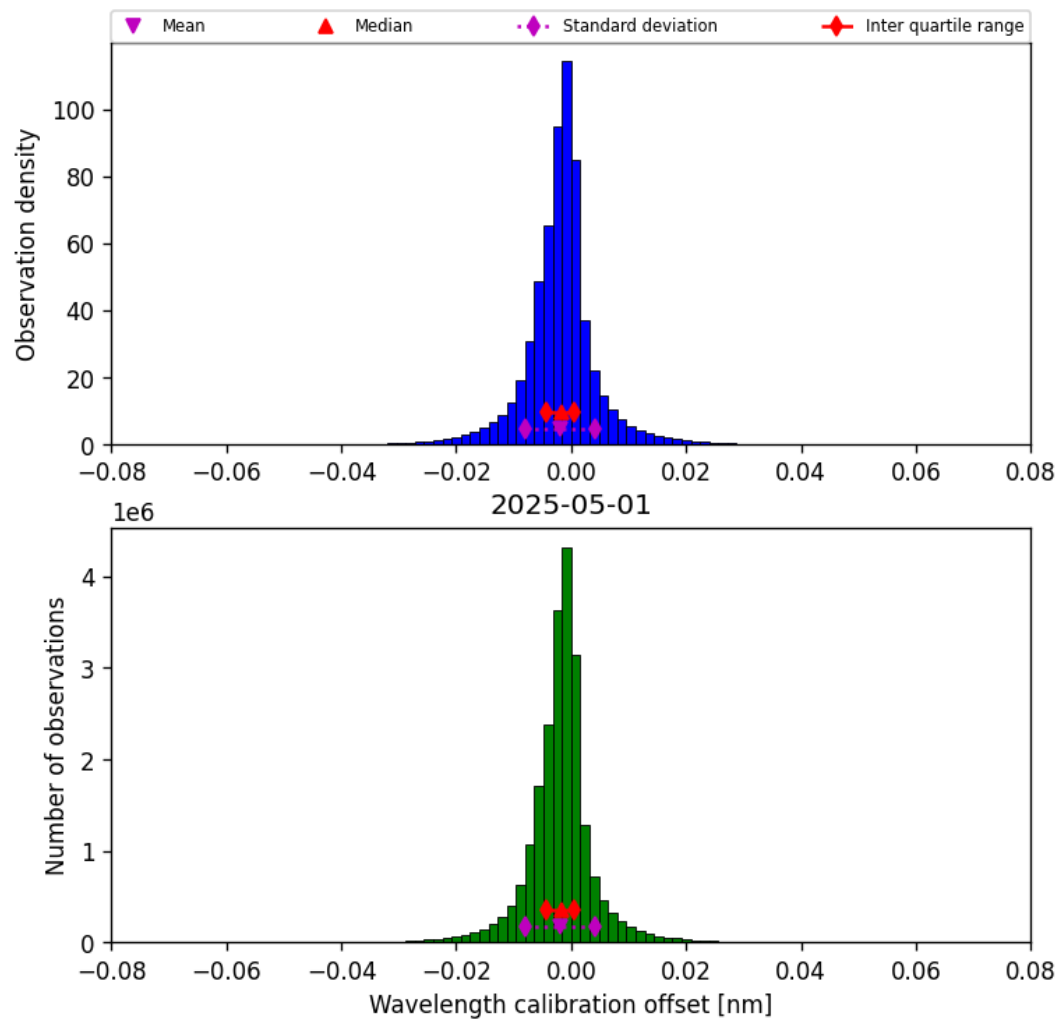
Figure 35: Histogram of “Wavelength calibration offset” for 2025-05-01 to 2025-05-02
