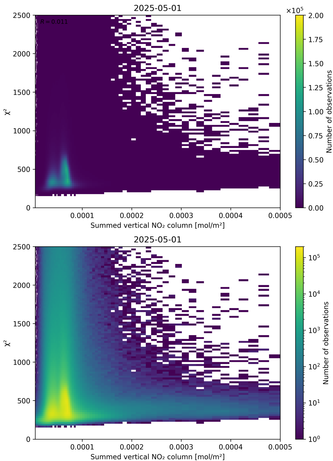
Figure 104: Scatter density plot of “Summed vertical NO 2 column” against “ \chi^2 ” for 2025-05-01 to 2025-05-02.
