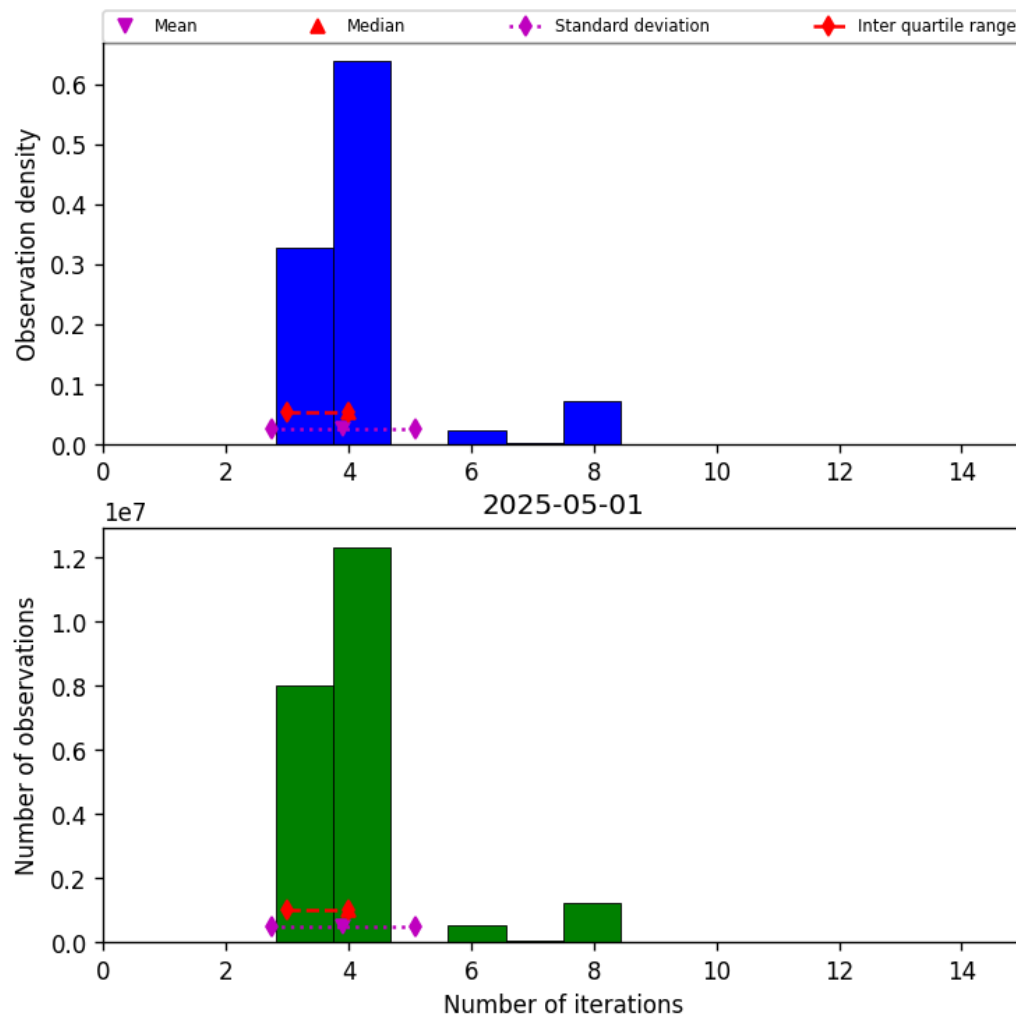
Figure 34: Histogram of “Number of iterations” for 2025-05-01 to 2025-05-02
