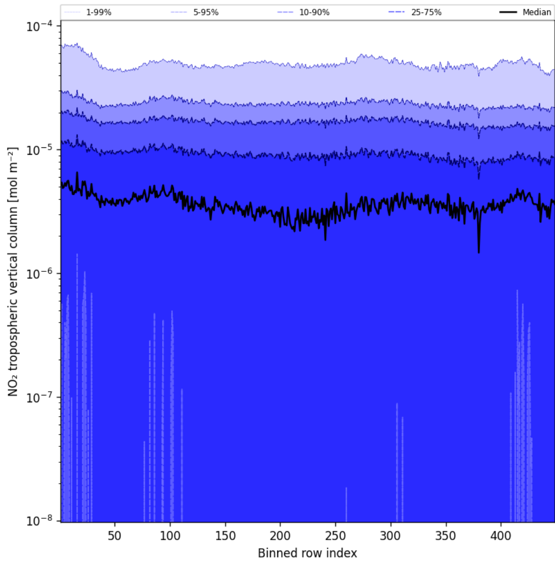
Figure 46: Along track statistics of “NO 2 tropospheric vertical column” for 2025-05-01 to 2025-05-02
