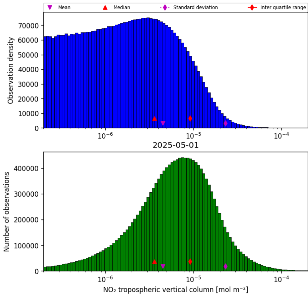
Figure 29: Histogram of “NO 2 tropospheric vertical column” for 2025-05-01 to 2025-05-02
