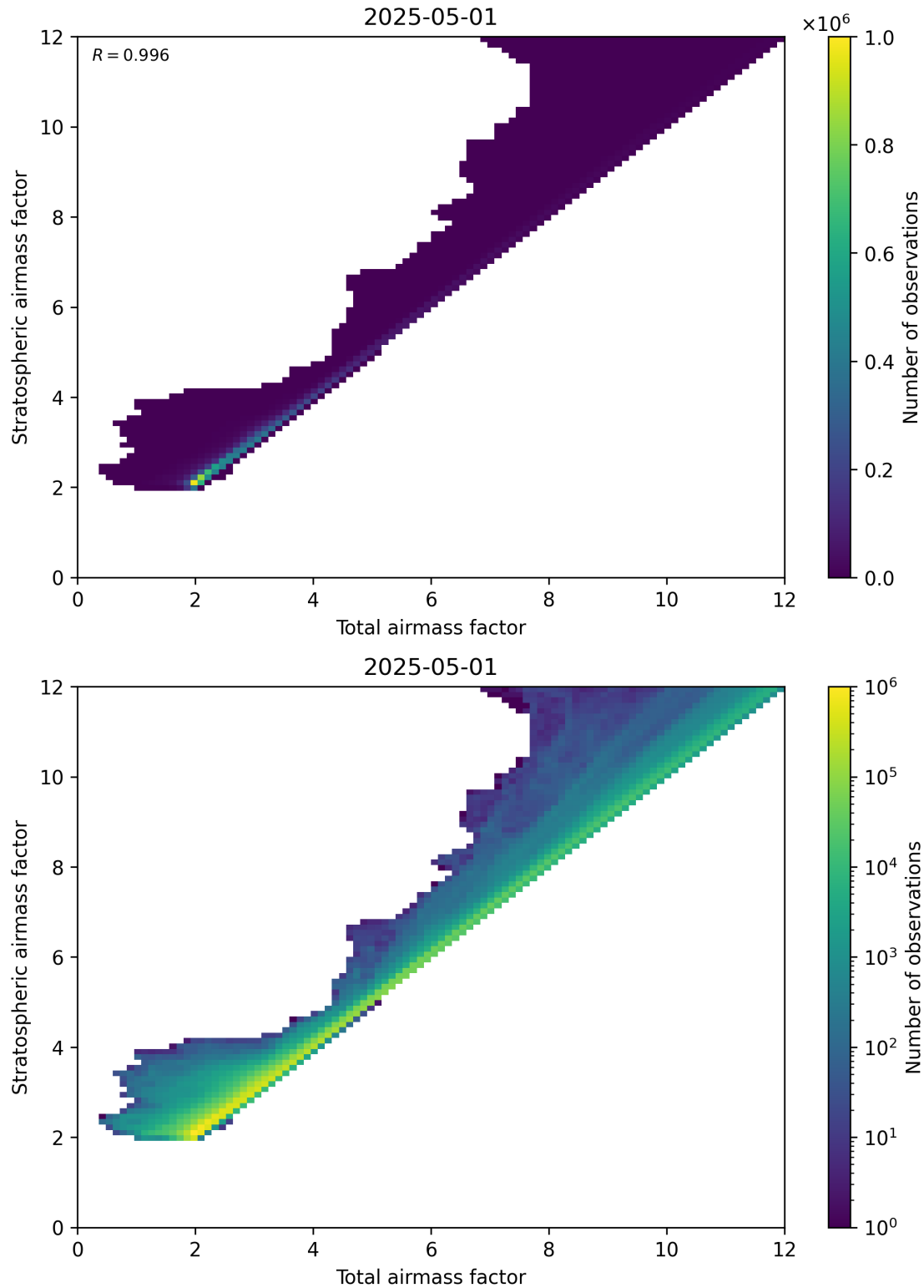
Figure 62: Scatter density plot of “Total airmass factor” against “Stratospheric airmass factor” for 2025-05-01 to 2025-05-02.
