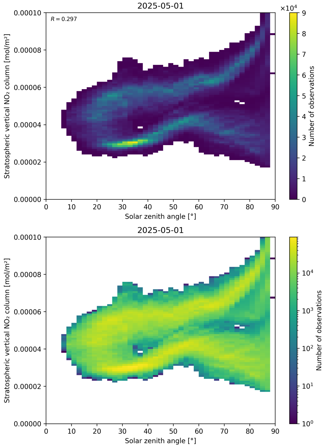
Figure 150: Scatter density plot of “Solar zenith angle” against “Stratospheric vertical NO 2 column” for 2025-05-01 to 2025-05-02.
