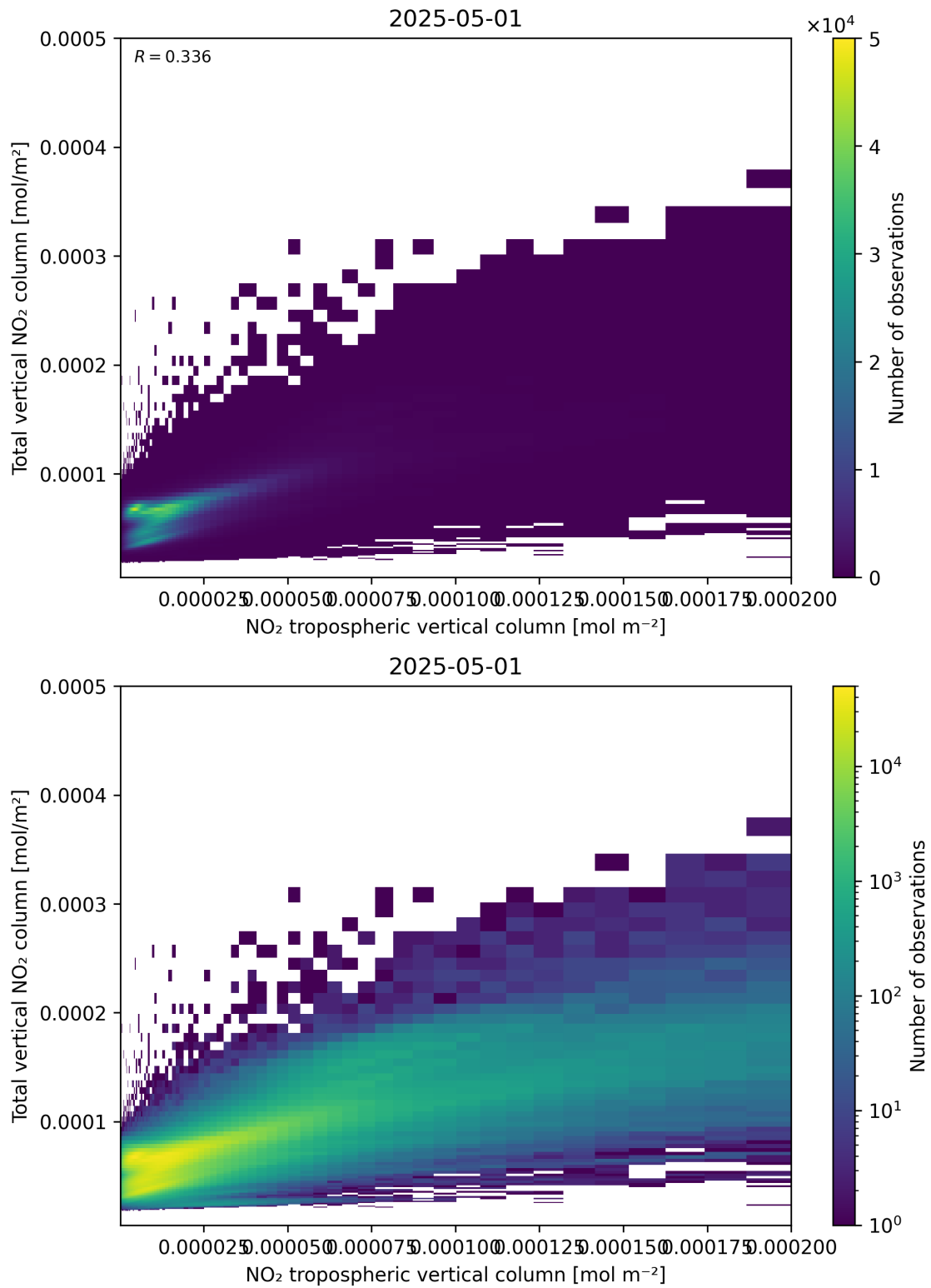
Figure 128: Scatter density plot of “NO 2 tropospheric vertical column” against “Total vertical NO 2 column” for 2025-05-01 to 2025-05-02.
