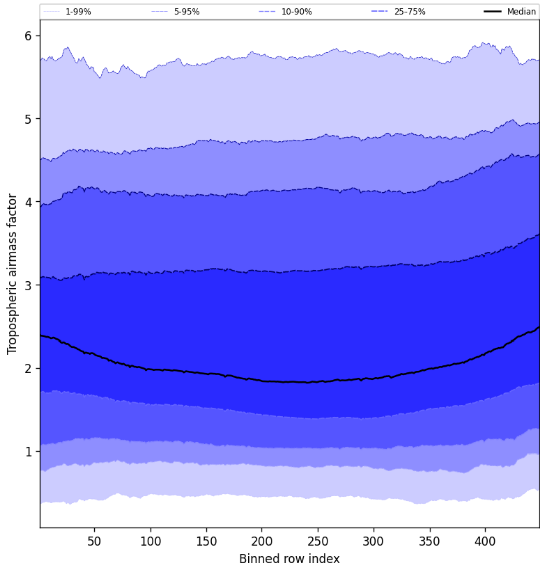
Figure 48: Along track statistics of “Tropospheric airmass factor” for 2025-05-01 to 2025-05-02
