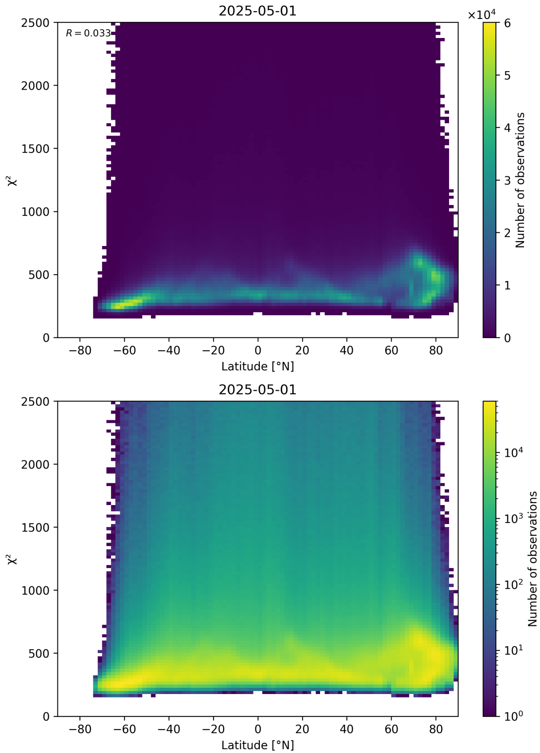
Figure 86: Scatter density plot of “Latitude” against “ \chi^2 ” for 2025-05-01 to 2025-05-02.
