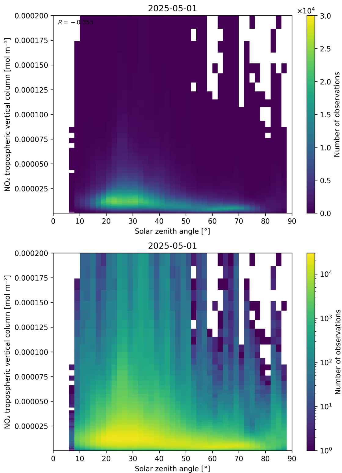
Figure 155: Scatter density plot of “Solar zenith angle” against “NO 2 tropospheric vertical column” for 2025-05-01 to 2025-05-02.
