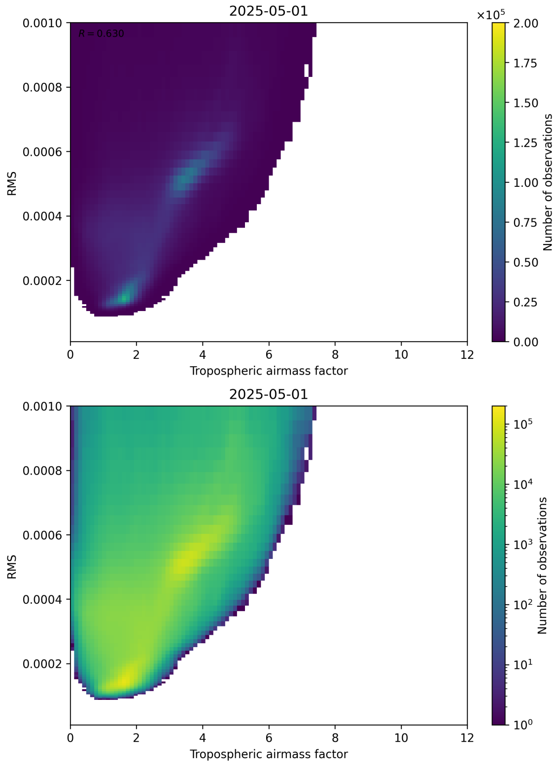
Figure 79: Scatter density plot of “Tropospheric airmass factor” against “RMS” for 2025-05-01 to 2025-05-02.
