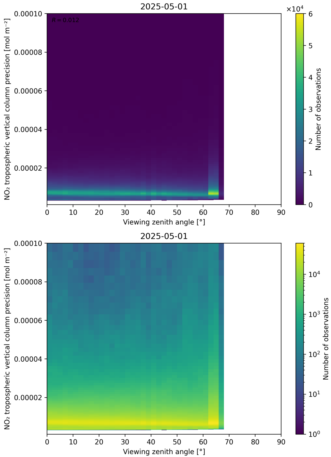
Figure 170: Scatter density plot of “Viewing zenith angle” against “NO 2 tropospheric vertical column precision” for 2025-05-01 to 2025-05-02.
