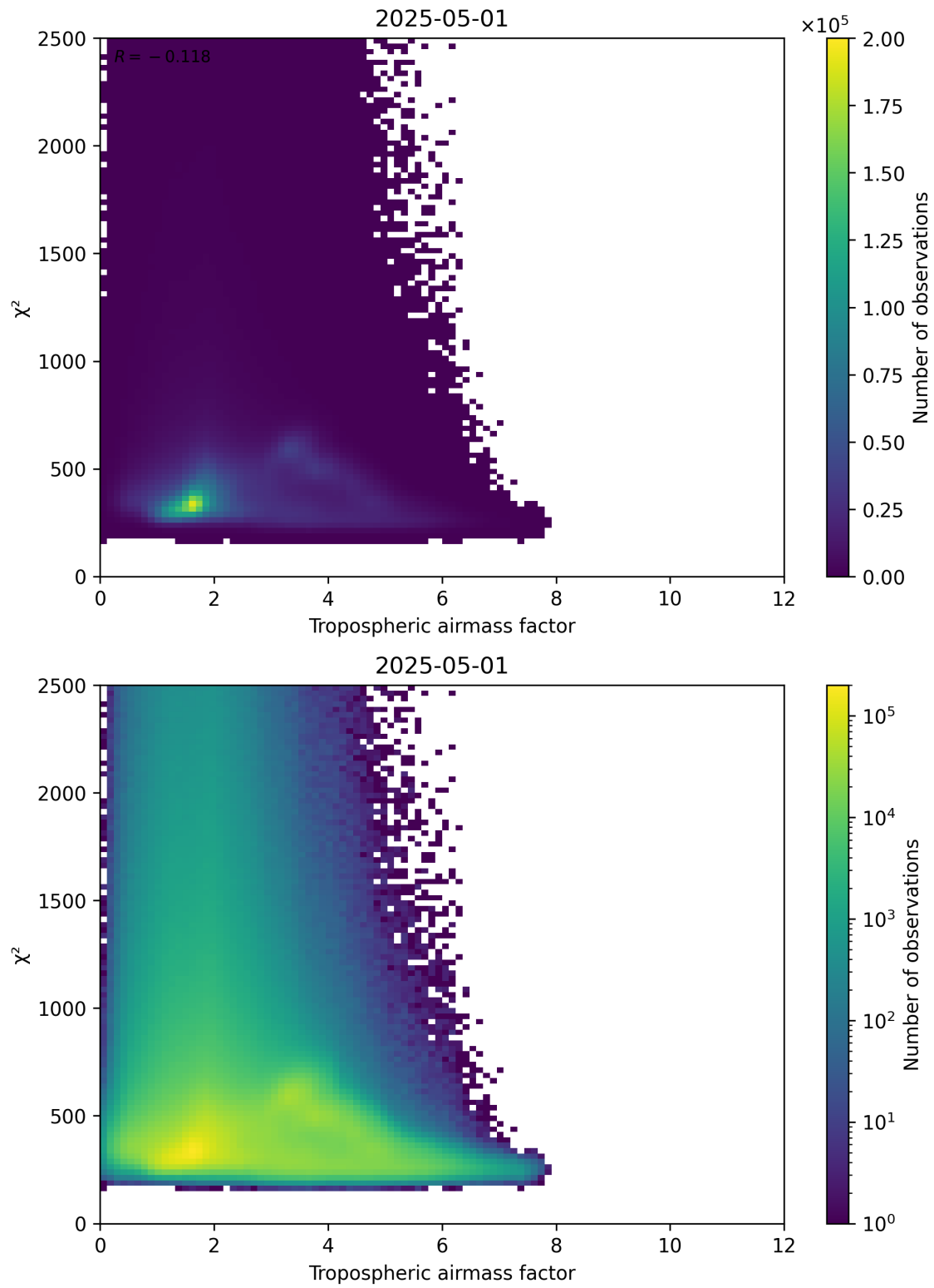
Figure 73: Scatter density plot of “Tropospheric airmass factor” against “ \chi^2 ” for 2025-05-01 to 2025-05-02.
