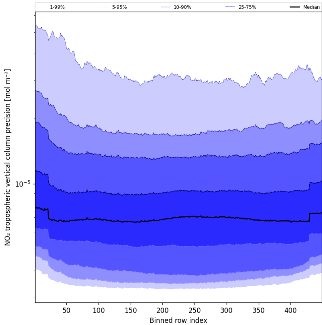
Figure 47: Along track statistics of “NO 2 tropospheric vertical column precision” for 2025-05-01 to 2025-05-02
