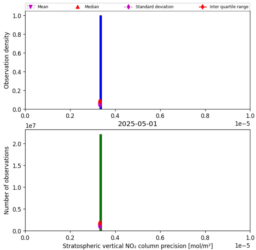
Figure 37: Histogram of “Stratospheric vertical NO 2 column precision” for 2025-05-01 to 2025-05-02
