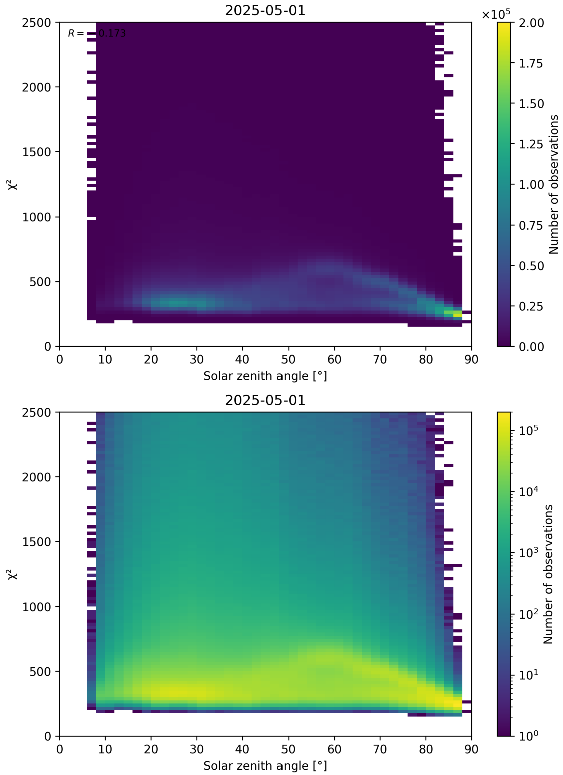
Figure 148: Scatter density plot of “Solar zenith angle” against “ \chi^2 ” for 2025-05-01 to 2025-05-02.
