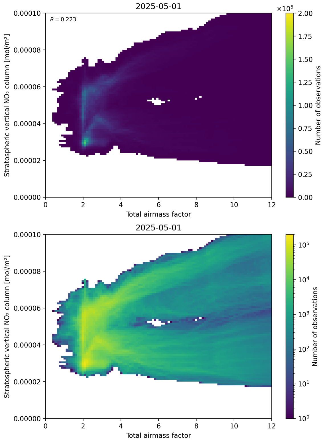
Figure 64: Scatter density plot of “Total airmass factor” against “Stratospheric vertical \text{NO}_2 column” for 2025-05-01 to 2025-05-02.
