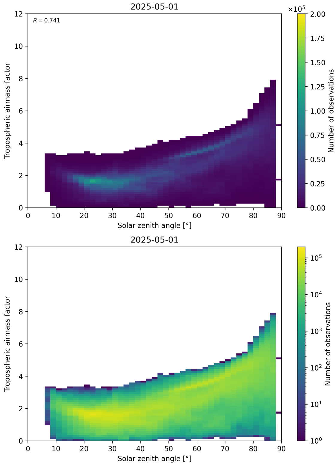
Figure 147: Scatter density plot of “Solar zenith angle” against “Tropospheric airmass factor” for 2025-05-01 to 2025-05-02.
