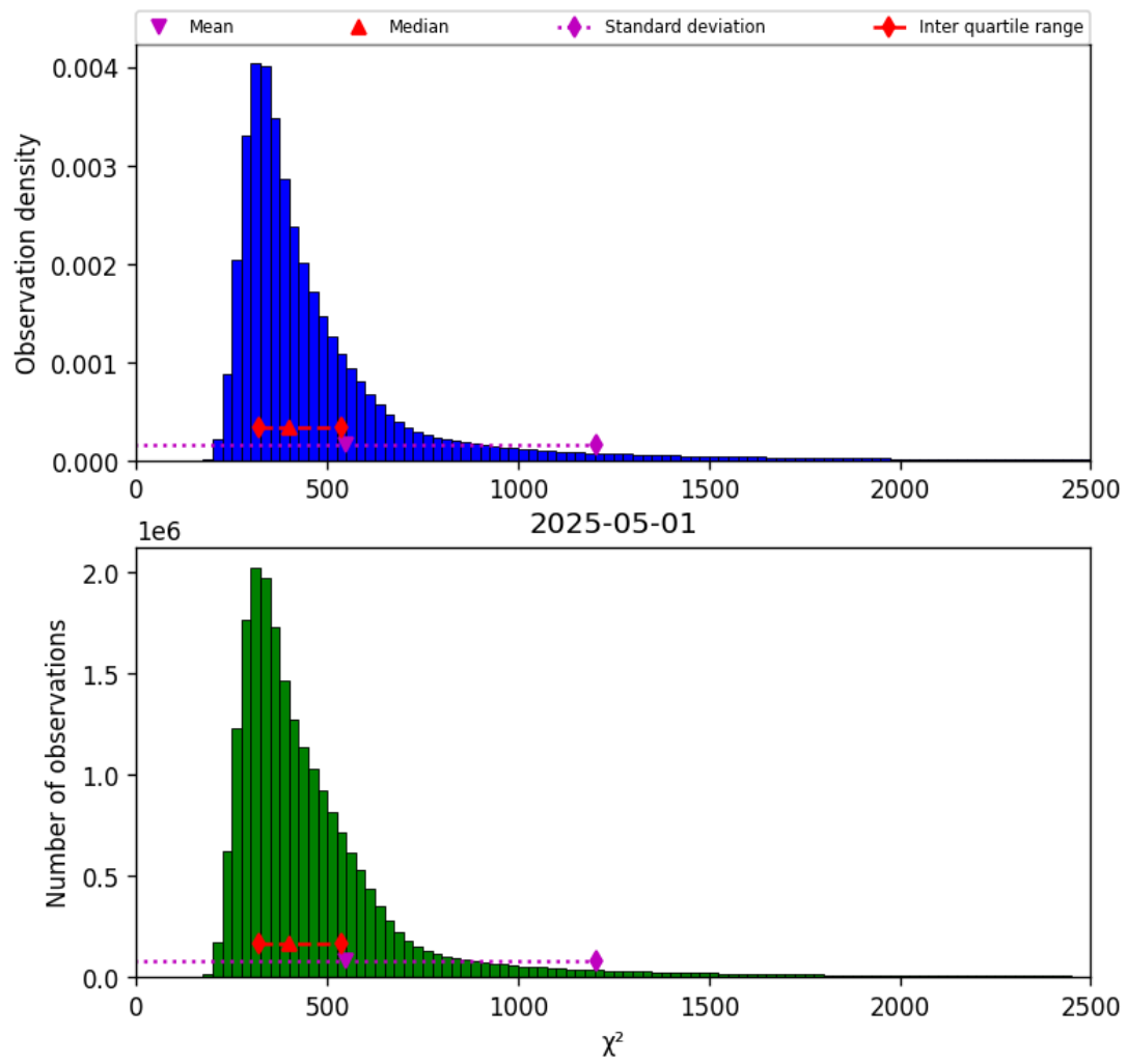
Figure 42: Histogram of “ \chi^2 ” for 2025-05-01 to 2025-05-02
