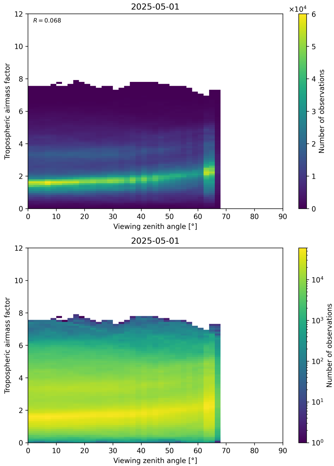
Figure 161: Scatter density plot of “Viewing zenith angle” against “Tropospheric airmass factor” for 2025-05-01 to 2025-05-02.
