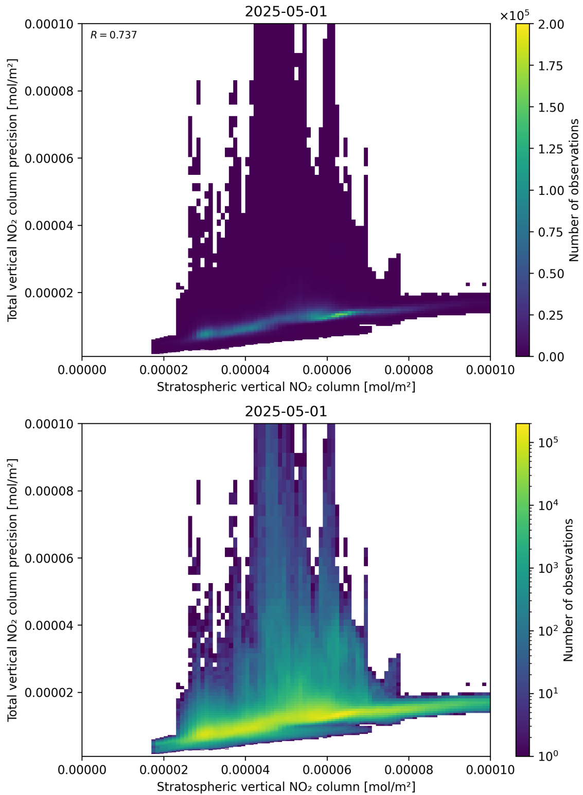
Figure 101: Scatter density plot of “Stratospheric vertical NO 2 column” against “Total vertical NO 2 column precision” for 2025-05-01 to 2025-05-02.
