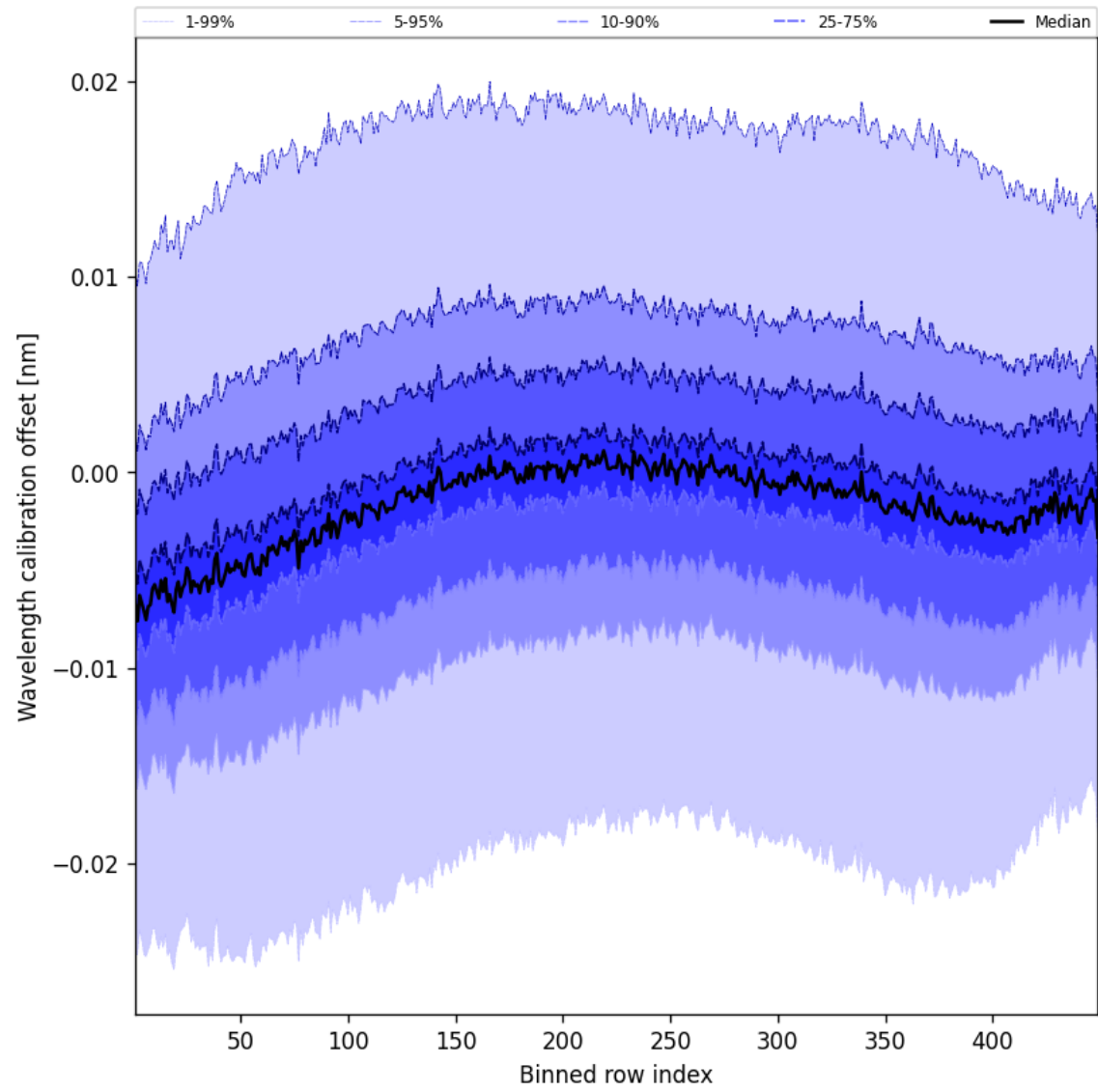
Figure 52: Along track statistics of “Wavelength calibration offset” for 2025-05-01 to 2025-05-02
