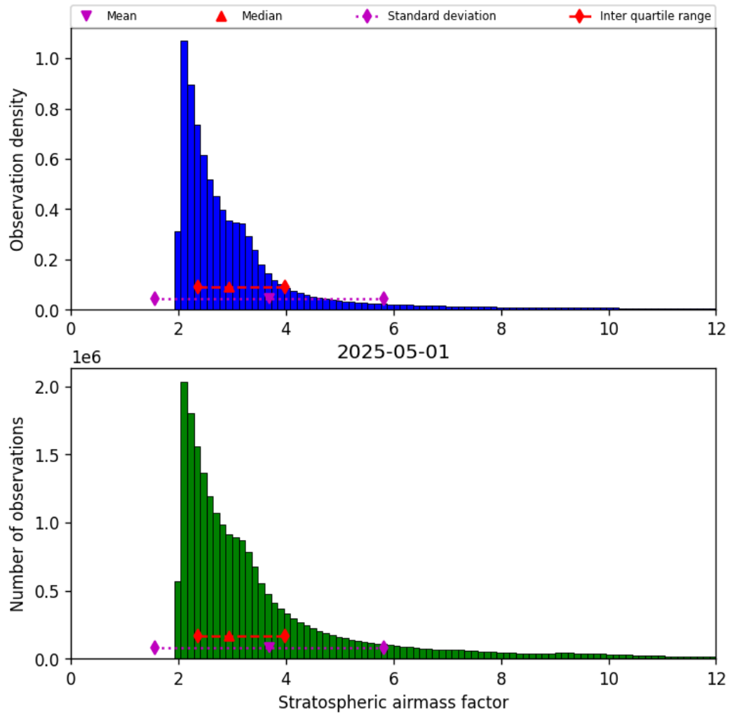
Figure 44: Histogram of “Stratospheric airmass factor” for 2025-05-01 to 2025-05-02
