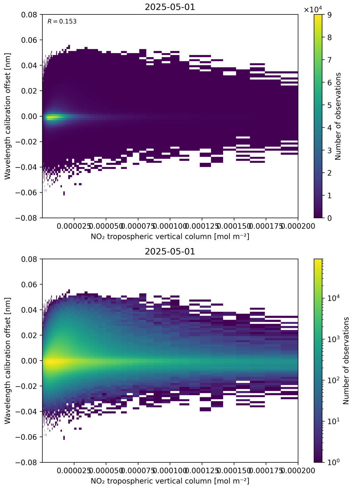
Figure 143: Scatter density plot of “NO 2 tropospheric vertical column” against “Wavelength calibration offset” for 2025-05-01 to 2025-05-02.
