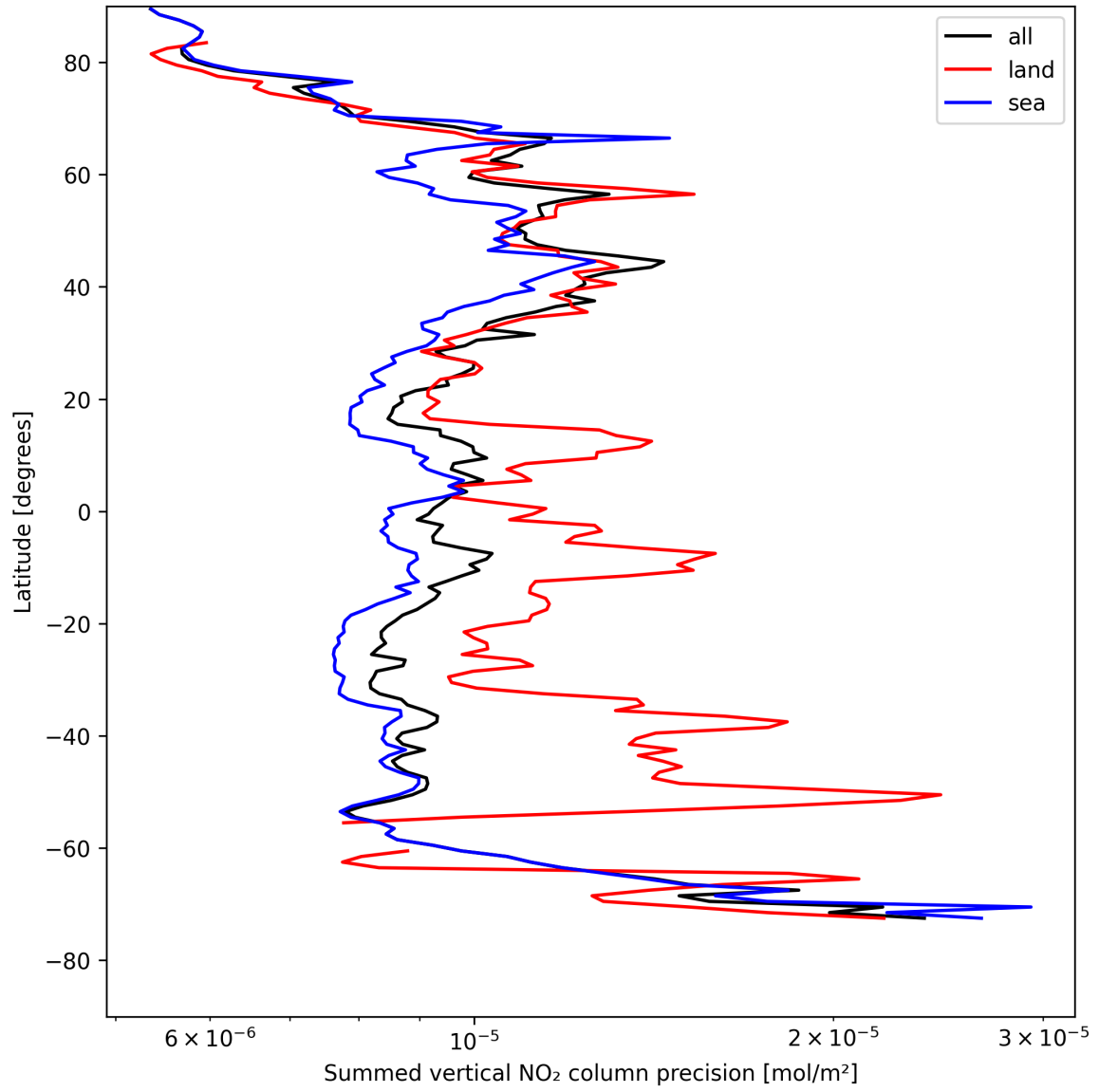
Figure 24: Zonal average of “Summed vertical NO 2 column precision” for 2025-05-01 to 2025-05-02.
