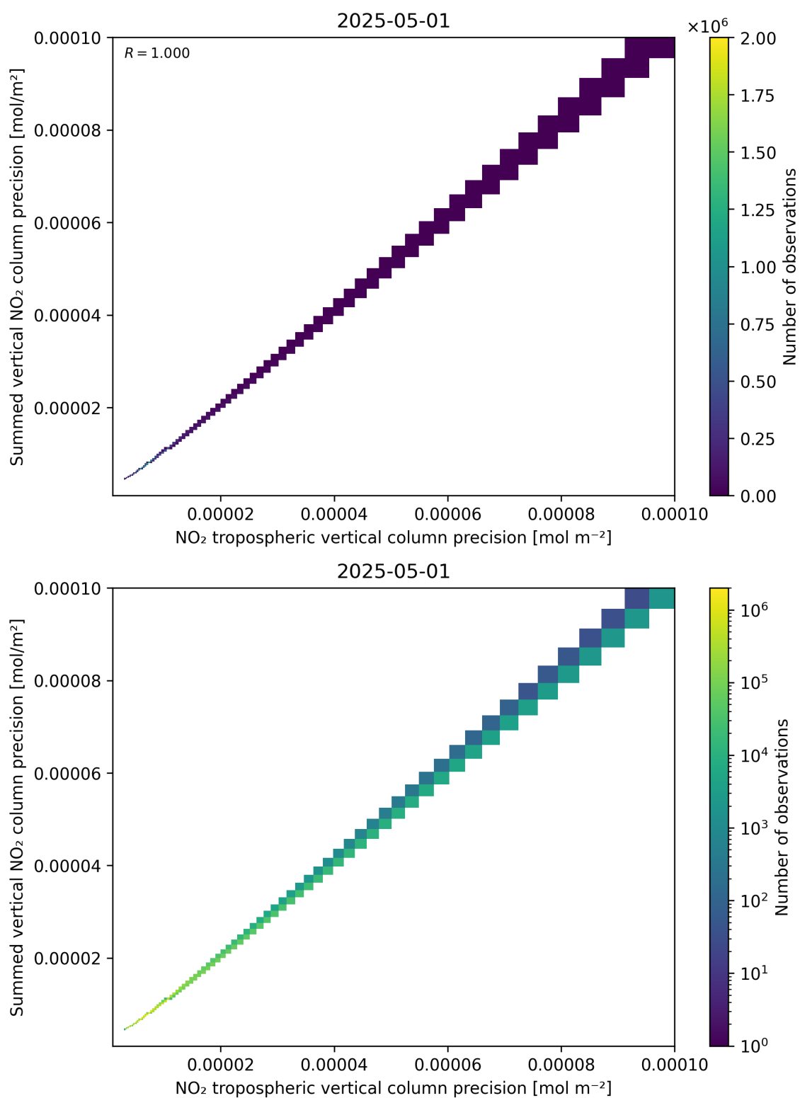
Figure 137: Scatter density plot of “NO 2 tropospheric vertical column precision” against “Summed vertical NO 2 column precision” for 2025-05-01 to 2025-05-02.
