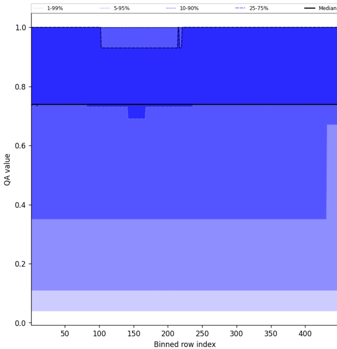
Figure 45: Along track statistics of “QA value” for 2025-05-01 to 2025-05-02
