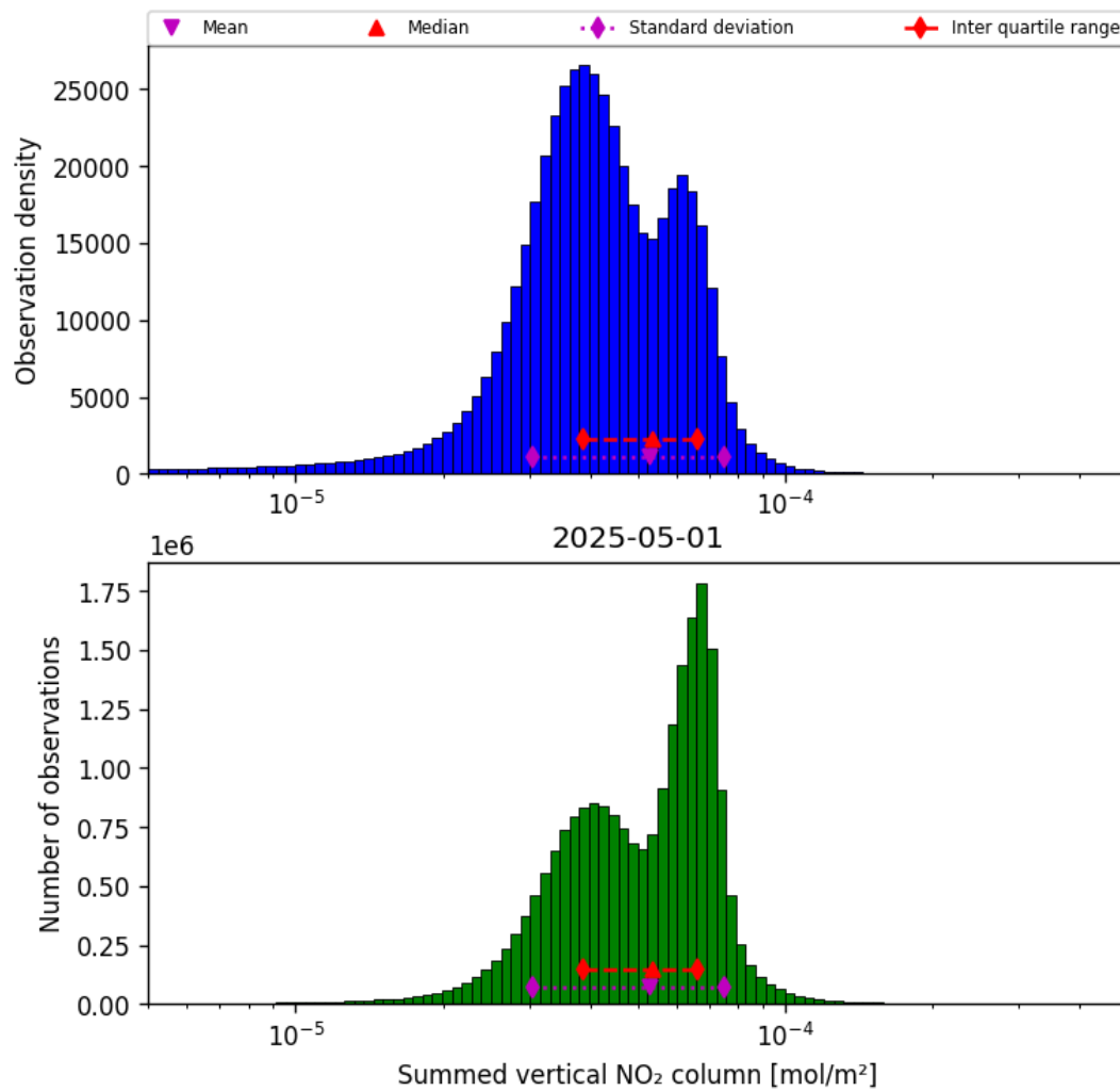
Figure 40: Histogram of “Summed vertical NO 2 column” for 2025-05-01 to 2025-05-02
