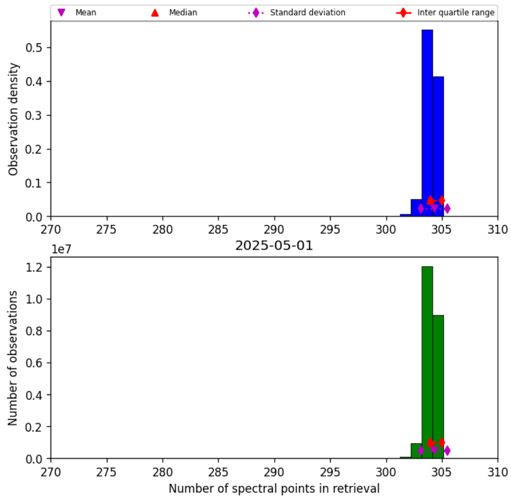
Figure 33: Histogram of “Number of spectral points in retrieval” for 2025-05-01 to 2025-05-02
