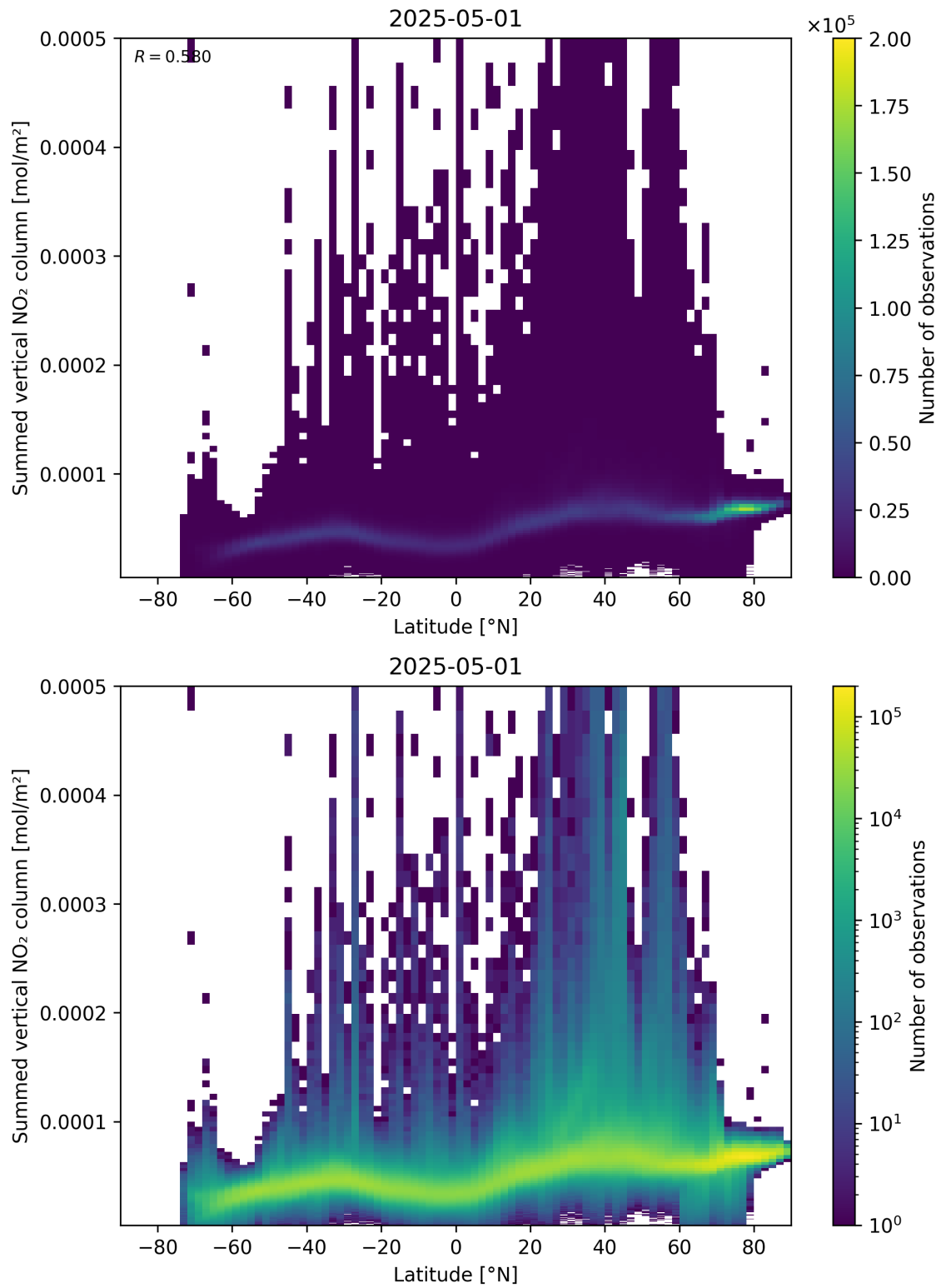
Figure 88: Scatter density plot of “Latitude” against “Summed vertical NO 2 column” for 2025-05-01 to 2025-05-02.
