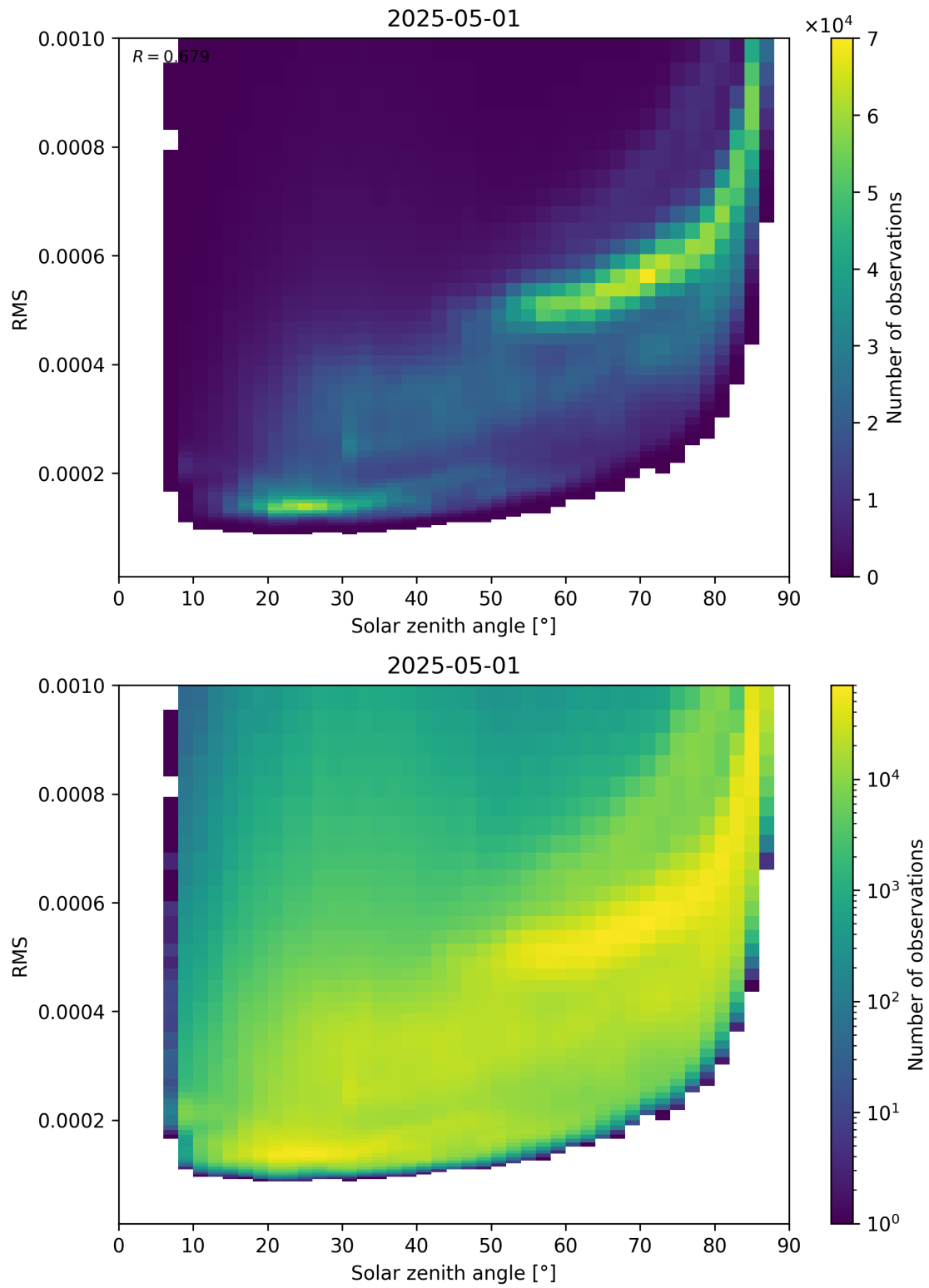
Figure 157: Scatter density plot of “Solar zenith angle” against “RMS” for 2025-05-01 to 2025-05-02.
