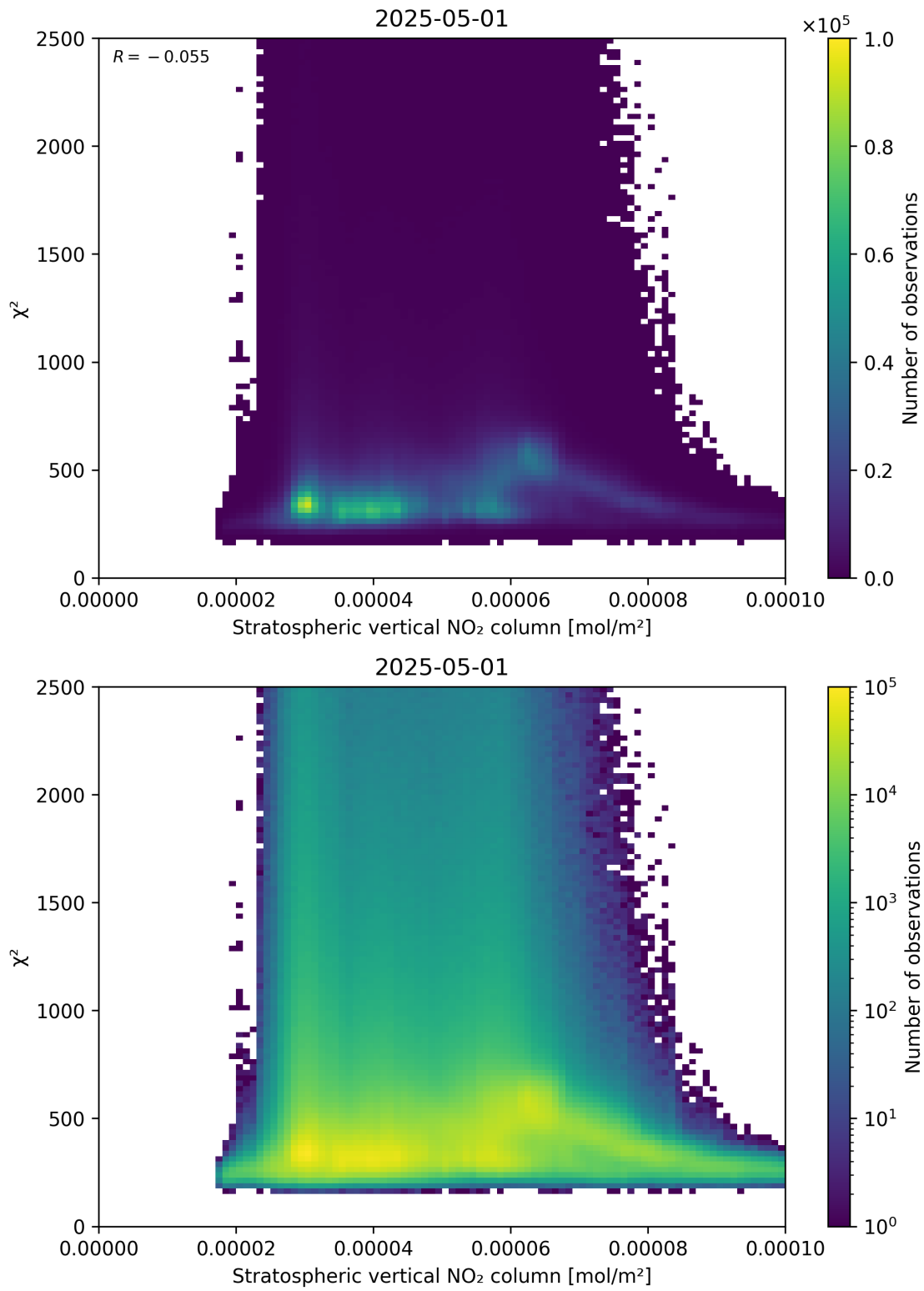
Figure 97: Scatter density plot of “Stratospheric vertical NO 2 column” against “ \chi^2 ” for 2025-05-01 to 2025-05-02.
