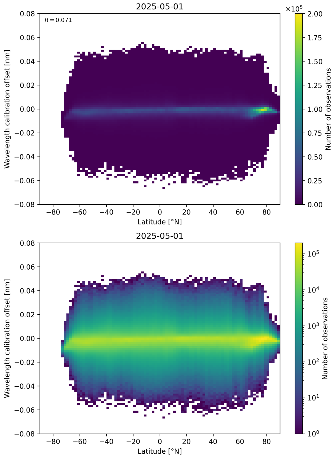
Figure 95: Scatter density plot of “Latitude” against “Wavelength calibration offset” for 2025-05-01 to 2025-05-02.
