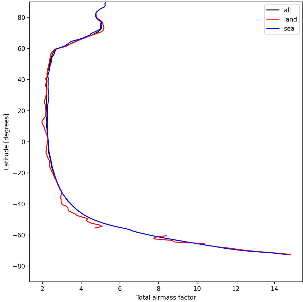
Figure 15: Zonal average of “Total airmass factor” for 2025-05-01 to 2025-05-02.
