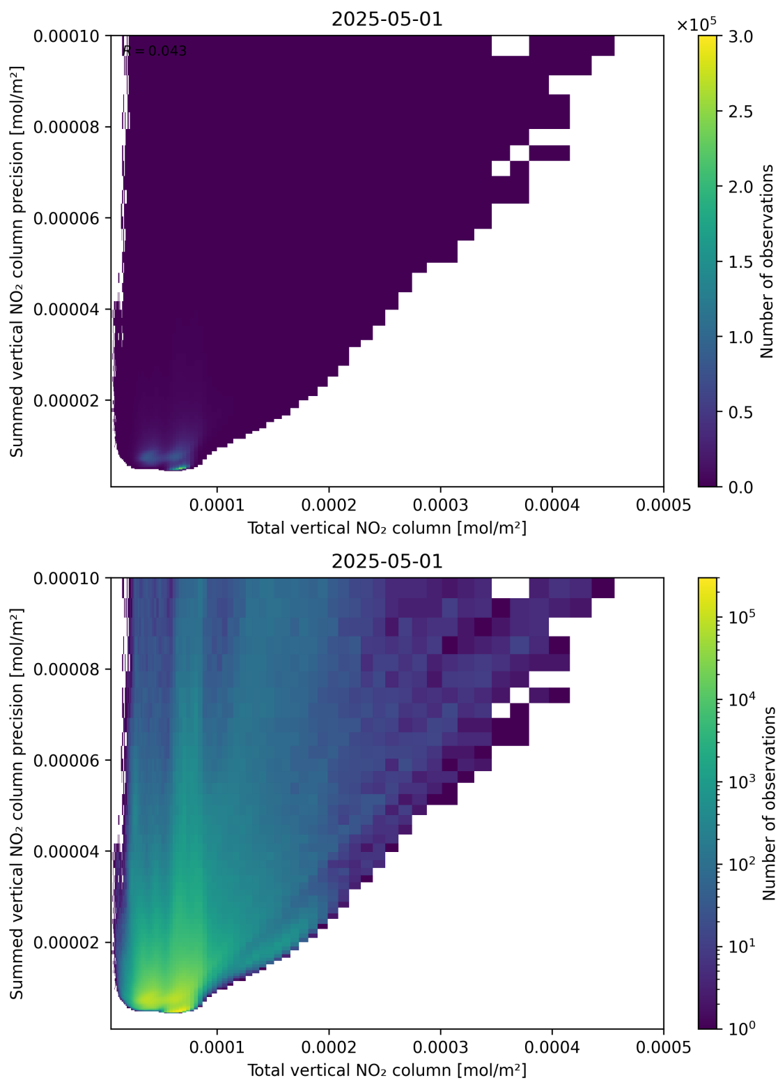
Figure 113: Scatter density plot of “Total vertical NO 2 column” against “Summed vertical NO 2 column precision” for 2025-05-01 to 2025-05-02.
