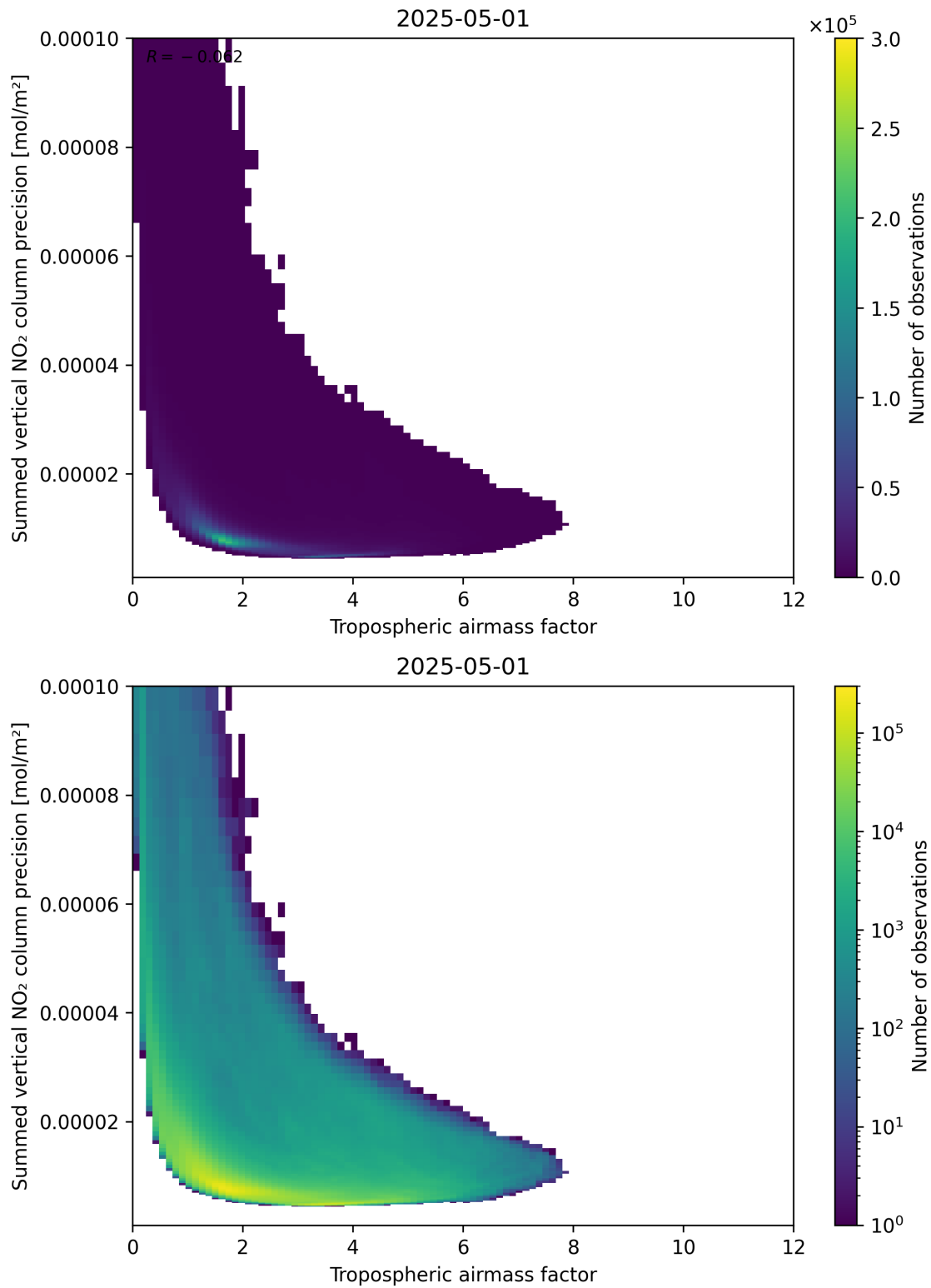
Figure 76: Scatter density plot of “Tropospheric air mass factor” against “Summed vertical NO 2 column precision” for 2025-05-01 to 2025-05-02.
