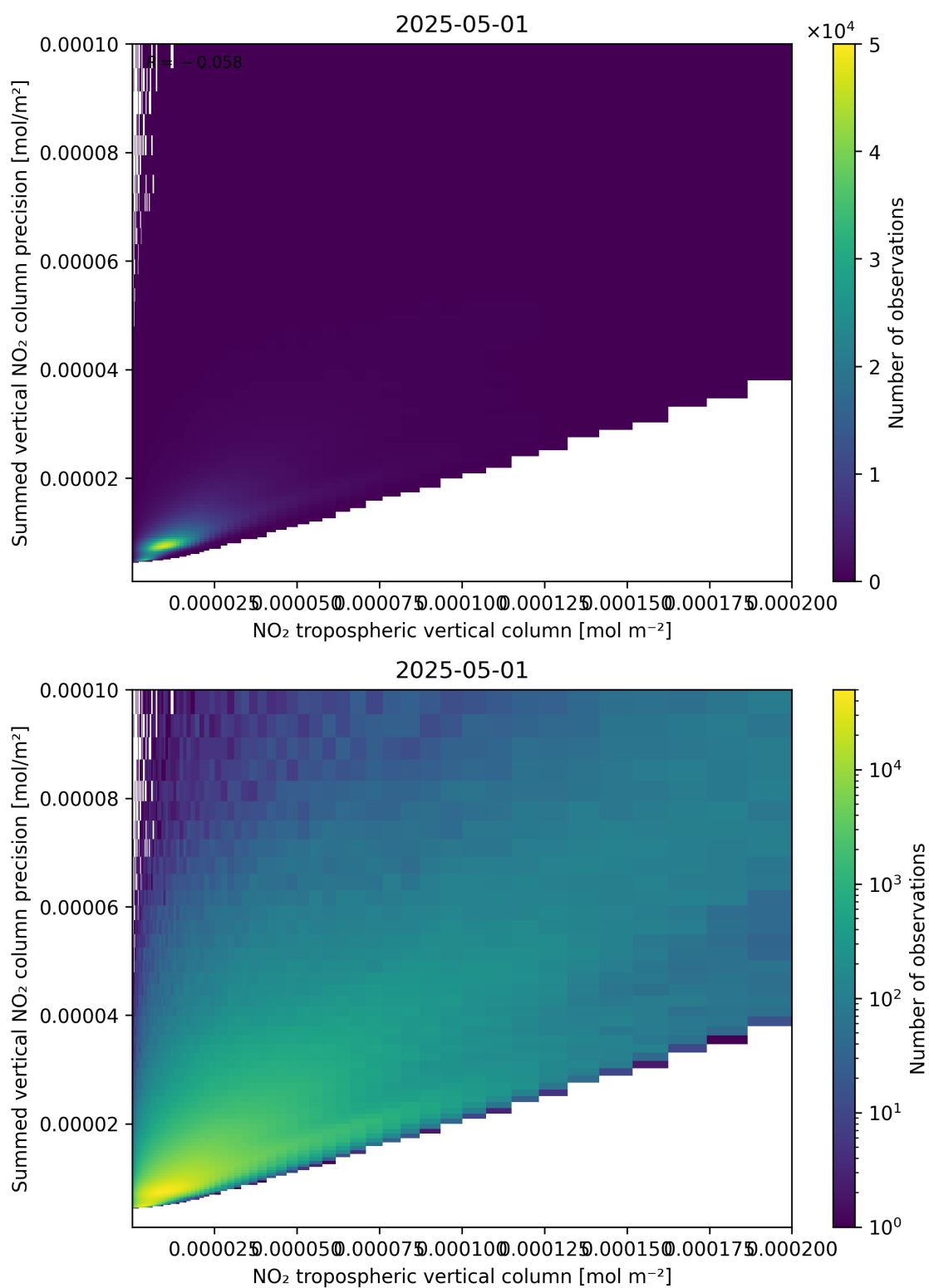
Figure 127: Scatter density plot of “NO 2 tropospheric vertical column” against “Summed vertical NO 2 column precision” for 2025-05-01 to 2025-05-02.
