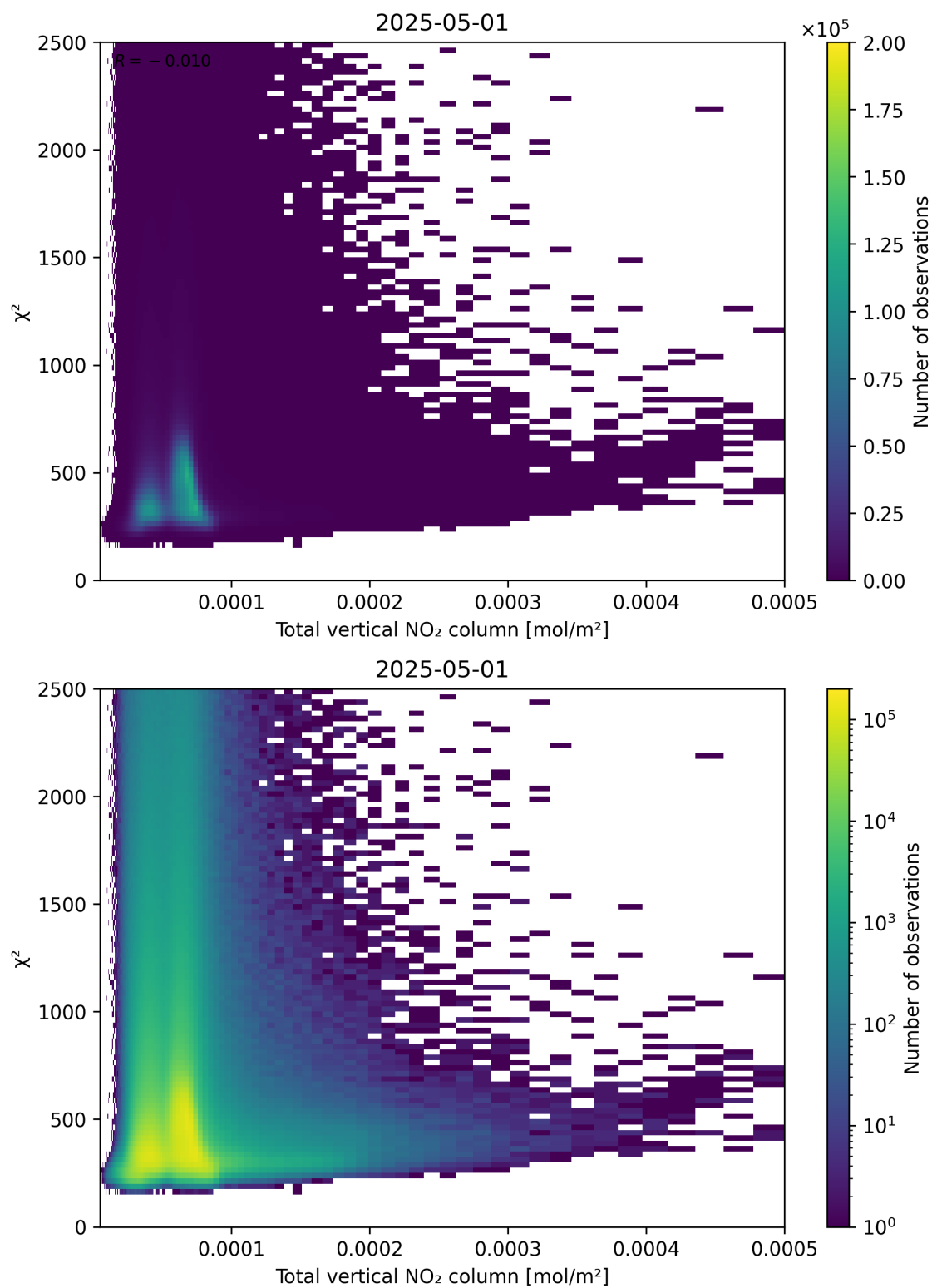
Figure 111: Scatter density plot of “Total vertical NO 2 column” against “ \chi^2 ” for 2025-05-01 to 2025-05-02.
