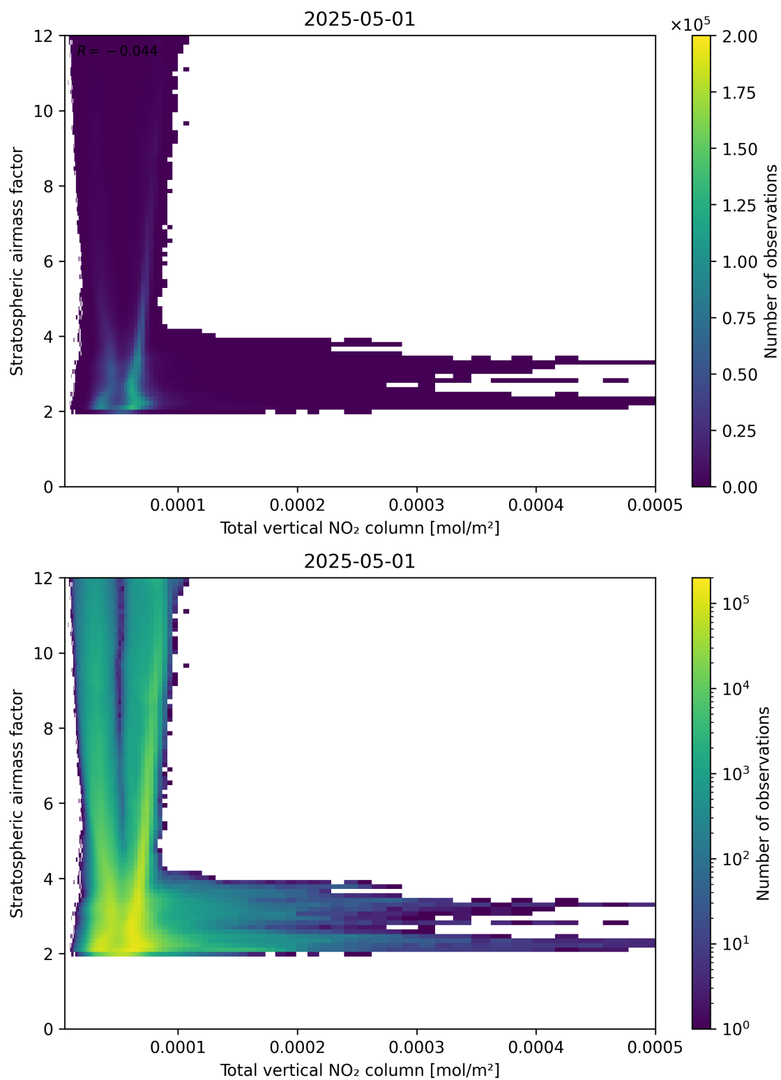
Figure 110: Scatter density plot of “Total vertical NO 2 column” against “Stratospheric airmass factor” for 2025-05-01 to 2025-05-02.
