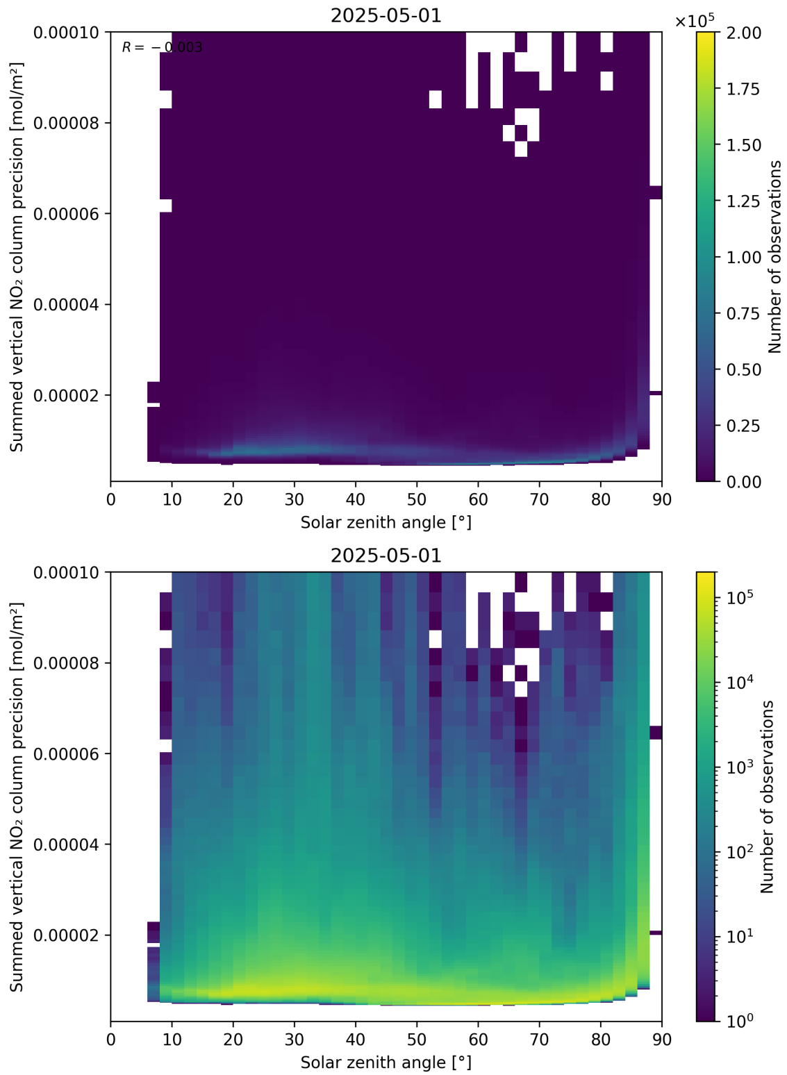
Figure 152: Scatter density plot of “Solar zenith angle” against “Summed vertical NO 2 column precision” for 2025-05-01 to 2025-05-02.
