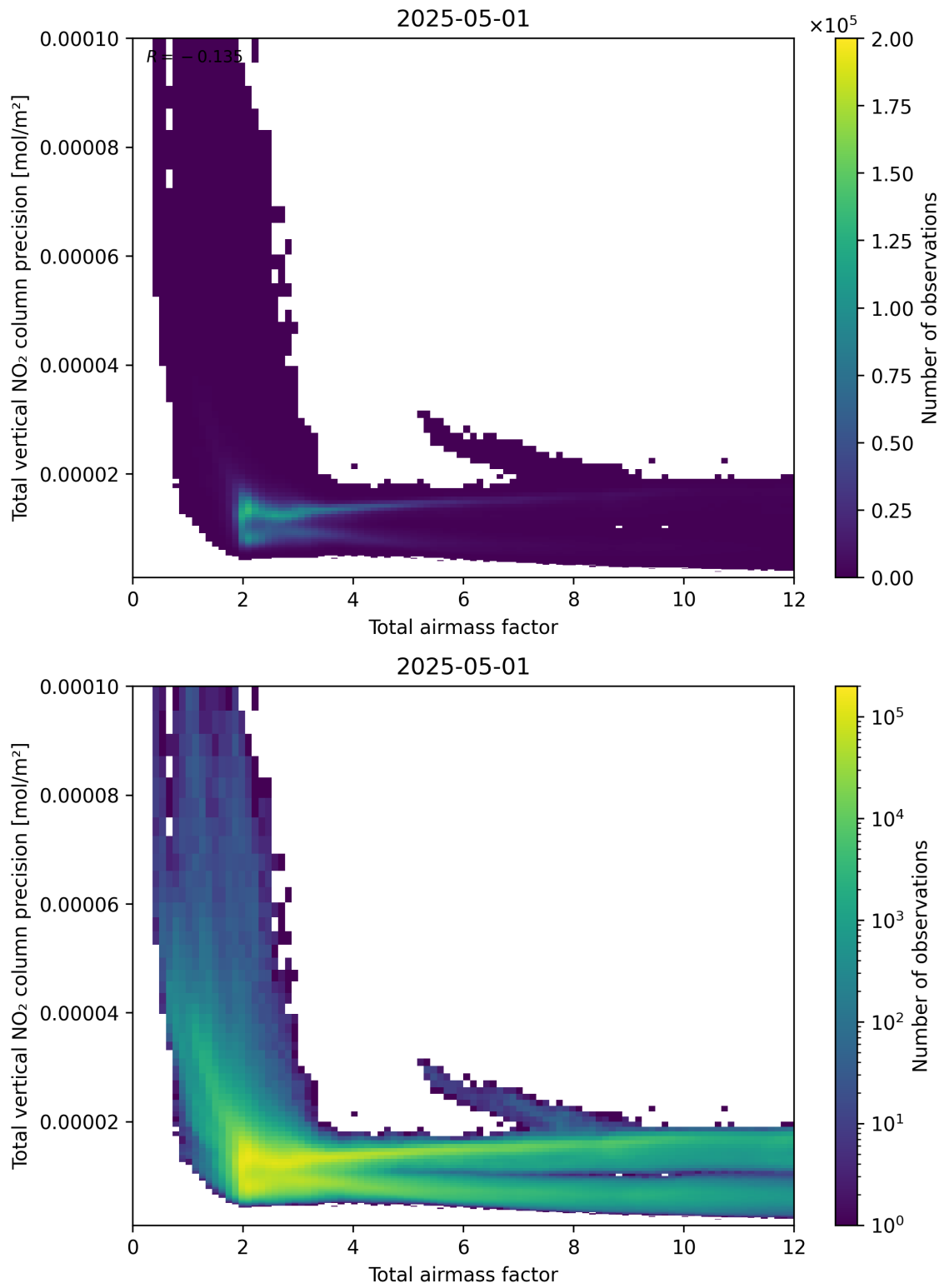
Figure 68: Scatter density plot of “Total airmass factor” against “Total vertical NO 2 column precision” for 2025-05-01 to 2025-05-02.
