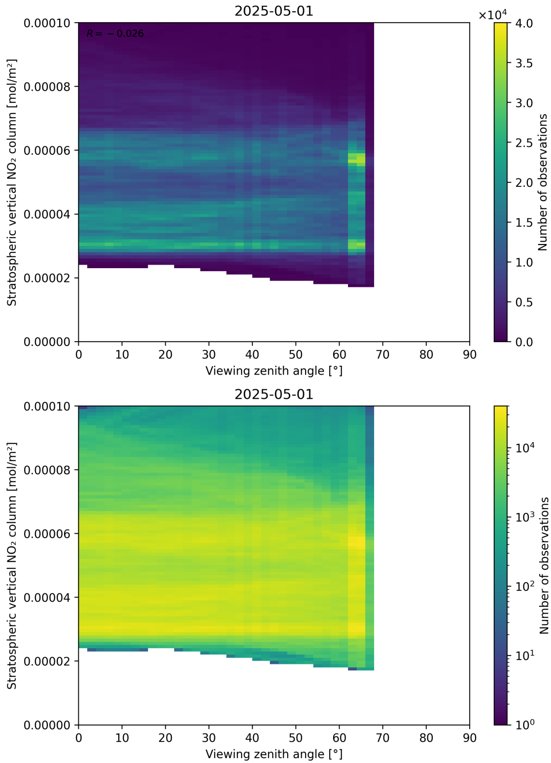
Figure 164: Scatter density plot of “Viewing zenith angle” against “Stratospheric vertical NO 2 column” for 2025-05-01 to 2025-05-02.
