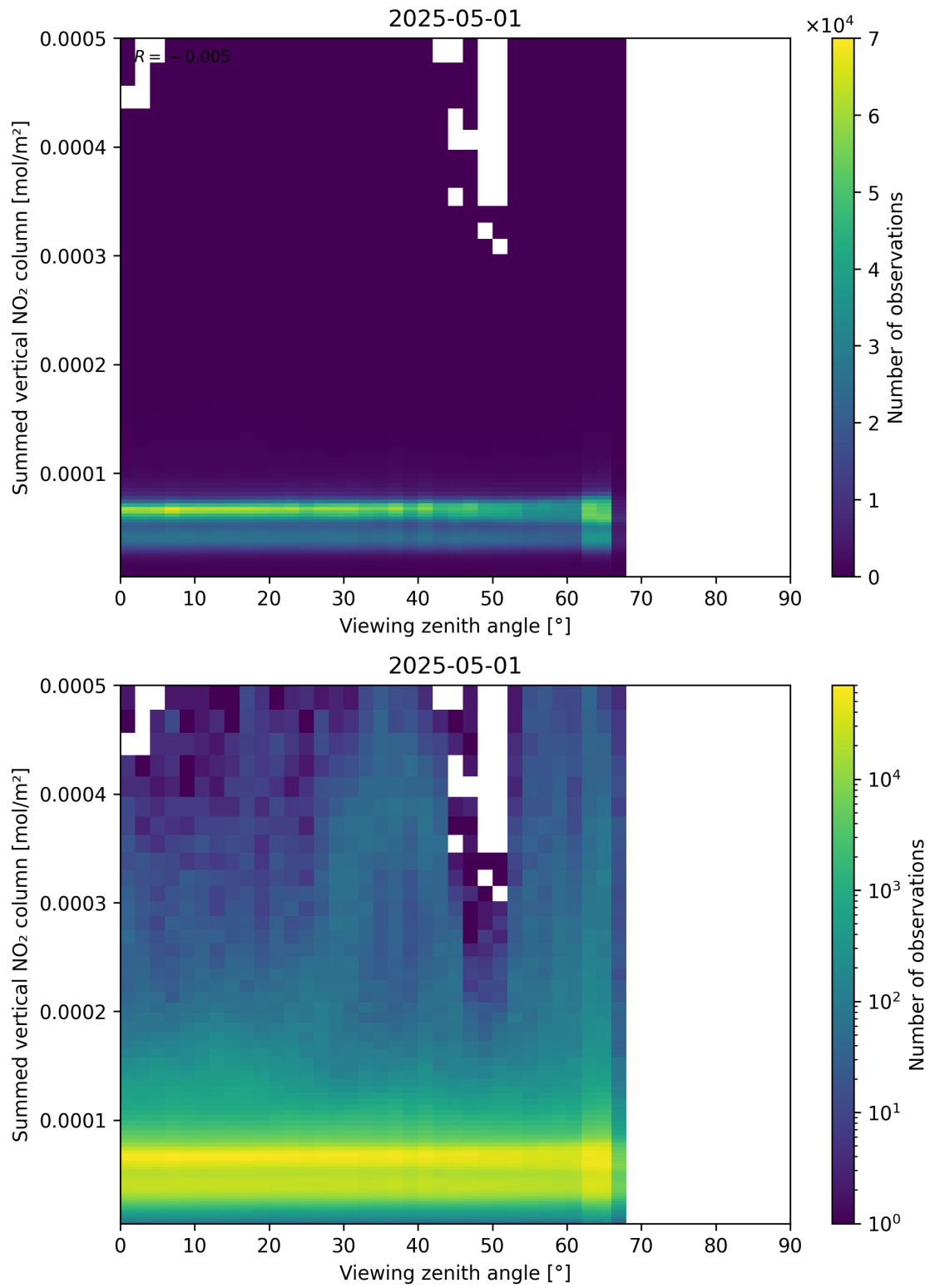
Figure 165: Scatter density plot of “Viewing zenith angle” against “Summed vertical NO 2 column” for 2025-05-01 to 2025-05-02.
