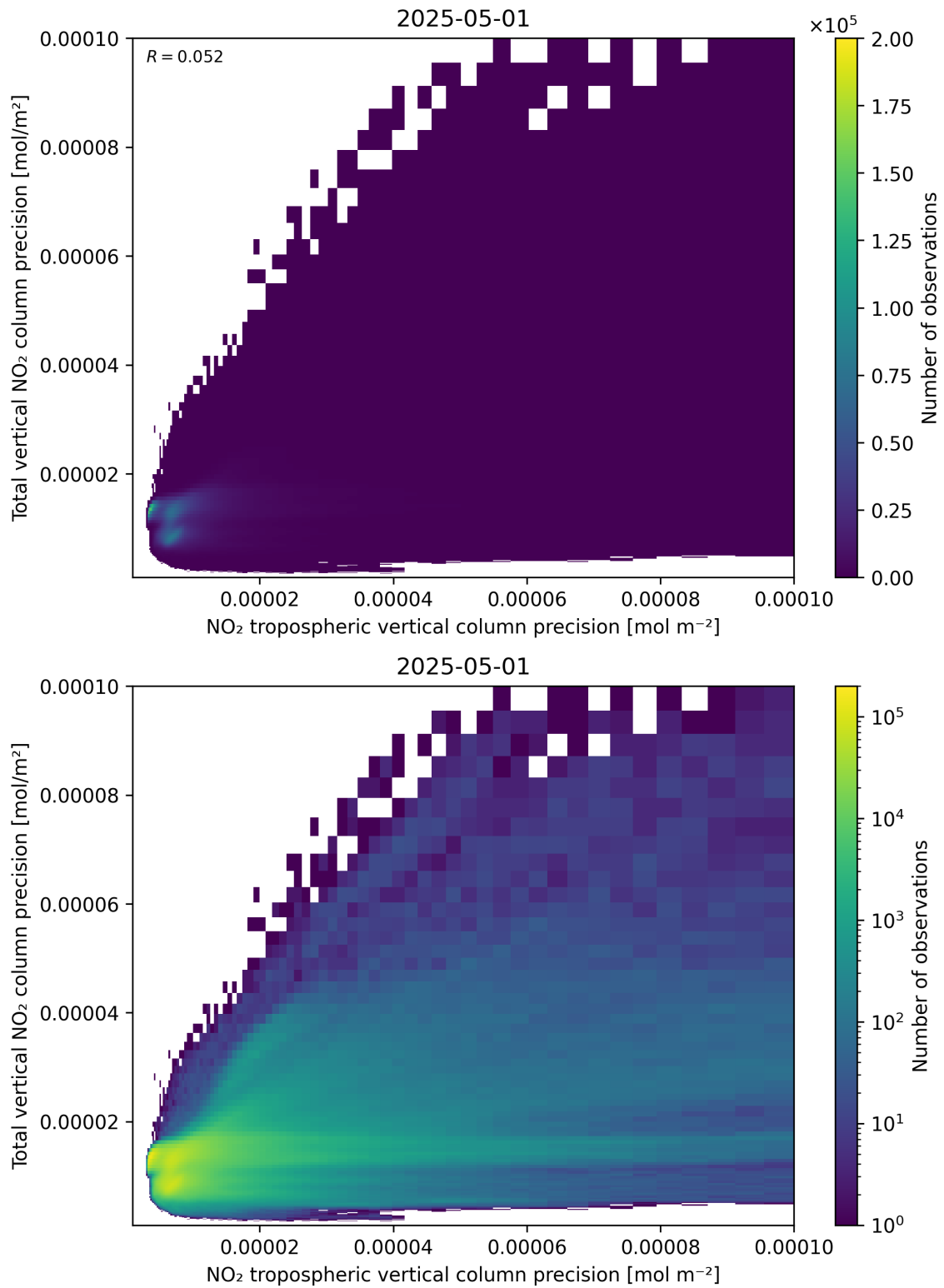
Figure 139: Scatter density plot of “NO 2 tropospheric vertical column precision” against “Total vertical NO 2 column precision” for 2025-05-01 to 2025-05-02.
