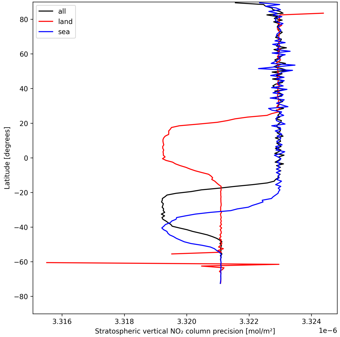
Figure 20: Zonal average of “Stratospheric vertical NO 2 column precision” for 2025-05-01 to 2025-05-02.
