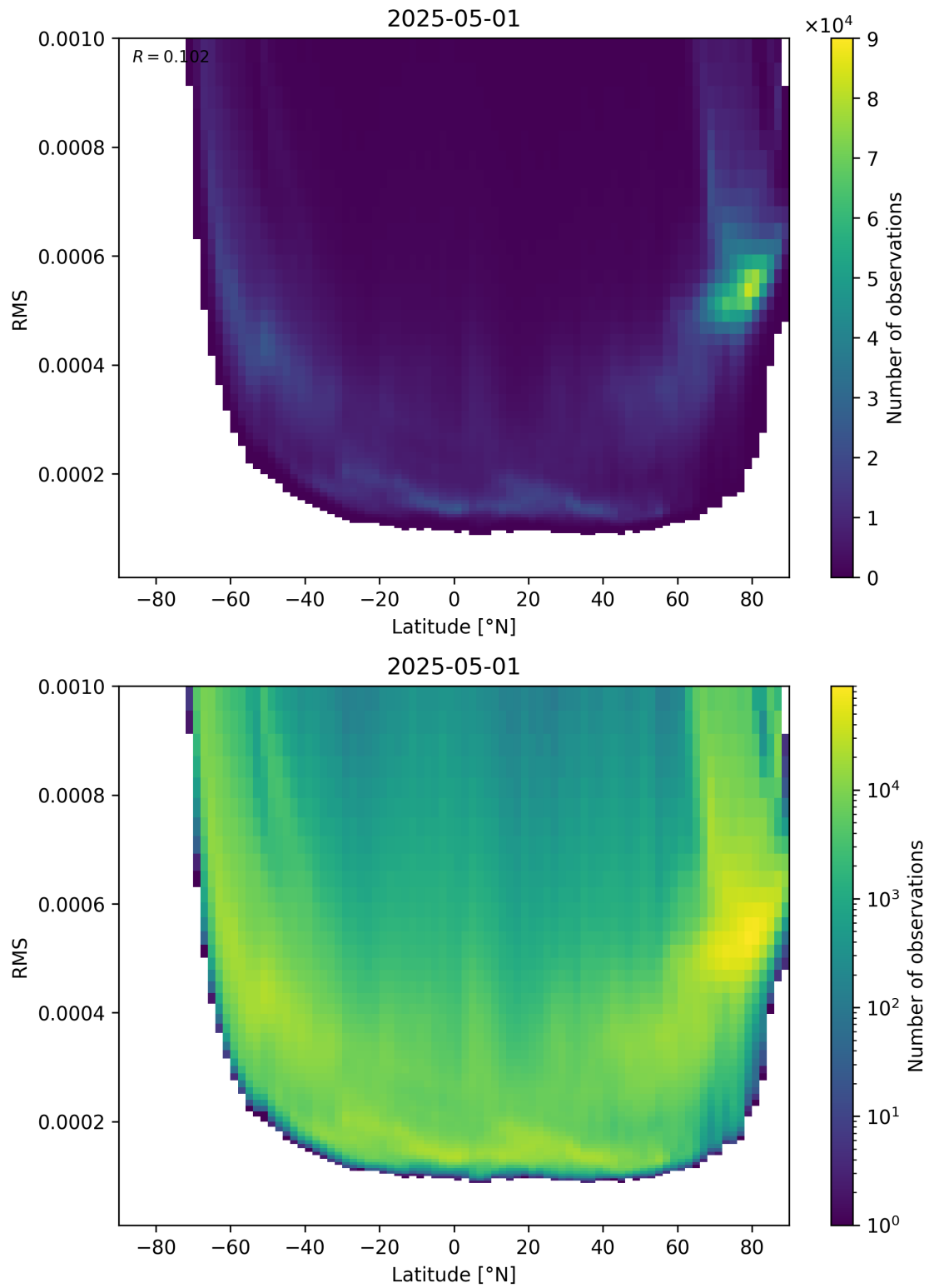
Figure 94: Scatter density plot of “Latitude” against “RMS” for 2025-05-01 to 2025-05-02.
