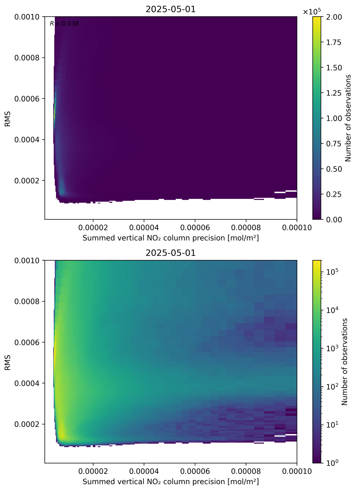
Figure 108: Scatter density plot of “Summed vertical NO 2 column precision” against “RMS” for 2025-05-01 to 2025-05-02.
