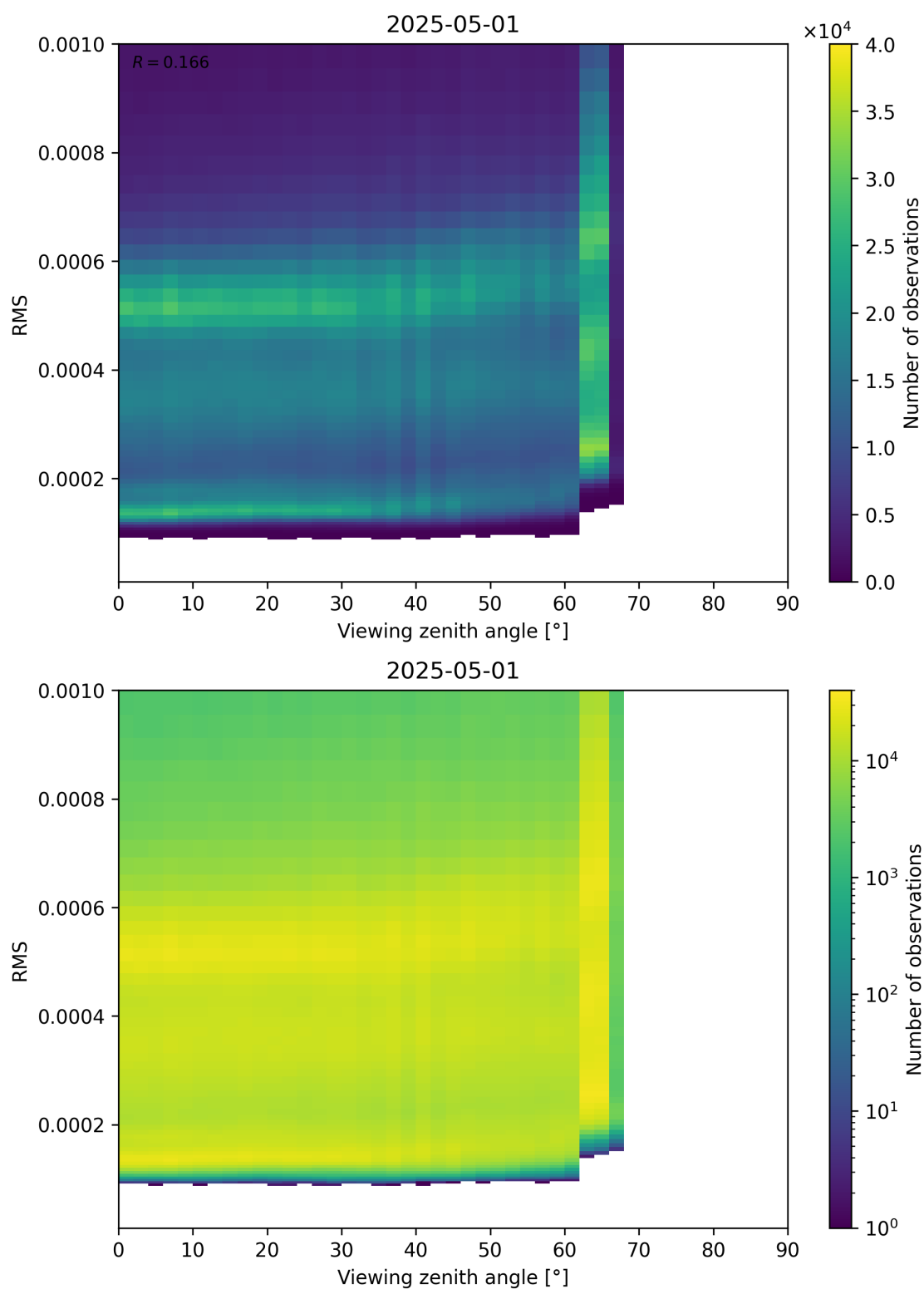
Figure 171: Scatter density plot of “Viewing zenith angle” against “RMS” for 2025-05-01 to 2025-05-02.
