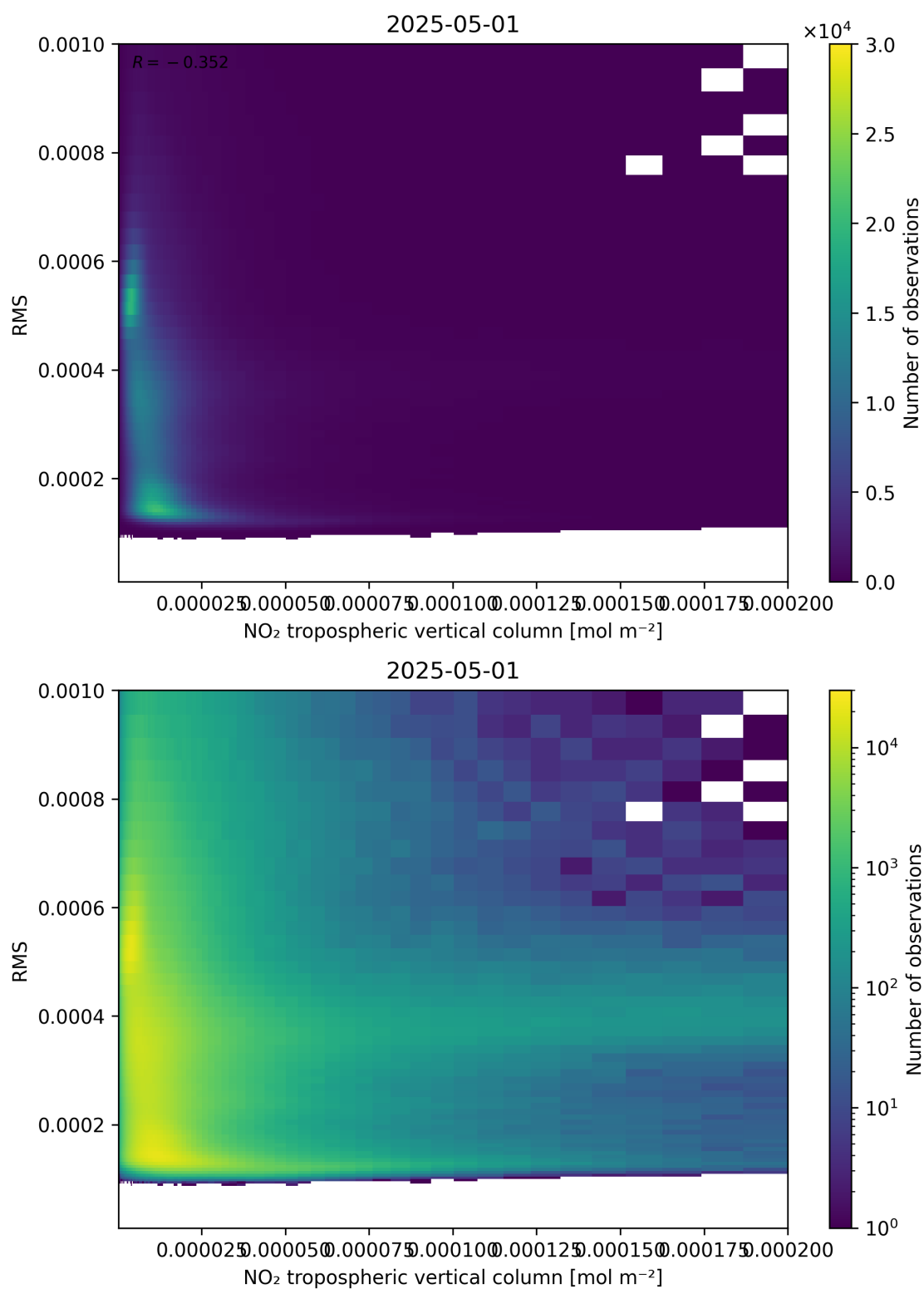
Figure 142: Scatter density plot of “NO 2 tropospheric vertical column” against “RMS” for 2025-05-01 to 2025-05-02.
