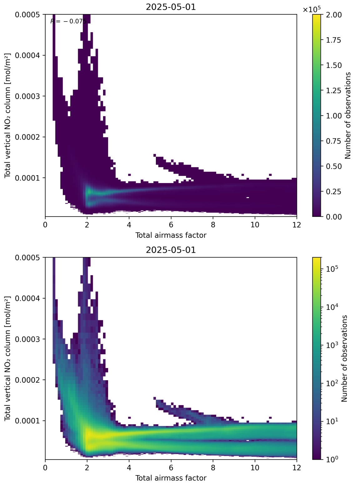
Figure 67: Scatter density plot of “Total airmass factor” against “Total vertical NO 2 column” for 2025-05-01 to 2025-05-02.
