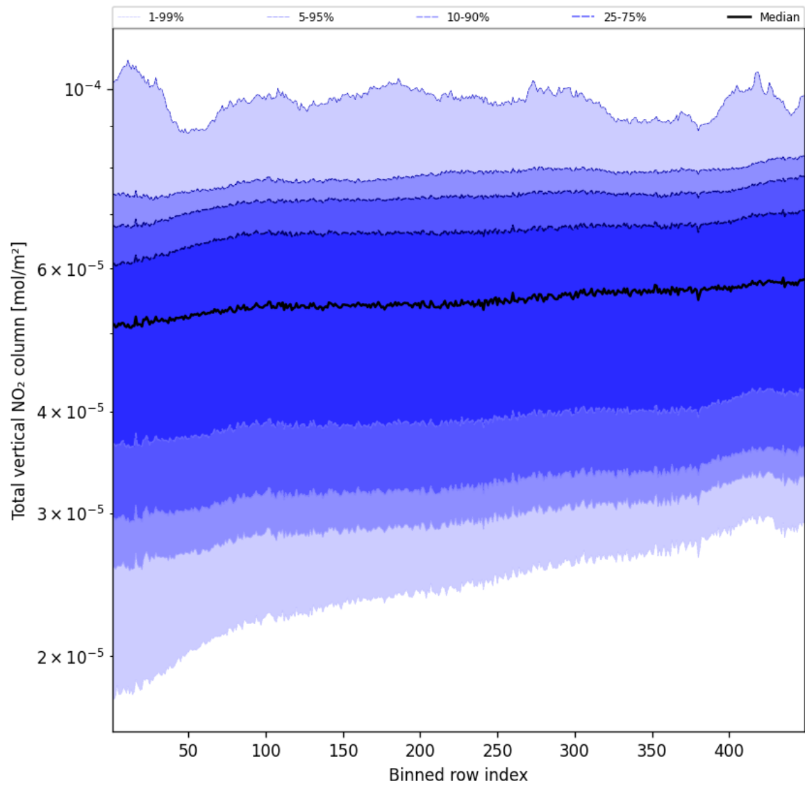
Figure 55: Along track statistics of “Total vertical NO 2 column” for 2025-05-01 to 2025-05-02
