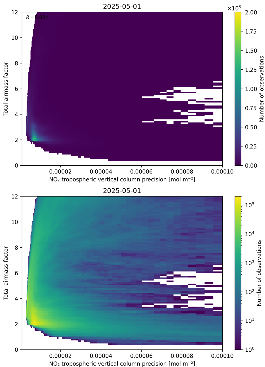
Figure 132: Scatter density plot of “NO 2 tropospheric vertical column precision” against “Total air mass factor” for 2025-05-01 to 2025-05-02.
