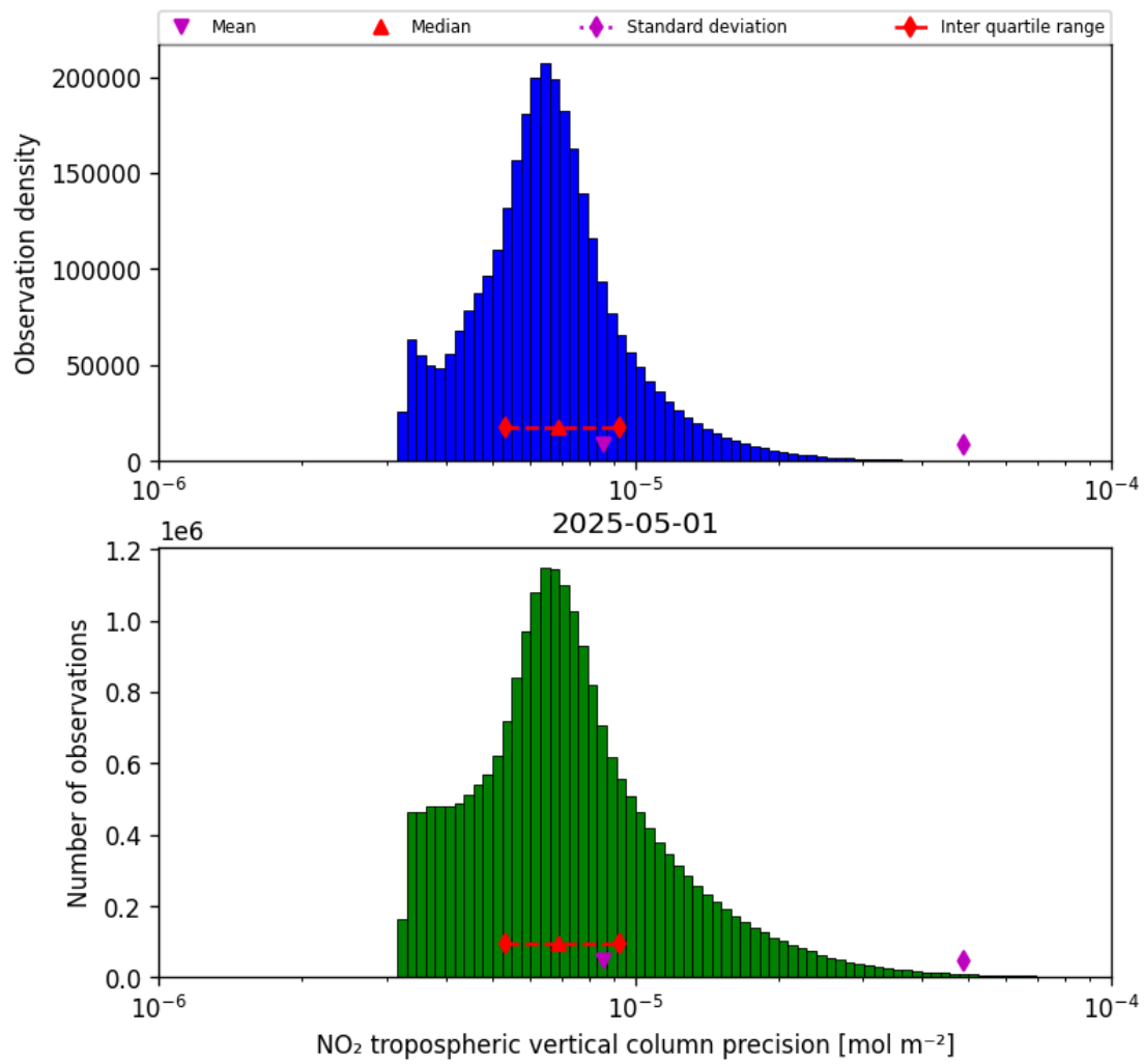
Figure 30: Histogram of “NO 2 tropospheric vertical column precision” for 2025-05-01 to 2025-05-02
