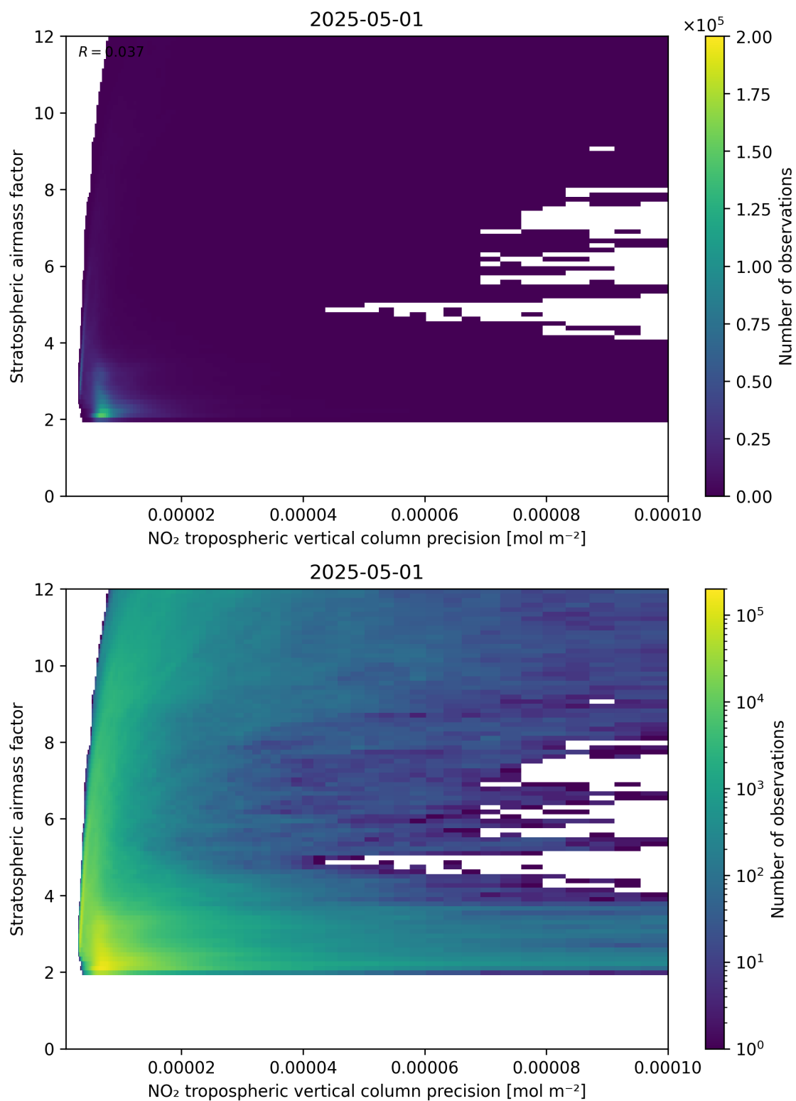
Figure 131: Scatter density plot of “NO 2 tropospheric vertical column precision” against “Stratospheric airmass factor” for 2025-05-01 to 2025-05-02.
