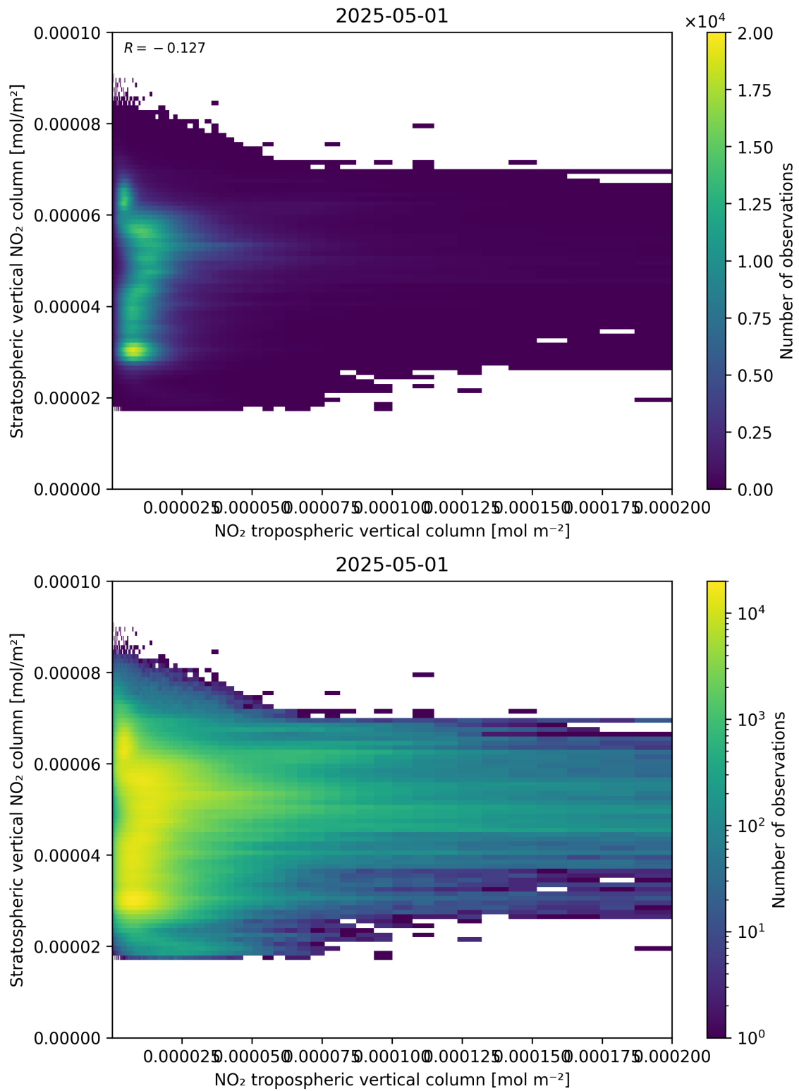
Figure 125: Scatter density plot of “NO 2 tropospheric vertical column” against “Stratospheric vertical NO 2 column” for 2025-05-01 to 2025-05-02.
