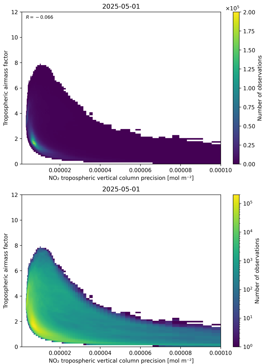
Figure 133: Scatter density plot of “NO 2 tropospheric vertical column precision” against “Tropospheric air mass factor” for 2025-05-01 to 2025-05-02.
