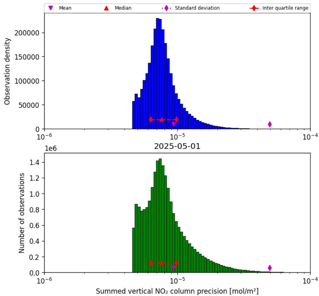
Figure 41: Histogram of “Summed vertical NO 2 column precision” for 2025-05-01 to 2025-05-02
