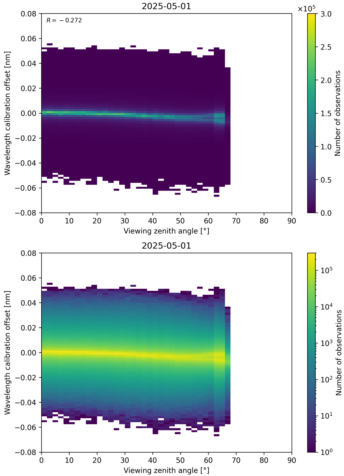
Figure 173: Scatter density plot of “Viewing zenith angle” against “Wavelength calibration offset” for 2025-05-01 to 2025-05-02.
