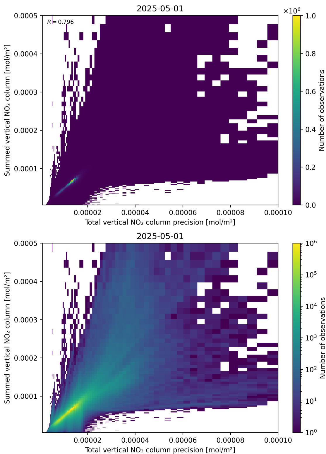
Figure 117: Scatter density plot of “Total vertical NO 2 column precision” against “Summed vertical NO 2 column” for 2025-05-01 to 2025-05-02.
