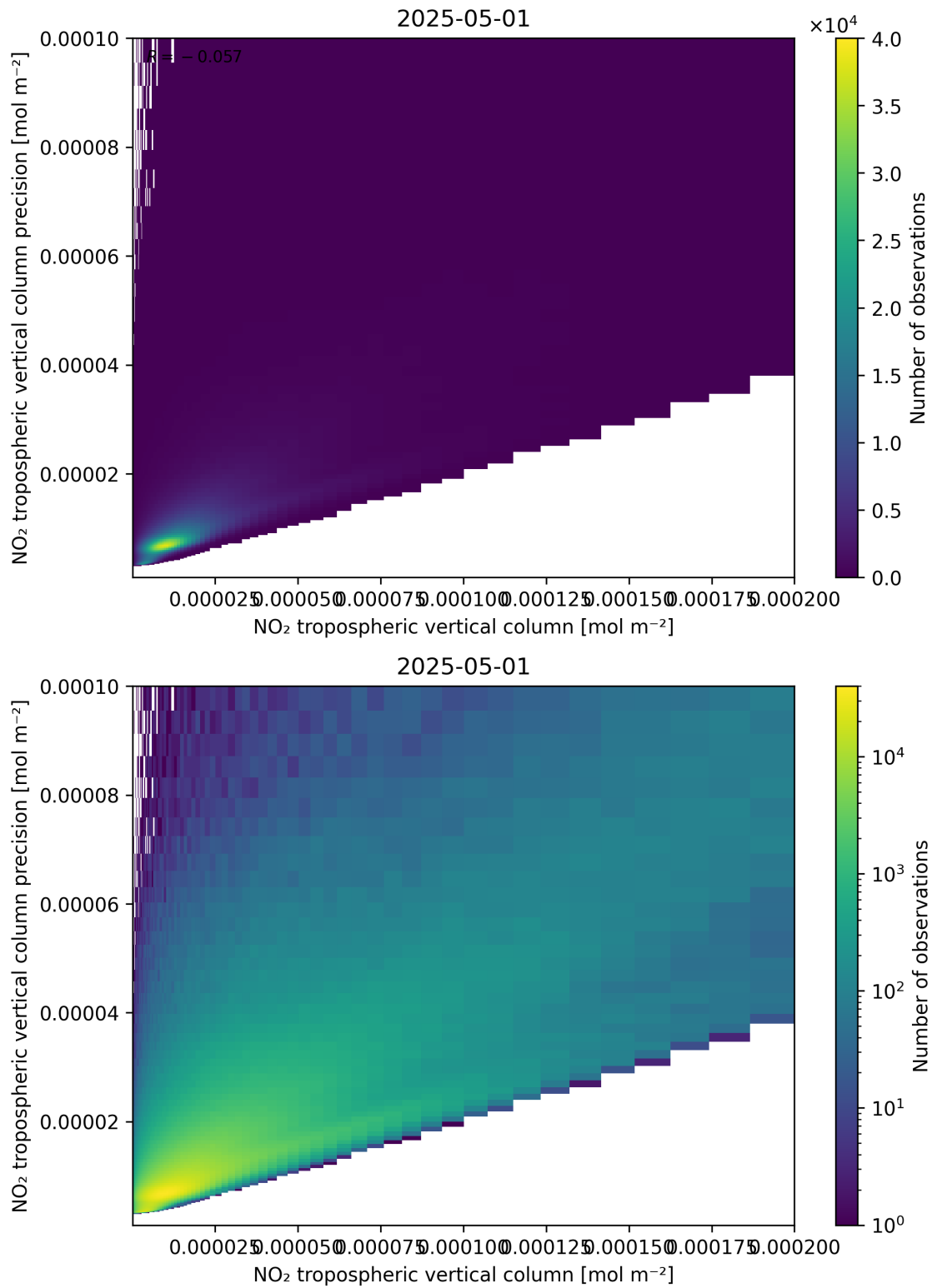
Figure 130: Scatter density plot of “NO 2 tropospheric vertical column” against “NO 2 tropospheric vertical column precision” for 2025-05-01 to 2025-05-02.
