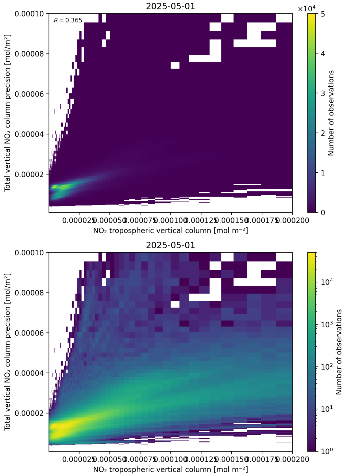
Figure 129: Scatter density plot of “NO 2 tropospheric vertical column” against “Total vertical NO 2 column precision” for 2025-05-01 to 2025-05-02.
