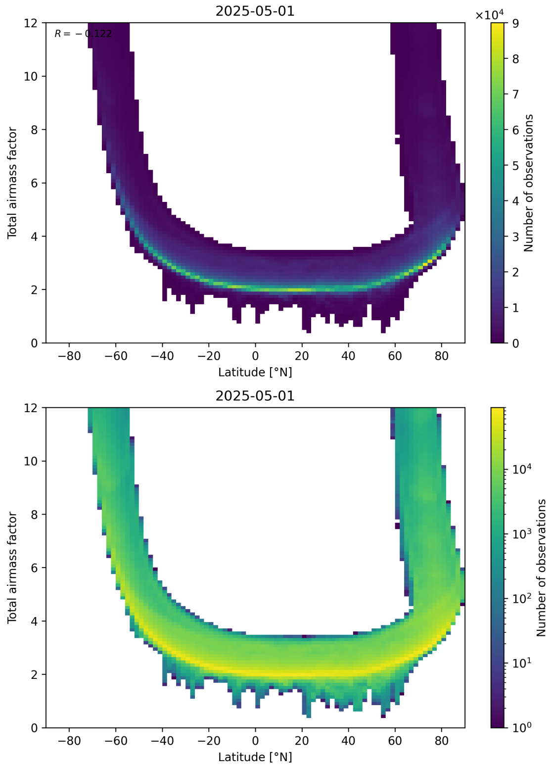
Figure 84: Scatter density plot of “Latitude” against “Total air mass factor” for 2025-05-01 to 2025-05-02.
