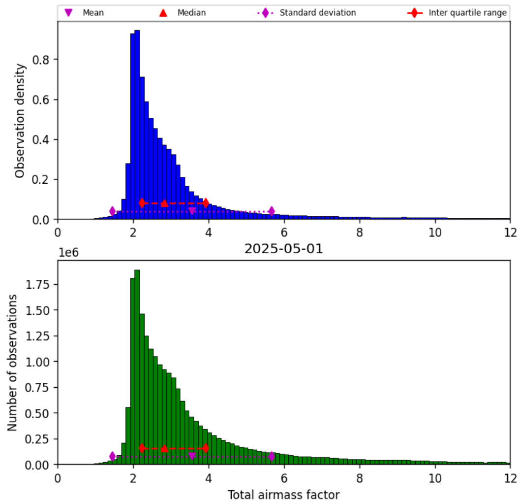
Figure 32: Histogram of “Total airmass factor” for 2025-05-01 to 2025-05-02
