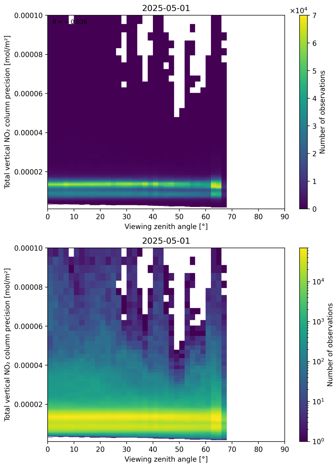
Figure 168: Scatter density plot of “Viewing zenith angle” against “Total vertical NO 2 column precision” for 2025-05-01 to 2025-05-02.
