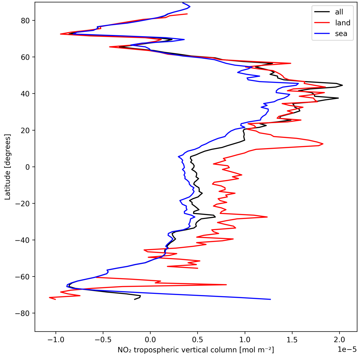
Figure 12: Zonal average of “NO 2 tropospheric vertical column” for 2025-05-01 to 2025-05-02.
