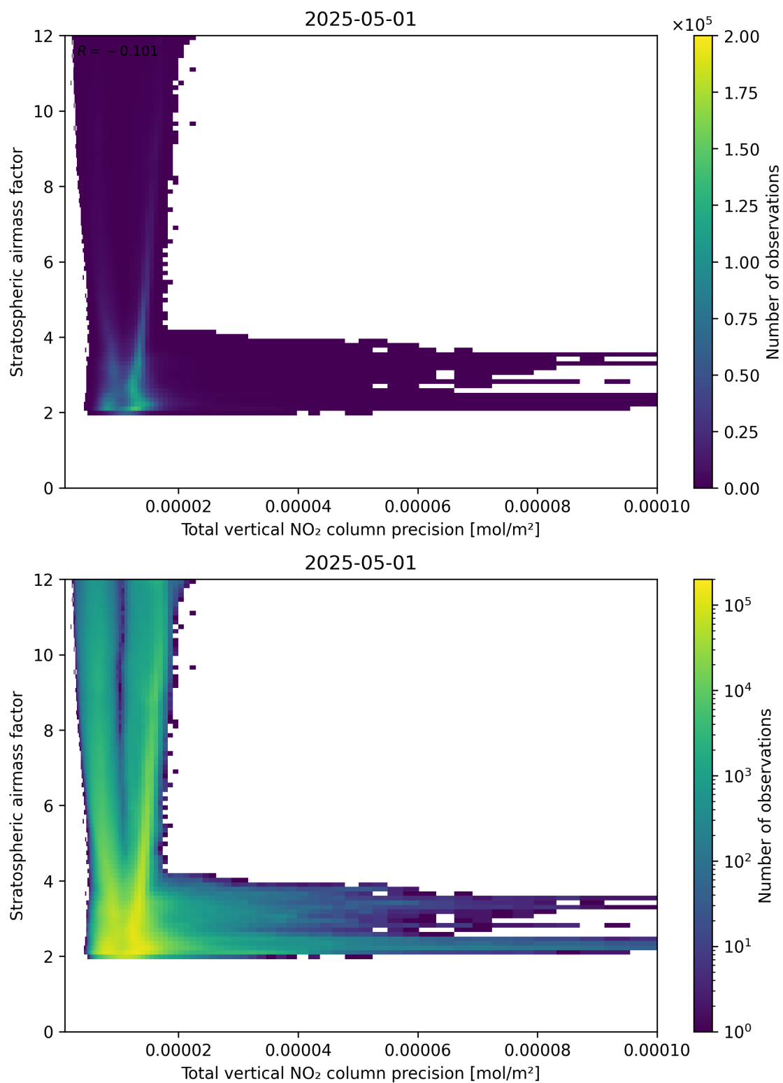
Figure 115: Scatter density plot of “Total vertical NO 2 column precision” against “Stratospheric air mass factor” for 2025-05-01 to 2025-05-02.
