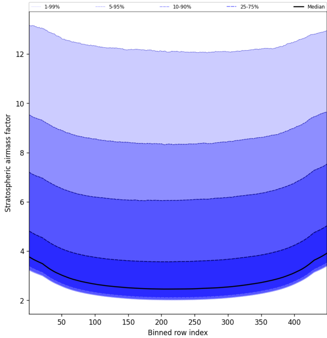
Figure 61: Along track statistics of “Stratospheric airmass factor” for 2025-05-01 to 2025-05-02
