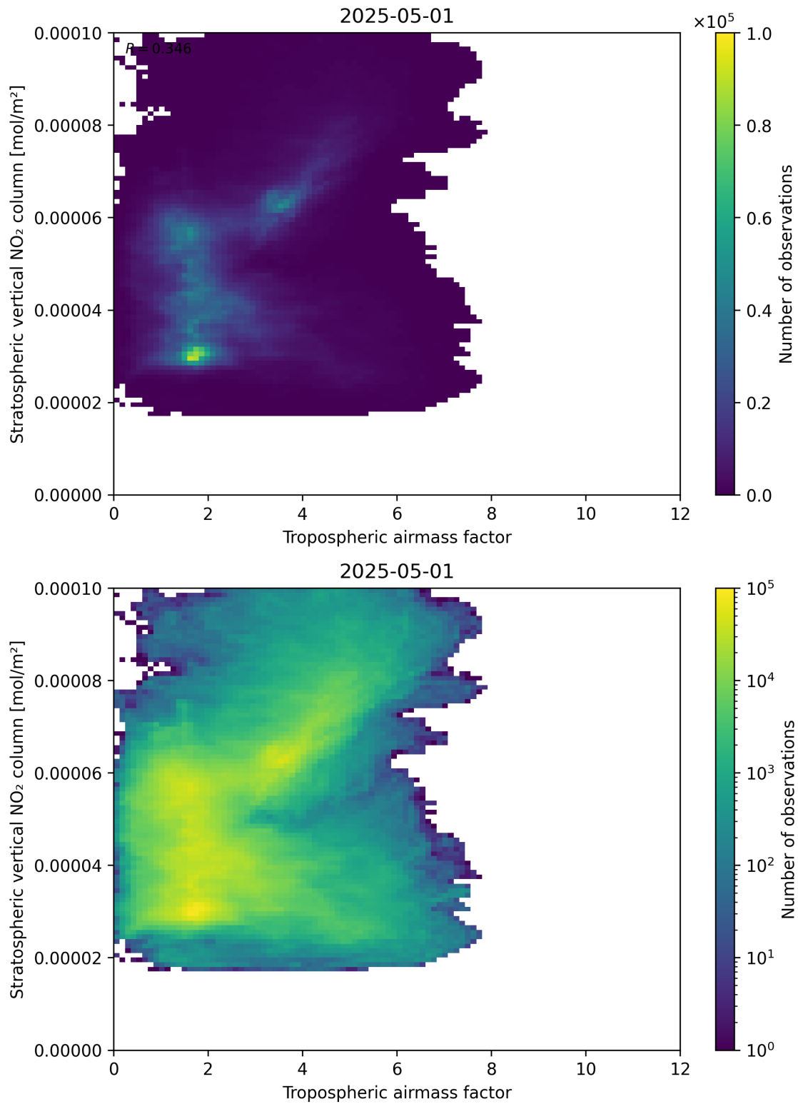
Figure 74: Scatter density plot of “Tropospheric air mass factor” against “Stratospheric vertical NO 2 column” for 2025-05-01 to 2025-05-02.
