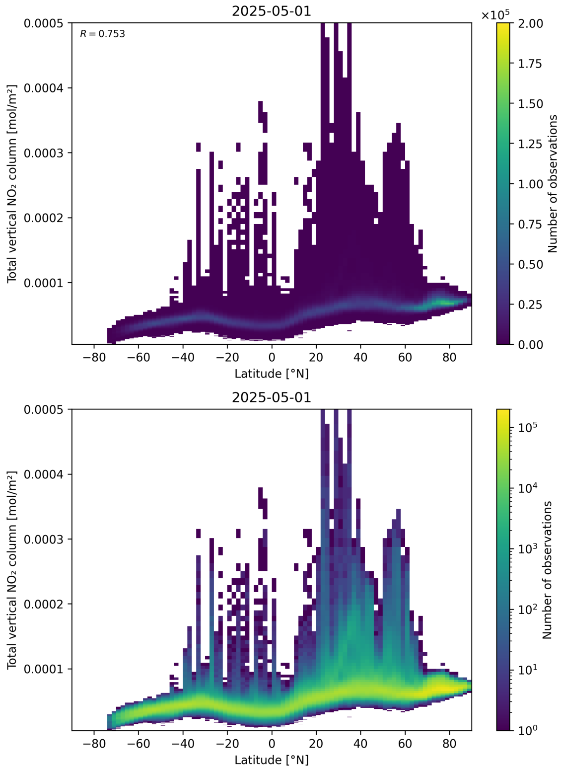
Figure 90: Scatter density plot of “Latitude” against “Total vertical NO 2 column” for 2025-05-01 to 2025-05-02.
