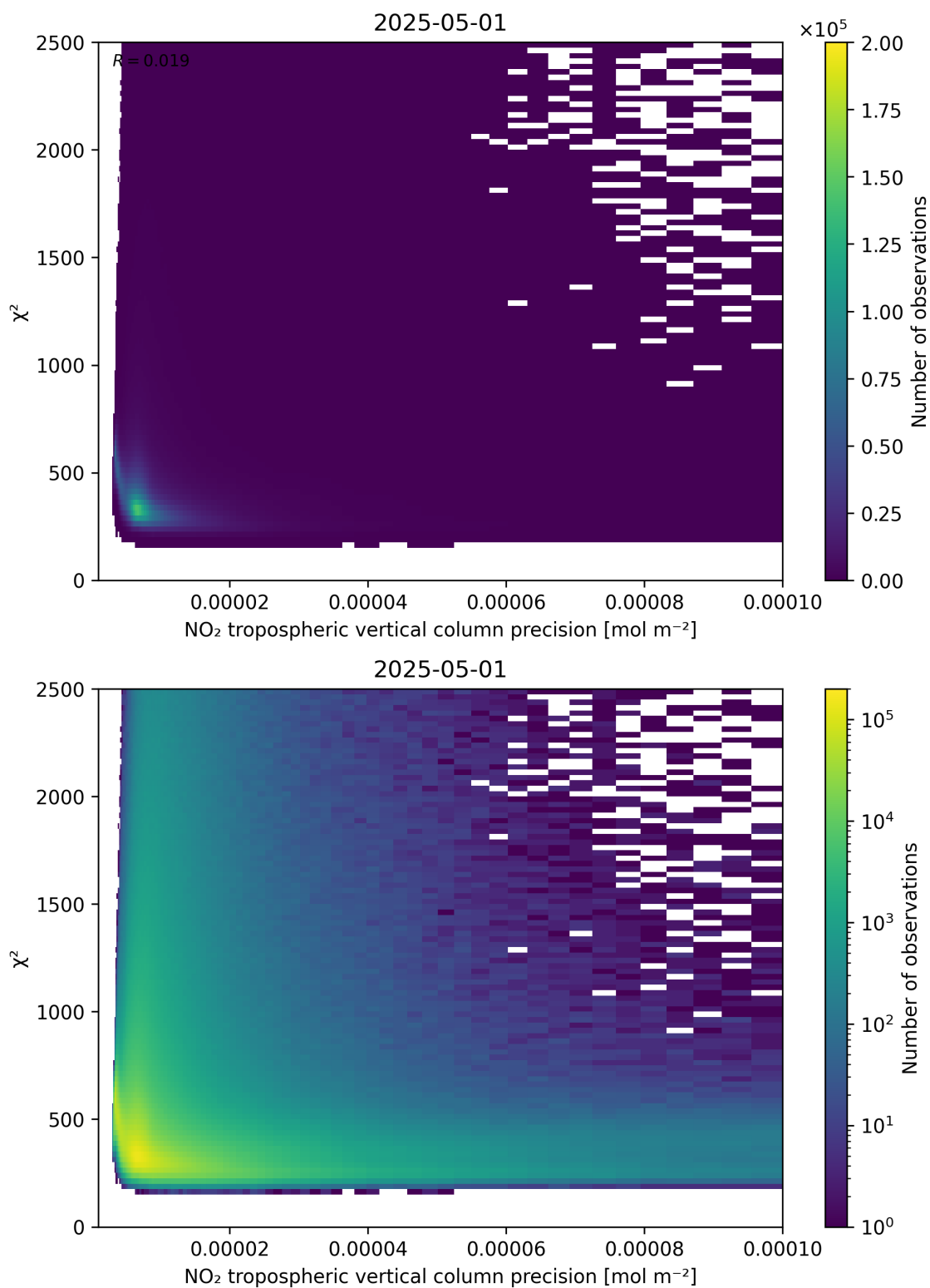
Figure 134: Scatter density plot of “NO 2 tropospheric vertical column precision” against “ \chi^2 ” for 2025-05-01 to 2025-05-02.
