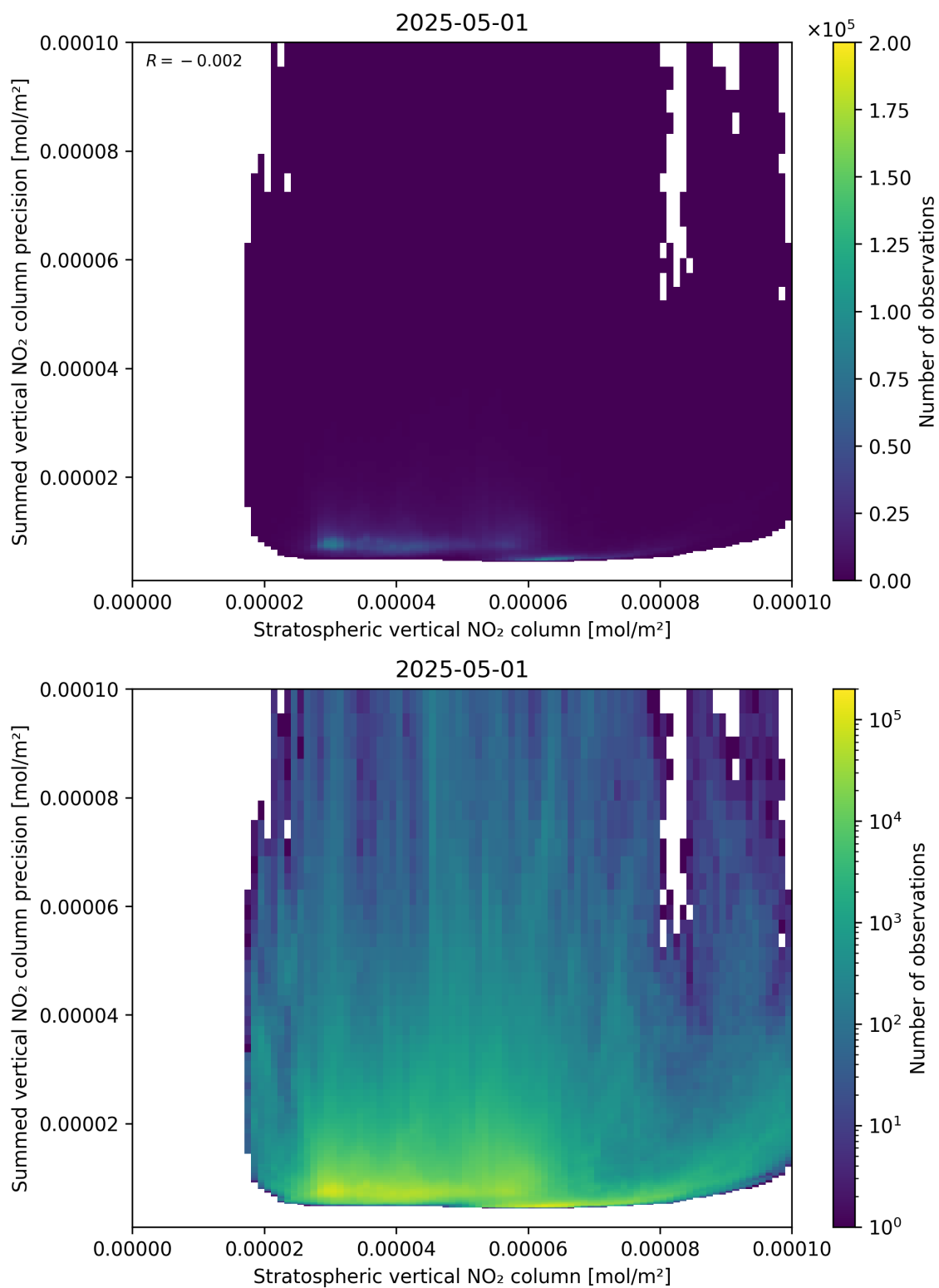
Figure 99: Scatter density plot of “Stratospheric vertical NO 2 column” against “Summed vertical NO 2 column precision” for 2025-05-01 to 2025-05-02.
