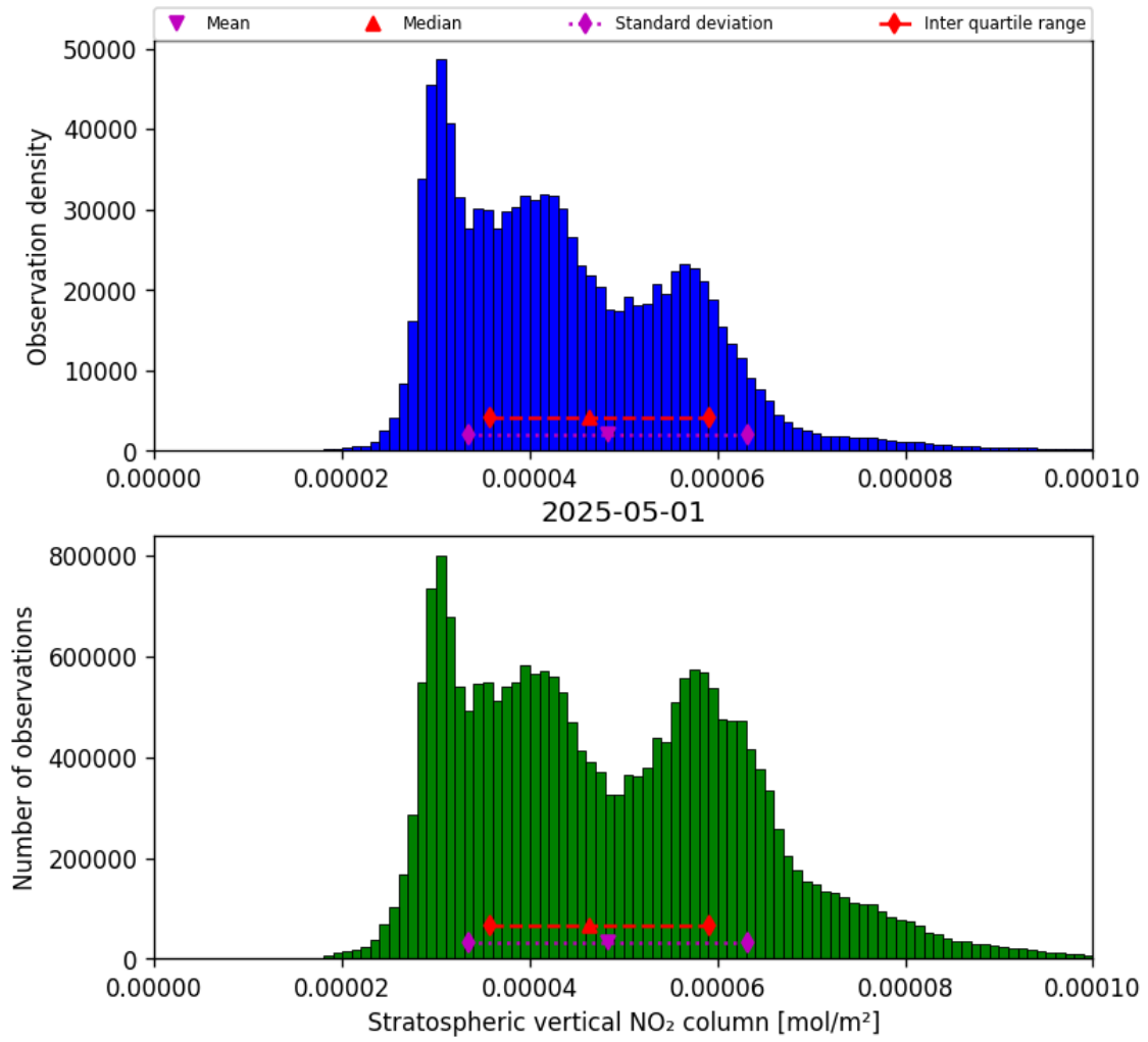
Figure 36: Histogram of “Stratospheric vertical NO 2 column” for 2025-05-01 to 2025-05-02
