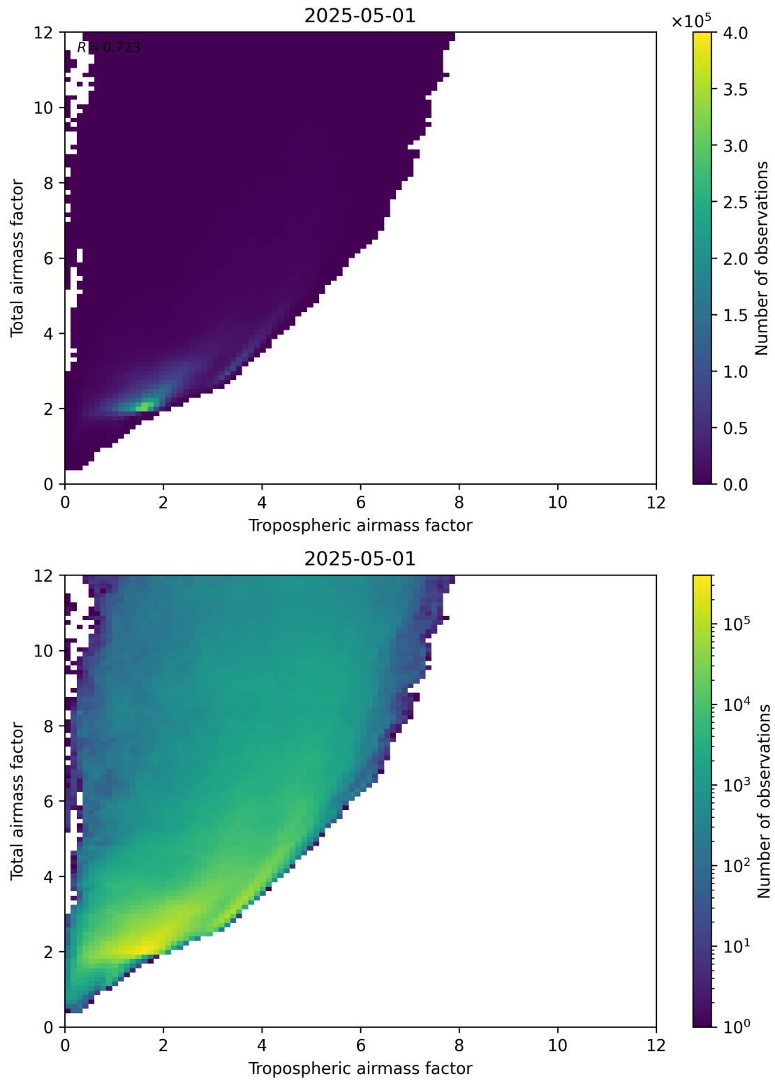
Figure 72: Scatter density plot of “Tropospheric airmass factor” against “Total airmass factor” for 2025-05-01 to 2025-05-02.
