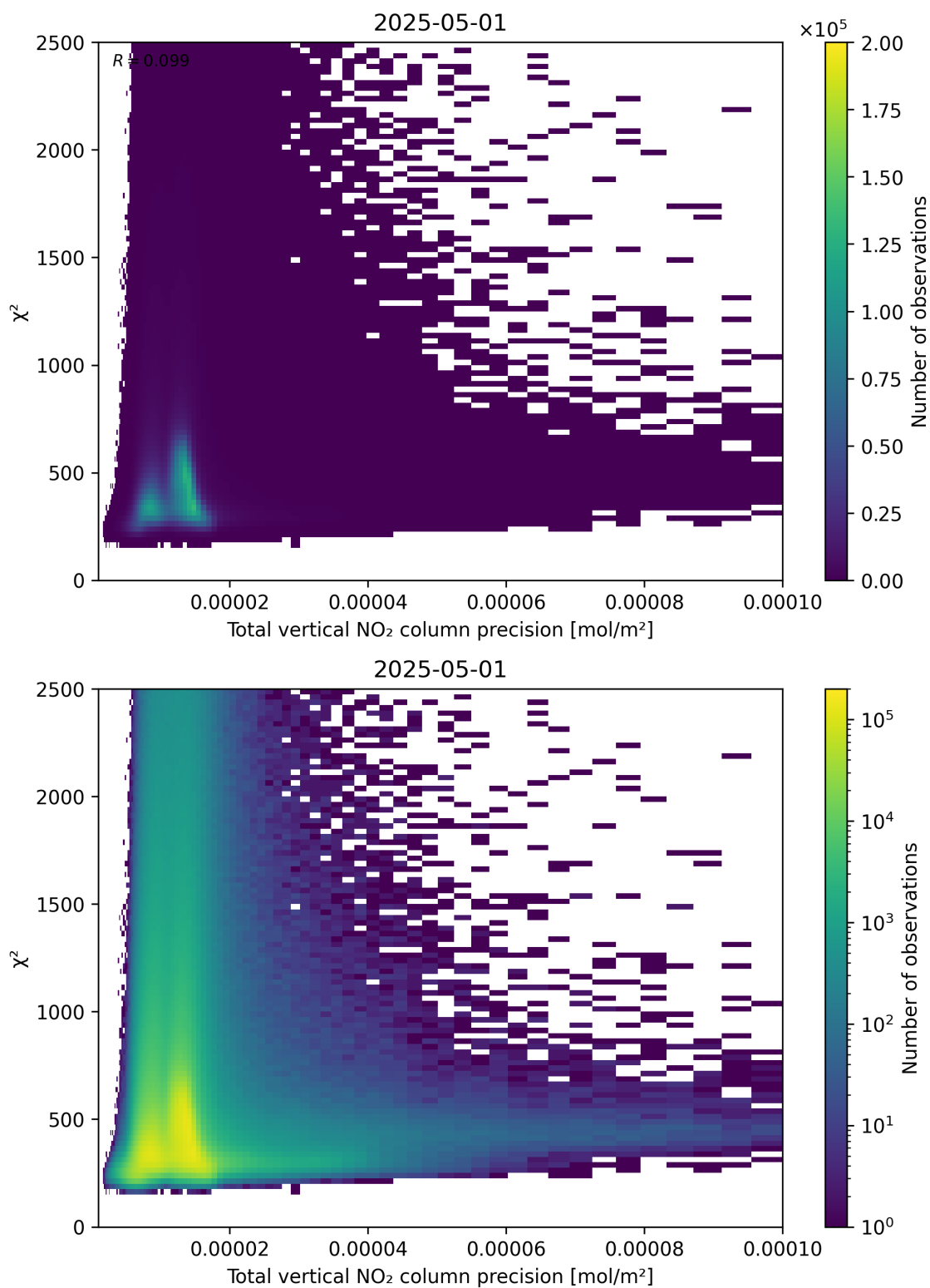
Figure 116: Scatter density plot of “Total vertical NO 2 column precision” against “ \chi^2 ” for 2025-05-01 to 2025-05-02.
