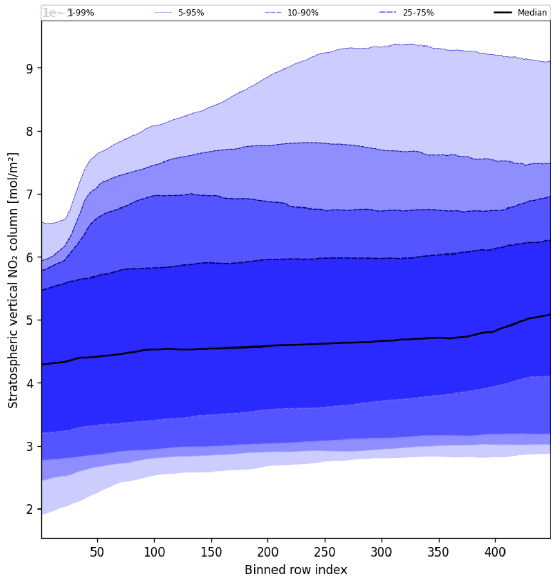
Figure 53: Along track statistics of “Stratospheric vertical NO 2 column” for 2025-05-01 to 2025-05-02
