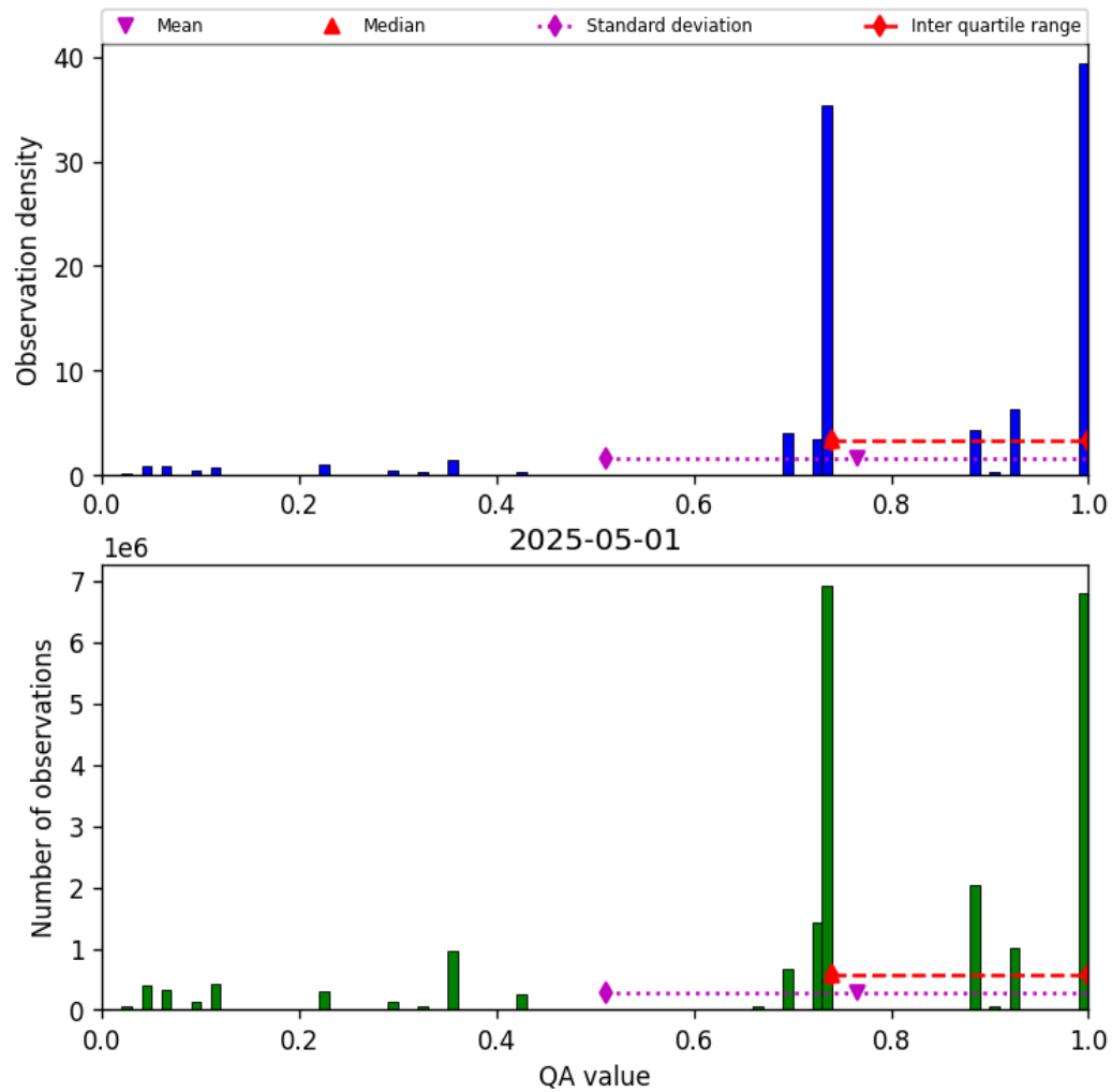
Figure 28: Histogram of “QA value” for 2025-05-01 to 2025-05-02
