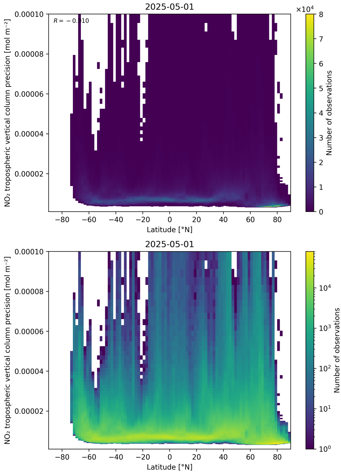
Figure 93: Scatter density plot of “Latitude” against “NO 2 tropospheric vertical column precision” for 2025-05-01 to 2025-05-02.
