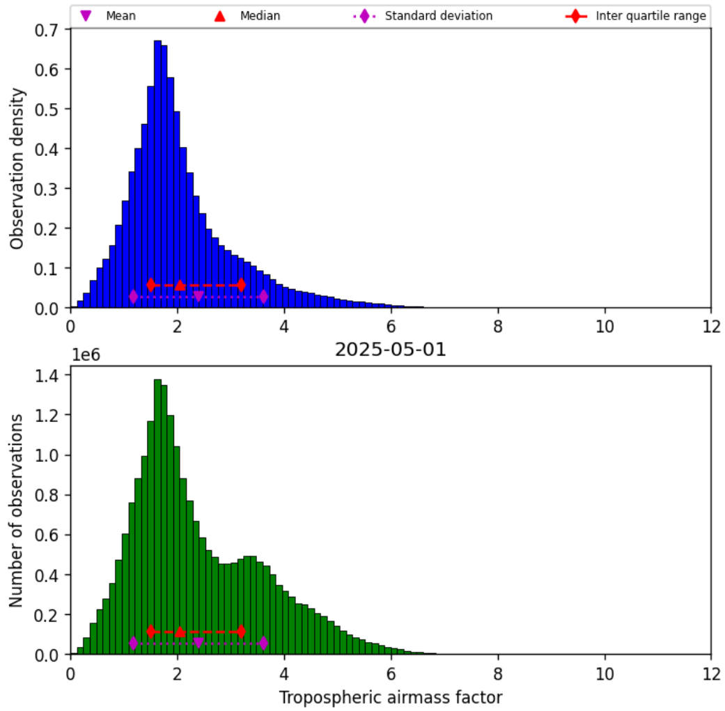
Figure 31: Histogram of “Tropospheric airmass factor” for 2025-05-01 to 2025-05-02
