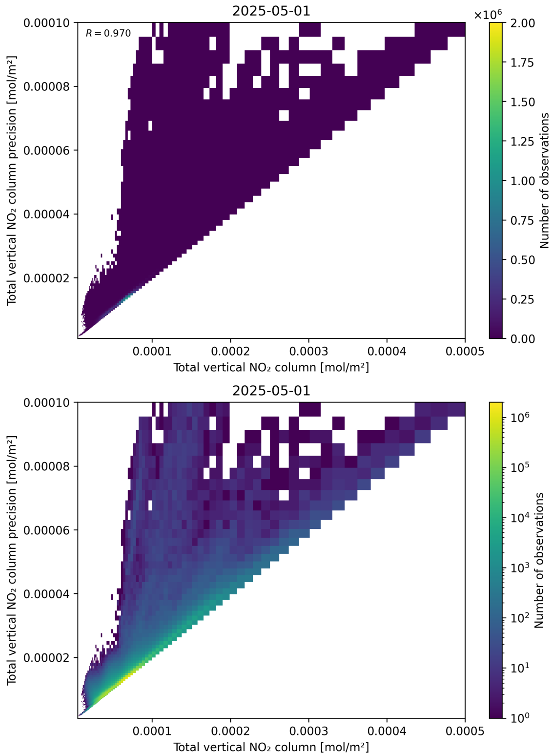
Figure 114: Scatter density plot of “Total vertical NO 2 column” against “Total vertical NO 2 column precision” for 2025-05-01 to 2025-05-02.
