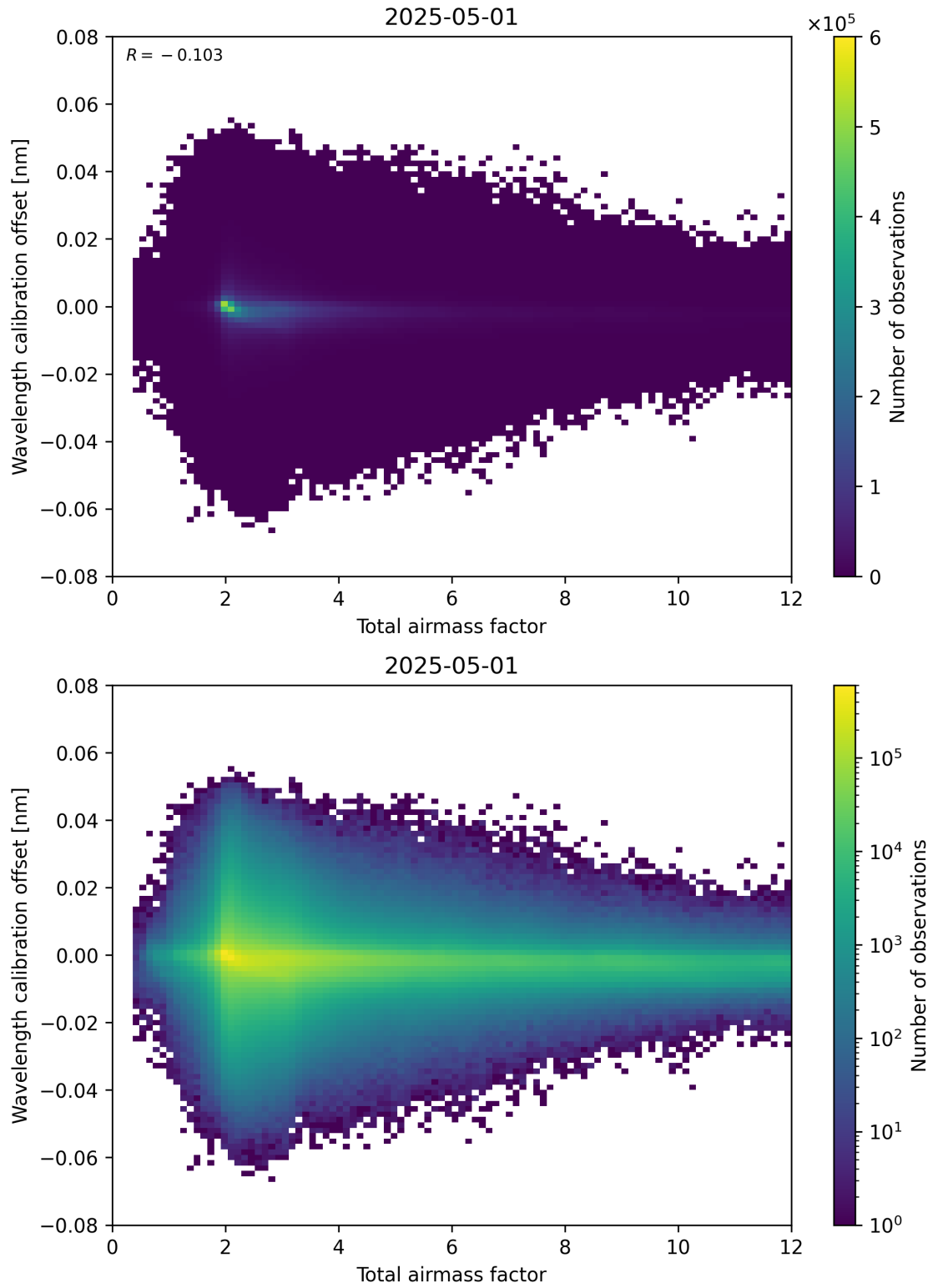
Figure 70: Scatter density plot of “Total airmass factor” against “Wavelength calibration offset” for 2025-05-01 to 2025-05-02.
