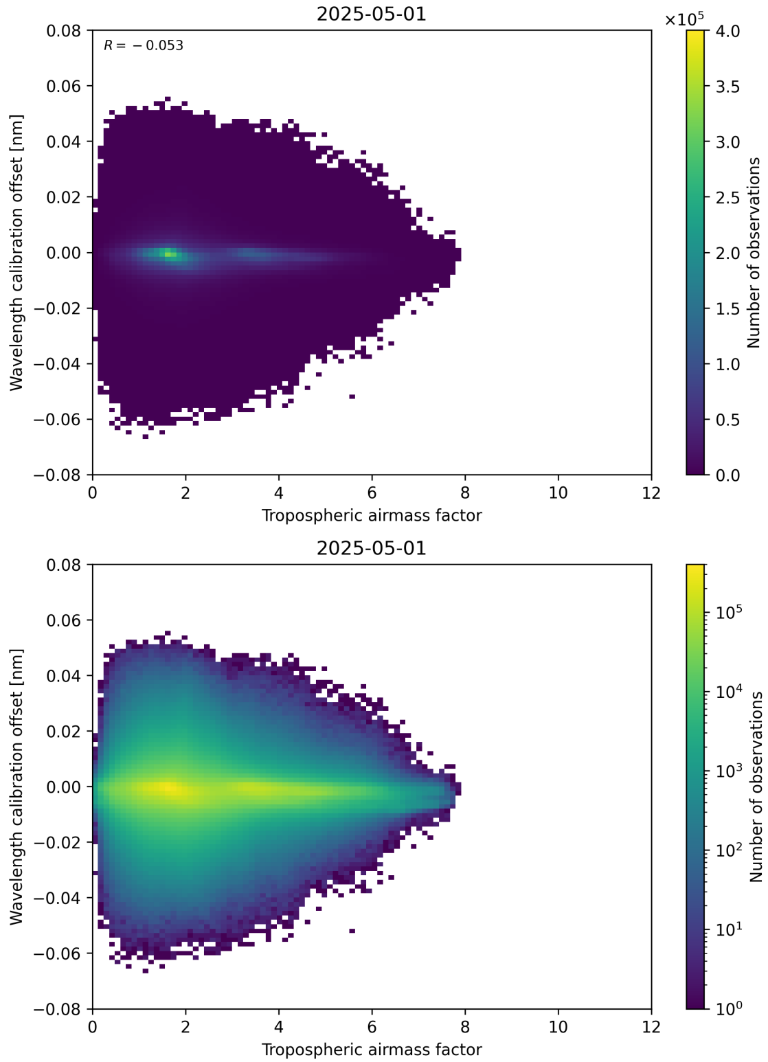
Figure 80: Scatter density plot of “Tropospheric airmass factor” against “Wavelength calibration offset” for 2025-05-01 to 2025-05-02.
