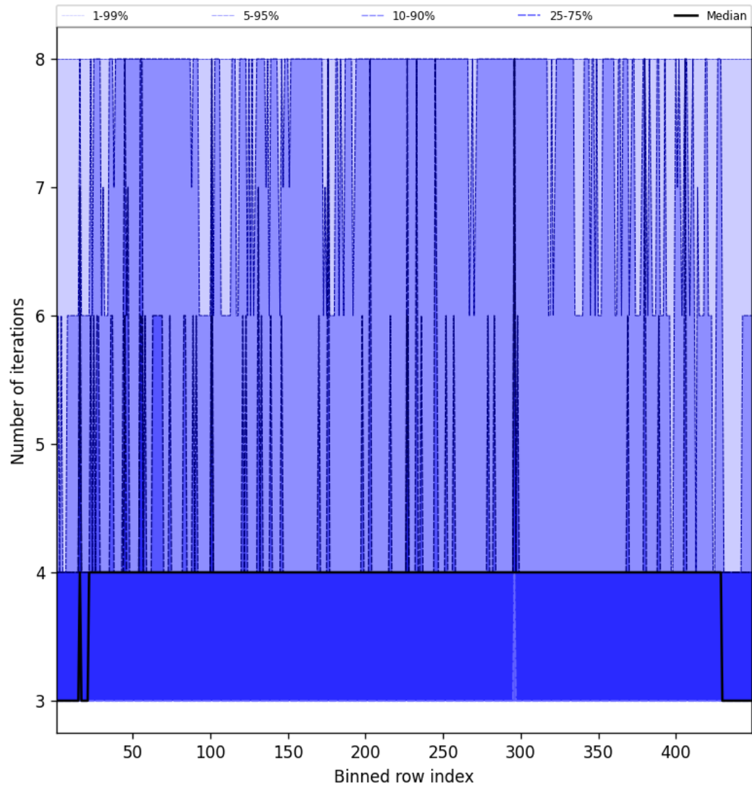
Figure 51: Along track statistics of “Number of iterations” for 2025-05-01 to 2025-05-02
