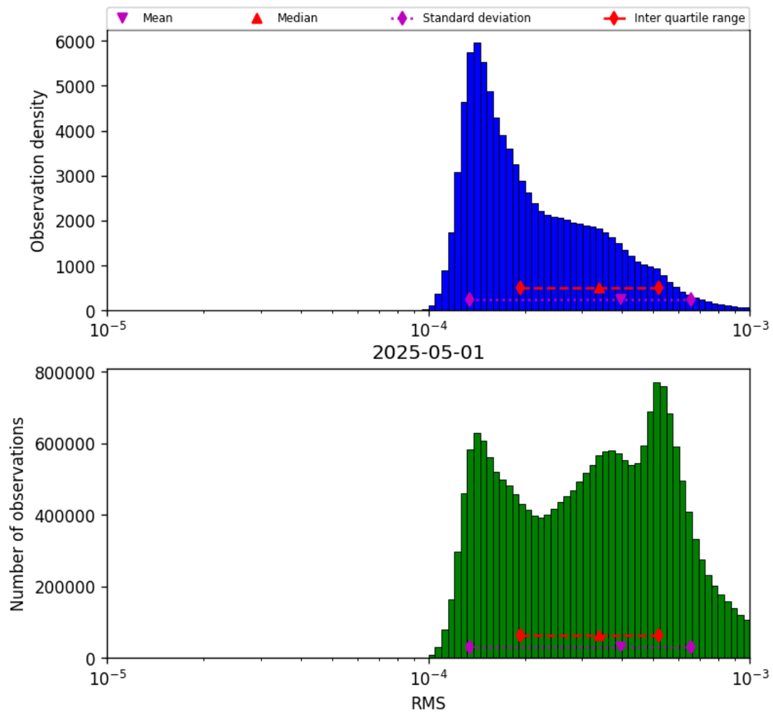
Figure 43: Histogram of “RMS” for 2025-05-01 to 2025-05-02
