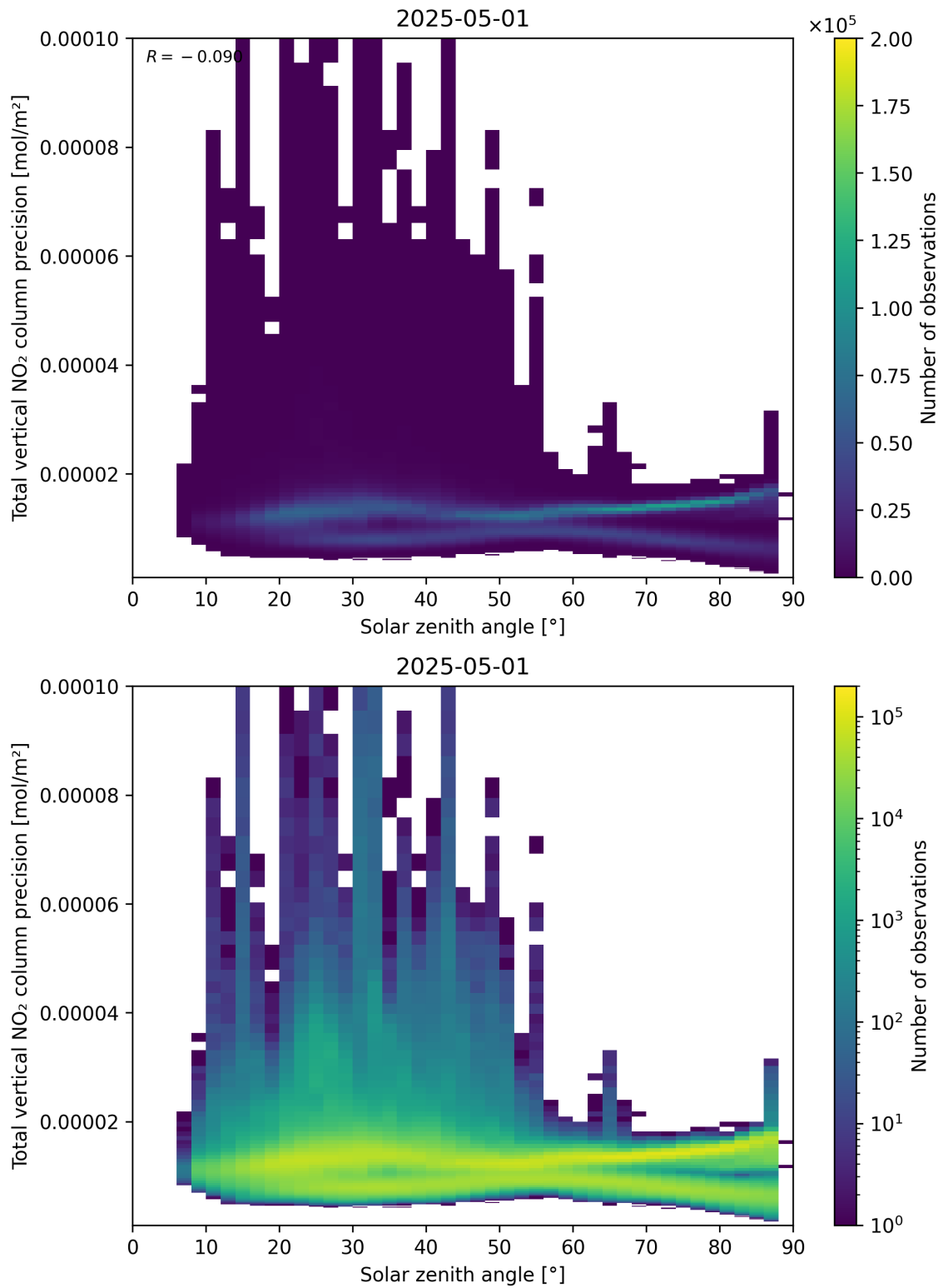
Figure 154: Scatter density plot of “Solar zenith angle” against “Total vertical NO 2 column precision” for 2025-05-01 to 2025-05-02.
