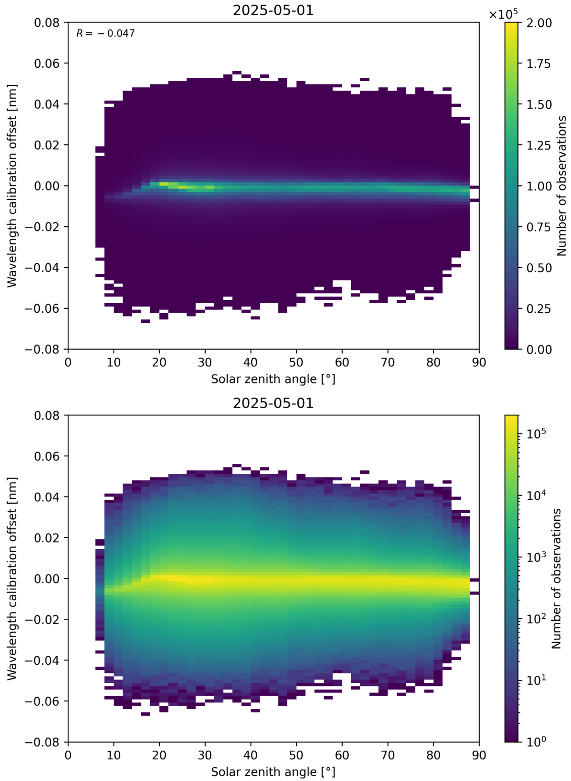
Figure 158: Scatter density plot of “Solar zenith angle” against “Wavelength calibration offset” for 2025-05-01 to 2025-05-02.
