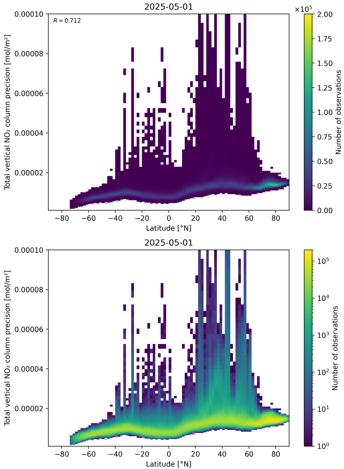
Figure 91: Scatter density plot of “Latitude” against “Total vertical NO 2 column precision” for 2025-05-01 to 2025-05-02.
