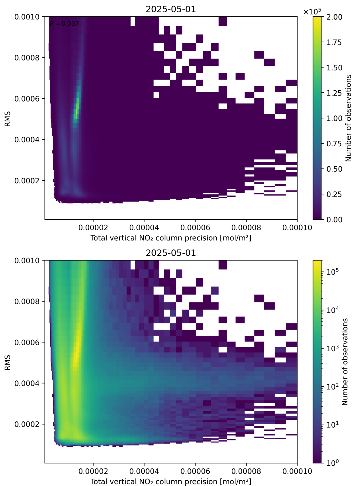
Figure 119: Scatter density plot of “Total vertical NO 2 column precision” against “RMS” for 2025-05-01 to 2025-05-02.
