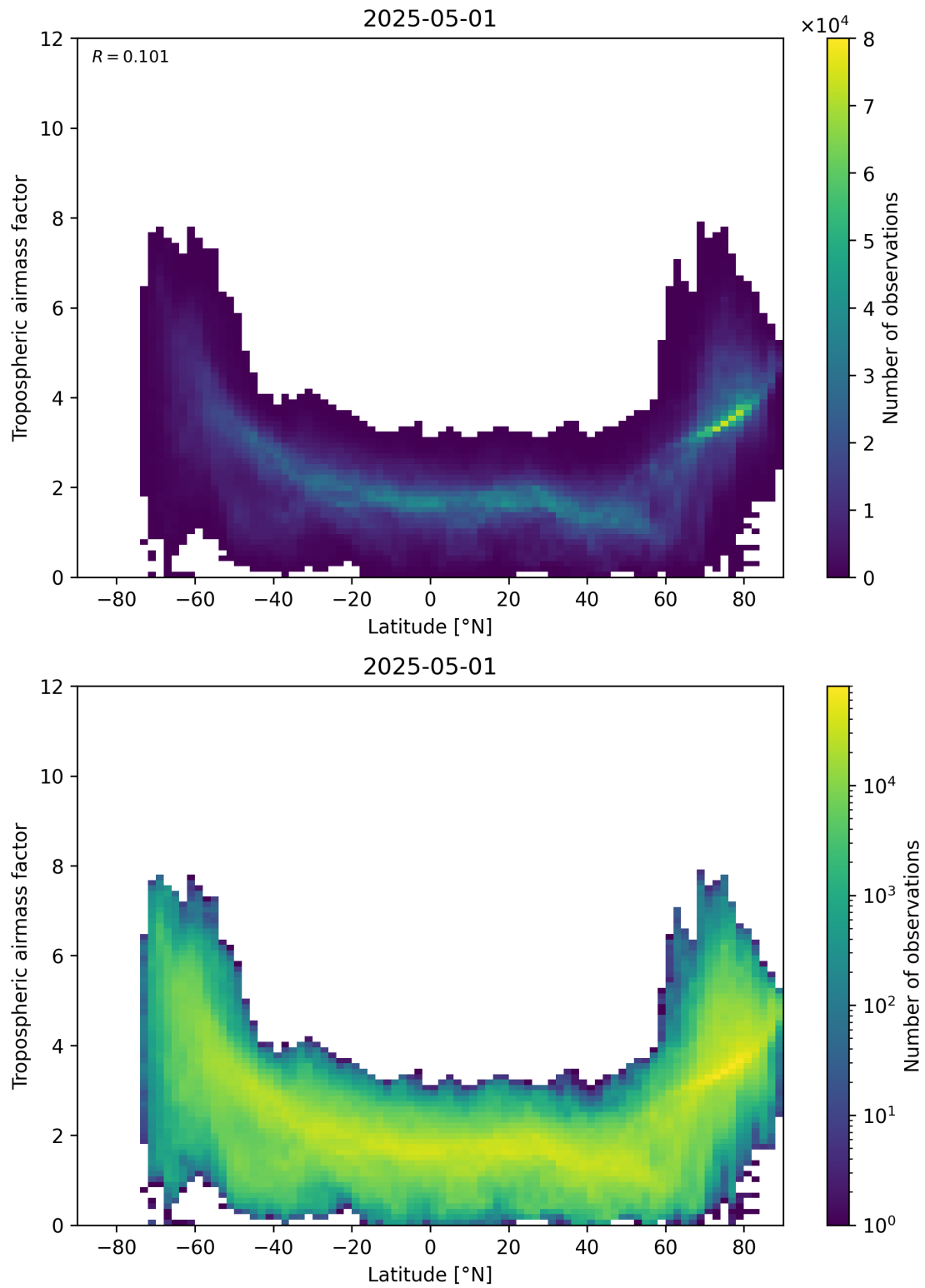
Figure 85: Scatter density plot of “Latitude” against “Tropospheric airmass factor” for 2025-05-01 to 2025-05-02.
