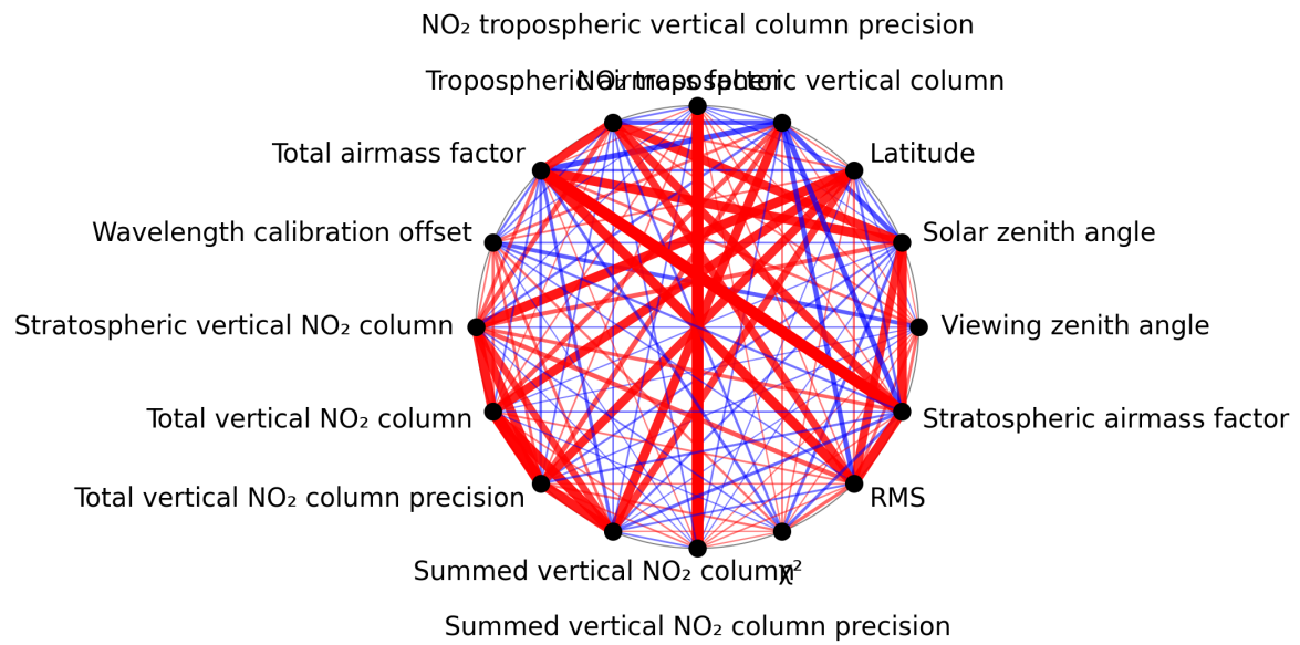
Figure 1: Map of correlation graph for 2025-05-01 to 2025-05-02.
