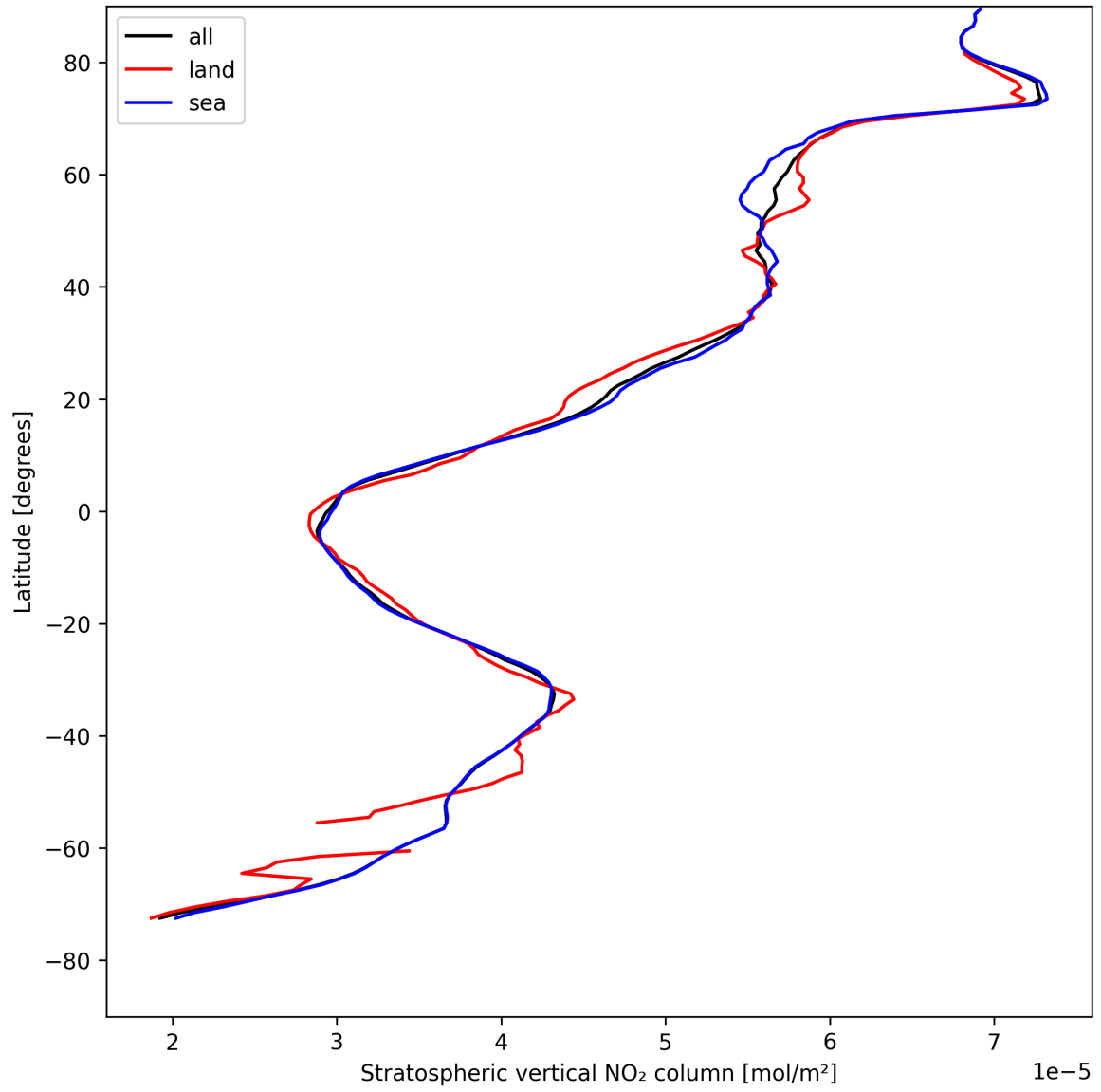
Figure 19: Zonal average of “Stratospheric vertical NO 2 column” for 2025-05-01 to 2025-05-02.
