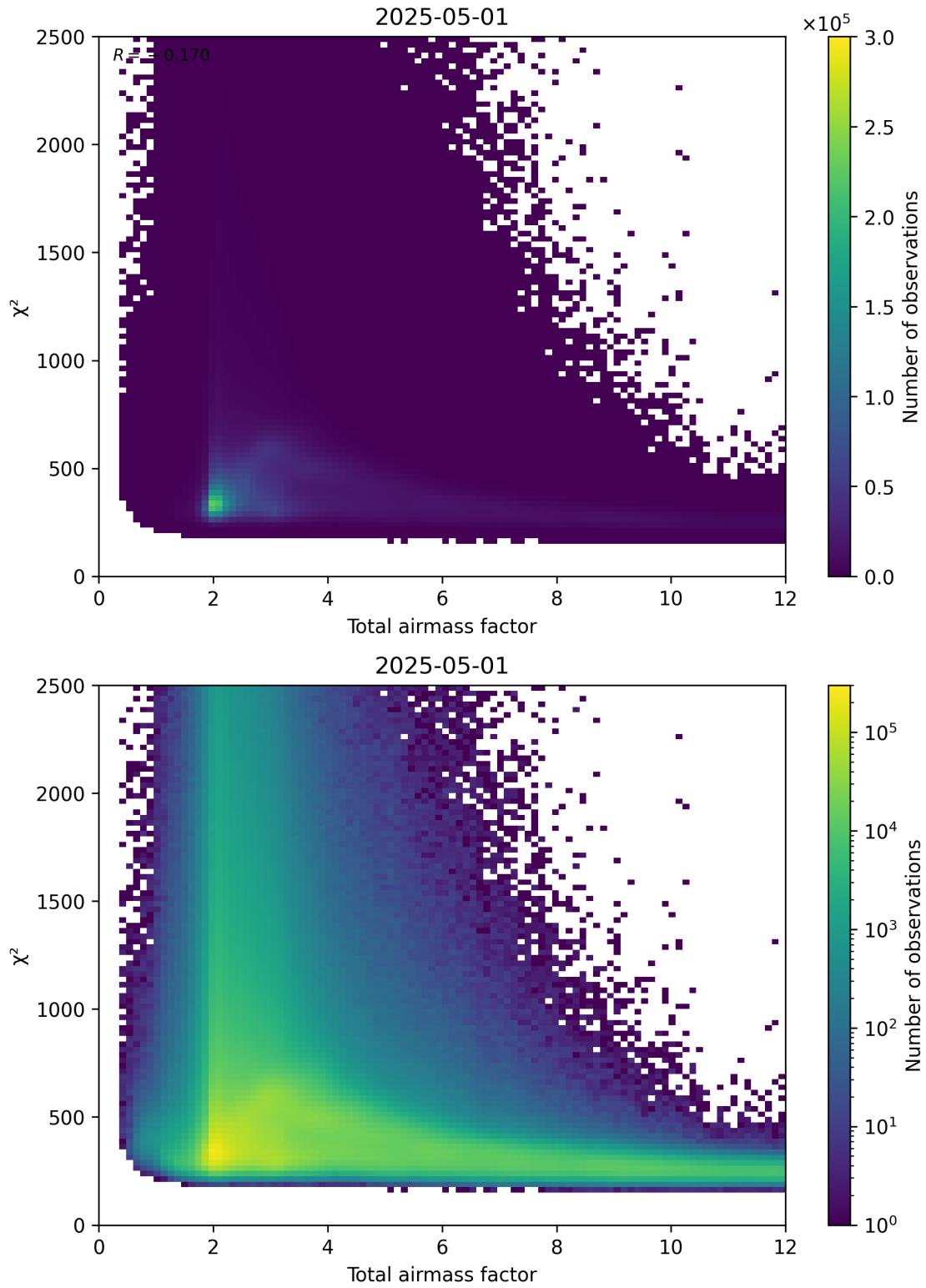
Figure 63: Scatter density plot of “Total airmass factor” against “ \chi^2 ” for 2025-05-01 to 2025-05-02.
