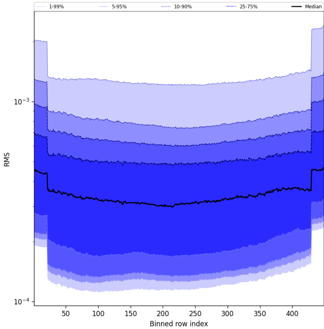
Figure 60: Along track statistics of “RMS” for 2025-05-01 to 2025-05-02
