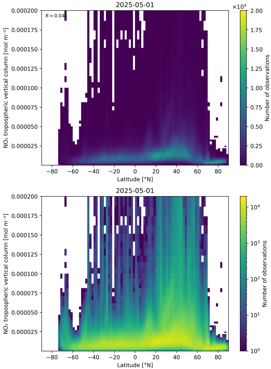
Figure 92: Scatter density plot of “Latitude” against “NO 2 tropospheric vertical column” for 2025-05-01 to 2025-05-02.
