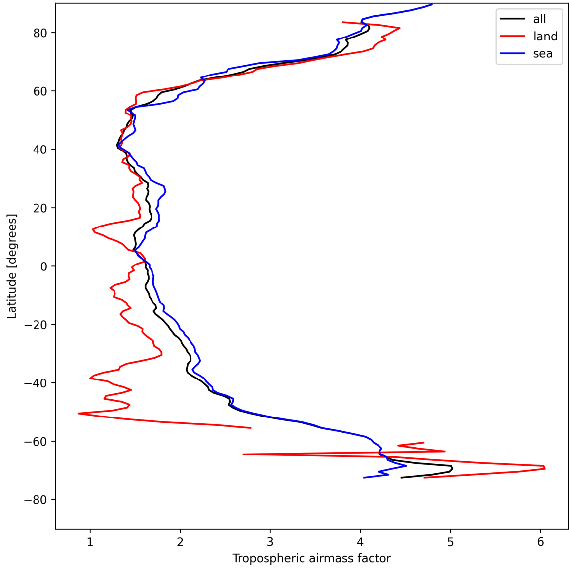
Figure 14: Zonal average of “Tropospheric air mass factor” for 2025-05-01 to 2025-05-02.
