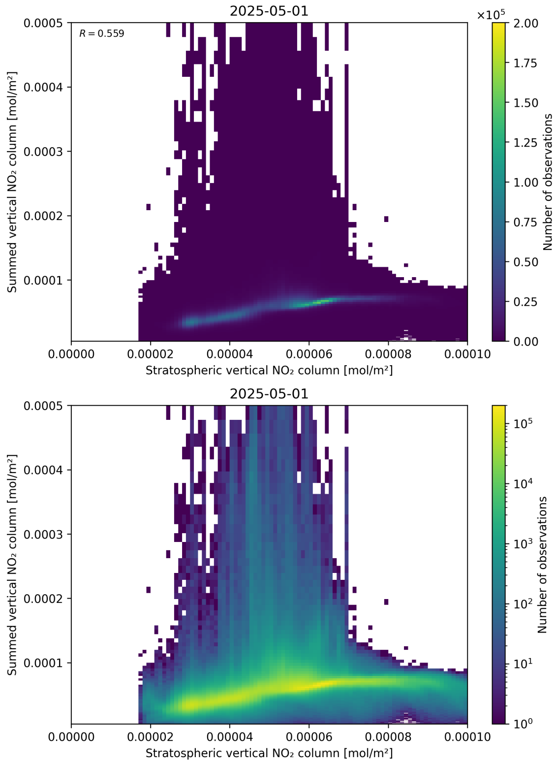
Figure 98: Scatter density plot of “Stratospheric vertical NO 2 column” against “Summed vertical NO 2 column” for 2025-05-01 to 2025-05-02.
