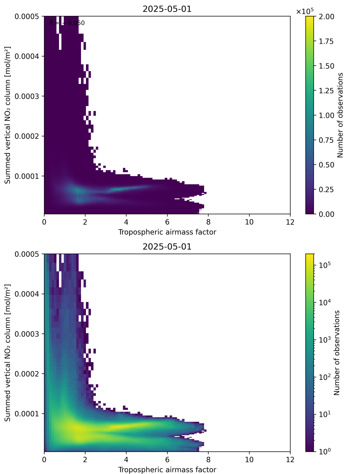
Figure 75: Scatter density plot of “Tropospheric air mass factor” against “Summed vertical NO 2 column” for 2025-05-01 to 2025-05-02.
