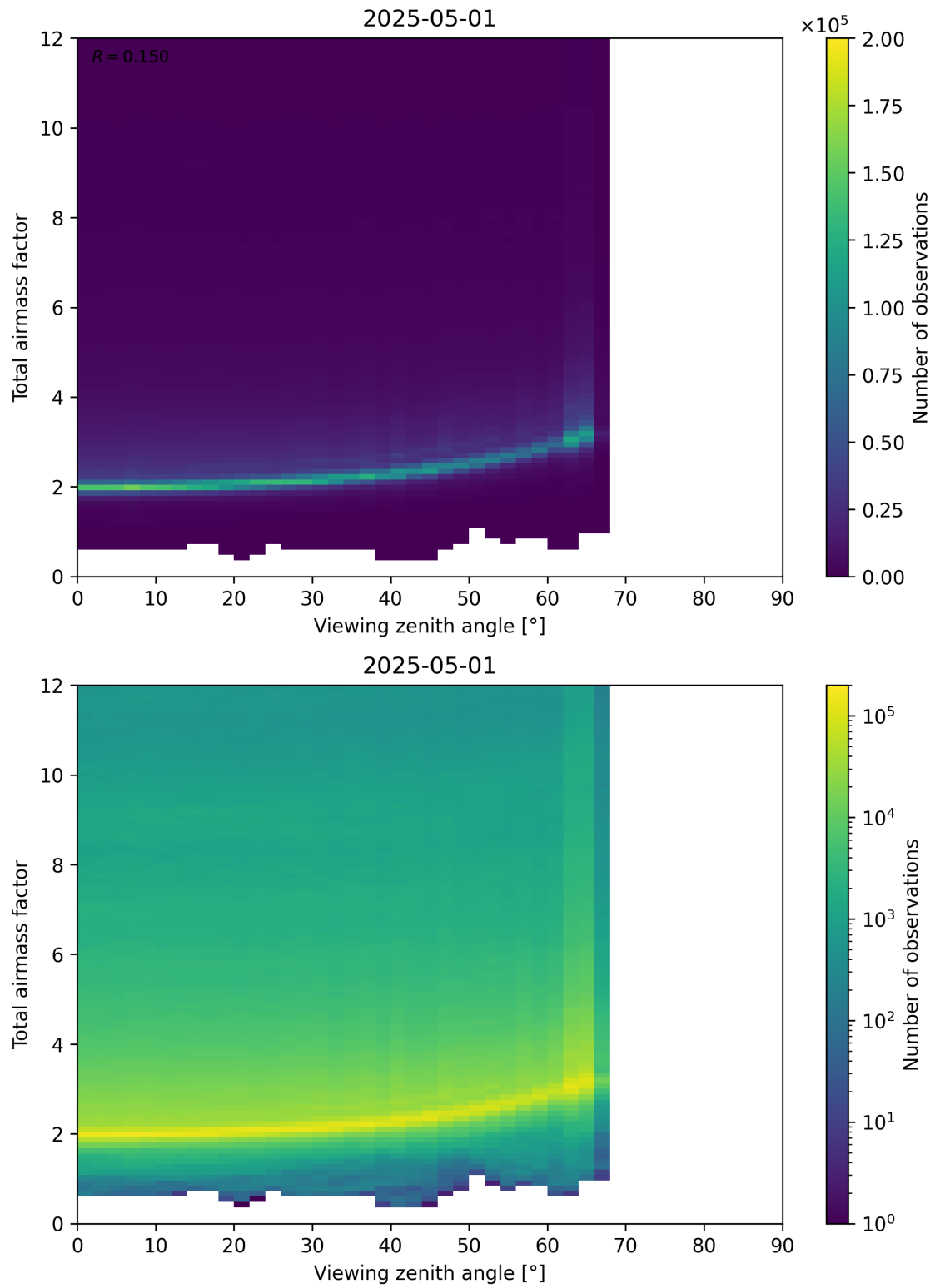
Figure 160: Scatter density plot of “Viewing zenith angle” against “Total airmass factor” for 2025-05-01 to 2025-05-02.
