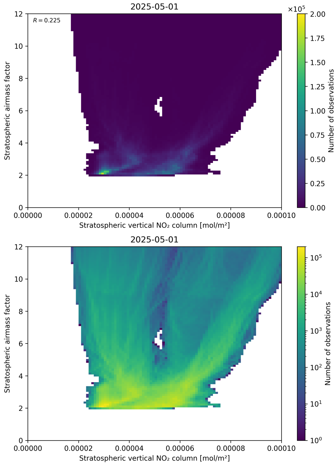
Figure 96: Scatter density plot of “Stratospheric vertical NO 2 column” against “Stratospheric airmass factor” for 2025-05-01 to 2025-05-02.
