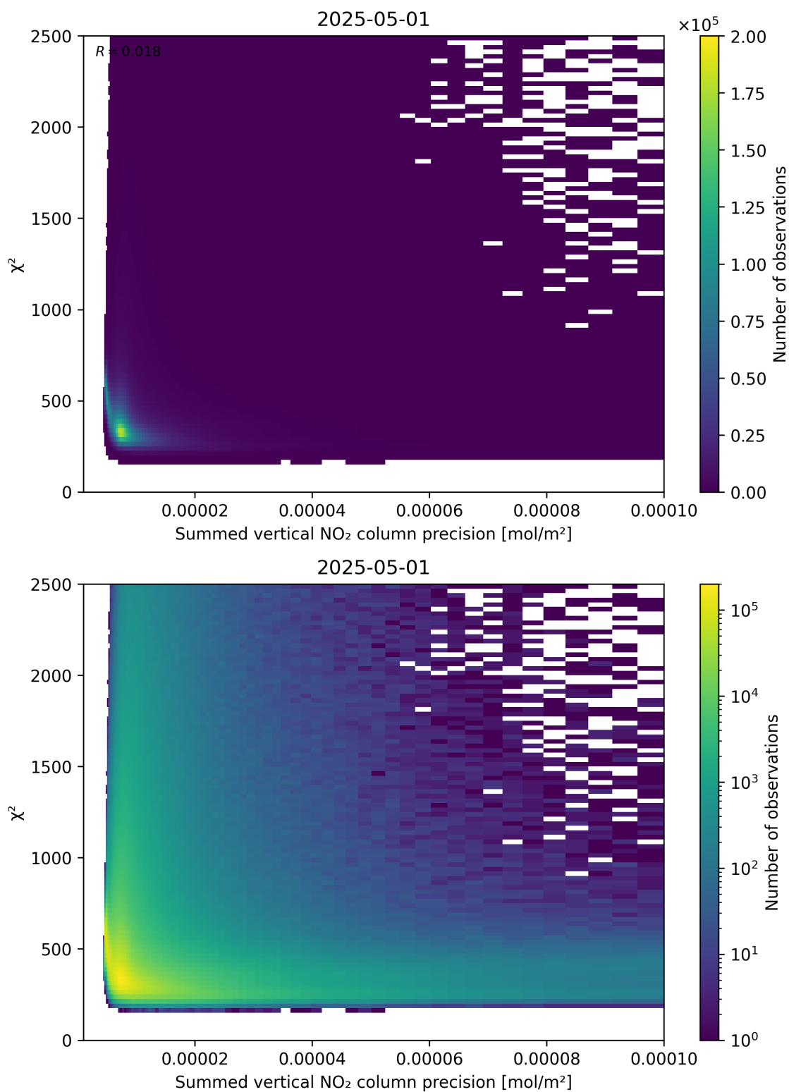
Figure 107: Scatter density plot of “Summed vertical NO 2 column precision” against “ \chi^2 ” for 2025-05-01 to 2025-05-02.
