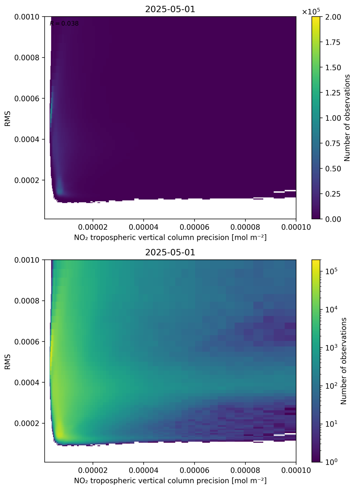
Figure 140: Scatter density plot of “NO 2 tropospheric vertical column precision” against “RMS” for 2025-05-01 to 2025-05-02.
