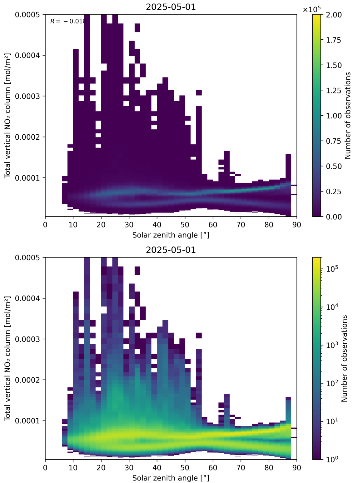
Figure 153: Scatter density plot of “Solar zenith angle” against “Total vertical NO 2 column” for 2025-05-01 to 2025-05-02.
