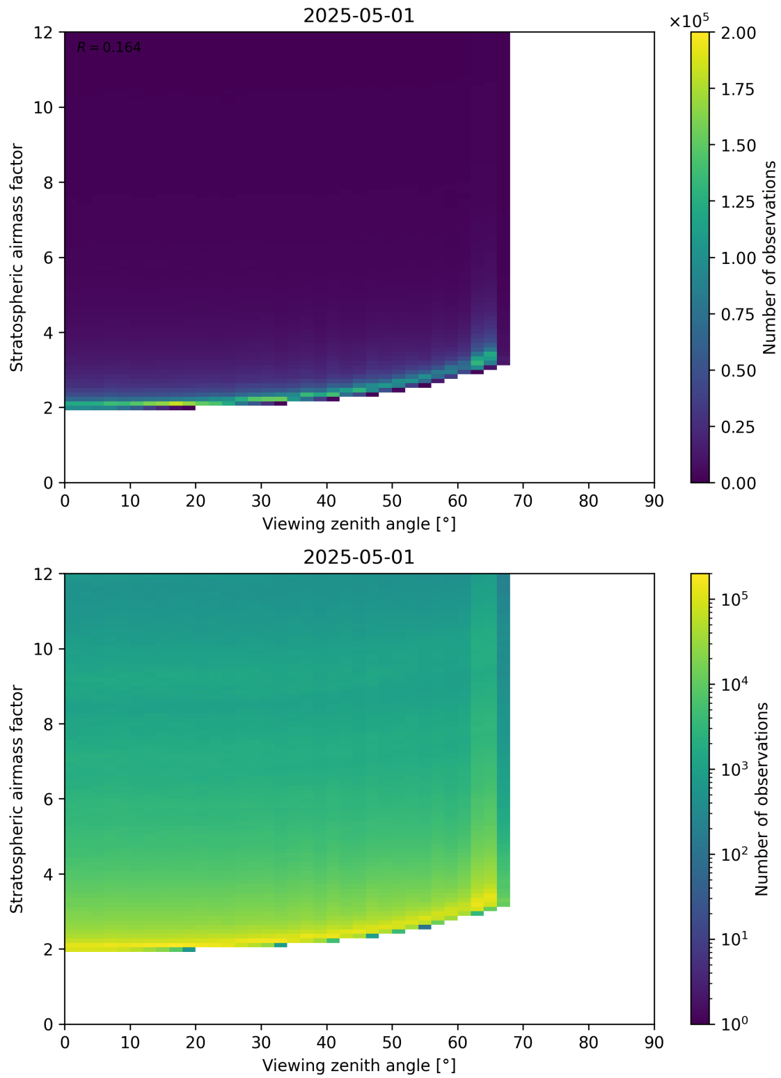
Figure 159: Scatter density plot of “Viewing zenith angle” against “Stratospheric airmass factor” for 2025-05-01 to 2025-05-02.
