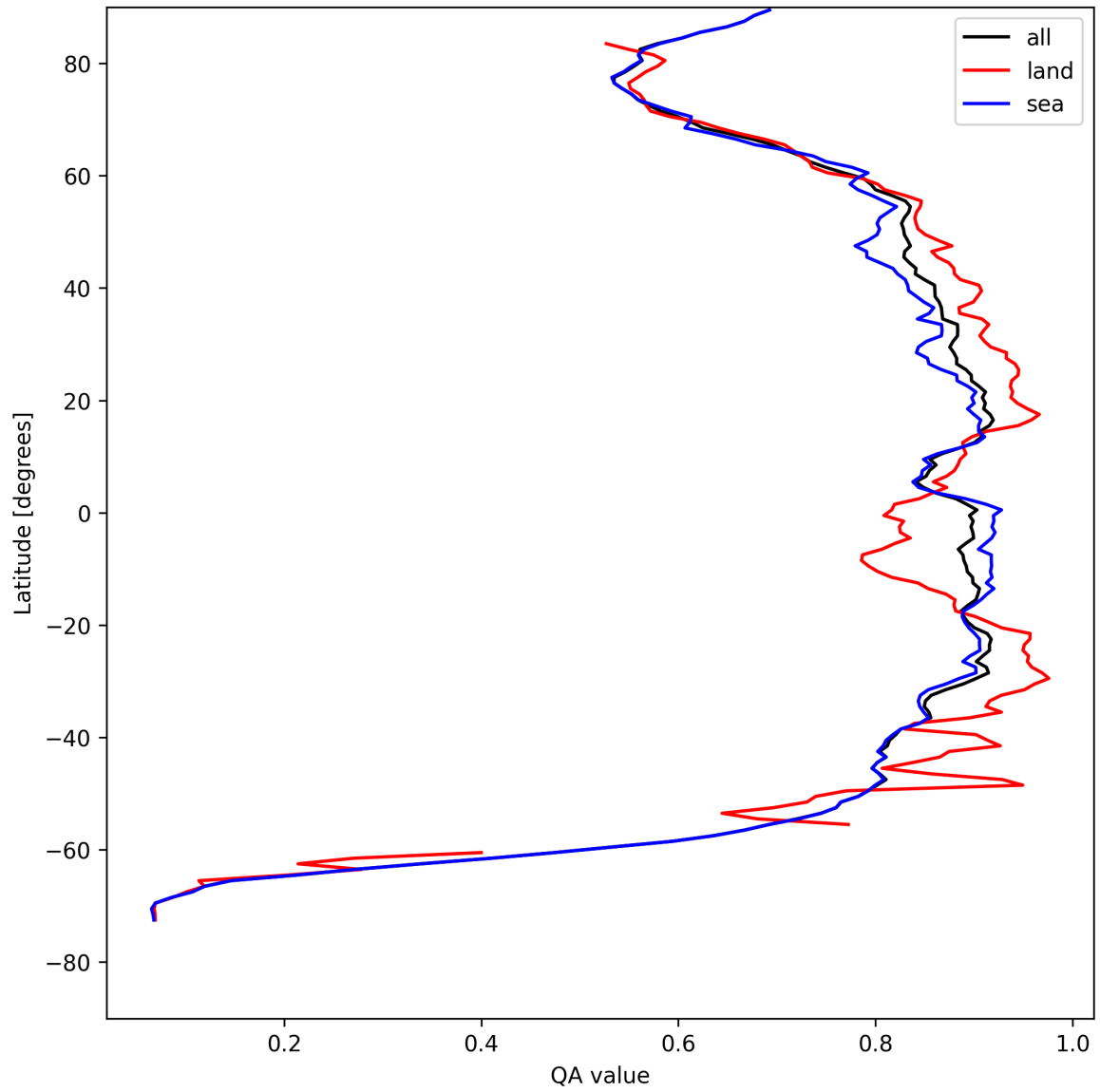
Figure 11: Zonal average of “QA value” for 2025-05-01 to 2025-05-02.
