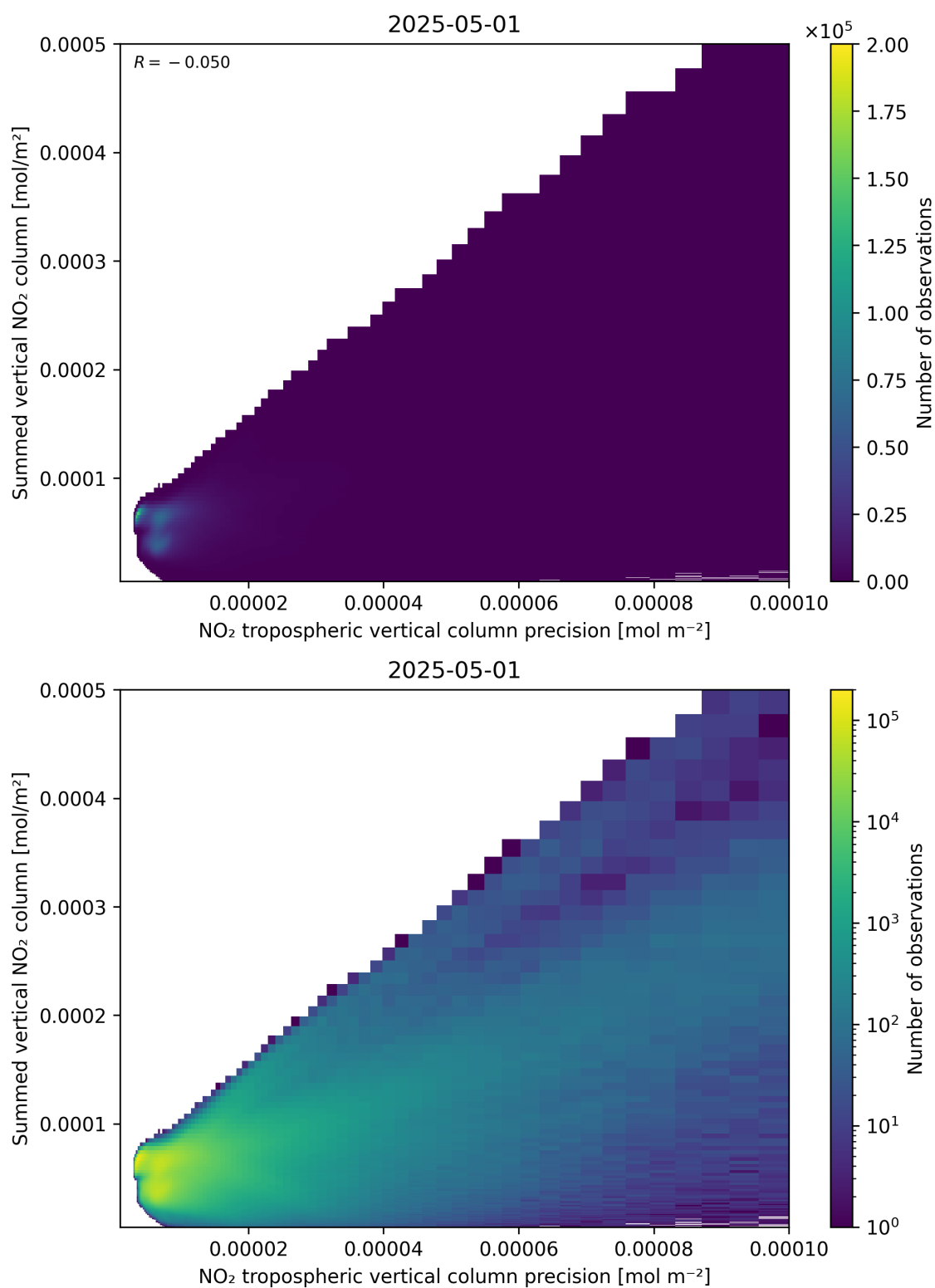
Figure 136: Scatter density plot of “NO 2 tropospheric vertical column precision” against “Summed vertical NO 2 column” for 2025-05-01 to 2025-05-02.
