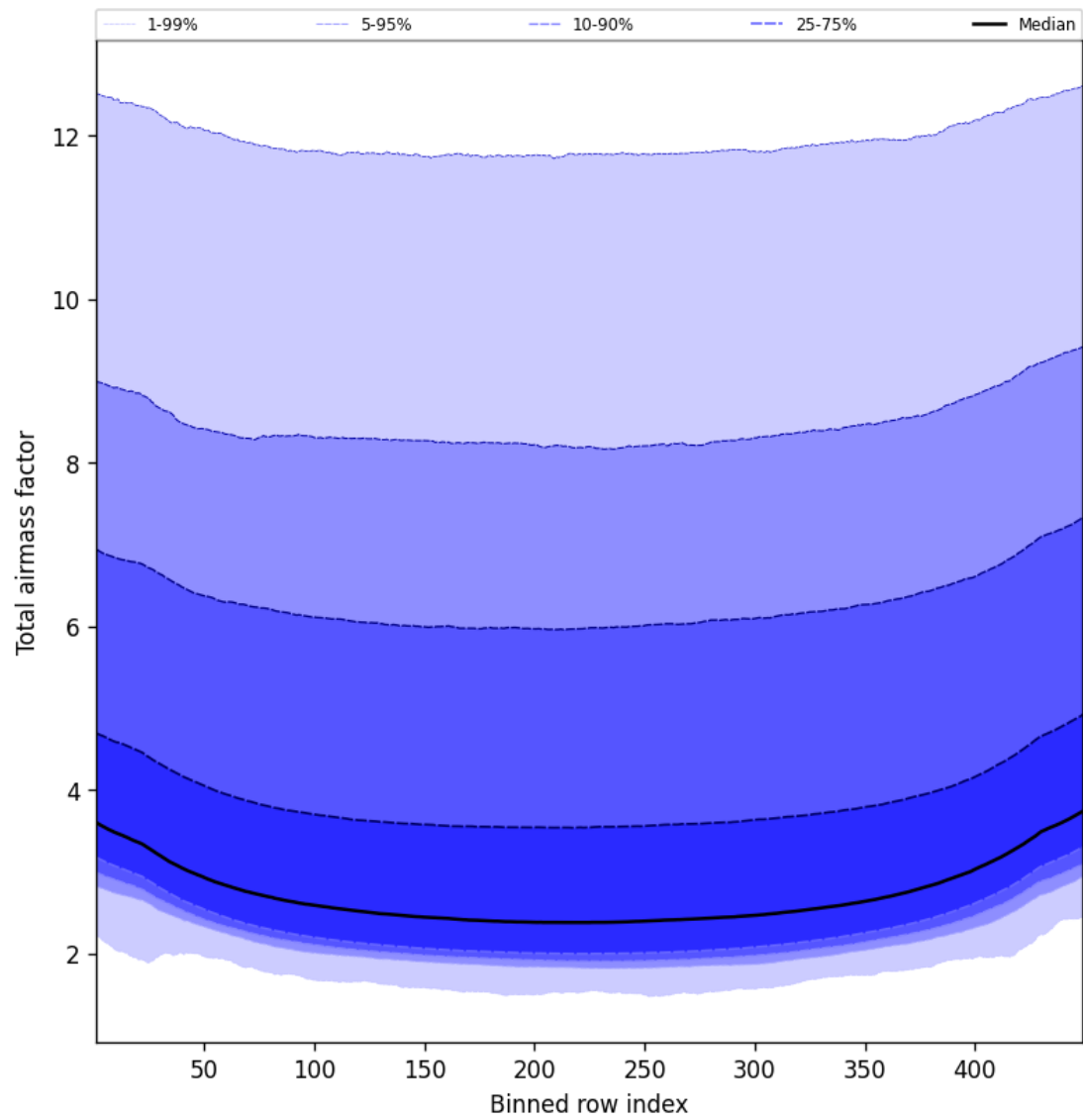
Figure 49: Along track statistics of “Total airmass factor” for 2025-05-01 to 2025-05-02
