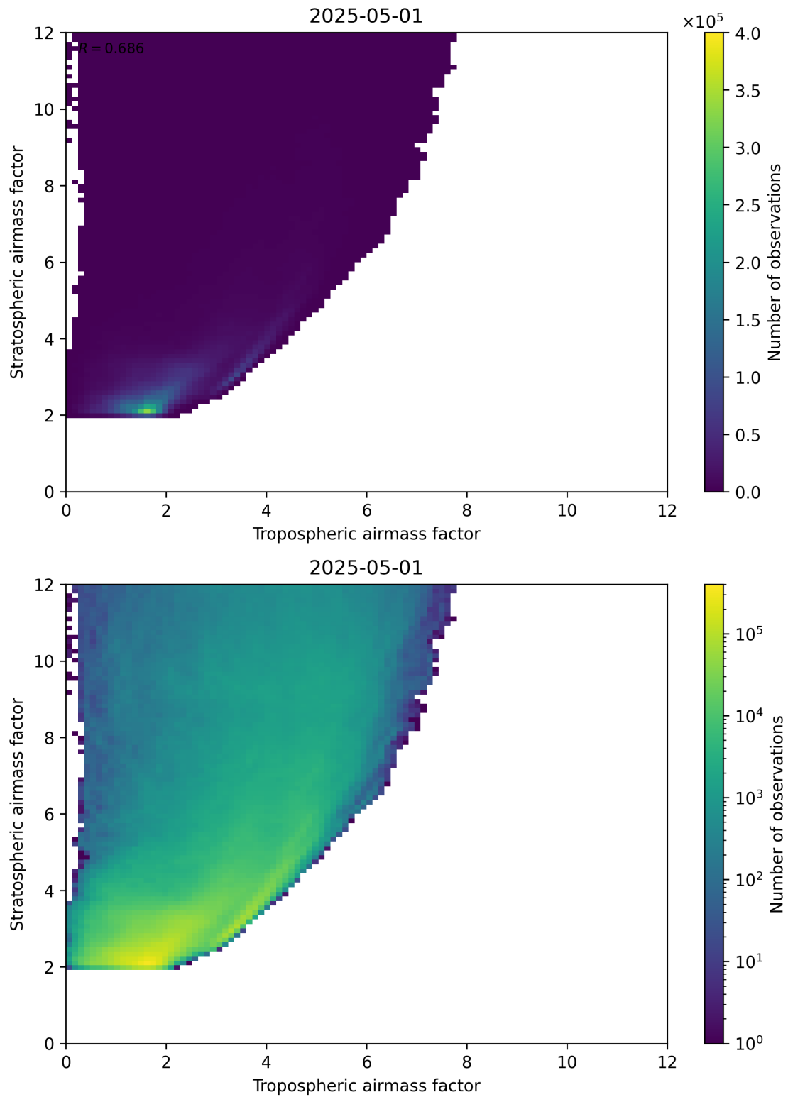
Figure 71: Scatter density plot of “Tropospheric airmass factor” against “Stratospheric airmass factor” for 2025-05-01 to 2025-05-02.
