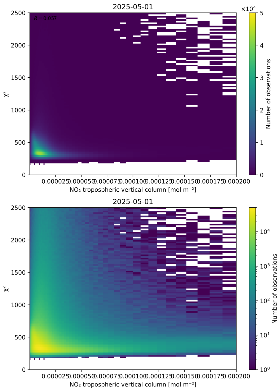
Figure 124: Scatter density plot of “NO 2 tropospheric vertical column” against “ \chi^2 ” for 2025-05-01 to 2025-05-02.
