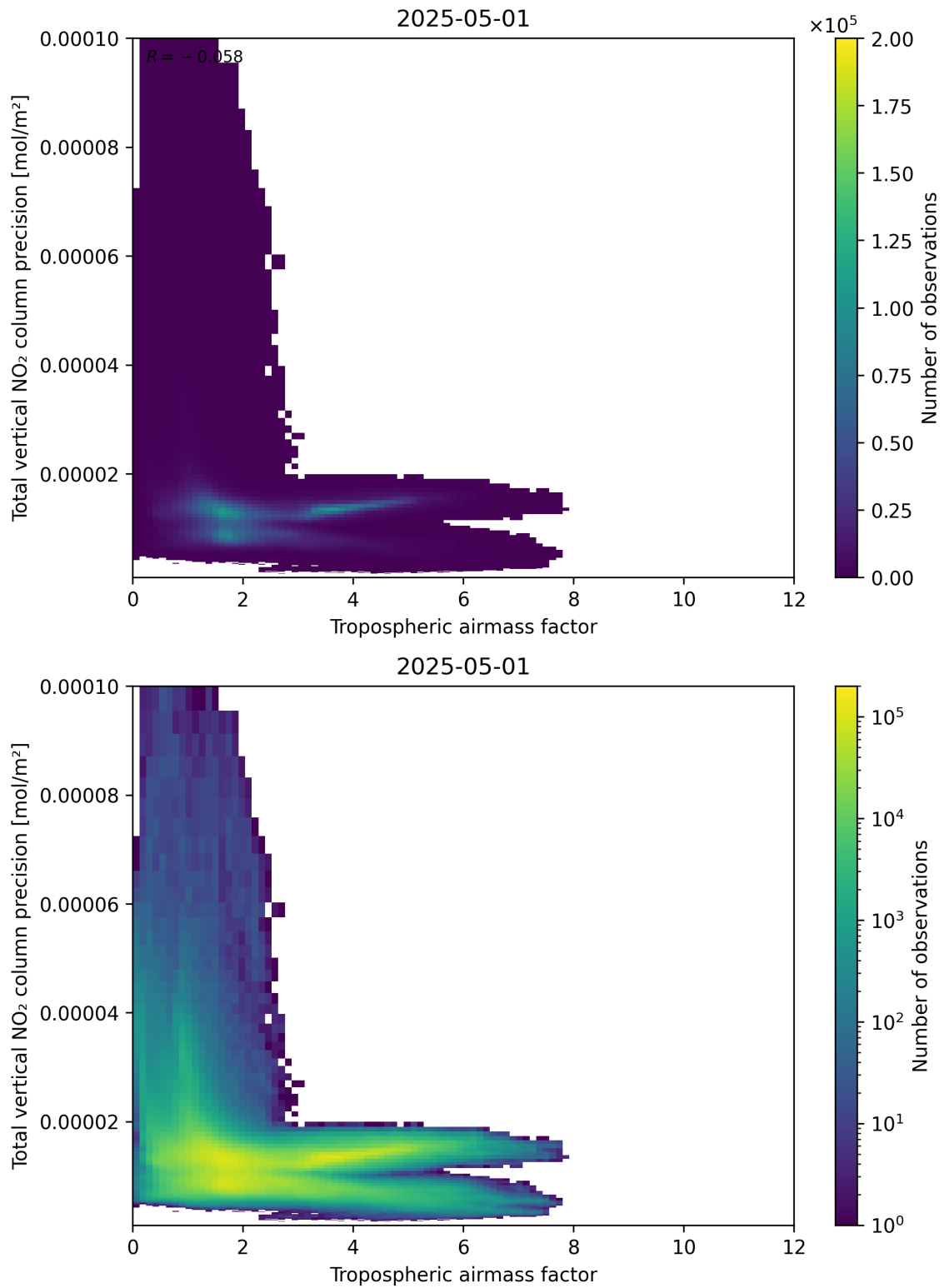
Figure 78: Scatter density plot of “Tropospheric airmass factor” against “Total vertical NO 2 column precision” for 2025-05-01 to 2025-05-02.
