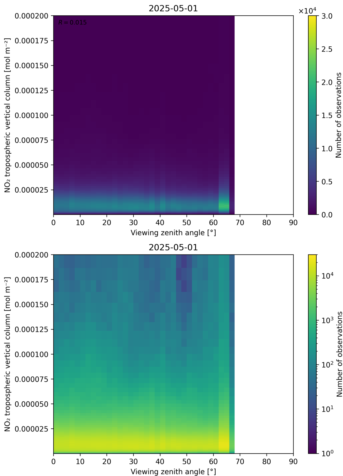
Figure 169: Scatter density plot of “Viewing zenith angle” against “NO 2 tropospheric vertical column” for 2025-05-01 to 2025-05-02.
