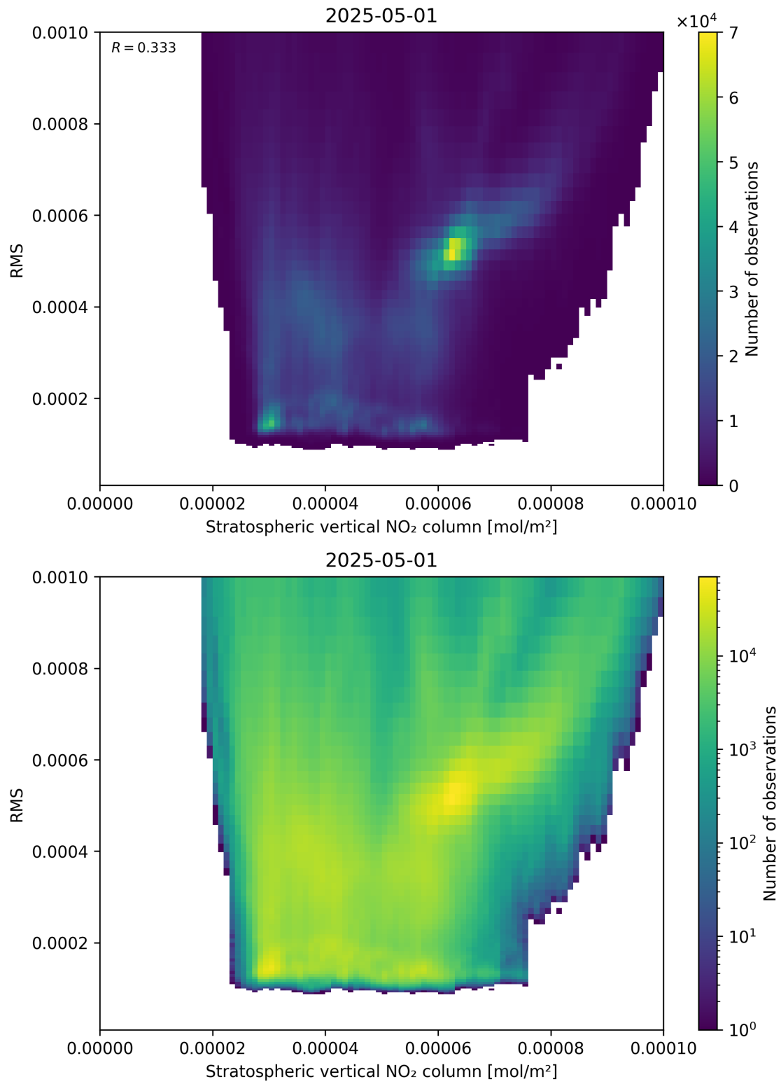
Figure 102: Scatter density plot of “Stratospheric vertical NO 2 column” against “RMS” for 2025-05-01 to 2025-05-02.
