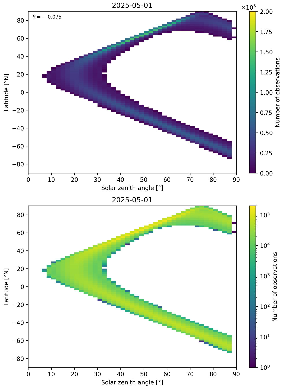
Figure 149: Scatter density plot of “Solar zenith angle” against “Latitude” for 2025-05-01 to 2025-05-02.
