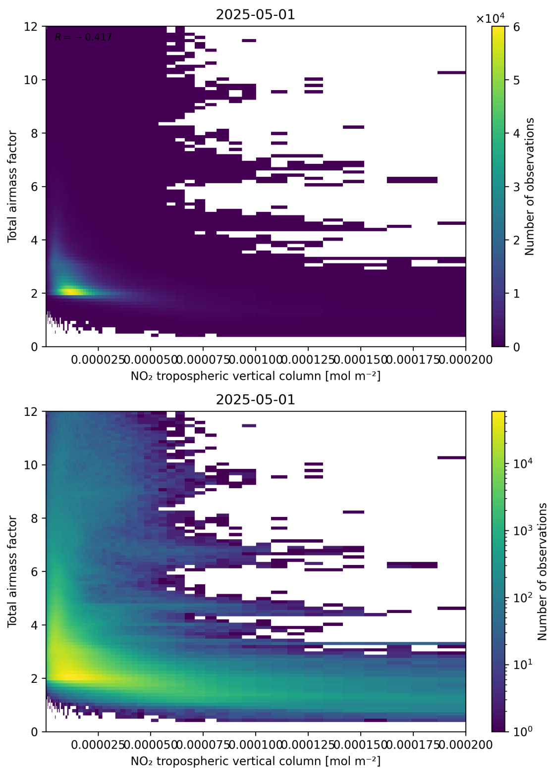
Figure 122: Scatter density plot of “NO 2 tropospheric vertical column” against “Total air mass factor” for 2025-05-01 to 2025-05-02.
