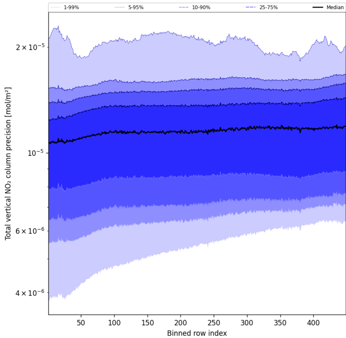
Figure 56: Along track statistics of “Total vertical NO 2 column precision” for 2025-05-01 to 2025-05-02
