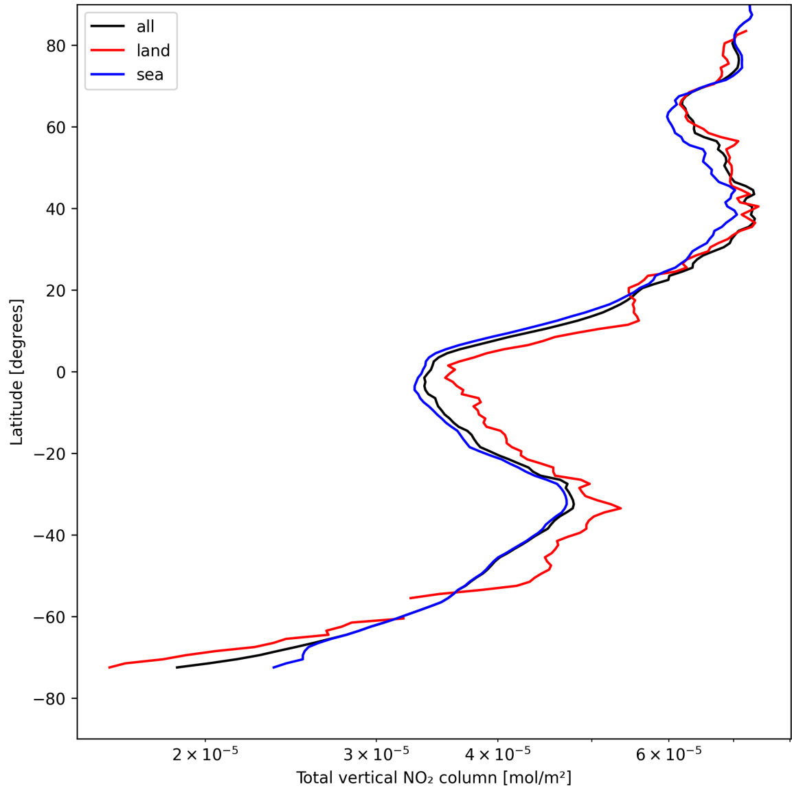
Figure 21: Zonal average of “Total vertical NO 2 column” for 2025-05-01 to 2025-05-02.
