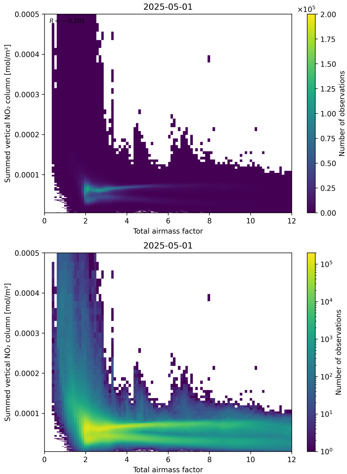
Figure 65: Scatter density plot of “Total airmass factor” against “Summed vertical NO 2 column” for 2025-05-01 to 2025-05-02.
