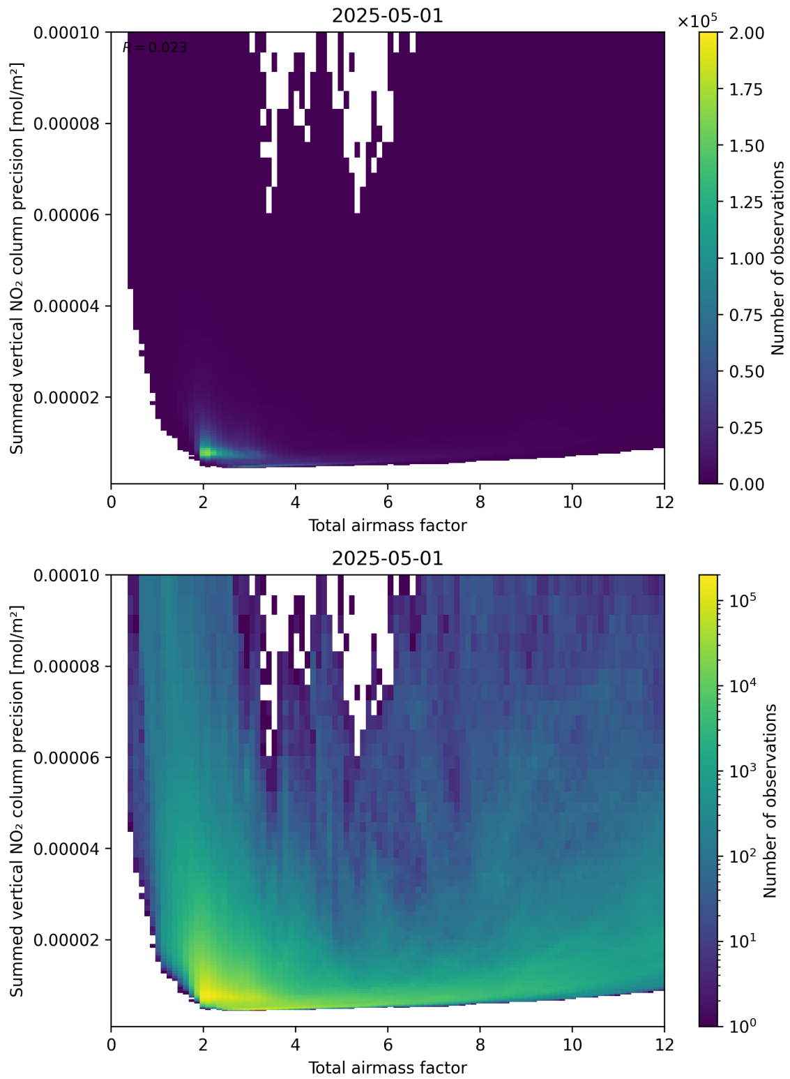
Figure 66: Scatter density plot of “Total airmass factor” against “Summed vertical NO 2 column precision” for 2025-05-01 to 2025-05-02.
