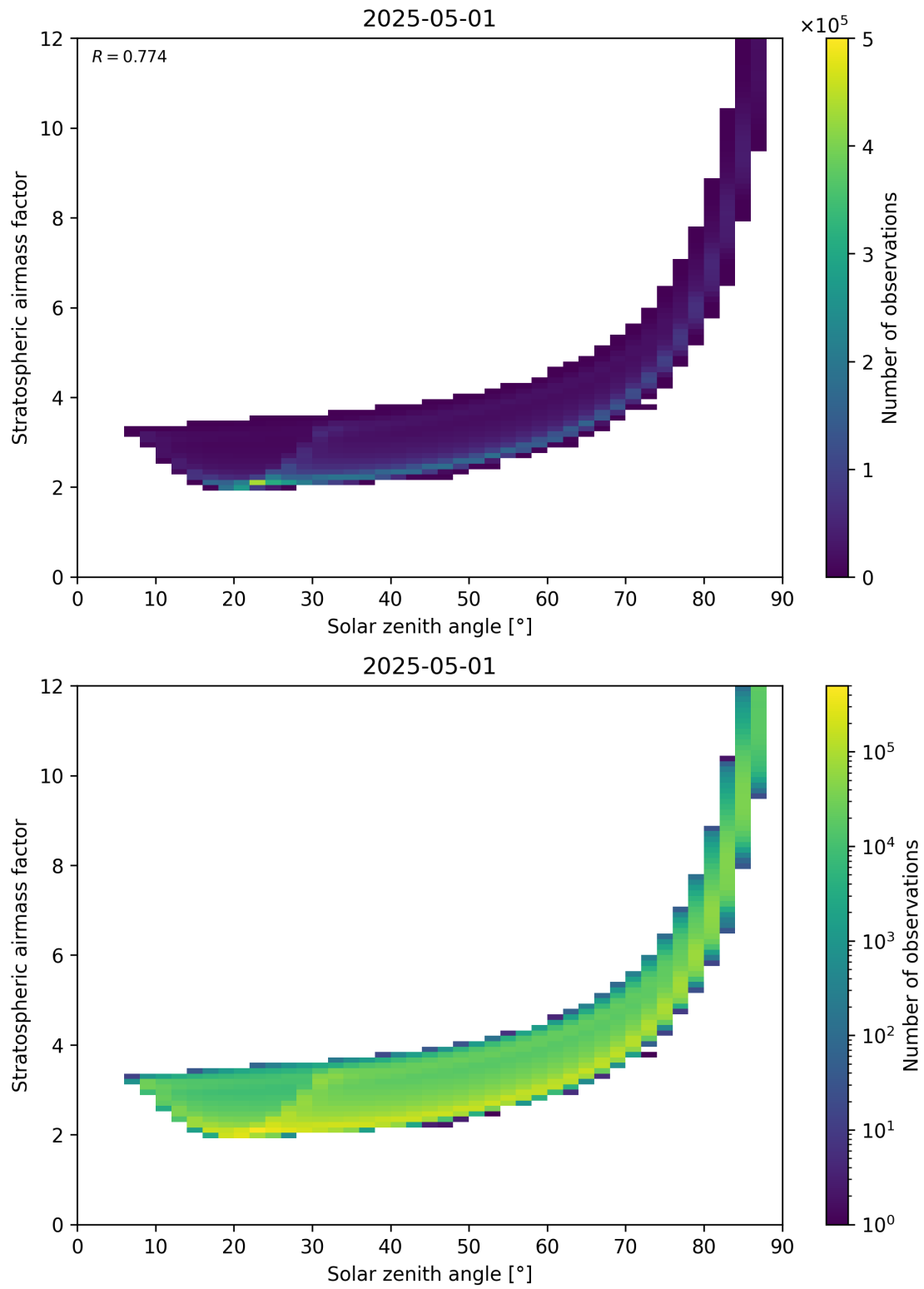
Figure 145: Scatter density plot of “Solar zenith angle” against “Stratospheric airmass factor” for 2025-05-01 to 2025-05-02.
