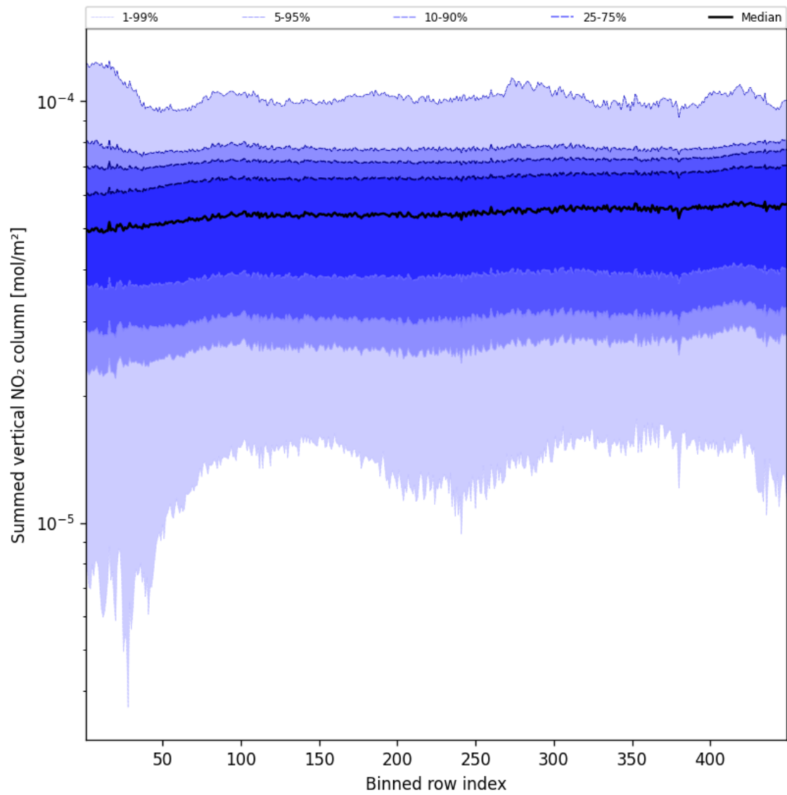
Figure 57: Along track statistics of “Summed vertical NO 2 column” for 2025-05-01 to 2025-05-02
