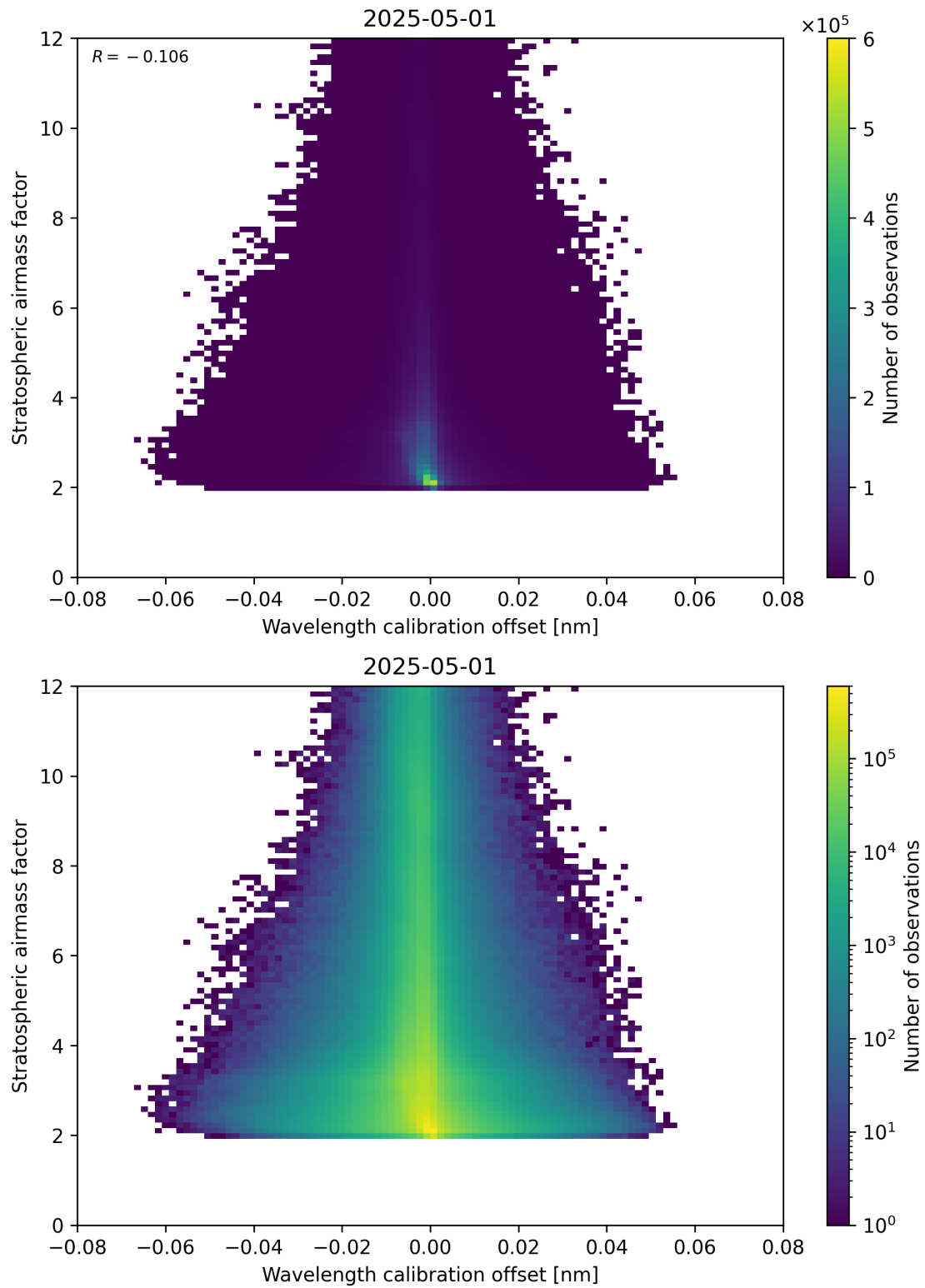
Figure 174: Scatter density plot of “Wavelength calibration offset” against “Stratospheric airmass factor” for 2025-05-01 to 2025-05-02.
