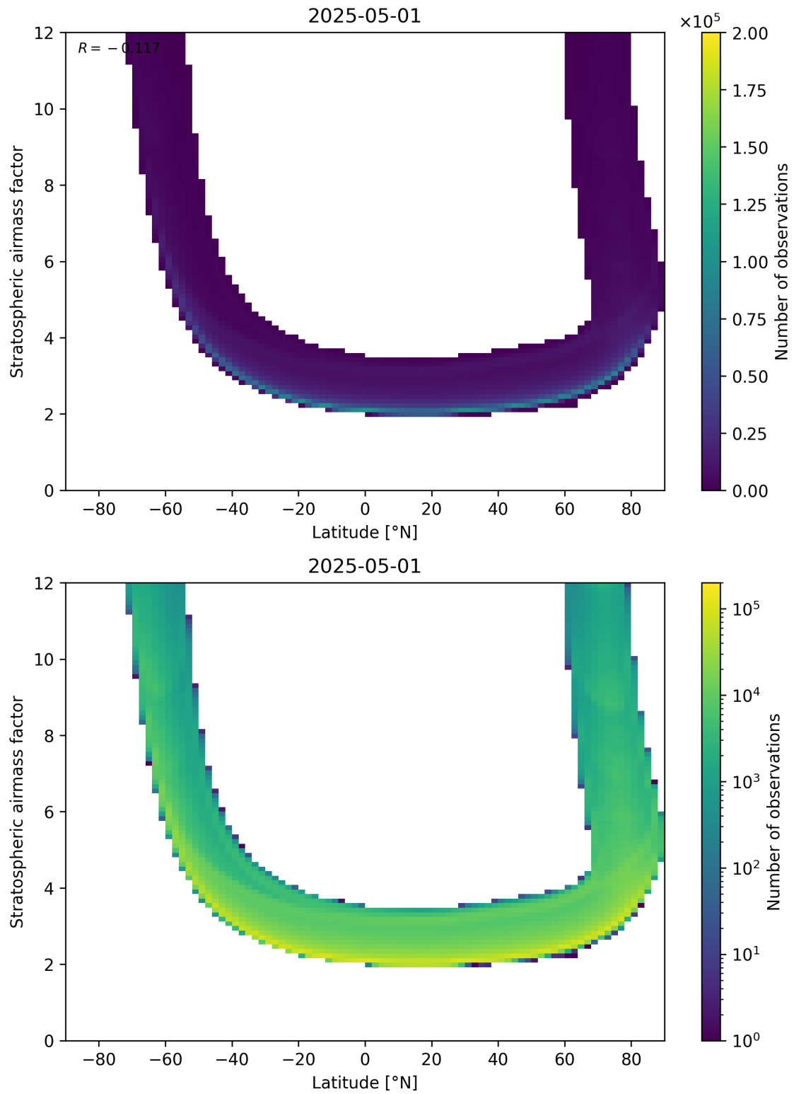
Figure 83: Scatter density plot of “Latitude” against “Stratospheric air mass factor” for 2025-05-01 to 2025-05-02.
