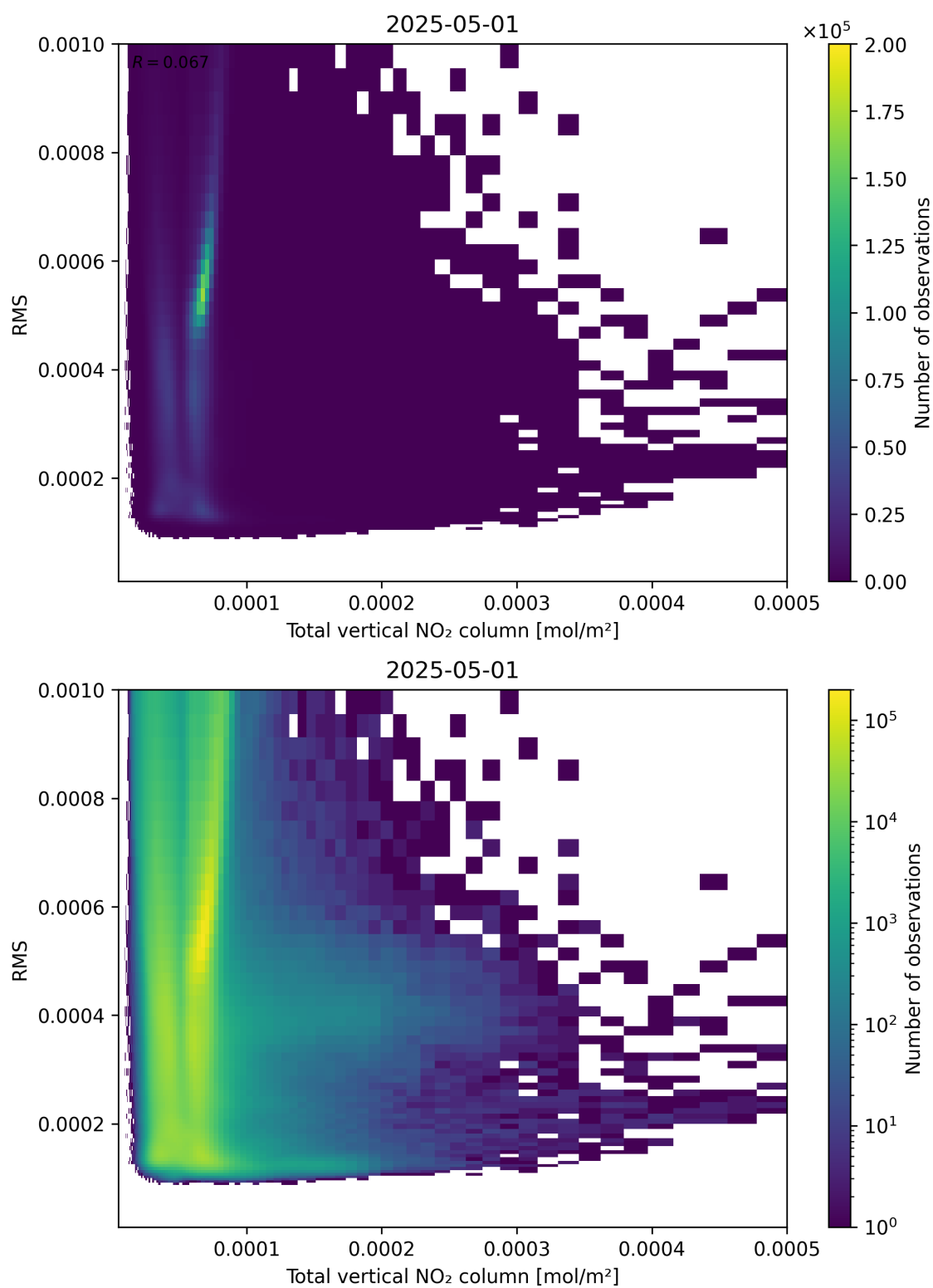
Figure 120: Scatter density plot of “Total vertical NO 2 column” against “RMS” for 2025-05-01 to 2025-05-02.
