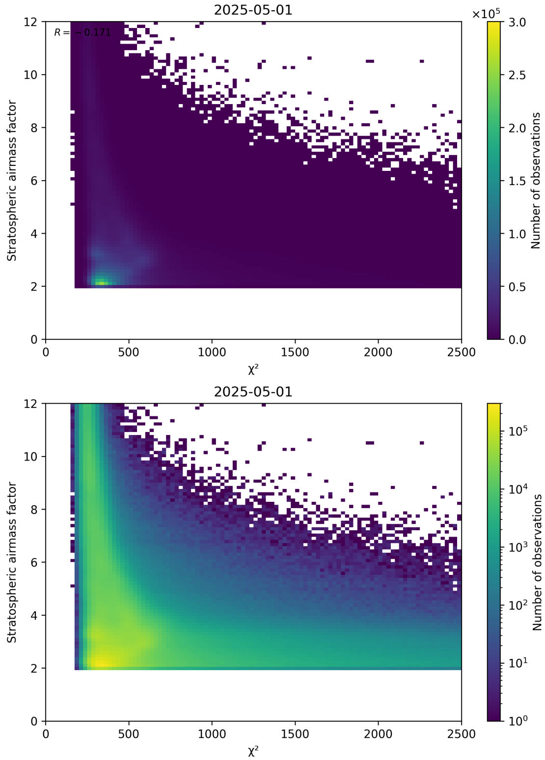
Figure 81: Scatter density plot of “ \chi^2 ” against “Stratospheric airmass factor” for 2025-05-01 to 2025-05-02.
