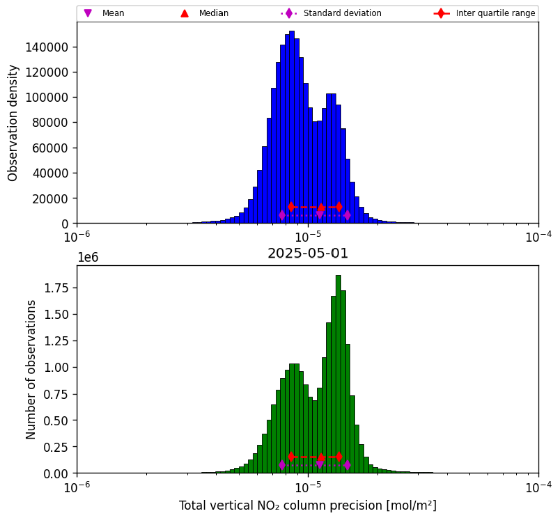
Figure 39: Histogram of “Total vertical NO 2 column precision” for 2025-05-01 to 2025-05-02
