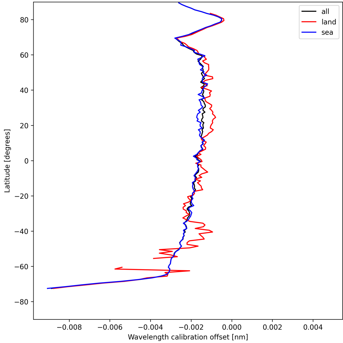
Figure 18: Zonal average of “Wavelength calibration offset” for 2025-05-01 to 2025-05-02.
