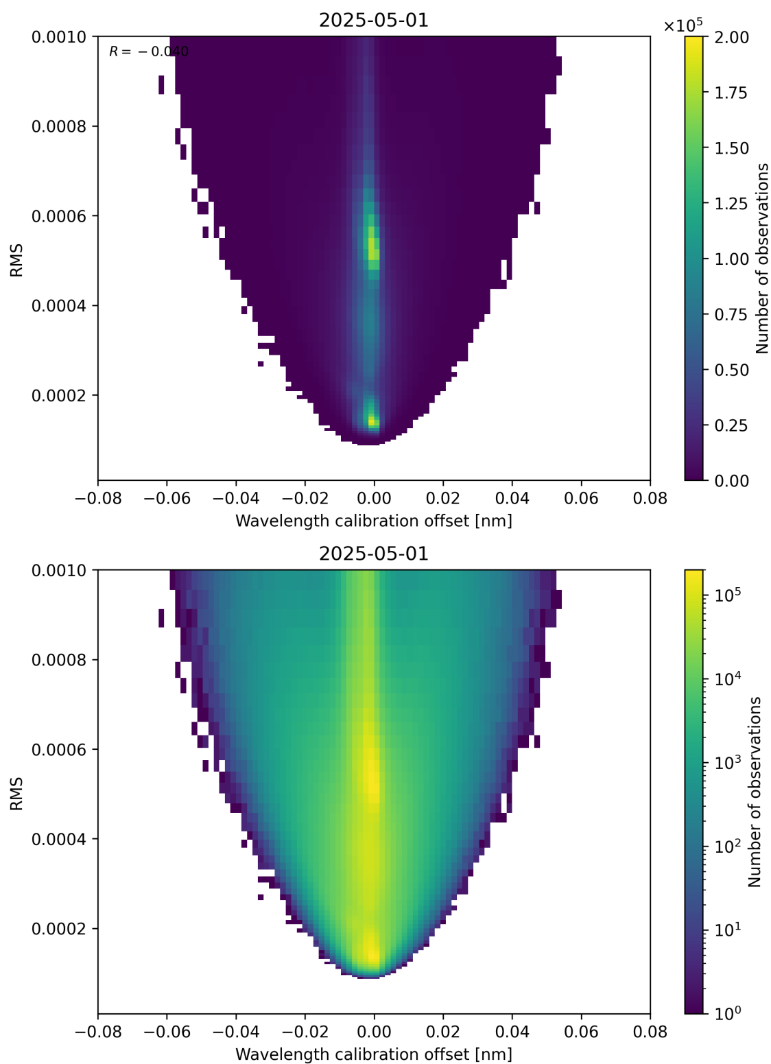
Figure 181: Scatter density plot of “Wavelength calibration offset” against “RMS” for 2025-05-01 to 2025-05-02.
