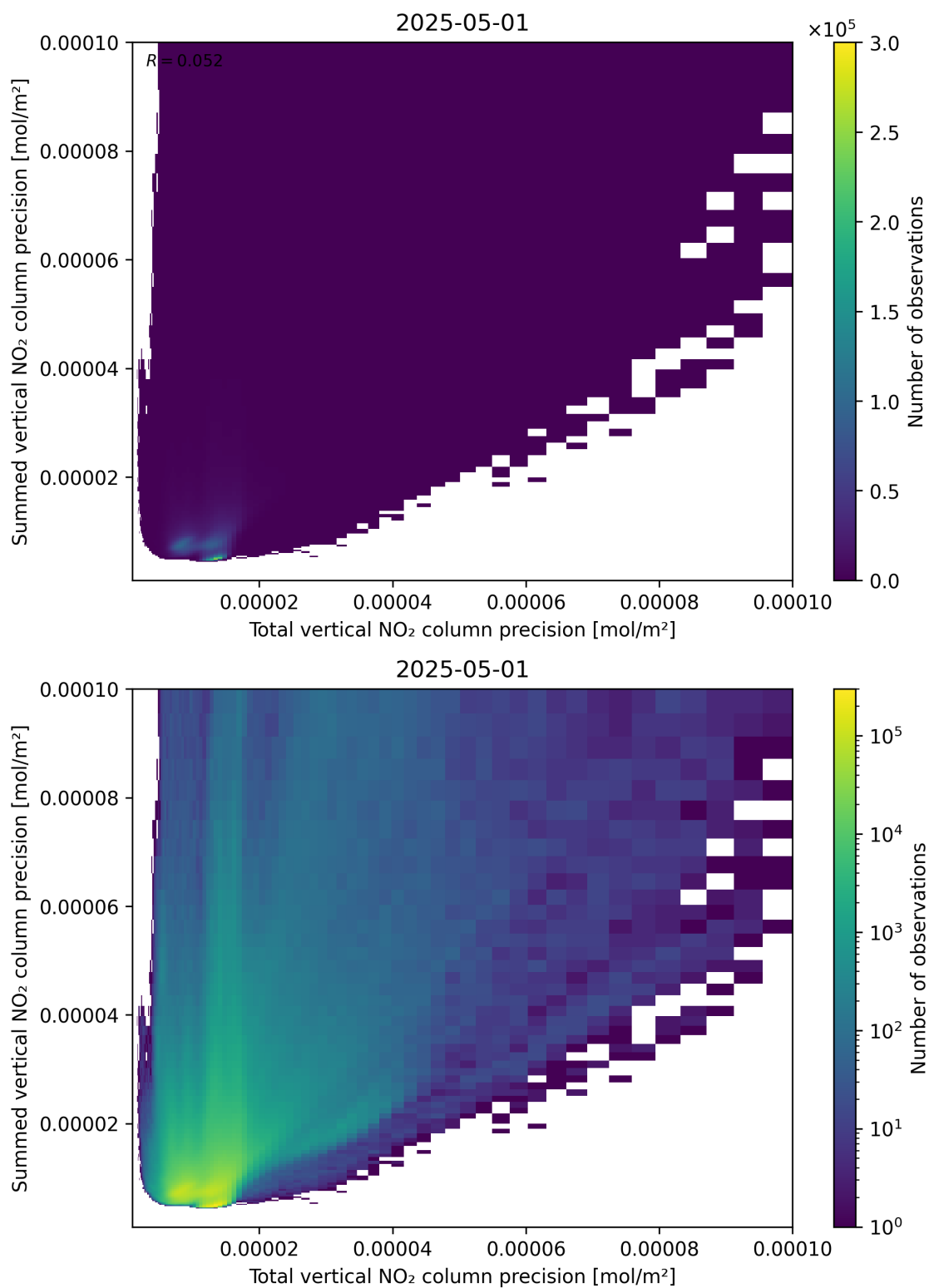
Figure 118: Scatter density plot of “Total vertical NO 2 column precision” against “Summed vertical NO 2 column precision” for 2025-05-01 to 2025-05-02.
