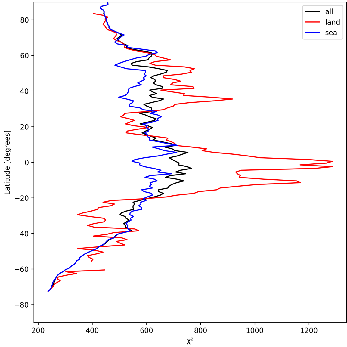
Figure 25: Zonal average of “ \chi^2 ” for 2025-05-01 to 2025-05-02.
