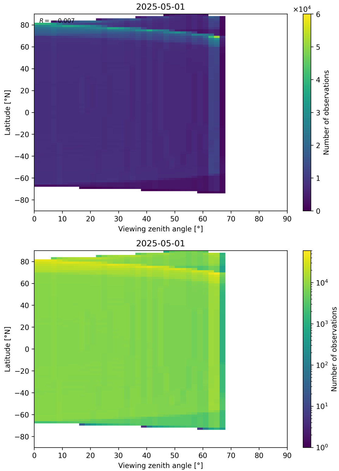
Figure 163: Scatter density plot of “Viewing zenith angle” against “Latitude” for 2025-05-01 to 2025-05-02.
