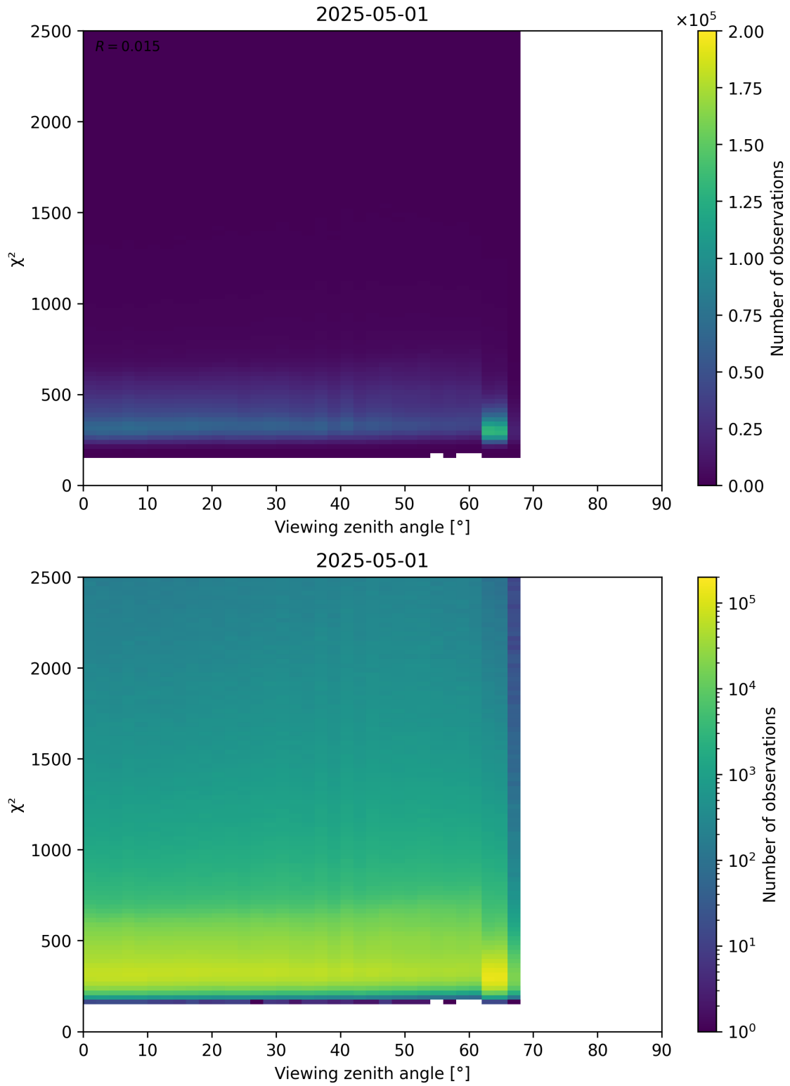
Figure 162: Scatter density plot of “Viewing zenith angle” against “ \chi^2 ” for 2025-05-01 to 2025-05-02.
