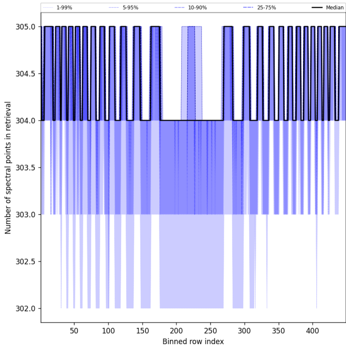
Figure 50: Along track statistics of “Number of spectral points in retrieval” for 2025-05-01 to 2025-05-02
