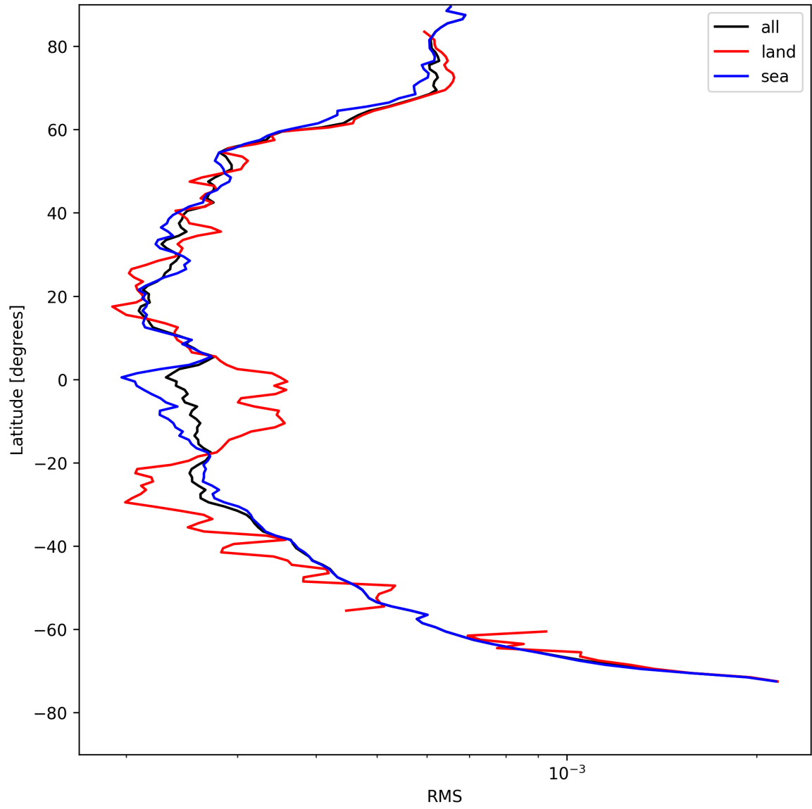
Figure 26: Zonal average of “RMS” for 2025-05-01 to 2025-05-02.
