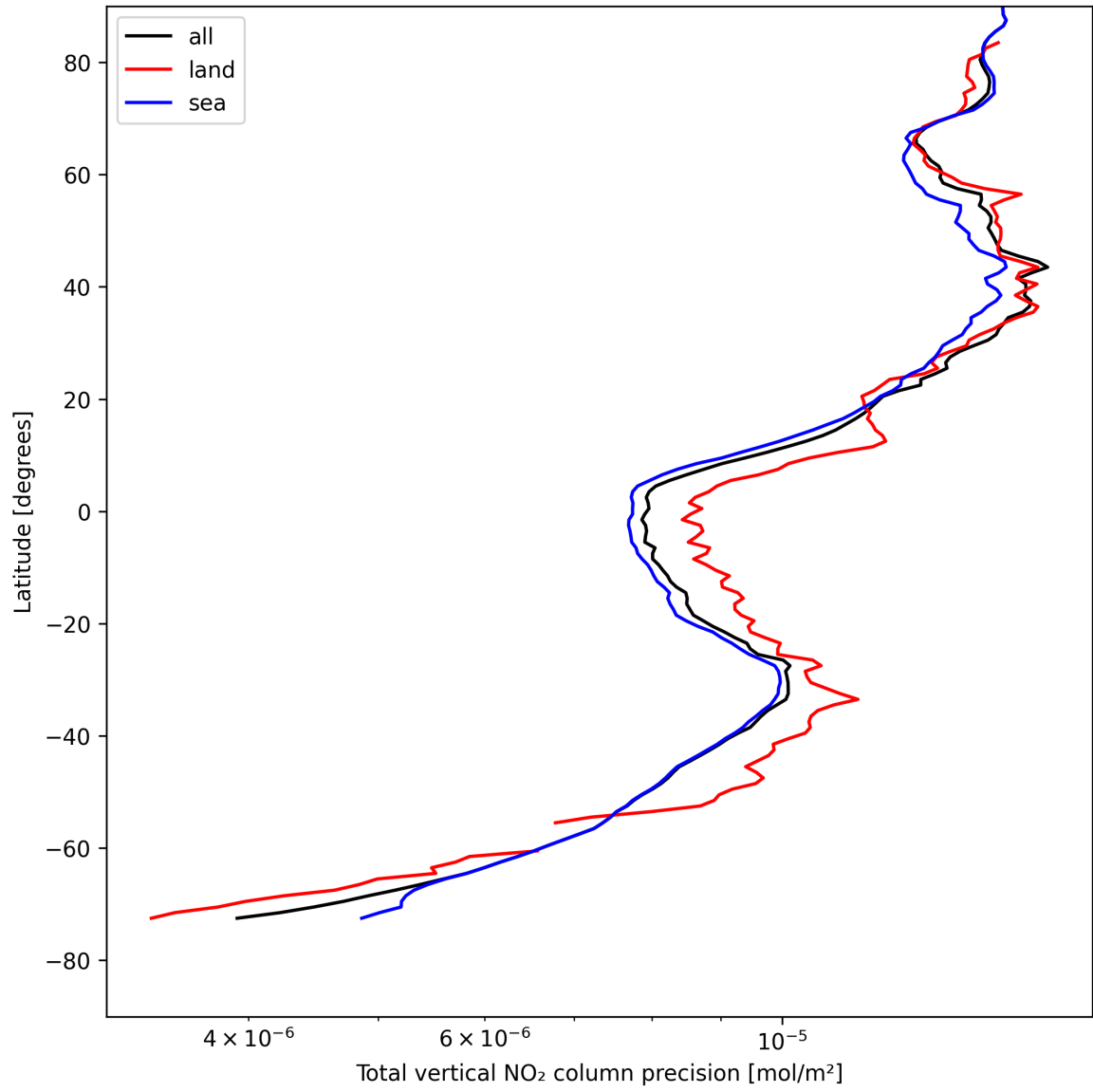
Figure 22: Zonal average of “Total vertical NO 2 column precision” for 2025-05-01 to 2025-05-02.
