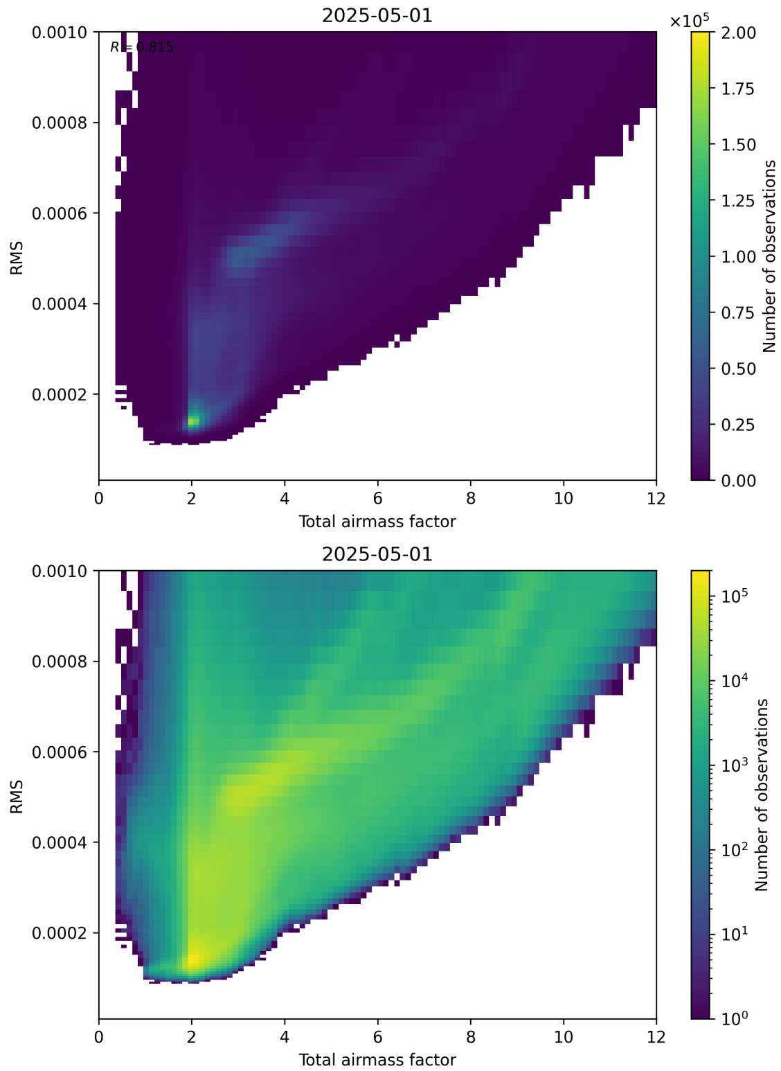
Figure 69: Scatter density plot of “Total airmass factor” against “RMS” for 2025-05-01 to 2025-05-02.
