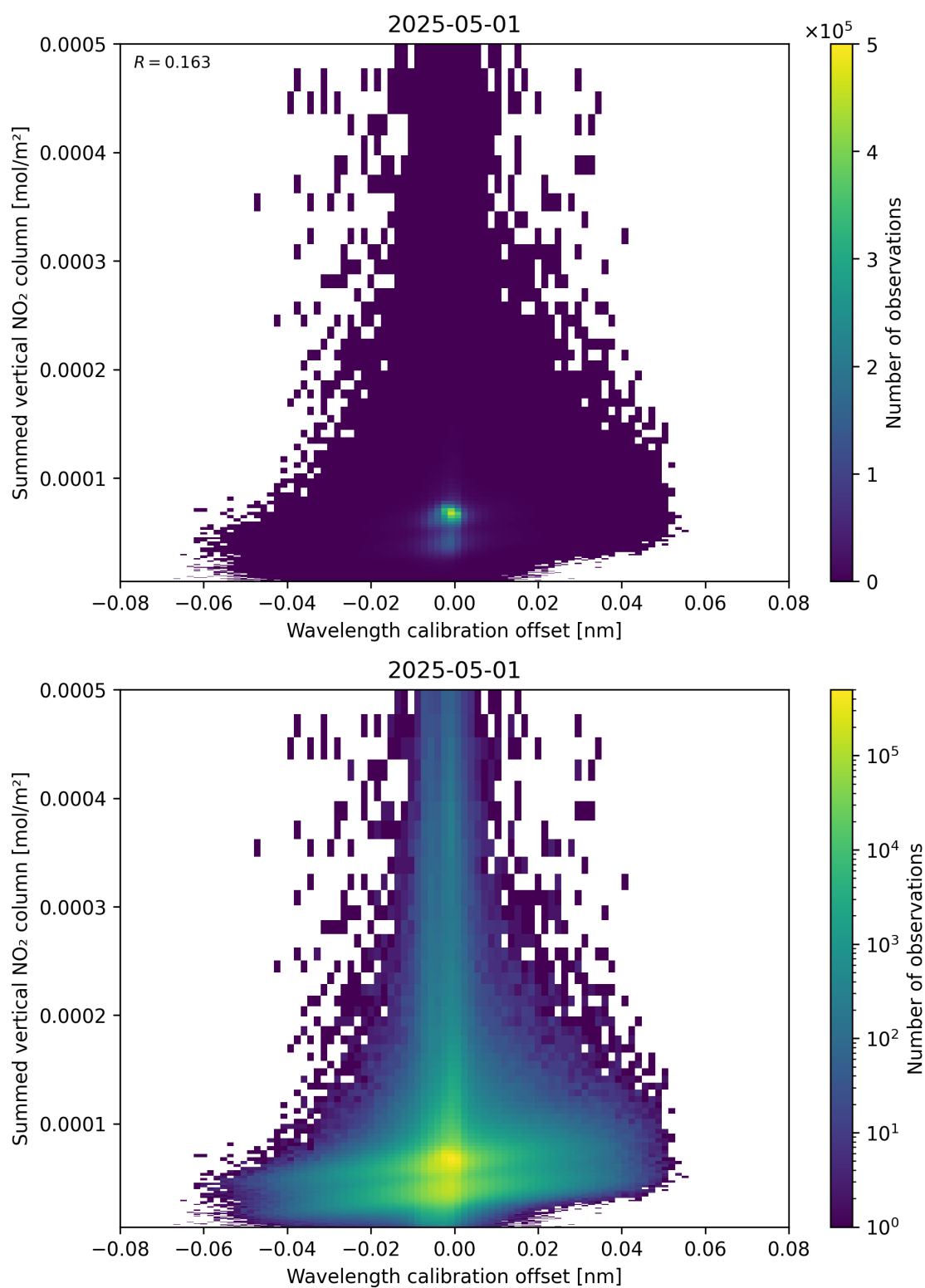
Figure 177: Scatter density plot of “Wavelength calibration offset” against “Summed vertical NO 2 column” for 2025-05-01 to 2025-05-02.
