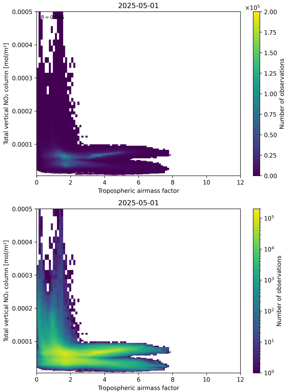
Figure 77: Scatter density plot of “Tropospheric airmass factor” against “Total vertical NO 2 column” for 2025-05-01 to 2025-05-02.
