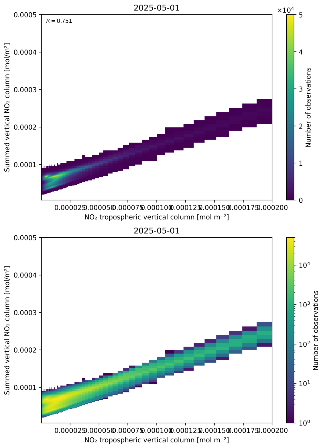
Figure 126: Scatter density plot of “NO 2 tropospheric vertical column” against “Summed vertical NO 2 column” for 2025-05-01 to 2025-05-02.
