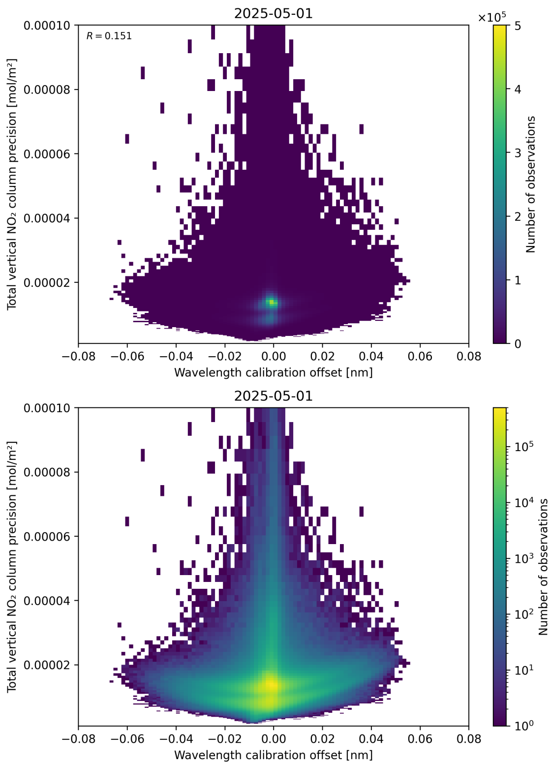
Figure 180: Scatter density plot of “Wavelength calibration offset” against “Total vertical NO 2 column precision” for 2025-05-01 to 2025-05-02.
