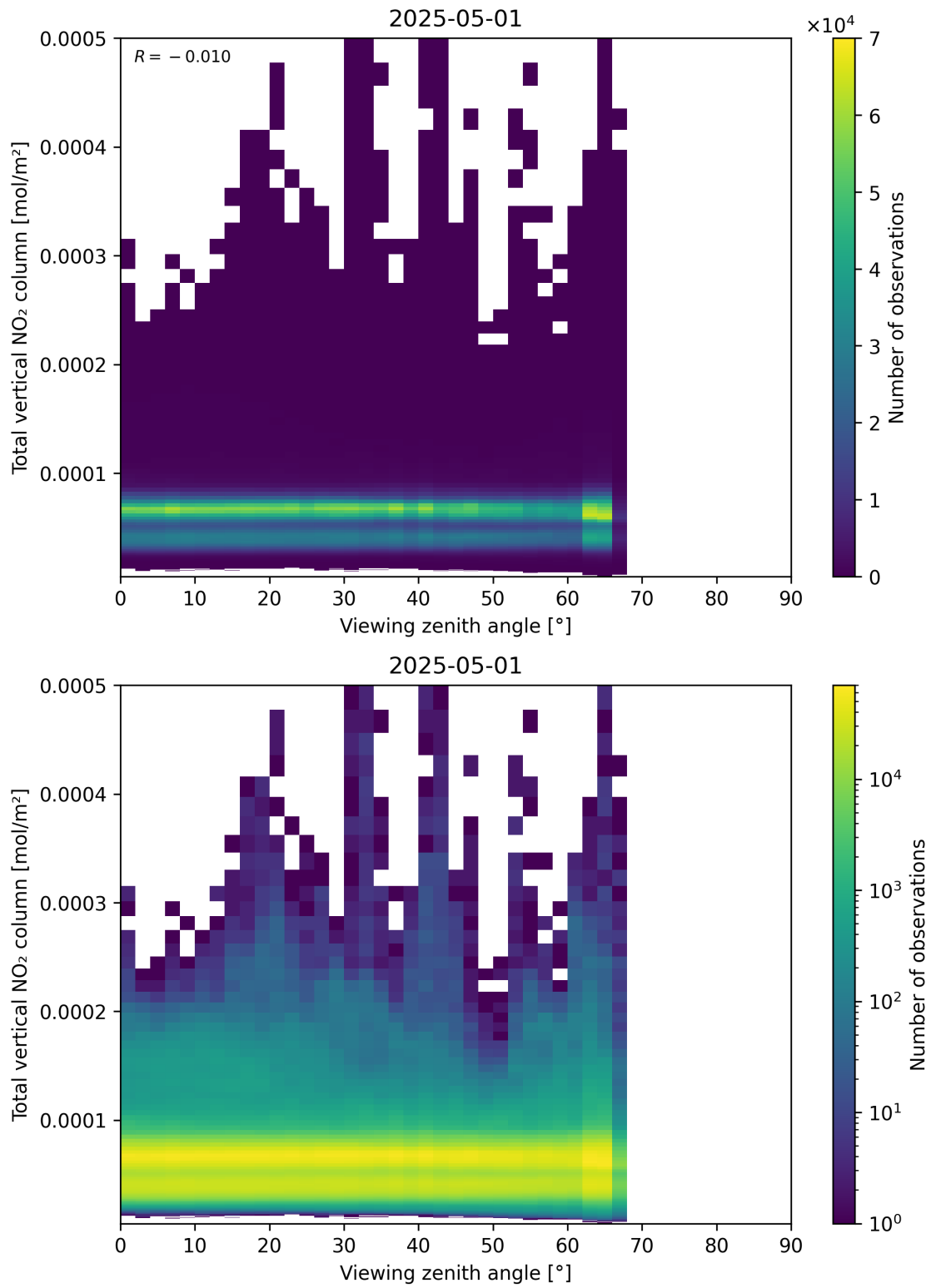
Figure 167: Scatter density plot of “Viewing zenith angle” against “Total vertical NO 2 column” for 2025-05-01 to 2025-05-02.
