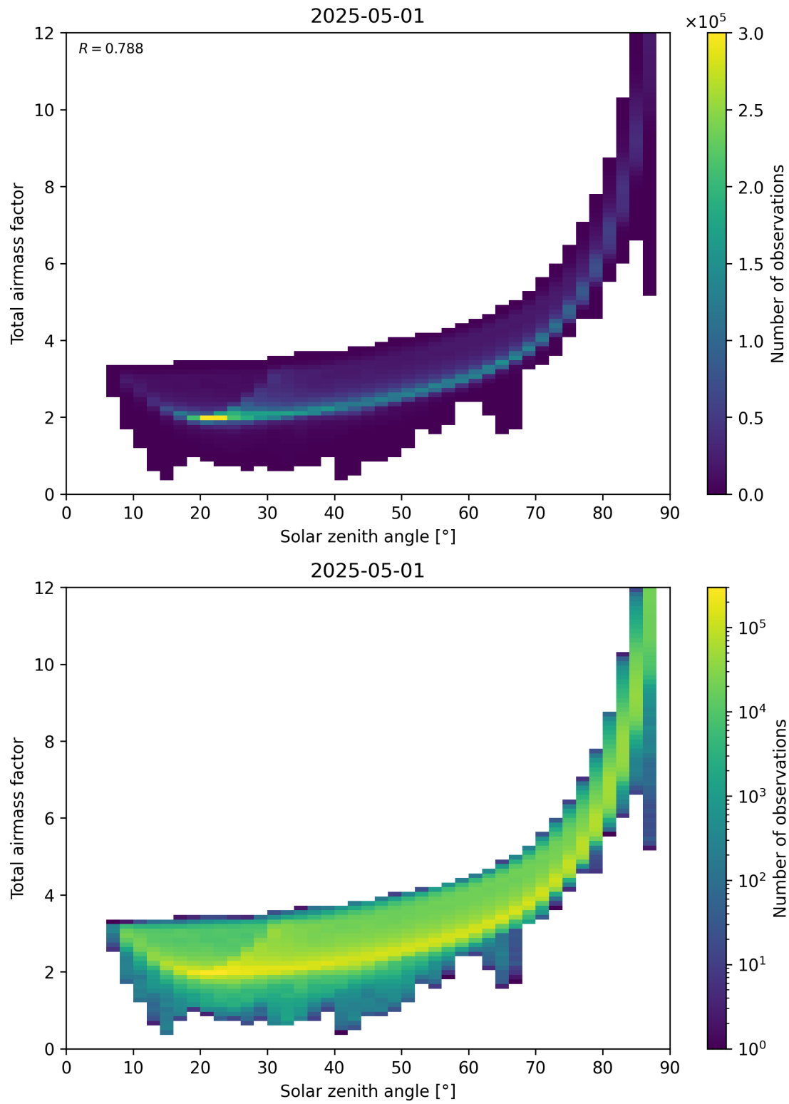
Figure 146: Scatter density plot of “Solar zenith angle” against “Total air mass factor” for 2025-05-01 to 2025-05-02.
