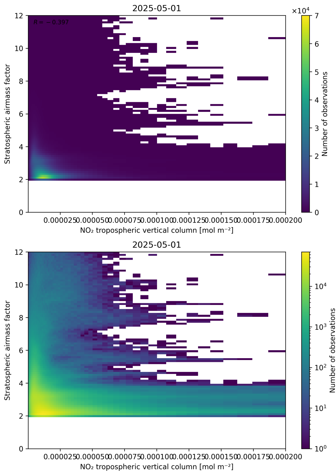
Figure 121: Scatter density plot of “NO 2 tropospheric vertical column” against “Stratospheric air mass factor” for 2025-05-01 to 2025-05-02.
