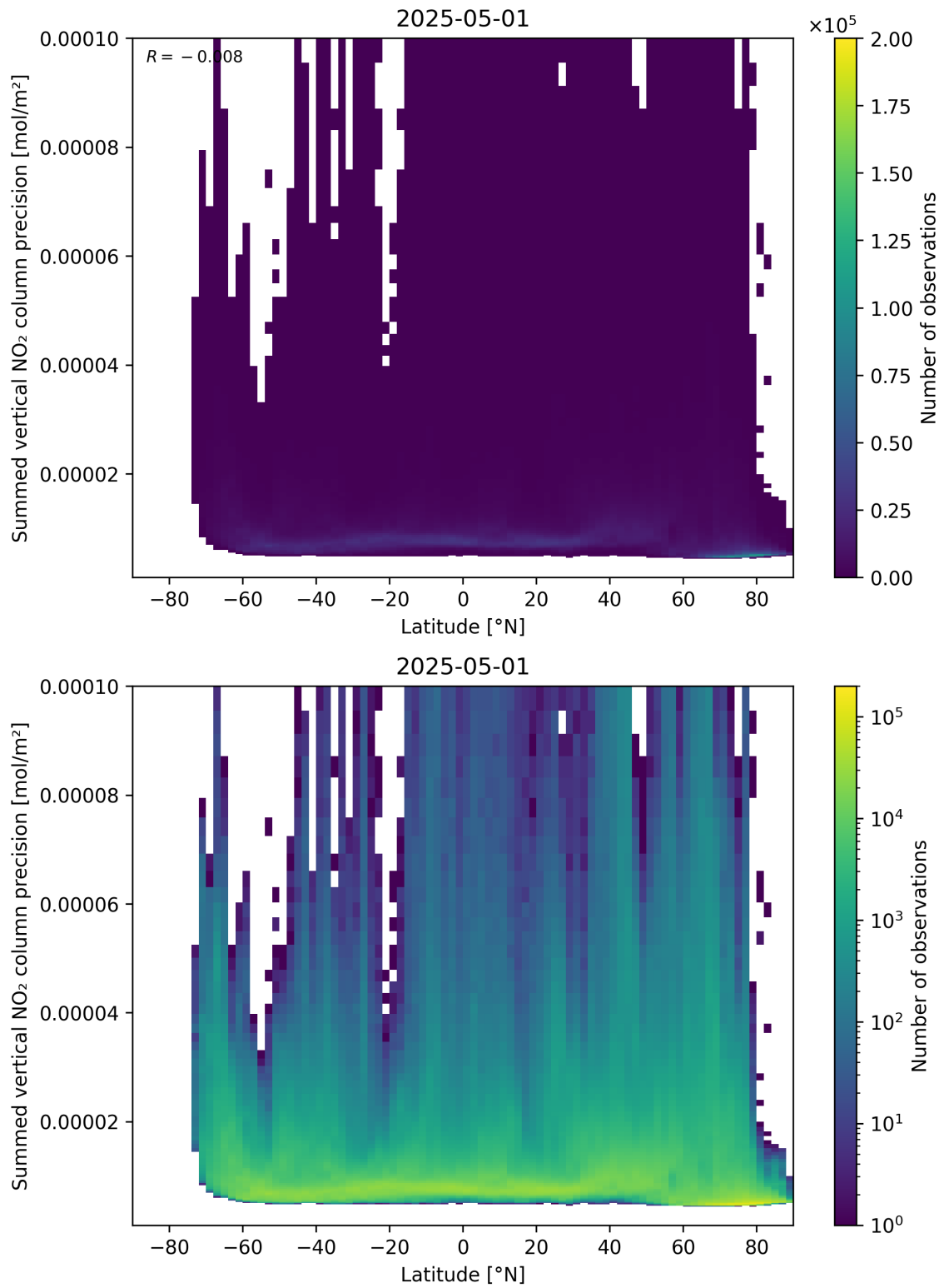
Figure 89: Scatter density plot of “Latitude” against “Summed vertical NO 2 column precision” for 2025-05-01 to 2025-05-02.
