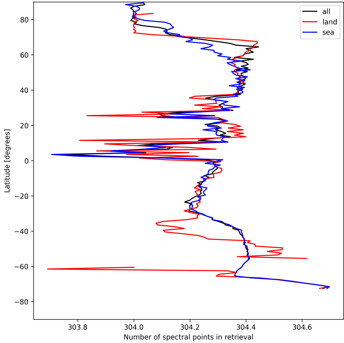
Figure 16: Zonal average of “Number of spectral points in retrieval” for 2025-05-01 to 2025-05-02.
