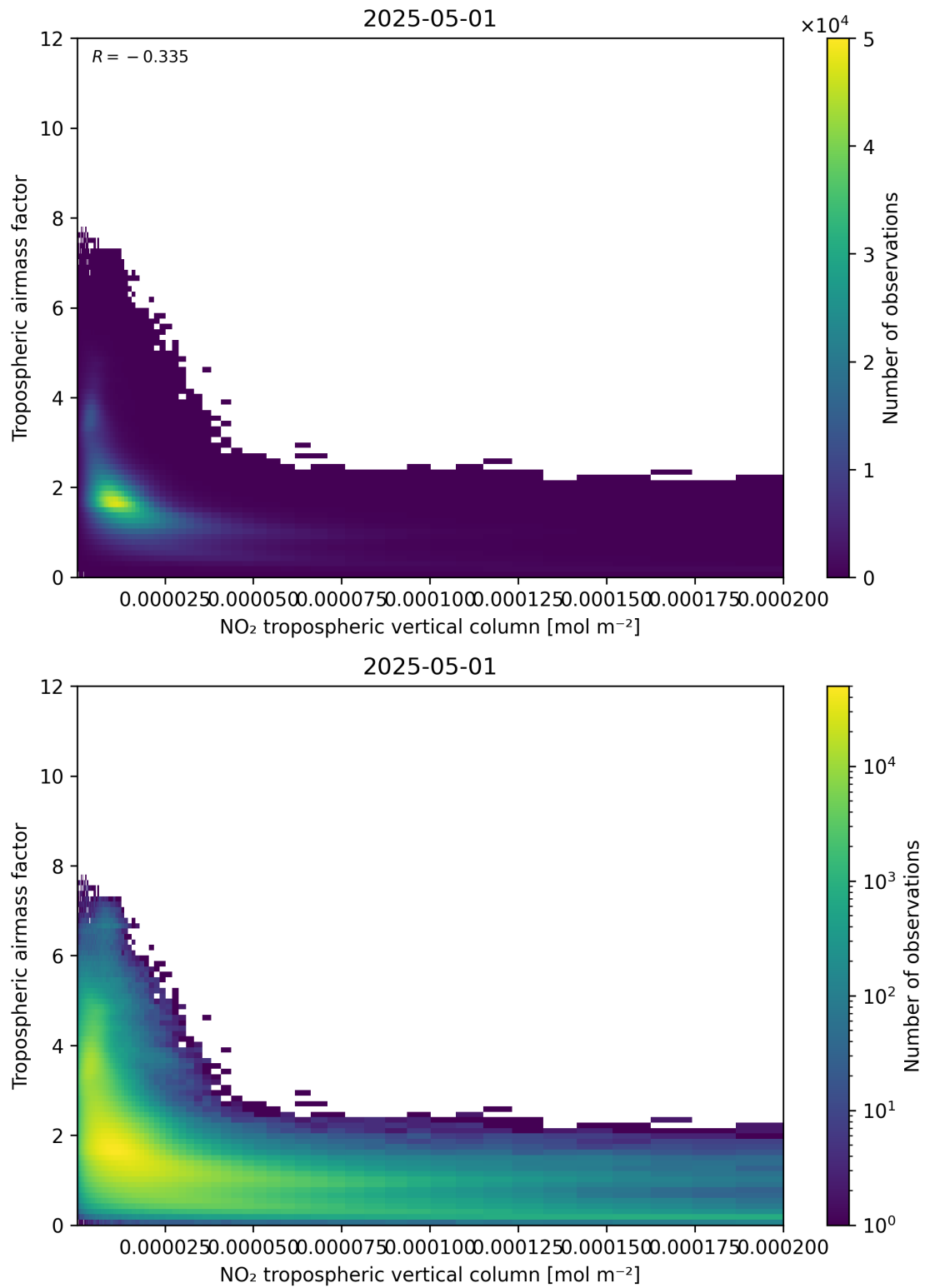
Figure 123: Scatter density plot of “NO 2 tropospheric vertical column” against “Tropospheric air mass factor” for 2025-05-01 to 2025-05-02.
