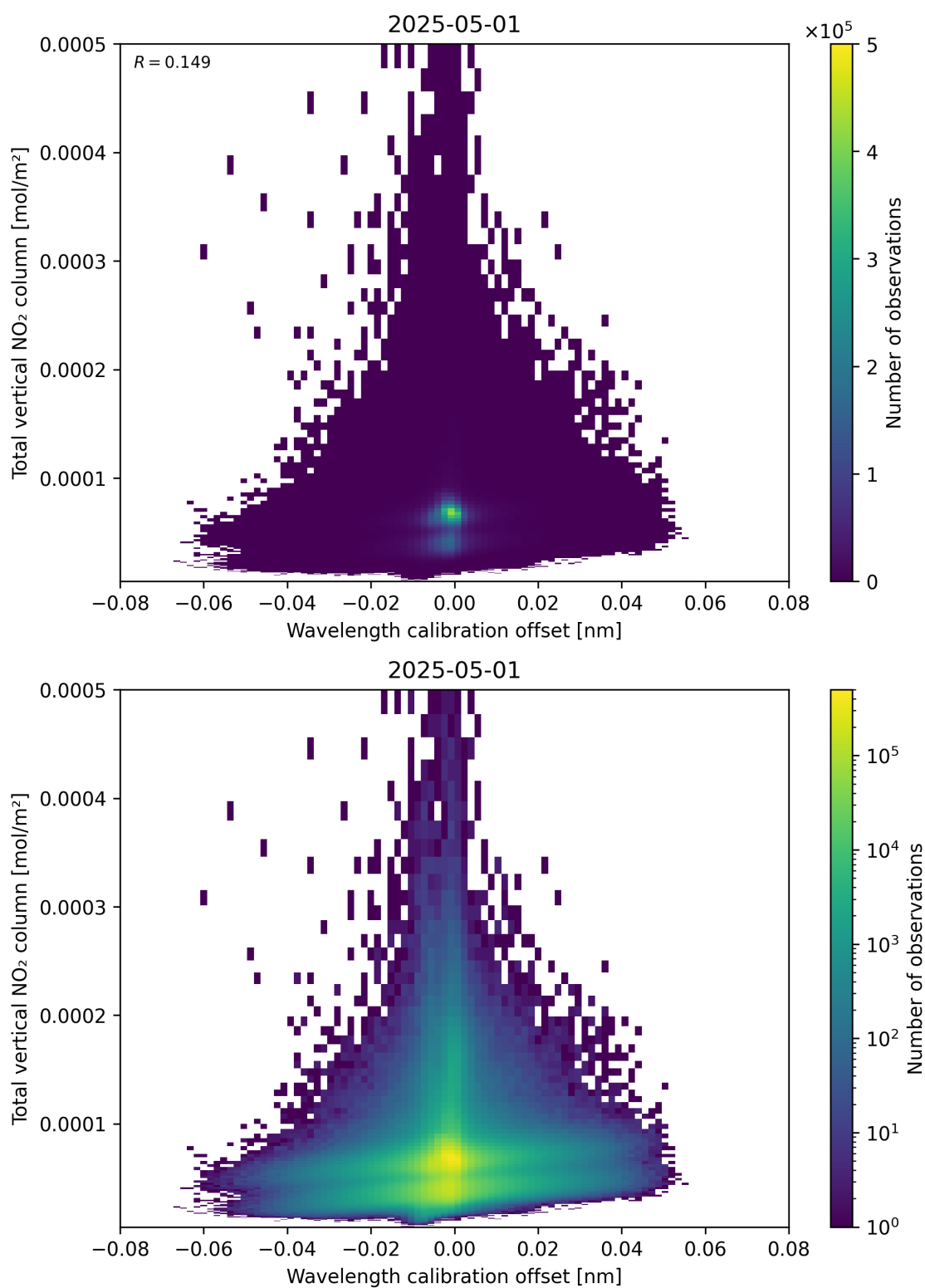
Figure 179: Scatter density plot of “Wavelength calibration offset” against “Total vertical NO 2 column” for 2025-05-01 to 2025-05-02.
