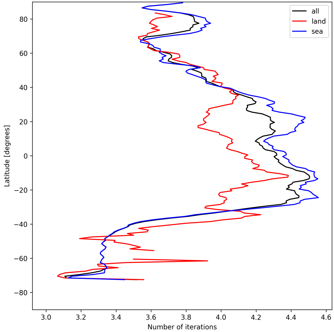
Figure 17: Zonal average of “Number of iterations” for 2025-05-01 to 2025-05-02.
