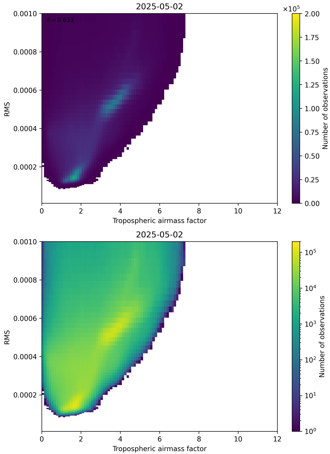
Figure 79: Scatter density plot of “Tropospheric airmass factor” against “RMS” for 2025-05-02 to 2025-05-02.
