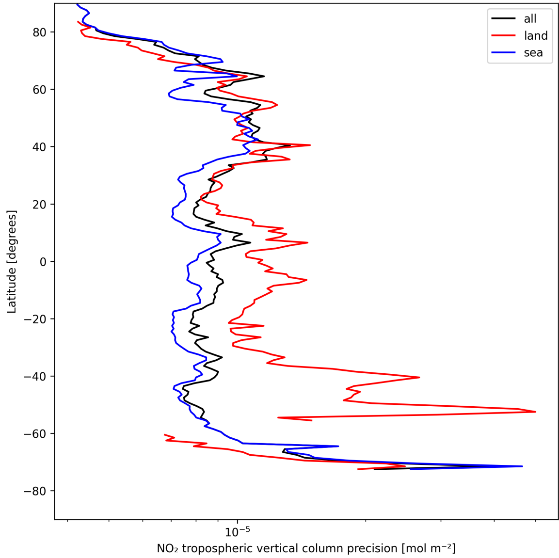
Figure 13: Zonal average of “NO 2 tropospheric vertical column precision” for 2025-05-02 to 2025-05-02.
