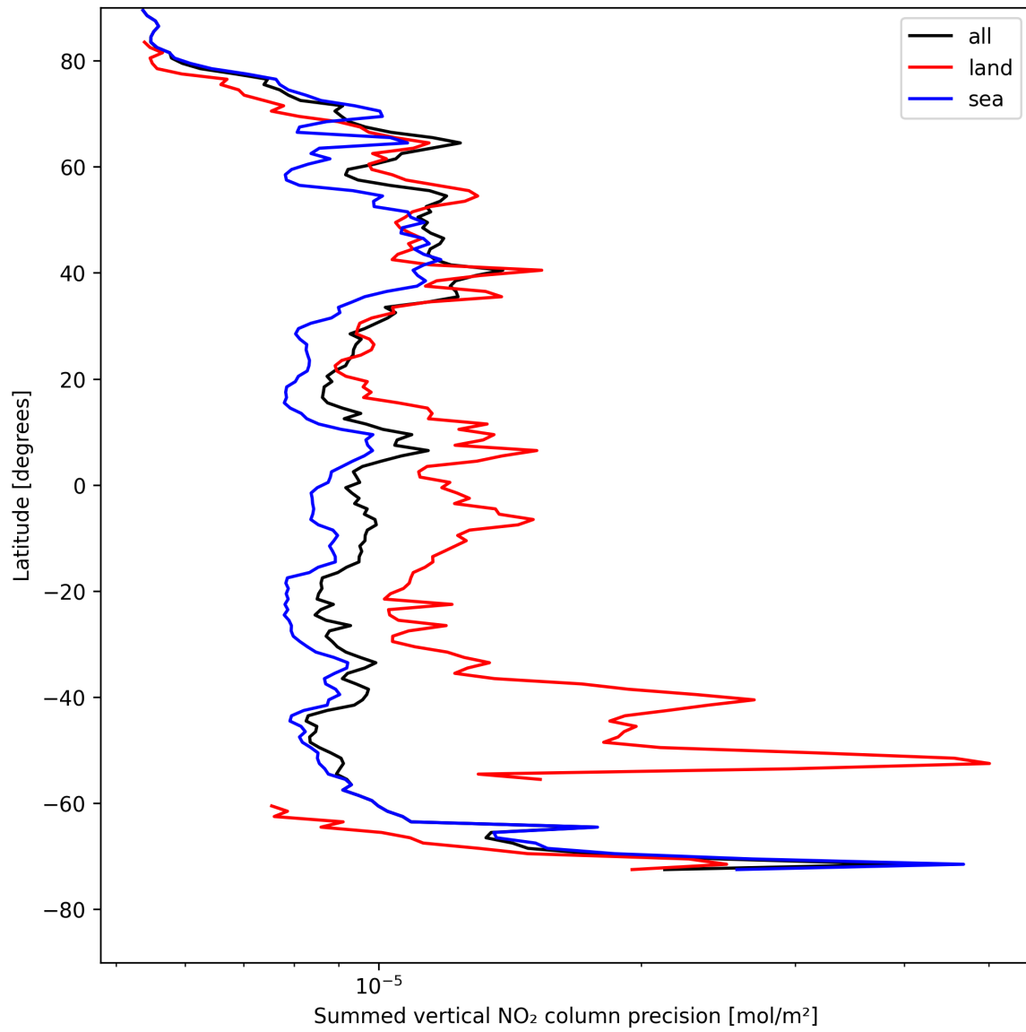
Figure 24: Zonal average of “Summed vertical NO 2 column precision” for 2025-05-02 to 2025-05-02.
