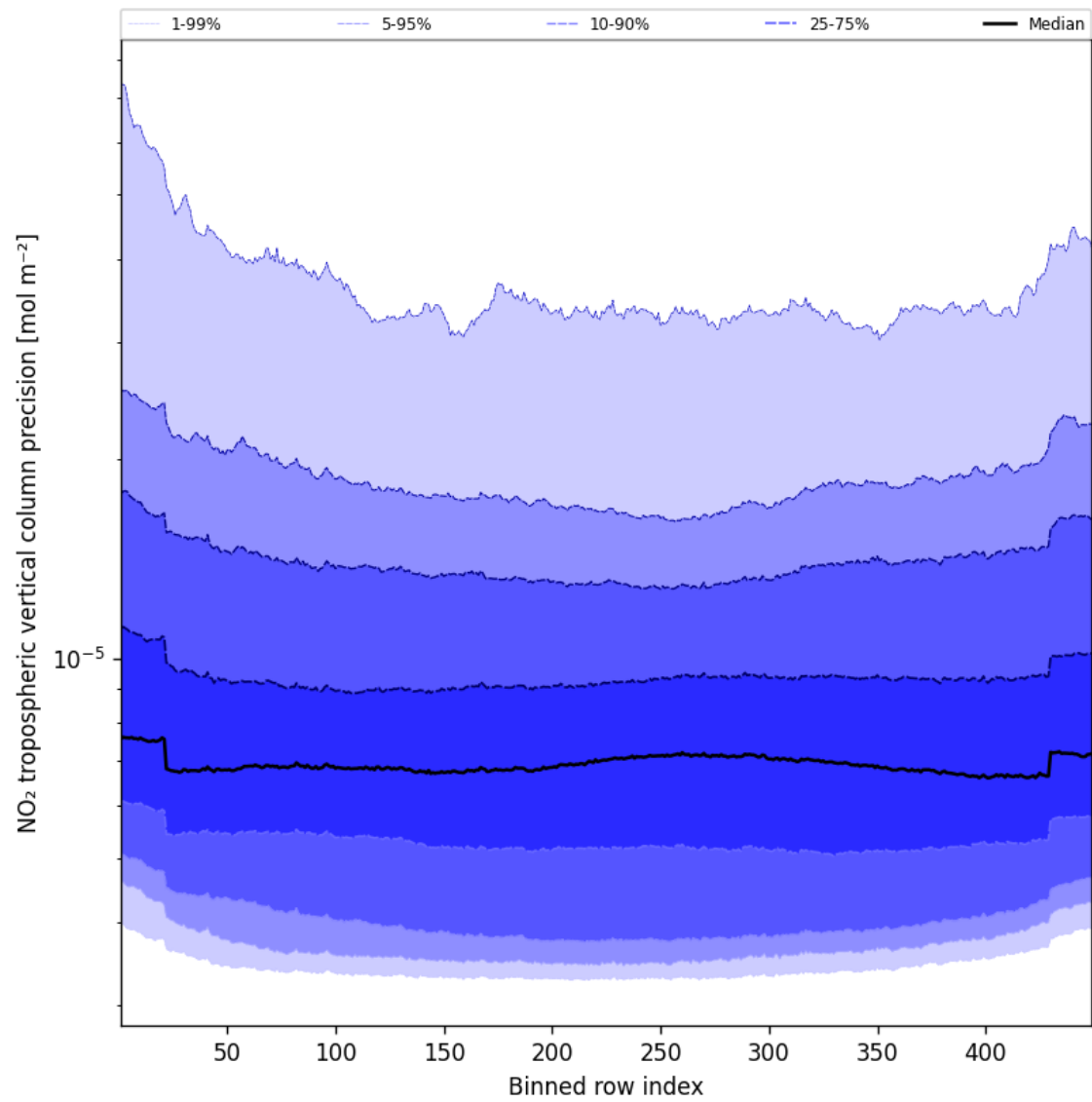
Figure 47: Along track statistics of “NO 2 tropospheric vertical column precision” for 2025-05-02 to 2025-05-02
