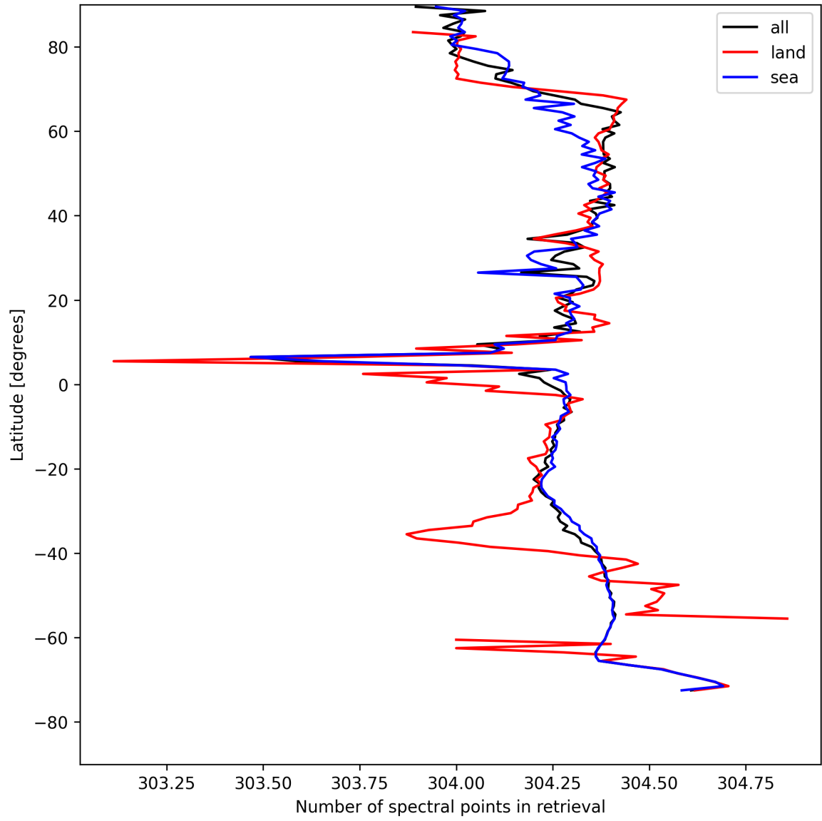
Figure 16: Zonal average of “Number of spectral points in retrieval” for 2025-05-02 to 2025-05-02.
