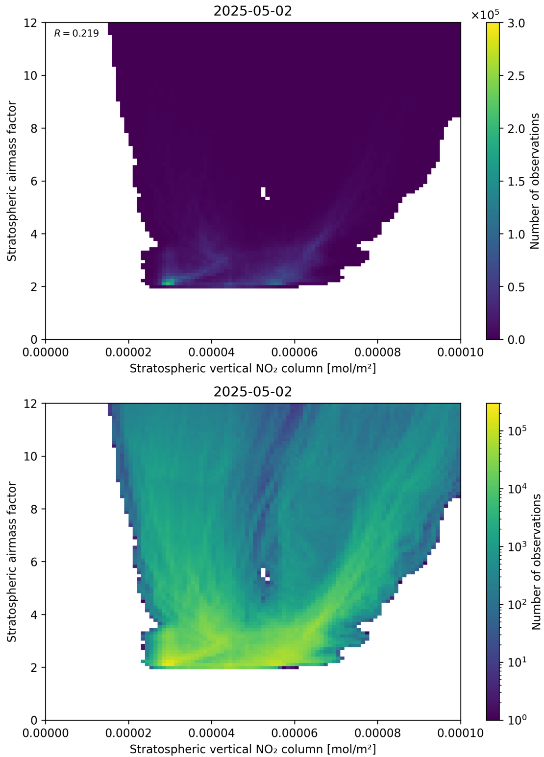
Figure 96: Scatter density plot of “Stratospheric vertical NO 2 column” against “Stratospheric airmass factor” for 2025-05-02 to 2025-05-02.
