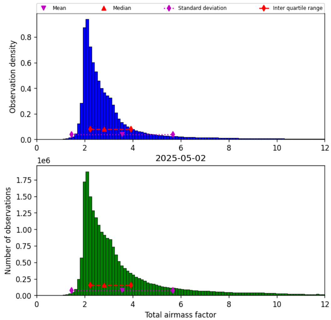
Figure 32: Histogram of “Total airmass factor” for 2025-05-02 to 2025-05-02
