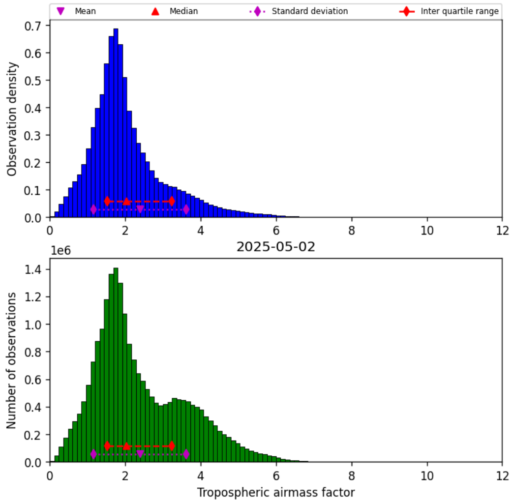
Figure 31: Histogram of “Tropospheric airmass factor” for 2025-05-02 to 2025-05-02
