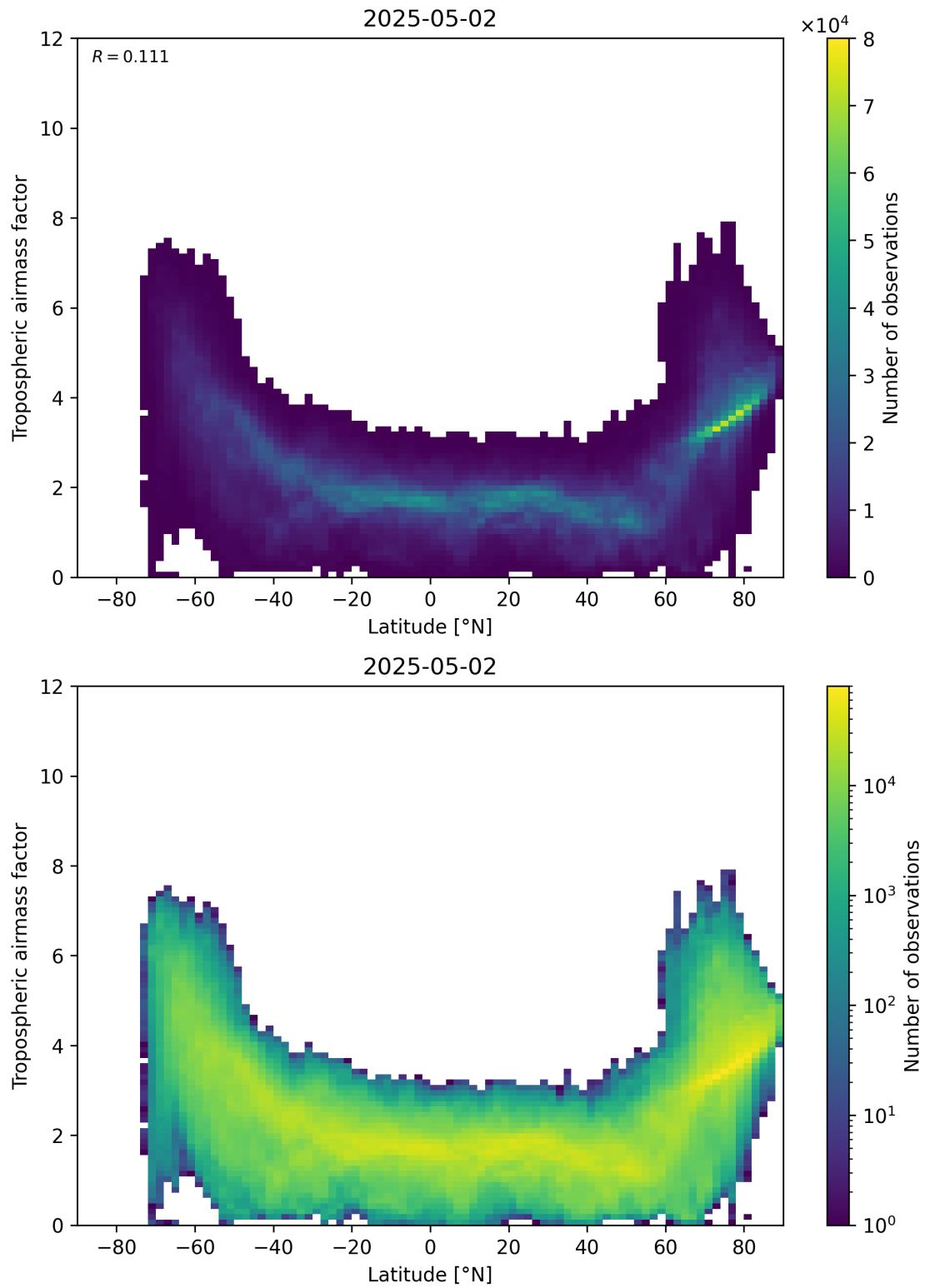
Figure 85: Scatter density plot of “Latitude” against “Tropospheric airmass factor” for 2025-05-02 to 2025-05-02.
