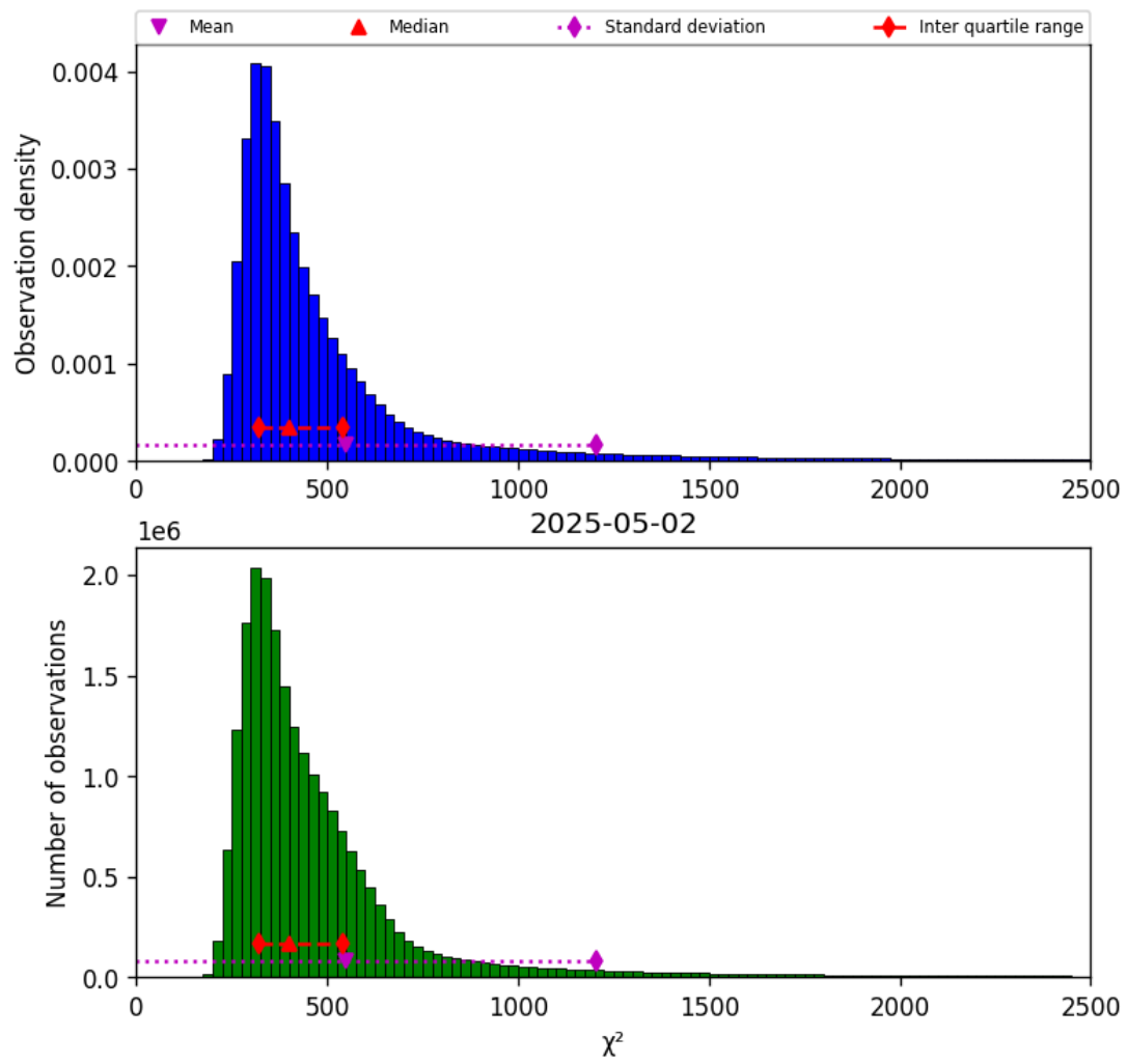
Figure 42: Histogram of " \chi^2 " for 2025-05-02 to 2025-05-02
