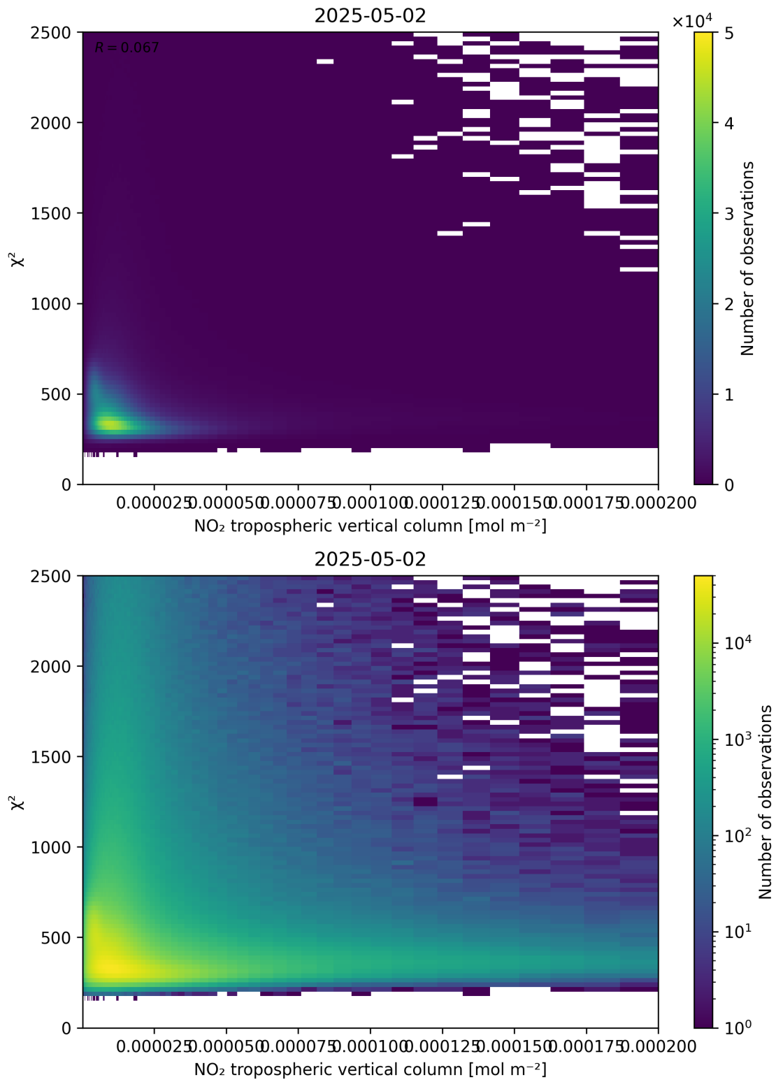
Figure 124: Scatter density plot of “NO 2 tropospheric vertical column” against “ \chi^2 ” for 2025-05-02 to 2025-05-02.
