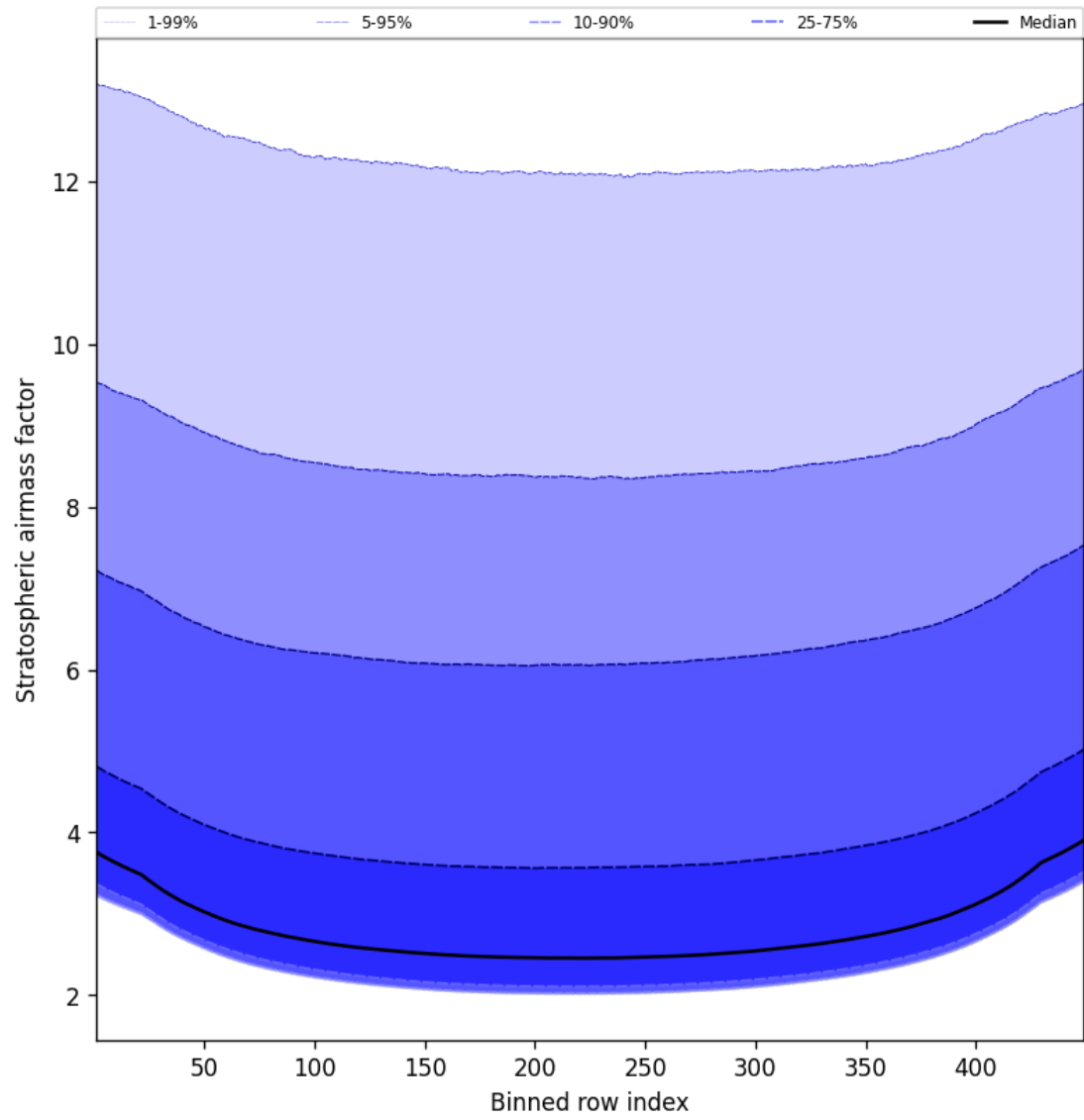
Figure 61: Along track statistics of “Stratospheric airmass factor” for 2025-05-02 to 2025-05-02
