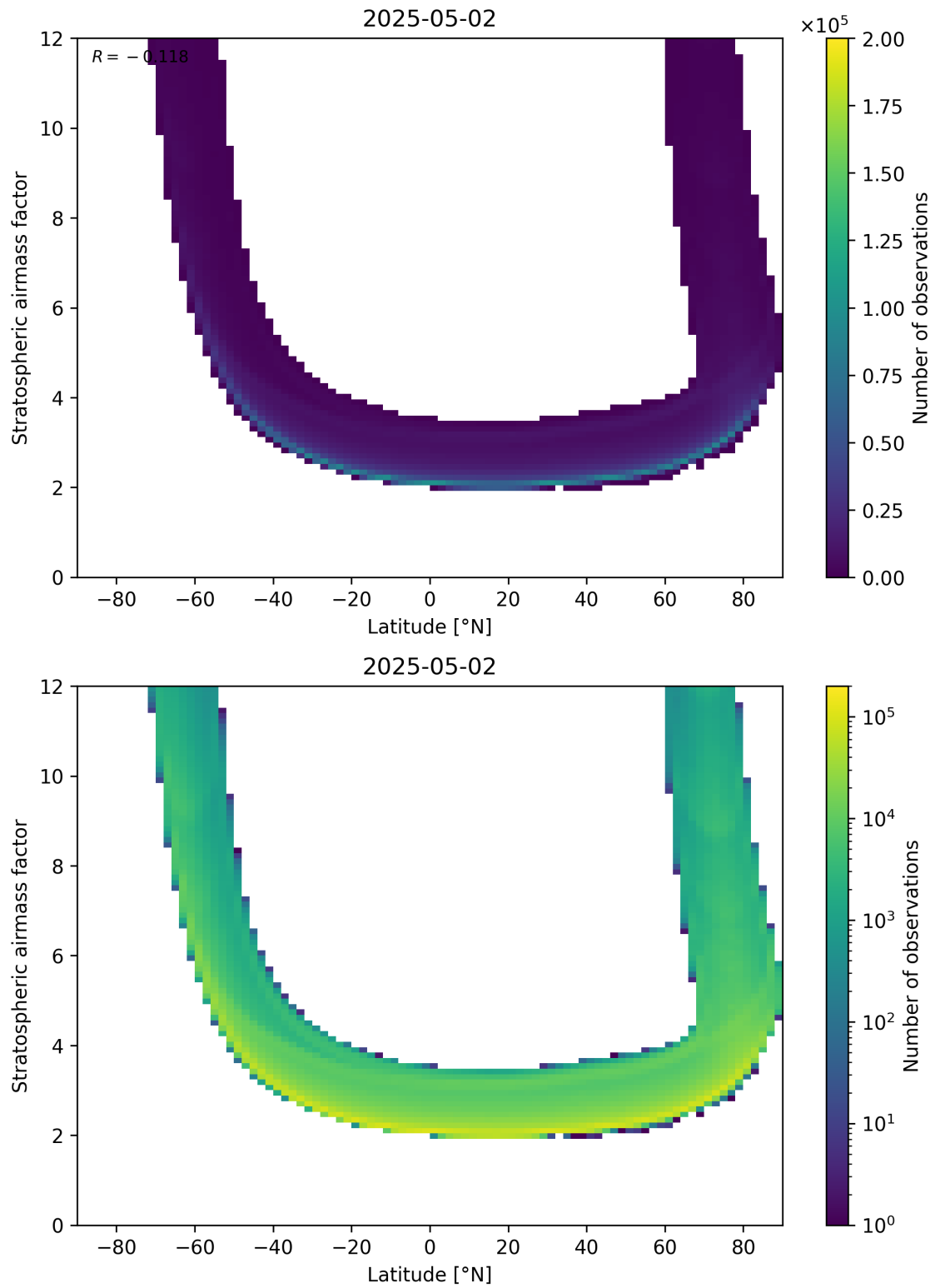
Figure 83: Scatter density plot of “Latitude” against “Stratospheric air mass factor” for 2025-05-02 to 2025-05-02.
