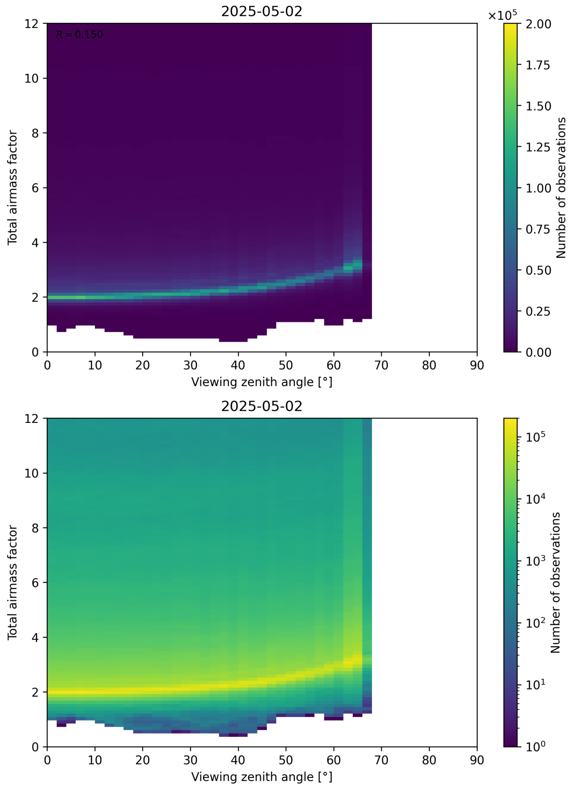
Figure 160: Scatter density plot of “Viewing zenith angle” against “Total airmass factor” for 2025-05-02 to 2025-05-02.
