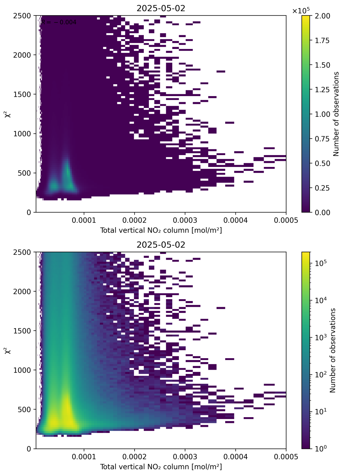
Figure 111: Scatter density plot of “Total vertical NO 2 column” against “ \chi^2 ” for 2025-05-02 to 2025-05-02.
