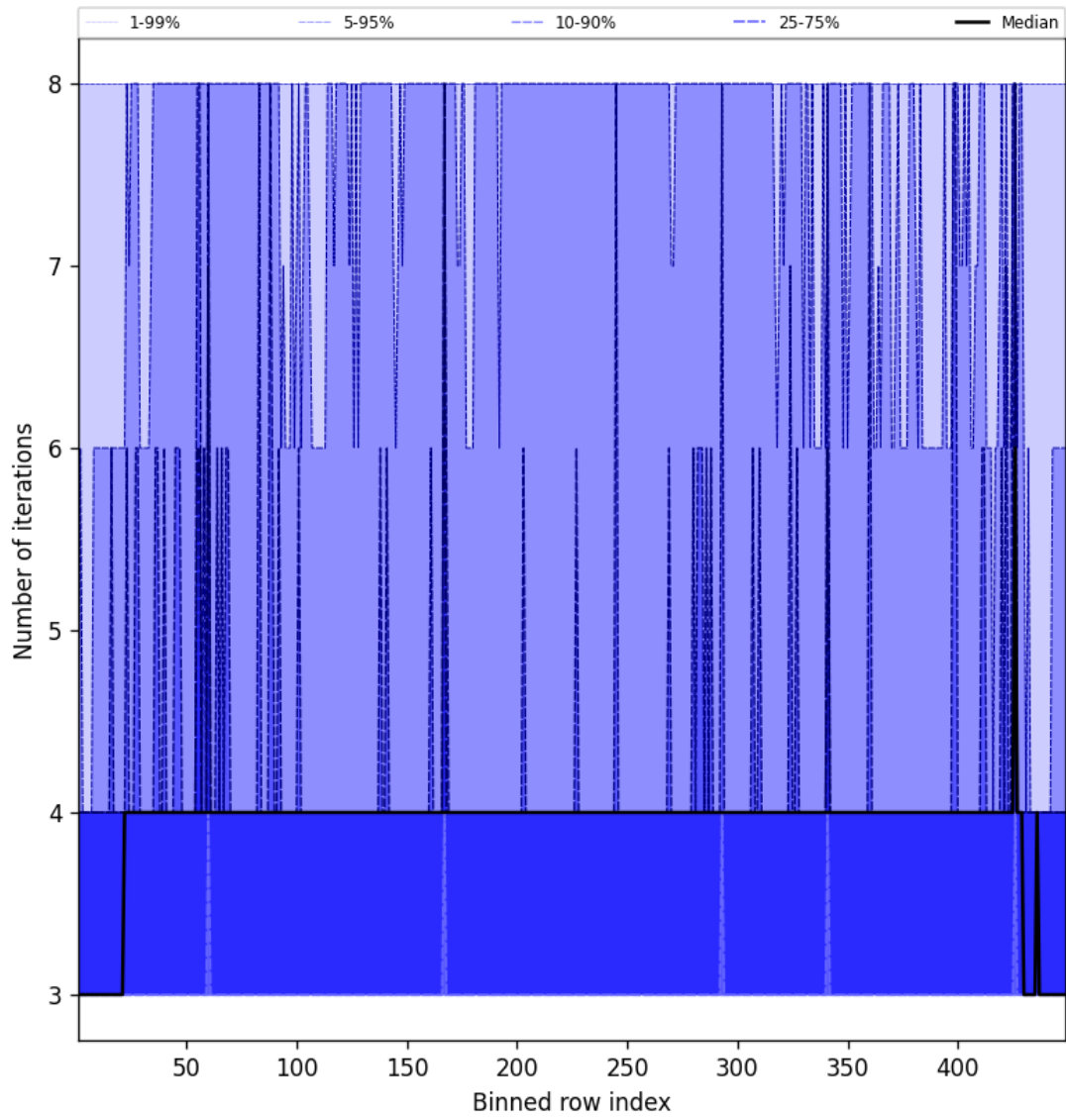
Figure 51: Along track statistics of “Number of iterations” for 2025-05-02 to 2025-05-02
