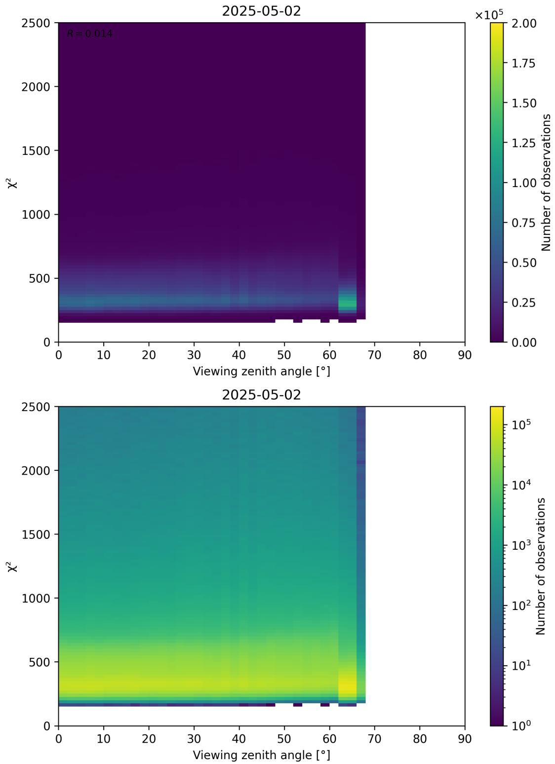
Figure 162: Scatter density plot of “Viewing zenith angle” against “ \chi^2 ” for 2025-05-02 to 2025-05-02.
