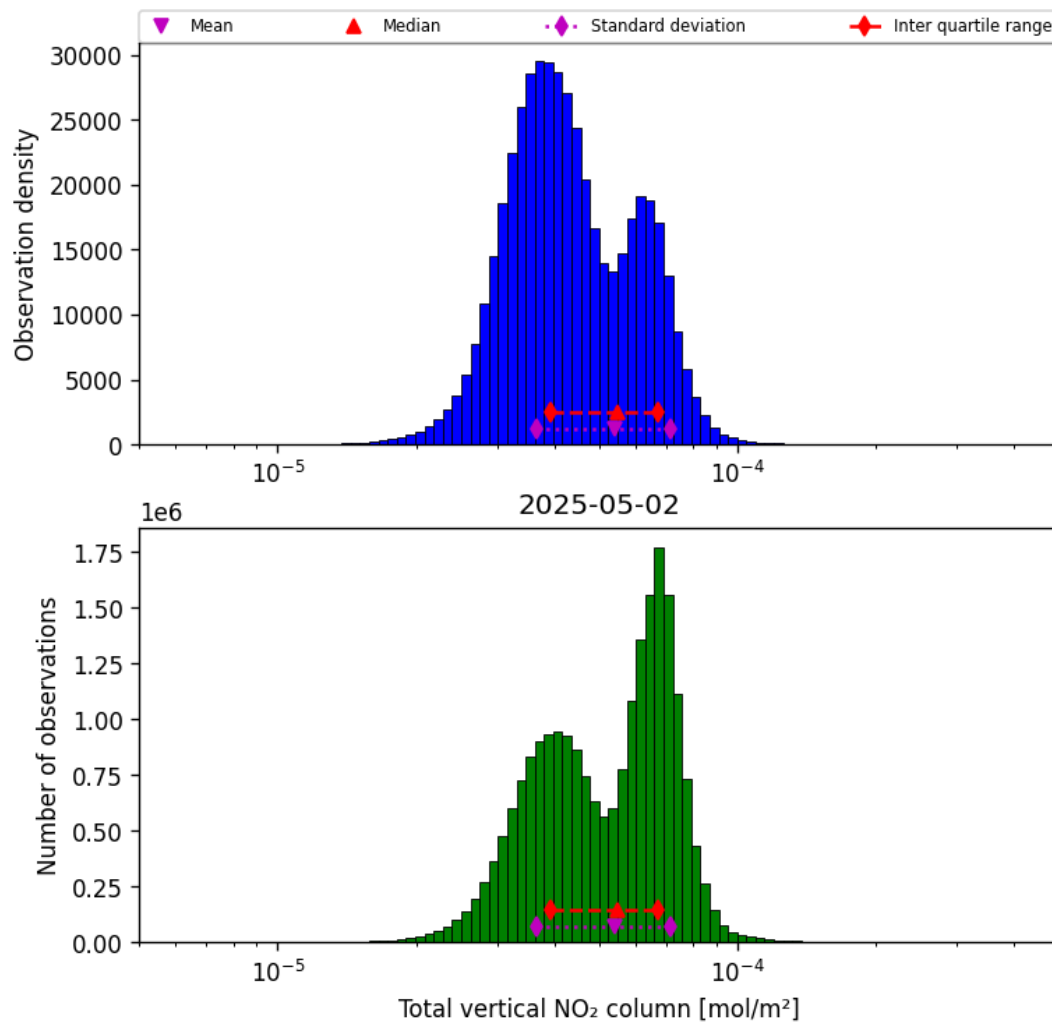
Figure 38: Histogram of "Total vertical NO 2 column" for 2025-05-02 to 2025-05-02
