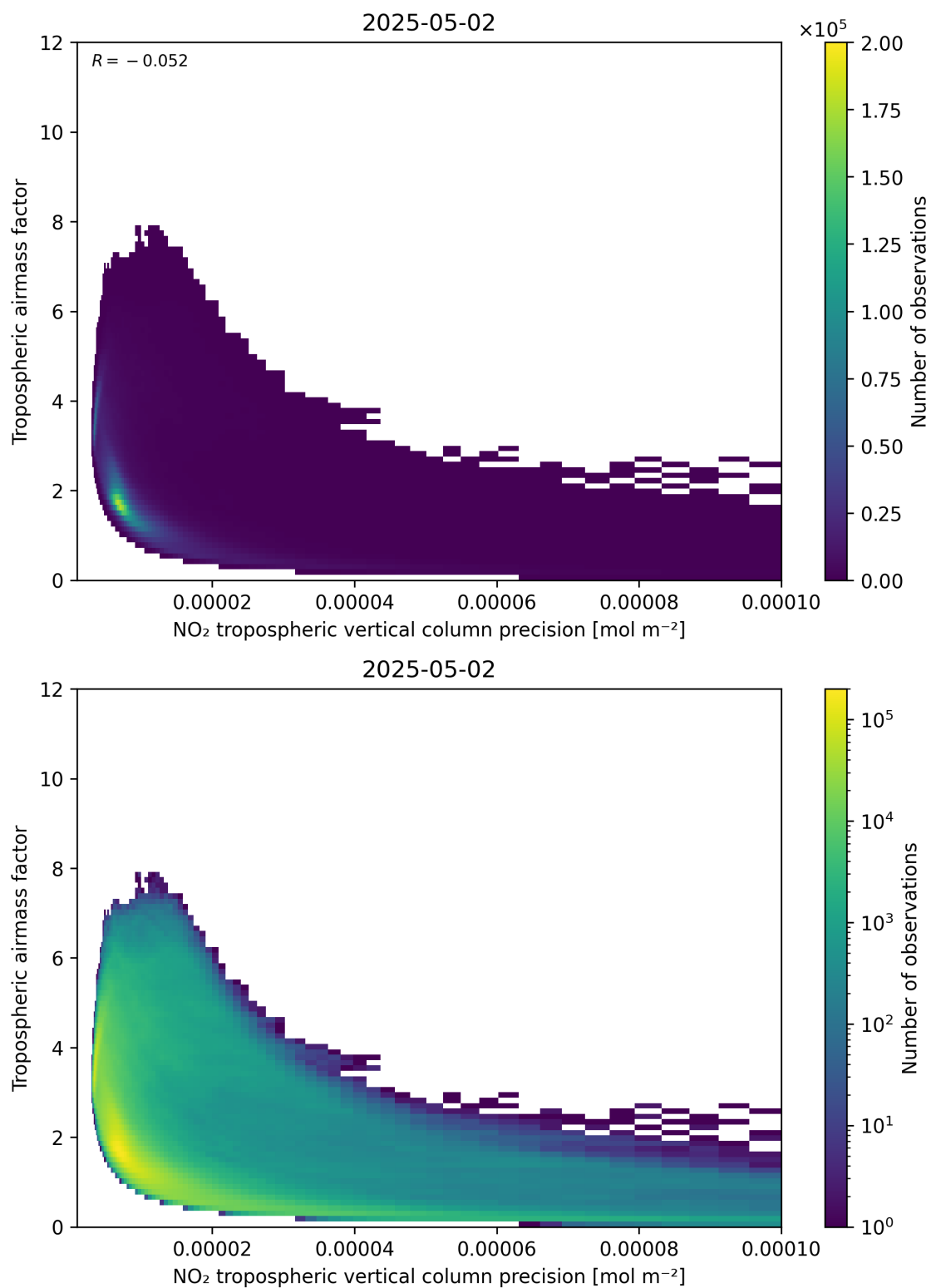
Figure 133: Scatter density plot of “NO 2 tropospheric vertical column precision” against “Tropospheric airmass factor” for 2025-05-02 to 2025-05-02.
