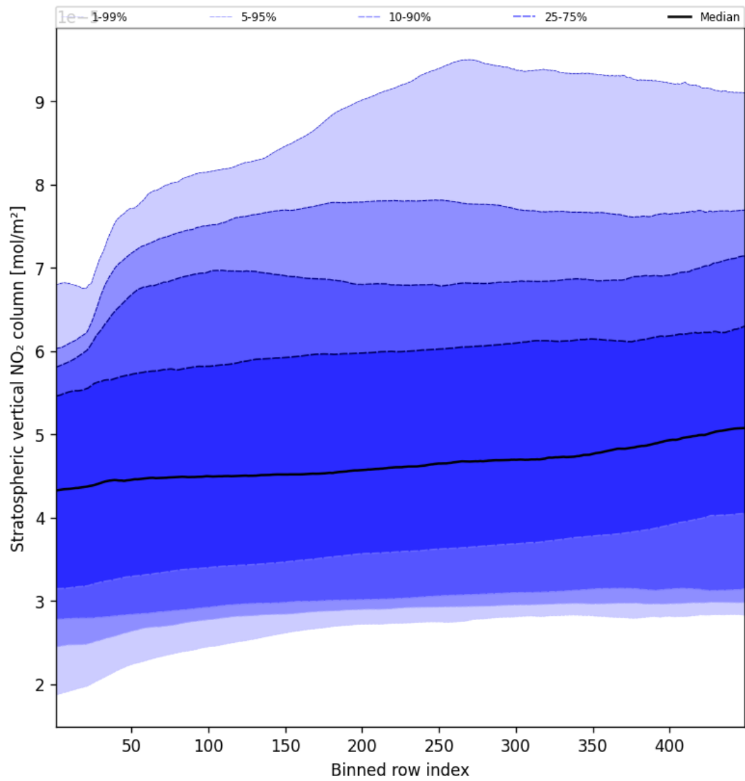
Figure 53: Along track statistics of “Stratospheric vertical NO 2 column” for 2025-05-02 to 2025-05-02
