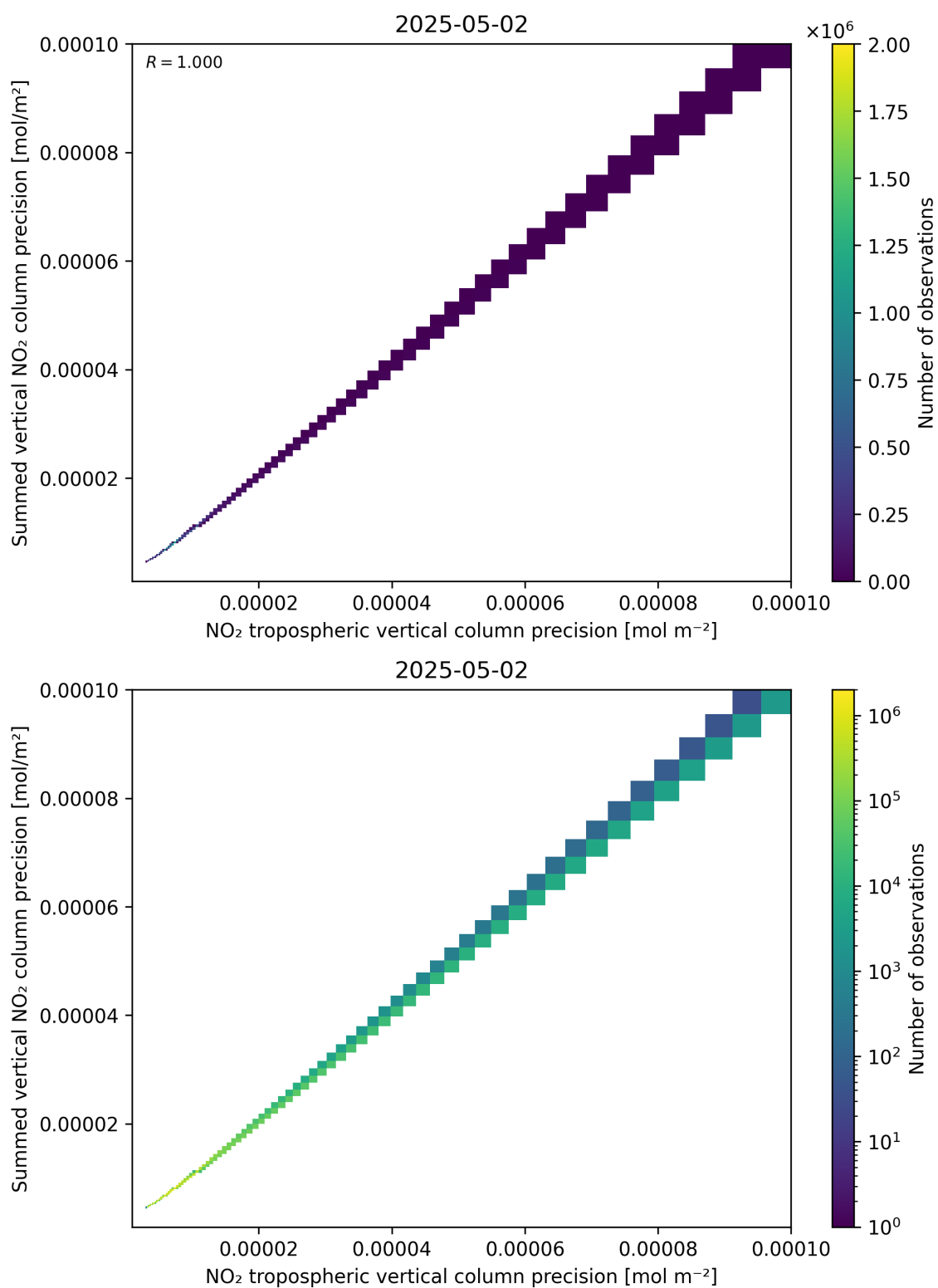
Figure 137: Scatter density plot of “NO 2 tropospheric vertical column precision” against “Summed vertical NO 2 column precision” for 2025-05-02 to 2025-05-02.
