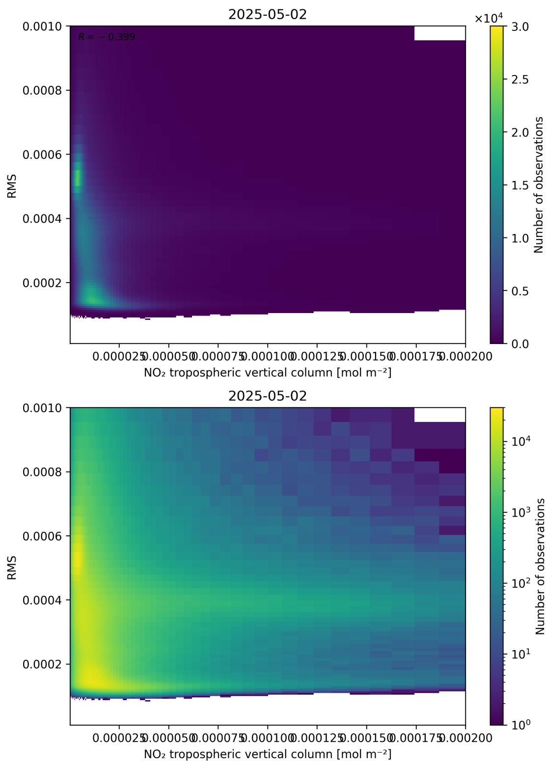
Figure 142: Scatter density plot of “NO 2 tropospheric vertical column” against “RMS” for 2025-05-02 to 2025-05-02.
