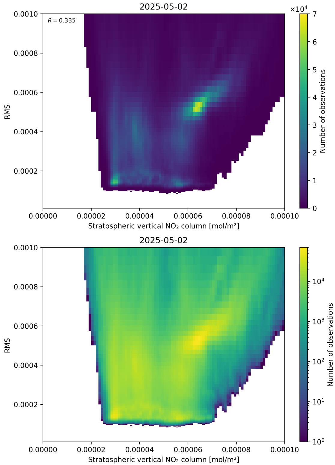
Figure 102: Scatter density plot of “Stratospheric vertical NO 2 column” against “RMS” for 2025-05-02 to 2025-05-02.
