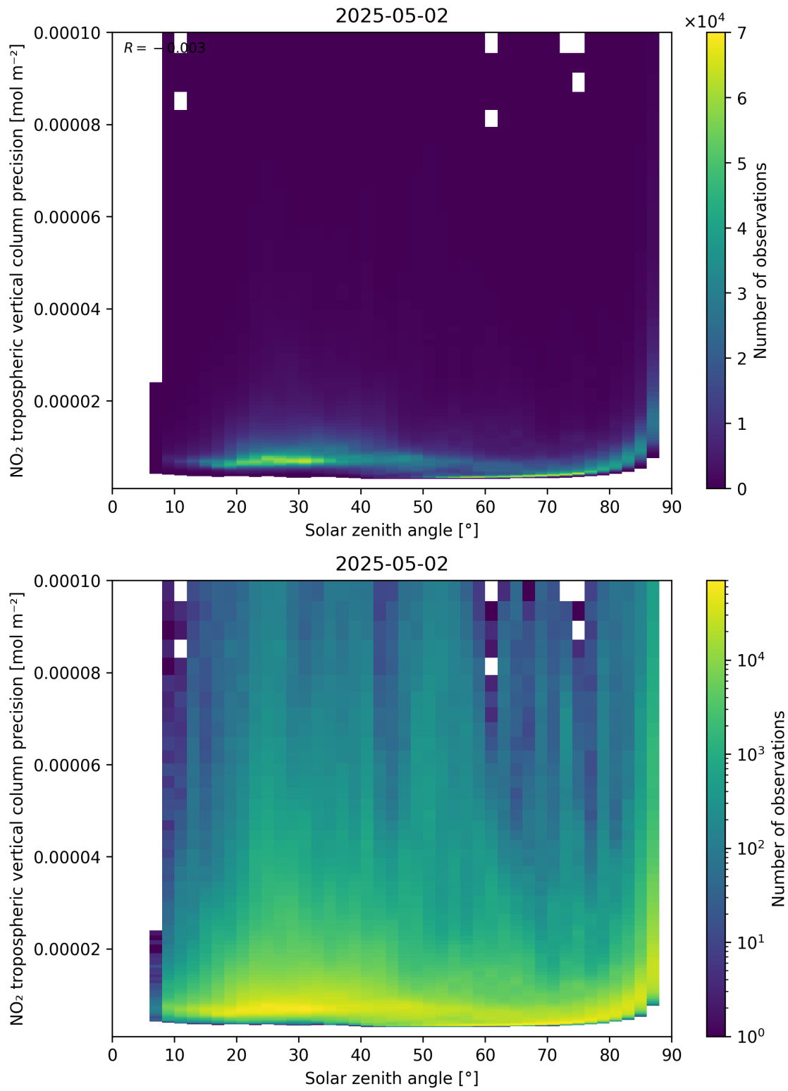
Figure 156: Scatter density plot of “Solar zenith angle” against “NO 2 tropospheric vertical column precision” for 2025-05-02 to 2025-05-02.
