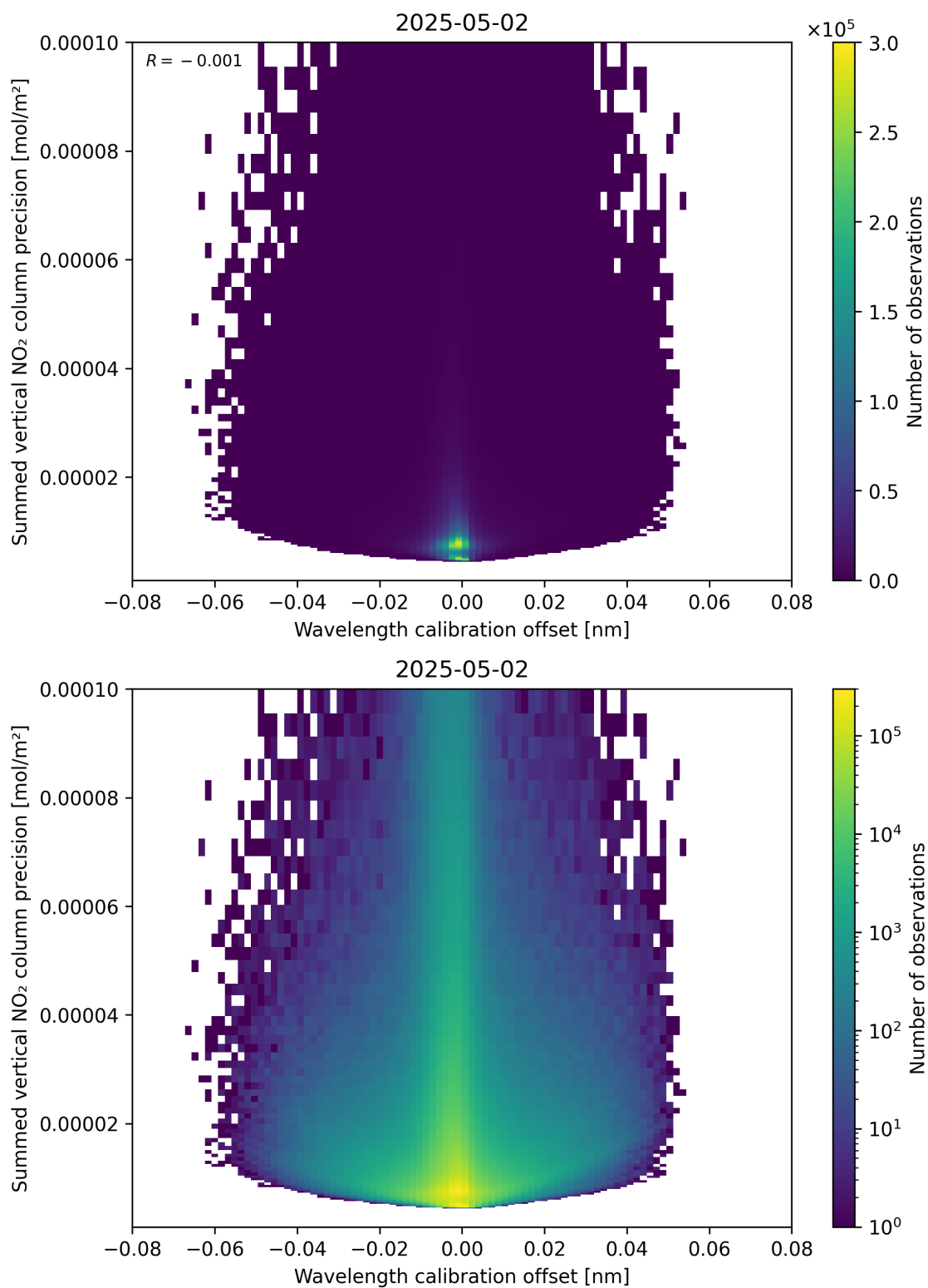
Figure 178: Scatter density plot of “Wavelength calibration offset” against “Summed vertical NO 2 column precision” for 2025-05-02 to 2025-05-02.
