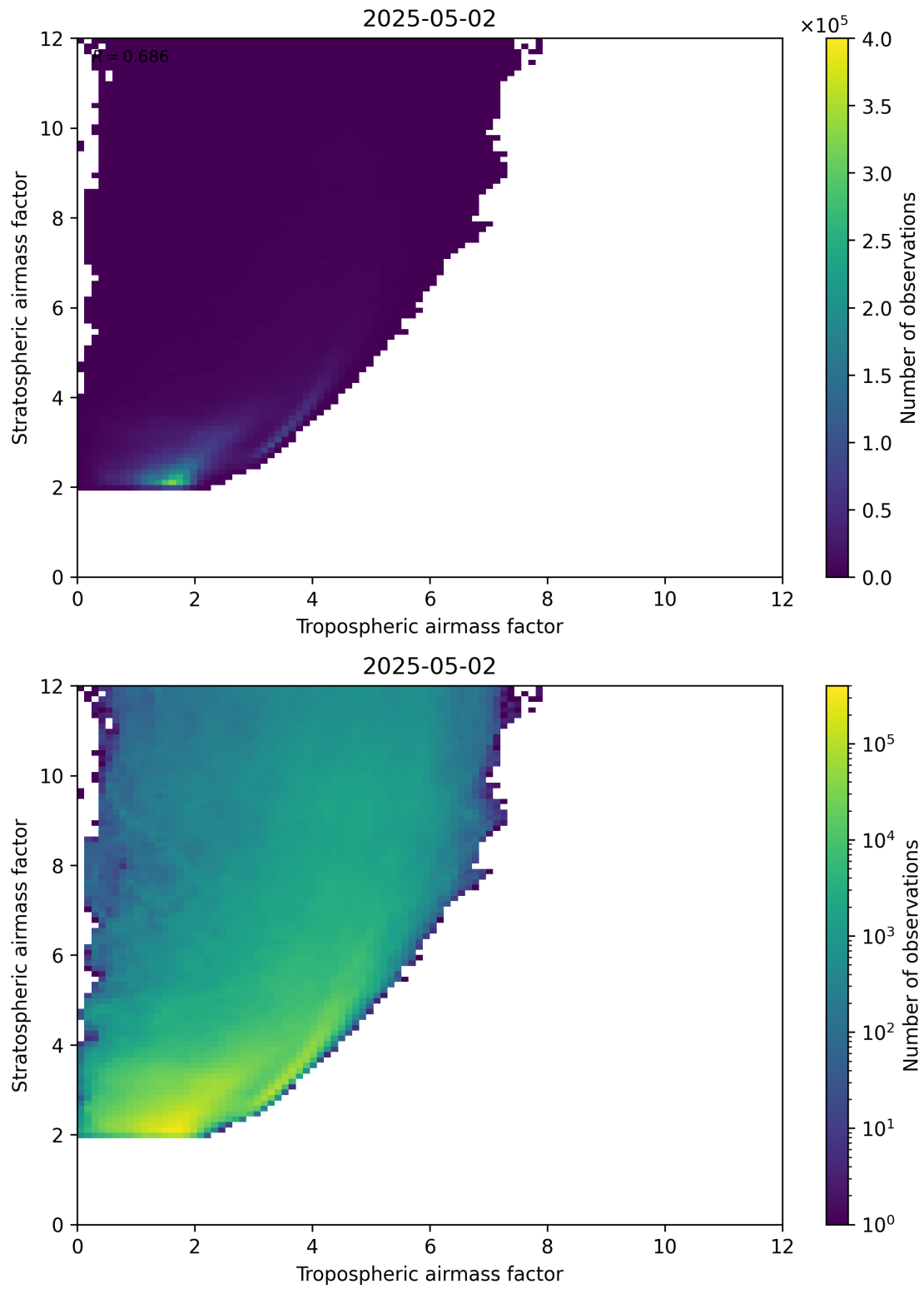
Figure 71: Scatter density plot of “Tropospheric airmass factor” against “Stratospheric airmass factor” for 2025-05-02 to 2025-05-02.
