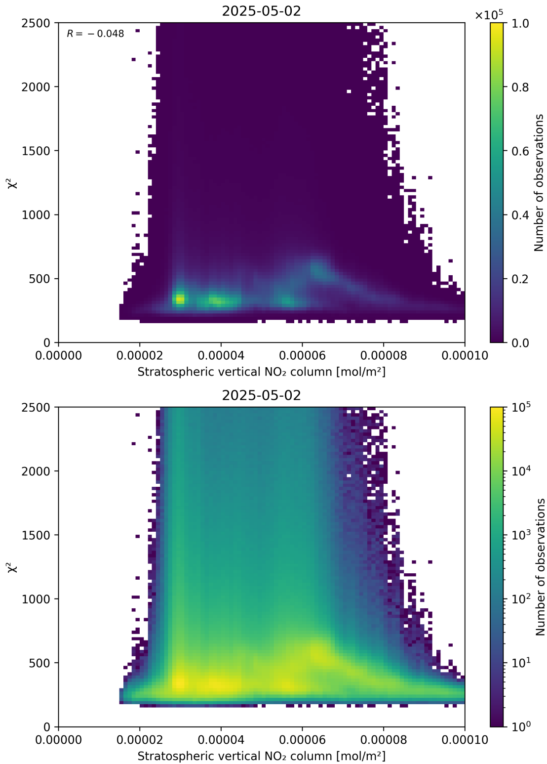
Figure 97: Scatter density plot of “Stratospheric vertical NO 2 column” against “ \chi^2 ” for 2025-05-02 to 2025-05-02.
