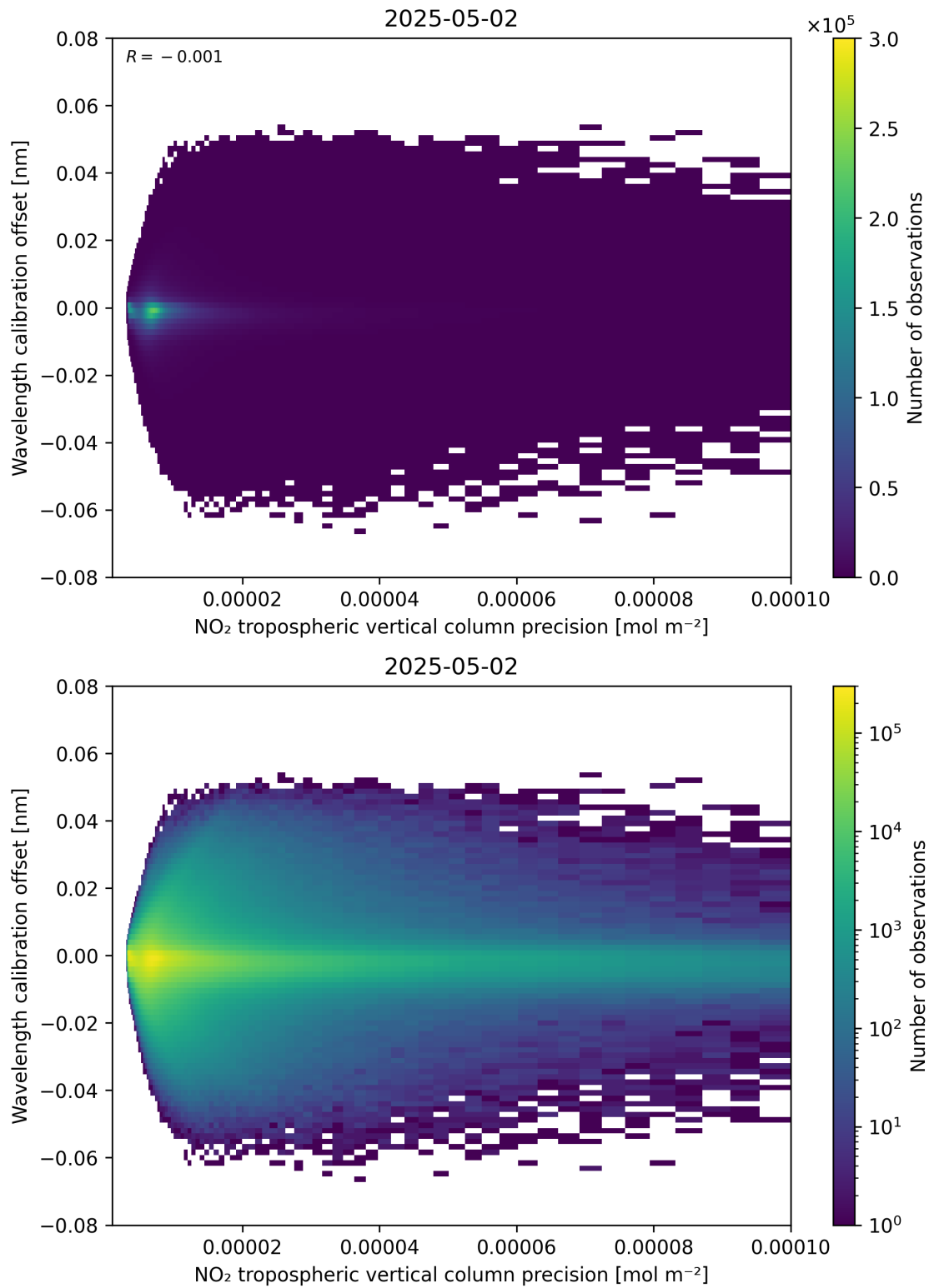
Figure 141: Scatter density plot of “NO 2 tropospheric vertical column precision” against “Wavelength calibration offset” for 2025-05-02 to 2025-05-02.
