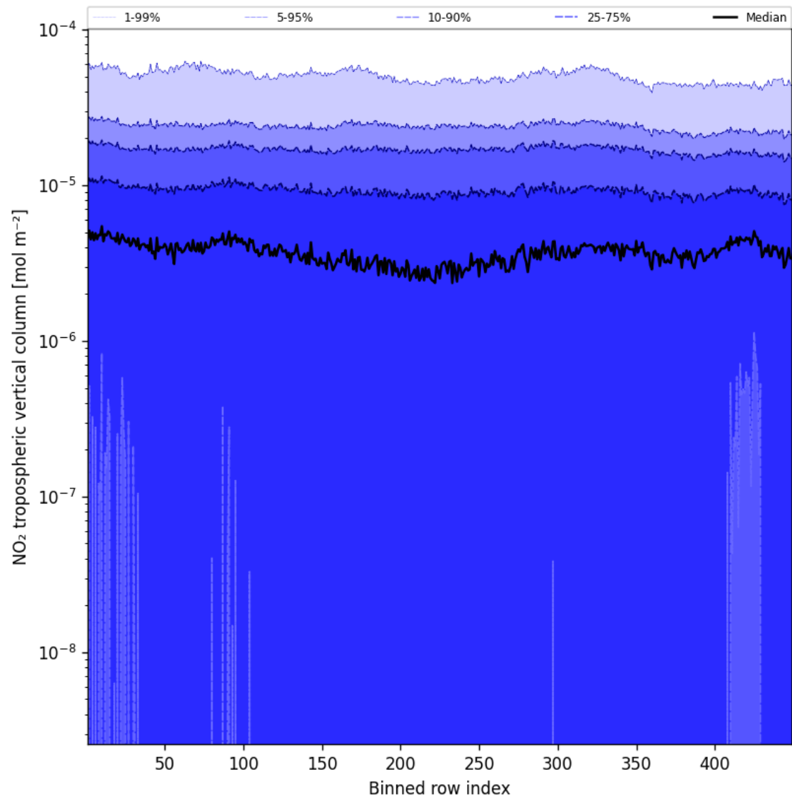
Figure 46: Along track statistics of "NO 2 tropospheric vertical column" for 2025-05-02 to 2025-05-02
