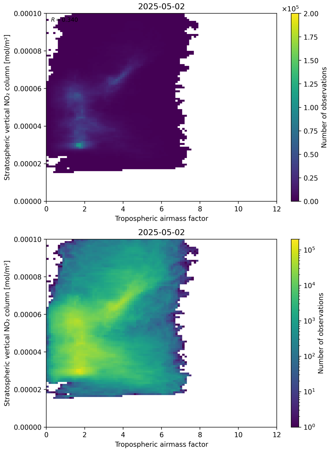
Figure 74: Scatter density plot of “Tropospheric air mass factor” against “Stratospheric vertical NO 2 column” for 2025-05-02 to 2025-05-02.
