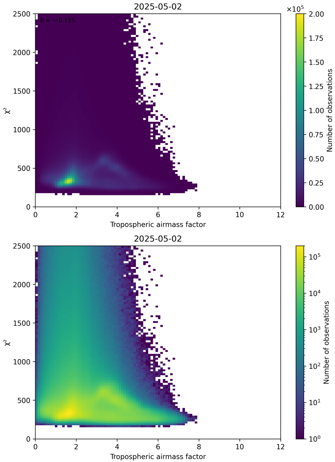
Figure 73: Scatter density plot of “Tropospheric airmass factor” against “ \chi^2 ” for 2025-05-02 to 2025-05-02.
