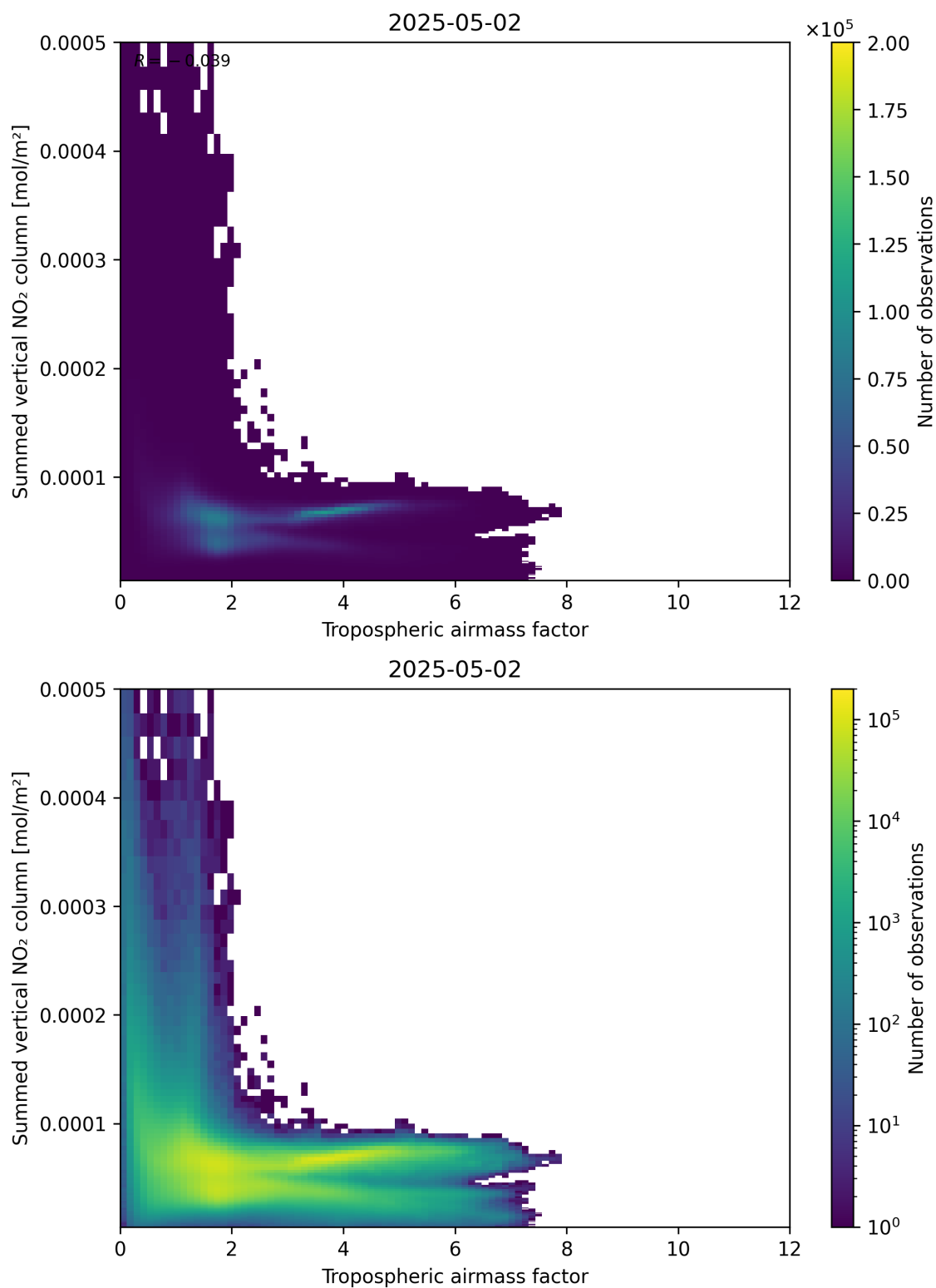
Figure 75: Scatter density plot of “Tropospheric airmass factor” against “Summed vertical NO 2 column” for 2025-05-02 to 2025-05-02.
