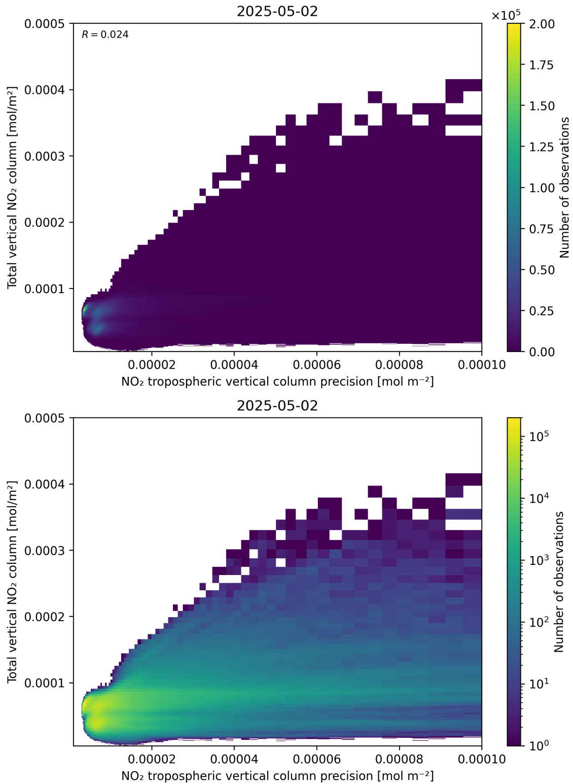
Figure 138: Scatter density plot of “NO 2 tropospheric vertical column precision” against “Total vertical NO 2 column” for 2025-05-02 to 2025-05-02.
