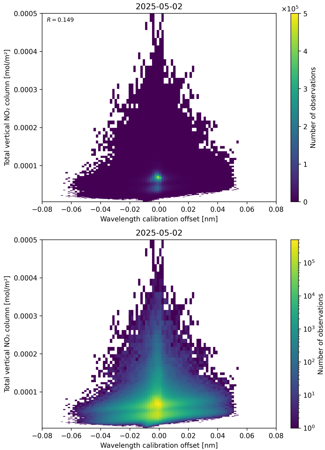
Figure 179: Scatter density plot of “Wavelength calibration offset” against “Total vertical NO 2 column” for 2025-05-02 to 2025-05-02.
