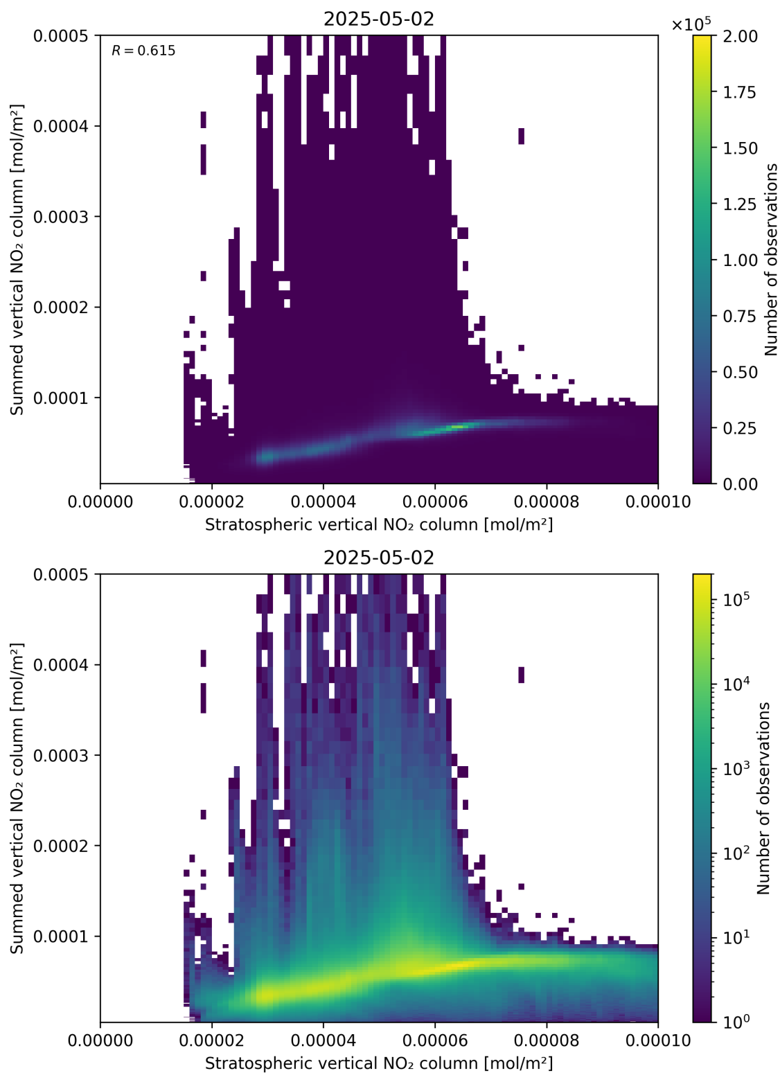
Figure 98: Scatter density plot of “Stratospheric vertical NO 2 column” against “Summed vertical NO 2 column” for 2025-05-02 to 2025-05-02.
