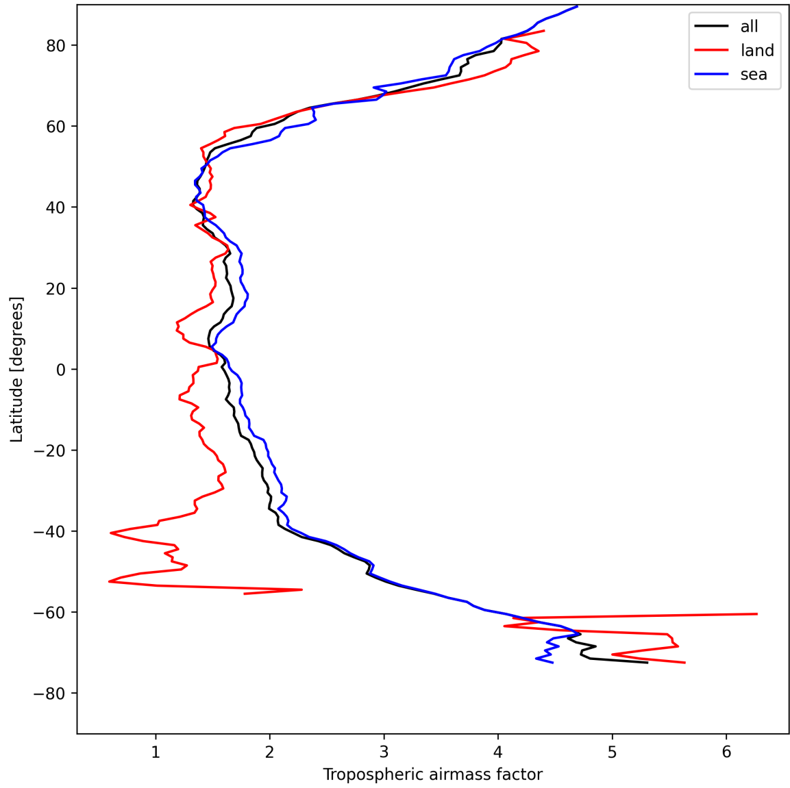
Figure 14: Zonal average of “Tropospheric airmass factor” for 2025-05-02 to 2025-05-02.
