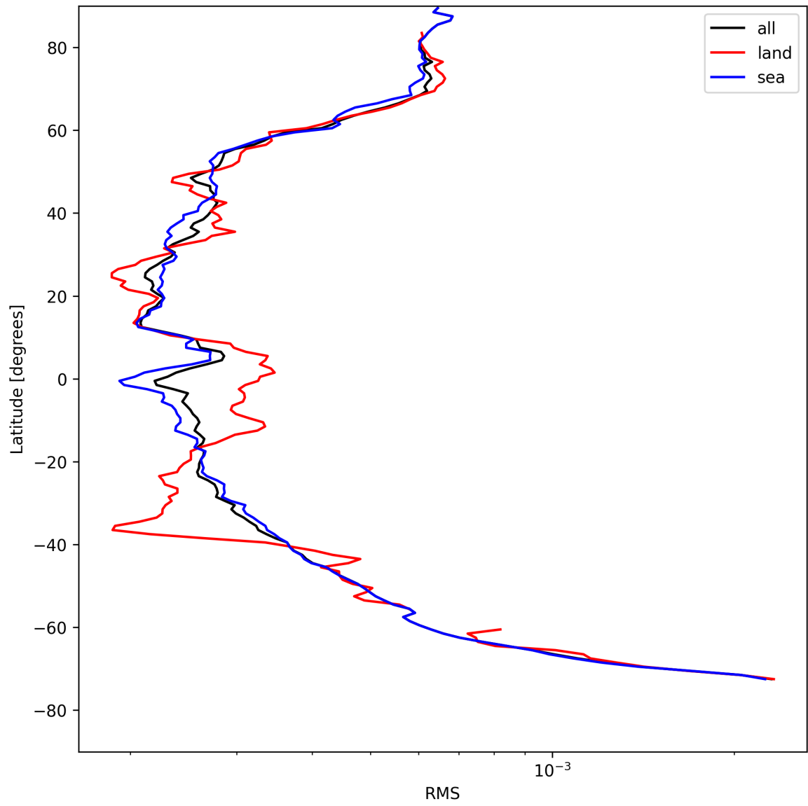
Figure 26: Zonal average of “RMS” for 2025-05-02 to 2025-05-02.
