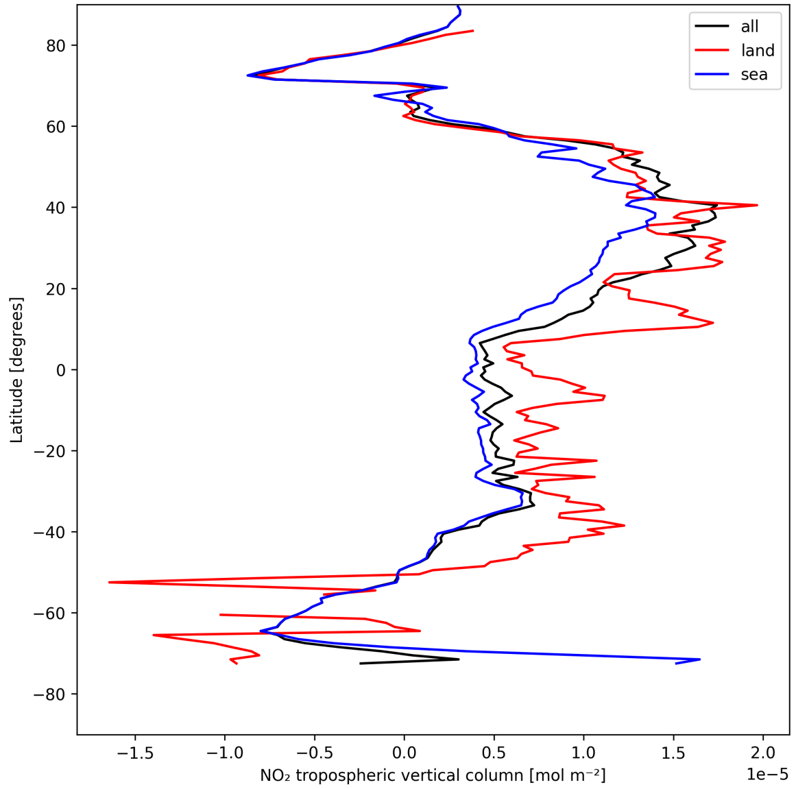
Figure 12: Zonal average of “NO 2 tropospheric vertical column” for 2025-05-02 to 2025-05-02.
