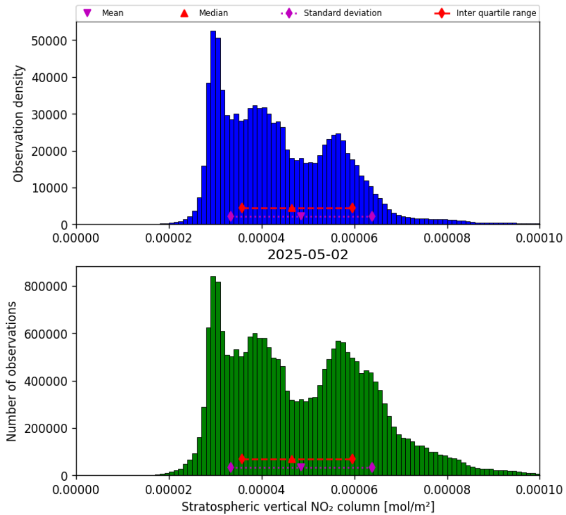
Figure 36: Histogram of “Stratospheric vertical NO 2 column” for 2025-05-02 to 2025-05-02
