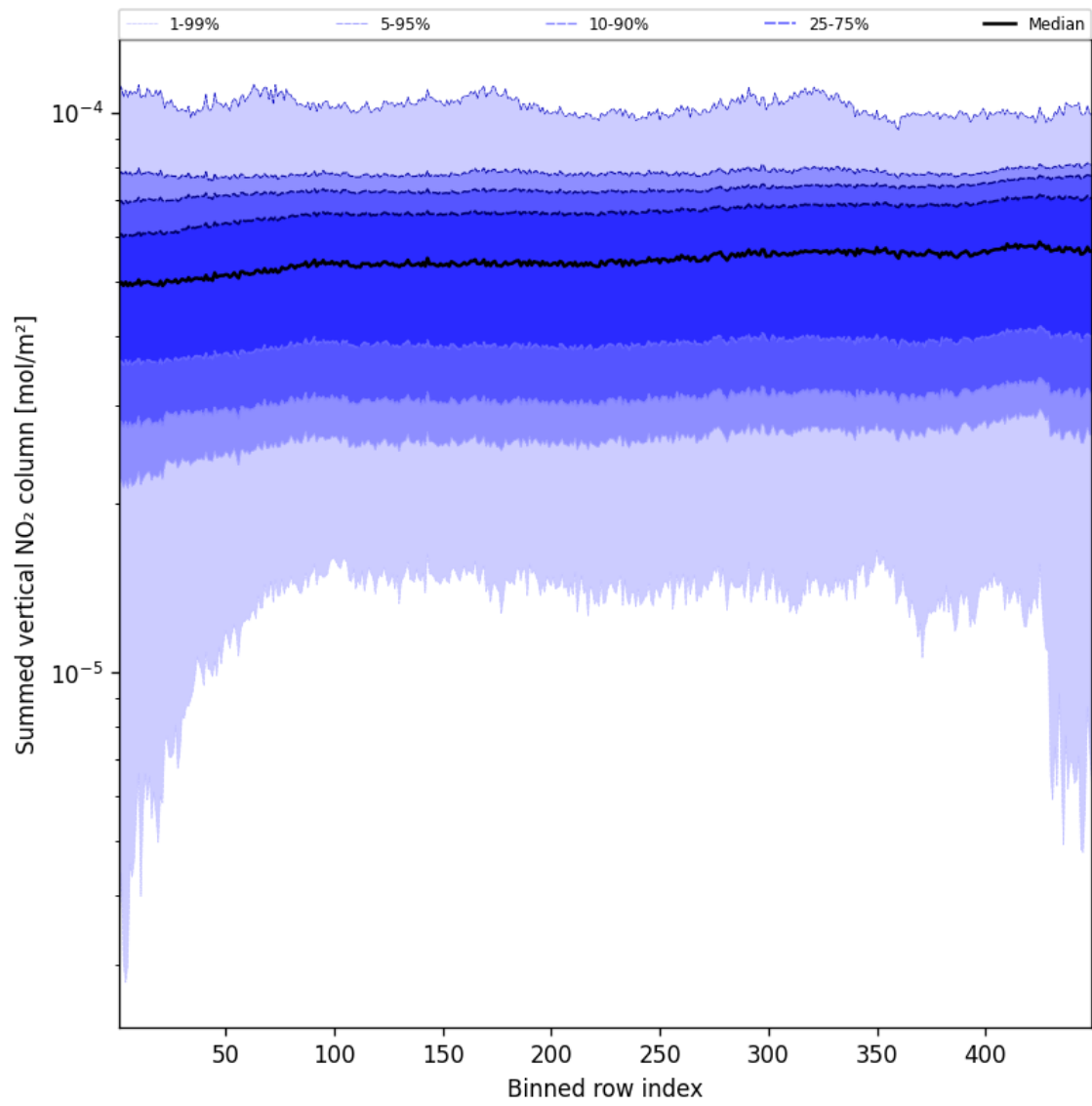
Figure 57: Along track statistics of “Summed vertical NO 2 column” for 2025-05-02 to 2025-05-02
