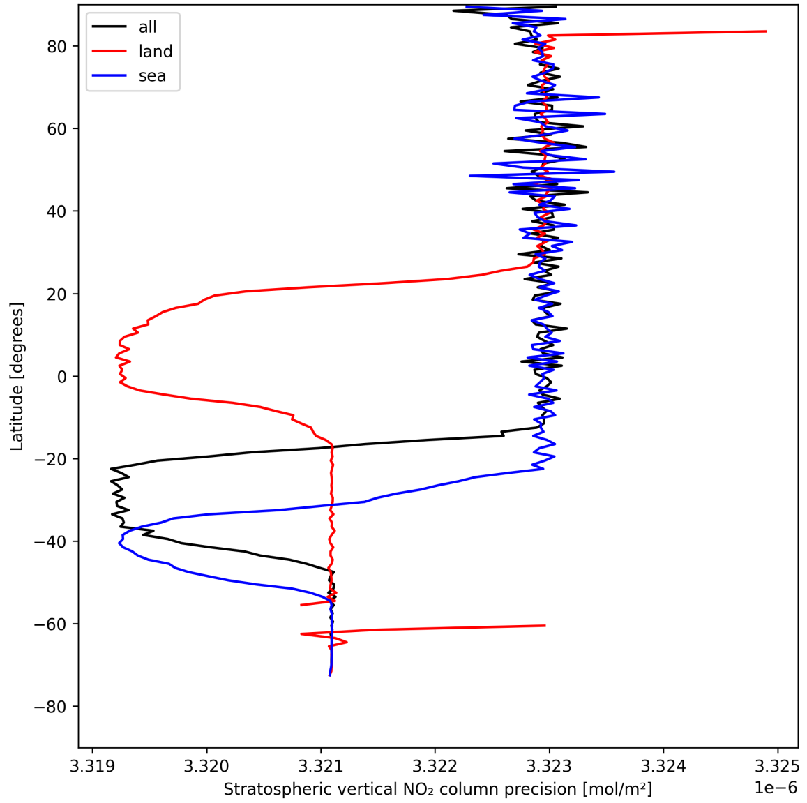
Figure 20: Zonal average of “Stratospheric vertical NO 2 column precision” for 2025-05-02 to 2025-05-02.
