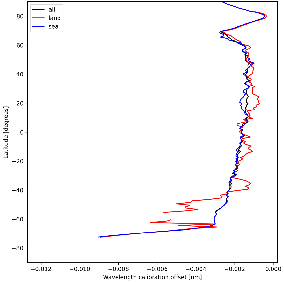
Figure 18: Zonal average of “Wavelength calibration offset” for 2025-05-02 to 2025-05-02.
