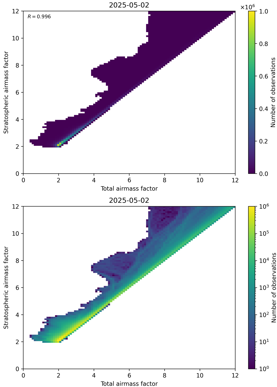
Figure 62: Scatter density plot of “Total airmass factor” against “Stratospheric airmass factor” for 2025-05-02 to 2025-05-02.
