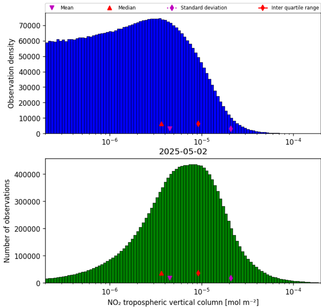
Figure 29: Histogram of “ \text{NO}_2 tropospheric vertical column” for 2025-05-02 to 2025-05-02
