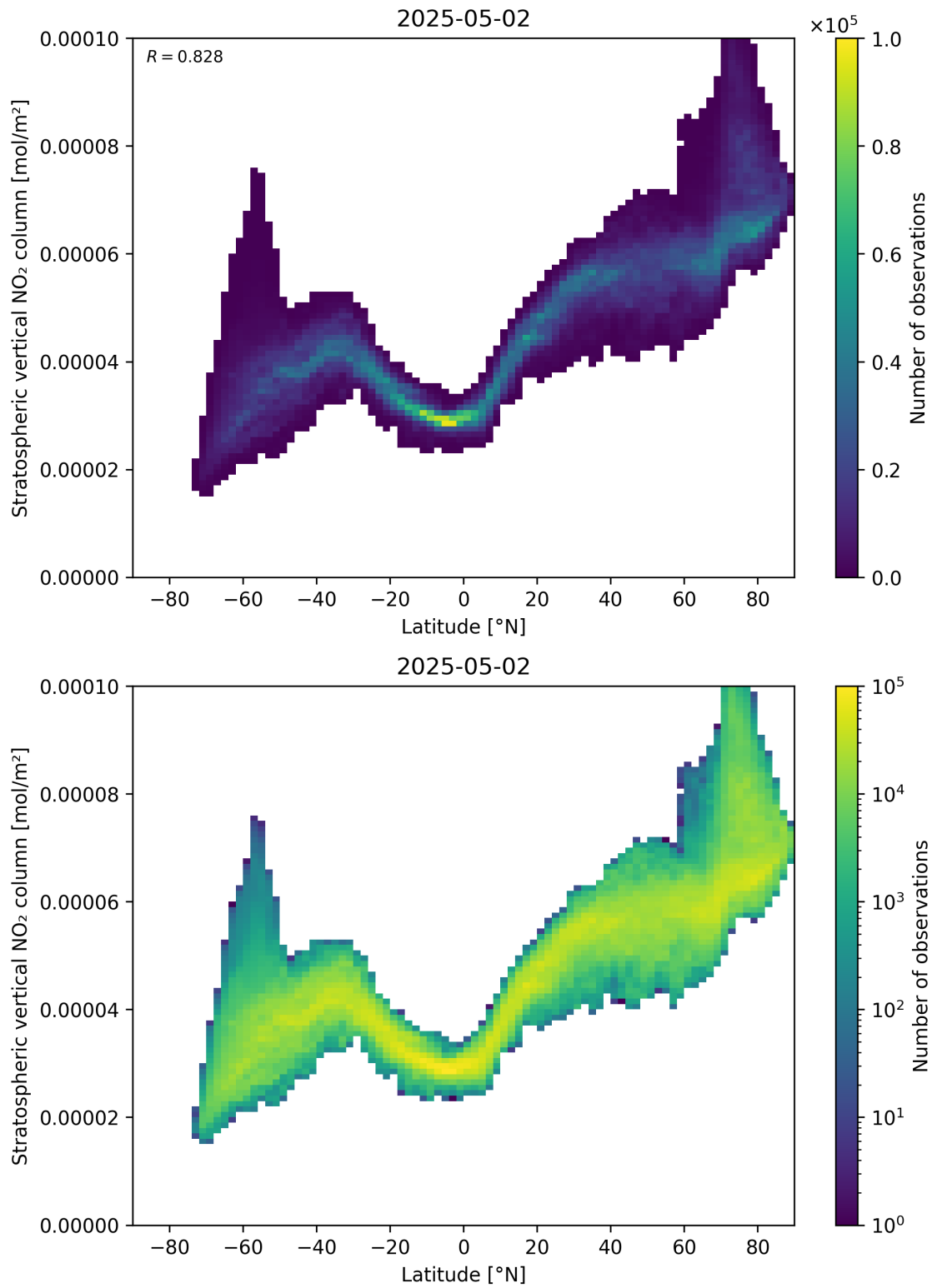
Figure 87: Scatter density plot of “Latitude” against “Stratospheric vertical NO 2 column” for 2025-05-02 to 2025-05-02.
