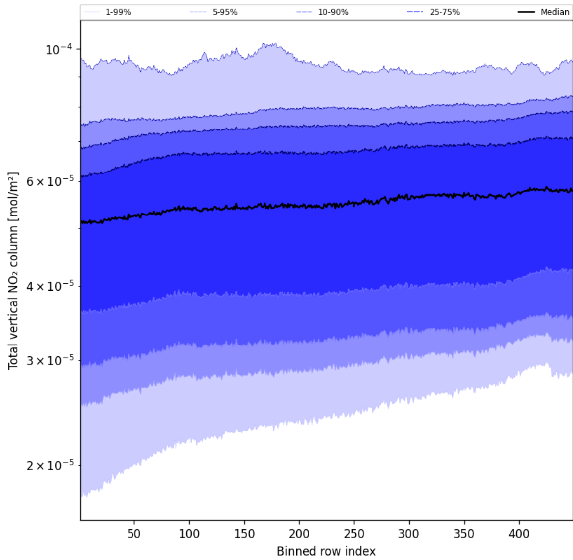
Figure 55: Along track statistics of “Total vertical NO 2 column” for 2025-05-02 to 2025-05-02
