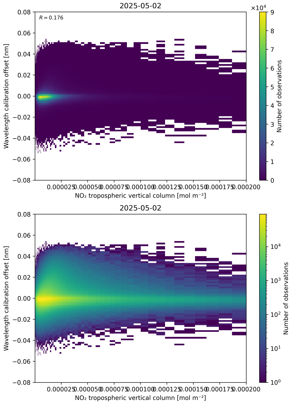
Figure 143: Scatter density plot of “NO 2 tropospheric vertical column” against “Wavelength calibration offset” for 2025-05-02 to 2025-05-02.
