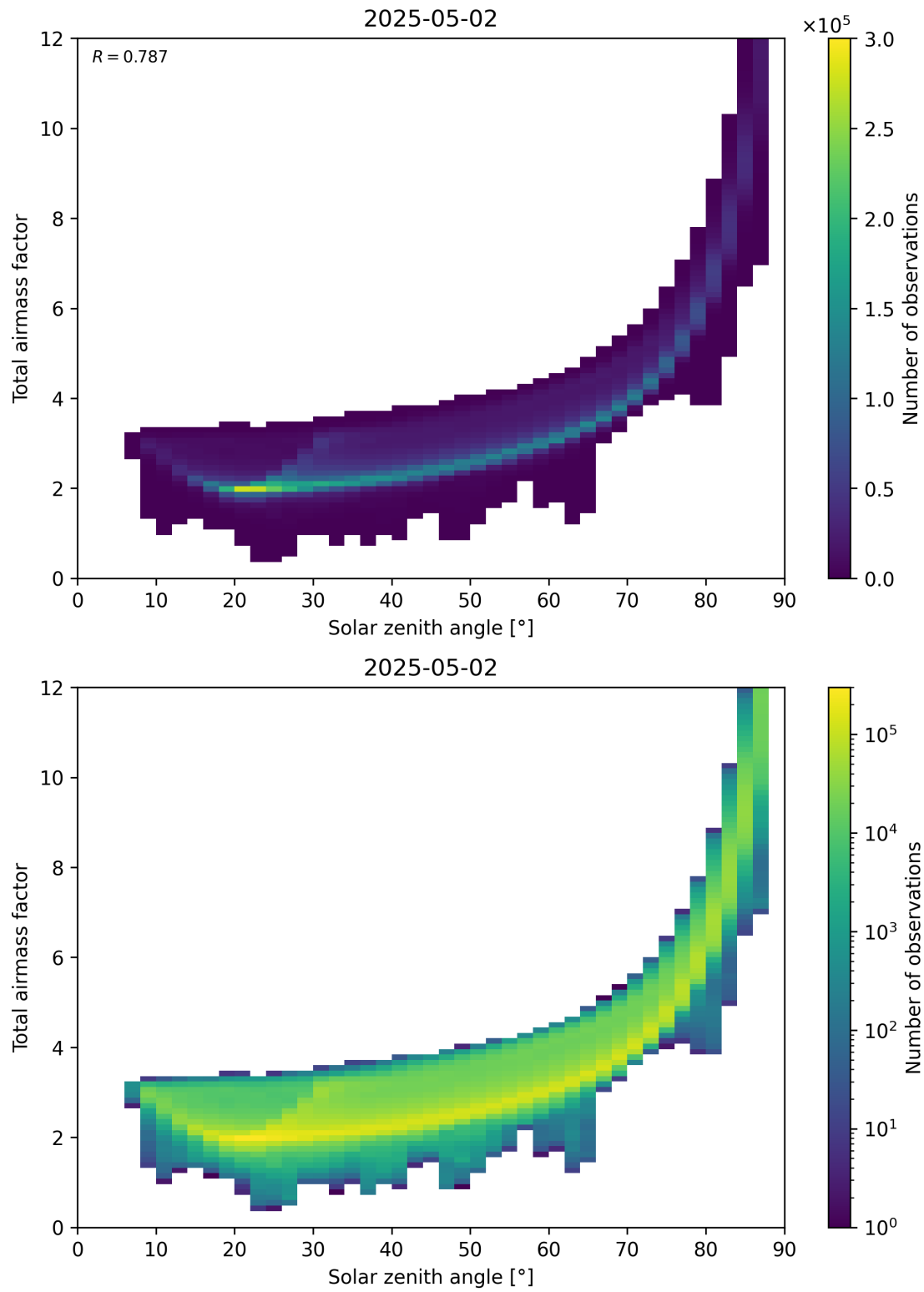
Figure 146: Scatter density plot of “Solar zenith angle” against “Total air mass factor” for 2025-05-02 to 2025-05-02.
