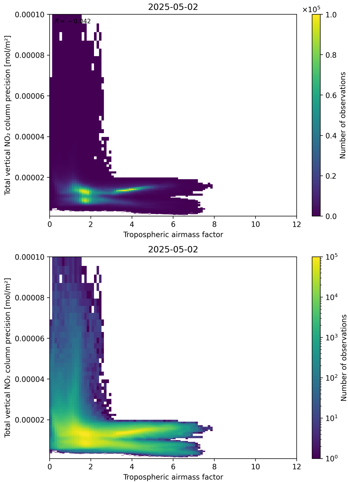
Figure 78: Scatter density plot of “Tropospheric air mass factor” against “Total vertical NO 2 column precision” for 2025-05-02 to 2025-05-02.
