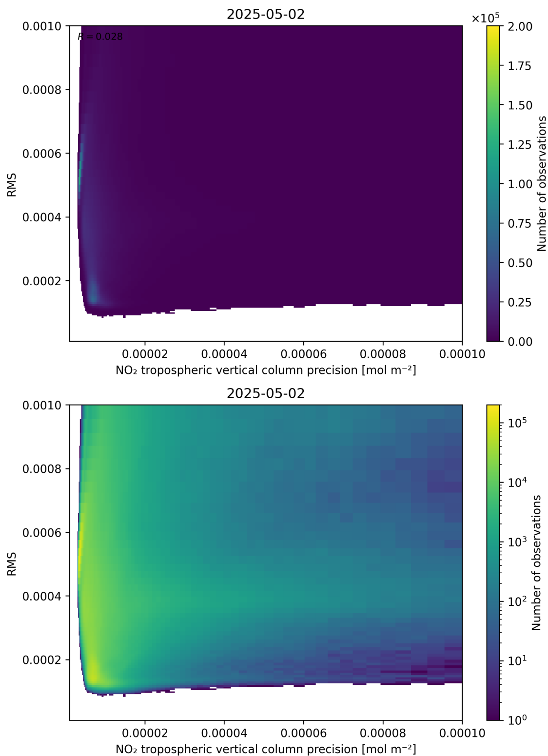
Figure 140: Scatter density plot of “NO 2 tropospheric vertical column precision” against “RMS” for 2025-05-02 to 2025-05-02.
