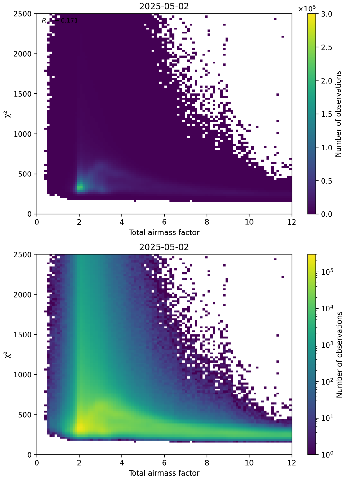
Figure 63: Scatter density plot of “Total airmass factor” against “ \chi^2 ” for 2025-05-02 to 2025-05-02.
