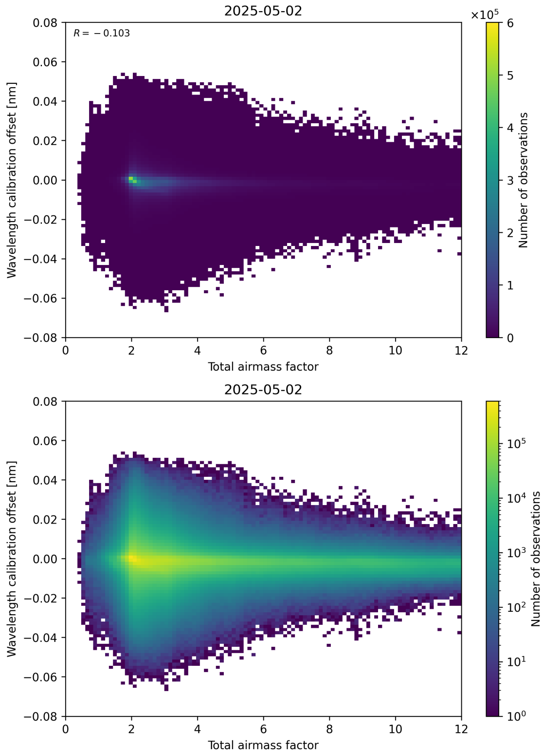
Figure 70: Scatter density plot of “Total airmass factor” against “Wavelength calibration offset” for 2025-05-02 to 2025-05-02.
