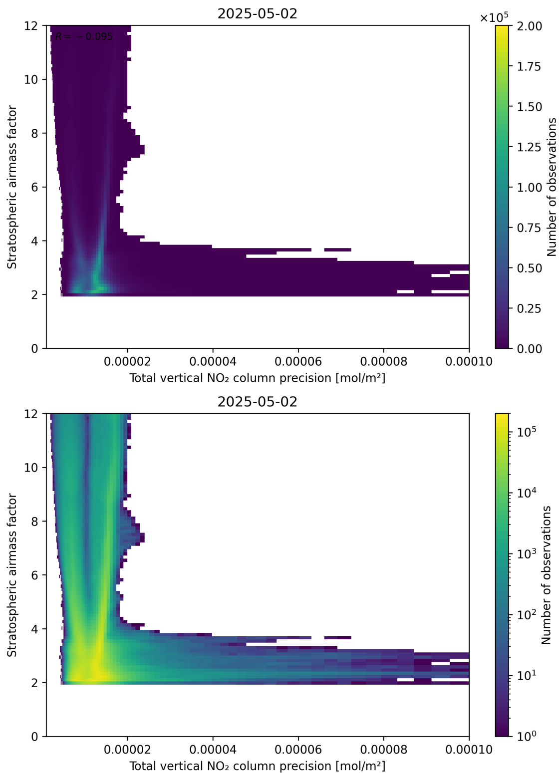
Figure 115: Scatter density plot of “Total vertical NO 2 column precision” against “Stratospheric air mass factor” for 2025-05-02 to 2025-05-02.
