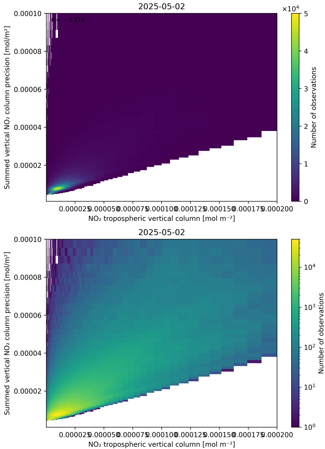
Figure 127: Scatter density plot of “NO 2 tropospheric vertical column” against “Summed vertical NO 2 column precision” for 2025-05-02 to 2025-05-02.
