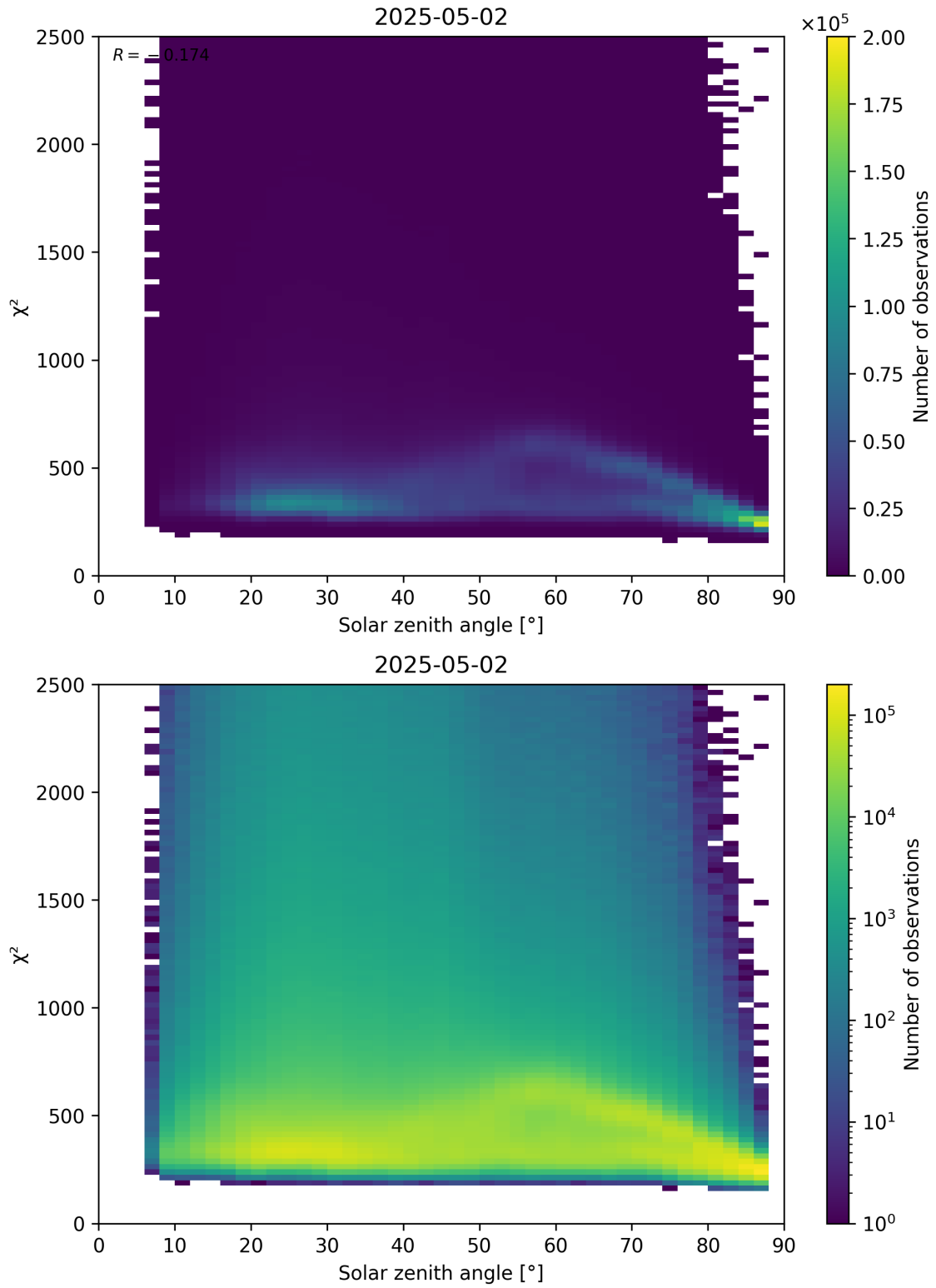
Figure 148: Scatter density plot of “Solar zenith angle” against “ \chi^2 ” for 2025-05-02 to 2025-05-02.
