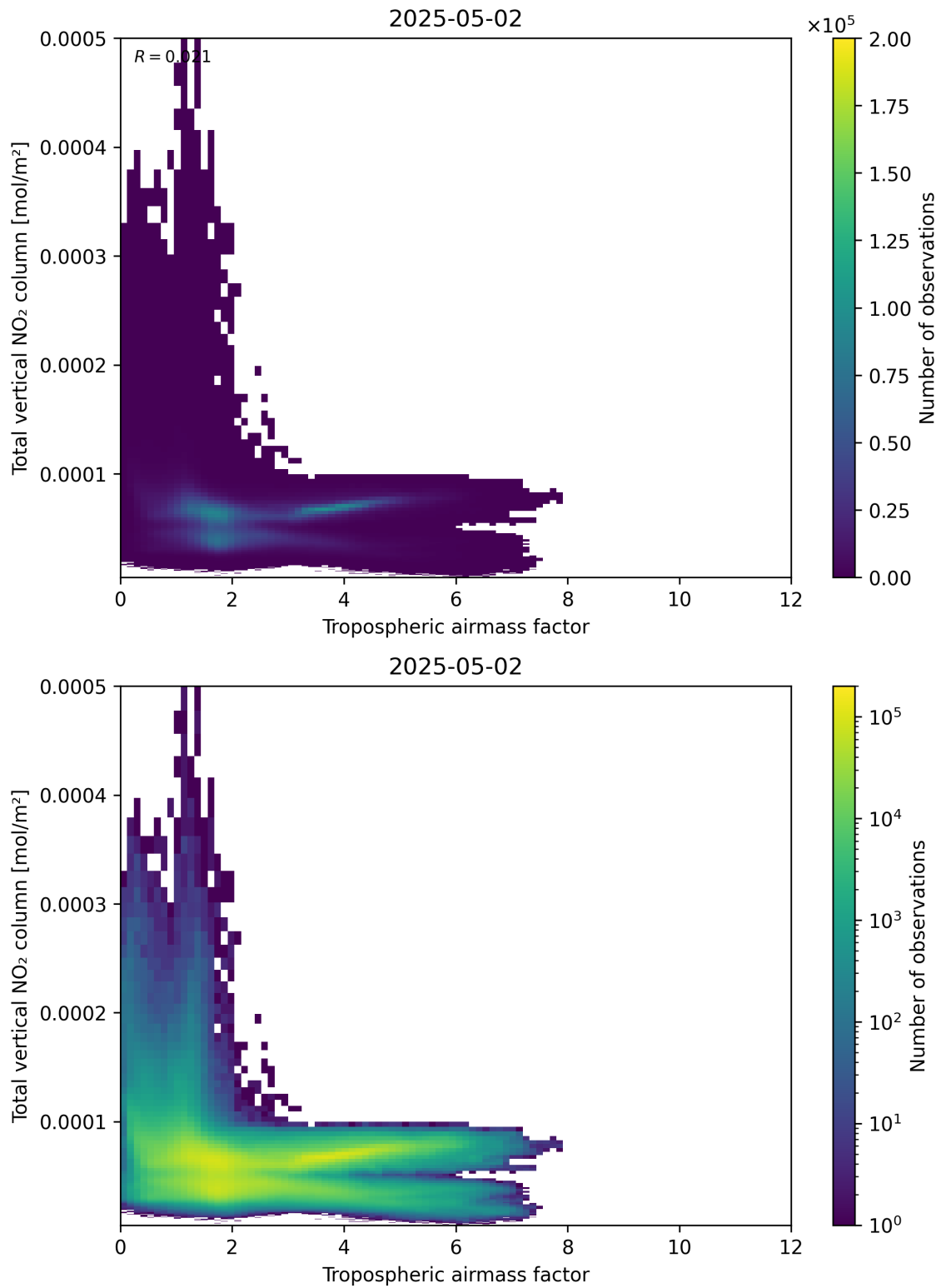
Figure 77: Scatter density plot of “Tropospheric airmass factor” against “Total vertical NO 2 column” for 2025-05-02 to 2025-05-02.
