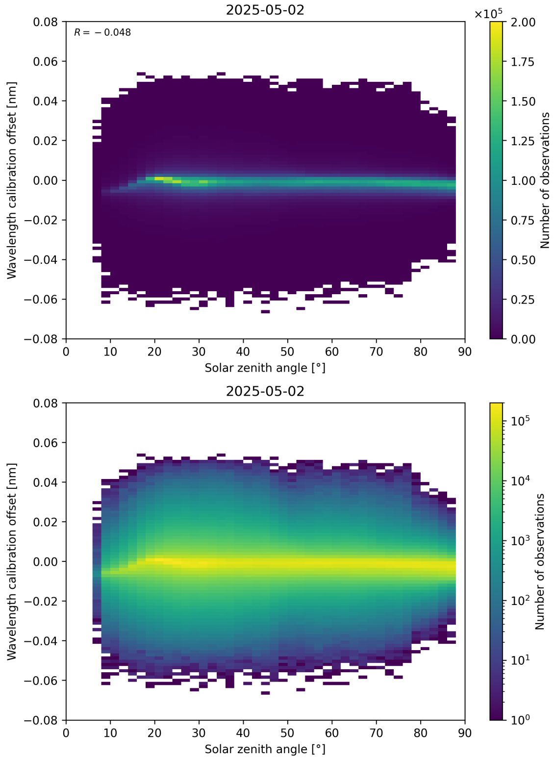
Figure 158: Scatter density plot of “Solar zenith angle” against “Wavelength calibration offset” for 2025-05-02 to 2025-05-02.
