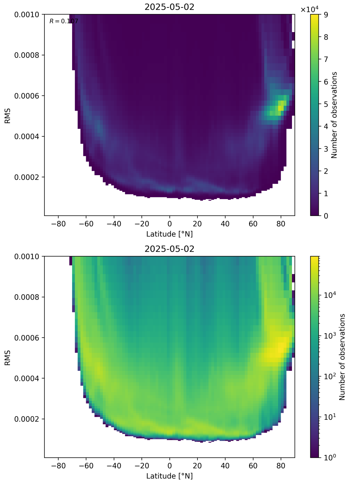
Figure 94: Scatter density plot of “Latitude” against “RMS” for 2025-05-02 to 2025-05-02.
