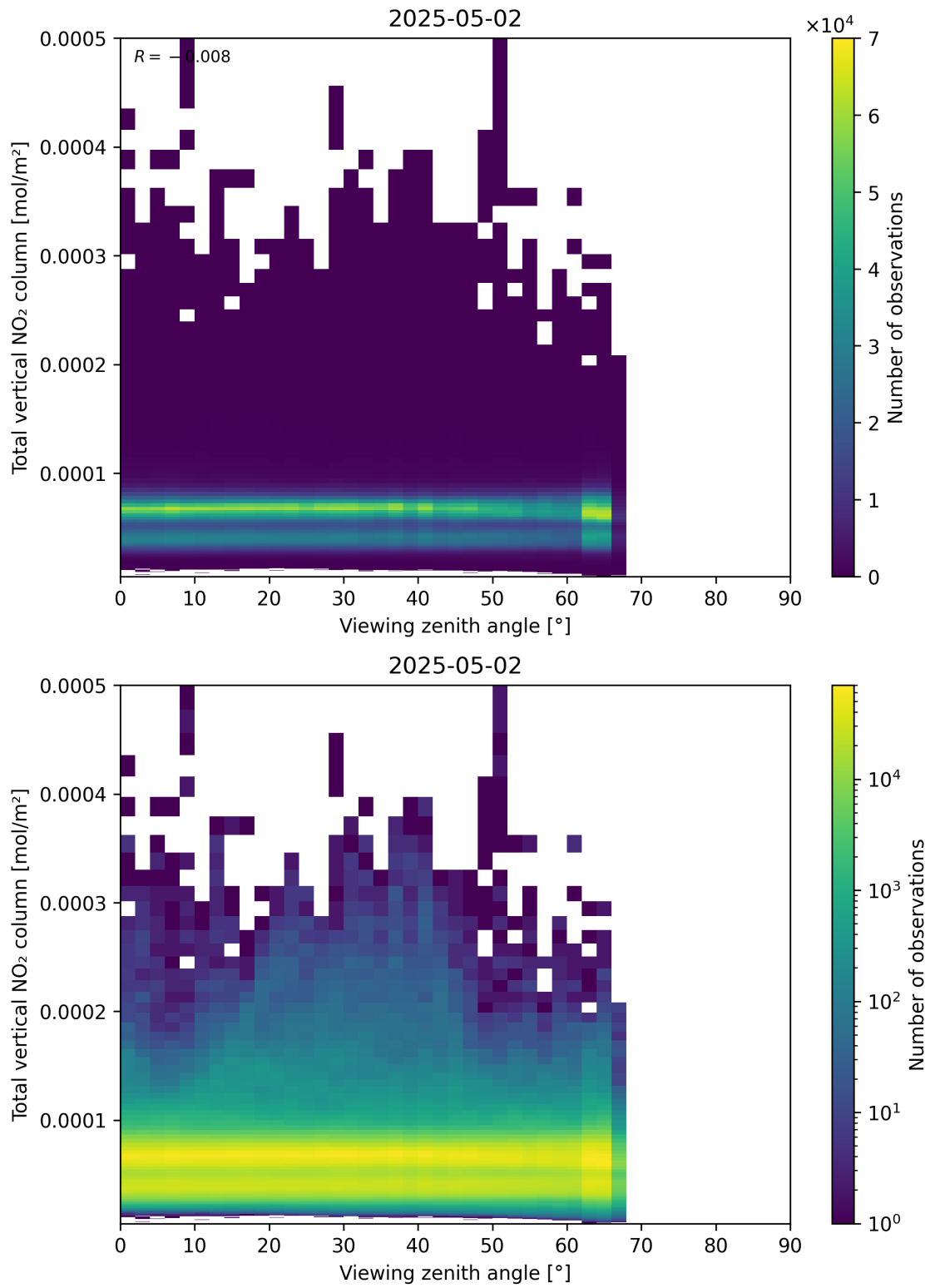
Figure 167: Scatter density plot of “Viewing zenith angle” against “Total vertical NO 2 column” for 2025-05-02 to 2025-05-02.
