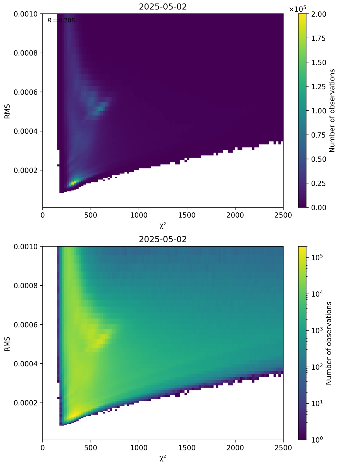
Figure 82: Scatter density plot of “ \chi^2 ” against “RMS” for 2025-05-02 to 2025-05-02.
