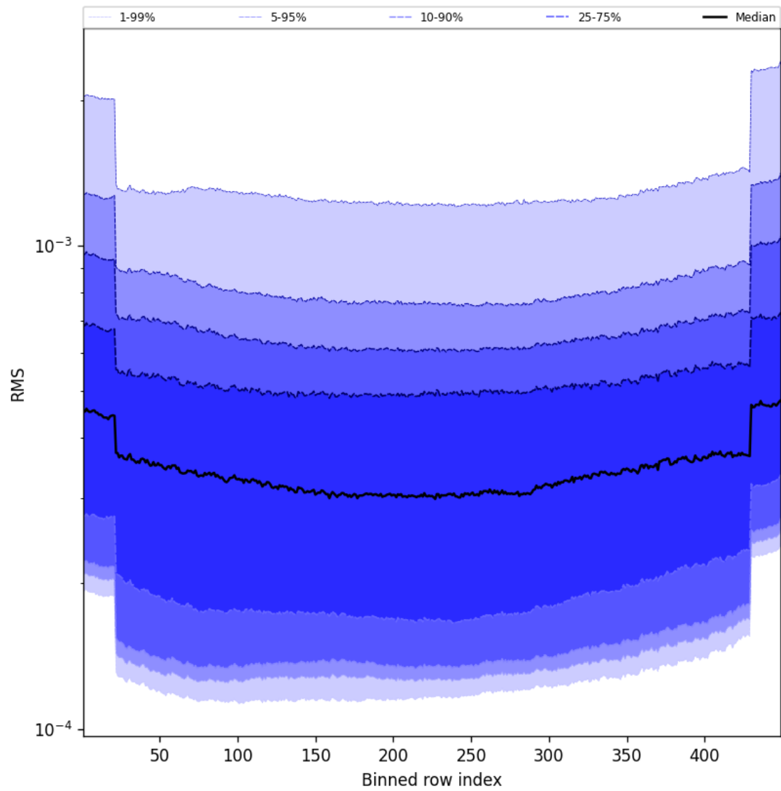
Figure 60: Along track statistics of “RMS” for 2025-05-02 to 2025-05-02
