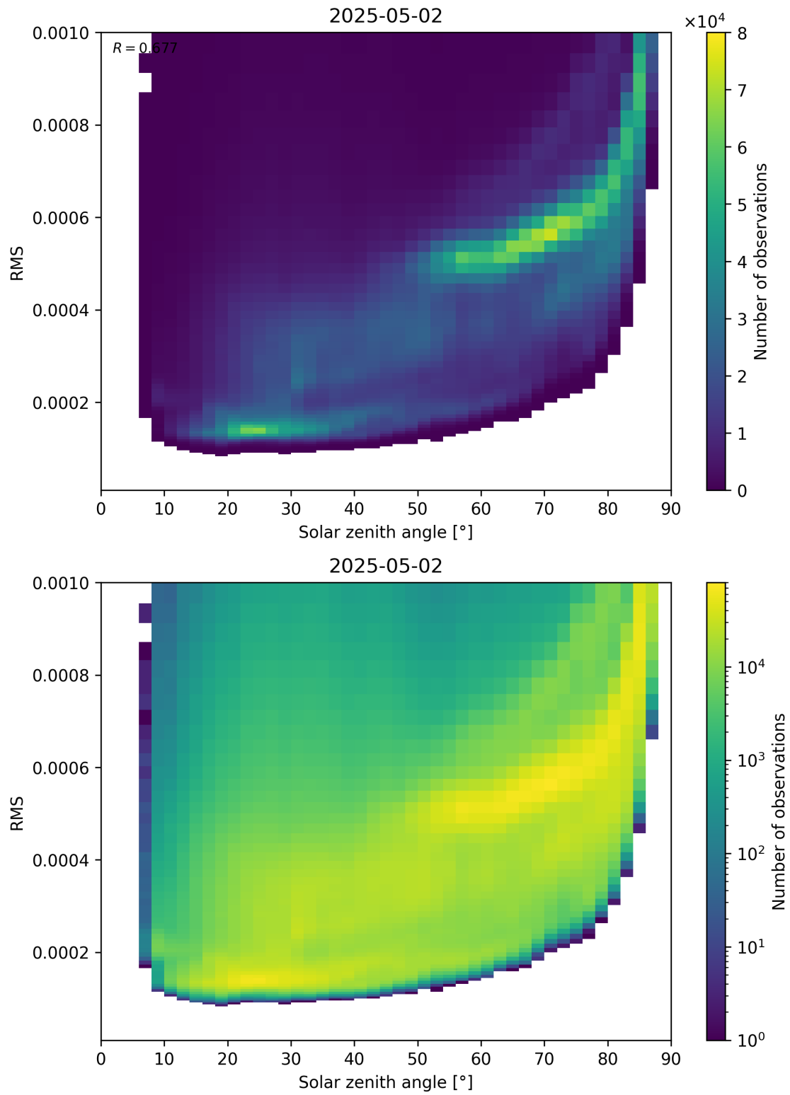
Figure 157: Scatter density plot of “Solar zenith angle” against “RMS” for 2025-05-02 to 2025-05-02.
