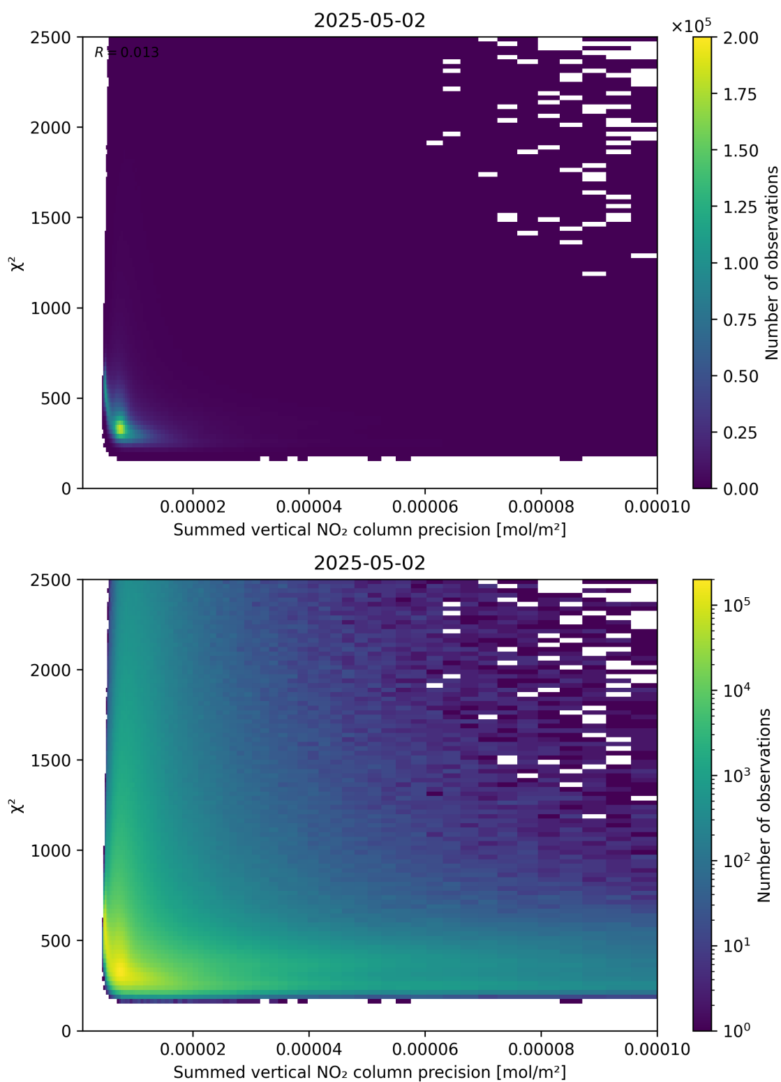
Figure 107: Scatter density plot of "Summed vertical NO 2 column precision" against " \chi^2 " for 2025-05-02 to 2025-05-02.
