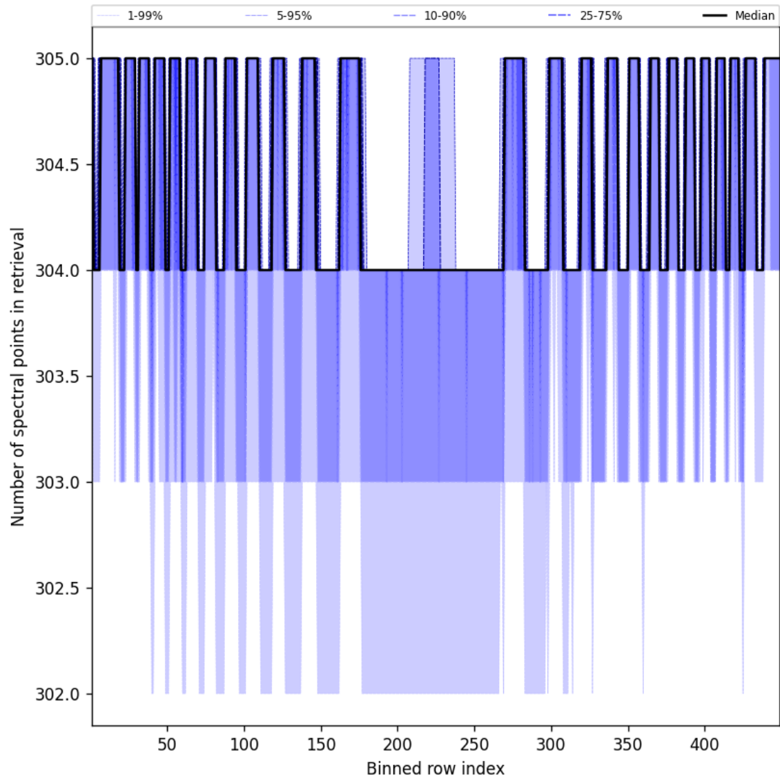
Figure 50: Along track statistics of “Number of spectral points in retrieval” for 2025-05-02 to 2025-05-02
