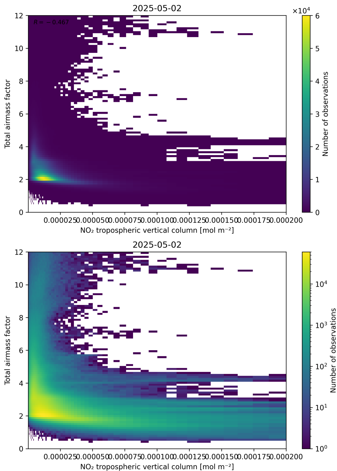
Figure 122: Scatter density plot of “NO 2 tropospheric vertical column” against “Total air mass factor” for 2025-05-02 to 2025-05-02.
