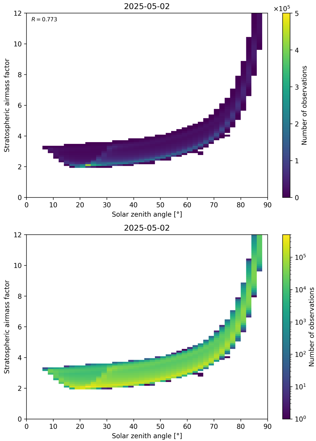
Figure 145: Scatter density plot of “Solar zenith angle” against “Stratospheric airmass factor” for 2025-05-02 to 2025-05-02.
