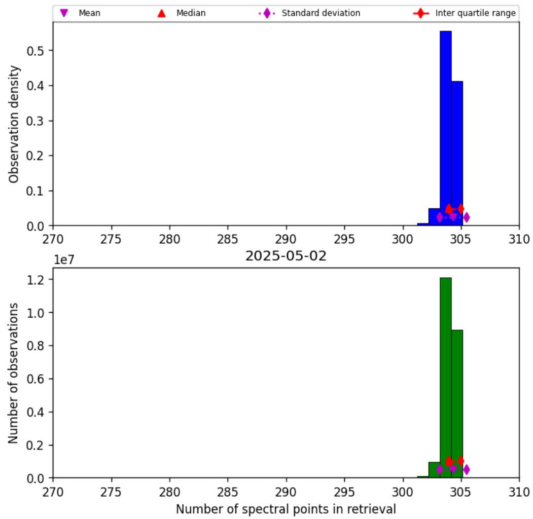
Figure 33: Histogram of “Number of spectral points in retrieval” for 2025-05-02 to 2025-05-02
