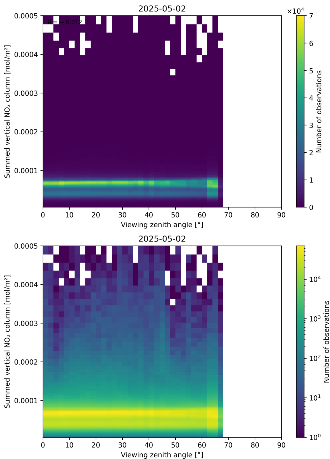
Figure 165: Scatter density plot of “Viewing zenith angle” against “Summed vertical NO 2 column” for 2025-05-02 to 2025-05-02.
