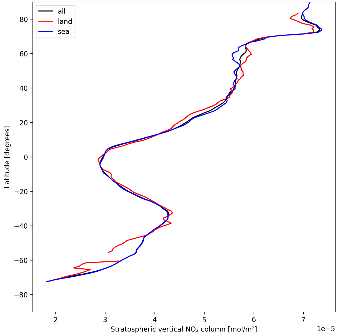
Figure 19: Zonal average of “Stratospheric vertical NO 2 column” for 2025-05-02 to 2025-05-02.
