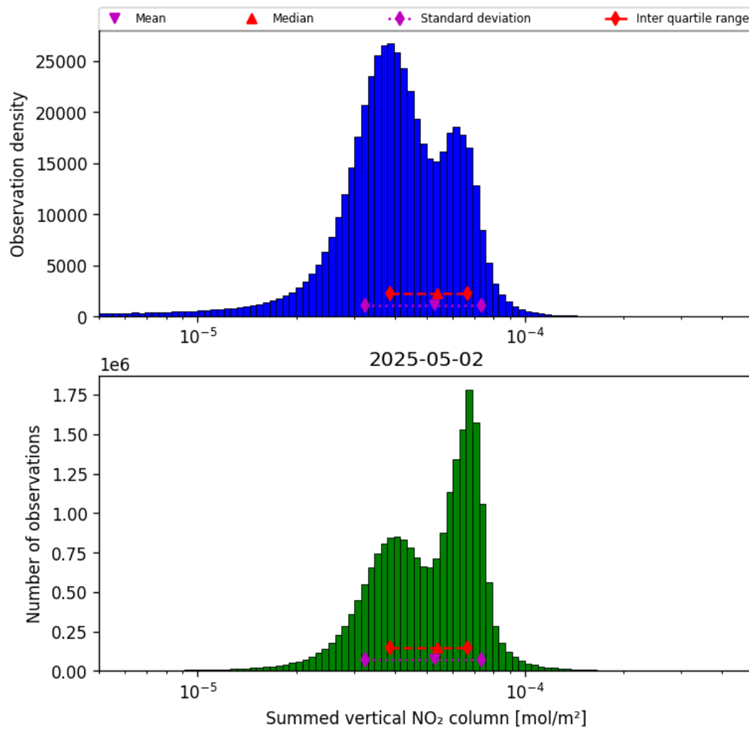
Figure 40: Histogram of “Summed vertical NO 2 column” for 2025-05-02 to 2025-05-02
