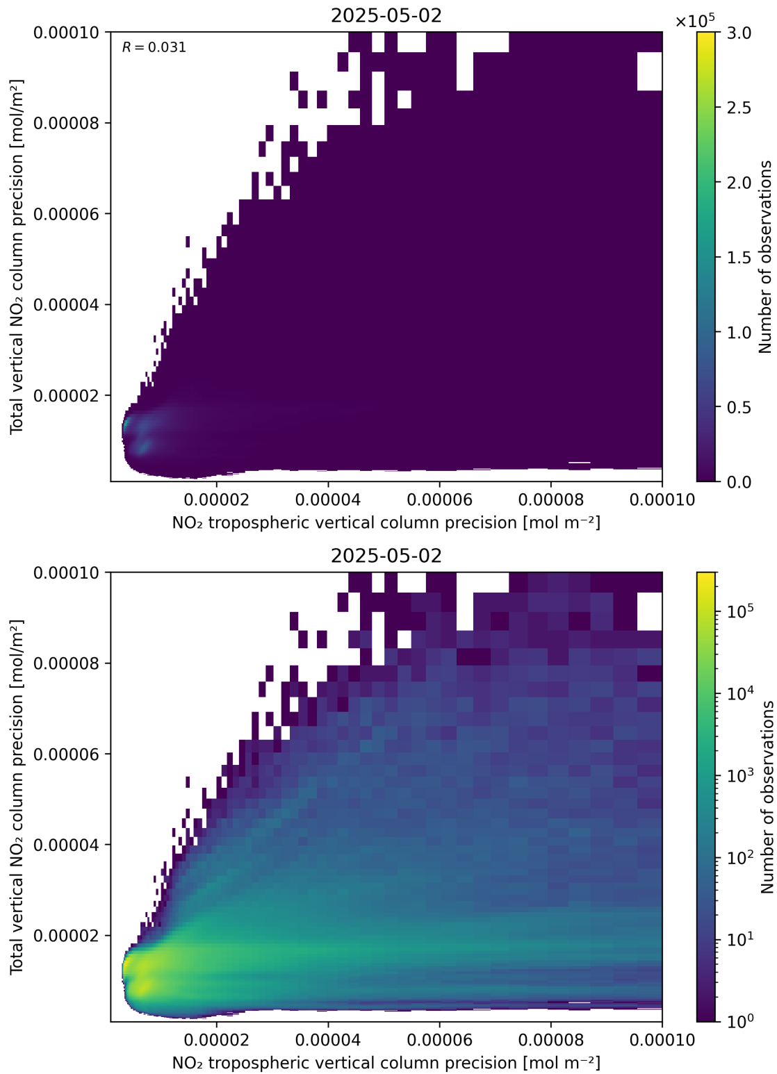
Figure 139: Scatter density plot of “NO 2 tropospheric vertical column precision” against “Total vertical NO 2 column precision” for 2025-05-02 to 2025-05-02.
