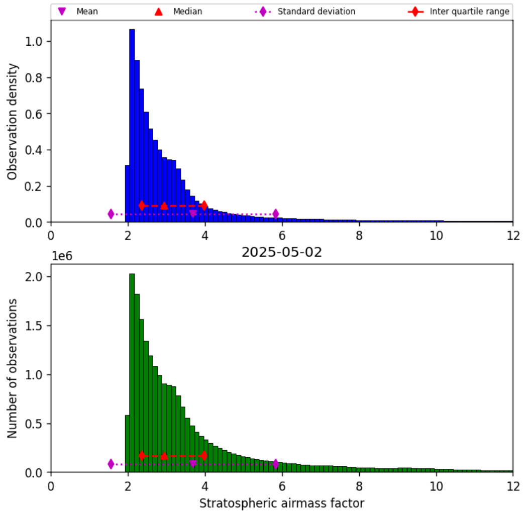
Figure 44: Histogram of “Stratospheric airmass factor” for 2025-05-02 to 2025-05-02
