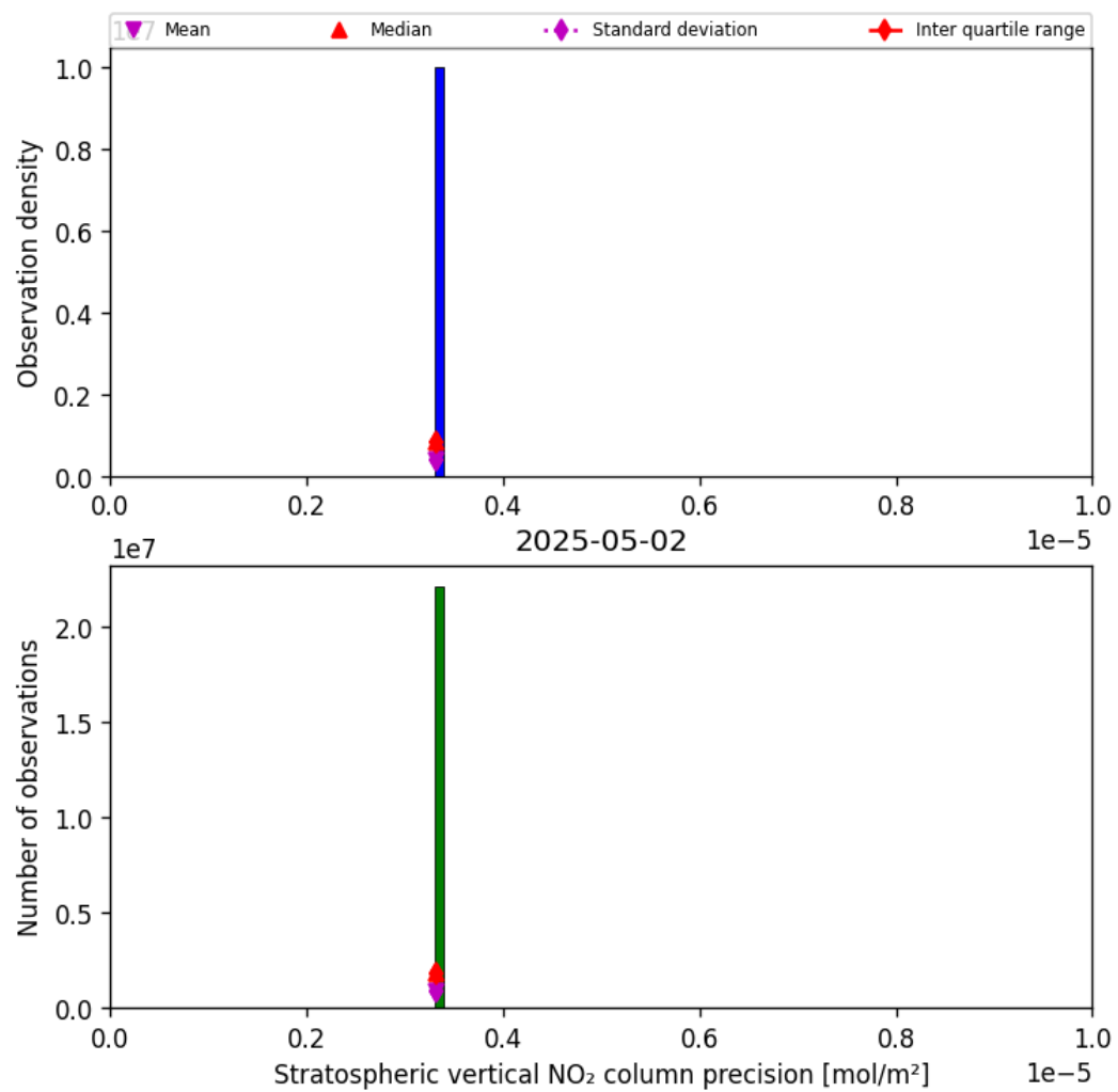
Figure 37: Histogram of “Stratospheric vertical NO 2 column precision” for 2025-05-02 to 2025-05-02
