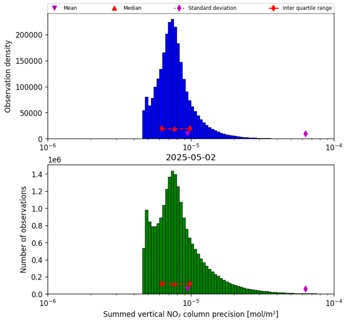
Figure 41: Histogram of "Summed vertical NO 2 column precision" for 2025-05-02 to 2025-05-02
