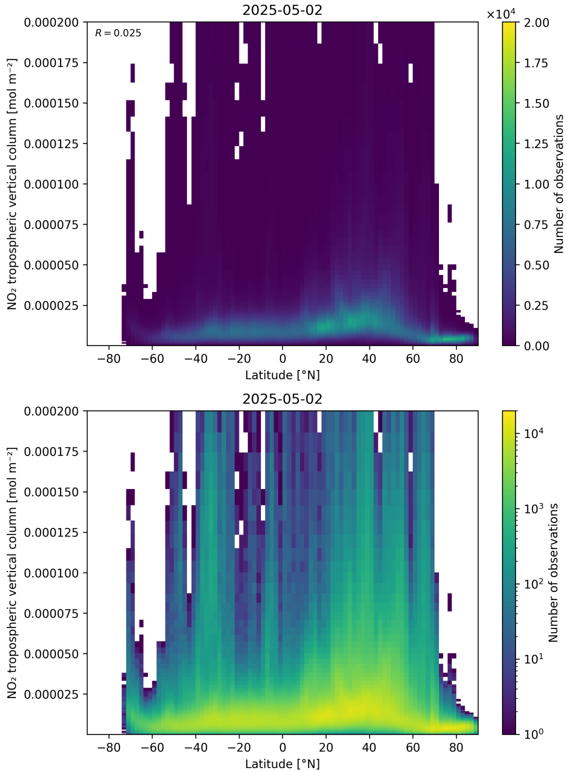
Figure 92: Scatter density plot of “Latitude” against “NO 2 tropospheric vertical column” for 2025-05-02 to 2025-05-02.
