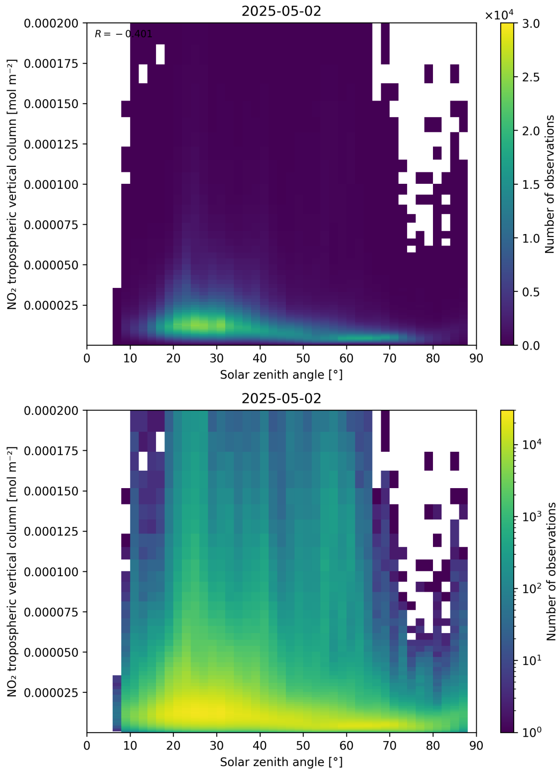
Figure 155: Scatter density plot of “Solar zenith angle” against “NO 2 tropospheric vertical column” for 2025-05-02 to 2025-05-02.
