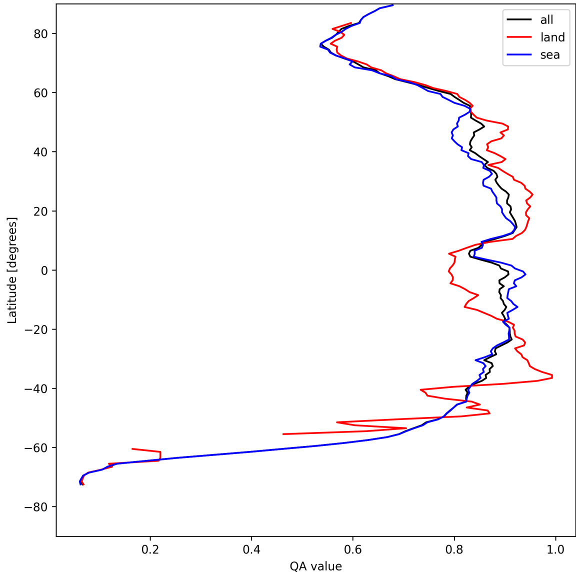
Figure 11: Zonal average of “QA value” for 2025-05-02 to 2025-05-02.
