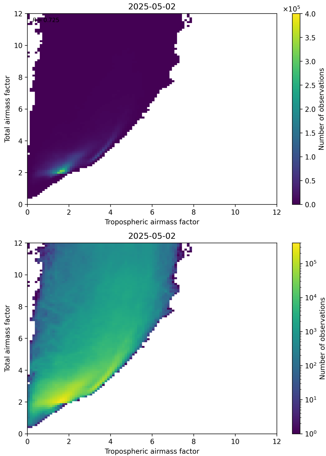
Figure 72: Scatter density plot of “Tropospheric airmass factor” against “Total airmass factor” for 2025-05-02 to 2025-05-02.
