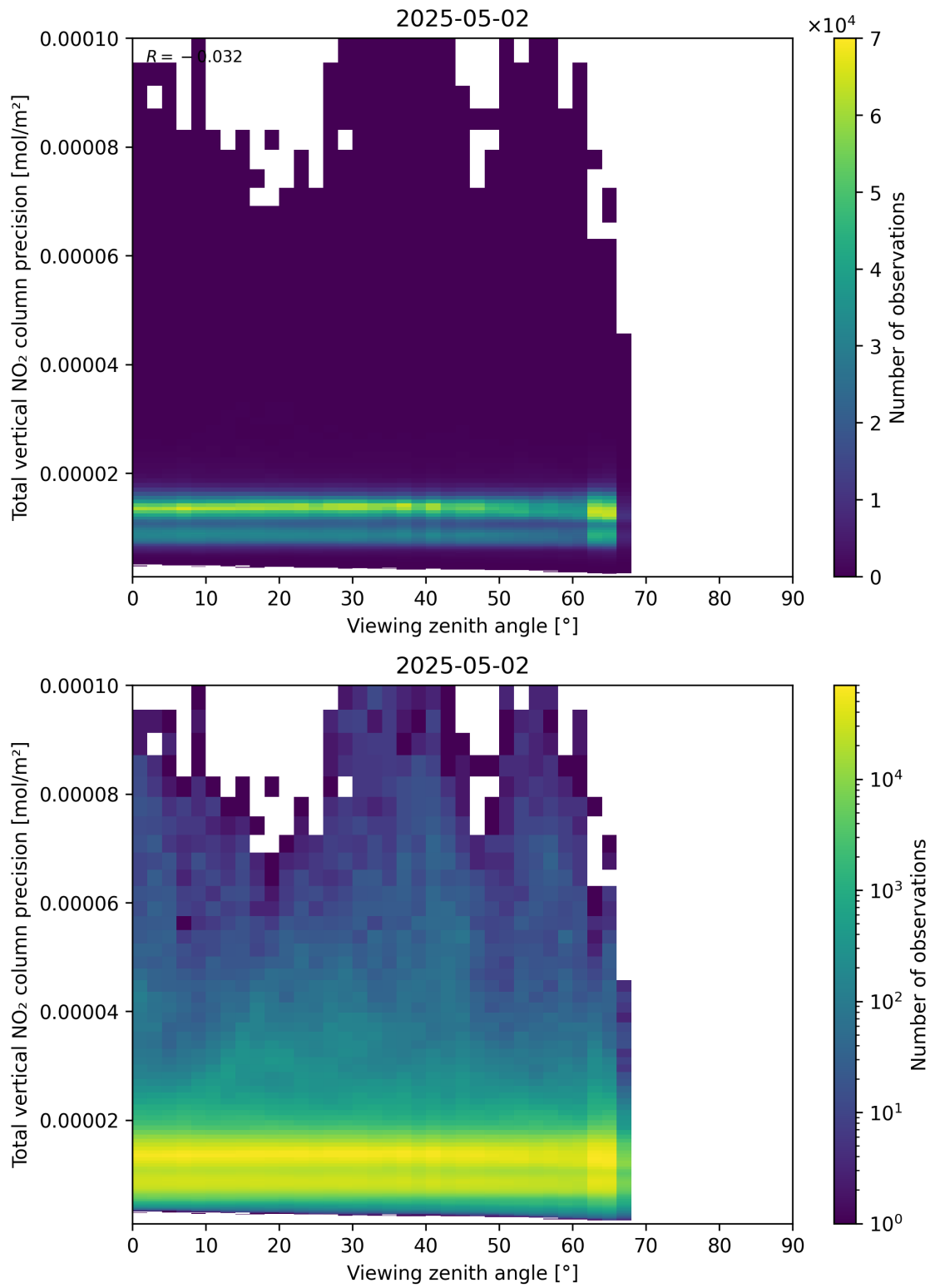
Figure 168: Scatter density plot of “Viewing zenith angle” against “Total vertical NO 2 column precision” for 2025-05-02 to 2025-05-02.
