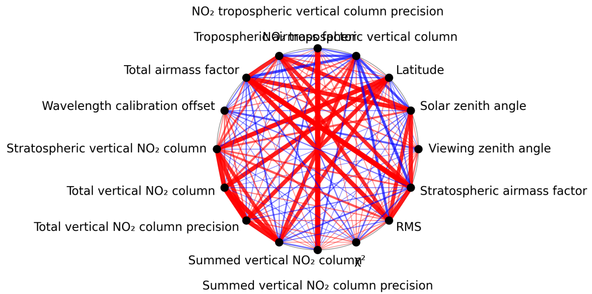
Figure 1: Map of correlation graph for 2025-05-02 to 2025-05-02.
