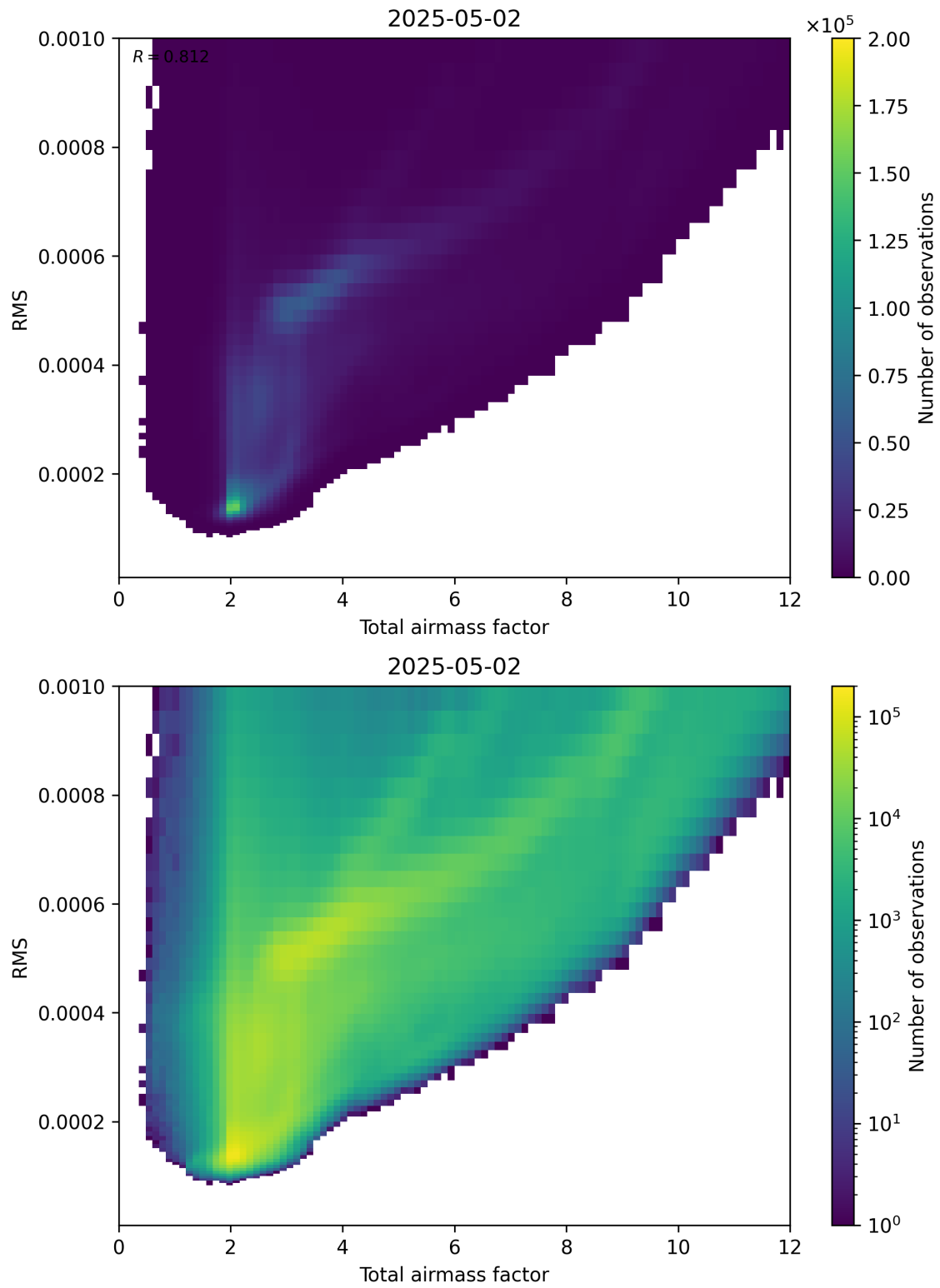
Figure 69: Scatter density plot of “Total airmass factor” against “RMS” for 2025-05-02 to 2025-05-02.
