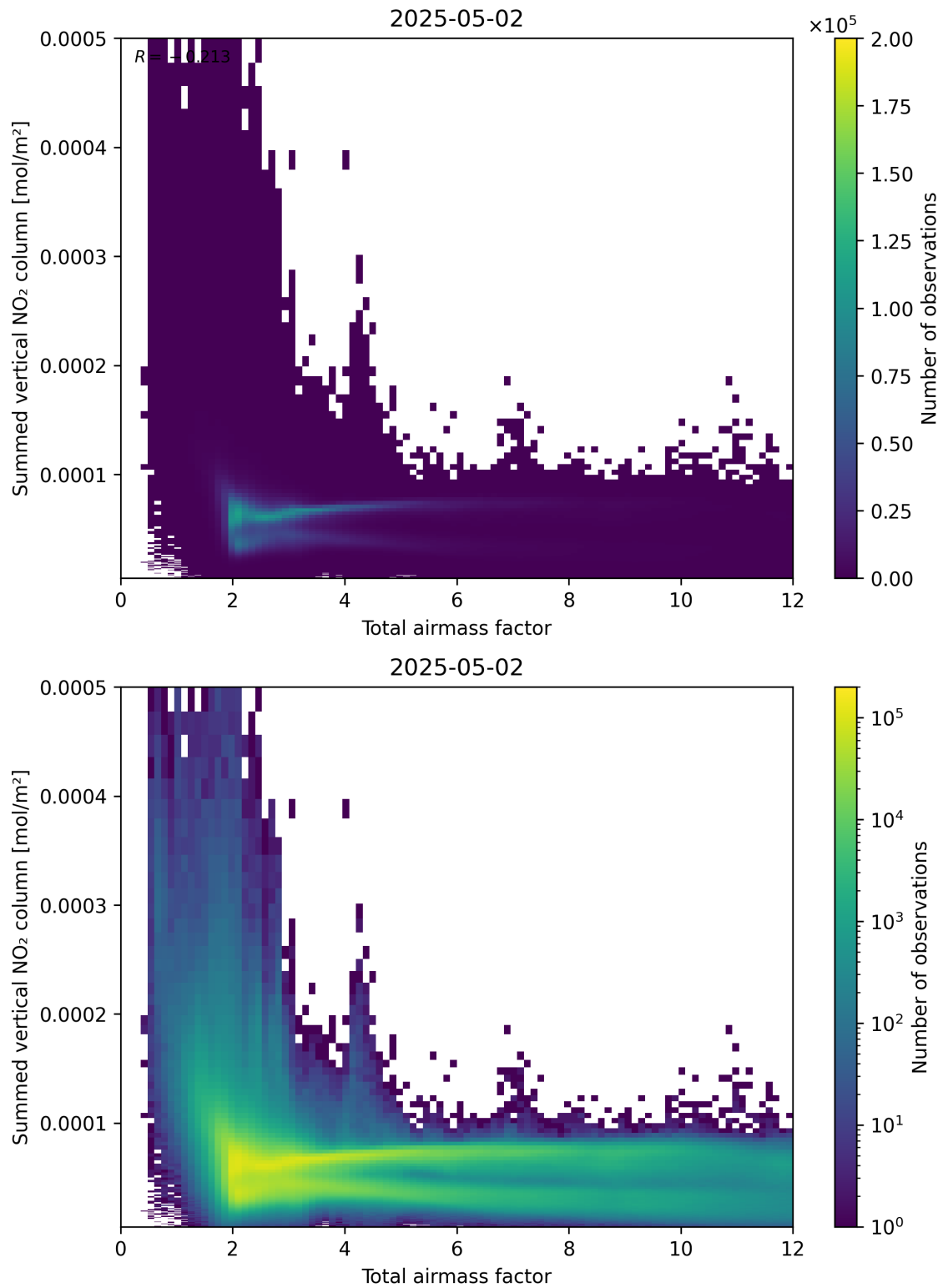
Figure 65: Scatter density plot of “Total airmass factor” against “Summed vertical NO 2 column” for 2025-05-02 to 2025-05-02.
