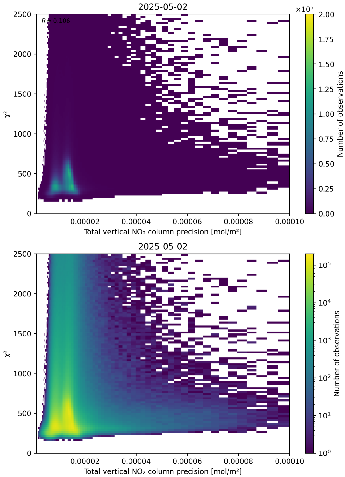
Figure 116: Scatter density plot of “Total vertical NO 2 column precision” against “ \chi^2 ” for 2025-05-02 to 2025-05-02.
