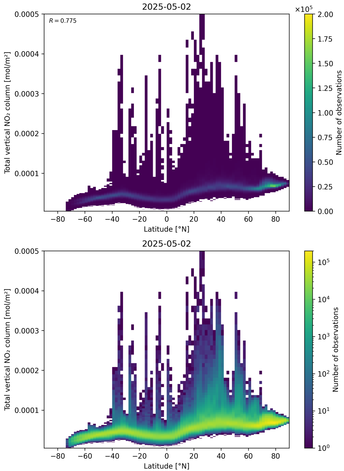
Figure 90: Scatter density plot of “Latitude” against “Total vertical NO 2 column” for 2025-05-02 to 2025-05-02.
