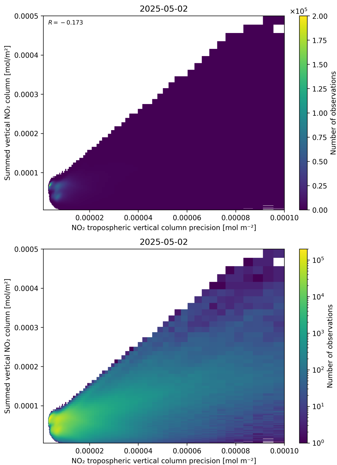
Figure 136: Scatter density plot of “NO 2 tropospheric vertical column precision” against “Summed vertical NO 2 column” for 2025-05-02 to 2025-05-02.
