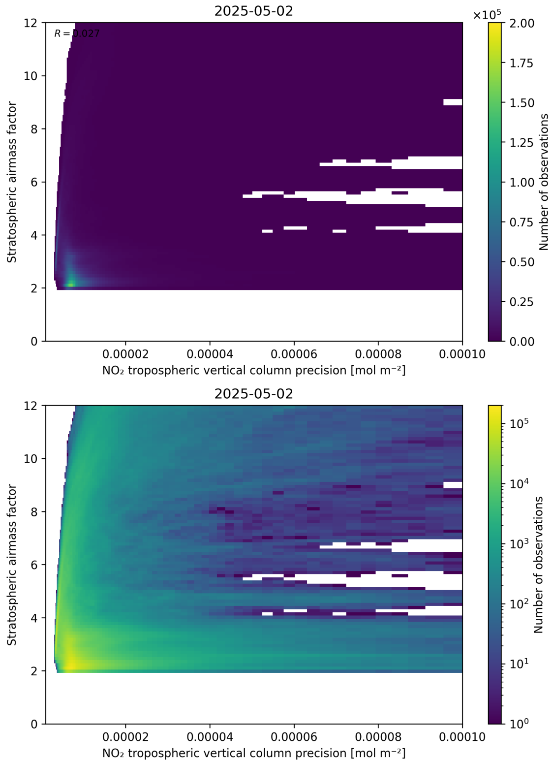
Figure 131: Scatter density plot of “NO 2 tropospheric vertical column precision” against “Stratospheric airmass factor” for 2025-05-02 to 2025-05-02.
