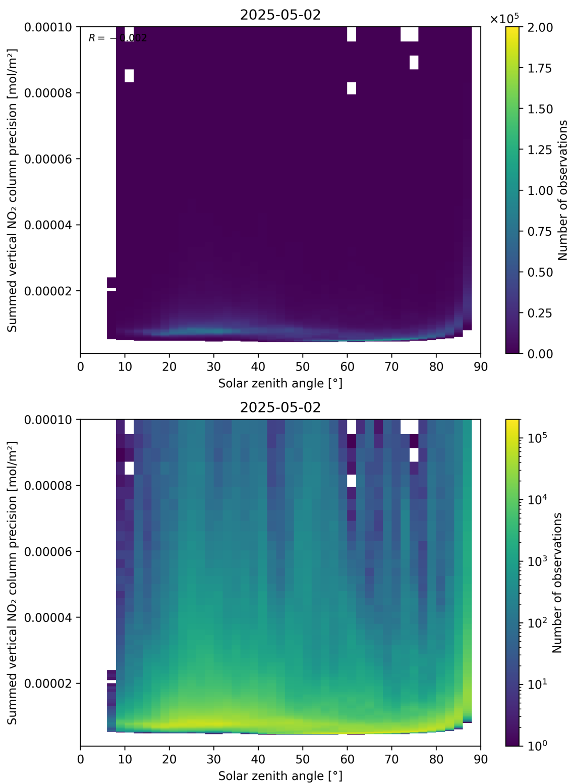
Figure 152: Scatter density plot of “Solar zenith angle” against “Summed vertical NO 2 column precision” for 2025-05-02 to 2025-05-02.
