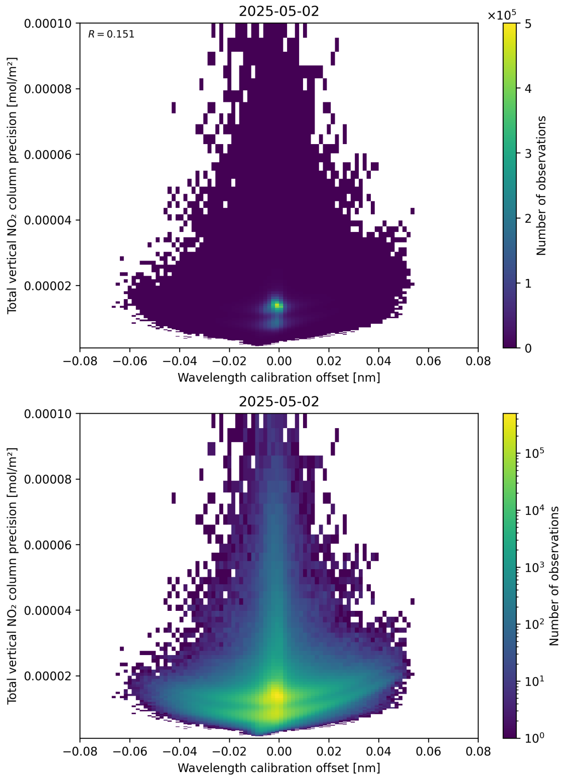
Figure 180: Scatter density plot of “Wavelength calibration offset” against “Total vertical NO 2 column precision” for 2025-05-02 to 2025-05-02.
