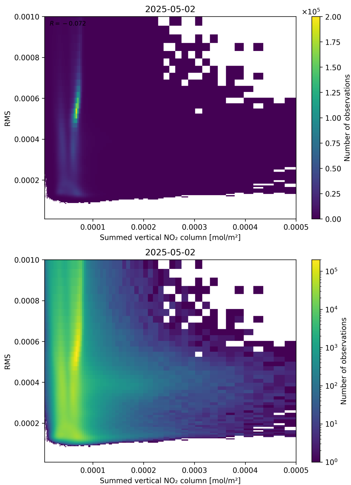
Figure 109: Scatter density plot of “Summed vertical NO 2 column” against “RMS” for 2025-05-02 to 2025-05-02.
