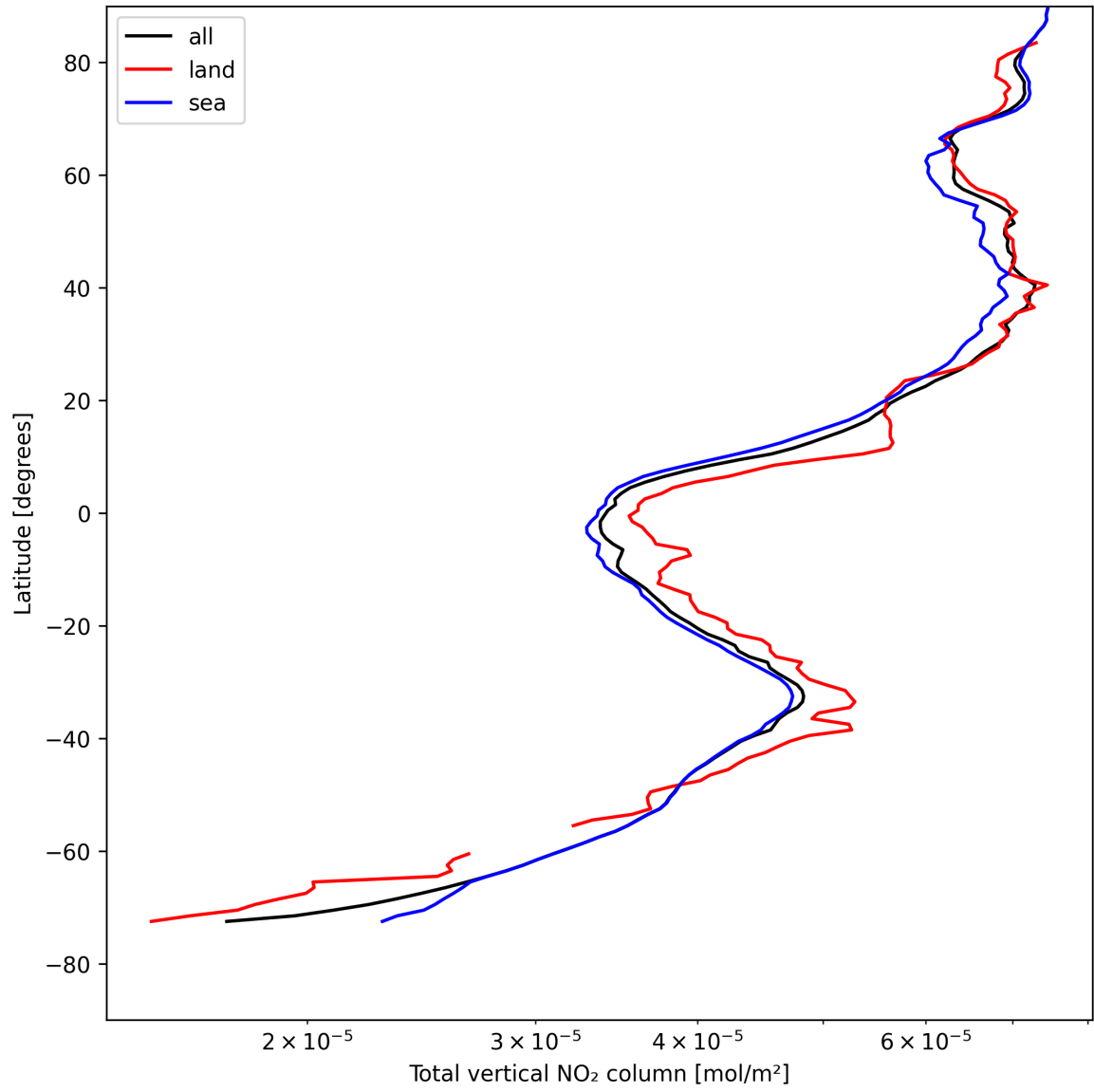
Figure 21: Zonal average of “Total vertical NO 2 column” for 2025-05-02 to 2025-05-02.
