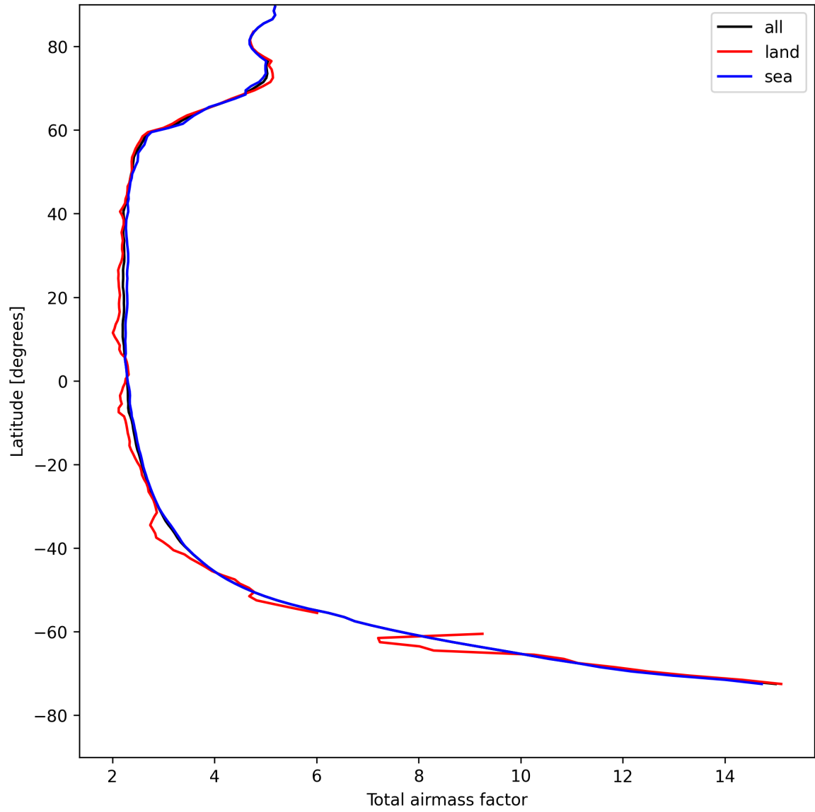
Figure 15: Zonal average of “Total airmass factor” for 2025-05-02 to 2025-05-02.
