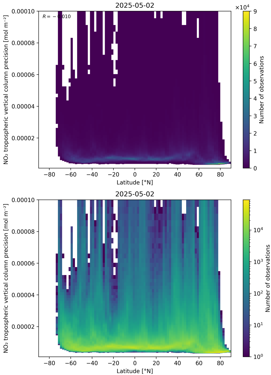
Figure 93: Scatter density plot of “Latitude” against “NO 2 tropospheric vertical column precision” for 2025-05-02 to 2025-05-02.
