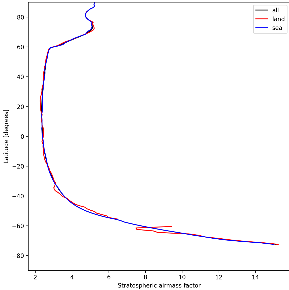
Figure 27: Zonal average of “Stratospheric airmass factor” for 2025-05-02 to 2025-05-02.
