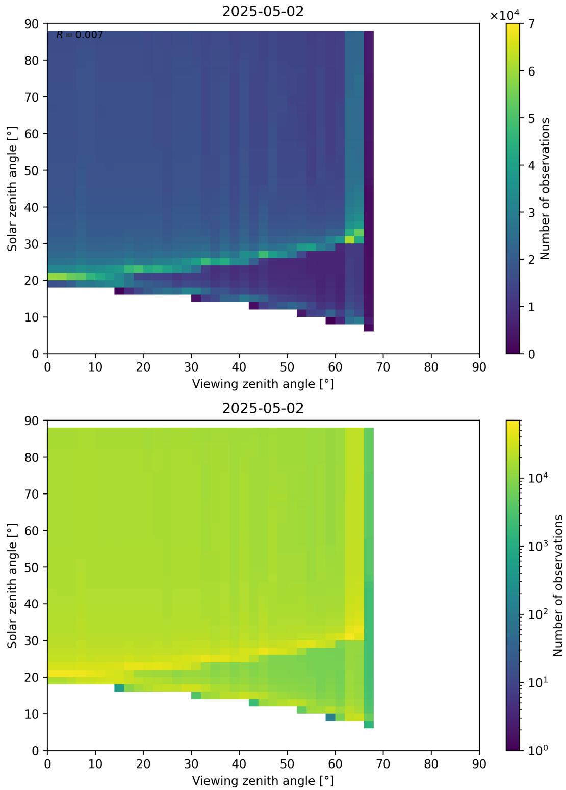
Figure 172: Scatter density plot of “Viewing zenith angle” against “Solar zenith angle” for 2025-05-02 to 2025-05-02.
