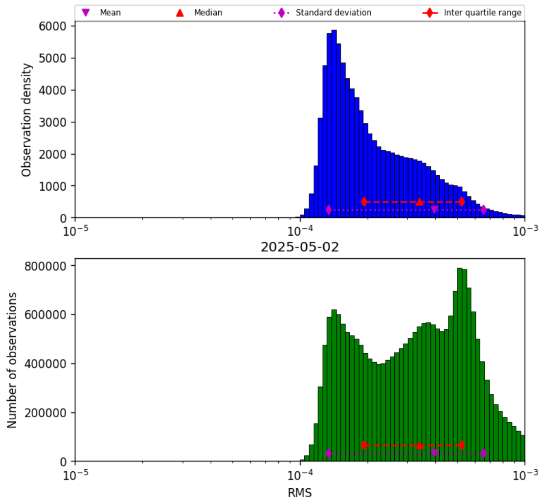
Figure 43: Histogram of “RMS” for 2025-05-02 to 2025-05-02
