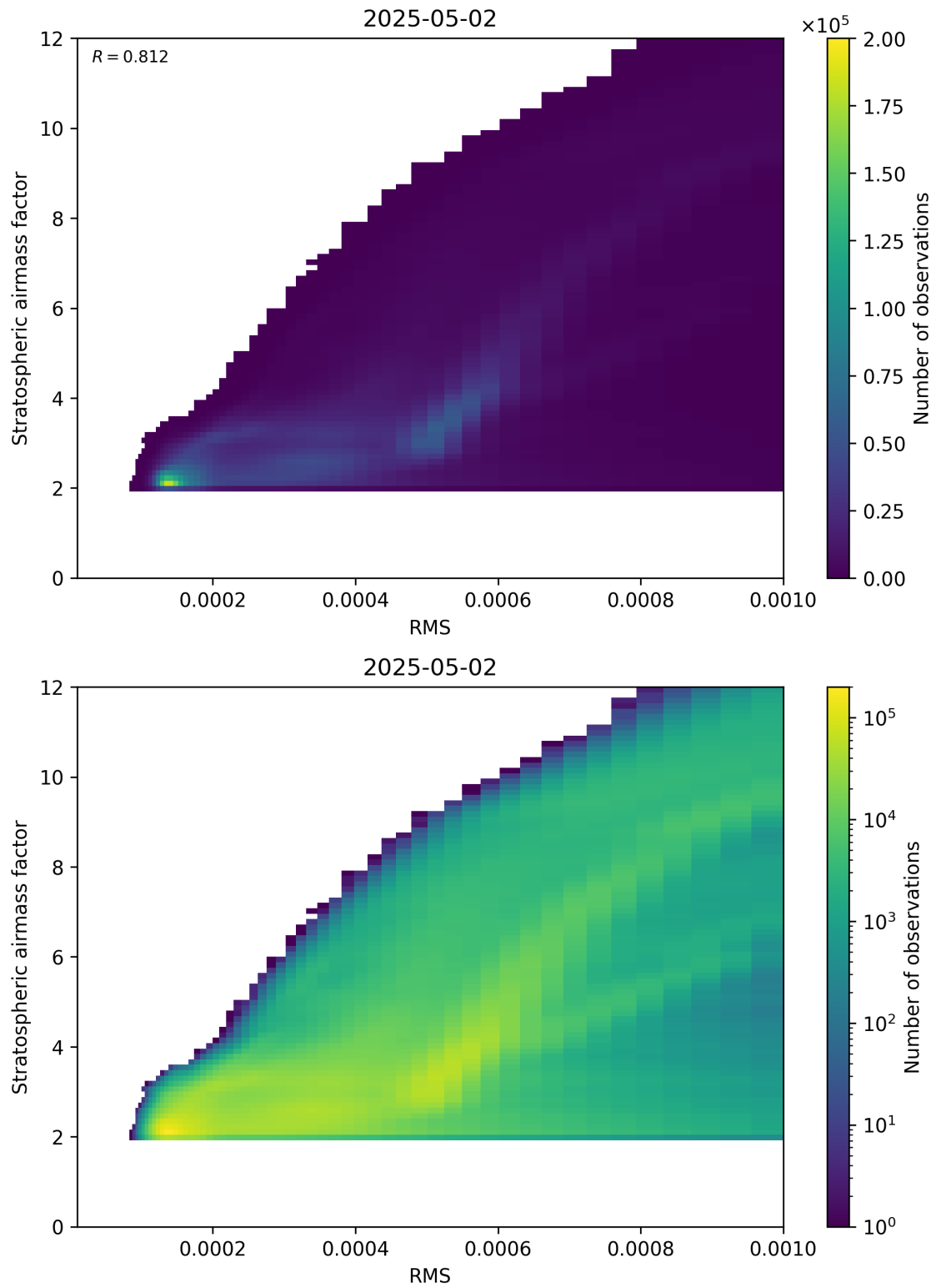
Figure 144: Scatter density plot of “RMS” against “Stratospheric airmass factor” for 2025-05-02 to 2025-05-02.
