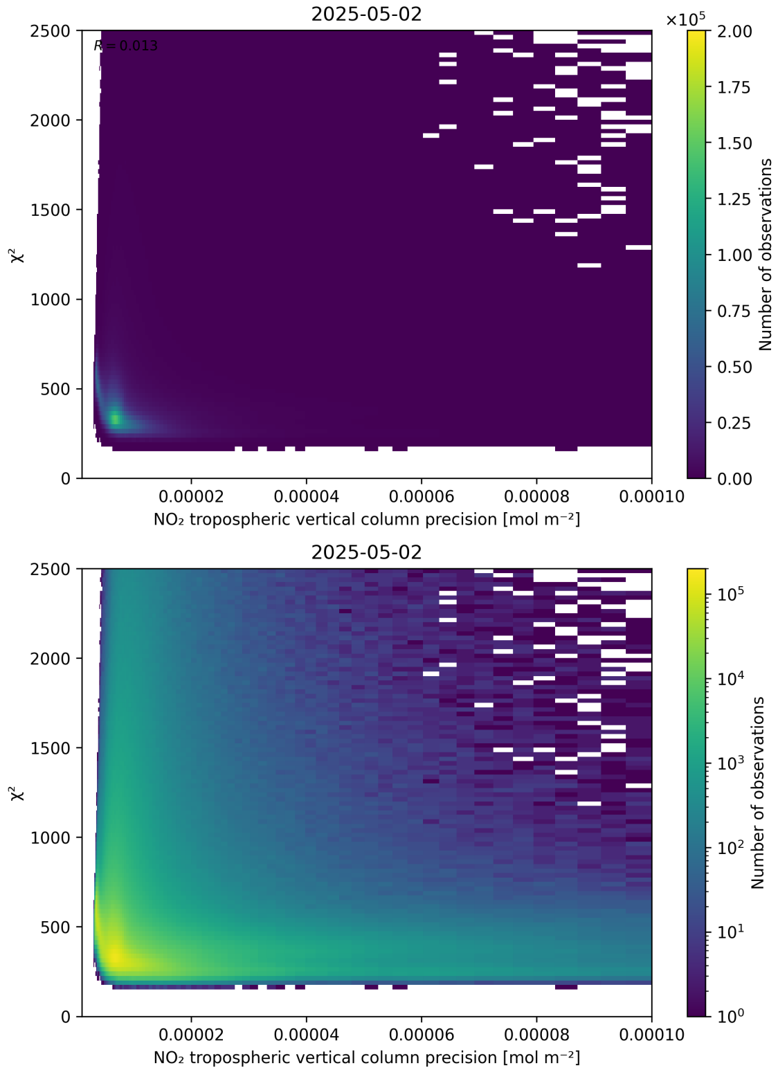
Figure 134: Scatter density plot of “NO 2 tropospheric vertical column precision” against “ \chi^2 ” for 2025-05-02 to 2025-05-02.
