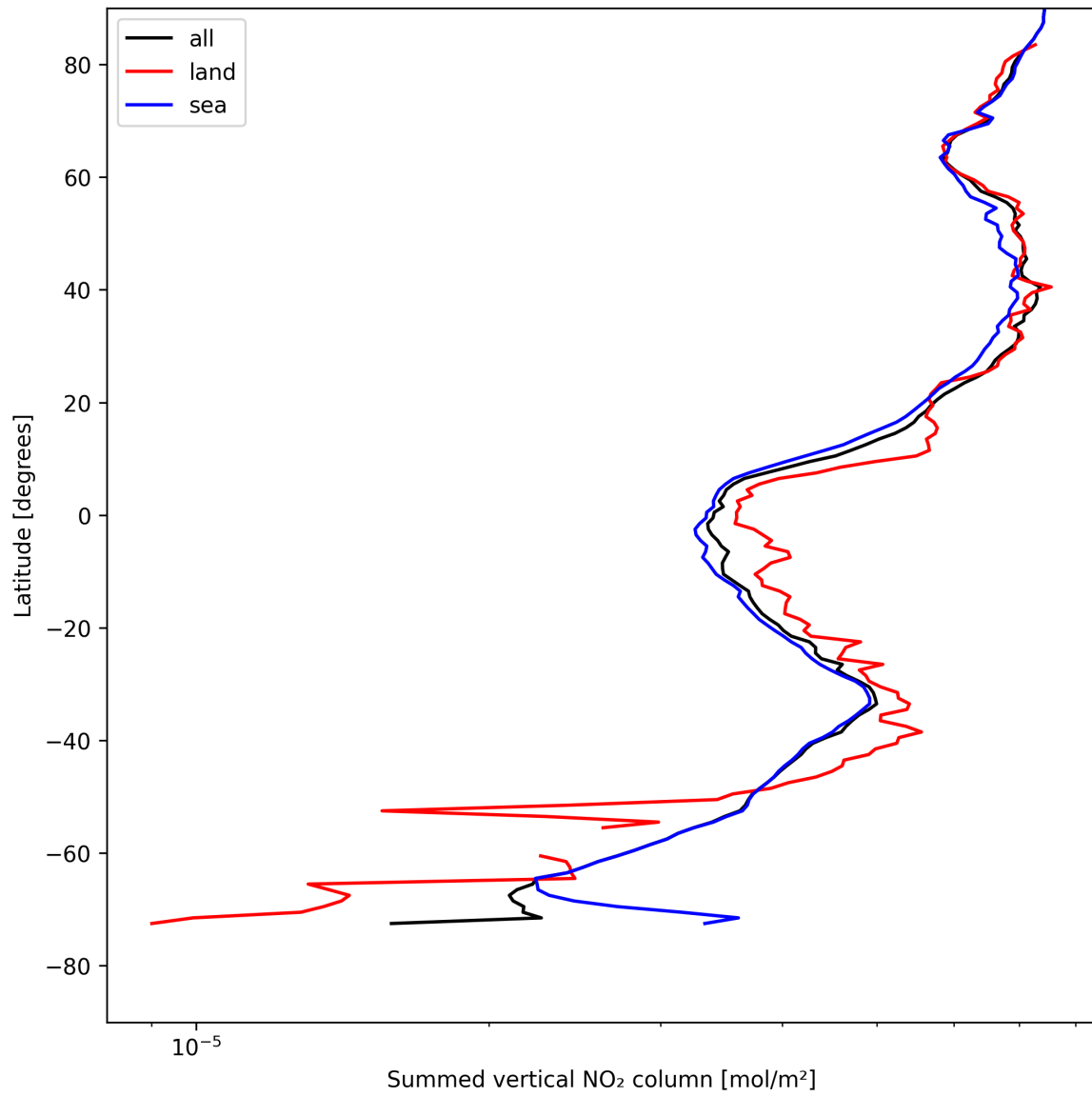
Figure 23: Zonal average of “Summed vertical NO 2 column” for 2025-05-02 to 2025-05-02.
