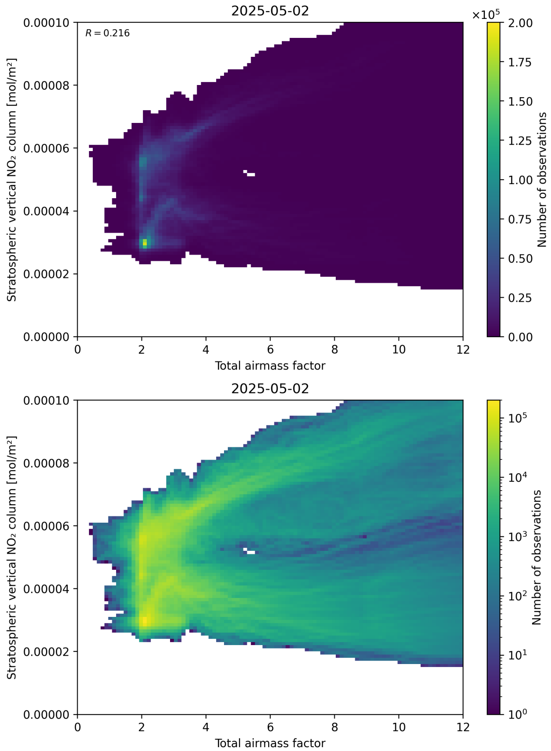
Figure 64: Scatter density plot of “Total airmass factor” against “Stratospheric vertical NO 2 column” for 2025-05-02 to 2025-05-02.
