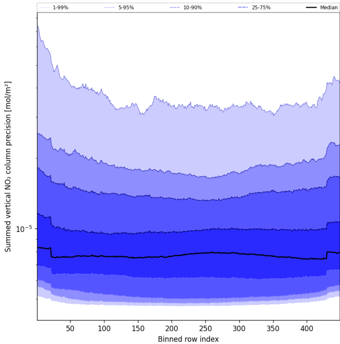
Figure 58: Along track statistics of “Summed vertical NO 2 column precision” for 2025-05-02 to 2025-05-02
