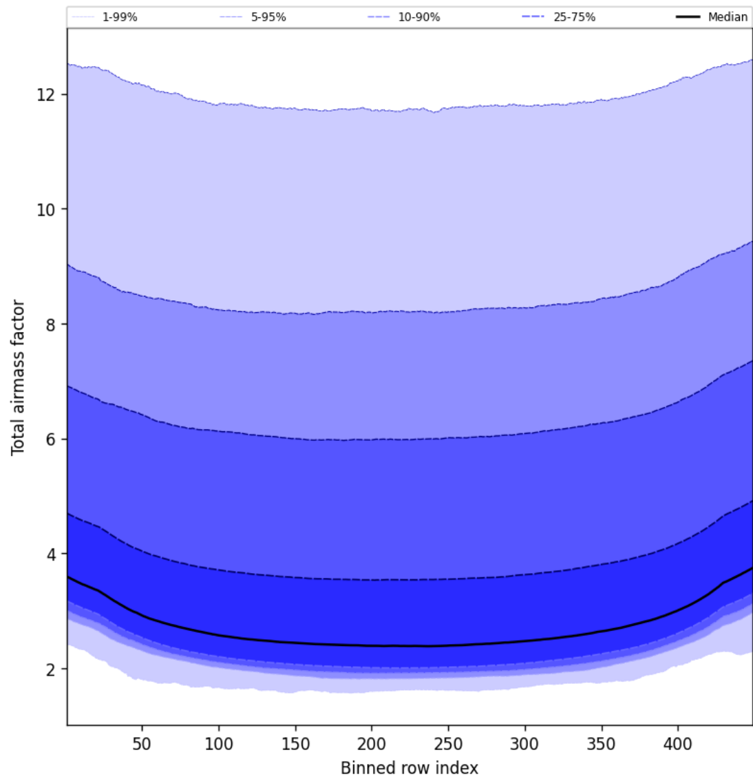
Figure 49: Along track statistics of “Total airmass factor” for 2025-05-02 to 2025-05-02
