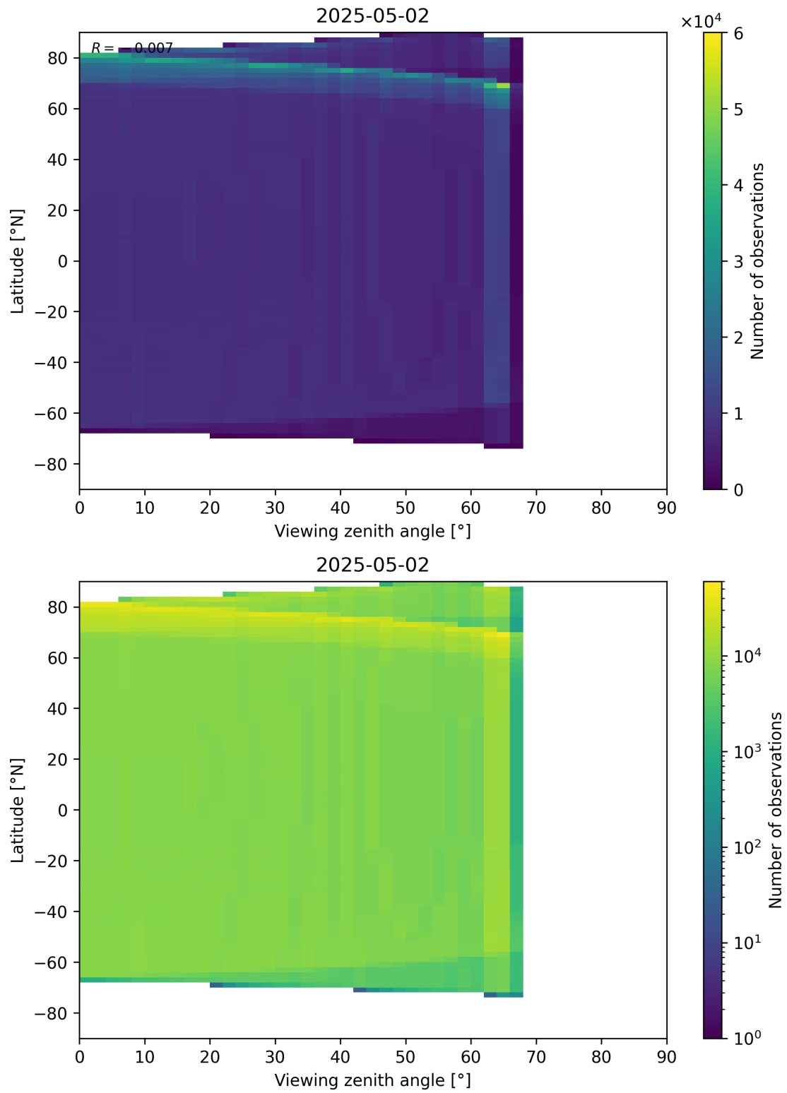
Figure 163: Scatter density plot of “Viewing zenith angle” against “Latitude” for 2025-05-02 to 2025-05-02.
