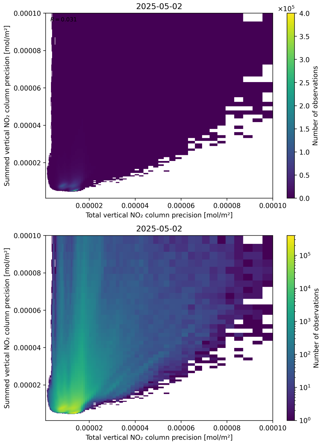
Figure 118: Scatter density plot of “Total vertical NO 2 column precision” against “Summed vertical NO 2 column precision” for 2025-05-02 to 2025-05-02.
