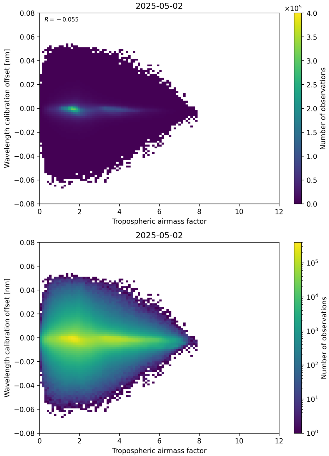
Figure 80: Scatter density plot of “Tropospheric airmass factor” against “Wavelength calibration offset” for 2025-05-02 to 2025-05-02.
