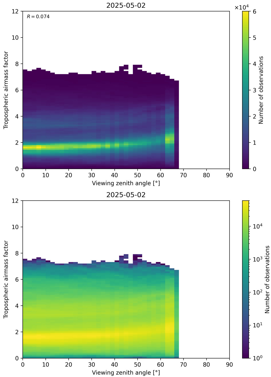
Figure 161: Scatter density plot of “Viewing zenith angle” against “Tropospheric airmass factor” for 2025-05-02 to 2025-05-02.
