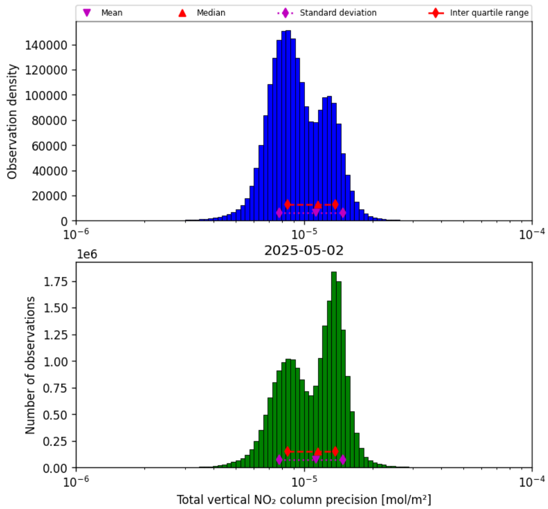
Figure 39: Histogram of “Total vertical NO 2 column precision” for 2025-05-02 to 2025-05-02
