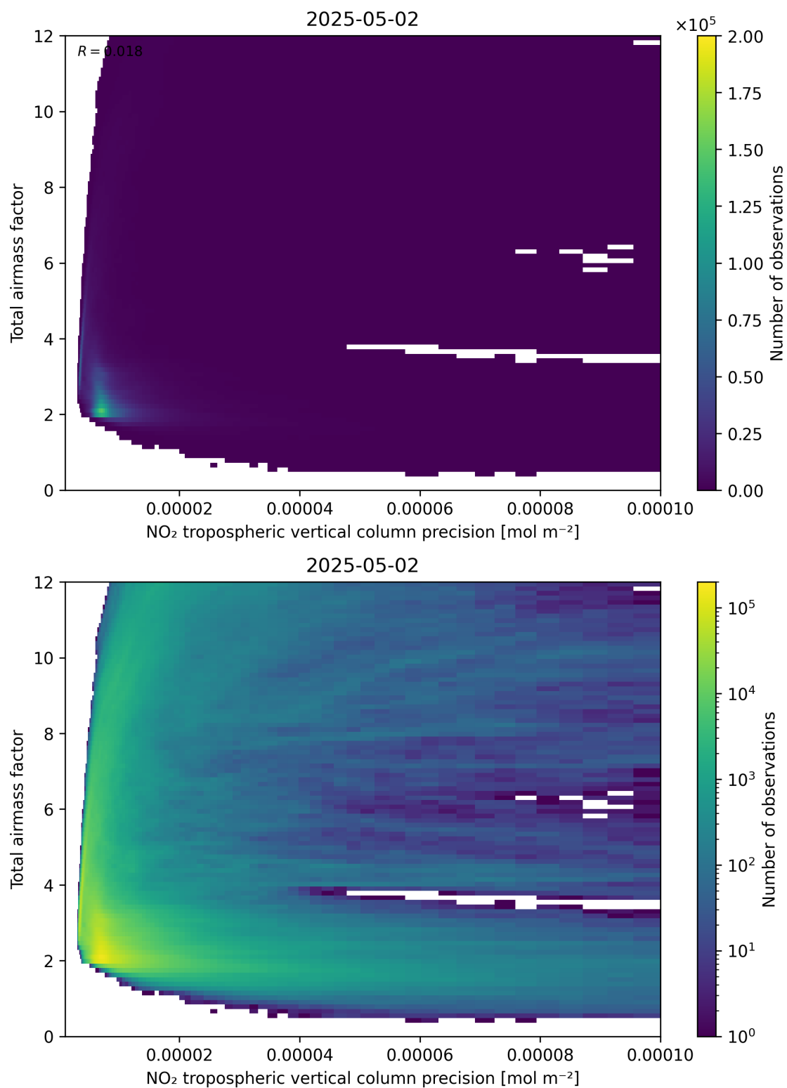
Figure 132: Scatter density plot of “NO 2 tropospheric vertical column precision” against “Total air mass factor” for 2025-05-02 to 2025-05-02.
