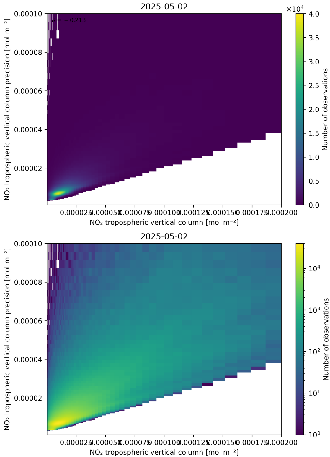
Figure 130: Scatter density plot of “NO 2 tropospheric vertical column” against “NO 2 tropospheric vertical column precision” for 2025-05-02 to 2025-05-02.
