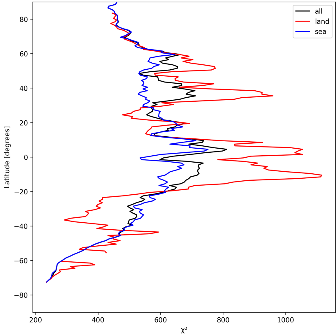
Figure 25: Zonal average of “ \chi^2 ” for 2025-05-02 to 2025-05-02.
