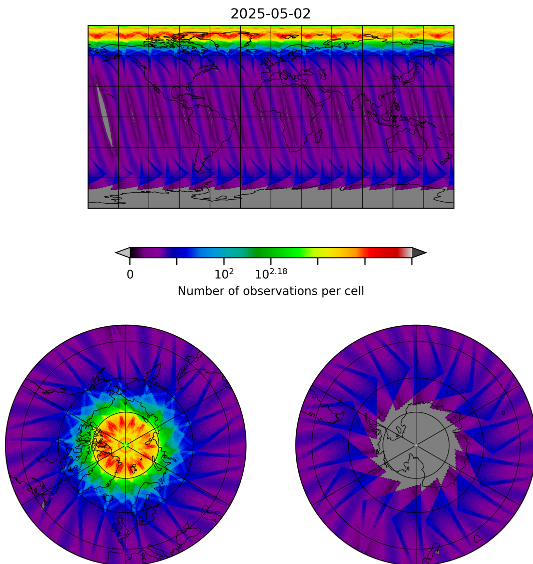
Figure 10: Map of the number of observations for 2025-05-02 to 2025-05-02
