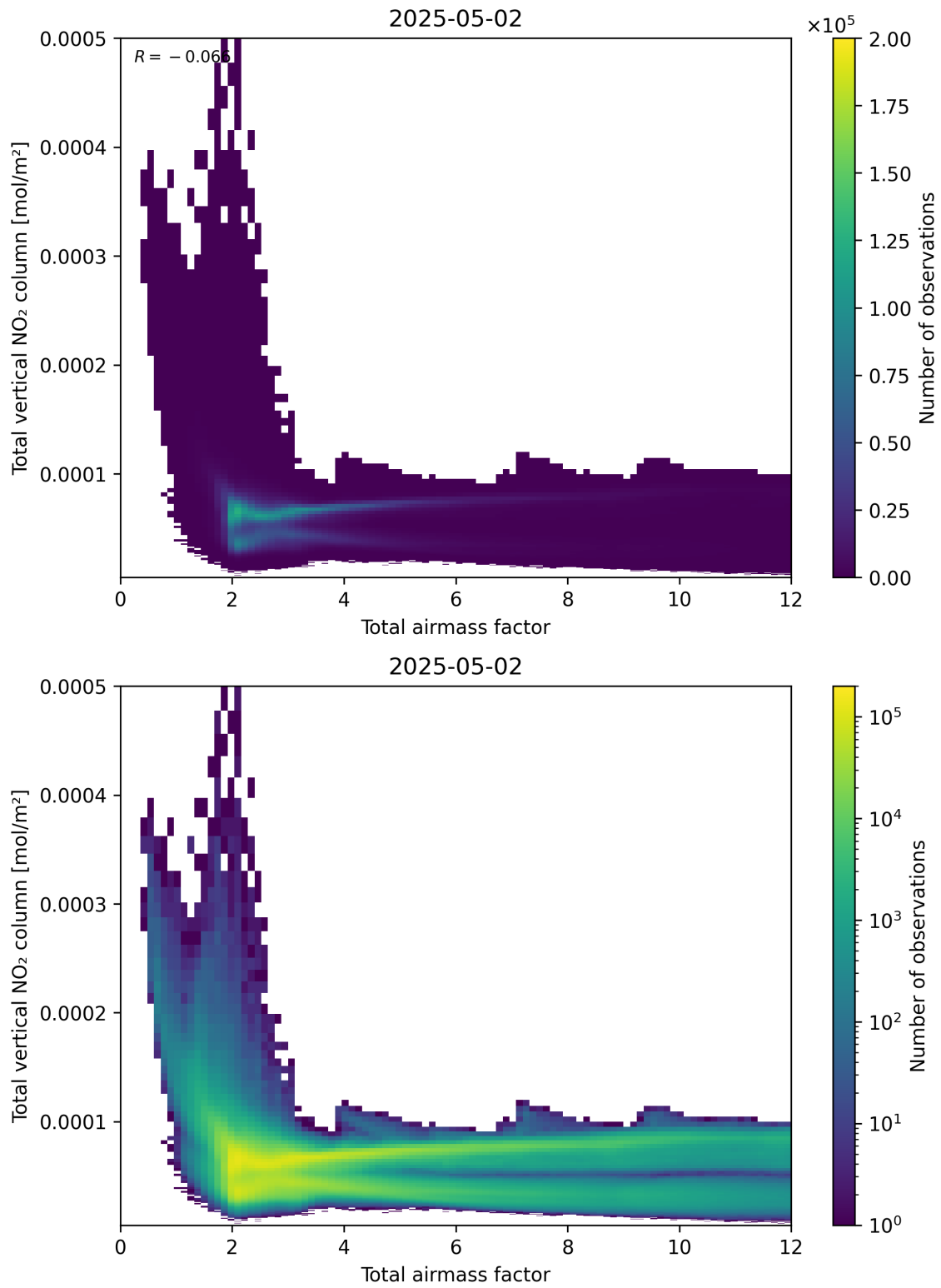
Figure 67: Scatter density plot of “Total airmass factor” against “Total vertical NO 2 column” for 2025-05-02 to 2025-05-02.
