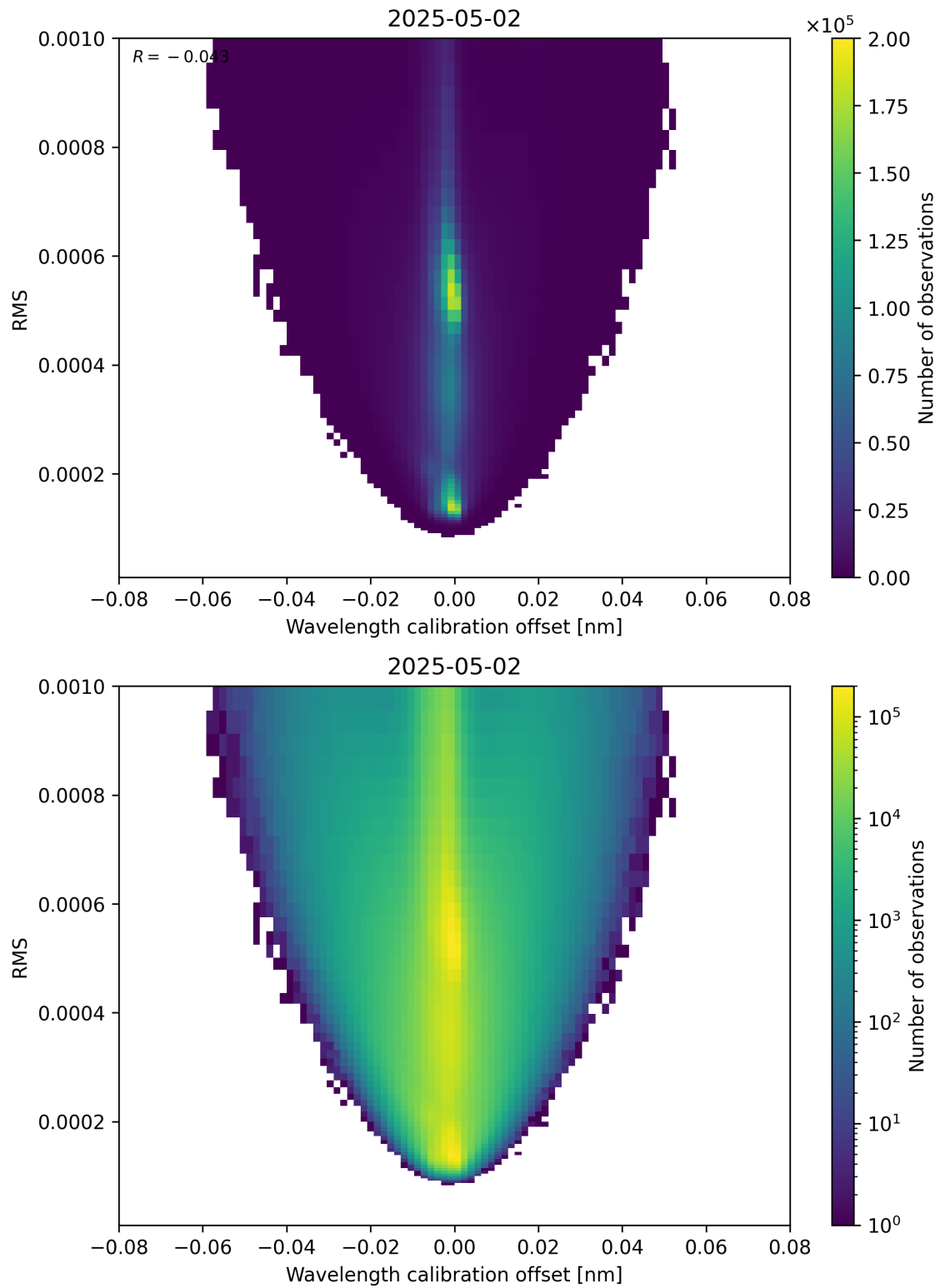
Figure 181: Scatter density plot of “Wavelength calibration offset” against “RMS” for 2025-05-02 to 2025-05-02.
