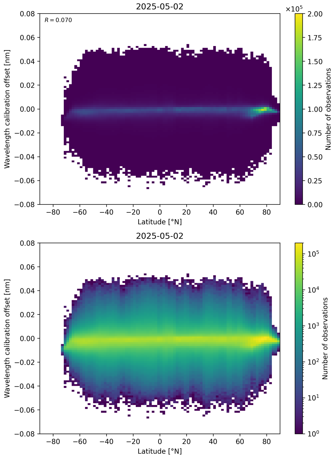
Figure 95: Scatter density plot of “Latitude” against “Wavelength calibration offset” for 2025-05-02 to 2025-05-02.
