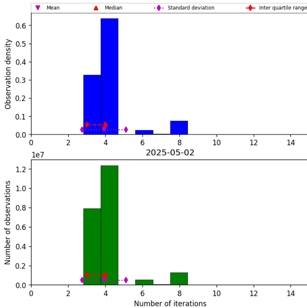
Figure 34: Histogram of “Number of iterations” for 2025-05-02 to 2025-05-02
