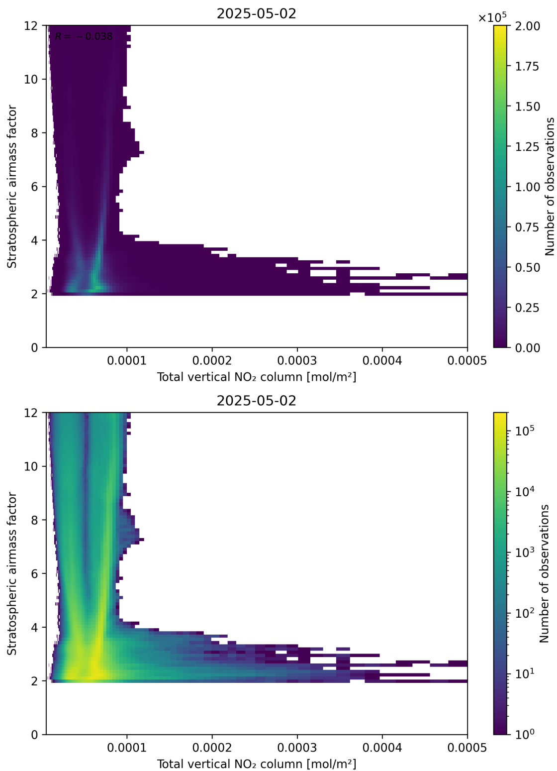
Figure 110: Scatter density plot of “Total vertical NO 2 column” against “Stratospheric airmass factor” for 2025-05-02 to 2025-05-02.
