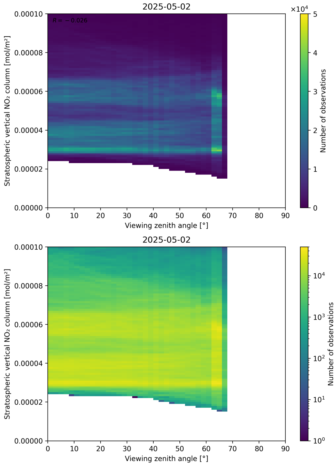
Figure 164: Scatter density plot of “Viewing zenith angle” against “Stratospheric vertical NO 2 column” for 2025-05-02 to 2025-05-02.
