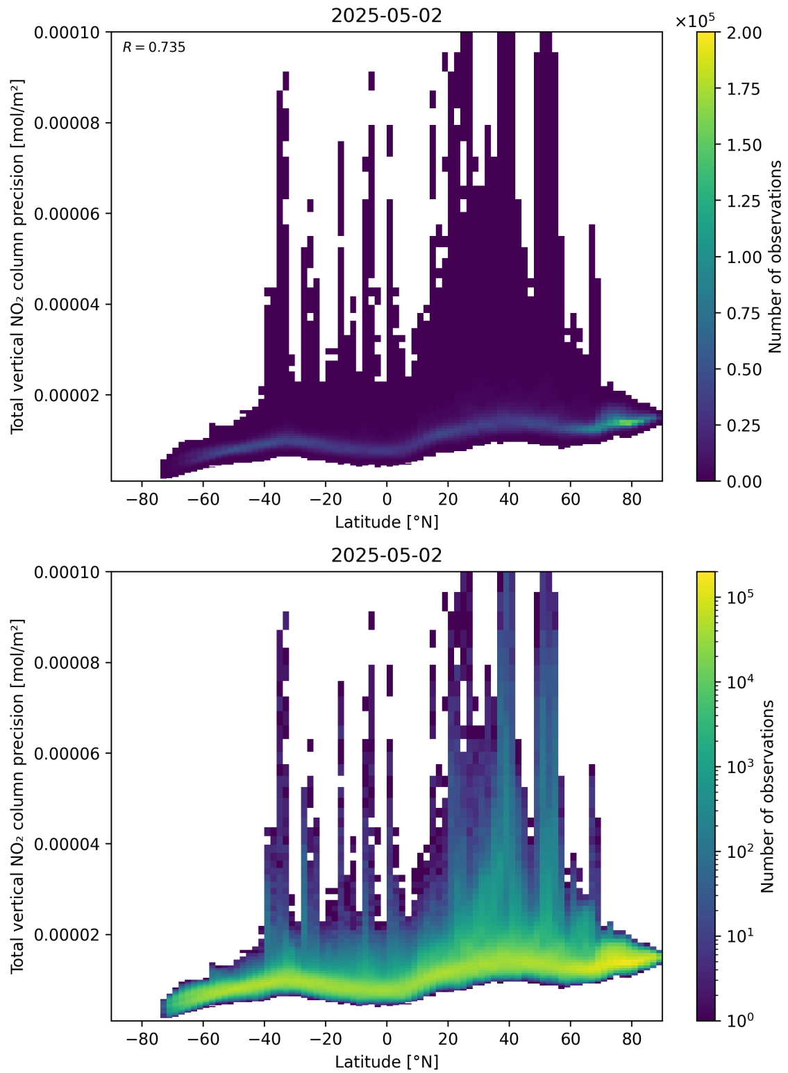
Figure 91: Scatter density plot of “Latitude” against “Total vertical NO 2 column precision” for 2025-05-02 to 2025-05-02.
