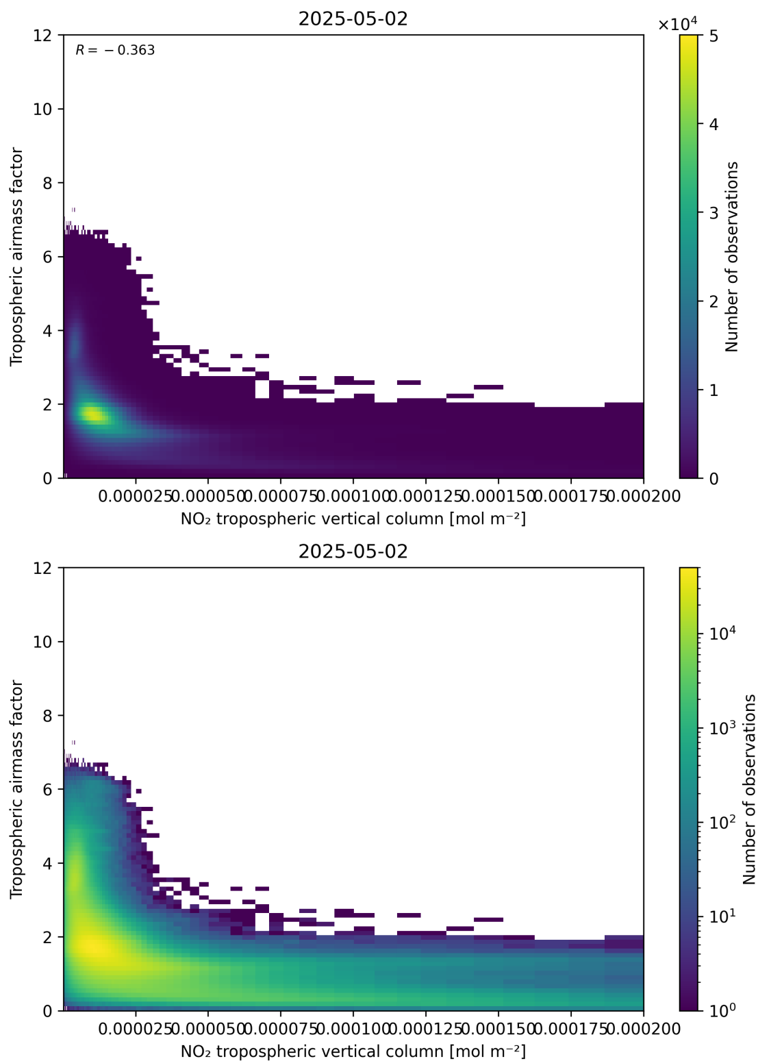
Figure 123: Scatter density plot of “NO 2 tropospheric vertical column” against “Tropospheric air mass factor” for 2025-05-02 to 2025-05-02.
