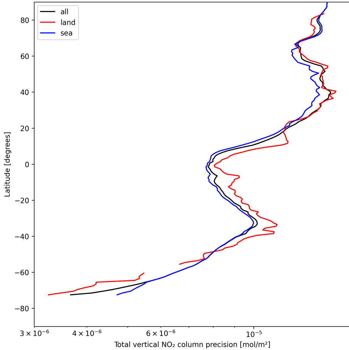
Figure 22: Zonal average of “Total vertical NO 2 column precision” for 2025-05-02 to 2025-05-02.
