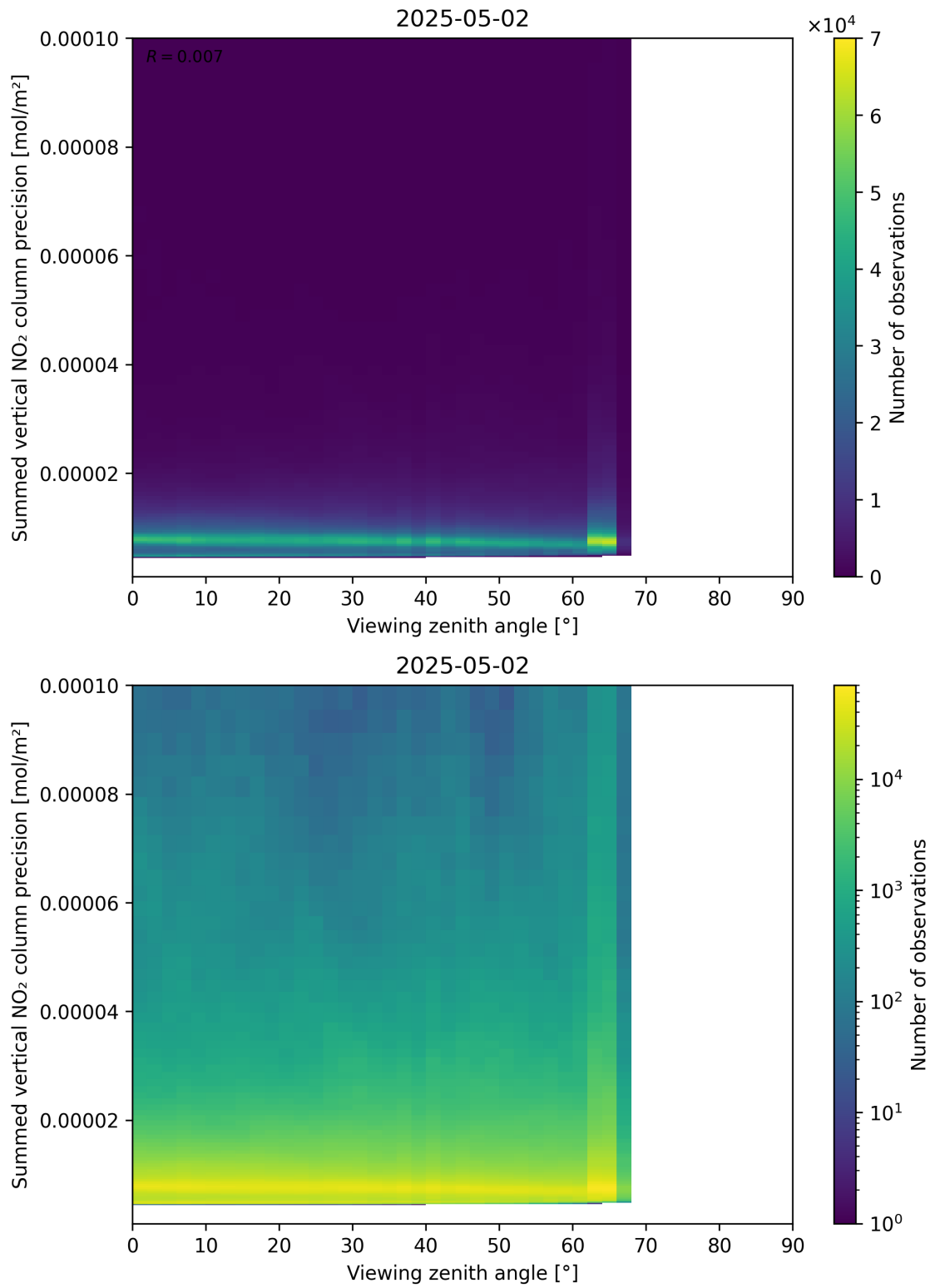
Figure 166: Scatter density plot of “Viewing zenith angle” against “Summed vertical NO 2 column precision” for 2025-05-02 to 2025-05-02.
