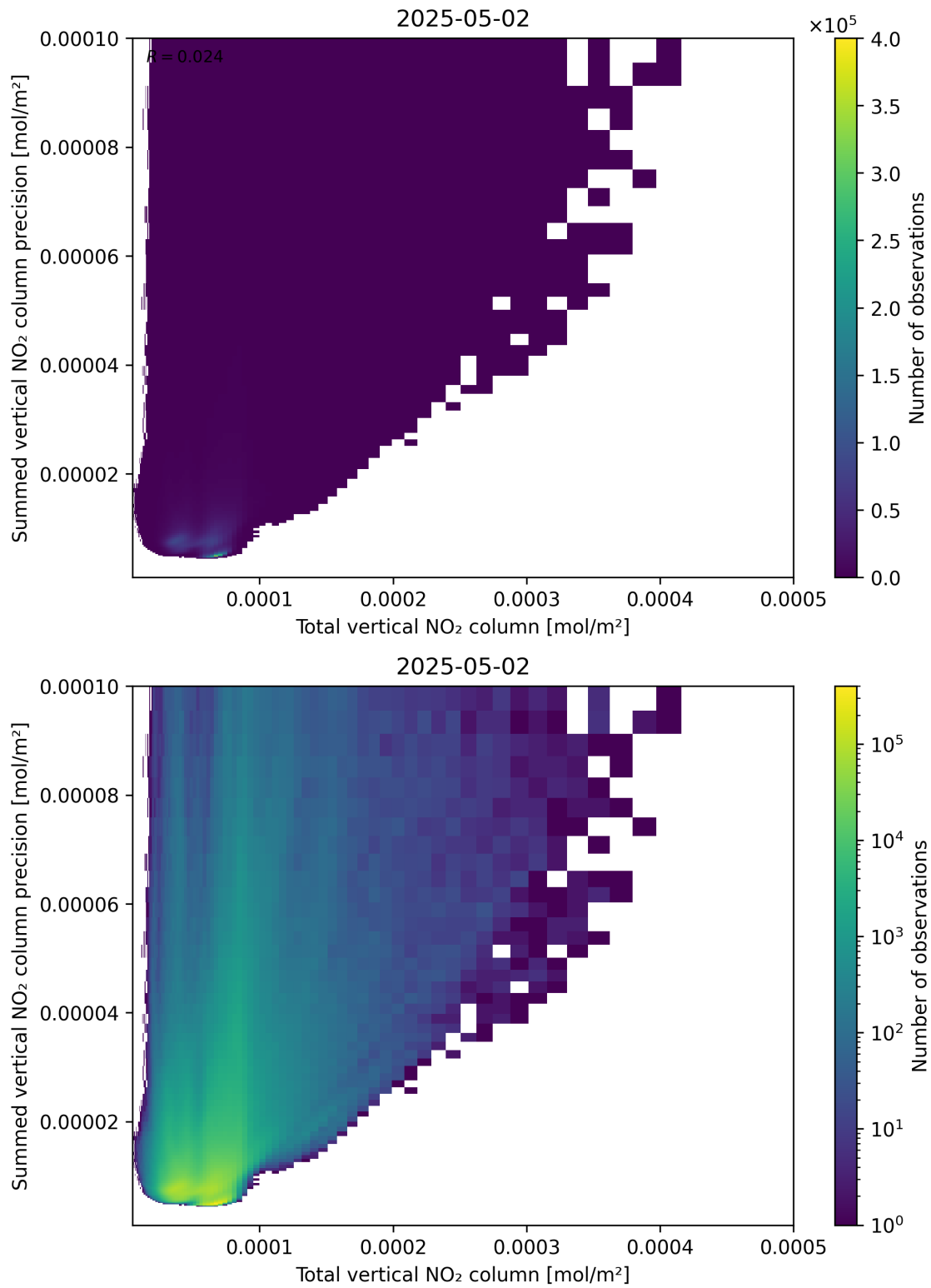
Figure 113: Scatter density plot of “Total vertical NO 2 column” against “Summed vertical NO 2 column precision” for 2025-05-02 to 2025-05-02.
