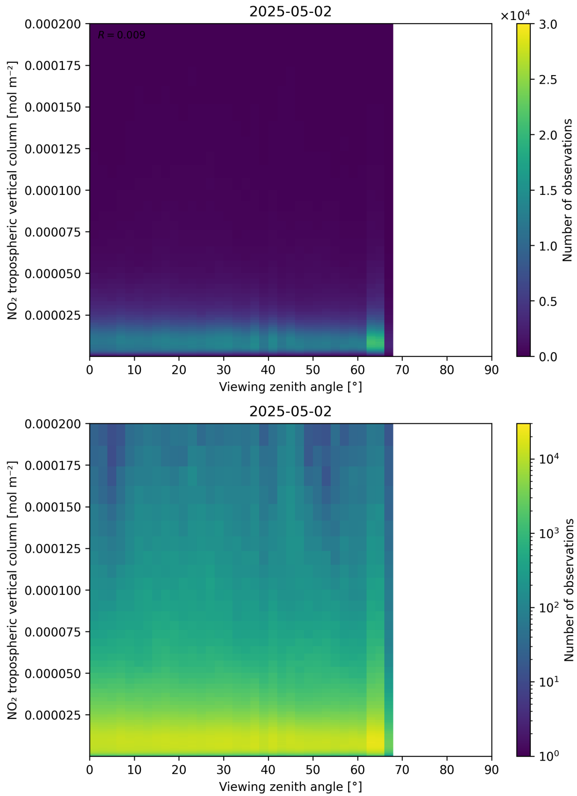
Figure 169: Scatter density plot of “Viewing zenith angle” against “NO 2 tropospheric vertical column” for 2025-05-02 to 2025-05-02.
