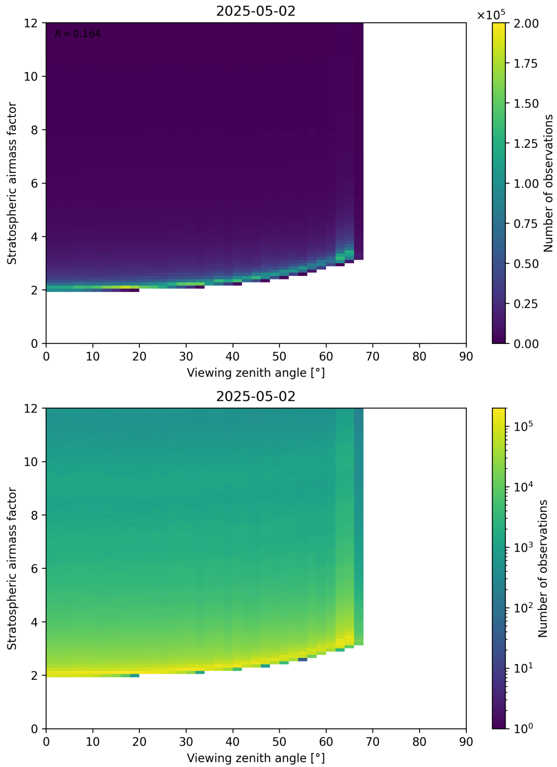
Figure 159: Scatter density plot of “Viewing zenith angle” against “Stratospheric airmass factor” for 2025-05-02 to 2025-05-02.
