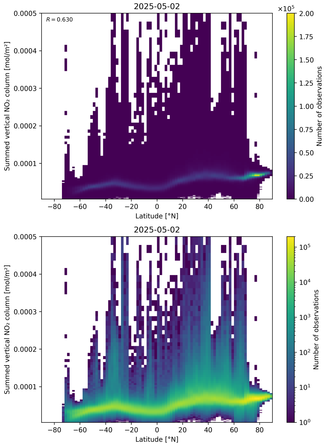
Figure 88: Scatter density plot of “Latitude” against “Summed vertical NO 2 column” for 2025-05-02 to 2025-05-02.
