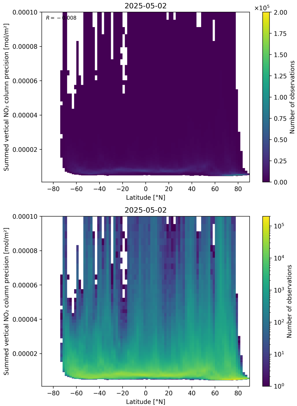
Figure 89: Scatter density plot of “Latitude” against “Summed vertical NO 2 column precision” for 2025-05-02 to 2025-05-02.
