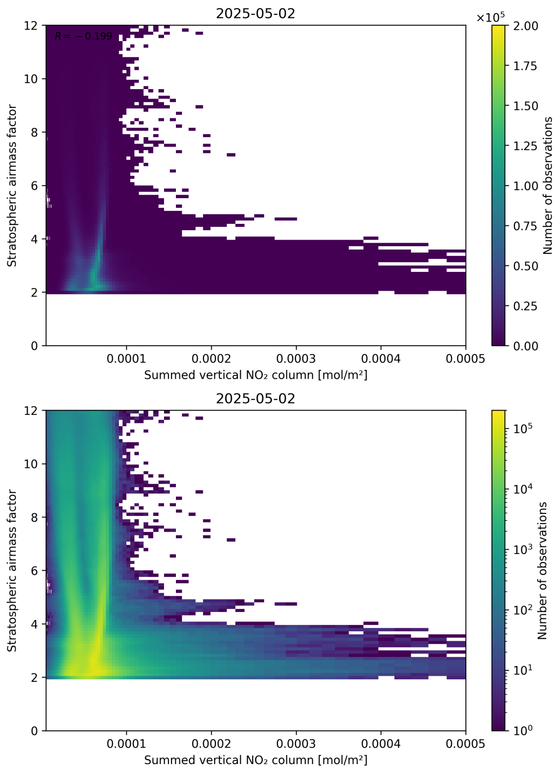
Figure 103: Scatter density plot of “Summed vertical NO 2 column” against “Stratospheric airmass factor” for 2025-05-02 to 2025-05-02.
