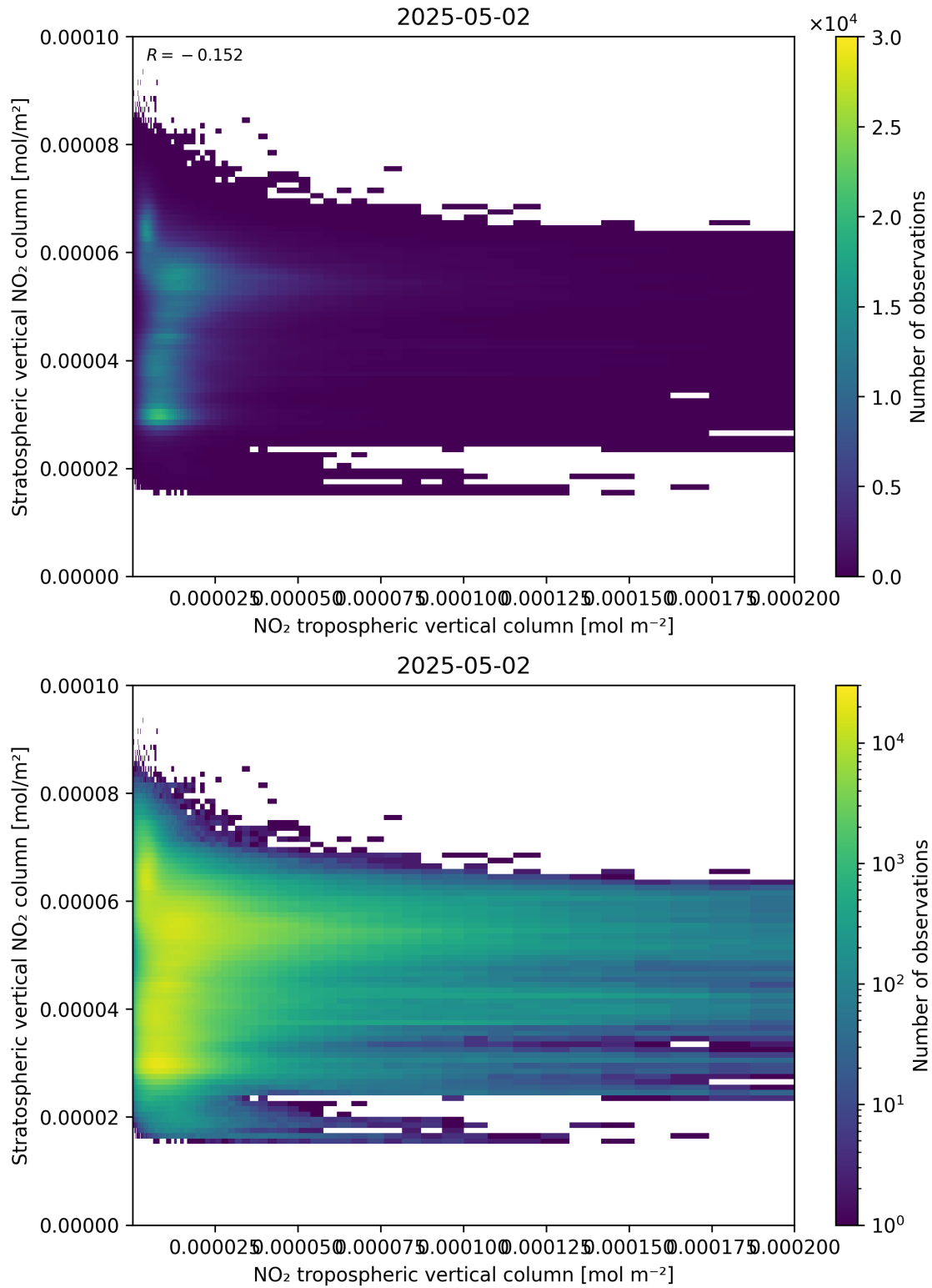
Figure 125: Scatter density plot of “NO 2 tropospheric vertical column” against “Stratospheric vertical NO 2 column” for 2025-05-02 to 2025-05-02.
