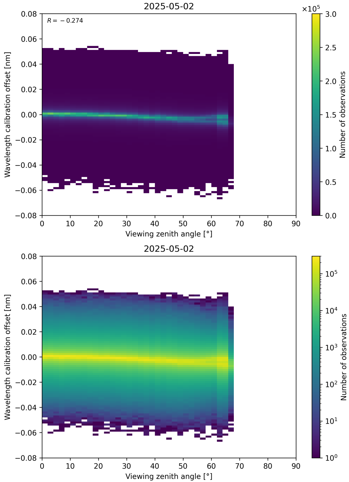
Figure 173: Scatter density plot of “Viewing zenith angle” against “Wavelength calibration offset” for 2025-05-02 to 2025-05-02.
