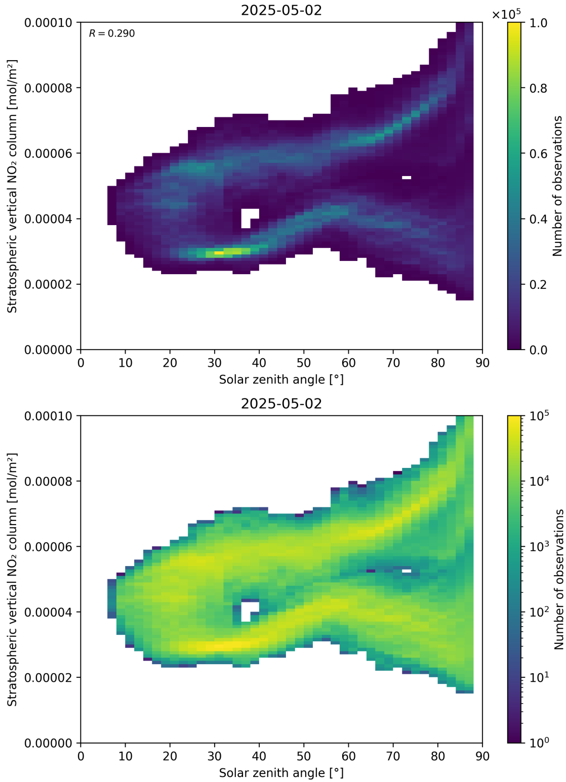
Figure 150: Scatter density plot of “Solar zenith angle” against “Stratospheric vertical NO 2 column” for 2025-05-02 to 2025-05-02.
