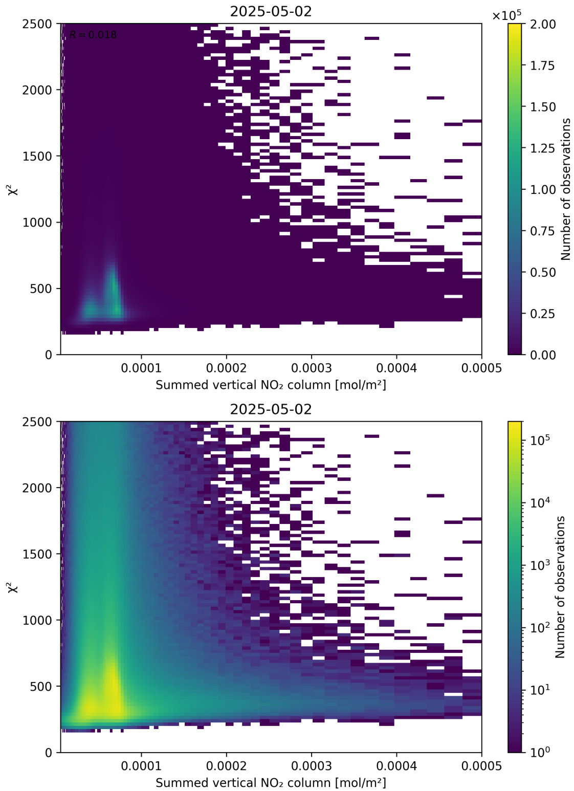
Figure 104: Scatter density plot of “Summed vertical NO 2 column” against “ \chi^2 ” for 2025-05-02 to 2025-05-02.
