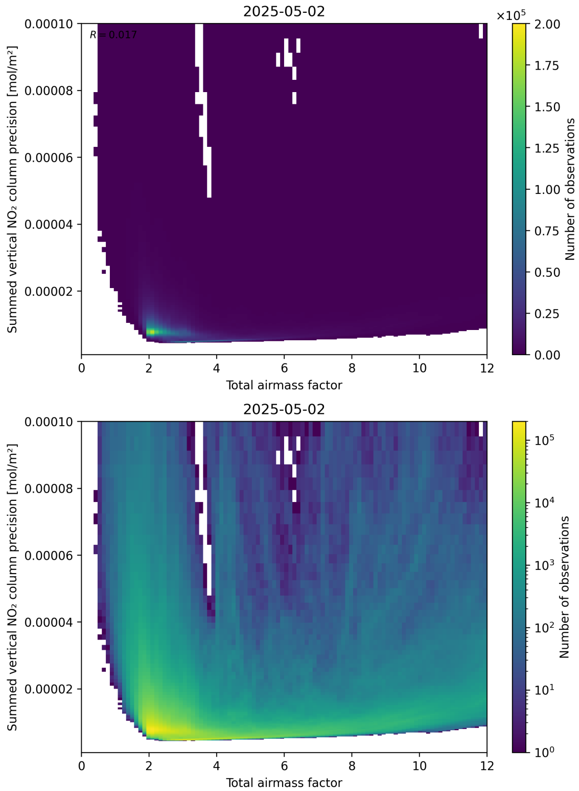
Figure 66: Scatter density plot of “Total airmass factor” against “Summed vertical NO 2 column precision” for 2025-05-02 to 2025-05-02.
