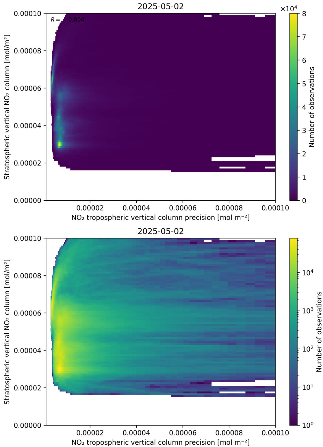
Figure 135: Scatter density plot of “NO 2 tropospheric vertical column precision” against “Stratospheric vertical NO 2 column” for 2025-05-02 to 2025-05-02.
