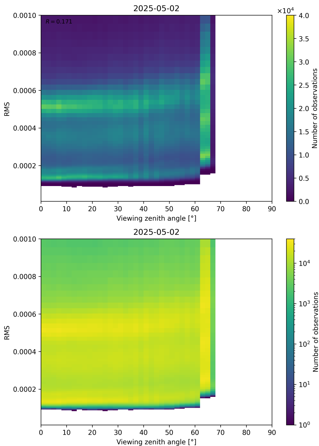
Figure 171: Scatter density plot of “Viewing zenith angle” against “RMS” for 2025-05-02 to 2025-05-02.
