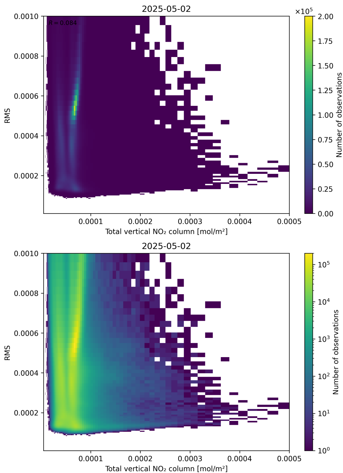
Figure 120: Scatter density plot of “Total vertical NO 2 column” against “RMS” for 2025-05-02 to 2025-05-02.
