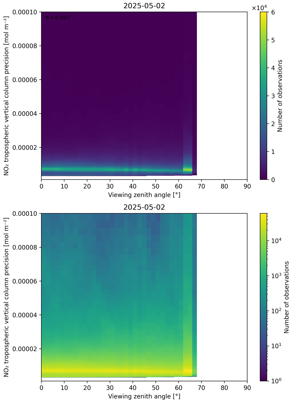
Figure 170: Scatter density plot of “Viewing zenith angle” against “NO 2 tropospheric vertical column precision” for 2025-05-02 to 2025-05-02.
