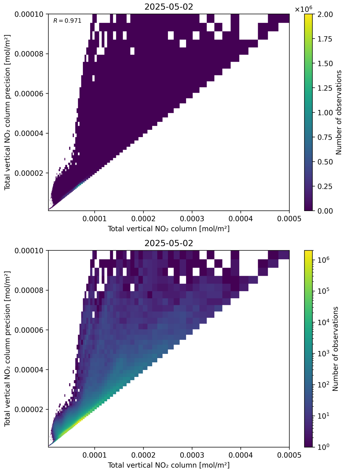
Figure 114: Scatter density plot of “Total vertical NO 2 column” against “Total vertical NO 2 column precision” for 2025-05-02 to 2025-05-02.
