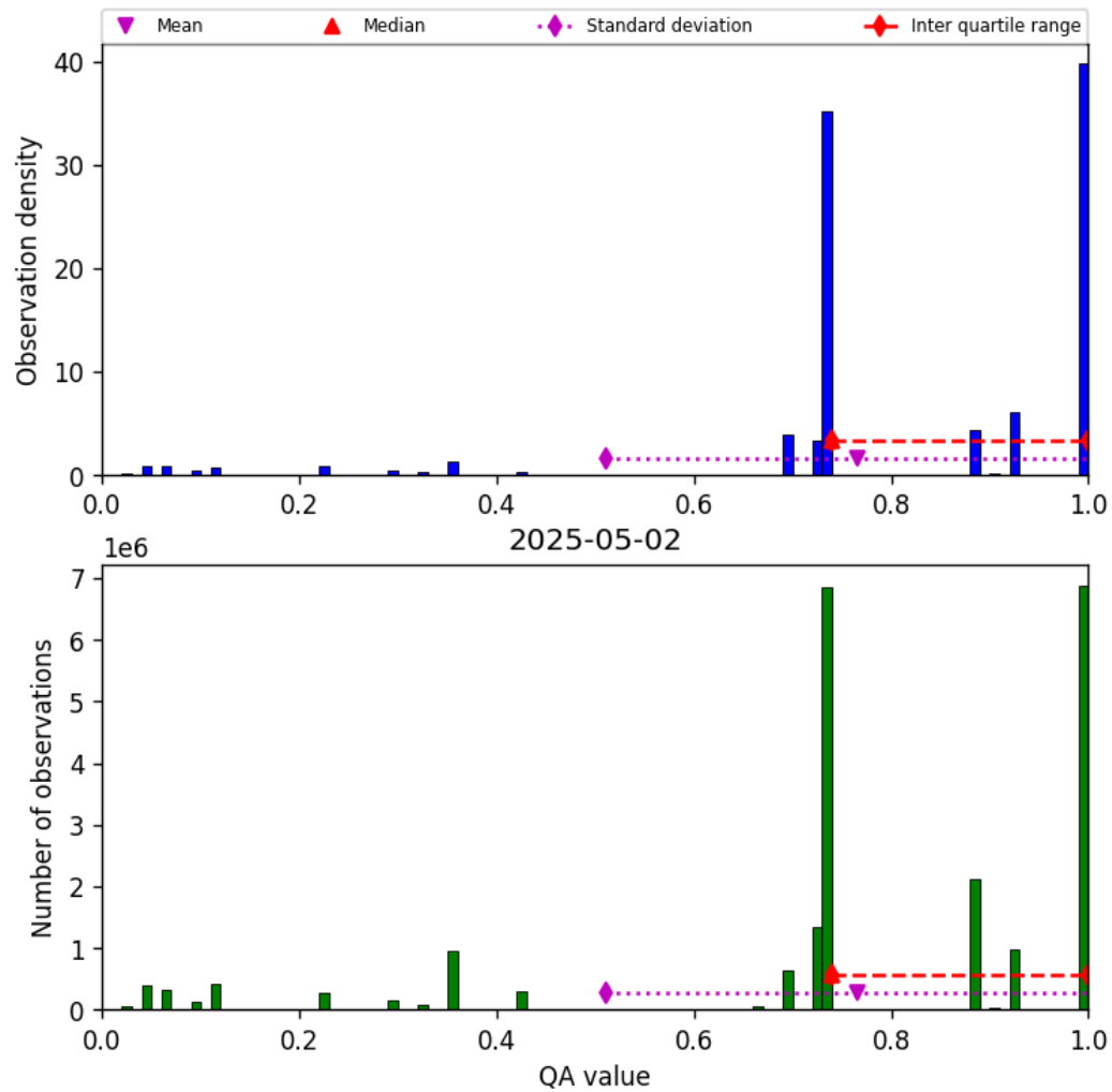
Figure 28: Histogram of “QA value” for 2025-05-02 to 2025-05-02
