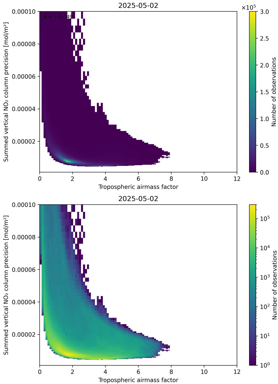
Figure 76: Scatter density plot of “Tropospheric air mass factor” against “Summed vertical NO 2 column precision” for 2025-05-02 to 2025-05-02.
