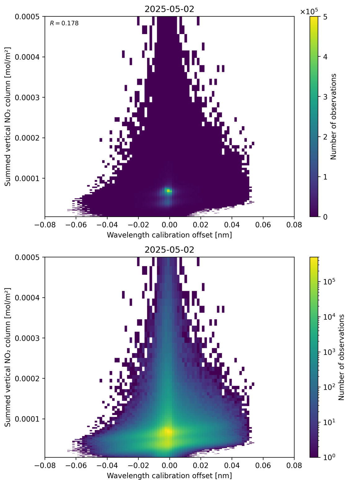
Figure 177: Scatter density plot of “Wavelength calibration offset” against “Summed vertical NO 2 column” for 2025-05-02 to 2025-05-02.
