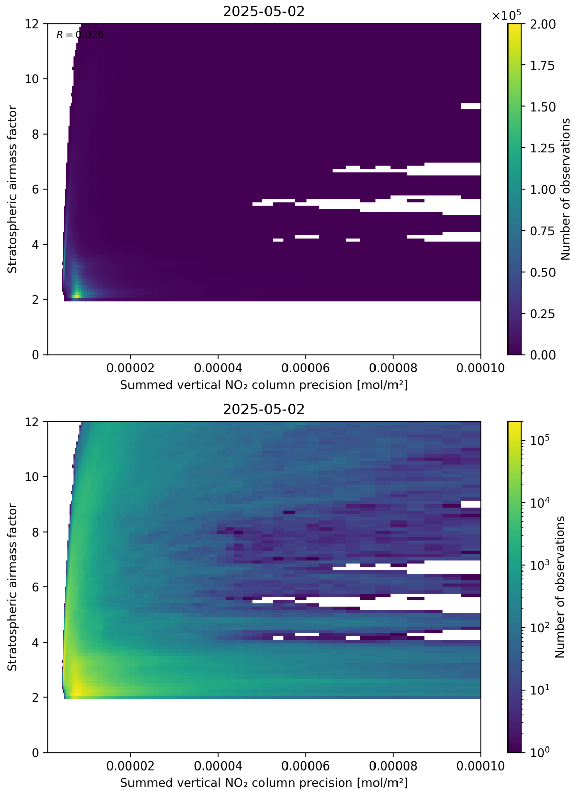
Figure 106: Scatter density plot of “Summed vertical NO 2 column precision” against “Stratospheric airmass factor” for 2025-05-02 to 2025-05-02.
