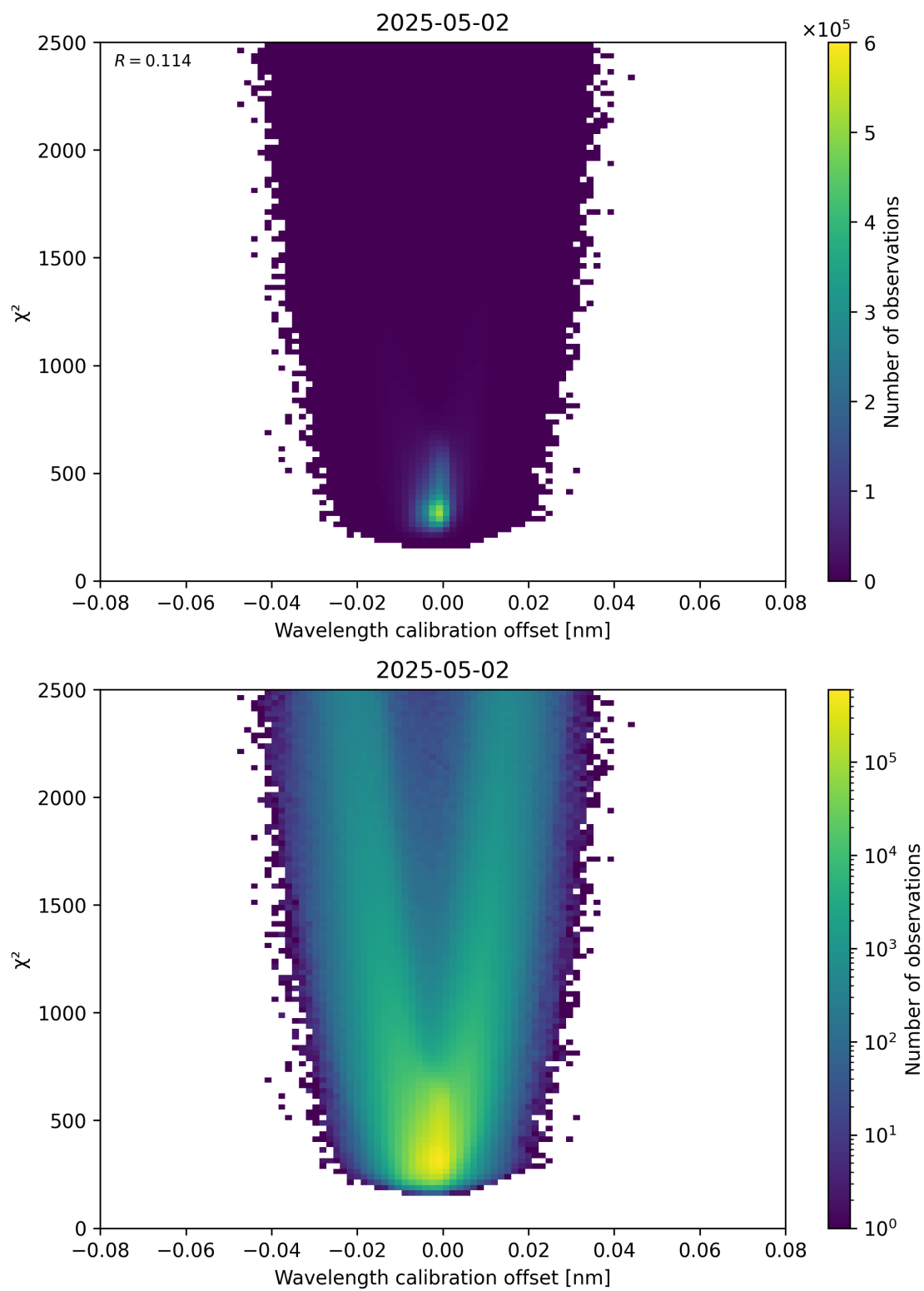
Figure 175: Scatter density plot of “Wavelength calibration offset” against “ \chi^2 ” for 2025-05-02 to 2025-05-02.
