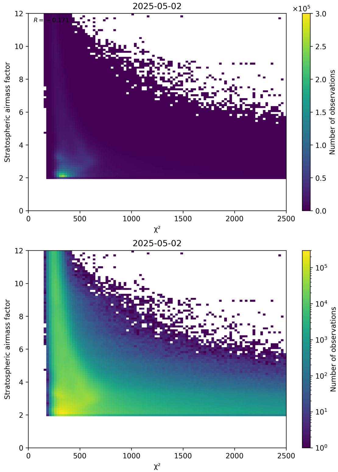
Figure 81: Scatter density plot of " \chi^2 " against "Stratospheric airmass factor" for 2025-05-02 to 2025-05-02.
