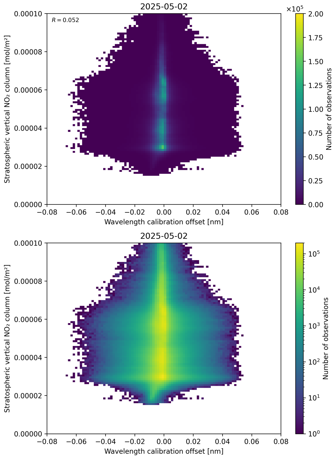
Figure 176: Scatter density plot of “Wavelength calibration offset” against “Stratospheric vertical NO 2 column” for 2025-05-02 to 2025-05-02.
