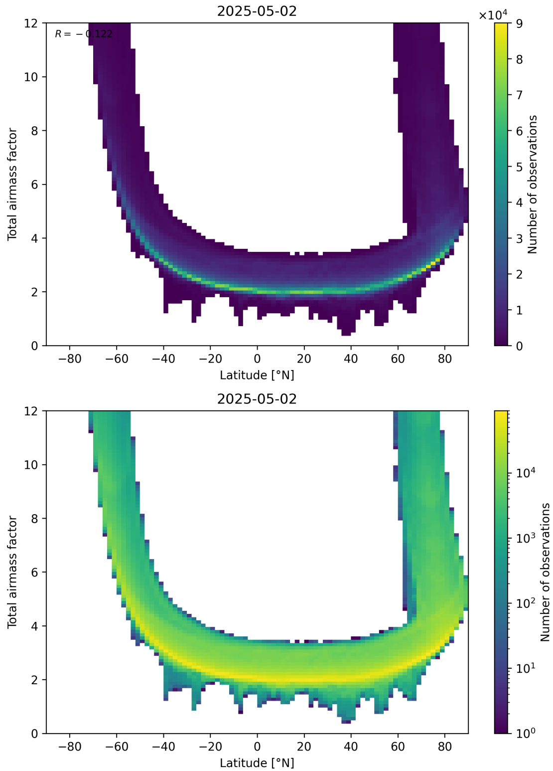
Figure 84: Scatter density plot of “Latitude” against “Total air mass factor” for 2025-05-02 to 2025-05-02.
