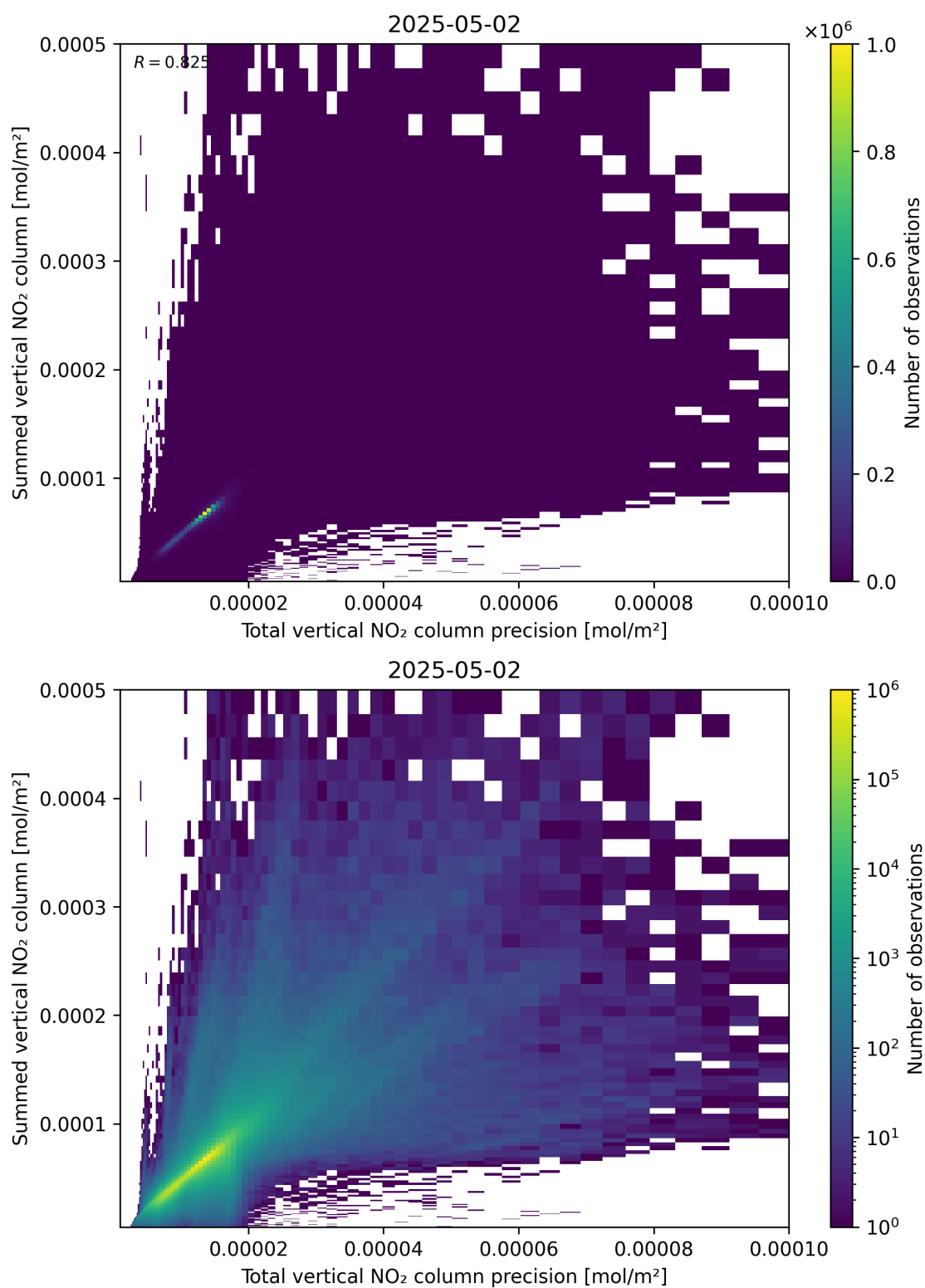
Figure 117: Scatter density plot of “Total vertical NO 2 column precision” against “Summed vertical NO 2 column” for 2025-05-02 to 2025-05-02.
