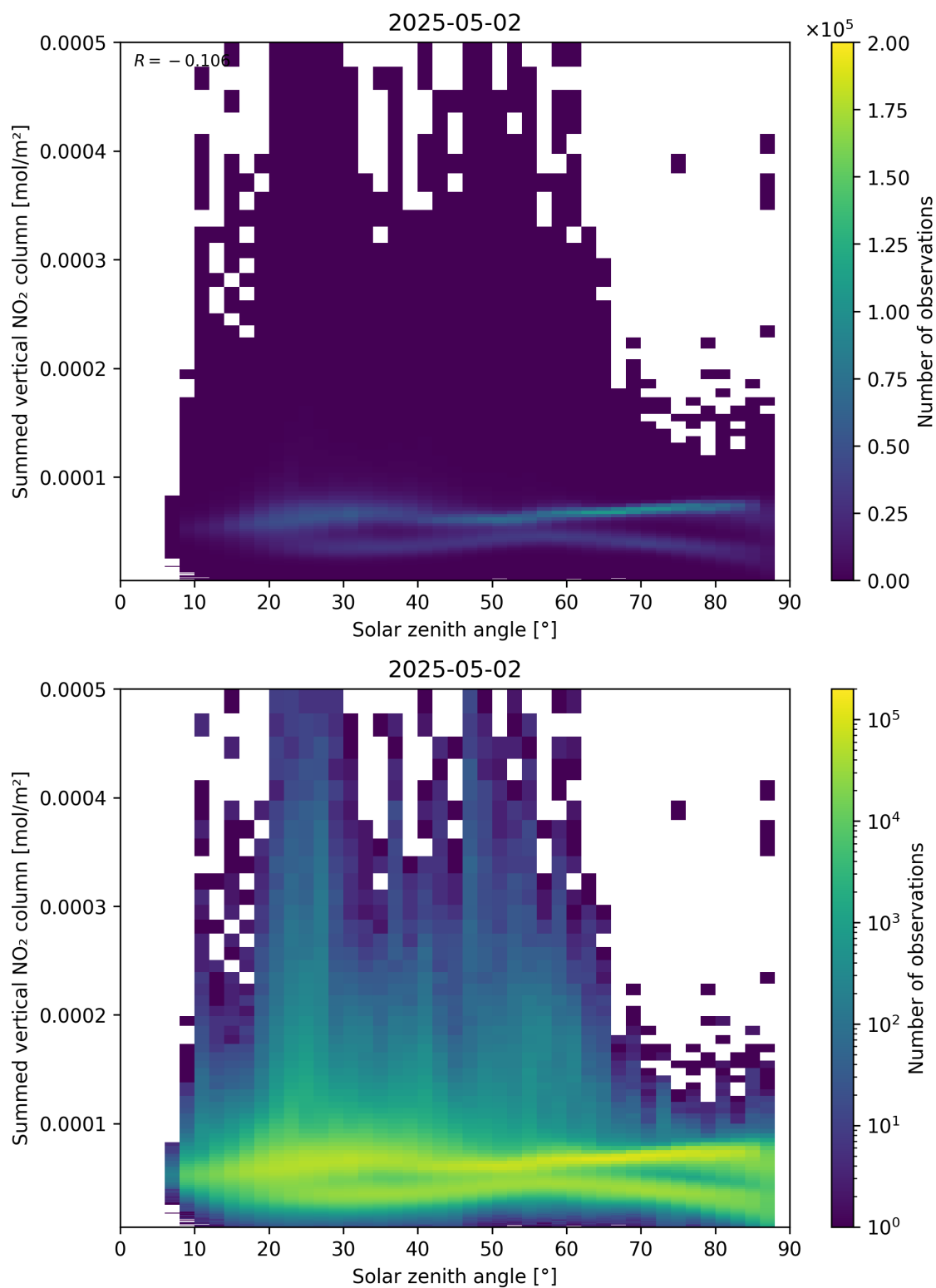
Figure 151: Scatter density plot of “Solar zenith angle” against “Summed vertical NO 2 column” for 2025-05-02 to 2025-05-02.
