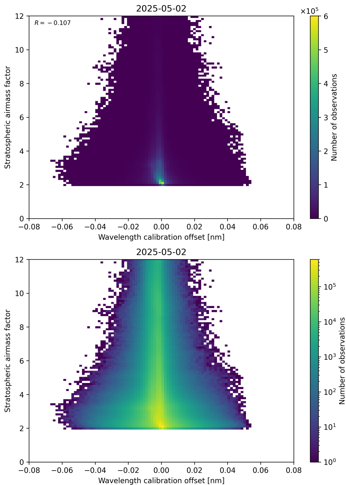
Figure 174: Scatter density plot of “Wavelength calibration offset” against “Stratospheric airmass factor” for 2025-05-02 to 2025-05-02.
