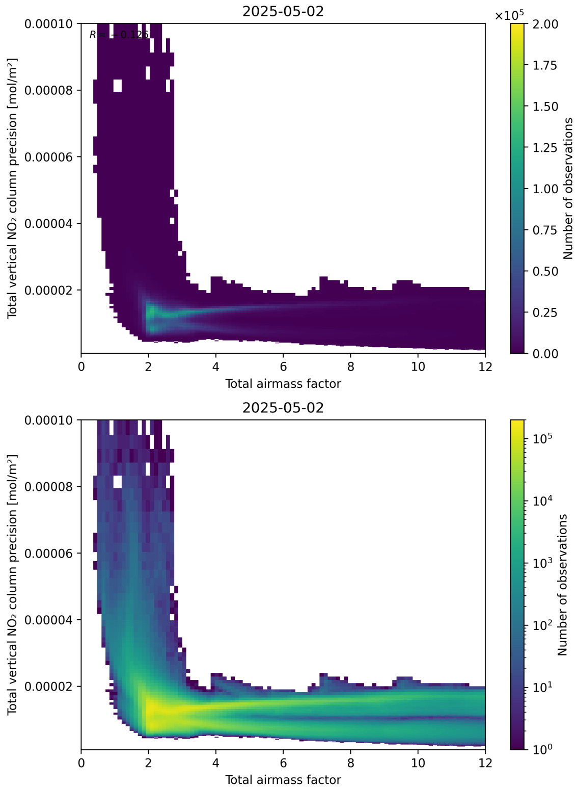
Figure 68: Scatter density plot of “Total airmass factor” against “Total vertical NO 2 column precision” for 2025-05-02 to 2025-05-02.
