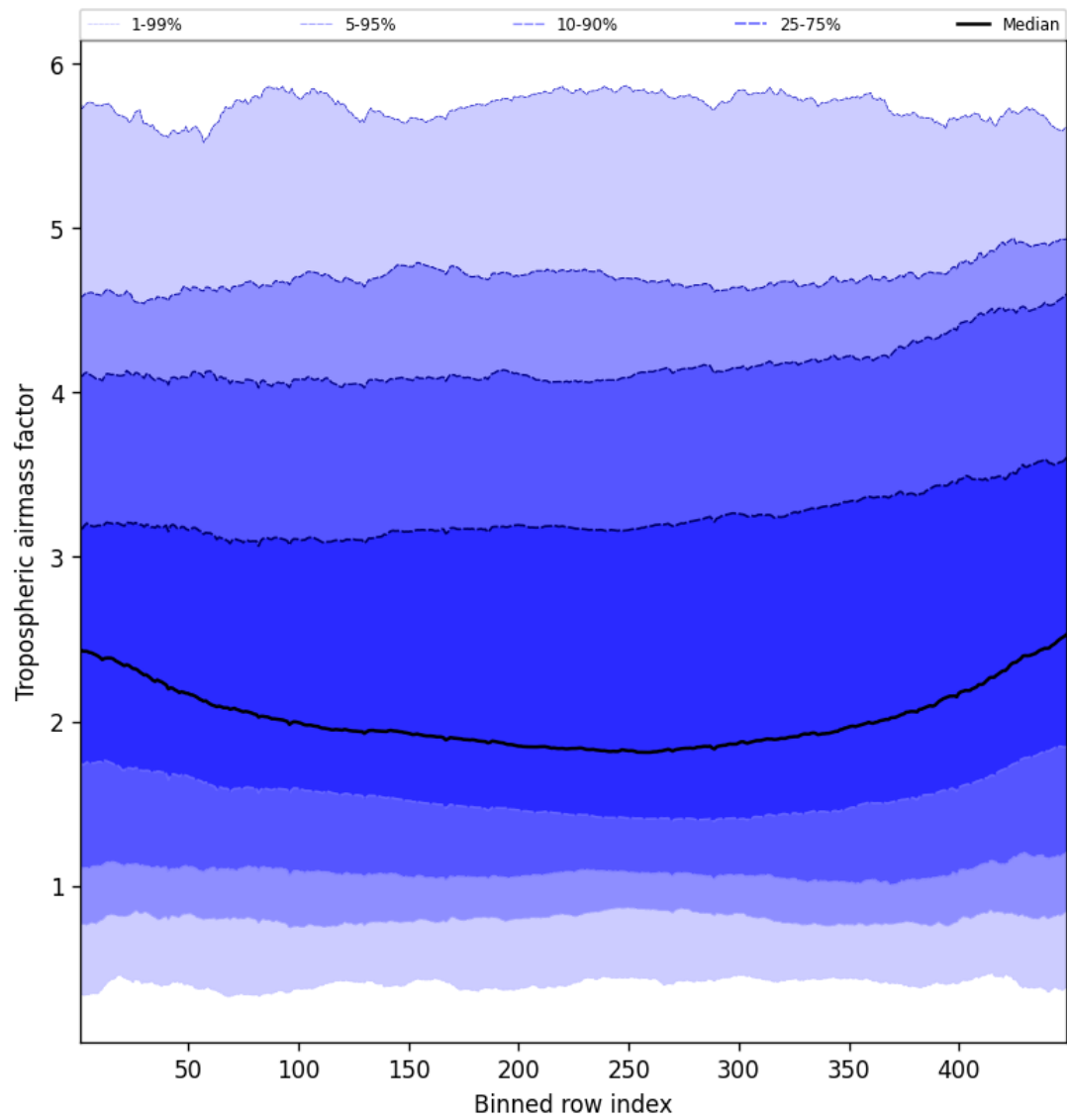
Figure 48: Along track statistics of “Tropospheric airmass factor” for 2025-05-02 to 2025-05-02
