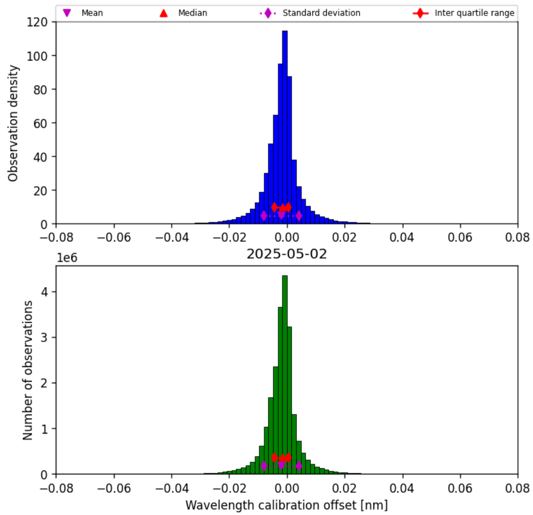
Figure 35: Histogram of “Wavelength calibration offset” for 2025-05-02 to 2025-05-02
