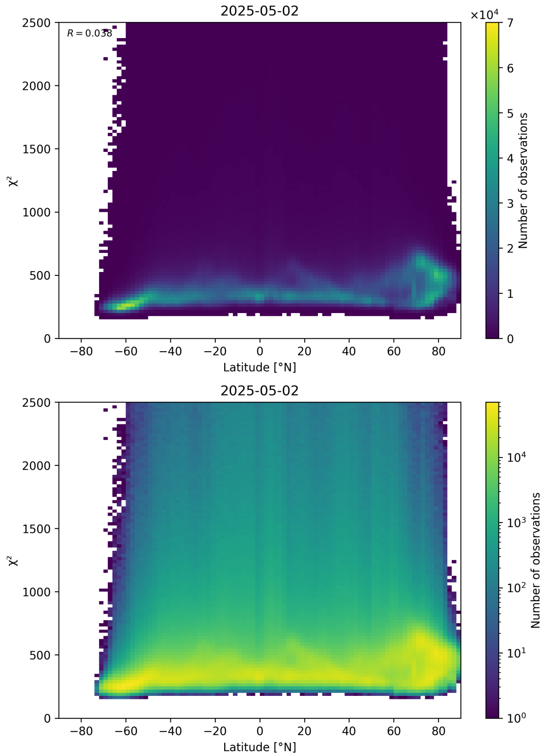
Figure 86: Scatter density plot of “Latitude” against “ \chi^2 ” for 2025-05-02 to 2025-05-02.
