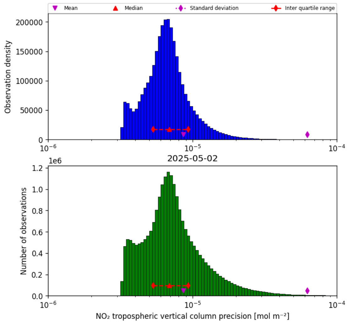
Figure 30: Histogram of “NO 2 tropospheric vertical column precision” for 2025-05-02 to 2025-05-02
