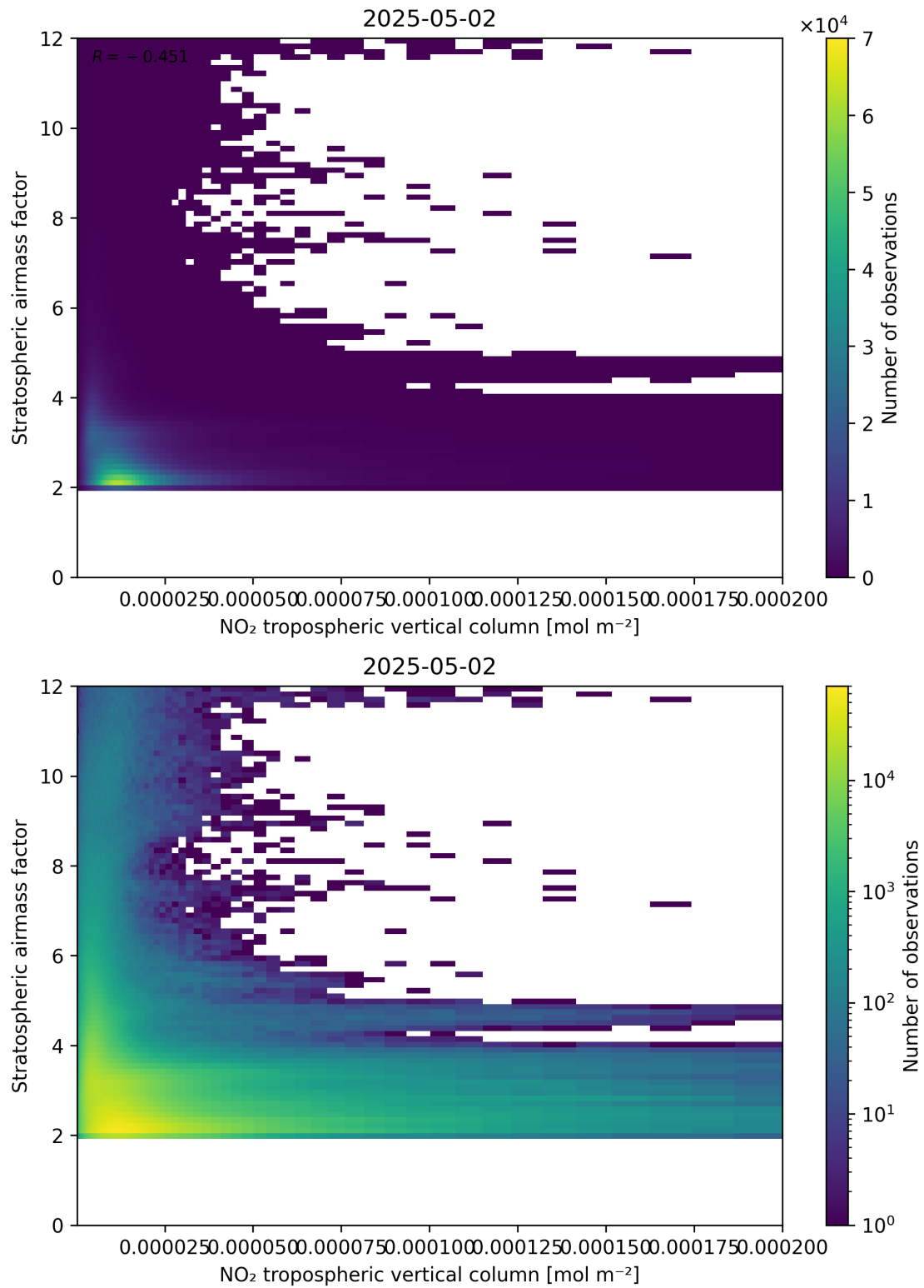
Figure 121: Scatter density plot of “NO 2 tropospheric vertical column” against “Stratospheric air mass factor” for 2025-05-02 to 2025-05-02.
