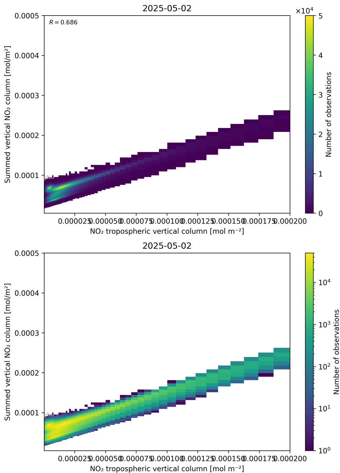
Figure 126: Scatter density plot of “NO 2 tropospheric vertical column” against “Summed vertical NO 2 column” for 2025-05-02 to 2025-05-02.
