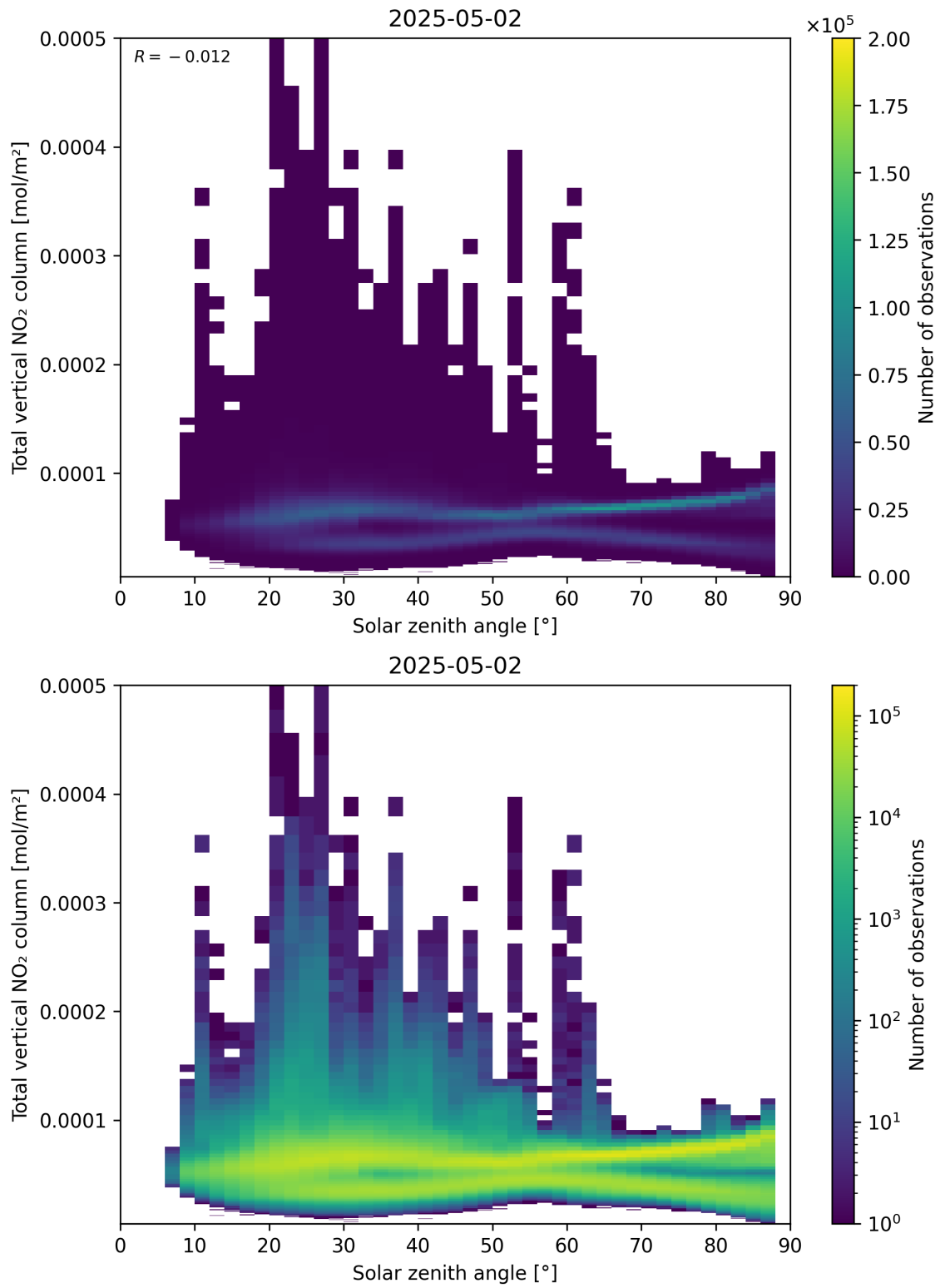
Figure 153: Scatter density plot of “Solar zenith angle” against “Total vertical NO 2 column” for 2025-05-02 to 2025-05-02.
