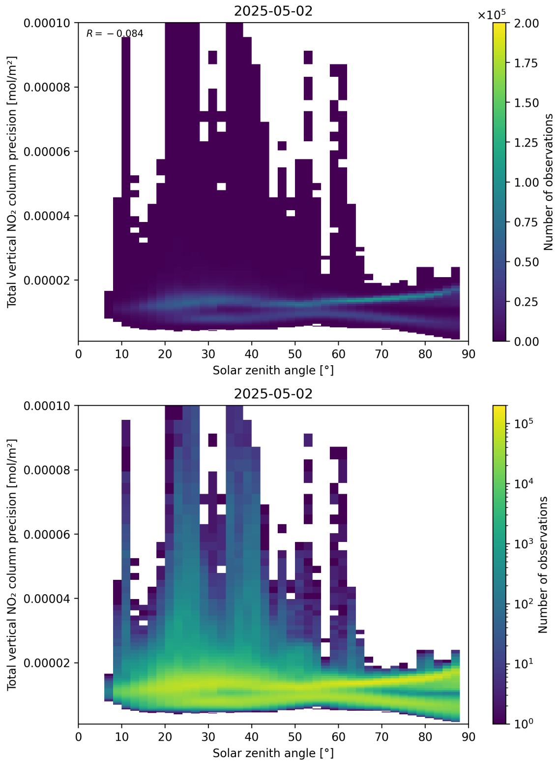
Figure 154: Scatter density plot of “Solar zenith angle” against “Total vertical NO 2 column precision” for 2025-05-02 to 2025-05-02.
