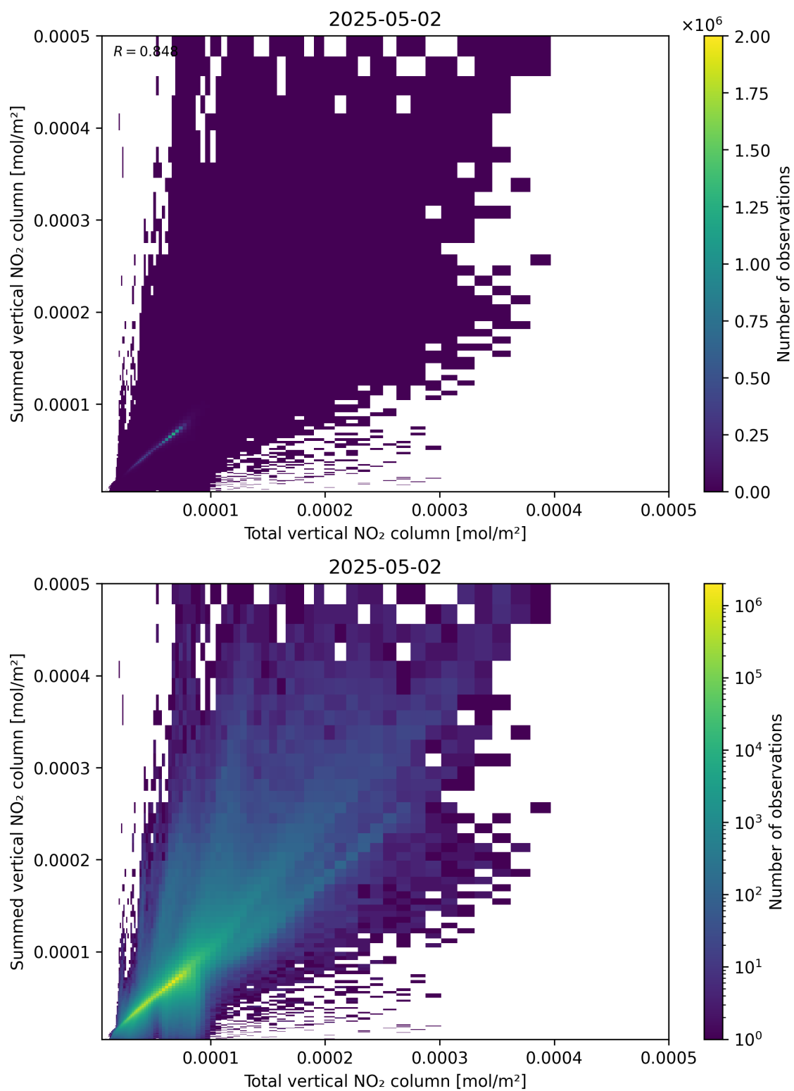
Figure 112: Scatter density plot of “Total vertical NO 2 column” against “Summed vertical NO 2 column” for 2025-05-02 to 2025-05-02.
