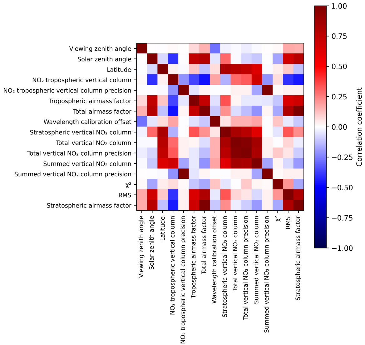
Figure 2: Map of correlation matrix for 2025-05-02 to 2025-05-02.
