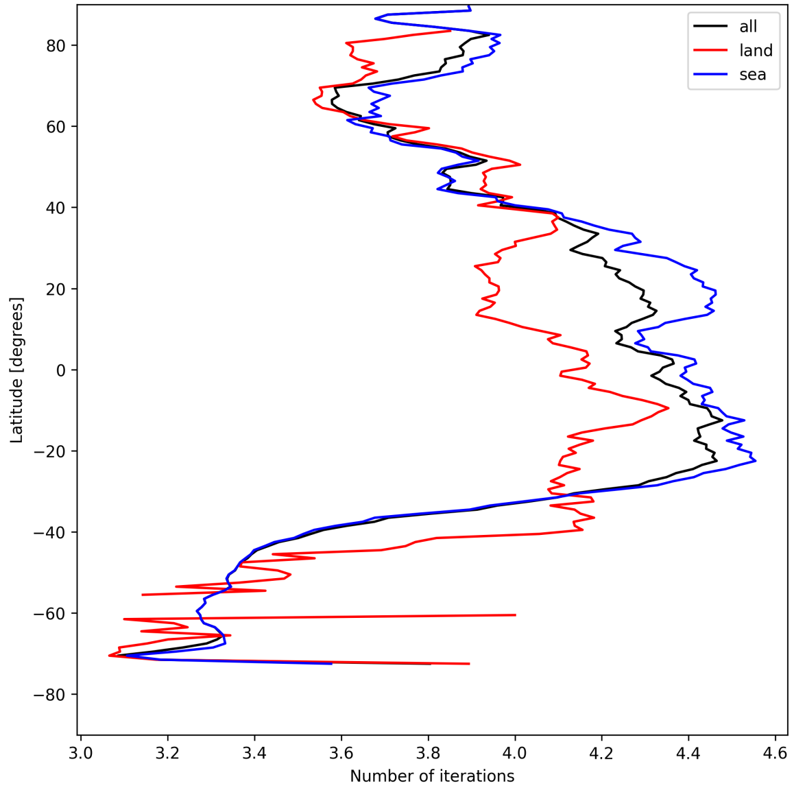
Figure 17: Zonal average of “Number of iterations” for 2025-05-02 to 2025-05-02.
