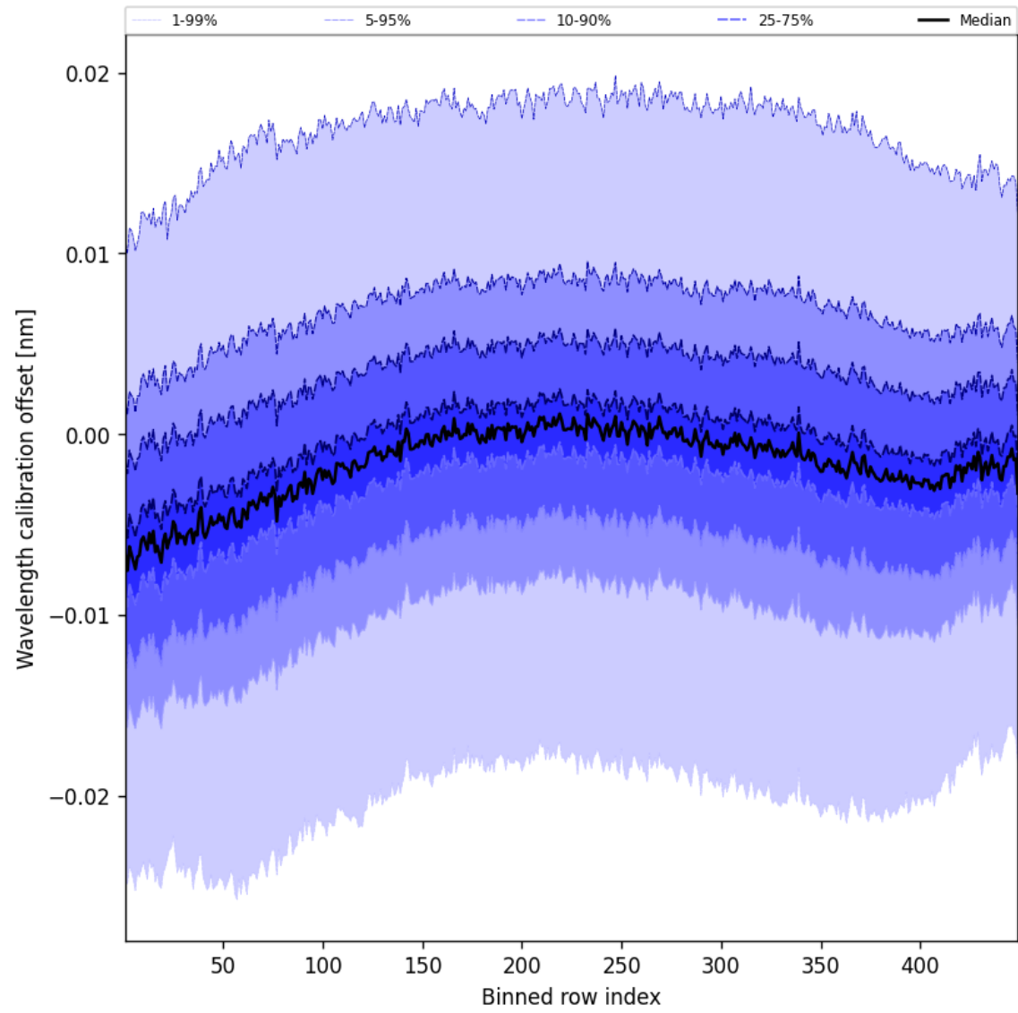
Figure 52: Along track statistics of “Wavelength calibration offset” for 2025-05-02 to 2025-05-02
