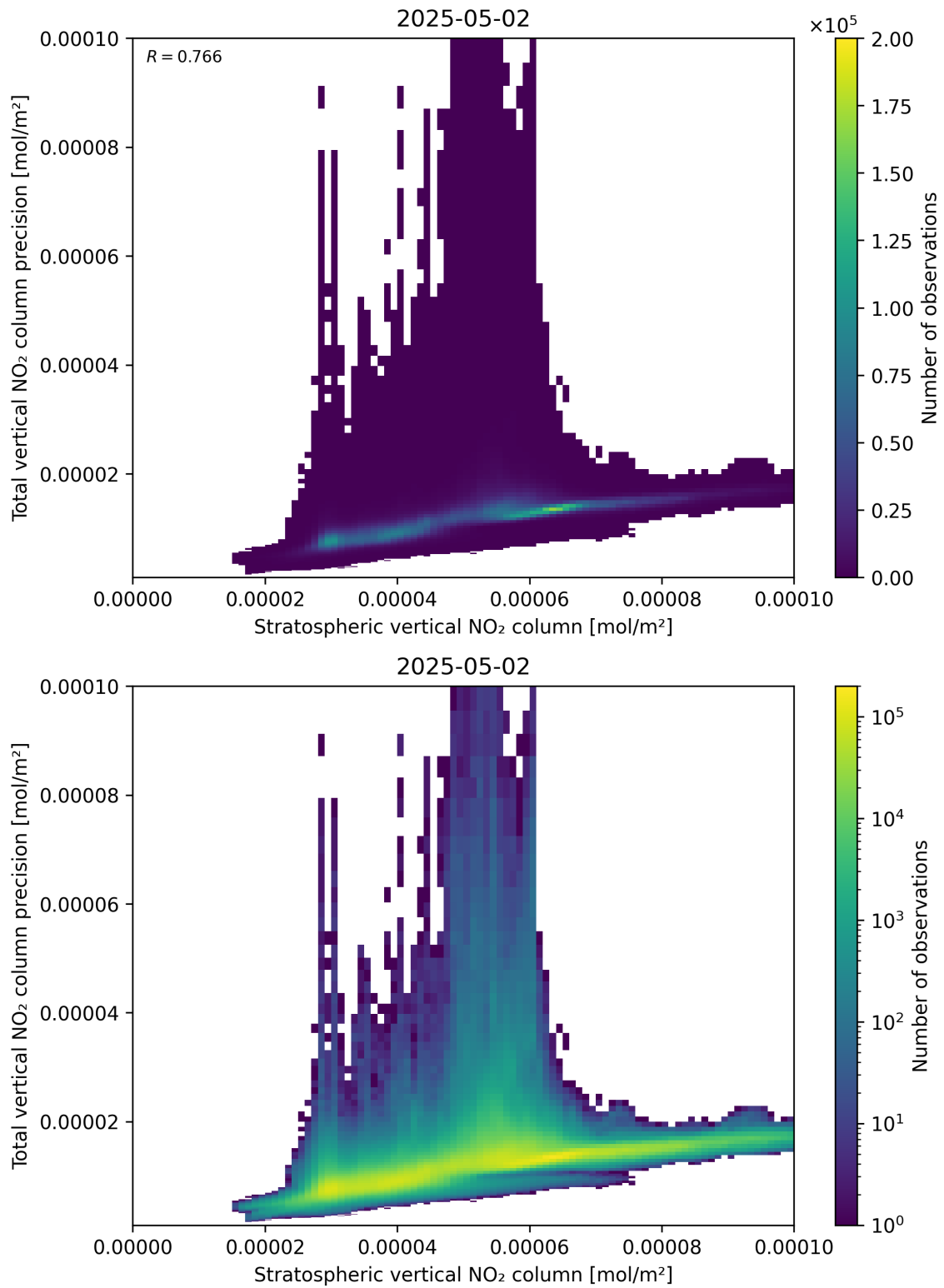
Figure 101: Scatter density plot of “Stratospheric vertical NO 2 column” against “Total vertical NO 2 column precision” for 2025-05-02 to 2025-05-02.
