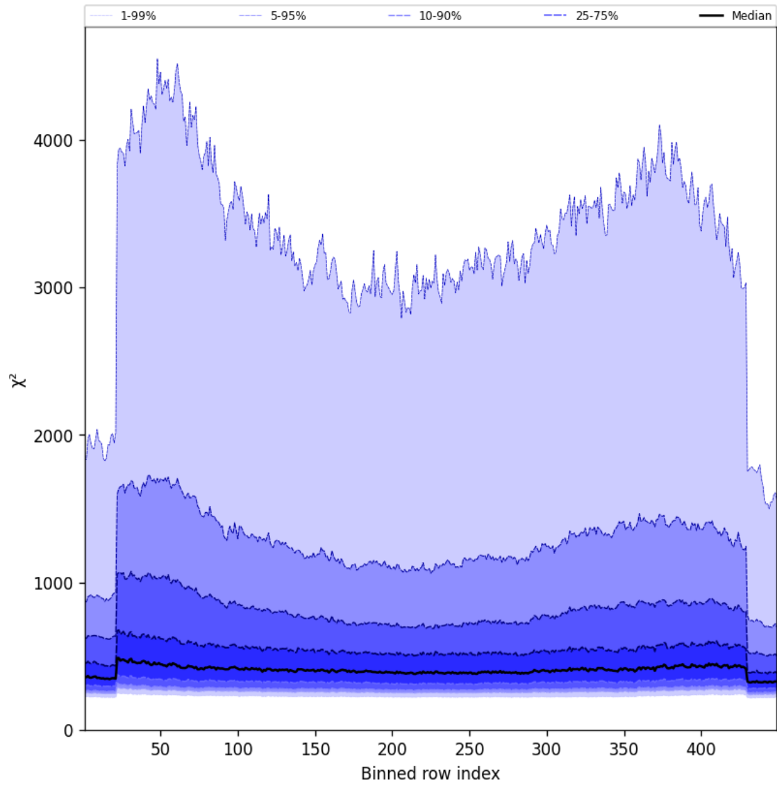
Figure 59: Along track statistics of “ \chi^2 ” for 2025-05-02 to 2025-05-02
