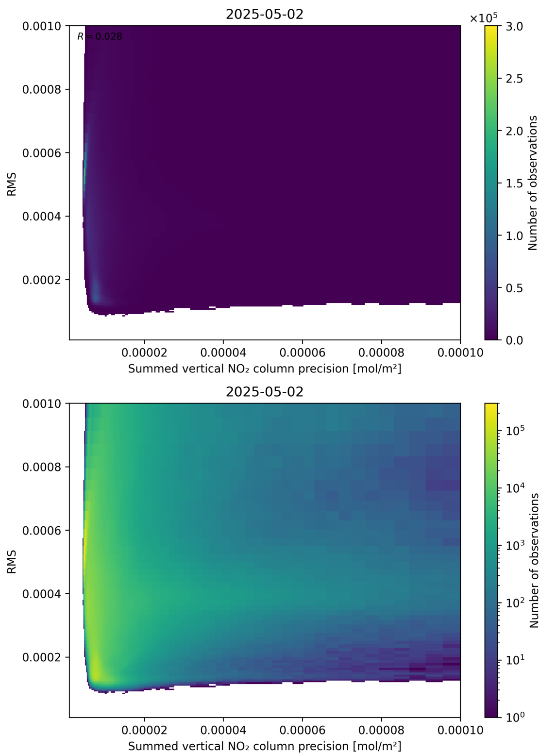
Figure 108: Scatter density plot of “Summed vertical NO 2 column precision” against “RMS” for 2025-05-02 to 2025-05-02.
