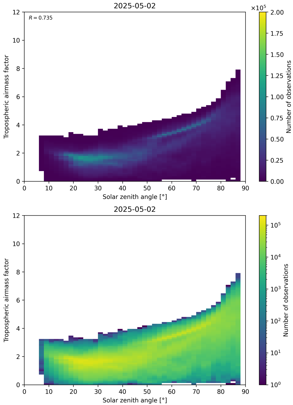
Figure 147: Scatter density plot of “Solar zenith angle” against “Tropospheric airmass factor” for 2025-05-02 to 2025-05-02.
