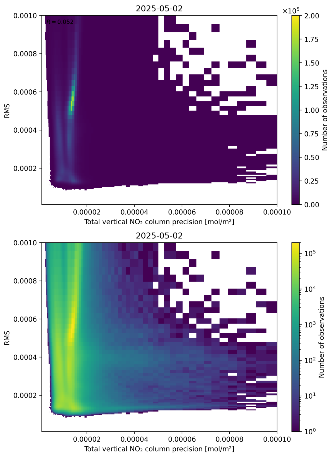
Figure 119: Scatter density plot of “Total vertical NO 2 column precision” against “RMS” for 2025-05-02 to 2025-05-02.
