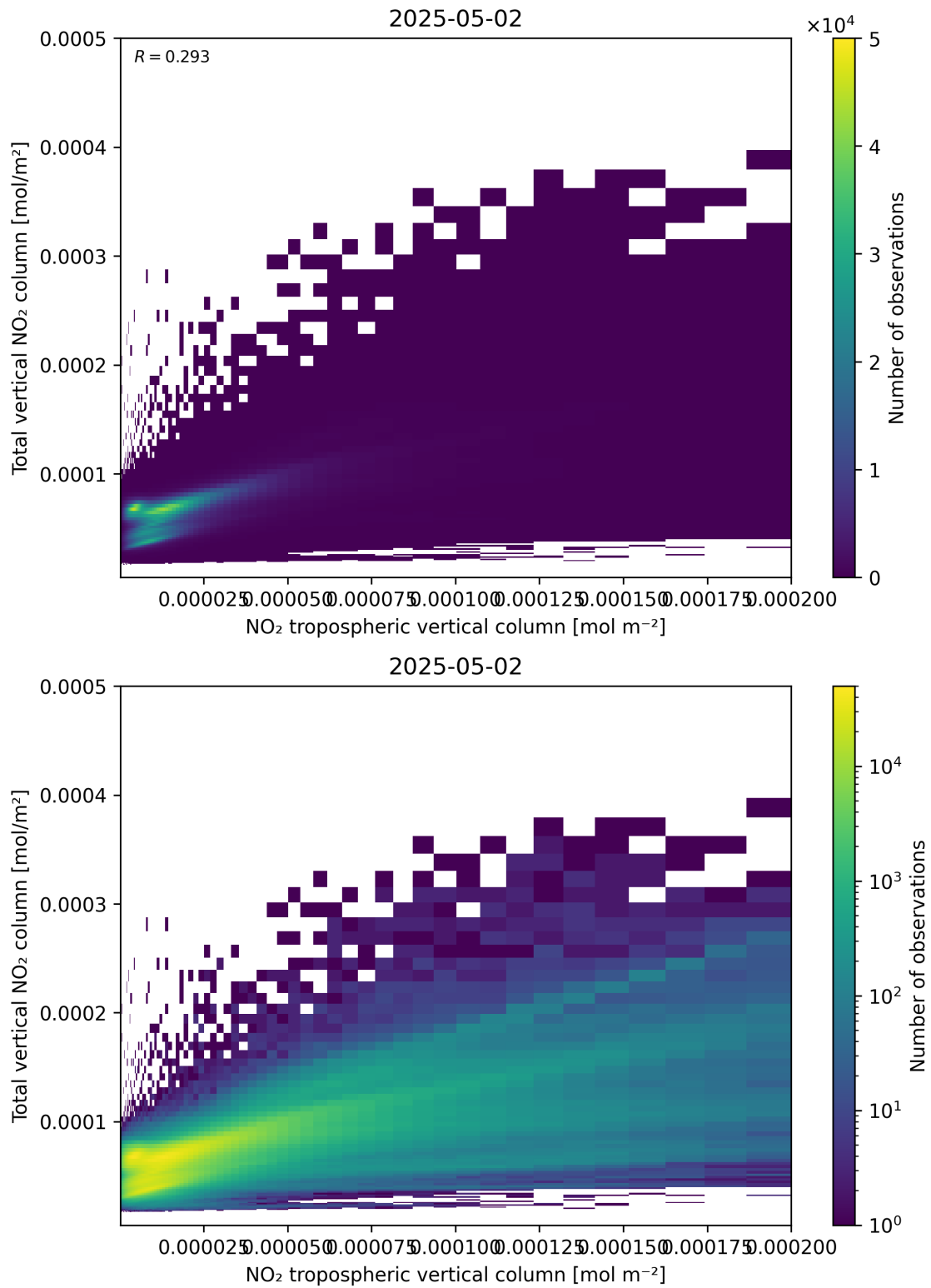
Figure 128: Scatter density plot of “NO 2 tropospheric vertical column” against “Total vertical NO 2 column” for 2025-05-02 to 2025-05-02.
