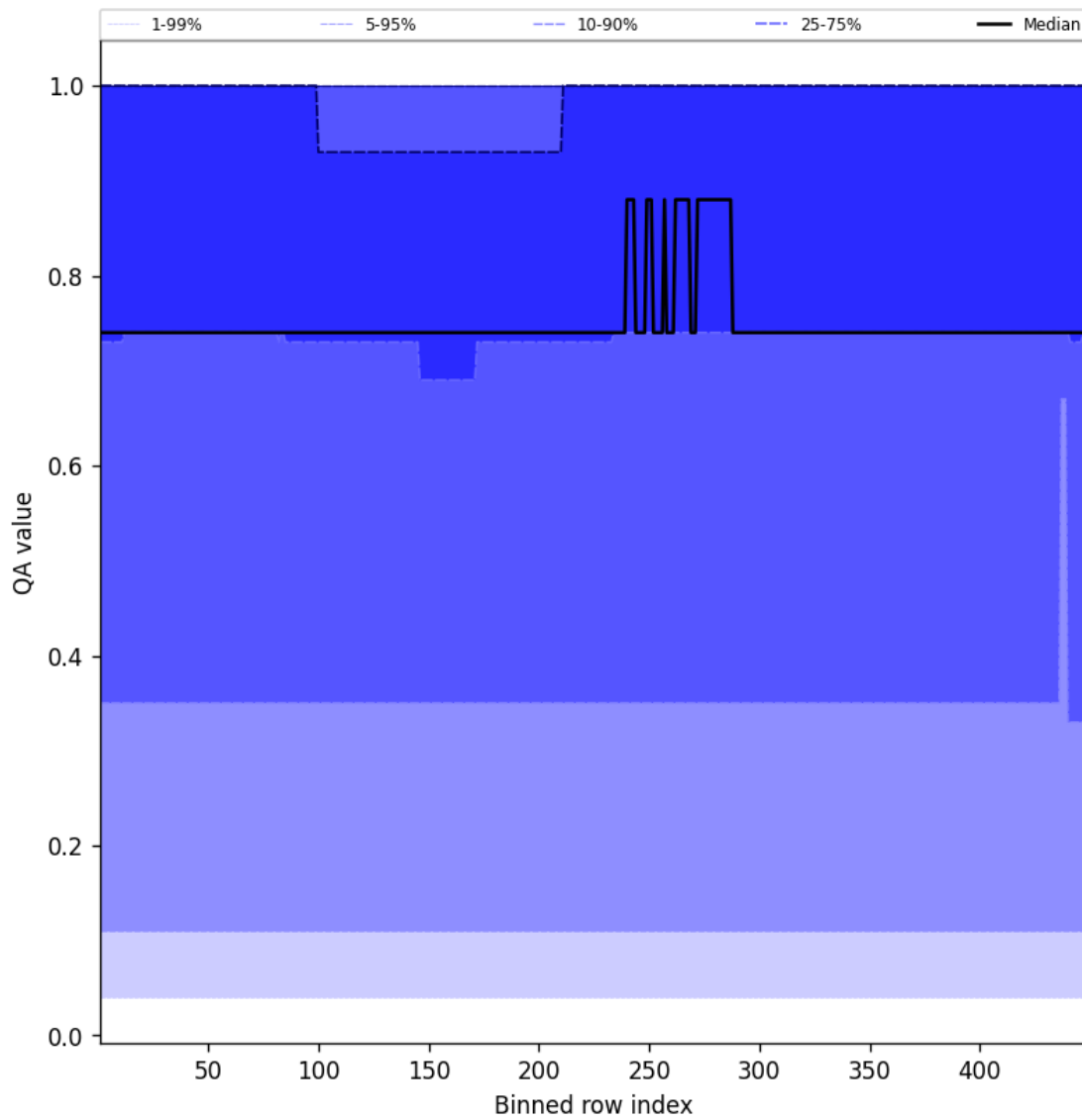
Figure 45: Along track statistics of “QA value” for 2025-05-02 to 2025-05-02
