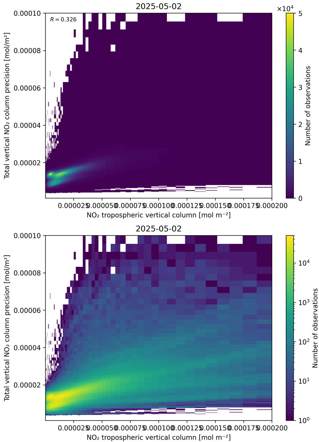
Figure 129: Scatter density plot of “NO 2 tropospheric vertical column” against “Total vertical NO 2 column precision” for 2025-05-02 to 2025-05-02.
