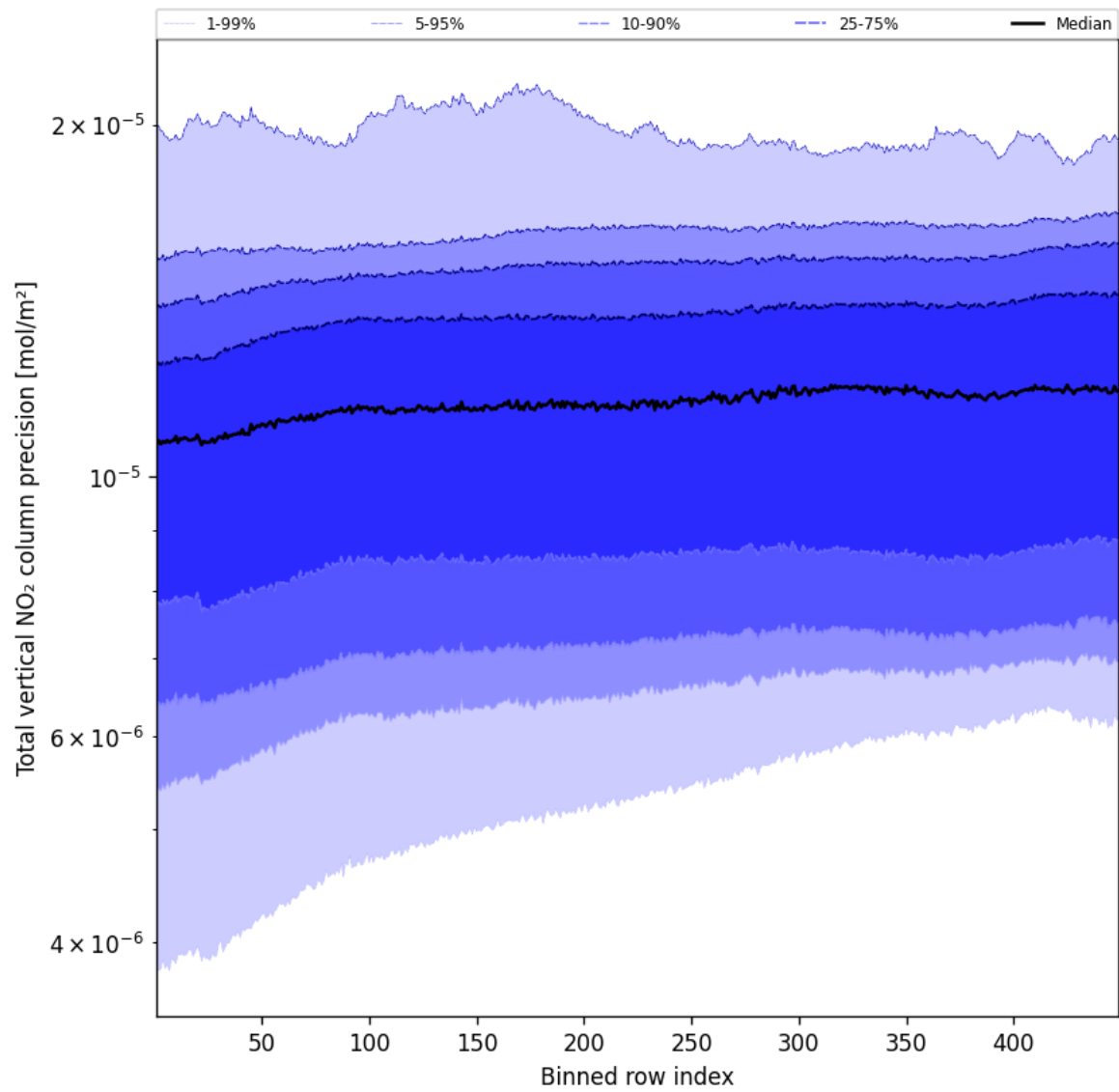
Figure 56: Along track statistics of "Total vertical NO 2 column precision" for 2025-05-02 to 2025-05-02
