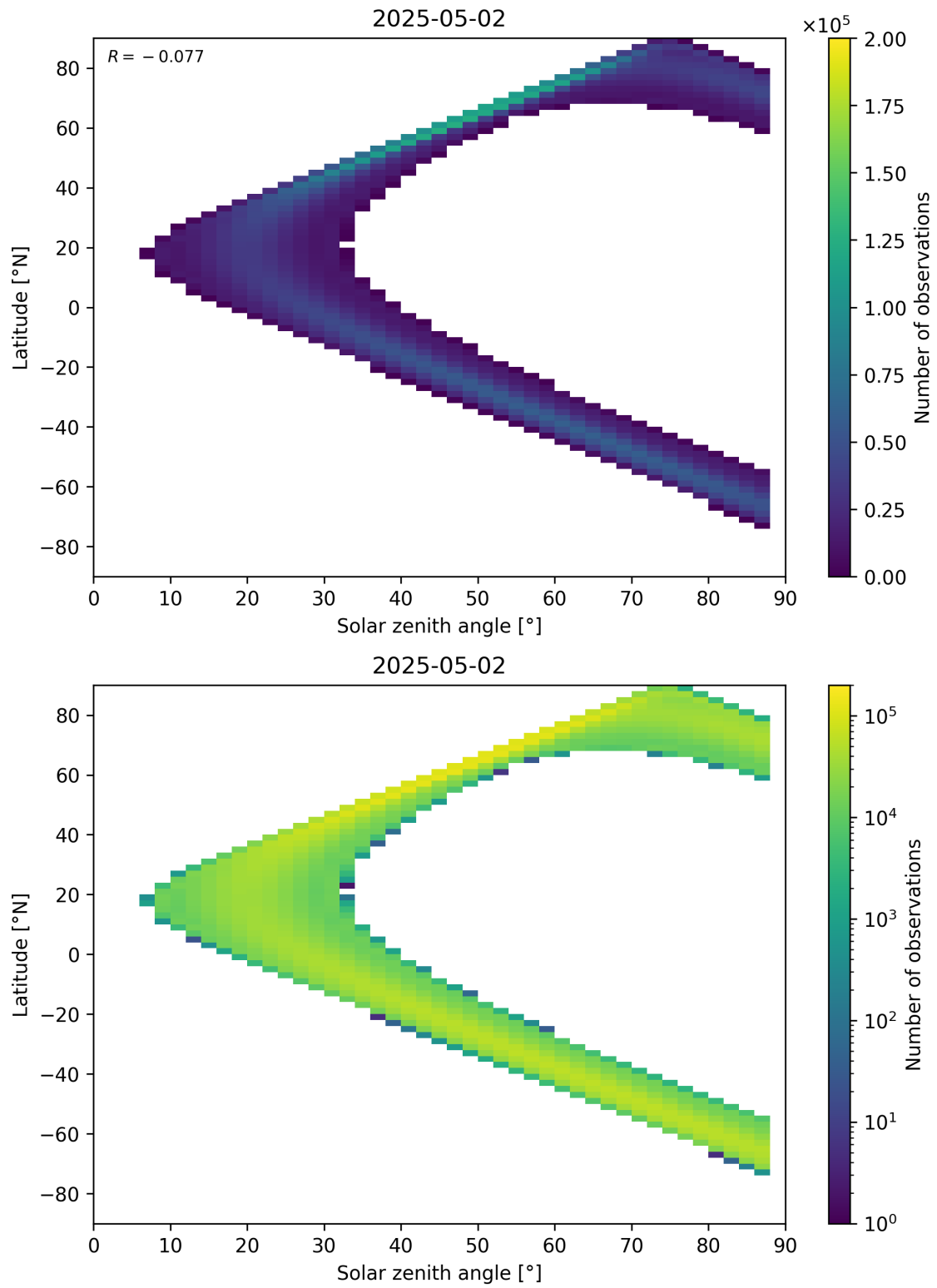
Figure 149: Scatter density plot of “Solar zenith angle” against “Latitude” for 2025-05-02 to 2025-05-02.
