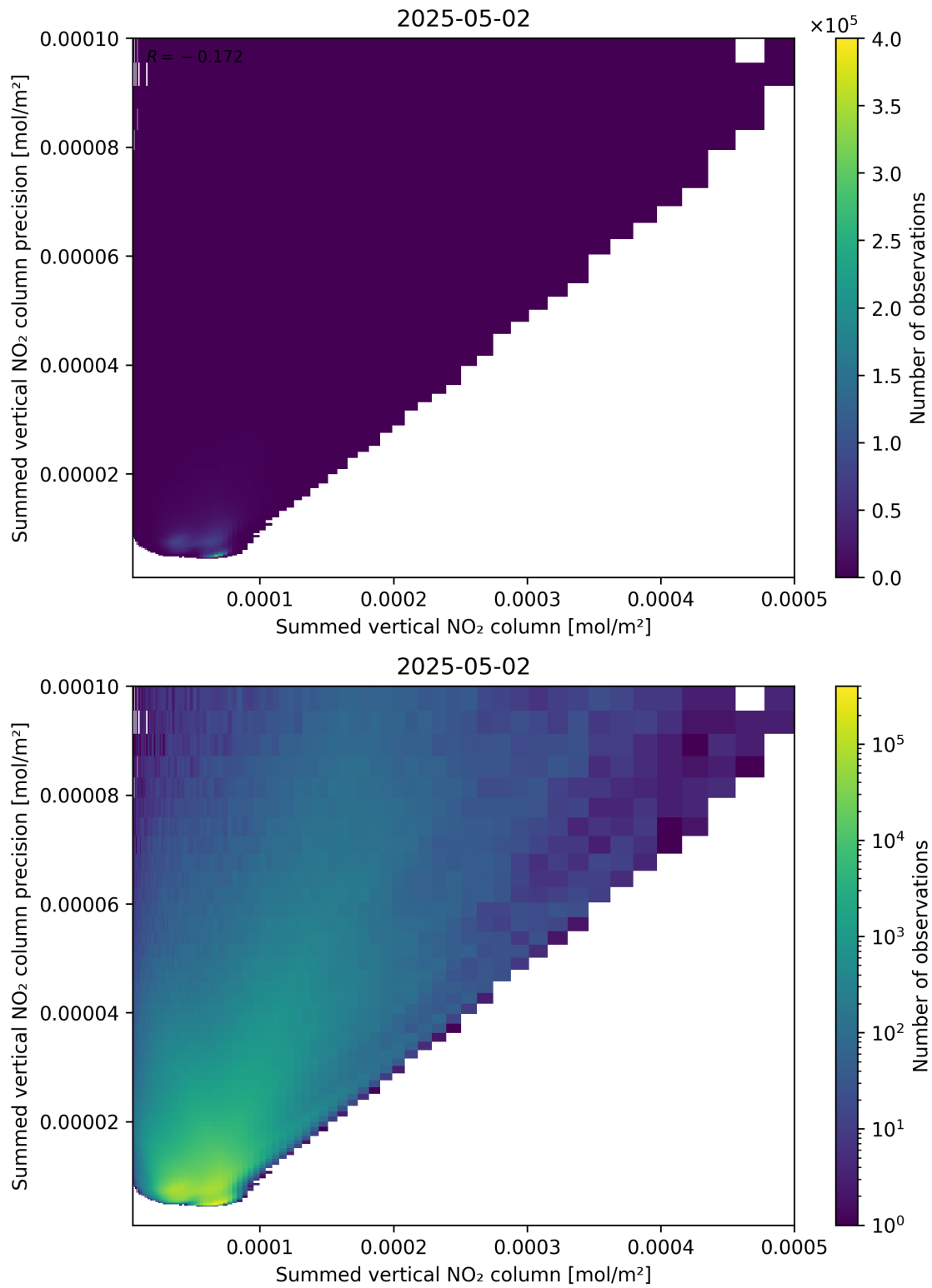
Figure 105: Scatter density plot of “Summed vertical NO 2 column” against “Summed vertical NO 2 column precision” for 2025-05-02 to 2025-05-02.
