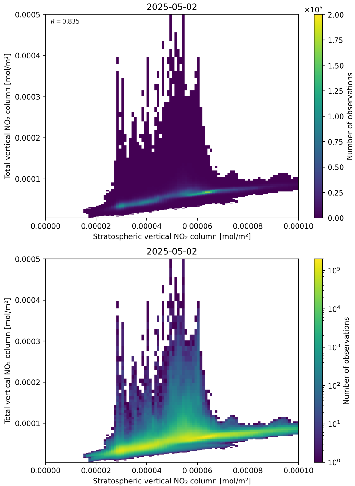
Figure 100: Scatter density plot of “Stratospheric vertical NO 2 column” against “Total vertical NO 2 column” for 2025-05-02 to 2025-05-02.
