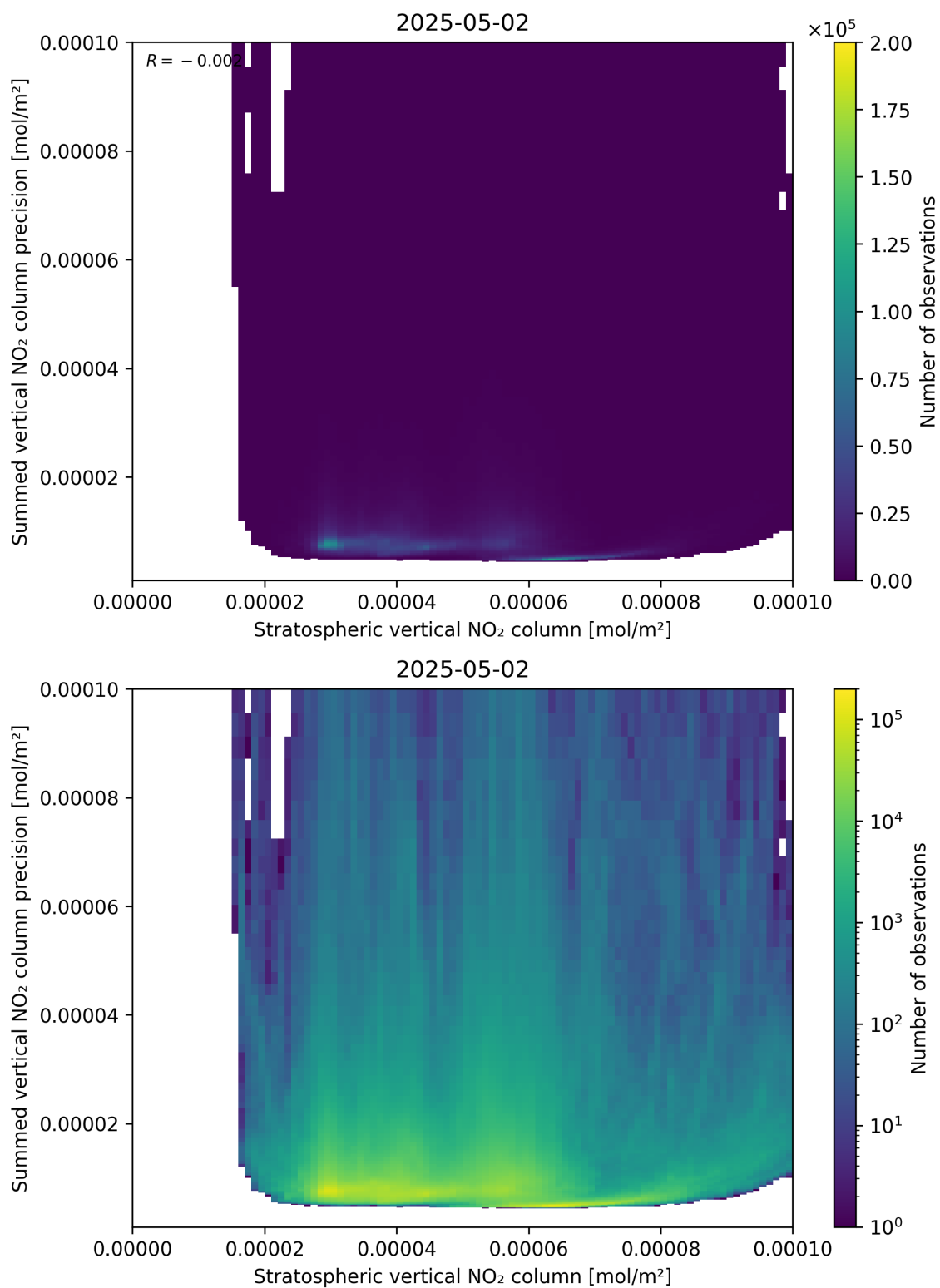
Figure 99: Scatter density plot of “Stratospheric vertical NO 2 column” against “Summed vertical NO 2 column precision” for 2025-05-02 to 2025-05-02.
