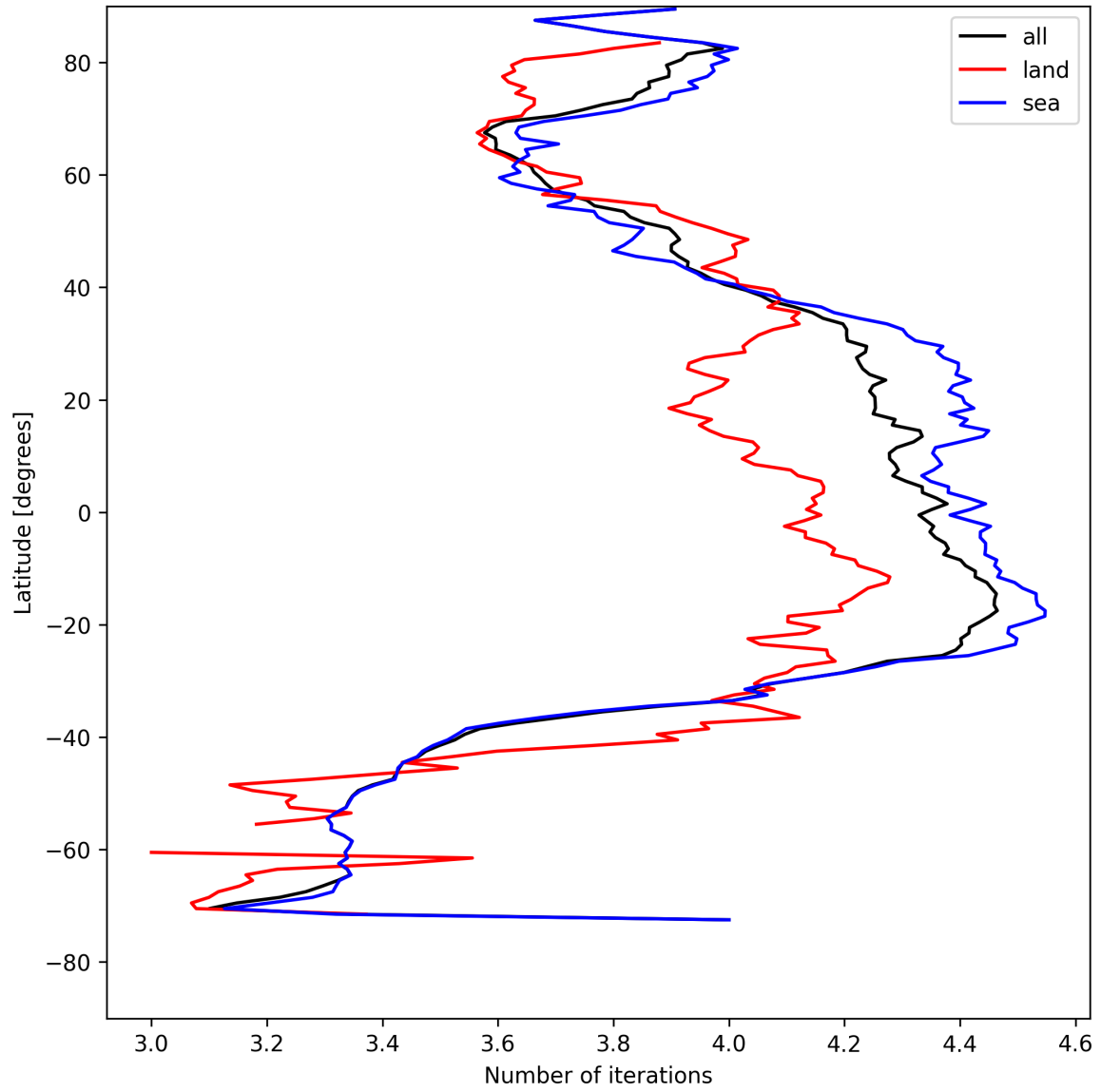
Figure 17: Zonal average of “Number of iterations” for 2025-05-03 to 2025-05-03.
