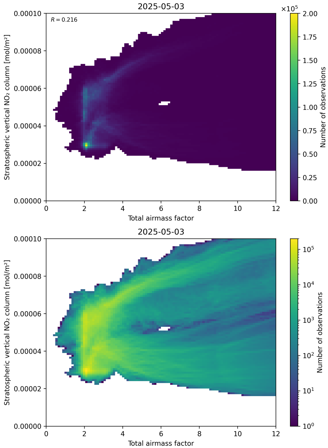
Figure 64: Scatter density plot of “Total airmass factor” against “Stratospheric vertical NO 2 column” for 2025-05-03 to 2025-05-03.
