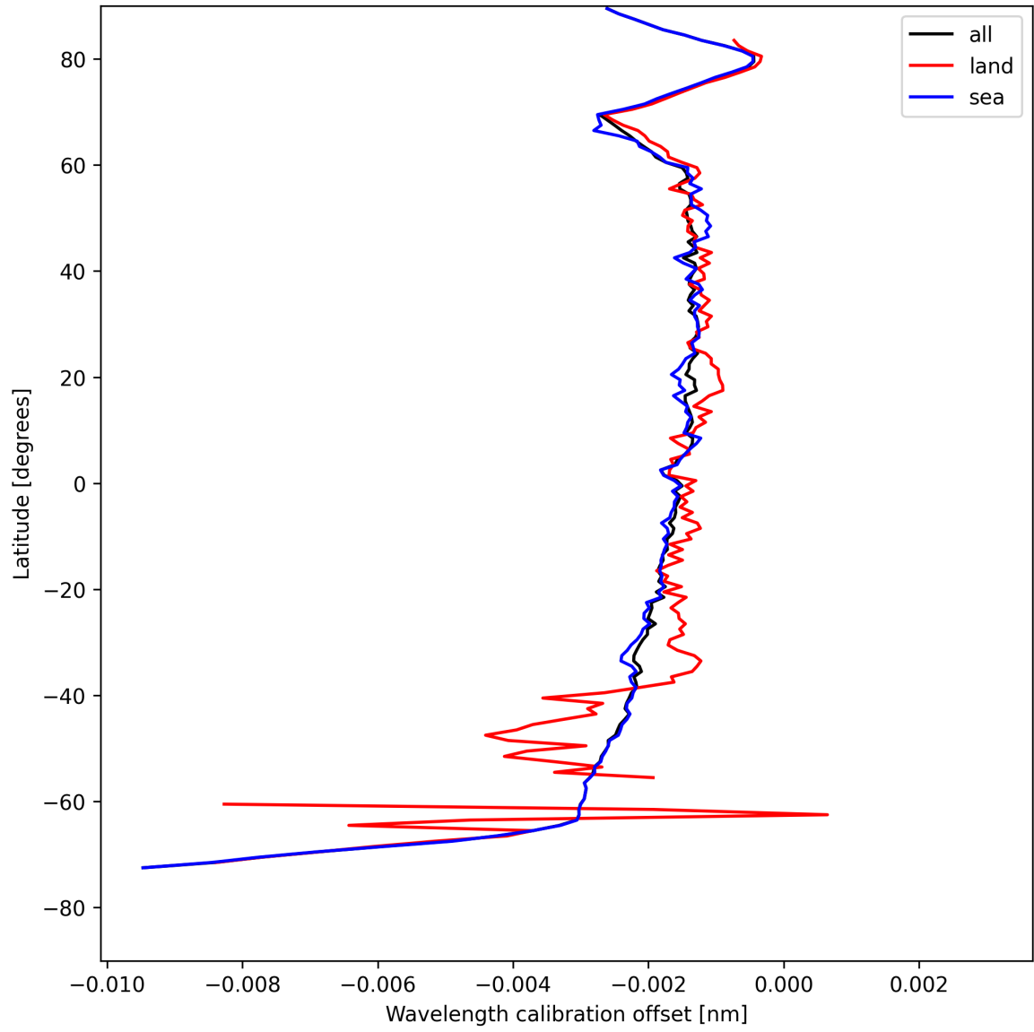
Figure 18: Zonal average of “Wavelength calibration offset” for 2025-05-03 to 2025-05-03.
