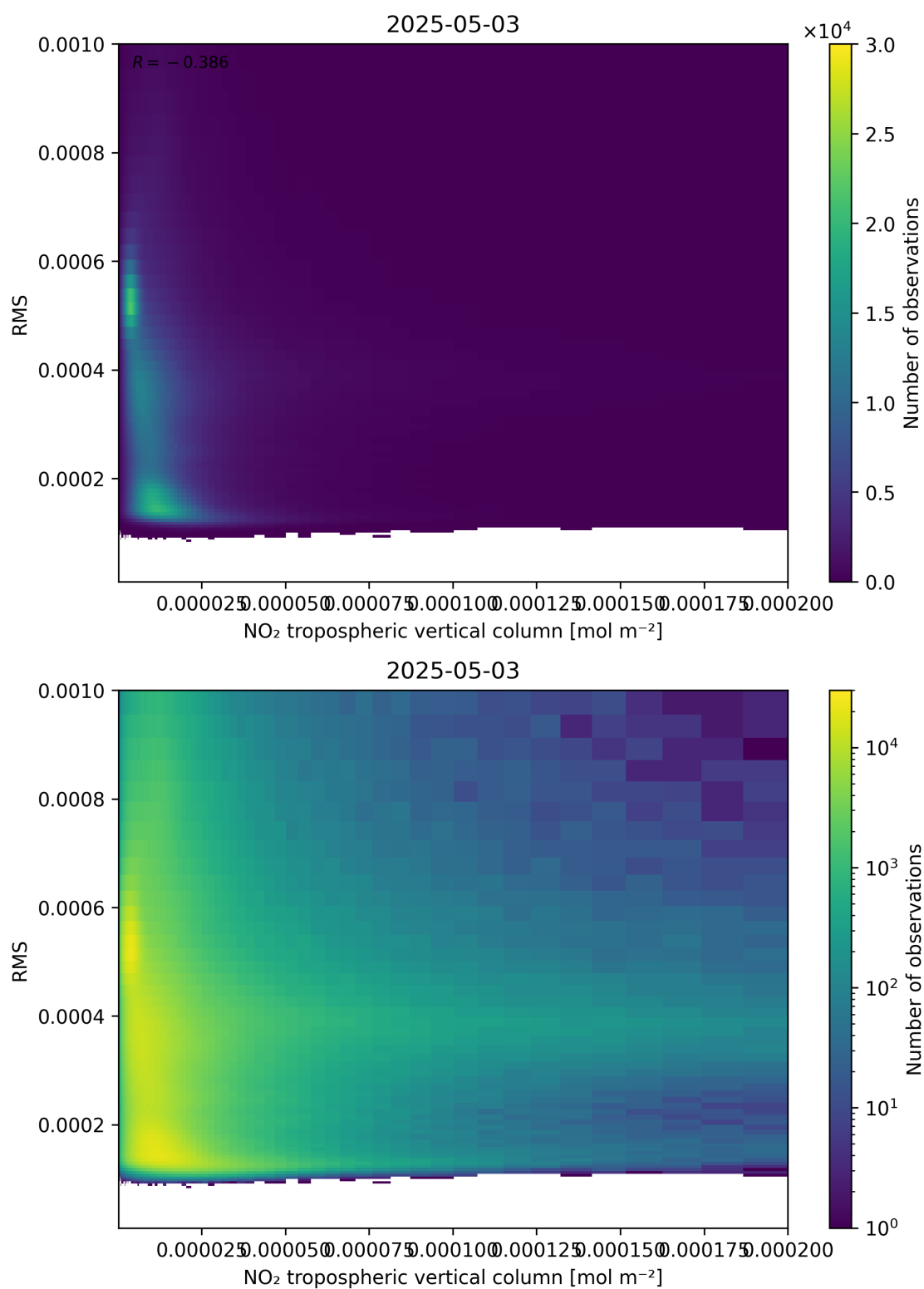
Figure 142: Scatter density plot of “NO 2 tropospheric vertical column” against “RMS” for 2025-05-03 to 2025-05-03.
