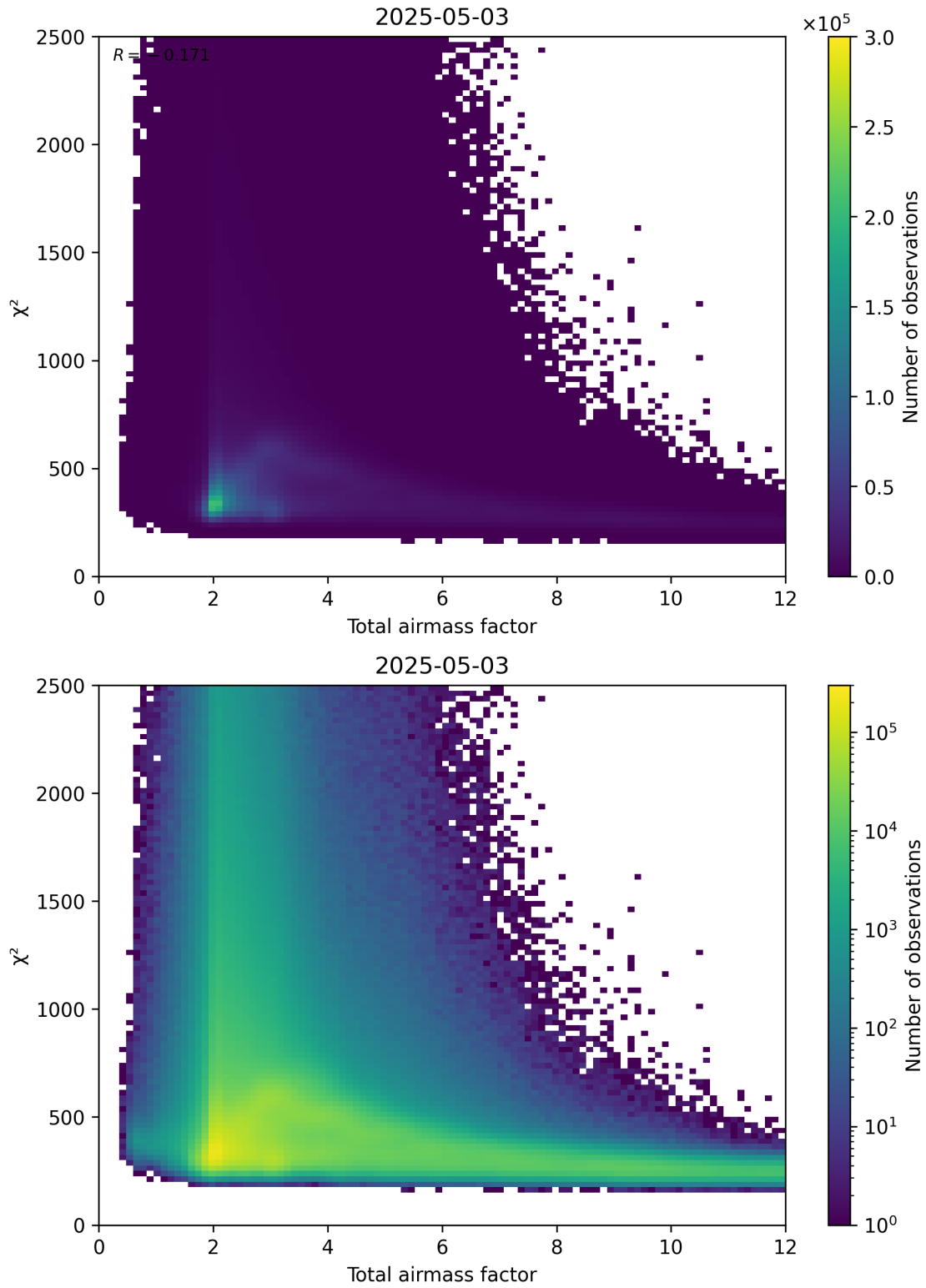
Figure 63: Scatter density plot of “Total airmass factor” against “ \chi^2 ” for 2025-05-03 to 2025-05-03.
