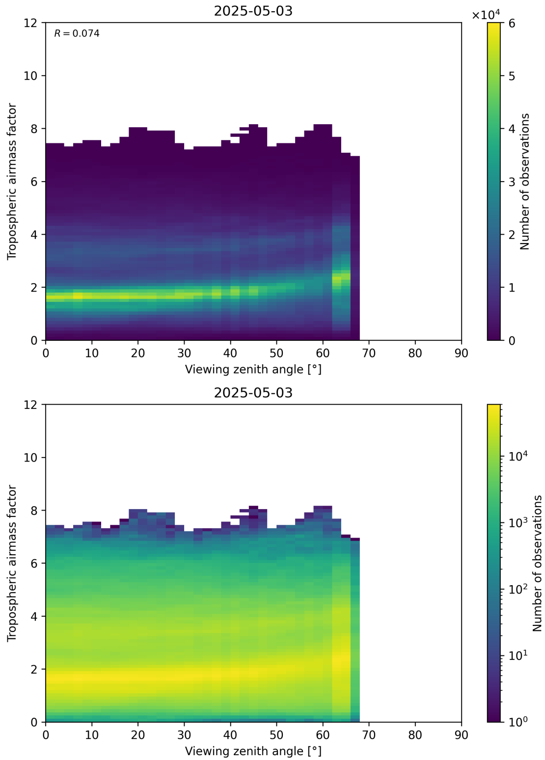
Figure 161: Scatter density plot of “Viewing zenith angle” against “Tropospheric airmass factor” for 2025-05-03 to 2025-05-03.
