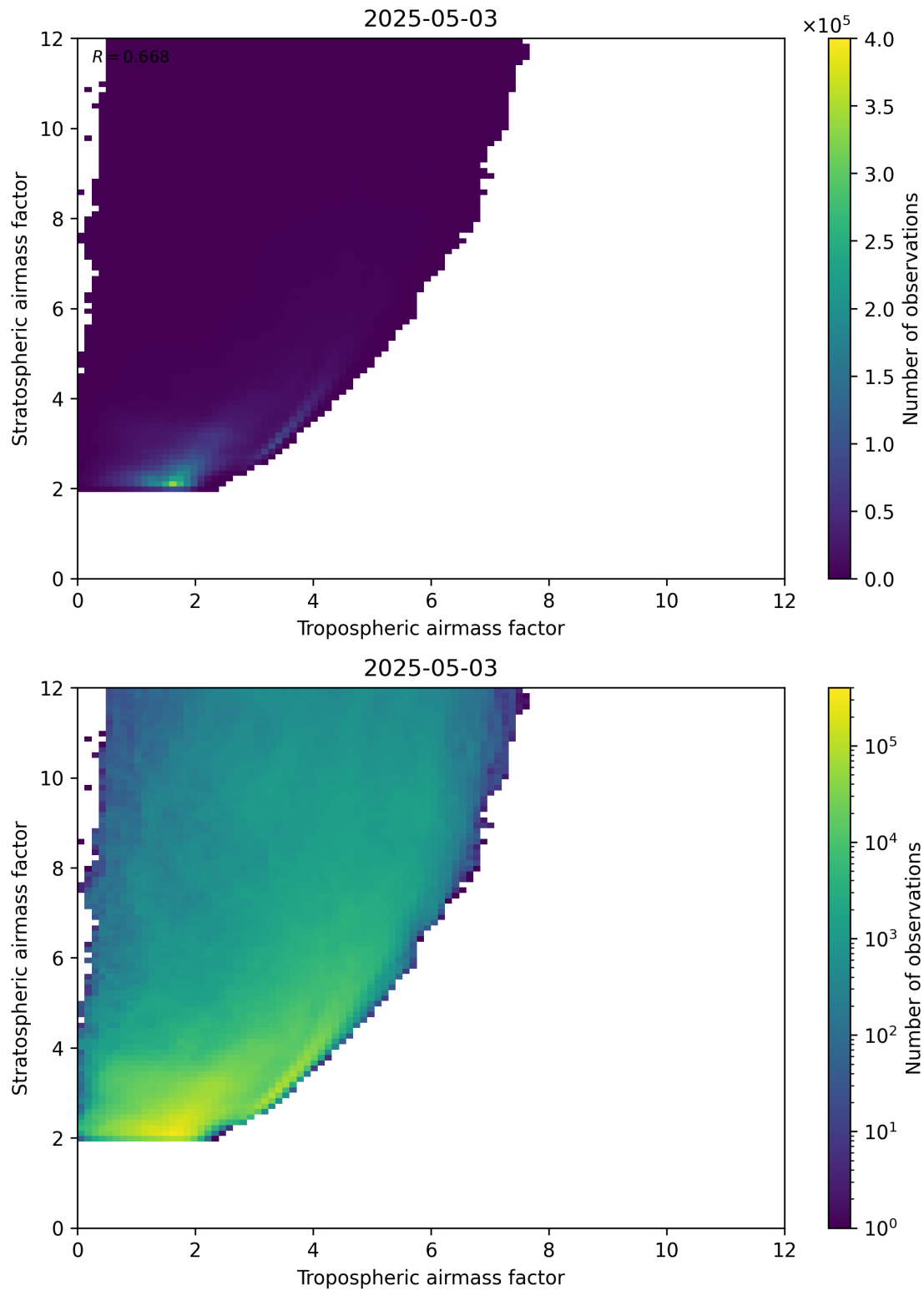
Figure 71: Scatter density plot of “Tropospheric airmass factor” against “Stratospheric airmass factor” for 2025-05-03 to 2025-05-03.
