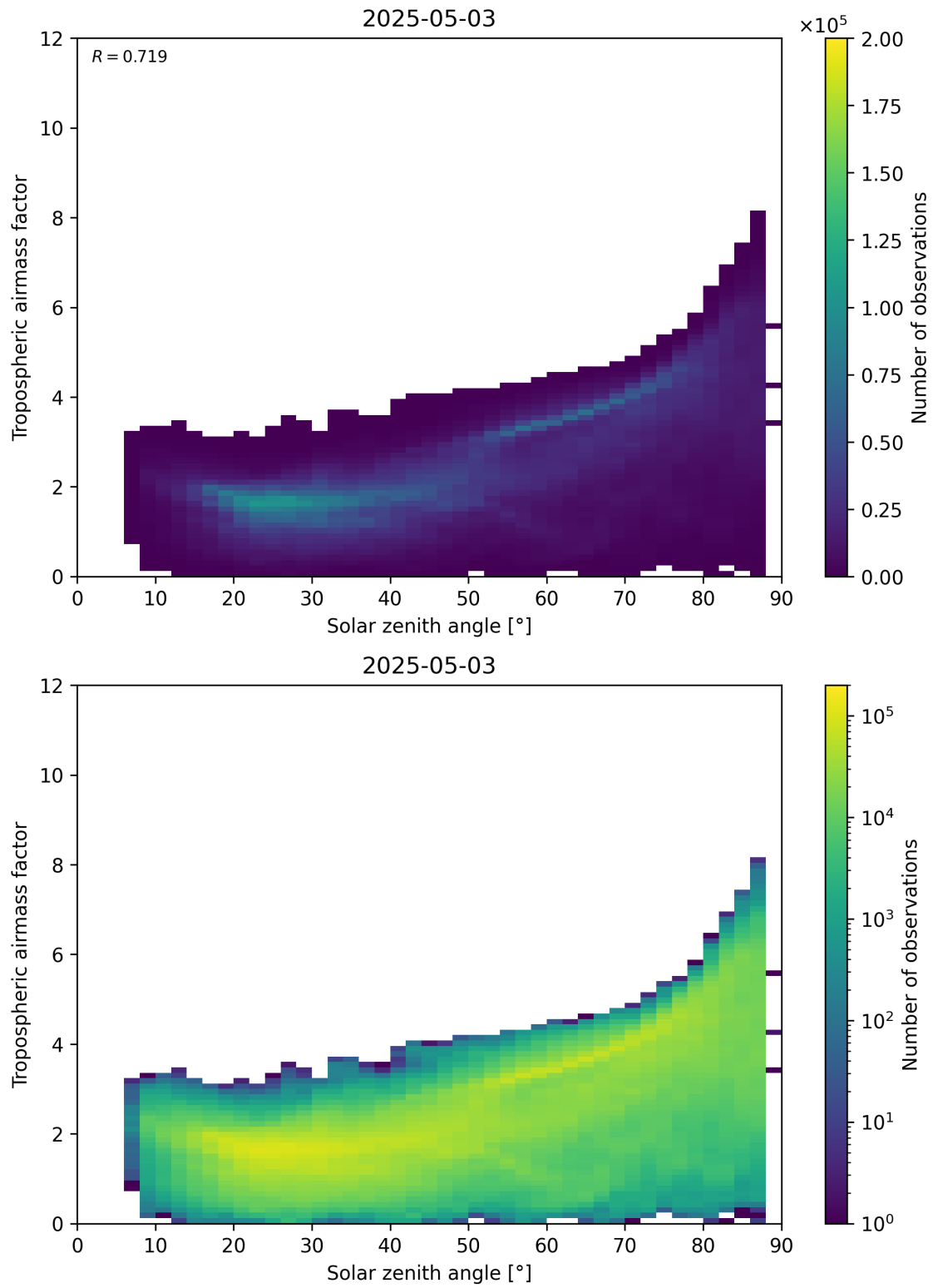
Figure 147: Scatter density plot of “Solar zenith angle” against “Tropospheric airmass factor” for 2025-05-03 to 2025-05-03.
