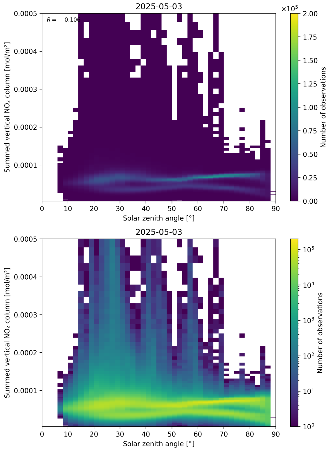
Figure 151: Scatter density plot of “Solar zenith angle” against “Summed vertical NO 2 column” for 2025-05-03 to 2025-05-03.
