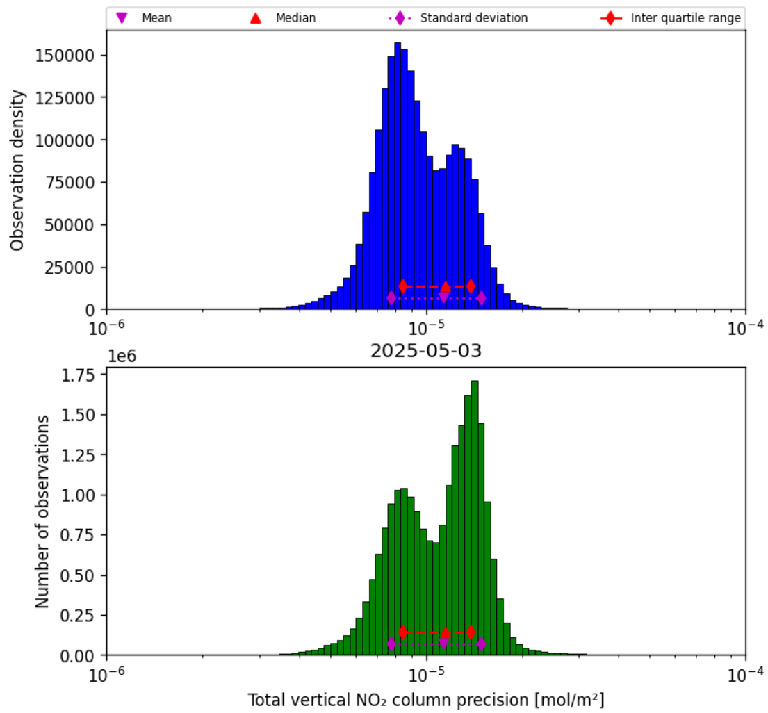
Figure 39: Histogram of “Total vertical NO 2 column precision” for 2025-05-03 to 2025-05-03
