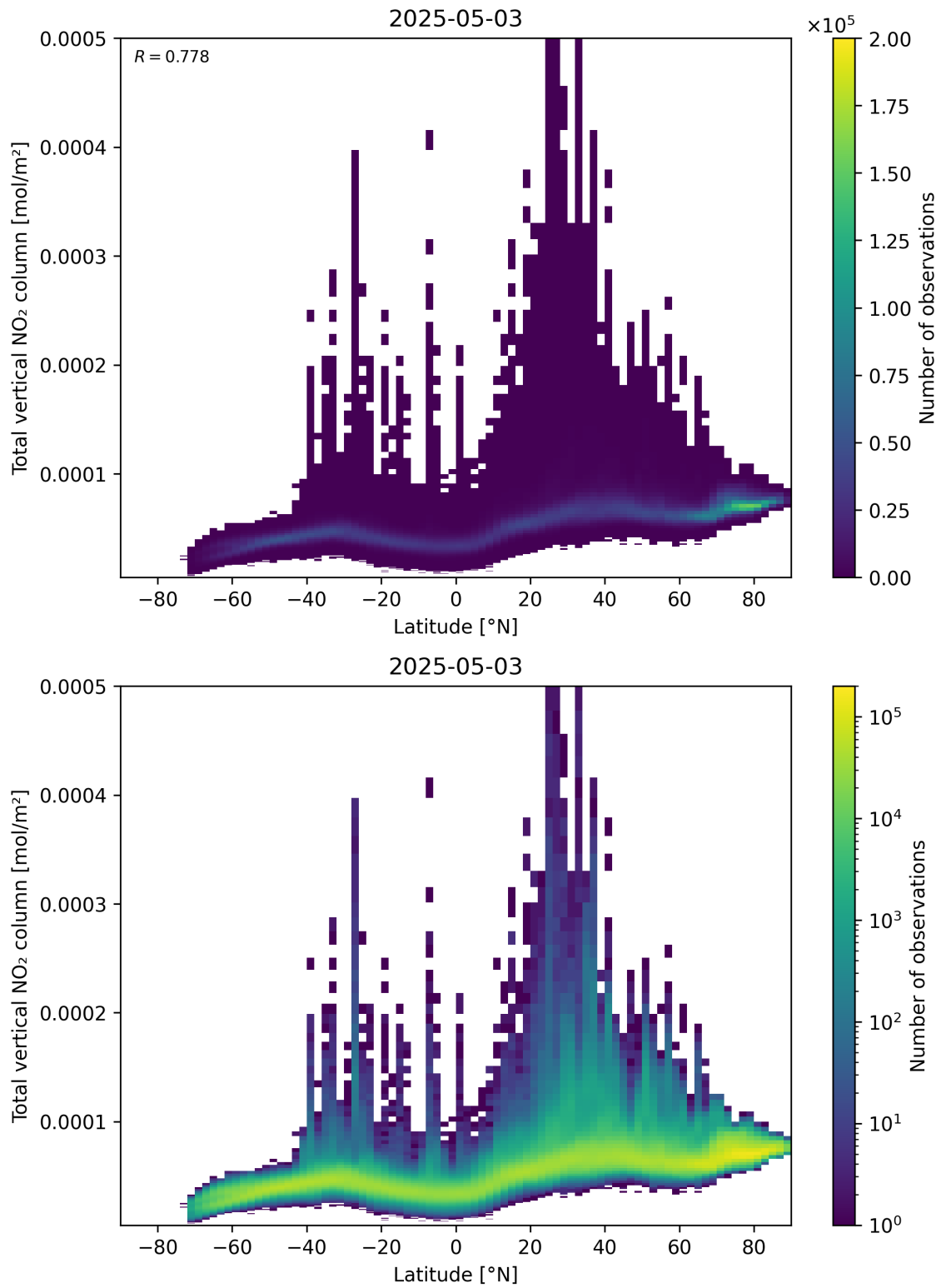
Figure 90: Scatter density plot of “Latitude” against “Total vertical NO 2 column” for 2025-05-03 to 2025-05-03.
