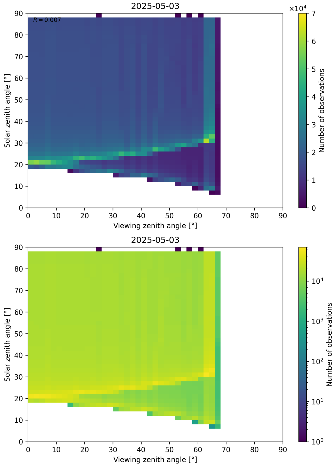
Figure 172: Scatter density plot of “Viewing zenith angle” against “Solar zenith angle” for 2025-05-03 to 2025-05-03.
