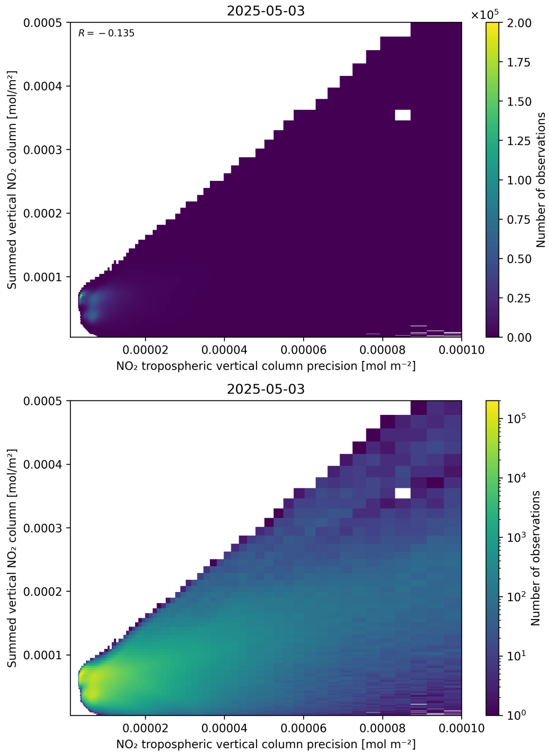
Figure 136: Scatter density plot of “NO 2 tropospheric vertical column precision” against “Summed vertical NO 2 column” for 2025-05-03 to 2025-05-03.
