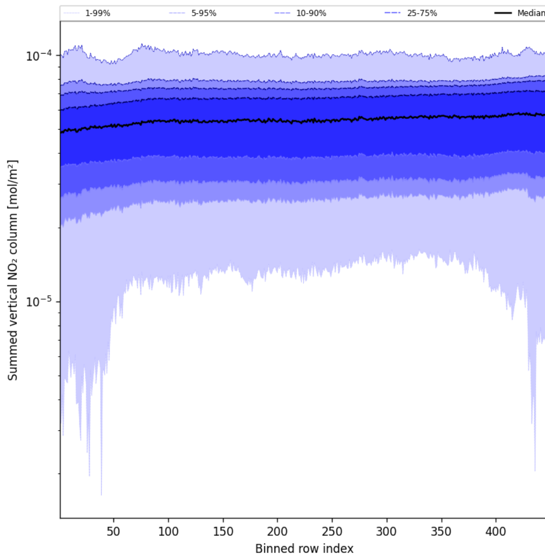
Figure 57: Along track statistics of “Summed vertical NO 2 column” for 2025-05-03 to 2025-05-03
