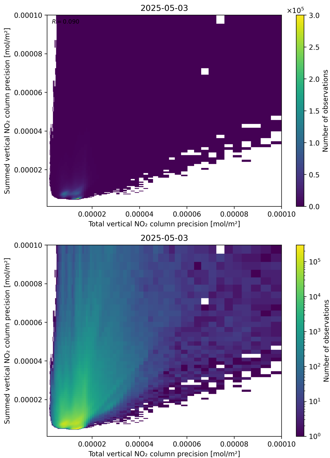
Figure 118: Scatter density plot of “Total vertical NO 2 column precision” against “Summed vertical NO 2 column precision” for 2025-05-03 to 2025-05-03.
