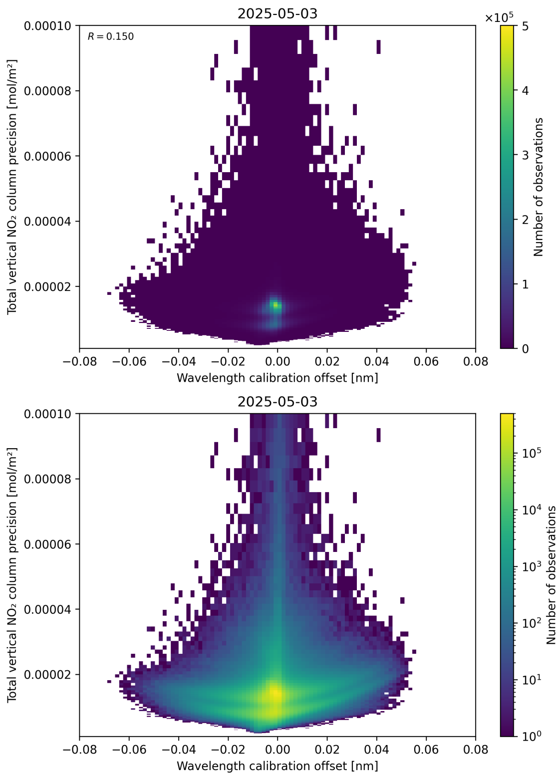
Figure 180: Scatter density plot of “Wavelength calibration offset” against “Total vertical NO 2 column precision” for 2025-05-03 to 2025-05-03.
