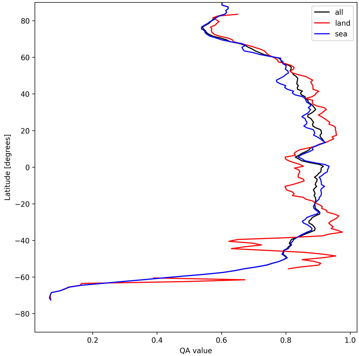
Figure 11: Zonal average of “QA value” for 2025-05-03 to 2025-05-03.
