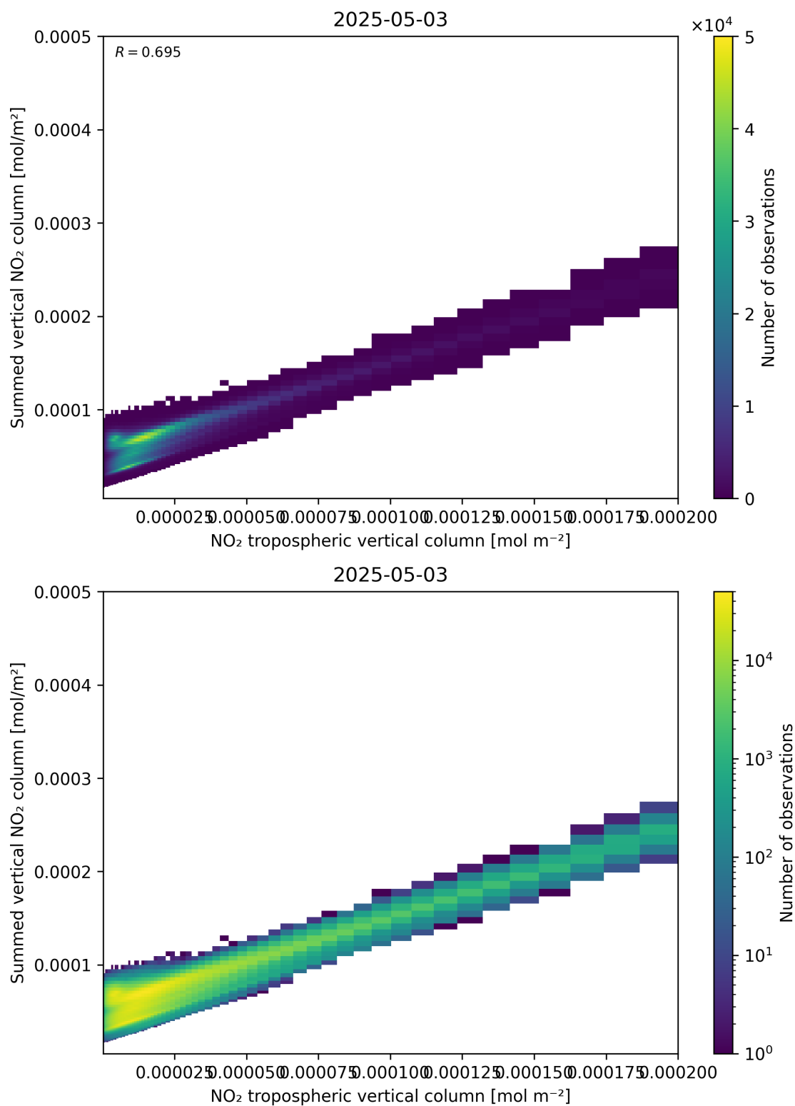
Figure 126: Scatter density plot of “NO 2 tropospheric vertical column” against “Summed vertical NO 2 column” for 2025-05-03 to 2025-05-03.
