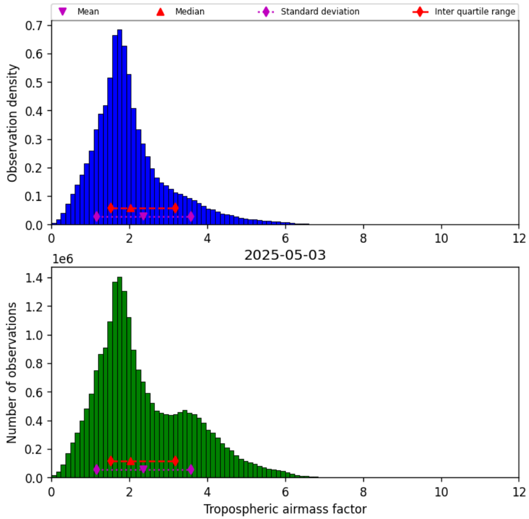
Figure 31: Histogram of “Tropospheric airmass factor” for 2025-05-03 to 2025-05-03
