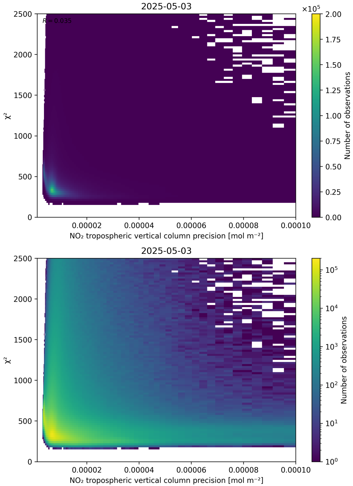
Figure 134: Scatter density plot of “NO 2 tropospheric vertical column precision” against “ \chi^2 ” for 2025-05-03 to 2025-05-03.
