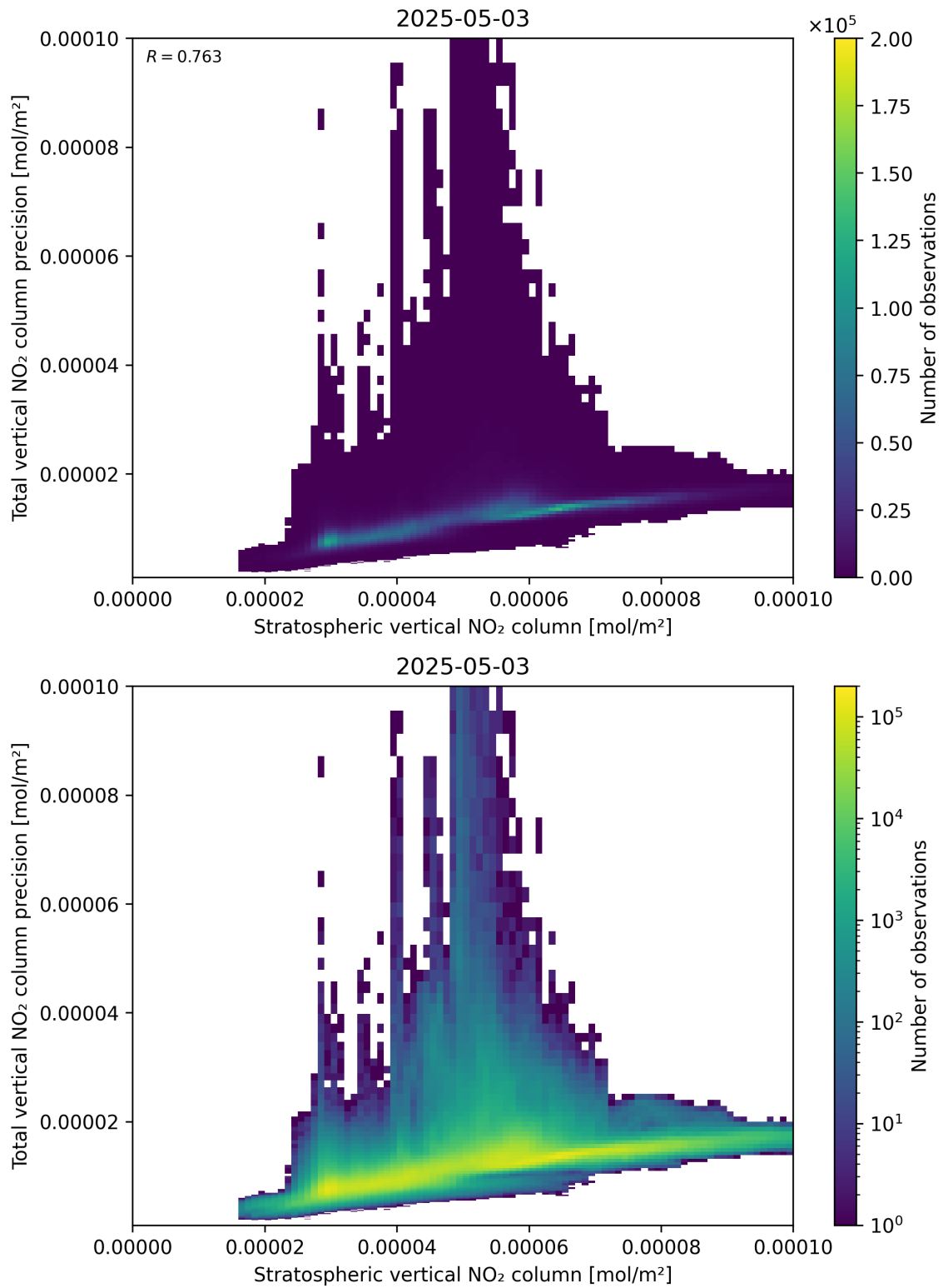
Figure 101: Scatter density plot of “Stratospheric vertical NO 2 column” against “Total vertical NO 2 column precision” for 2025-05-03 to 2025-05-03.
