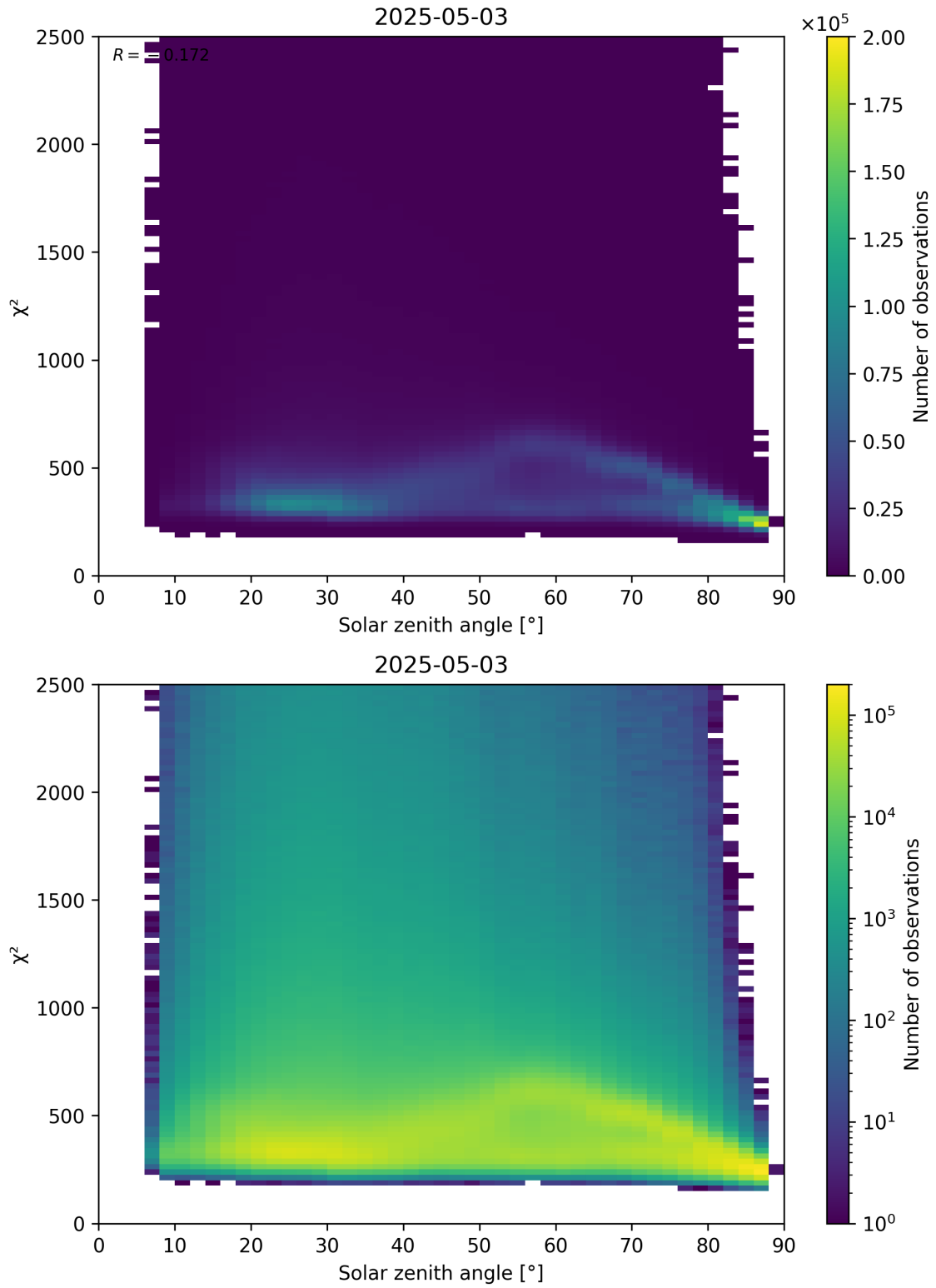
Figure 148: Scatter density plot of “Solar zenith angle” against “ \chi^2 ” for 2025-05-03 to 2025-05-03.
