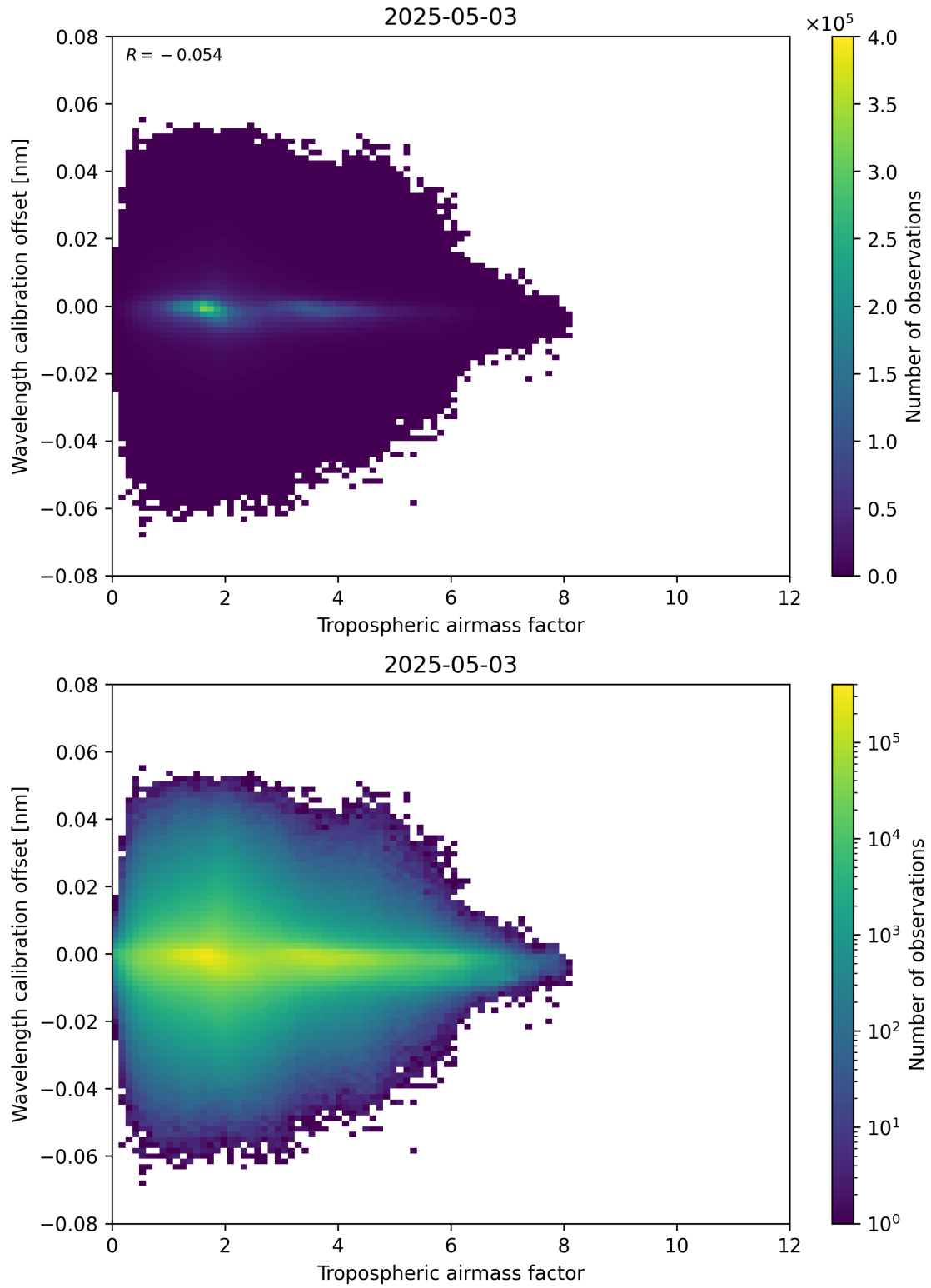
Figure 80: Scatter density plot of “Tropospheric airmass factor” against “Wavelength calibration offset” for 2025-05-03 to 2025-05-03.
