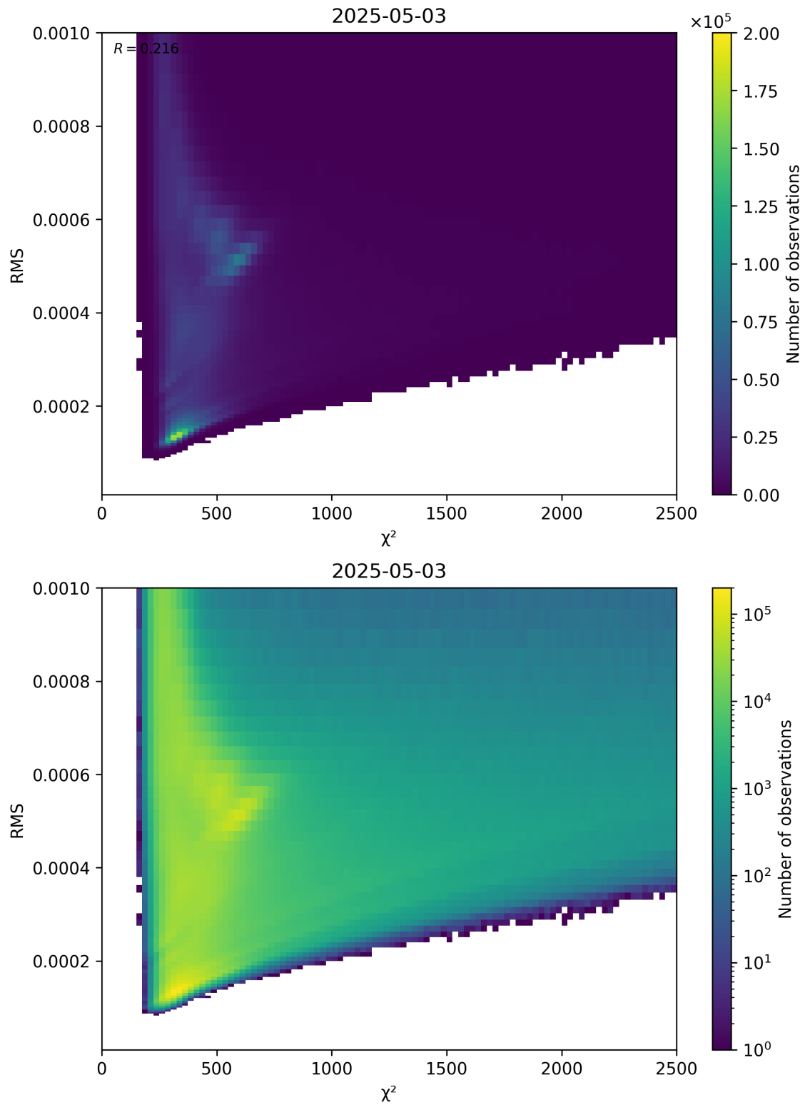
Figure 82: Scatter density plot of “ \chi^2 ” against “RMS” for 2025-05-03 to 2025-05-03.
