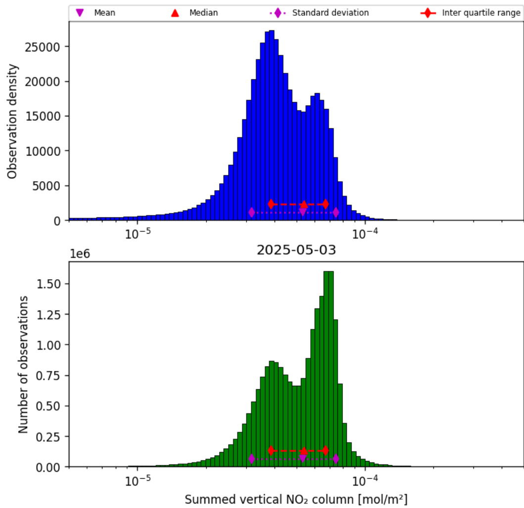
Figure 40: Histogram of “Summed vertical NO 2 column” for 2025-05-03 to 2025-05-03
