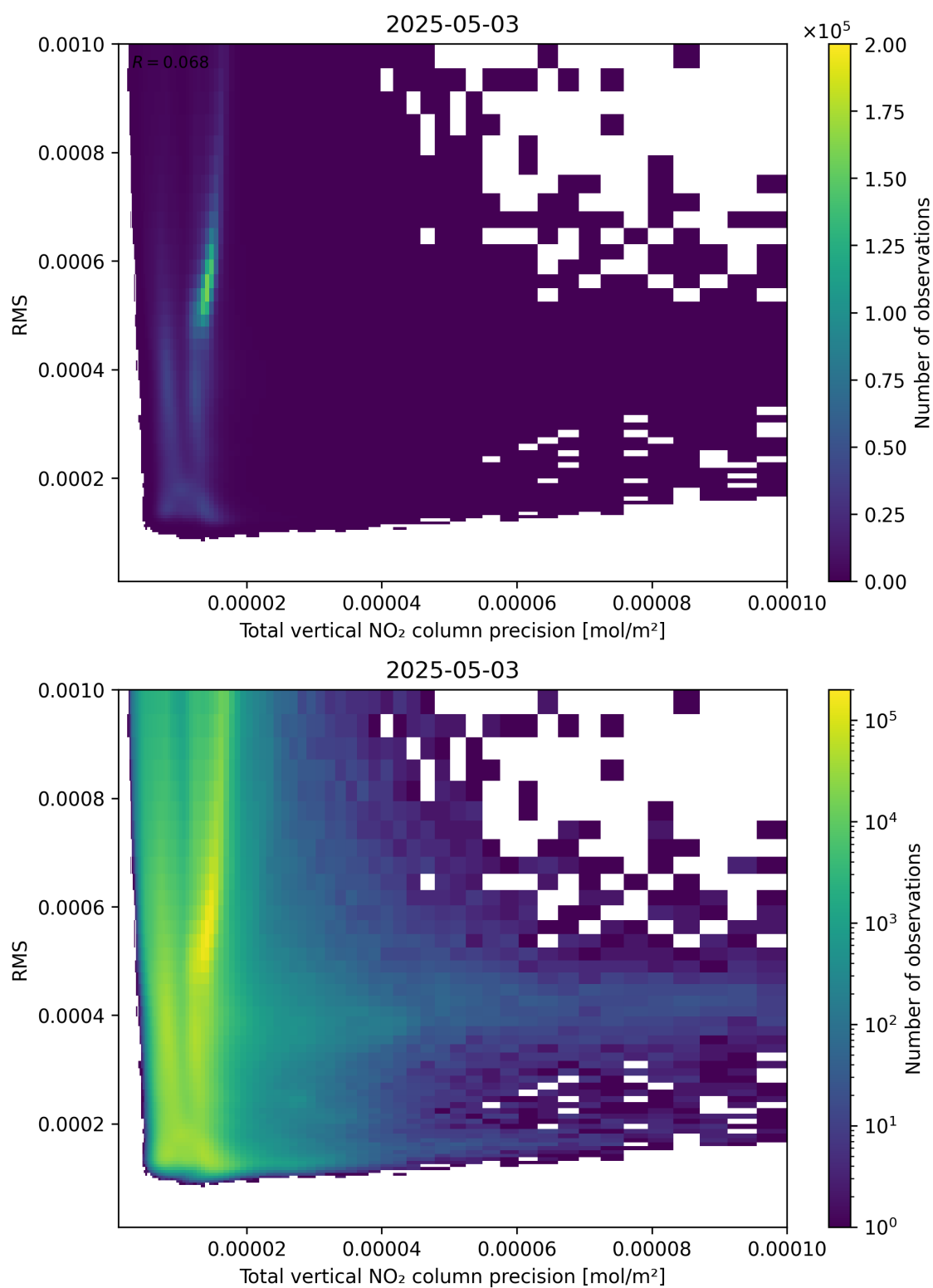
Figure 119: Scatter density plot of “Total vertical NO 2 column precision” against “RMS” for 2025-05-03 to 2025-05-03.
