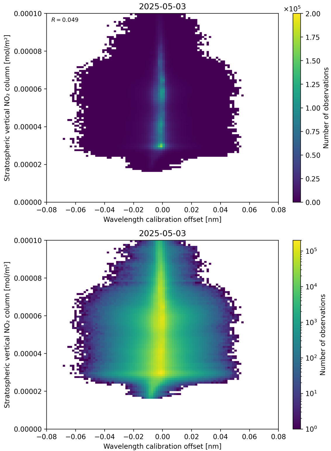
Figure 176: Scatter density plot of “Wavelength calibration offset” against “Stratospheric vertical NO 2 column” for 2025-05-03 to 2025-05-03.
