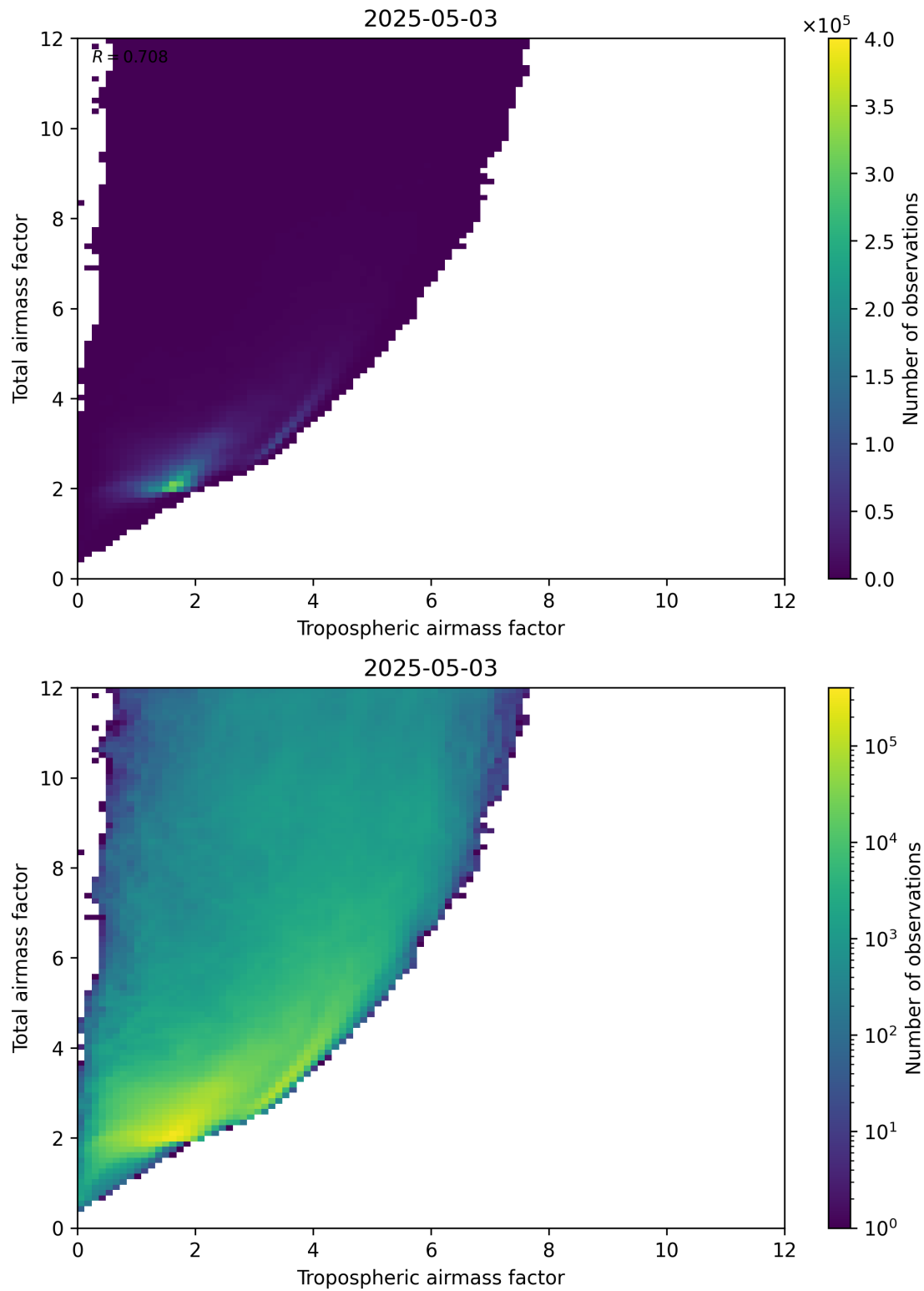
Figure 72: Scatter density plot of “Tropospheric airmass factor” against “Total airmass factor” for 2025-05-03 to 2025-05-03.
