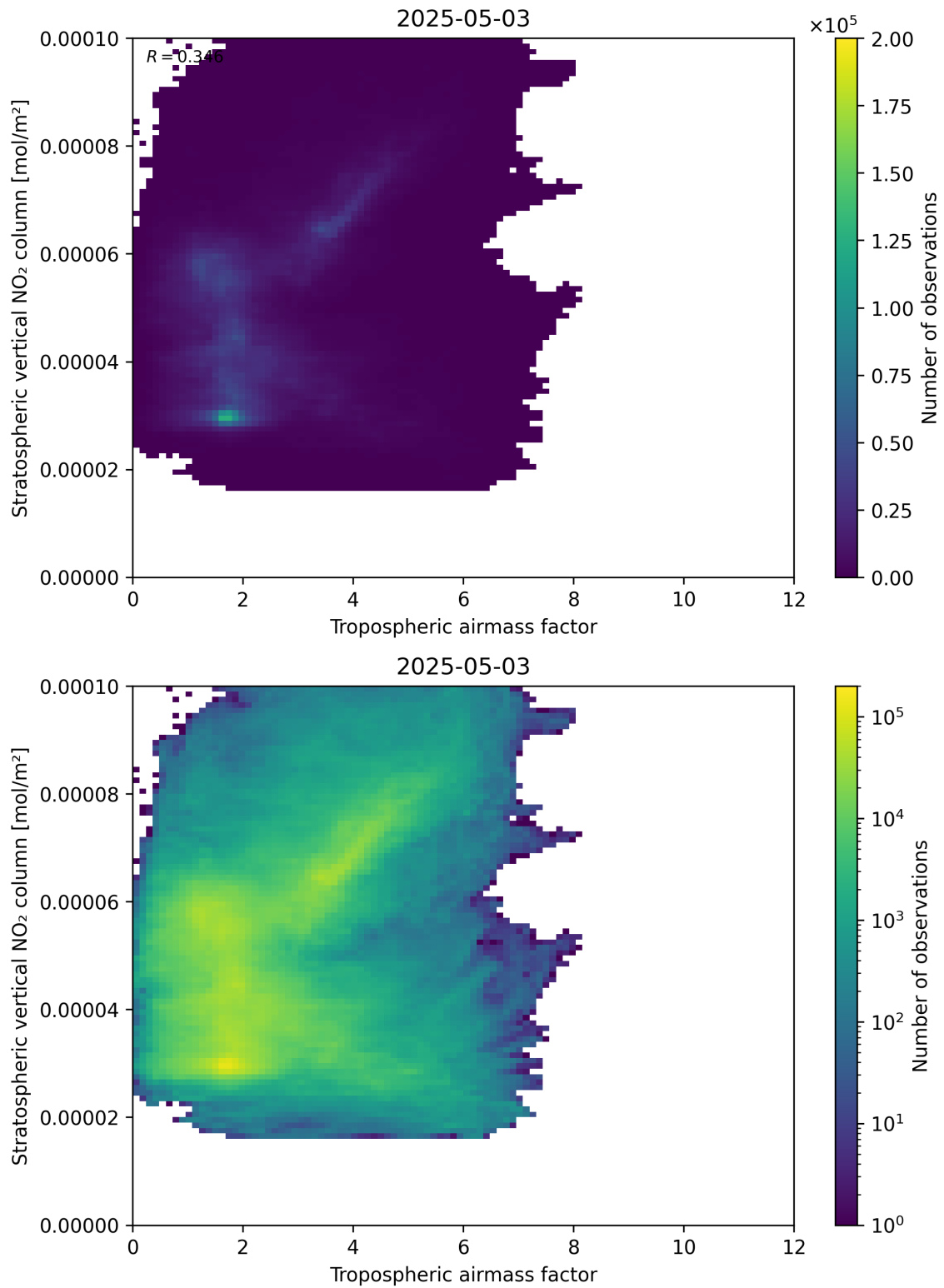
Figure 74: Scatter density plot of “Tropospheric air mass factor” against “Stratospheric vertical NO 2 column” for 2025-05-03 to 2025-05-03.
