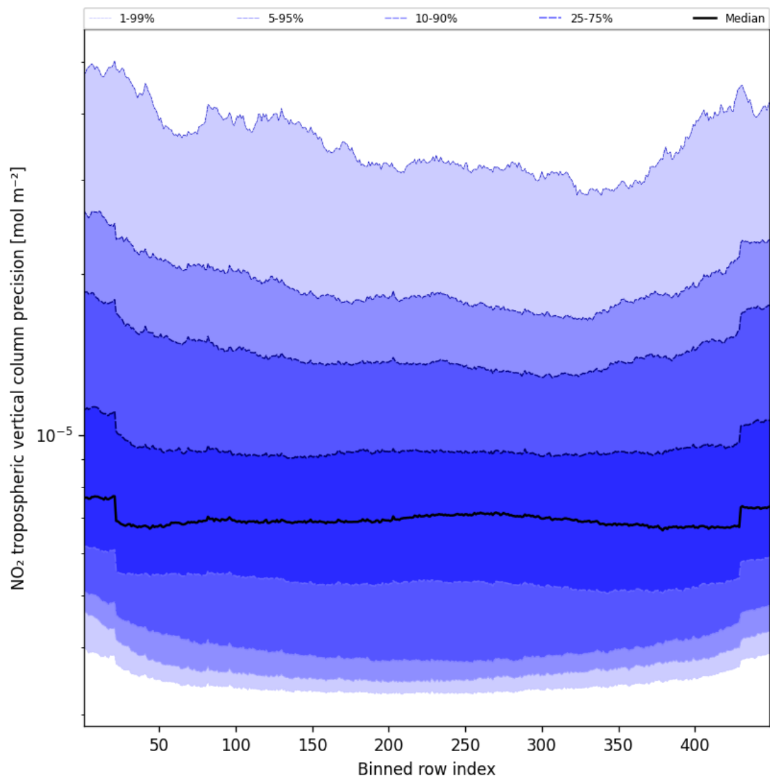
Figure 47: Along track statistics of “NO 2 tropospheric vertical column precision” for 2025-05-03 to 2025-05-03
