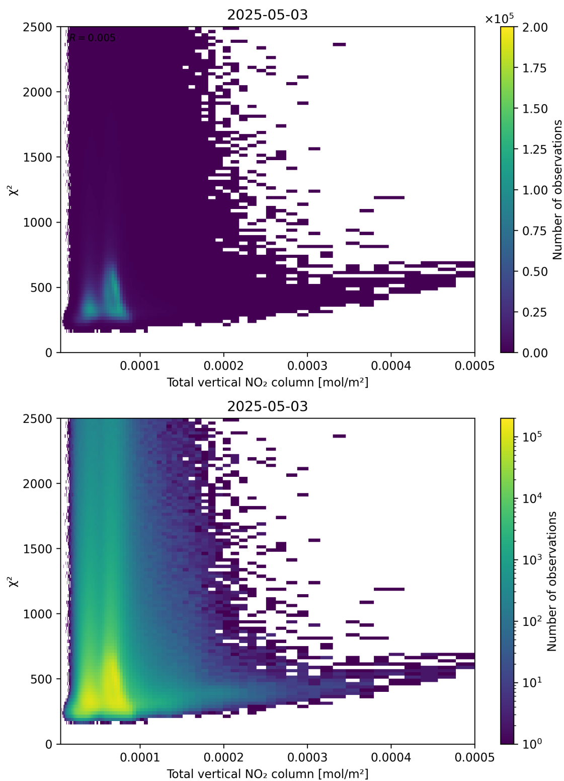
Figure 111: Scatter density plot of “Total vertical NO 2 column” against “ \chi^2 ” for 2025-05-03 to 2025-05-03.
