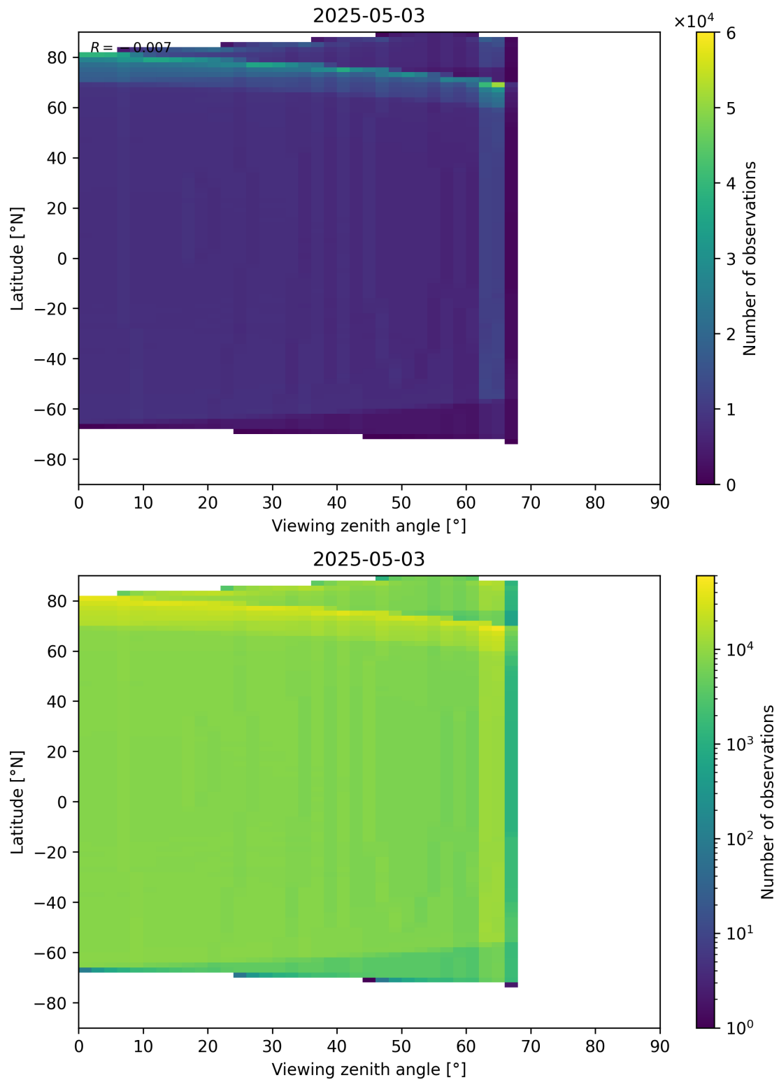
Figure 163: Scatter density plot of “Viewing zenith angle” against “Latitude” for 2025-05-03 to 2025-05-03.
