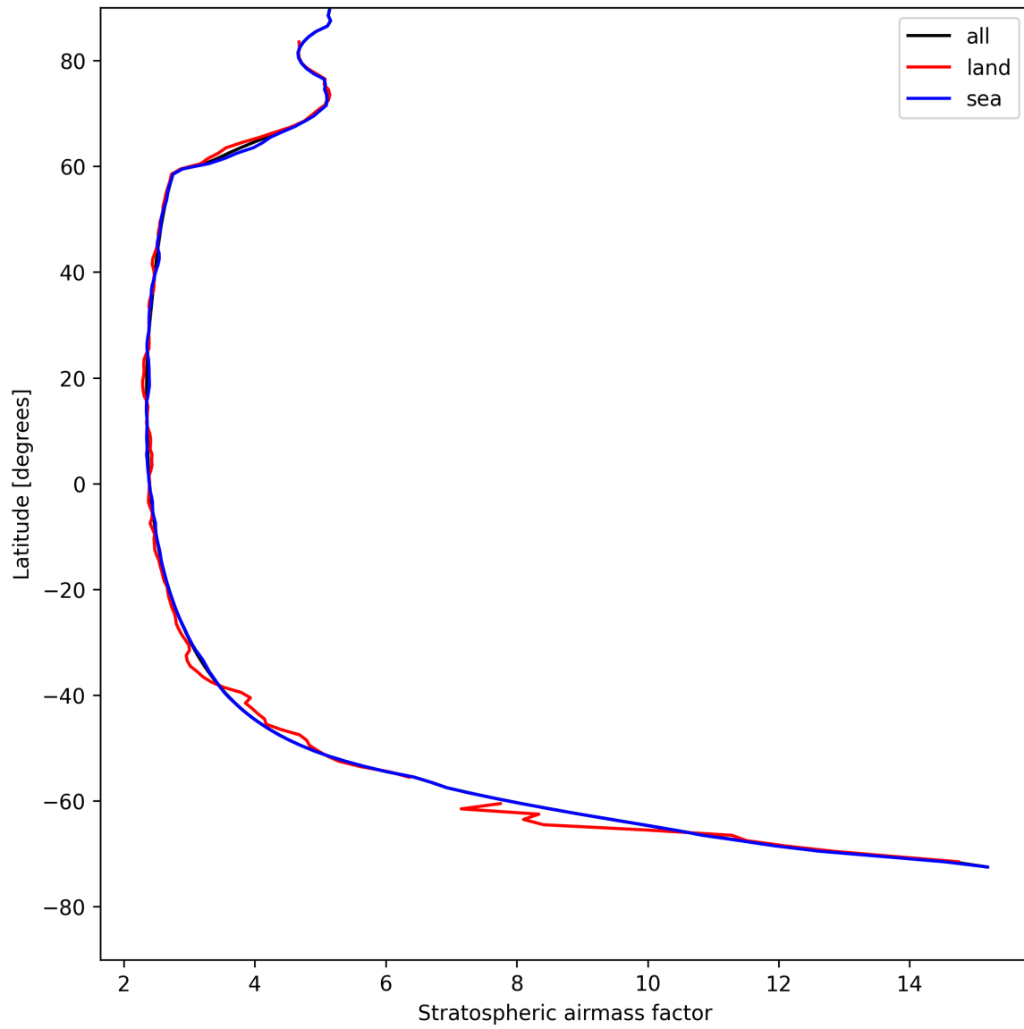
Figure 27: Zonal average of “Stratospheric airmass factor” for 2025-05-03 to 2025-05-03.
