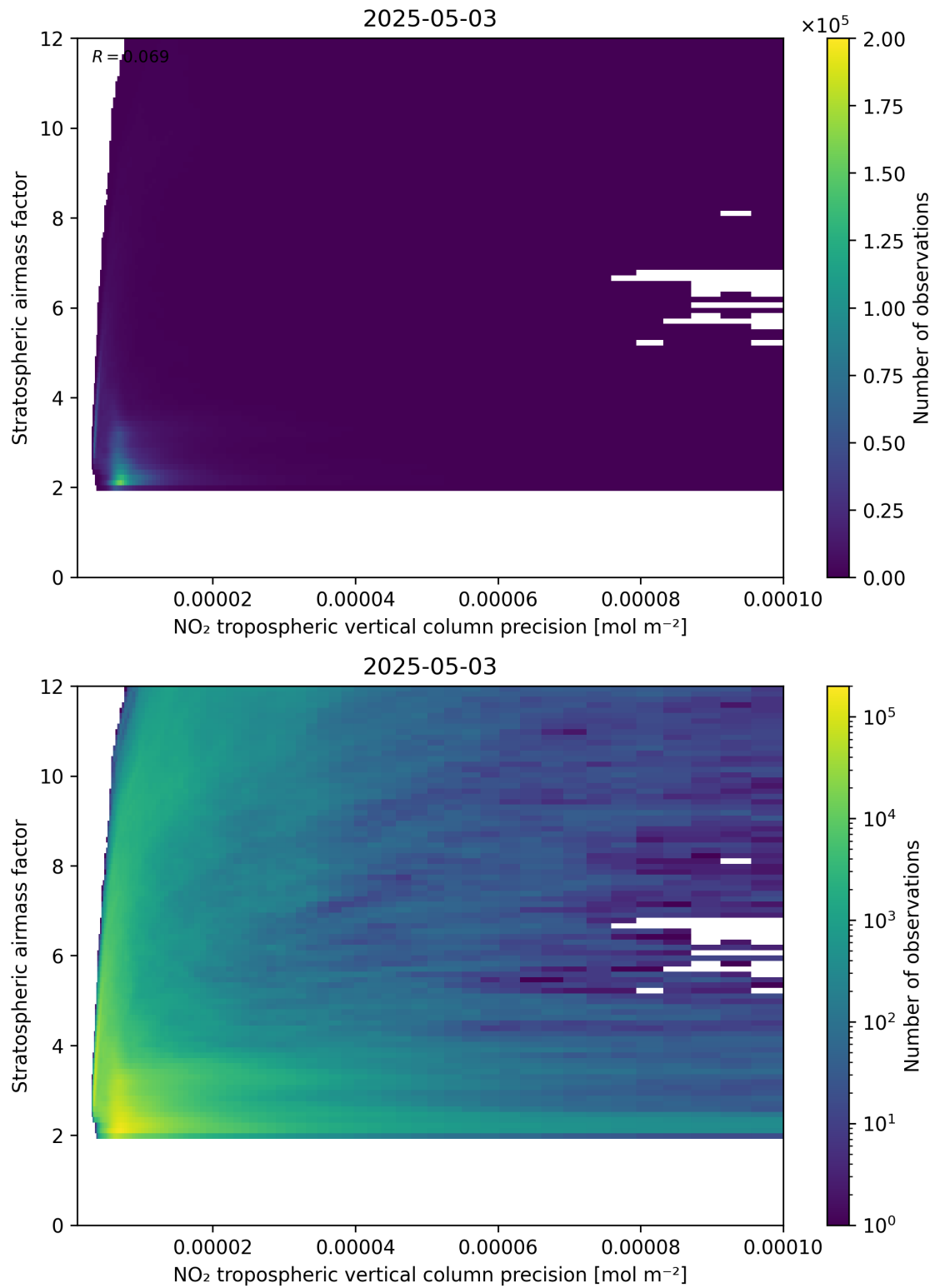
Figure 131: Scatter density plot of “NO 2 tropospheric vertical column precision” against “Stratospheric airmass factor” for 2025-05-03 to 2025-05-03.
