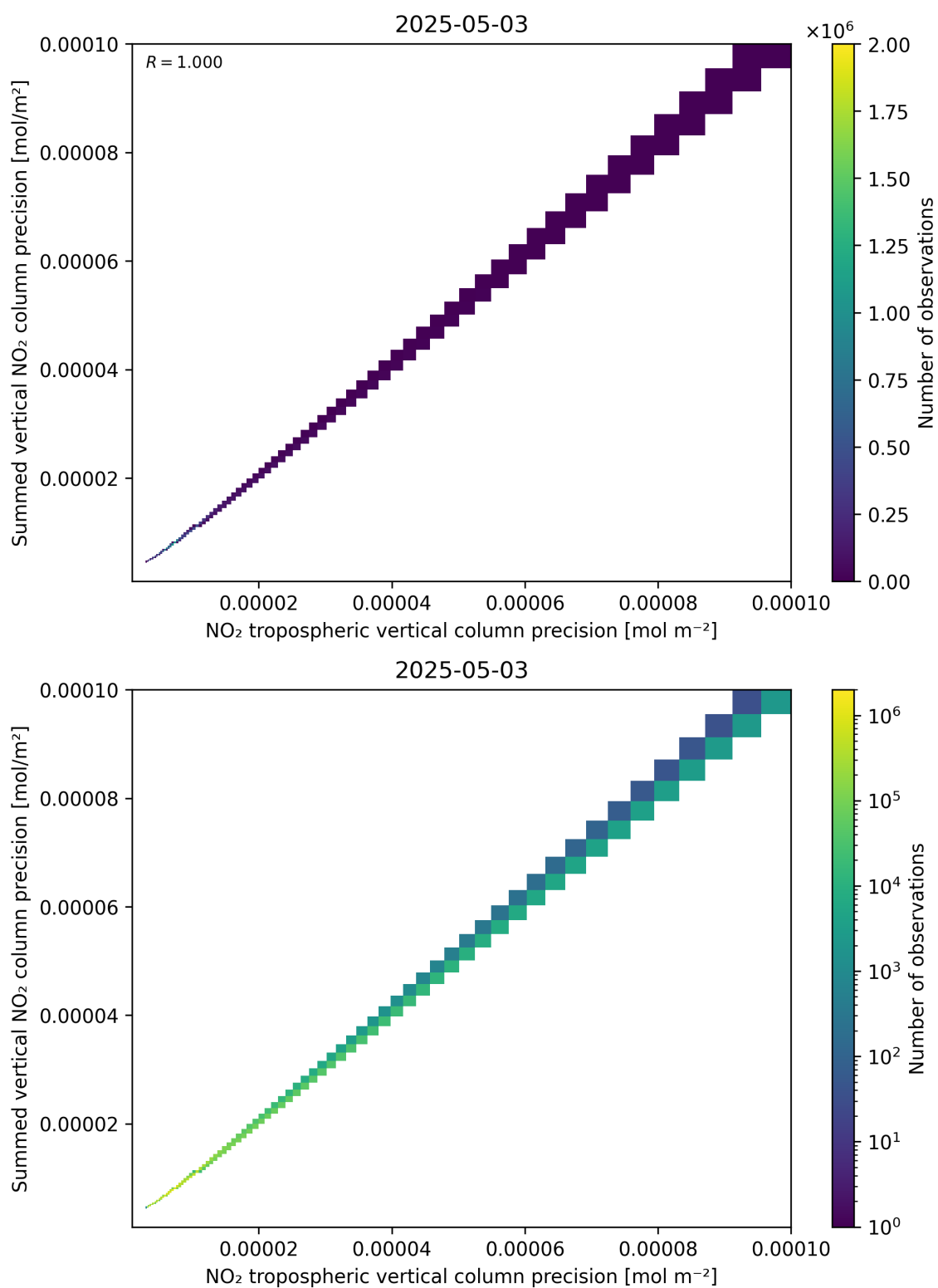
Figure 137: Scatter density plot of “NO 2 tropospheric vertical column precision” against “Summed vertical NO 2 column precision” for 2025-05-03 to 2025-05-03.
