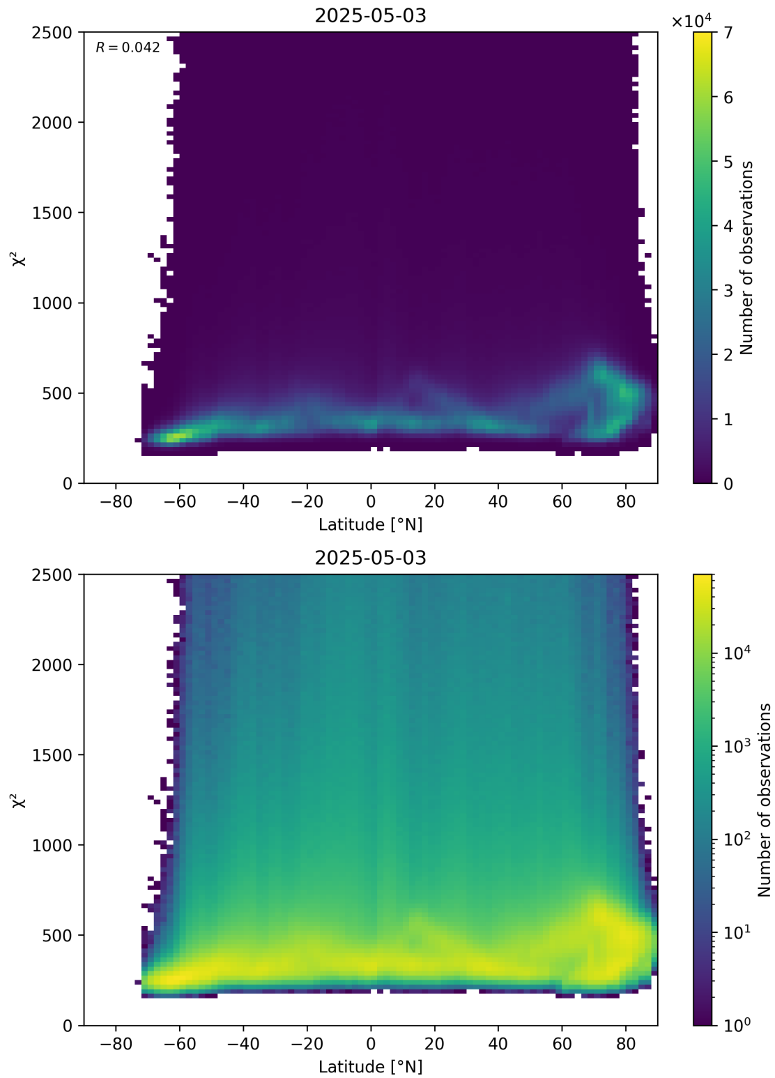
Figure 86: Scatter density plot of “Latitude” against “ \chi^2 ” for 2025-05-03 to 2025-05-03.
