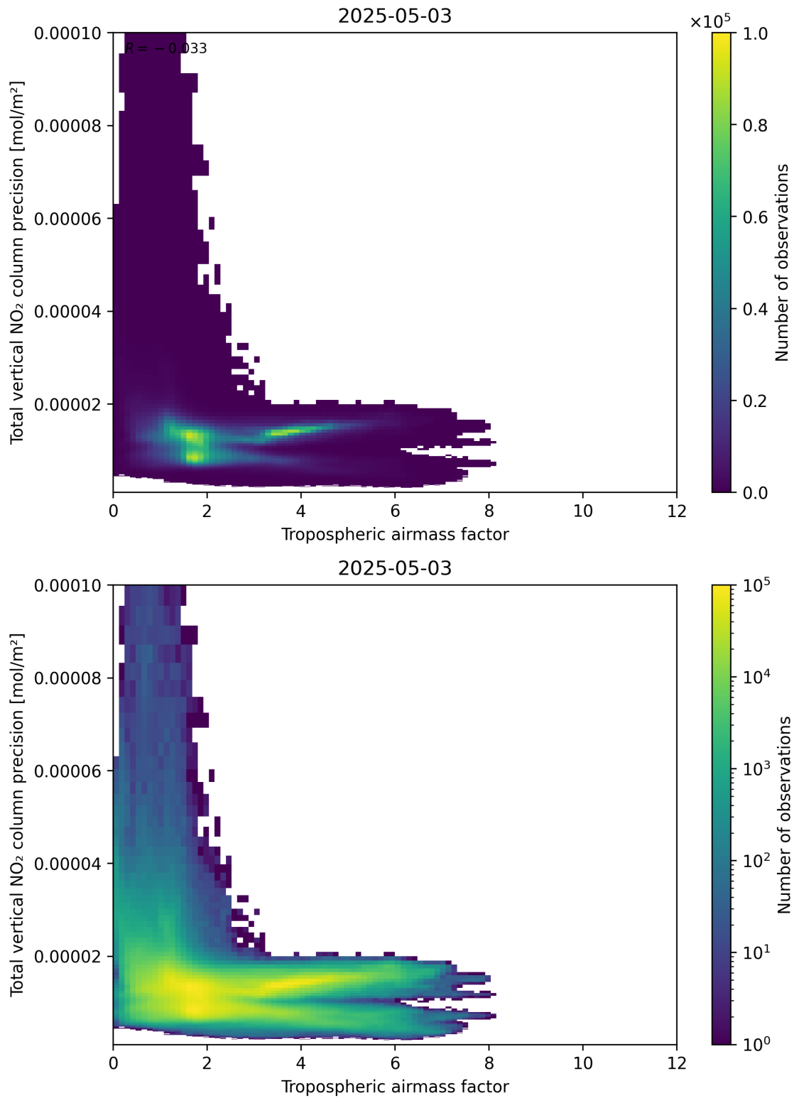
Figure 78: Scatter density plot of “Tropospheric air mass factor” against “Total vertical NO 2 column precision” for 2025-05-03 to 2025-05-03.
