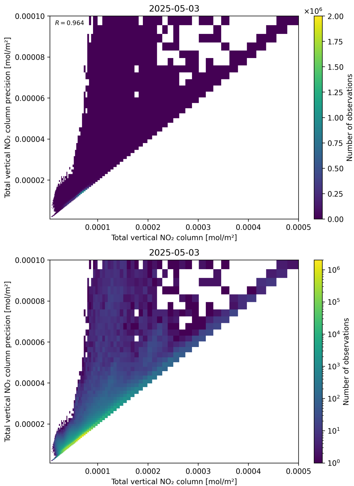
Figure 114: Scatter density plot of “Total vertical NO 2 column” against “Total vertical NO 2 column precision” for 2025-05-03 to 2025-05-03.
