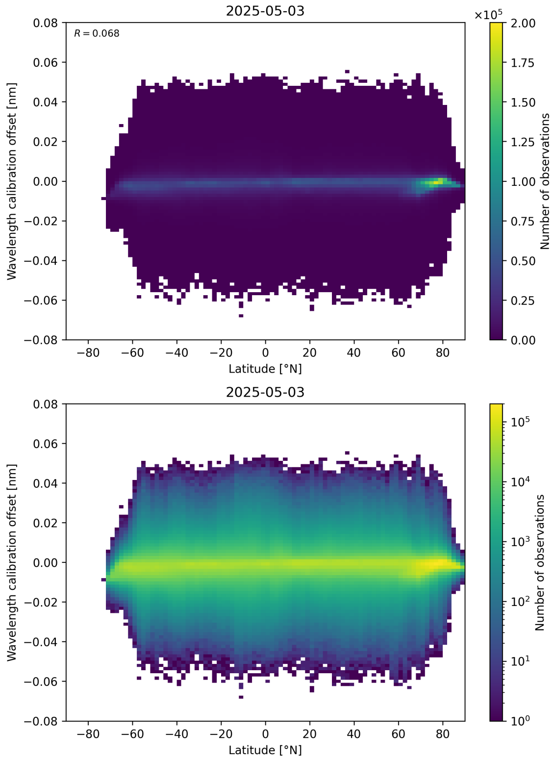
Figure 95: Scatter density plot of “Latitude” against “Wavelength calibration offset” for 2025-05-03 to 2025-05-03.
