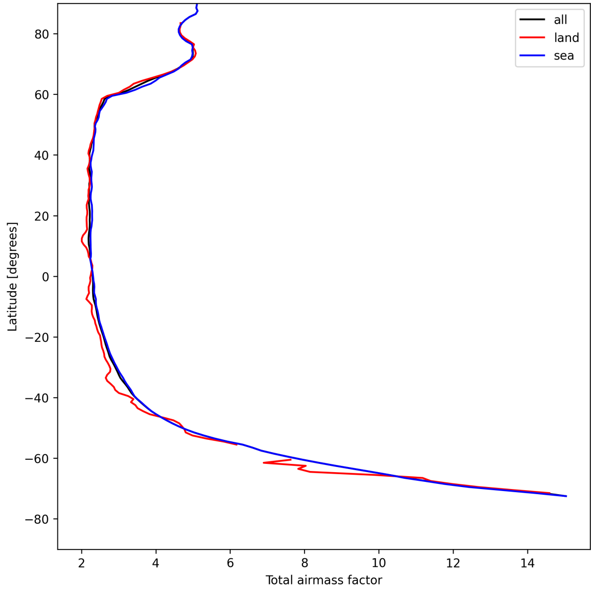
Figure 15: Zonal average of “Total airmass factor” for 2025-05-03 to 2025-05-03.
