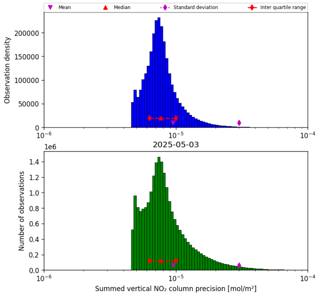
Figure 41: Histogram of "Summed vertical NO 2 column precision" for 2025-05-03 to 2025-05-03
