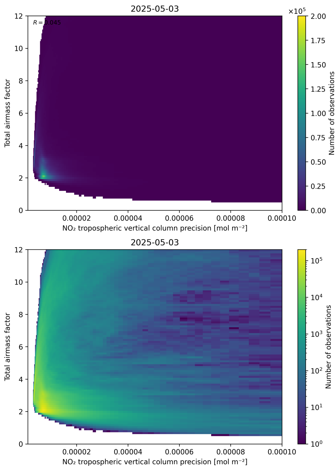
Figure 132: Scatter density plot of “NO 2 tropospheric vertical column precision” against “Total air mass factor” for 2025-05-03 to 2025-05-03.
