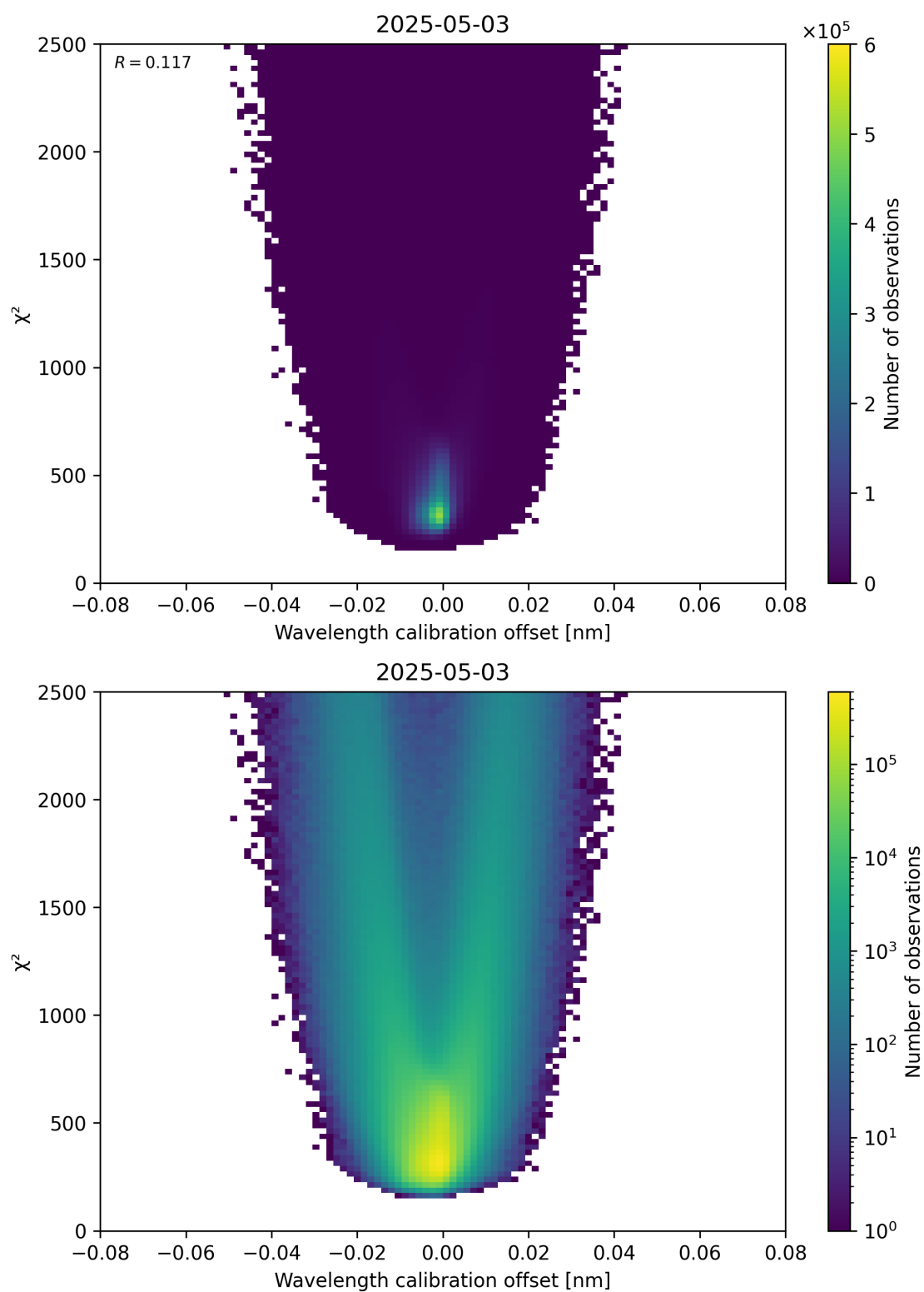
Figure 175: Scatter density plot of “Wavelength calibration offset” against “ \chi^2 ” for 2025-05-03 to 2025-05-03.
