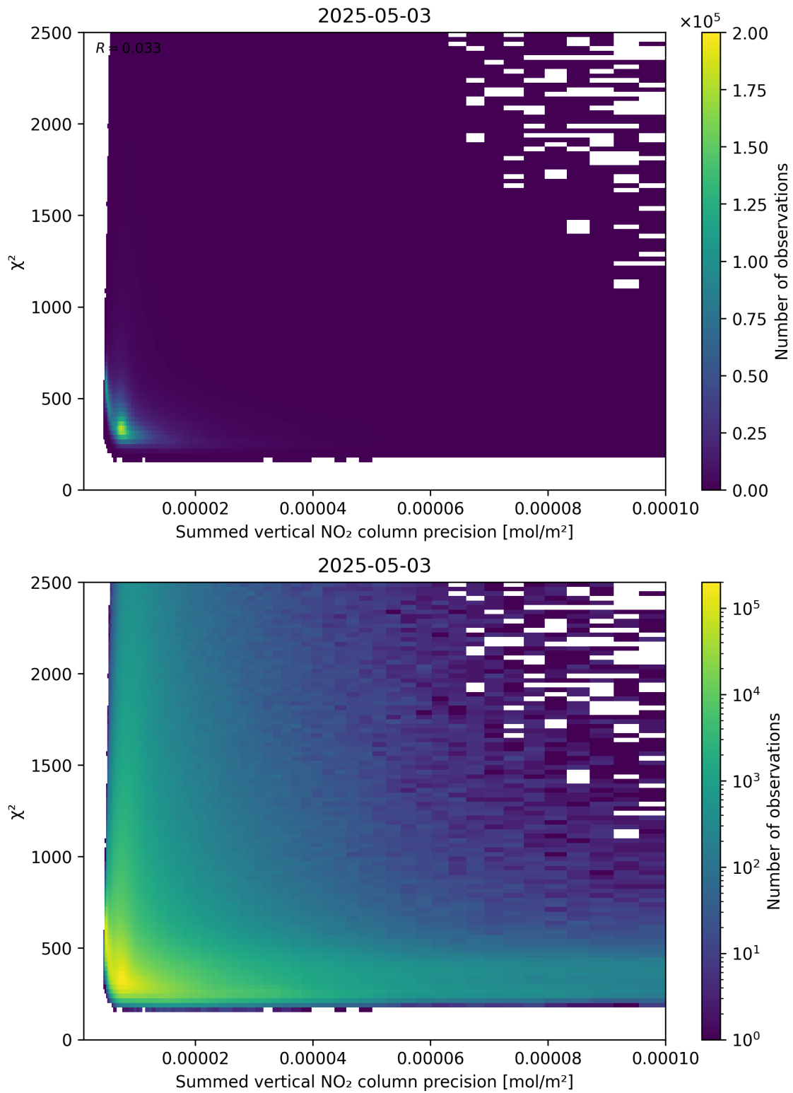
Figure 107: Scatter density plot of “Summed vertical NO 2 column precision” against “ \chi^2 ” for 2025-05-03 to 2025-05-03.
