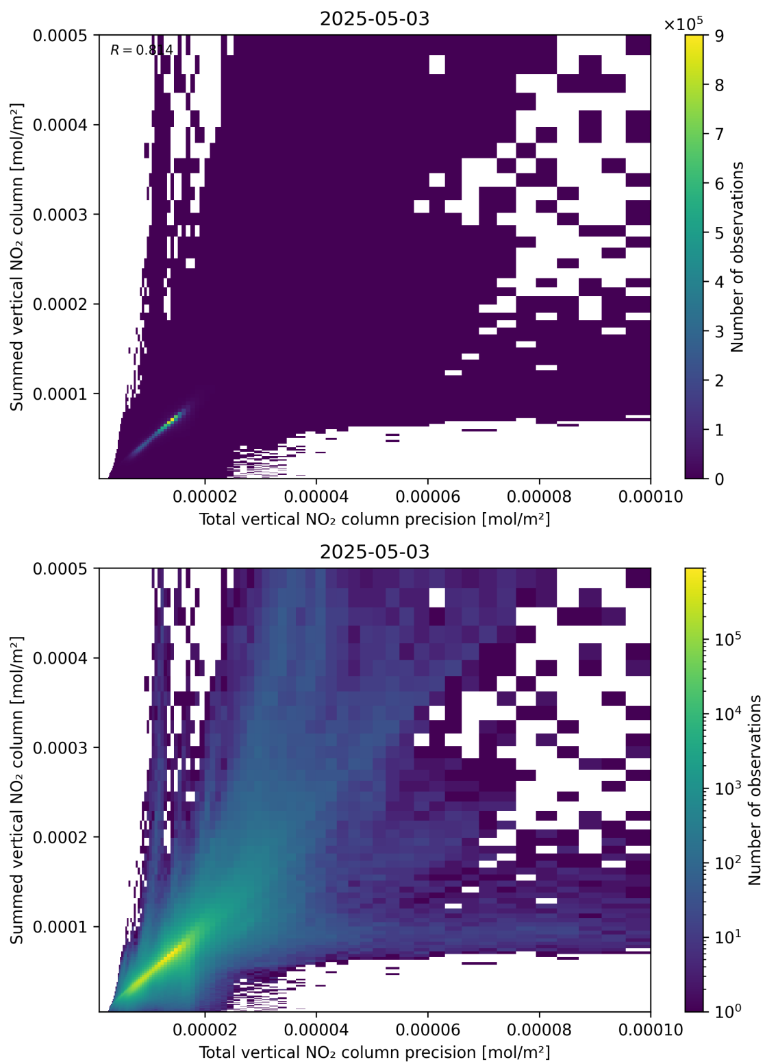
Figure 117: Scatter density plot of “Total vertical NO 2 column precision” against “Summed vertical NO 2 column” for 2025-05-03 to 2025-05-03.
