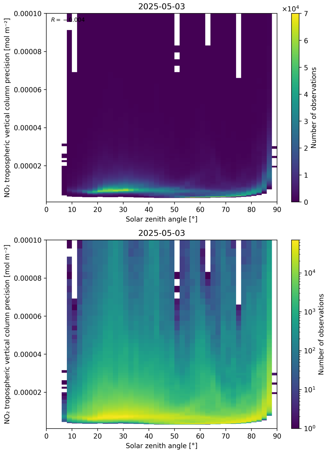
Figure 156: Scatter density plot of “Solar zenith angle” against “NO 2 tropospheric vertical column precision” for 2025-05-03 to 2025-05-03.
