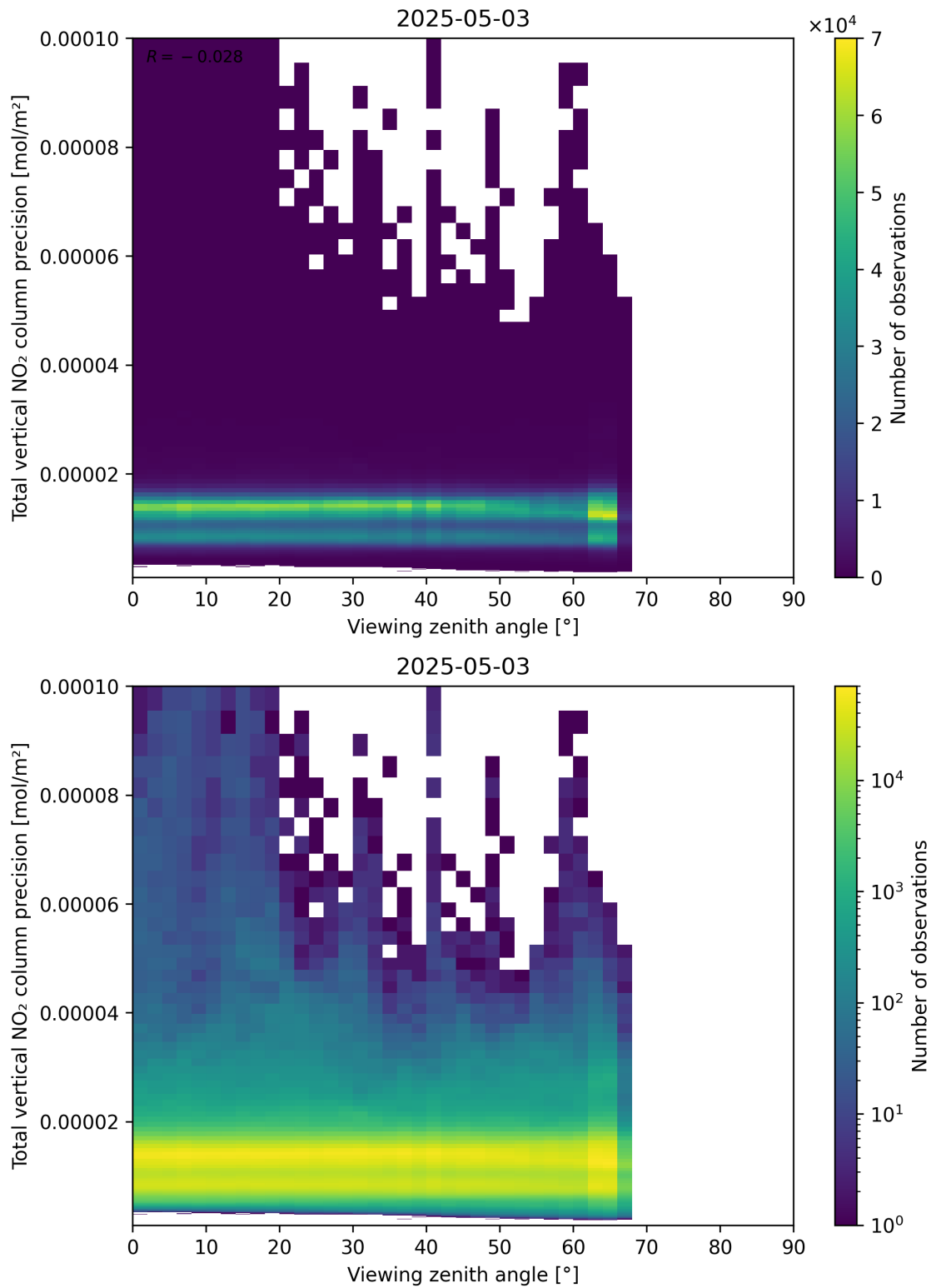
Figure 168: Scatter density plot of “Viewing zenith angle” against “Total vertical NO 2 column precision” for 2025-05-03 to 2025-05-03.
