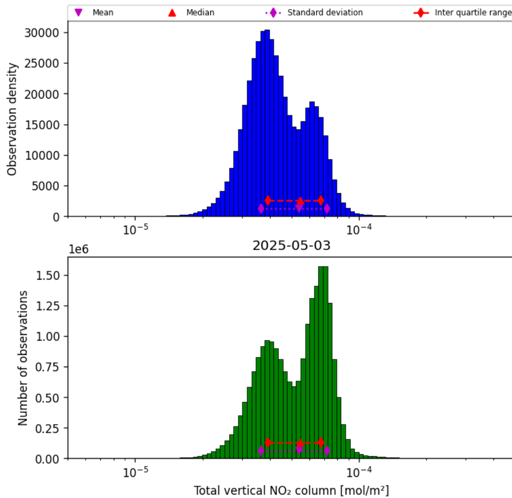
Figure 38: Histogram of “Total vertical NO 2 column” for 2025-05-03 to 2025-05-03
