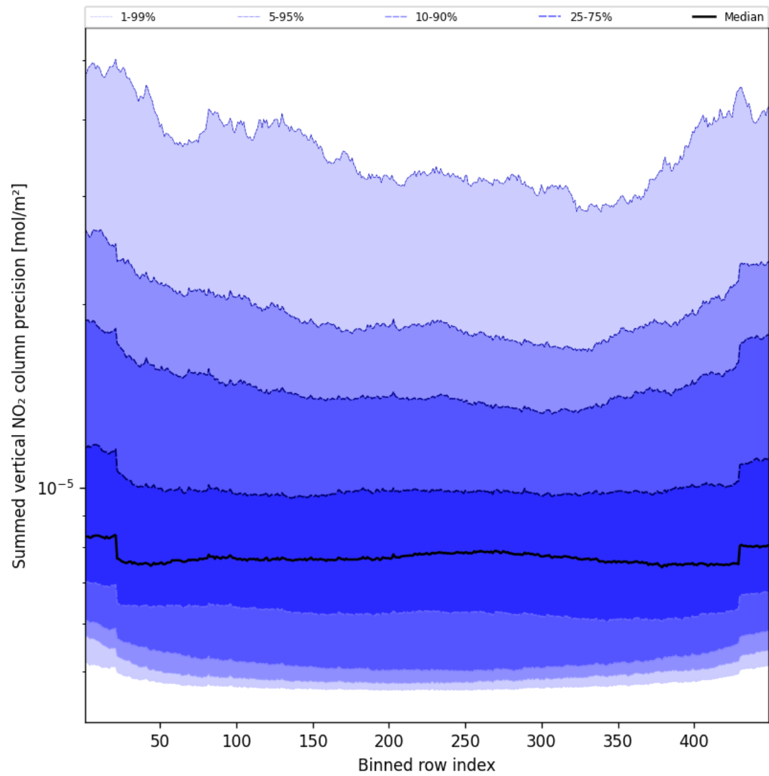
Figure 58: Along track statistics of “Summed vertical NO 2 column precision” for 2025-05-03 to 2025-05-03
