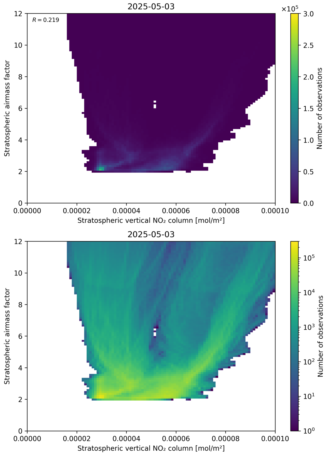
Figure 96: Scatter density plot of “Stratospheric vertical NO 2 column” against “Stratospheric airmass factor” for 2025-05-03 to 2025-05-03.
