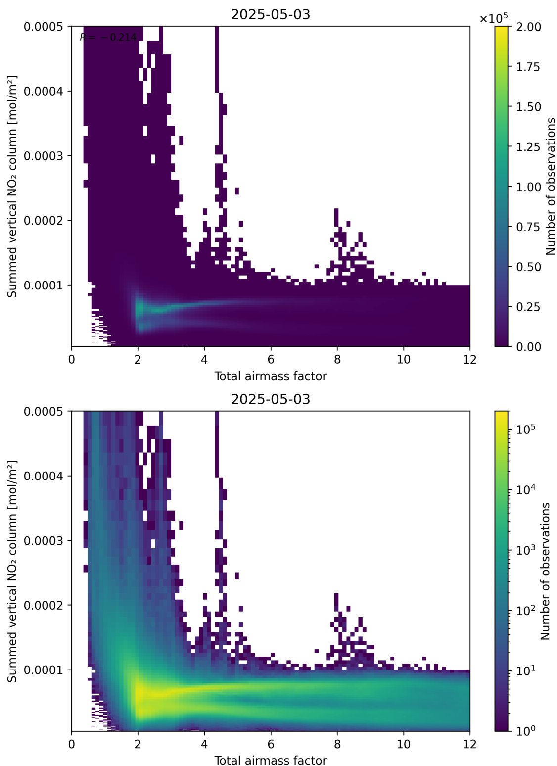
Figure 65: Scatter density plot of “Total airmass factor” against “Summed vertical NO 2 column” for 2025-05-03 to 2025-05-03.
