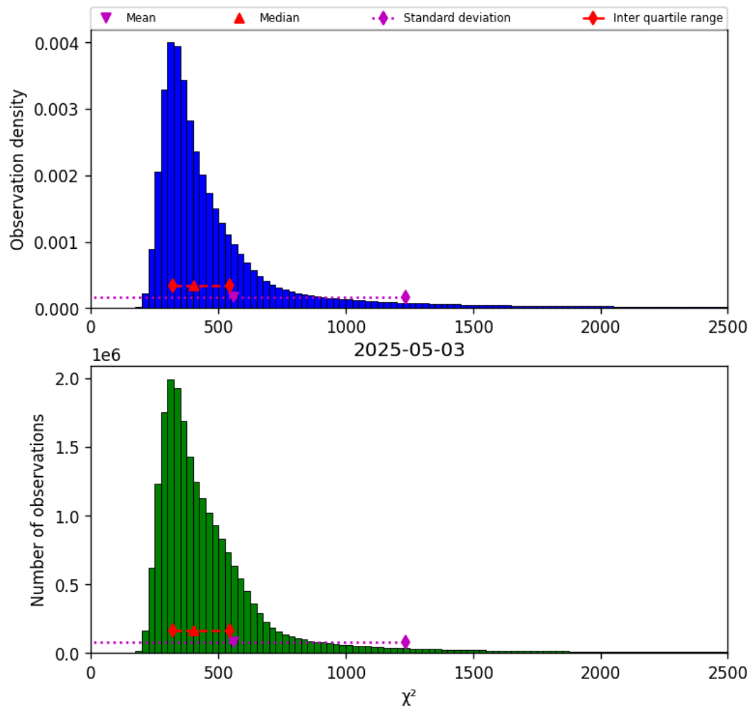
Figure 42: Histogram of “ \chi^2 ” for 2025-05-03 to 2025-05-03
