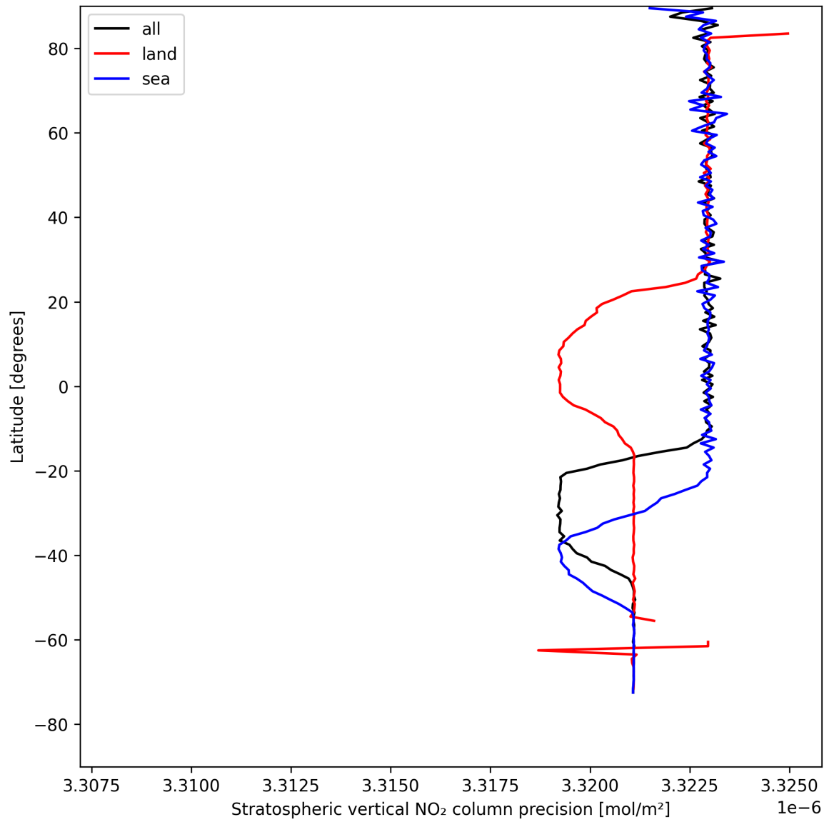
Figure 20: Zonal average of “Stratospheric vertical NO 2 column precision” for 2025-05-03 to 2025-05-03.
