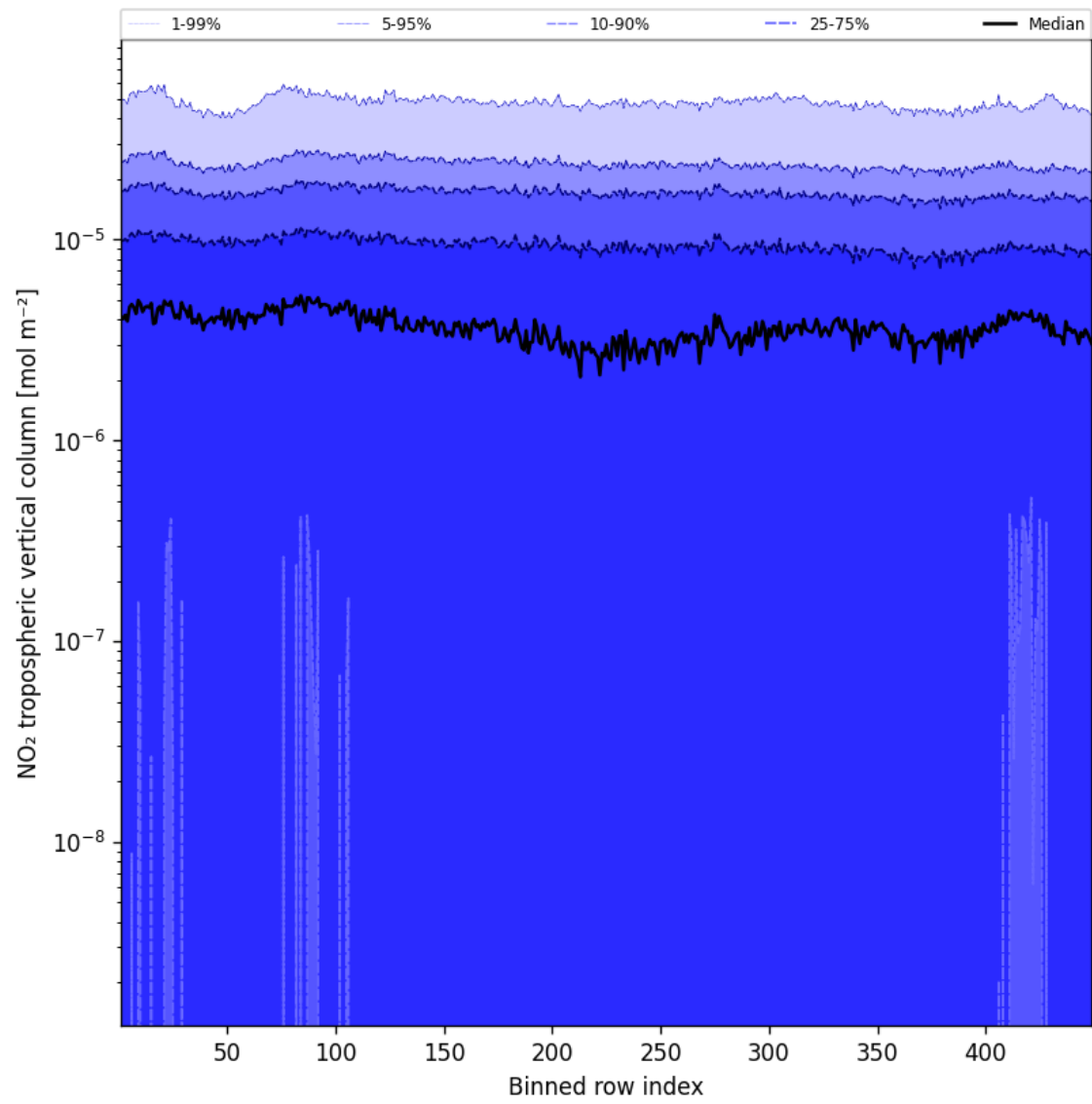
Figure 46: Along track statistics of "NO 2 tropospheric vertical column" for 2025-05-03 to 2025-05-03
