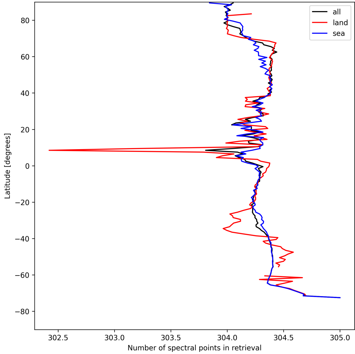
Figure 16: Zonal average of “Number of spectral points in retrieval” for 2025-05-03 to 2025-05-03.
