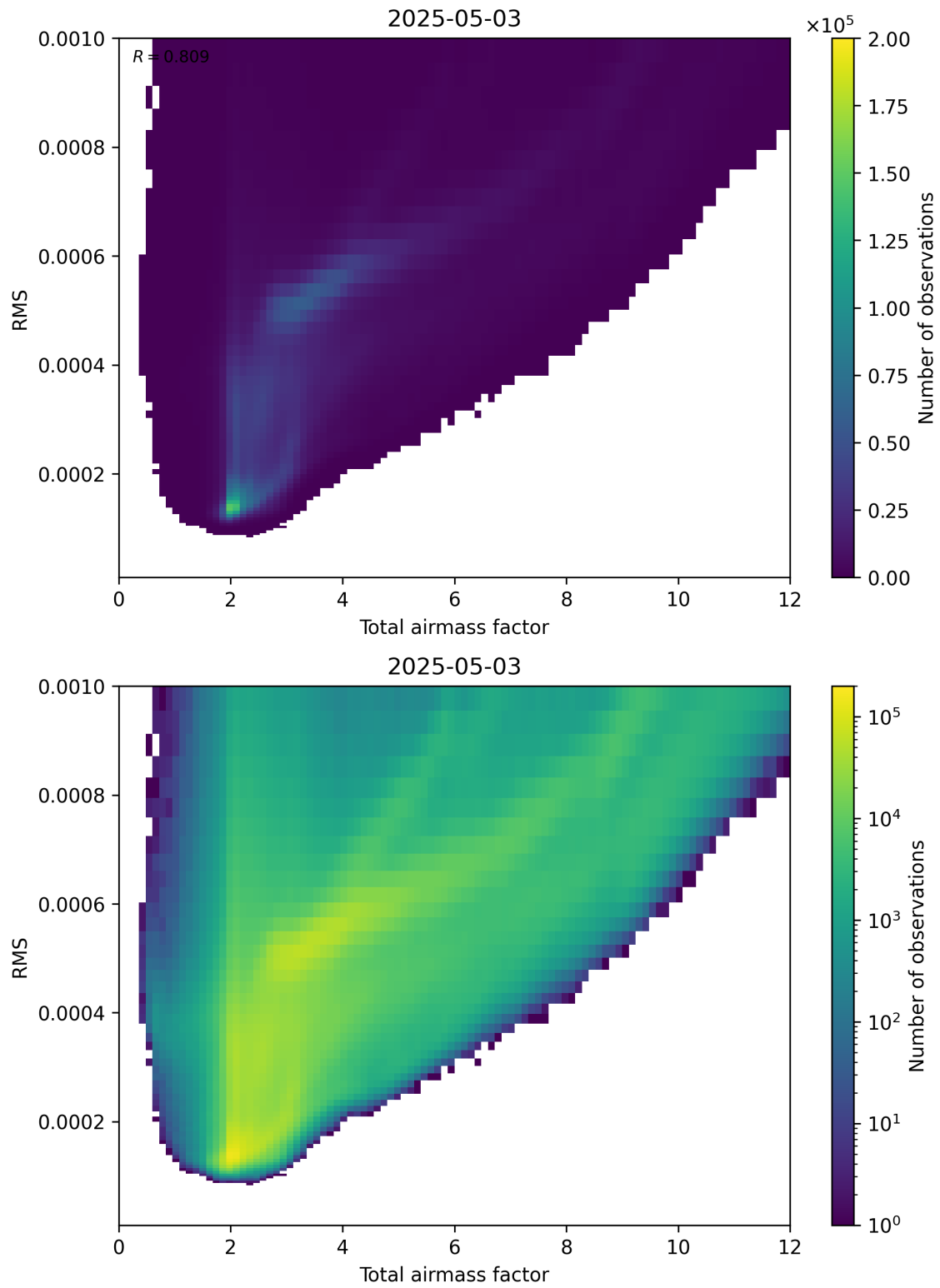
Figure 69: Scatter density plot of “Total airmass factor” against “RMS” for 2025-05-03 to 2025-05-03.
