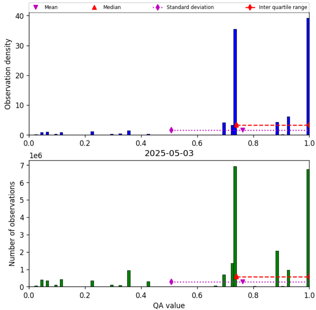
Figure 28: Histogram of “QA value” for 2025-05-03 to 2025-05-03
