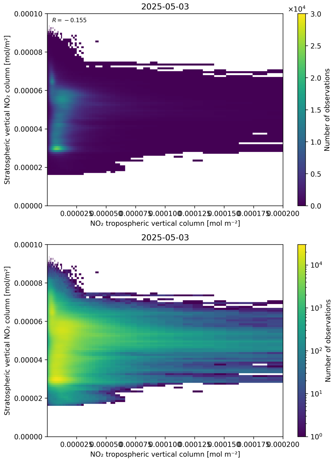
Figure 125: Scatter density plot of “NO 2 tropospheric vertical column” against “Stratospheric vertical NO 2 column” for 2025-05-03 to 2025-05-03.
