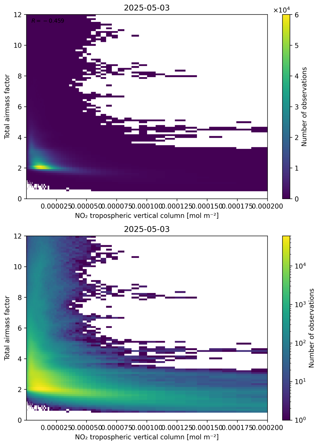
Figure 122: Scatter density plot of “NO 2 tropospheric vertical column” against “Total air mass factor” for 2025-05-03 to 2025-05-03.
