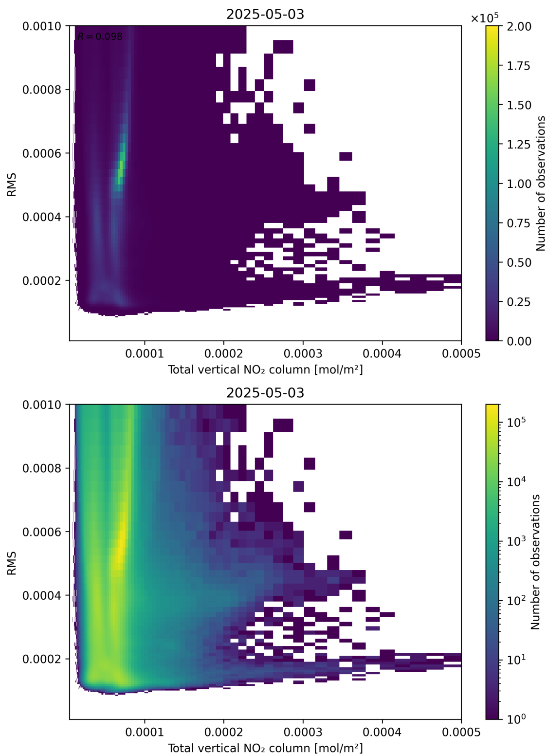
Figure 120: Scatter density plot of “Total vertical NO 2 column” against “RMS” for 2025-05-03 to 2025-05-03.
