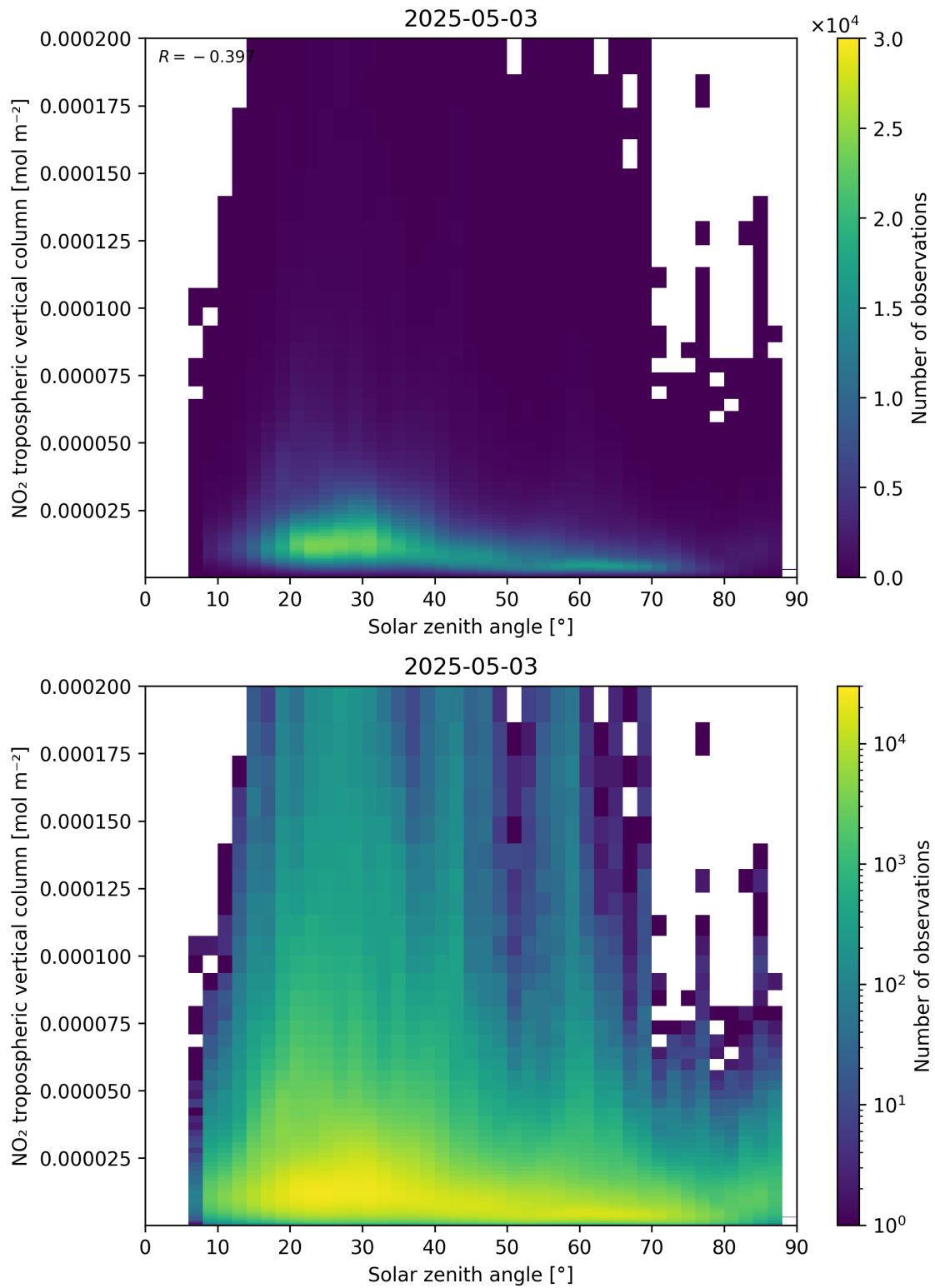
Figure 155: Scatter density plot of “Solar zenith angle” against “NO 2 tropospheric vertical column” for 2025-05-03 to 2025-05-03.
