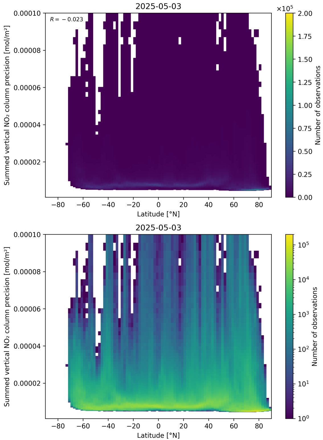
Figure 89: Scatter density plot of “Latitude” against “Summed vertical NO 2 column precision” for 2025-05-03 to 2025-05-03.
