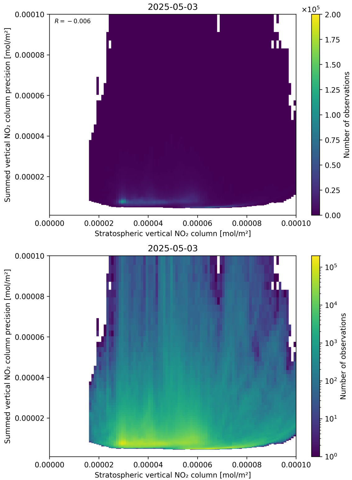
Figure 99: Scatter density plot of “Stratospheric vertical NO 2 column” against “Summed vertical NO 2 column precision” for 2025-05-03 to 2025-05-03.
