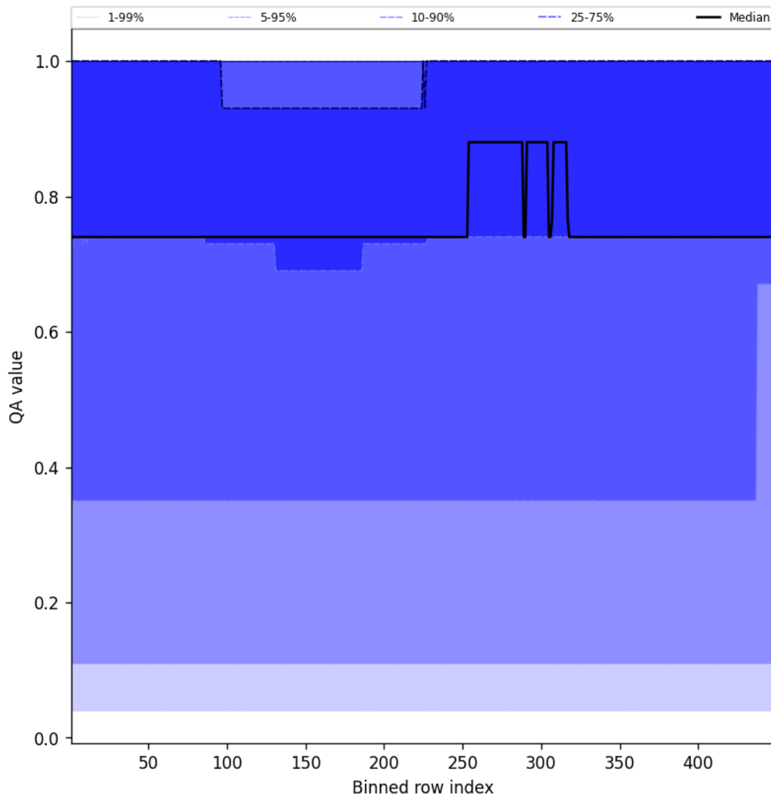
Figure 45: Along track statistics of “QA value” for 2025-05-03 to 2025-05-03
