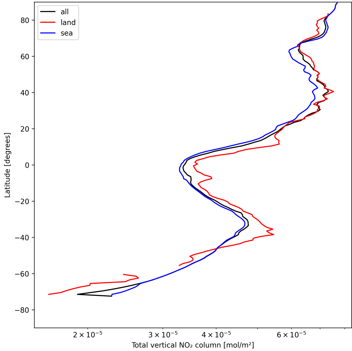
Figure 21: Zonal average of “Total vertical NO 2 column” for 2025-05-03 to 2025-05-03.
