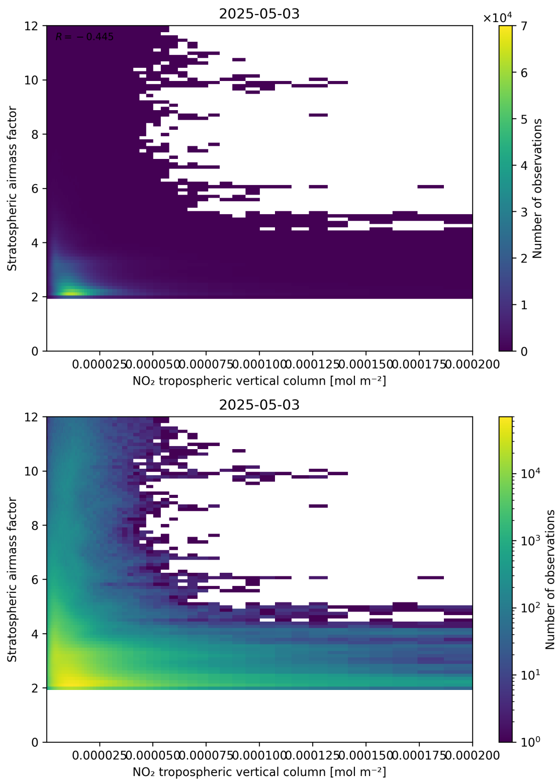
Figure 121: Scatter density plot of “NO 2 tropospheric vertical column” against “Stratospheric air mass factor” for 2025-05-03 to 2025-05-03.
