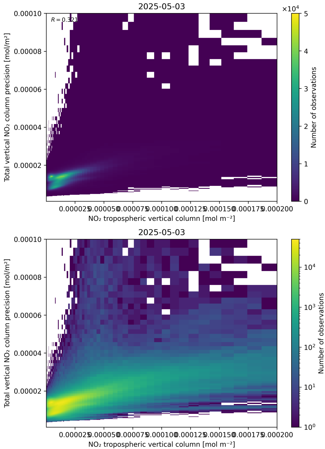
Figure 129: Scatter density plot of “NO 2 tropospheric vertical column” against “Total vertical NO 2 column precision” for 2025-05-03 to 2025-05-03.
