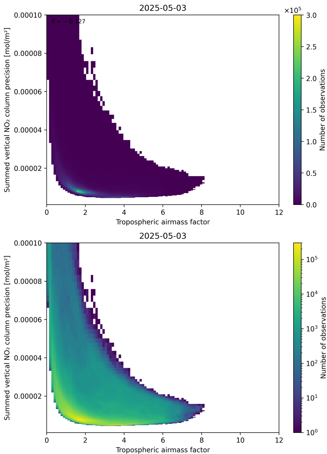
Figure 76: Scatter density plot of “Tropospheric air mass factor” against “Summed vertical NO 2 column precision” for 2025-05-03 to 2025-05-03.
