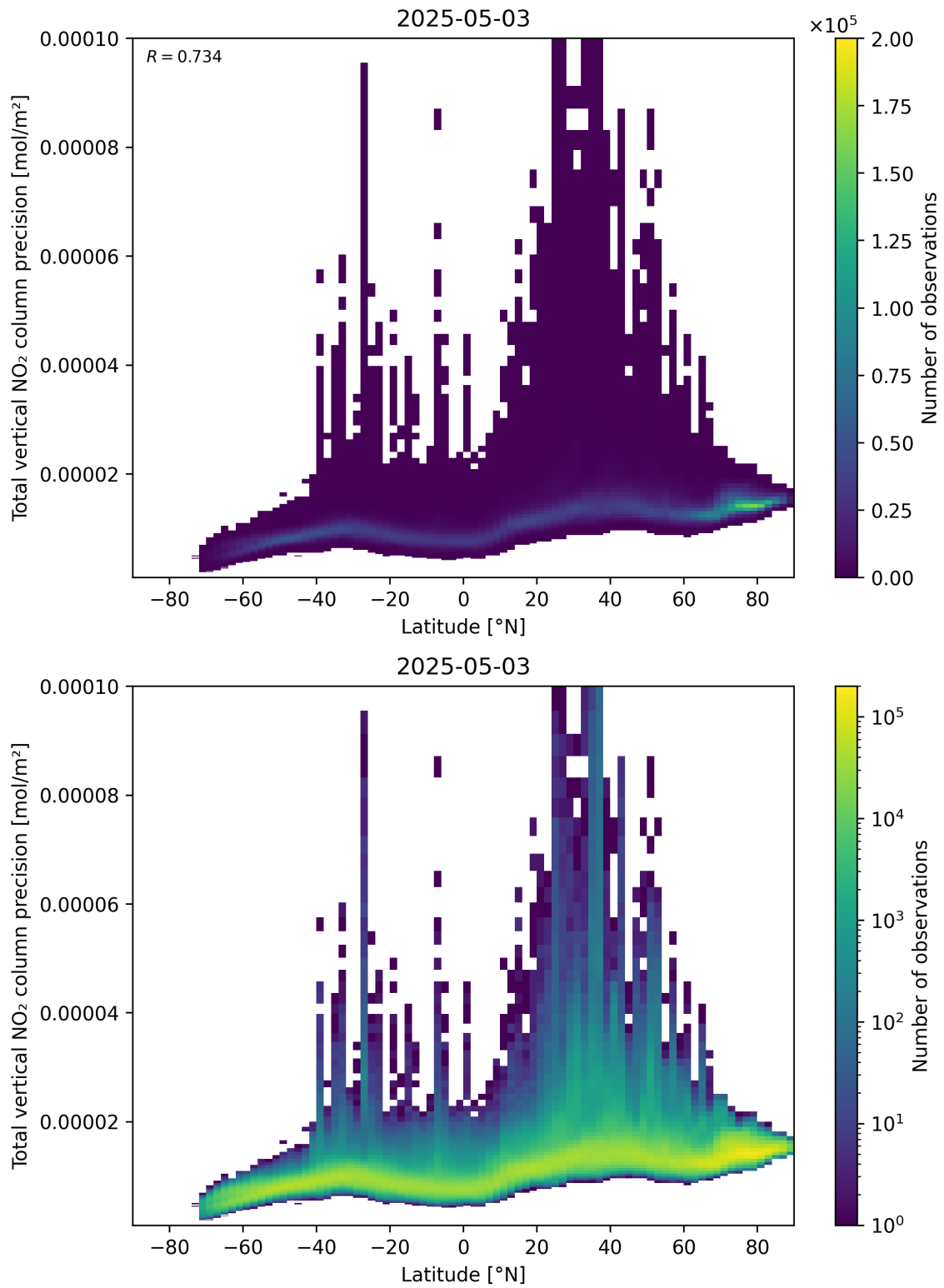
Figure 91: Scatter density plot of “Latitude” against “Total vertical NO 2 column precision” for 2025-05-03 to 2025-05-03.
