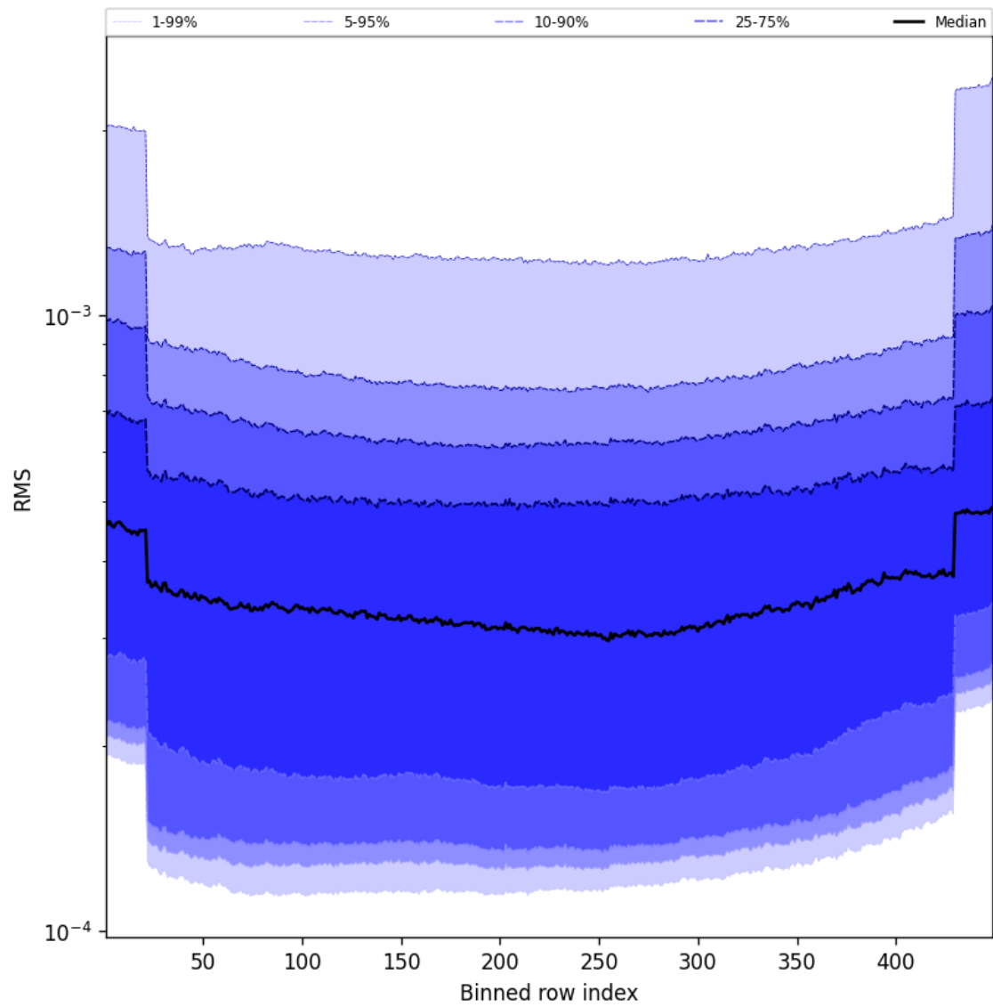
Figure 60: Along track statistics of “RMS” for 2025-05-03 to 2025-05-03
