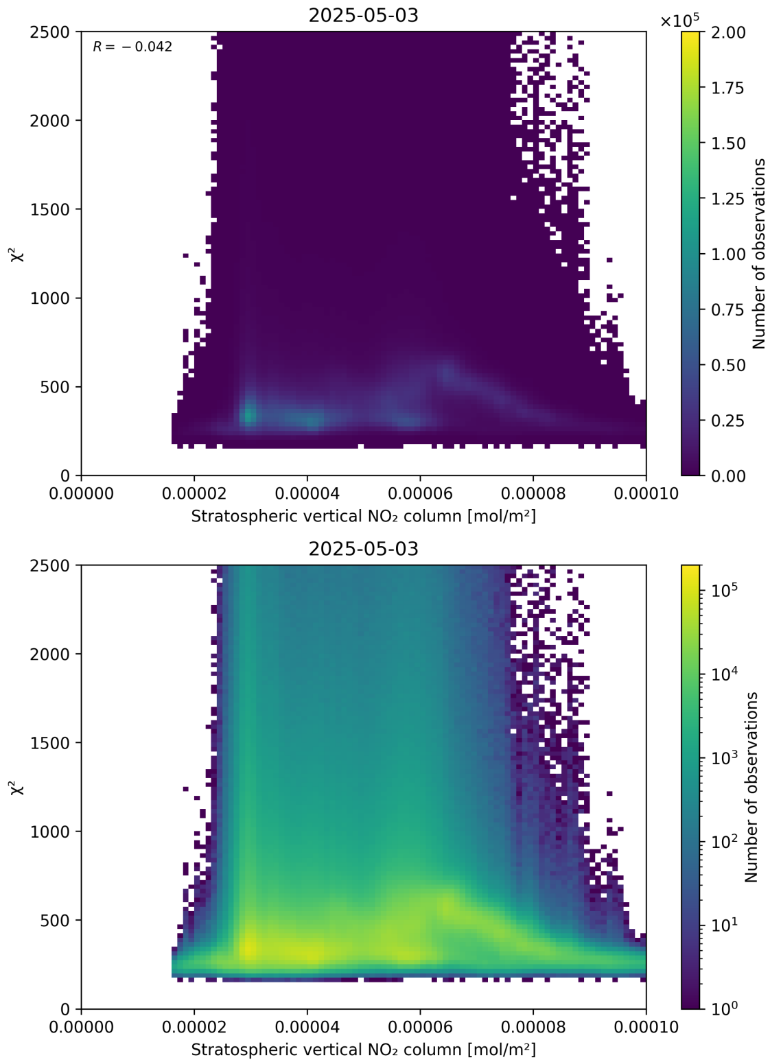
Figure 97: Scatter density plot of “Stratospheric vertical NO 2 column” against “ \chi^2 ” for 2025-05-03 to 2025-05-03.
