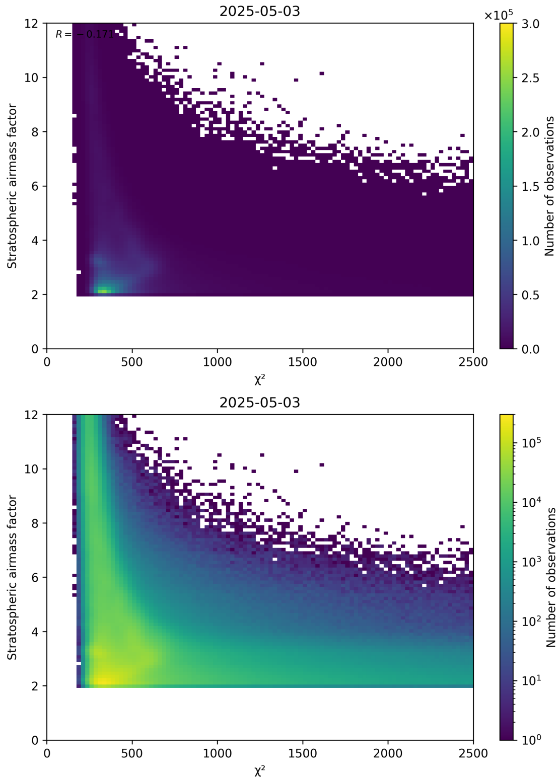
Figure 81: Scatter density plot of “ \chi^2 ” against “Stratospheric airmass factor” for 2025-05-03 to 2025-05-03.
