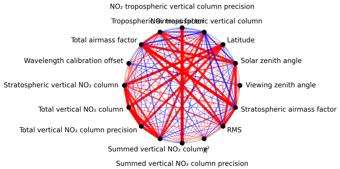
Figure 1: Map of correlation graph for 2025-05-03 to 2025-05-03.
