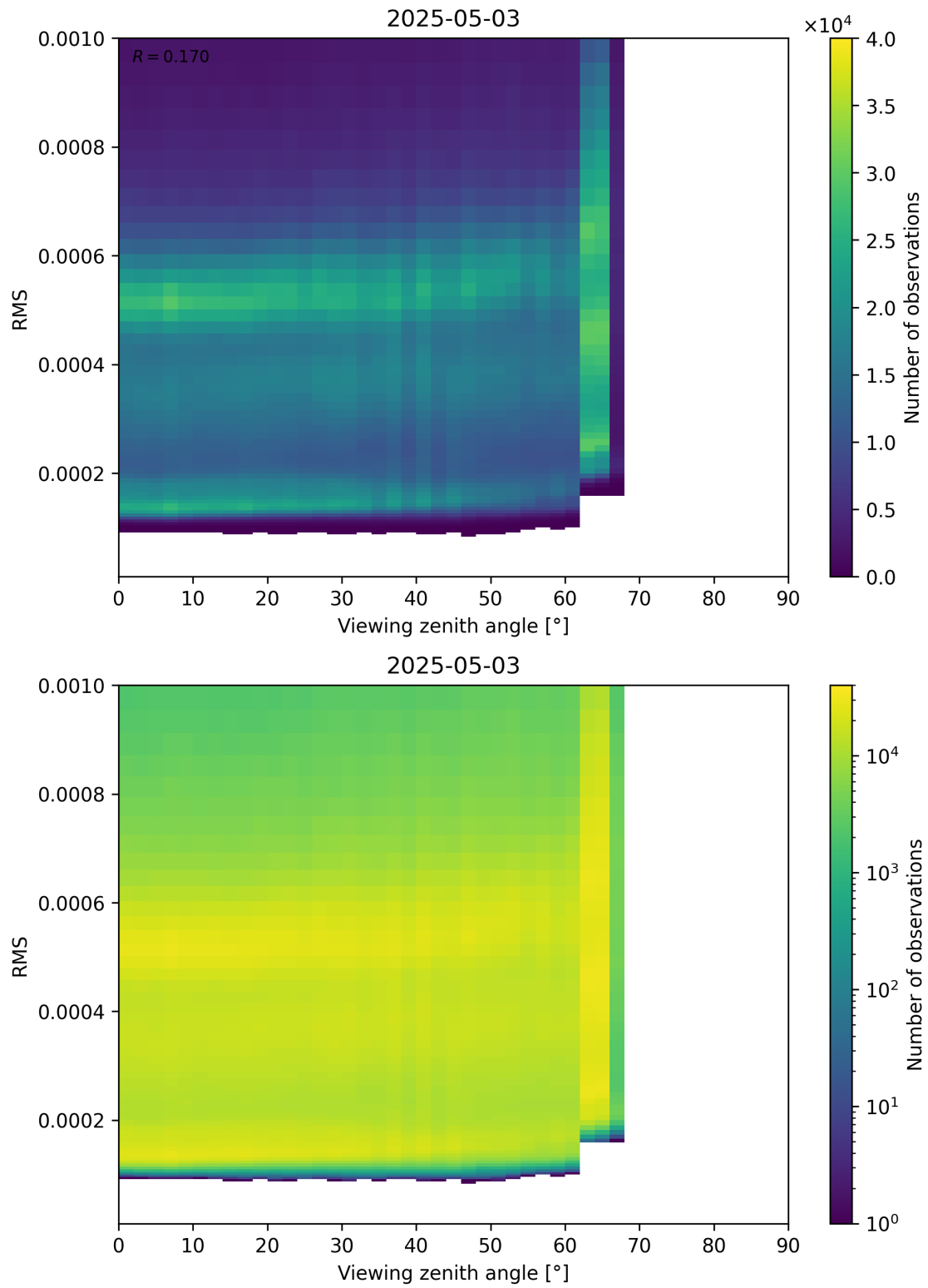
Figure 171: Scatter density plot of “Viewing zenith angle” against “RMS” for 2025-05-03 to 2025-05-03.
