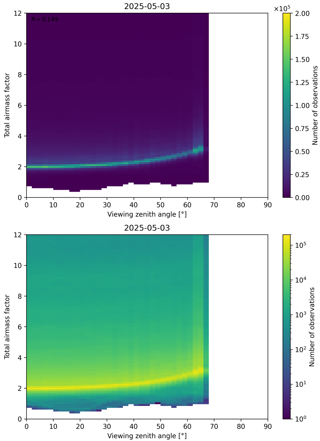
Figure 160: Scatter density plot of “Viewing zenith angle” against “Total airmass factor” for 2025-05-03 to 2025-05-03.
