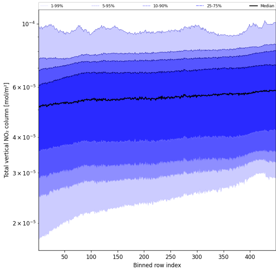
Figure 55: Along track statistics of “Total vertical NO 2 column” for 2025-05-03 to 2025-05-03
