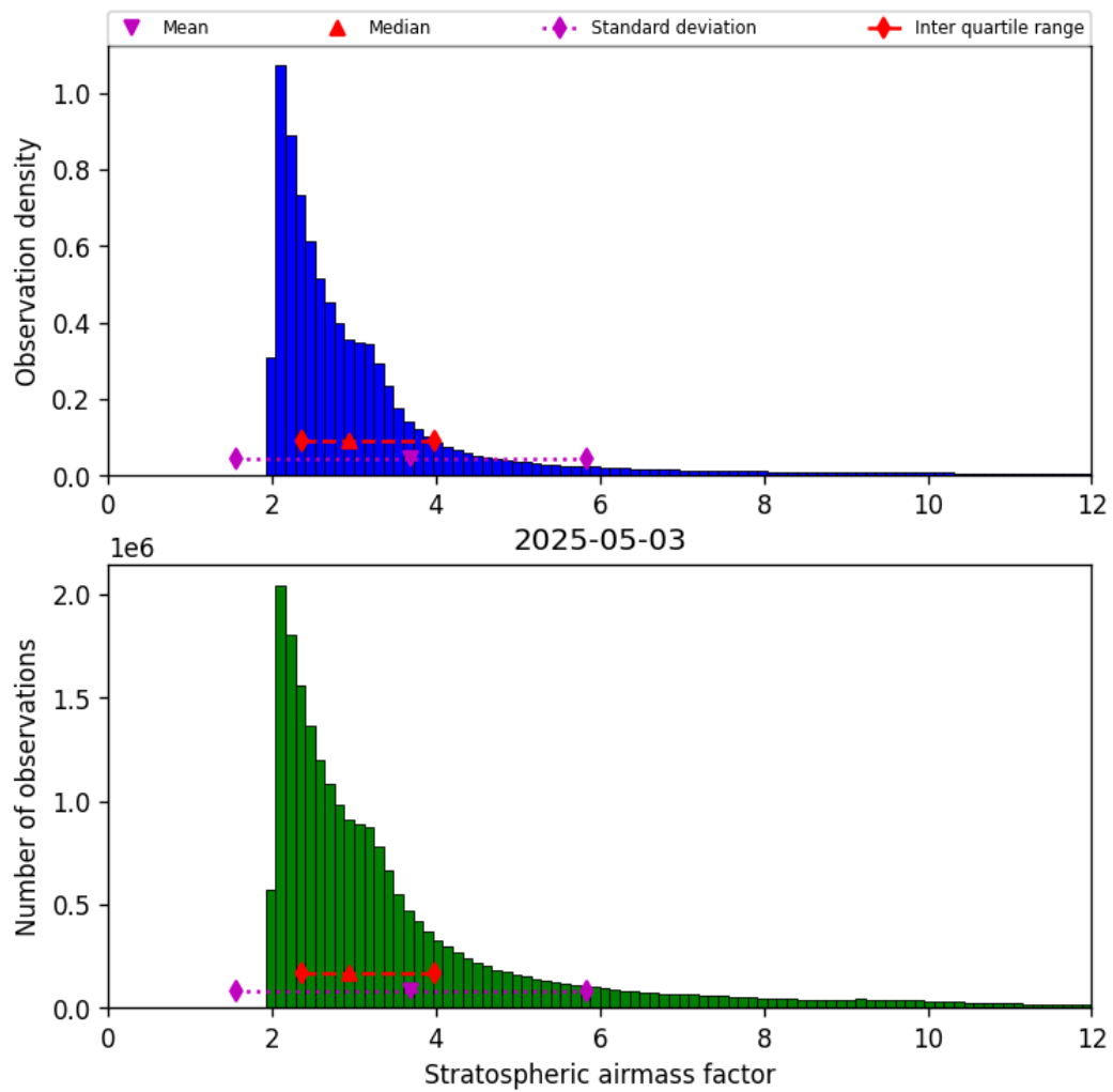
Figure 44: Histogram of “Stratospheric airmass factor” for 2025-05-03 to 2025-05-03
