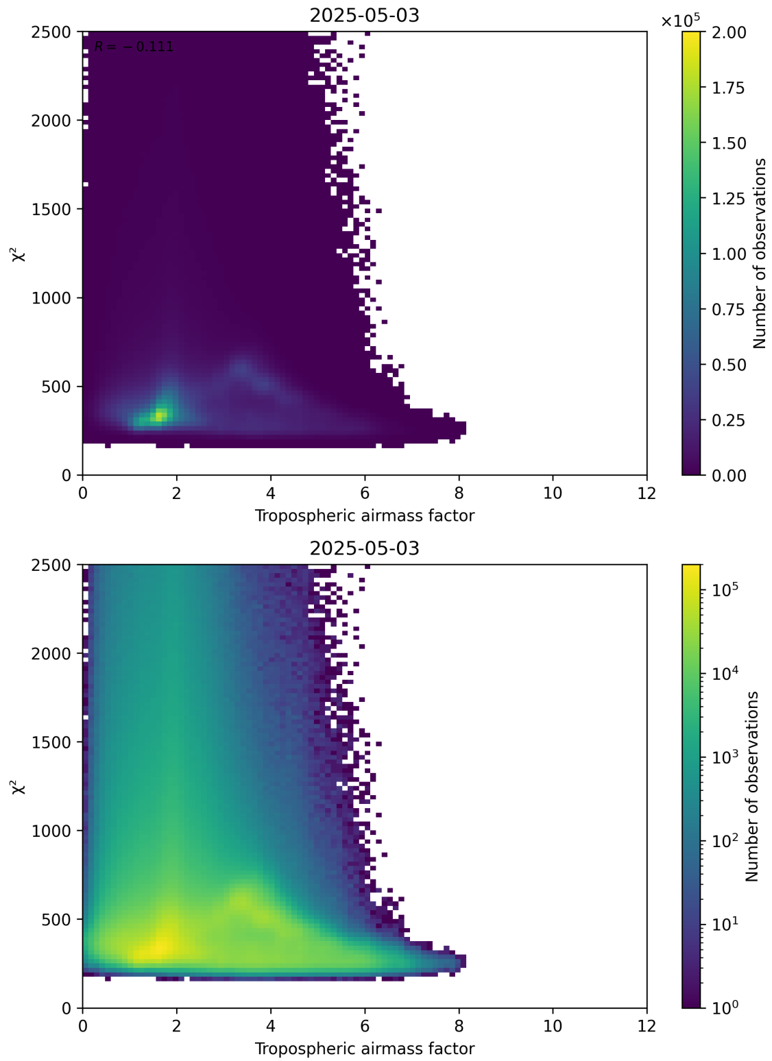
Figure 73: Scatter density plot of “Tropospheric airmass factor” against “ \chi^2 ” for 2025-05-03 to 2025-05-03.
