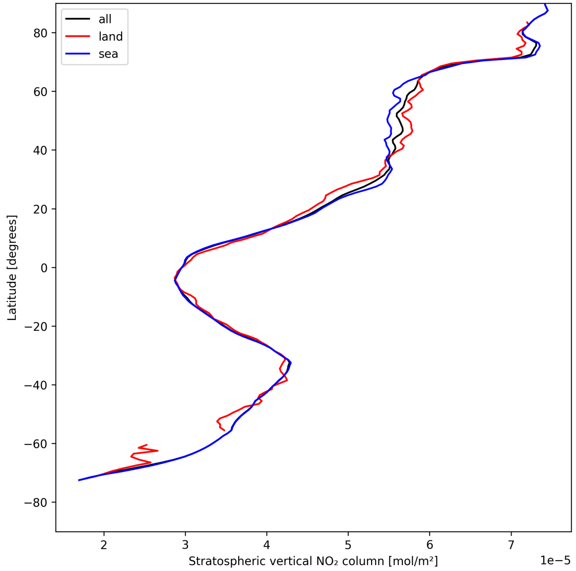
Figure 19: Zonal average of “Stratospheric vertical NO 2 column” for 2025-05-03 to 2025-05-03.
