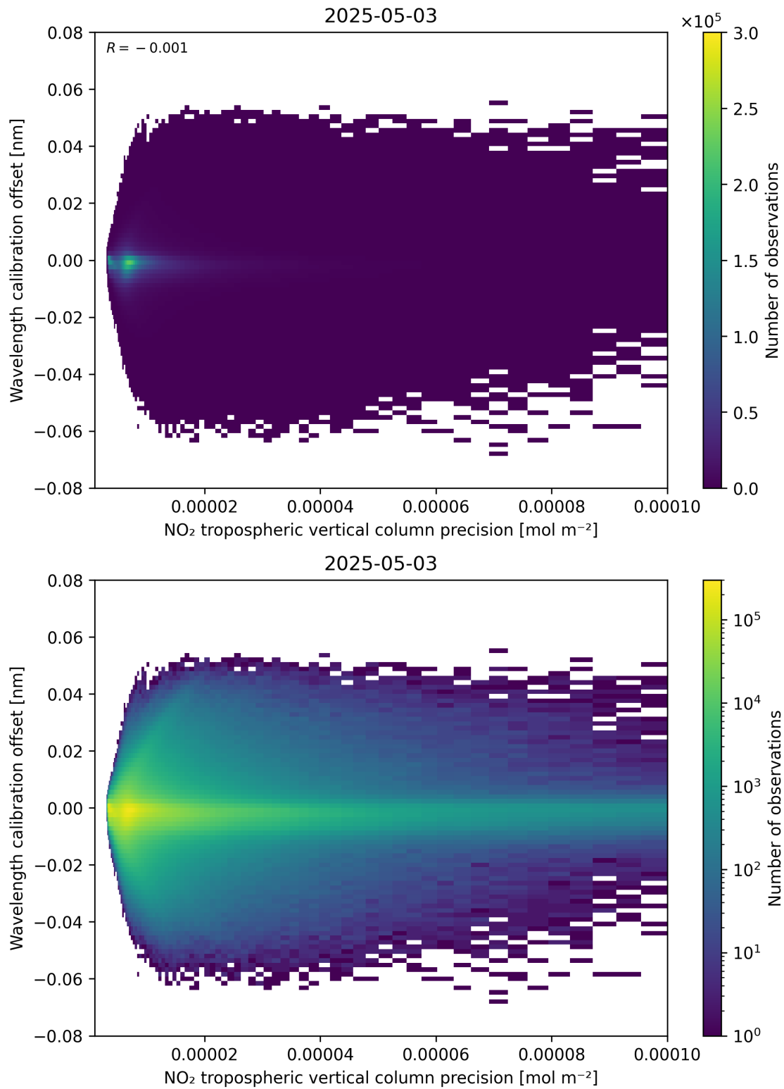
Figure 141: Scatter density plot of “NO 2 tropospheric vertical column precision” against “Wavelength calibration offset” for 2025-05-03 to 2025-05-03.
