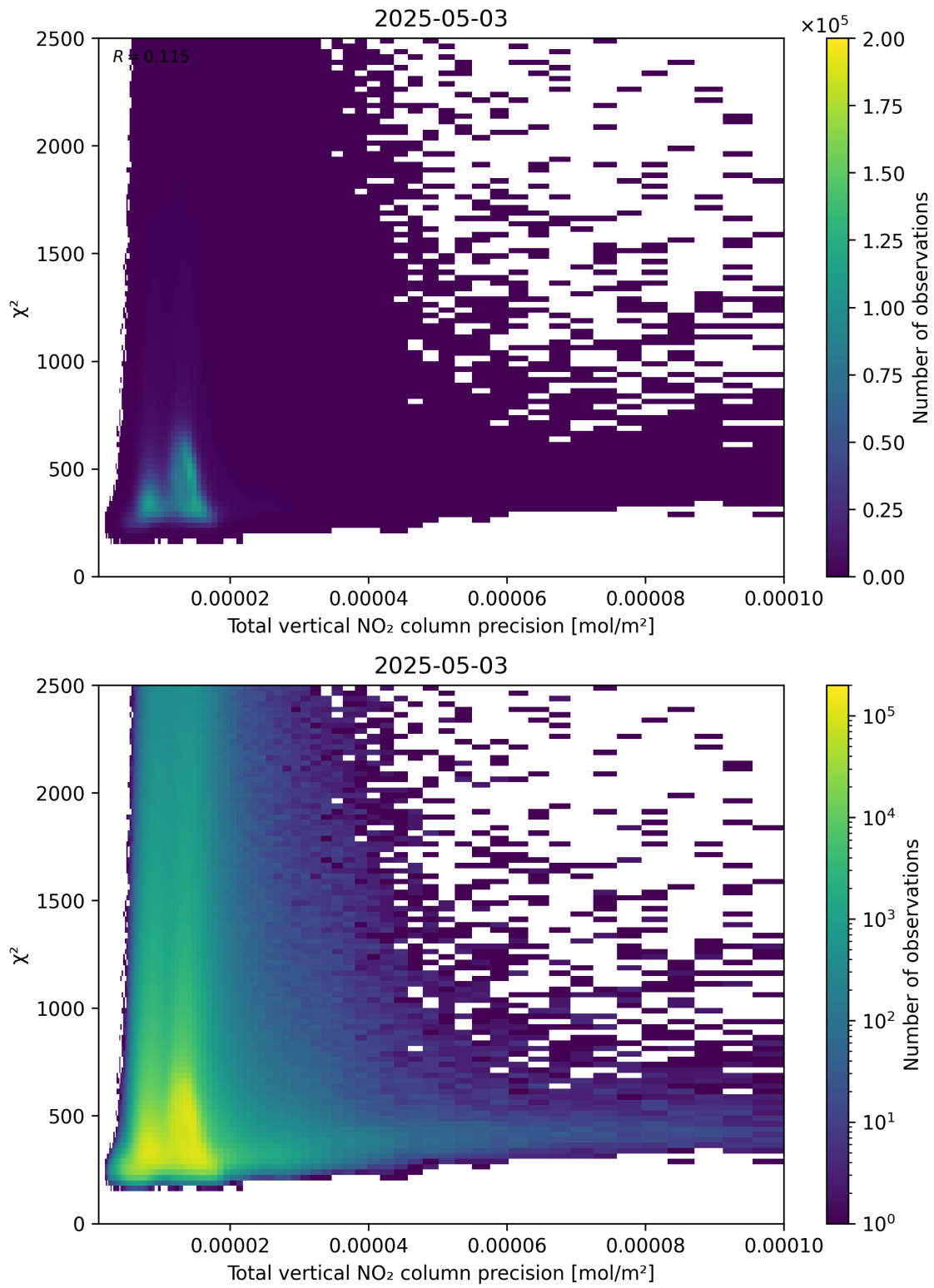
Figure 116: Scatter density plot of “Total vertical NO 2 column precision” against “ \chi^2 ” for 2025-05-03 to 2025-05-03.
