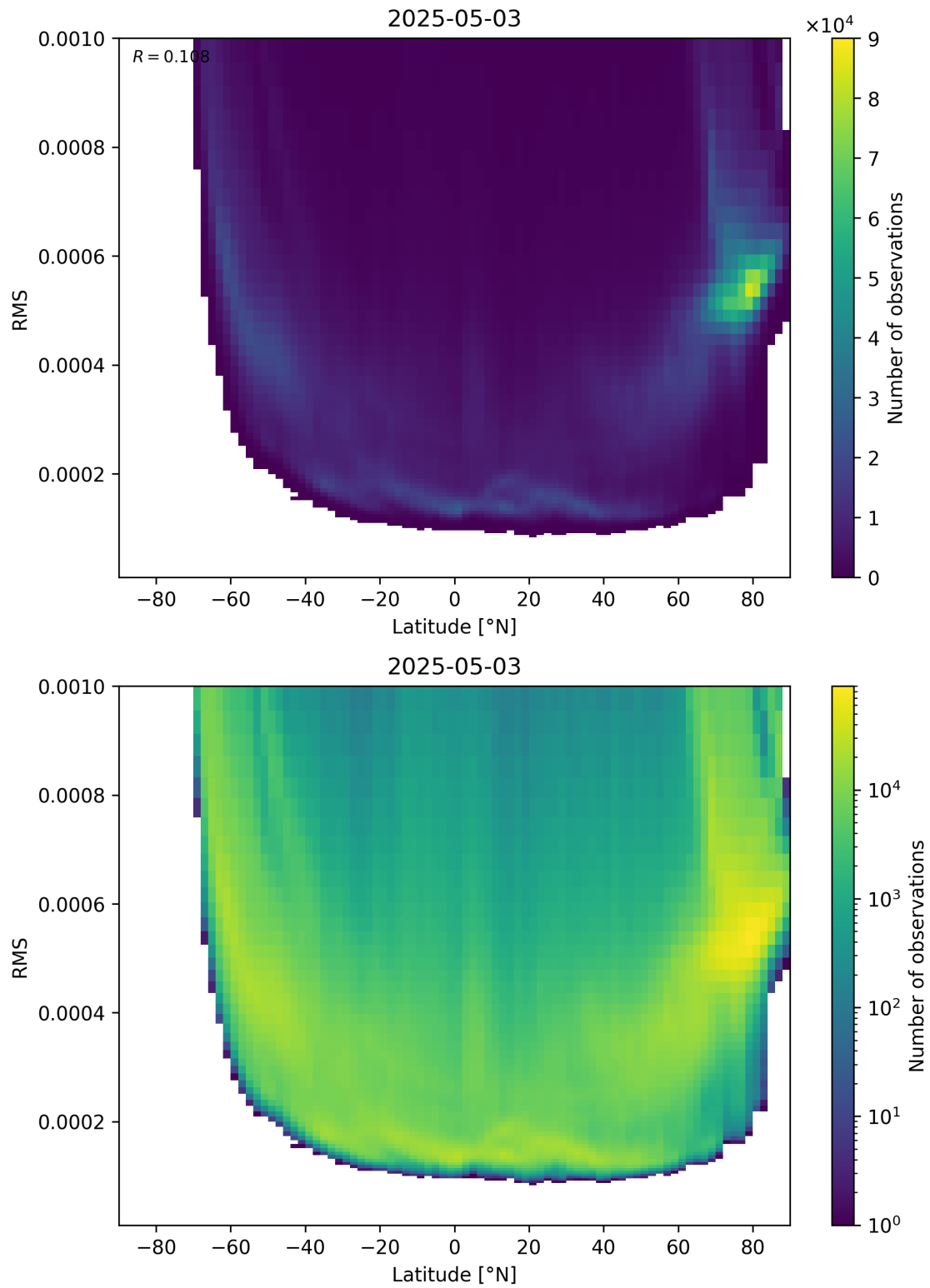
Figure 94: Scatter density plot of “Latitude” against “RMS” for 2025-05-03 to 2025-05-03.
