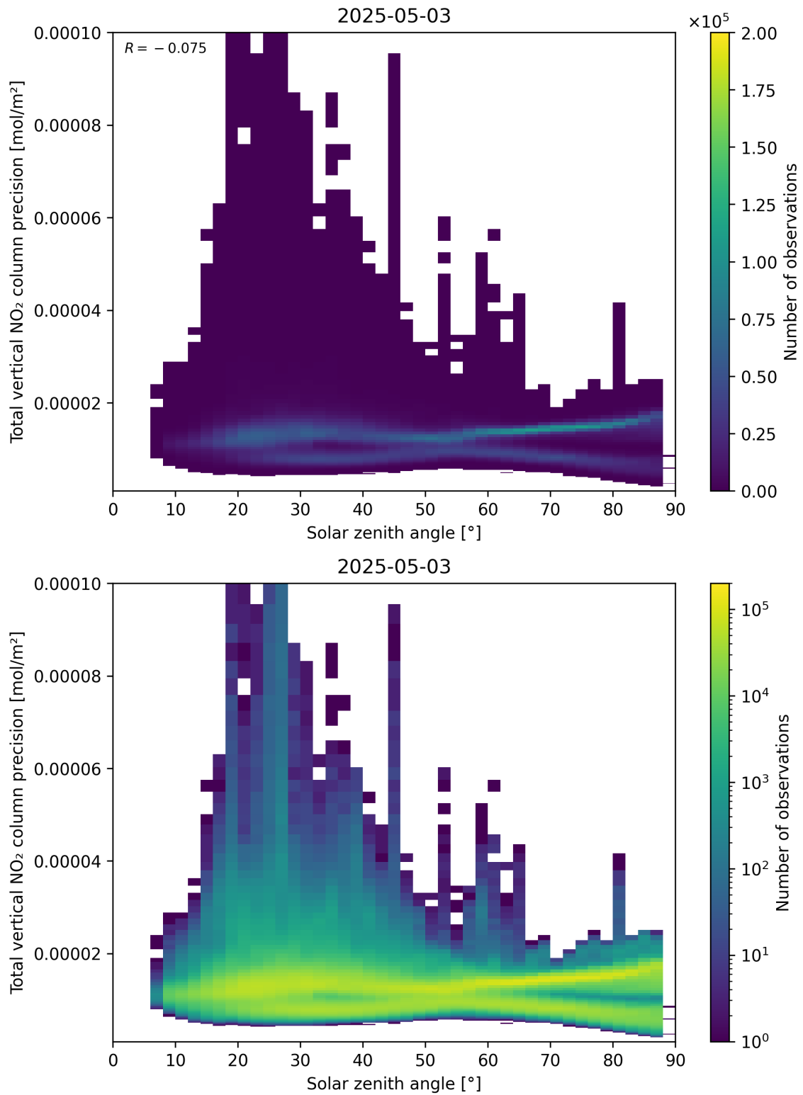
Figure 154: Scatter density plot of “Solar zenith angle” against “Total vertical NO 2 column precision” for 2025-05-03 to 2025-05-03.
