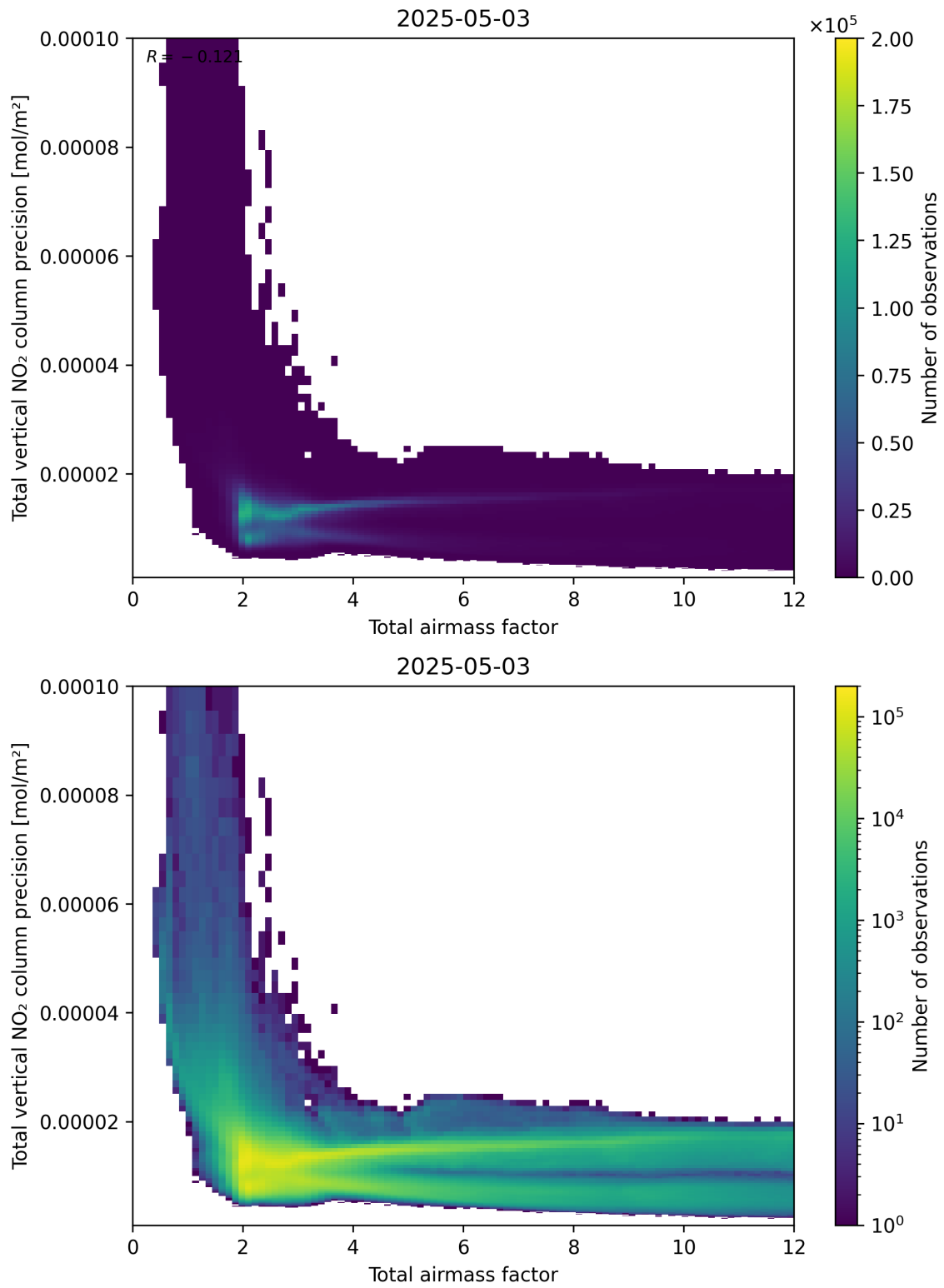
Figure 68: Scatter density plot of “Total airmass factor” against “Total vertical NO 2 column precision” for 2025-05-03 to 2025-05-03.
