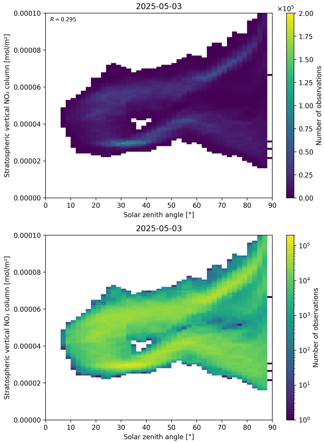
Figure 150: Scatter density plot of “Solar zenith angle” against “Stratospheric vertical NO 2 column” for 2025-05-03 to 2025-05-03.
