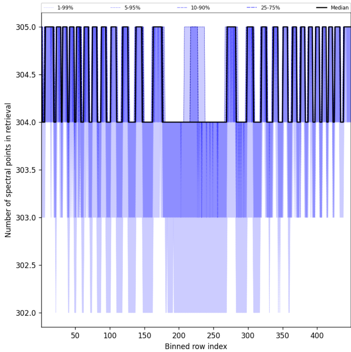
Figure 50: Along track statistics of “Number of spectral points in retrieval” for 2025-05-03 to 2025-05-03
