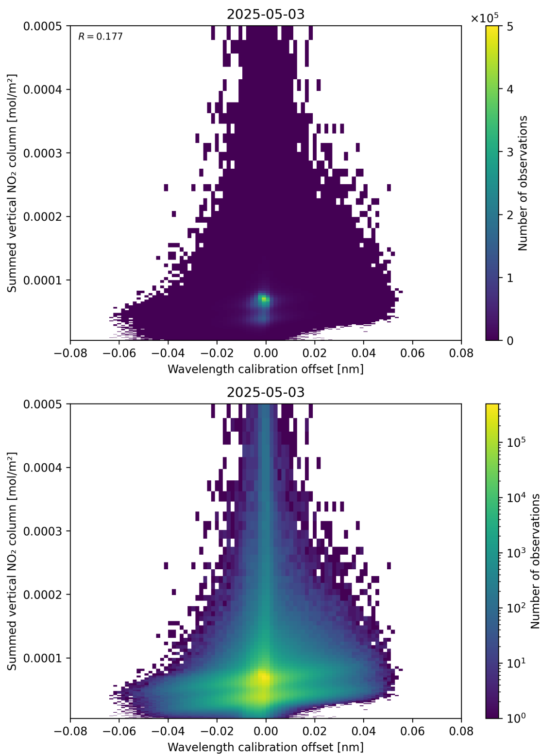
Figure 177: Scatter density plot of “Wavelength calibration offset” against “Summed vertical NO 2 column” for 2025-05-03 to 2025-05-03.
