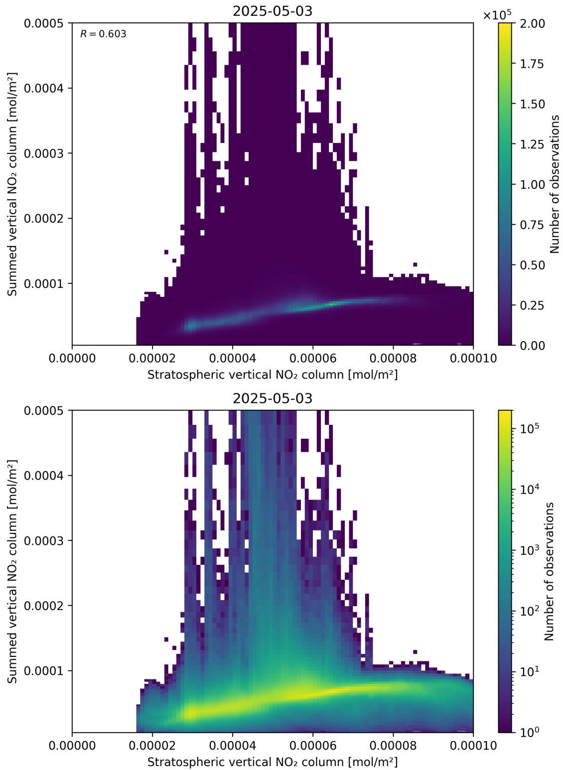
Figure 98: Scatter density plot of “Stratospheric vertical NO 2 column” against “Summed vertical NO 2 column” for 2025-05-03 to 2025-05-03.
