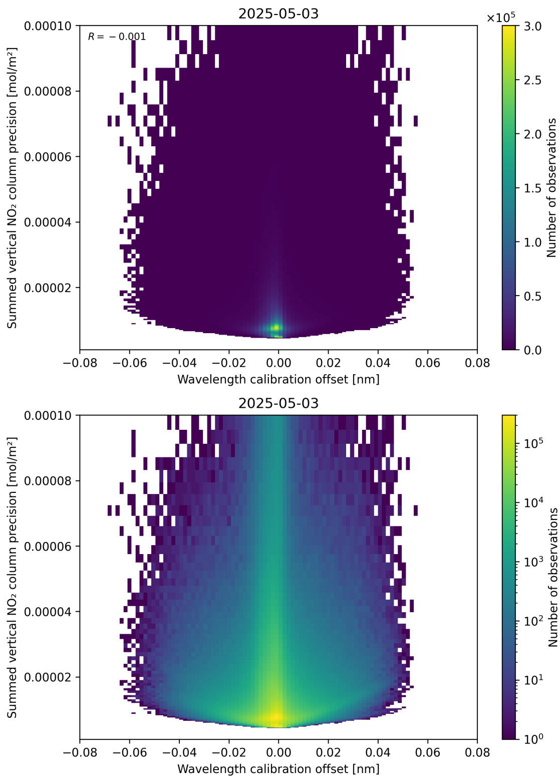
Figure 178: Scatter density plot of “Wavelength calibration offset” against “Summed vertical NO 2 column precision” for 2025-05-03 to 2025-05-03.
