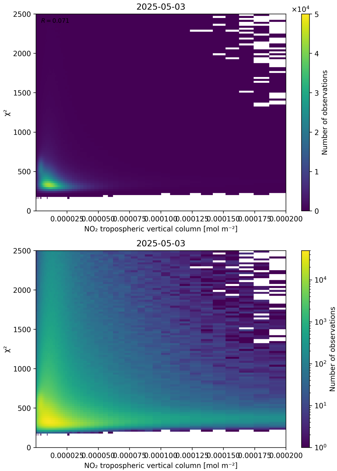
Figure 124: Scatter density plot of “NO 2 tropospheric vertical column” against “ \chi^2 ” for 2025-05-03 to 2025-05-03.
