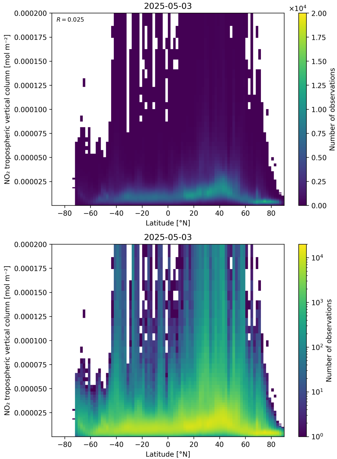
Figure 92: Scatter density plot of “Latitude” against “NO 2 tropospheric vertical column” for 2025-05-03 to 2025-05-03.
