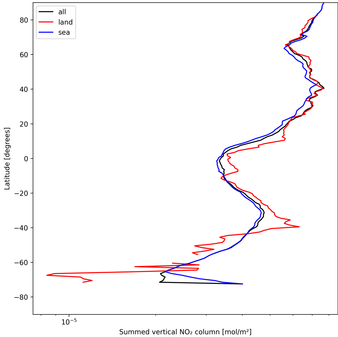
Figure 23: Zonal average of “Summed vertical NO 2 column” for 2025-05-03 to 2025-05-03.
