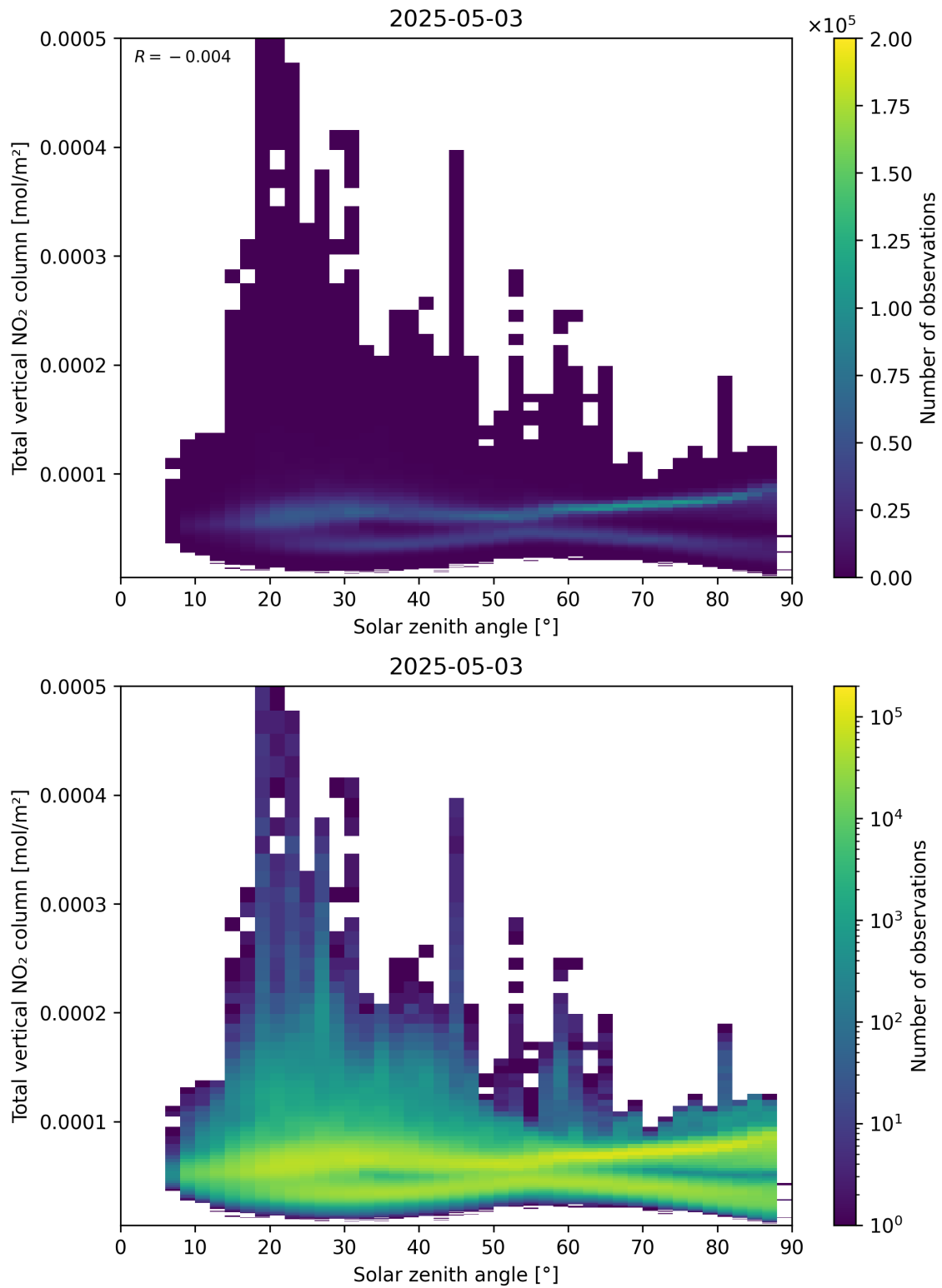
Figure 153: Scatter density plot of “Solar zenith angle” against “Total vertical NO 2 column” for 2025-05-03 to 2025-05-03.
