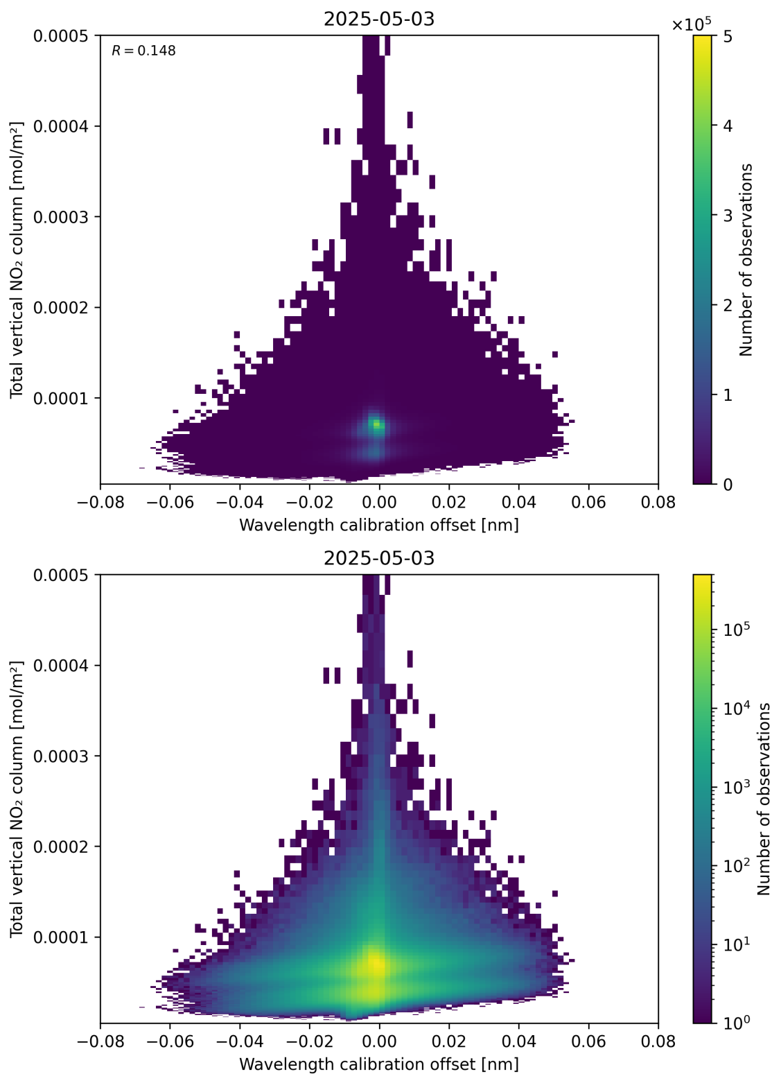
Figure 179: Scatter density plot of “Wavelength calibration offset” against “Total vertical NO 2 column” for 2025-05-03 to 2025-05-03.
