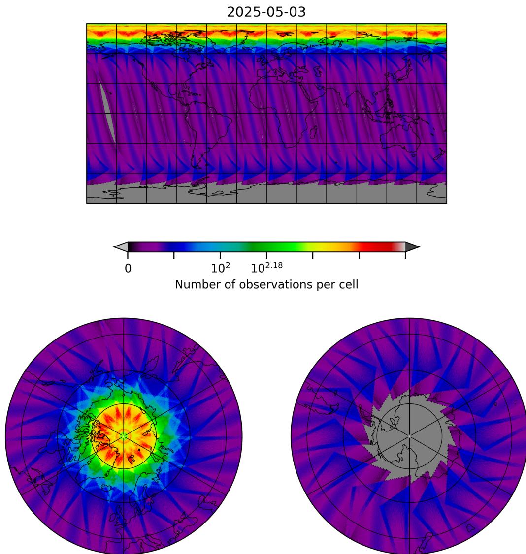
Figure 10: Map of the number of observations for 2025-05-03 to 2025-05-03
