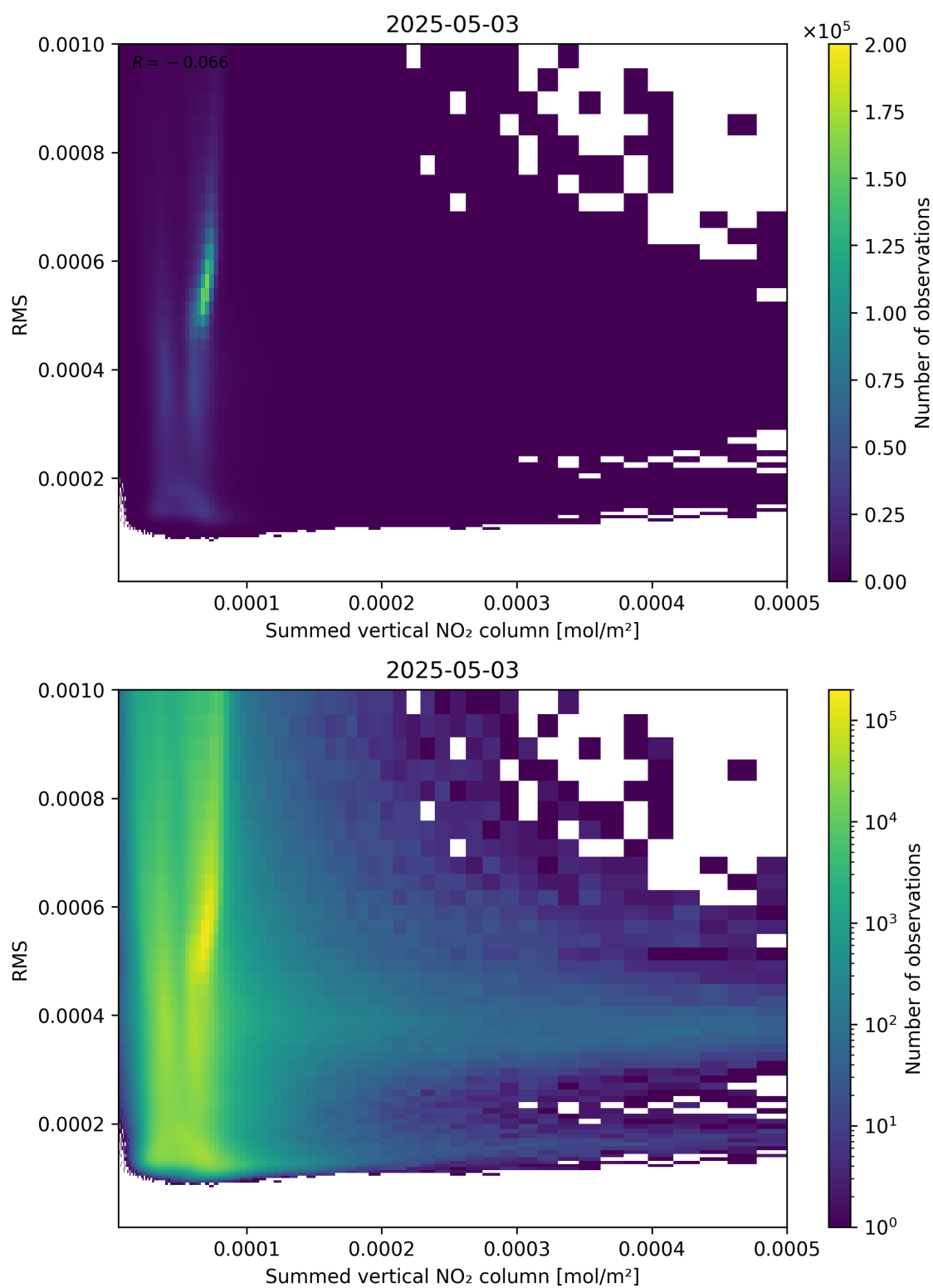
Figure 109: Scatter density plot of “Summed vertical NO 2 column” against “RMS” for 2025-05-03 to 2025-05-03.
