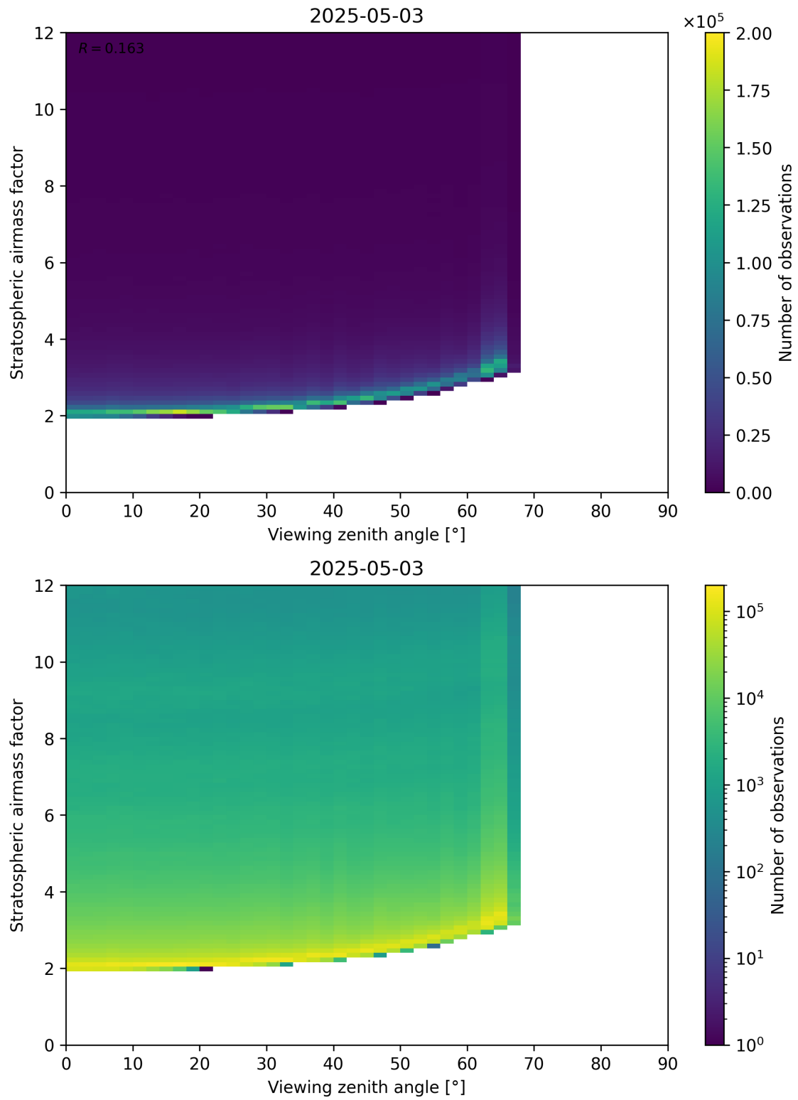
Figure 159: Scatter density plot of “Viewing zenith angle” against “Stratospheric airmass factor” for 2025-05-03 to 2025-05-03.
