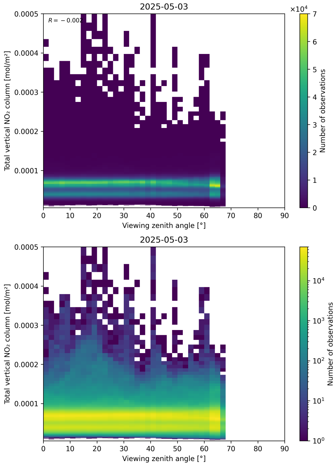
Figure 167: Scatter density plot of “Viewing zenith angle” against “Total vertical NO 2 column” for 2025-05-03 to 2025-05-03.
