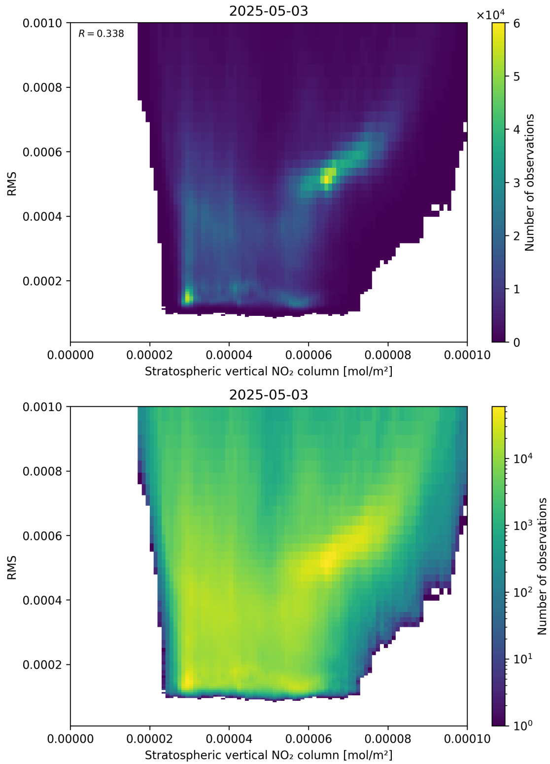
Figure 102: Scatter density plot of “Stratospheric vertical NO 2 column” against “RMS” for 2025-05-03 to 2025-05-03.
