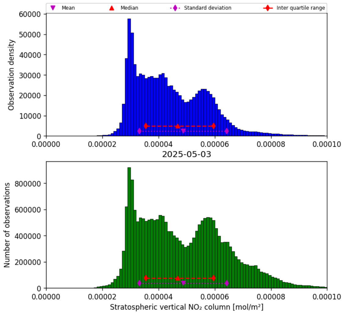
Figure 36: Histogram of “Stratospheric vertical NO 2 column” for 2025-05-03 to 2025-05-03
