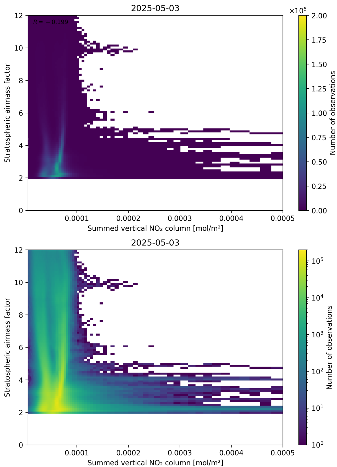
Figure 103: Scatter density plot of “Summed vertical NO 2 column” against “Stratospheric airmass factor” for 2025-05-03 to 2025-05-03.
