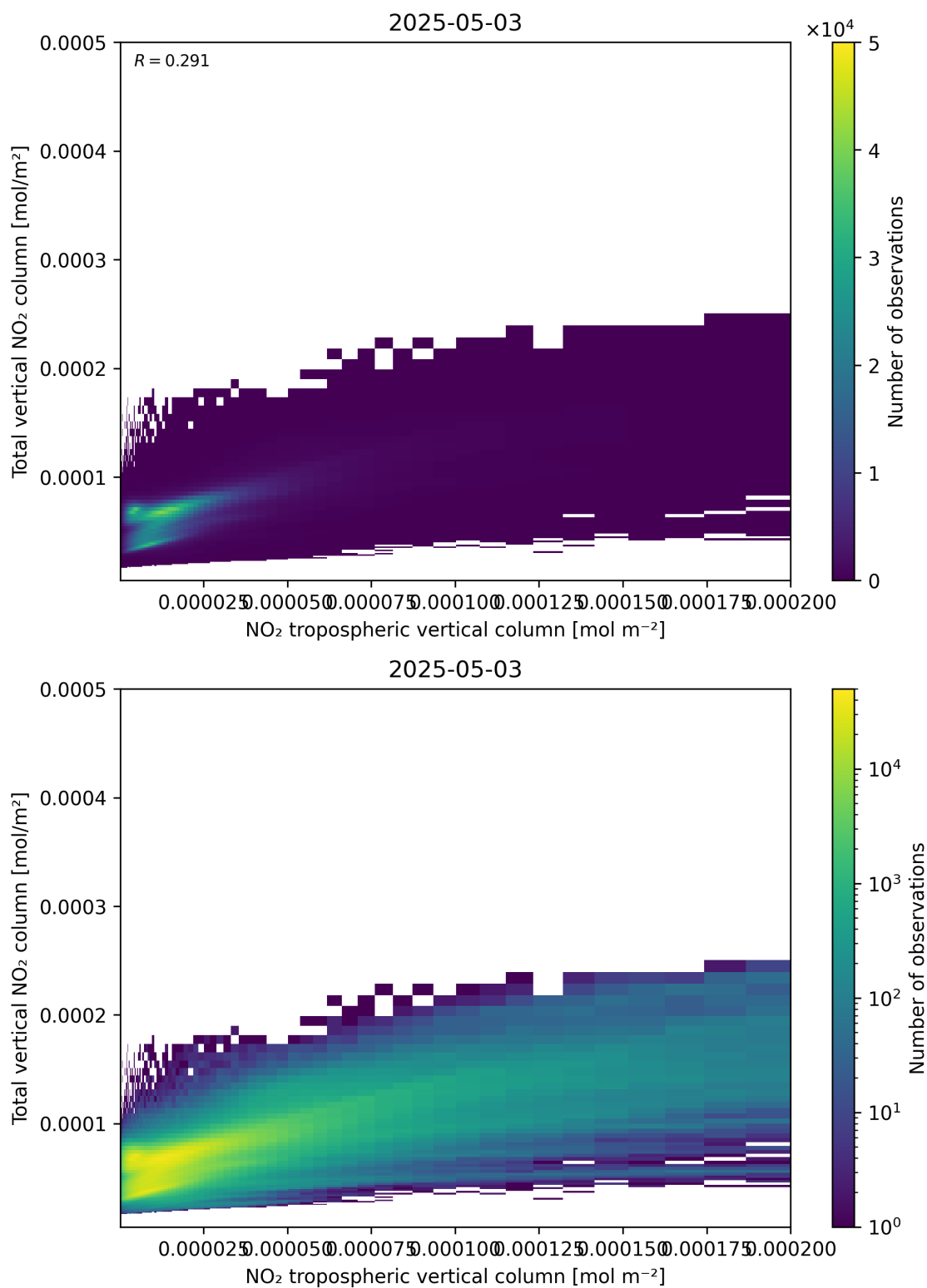
Figure 128: Scatter density plot of “NO 2 tropospheric vertical column” against “Total vertical NO 2 column” for 2025-05-03 to 2025-05-03.
