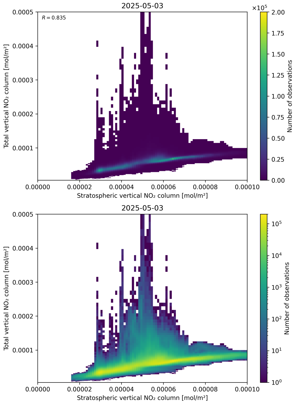
Figure 100: Scatter density plot of “Stratospheric vertical NO 2 column” against “Total vertical NO 2 column” for 2025-05-03 to 2025-05-03.
