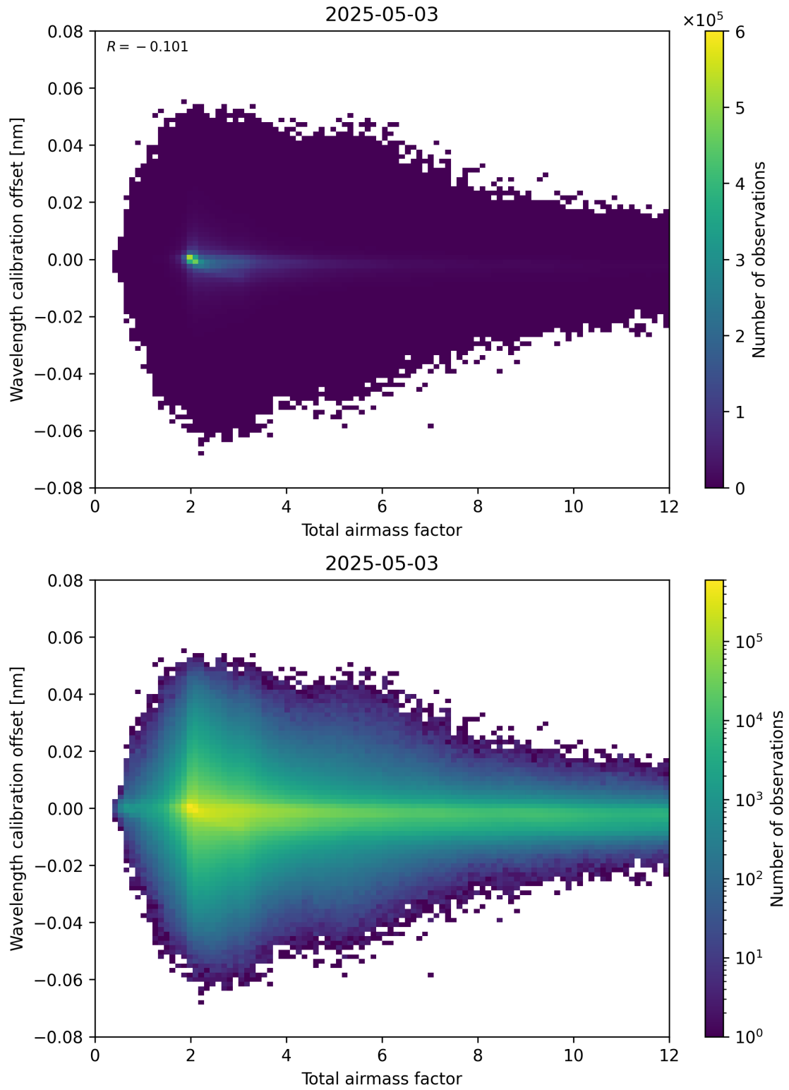
Figure 70: Scatter density plot of “Total airmass factor” against “Wavelength calibration offset” for 2025-05-03 to 2025-05-03.
