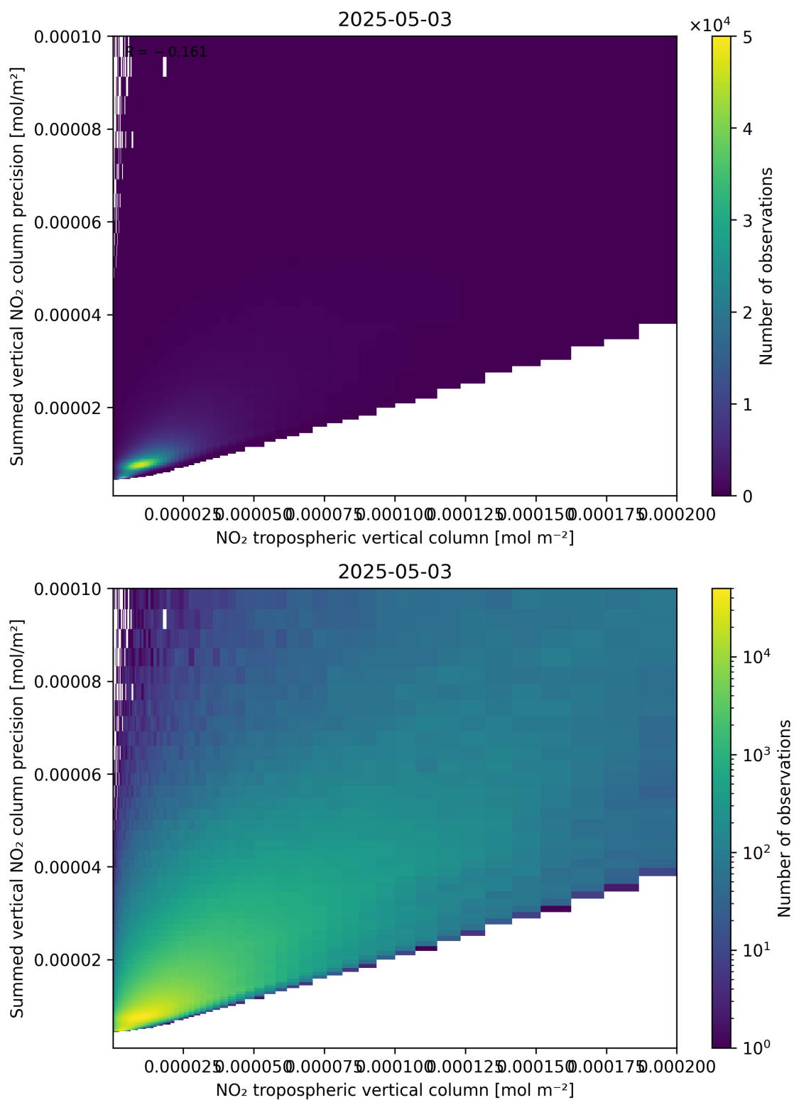
Figure 127: Scatter density plot of “NO 2 tropospheric vertical column” against “Summed vertical NO 2 column precision” for 2025-05-03 to 2025-05-03.
