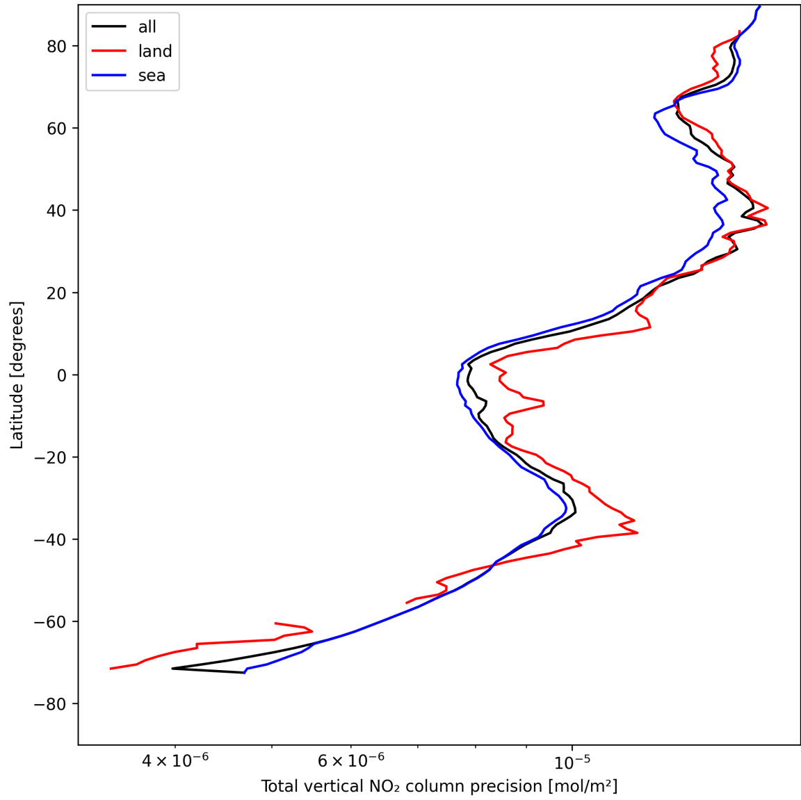
Figure 22: Zonal average of “Total vertical NO 2 column precision” for 2025-05-03 to 2025-05-03.
