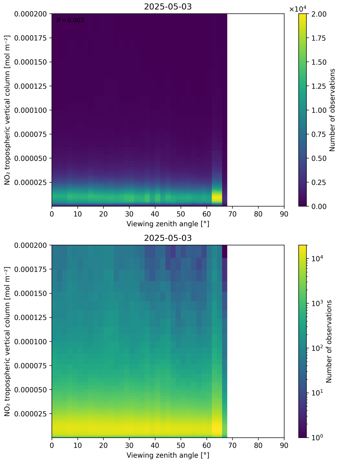
Figure 169: Scatter density plot of “Viewing zenith angle” against “NO 2 tropospheric vertical column” for 2025-05-03 to 2025-05-03.
