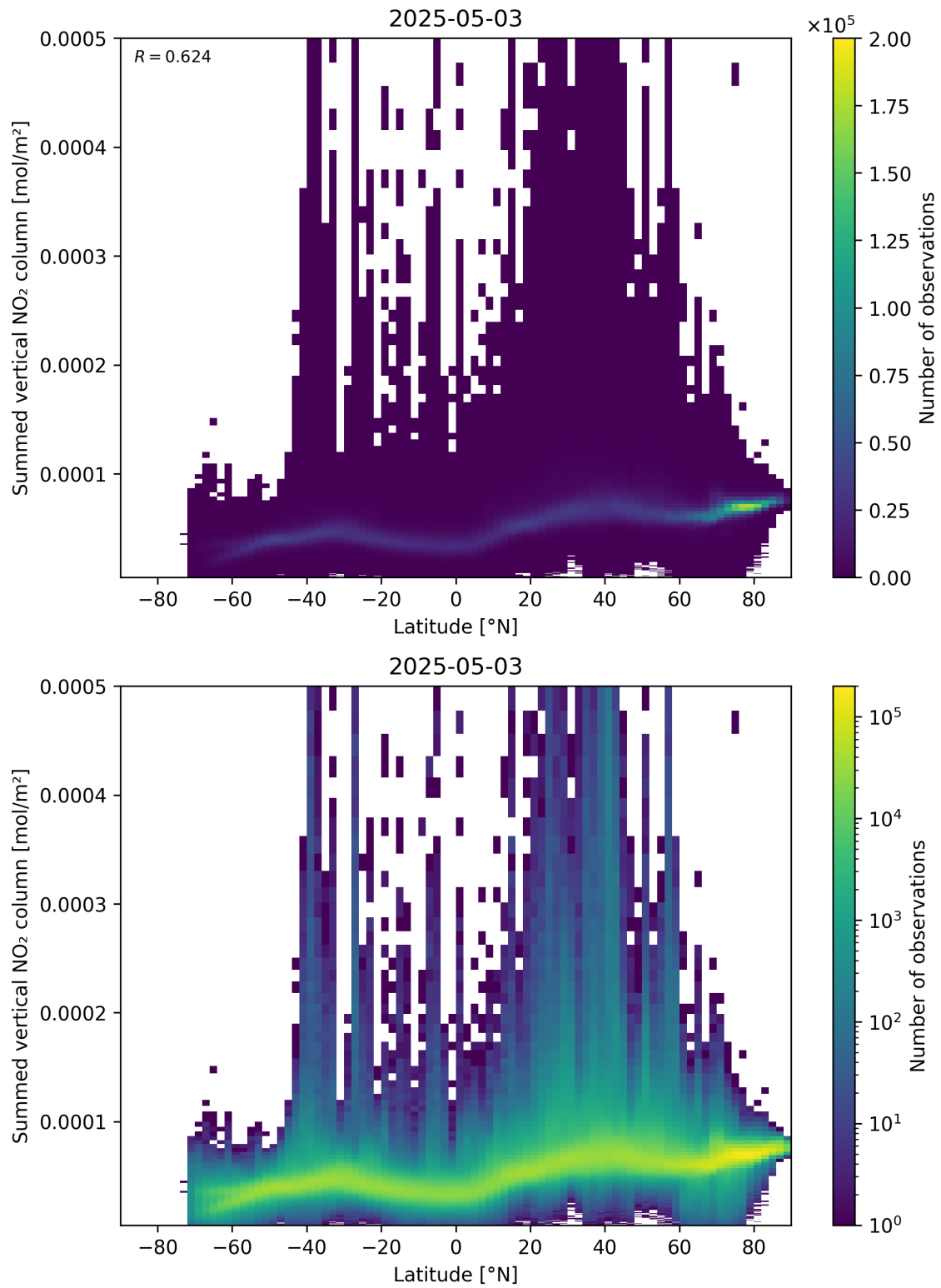
Figure 88: Scatter density plot of “Latitude” against “Summed vertical NO 2 column” for 2025-05-03 to 2025-05-03.
