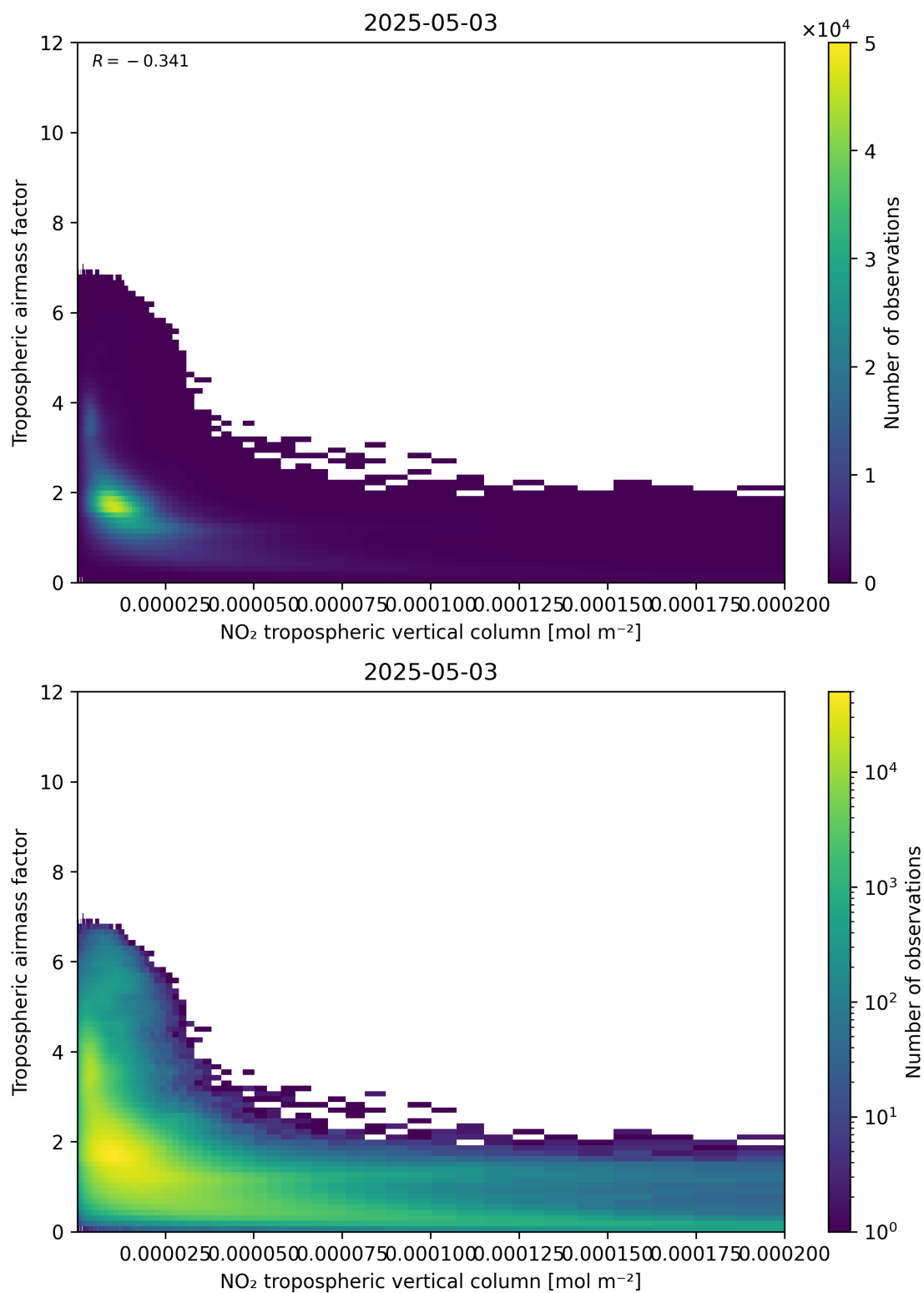
Figure 123: Scatter density plot of “NO 2 tropospheric vertical column” against “Tropospheric air mass factor” for 2025-05-03 to 2025-05-03.
