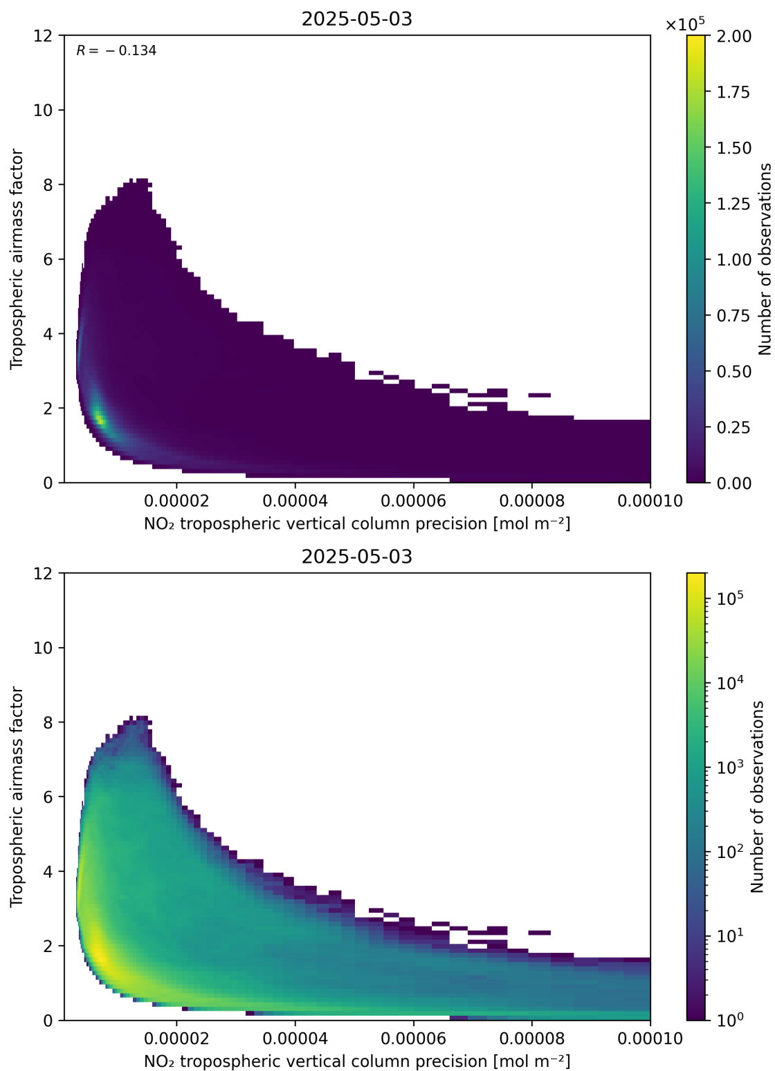
Figure 133: Scatter density plot of “NO 2 tropospheric vertical column precision” against “Tropospheric airmass factor” for 2025-05-03 to 2025-05-03.
