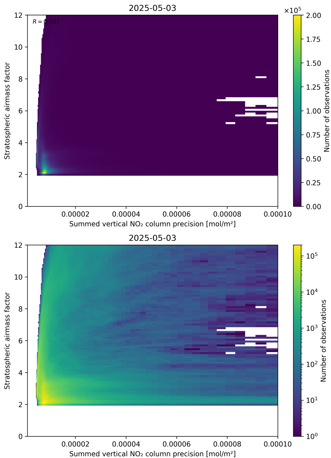
Figure 106: Scatter density plot of “Summed vertical NO 2 column precision” against “Stratospheric airmass factor” for 2025-05-03 to 2025-05-03.
