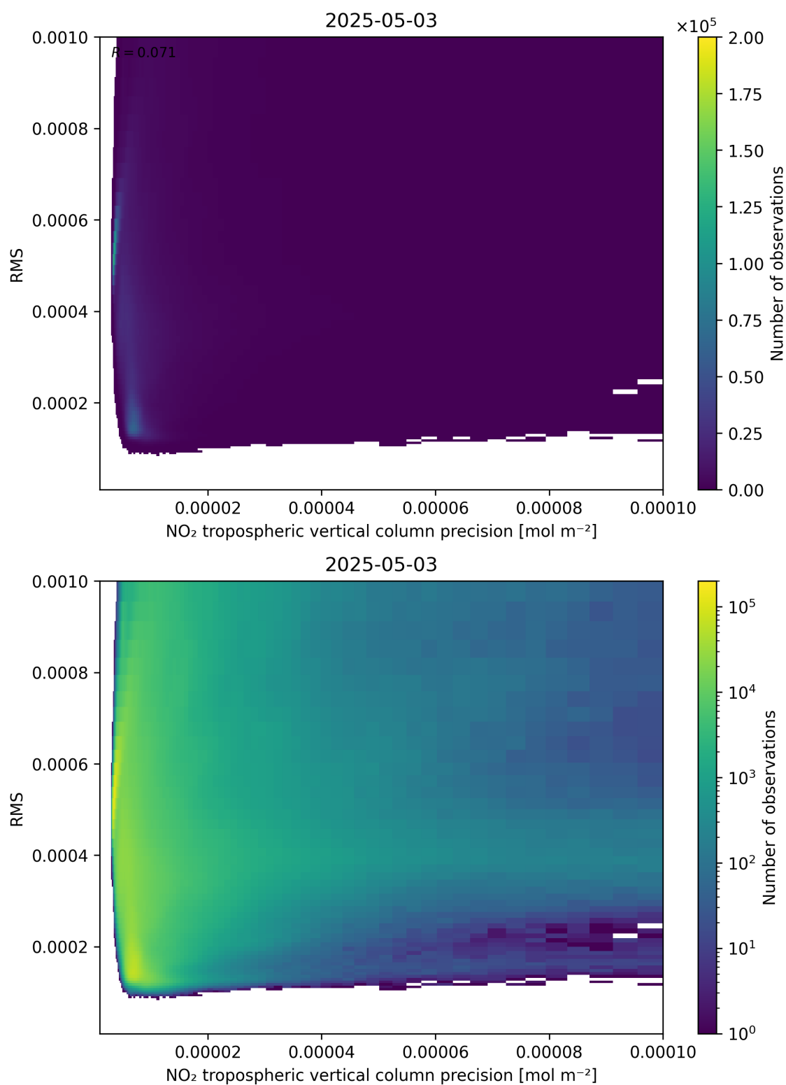
Figure 140: Scatter density plot of “NO 2 tropospheric vertical column precision” against “RMS” for 2025-05-03 to 2025-05-03.
