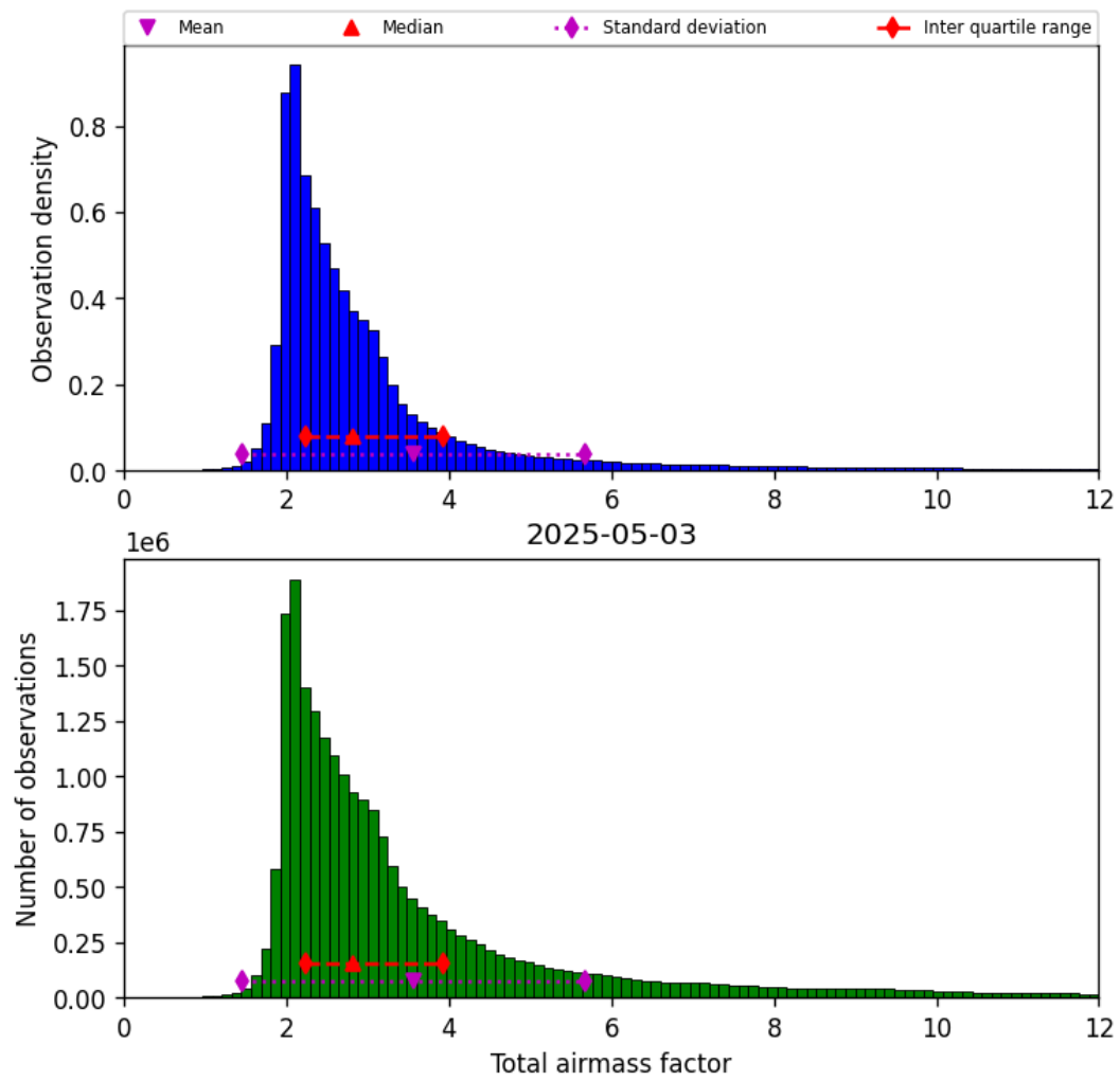
Figure 32: Histogram of “Total airmass factor” for 2025-05-03 to 2025-05-03
