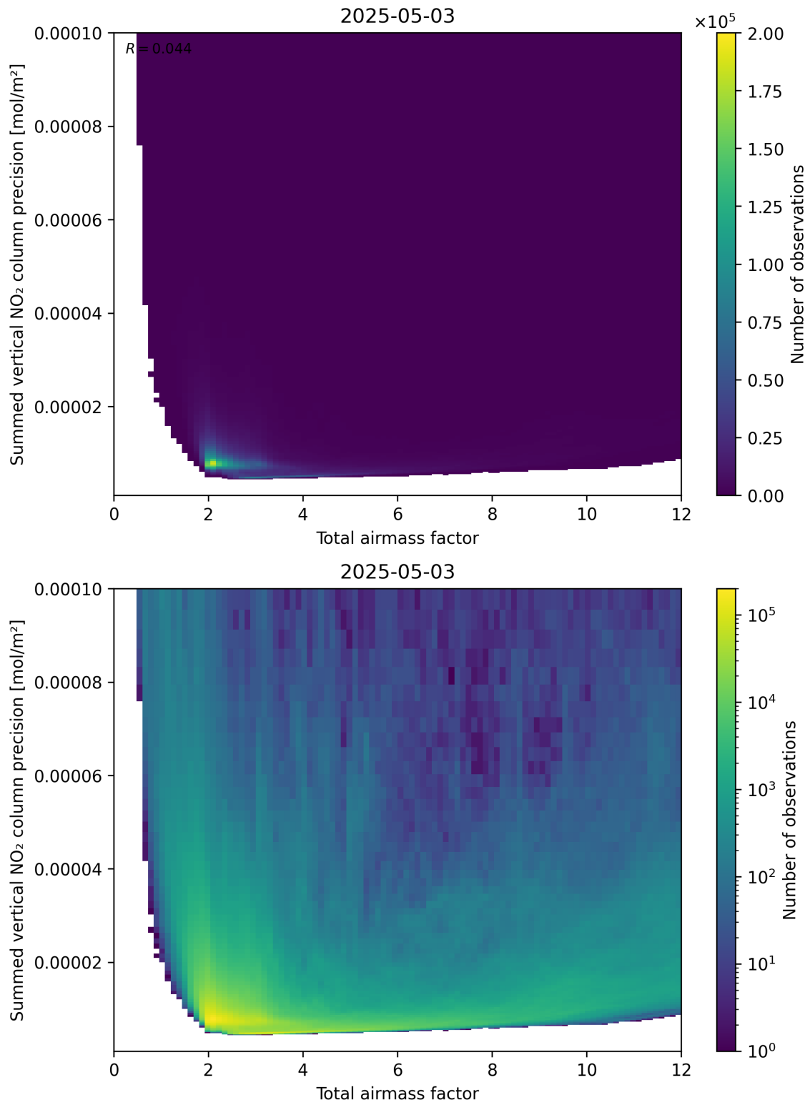
Figure 66: Scatter density plot of “Total airmass factor” against “Summed vertical NO 2 column precision” for 2025-05-03 to 2025-05-03.
