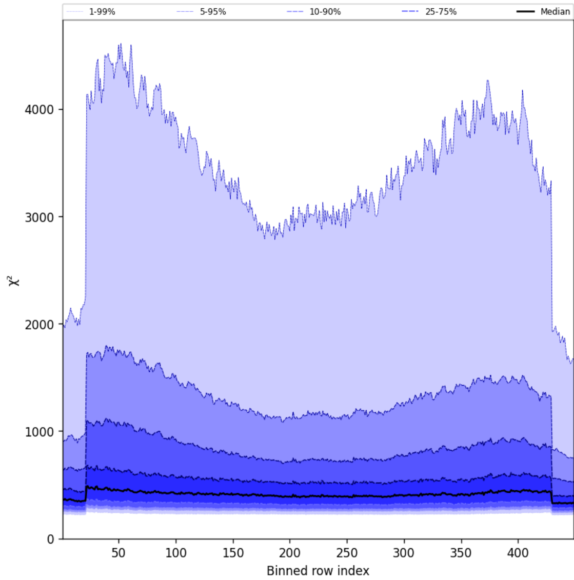
Figure 59: Along track statistics of “ \chi^2 ” for 2025-05-03 to 2025-05-03
