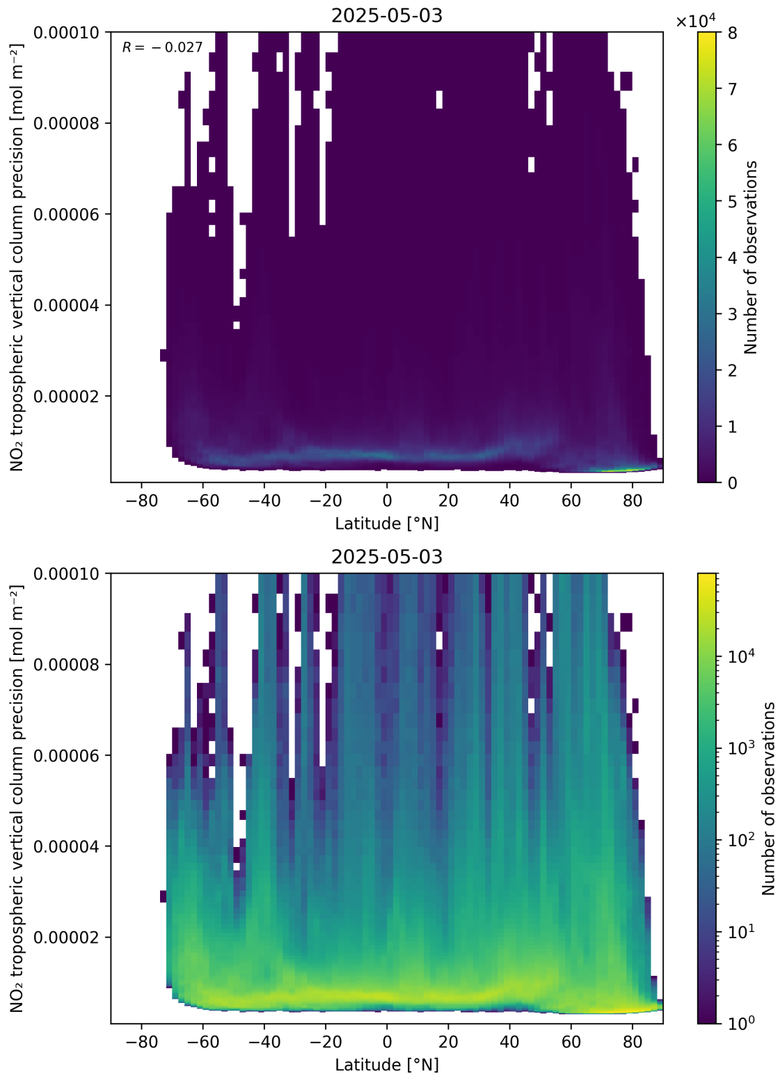
Figure 93: Scatter density plot of “Latitude” against “NO 2 tropospheric vertical column precision” for 2025-05-03 to 2025-05-03.
