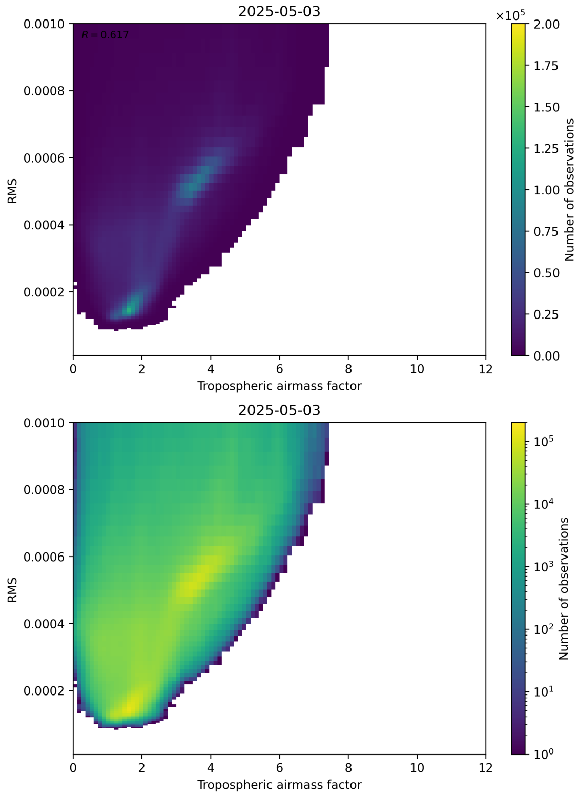
Figure 79: Scatter density plot of “Tropospheric airmass factor” against “RMS” for 2025-05-03 to 2025-05-03.
