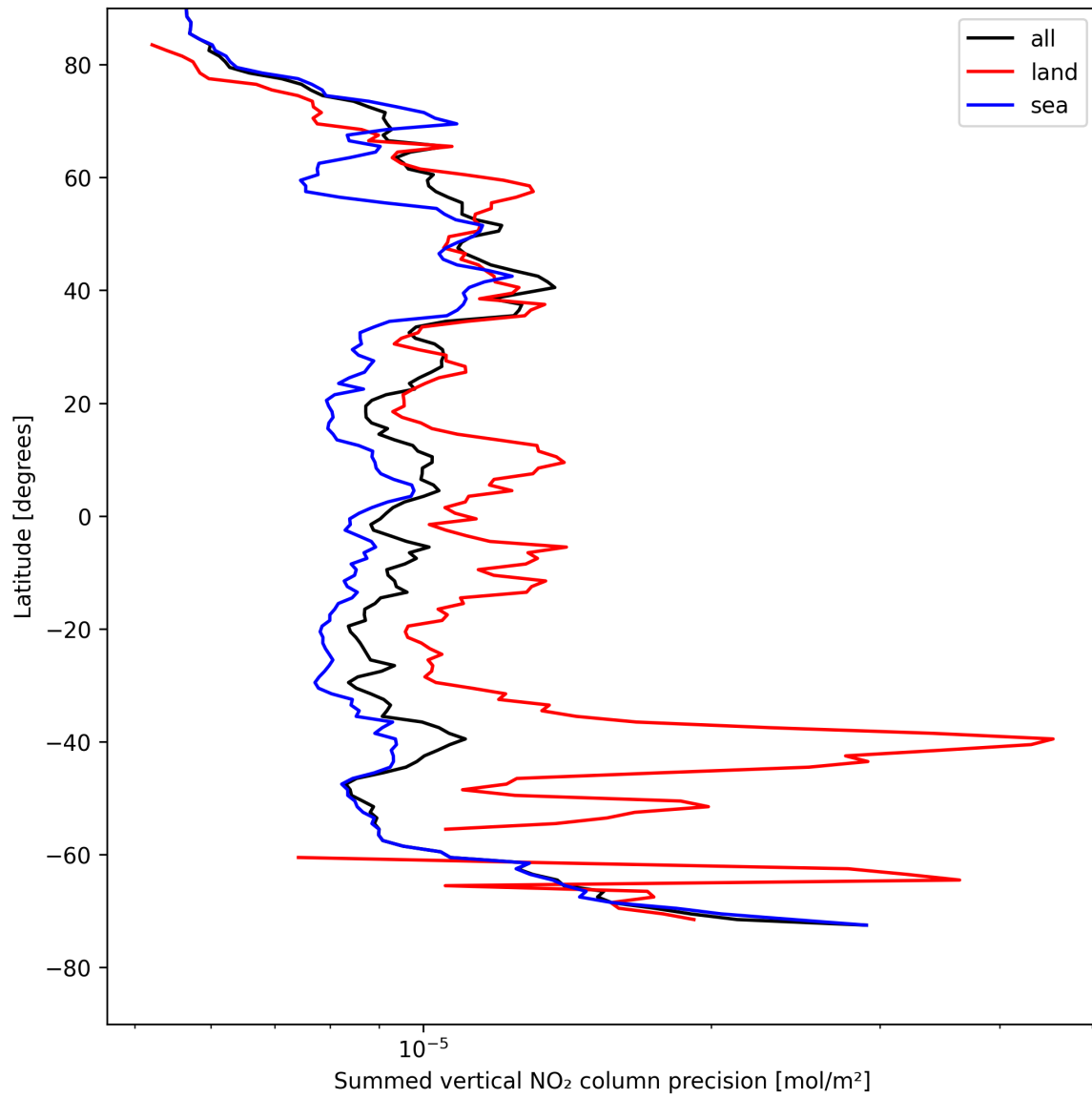
Figure 24: Zonal average of “Summed vertical NO 2 column precision” for 2025-05-03 to 2025-05-03.
