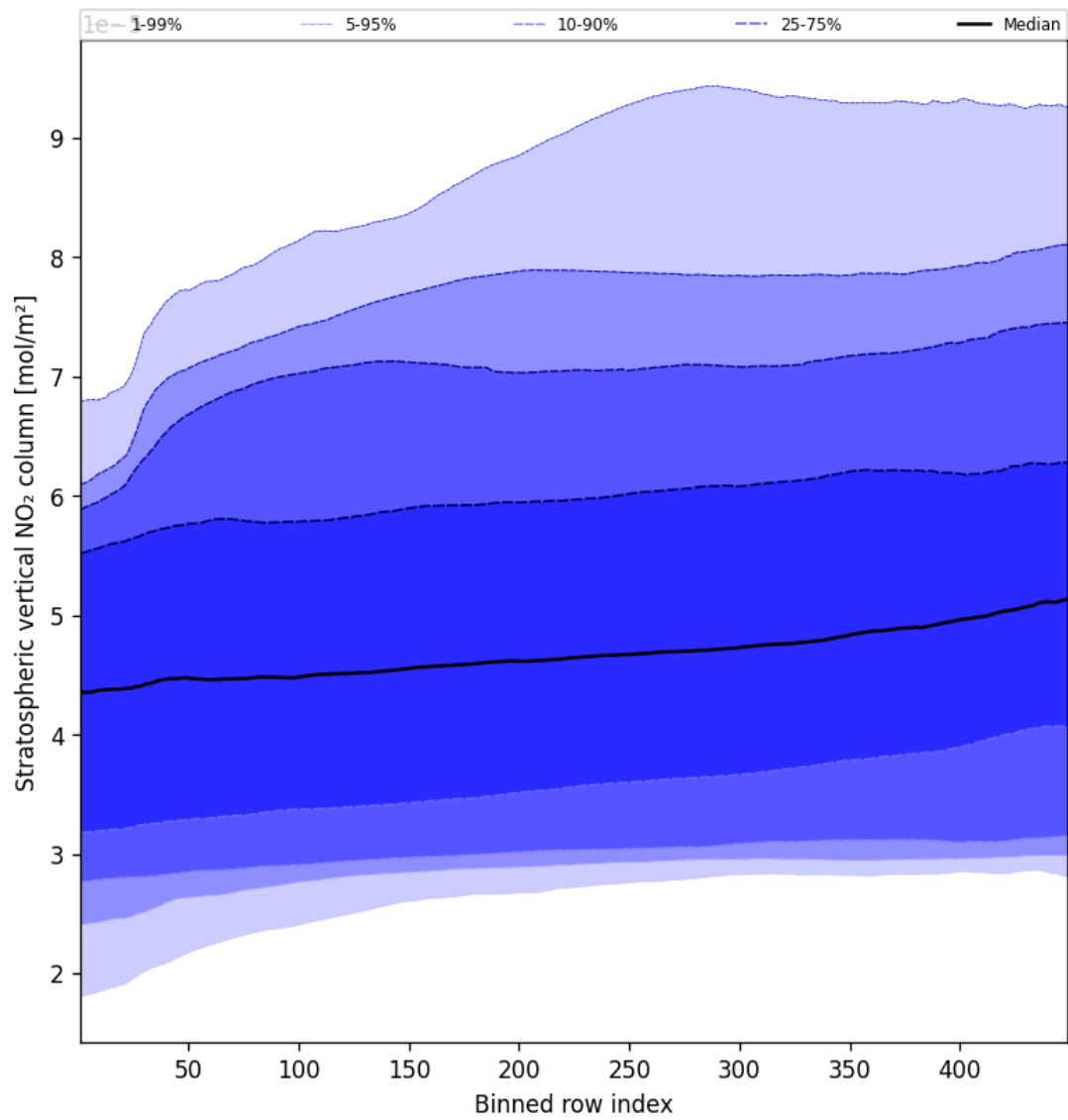
Figure 53: Along track statistics of “Stratospheric vertical NO 2 column” for 2025-05-03 to 2025-05-03
