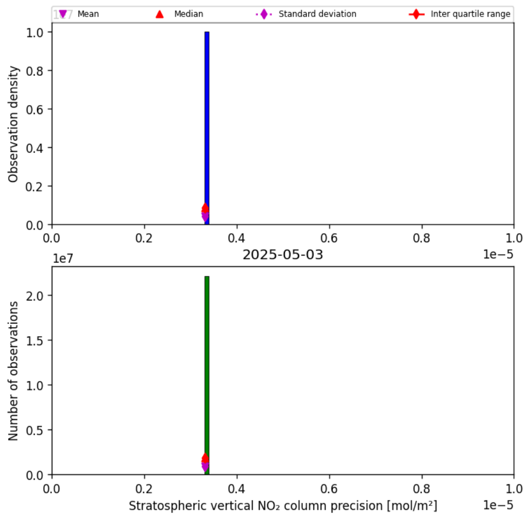
Figure 37: Histogram of “Stratospheric vertical NO 2 column precision” for 2025-05-03 to 2025-05-03
