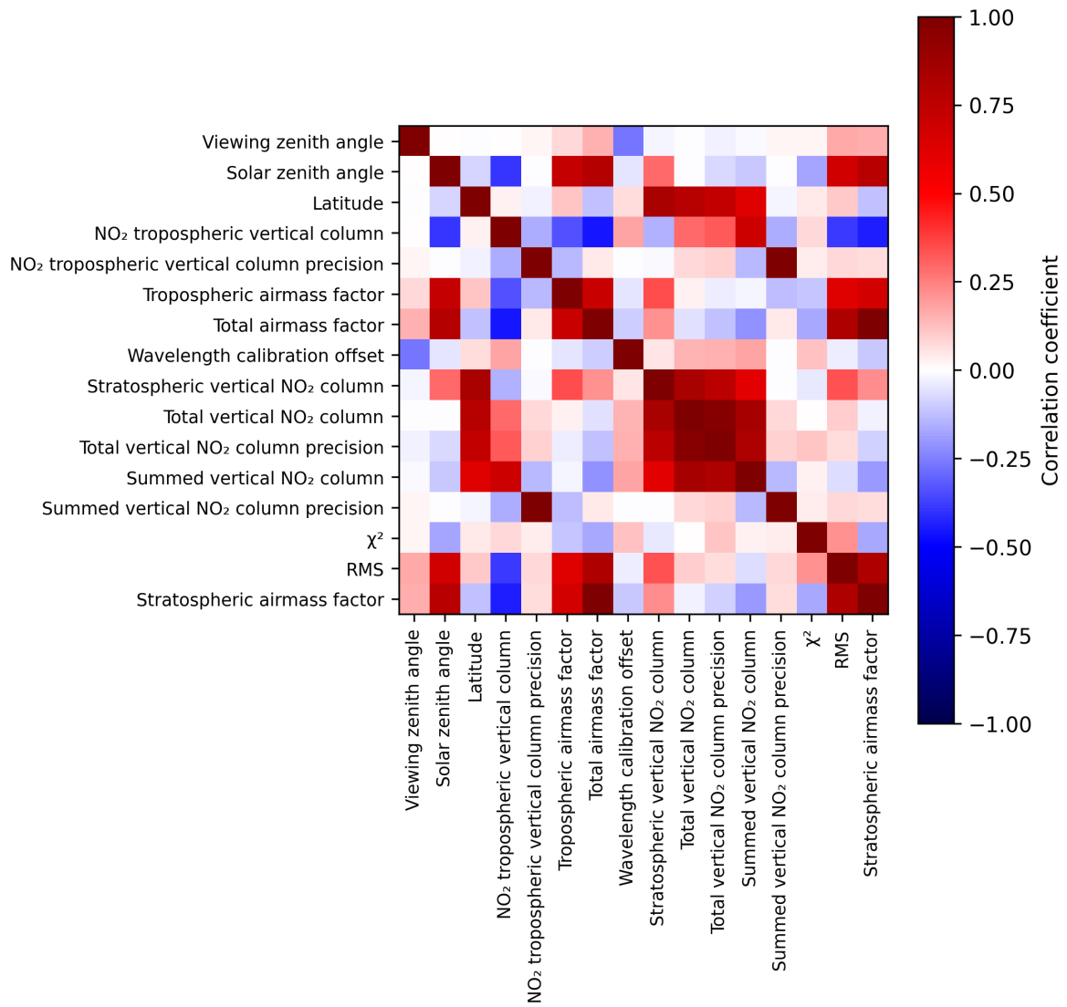
Figure 2: Map of correlation matrix for 2025-05-03 to 2025-05-03.
