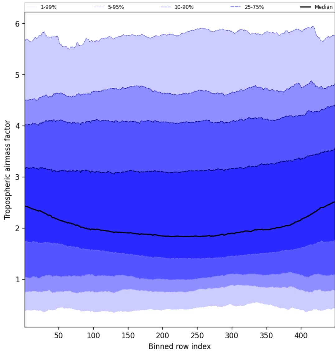
Figure 48: Along track statistics of “Tropospheric airmass factor” for 2025-05-03 to 2025-05-03
