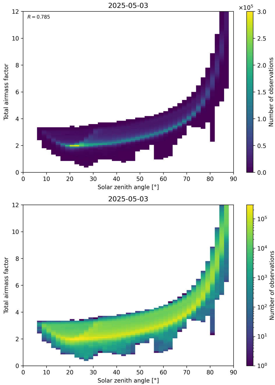
Figure 146: Scatter density plot of “Solar zenith angle” against “Total air mass factor” for 2025-05-03 to 2025-05-03.
