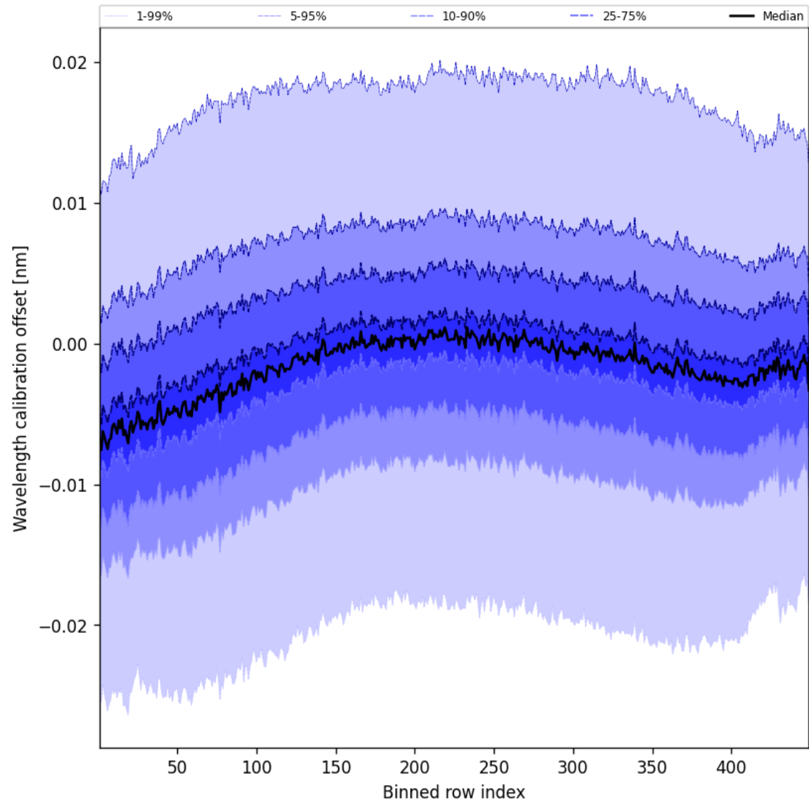
Figure 52: Along track statistics of “Wavelength calibration offset” for 2025-05-03 to 2025-05-03
