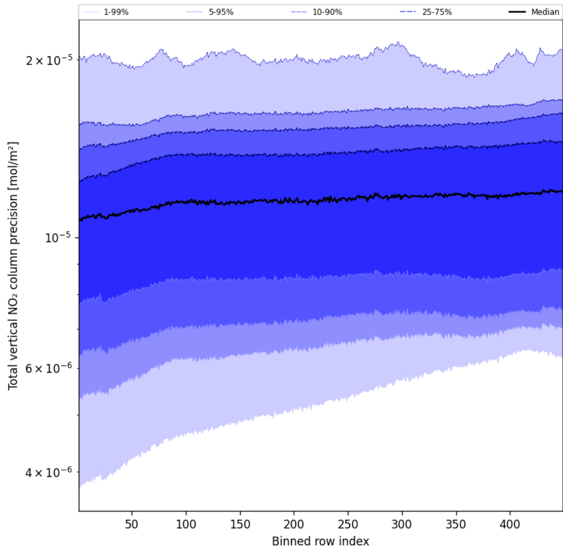
Figure 56: Along track statistics of “Total vertical NO 2 column precision” for 2025-05-03 to 2025-05-03
