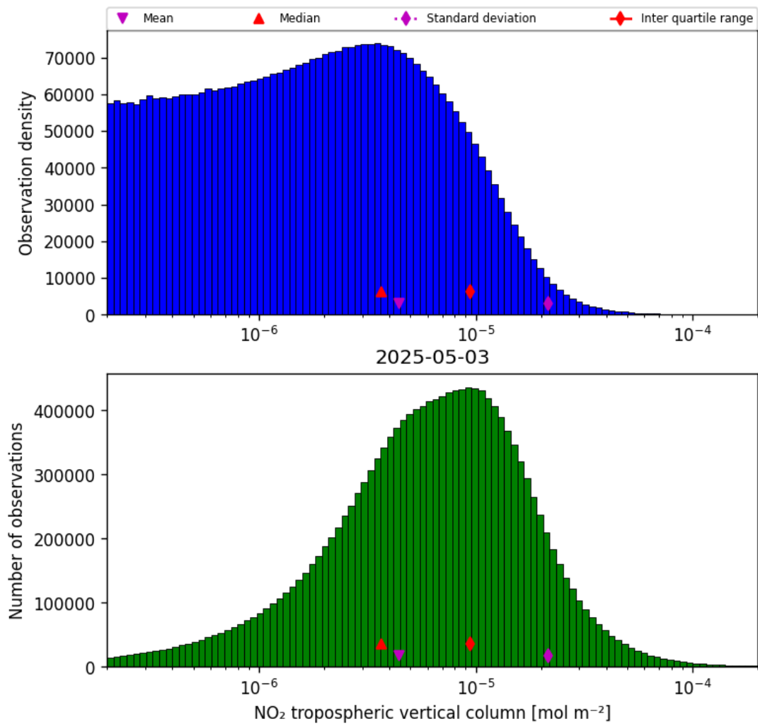
Figure 29: Histogram of “NO 2 tropospheric vertical column” for 2025-05-03 to 2025-05-03
