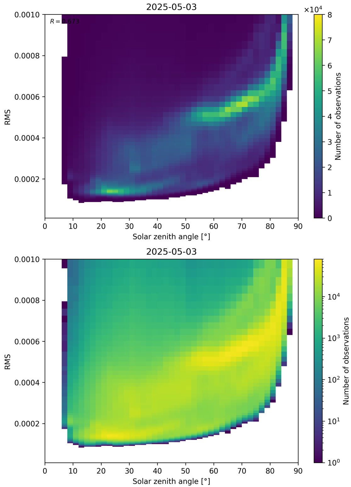
Figure 157: Scatter density plot of “Solar zenith angle” against “RMS” for 2025-05-03 to 2025-05-03.
