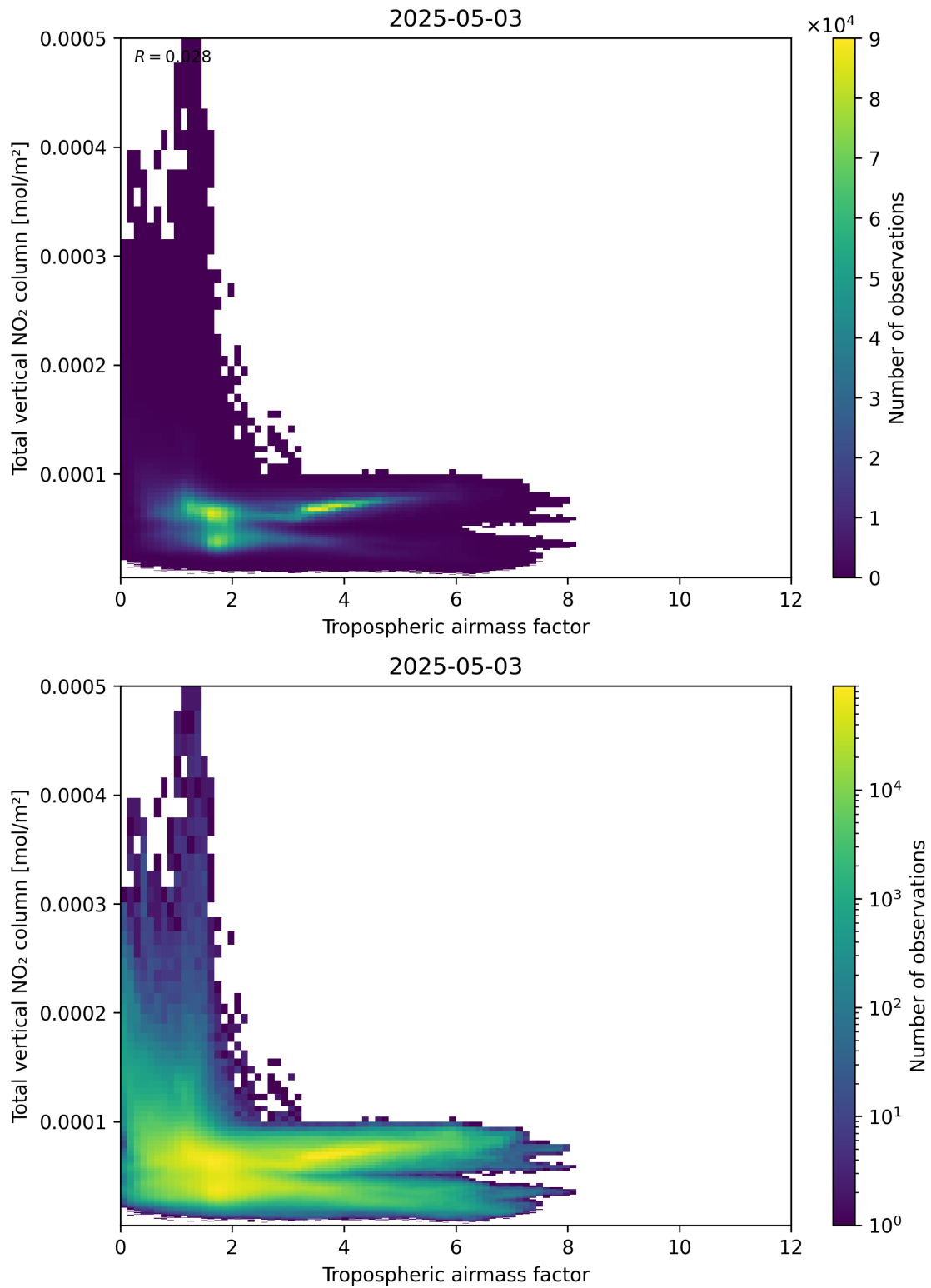
Figure 77: Scatter density plot of “Tropospheric airmass factor” against “Total vertical NO 2 column” for 2025-05-03 to 2025-05-03.
