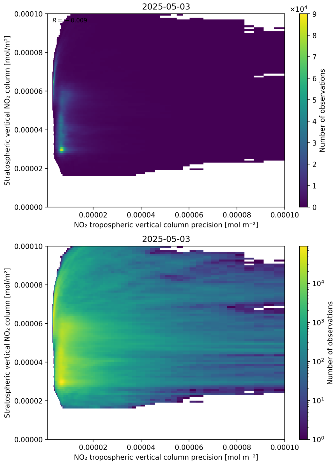
Figure 135: Scatter density plot of “NO 2 tropospheric vertical column precision” against “Stratospheric vertical NO 2 column” for 2025-05-03 to 2025-05-03.
