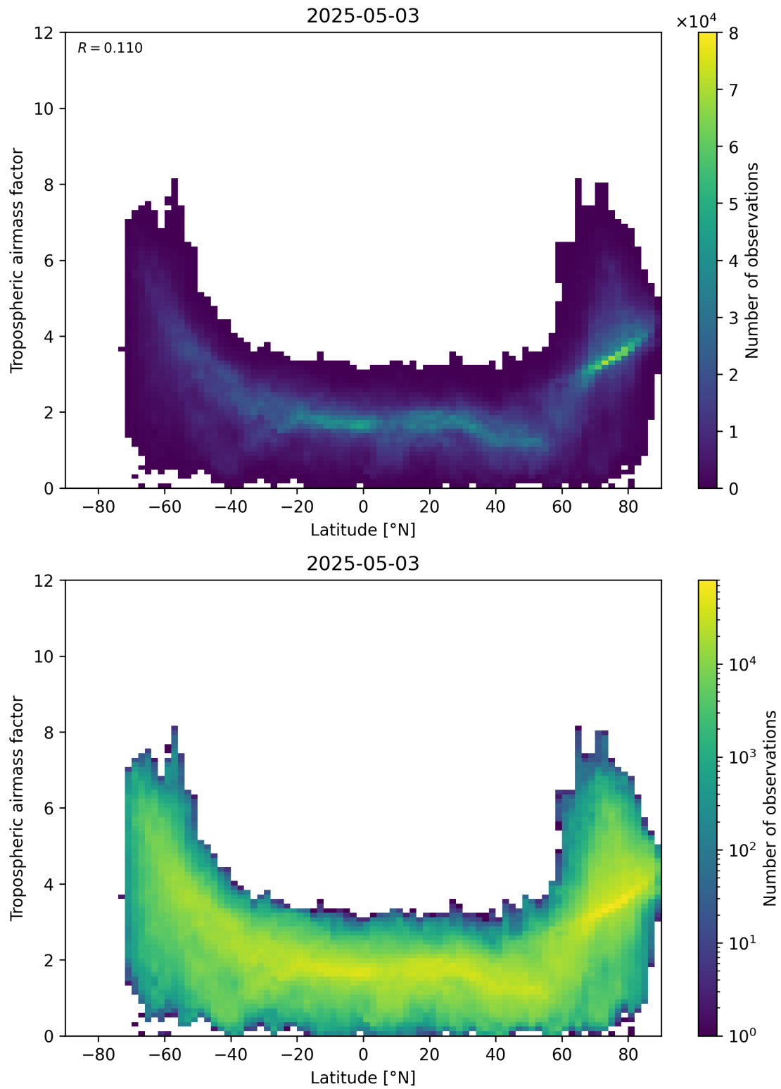
Figure 85: Scatter density plot of “Latitude” against “Tropospheric airmass factor” for 2025-05-03 to 2025-05-03.
