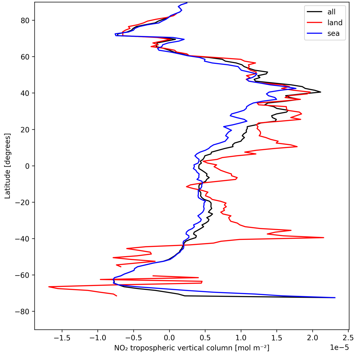
Figure 12: Zonal average of “NO 2 tropospheric vertical column” for 2025-05-03 to 2025-05-03.
