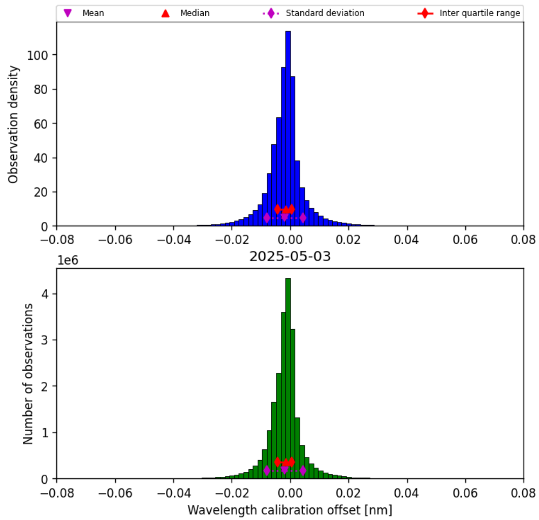
Figure 35: Histogram of “Wavelength calibration offset” for 2025-05-03 to 2025-05-03
