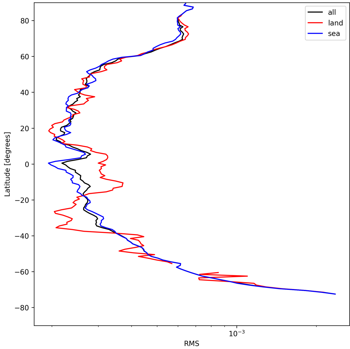
Figure 26: Zonal average of “RMS” for 2025-05-03 to 2025-05-03.
