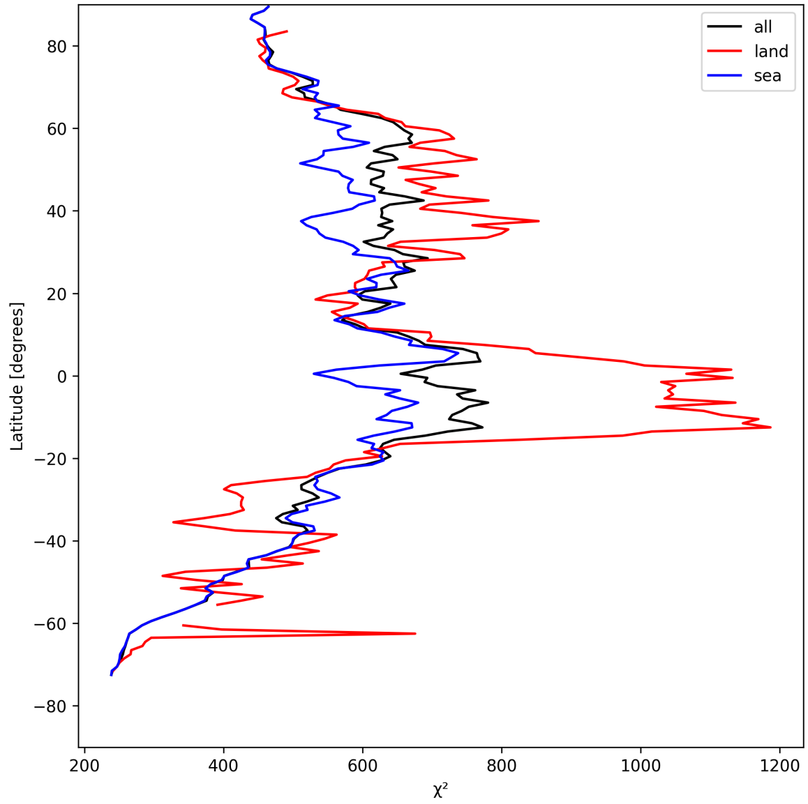
Figure 25: Zonal average of “ \chi^2 ” for 2025-05-03 to 2025-05-03.
