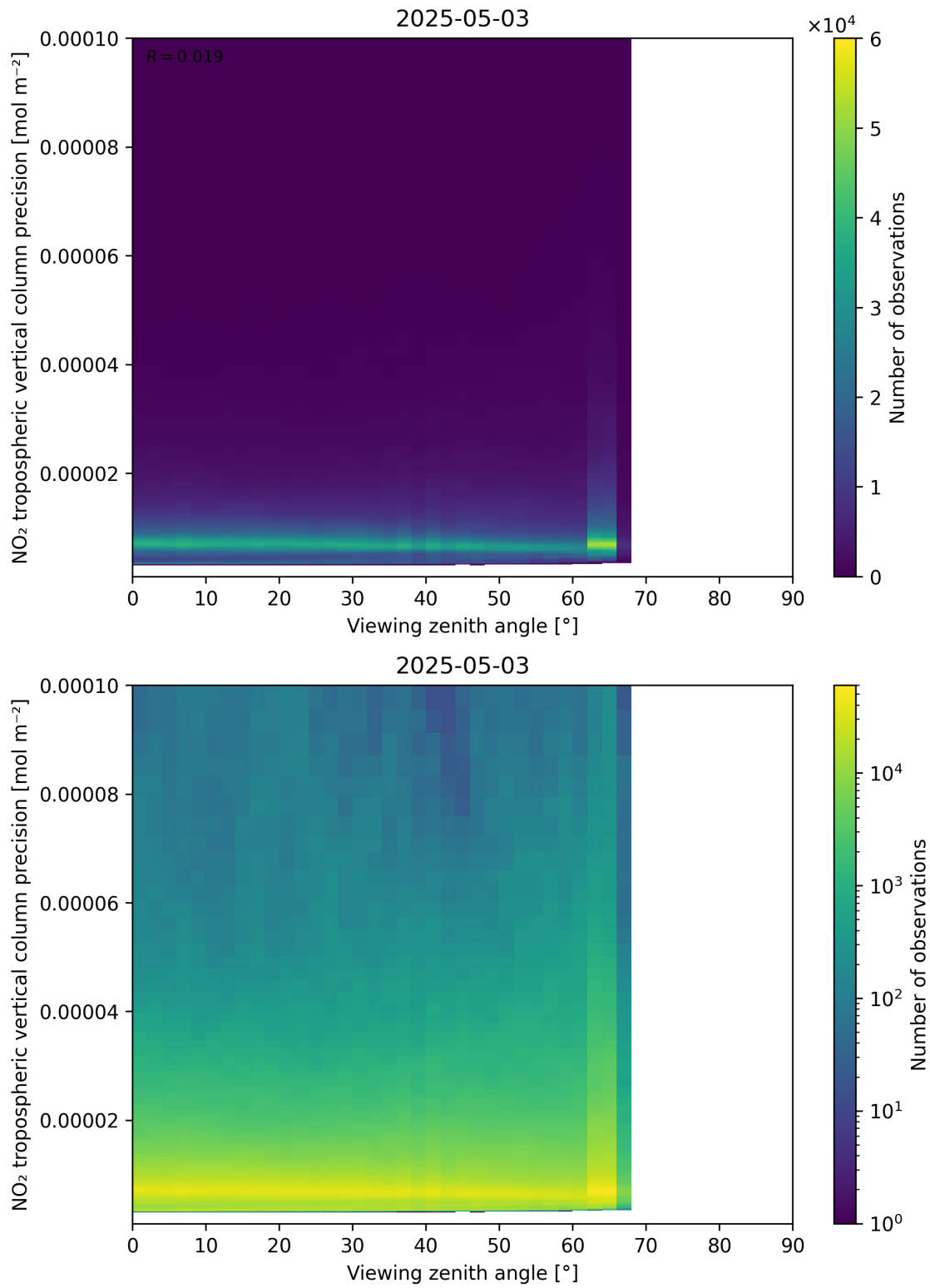
Figure 170: Scatter density plot of “Viewing zenith angle” against “NO 2 tropospheric vertical column precision” for 2025-05-03 to 2025-05-03.
