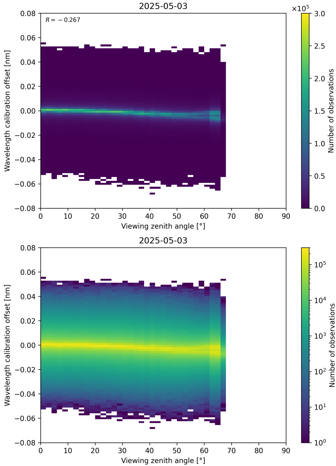
Figure 173: Scatter density plot of “Viewing zenith angle” against “Wavelength calibration offset” for 2025-05-03 to 2025-05-03.
