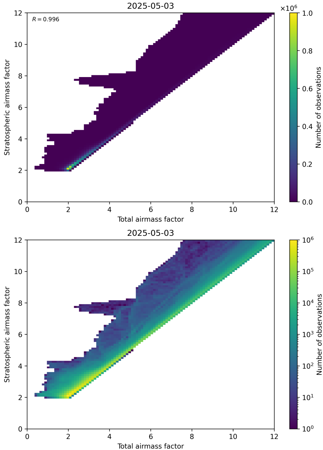
Figure 62: Scatter density plot of “Total airmass factor” against “Stratospheric airmass factor” for 2025-05-03 to 2025-05-03.
