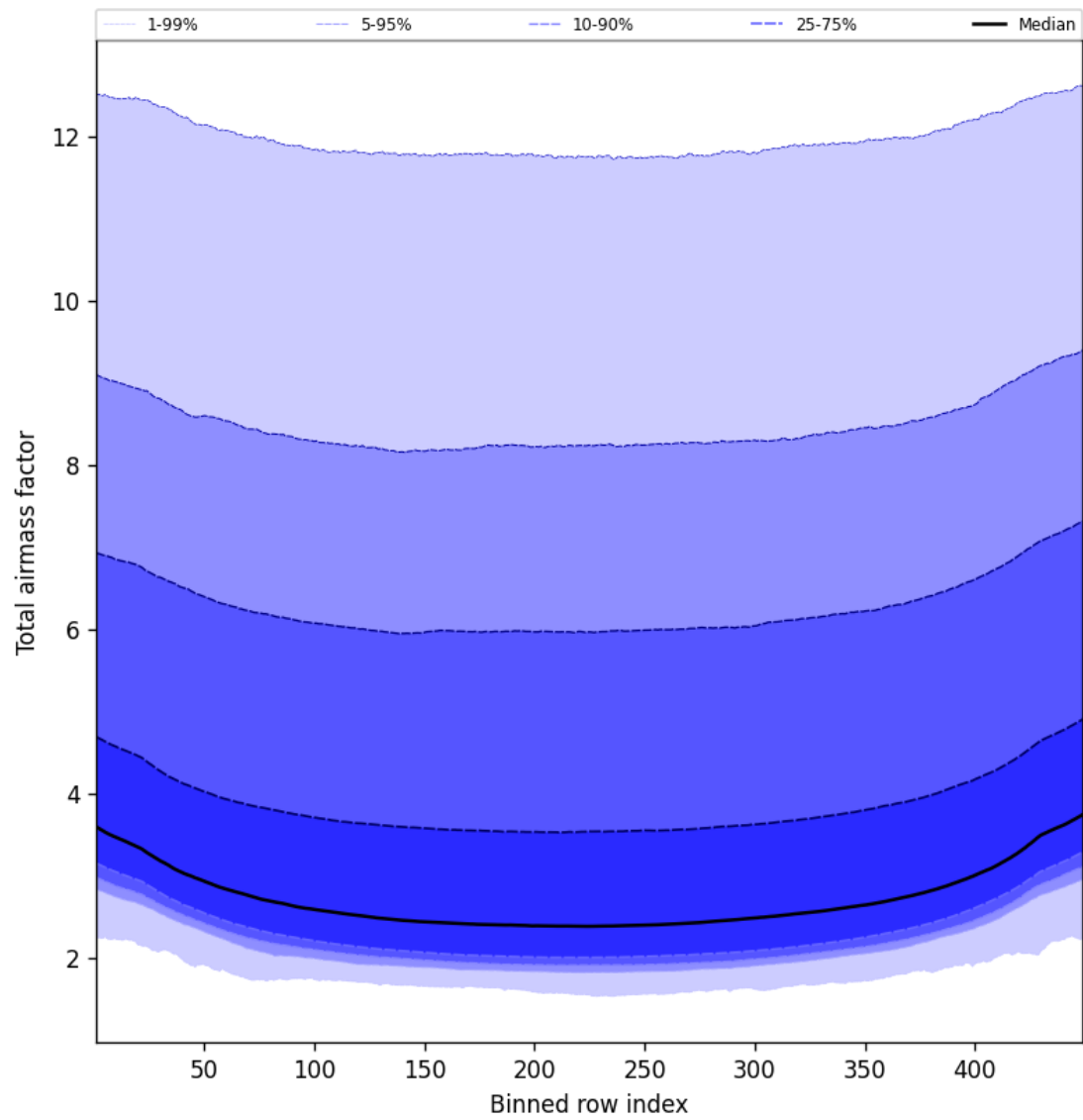
Figure 49: Along track statistics of “Total airmass factor” for 2025-05-03 to 2025-05-03
