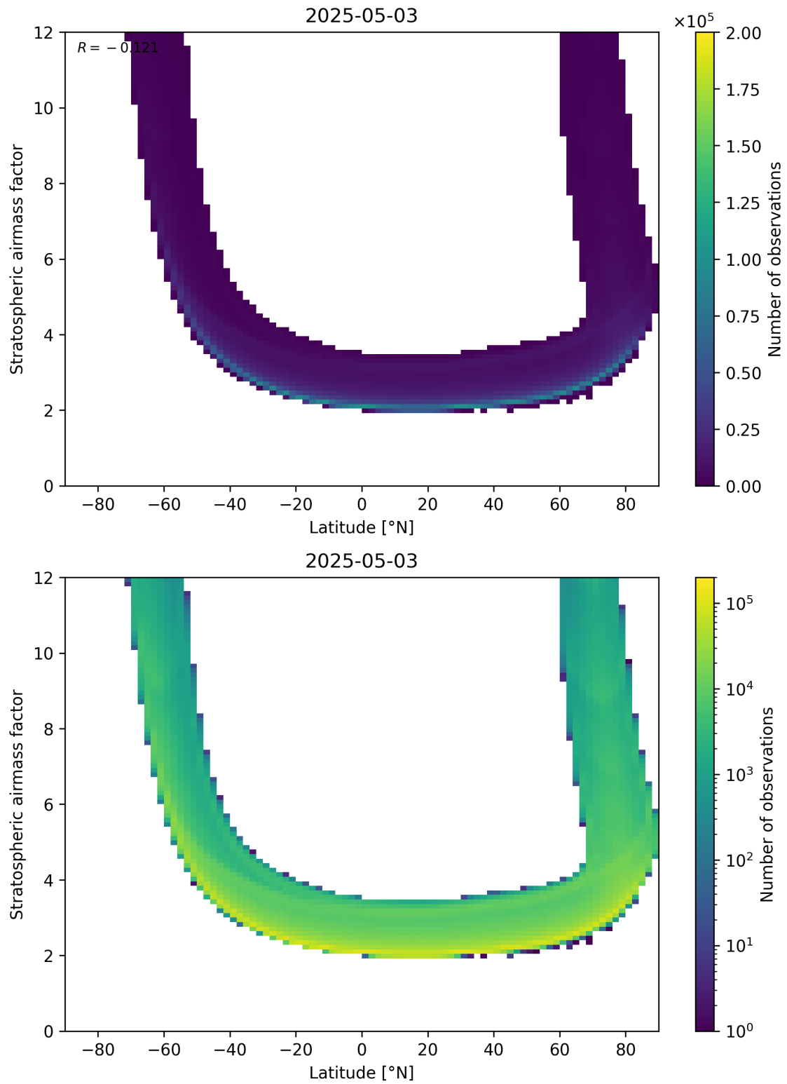
Figure 83: Scatter density plot of “Latitude” against “Stratospheric air mass factor” for 2025-05-03 to 2025-05-03.
