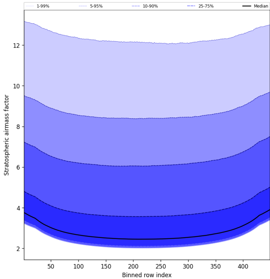
Figure 61: Along track statistics of “Stratospheric air mass factor” for 2025-05-03 to 2025-05-03
