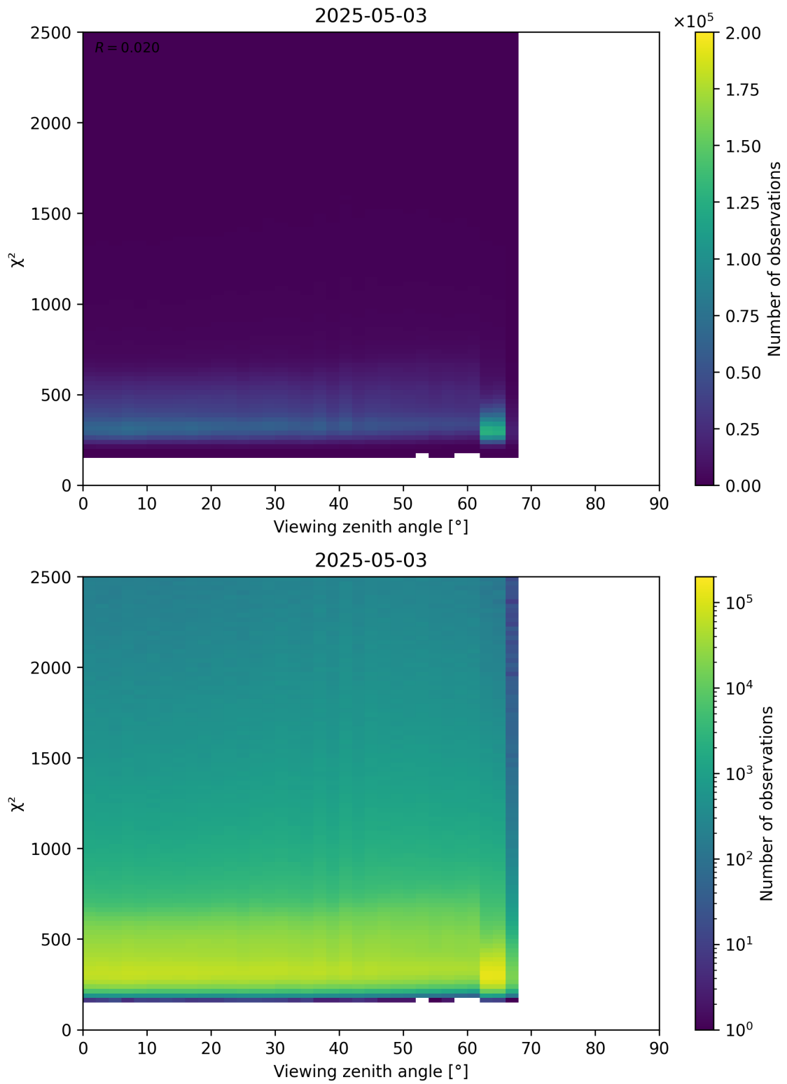
Figure 162: Scatter density plot of “Viewing zenith angle” against “ \chi^2 ” for 2025-05-03 to 2025-05-03.
