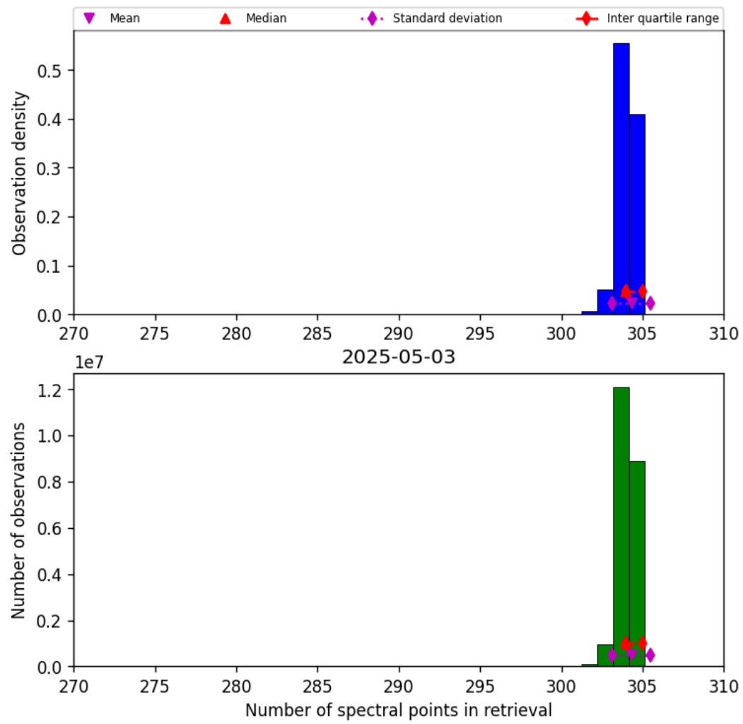
Figure 33: Histogram of “Number of spectral points in retrieval” for 2025-05-03 to 2025-05-03
