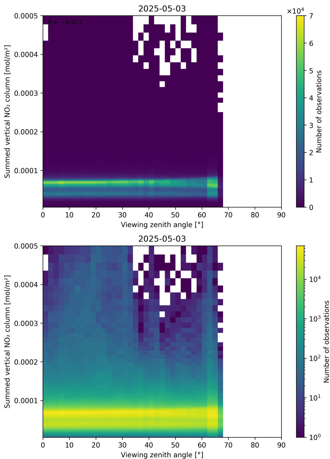
Figure 165: Scatter density plot of “Viewing zenith angle” against “Summed vertical NO 2 column” for 2025-05-03 to 2025-05-03.
