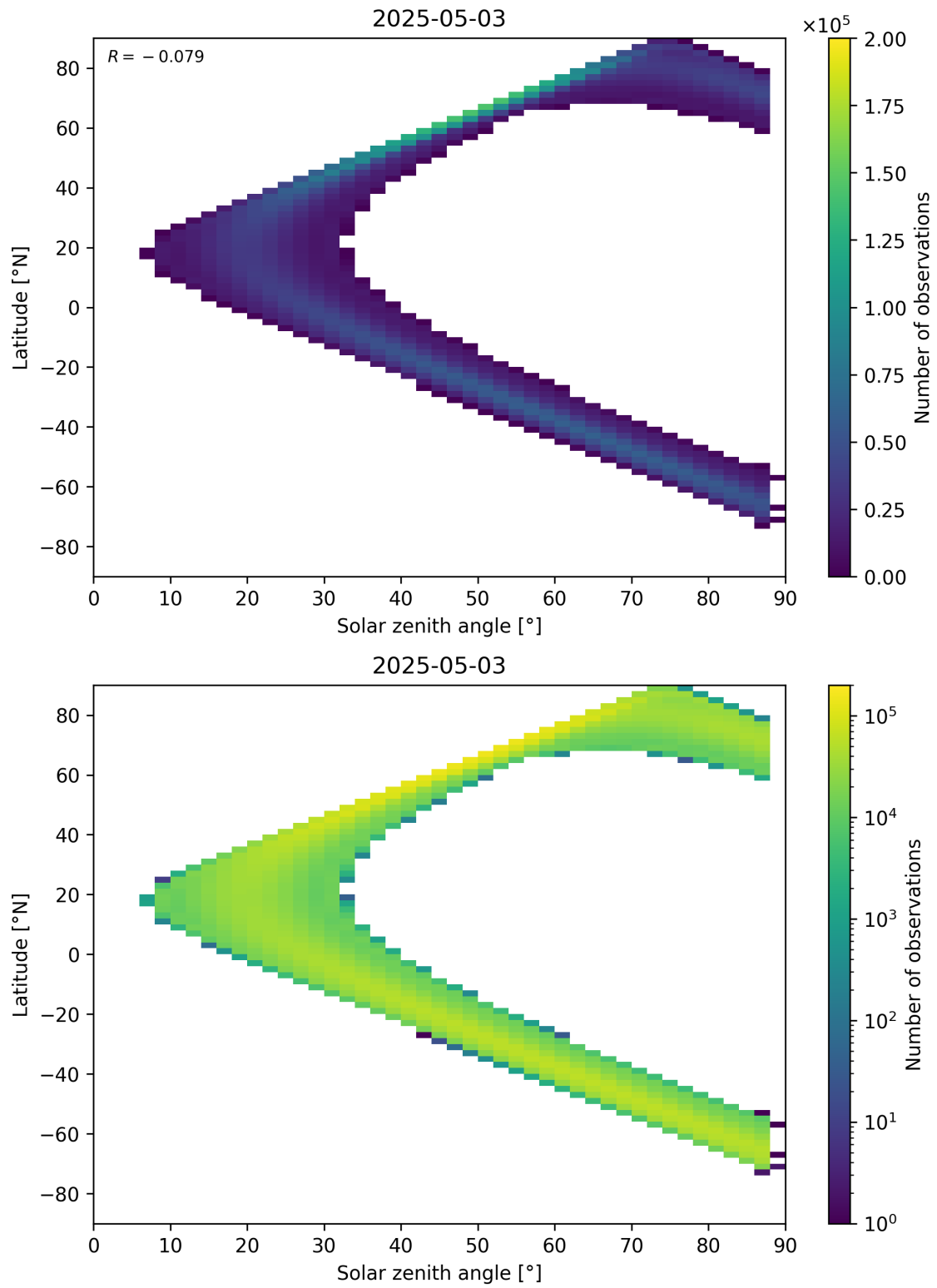
Figure 149: Scatter density plot of “Solar zenith angle” against “Latitude” for 2025-05-03 to 2025-05-03.
