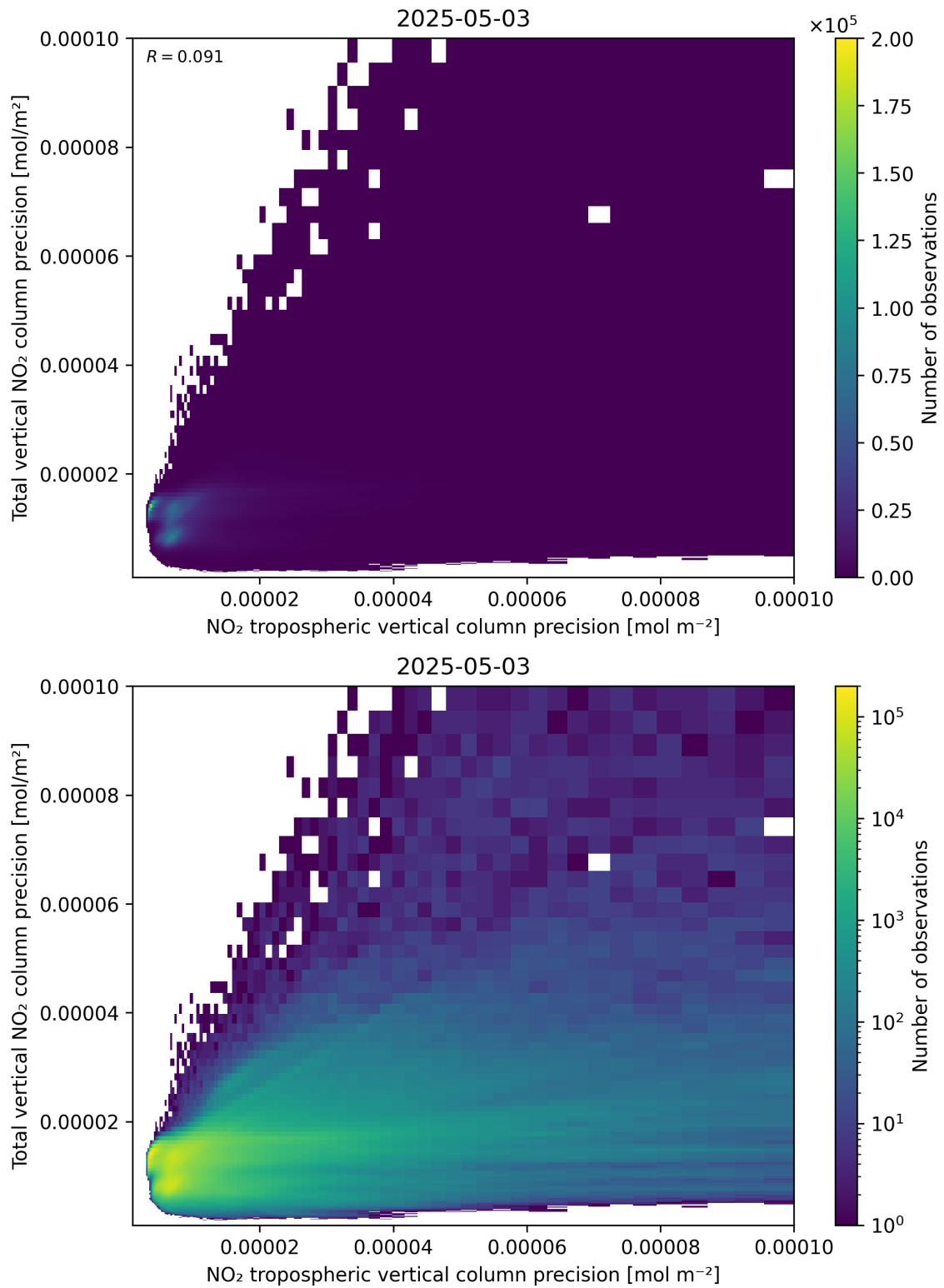
Figure 139: Scatter density plot of “NO 2 tropospheric vertical column precision” against “Total vertical NO 2 column precision” for 2025-05-03 to 2025-05-03.
