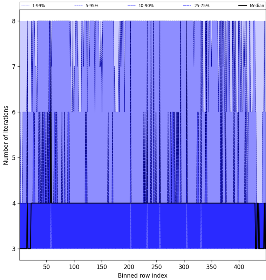
Figure 51: Along track statistics of “Number of iterations” for 2025-05-03 to 2025-05-03
