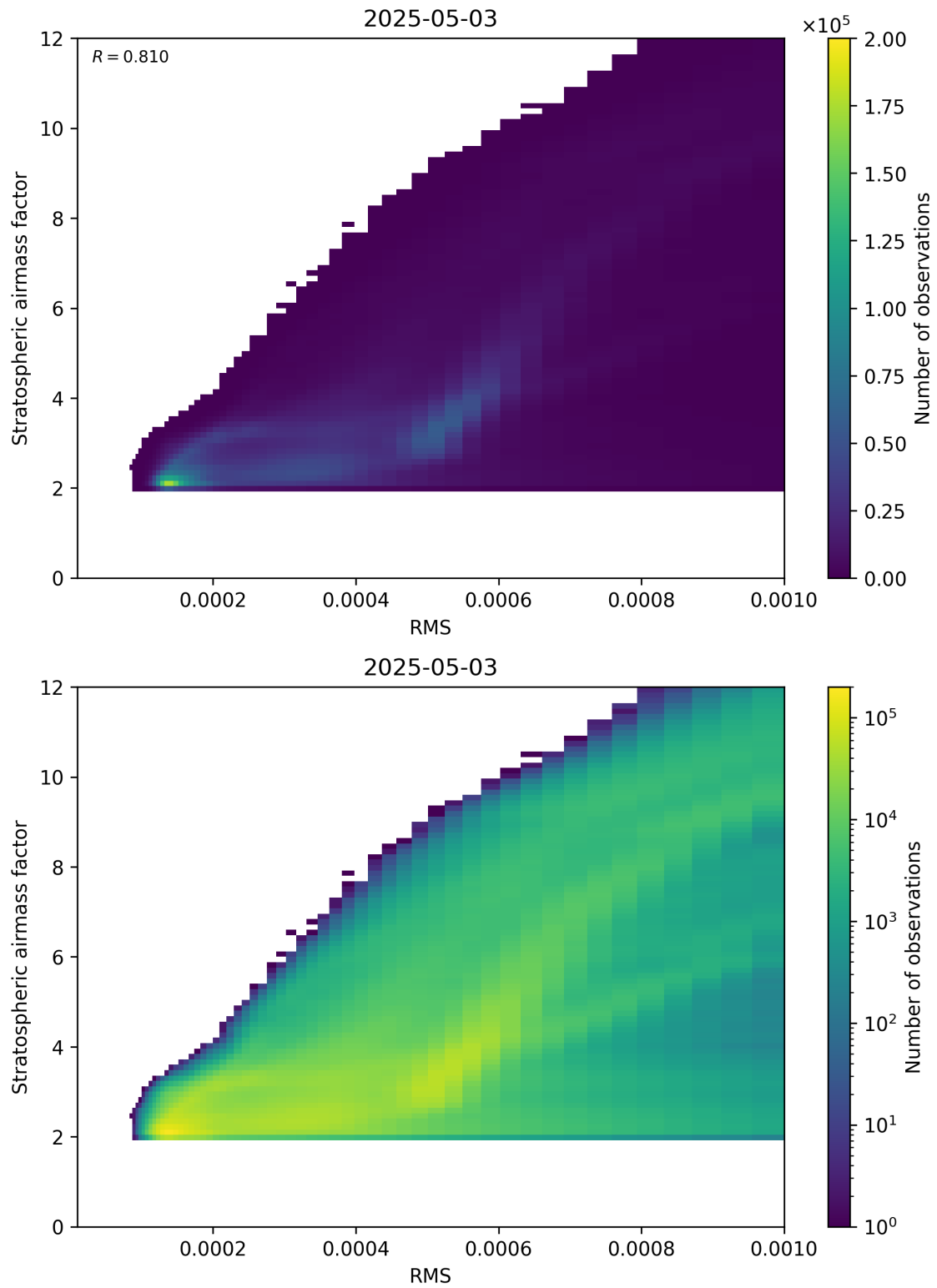
Figure 144: Scatter density plot of “RMS” against “Stratospheric airmass factor” for 2025-05-03 to 2025-05-03.
