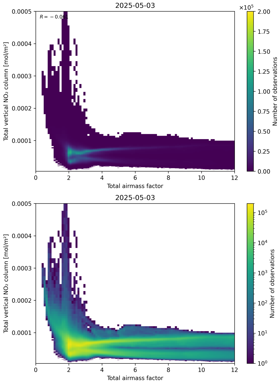
Figure 67: Scatter density plot of “Total airmass factor” against “Total vertical NO 2 column” for 2025-05-03 to 2025-05-03.
