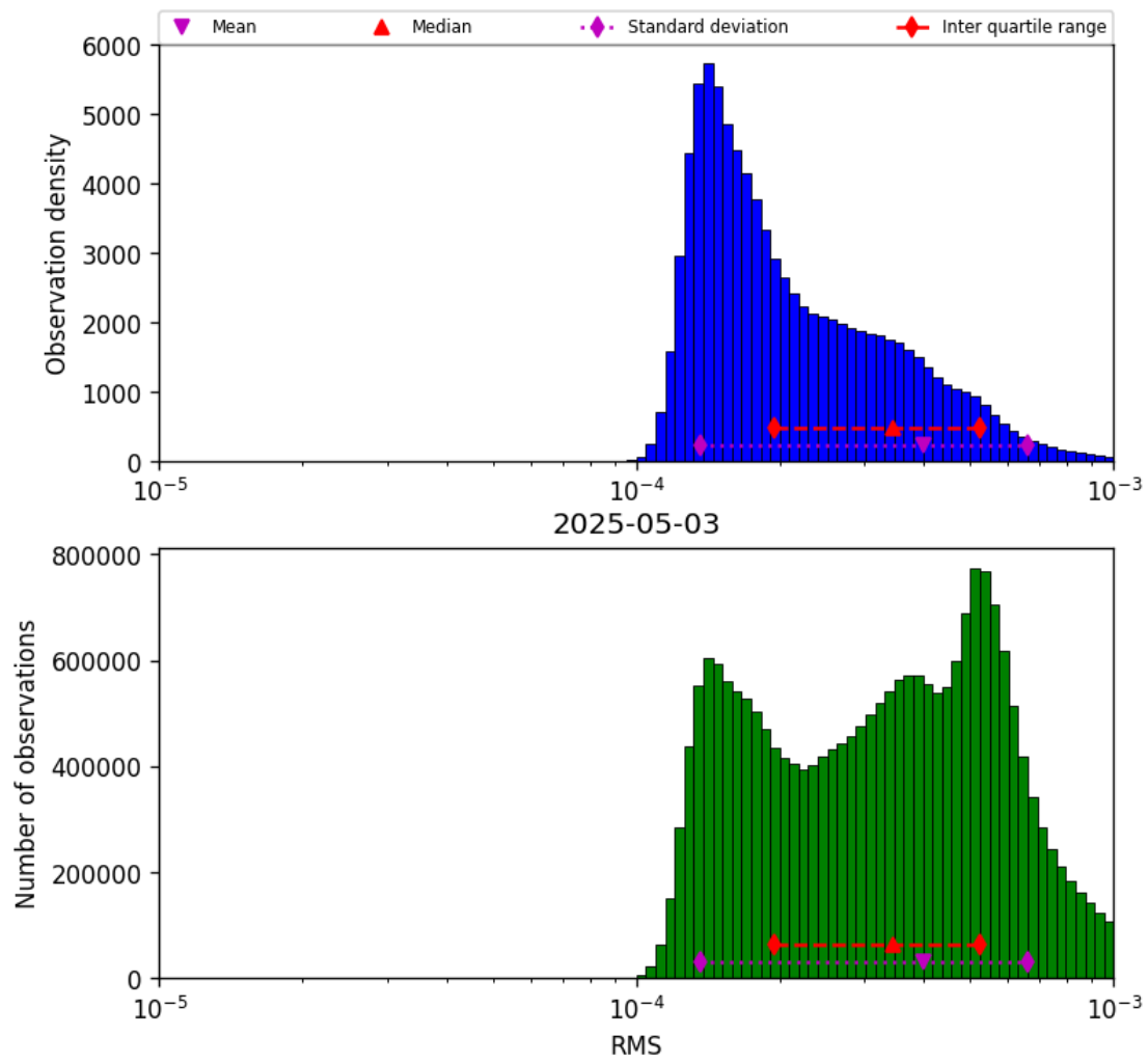
Figure 43: Histogram of “RMS” for 2025-05-03 to 2025-05-03
