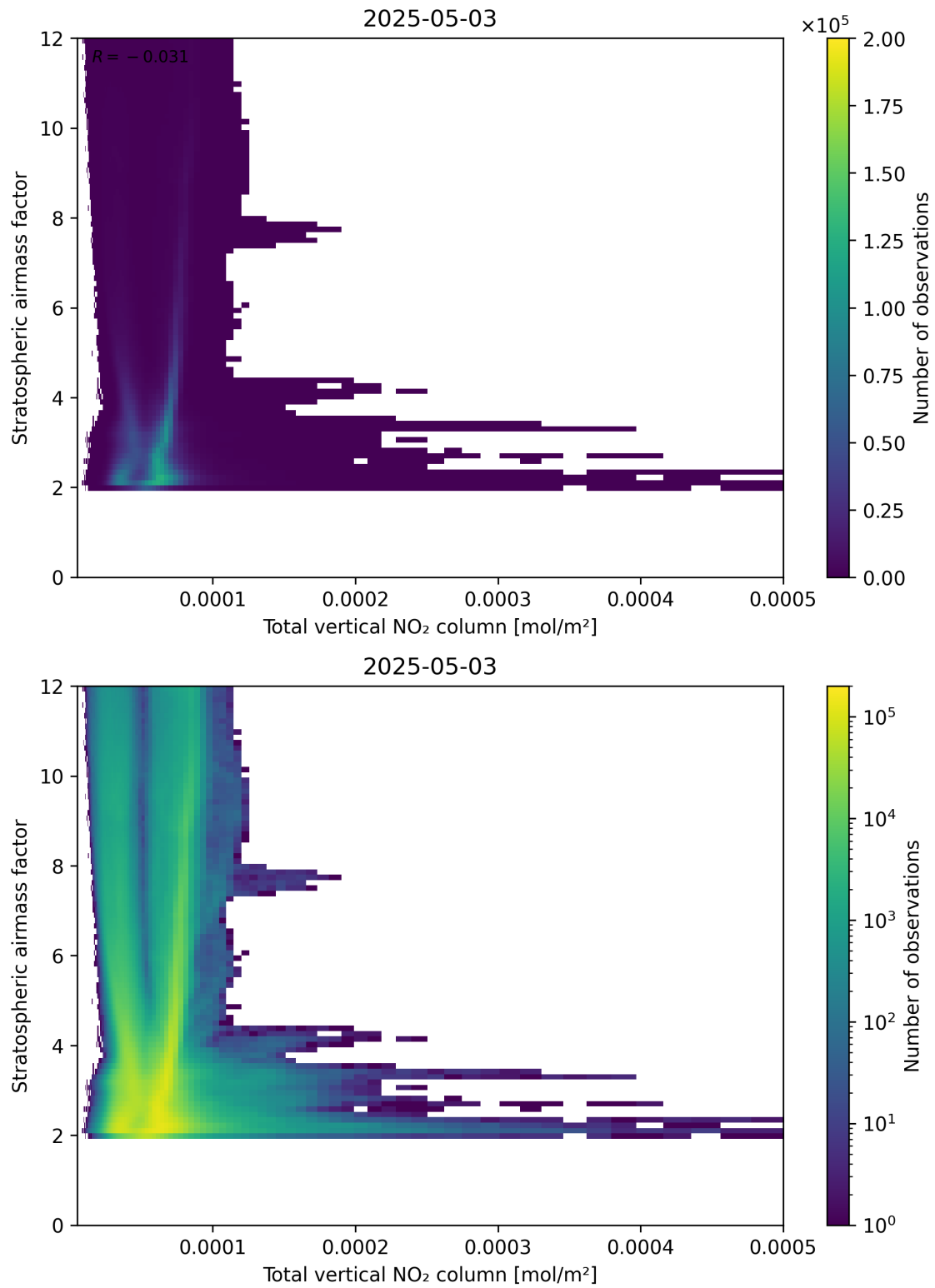
Figure 110: Scatter density plot of “Total vertical NO 2 column” against “Stratospheric airmass factor” for 2025-05-03 to 2025-05-03.
