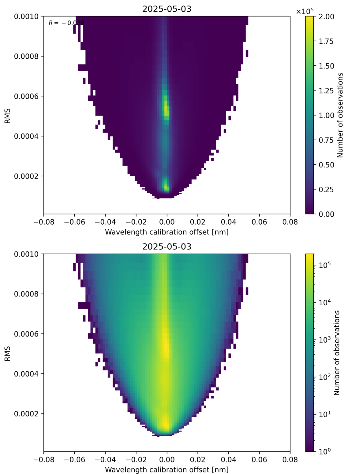
Figure 181: Scatter density plot of “Wavelength calibration offset” against “RMS” for 2025-05-03 to 2025-05-03.
