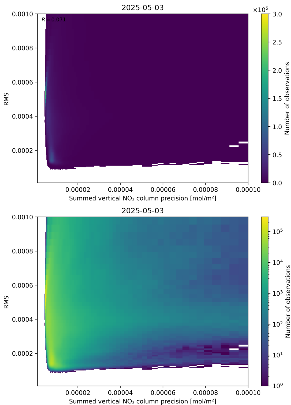
Figure 108: Scatter density plot of “Summed vertical NO 2 column precision” against “RMS” for 2025-05-03 to 2025-05-03.
