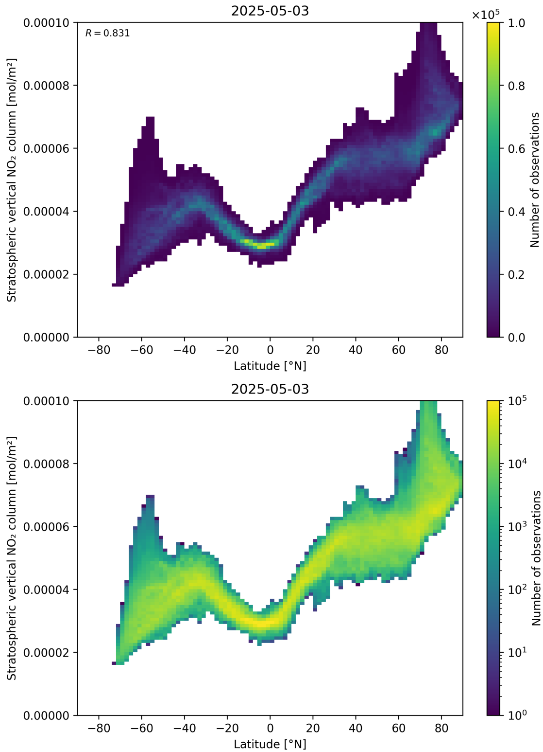
Figure 87: Scatter density plot of “Latitude” against “Stratospheric vertical NO 2 column” for 2025-05-03 to 2025-05-03.
