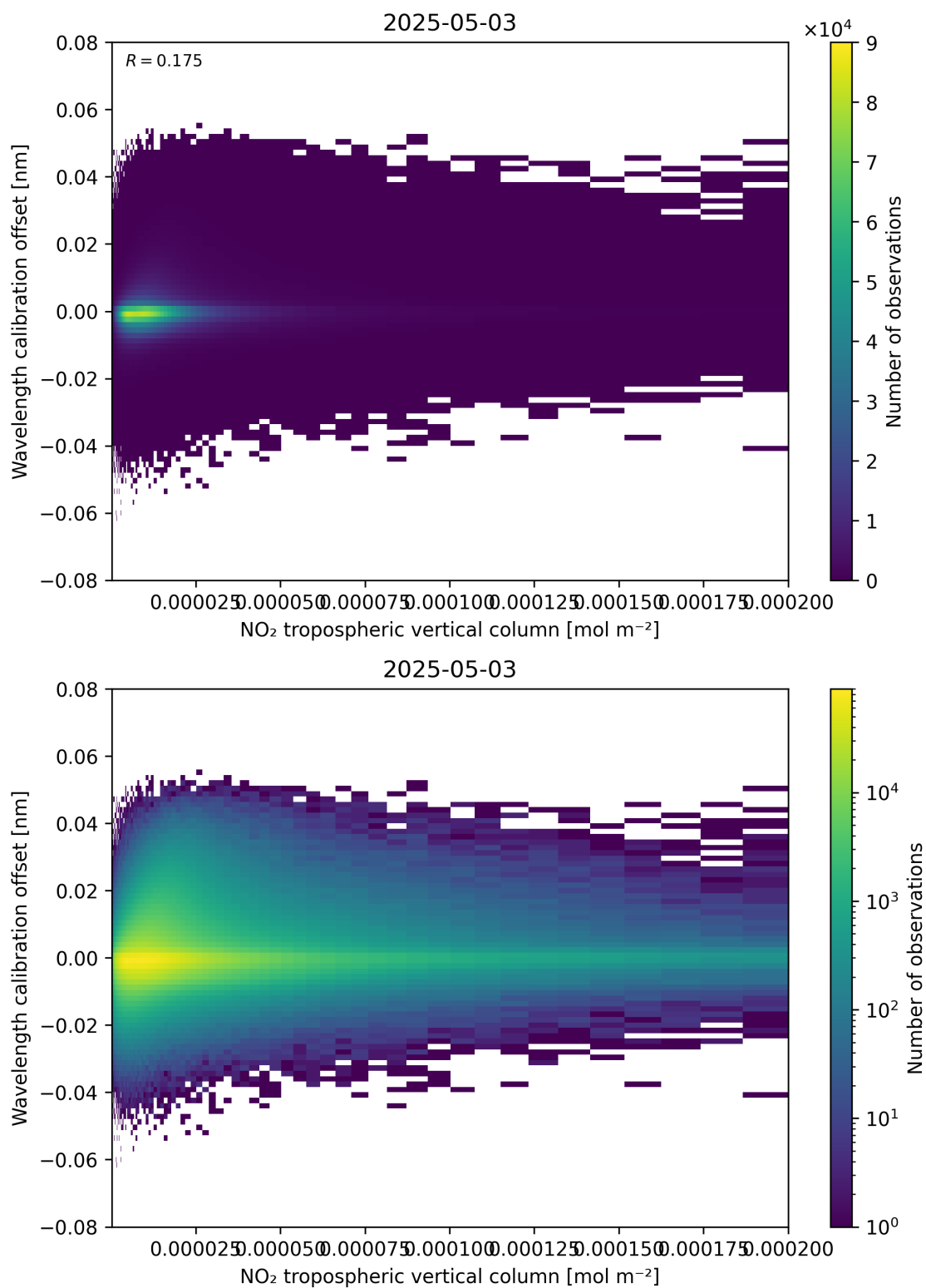
Figure 143: Scatter density plot of “NO 2 tropospheric vertical column” against “Wavelength calibration offset” for 2025-05-03 to 2025-05-03.
