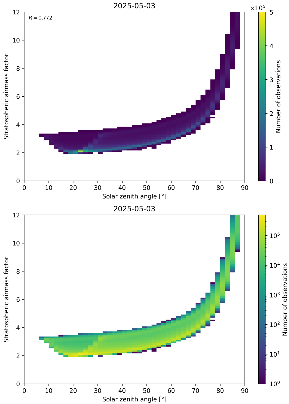
Figure 145: Scatter density plot of “Solar zenith angle” against “Stratospheric airmass factor” for 2025-05-03 to 2025-05-03.
