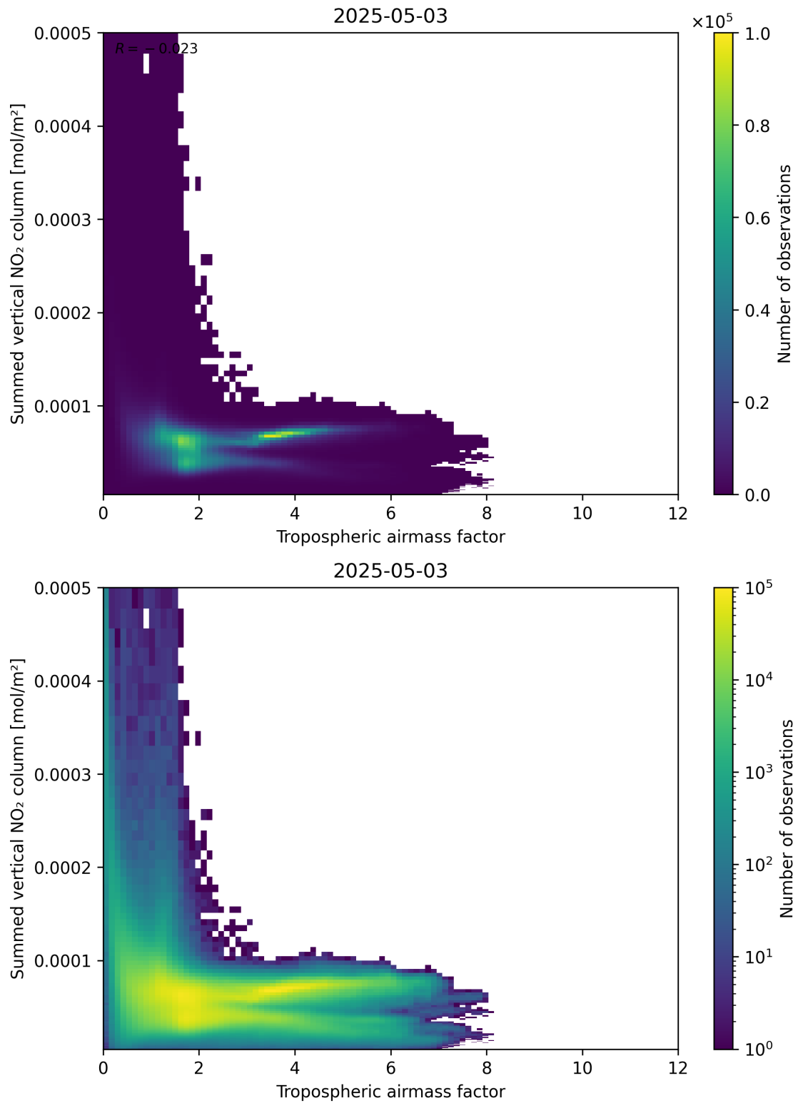
Figure 75: Scatter density plot of “Tropospheric air mass factor” against “Summed vertical NO 2 column” for 2025-05-03 to 2025-05-03.
