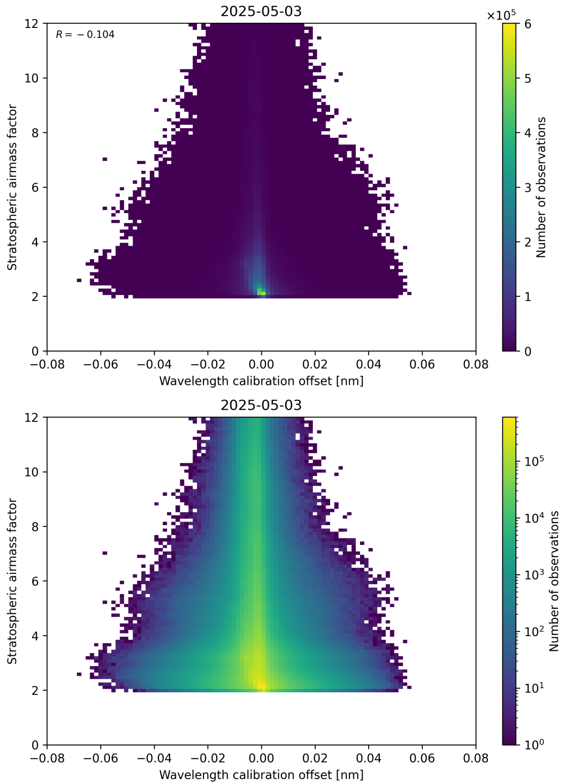
Figure 174: Scatter density plot of “Wavelength calibration offset” against “Stratospheric airmass factor” for 2025-05-03 to 2025-05-03.
