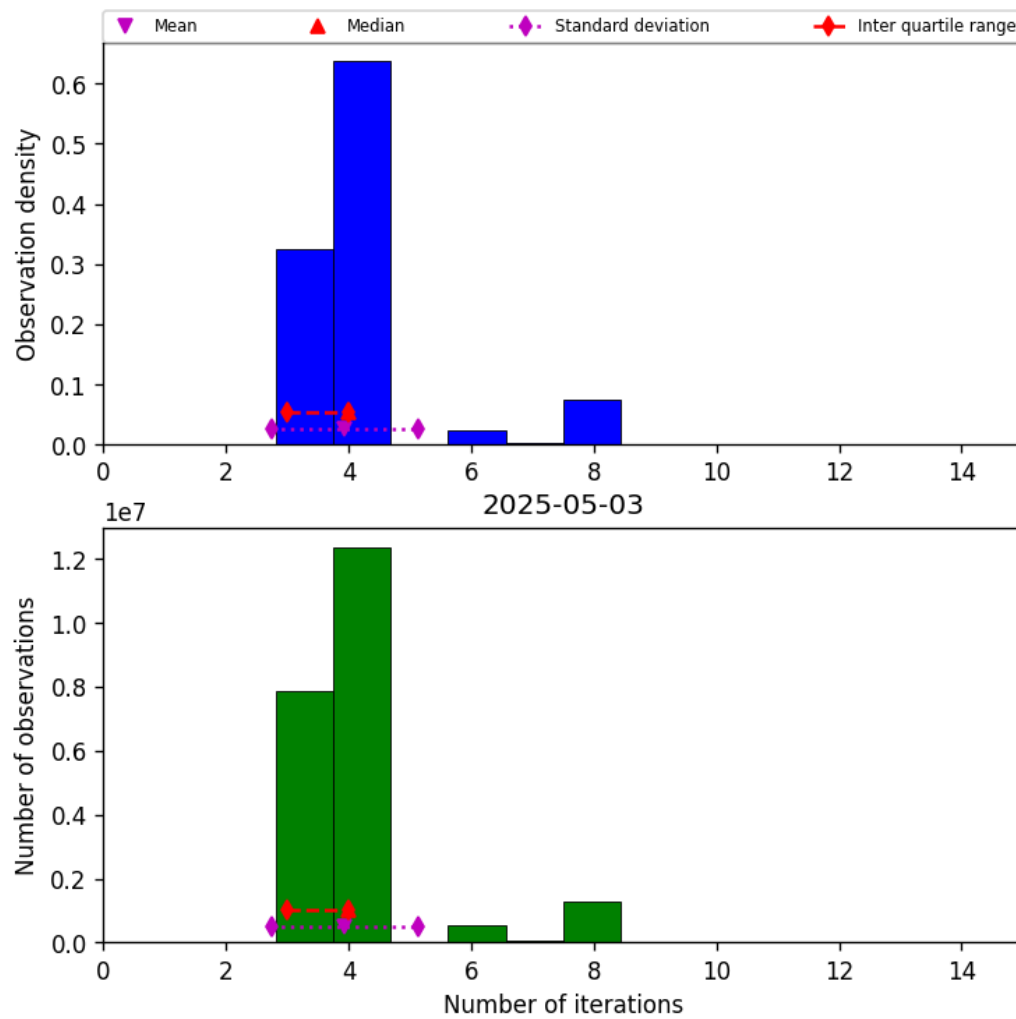
Figure 34: Histogram of “Number of iterations” for 2025-05-03 to 2025-05-03
