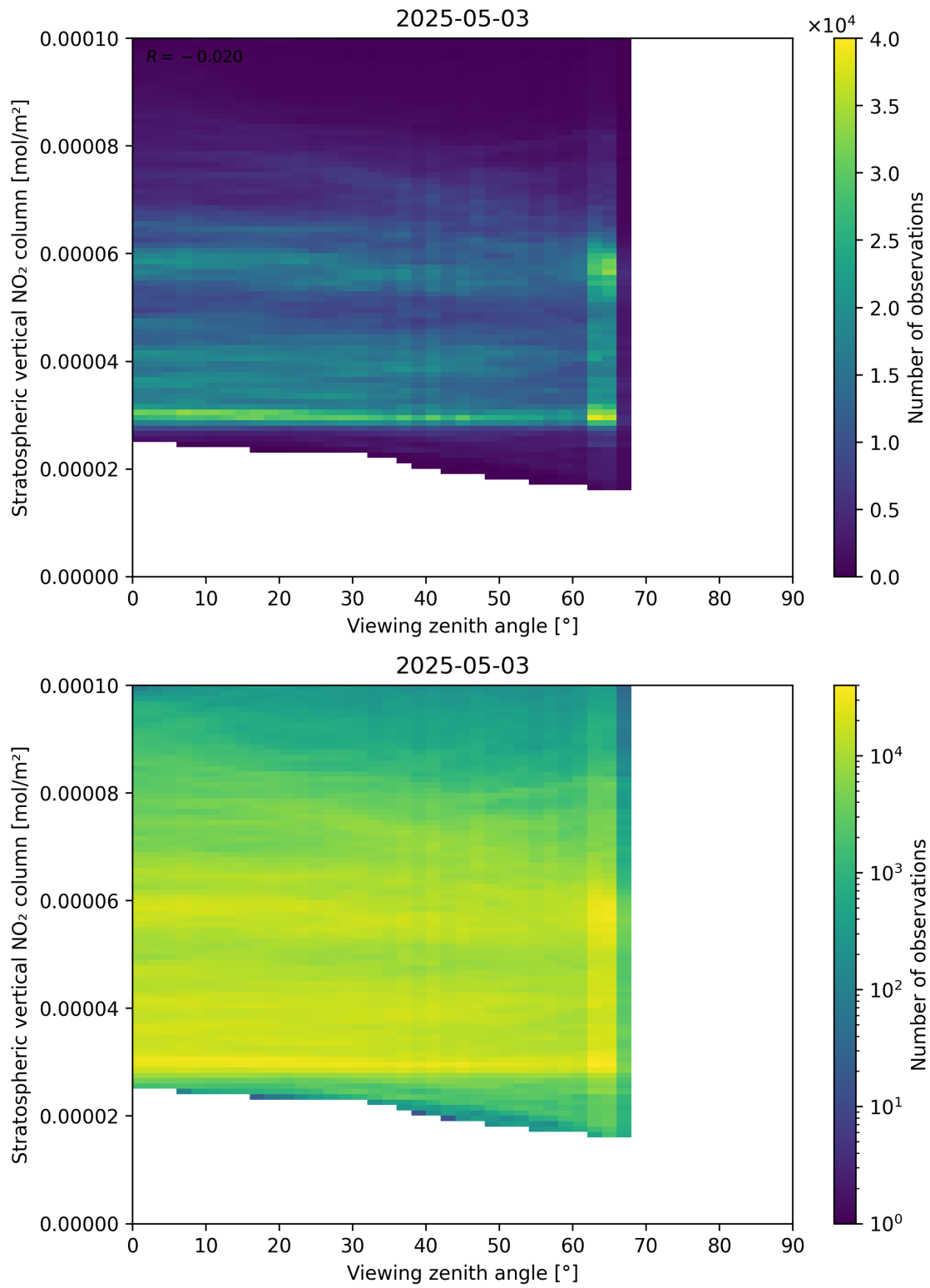
Figure 164: Scatter density plot of “Viewing zenith angle” against “Stratospheric vertical NO 2 column” for 2025-05-03 to 2025-05-03.
