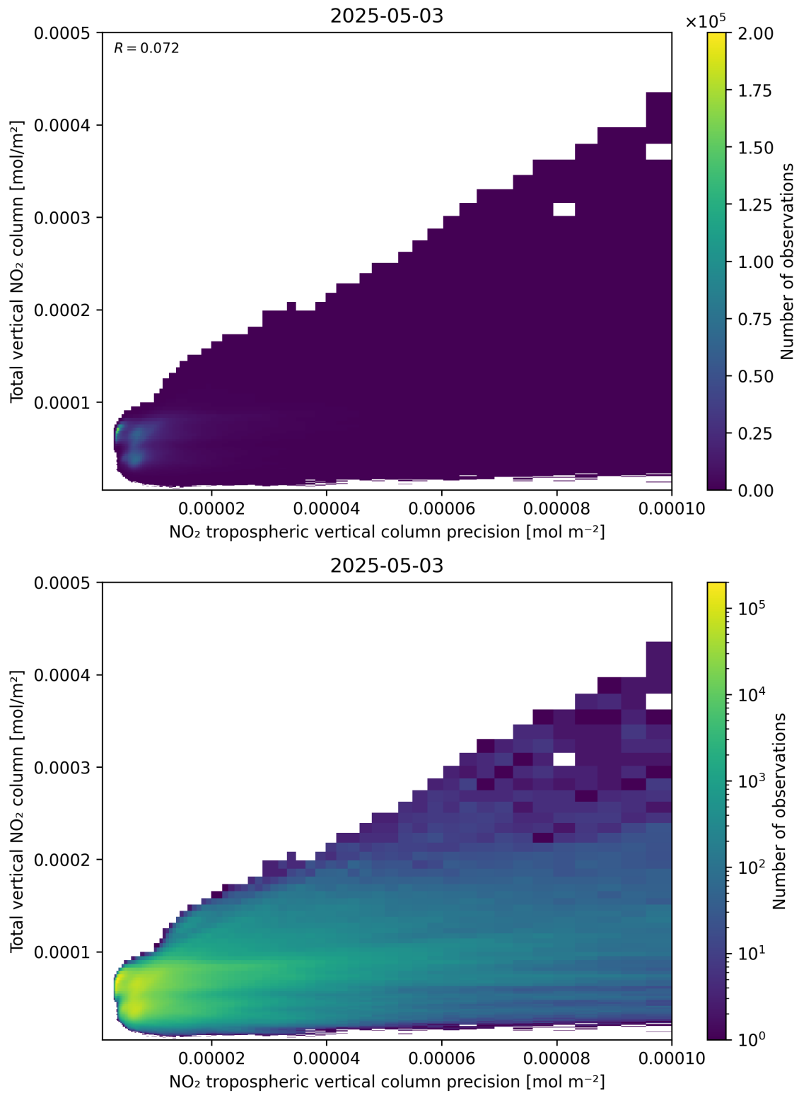
Figure 138: Scatter density plot of “NO 2 tropospheric vertical column precision” against “Total vertical NO 2 column” for 2025-05-03 to 2025-05-03.
