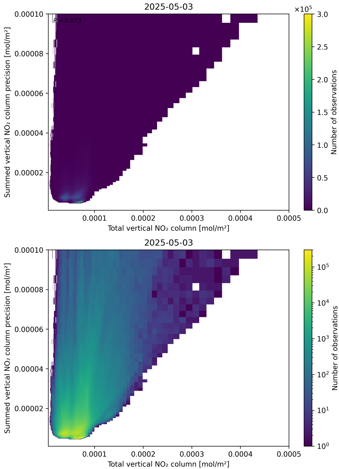
Figure 113: Scatter density plot of “Total vertical NO 2 column” against “Summed vertical NO 2 column precision” for 2025-05-03 to 2025-05-03.
