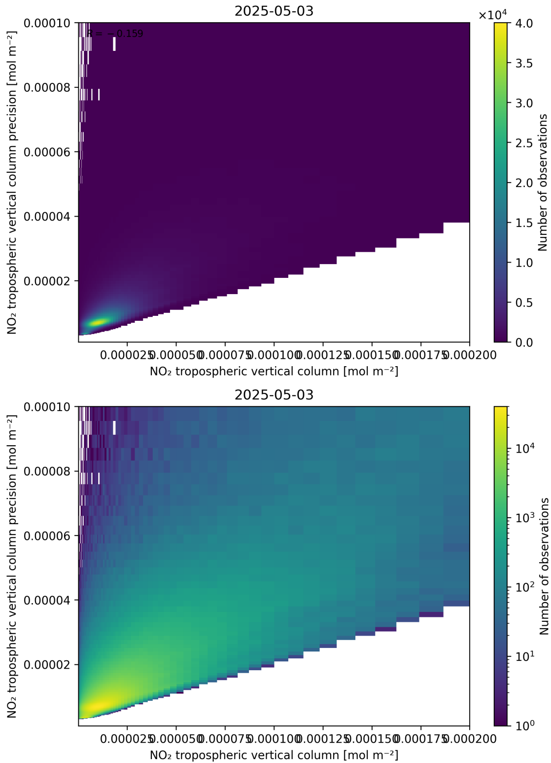
Figure 130: Scatter density plot of “NO 2 tropospheric vertical column” against “NO 2 tropospheric vertical column precision” for 2025-05-03 to 2025-05-03.
