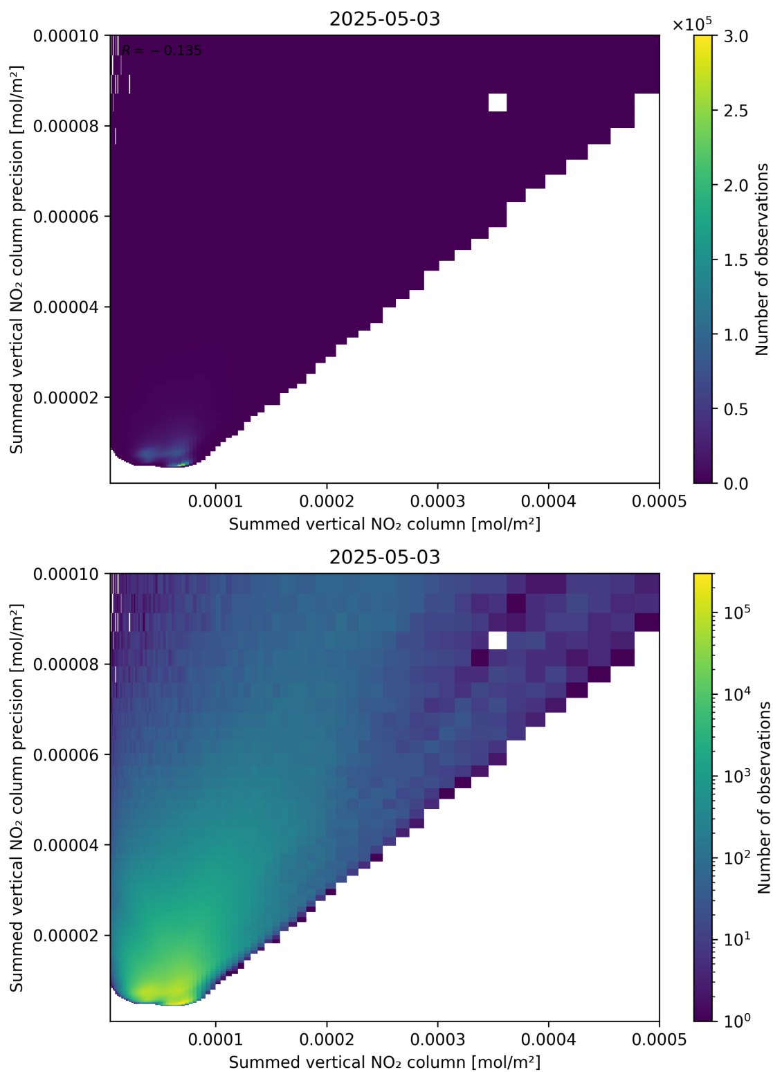
Figure 105: Scatter density plot of “Summed vertical NO 2 column” against “Summed vertical NO 2 column precision” for 2025-05-03 to 2025-05-03.
