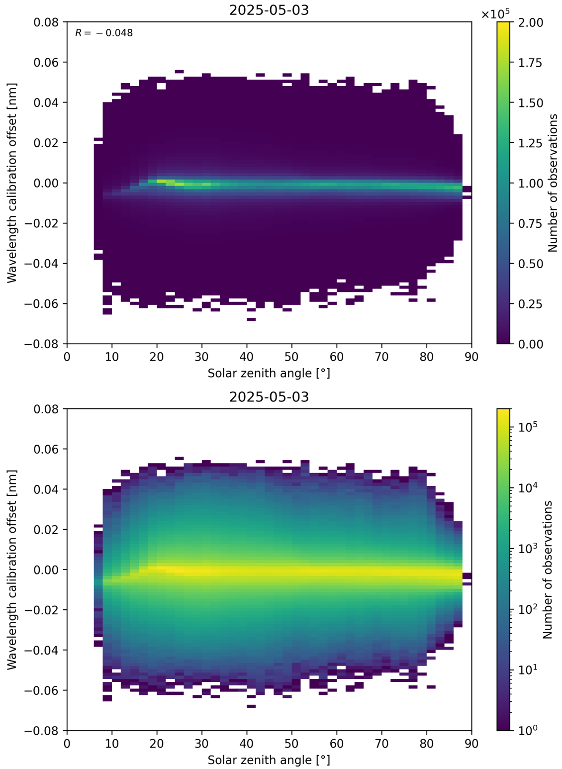
Figure 158: Scatter density plot of “Solar zenith angle” against “Wavelength calibration offset” for 2025-05-03 to 2025-05-03.
