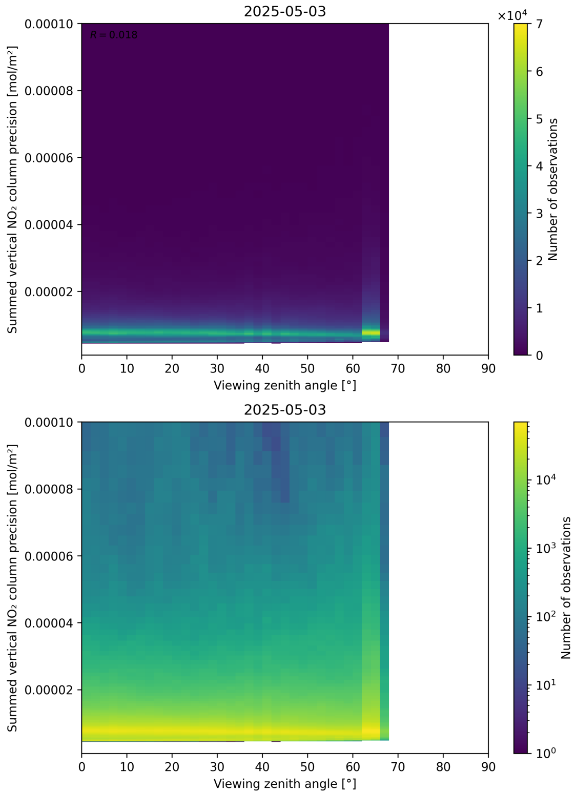
Figure 166: Scatter density plot of “Viewing zenith angle” against “Summed vertical NO 2 column precision” for 2025-05-03 to 2025-05-03.
