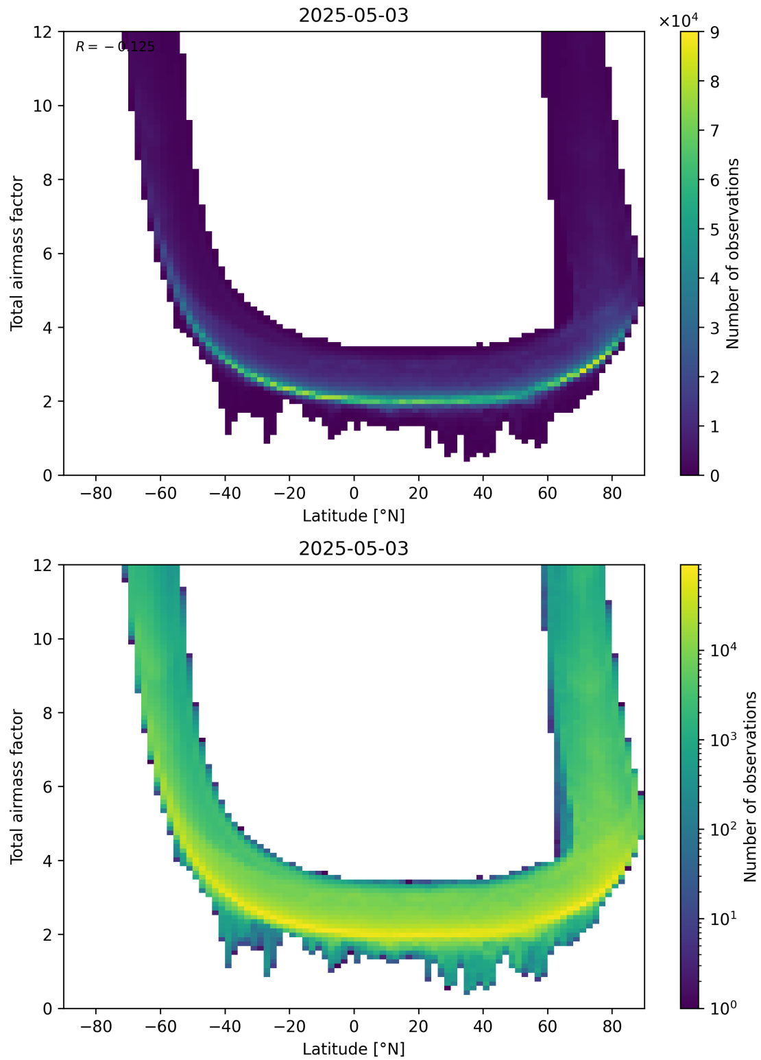
Figure 84: Scatter density plot of “Latitude” against “Total air mass factor” for 2025-05-03 to 2025-05-03.
