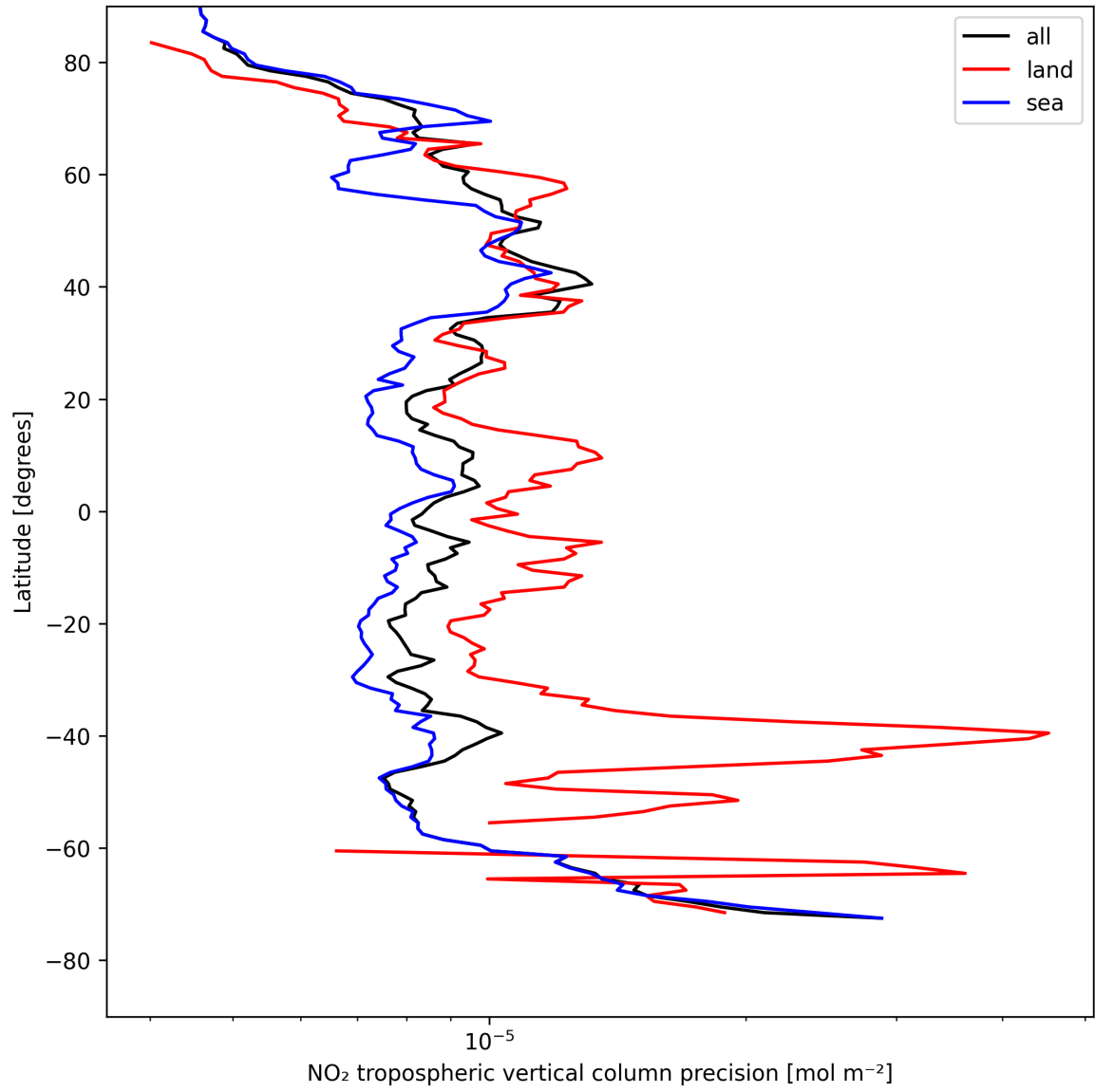
Figure 13: Zonal average of “NO 2 tropospheric vertical column precision” for 2025-05-03 to 2025-05-03.
