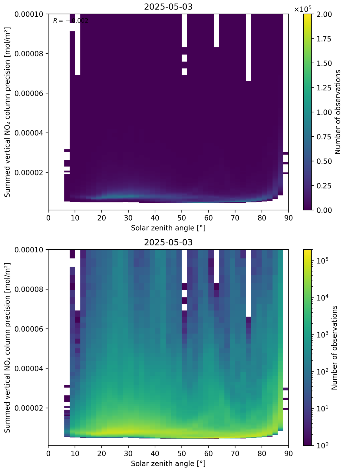
Figure 152: Scatter density plot of “Solar zenith angle” against “Summed vertical NO 2 column precision” for 2025-05-03 to 2025-05-03.
