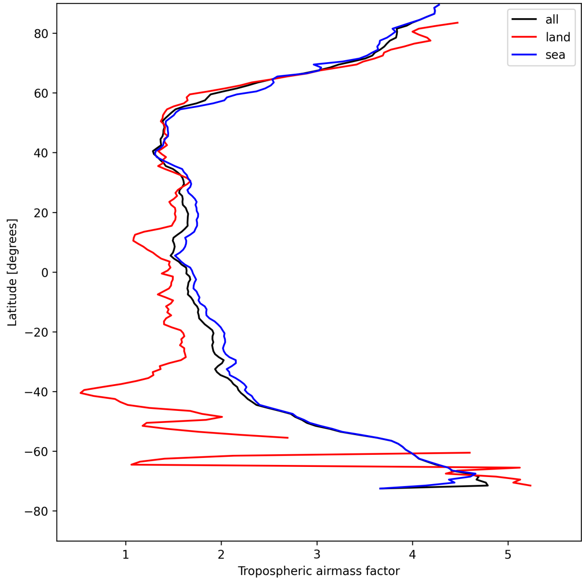
Figure 14: Zonal average of “Tropospheric airmass factor” for 2025-05-03 to 2025-05-03.
