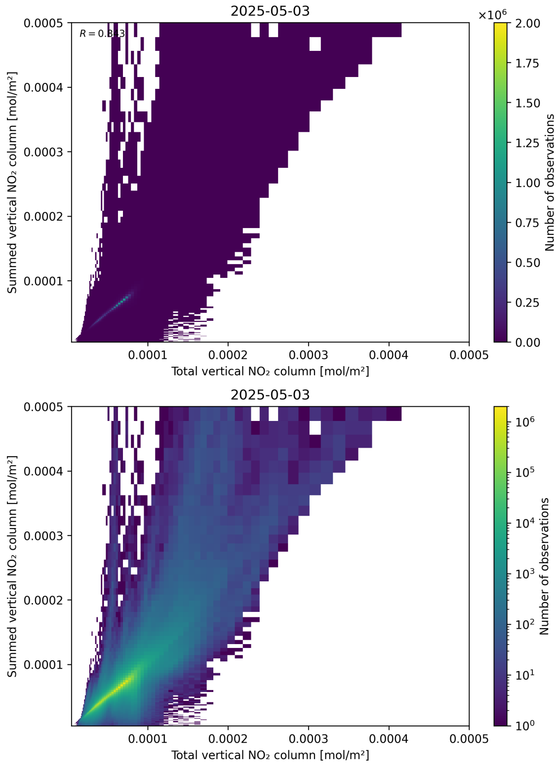
Figure 112: Scatter density plot of “Total vertical NO 2 column” against “Summed vertical NO 2 column” for 2025-05-03 to 2025-05-03.
