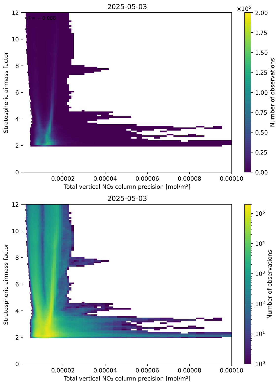
Figure 115: Scatter density plot of “Total vertical NO 2 column precision” against “Stratospheric air mass factor” for 2025-05-03 to 2025-05-03.
