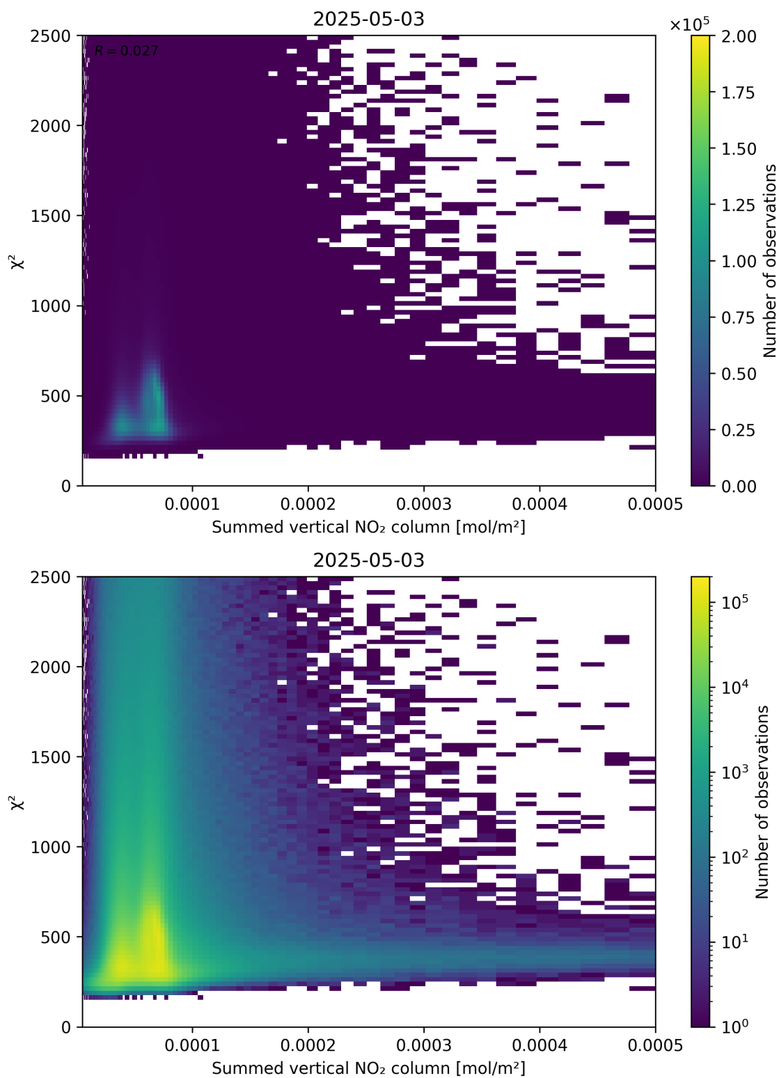
Figure 104: Scatter density plot of “Summed vertical NO 2 column” against “ \chi^2 ” for 2025-05-03 to 2025-05-03.
