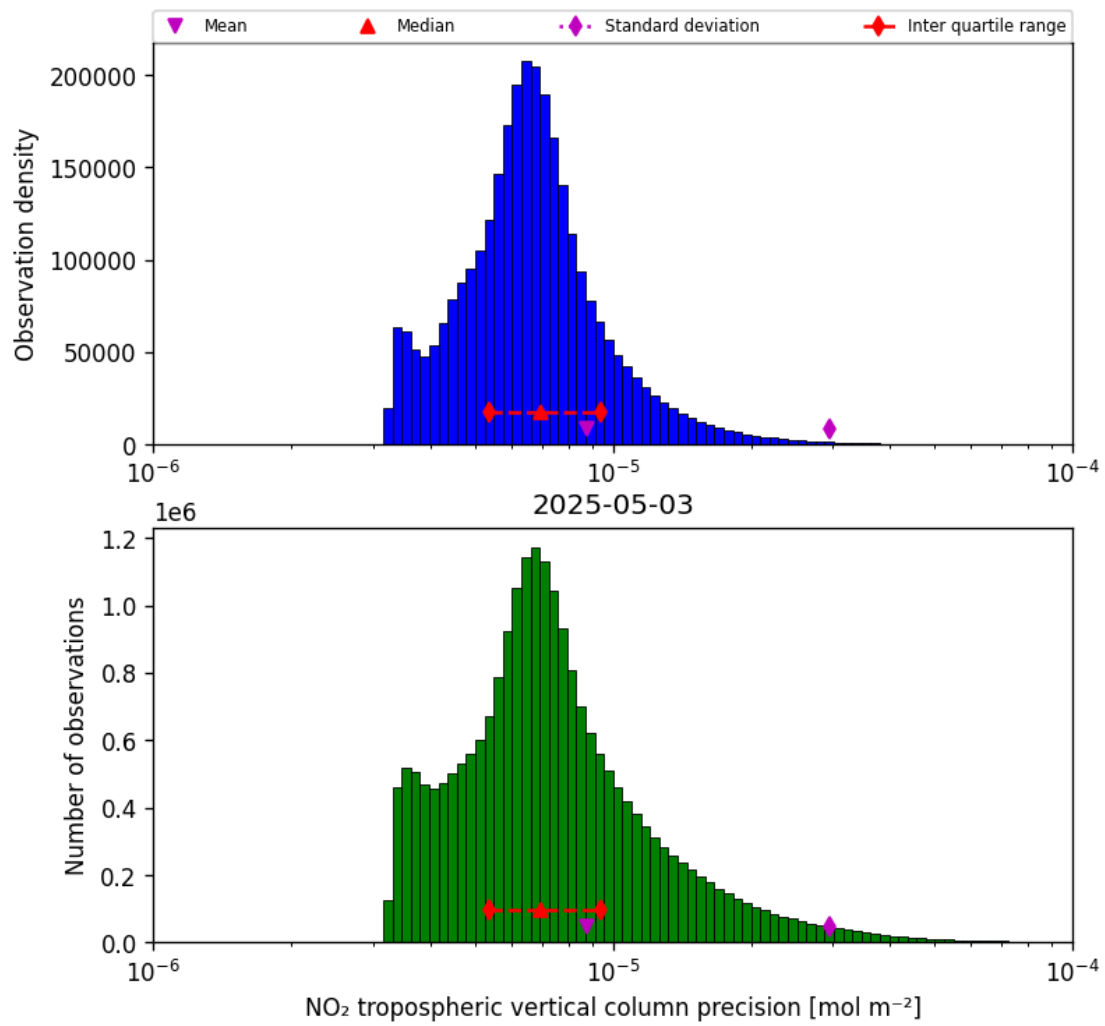
Figure 30: Histogram of “NO 2 tropospheric vertical column precision” for 2025-05-03 to 2025-05-03
