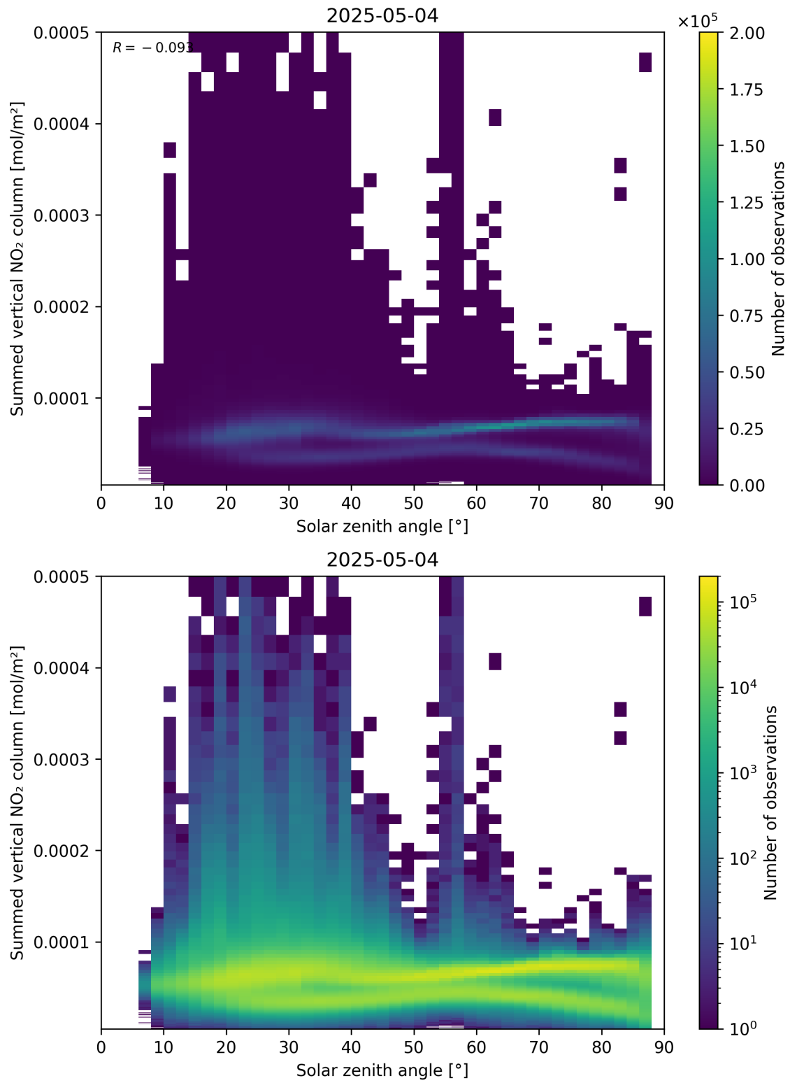
Figure 151: Scatter density plot of “Solar zenith angle” against “Summed vertical NO 2 column” for 2025-05-04 to 2025-05-05.
