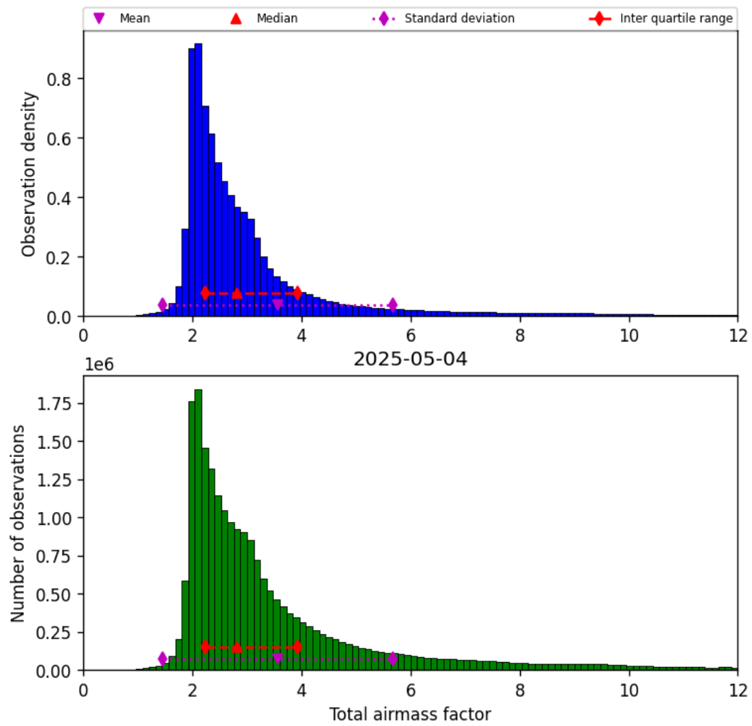
Figure 32: Histogram of “Total airmass factor” for 2025-05-04 to 2025-05-05
