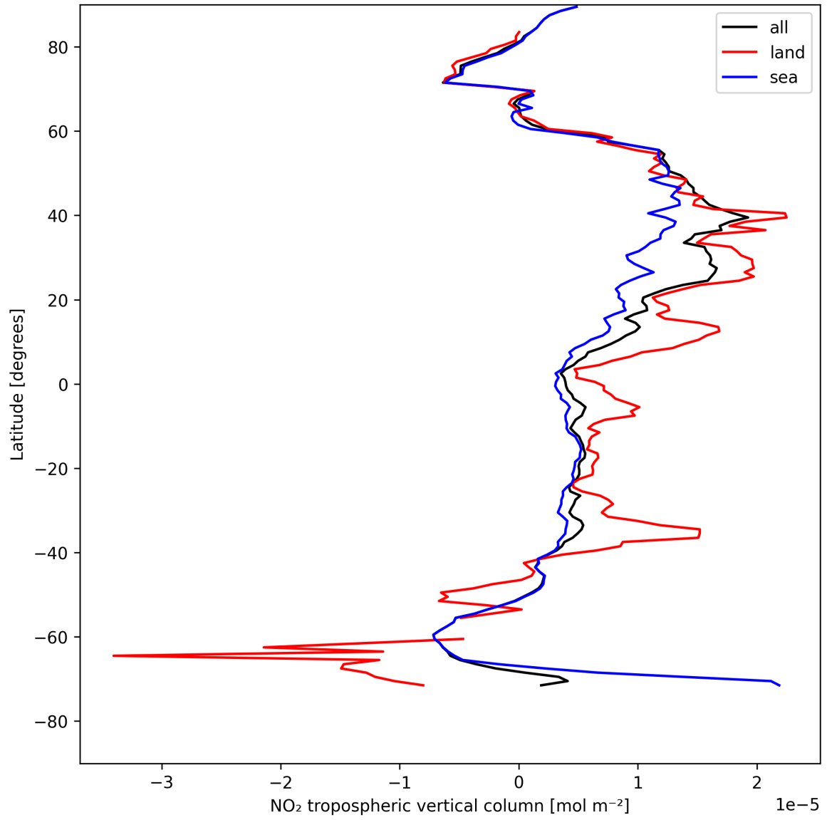
Figure 12: Zonal average of “NO 2 tropospheric vertical column” for 2025-05-04 to 2025-05-05.
