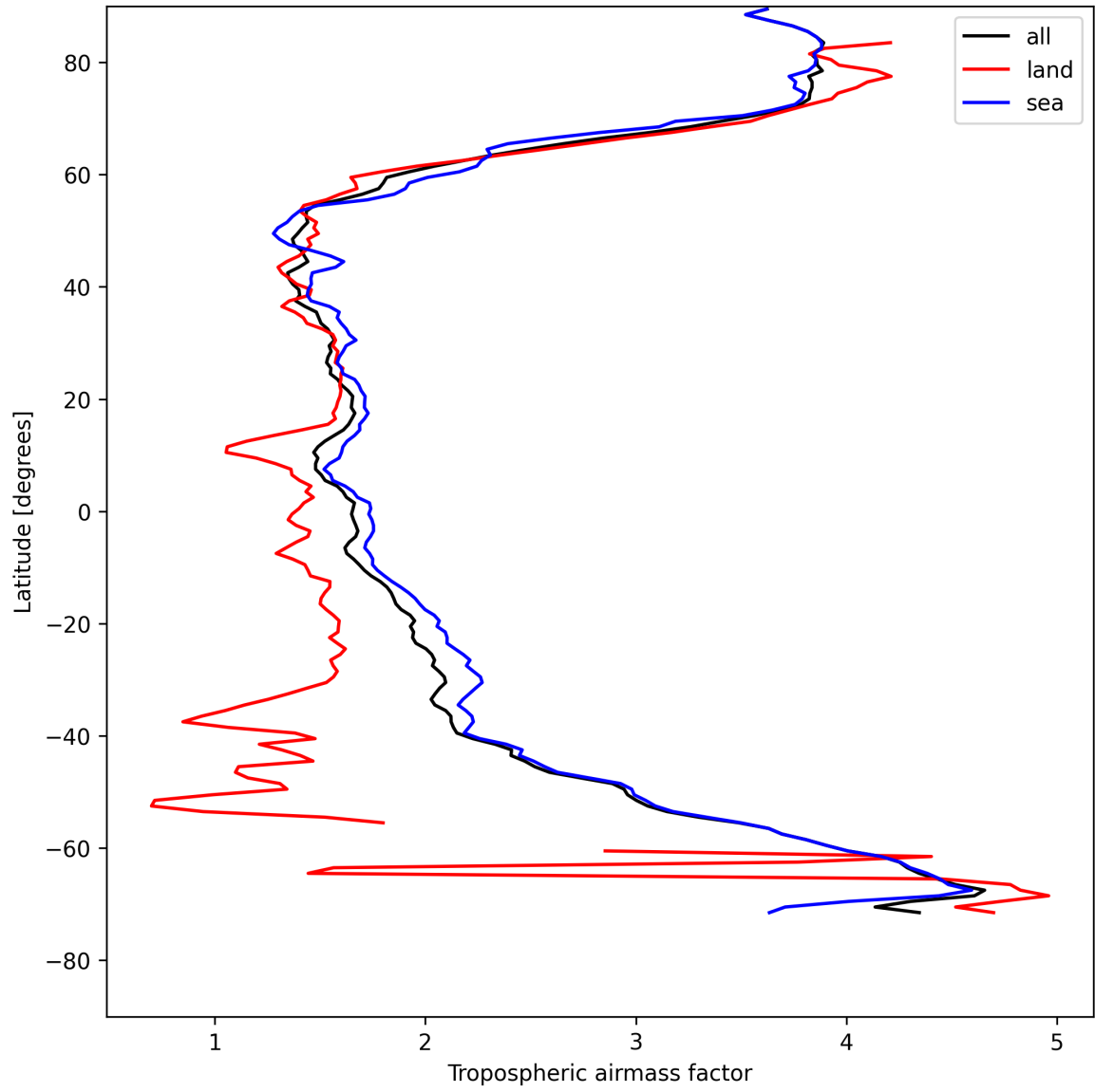
Figure 14: Zonal average of “Tropospheric airmass factor” for 2025-05-04 to 2025-05-05.
