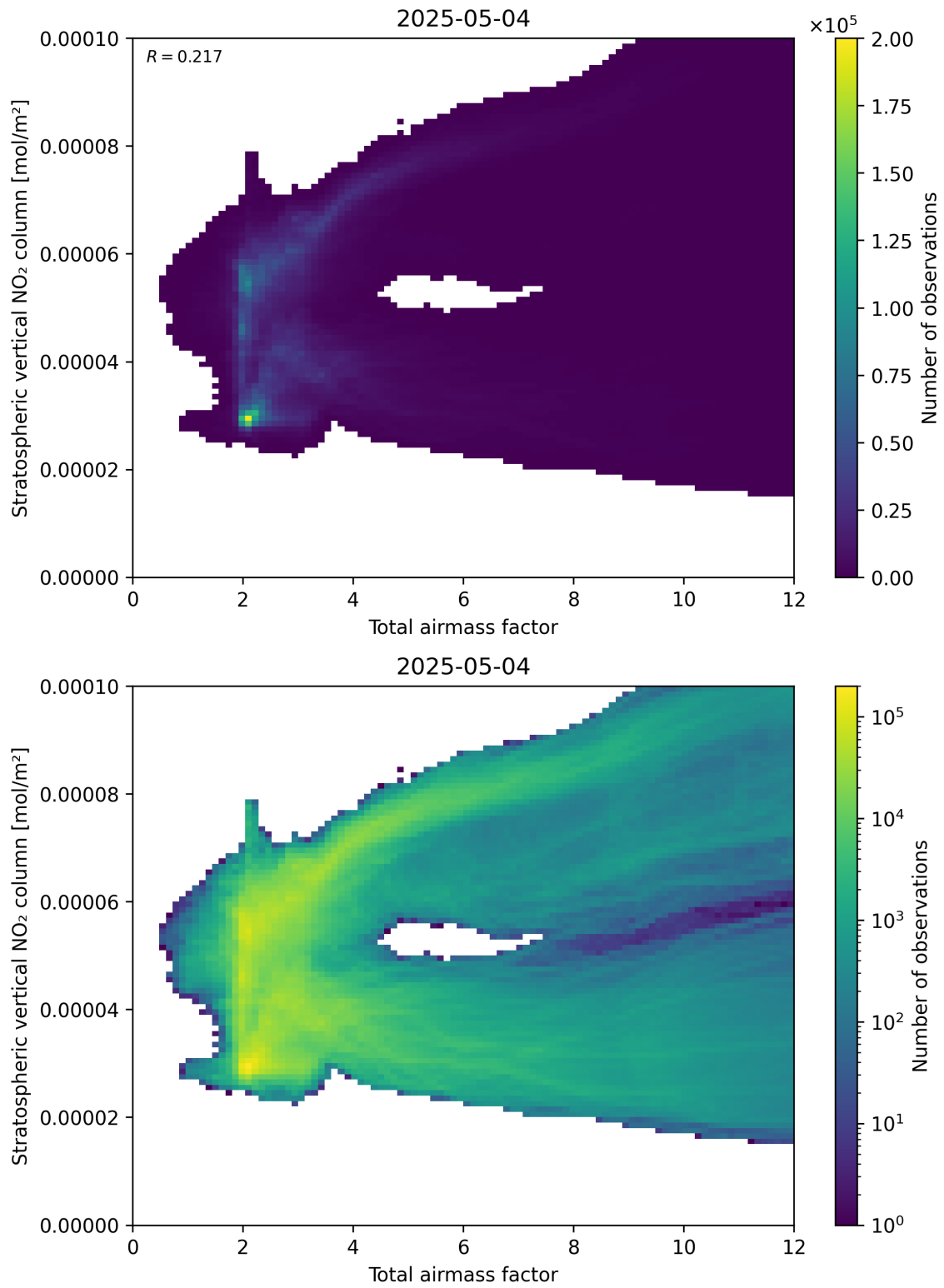
Figure 64: Scatter density plot of “Total airmass factor” against “Stratospheric vertical \text{NO}_2 column” for 2025-05-04 to 2025-05-05.
