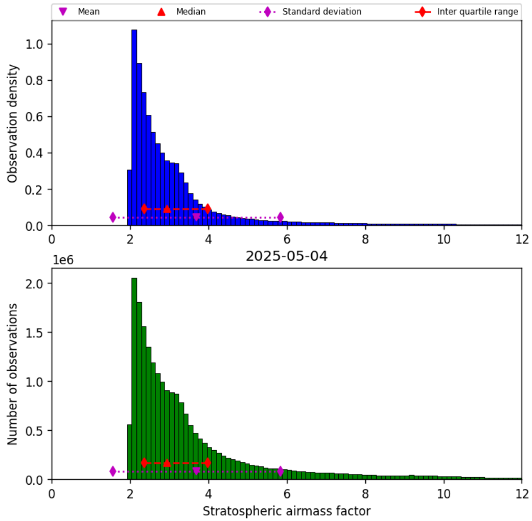
Figure 44: Histogram of “Stratospheric airmass factor” for 2025-05-04 to 2025-05-05
