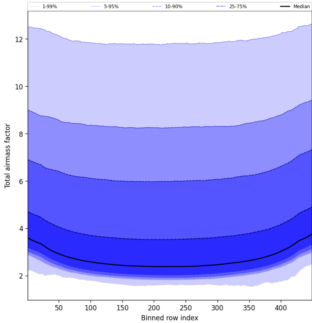
Figure 49: Along track statistics of “Total airmass factor” for 2025-05-04 to 2025-05-05
