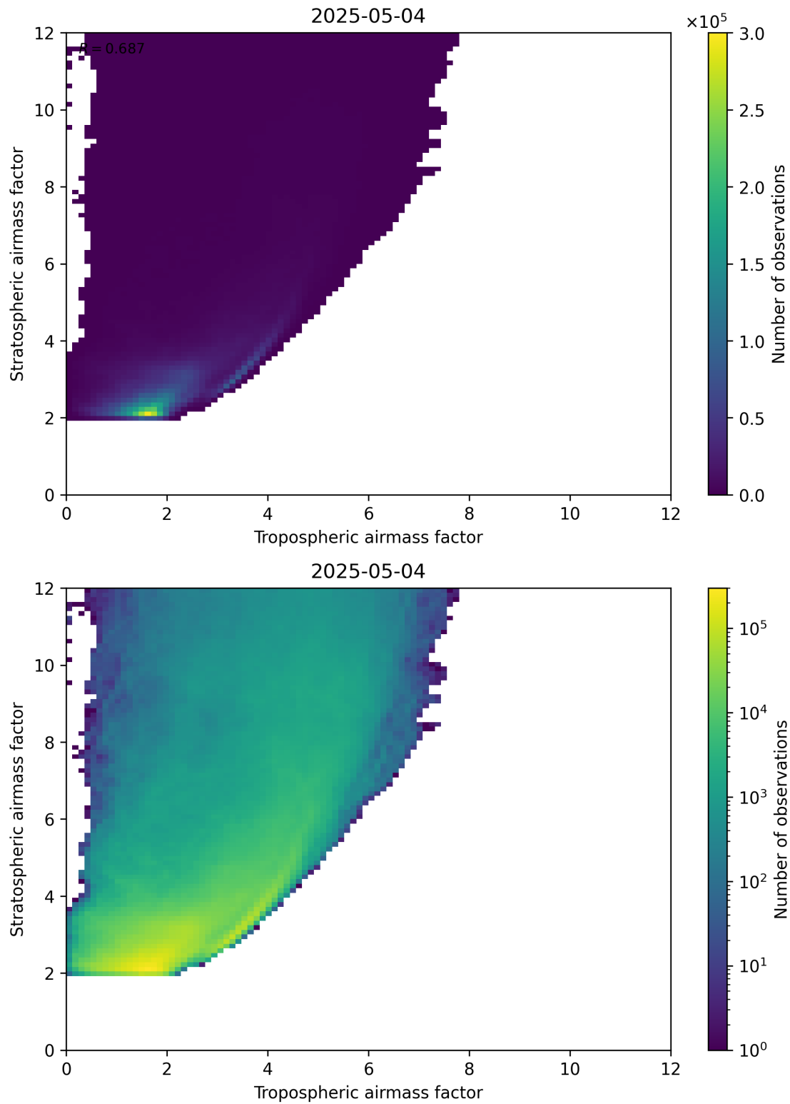
Figure 71: Scatter density plot of “Tropospheric airmass factor” against “Stratospheric airmass factor” for 2025-05-04 to 2025-05-05.
