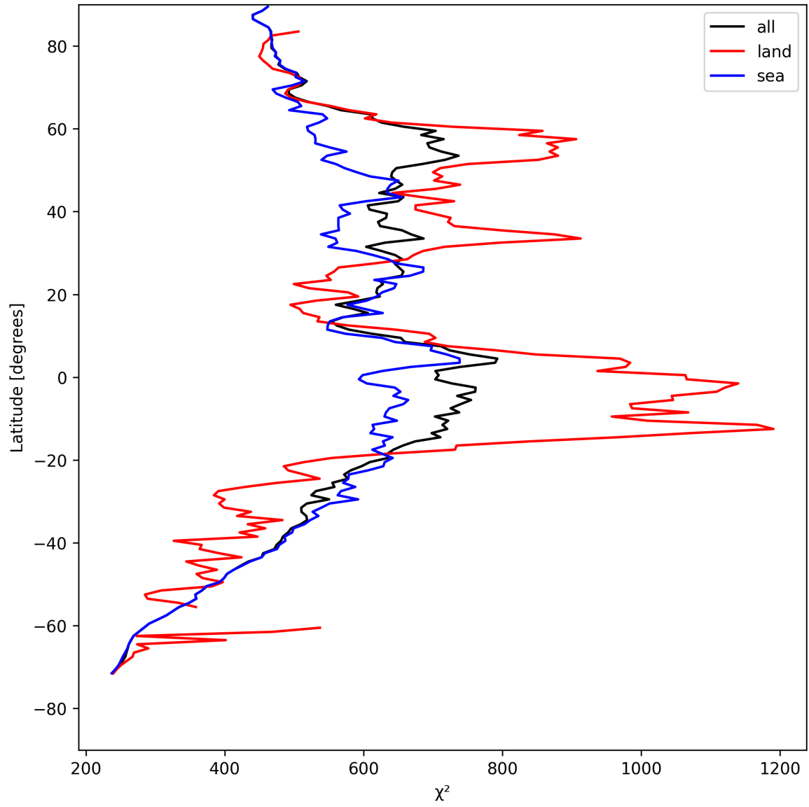
Figure 25: Zonal average of “ \chi^2 ” for 2025-05-04 to 2025-05-05.
