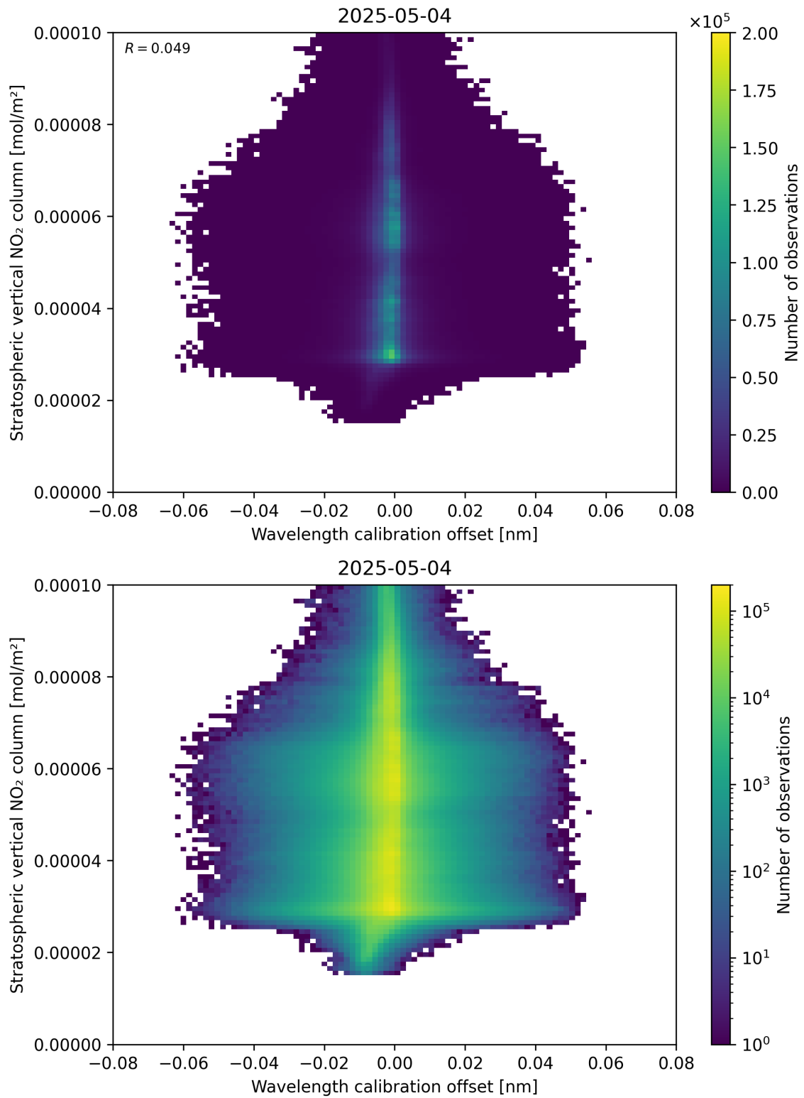
Figure 176: Scatter density plot of “Wavelength calibration offset” against “Stratospheric vertical NO 2 column” for 2025-05-04 to 2025-05-05.
