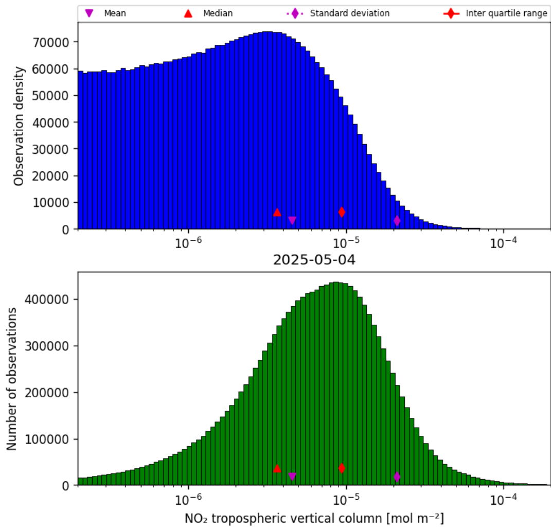
Figure 29: Histogram of “NO 2 tropospheric vertical column” for 2025-05-04 to 2025-05-05
