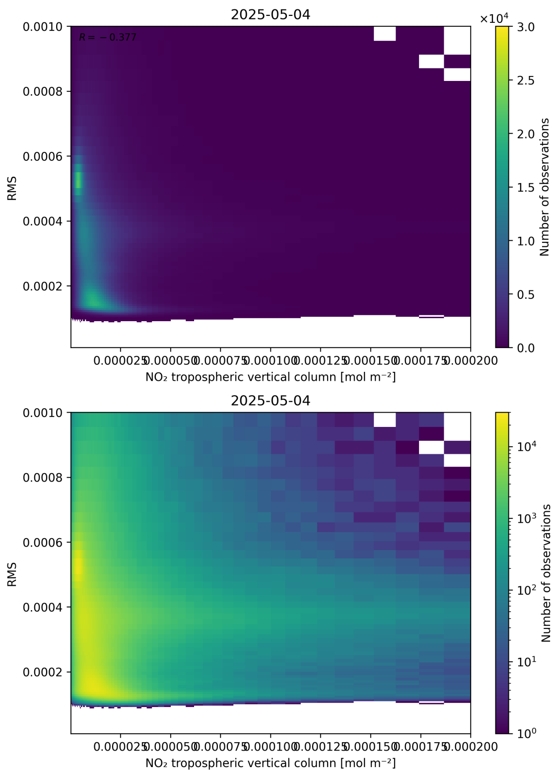
Figure 142: Scatter density plot of “NO 2 tropospheric vertical column” against “RMS” for 2025-05-04 to 2025-05-05.
