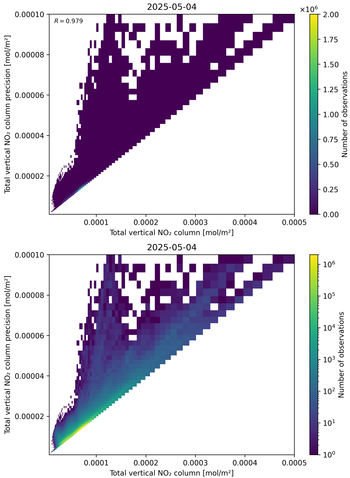
Figure 114: Scatter density plot of “Total vertical NO 2 column” against “Total vertical NO 2 column precision” for 2025-05-04 to 2025-05-05.
