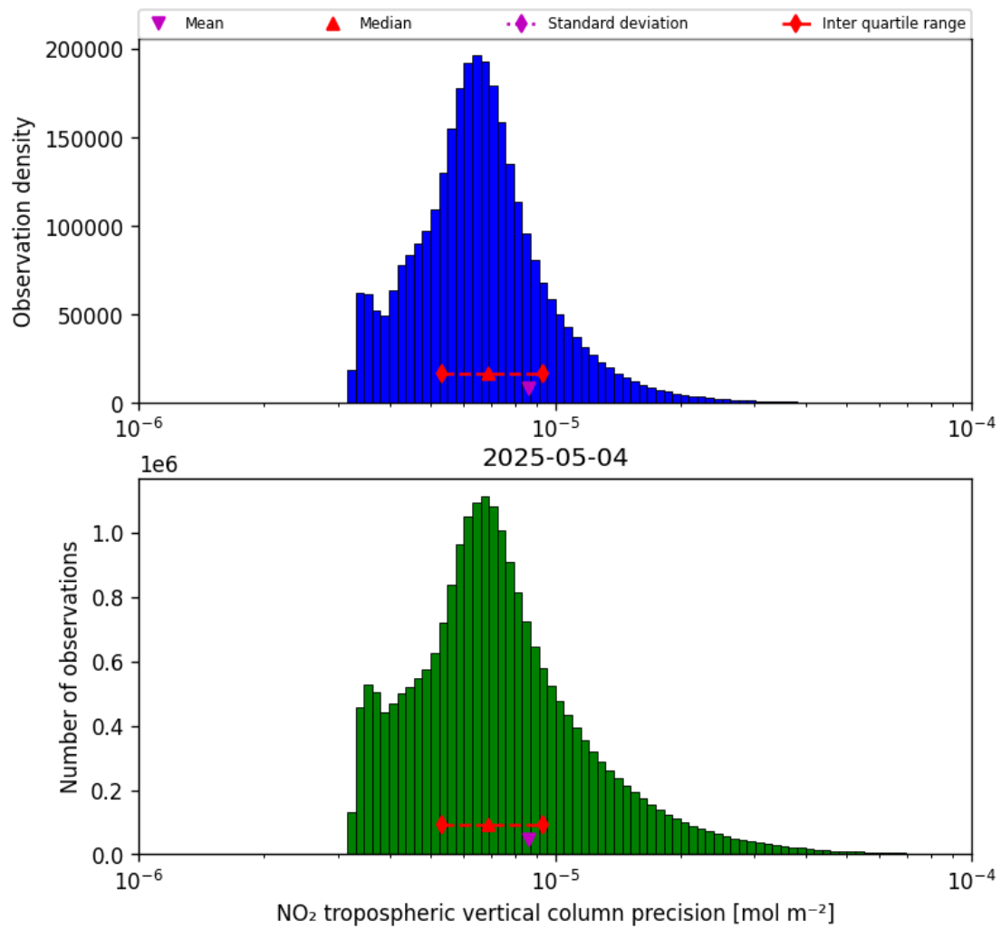
Figure 30: Histogram of “NO 2 tropospheric vertical column precision” for 2025-05-04 to 2025-05-05
