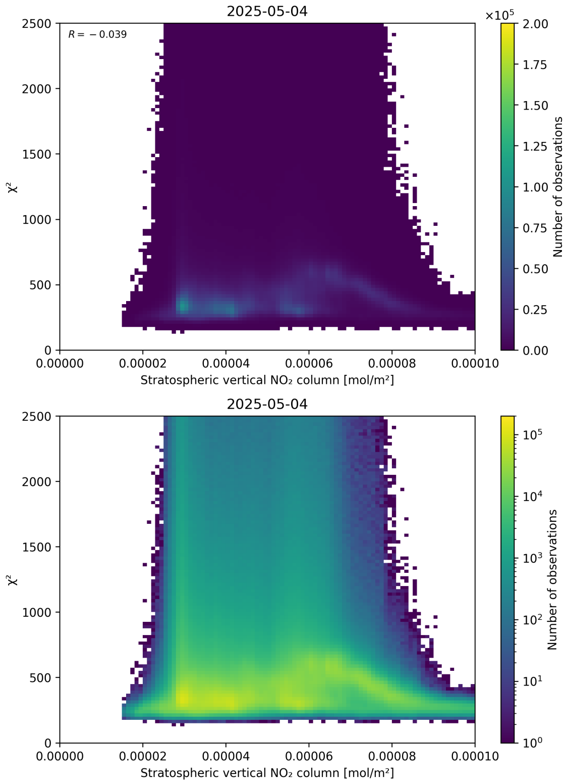
Figure 97: Scatter density plot of “Stratospheric vertical NO 2 column” against “ \chi^2 ” for 2025-05-04 to 2025-05-05.
