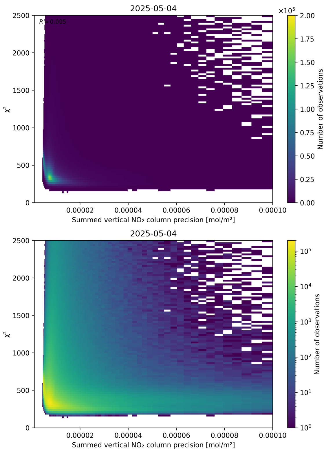
Figure 107: Scatter density plot of “Summed vertical NO 2 column precision” against “ \chi^2 ” for 2025-05-04 to 2025-05-05.
