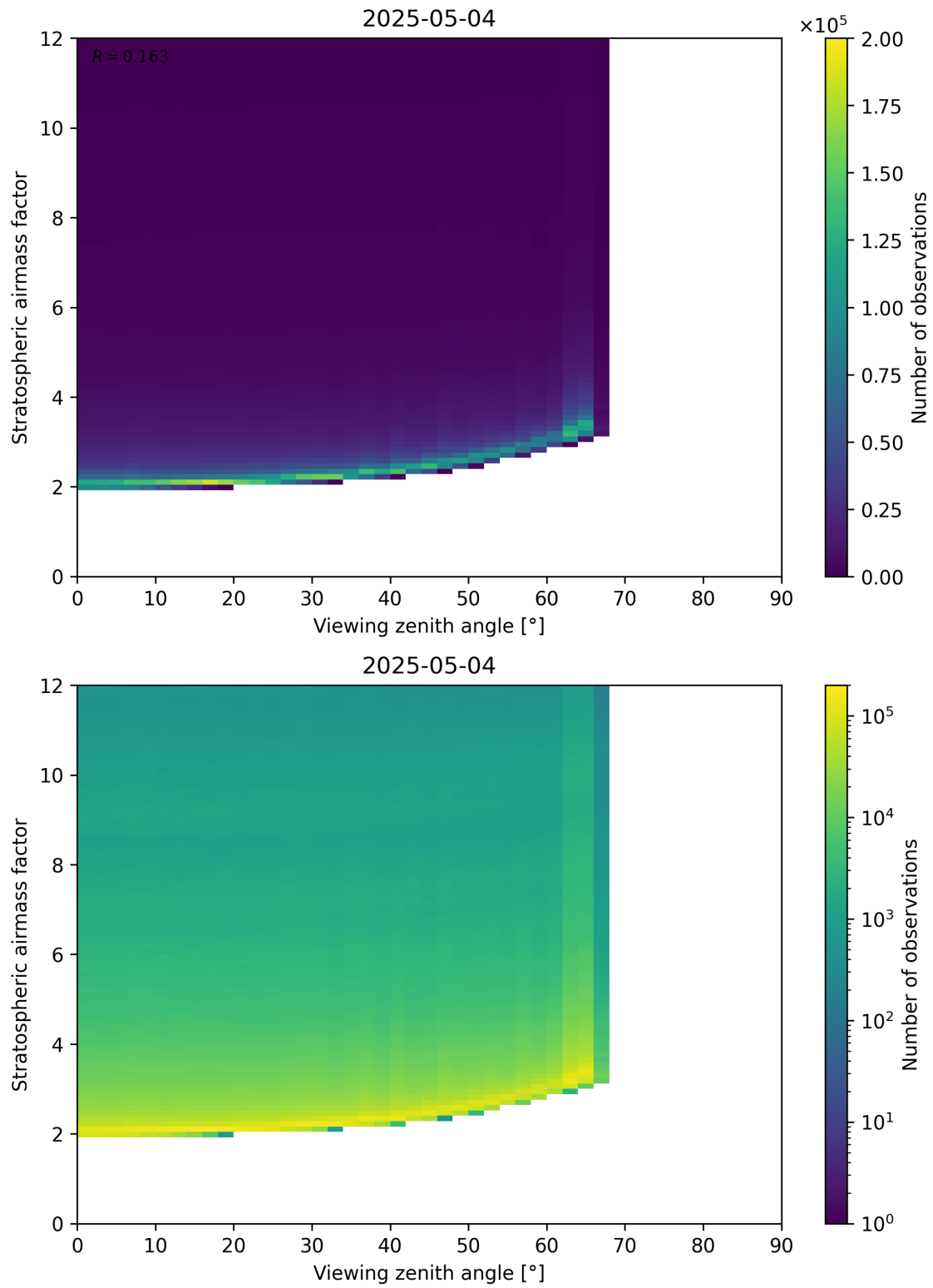
Figure 159: Scatter density plot of “Viewing zenith angle” against “Stratospheric airmass factor” for 2025-05-04 to 2025-05-05.
