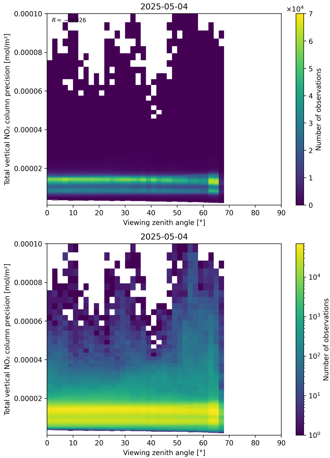
Figure 168: Scatter density plot of “Viewing zenith angle” against “Total vertical NO 2 column precision” for 2025-05-04 to 2025-05-05.
