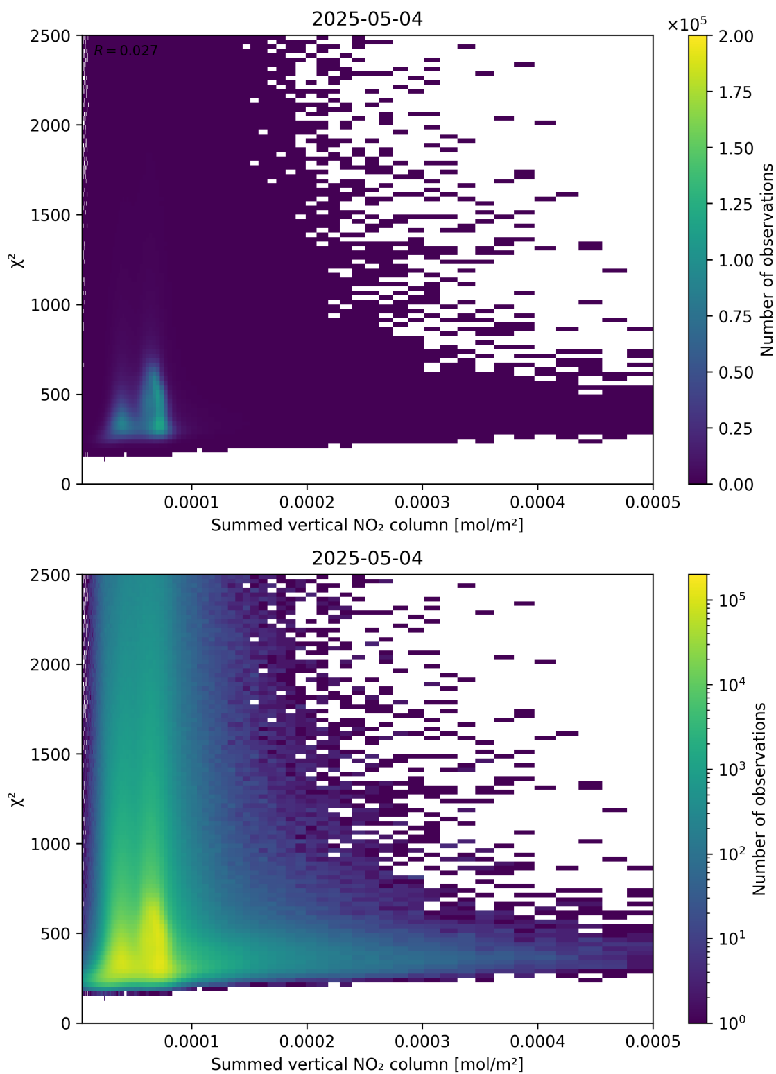
Figure 104: Scatter density plot of “Summed vertical NO 2 column” against “ \chi^2 ” for 2025-05-04 to 2025-05-05.
