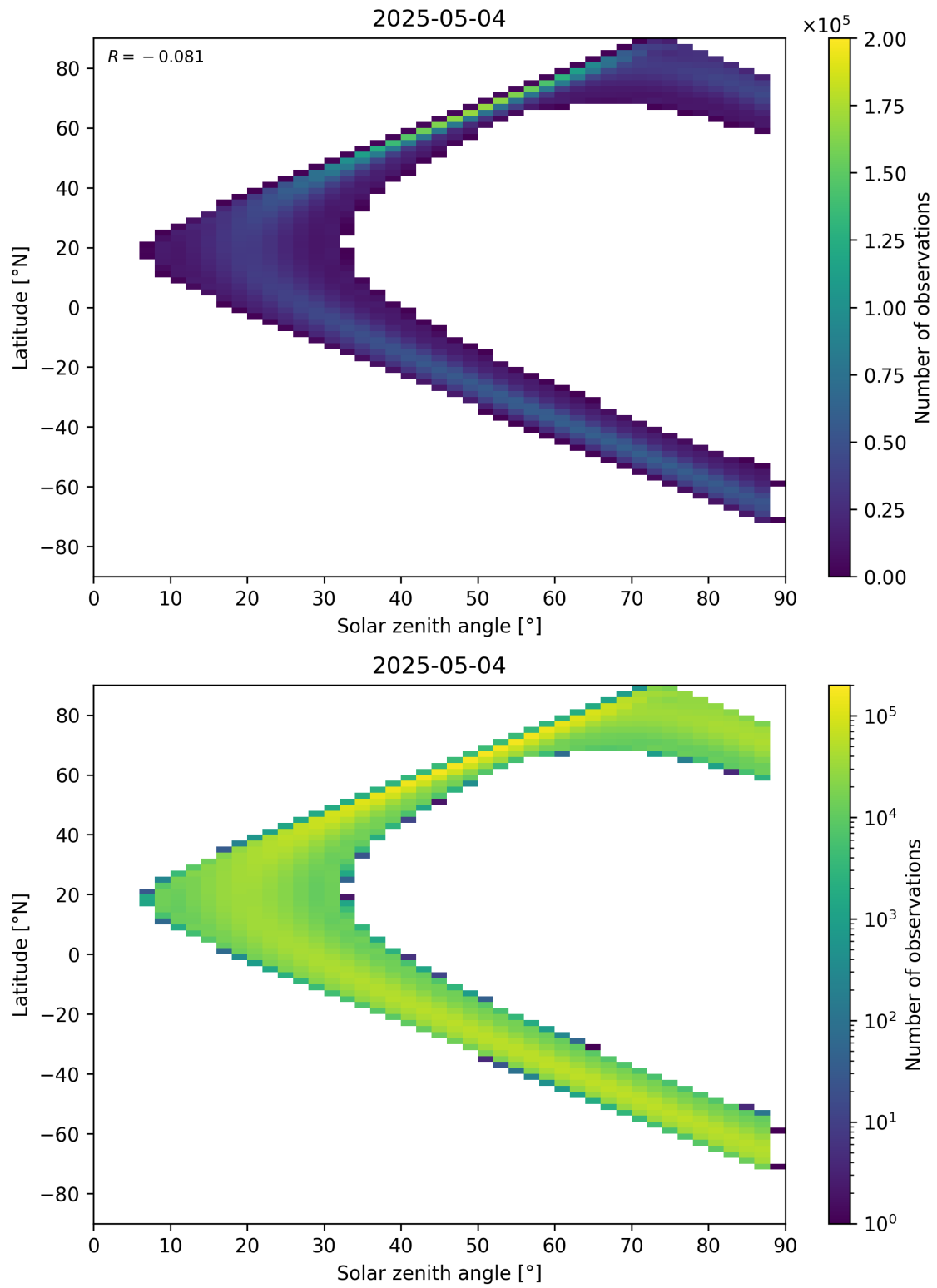
Figure 149: Scatter density plot of “Solar zenith angle” against “Latitude” for 2025-05-04 to 2025-05-05.
