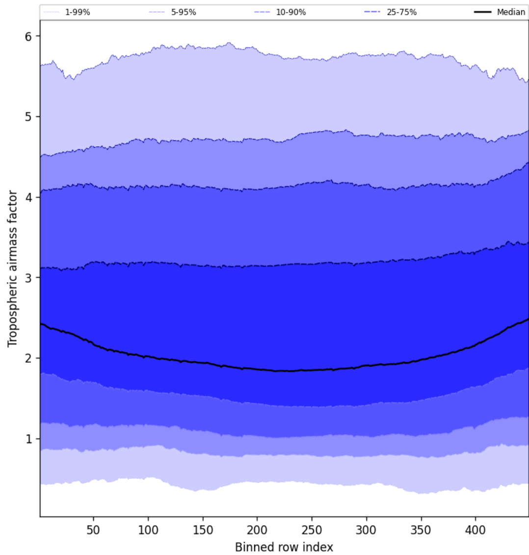
Figure 48: Along track statistics of “Tropospheric airmass factor” for 2025-05-04 to 2025-05-05
