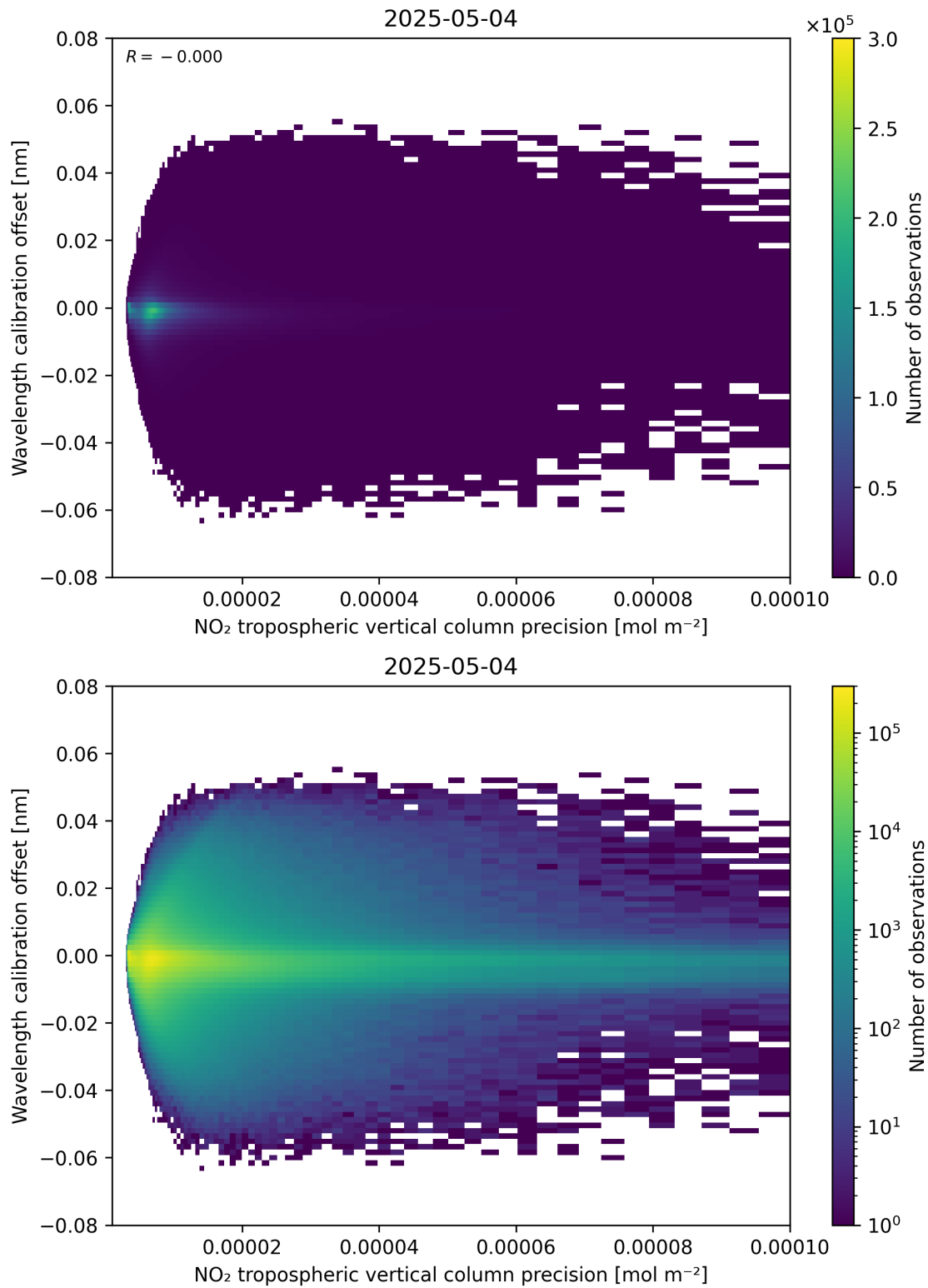
Figure 141: Scatter density plot of “NO 2 tropospheric vertical column precision” against “Wavelength calibration offset” for 2025-05-04 to 2025-05-05.
