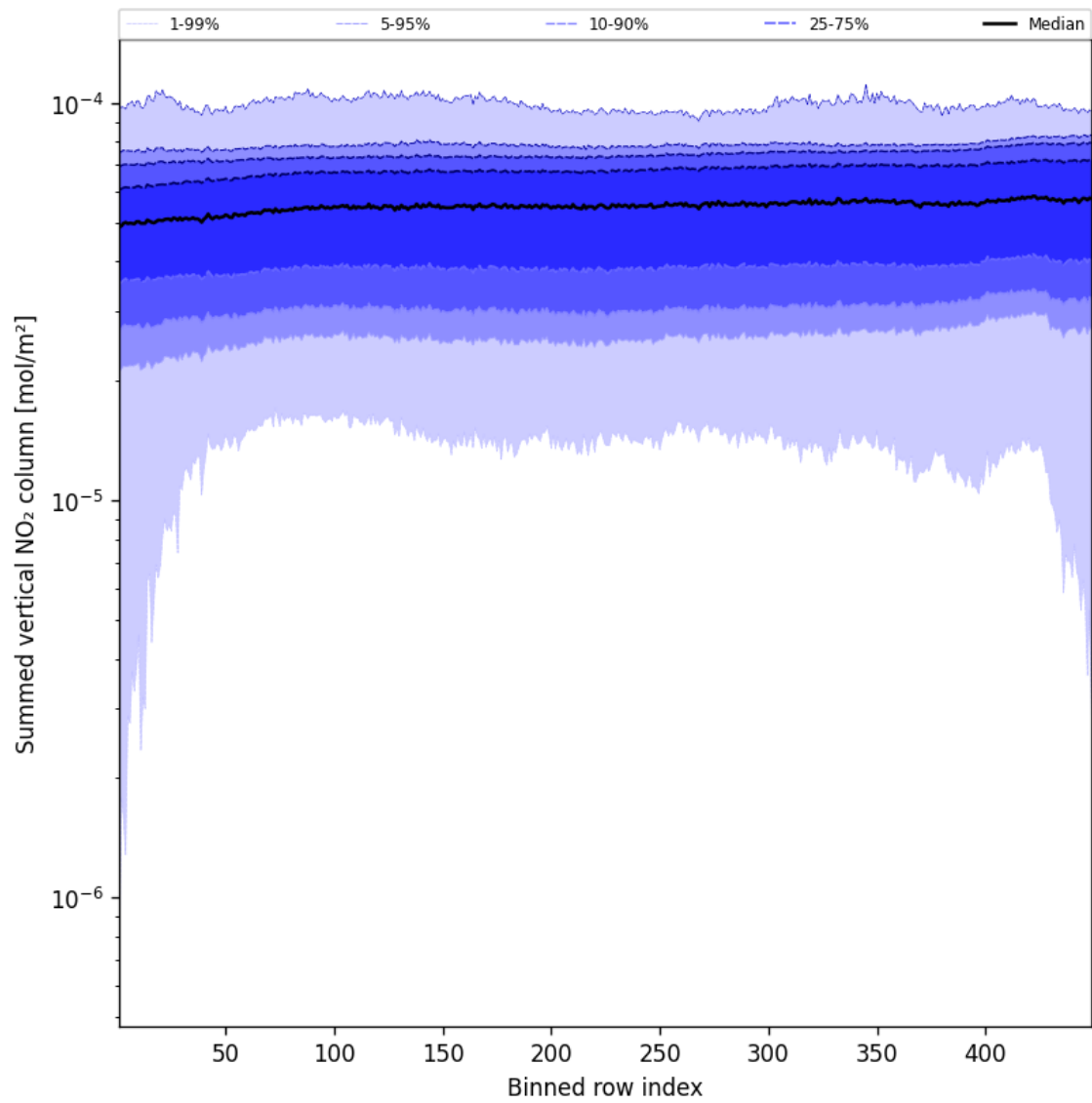
Figure 57: Along track statistics of “Summed vertical NO 2 column” for 2025-05-04 to 2025-05-05
