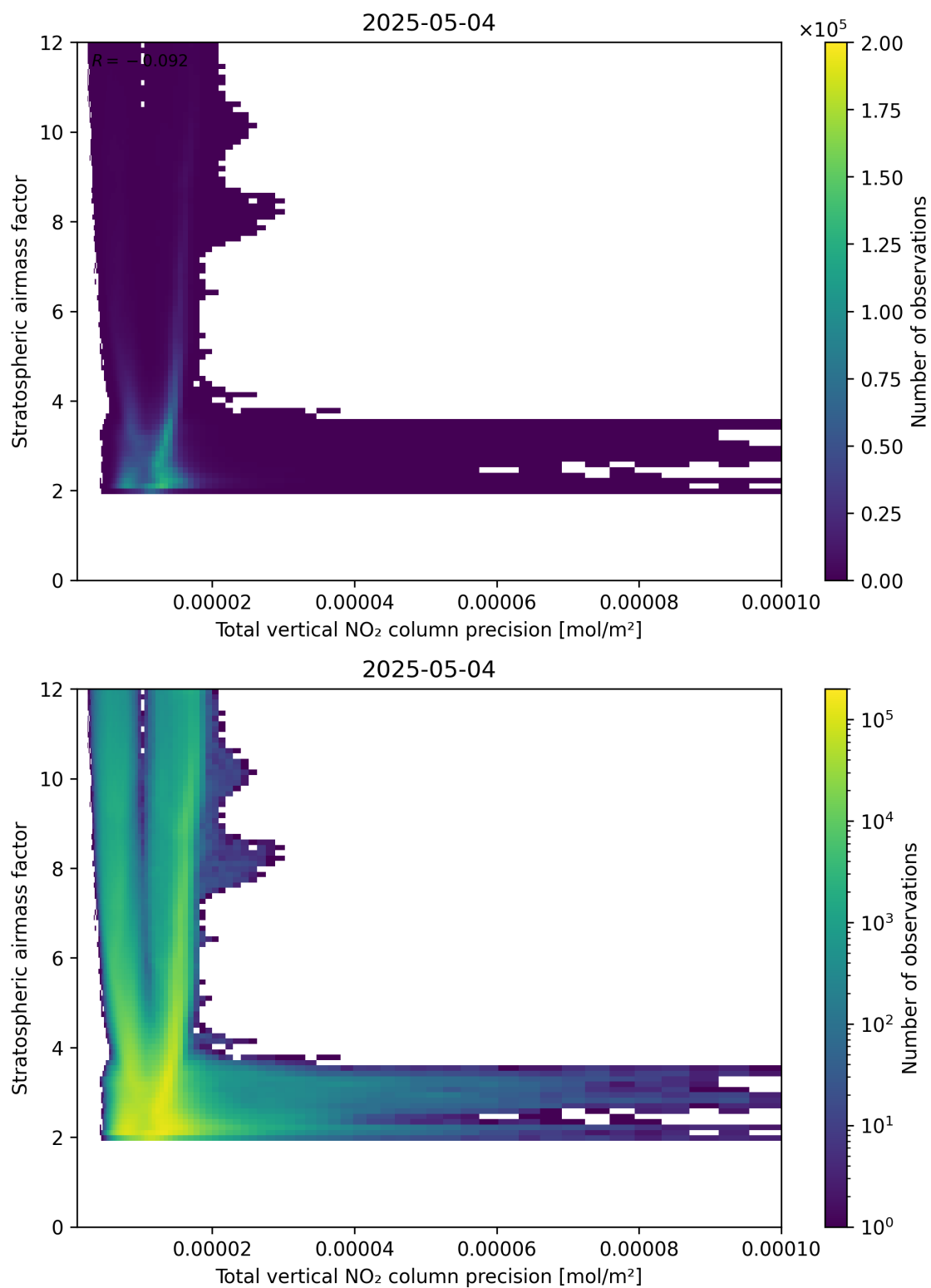
Figure 115: Scatter density plot of “Total vertical NO 2 column precision” against “Stratospheric air mass factor” for 2025-05-04 to 2025-05-05.
