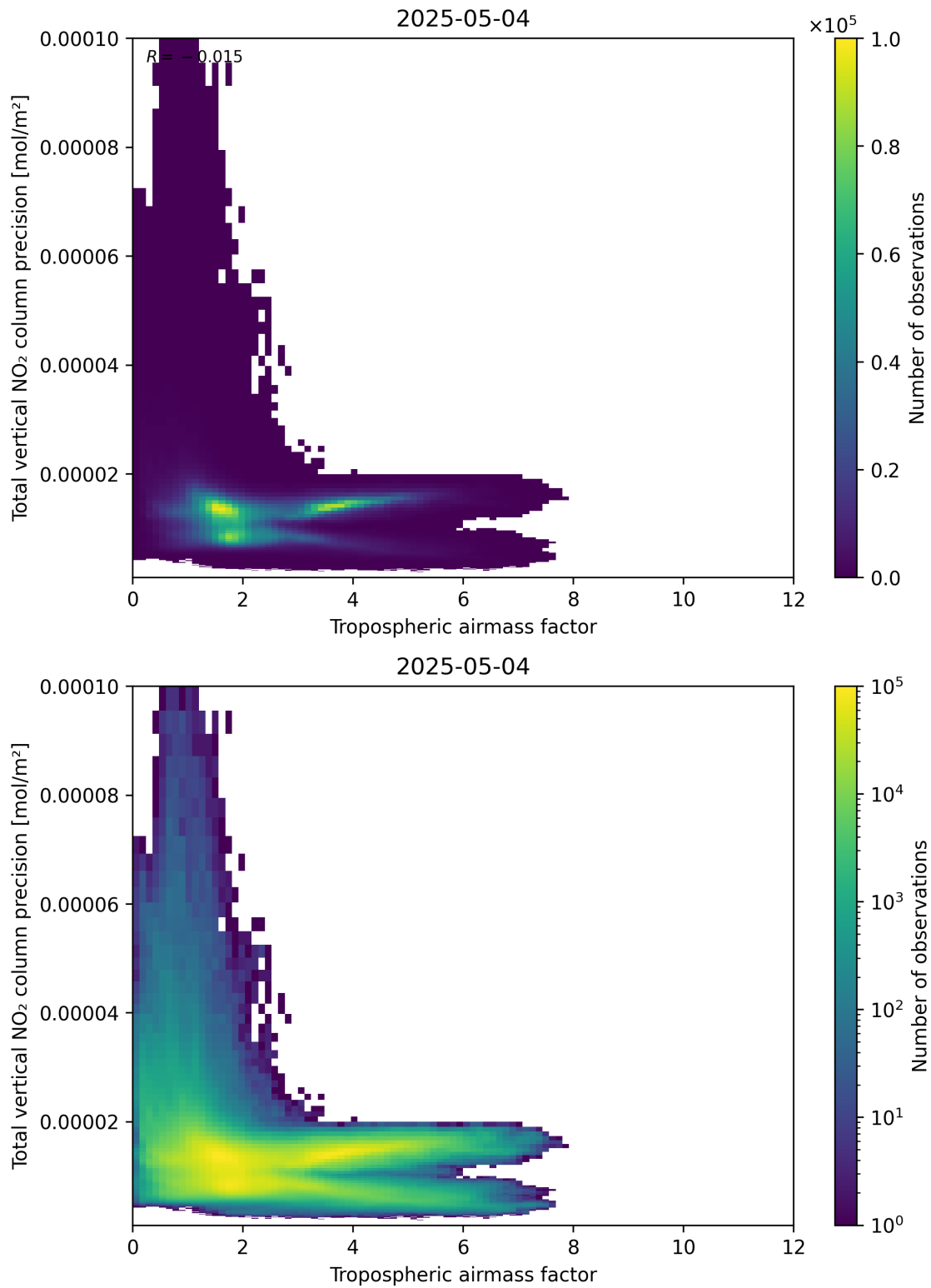
Figure 78: Scatter density plot of “Tropospheric airmass factor” against “Total vertical NO 2 column precision” for 2025-05-04 to 2025-05-05.
