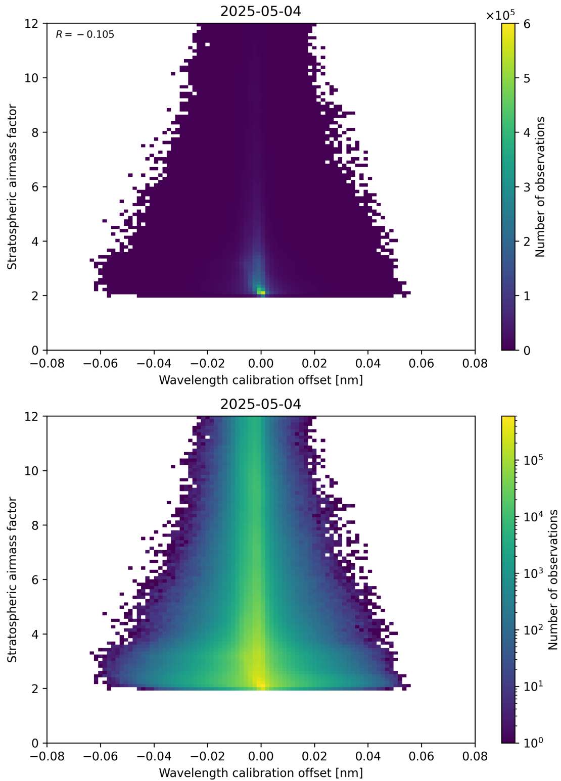
Figure 174: Scatter density plot of “Wavelength calibration offset” against “Stratospheric airmass factor” for 2025-05-04 to 2025-05-05.
