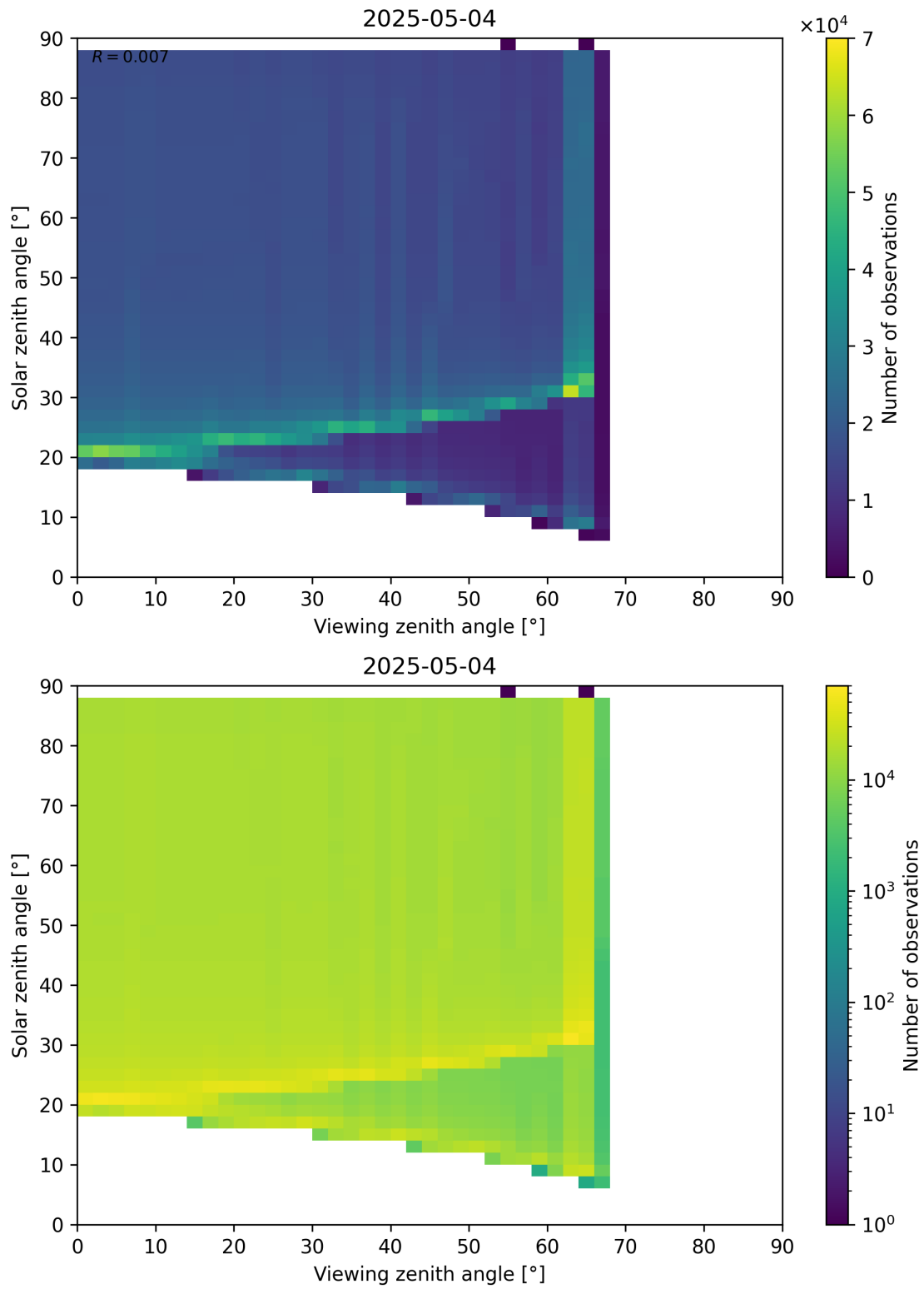
Figure 172: Scatter density plot of “Viewing zenith angle” against “Solar zenith angle” for 2025-05-04 to 2025-05-05.
