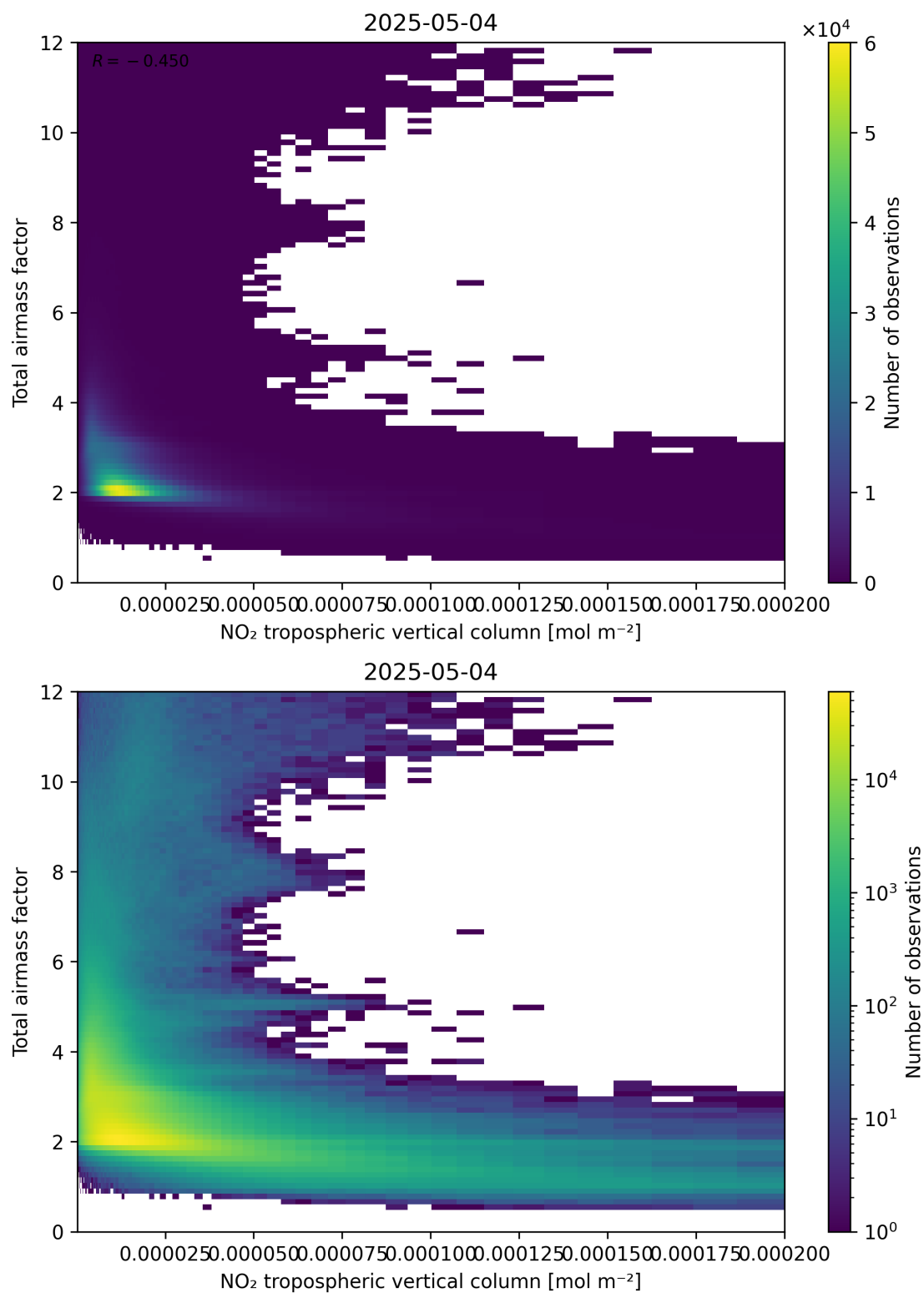
Figure 122: Scatter density plot of “NO 2 tropospheric vertical column” against “Total air mass factor” for 2025-05-04 to 2025-05-05.
