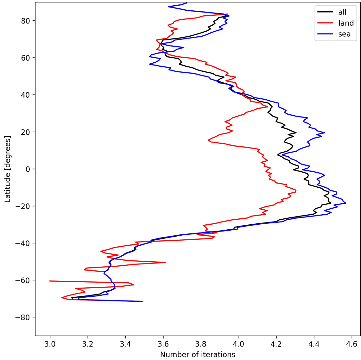
Figure 17: Zonal average of “Number of iterations” for 2025-05-04 to 2025-05-05.
