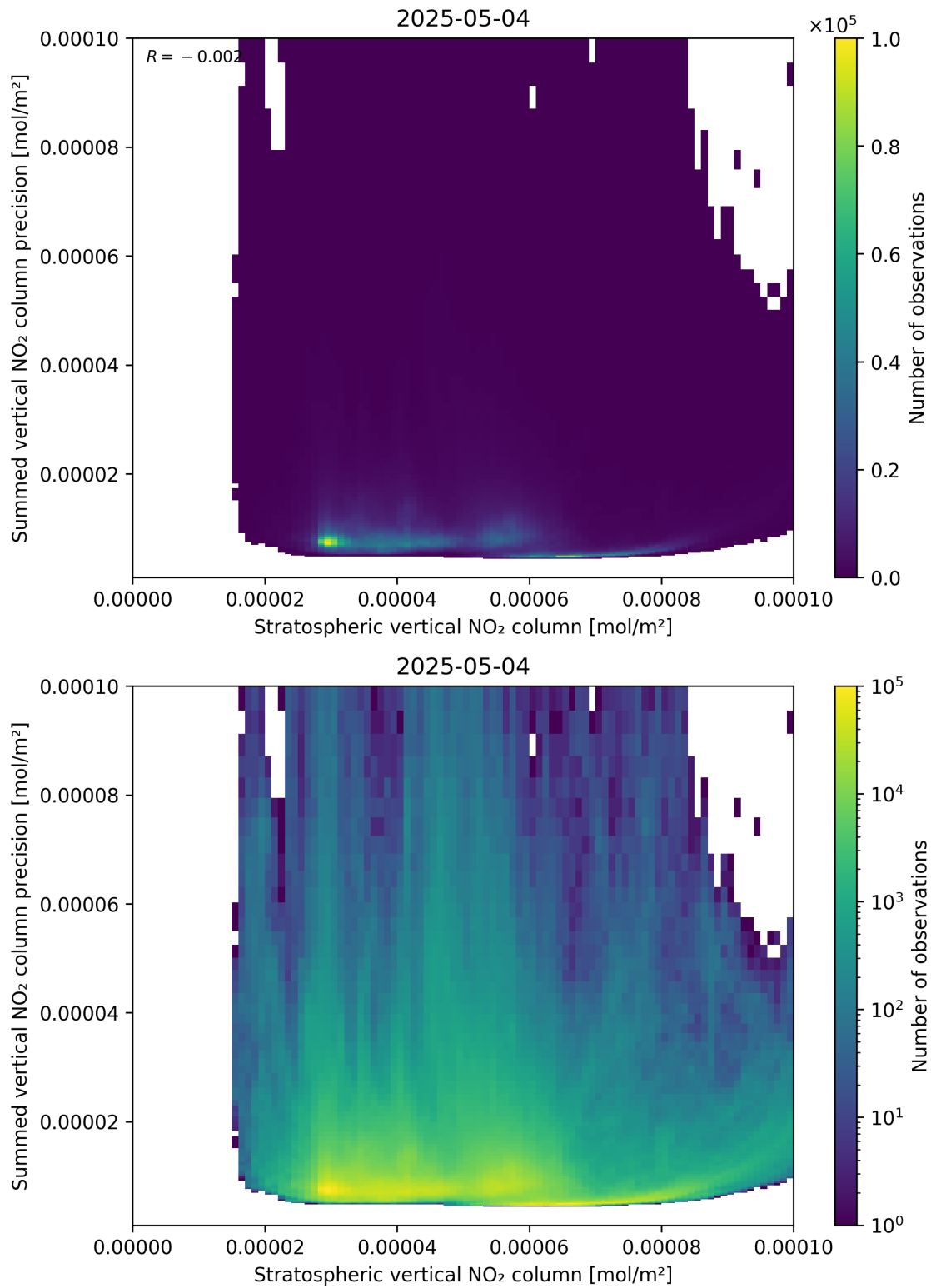
Figure 99: Scatter density plot of “Stratospheric vertical NO 2 column” against “Summed vertical NO 2 column precision” for 2025-05-04 to 2025-05-05.
