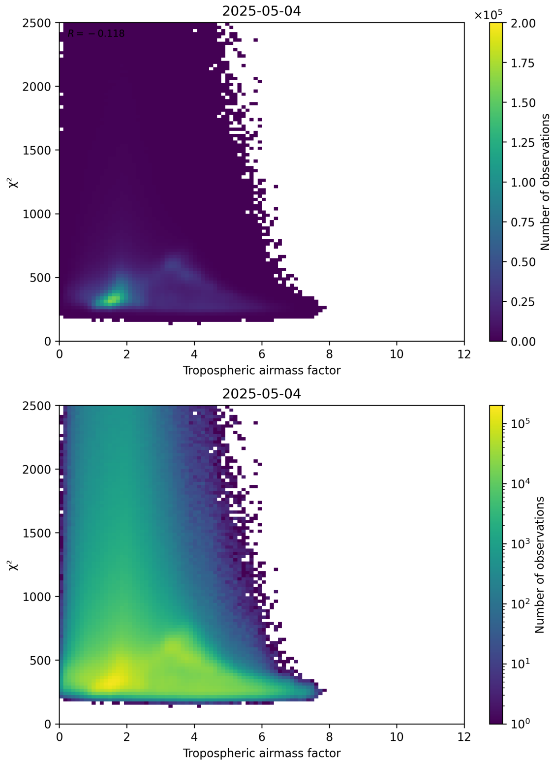
Figure 73: Scatter density plot of “Tropospheric airmass factor” against “ \chi^2 ” for 2025-05-04 to 2025-05-05.
