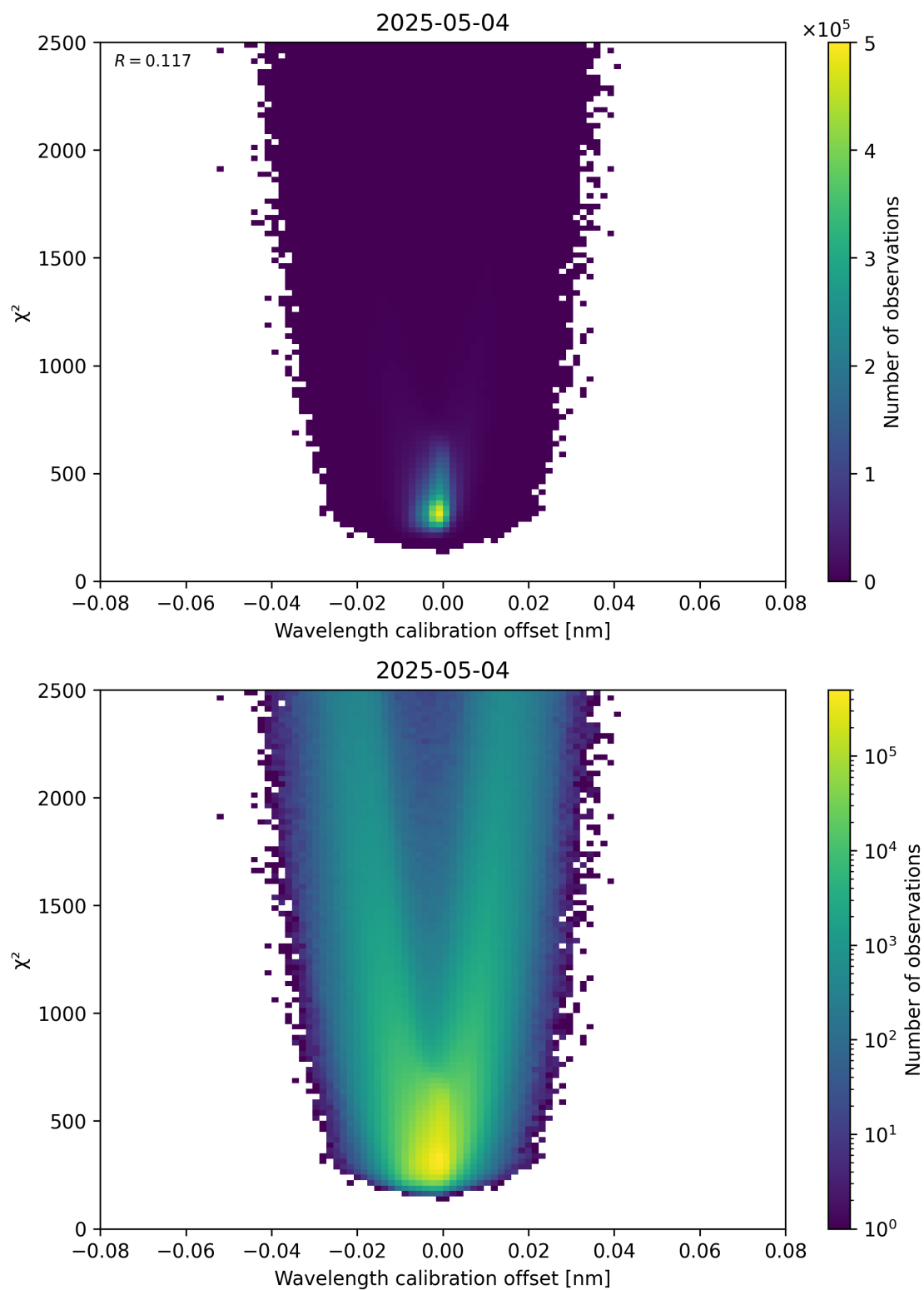
Figure 175: Scatter density plot of “Wavelength calibration offset” against “ \chi^2 ” for 2025-05-04 to 2025-05-05.
