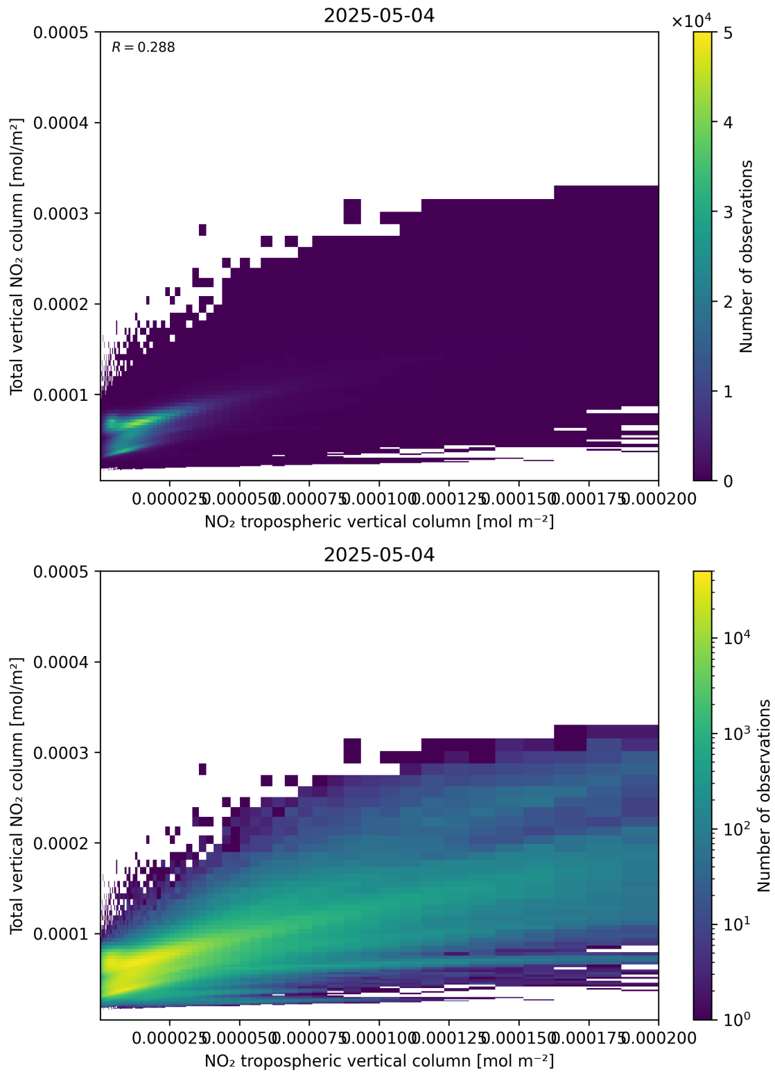
Figure 128: Scatter density plot of “NO 2 tropospheric vertical column” against “Total vertical NO 2 column” for 2025-05-04 to 2025-05-05.
