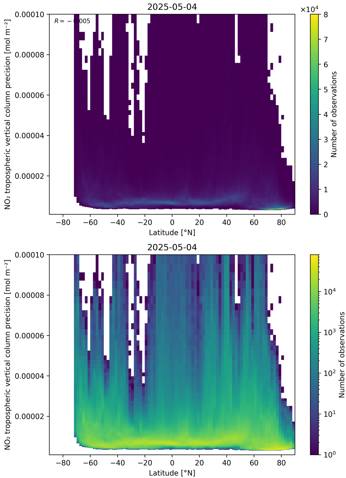
Figure 93: Scatter density plot of “Latitude” against “NO 2 tropospheric vertical column precision” for 2025-05-04 to 2025-05-05.
