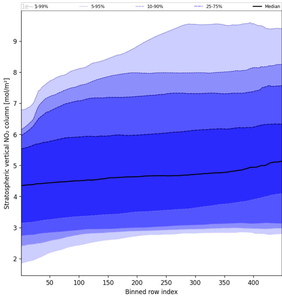
Figure 53: Along track statistics of “Stratospheric vertical NO 2 column” for 2025-05-04 to 2025-05-05
