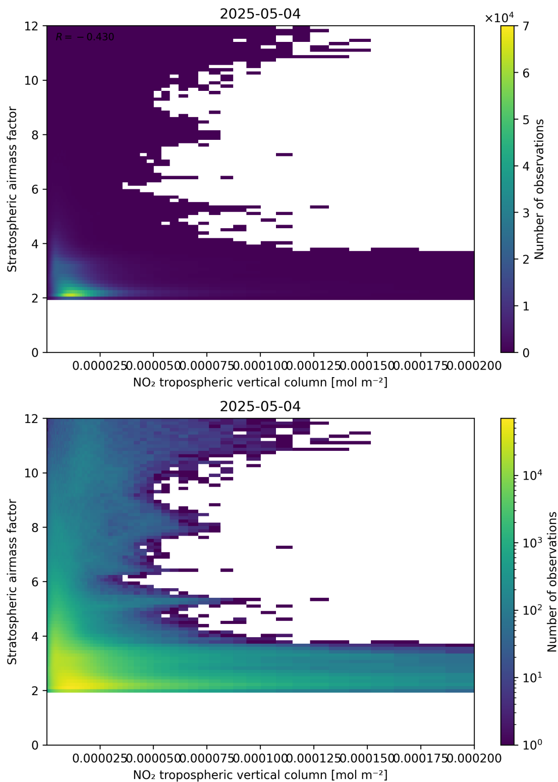
Figure 121: Scatter density plot of “NO 2 tropospheric vertical column” against “Stratospheric air mass factor” for 2025-05-04 to 2025-05-05.
