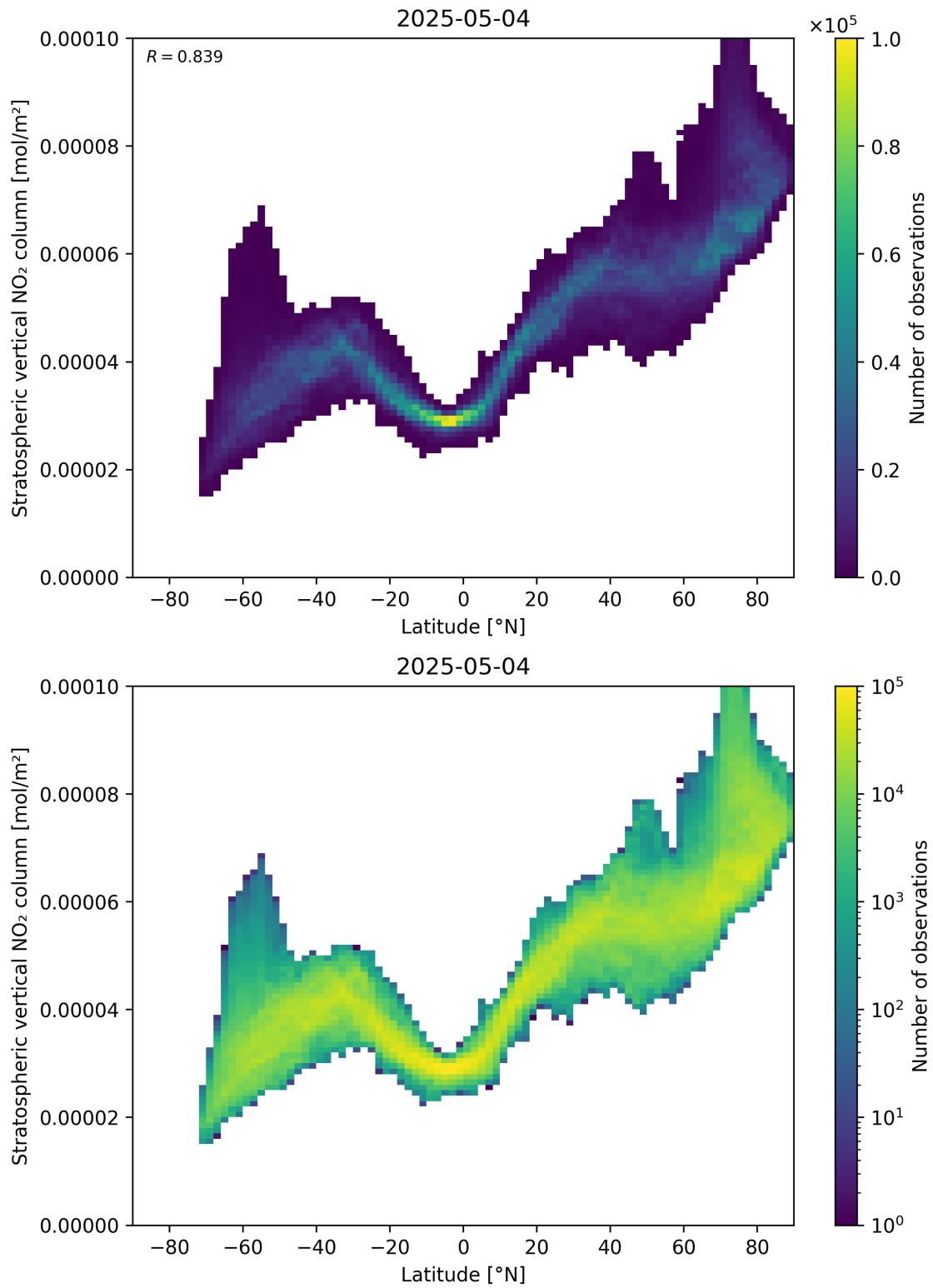
Figure 87: Scatter density plot of “Latitude” against “Stratospheric vertical \text{NO}_2 column” for 2025-05-04 to 2025-05-05.
