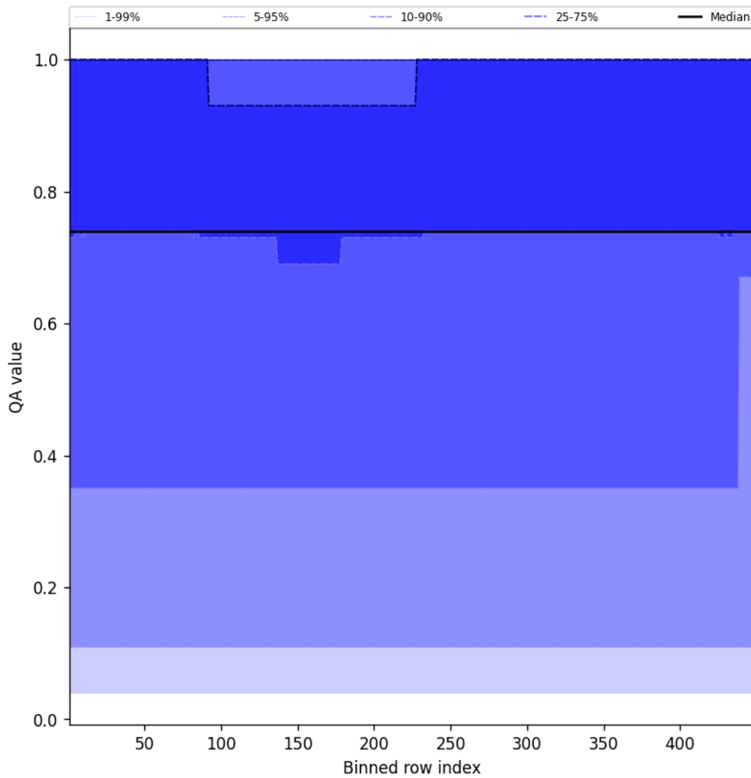
Figure 45: Along track statistics of “QA value” for 2025-05-04 to 2025-05-05
