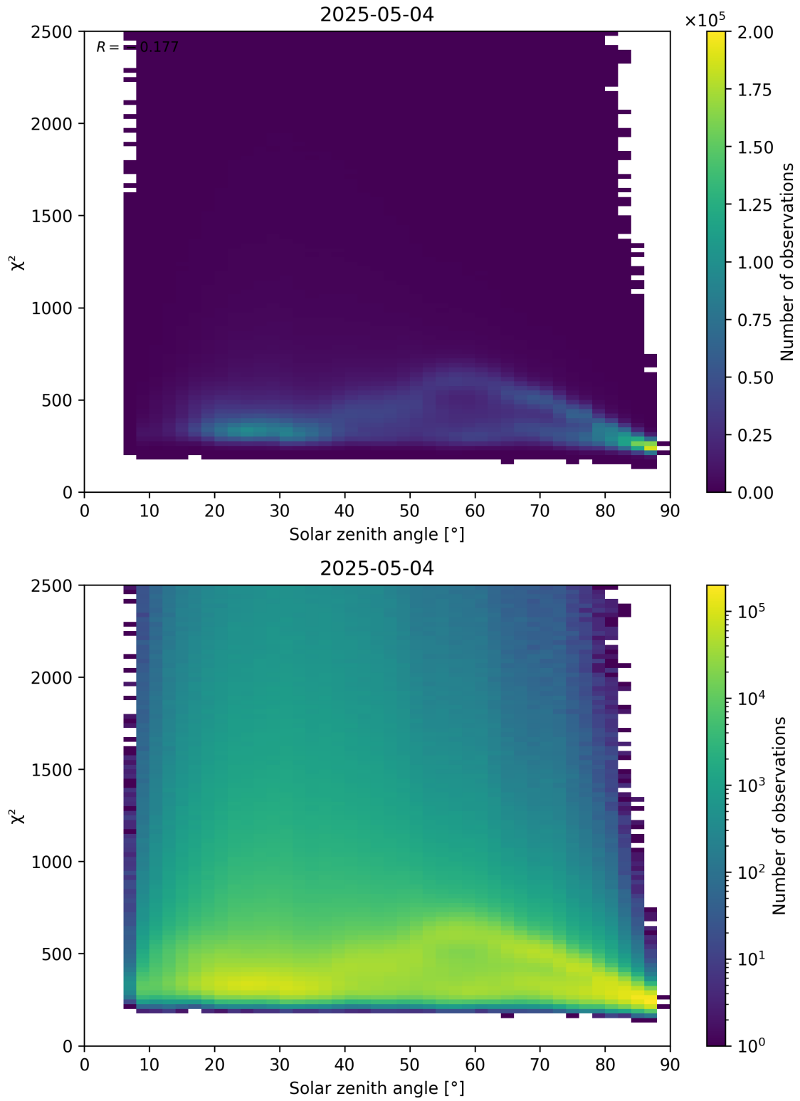
Figure 148: Scatter density plot of “Solar zenith angle” against “ \chi^2 ” for 2025-05-04 to 2025-05-05.
