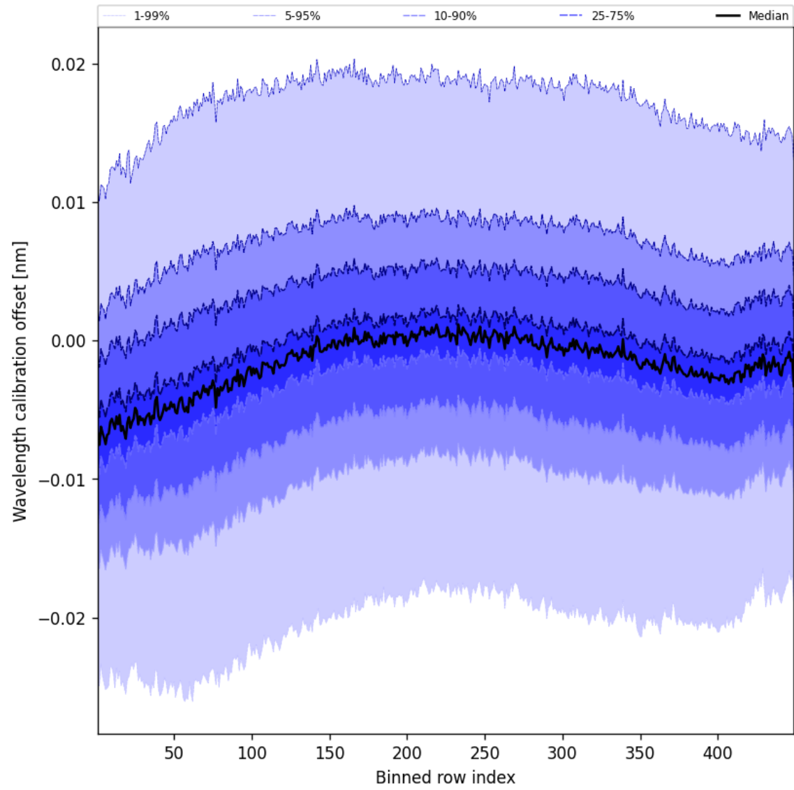
Figure 52: Along track statistics of “Wavelength calibration offset” for 2025-05-04 to 2025-05-05
