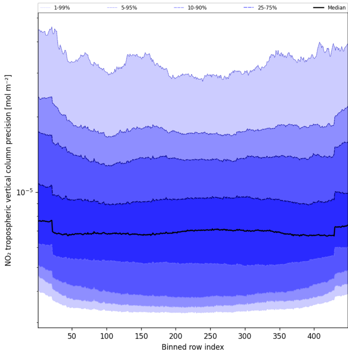
Figure 47: Along track statistics of “NO 2 tropospheric vertical column precision” for 2025-05-04 to 2025-05-05
