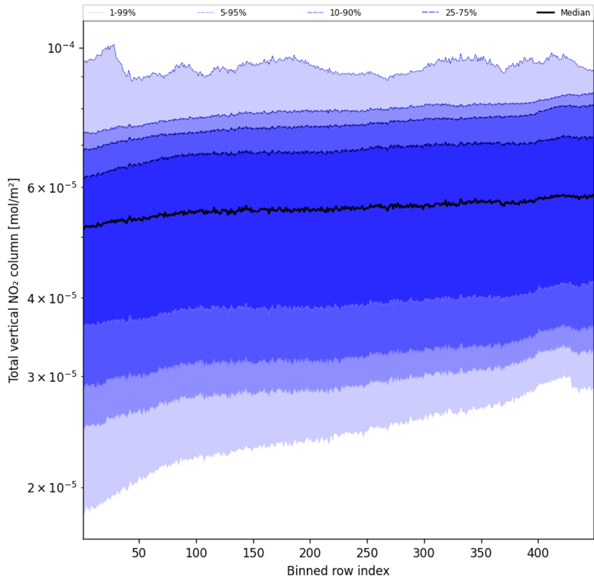
Figure 55: Along track statistics of “Total vertical NO 2 column” for 2025-05-04 to 2025-05-05
