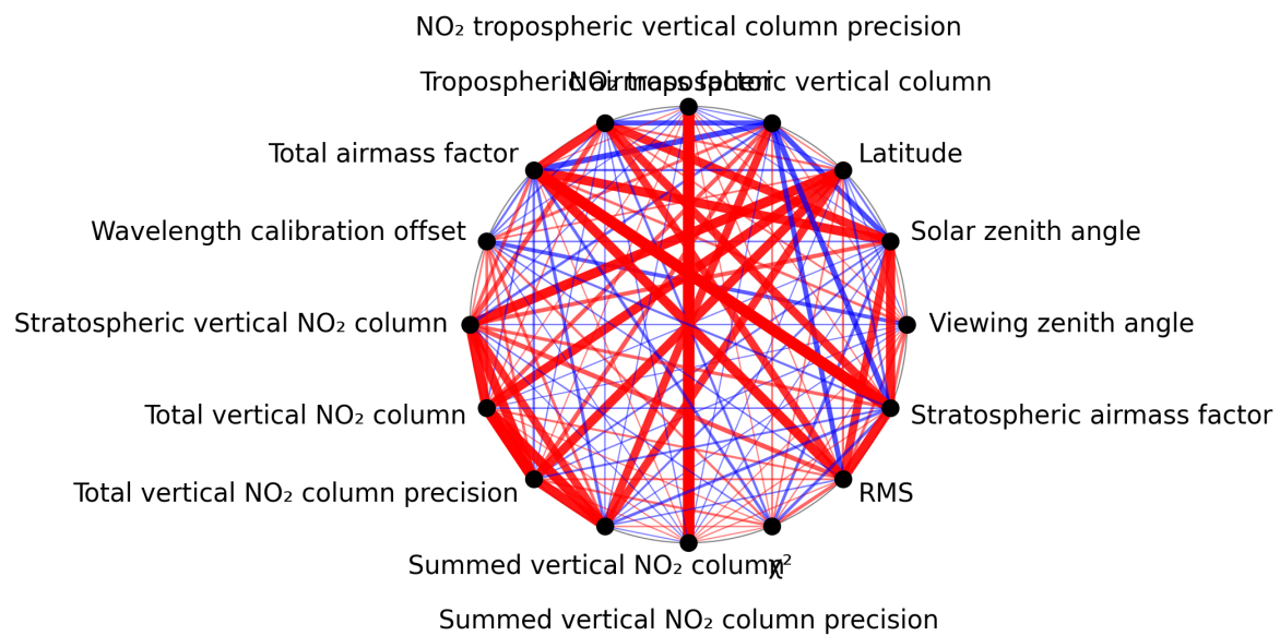
Figure 1: Map of correlation graph for 2025-05-04 to 2025-05-05.
