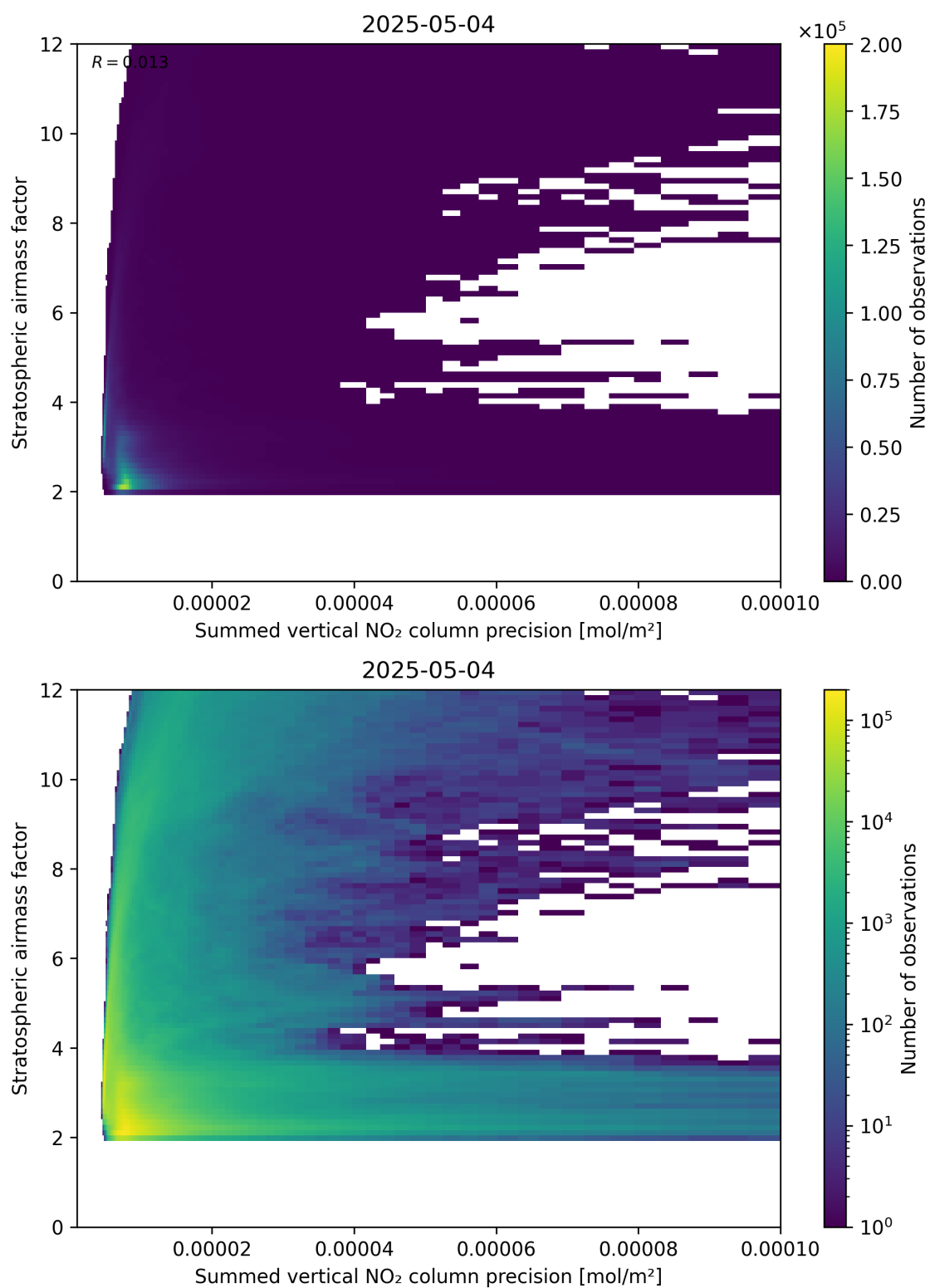
Figure 106: Scatter density plot of “Summed vertical NO 2 column precision” against “Stratospheric airmass factor” for 2025-05-04 to 2025-05-05.
