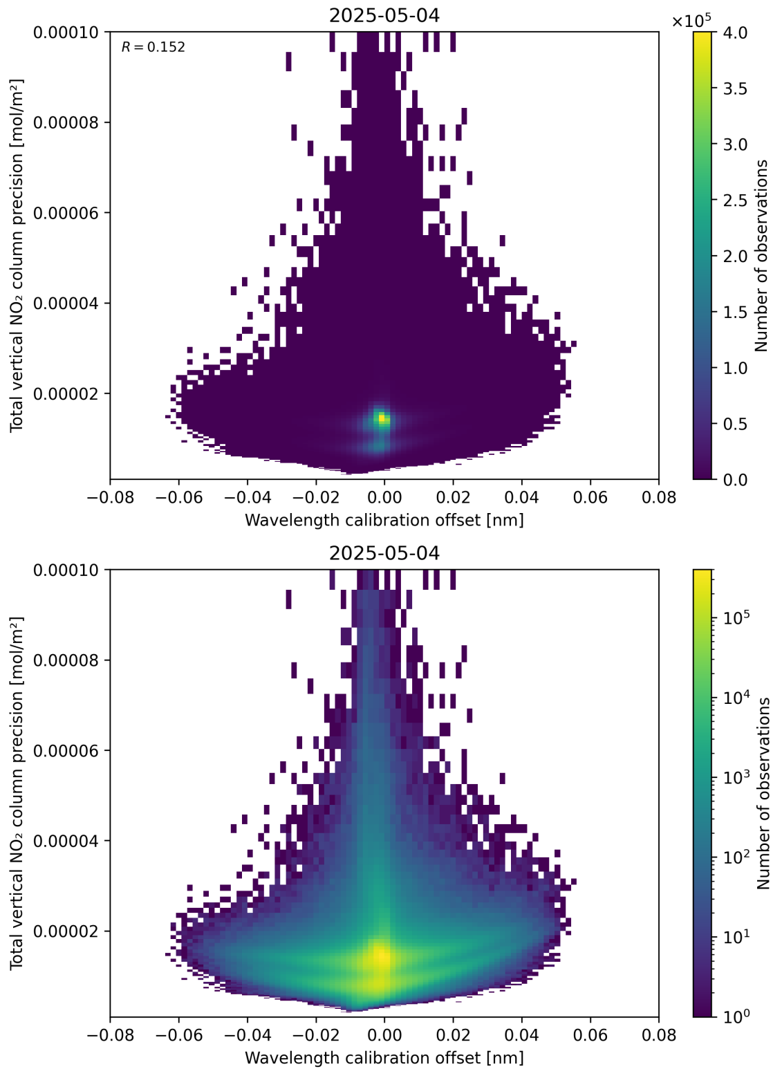
Figure 180: Scatter density plot of “Wavelength calibration offset” against “Total vertical NO 2 column precision” for 2025-05-04 to 2025-05-05.
