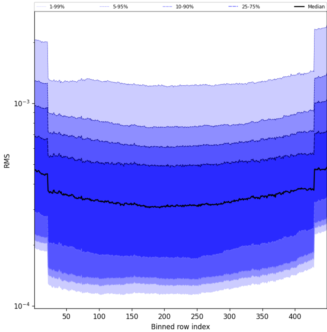
Figure 60: Along track statistics of “RMS” for 2025-05-04 to 2025-05-05
