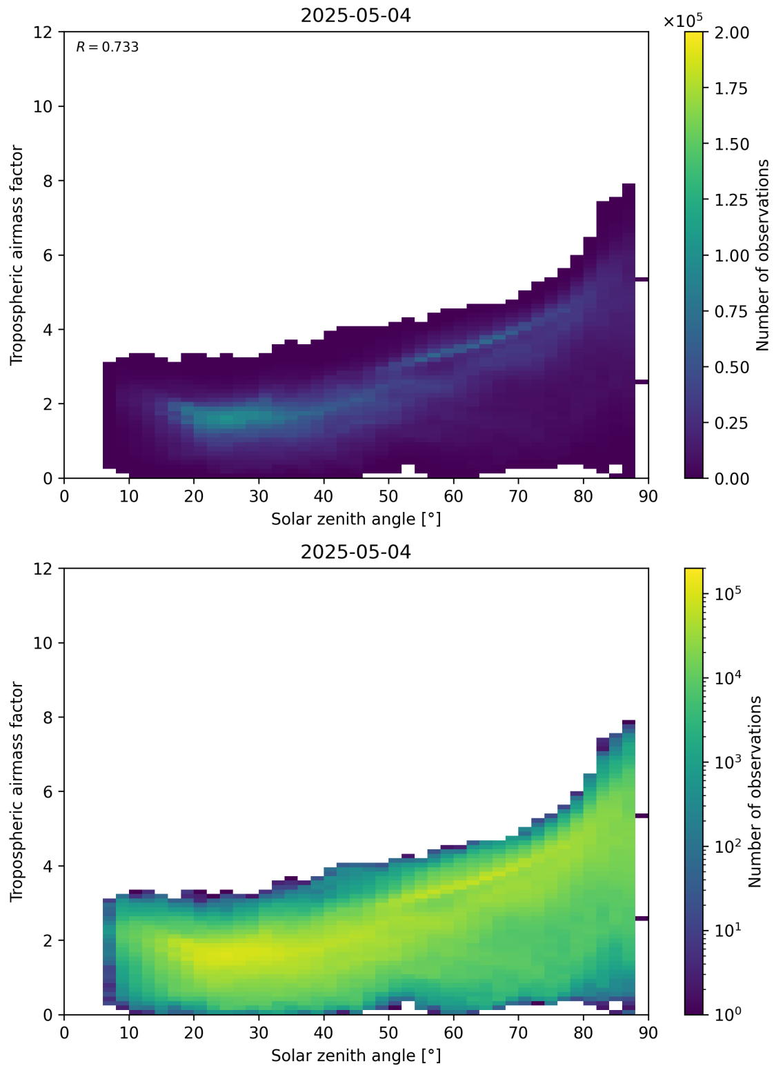
Figure 147: Scatter density plot of “Solar zenith angle” against “Tropospheric airmass factor” for 2025-05-04 to 2025-05-05.
