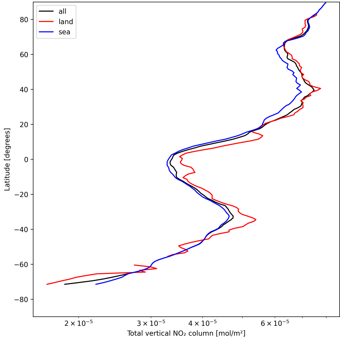
Figure 21: Zonal average of “Total vertical NO 2 column” for 2025-05-04 to 2025-05-05.
