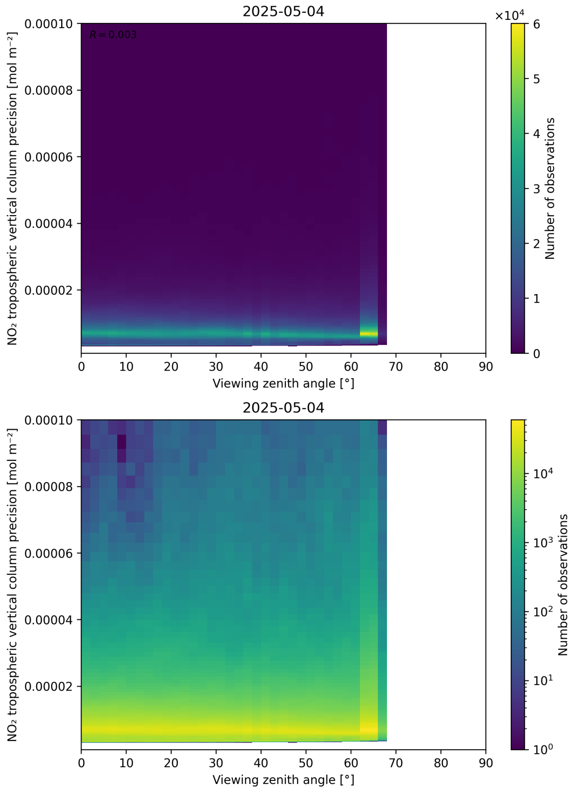
Figure 170: Scatter density plot of “Viewing zenith angle” against “NO 2 tropospheric vertical column precision” for 2025-05-04 to 2025-05-05.
