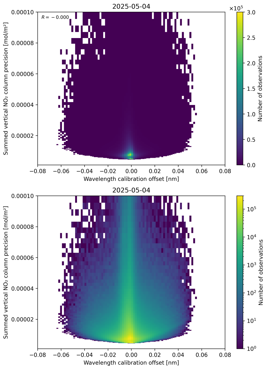
Figure 178: Scatter density plot of “Wavelength calibration offset” against “Summed vertical NO 2 column precision” for 2025-05-04 to 2025-05-05.
