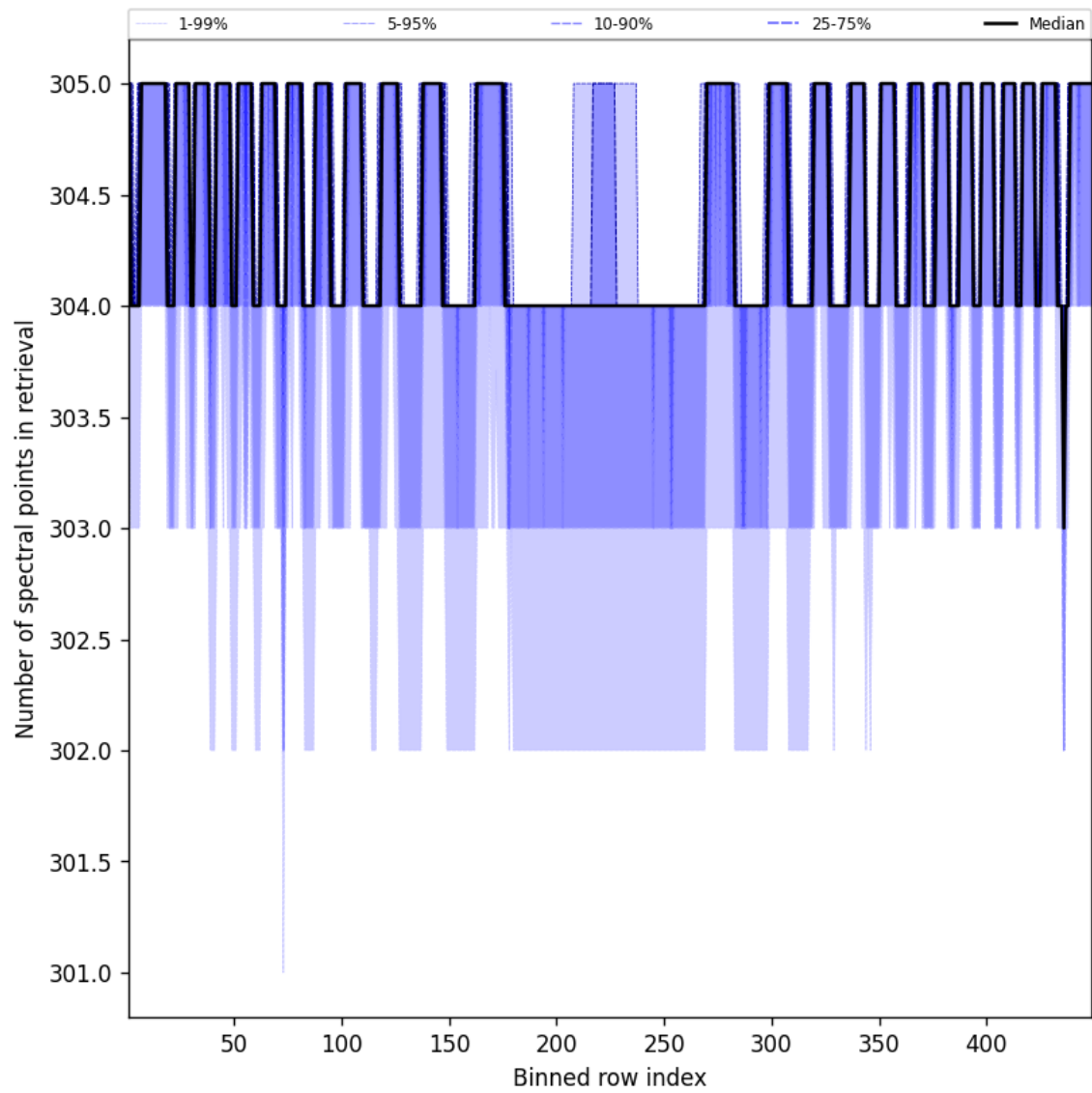
Figure 50: Along track statistics of “Number of spectral points in retrieval” for 2025-05-04 to 2025-05-05
