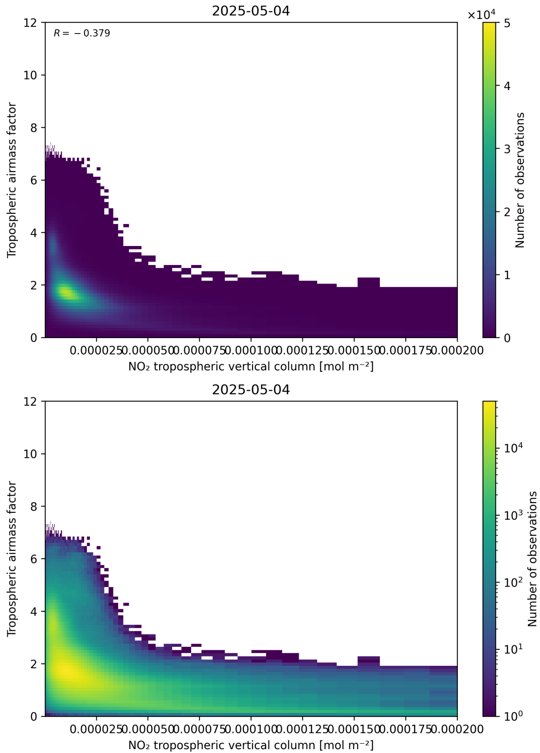
Figure 123: Scatter density plot of “NO 2 tropospheric vertical column” against “Tropospheric air mass factor” for 2025-05-04 to 2025-05-05.
