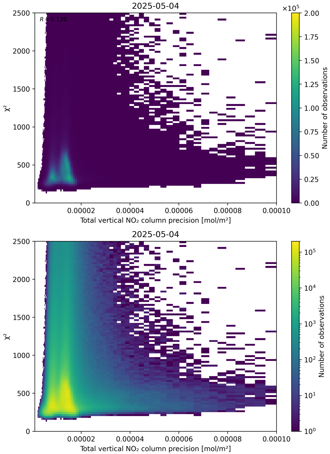
Figure 116: Scatter density plot of “Total vertical NO 2 column precision” against “ \chi^2 ” for 2025-05-04 to 2025-05-05.
