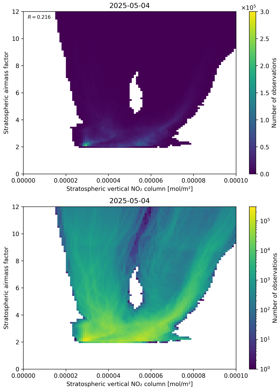
Figure 96: Scatter density plot of “Stratospheric vertical \text{NO}_2 column” against “Stratospheric airmass factor” for 2025-05-04 to 2025-05-05.
