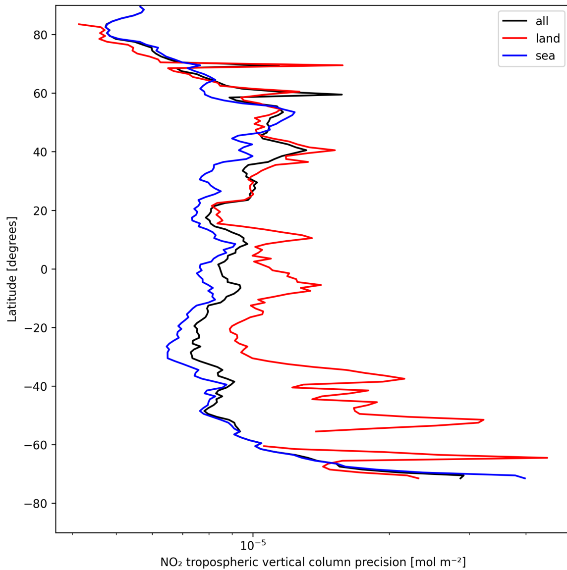
Figure 13: Zonal average of “NO 2 tropospheric vertical column precision” for 2025-05-04 to 2025-05-05.
