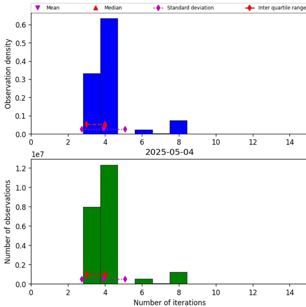
Figure 34: Histogram of “Number of iterations” for 2025-05-04 to 2025-05-05
