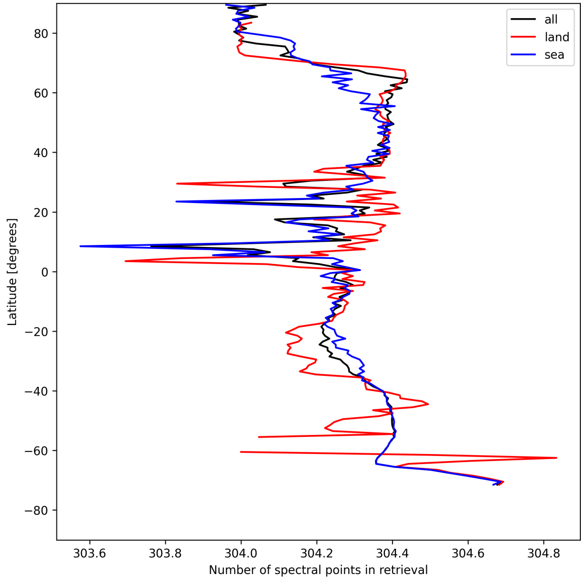
Figure 16: Zonal average of “Number of spectral points in retrieval” for 2025-05-04 to 2025-05-05.
