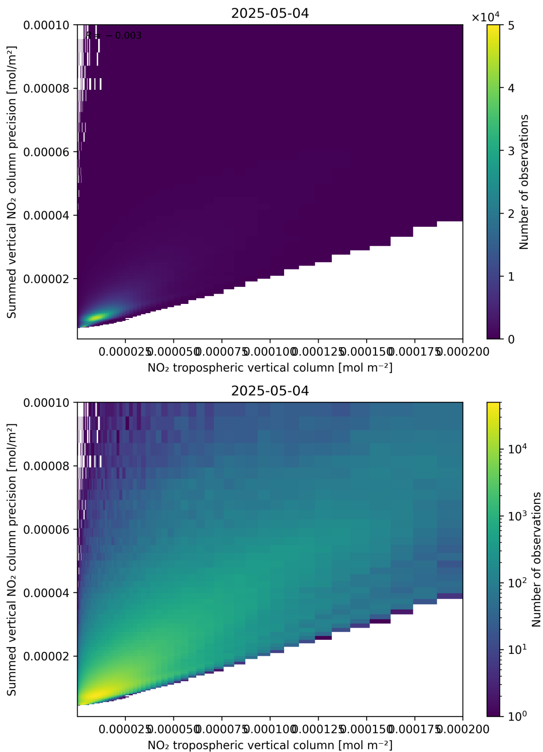
Figure 127: Scatter density plot of “NO 2 tropospheric vertical column” against “Summed vertical NO 2 column precision” for 2025-05-04 to 2025-05-05.
