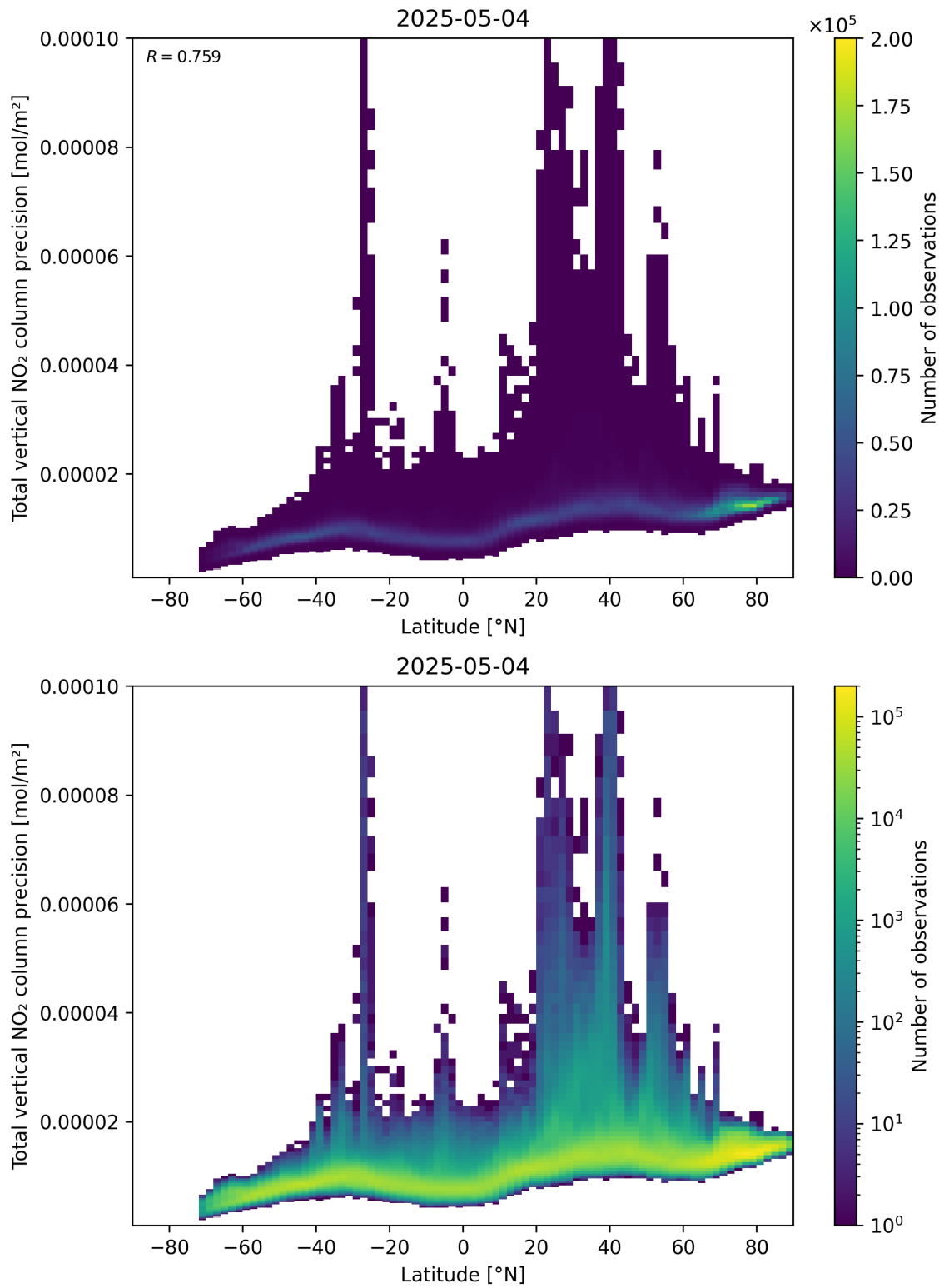
Figure 91: Scatter density plot of “Latitude” against “Total vertical NO 2 column precision” for 2025-05-04 to 2025-05-05.
