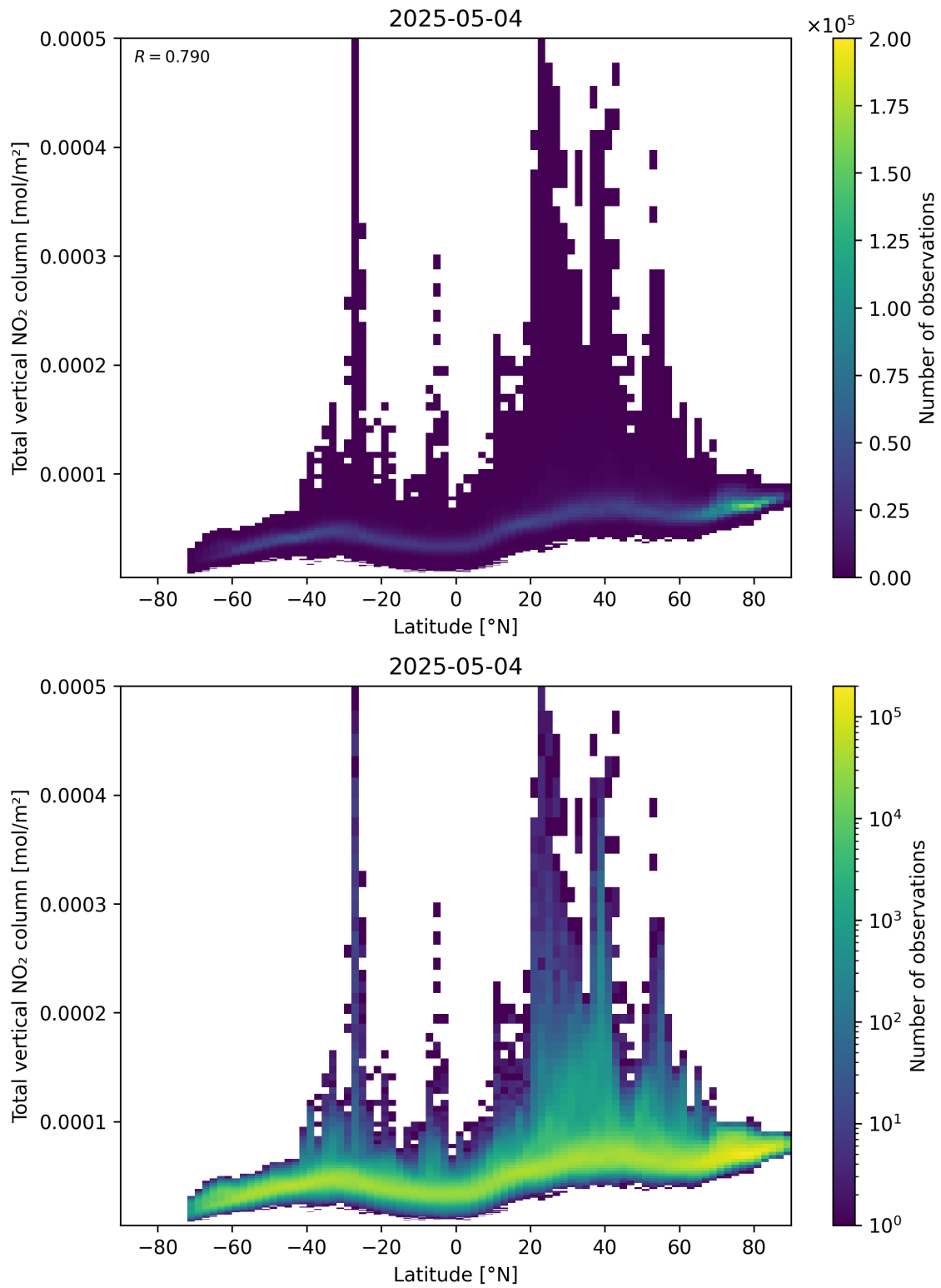
Figure 90: Scatter density plot of “Latitude” against “Total vertical NO 2 column” for 2025-05-04 to 2025-05-05.
