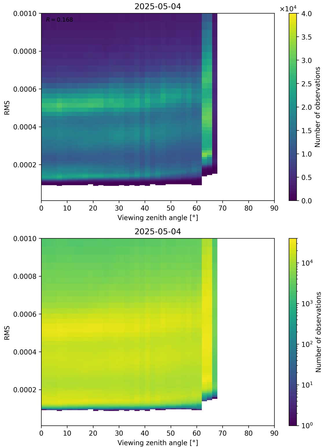
Figure 171: Scatter density plot of “Viewing zenith angle” against “RMS” for 2025-05-04 to 2025-05-05.
