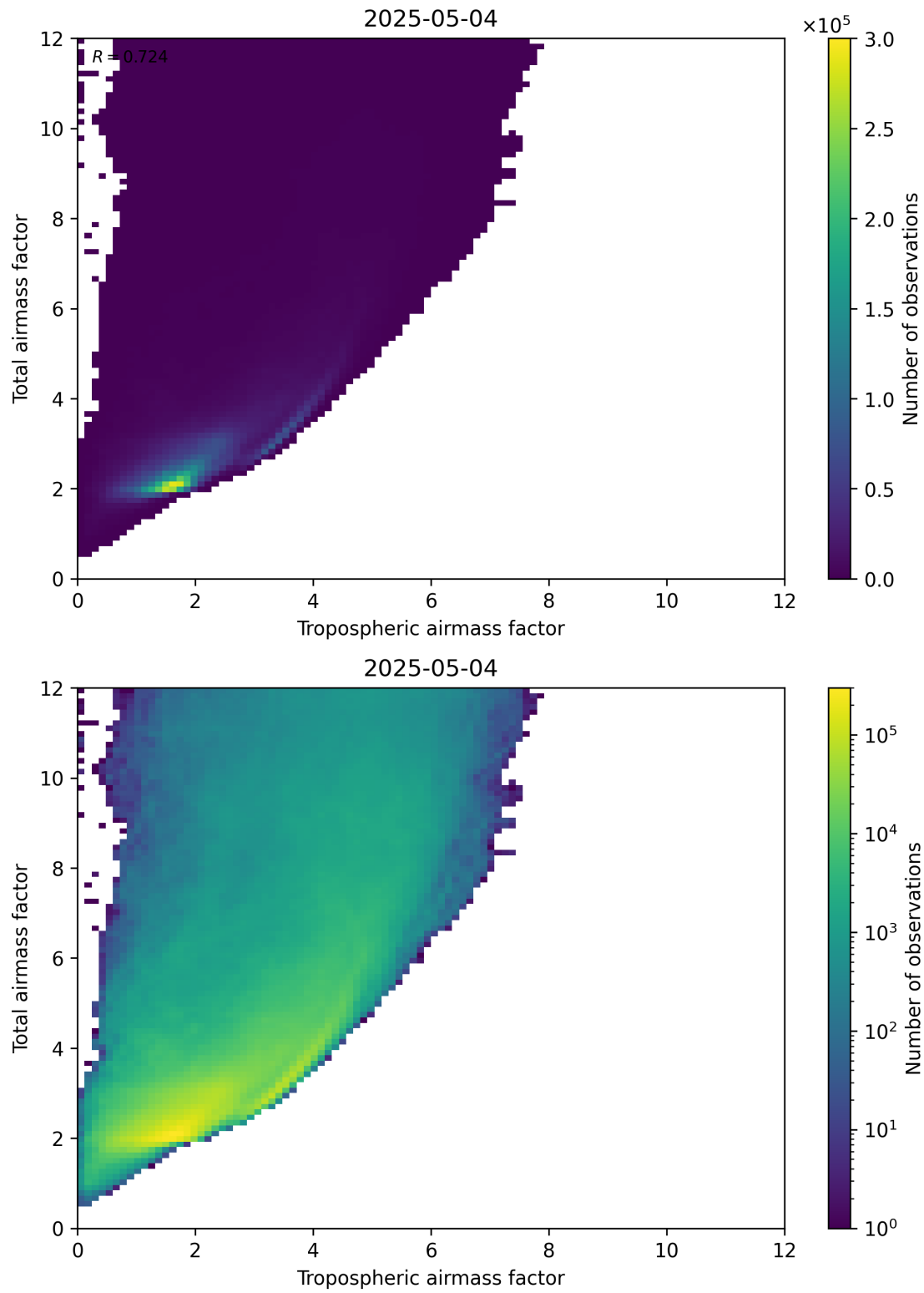
Figure 72: Scatter density plot of “Tropospheric airmass factor” against “Total airmass factor” for 2025-05-04 to 2025-05-05.
