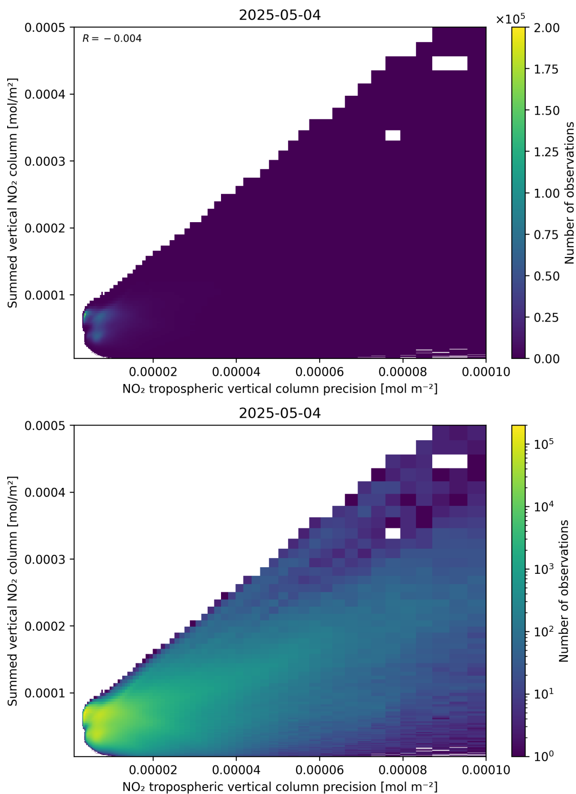
Figure 136: Scatter density plot of “NO 2 tropospheric vertical column precision” against “Summed vertical NO 2 column” for 2025-05-04 to 2025-05-05.
