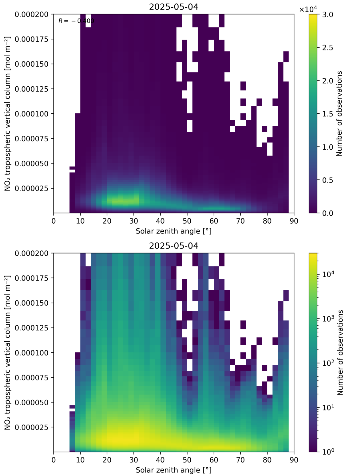
Figure 155: Scatter density plot of “Solar zenith angle” against “NO 2 tropospheric vertical column” for 2025-05-04 to 2025-05-05.
