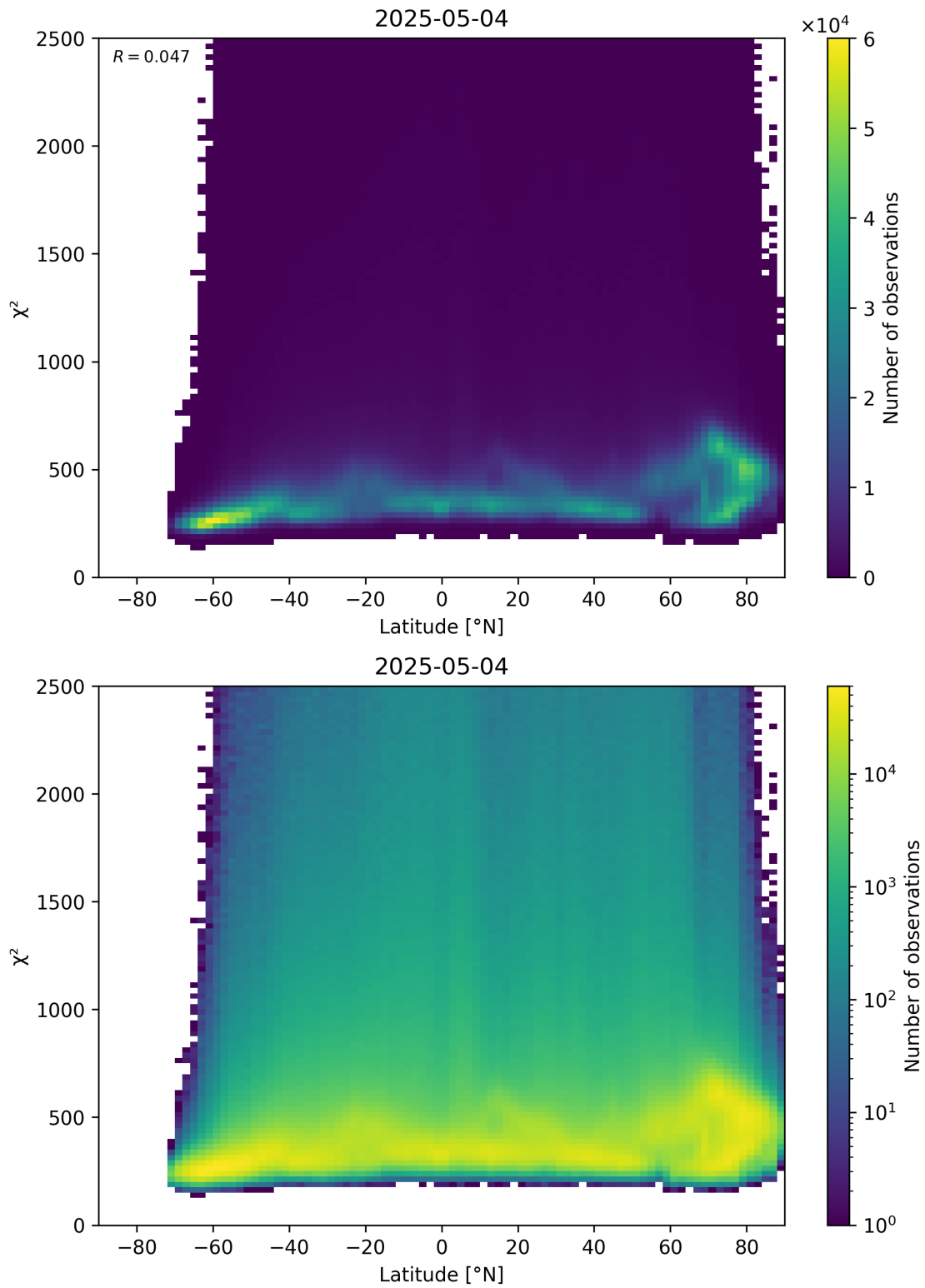
Figure 86: Scatter density plot of “Latitude” against “ \chi^2 ” for 2025-05-04 to 2025-05-05.
