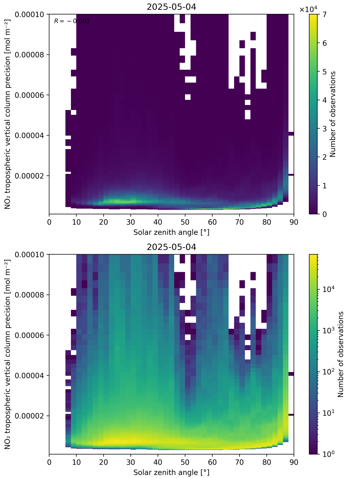
Figure 156: Scatter density plot of “Solar zenith angle” against “NO 2 tropospheric vertical column precision” for 2025-05-04 to 2025-05-05.
