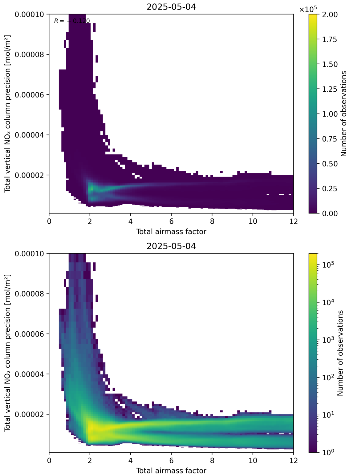
Figure 68: Scatter density plot of “Total airmass factor” against “Total vertical NO 2 column precision” for 2025-05-04 to 2025-05-05.
