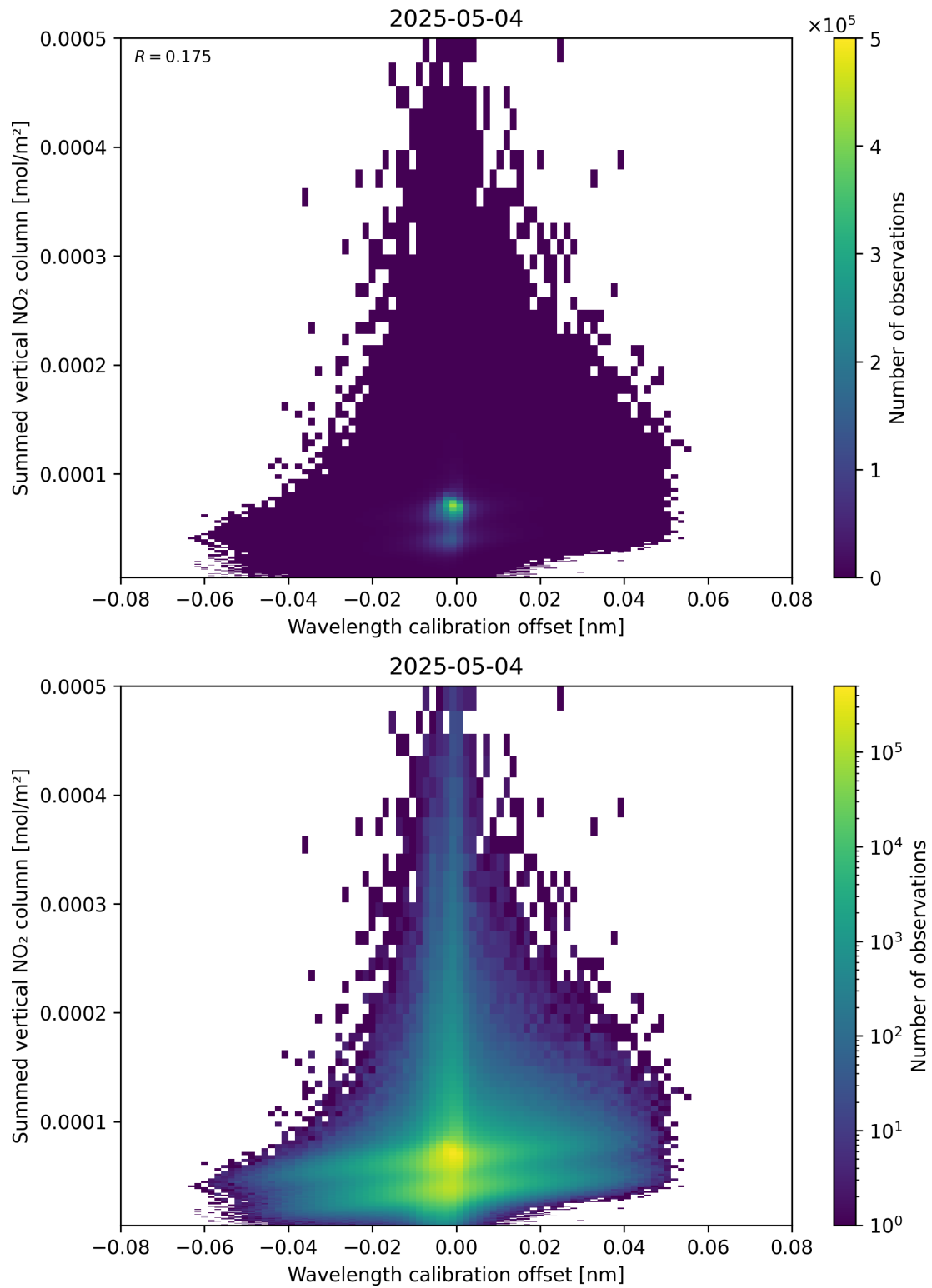
Figure 177: Scatter density plot of “Wavelength calibration offset” against “Summed vertical NO 2 column” for 2025-05-04 to 2025-05-05.
