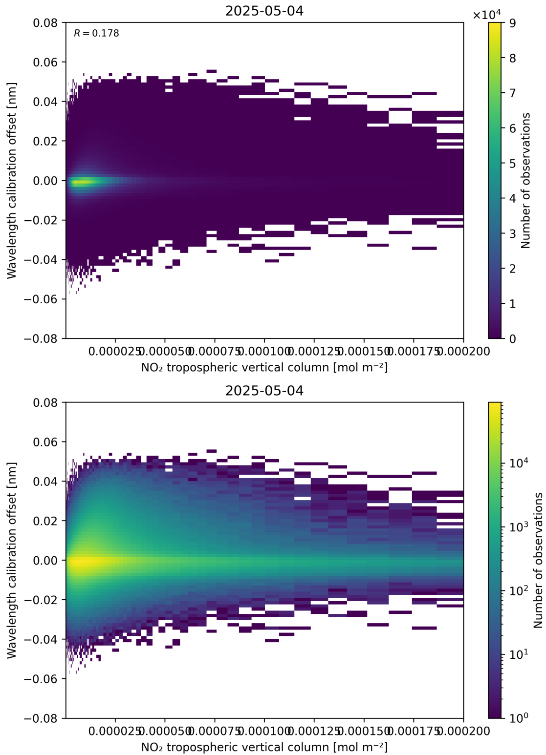
Figure 143: Scatter density plot of “NO 2 tropospheric vertical column” against “Wavelength calibration offset” for 2025-05-04 to 2025-05-05.
