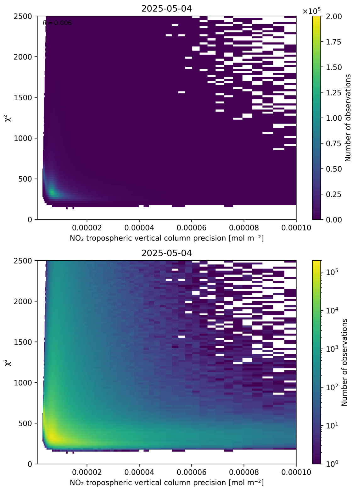
Figure 134: Scatter density plot of “NO 2 tropospheric vertical column precision” against “ \chi^2 ” for 2025-05-04 to 2025-05-05.
