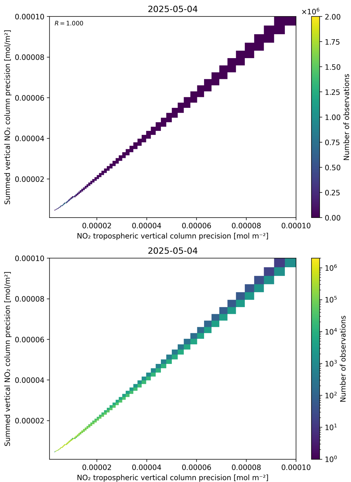
Figure 137: Scatter density plot of “NO 2 tropospheric vertical column precision” against “Summed vertical NO 2 column precision” for 2025-05-04 to 2025-05-05.
