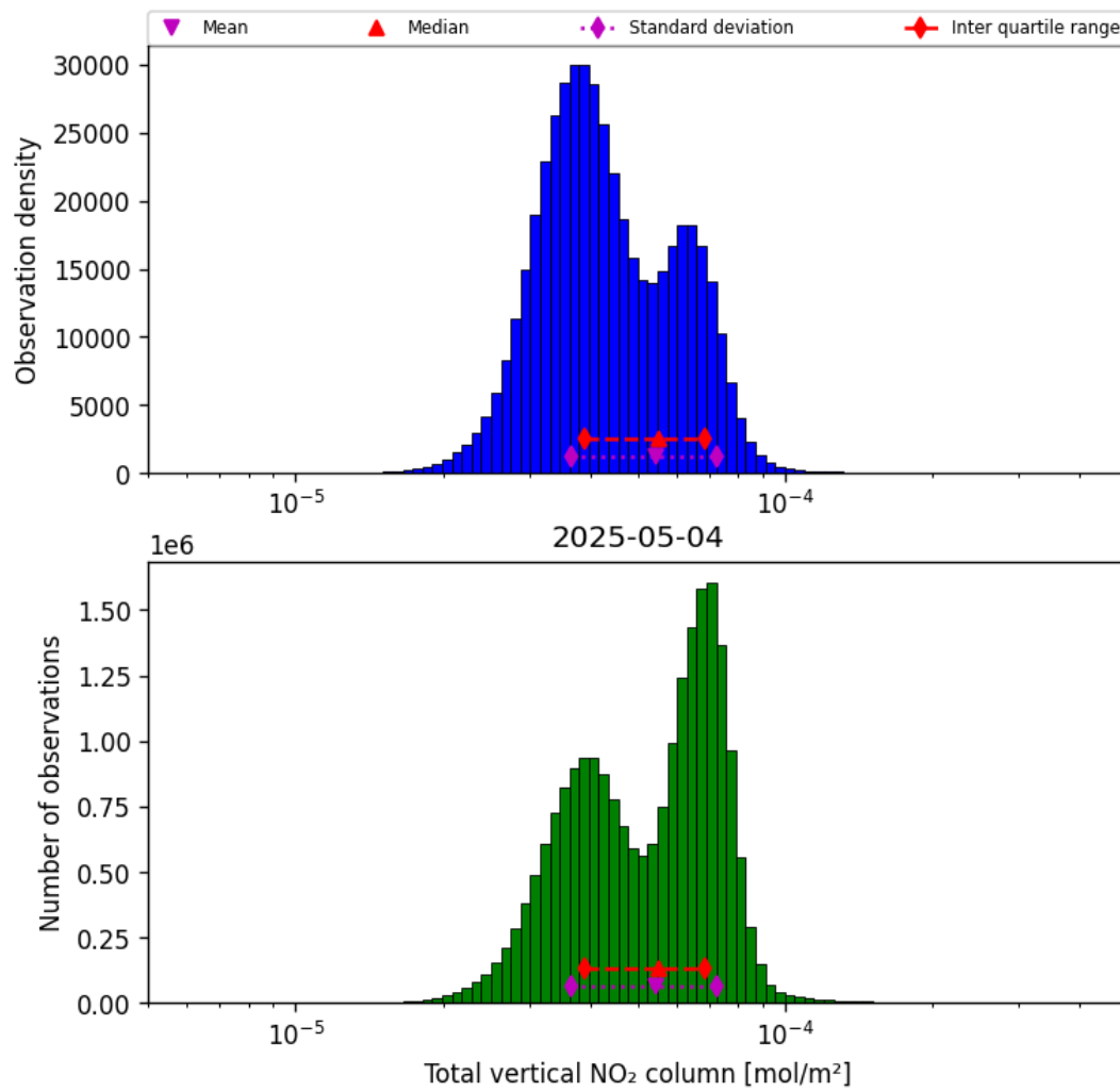
Figure 38: Histogram of “Total vertical NO 2 column” for 2025-05-04 to 2025-05-05
