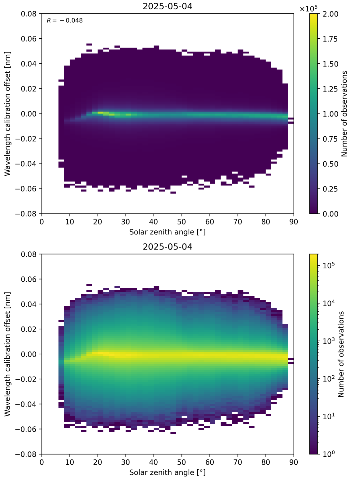
Figure 158: Scatter density plot of “Solar zenith angle” against “Wavelength calibration offset” for 2025-05-04 to 2025-05-05.
