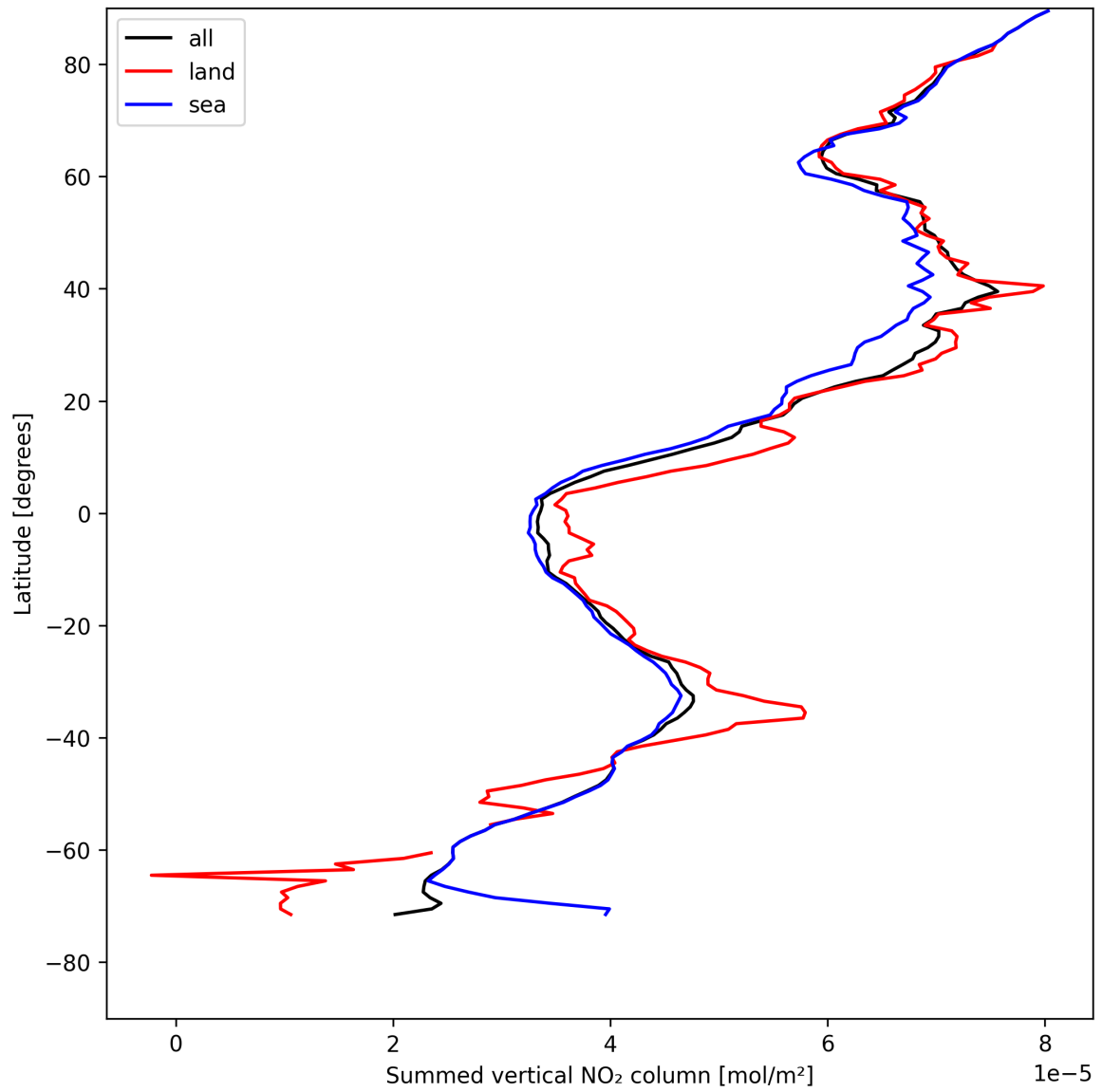
Figure 23: Zonal average of “Summed vertical NO 2 column” for 2025-05-04 to 2025-05-05.
