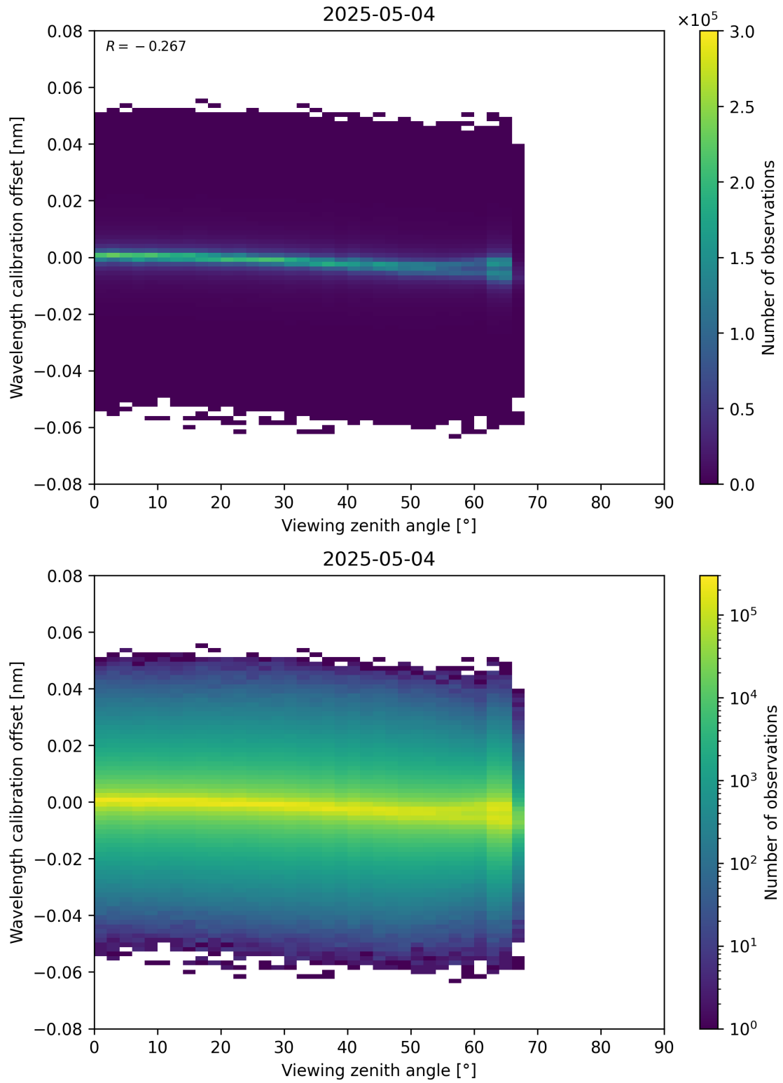
Figure 173: Scatter density plot of “Viewing zenith angle” against “Wavelength calibration offset” for 2025-05-04 to 2025-05-05.
