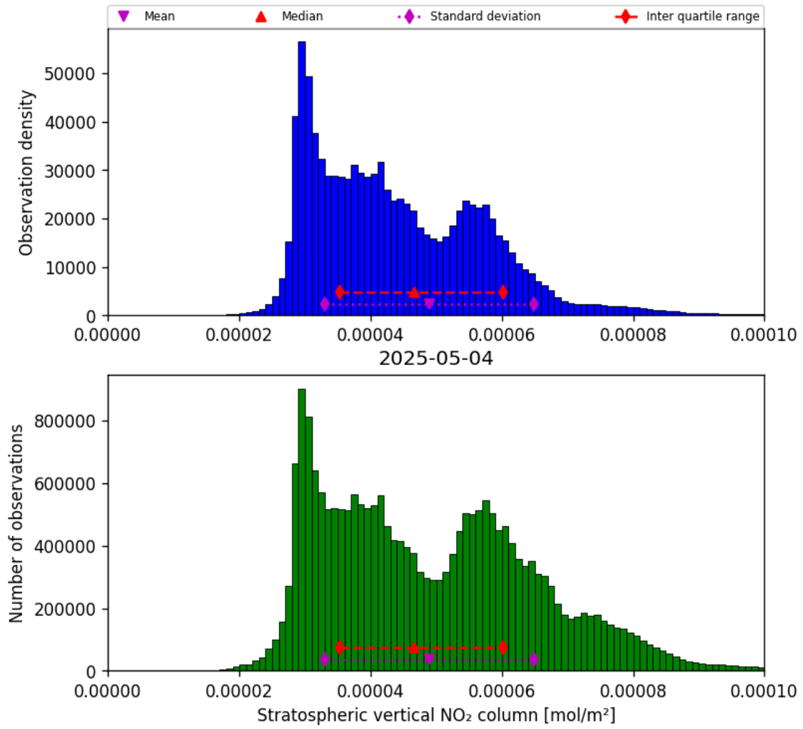
Figure 36: Histogram of “Stratospheric vertical NO 2 column” for 2025-05-04 to 2025-05-05
