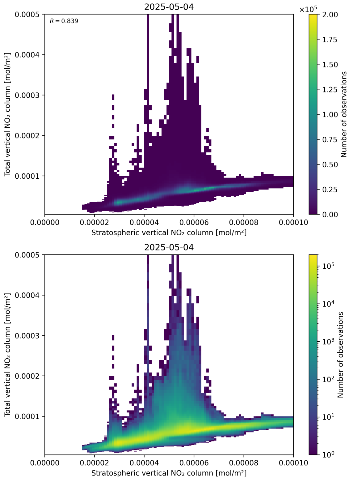
Figure 100: Scatter density plot of “Stratospheric vertical NO 2 column” against “Total vertical NO 2 column” for 2025-05-04 to 2025-05-05.
