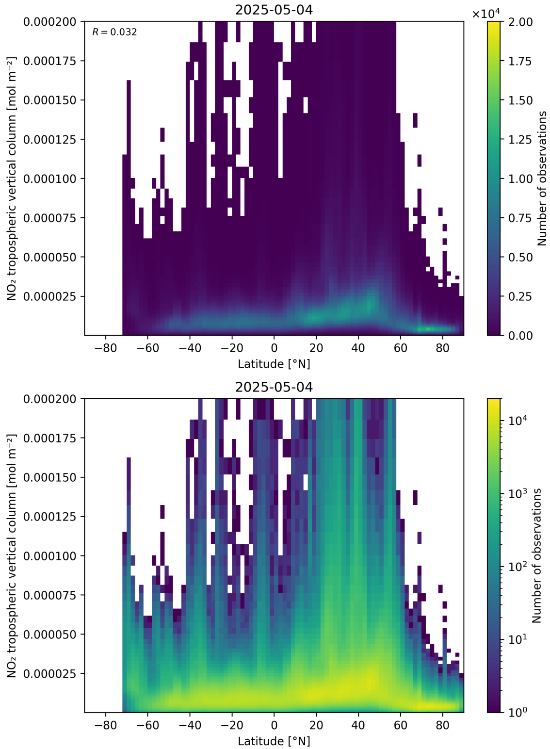
Figure 92: Scatter density plot of “Latitude” against “NO 2 tropospheric vertical column” for 2025-05-04 to 2025-05-05.
