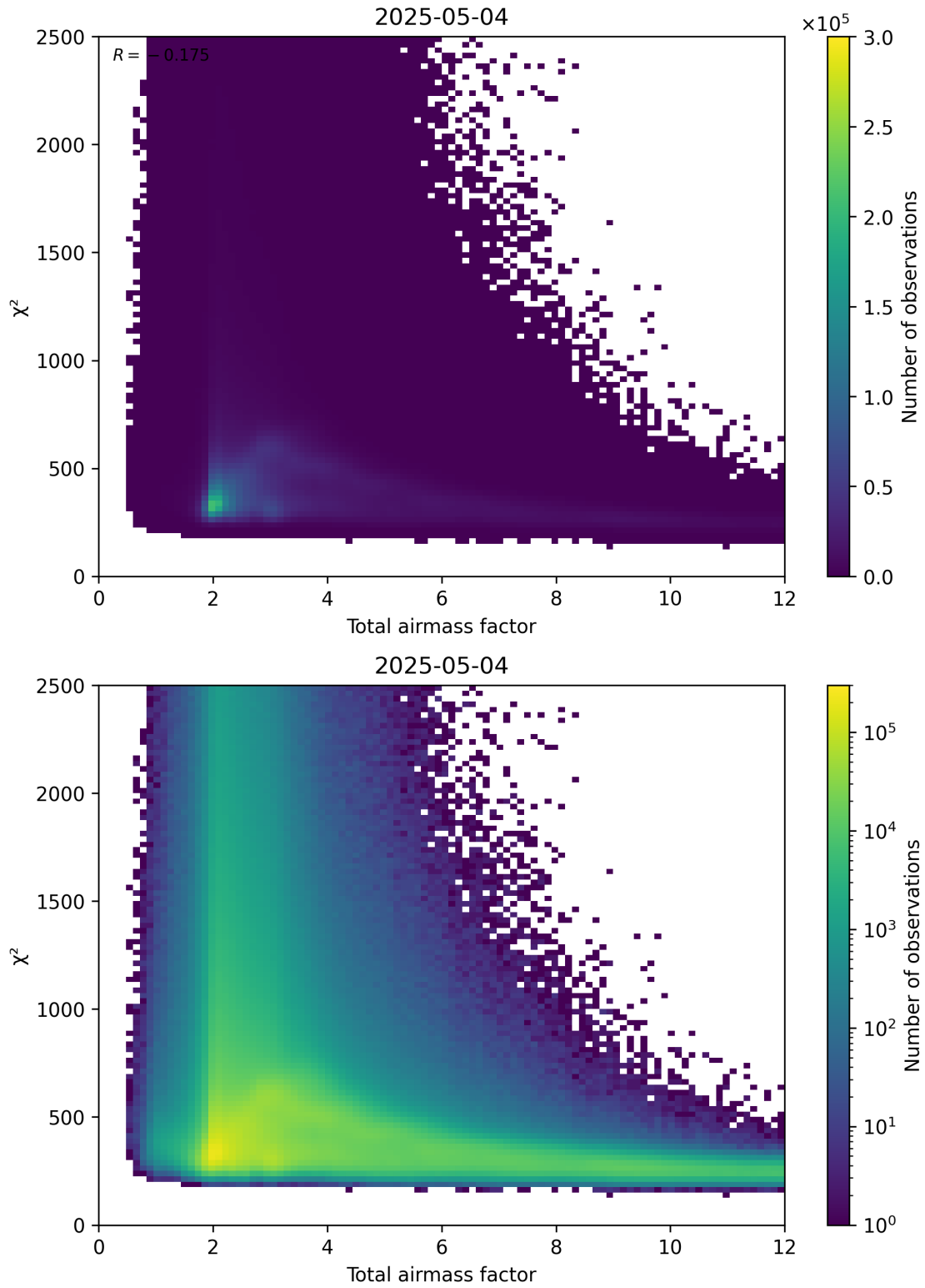
Figure 63: Scatter density plot of “Total airmass factor” against “ \chi^2 ” for 2025-05-04 to 2025-05-05.
