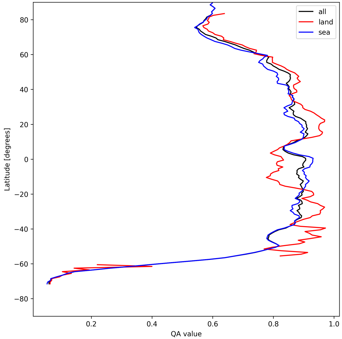
Figure 11: Zonal average of “QA value” for 2025-05-04 to 2025-05-05.
