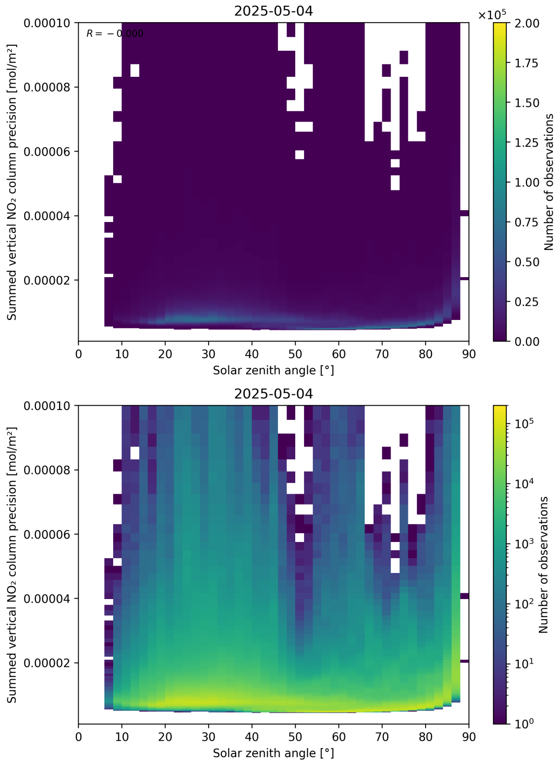
Figure 152: Scatter density plot of “Solar zenith angle” against “Summed vertical NO 2 column precision” for 2025-05-04 to 2025-05-05.
