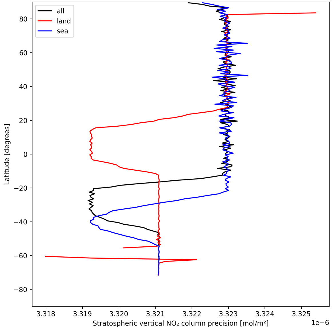
Figure 20: Zonal average of “Stratospheric vertical NO 2 column precision” for 2025-05-04 to 2025-05-05.
