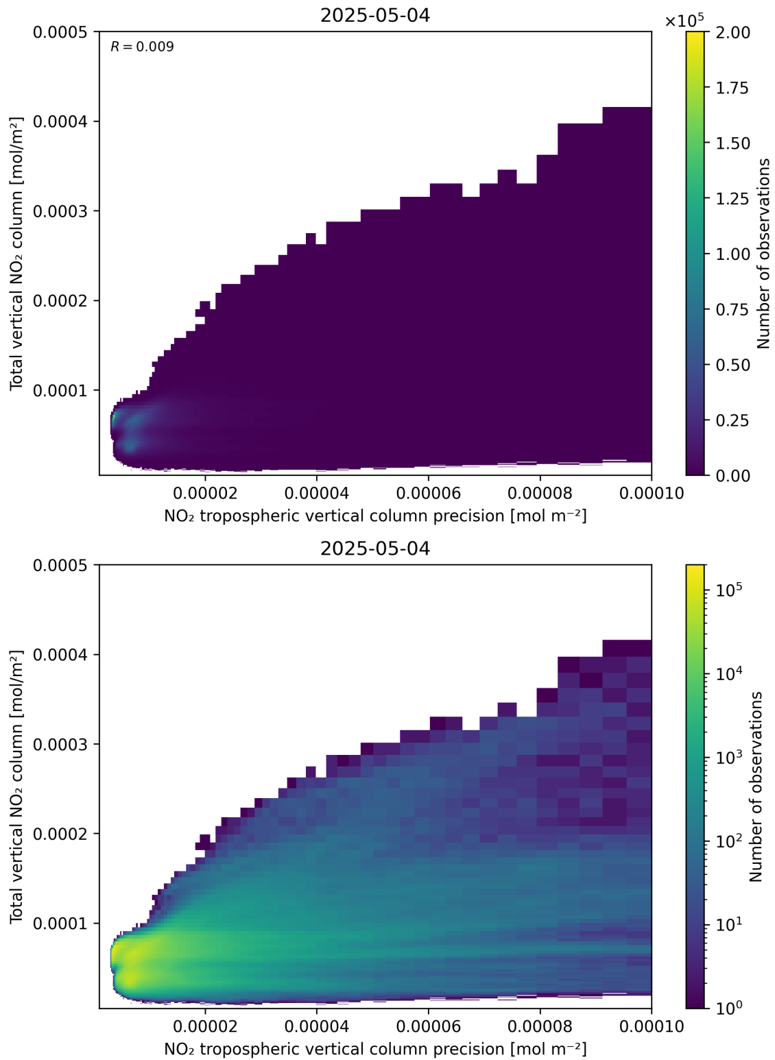
Figure 138: Scatter density plot of “NO 2 tropospheric vertical column precision” against “Total vertical NO 2 column” for 2025-05-04 to 2025-05-05.
