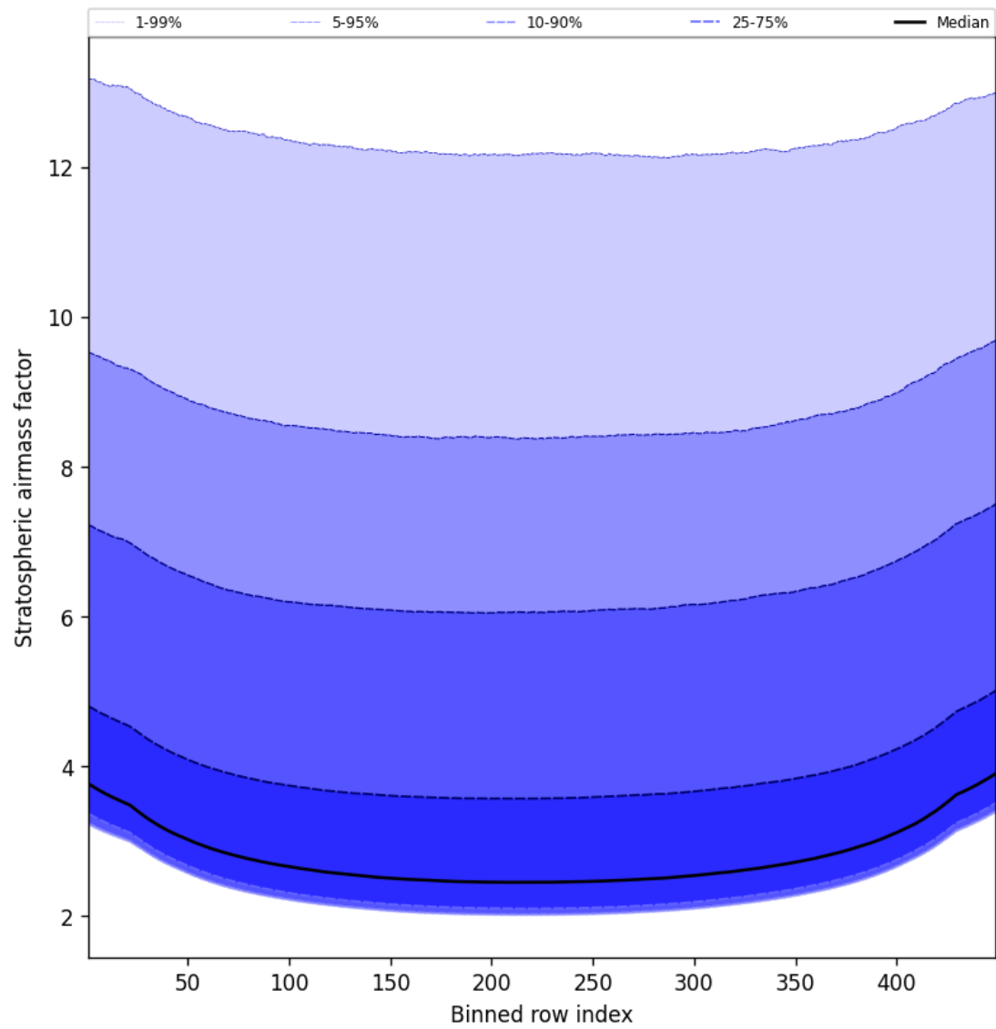
Figure 61: Along track statistics of “Stratospheric airmass factor” for 2025-05-04 to 2025-05-05
