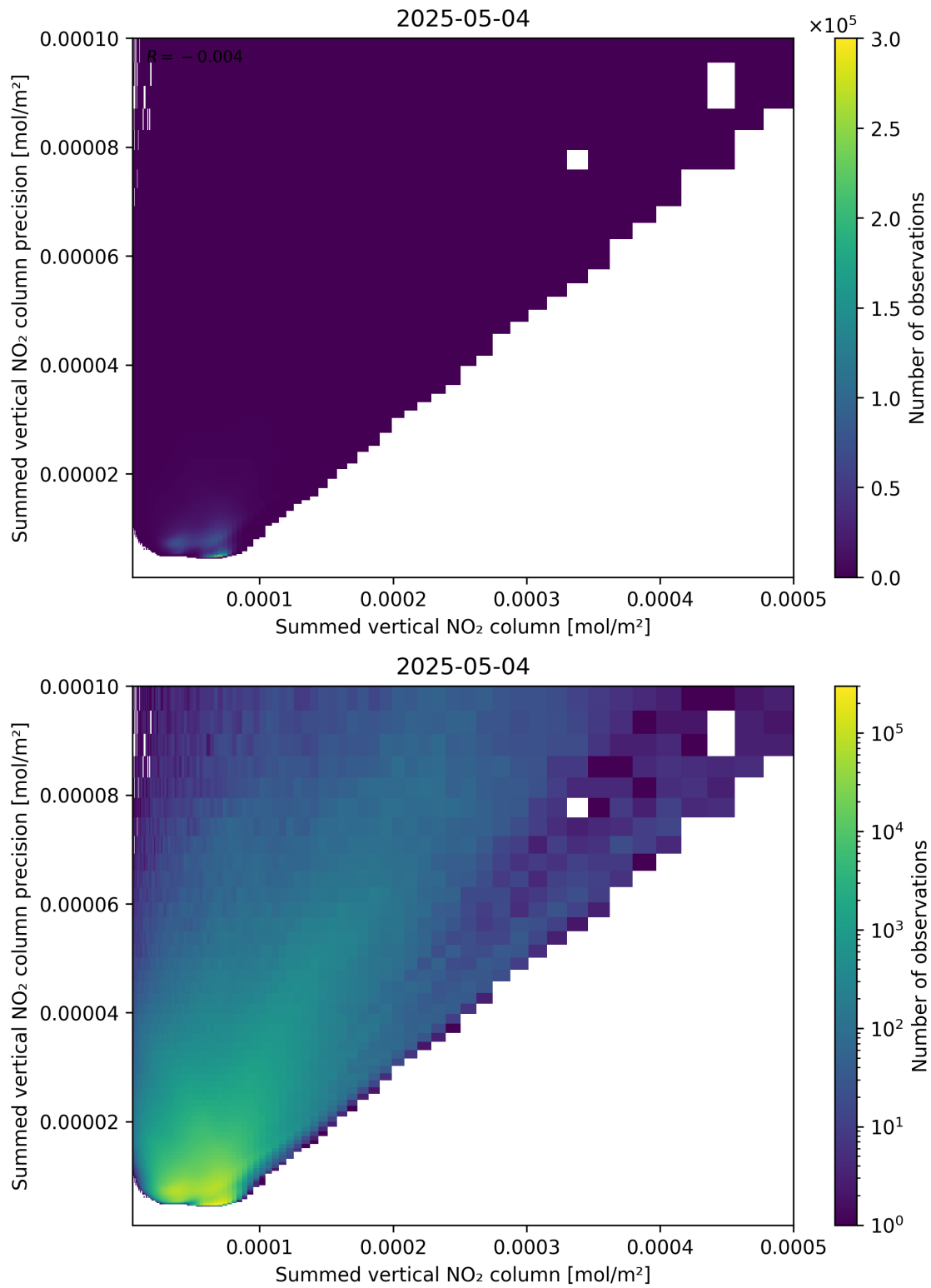
Figure 105: Scatter density plot of “Summed vertical NO 2 column” against “Summed vertical NO 2 column precision” for 2025-05-04 to 2025-05-05.
