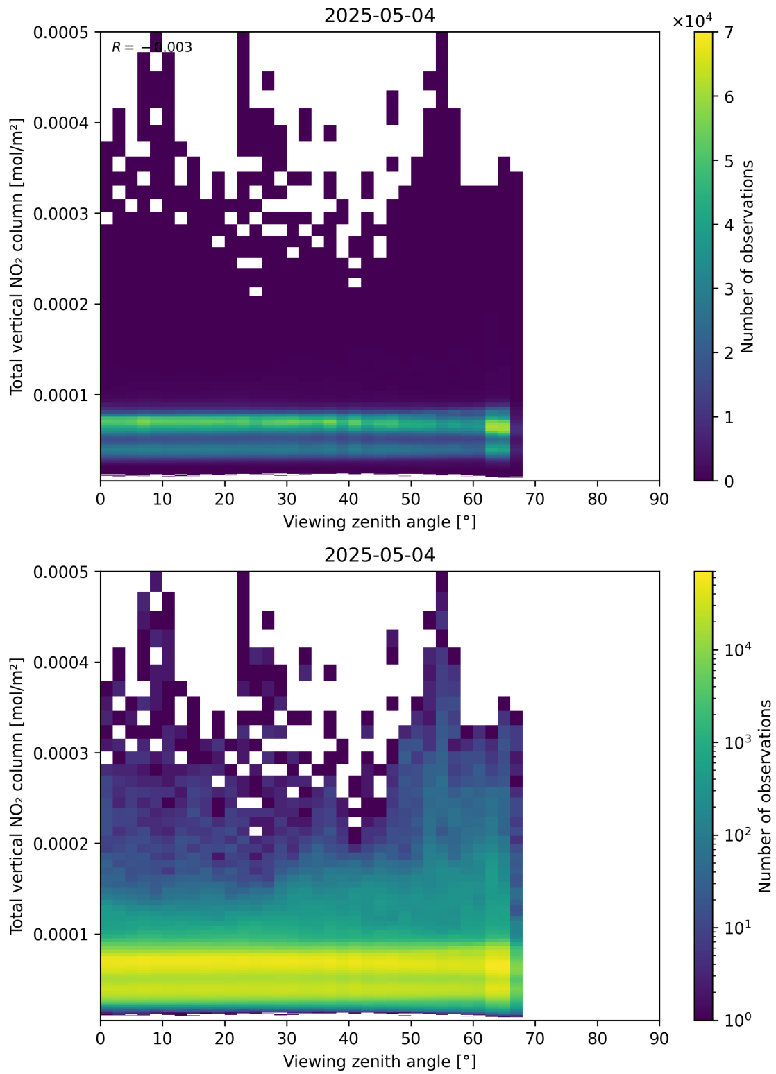
Figure 167: Scatter density plot of “Viewing zenith angle” against “Total vertical NO 2 column” for 2025-05-04 to 2025-05-05.
