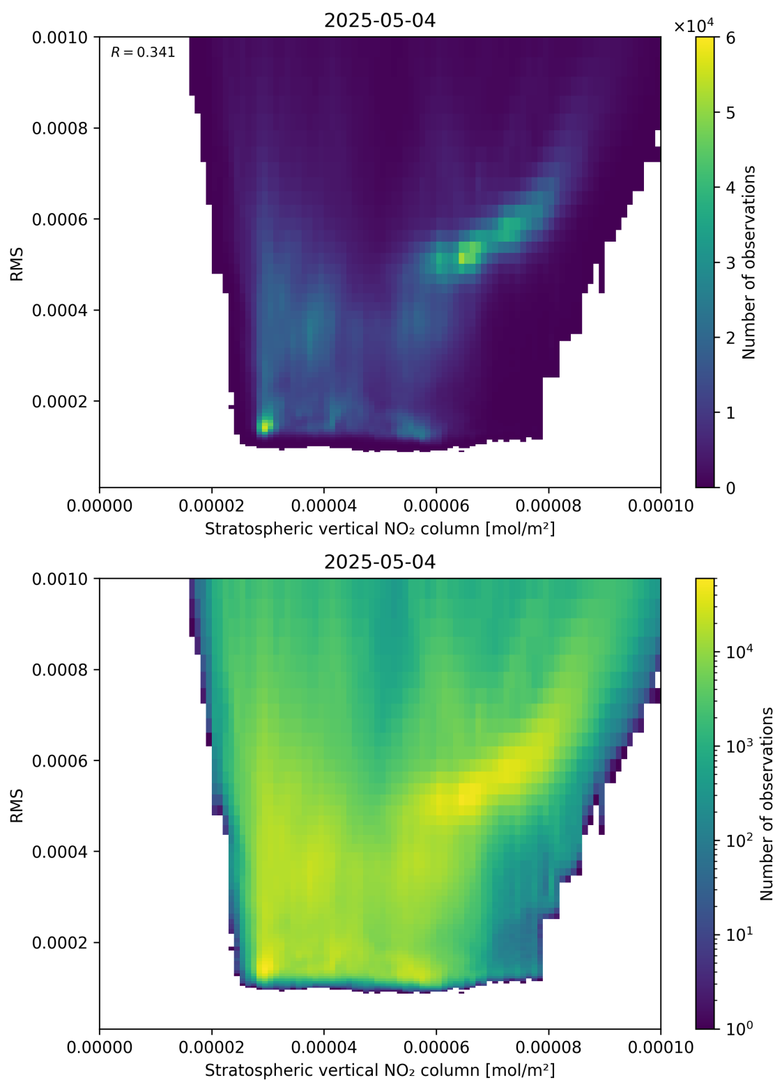
Figure 102: Scatter density plot of “Stratospheric vertical NO 2 column” against “RMS” for 2025-05-04 to 2025-05-05.
