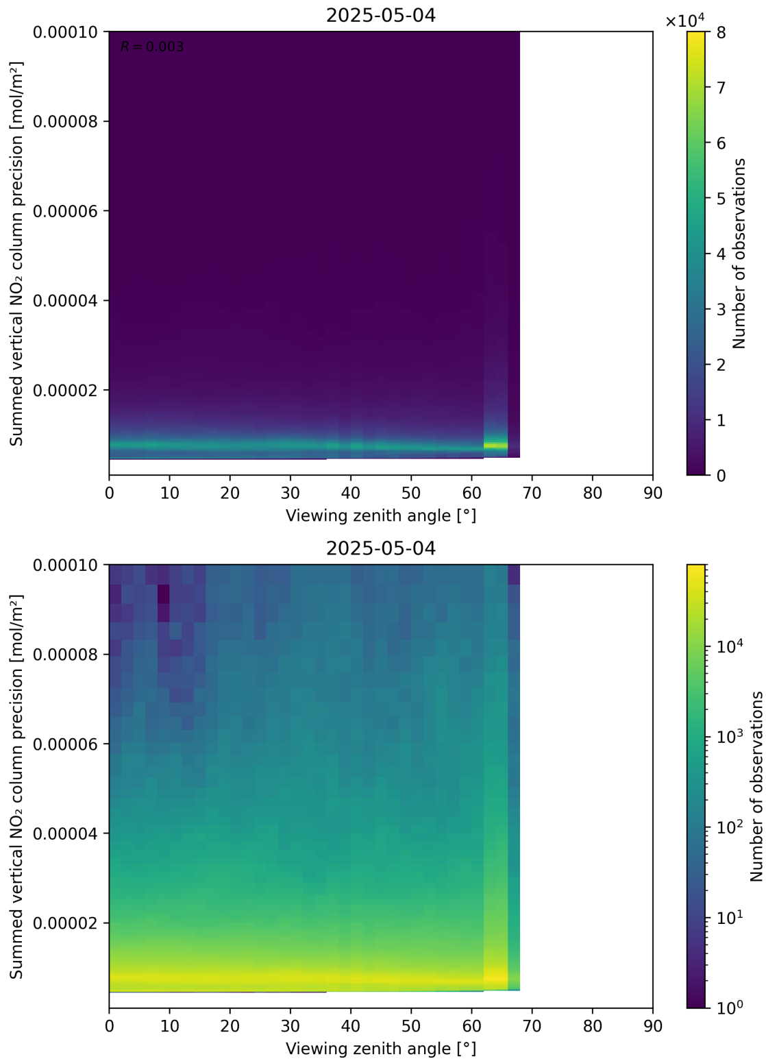
Figure 166: Scatter density plot of “Viewing zenith angle” against “Summed vertical NO 2 column precision” for 2025-05-04 to 2025-05-05.
