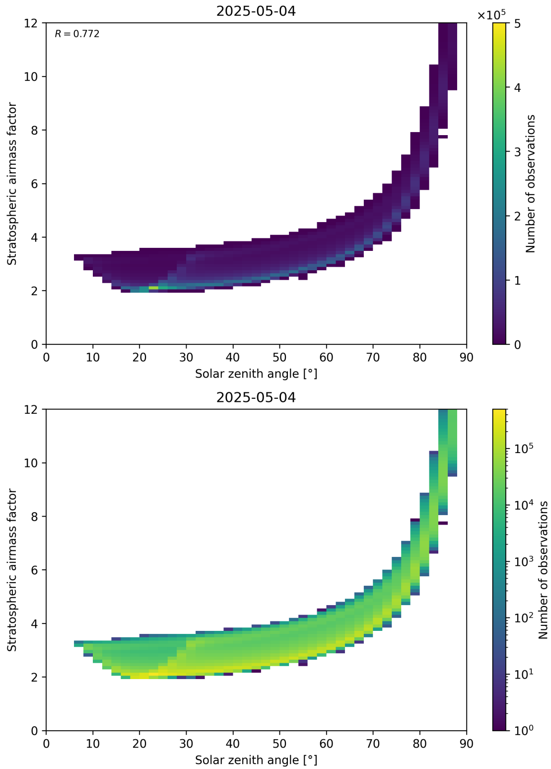
Figure 145: Scatter density plot of “Solar zenith angle” against “Stratospheric airmass factor” for 2025-05-04 to 2025-05-05.
