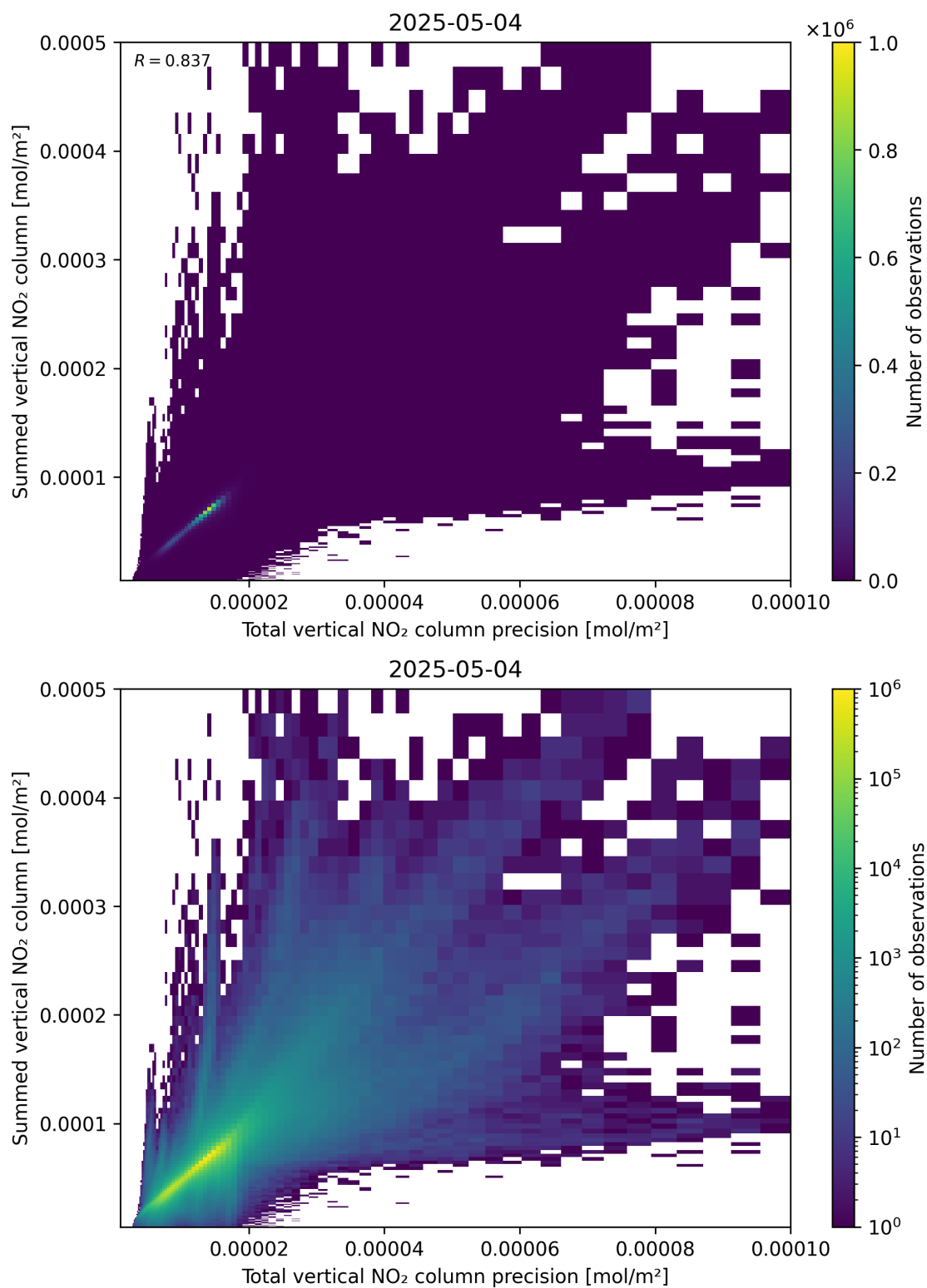
Figure 117: Scatter density plot of “Total vertical NO 2 column precision” against “Summed vertical NO 2 column” for 2025-05-04 to 2025-05-05.
