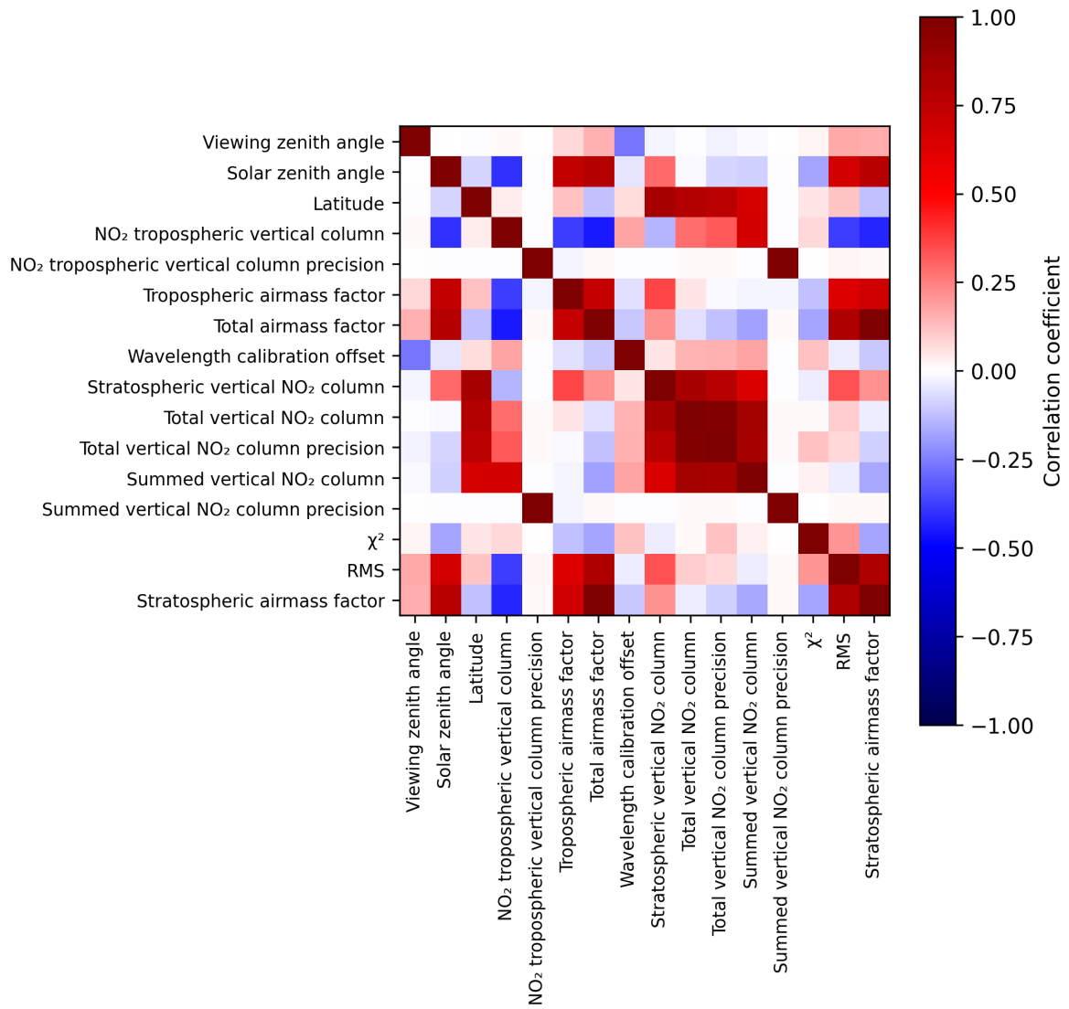
Figure 2: Map of correlation matrix for 2025-05-04 to 2025-05-05.
