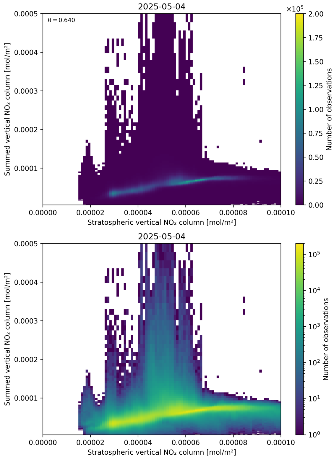
Figure 98: Scatter density plot of “Stratospheric vertical NO 2 column” against “Summed vertical NO 2 column” for 2025-05-04 to 2025-05-05.
