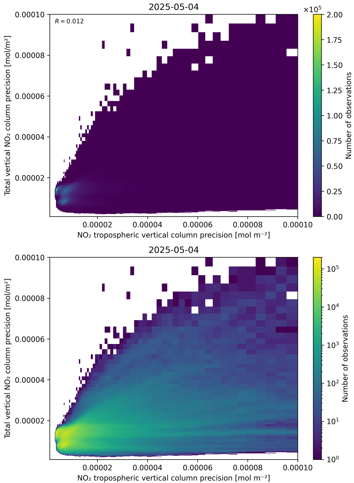
Figure 139: Scatter density plot of “NO 2 tropospheric vertical column precision” against “Total vertical NO 2 column precision” for 2025-05-04 to 2025-05-05.
