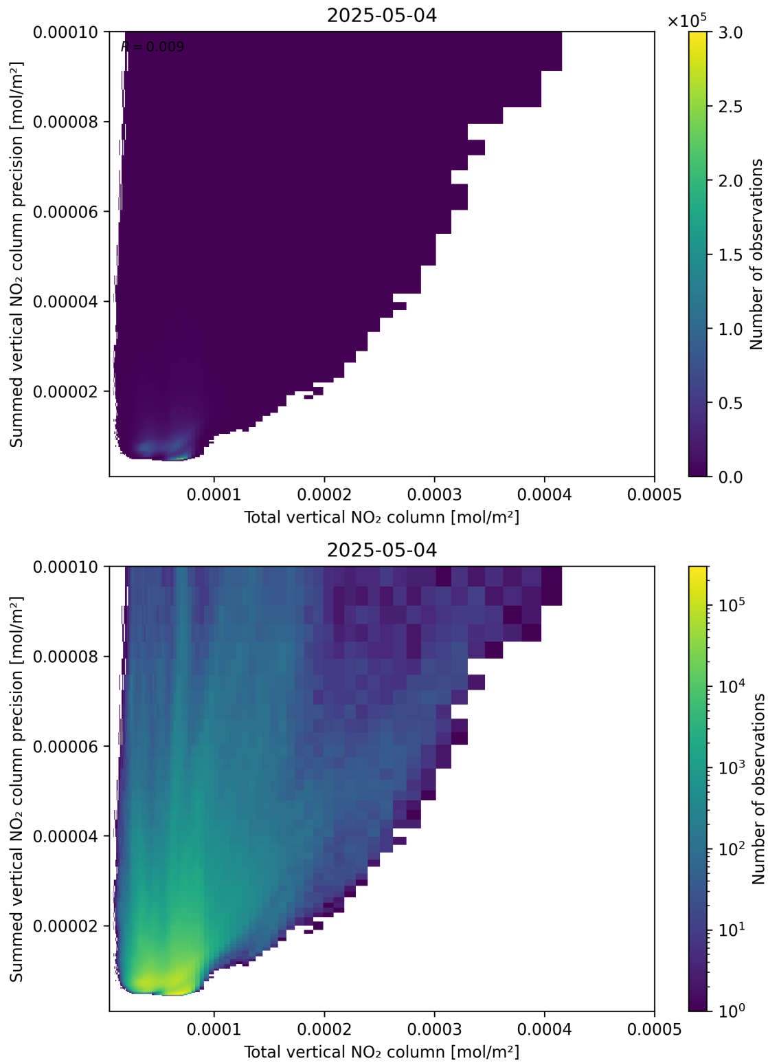
Figure 113: Scatter density plot of “Total vertical NO 2 column” against “Summed vertical NO 2 column precision” for 2025-05-04 to 2025-05-05.
