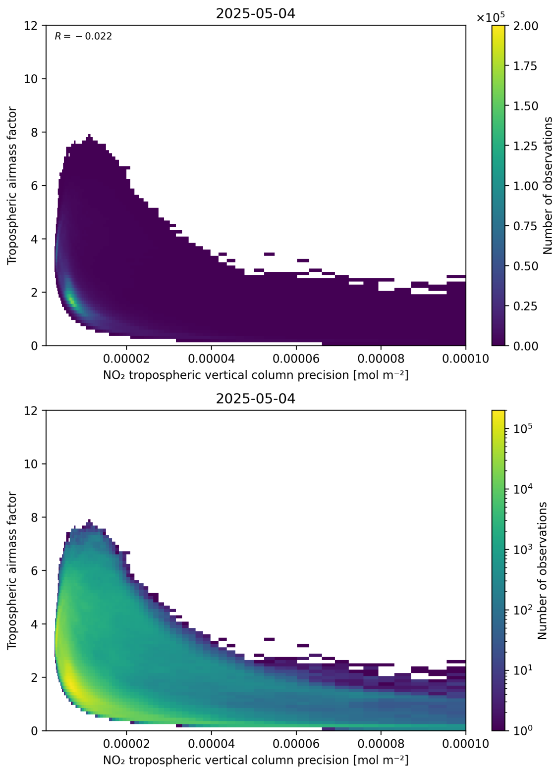
Figure 133: Scatter density plot of “NO 2 tropospheric vertical column precision” against “Tropospheric air mass factor” for 2025-05-04 to 2025-05-05.
