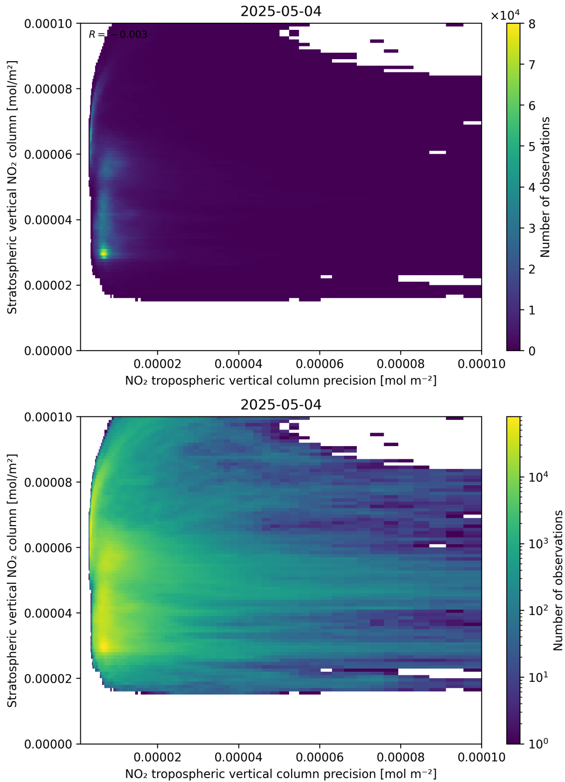
Figure 135: Scatter density plot of “NO 2 tropospheric vertical column precision” against “Stratospheric vertical NO 2 column” for 2025-05-04 to 2025-05-05.
