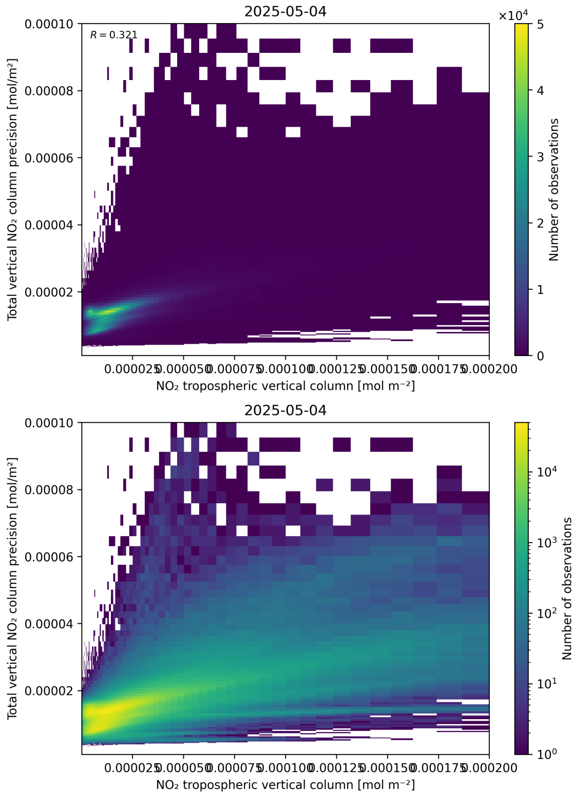
Figure 129: Scatter density plot of “NO 2 tropospheric vertical column” against “Total vertical NO 2 column precision” for 2025-05-04 to 2025-05-05.
