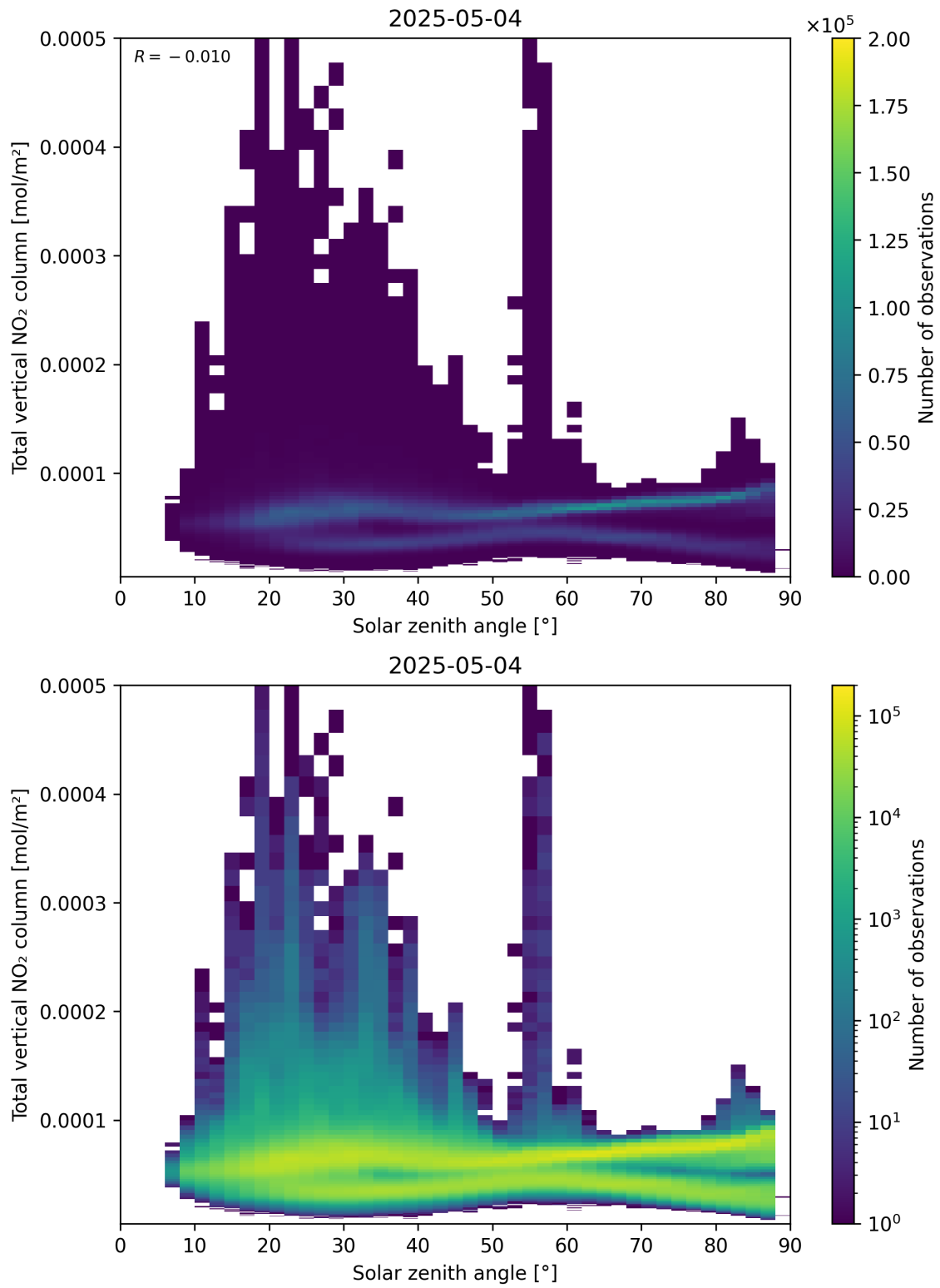
Figure 153: Scatter density plot of “Solar zenith angle” against “Total vertical NO 2 column” for 2025-05-04 to 2025-05-05.
