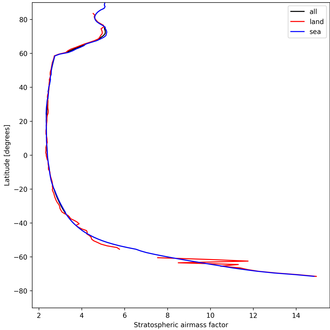
Figure 27: Zonal average of “Stratospheric air mass factor” for 2025-05-04 to 2025-05-05.
