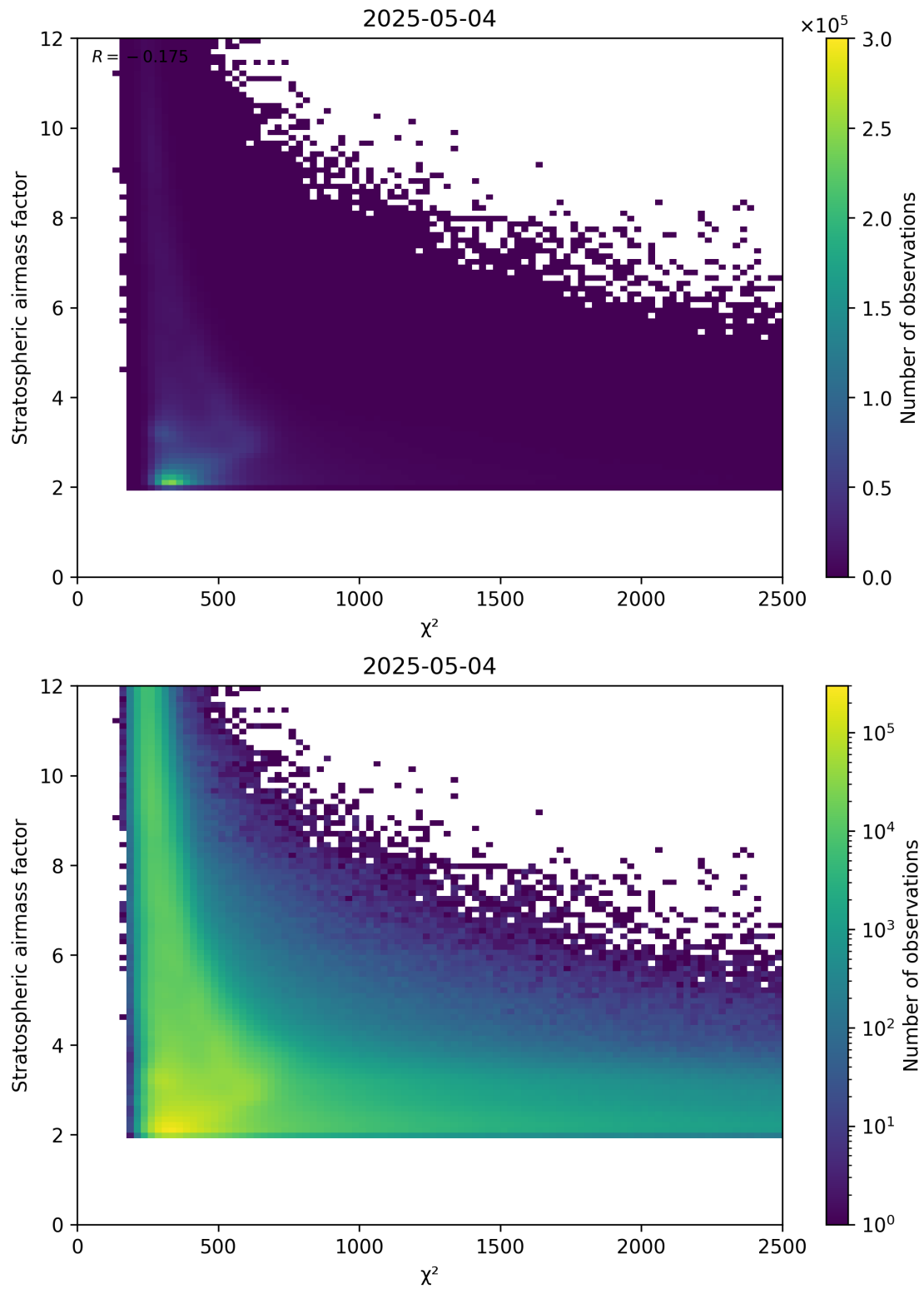
Figure 81: Scatter density plot of “ \chi^2 ” against “Stratospheric airmass factor” for 2025-05-04 to 2025-05-05.
