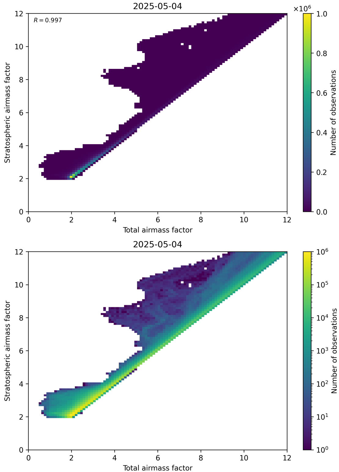
Figure 62: Scatter density plot of “Total airmass factor” against “Stratospheric airmass factor” for 2025-05-04 to 2025-05-05.
