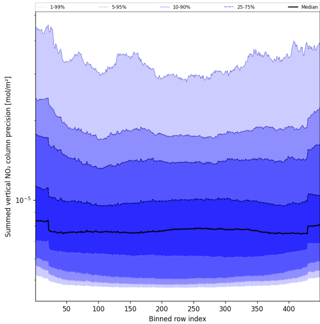
Figure 58: Along track statistics of “Summed vertical NO 2 column precision” for 2025-05-04 to 2025-05-05
