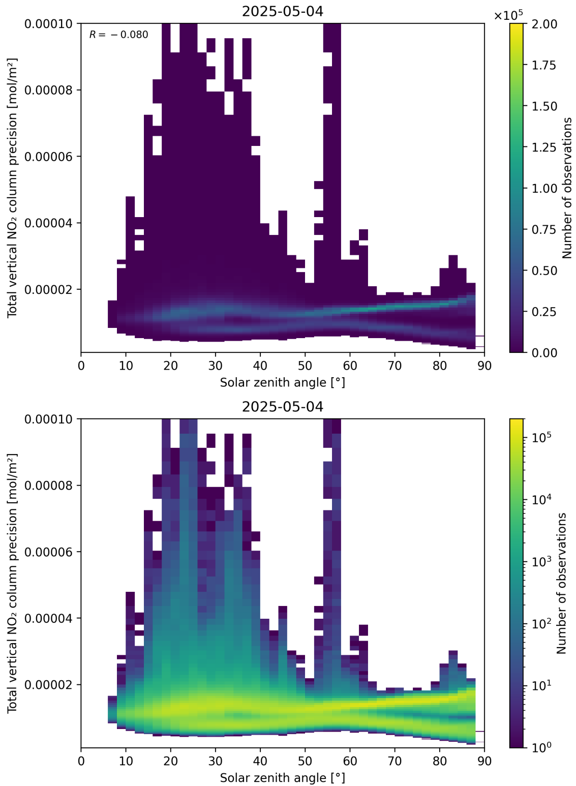
Figure 154: Scatter density plot of “Solar zenith angle” against “Total vertical NO 2 column precision” for 2025-05-04 to 2025-05-05.
