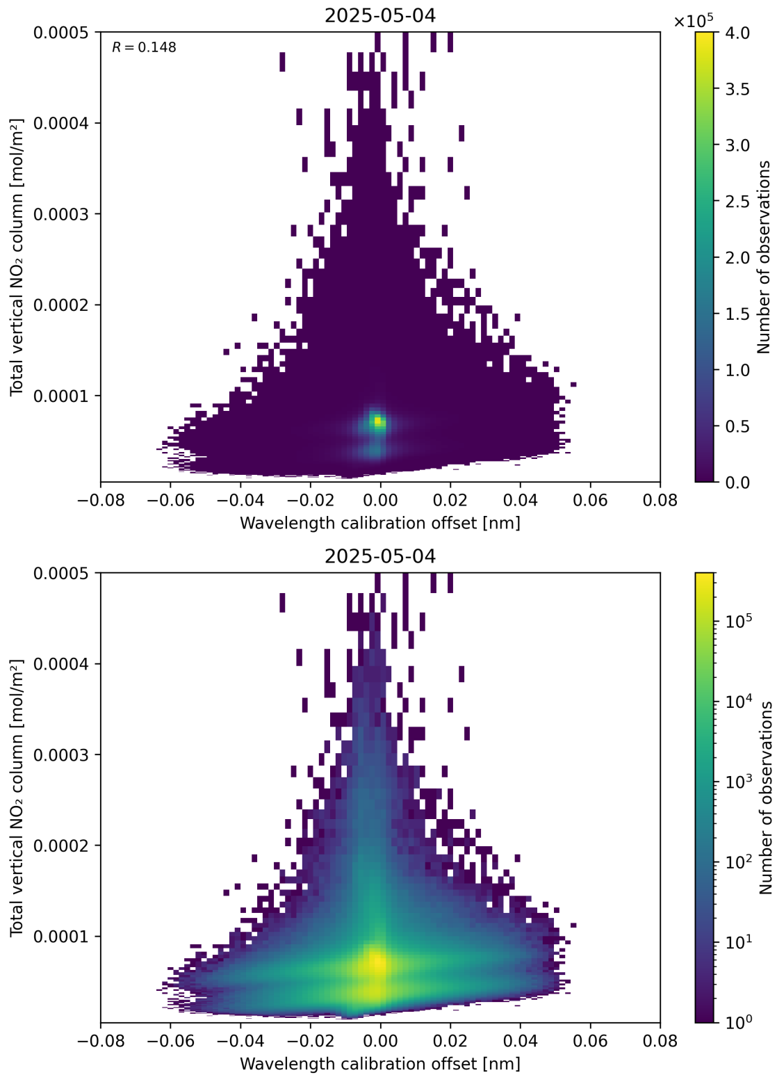
Figure 179: Scatter density plot of “Wavelength calibration offset” against “Total vertical NO 2 column” for 2025-05-04 to 2025-05-05.
