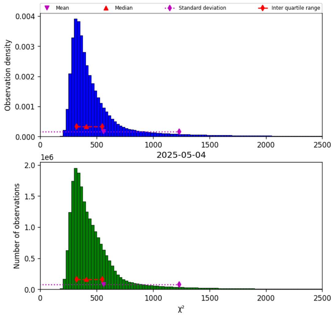
Figure 42: Histogram of “ \chi^2 ” for 2025-05-04 to 2025-05-05
