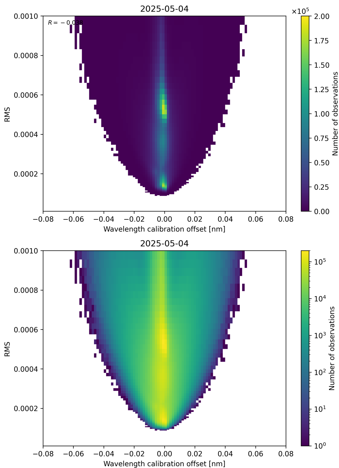
Figure 181: Scatter density plot of “Wavelength calibration offset” against “RMS” for 2025-05-04 to 2025-05-05.
