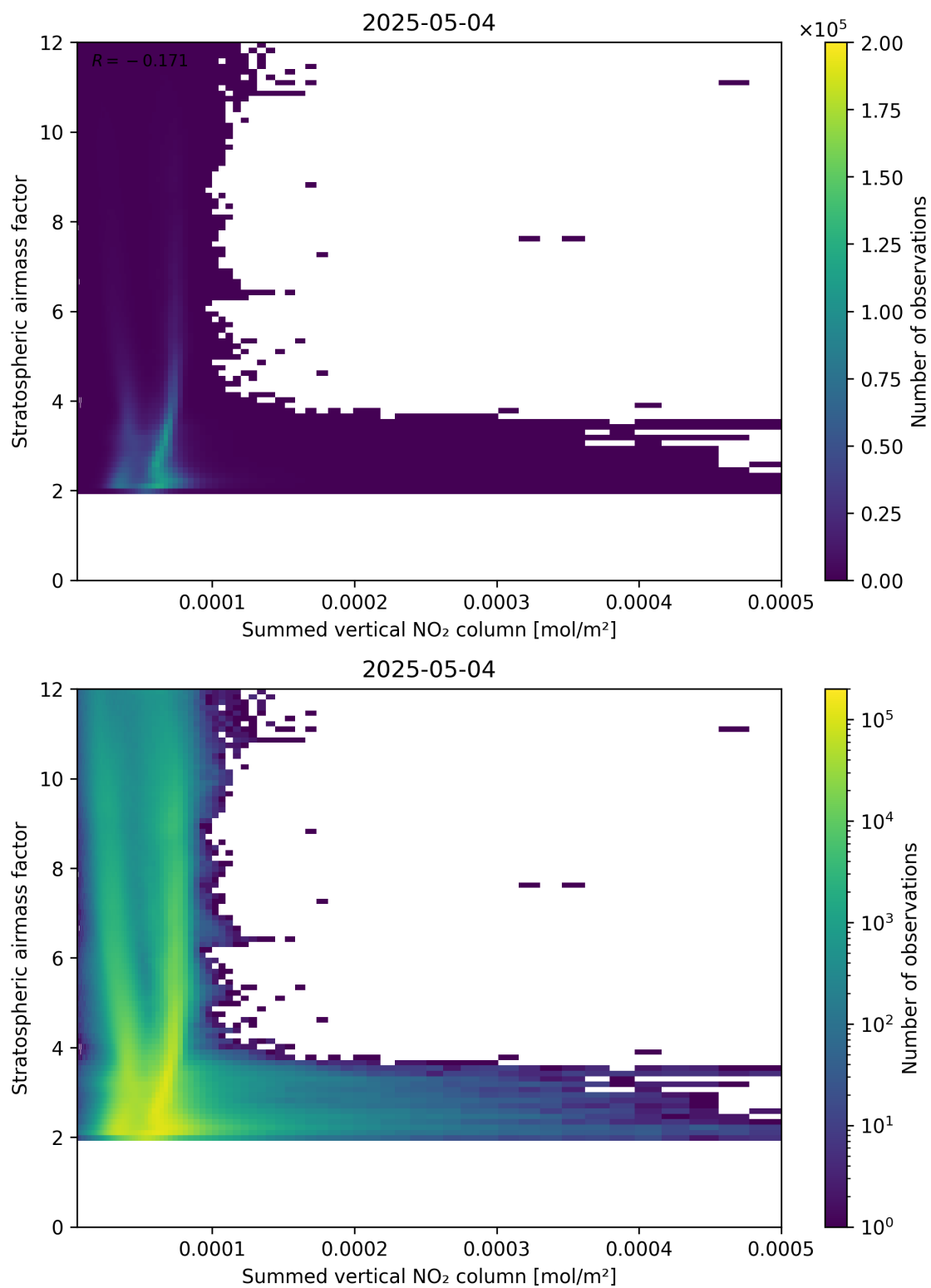
Figure 103: Scatter density plot of “Summed vertical NO 2 column” against “Stratospheric air mass factor” for 2025-05-04 to 2025-05-05.
