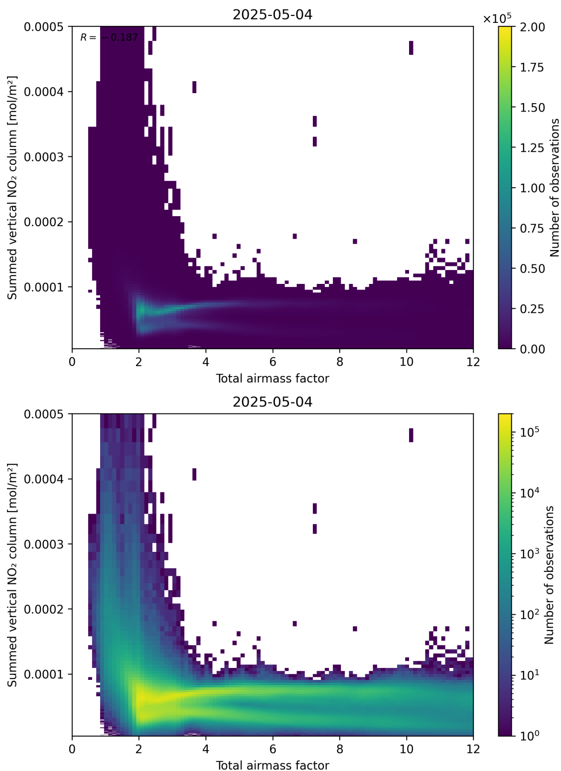
Figure 65: Scatter density plot of “Total airmass factor” against “Summed vertical NO 2 column” for 2025-05-04 to 2025-05-05.
