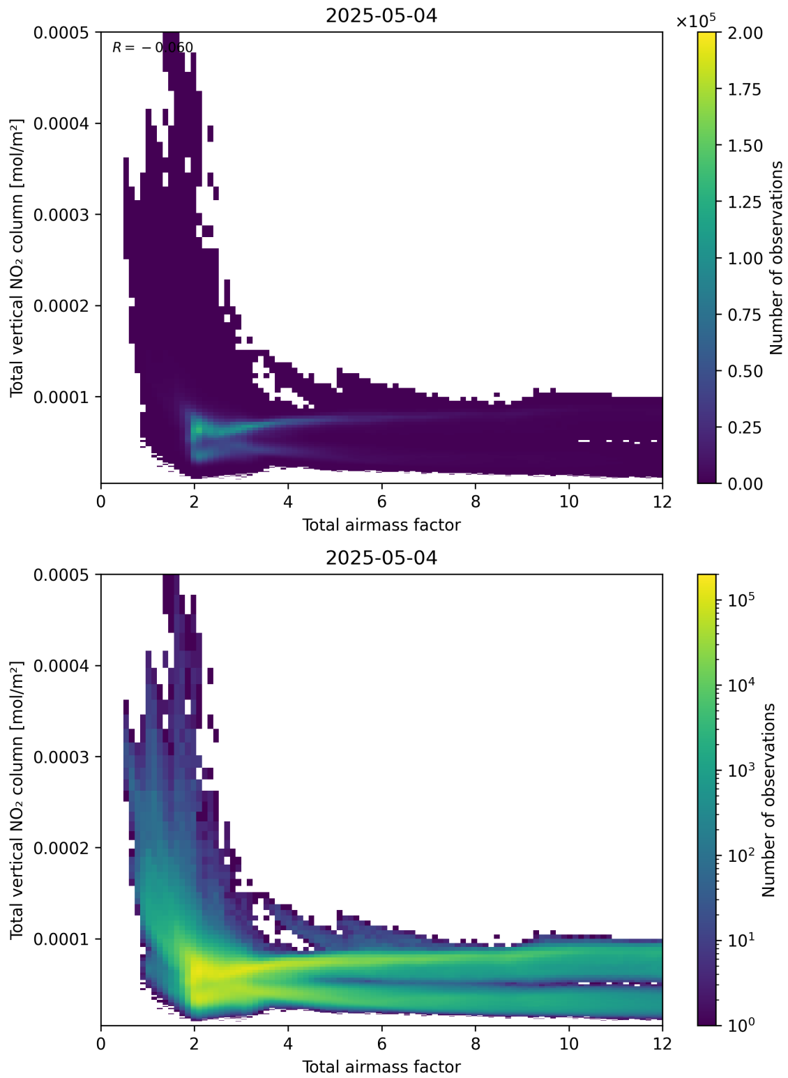
Figure 67: Scatter density plot of “Total airmass factor” against “Total vertical NO 2 column” for 2025-05-04 to 2025-05-05.
