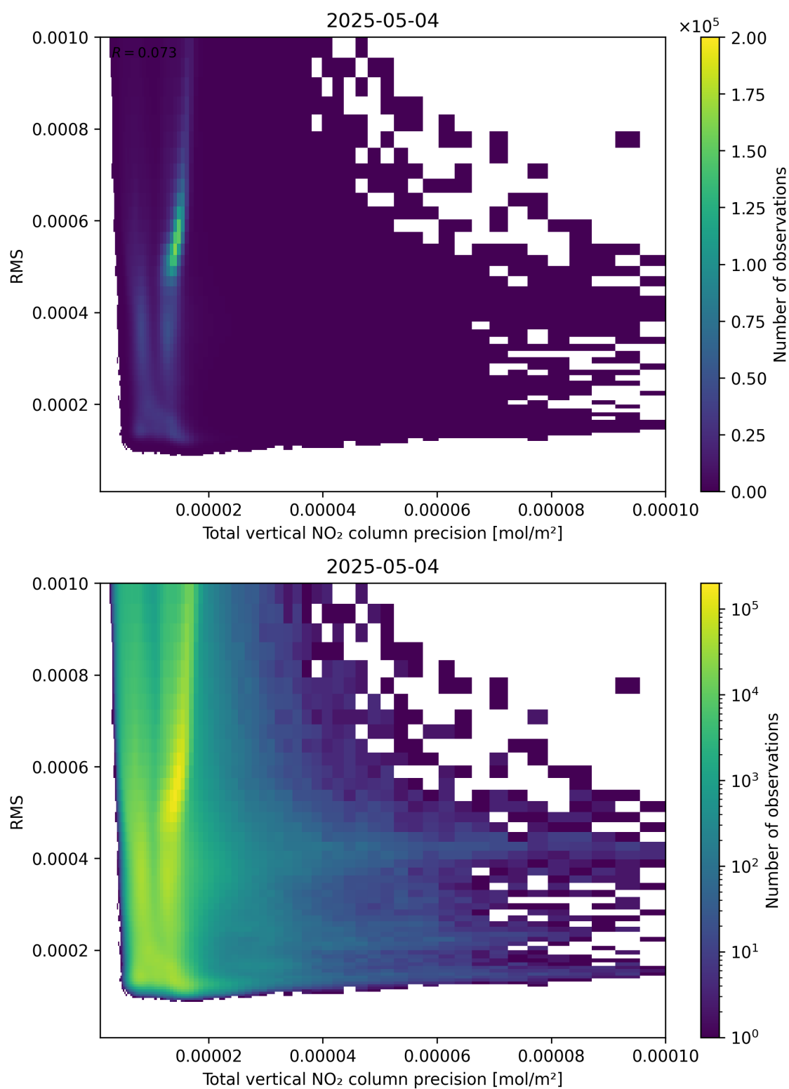
Figure 119: Scatter density plot of “Total vertical NO 2 column precision” against “RMS” for 2025-05-04 to 2025-05-05.
