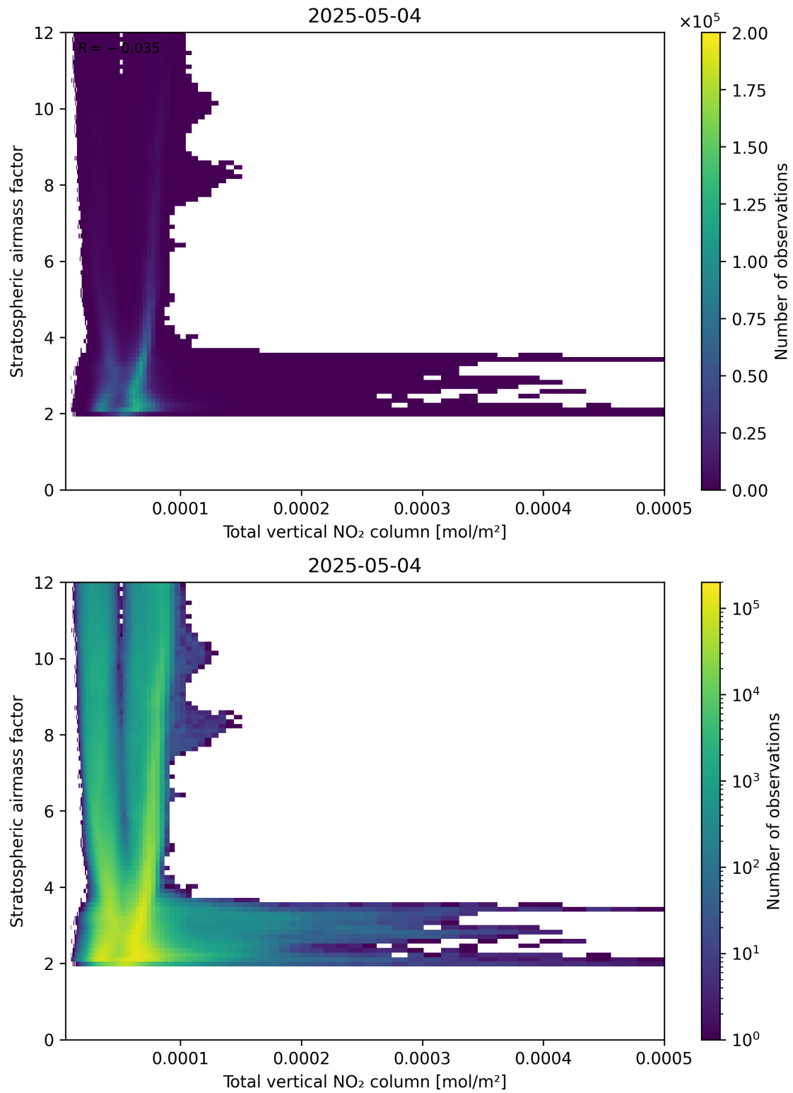
Figure 110: Scatter density plot of “Total vertical NO 2 column” against “Stratospheric airmass factor” for 2025-05-04 to 2025-05-05.
