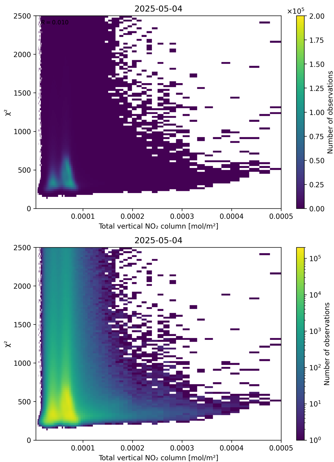
Figure 111: Scatter density plot of “Total vertical NO 2 column” against “ \chi^2 ” for 2025-05-04 to 2025-05-05.
