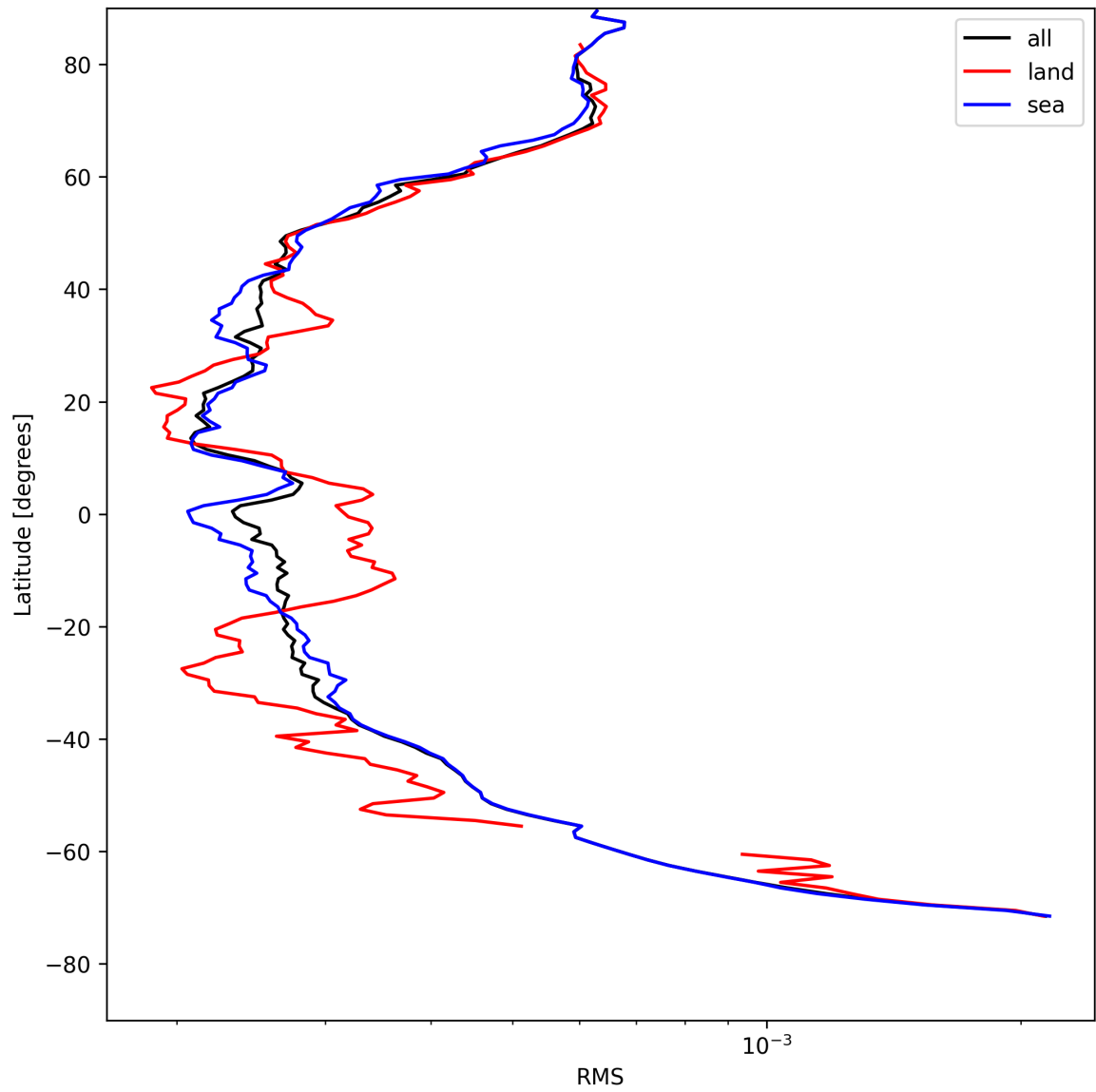
Figure 26: Zonal average of “RMS” for 2025-05-04 to 2025-05-05.
