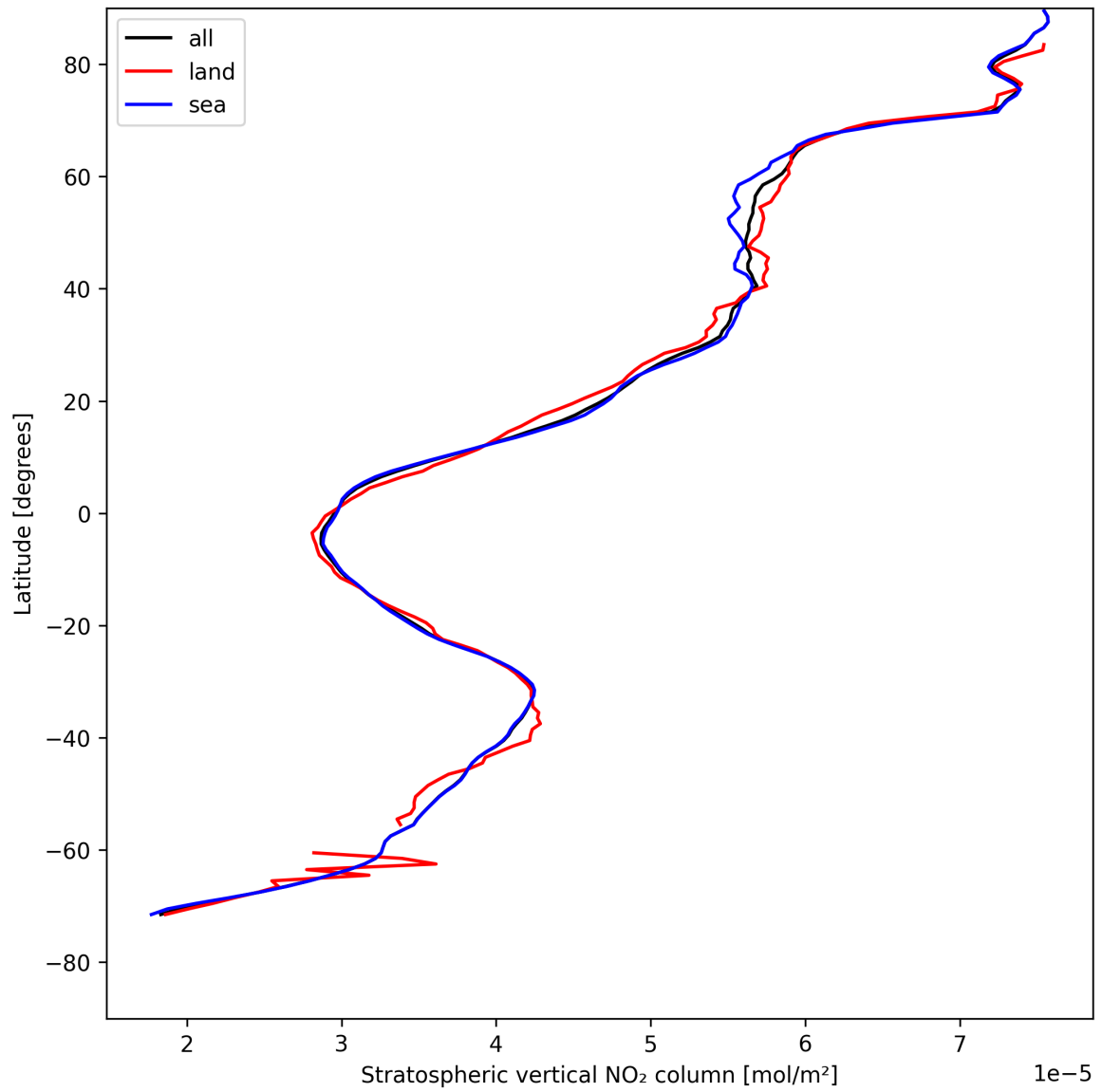
Figure 19: Zonal average of “Stratospheric vertical NO 2 column” for 2025-05-04 to 2025-05-05.
