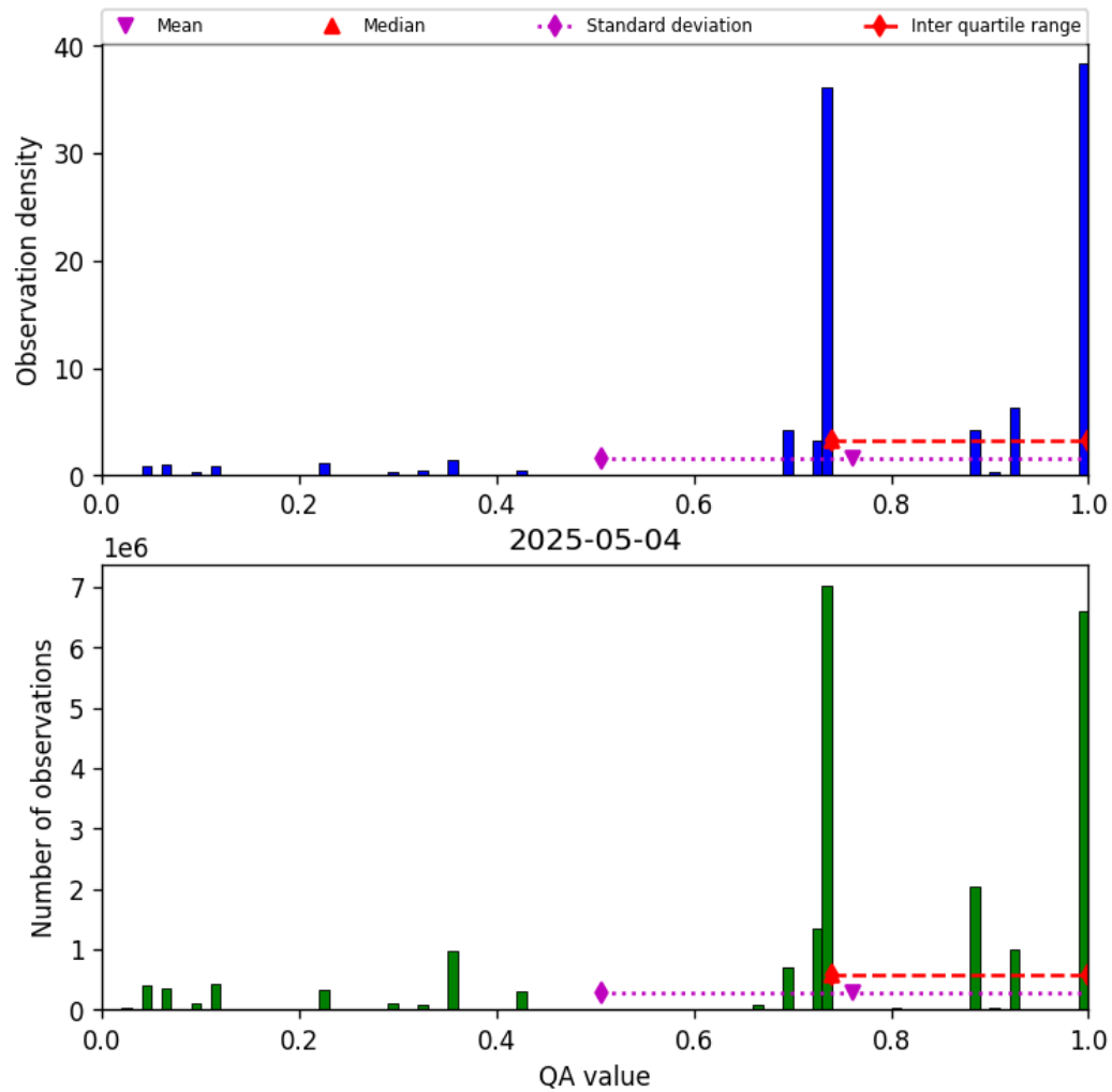
Figure 28: Histogram of “QA value” for 2025-05-04 to 2025-05-05
