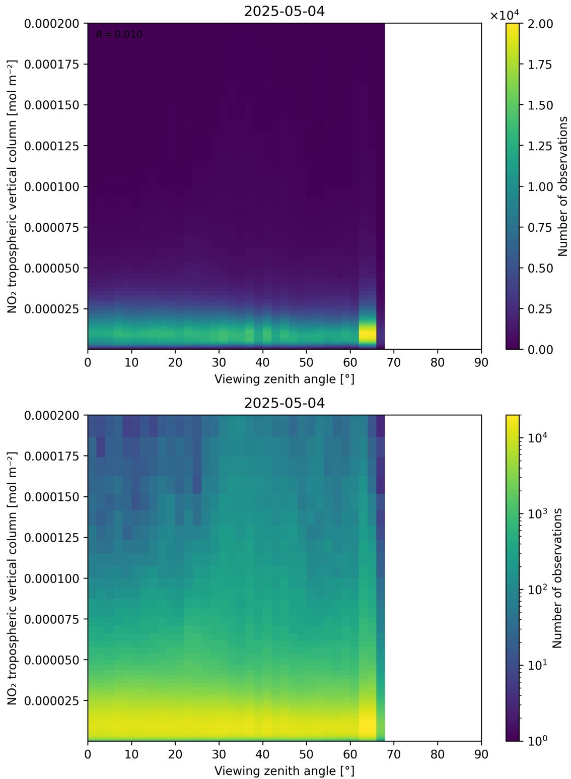
Figure 169: Scatter density plot of “Viewing zenith angle” against “NO 2 tropospheric vertical column” for 2025-05-04 to 2025-05-05.
