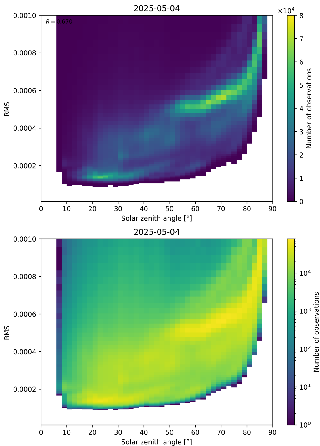
Figure 157: Scatter density plot of “Solar zenith angle” against “RMS” for 2025-05-04 to 2025-05-05.
