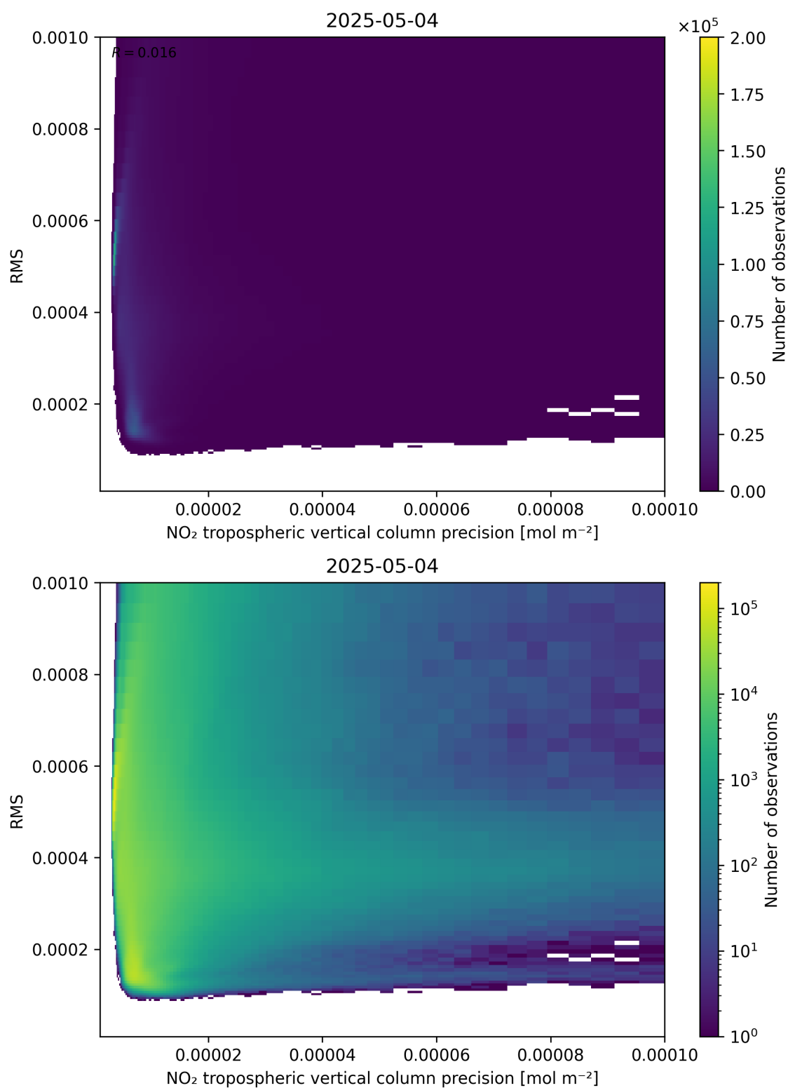
Figure 140: Scatter density plot of “NO 2 tropospheric vertical column precision” against “RMS” for 2025-05-04 to 2025-05-05.
