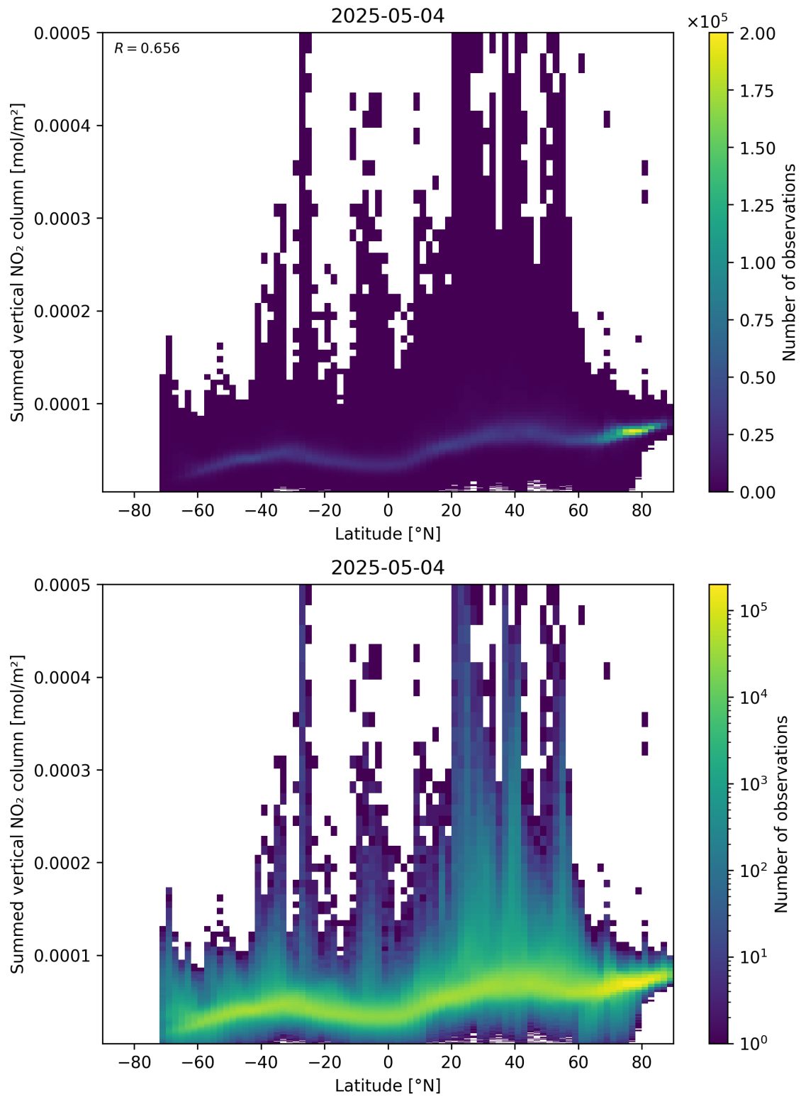
Figure 88: Scatter density plot of “Latitude” against “Summed vertical NO 2 column” for 2025-05-04 to 2025-05-05.
