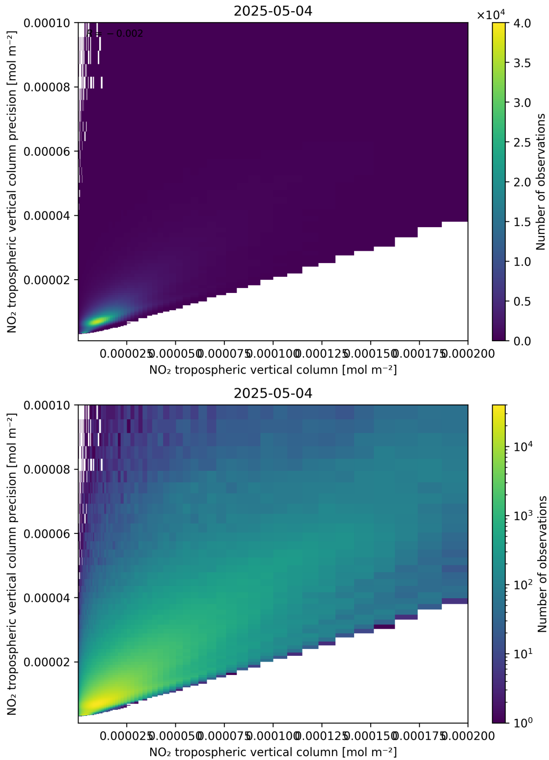
Figure 130: Scatter density plot of “NO 2 tropospheric vertical column” against “NO 2 tropospheric vertical column precision” for 2025-05-04 to 2025-05-05.
