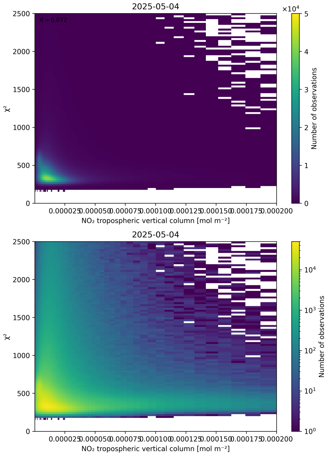
Figure 124: Scatter density plot of “NO 2 tropospheric vertical column” against “ \chi^2 ” for 2025-05-04 to 2025-05-05.
