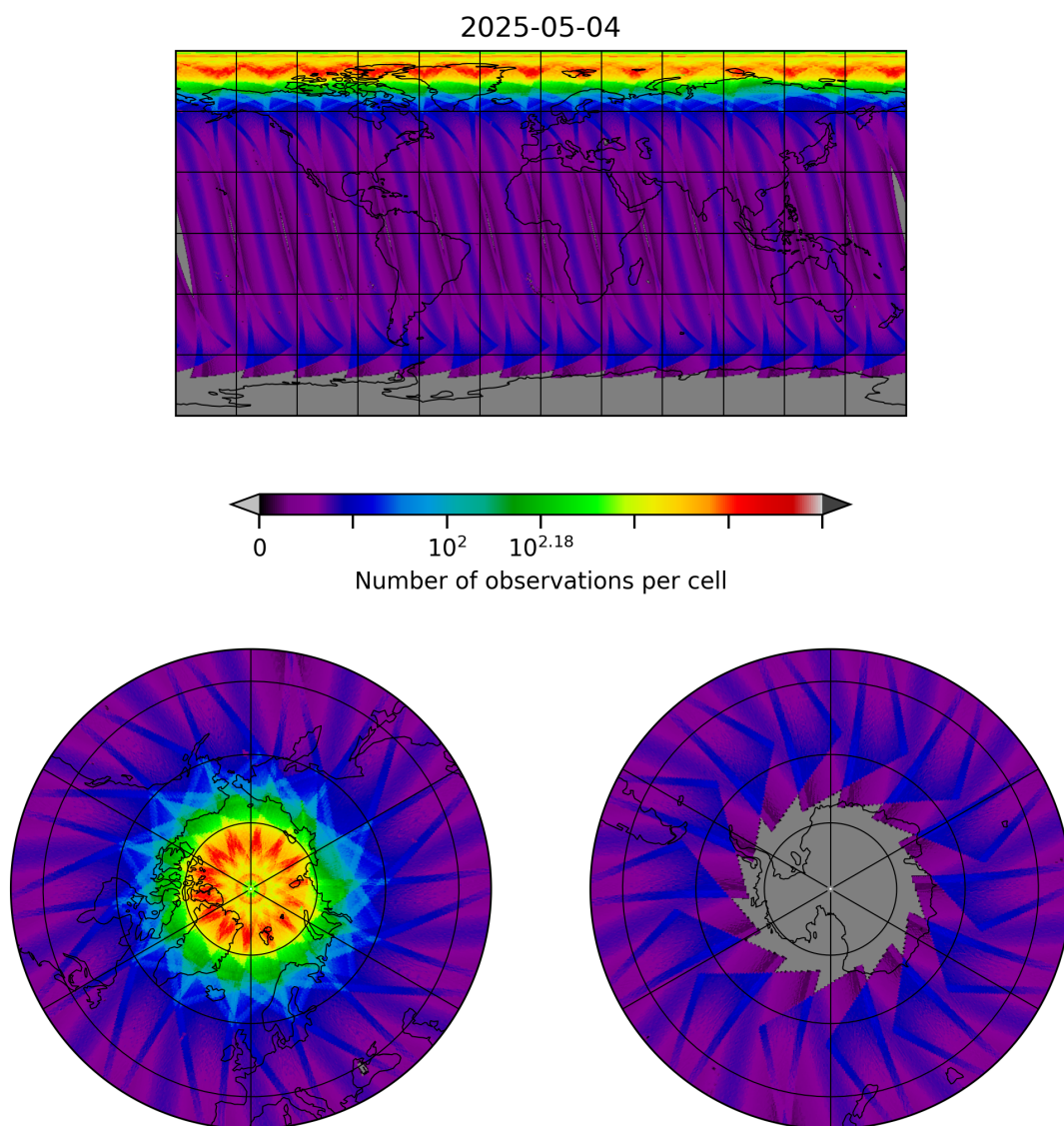
Figure 10: Map of the number of observations for 2025-05-04 to 2025-05-05
