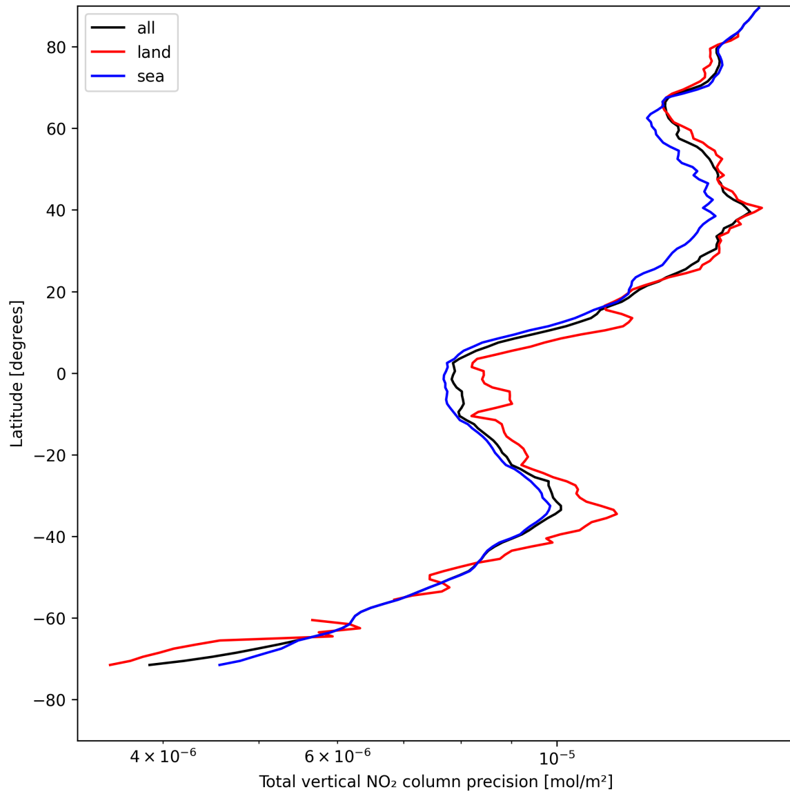
Figure 22: Zonal average of “Total vertical NO 2 column precision” for 2025-05-04 to 2025-05-05.
