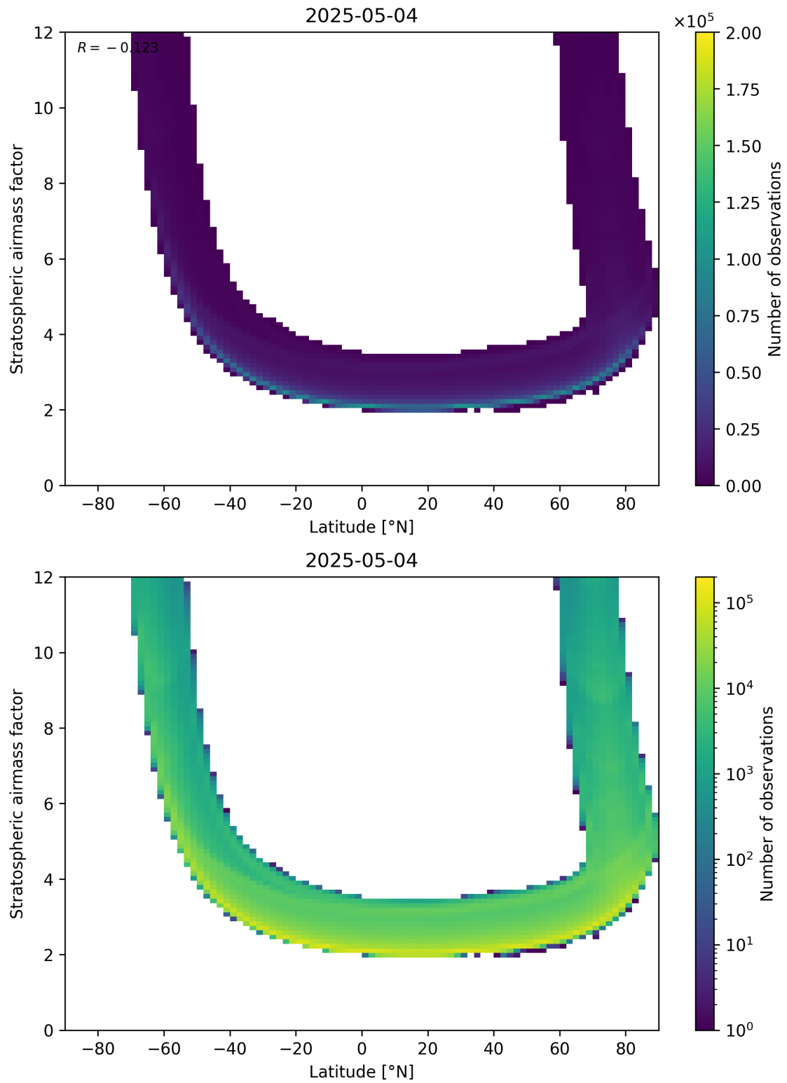
Figure 83: Scatter density plot of “Latitude” against “Stratospheric air mass factor” for 2025-05-04 to 2025-05-05.
