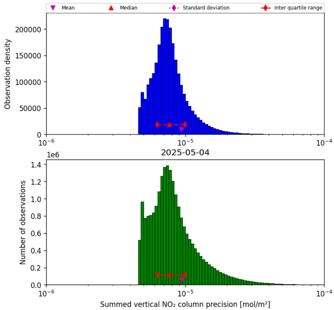
Figure 41: Histogram of "Summed vertical NO 2 column precision" for 2025-05-04 to 2025-05-05
