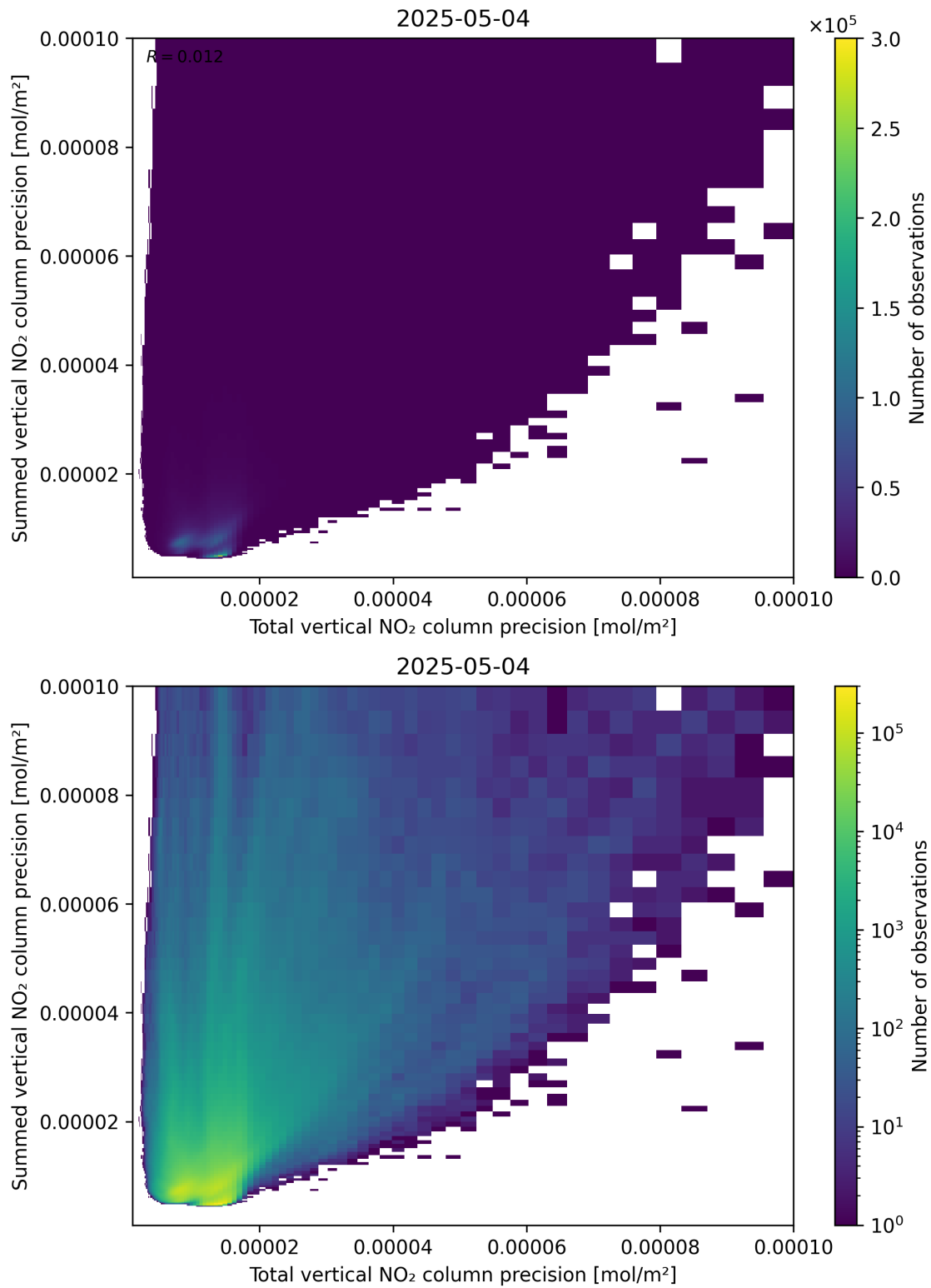
Figure 118: Scatter density plot of “Total vertical NO 2 column precision” against “Summed vertical NO 2 column precision” for 2025-05-04 to 2025-05-05.
