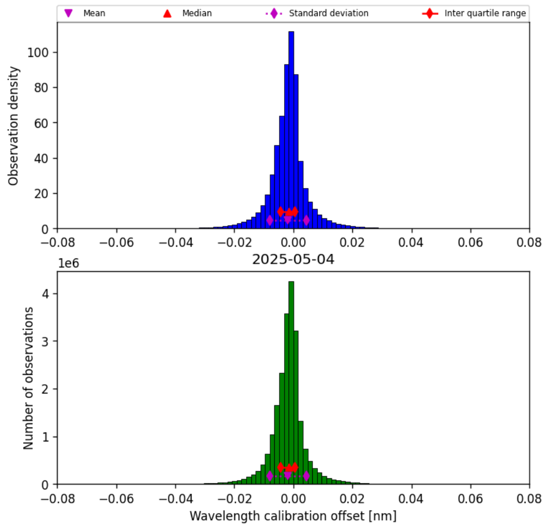
Figure 35: Histogram of “Wavelength calibration offset” for 2025-05-04 to 2025-05-05
