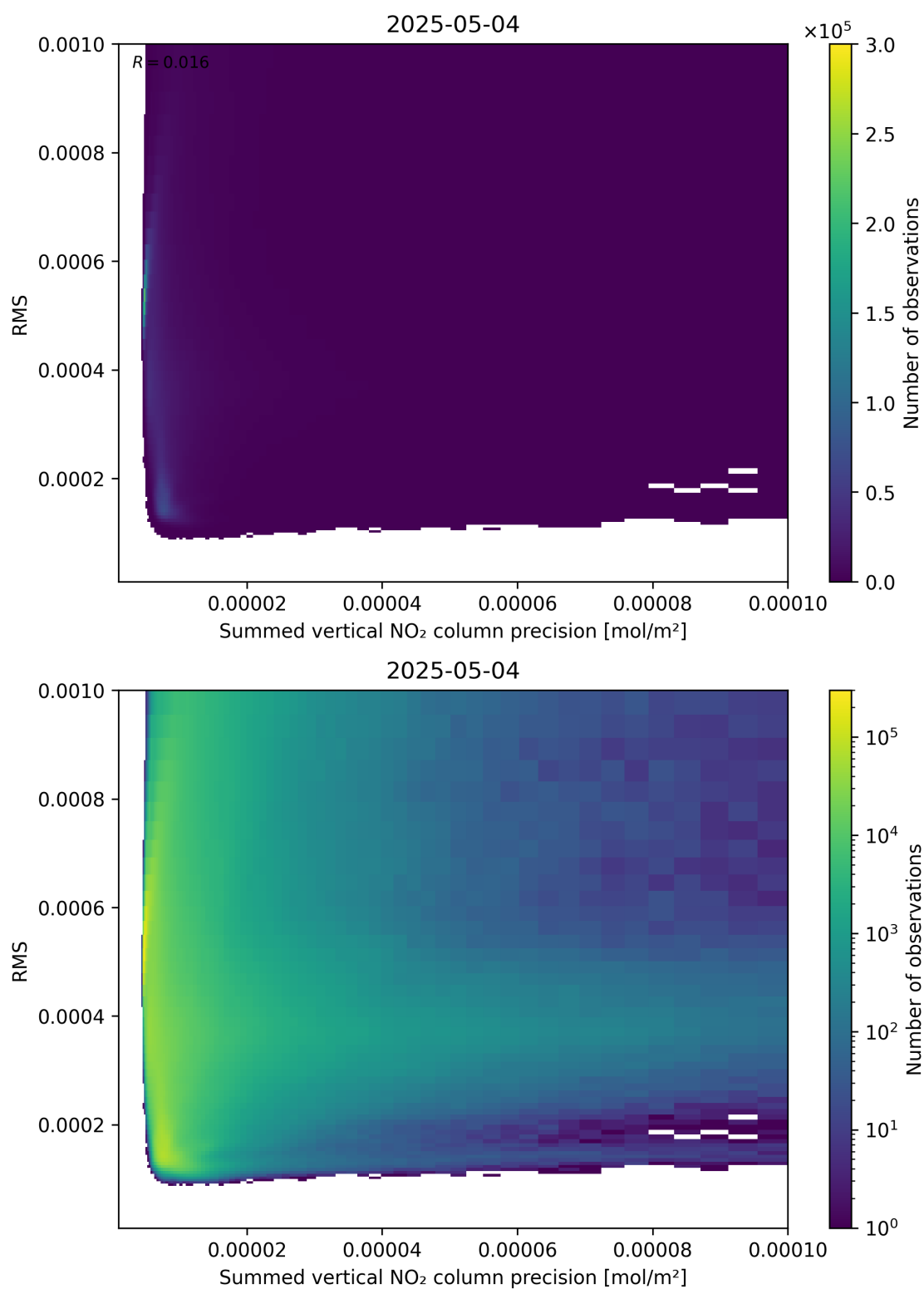
Figure 108: Scatter density plot of “Summed vertical NO 2 column precision” against “RMS” for 2025-05-04 to 2025-05-05.
