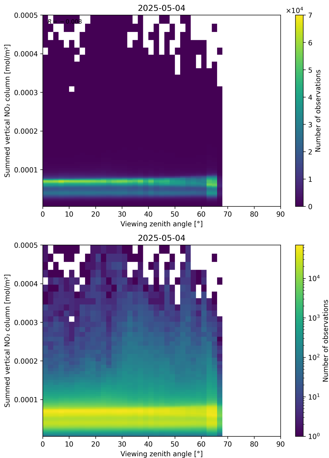
Figure 165: Scatter density plot of “Viewing zenith angle” against “Summed vertical NO 2 column” for 2025-05-04 to 2025-05-05.
