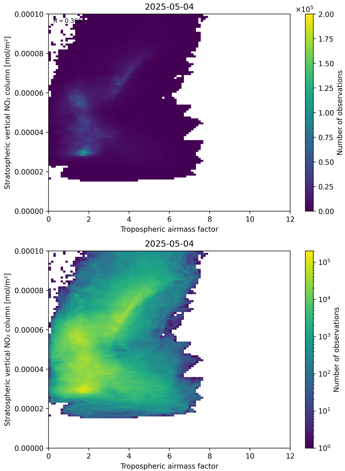
Figure 74: Scatter density plot of “Tropospheric air mass factor” against “Stratospheric vertical NO 2 column” for 2025-05-04 to 2025-05-05.
