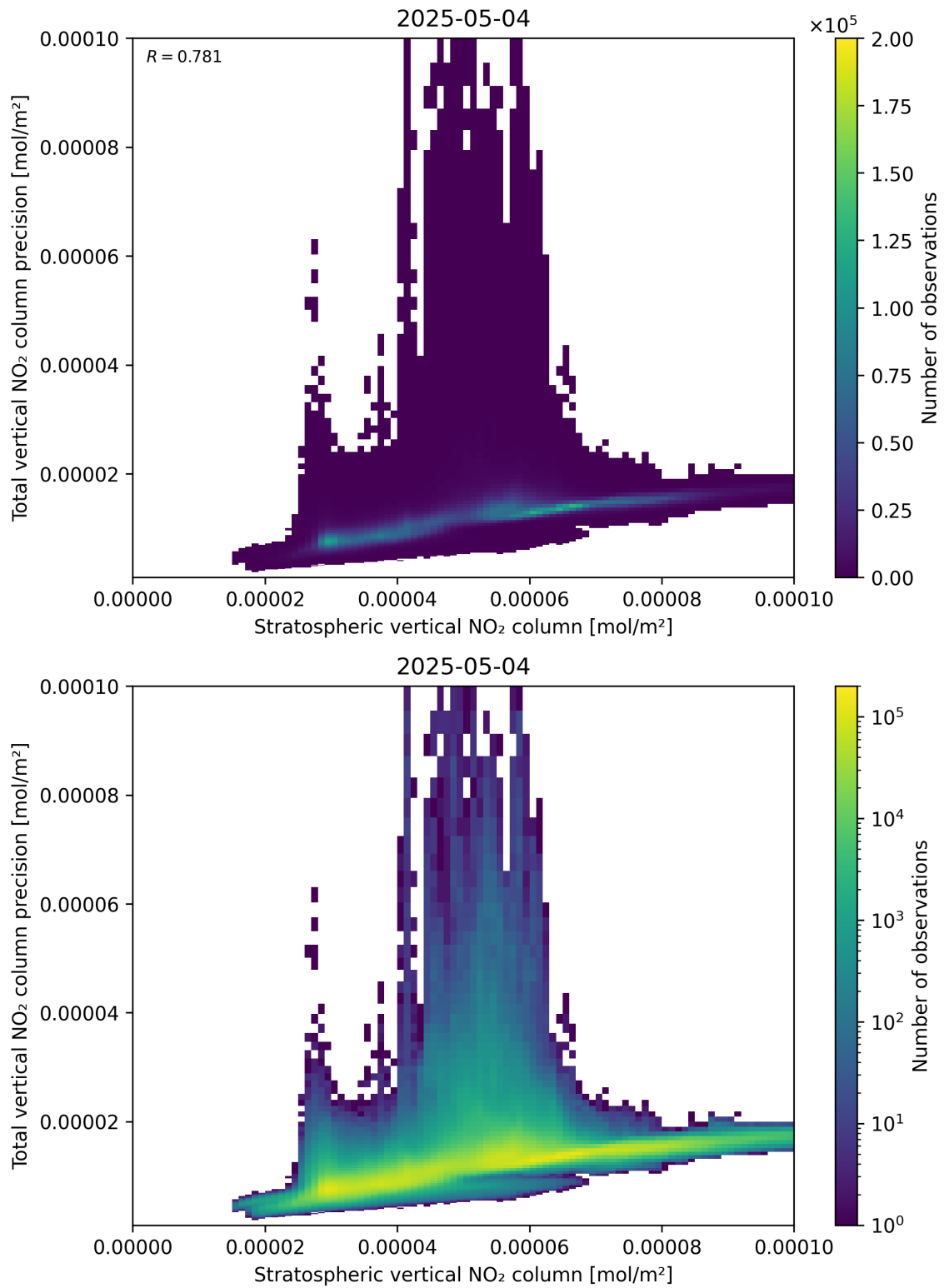
Figure 101: Scatter density plot of “Stratospheric vertical NO 2 column” against “Total vertical NO 2 column precision” for 2025-05-04 to 2025-05-05.
