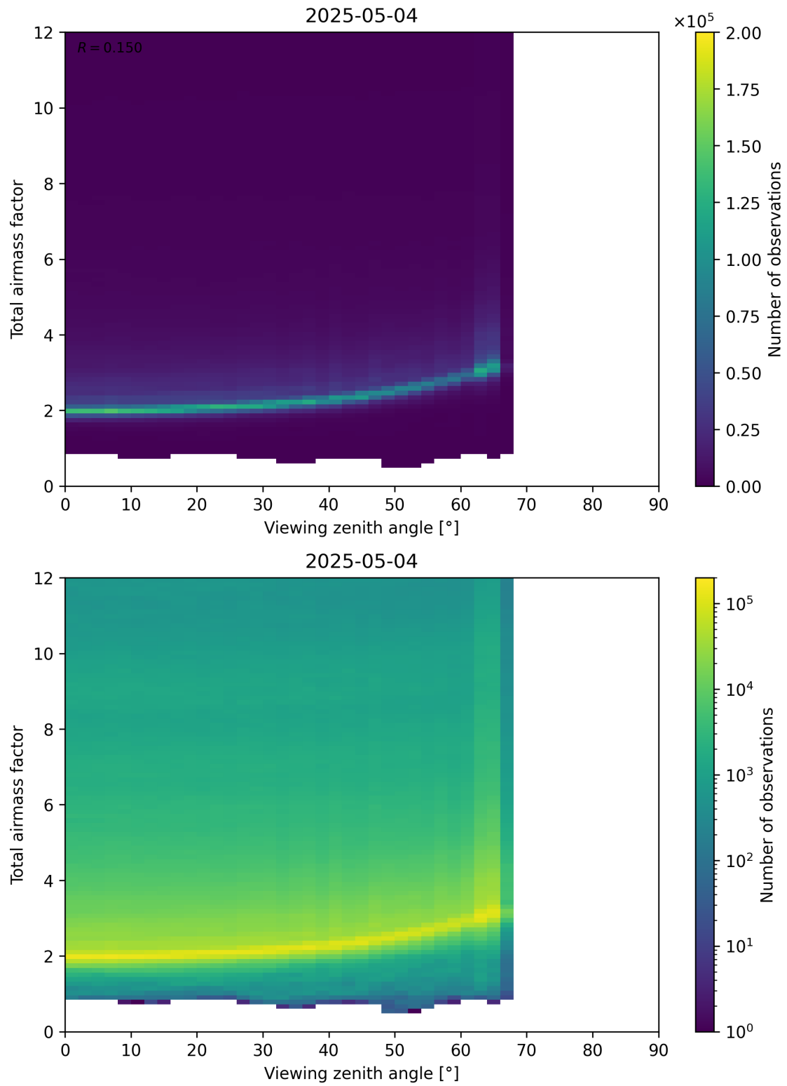
Figure 160: Scatter density plot of “Viewing zenith angle” against “Total airmass factor” for 2025-05-04 to 2025-05-05.
