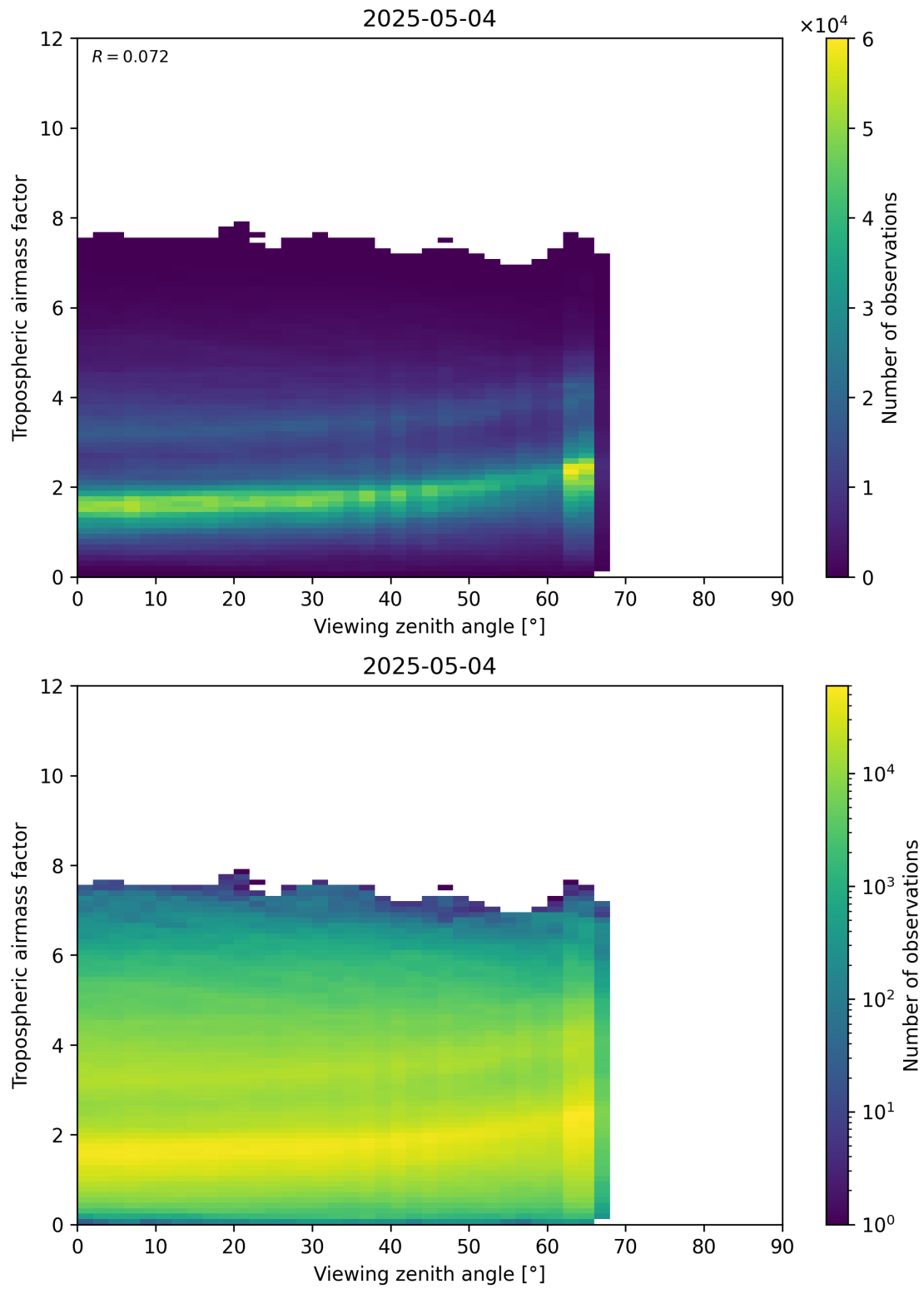
Figure 161: Scatter density plot of “Viewing zenith angle” against “Tropospheric airmass factor” for 2025-05-04 to 2025-05-05.
