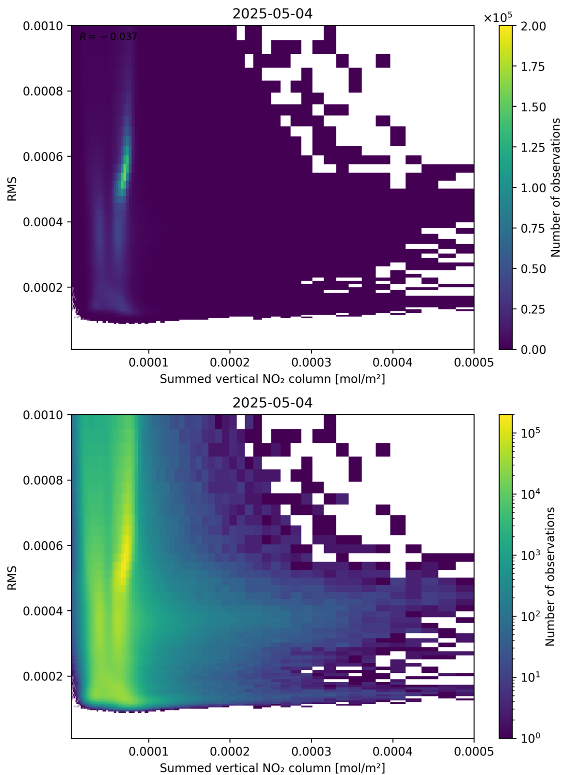
Figure 109: Scatter density plot of “Summed vertical NO 2 column” against “RMS” for 2025-05-04 to 2025-05-05.
