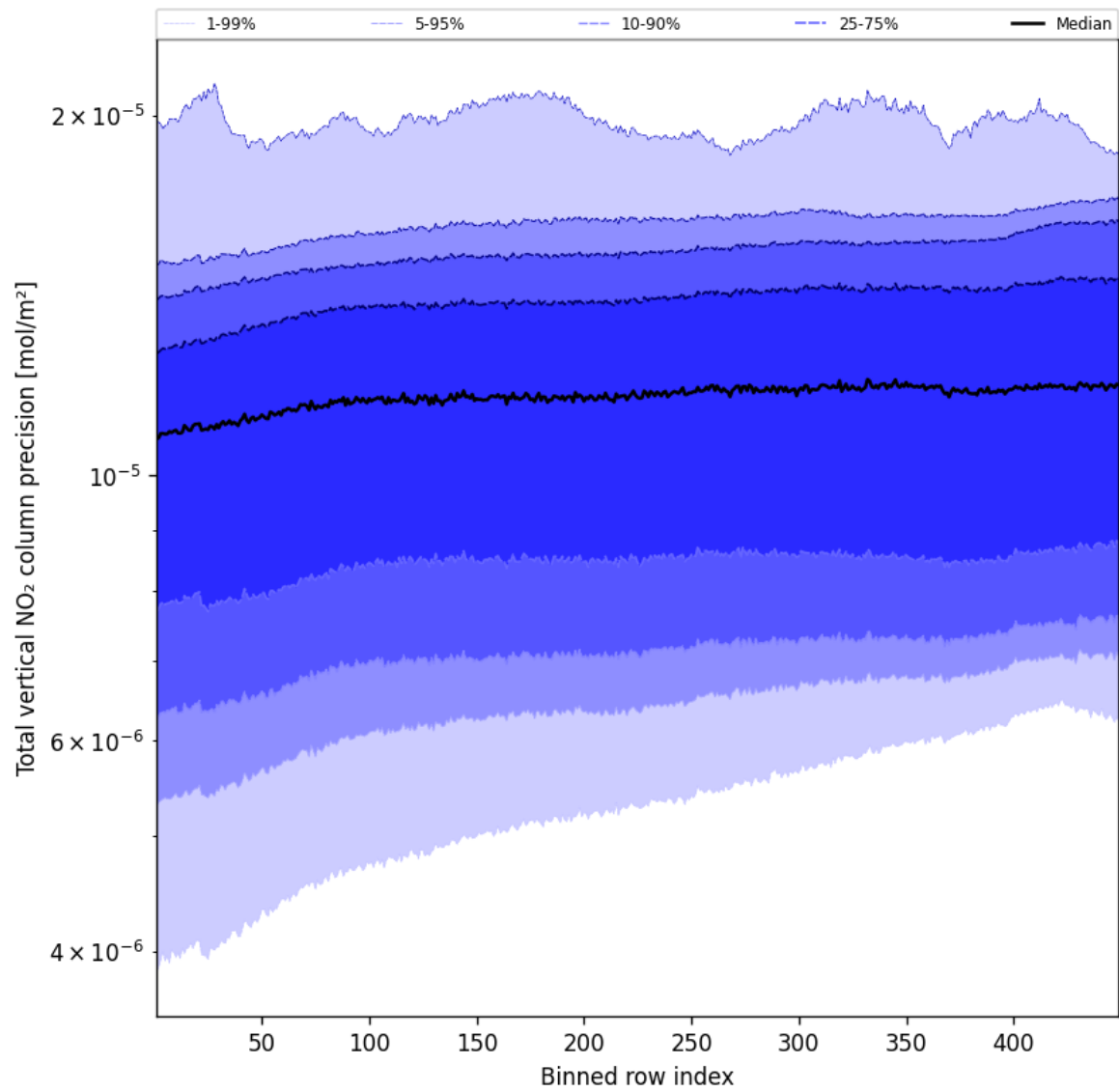
Figure 56: Along track statistics of “Total vertical NO 2 column precision” for 2025-05-04 to 2025-05-05
