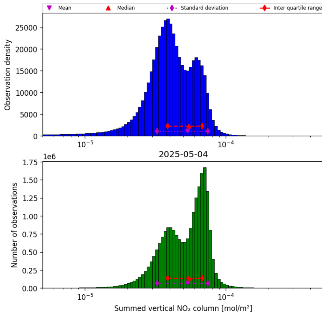
Figure 40: Histogram of “Summed vertical NO 2 column” for 2025-05-04 to 2025-05-05
