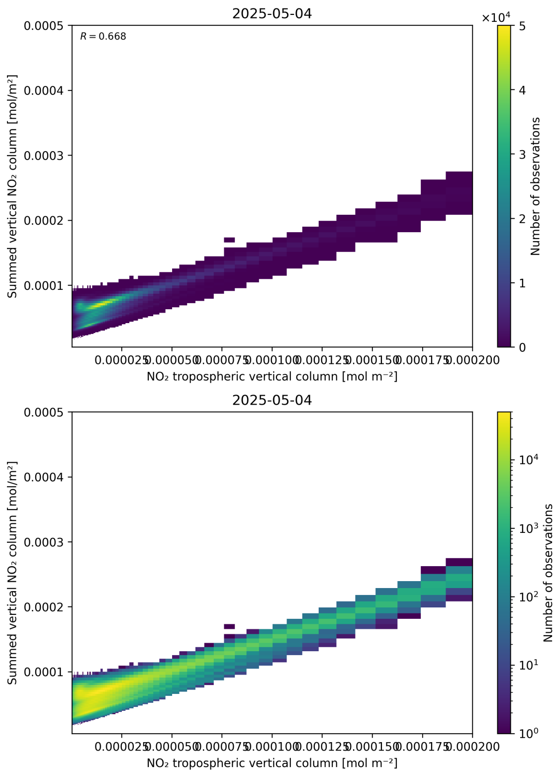
Figure 126: Scatter density plot of “NO 2 tropospheric vertical column” against “Summed vertical NO 2 column” for 2025-05-04 to 2025-05-05.
