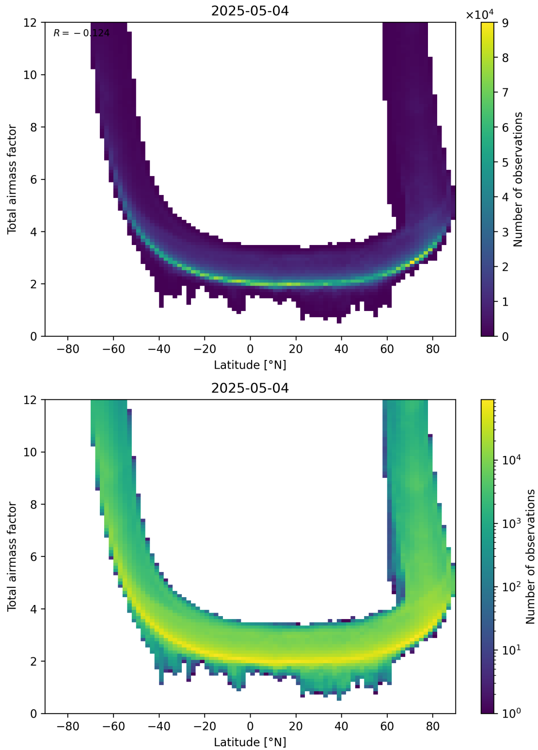
Figure 84: Scatter density plot of “Latitude” against “Total airmass factor” for 2025-05-04 to 2025-05-05.
