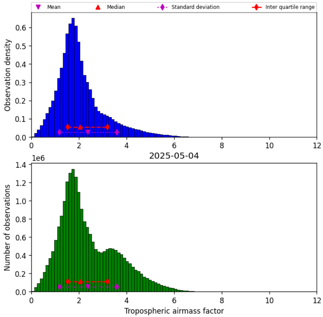
Figure 31: Histogram of “Tropospheric airmass factor” for 2025-05-04 to 2025-05-05
