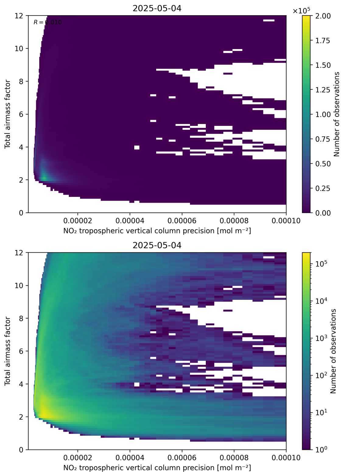
Figure 132: Scatter density plot of “NO 2 tropospheric vertical column precision” against “Total air mass factor” for 2025-05-04 to 2025-05-05.
