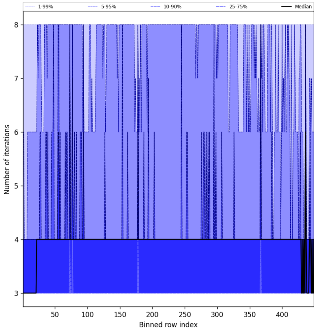
Figure 51: Along track statistics of “Number of iterations” for 2025-05-04 to 2025-05-05
