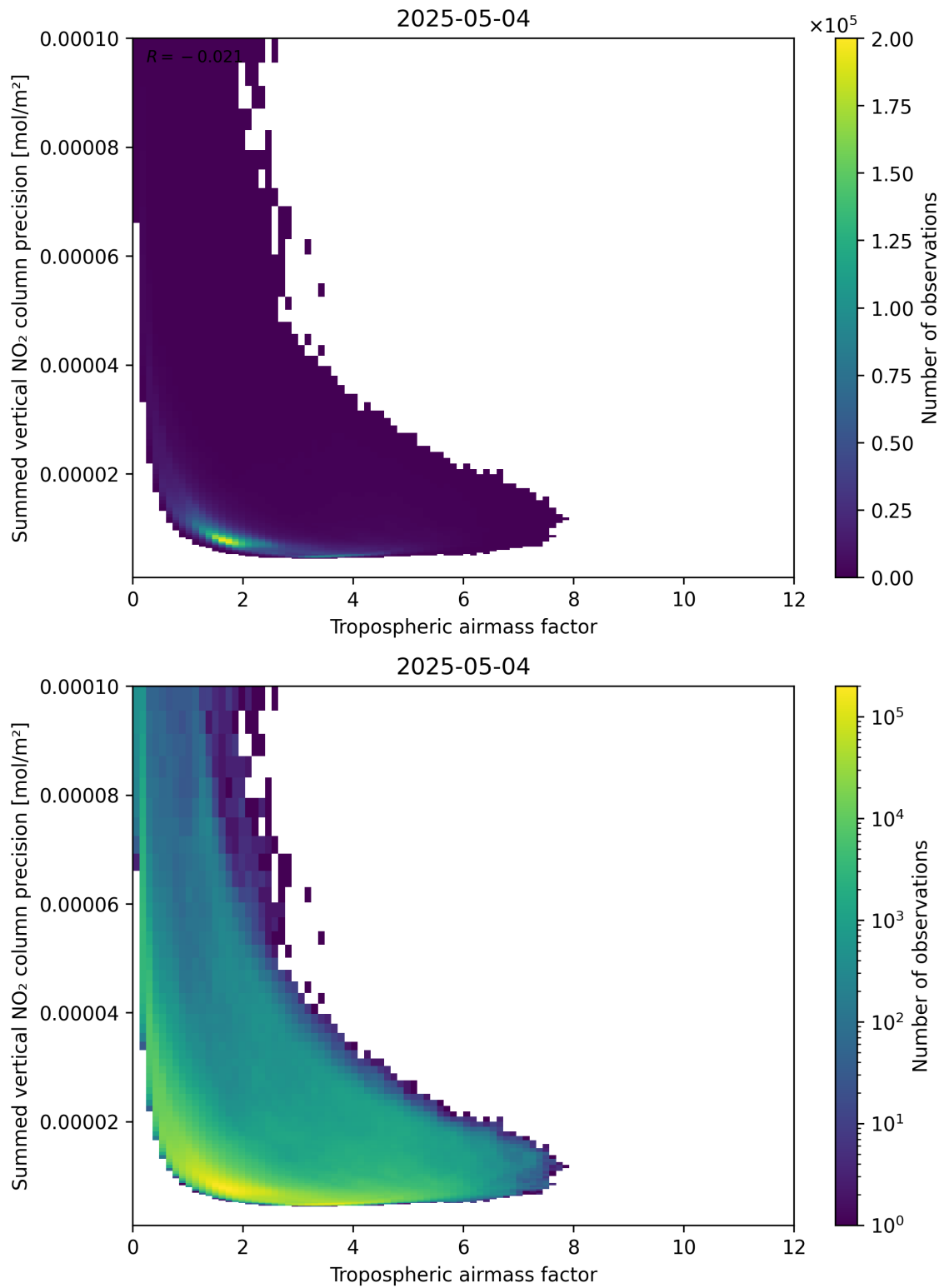
Figure 76: Scatter density plot of “Tropospheric air mass factor” against “Summed vertical NO 2 column precision” for 2025-05-04 to 2025-05-05.
