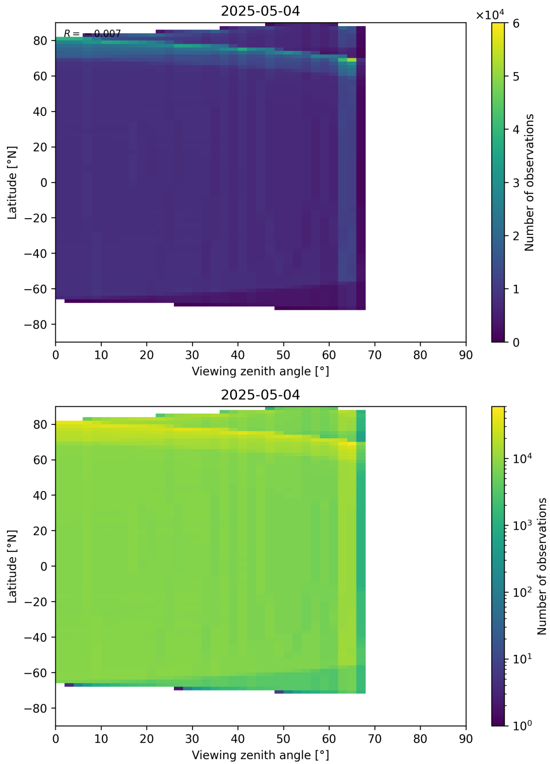
Figure 163: Scatter density plot of “Viewing zenith angle” against “Latitude” for 2025-05-04 to 2025-05-05.
