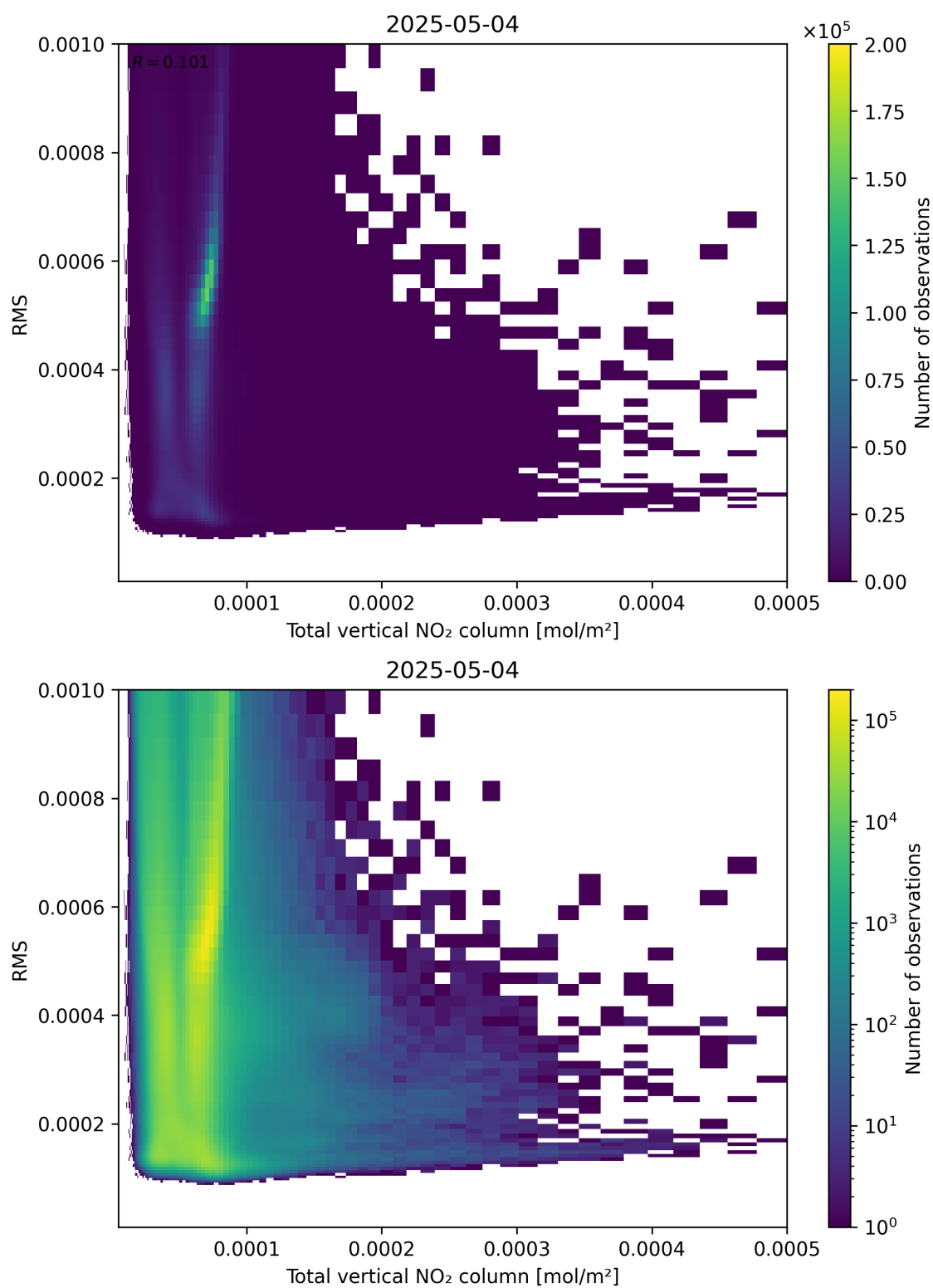
Figure 120: Scatter density plot of “Total vertical NO 2 column” against “RMS” for 2025-05-04 to 2025-05-05.
