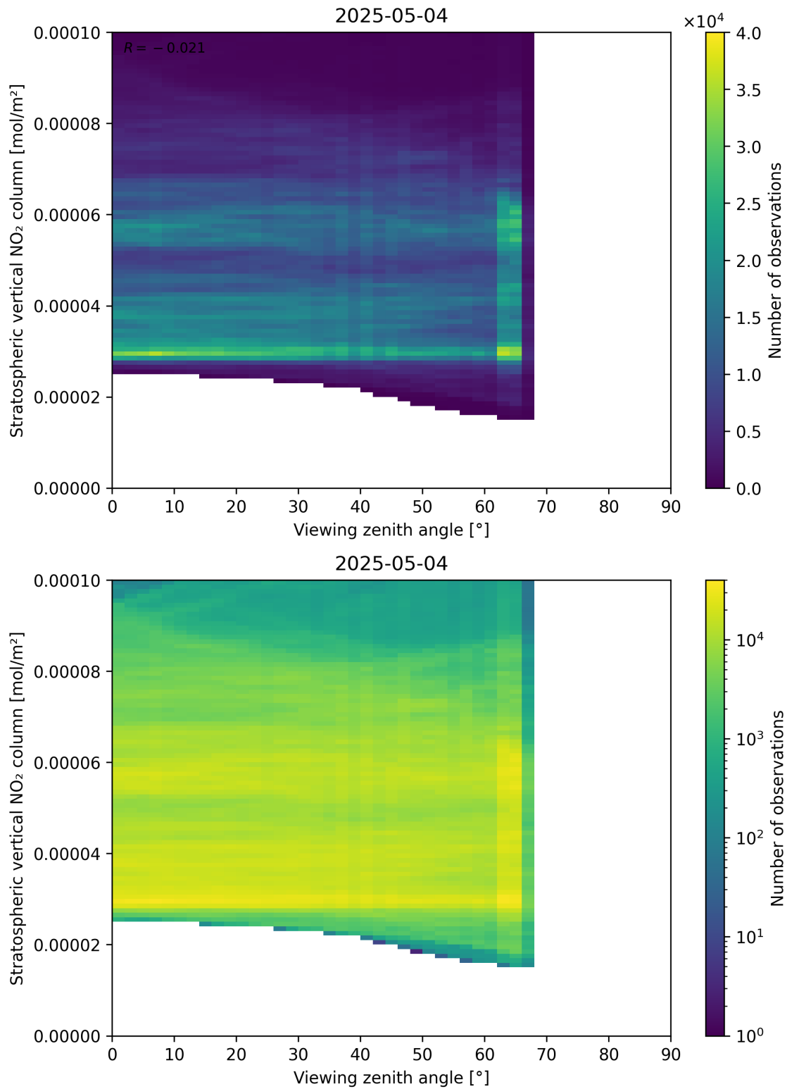
Figure 164: Scatter density plot of “Viewing zenith angle” against “Stratospheric vertical NO 2 column” for 2025-05-04 to 2025-05-05.
