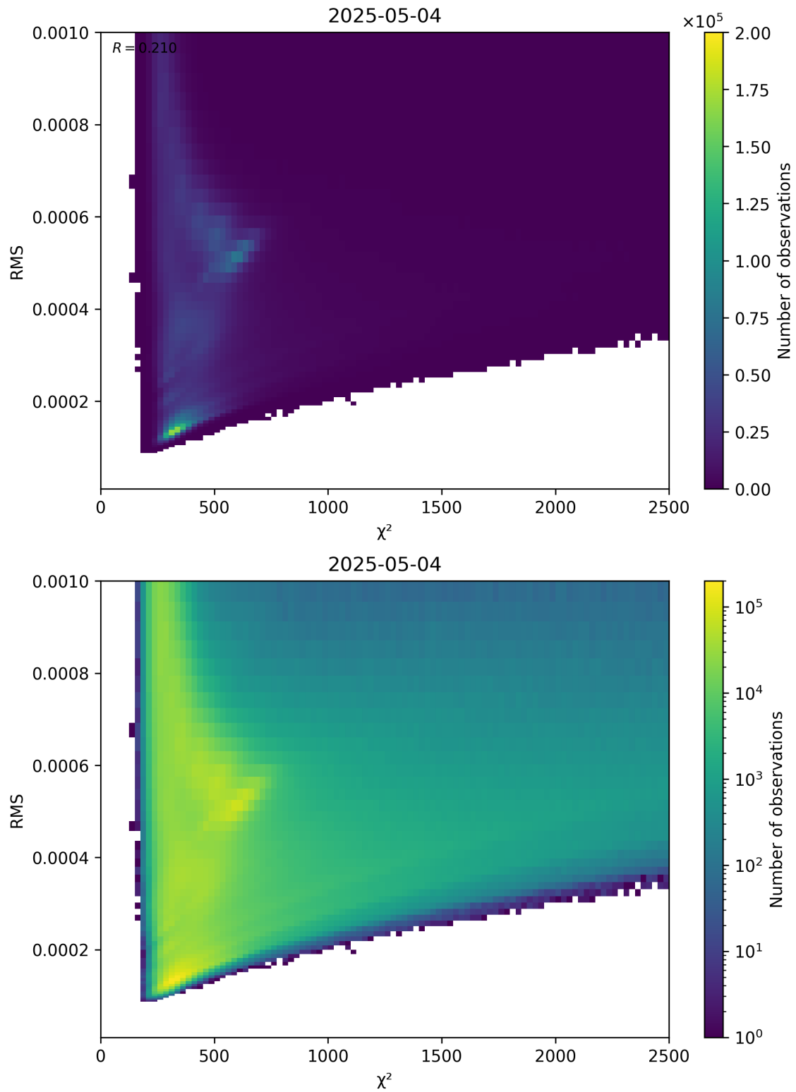
Figure 82: Scatter density plot of “ \chi^2 ” against “RMS” for 2025-05-04 to 2025-05-05.
