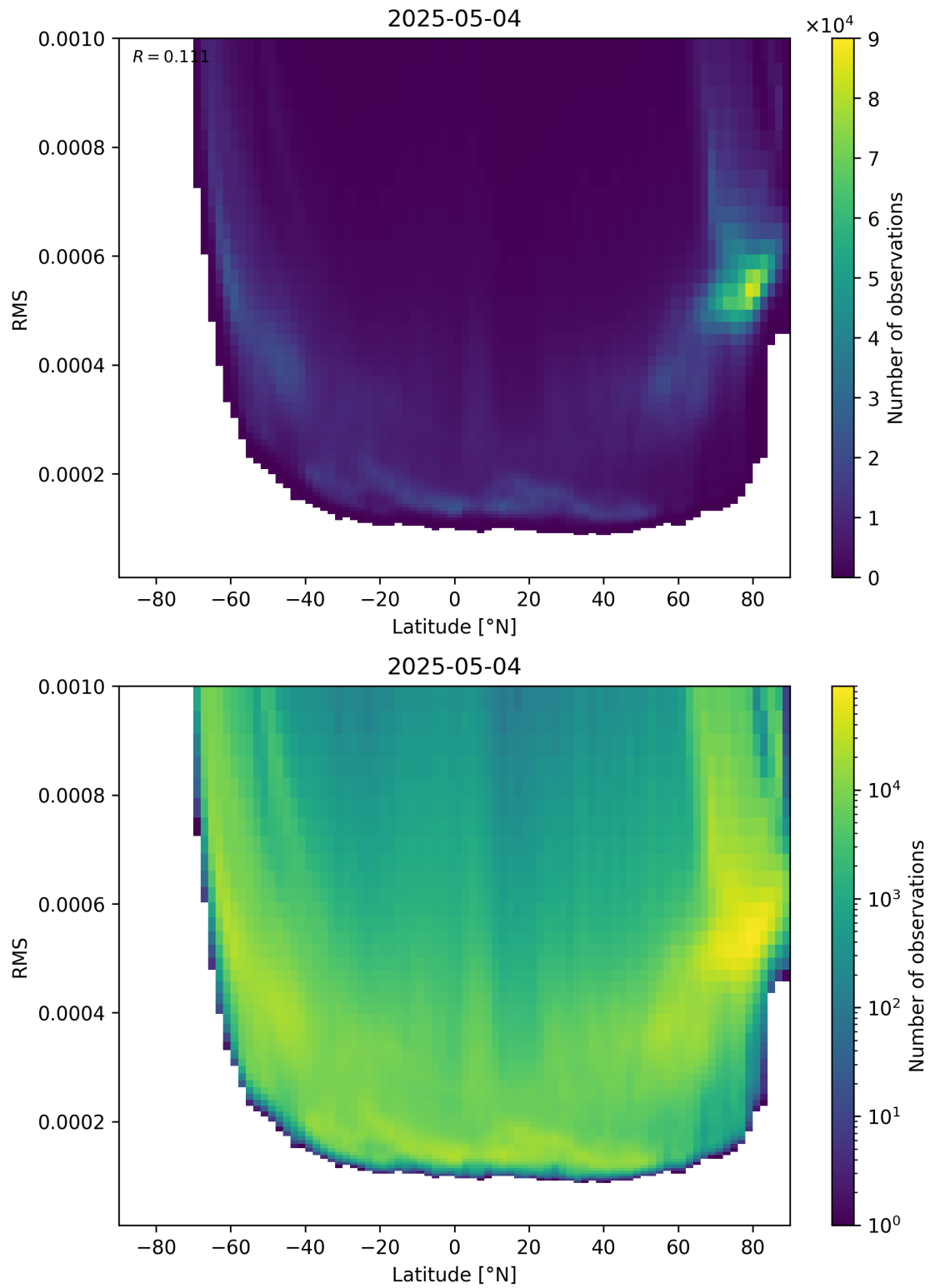
Figure 94: Scatter density plot of “Latitude” against “RMS” for 2025-05-04 to 2025-05-05.
