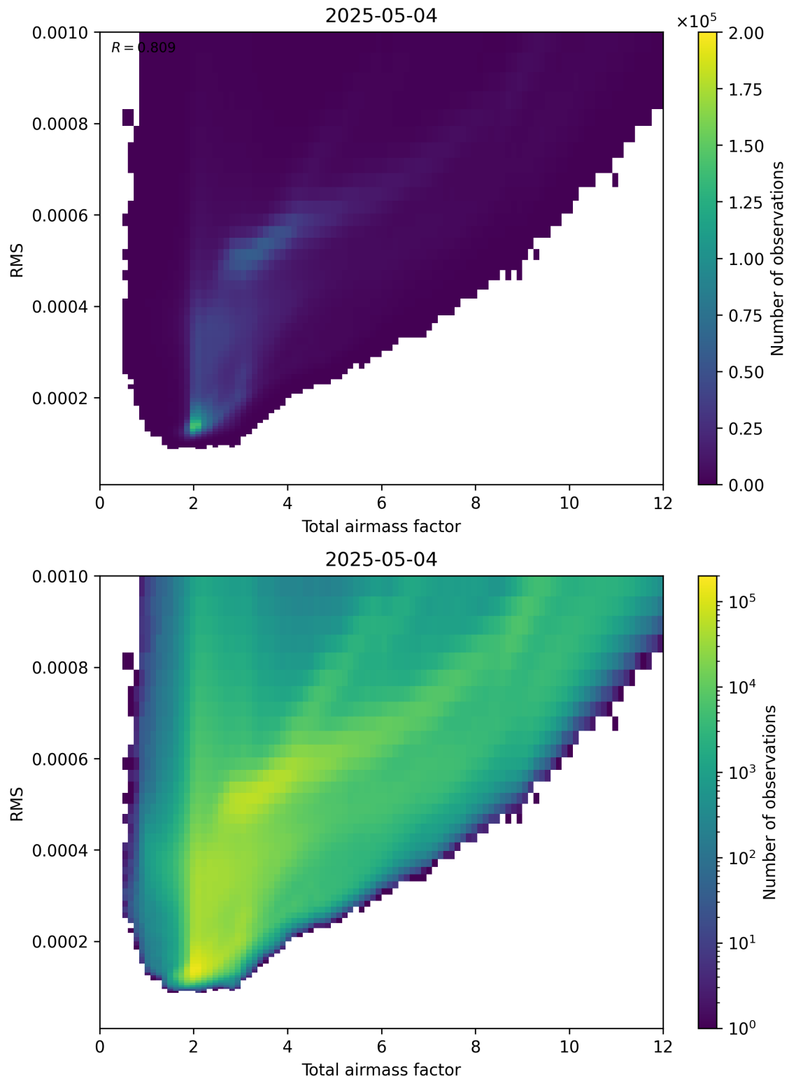
Figure 69: Scatter density plot of “Total airmass factor” against “RMS” for 2025-05-04 to 2025-05-05.
