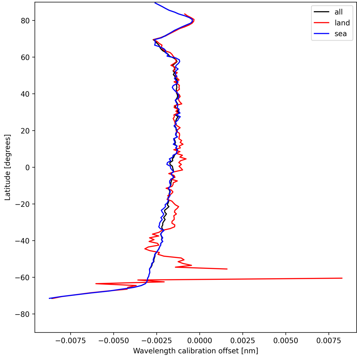
Figure 18: Zonal average of “Wavelength calibration offset” for 2025-05-04 to 2025-05-05.
