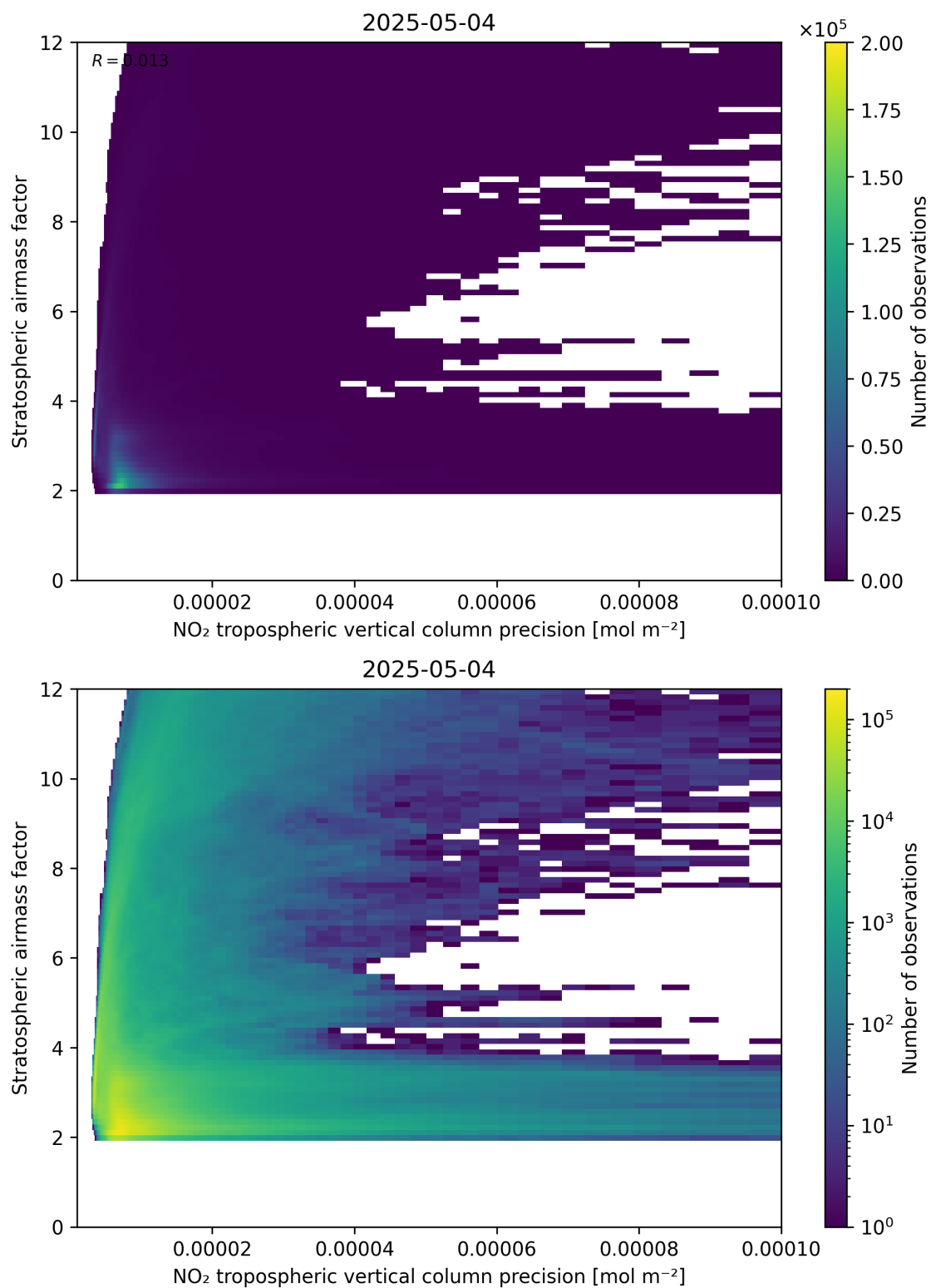
Figure 131: Scatter density plot of “NO 2 tropospheric vertical column precision” against “Stratospheric airmass factor” for 2025-05-04 to 2025-05-05.
