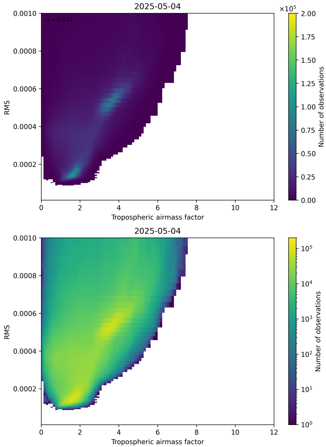
Figure 79: Scatter density plot of “Tropospheric airmass factor” against “RMS” for 2025-05-04 to 2025-05-05.
