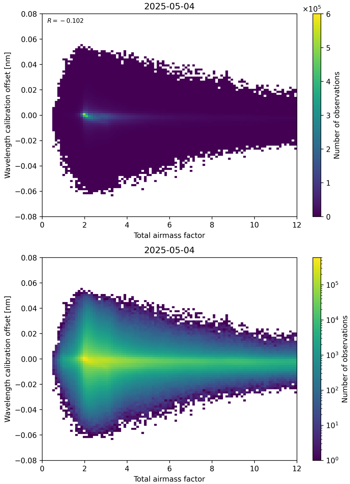
Figure 70: Scatter density plot of “Total airmass factor” against “Wavelength calibration offset” for 2025-05-04 to 2025-05-05.
