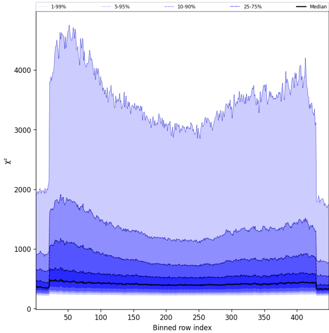
Figure 59: Along track statistics of “ \chi^2 ” for 2025-05-04 to 2025-05-05
