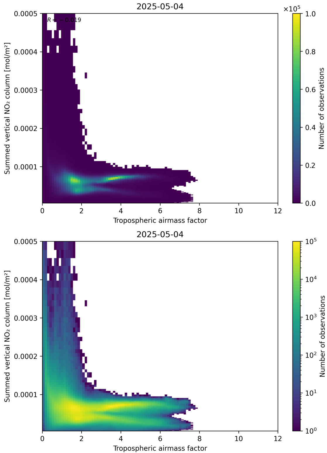
Figure 75: Scatter density plot of “Tropospheric air mass factor” against “Summed vertical NO 2 column” for 2025-05-04 to 2025-05-05.
