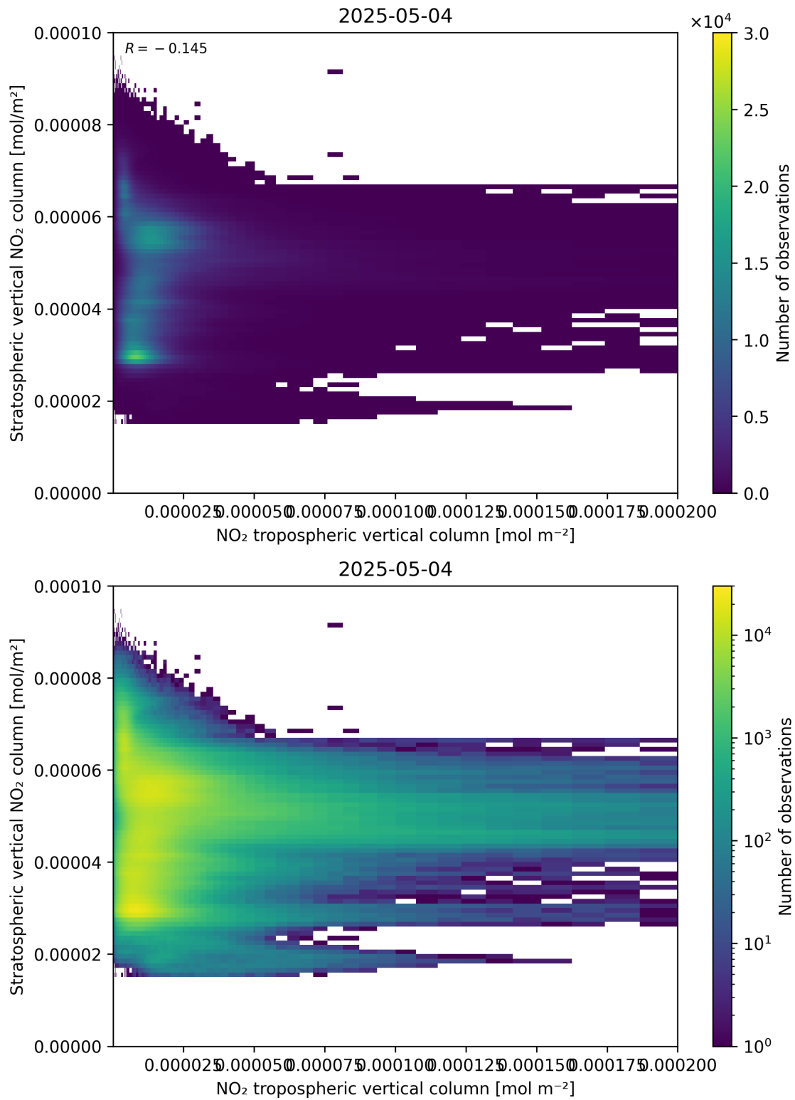
Figure 125: Scatter density plot of “NO 2 tropospheric vertical column” against “Stratospheric vertical NO 2 column” for 2025-05-04 to 2025-05-05.
