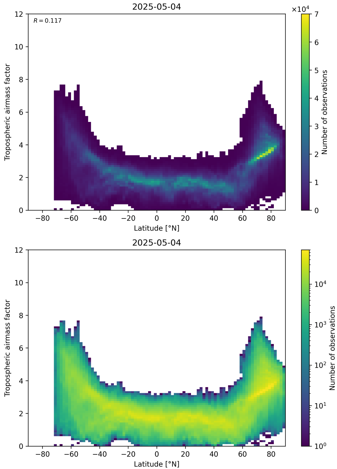
Figure 85: Scatter density plot of “Latitude” against “Tropospheric air mass factor” for 2025-05-04 to 2025-05-05.
