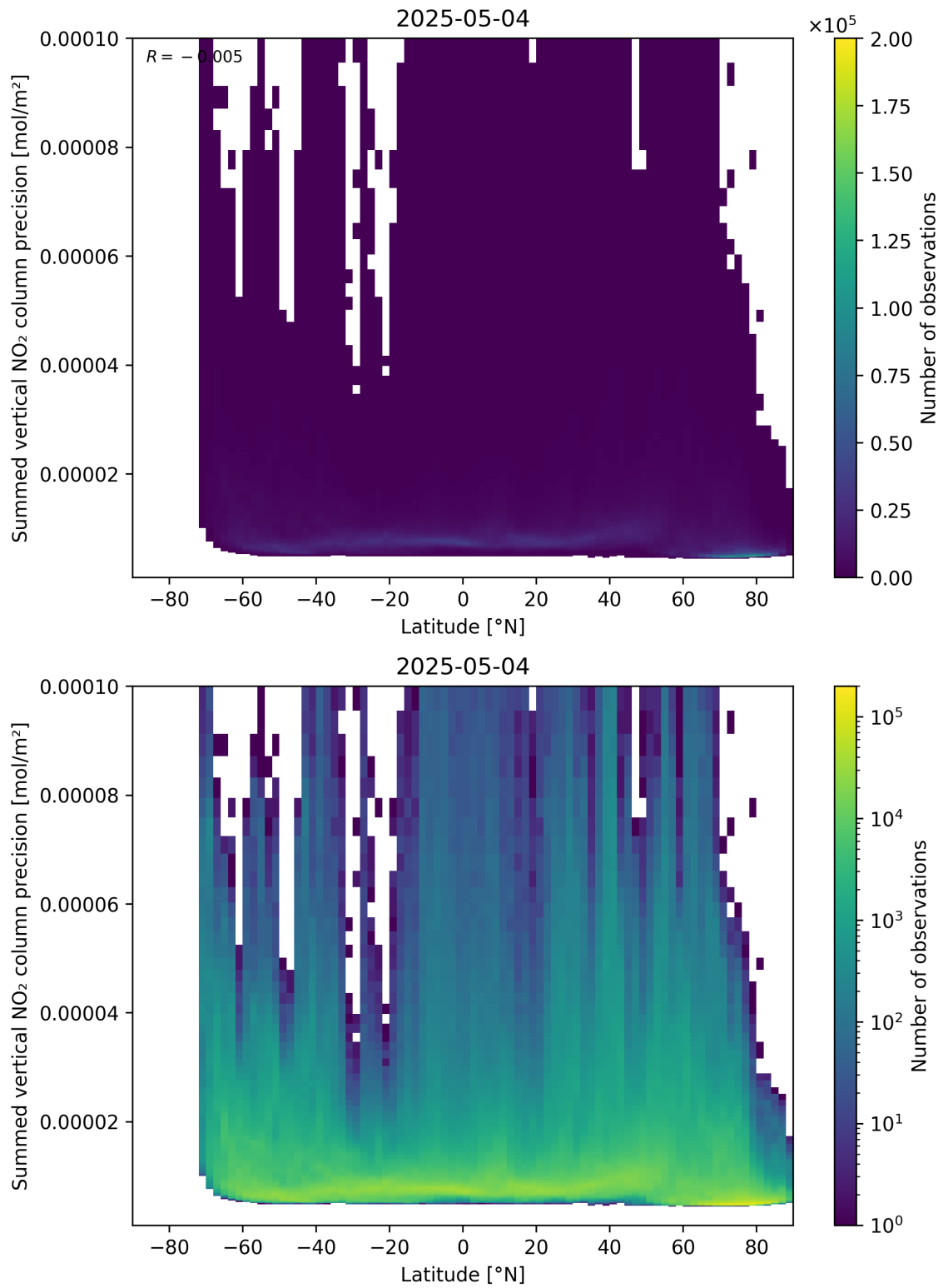
Figure 89: Scatter density plot of “Latitude” against “Summed vertical NO 2 column precision” for 2025-05-04 to 2025-05-05.
