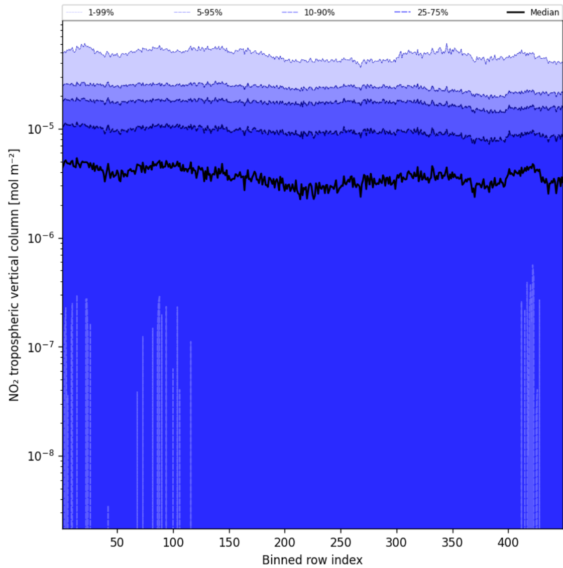
Figure 46: Along track statistics of “NO 2 tropospheric vertical column” for 2025-05-04 to 2025-05-05
