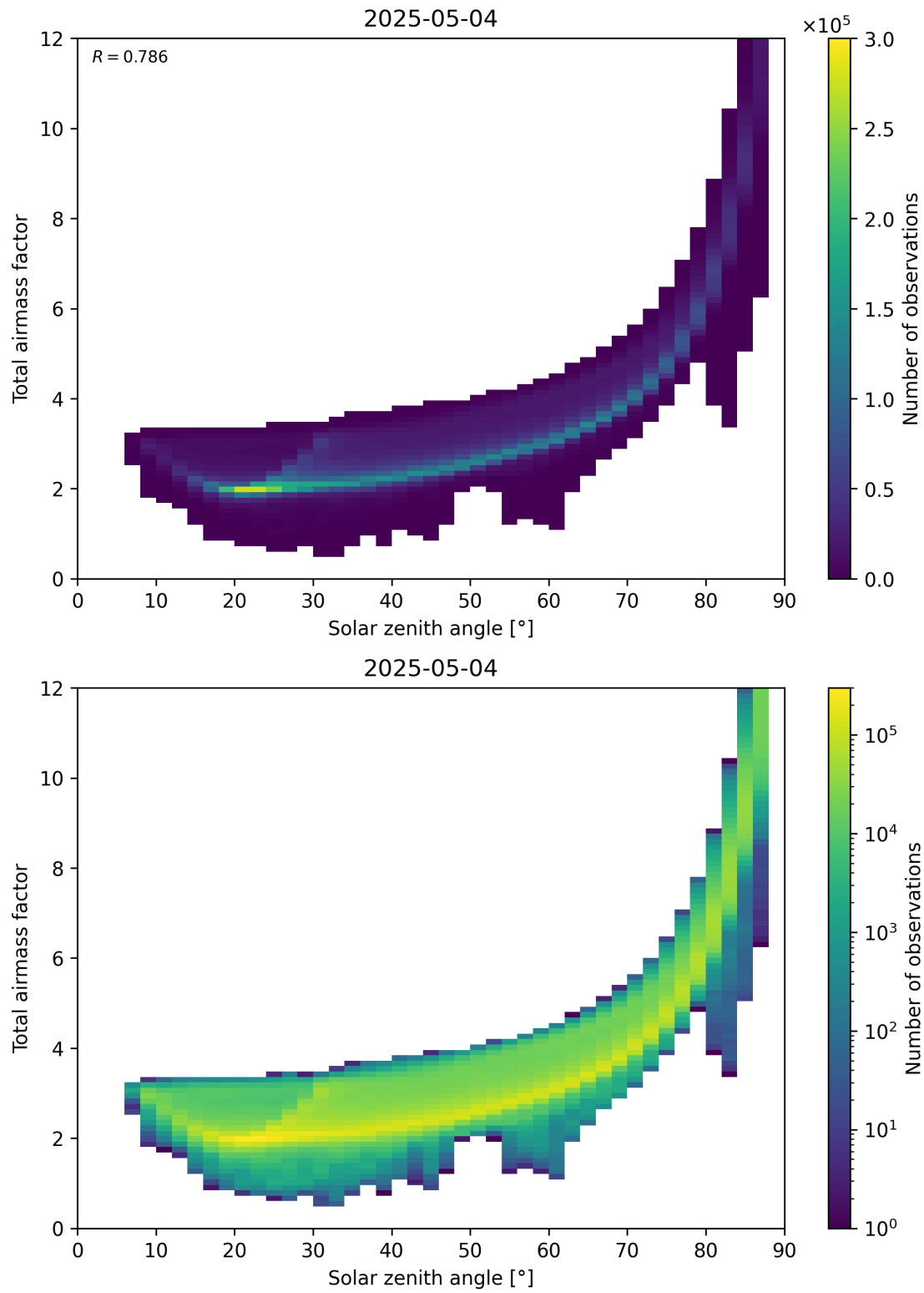
Figure 146: Scatter density plot of “Solar zenith angle” against “Total airmass factor” for 2025-05-04 to 2025-05-05.
