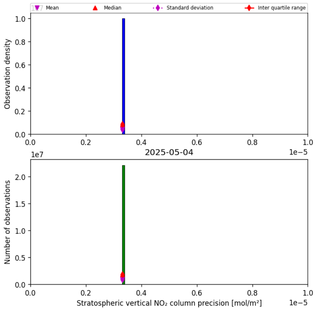
Figure 37: Histogram of “Stratospheric vertical NO 2 column precision” for 2025-05-04 to 2025-05-05
