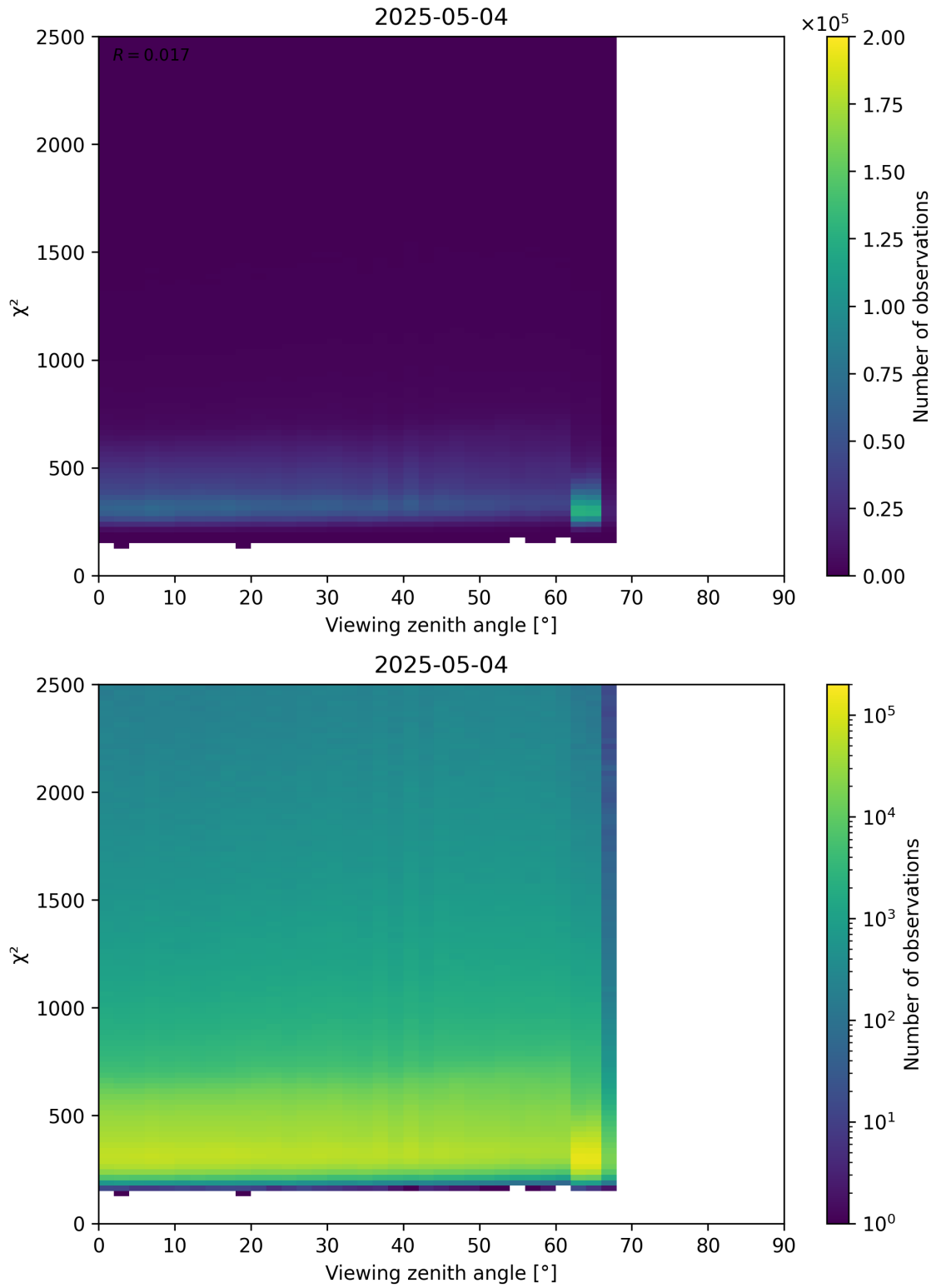
Figure 162: Scatter density plot of “Viewing zenith angle” against “ \chi^2 ” for 2025-05-04 to 2025-05-05.
