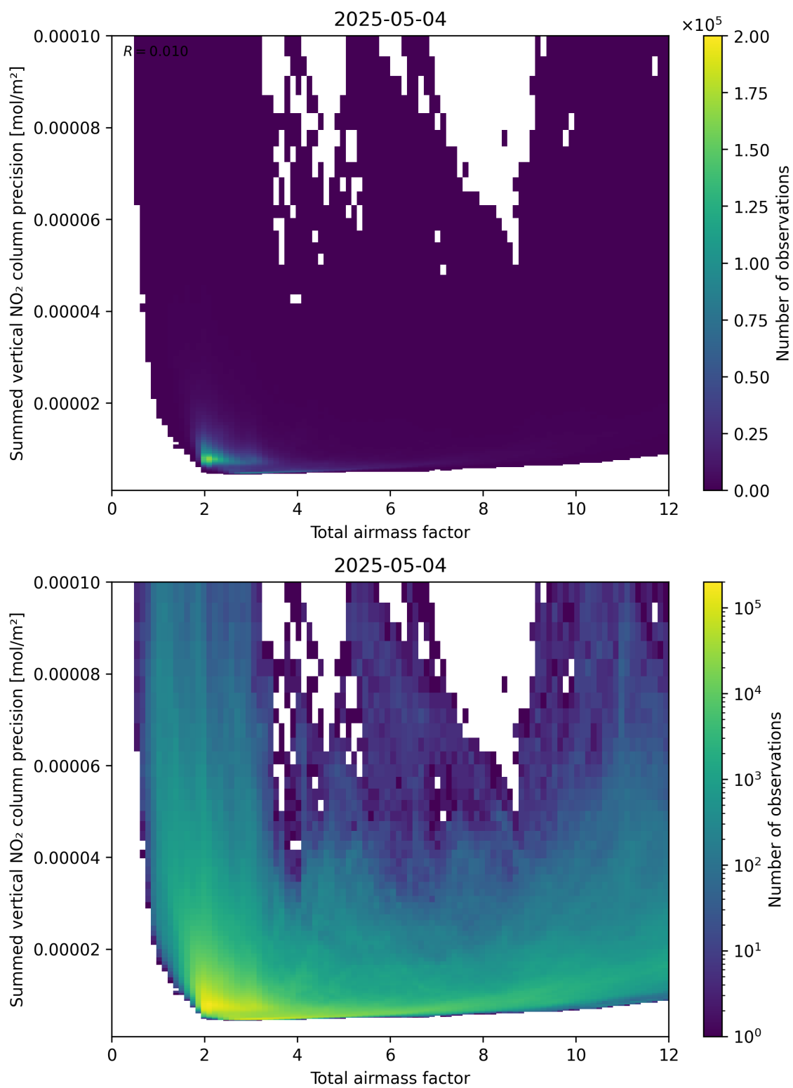
Figure 66: Scatter density plot of “Total airmass factor” against “Summed vertical NO 2 column precision” for 2025-05-04 to 2025-05-05.
