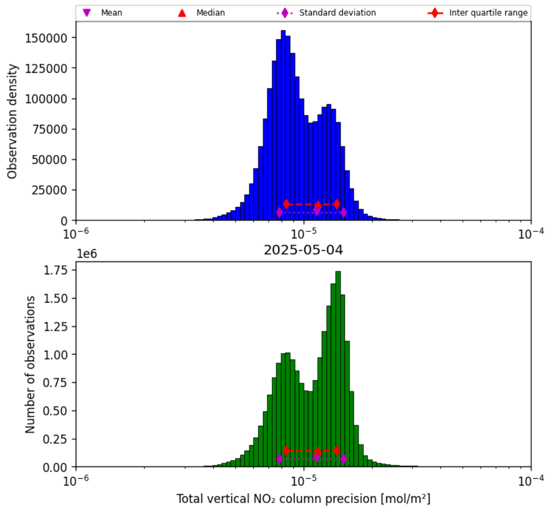
Figure 39: Histogram of “Total vertical NO 2 column precision” for 2025-05-04 to 2025-05-05
