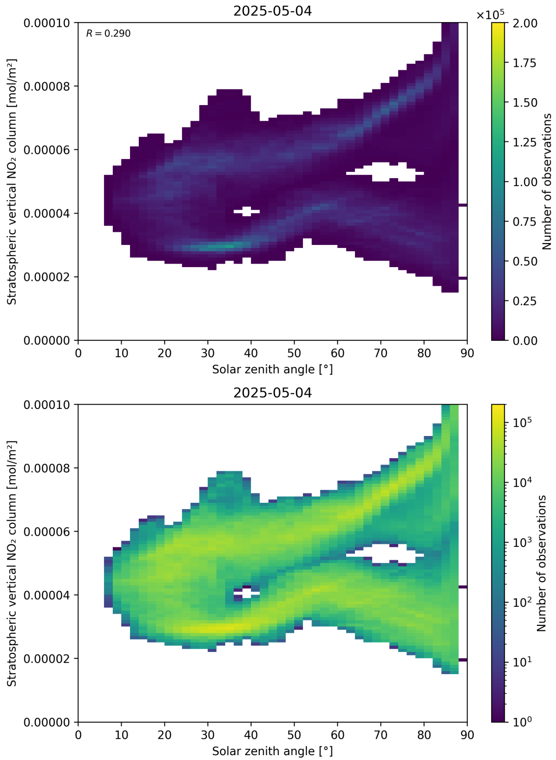
Figure 150: Scatter density plot of “Solar zenith angle” against “Stratospheric vertical NO 2 column” for 2025-05-04 to 2025-05-05.
