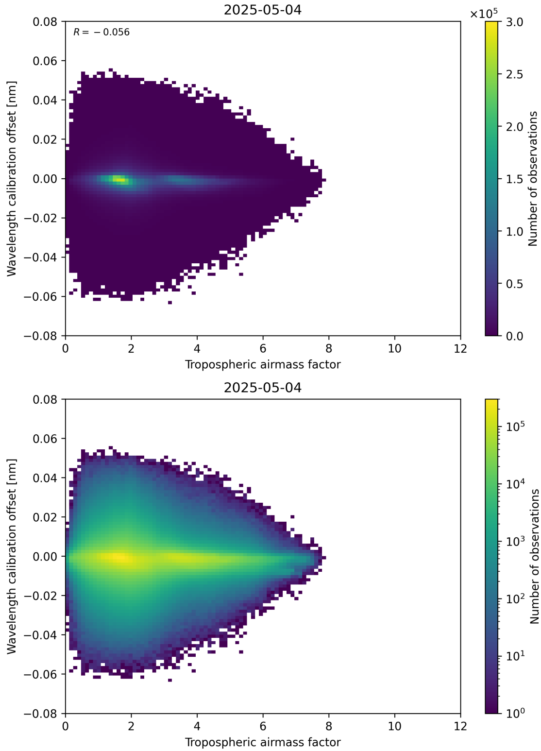
Figure 80: Scatter density plot of “Tropospheric airmass factor” against “Wavelength calibration offset” for 2025-05-04 to 2025-05-05.
