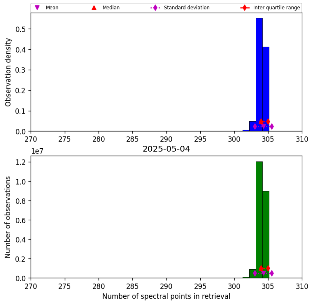
Figure 33: Histogram of “Number of spectral points in retrieval” for 2025-05-04 to 2025-05-05
