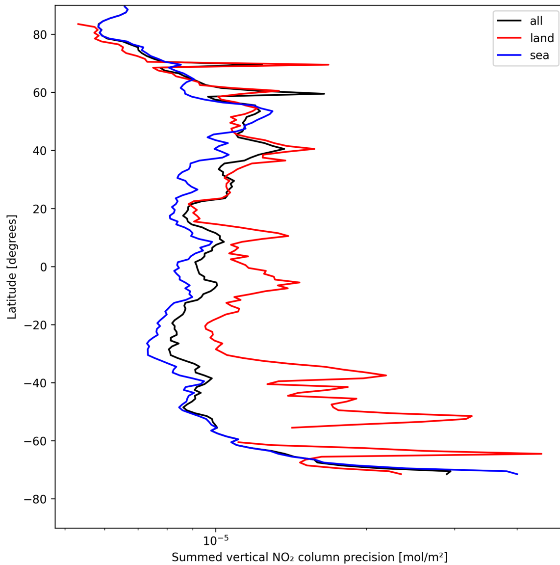
Figure 24: Zonal average of “Summed vertical NO 2 column precision” for 2025-05-04 to 2025-05-05.
