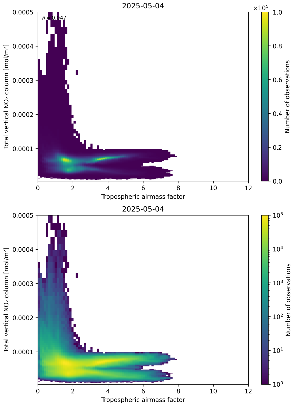
Figure 77: Scatter density plot of “Tropospheric airmass factor” against “Total vertical NO 2 column” for 2025-05-04 to 2025-05-05.
