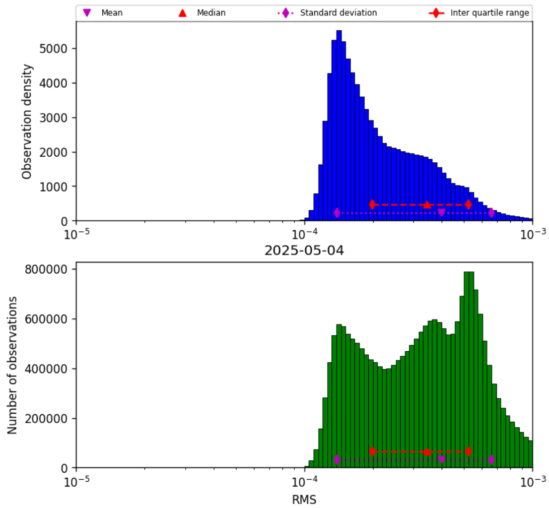
Figure 43: Histogram of “RMS” for 2025-05-04 to 2025-05-05
