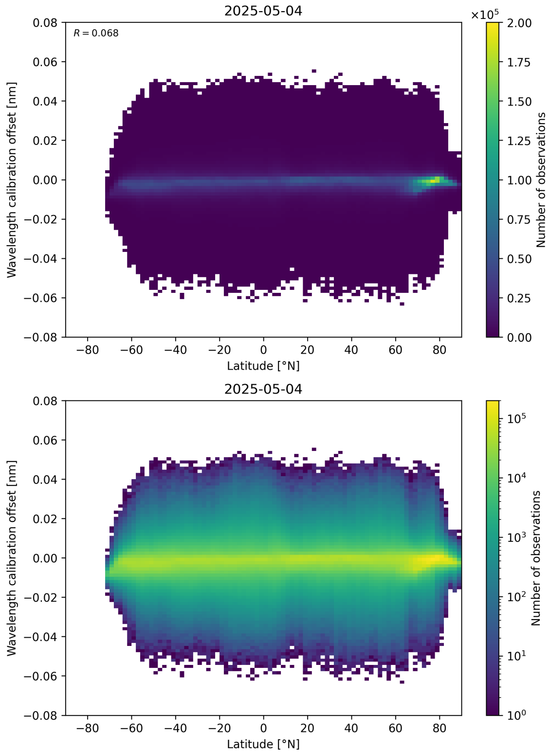
Figure 95: Scatter density plot of “Latitude” against “Wavelength calibration offset” for 2025-05-04 to 2025-05-05.
