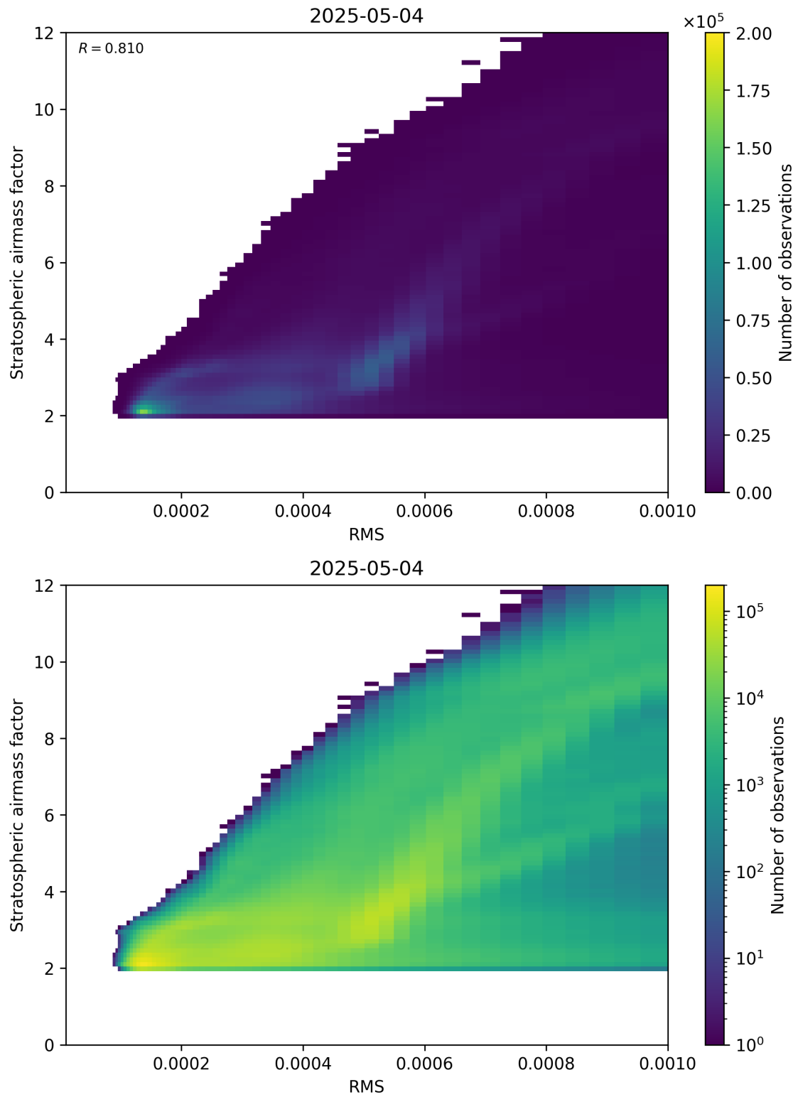
Figure 144: Scatter density plot of “RMS” against “Stratospheric airmass factor” for 2025-05-04 to 2025-05-05.
