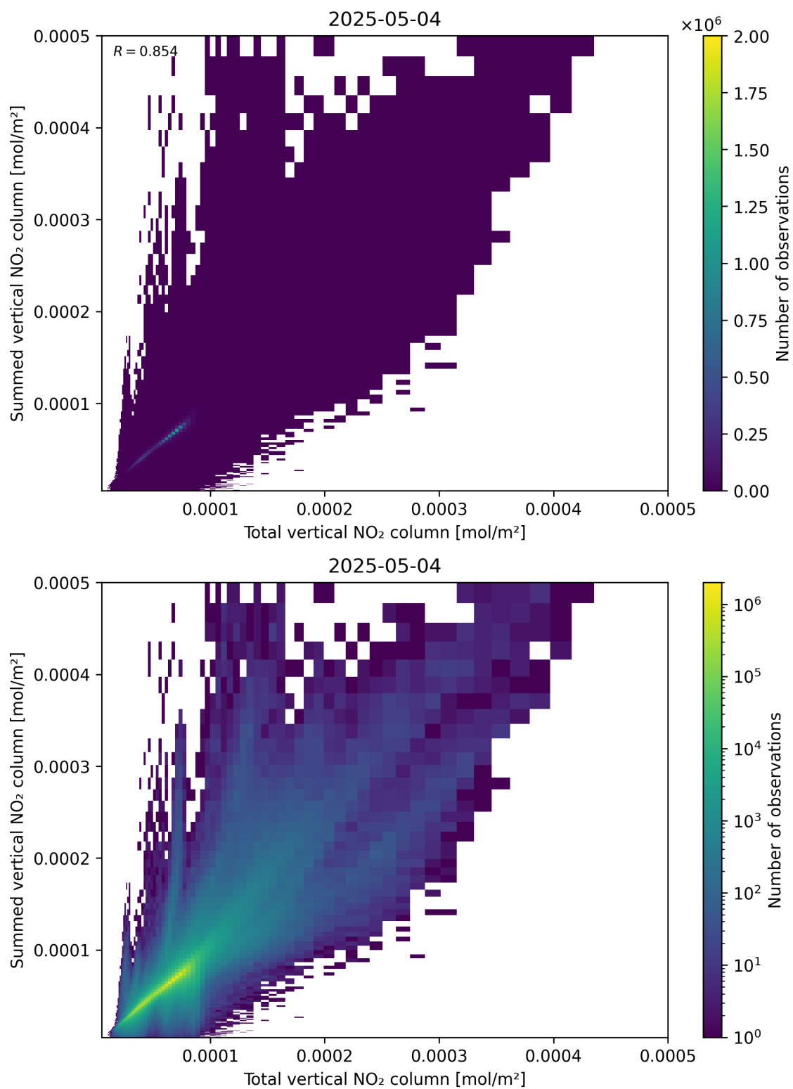
Figure 112: Scatter density plot of “Total vertical NO 2 column” against “Summed vertical NO 2 column” for 2025-05-04 to 2025-05-05.
