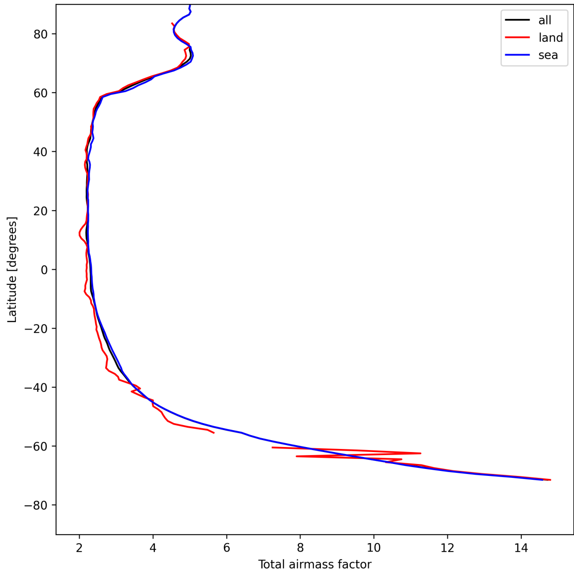
Figure 15: Zonal average of “Total airmass factor” for 2025-05-04 to 2025-05-05.
