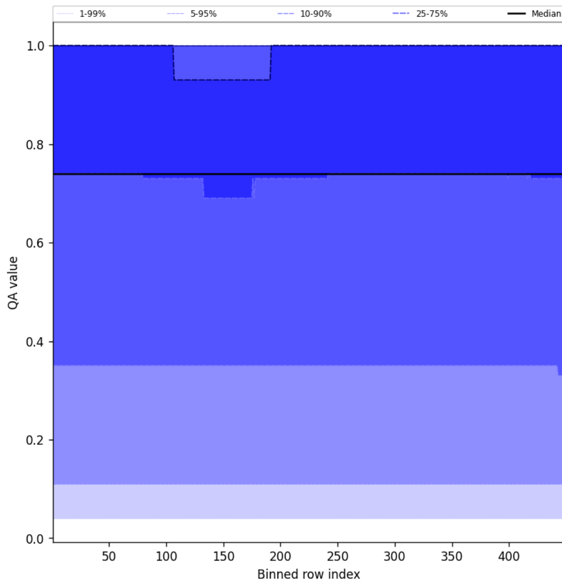
Figure 45: Along track statistics of “QA value” for 2025-05-07 to 2025-05-08
