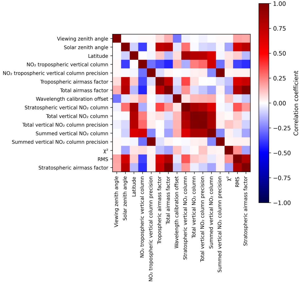
Figure 2: Map of correlation matrix for 2025-05-07 to 2025-05-08.
