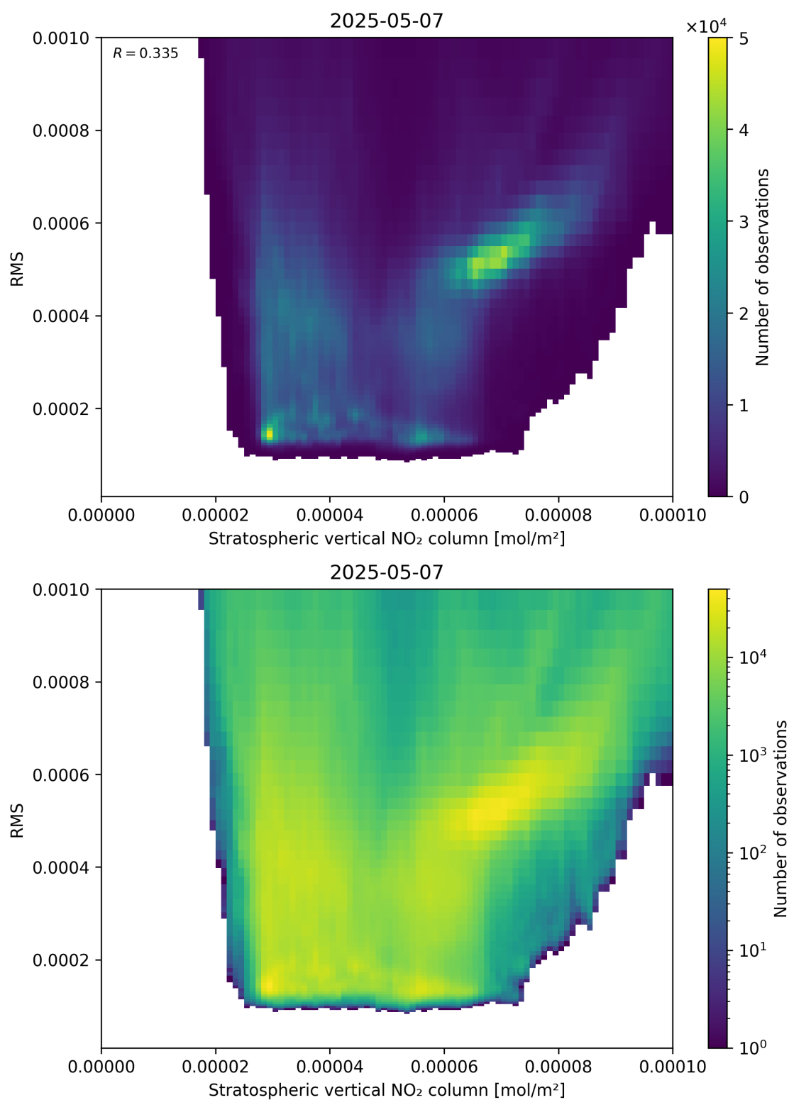
Figure 102: Scatter density plot of “Stratospheric vertical NO 2 column” against “RMS” for 2025-05-07 to 2025-05-08.
