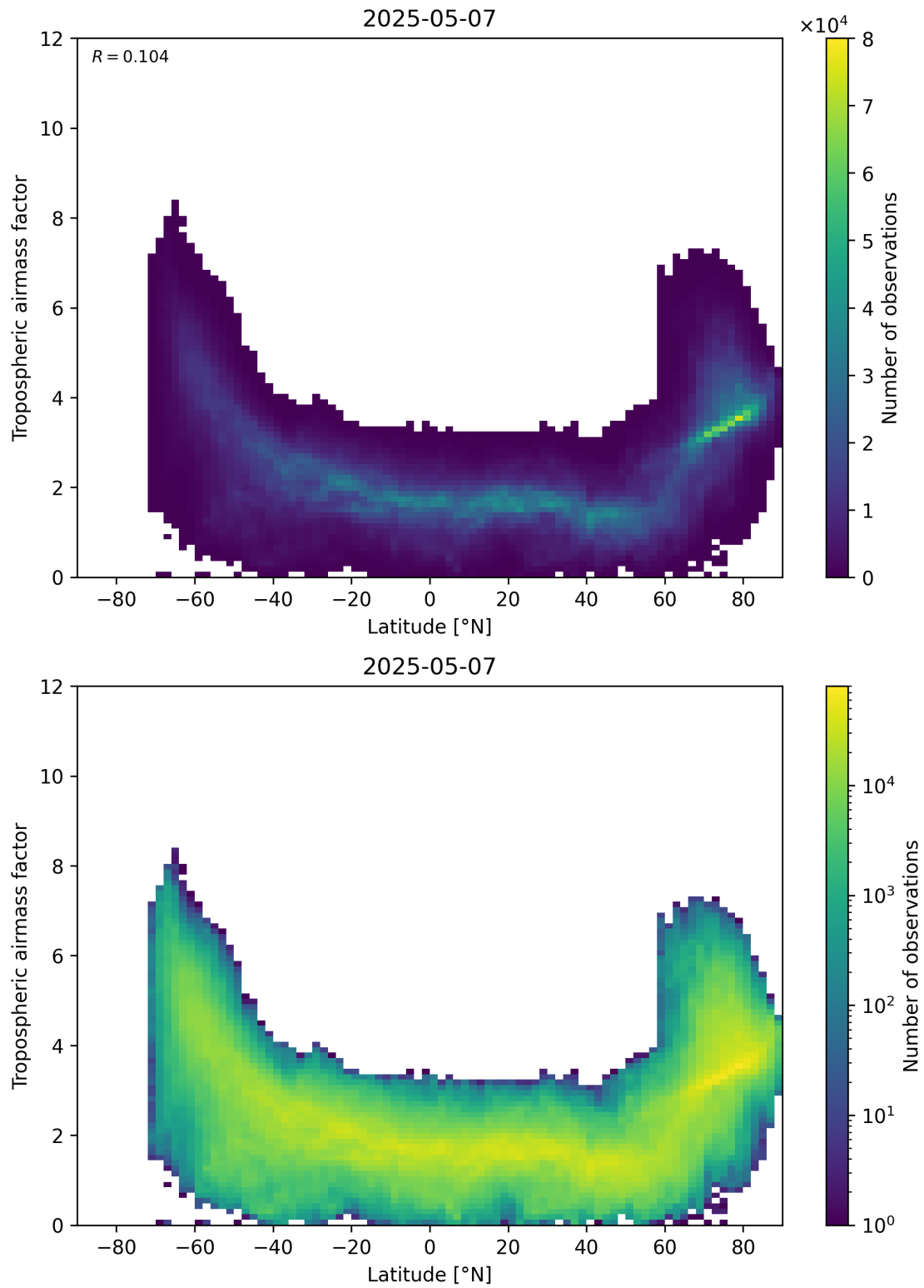
Figure 85: Scatter density plot of “Latitude” against “Tropospheric air mass factor” for 2025-05-07 to 2025-05-08.
