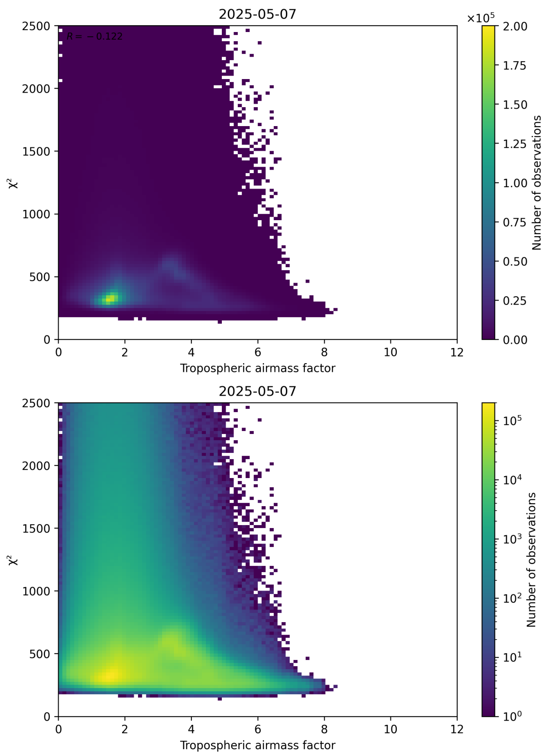
Figure 73: Scatter density plot of “Tropospheric airmass factor” against “ \chi^2 ” for 2025-05-07 to 2025-05-08.
