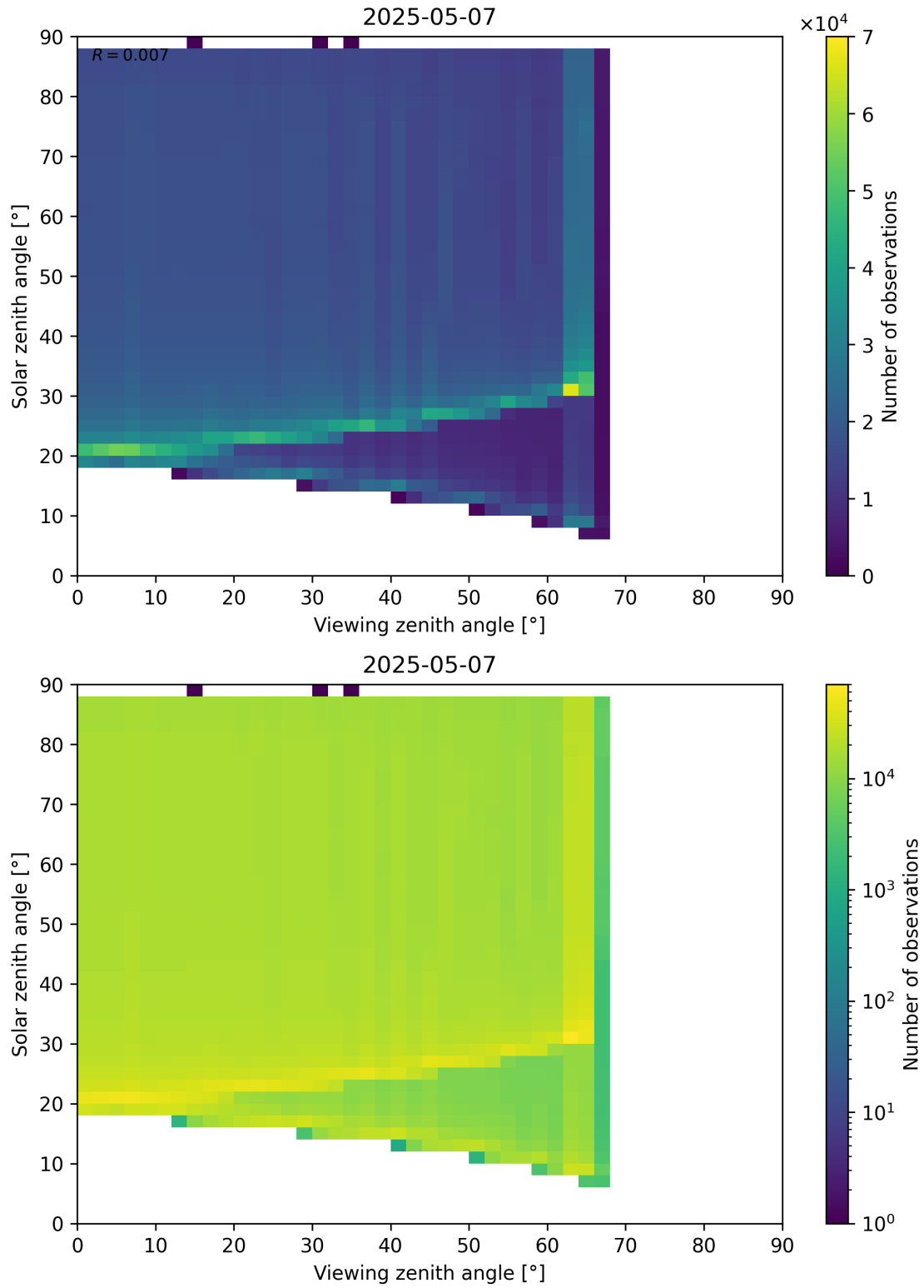
Figure 172: Scatter density plot of “Viewing zenith angle” against “Solar zenith angle” for 2025-05-07 to 2025-05-08.
