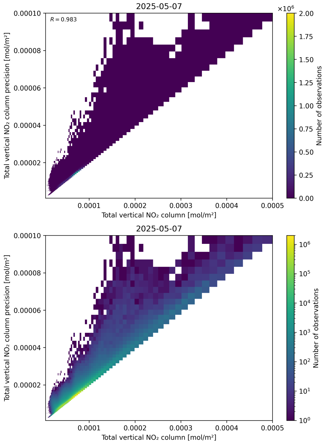
Figure 114: Scatter density plot of “Total vertical NO 2 column” against “Total vertical NO 2 column precision” for 2025-05-07 to 2025-05-08.
