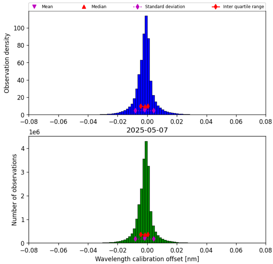
Figure 35: Histogram of “Wavelength calibration offset” for 2025-05-07 to 2025-05-08
