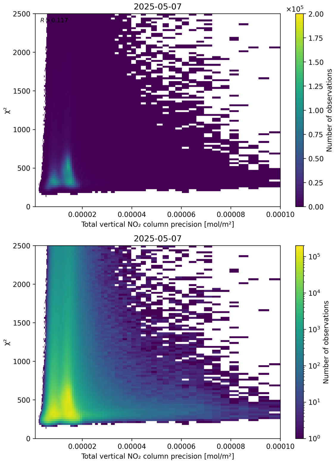
Figure 116: Scatter density plot of “Total vertical NO 2 column precision” against “ \chi^2 ” for 2025-05-07 to 2025-05-08.
