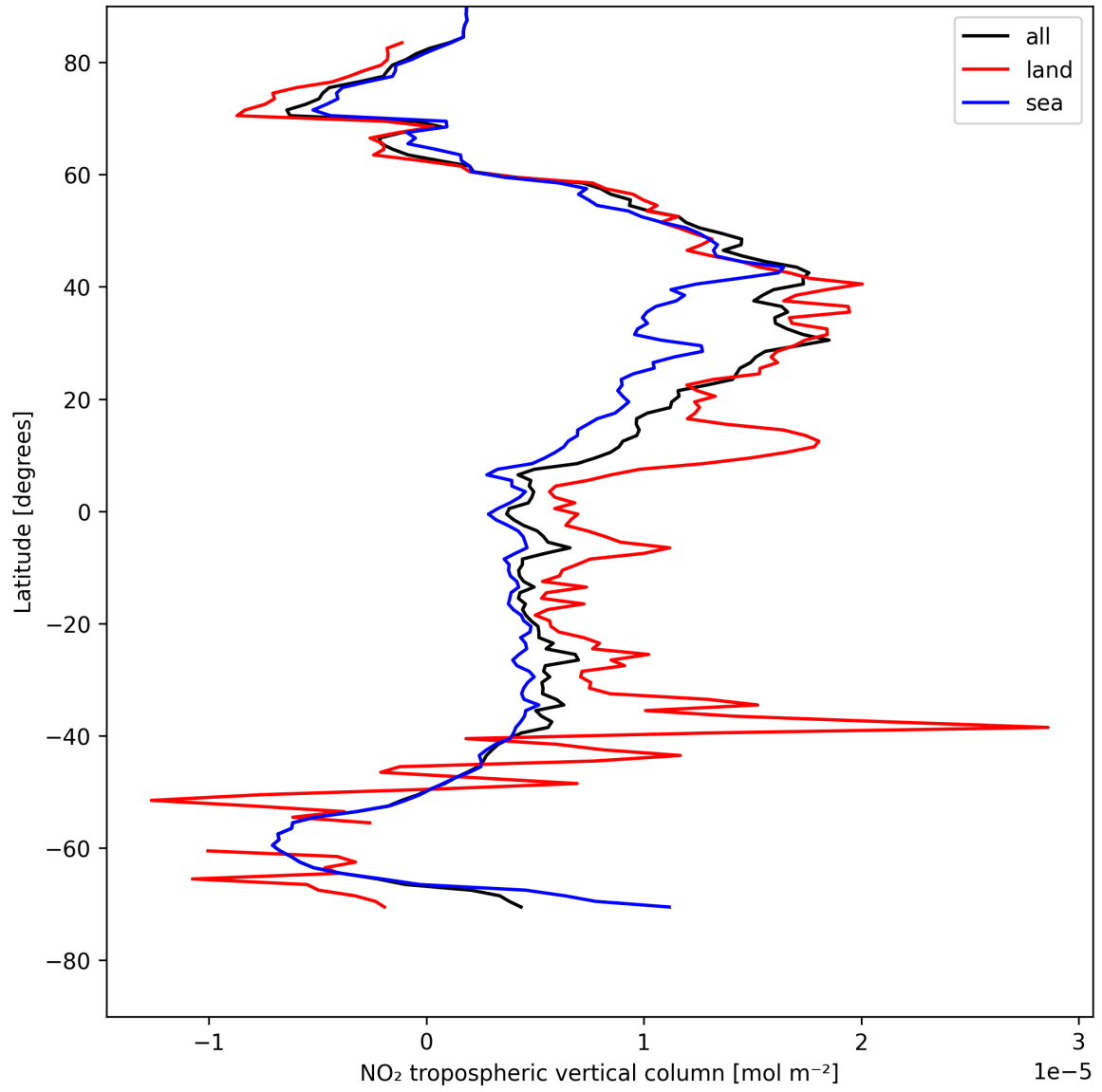
Figure 12: Zonal average of “NO 2 tropospheric vertical column” for 2025-05-07 to 2025-05-08.
