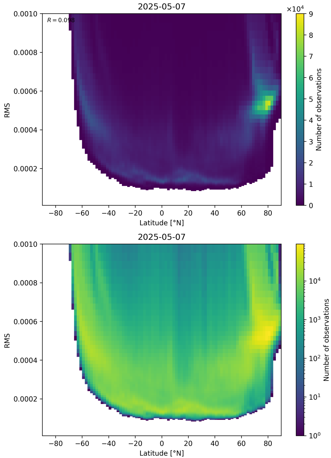
Figure 94: Scatter density plot of “Latitude” against “RMS” for 2025-05-07 to 2025-05-08.
