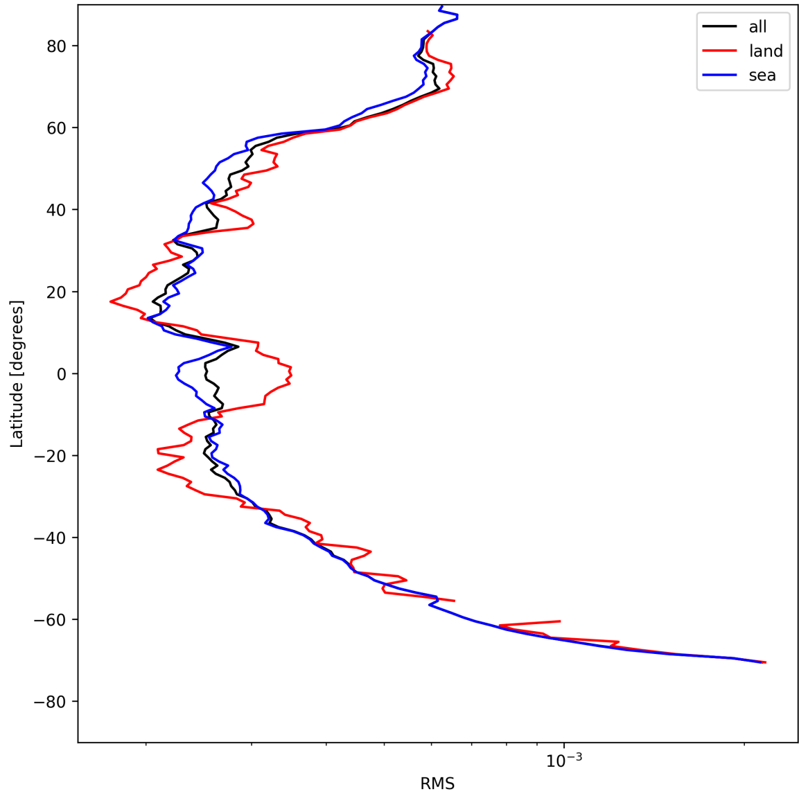
Figure 26: Zonal average of “RMS” for 2025-05-07 to 2025-05-08.
