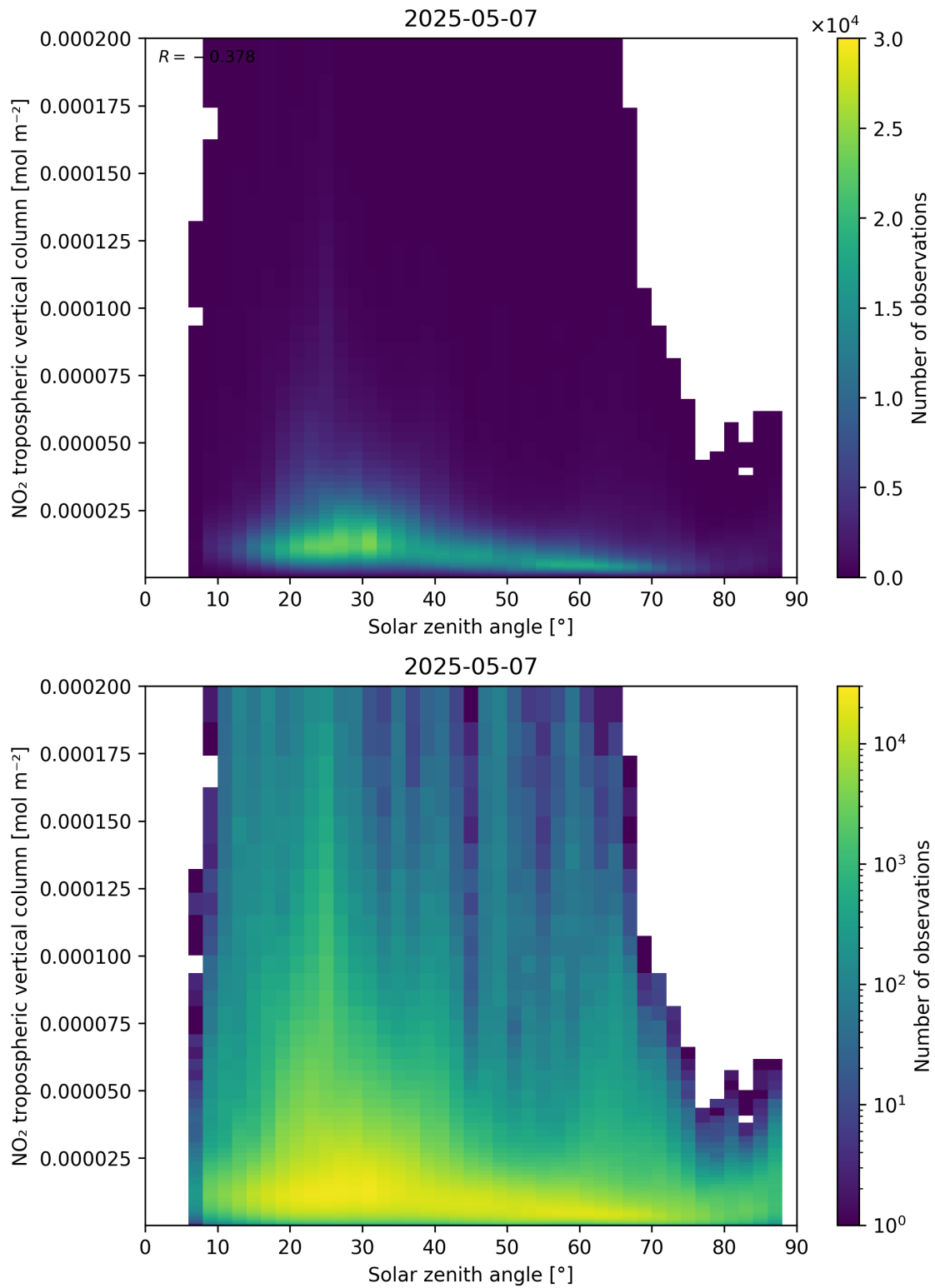
Figure 155: Scatter density plot of “Solar zenith angle” against “NO 2 tropospheric vertical column” for 2025-05-07 to 2025-05-08.
