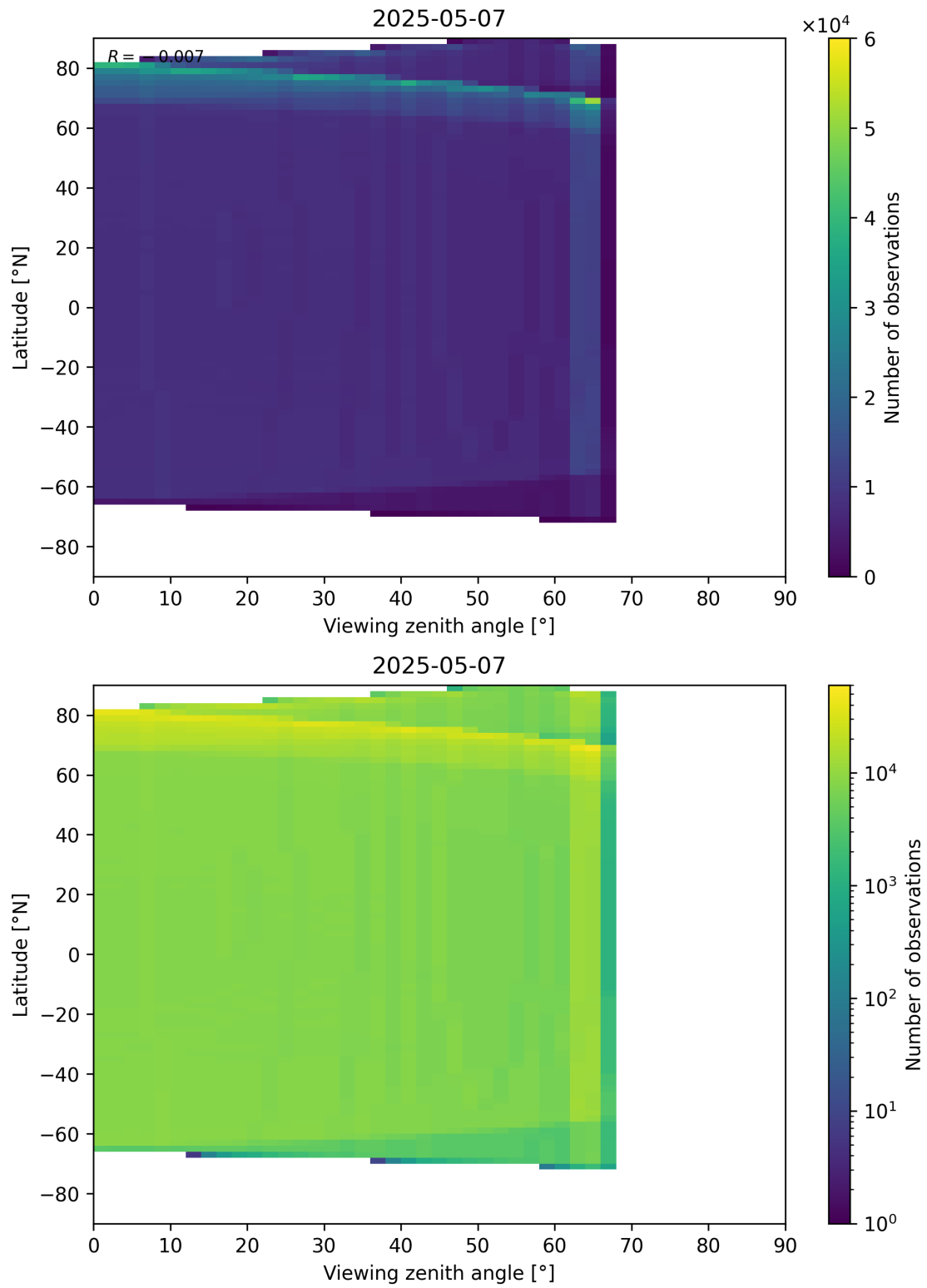
Figure 163: Scatter density plot of “Viewing zenith angle” against “Latitude” for 2025-05-07 to 2025-05-08.
