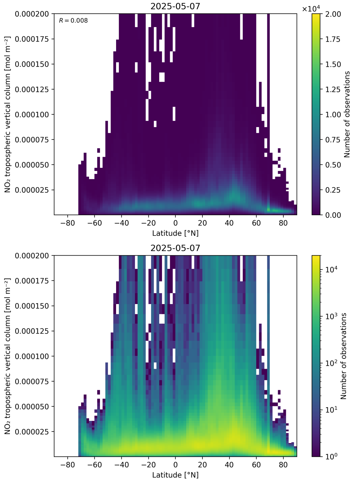
Figure 92: Scatter density plot of “Latitude” against “NO 2 tropospheric vertical column” for 2025-05-07 to 2025-05-08.
