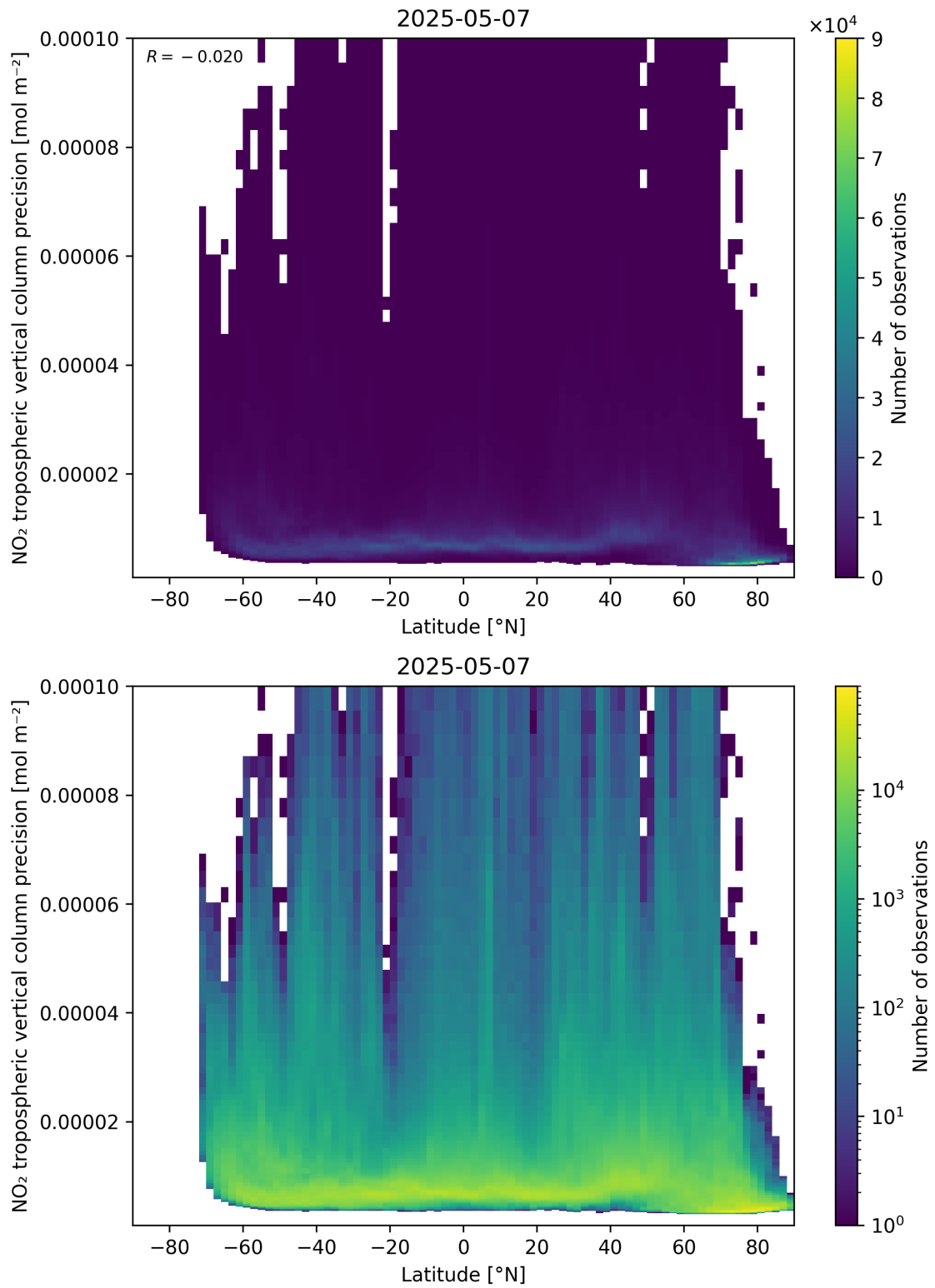
Figure 93: Scatter density plot of “Latitude” against “NO 2 tropospheric vertical column precision” for 2025-05-07 to 2025-05-08.
