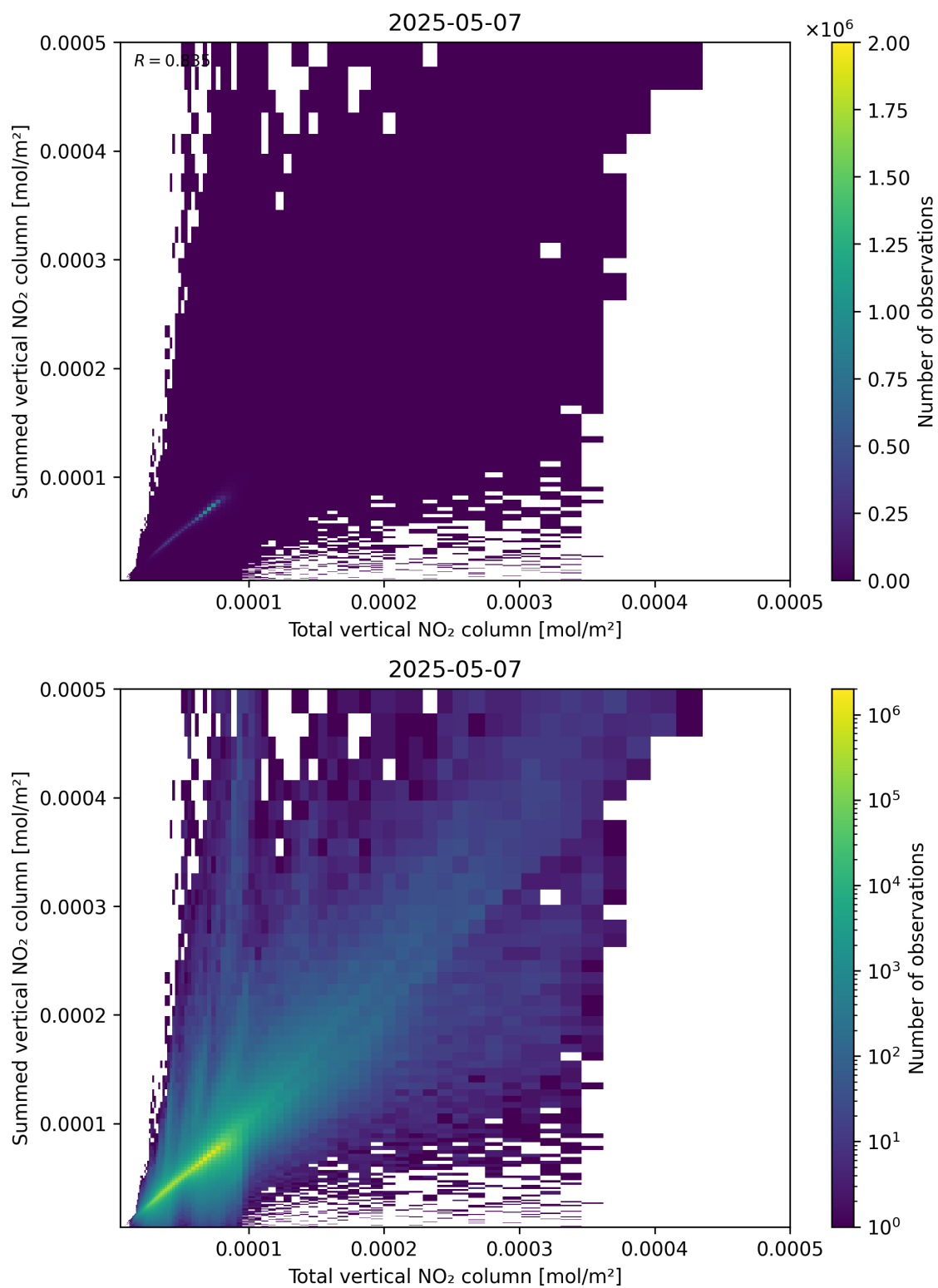
Figure 112: Scatter density plot of “Total vertical NO 2 column” against “Summed vertical NO 2 column” for 2025-05-07 to 2025-05-08.
