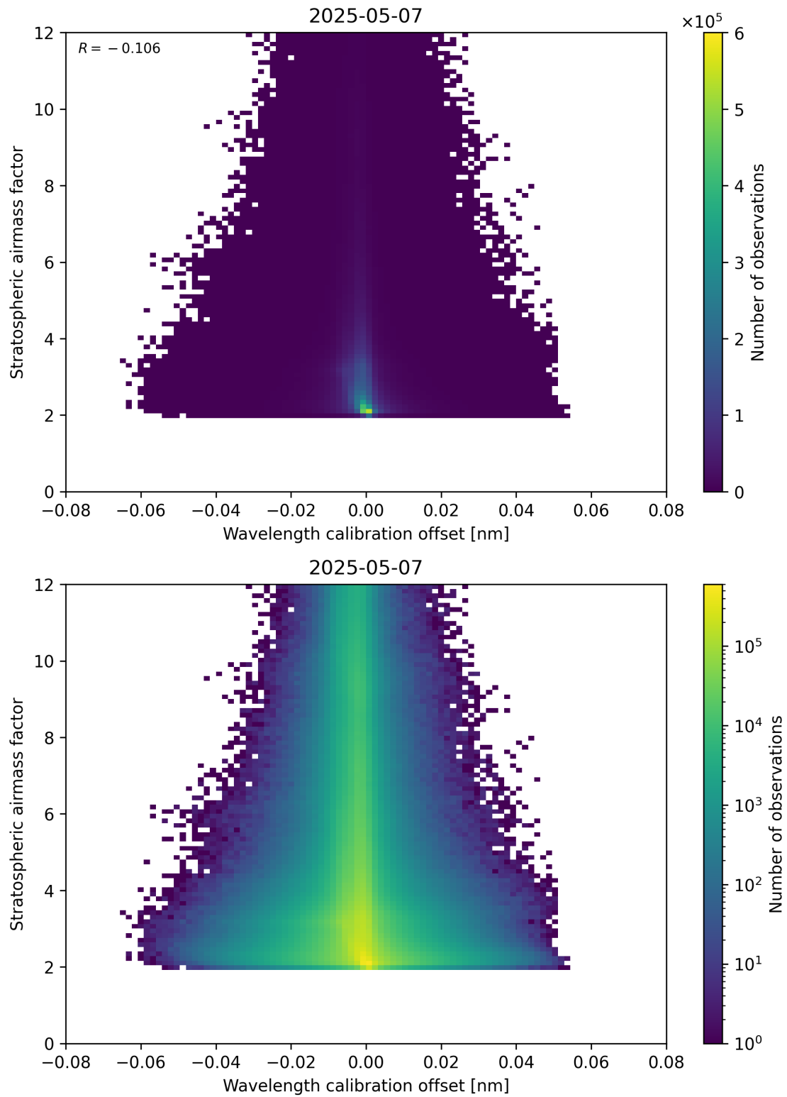
Figure 174: Scatter density plot of “Wavelength calibration offset” against “Stratospheric airmass factor” for 2025-05-07 to 2025-05-08.
