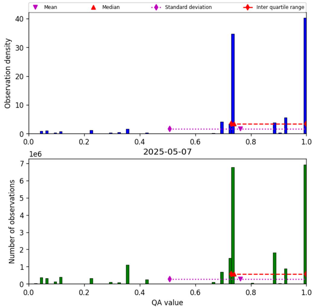
Figure 28: Histogram of “QA value” for 2025-05-07 to 2025-05-08
