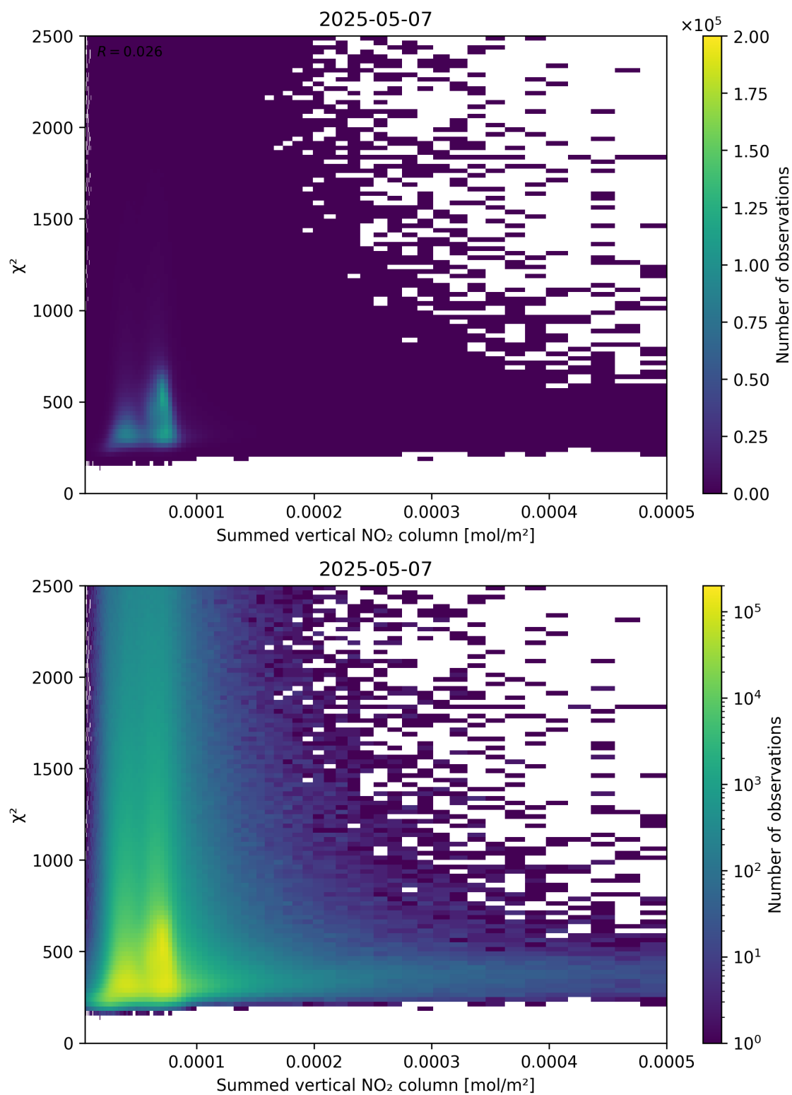
Figure 104: Scatter density plot of “Summed vertical NO 2 column” against “ \chi^2 ” for 2025-05-07 to 2025-05-08.
