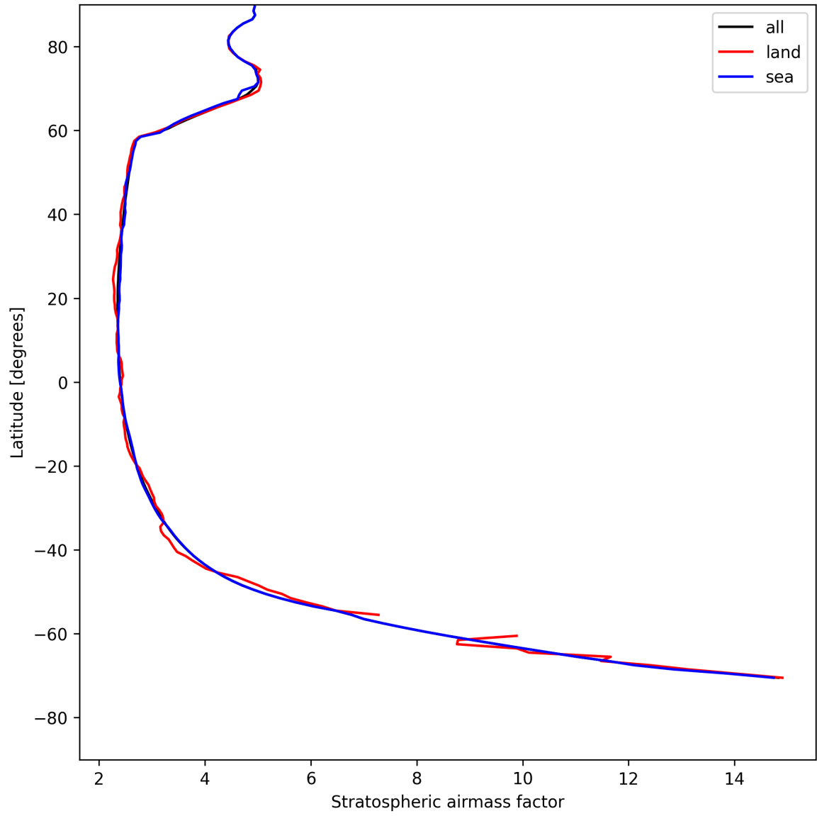
Figure 27: Zonal average of “Stratospheric airmass factor” for 2025-05-07 to 2025-05-08.
