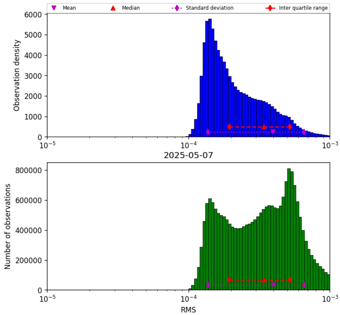
Figure 43: Histogram of “RMS” for 2025-05-07 to 2025-05-08
