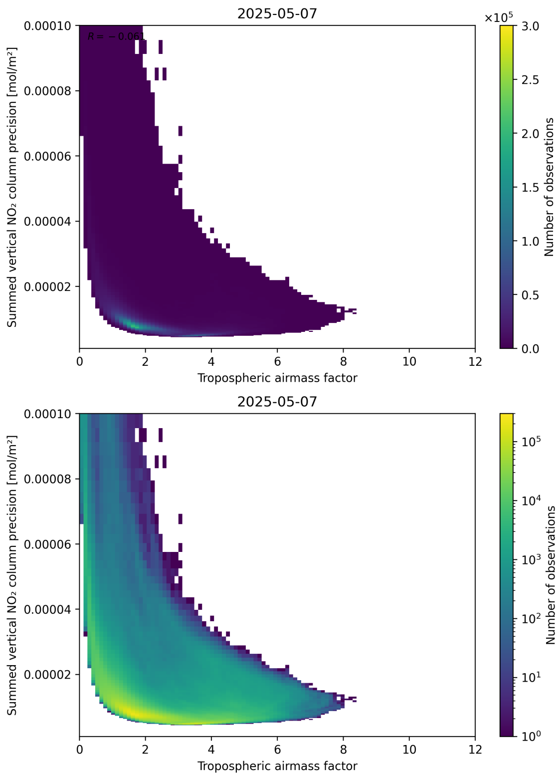
Figure 76: Scatter density plot of “Tropospheric air mass factor” against “Summed vertical NO 2 column precision” for 2025-05-07 to 2025-05-08.
