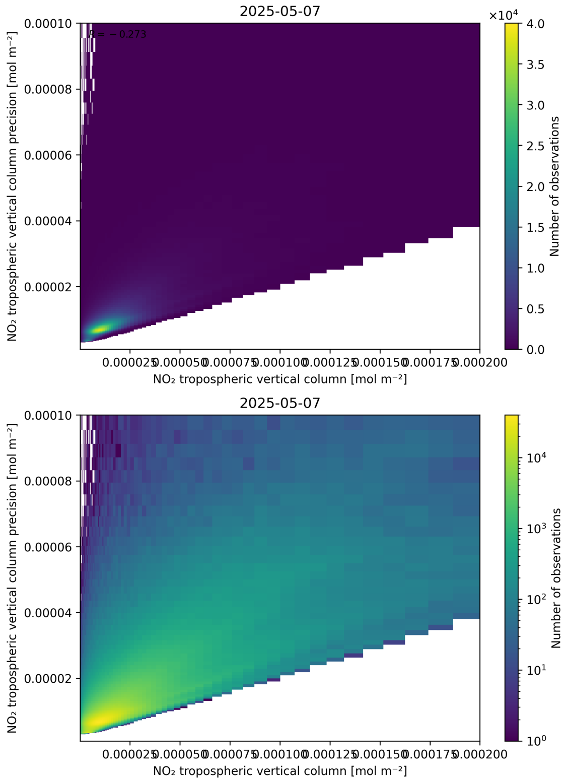
Figure 130: Scatter density plot of “NO 2 tropospheric vertical column” against “NO 2 tropospheric vertical column precision” for 2025-05-07 to 2025-05-08.
