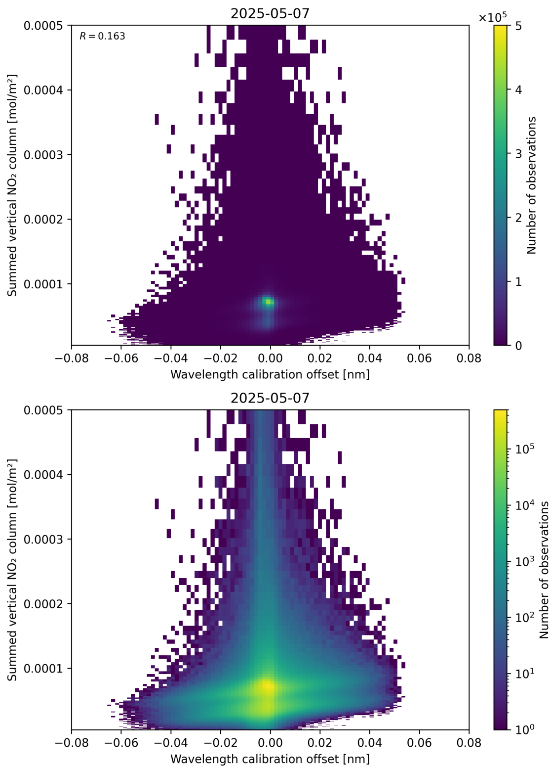
Figure 177: Scatter density plot of “Wavelength calibration offset” against “Summed vertical NO 2 column” for 2025-05-07 to 2025-05-08.
