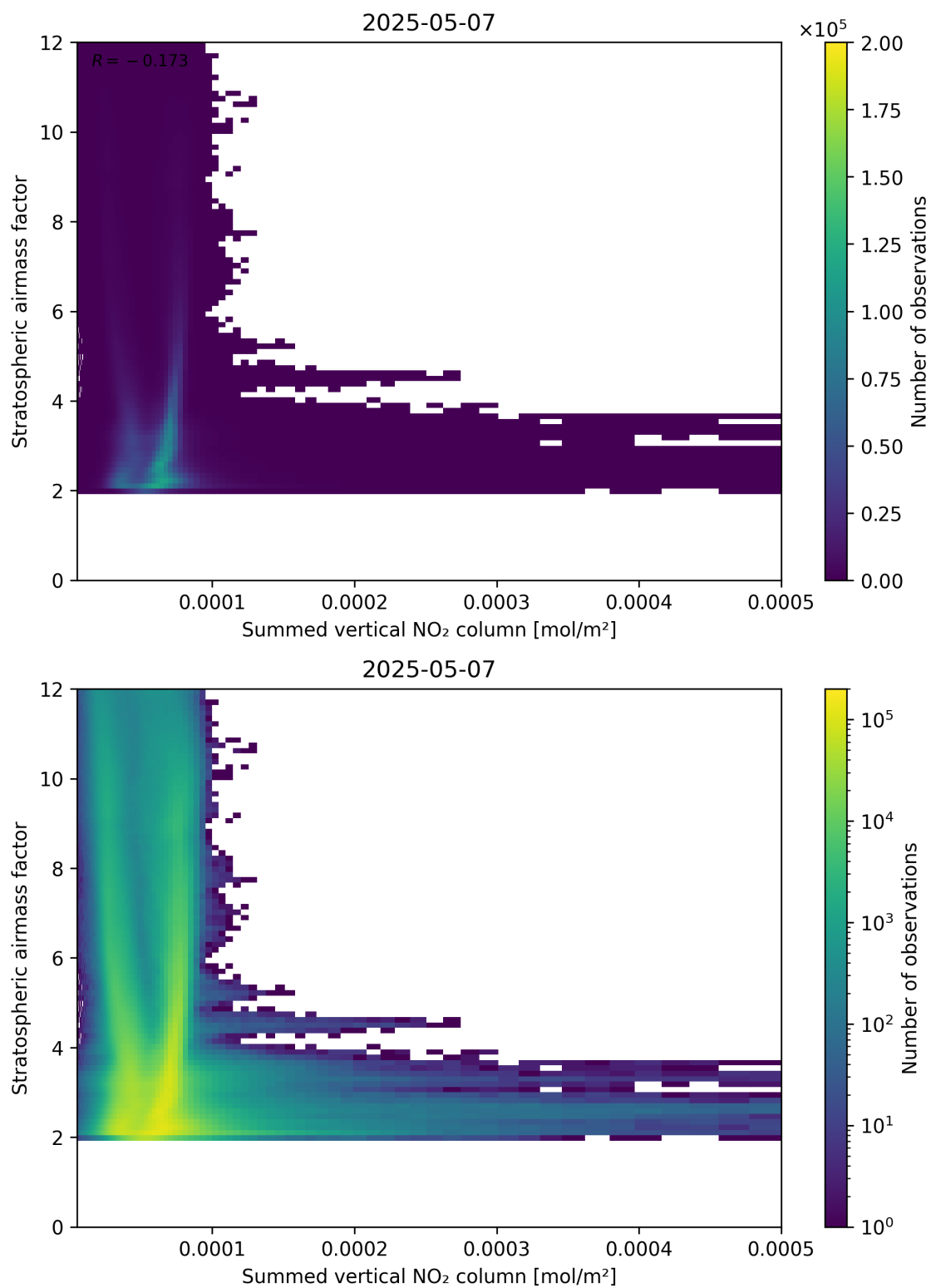
Figure 103: Scatter density plot of “Summed vertical NO 2 column” against “Stratospheric airmass factor” for 2025-05-07 to 2025-05-08.
