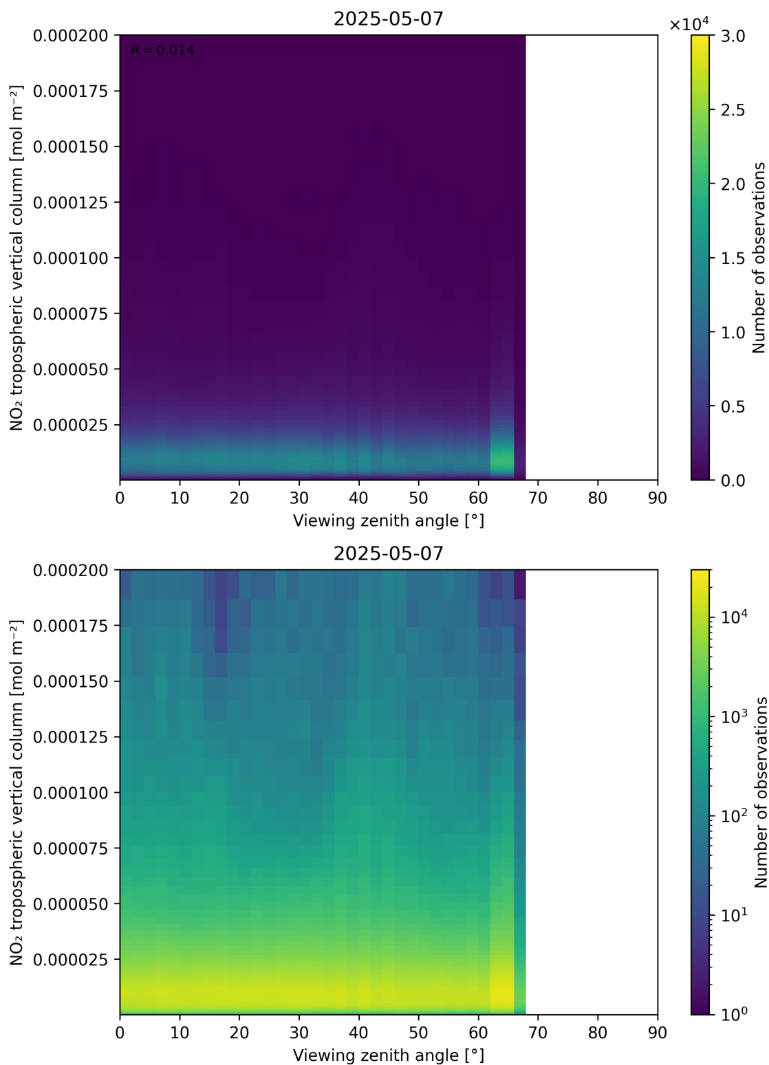
Figure 169: Scatter density plot of “Viewing zenith angle” against “NO 2 tropospheric vertical column” for 2025-05-07 to 2025-05-08.
