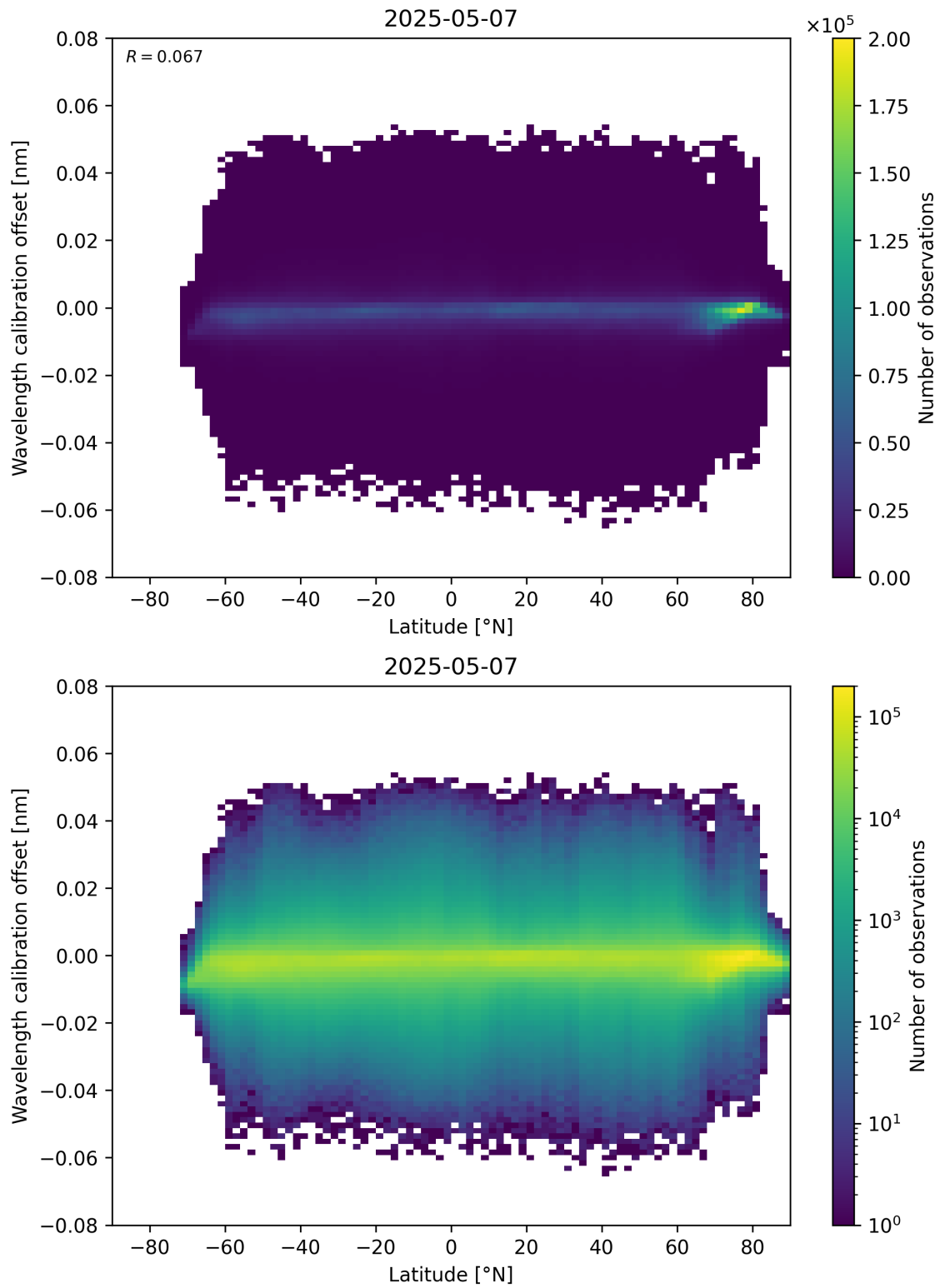
Figure 95: Scatter density plot of “Latitude” against “Wavelength calibration offset” for 2025-05-07 to 2025-05-08.
