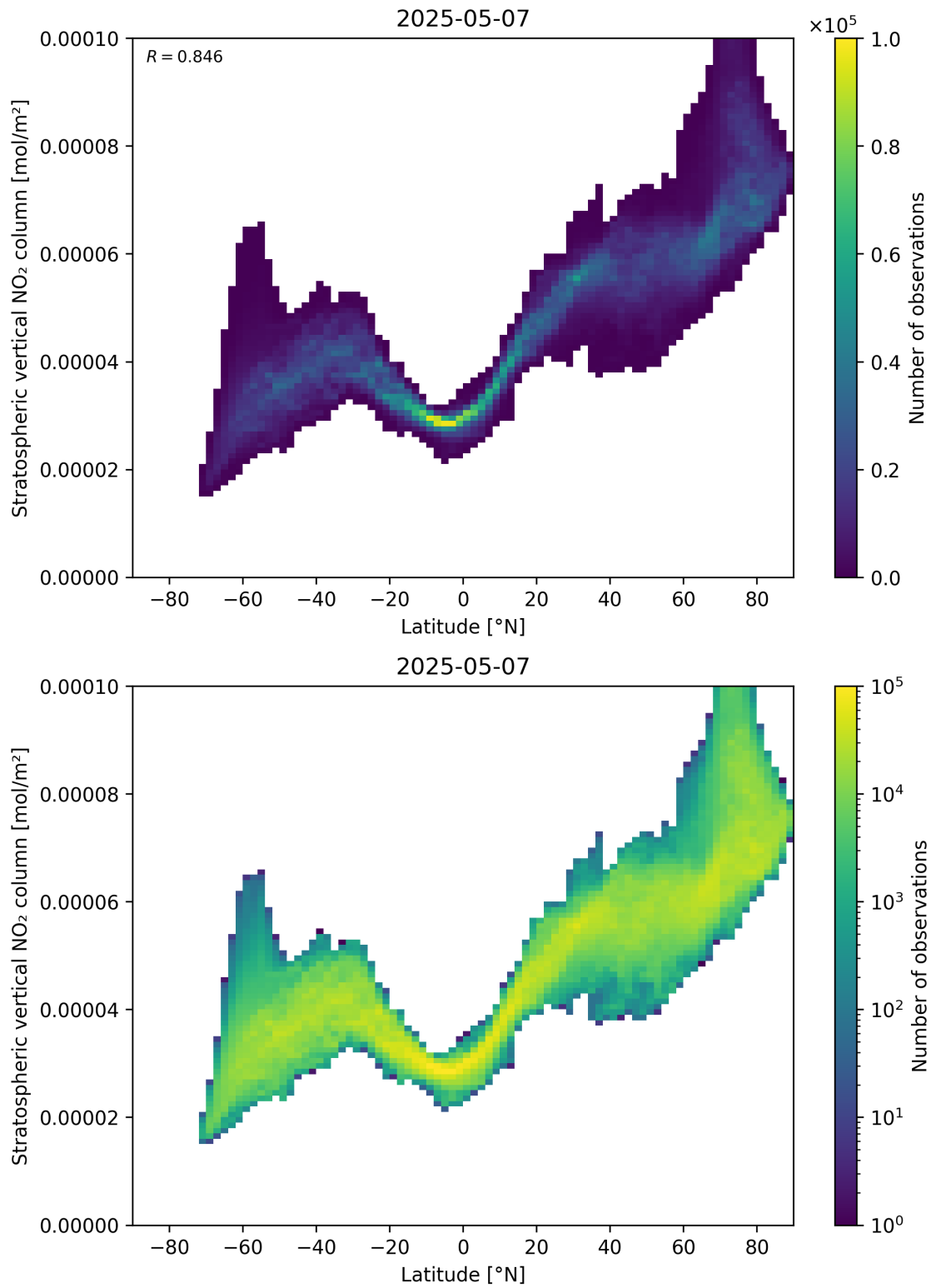
Figure 87: Scatter density plot of “Latitude” against “Stratospheric vertical \text{NO}_2 column” for 2025-05-07 to 2025-05-08.
