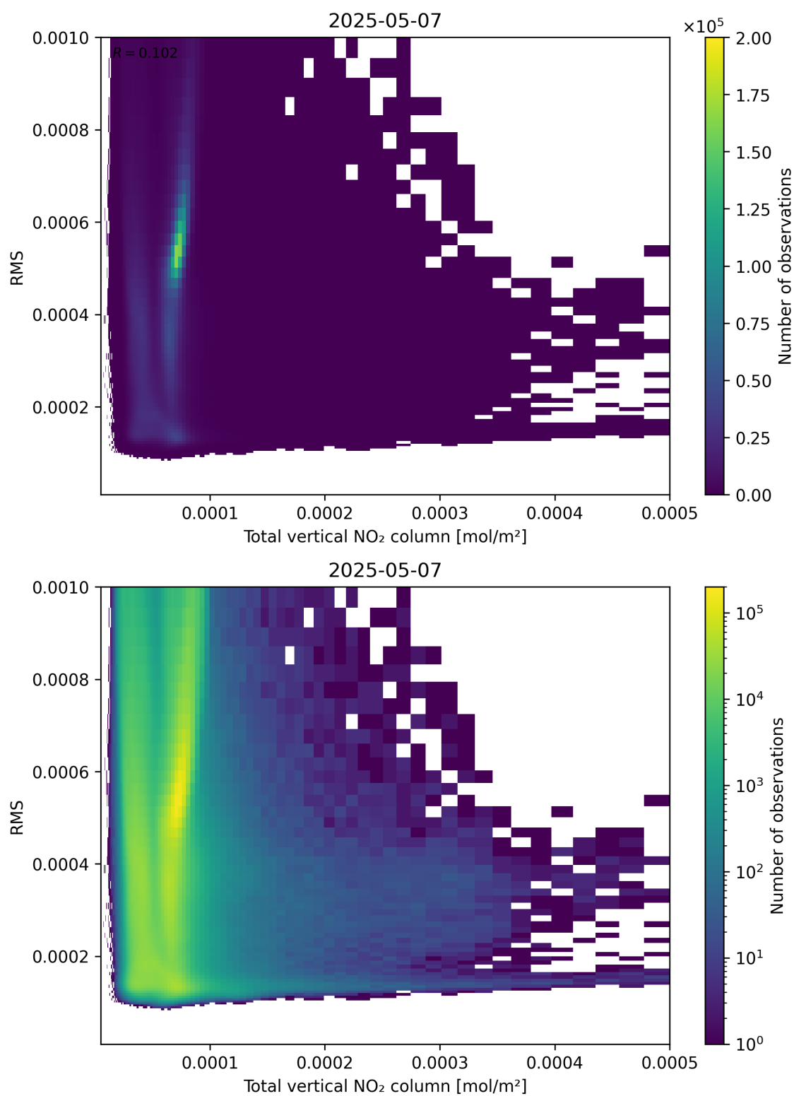
Figure 120: Scatter density plot of “Total vertical NO 2 column” against “RMS” for 2025-05-07 to 2025-05-08.
