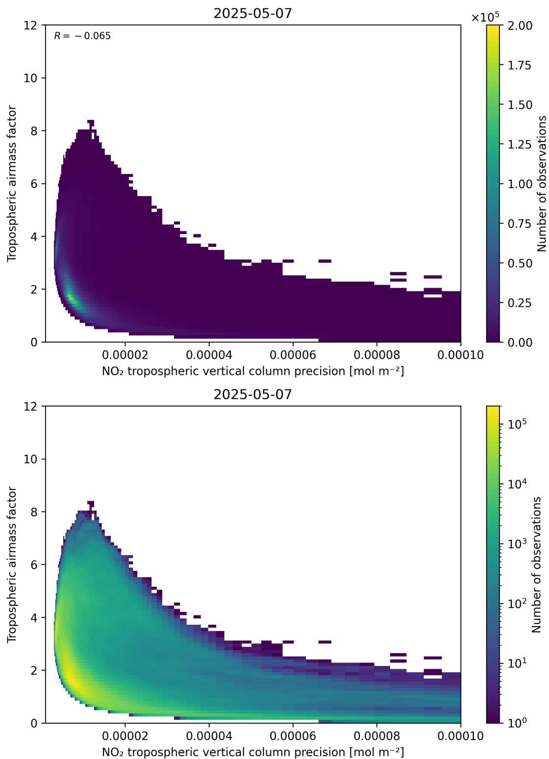
Figure 133: Scatter density plot of “NO 2 tropospheric vertical column precision” against “Tropospheric air mass factor” for 2025-05-07 to 2025-05-08.
