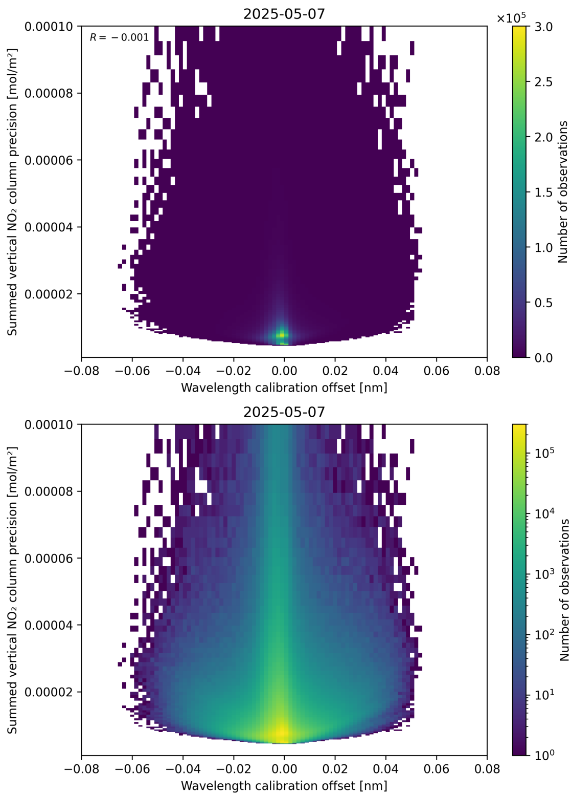
Figure 178: Scatter density plot of “Wavelength calibration offset” against “Summed vertical NO 2 column precision” for 2025-05-07 to 2025-05-08.
