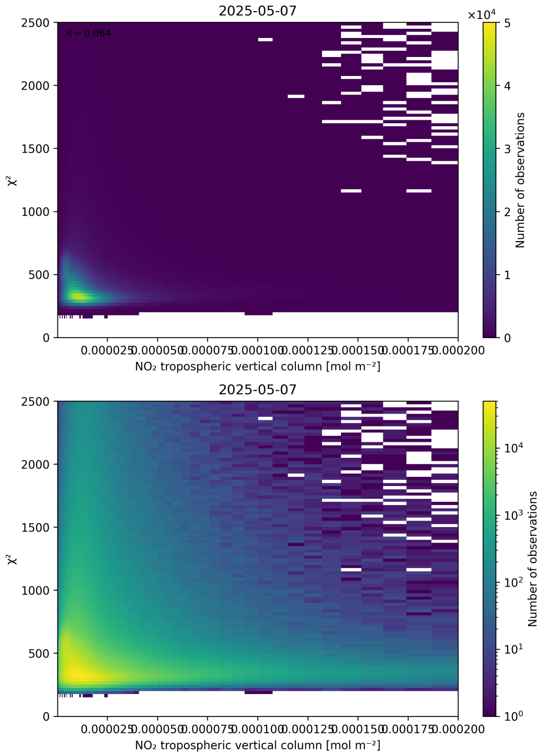
Figure 124: Scatter density plot of “NO 2 tropospheric vertical column” against “ \chi^2 ” for 2025-05-07 to 2025-05-08.
