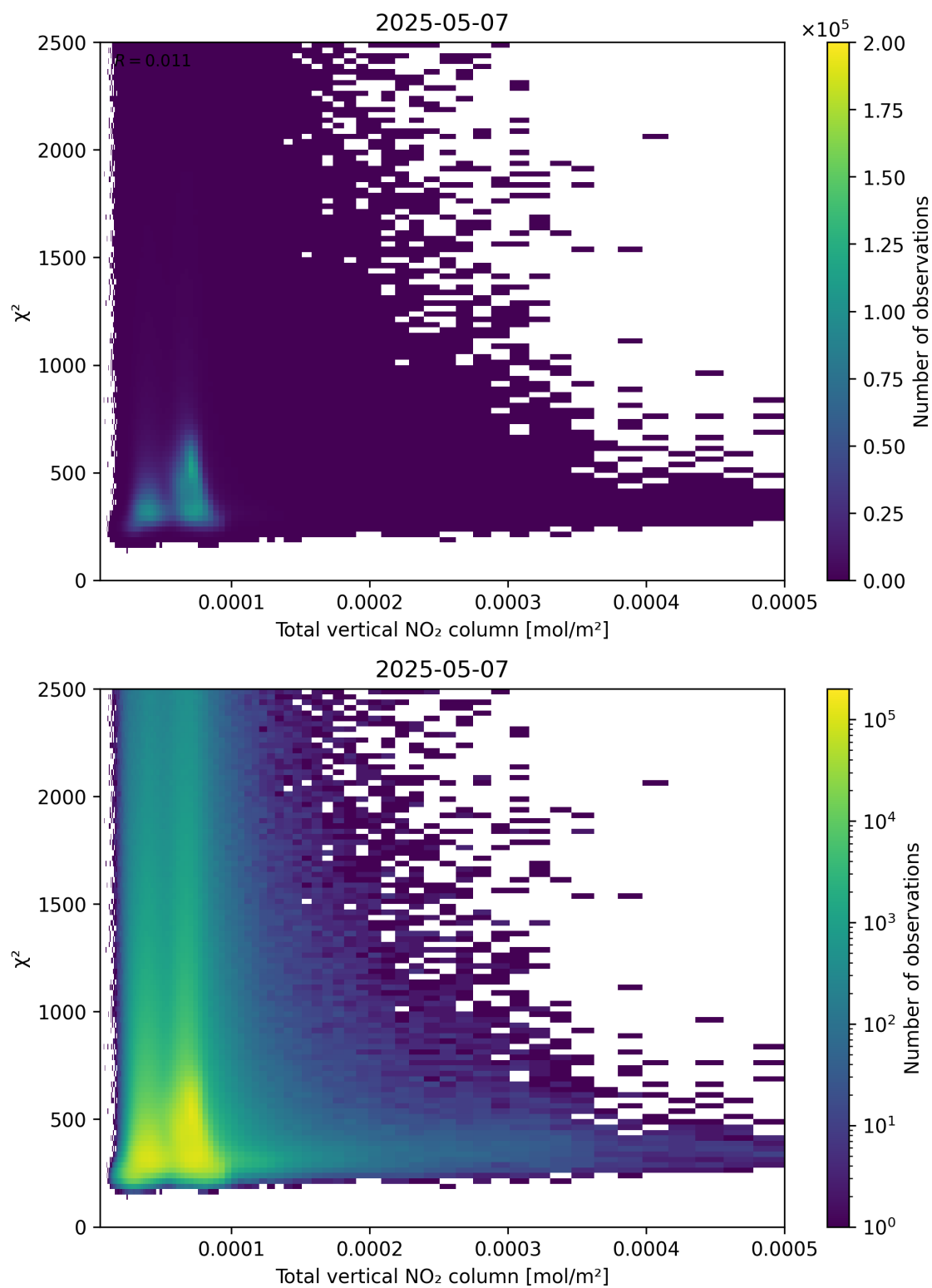
Figure 111: Scatter density plot of “Total vertical NO 2 column” against “ \chi^2 ” for 2025-05-07 to 2025-05-08.
