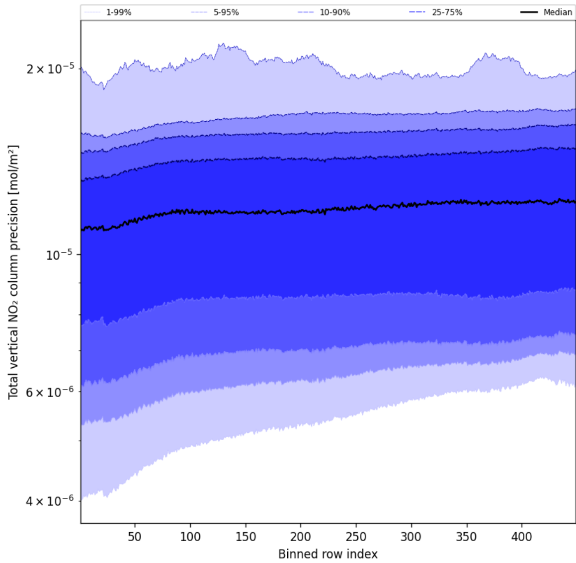
Figure 56: Along track statistics of “Total vertical NO 2 column precision” for 2025-05-07 to 2025-05-08
