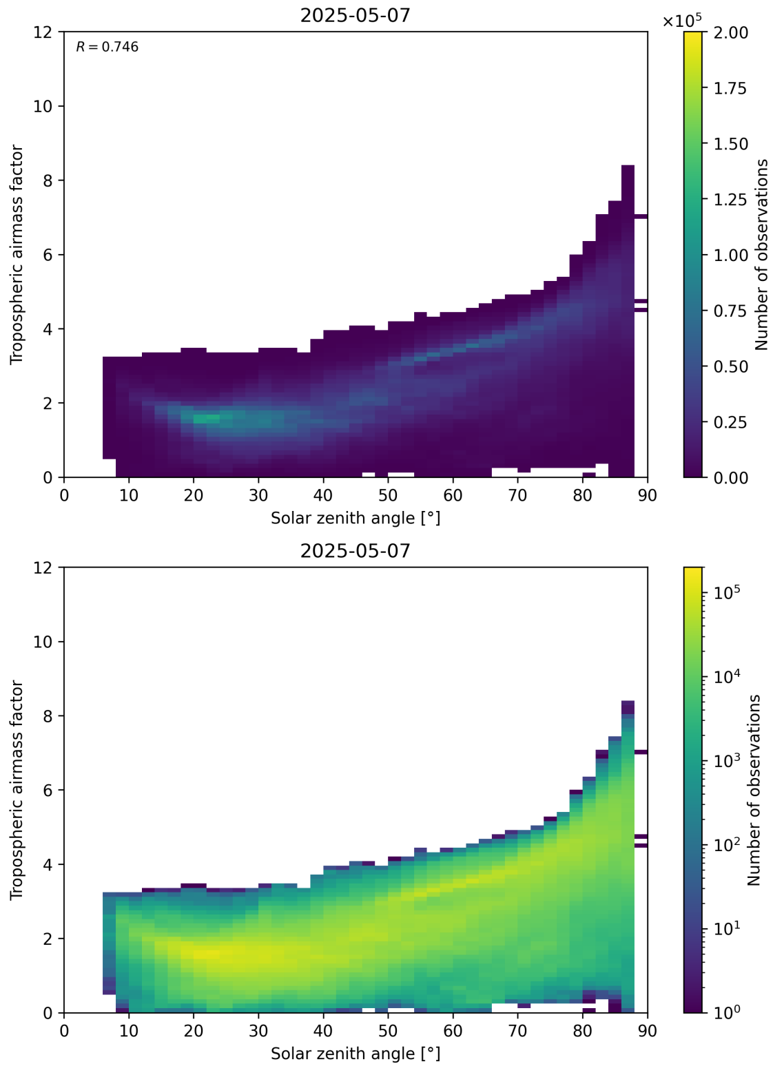
Figure 147: Scatter density plot of “Solar zenith angle” against “Tropospheric airmass factor” for 2025-05-07 to 2025-05-08.
