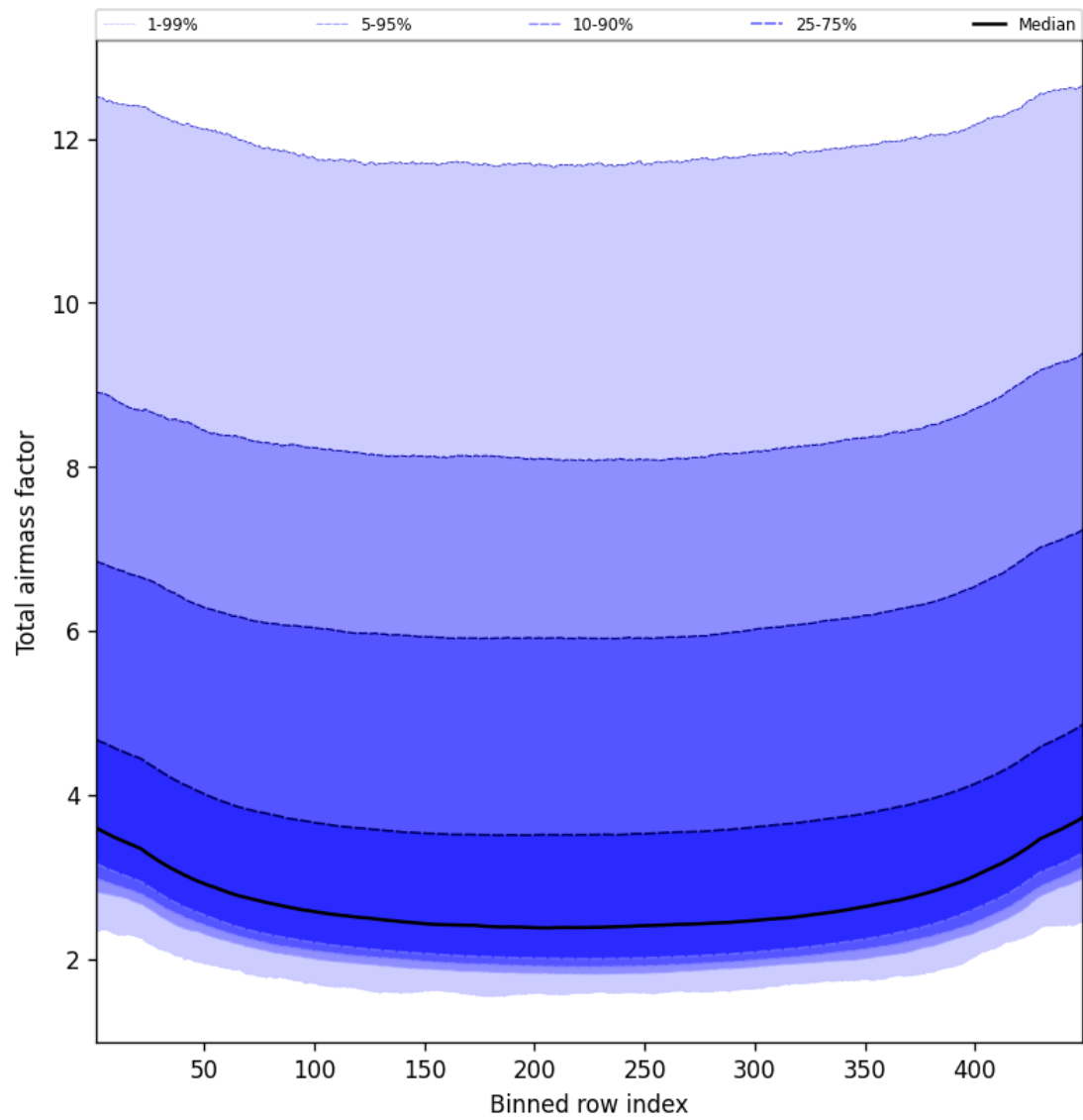
Figure 49: Along track statistics of “Total airmass factor” for 2025-05-07 to 2025-05-08
