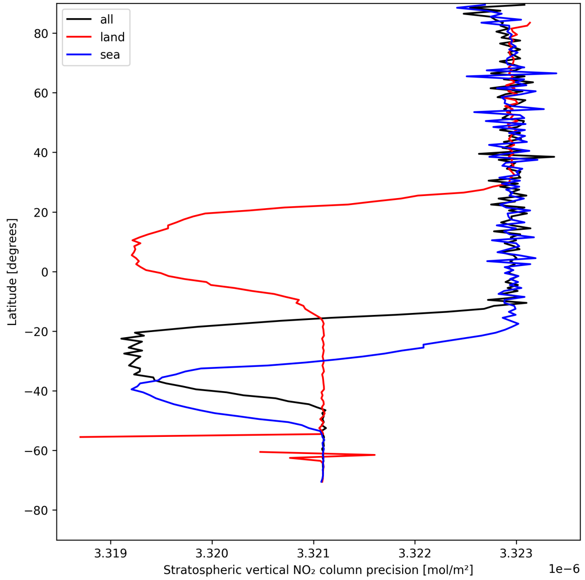
Figure 20: Zonal average of “Stratospheric vertical NO 2 column precision” for 2025-05-07 to 2025-05-08.
