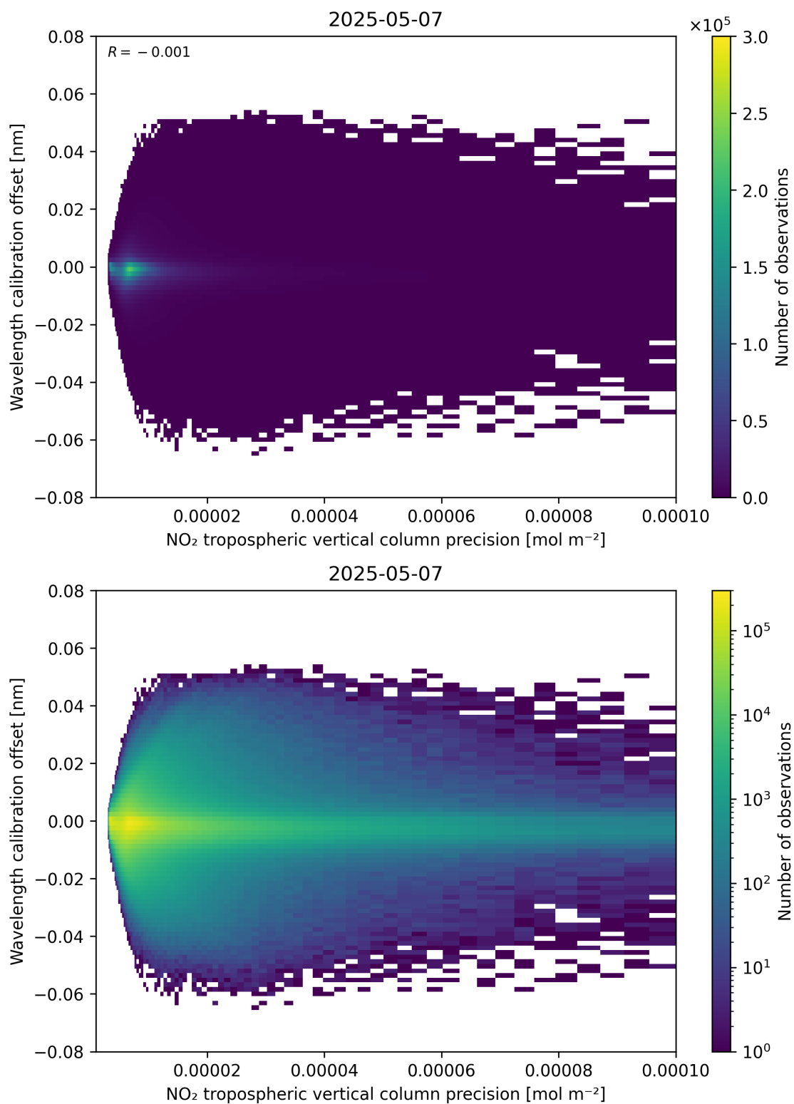
Figure 141: Scatter density plot of “NO 2 tropospheric vertical column precision” against “Wavelength calibration offset” for 2025-05-07 to 2025-05-08.
