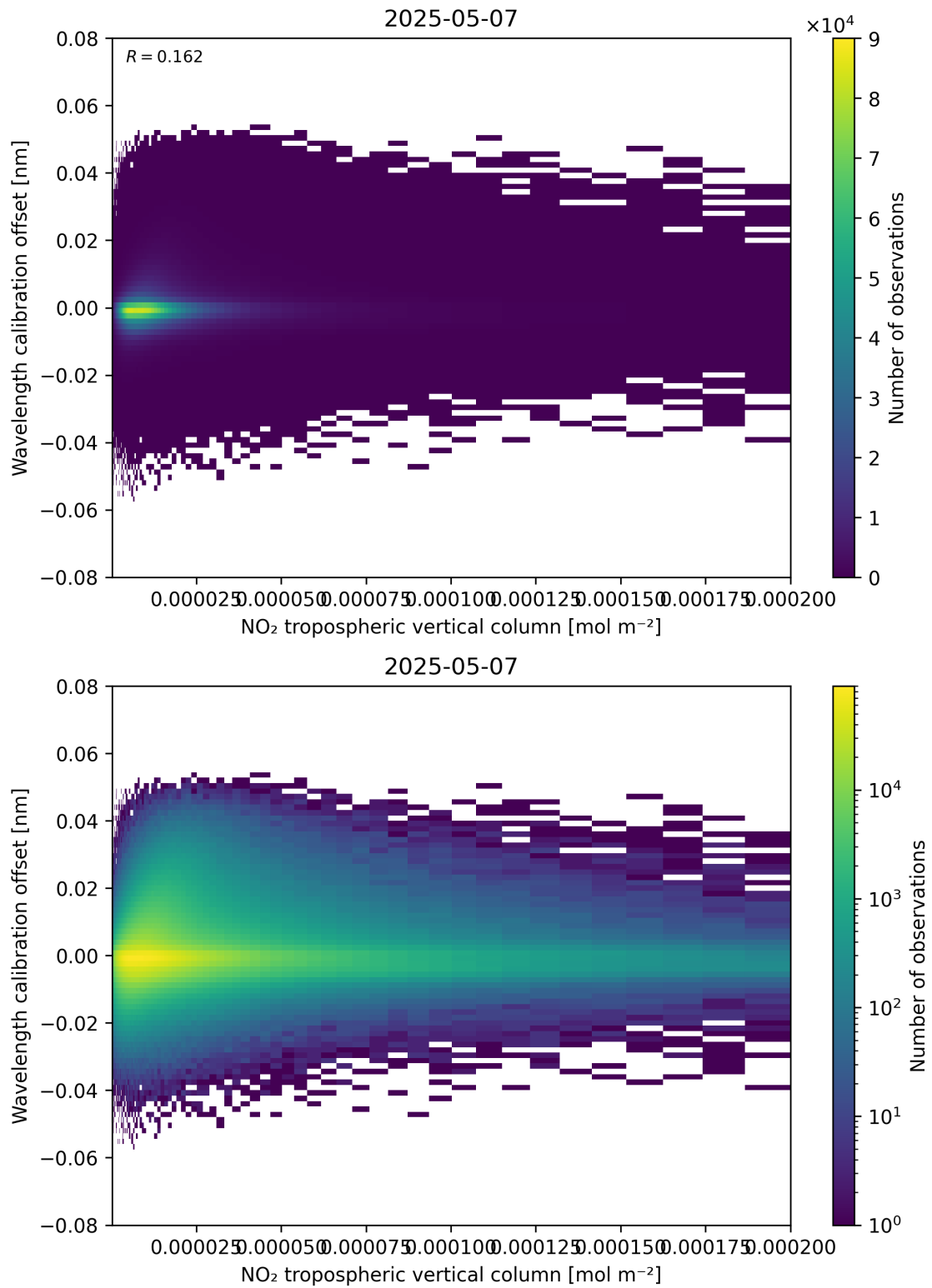
Figure 143: Scatter density plot of “NO 2 tropospheric vertical column” against “Wavelength calibration offset” for 2025-05-07 to 2025-05-08.
