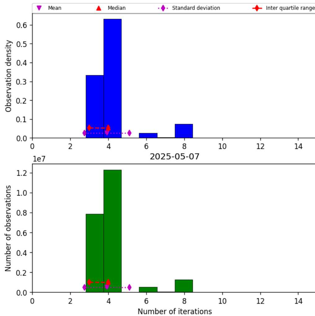
Figure 34: Histogram of “Number of iterations” for 2025-05-07 to 2025-05-08
