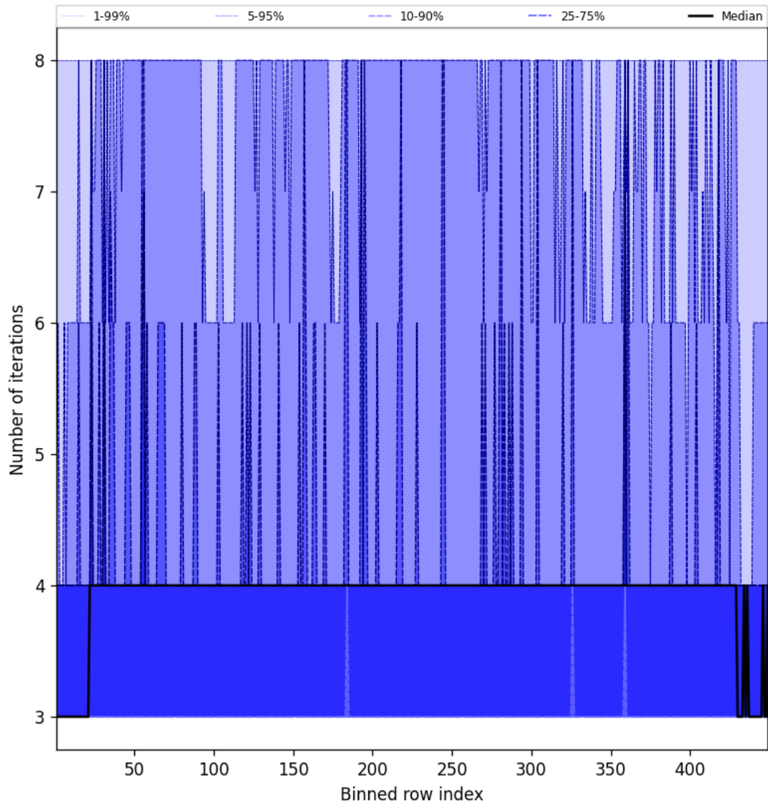
Figure 51: Along track statistics of “Number of iterations” for 2025-05-07 to 2025-05-08
