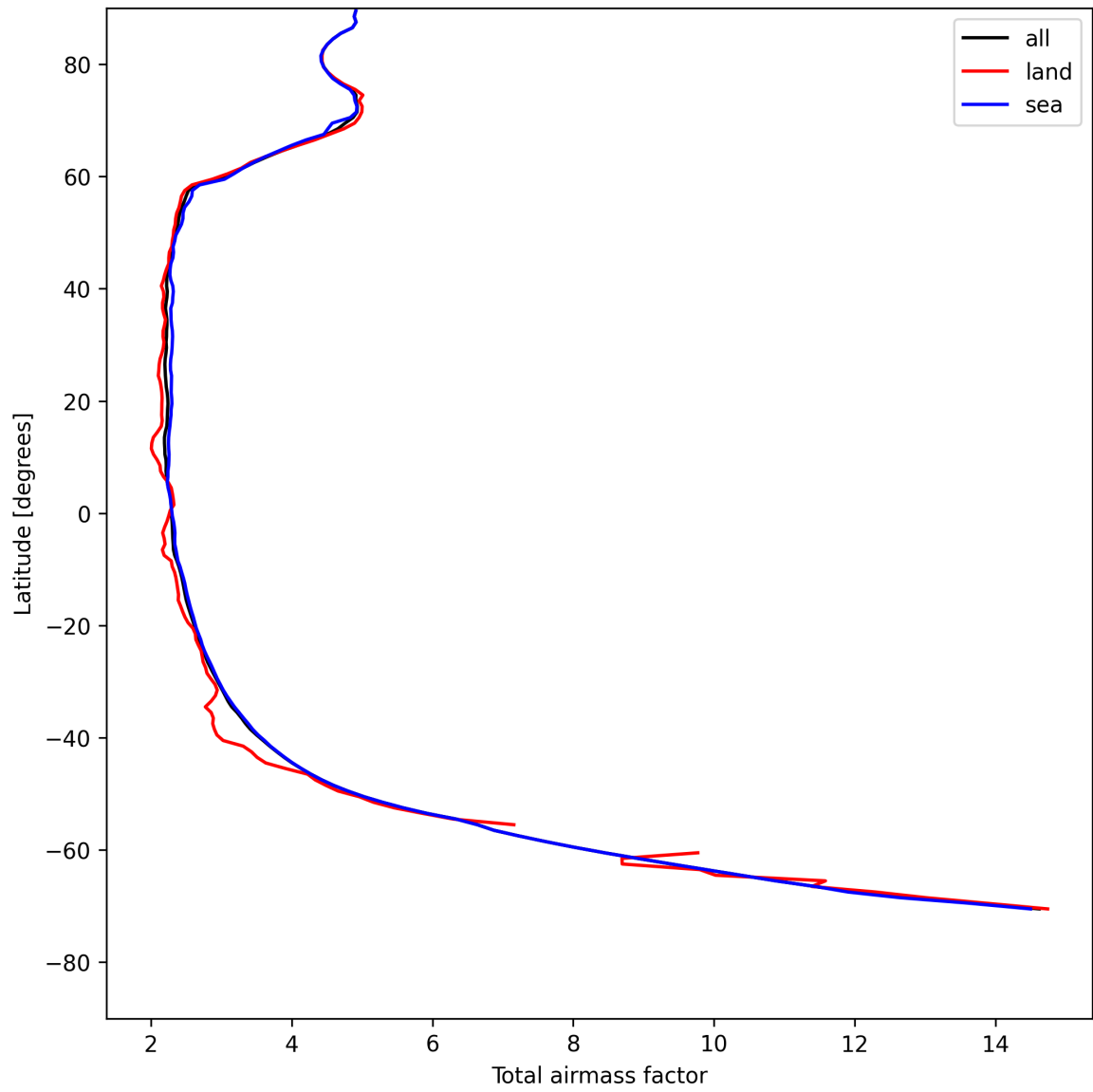
Figure 15: Zonal average of “Total airmass factor” for 2025-05-07 to 2025-05-08.
