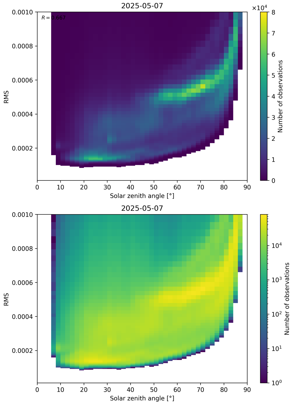
Figure 157: Scatter density plot of “Solar zenith angle” against “RMS” for 2025-05-07 to 2025-05-08.
