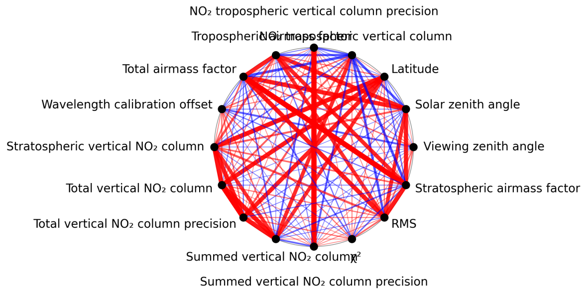
Figure 1: Map of correlation graph for 2025-05-07 to 2025-05-08.
