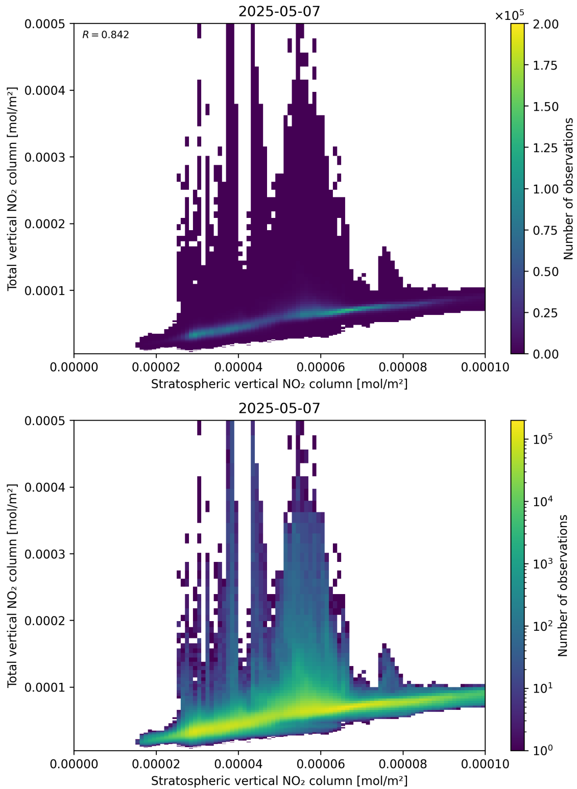
Figure 100: Scatter density plot of “Stratospheric vertical NO 2 column” against “Total vertical NO 2 column” for 2025-05-07 to 2025-05-08.
