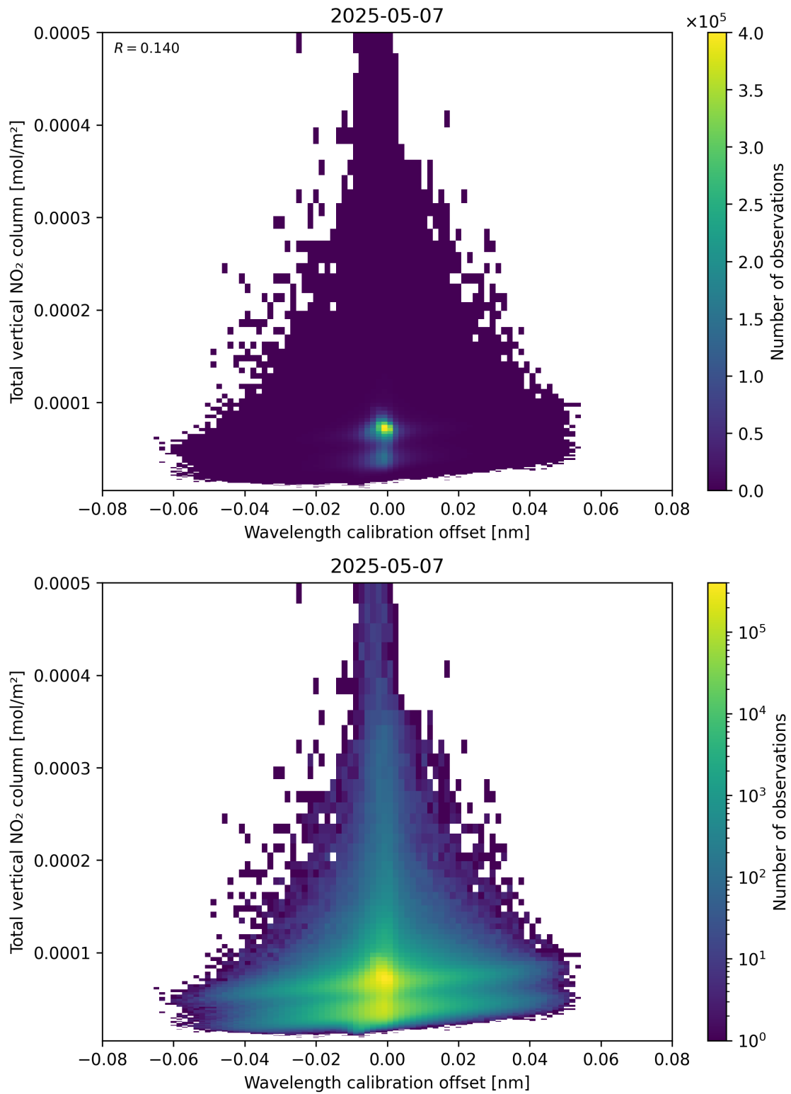
Figure 179: Scatter density plot of “Wavelength calibration offset” against “Total vertical NO 2 column” for 2025-05-07 to 2025-05-08.
