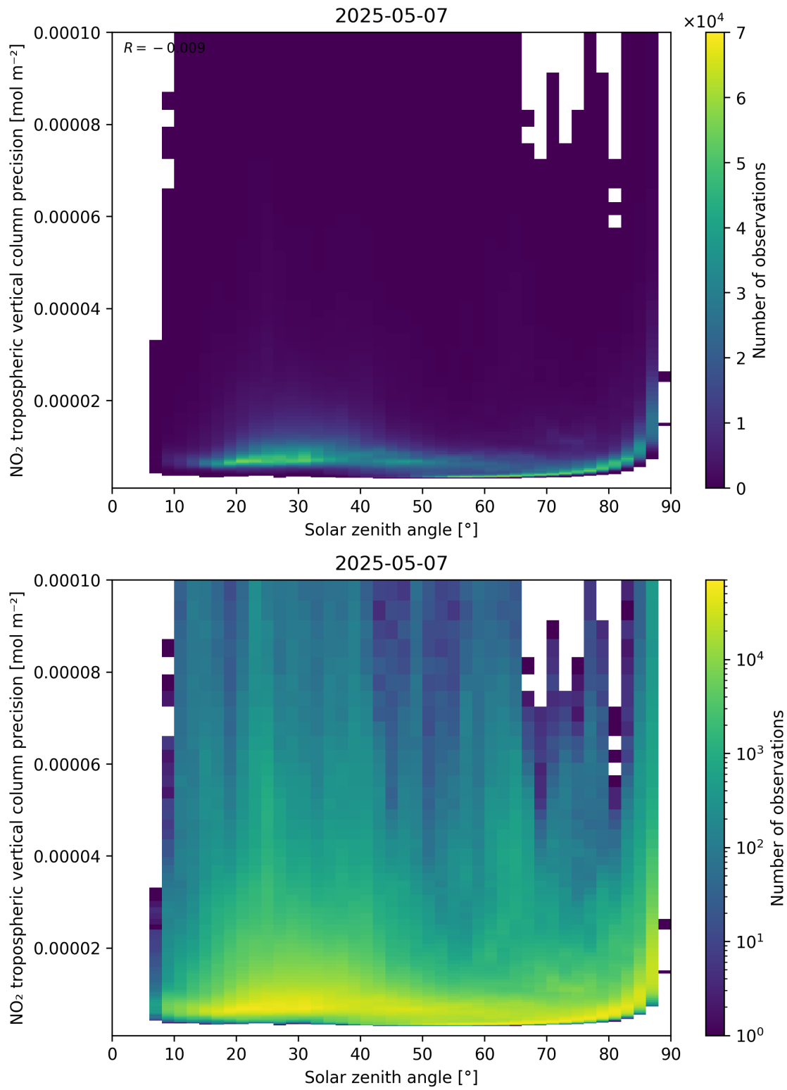
Figure 156: Scatter density plot of “Solar zenith angle” against “NO 2 tropospheric vertical column precision” for 2025-05-07 to 2025-05-08.
