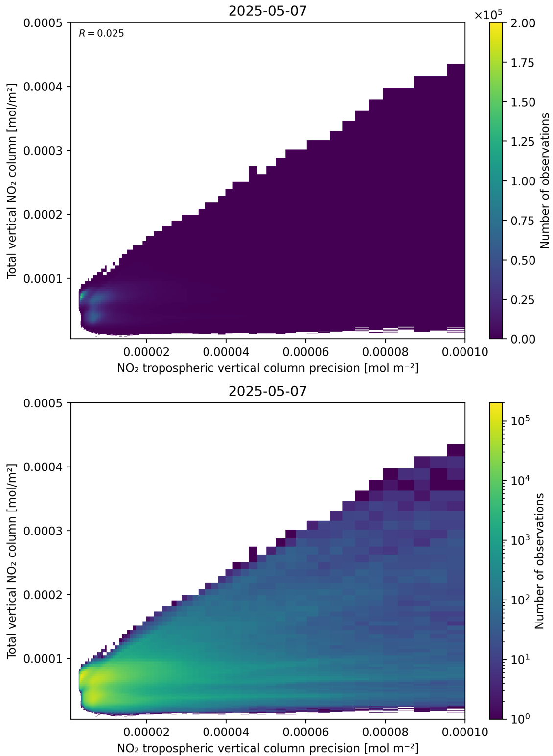
Figure 138: Scatter density plot of “NO 2 tropospheric vertical column precision” against “Total vertical NO 2 column” for 2025-05-07 to 2025-05-08.
