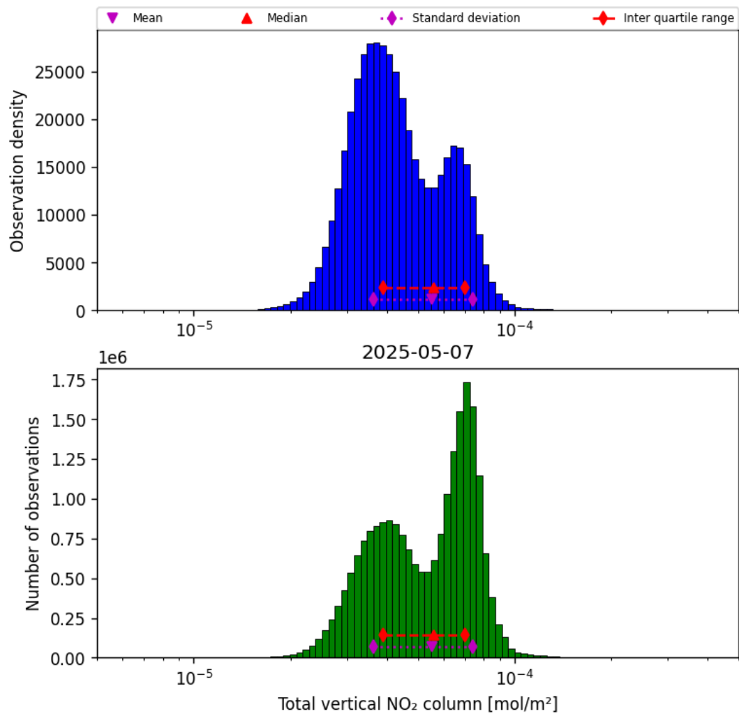
Figure 38: Histogram of “Total vertical NO 2 column” for 2025-05-07 to 2025-05-08
