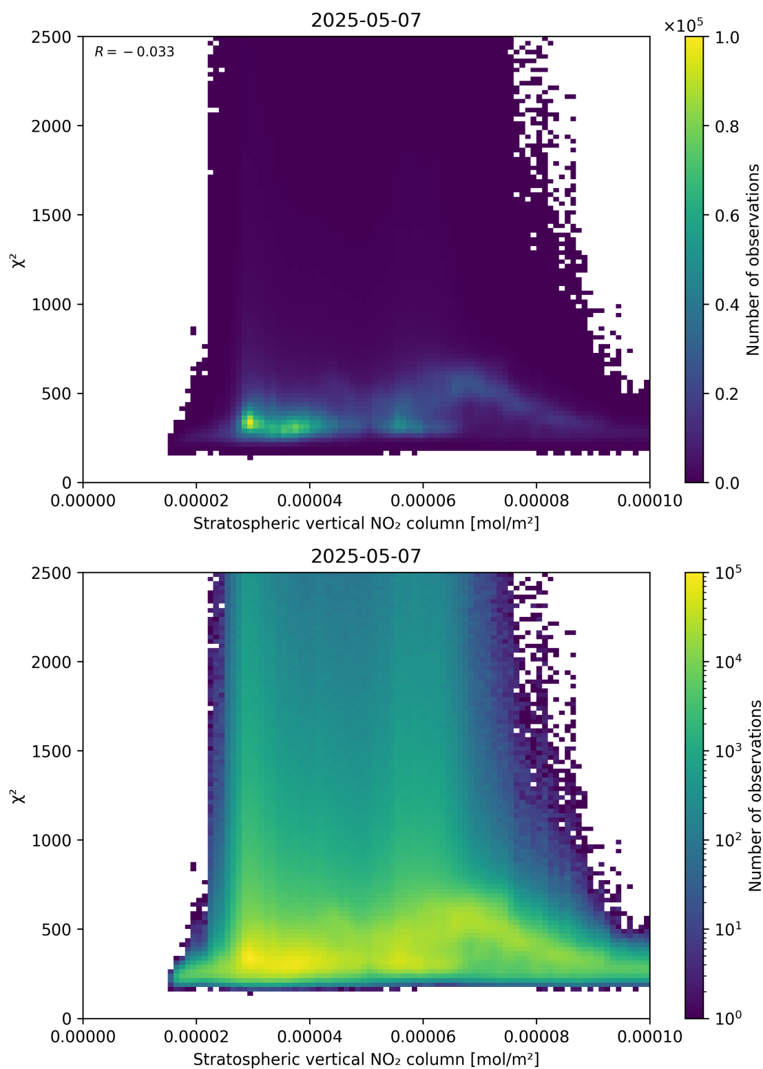
Figure 97: Scatter density plot of “Stratospheric vertical NO 2 column” against “ \chi^2 ” for 2025-05-07 to 2025-05-08.
