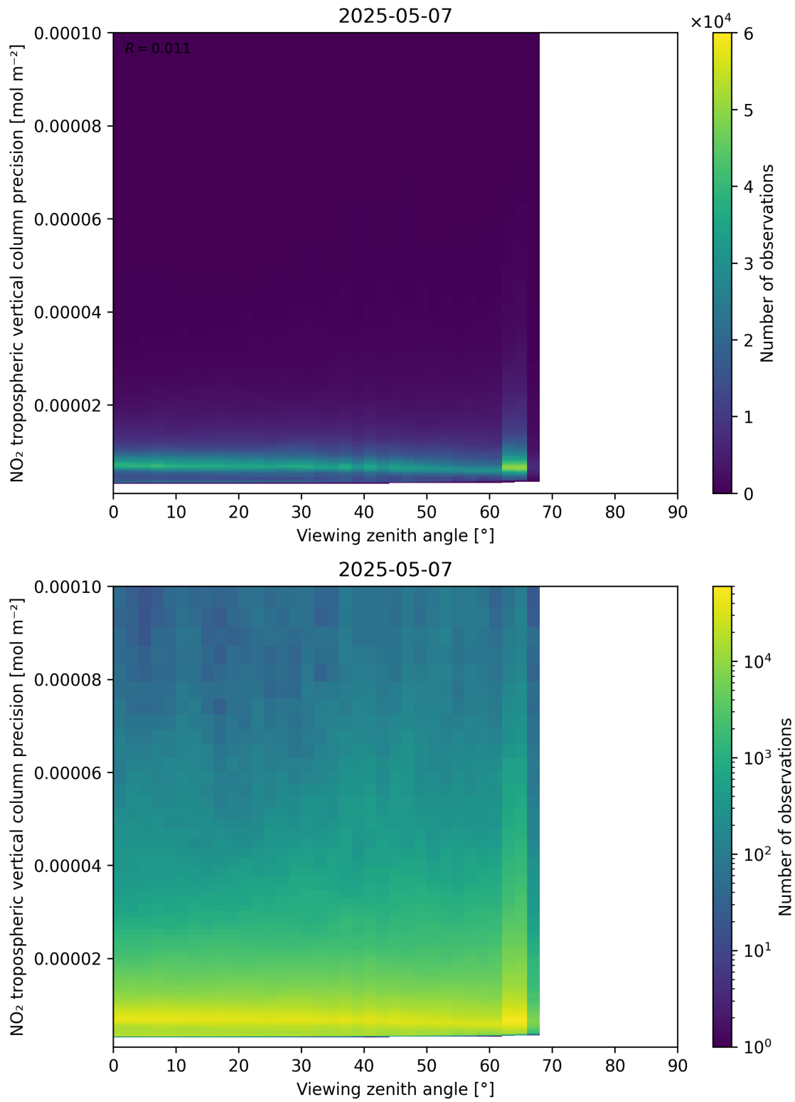
Figure 170: Scatter density plot of “Viewing zenith angle” against “NO 2 tropospheric vertical column precision” for 2025-05-07 to 2025-05-08.
