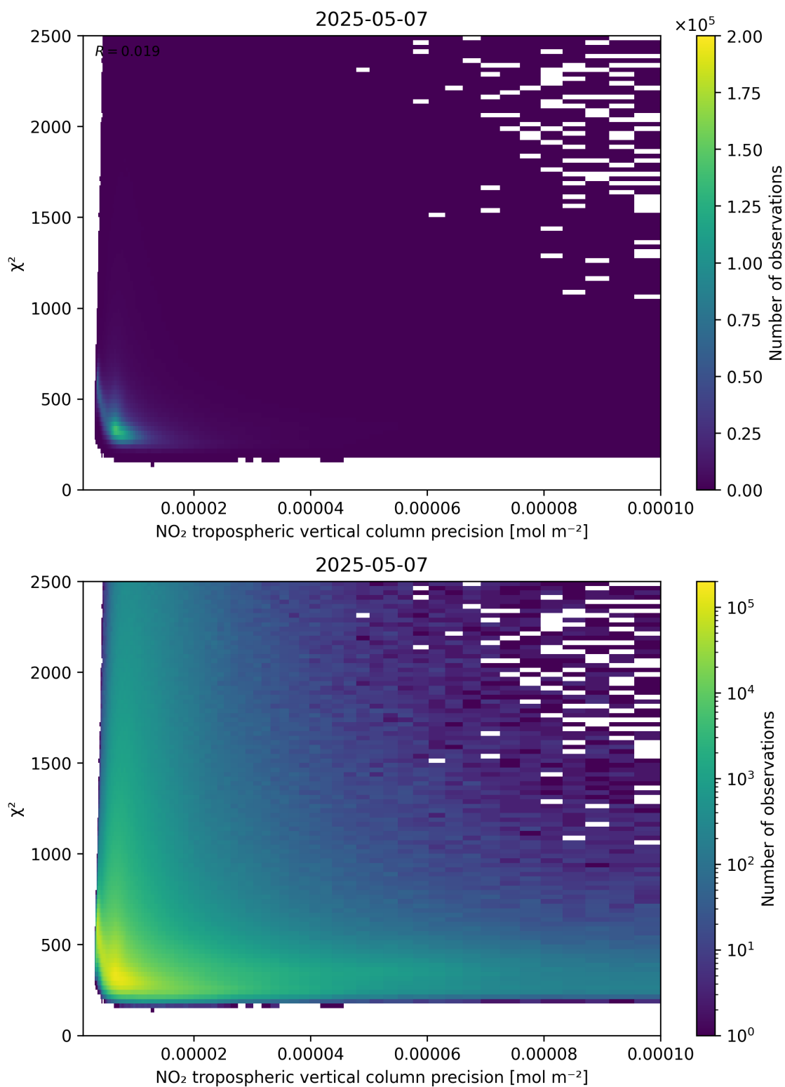
Figure 134: Scatter density plot of “NO 2 tropospheric vertical column precision” against “ \chi^2 ” for 2025-05-07 to 2025-05-08.
