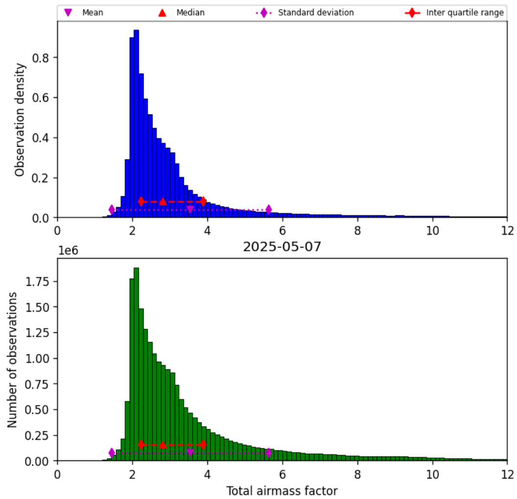
Figure 32: Histogram of “Total airmass factor” for 2025-05-07 to 2025-05-08
