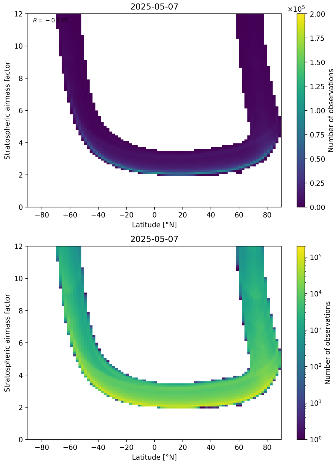
Figure 83: Scatter density plot of “Latitude” against “Stratospheric air mass factor” for 2025-05-07 to 2025-05-08.
