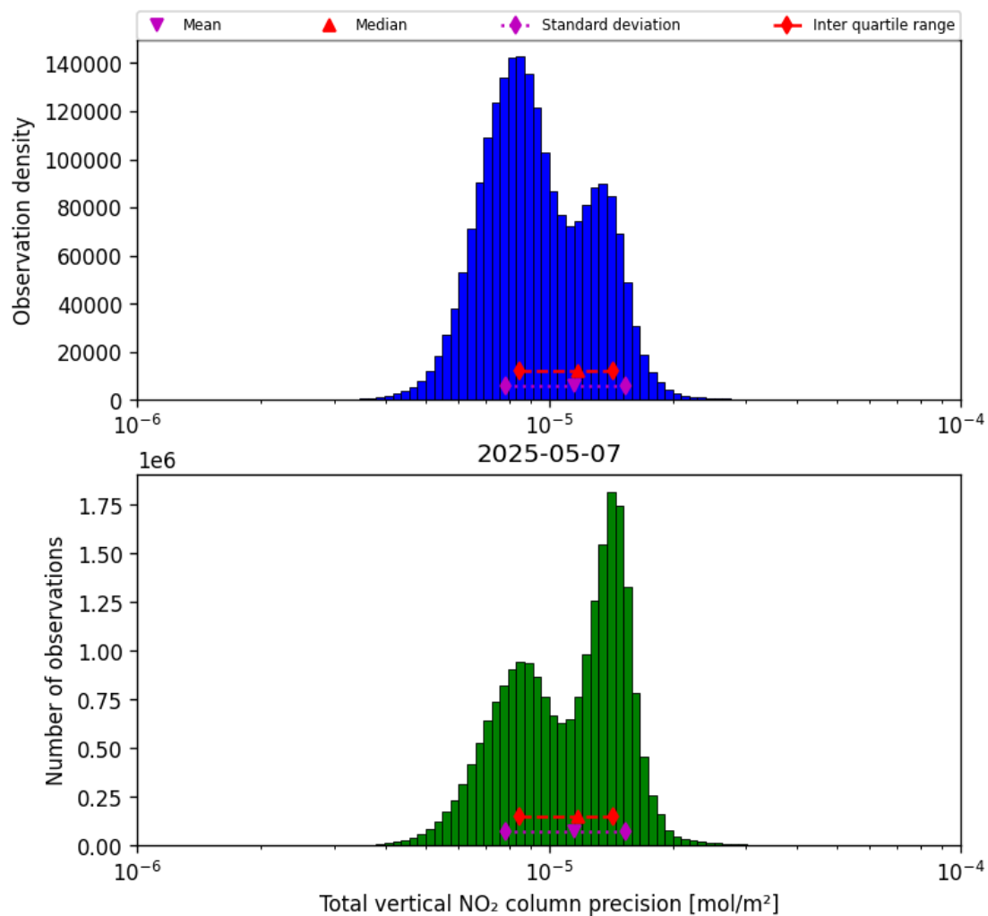
Figure 39: Histogram of “Total vertical NO 2 column precision” for 2025-05-07 to 2025-05-08
