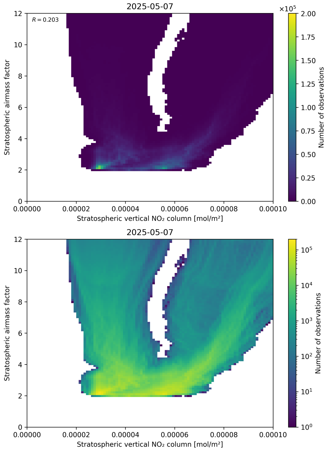
Figure 96: Scatter density plot of “Stratospheric vertical NO 2 column” against “Stratospheric airmass factor” for 2025-05-07 to 2025-05-08.
