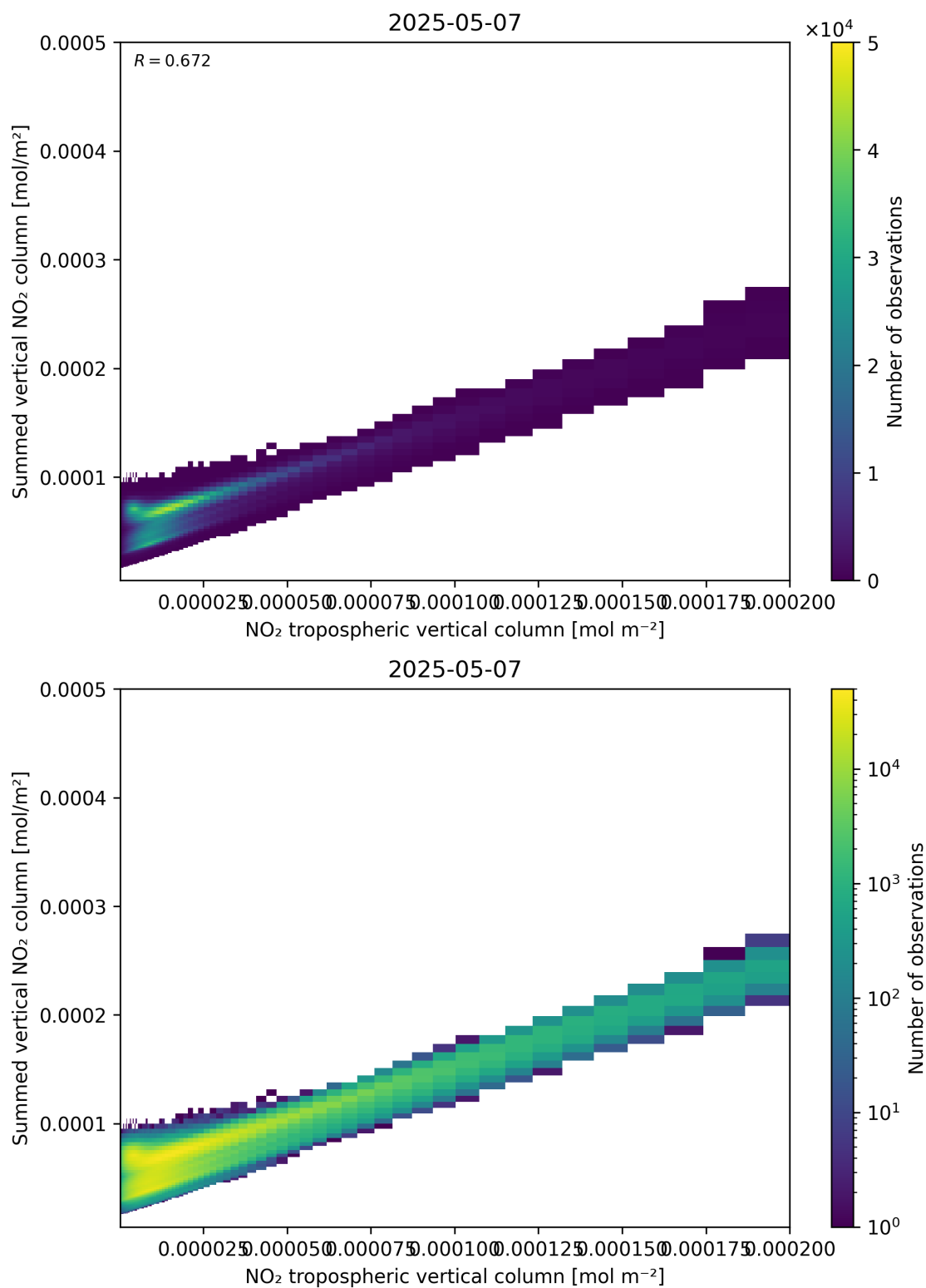
Figure 126: Scatter density plot of “NO 2 tropospheric vertical column” against “Summed vertical NO 2 column” for 2025-05-07 to 2025-05-08.
