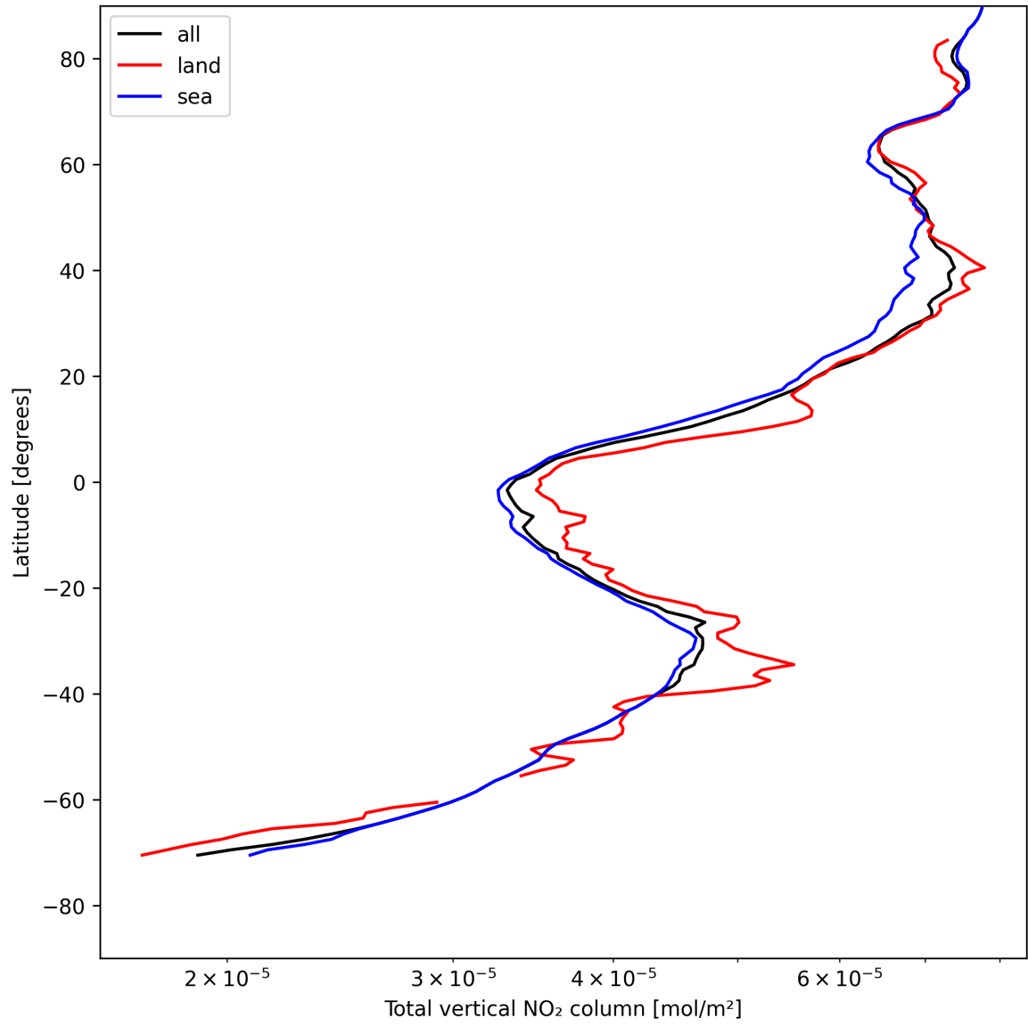
Figure 21: Zonal average of “Total vertical NO 2 column” for 2025-05-07 to 2025-05-08.
