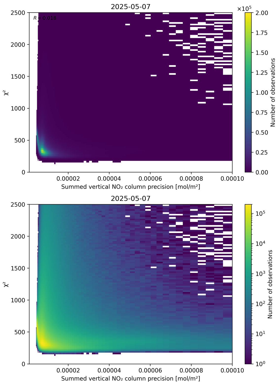
Figure 107: Scatter density plot of “Summed vertical NO 2 column precision” against “ \chi^2 ” for 2025-05-07 to 2025-05-08.
