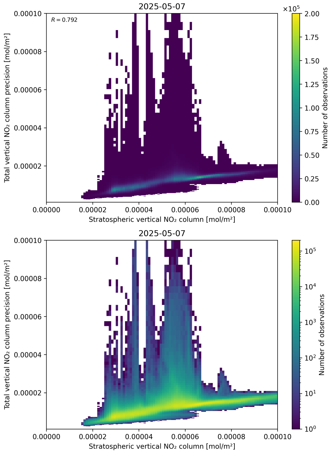
Figure 101: Scatter density plot of “Stratospheric vertical NO 2 column” against “Total vertical NO 2 column precision” for 2025-05-07 to 2025-05-08.
