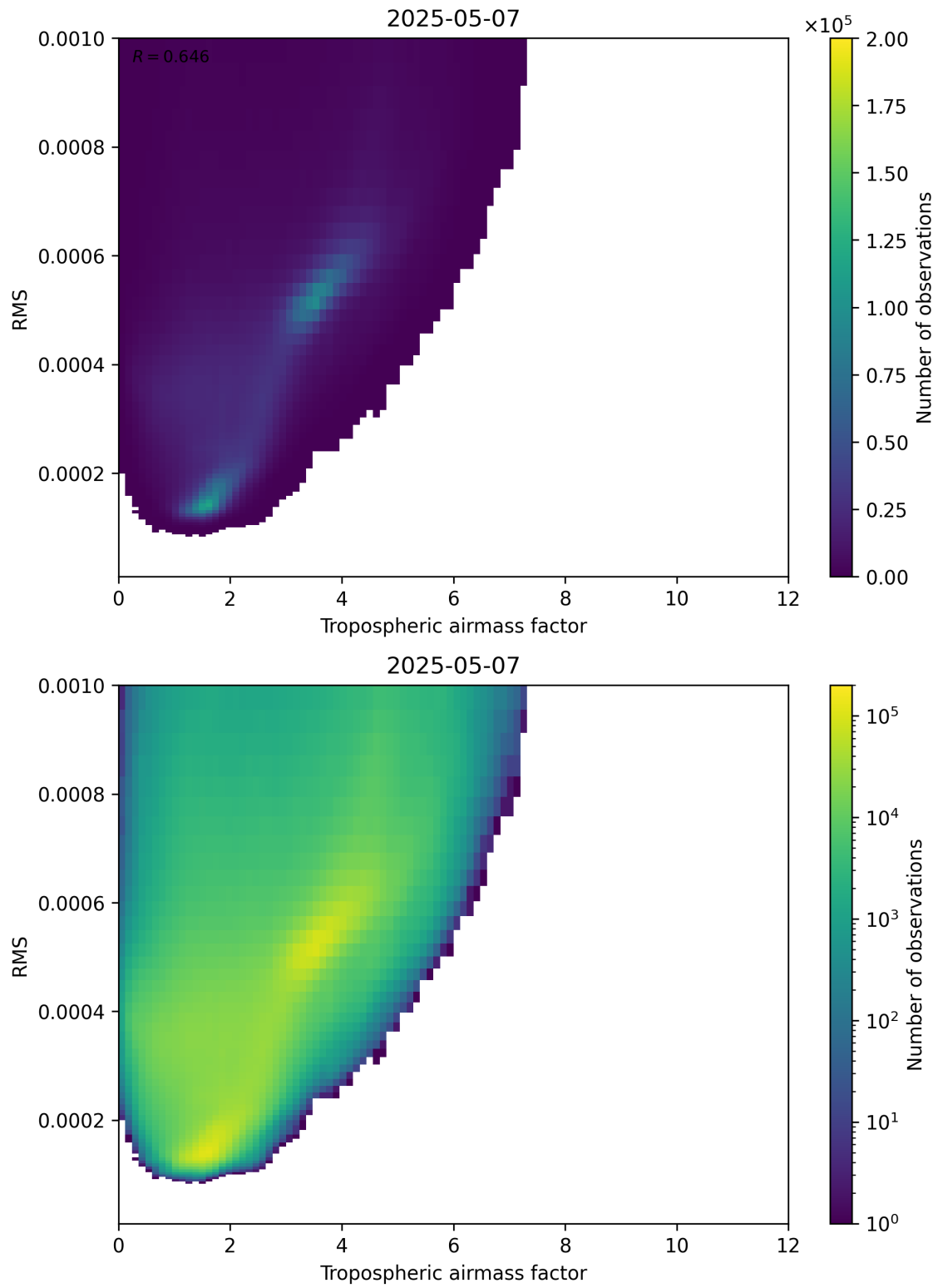
Figure 79: Scatter density plot of “Tropospheric airmass factor” against “RMS” for 2025-05-07 to 2025-05-08.
