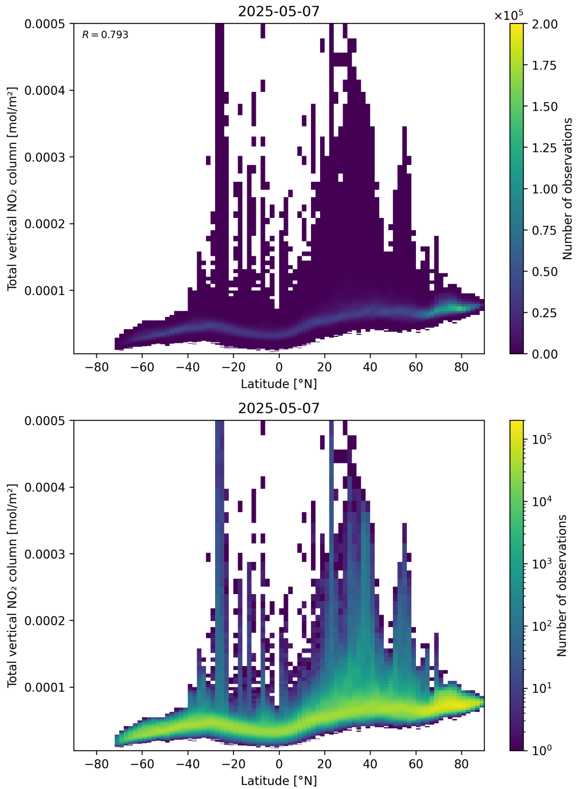
Figure 90: Scatter density plot of “Latitude” against “Total vertical NO 2 column” for 2025-05-07 to 2025-05-08.
