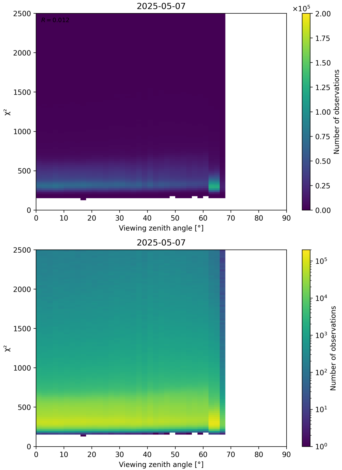
Figure 162: Scatter density plot of “Viewing zenith angle” against “ \chi^2 ” for 2025-05-07 to 2025-05-08.
