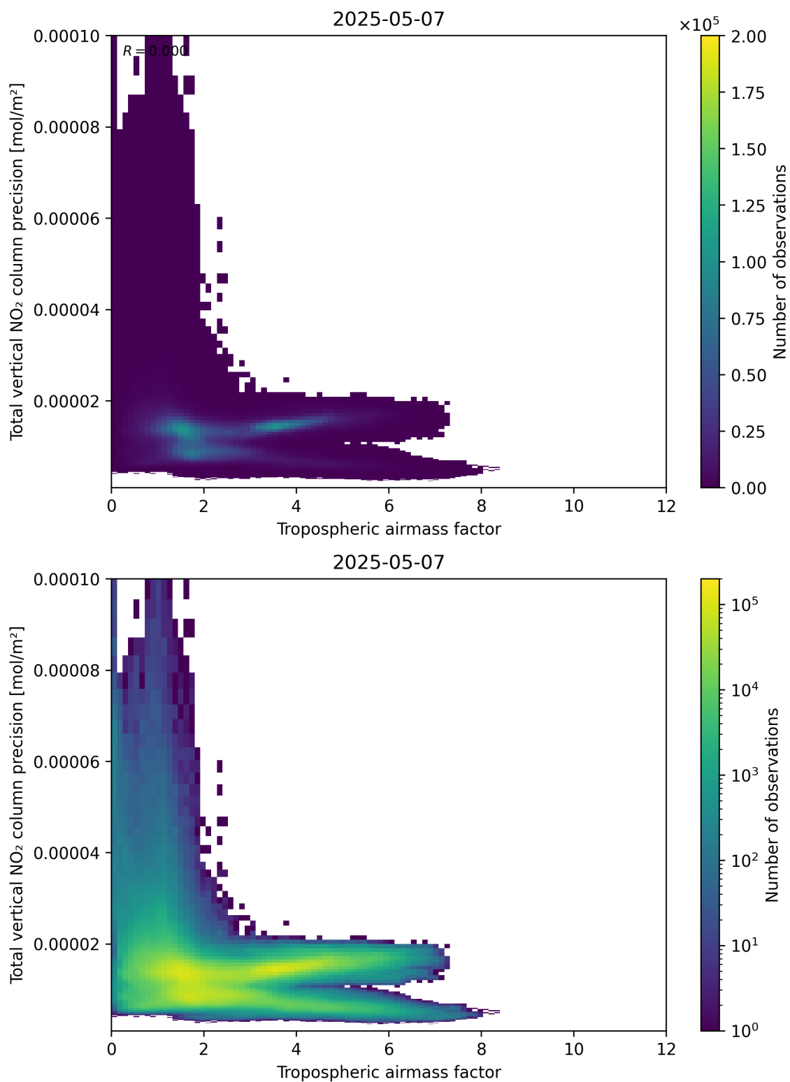
Figure 78: Scatter density plot of “Tropospheric air mass factor” against “Total vertical NO 2 column precision” for 2025-05-07 to 2025-05-08.
