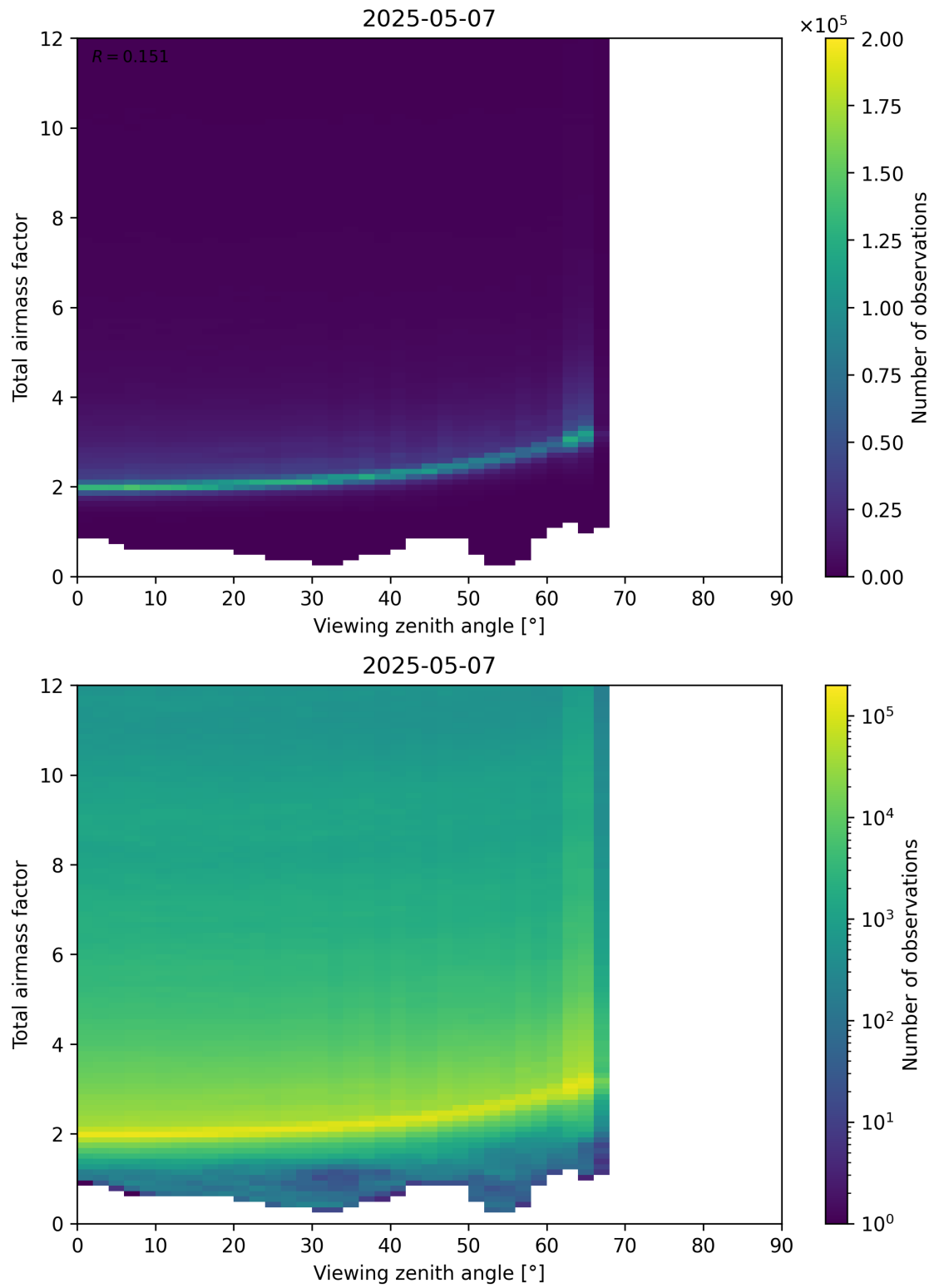
Figure 160: Scatter density plot of “Viewing zenith angle” against “Total airmass factor” for 2025-05-07 to 2025-05-08.
