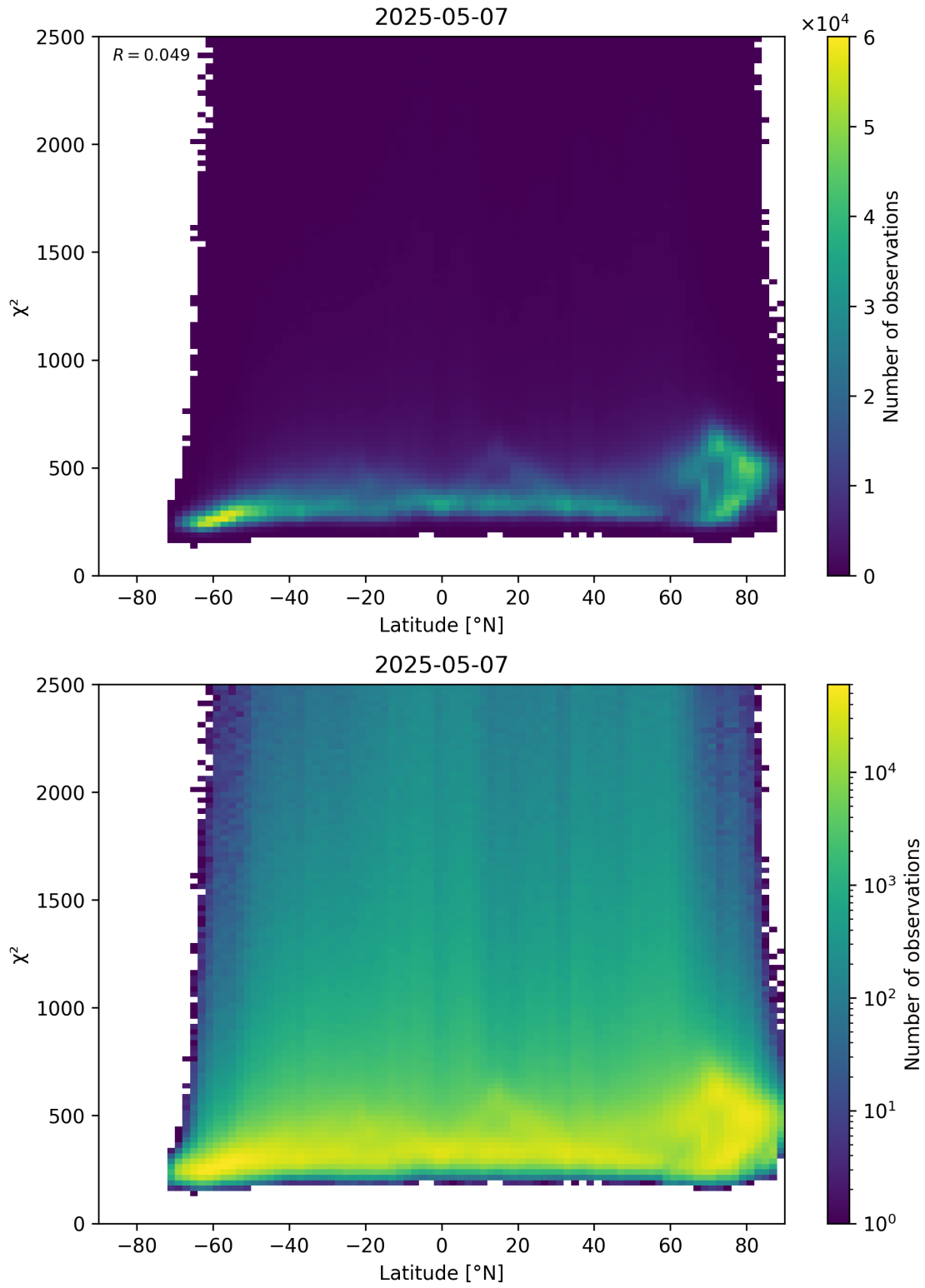
Figure 86: Scatter density plot of “Latitude” against “ \chi^2 ” for 2025-05-07 to 2025-05-08.
