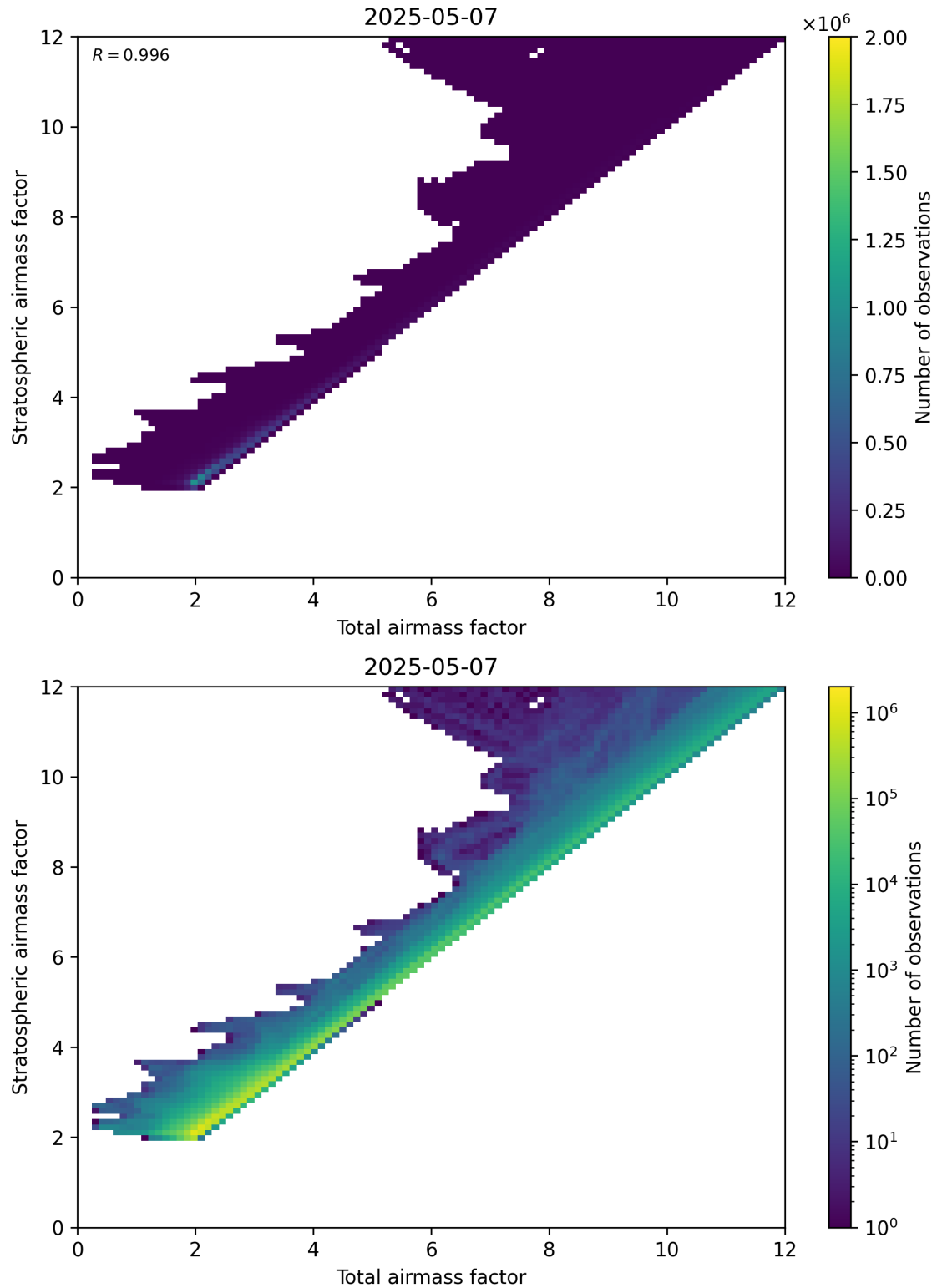
Figure 62: Scatter density plot of “Total airmass factor” against “Stratospheric airmass factor” for 2025-05-07 to 2025-05-08.
