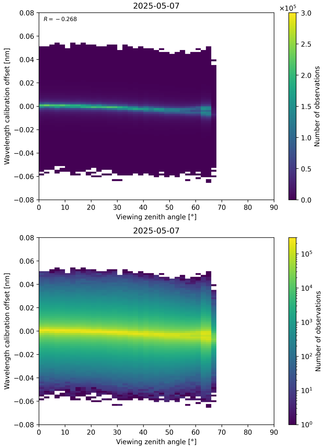
Figure 173: Scatter density plot of “Viewing zenith angle” against “Wavelength calibration offset” for 2025-05-07 to 2025-05-08.
