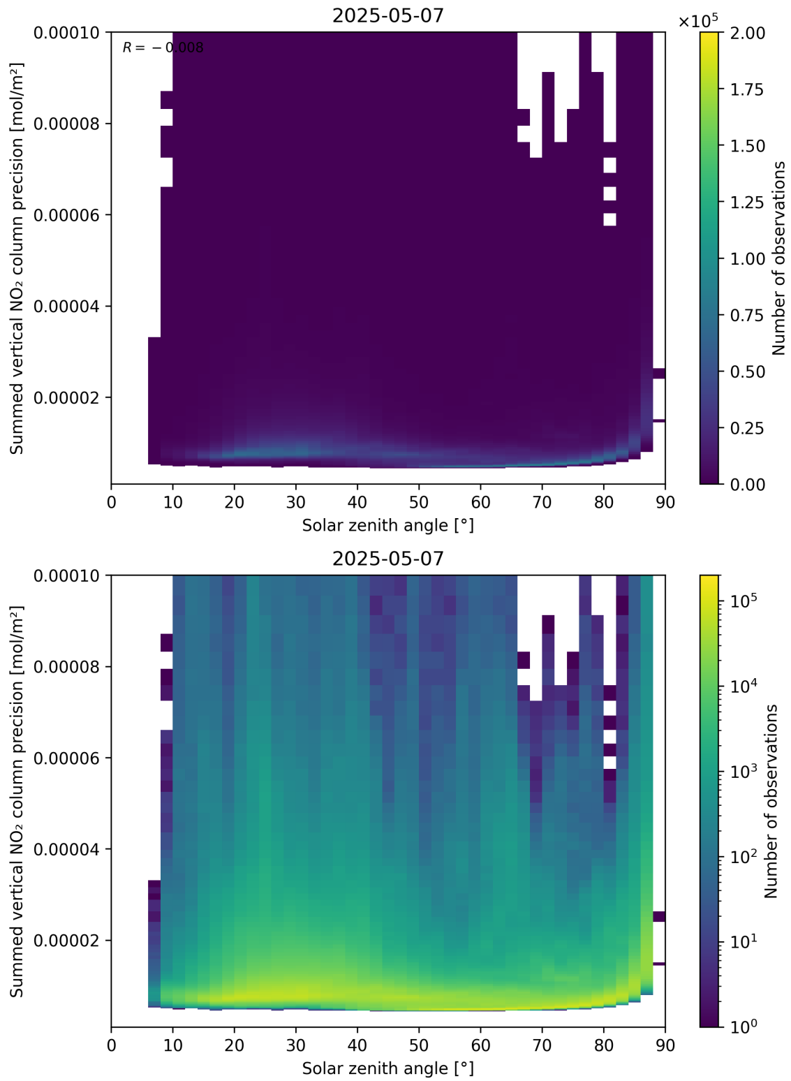
Figure 152: Scatter density plot of “Solar zenith angle” against “Summed vertical NO 2 column precision” for 2025-05-07 to 2025-05-08.
