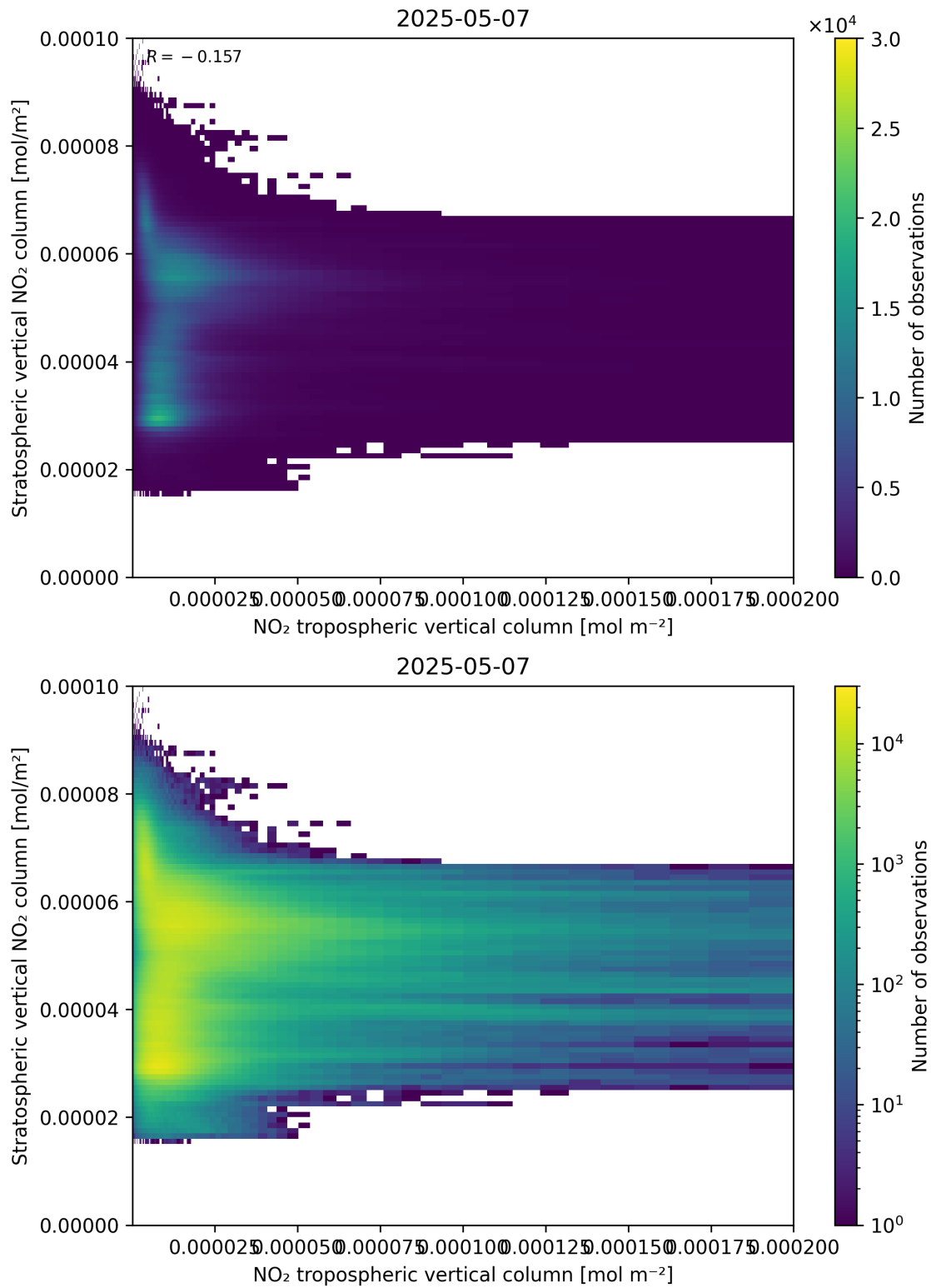
Figure 125: Scatter density plot of “NO 2 tropospheric vertical column” against “Stratospheric vertical NO 2 column” for 2025-05-07 to 2025-05-08.
