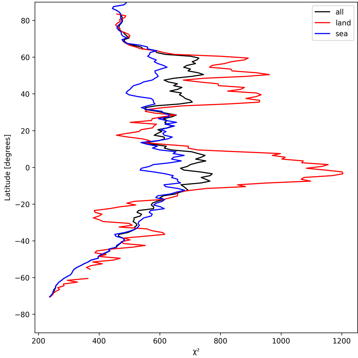
Figure 25: Zonal average of “ \chi^2 ” for 2025-05-07 to 2025-05-08.
