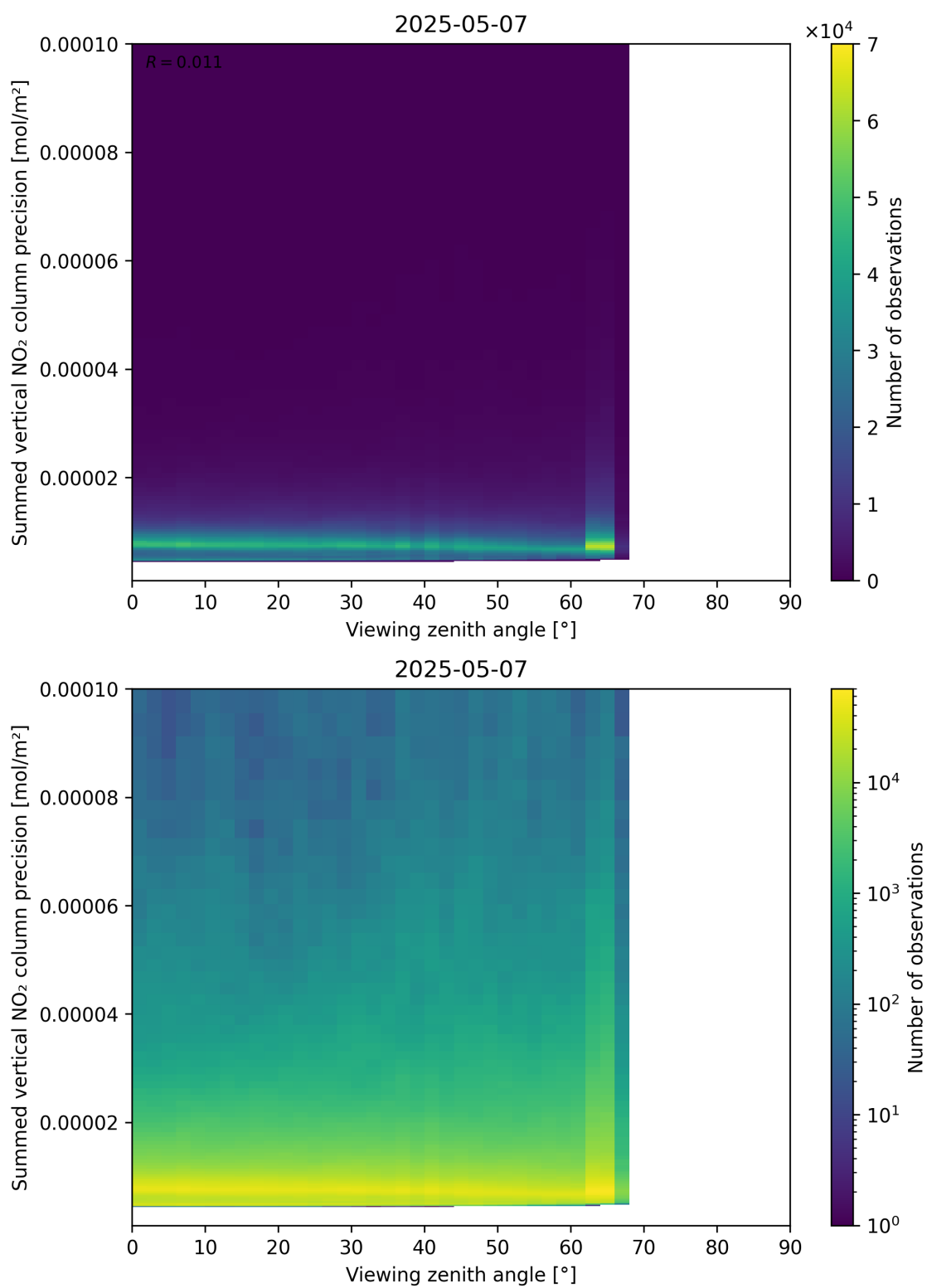
Figure 166: Scatter density plot of “Viewing zenith angle” against “Summed vertical NO 2 column precision” for 2025-05-07 to 2025-05-08.
