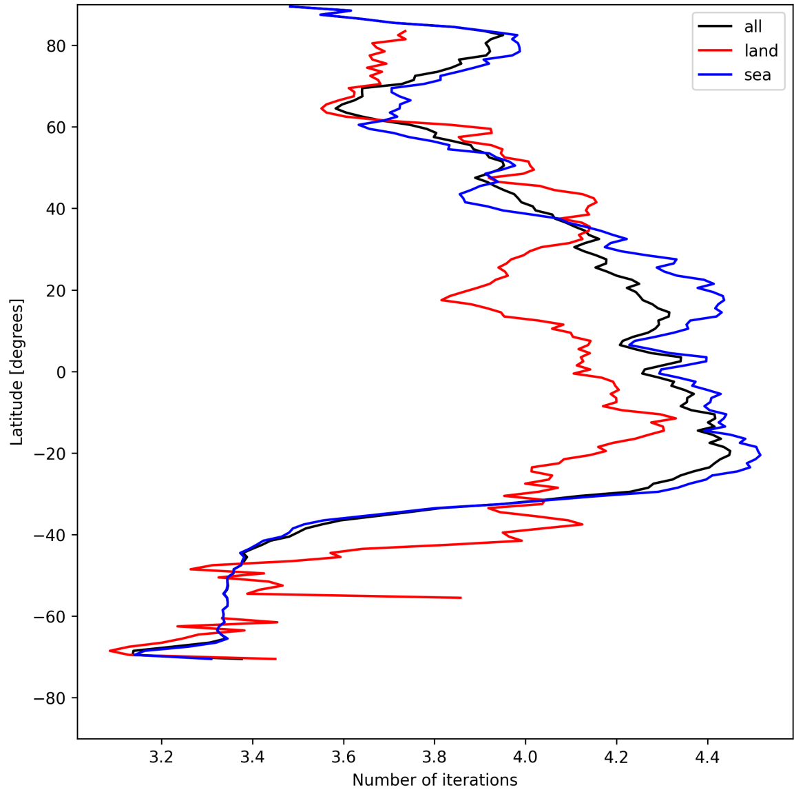
Figure 17: Zonal average of “Number of iterations” for 2025-05-07 to 2025-05-08.
