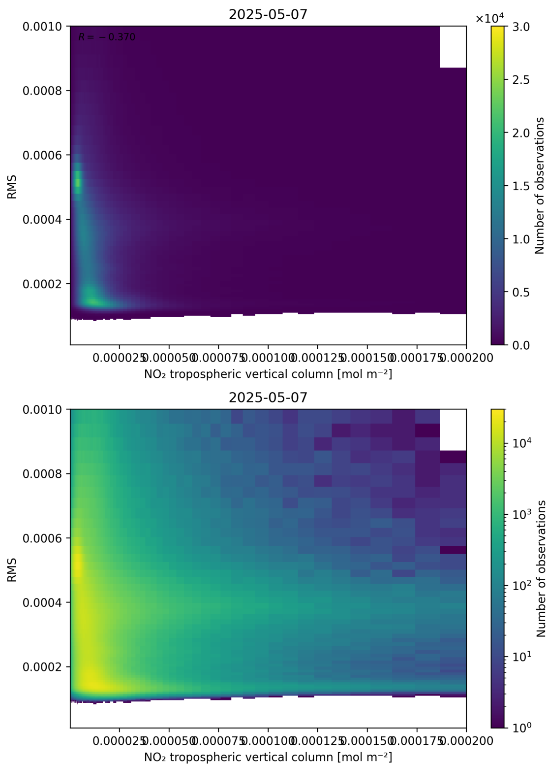
Figure 142: Scatter density plot of “NO 2 tropospheric vertical column” against “RMS” for 2025-05-07 to 2025-05-08.
