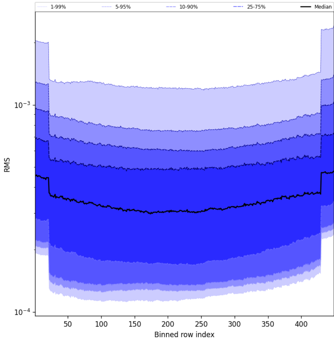
Figure 60: Along track statistics of “RMS” for 2025-05-07 to 2025-05-08
