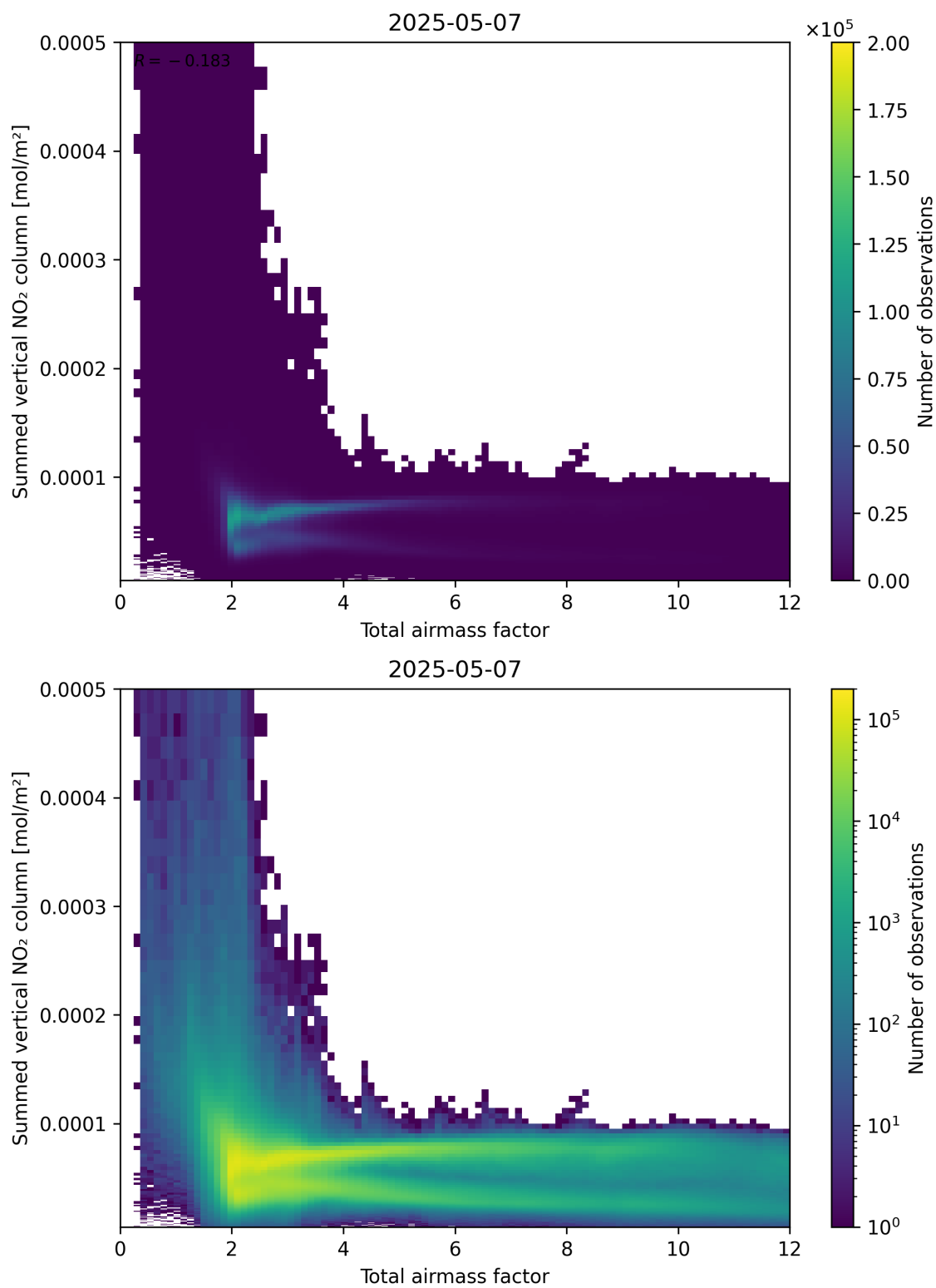
Figure 65: Scatter density plot of “Total airmass factor” against “Summed vertical NO 2 column” for 2025-05-07 to 2025-05-08.
