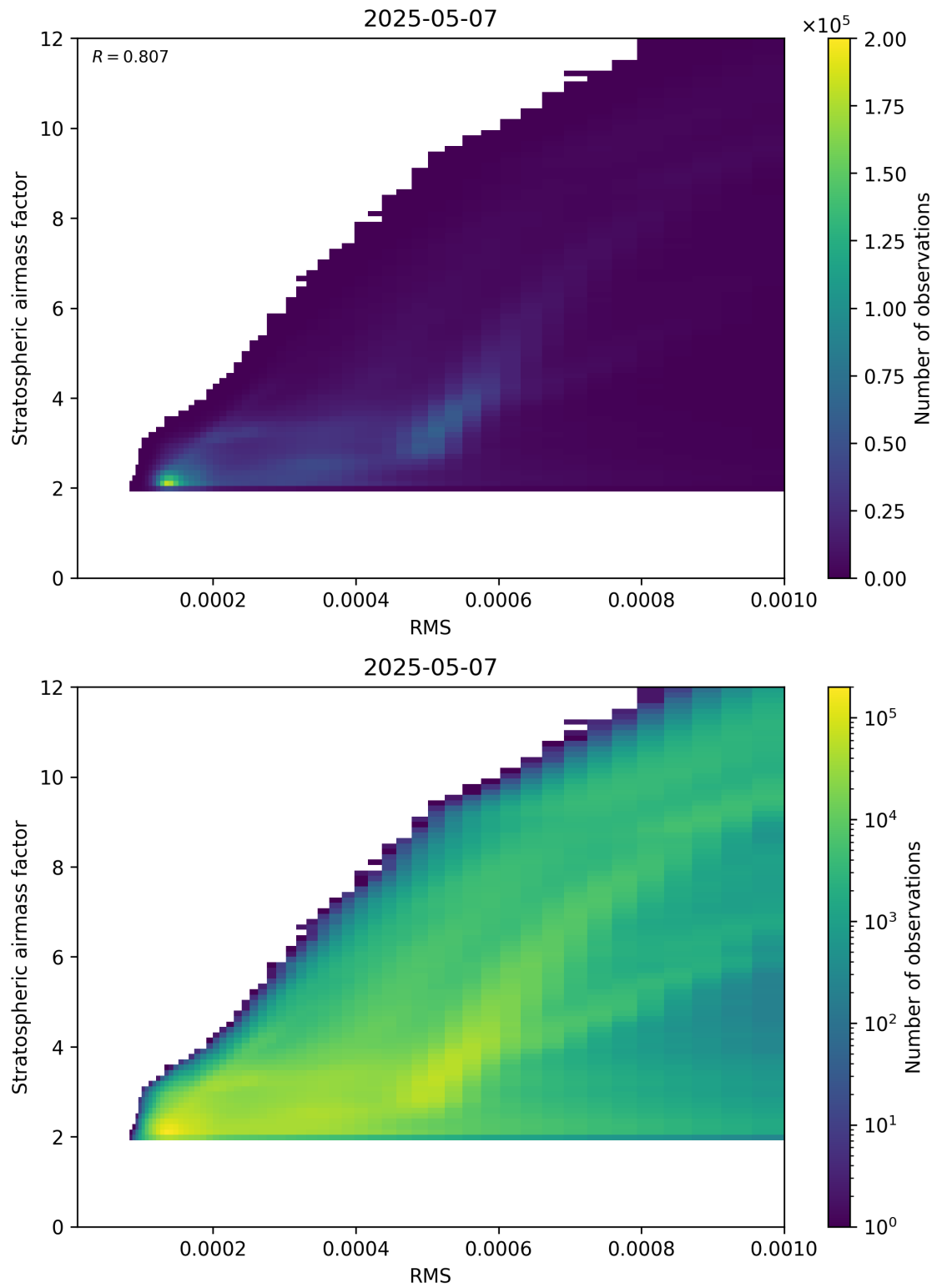
Figure 144: Scatter density plot of “RMS” against “Stratospheric airmass factor” for 2025-05-07 to 2025-05-08.
