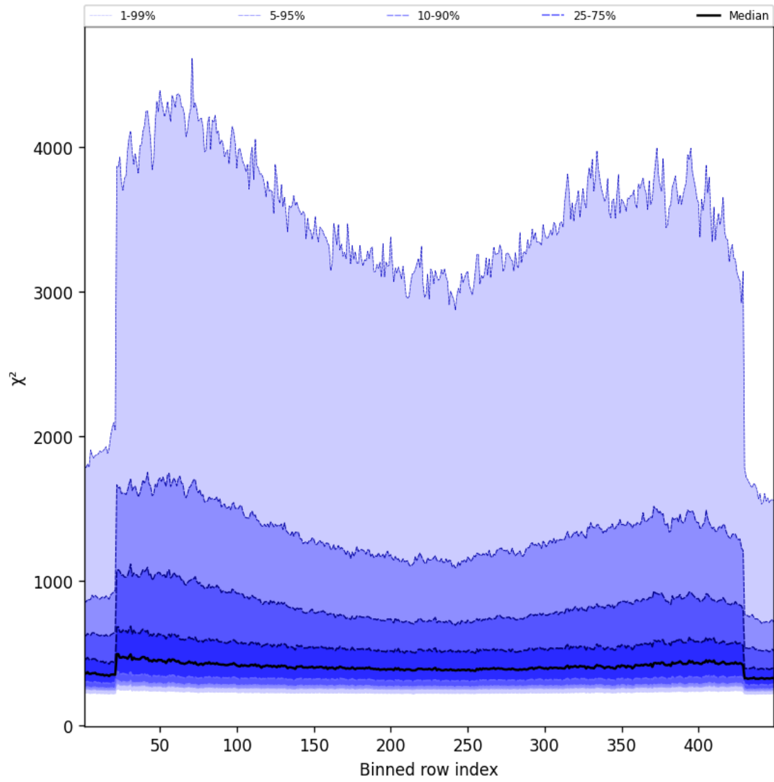
Figure 59: Along track statistics of “ \chi^2 ” for 2025-05-07 to 2025-05-08
