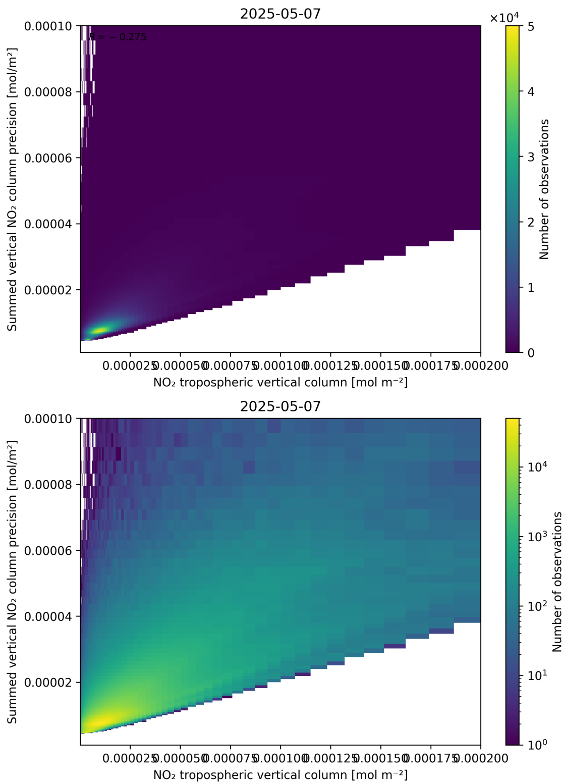
Figure 127: Scatter density plot of “NO 2 tropospheric vertical column” against “Summed vertical NO 2 column precision” for 2025-05-07 to 2025-05-08.
