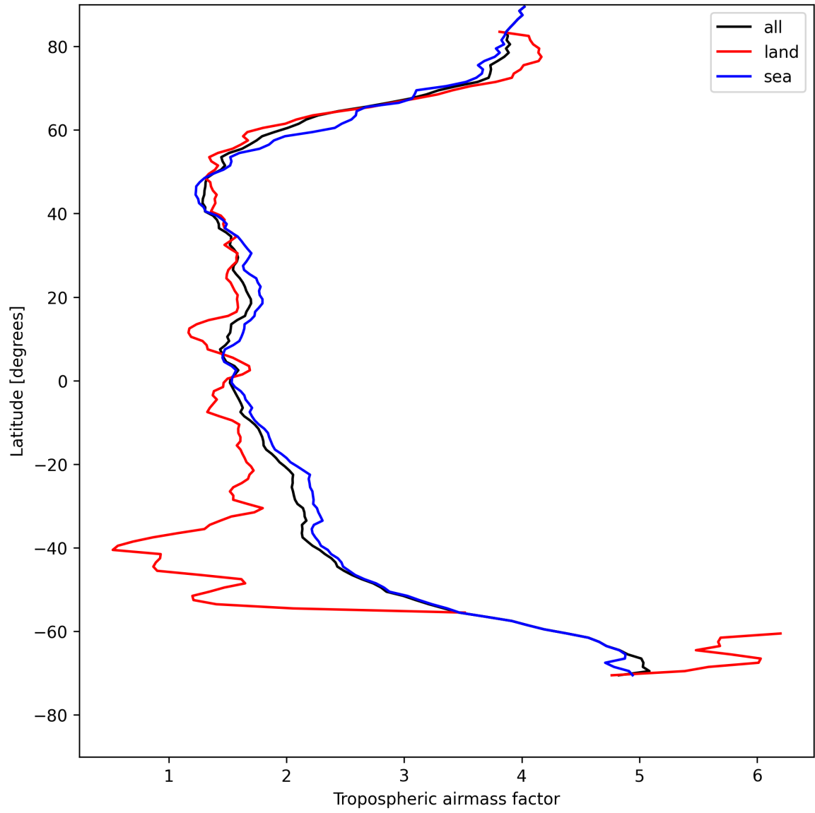
Figure 14: Zonal average of “Tropospheric air mass factor” for 2025-05-07 to 2025-05-08.
