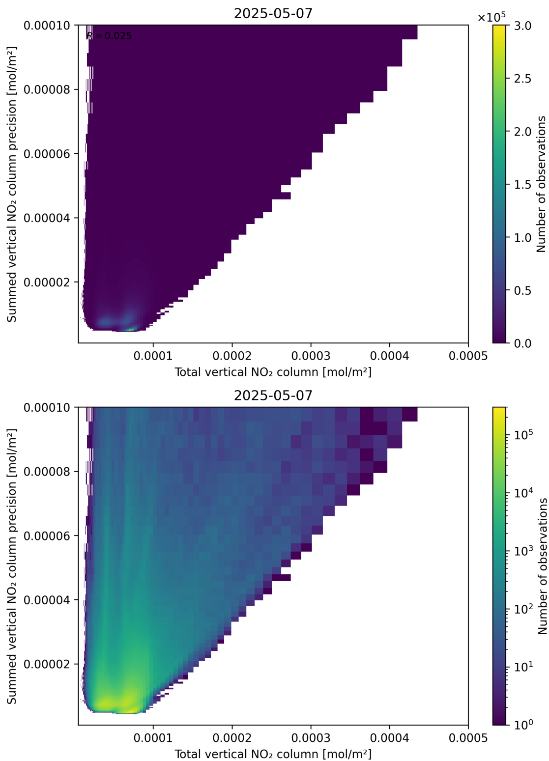
Figure 113: Scatter density plot of “Total vertical NO 2 column” against “Summed vertical NO 2 column precision” for 2025-05-07 to 2025-05-08.
