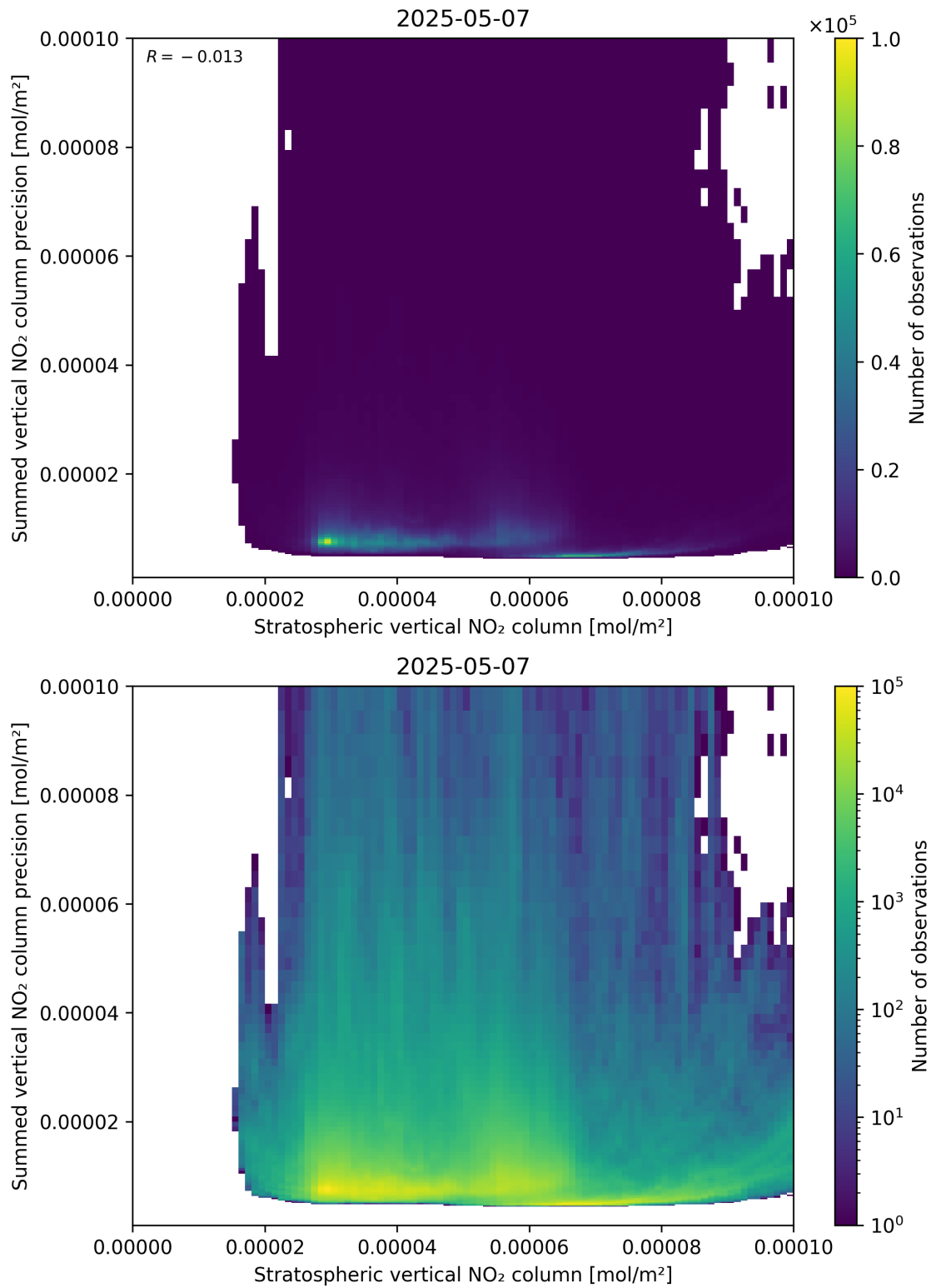
Figure 99: Scatter density plot of “Stratospheric vertical NO 2 column” against “Summed vertical NO 2 column precision” for 2025-05-07 to 2025-05-08.
