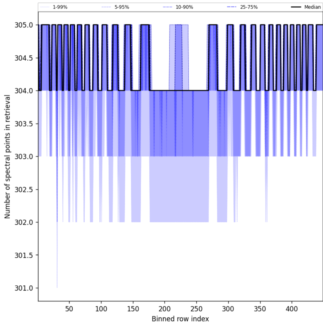
Figure 50: Along track statistics of “Number of spectral points in retrieval” for 2025-05-07 to 2025-05-08
