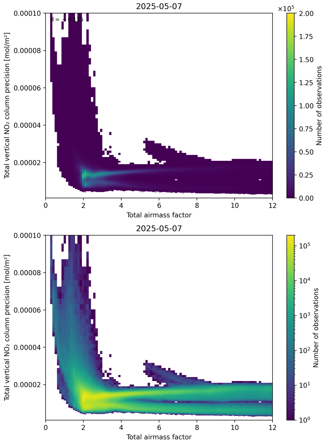
Figure 68: Scatter density plot of “Total airmass factor” against “Total vertical NO 2 column precision” for 2025-05-07 to 2025-05-08.
