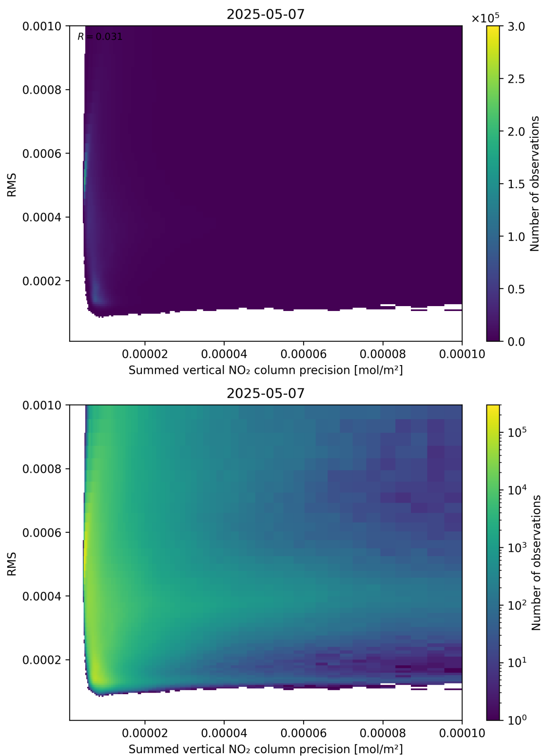
Figure 108: Scatter density plot of “Summed vertical NO 2 column precision” against “RMS” for 2025-05-07 to 2025-05-08.
