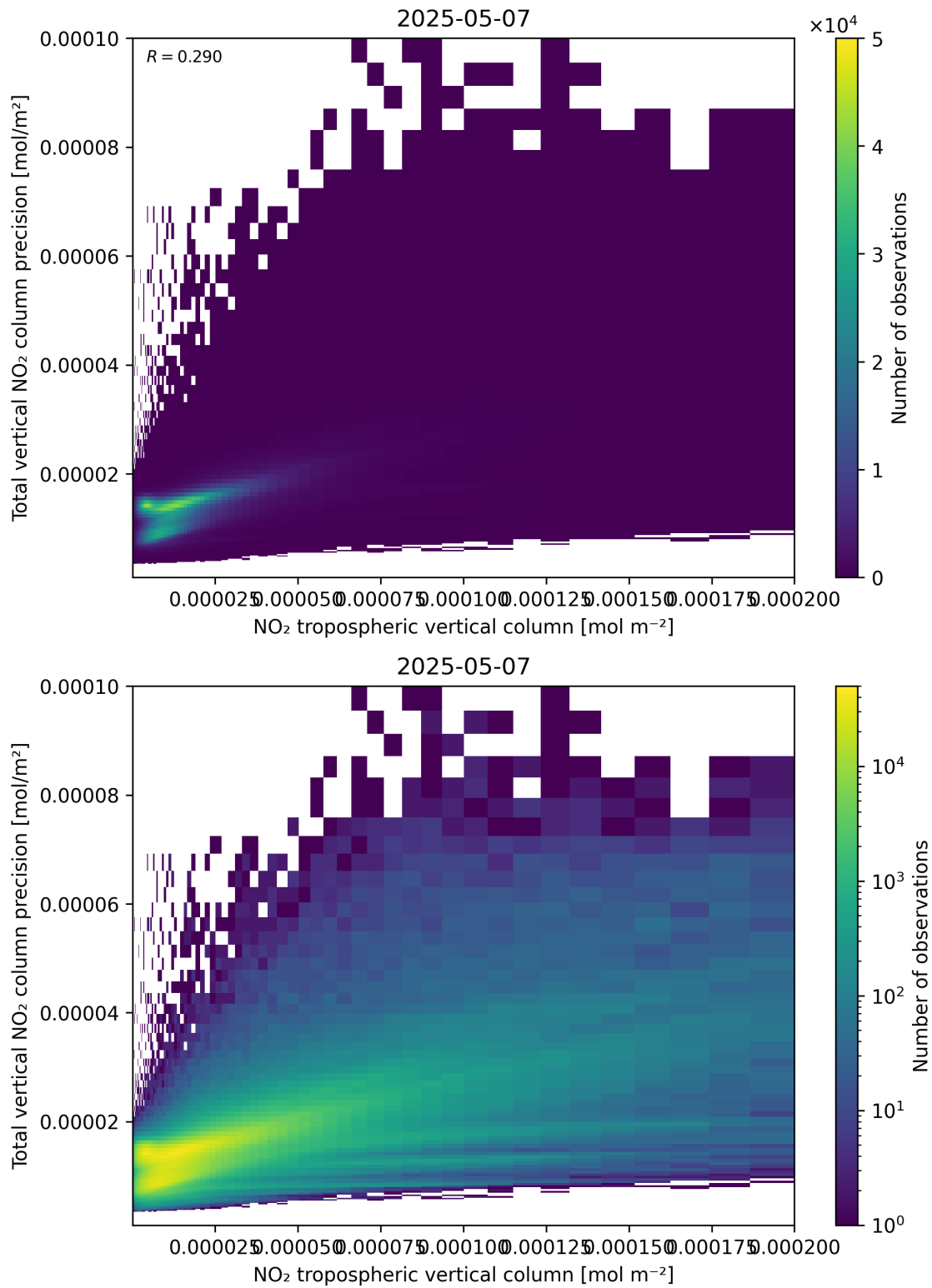
Figure 129: Scatter density plot of “NO 2 tropospheric vertical column” against “Total vertical NO 2 column precision” for 2025-05-07 to 2025-05-08.
