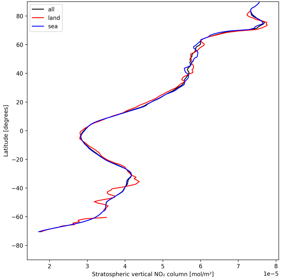
Figure 19: Zonal average of “Stratospheric vertical NO 2 column” for 2025-05-07 to 2025-05-08.
