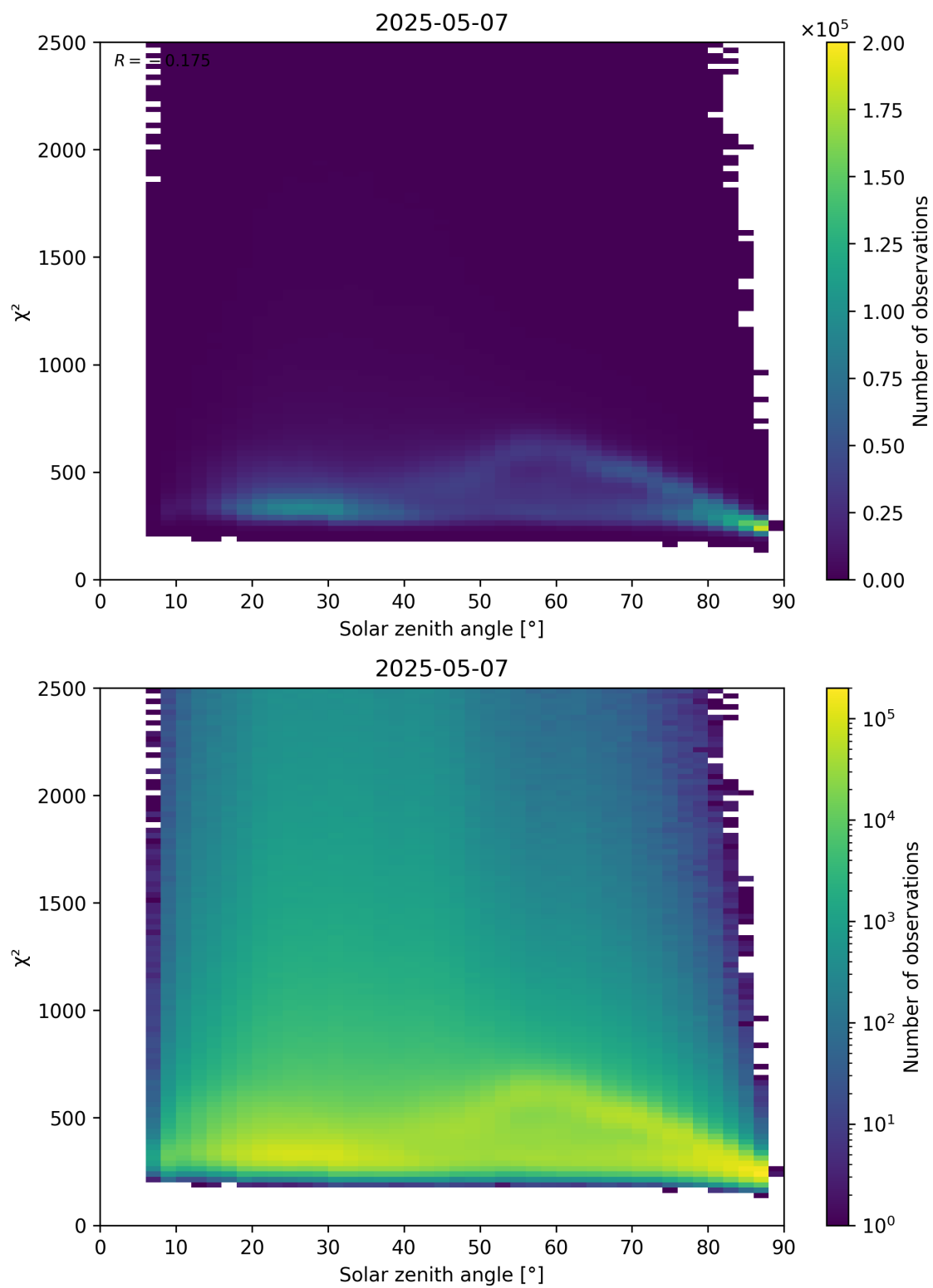
Figure 148: Scatter density plot of “Solar zenith angle” against “ \chi^2 ” for 2025-05-07 to 2025-05-08.
