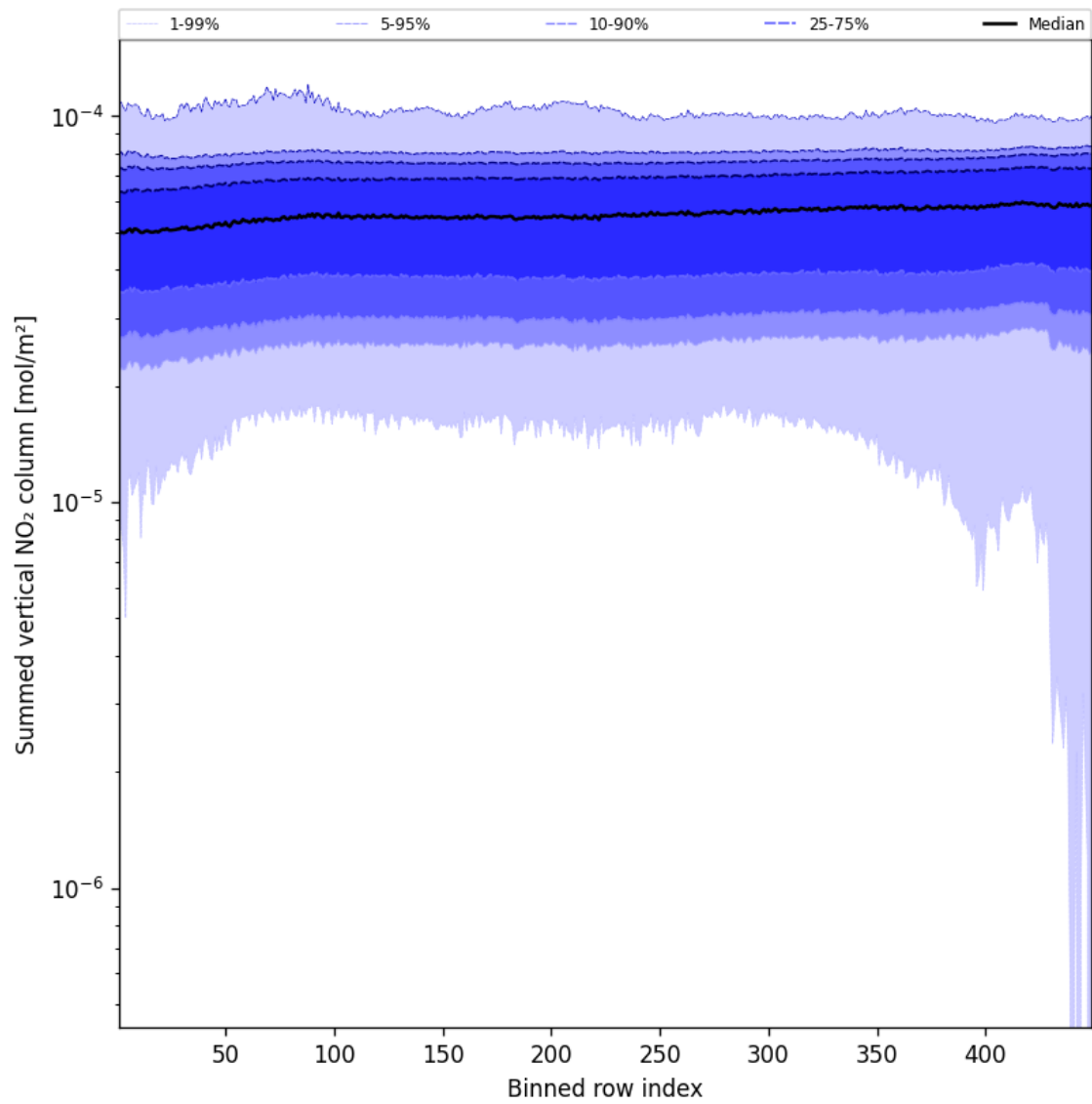
Figure 57: Along track statistics of “Summed vertical NO 2 column” for 2025-05-07 to 2025-05-08
