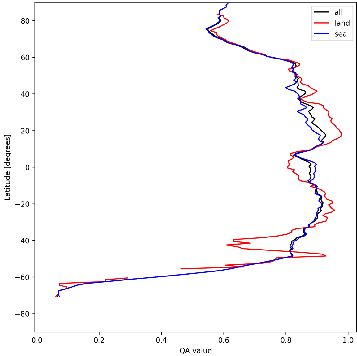
Figure 11: Zonal average of “QA value” for 2025-05-07 to 2025-05-08.
