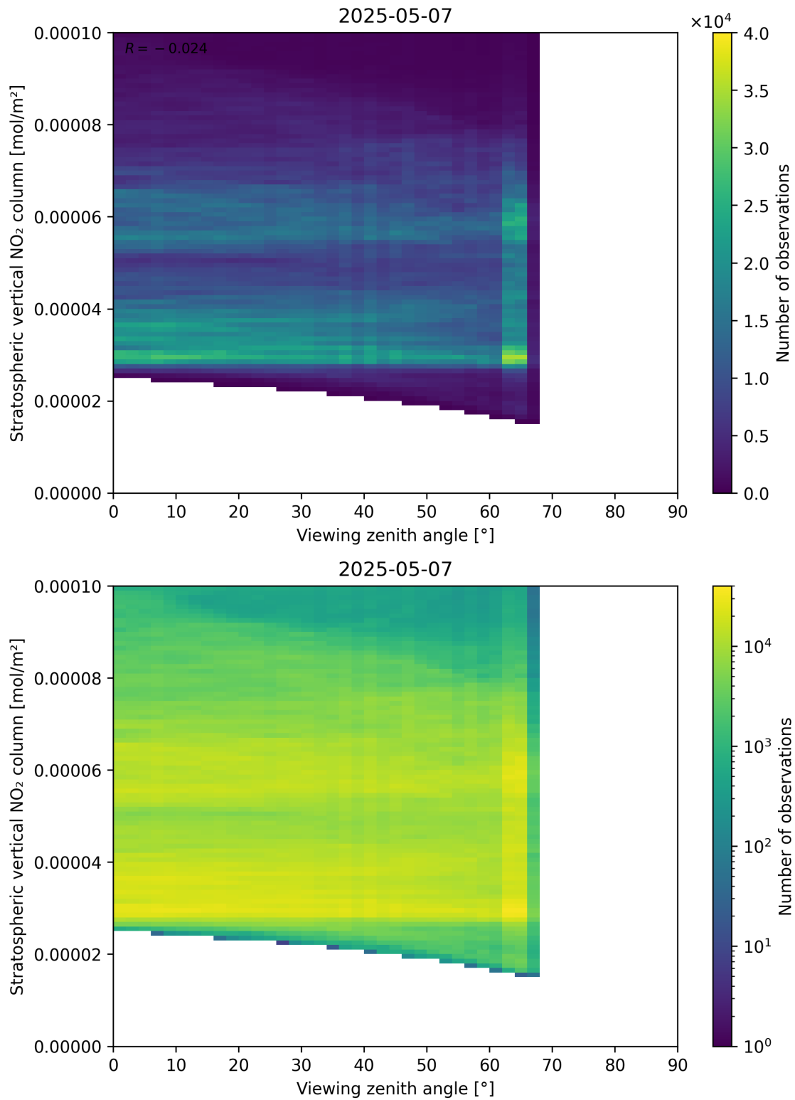
Figure 164: Scatter density plot of “Viewing zenith angle” against “Stratospheric vertical NO 2 column” for 2025-05-07 to 2025-05-08.
