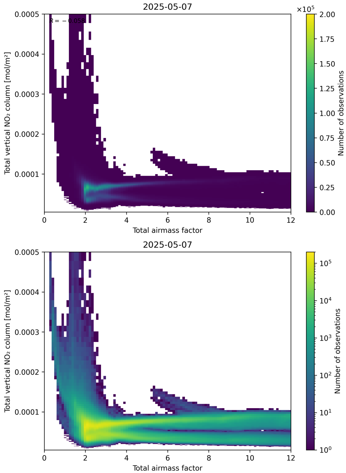
Figure 67: Scatter density plot of “Total airmass factor” against “Total vertical NO 2 column” for 2025-05-07 to 2025-05-08.
