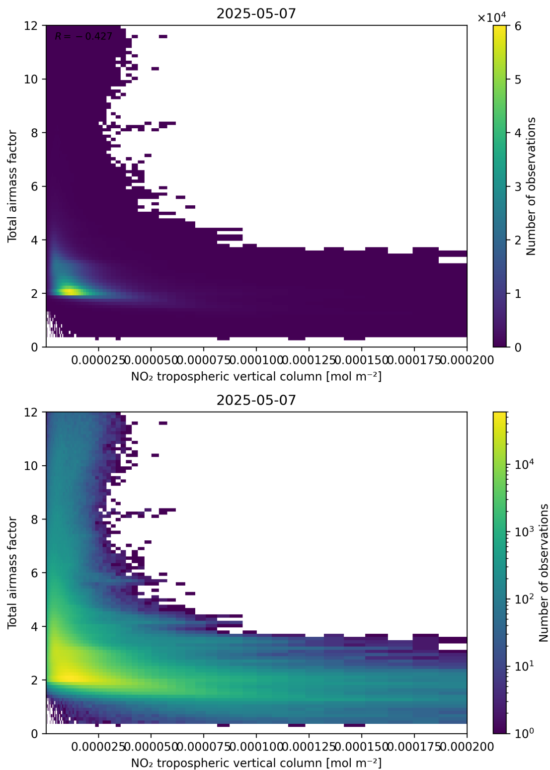
Figure 122: Scatter density plot of “NO 2 tropospheric vertical column” against “Total air mass factor” for 2025-05-07 to 2025-05-08.
