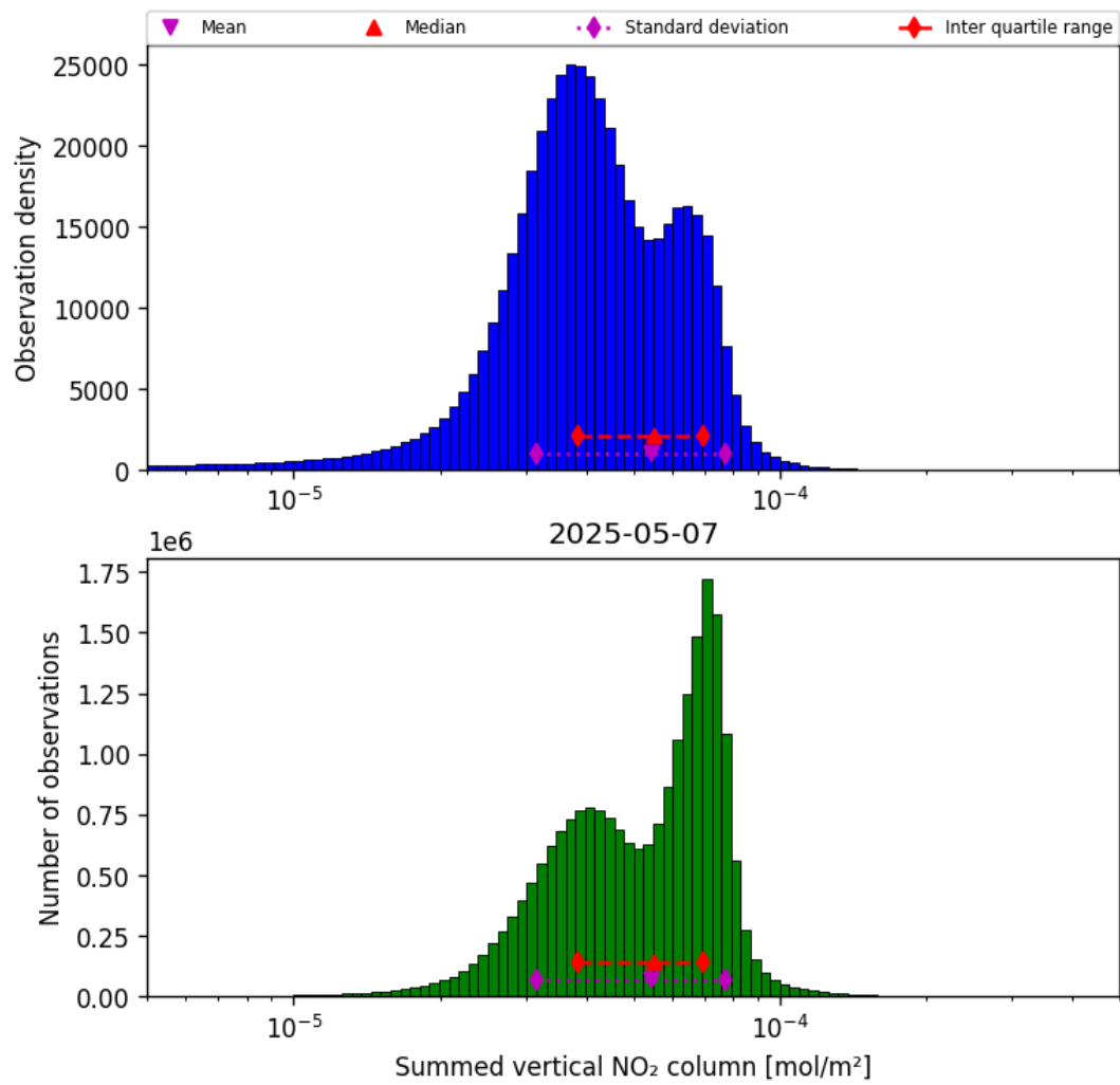
Figure 40: Histogram of “Summed vertical NO 2 column” for 2025-05-07 to 2025-05-08
