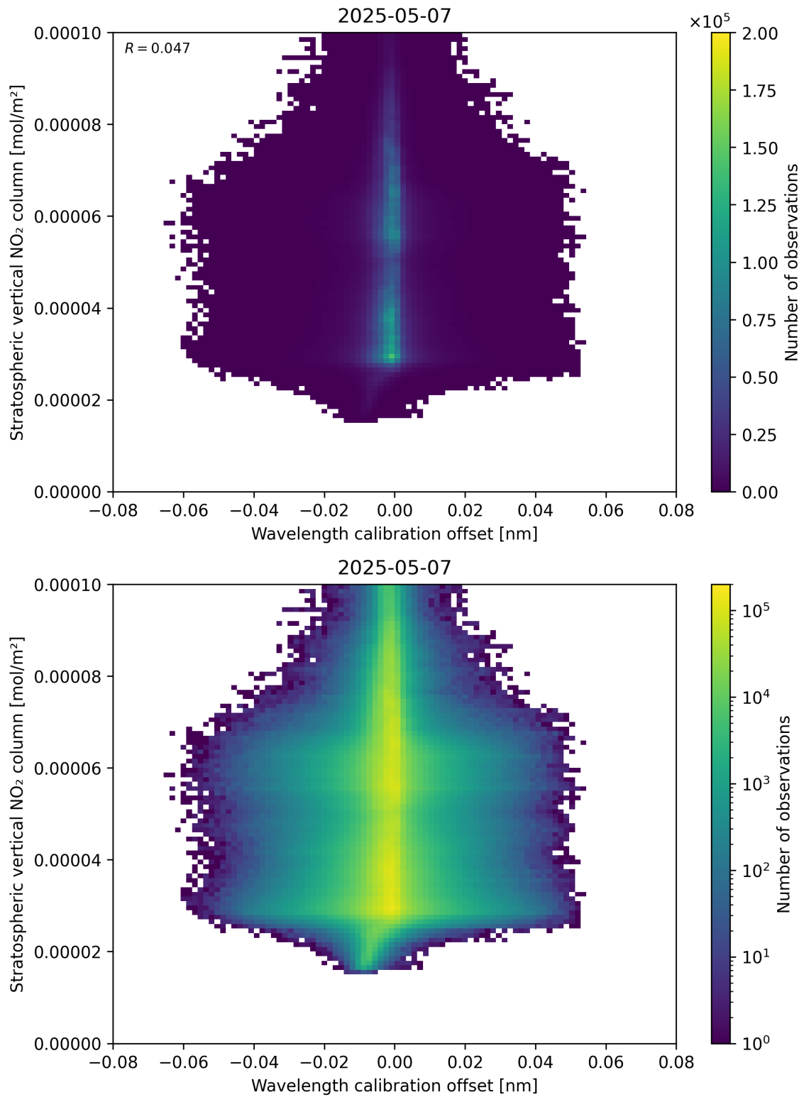
Figure 176: Scatter density plot of “Wavelength calibration offset” against “Stratospheric vertical NO 2 column” for 2025-05-07 to 2025-05-08.
