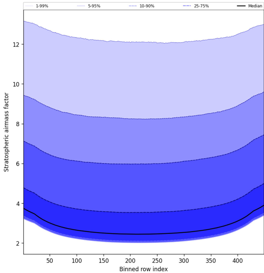
Figure 61: Along track statistics of “Stratospheric airmass factor” for 2025-05-07 to 2025-05-08
