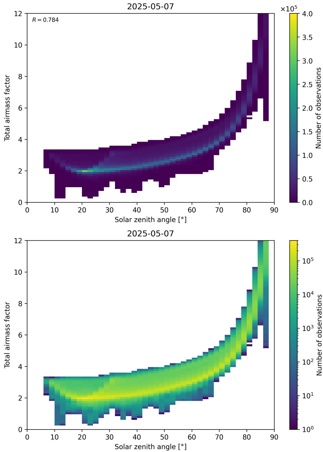
Figure 146: Scatter density plot of “Solar zenith angle” against “Total air mass factor” for 2025-05-07 to 2025-05-08.
