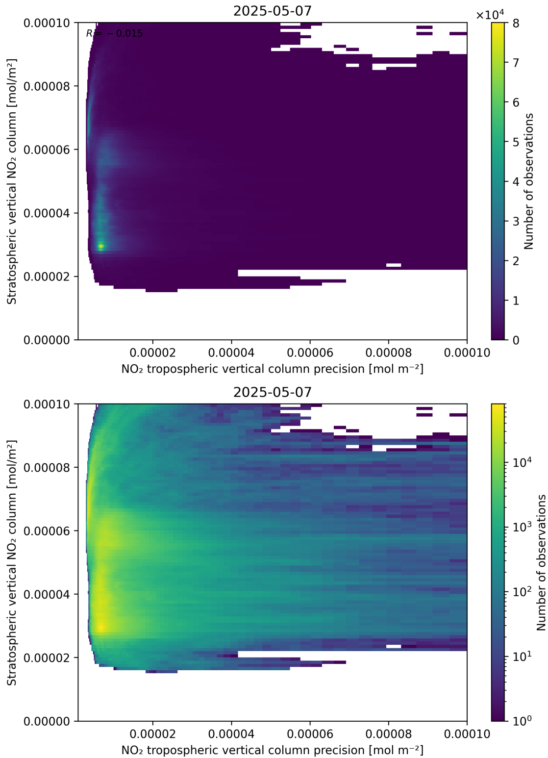
Figure 135: Scatter density plot of “NO 2 tropospheric vertical column precision” against “Stratospheric vertical NO 2 column” for 2025-05-07 to 2025-05-08.
