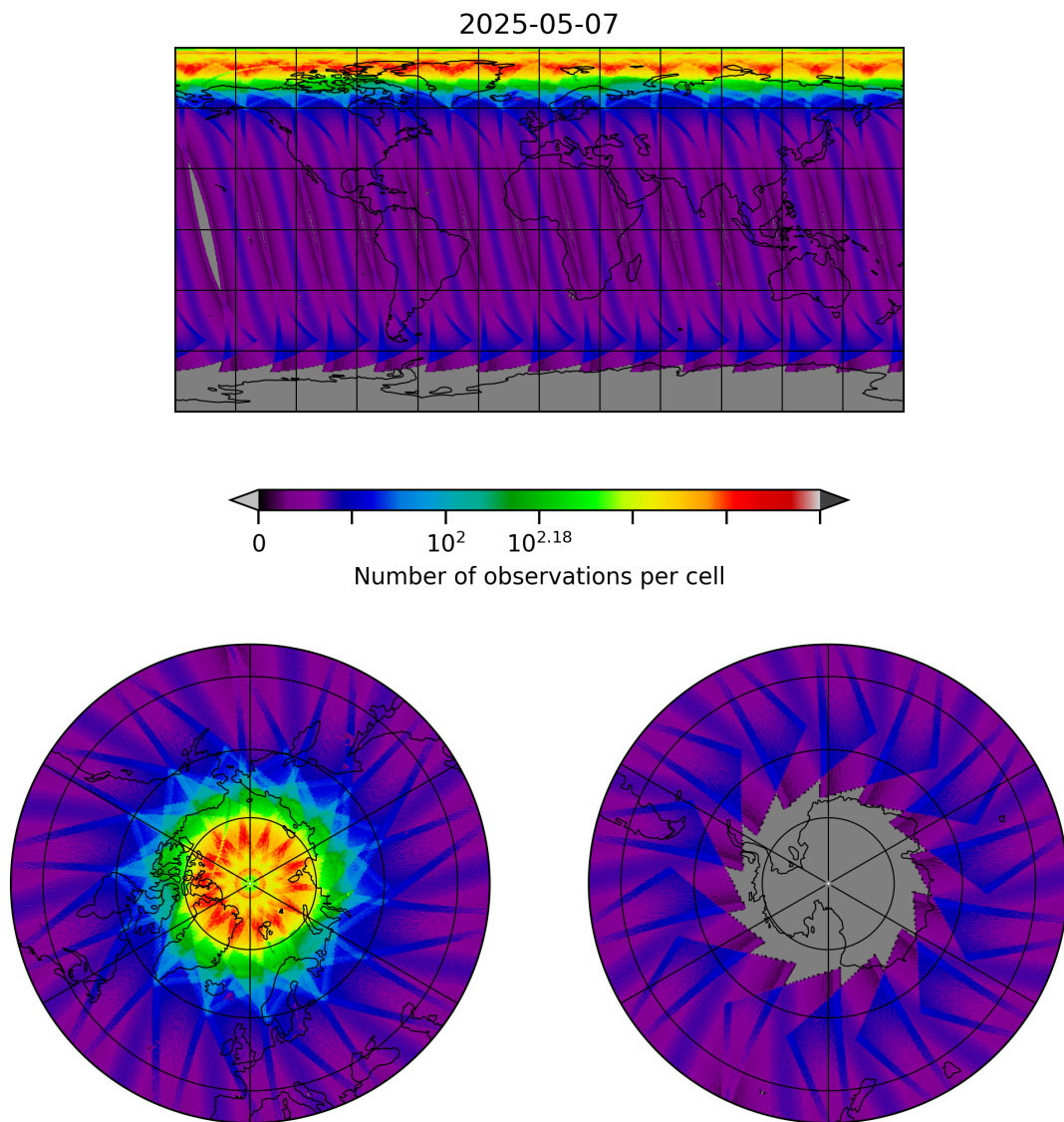
Figure 10: Map of the number of observations for 2025-05-07 to 2025-05-08
