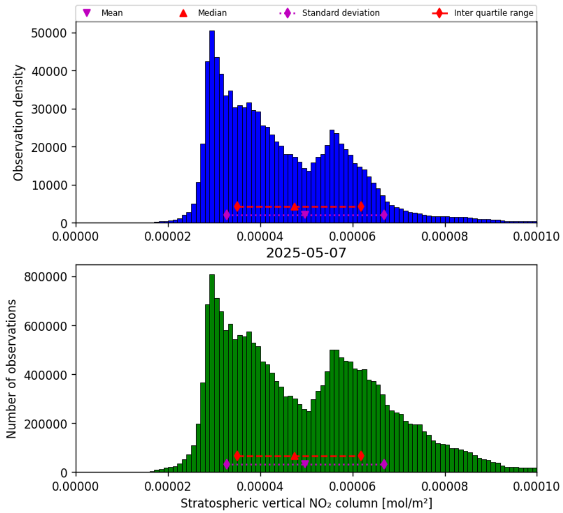
Figure 36: Histogram of “Stratospheric vertical NO 2 column” for 2025-05-07 to 2025-05-08
