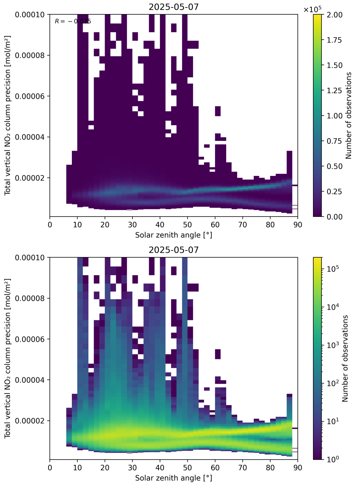
Figure 154: Scatter density plot of “Solar zenith angle” against “Total vertical NO 2 column precision” for 2025-05-07 to 2025-05-08.
