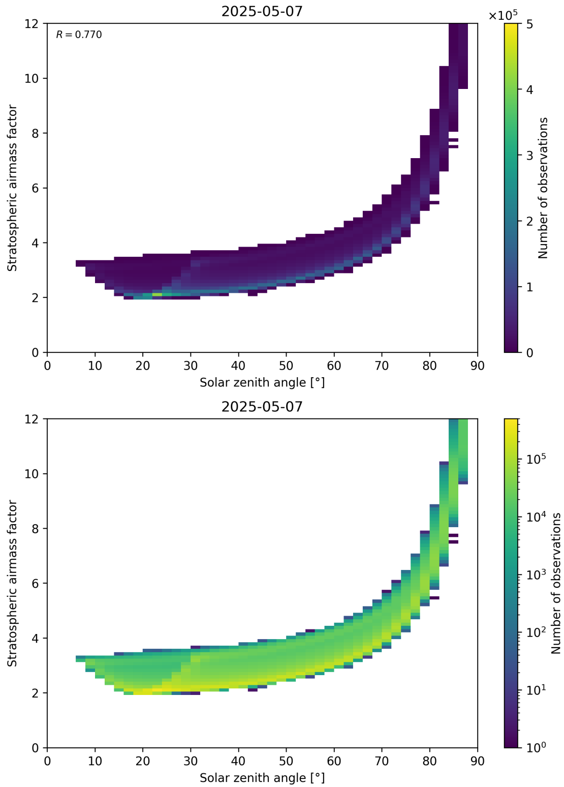
Figure 145: Scatter density plot of “Solar zenith angle” against “Stratospheric airmass factor” for 2025-05-07 to 2025-05-08.
