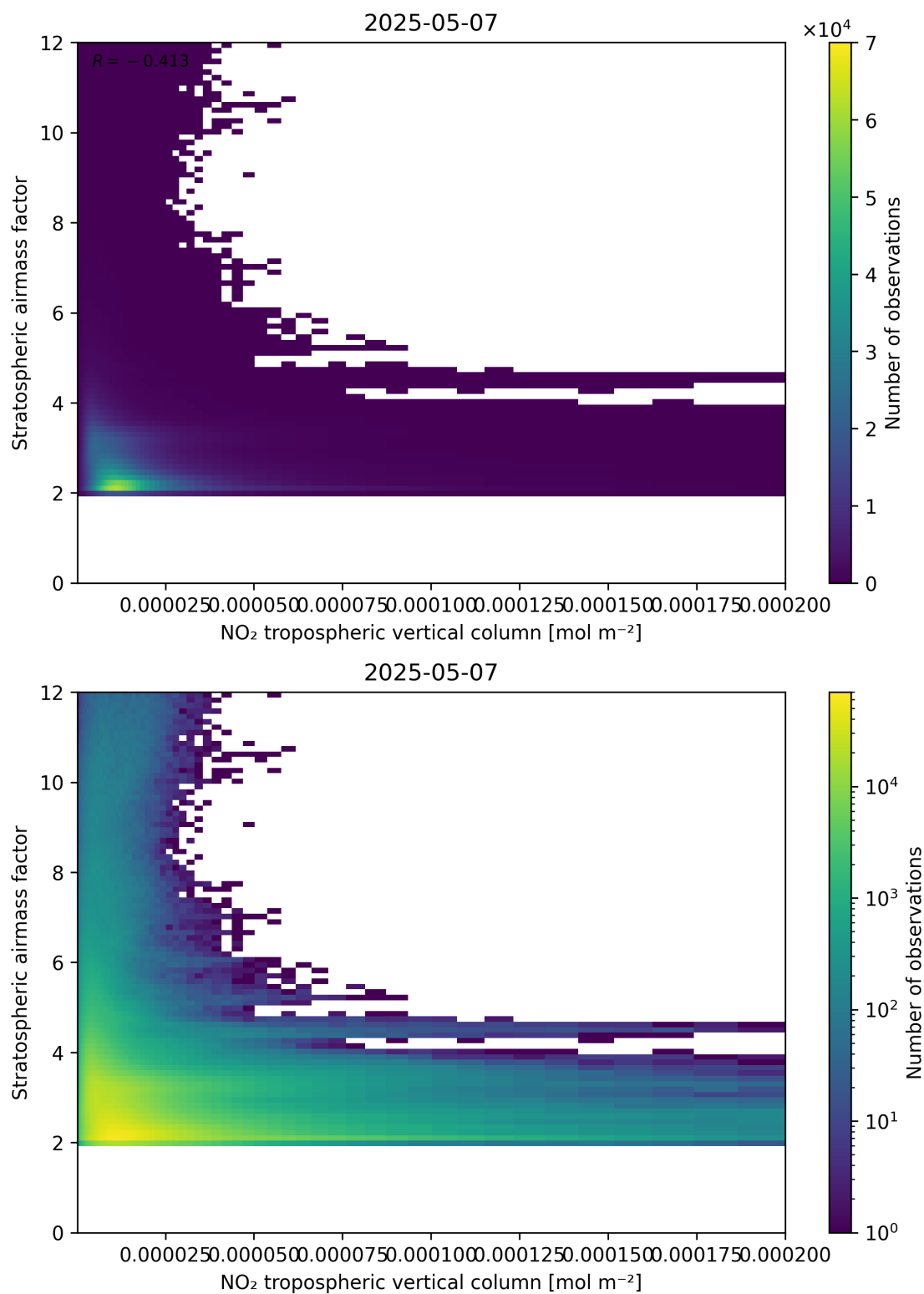
Figure 121: Scatter density plot of “NO 2 tropospheric vertical column” against “Stratospheric air mass factor” for 2025-05-07 to 2025-05-08.
