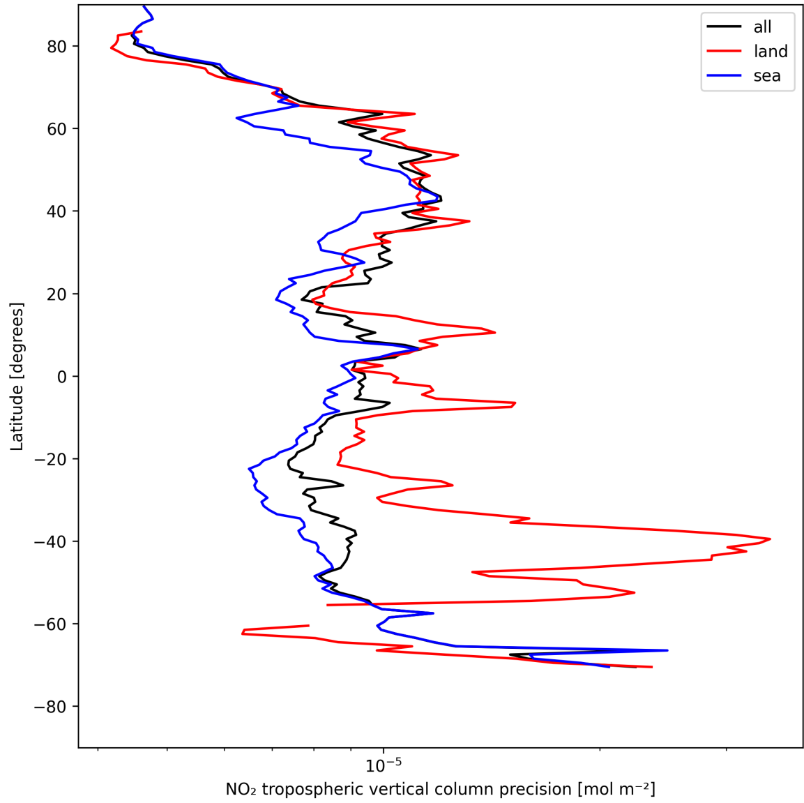
Figure 13: Zonal average of “NO 2 tropospheric vertical column precision” for 2025-05-07 to 2025-05-08.
