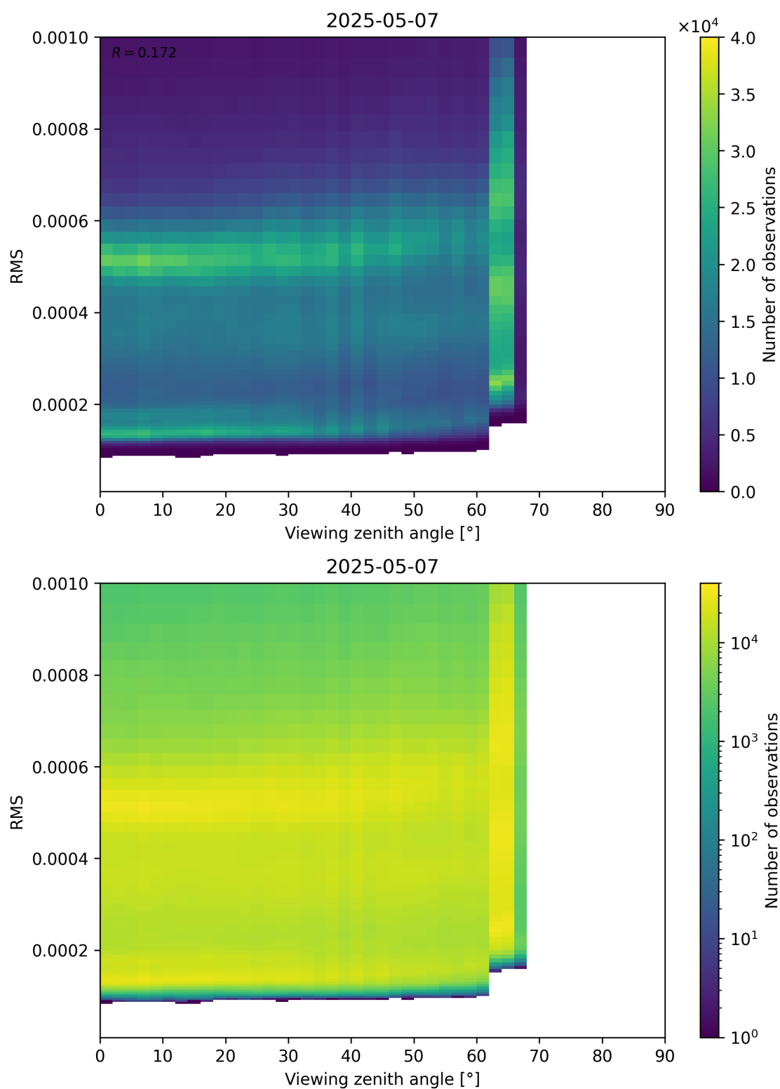
Figure 171: Scatter density plot of “Viewing zenith angle” against “RMS” for 2025-05-07 to 2025-05-08.
