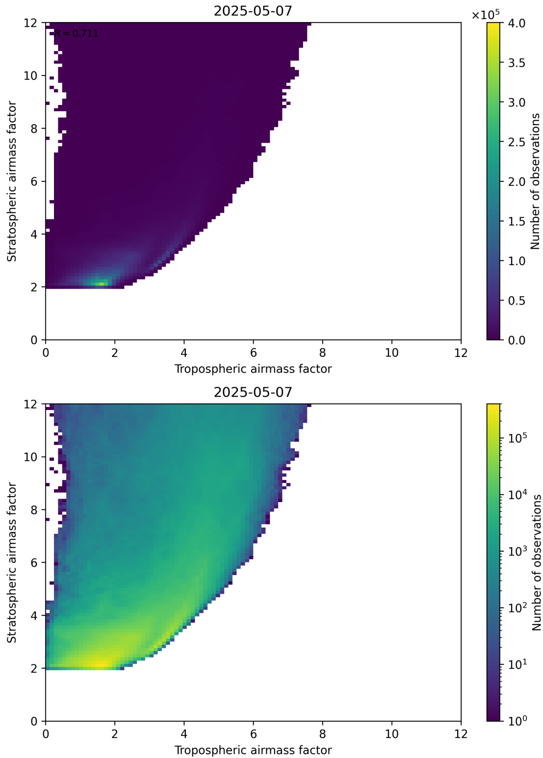
Figure 71: Scatter density plot of “Tropospheric airmass factor” against “Stratospheric airmass factor” for 2025-05-07 to 2025-05-08.
