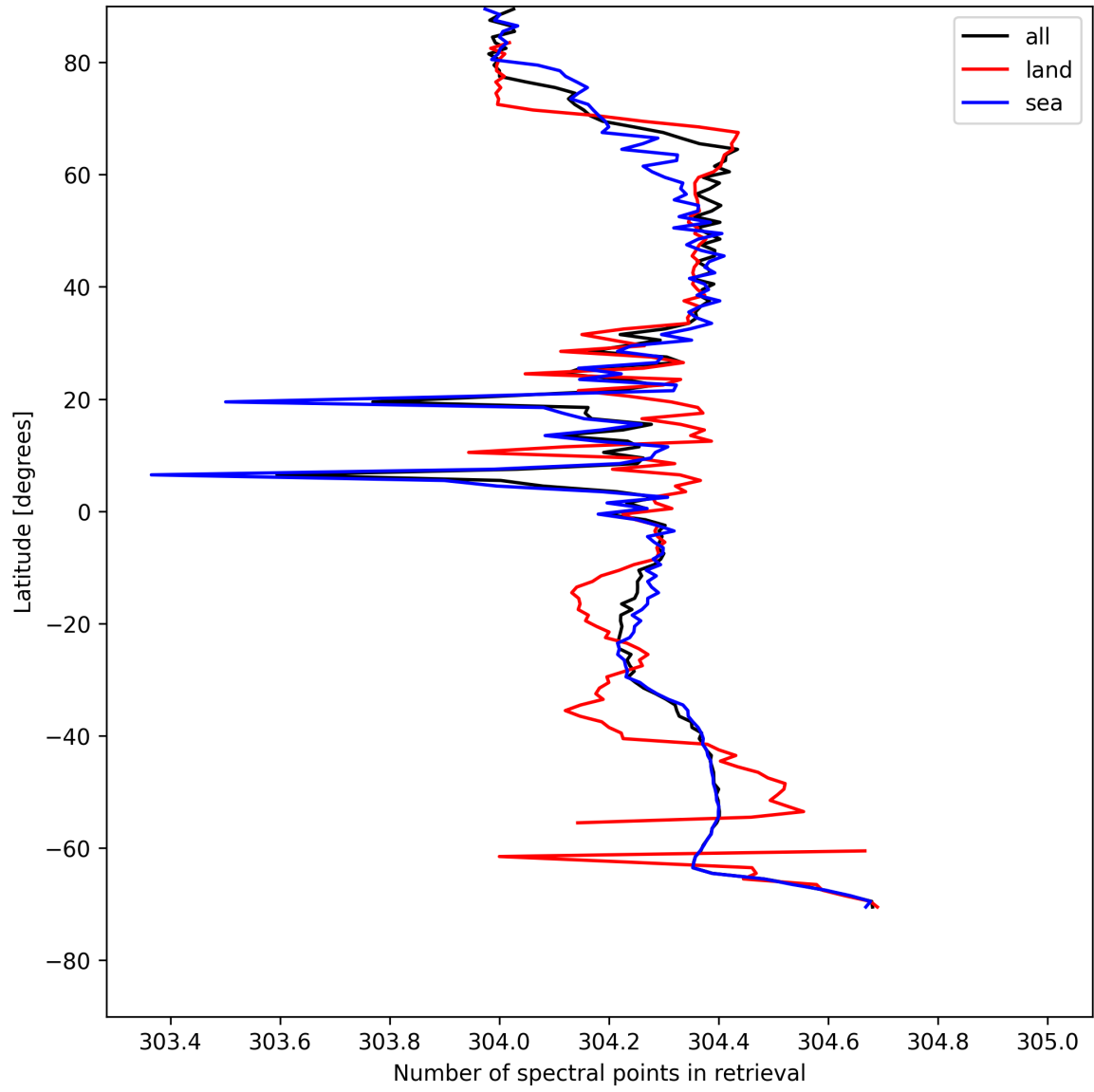
Figure 16: Zonal average of “Number of spectral points in retrieval” for 2025-05-07 to 2025-05-08.
