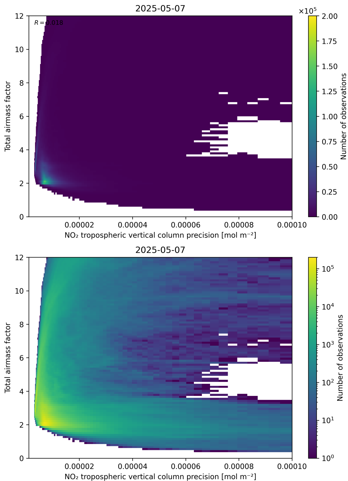
Figure 132: Scatter density plot of “NO 2 tropospheric vertical column precision” against “Total air mass factor” for 2025-05-07 to 2025-05-08.
