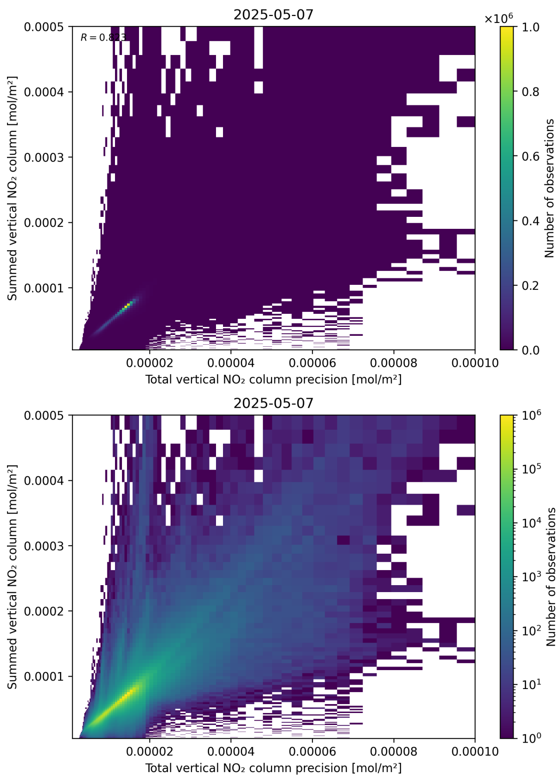
Figure 117: Scatter density plot of “Total vertical NO 2 column precision” against “Summed vertical NO 2 column” for 2025-05-07 to 2025-05-08.
