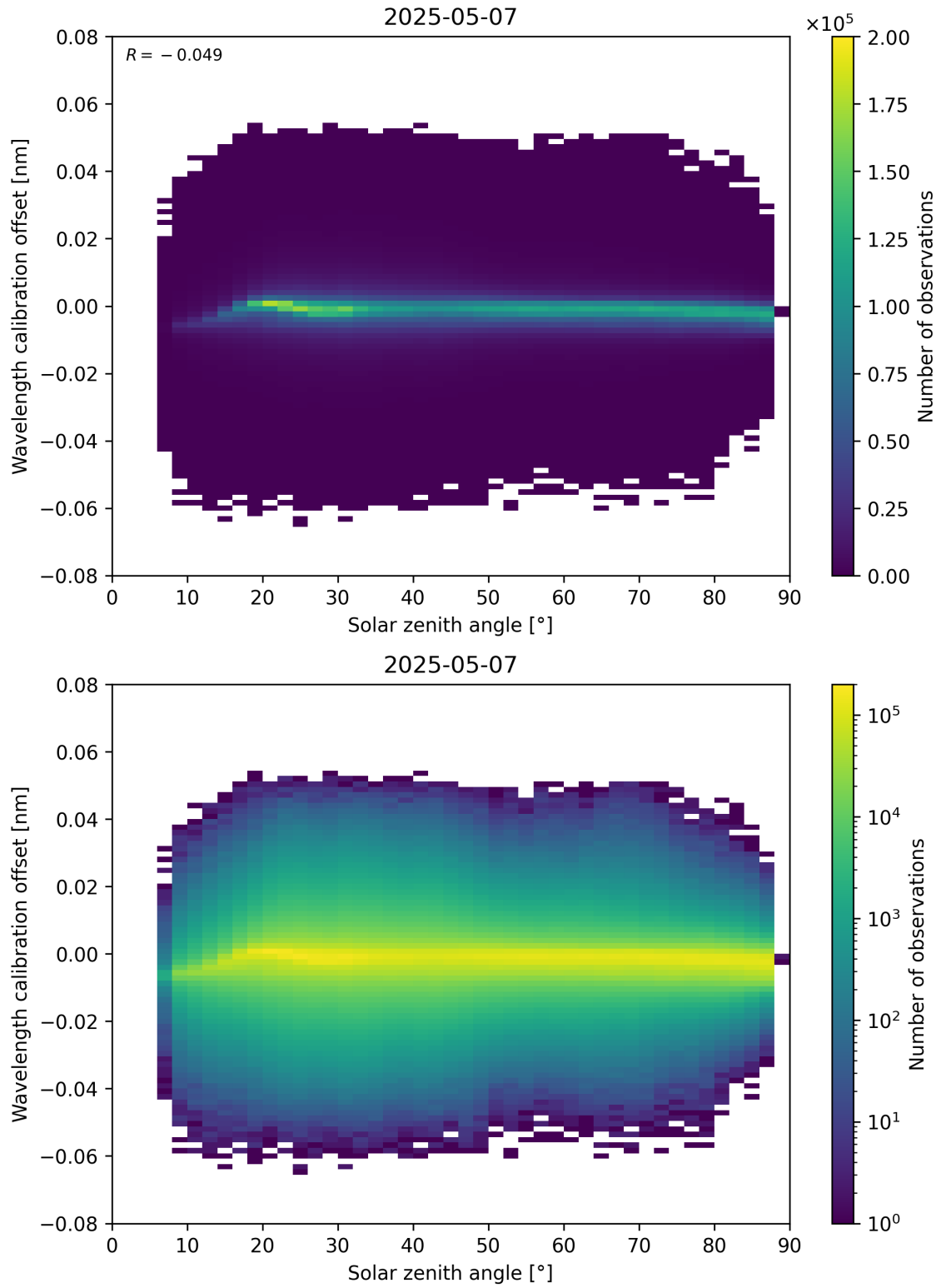
Figure 158: Scatter density plot of “Solar zenith angle” against “Wavelength calibration offset” for 2025-05-07 to 2025-05-08.
