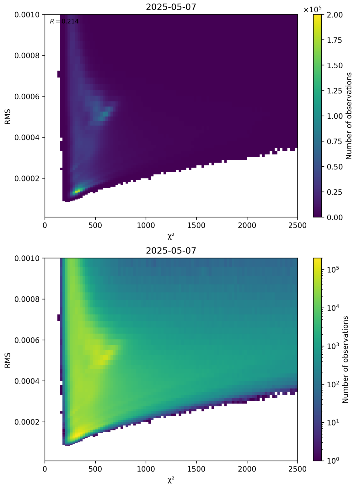
Figure 82: Scatter density plot of “ \chi^2 ” against “RMS” for 2025-05-07 to 2025-05-08.
