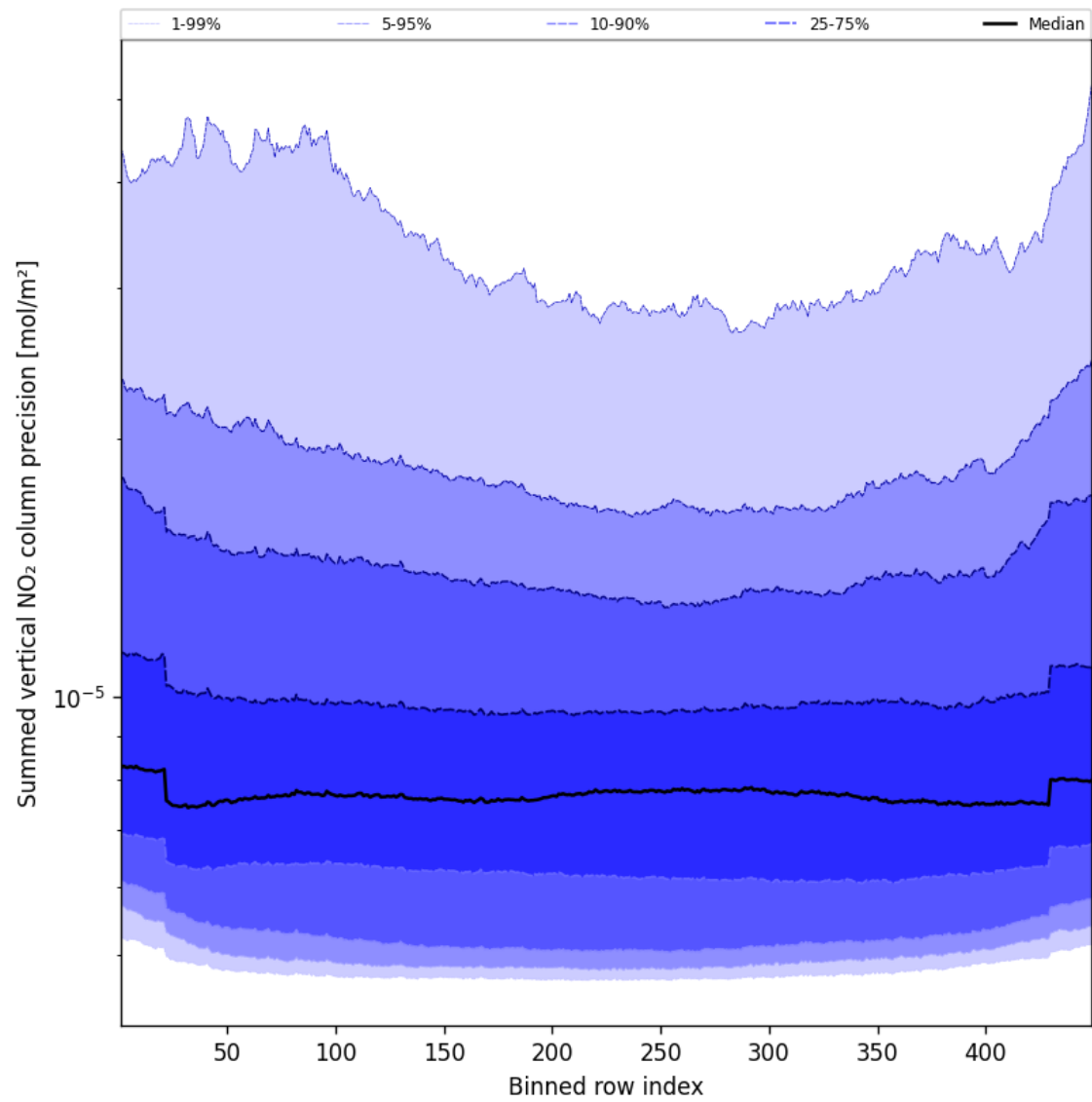
Figure 58: Along track statistics of “Summed vertical NO 2 column precision” for 2025-05-07 to 2025-05-08
