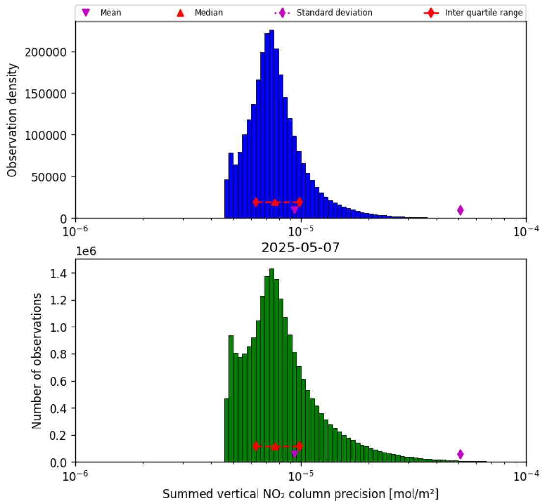
Figure 41: Histogram of “Summed vertical NO 2 column precision” for 2025-05-07 to 2025-05-08
