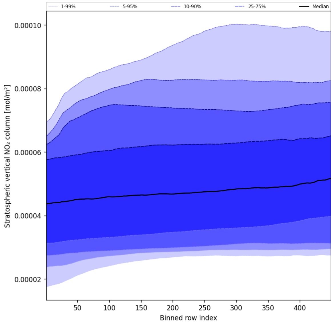
Figure 53: Along track statistics of “Stratospheric vertical NO 2 column” for 2025-05-07 to 2025-05-08
