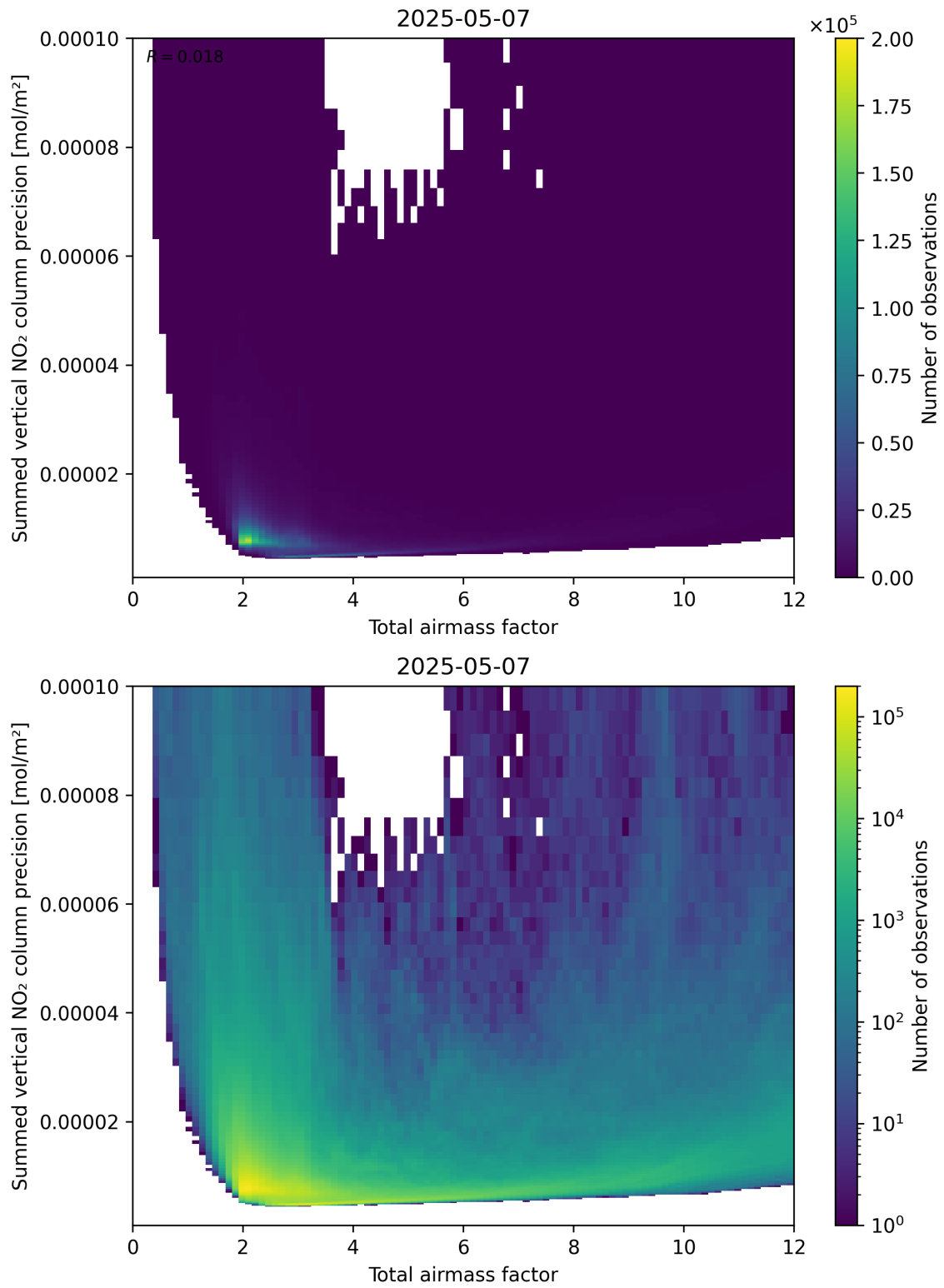
Figure 66: Scatter density plot of “Total airmass factor” against “Summed vertical NO 2 column precision” for 2025-05-07 to 2025-05-08.
