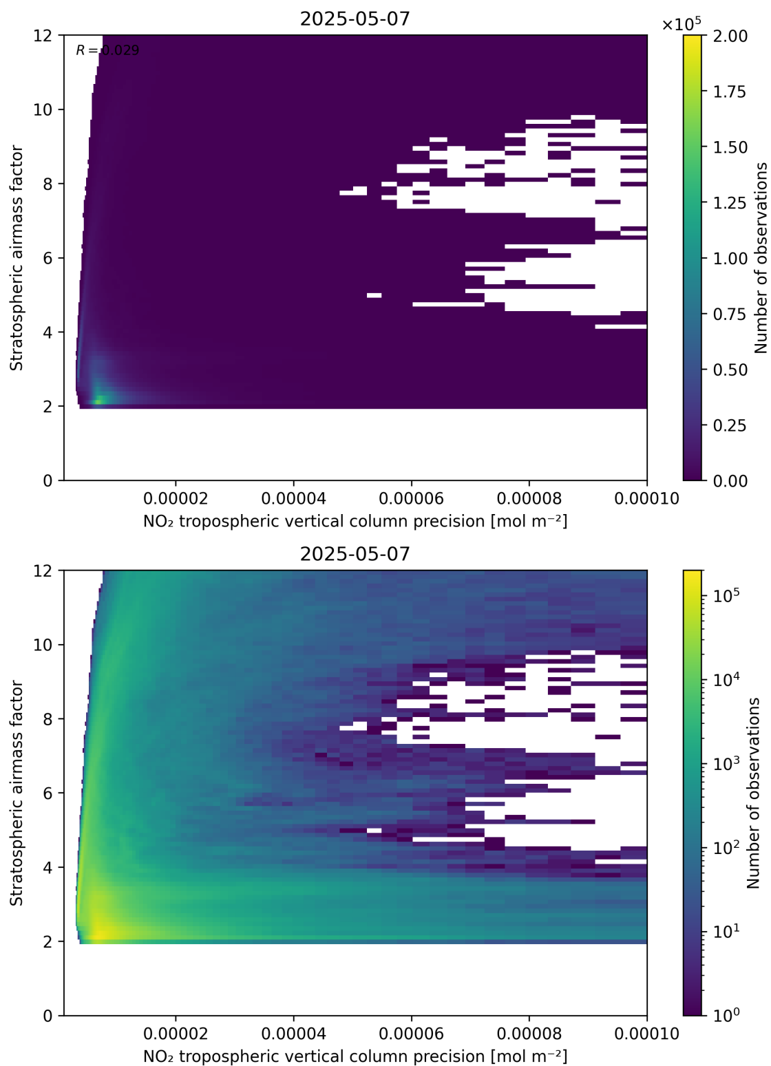
Figure 131: Scatter density plot of “NO 2 tropospheric vertical column precision” against “Stratospheric airmass factor” for 2025-05-07 to 2025-05-08.
