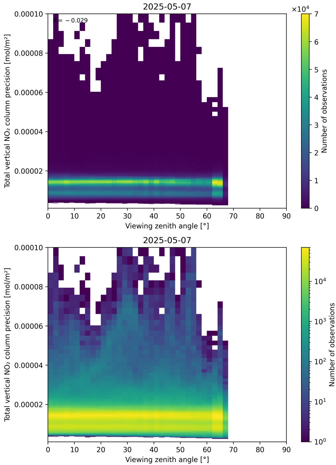
Figure 168: Scatter density plot of “Viewing zenith angle” against “Total vertical NO 2 column precision” for 2025-05-07 to 2025-05-08.
