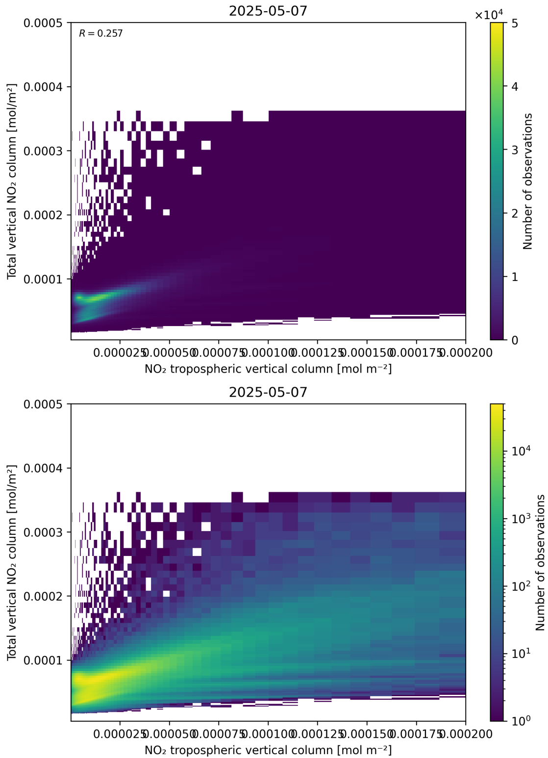
Figure 128: Scatter density plot of “NO 2 tropospheric vertical column” against “Total vertical NO 2 column” for 2025-05-07 to 2025-05-08.
