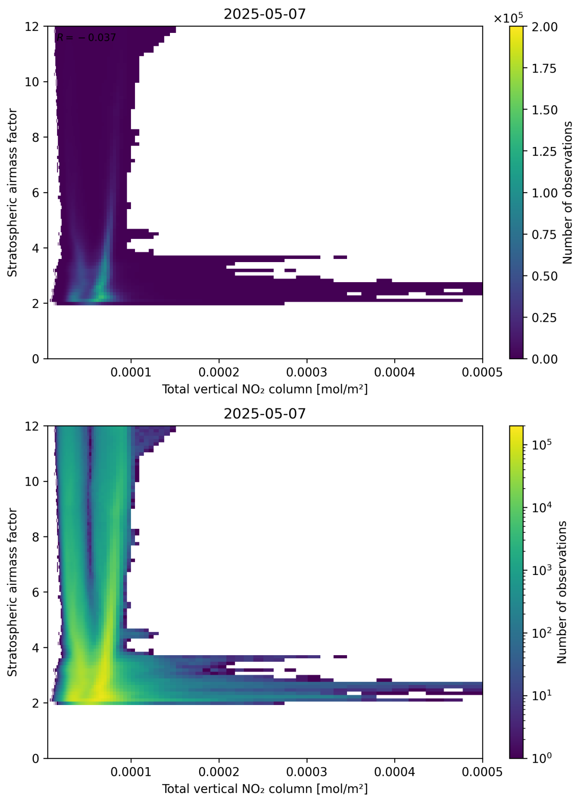
Figure 110: Scatter density plot of “Total vertical NO 2 column” against “Stratospheric airmass factor” for 2025-05-07 to 2025-05-08.
