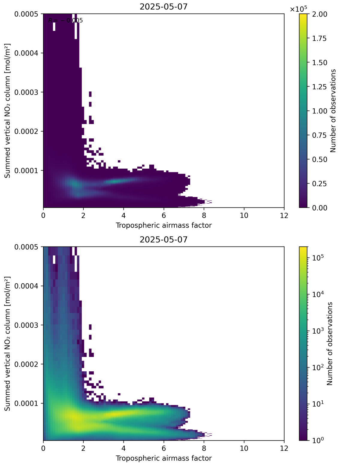
Figure 75: Scatter density plot of “Tropospheric airmass factor” against “Summed vertical NO 2 column” for 2025-05-07 to 2025-05-08.
