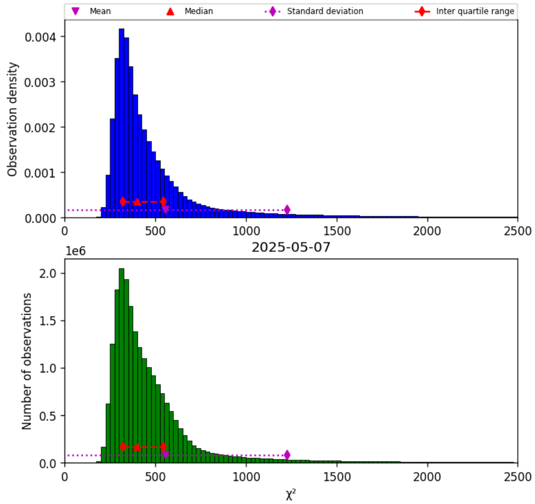
Figure 42: Histogram of " \chi^2 " for 2025-05-07 to 2025-05-08
