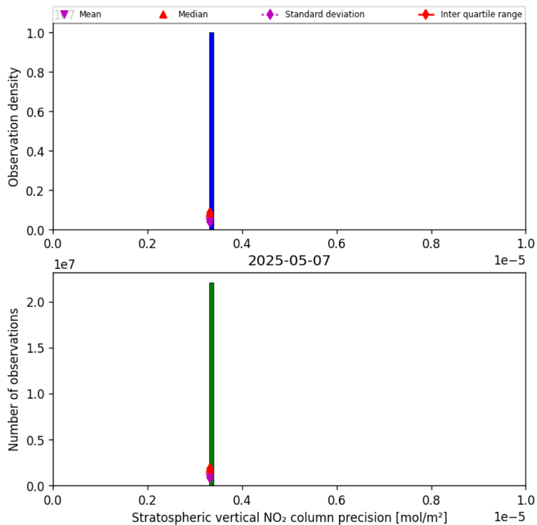
Figure 37: Histogram of “Stratospheric vertical NO 2 column precision” for 2025-05-07 to 2025-05-08
