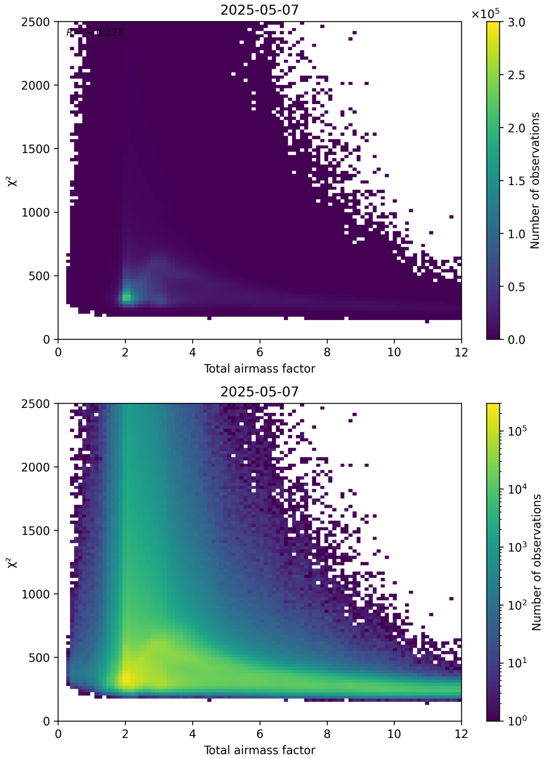
Figure 63: Scatter density plot of “Total airmass factor” against “ \chi^2 ” for 2025-05-07 to 2025-05-08.
