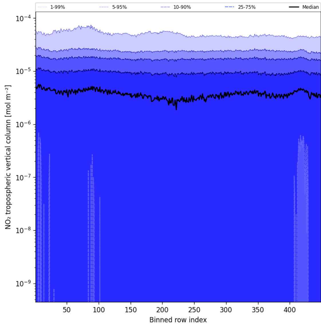
Figure 46: Along track statistics of “NO 2 tropospheric vertical column” for 2025-05-07 to 2025-05-08
