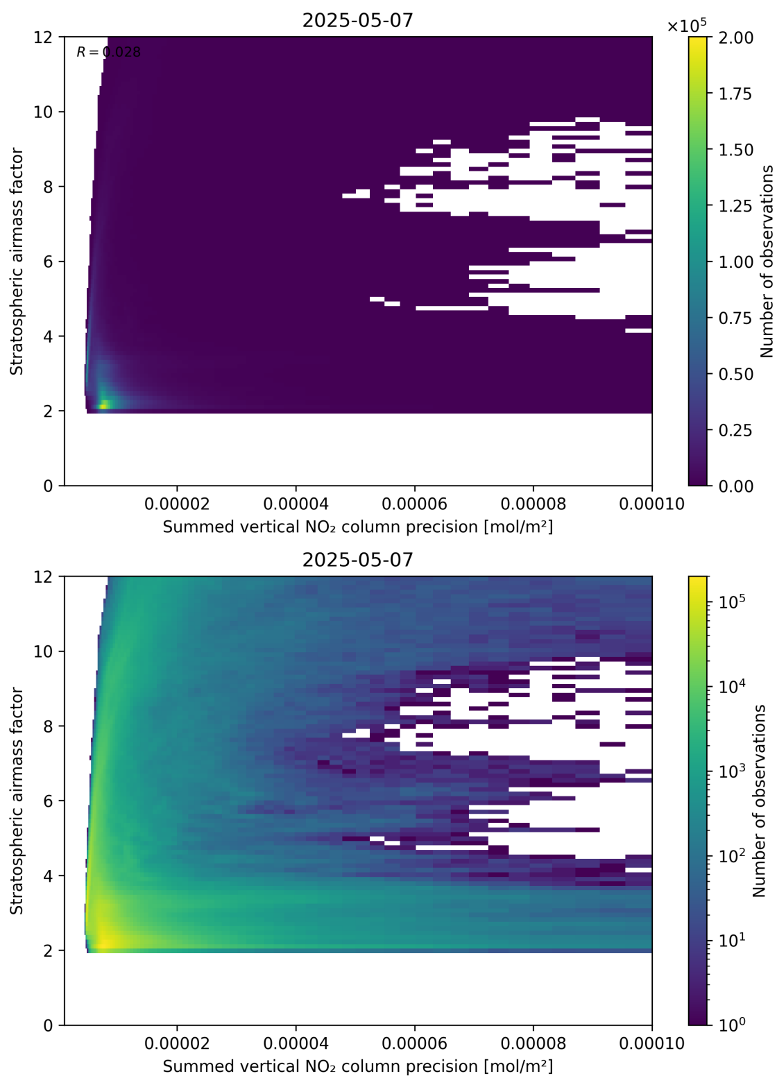
Figure 106: Scatter density plot of “Summed vertical NO 2 column precision” against “Stratospheric airmass factor” for 2025-05-07 to 2025-05-08.
