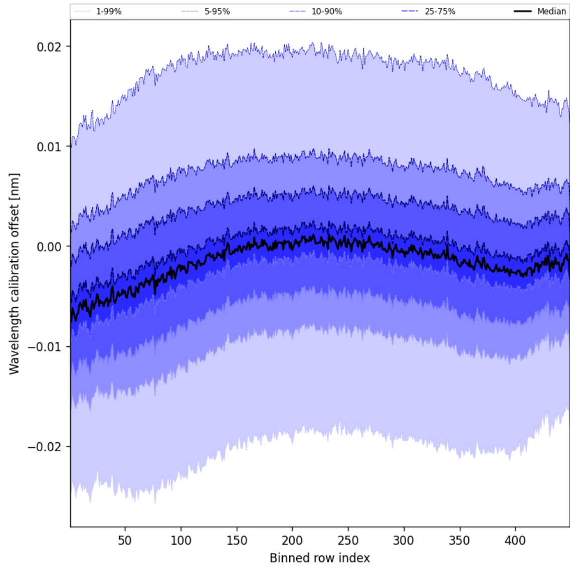
Figure 52: Along track statistics of “Wavelength calibration offset” for 2025-05-07 to 2025-05-08
