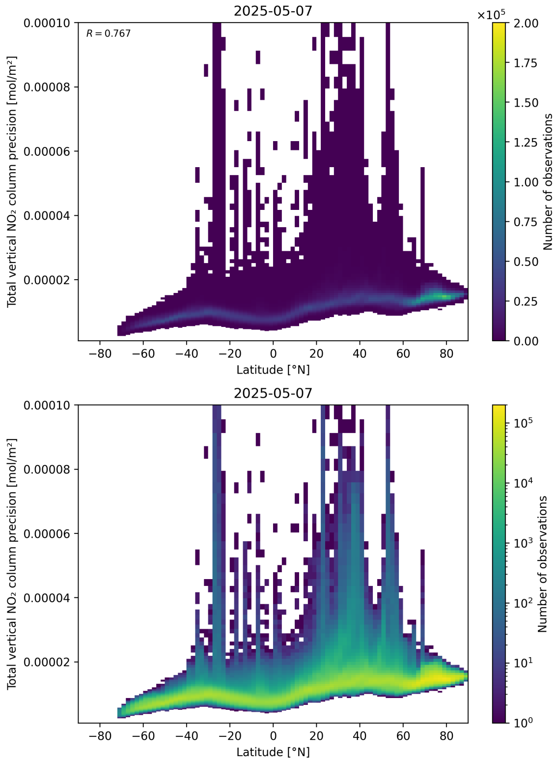
Figure 91: Scatter density plot of “Latitude” against “Total vertical NO 2 column precision” for 2025-05-07 to 2025-05-08.
