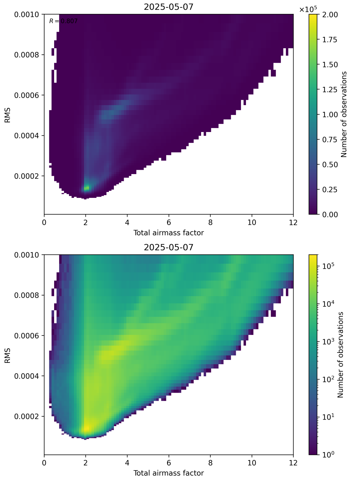
Figure 69: Scatter density plot of “Total airmass factor” against “RMS” for 2025-05-07 to 2025-05-08.
