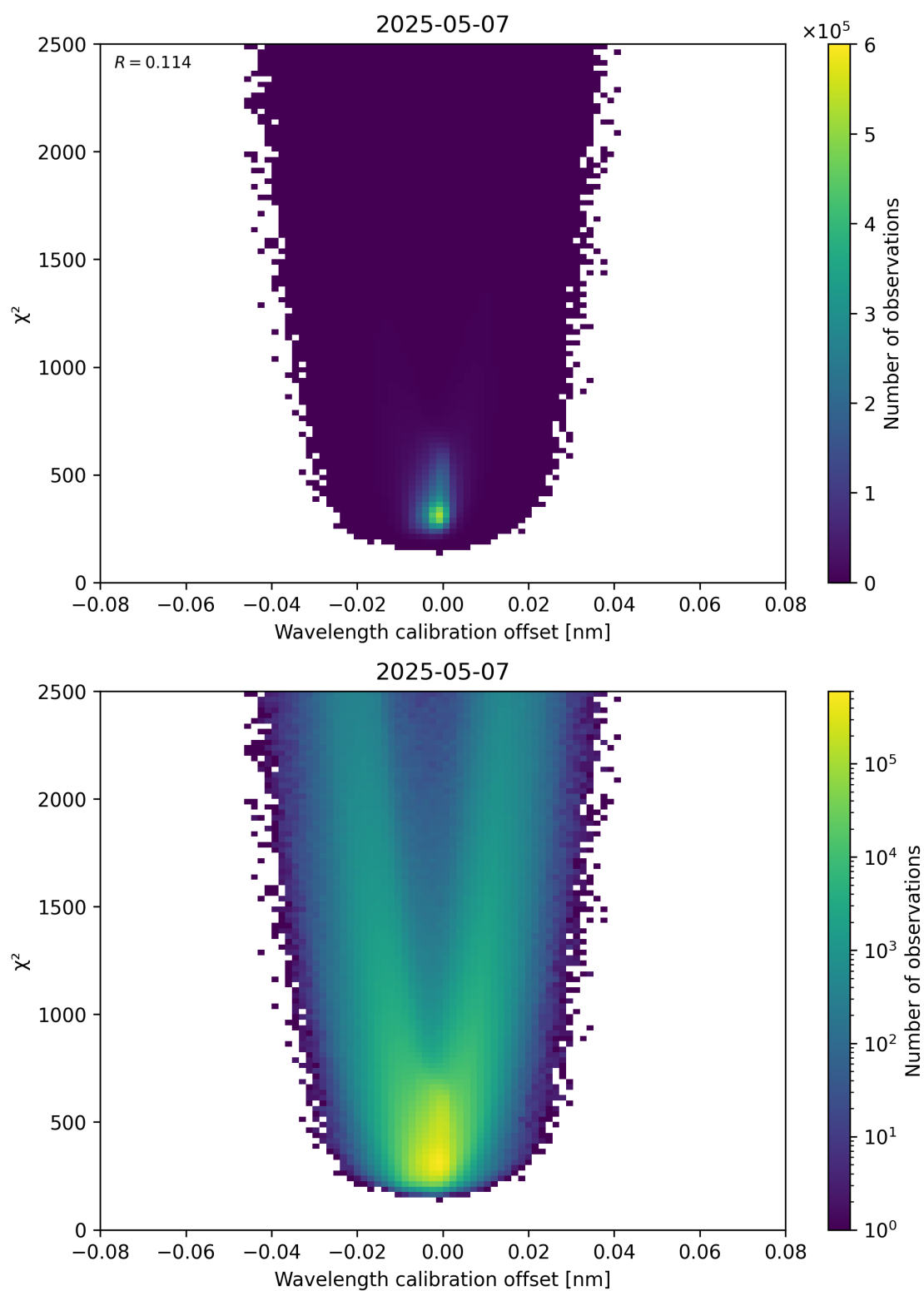
Figure 175: Scatter density plot of “Wavelength calibration offset” against “ \chi^2 ” for 2025-05-07 to 2025-05-08.
