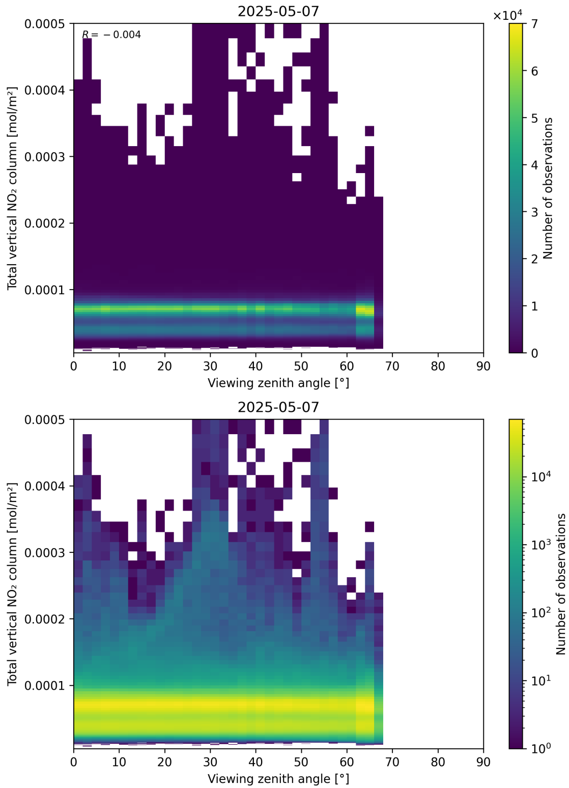
Figure 167: Scatter density plot of “Viewing zenith angle” against “Total vertical NO 2 column” for 2025-05-07 to 2025-05-08.
