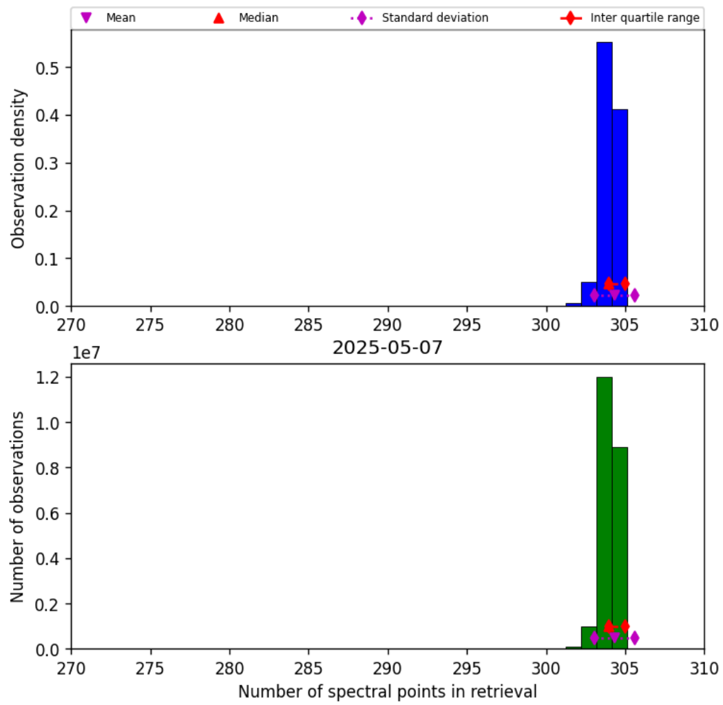
Figure 33: Histogram of “Number of spectral points in retrieval” for 2025-05-07 to 2025-05-08
