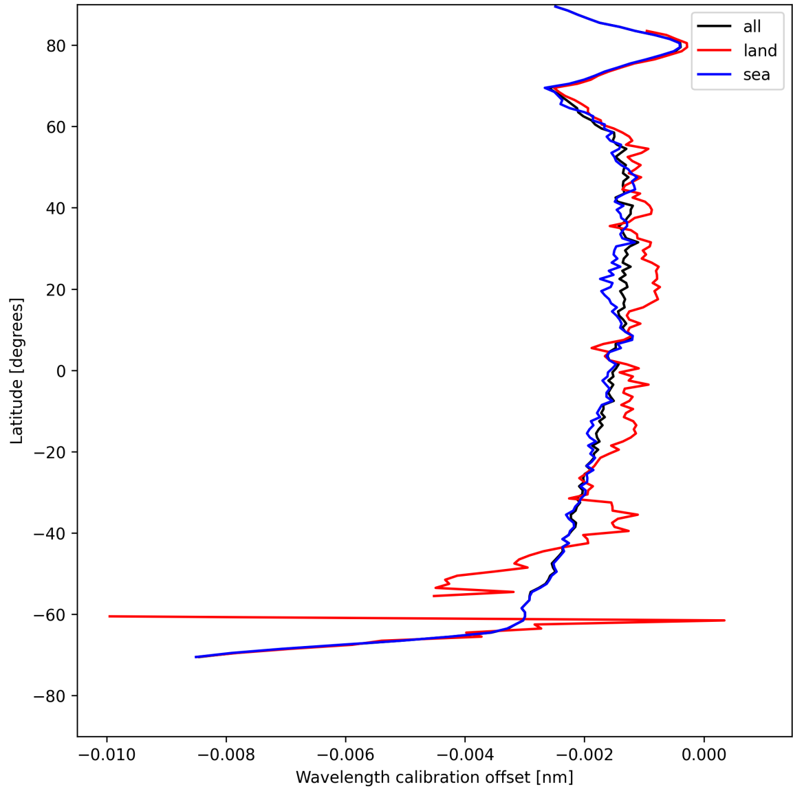
Figure 18: Zonal average of “Wavelength calibration offset” for 2025-05-07 to 2025-05-08.
