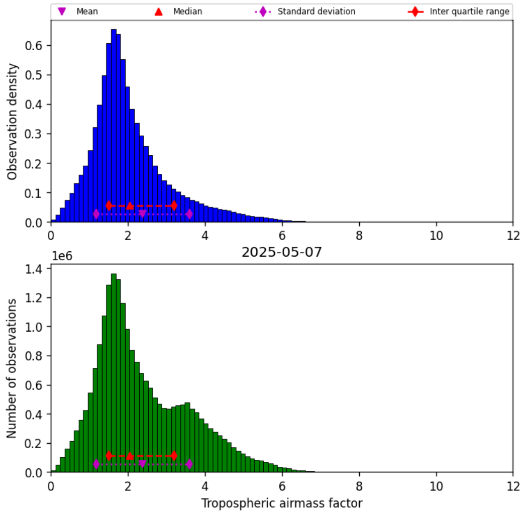
Figure 31: Histogram of “Tropospheric airmass factor” for 2025-05-07 to 2025-05-08
