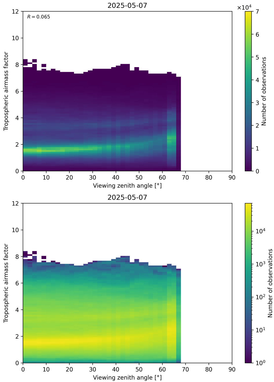
Figure 161: Scatter density plot of “Viewing zenith angle” against “Tropospheric airmass factor” for 2025-05-07 to 2025-05-08.
