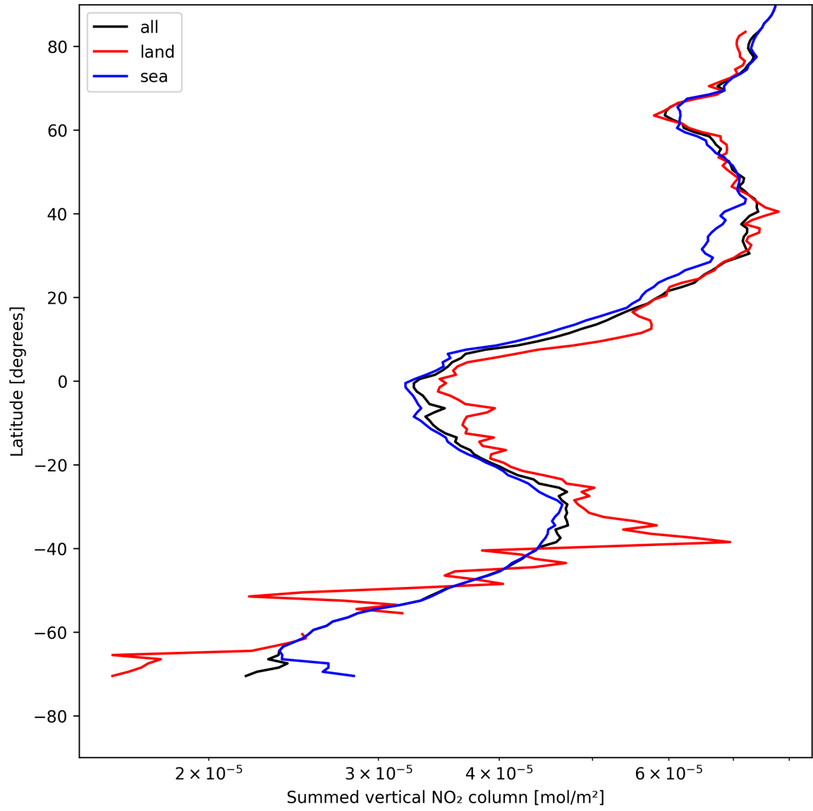
Figure 23: Zonal average of “Summed vertical NO 2 column” for 2025-05-07 to 2025-05-08.
