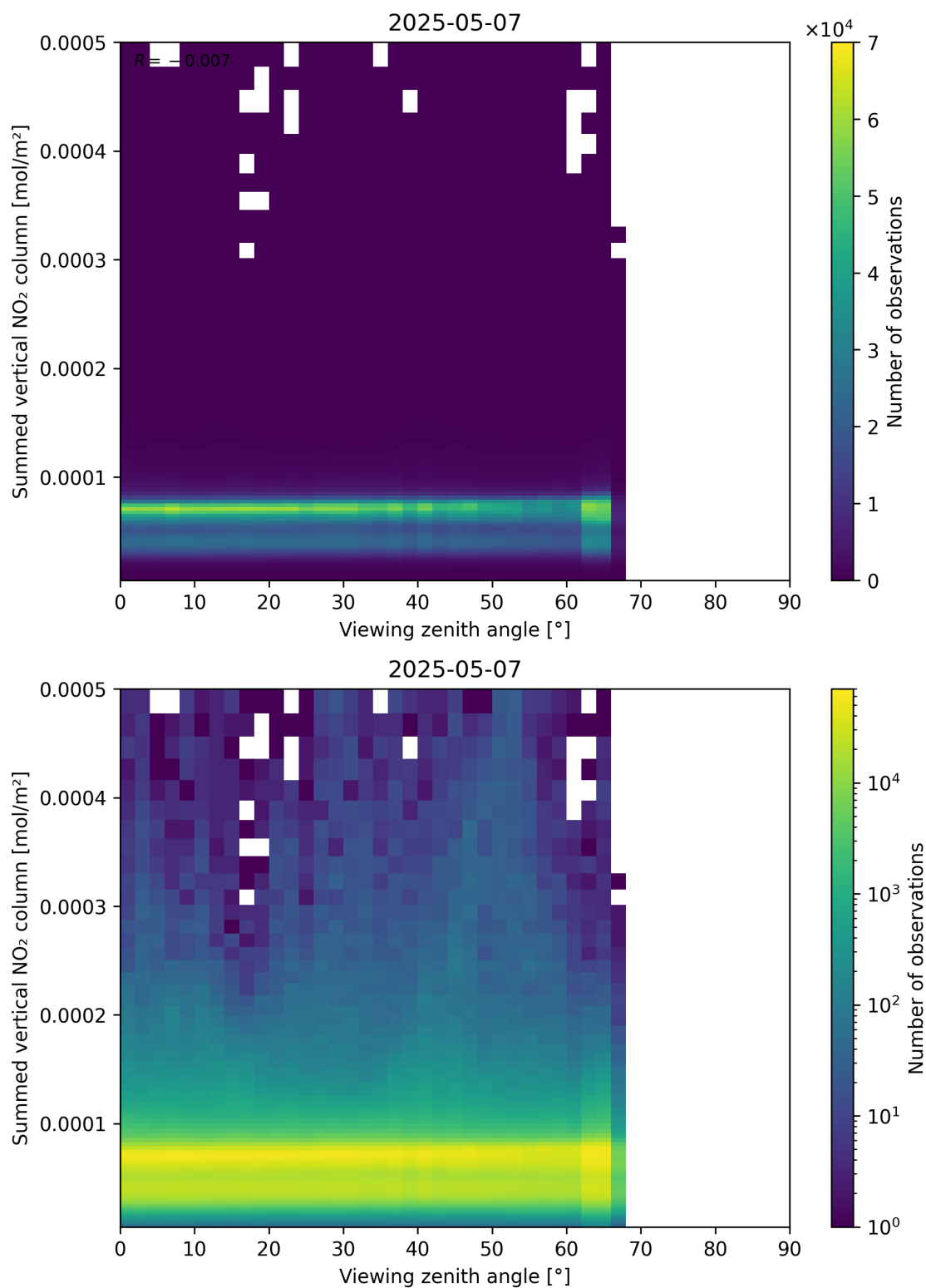
Figure 165: Scatter density plot of “Viewing zenith angle” against “Summed vertical NO 2 column” for 2025-05-07 to 2025-05-08.
