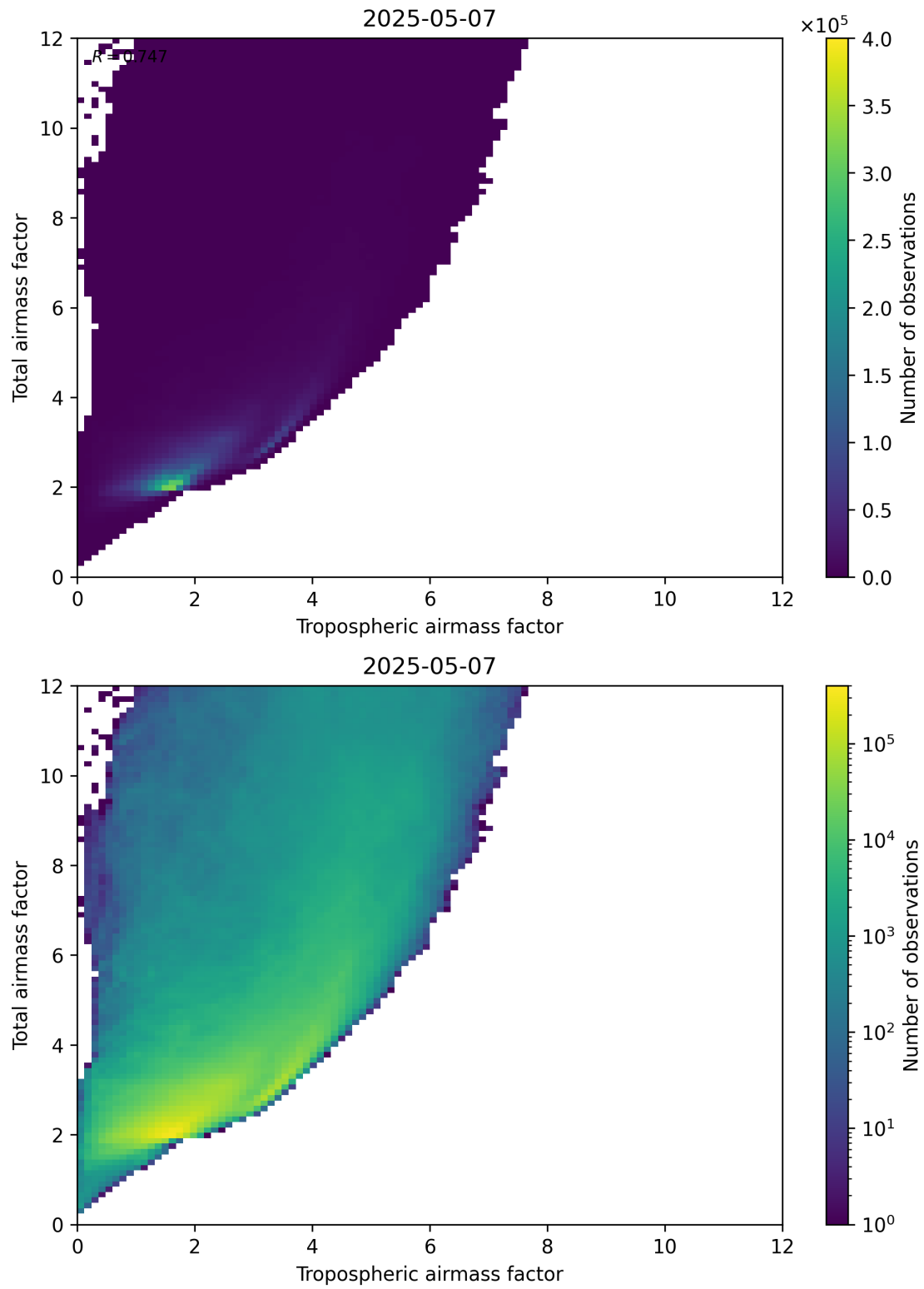
Figure 72: Scatter density plot of “Tropospheric airmass factor” against “Total airmass factor” for 2025-05-07 to 2025-05-08.
