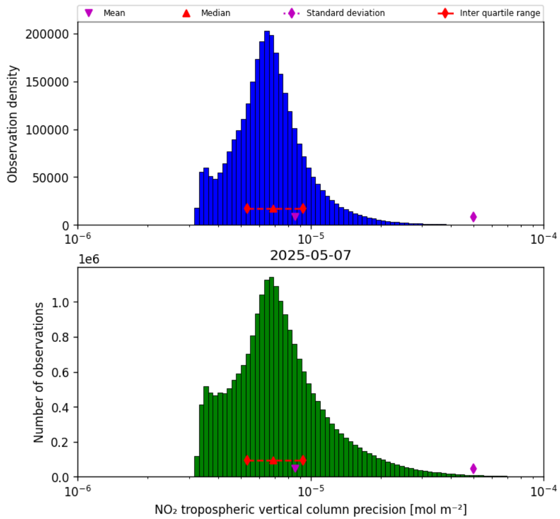
Figure 30: Histogram of “NO 2 tropospheric vertical column precision” for 2025-05-07 to 2025-05-08
