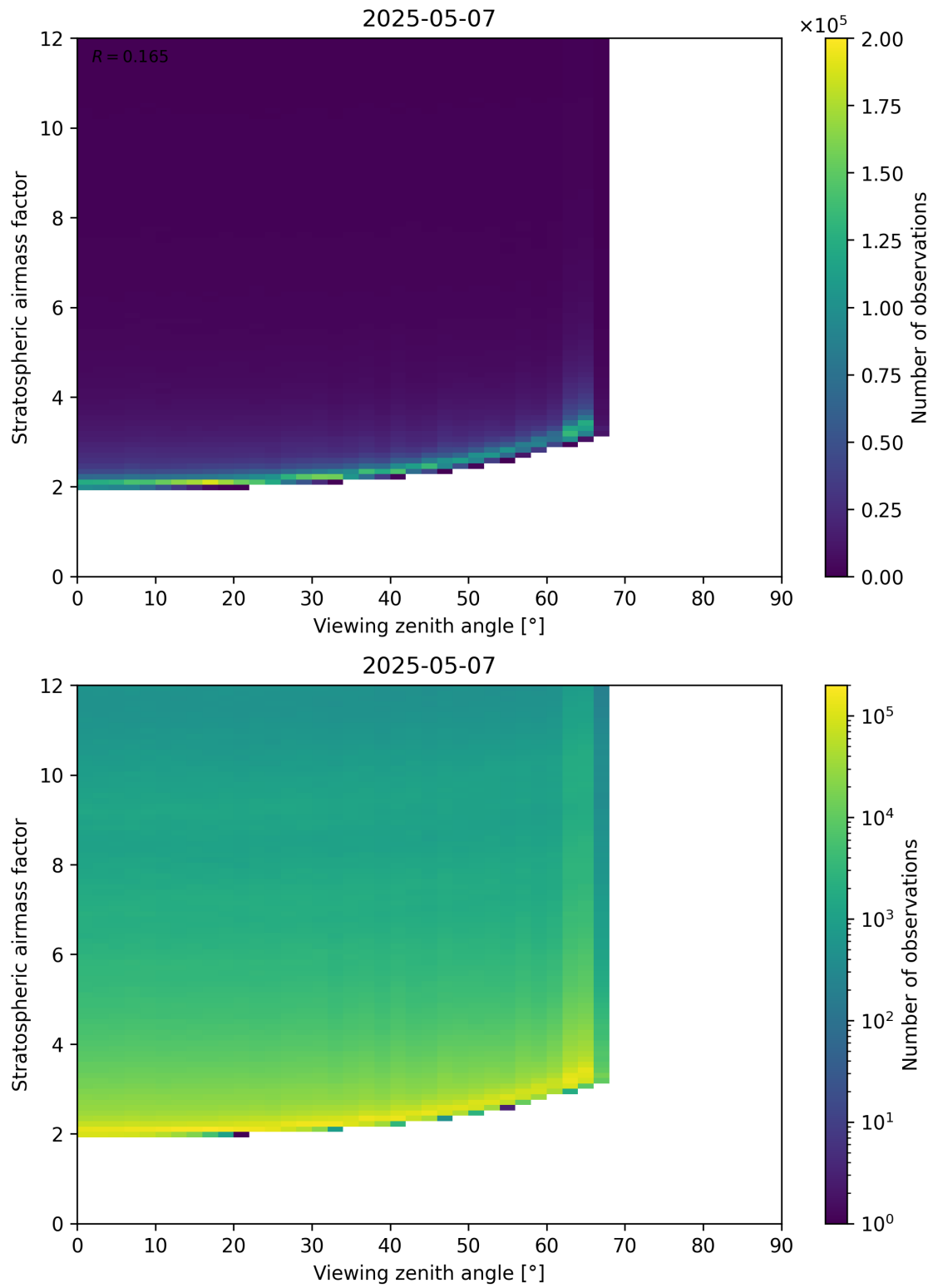
Figure 159: Scatter density plot of “Viewing zenith angle” against “Stratospheric airmass factor” for 2025-05-07 to 2025-05-08.
