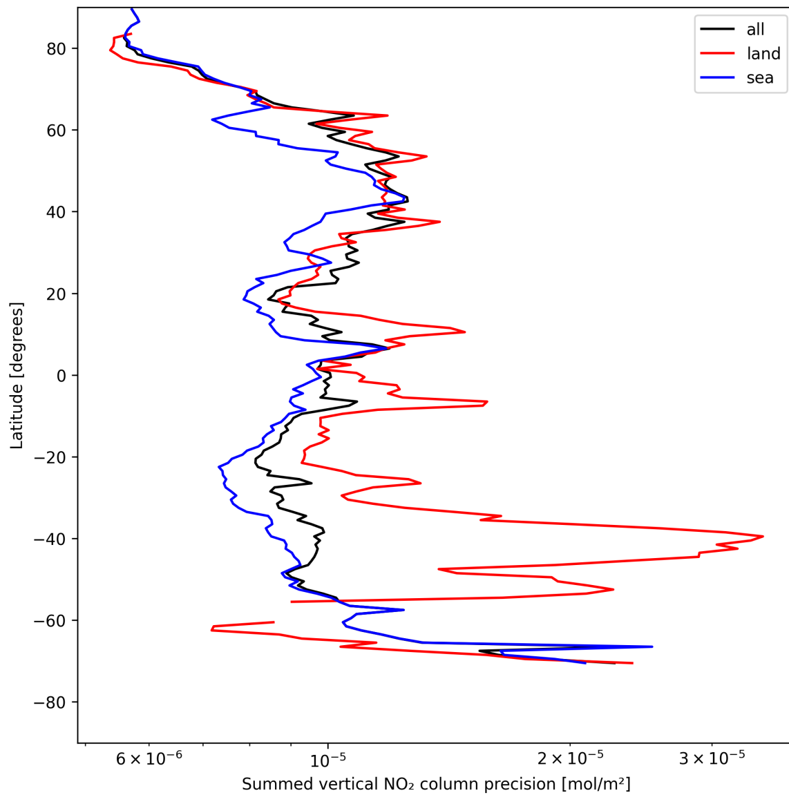
Figure 24: Zonal average of “Summed vertical NO 2 column precision” for 2025-05-07 to 2025-05-08.
