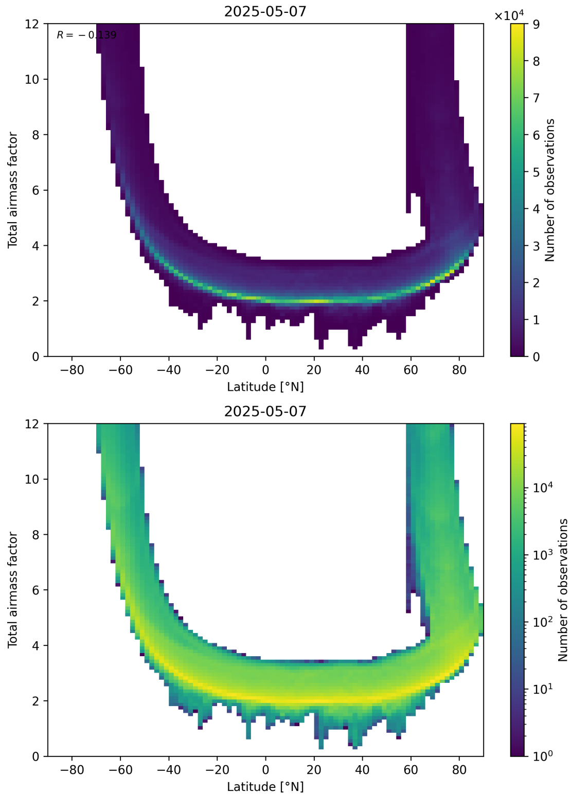
Figure 84: Scatter density plot of “Latitude” against “Total airmass factor” for 2025-05-07 to 2025-05-08.
