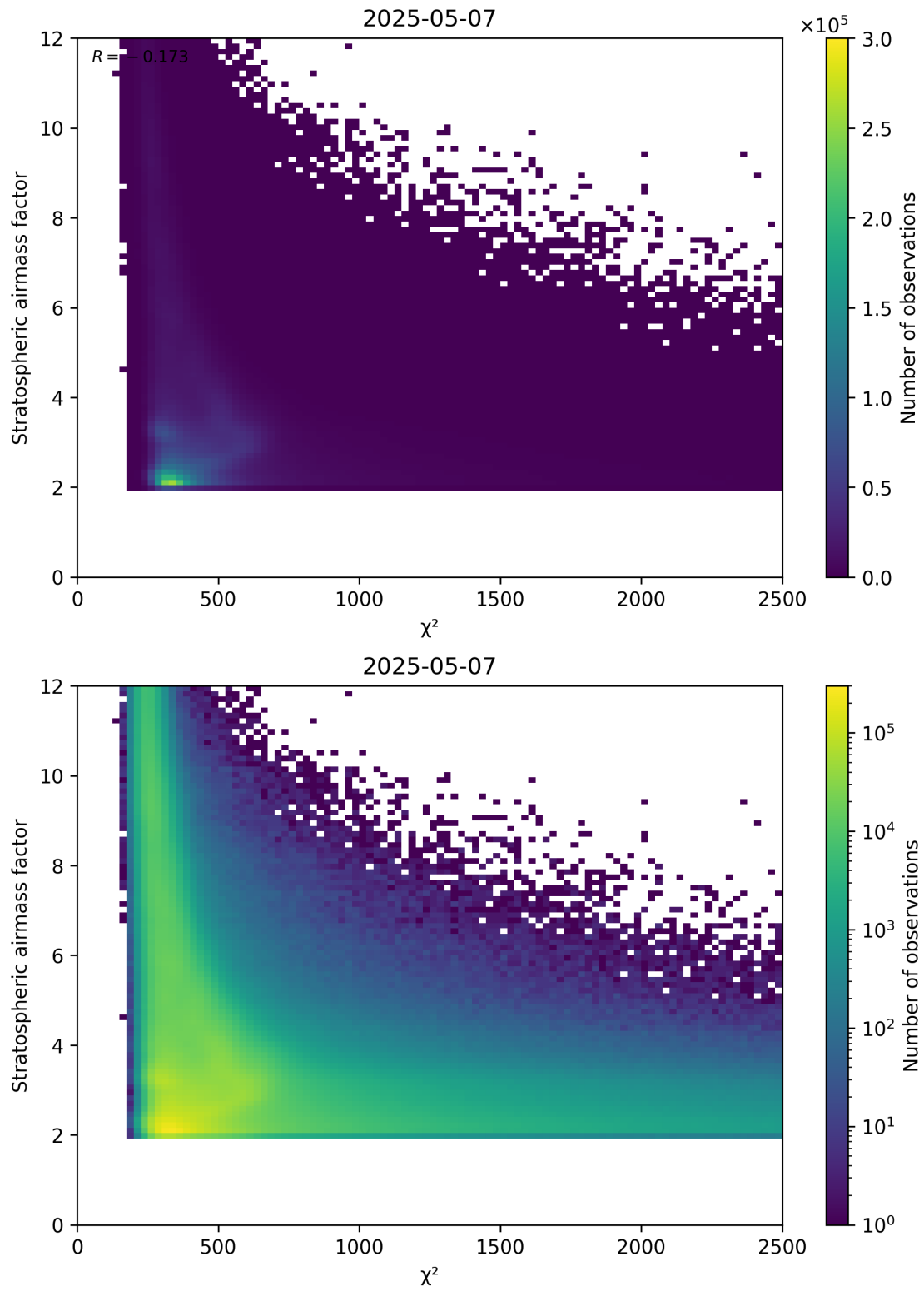
Figure 81: Scatter density plot of “ \chi^2 ” against “Stratospheric airmass factor” for 2025-05-07 to 2025-05-08.
