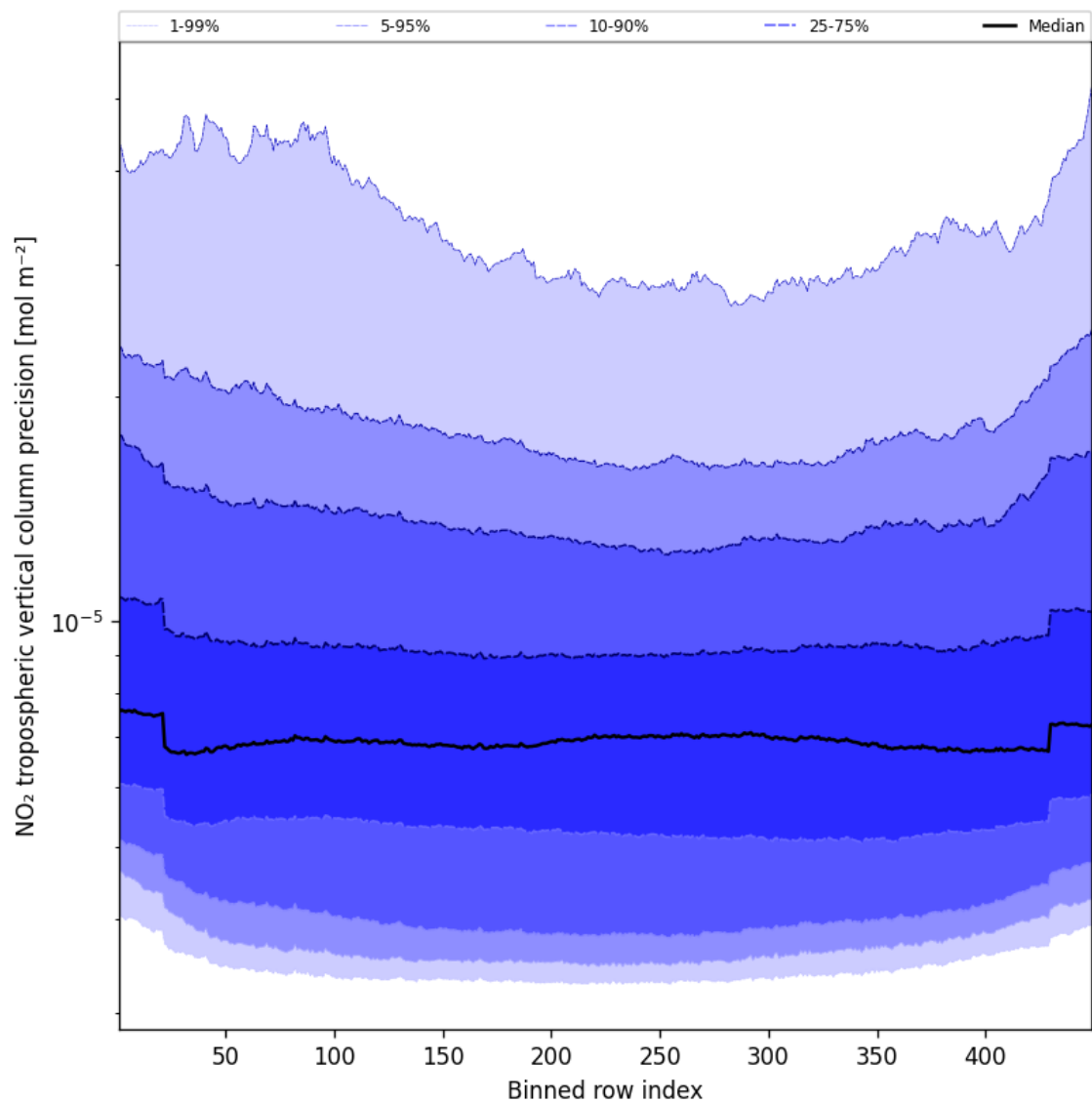
Figure 47: Along track statistics of “NO 2 tropospheric vertical column precision” for 2025-05-07 to 2025-05-08
