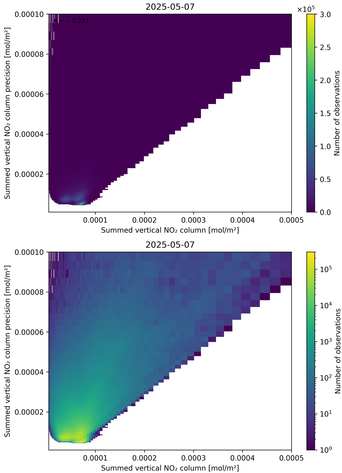
Figure 105: Scatter density plot of “Summed vertical NO 2 column” against “Summed vertical NO 2 column precision” for 2025-05-07 to 2025-05-08.
