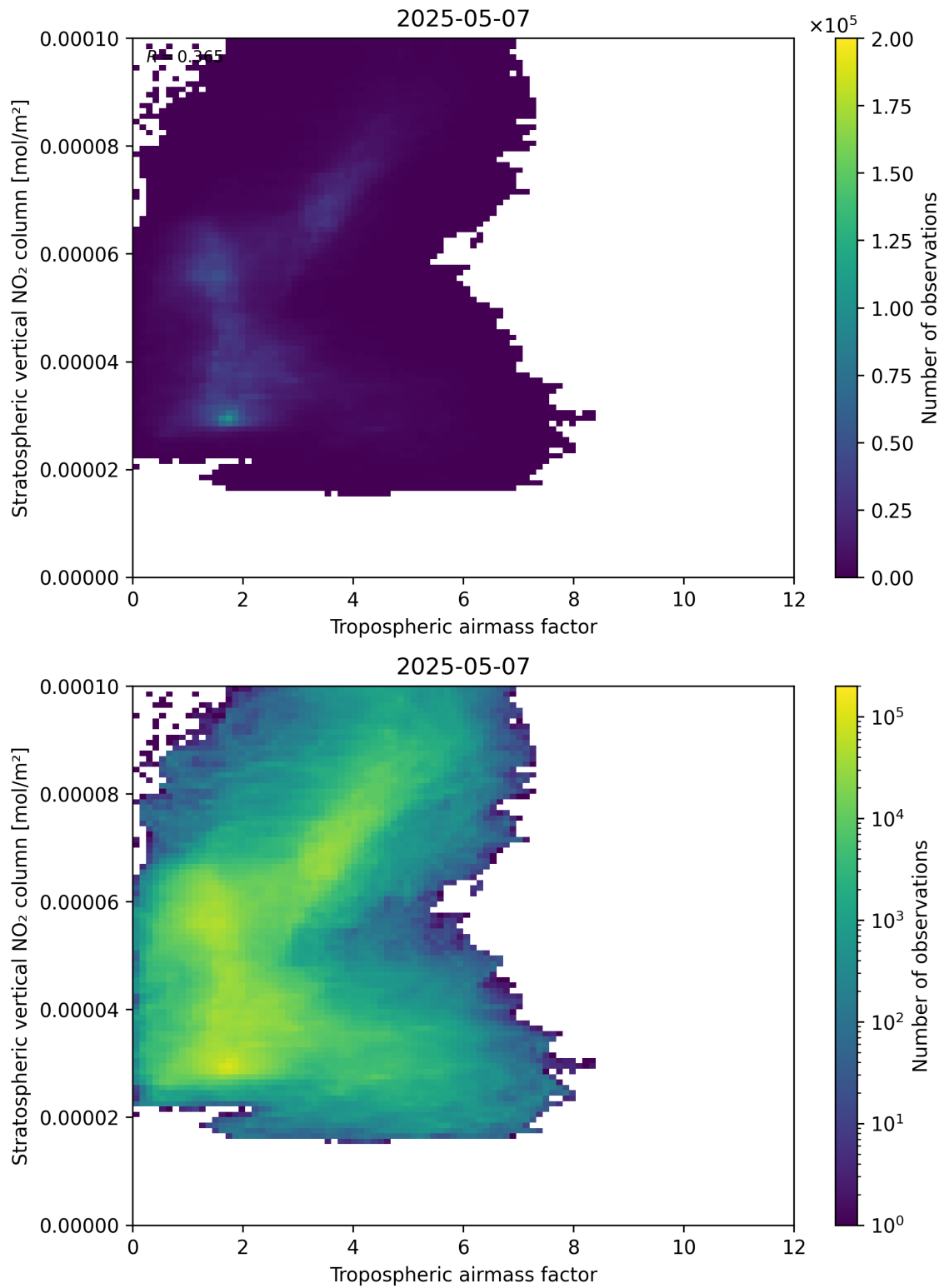
Figure 74: Scatter density plot of “Tropospheric airmass factor” against “Stratospheric vertical NO 2 column” for 2025-05-07 to 2025-05-08.
