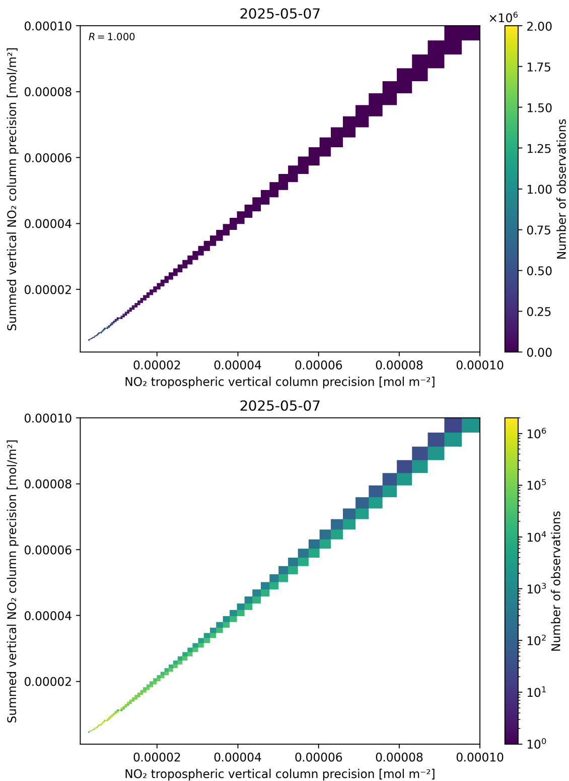
Figure 137: Scatter density plot of “NO 2 tropospheric vertical column precision” against “Summed vertical NO 2 column precision” for 2025-05-07 to 2025-05-08.
