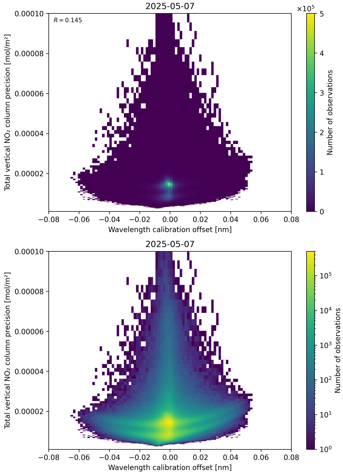
Figure 180: Scatter density plot of “Wavelength calibration offset” against “Total vertical NO 2 column precision” for 2025-05-07 to 2025-05-08.
