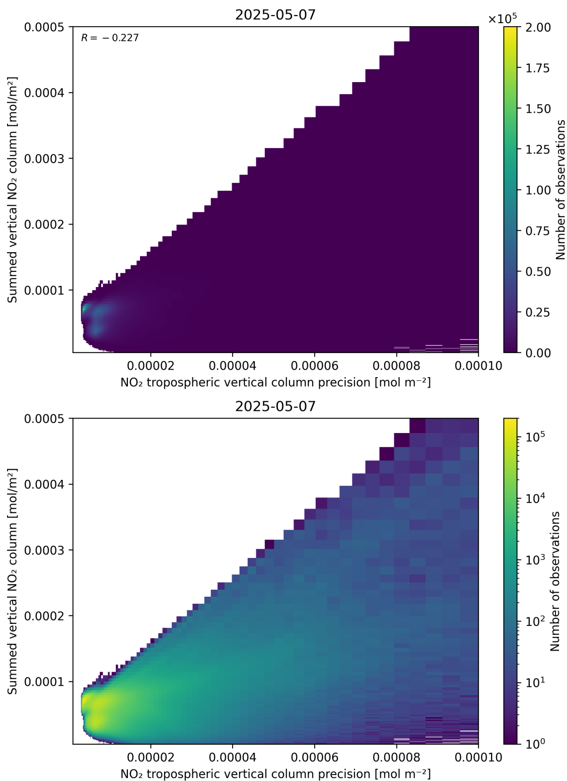
Figure 136: Scatter density plot of “NO 2 tropospheric vertical column precision” against “Summed vertical NO 2 column” for 2025-05-07 to 2025-05-08.
