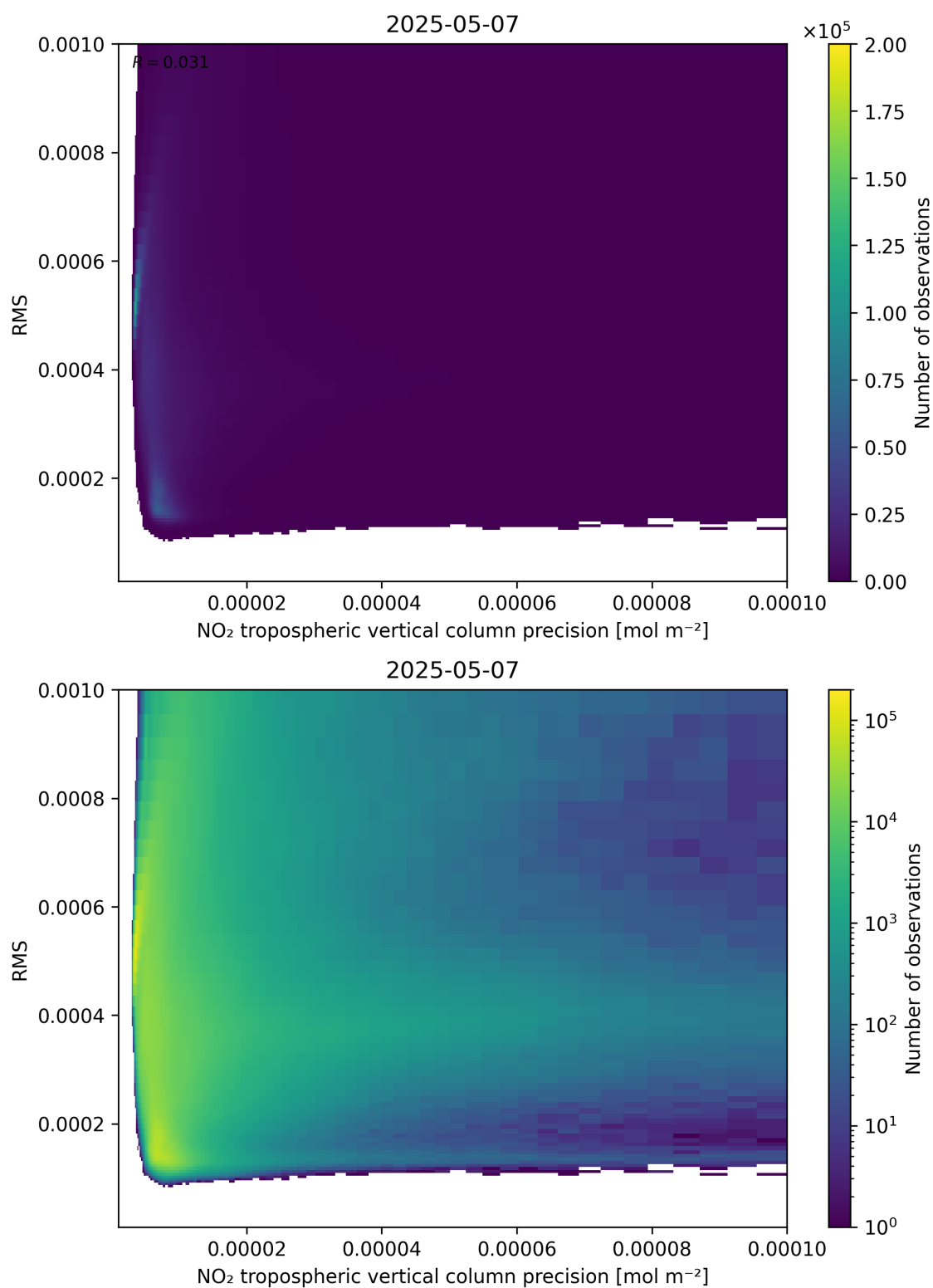
Figure 140: Scatter density plot of “NO 2 tropospheric vertical column precision” against “RMS” for 2025-05-07 to 2025-05-08.
