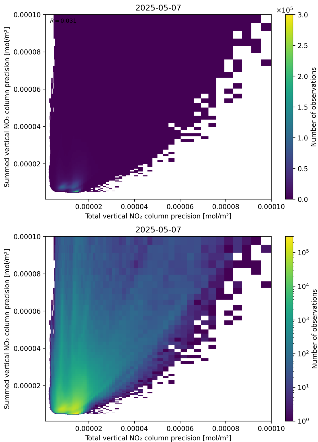
Figure 118: Scatter density plot of “Total vertical NO 2 column precision” against “Summed vertical NO 2 column precision” for 2025-05-07 to 2025-05-08.
