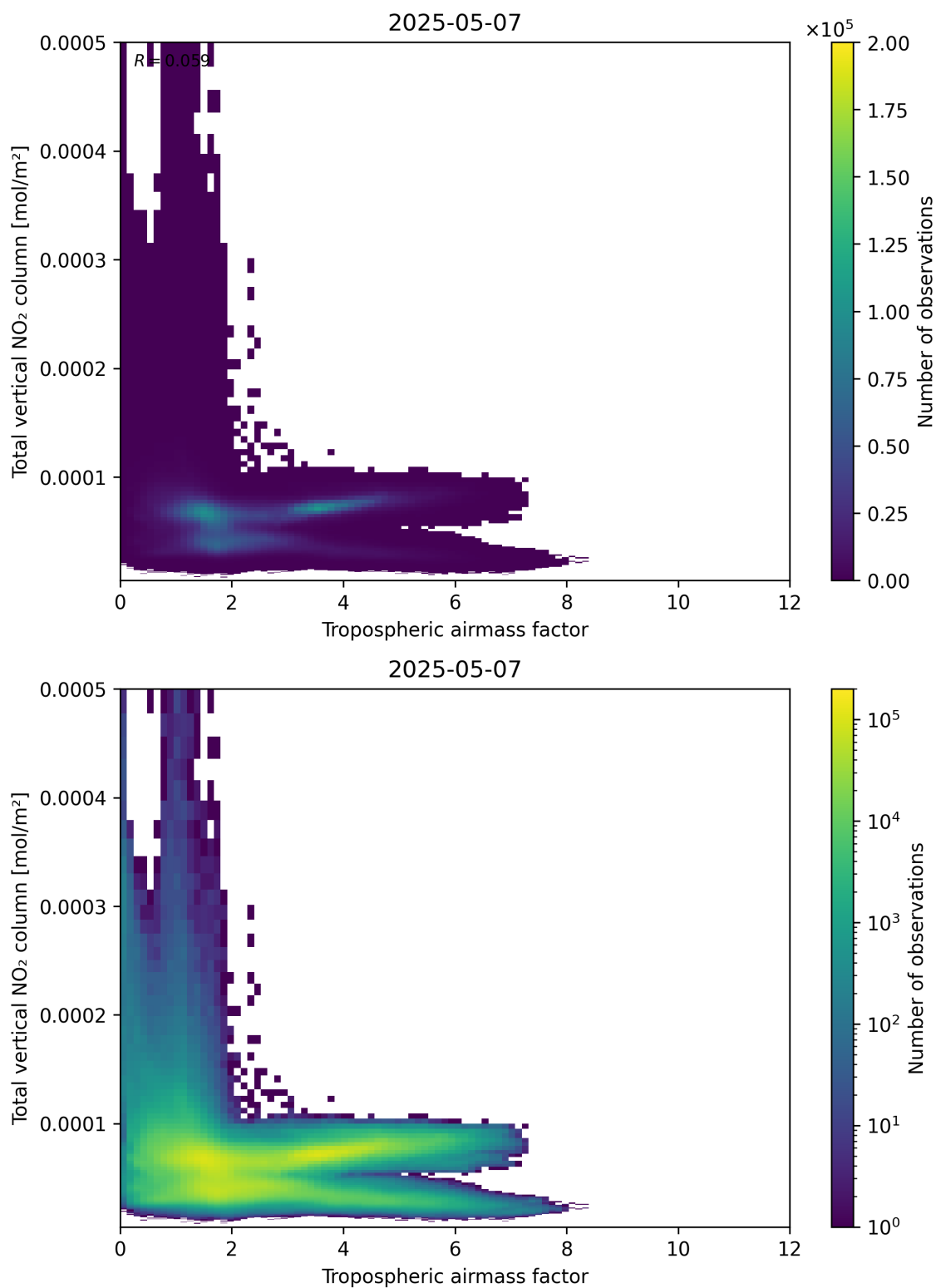
Figure 77: Scatter density plot of “Tropospheric airmass factor” against “Total vertical NO 2 column” for 2025-05-07 to 2025-05-08.
