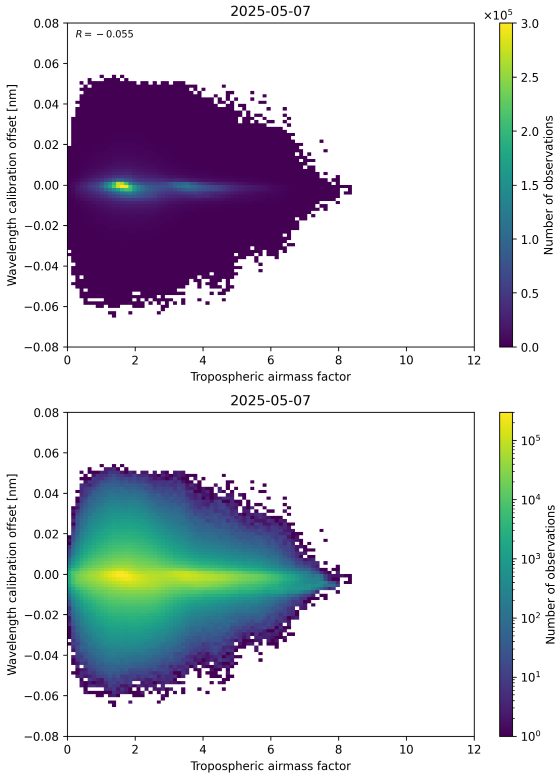
Figure 80: Scatter density plot of “Tropospheric airmass factor” against “Wavelength calibration offset” for 2025-05-07 to 2025-05-08.
