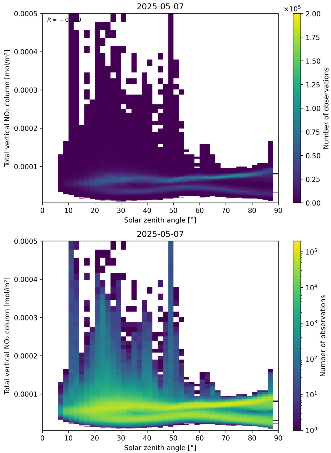
Figure 153: Scatter density plot of “Solar zenith angle” against “Total vertical NO 2 column” for 2025-05-07 to 2025-05-08.
