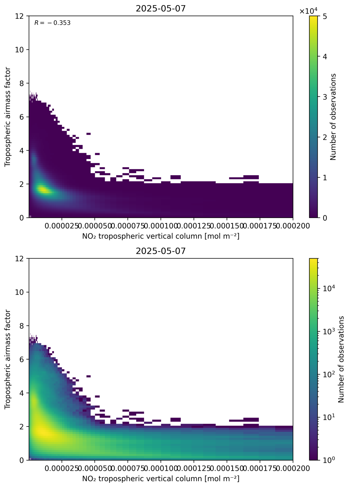
Figure 123: Scatter density plot of “NO 2 tropospheric vertical column” against “Tropospheric air mass factor” for 2025-05-07 to 2025-05-08.
