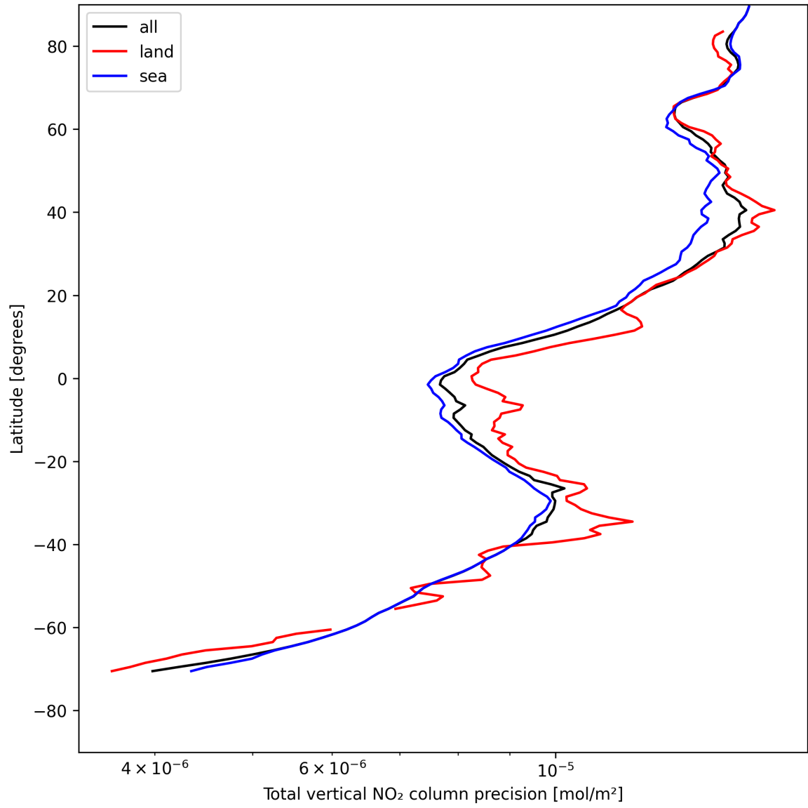
Figure 22: Zonal average of “Total vertical NO 2 column precision” for 2025-05-07 to 2025-05-08.
