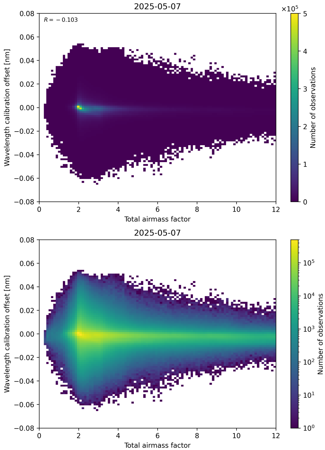
Figure 70: Scatter density plot of “Total airmass factor” against “Wavelength calibration offset” for 2025-05-07 to 2025-05-08.
