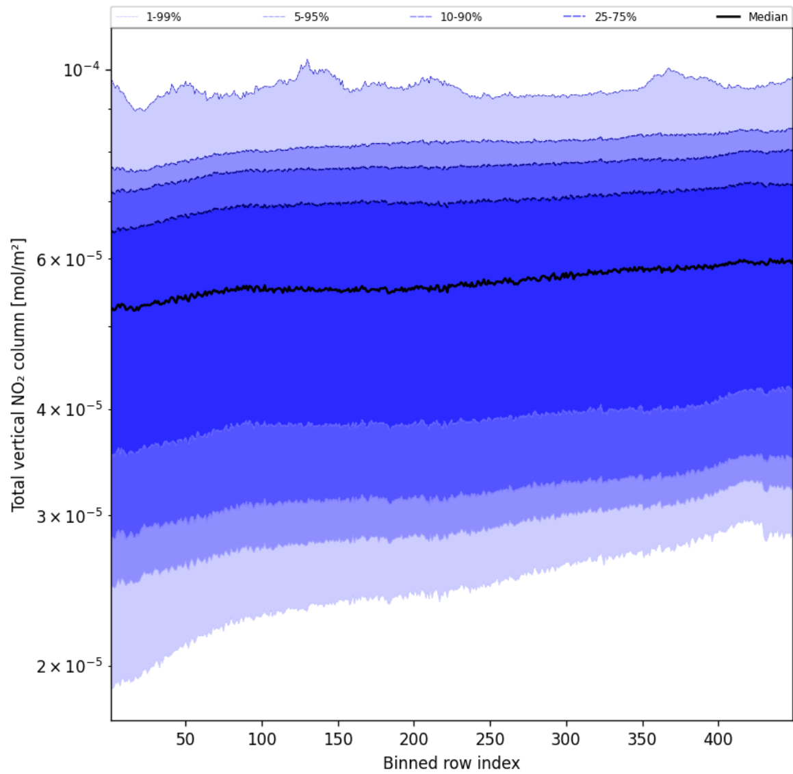
Figure 55: Along track statistics of “Total vertical NO 2 column” for 2025-05-07 to 2025-05-08
