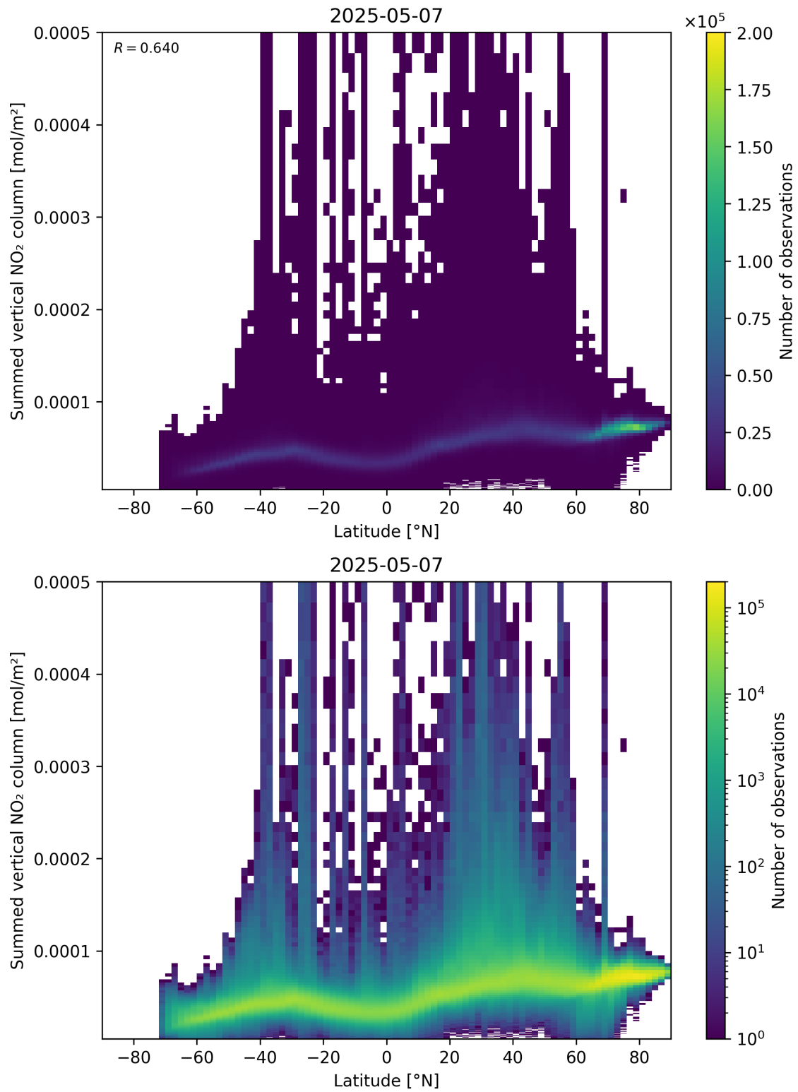
Figure 88: Scatter density plot of “Latitude” against “Summed vertical NO 2 column” for 2025-05-07 to 2025-05-08.
