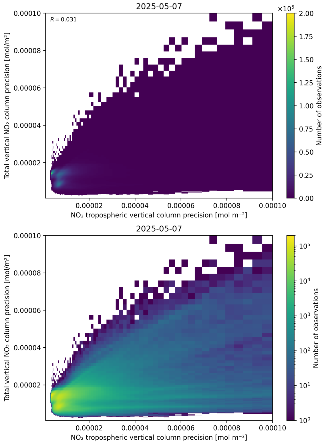
Figure 139: Scatter density plot of “NO 2 tropospheric vertical column precision” against “Total vertical NO 2 column precision” for 2025-05-07 to 2025-05-08.
