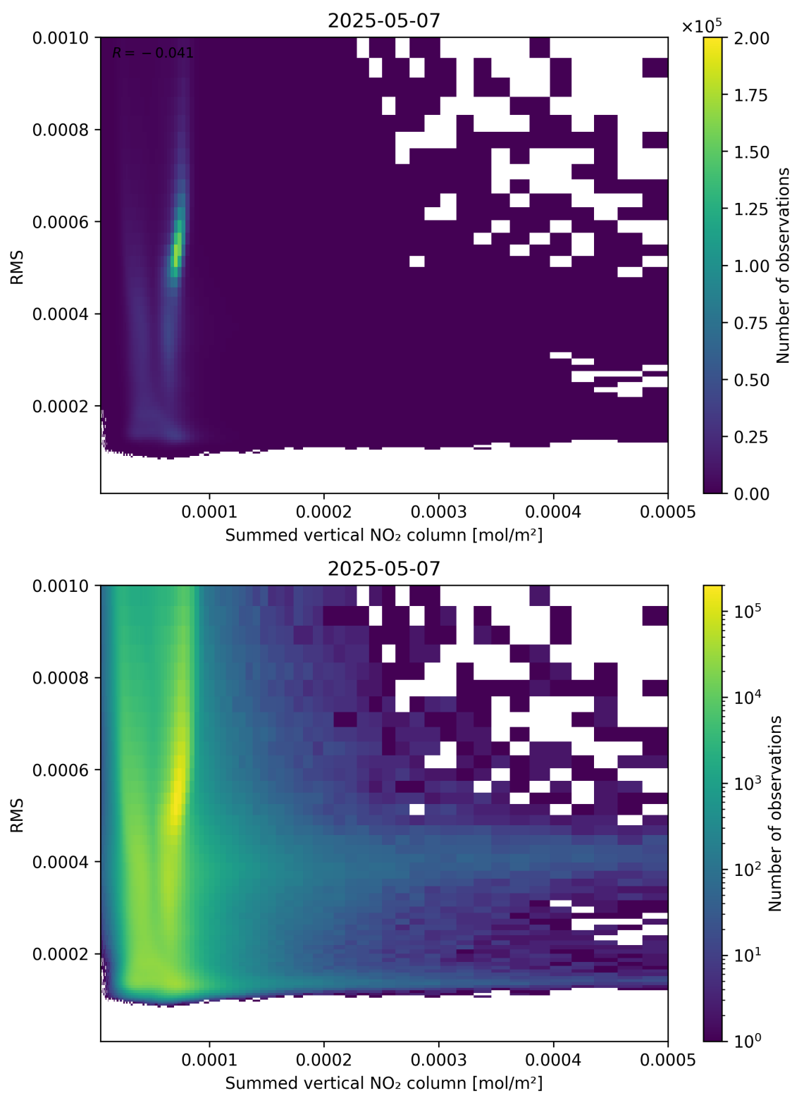
Figure 109: Scatter density plot of “Summed vertical NO 2 column” against “RMS” for 2025-05-07 to 2025-05-08.
