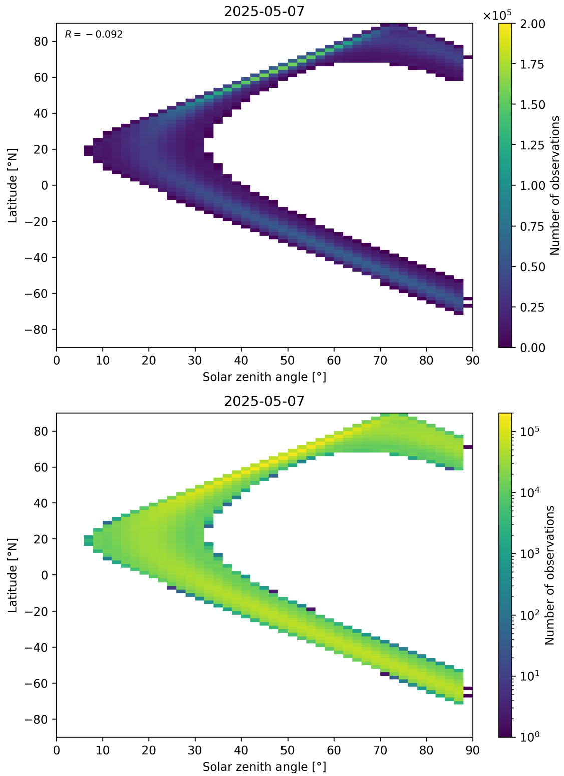
Figure 149: Scatter density plot of “Solar zenith angle” against “Latitude” for 2025-05-07 to 2025-05-08.
