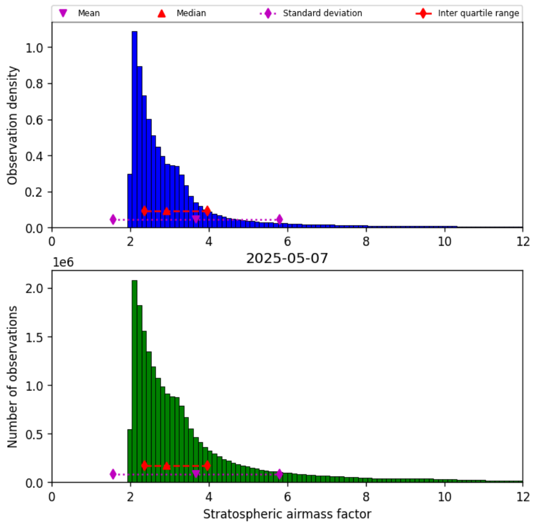
Figure 44: Histogram of “Stratospheric airmass factor” for 2025-05-07 to 2025-05-08
