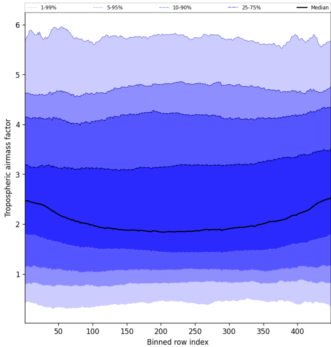
Figure 48: Along track statistics of “Tropospheric airmass factor” for 2025-05-07 to 2025-05-08
