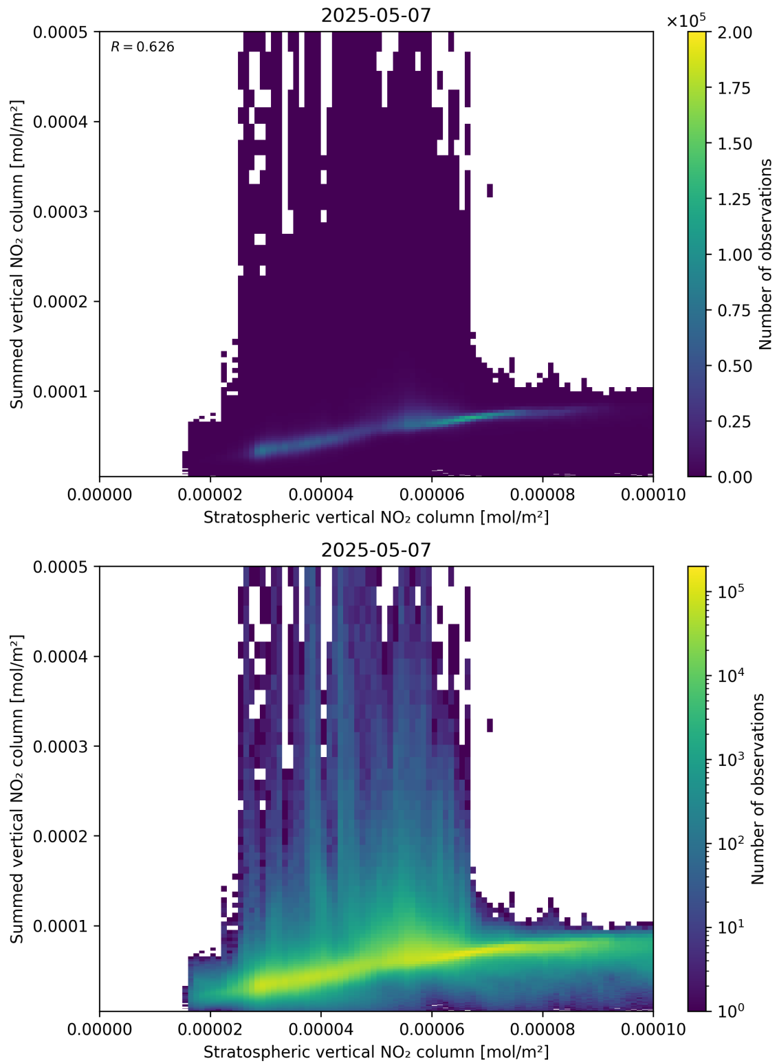
Figure 98: Scatter density plot of “Stratospheric vertical NO 2 column” against “Summed vertical NO 2 column” for 2025-05-07 to 2025-05-08.
