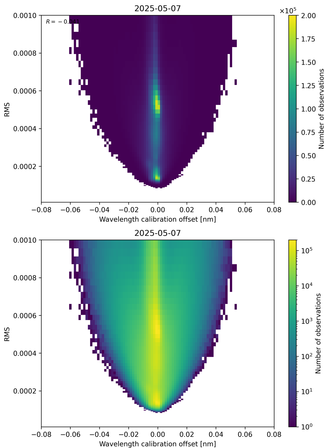
Figure 181: Scatter density plot of “Wavelength calibration offset” against “RMS” for 2025-05-07 to 2025-05-08.
