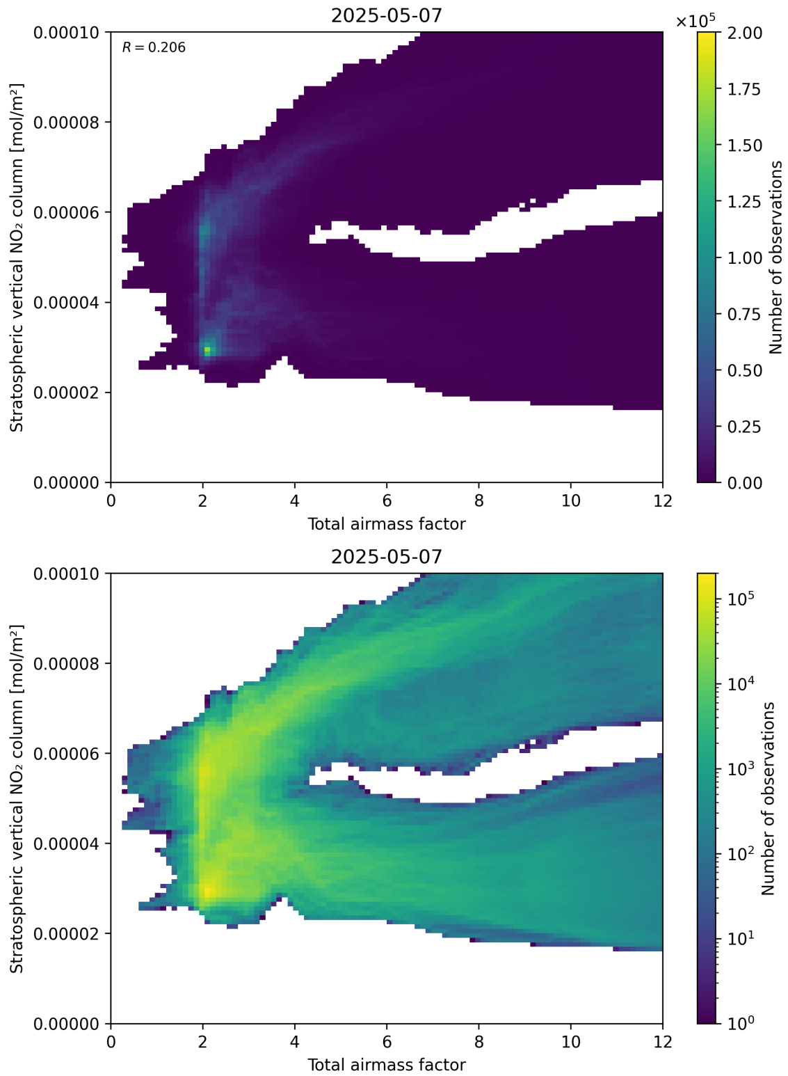
Figure 64: Scatter density plot of “Total airmass factor” against “Stratospheric vertical \text{NO}_2 column” for 2025-05-07 to 2025-05-08.
