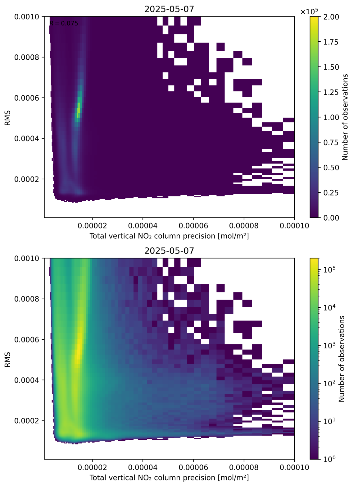
Figure 119: Scatter density plot of “Total vertical NO 2 column precision” against “RMS” for 2025-05-07 to 2025-05-08.
