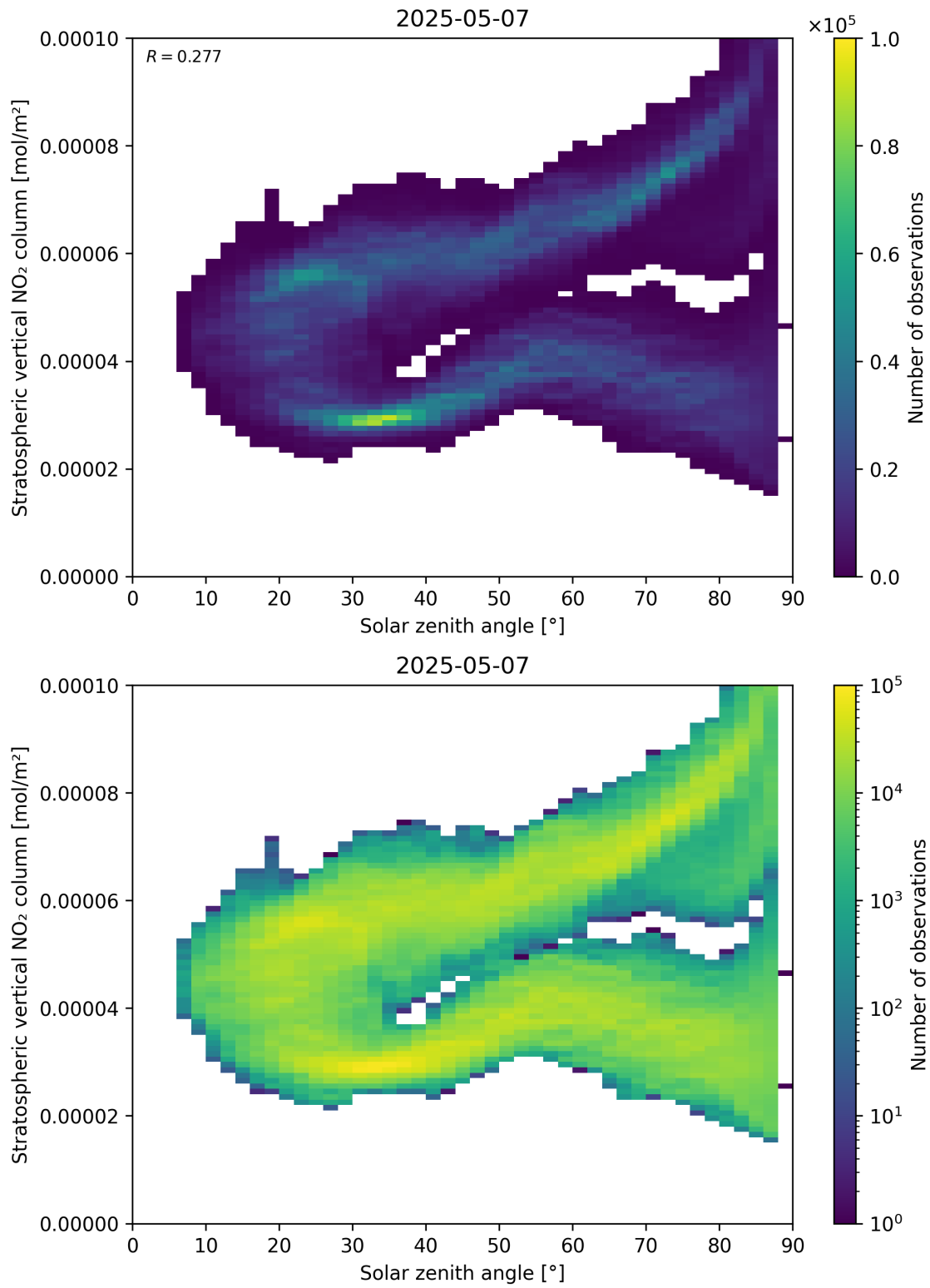
Figure 150: Scatter density plot of “Solar zenith angle” against “Stratospheric vertical NO 2 column” for 2025-05-07 to 2025-05-08.
