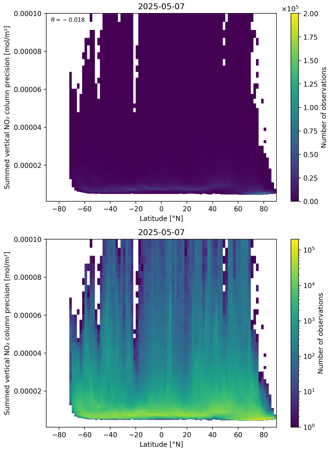
Figure 89: Scatter density plot of “Latitude” against “Summed vertical NO 2 column precision” for 2025-05-07 to 2025-05-08.
