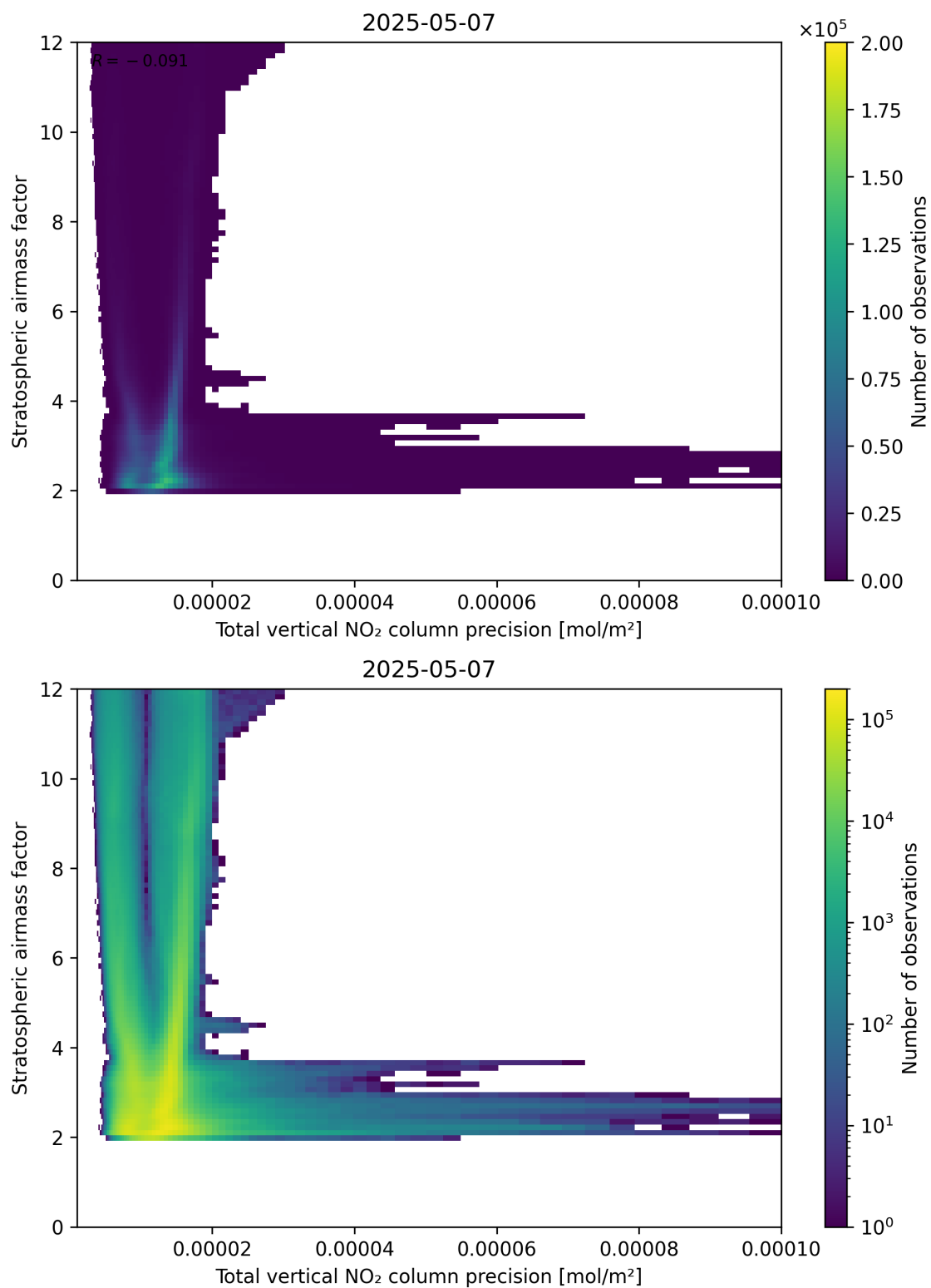
Figure 115: Scatter density plot of “Total vertical NO 2 column precision” against “Stratospheric air mass factor” for 2025-05-07 to 2025-05-08.
