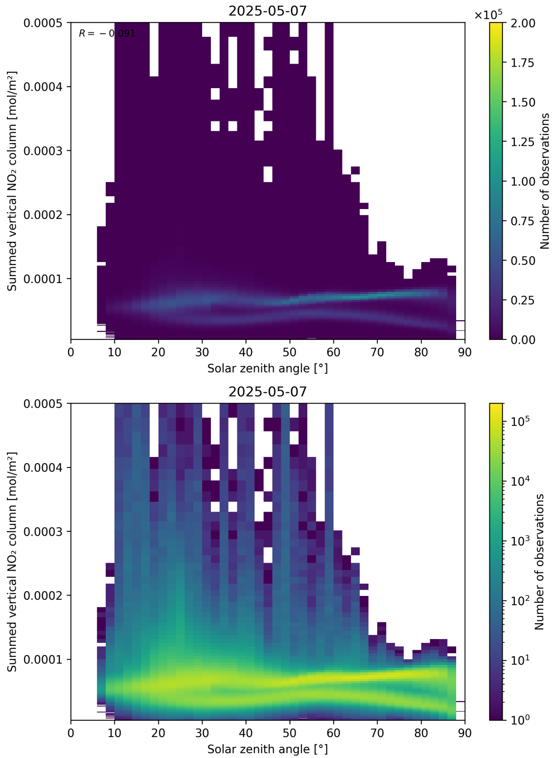
Figure 151: Scatter density plot of “Solar zenith angle” against “Summed vertical NO 2 column” for 2025-05-07 to 2025-05-08.
