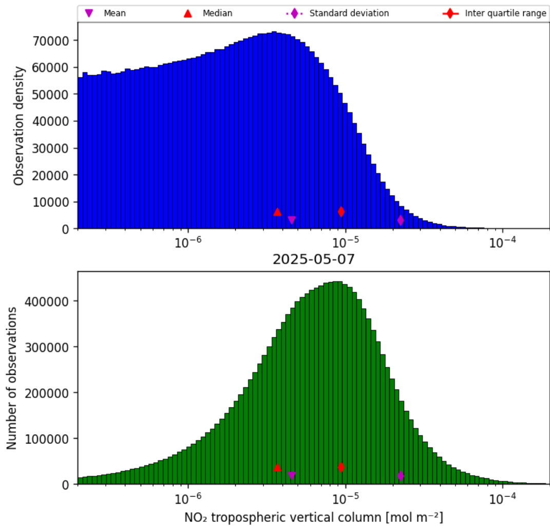
Figure 29: Histogram of “NO 2 tropospheric vertical column” for 2025-05-07 to 2025-05-08
