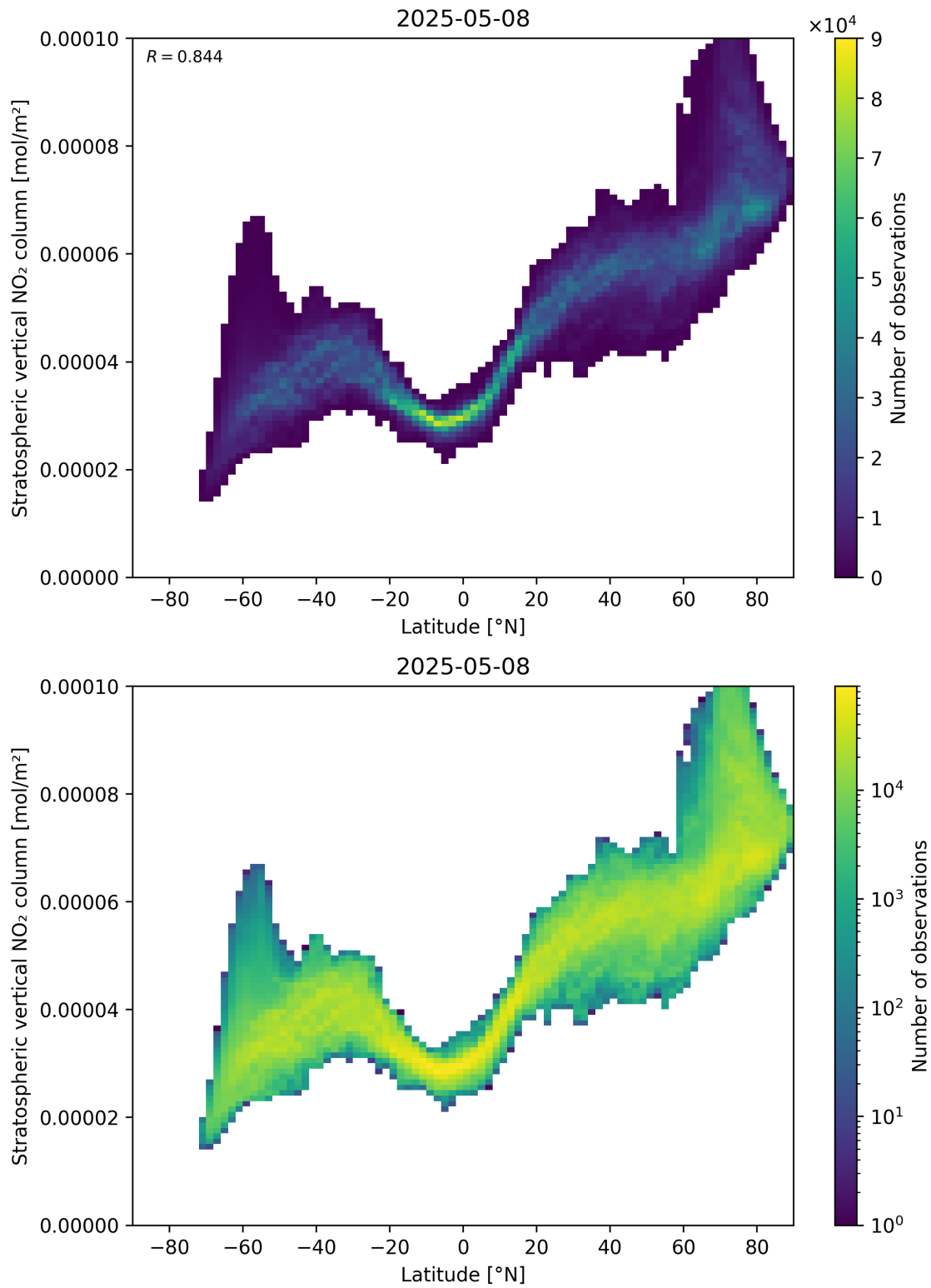
Figure 87: Scatter density plot of “Latitude” against “Stratospheric vertical NO 2 column” for 2025-05-08 to 2025-05-08.
