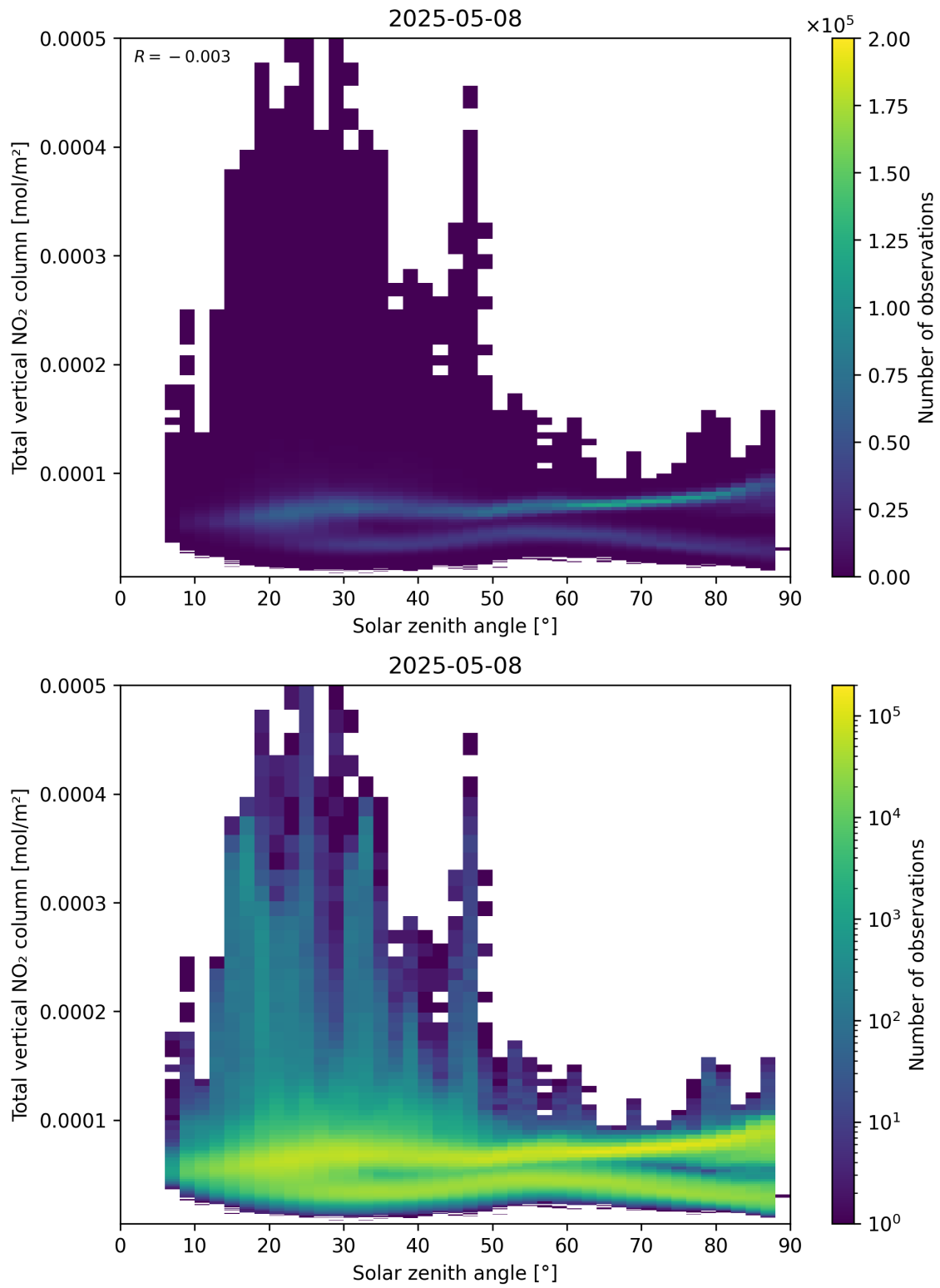
Figure 153: Scatter density plot of “Solar zenith angle” against “Total vertical NO 2 column” for 2025-05-08 to 2025-05-08.
