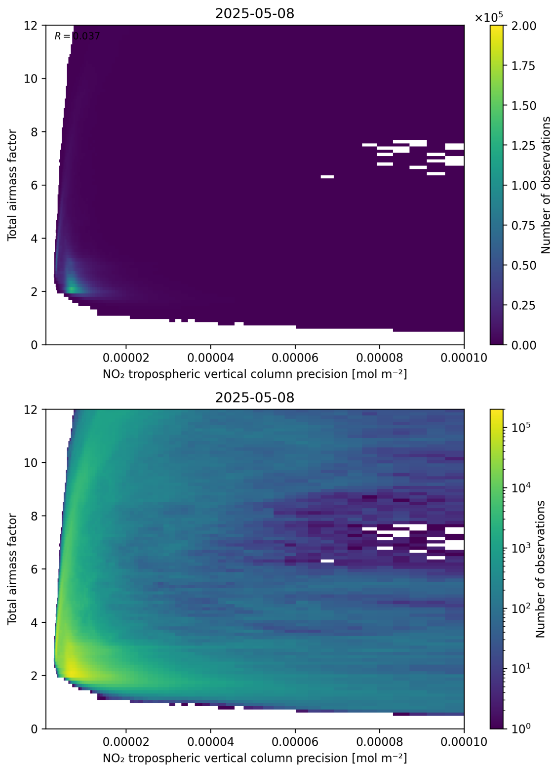
Figure 132: Scatter density plot of “NO 2 tropospheric vertical column precision” against “Total air mass factor” for 2025-05-08 to 2025-05-08.
