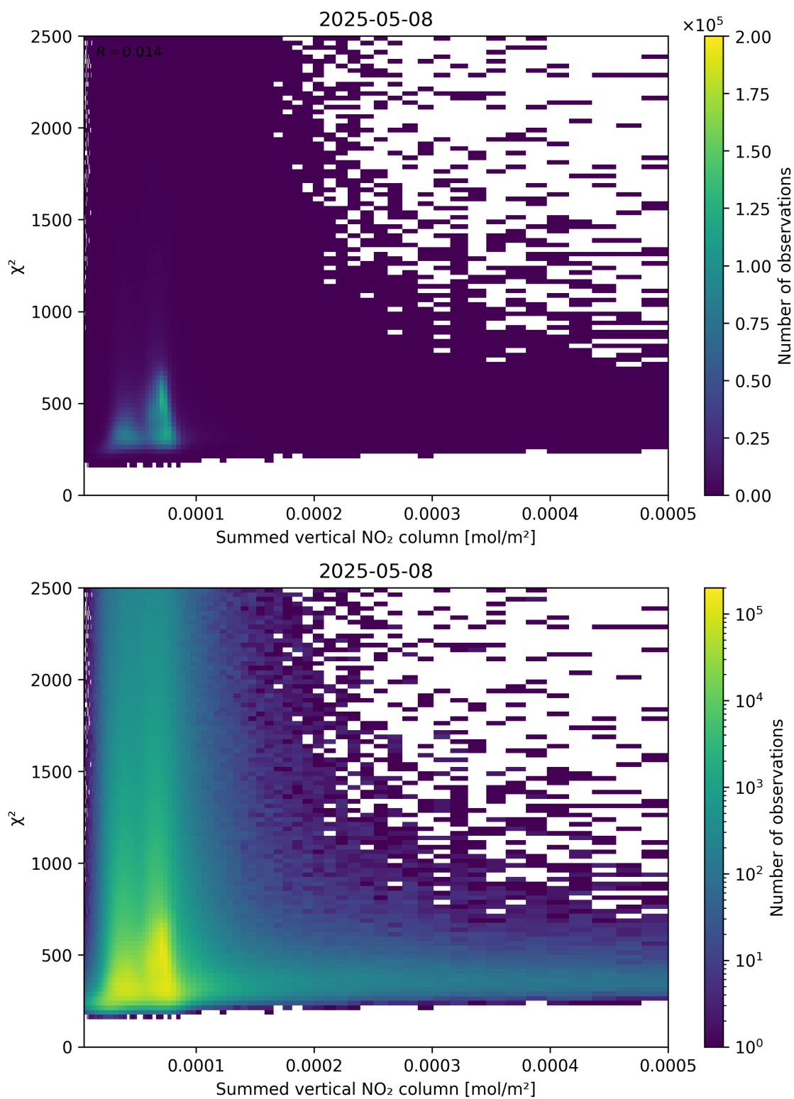
Figure 104: Scatter density plot of “Summed vertical NO 2 column” against “ \chi^2 ” for 2025-05-08 to 2025-05-08.
