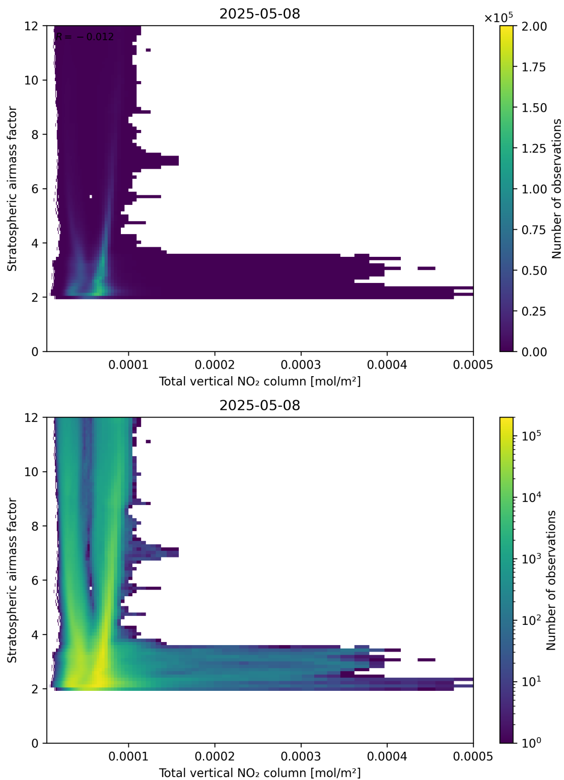
Figure 110: Scatter density plot of “Total vertical NO 2 column” against “Stratospheric airmass factor” for 2025-05-08 to 2025-05-08.
