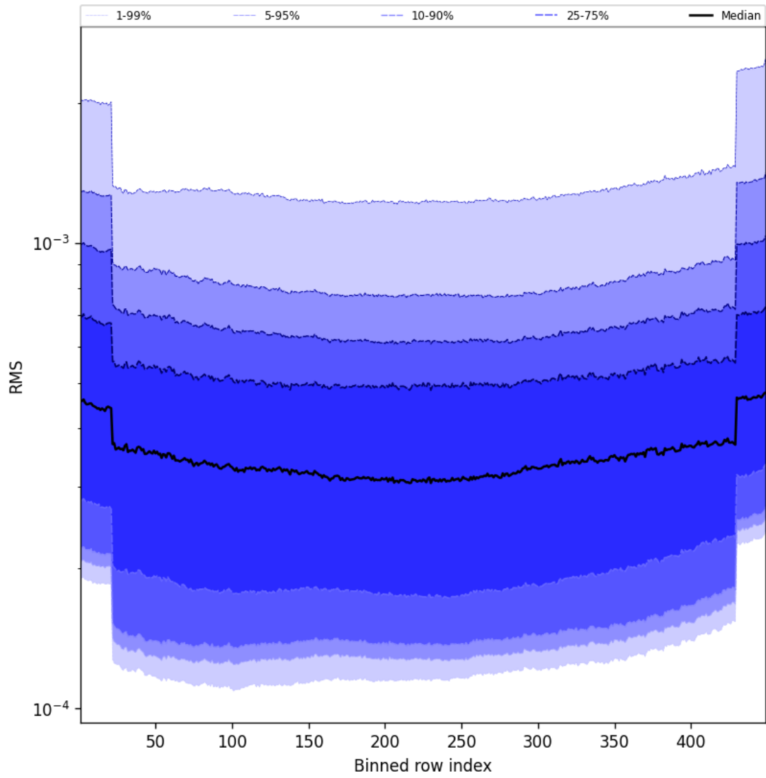
Figure 60: Along track statistics of “RMS” for 2025-05-08 to 2025-05-08
