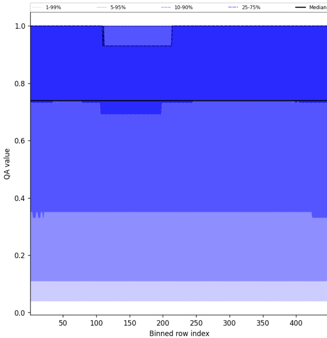
Figure 45: Along track statistics of “QA value” for 2025-05-08 to 2025-05-08
