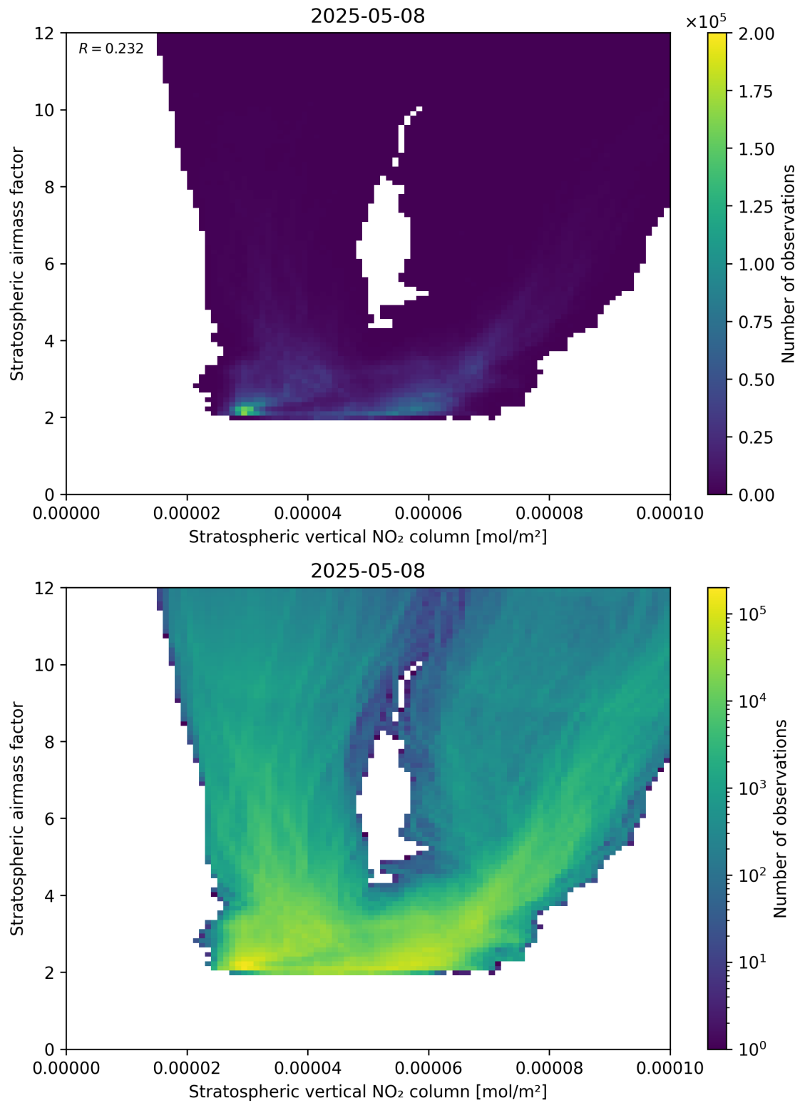
Figure 96: Scatter density plot of “Stratospheric vertical NO 2 column” against “Stratospheric airmass factor” for 2025-05-08 to 2025-05-08.
