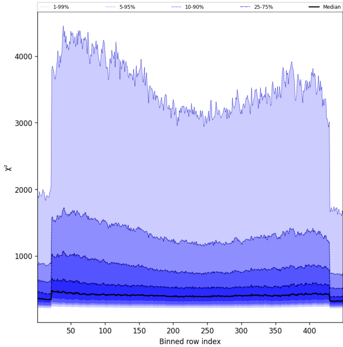
Figure 59: Along track statistics of “ \chi^2 ” for 2025-05-08 to 2025-05-08
