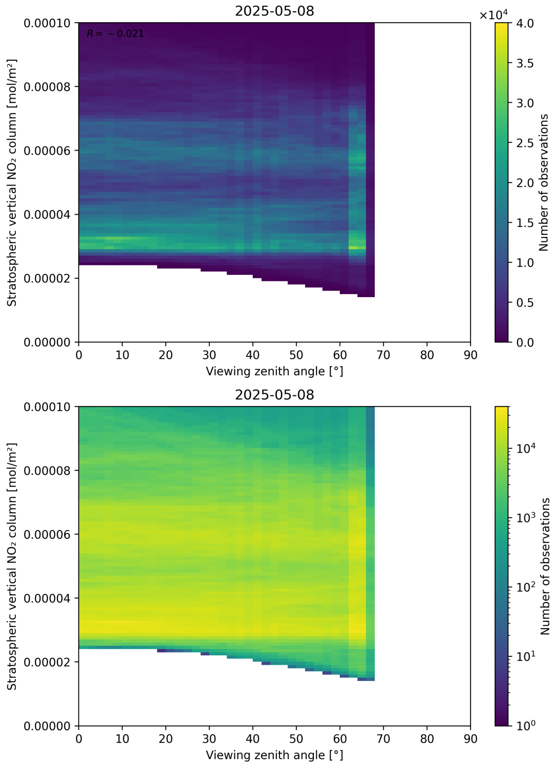
Figure 164: Scatter density plot of “Viewing zenith angle” against “Stratospheric vertical NO 2 column” for 2025-05-08 to 2025-05-08.
