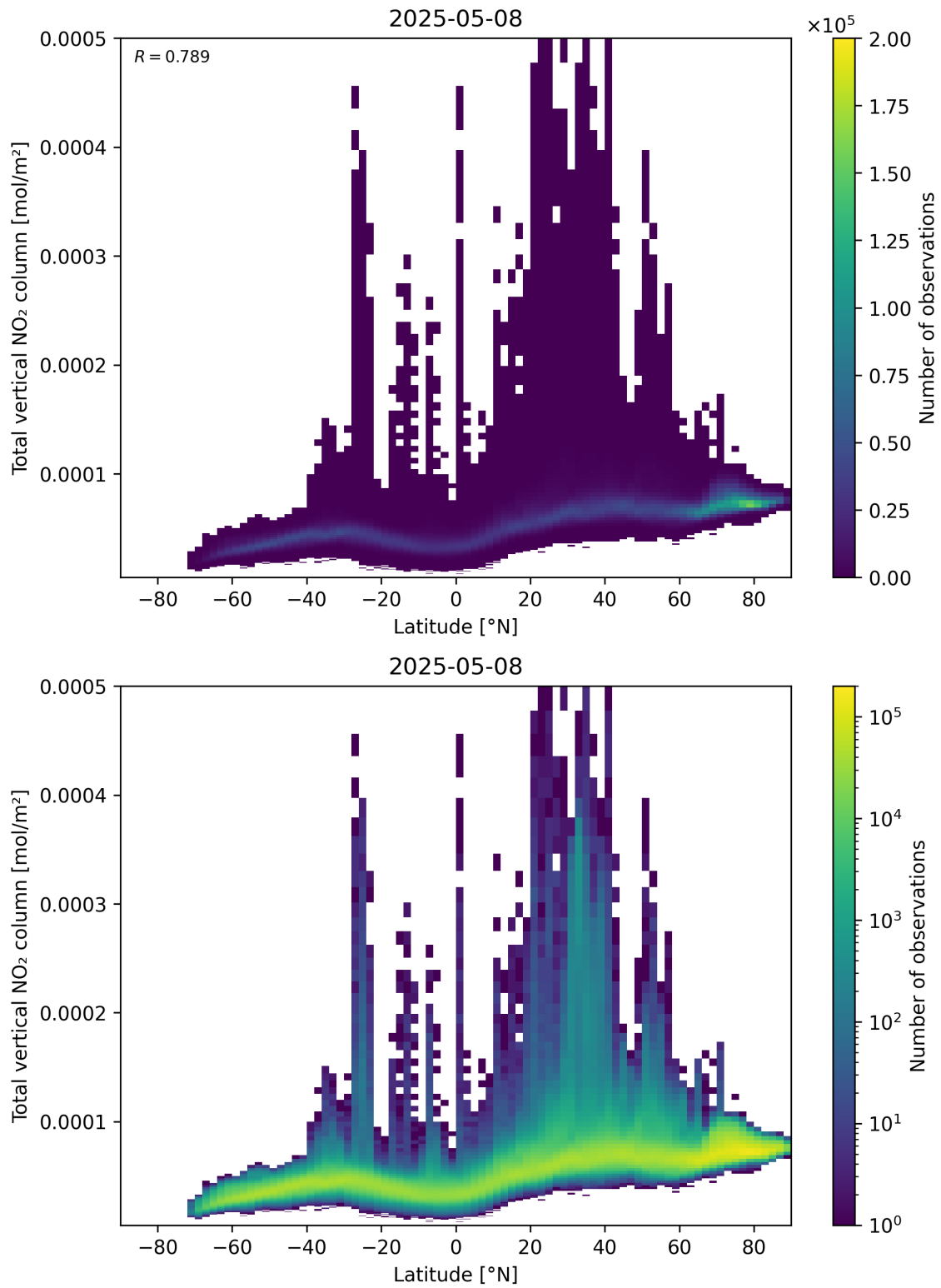
Figure 90: Scatter density plot of “Latitude” against “Total vertical NO 2 column” for 2025-05-08 to 2025-05-08.
