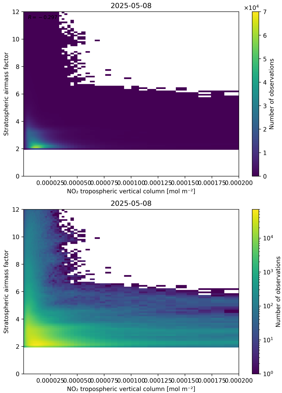
Figure 121: Scatter density plot of “NO 2 tropospheric vertical column” against “Stratospheric air mass factor” for 2025-05-08 to 2025-05-08.
