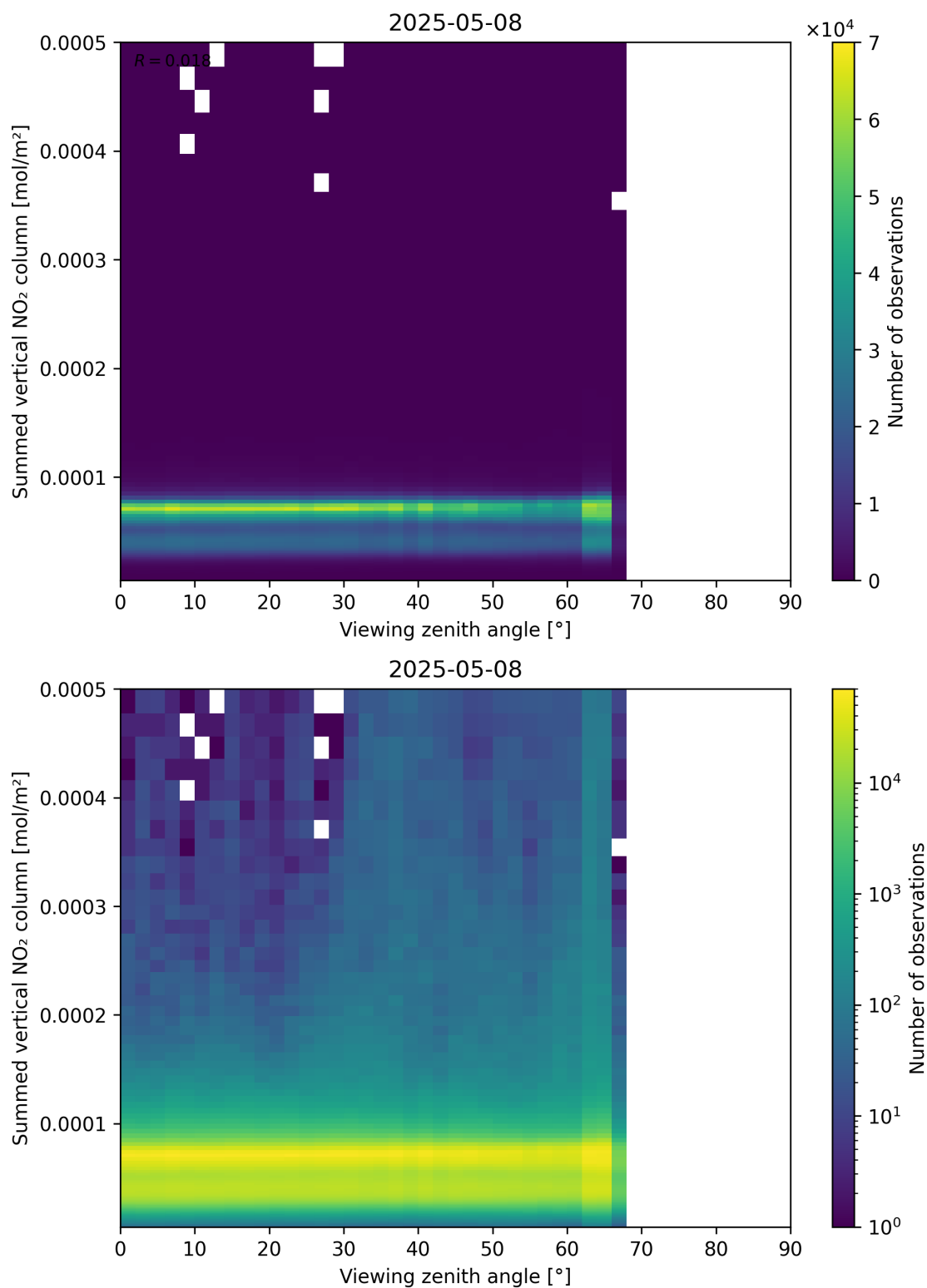
Figure 165: Scatter density plot of “Viewing zenith angle” against “Summed vertical NO 2 column” for 2025-05-08 to 2025-05-08.
