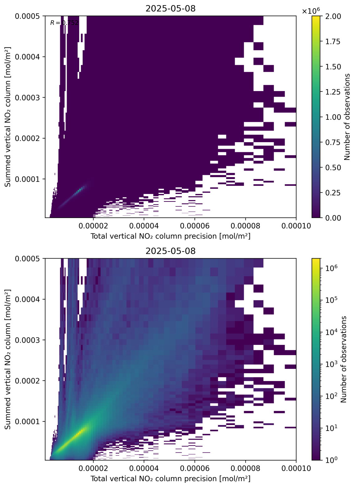
Figure 117: Scatter density plot of “Total vertical NO 2 column precision” against “Summed vertical NO 2 column” for 2025-05-08 to 2025-05-08.
