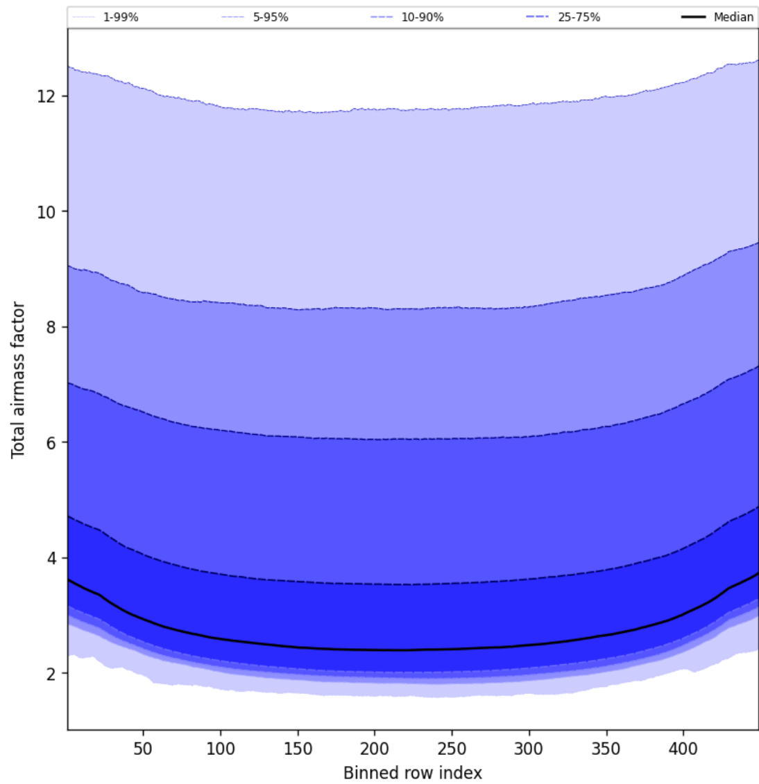
Figure 49: Along track statistics of “Total airmass factor” for 2025-05-08 to 2025-05-08
