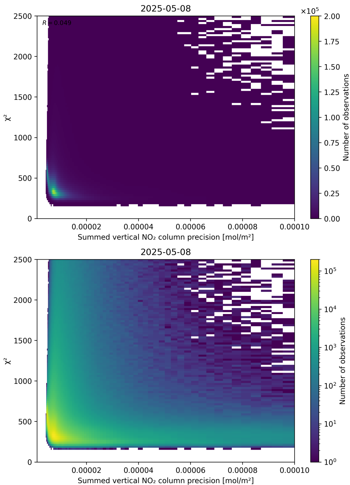
Figure 107: Scatter density plot of “Summed vertical NO 2 column precision” against “ \chi^2 ” for 2025-05-08 to 2025-05-08.
