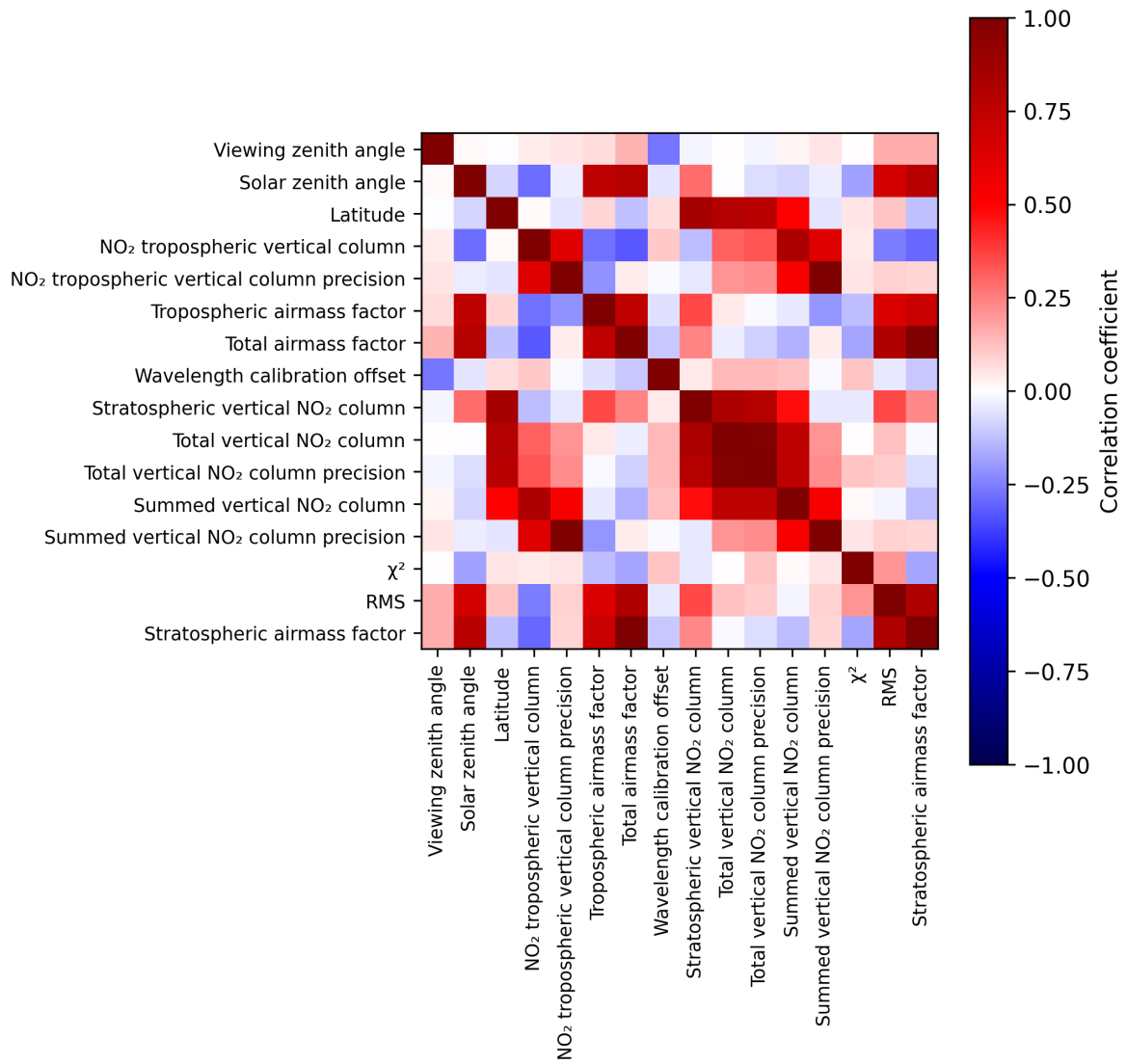
Figure 2: Map of correlation matrix for 2025-05-08 to 2025-05-08.
