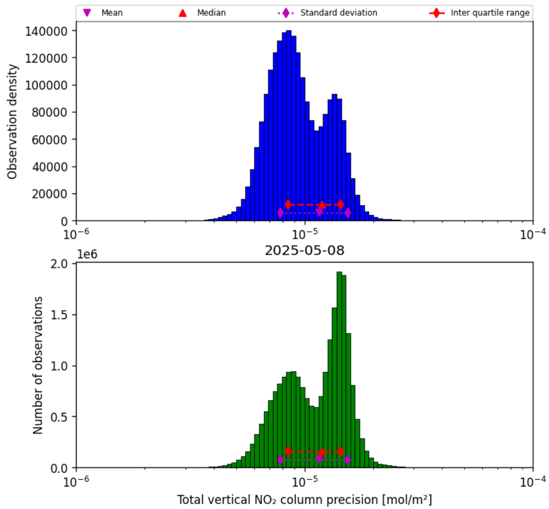
Figure 39: Histogram of "Total vertical NO 2 column precision" for 2025-05-08 to 2025-05-08
