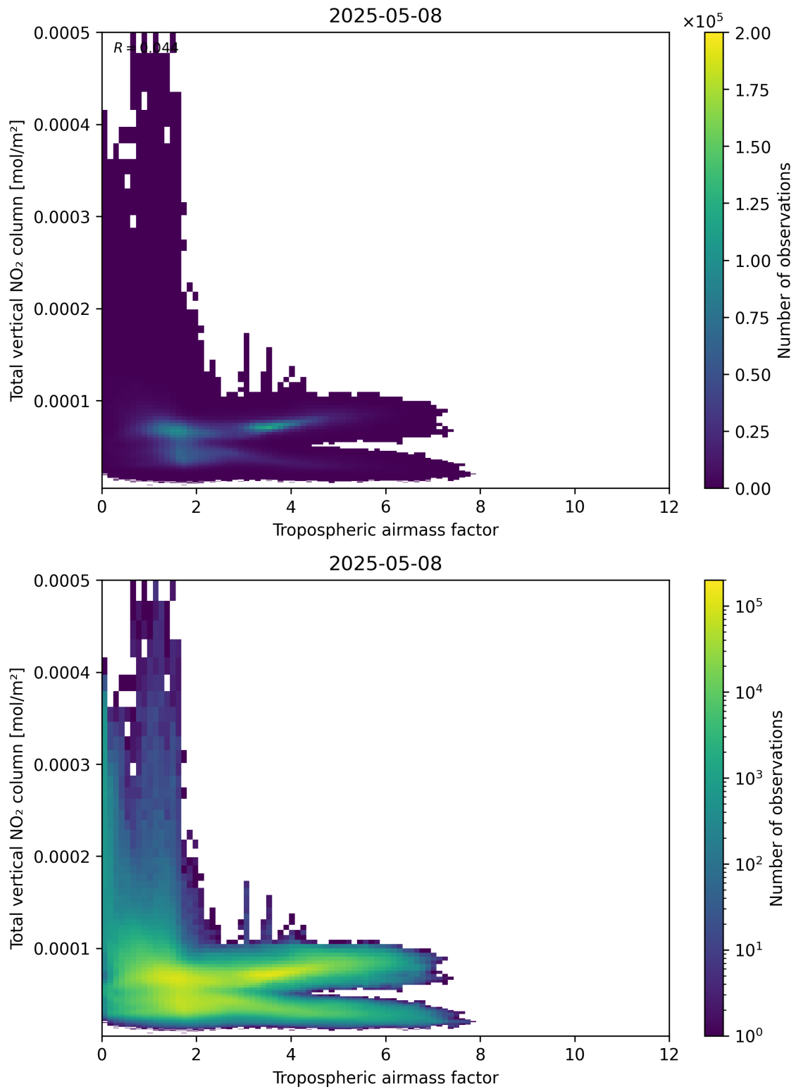
Figure 77: Scatter density plot of “Tropospheric airmass factor” against “Total vertical NO 2 column” for 2025-05-08 to 2025-05-08.
