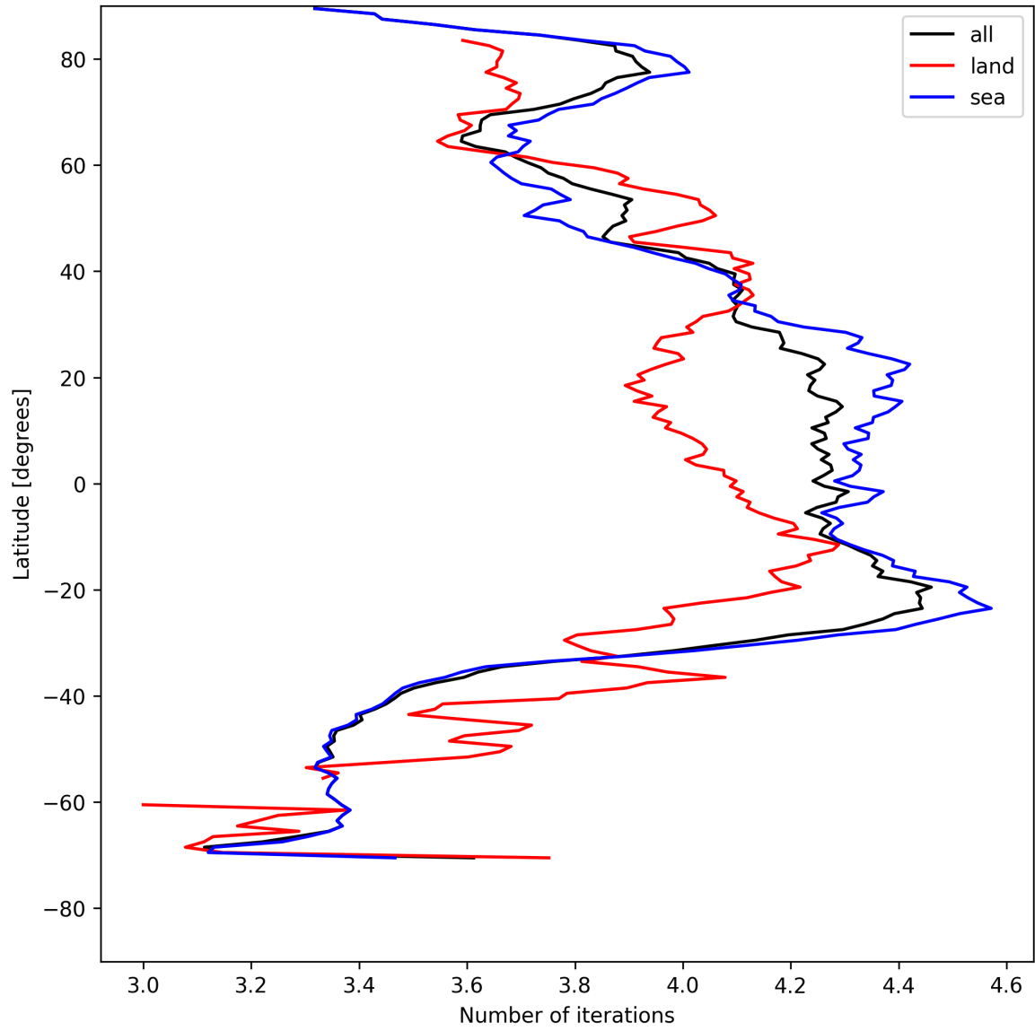
Figure 17: Zonal average of “Number of iterations” for 2025-05-08 to 2025-05-08.
