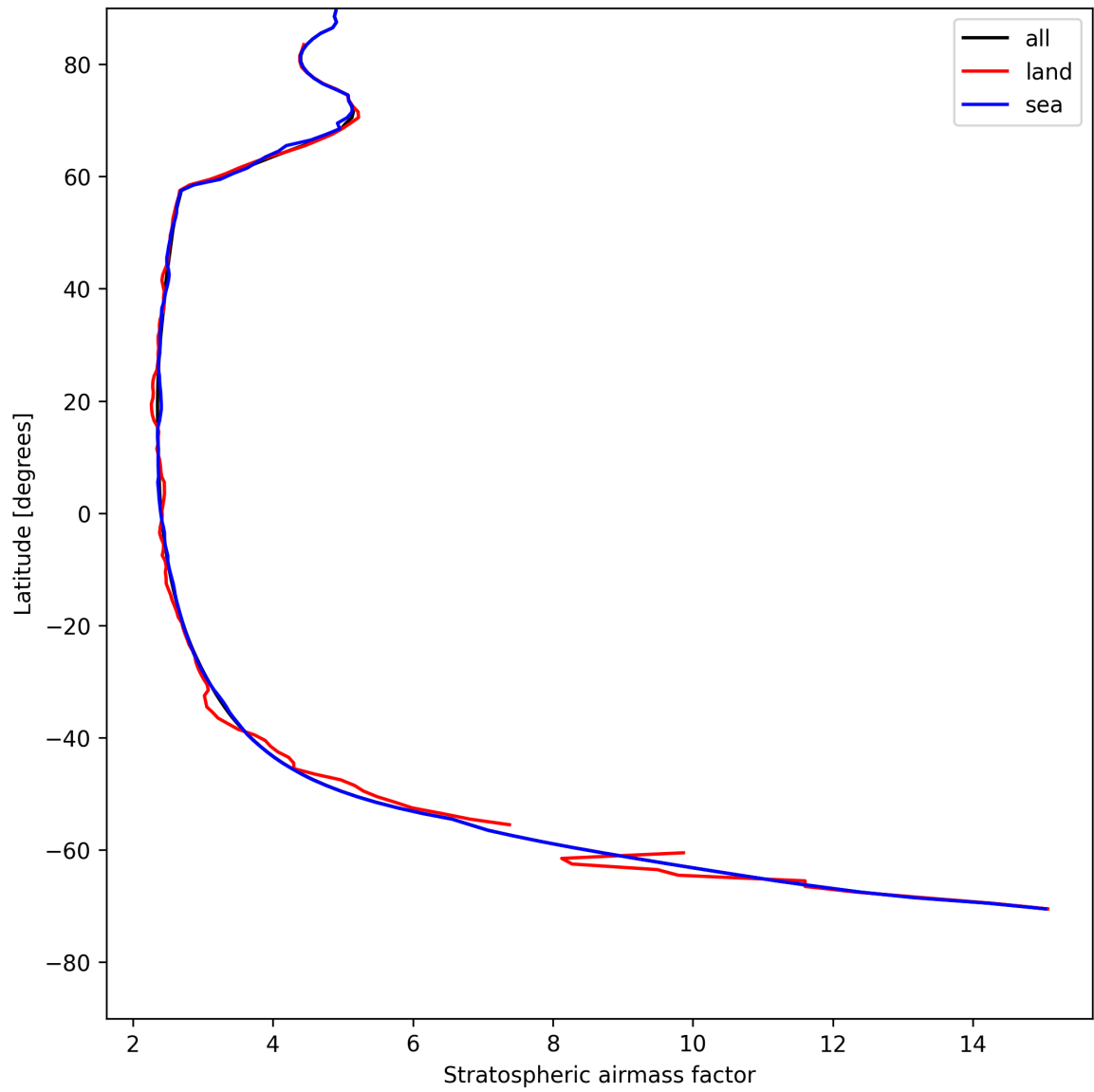
Figure 27: Zonal average of “Stratospheric air mass factor” for 2025-05-08 to 2025-05-08.
