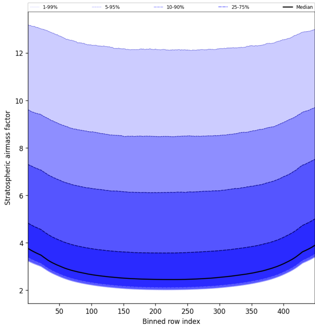
Figure 61: Along track statistics of “Stratospheric airmass factor” for 2025-05-08 to 2025-05-08
