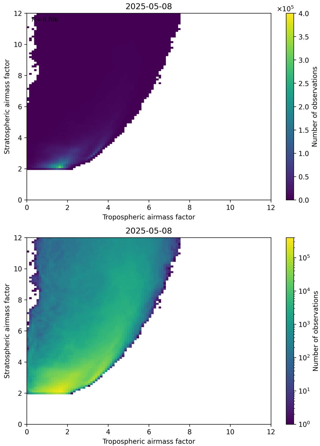
Figure 71: Scatter density plot of “Tropospheric airmass factor” against “Stratospheric airmass factor” for 2025-05-08 to 2025-05-08.
