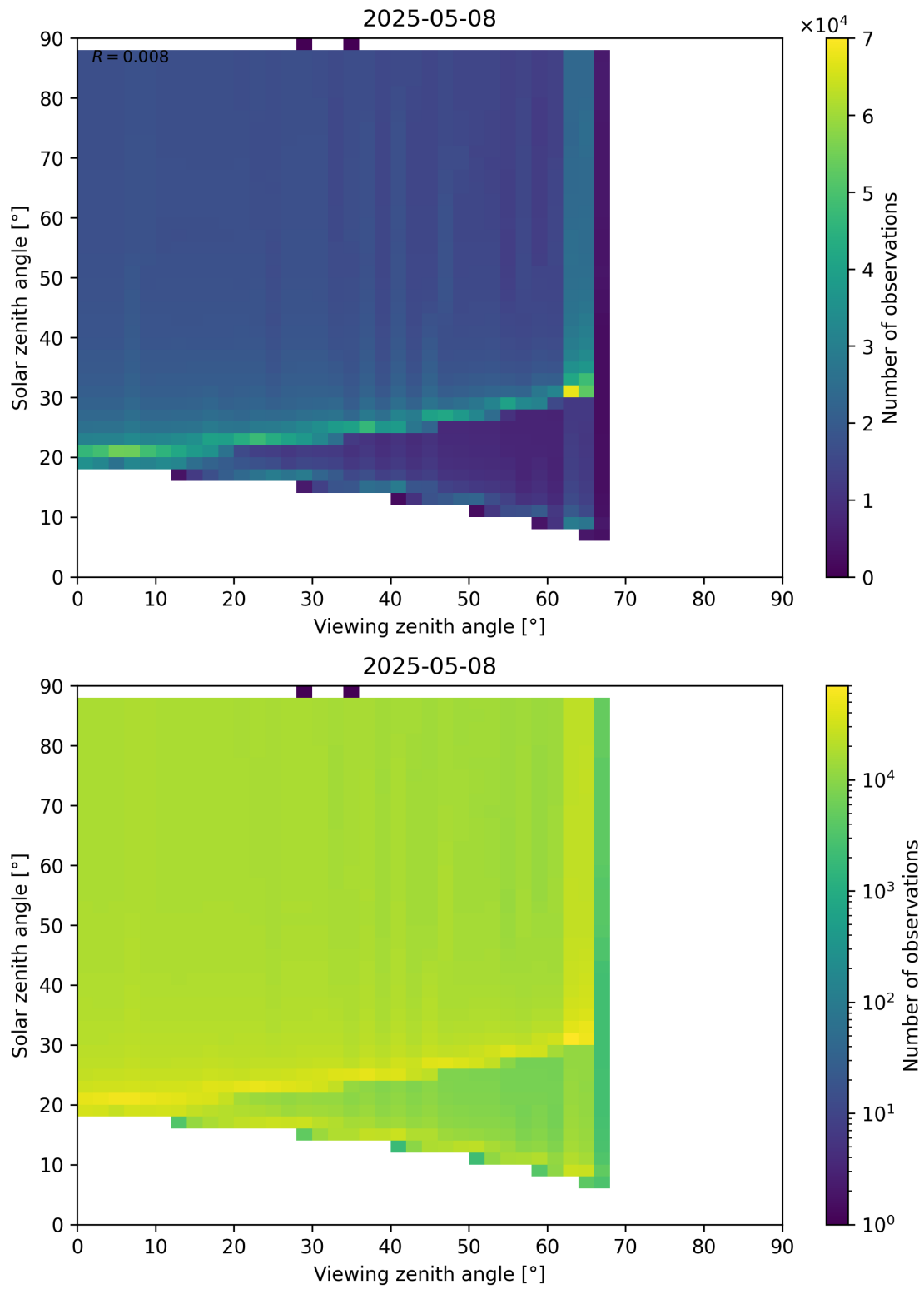
Figure 172: Scatter density plot of “Viewing zenith angle” against “Solar zenith angle” for 2025-05-08 to 2025-05-08.
