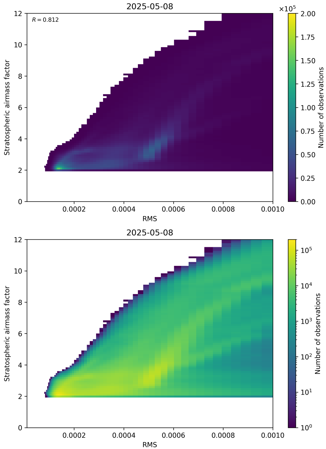
Figure 144: Scatter density plot of “RMS” against “Stratospheric airmass factor” for 2025-05-08 to 2025-05-08.
