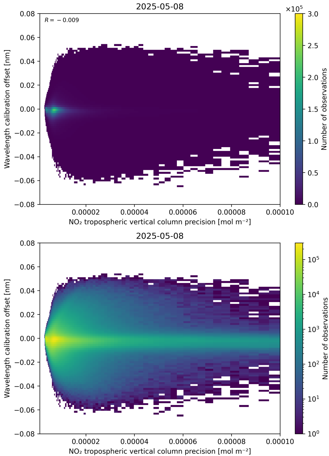
Figure 141: Scatter density plot of “NO 2 tropospheric vertical column precision” against “Wavelength calibration offset” for 2025-05-08 to 2025-05-08.
