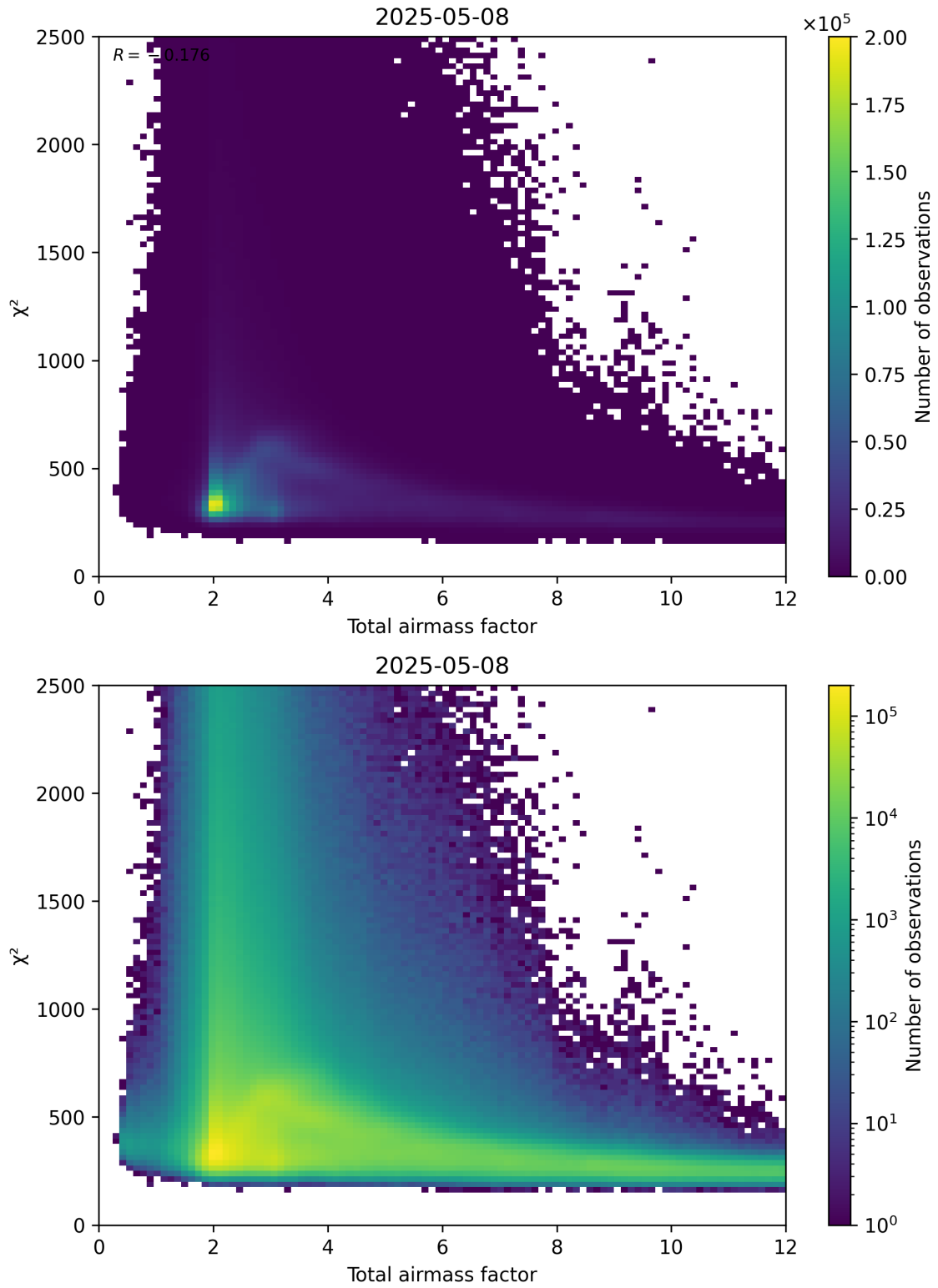
Figure 63: Scatter density plot of “Total airmass factor” against “ \chi^2 ” for 2025-05-08 to 2025-05-08.
