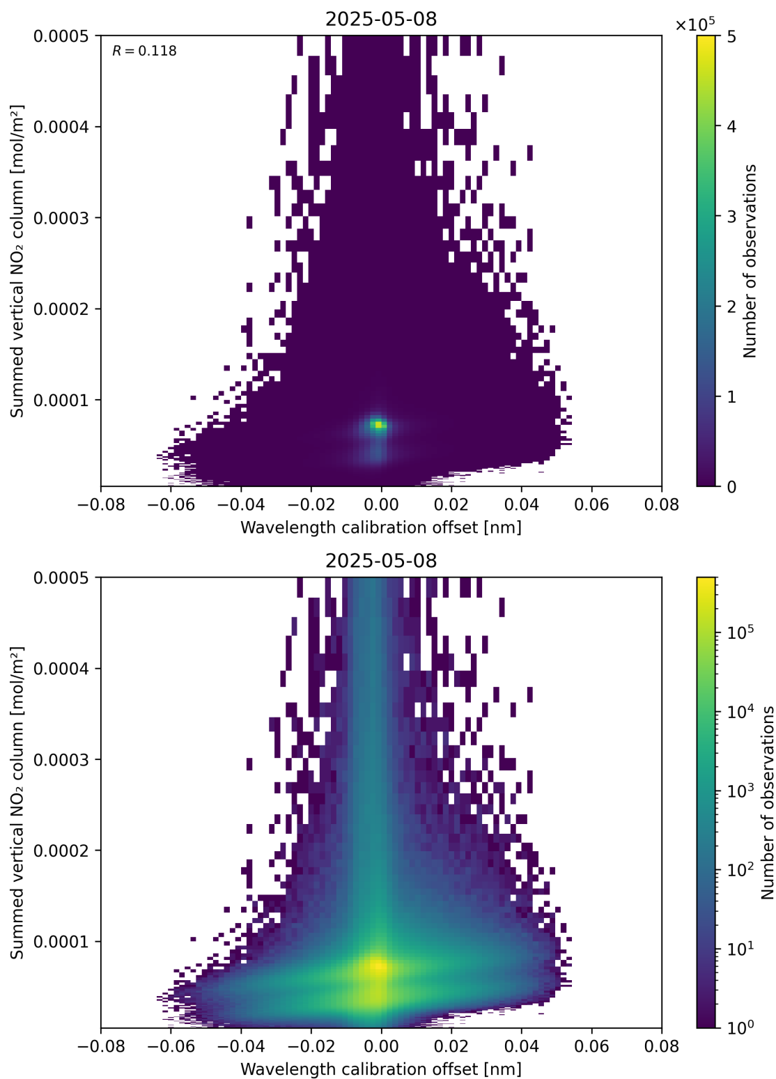
Figure 177: Scatter density plot of “Wavelength calibration offset” against “Summed vertical NO 2 column” for 2025-05-08 to 2025-05-08.
