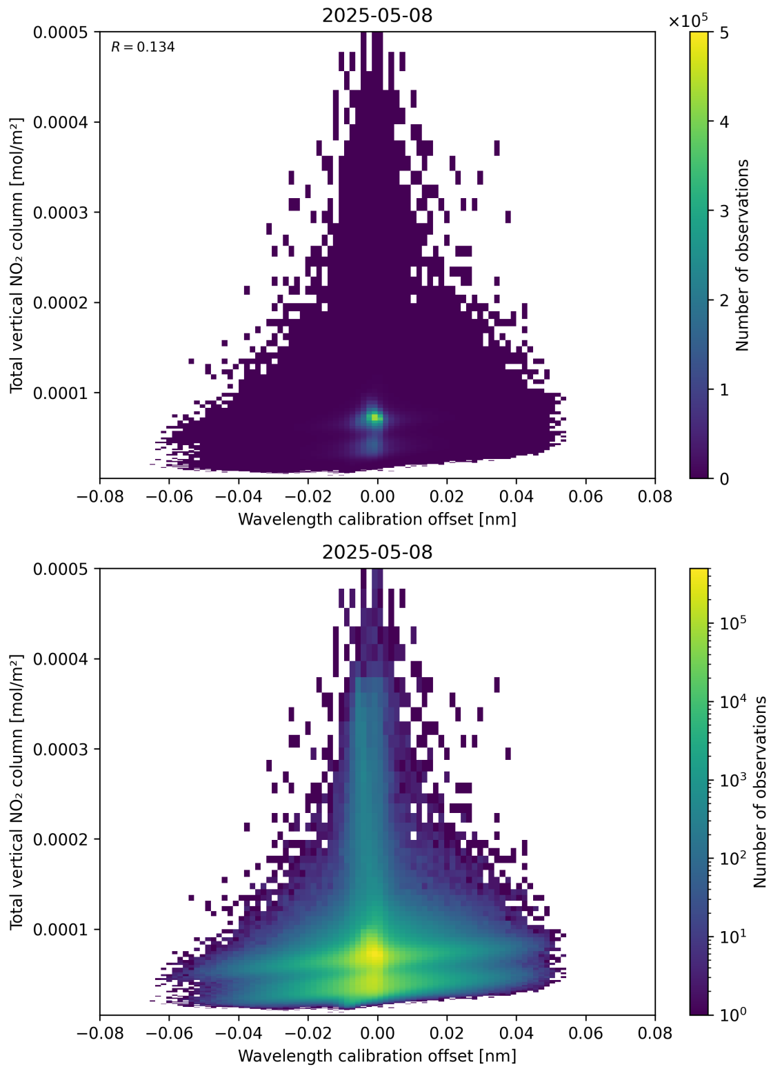
Figure 179: Scatter density plot of “Wavelength calibration offset” against “Total vertical NO 2 column” for 2025-05-08 to 2025-05-08.
