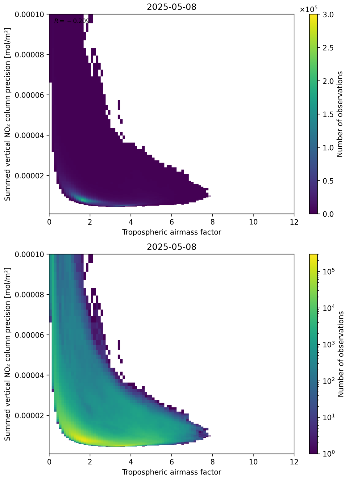
Figure 76: Scatter density plot of “Tropospheric air mass factor” against “Summed vertical NO 2 column precision” for 2025-05-08 to 2025-05-08.
