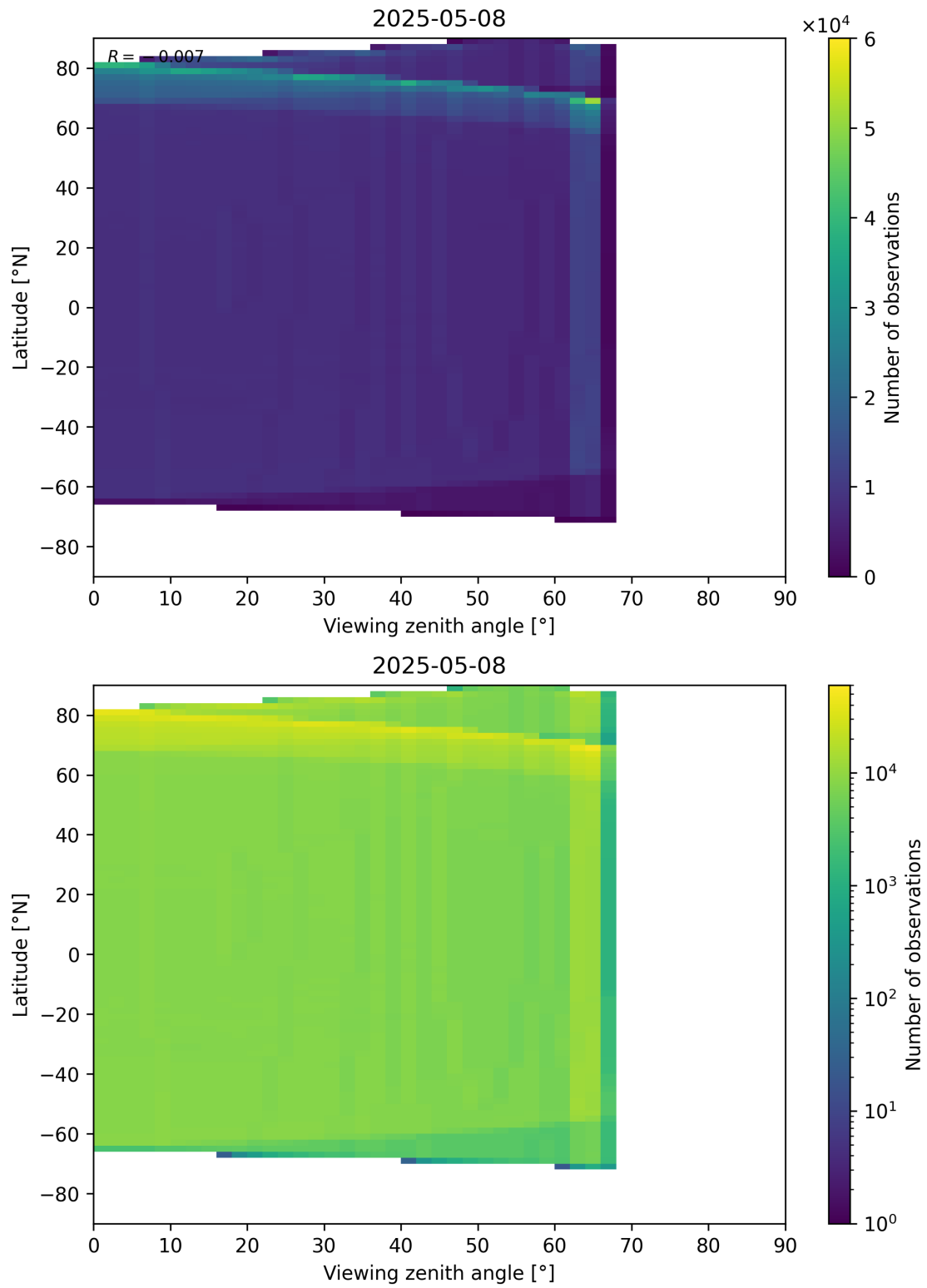
Figure 163: Scatter density plot of “Viewing zenith angle” against “Latitude” for 2025-05-08 to 2025-05-08.
