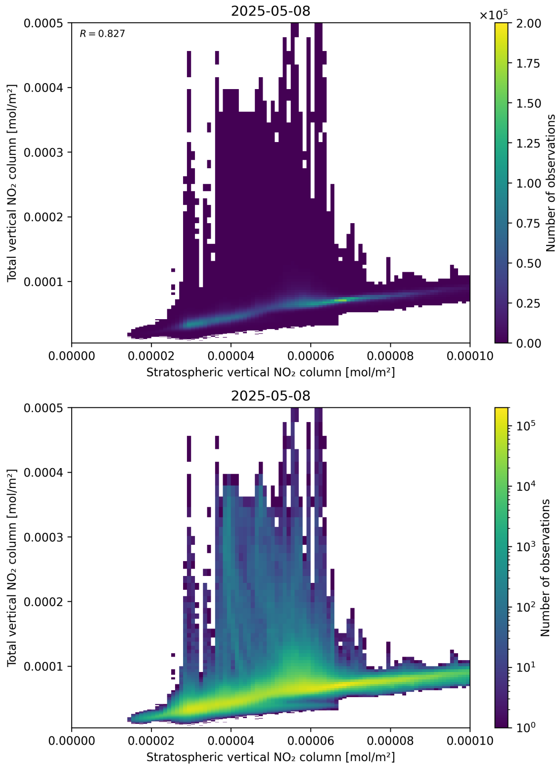
Figure 100: Scatter density plot of “Stratospheric vertical NO 2 column” against “Total vertical NO 2 column” for 2025-05-08 to 2025-05-08.
