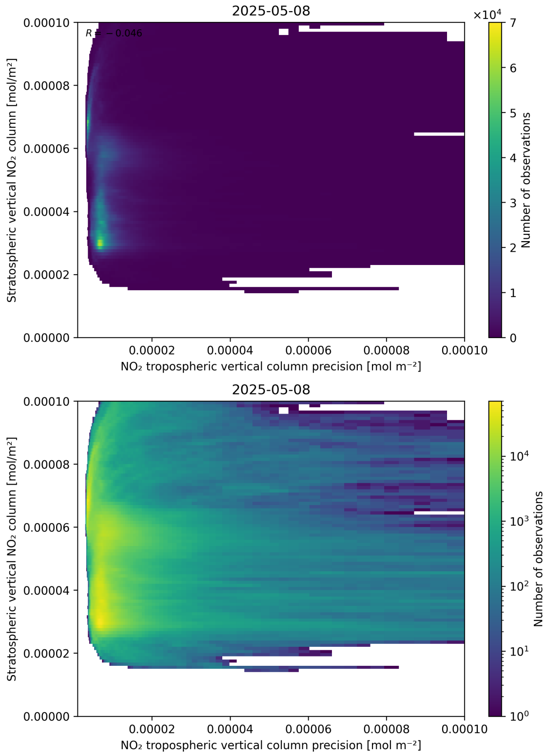
Figure 135: Scatter density plot of “NO 2 tropospheric vertical column precision” against “Stratospheric vertical NO 2 column” for 2025-05-08 to 2025-05-08.
