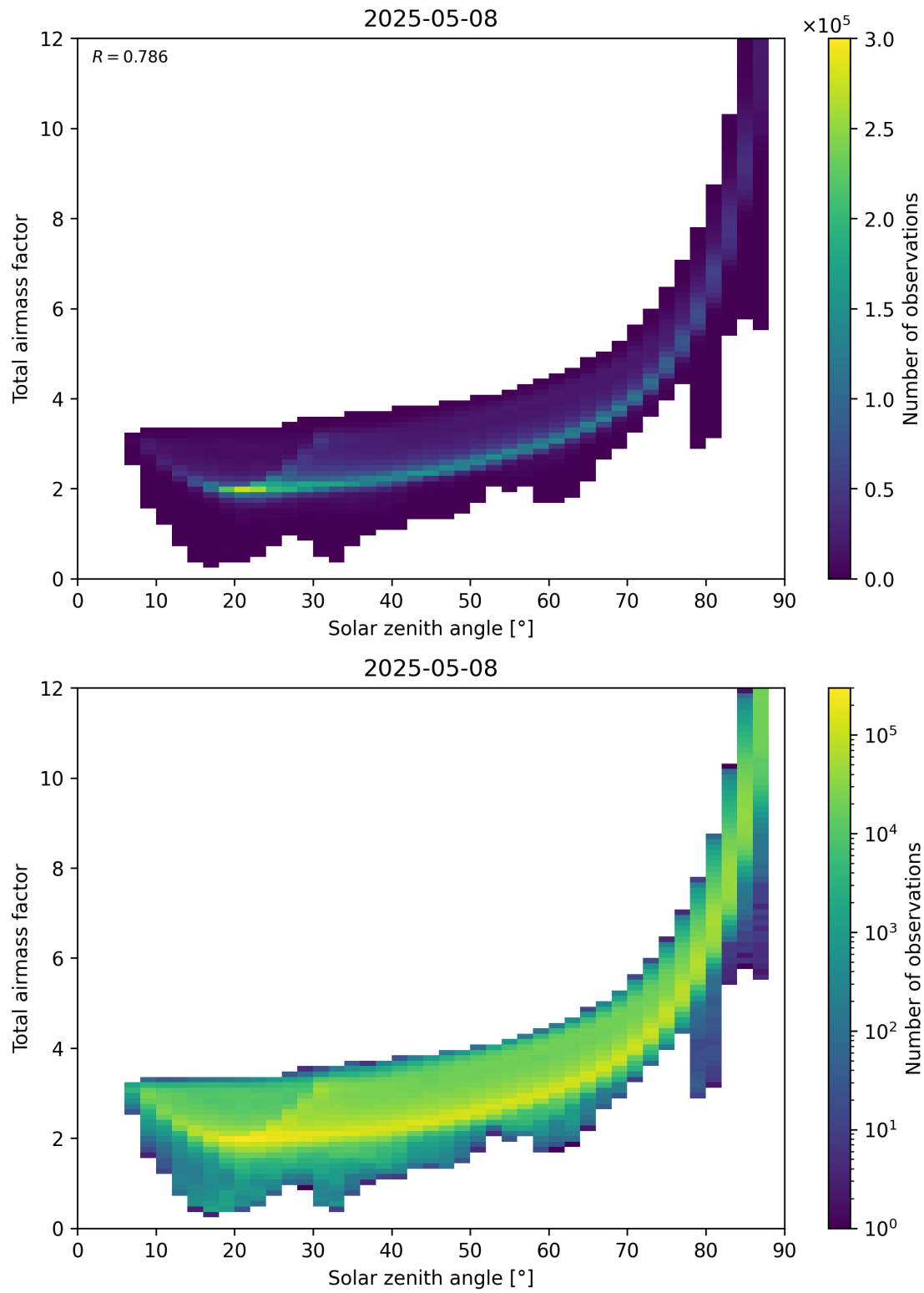
Figure 146: Scatter density plot of “Solar zenith angle” against “Total airmass factor” for 2025-05-08 to 2025-05-08.
