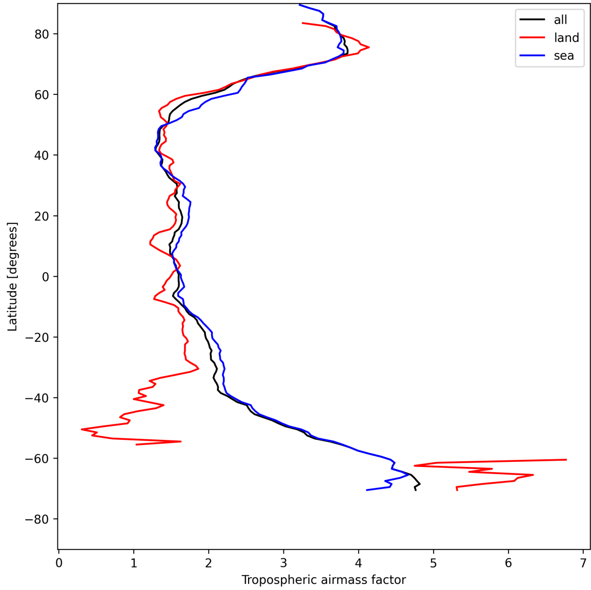
Figure 14: Zonal average of “Tropospheric airmass factor” for 2025-05-08 to 2025-05-08.
