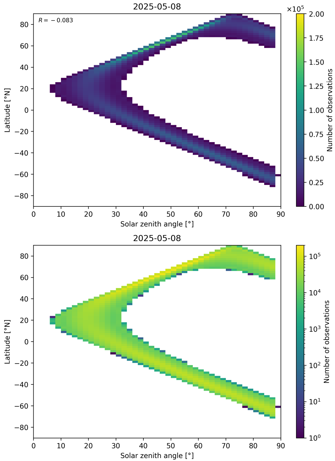
Figure 149: Scatter density plot of “Solar zenith angle” against “Latitude” for 2025-05-08 to 2025-05-08.
