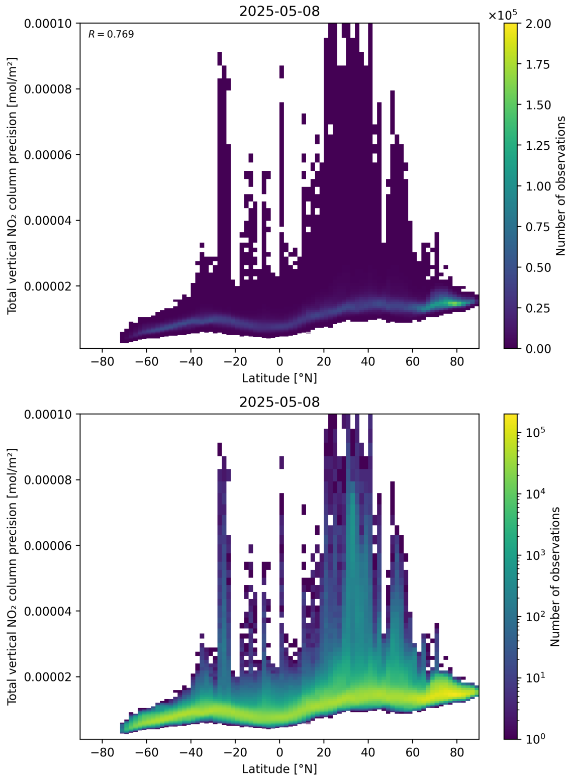
Figure 91: Scatter density plot of “Latitude” against “Total vertical NO 2 column precision” for 2025-05-08 to 2025-05-08.
