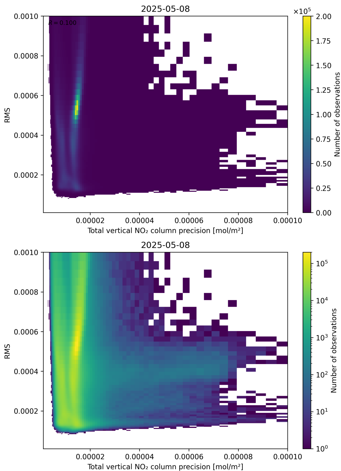
Figure 119: Scatter density plot of “Total vertical NO 2 column precision” against “RMS” for 2025-05-08 to 2025-05-08.
