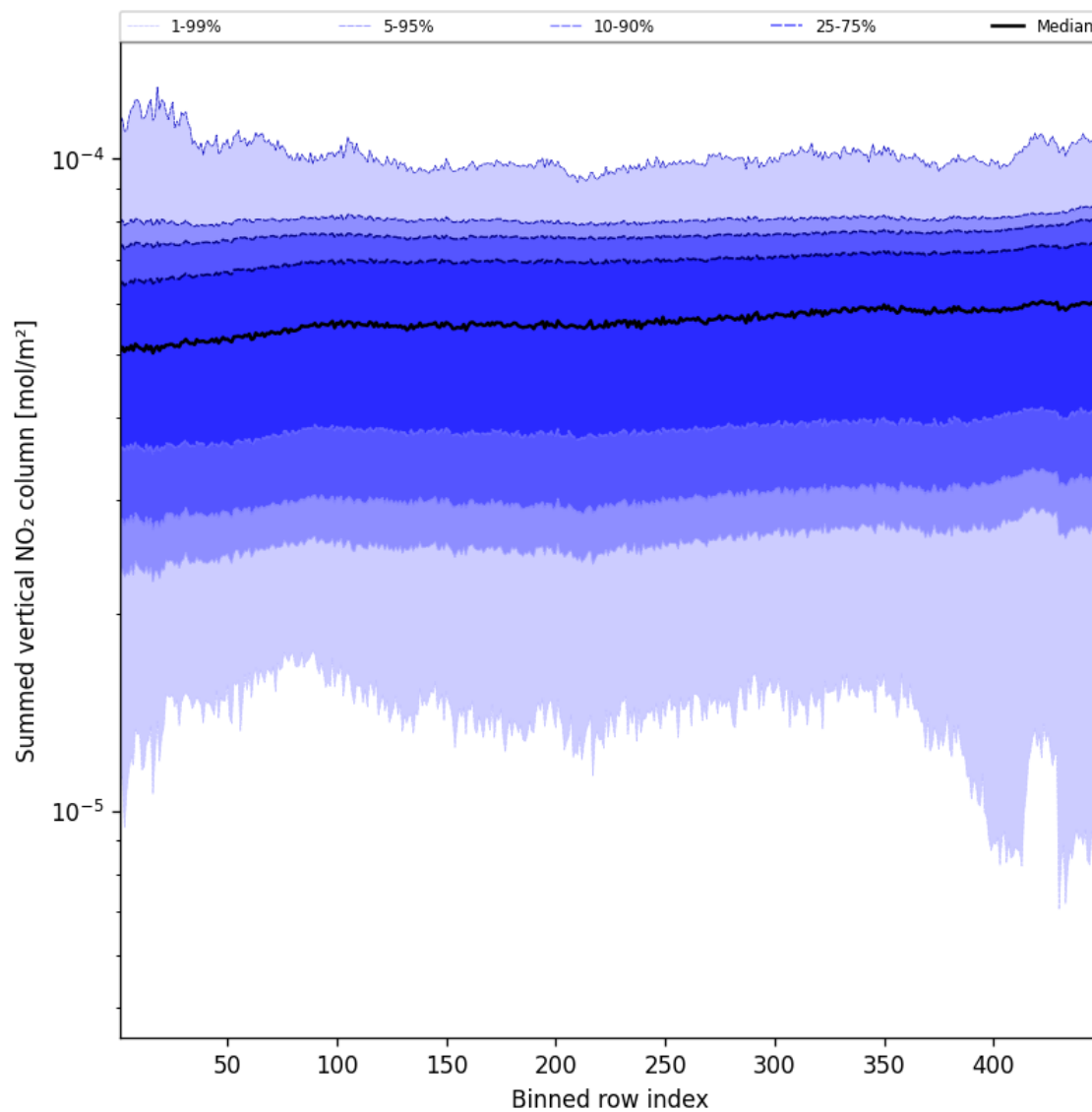
Figure 57: Along track statistics of “Summed vertical NO 2 column” for 2025-05-08 to 2025-05-08
