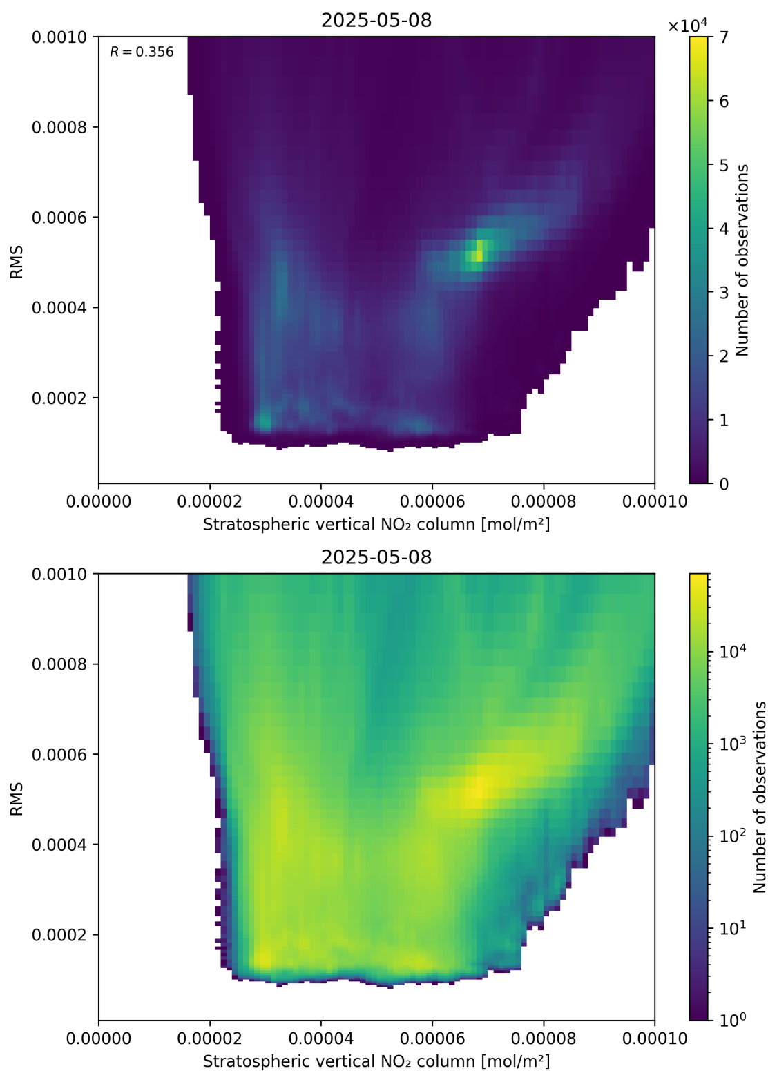
Figure 102: Scatter density plot of “Stratospheric vertical NO 2 column” against “RMS” for 2025-05-08 to 2025-05-08.
