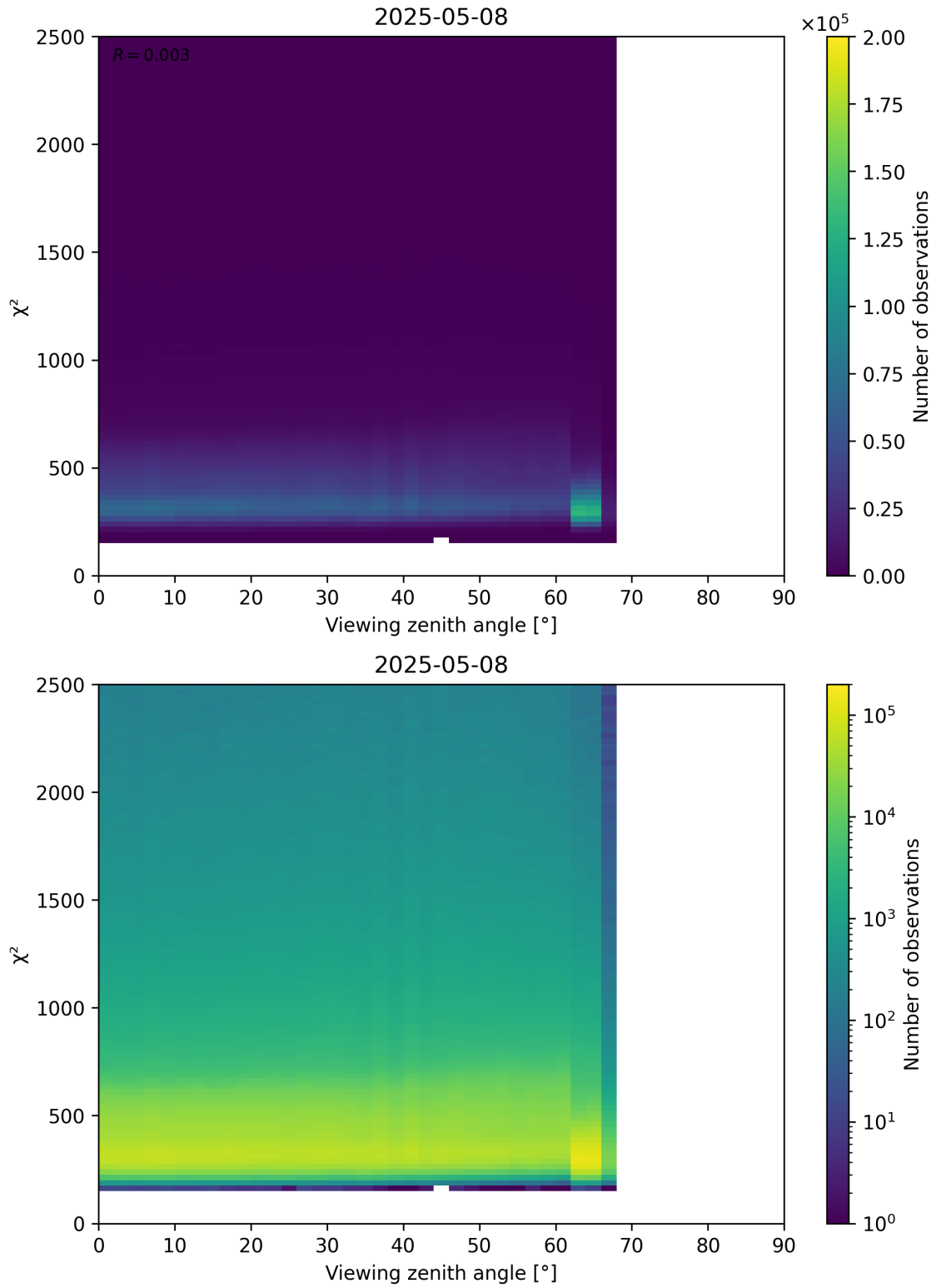
Figure 162: Scatter density plot of “Viewing zenith angle” against “ \chi^2 ” for 2025-05-08 to 2025-05-08.
