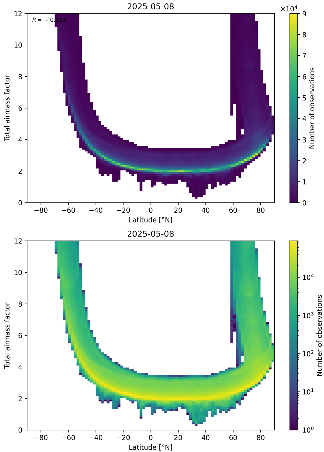
Figure 84: Scatter density plot of “Latitude” against “Total air mass factor” for 2025-05-08 to 2025-05-08.
