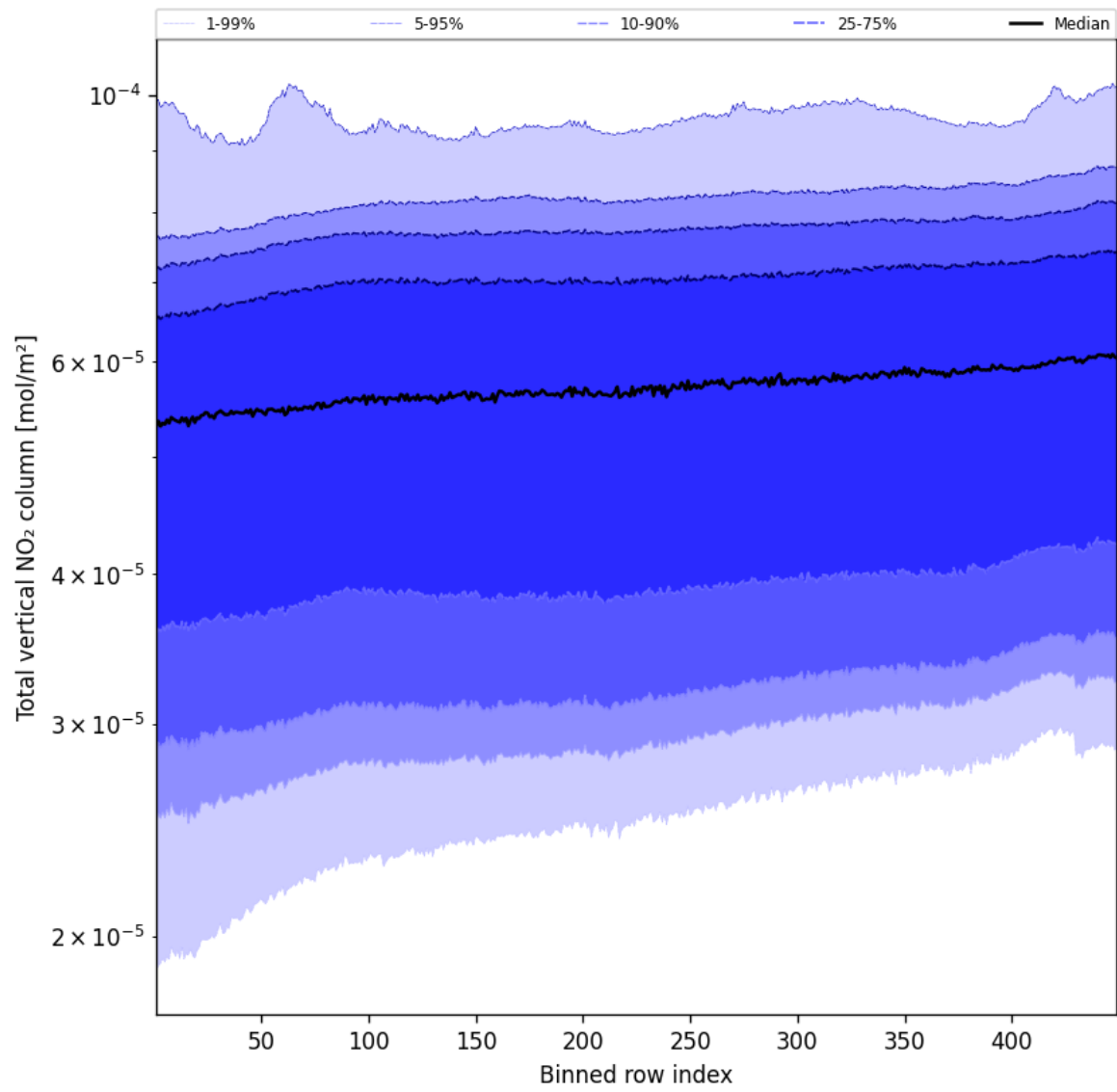
Figure 55: Along track statistics of “Total vertical NO 2 column” for 2025-05-08 to 2025-05-08
