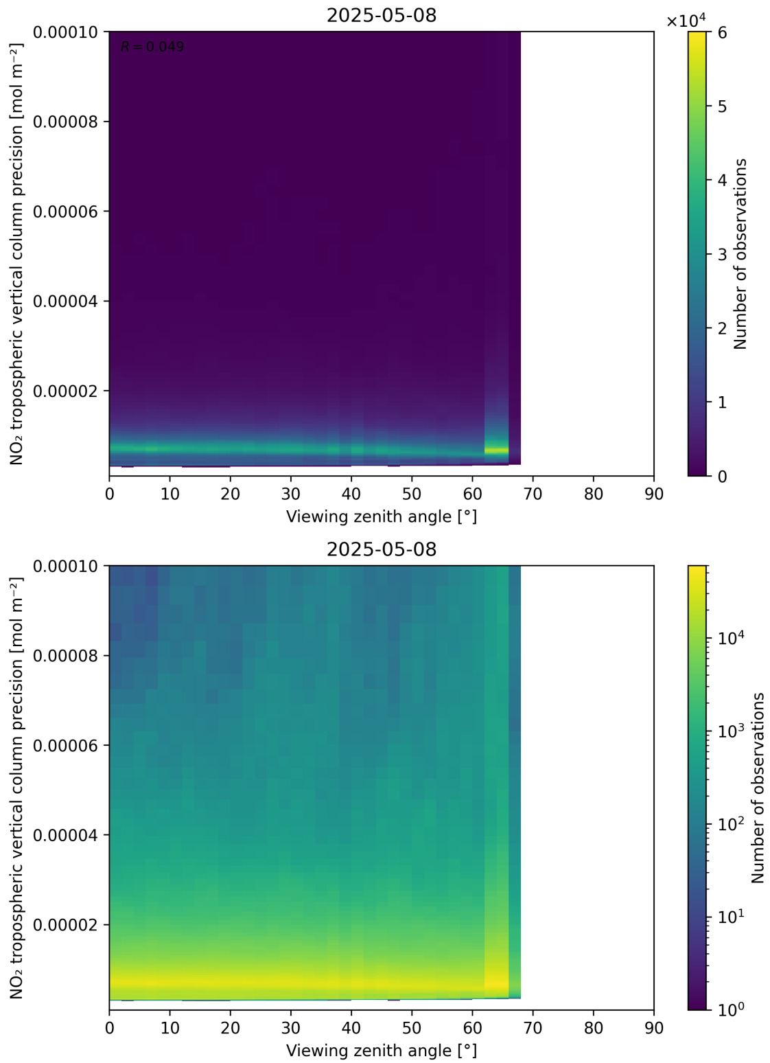
Figure 170: Scatter density plot of “Viewing zenith angle” against “NO 2 tropospheric vertical column precision” for 2025-05-08 to 2025-05-08.
