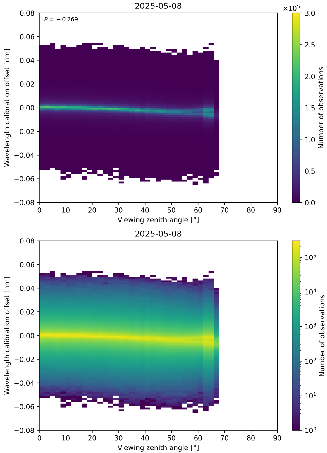
Figure 173: Scatter density plot of “Viewing zenith angle” against “Wavelength calibration offset” for 2025-05-08 to 2025-05-08.
