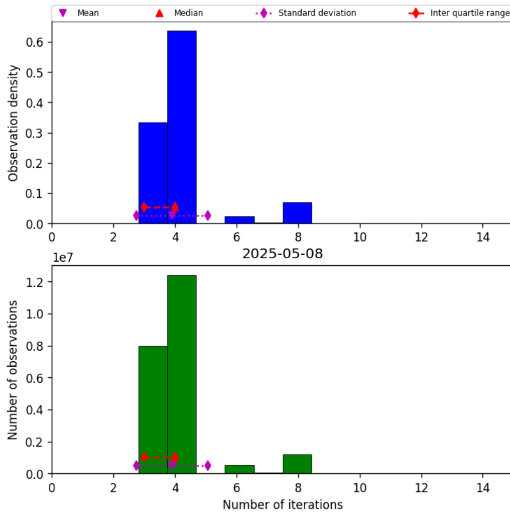
Figure 34: Histogram of “Number of iterations” for 2025-05-08 to 2025-05-08
