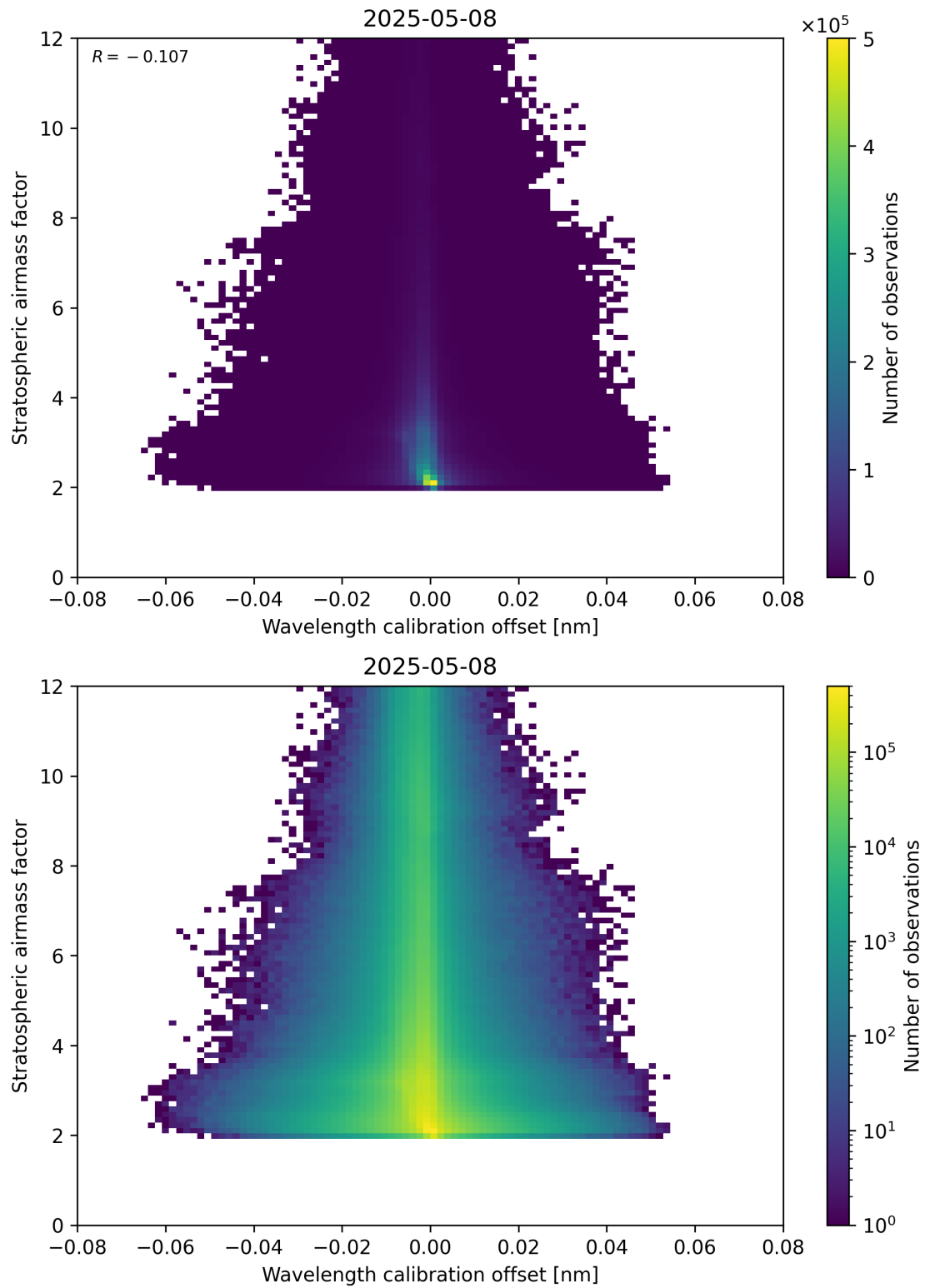
Figure 174: Scatter density plot of “Wavelength calibration offset” against “Stratospheric airmass factor” for 2025-05-08 to 2025-05-08.
