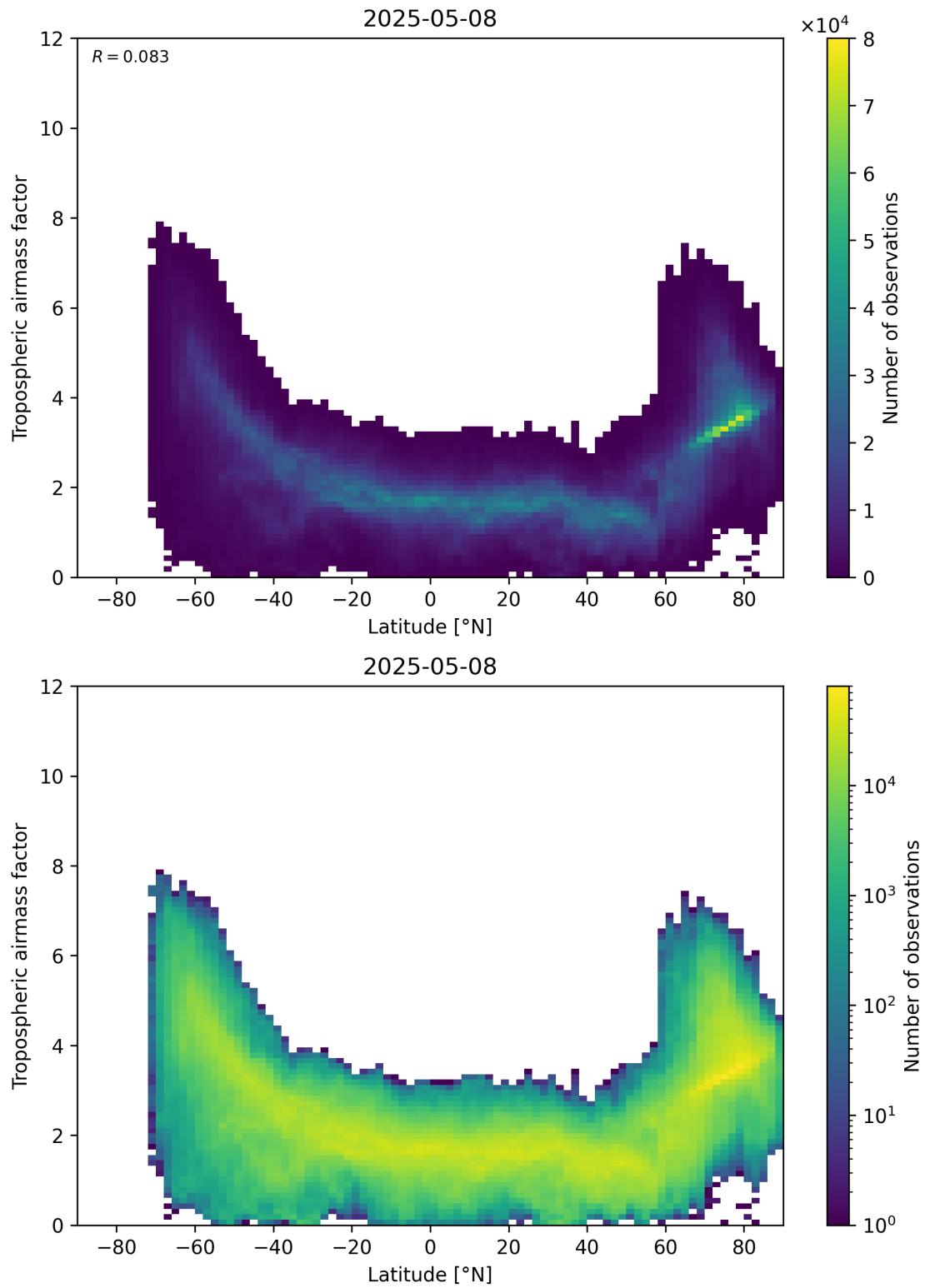
Figure 85: Scatter density plot of “Latitude” against “Tropospheric airmass factor” for 2025-05-08 to 2025-05-08.
