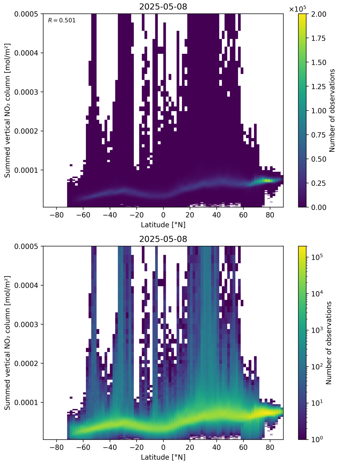
Figure 88: Scatter density plot of “Latitude” against “Summed vertical NO 2 column” for 2025-05-08 to 2025-05-08.
