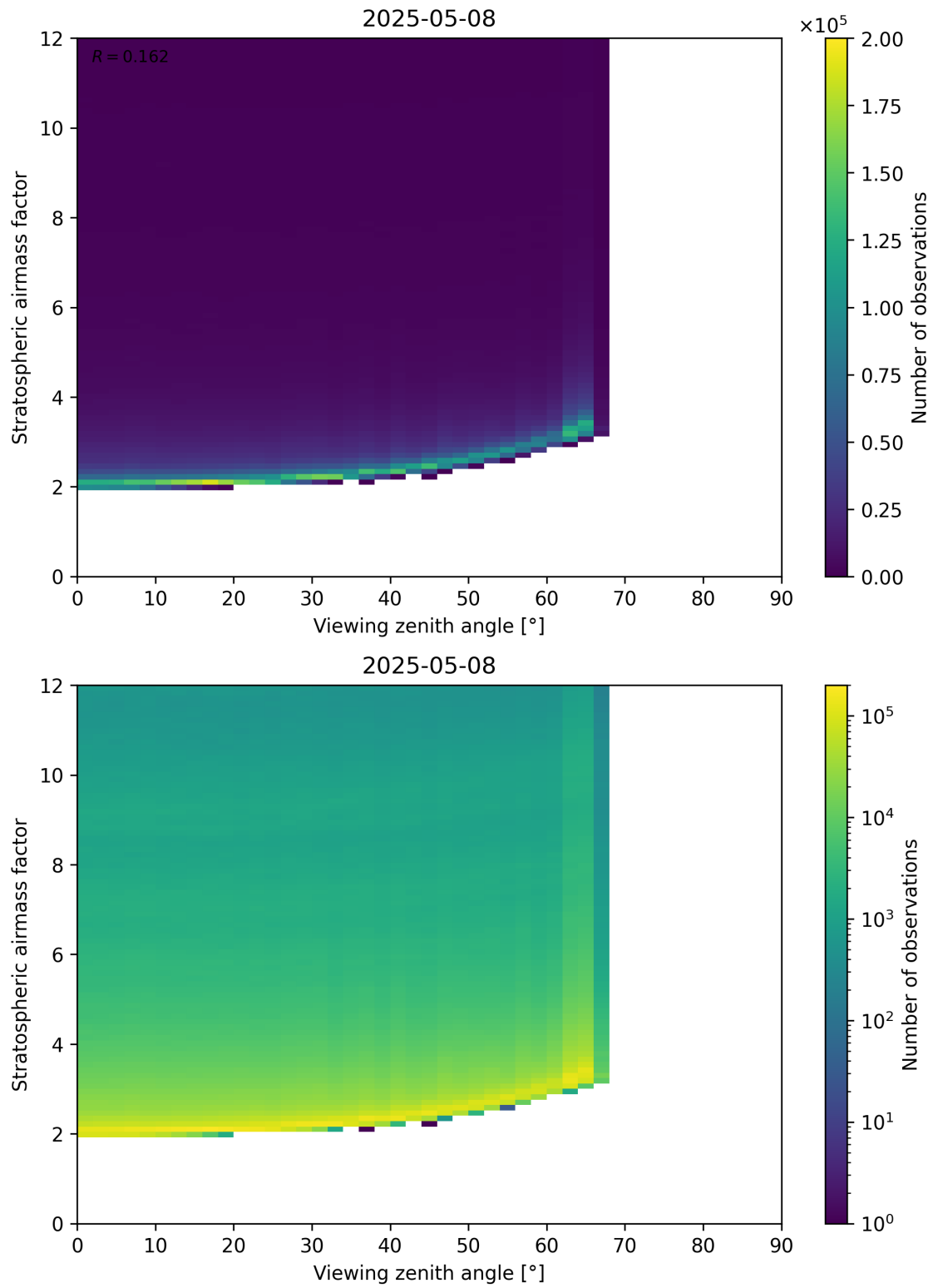
Figure 159: Scatter density plot of “Viewing zenith angle” against “Stratospheric airmass factor” for 2025-05-08 to 2025-05-08.
