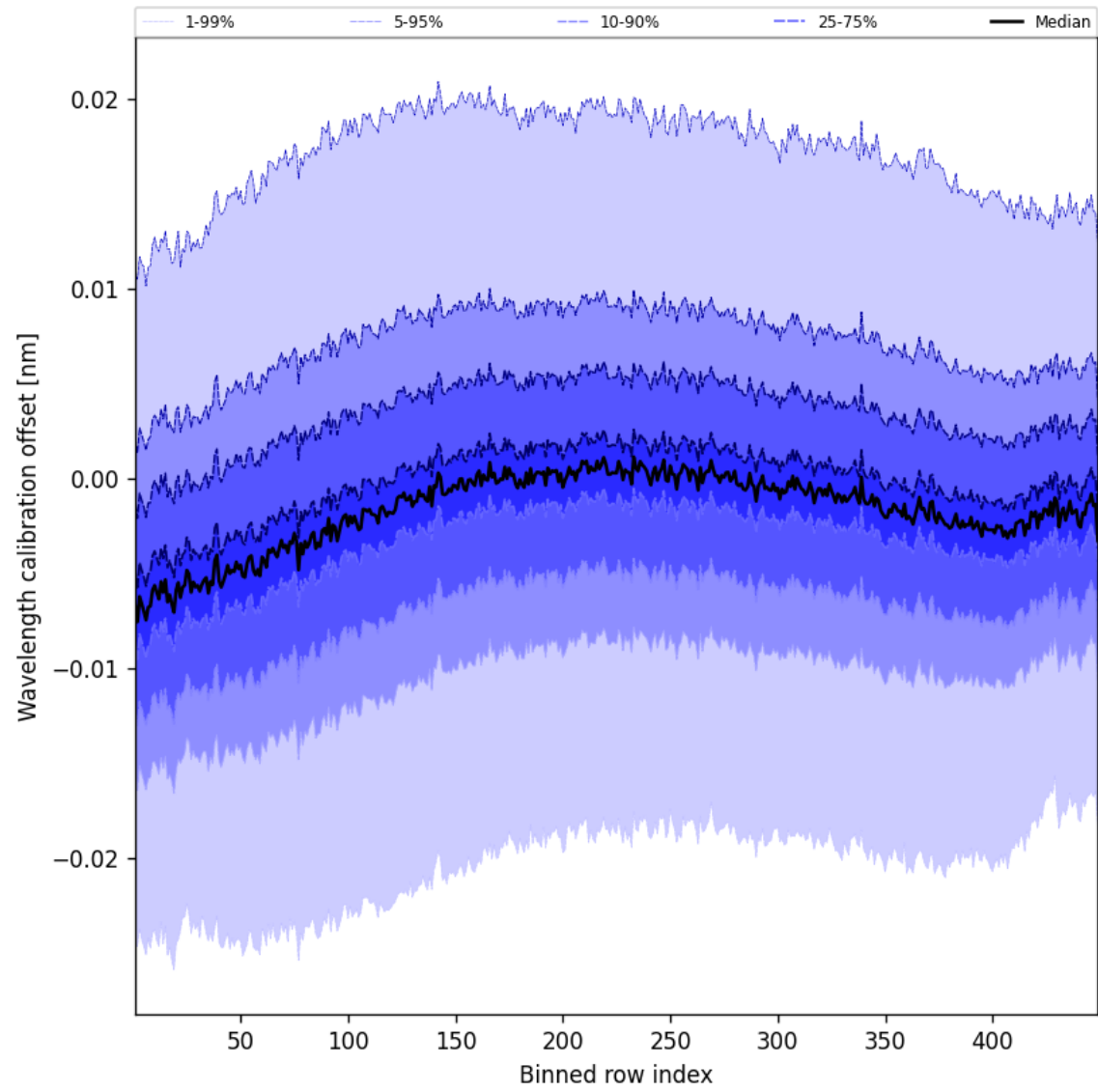
Figure 52: Along track statistics of “Wavelength calibration offset” for 2025-05-08 to 2025-05-08
