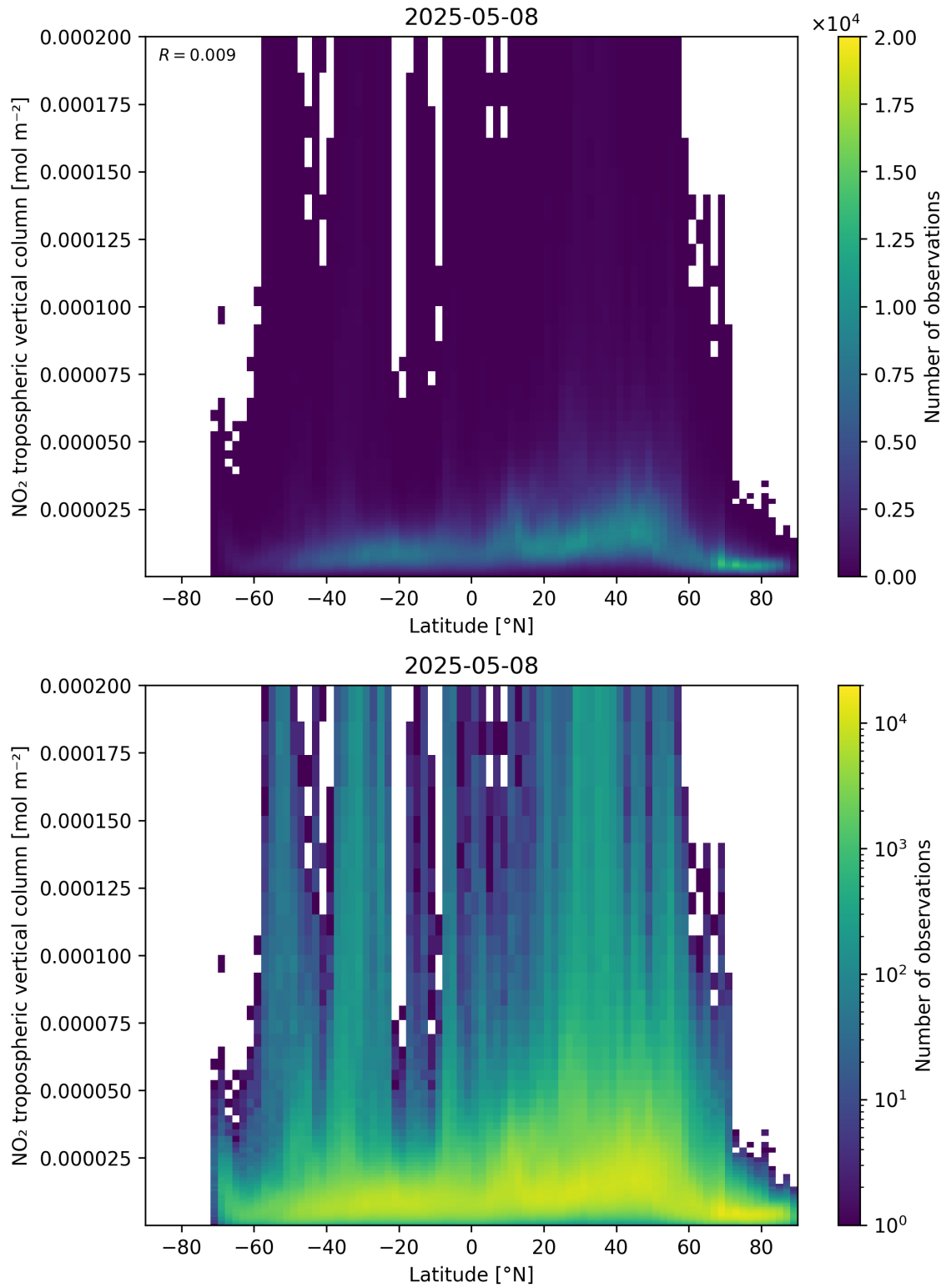
Figure 92: Scatter density plot of “Latitude” against “NO 2 tropospheric vertical column” for 2025-05-08 to 2025-05-08.
