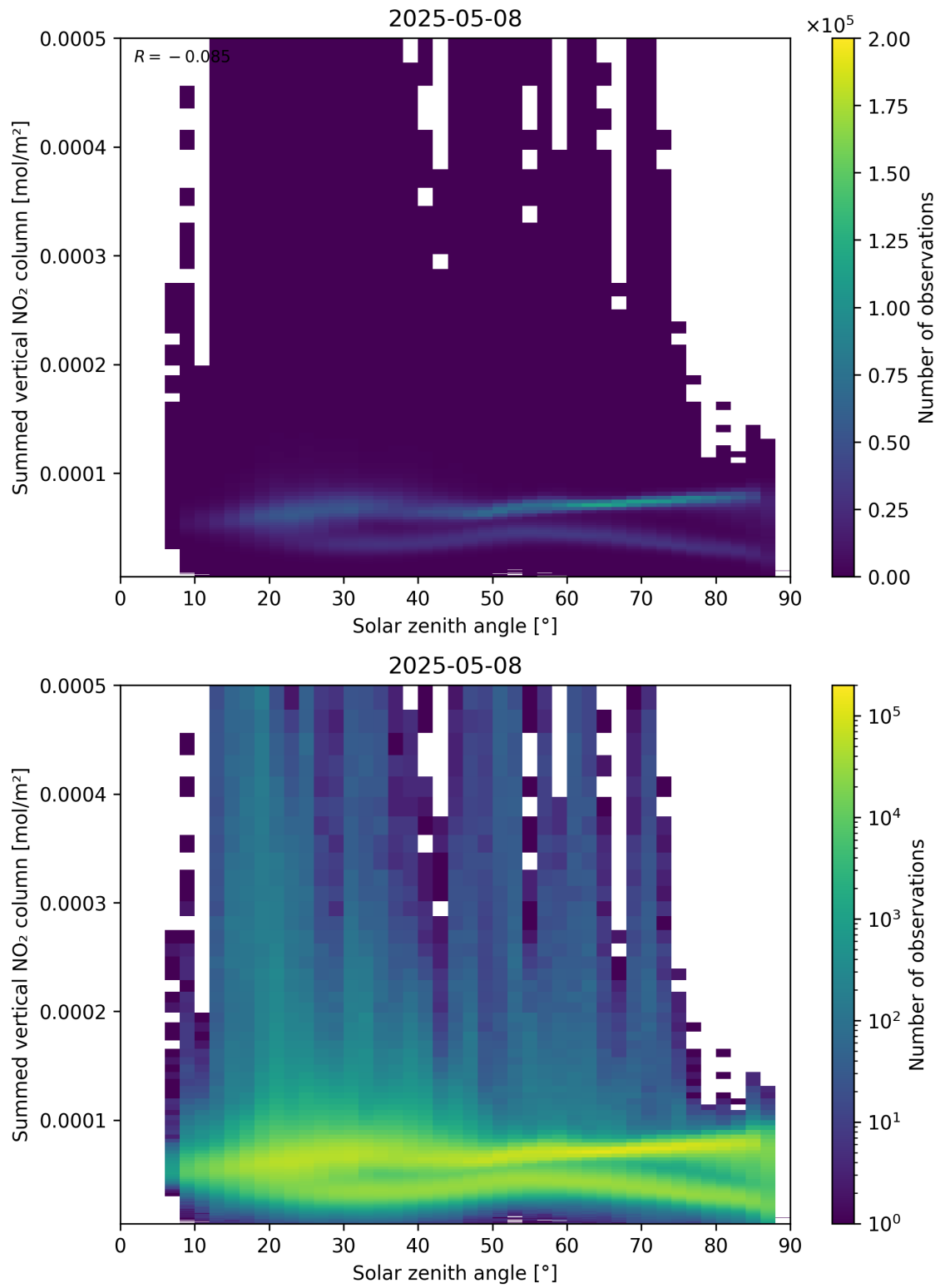
Figure 151: Scatter density plot of “Solar zenith angle” against “Summed vertical NO 2 column” for 2025-05-08 to 2025-05-08.
