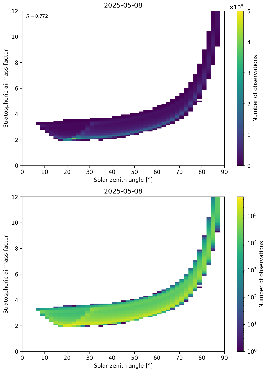
Figure 145: Scatter density plot of “Solar zenith angle” against “Stratospheric airmass factor” for 2025-05-08 to 2025-05-08.
