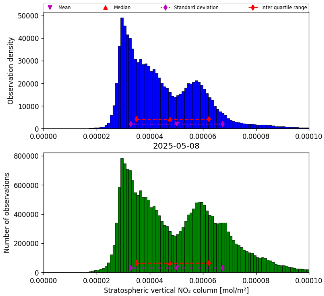
Figure 36: Histogram of “Stratospheric vertical NO 2 column” for 2025-05-08 to 2025-05-08
