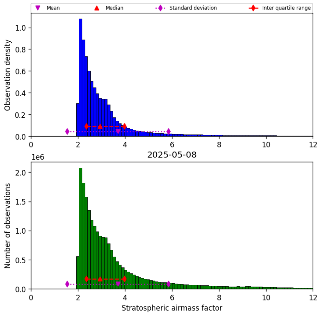
Figure 44: Histogram of “Stratospheric airmass factor” for 2025-05-08 to 2025-05-08
