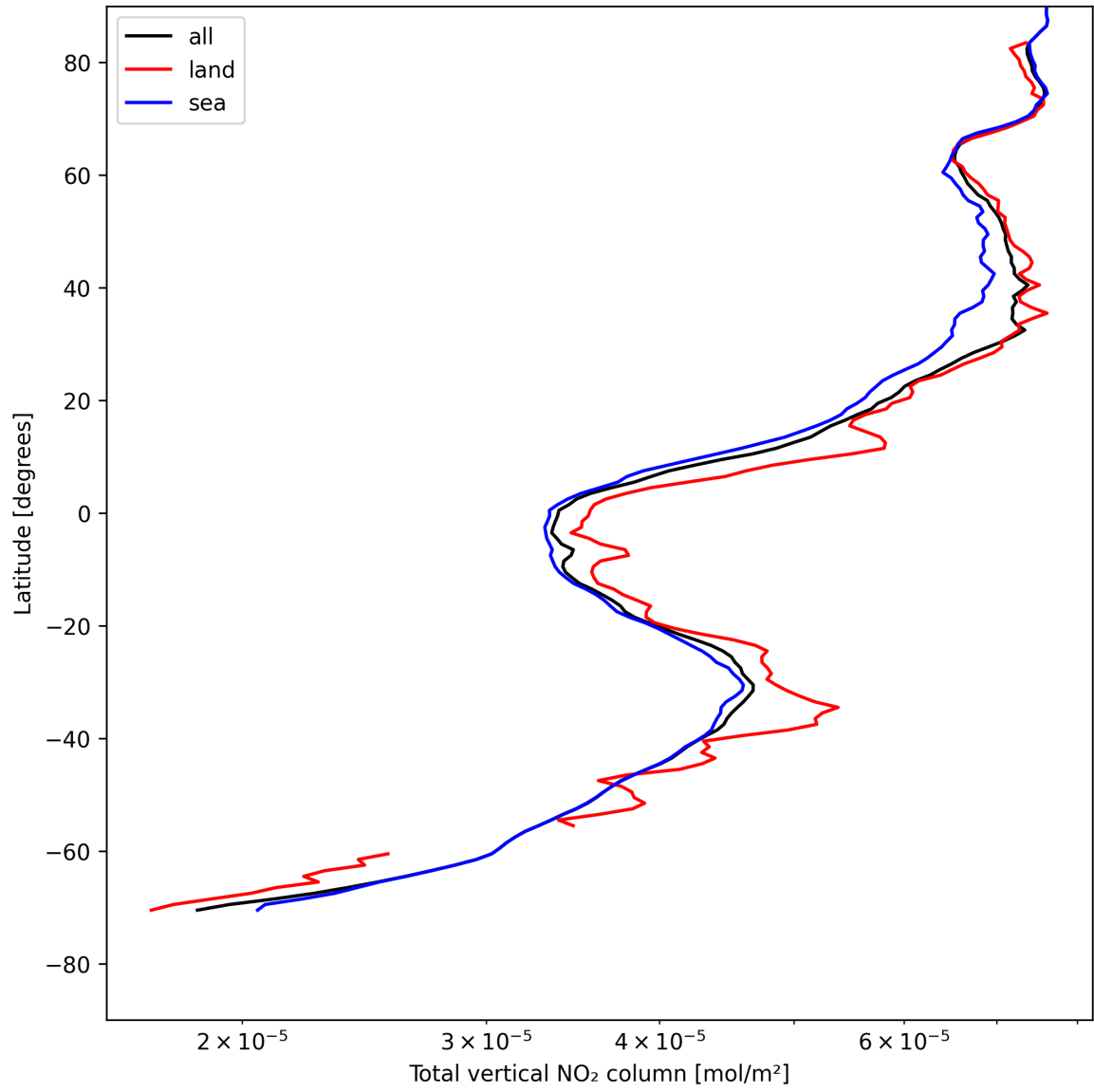
Figure 21: Zonal average of “Total vertical NO 2 column” for 2025-05-08 to 2025-05-08.
