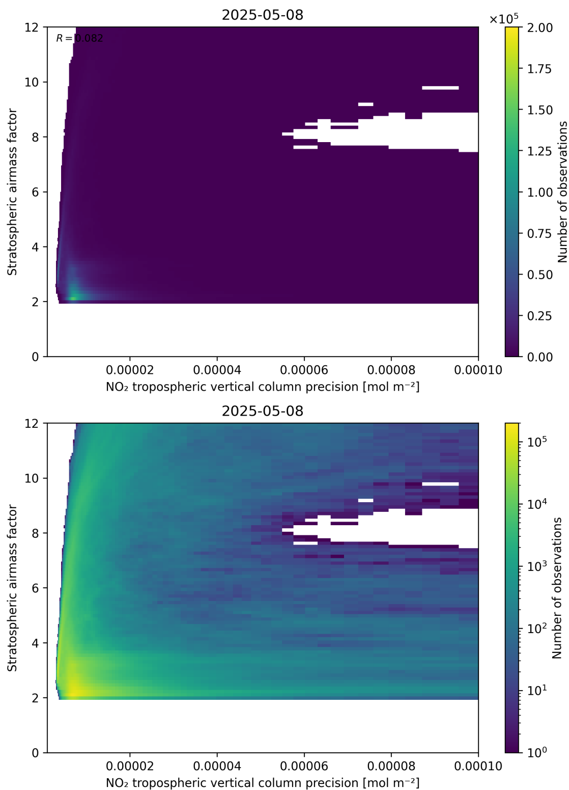
Figure 131: Scatter density plot of “NO 2 tropospheric vertical column precision” against “Stratospheric airmass factor” for 2025-05-08 to 2025-05-08.
