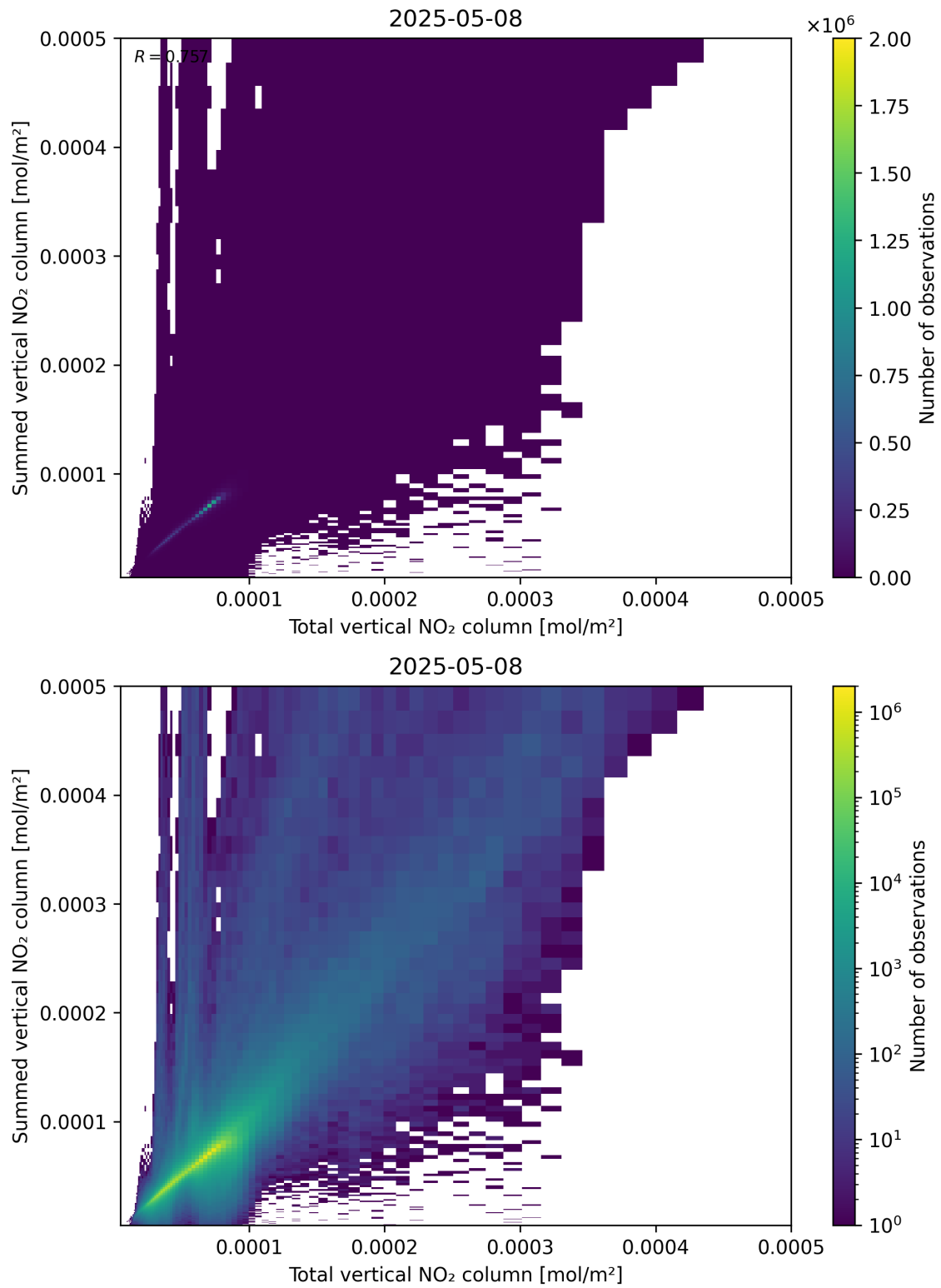
Figure 112: Scatter density plot of “Total vertical NO 2 column” against “Summed vertical NO 2 column” for 2025-05-08 to 2025-05-08.
