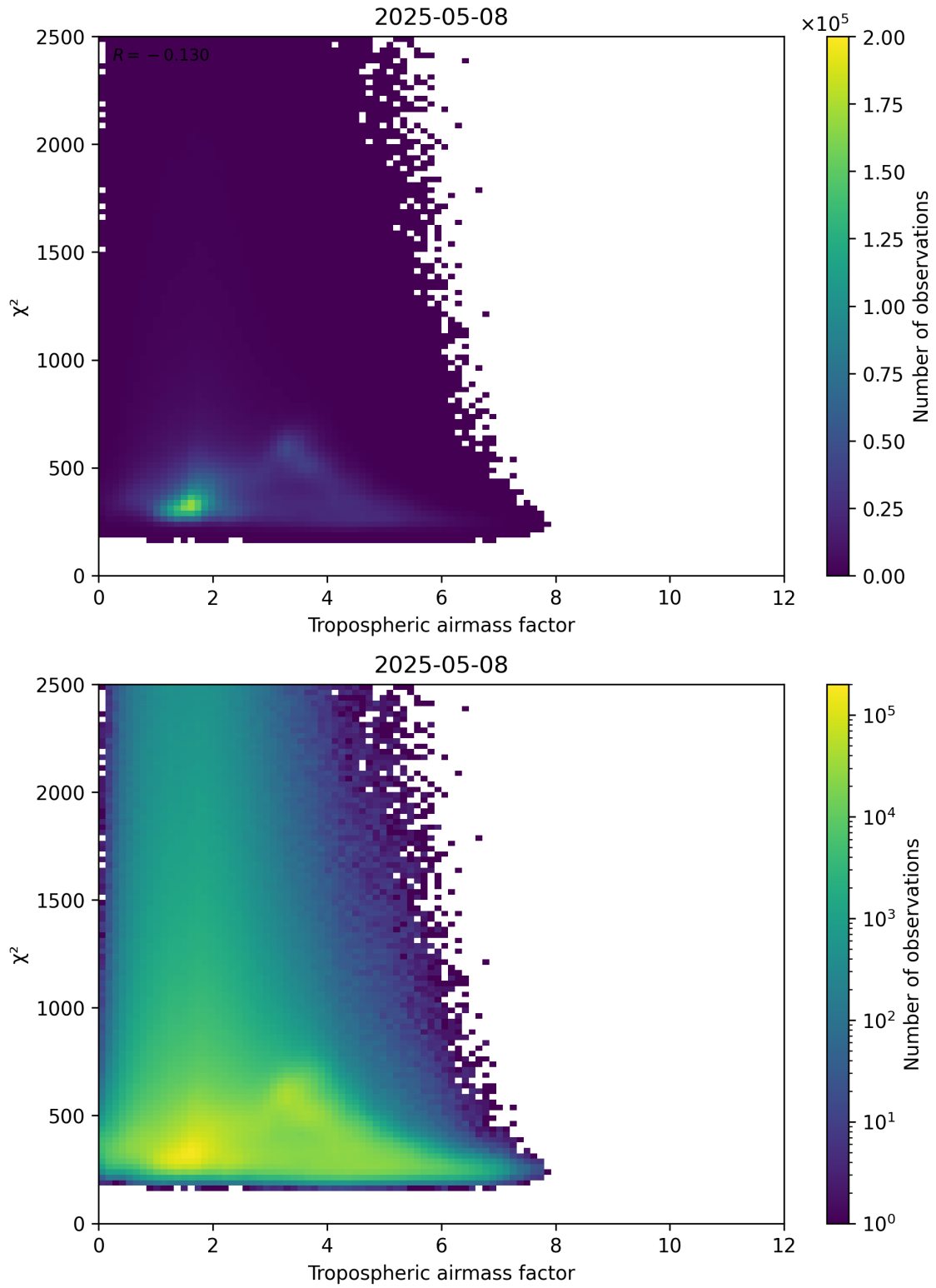
Figure 73: Scatter density plot of “Tropospheric airmass factor” against “ \chi^2 ” for 2025-05-08 to 2025-05-08.
