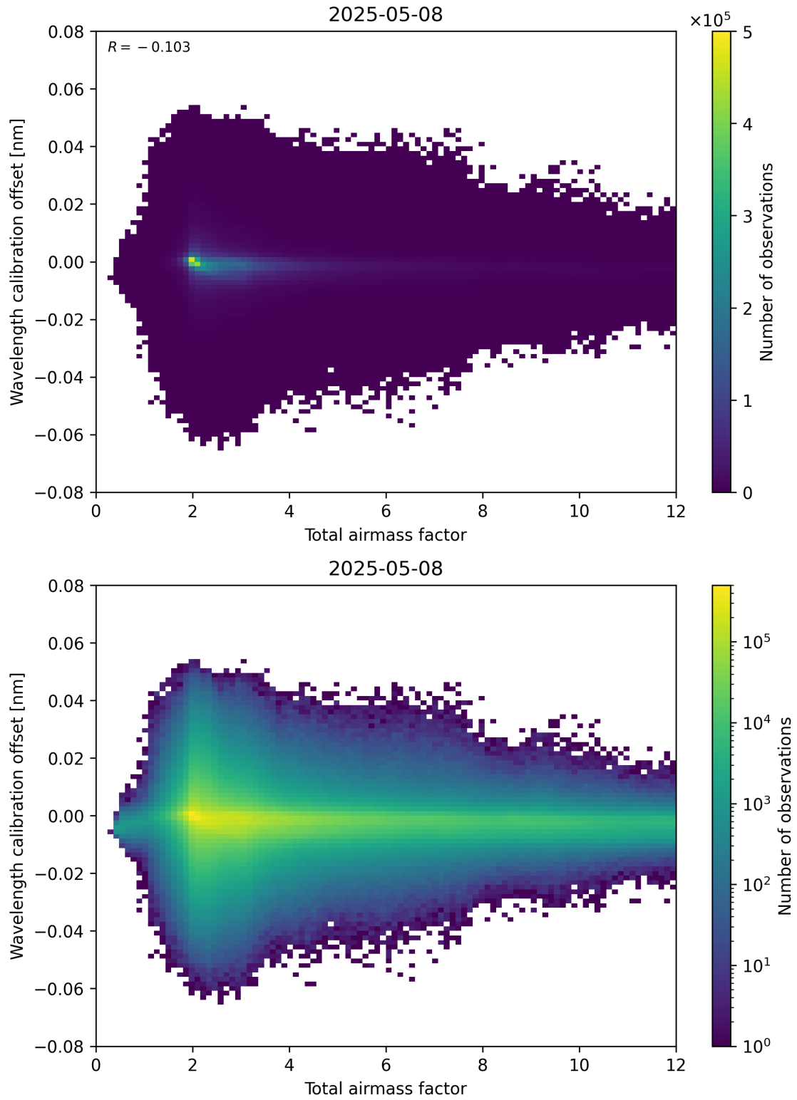
Figure 70: Scatter density plot of “Total airmass factor” against “Wavelength calibration offset” for 2025-05-08 to 2025-05-08.
