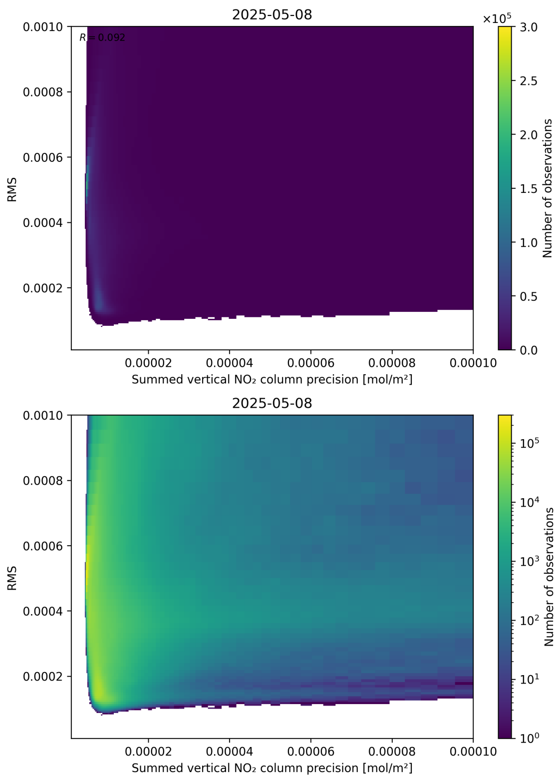
Figure 108: Scatter density plot of “Summed vertical NO 2 column precision” against “RMS” for 2025-05-08 to 2025-05-08.
