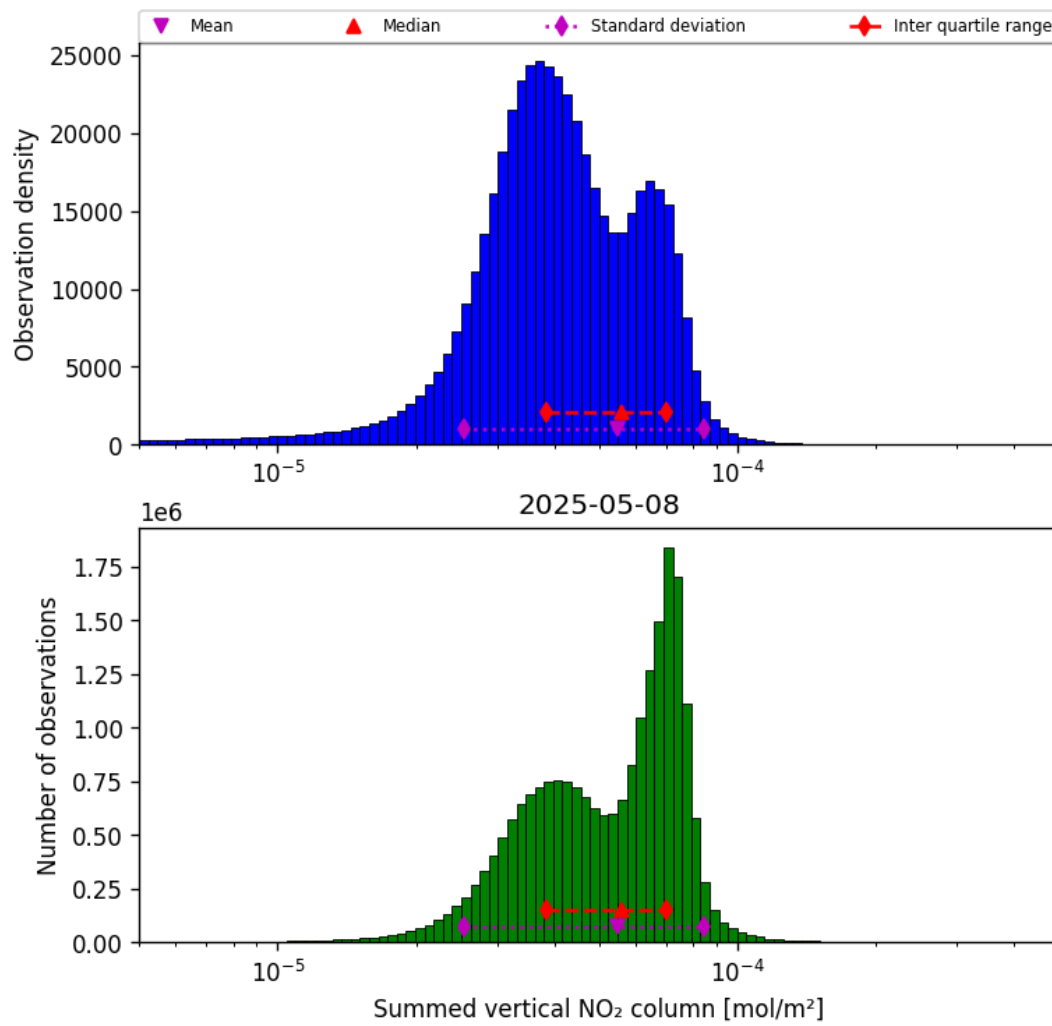
Figure 40: Histogram of "Summed vertical NO 2 column" for 2025-05-08 to 2025-05-08
