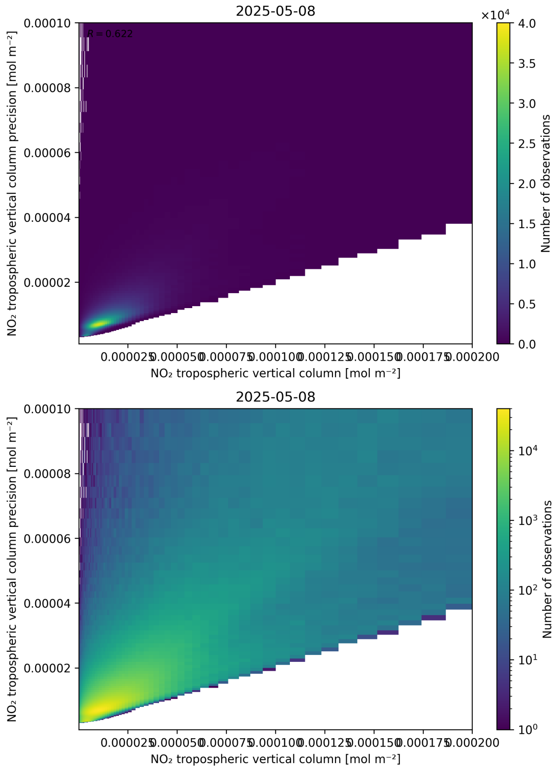
Figure 130: Scatter density plot of “NO 2 tropospheric vertical column” against “NO 2 tropospheric vertical column precision” for 2025-05-08 to 2025-05-08.
