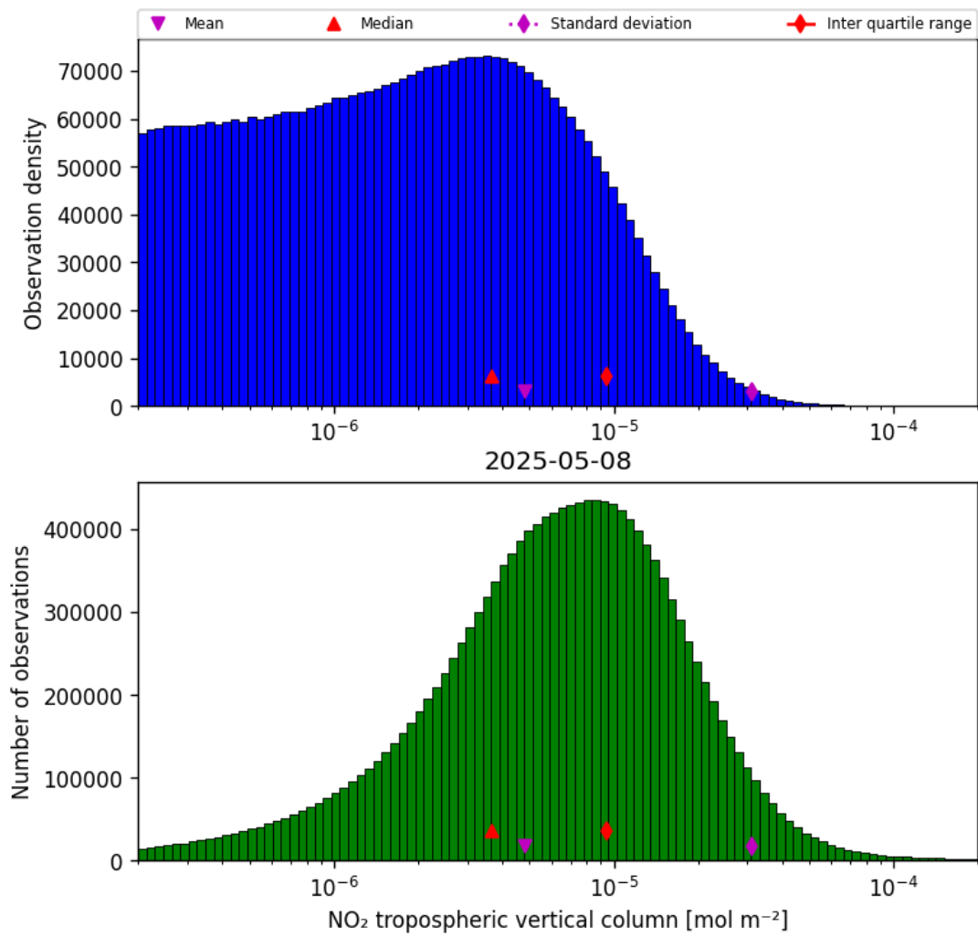
Figure 29: Histogram of “ \text{NO}_2 tropospheric vertical column” for 2025-05-08 to 2025-05-08
