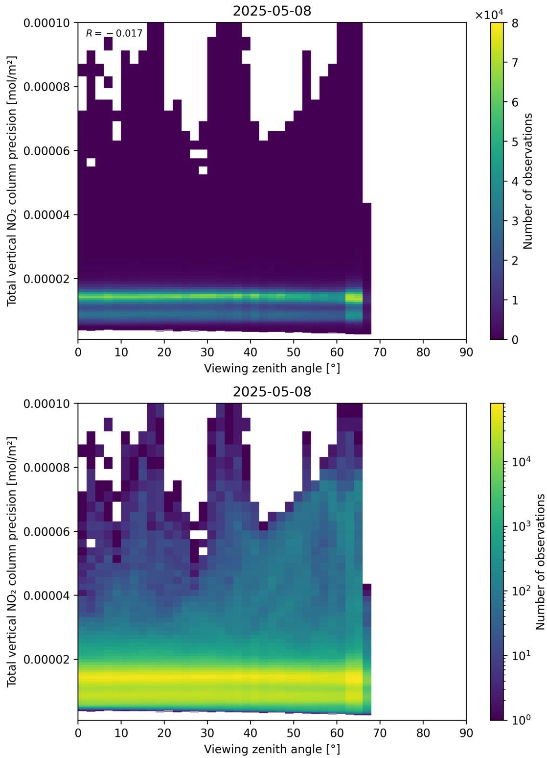
Figure 168: Scatter density plot of “Viewing zenith angle” against “Total vertical NO 2 column precision” for 2025-05-08 to 2025-05-08.
