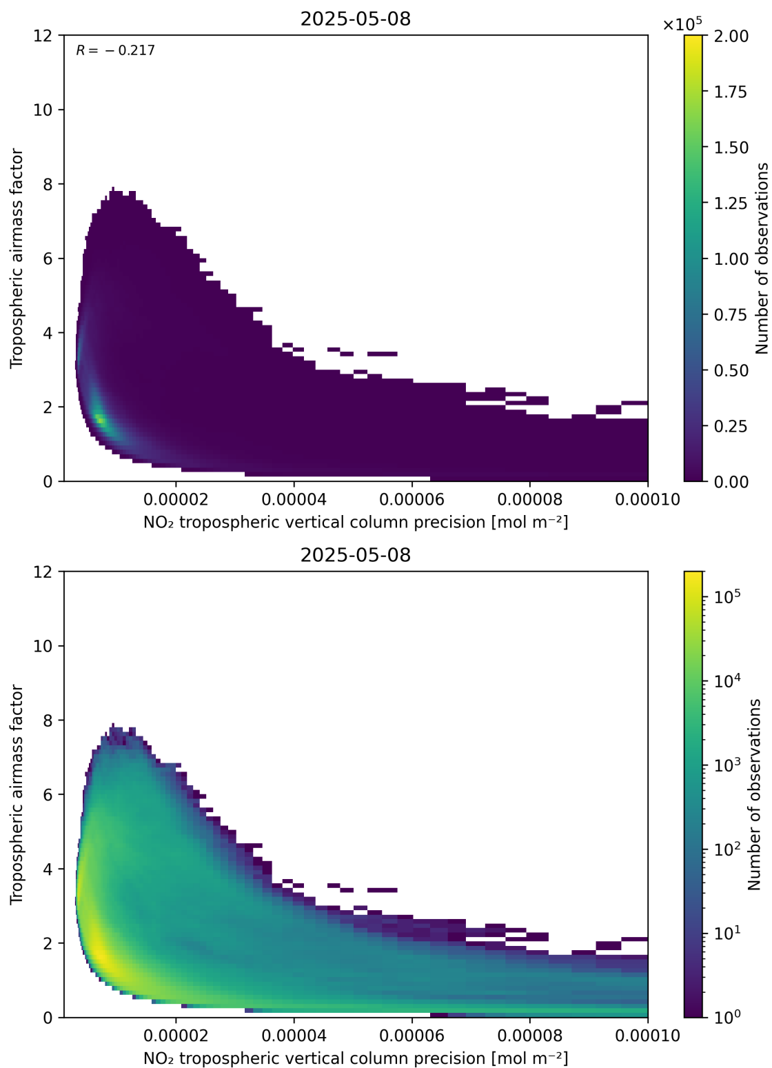
Figure 133: Scatter density plot of “NO 2 tropospheric vertical column precision” against “Tropospheric air mass factor” for 2025-05-08 to 2025-05-08.
