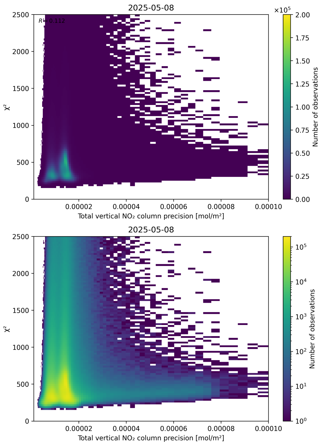
Figure 116: Scatter density plot of “Total vertical NO 2 column precision” against “ \chi^2 ” for 2025-05-08 to 2025-05-08.
