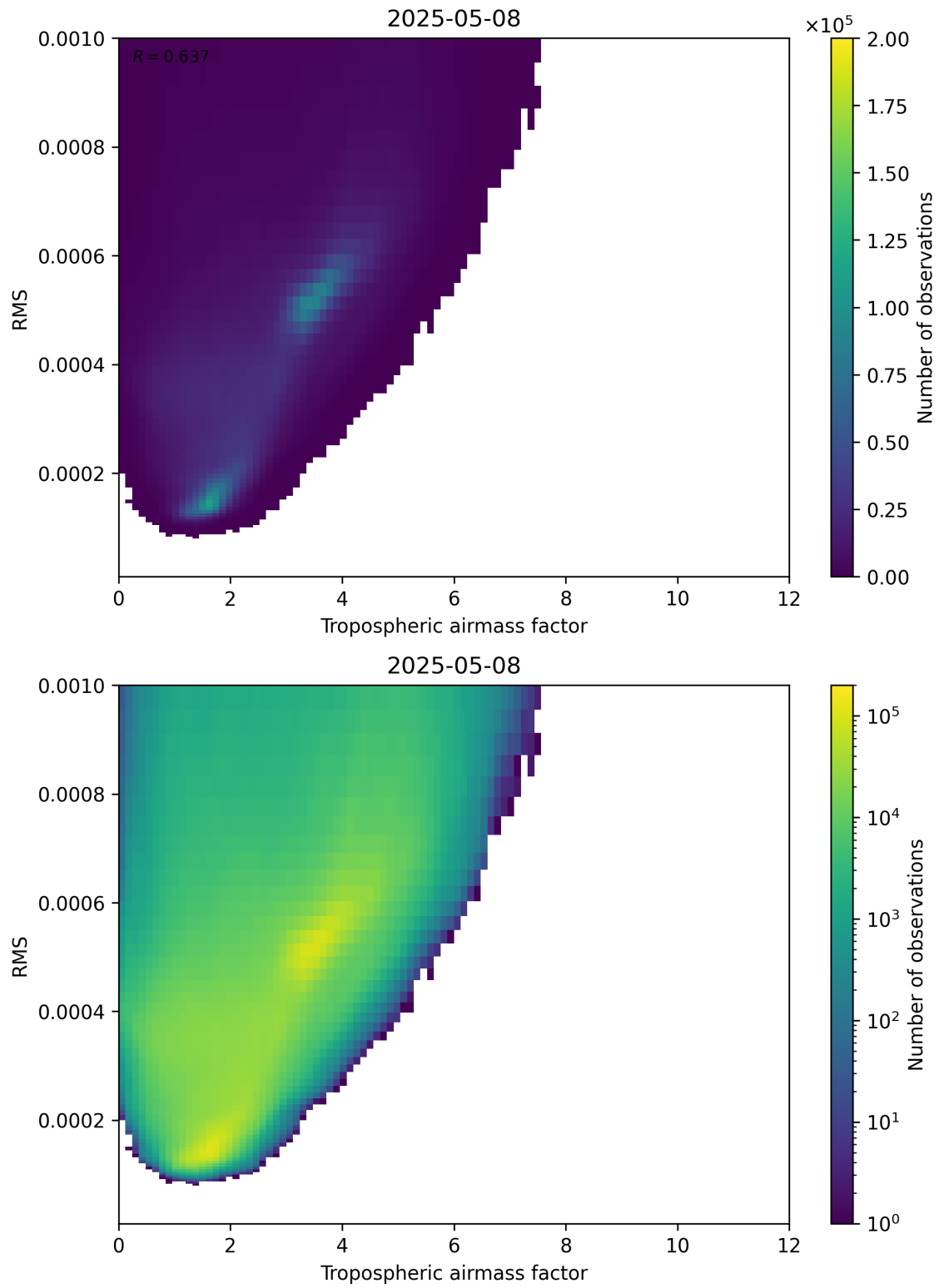
Figure 79: Scatter density plot of “Tropospheric airmass factor” against “RMS” for 2025-05-08 to 2025-05-08.
