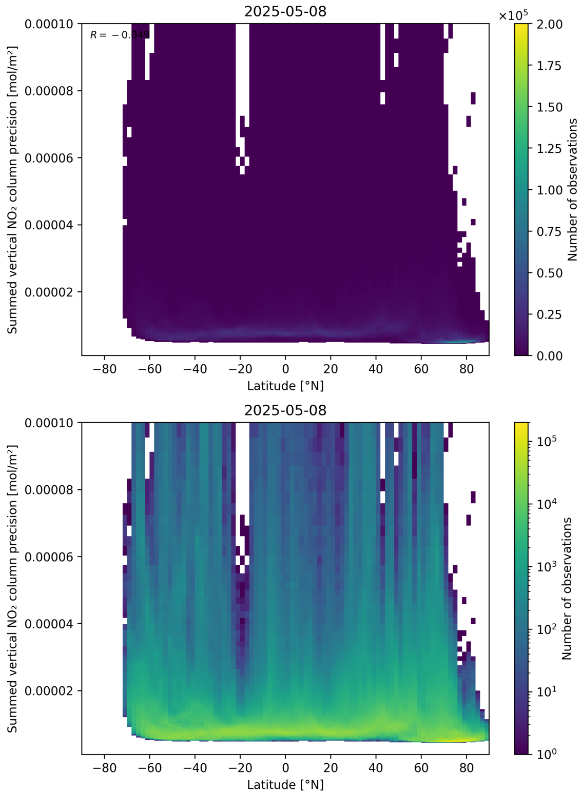
Figure 89: Scatter density plot of “Latitude” against “Summed vertical NO 2 column precision” for 2025-05-08 to 2025-05-08.
