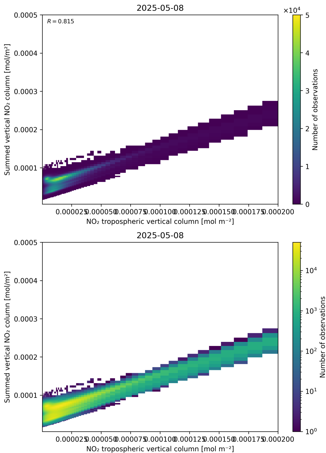
Figure 126: Scatter density plot of “NO 2 tropospheric vertical column” against “Summed vertical NO 2 column” for 2025-05-08 to 2025-05-08.
