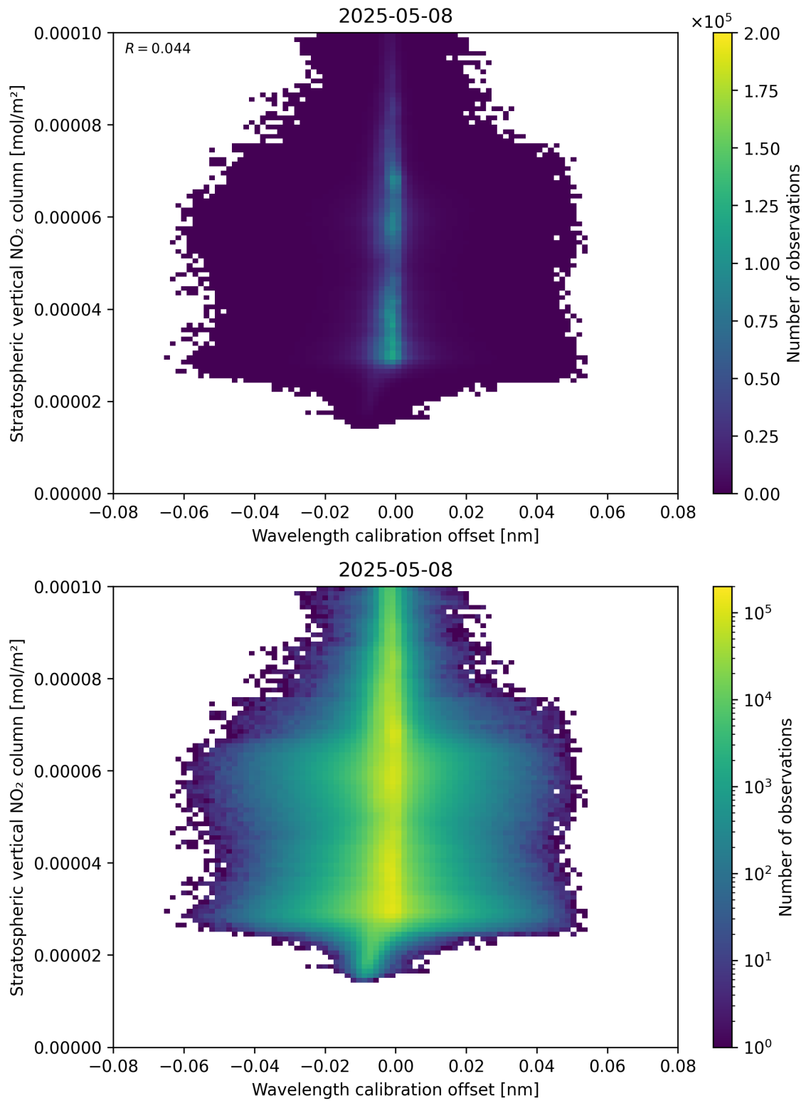
Figure 176: Scatter density plot of “Wavelength calibration offset” against “Stratospheric vertical NO 2 column” for 2025-05-08 to 2025-05-08.
