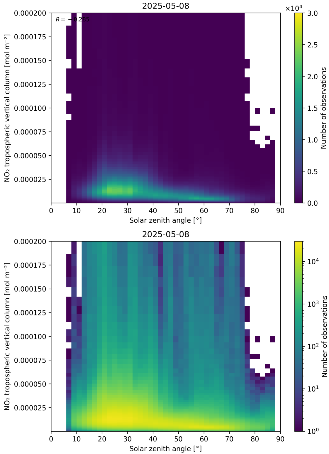
Figure 155: Scatter density plot of “Solar zenith angle” against “NO 2 tropospheric vertical column” for 2025-05-08 to 2025-05-08.
