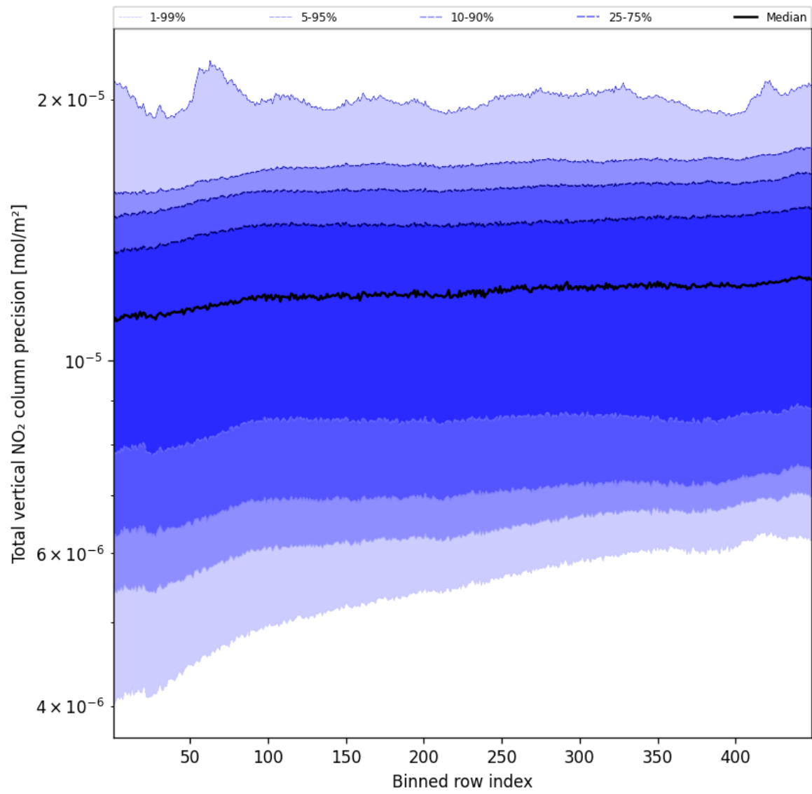
Figure 56: Along track statistics of “Total vertical NO 2 column precision” for 2025-05-08 to 2025-05-08
