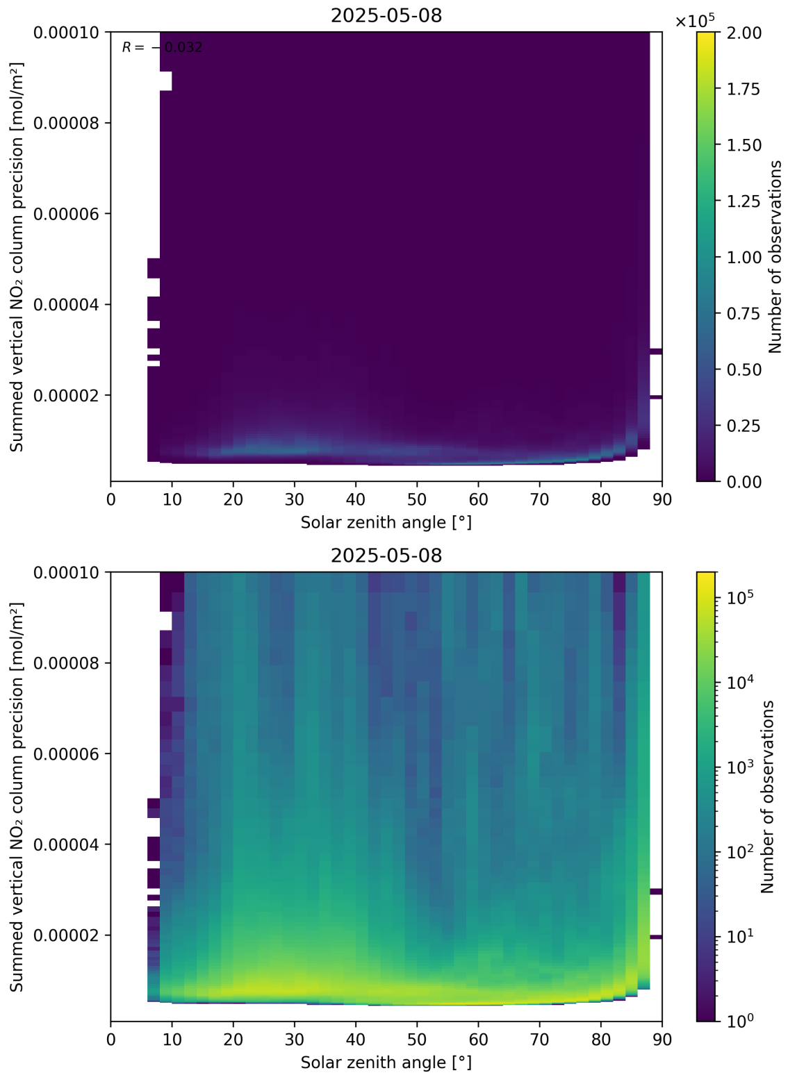
Figure 152: Scatter density plot of “Solar zenith angle” against “Summed vertical NO 2 column precision” for 2025-05-08 to 2025-05-08.
