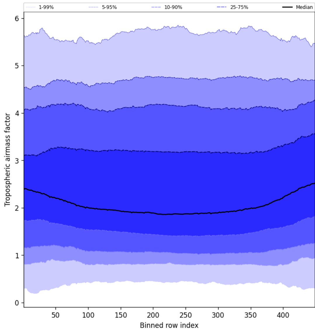
Figure 48: Along track statistics of “Tropospheric airmass factor” for 2025-05-08 to 2025-05-08
