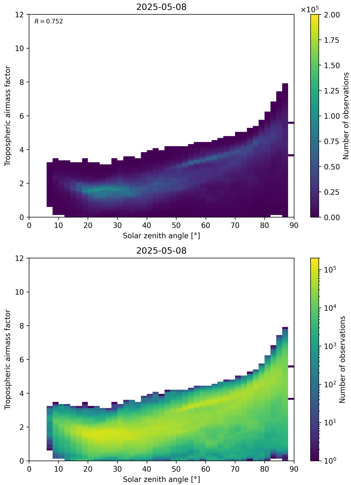
Figure 147: Scatter density plot of “Solar zenith angle” against “Tropospheric airmass factor” for 2025-05-08 to 2025-05-08.
