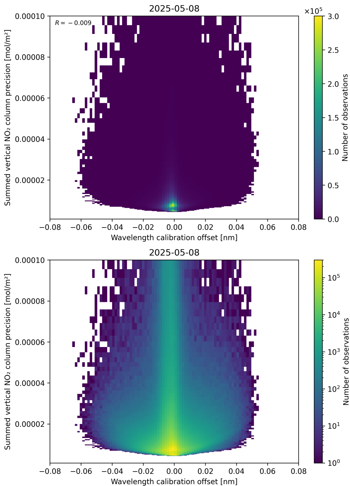
Figure 178: Scatter density plot of “Wavelength calibration offset” against “Summed vertical NO 2 column precision” for 2025-05-08 to 2025-05-08.
