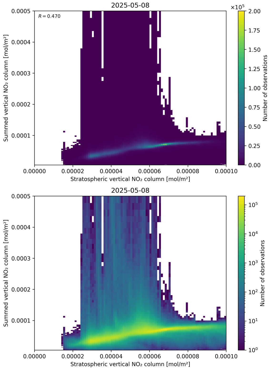
Figure 98: Scatter density plot of “Stratospheric vertical NO 2 column” against “Summed vertical NO 2 column” for 2025-05-08 to 2025-05-08.
