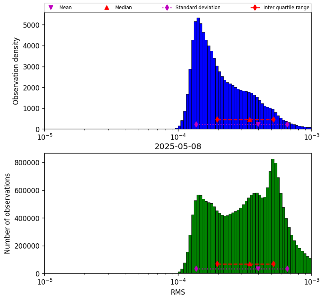
Figure 43: Histogram of “RMS” for 2025-05-08 to 2025-05-08
