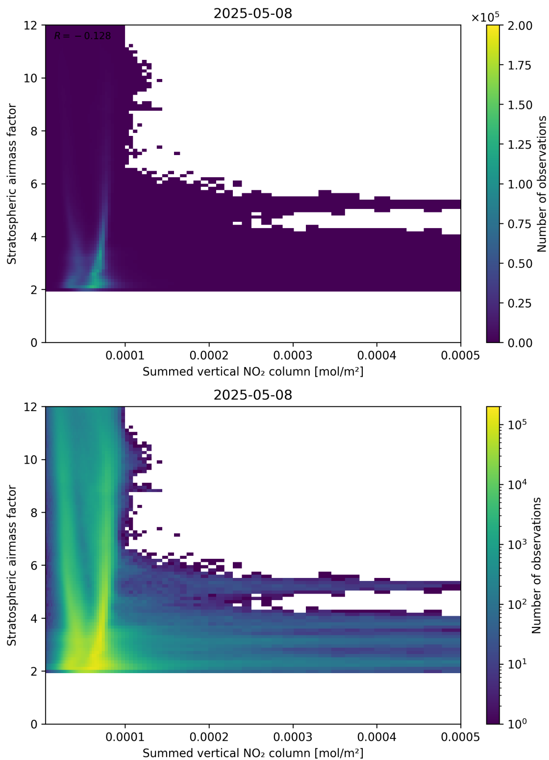
Figure 103: Scatter density plot of “Summed vertical NO 2 column” against “Stratospheric air mass factor” for 2025-05-08 to 2025-05-08.
