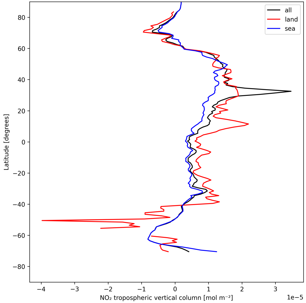
Figure 12: Zonal average of “NO 2 tropospheric vertical column” for 2025-05-08 to 2025-05-08.
