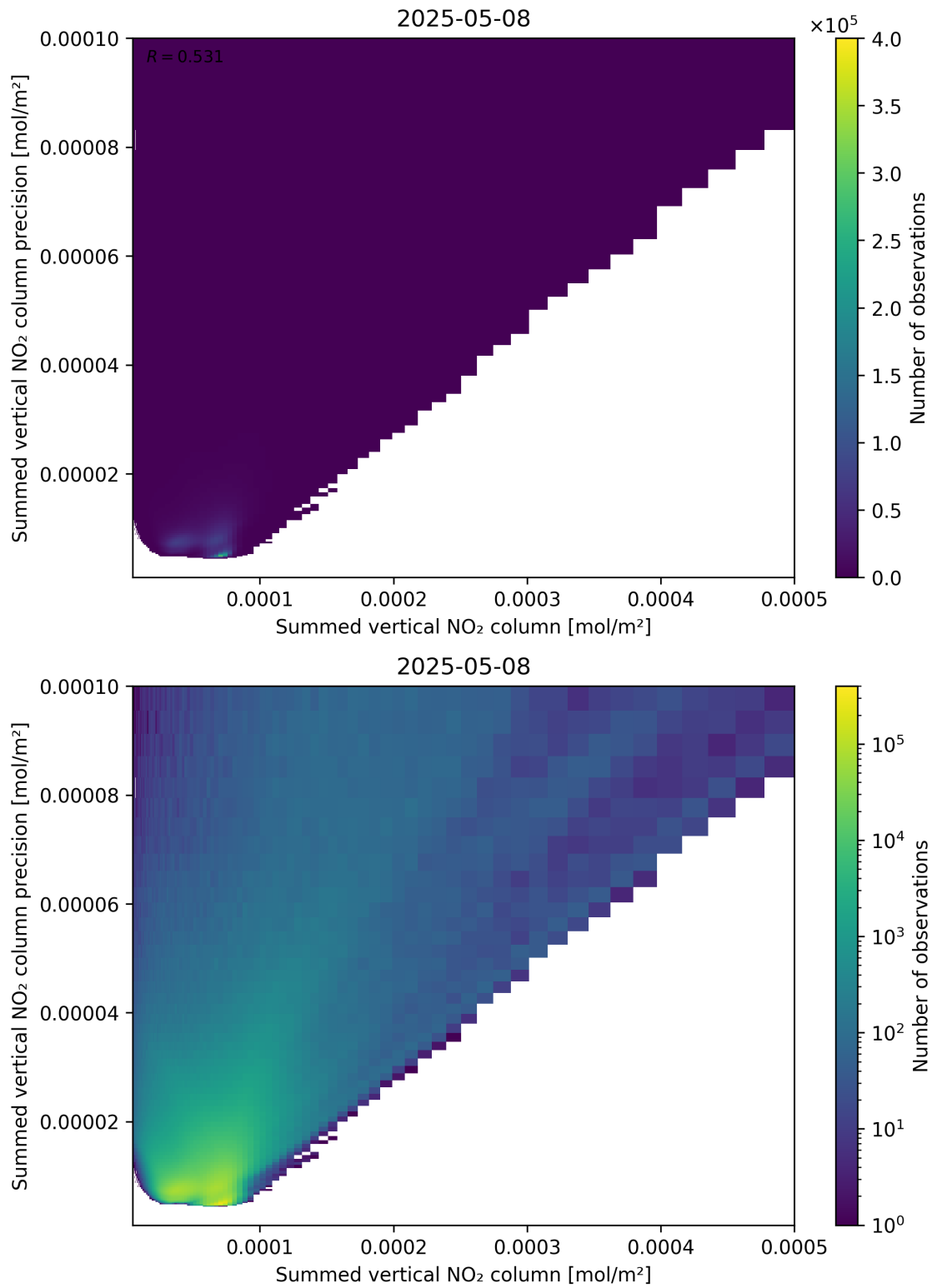
Figure 105: Scatter density plot of “Summed vertical NO 2 column” against “Summed vertical NO 2 column precision” for 2025-05-08 to 2025-05-08.
