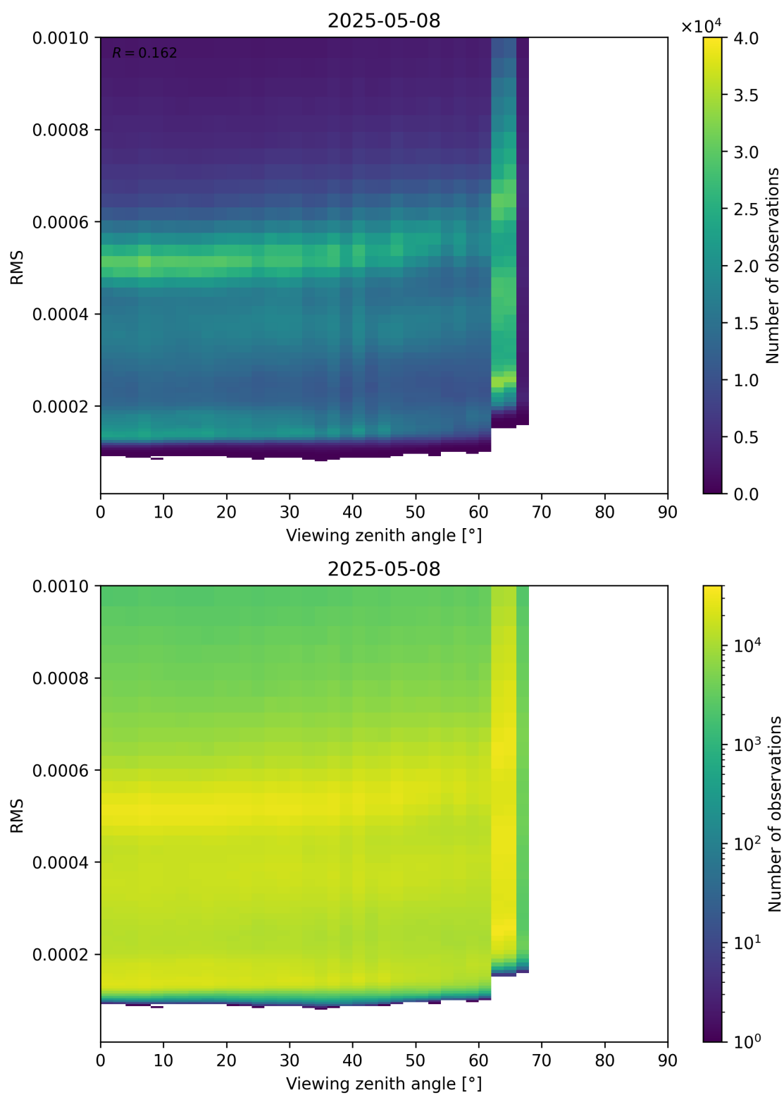
Figure 171: Scatter density plot of “Viewing zenith angle” against “RMS” for 2025-05-08 to 2025-05-08.
