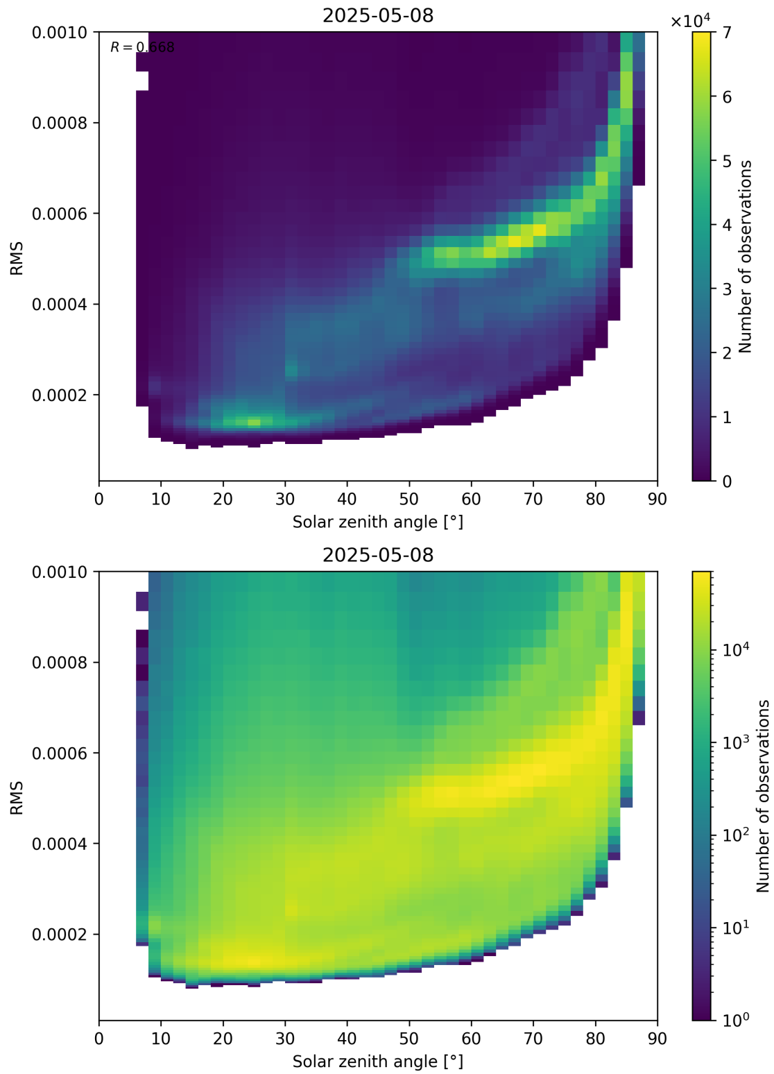
Figure 157: Scatter density plot of “Solar zenith angle” against “RMS” for 2025-05-08 to 2025-05-08.
