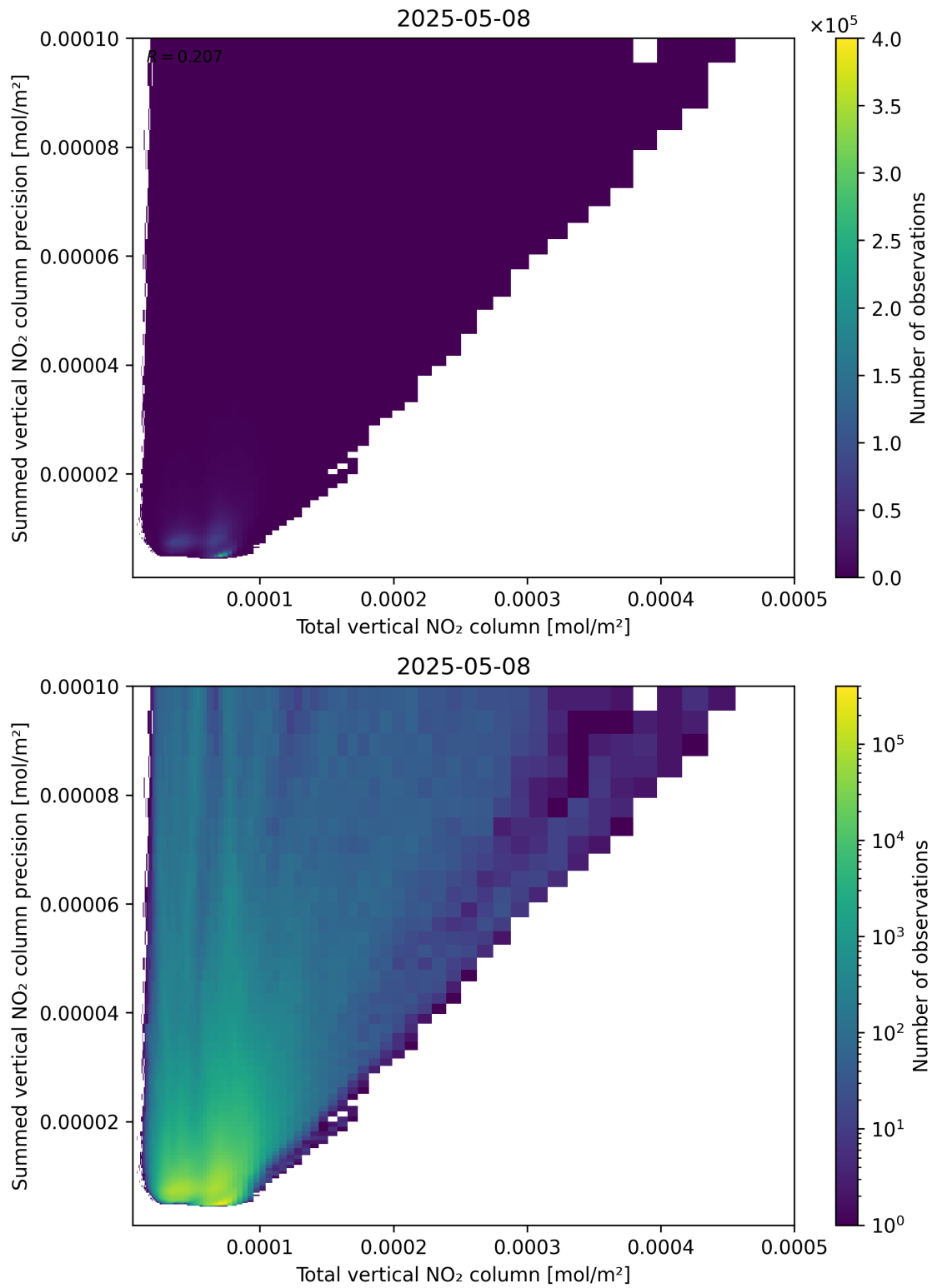
Figure 113: Scatter density plot of “Total vertical NO 2 column” against “Summed vertical NO 2 column precision” for 2025-05-08 to 2025-05-08.
