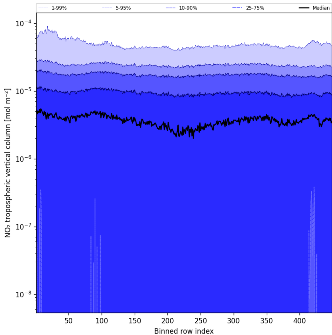
Figure 46: Along track statistics of “NO 2 tropospheric vertical column” for 2025-05-08 to 2025-05-08
