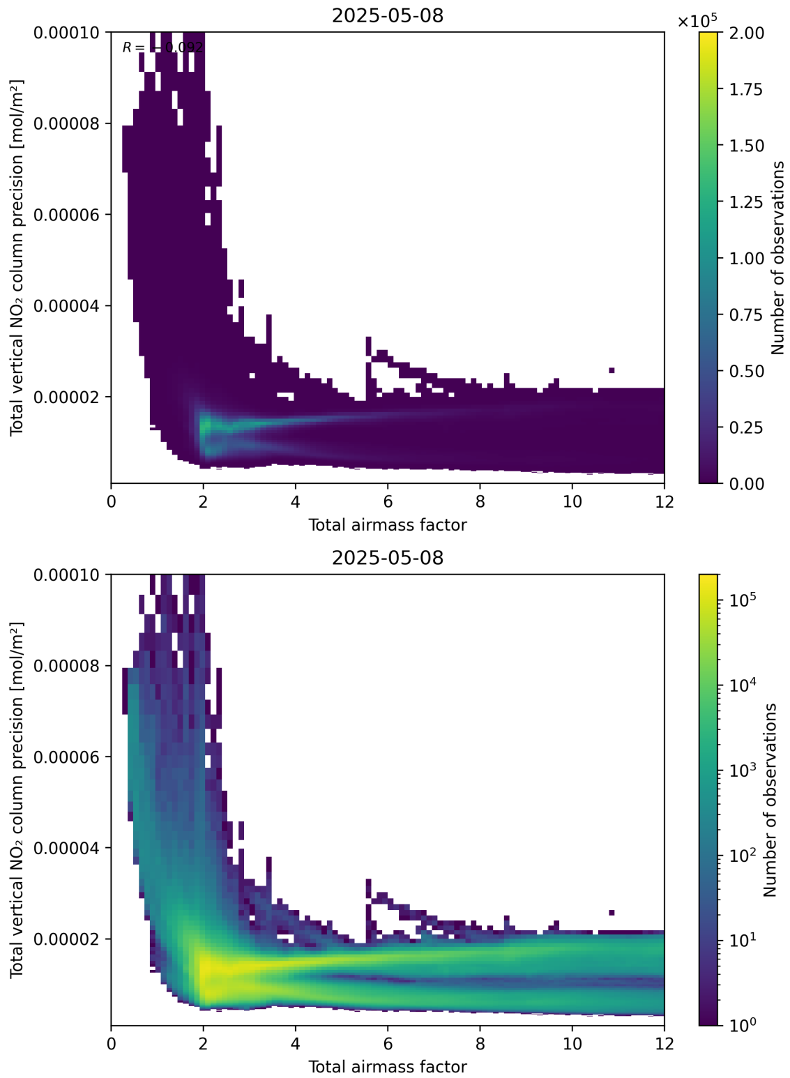
Figure 68: Scatter density plot of “Total airmass factor” against “Total vertical NO 2 column precision” for 2025-05-08 to 2025-05-08.
