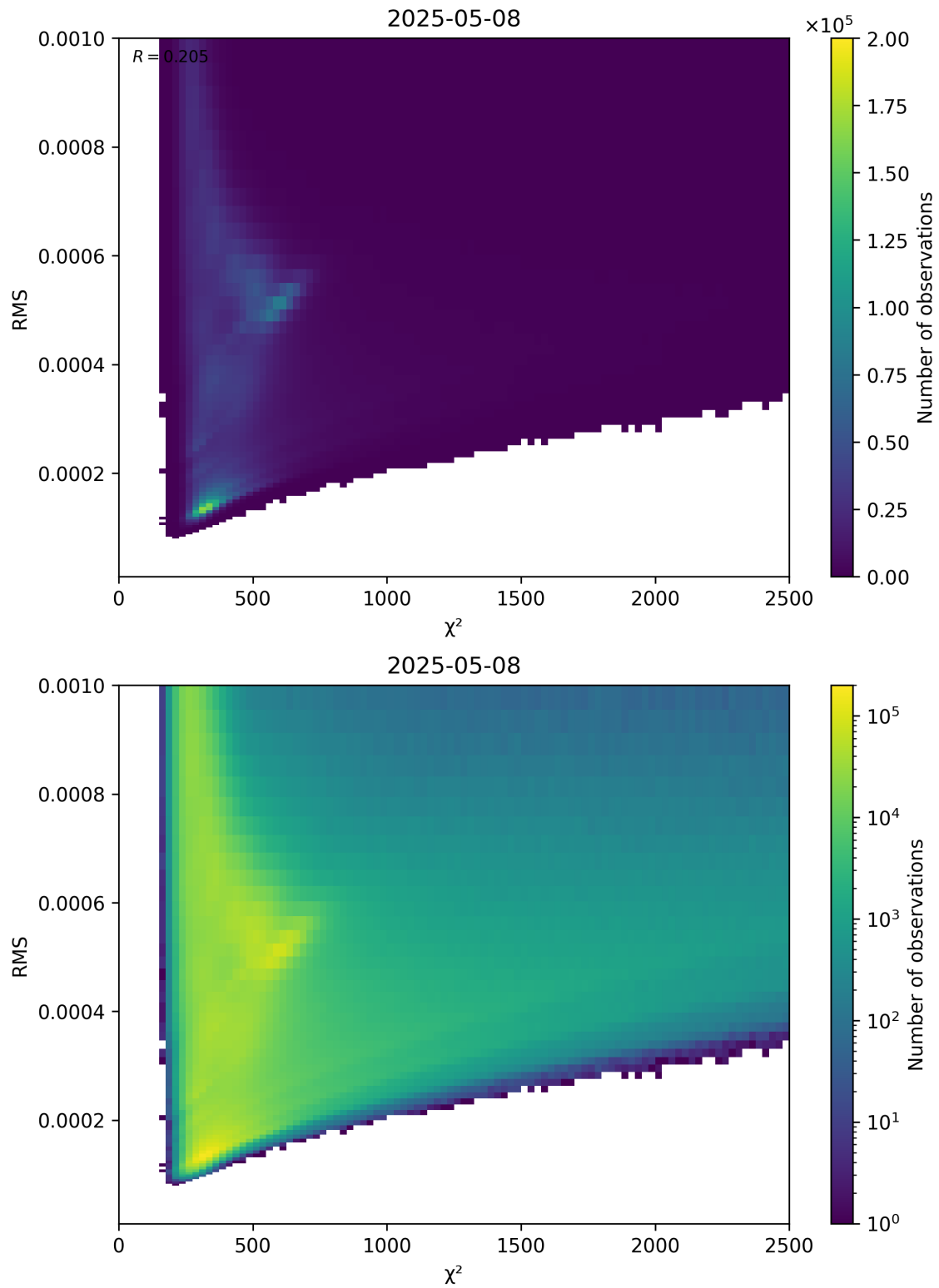
Figure 82: Scatter density plot of “ \chi^2 ” against “RMS” for 2025-05-08 to 2025-05-08.
