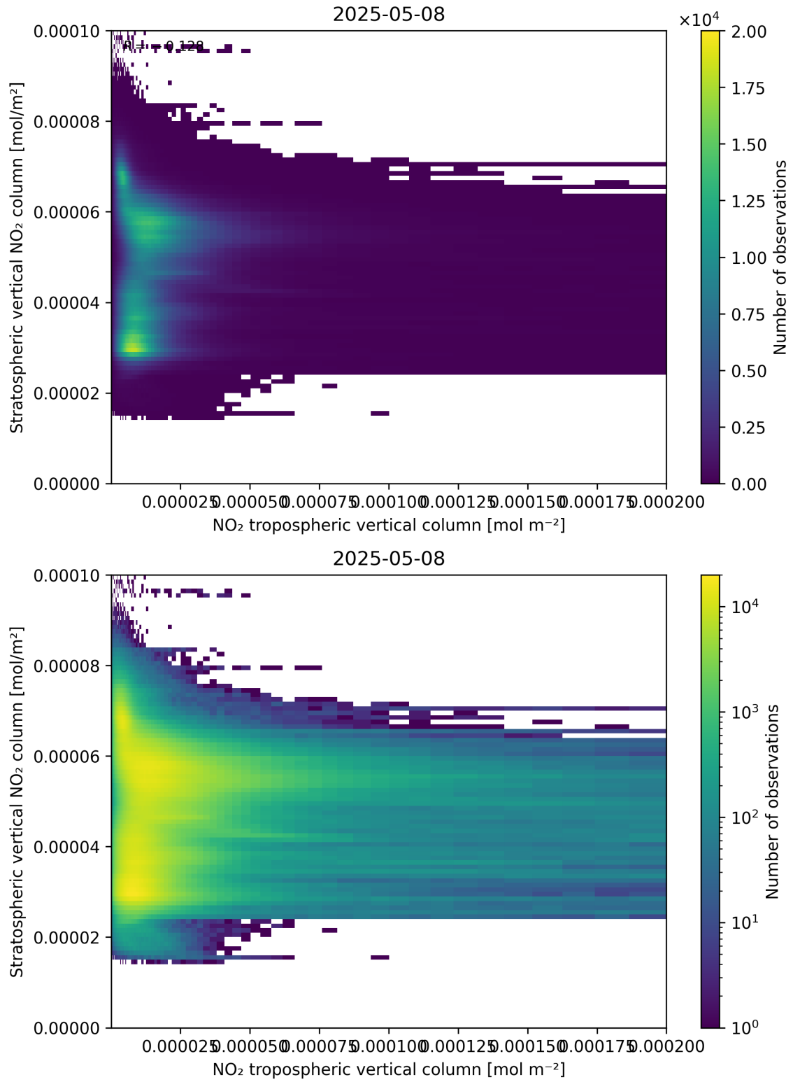
Figure 125: Scatter density plot of “NO 2 tropospheric vertical column” against “Stratospheric vertical NO 2 column” for 2025-05-08 to 2025-05-08.
