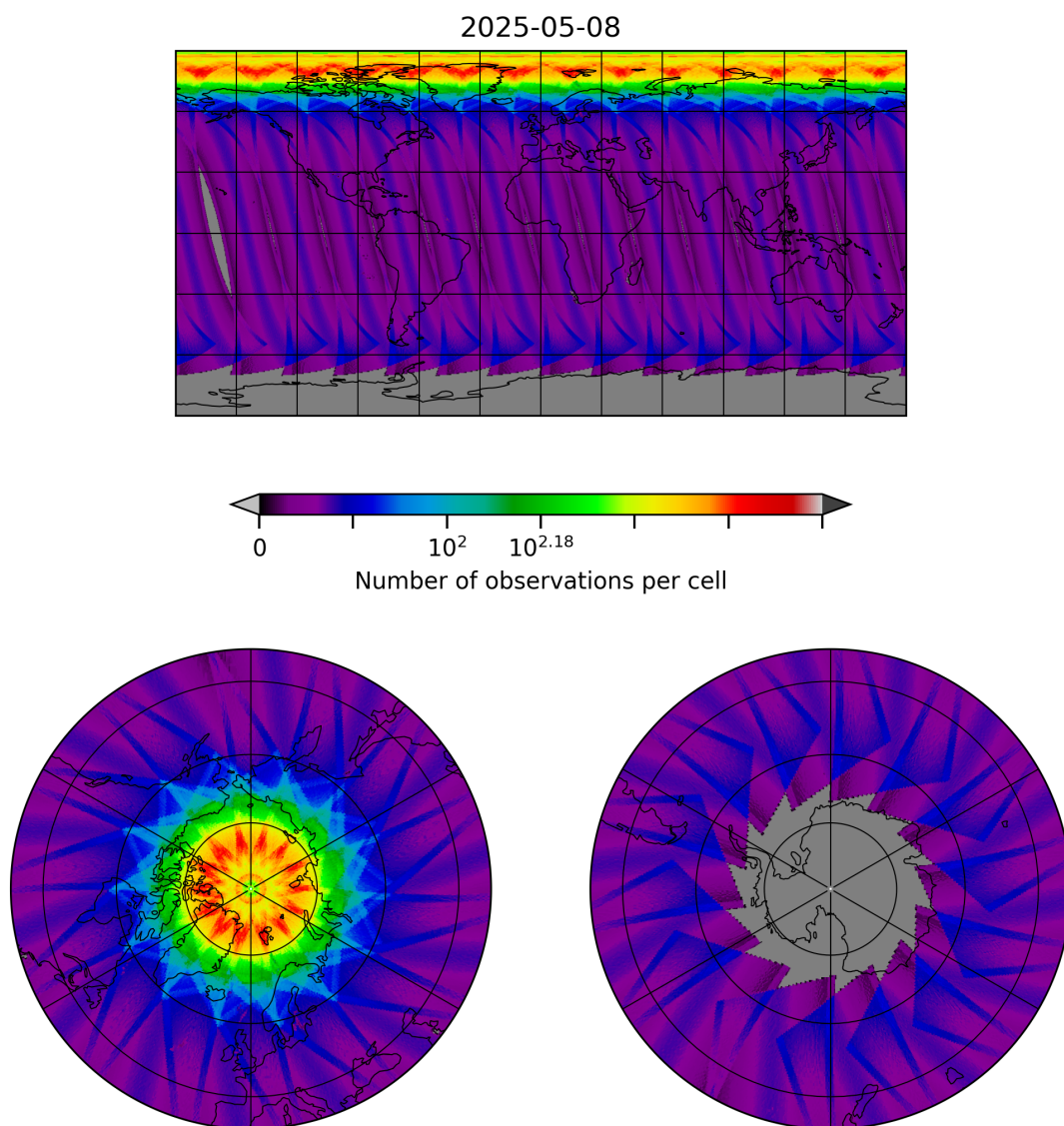
Figure 10: Map of the number of observations for 2025-05-08 to 2025-05-08
