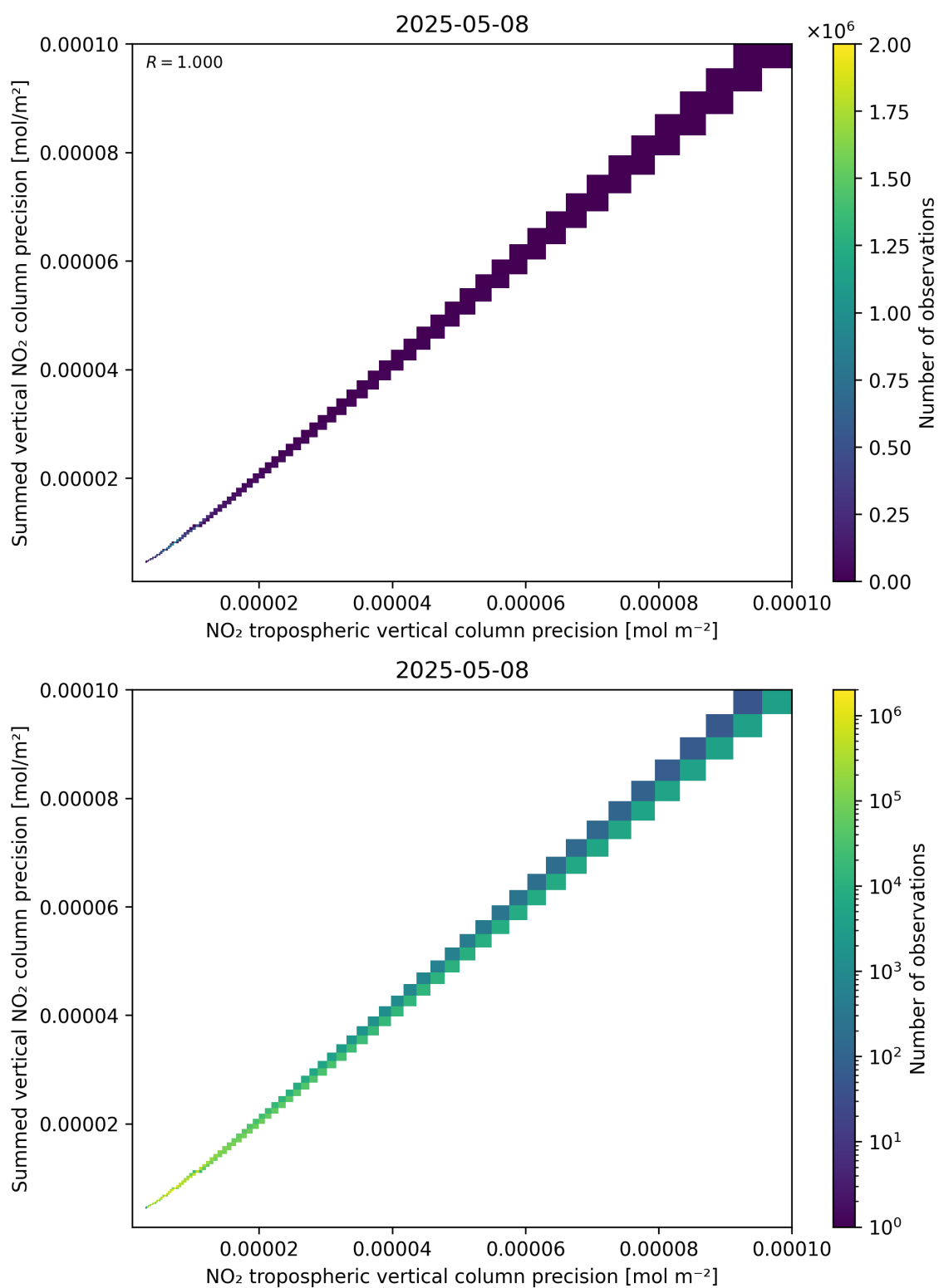
Figure 137: Scatter density plot of “NO 2 tropospheric vertical column precision” against “Summed vertical NO 2 column precision” for 2025-05-08 to 2025-05-08.
