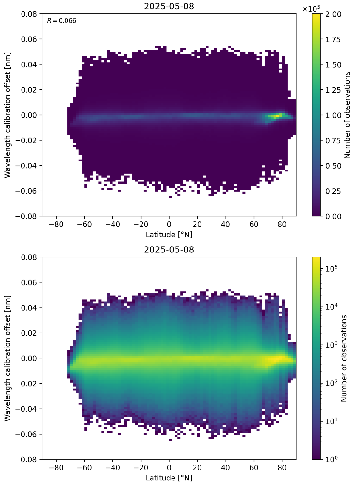
Figure 95: Scatter density plot of “Latitude” against “Wavelength calibration offset” for 2025-05-08 to 2025-05-08.
