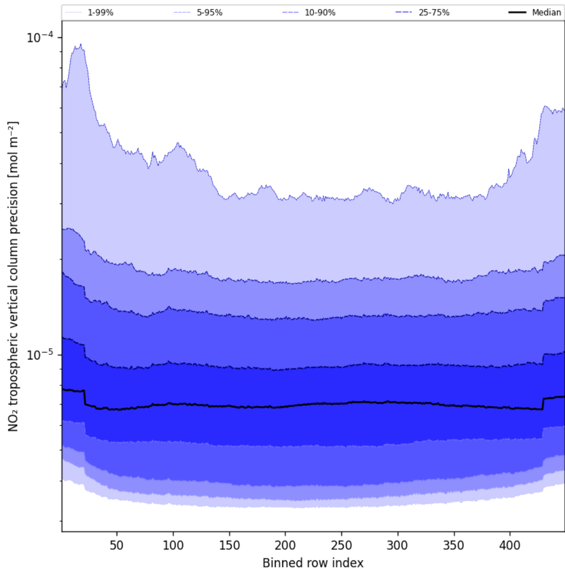
Figure 47: Along track statistics of “NO 2 tropospheric vertical column precision” for 2025-05-08 to 2025-05-08
