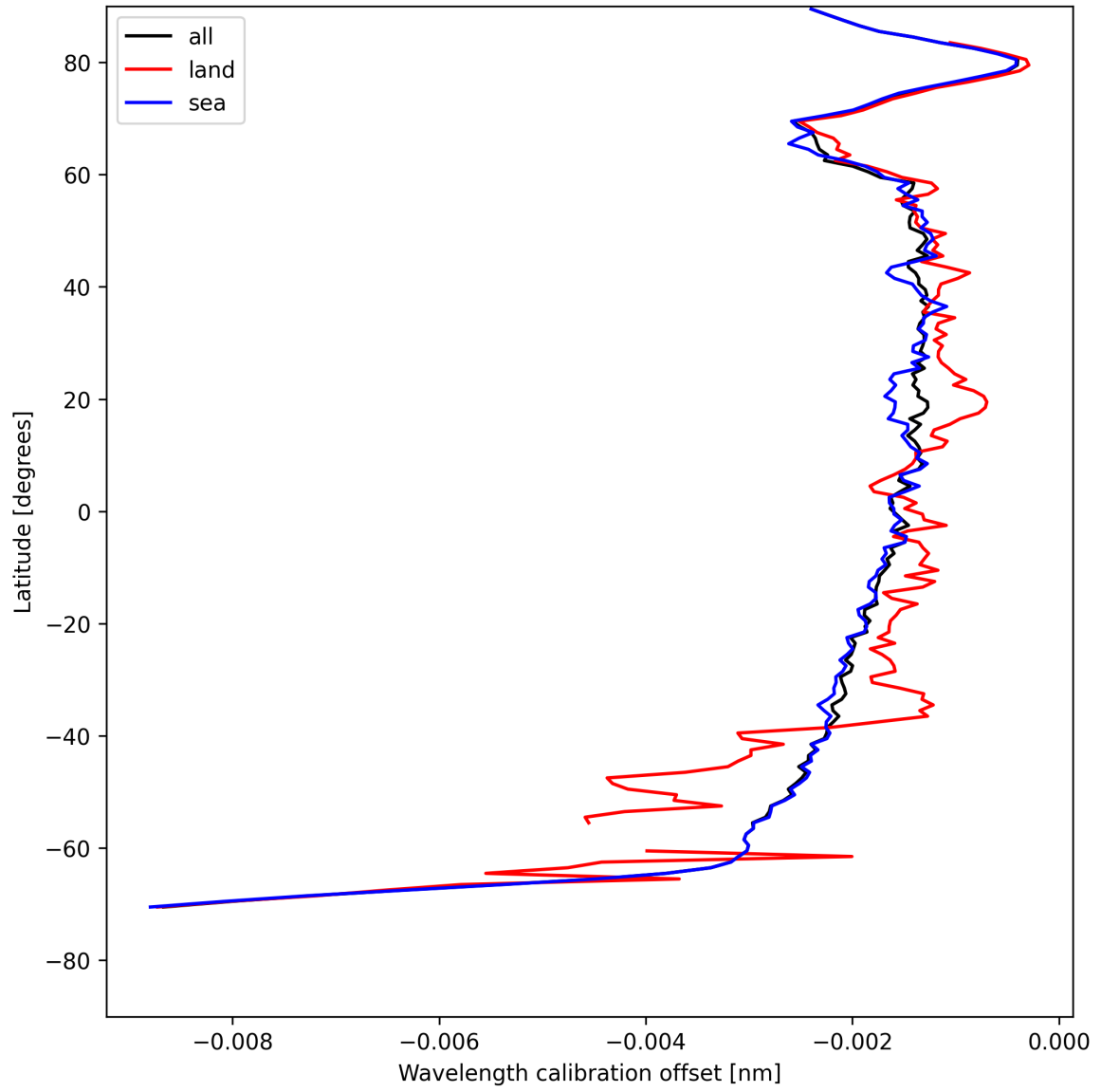
Figure 18: Zonal average of “Wavelength calibration offset” for 2025-05-08 to 2025-05-08.
