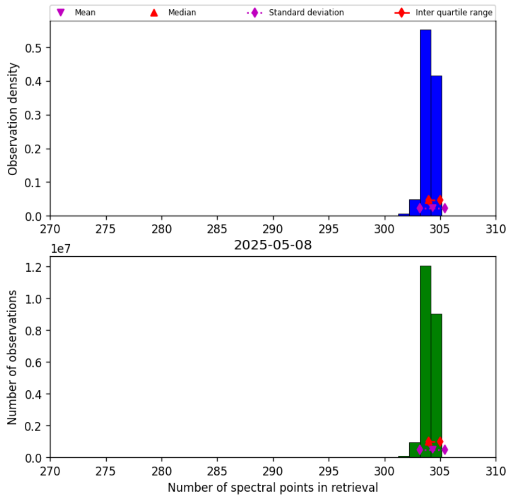
Figure 33: Histogram of “Number of spectral points in retrieval” for 2025-05-08 to 2025-05-08
