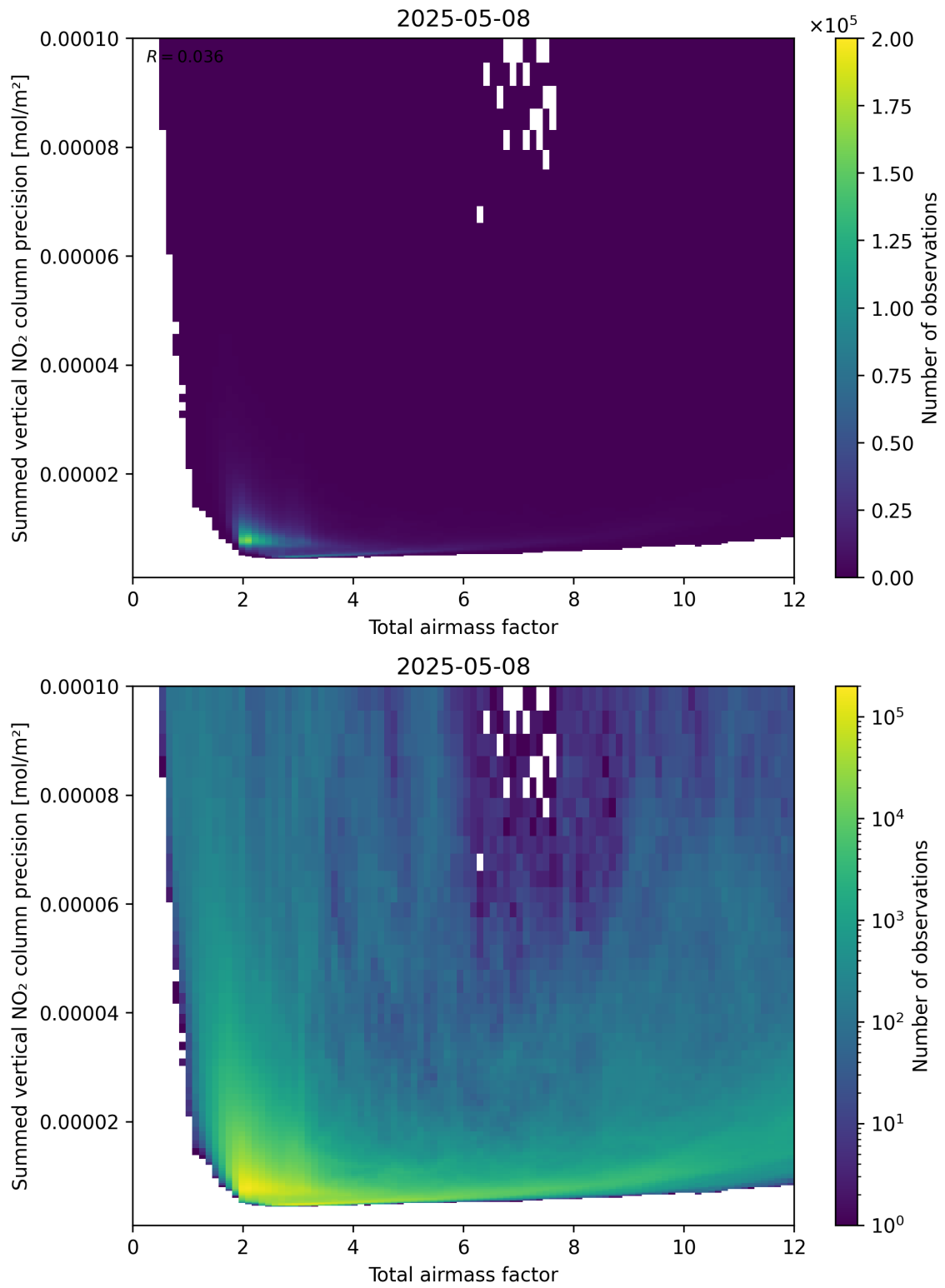
Figure 66: Scatter density plot of “Total airmass factor” against “Summed vertical NO 2 column precision” for 2025-05-08 to 2025-05-08.
