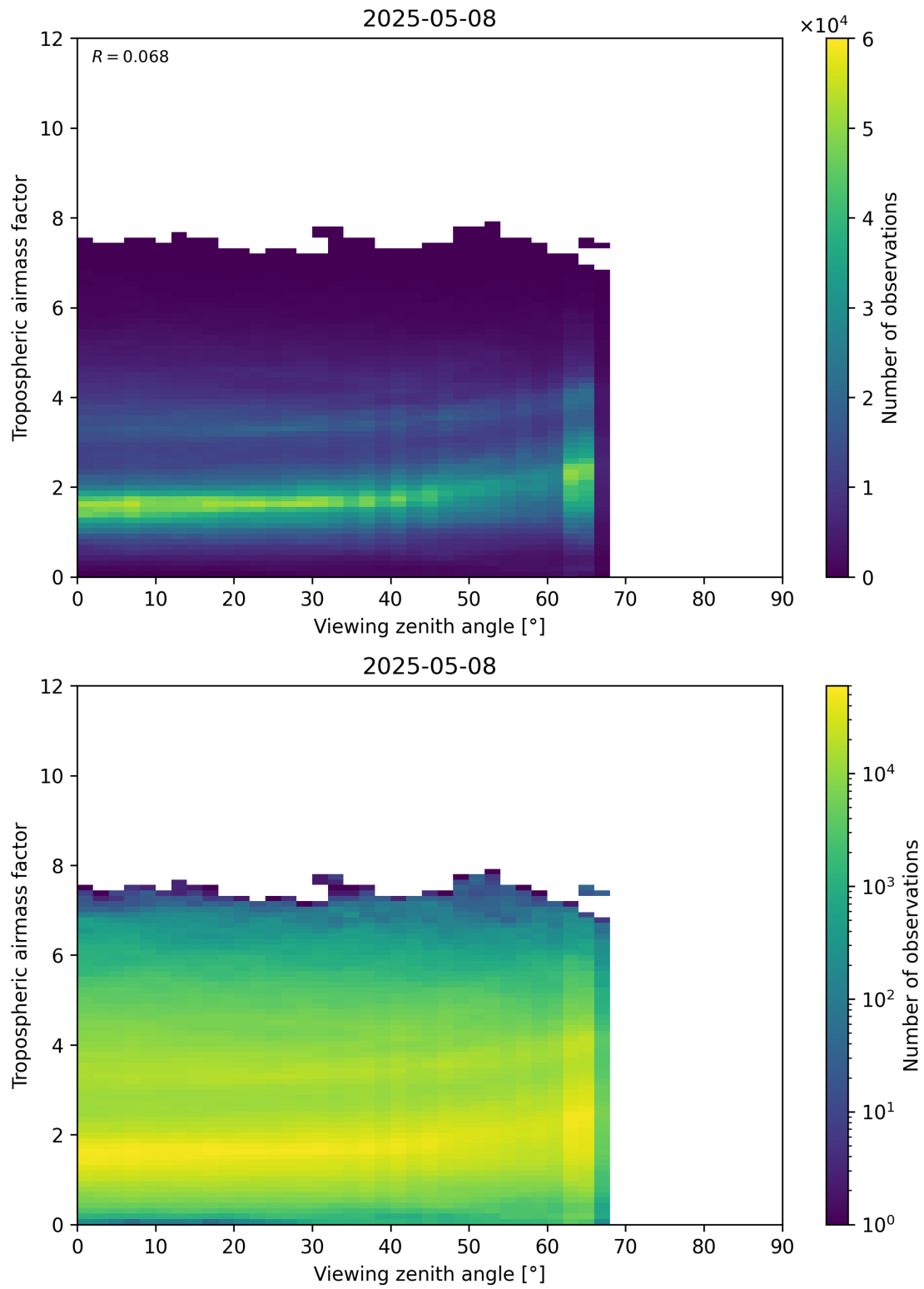
Figure 161: Scatter density plot of “Viewing zenith angle” against “Tropospheric airmass factor” for 2025-05-08 to 2025-05-08.
