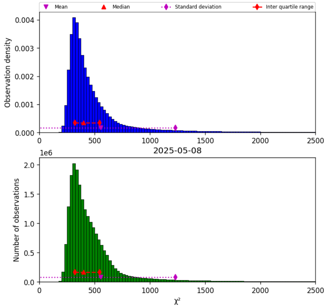
Figure 42: Histogram of " \chi^2 " for 2025-05-08 to 2025-05-08
