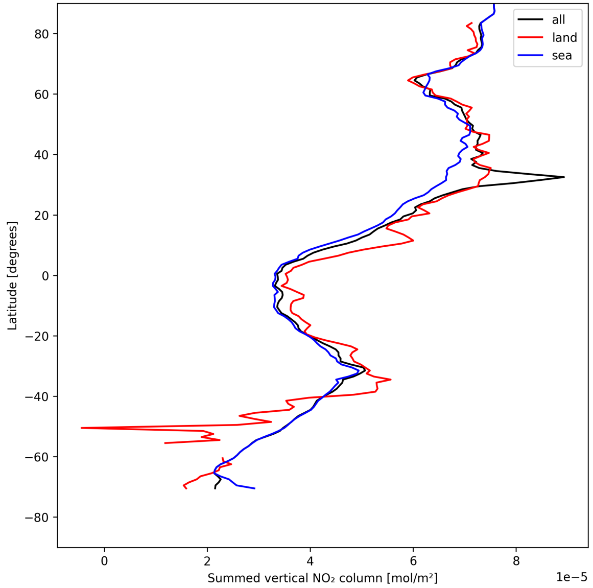
Figure 23: Zonal average of “Summed vertical NO 2 column” for 2025-05-08 to 2025-05-08.
