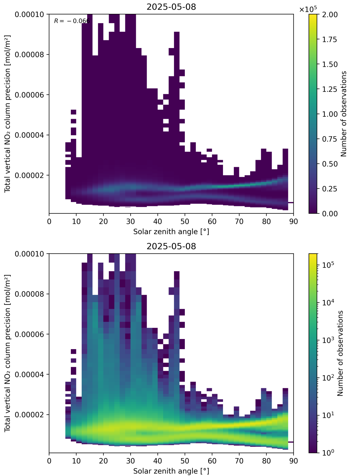
Figure 154: Scatter density plot of “Solar zenith angle” against “Total vertical NO 2 column precision” for 2025-05-08 to 2025-05-08.
