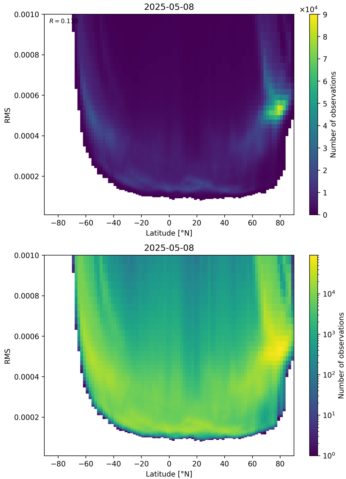
Figure 94: Scatter density plot of “Latitude” against “RMS” for 2025-05-08 to 2025-05-08.
