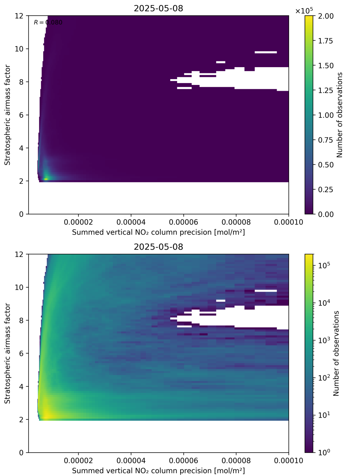
Figure 106: Scatter density plot of “Summed vertical NO 2 column precision” against “Stratospheric airmass factor” for 2025-05-08 to 2025-05-08.
