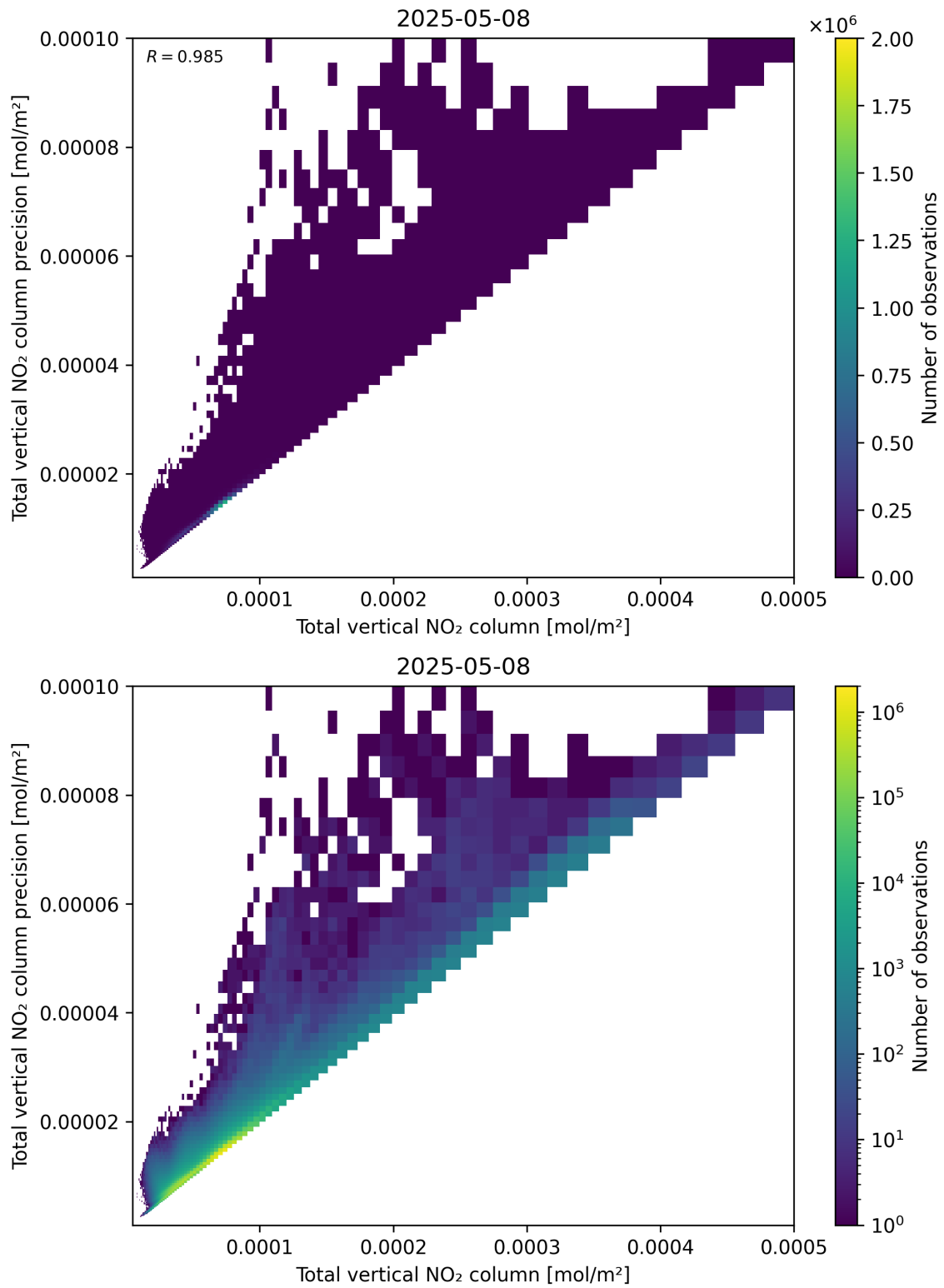
Figure 114: Scatter density plot of “Total vertical NO 2 column” against “Total vertical NO 2 column precision” for 2025-05-08 to 2025-05-08.
