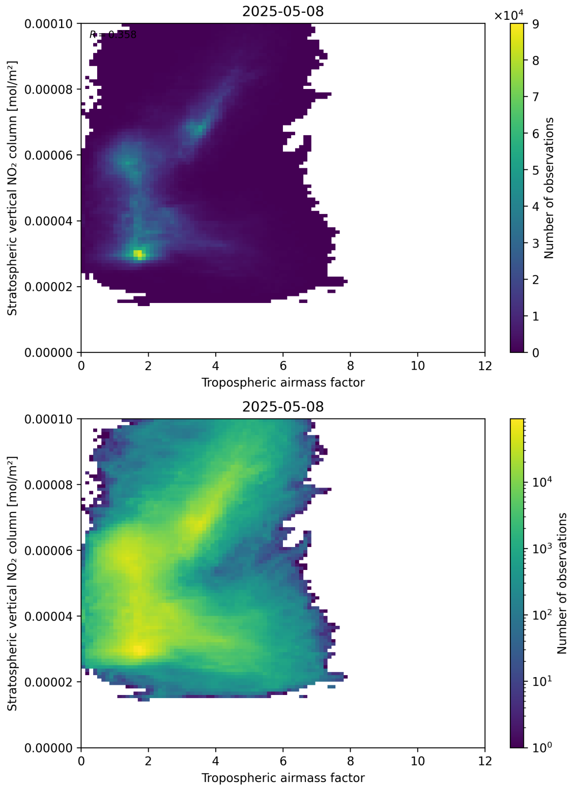
Figure 74: Scatter density plot of “Tropospheric air mass factor” against “Stratospheric vertical NO 2 column” for 2025-05-08 to 2025-05-08.
