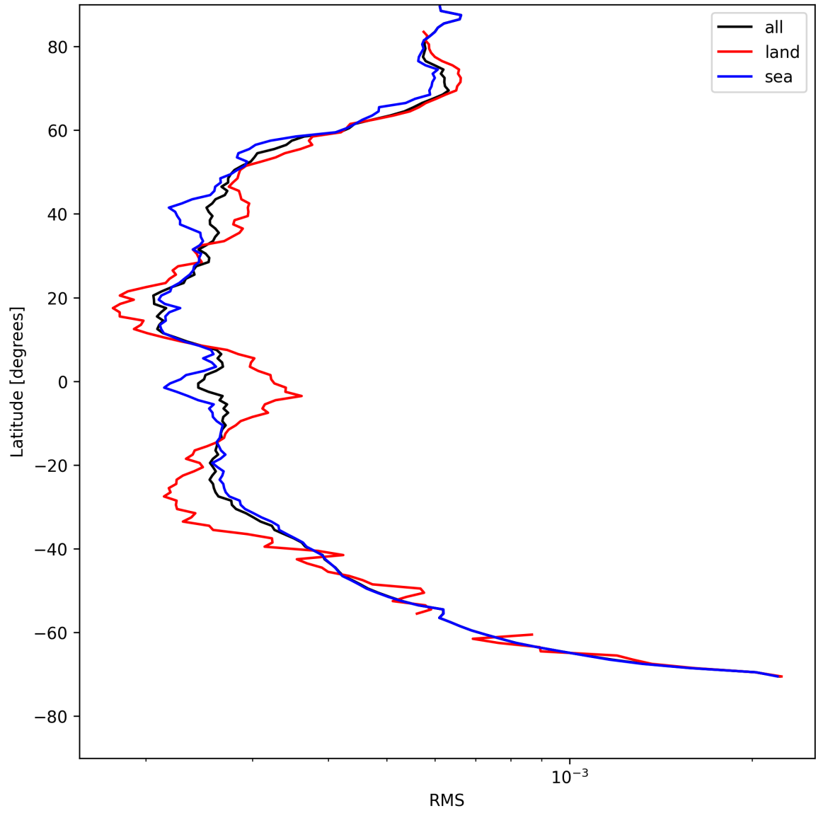
Figure 26: Zonal average of “RMS” for 2025-05-08 to 2025-05-08.
