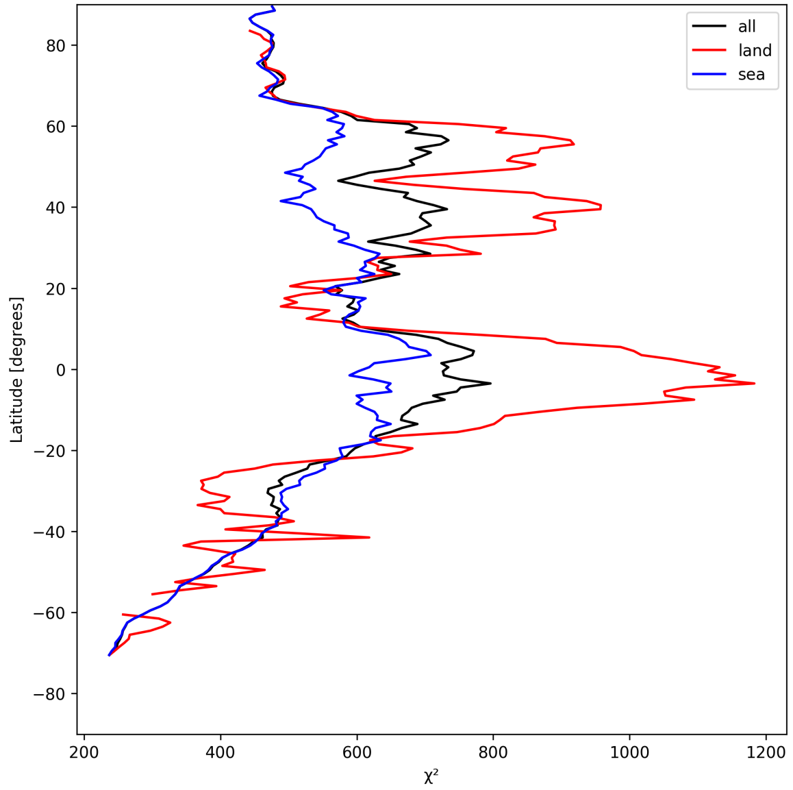
Figure 25: Zonal average of “ \chi^2 ” for 2025-05-08 to 2025-05-08.
