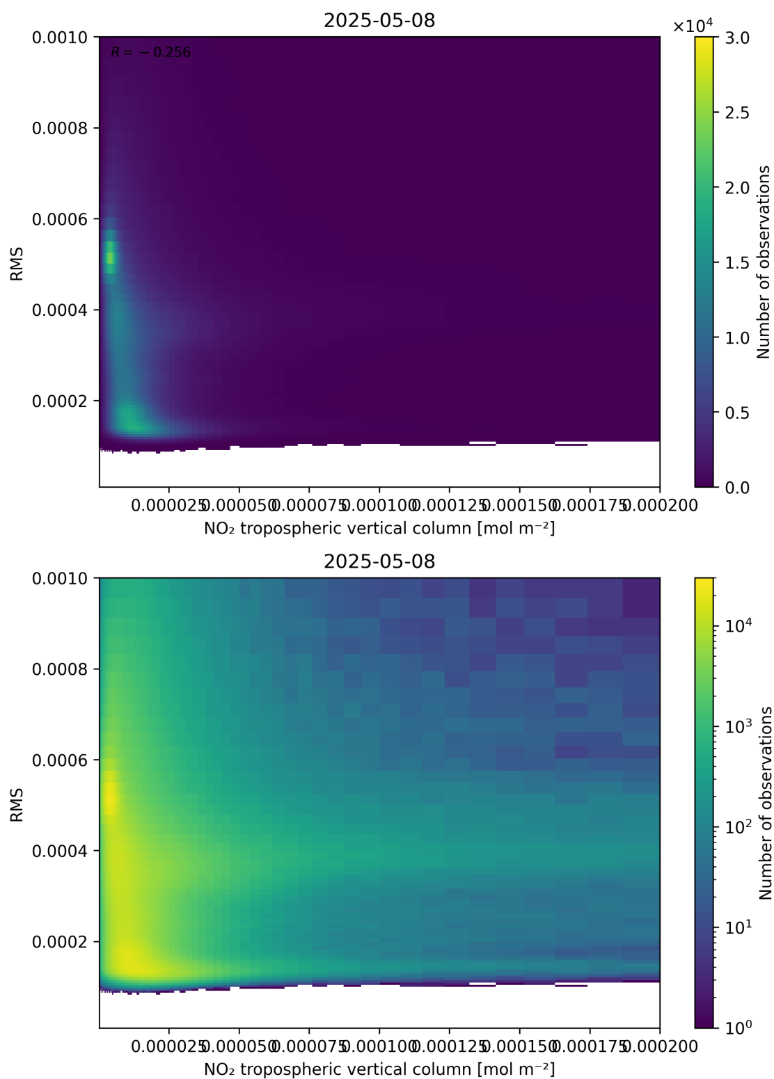
Figure 142: Scatter density plot of “NO 2 tropospheric vertical column” against “RMS” for 2025-05-08 to 2025-05-08.
