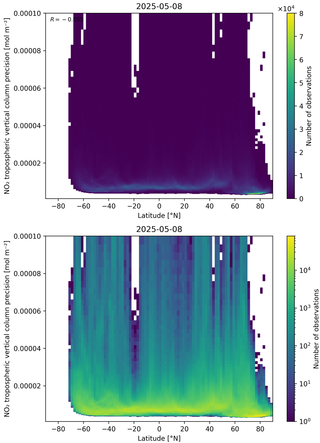
Figure 93: Scatter density plot of “Latitude” against “NO 2 tropospheric vertical column precision” for 2025-05-08 to 2025-05-08.
