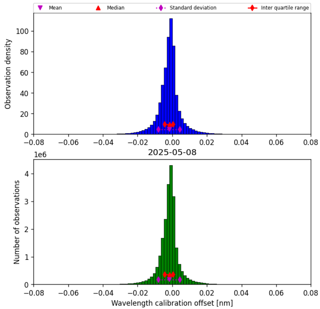
Figure 35: Histogram of “Wavelength calibration offset” for 2025-05-08 to 2025-05-08
