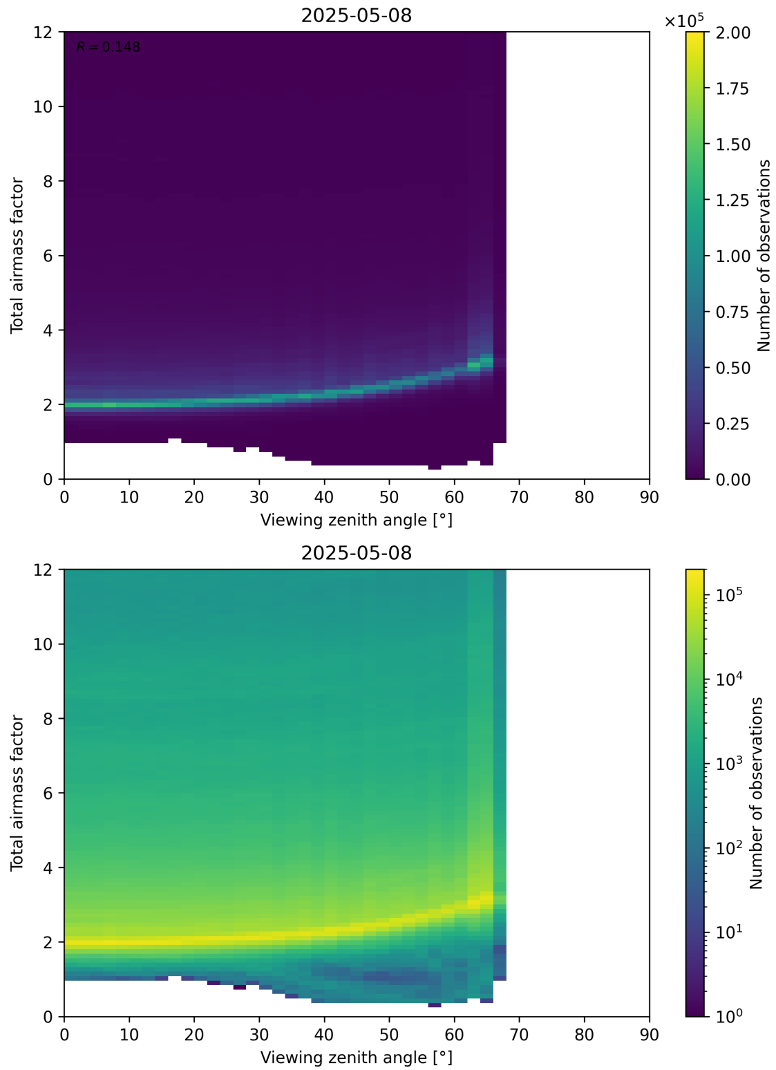
Figure 160: Scatter density plot of “Viewing zenith angle” against “Total airmass factor” for 2025-05-08 to 2025-05-08.
