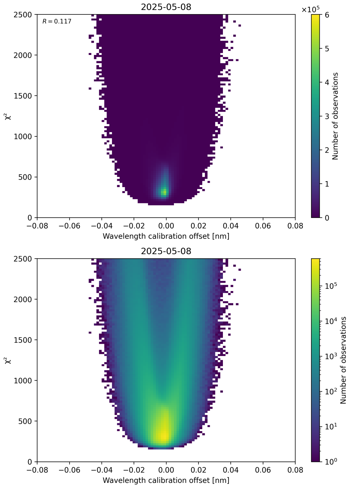
Figure 175: Scatter density plot of “Wavelength calibration offset” against “ \chi^2 ” for 2025-05-08 to 2025-05-08.
