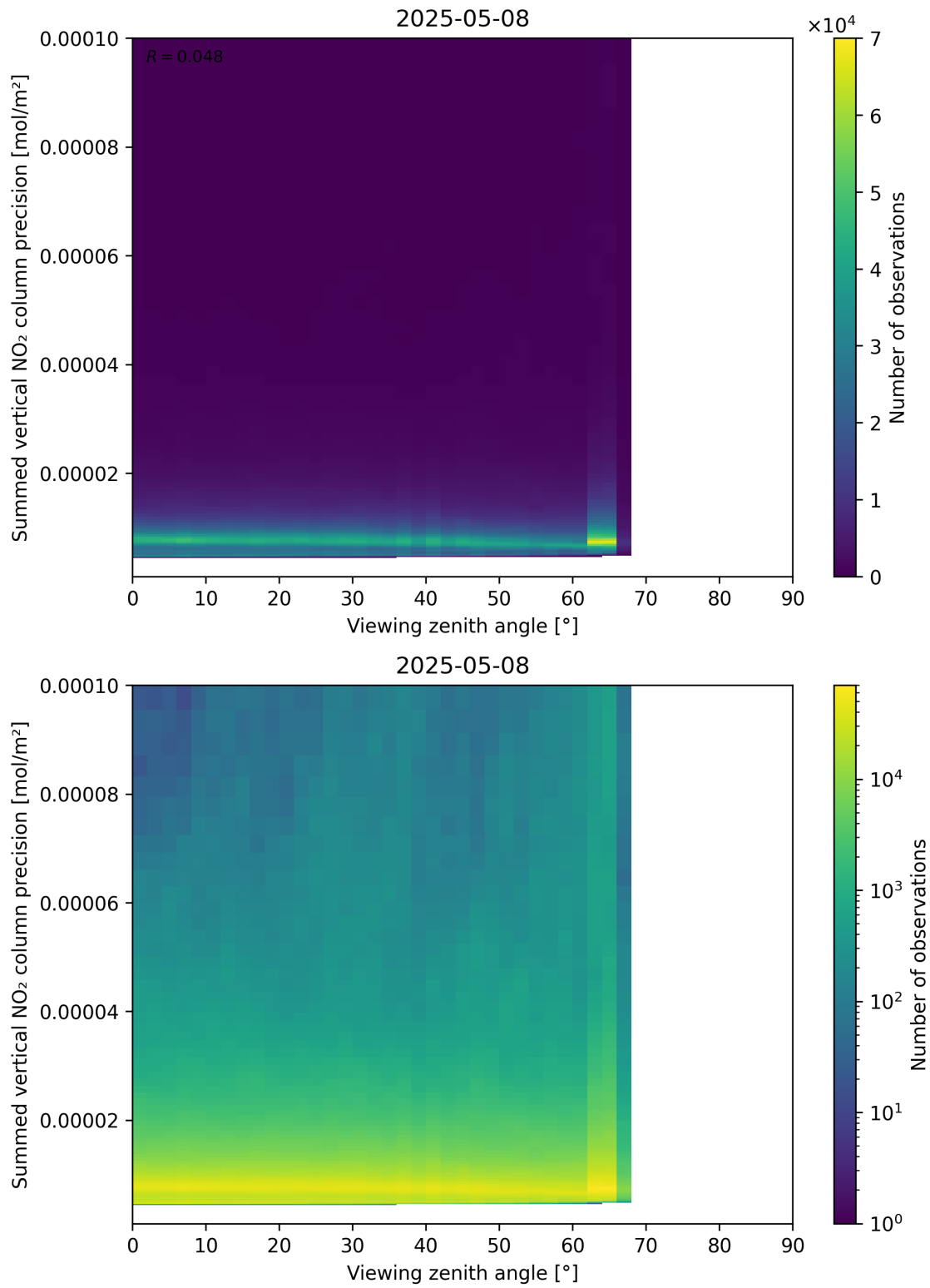
Figure 166: Scatter density plot of “Viewing zenith angle” against “Summed vertical NO 2 column precision” for 2025-05-08 to 2025-05-08.
