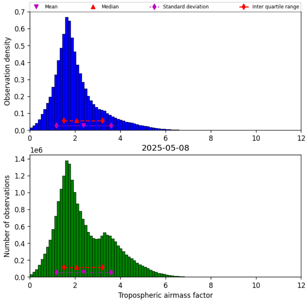
Figure 31: Histogram of “Tropospheric airmass factor” for 2025-05-08 to 2025-05-08
