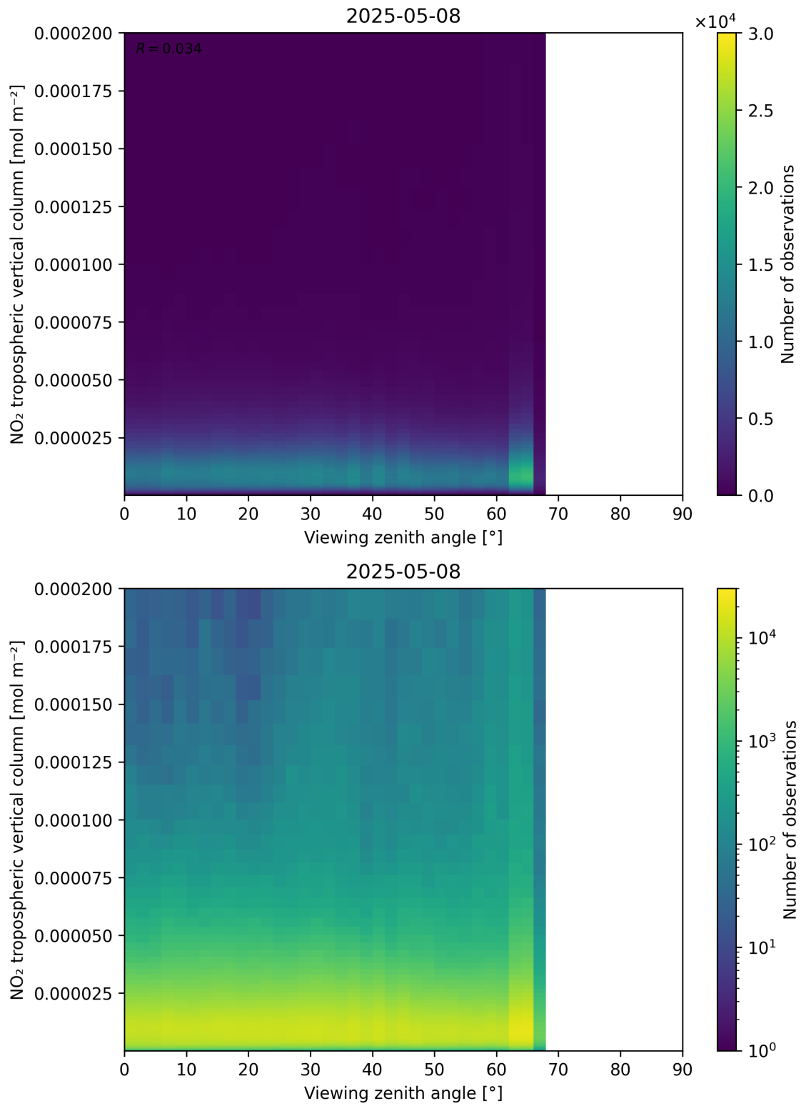
Figure 169: Scatter density plot of “Viewing zenith angle” against “NO 2 tropospheric vertical column” for 2025-05-08 to 2025-05-08.
