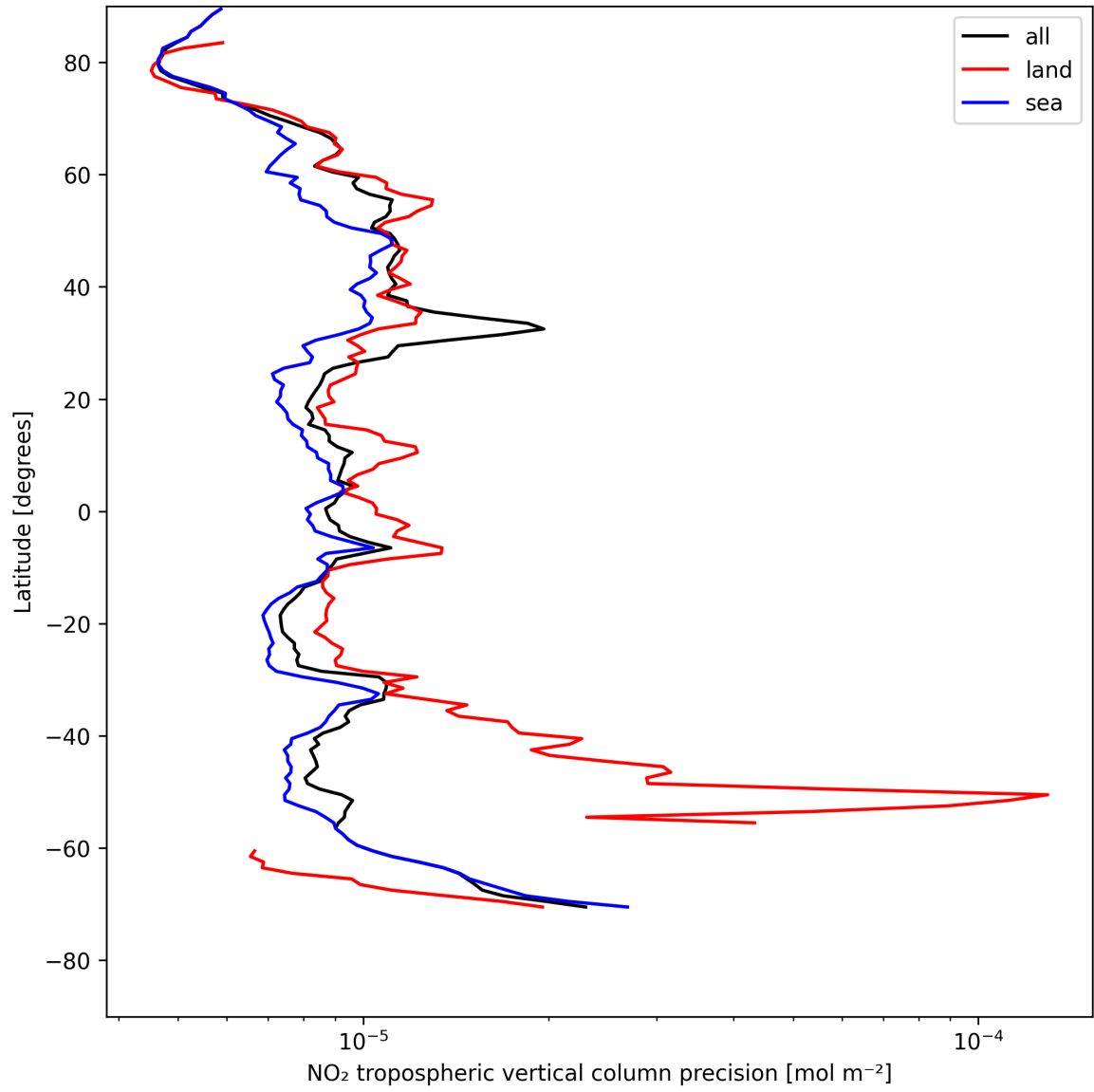
Figure 13: Zonal average of “NO 2 tropospheric vertical column precision” for 2025-05-08 to 2025-05-08.
