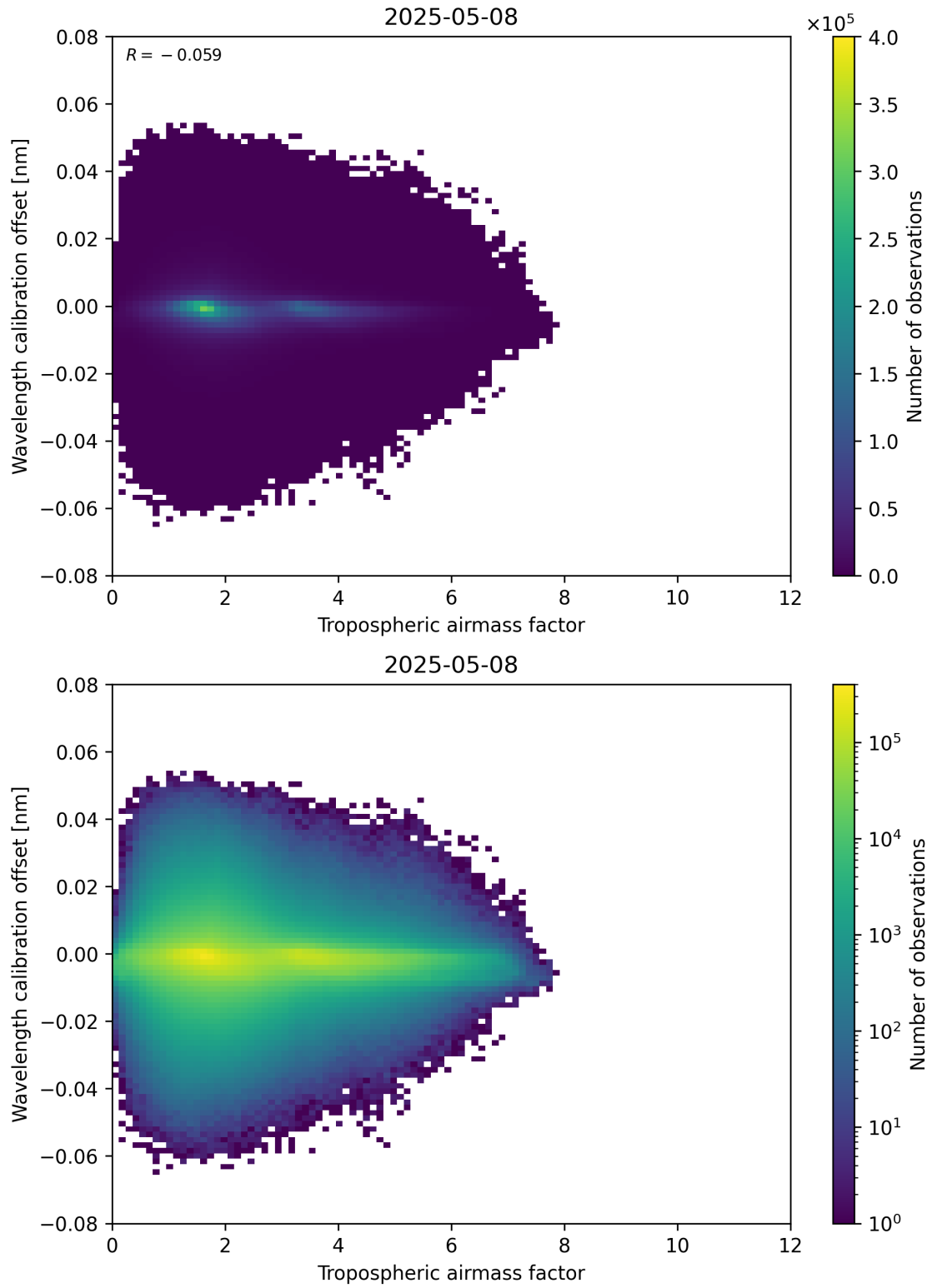
Figure 80: Scatter density plot of “Tropospheric airmass factor” against “Wavelength calibration offset” for 2025-05-08 to 2025-05-08.
