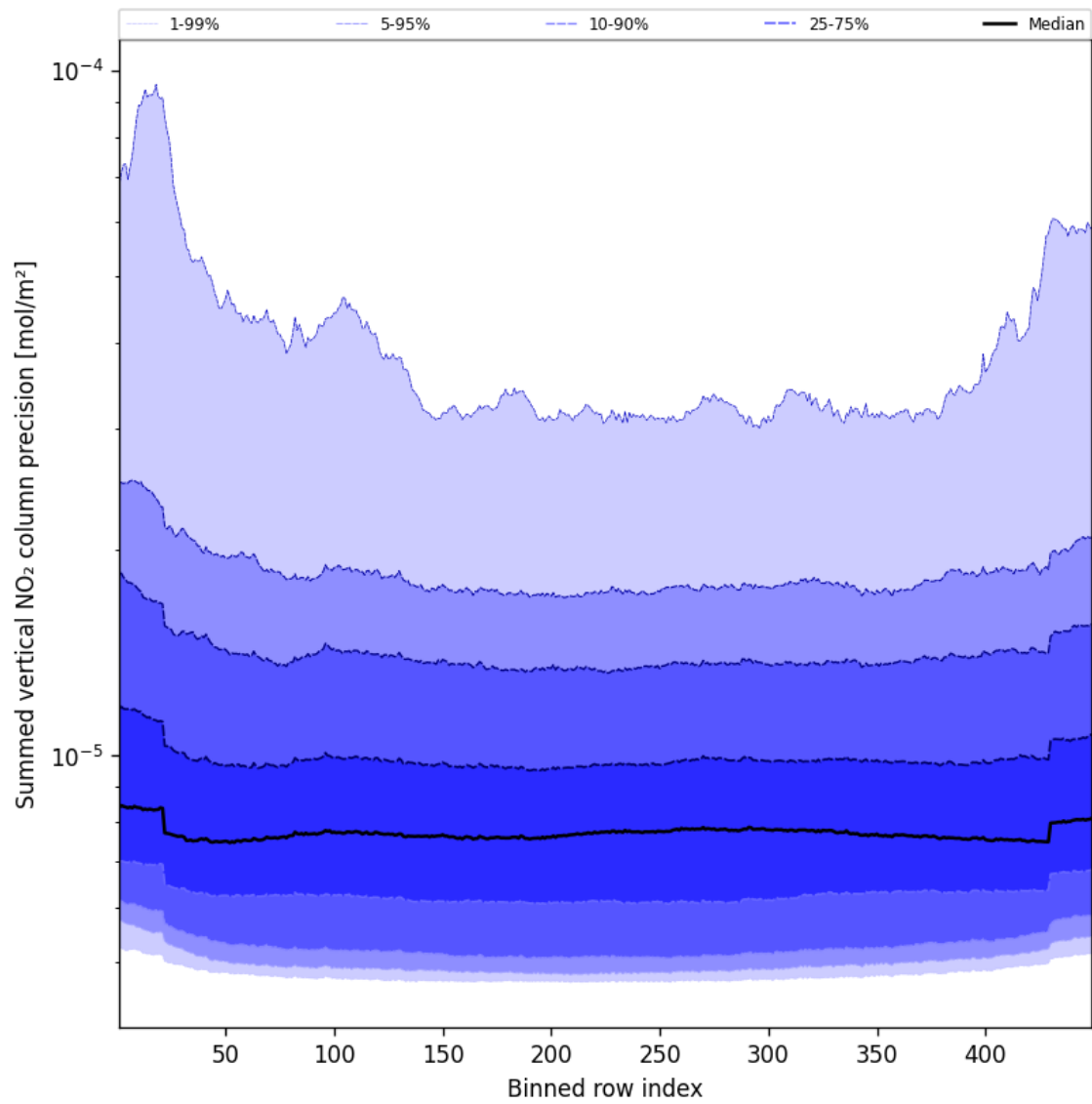
Figure 58: Along track statistics of “Summed vertical NO 2 column precision” for 2025-05-08 to 2025-05-08
