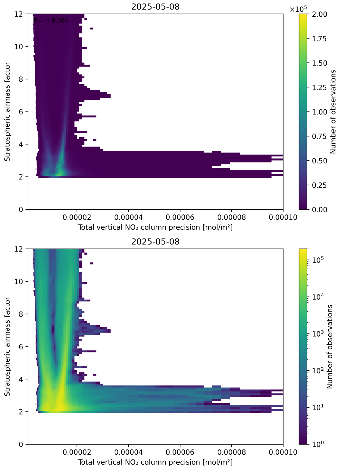
Figure 115: Scatter density plot of “Total vertical NO 2 column precision” against “Stratospheric air mass factor” for 2025-05-08 to 2025-05-08.
