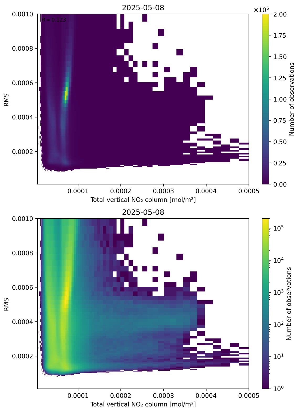
Figure 120: Scatter density plot of “Total vertical NO 2 column” against “RMS” for 2025-05-08 to 2025-05-08.
