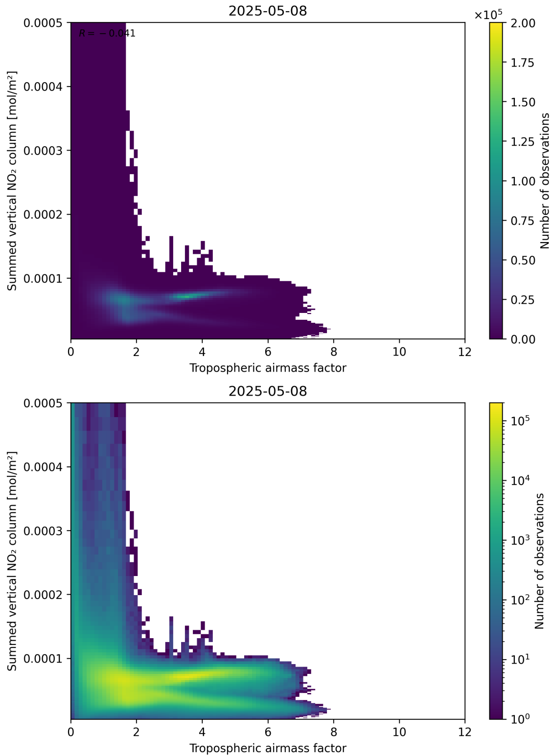
Figure 75: Scatter density plot of “Tropospheric airmass factor” against “Summed vertical NO 2 column” for 2025-05-08 to 2025-05-08.
