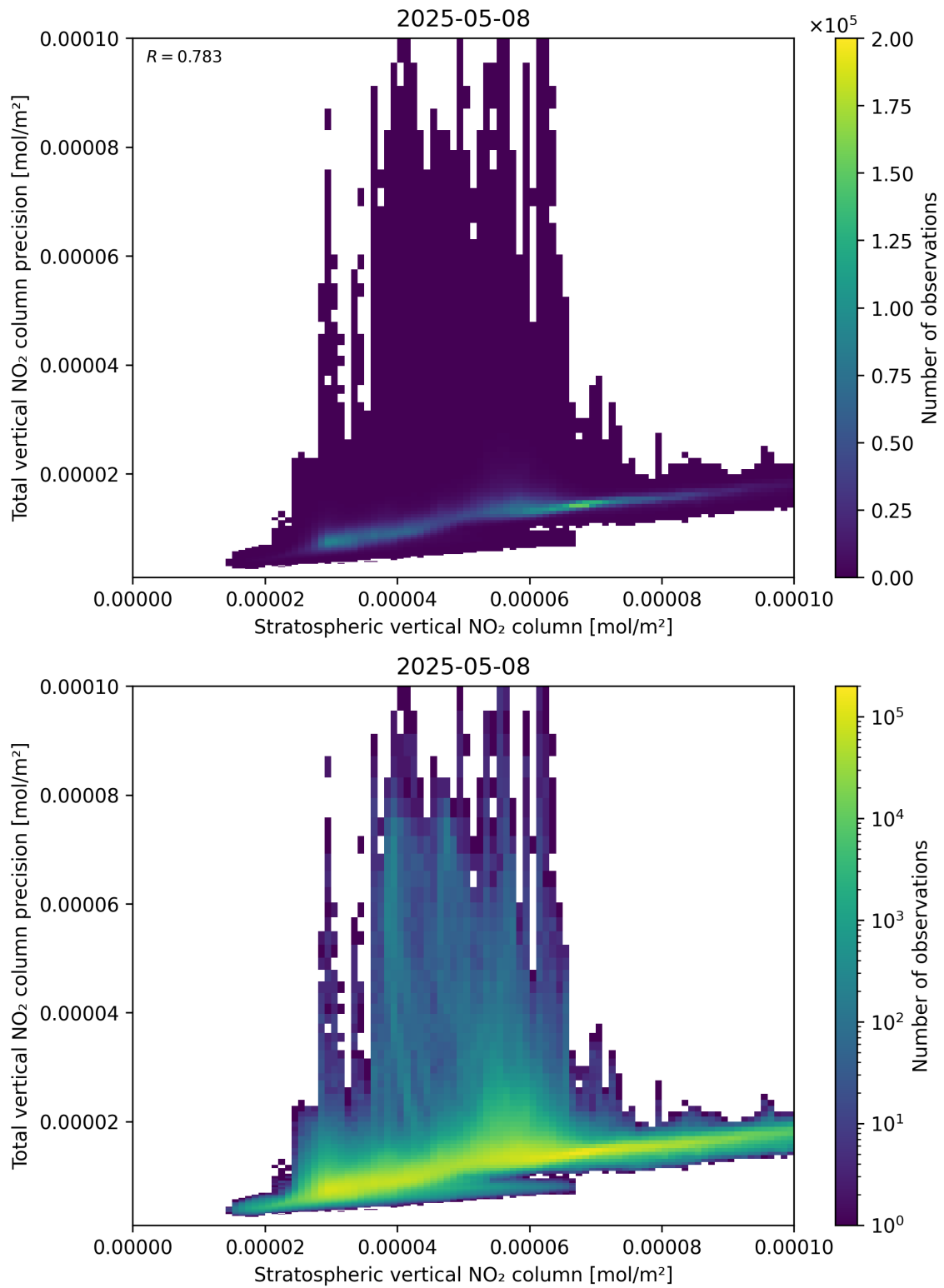
Figure 101: Scatter density plot of “Stratospheric vertical NO 2 column” against “Total vertical NO 2 column precision” for 2025-05-08 to 2025-05-08.
