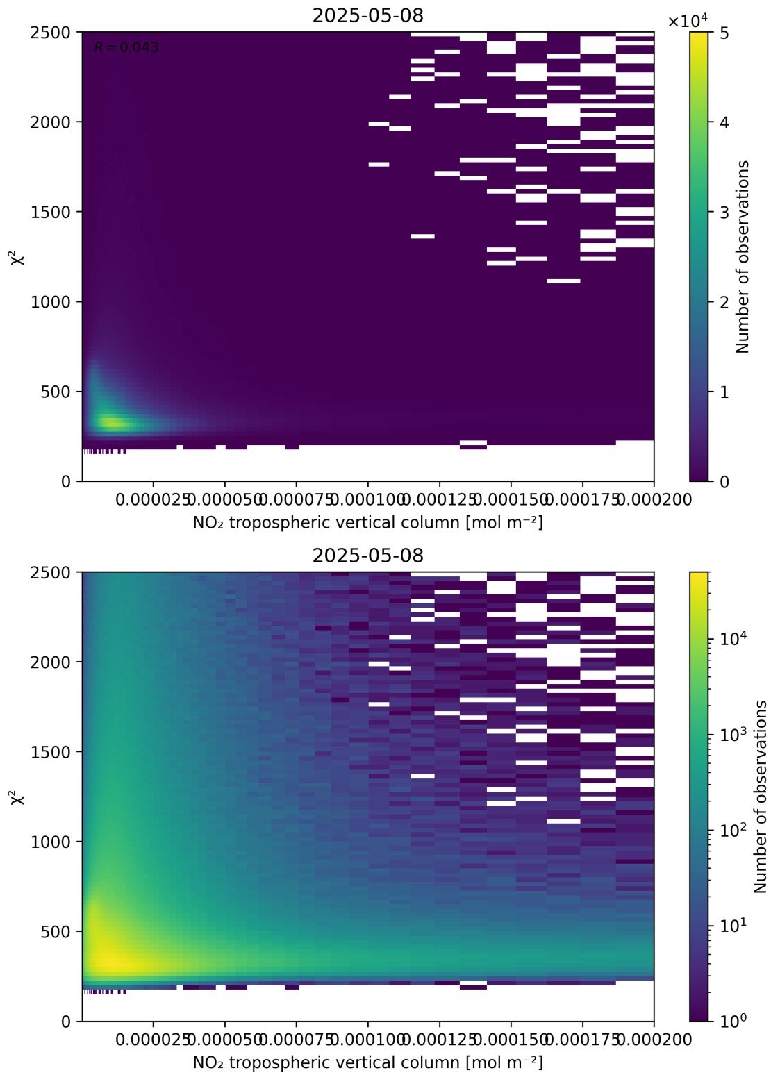
Figure 124: Scatter density plot of “NO 2 tropospheric vertical column” against “ \chi^2 ” for 2025-05-08 to 2025-05-08.
