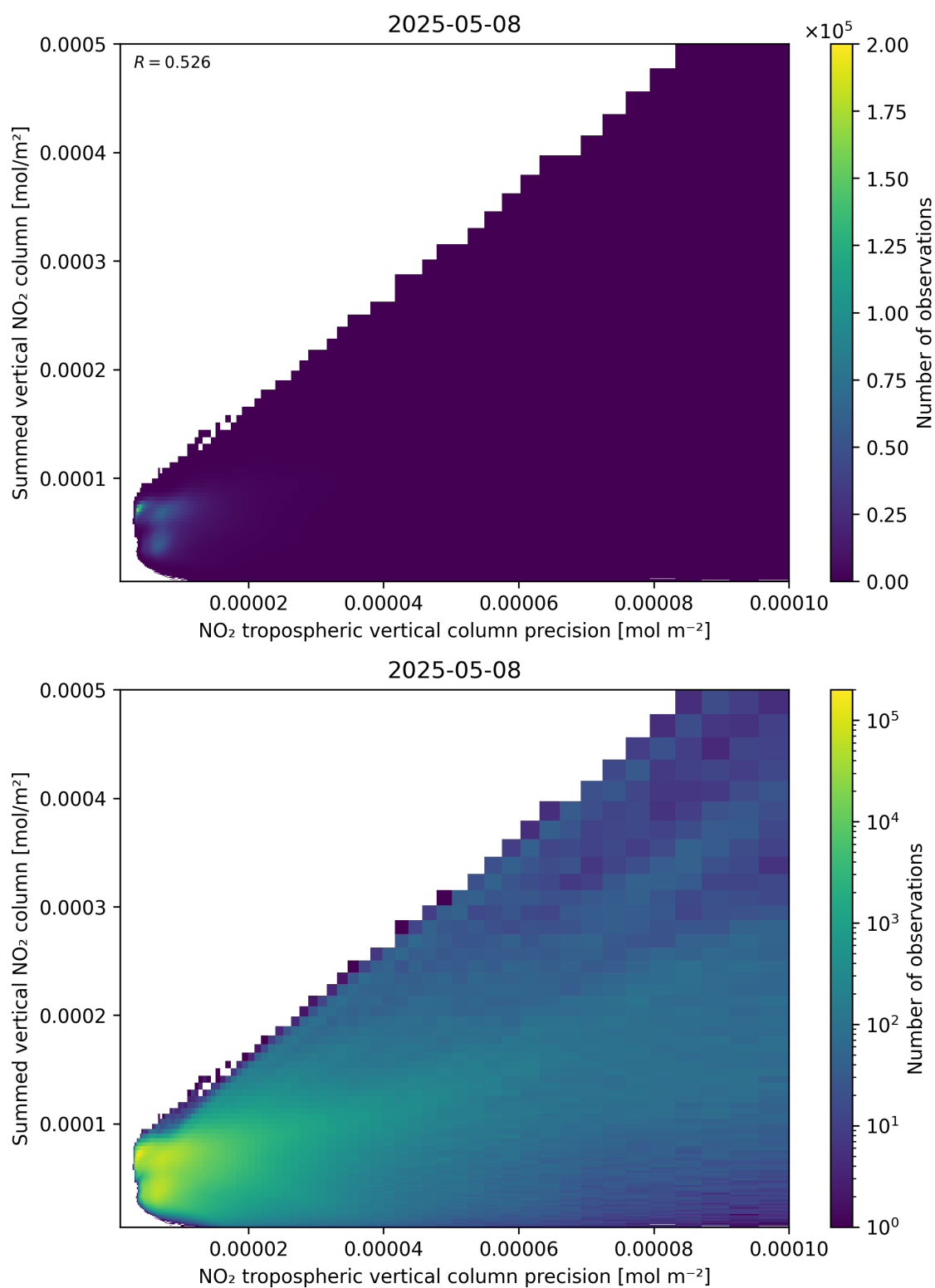
Figure 136: Scatter density plot of “NO 2 tropospheric vertical column precision” against “Summed vertical NO 2 column” for 2025-05-08 to 2025-05-08.
