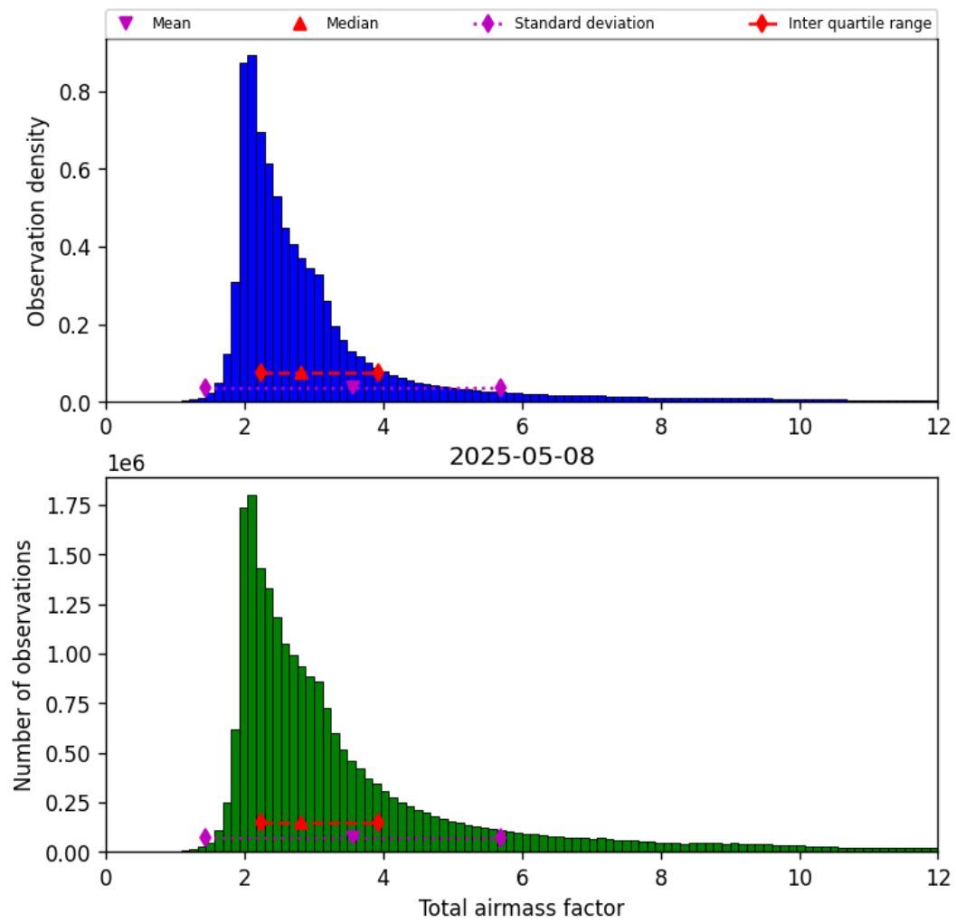
Figure 32: Histogram of “Total airmass factor” for 2025-05-08 to 2025-05-08
