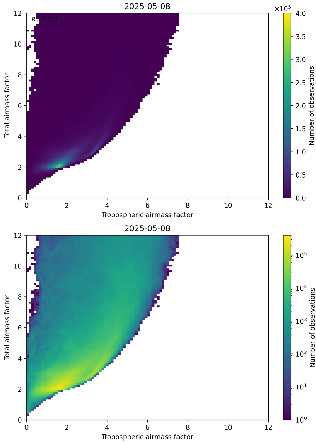
Figure 72: Scatter density plot of “Tropospheric airmass factor” against “Total airmass factor” for 2025-05-08 to 2025-05-08.
