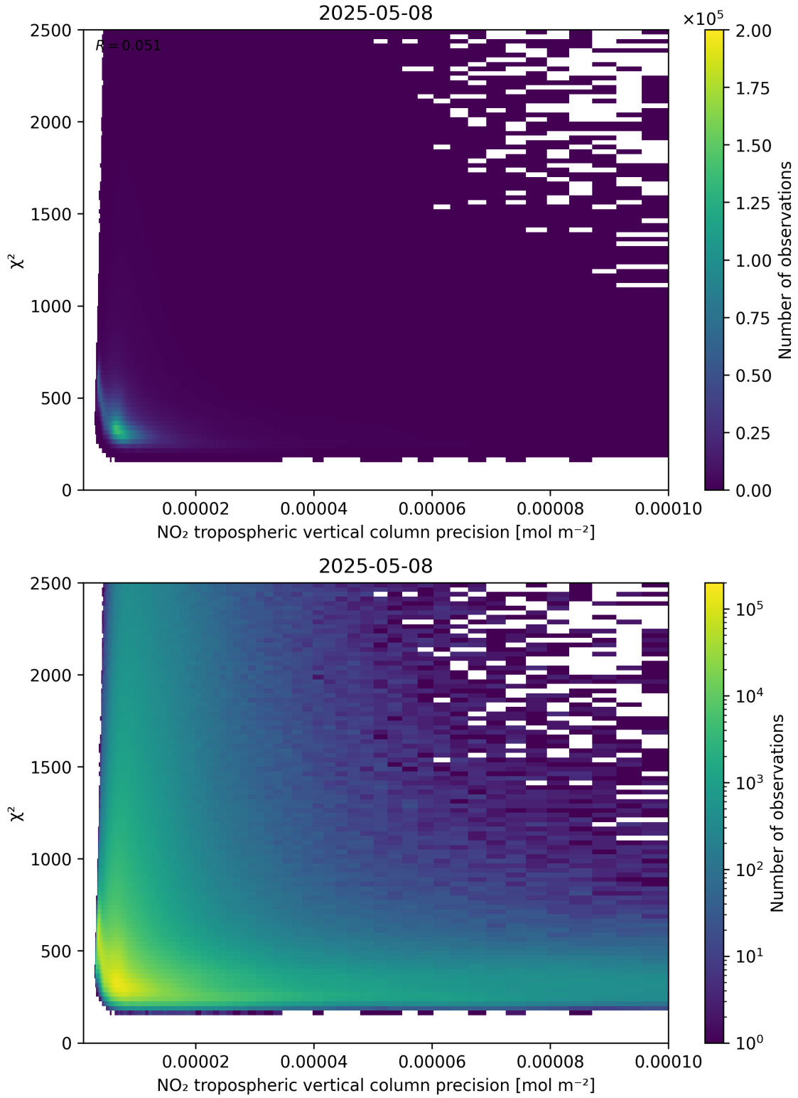
Figure 134: Scatter density plot of “NO 2 tropospheric vertical column precision” against “ \chi^2 ” for 2025-05-08 to 2025-05-08.
