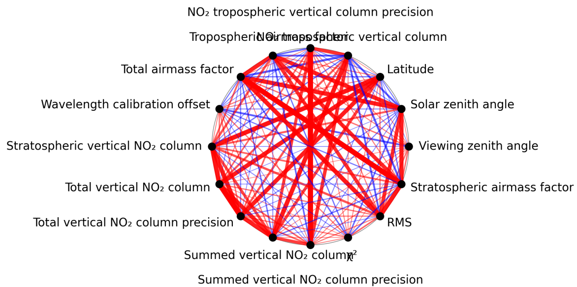
Figure 1: Map of correlation graph for 2025-05-08 to 2025-05-08.
