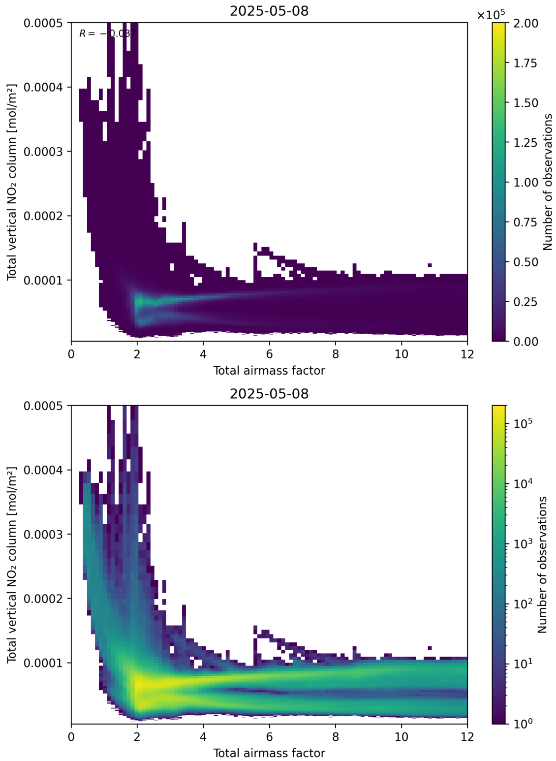
Figure 67: Scatter density plot of “Total airmass factor” against “Total vertical NO 2 column” for 2025-05-08 to 2025-05-08.
