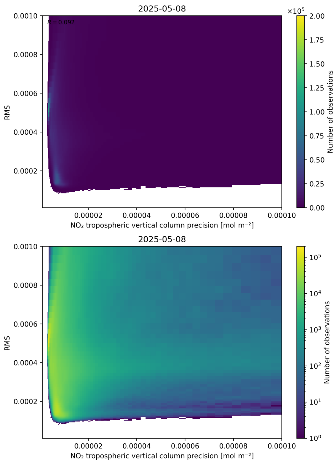
Figure 140: Scatter density plot of “NO 2 tropospheric vertical column precision” against “RMS” for 2025-05-08 to 2025-05-08.
