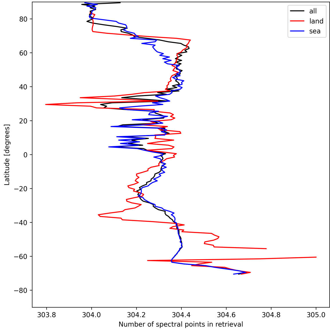
Figure 16: Zonal average of “Number of spectral points in retrieval” for 2025-05-08 to 2025-05-08.
