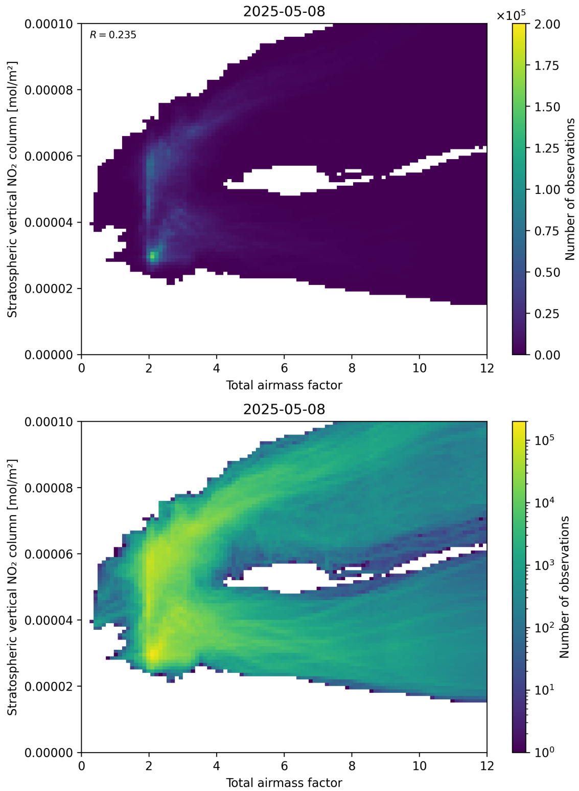
Figure 64: Scatter density plot of “Total airmass factor” against “Stratospheric vertical NO 2 column” for 2025-05-08 to 2025-05-08.
