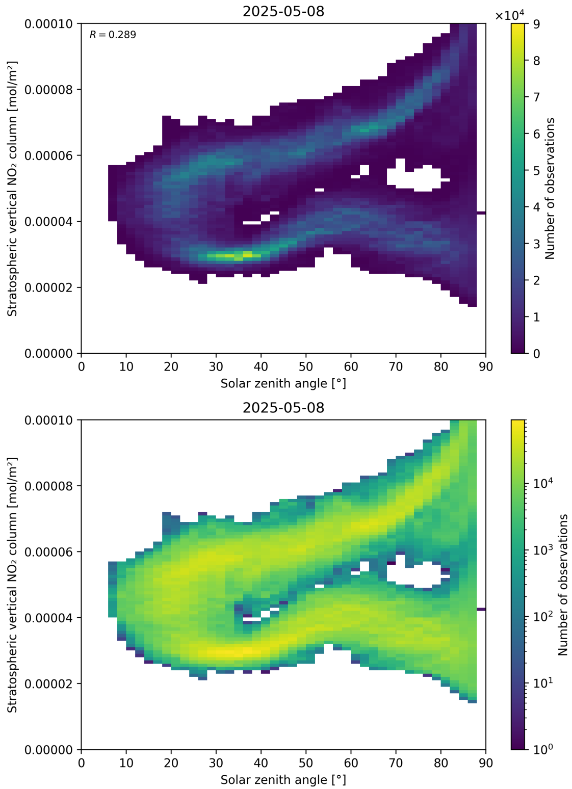
Figure 150: Scatter density plot of “Solar zenith angle” against “Stratospheric vertical NO 2 column” for 2025-05-08 to 2025-05-08.
