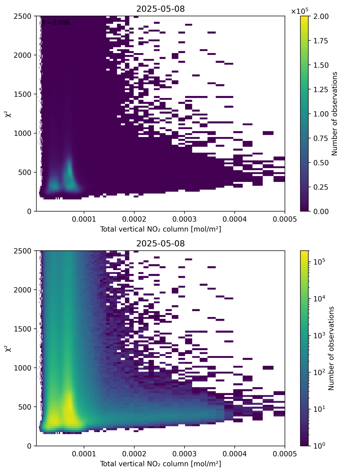
Figure 111: Scatter density plot of “Total vertical NO 2 column” against “ \chi^2 ” for 2025-05-08 to 2025-05-08.
