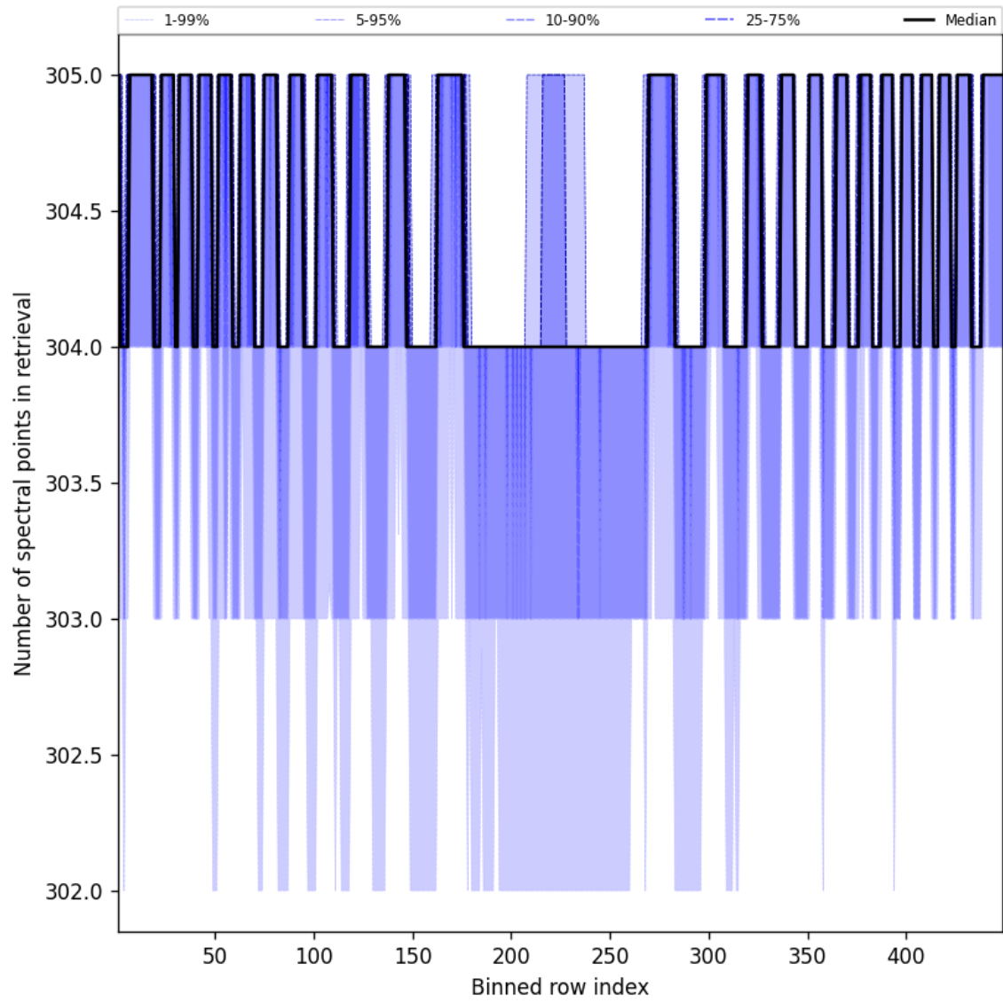
Figure 50: Along track statistics of “Number of spectral points in retrieval” for 2025-05-08 to 2025-05-08
