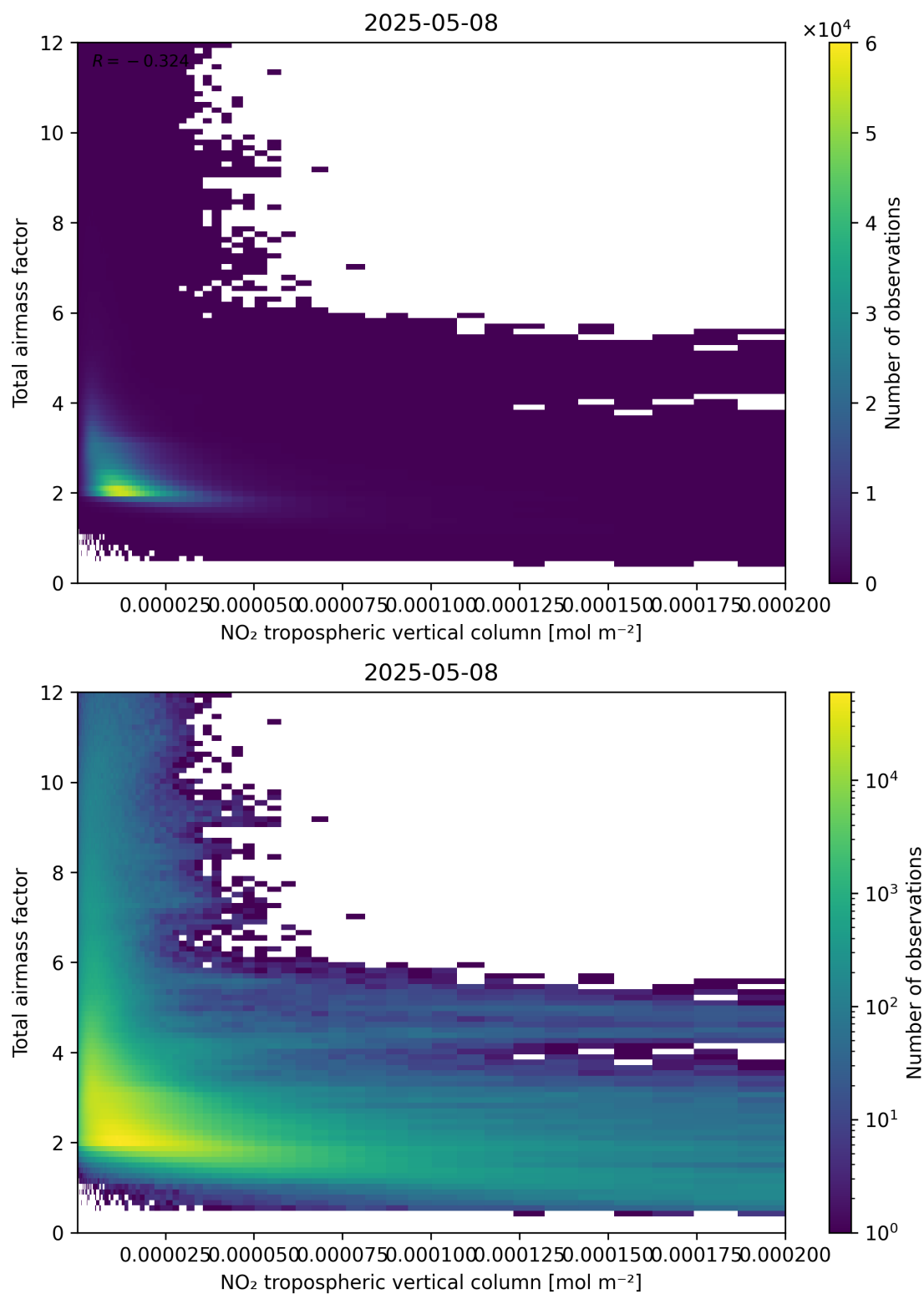
Figure 122: Scatter density plot of “NO 2 tropospheric vertical column” against “Total air mass factor” for 2025-05-08 to 2025-05-08.
