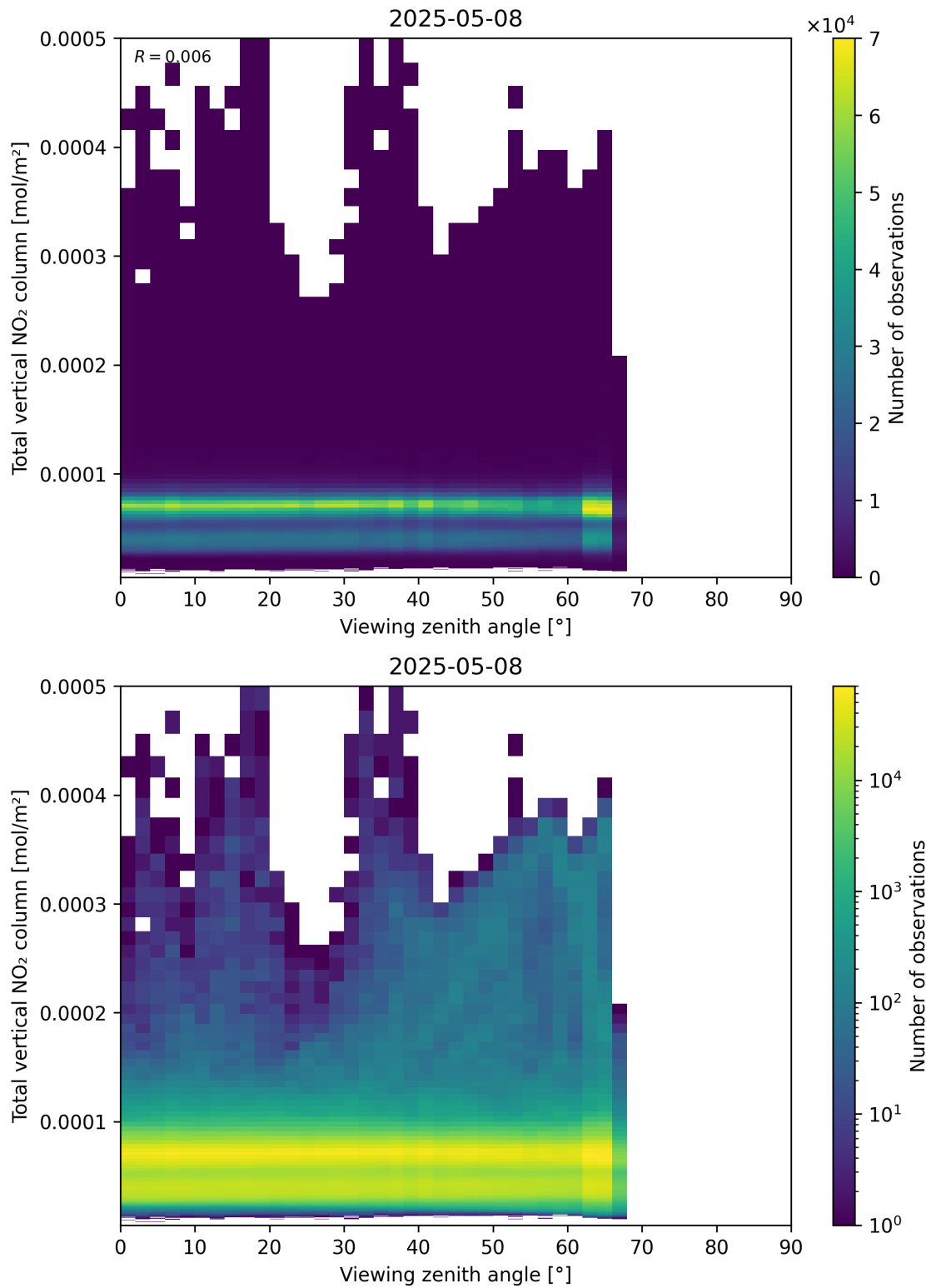
Figure 167: Scatter density plot of “Viewing zenith angle” against “Total vertical NO 2 column” for 2025-05-08 to 2025-05-08.
