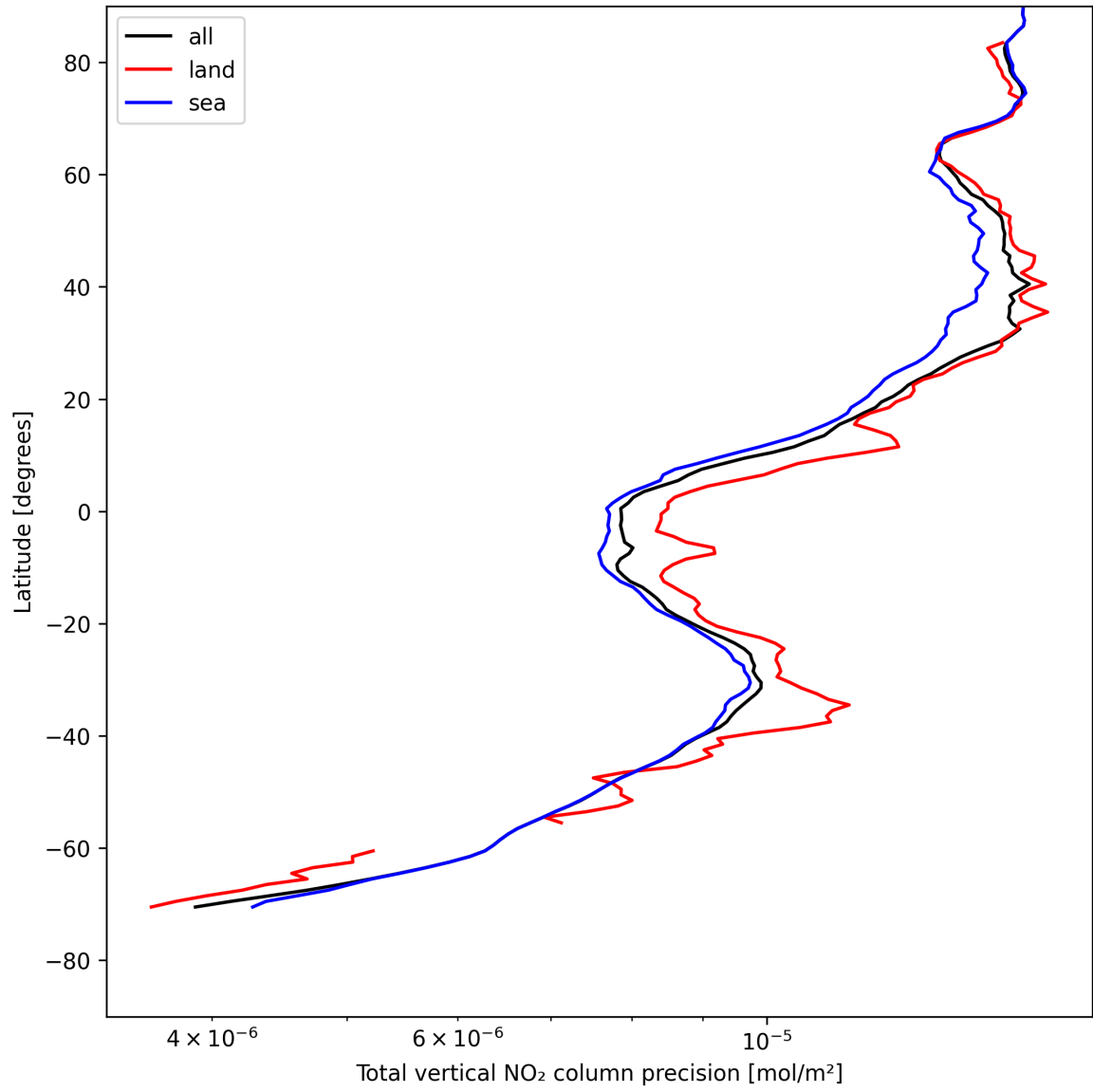
Figure 22: Zonal average of “Total vertical NO 2 column precision” for 2025-05-08 to 2025-05-08.
