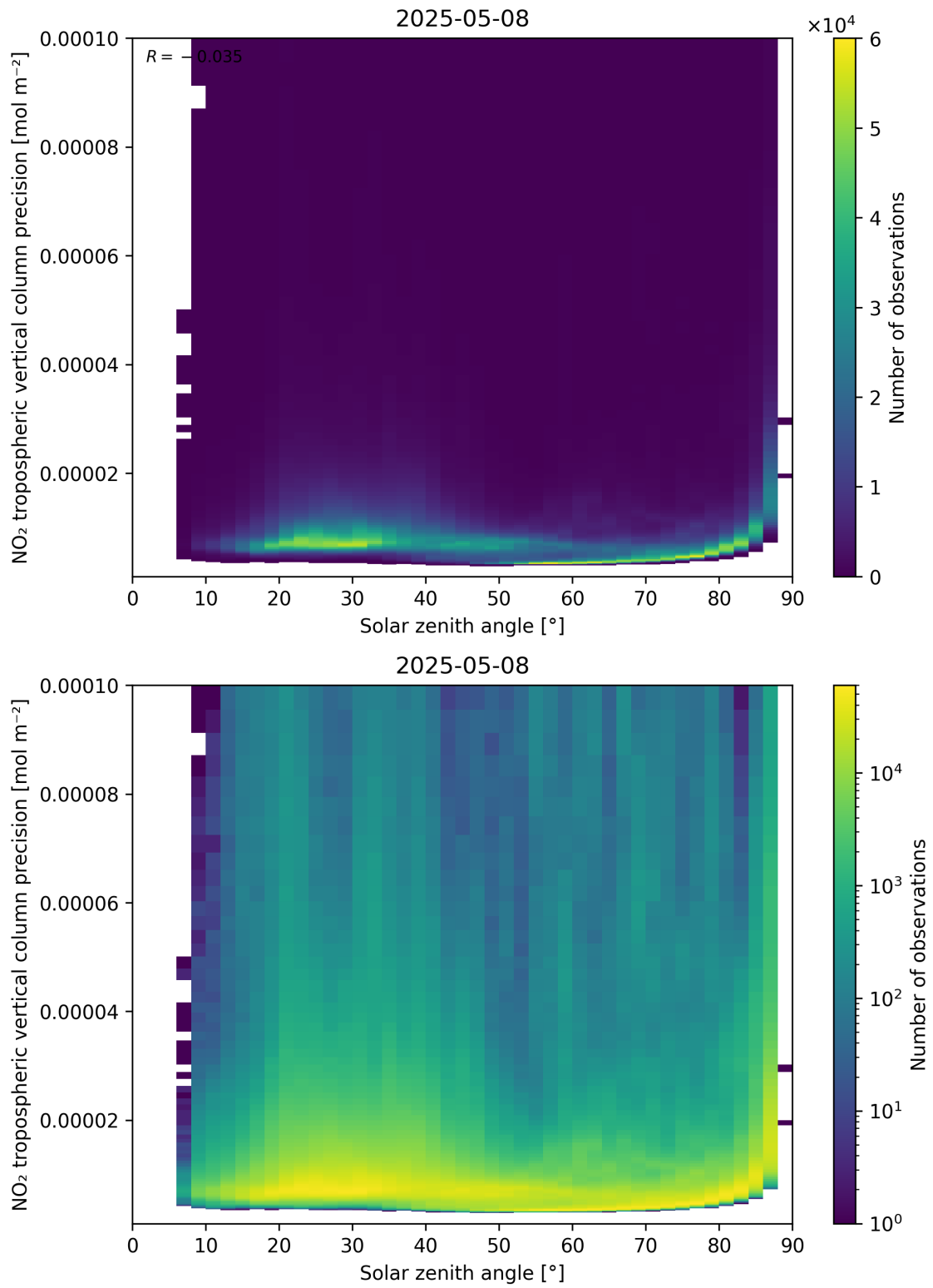
Figure 156: Scatter density plot of “Solar zenith angle” against “NO 2 tropospheric vertical column precision” for 2025-05-08 to 2025-05-08.
