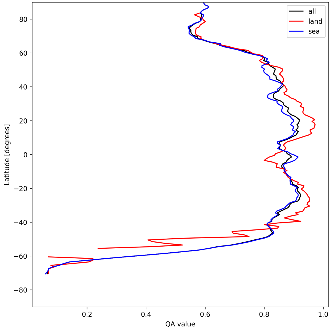
Figure 11: Zonal average of “QA value” for 2025-05-08 to 2025-05-08.
