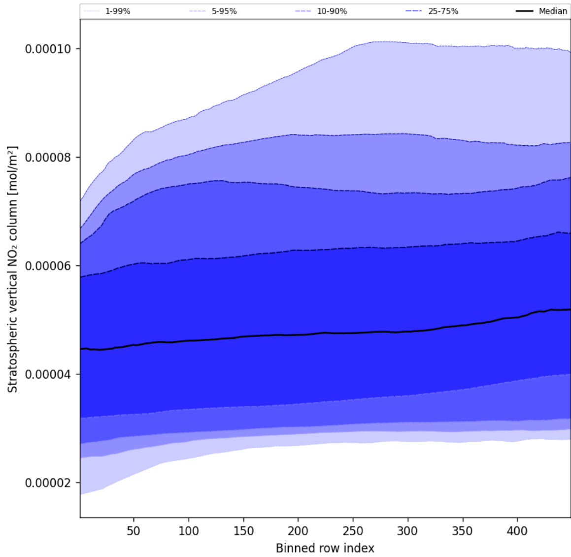
Figure 53: Along track statistics of “Stratospheric vertical NO 2 column” for 2025-05-08 to 2025-05-08
