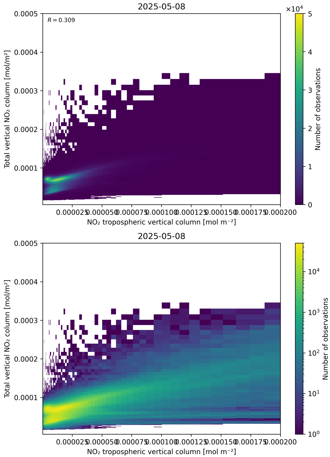
Figure 128: Scatter density plot of “NO 2 tropospheric vertical column” against “Total vertical NO 2 column” for 2025-05-08 to 2025-05-08.
