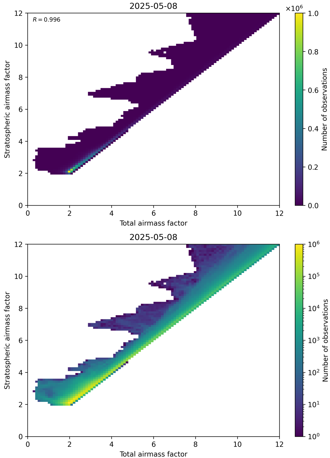
Figure 62: Scatter density plot of “Total airmass factor” against “Stratospheric airmass factor” for 2025-05-08 to 2025-05-08.
