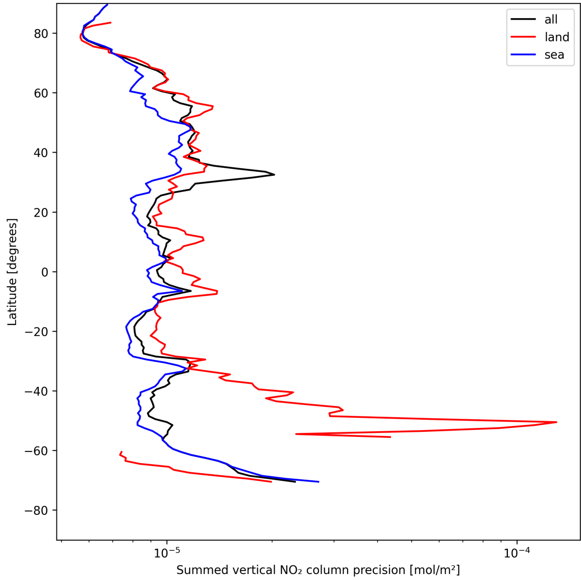
Figure 24: Zonal average of “Summed vertical NO 2 column precision” for 2025-05-08 to 2025-05-08.
