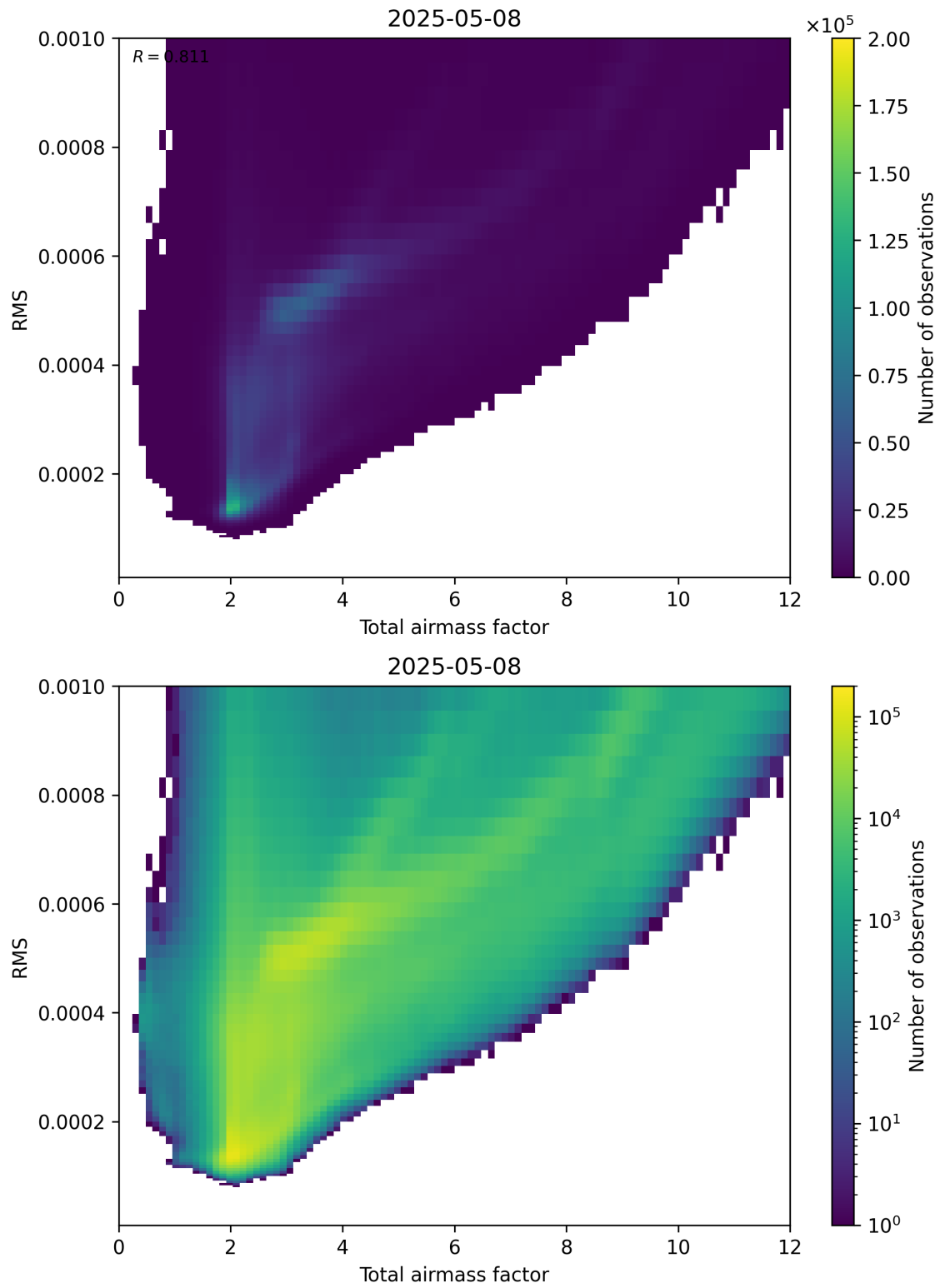
Figure 69: Scatter density plot of “Total airmass factor” against “RMS” for 2025-05-08 to 2025-05-08.
