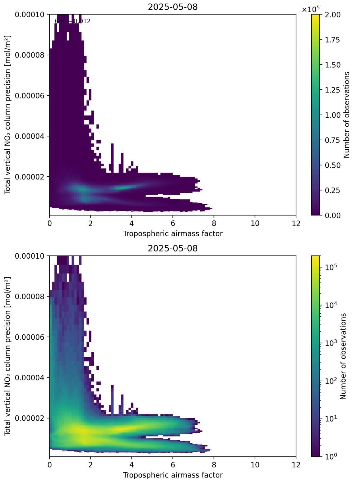
Figure 78: Scatter density plot of “Tropospheric air mass factor” against “Total vertical NO 2 column precision” for 2025-05-08 to 2025-05-08.
