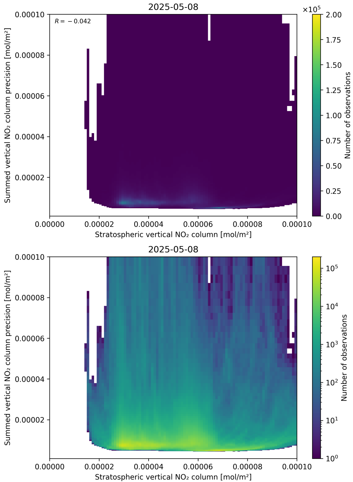
Figure 99: Scatter density plot of “Stratospheric vertical NO 2 column” against “Summed vertical NO 2 column precision” for 2025-05-08 to 2025-05-08.
