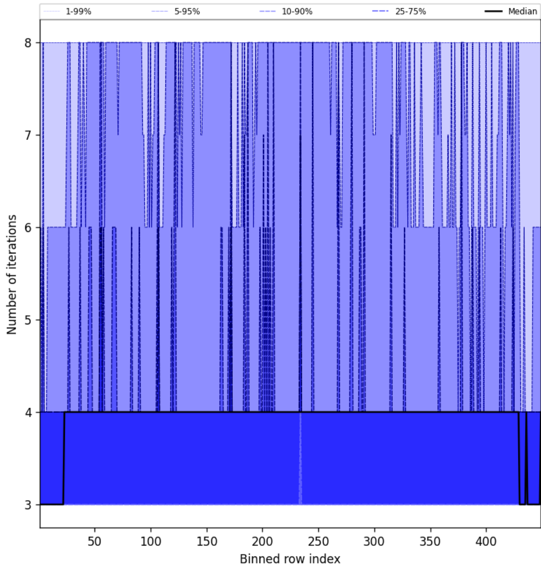
Figure 51: Along track statistics of "Number of iterations" for 2025-05-08 to 2025-05-08
