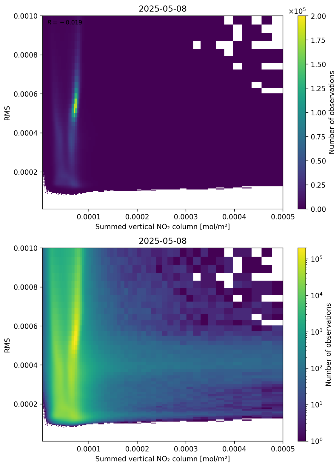
Figure 109: Scatter density plot of “Summed vertical NO 2 column” against “RMS” for 2025-05-08 to 2025-05-08.
