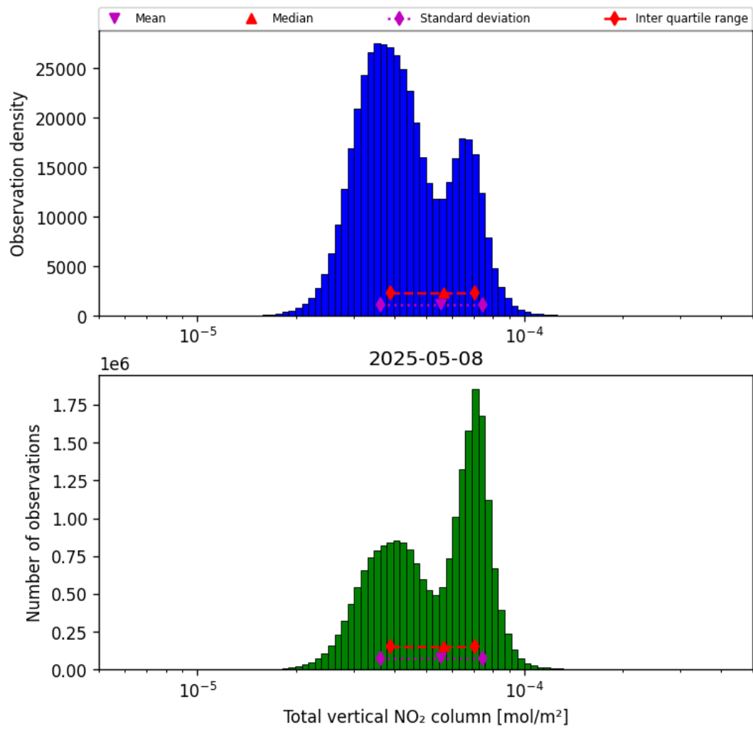
Figure 38: Histogram of “Total vertical NO 2 column” for 2025-05-08 to 2025-05-08
