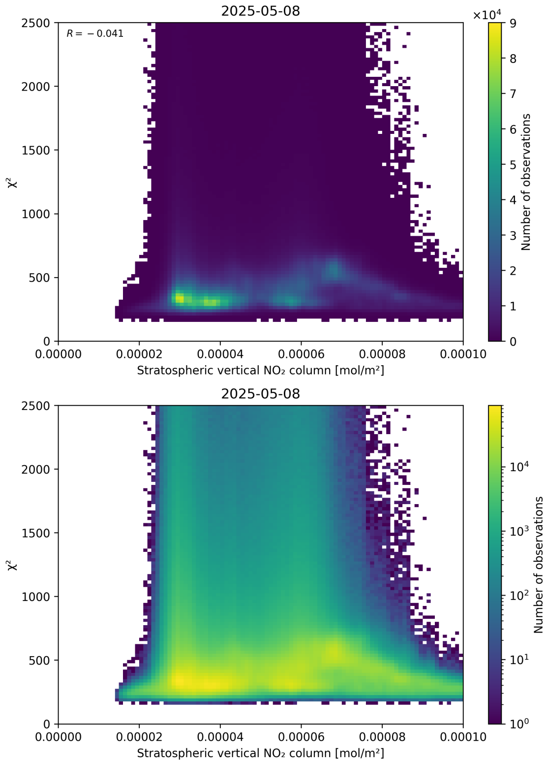
Figure 97: Scatter density plot of “Stratospheric vertical NO 2 column” against “ \chi^2 ” for 2025-05-08 to 2025-05-08.
