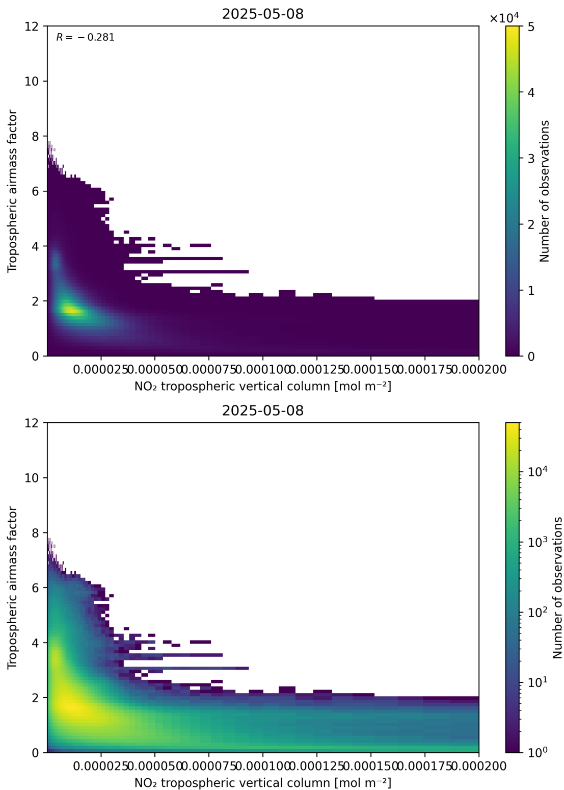
Figure 123: Scatter density plot of “NO 2 tropospheric vertical column” against “Tropospheric air mass factor” for 2025-05-08 to 2025-05-08.
