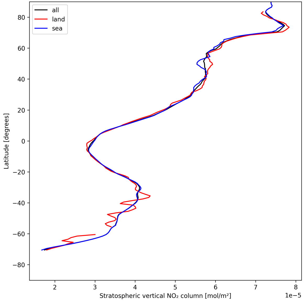
Figure 19: Zonal average of “Stratospheric vertical NO 2 column” for 2025-05-08 to 2025-05-08.
