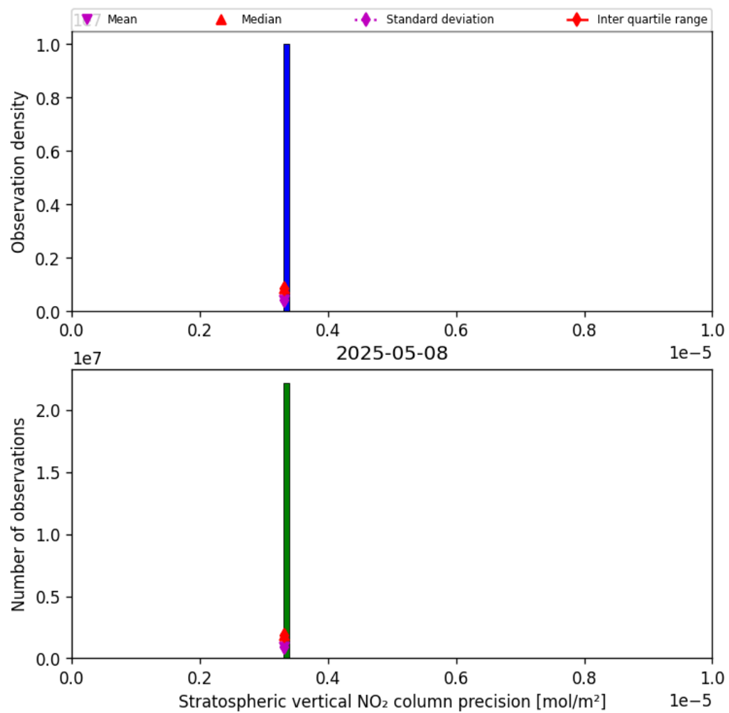
Figure 37: Histogram of “Stratospheric vertical NO 2 column precision” for 2025-05-08 to 2025-05-08
