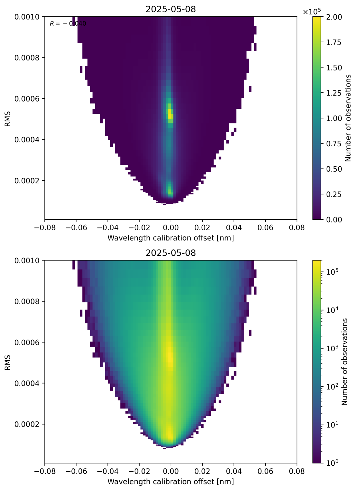
Figure 181: Scatter density plot of “Wavelength calibration offset” against “RMS” for 2025-05-08 to 2025-05-08.
