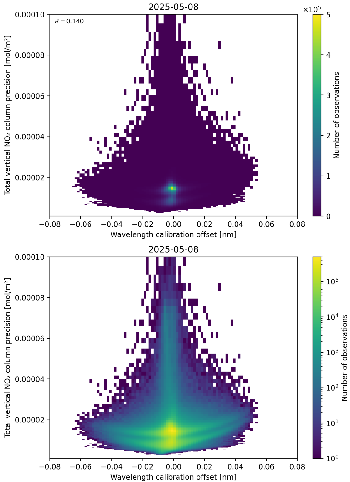
Figure 180: Scatter density plot of “Wavelength calibration offset” against “Total vertical NO 2 column precision” for 2025-05-08 to 2025-05-08.
