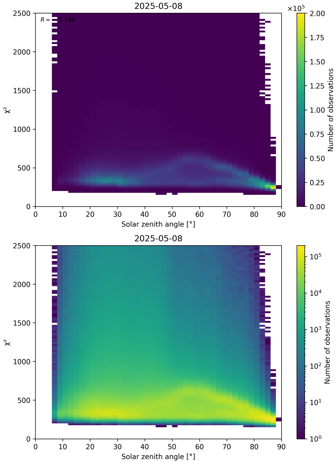
Figure 148: Scatter density plot of “Solar zenith angle” against “ \chi^2 ” for 2025-05-08 to 2025-05-08.
