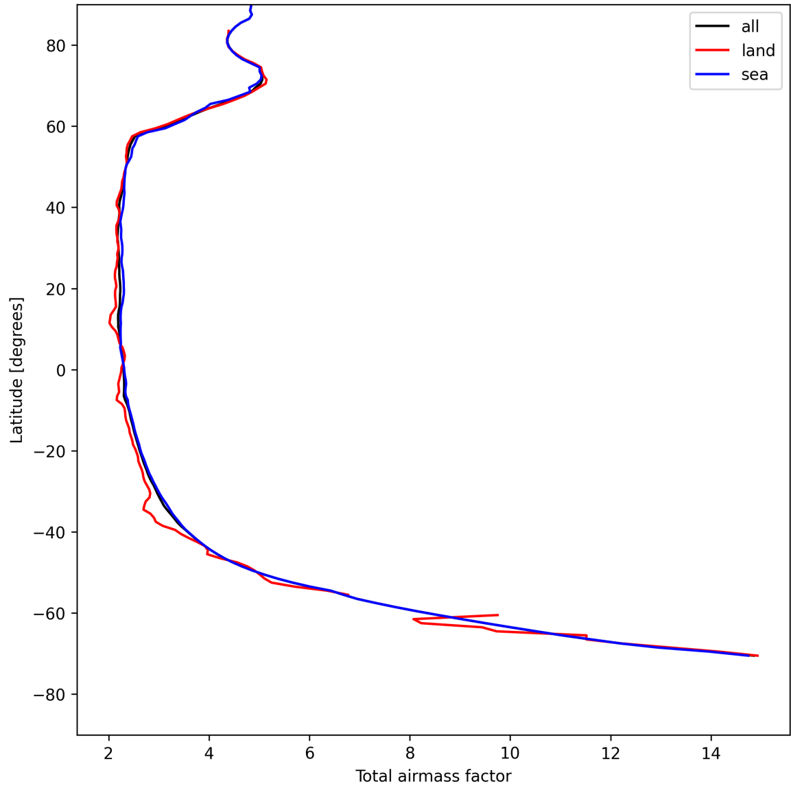
Figure 15: Zonal average of “Total airmass factor” for 2025-05-08 to 2025-05-08.
