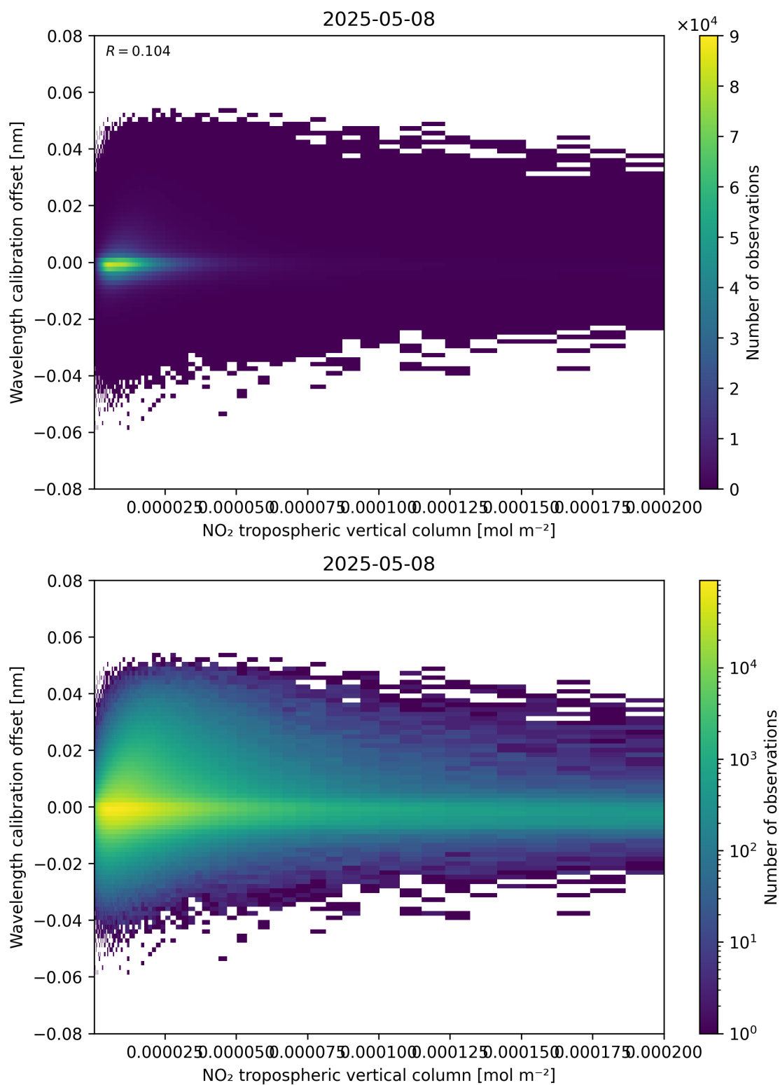
Figure 143: Scatter density plot of “NO 2 tropospheric vertical column” against “Wavelength calibration offset” for 2025-05-08 to 2025-05-08.
