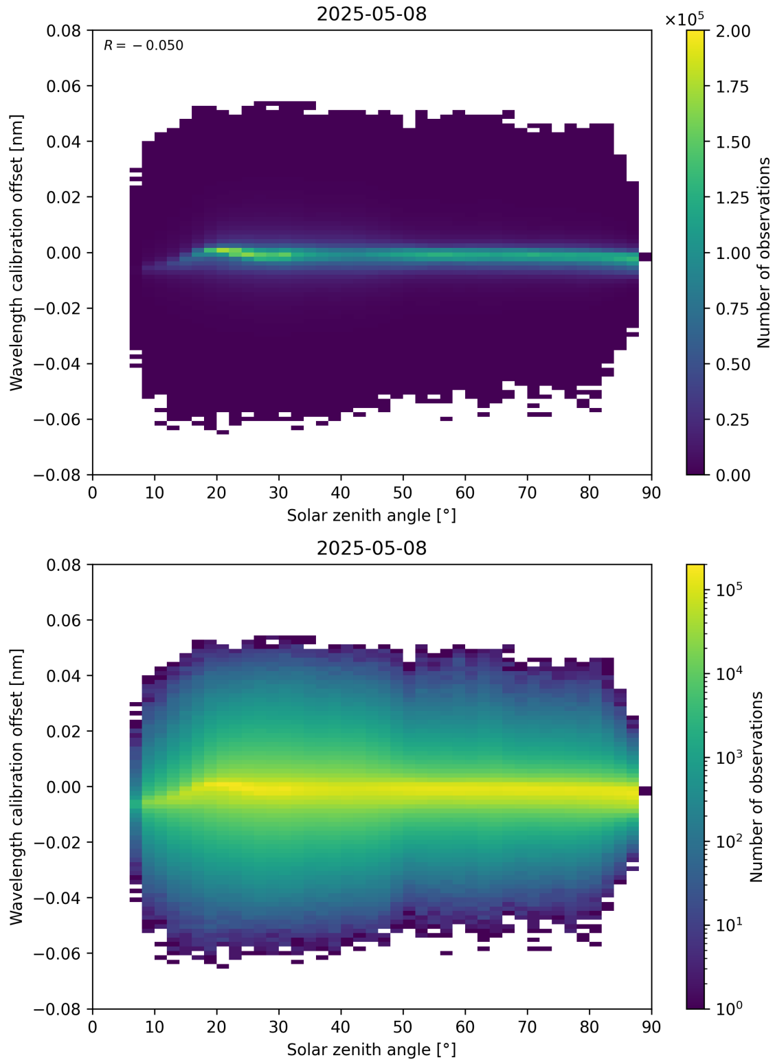
Figure 158: Scatter density plot of “Solar zenith angle” against “Wavelength calibration offset” for 2025-05-08 to 2025-05-08.
