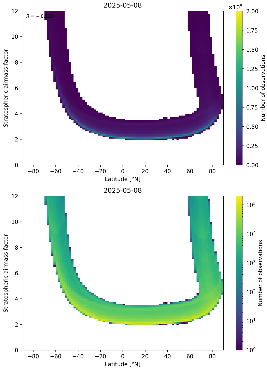
Figure 83: Scatter density plot of “Latitude” against “Stratospheric air mass factor” for 2025-05-08 to 2025-05-08.
