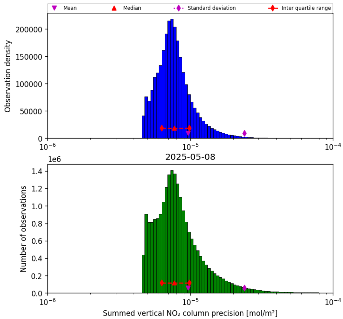
Figure 41: Histogram of "Summed vertical NO 2 column precision" for 2025-05-08 to 2025-05-08
