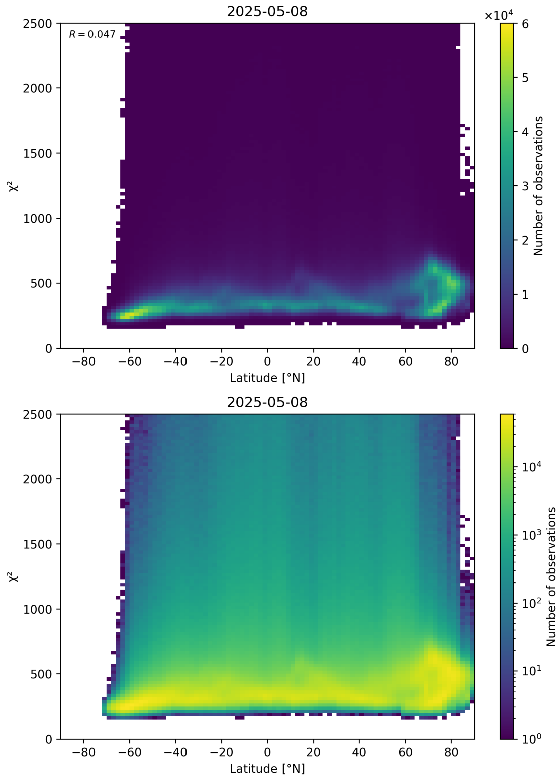
Figure 86: Scatter density plot of “Latitude” against “ \chi^2 ” for 2025-05-08 to 2025-05-08.
