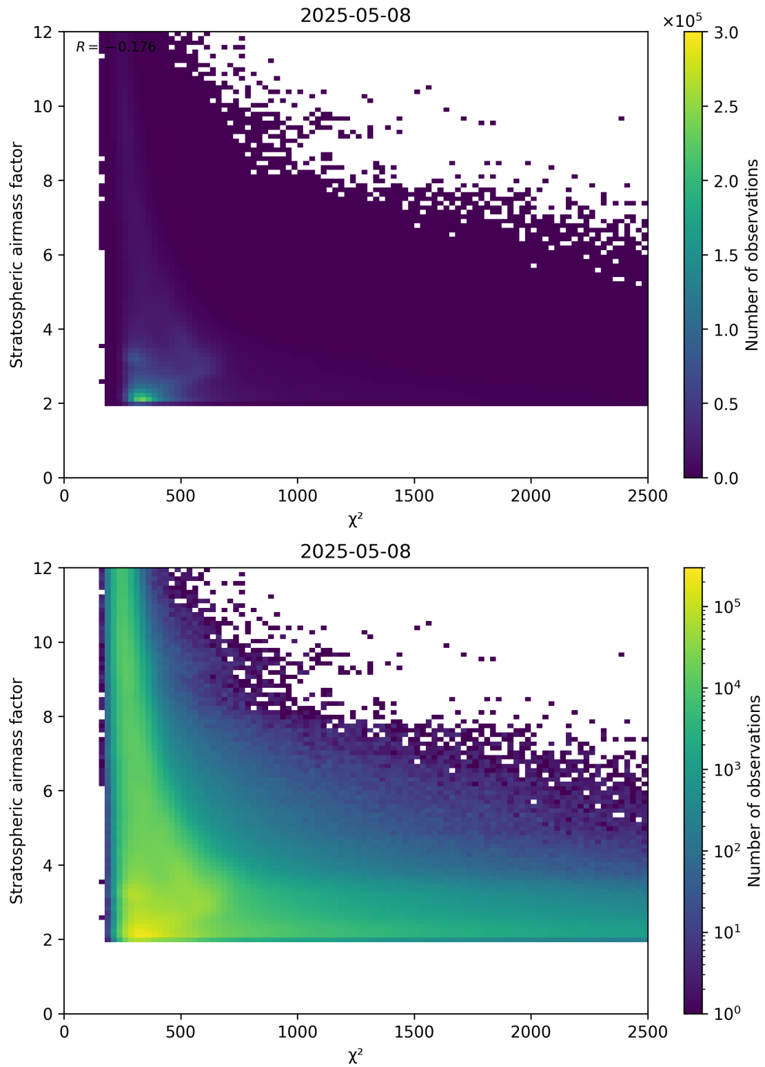
Figure 81: Scatter density plot of “ \chi^2 ” against “Stratospheric airmass factor” for 2025-05-08 to 2025-05-08.
