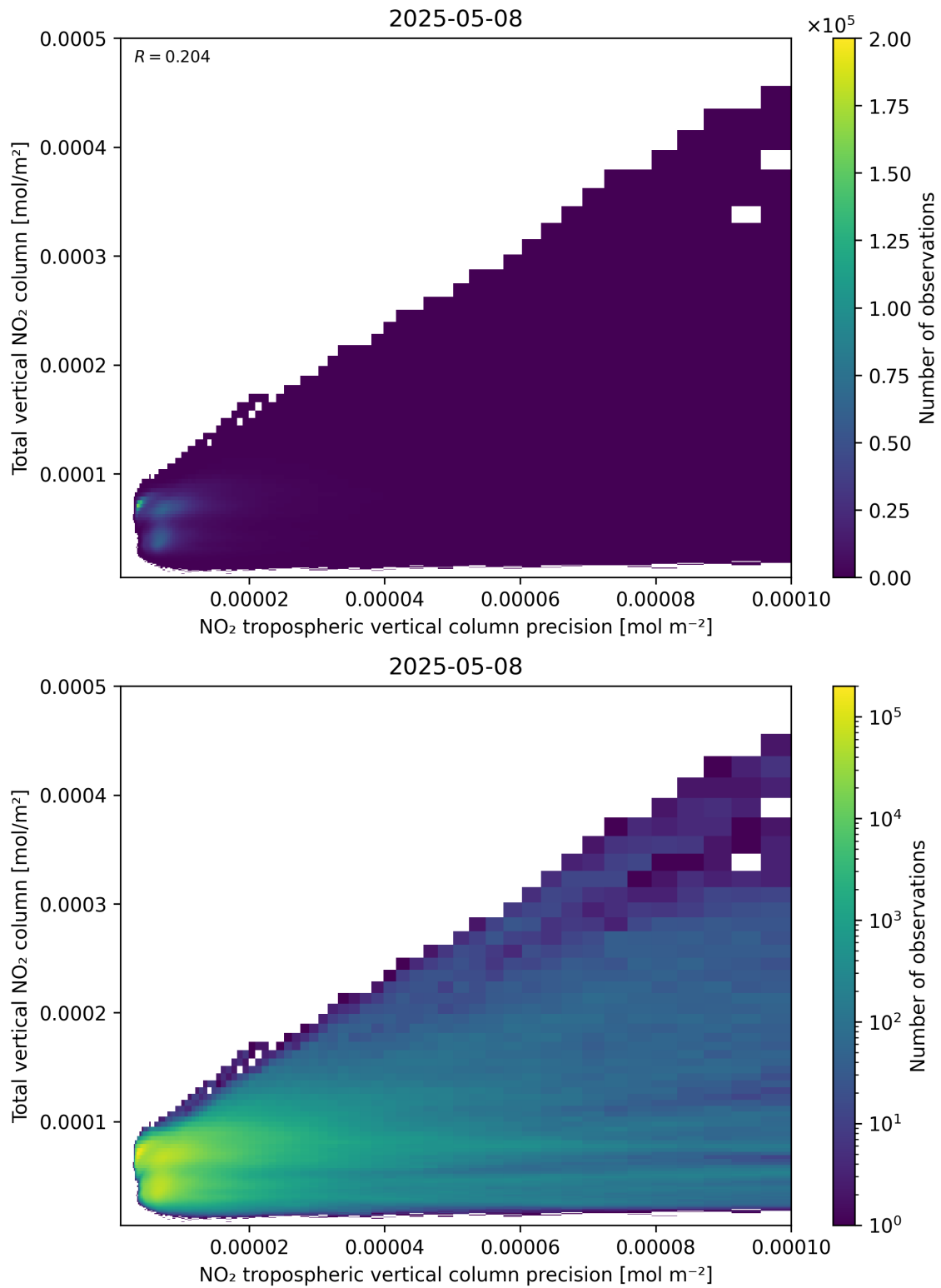
Figure 138: Scatter density plot of “NO 2 tropospheric vertical column precision” against “Total vertical NO 2 column” for 2025-05-08 to 2025-05-08.
