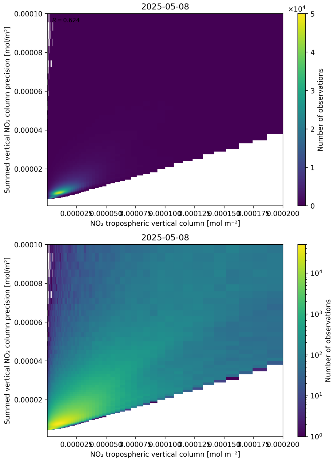
Figure 127: Scatter density plot of “NO 2 tropospheric vertical column” against “Summed vertical NO 2 column precision” for 2025-05-08 to 2025-05-08.
