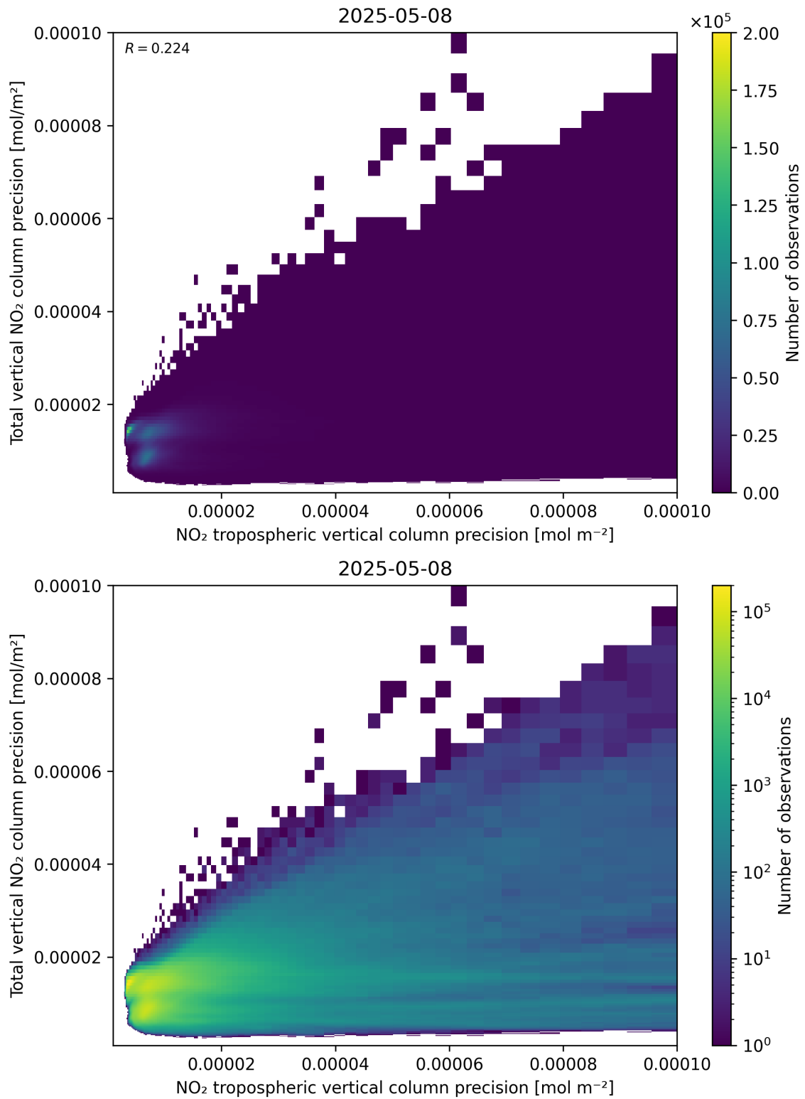
Figure 139: Scatter density plot of “NO 2 tropospheric vertical column precision” against “Total vertical NO 2 column precision” for 2025-05-08 to 2025-05-08.
