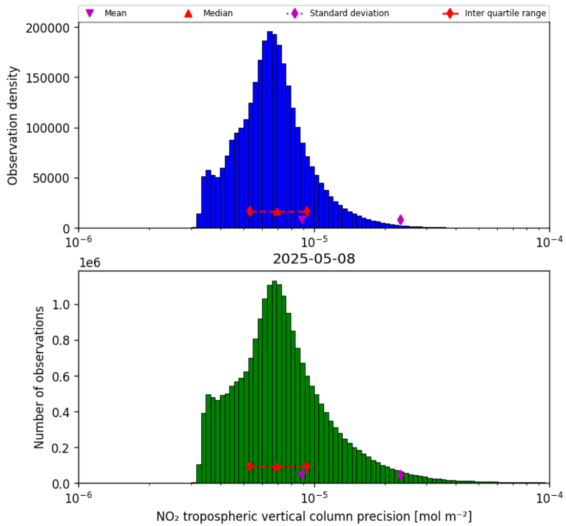
Figure 30: Histogram of “NO 2 tropospheric vertical column precision” for 2025-05-08 to 2025-05-08
