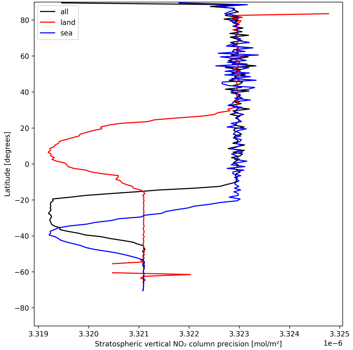
Figure 20: Zonal average of “Stratospheric vertical NO 2 column precision” for 2025-05-08 to 2025-05-08.
