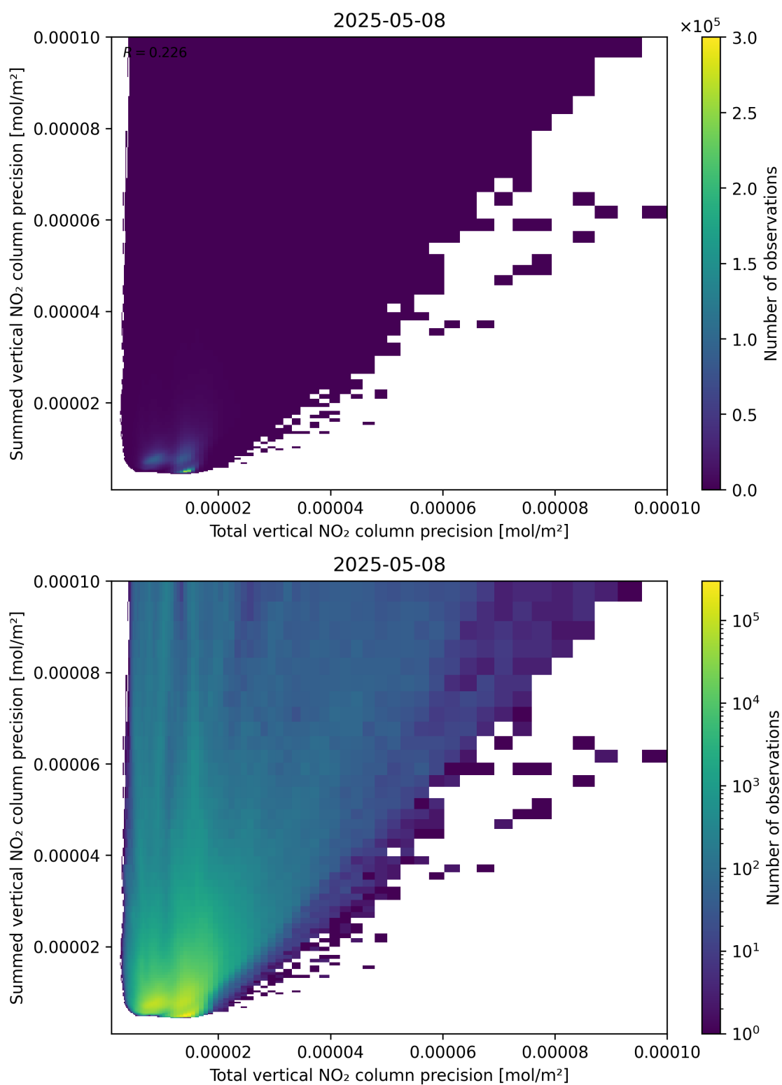
Figure 118: Scatter density plot of “Total vertical NO 2 column precision” against “Summed vertical NO 2 column precision” for 2025-05-08 to 2025-05-08.
