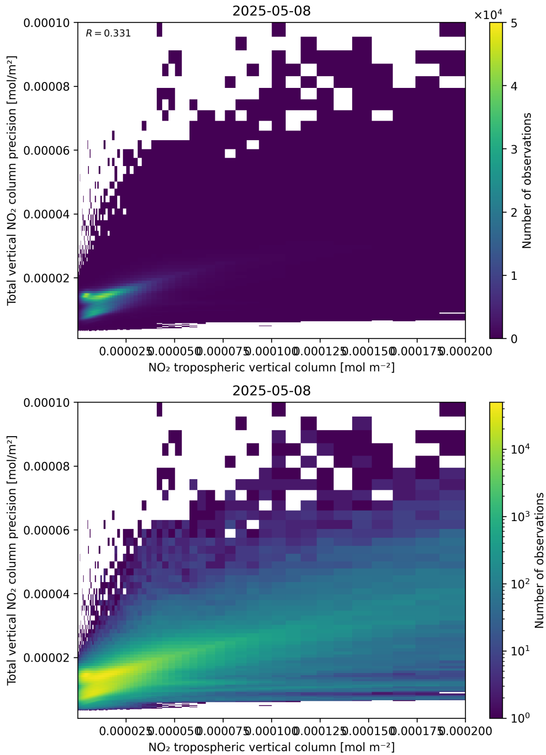
Figure 129: Scatter density plot of “NO 2 tropospheric vertical column” against “Total vertical NO 2 column precision” for 2025-05-08 to 2025-05-08.
