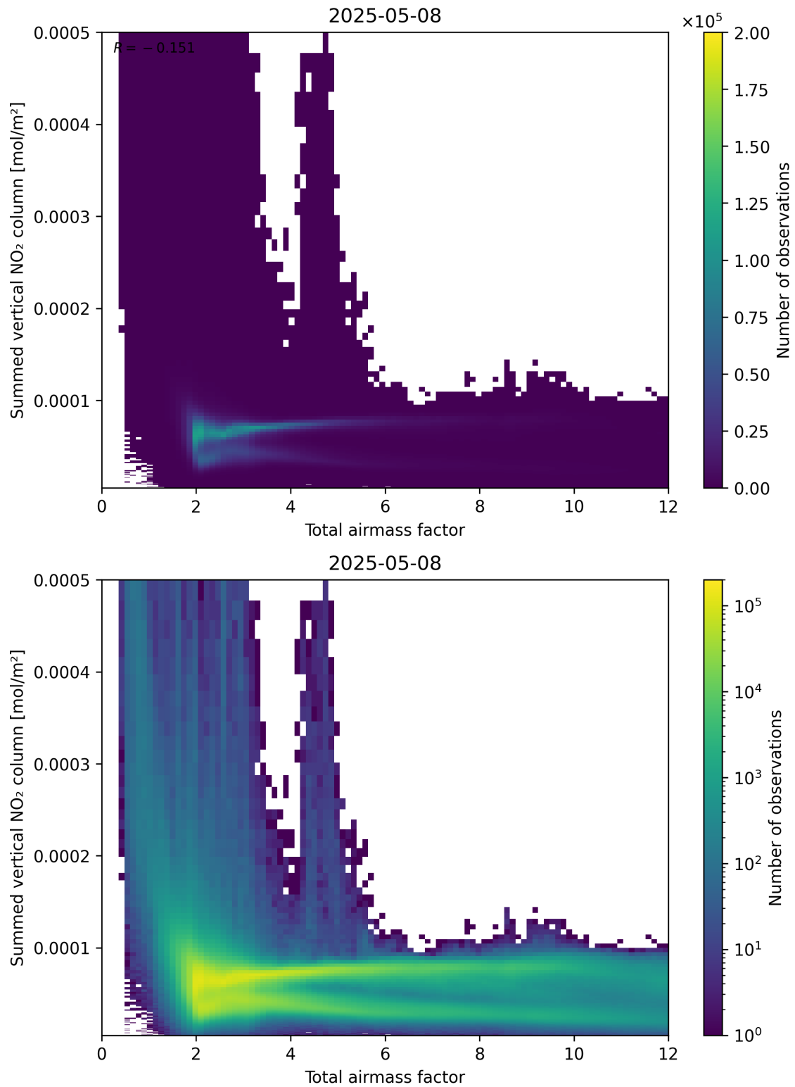
Figure 65: Scatter density plot of “Total airmass factor” against “Summed vertical NO 2 column” for 2025-05-08 to 2025-05-08.
