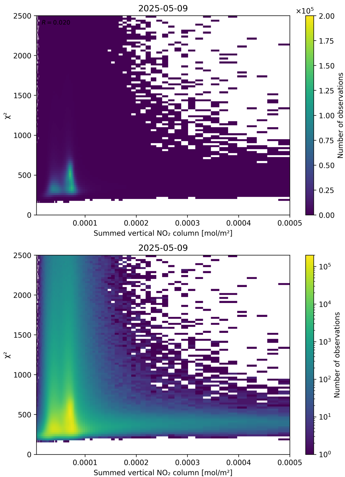
Figure 104: Scatter density plot of “Summed vertical NO 2 column” against “ \chi^2 ” for 2025-05-09 to 2025-05-10.
