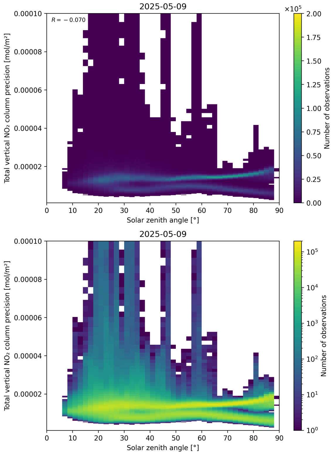
Figure 154: Scatter density plot of “Solar zenith angle” against “Total vertical NO 2 column precision” for 2025-05-09 to 2025-05-10.
