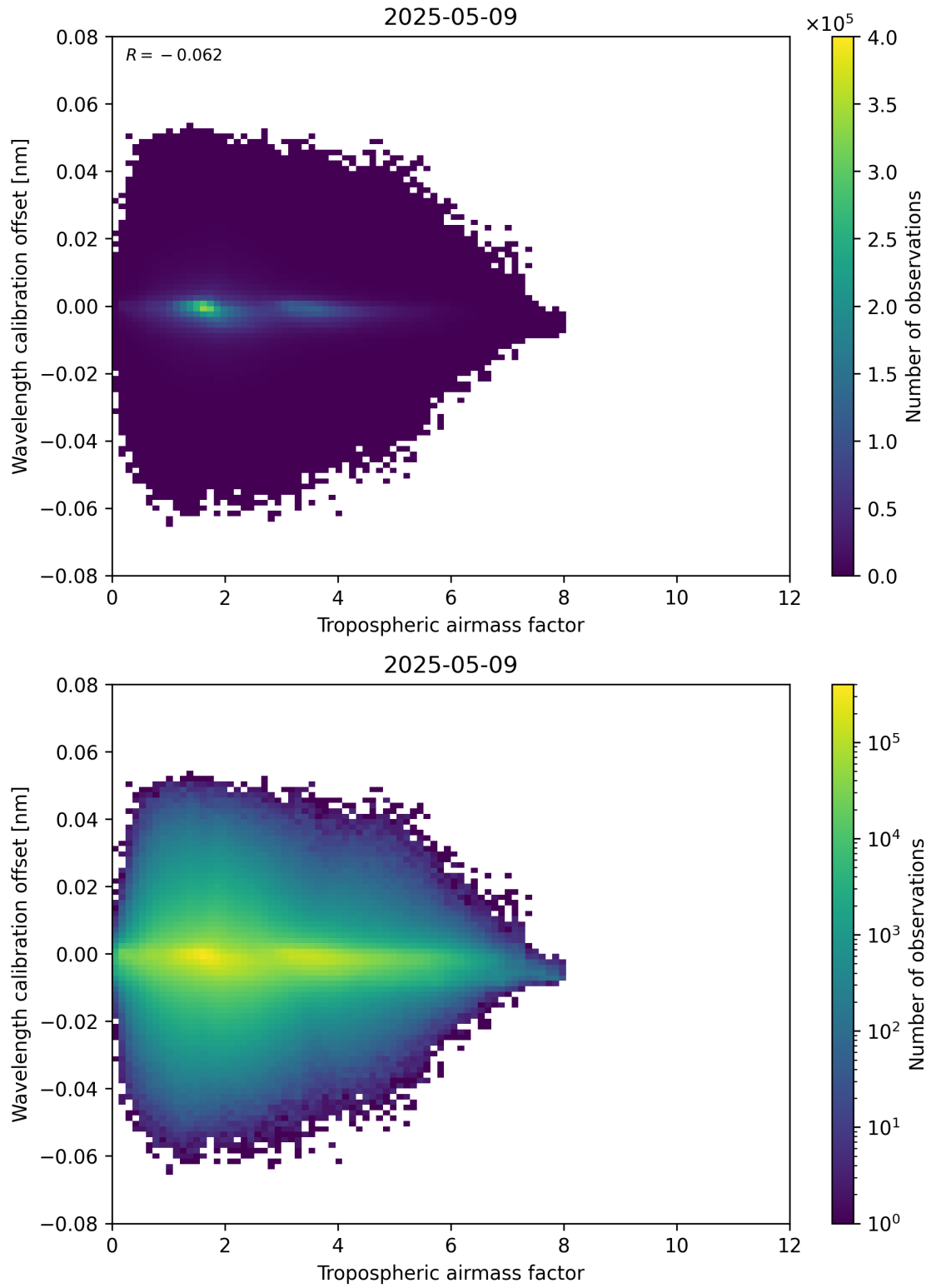
Figure 80: Scatter density plot of “Tropospheric airmass factor” against “Wavelength calibration offset” for 2025-05-09 to 2025-05-10.
