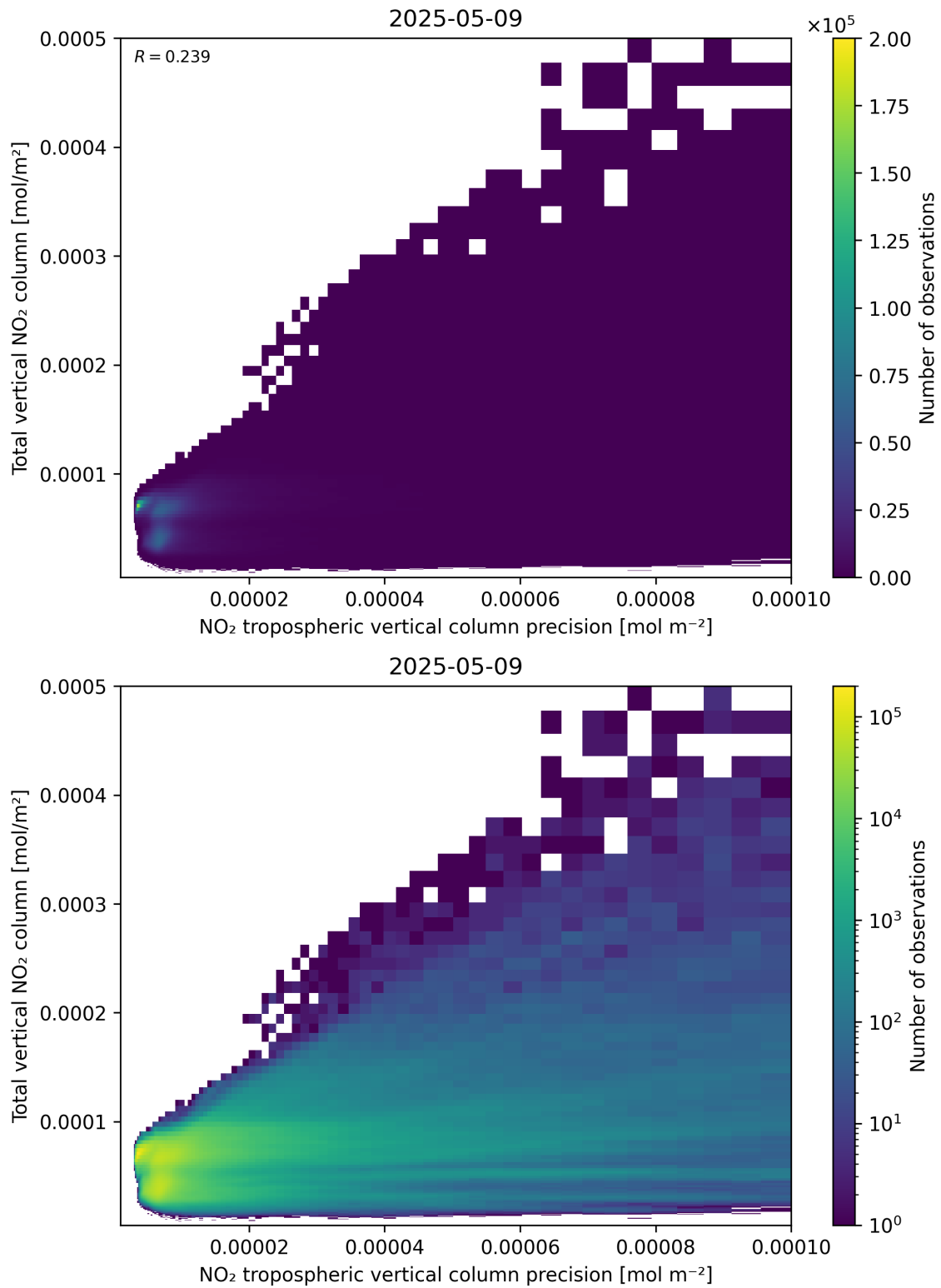
Figure 138: Scatter density plot of “NO 2 tropospheric vertical column precision” against “Total vertical NO 2 column” for 2025-05-09 to 2025-05-10.
