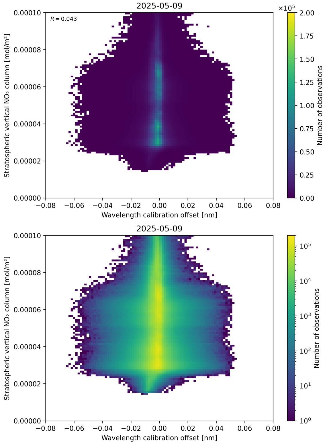
Figure 176: Scatter density plot of “Wavelength calibration offset” against “Stratospheric vertical NO 2 column” for 2025-05-09 to 2025-05-10.
