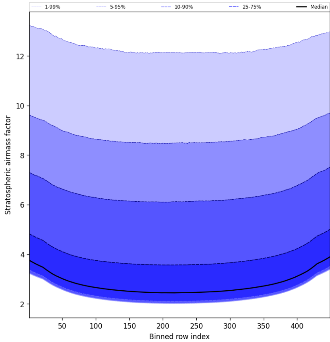
Figure 61: Along track statistics of “Stratospheric airmass factor” for 2025-05-09 to 2025-05-10
