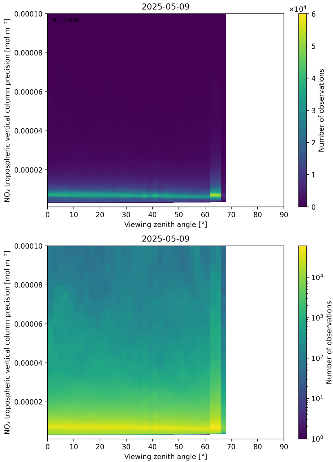
Figure 170: Scatter density plot of “Viewing zenith angle” against “NO 2 tropospheric vertical column precision” for 2025-05-09 to 2025-05-10.
