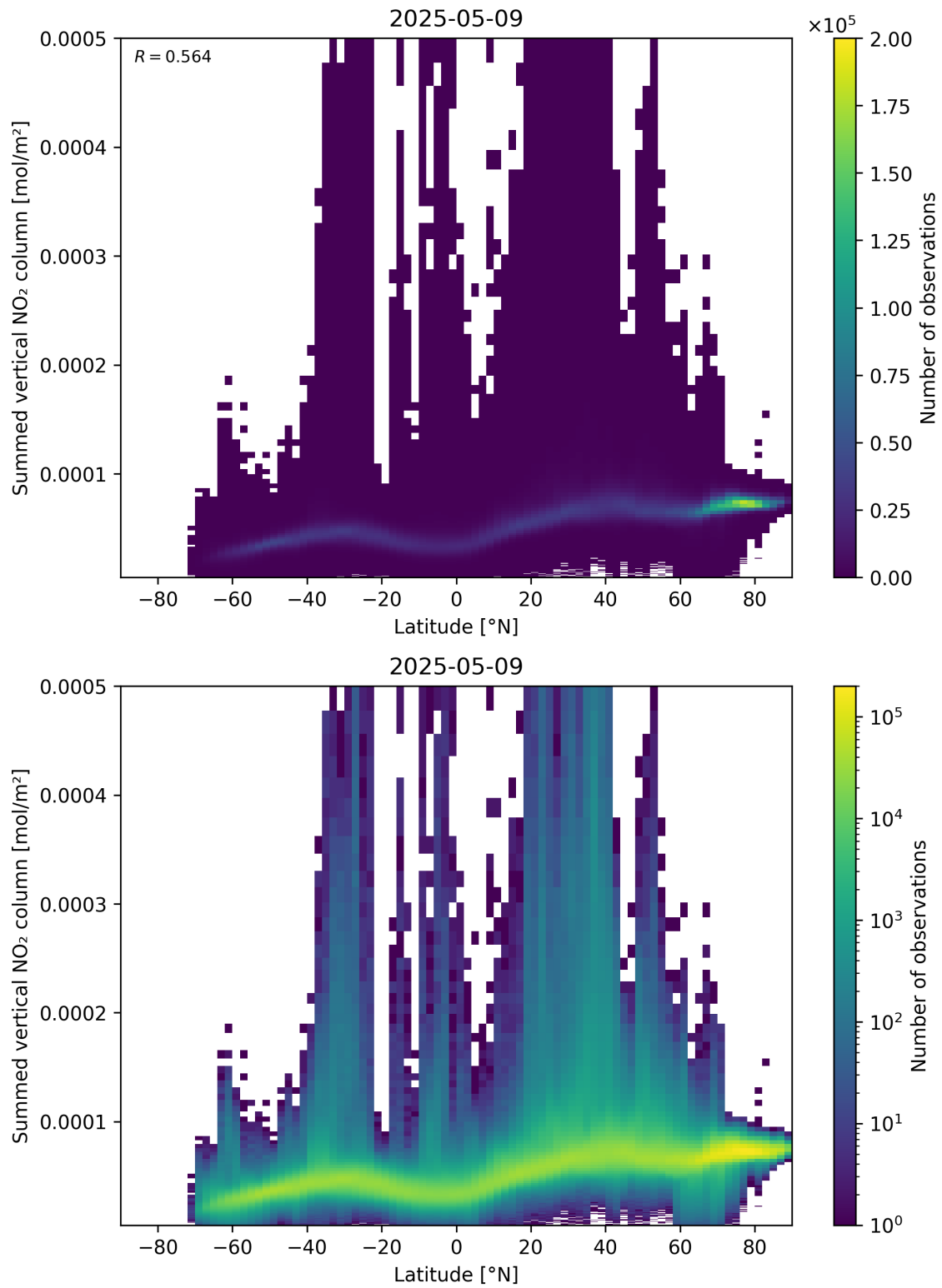
Figure 88: Scatter density plot of “Latitude” against “Summed vertical NO 2 column” for 2025-05-09 to 2025-05-10.
