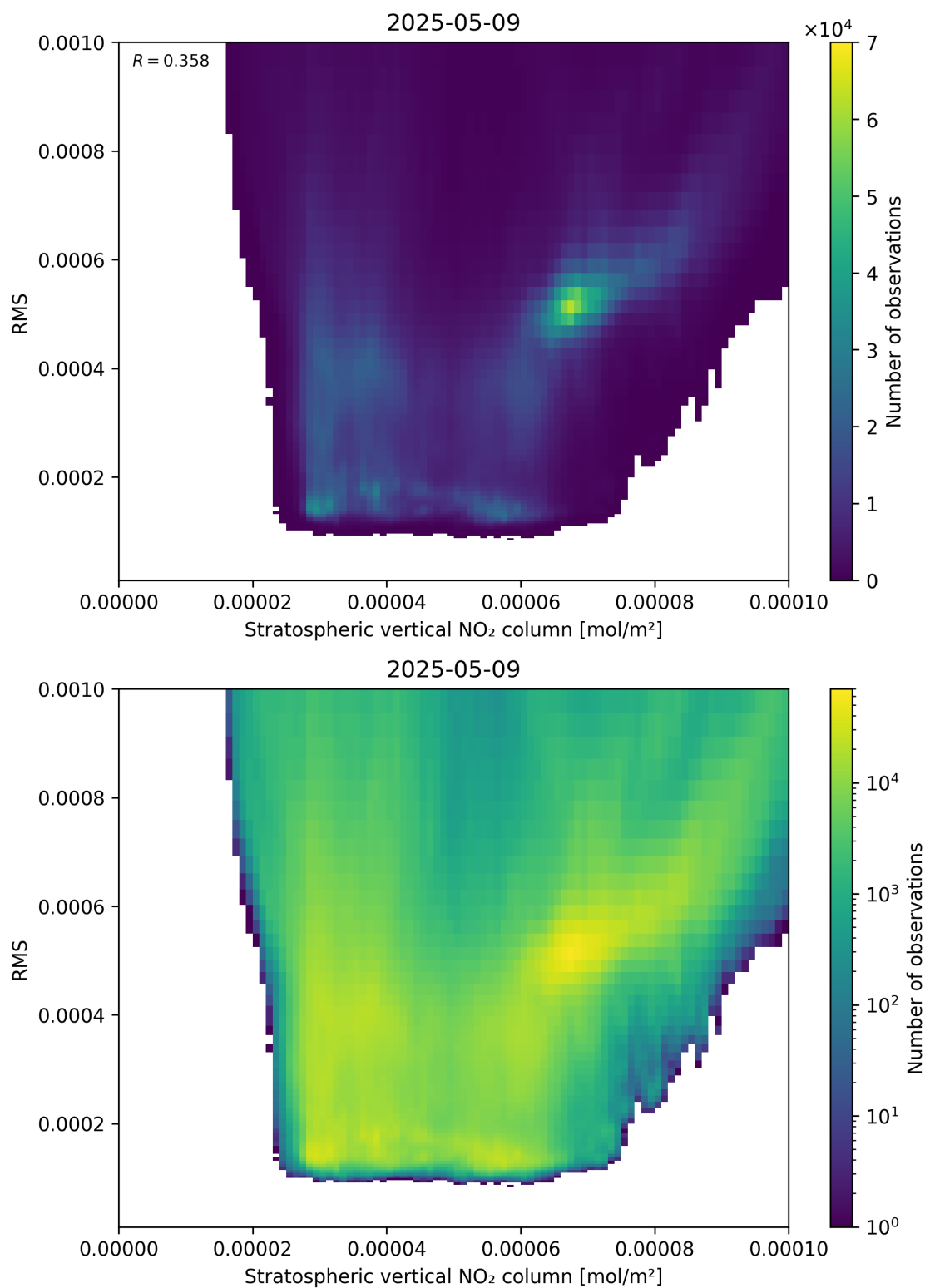
Figure 102: Scatter density plot of “Stratospheric vertical NO 2 column” against “RMS” for 2025-05-09 to 2025-05-10.
