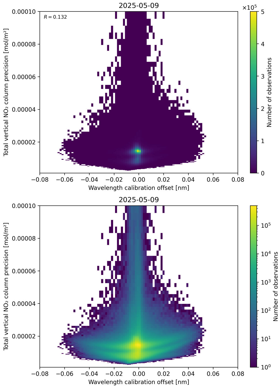
Figure 180: Scatter density plot of “Wavelength calibration offset” against “Total vertical NO 2 column precision” for 2025-05-09 to 2025-05-10.
