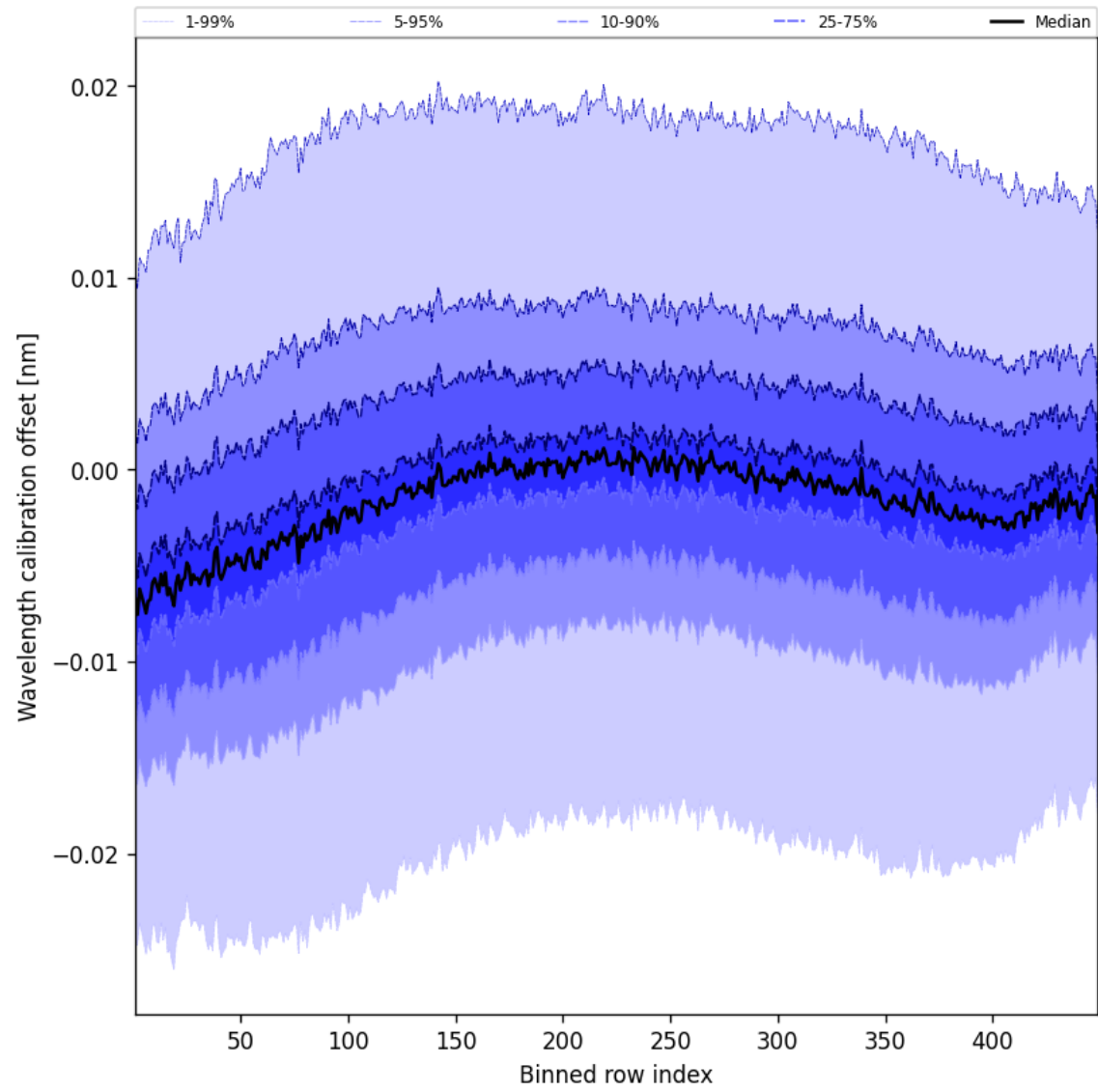
Figure 52: Along track statistics of “Wavelength calibration offset” for 2025-05-09 to 2025-05-10
