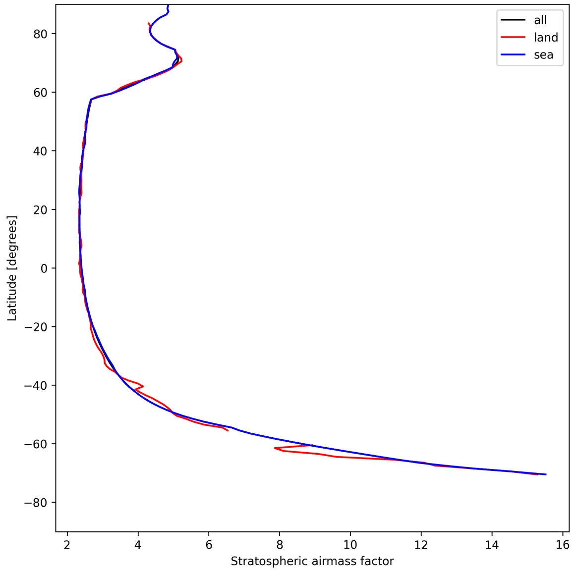
Figure 27: Zonal average of “Stratospheric airmass factor” for 2025-05-09 to 2025-05-10.
