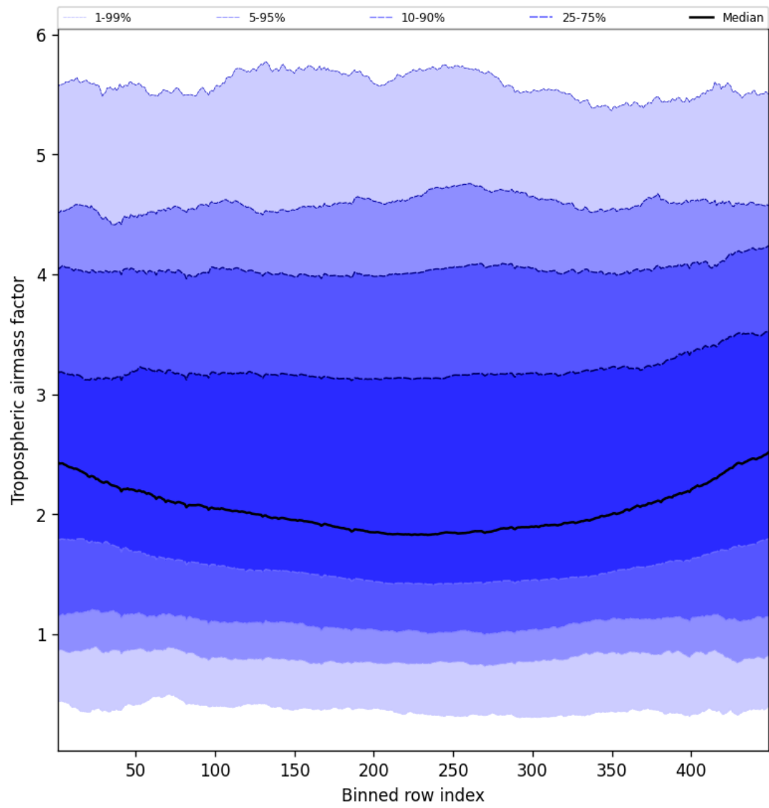
Figure 48: Along track statistics of "Tropospheric airmass factor" for 2025-05-09 to 2025-05-10
