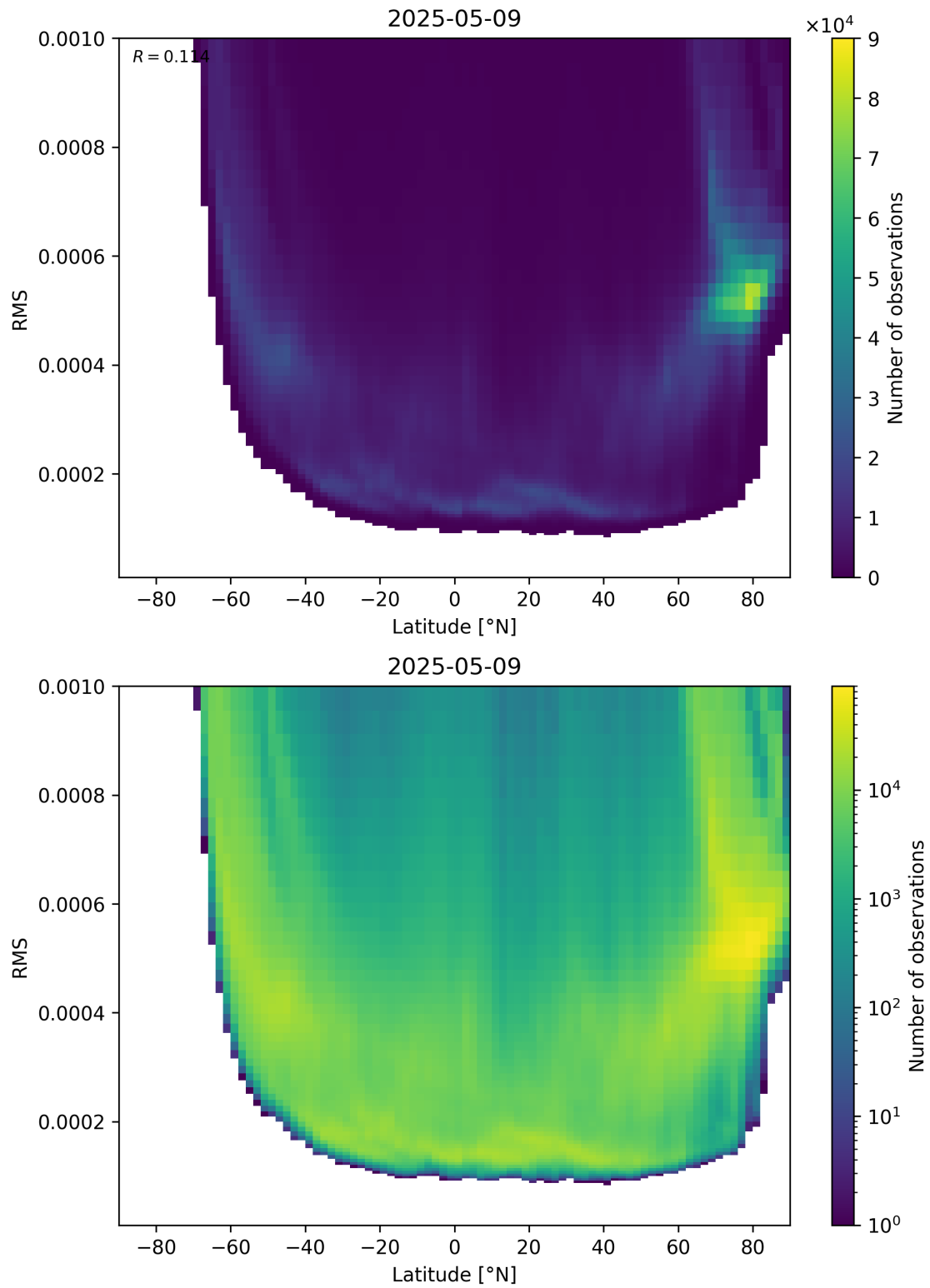
Figure 94: Scatter density plot of “Latitude” against “RMS” for 2025-05-09 to 2025-05-10.
