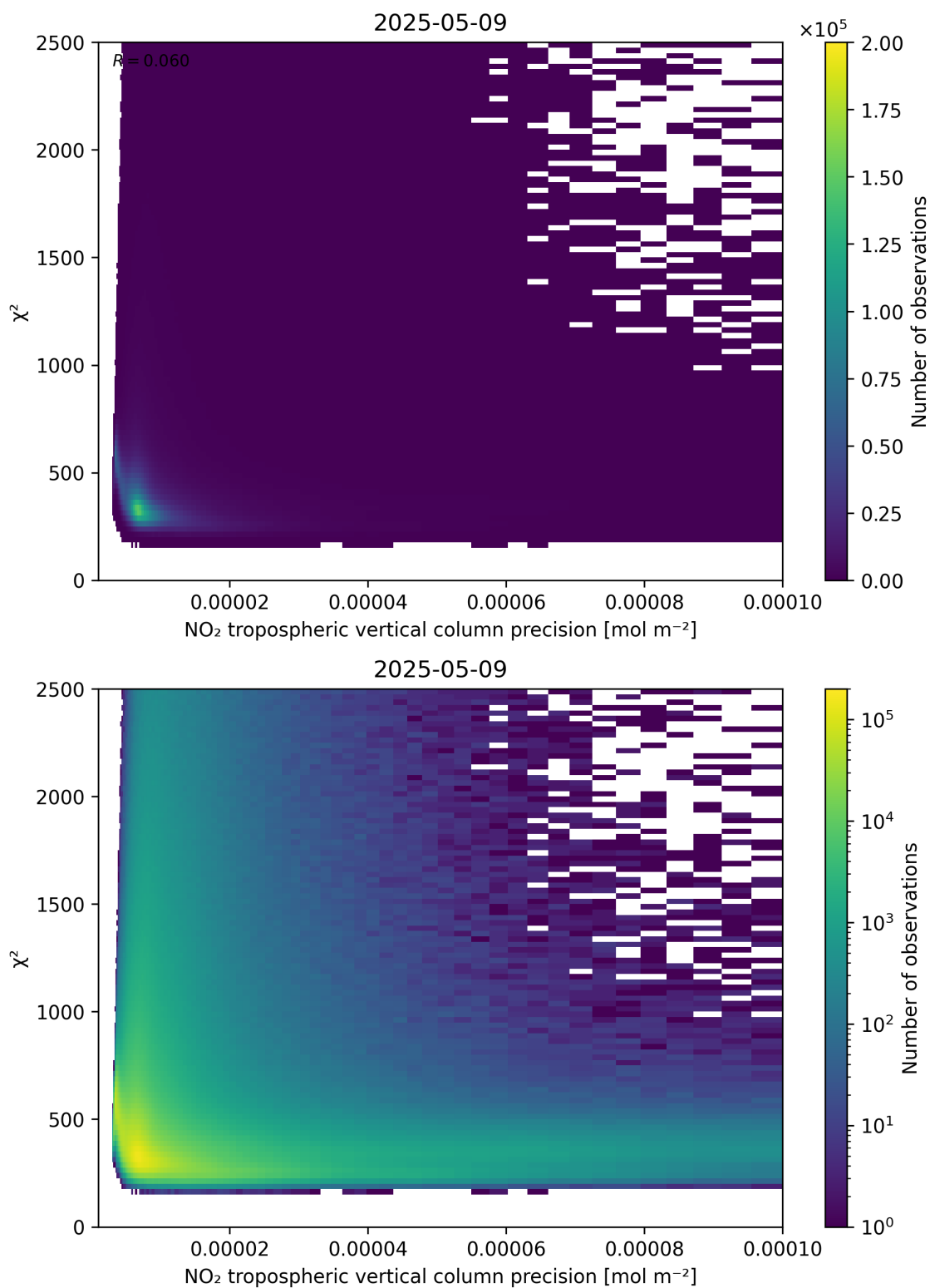
Figure 134: Scatter density plot of “NO 2 tropospheric vertical column precision” against “ \chi^2 ” for 2025-05-09 to 2025-05-10.
