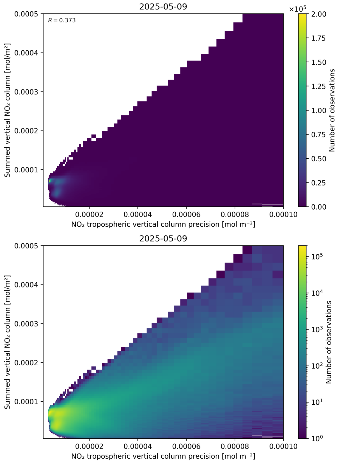
Figure 136: Scatter density plot of “NO 2 tropospheric vertical column precision” against “Summed vertical NO 2 column” for 2025-05-09 to 2025-05-10.
