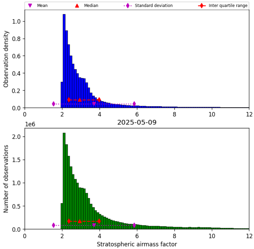
Figure 44: Histogram of “Stratospheric airmass factor” for 2025-05-09 to 2025-05-10
