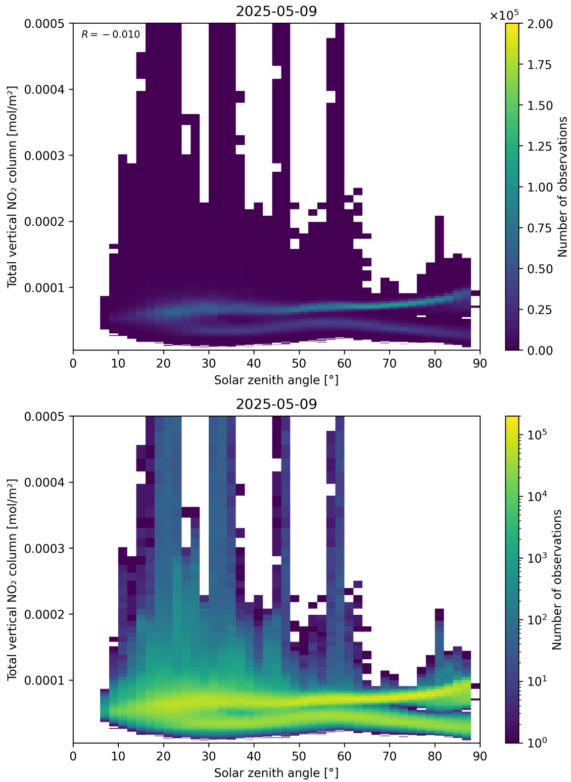
Figure 153: Scatter density plot of “Solar zenith angle” against “Total vertical NO 2 column” for 2025-05-09 to 2025-05-10.
