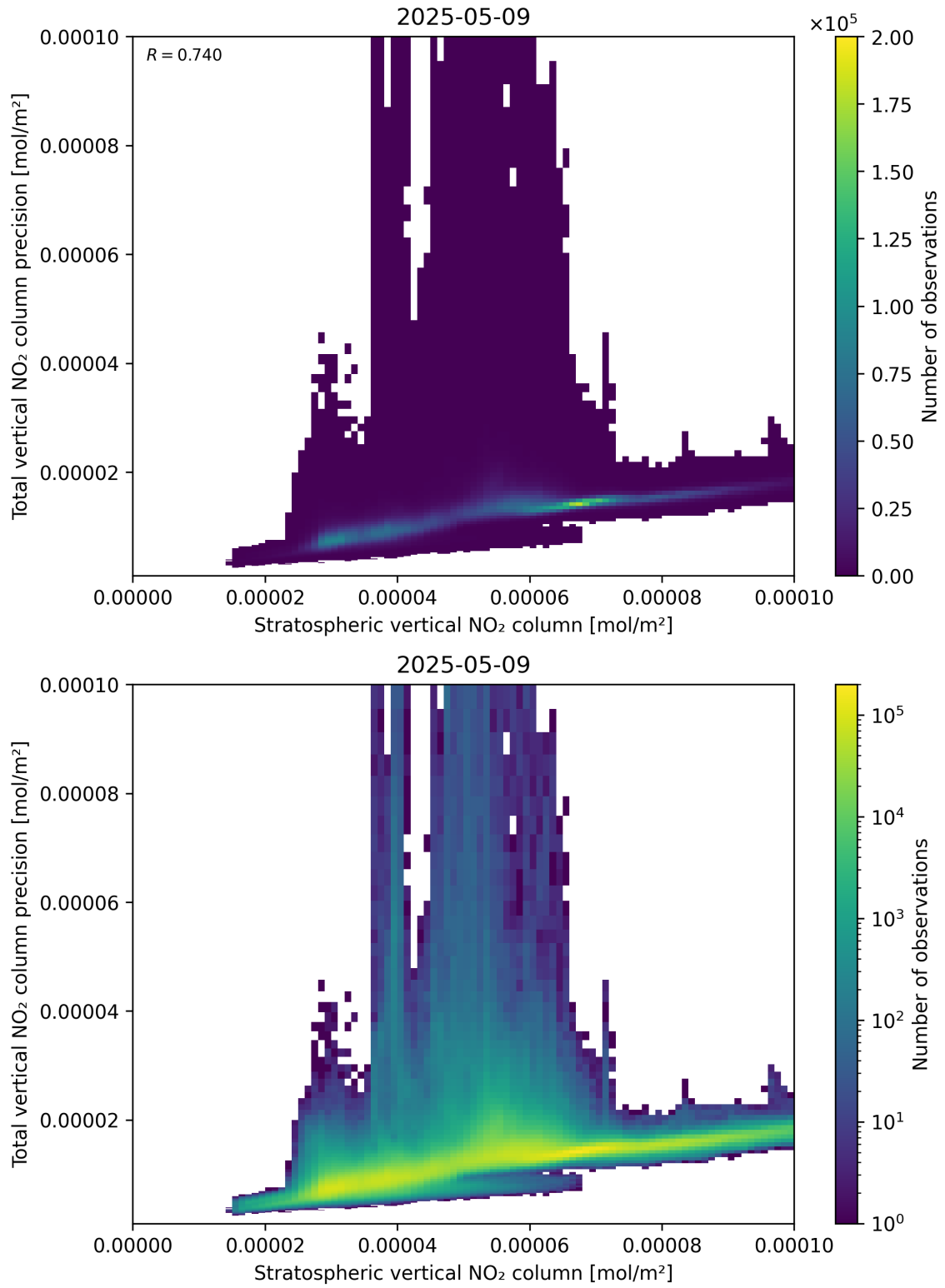
Figure 101: Scatter density plot of “Stratospheric vertical NO 2 column” against “Total vertical NO 2 column precision” for 2025-05-09 to 2025-05-10.
