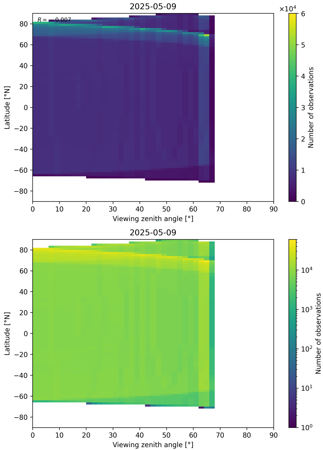
Figure 163: Scatter density plot of “Viewing zenith angle” against “Latitude” for 2025-05-09 to 2025-05-10.
