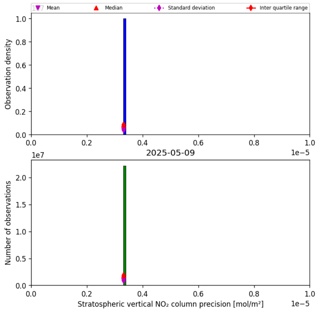
Figure 37: Histogram of “Stratospheric vertical NO 2 column precision” for 2025-05-09 to 2025-05-10
