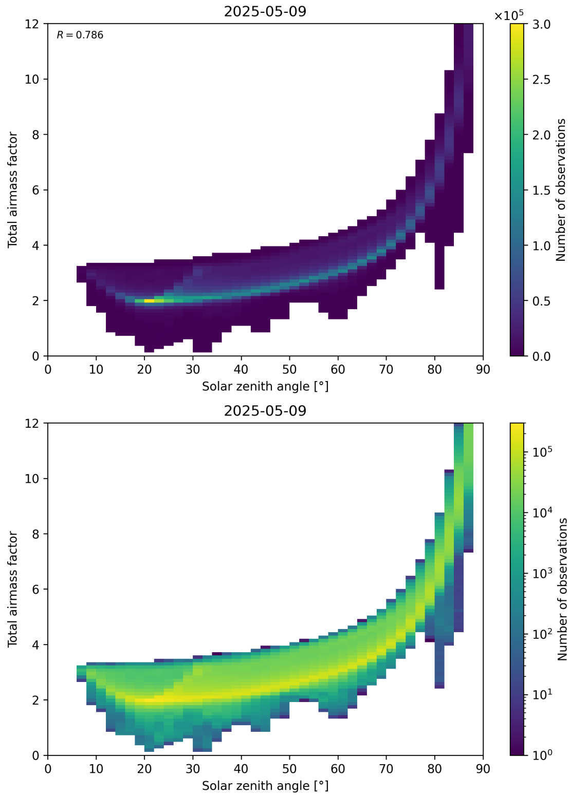
Figure 146: Scatter density plot of “Solar zenith angle” against “Total airmass factor” for 2025-05-09 to 2025-05-10.
