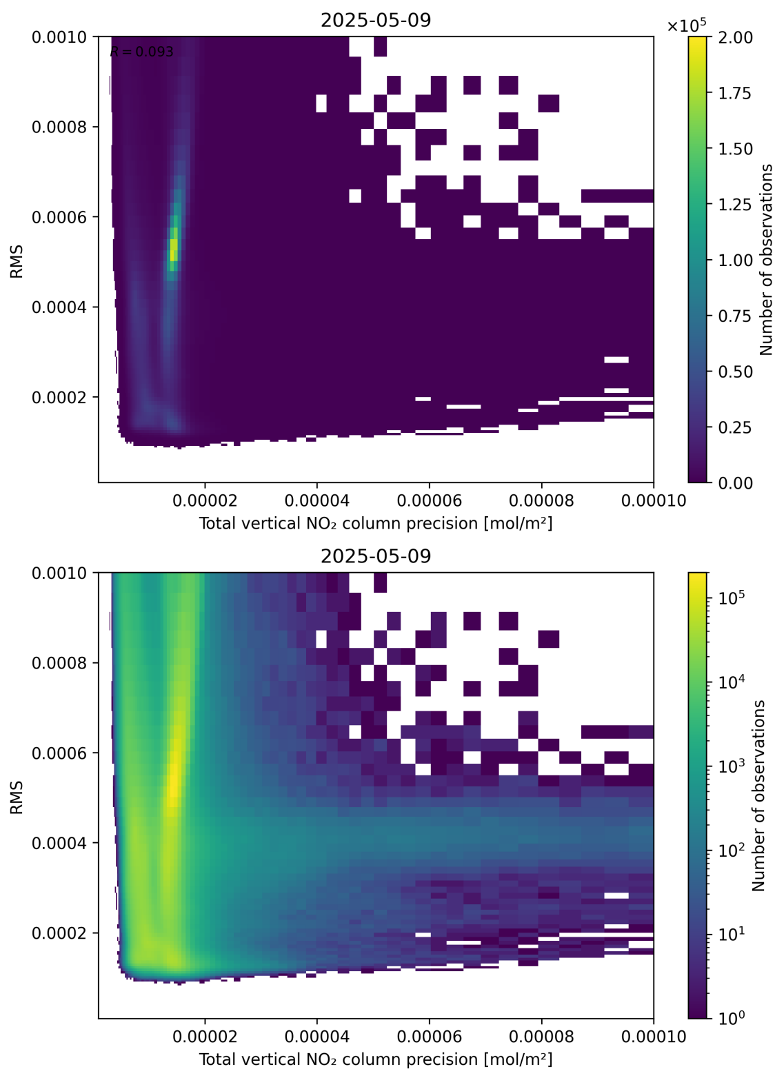
Figure 119: Scatter density plot of “Total vertical NO 2 column precision” against “RMS” for 2025-05-09 to 2025-05-10.
