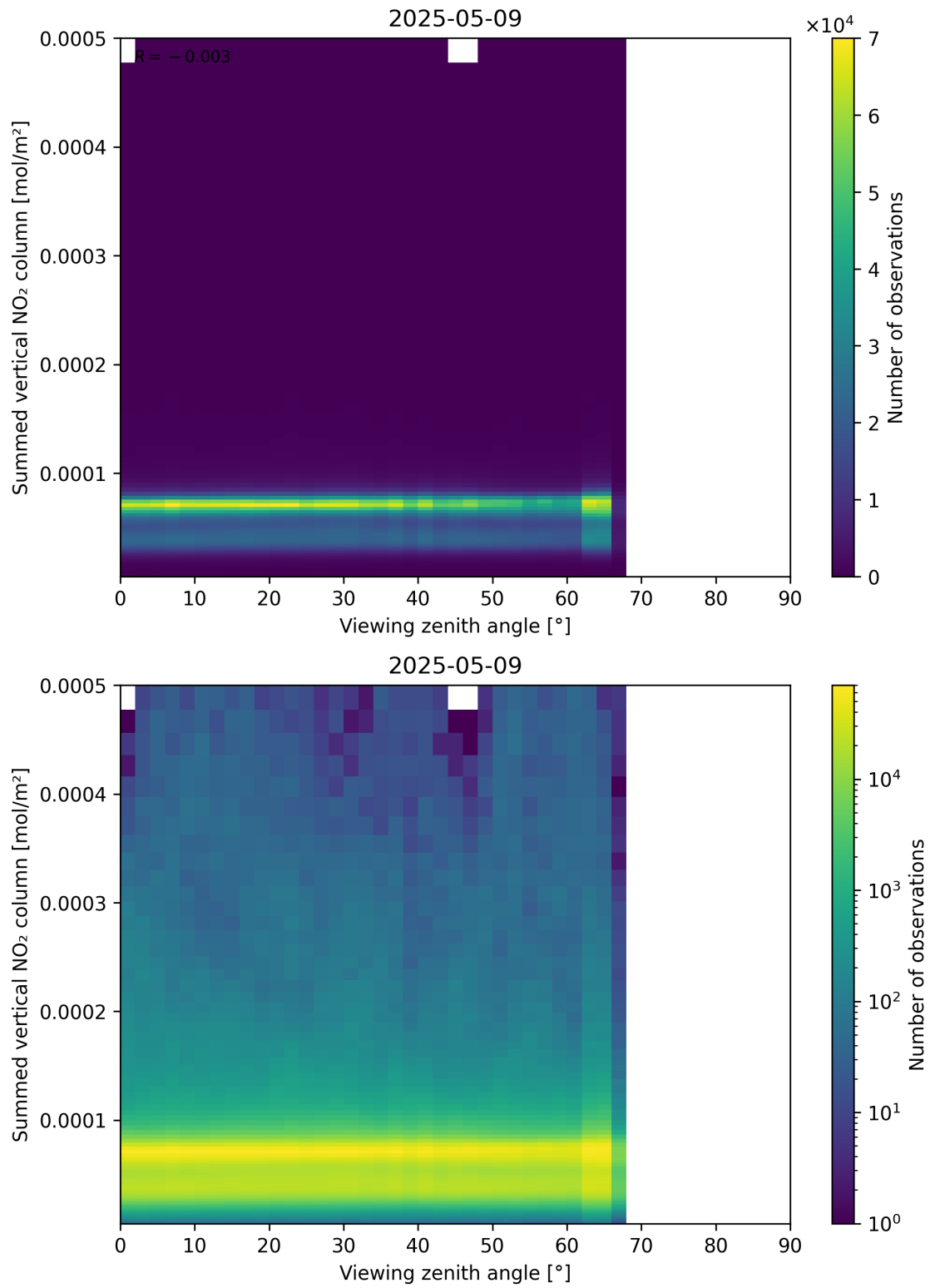
Figure 165: Scatter density plot of “Viewing zenith angle” against “Summed vertical NO 2 column” for 2025-05-09 to 2025-05-10.
