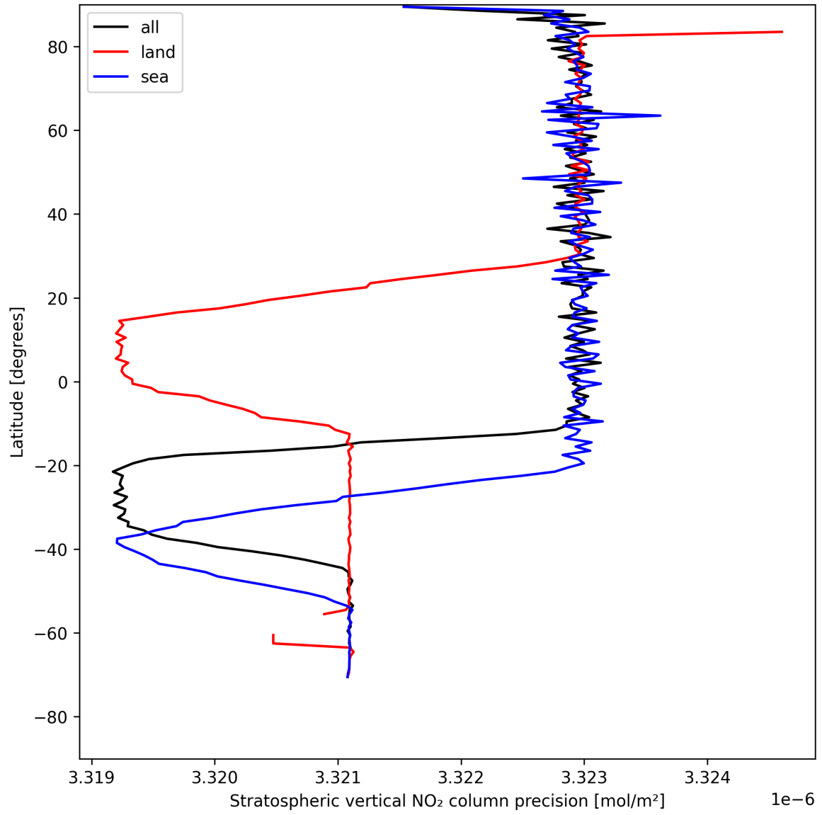
Figure 20: Zonal average of “Stratospheric vertical NO 2 column precision” for 2025-05-09 to 2025-05-10.
