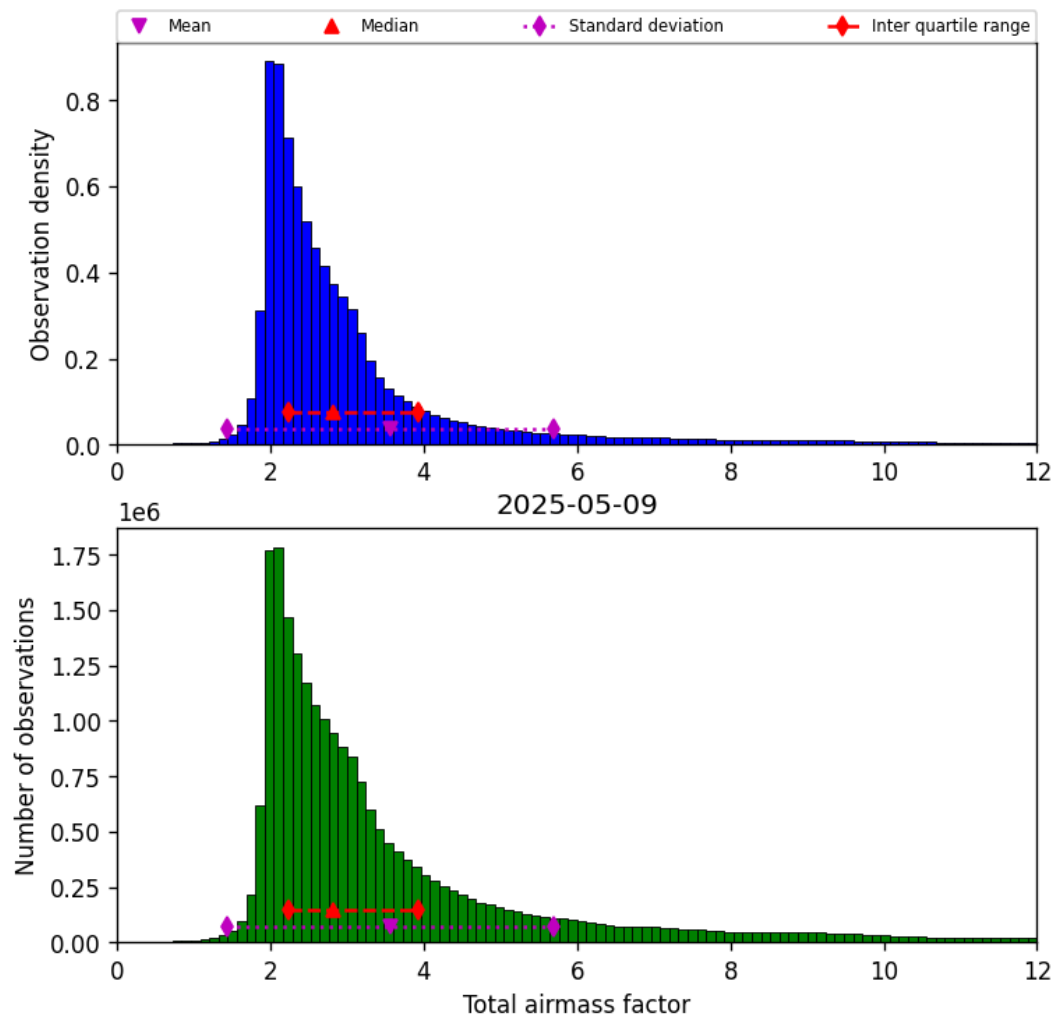
Figure 32: Histogram of “Total airmass factor” for 2025-05-09 to 2025-05-10
