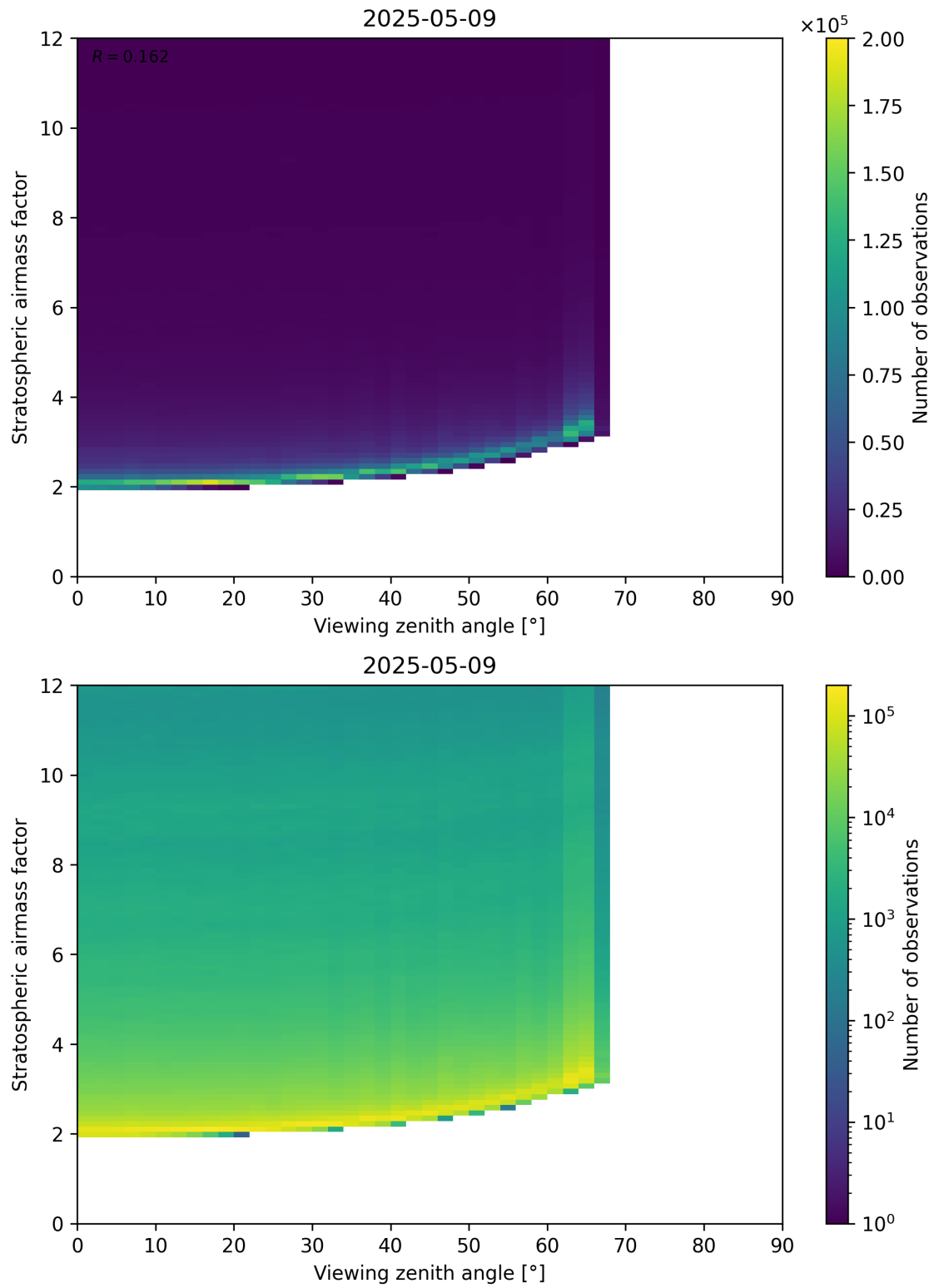
Figure 159: Scatter density plot of “Viewing zenith angle” against “Stratospheric airmass factor” for 2025-05-09 to 2025-05-10.
