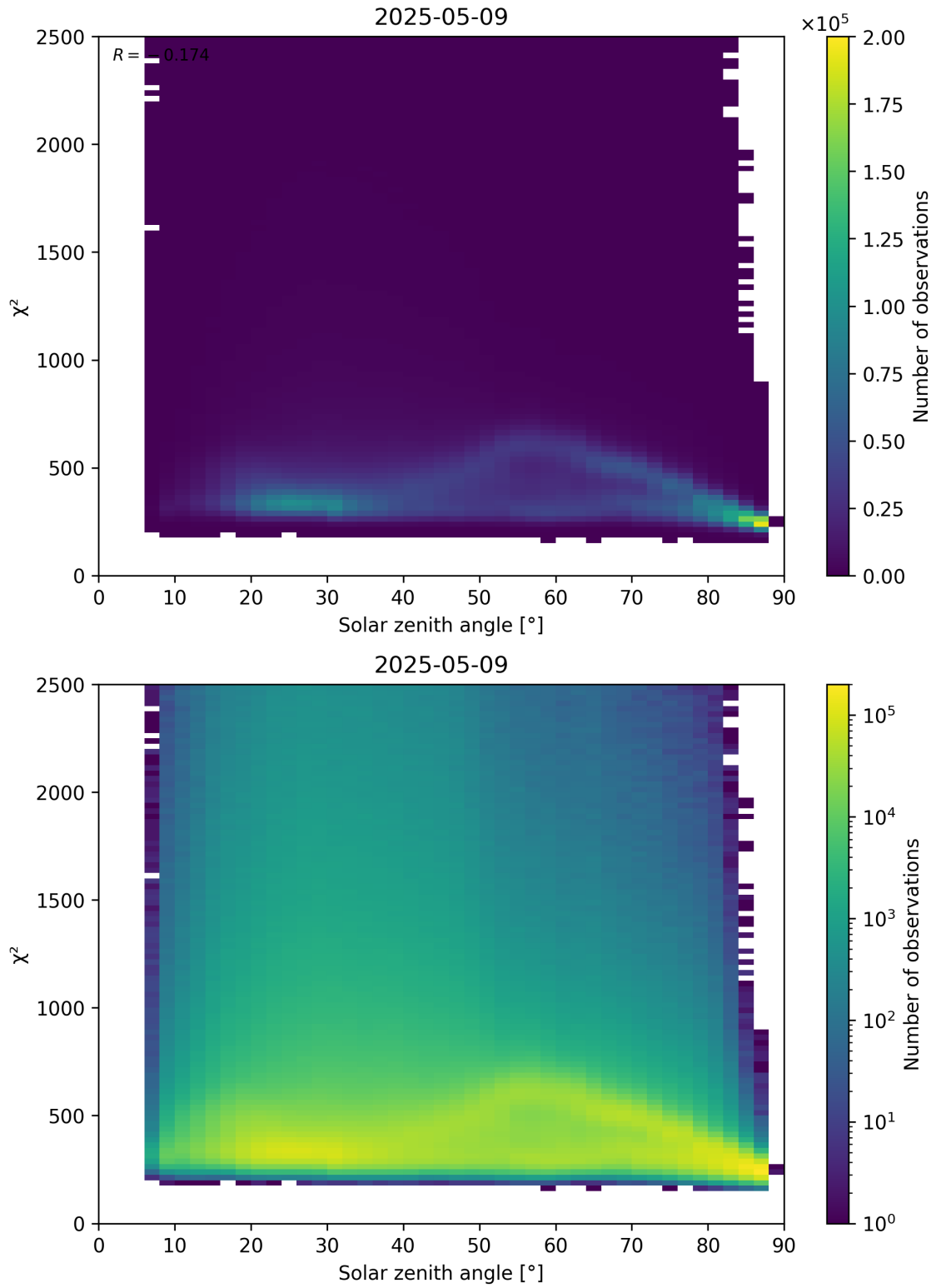
Figure 148: Scatter density plot of “Solar zenith angle” against “ \chi^2 ” for 2025-05-09 to 2025-05-10.
