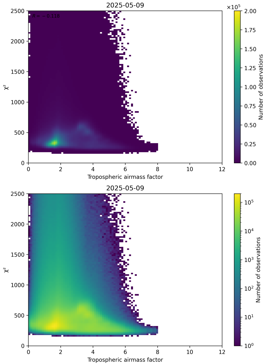
Figure 73: Scatter density plot of “Tropospheric airmass factor” against “ \chi^2 ” for 2025-05-09 to 2025-05-10.
