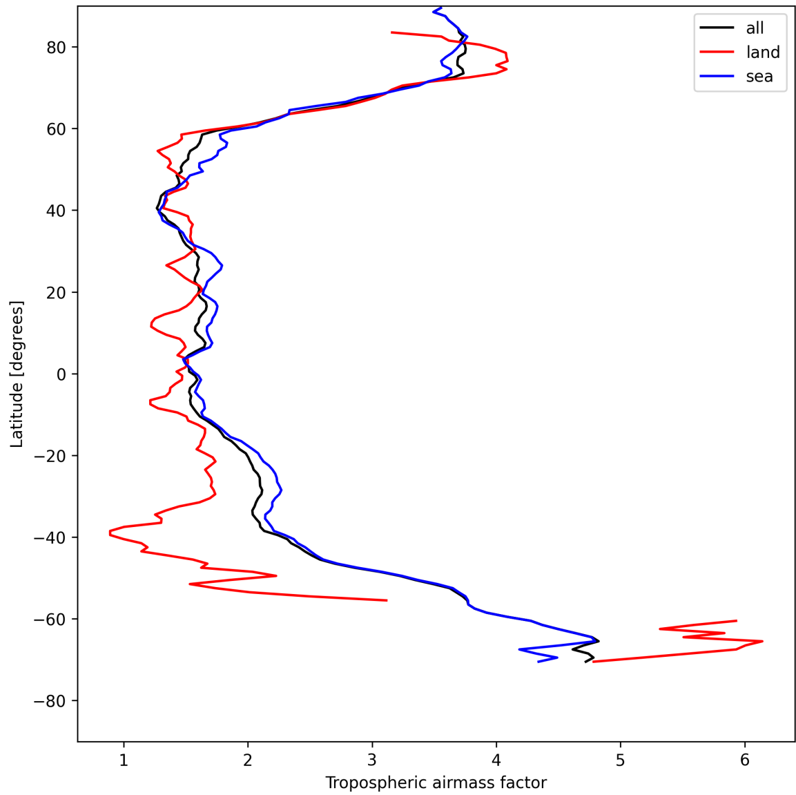
Figure 14: Zonal average of “Tropospheric airmass factor” for 2025-05-09 to 2025-05-10.
