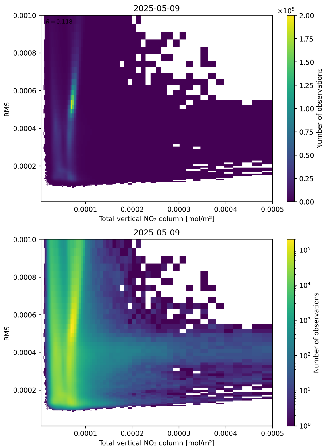
Figure 120: Scatter density plot of “Total vertical NO 2 column” against “RMS” for 2025-05-09 to 2025-05-10.
