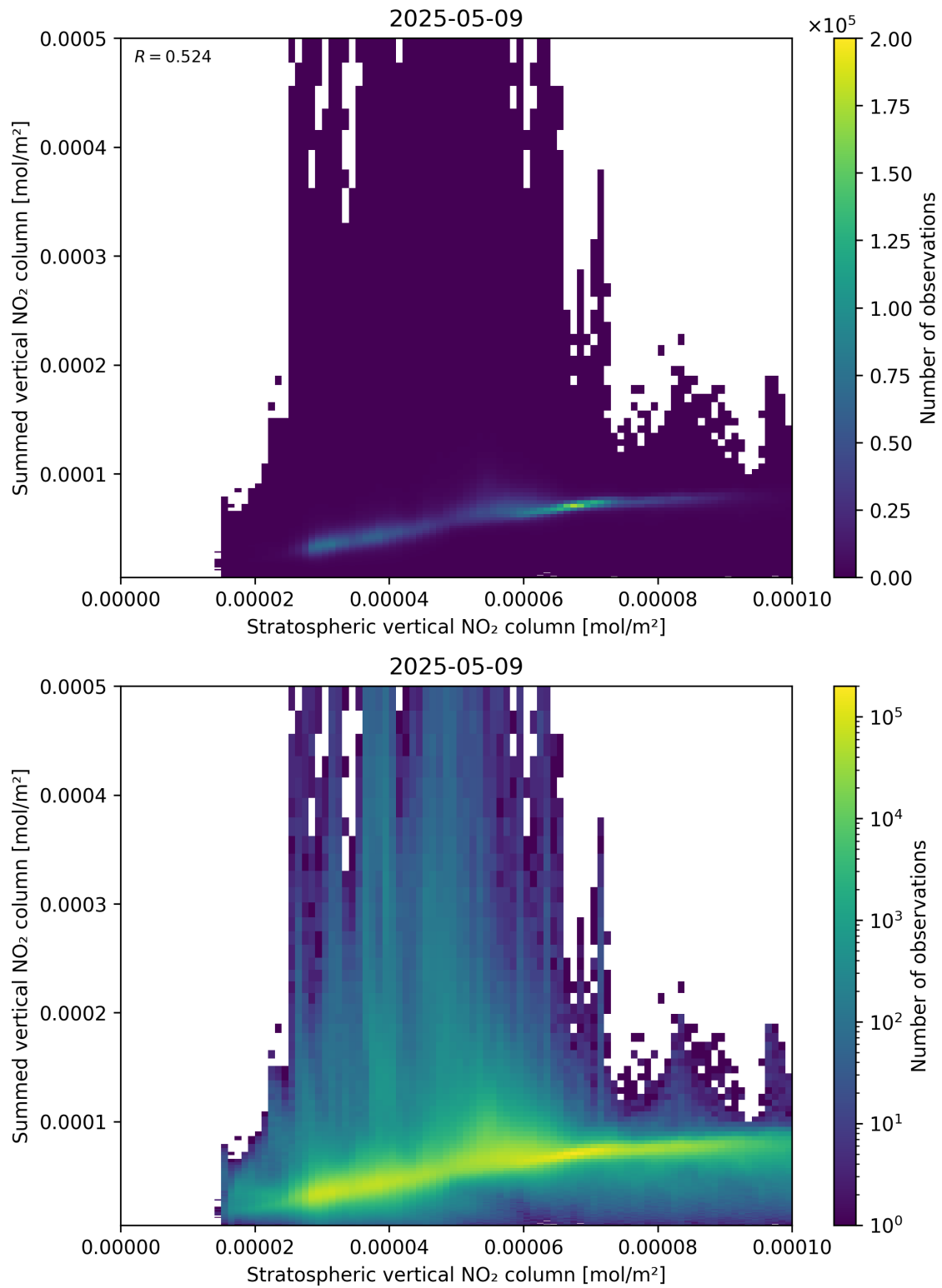
Figure 98: Scatter density plot of “Stratospheric vertical NO 2 column” against “Summed vertical NO 2 column” for 2025-05-09 to 2025-05-10.
