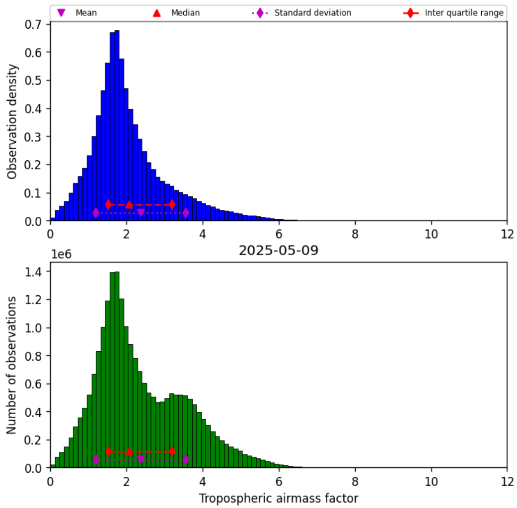
Figure 31: Histogram of “Tropospheric airmass factor” for 2025-05-09 to 2025-05-10
