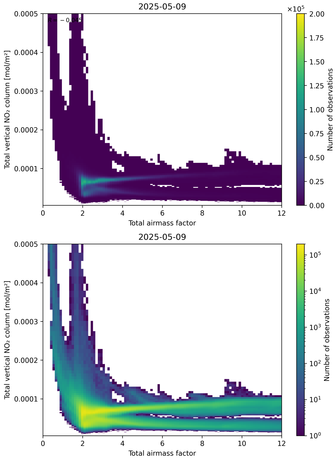
Figure 67: Scatter density plot of “Total airmass factor” against “Total vertical NO 2 column” for 2025-05-09 to 2025-05-10.
