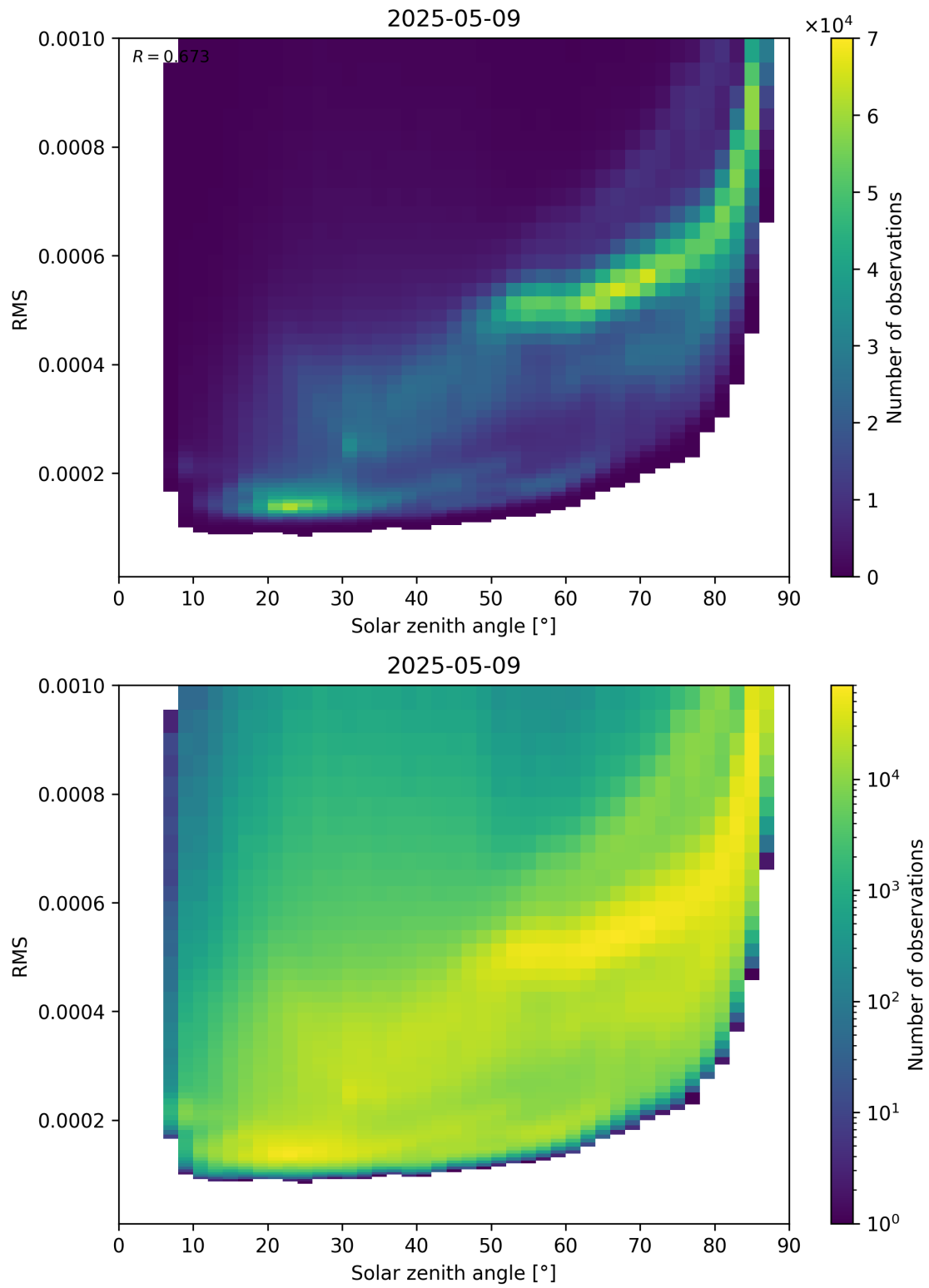
Figure 157: Scatter density plot of “Solar zenith angle” against “RMS” for 2025-05-09 to 2025-05-10.
