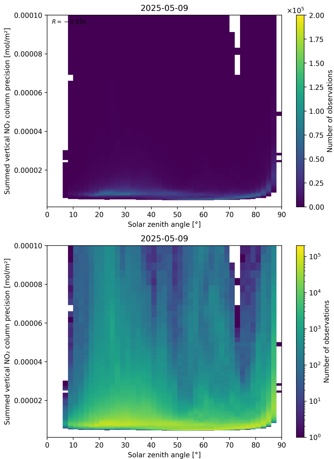
Figure 152: Scatter density plot of “Solar zenith angle” against “Summed vertical NO 2 column precision” for 2025-05-09 to 2025-05-10.
