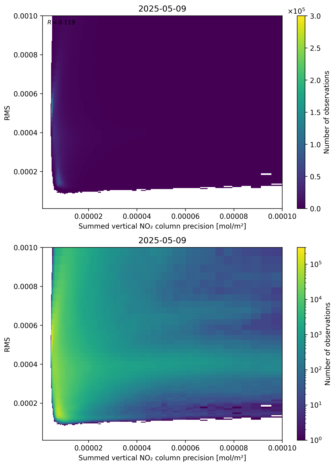
Figure 108: Scatter density plot of “Summed vertical NO 2 column precision” against “RMS” for 2025-05-09 to 2025-05-10.
