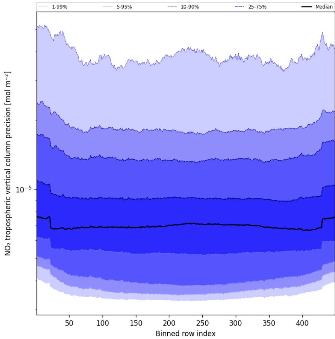
Figure 47: Along track statistics of “NO 2 tropospheric vertical column precision” for 2025-05-09 to 2025-05-10
