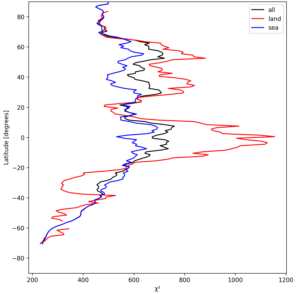
Figure 25: Zonal average of “ \chi^2 ” for 2025-05-09 to 2025-05-10.
