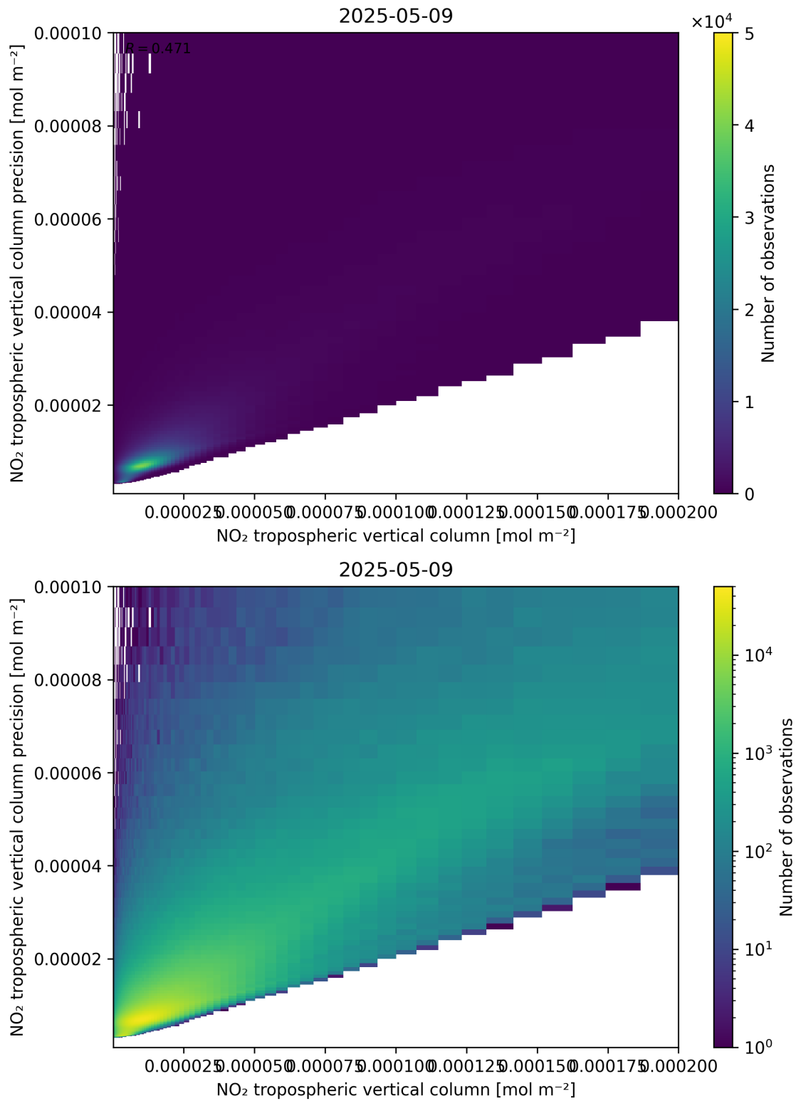
Figure 130: Scatter density plot of “NO 2 tropospheric vertical column” against “NO 2 tropospheric vertical column precision” for 2025-05-09 to 2025-05-10.
