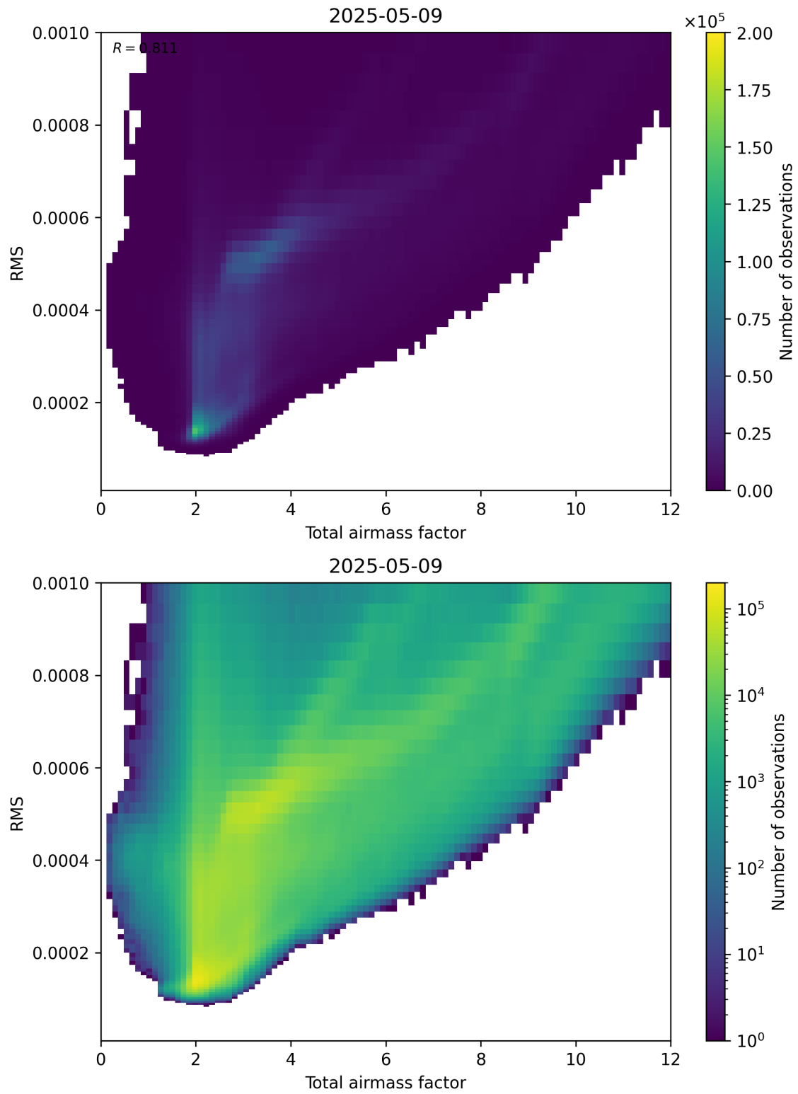
Figure 69: Scatter density plot of “Total airmass factor” against “RMS” for 2025-05-09 to 2025-05-10.
