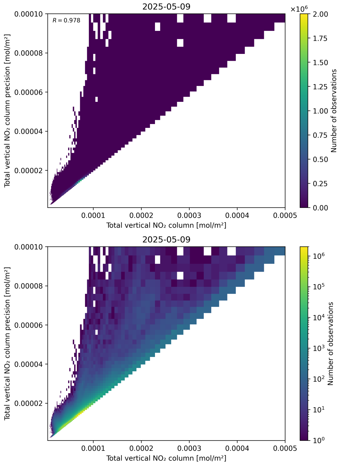
Figure 114: Scatter density plot of “Total vertical NO 2 column” against “Total vertical NO 2 column precision” for 2025-05-09 to 2025-05-10.
