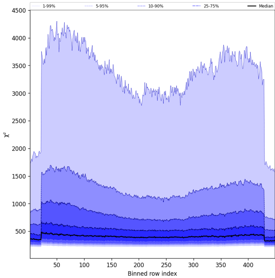
Figure 59: Along track statistics of “ \chi^2 ” for 2025-05-09 to 2025-05-10
