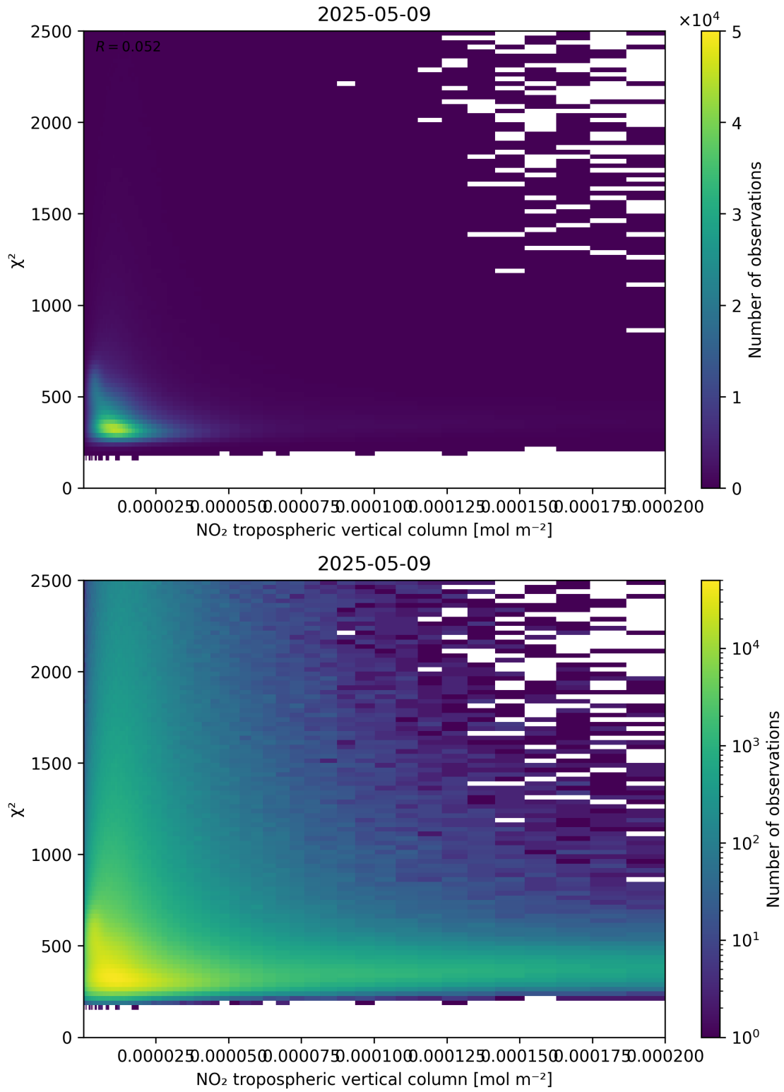
Figure 124: Scatter density plot of “NO 2 tropospheric vertical column” against “ \chi^2 ” for 2025-05-09 to 2025-05-10.
