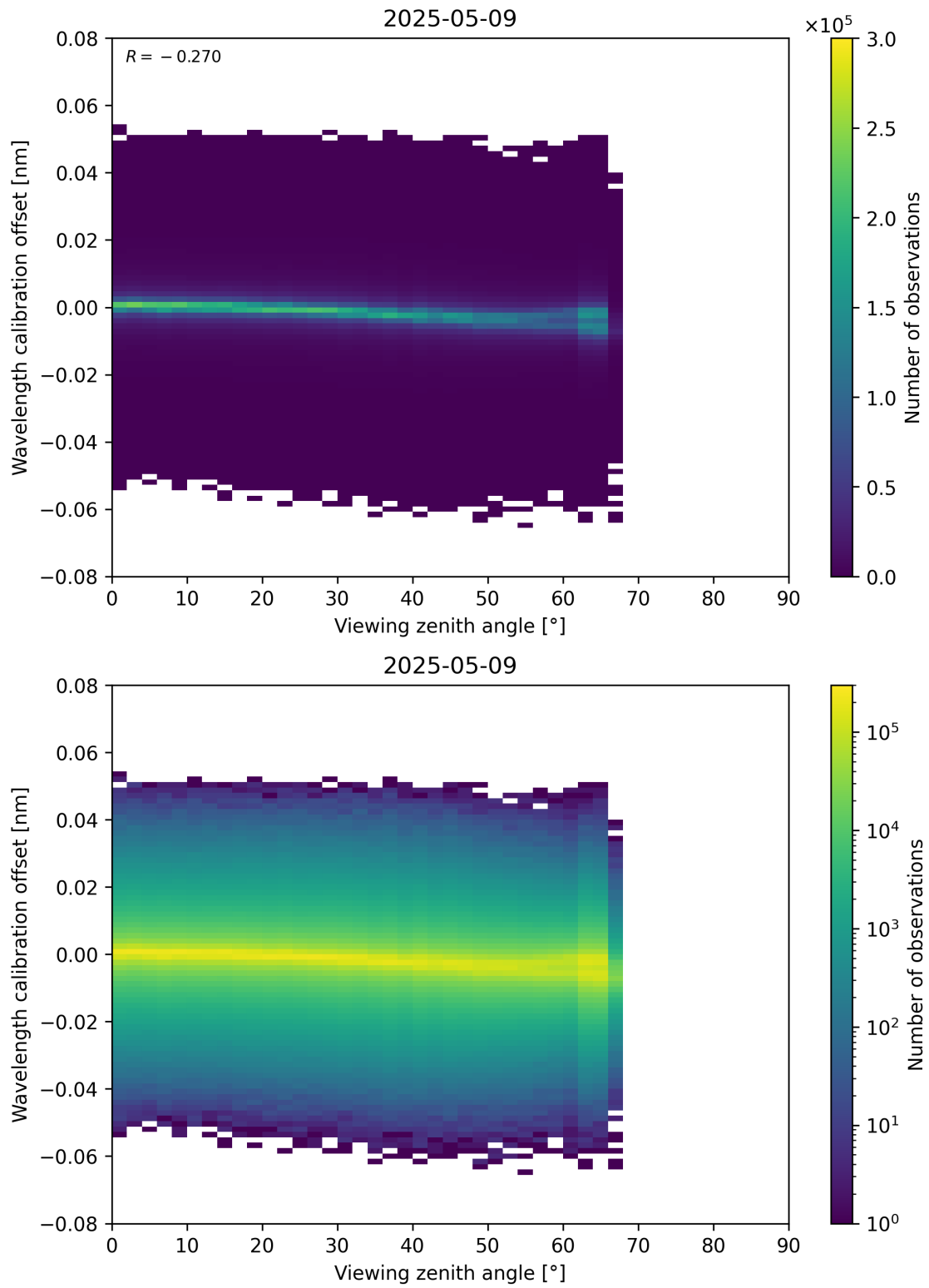
Figure 173: Scatter density plot of “Viewing zenith angle” against “Wavelength calibration offset” for 2025-05-09 to 2025-05-10.
