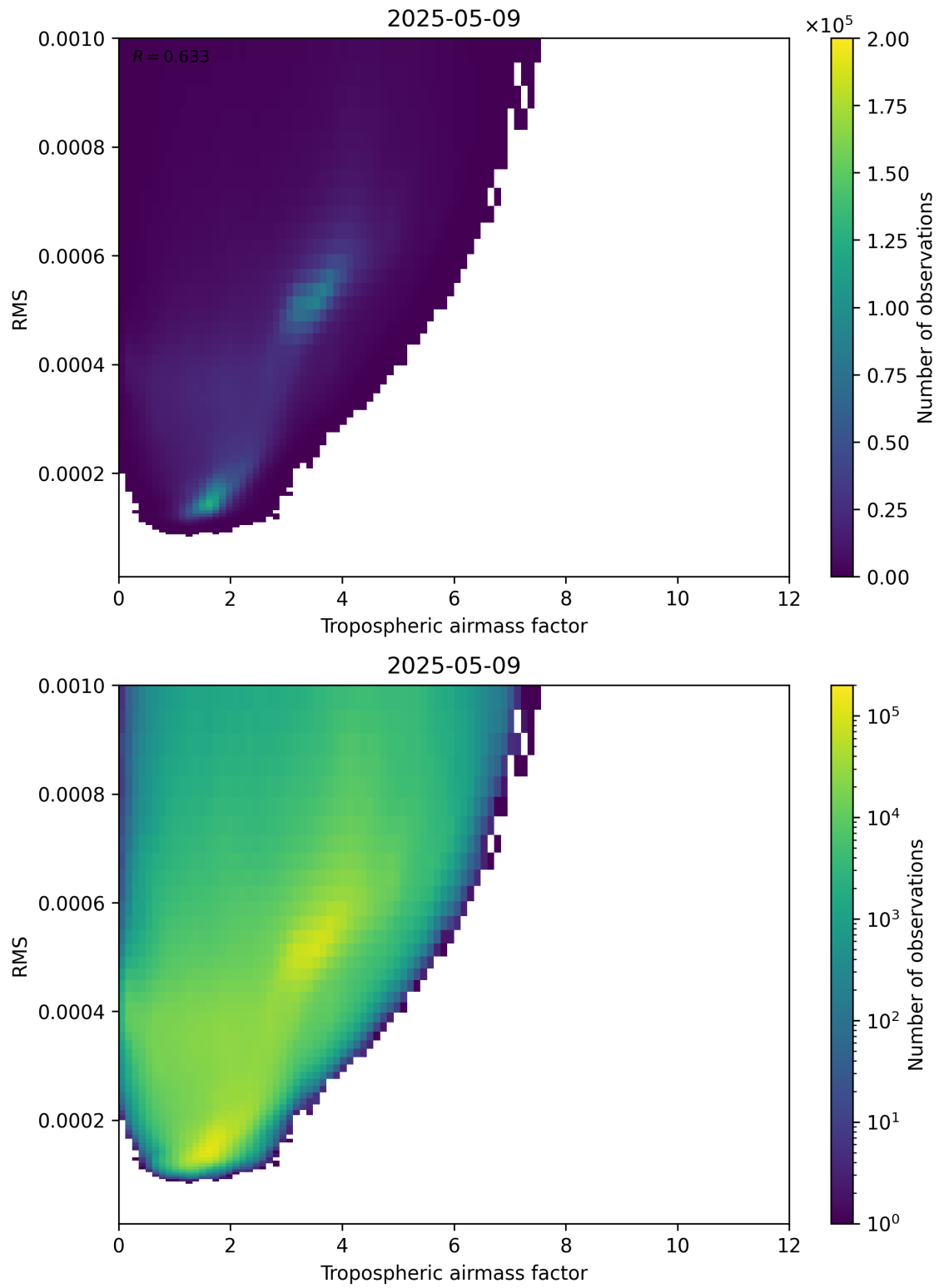
Figure 79: Scatter density plot of “Tropospheric airmass factor” against “RMS” for 2025-05-09 to 2025-05-10.
