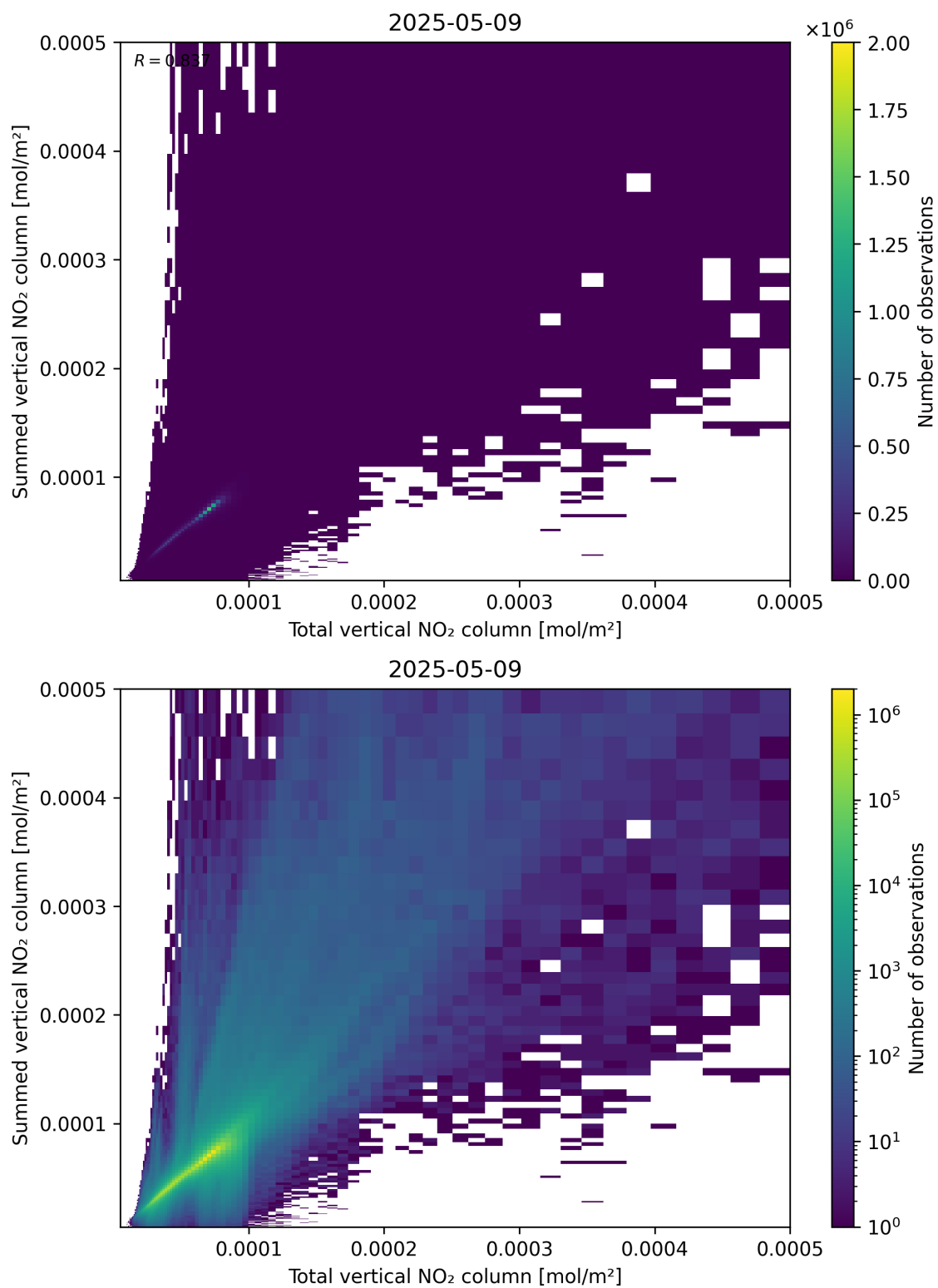
Figure 112: Scatter density plot of “Total vertical NO 2 column” against “Summed vertical NO 2 column” for 2025-05-09 to 2025-05-10.
