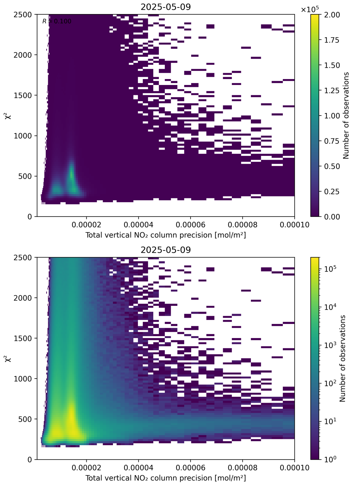
Figure 116: Scatter density plot of “Total vertical NO 2 column precision” against “ \chi^2 ” for 2025-05-09 to 2025-05-10.
