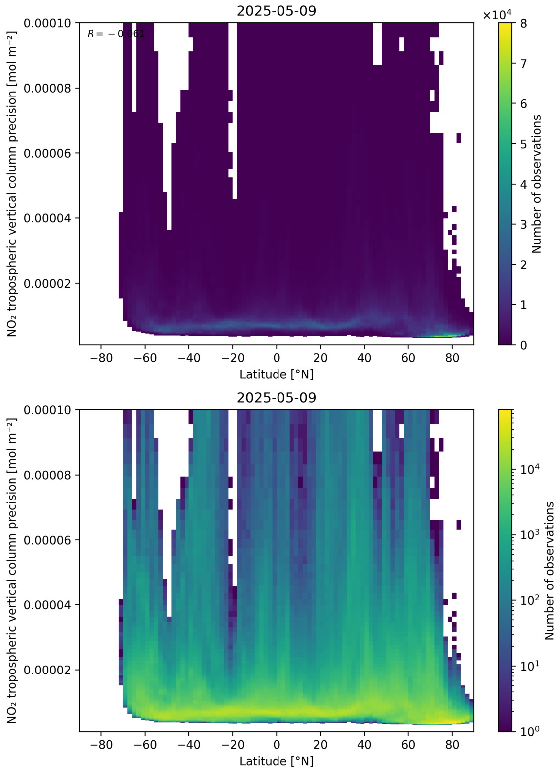
Figure 93: Scatter density plot of “Latitude” against “NO 2 tropospheric vertical column precision” for 2025-05-09 to 2025-05-10.
