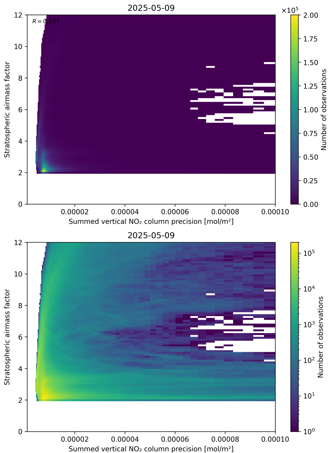
Figure 106: Scatter density plot of “Summed vertical NO 2 column precision” against “Stratospheric airmass factor” for 2025-05-09 to 2025-05-10.
