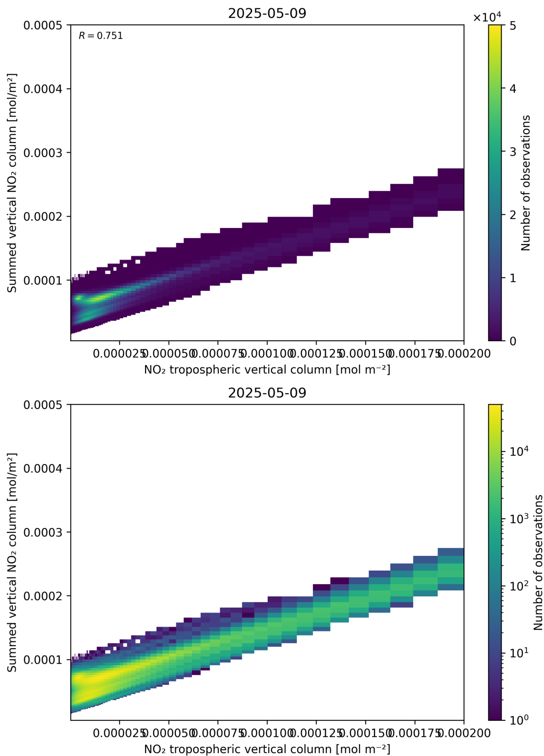
Figure 126: Scatter density plot of “NO 2 tropospheric vertical column” against “Summed vertical NO 2 column” for 2025-05-09 to 2025-05-10.
