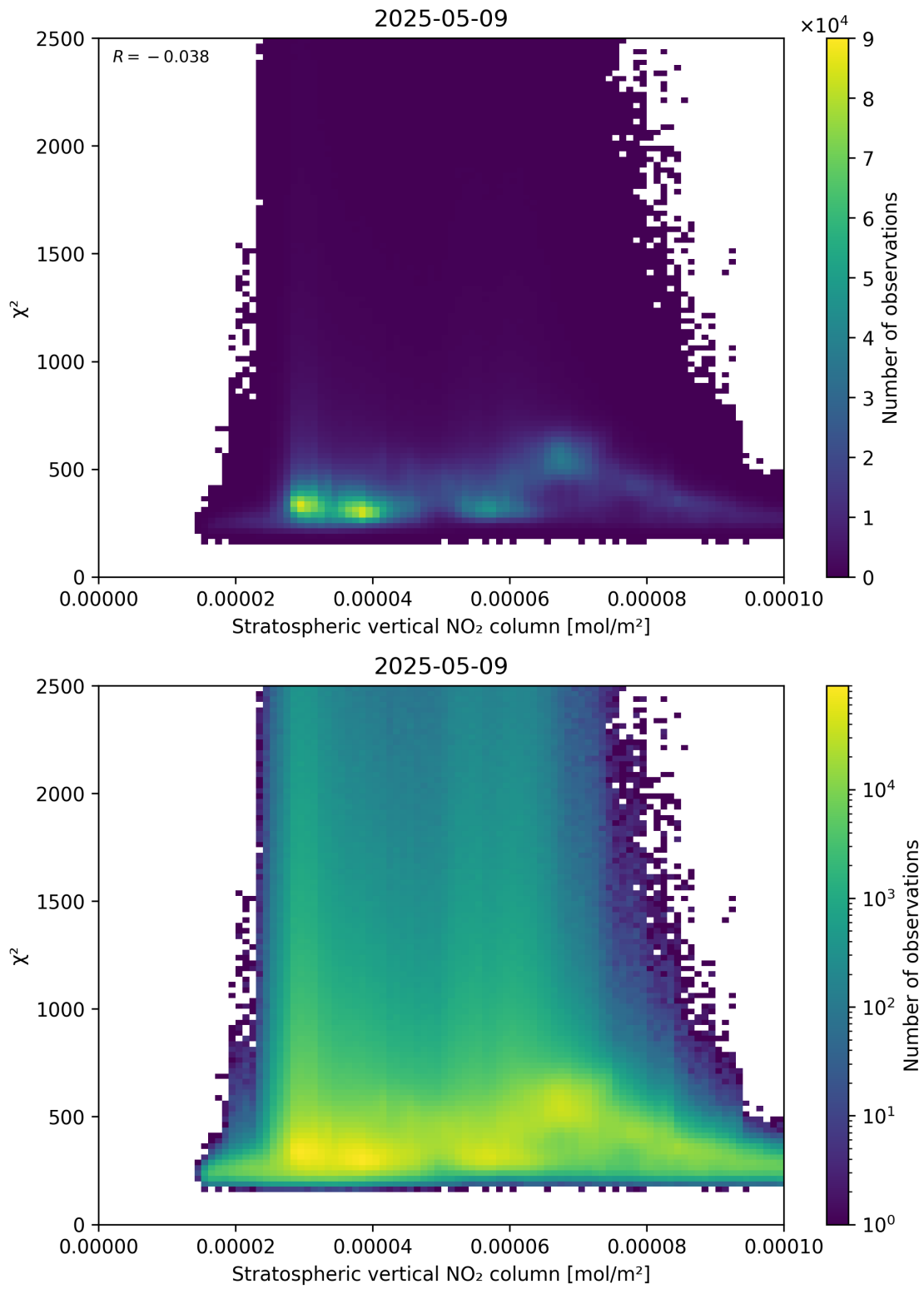
Figure 97: Scatter density plot of “Stratospheric vertical NO 2 column” against “ \chi^2 ” for 2025-05-09 to 2025-05-10.
