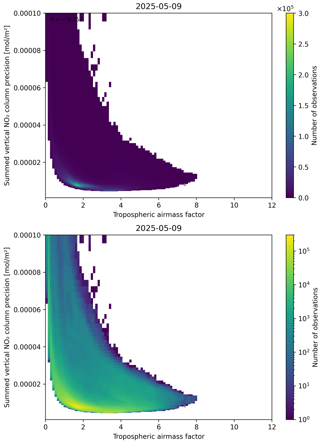
Figure 76: Scatter density plot of “Tropospheric air mass factor” against “Summed vertical NO 2 column precision” for 2025-05-09 to 2025-05-10.
