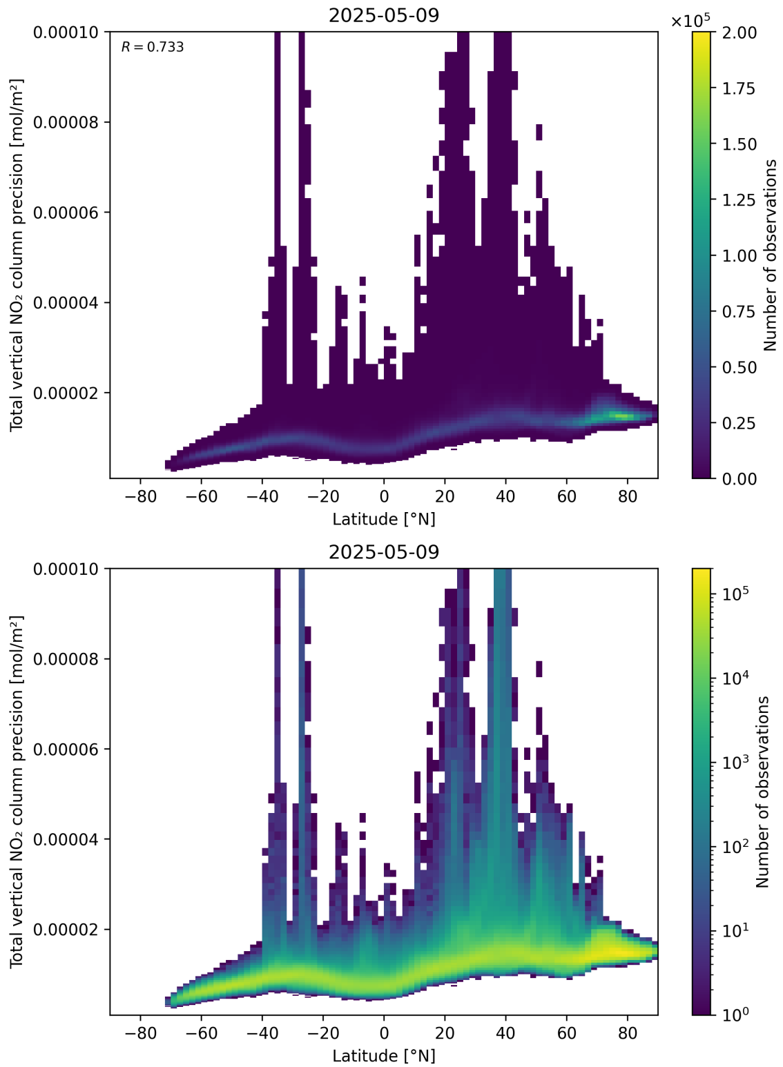
Figure 91: Scatter density plot of “Latitude” against “Total vertical NO 2 column precision” for 2025-05-09 to 2025-05-10.
