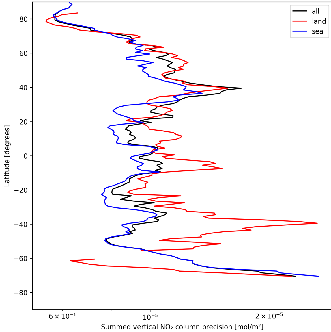
Figure 24: Zonal average of “Summed vertical NO 2 column precision” for 2025-05-09 to 2025-05-10.
