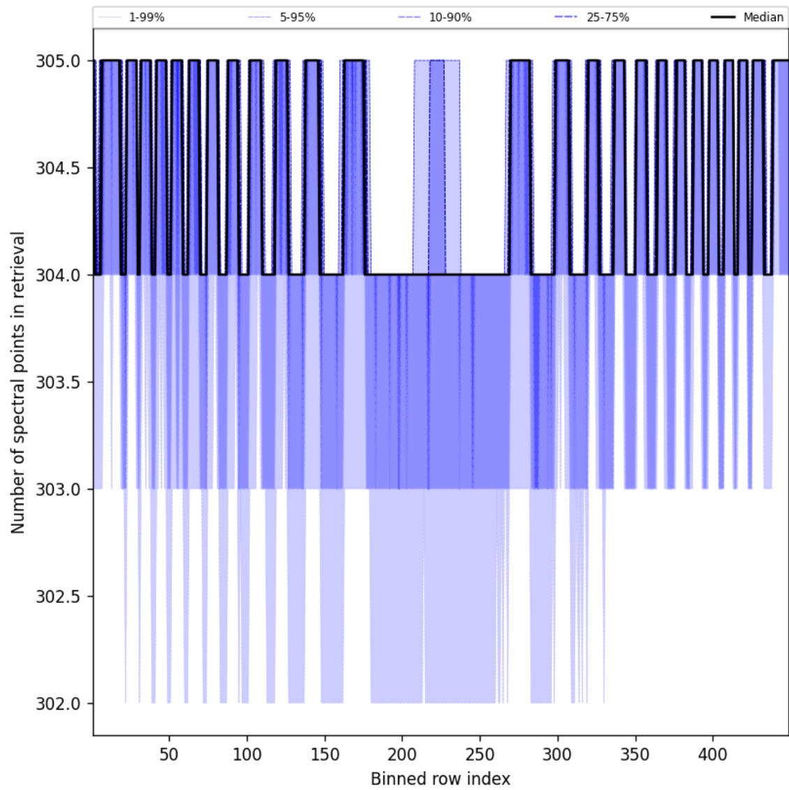
Figure 50: Along track statistics of “Number of spectral points in retrieval” for 2025-05-09 to 2025-05-10
