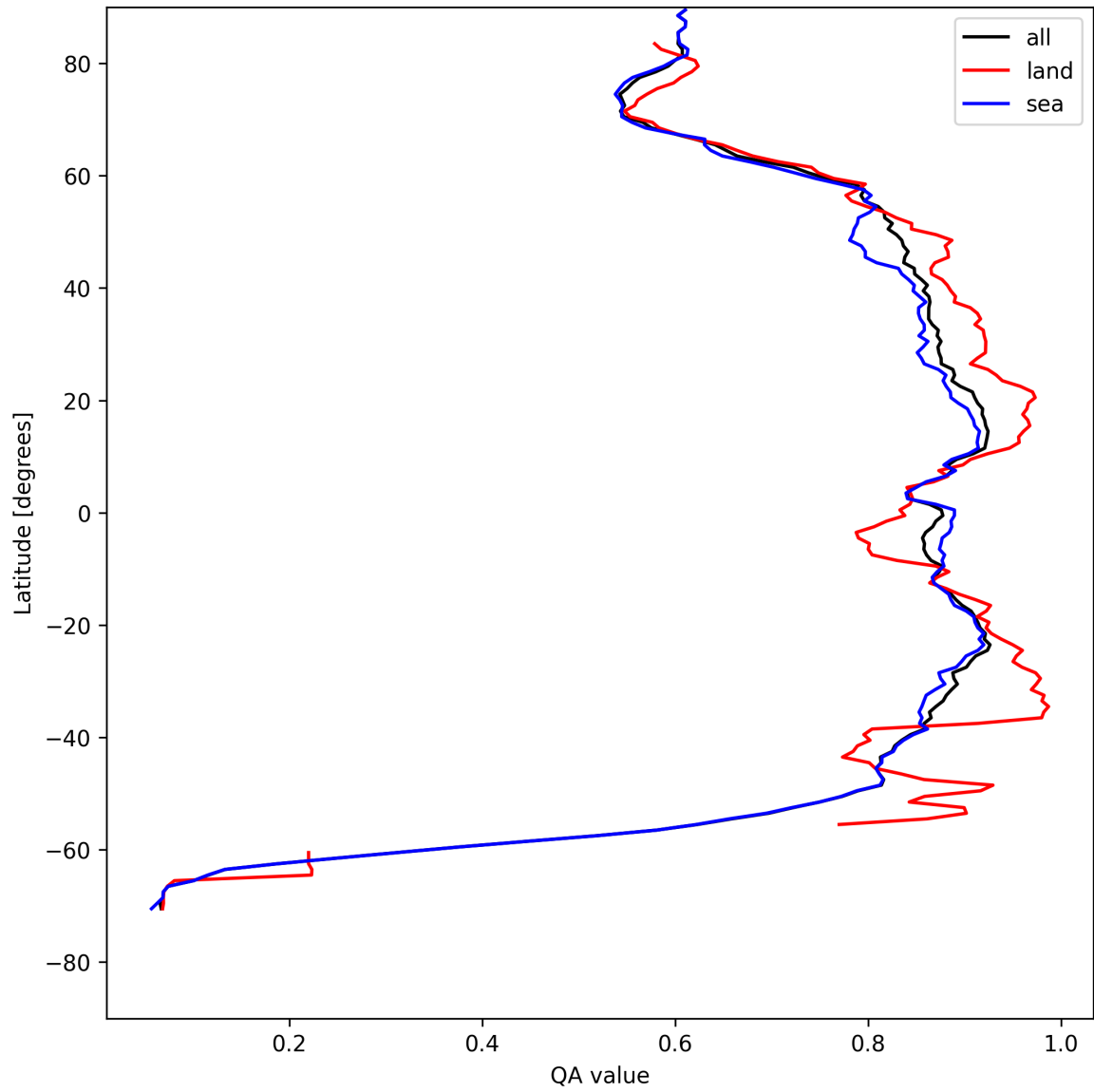
Figure 11: Zonal average of “QA value” for 2025-05-09 to 2025-05-10.
