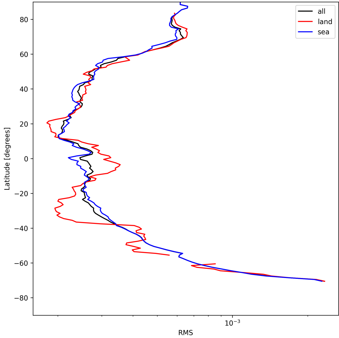
Figure 26: Zonal average of “RMS” for 2025-05-09 to 2025-05-10.
