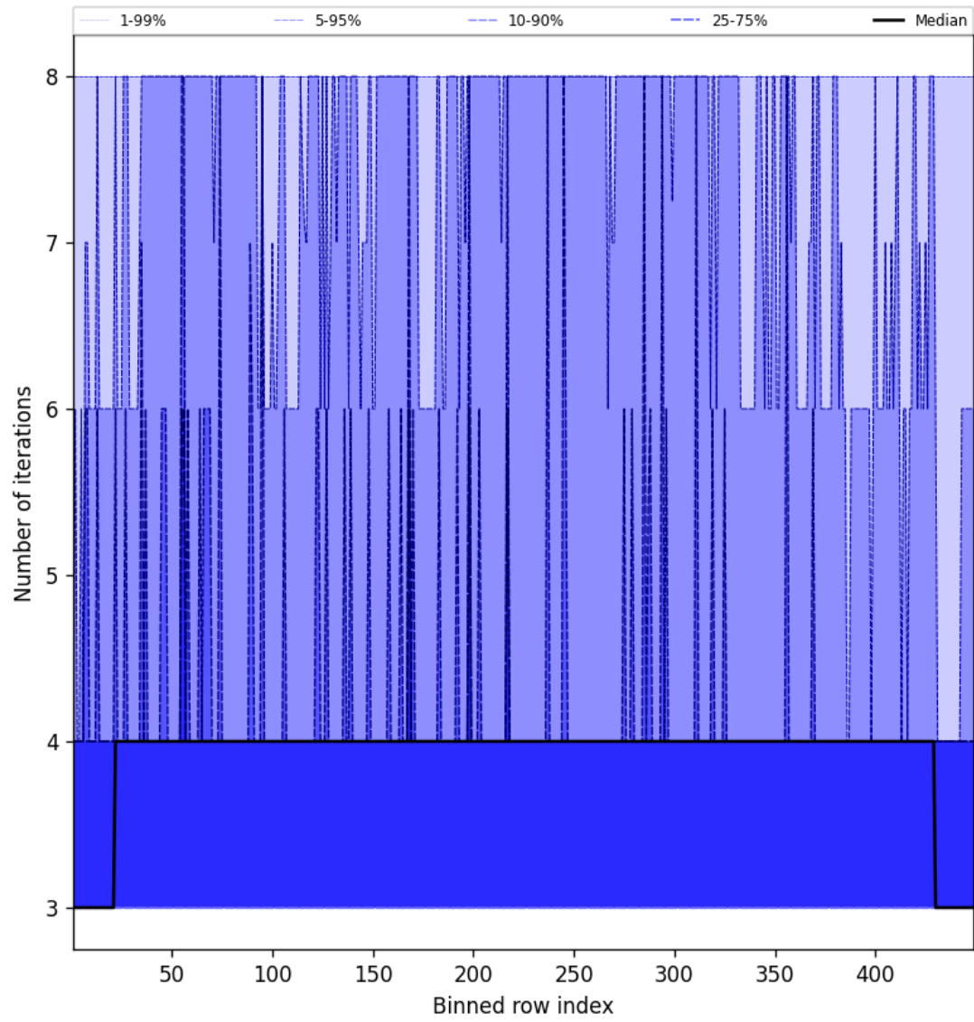
Figure 51: Along track statistics of “Number of iterations” for 2025-05-09 to 2025-05-10
