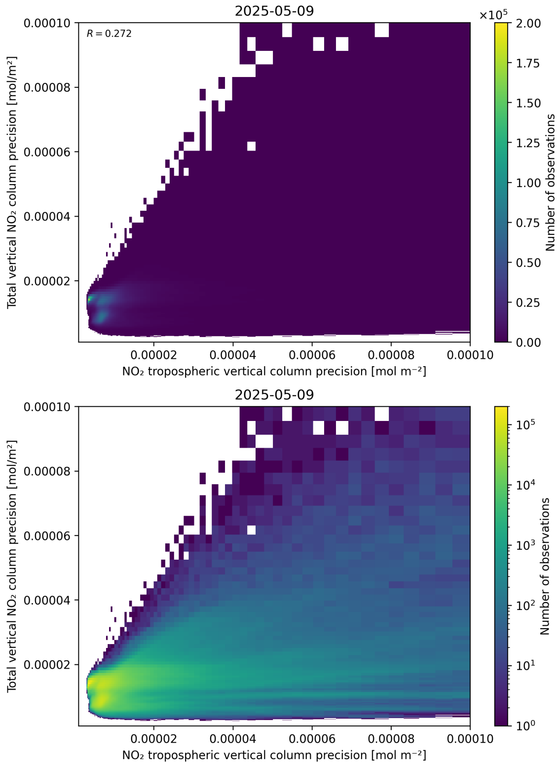
Figure 139: Scatter density plot of “NO 2 tropospheric vertical column precision” against “Total vertical NO 2 column precision” for 2025-05-09 to 2025-05-10.
