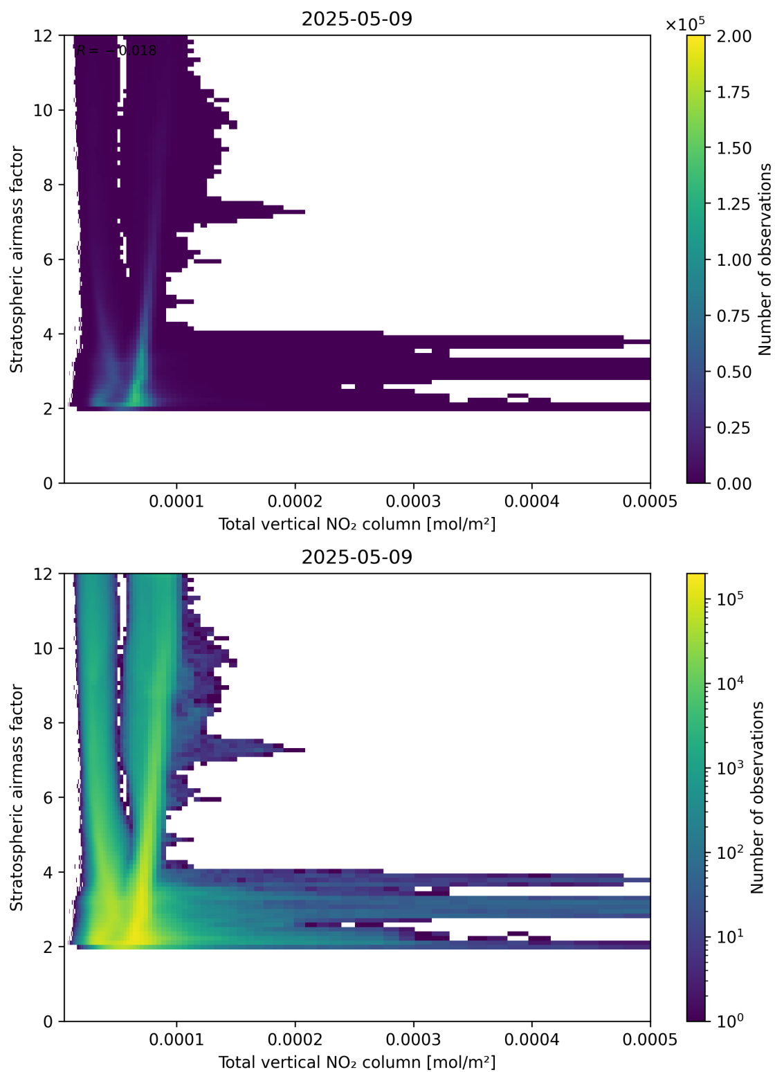
Figure 110: Scatter density plot of “Total vertical NO 2 column” against “Stratospheric airmass factor” for 2025-05-09 to 2025-05-10.
