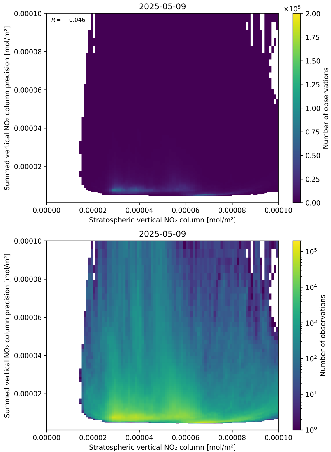
Figure 99: Scatter density plot of “Stratospheric vertical NO 2 column” against “Summed vertical NO 2 column precision” for 2025-05-09 to 2025-05-10.
