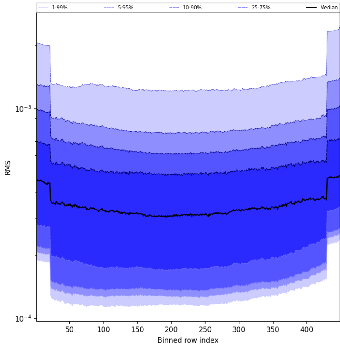
Figure 60: Along track statistics of “RMS” for 2025-05-09 to 2025-05-10
