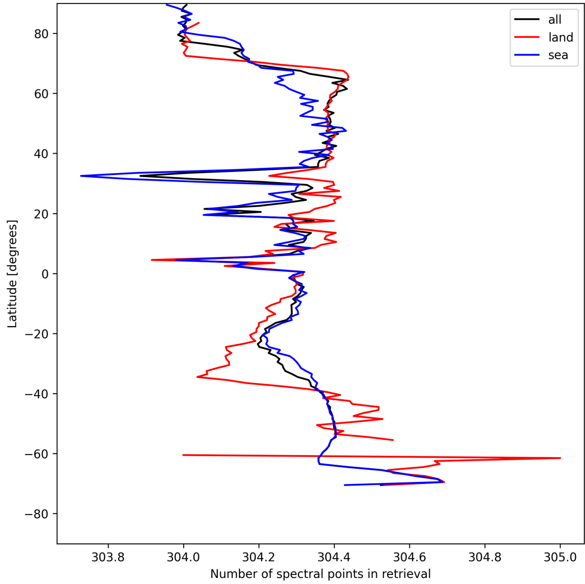
Figure 16: Zonal average of “Number of spectral points in retrieval” for 2025-05-09 to 2025-05-10.
