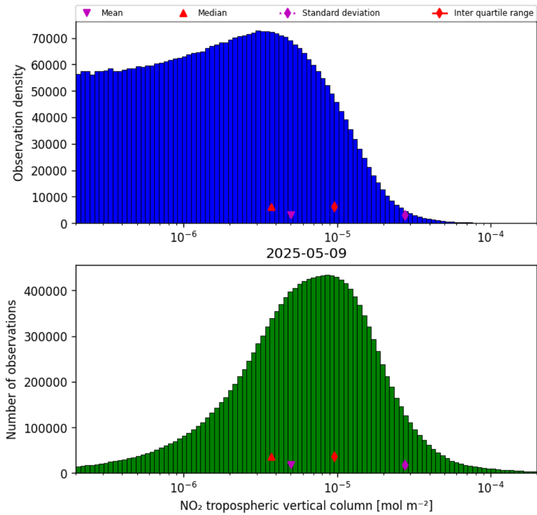
Figure 29: Histogram of “NO 2 tropospheric vertical column” for 2025-05-09 to 2025-05-10
