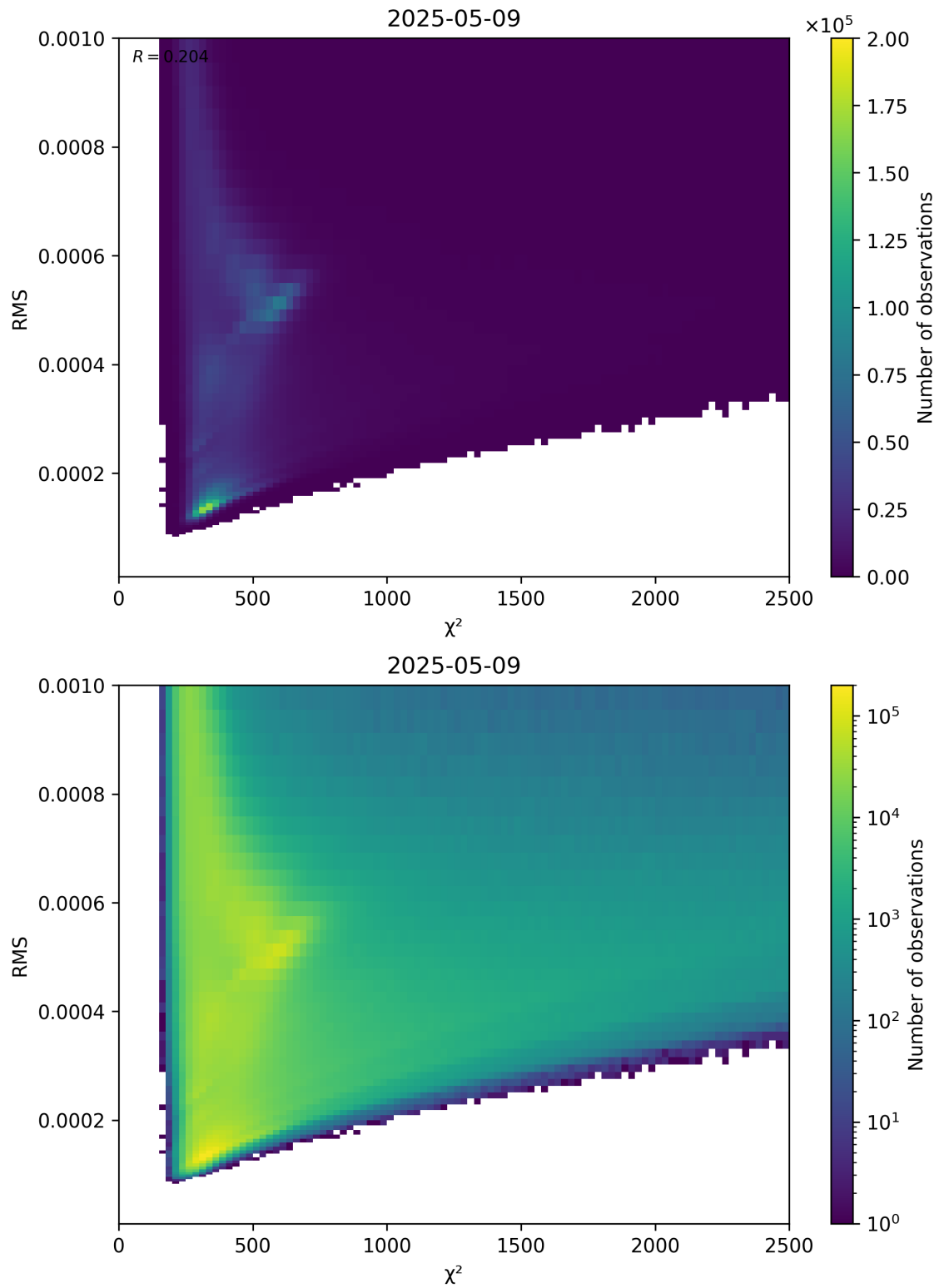
Figure 82: Scatter density plot of “ \chi^2 ” against “RMS” for 2025-05-09 to 2025-05-10.
