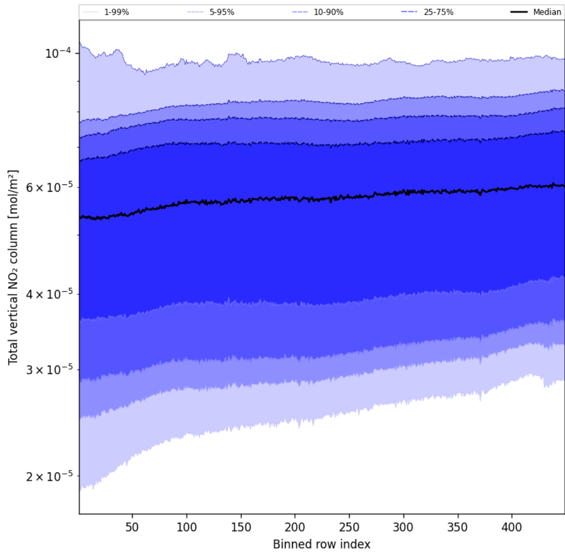
Figure 55: Along track statistics of “Total vertical NO 2 column” for 2025-05-09 to 2025-05-10
