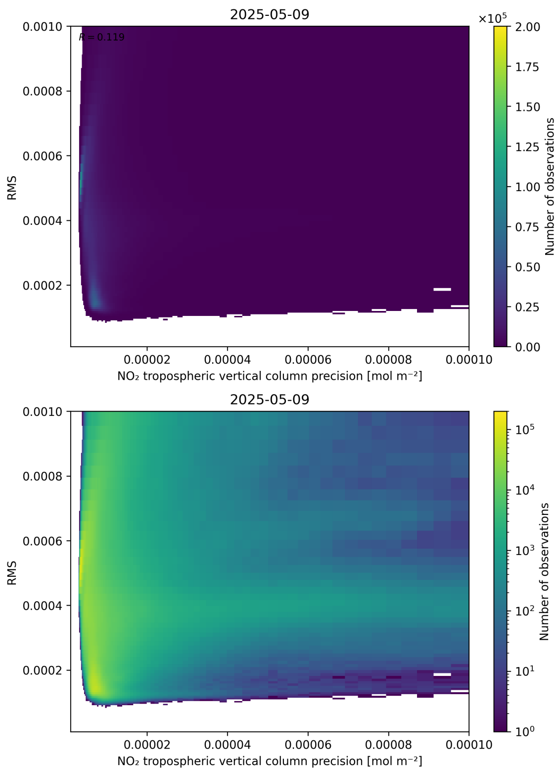
Figure 140: Scatter density plot of “NO 2 tropospheric vertical column precision” against “RMS” for 2025-05-09 to 2025-05-10.
