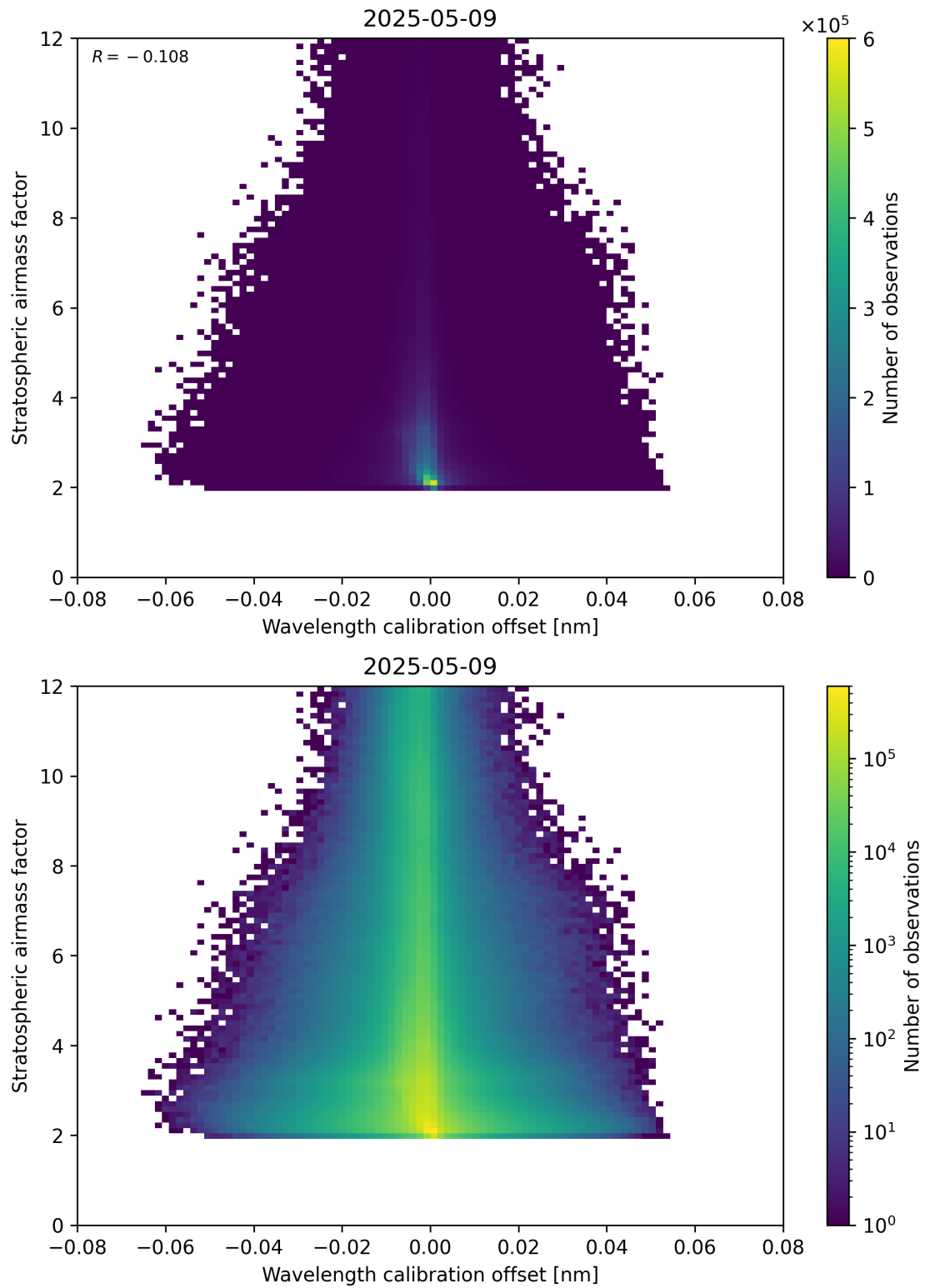
Figure 174: Scatter density plot of “Wavelength calibration offset” against “Stratospheric airmass factor” for 2025-05-09 to 2025-05-10.
