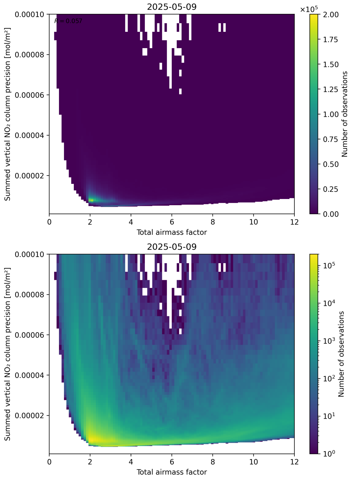
Figure 66: Scatter density plot of “Total airmass factor” against “Summed vertical NO 2 column precision” for 2025-05-09 to 2025-05-10.
