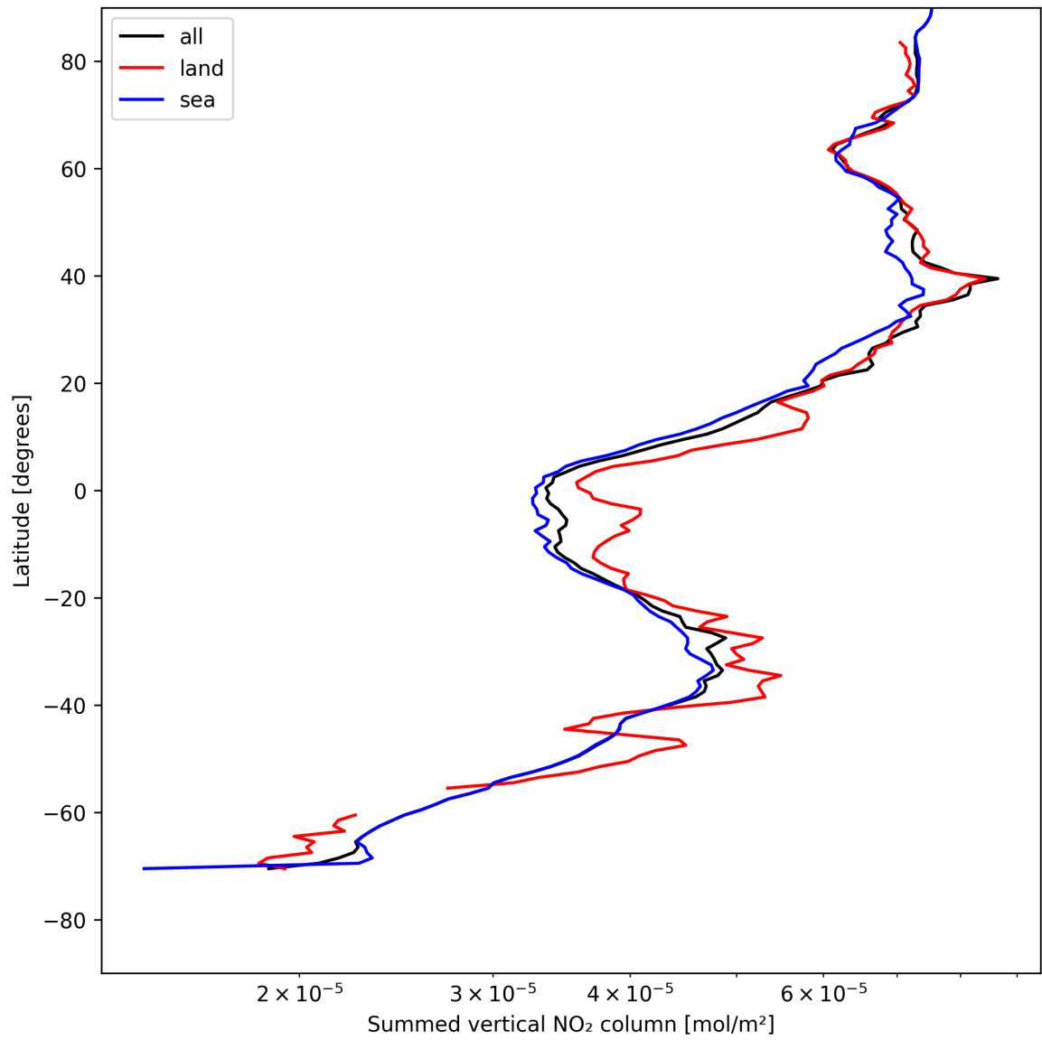
Figure 23: Zonal average of “Summed vertical NO 2 column” for 2025-05-09 to 2025-05-10.
