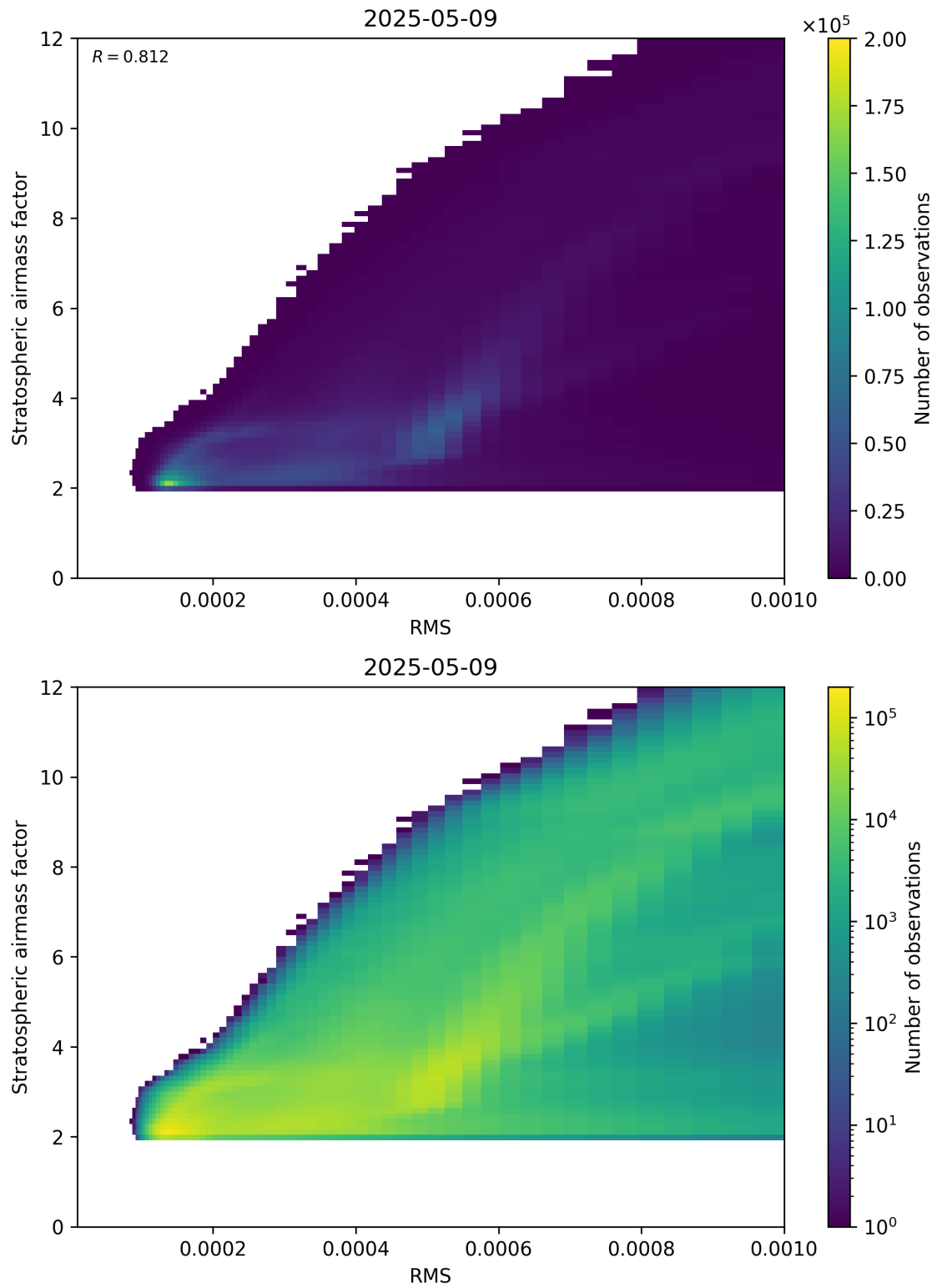
Figure 144: Scatter density plot of “RMS” against “Stratospheric airmass factor” for 2025-05-09 to 2025-05-10.
