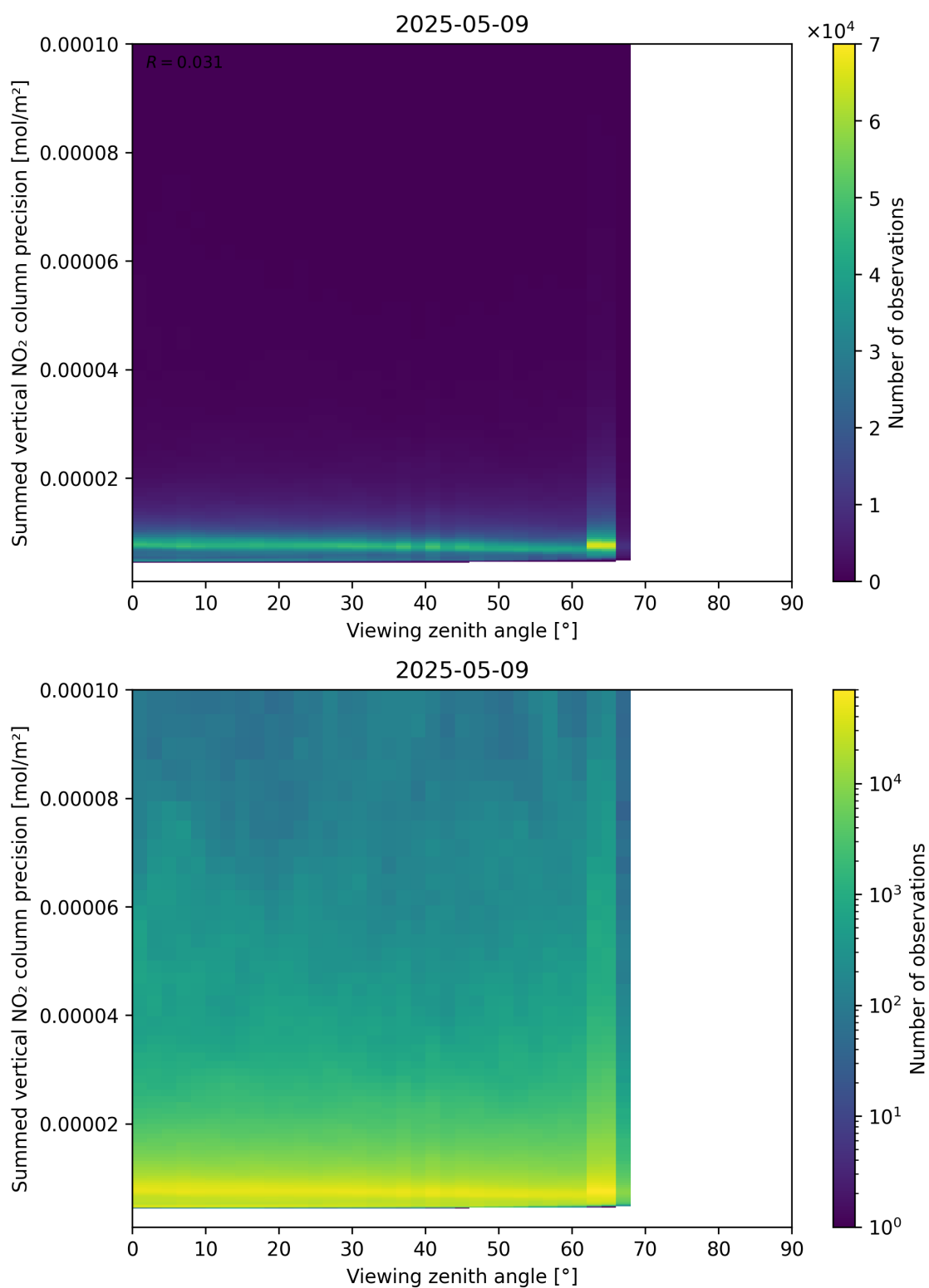
Figure 166: Scatter density plot of “Viewing zenith angle” against “Summed vertical NO 2 column precision” for 2025-05-09 to 2025-05-10.
