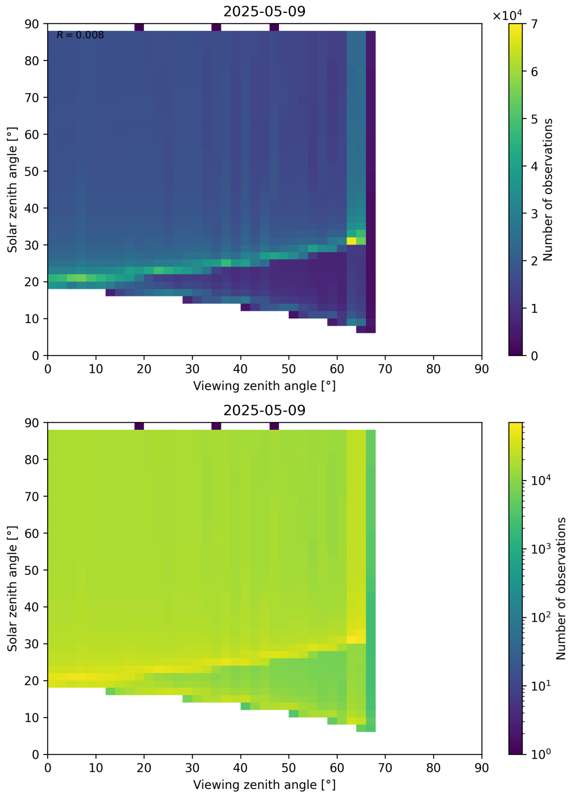
Figure 172: Scatter density plot of “Viewing zenith angle” against “Solar zenith angle” for 2025-05-09 to 2025-05-10.
