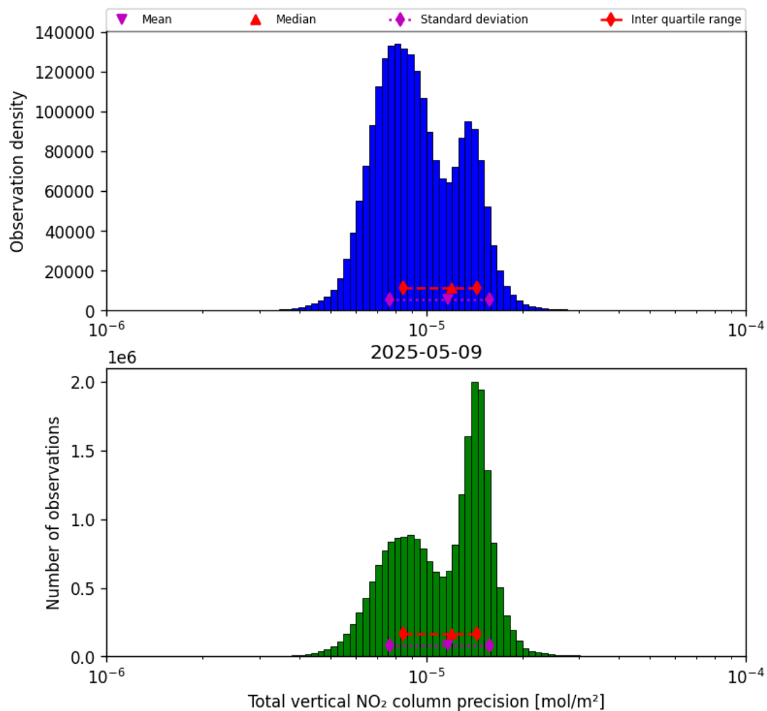
Figure 39: Histogram of “Total vertical NO 2 column precision” for 2025-05-09 to 2025-05-10
