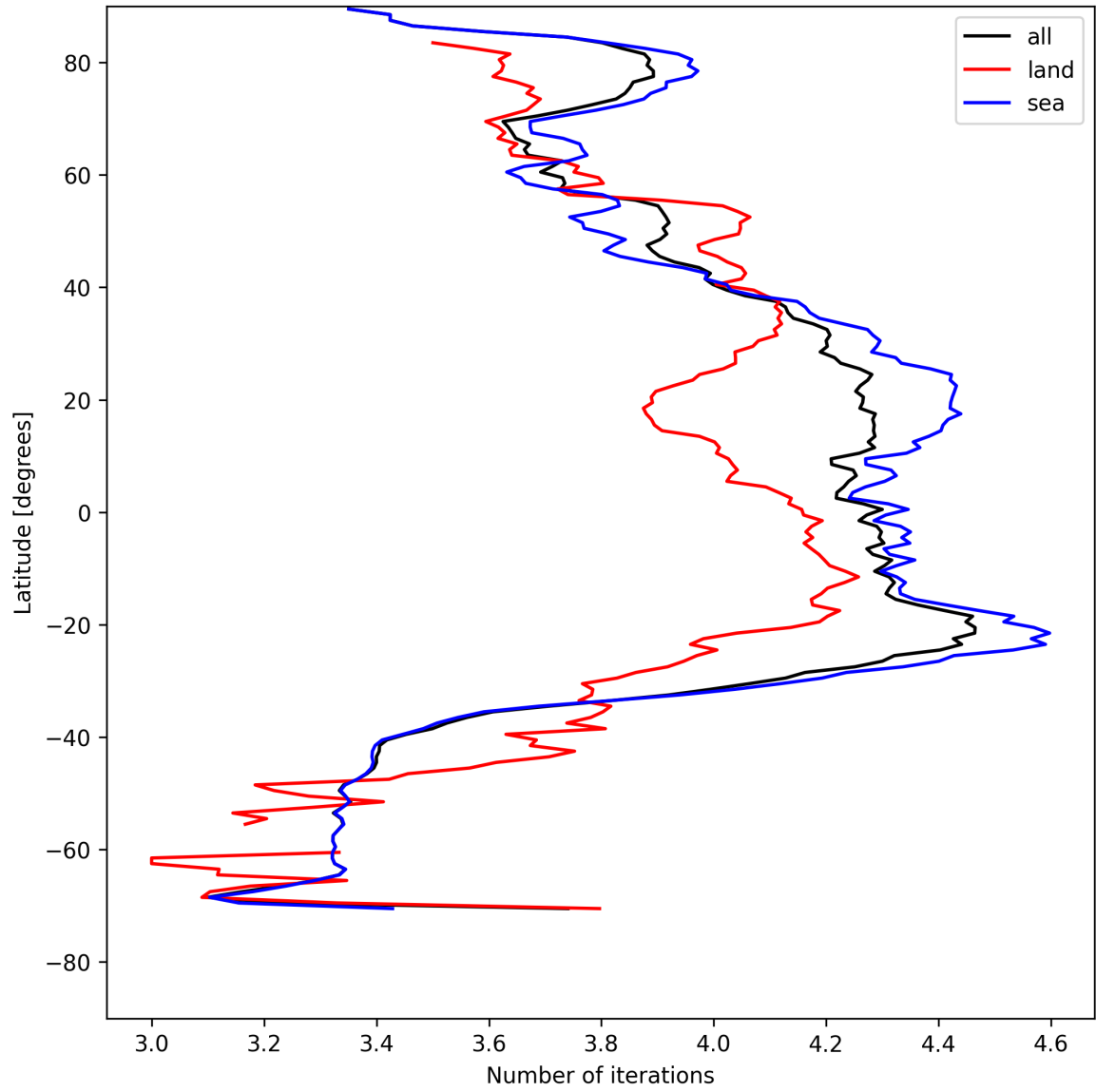
Figure 17: Zonal average of “Number of iterations” for 2025-05-09 to 2025-05-10.
