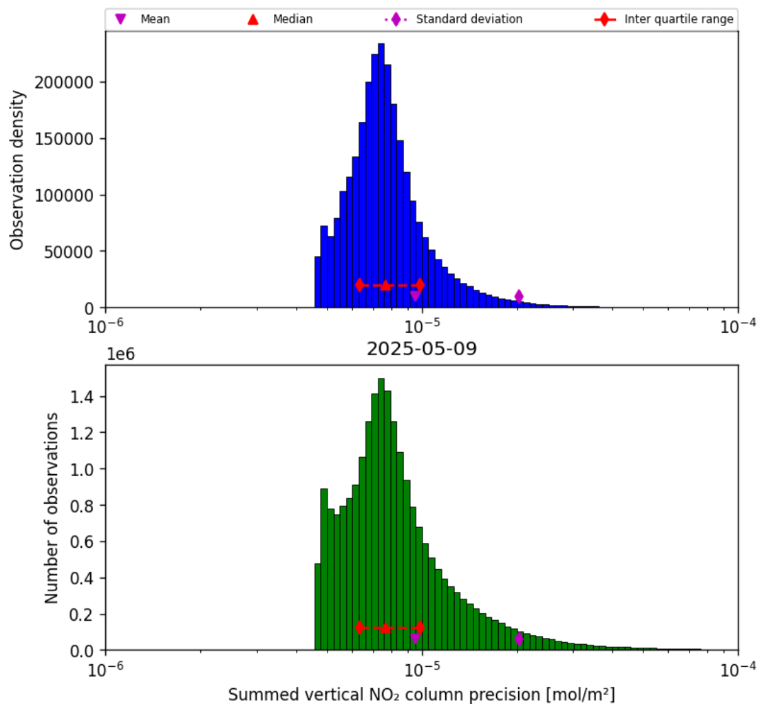
Figure 41: Histogram of "Summed vertical NO 2 column precision" for 2025-05-09 to 2025-05-10
