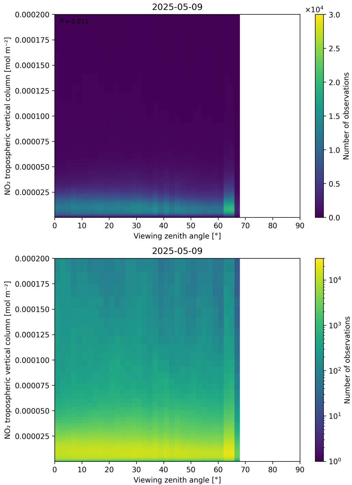
Figure 169: Scatter density plot of “Viewing zenith angle” against “NO 2 tropospheric vertical column” for 2025-05-09 to 2025-05-10.
