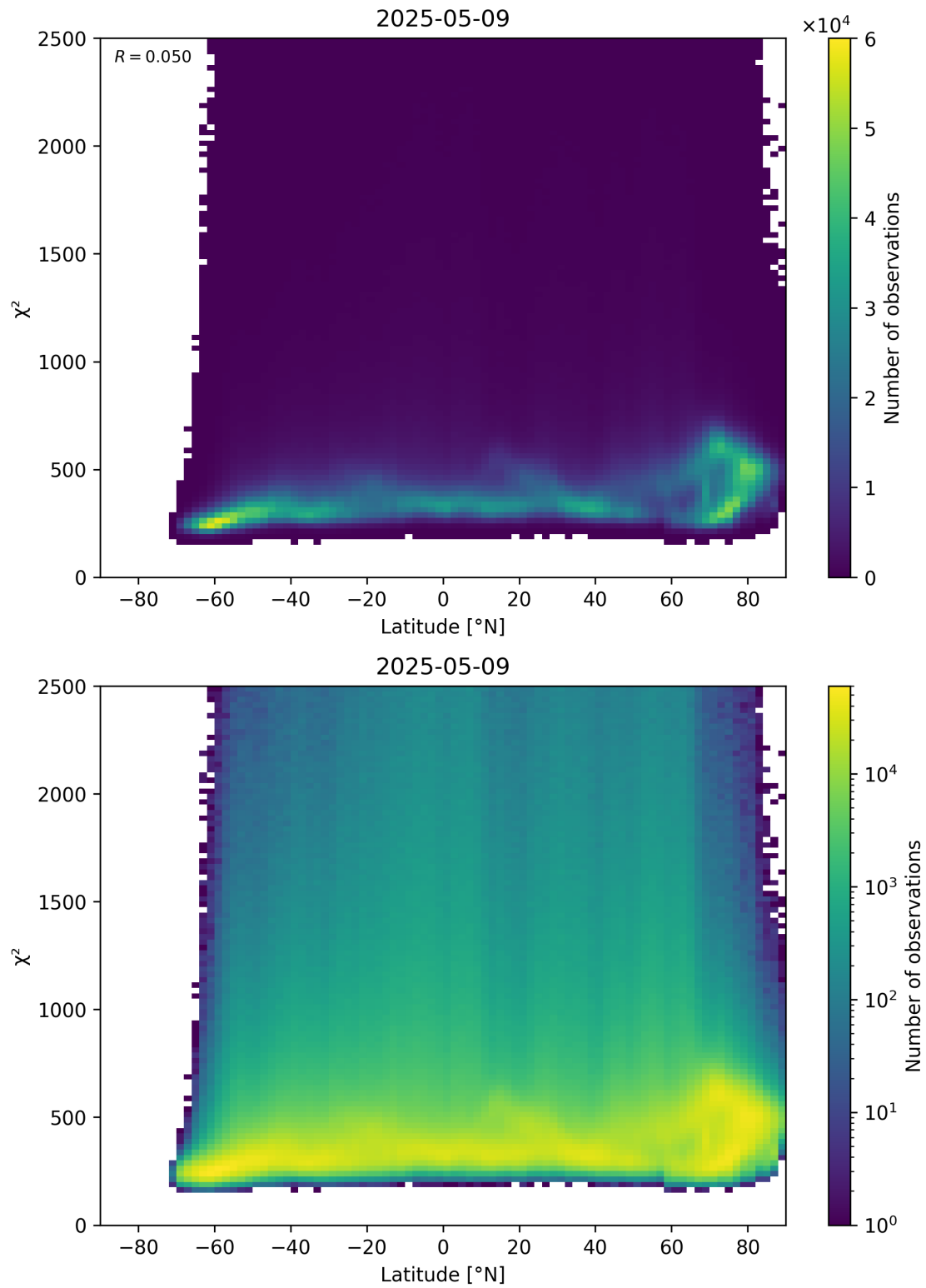
Figure 86: Scatter density plot of “Latitude” against “ \chi^2 ” for 2025-05-09 to 2025-05-10.
