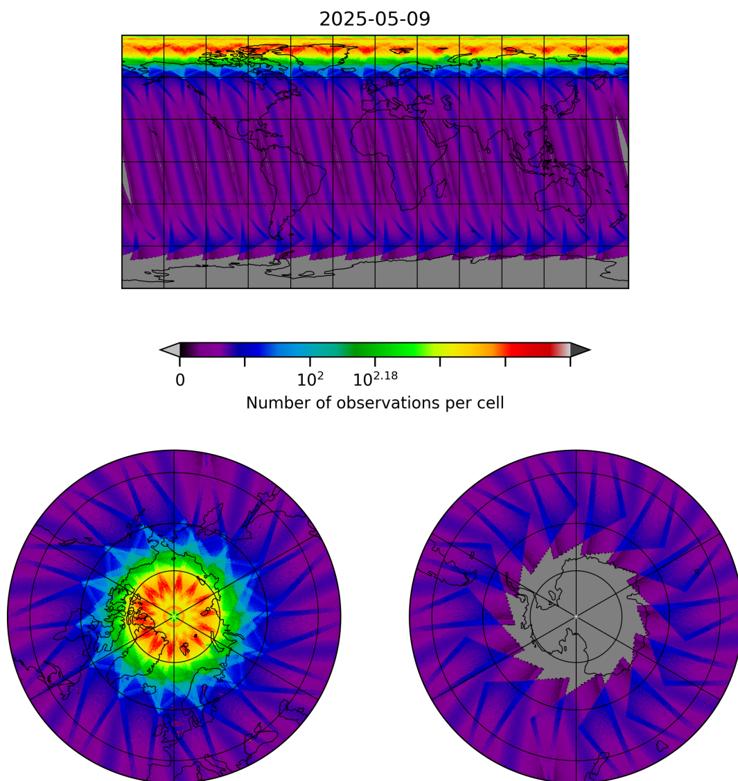
Figure 10: Map of the number of observations for 2025-05-09 to 2025-05-10
