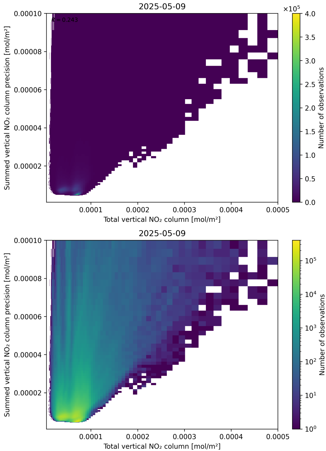
Figure 113: Scatter density plot of “Total vertical NO 2 column” against “Summed vertical NO 2 column precision” for 2025-05-09 to 2025-05-10.
