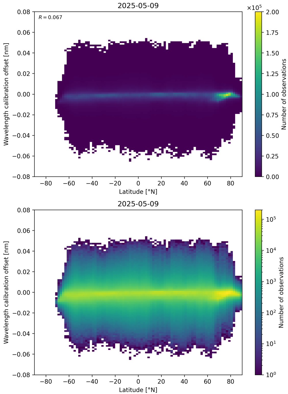
Figure 95: Scatter density plot of “Latitude” against “Wavelength calibration offset” for 2025-05-09 to 2025-05-10.
