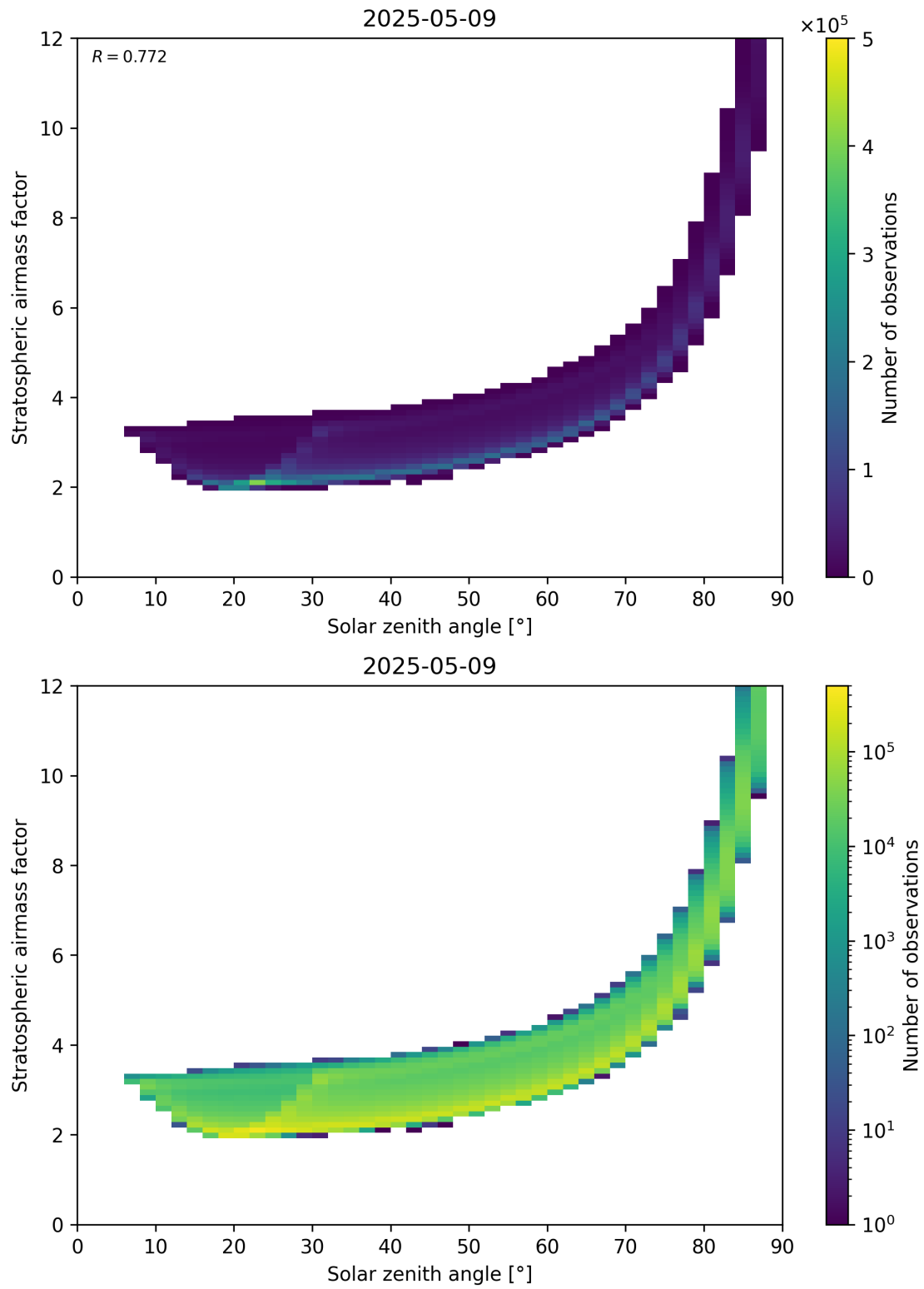
Figure 145: Scatter density plot of “Solar zenith angle” against “Stratospheric airmass factor” for 2025-05-09 to 2025-05-10.
