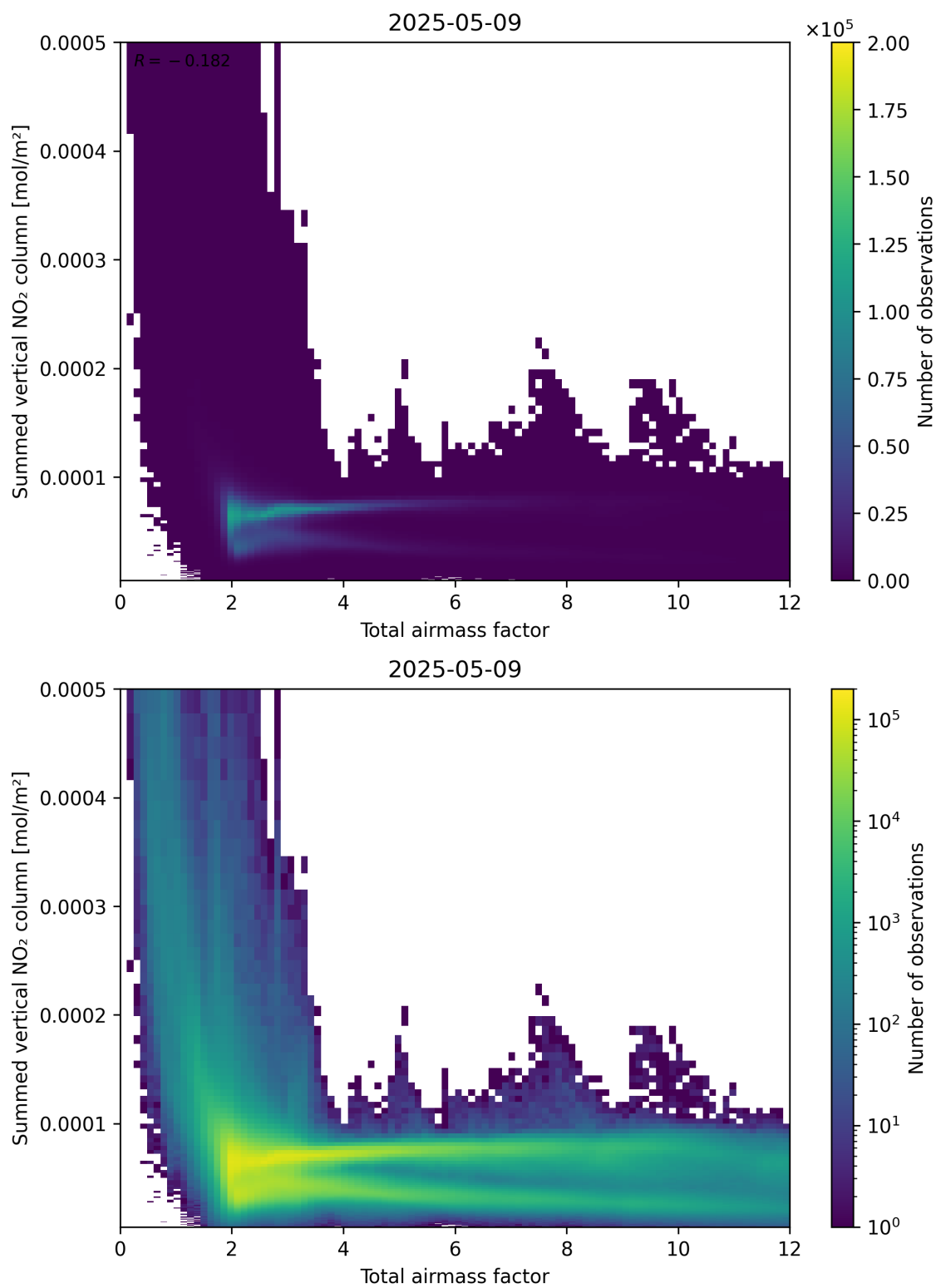
Figure 65: Scatter density plot of “Total airmass factor” against “Summed vertical NO 2 column” for 2025-05-09 to 2025-05-10.
