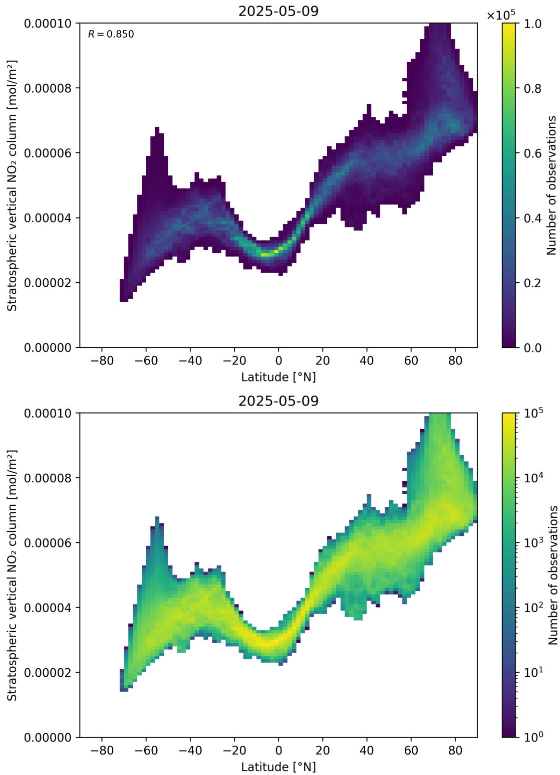
Figure 87: Scatter density plot of “Latitude” against “Stratospheric vertical NO 2 column” for 2025-05-09 to 2025-05-10.
