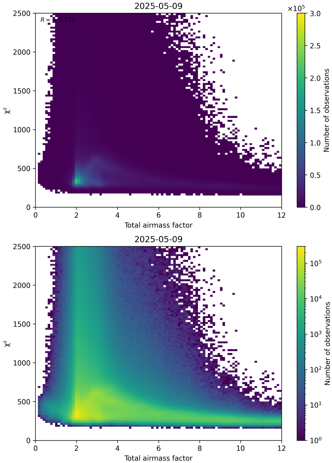
Figure 63: Scatter density plot of “Total airmass factor” against “ \chi^2 ” for 2025-05-09 to 2025-05-10.
