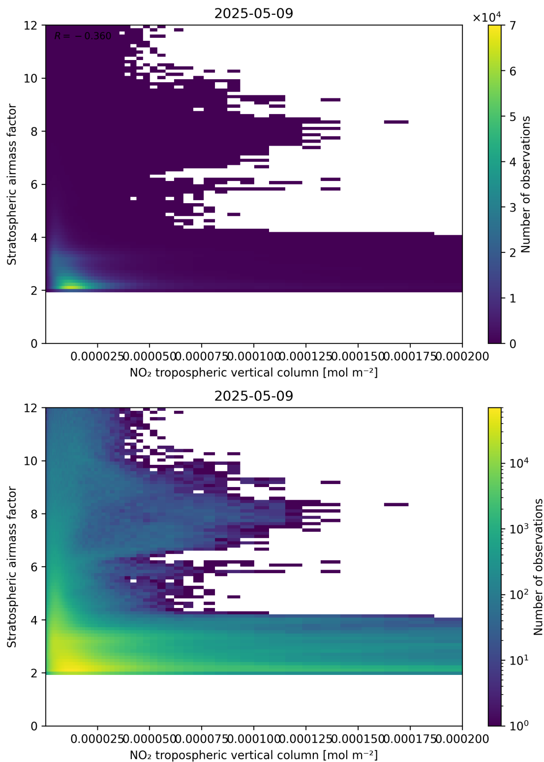
Figure 121: Scatter density plot of “NO 2 tropospheric vertical column” against “Stratospheric air mass factor” for 2025-05-09 to 2025-05-10.
