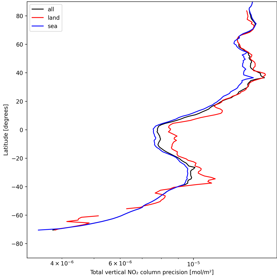
Figure 22: Zonal average of “Total vertical NO 2 column precision” for 2025-05-09 to 2025-05-10.
