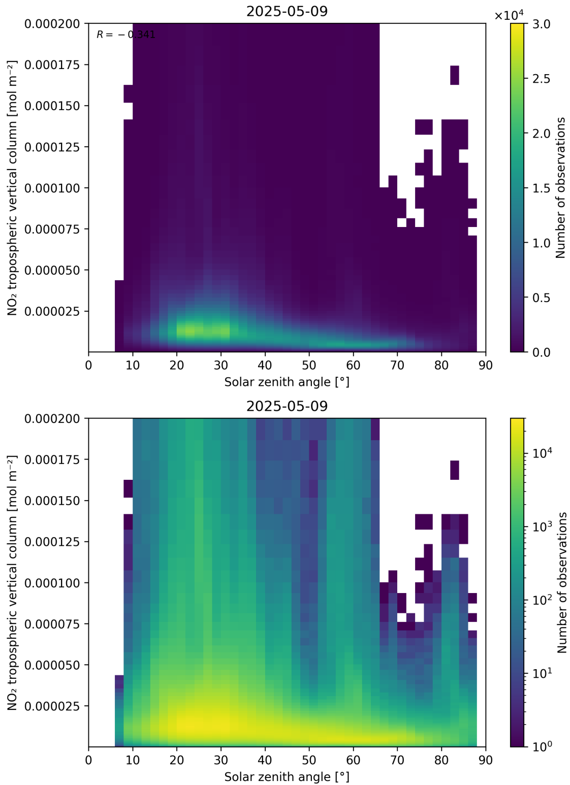
Figure 155: Scatter density plot of “Solar zenith angle” against “NO 2 tropospheric vertical column” for 2025-05-09 to 2025-05-10.
