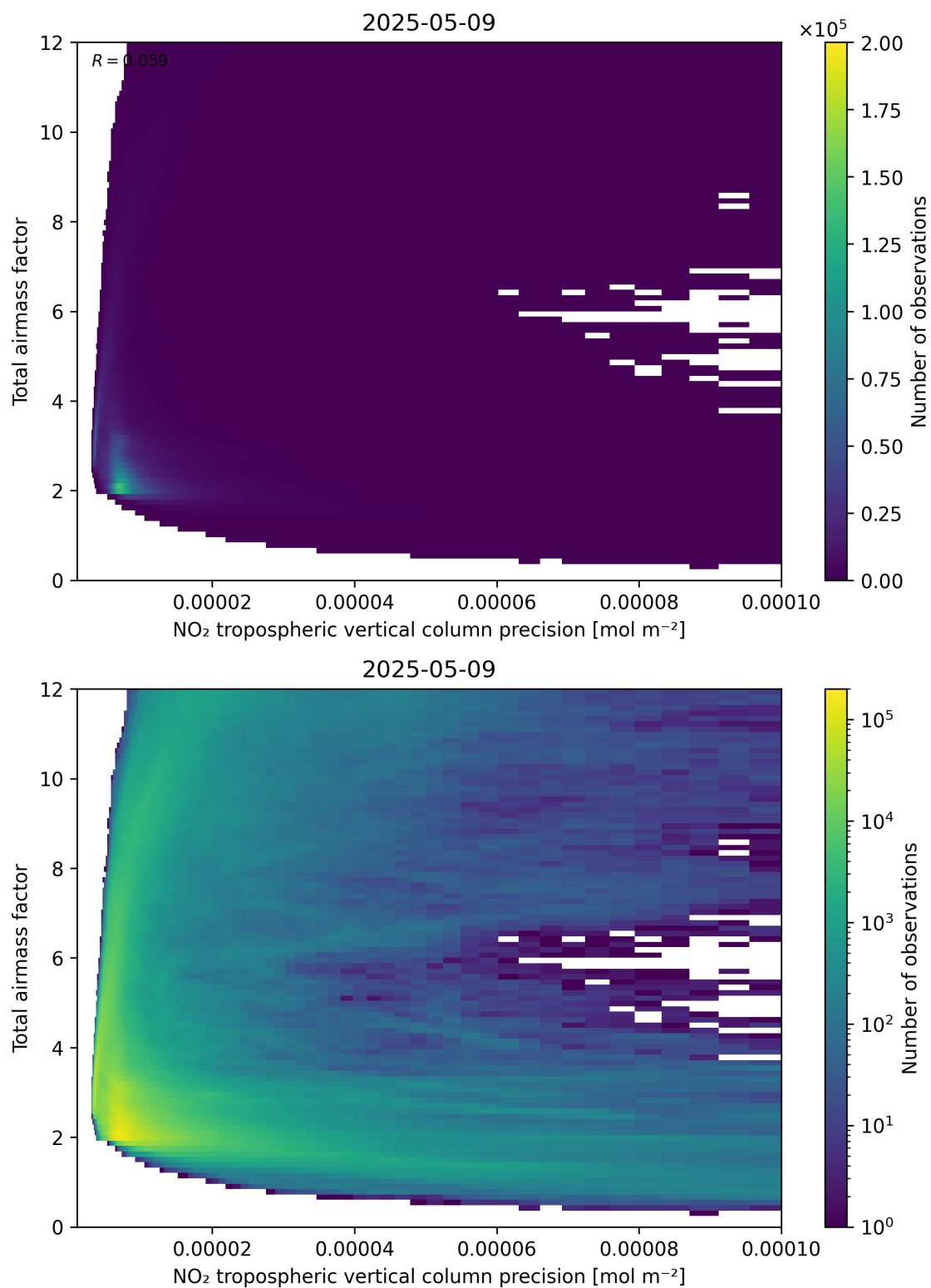
Figure 132: Scatter density plot of “NO 2 tropospheric vertical column precision” against “Total air mass factor” for 2025-05-09 to 2025-05-10.
