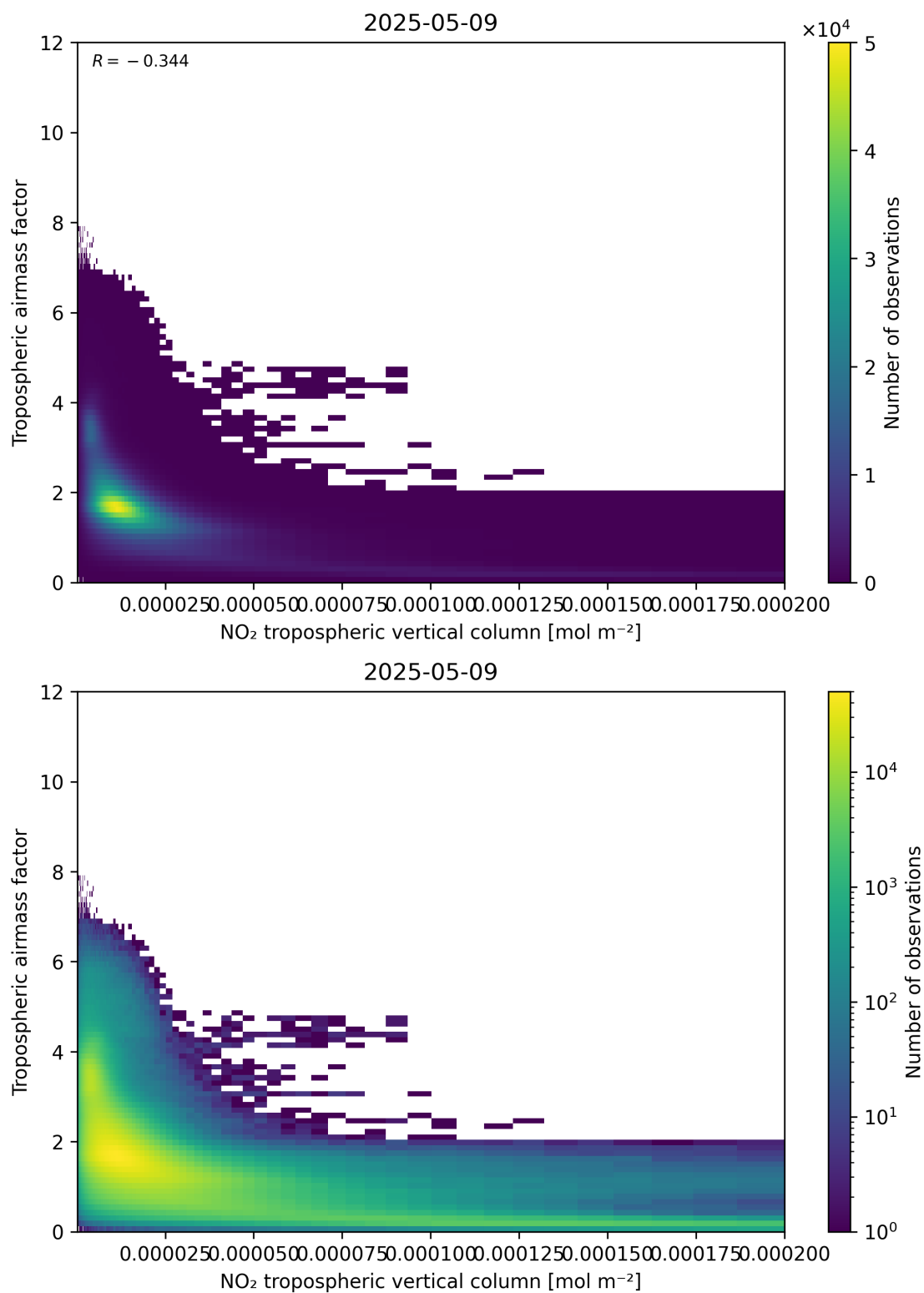
Figure 123: Scatter density plot of “NO 2 tropospheric vertical column” against “Tropospheric air mass factor” for 2025-05-09 to 2025-05-10.
