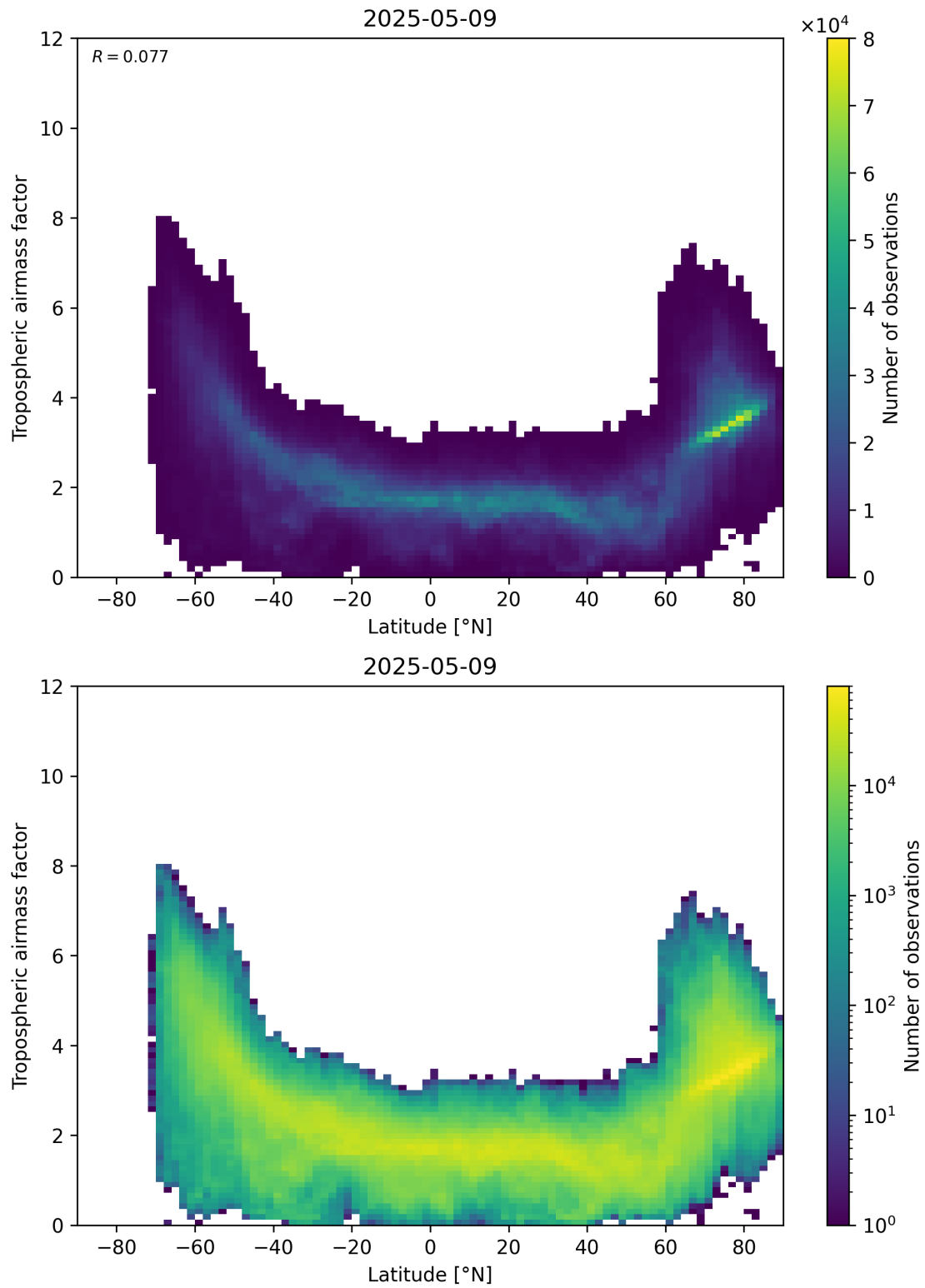
Figure 85: Scatter density plot of “Latitude” against “Tropospheric airmass factor” for 2025-05-09 to 2025-05-10.
