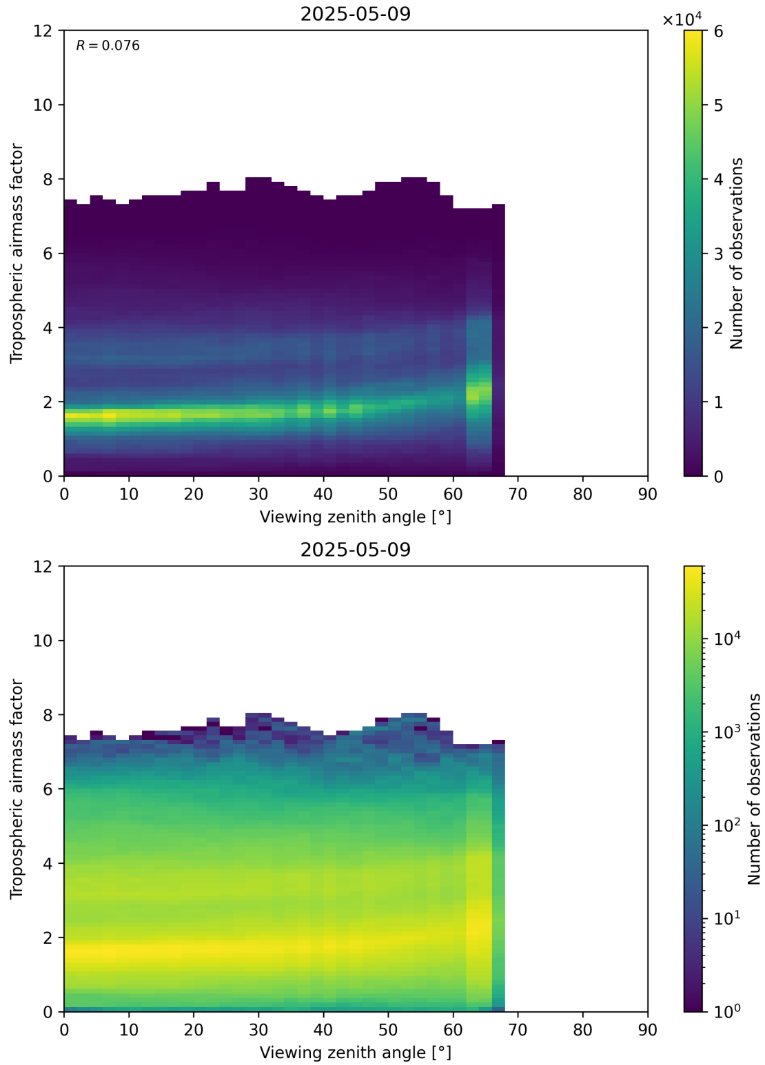
Figure 161: Scatter density plot of “Viewing zenith angle” against “Tropospheric airmass factor” for 2025-05-09 to 2025-05-10.
