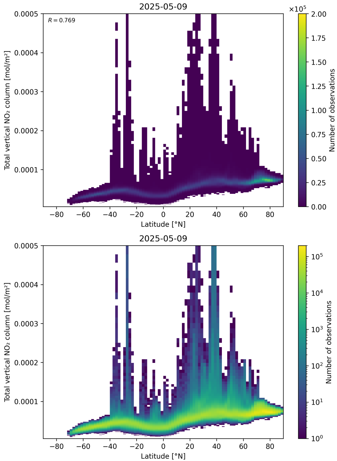
Figure 90: Scatter density plot of “Latitude” against “Total vertical NO 2 column” for 2025-05-09 to 2025-05-10.
