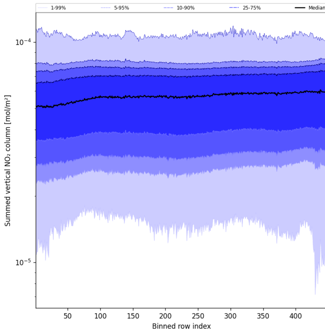
Figure 57: Along track statistics of “Summed vertical NO 2 column” for 2025-05-09 to 2025-05-10
