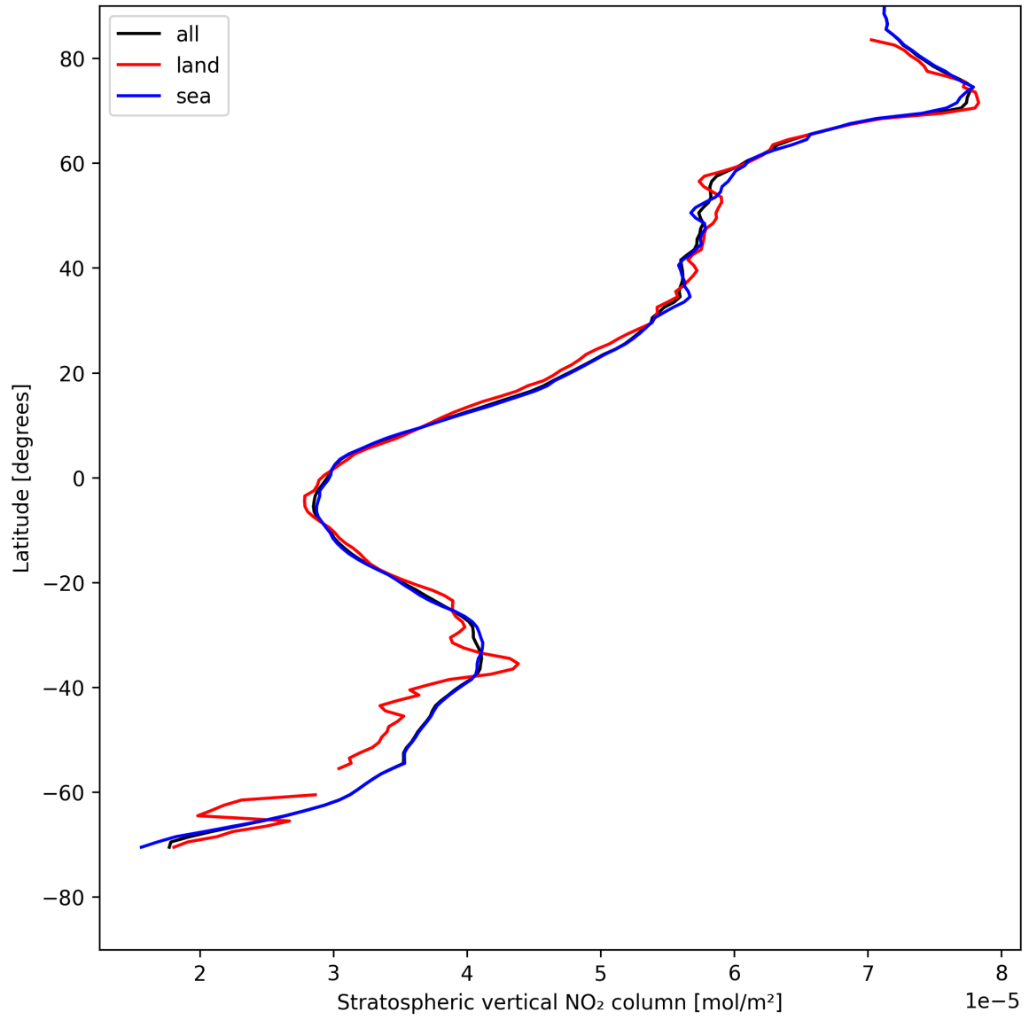
Figure 19: Zonal average of “Stratospheric vertical NO 2 column” for 2025-05-09 to 2025-05-10.
