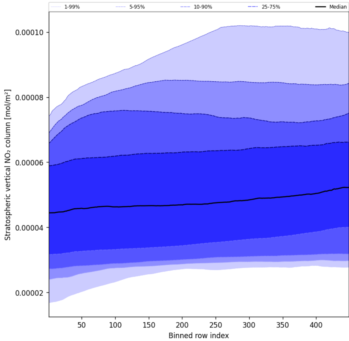
Figure 53: Along track statistics of “Stratospheric vertical NO 2 column” for 2025-05-09 to 2025-05-10
