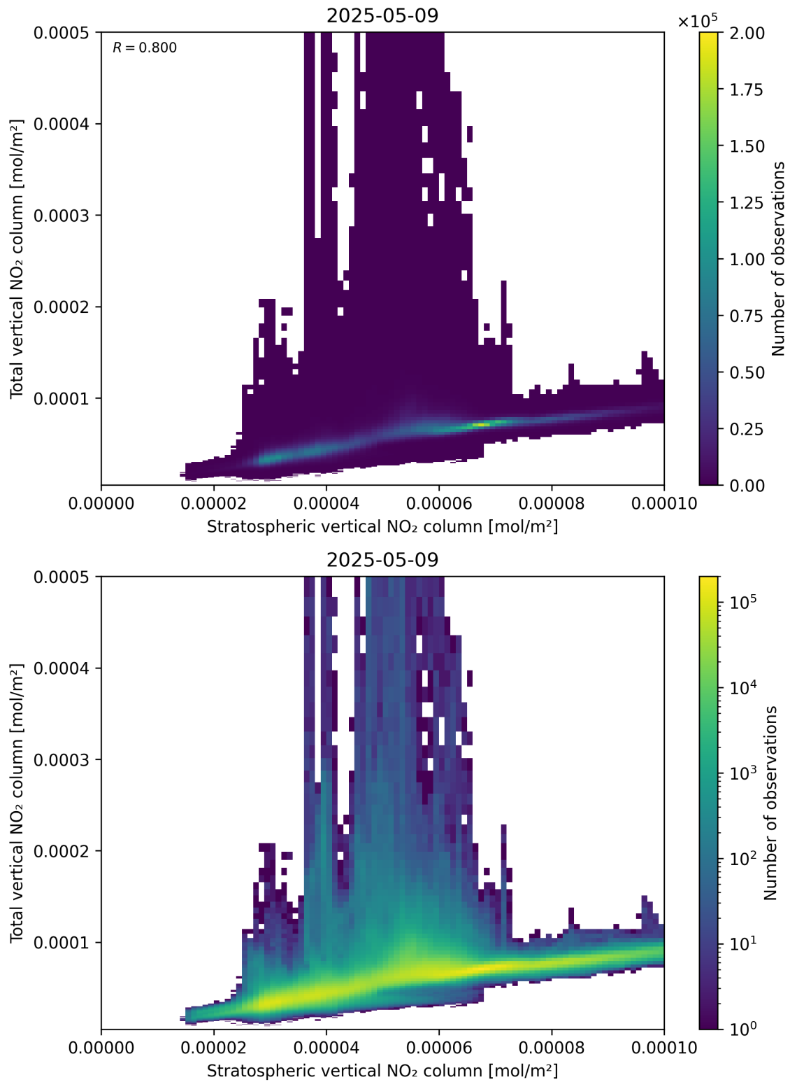
Figure 100: Scatter density plot of “Stratospheric vertical NO 2 column” against “Total vertical NO 2 column” for 2025-05-09 to 2025-05-10.
