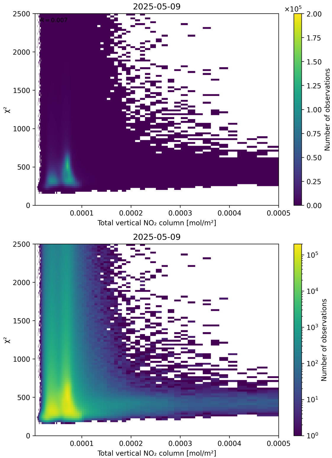
Figure 111: Scatter density plot of “Total vertical NO 2 column” against “ \chi^2 ” for 2025-05-09 to 2025-05-10.
