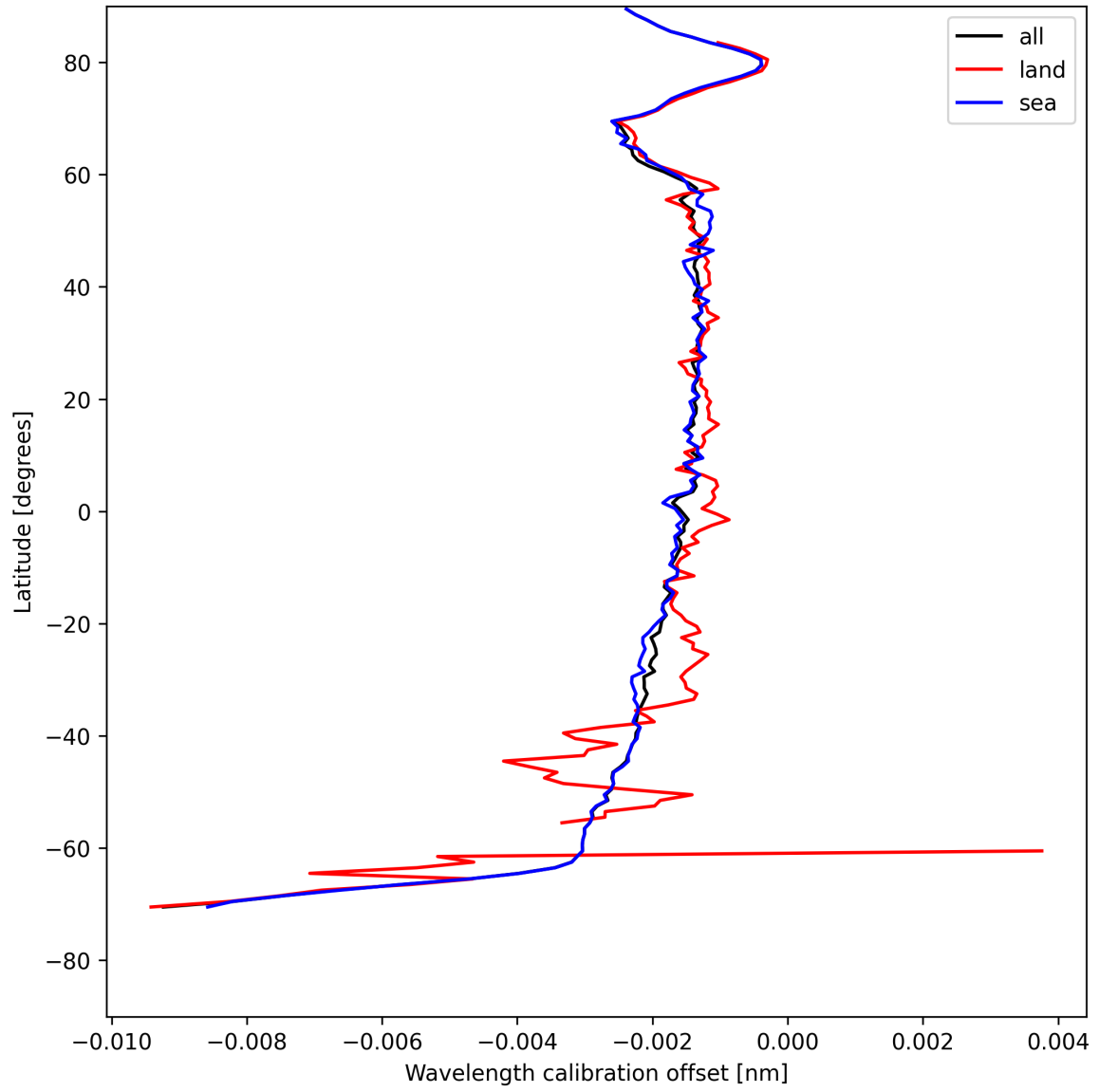
Figure 18: Zonal average of “Wavelength calibration offset” for 2025-05-09 to 2025-05-10.
