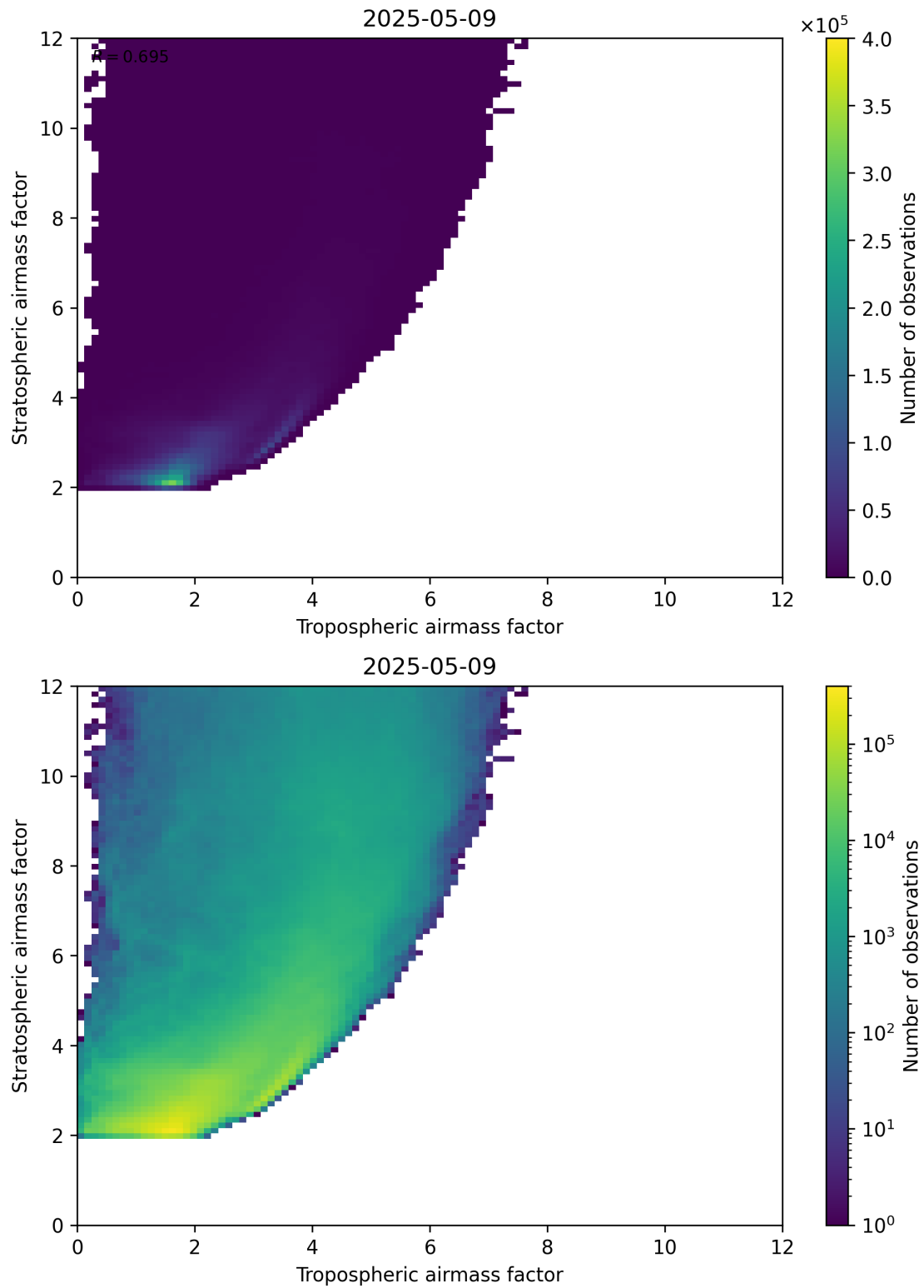
Figure 71: Scatter density plot of “Tropospheric airmass factor” against “Stratospheric airmass factor” for 2025-05-09 to 2025-05-10.
