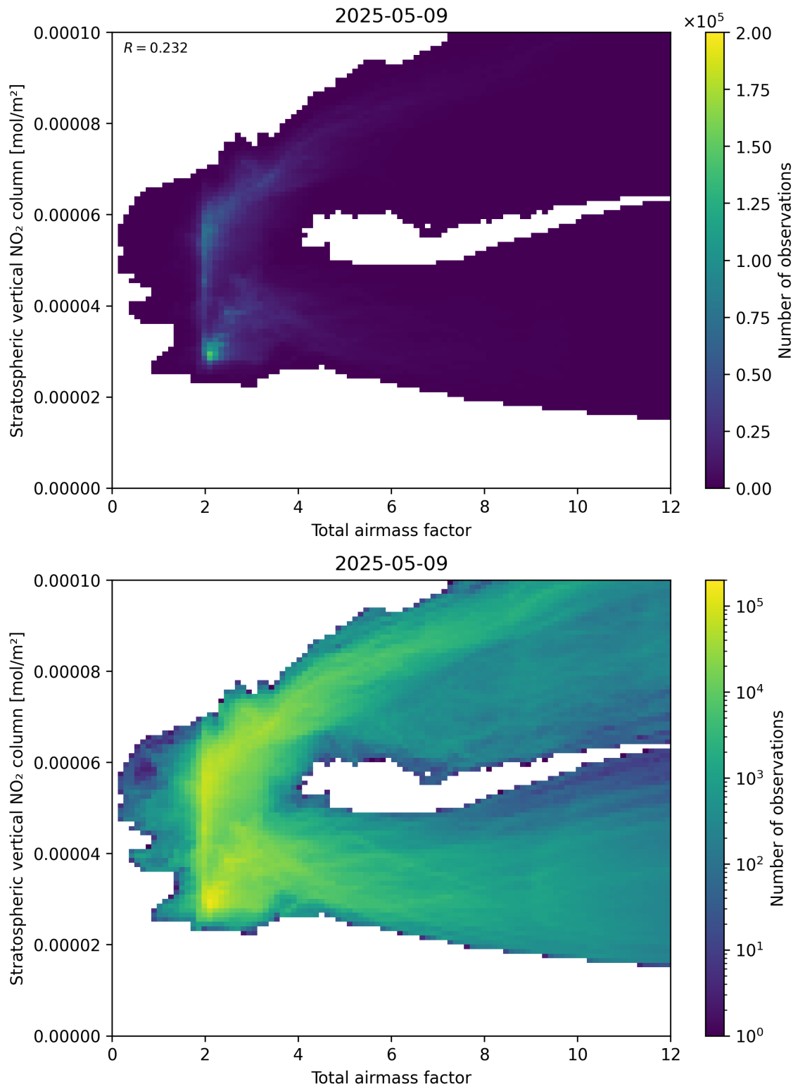
Figure 64: Scatter density plot of “Total airmass factor” against “Stratospheric vertical \text{NO}_2 column” for 2025-05-09 to 2025-05-10.
