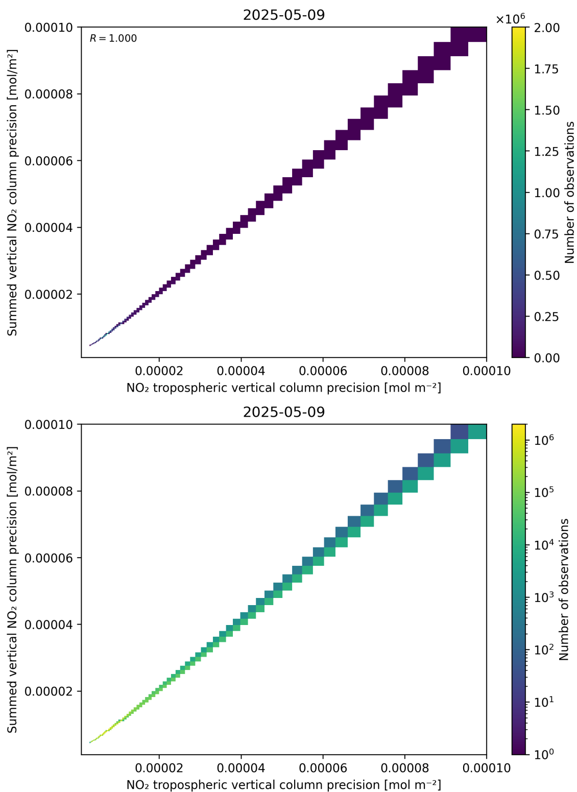
Figure 137: Scatter density plot of “NO 2 tropospheric vertical column precision” against “Summed vertical NO 2 column precision” for 2025-05-09 to 2025-05-10.
