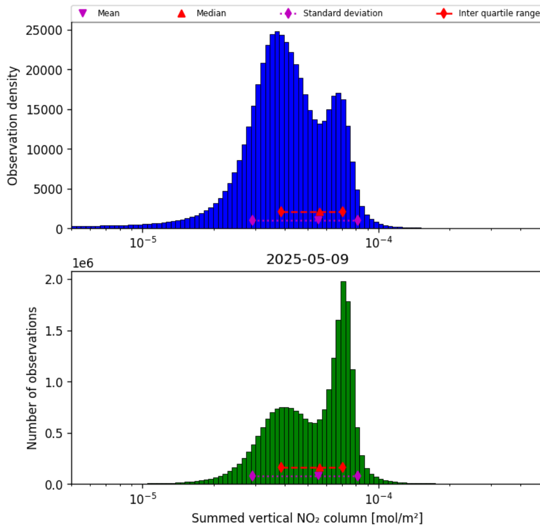
Figure 40: Histogram of “Summed vertical NO 2 column” for 2025-05-09 to 2025-05-10
