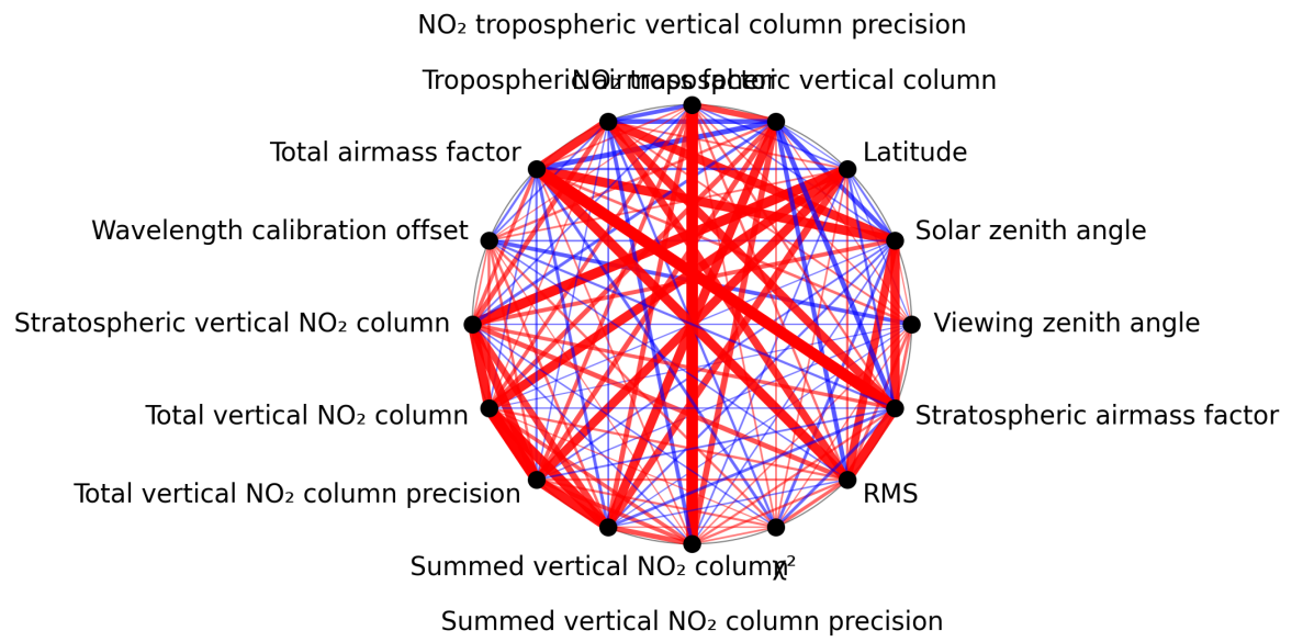
Figure 1: Map of correlation graph for 2025-05-09 to 2025-05-10.
