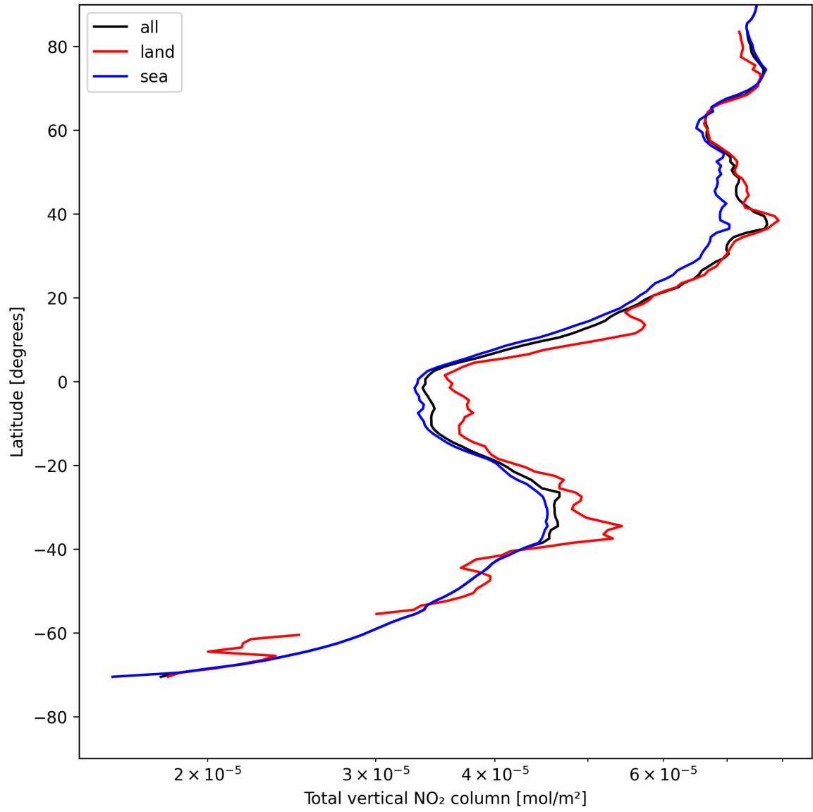
Figure 21: Zonal average of “Total vertical NO 2 column” for 2025-05-09 to 2025-05-10.
