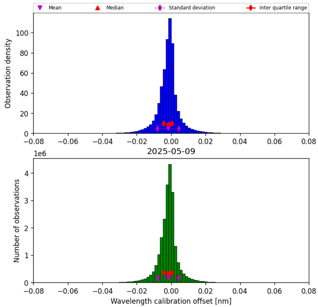
Figure 35: Histogram of “Wavelength calibration offset” for 2025-05-09 to 2025-05-10
