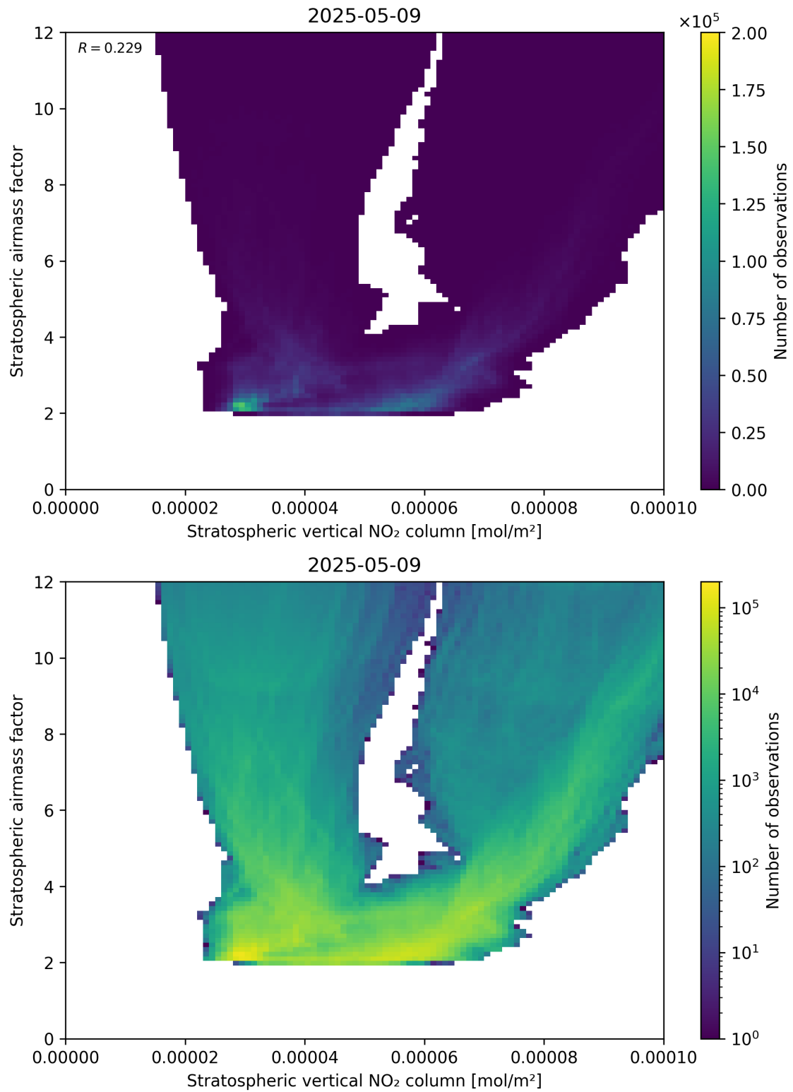
Figure 96: Scatter density plot of “Stratospheric vertical NO 2 column” against “Stratospheric airmass factor” for 2025-05-09 to 2025-05-10.
