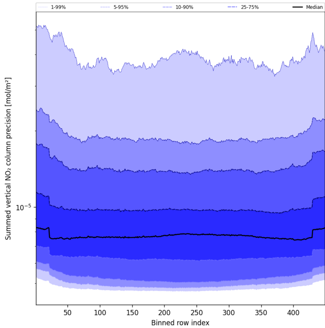
Figure 58: Along track statistics of “Summed vertical NO 2 column precision” for 2025-05-09 to 2025-05-10
