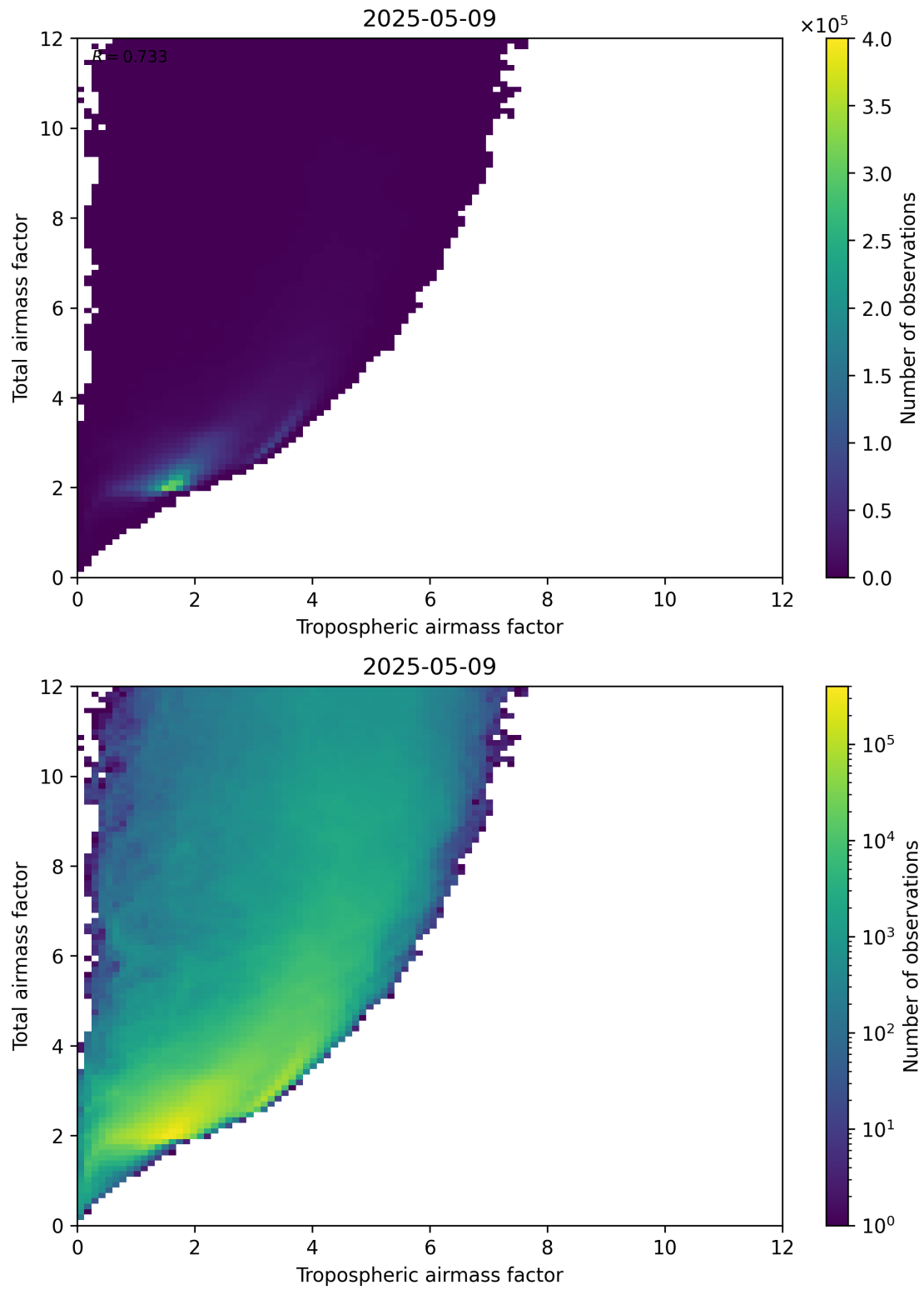
Figure 72: Scatter density plot of “Tropospheric airmass factor” against “Total airmass factor” for 2025-05-09 to 2025-05-10.
