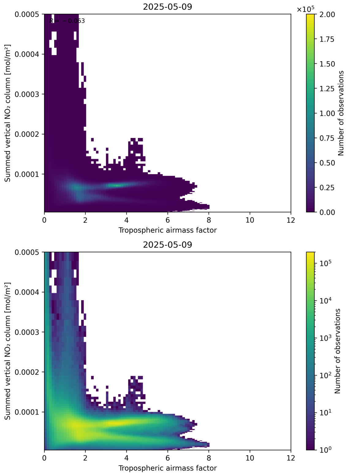
Figure 75: Scatter density plot of “Tropospheric airmass factor” against “Summed vertical NO 2 column” for 2025-05-09 to 2025-05-10.
