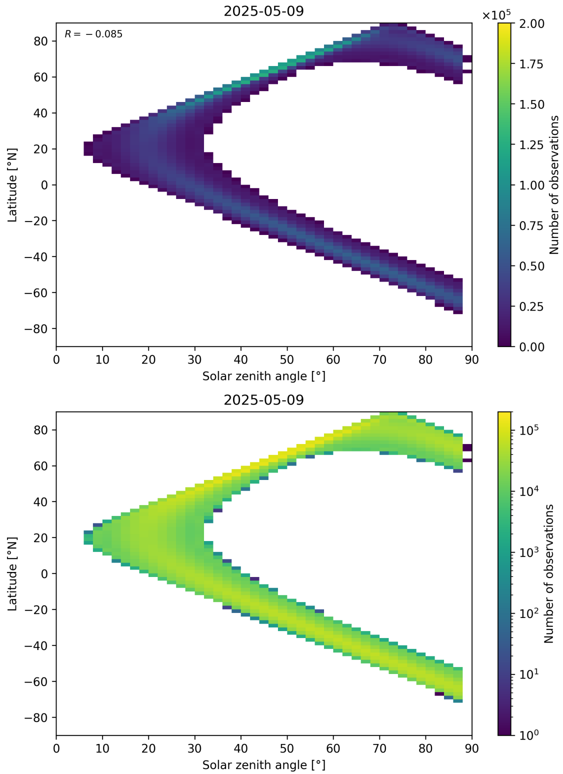
Figure 149: Scatter density plot of “Solar zenith angle” against “Latitude” for 2025-05-09 to 2025-05-10.
