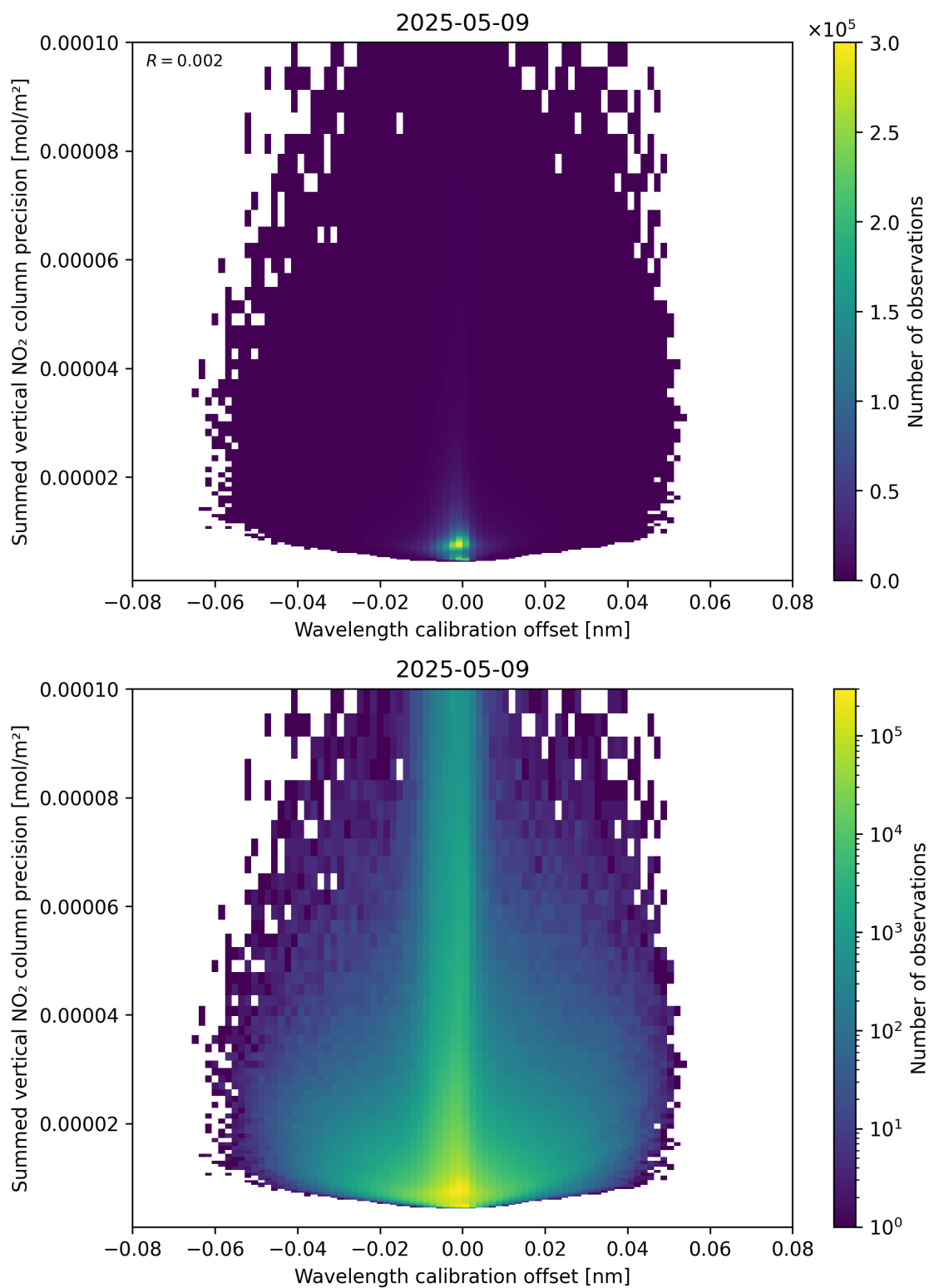
Figure 178: Scatter density plot of “Wavelength calibration offset” against “Summed vertical NO 2 column precision” for 2025-05-09 to 2025-05-10.
