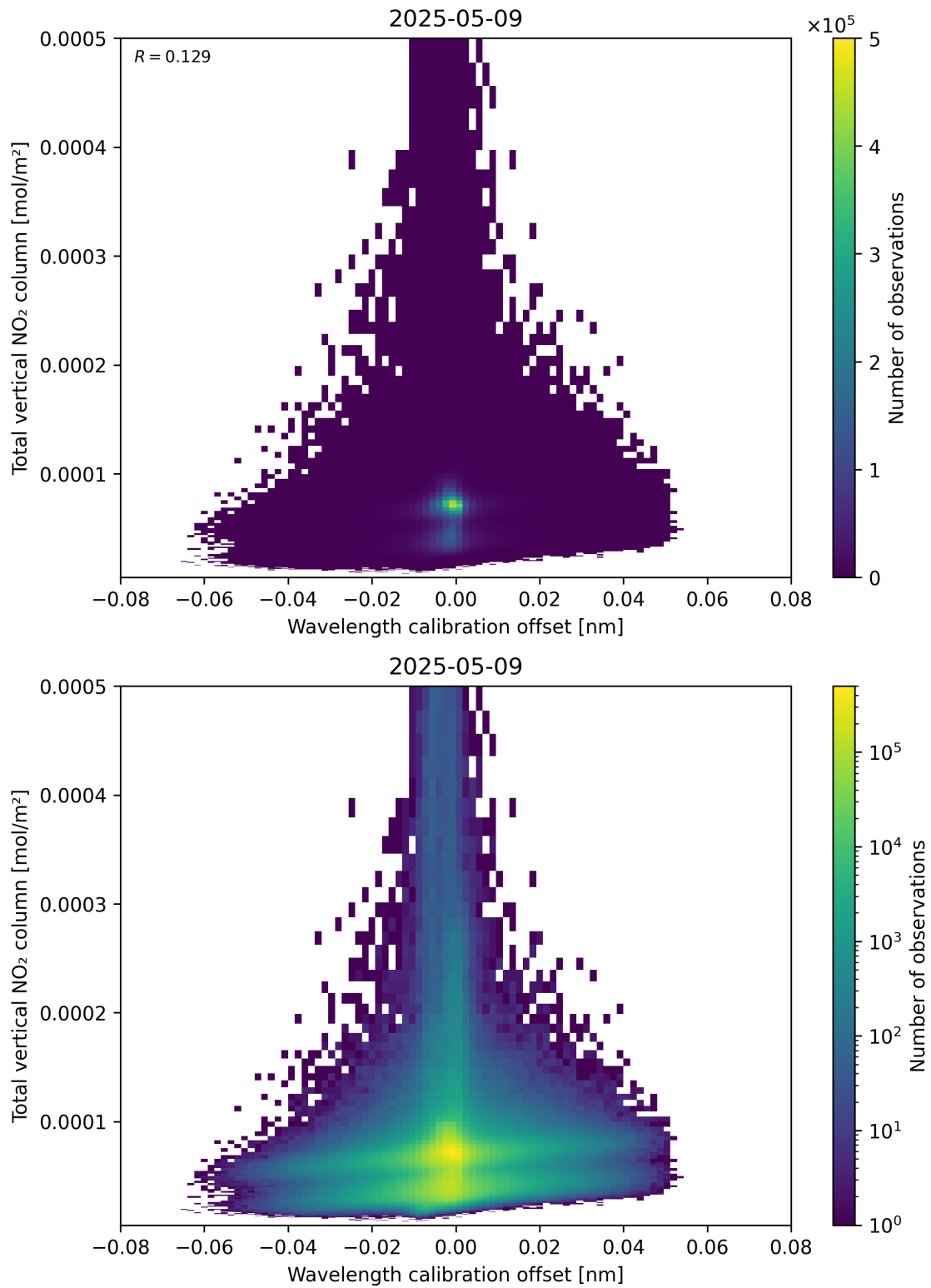
Figure 179: Scatter density plot of “Wavelength calibration offset” against “Total vertical NO 2 column” for 2025-05-09 to 2025-05-10.
