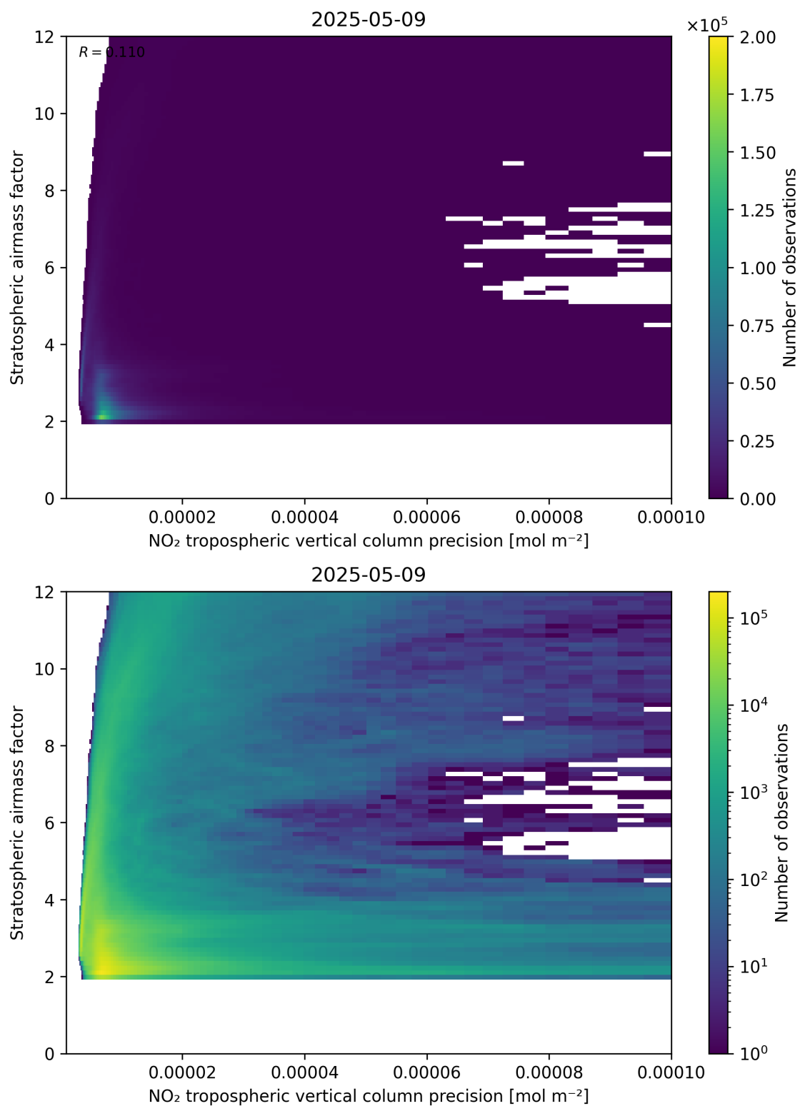
Figure 131: Scatter density plot of “NO 2 tropospheric vertical column precision” against “Stratospheric airmass factor” for 2025-05-09 to 2025-05-10.
