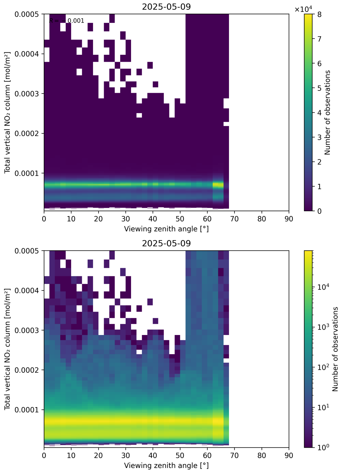
Figure 167: Scatter density plot of “Viewing zenith angle” against “Total vertical NO 2 column” for 2025-05-09 to 2025-05-10.
