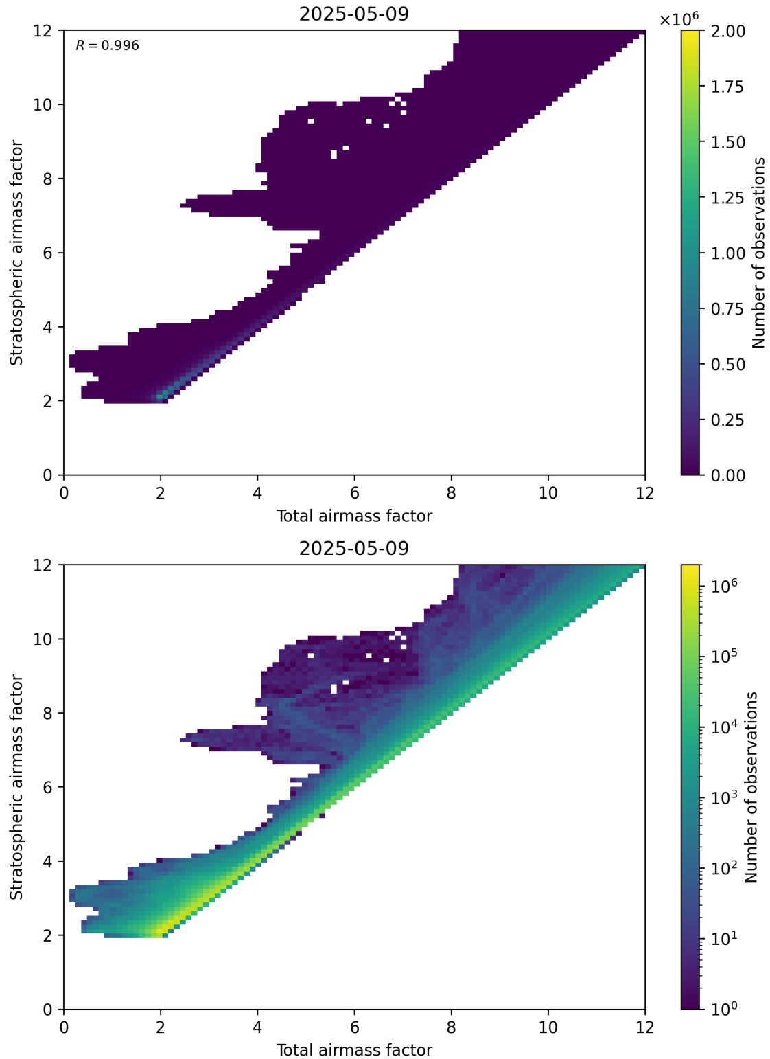
Figure 62: Scatter density plot of “Total airmass factor” against “Stratospheric airmass factor” for 2025-05-09 to 2025-05-10.
