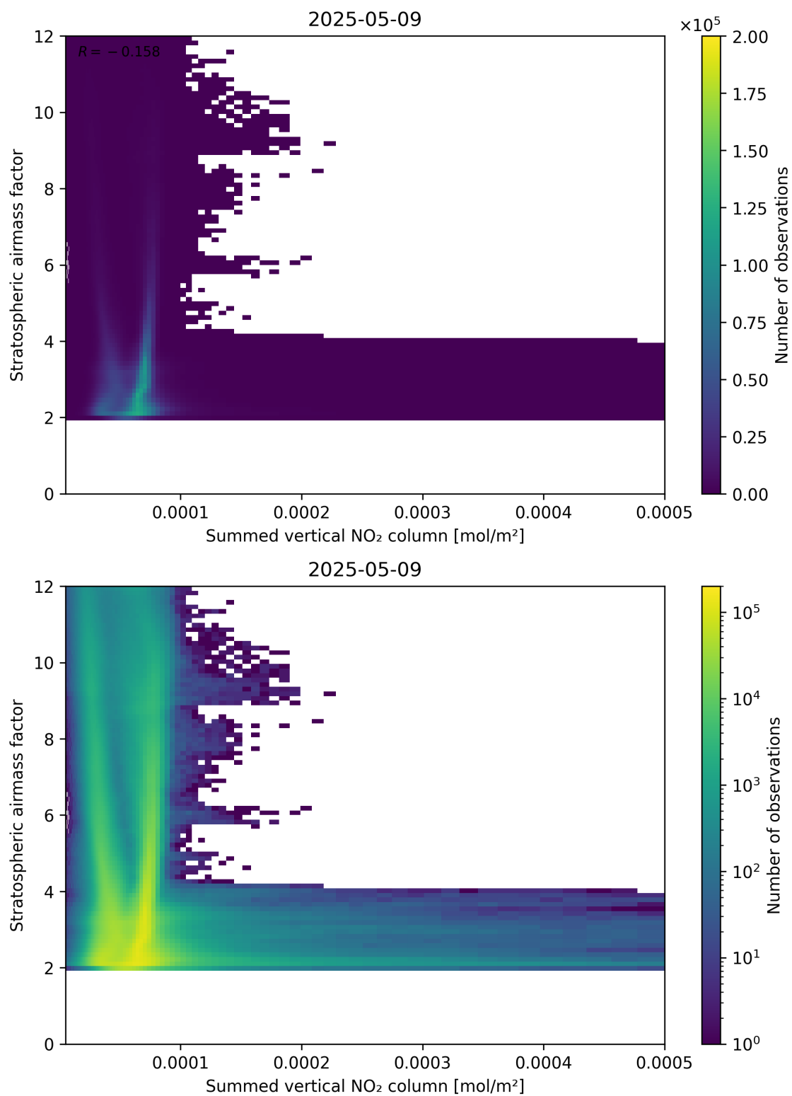
Figure 103: Scatter density plot of “Summed vertical NO 2 column” against “Stratospheric air mass factor” for 2025-05-09 to 2025-05-10.
