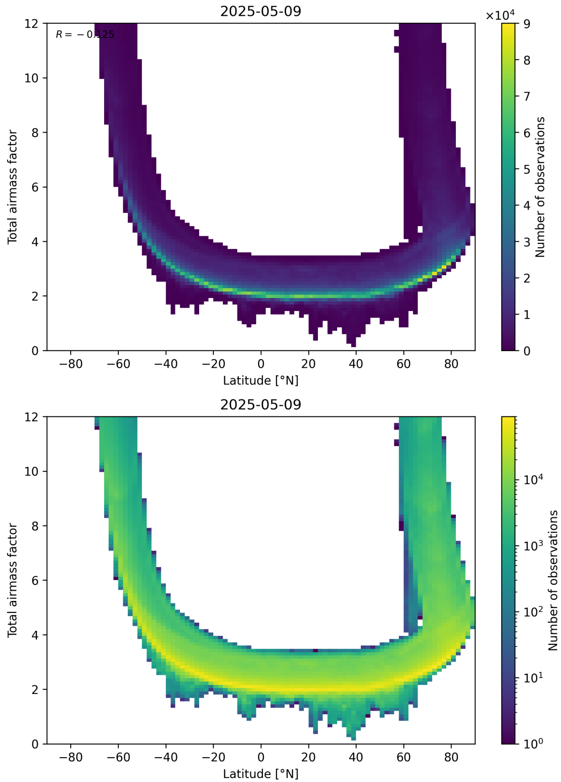
Figure 84: Scatter density plot of “Latitude” against “Total airmass factor” for 2025-05-09 to 2025-05-10.
