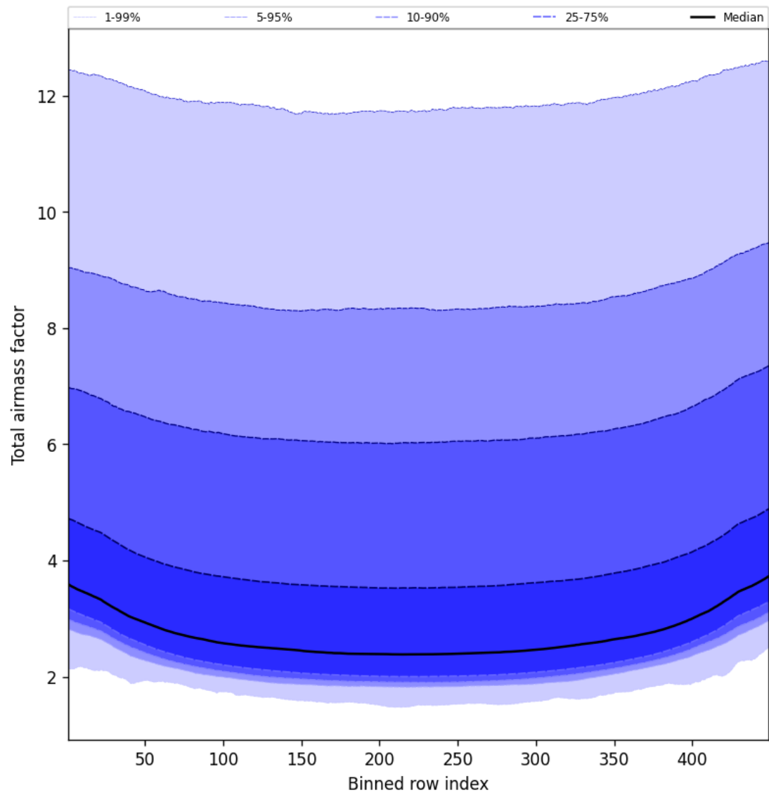
Figure 49: Along track statistics of “Total airmass factor” for 2025-05-09 to 2025-05-10
