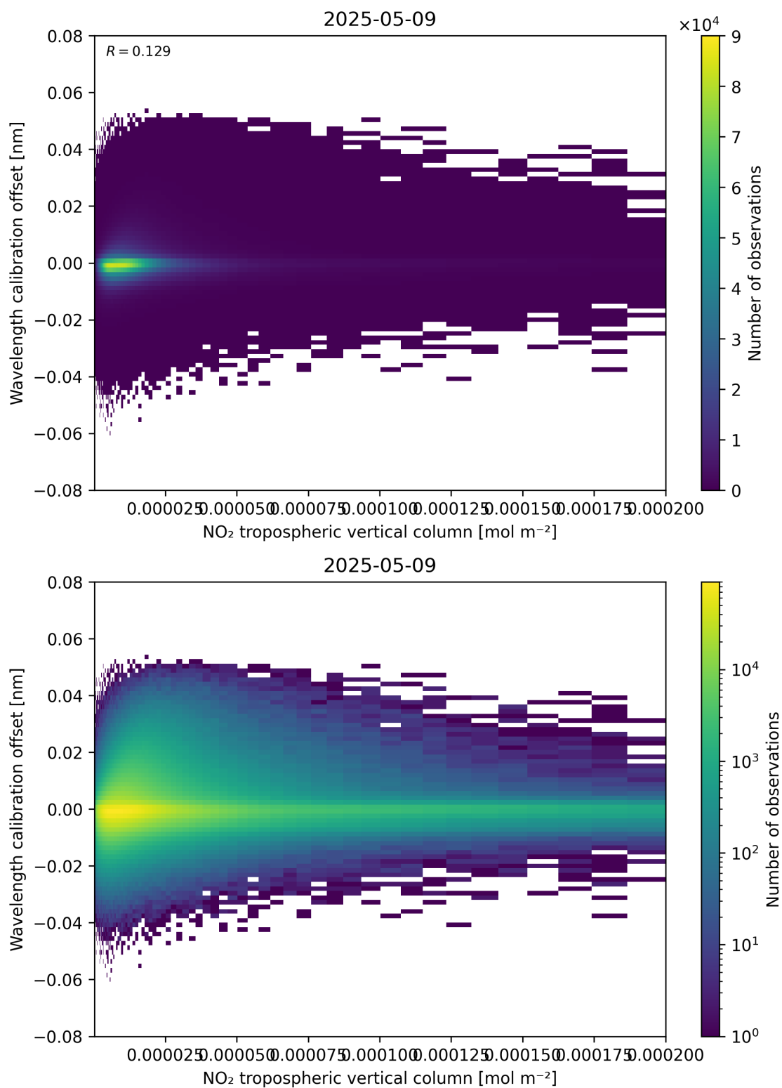
Figure 143: Scatter density plot of “NO 2 tropospheric vertical column” against “Wavelength calibration offset” for 2025-05-09 to 2025-05-10.
