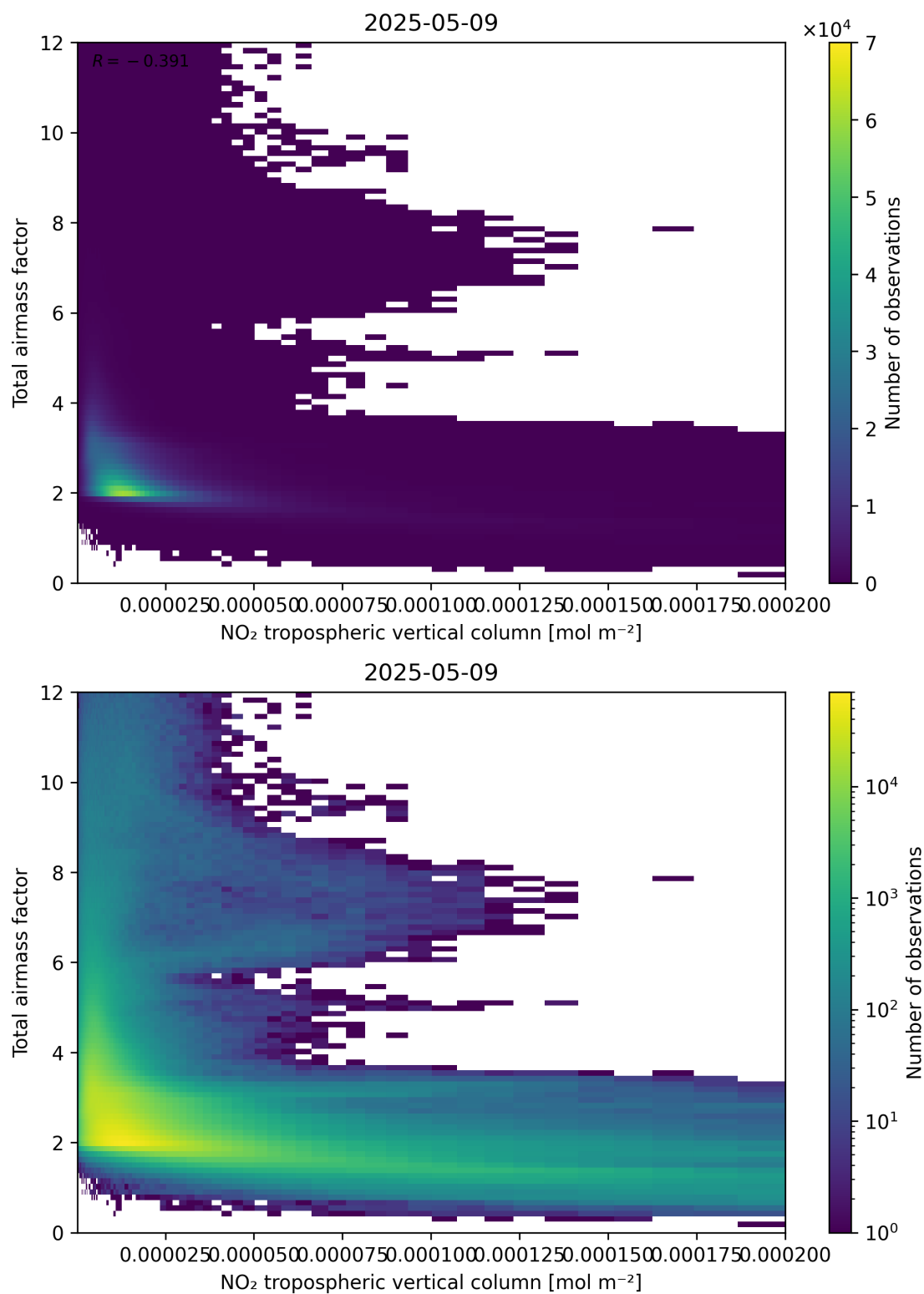
Figure 122: Scatter density plot of “NO 2 tropospheric vertical column” against “Total air mass factor” for 2025-05-09 to 2025-05-10.
