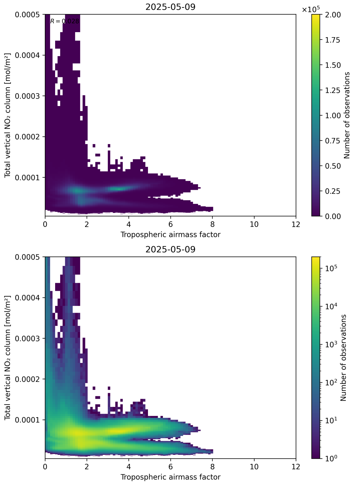
Figure 77: Scatter density plot of “Tropospheric airmass factor” against “Total vertical NO 2 column” for 2025-05-09 to 2025-05-10.
