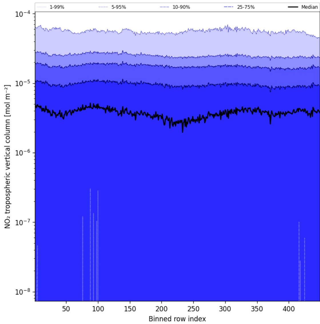
Figure 46: Along track statistics of “NO 2 tropospheric vertical column” for 2025-05-09 to 2025-05-10
