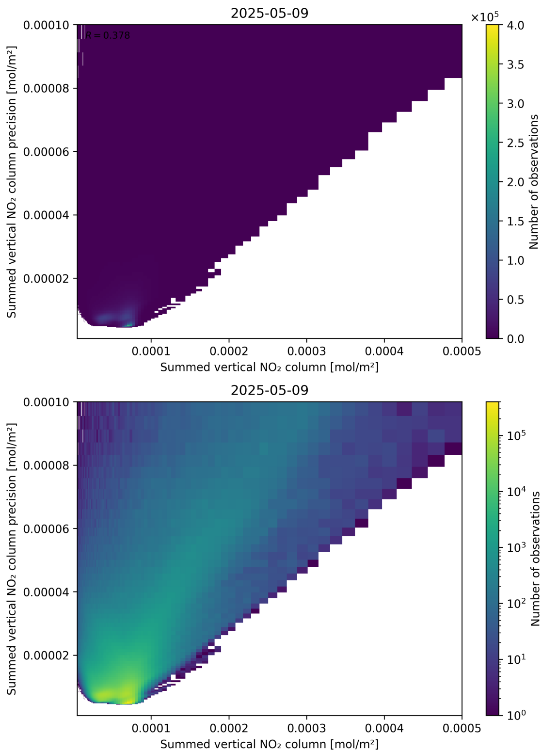
Figure 105: Scatter density plot of “Summed vertical NO 2 column” against “Summed vertical NO 2 column precision” for 2025-05-09 to 2025-05-10.
