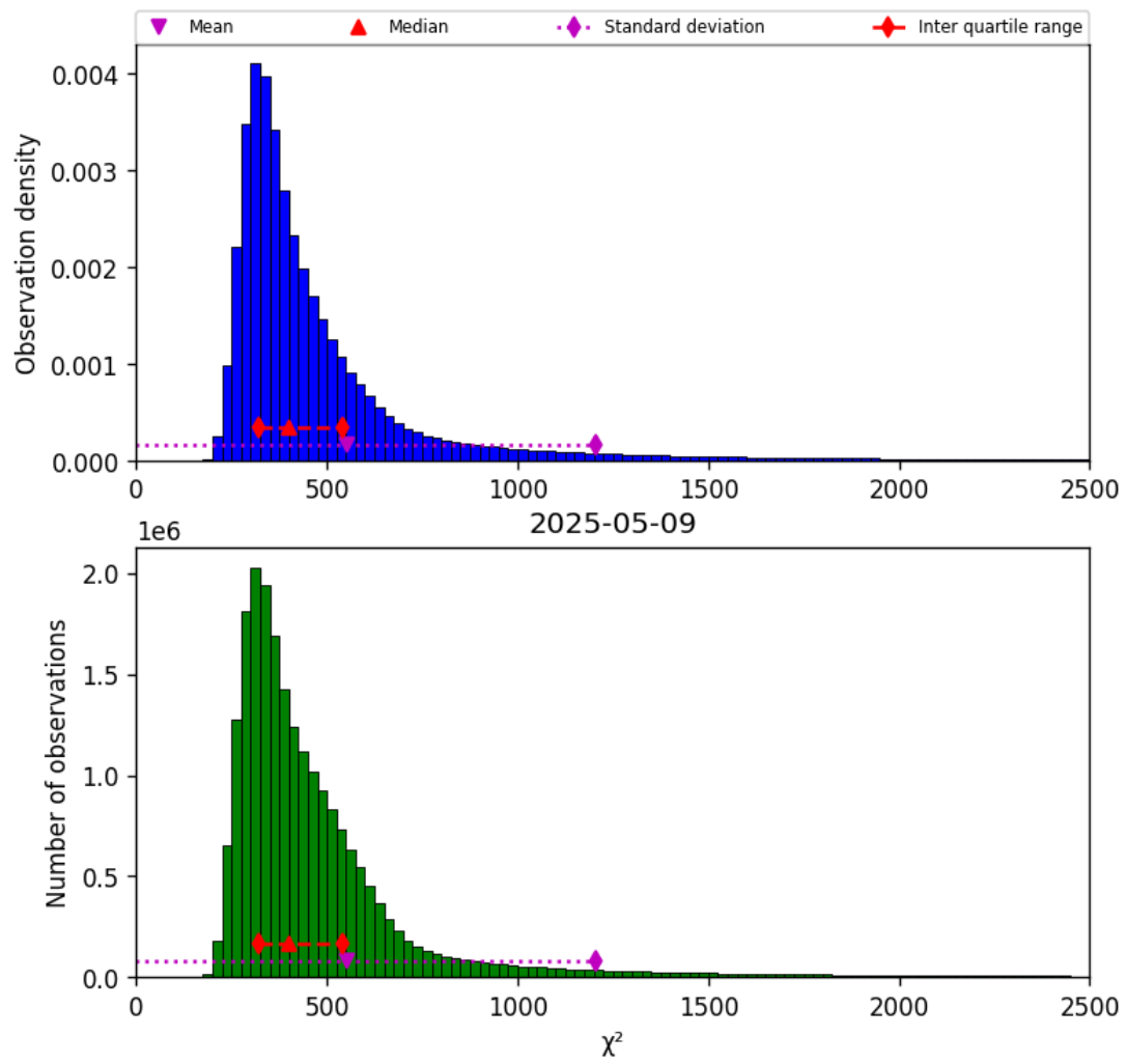
Figure 42: Histogram of “ \chi^2 ” for 2025-05-09 to 2025-05-10
