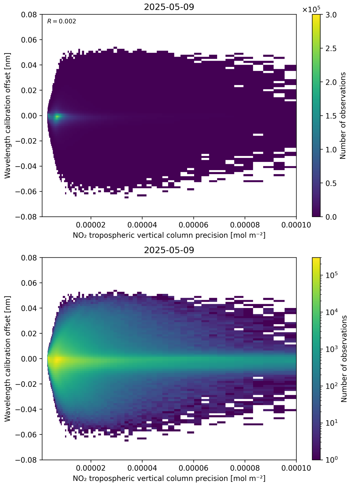
Figure 141: Scatter density plot of “NO 2 tropospheric vertical column precision” against “Wavelength calibration offset” for 2025-05-09 to 2025-05-10.
