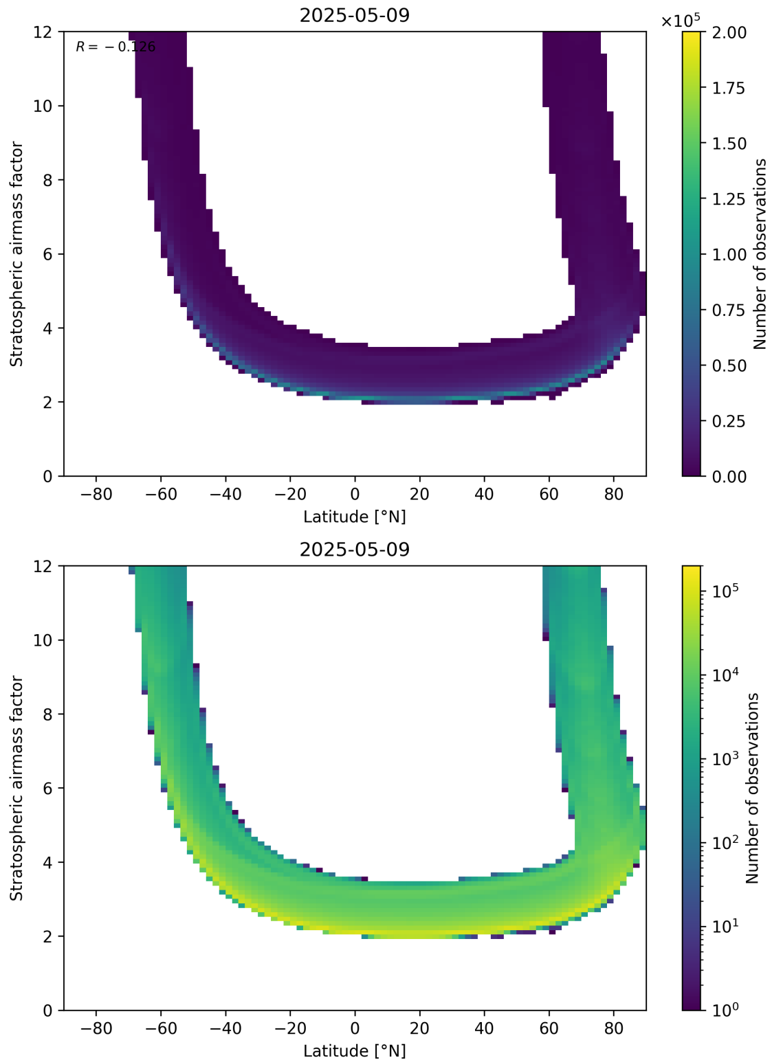
Figure 83: Scatter density plot of “Latitude” against “Stratospheric air mass factor” for 2025-05-09 to 2025-05-10.
