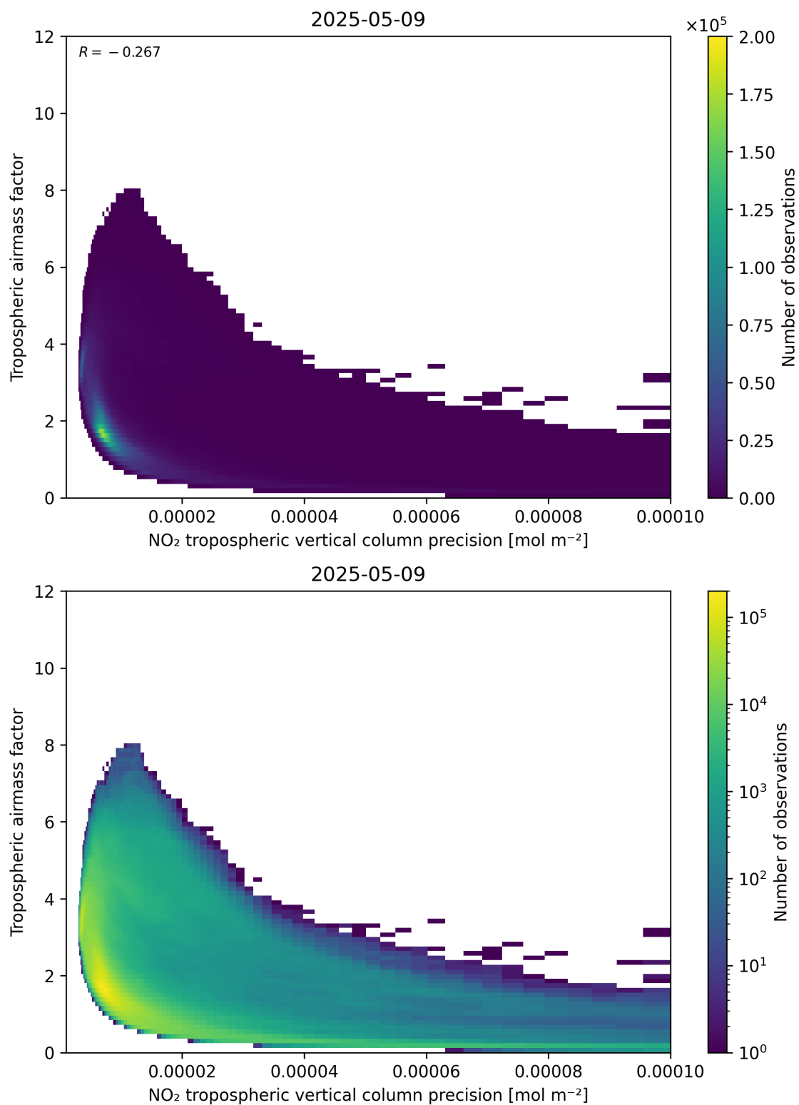
Figure 133: Scatter density plot of “NO 2 tropospheric vertical column precision” against “Tropospheric air mass factor” for 2025-05-09 to 2025-05-10.
