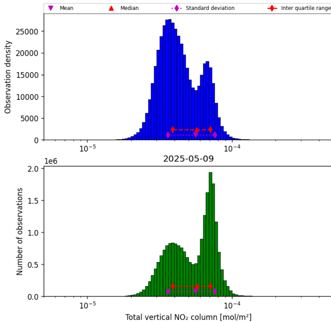
Figure 38: Histogram of “Total vertical NO 2 column” for 2025-05-09 to 2025-05-10
