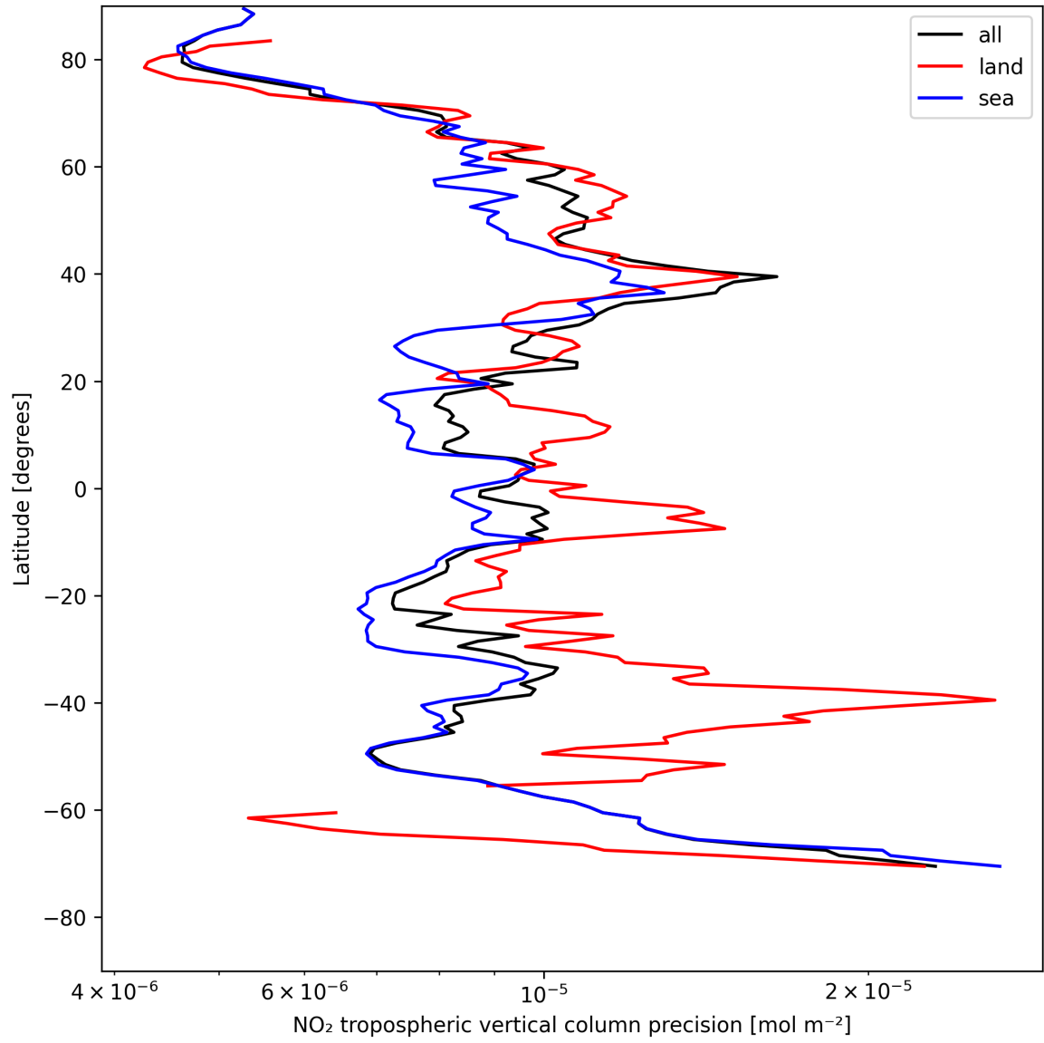
Figure 13: Zonal average of “NO 2 tropospheric vertical column precision” for 2025-05-09 to 2025-05-10.
