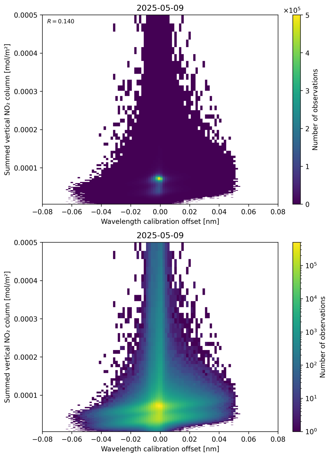
Figure 177: Scatter density plot of “Wavelength calibration offset” against “Summed vertical NO 2 column” for 2025-05-09 to 2025-05-10.
