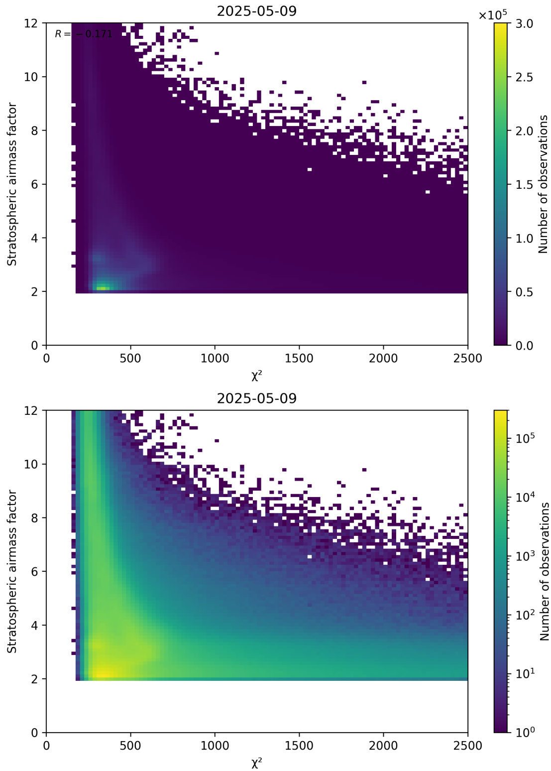
Figure 81: Scatter density plot of “ \chi^2 ” against “Stratospheric airmass factor” for 2025-05-09 to 2025-05-10.
