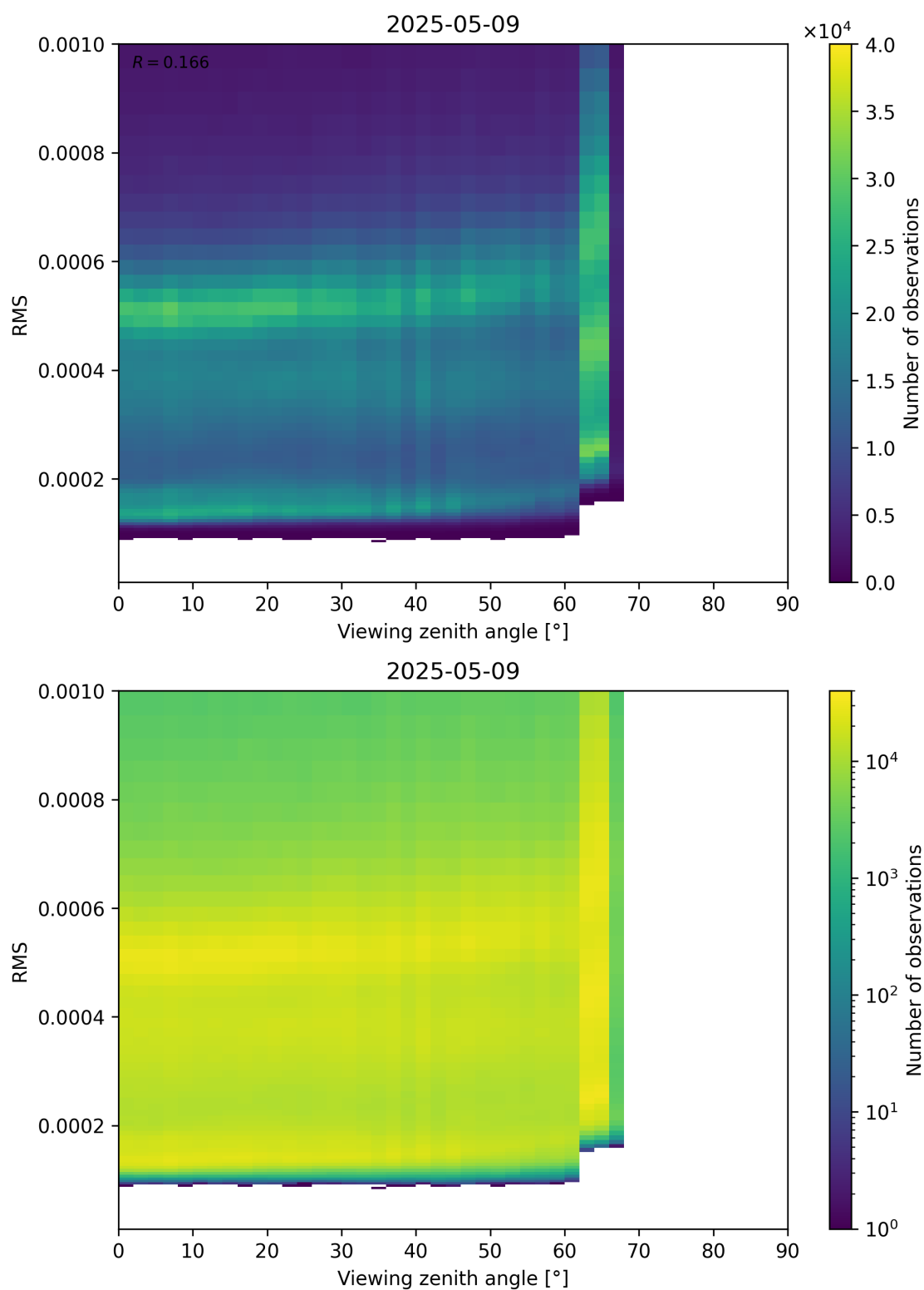
Figure 171: Scatter density plot of “Viewing zenith angle” against “RMS” for 2025-05-09 to 2025-05-10.
