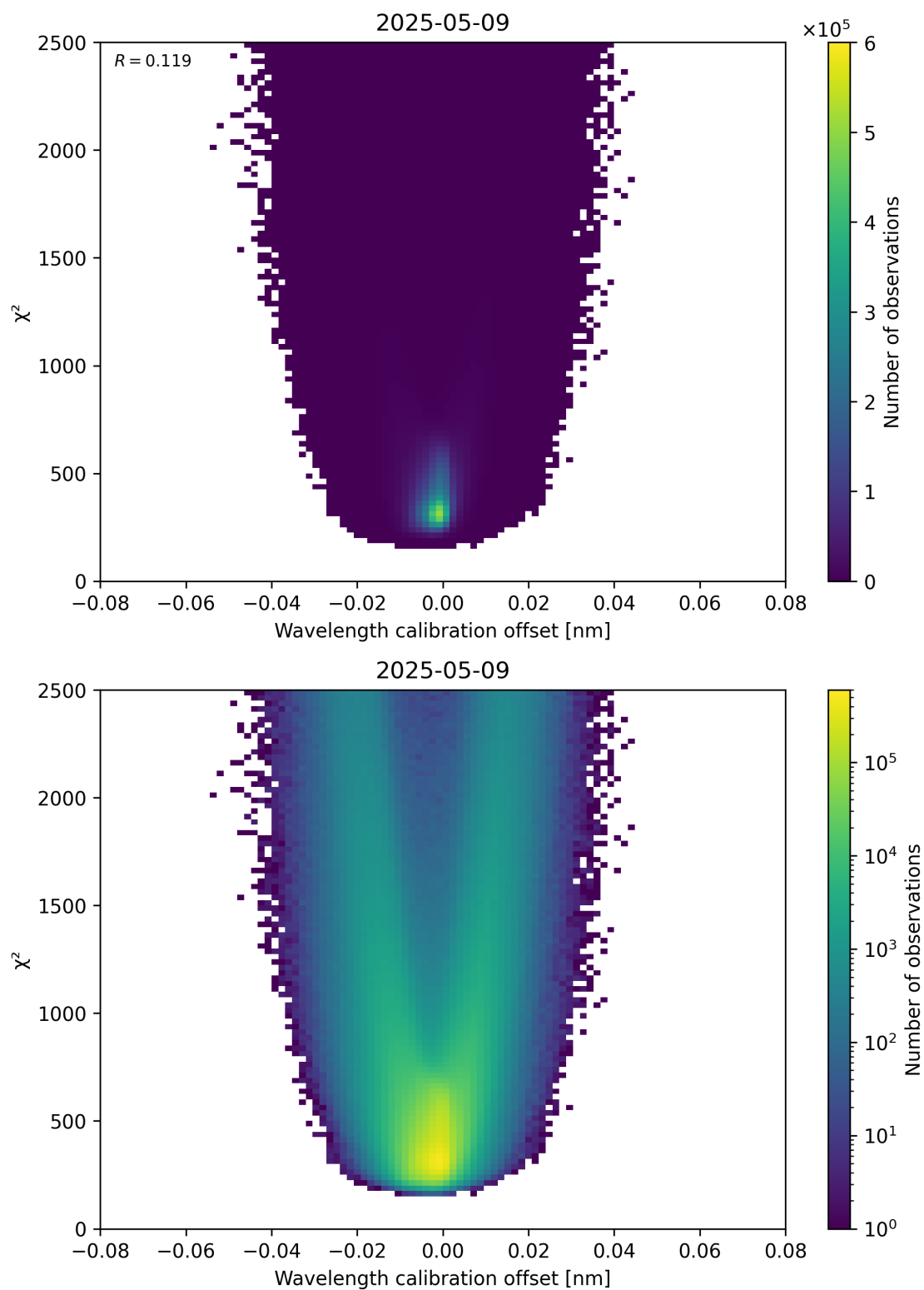
Figure 175: Scatter density plot of “Wavelength calibration offset” against “ \chi^2 ” for 2025-05-09 to 2025-05-10.
