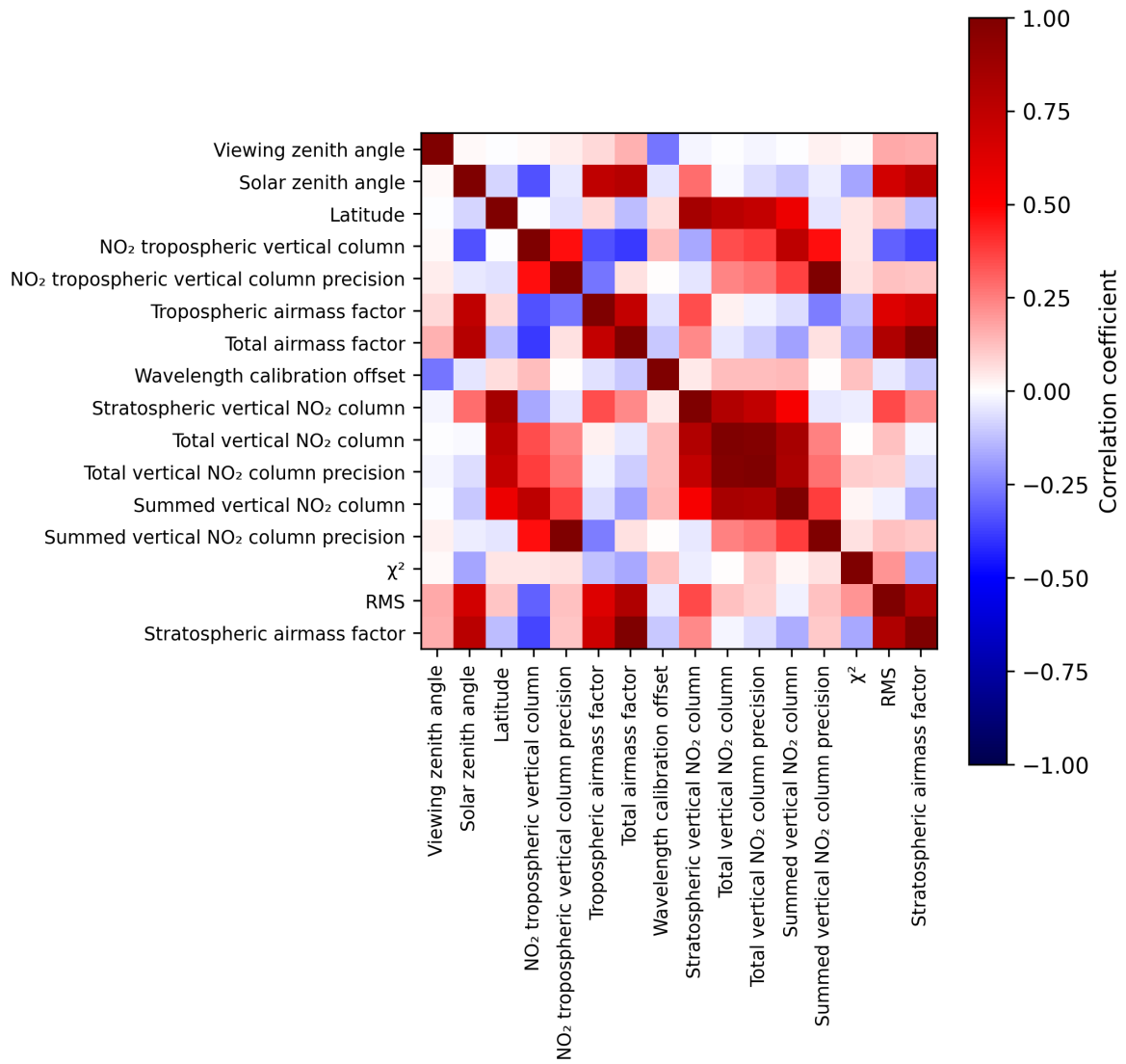
Figure 2: Map of correlation matrix for 2025-05-09 to 2025-05-10.
