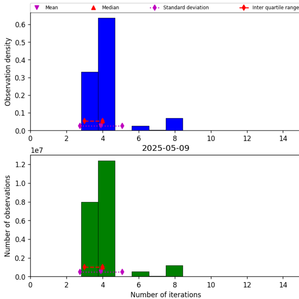
Figure 34: Histogram of “Number of iterations” for 2025-05-09 to 2025-05-10
