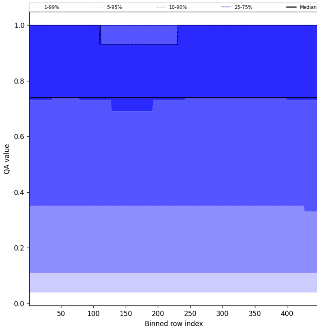
Figure 45: Along track statistics of “QA value” for 2025-05-09 to 2025-05-10
