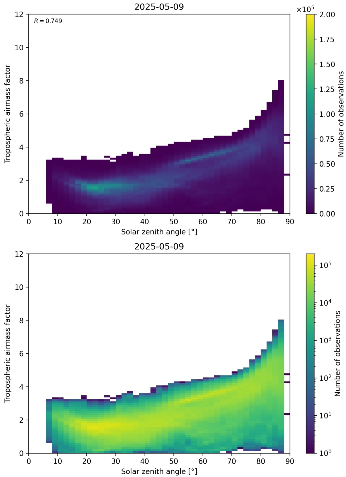
Figure 147: Scatter density plot of “Solar zenith angle” against “Tropospheric airmass factor” for 2025-05-09 to 2025-05-10.
