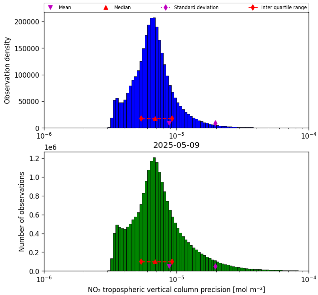
Figure 30: Histogram of “NO 2 tropospheric vertical column precision” for 2025-05-09 to 2025-05-10
