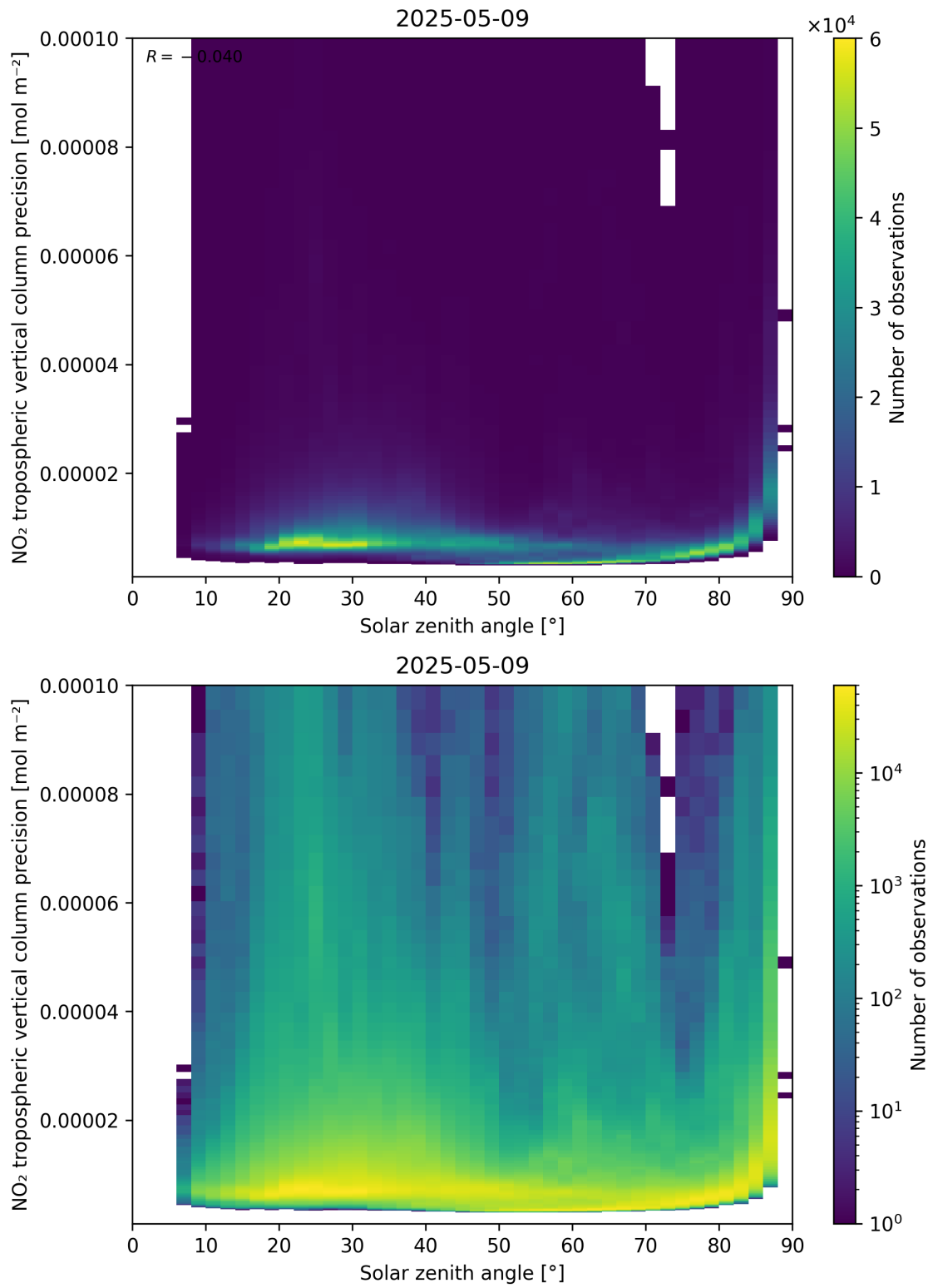
Figure 156: Scatter density plot of “Solar zenith angle” against “NO 2 tropospheric vertical column precision” for 2025-05-09 to 2025-05-10.
