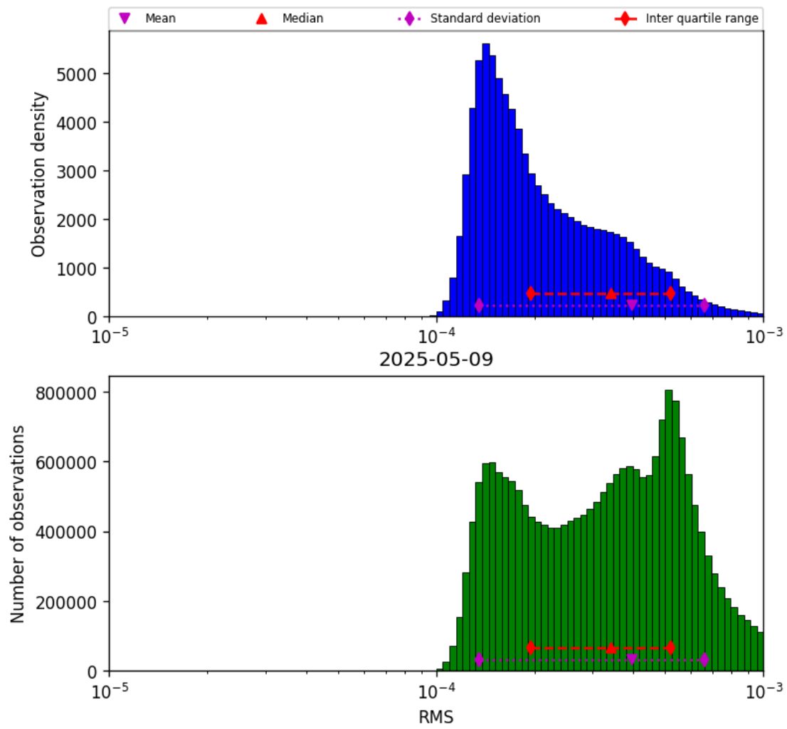
Figure 43: Histogram of “RMS” for 2025-05-09 to 2025-05-10
