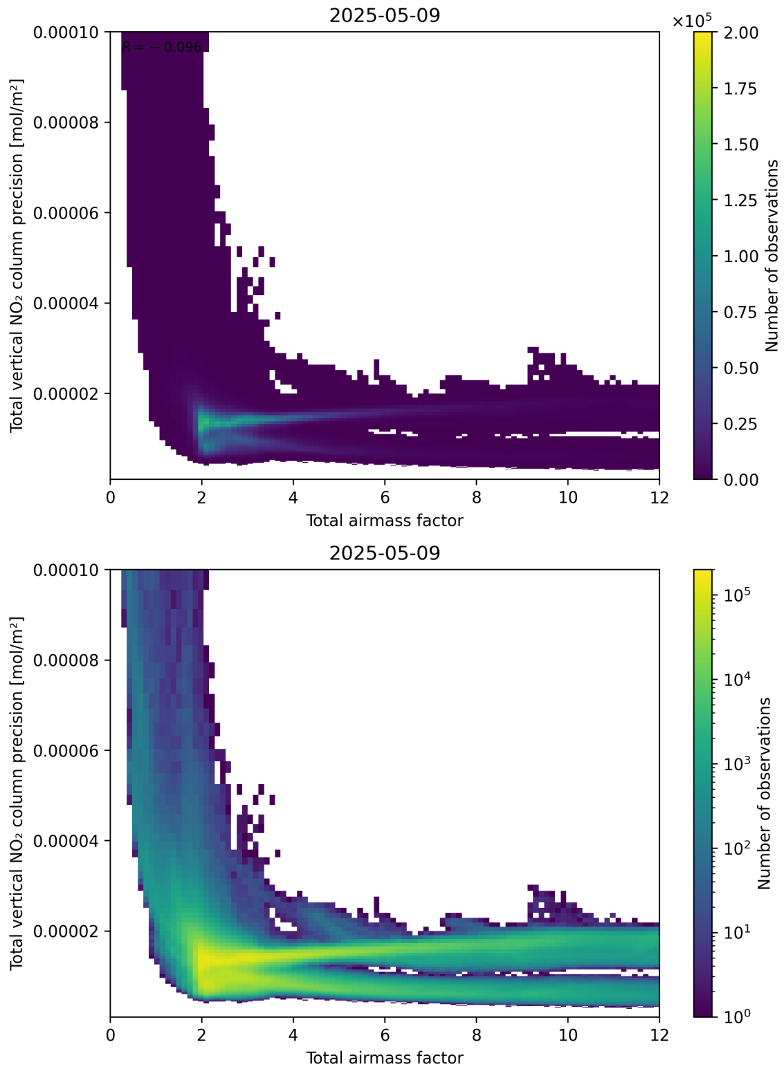
Figure 68: Scatter density plot of “Total airmass factor” against “Total vertical NO 2 column precision” for 2025-05-09 to 2025-05-10.
