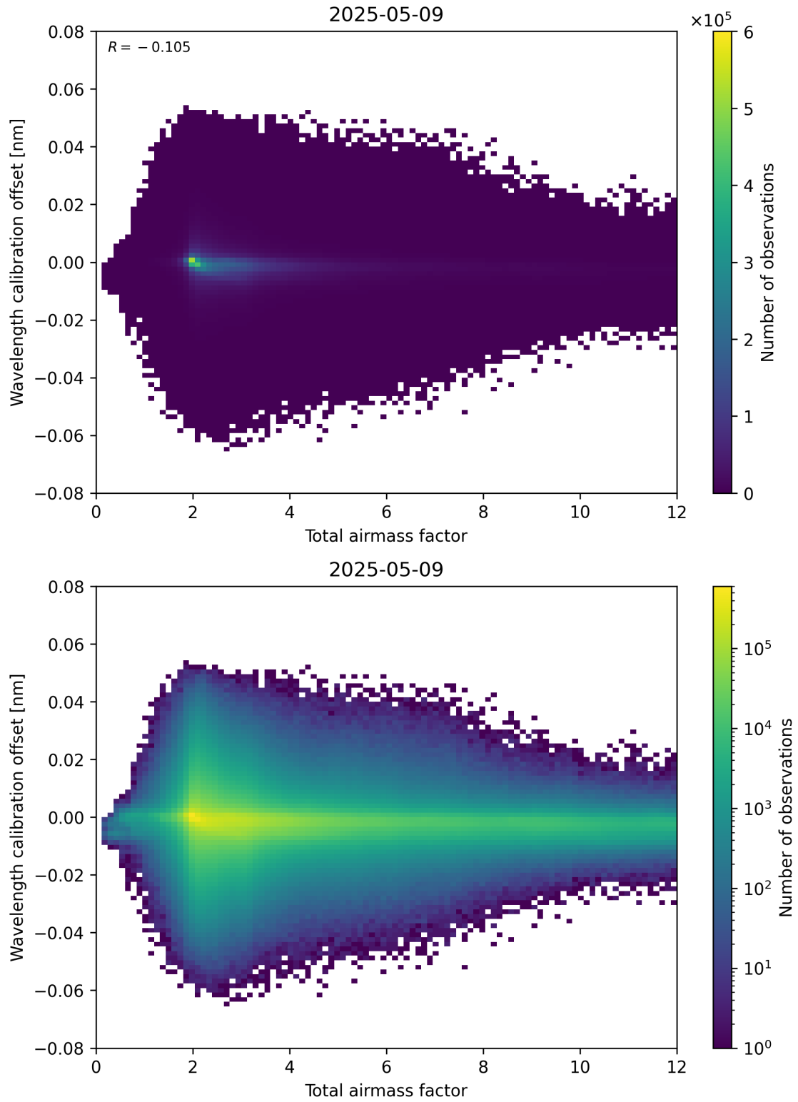
Figure 70: Scatter density plot of “Total airmass factor” against “Wavelength calibration offset” for 2025-05-09 to 2025-05-10.
