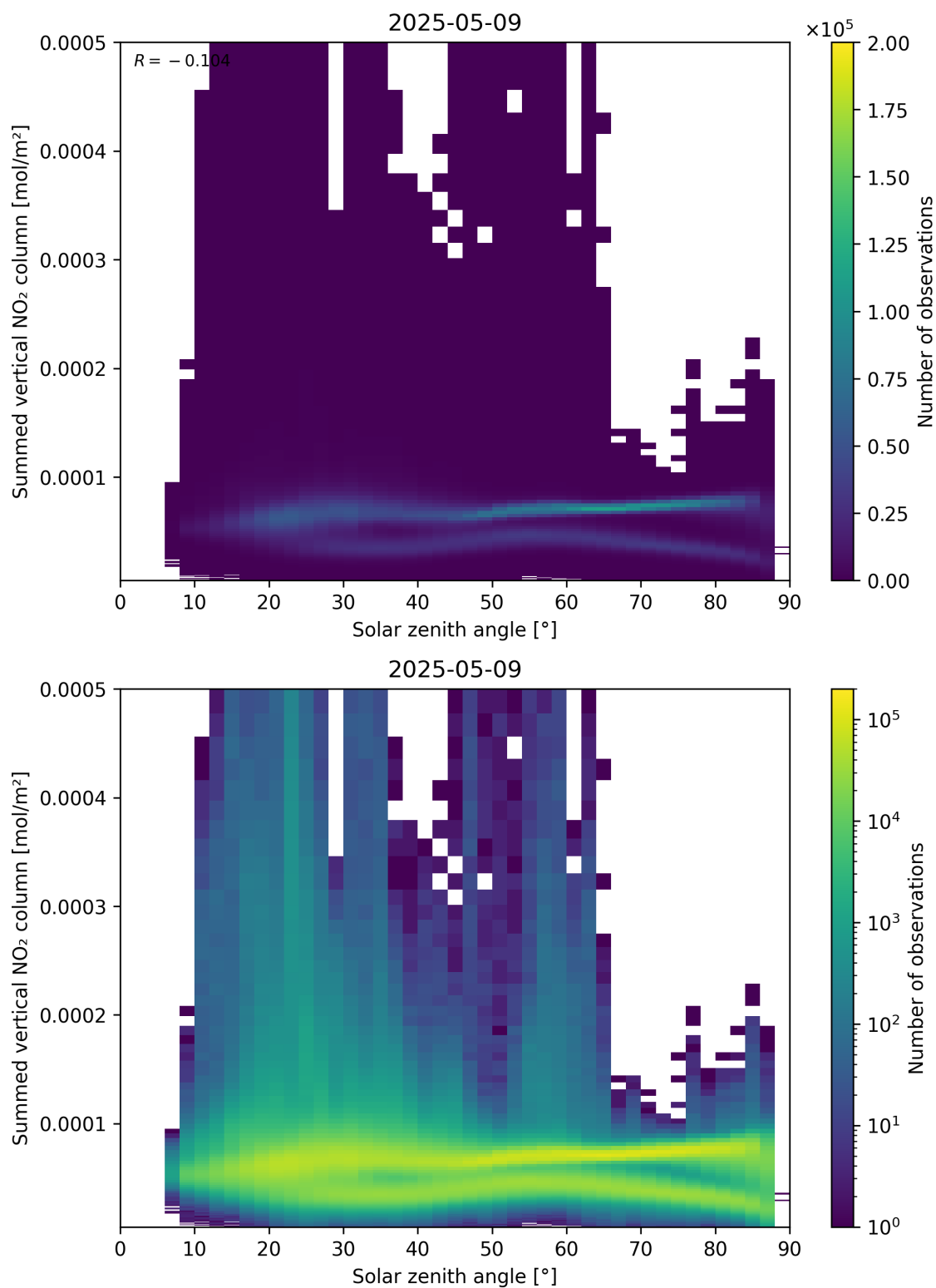
Figure 151: Scatter density plot of “Solar zenith angle” against “Summed vertical NO 2 column” for 2025-05-09 to 2025-05-10.
