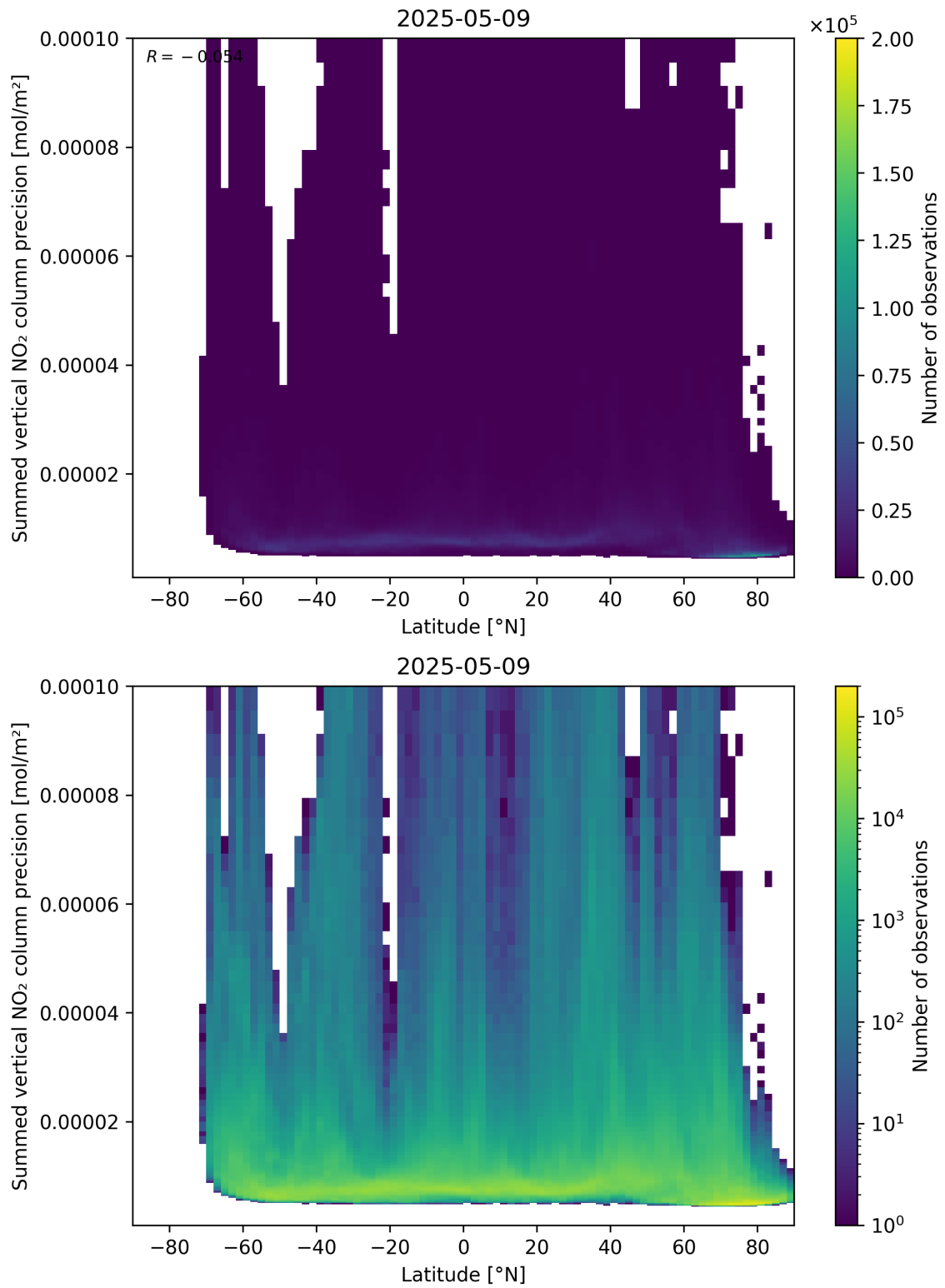
Figure 89: Scatter density plot of “Latitude” against “Summed vertical NO 2 column precision” for 2025-05-09 to 2025-05-10.
