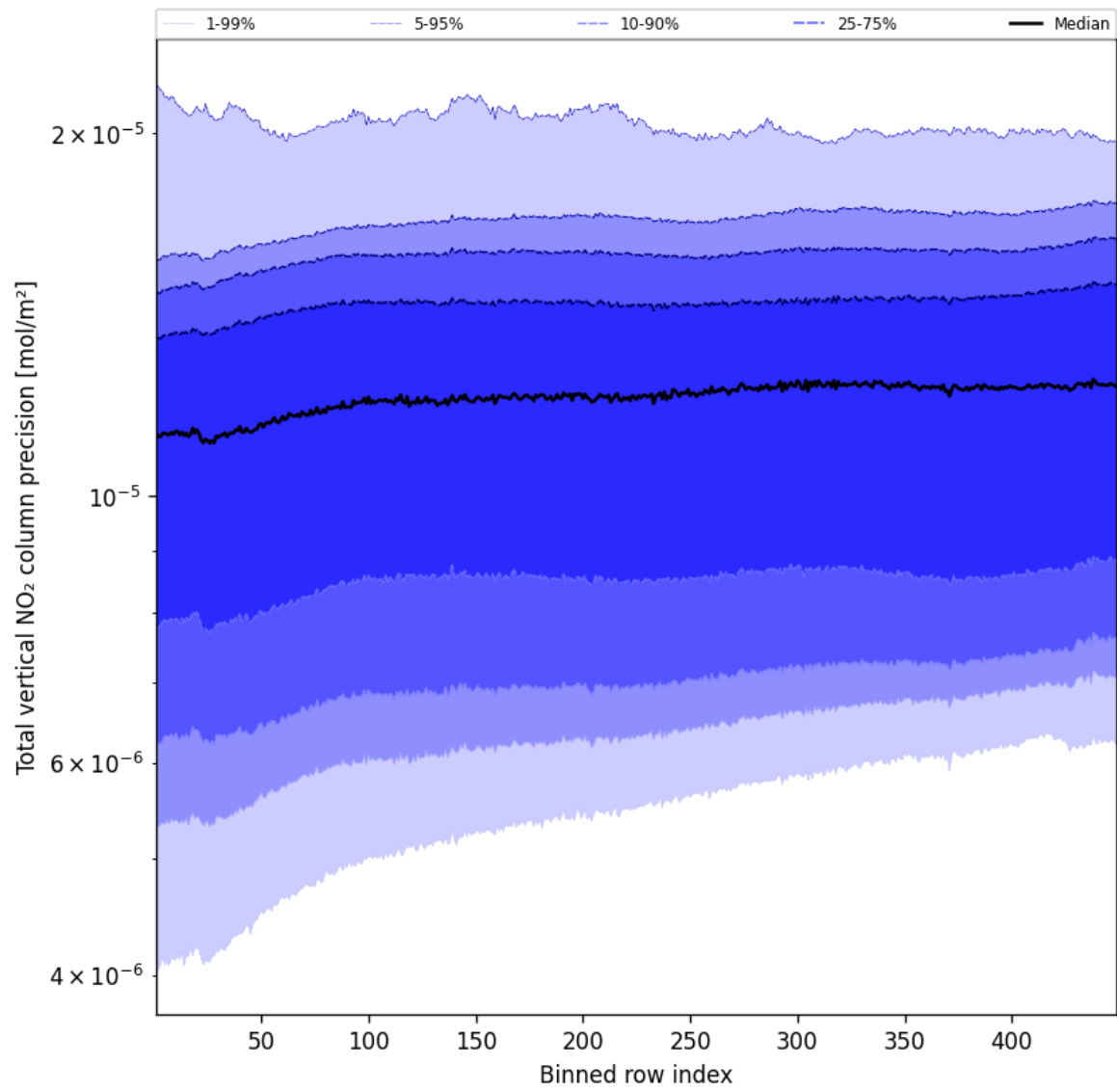
Figure 56: Along track statistics of “Total vertical NO 2 column precision” for 2025-05-09 to 2025-05-10
