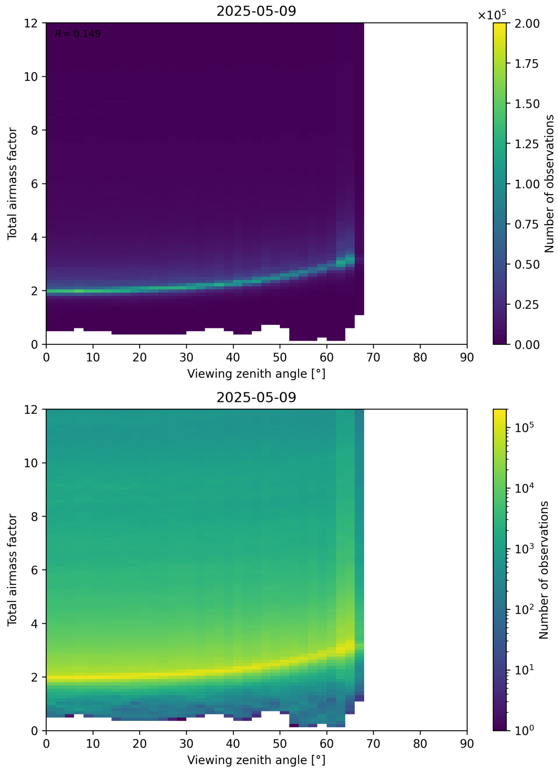
Figure 160: Scatter density plot of “Viewing zenith angle” against “Total airmass factor” for 2025-05-09 to 2025-05-10.
