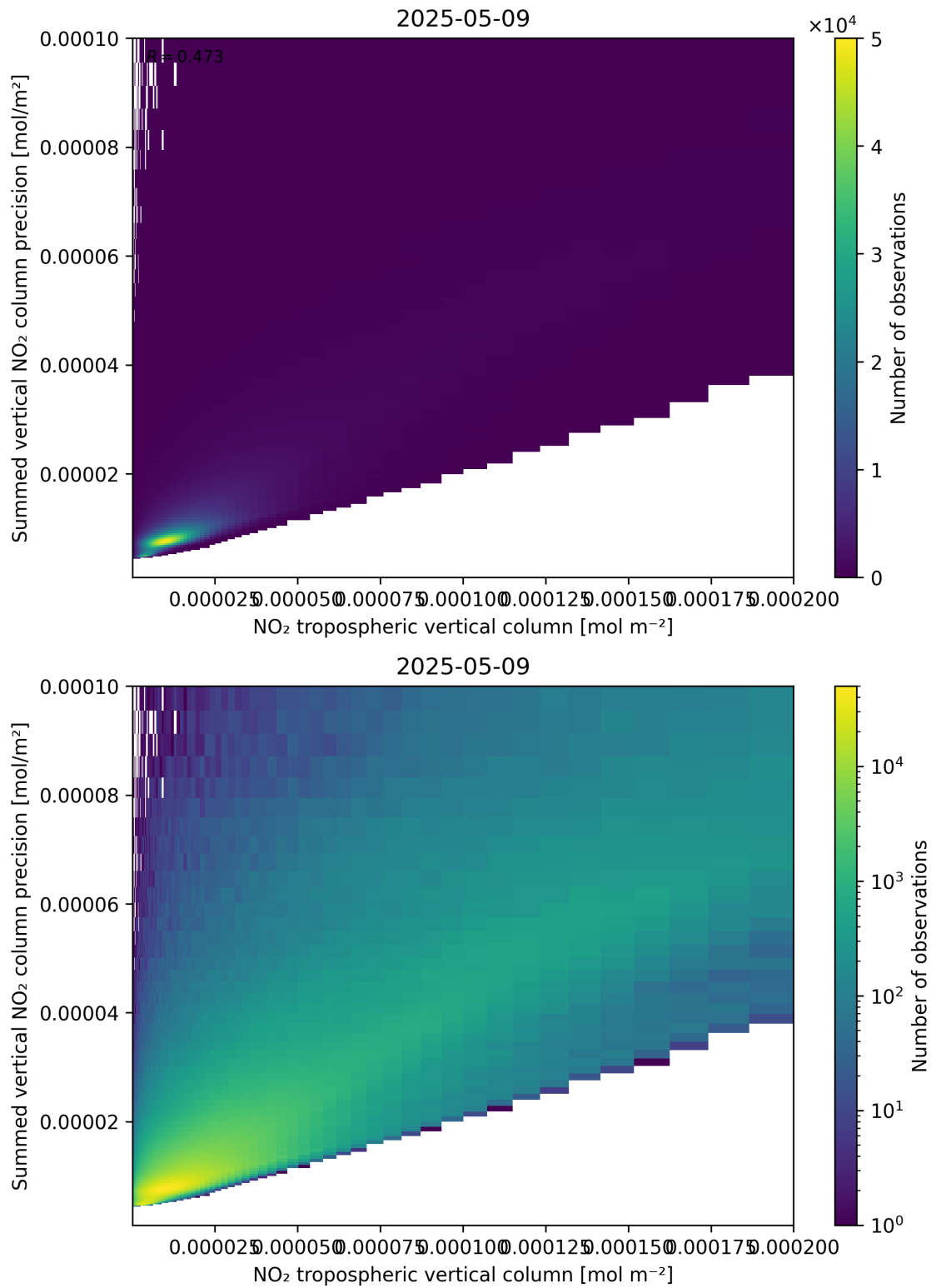
Figure 127: Scatter density plot of “NO 2 tropospheric vertical column” against “Summed vertical NO 2 column precision” for 2025-05-09 to 2025-05-10.
