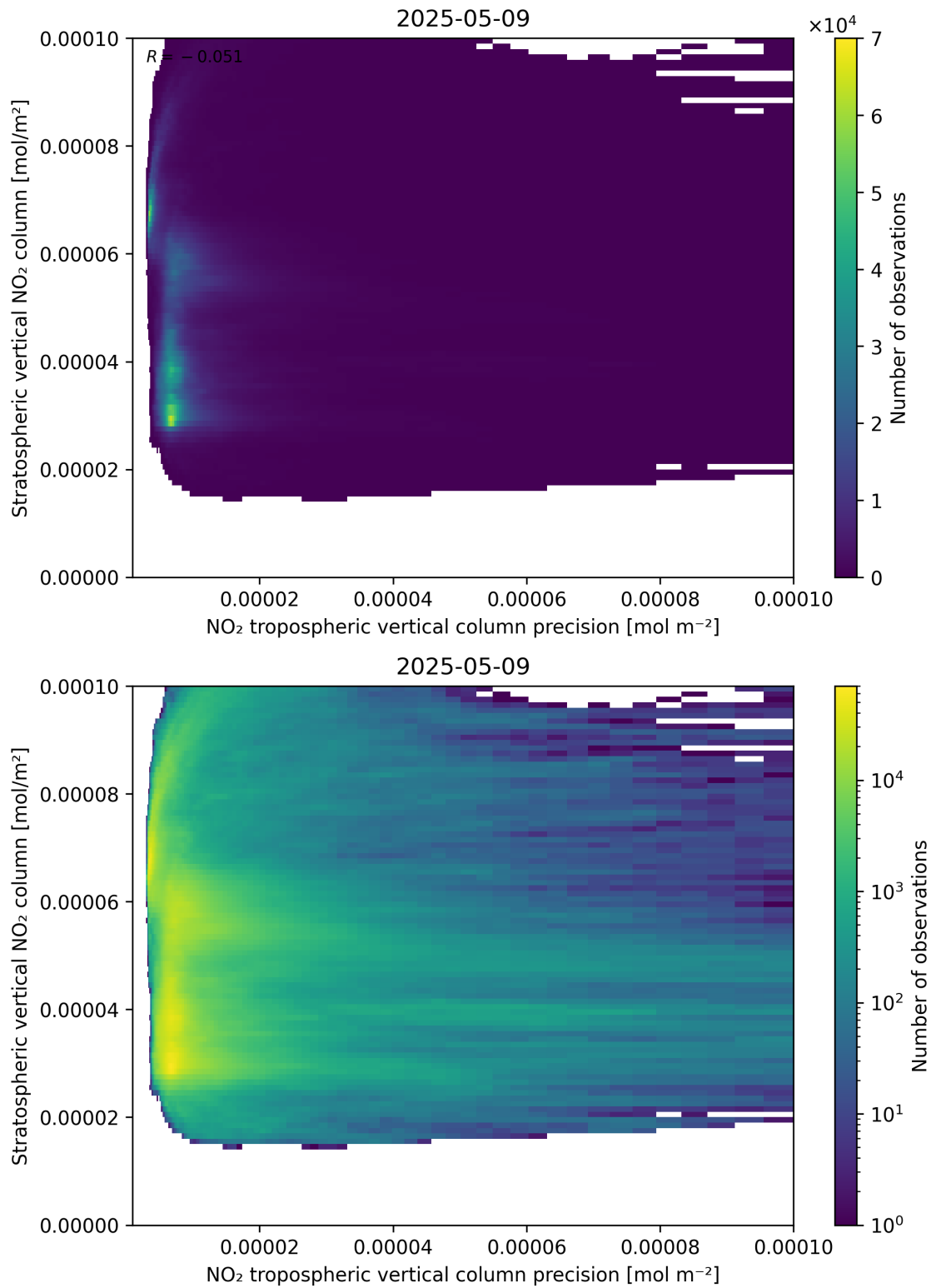
Figure 135: Scatter density plot of “NO 2 tropospheric vertical column precision” against “Stratospheric vertical NO 2 column” for 2025-05-09 to 2025-05-10.
