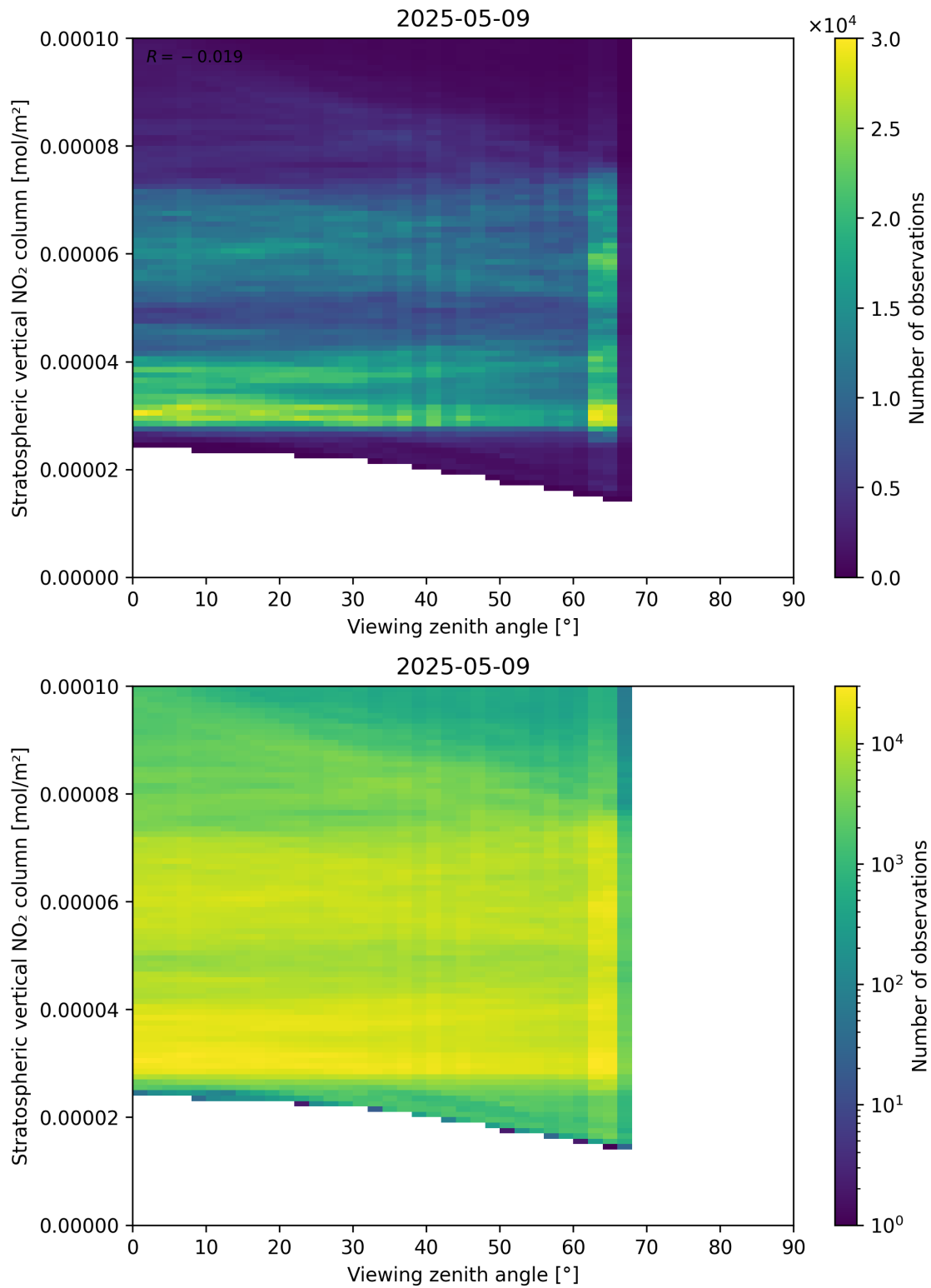
Figure 164: Scatter density plot of “Viewing zenith angle” against “Stratospheric vertical NO 2 column” for 2025-05-09 to 2025-05-10.
