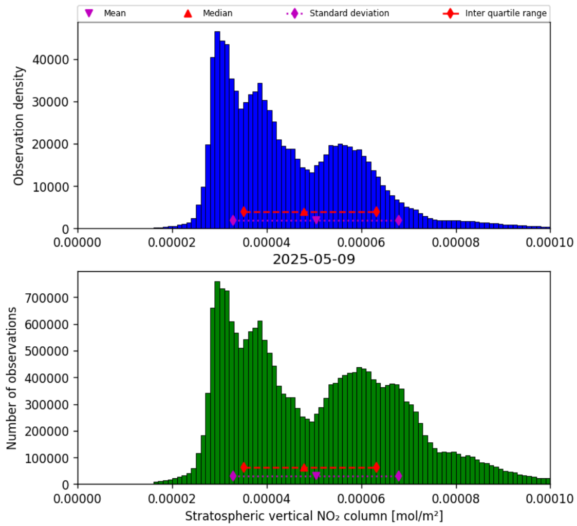
Figure 36: Histogram of “Stratospheric vertical NO 2 column” for 2025-05-09 to 2025-05-10
