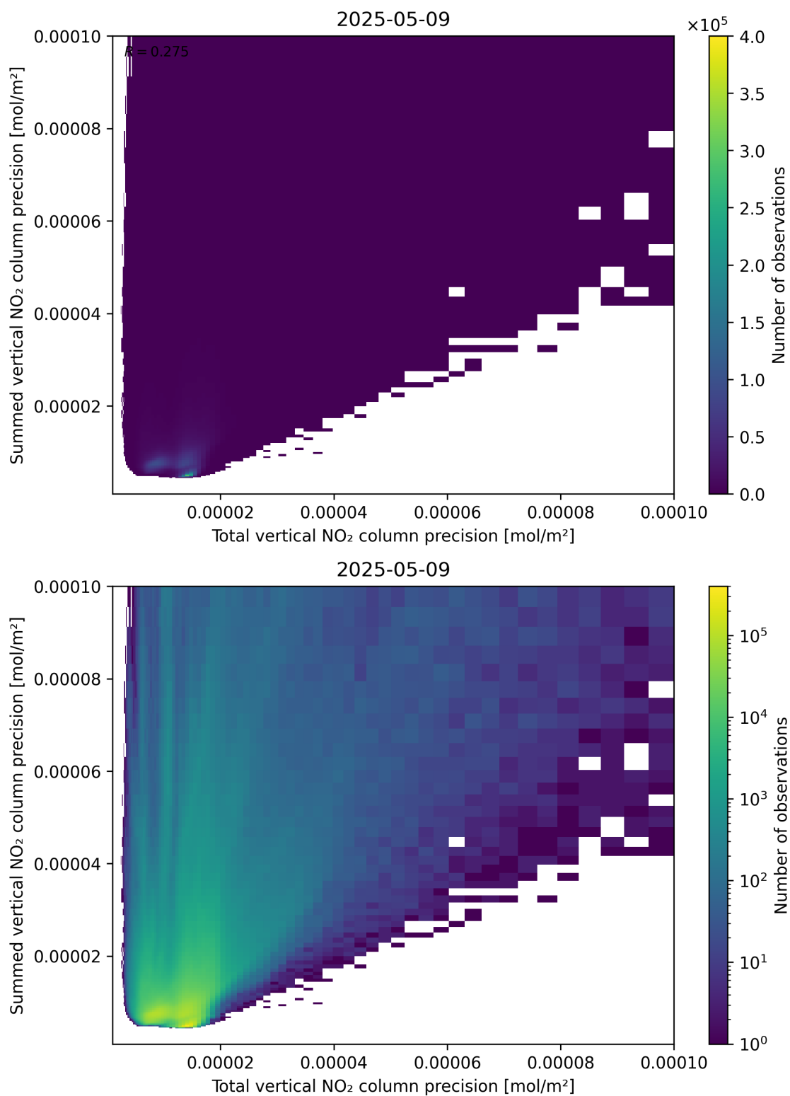
Figure 118: Scatter density plot of “Total vertical NO 2 column precision” against “Summed vertical NO 2 column precision” for 2025-05-09 to 2025-05-10.
