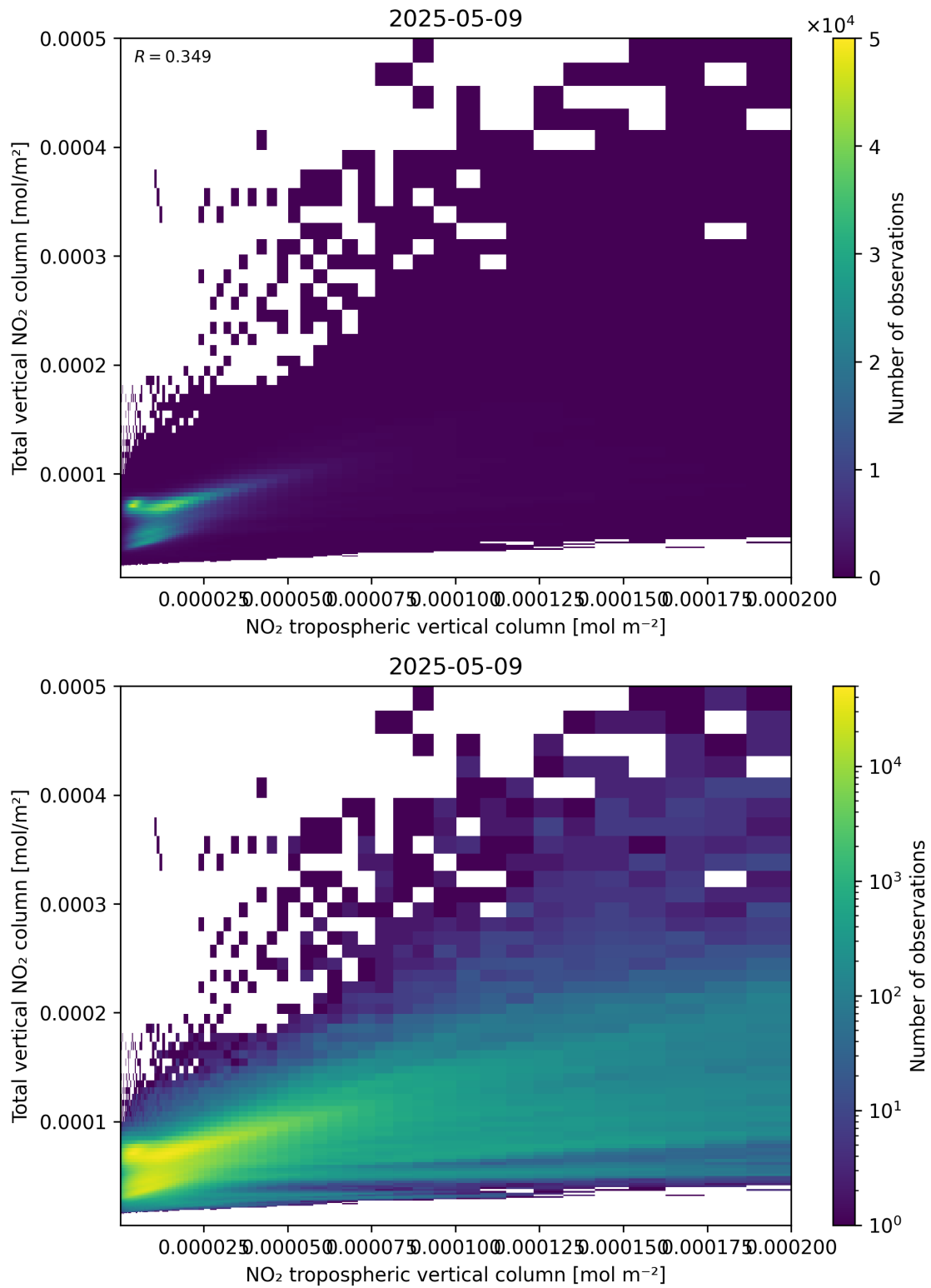
Figure 128: Scatter density plot of “NO 2 tropospheric vertical column” against “Total vertical NO 2 column” for 2025-05-09 to 2025-05-10.
