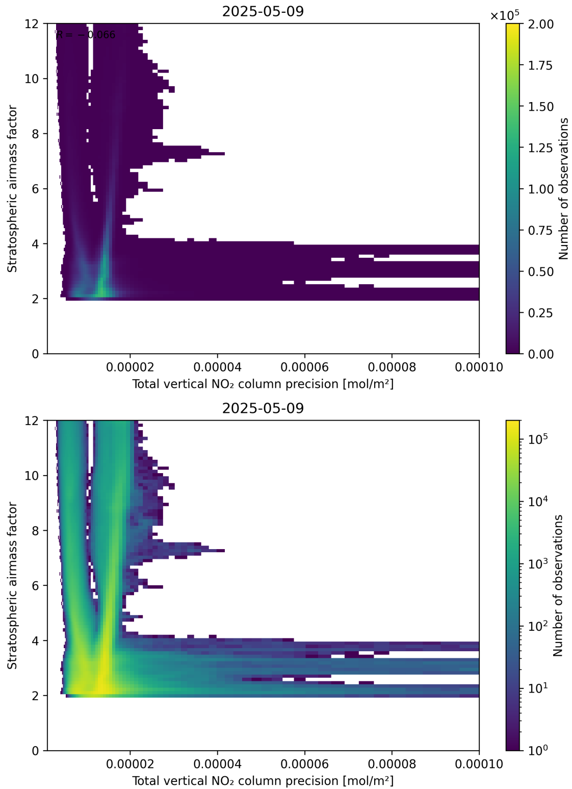
Figure 115: Scatter density plot of “Total vertical NO 2 column precision” against “Stratospheric air mass factor” for 2025-05-09 to 2025-05-10.
