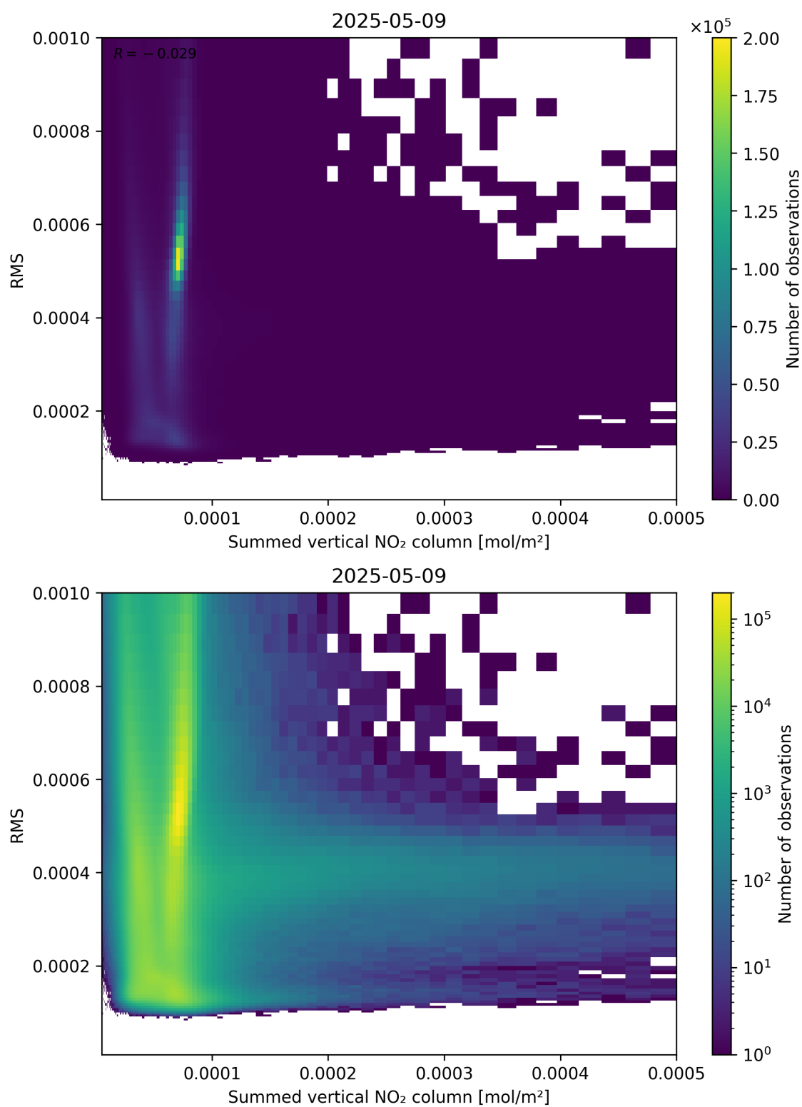
Figure 109: Scatter density plot of “Summed vertical NO 2 column” against “RMS” for 2025-05-09 to 2025-05-10.
