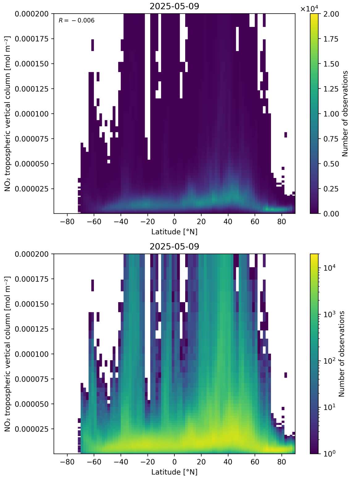
Figure 92: Scatter density plot of “Latitude” against “NO 2 tropospheric vertical column” for 2025-05-09 to 2025-05-10.
