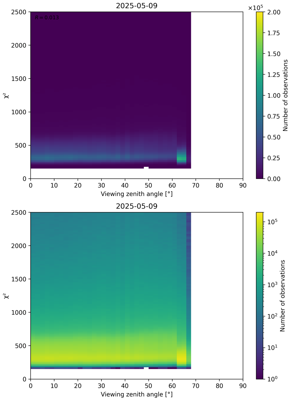
Figure 162: Scatter density plot of “Viewing zenith angle” against “ \chi^2 ” for 2025-05-09 to 2025-05-10.
