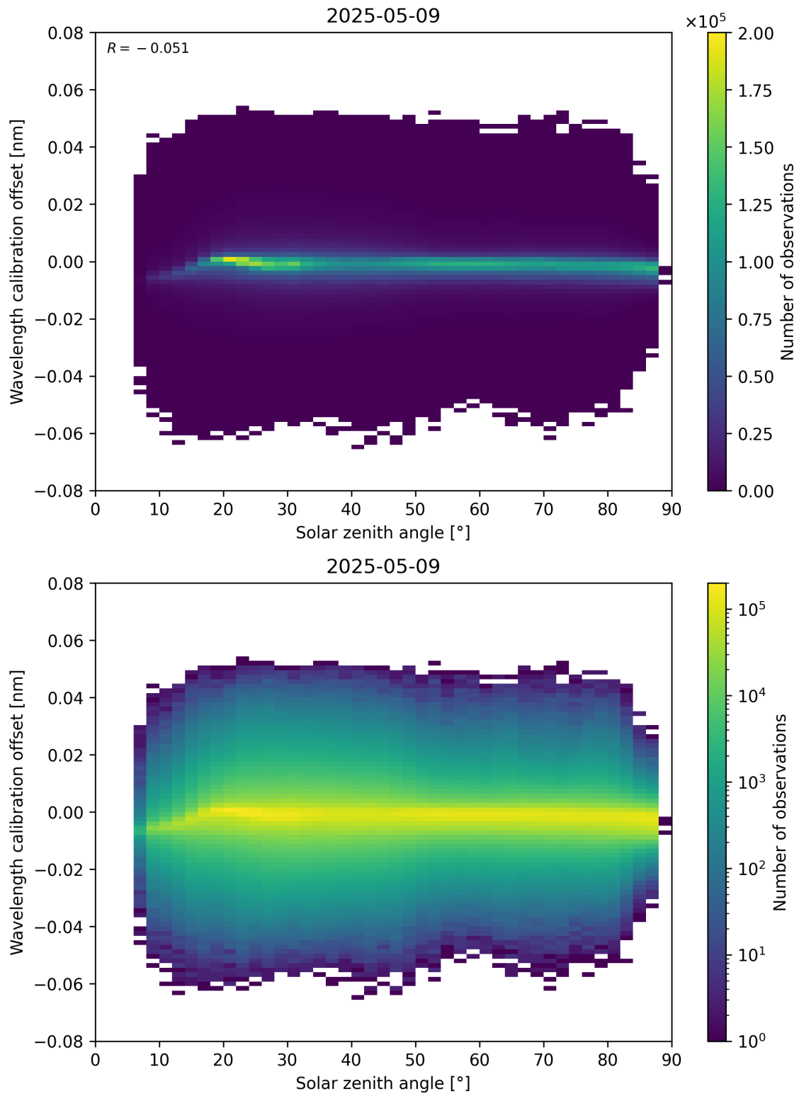
Figure 158: Scatter density plot of “Solar zenith angle” against “Wavelength calibration offset” for 2025-05-09 to 2025-05-10.
