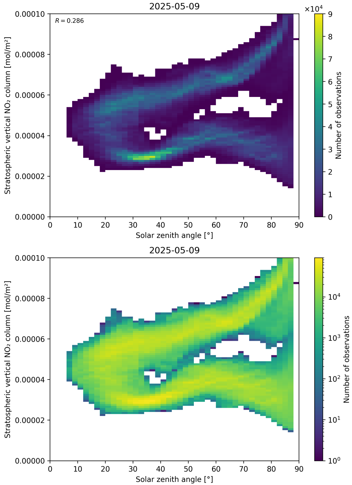
Figure 150: Scatter density plot of “Solar zenith angle” against “Stratospheric vertical NO 2 column” for 2025-05-09 to 2025-05-10.
