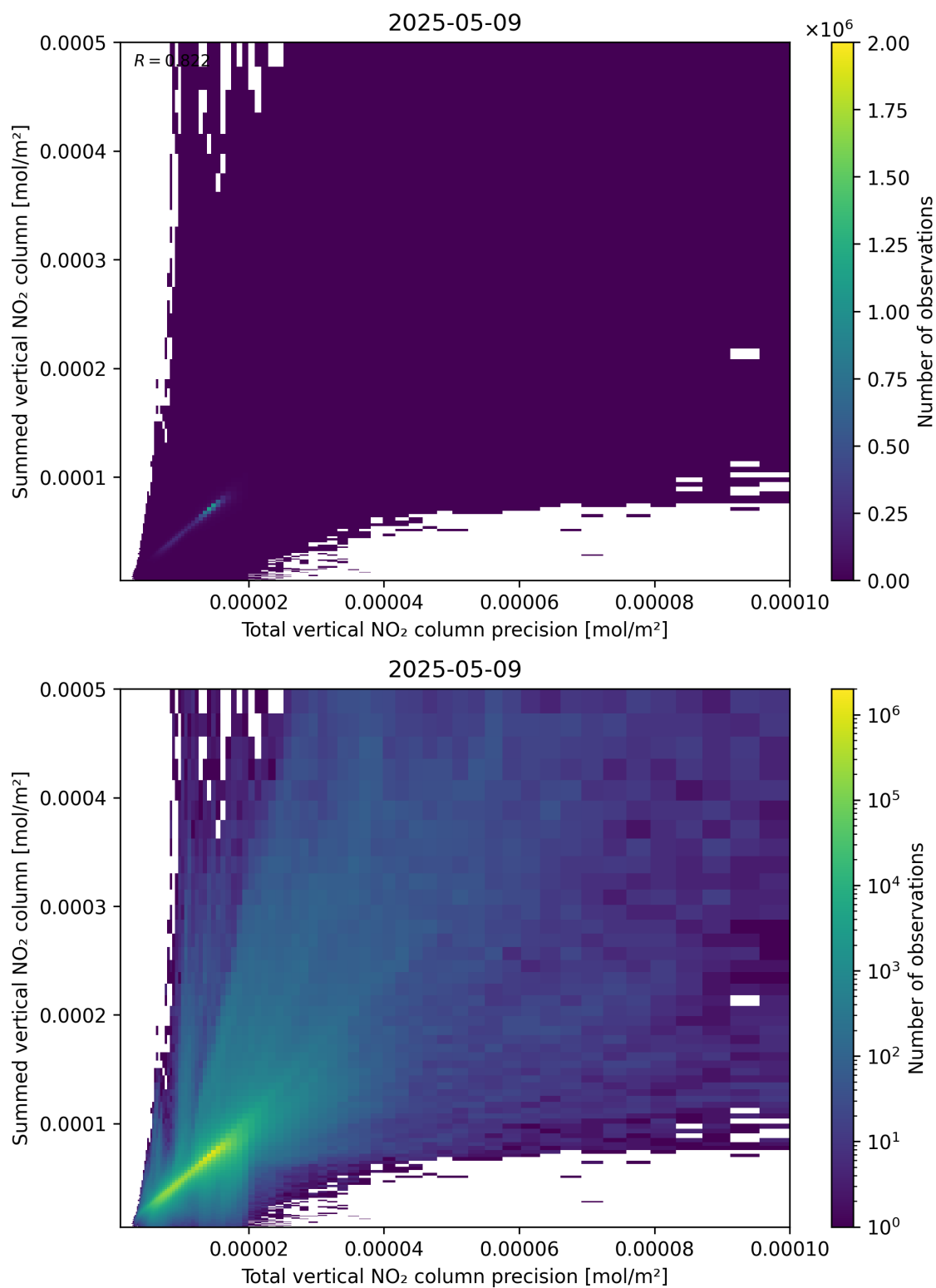
Figure 117: Scatter density plot of “Total vertical NO 2 column precision” against “Summed vertical NO 2 column” for 2025-05-09 to 2025-05-10.
