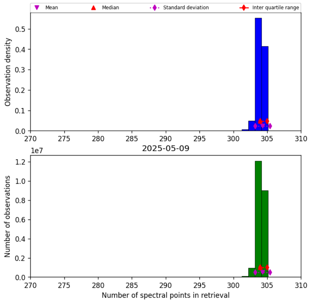
Figure 33: Histogram of “Number of spectral points in retrieval” for 2025-05-09 to 2025-05-10
