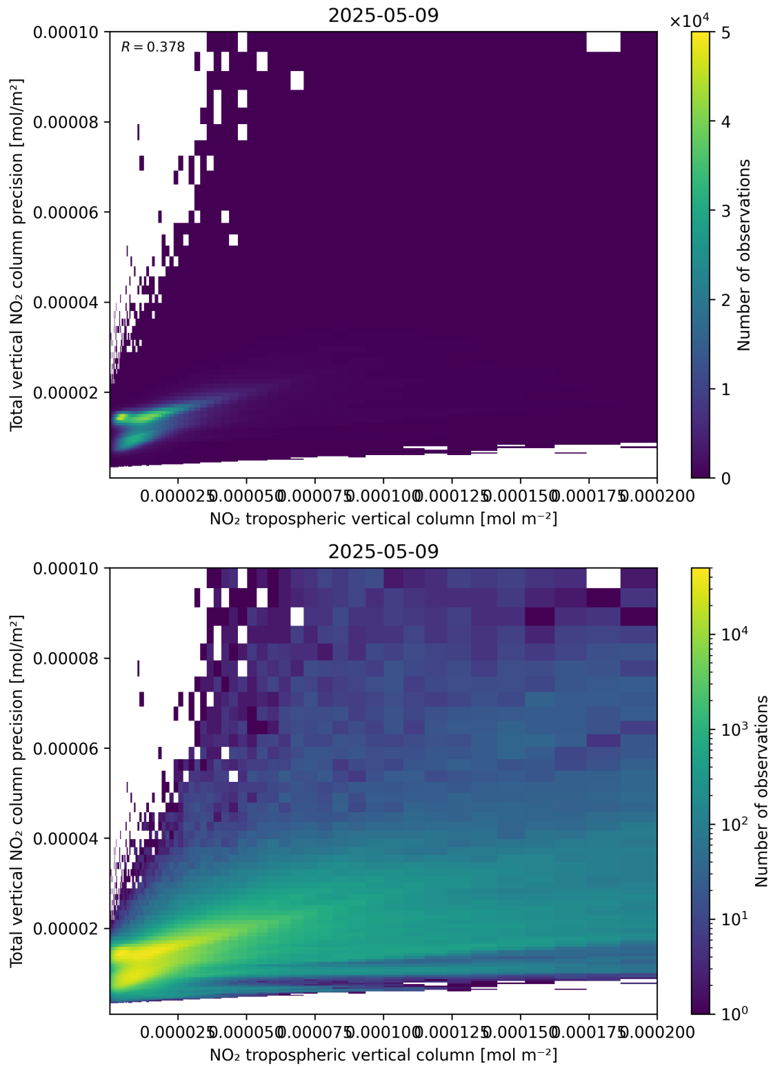
Figure 129: Scatter density plot of “NO 2 tropospheric vertical column” against “Total vertical NO 2 column precision” for 2025-05-09 to 2025-05-10.
