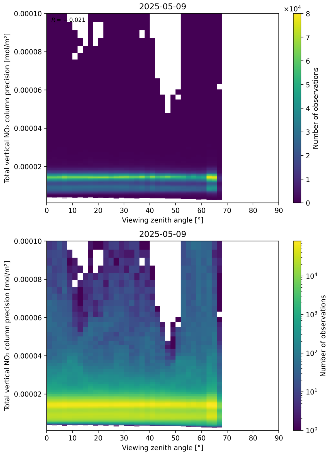
Figure 168: Scatter density plot of “Viewing zenith angle” against “Total vertical NO 2 column precision” for 2025-05-09 to 2025-05-10.
