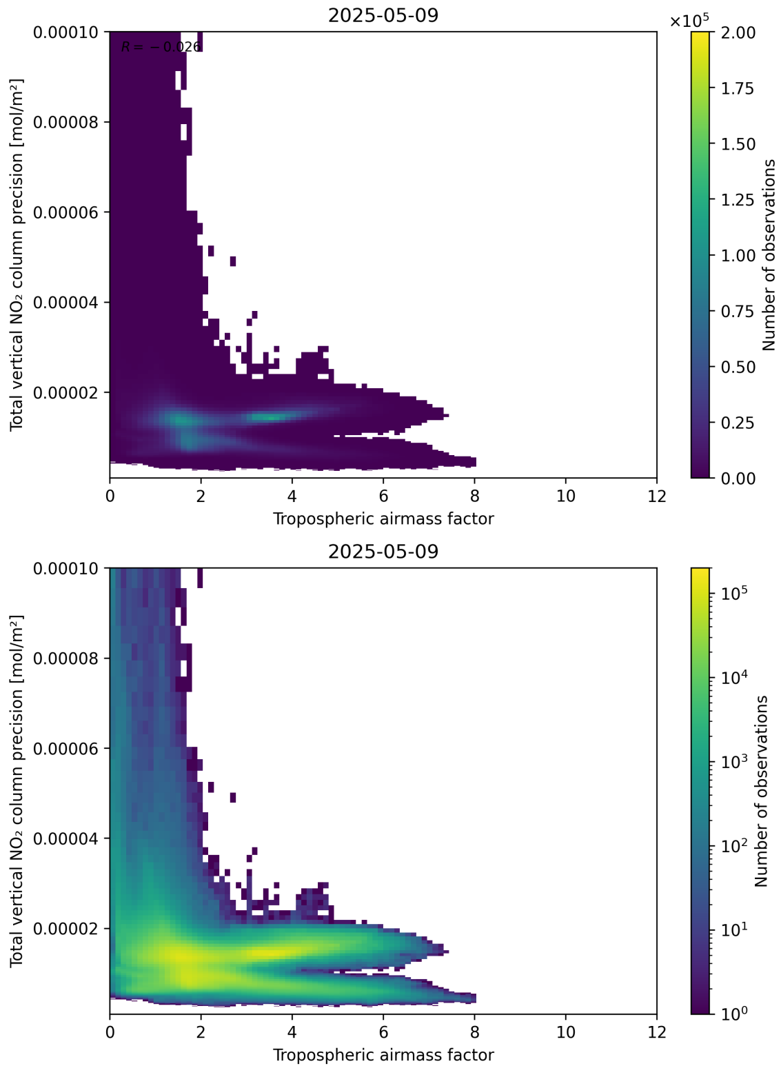
Figure 78: Scatter density plot of “Tropospheric air mass factor” against “Total vertical NO 2 column precision” for 2025-05-09 to 2025-05-10.
