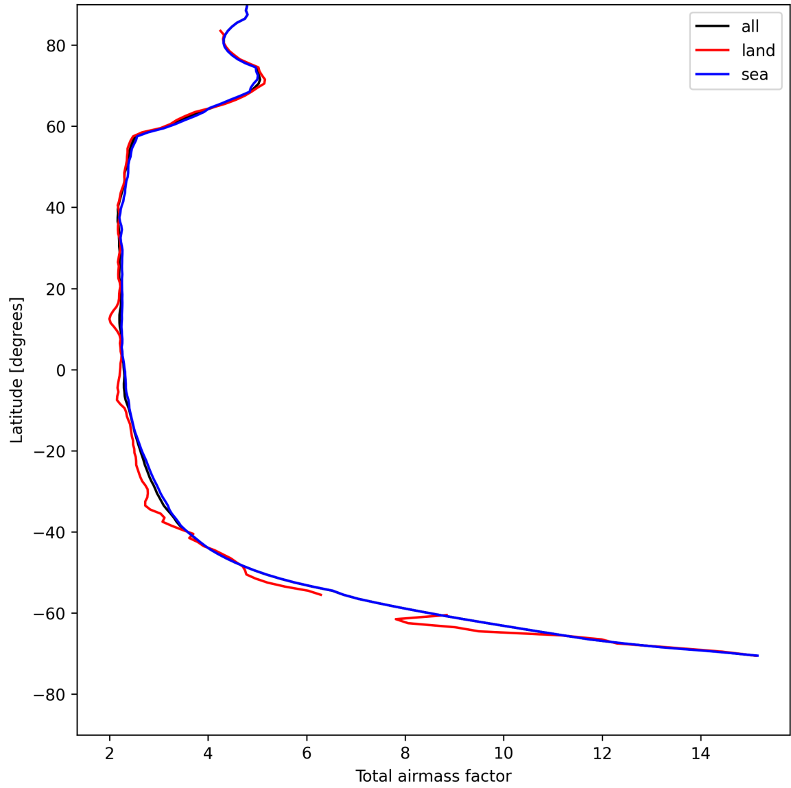
Figure 15: Zonal average of “Total airmass factor” for 2025-05-09 to 2025-05-10.
