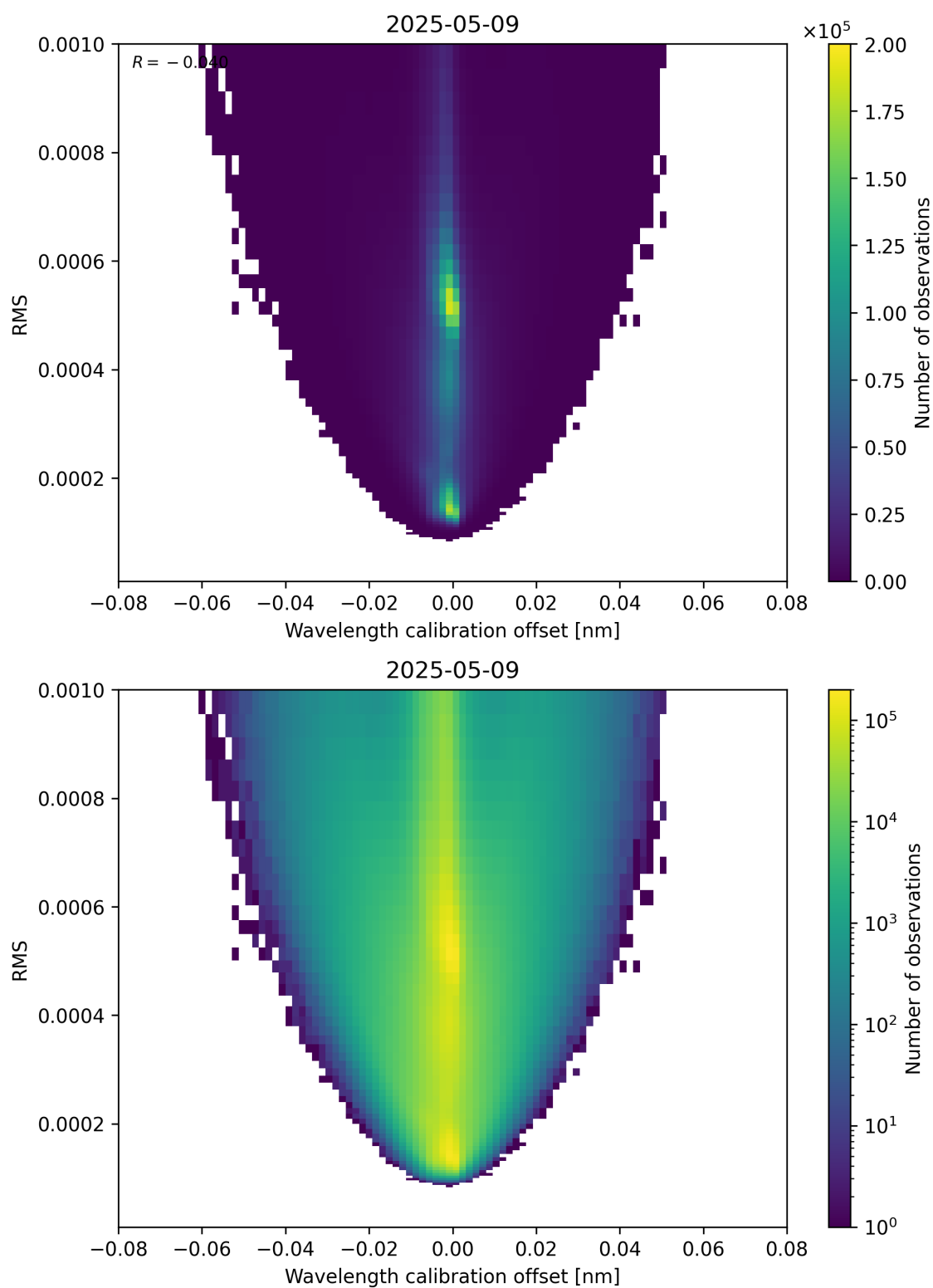
Figure 181: Scatter density plot of “Wavelength calibration offset” against “RMS” for 2025-05-09 to 2025-05-10.
