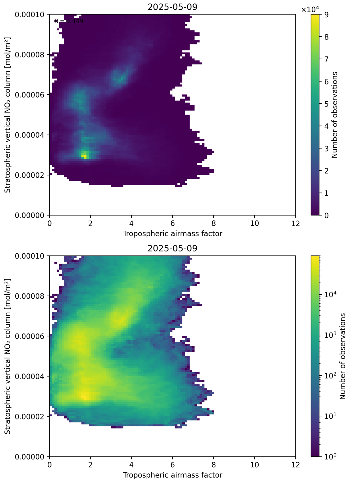
Figure 74: Scatter density plot of “Tropospheric air mass factor” against “Stratospheric vertical NO 2 column” for 2025-05-09 to 2025-05-10.
