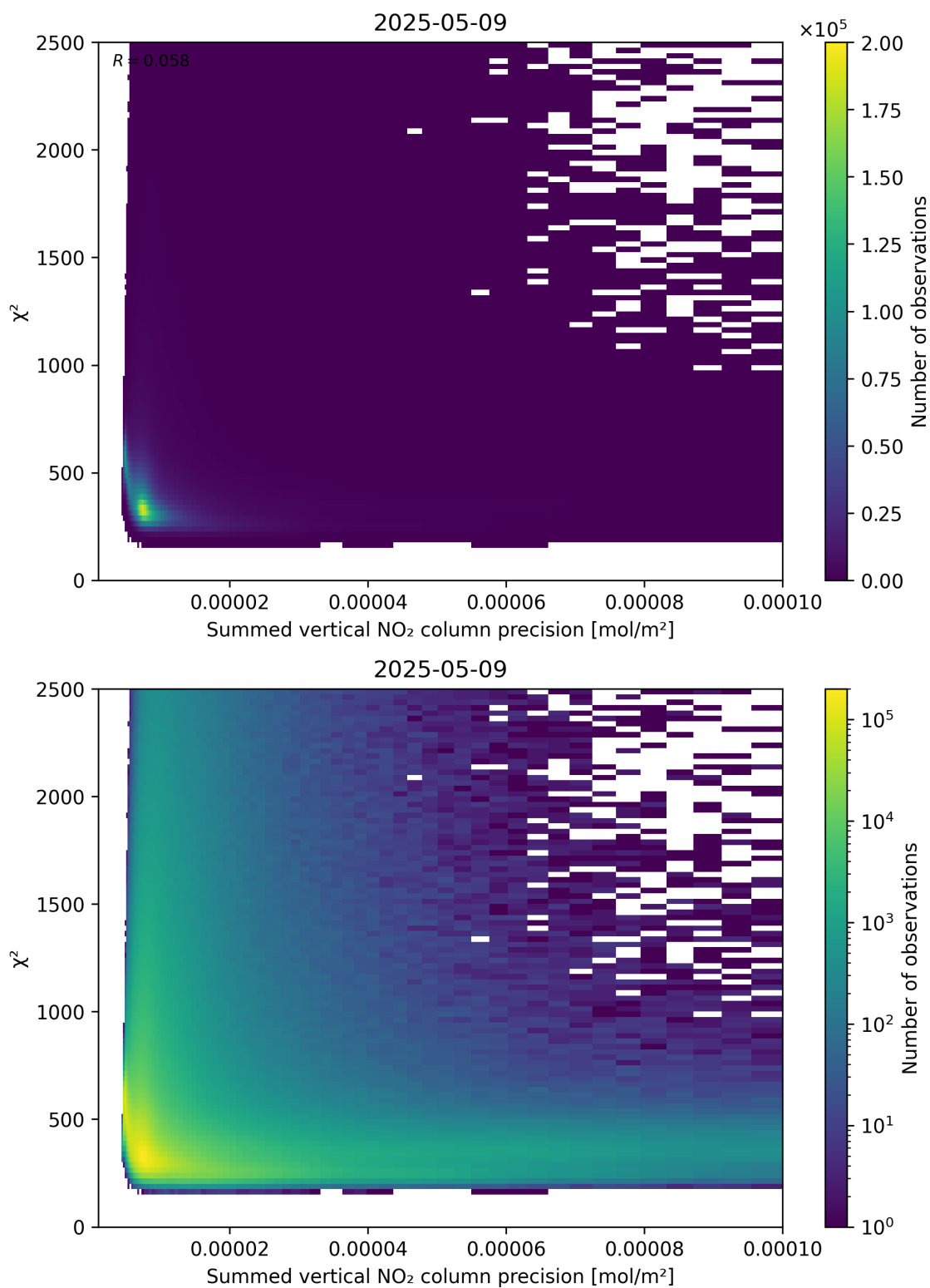
Figure 107: Scatter density plot of “Summed vertical NO 2 column precision” against “ \chi^2 ” for 2025-05-09 to 2025-05-10.
