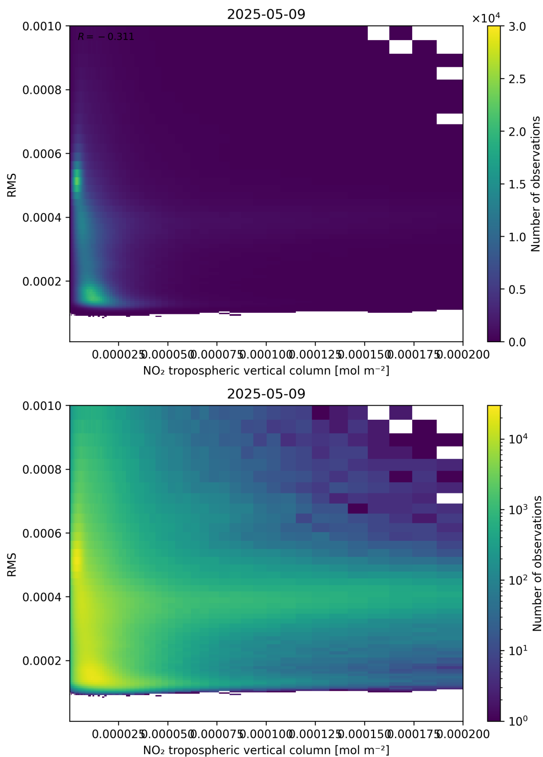
Figure 142: Scatter density plot of “NO 2 tropospheric vertical column” against “RMS” for 2025-05-09 to 2025-05-10.
