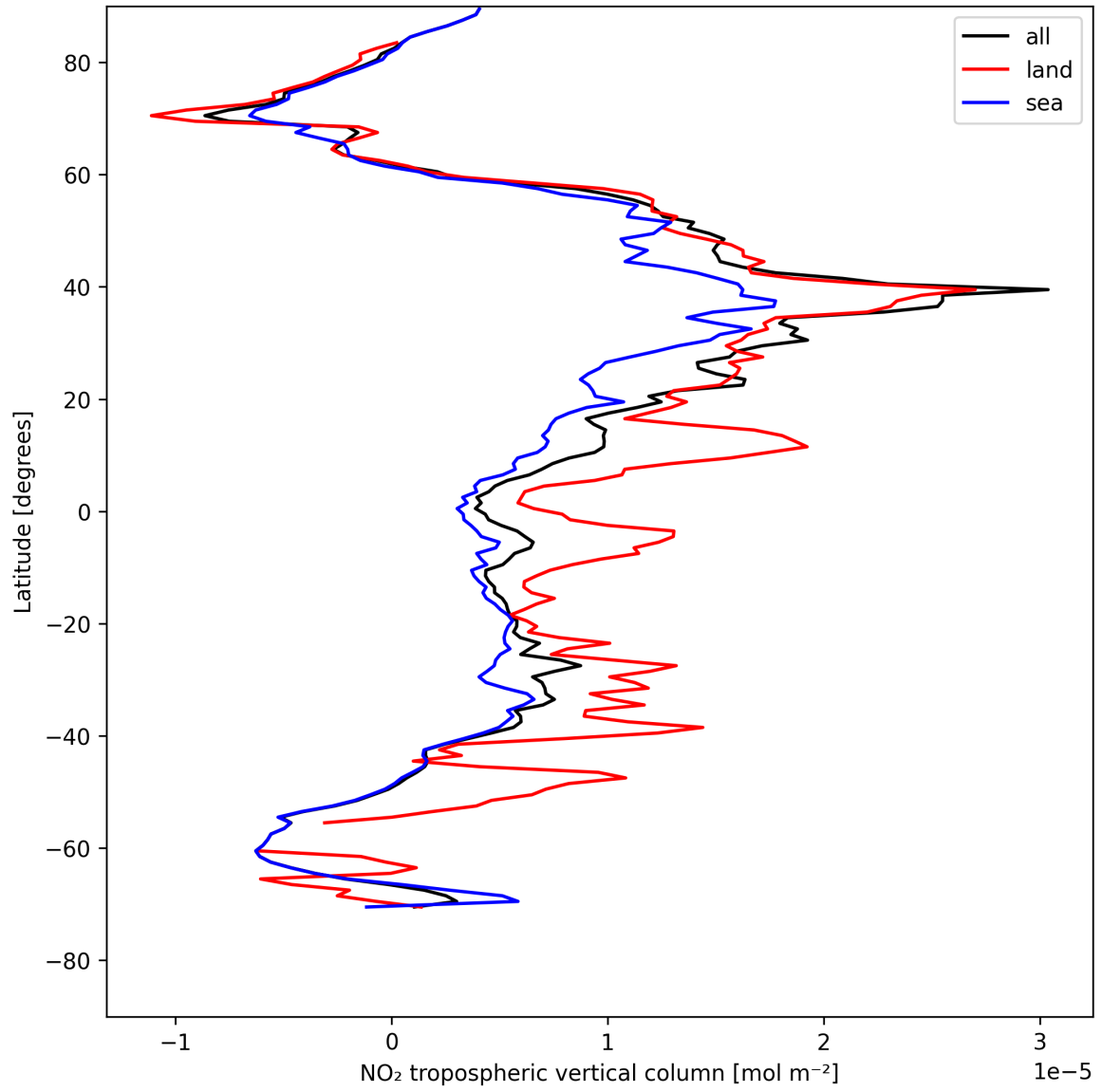
Figure 12: Zonal average of “NO 2 tropospheric vertical column” for 2025-05-09 to 2025-05-10.
