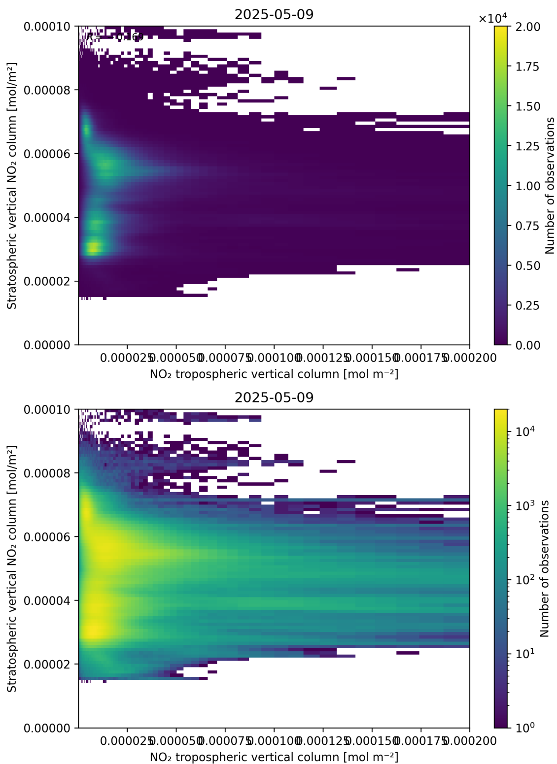
Figure 125: Scatter density plot of “NO 2 tropospheric vertical column” against “Stratospheric vertical NO 2 column” for 2025-05-09 to 2025-05-10.
