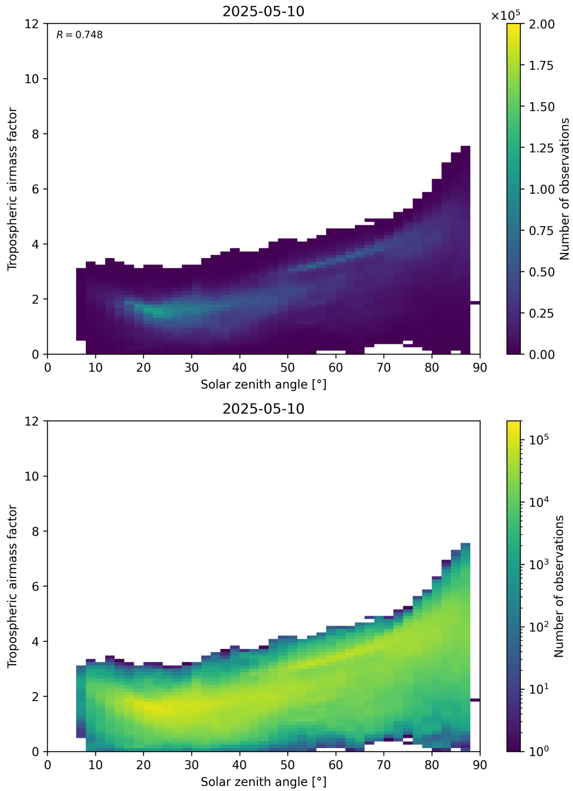
Figure 147: Scatter density plot of “Solar zenith angle” against “Tropospheric airmass factor” for 2025-05-10 to 2025-05-11.
