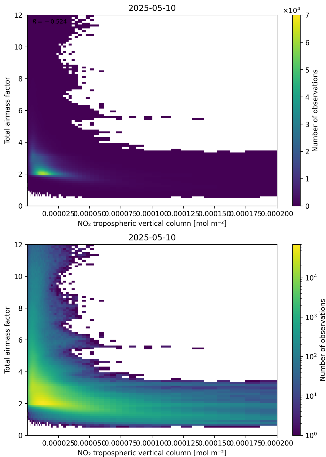
Figure 122: Scatter density plot of “NO 2 tropospheric vertical column” against “Total air mass factor” for 2025-05-10 to 2025-05-11.
