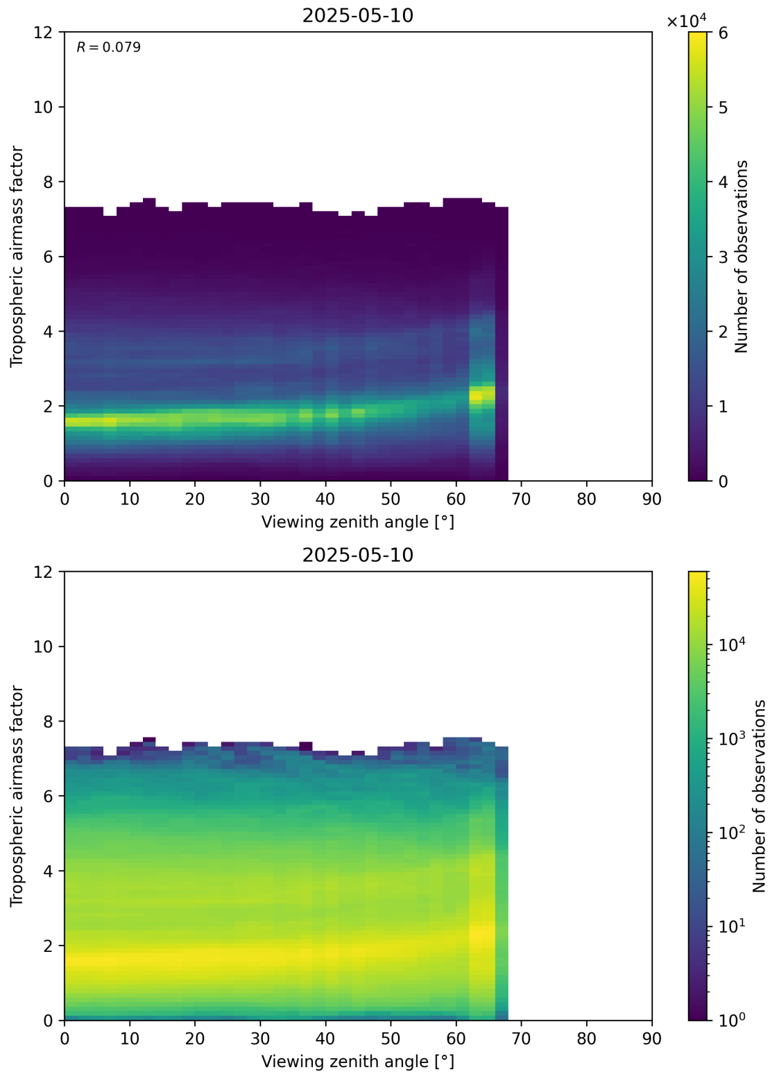
Figure 161: Scatter density plot of “Viewing zenith angle” against “Tropospheric airmass factor” for 2025-05-10 to 2025-05-11.
