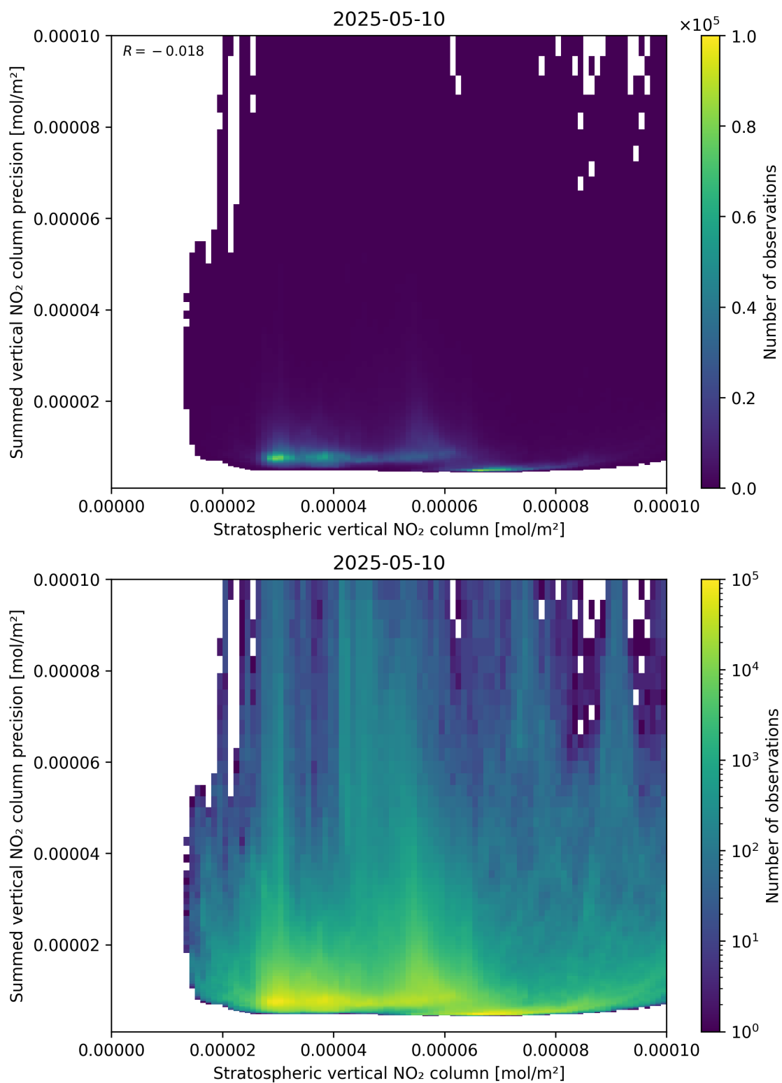
Figure 99: Scatter density plot of “Stratospheric vertical NO 2 column” against “Summed vertical NO 2 column precision” for 2025-05-10 to 2025-05-11.
