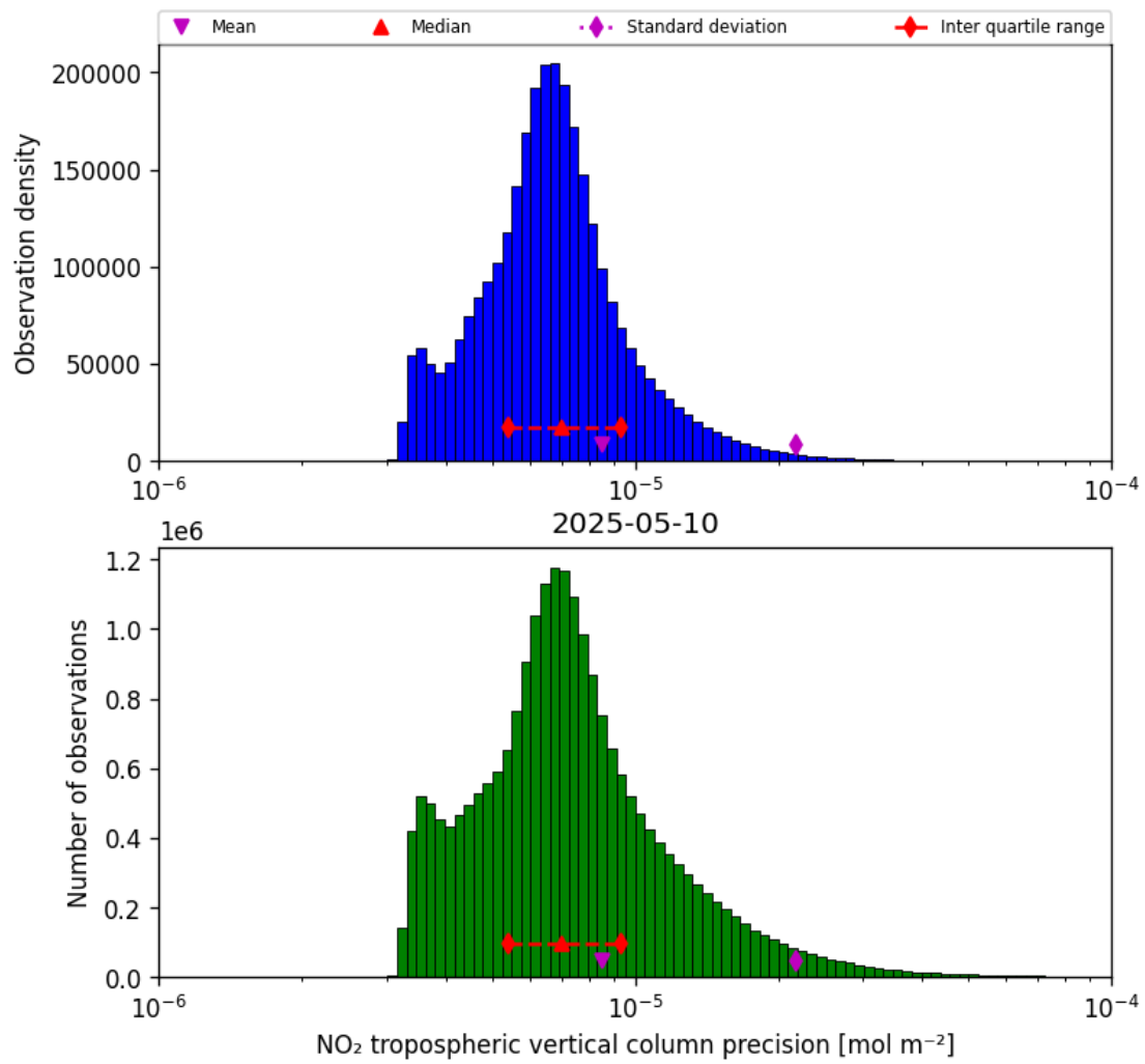
Figure 30: Histogram of “NO 2 tropospheric vertical column precision” for 2025-05-10 to 2025-05-11
