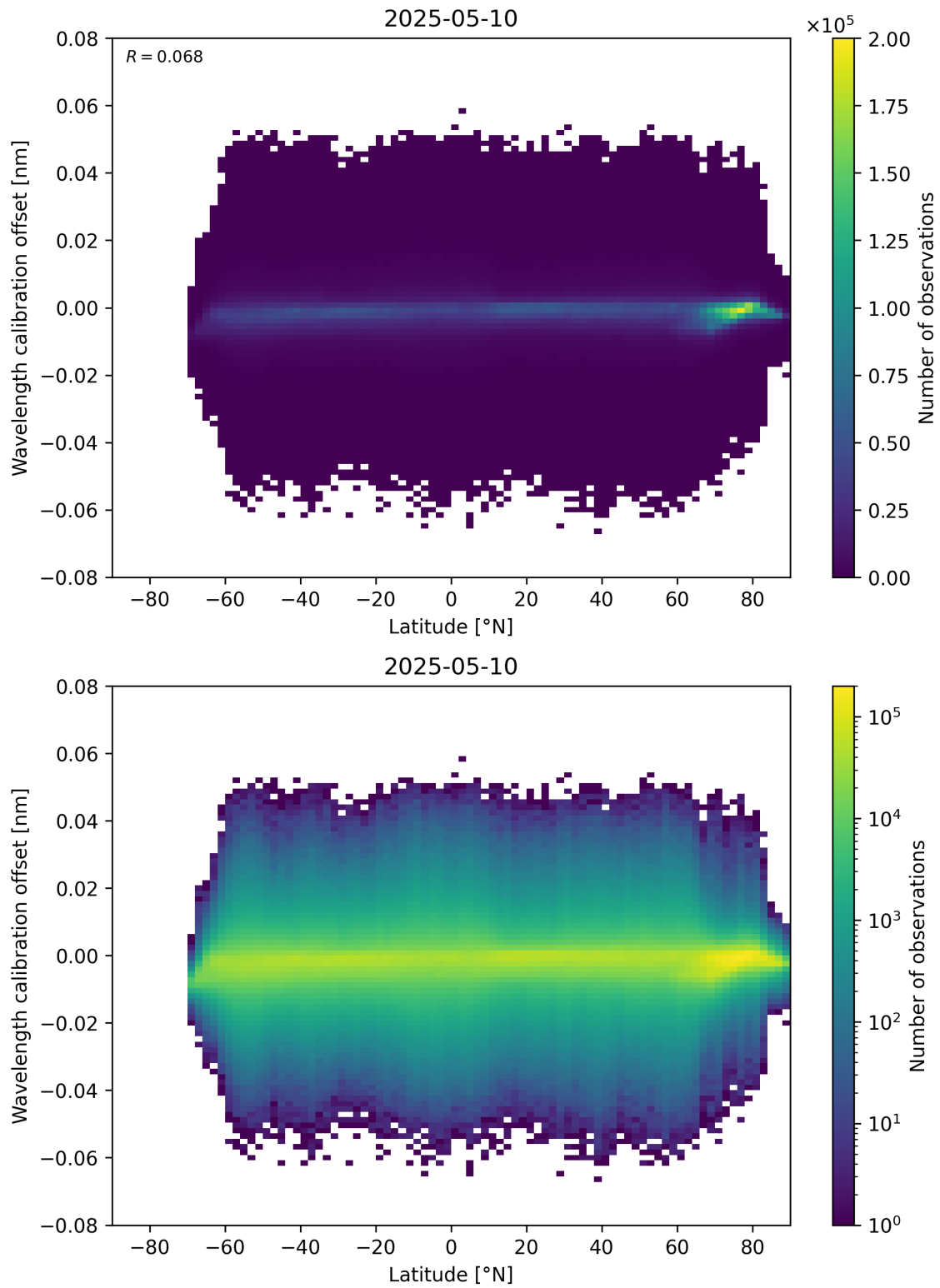
Figure 95: Scatter density plot of “Latitude” against “Wavelength calibration offset” for 2025-05-10 to 2025-05-11.
