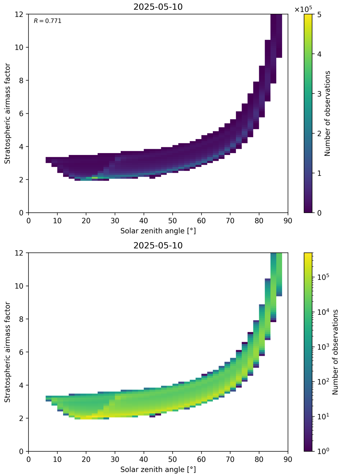
Figure 145: Scatter density plot of “Solar zenith angle” against “Stratospheric airmass factor” for 2025-05-10 to 2025-05-11.
