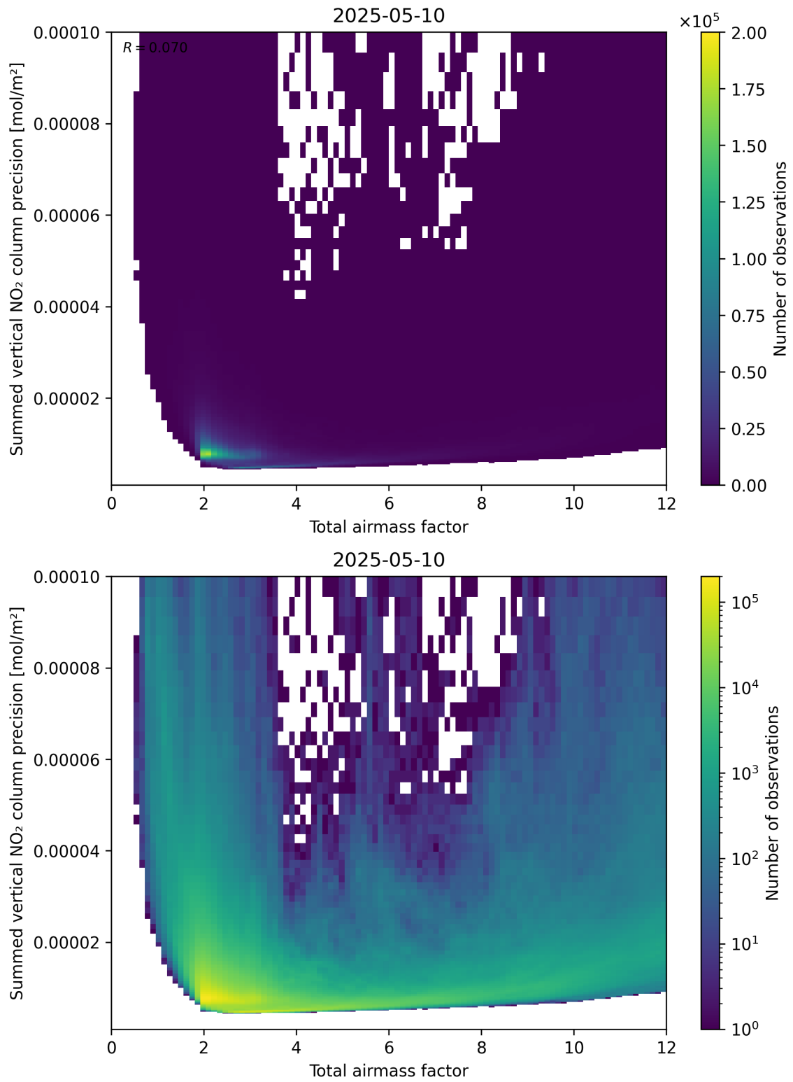
Figure 66: Scatter density plot of “Total airmass factor” against “Summed vertical NO 2 column precision” for 2025-05-10 to 2025-05-11.
