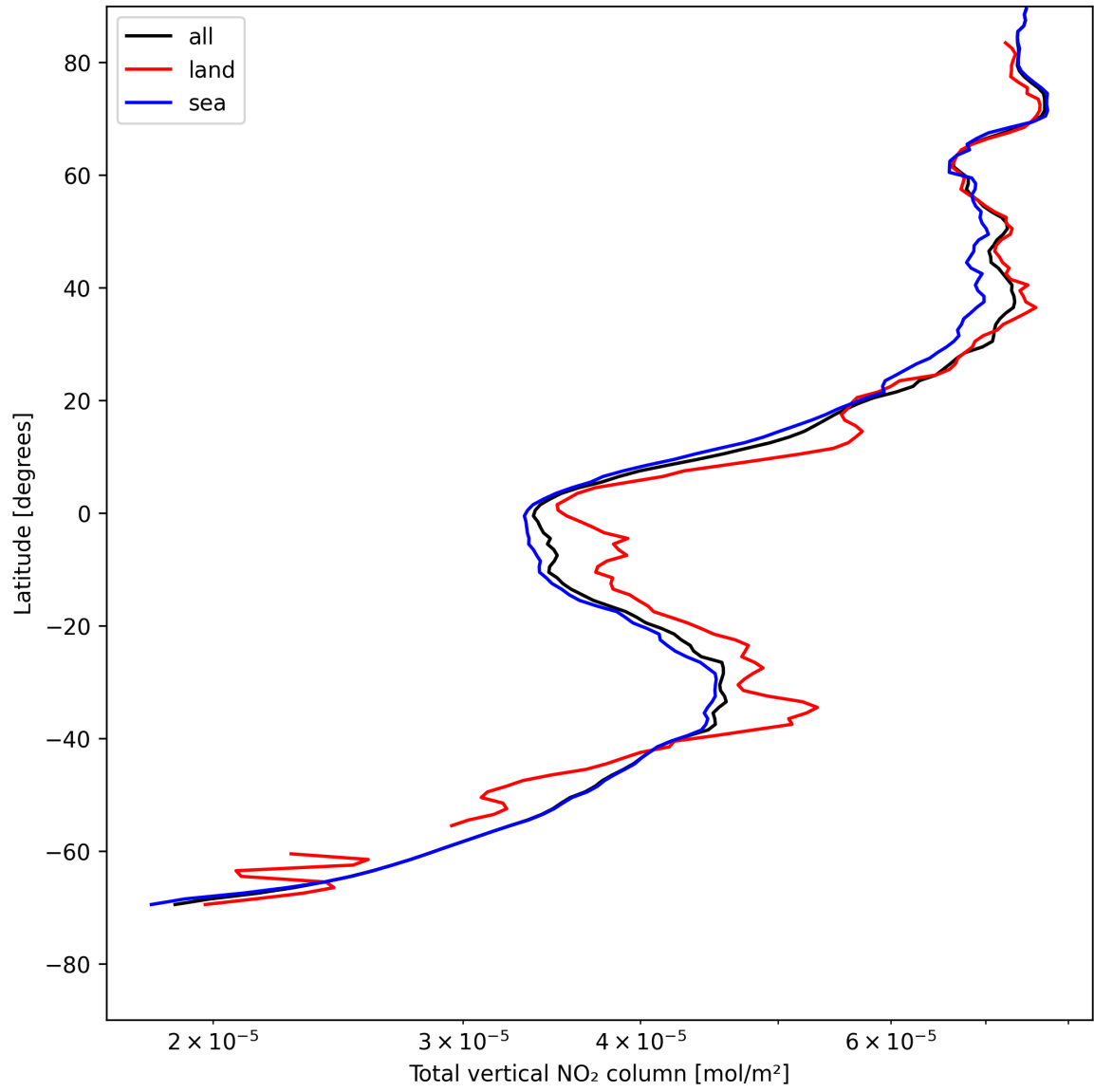
Figure 21: Zonal average of “Total vertical NO 2 column” for 2025-05-10 to 2025-05-11.
