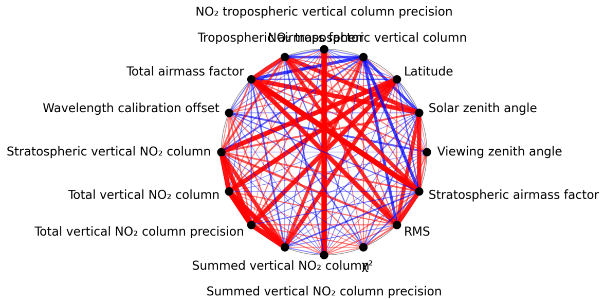
Figure 1: Map of correlation graph for 2025-05-10 to 2025-05-11.
