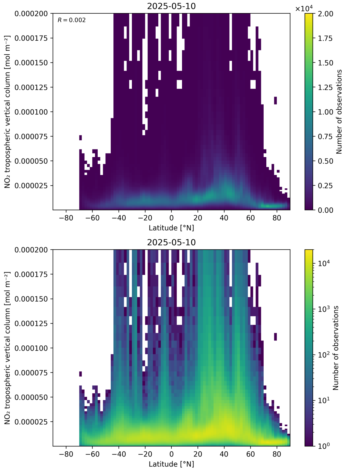
Figure 92: Scatter density plot of “Latitude” against “NO 2 tropospheric vertical column” for 2025-05-10 to 2025-05-11.
