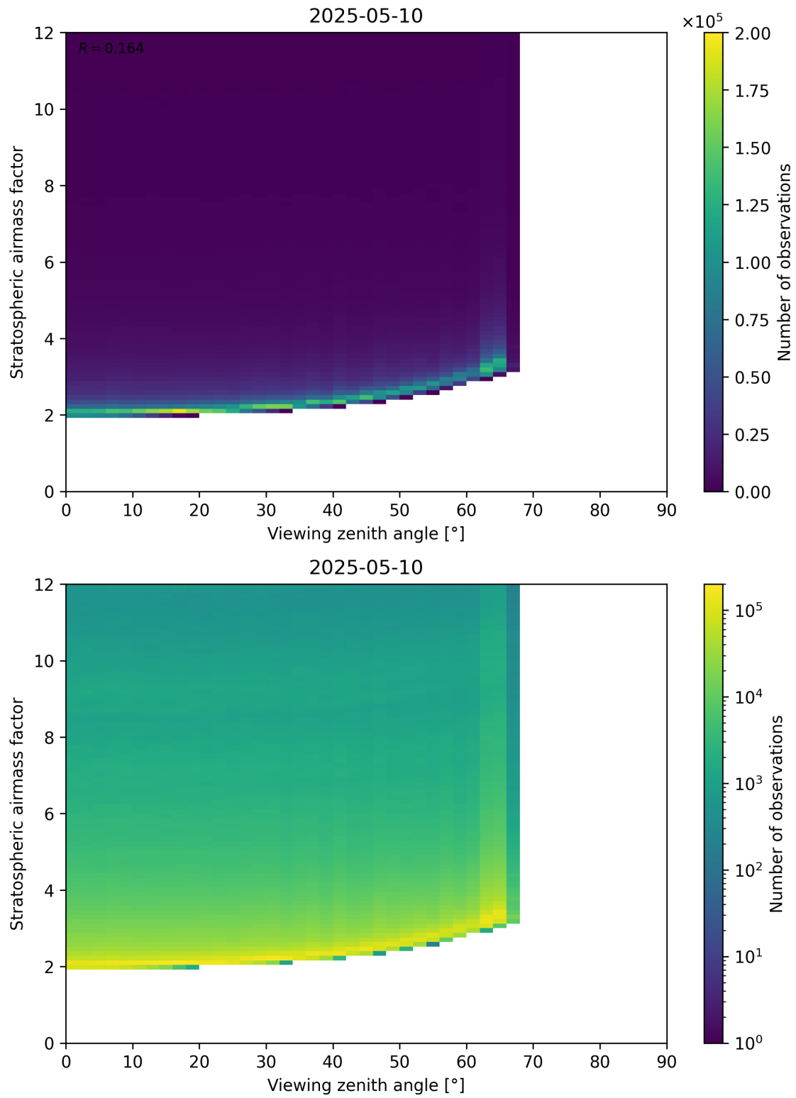
Figure 159: Scatter density plot of “Viewing zenith angle” against “Stratospheric airmass factor” for 2025-05-10 to 2025-05-11.
