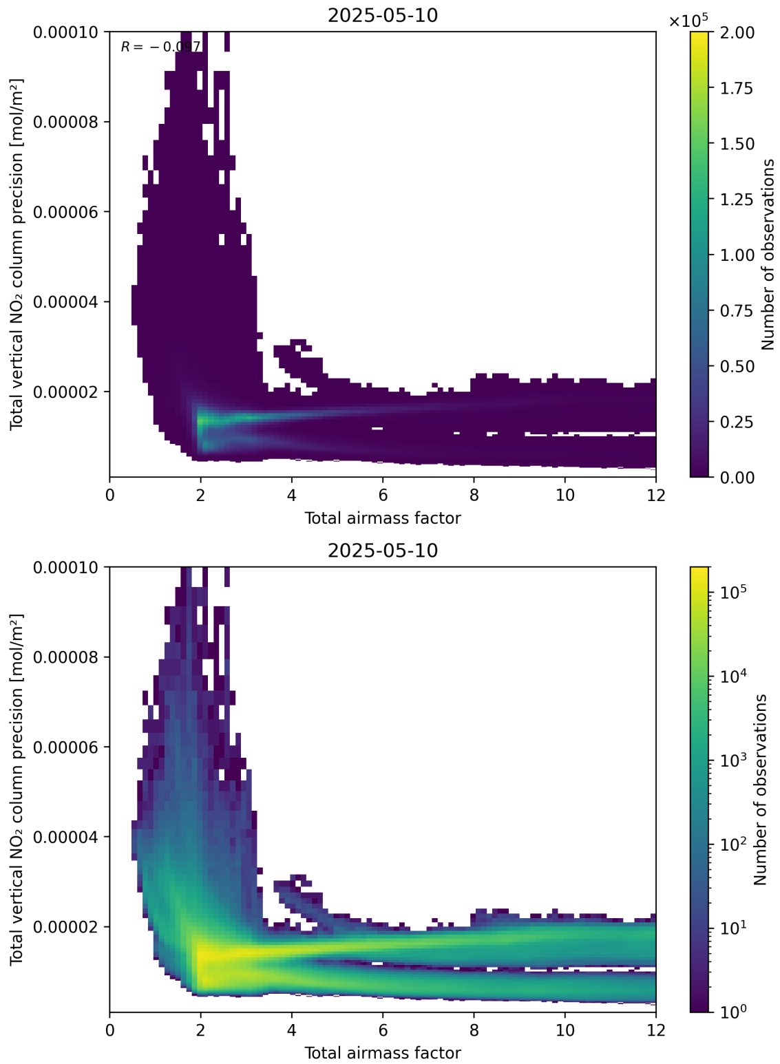
Figure 68: Scatter density plot of “Total airmass factor” against “Total vertical NO 2 column precision” for 2025-05-10 to 2025-05-11.
