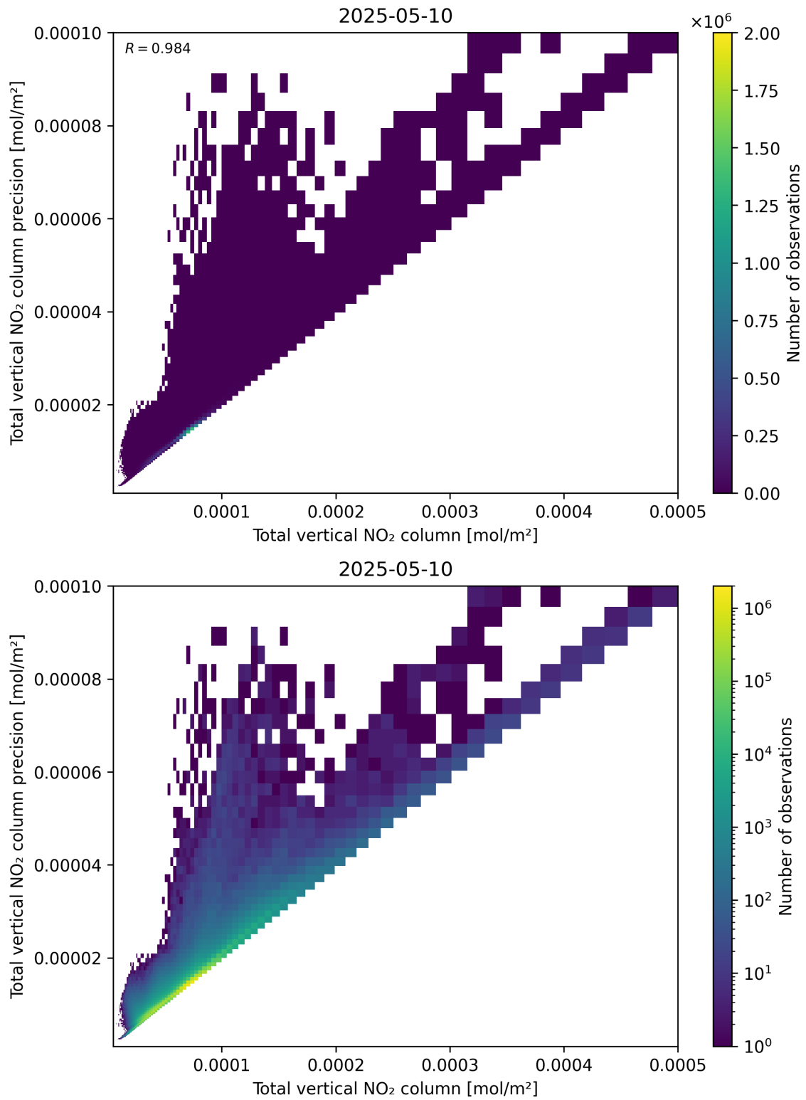
Figure 114: Scatter density plot of “Total vertical NO 2 column” against “Total vertical NO 2 column precision” for 2025-05-10 to 2025-05-11.
