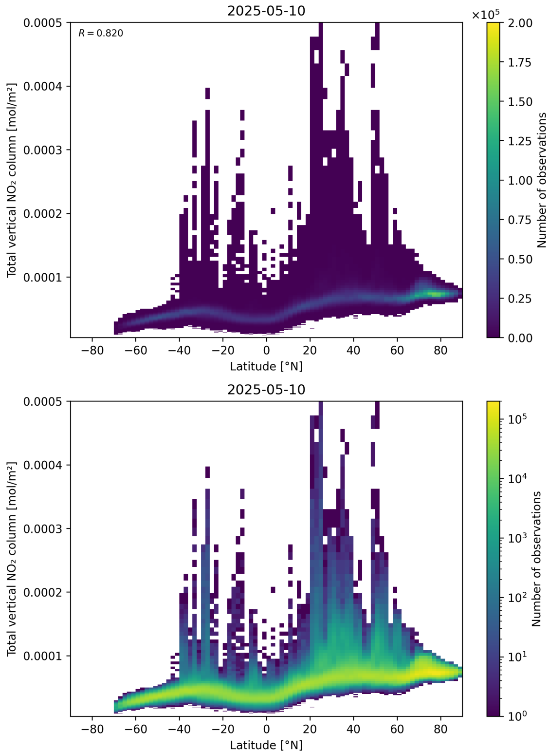
Figure 90: Scatter density plot of “Latitude” against “Total vertical NO 2 column” for 2025-05-10 to 2025-05-11.
