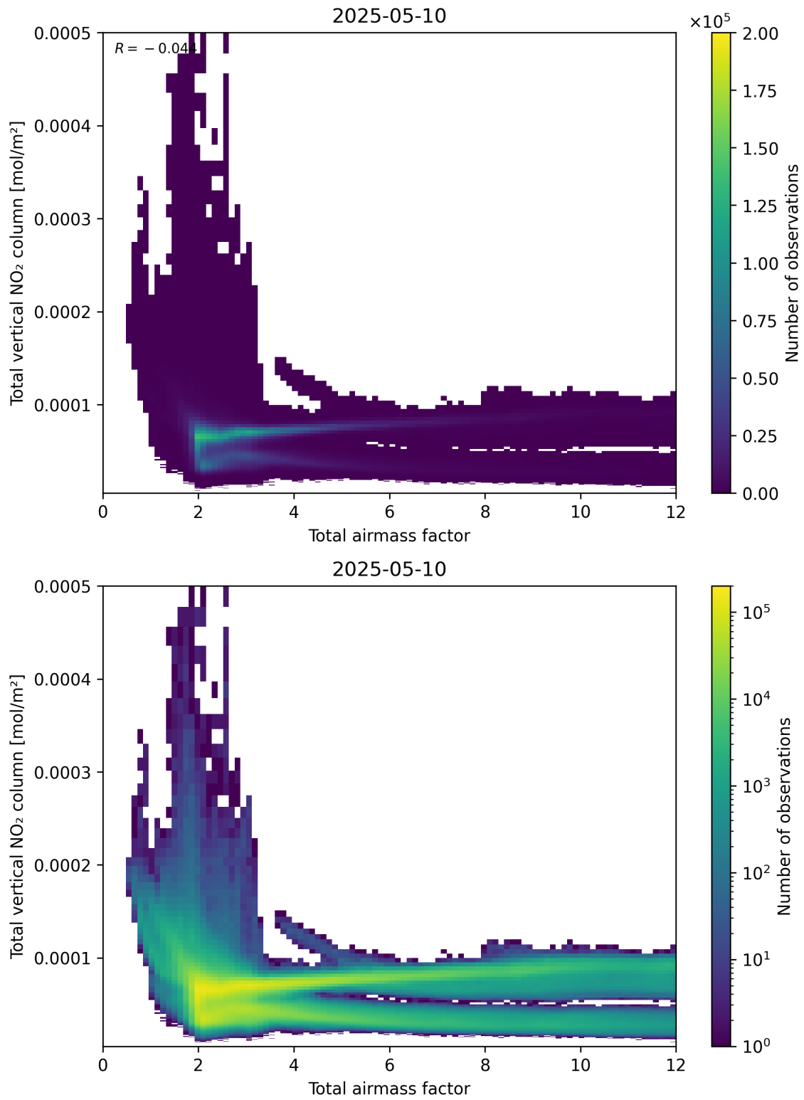
Figure 67: Scatter density plot of “Total air mass factor” against “Total vertical NO 2 column” for 2025-05-10 to 2025-05-11.
