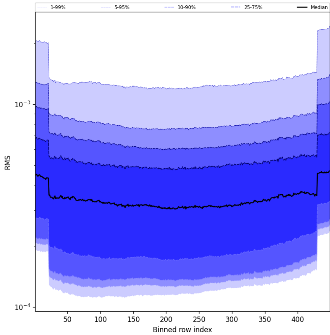
Figure 60: Along track statistics of “RMS” for 2025-05-10 to 2025-05-11
