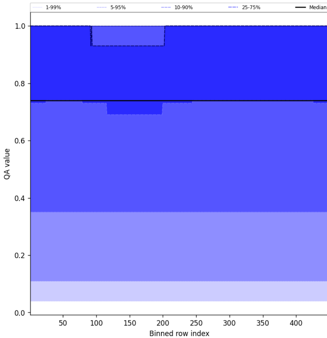
Figure 45: Along track statistics of “QA value” for 2025-05-10 to 2025-05-11
