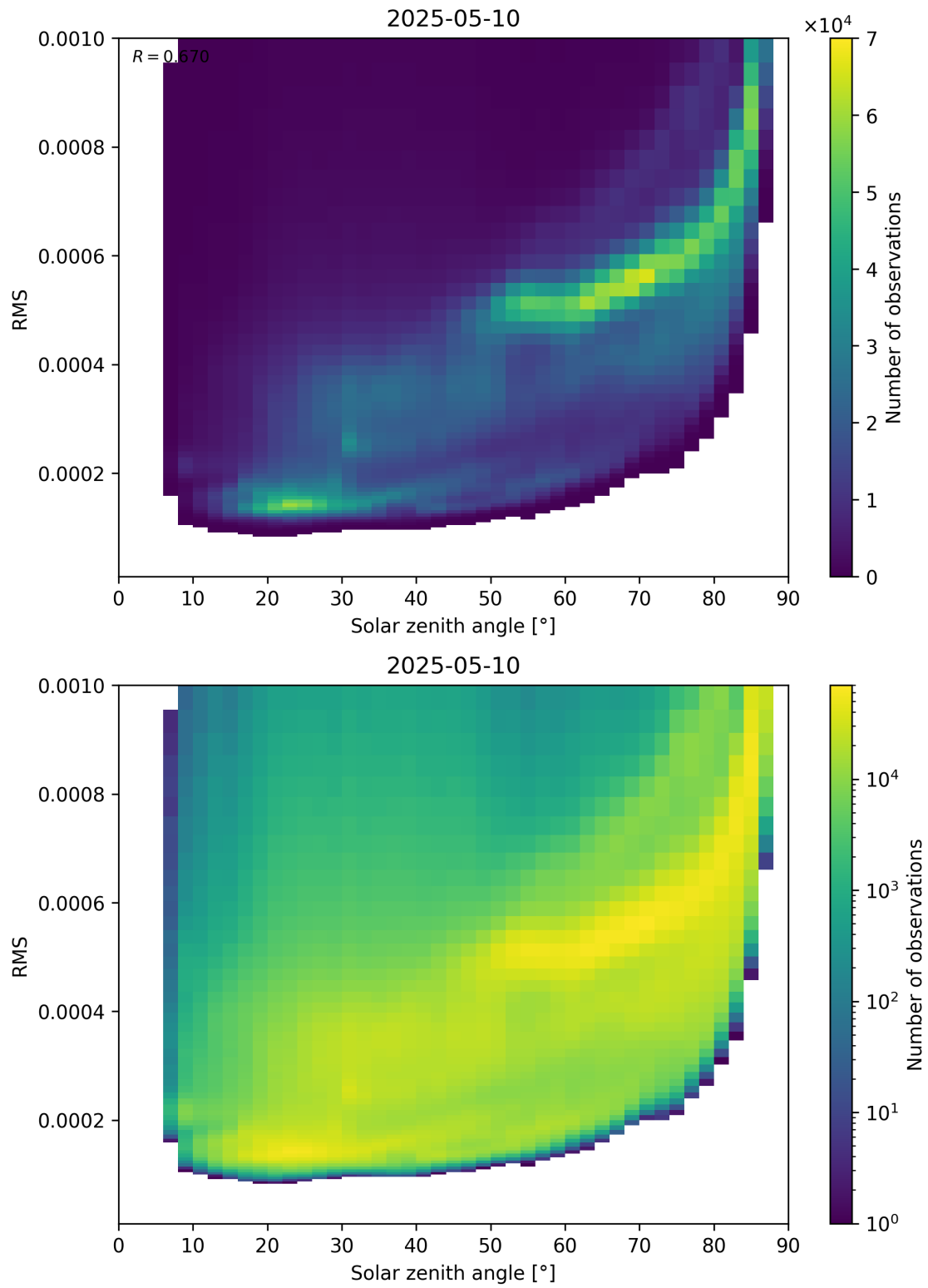
Figure 157: Scatter density plot of “Solar zenith angle” against “RMS” for 2025-05-10 to 2025-05-11.
