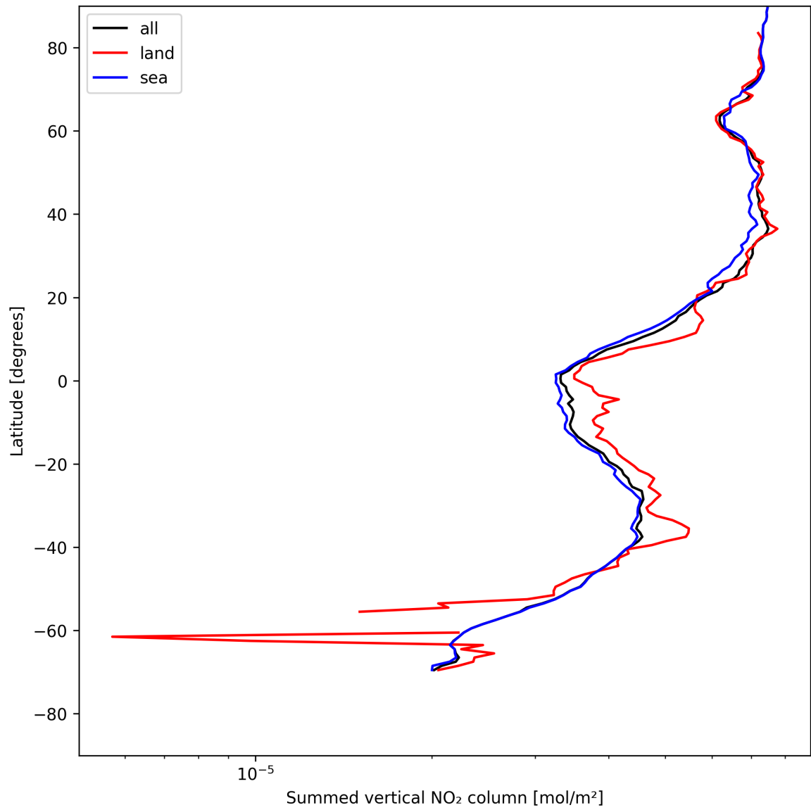
Figure 23: Zonal average of “Summed vertical NO 2 column” for 2025-05-10 to 2025-05-11.
