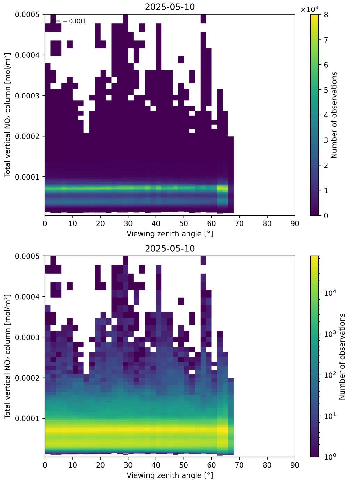
Figure 167: Scatter density plot of “Viewing zenith angle” against “Total vertical NO 2 column” for 2025-05-10 to 2025-05-11.
