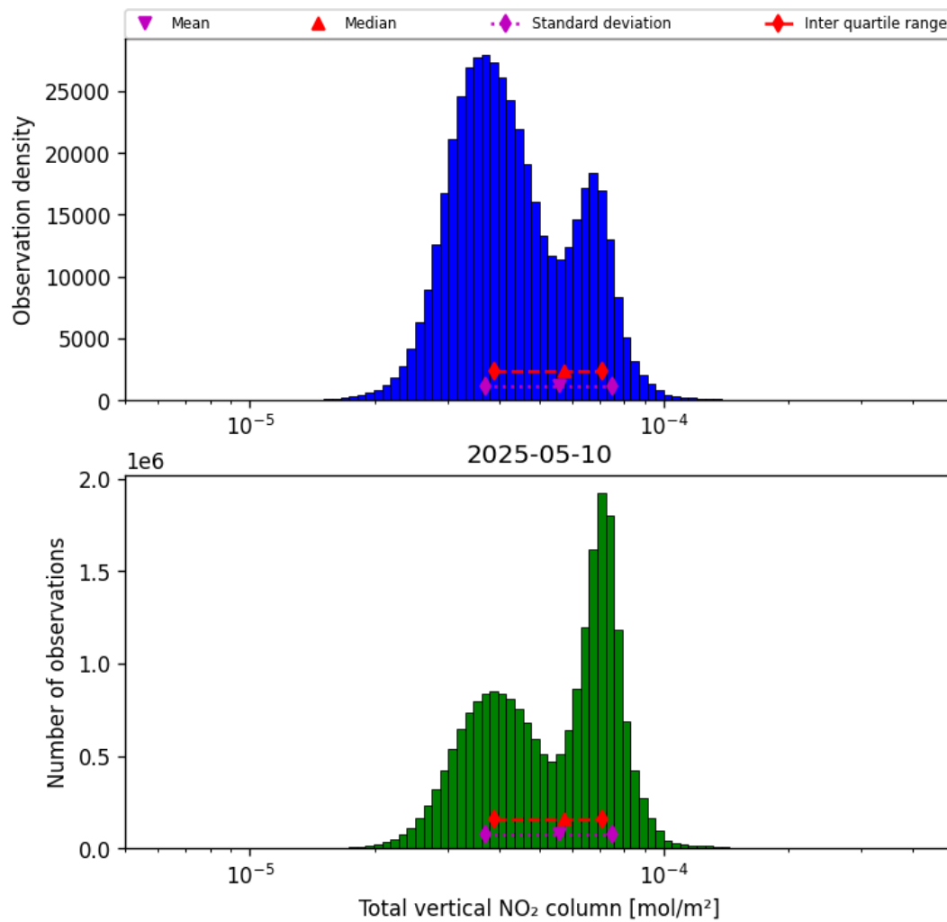
Figure 38: Histogram of “Total vertical NO 2 column” for 2025-05-10 to 2025-05-11
