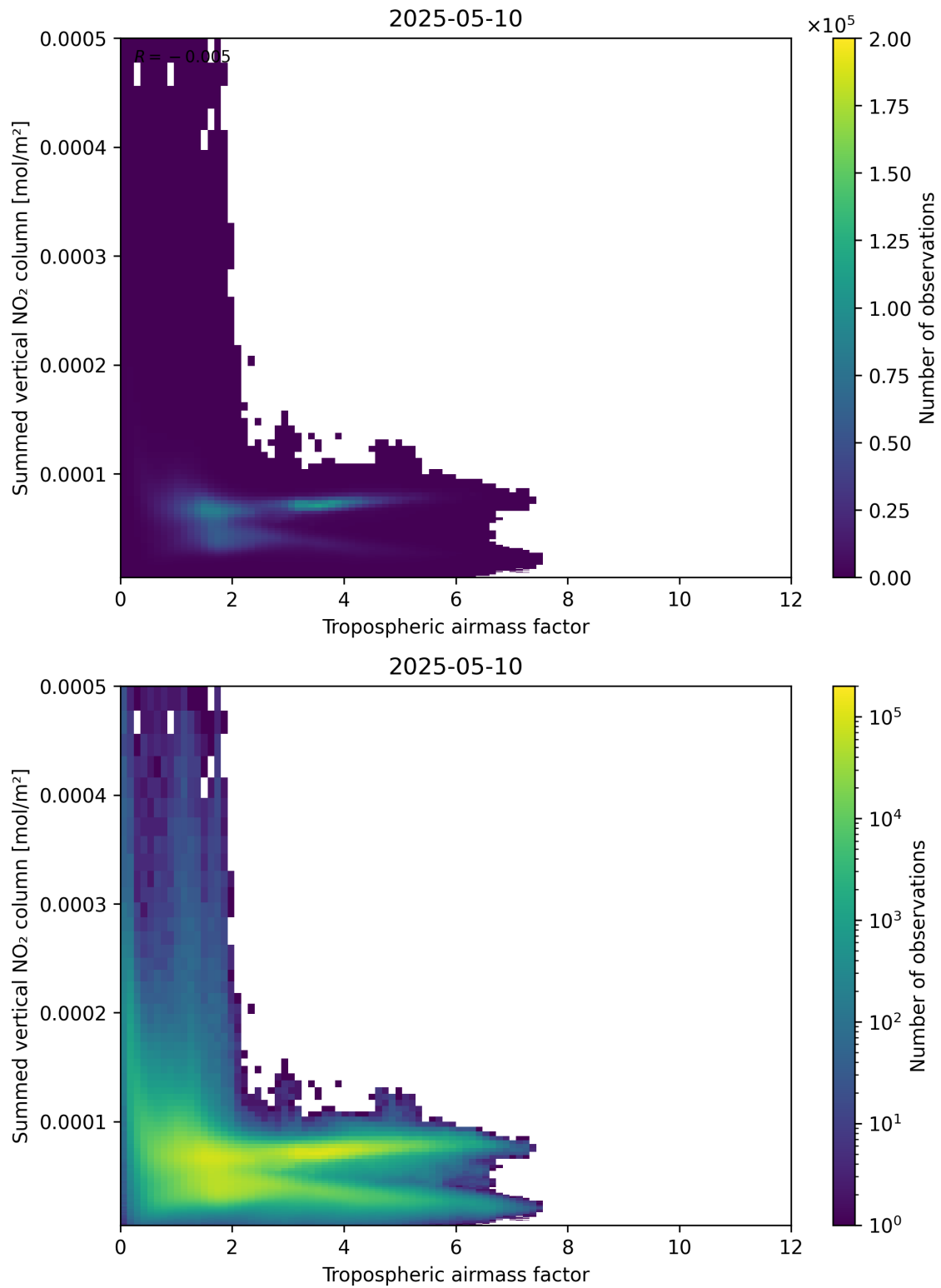
Figure 75: Scatter density plot of “Tropospheric airmass factor” against “Summed vertical NO 2 column” for 2025-05-10 to 2025-05-11.
