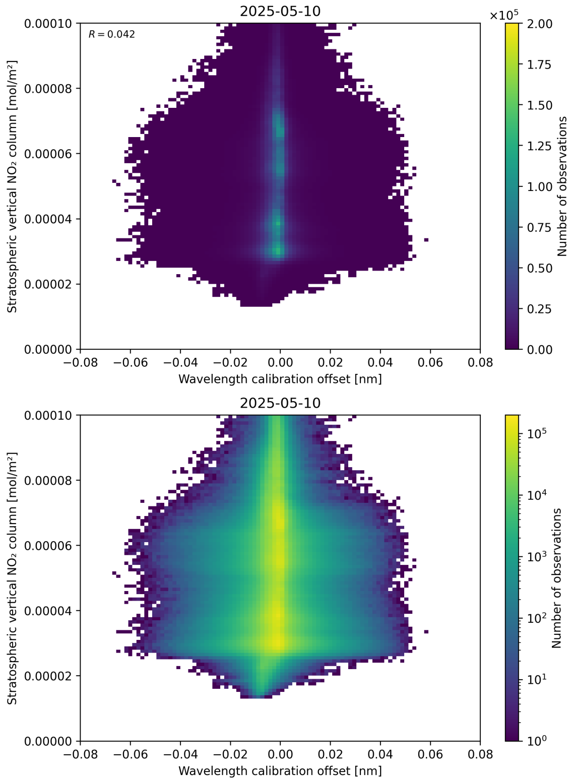
Figure 176: Scatter density plot of “Wavelength calibration offset” against “Stratospheric vertical NO 2 column” for 2025-05-10 to 2025-05-11.
