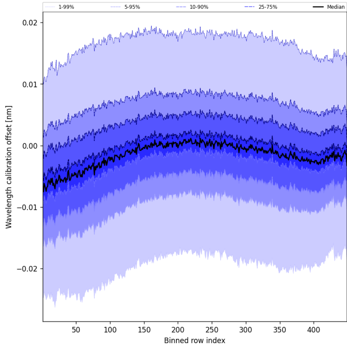
Figure 52: Along track statistics of “Wavelength calibration offset” for 2025-05-10 to 2025-05-11
