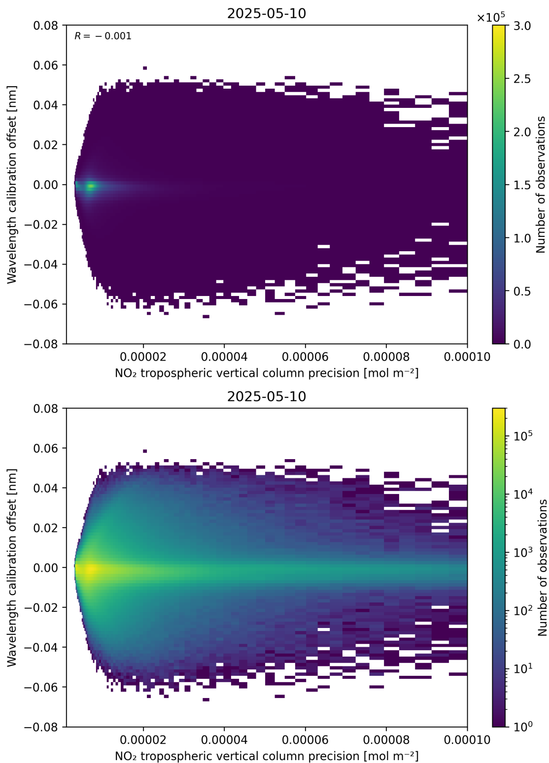
Figure 141: Scatter density plot of “NO 2 tropospheric vertical column precision” against “Wavelength calibration offset” for 2025-05-10 to 2025-05-11.
