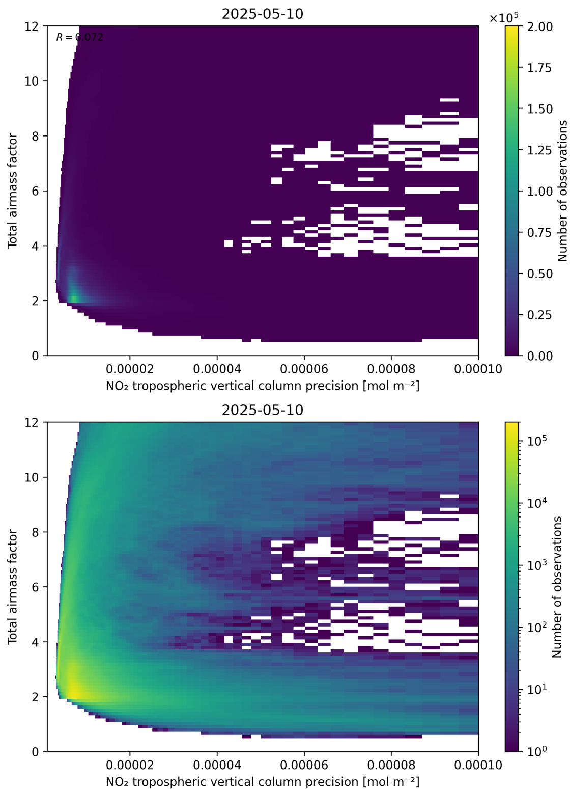
Figure 132: Scatter density plot of “NO 2 tropospheric vertical column precision” against “Total air mass factor” for 2025-05-10 to 2025-05-11.
