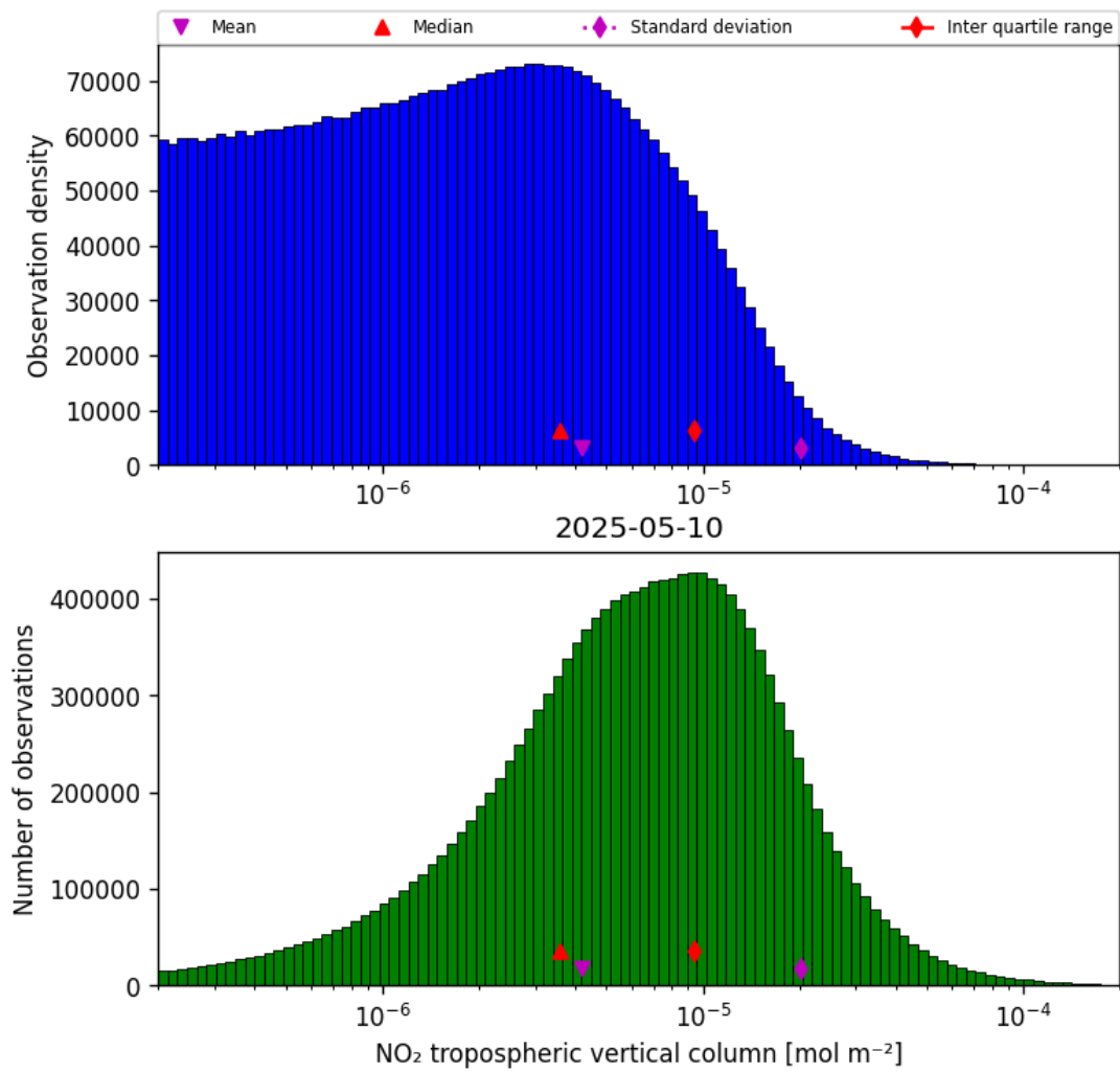
Figure 29: Histogram of “NO 2 tropospheric vertical column” for 2025-05-10 to 2025-05-11
