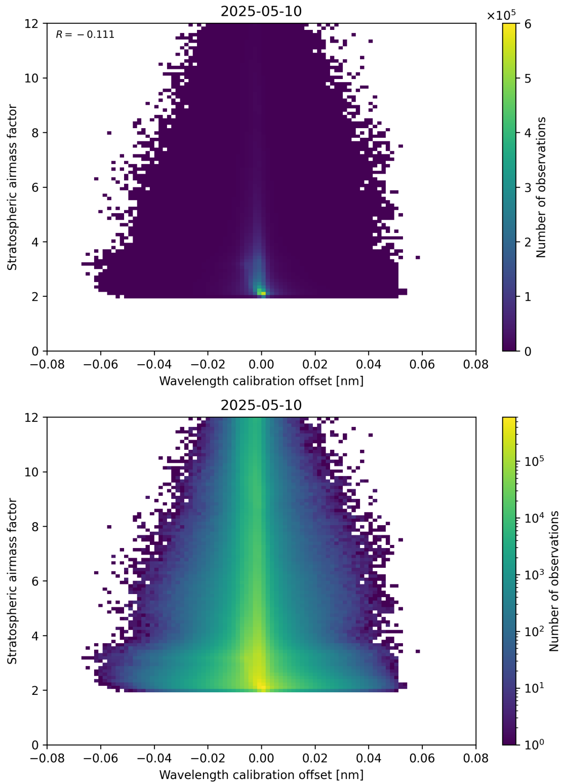
Figure 174: Scatter density plot of “Wavelength calibration offset” against “Stratospheric airmass factor” for 2025-05-10 to 2025-05-11.
