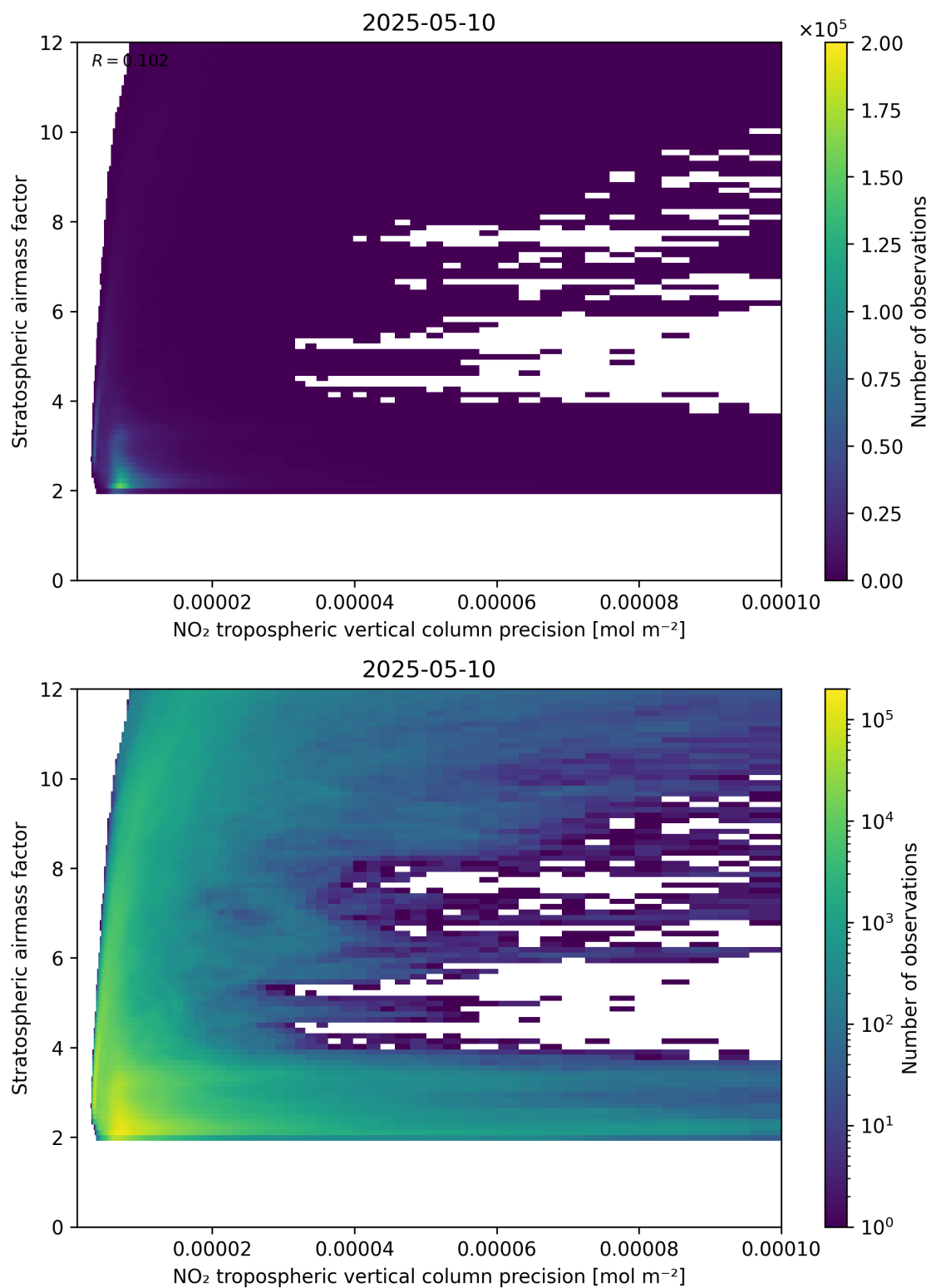
Figure 131: Scatter density plot of “NO 2 tropospheric vertical column precision” against “Stratospheric airmass factor” for 2025-05-10 to 2025-05-11.
