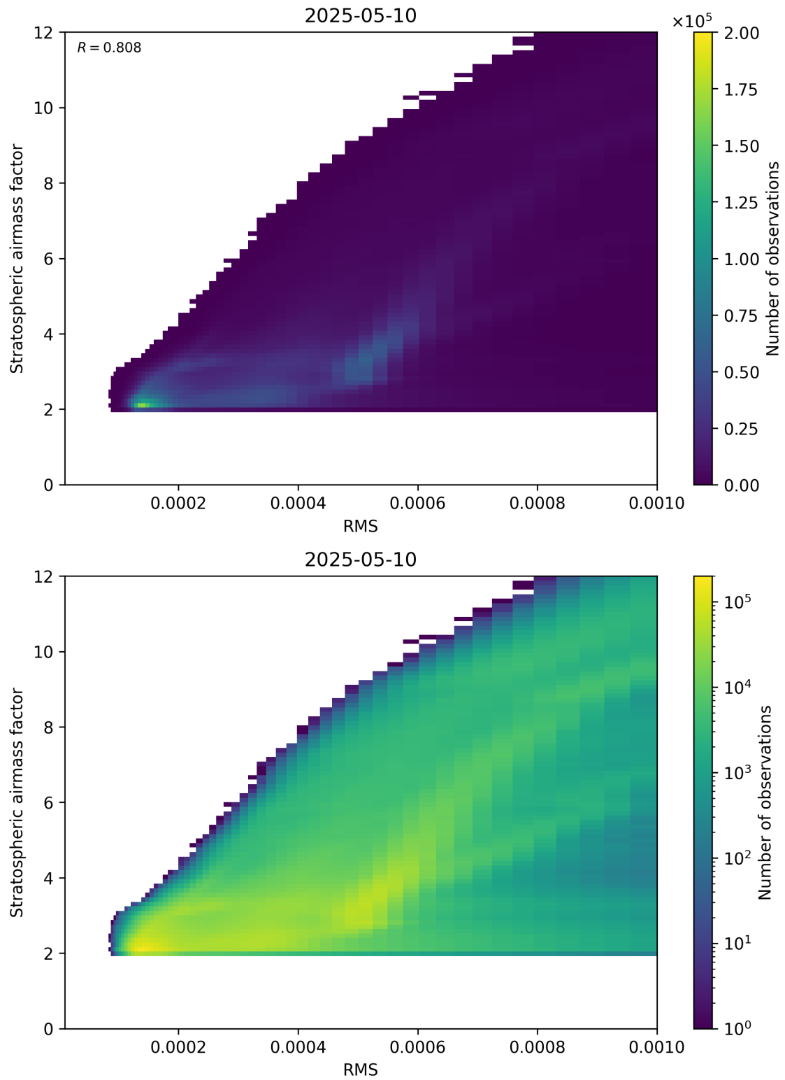
Figure 144: Scatter density plot of “RMS” against “Stratospheric airmass factor” for 2025-05-10 to 2025-05-11.
