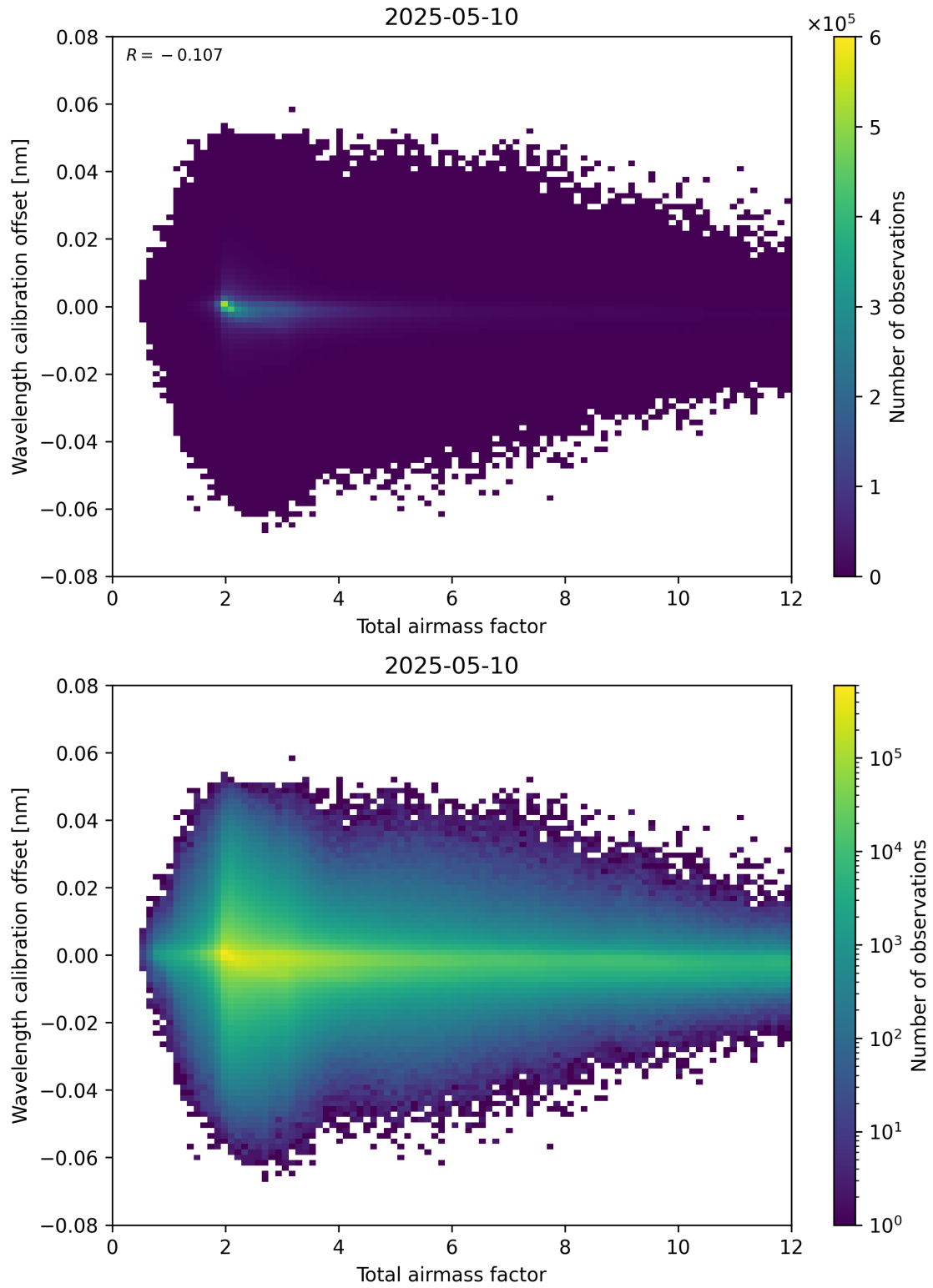
Figure 70: Scatter density plot of “Total airmass factor” against “Wavelength calibration offset” for 2025-05-10 to 2025-05-11.
