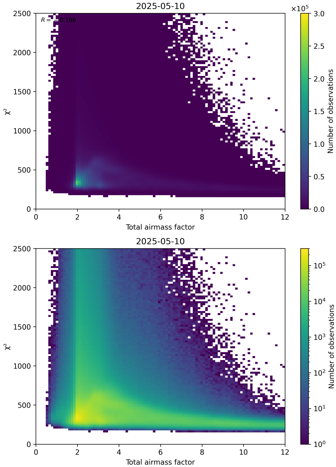
Figure 63: Scatter density plot of “Total airmass factor” against “ \chi^2 ” for 2025-05-10 to 2025-05-11.
