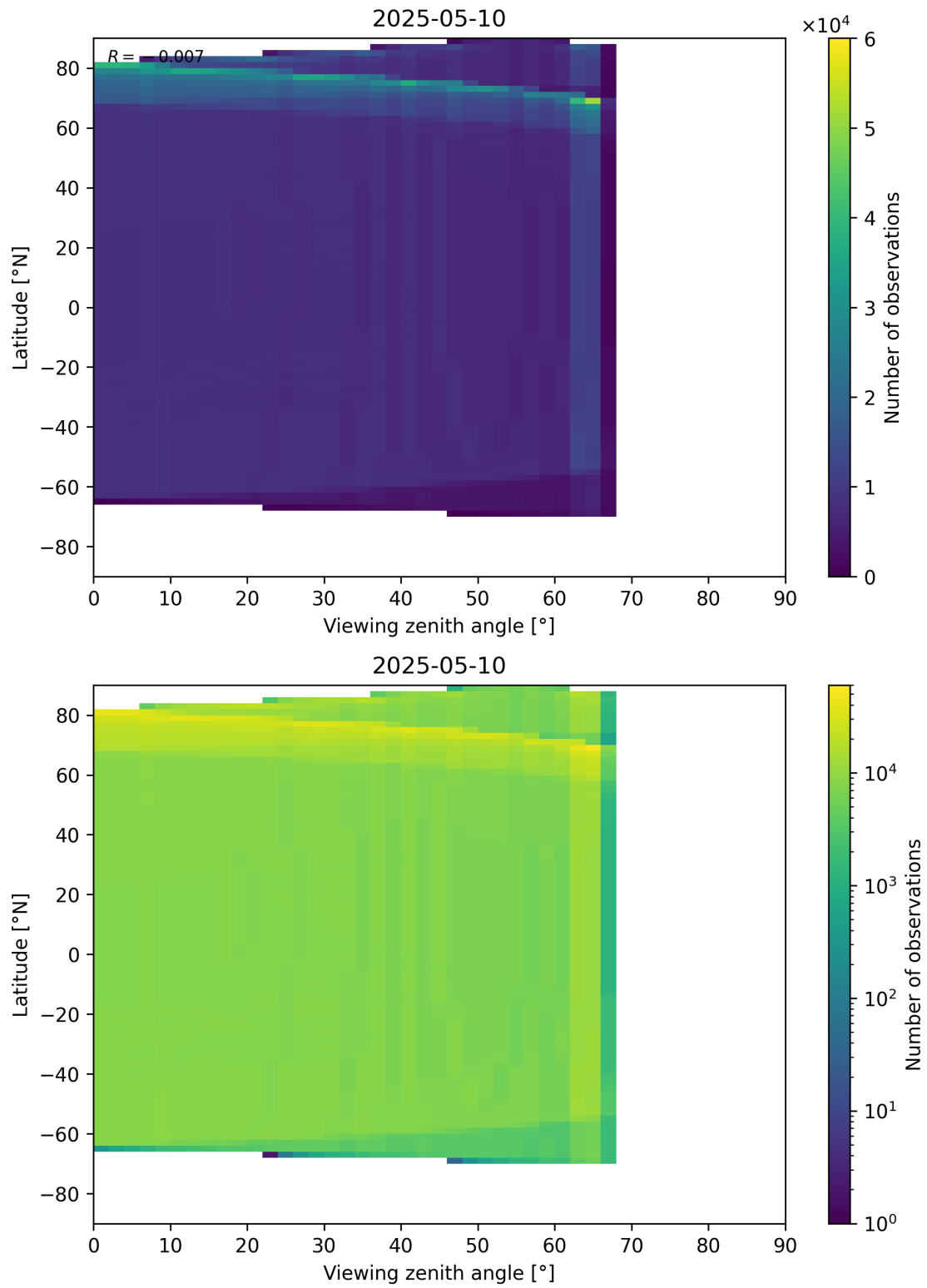
Figure 163: Scatter density plot of “Viewing zenith angle” against “Latitude” for 2025-05-10 to 2025-05-11.
