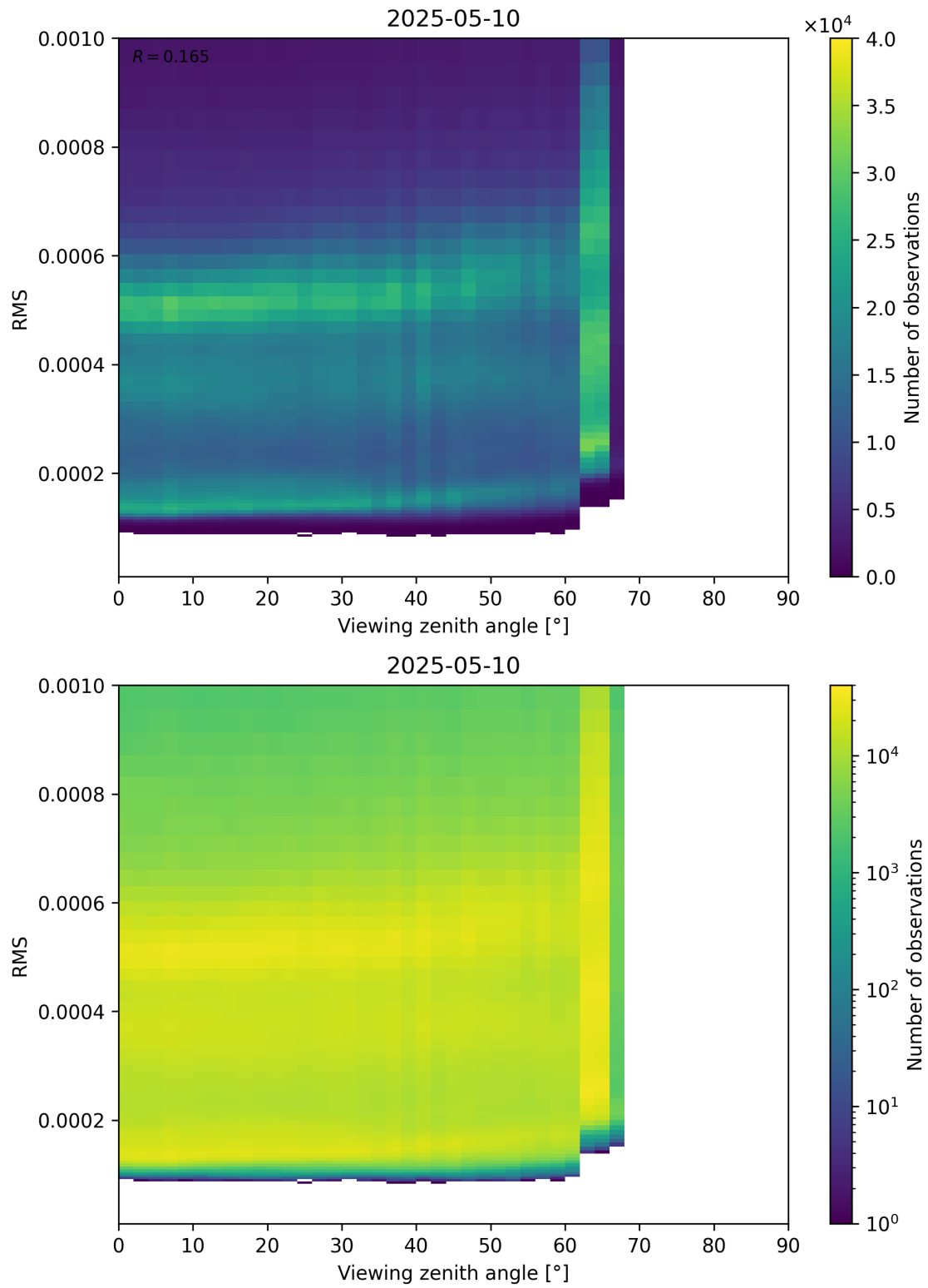
Figure 171: Scatter density plot of “Viewing zenith angle” against “RMS” for 2025-05-10 to 2025-05-11.
