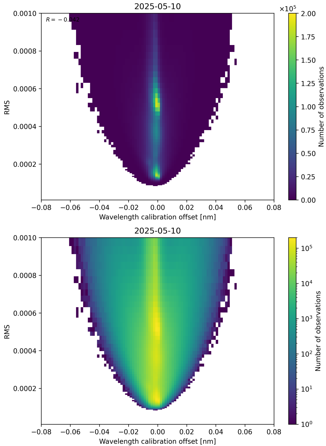
Figure 181: Scatter density plot of “Wavelength calibration offset” against “RMS” for 2025-05-10 to 2025-05-11.
