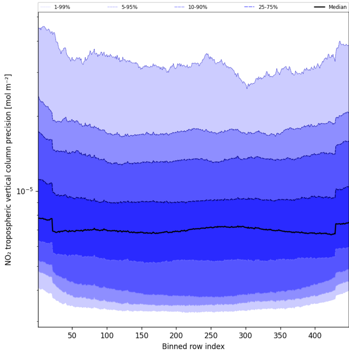
Figure 47: Along track statistics of “NO 2 tropospheric vertical column precision” for 2025-05-10 to 2025-05-11
