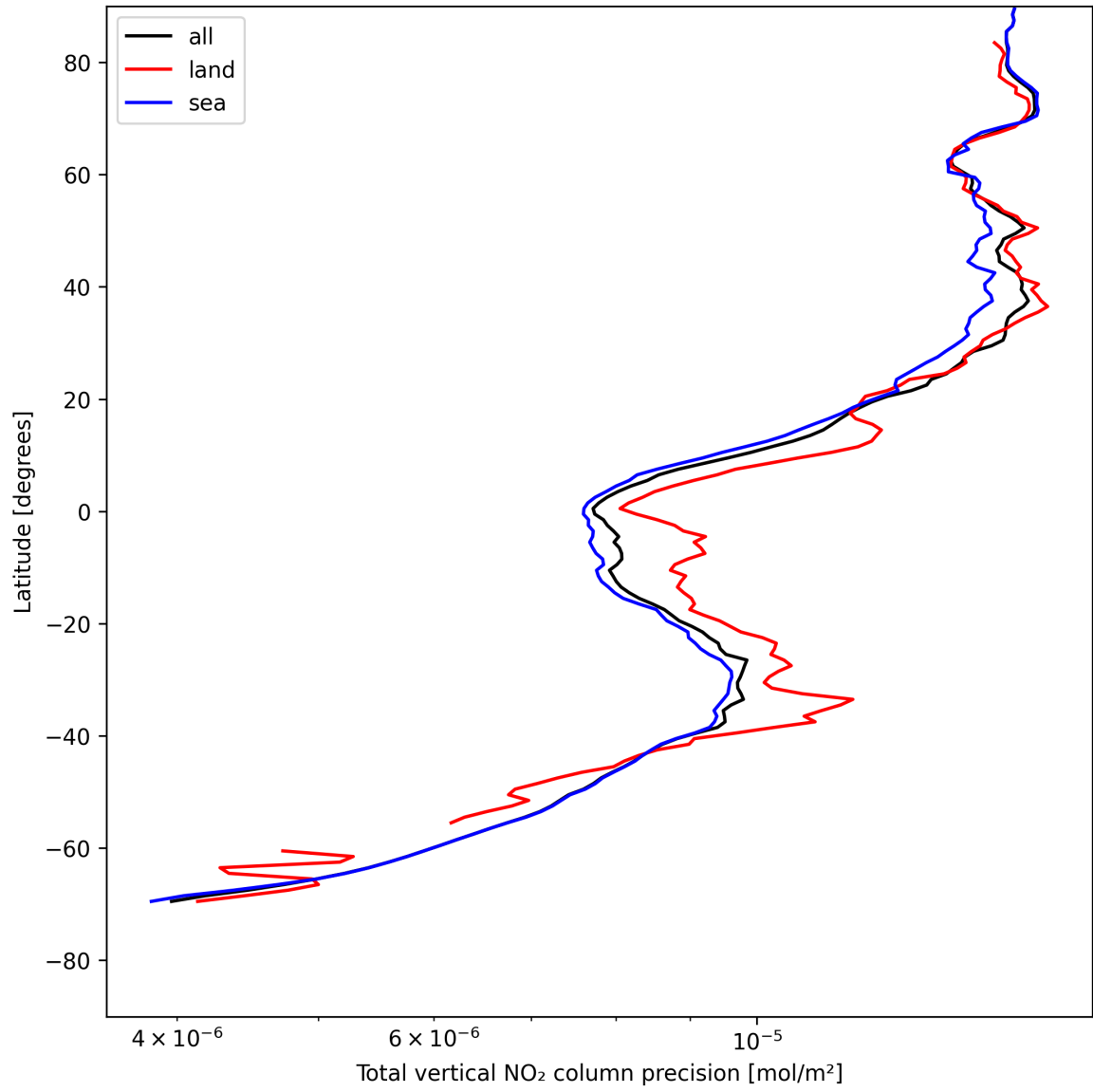
Figure 22: Zonal average of “Total vertical NO 2 column precision” for 2025-05-10 to 2025-05-11.
