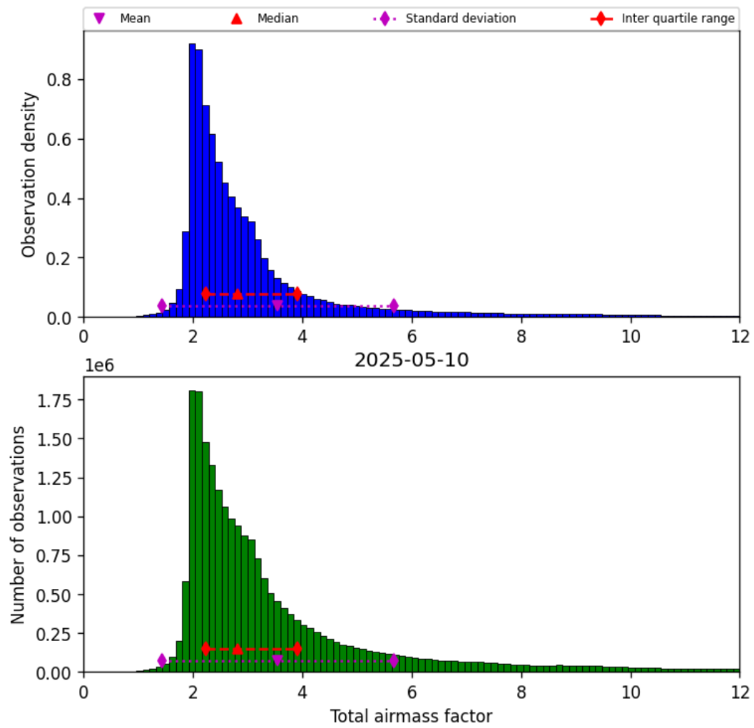
Figure 32: Histogram of “Total airmass factor” for 2025-05-10 to 2025-05-11
