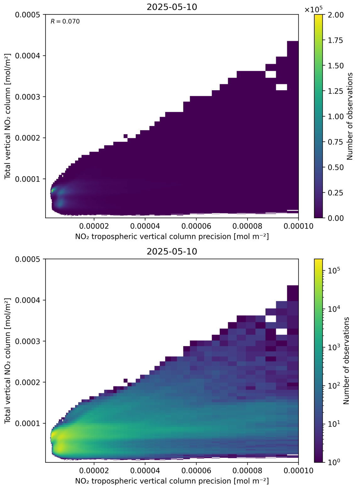
Figure 138: Scatter density plot of “NO 2 tropospheric vertical column precision” against “Total vertical NO 2 column” for 2025-05-10 to 2025-05-11.
