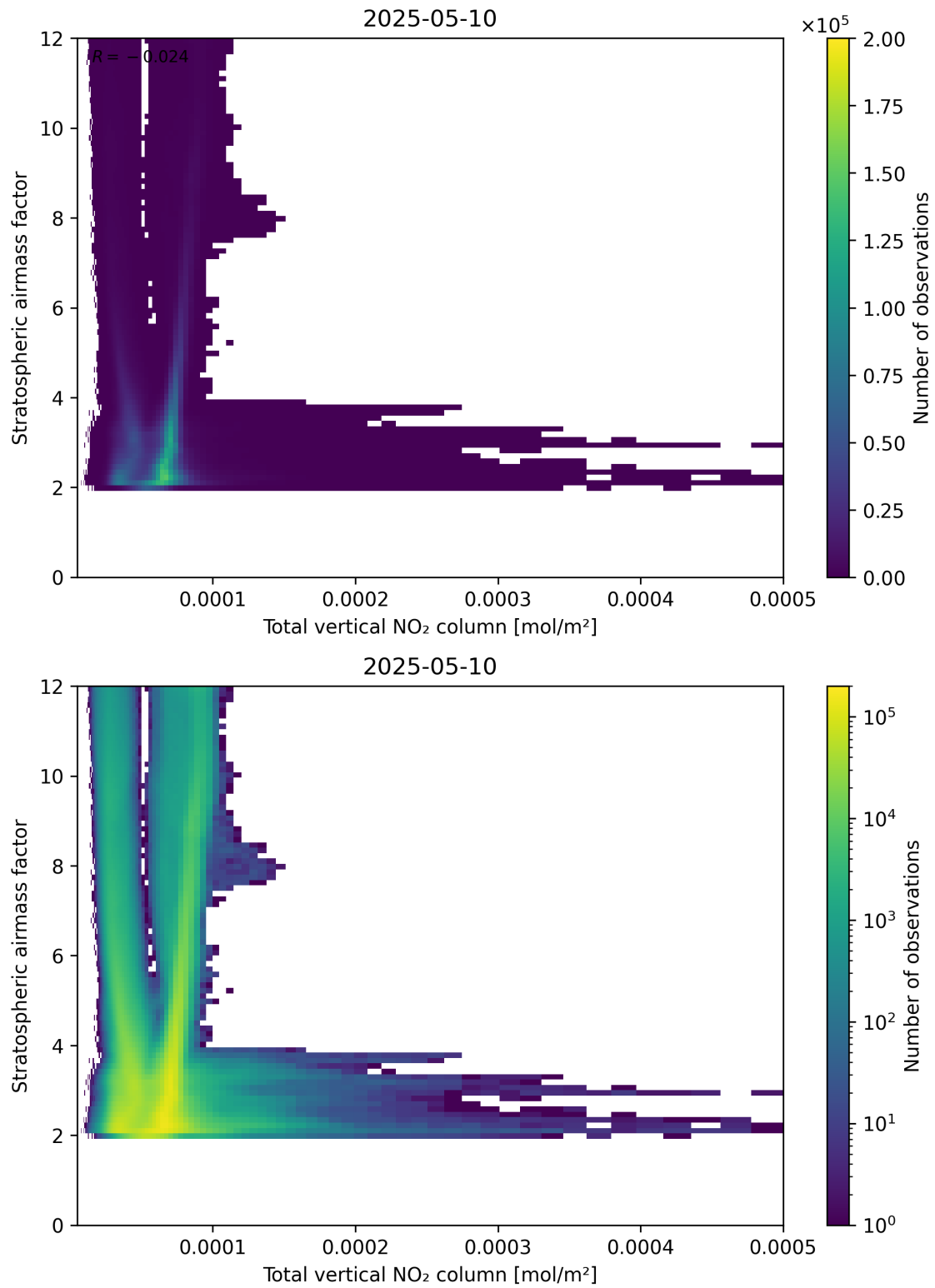
Figure 110: Scatter density plot of “Total vertical NO 2 column” against “Stratospheric airmass factor” for 2025-05-10 to 2025-05-11.
