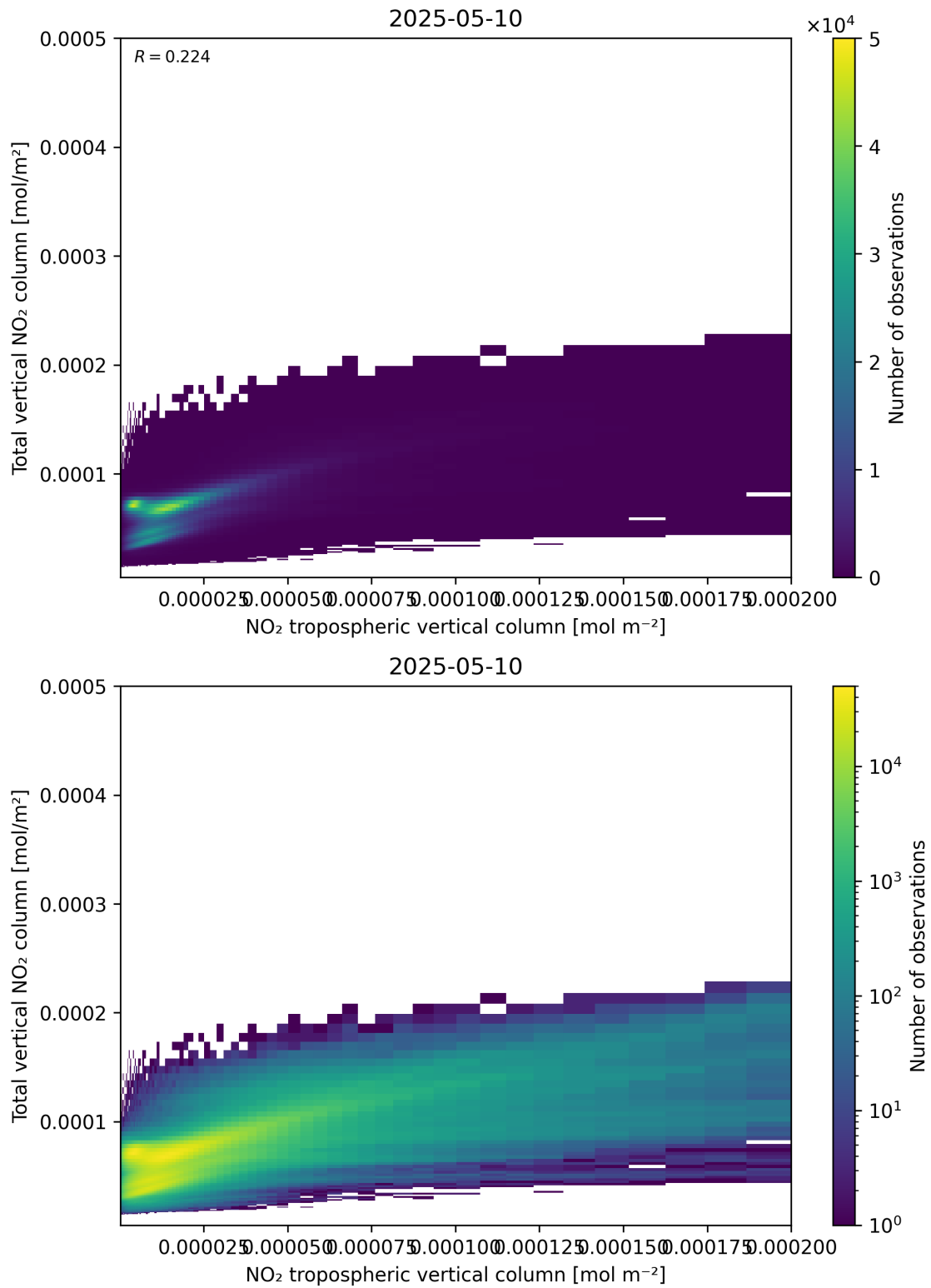
Figure 128: Scatter density plot of “NO 2 tropospheric vertical column” against “Total vertical NO 2 column” for 2025-05-10 to 2025-05-11.
