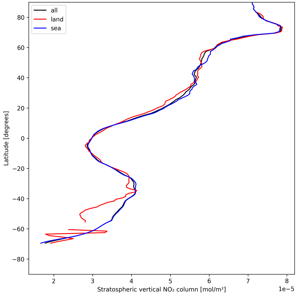
Figure 19: Zonal average of “Stratospheric vertical NO 2 column” for 2025-05-10 to 2025-05-11.
