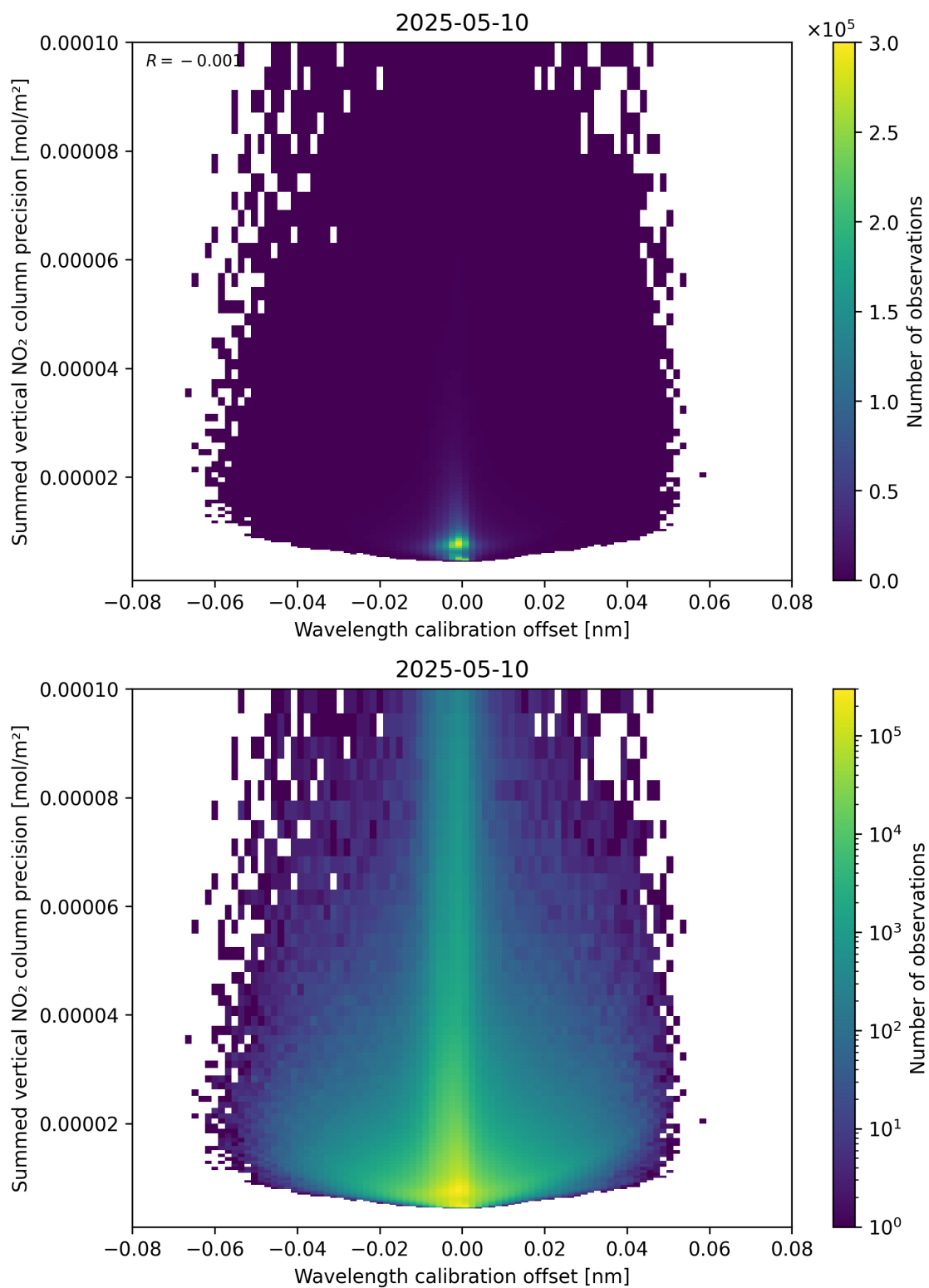
Figure 178: Scatter density plot of “Wavelength calibration offset” against “Summed vertical NO 2 column precision” for 2025-05-10 to 2025-05-11.
