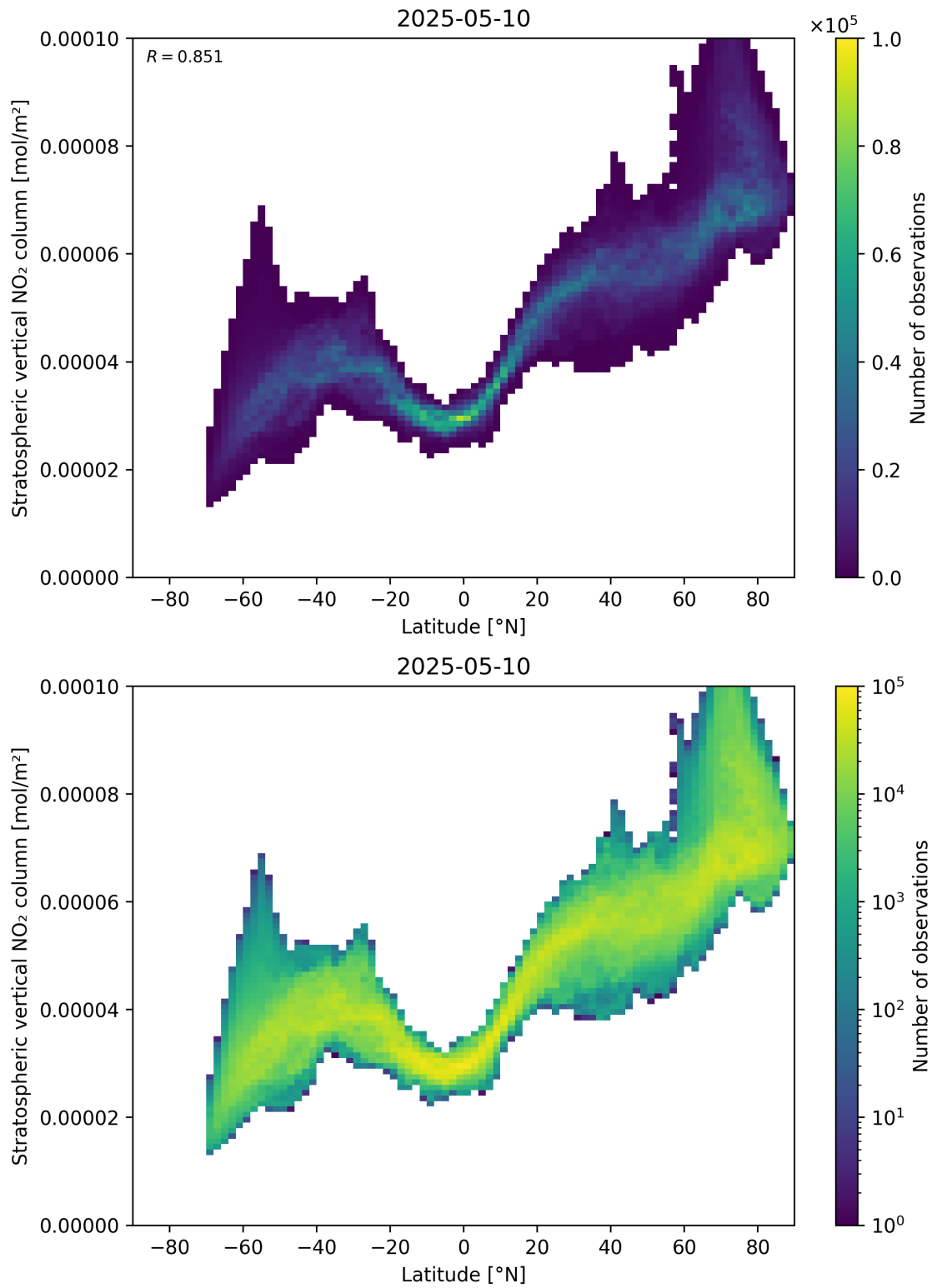
Figure 87: Scatter density plot of “Latitude” against “Stratospheric vertical \text{NO}_2 column” for 2025-05-10 to 2025-05-11.
