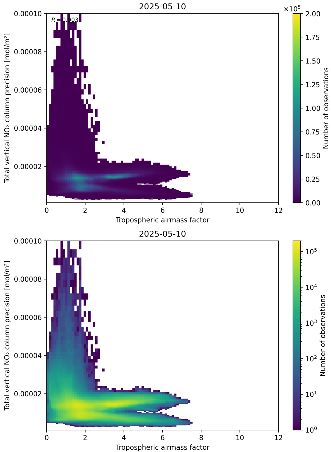
Figure 78: Scatter density plot of “Tropospheric airmass factor” against “Total vertical NO 2 column precision” for 2025-05-10 to 2025-05-11.
