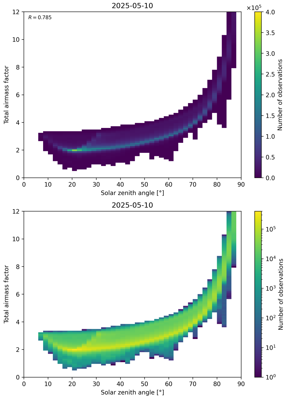
Figure 146: Scatter density plot of “Solar zenith angle” against “Total air mass factor” for 2025-05-10 to 2025-05-11.
