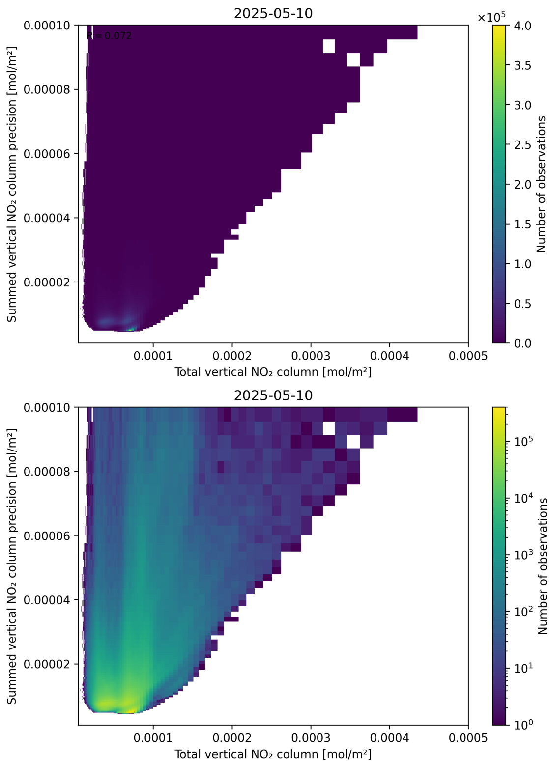
Figure 113: Scatter density plot of “Total vertical NO 2 column” against “Summed vertical NO 2 column precision” for 2025-05-10 to 2025-05-11.
