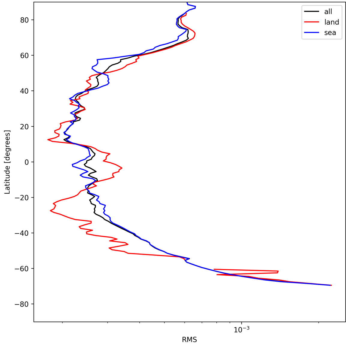
Figure 26: Zonal average of “RMS” for 2025-05-10 to 2025-05-11.
