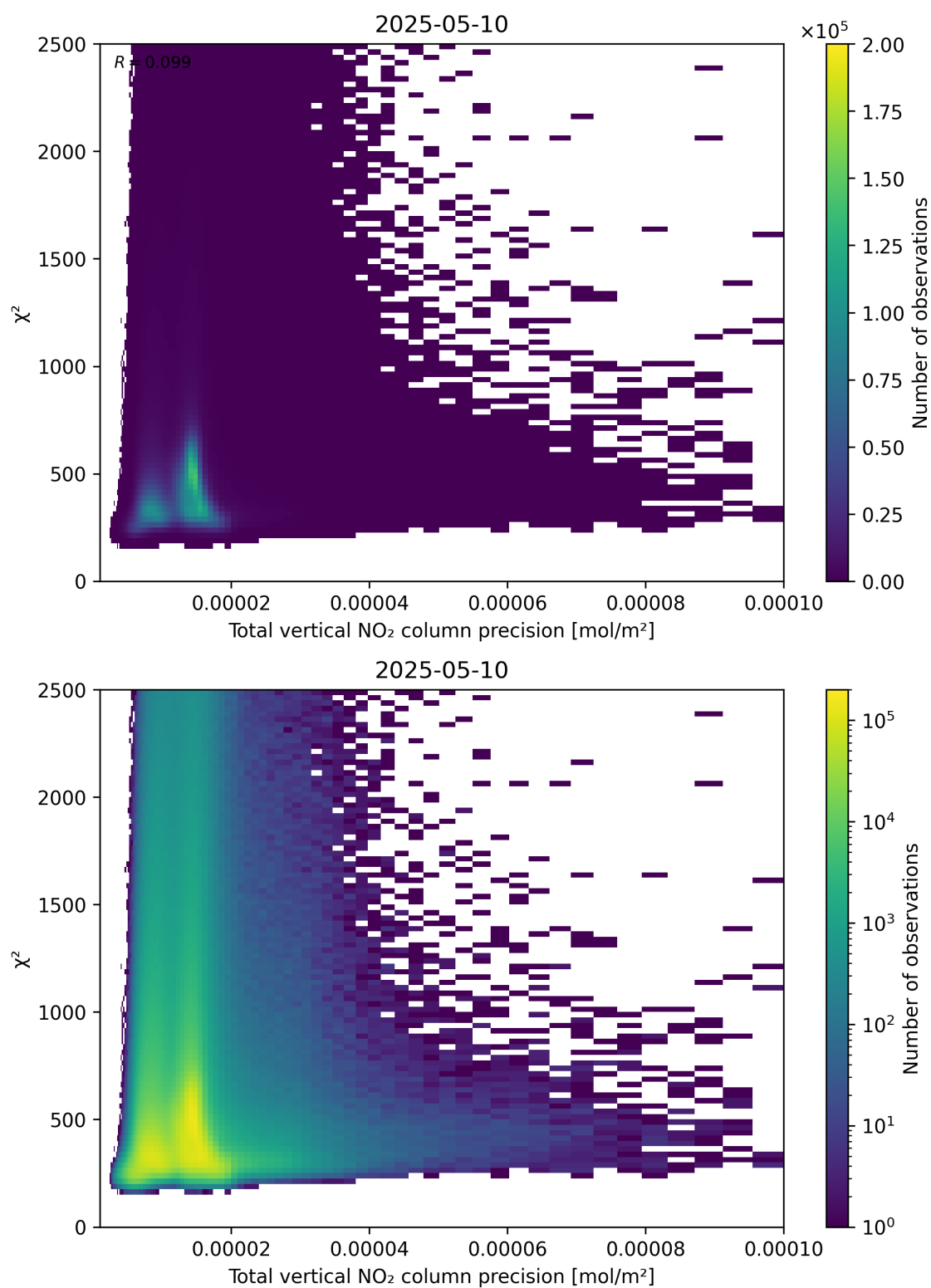
Figure 116: Scatter density plot of “Total vertical NO 2 column precision” against “ \chi^2 ” for 2025-05-10 to 2025-05-11.
