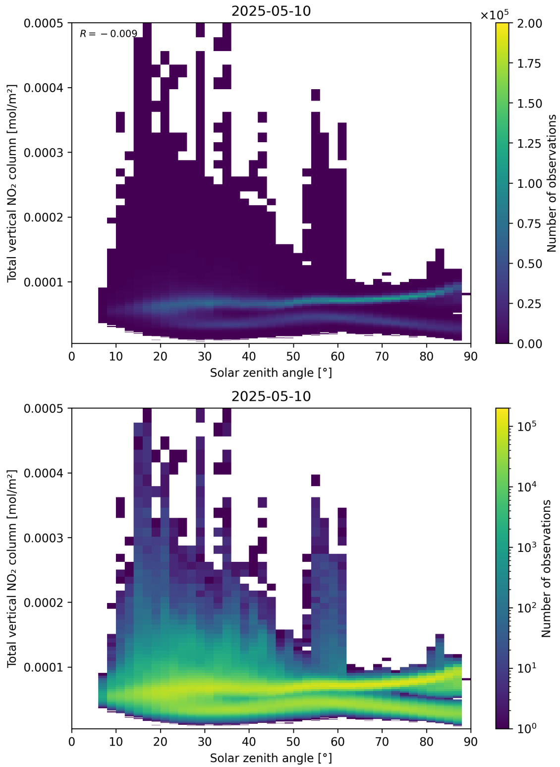
Figure 153: Scatter density plot of “Solar zenith angle” against “Total vertical NO 2 column” for 2025-05-10 to 2025-05-11.
