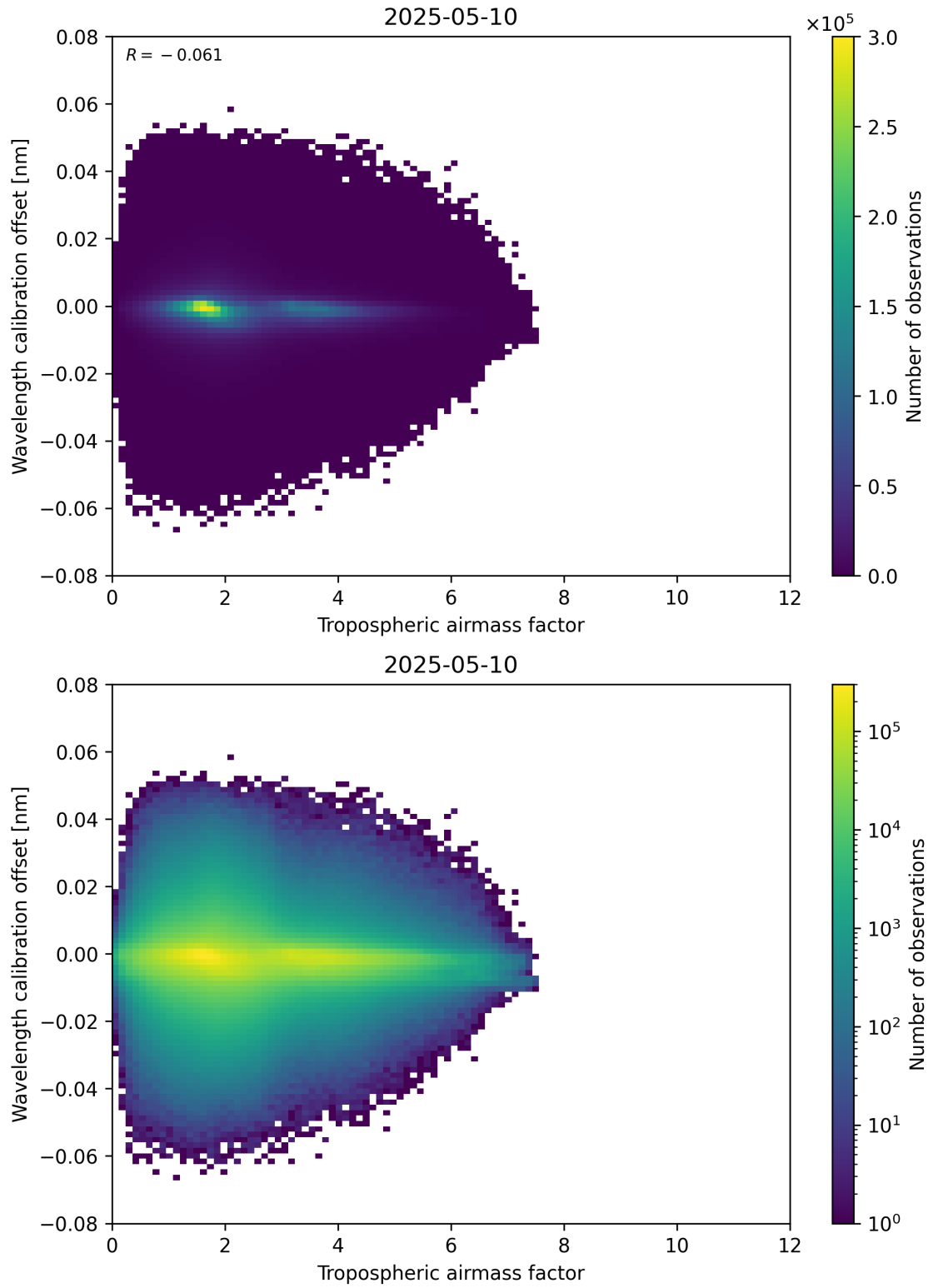
Figure 80: Scatter density plot of “Tropospheric airmass factor” against “Wavelength calibration offset” for 2025-05-10 to 2025-05-11.
