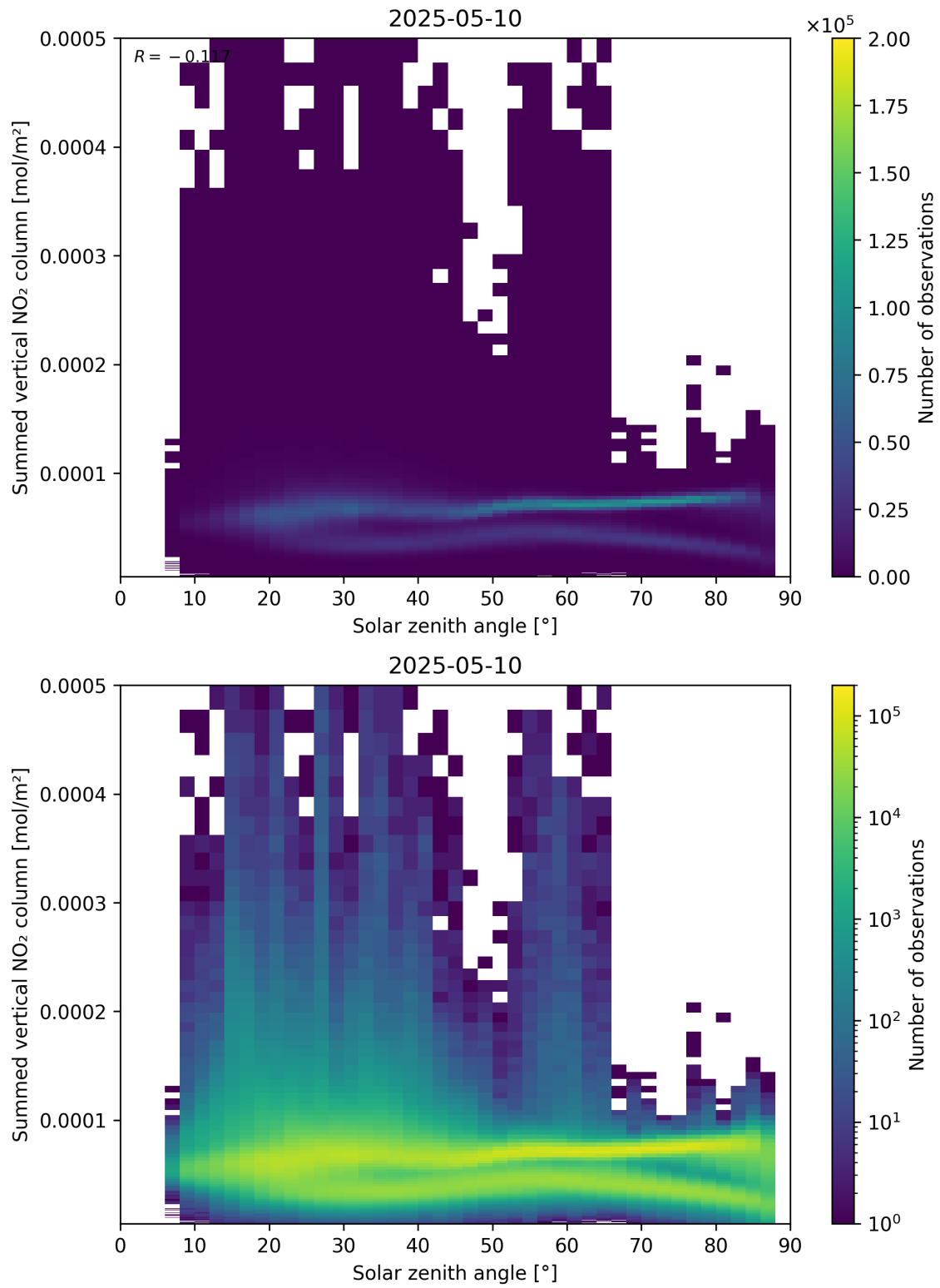
Figure 151: Scatter density plot of “Solar zenith angle” against “Summed vertical NO 2 column” for 2025-05-10 to 2025-05-11.
