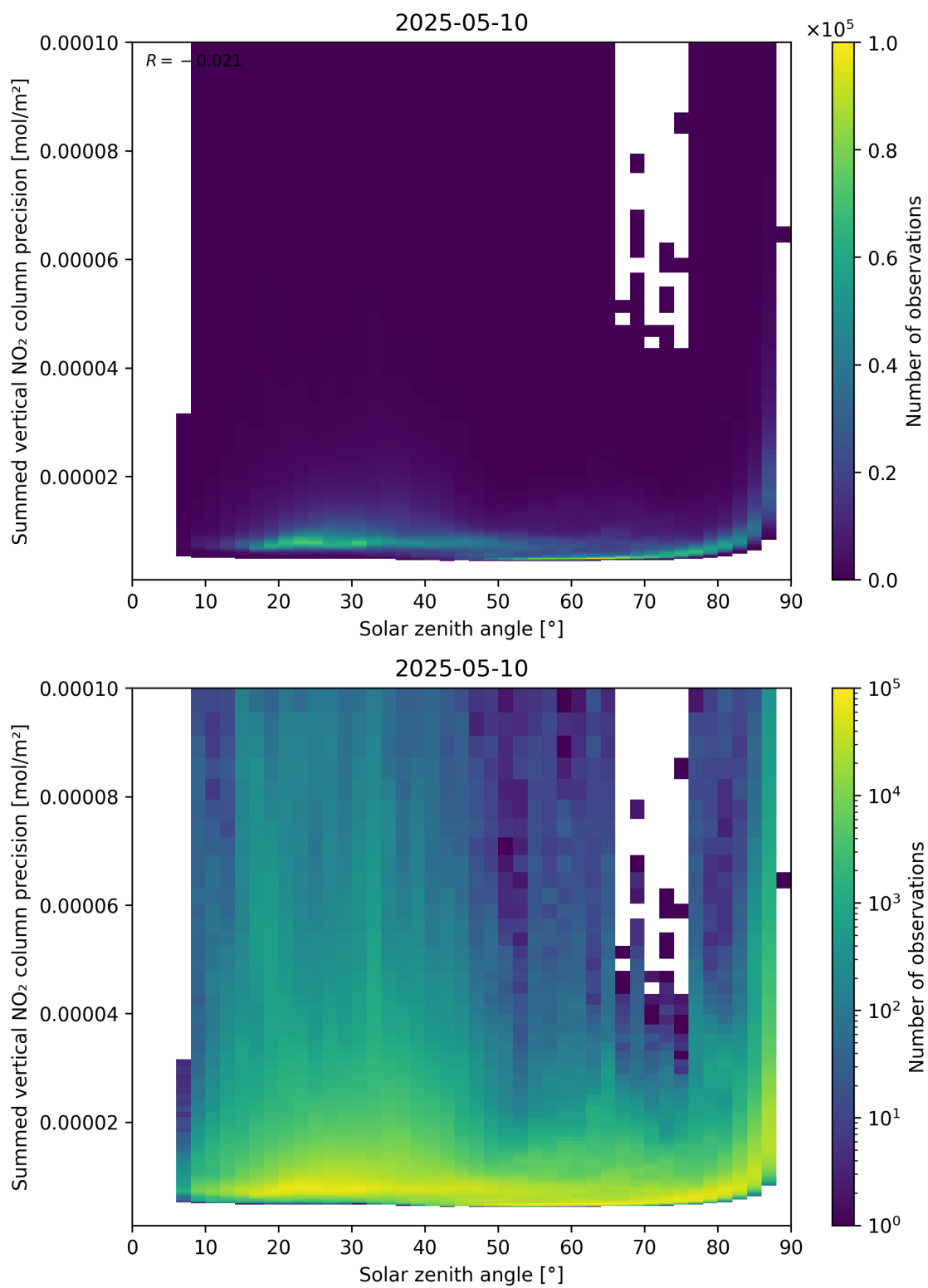
Figure 152: Scatter density plot of “Solar zenith angle” against “Summed vertical NO 2 column precision” for 2025-05-10 to 2025-05-11.
