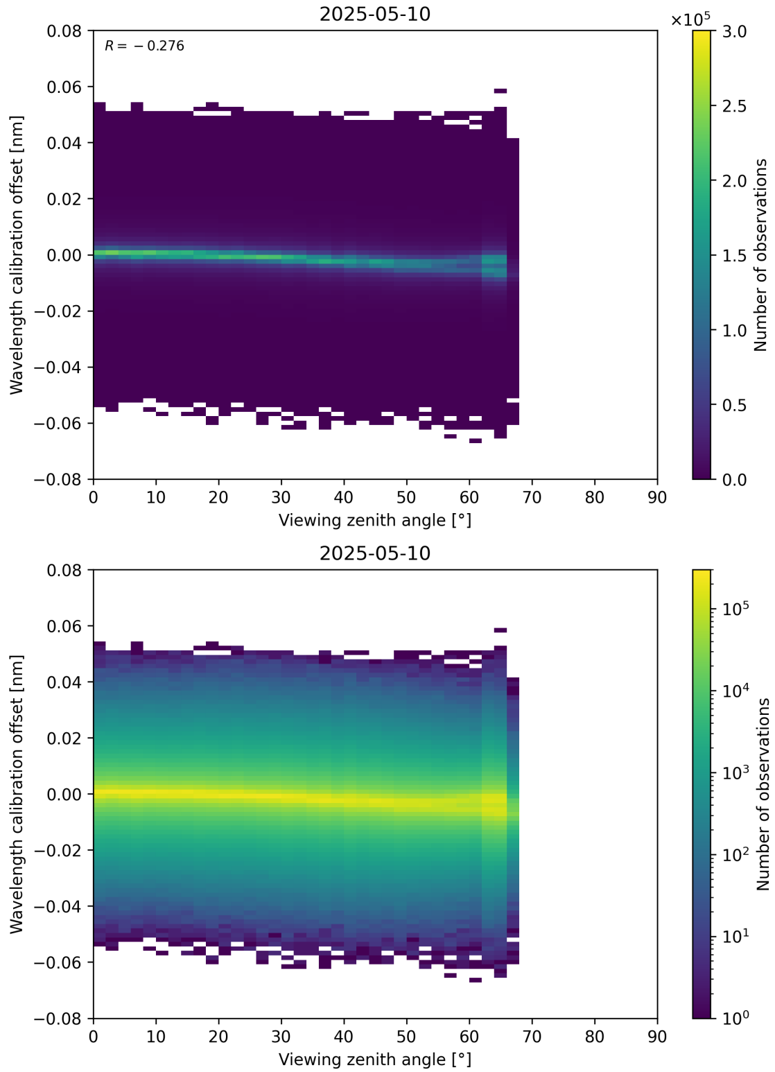
Figure 173: Scatter density plot of “Viewing zenith angle” against “Wavelength calibration offset” for 2025-05-10 to 2025-05-11.
