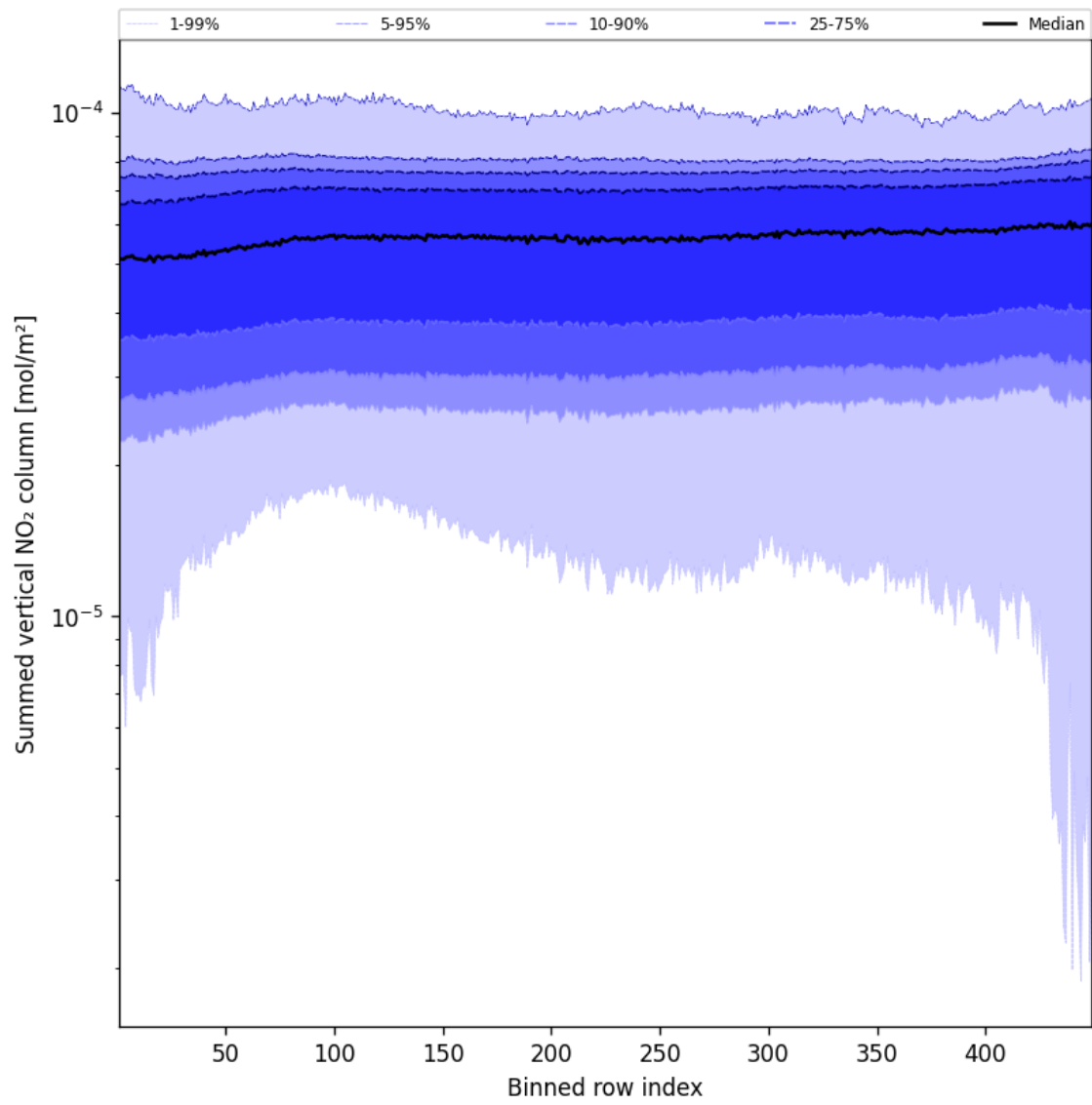
Figure 57: Along track statistics of “Summed vertical NO 2 column” for 2025-05-10 to 2025-05-11
