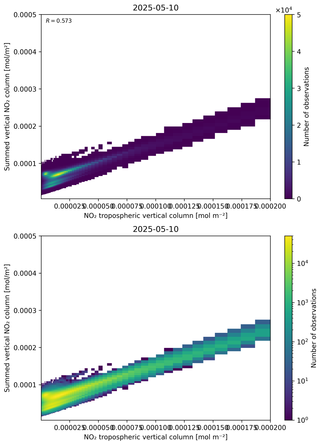
Figure 126: Scatter density plot of “NO 2 tropospheric vertical column” against “Summed vertical NO 2 column” for 2025-05-10 to 2025-05-11.
