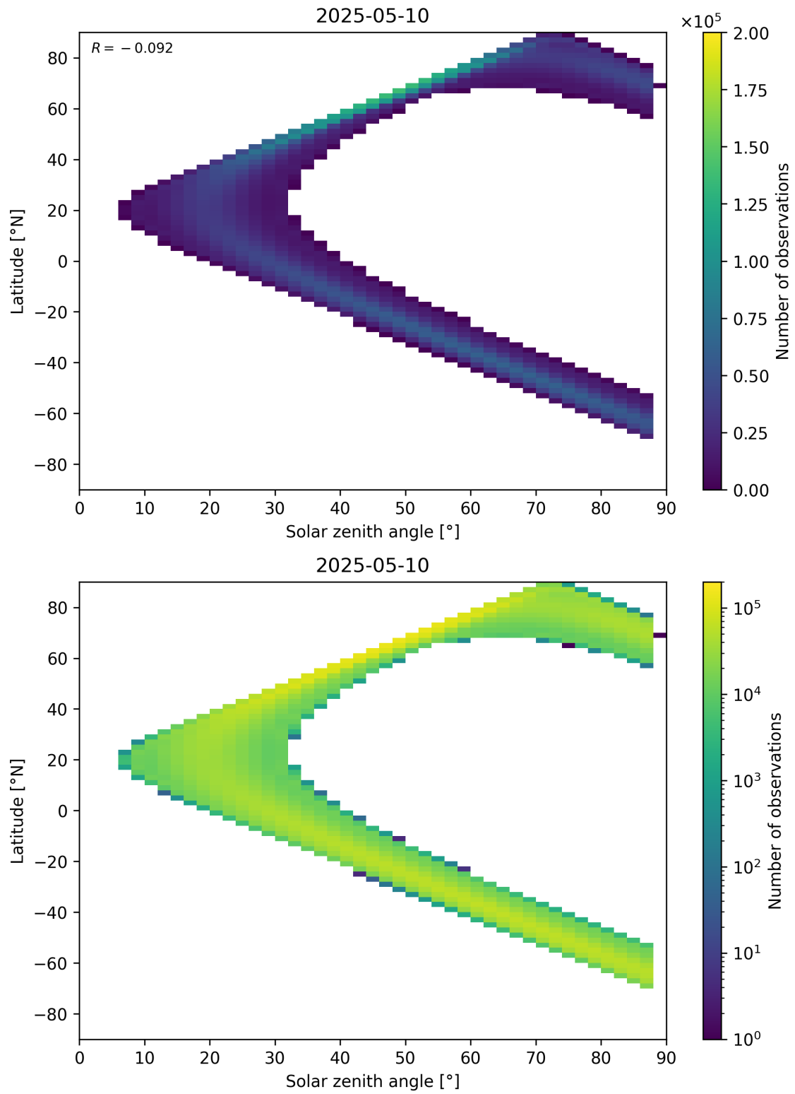
Figure 149: Scatter density plot of “Solar zenith angle” against “Latitude” for 2025-05-10 to 2025-05-11.
