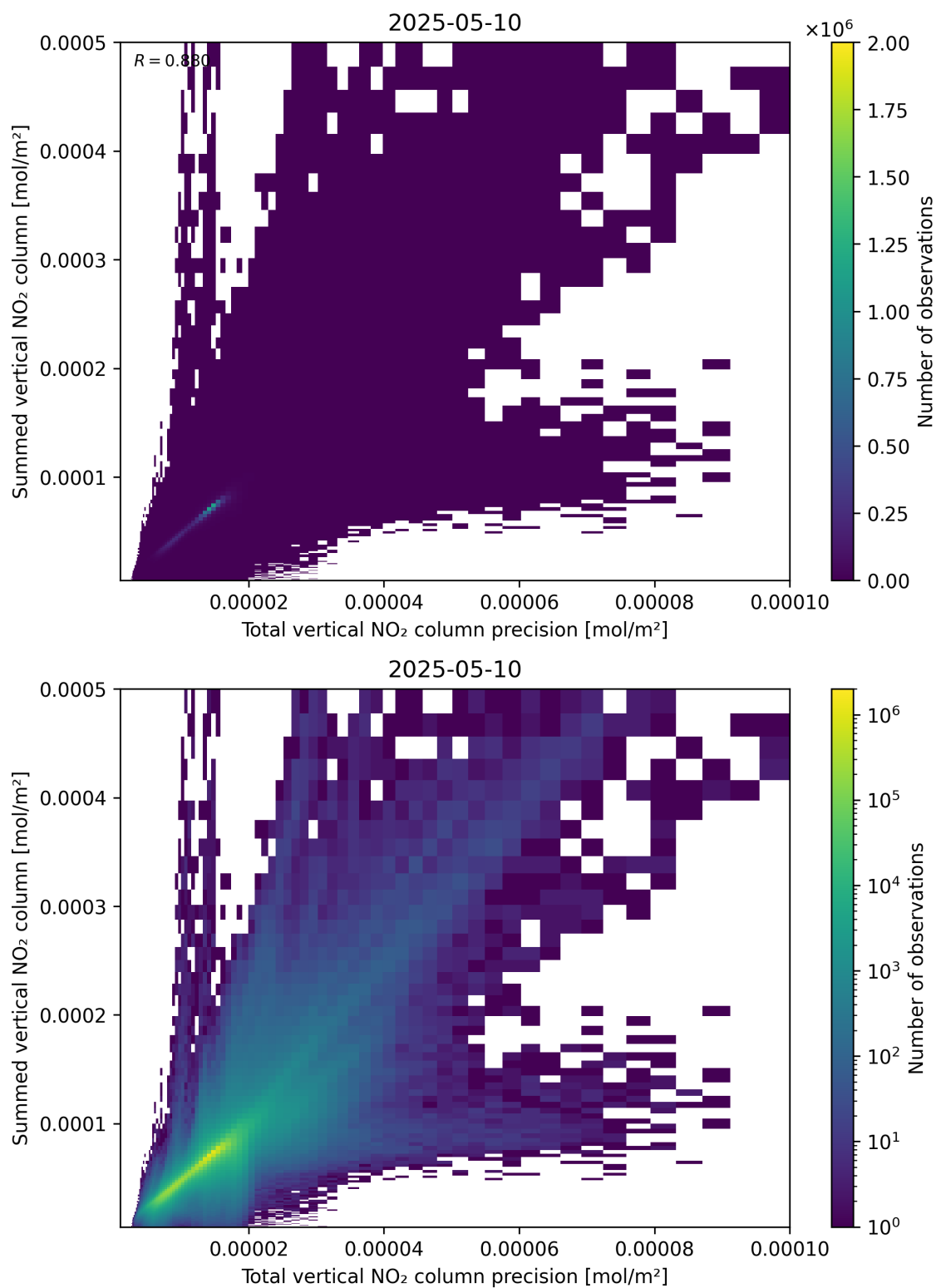
Figure 117: Scatter density plot of “Total vertical NO 2 column precision” against “Summed vertical NO 2 column” for 2025-05-10 to 2025-05-11.
