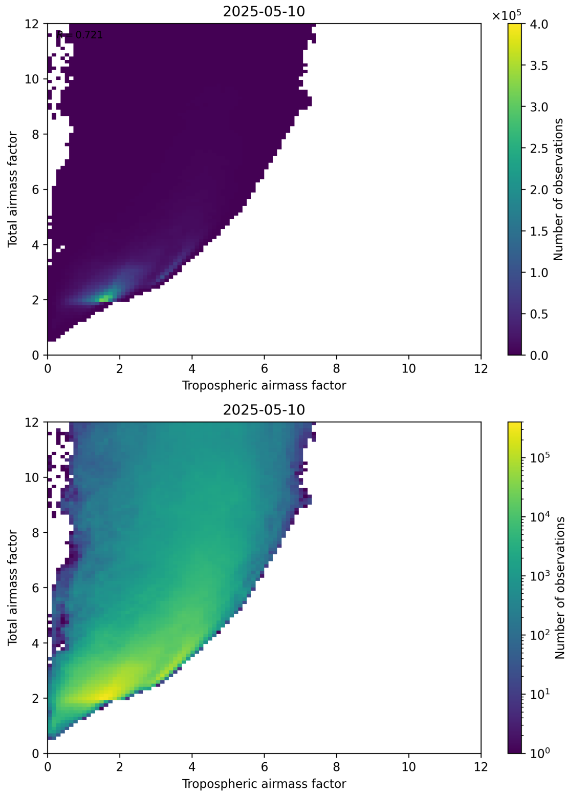
Figure 72: Scatter density plot of “Tropospheric airmass factor” against “Total airmass factor” for 2025-05-10 to 2025-05-11.
