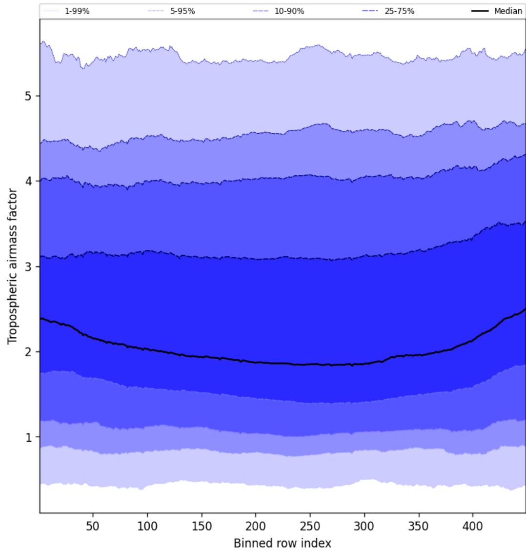
Figure 48: Along track statistics of “Tropospheric airmass factor” for 2025-05-10 to 2025-05-11
