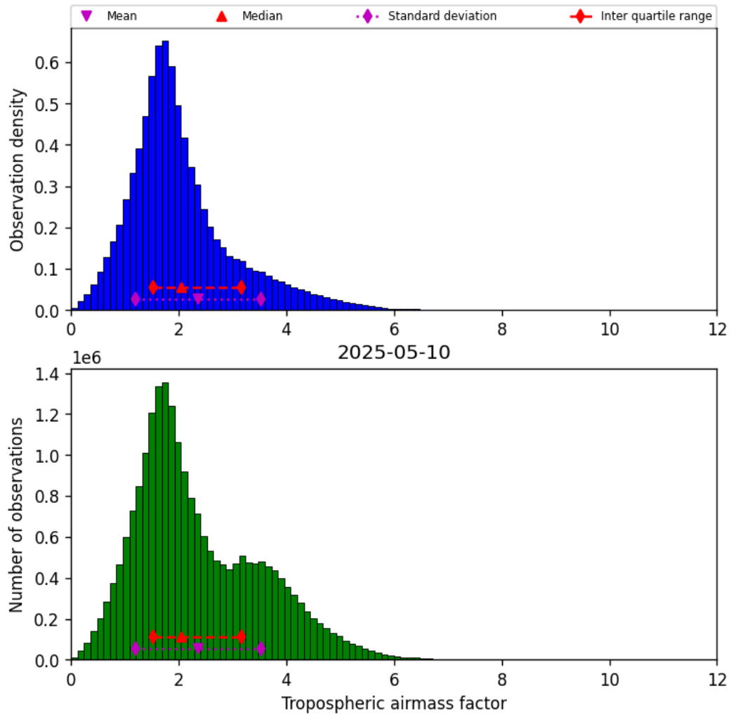
Figure 31: Histogram of “Tropospheric airmass factor” for 2025-05-10 to 2025-05-11
