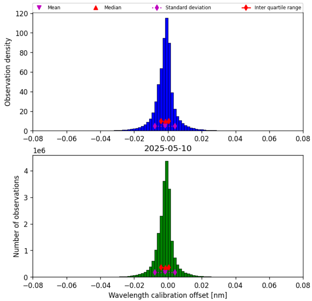
Figure 35: Histogram of “Wavelength calibration offset” for 2025-05-10 to 2025-05-11
