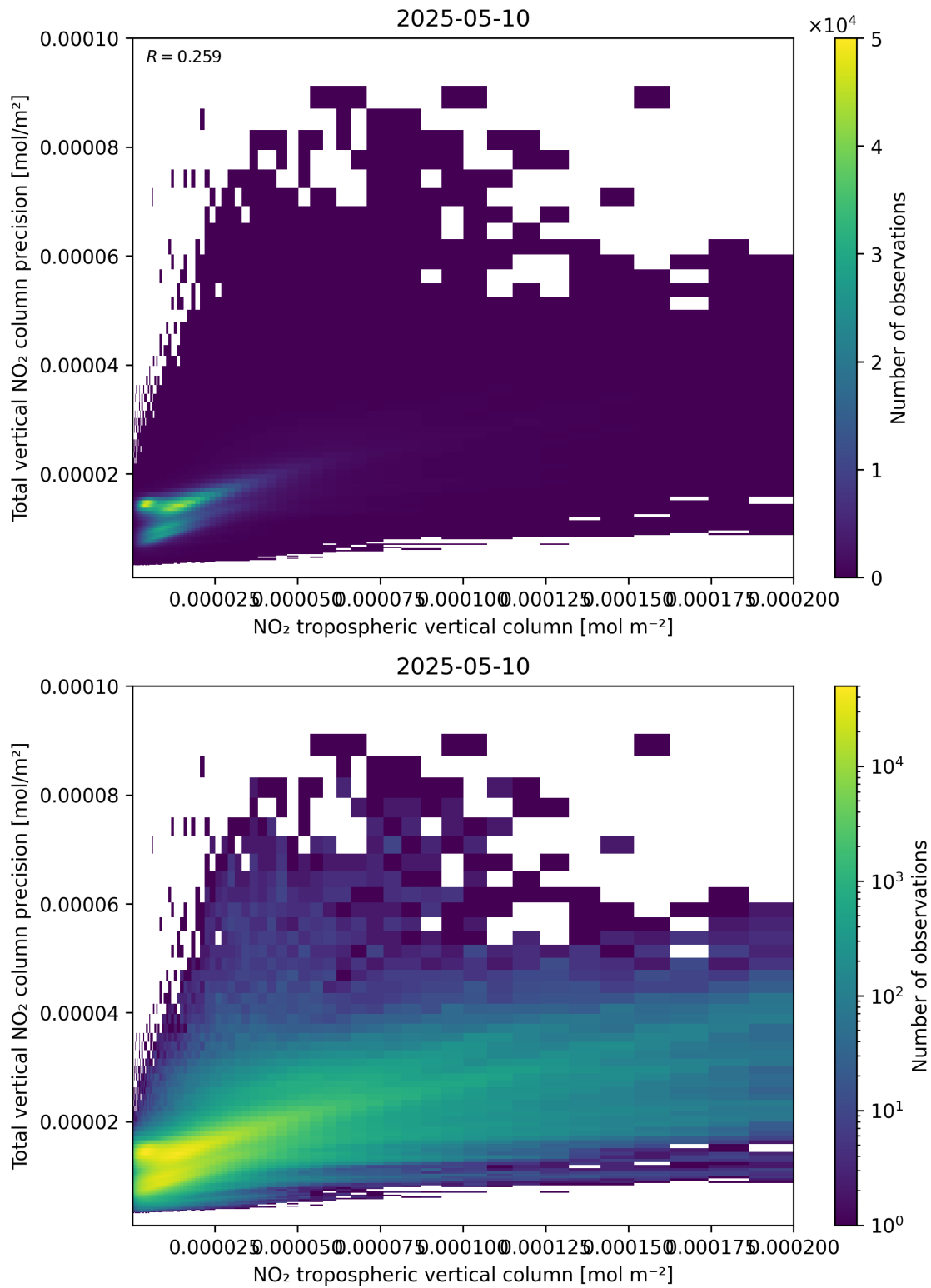
Figure 129: Scatter density plot of “NO 2 tropospheric vertical column” against “Total vertical NO 2 column precision” for 2025-05-10 to 2025-05-11.
