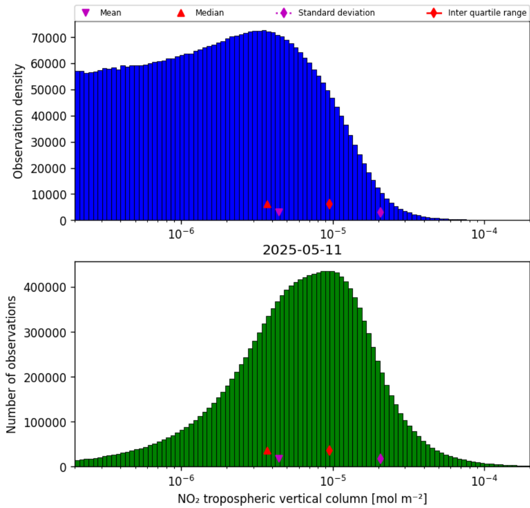
Figure 29: Histogram of “NO 2 tropospheric vertical column” for 2025-05-11 to 2025-05-12
