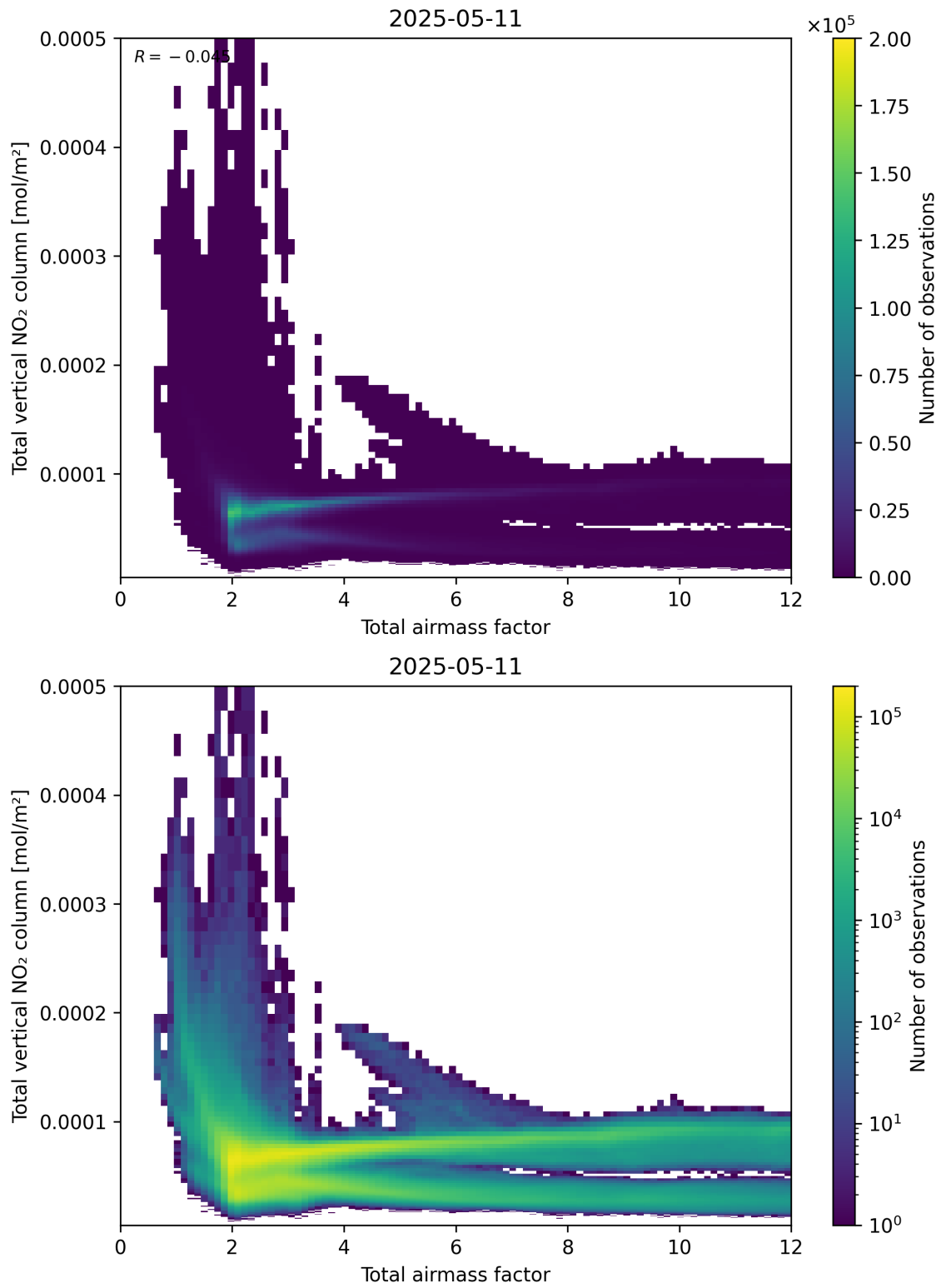
Figure 67: Scatter density plot of “Total airmass factor” against “Total vertical NO 2 column” for 2025-05-11 to 2025-05-12.
