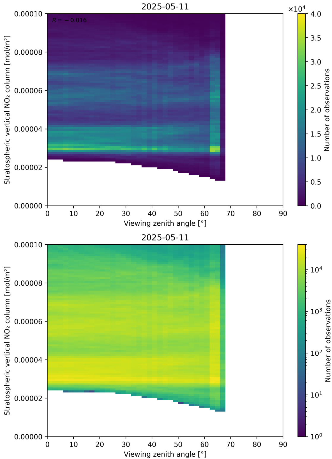
Figure 164: Scatter density plot of “Viewing zenith angle” against “Stratospheric vertical NO 2 column” for 2025-05-11 to 2025-05-12.
