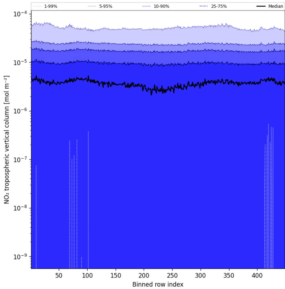
Figure 46: Along track statistics of “NO 2 tropospheric vertical column” for 2025-05-11 to 2025-05-12
