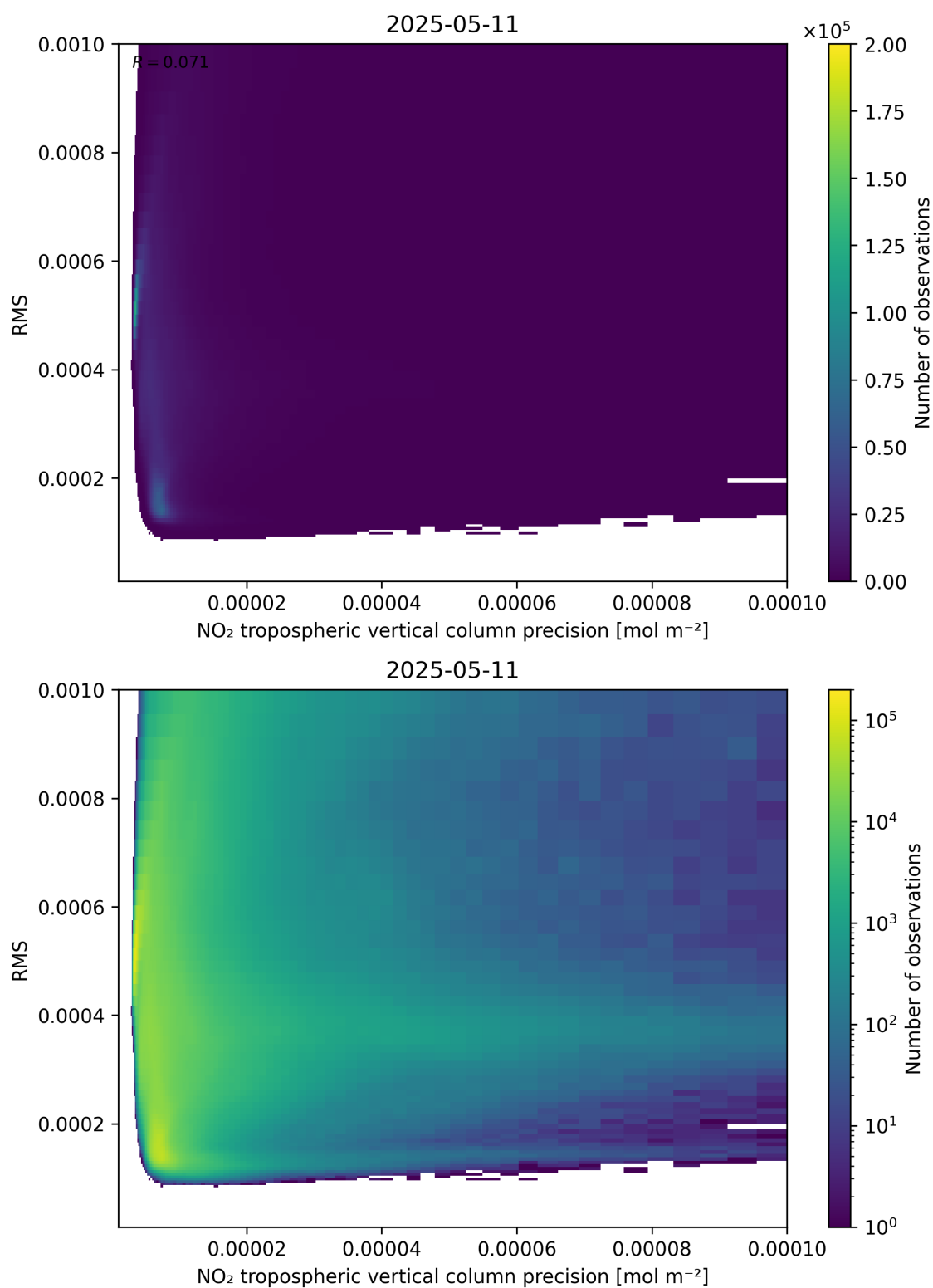
Figure 140: Scatter density plot of “NO 2 tropospheric vertical column precision” against “RMS” for 2025-05-11 to 2025-05-12.
