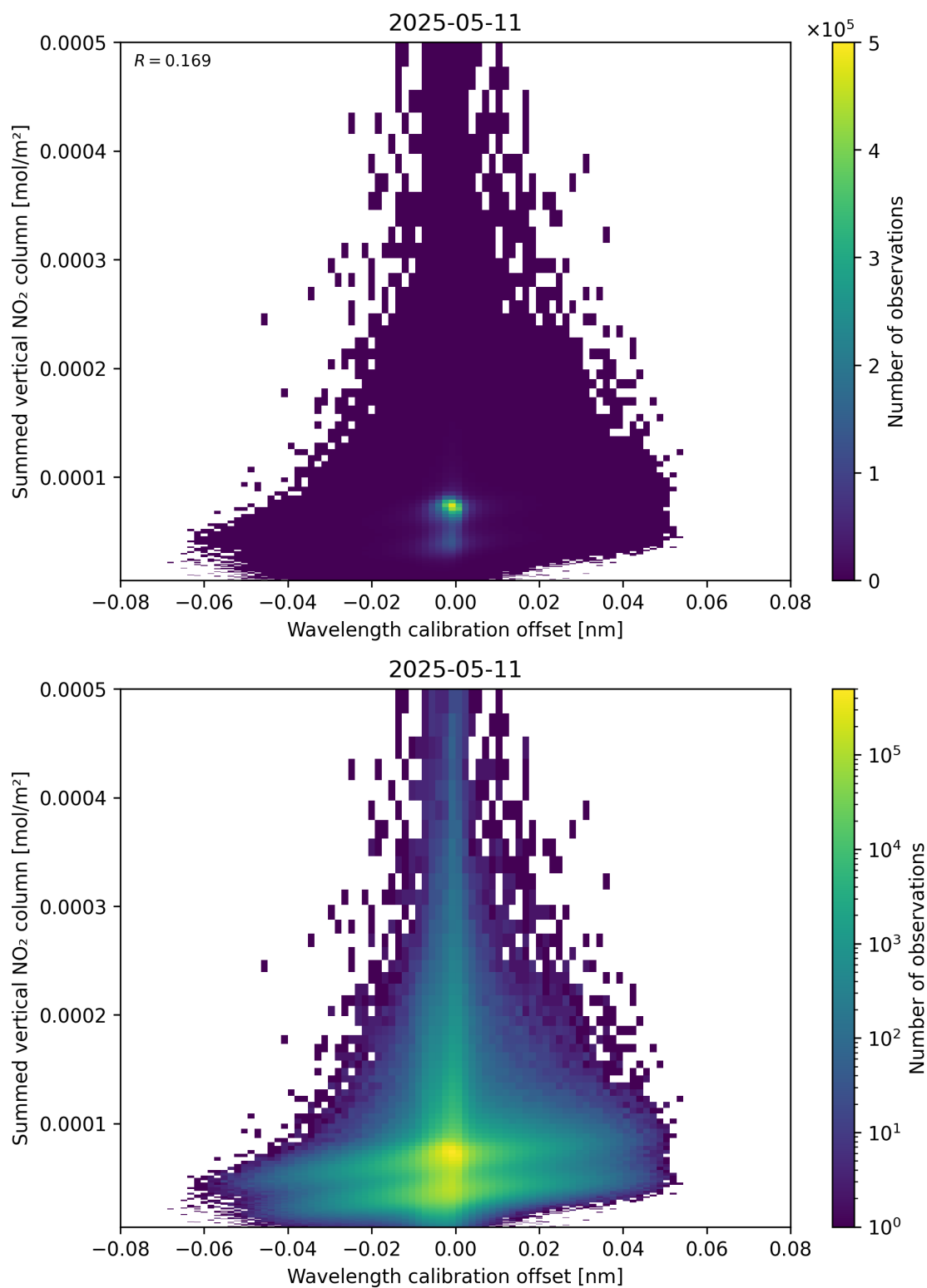
Figure 177: Scatter density plot of “Wavelength calibration offset” against “Summed vertical NO 2 column” for 2025-05-11 to 2025-05-12.
