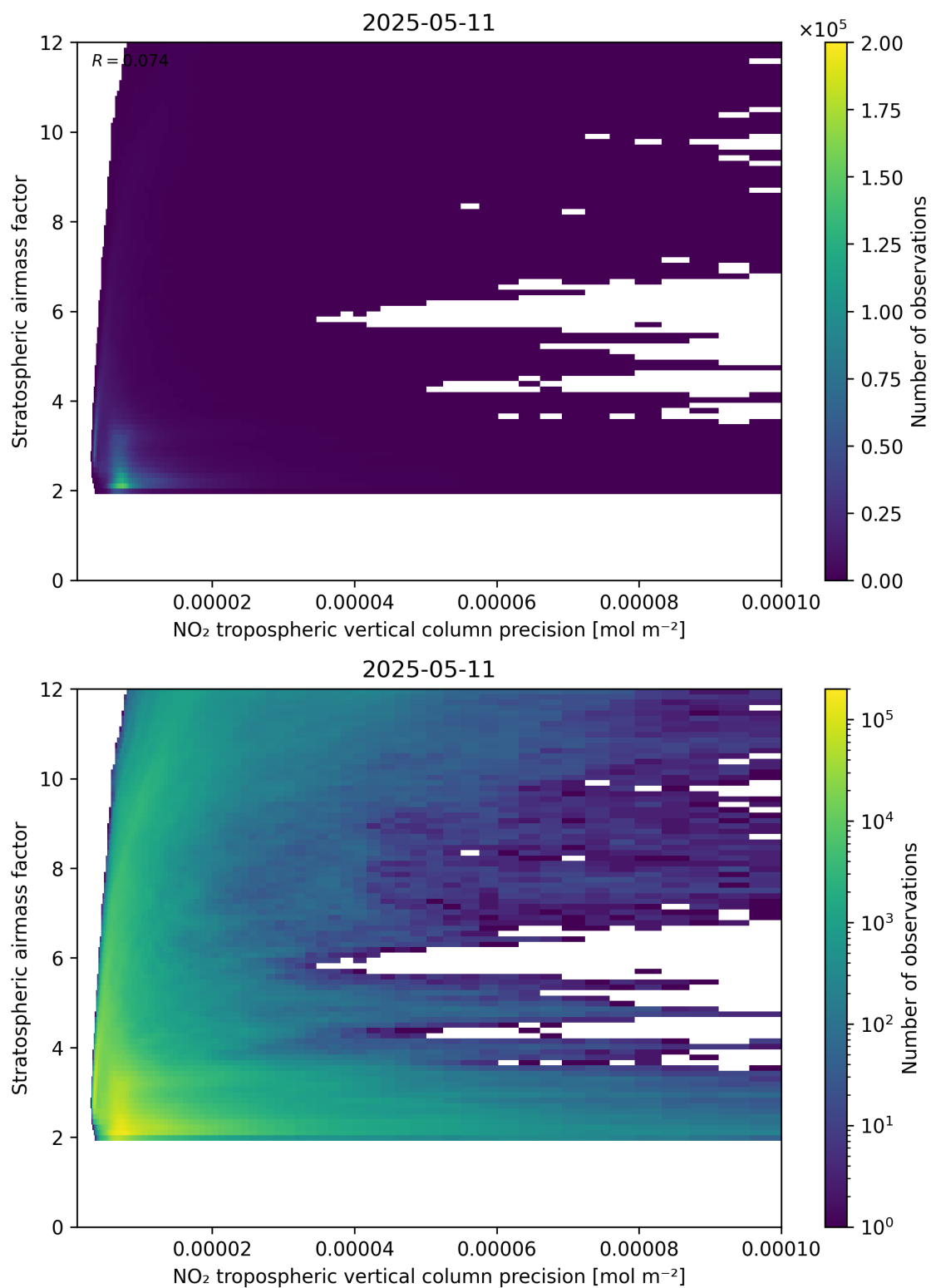
Figure 131: Scatter density plot of “NO 2 tropospheric vertical column precision” against “Stratospheric airmass factor” for 2025-05-11 to 2025-05-12.
