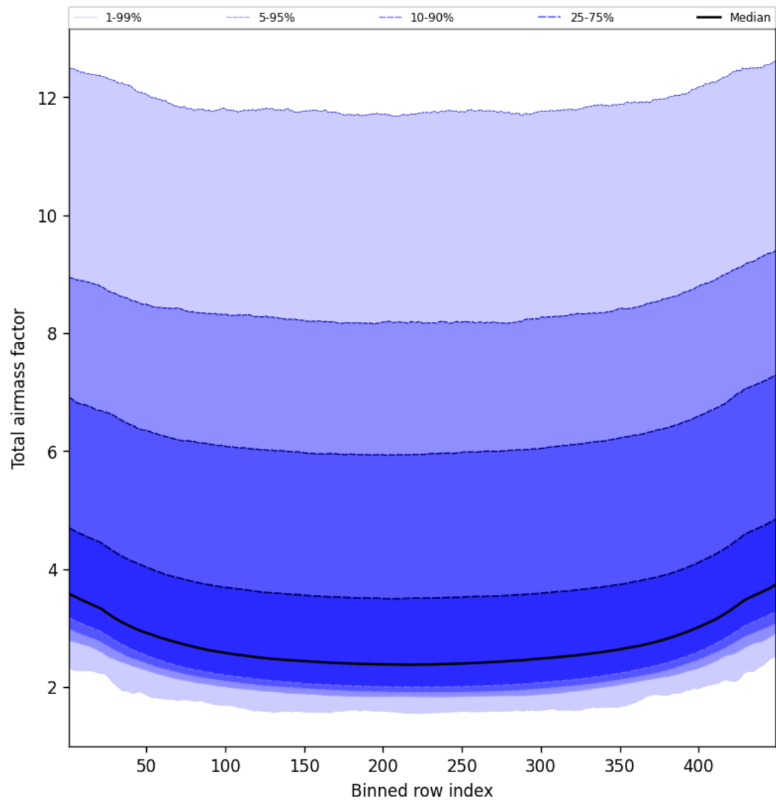
Figure 49: Along track statistics of “Total airmass factor” for 2025-05-11 to 2025-05-12
