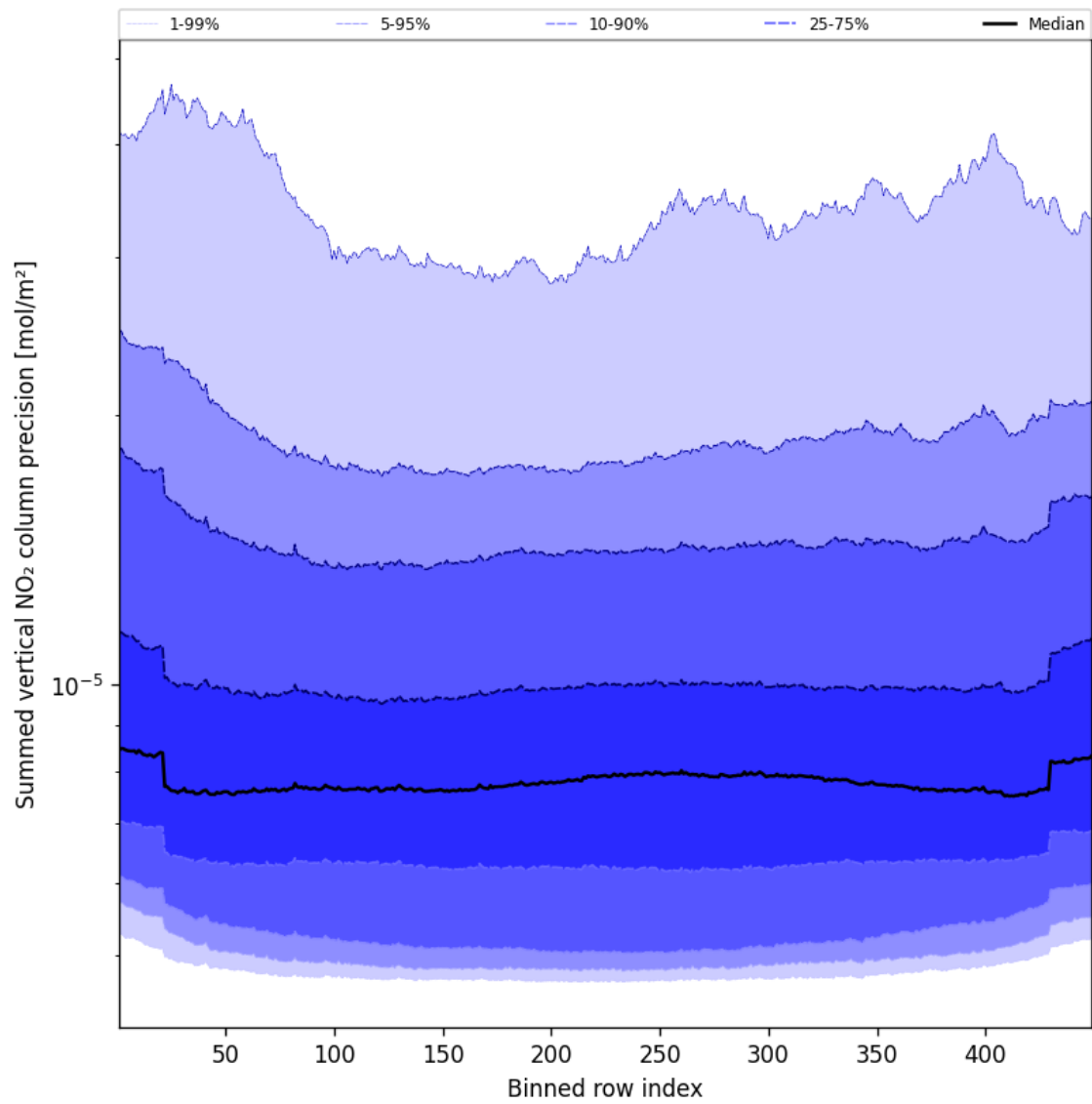
Figure 58: Along track statistics of “Summed vertical NO 2 column precision” for 2025-05-11 to 2025-05-12
