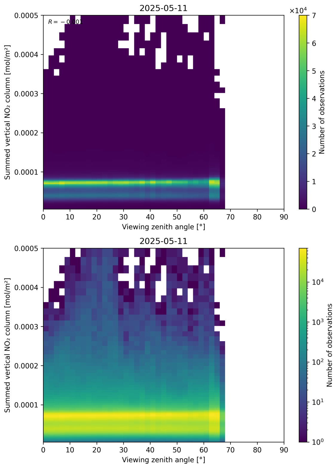
Figure 165: Scatter density plot of “Viewing zenith angle” against “Summed vertical NO 2 column” for 2025-05-11 to 2025-05-12.
