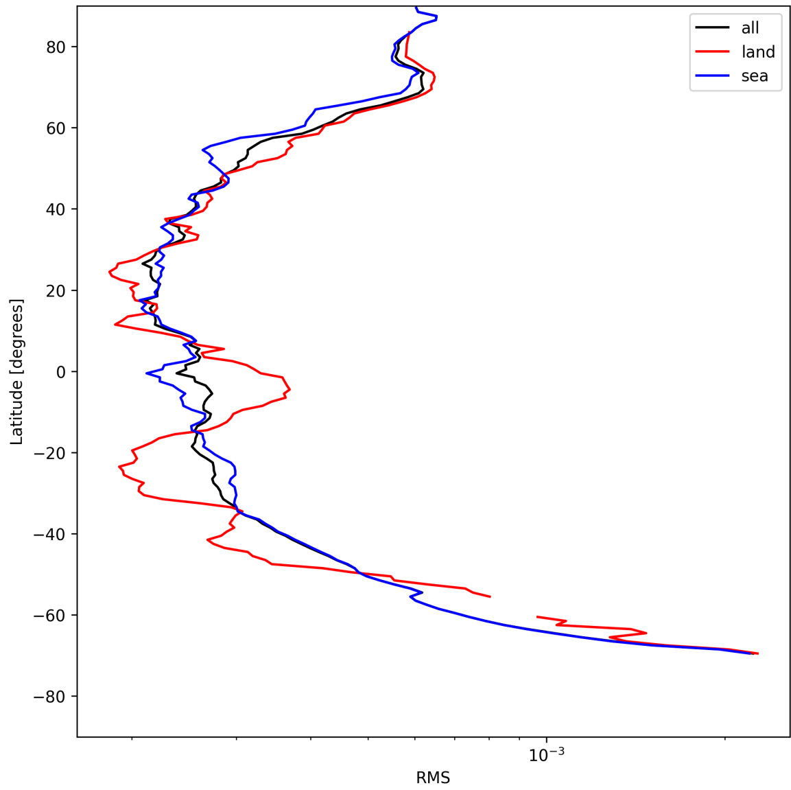
Figure 26: Zonal average of “RMS” for 2025-05-11 to 2025-05-12.
