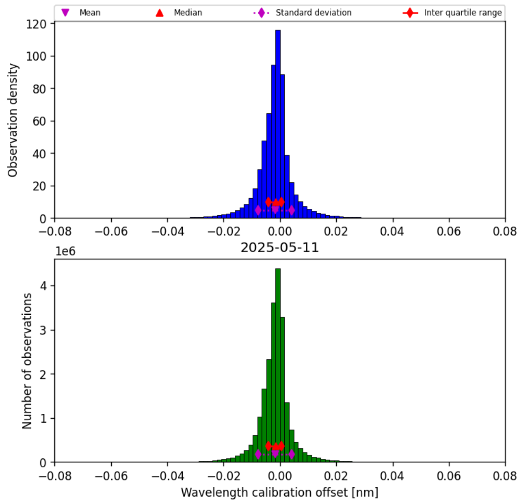
Figure 35: Histogram of “Wavelength calibration offset” for 2025-05-11 to 2025-05-12
