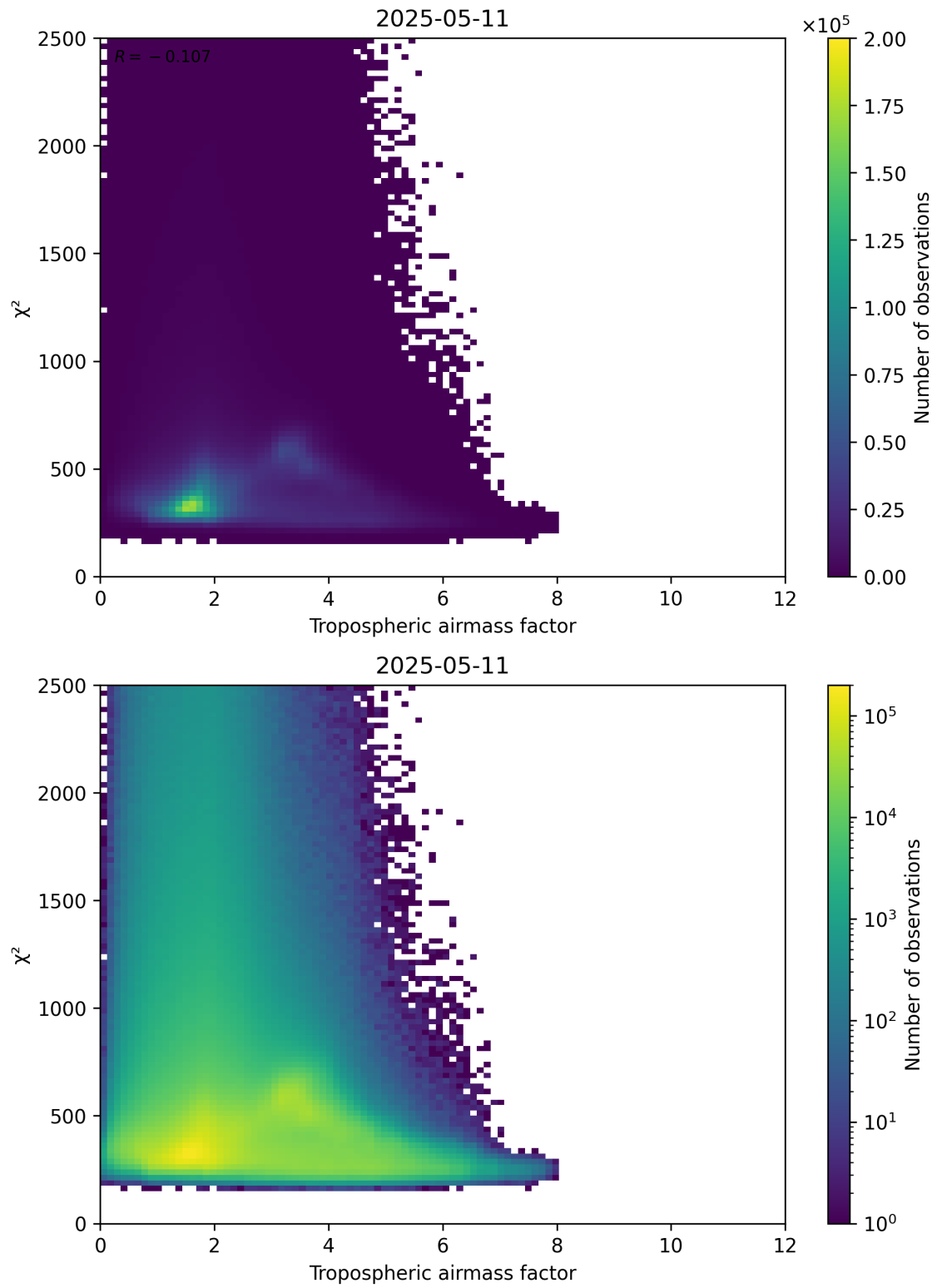
Figure 73: Scatter density plot of “Tropospheric airmass factor” against “ \chi^2 ” for 2025-05-11 to 2025-05-12.
