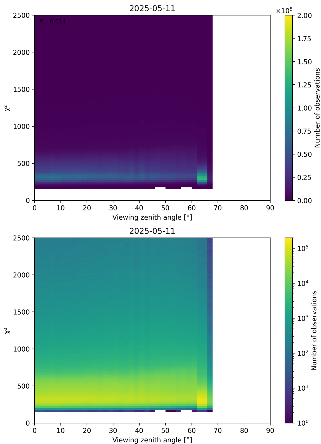
Figure 162: Scatter density plot of “Viewing zenith angle” against “ \chi^2 ” for 2025-05-11 to 2025-05-12.
