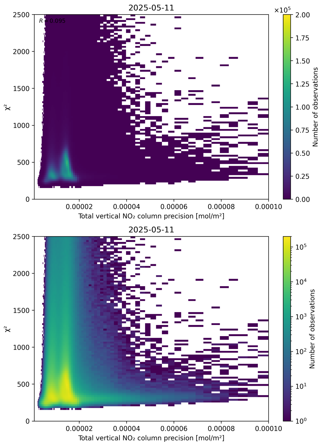
Figure 116: Scatter density plot of “Total vertical NO 2 column precision” against “ \chi^2 ” for 2025-05-11 to 2025-05-12.
