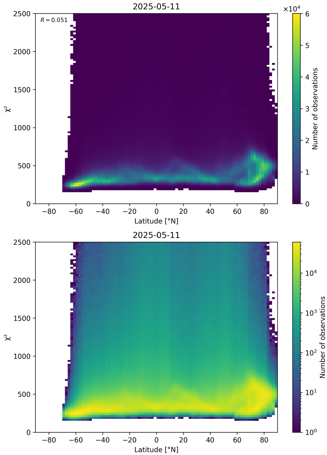
Figure 86: Scatter density plot of “Latitude” against “ \chi^2 ” for 2025-05-11 to 2025-05-12.
