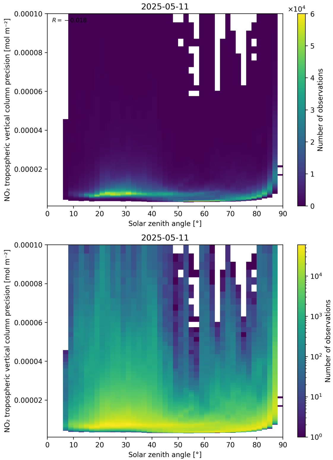
Figure 156: Scatter density plot of “Solar zenith angle” against “NO 2 tropospheric vertical column precision” for 2025-05-11 to 2025-05-12.
