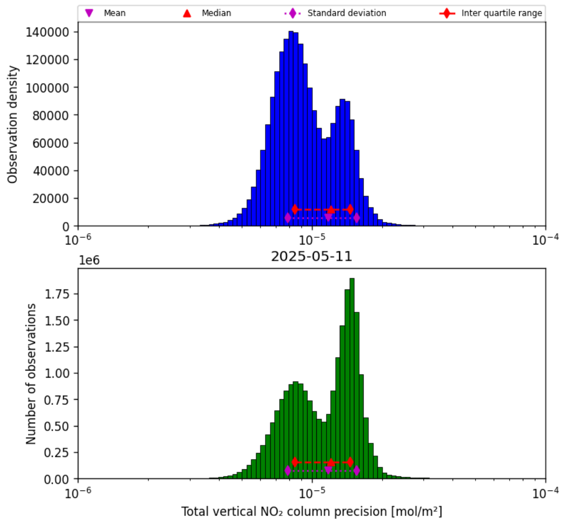
Figure 39: Histogram of “Total vertical NO 2 column precision” for 2025-05-11 to 2025-05-12
