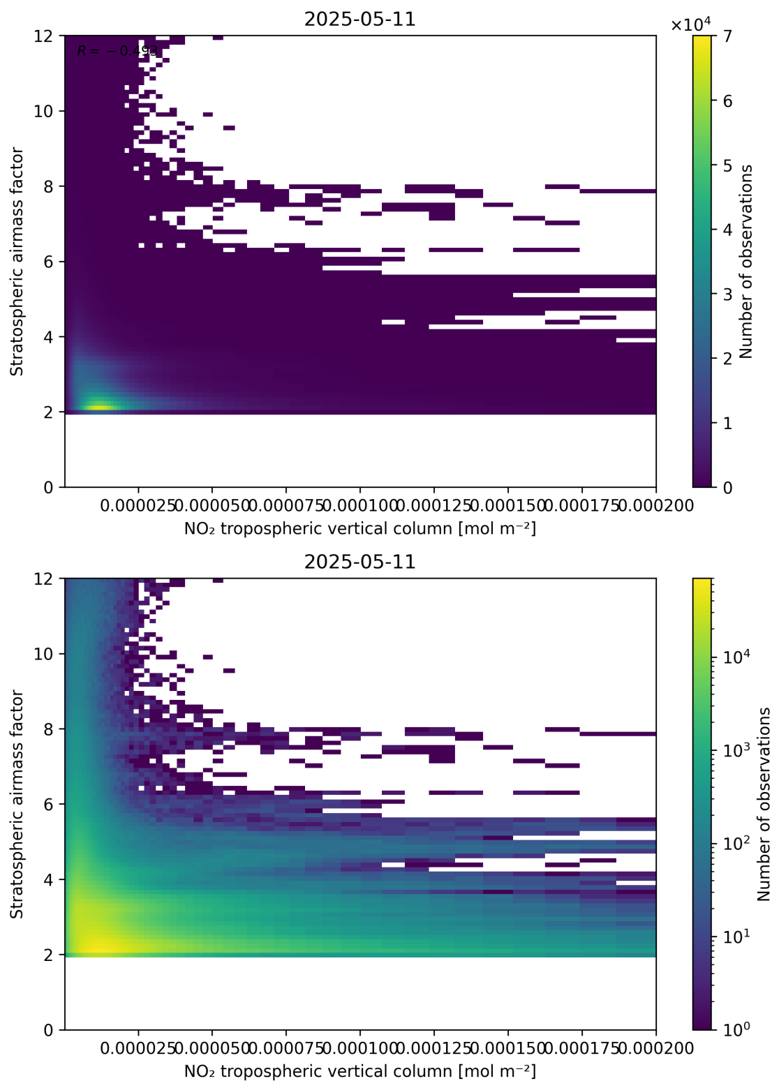
Figure 121: Scatter density plot of “NO 2 tropospheric vertical column” against “Stratospheric air mass factor” for 2025-05-11 to 2025-05-12.
