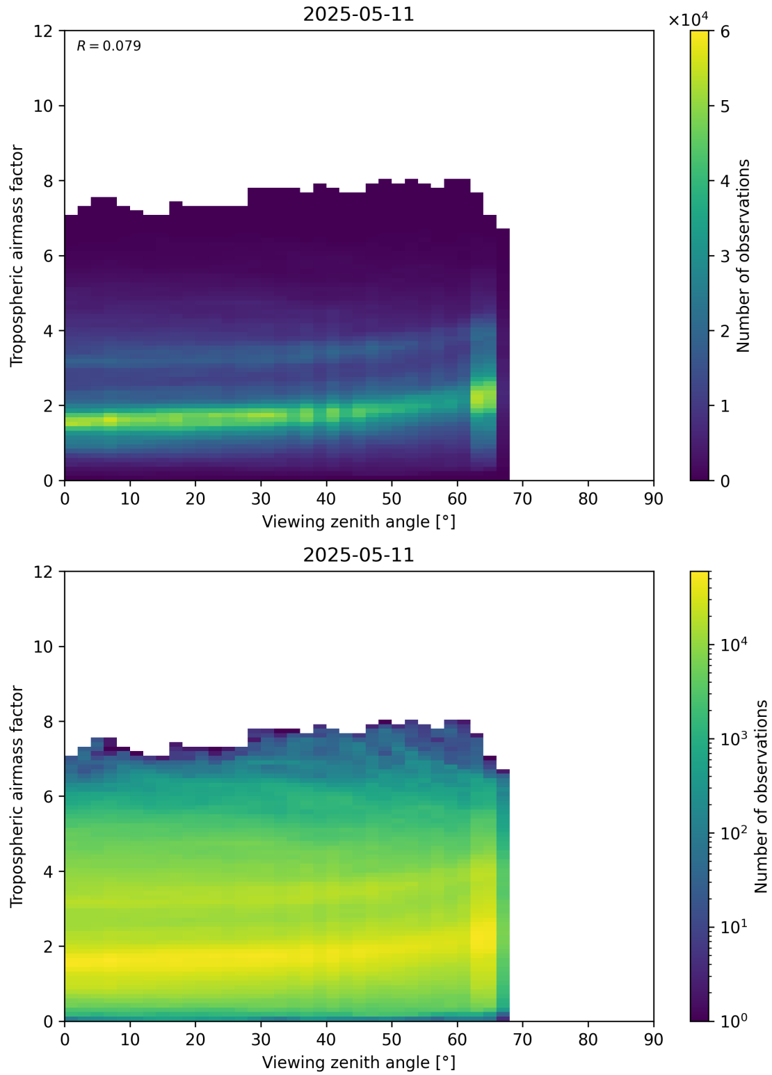
Figure 161: Scatter density plot of “Viewing zenith angle” against “Tropospheric airmass factor” for 2025-05-11 to 2025-05-12.
