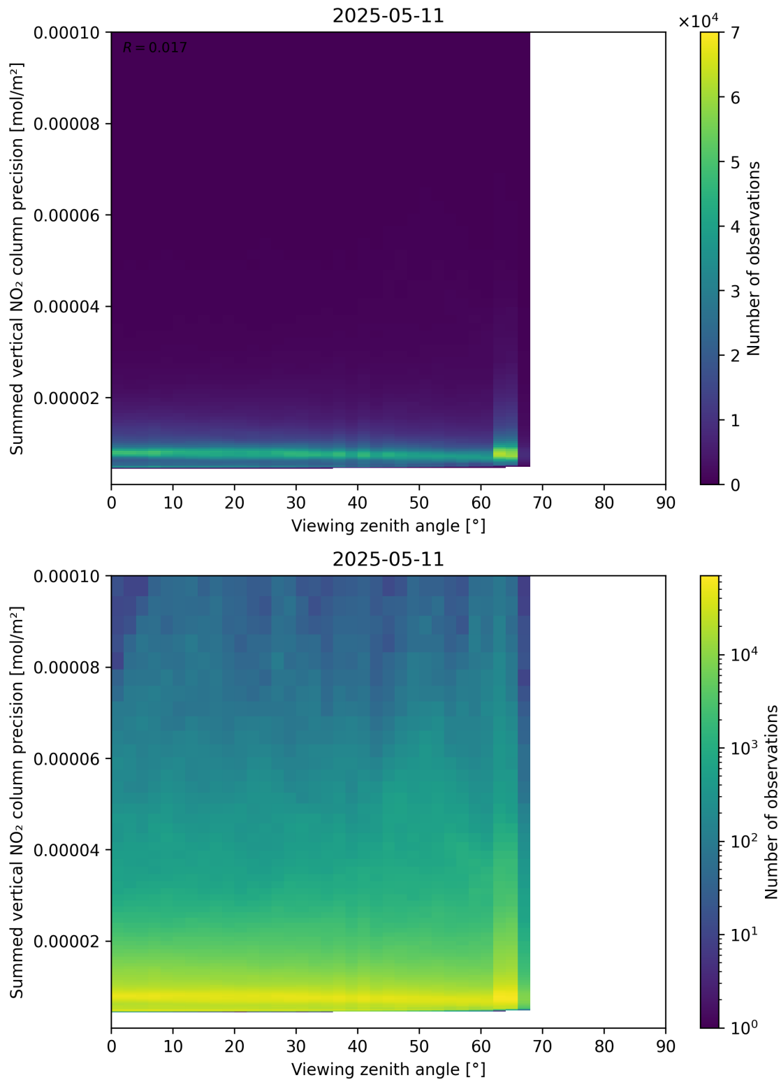
Figure 166: Scatter density plot of “Viewing zenith angle” against “Summed vertical NO 2 column precision” for 2025-05-11 to 2025-05-12.
