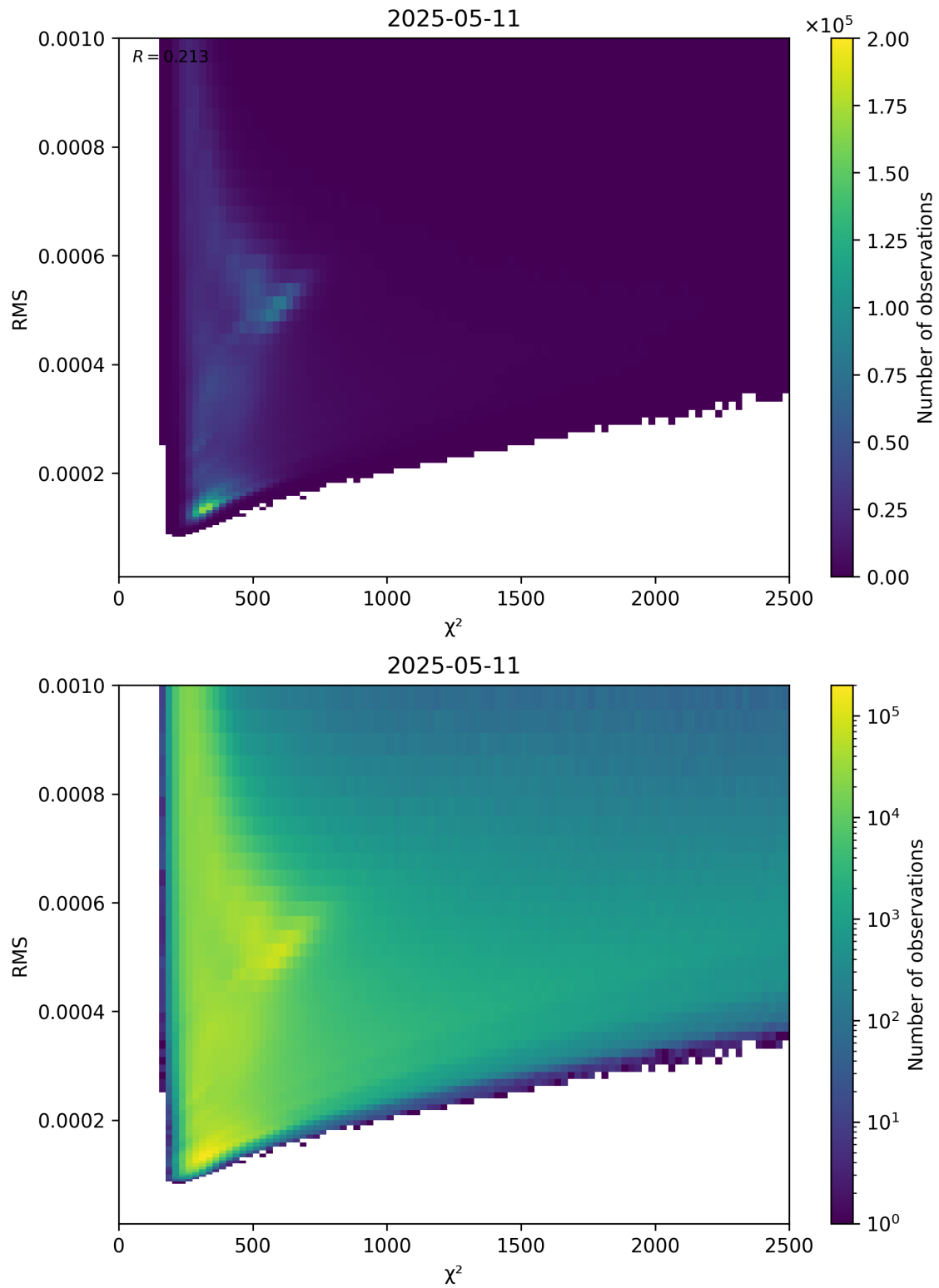
Figure 82: Scatter density plot of “ \chi^2 ” against “RMS” for 2025-05-11 to 2025-05-12.
