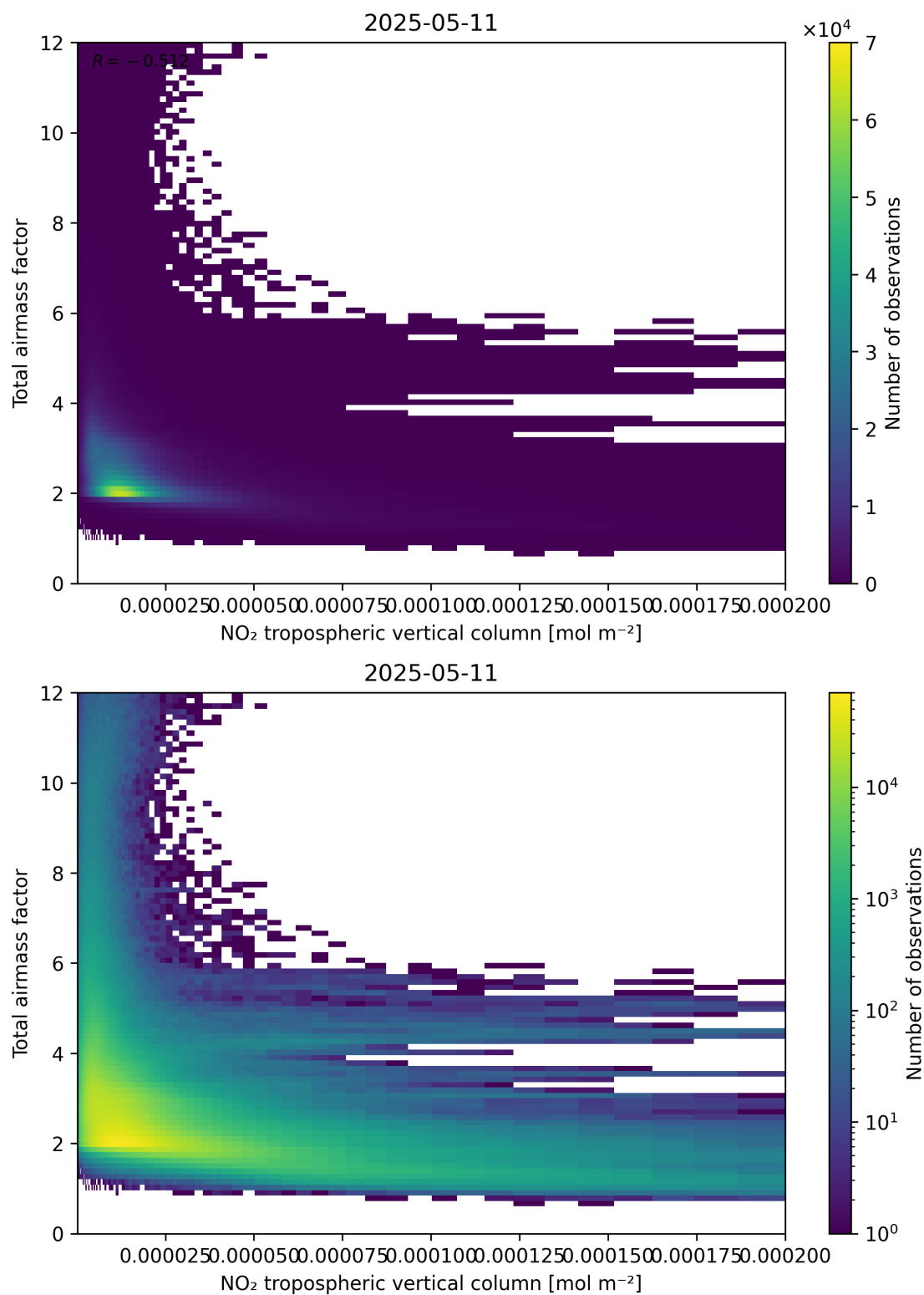
Figure 122: Scatter density plot of “NO 2 tropospheric vertical column” against “Total air mass factor” for 2025-05-11 to 2025-05-12.
