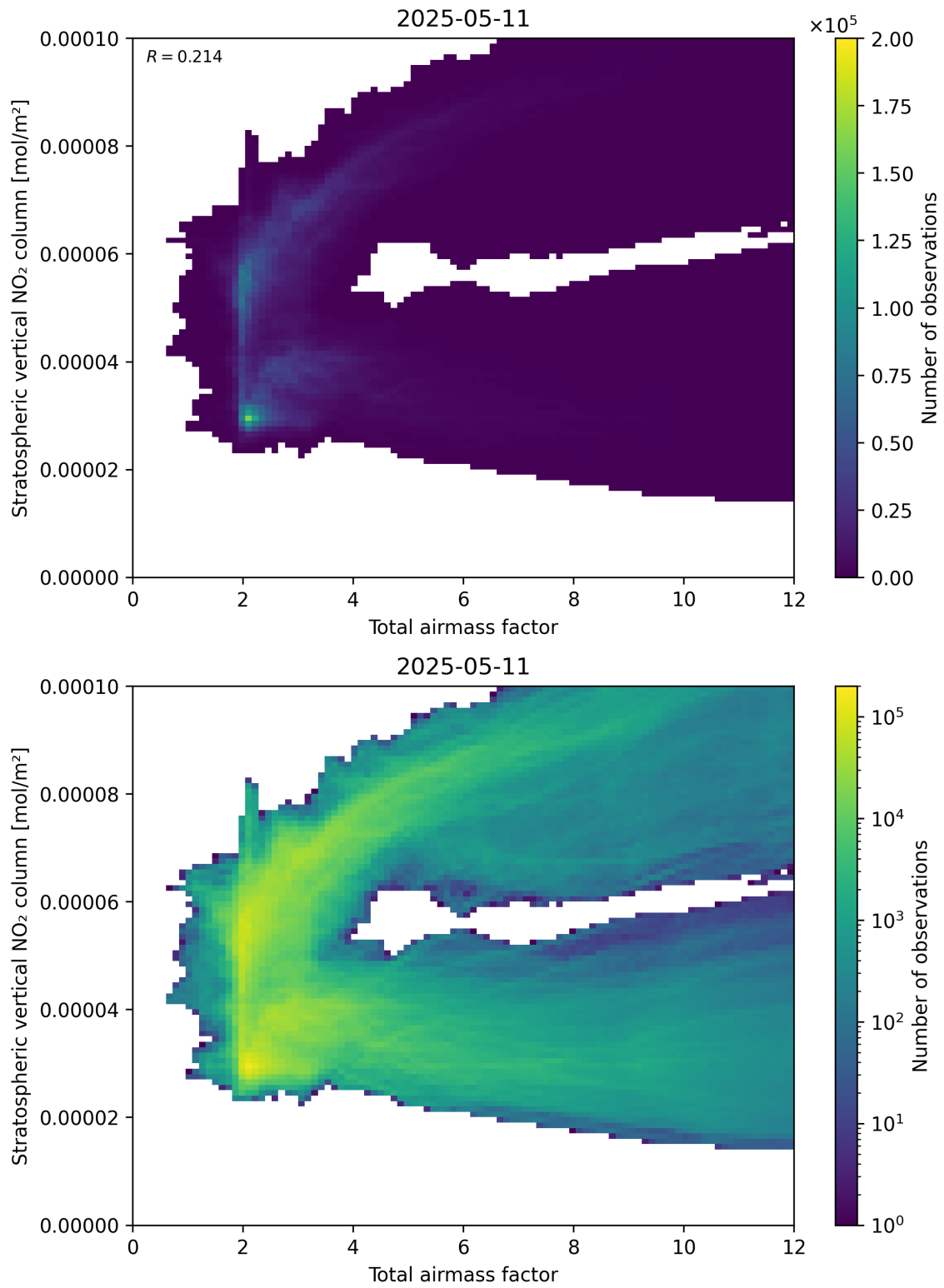
Figure 64: Scatter density plot of “Total airmass factor” against “Stratospheric vertical NO 2 column” for 2025-05-11 to 2025-05-12.
