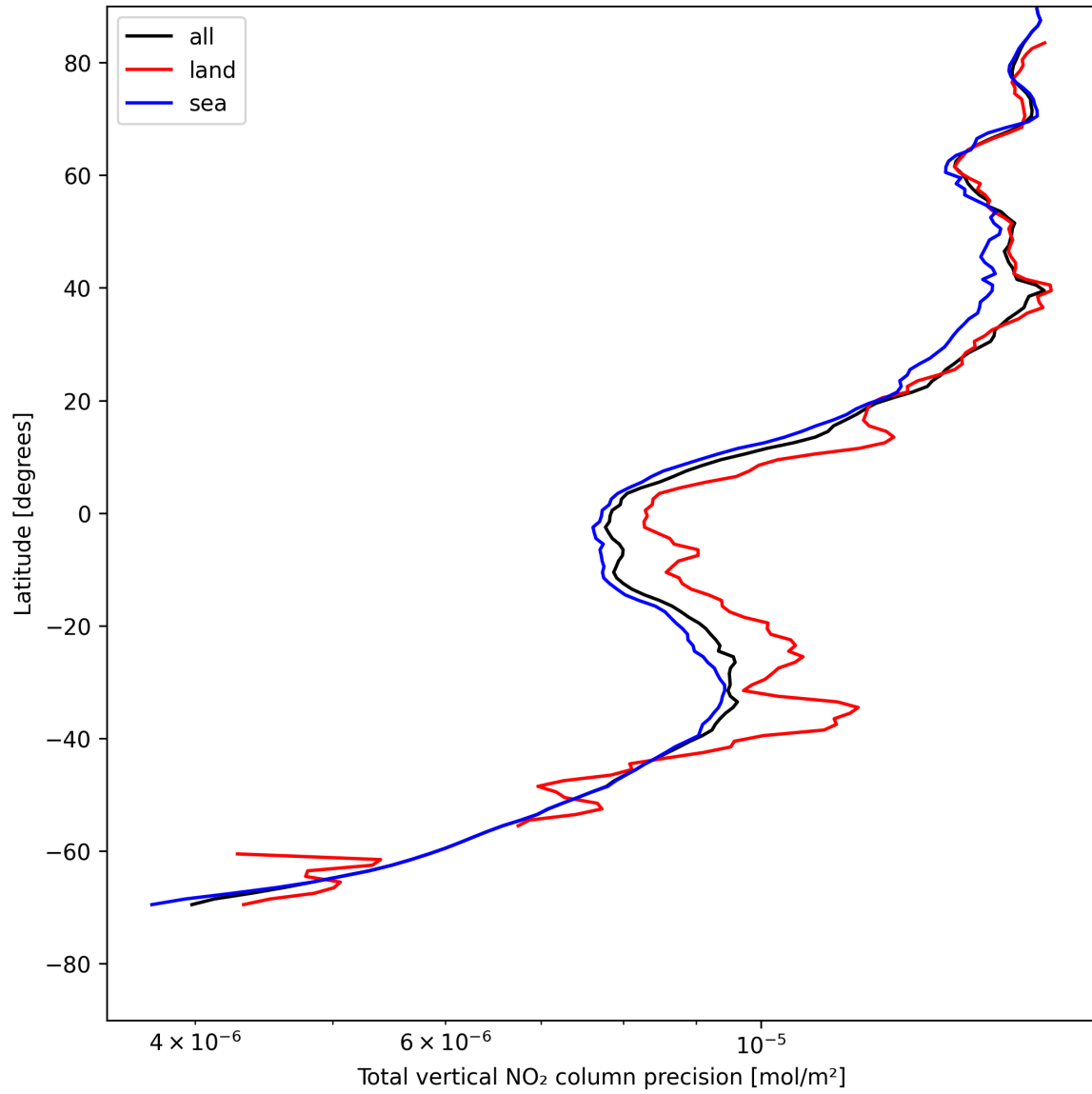
Figure 22: Zonal average of “Total vertical NO 2 column precision” for 2025-05-11 to 2025-05-12.
