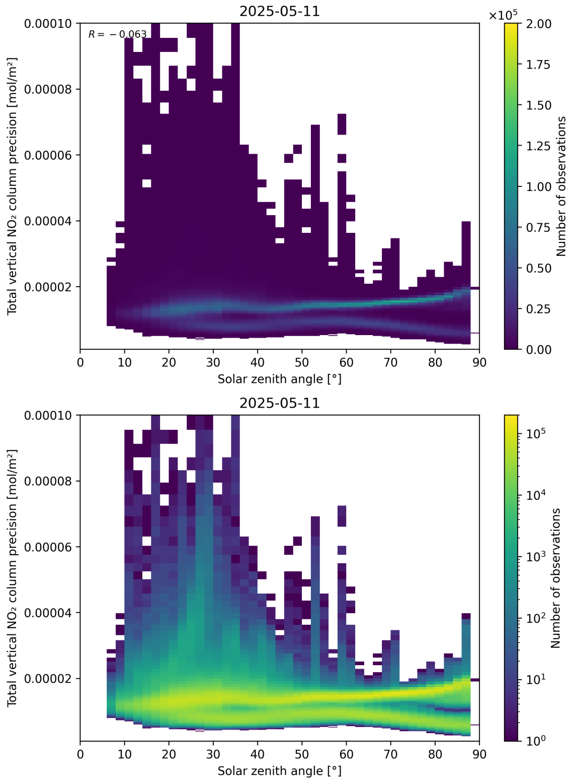
Figure 154: Scatter density plot of “Solar zenith angle” against “Total vertical NO 2 column precision” for 2025-05-11 to 2025-05-12.
