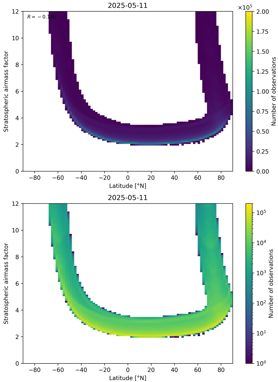
Figure 83: Scatter density plot of “Latitude” against “Stratospheric air mass factor” for 2025-05-11 to 2025-05-12.
