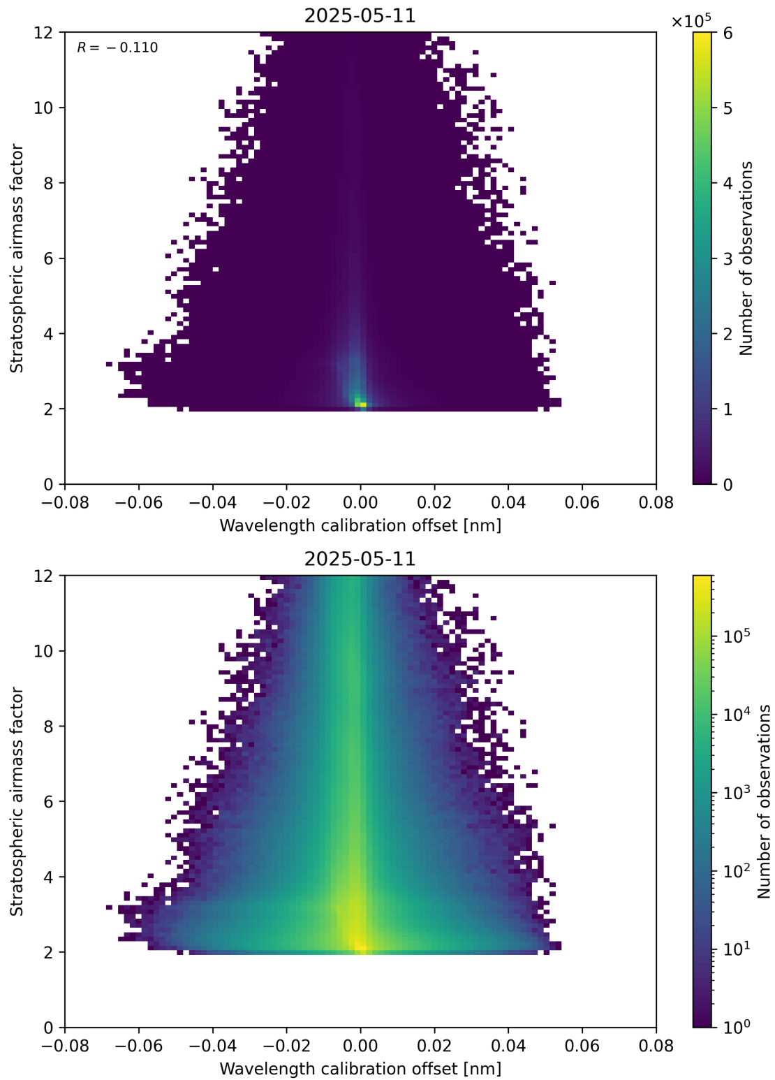
Figure 174: Scatter density plot of “Wavelength calibration offset” against “Stratospheric airmass factor” for 2025-05-11 to 2025-05-12.
