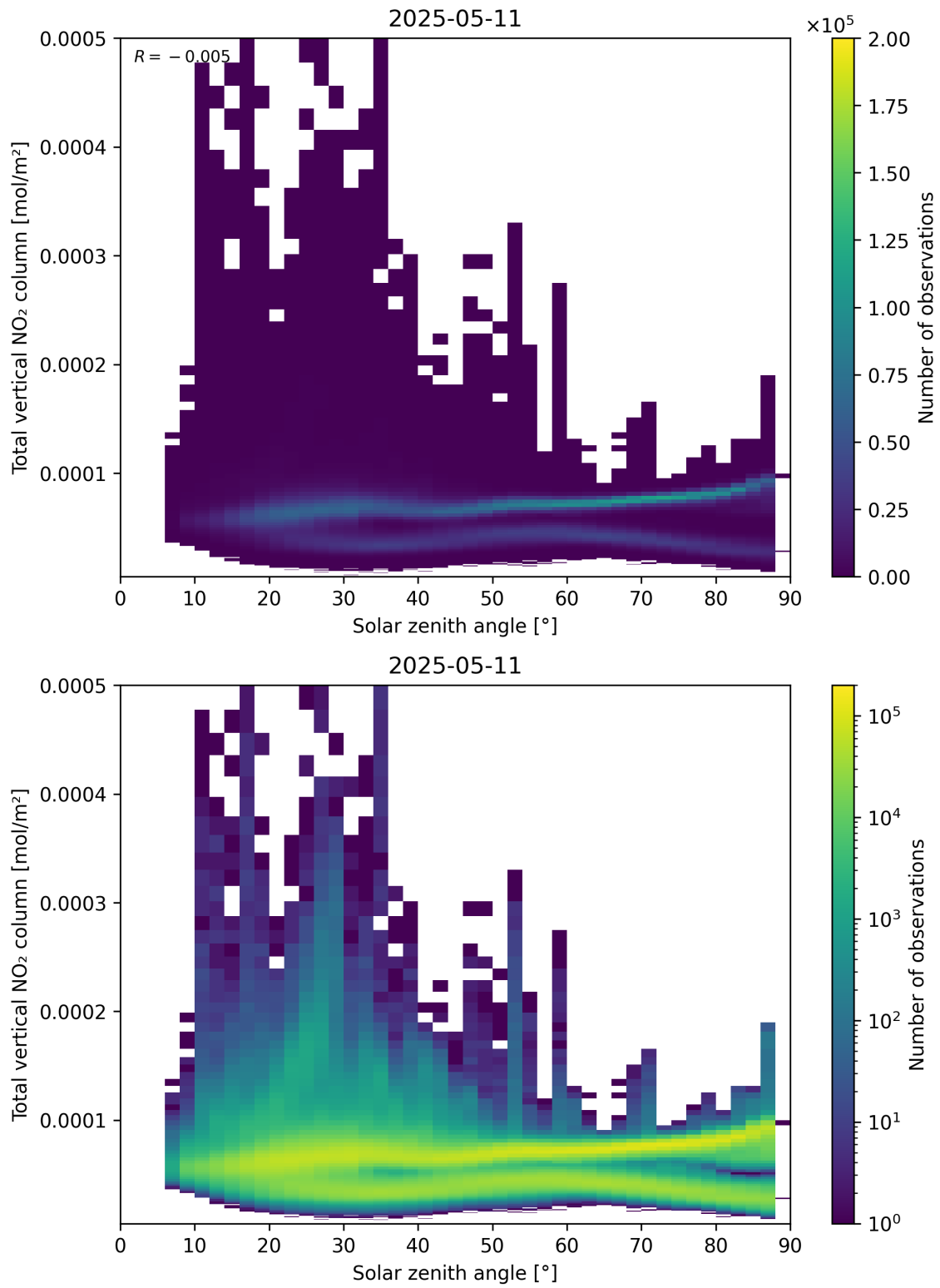
Figure 153: Scatter density plot of “Solar zenith angle” against “Total vertical NO 2 column” for 2025-05-11 to 2025-05-12.
