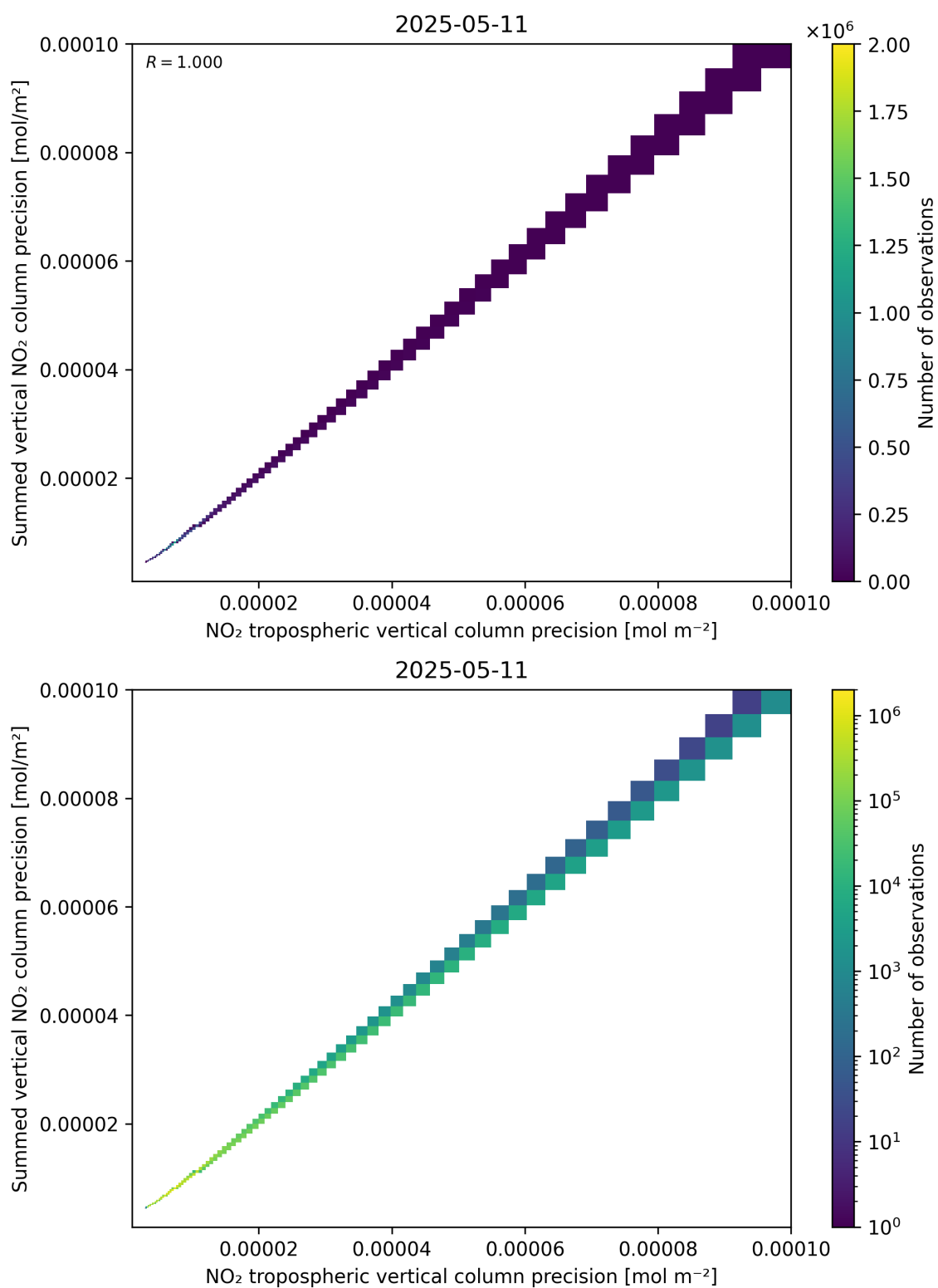
Figure 137: Scatter density plot of “NO 2 tropospheric vertical column precision” against “Summed vertical NO 2 column precision” for 2025-05-11 to 2025-05-12.
