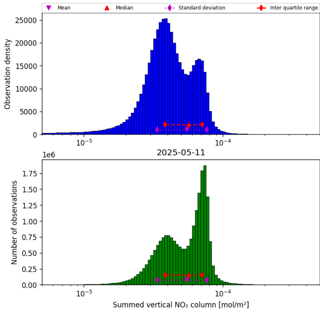
Figure 40: Histogram of “Summed vertical NO 2 column” for 2025-05-11 to 2025-05-12
