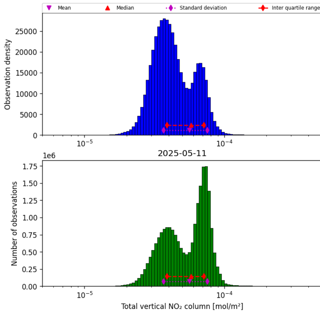
Figure 38: Histogram of “Total vertical NO 2 column” for 2025-05-11 to 2025-05-12
