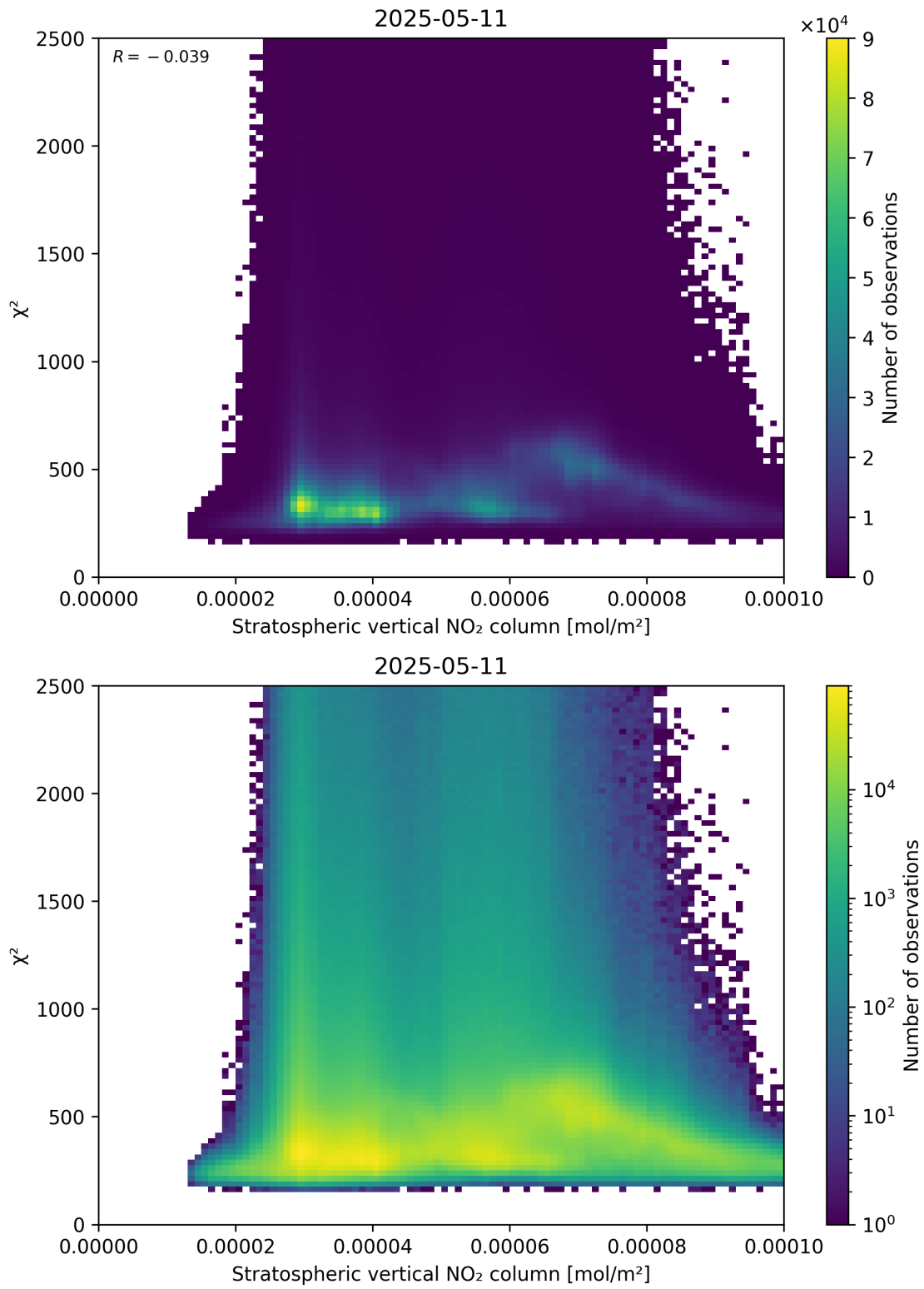
Figure 97: Scatter density plot of “Stratospheric vertical NO 2 column” against “ \chi^2 ” for 2025-05-11 to 2025-05-12.
