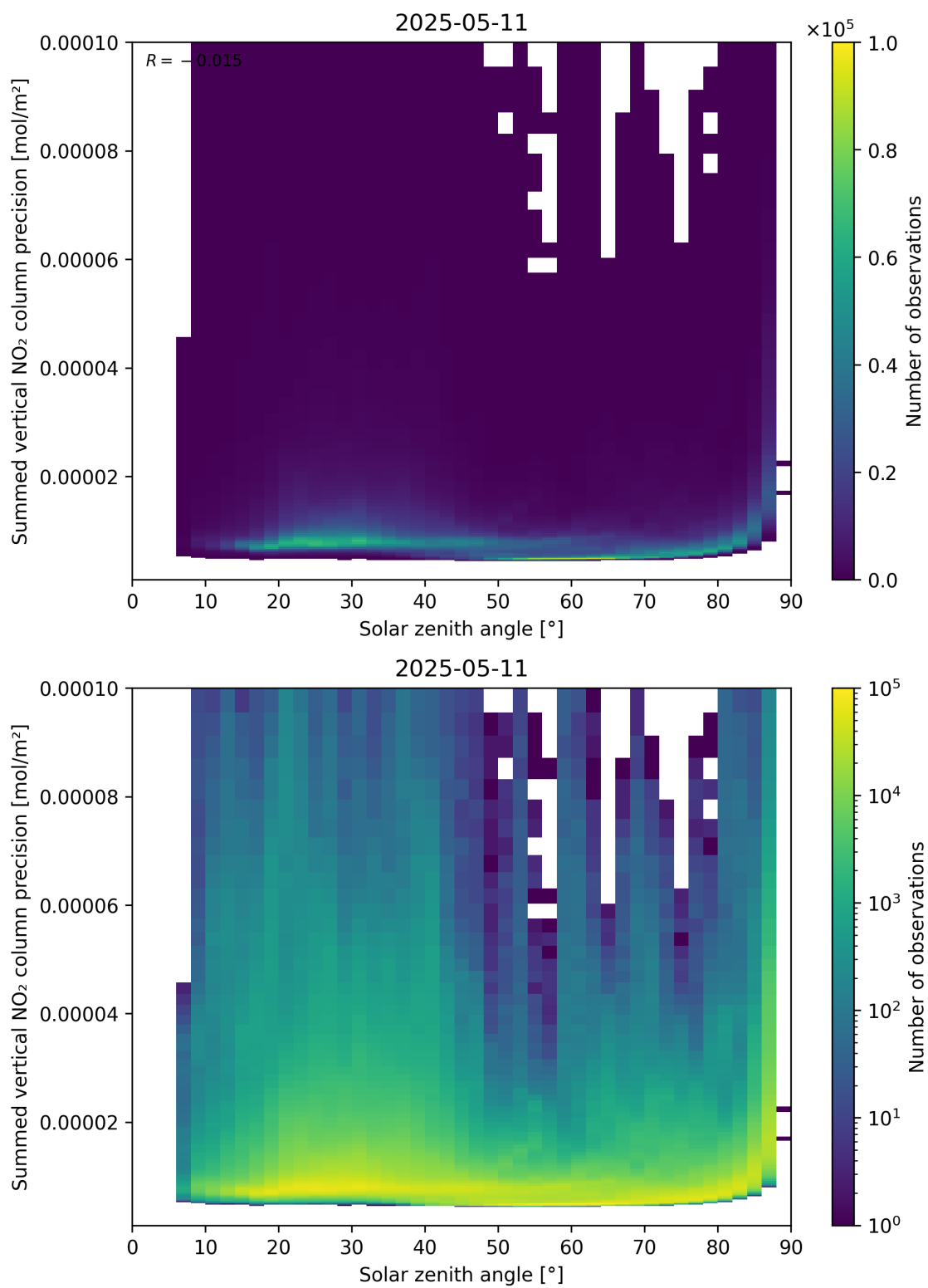
Figure 152: Scatter density plot of “Solar zenith angle” against “Summed vertical NO 2 column precision” for 2025-05-11 to 2025-05-12.
