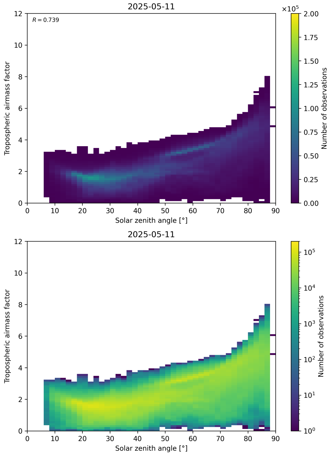
Figure 147: Scatter density plot of “Solar zenith angle” against “Tropospheric airmass factor” for 2025-05-11 to 2025-05-12.
