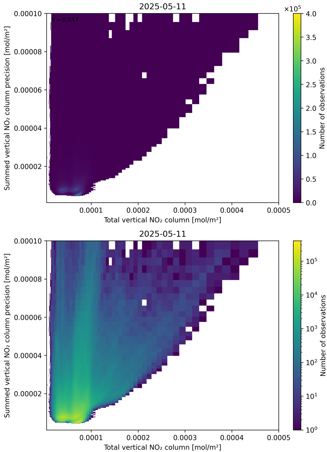
Figure 113: Scatter density plot of “Total vertical NO 2 column” against “Summed vertical NO 2 column precision” for 2025-05-11 to 2025-05-12.
