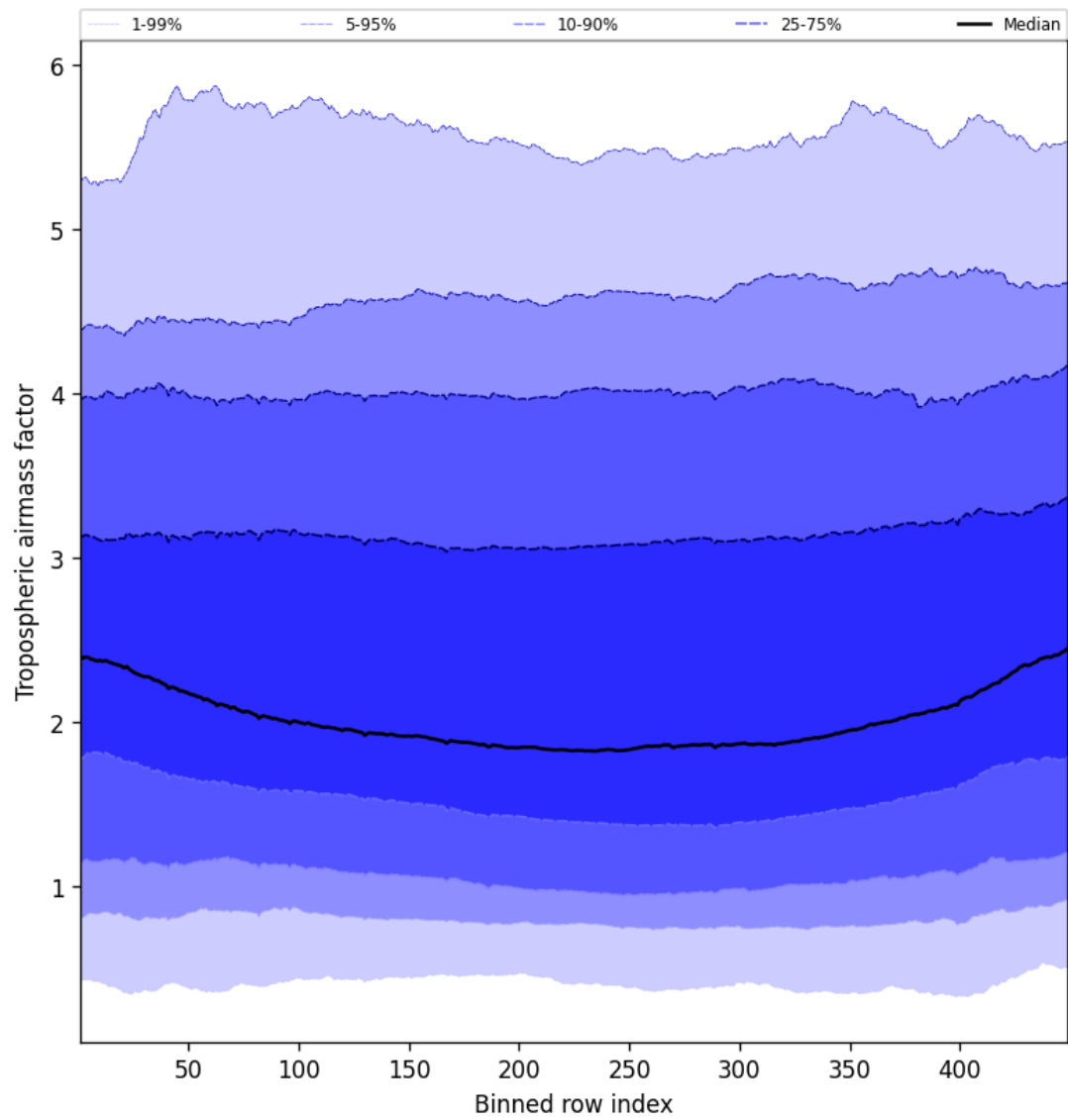
Figure 48: Along track statistics of “Tropospheric air mass factor” for 2025-05-11 to 2025-05-12
