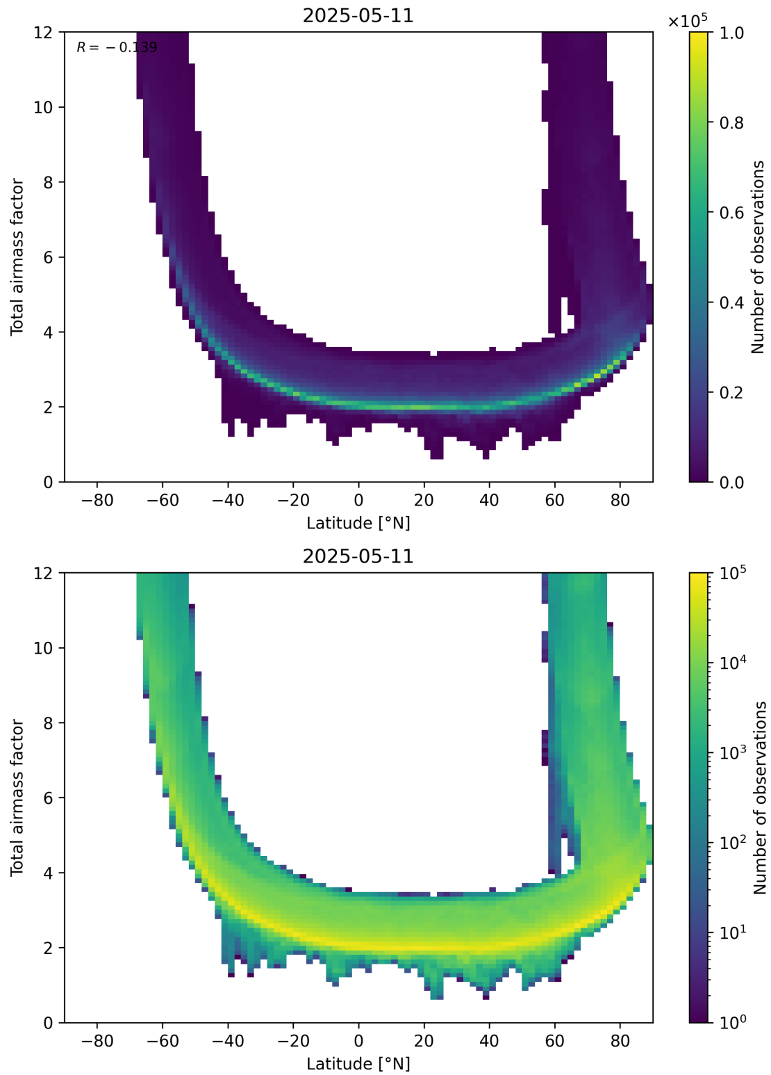
Figure 84: Scatter density plot of “Latitude” against “Total airmass factor” for 2025-05-11 to 2025-05-12.
