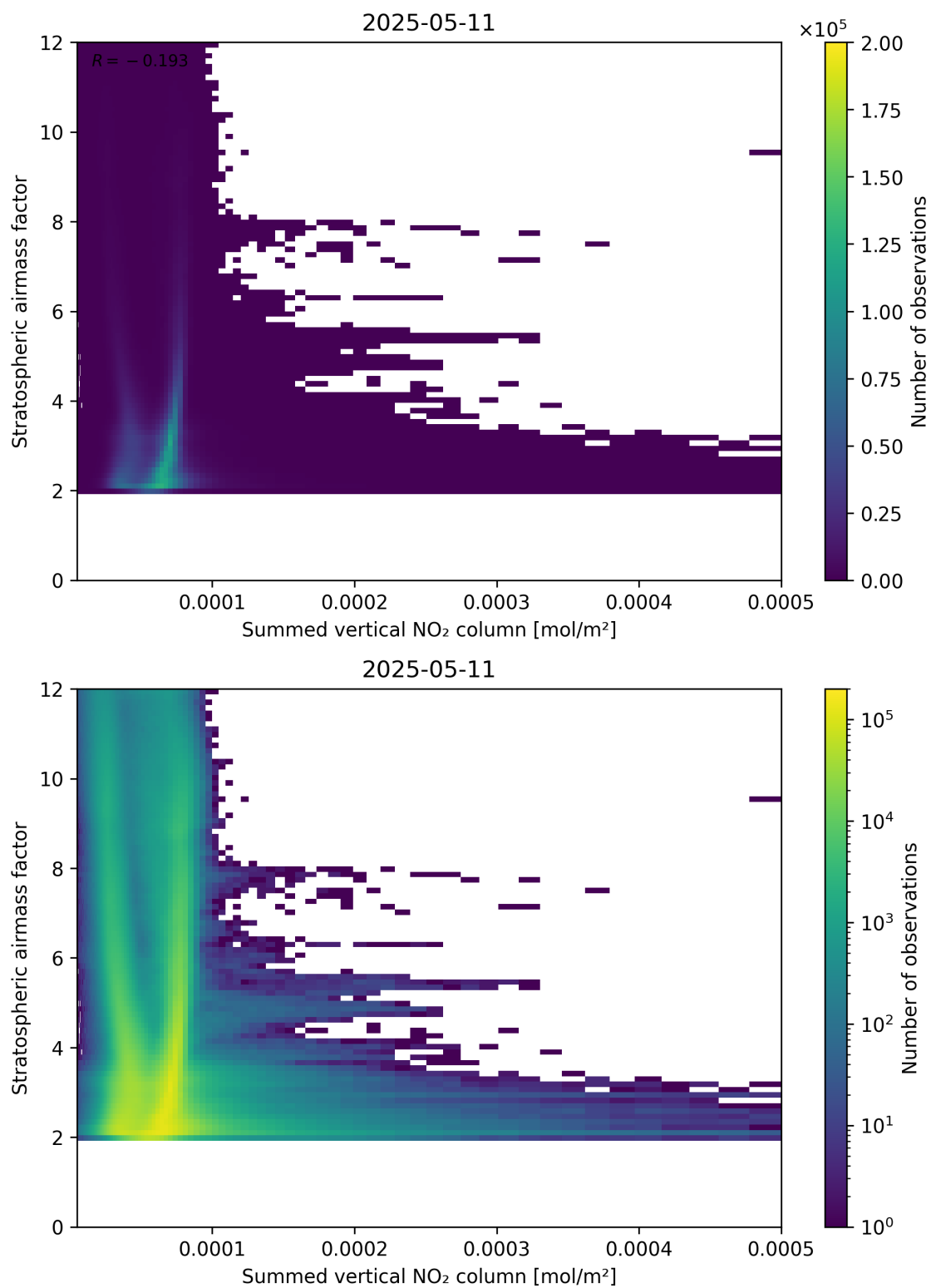
Figure 103: Scatter density plot of “Summed vertical NO 2 column” against “Stratospheric air mass factor” for 2025-05-11 to 2025-05-12.
