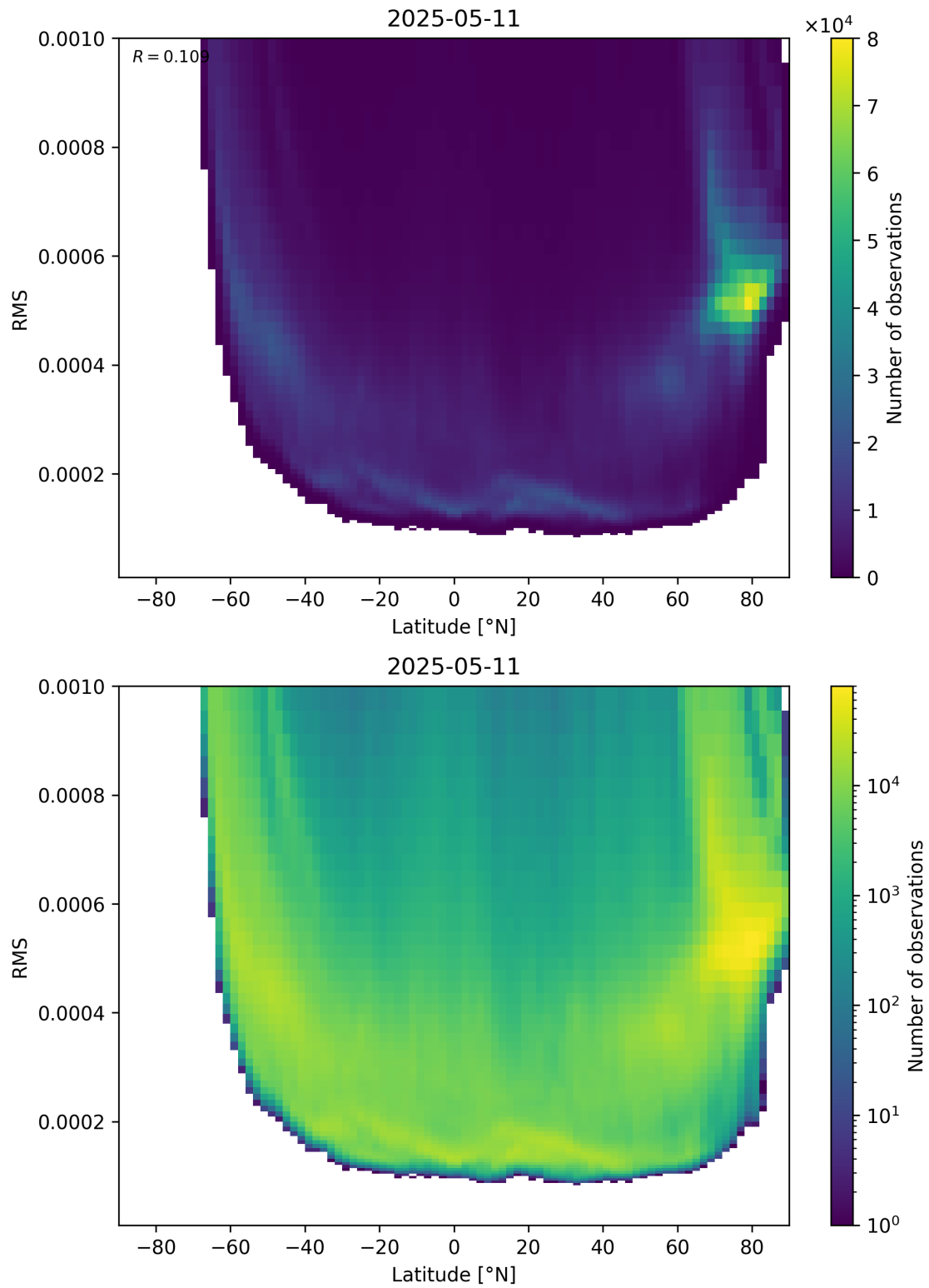
Figure 94: Scatter density plot of “Latitude” against “RMS” for 2025-05-11 to 2025-05-12.
