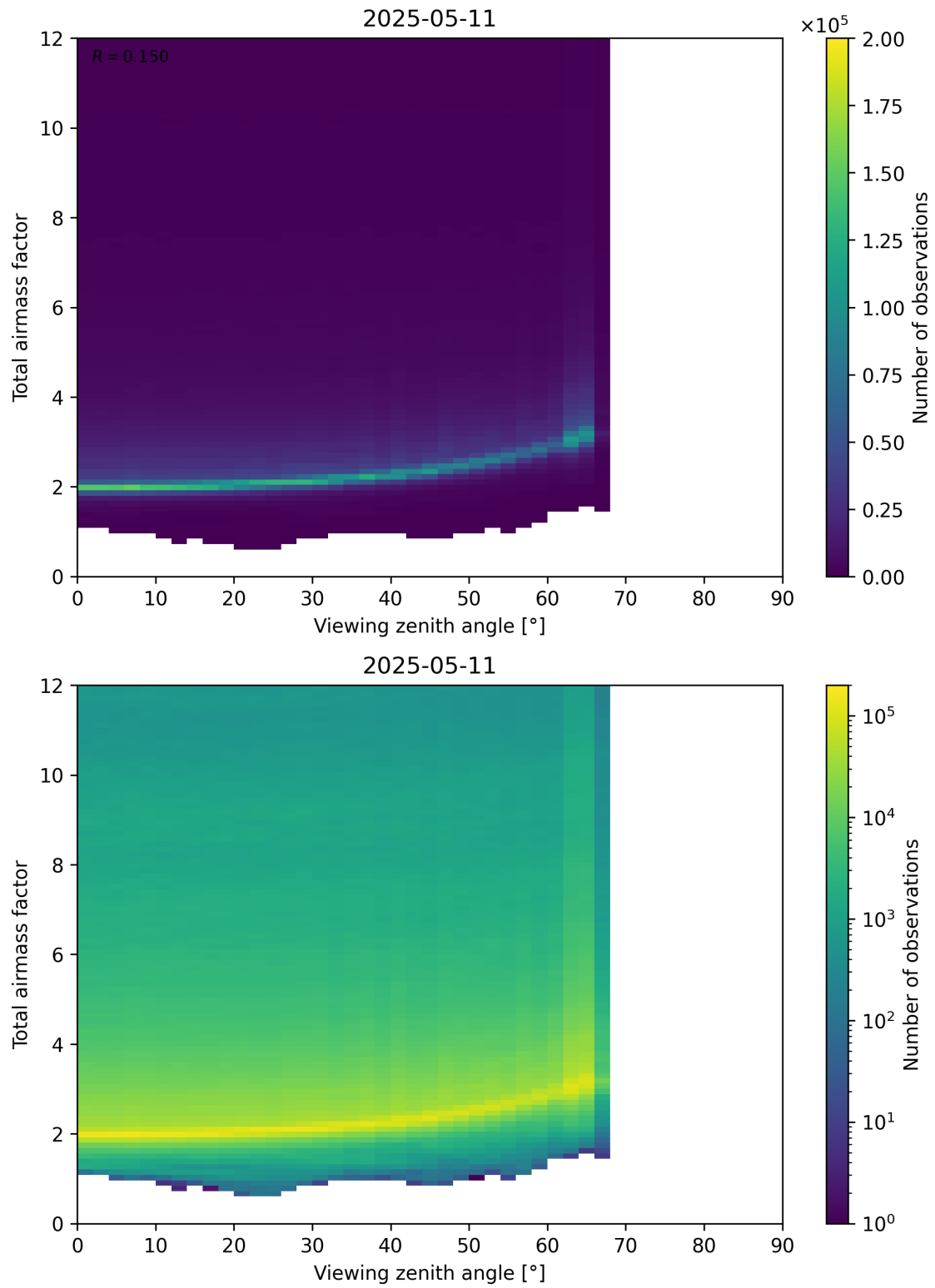
Figure 160: Scatter density plot of “Viewing zenith angle” against “Total airmass factor” for 2025-05-11 to 2025-05-12.
