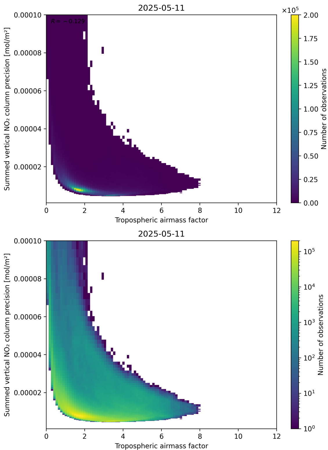
Figure 76: Scatter density plot of “Tropospheric air mass factor” against “Summed vertical NO 2 column precision” for 2025-05-11 to 2025-05-12.
