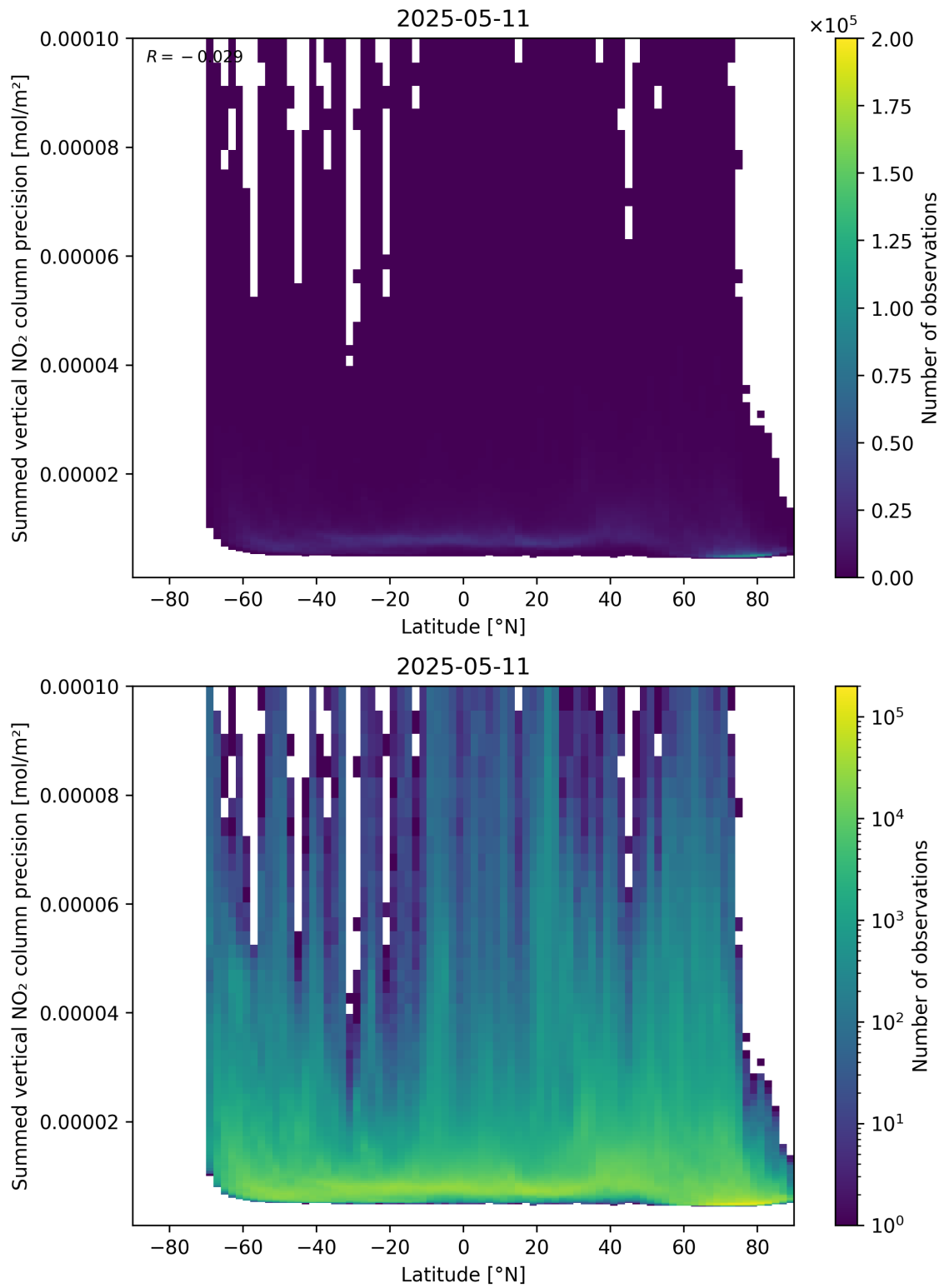
Figure 89: Scatter density plot of “Latitude” against “Summed vertical NO 2 column precision” for 2025-05-11 to 2025-05-12.
