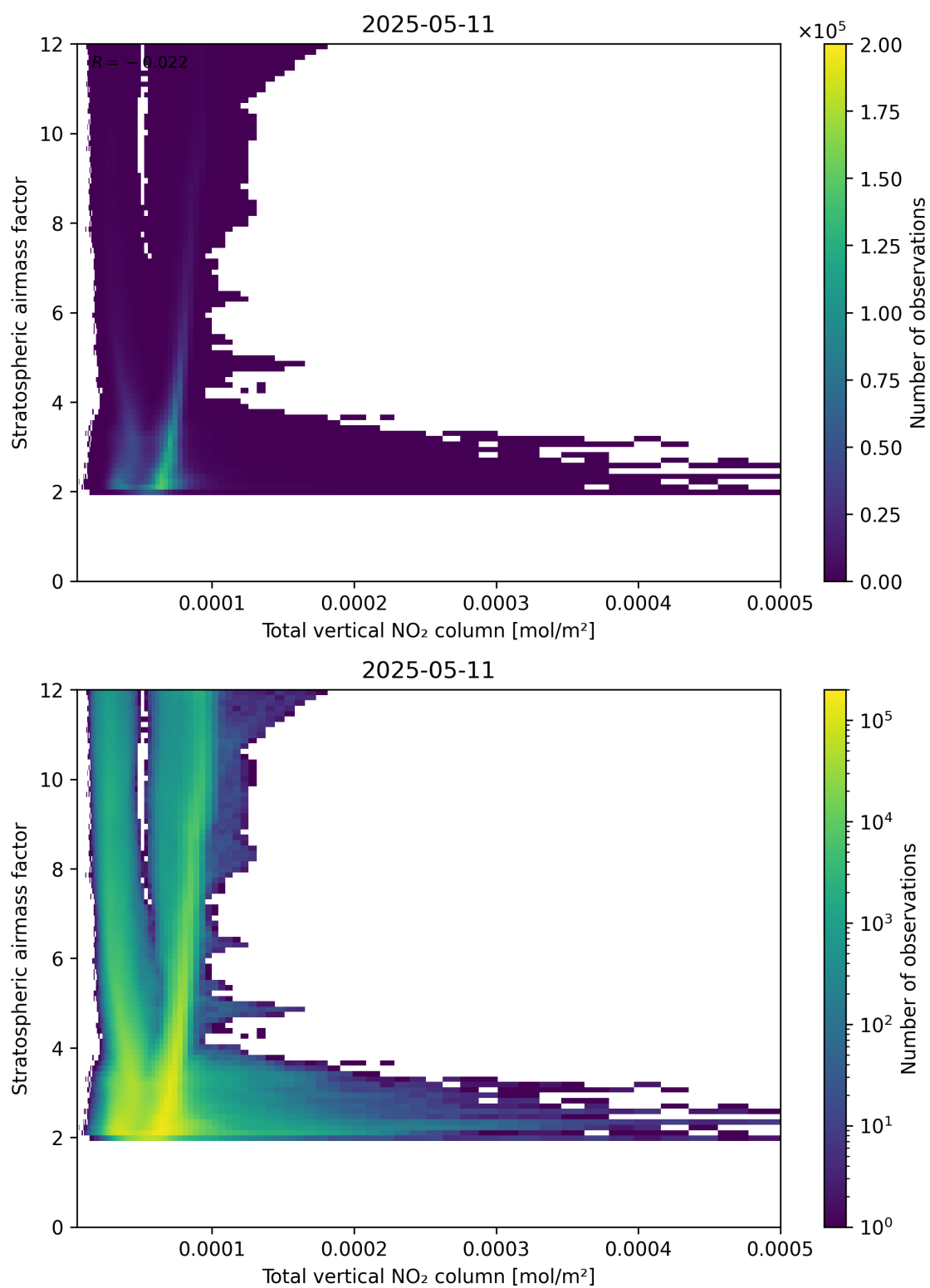
Figure 110: Scatter density plot of “Total vertical NO 2 column” against “Stratospheric airmass factor” for 2025-05-11 to 2025-05-12.
