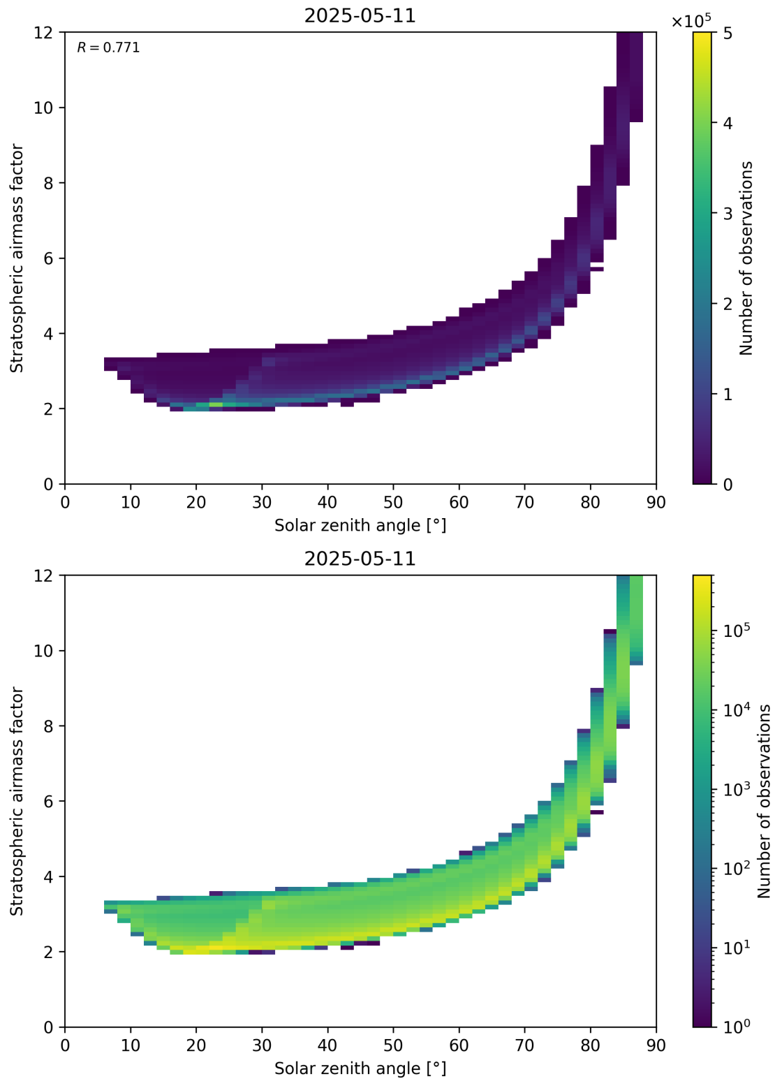
Figure 145: Scatter density plot of “Solar zenith angle” against “Stratospheric airmass factor” for 2025-05-11 to 2025-05-12.
