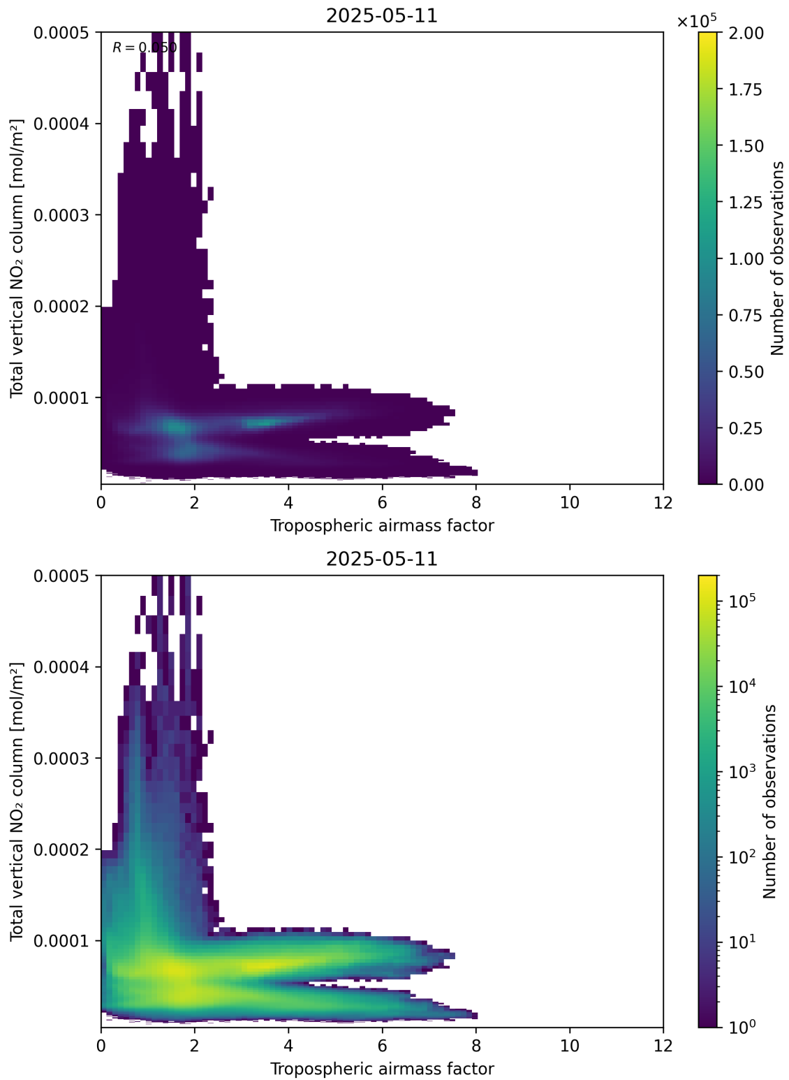
Figure 77: Scatter density plot of “Tropospheric airmass factor” against “Total vertical NO 2 column” for 2025-05-11 to 2025-05-12.
