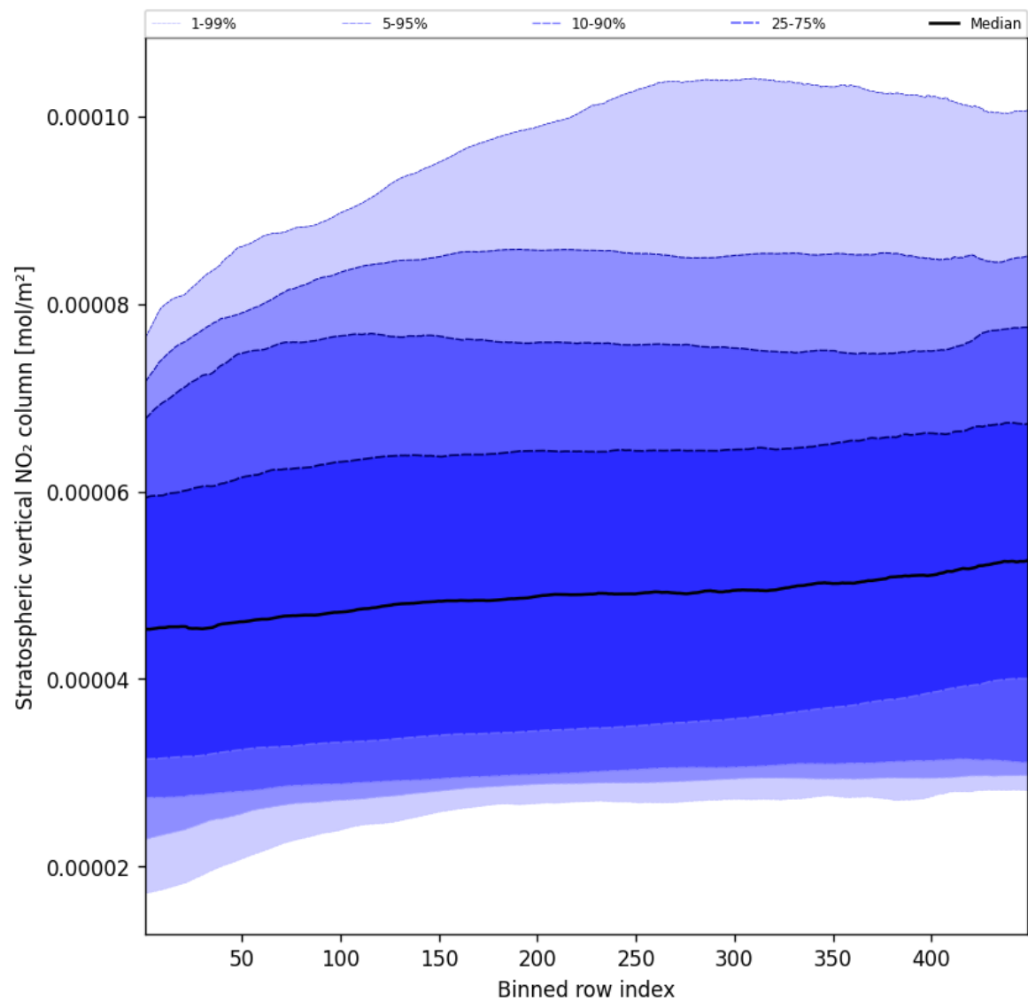
Figure 53: Along track statistics of “Stratospheric vertical NO 2 column” for 2025-05-11 to 2025-05-12
