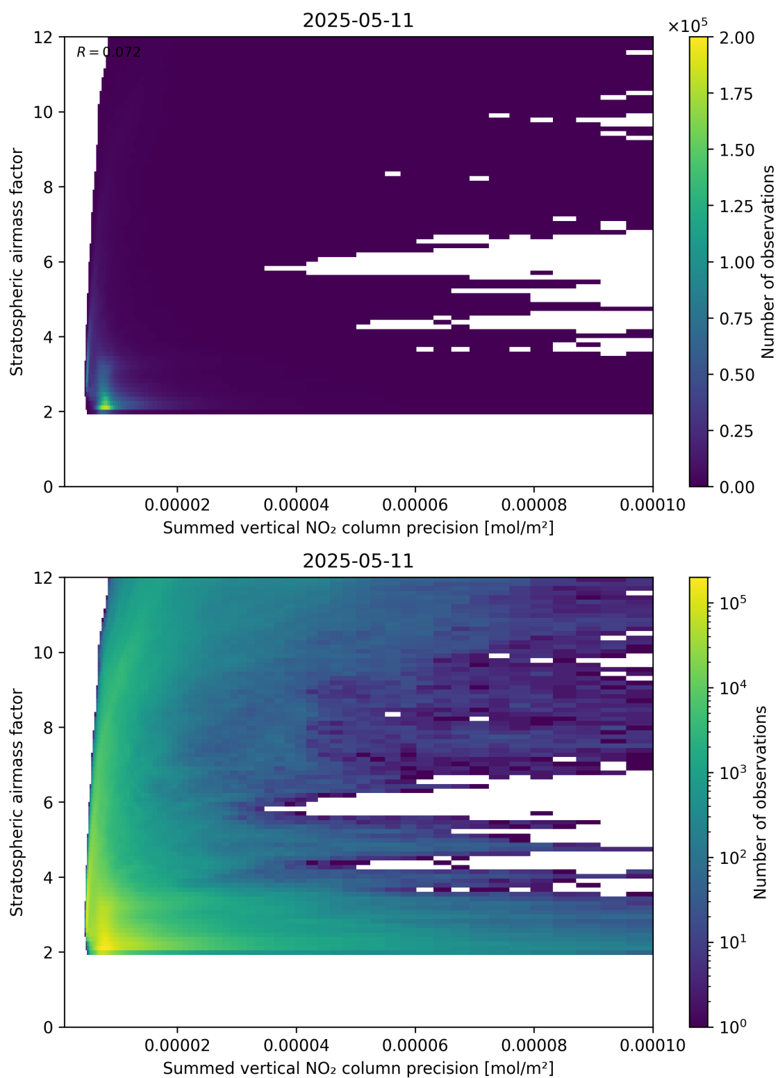
Figure 106: Scatter density plot of “Summed vertical NO 2 column precision” against “Stratospheric airmass factor” for 2025-05-11 to 2025-05-12.
