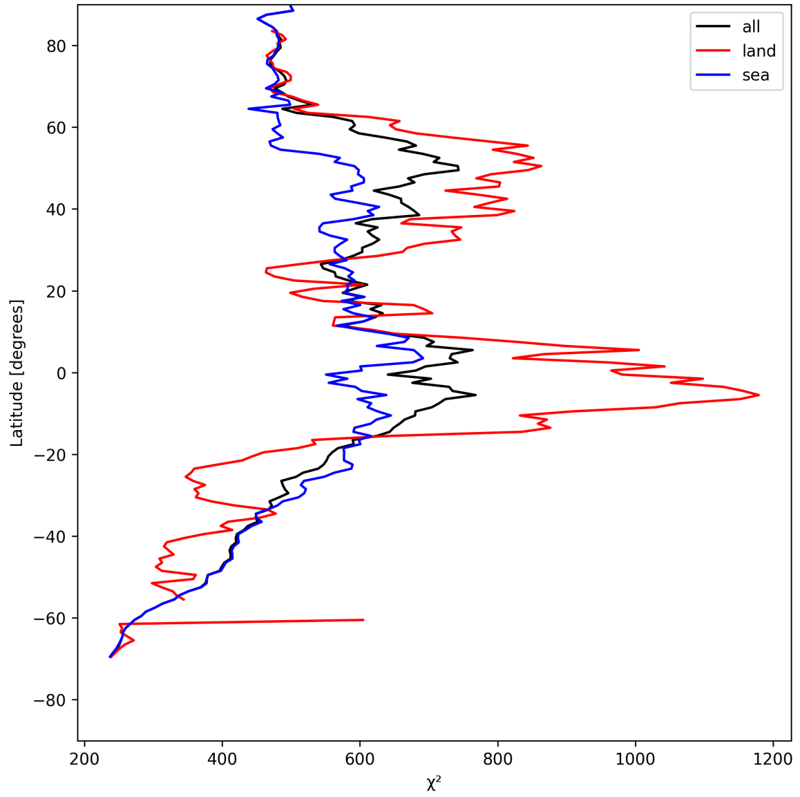
Figure 25: Zonal average of “ \chi^2 ” for 2025-05-11 to 2025-05-12.
