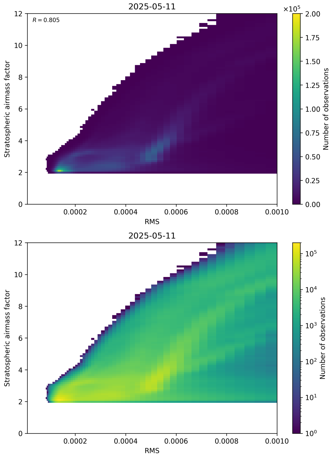
Figure 144: Scatter density plot of “RMS” against “Stratospheric airmass factor” for 2025-05-11 to 2025-05-12.
