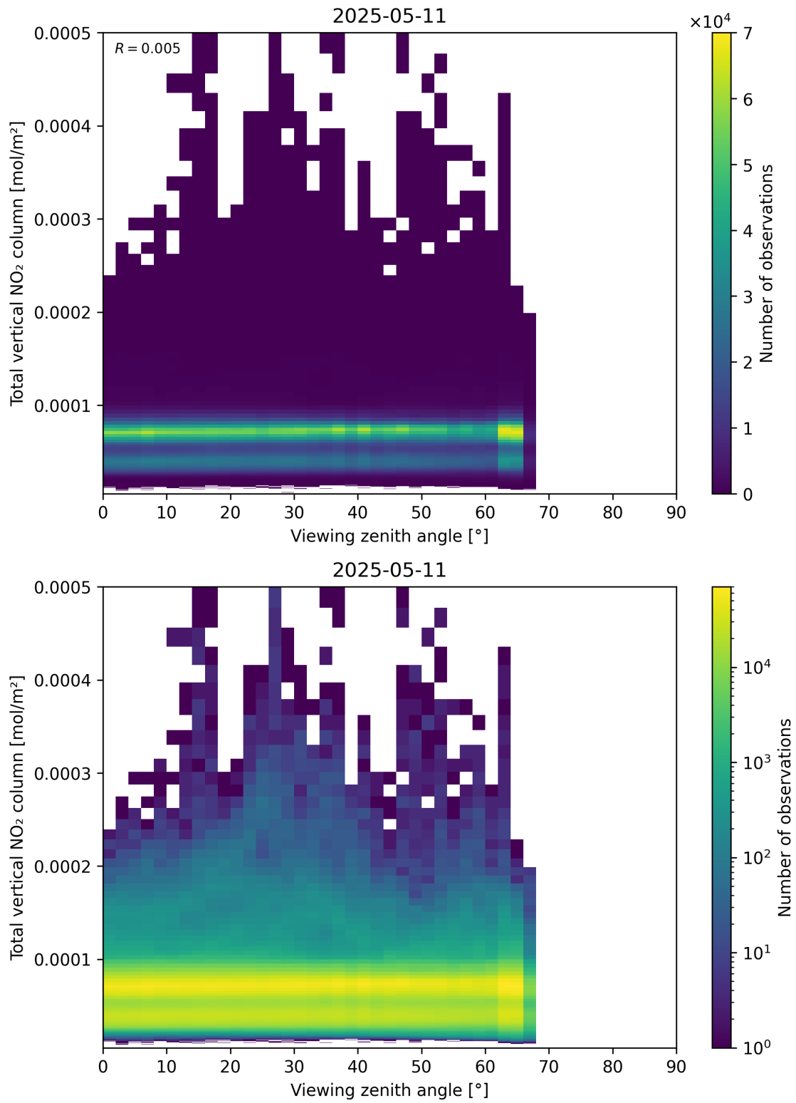
Figure 167: Scatter density plot of “Viewing zenith angle” against “Total vertical NO 2 column” for 2025-05-11 to 2025-05-12.
