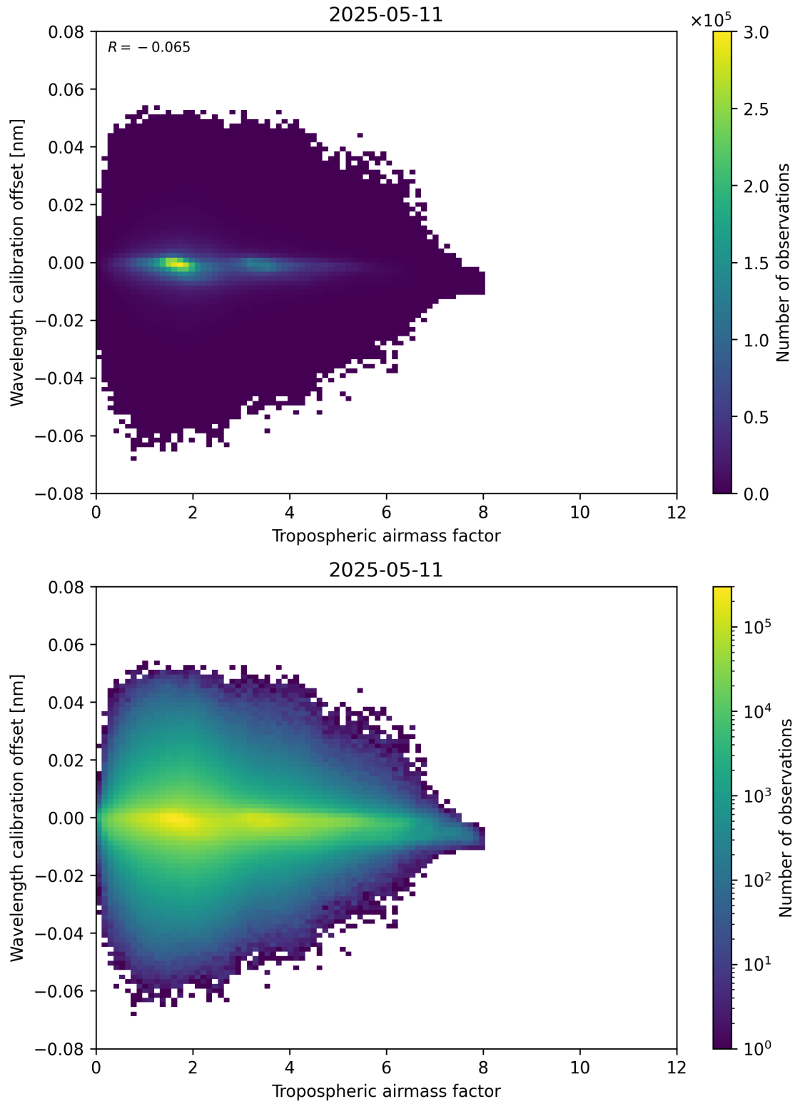
Figure 80: Scatter density plot of “Tropospheric airmass factor” against “Wavelength calibration offset” for 2025-05-11 to 2025-05-12.
