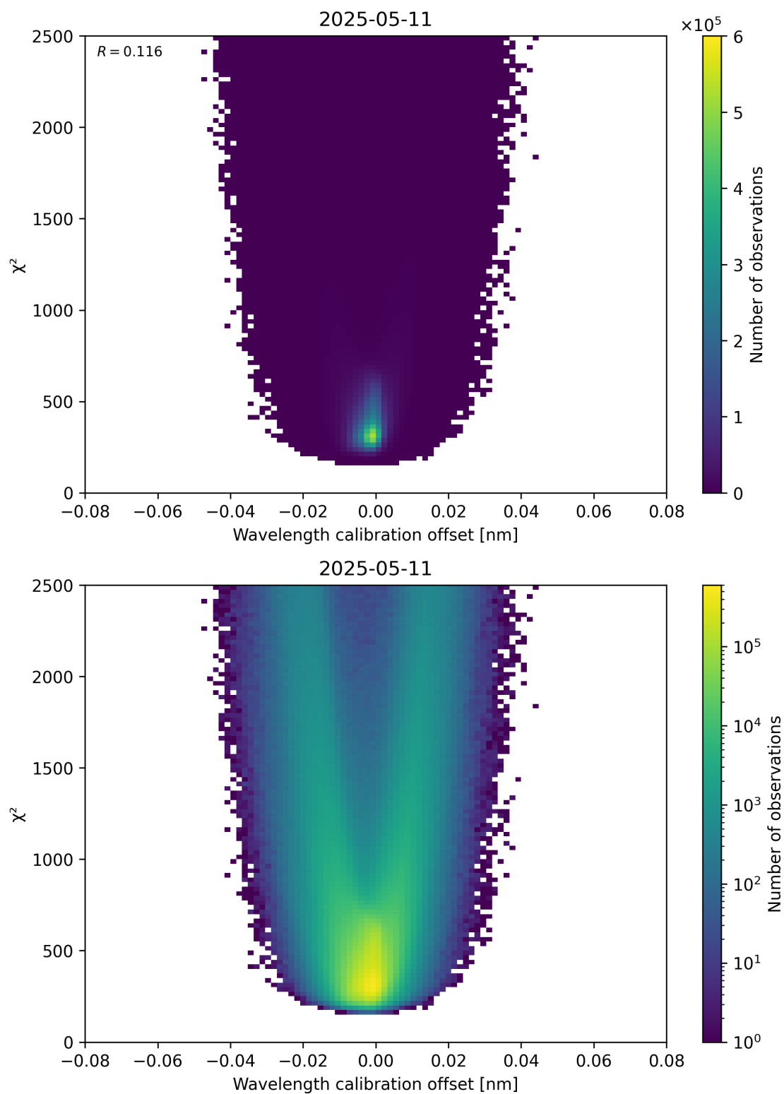
Figure 175: Scatter density plot of “Wavelength calibration offset” against “ \chi^2 ” for 2025-05-11 to 2025-05-12.
