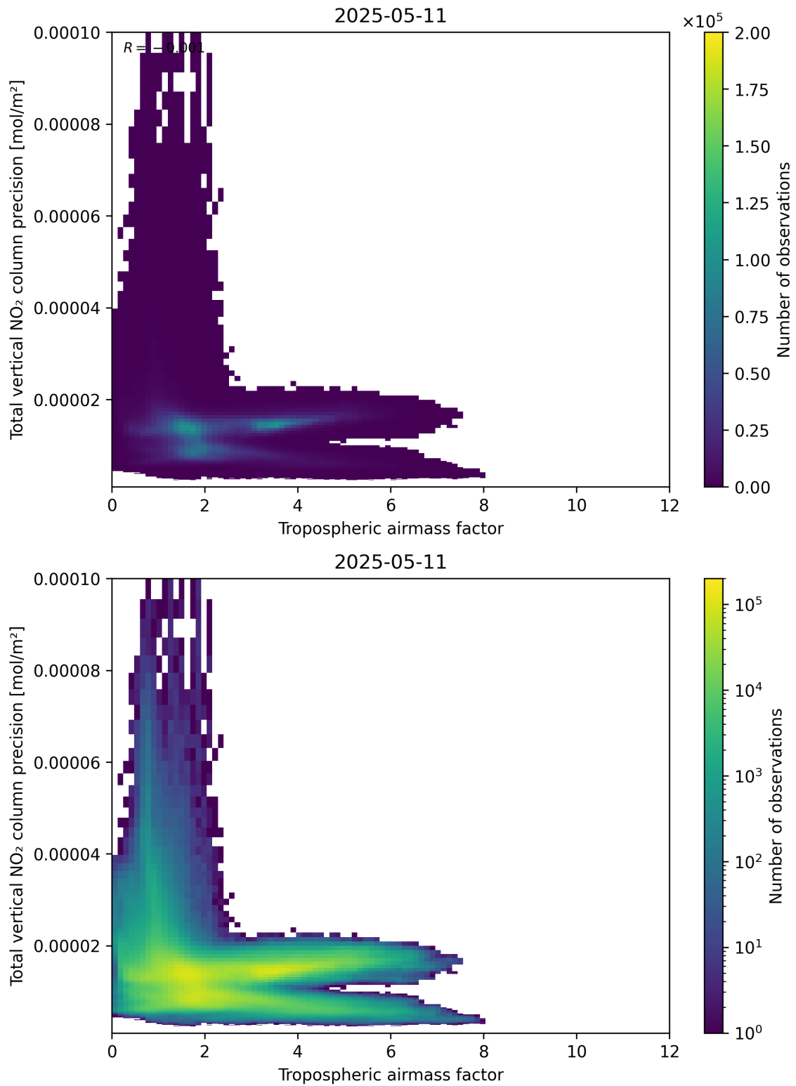
Figure 78: Scatter density plot of “Tropospheric air mass factor” against “Total vertical NO 2 column precision” for 2025-05-11 to 2025-05-12.
