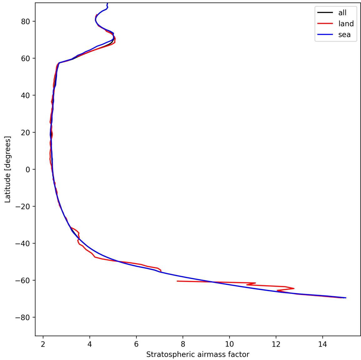
Figure 27: Zonal average of “Stratospheric airmass factor” for 2025-05-11 to 2025-05-12.
