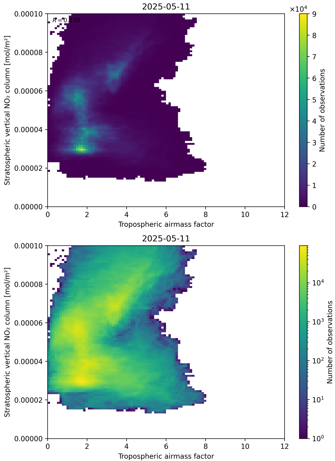
Figure 74: Scatter density plot of “Tropospheric airmass factor” against “Stratospheric vertical NO 2 column” for 2025-05-11 to 2025-05-12.
