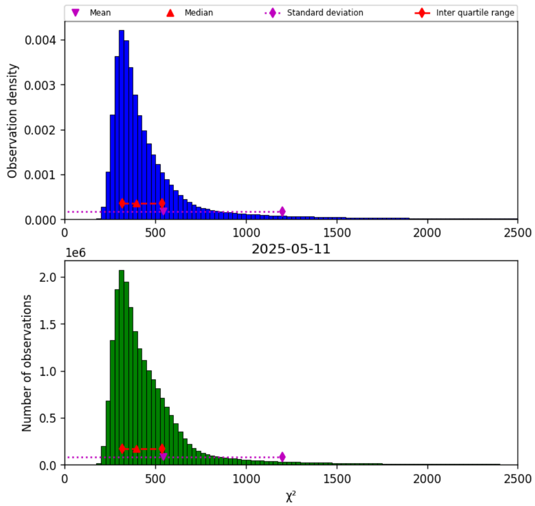
Figure 42: Histogram of “ \chi^2 ” for 2025-05-11 to 2025-05-12
