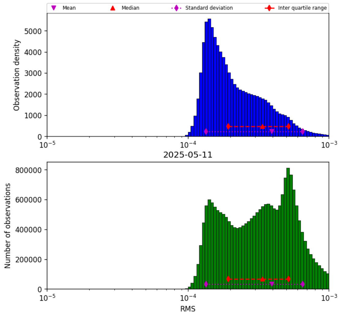
Figure 43: Histogram of “RMS” for 2025-05-11 to 2025-05-12
