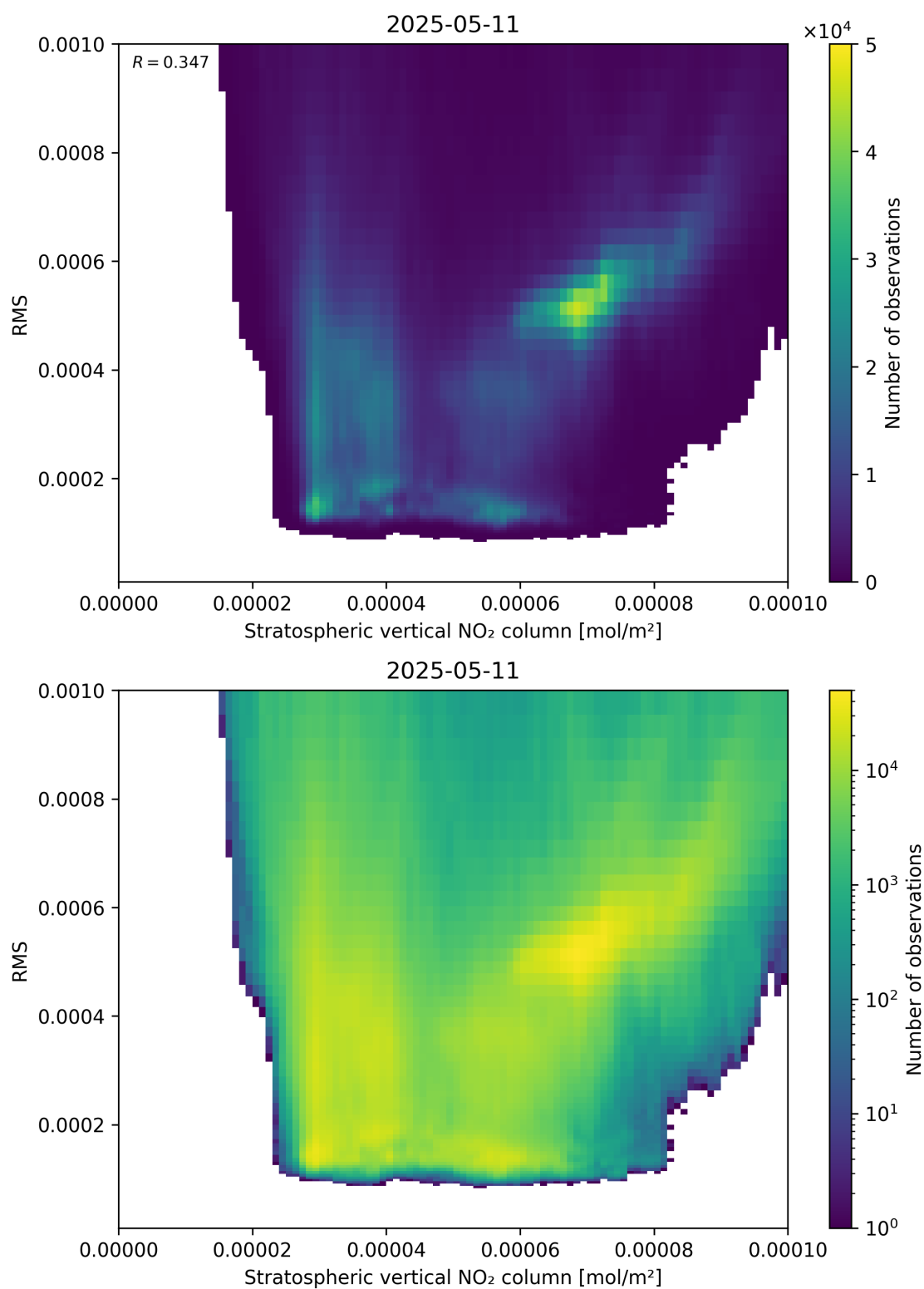
Figure 102: Scatter density plot of “Stratospheric vertical NO 2 column” against “RMS” for 2025-05-11 to 2025-05-12.
