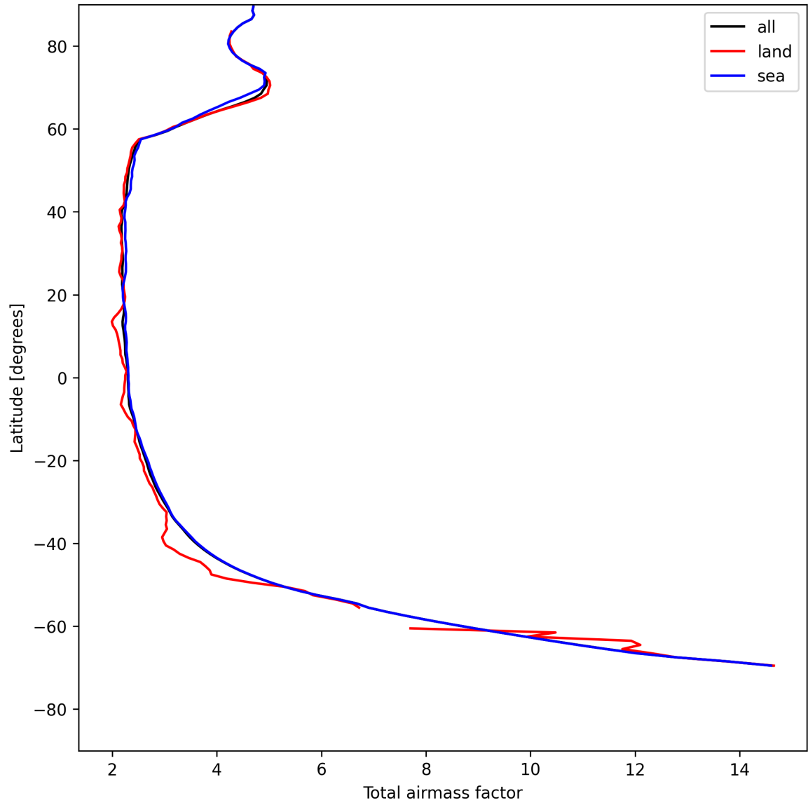
Figure 15: Zonal average of “Total airmass factor” for 2025-05-11 to 2025-05-12.
