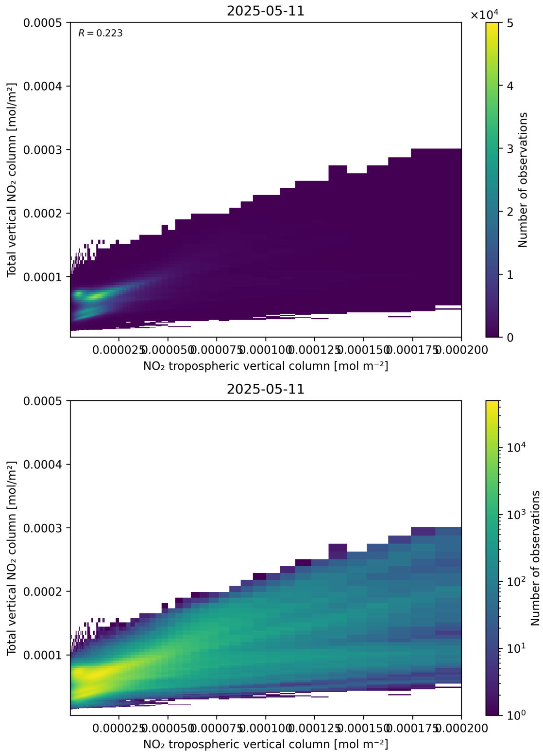
Figure 128: Scatter density plot of “NO 2 tropospheric vertical column” against “Total vertical NO 2 column” for 2025-05-11 to 2025-05-12.
