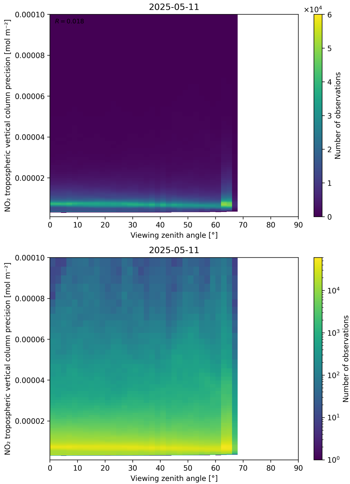
Figure 170: Scatter density plot of “Viewing zenith angle” against “NO 2 tropospheric vertical column precision” for 2025-05-11 to 2025-05-12.
