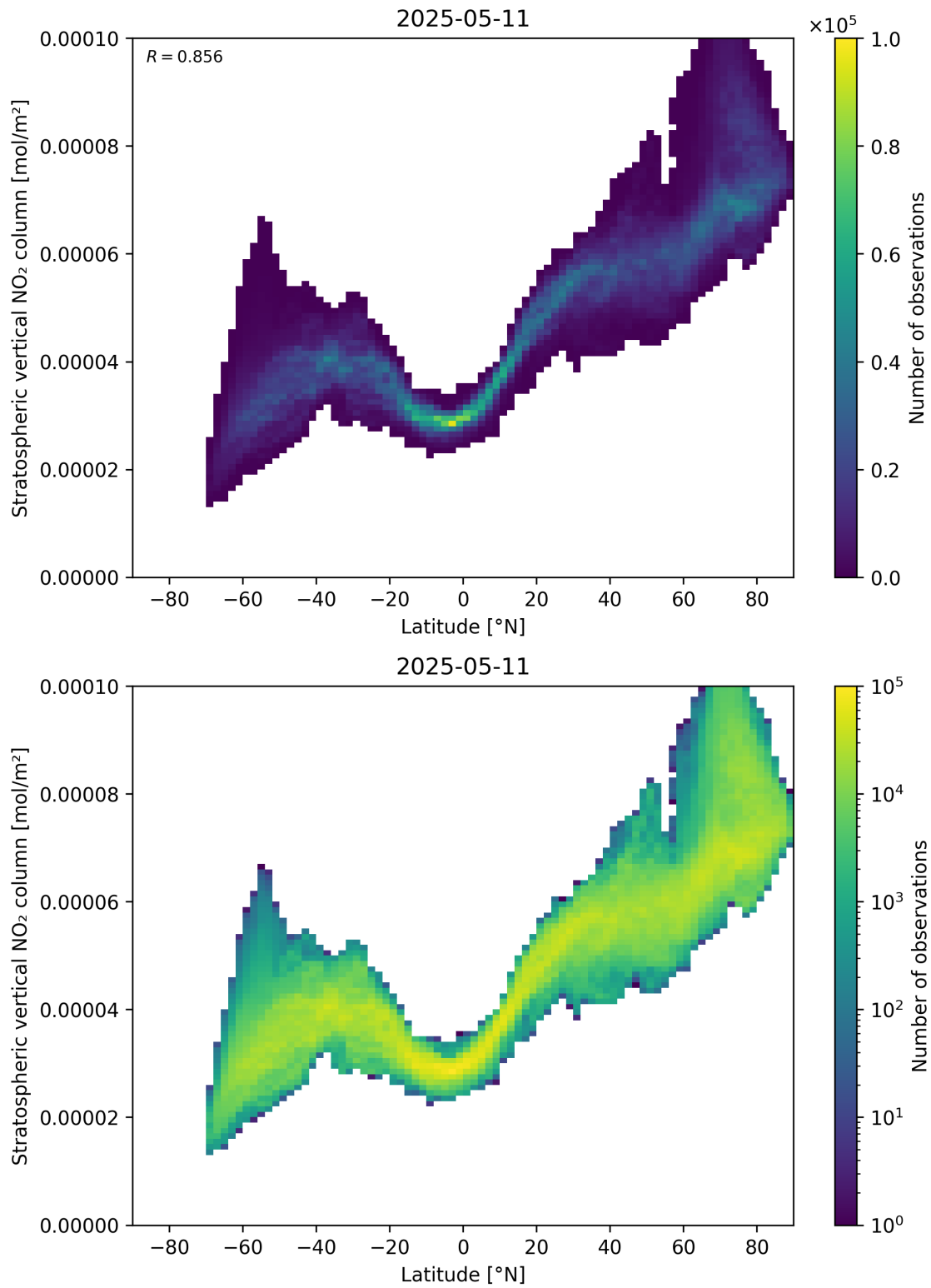
Figure 87: Scatter density plot of “Latitude” against “Stratospheric vertical NO 2 column” for 2025-05-11 to 2025-05-12.
