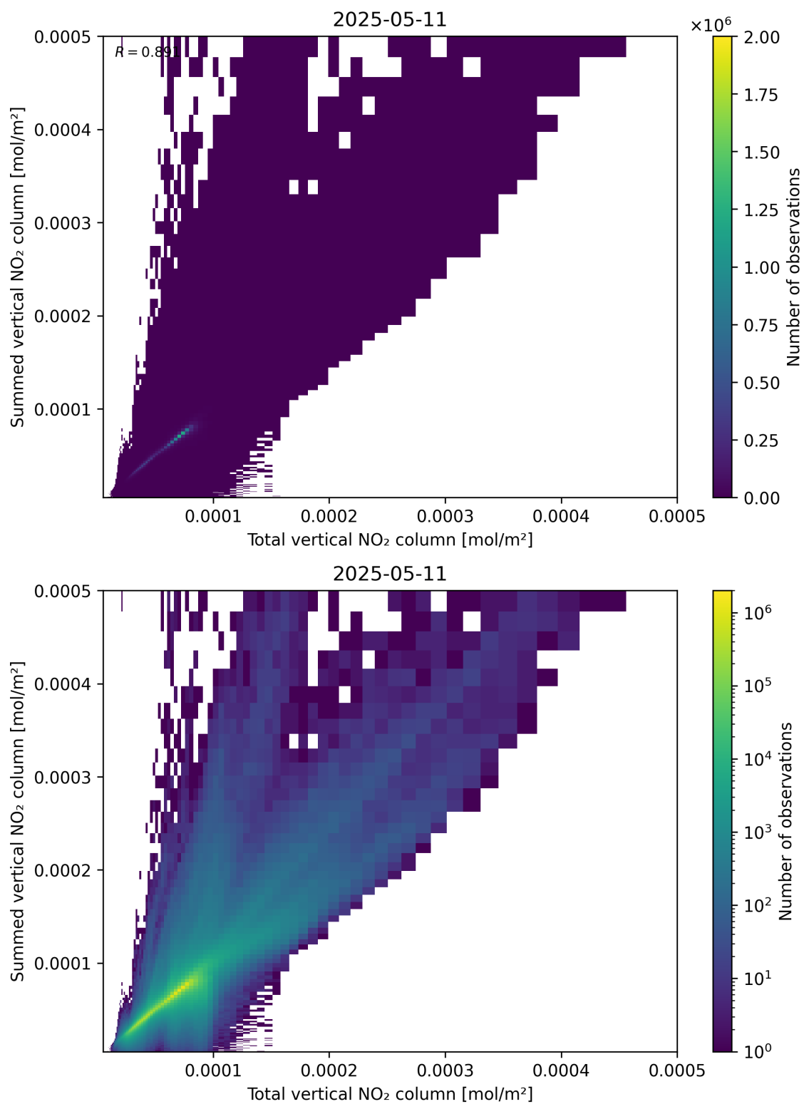
Figure 112: Scatter density plot of “Total vertical NO 2 column” against “Summed vertical NO 2 column” for 2025-05-11 to 2025-05-12.
