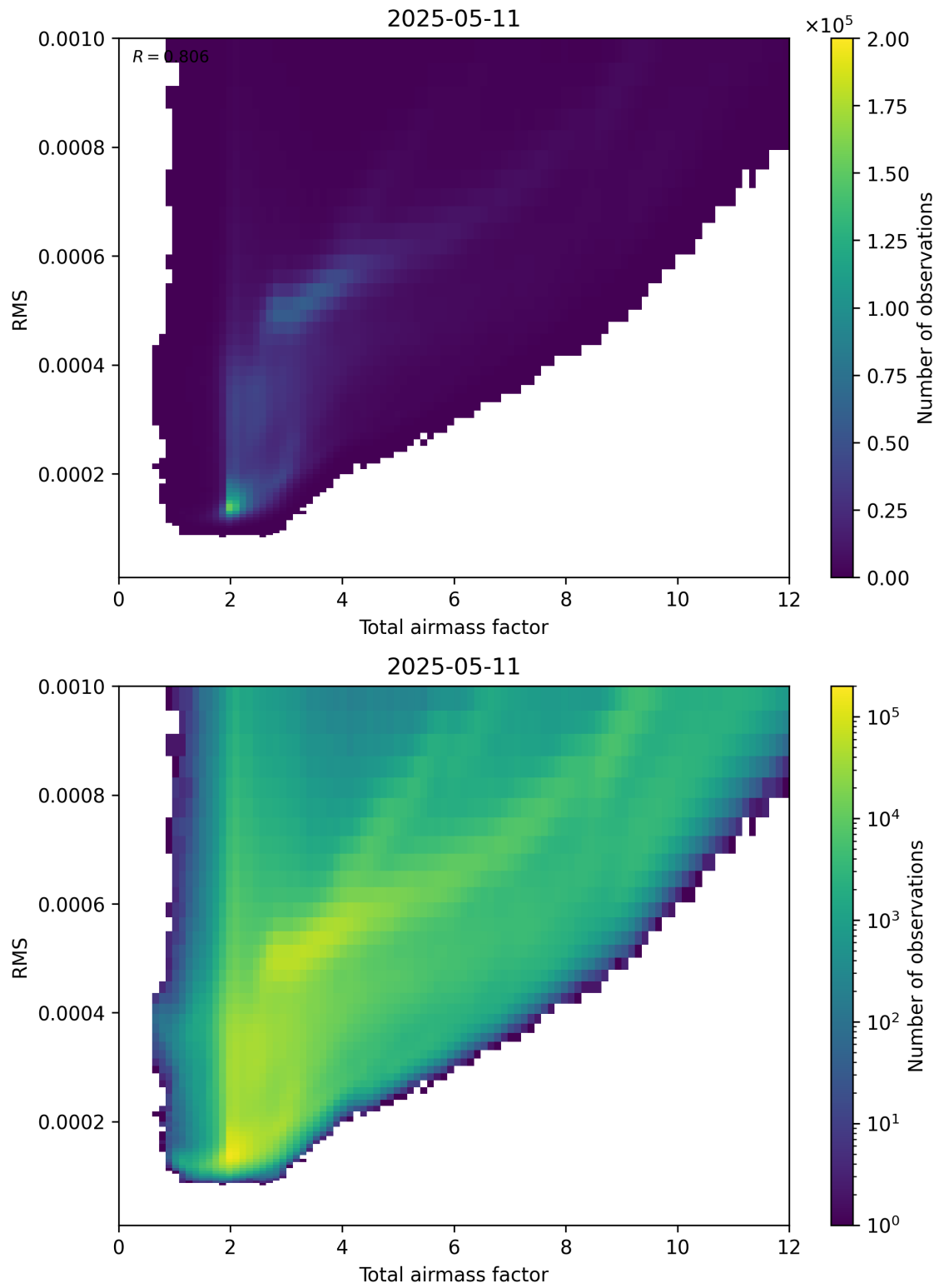
Figure 69: Scatter density plot of “Total airmass factor” against “RMS” for 2025-05-11 to 2025-05-12.
