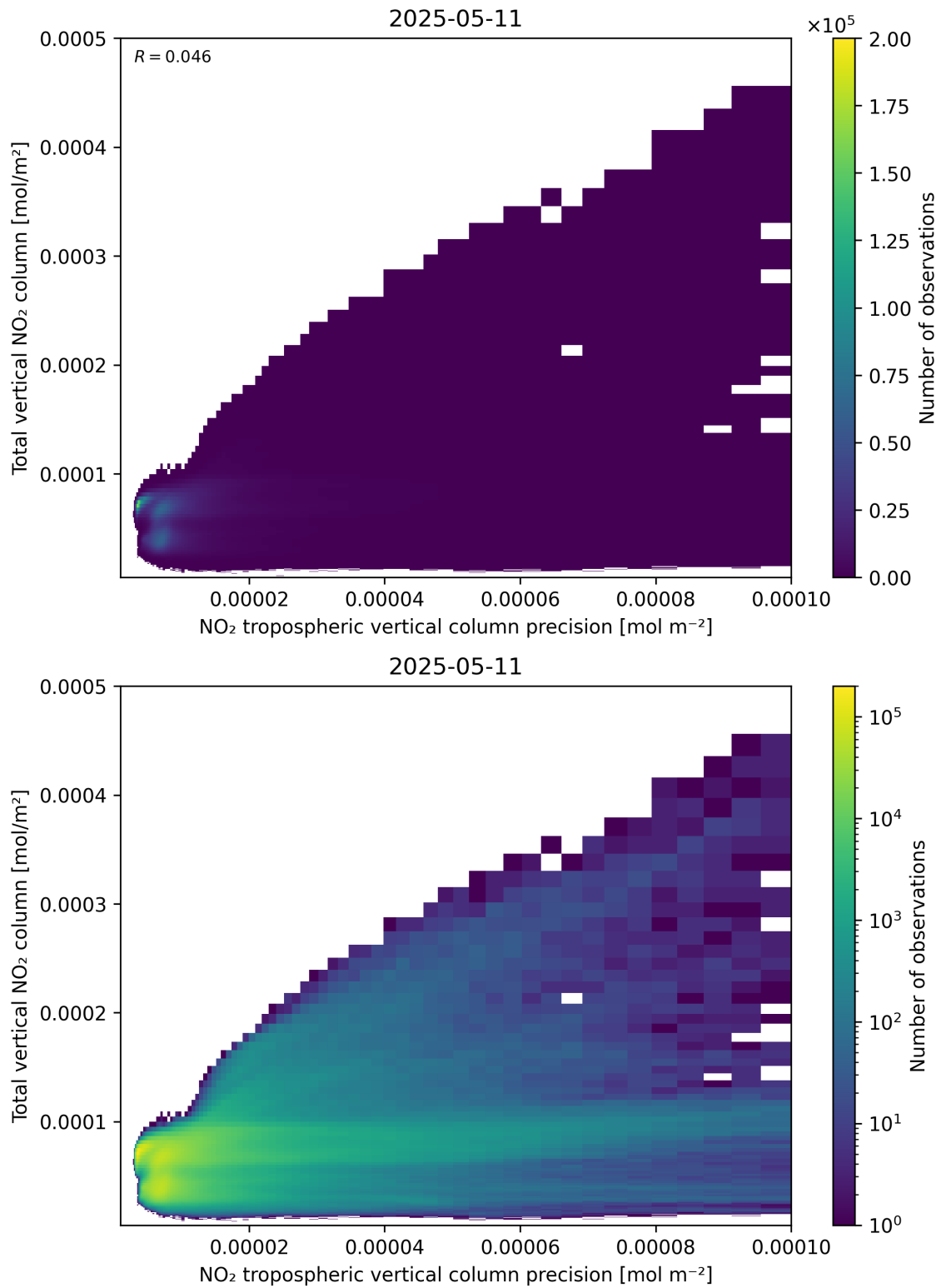
Figure 138: Scatter density plot of “NO 2 tropospheric vertical column precision” against “Total vertical NO 2 column” for 2025-05-11 to 2025-05-12.
