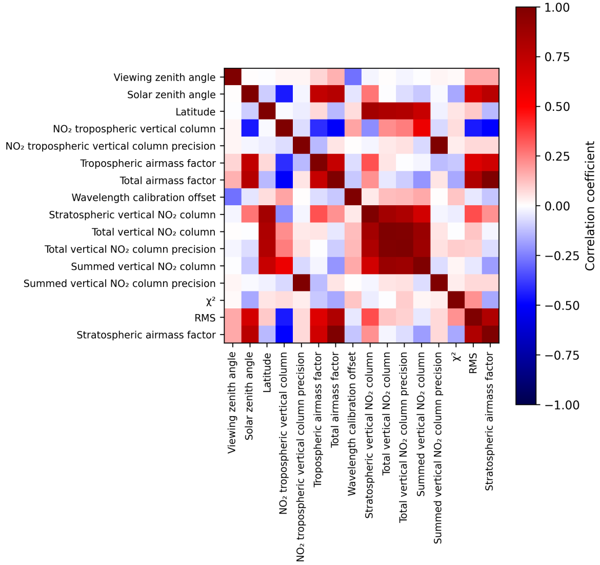
Figure 2: Map of correlation matrix for 2025-05-11 to 2025-05-12.
