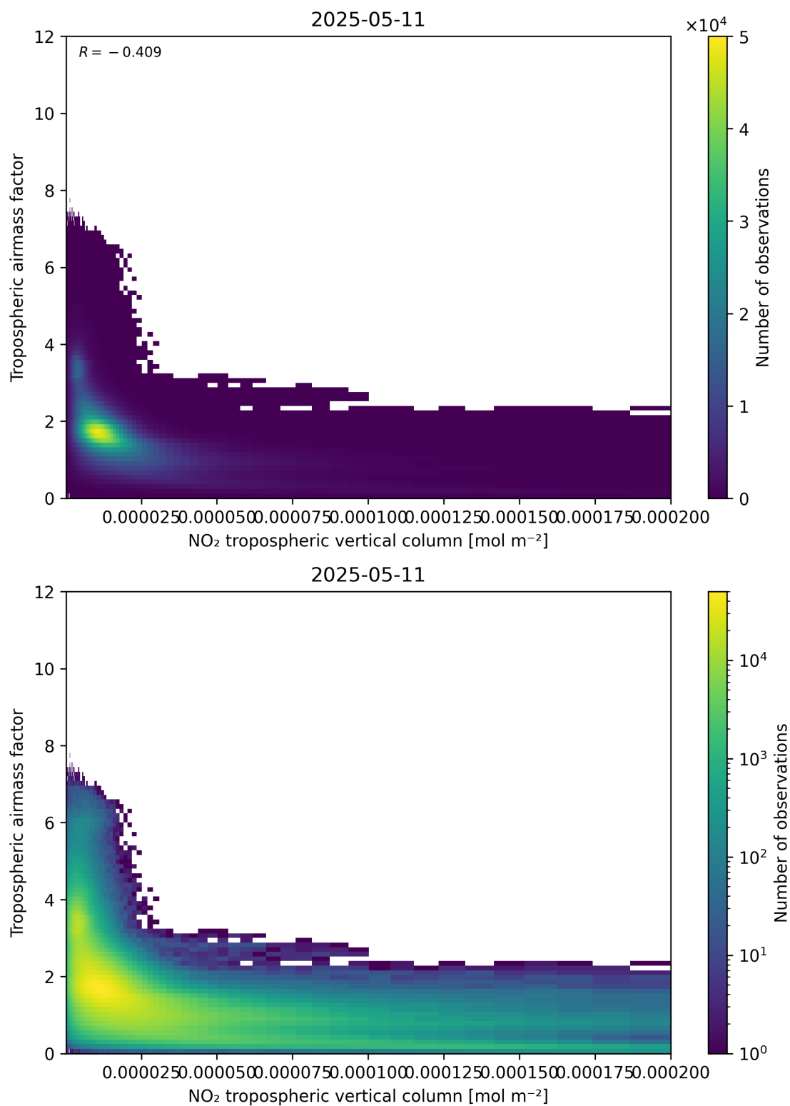
Figure 123: Scatter density plot of “NO 2 tropospheric vertical column” against “Tropospheric air mass factor” for 2025-05-11 to 2025-05-12.
