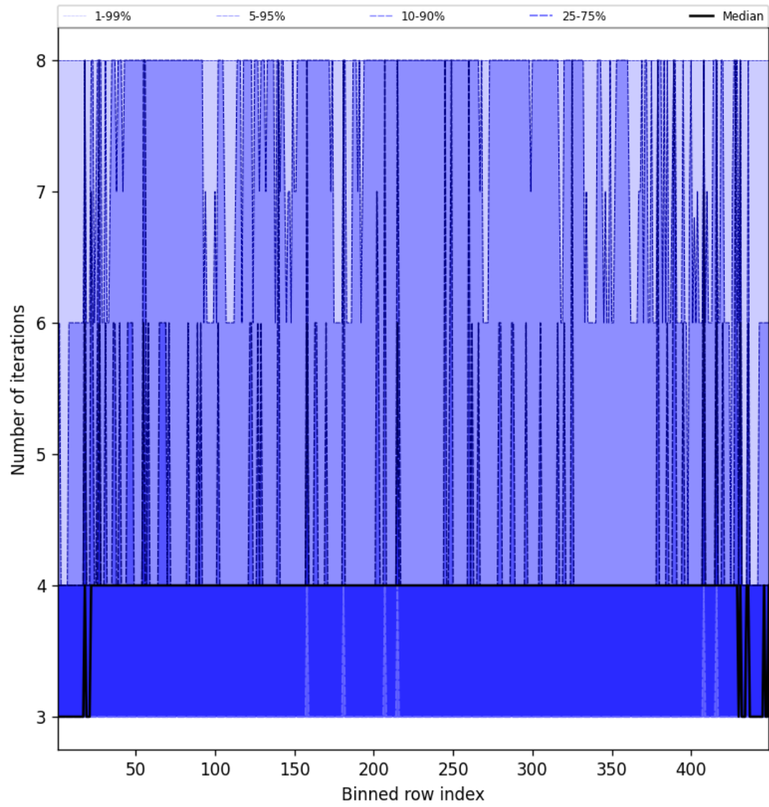
Figure 51: Along track statistics of “Number of iterations” for 2025-05-11 to 2025-05-12
