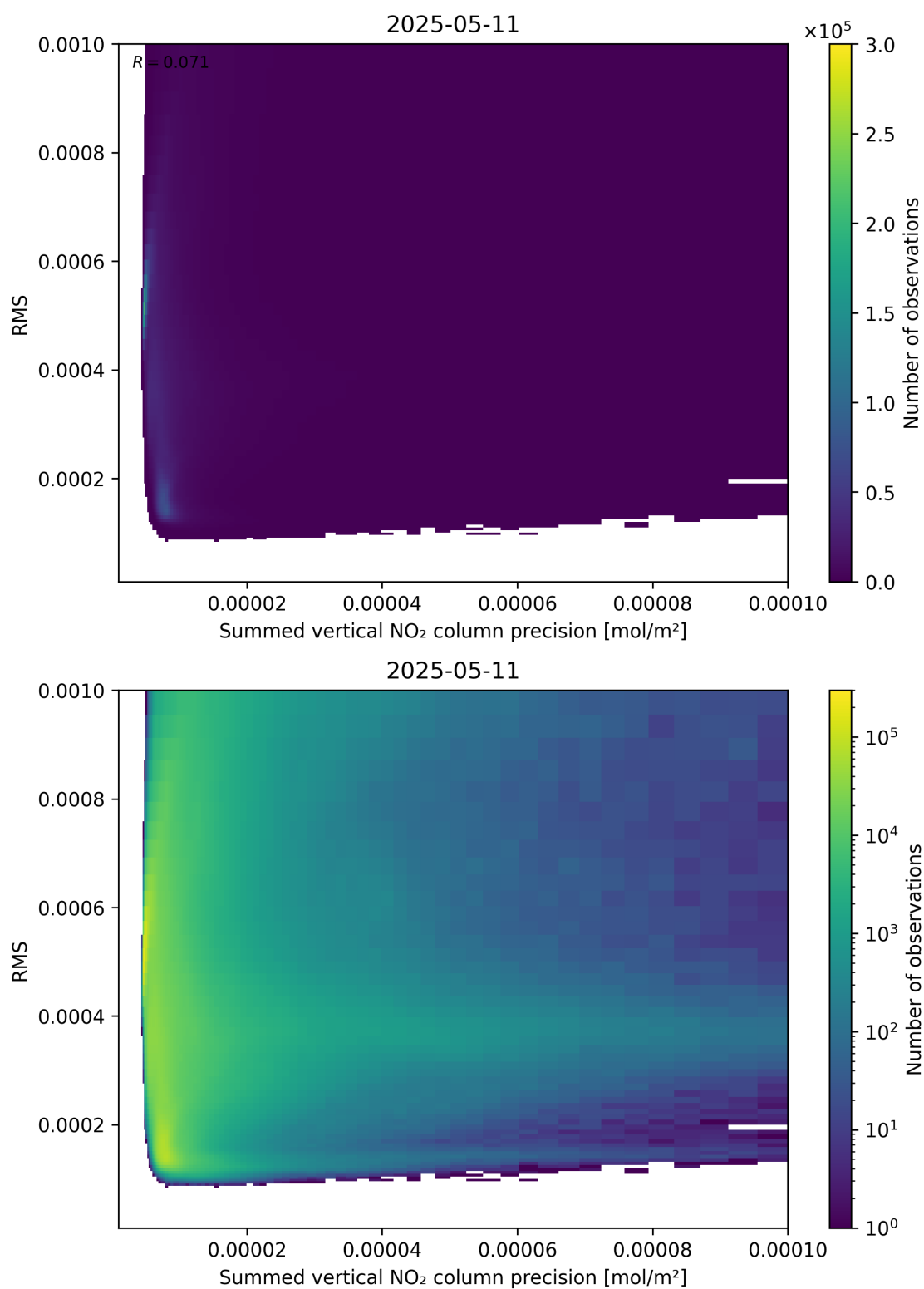
Figure 108: Scatter density plot of “Summed vertical NO 2 column precision” against “RMS” for 2025-05-11 to 2025-05-12.
