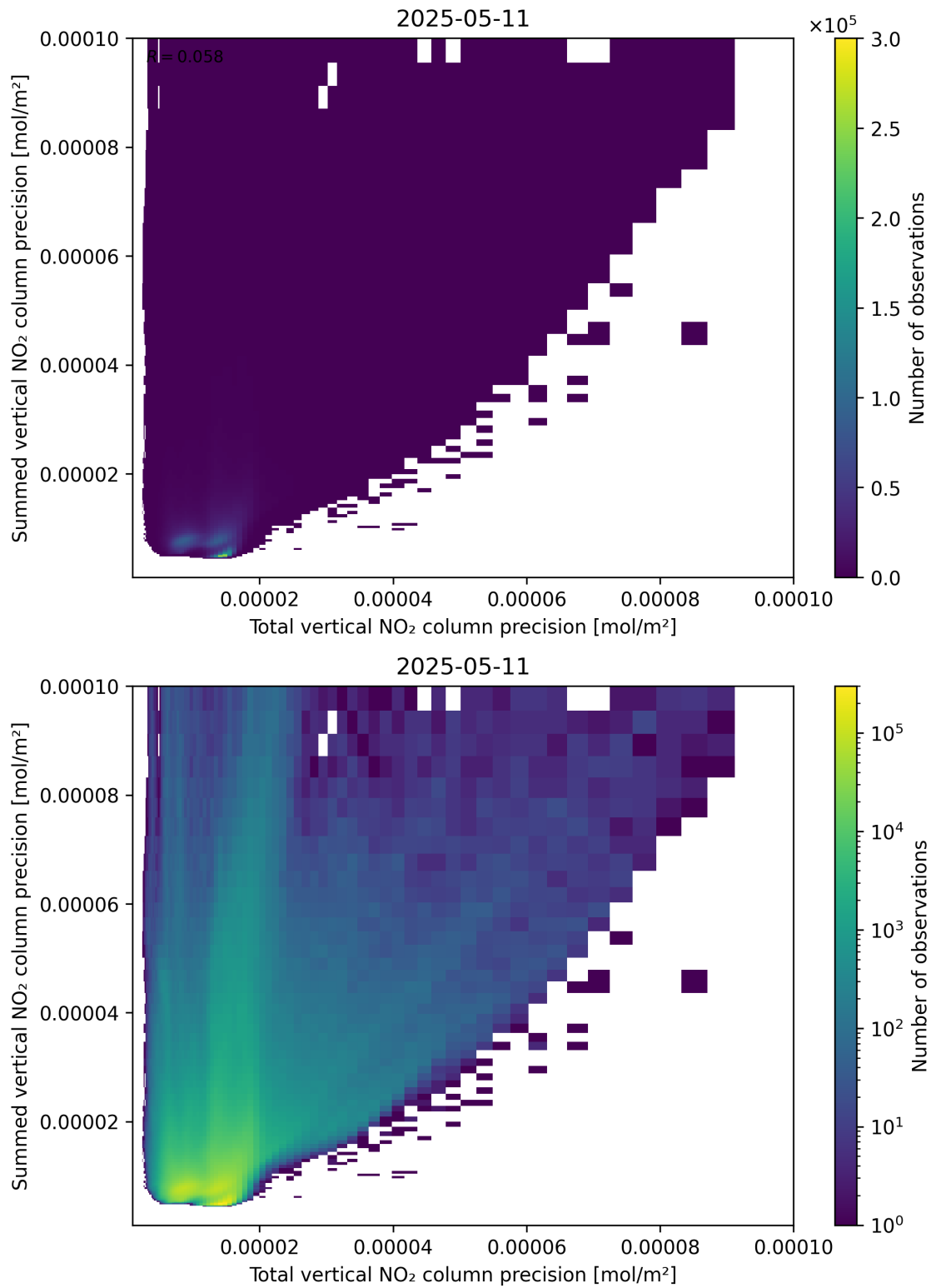
Figure 118: Scatter density plot of “Total vertical NO 2 column precision” against “Summed vertical NO 2 column precision” for 2025-05-11 to 2025-05-12.
