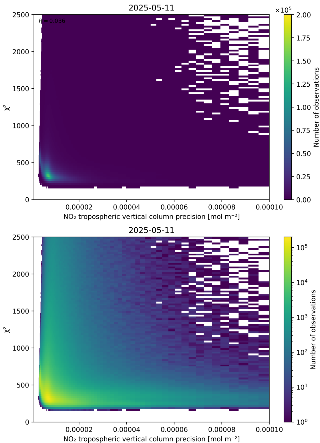
Figure 134: Scatter density plot of “NO 2 tropospheric vertical column precision” against “ \chi^2 ” for 2025-05-11 to 2025-05-12.
