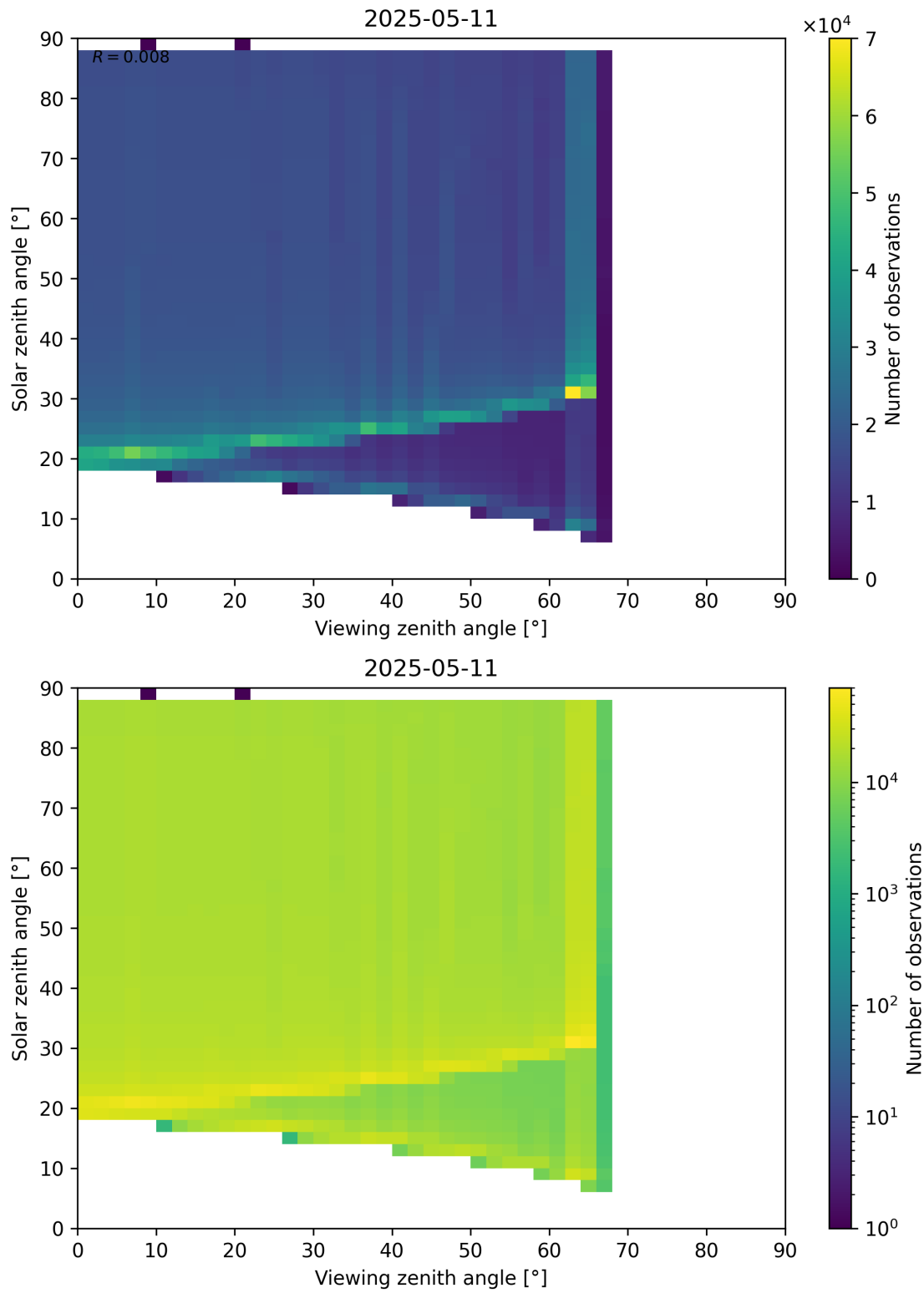
Figure 172: Scatter density plot of “Viewing zenith angle” against “Solar zenith angle” for 2025-05-11 to 2025-05-12.
