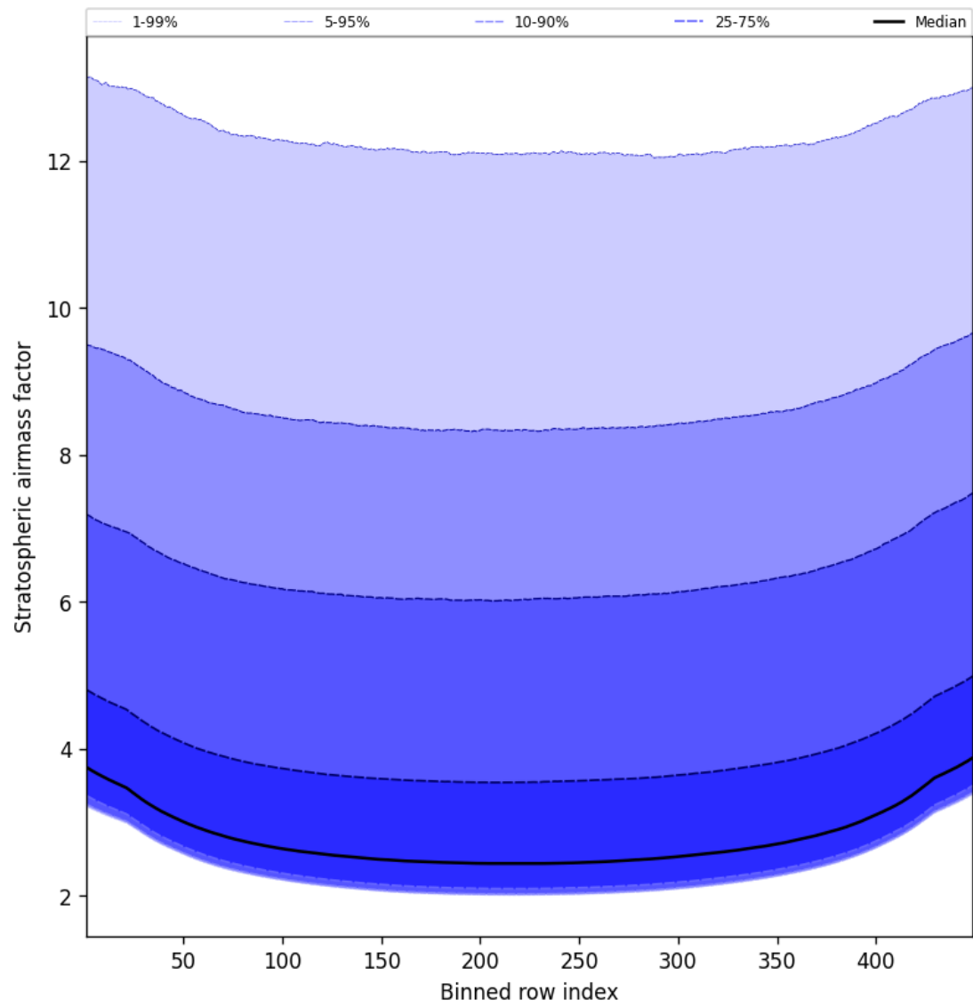
Figure 61: Along track statistics of “Stratospheric airmass factor” for 2025-05-11 to 2025-05-12
