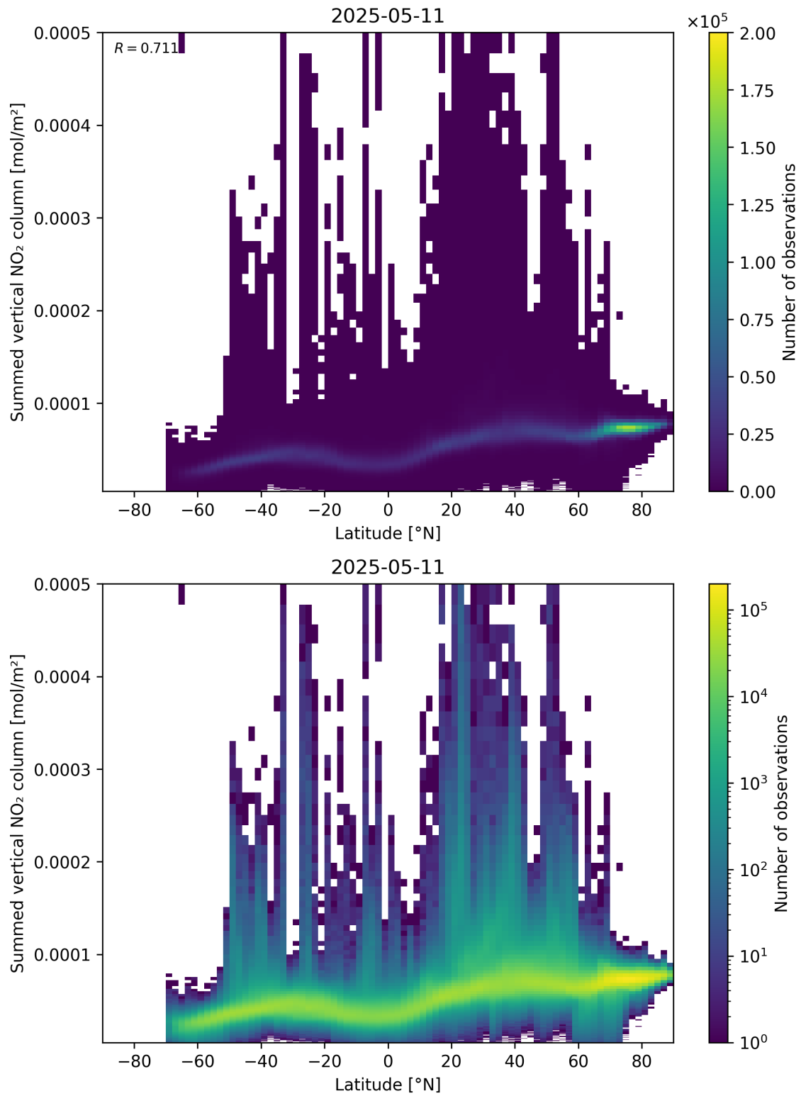
Figure 88: Scatter density plot of “Latitude” against “Summed vertical NO 2 column” for 2025-05-11 to 2025-05-12.
