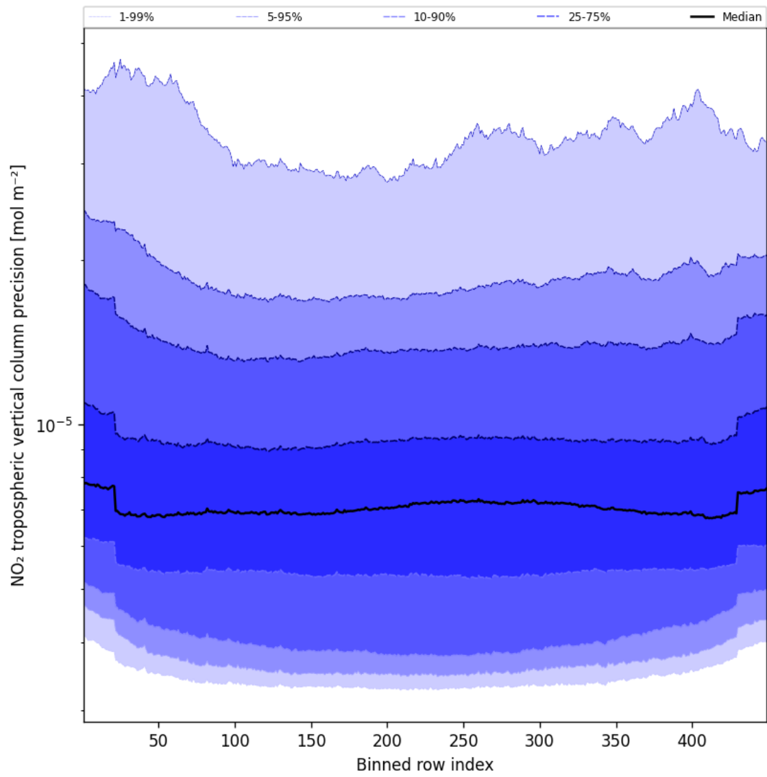
Figure 47: Along track statistics of “NO 2 tropospheric vertical column precision” for 2025-05-11 to 2025-05-12
