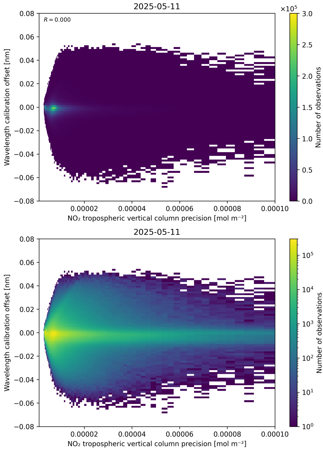
Figure 141: Scatter density plot of “NO 2 tropospheric vertical column precision” against “Wavelength calibration offset” for 2025-05-11 to 2025-05-12.
