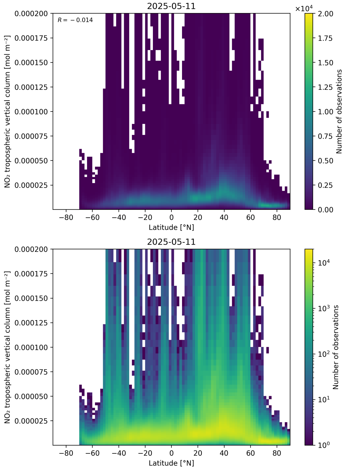
Figure 92: Scatter density plot of “Latitude” against “NO 2 tropospheric vertical column” for 2025-05-11 to 2025-05-12.
