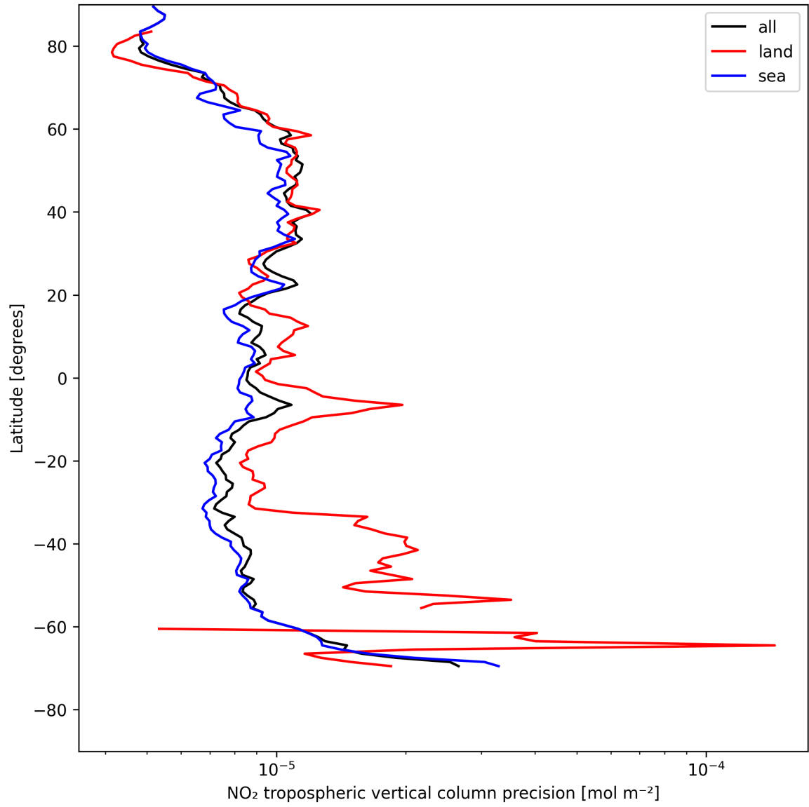
Figure 13: Zonal average of “NO 2 tropospheric vertical column precision” for 2025-05-11 to 2025-05-12.
