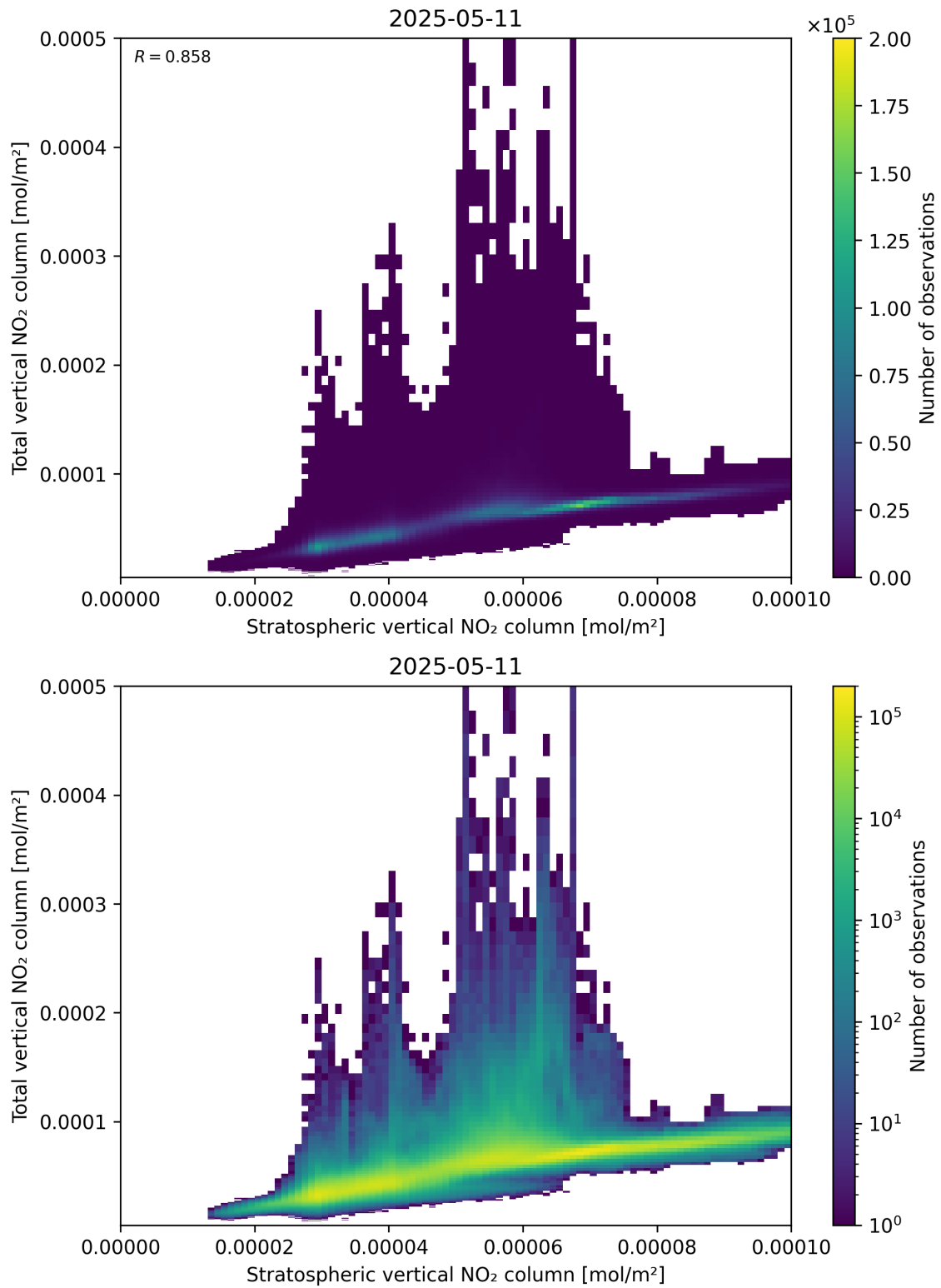
Figure 100: Scatter density plot of “Stratospheric vertical NO 2 column” against “Total vertical NO 2 column” for 2025-05-11 to 2025-05-12.
