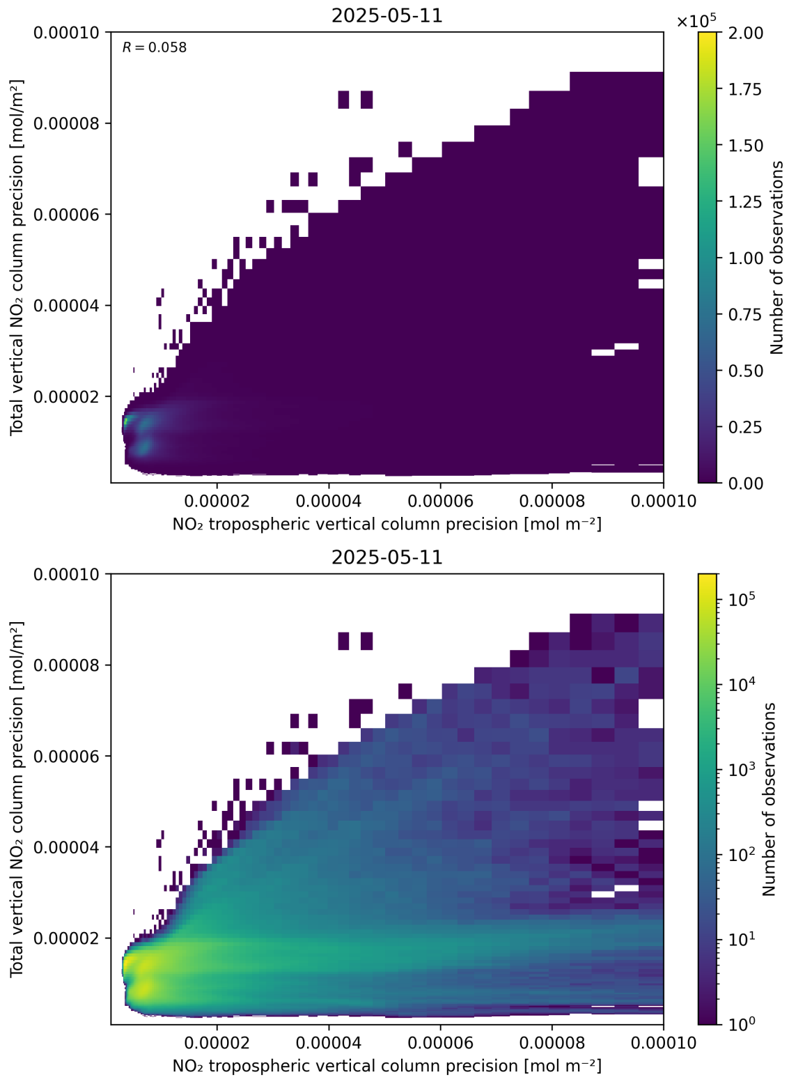
Figure 139: Scatter density plot of “NO 2 tropospheric vertical column precision” against “Total vertical NO 2 column precision” for 2025-05-11 to 2025-05-12.
