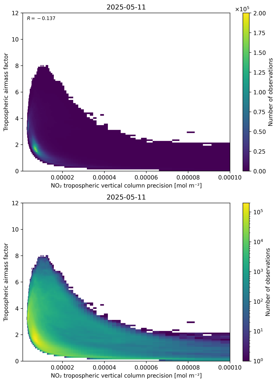
Figure 133: Scatter density plot of “NO 2 tropospheric vertical column precision” against “Tropospheric airmass factor” for 2025-05-11 to 2025-05-12.
