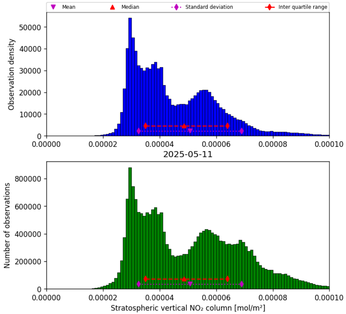
Figure 36: Histogram of “Stratospheric vertical NO 2 column” for 2025-05-11 to 2025-05-12
