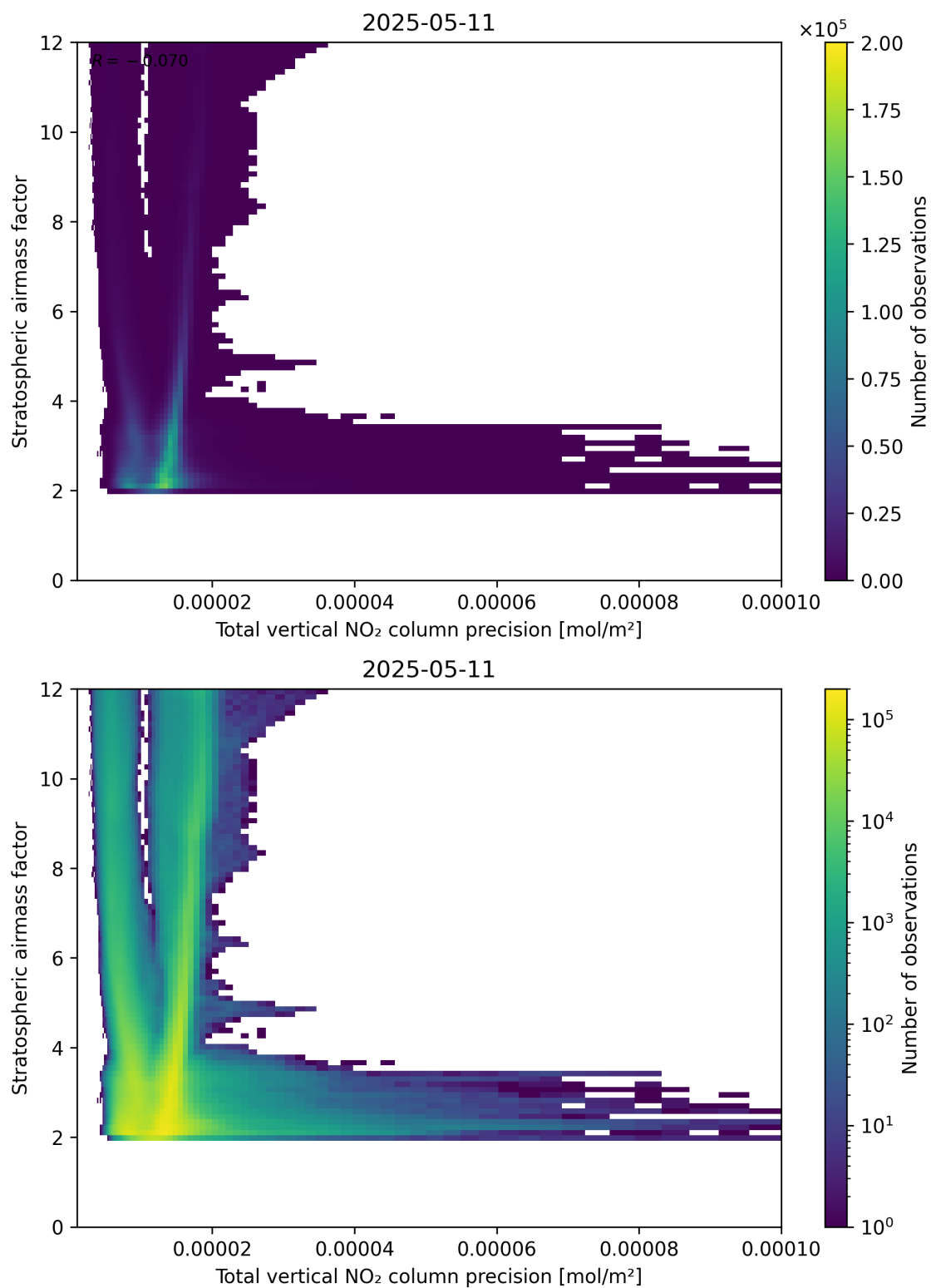
Figure 115: Scatter density plot of “Total vertical NO 2 column precision” against “Stratospheric air mass factor” for 2025-05-11 to 2025-05-12.
