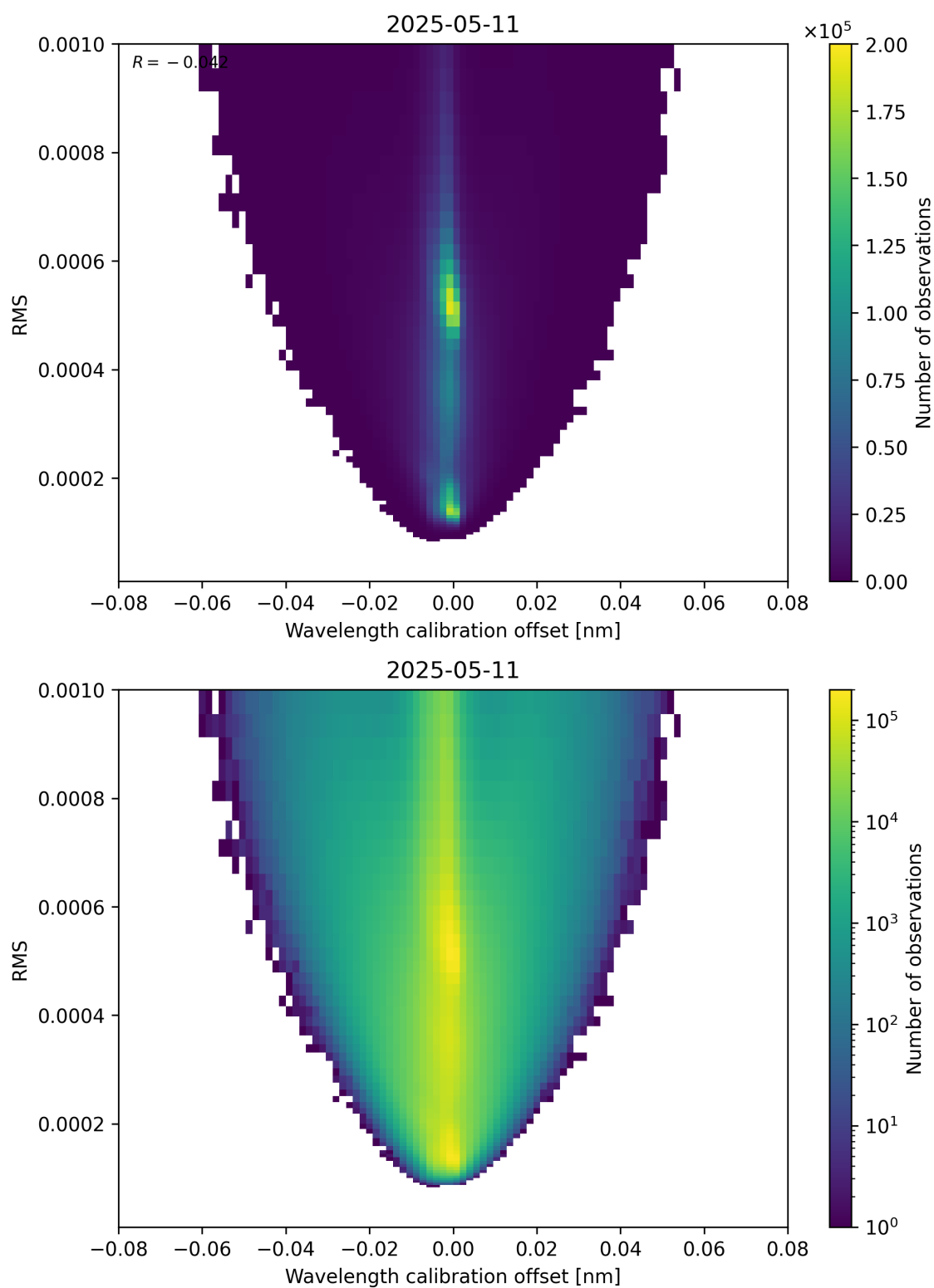
Figure 181: Scatter density plot of “Wavelength calibration offset” against “RMS” for 2025-05-11 to 2025-05-12.
