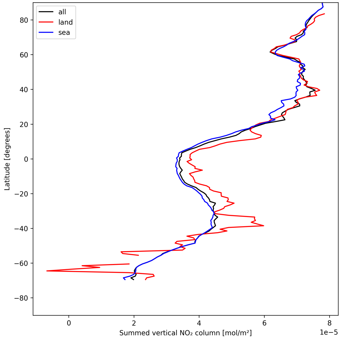
Figure 23: Zonal average of “Summed vertical NO 2 column” for 2025-05-11 to 2025-05-12.
