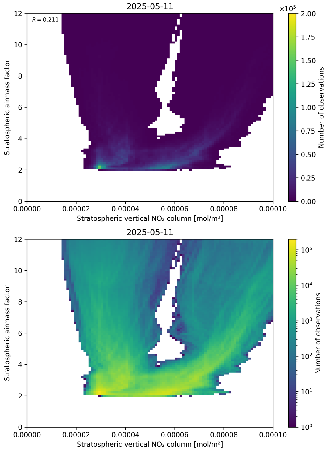
Figure 96: Scatter density plot of “Stratospheric vertical NO 2 column” against “Stratospheric airmass factor” for 2025-05-11 to 2025-05-12.
