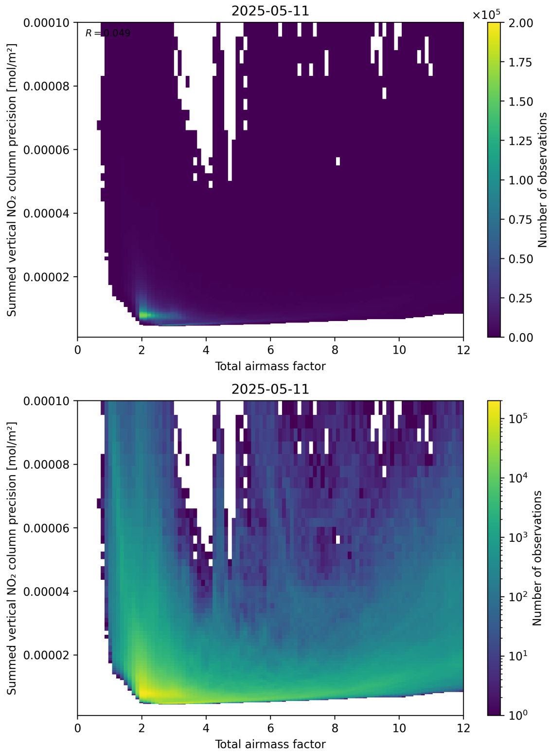
Figure 66: Scatter density plot of “Total airmass factor” against “Summed vertical NO 2 column precision” for 2025-05-11 to 2025-05-12.
