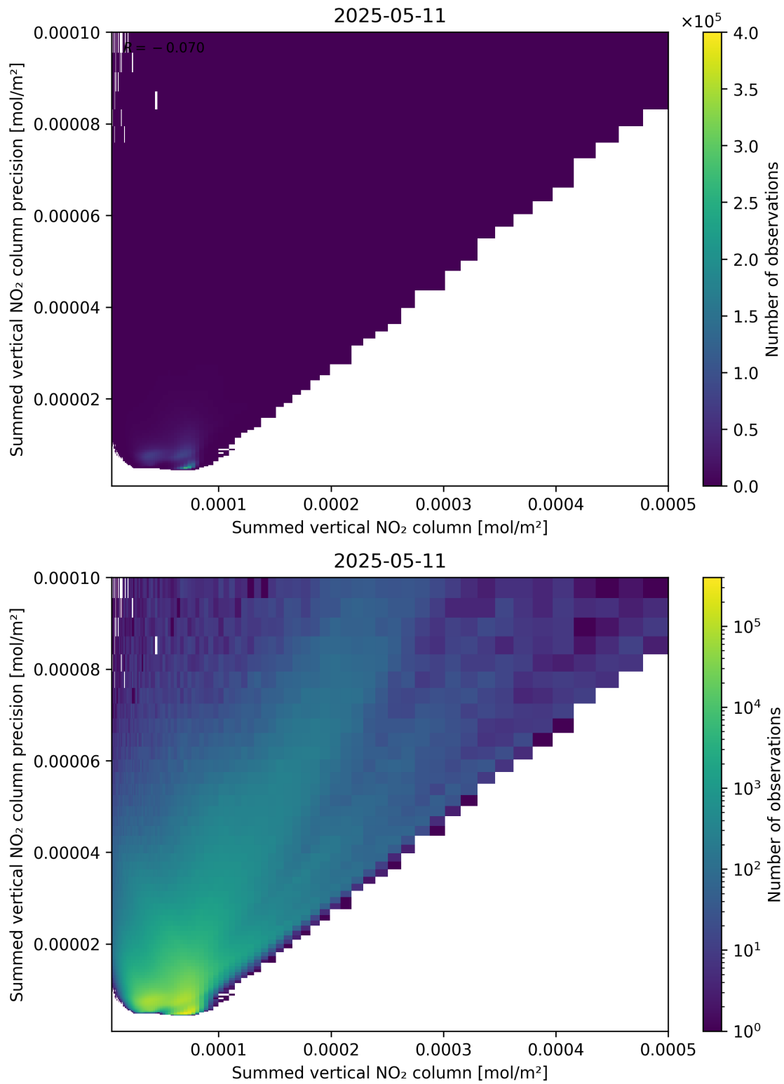
Figure 105: Scatter density plot of “Summed vertical NO 2 column” against “Summed vertical NO 2 column precision” for 2025-05-11 to 2025-05-12.
