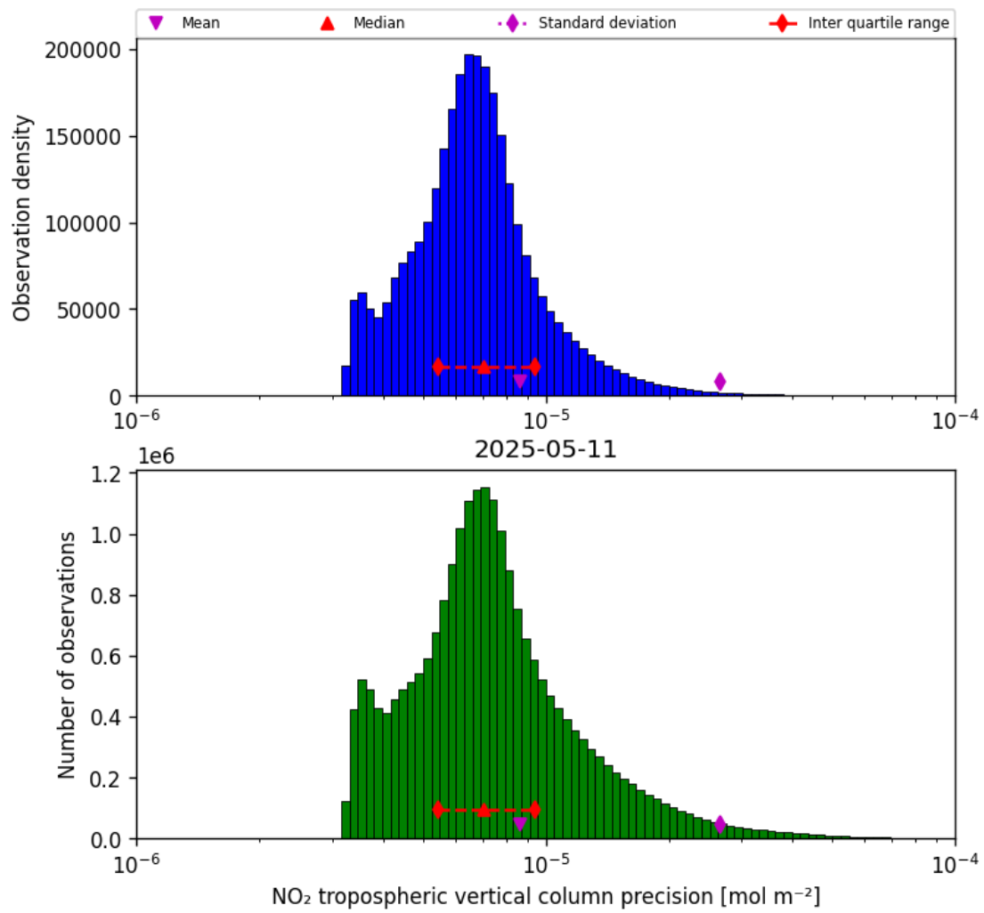
Figure 30: Histogram of “NO 2 tropospheric vertical column precision” for 2025-05-11 to 2025-05-12
