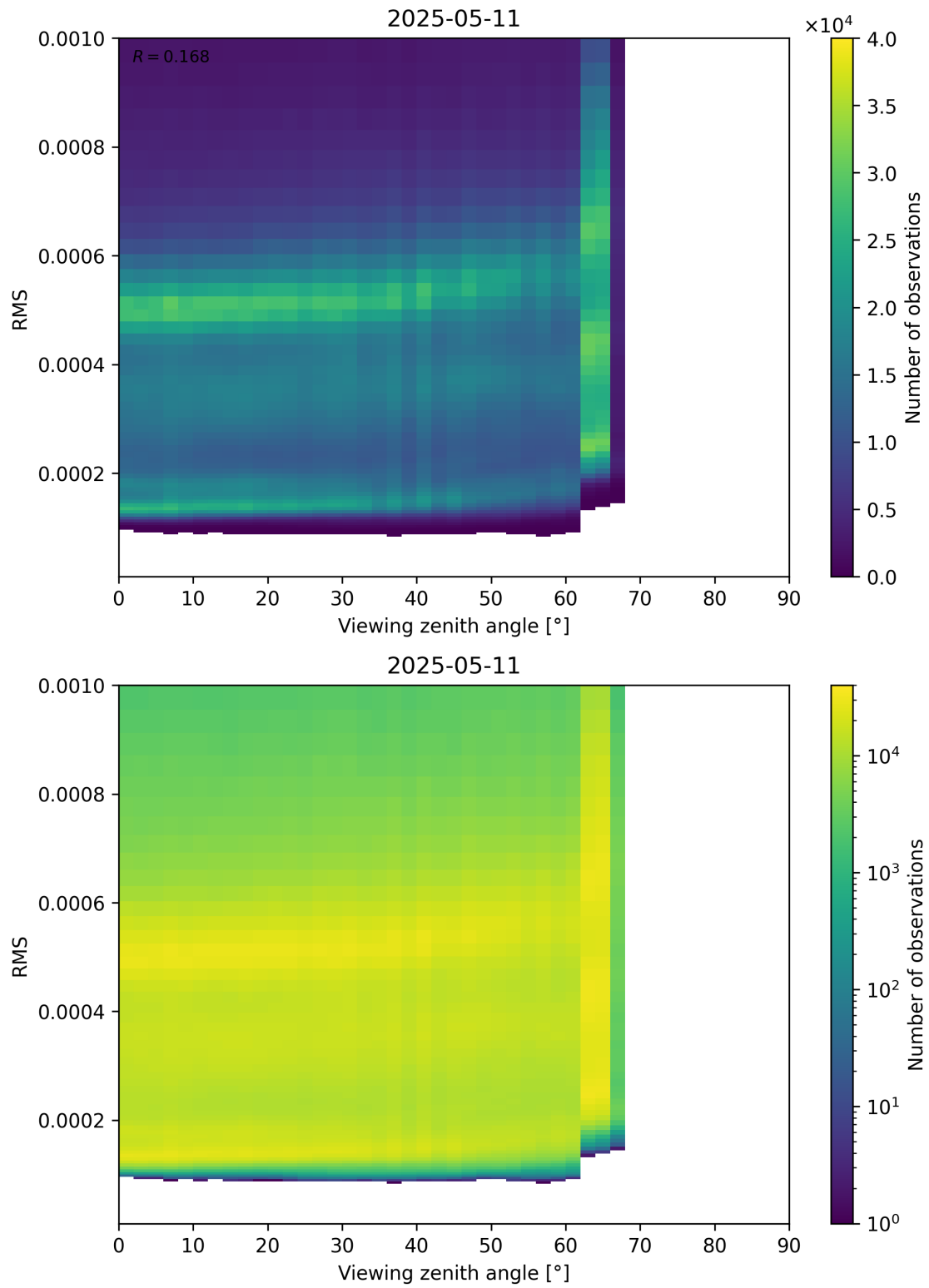
Figure 171: Scatter density plot of “Viewing zenith angle” against “RMS” for 2025-05-11 to 2025-05-12.
