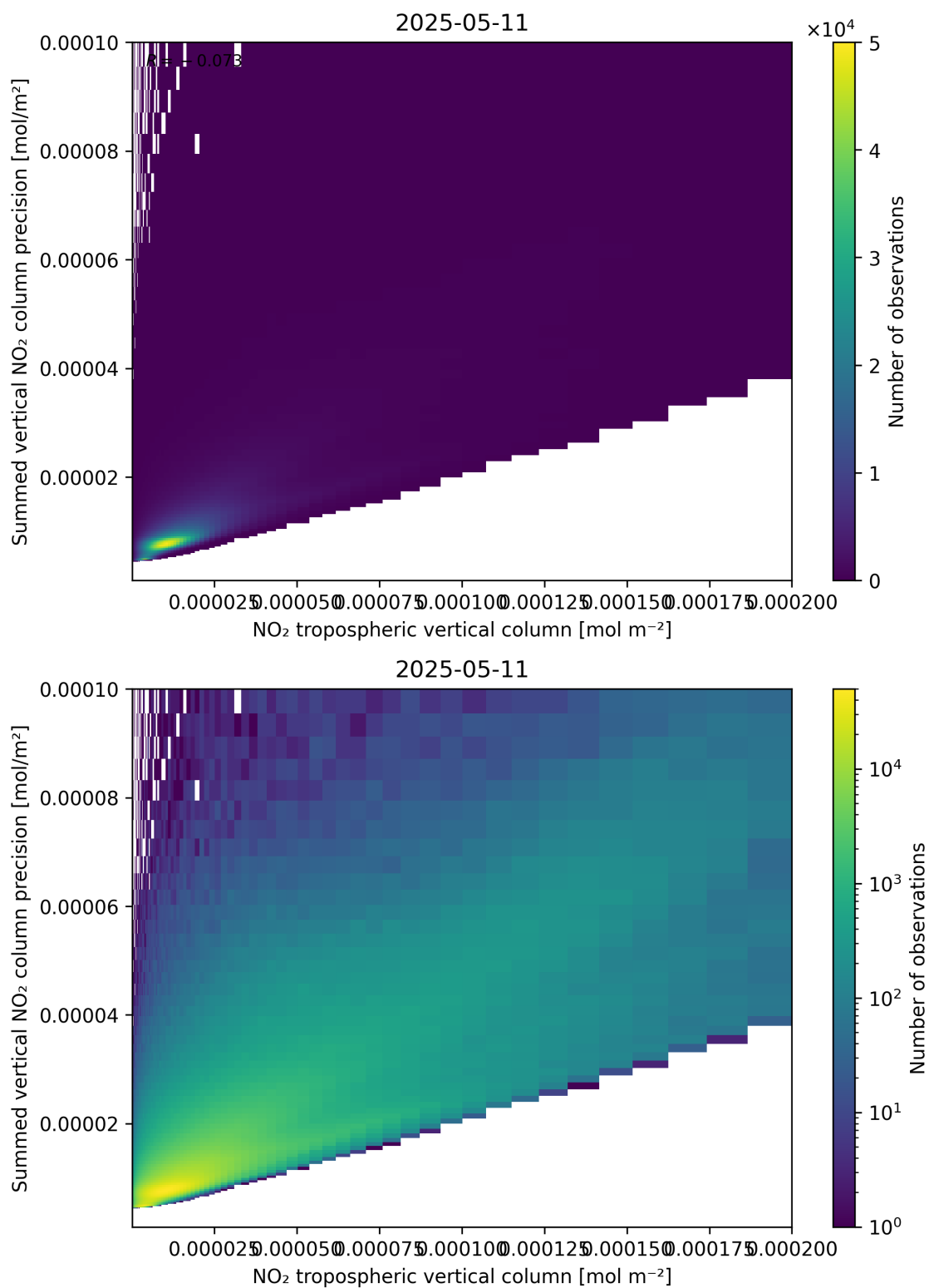
Figure 127: Scatter density plot of “NO 2 tropospheric vertical column” against “Summed vertical NO 2 column precision” for 2025-05-11 to 2025-05-12.
