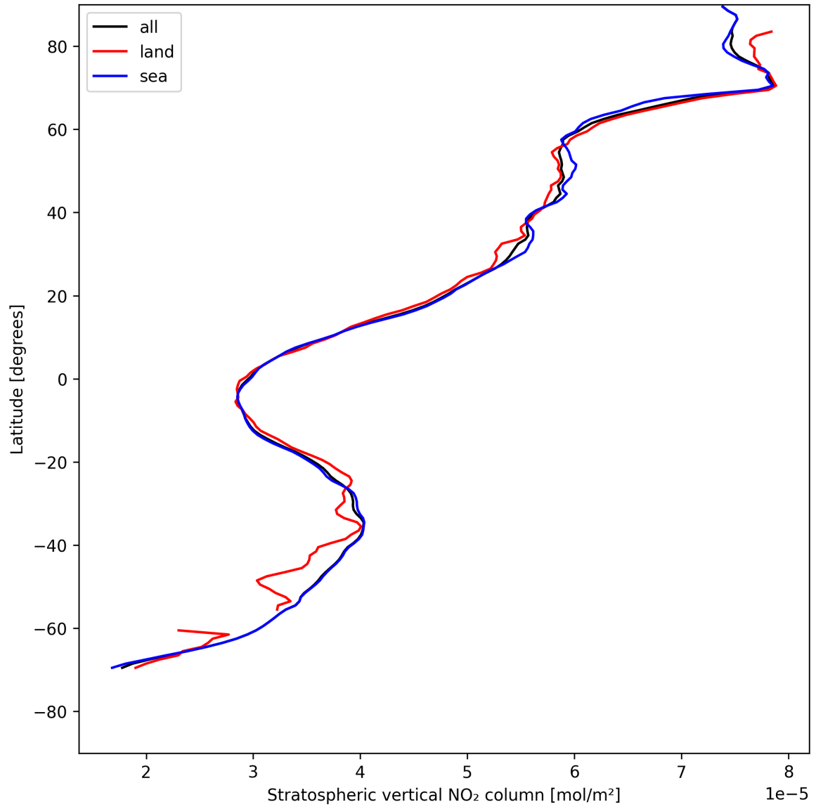
Figure 19: Zonal average of “Stratospheric vertical NO 2 column” for 2025-05-11 to 2025-05-12.
