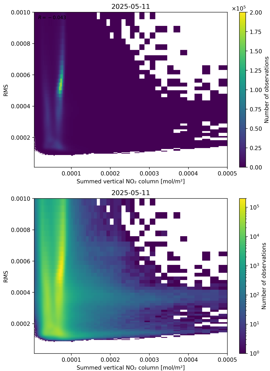
Figure 109: Scatter density plot of “Summed vertical NO 2 column” against “RMS” for 2025-05-11 to 2025-05-12.
