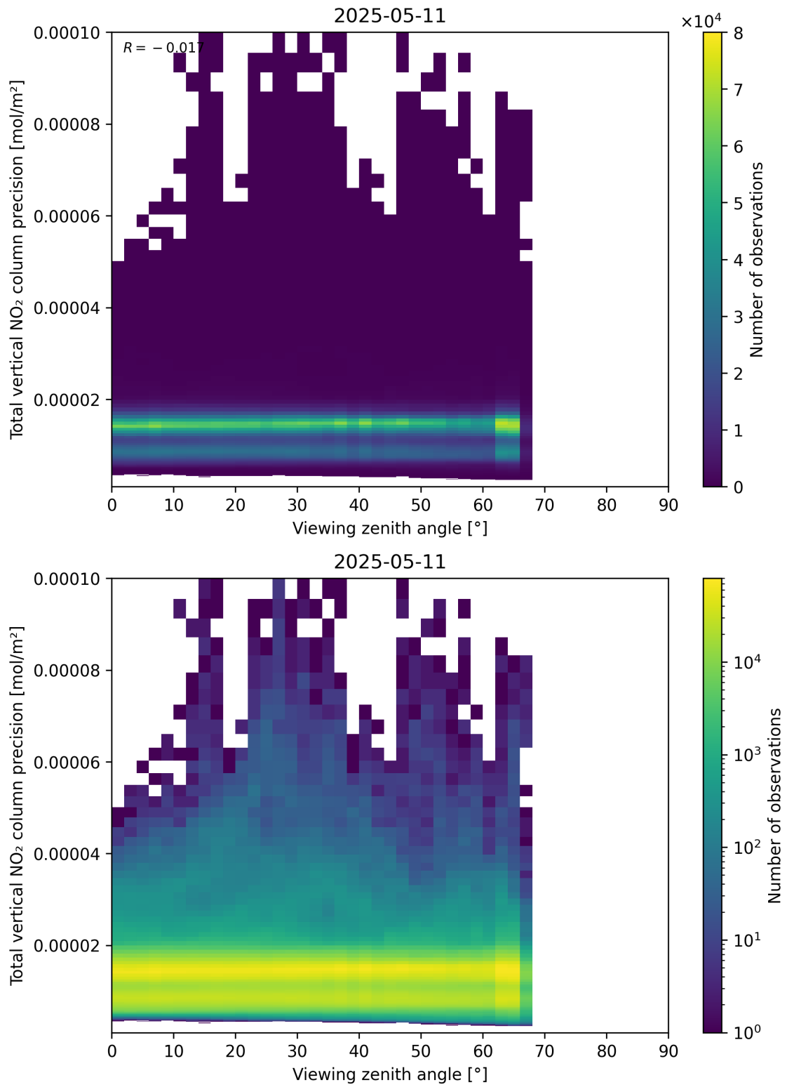
Figure 168: Scatter density plot of “Viewing zenith angle” against “Total vertical NO 2 column precision” for 2025-05-11 to 2025-05-12.
