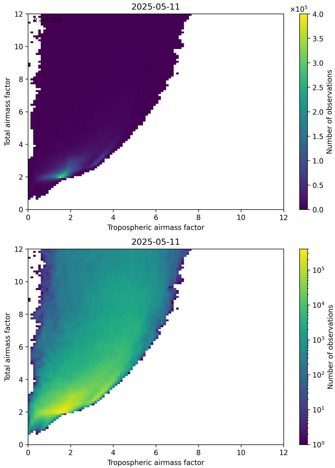
Figure 72: Scatter density plot of “Tropospheric airmass factor” against “Total airmass factor” for 2025-05-11 to 2025-05-12.
