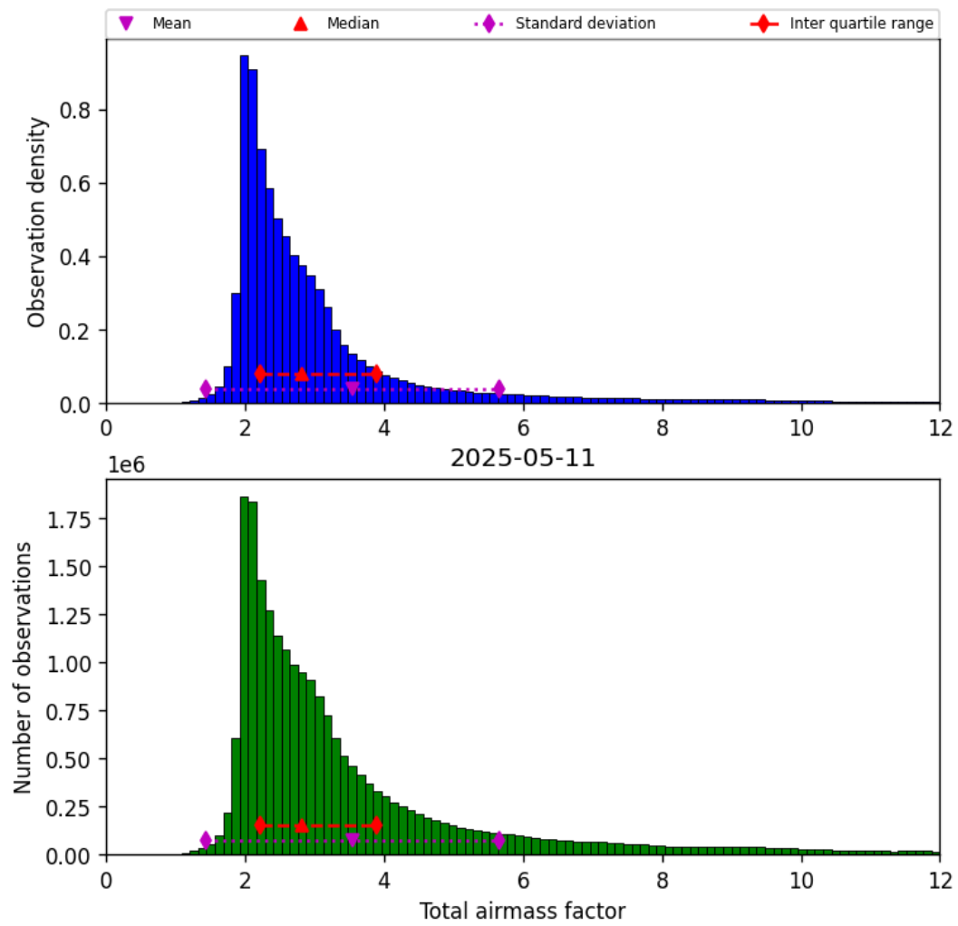
Figure 32: Histogram of “Total airmass factor” for 2025-05-11 to 2025-05-12
