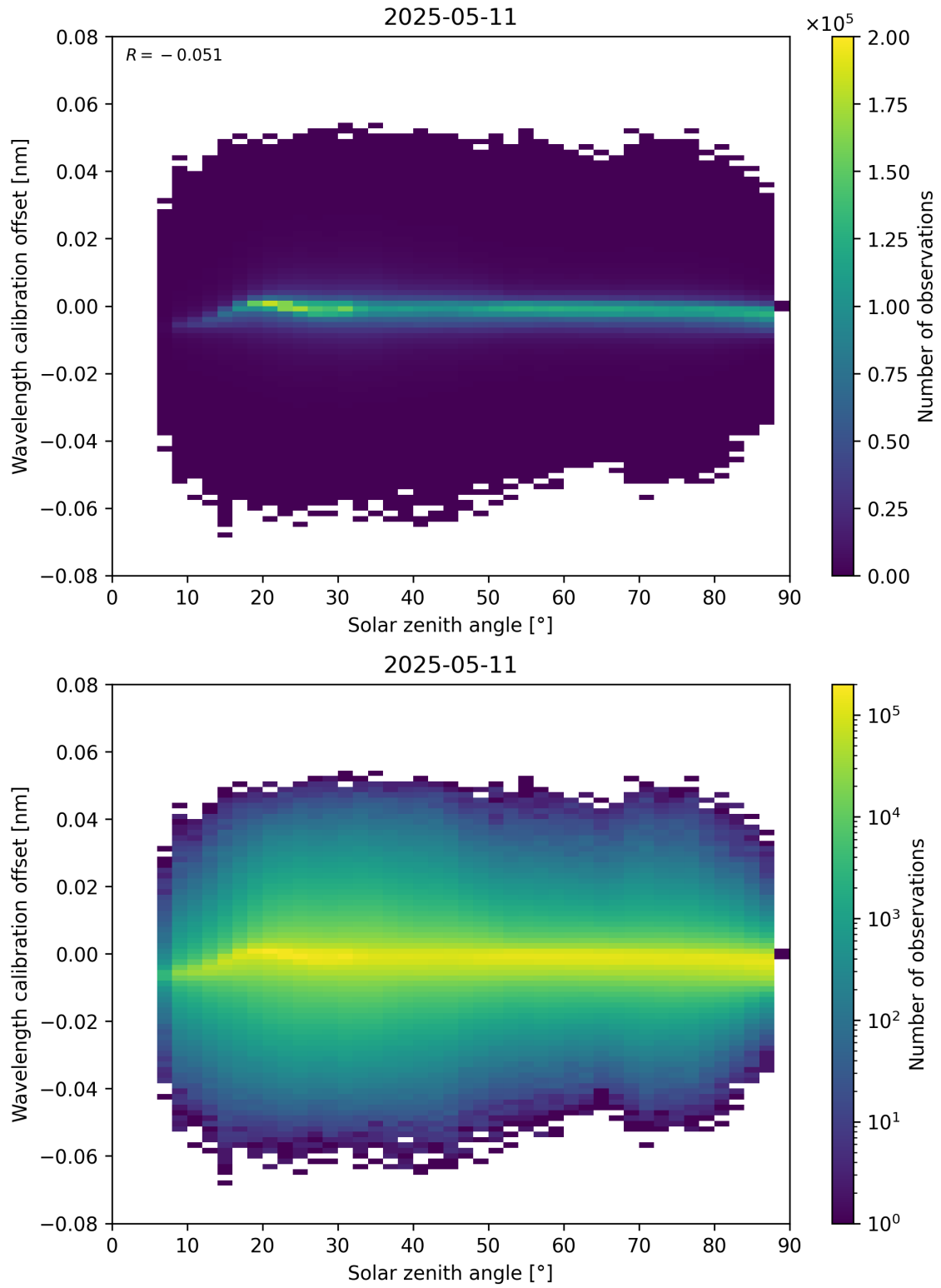
Figure 158: Scatter density plot of “Solar zenith angle” against “Wavelength calibration offset” for 2025-05-11 to 2025-05-12.
