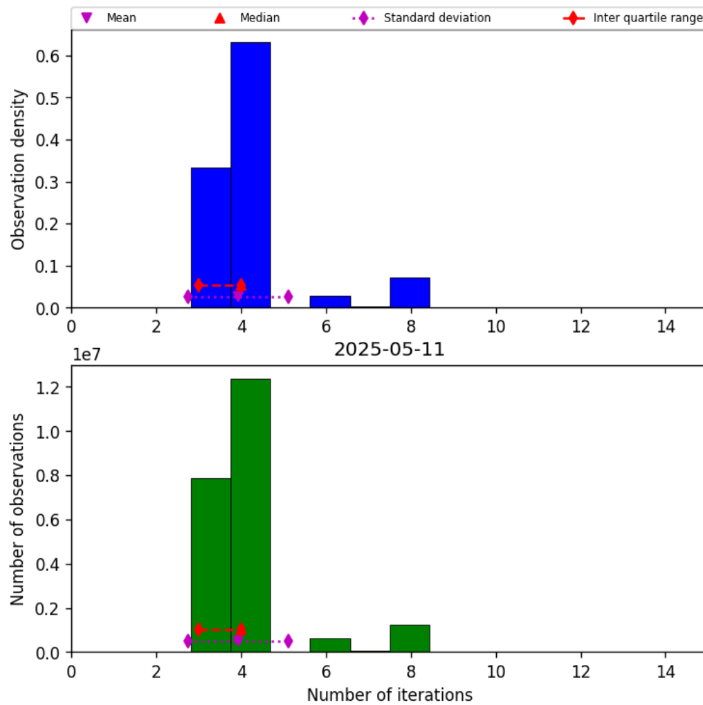
Figure 34: Histogram of “Number of iterations” for 2025-05-11 to 2025-05-12
