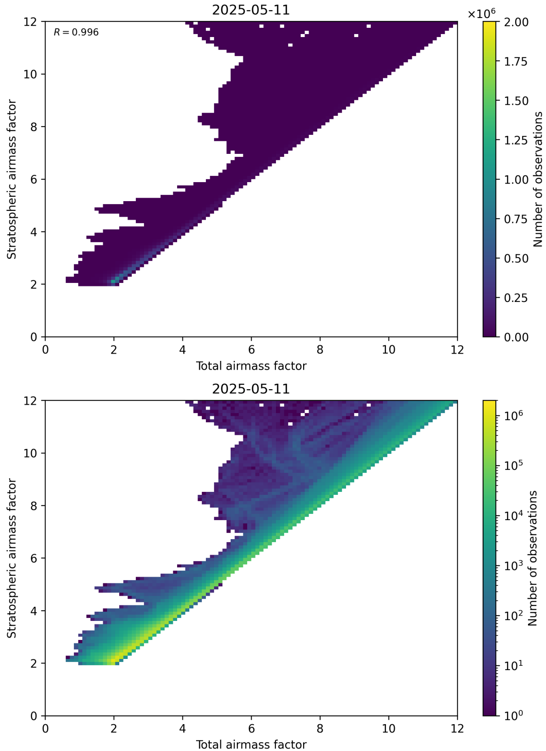
Figure 62: Scatter density plot of “Total airmass factor” against “Stratospheric airmass factor” for 2025-05-11 to 2025-05-12.
