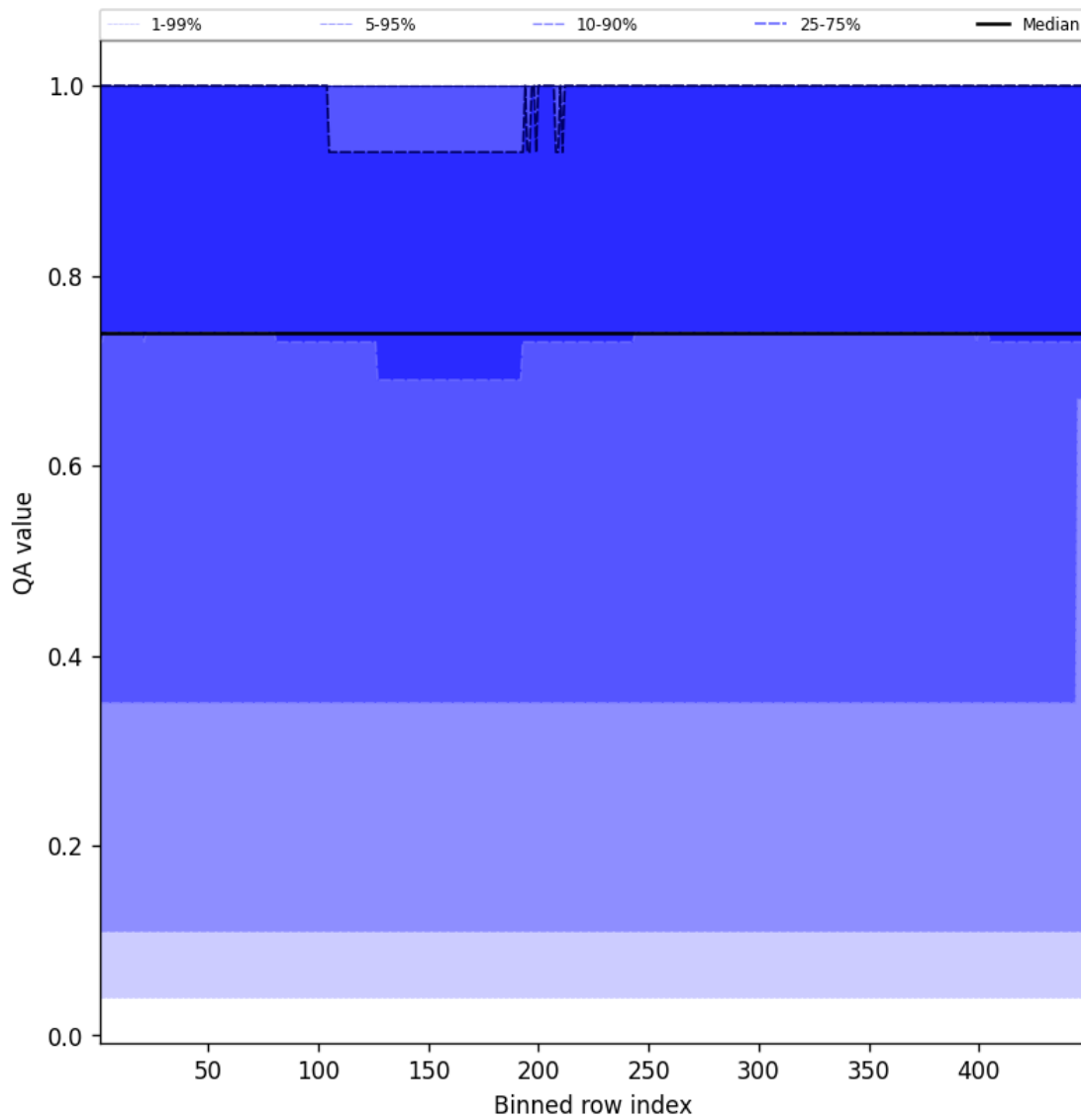
Figure 45: Along track statistics of “QA value” for 2025-05-11 to 2025-05-12
