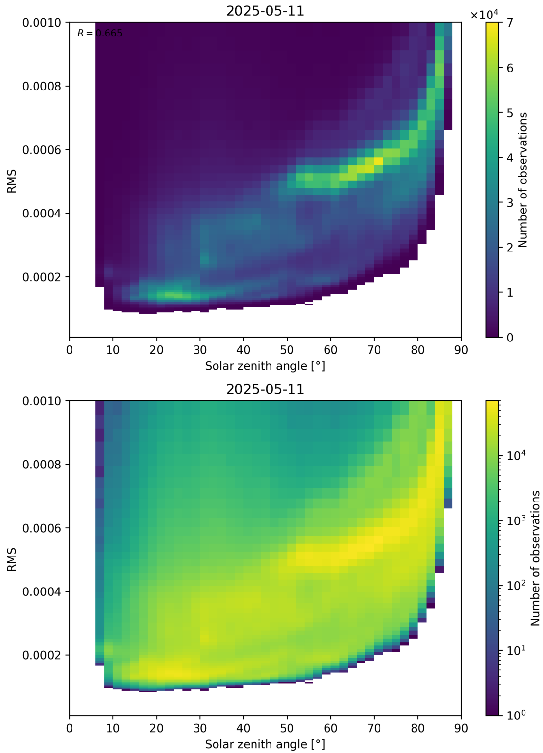
Figure 157: Scatter density plot of “Solar zenith angle” against “RMS” for 2025-05-11 to 2025-05-12.
