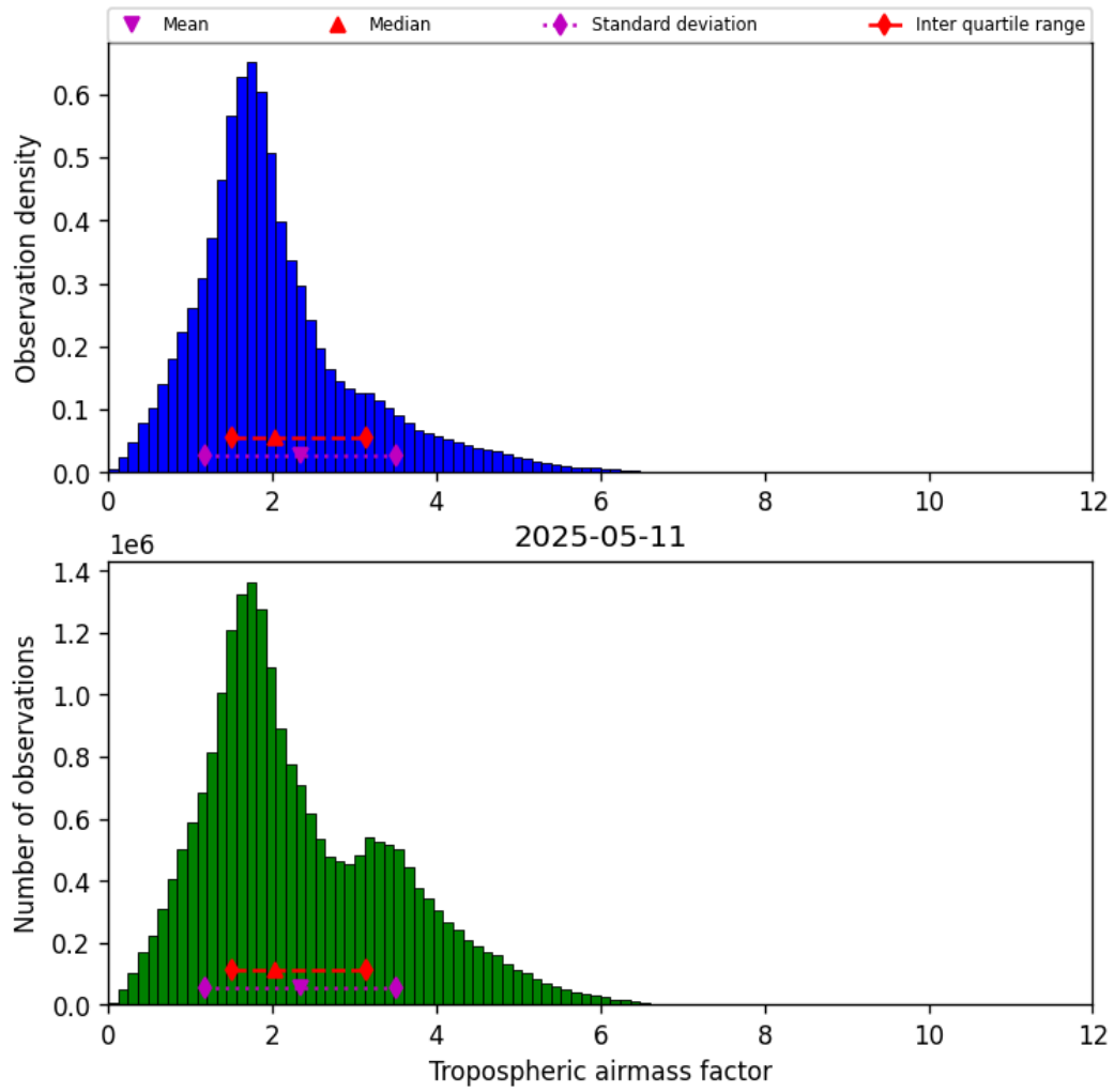
Figure 31: Histogram of “Tropospheric airmass factor” for 2025-05-11 to 2025-05-12
