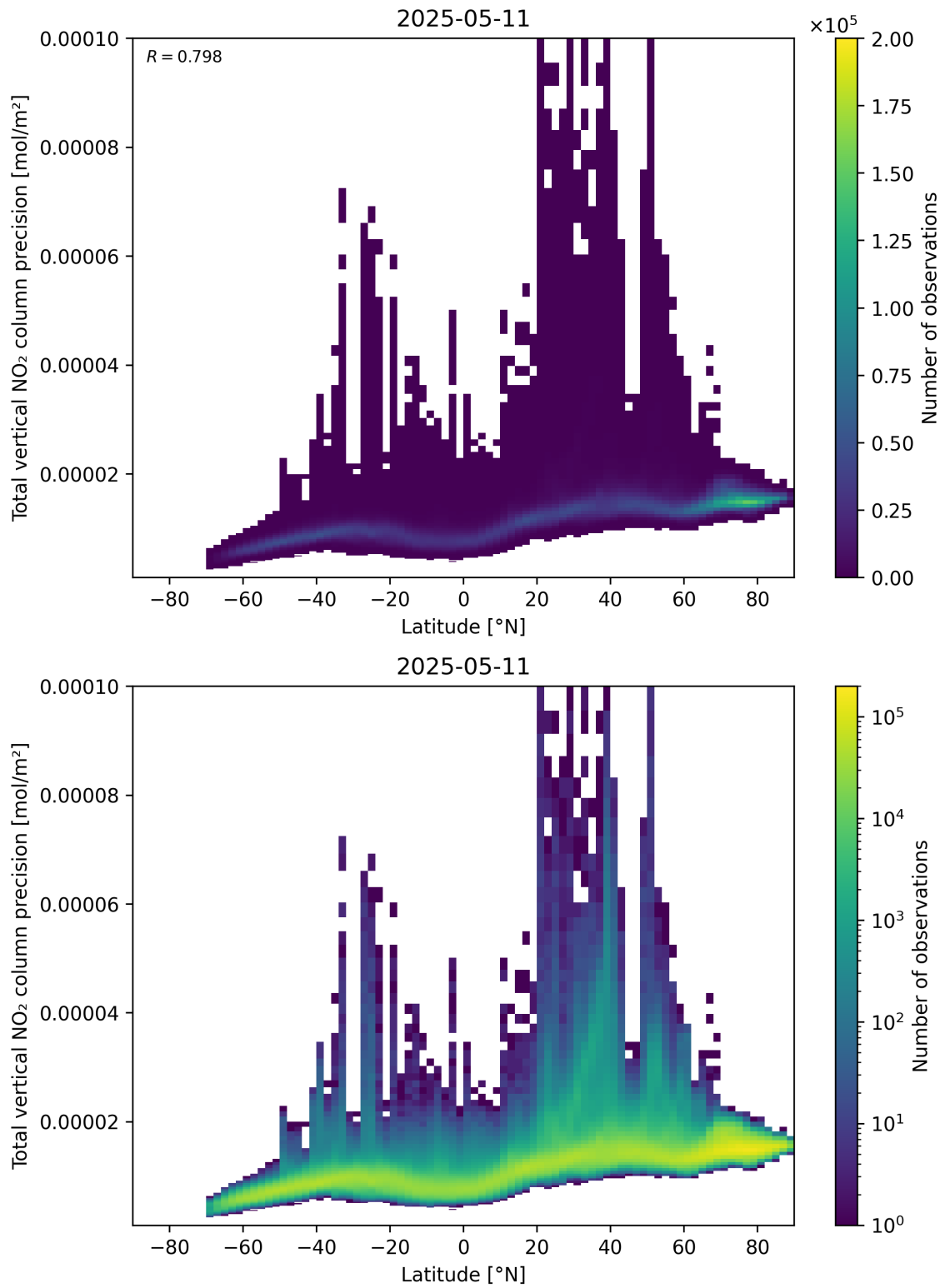
Figure 91: Scatter density plot of “Latitude” against “Total vertical NO 2 column precision” for 2025-05-11 to 2025-05-12.
