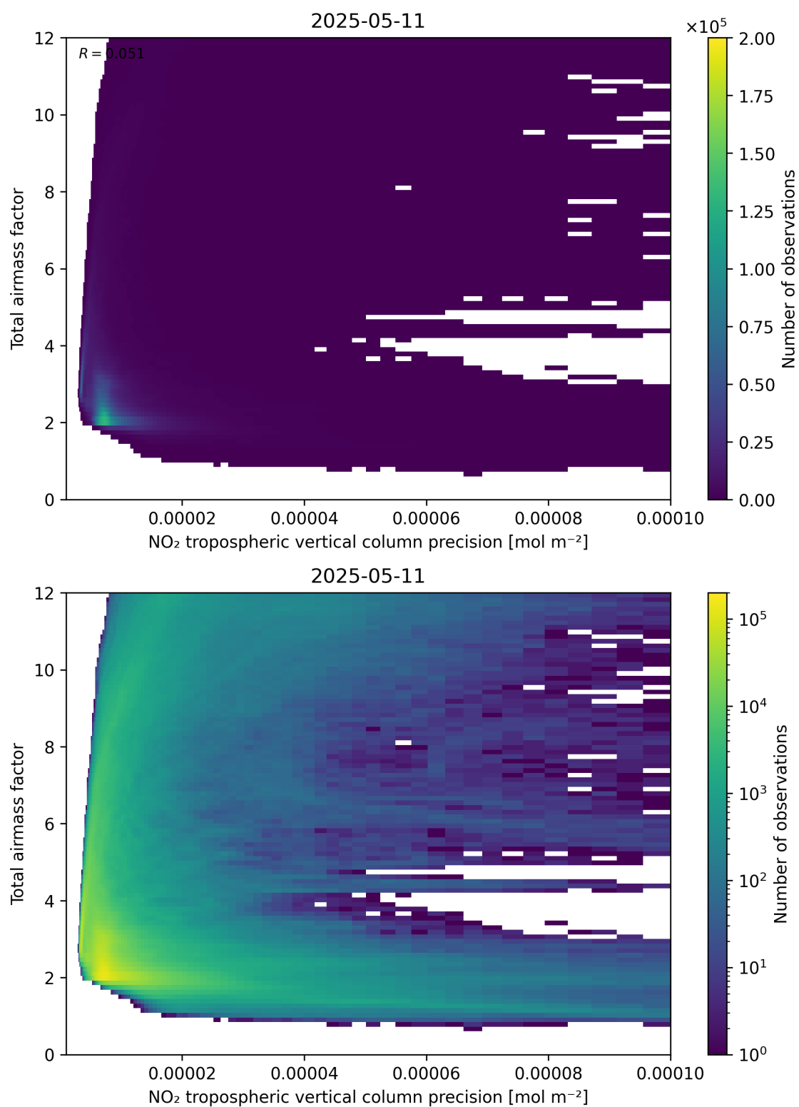
Figure 132: Scatter density plot of “NO 2 tropospheric vertical column precision” against “Total air mass factor” for 2025-05-11 to 2025-05-12.
