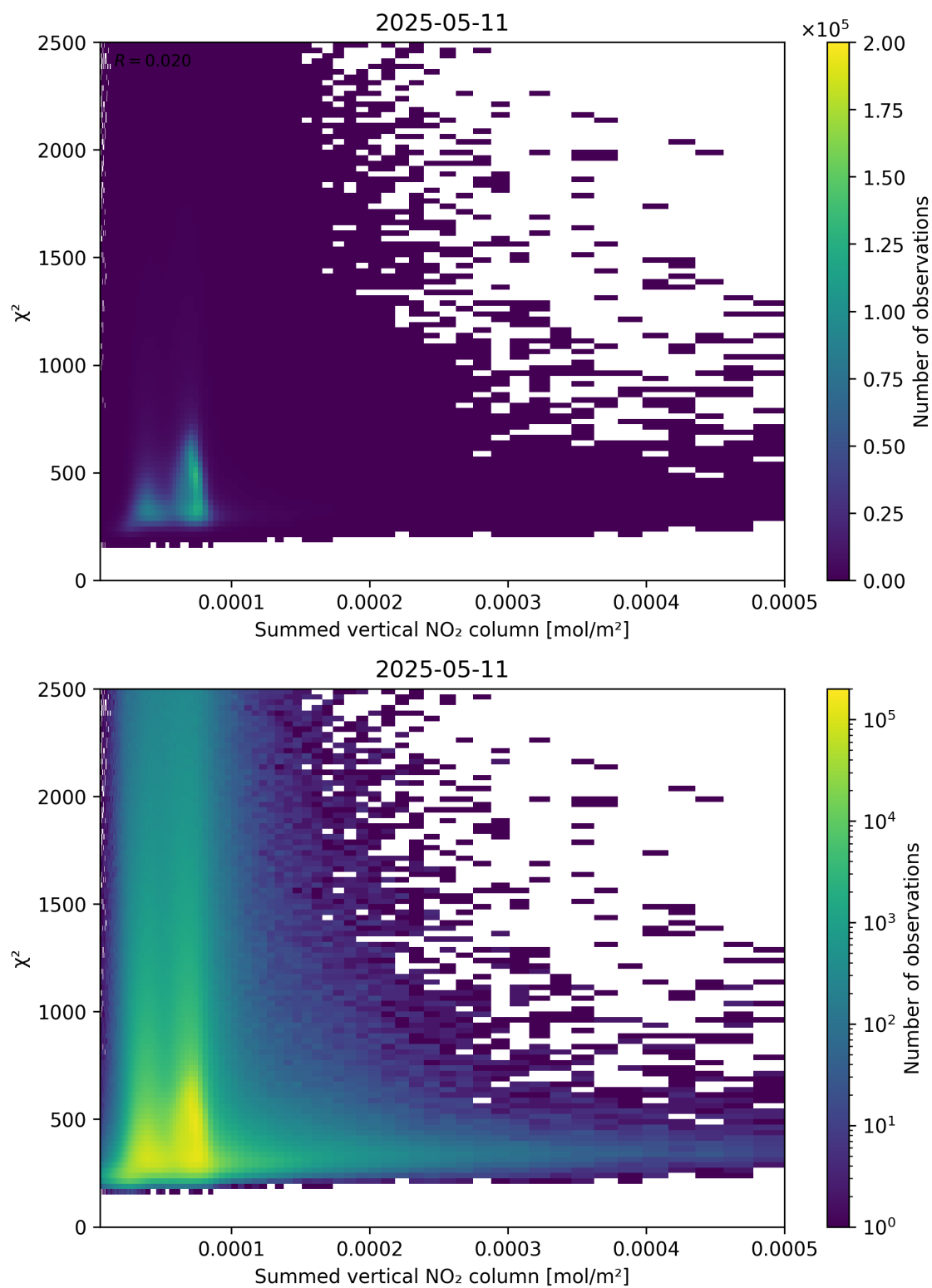
Figure 104: Scatter density plot of “Summed vertical NO 2 column” against “ \chi^2 ” for 2025-05-11 to 2025-05-12.
