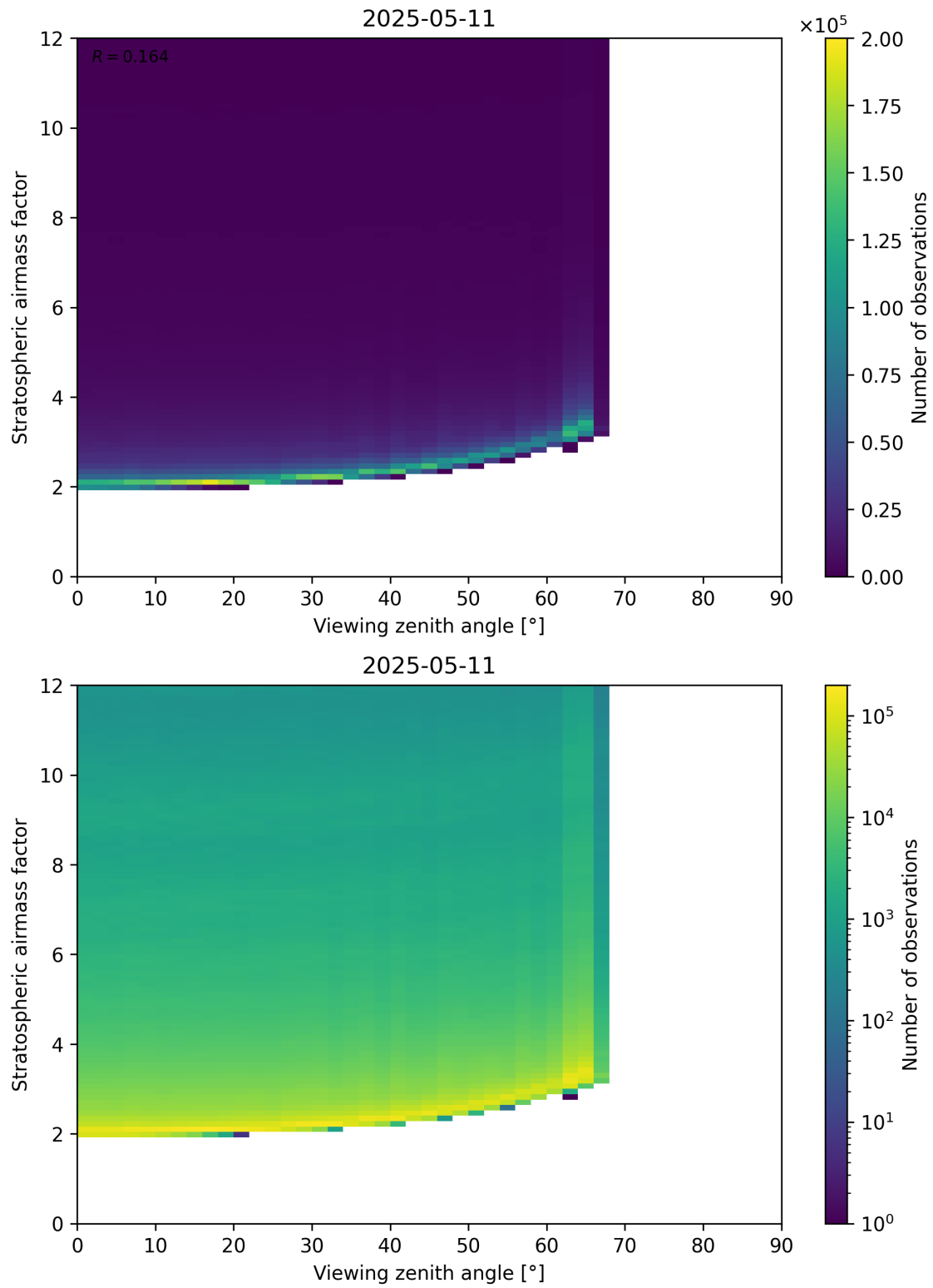
Figure 159: Scatter density plot of “Viewing zenith angle” against “Stratospheric airmass factor” for 2025-05-11 to 2025-05-12.
