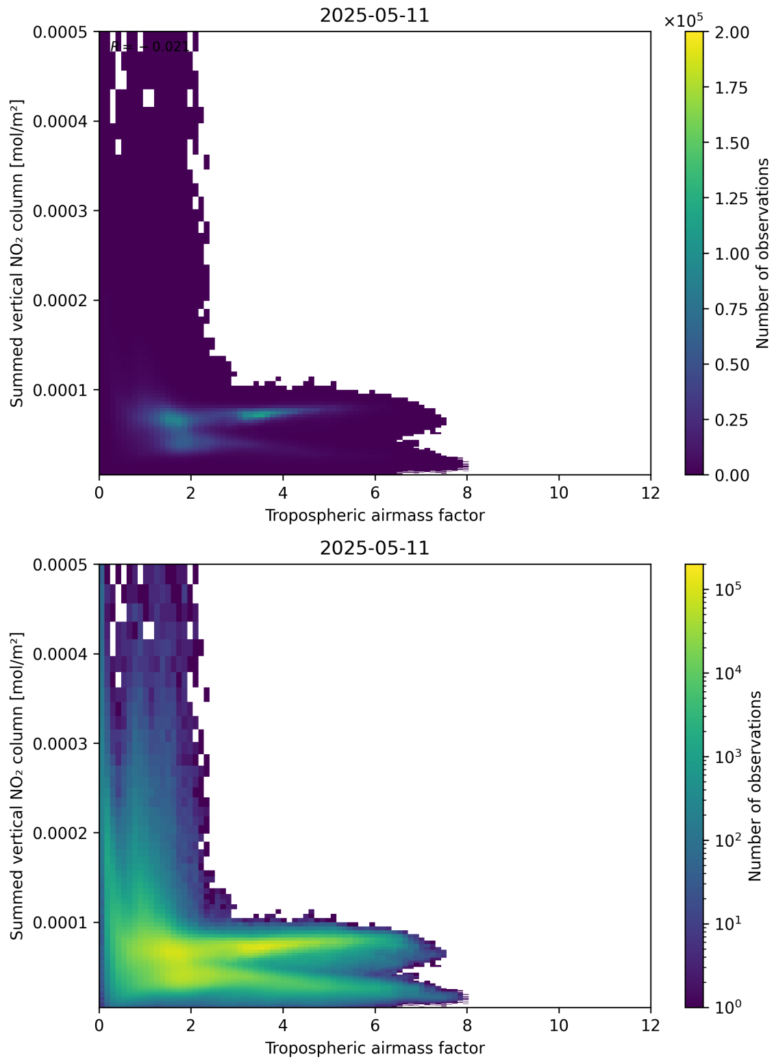
Figure 75: Scatter density plot of “Tropospheric air mass factor” against “Summed vertical NO 2 column” for 2025-05-11 to 2025-05-12.
