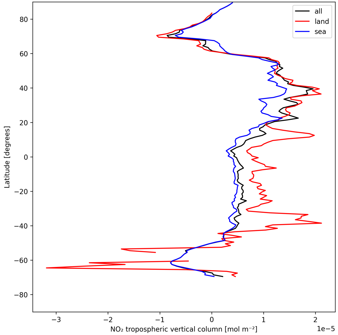
Figure 12: Zonal average of “NO 2 tropospheric vertical column” for 2025-05-11 to 2025-05-12.
