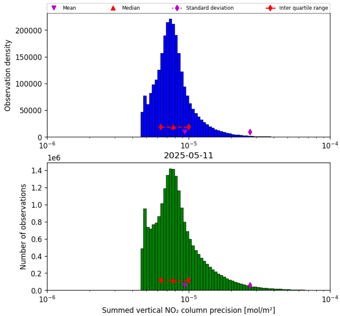
Figure 41: Histogram of “Summed vertical NO 2 column precision” for 2025-05-11 to 2025-05-12
