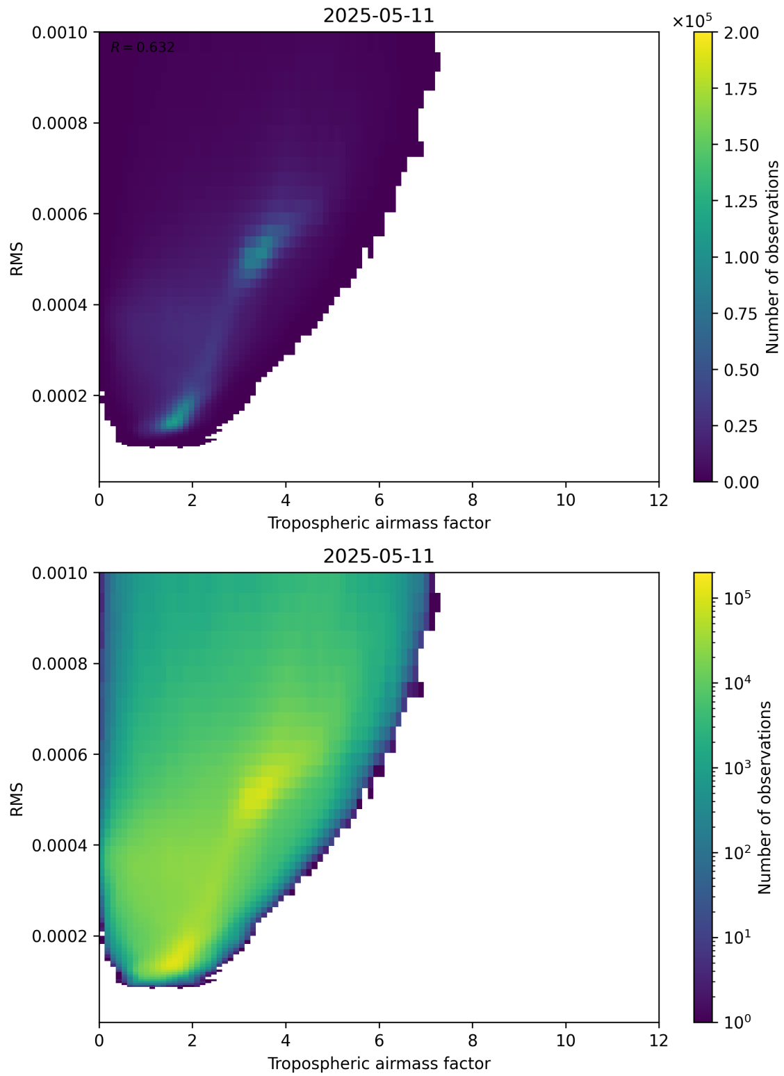
Figure 79: Scatter density plot of “Tropospheric airmass factor” against “RMS” for 2025-05-11 to 2025-05-12.
