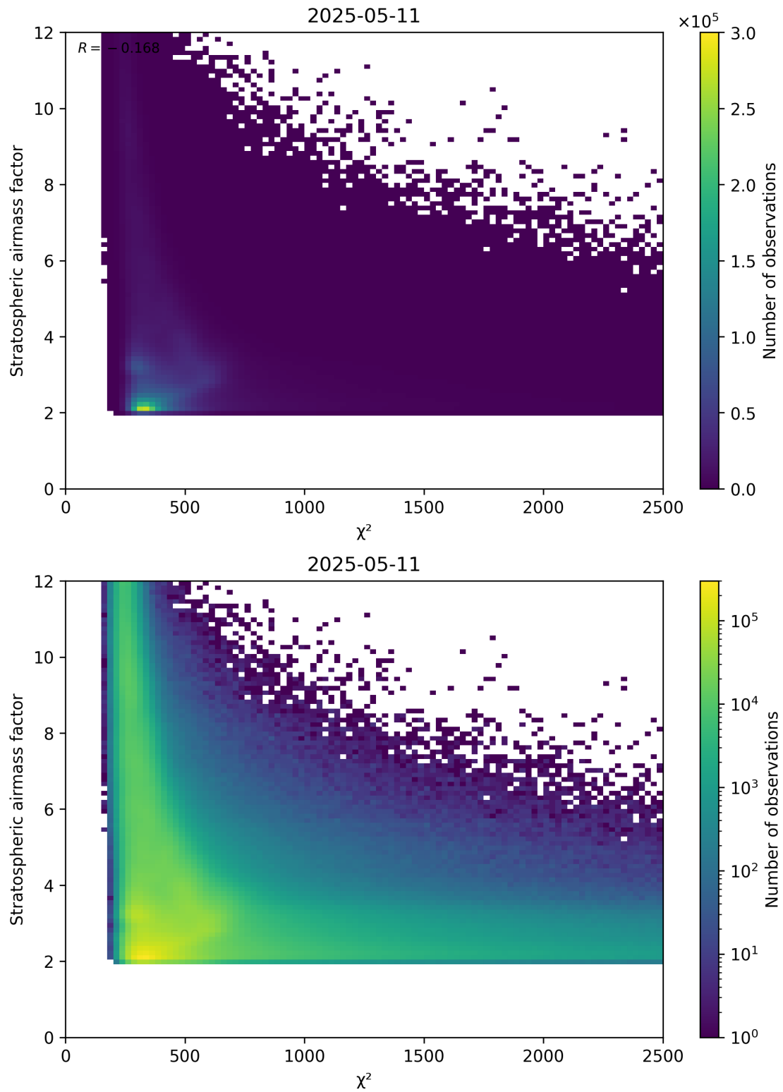
Figure 81: Scatter density plot of " \chi^2 " against "Stratospheric airmass factor" for 2025-05-11 to 2025-05-12.
