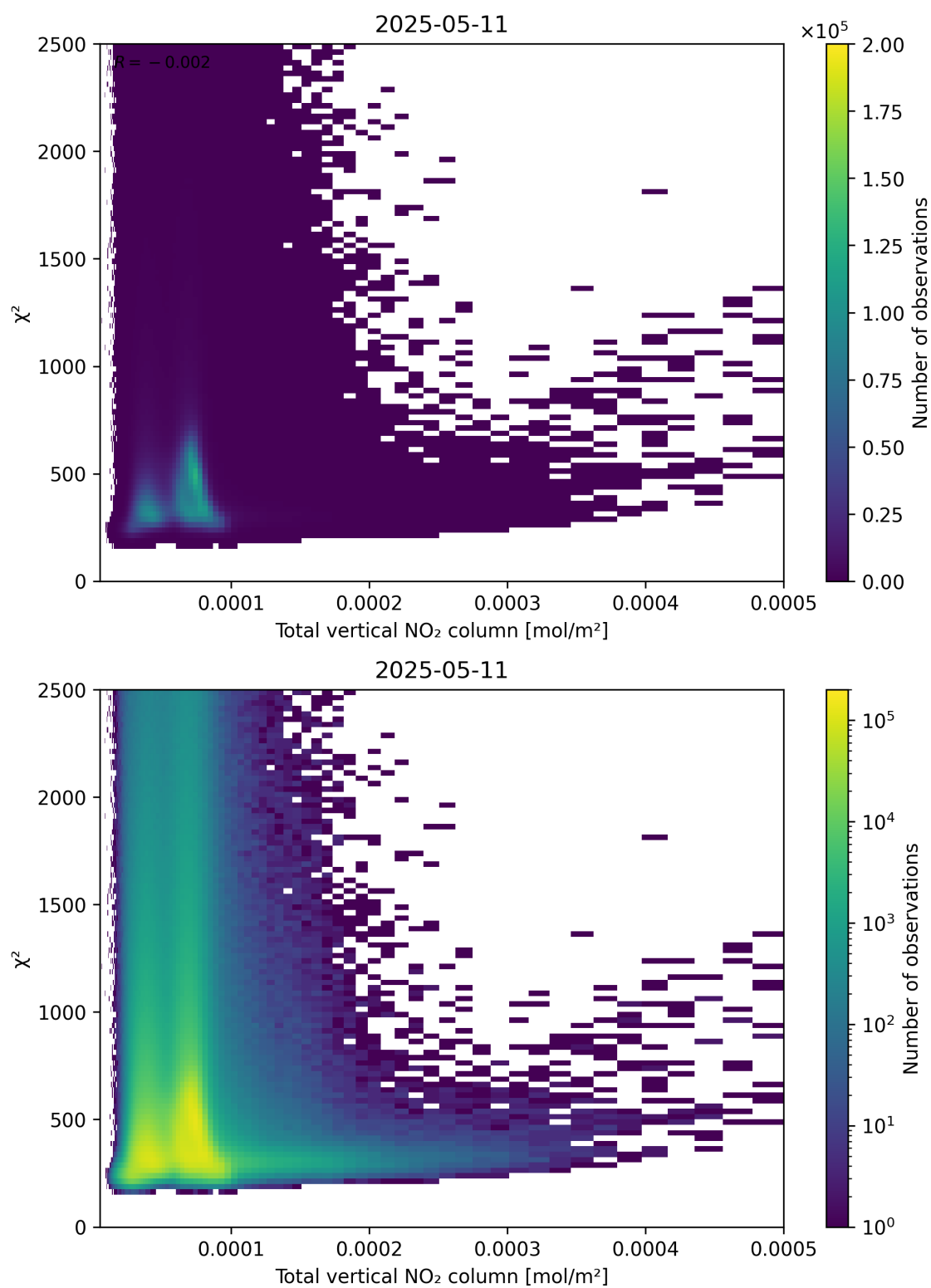
Figure 111: Scatter density plot of “Total vertical NO 2 column” against “ \chi^2 ” for 2025-05-11 to 2025-05-12.
