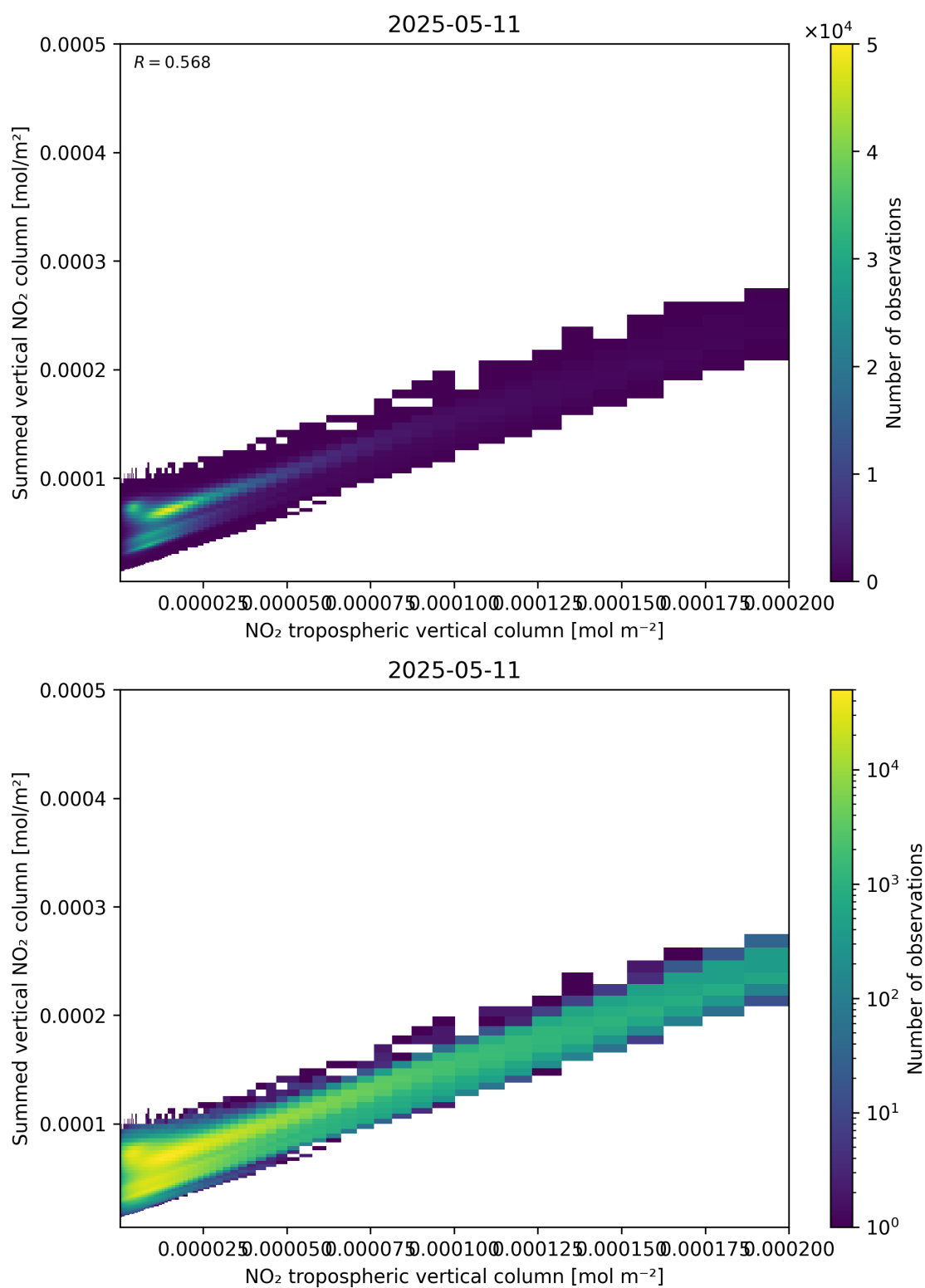
Figure 126: Scatter density plot of “NO 2 tropospheric vertical column” against “Summed vertical NO 2 column” for 2025-05-11 to 2025-05-12.
