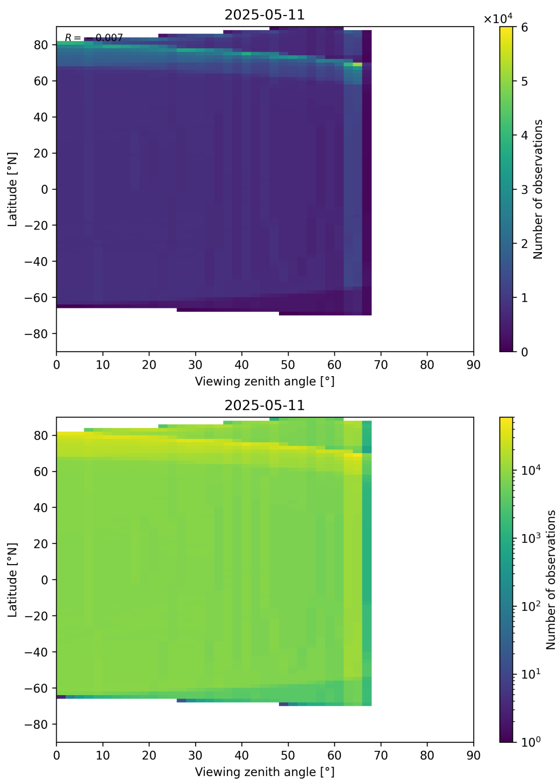
Figure 163: Scatter density plot of “Viewing zenith angle” against “Latitude” for 2025-05-11 to 2025-05-12.
