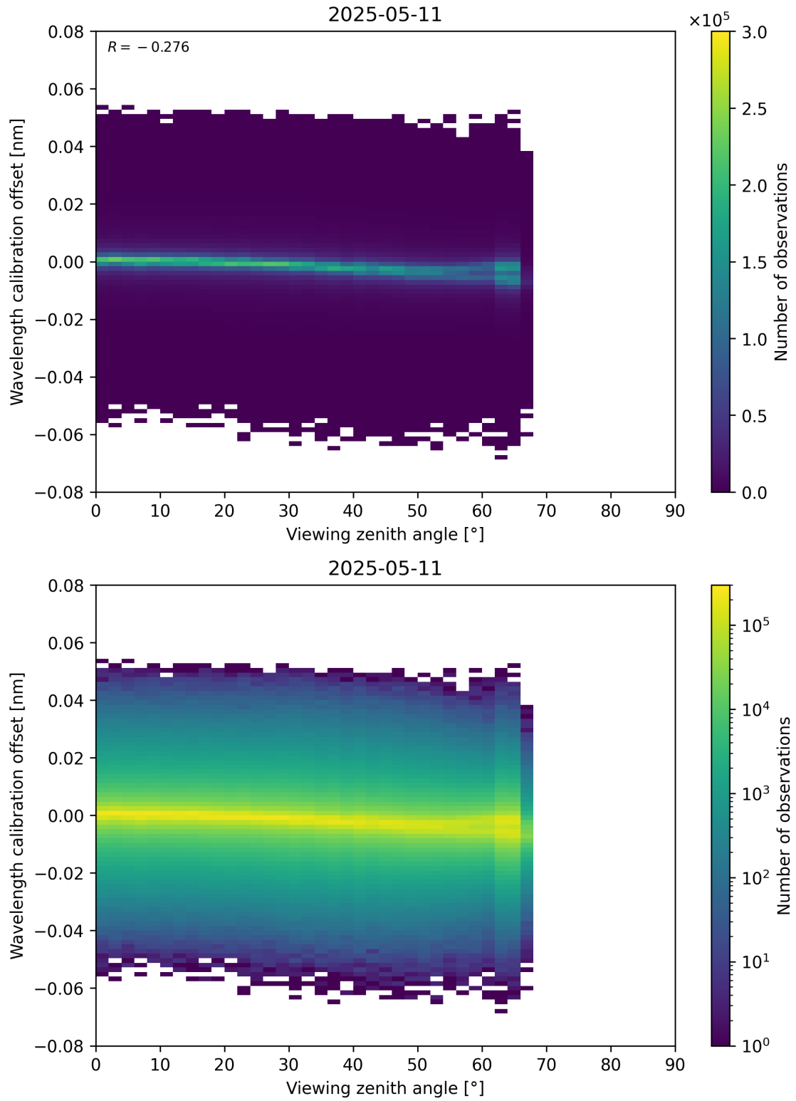
Figure 173: Scatter density plot of “Viewing zenith angle” against “Wavelength calibration offset” for 2025-05-11 to 2025-05-12.
