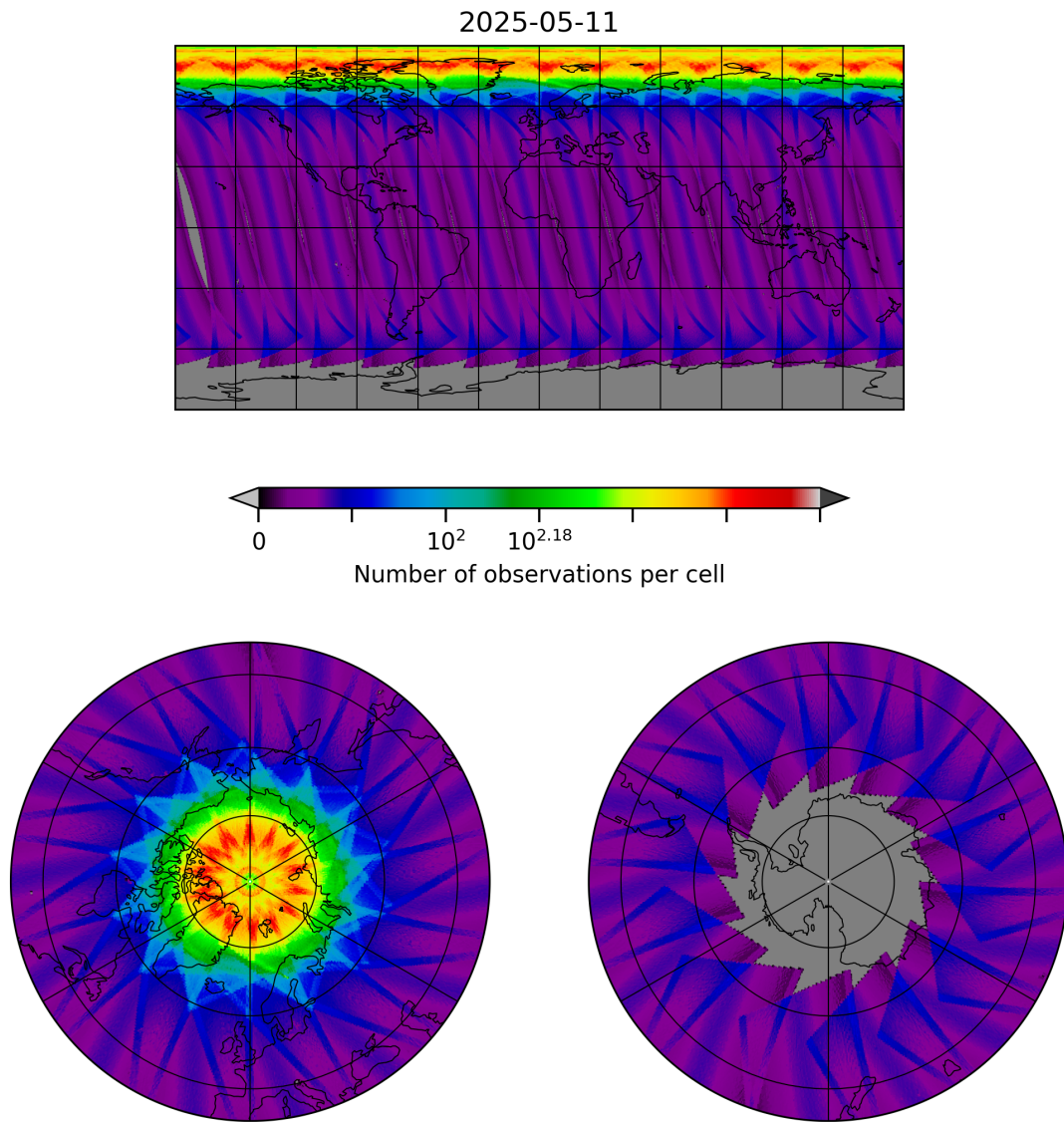
Figure 10: Map of the number of observations for 2025-05-11 to 2025-05-12
