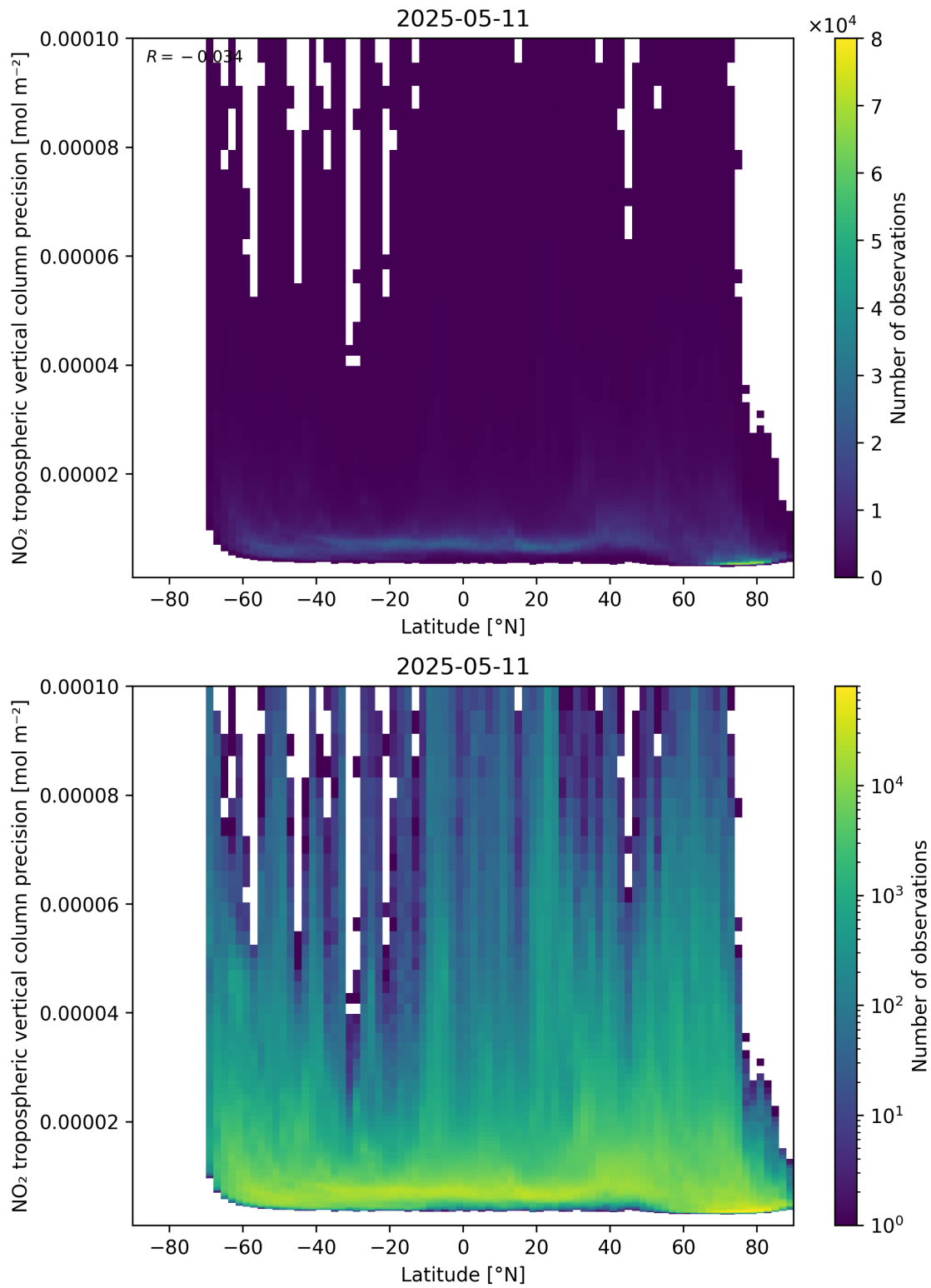
Figure 93: Scatter density plot of “Latitude” against “NO 2 tropospheric vertical column precision” for 2025-05-11 to 2025-05-12.
