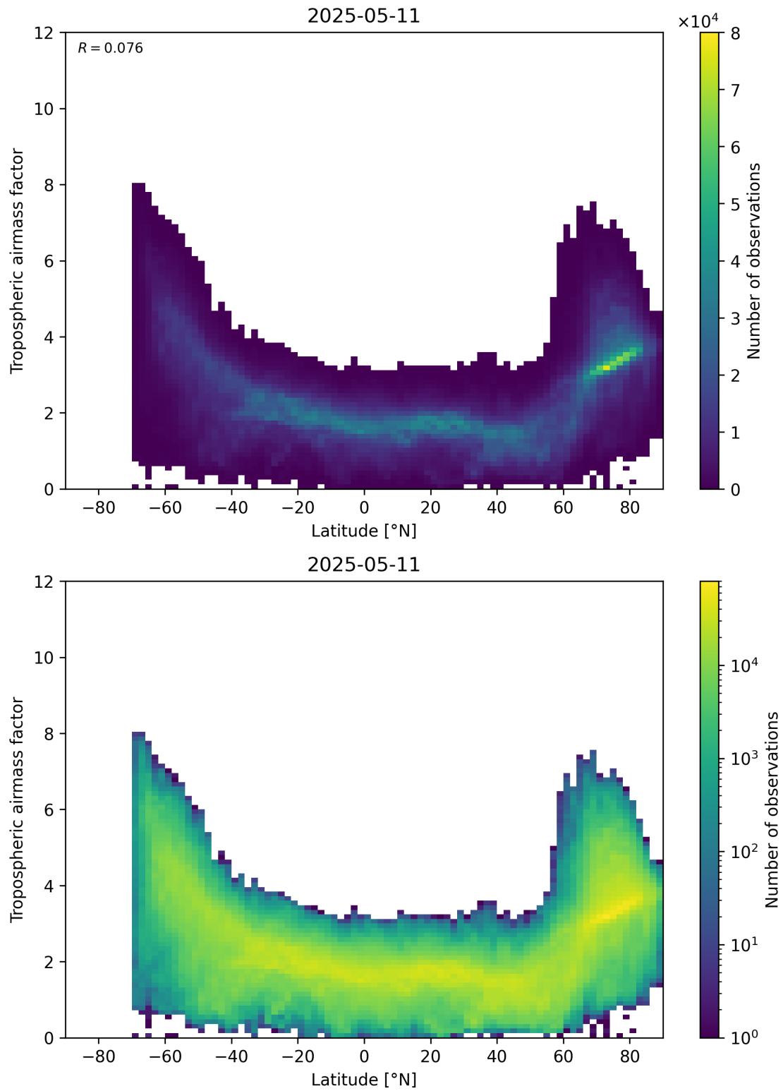
Figure 85: Scatter density plot of “Latitude” against “Tropospheric air mass factor” for 2025-05-11 to 2025-05-12.
