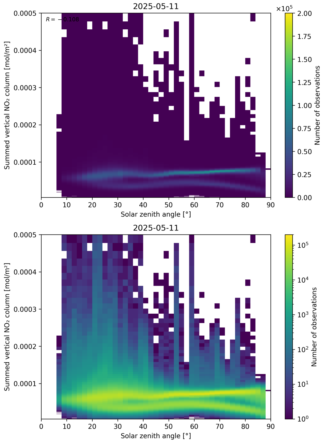
Figure 151: Scatter density plot of “Solar zenith angle” against “Summed vertical NO 2 column” for 2025-05-11 to 2025-05-12.
