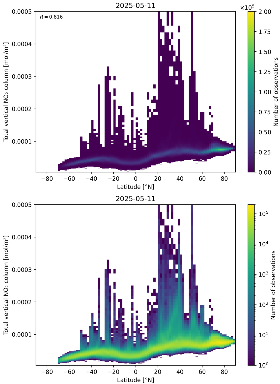
Figure 90: Scatter density plot of “Latitude” against “Total vertical NO 2 column” for 2025-05-11 to 2025-05-12.
