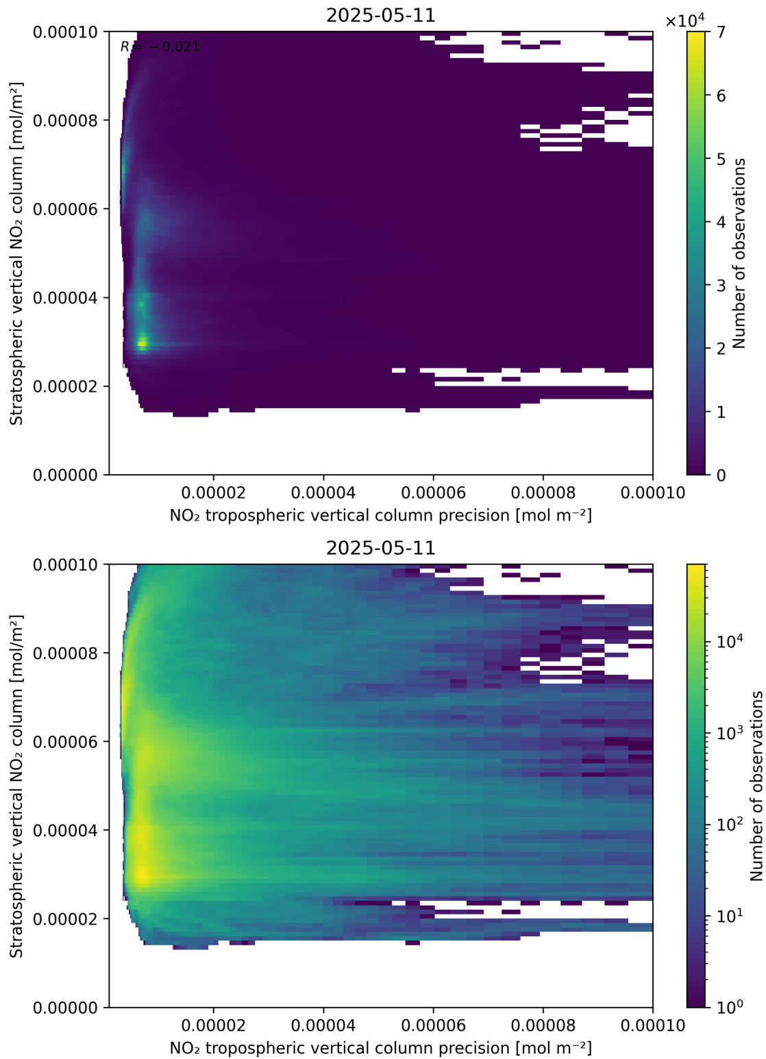
Figure 135: Scatter density plot of “NO 2 tropospheric vertical column precision” against “Stratospheric vertical NO 2 column” for 2025-05-11 to 2025-05-12.
