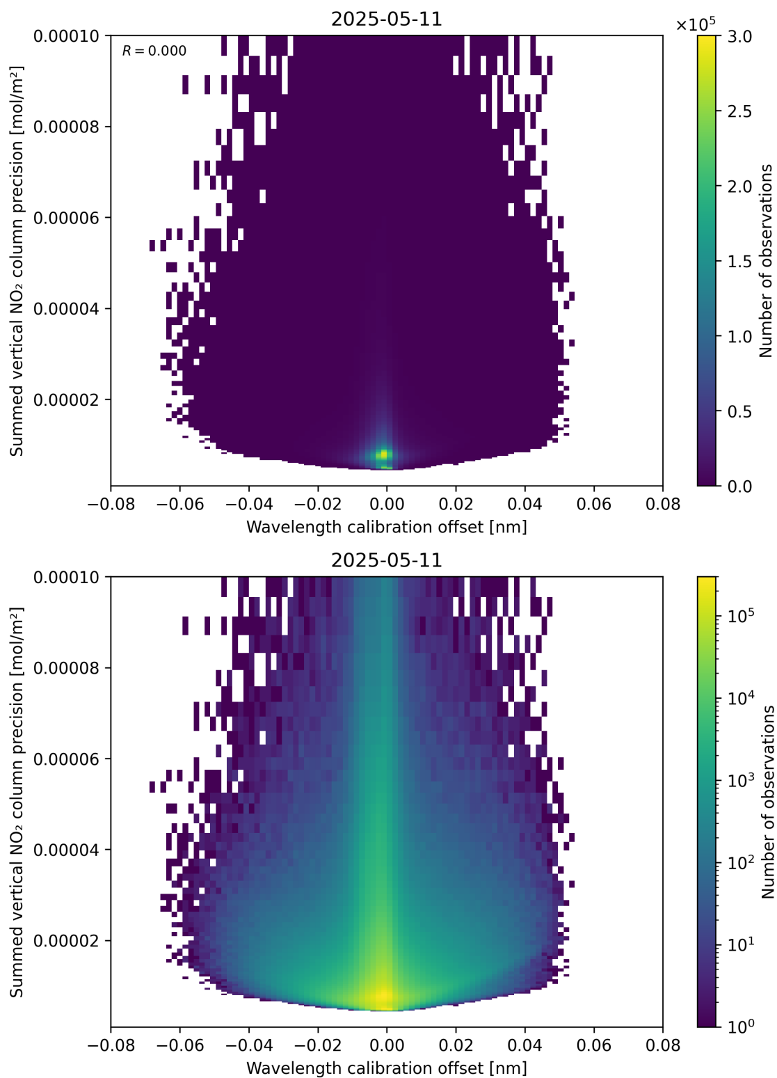
Figure 178: Scatter density plot of “Wavelength calibration offset” against “Summed vertical NO 2 column precision” for 2025-05-11 to 2025-05-12.
