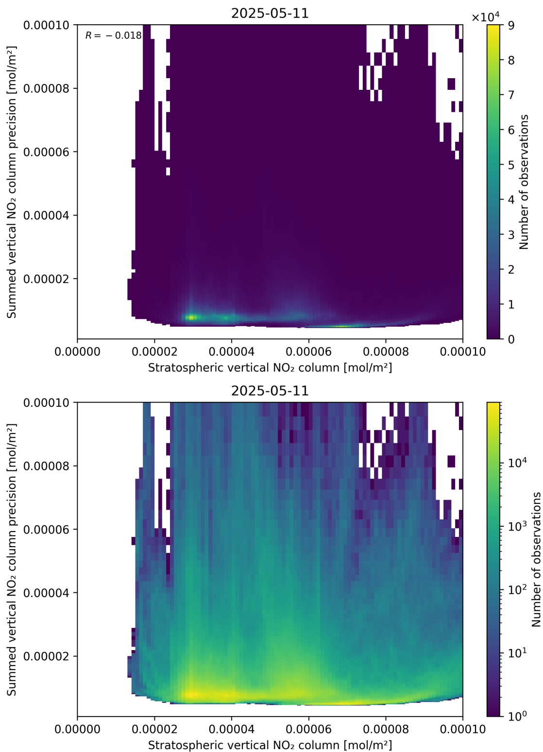
Figure 99: Scatter density plot of “Stratospheric vertical NO 2 column” against “Summed vertical NO 2 column precision” for 2025-05-11 to 2025-05-12.
