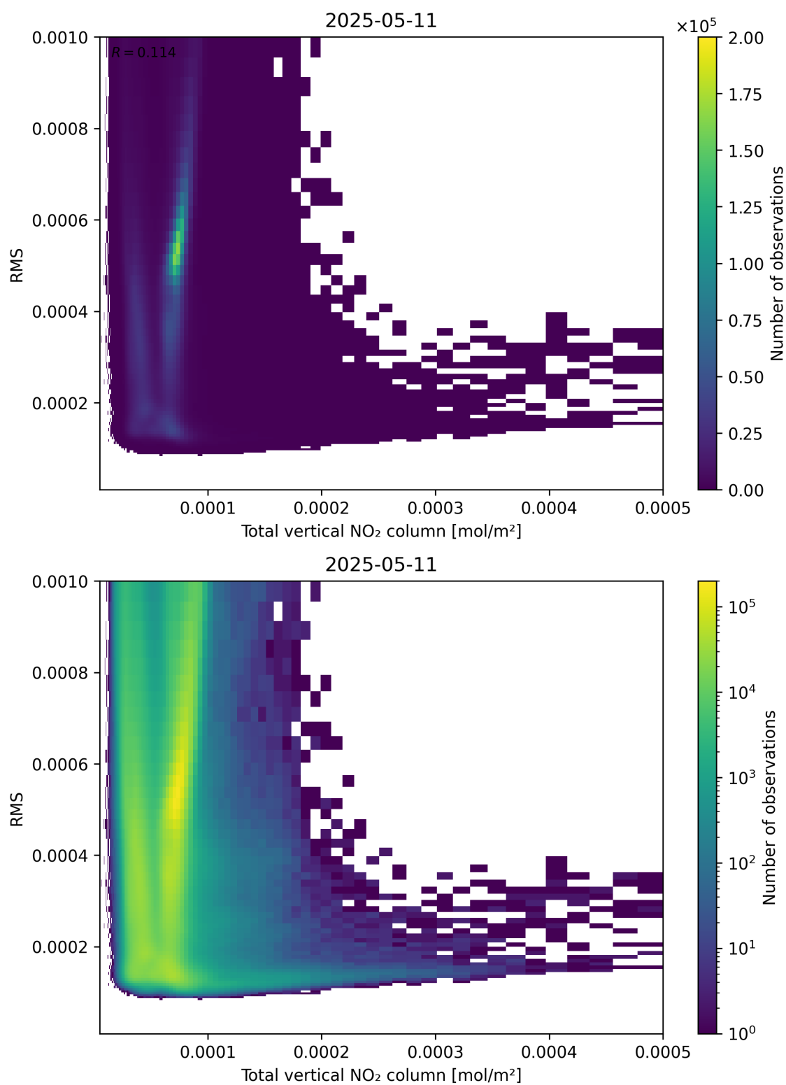
Figure 120: Scatter density plot of “Total vertical NO 2 column” against “RMS” for 2025-05-11 to 2025-05-12.
