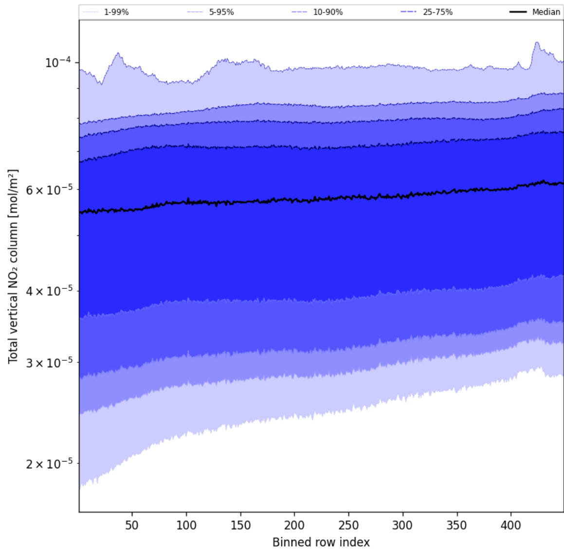
Figure 55: Along track statistics of “Total vertical NO 2 column” for 2025-05-11 to 2025-05-12
