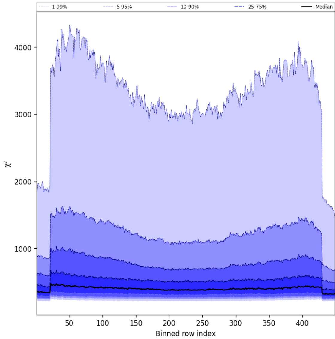
Figure 59: Along track statistics of “ \chi^2 ” for 2025-05-11 to 2025-05-12
