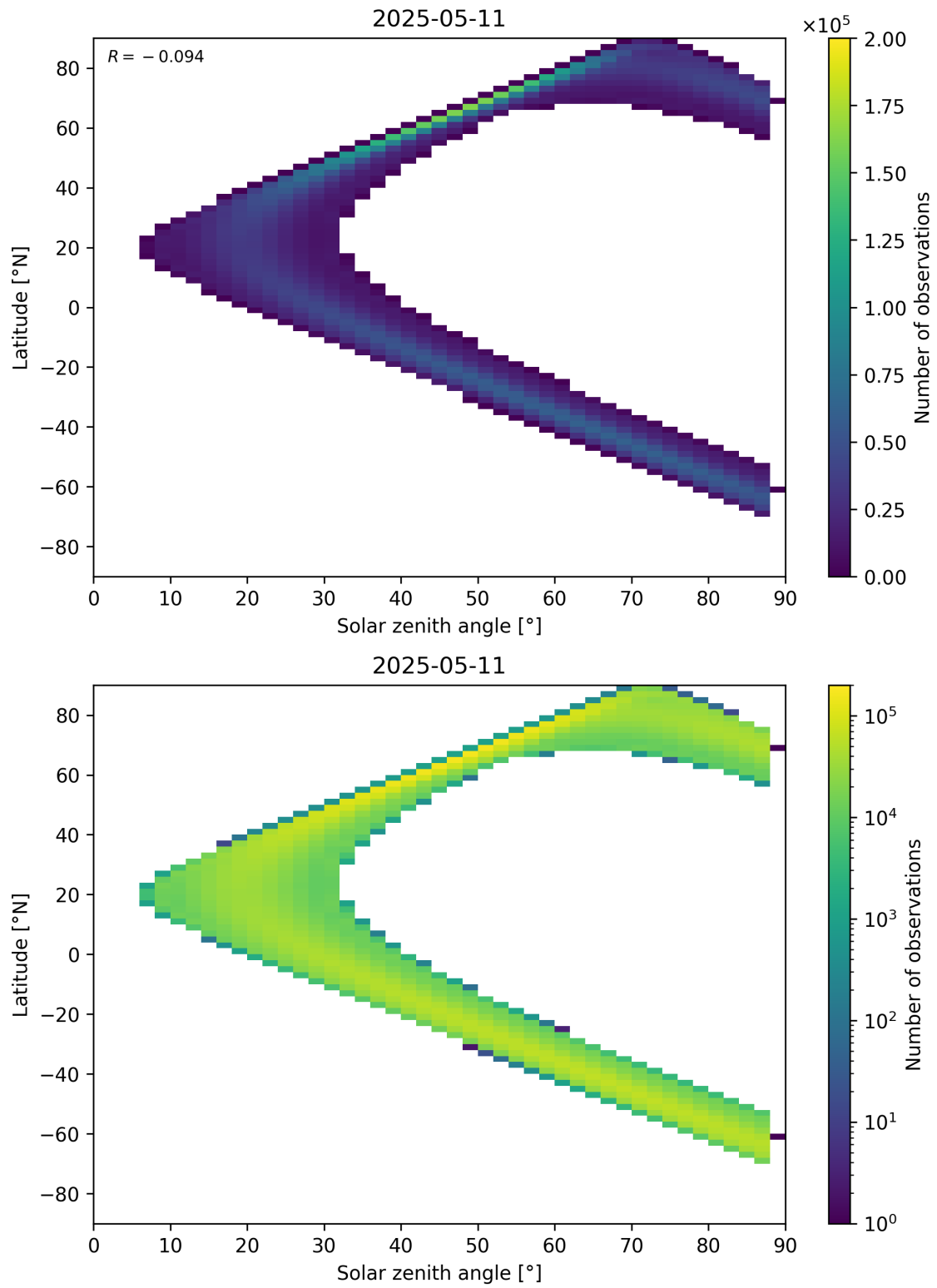
Figure 149: Scatter density plot of “Solar zenith angle” against “Latitude” for 2025-05-11 to 2025-05-12.
