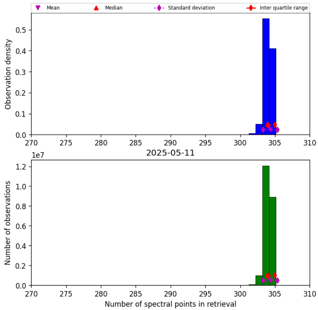
Figure 33: Histogram of “Number of spectral points in retrieval” for 2025-05-11 to 2025-05-12
