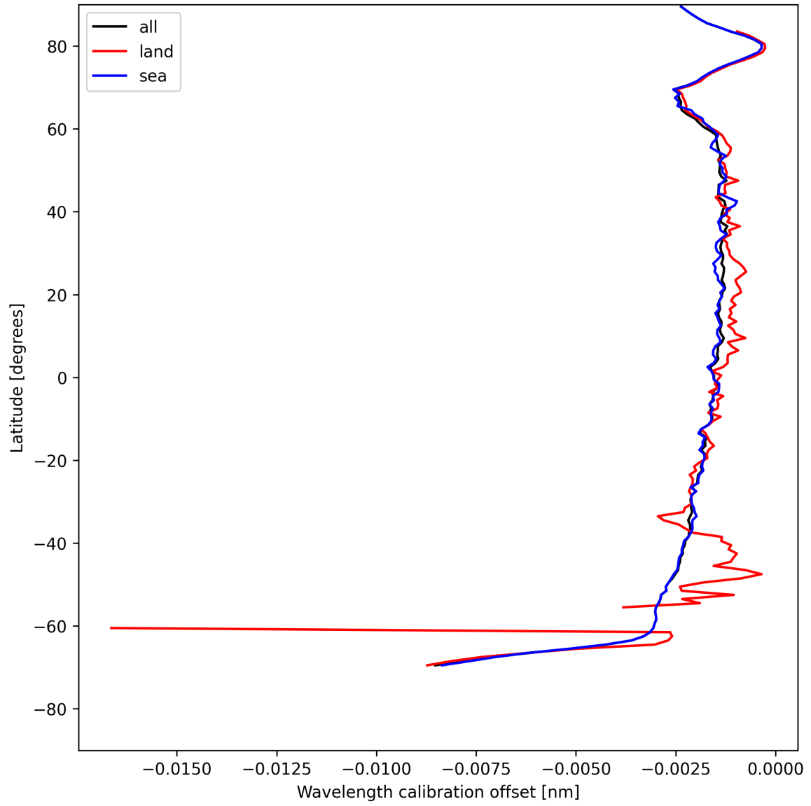
Figure 18: Zonal average of “Wavelength calibration offset” for 2025-05-11 to 2025-05-12.
