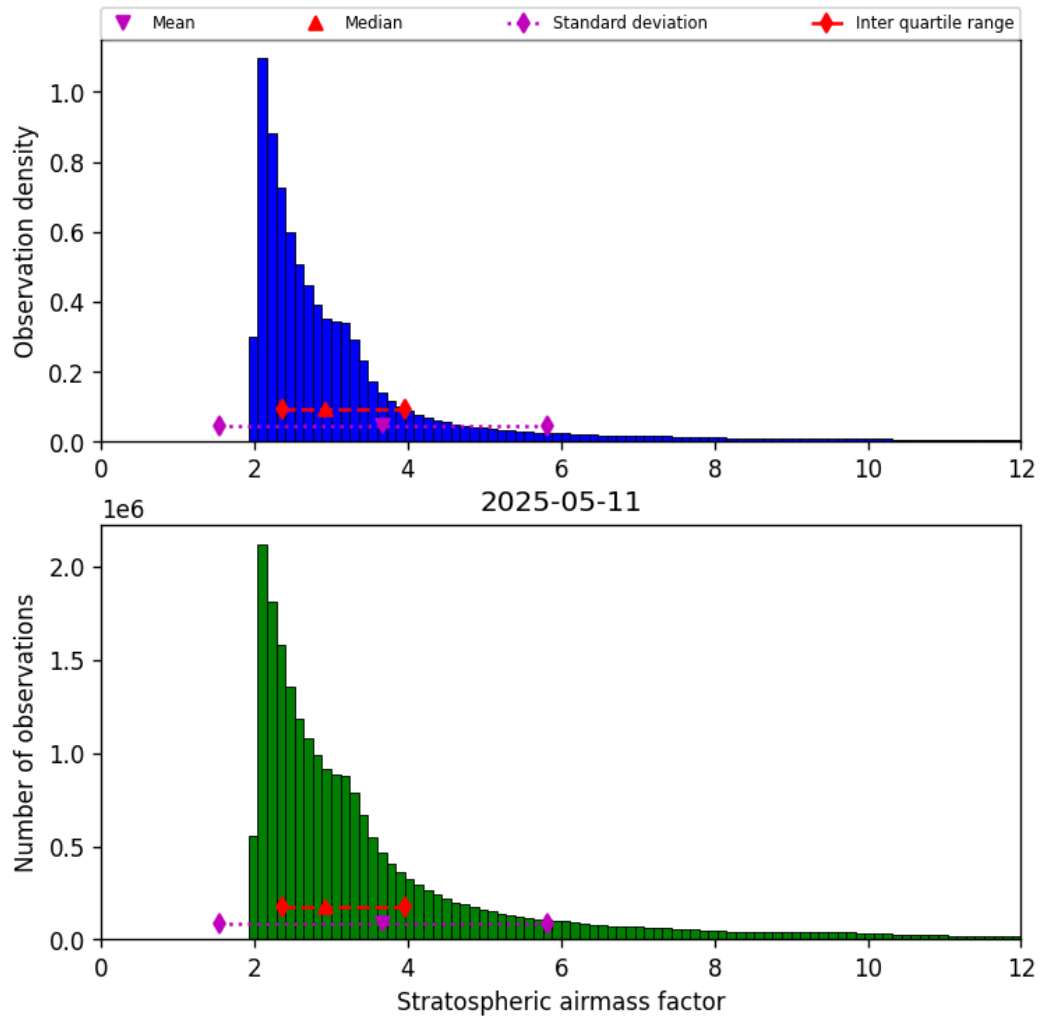
Figure 44: Histogram of “Stratospheric airmass factor” for 2025-05-11 to 2025-05-12
