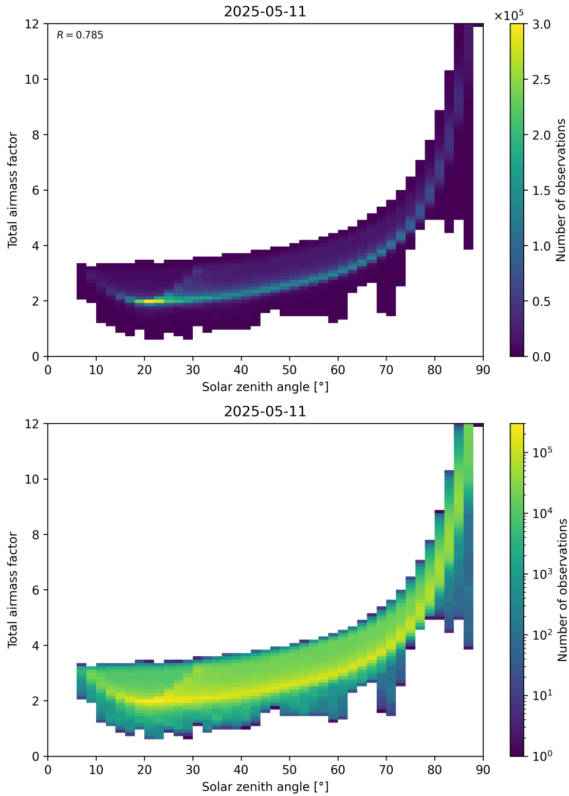
Figure 146: Scatter density plot of “Solar zenith angle” against “Total airmass factor” for 2025-05-11 to 2025-05-12.
