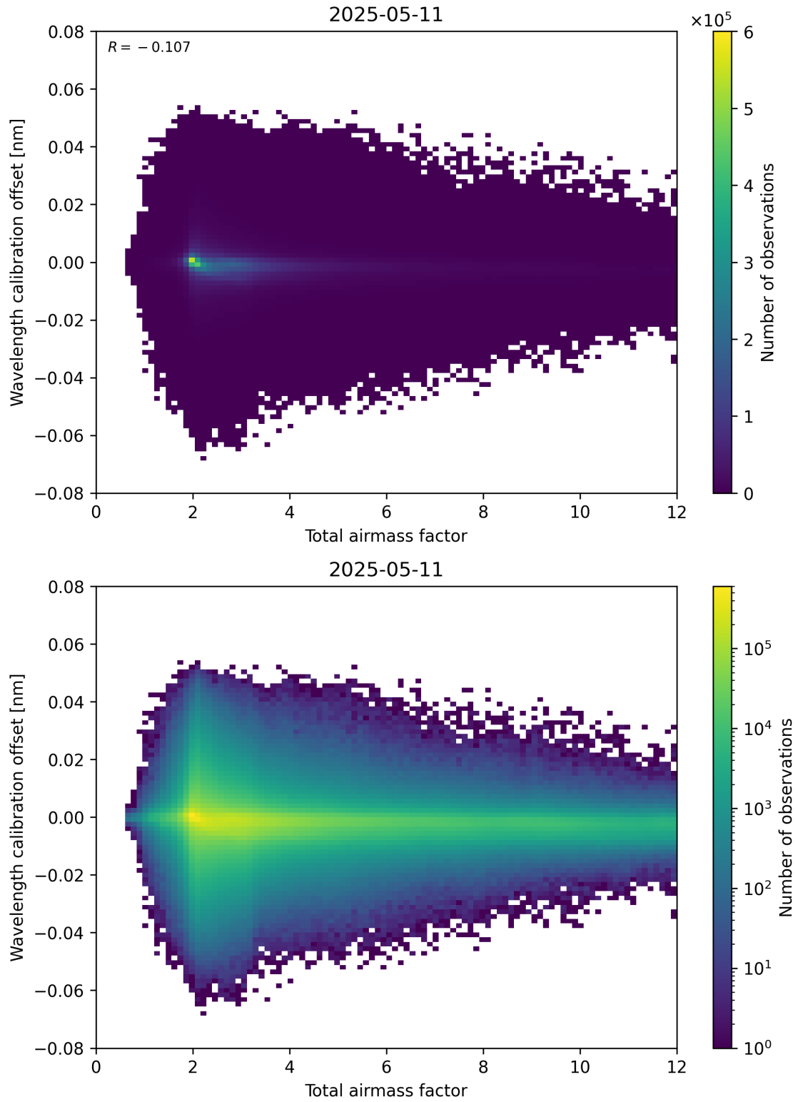
Figure 70: Scatter density plot of “Total airmass factor” against “Wavelength calibration offset” for 2025-05-11 to 2025-05-12.
