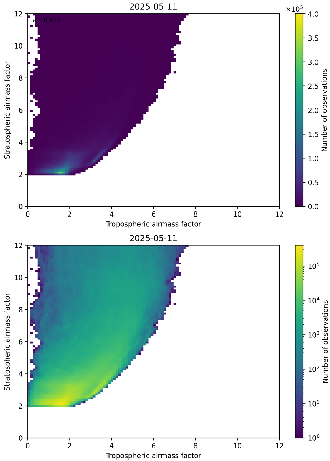
Figure 71: Scatter density plot of “Tropospheric airmass factor” against “Stratospheric airmass factor” for 2025-05-11 to 2025-05-12.
