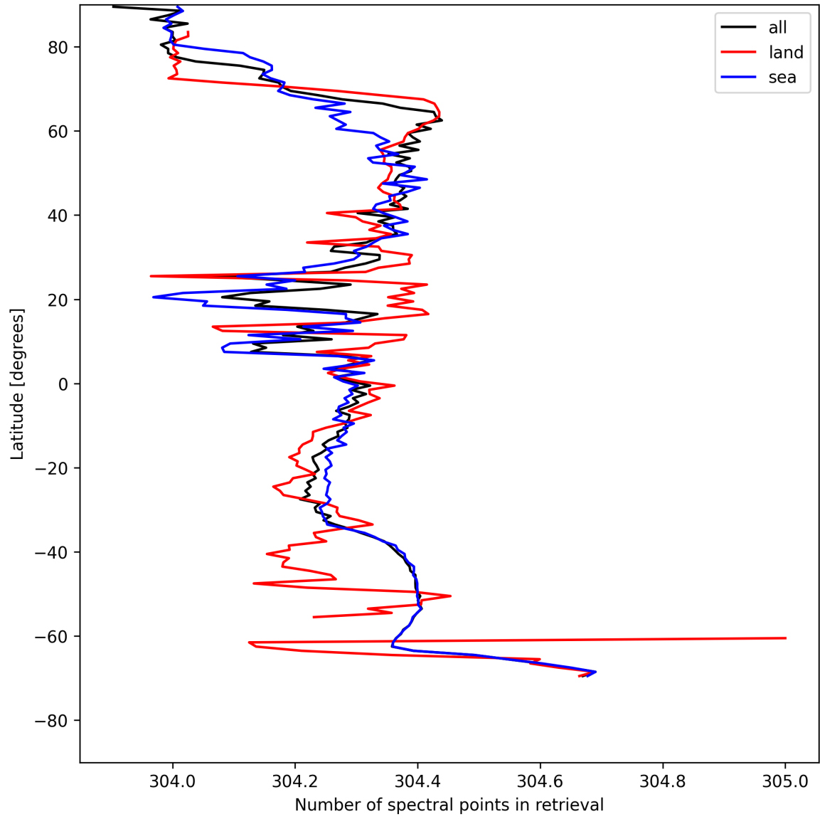
Figure 16: Zonal average of “Number of spectral points in retrieval” for 2025-05-11 to 2025-05-12.
