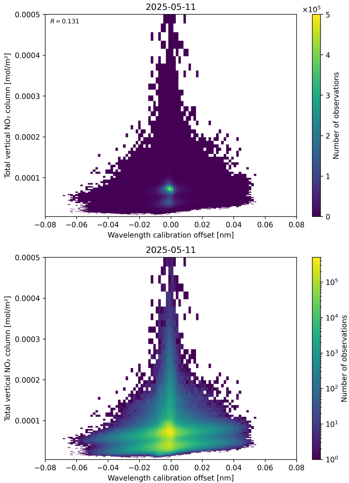
Figure 179: Scatter density plot of “Wavelength calibration offset” against “Total vertical NO 2 column” for 2025-05-11 to 2025-05-12.
