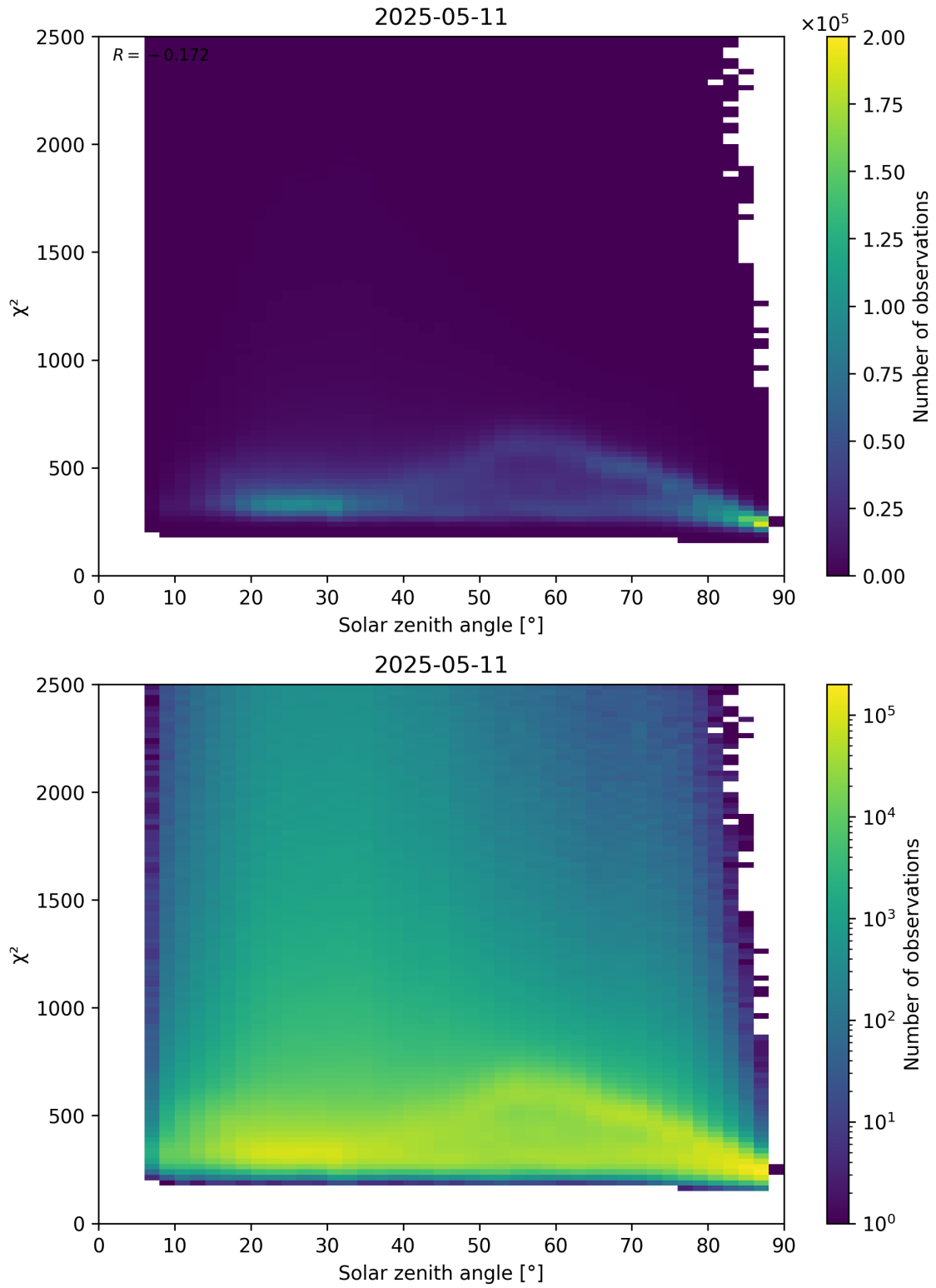
Figure 148: Scatter density plot of “Solar zenith angle” against “ \chi^2 ” for 2025-05-11 to 2025-05-12.
