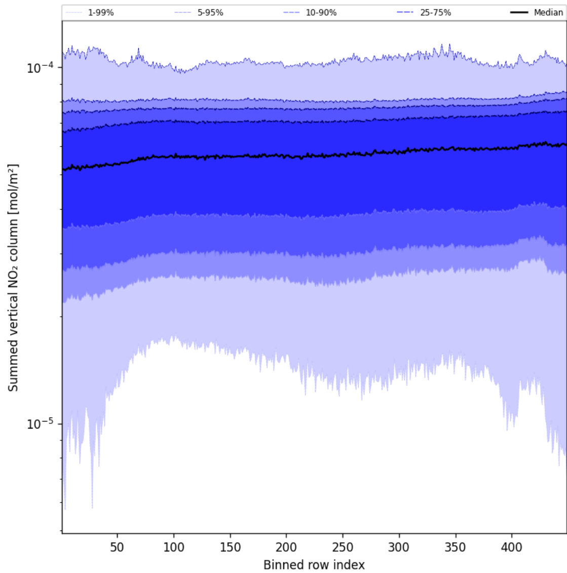
Figure 57: Along track statistics of “Summed vertical NO 2 column” for 2025-05-11 to 2025-05-12
