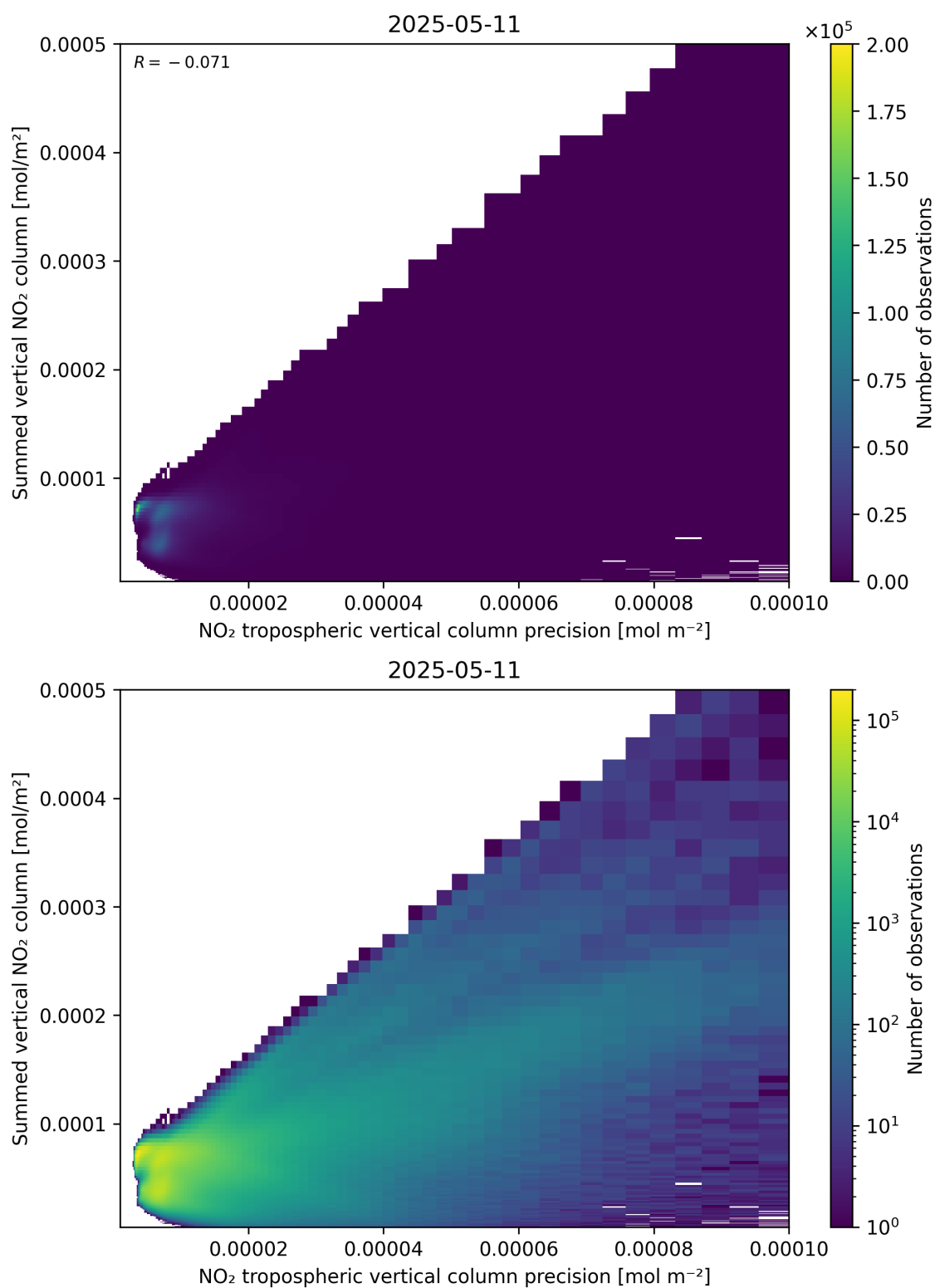
Figure 136: Scatter density plot of “NO 2 tropospheric vertical column precision” against “Summed vertical NO 2 column” for 2025-05-11 to 2025-05-12.
