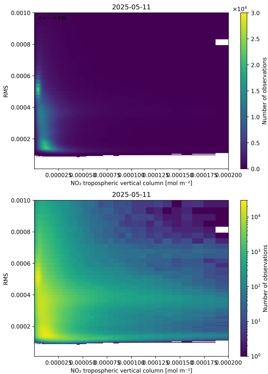
Figure 142: Scatter density plot of “NO 2 tropospheric vertical column” against “RMS” for 2025-05-11 to 2025-05-12.
