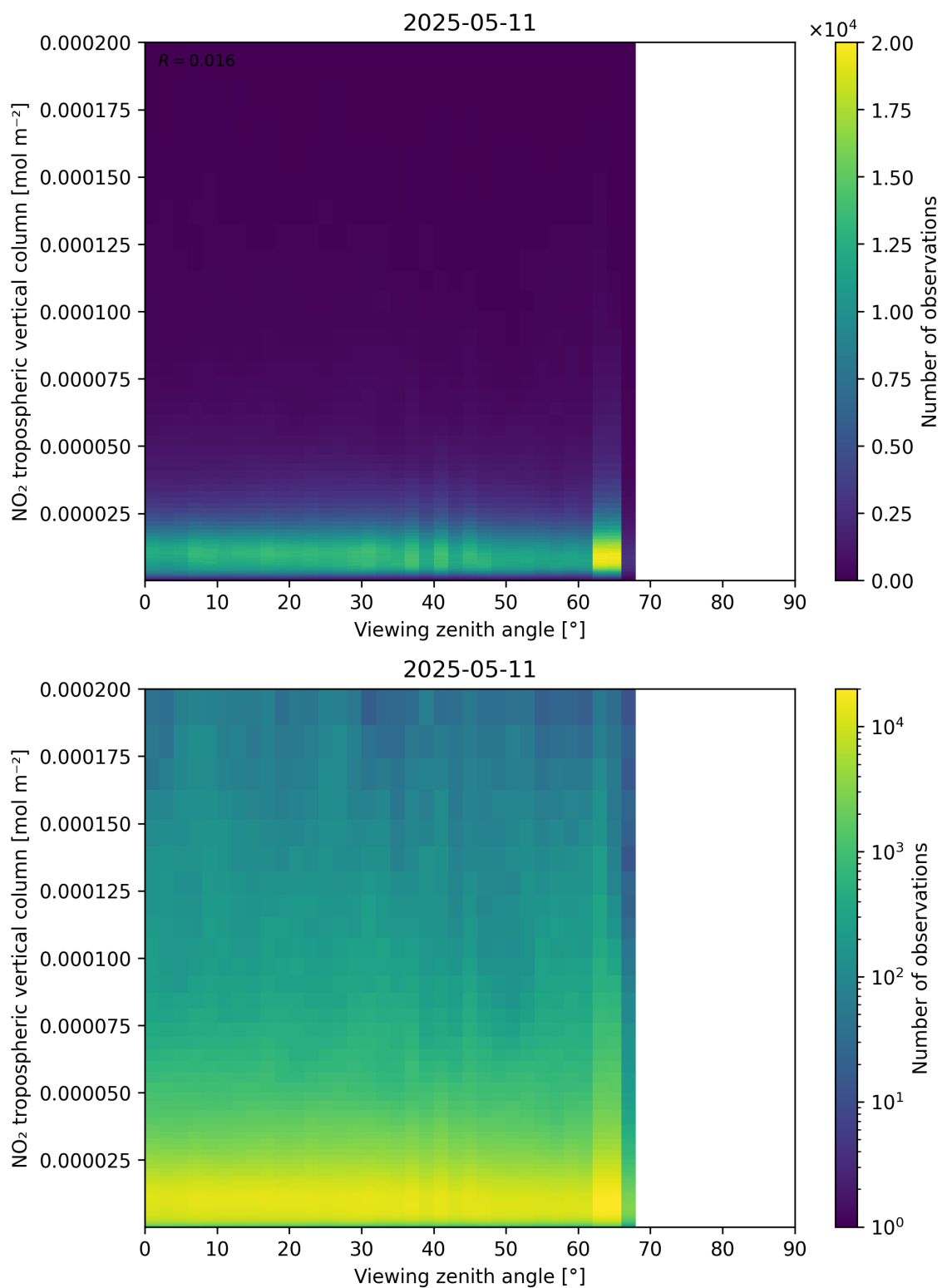
Figure 169: Scatter density plot of “Viewing zenith angle” against “NO 2 tropospheric vertical column” for 2025-05-11 to 2025-05-12.
