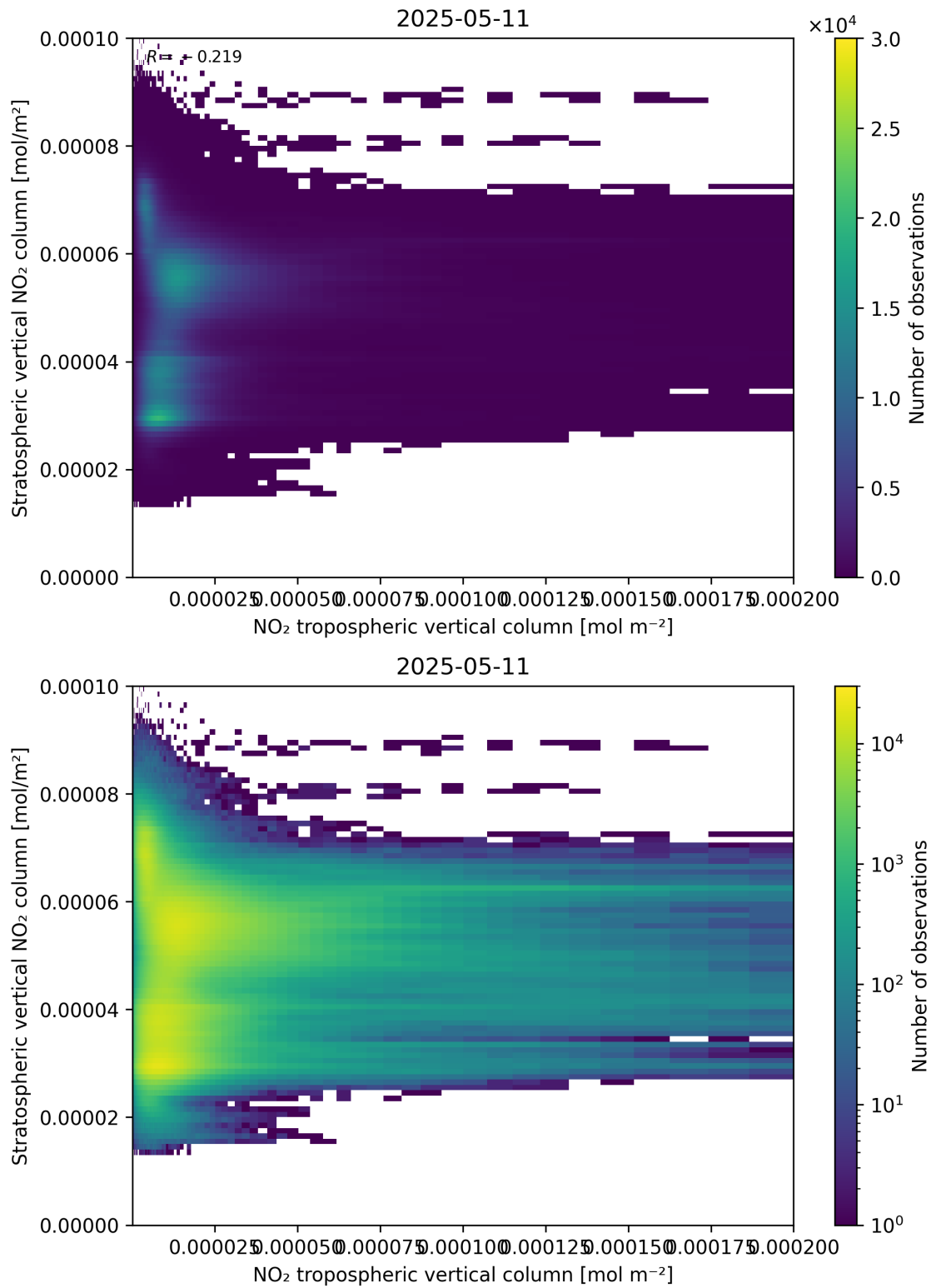
Figure 125: Scatter density plot of “NO 2 tropospheric vertical column” against “Stratospheric vertical NO 2 column” for 2025-05-11 to 2025-05-12.
