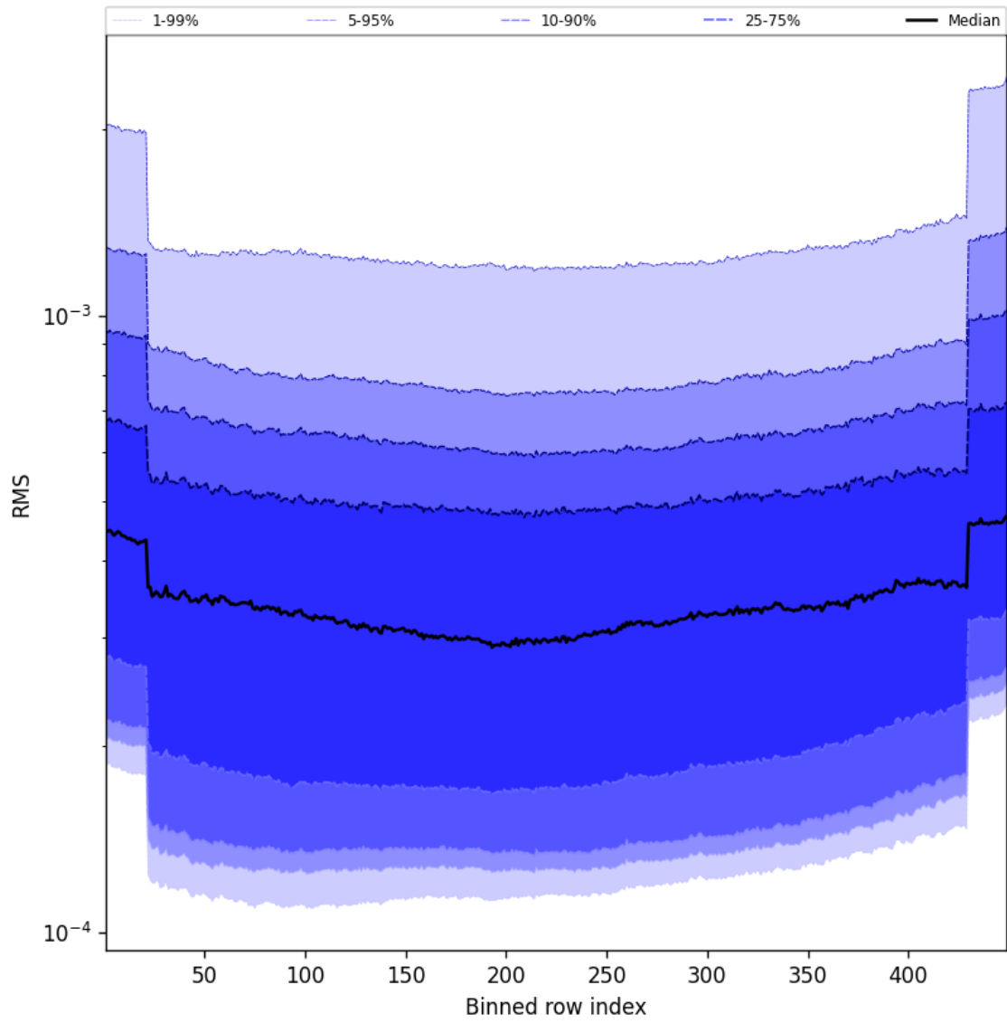
Figure 60: Along track statistics of “RMS” for 2025-05-11 to 2025-05-12
