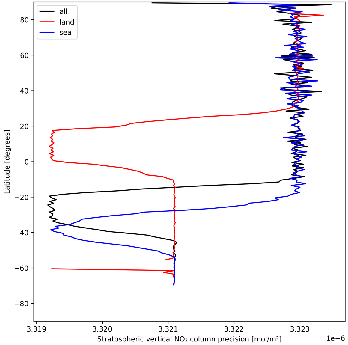
Figure 20: Zonal average of “Stratospheric vertical NO 2 column precision” for 2025-05-11 to 2025-05-12.
