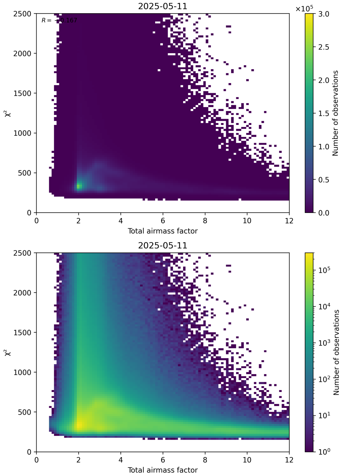
Figure 63: Scatter density plot of “Total airmass factor” against “ \chi^2 ” for 2025-05-11 to 2025-05-12.
