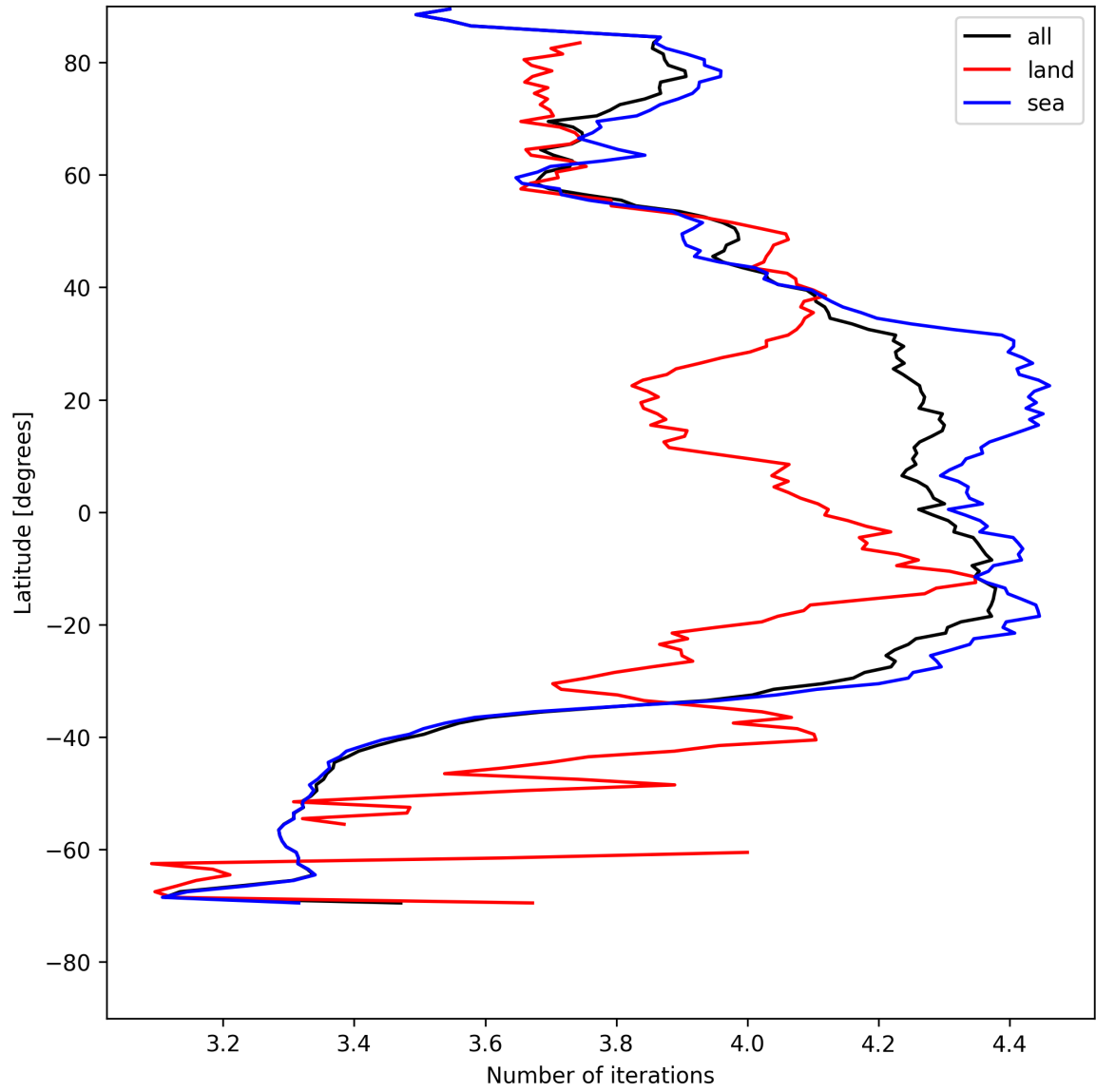
Figure 17: Zonal average of “Number of iterations” for 2025-05-11 to 2025-05-12.
