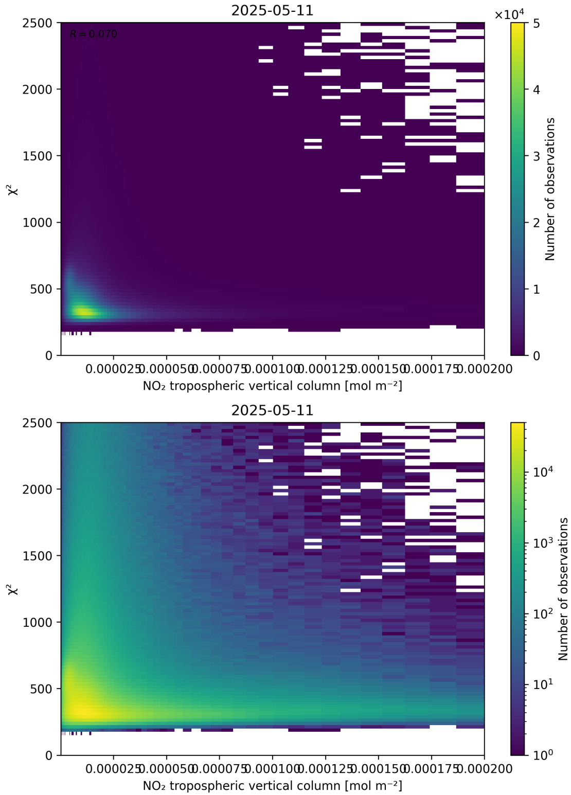
Figure 124: Scatter density plot of “NO 2 tropospheric vertical column” against “ \chi^2 ” for 2025-05-11 to 2025-05-12.
