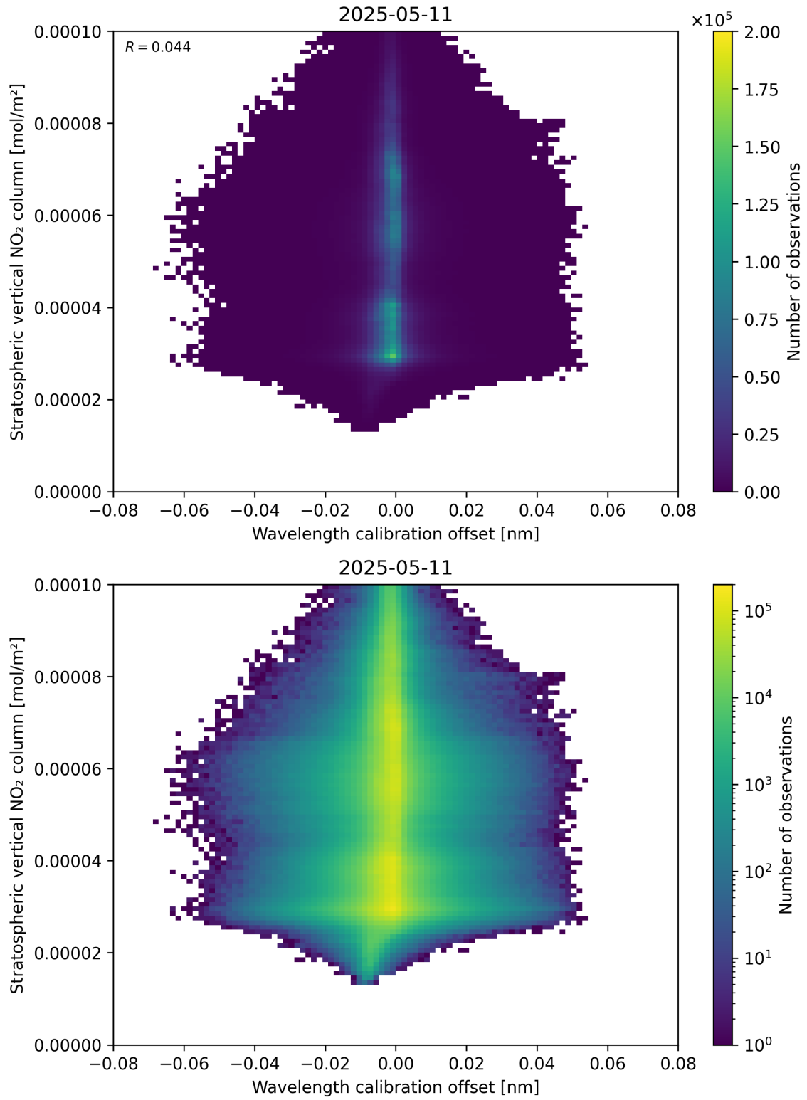
Figure 176: Scatter density plot of “Wavelength calibration offset” against “Stratospheric vertical NO 2 column” for 2025-05-11 to 2025-05-12.
