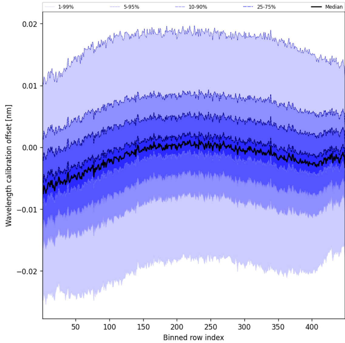
Figure 52: Along track statistics of “Wavelength calibration offset” for 2025-05-11 to 2025-05-12
