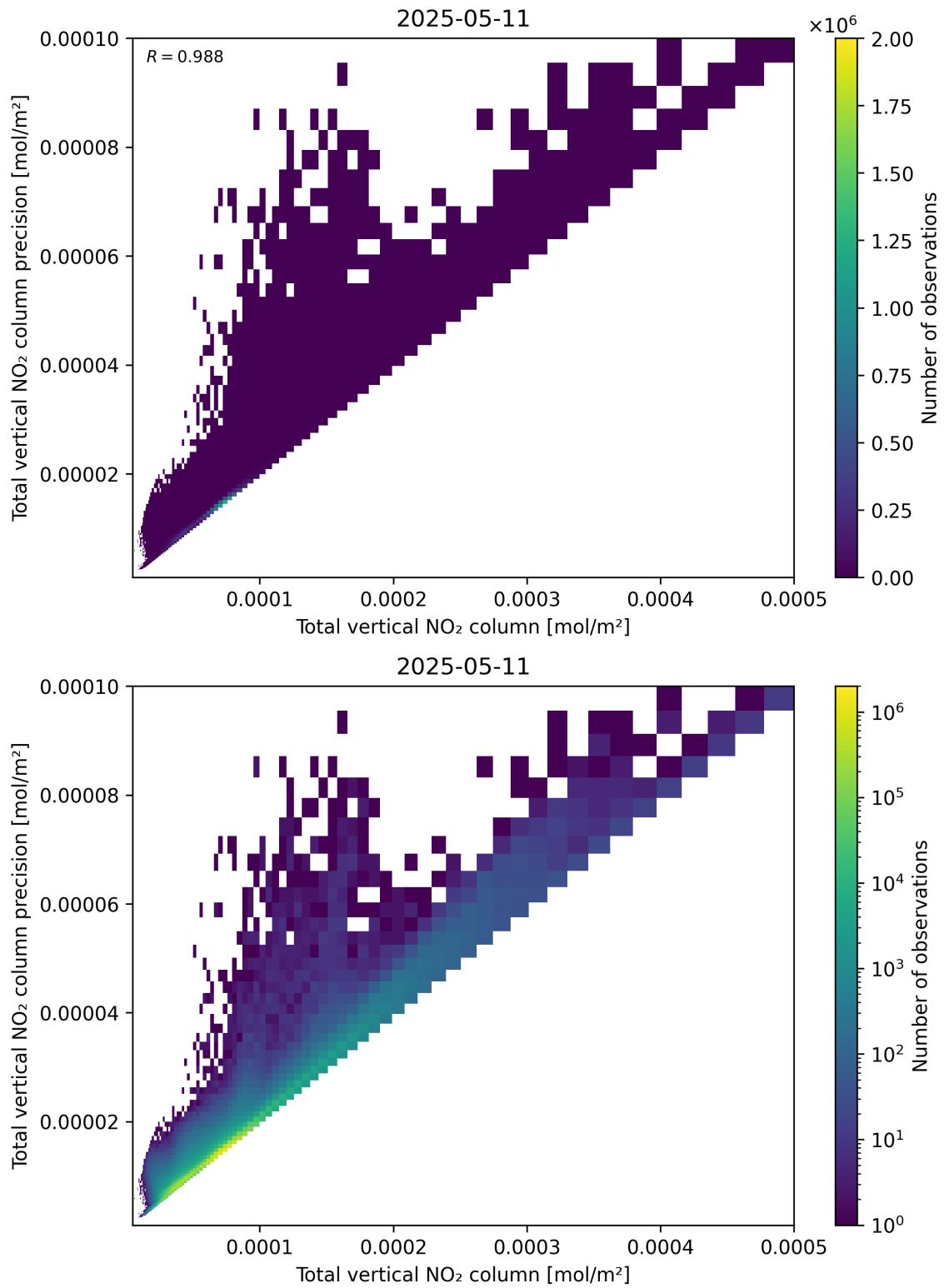
Figure 114: Scatter density plot of “Total vertical NO 2 column” against “Total vertical NO 2 column precision” for 2025-05-11 to 2025-05-12.
