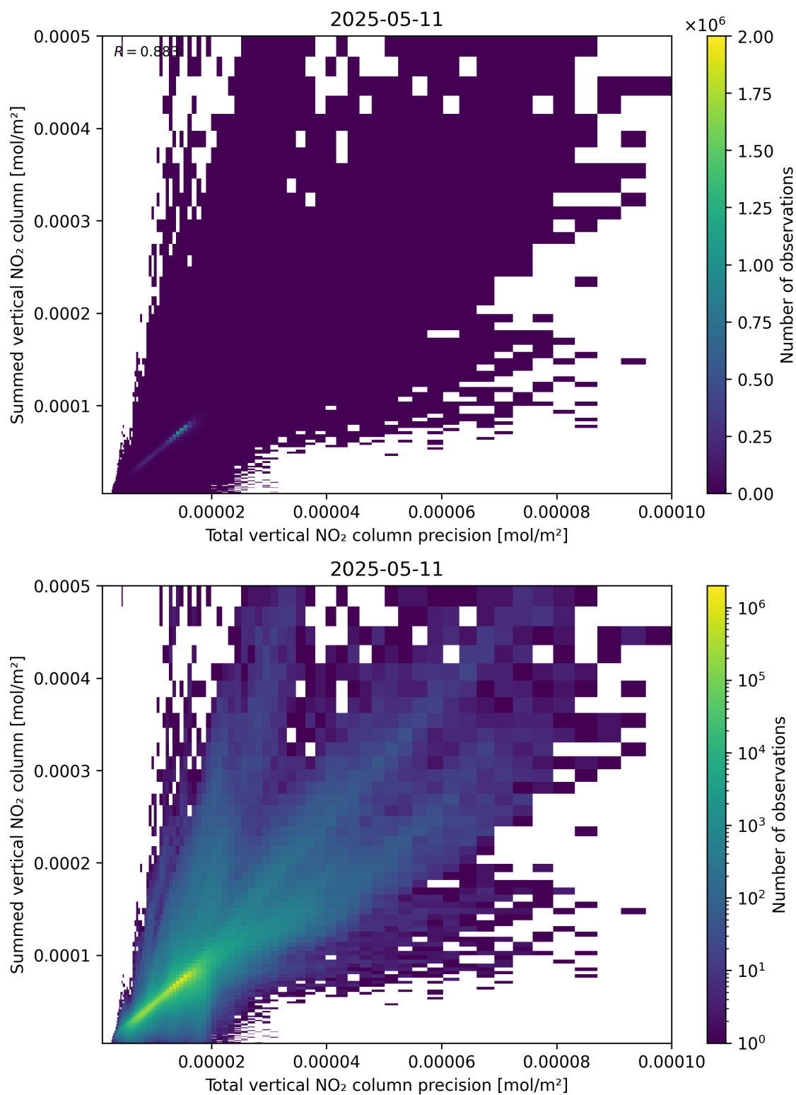
Figure 117: Scatter density plot of “Total vertical NO 2 column precision” against “Summed vertical NO 2 column” for 2025-05-11 to 2025-05-12.
