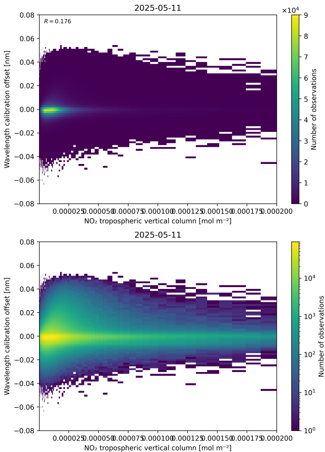
Figure 143: Scatter density plot of “NO 2 tropospheric vertical column” against “Wavelength calibration offset” for 2025-05-11 to 2025-05-12.
