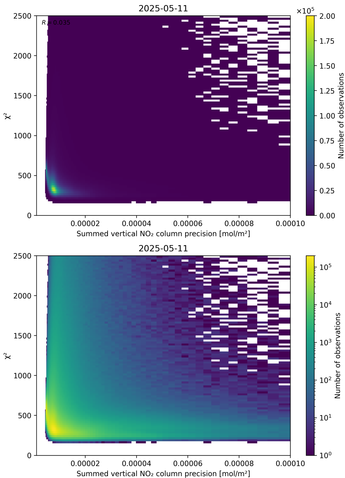
Figure 107: Scatter density plot of “Summed vertical NO 2 column precision” against “ \chi^2 ” for 2025-05-11 to 2025-05-12.
