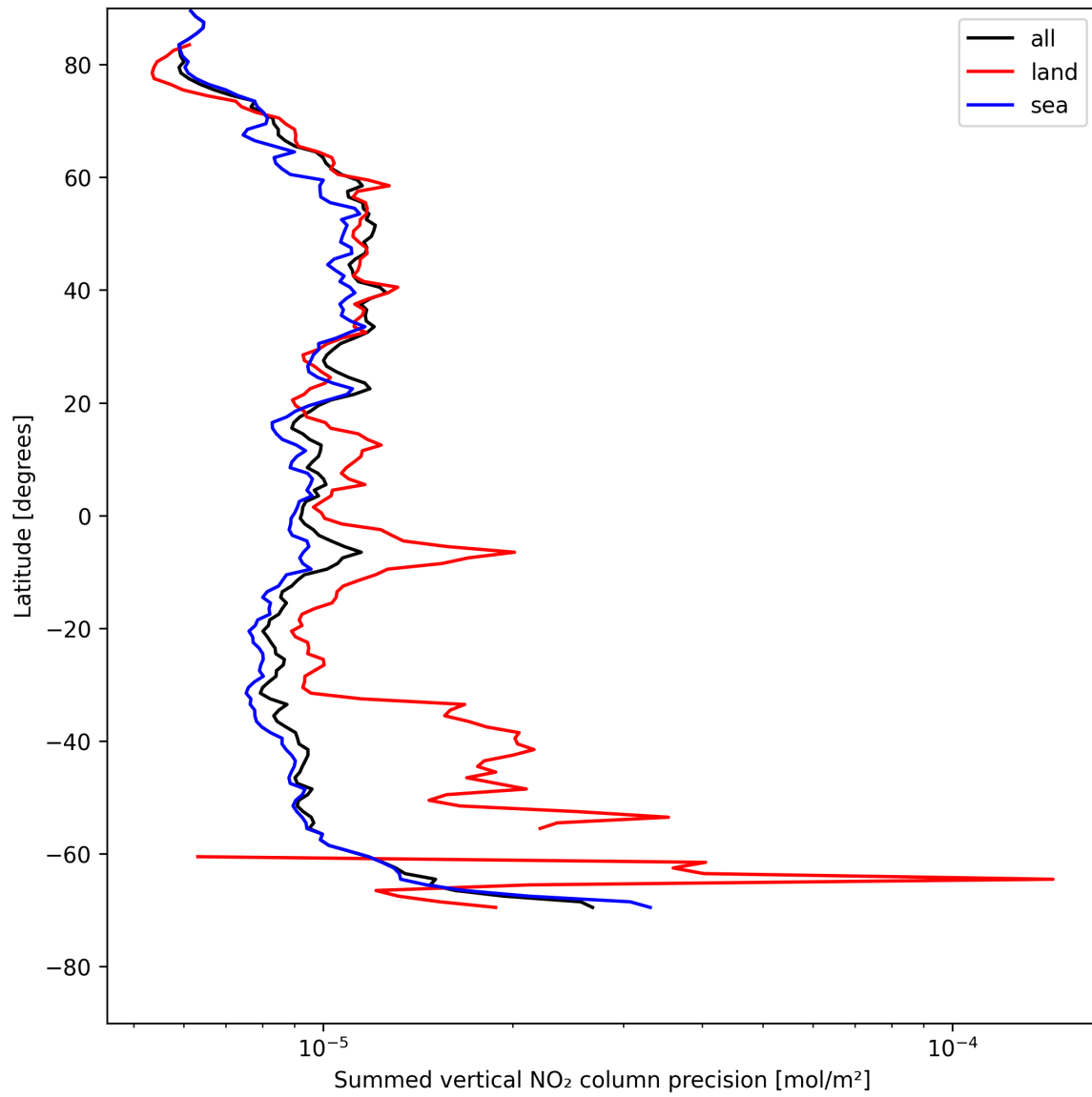
Figure 24: Zonal average of “Summed vertical NO 2 column precision” for 2025-05-11 to 2025-05-12.
