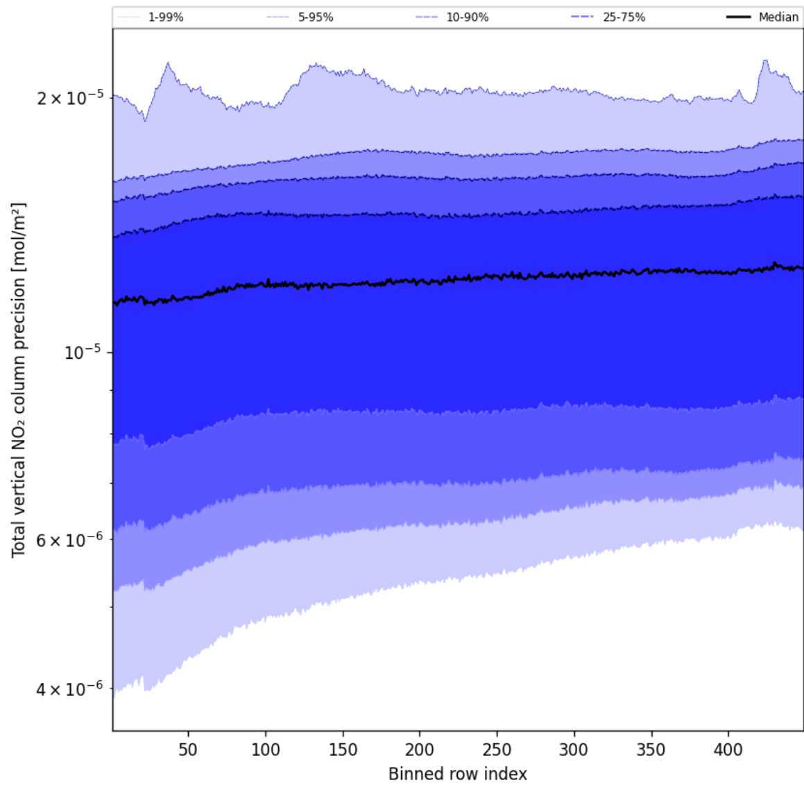
Figure 56: Along track statistics of “Total vertical NO 2 column precision” for 2025-05-11 to 2025-05-12
