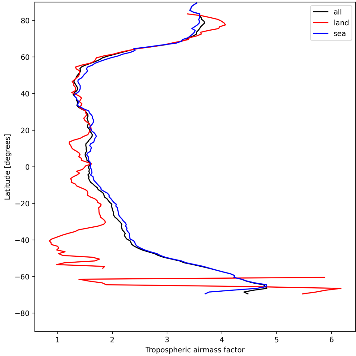
Figure 14: Zonal average of “Tropospheric airmass factor” for 2025-05-11 to 2025-05-12.
