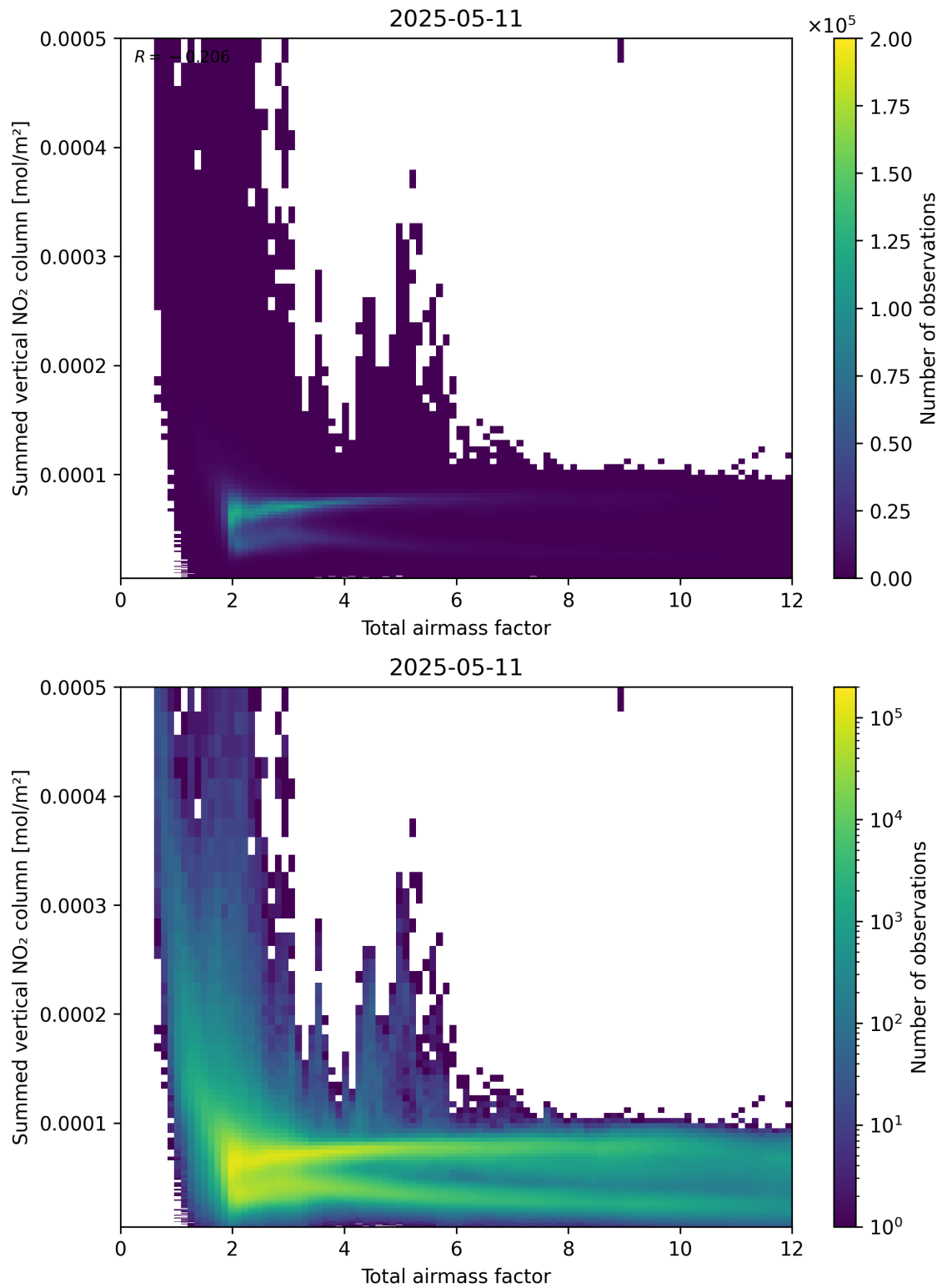
Figure 65: Scatter density plot of “Total airmass factor” against “Summed vertical NO 2 column” for 2025-05-11 to 2025-05-12.
