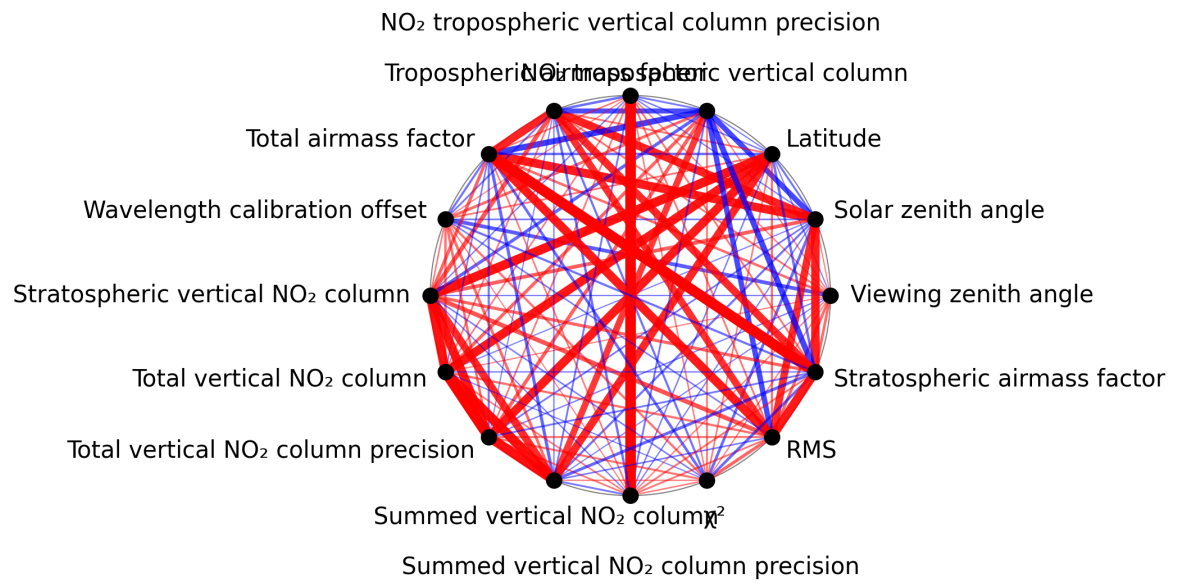
Figure 1: Map of correlation graph for 2025-05-11 to 2025-05-12.
