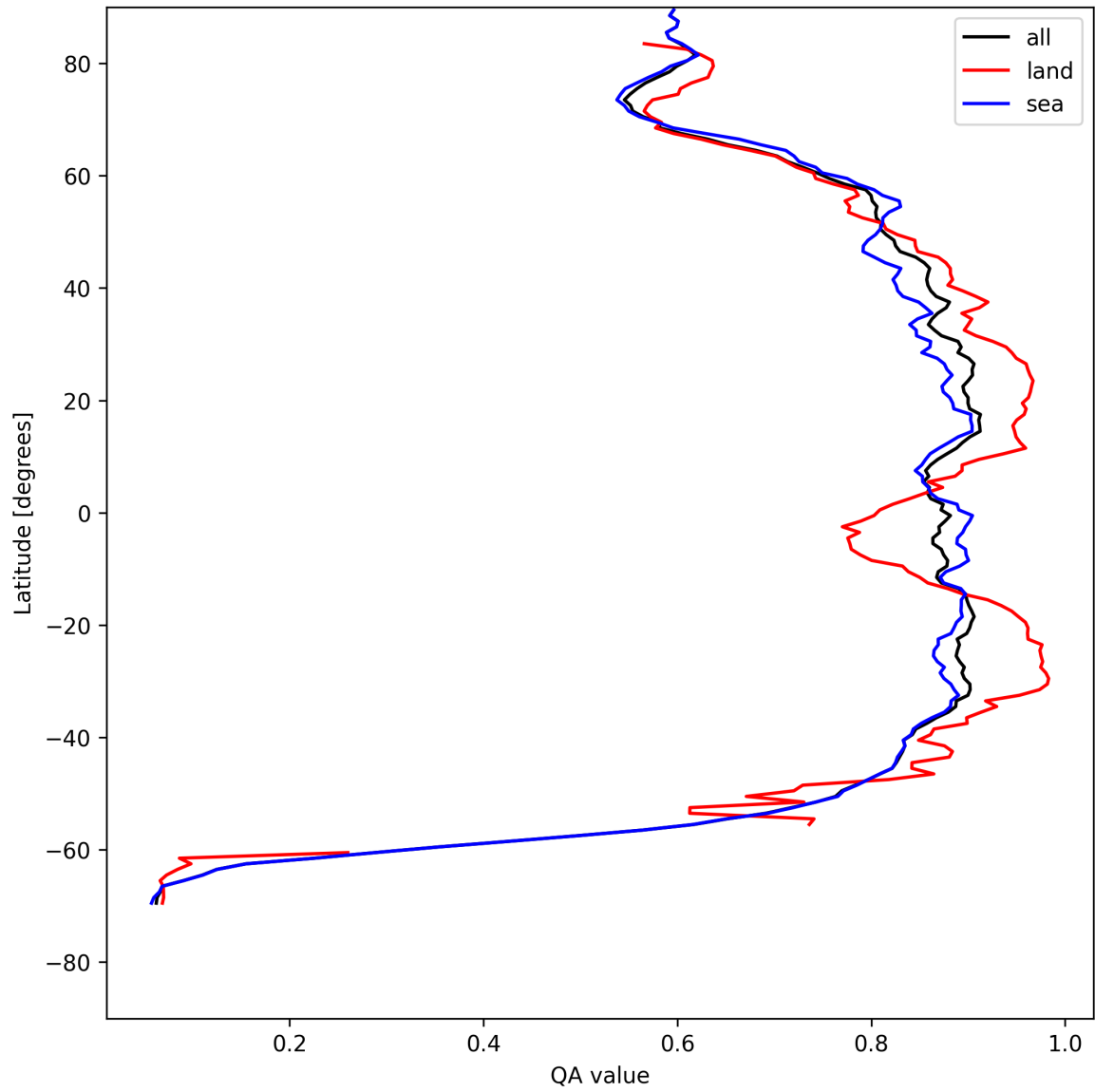
Figure 11: Zonal average of “QA value” for 2025-05-11 to 2025-05-12.
