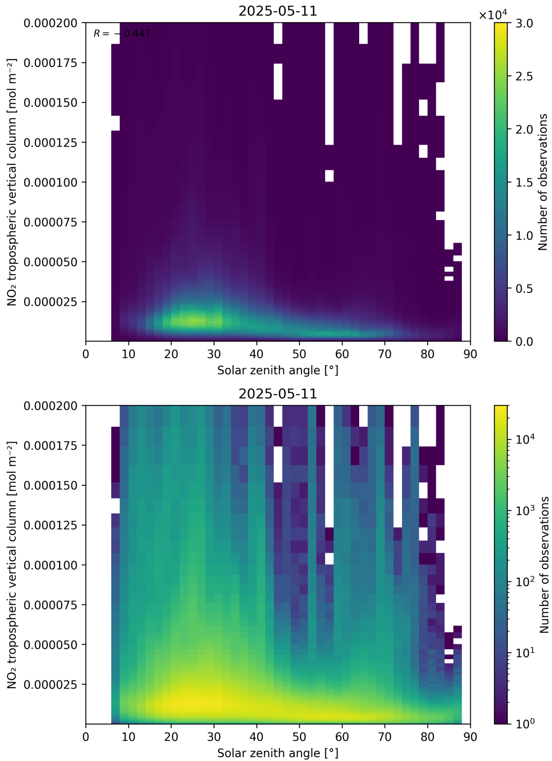
Figure 155: Scatter density plot of “Solar zenith angle” against “NO 2 tropospheric vertical column” for 2025-05-11 to 2025-05-12.
