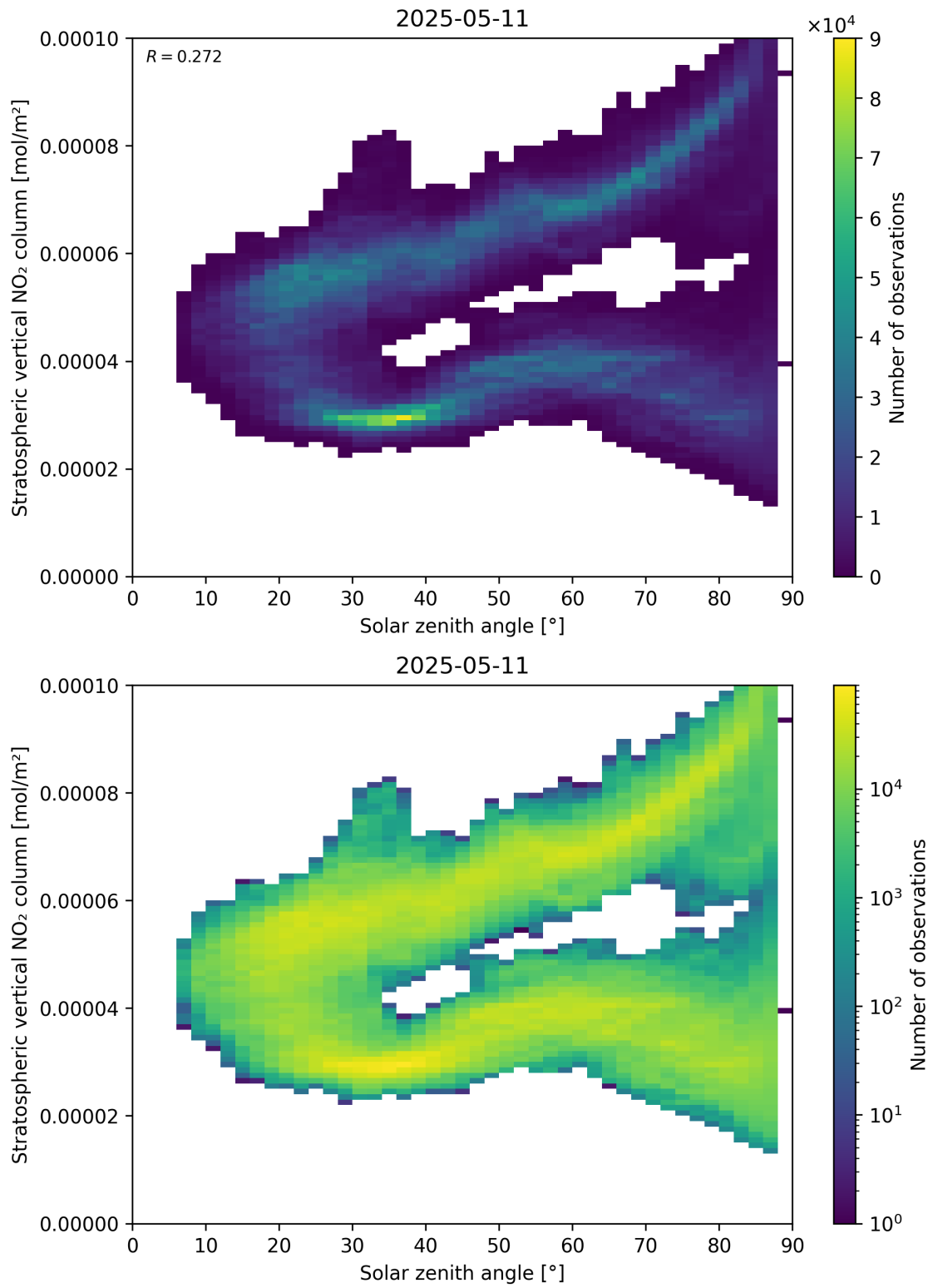
Figure 150: Scatter density plot of “Solar zenith angle” against “Stratospheric vertical NO 2 column” for 2025-05-11 to 2025-05-12.
