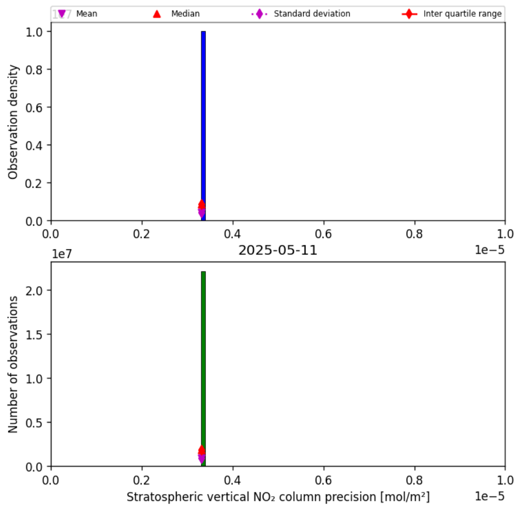
Figure 37: Histogram of “Stratospheric vertical NO 2 column precision” for 2025-05-11 to 2025-05-12
