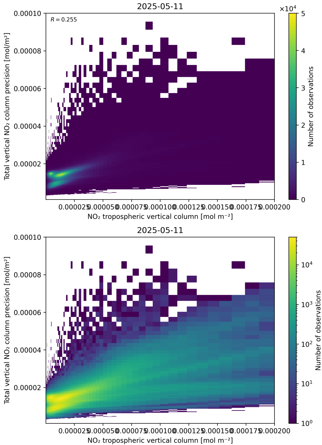
Figure 129: Scatter density plot of “NO 2 tropospheric vertical column” against “Total vertical NO 2 column precision” for 2025-05-11 to 2025-05-12.
