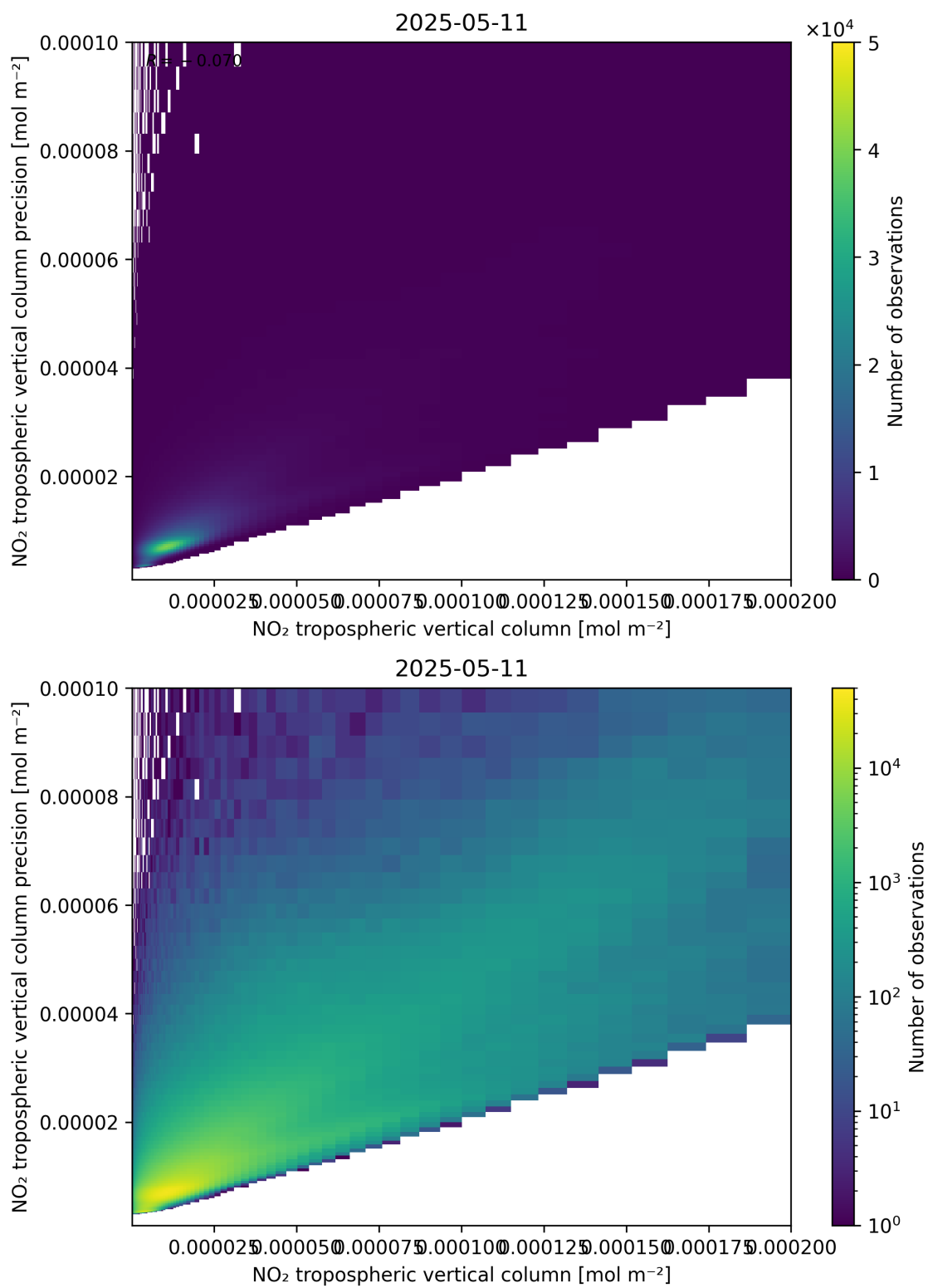
Figure 130: Scatter density plot of “NO 2 tropospheric vertical column” against “NO 2 tropospheric vertical column precision” for 2025-05-11 to 2025-05-12.
