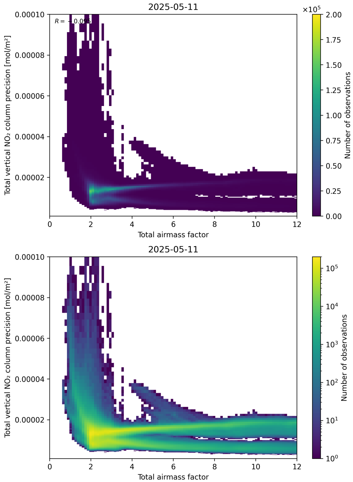
Figure 68: Scatter density plot of “Total airmass factor” against “Total vertical NO 2 column precision” for 2025-05-11 to 2025-05-12.
