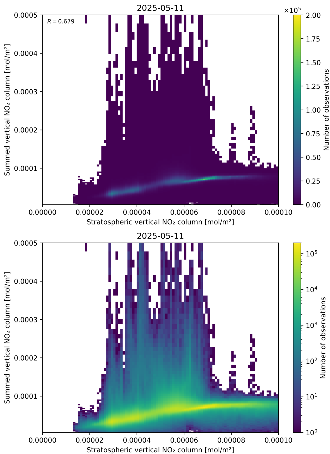
Figure 98: Scatter density plot of “Stratospheric vertical NO 2 column” against “Summed vertical NO 2 column” for 2025-05-11 to 2025-05-12.
