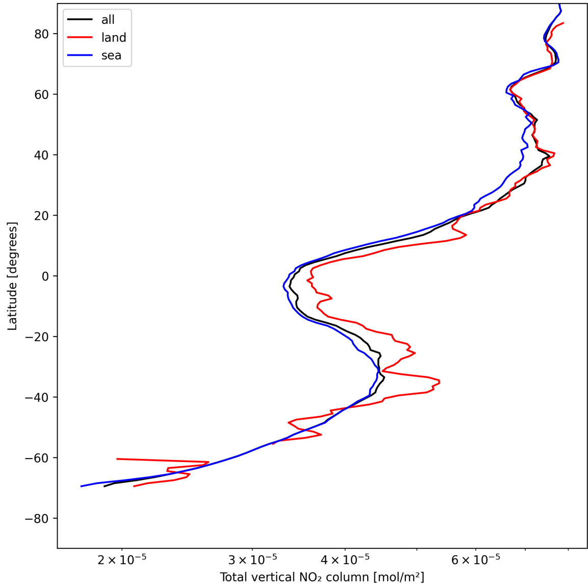
Figure 21: Zonal average of “Total vertical NO 2 column” for 2025-05-11 to 2025-05-12.
