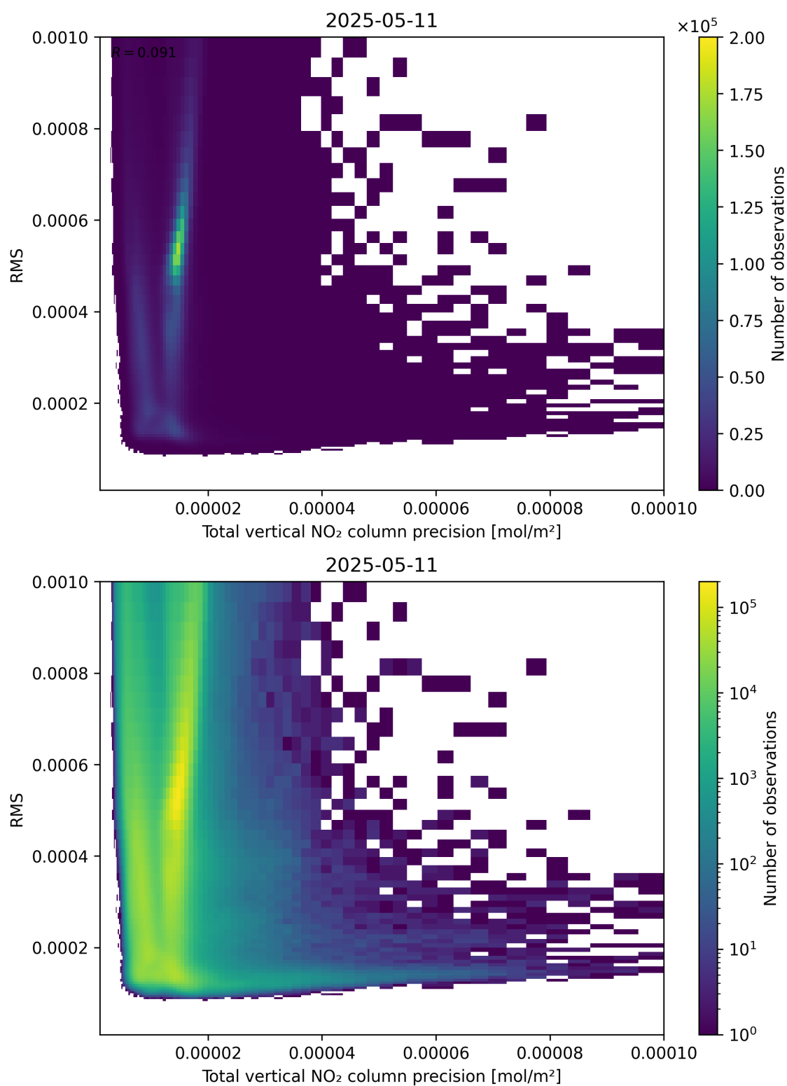
Figure 119: Scatter density plot of “Total vertical NO 2 column precision” against “RMS” for 2025-05-11 to 2025-05-12.
