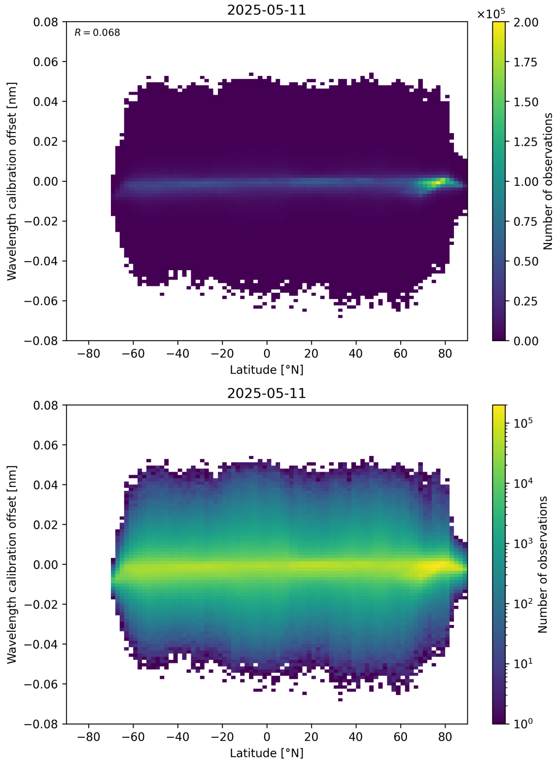
Figure 95: Scatter density plot of “Latitude” against “Wavelength calibration offset” for 2025-05-11 to 2025-05-12.
