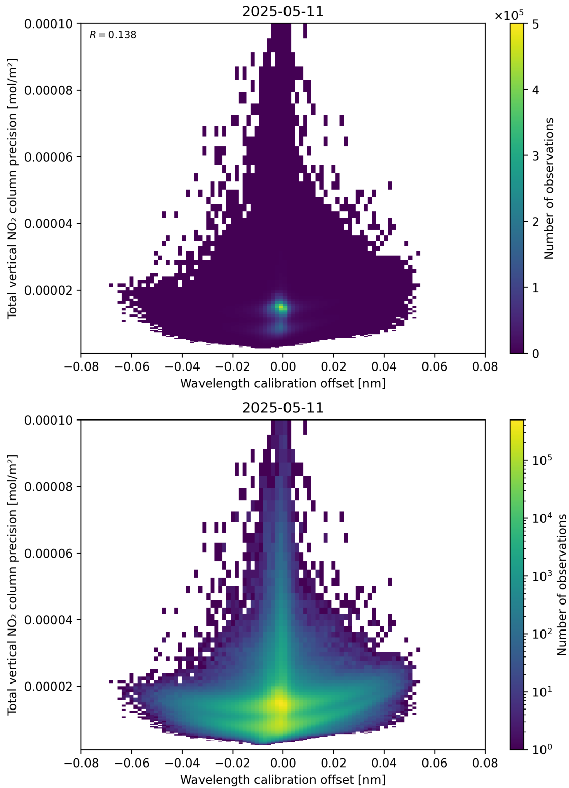
Figure 180: Scatter density plot of “Wavelength calibration offset” against “Total vertical NO 2 column precision” for 2025-05-11 to 2025-05-12.
