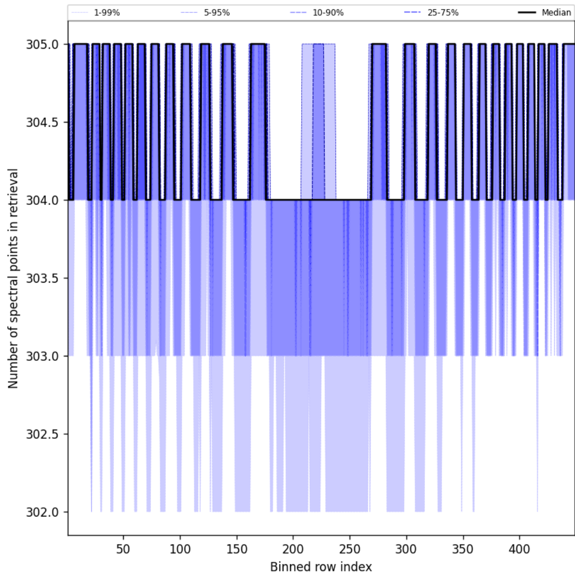
Figure 50: Along track statistics of “Number of spectral points in retrieval” for 2025-05-11 to 2025-05-12
