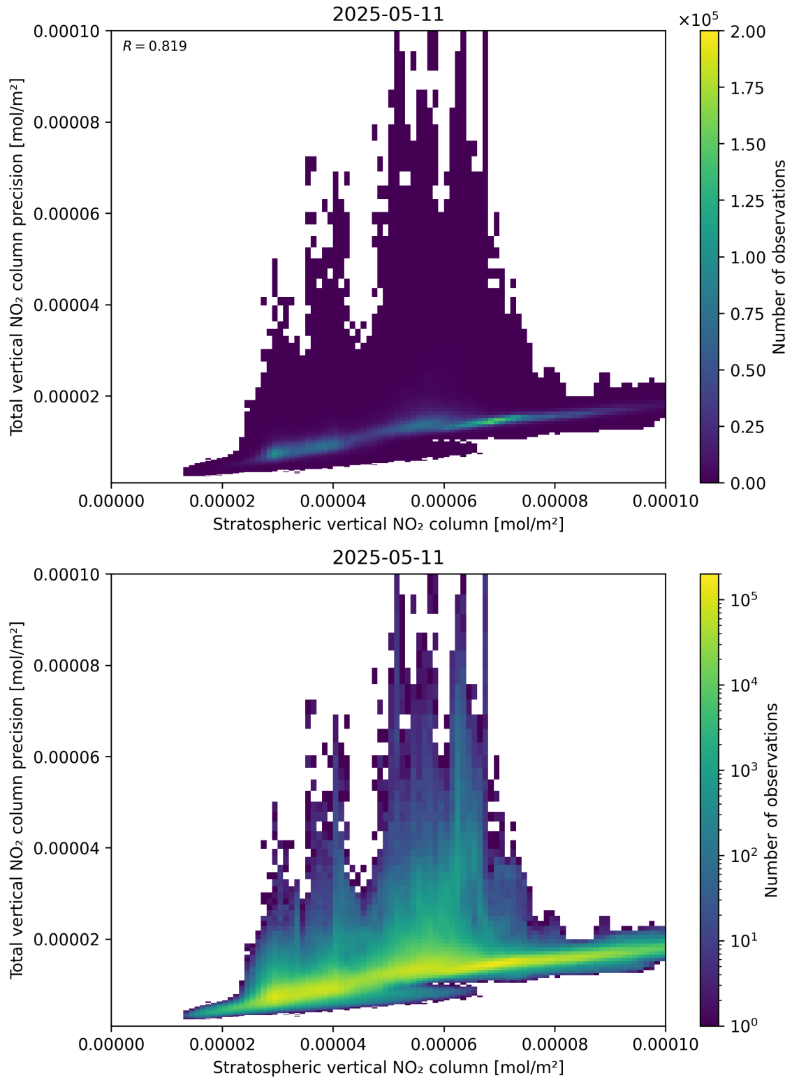
Figure 101: Scatter density plot of “Stratospheric vertical NO 2 column” against “Total vertical NO 2 column precision” for 2025-05-11 to 2025-05-12.
