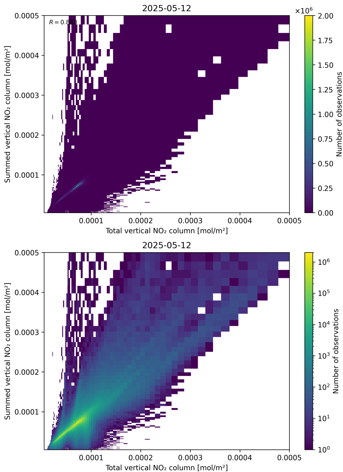
Figure 112: Scatter density plot of “Total vertical NO 2 column” against “Summed vertical NO 2 column” for 2025-05-12 to 2025-05-13.
