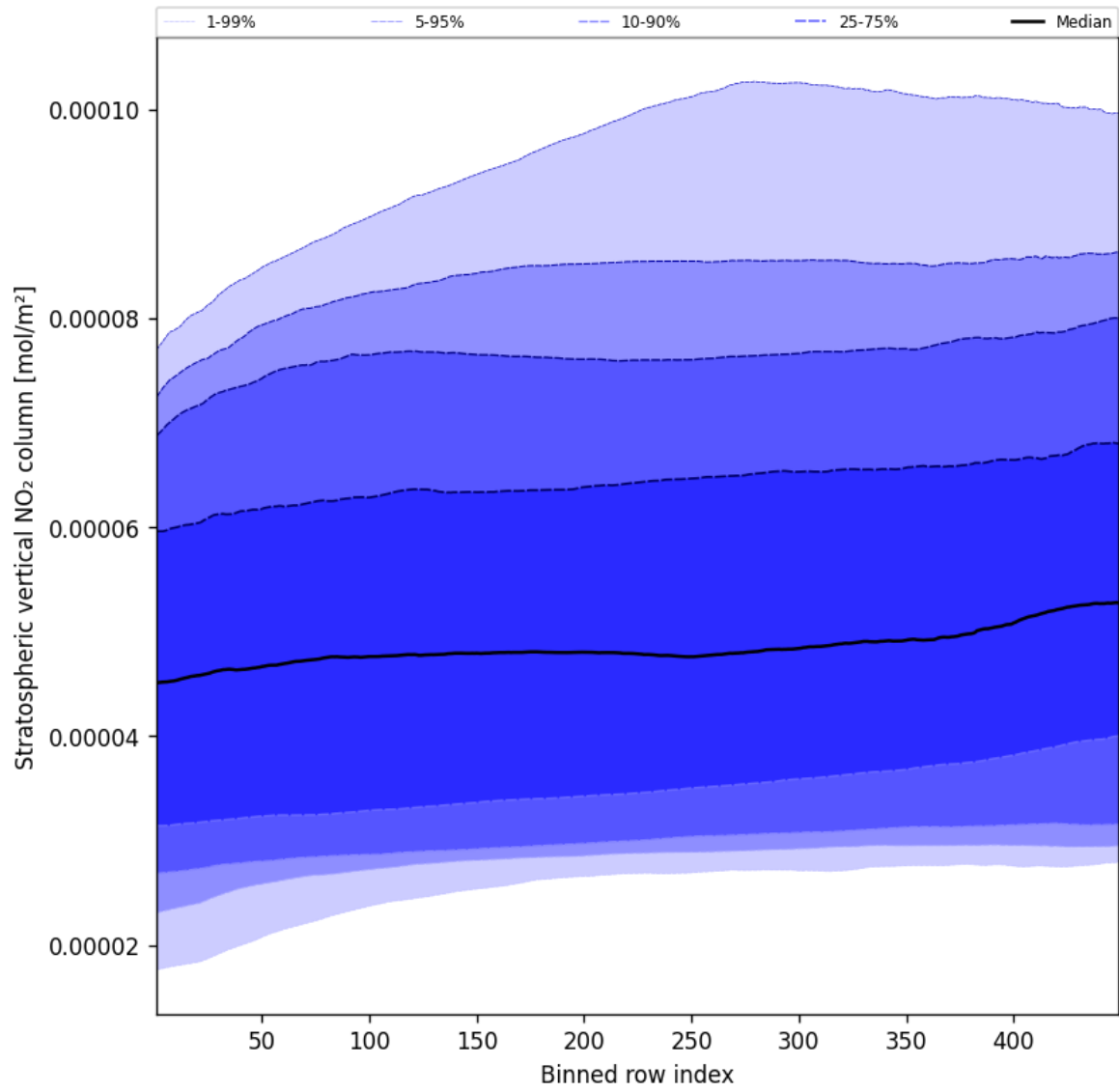
Figure 53: Along track statistics of “Stratospheric vertical NO 2 column” for 2025-05-12 to 2025-05-13
