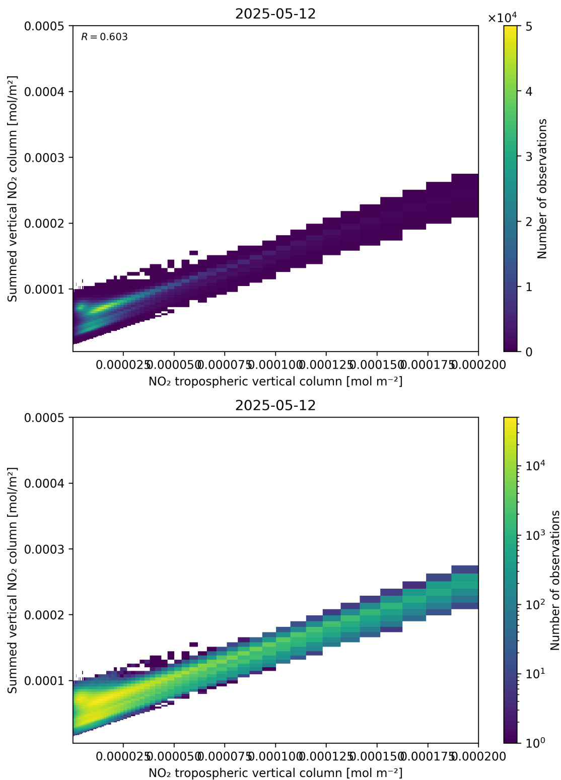
Figure 126: Scatter density plot of “NO 2 tropospheric vertical column” against “Summed vertical NO 2 column” for 2025-05-12 to 2025-05-13.
