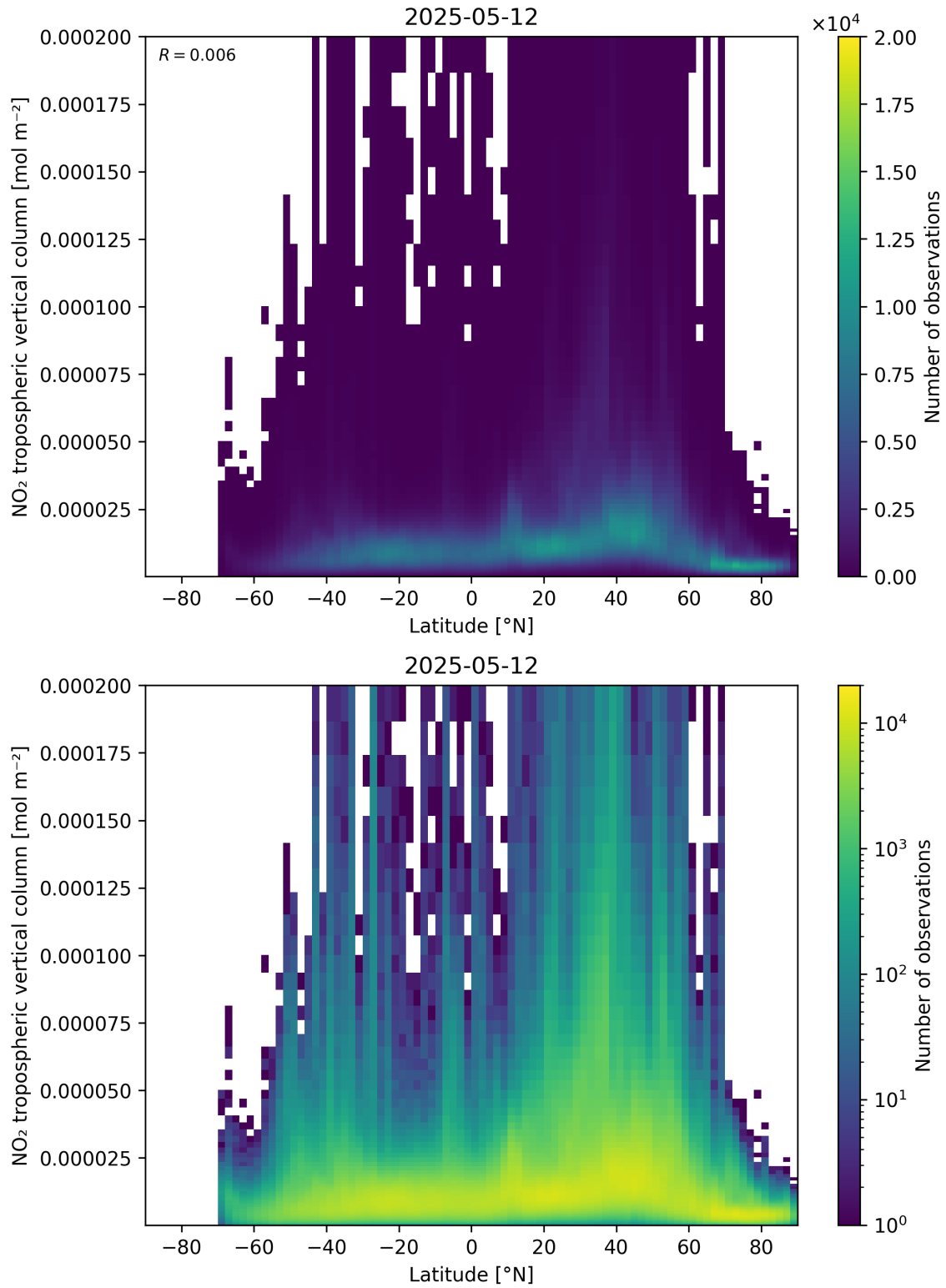
Figure 92: Scatter density plot of “Latitude” against “NO 2 tropospheric vertical column” for 2025-05-12 to 2025-05-13.
