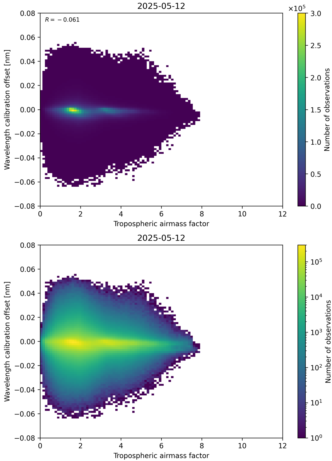
Figure 80: Scatter density plot of “Tropospheric airmass factor” against “Wavelength calibration offset” for 2025-05-12 to 2025-05-13.
