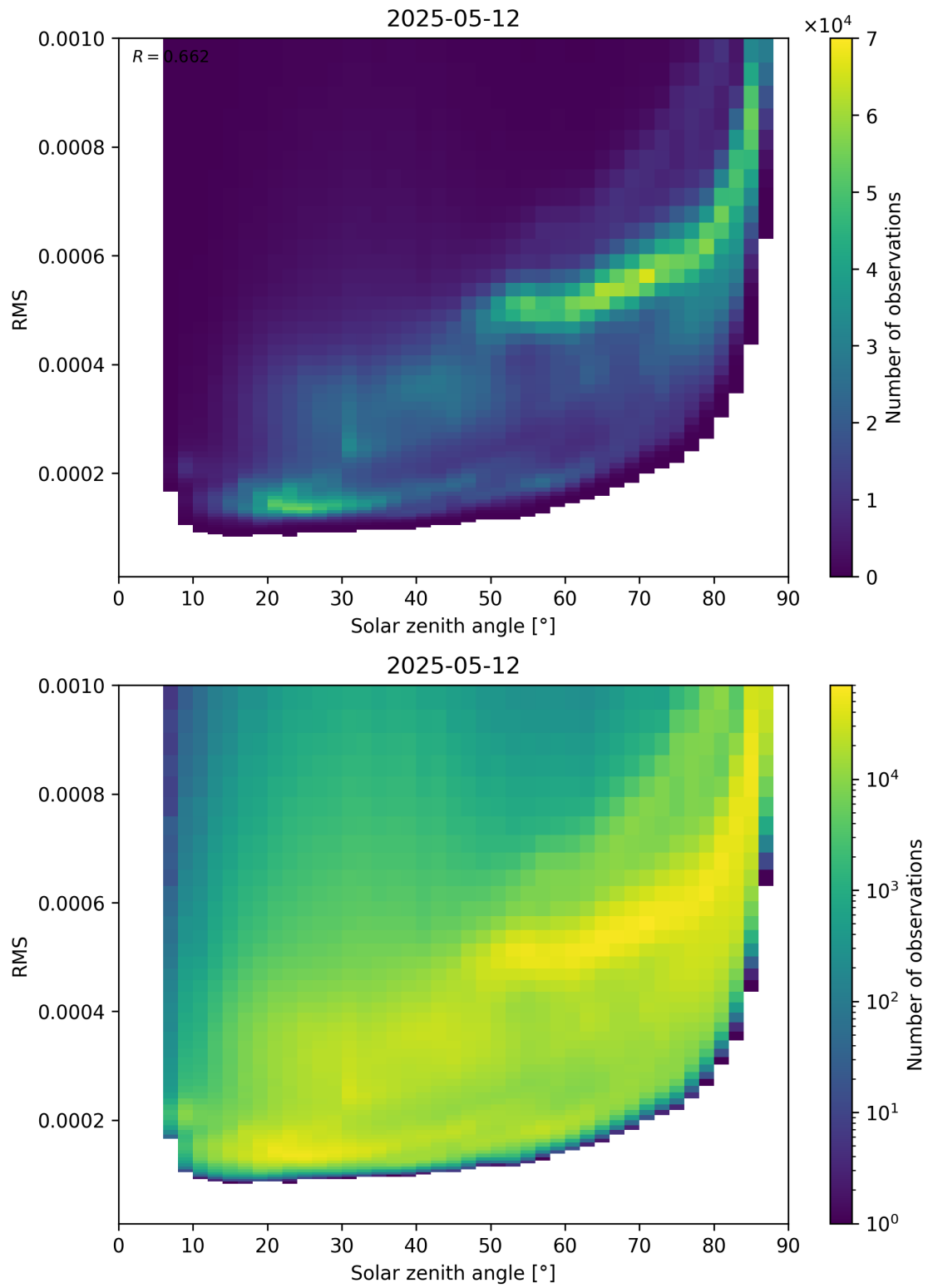
Figure 157: Scatter density plot of “Solar zenith angle” against “RMS” for 2025-05-12 to 2025-05-13.
