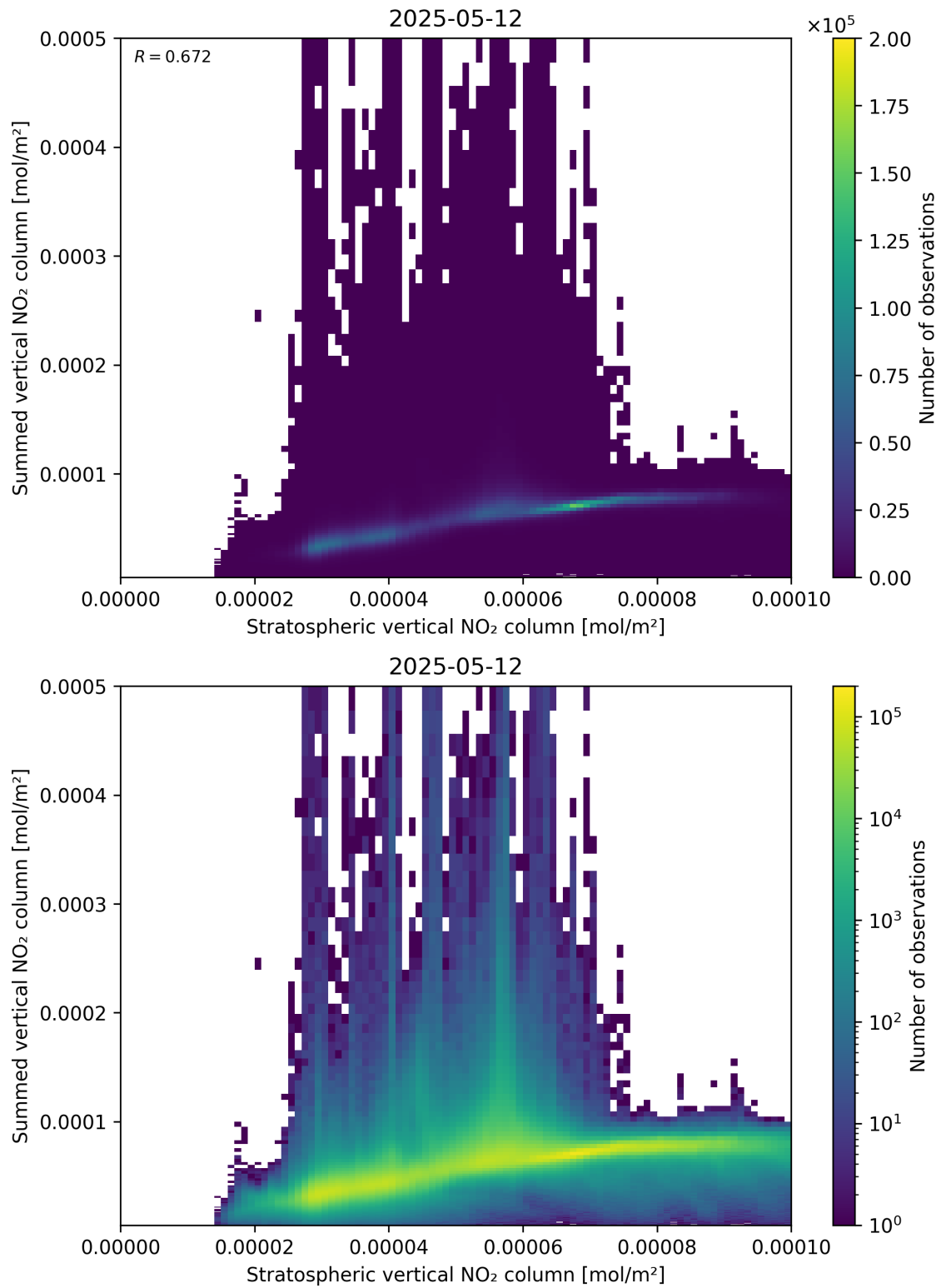
Figure 98: Scatter density plot of “Stratospheric vertical NO 2 column” against “Summed vertical NO 2 column” for 2025-05-12 to 2025-05-13.
