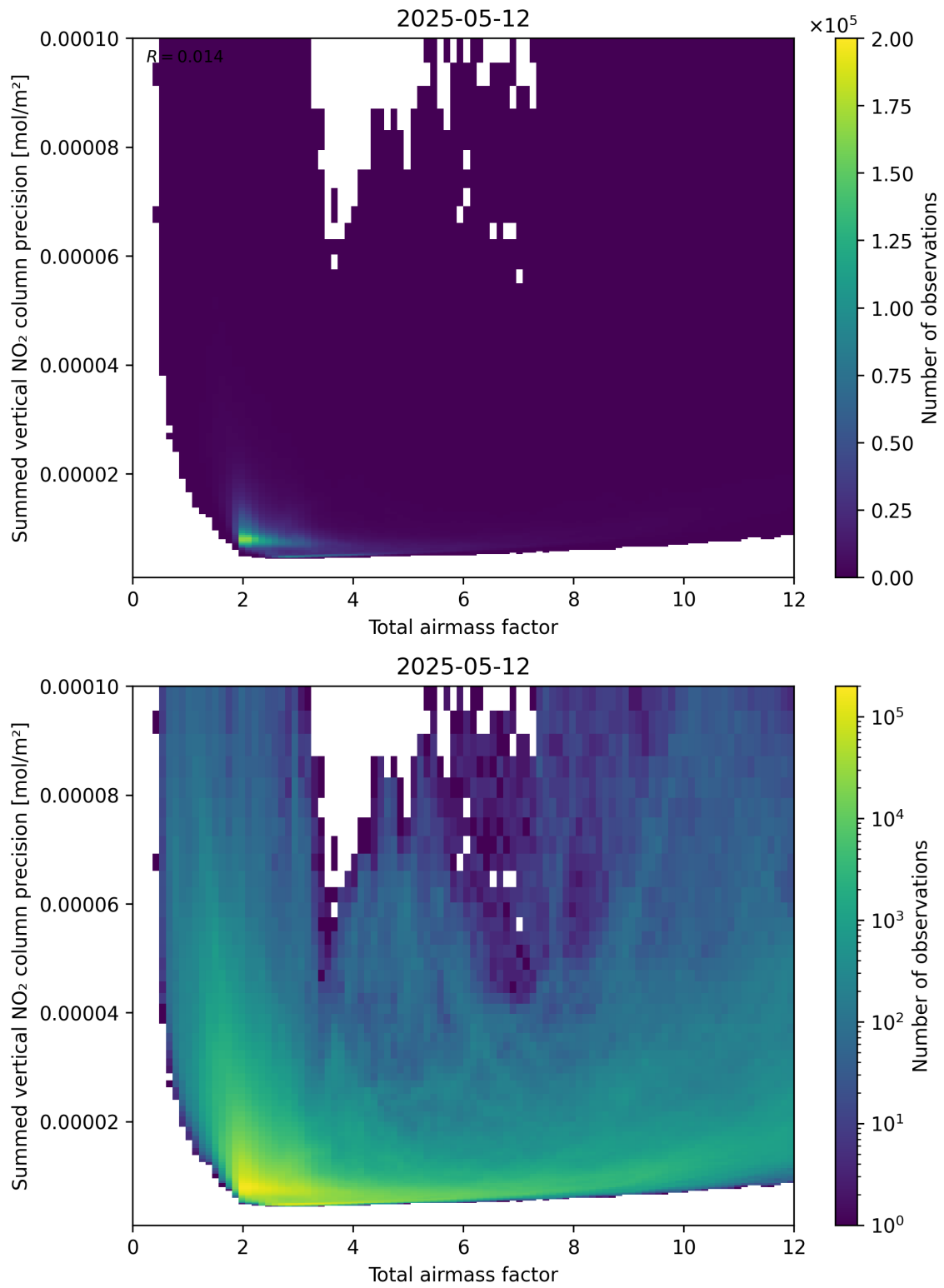
Figure 66: Scatter density plot of “Total airmass factor” against “Summed vertical NO 2 column precision” for 2025-05-12 to 2025-05-13.
