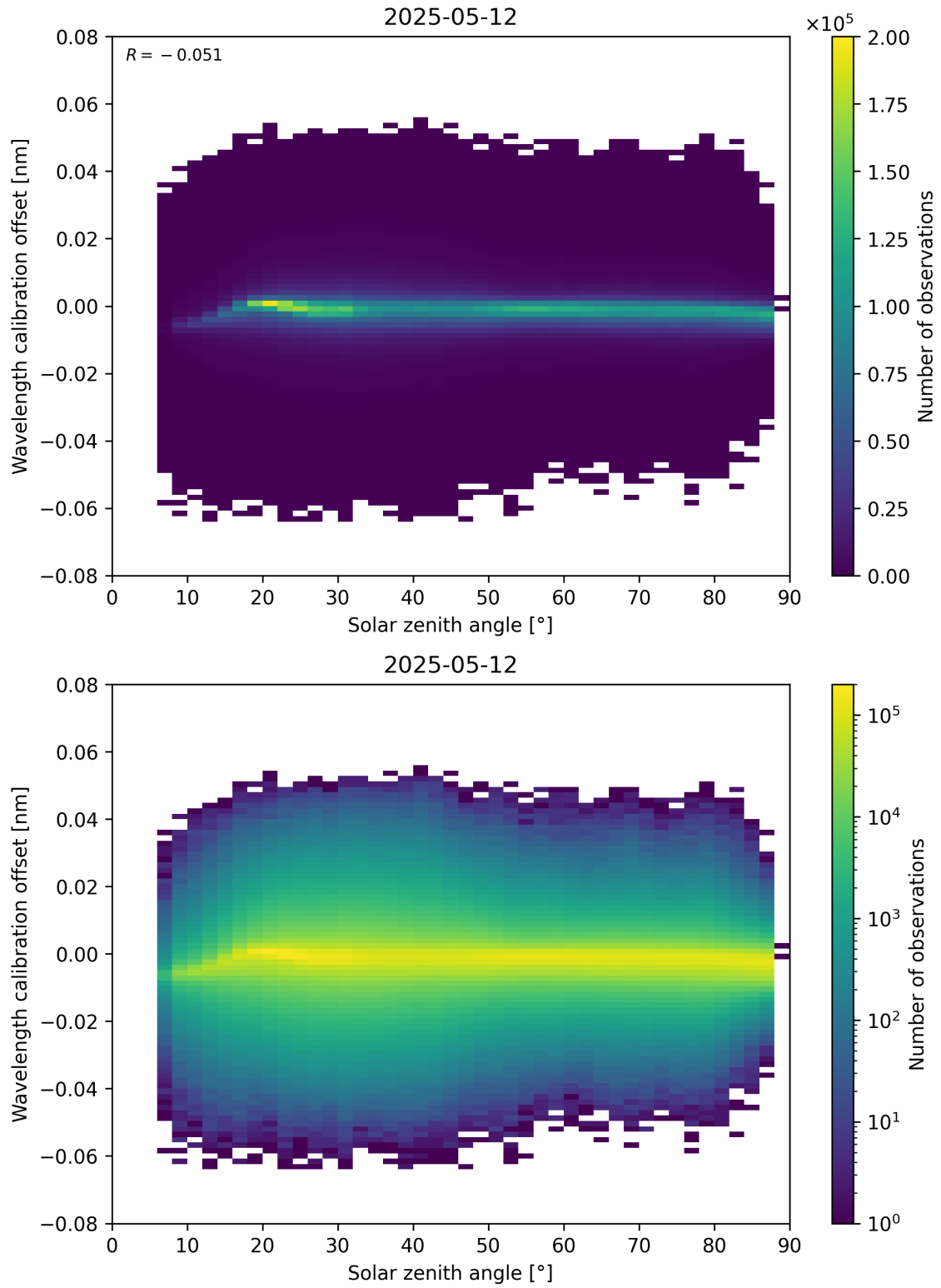
Figure 158: Scatter density plot of “Solar zenith angle” against “Wavelength calibration offset” for 2025-05-12 to 2025-05-13.
