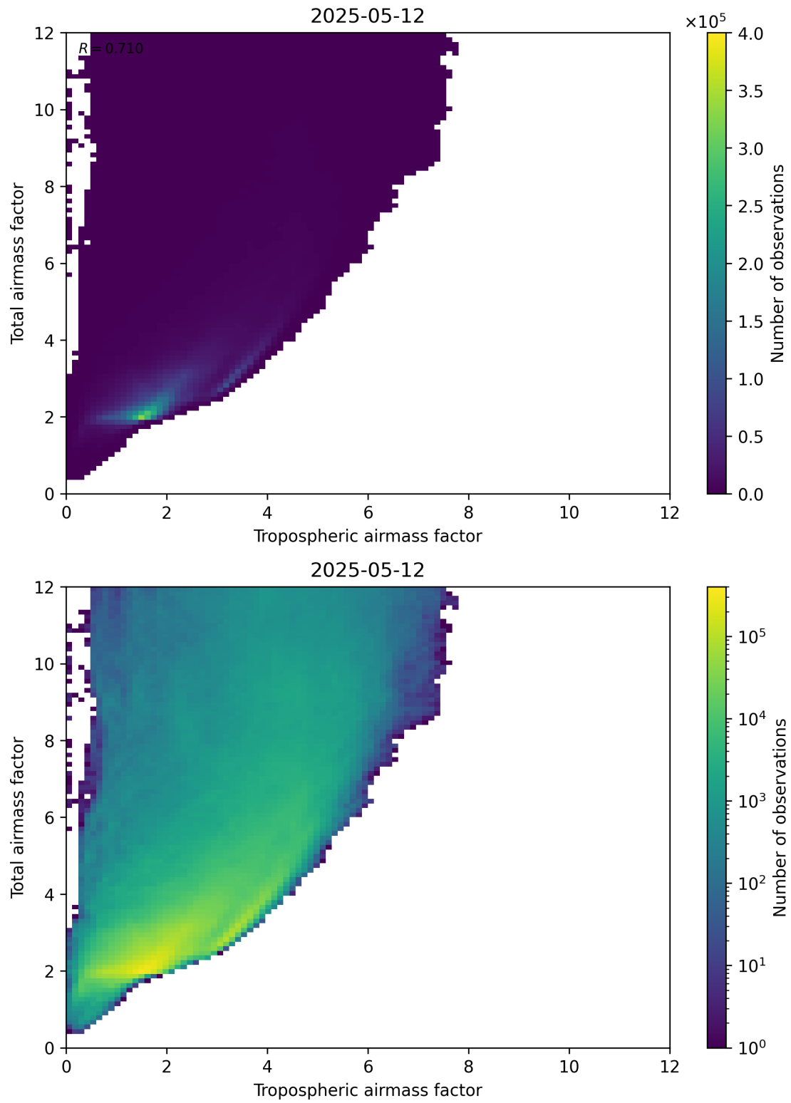
Figure 72: Scatter density plot of “Tropospheric airmass factor” against “Total airmass factor” for 2025-05-12 to 2025-05-13.
