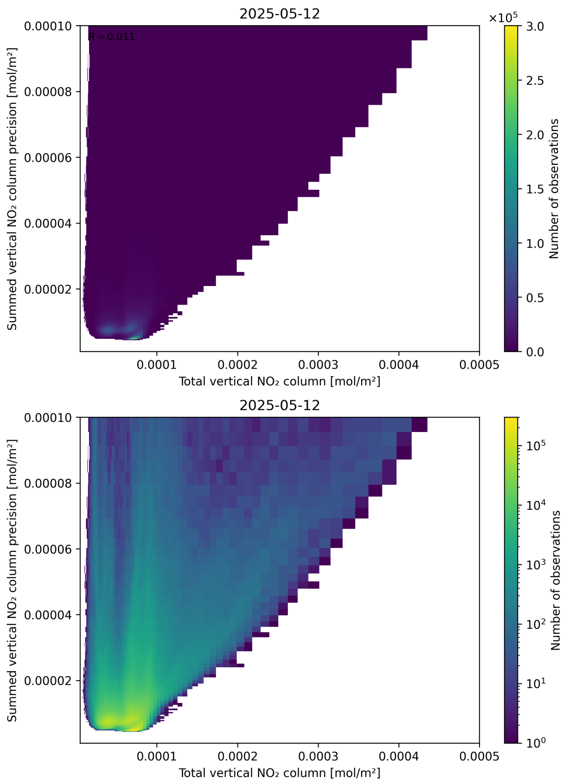
Figure 113: Scatter density plot of “Total vertical NO 2 column” against “Summed vertical NO 2 column precision” for 2025-05-12 to 2025-05-13.
