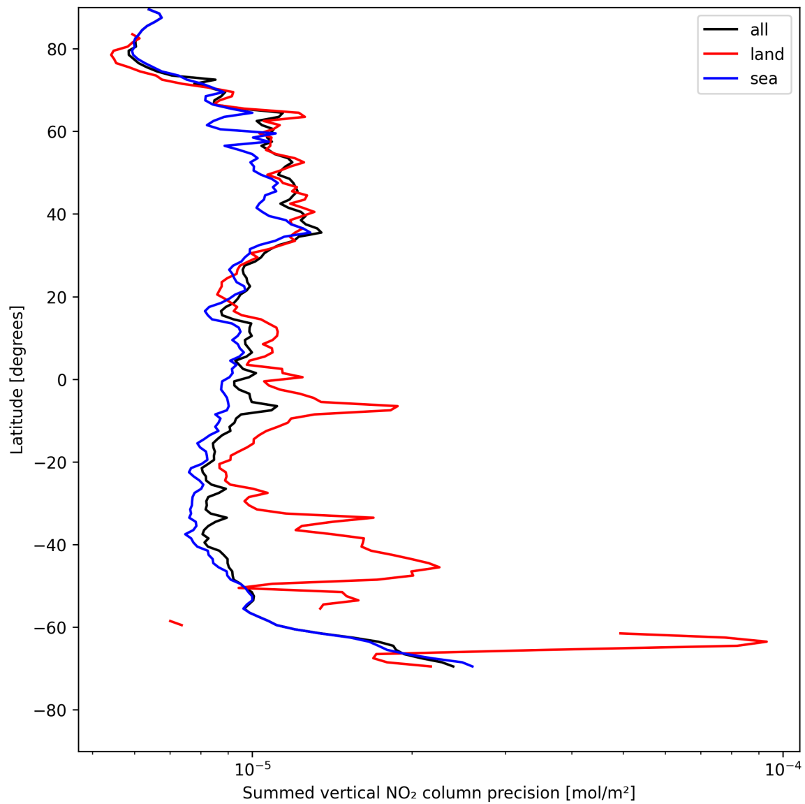
Figure 24: Zonal average of “Summed vertical NO 2 column precision” for 2025-05-12 to 2025-05-13.
