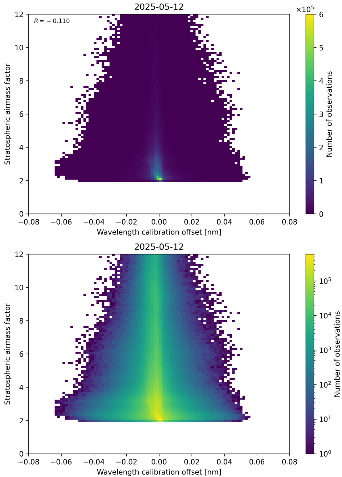
Figure 174: Scatter density plot of “Wavelength calibration offset” against “Stratospheric airmass factor” for 2025-05-12 to 2025-05-13.
