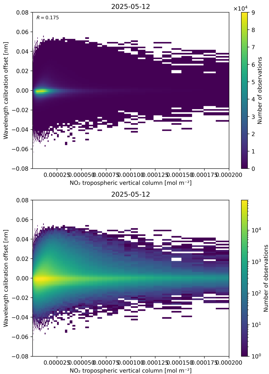
Figure 143: Scatter density plot of “NO 2 tropospheric vertical column” against “Wavelength calibration offset” for 2025-05-12 to 2025-05-13.
