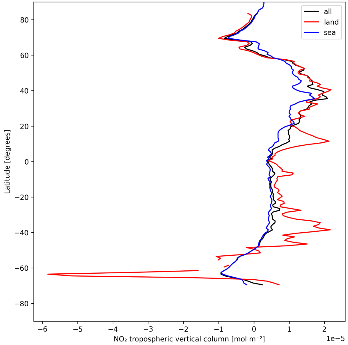
Figure 12: Zonal average of “NO 2 tropospheric vertical column” for 2025-05-12 to 2025-05-13.
