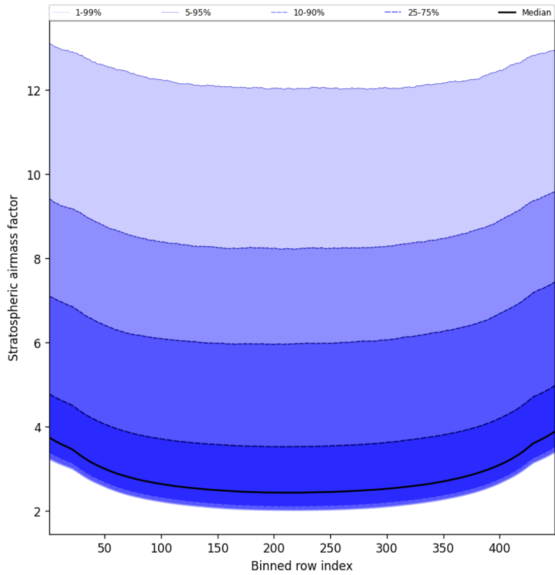
Figure 61: Along track statistics of “Stratospheric airmass factor” for 2025-05-12 to 2025-05-13
