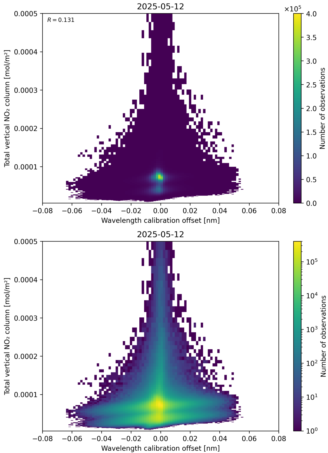
Figure 179: Scatter density plot of “Wavelength calibration offset” against “Total vertical NO 2 column” for 2025-05-12 to 2025-05-13.
