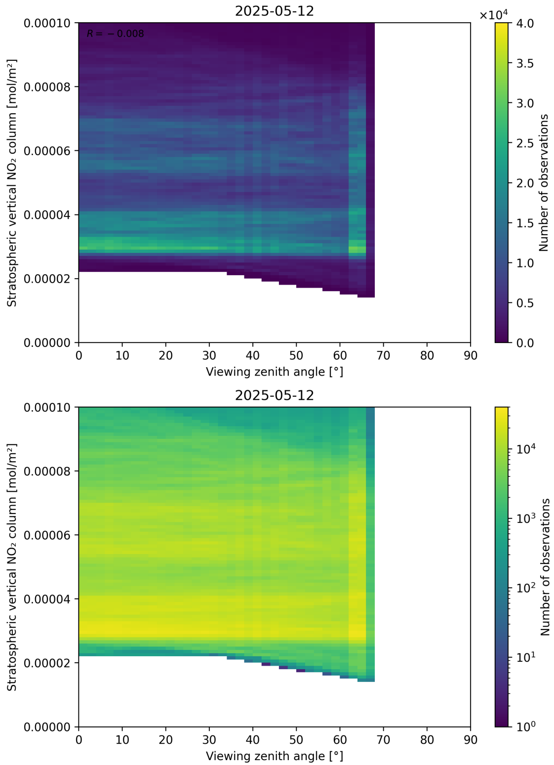
Figure 164: Scatter density plot of “Viewing zenith angle” against “Stratospheric vertical NO 2 column” for 2025-05-12 to 2025-05-13.
