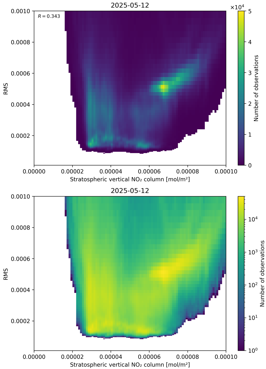
Figure 102: Scatter density plot of “Stratospheric vertical NO 2 column” against “RMS” for 2025-05-12 to 2025-05-13.
