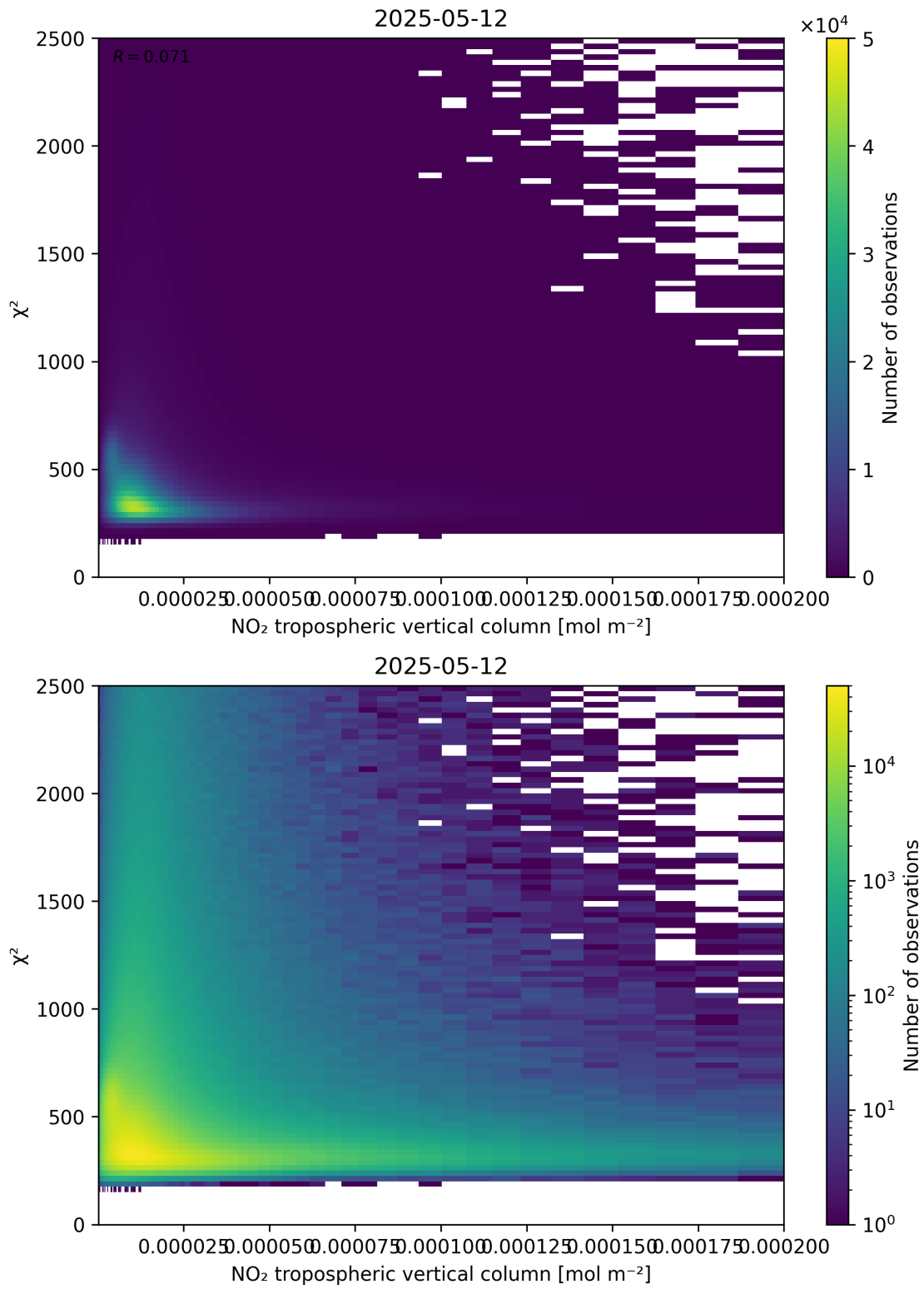
Figure 124: Scatter density plot of “NO 2 tropospheric vertical column” against “ \chi^2 ” for 2025-05-12 to 2025-05-13.
