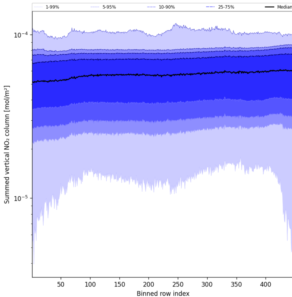
Figure 57: Along track statistics of “Summed vertical NO 2 column” for 2025-05-12 to 2025-05-13
