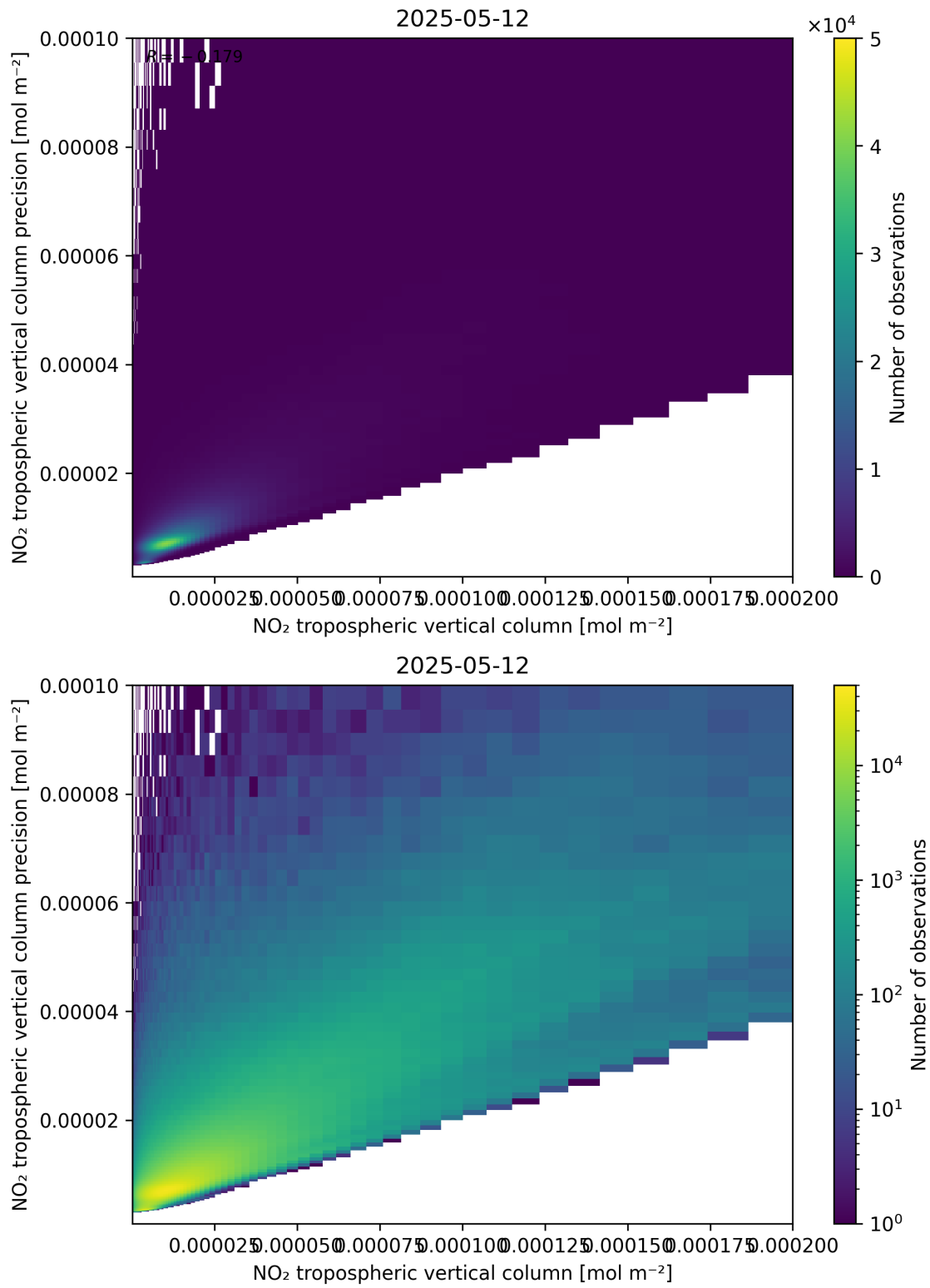
Figure 130: Scatter density plot of “NO 2 tropospheric vertical column” against “NO 2 tropospheric vertical column precision” for 2025-05-12 to 2025-05-13.
