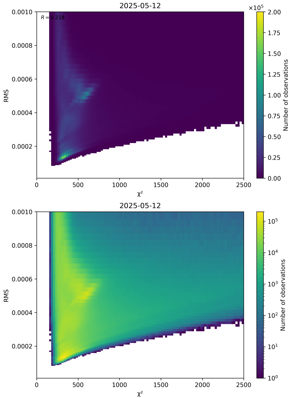
Figure 82: Scatter density plot of “ \chi^2 ” against “RMS” for 2025-05-12 to 2025-05-13.
