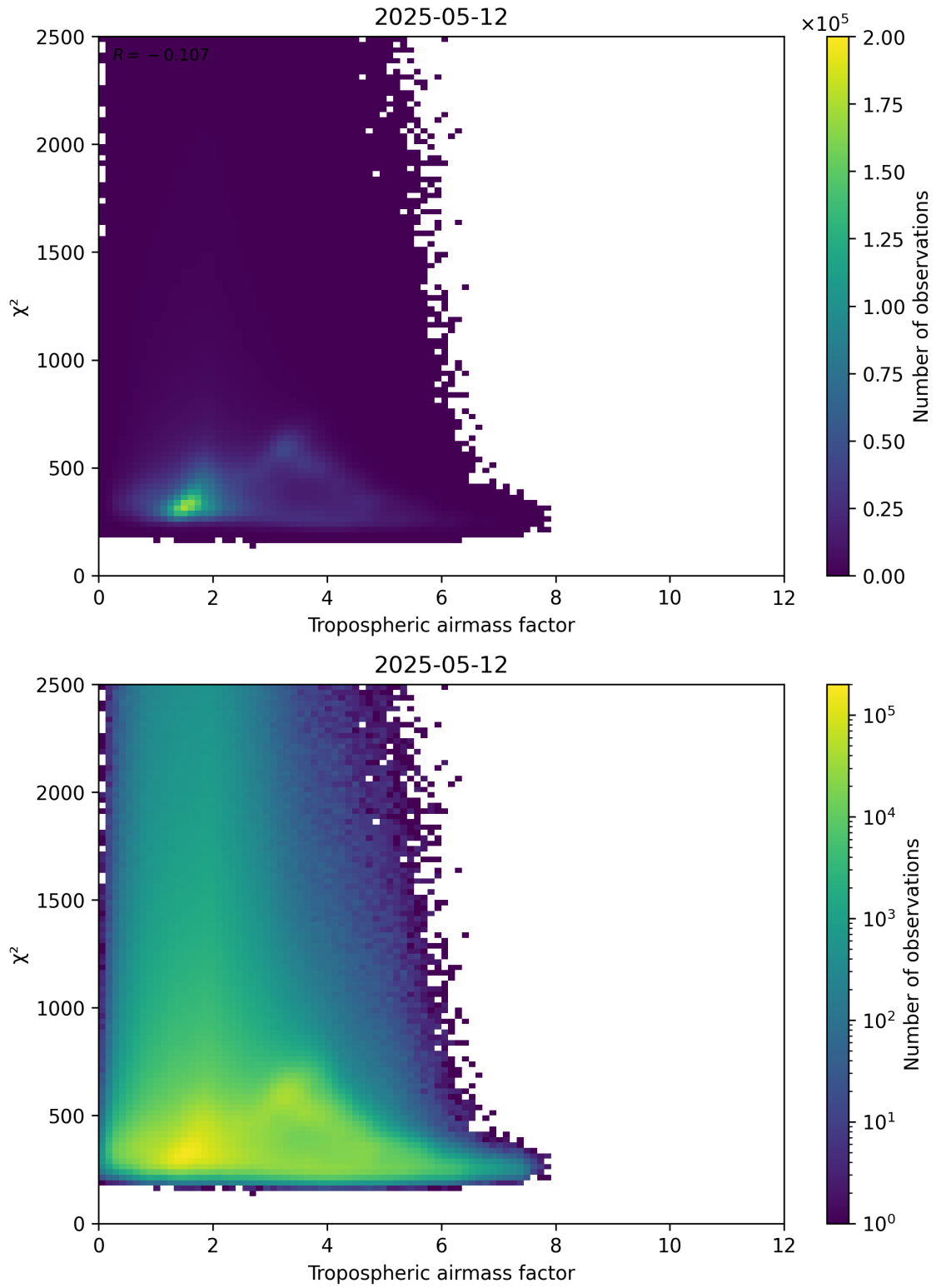
Figure 73: Scatter density plot of “Tropospheric airmass factor” against “ \chi^2 ” for 2025-05-12 to 2025-05-13.
