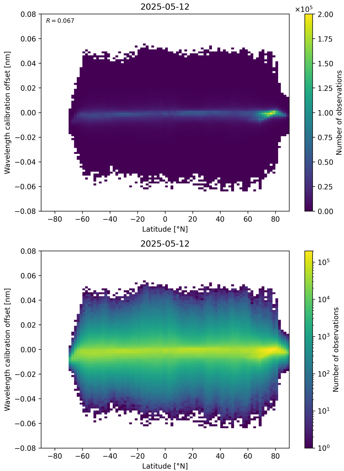
Figure 95: Scatter density plot of “Latitude” against “Wavelength calibration offset” for 2025-05-12 to 2025-05-13.
