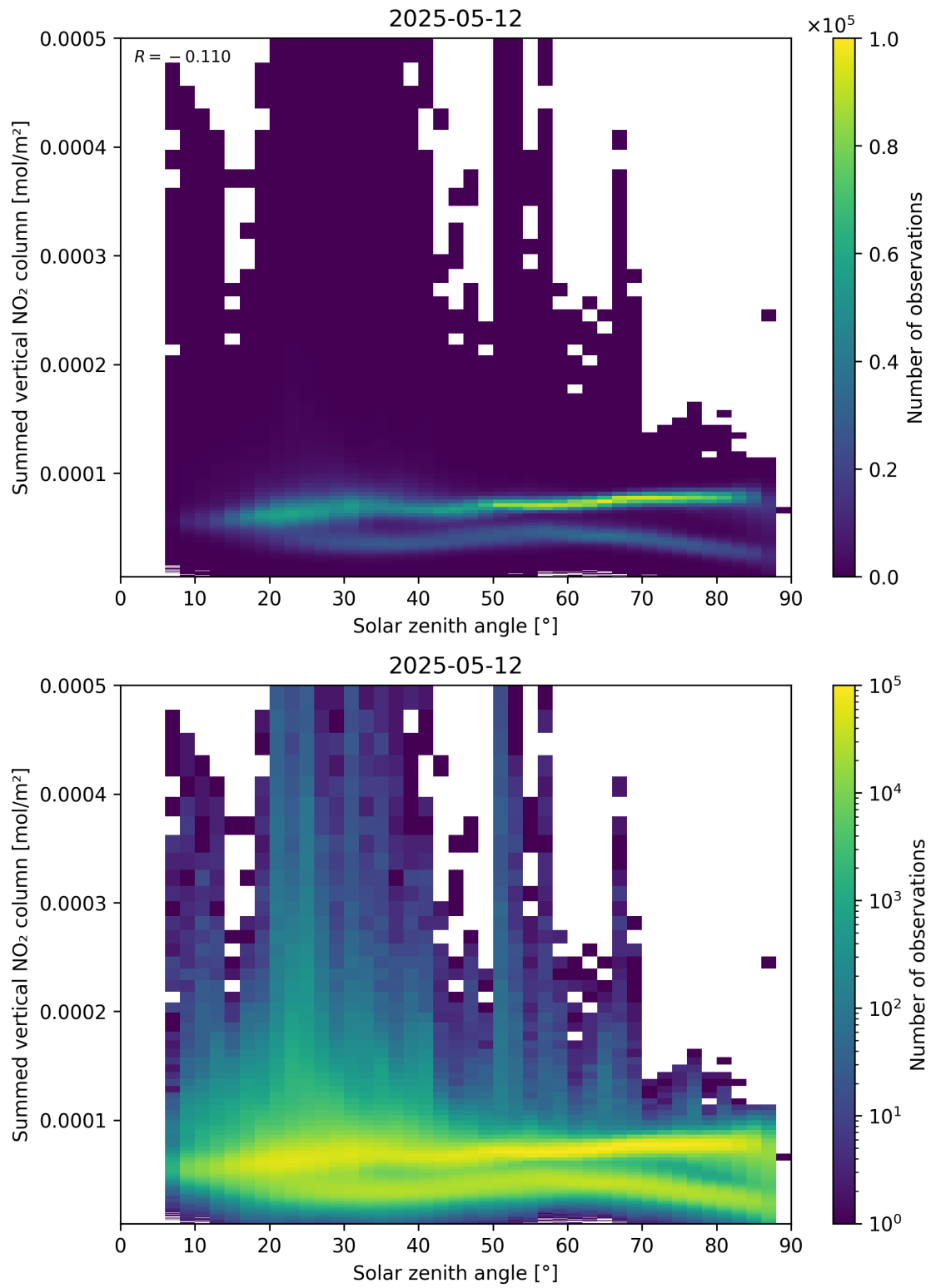
Figure 151: Scatter density plot of “Solar zenith angle” against “Summed vertical NO 2 column” for 2025-05-12 to 2025-05-13.
