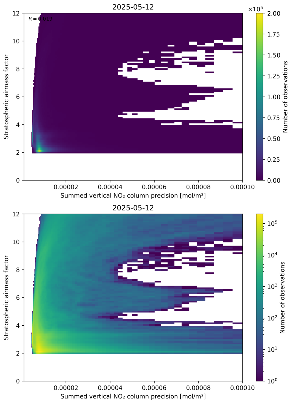
Figure 106: Scatter density plot of “Summed vertical NO 2 column precision” against “Stratospheric airmass factor” for 2025-05-12 to 2025-05-13.
