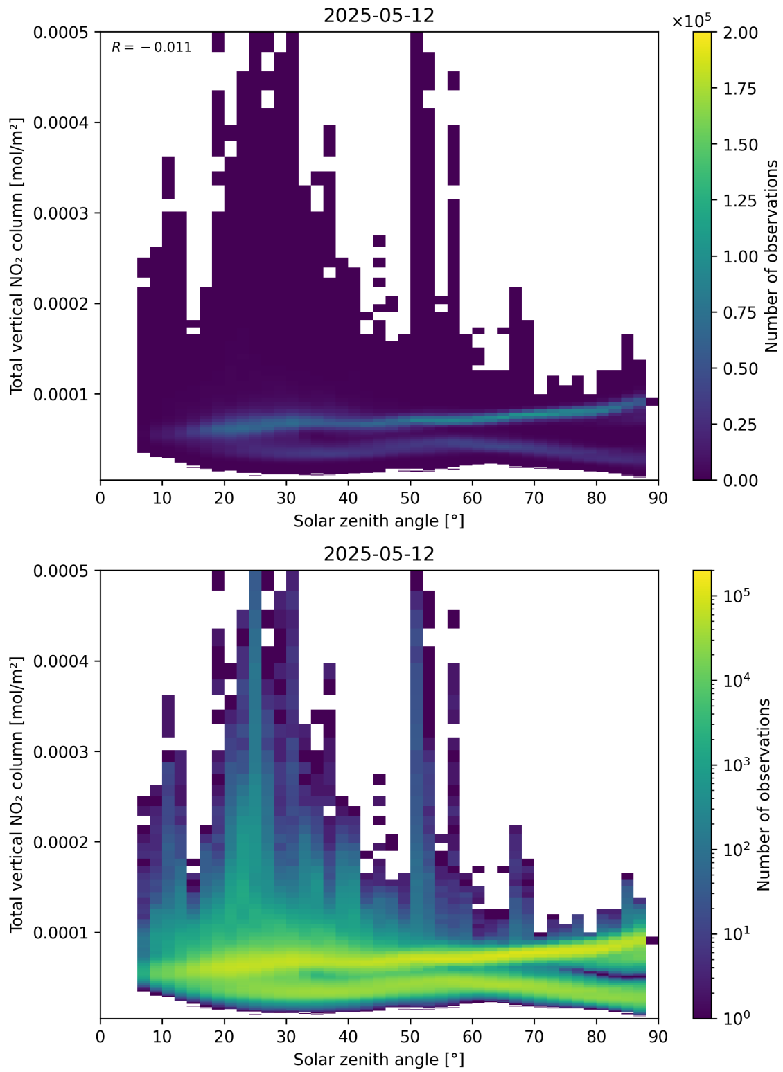
Figure 153: Scatter density plot of “Solar zenith angle” against “Total vertical NO 2 column” for 2025-05-12 to 2025-05-13.
