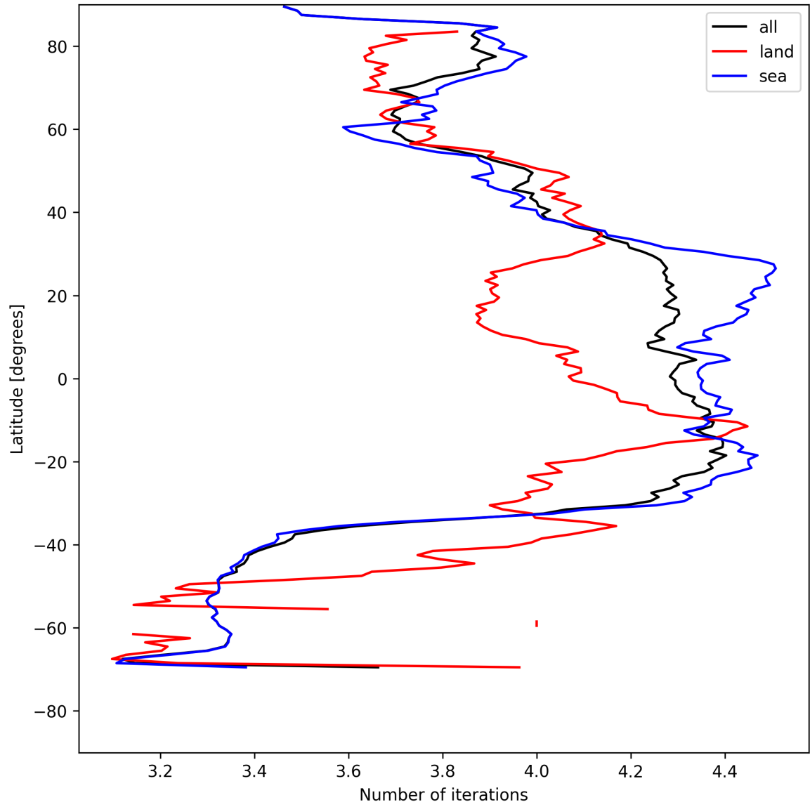
Figure 17: Zonal average of “Number of iterations” for 2025-05-12 to 2025-05-13.
