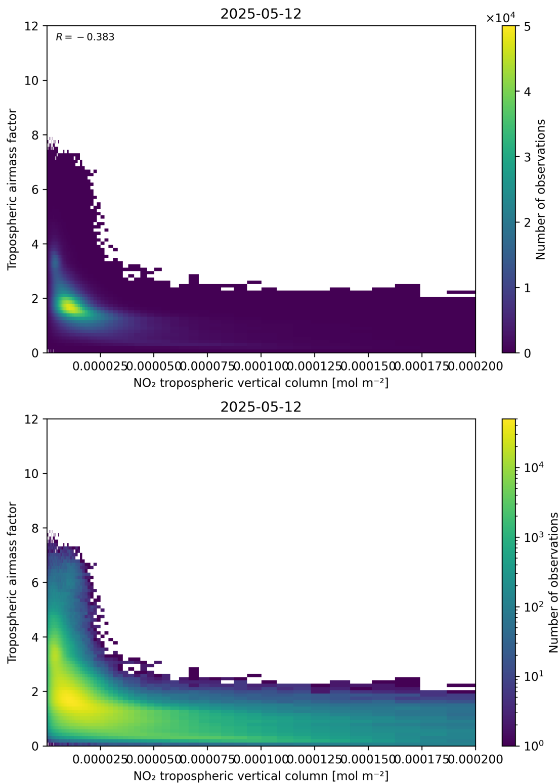
Figure 123: Scatter density plot of “NO 2 tropospheric vertical column” against “Tropospheric air mass factor” for 2025-05-12 to 2025-05-13.
