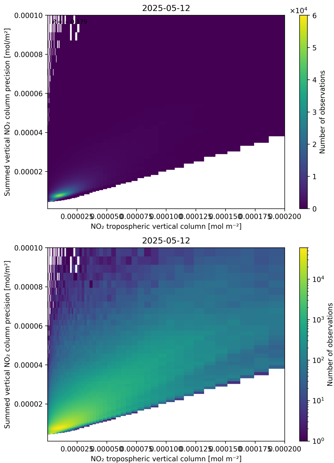
Figure 127: Scatter density plot of “NO 2 tropospheric vertical column” against “Summed vertical NO 2 column precision” for 2025-05-12 to 2025-05-13.
