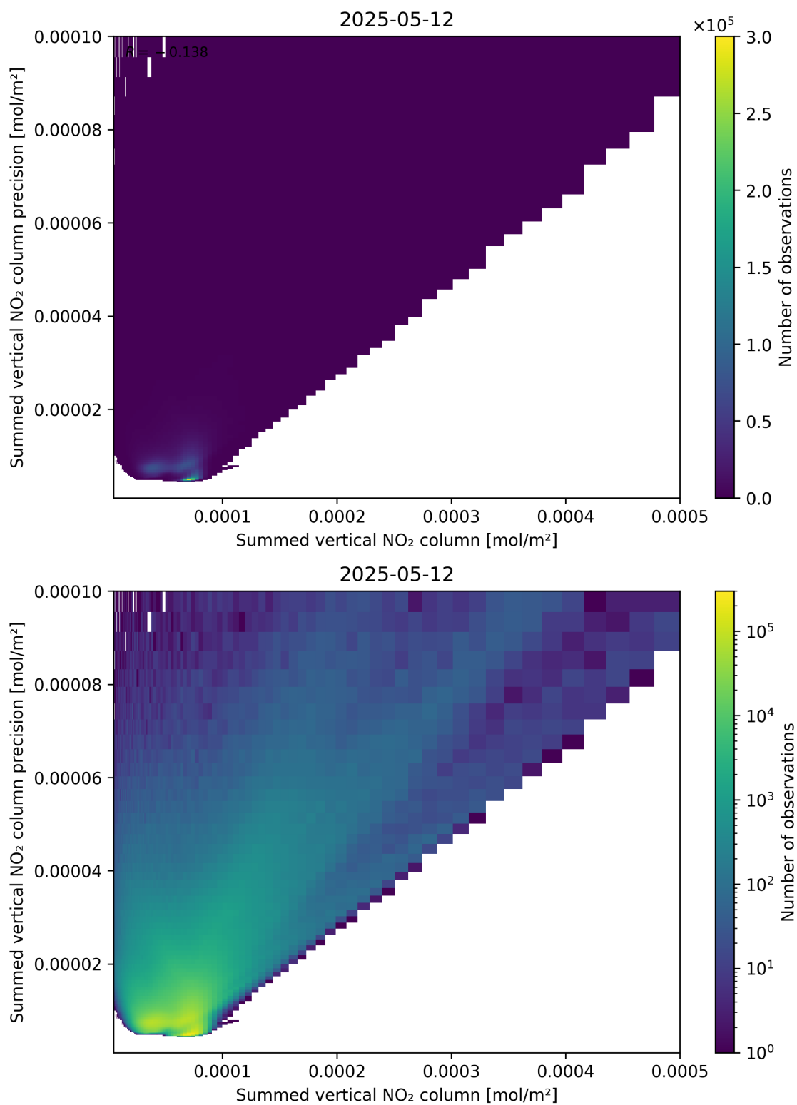
Figure 105: Scatter density plot of “Summed vertical NO 2 column” against “Summed vertical NO 2 column precision” for 2025-05-12 to 2025-05-13.
