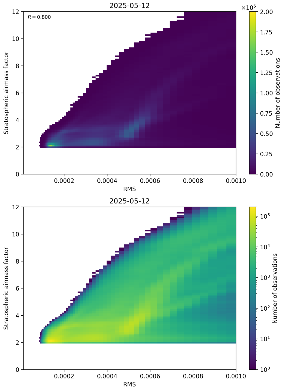
Figure 144: Scatter density plot of “RMS” against “Stratospheric airmass factor” for 2025-05-12 to 2025-05-13.
