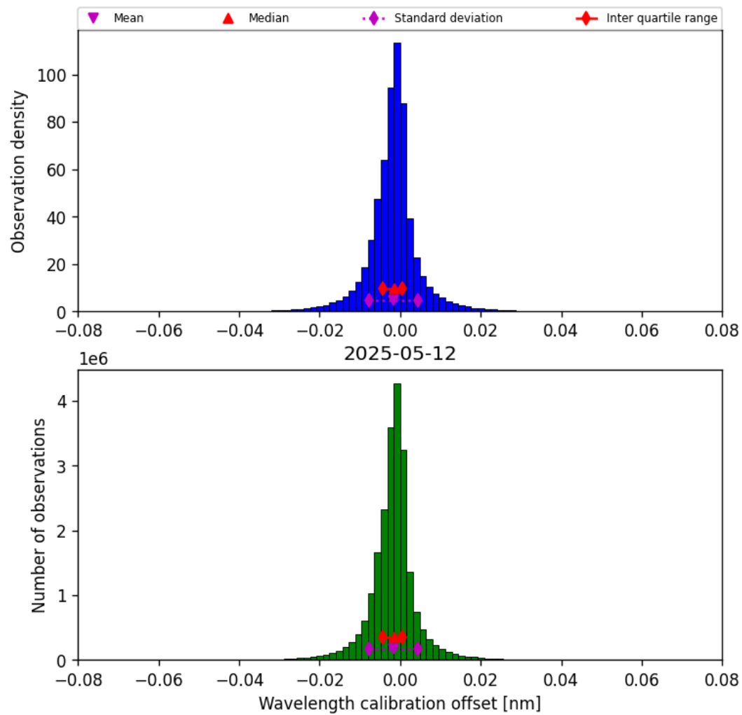
Figure 35: Histogram of “Wavelength calibration offset” for 2025-05-12 to 2025-05-13
