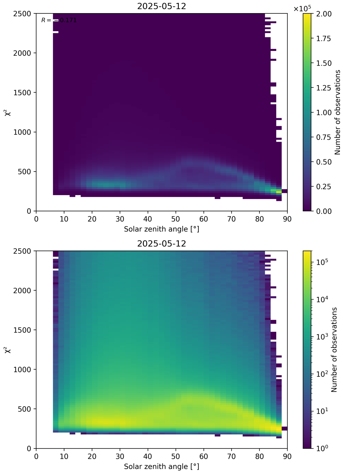
Figure 148: Scatter density plot of “Solar zenith angle” against “ \chi^2 ” for 2025-05-12 to 2025-05-13.
