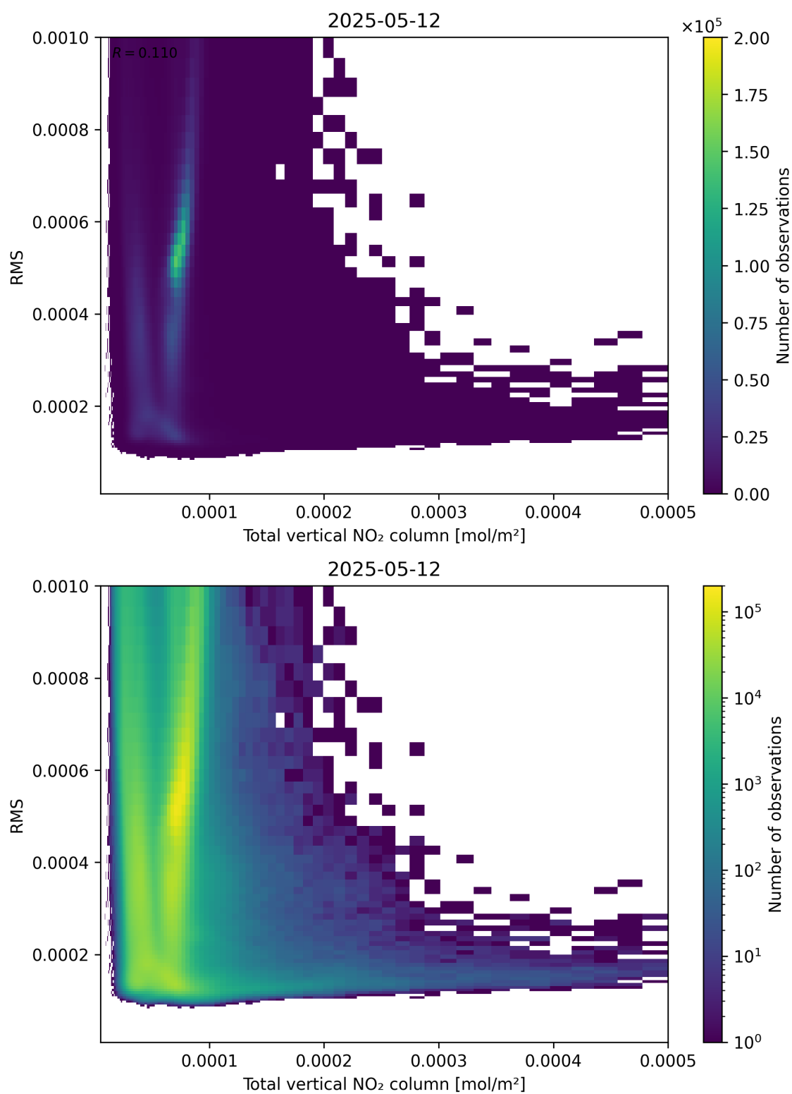
Figure 120: Scatter density plot of “Total vertical NO 2 column” against “RMS” for 2025-05-12 to 2025-05-13.
