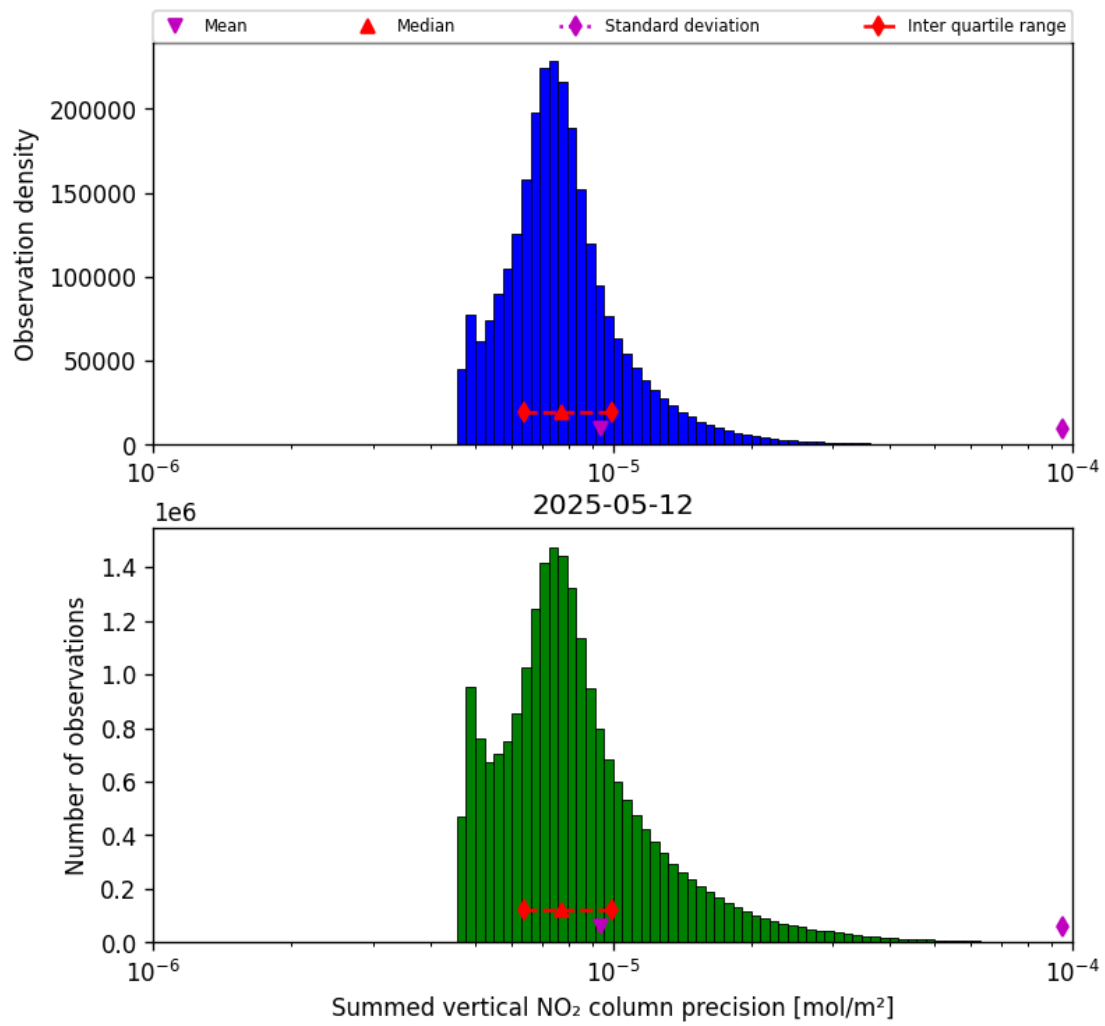
Figure 41: Histogram of "Summed vertical NO 2 column precision" for 2025-05-12 to 2025-05-13
