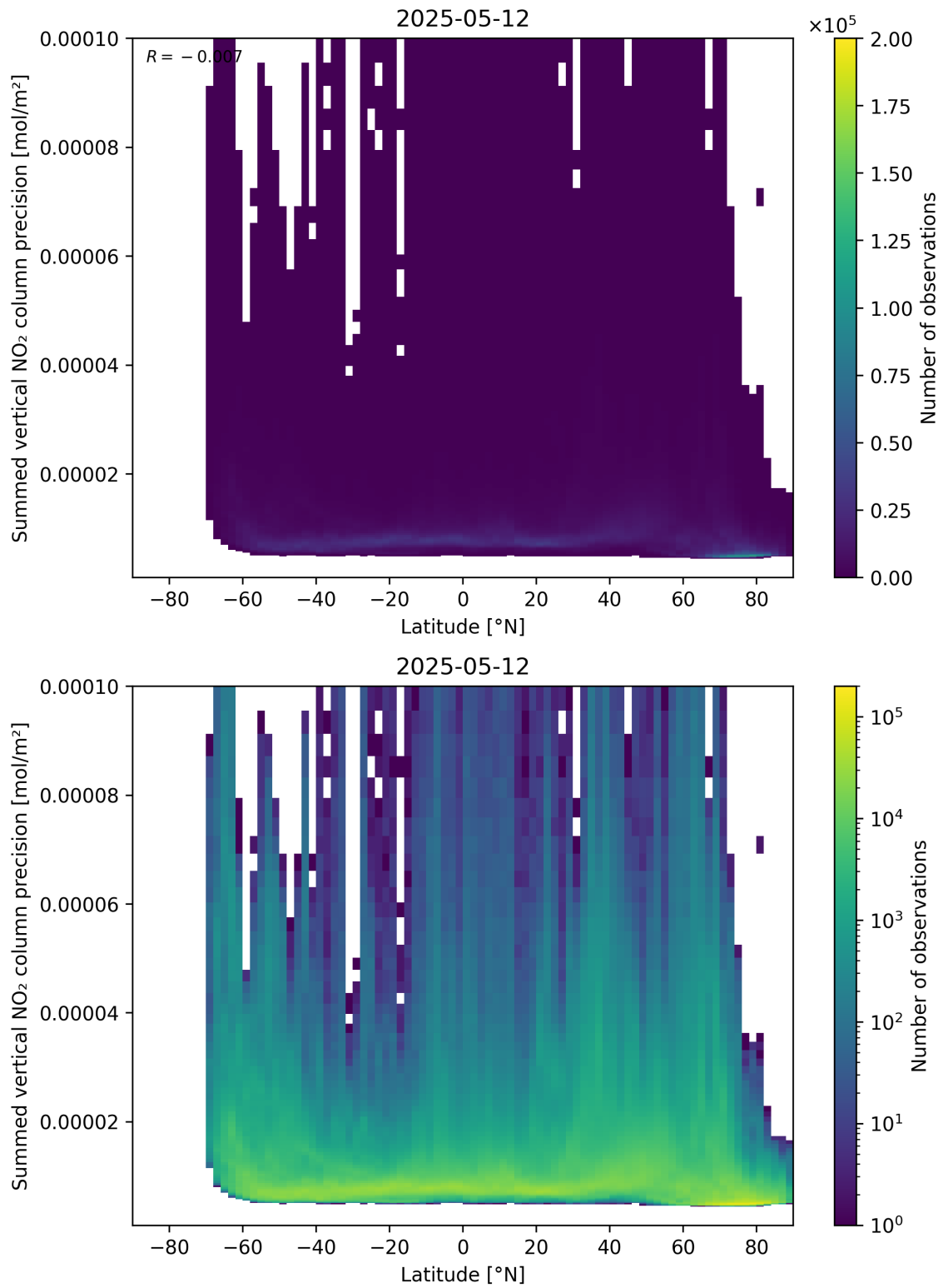
Figure 89: Scatter density plot of “Latitude” against “Summed vertical NO 2 column precision” for 2025-05-12 to 2025-05-13.
