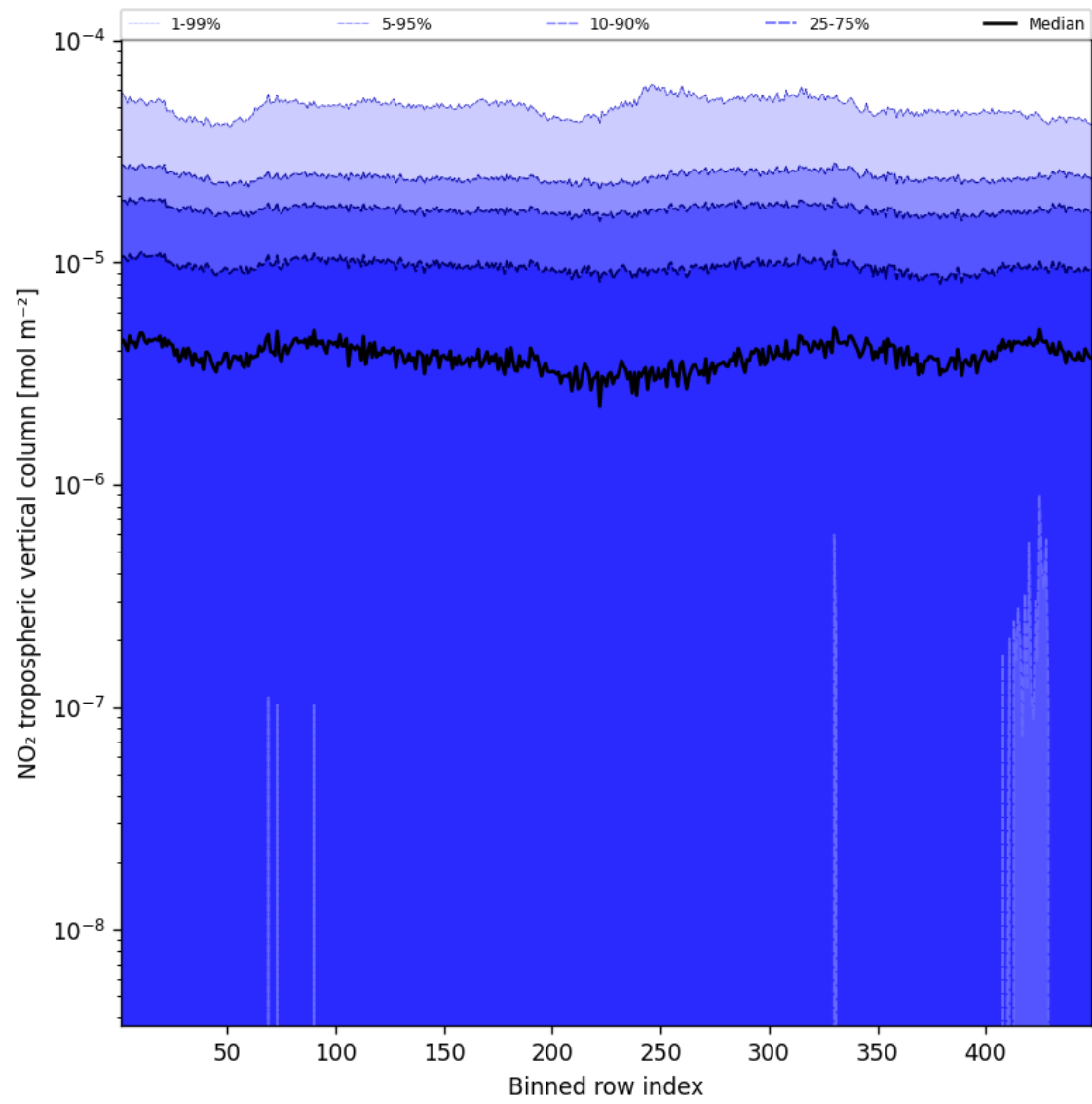
Figure 46: Along track statistics of “NO 2 tropospheric vertical column” for 2025-05-12 to 2025-05-13
