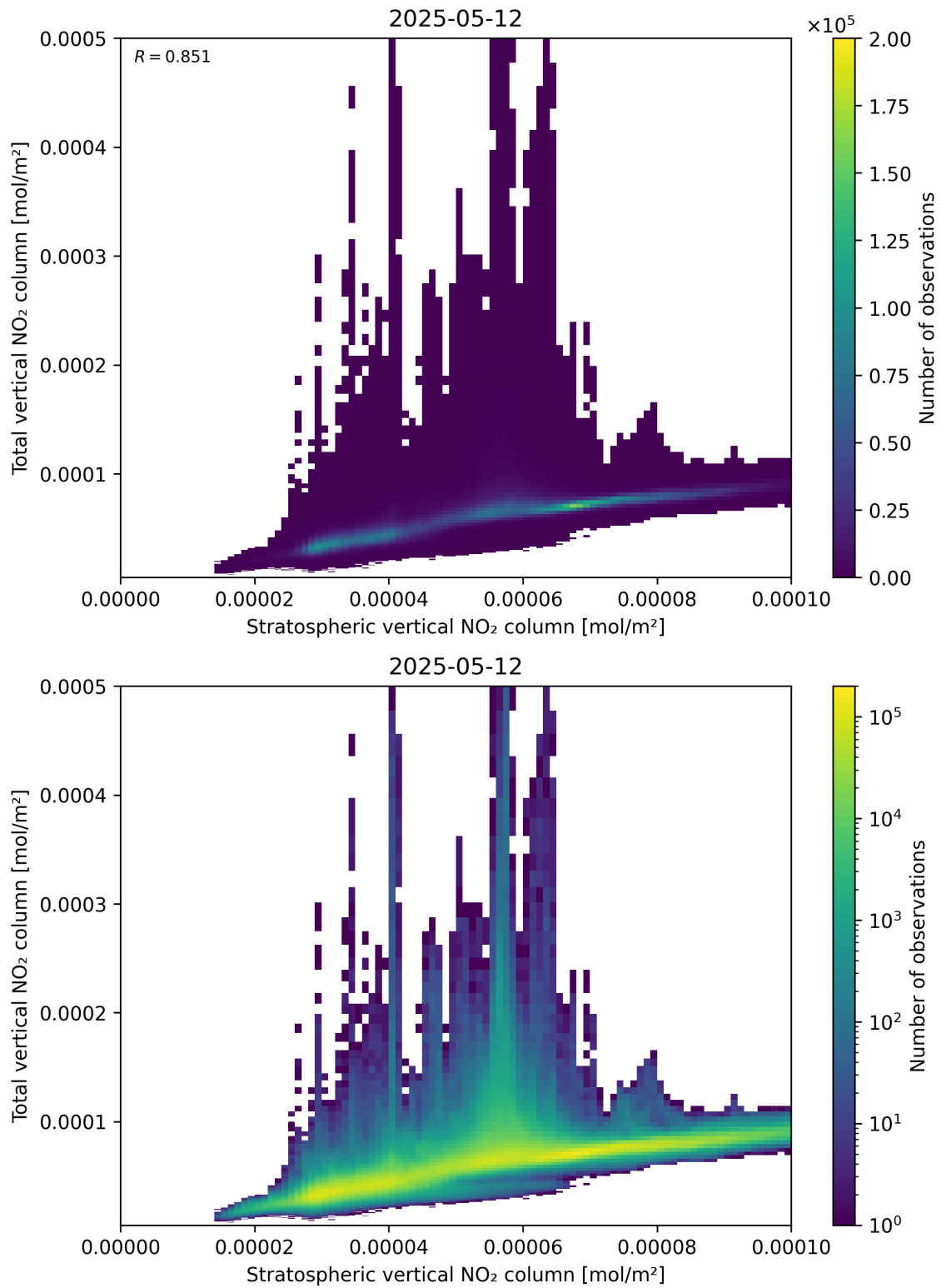
Figure 100: Scatter density plot of “Stratospheric vertical NO 2 column” against “Total vertical NO 2 column” for 2025-05-12 to 2025-05-13.
