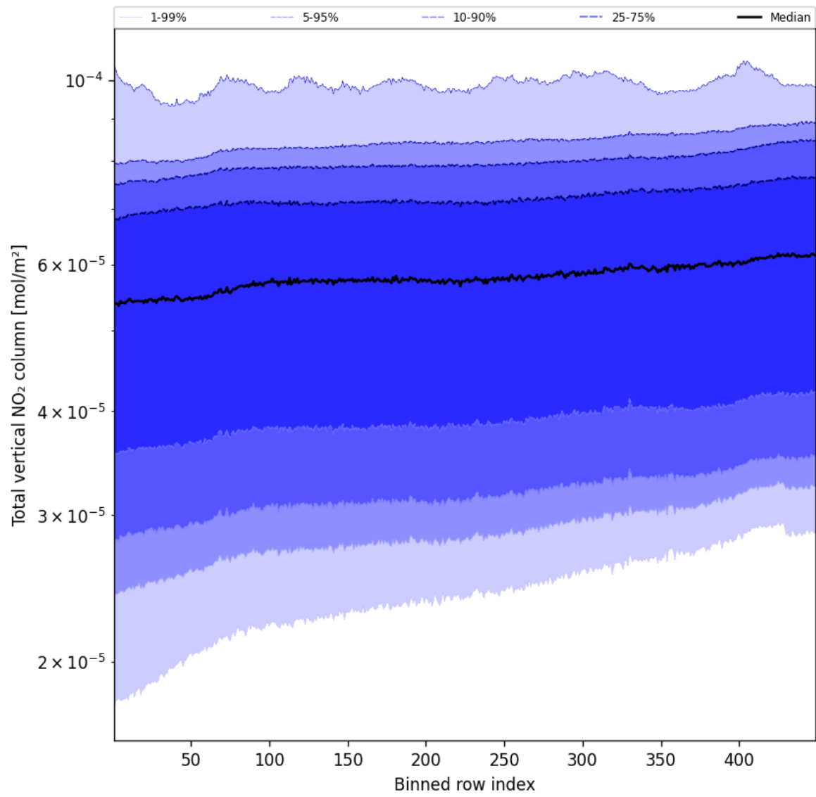
Figure 55: Along track statistics of “Total vertical NO 2 column” for 2025-05-12 to 2025-05-13
