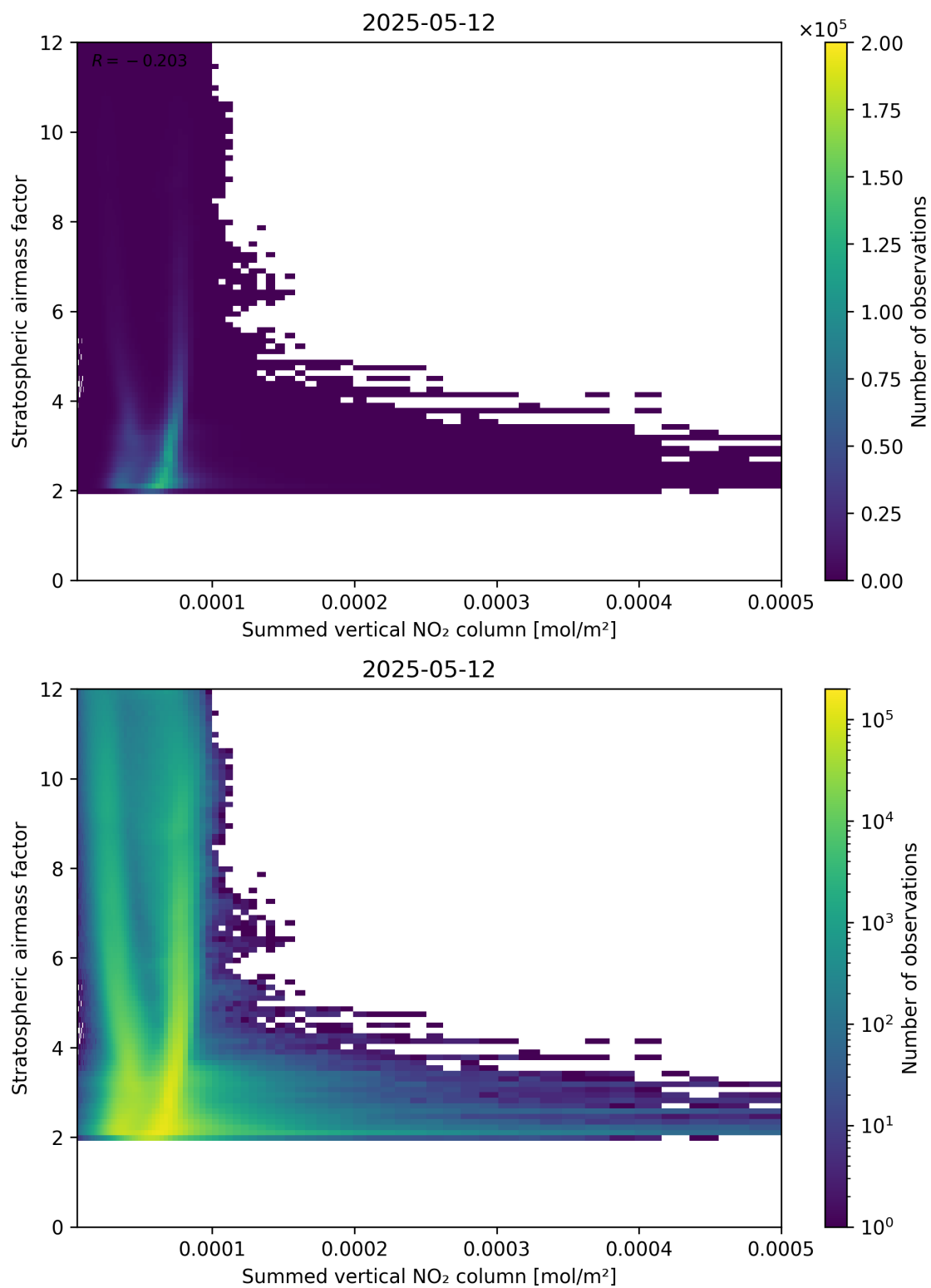
Figure 103: Scatter density plot of “Summed vertical NO 2 column” against “Stratospheric airmass factor” for 2025-05-12 to 2025-05-13.
