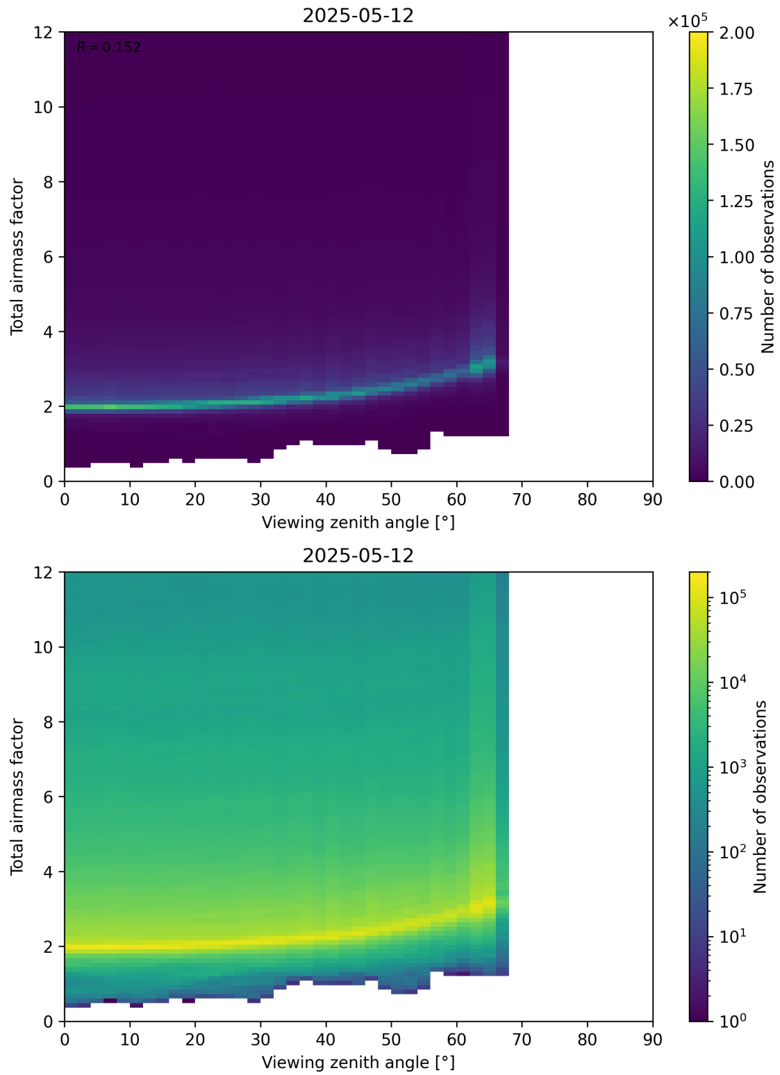
Figure 160: Scatter density plot of “Viewing zenith angle” against “Total airmass factor” for 2025-05-12 to 2025-05-13.
