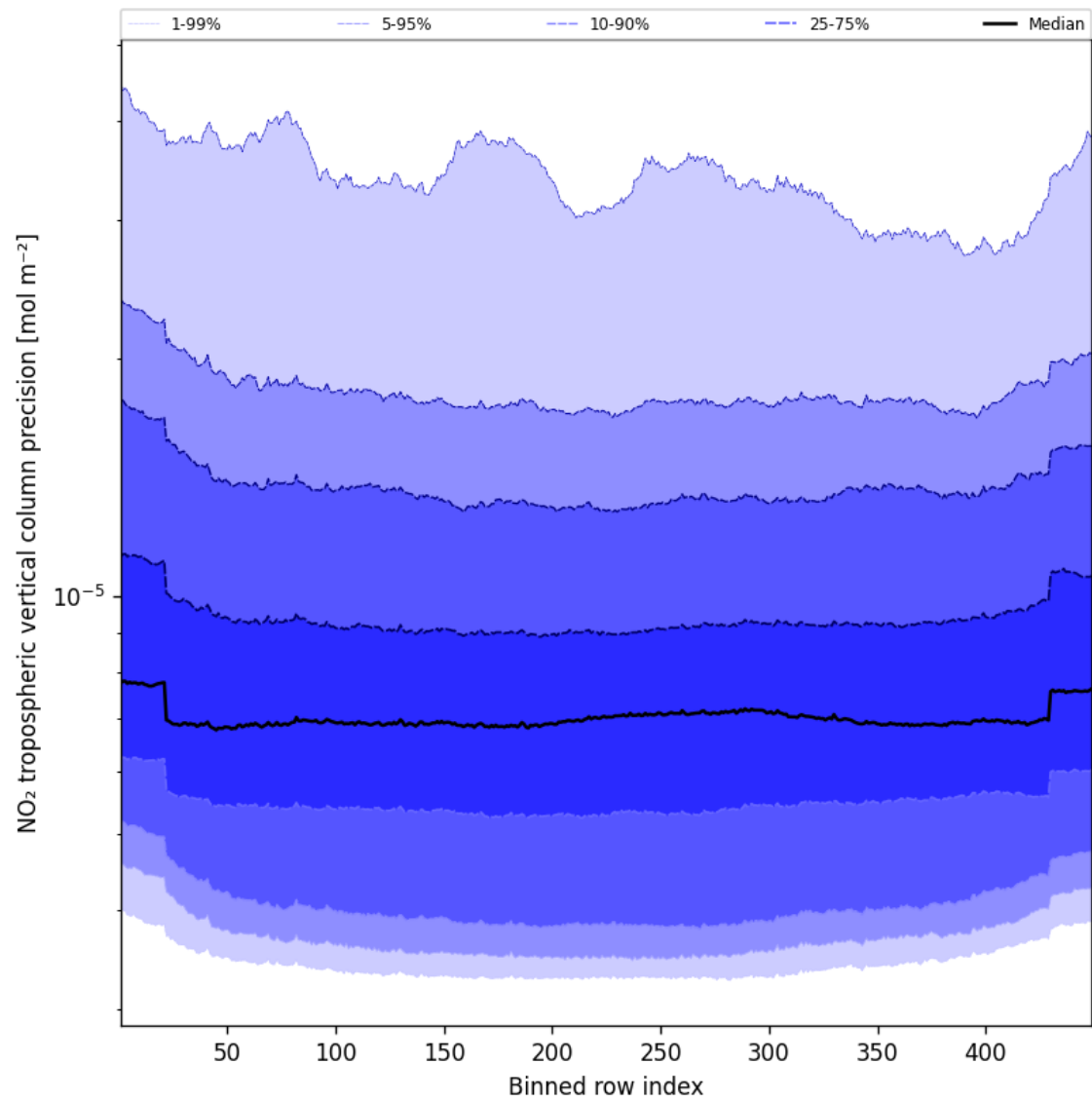
Figure 47: Along track statistics of “NO 2 tropospheric vertical column precision” for 2025-05-12 to 2025-05-13
