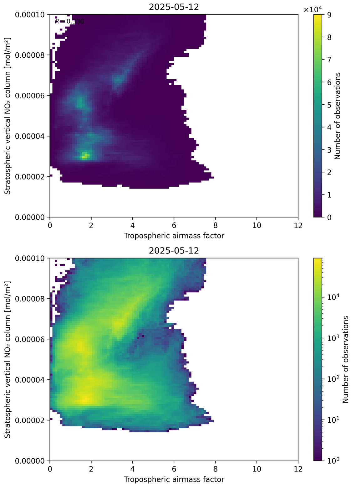
Figure 74: Scatter density plot of “Tropospheric air mass factor” against “Stratospheric vertical NO 2 column” for 2025-05-12 to 2025-05-13.
