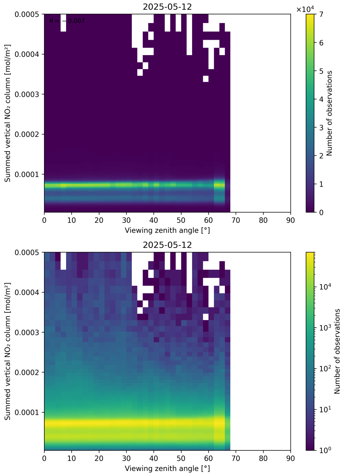
Figure 165: Scatter density plot of “Viewing zenith angle” against “Summed vertical NO 2 column” for 2025-05-12 to 2025-05-13.
