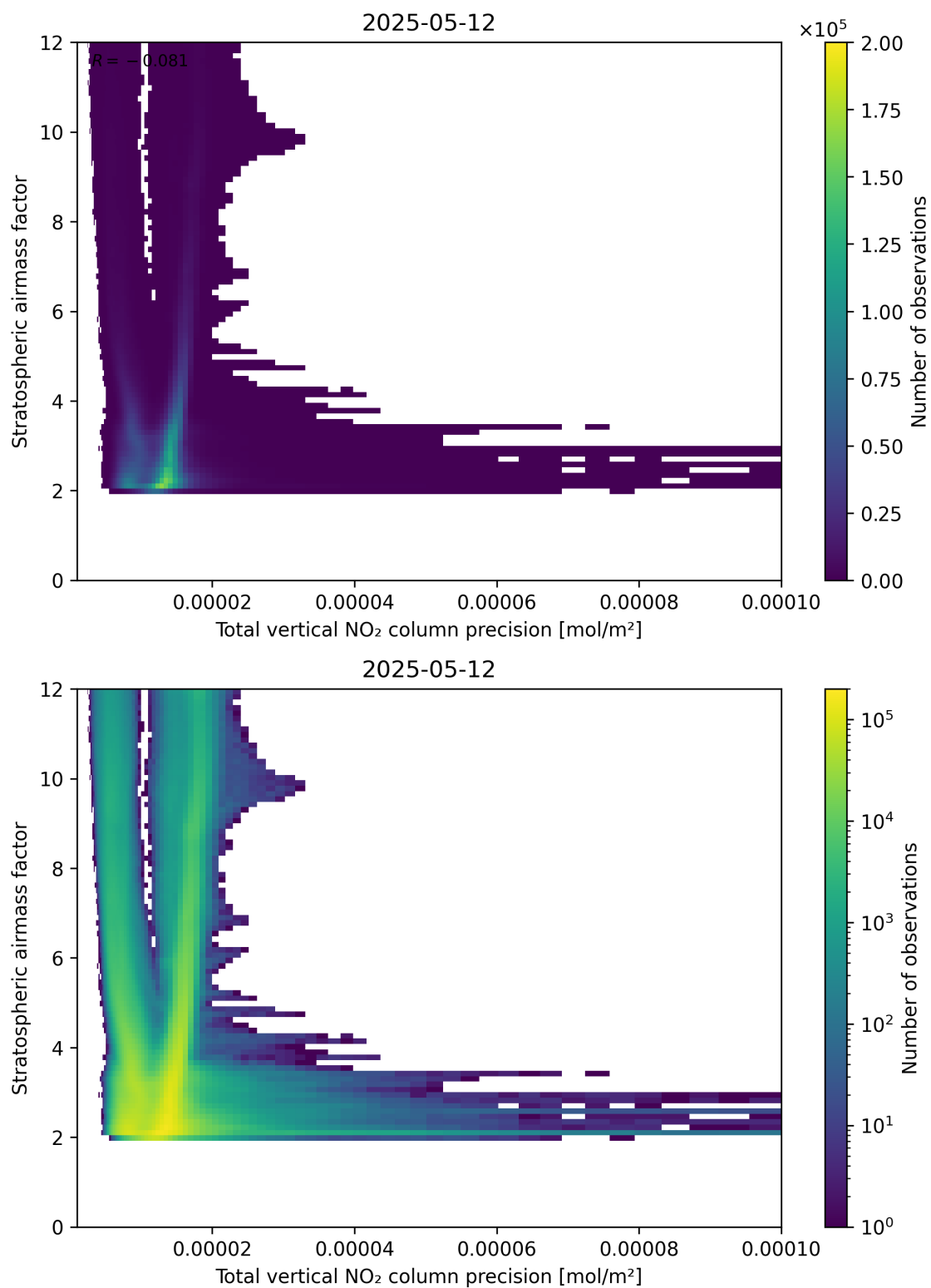
Figure 115: Scatter density plot of “Total vertical NO 2 column precision” against “Stratospheric air mass factor” for 2025-05-12 to 2025-05-13.
