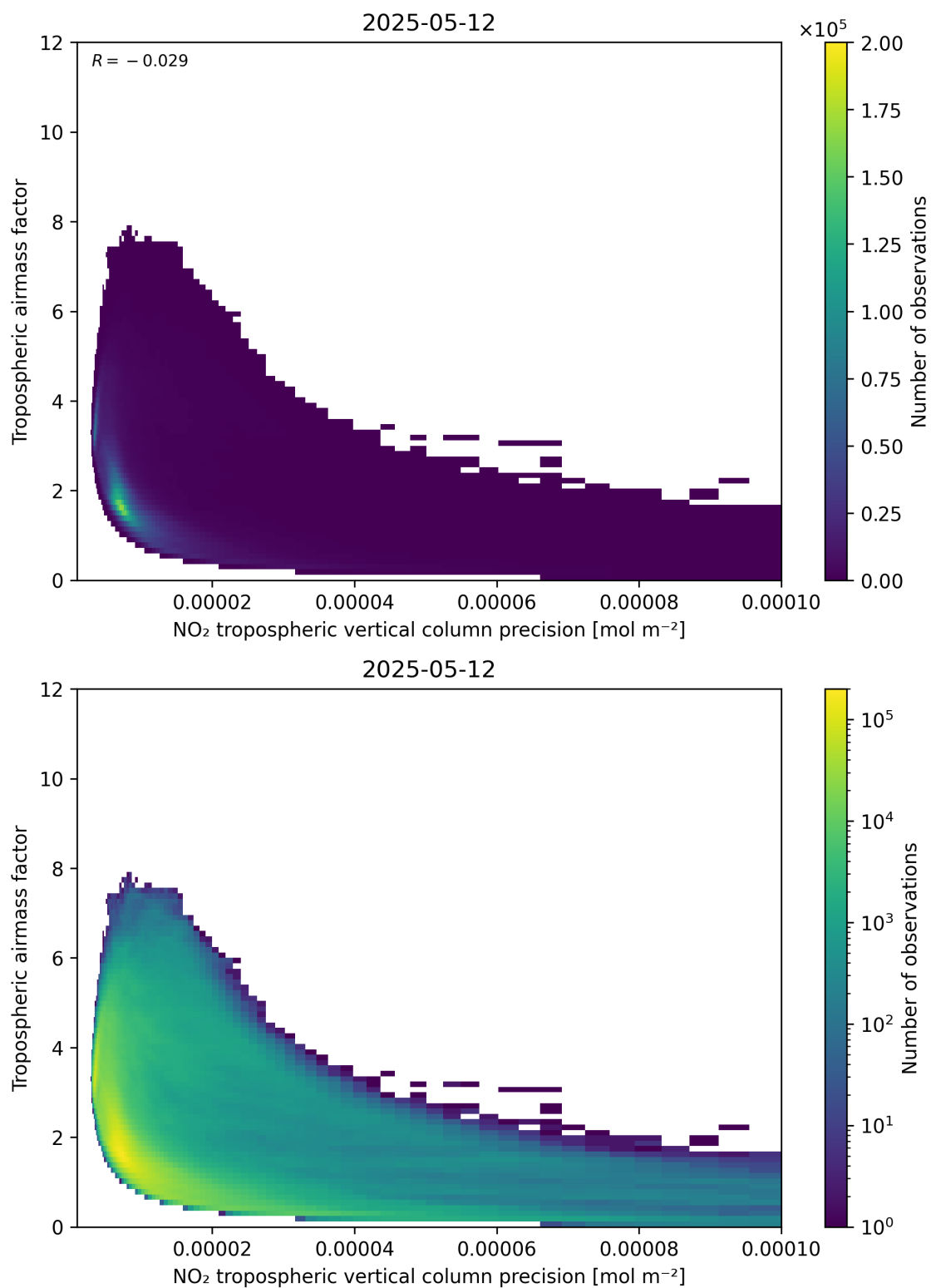
Figure 133: Scatter density plot of “NO 2 tropospheric vertical column precision” against “Tropospheric air mass factor” for 2025-05-12 to 2025-05-13.
