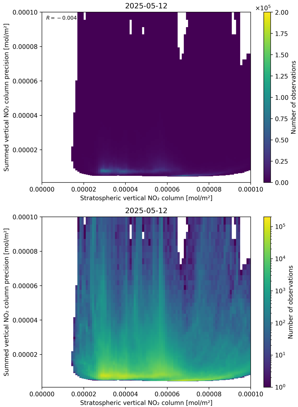
Figure 99: Scatter density plot of “Stratospheric vertical NO 2 column” against “Summed vertical NO 2 column precision” for 2025-05-12 to 2025-05-13.
