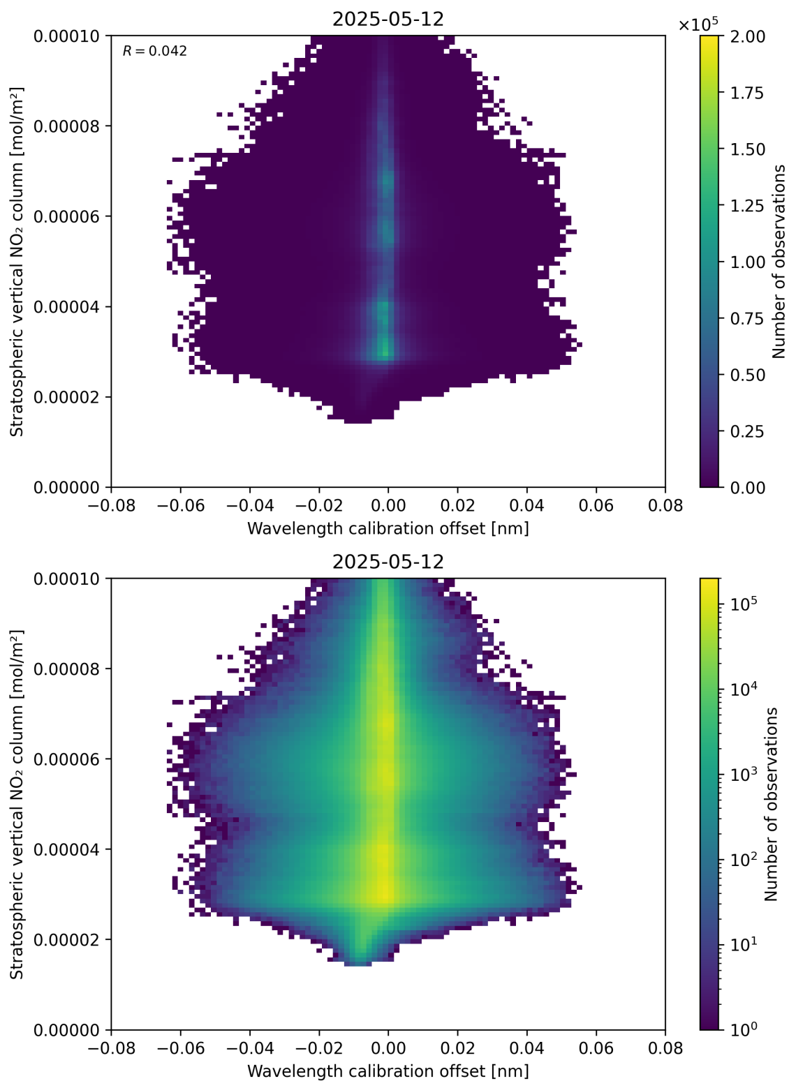
Figure 176: Scatter density plot of “Wavelength calibration offset” against “Stratospheric vertical NO 2 column” for 2025-05-12 to 2025-05-13.
