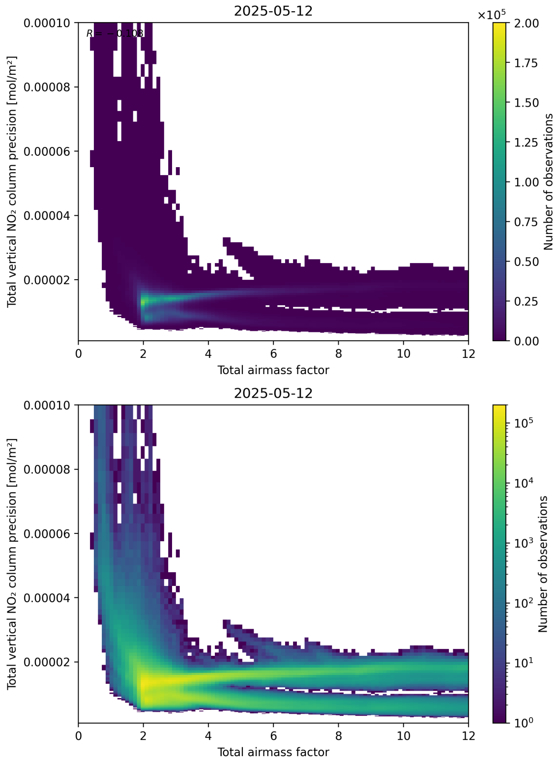
Figure 68: Scatter density plot of “Total airmass factor” against “Total vertical NO 2 column precision” for 2025-05-12 to 2025-05-13.
