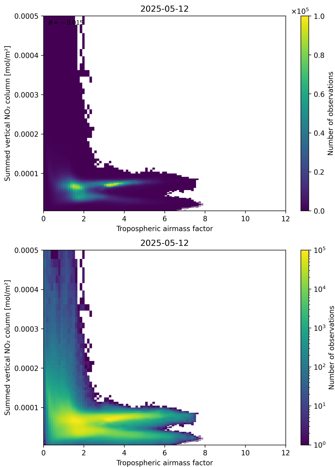
Figure 75: Scatter density plot of “Tropospheric air mass factor” against “Summed vertical NO 2 column” for 2025-05-12 to 2025-05-13.
