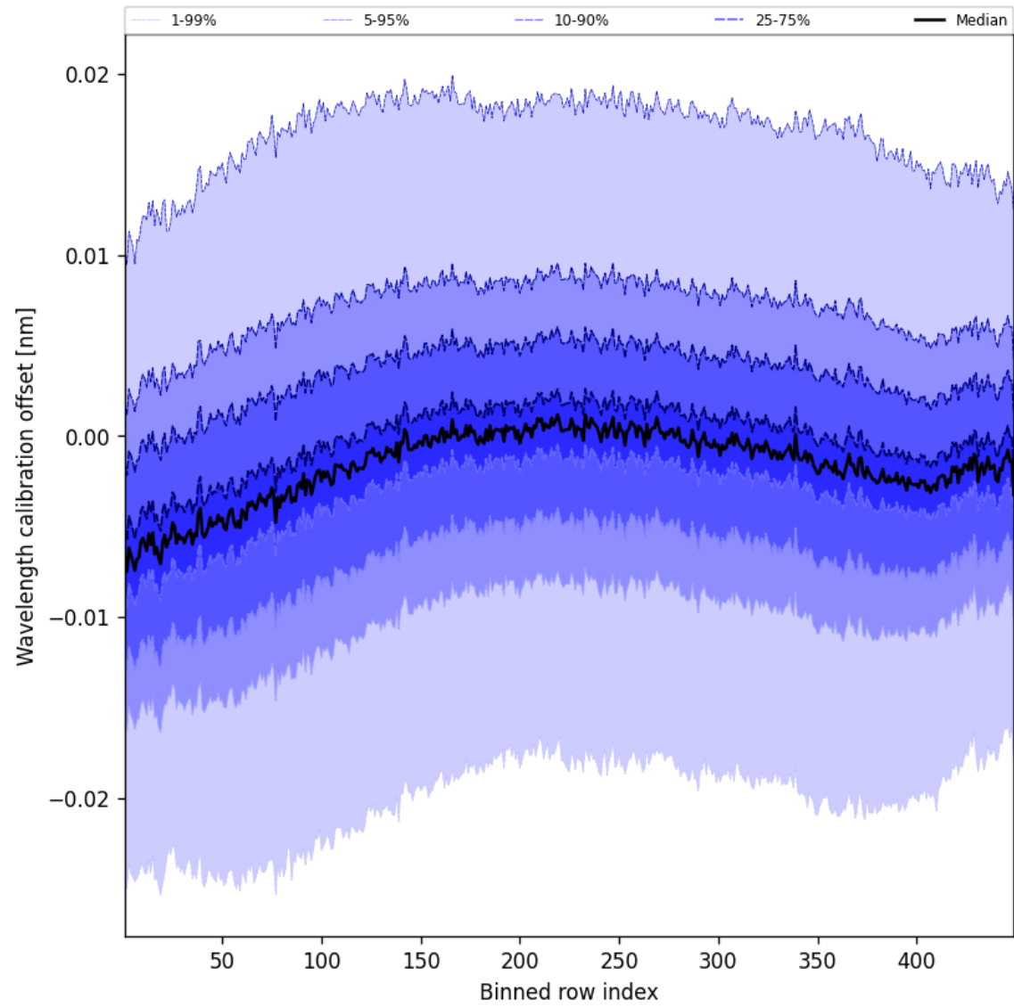
Figure 52: Along track statistics of “Wavelength calibration offset” for 2025-05-12 to 2025-05-13
