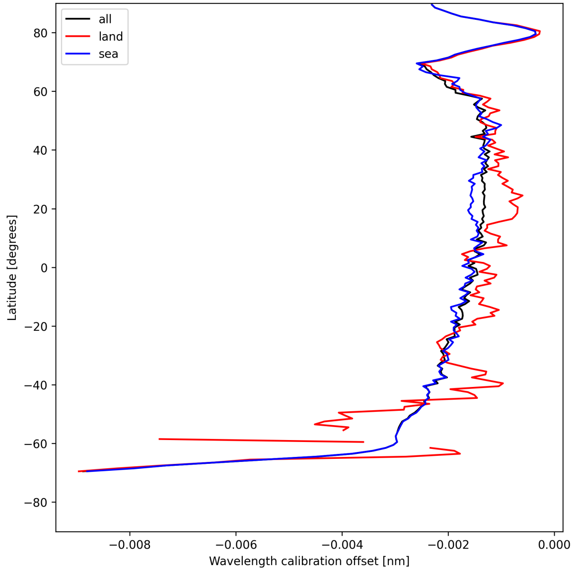
Figure 18: Zonal average of “Wavelength calibration offset” for 2025-05-12 to 2025-05-13.
