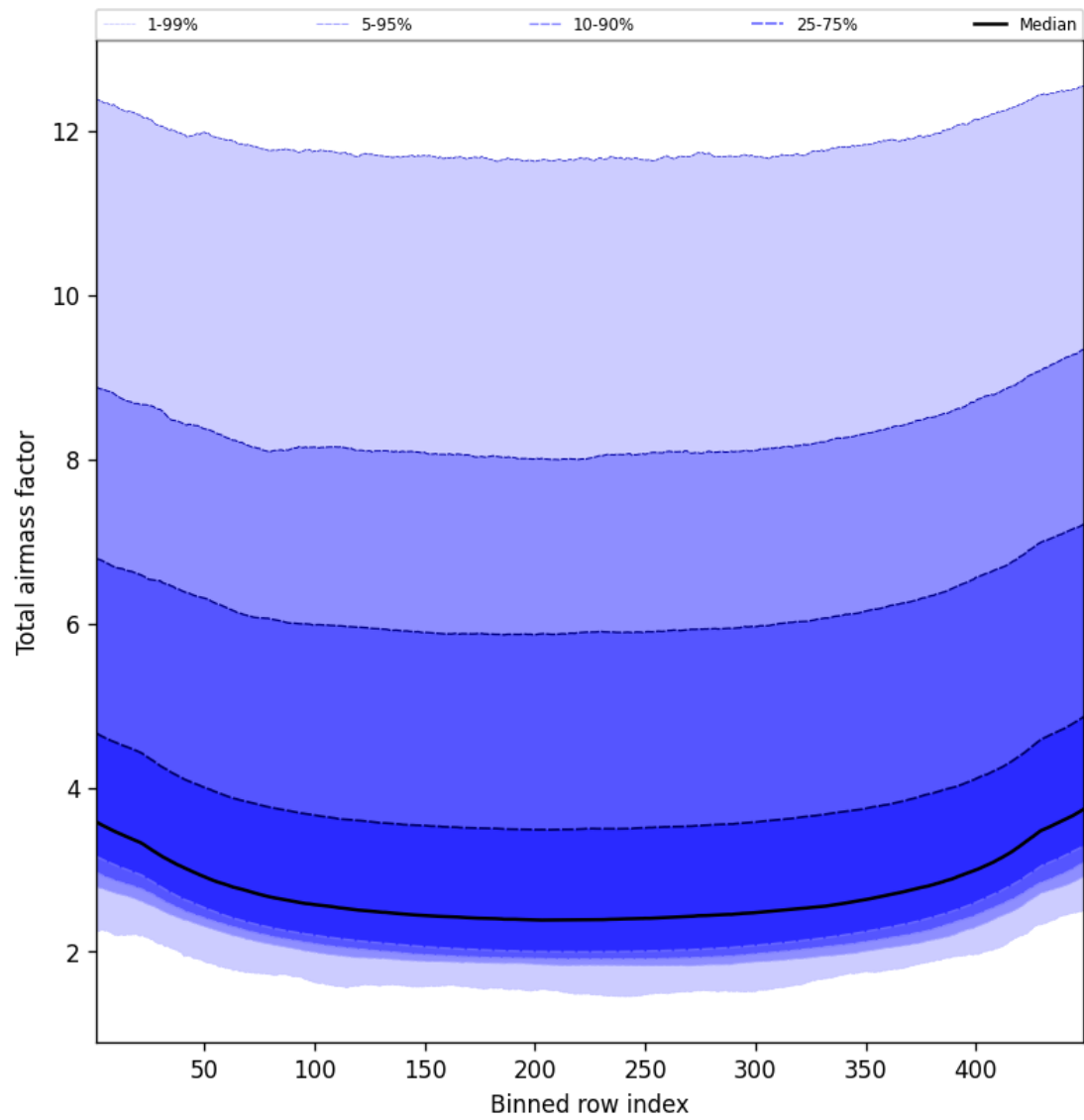
Figure 49: Along track statistics of “Total airmass factor” for 2025-05-12 to 2025-05-13
