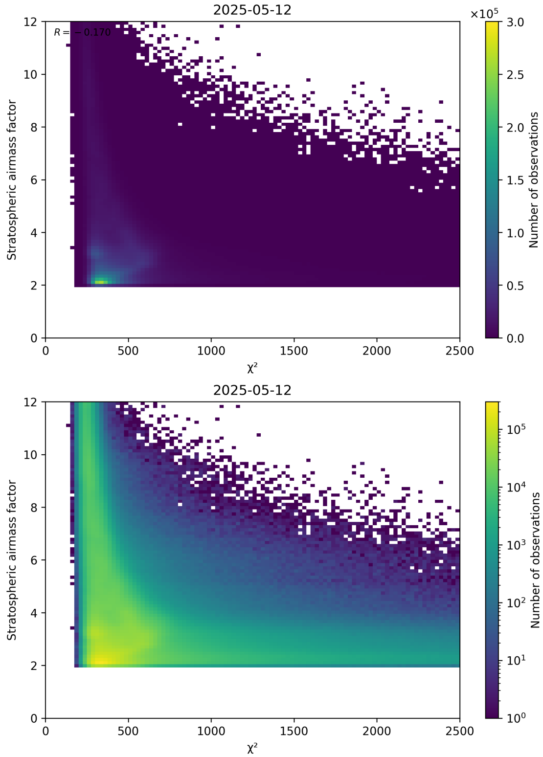
Figure 81: Scatter density plot of “ \chi^2 ” against “Stratospheric airmass factor” for 2025-05-12 to 2025-05-13.
