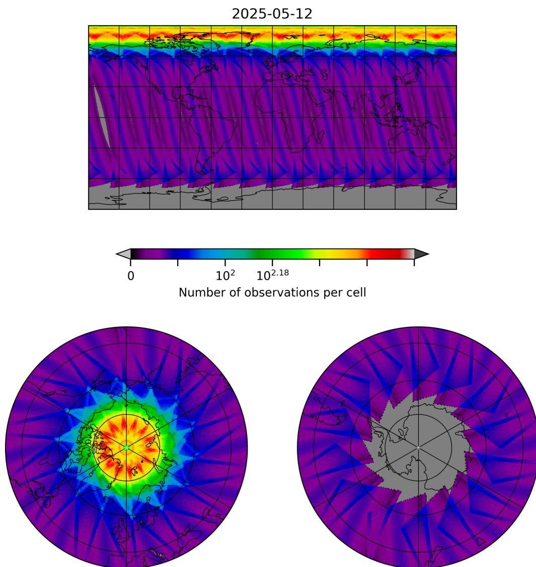
Figure 10: Map of the number of observations for 2025-05-12 to 2025-05-13
