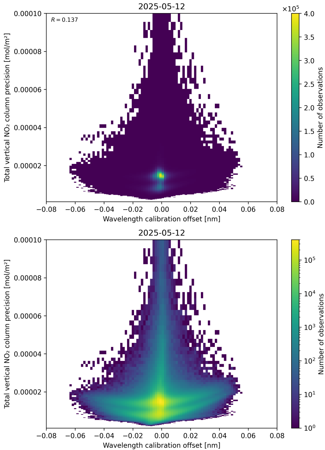
Figure 180: Scatter density plot of “Wavelength calibration offset” against “Total vertical NO 2 column precision” for 2025-05-12 to 2025-05-13.
