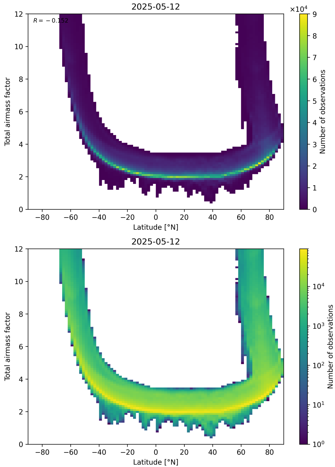
Figure 84: Scatter density plot of “Latitude” against “Total airmass factor” for 2025-05-12 to 2025-05-13.
