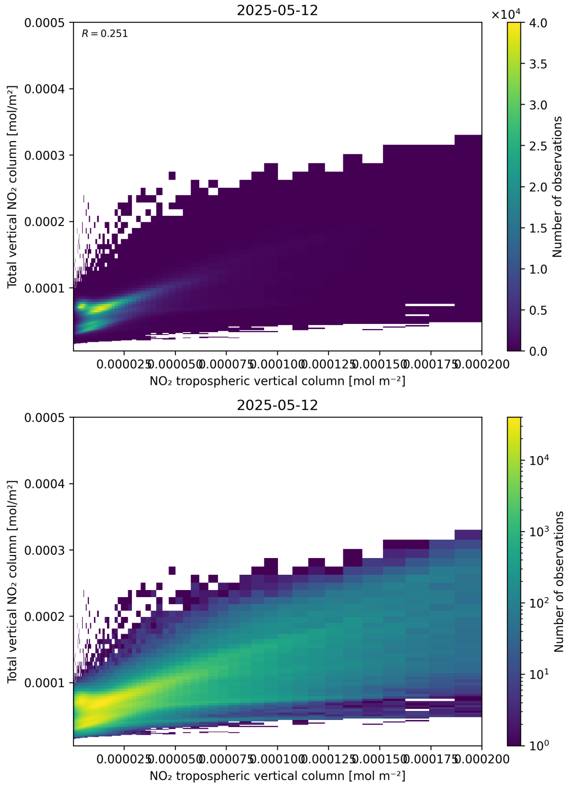
Figure 128: Scatter density plot of “NO 2 tropospheric vertical column” against “Total vertical NO 2 column” for 2025-05-12 to 2025-05-13.
