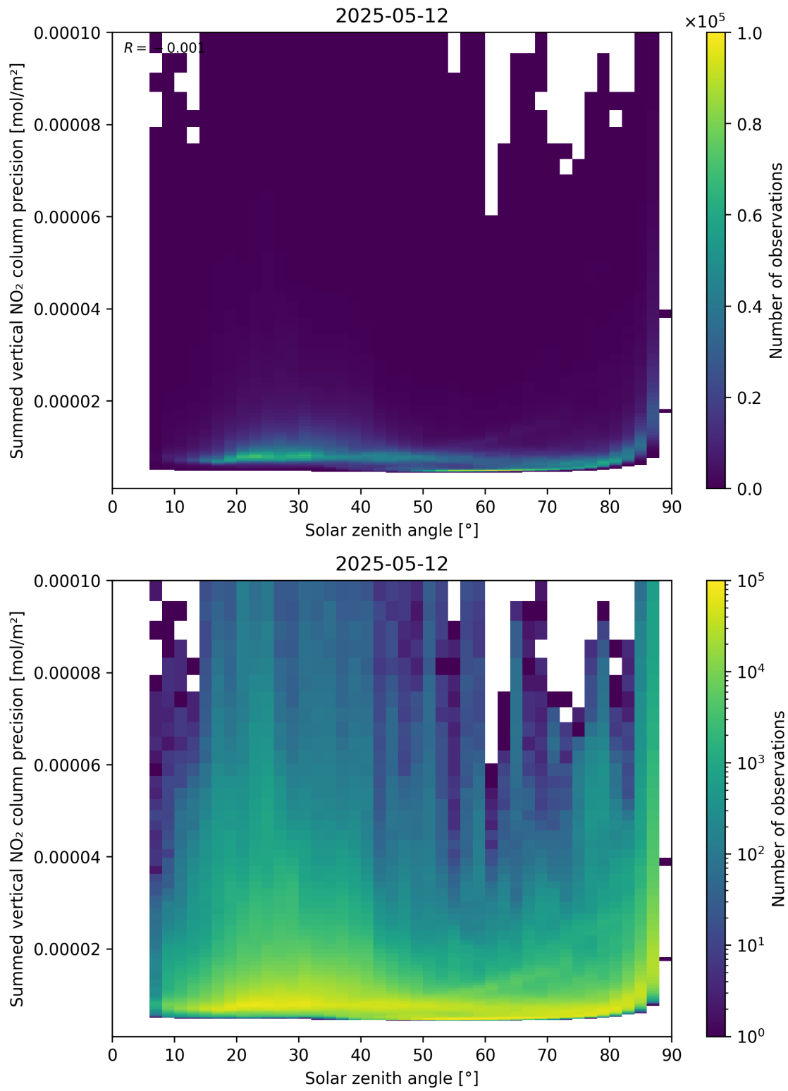
Figure 152: Scatter density plot of “Solar zenith angle” against “Summed vertical NO 2 column precision” for 2025-05-12 to 2025-05-13.
