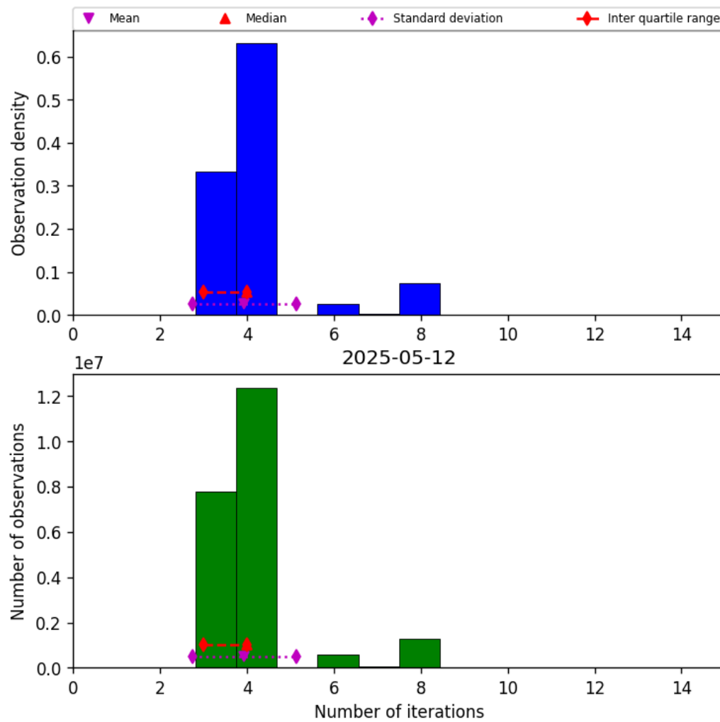
Figure 34: Histogram of “Number of iterations” for 2025-05-12 to 2025-05-13
