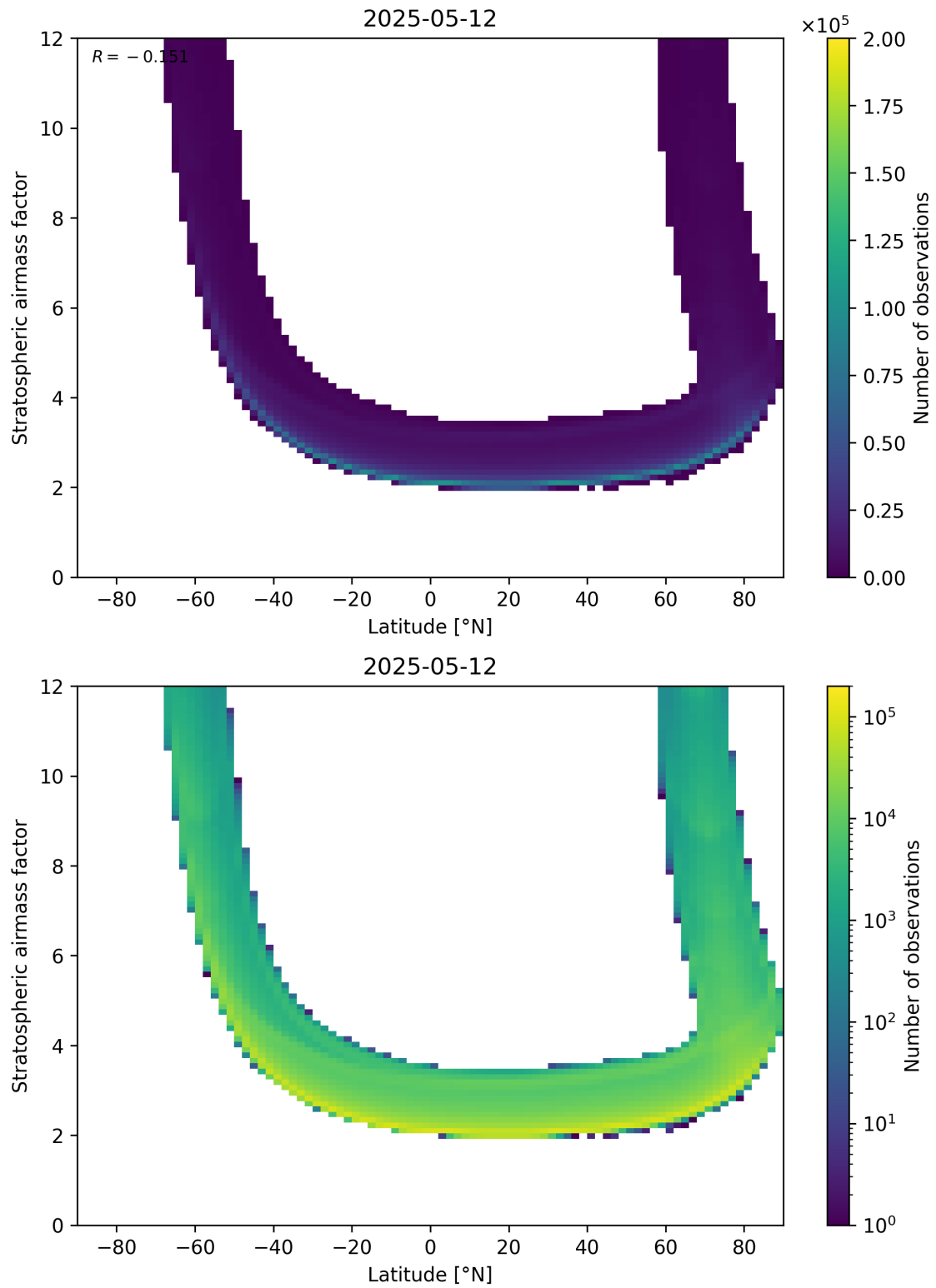
Figure 83: Scatter density plot of “Latitude” against “Stratospheric air mass factor” for 2025-05-12 to 2025-05-13.
