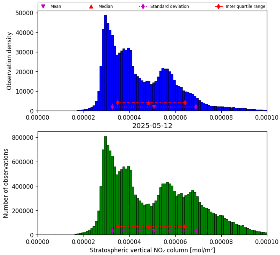
Figure 36: Histogram of “Stratospheric vertical NO 2 column” for 2025-05-12 to 2025-05-13
