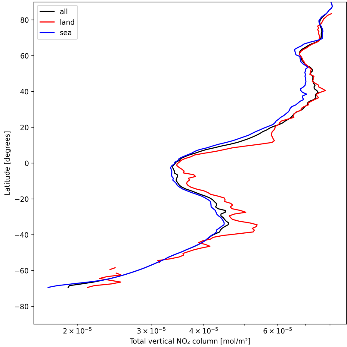
Figure 21: Zonal average of “Total vertical NO 2 column” for 2025-05-12 to 2025-05-13.
