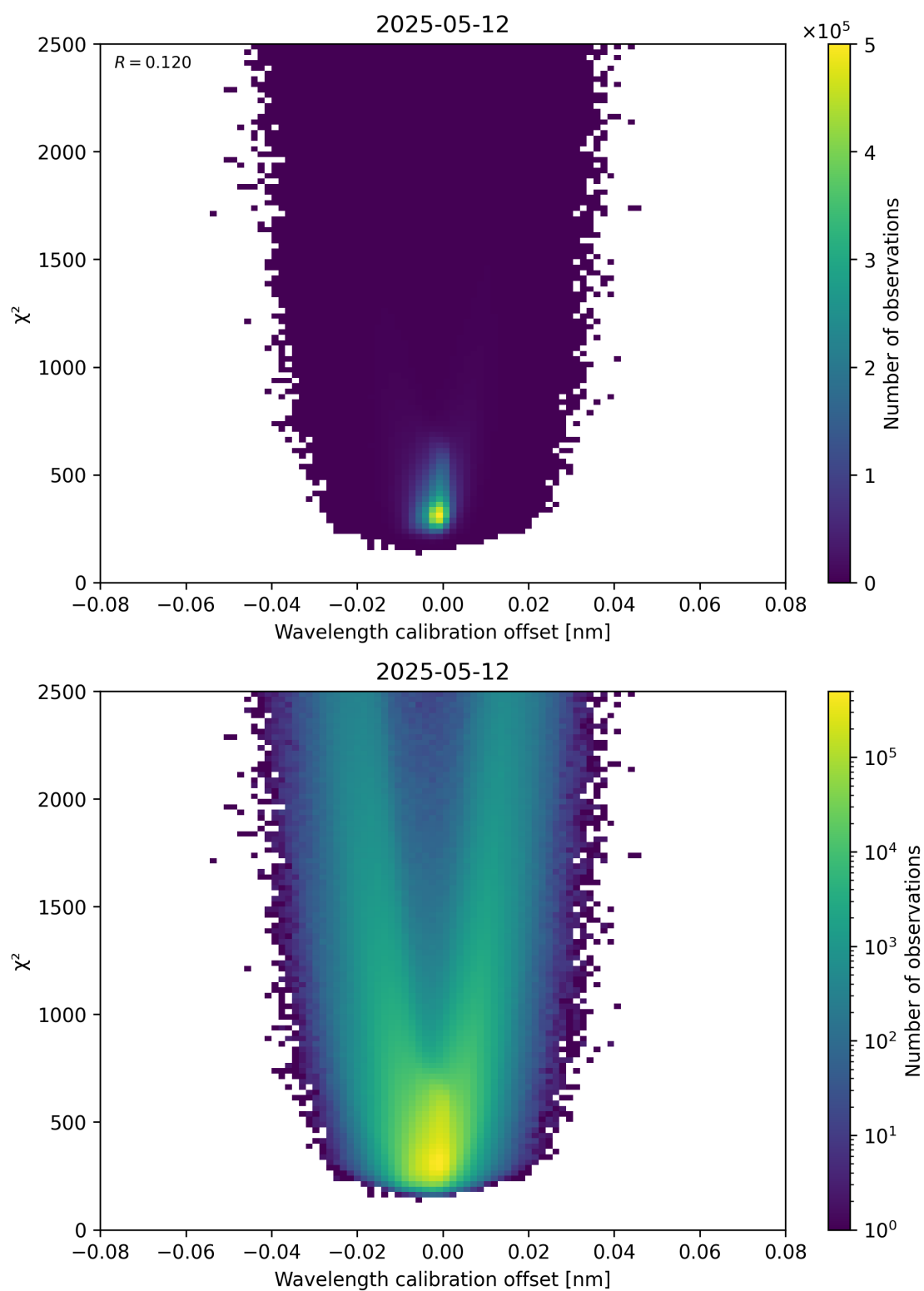
Figure 175: Scatter density plot of “Wavelength calibration offset” against “ \chi^2 ” for 2025-05-12 to 2025-05-13.
