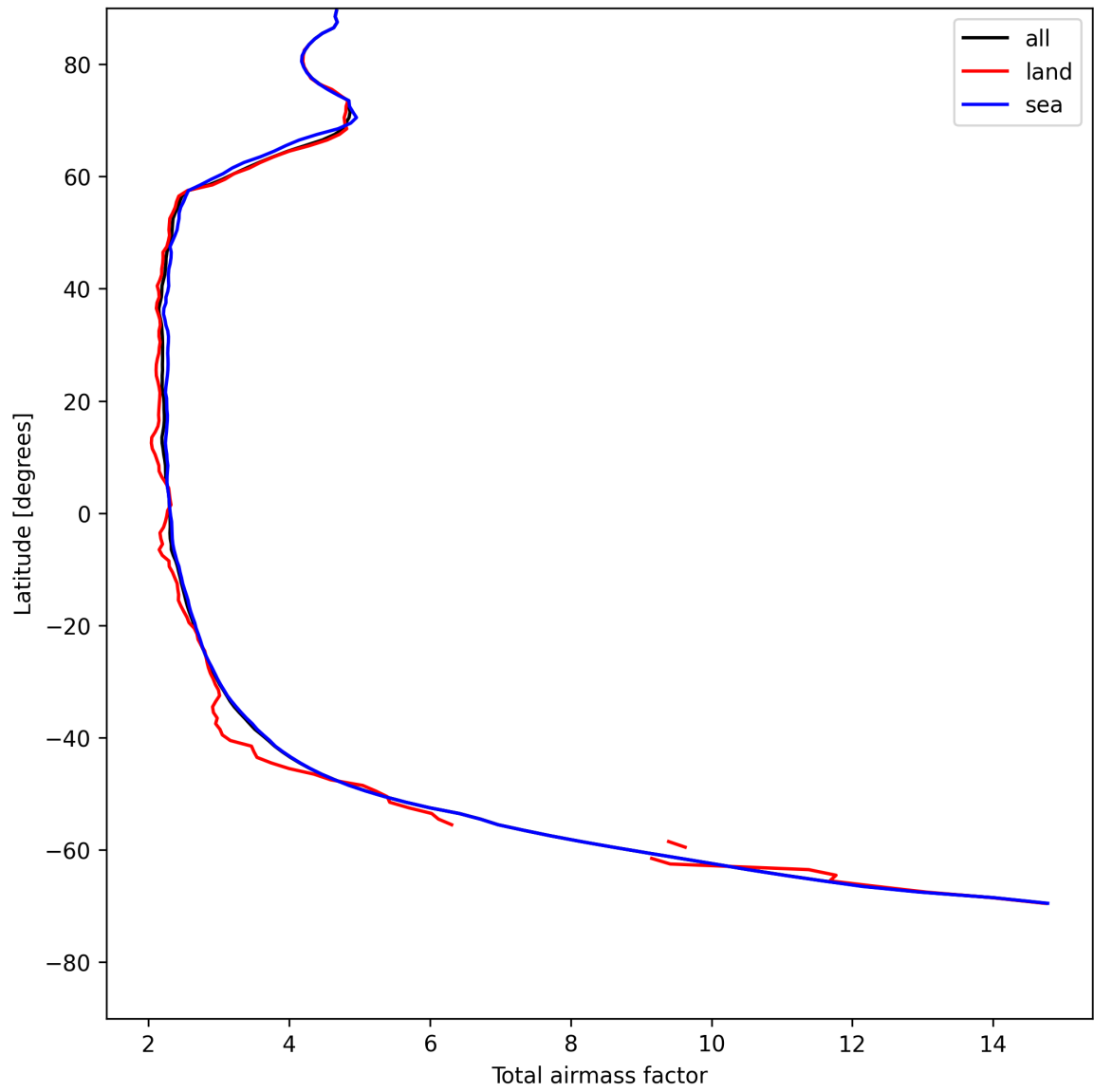
Figure 15: Zonal average of “Total airmass factor” for 2025-05-12 to 2025-05-13.
