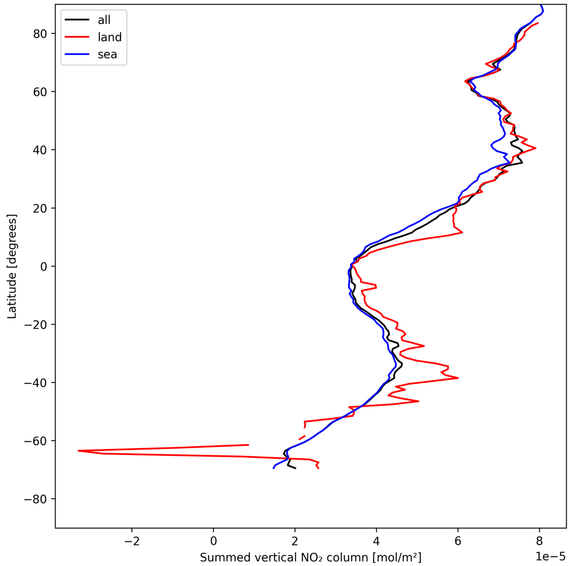
Figure 23: Zonal average of “Summed vertical NO 2 column” for 2025-05-12 to 2025-05-13.
