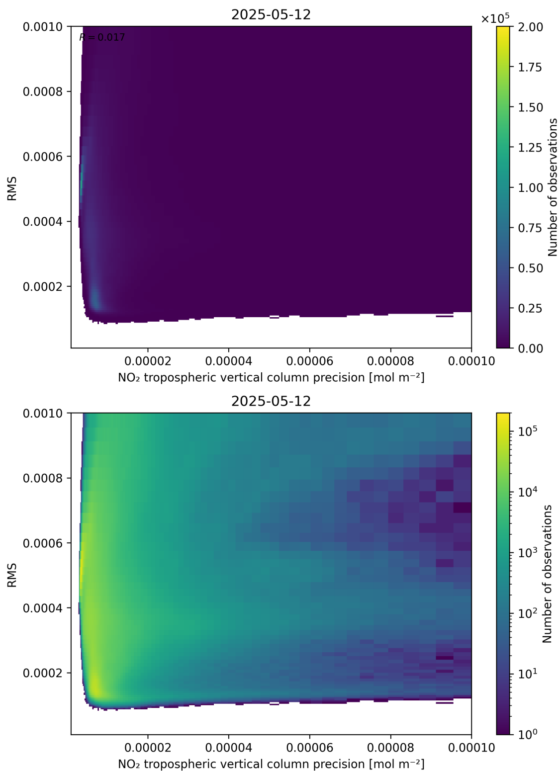
Figure 140: Scatter density plot of “NO 2 tropospheric vertical column precision” against “RMS” for 2025-05-12 to 2025-05-13.
