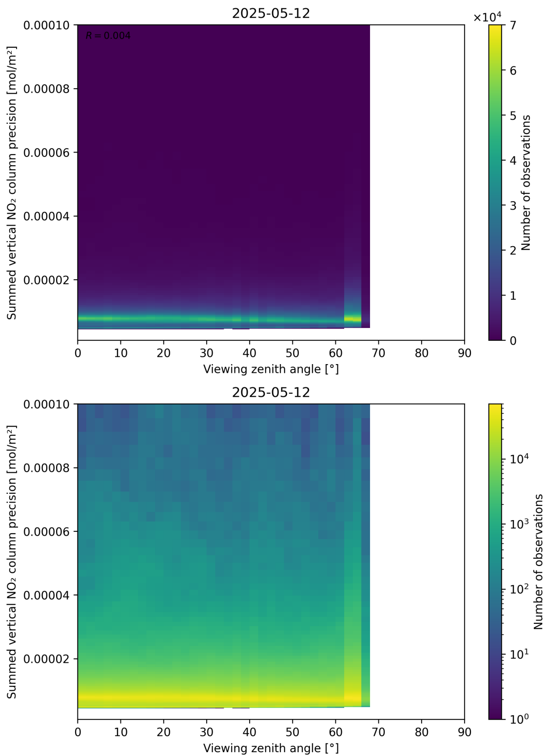
Figure 166: Scatter density plot of “Viewing zenith angle” against “Summed vertical NO 2 column precision” for 2025-05-12 to 2025-05-13.
