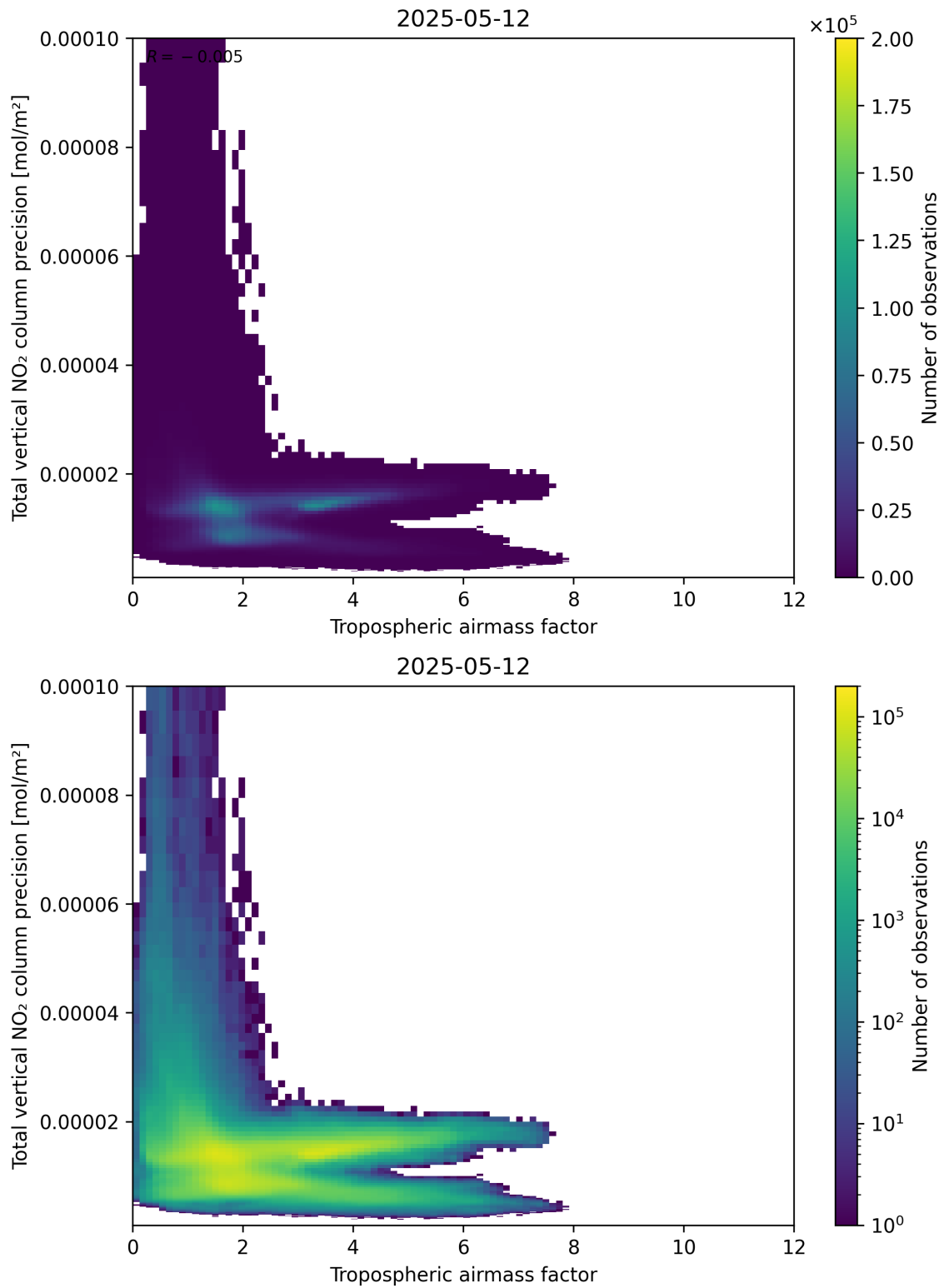
Figure 78: Scatter density plot of “Tropospheric air mass factor” against “Total vertical NO 2 column precision” for 2025-05-12 to 2025-05-13.
