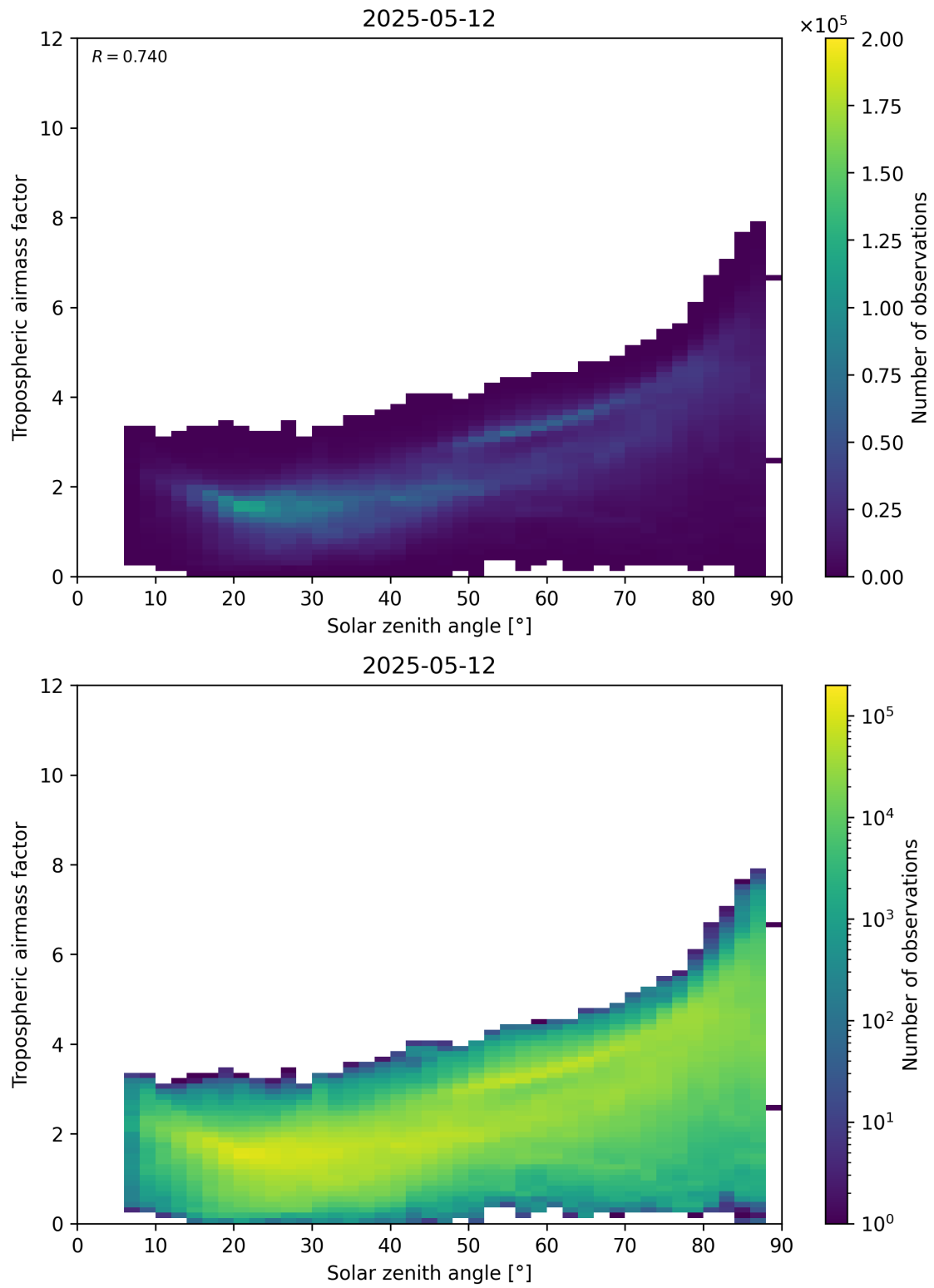
Figure 147: Scatter density plot of “Solar zenith angle” against “Tropospheric airmass factor” for 2025-05-12 to 2025-05-13.
