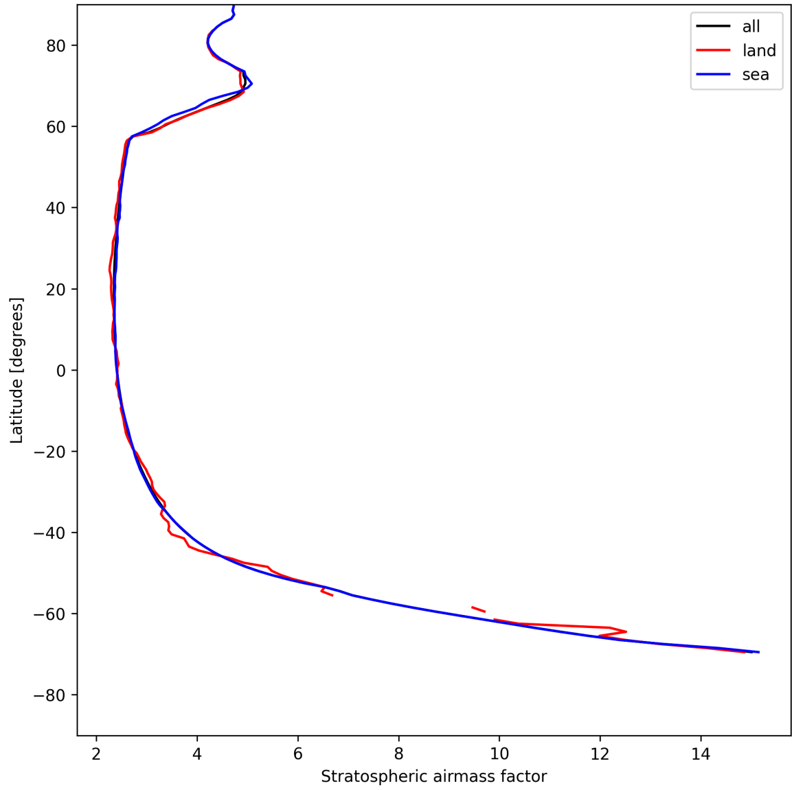
Figure 27: Zonal average of “Stratospheric air mass factor” for 2025-05-12 to 2025-05-13.
