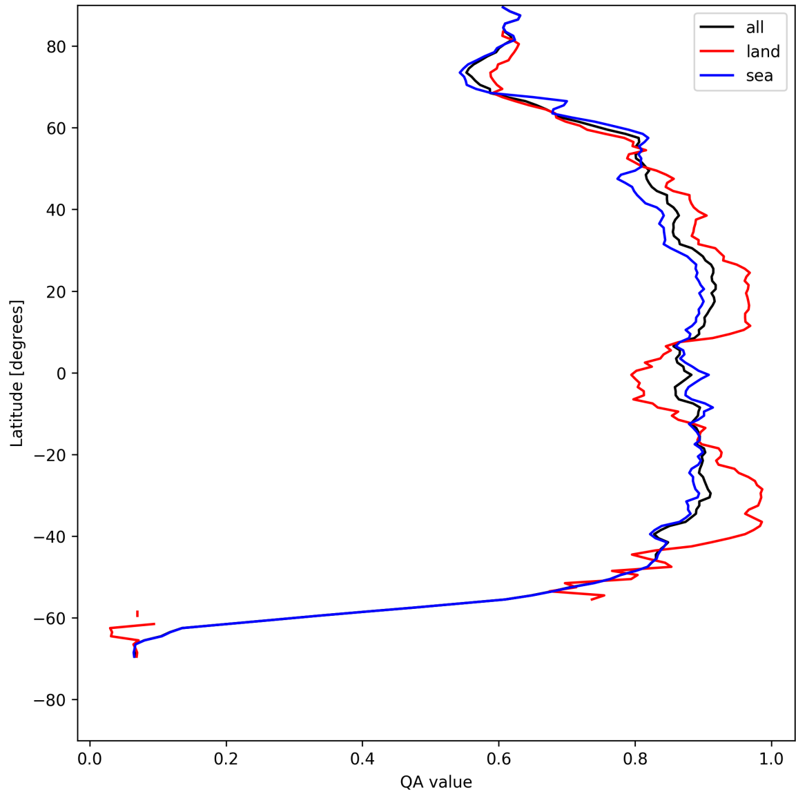
Figure 11: Zonal average of “QA value” for 2025-05-12 to 2025-05-13.
