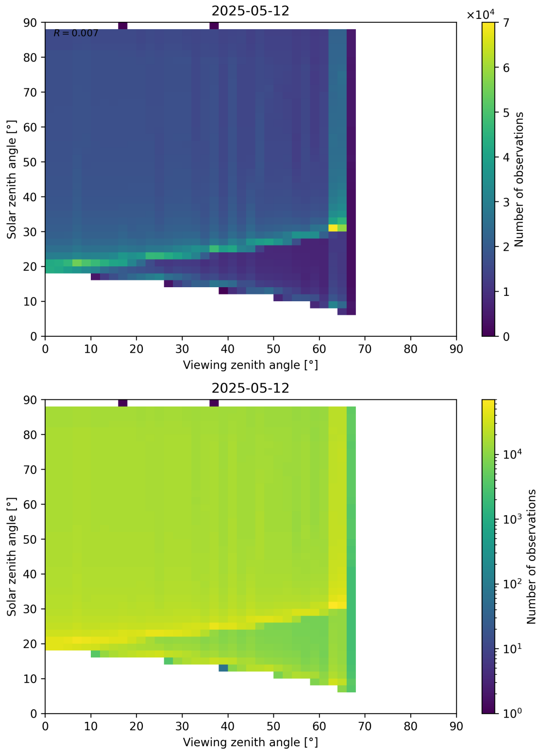
Figure 172: Scatter density plot of “Viewing zenith angle” against “Solar zenith angle” for 2025-05-12 to 2025-05-13.
