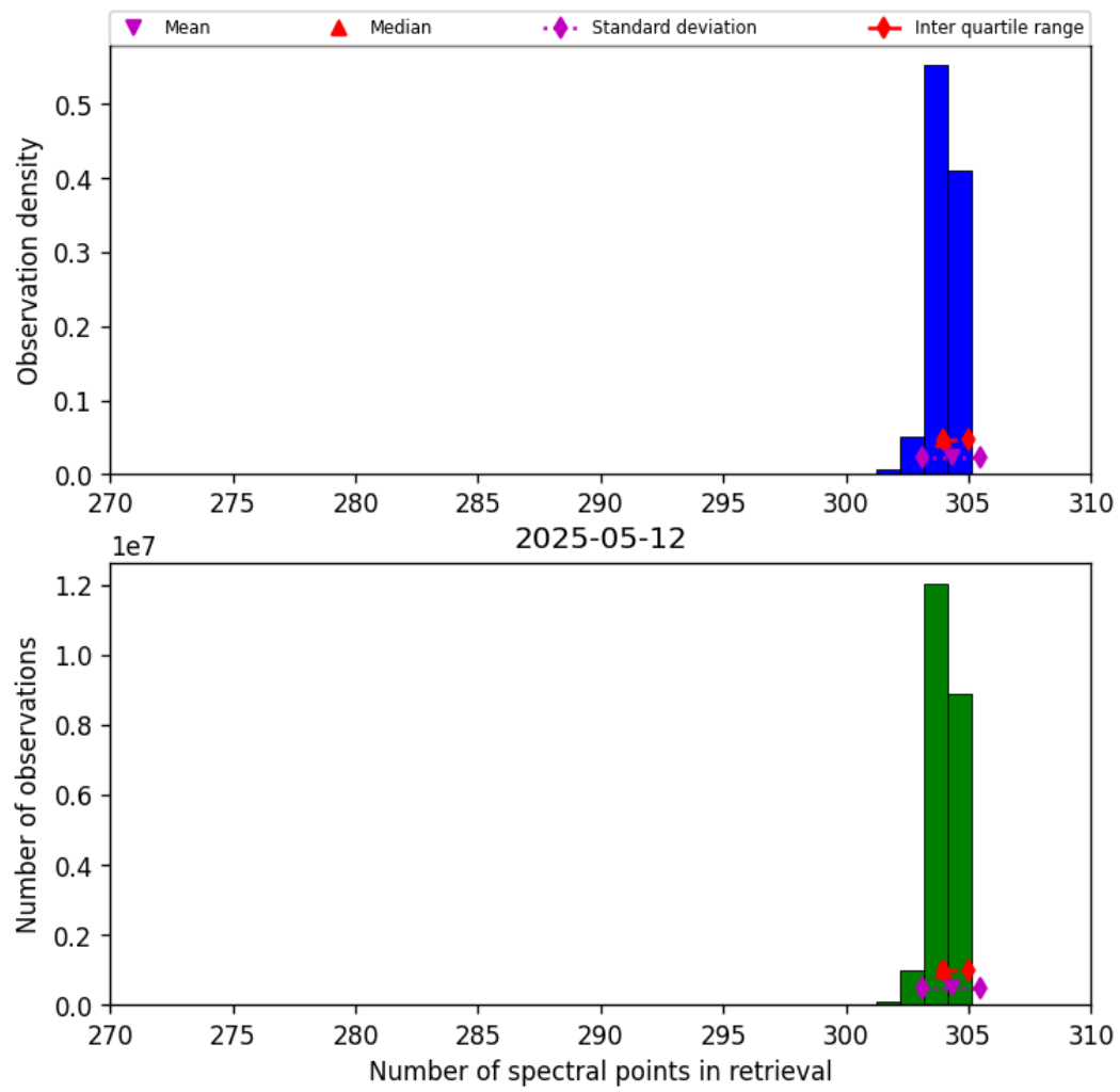
Figure 33: Histogram of “Number of spectral points in retrieval” for 2025-05-12 to 2025-05-13
