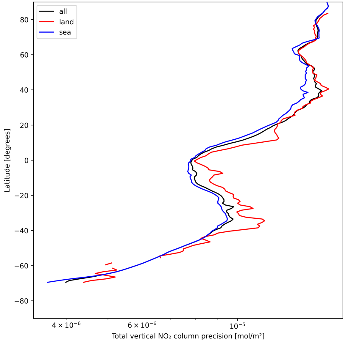
Figure 22: Zonal average of “Total vertical NO 2 column precision” for 2025-05-12 to 2025-05-13.
