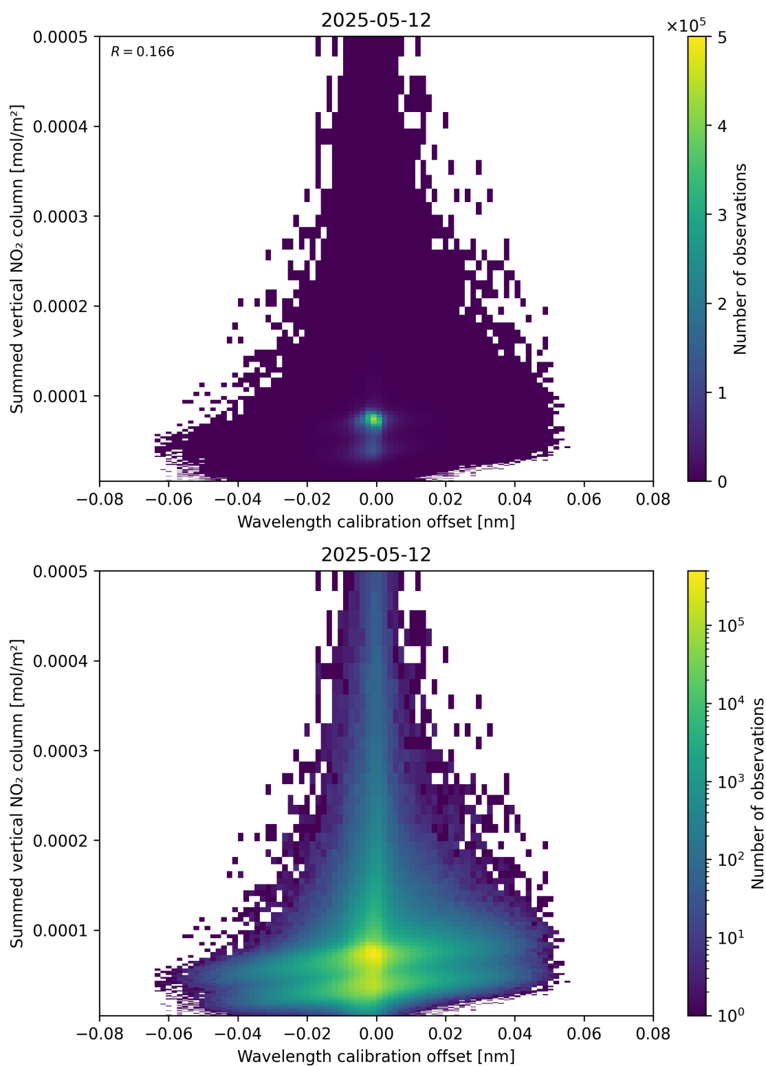
Figure 177: Scatter density plot of “Wavelength calibration offset” against “Summed vertical NO 2 column” for 2025-05-12 to 2025-05-13.
