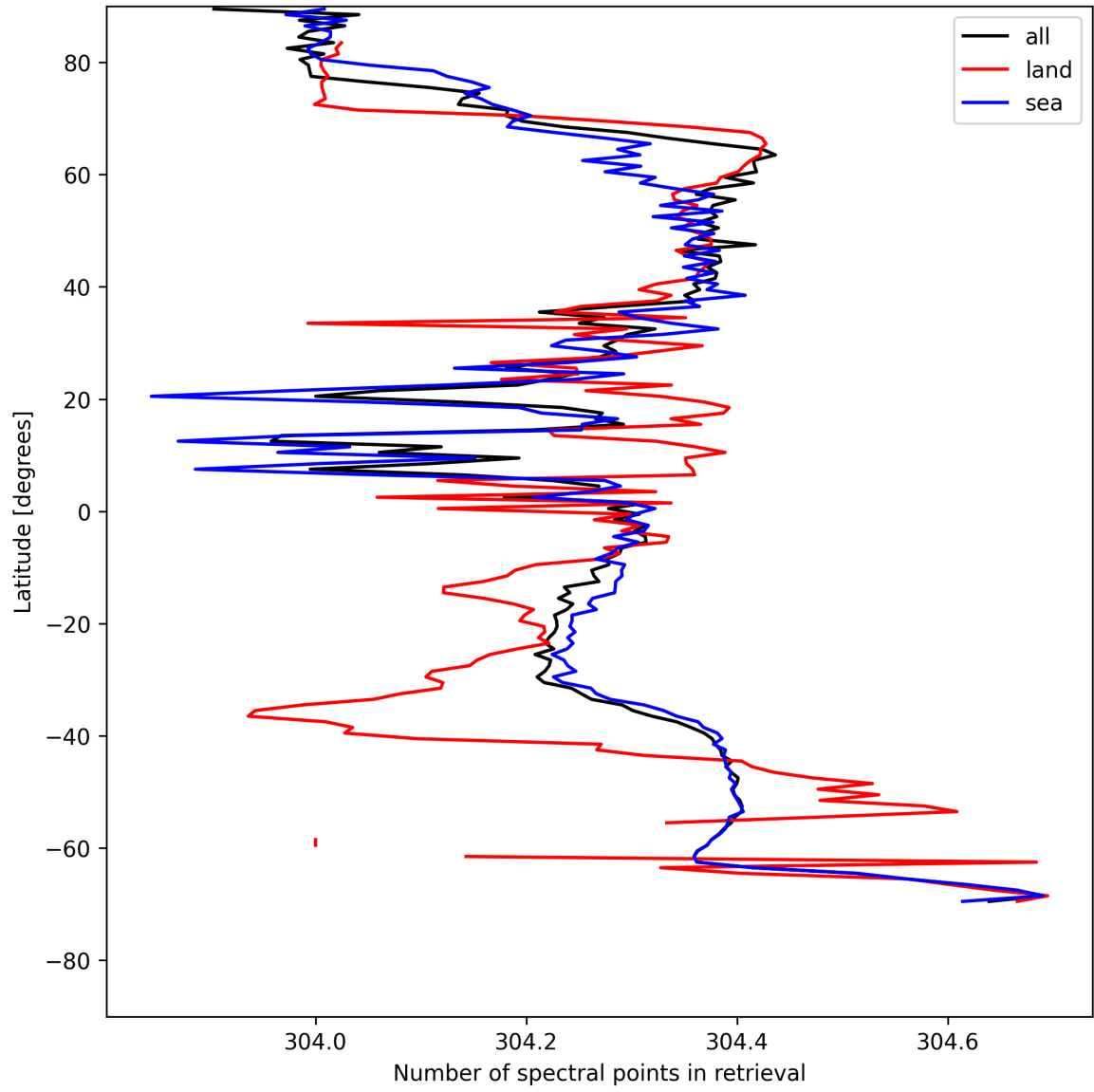
Figure 16: Zonal average of “Number of spectral points in retrieval” for 2025-05-12 to 2025-05-13.
