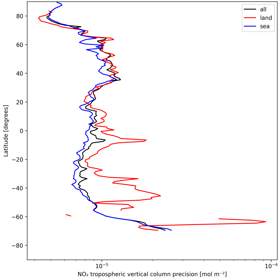
Figure 13: Zonal average of “NO 2 tropospheric vertical column precision” for 2025-05-12 to 2025-05-13.
