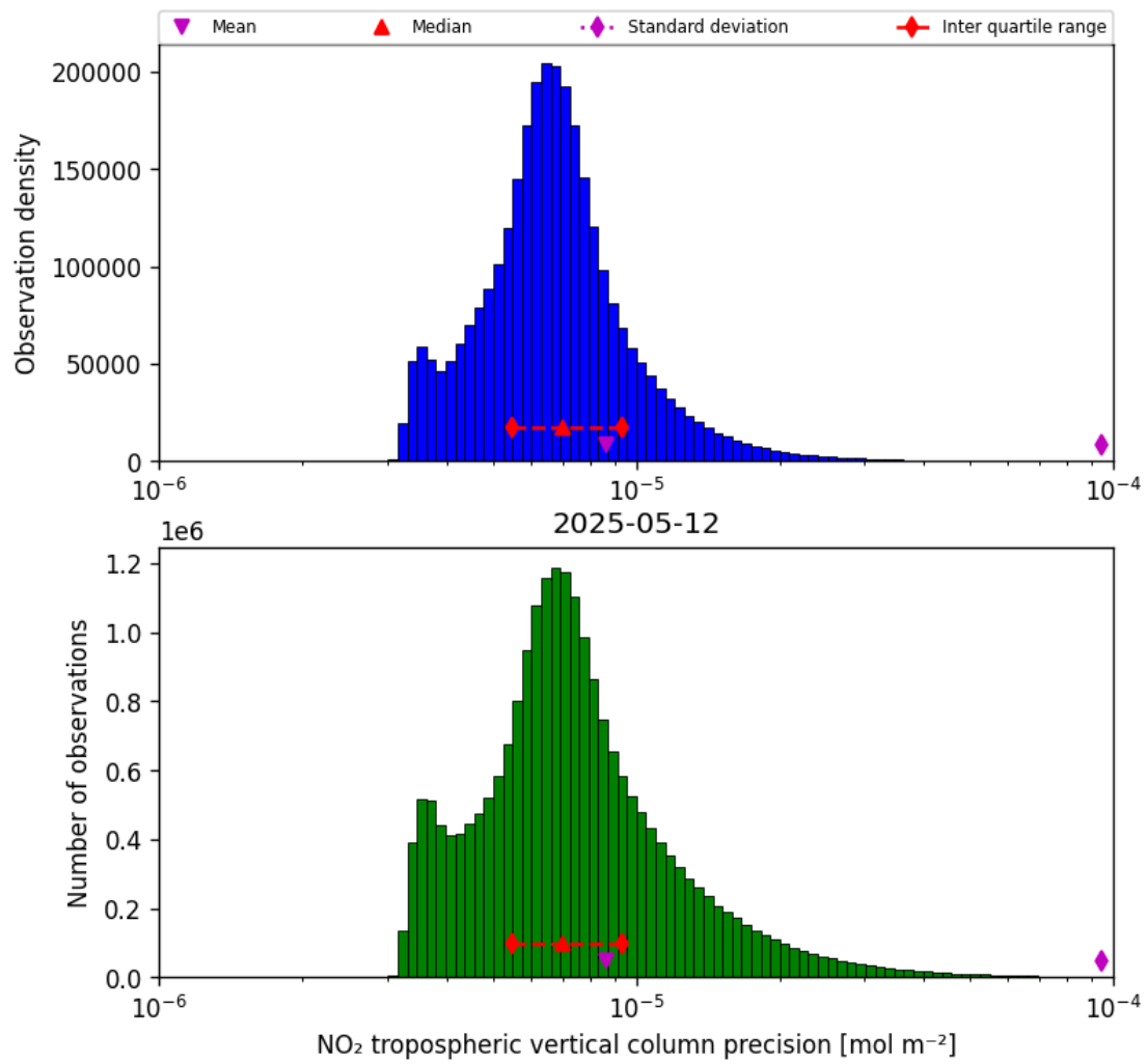
Figure 30: Histogram of “NO 2 tropospheric vertical column precision” for 2025-05-12 to 2025-05-13
