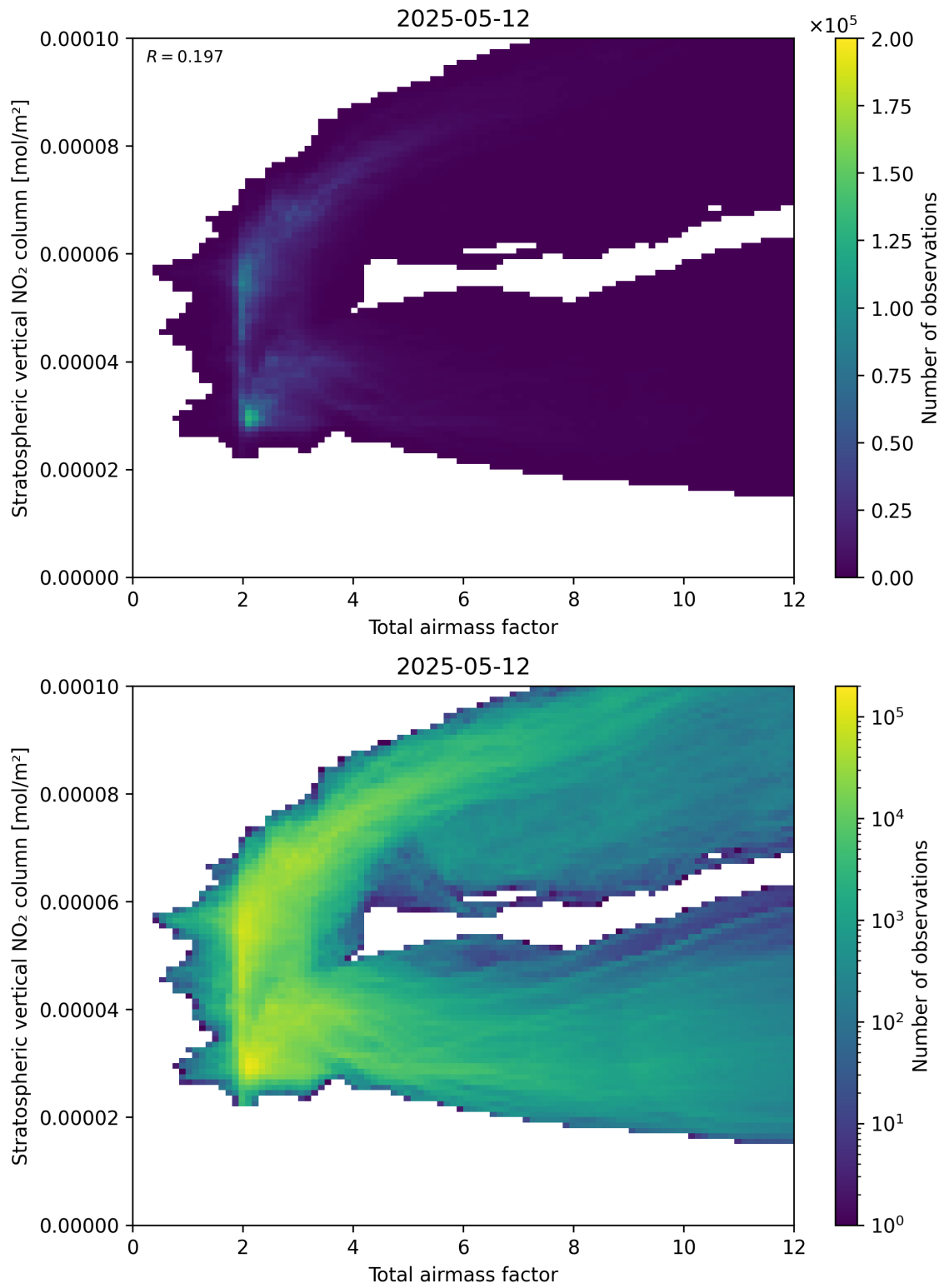
Figure 64: Scatter density plot of “Total airmass factor” against “Stratospheric vertical NO 2 column” for 2025-05-12 to 2025-05-13.
