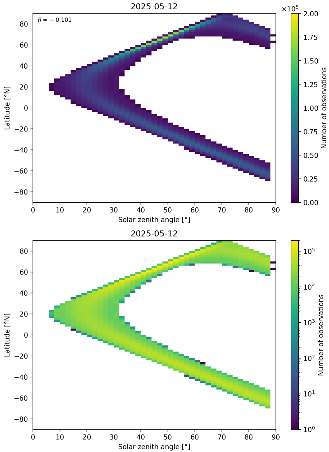
Figure 149: Scatter density plot of “Solar zenith angle” against “Latitude” for 2025-05-12 to 2025-05-13.
