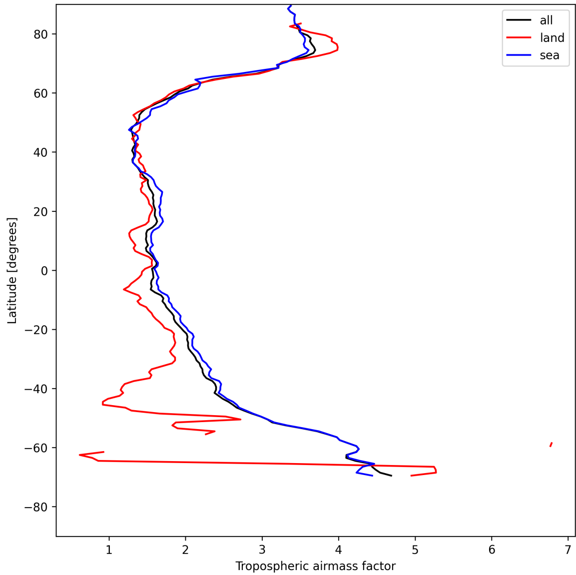
Figure 14: Zonal average of “Tropospheric airmass factor” for 2025-05-12 to 2025-05-13.
