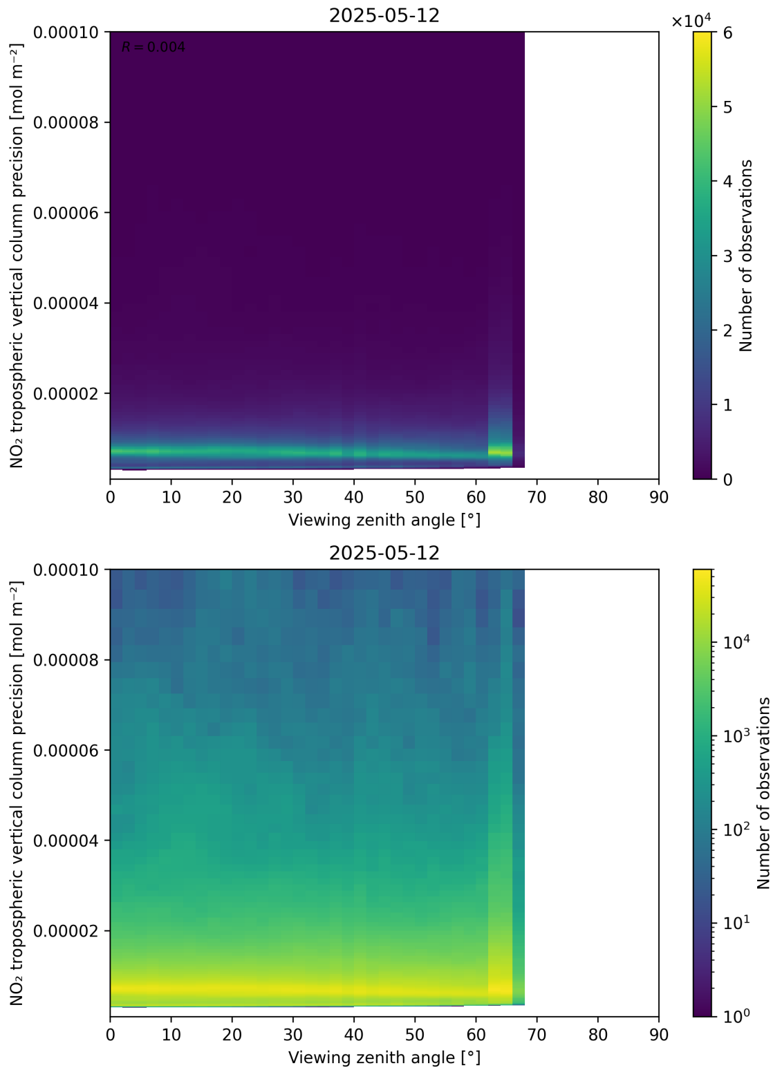
Figure 170: Scatter density plot of “Viewing zenith angle” against “NO 2 tropospheric vertical column precision” for 2025-05-12 to 2025-05-13.
