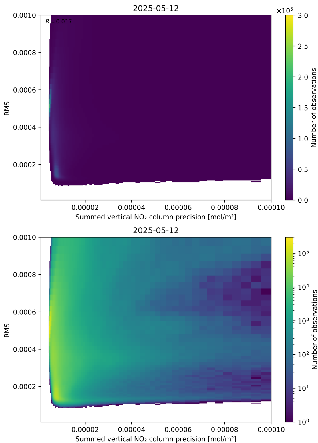
Figure 108: Scatter density plot of “Summed vertical NO 2 column precision” against “RMS” for 2025-05-12 to 2025-05-13.
