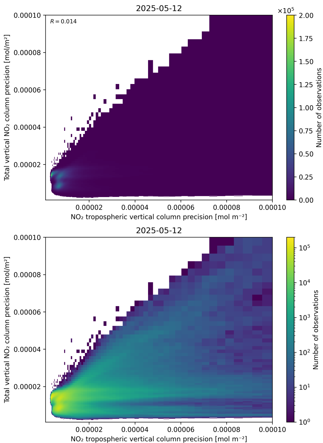
Figure 139: Scatter density plot of “NO 2 tropospheric vertical column precision” against “Total vertical NO 2 column precision” for 2025-05-12 to 2025-05-13.
