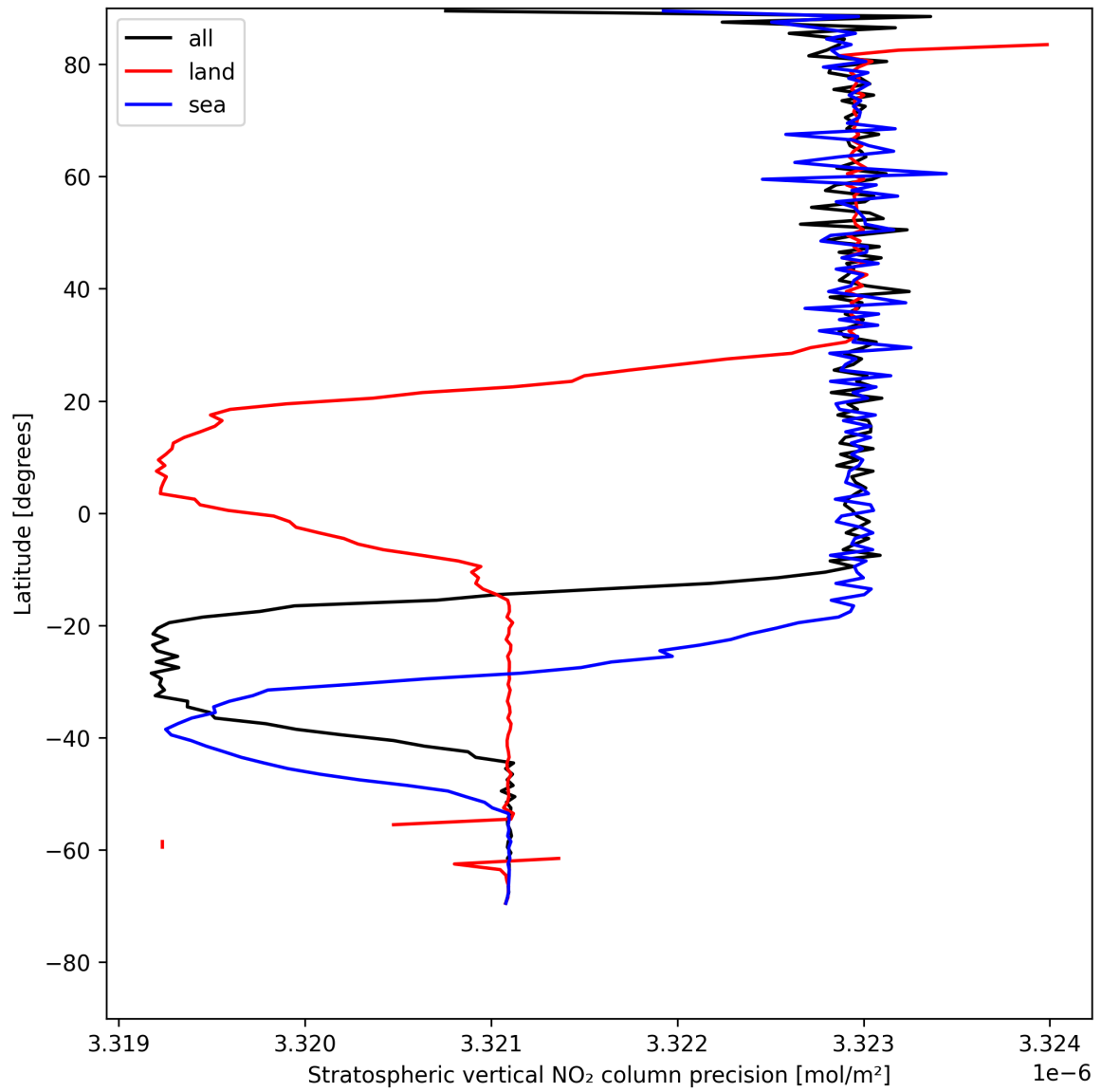
Figure 20: Zonal average of “Stratospheric vertical NO 2 column precision” for 2025-05-12 to 2025-05-13.
