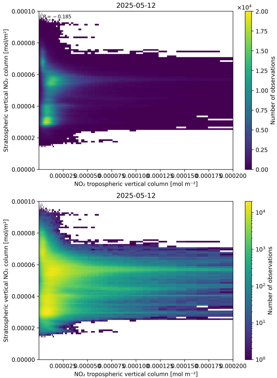
Figure 125: Scatter density plot of “NO 2 tropospheric vertical column” against “Stratospheric vertical NO 2 column” for 2025-05-12 to 2025-05-13.
