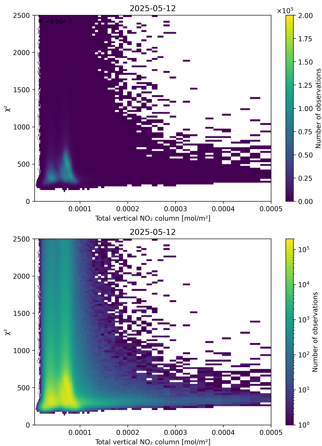
Figure 111: Scatter density plot of “Total vertical NO 2 column” against “ \chi^2 ” for 2025-05-12 to 2025-05-13.
