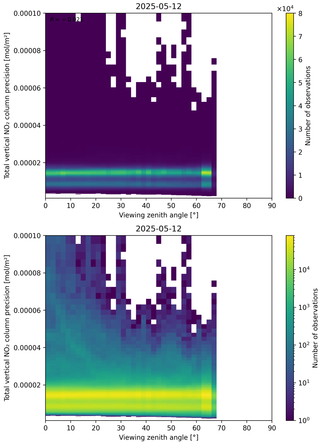
Figure 168: Scatter density plot of “Viewing zenith angle” against “Total vertical NO 2 column precision” for 2025-05-12 to 2025-05-13.
