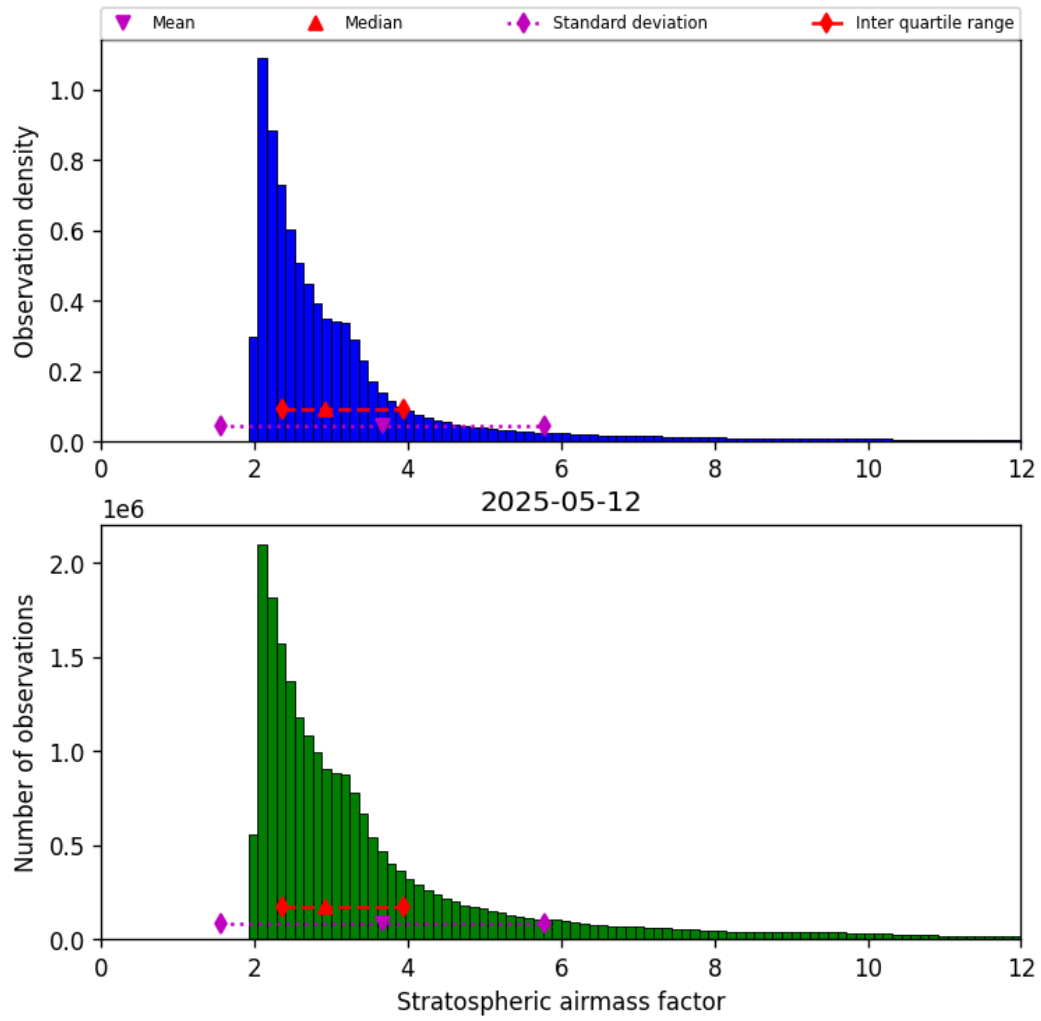
Figure 44: Histogram of “Stratospheric airmass factor” for 2025-05-12 to 2025-05-13
