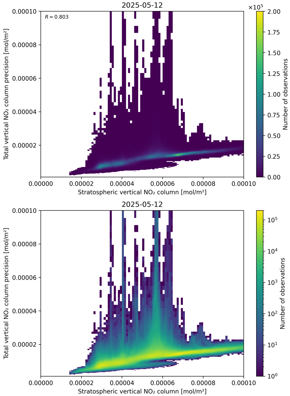
Figure 101: Scatter density plot of “Stratospheric vertical NO 2 column” against “Total vertical NO 2 column precision” for 2025-05-12 to 2025-05-13.
