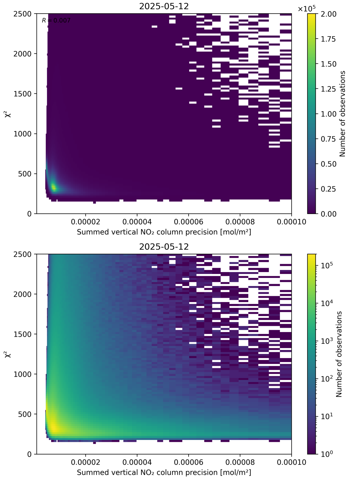
Figure 107: Scatter density plot of “Summed vertical NO 2 column precision” against “ \chi^2 ” for 2025-05-12 to 2025-05-13.
