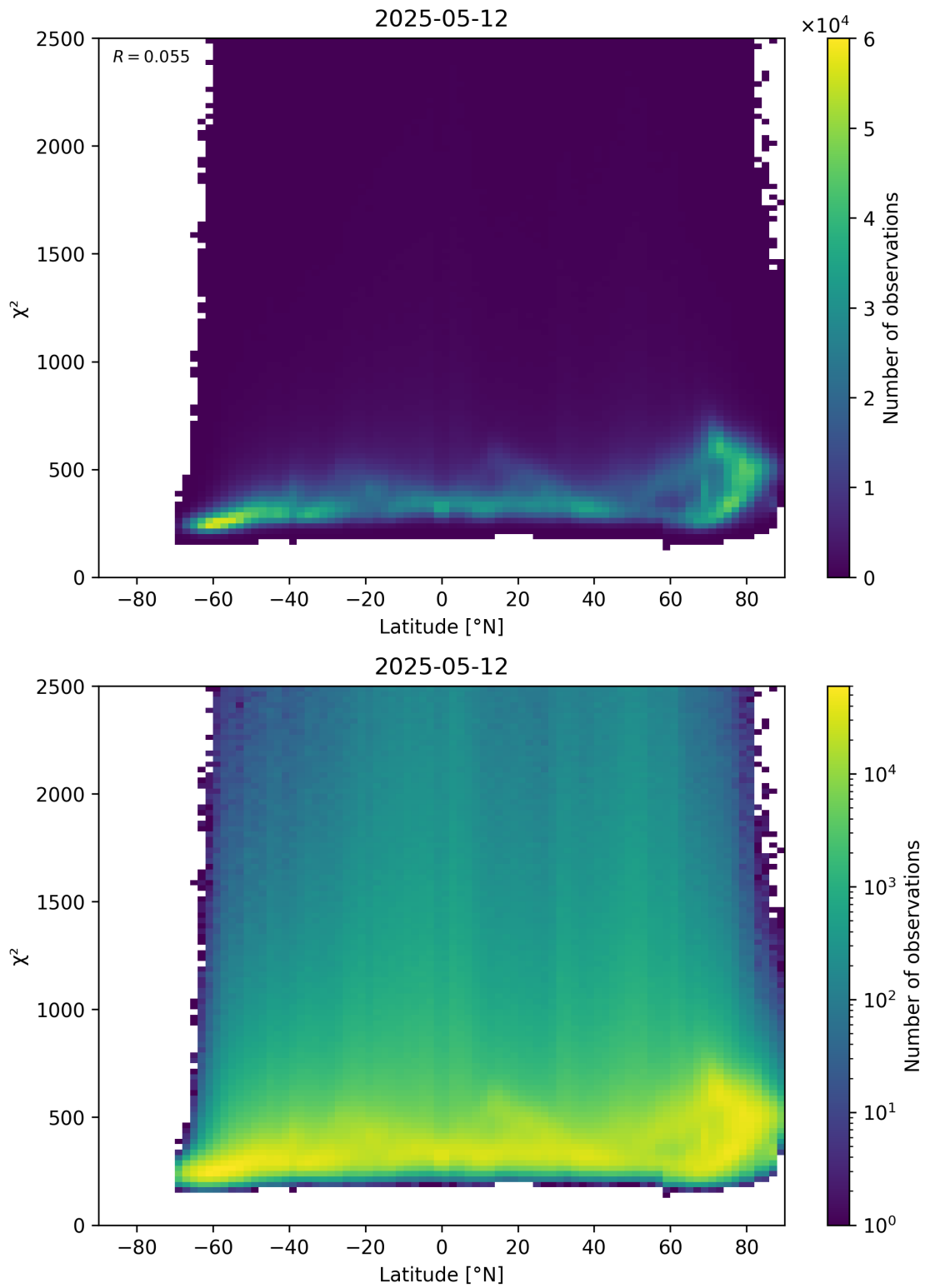
Figure 86: Scatter density plot of “Latitude” against “ \chi^2 ” for 2025-05-12 to 2025-05-13.
