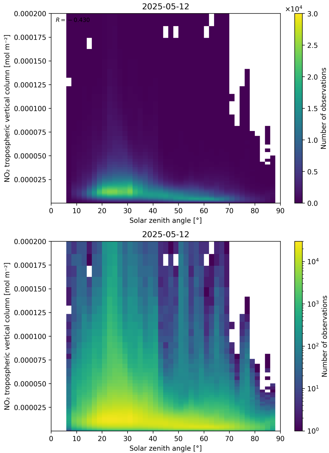
Figure 155: Scatter density plot of “Solar zenith angle” against “NO 2 tropospheric vertical column” for 2025-05-12 to 2025-05-13.
