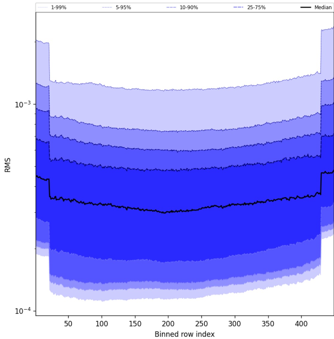
Figure 60: Along track statistics of “RMS” for 2025-05-12 to 2025-05-13
