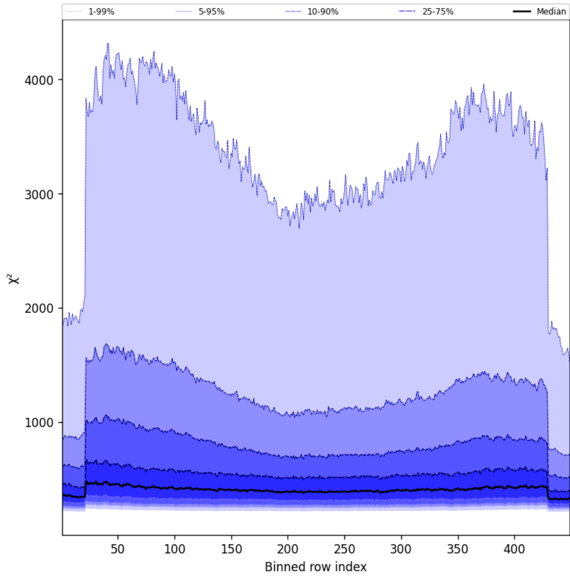
Figure 59: Along track statistics of “ \chi^2 ” for 2025-05-12 to 2025-05-13
