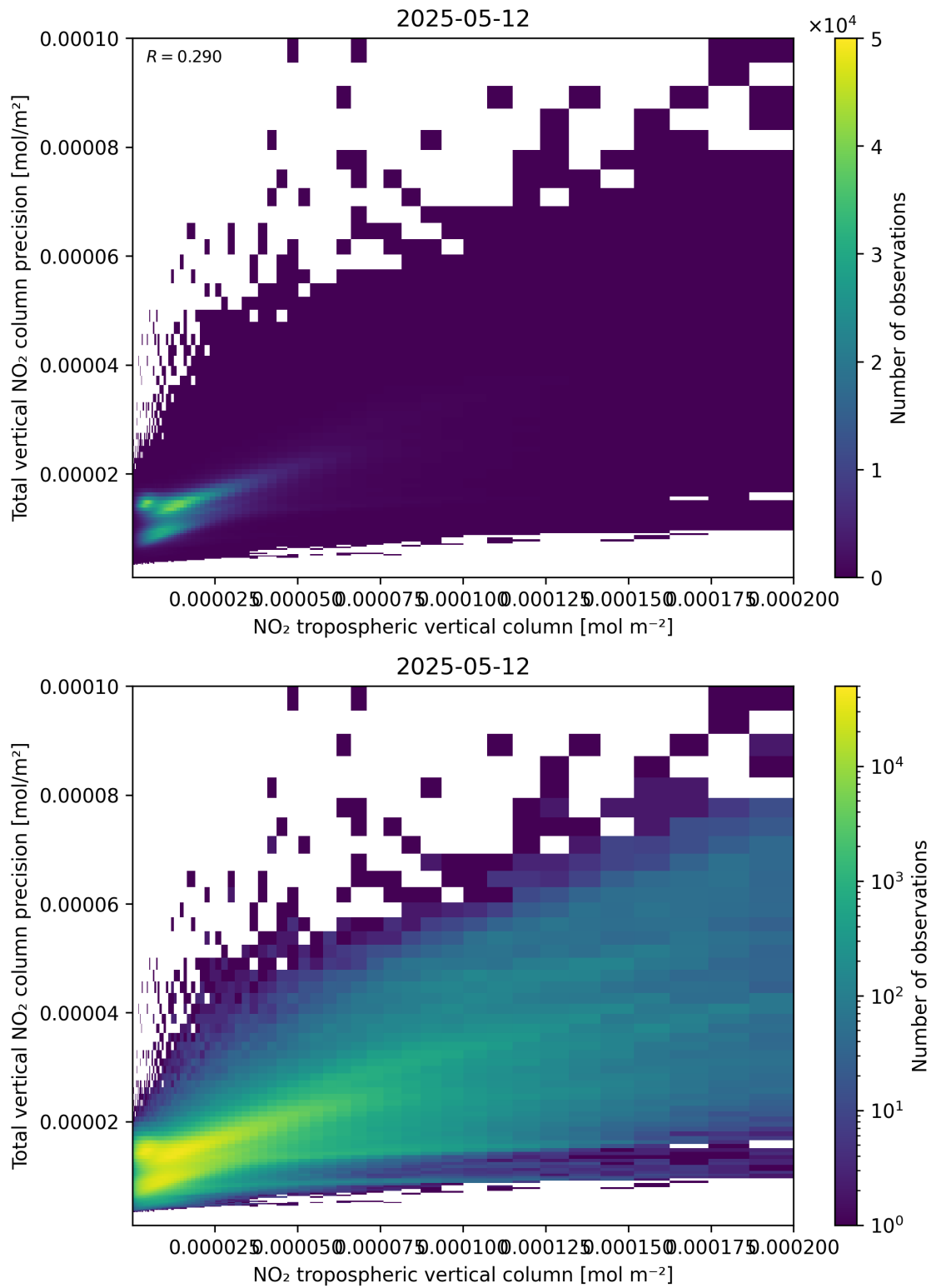
Figure 129: Scatter density plot of “NO 2 tropospheric vertical column” against “Total vertical NO 2 column precision” for 2025-05-12 to 2025-05-13.
