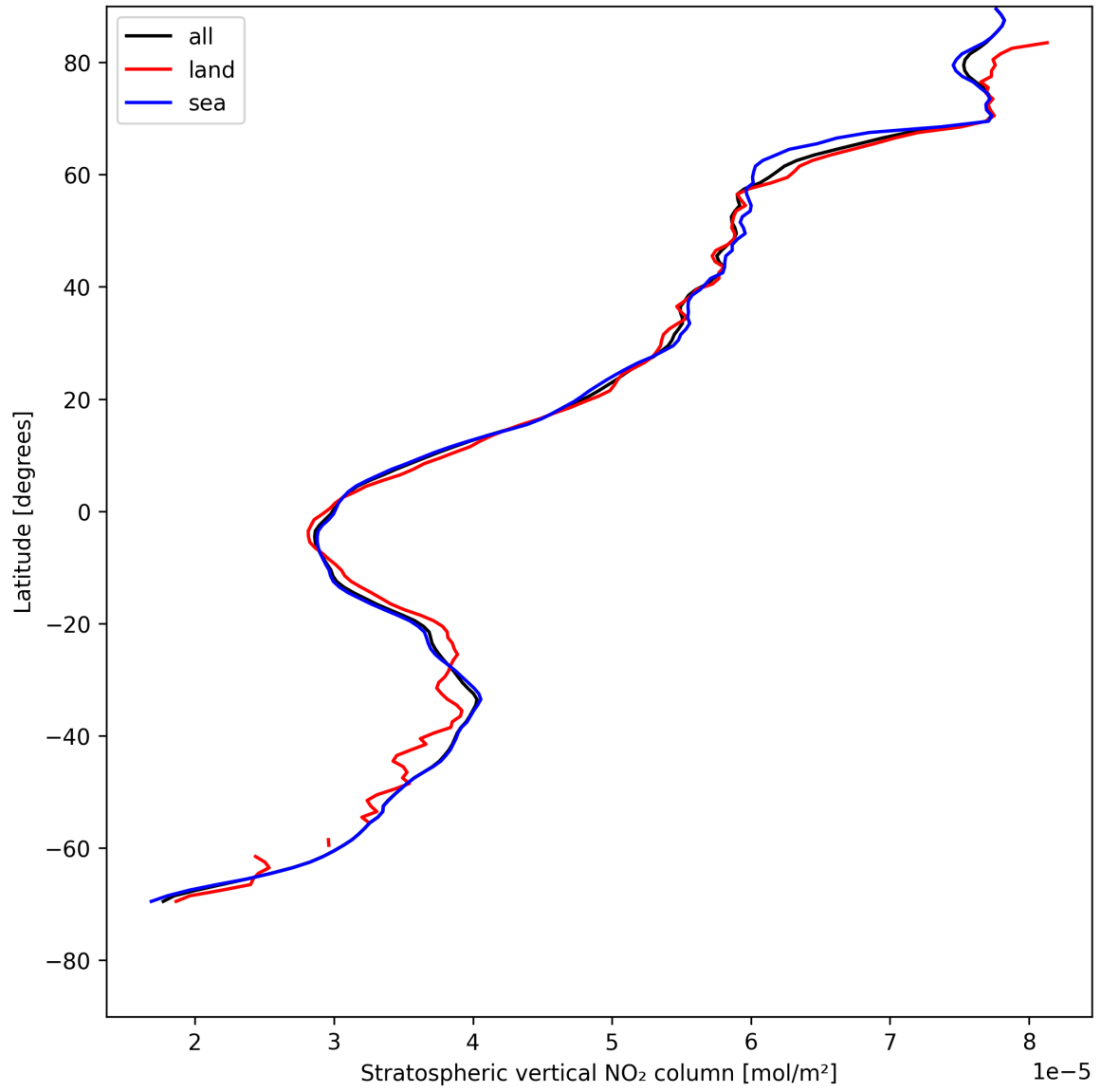
Figure 19: Zonal average of “Stratospheric vertical NO 2 column” for 2025-05-12 to 2025-05-13.
