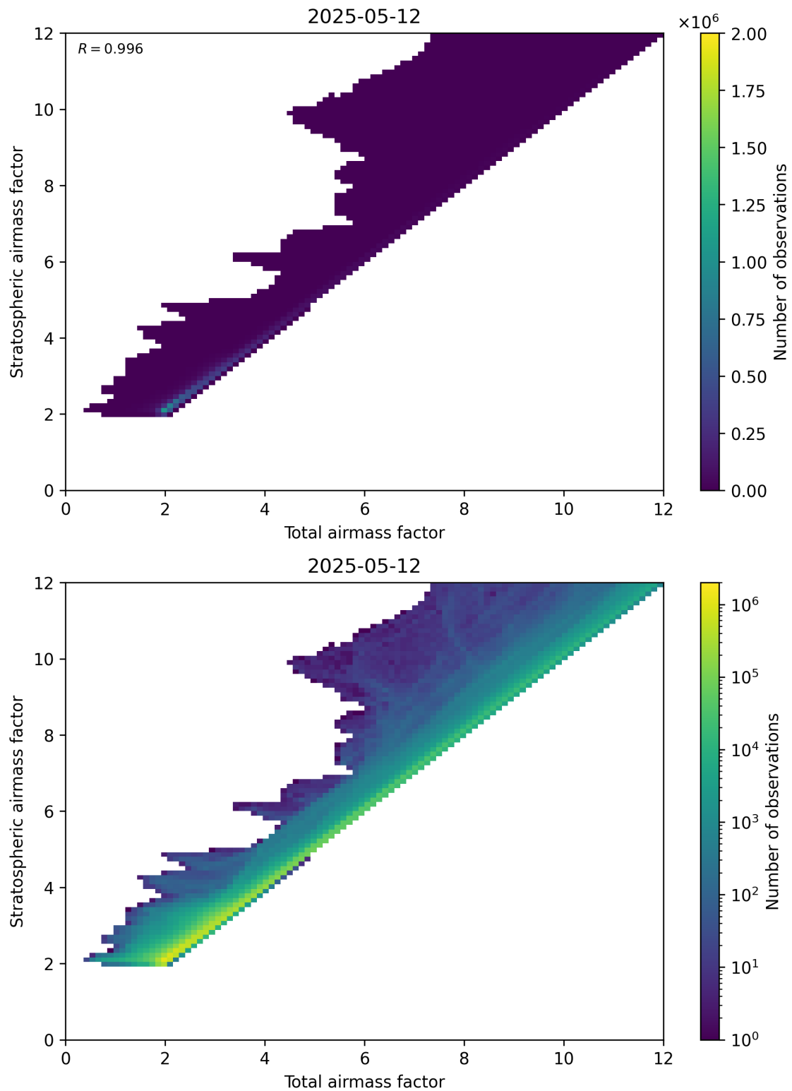
Figure 62: Scatter density plot of “Total airmass factor” against “Stratospheric airmass factor” for 2025-05-12 to 2025-05-13.
