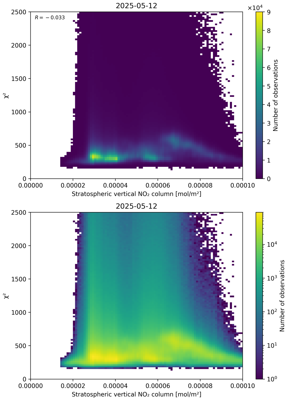
Figure 97: Scatter density plot of “Stratospheric vertical NO 2 column” against “ \chi^2 ” for 2025-05-12 to 2025-05-13.
