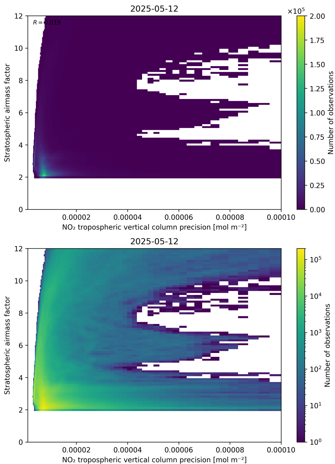
Figure 131: Scatter density plot of “NO 2 tropospheric vertical column precision” against “Stratospheric airmass factor” for 2025-05-12 to 2025-05-13.
