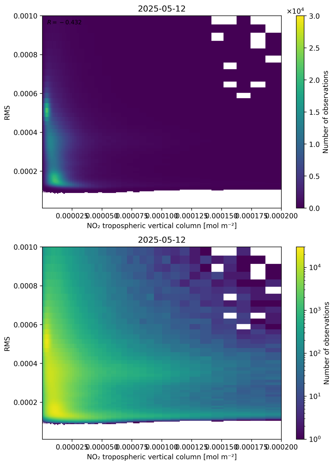
Figure 142: Scatter density plot of “NO 2 tropospheric vertical column” against “RMS” for 2025-05-12 to 2025-05-13.
