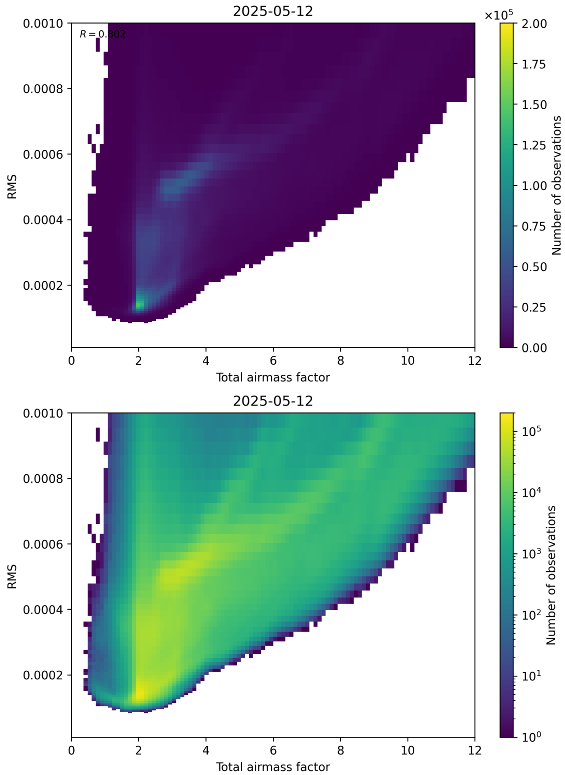
Figure 69: Scatter density plot of “Total airmass factor” against “RMS” for 2025-05-12 to 2025-05-13.
