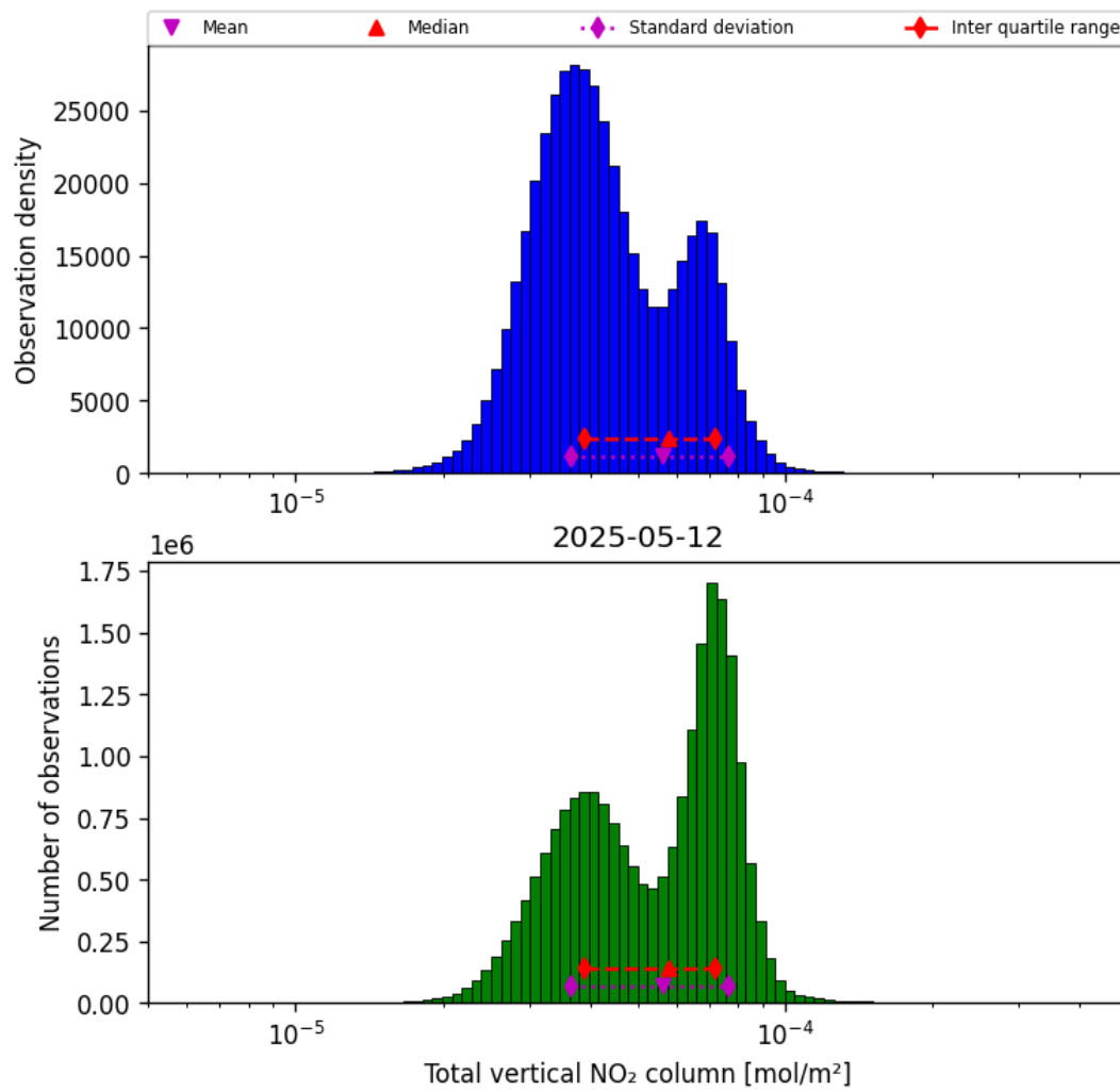
Figure 38: Histogram of “Total vertical NO 2 column” for 2025-05-12 to 2025-05-13
