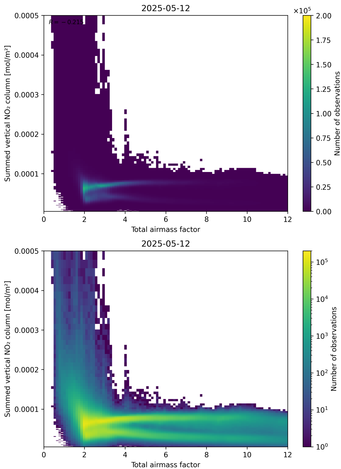
Figure 65: Scatter density plot of “Total airmass factor” against “Summed vertical NO 2 column” for 2025-05-12 to 2025-05-13.
