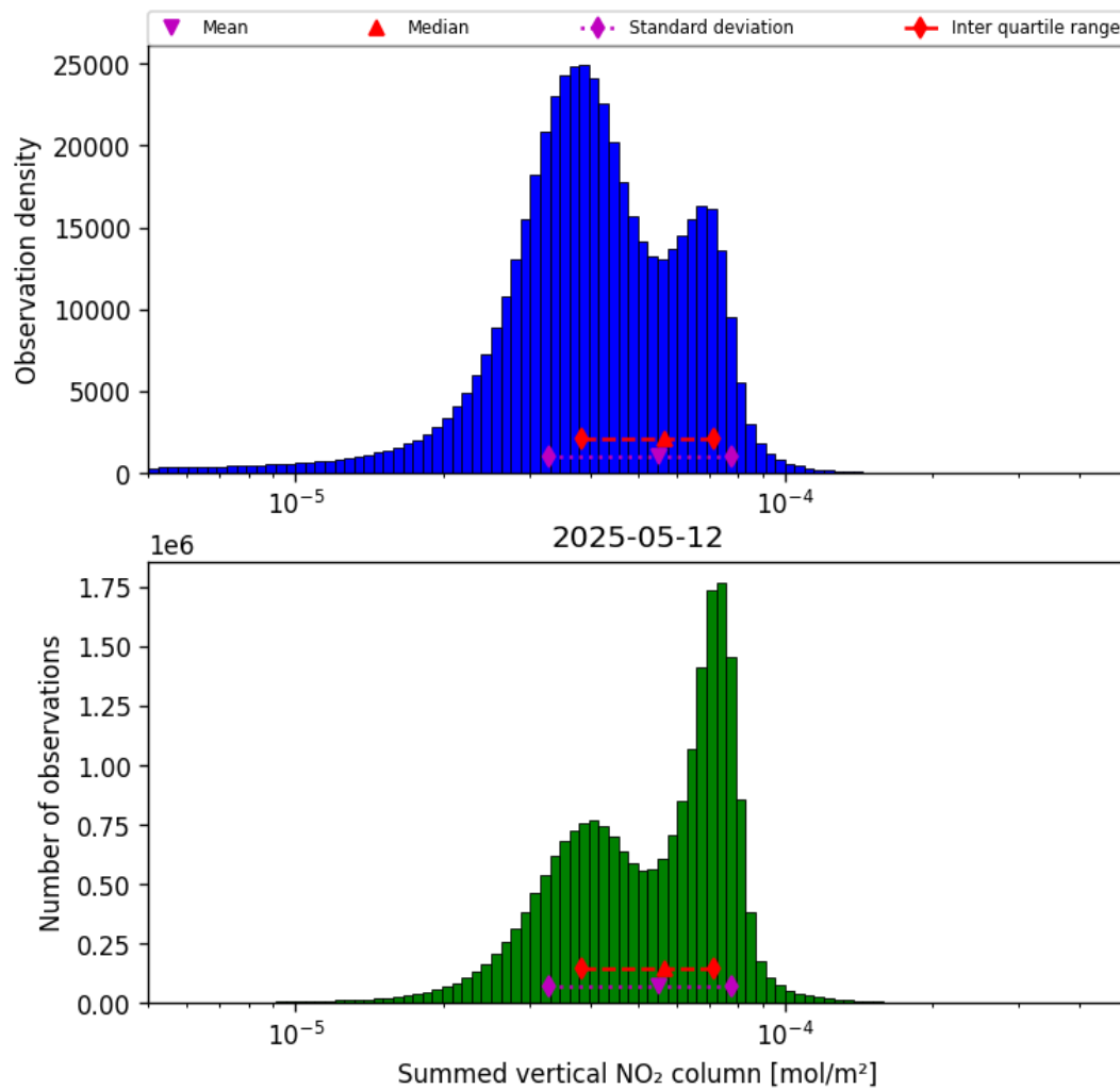
Figure 40: Histogram of “Summed vertical NO 2 column” for 2025-05-12 to 2025-05-13
