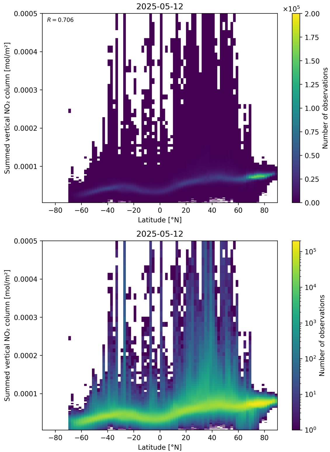
Figure 88: Scatter density plot of “Latitude” against “Summed vertical NO 2 column” for 2025-05-12 to 2025-05-13.
