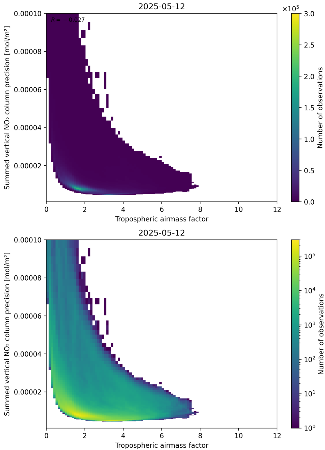
Figure 76: Scatter density plot of “Tropospheric air mass factor” against “Summed vertical NO 2 column precision” for 2025-05-12 to 2025-05-13.
