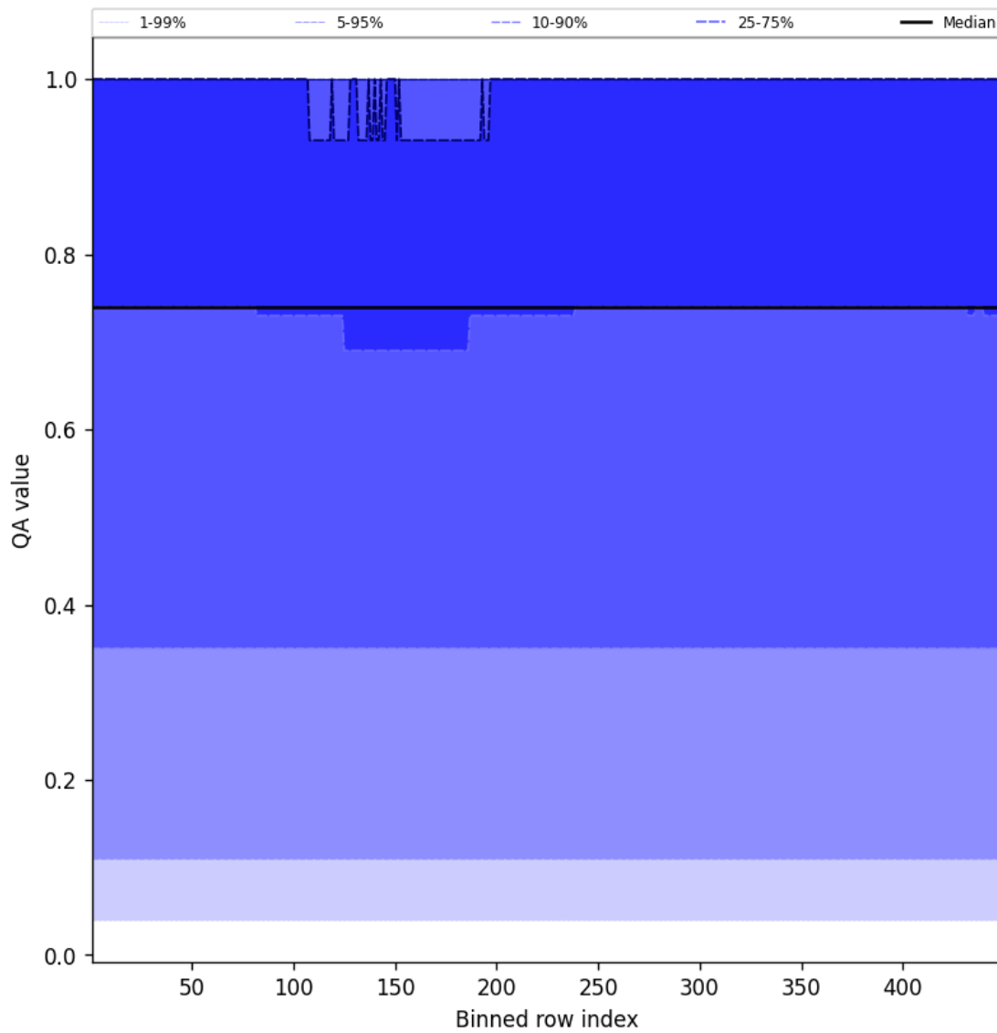
Figure 45: Along track statistics of “QA value” for 2025-05-12 to 2025-05-13
