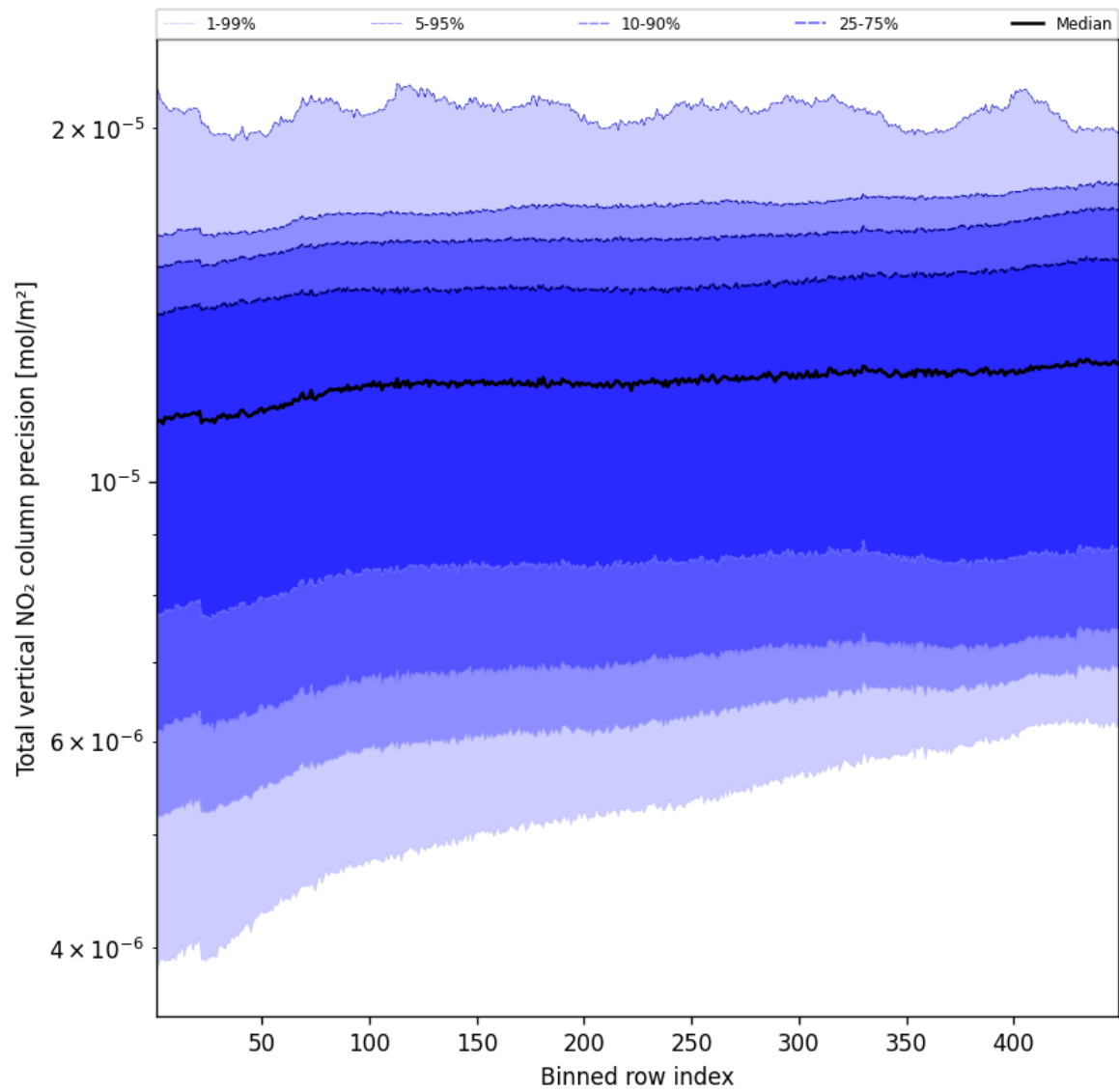
Figure 56: Along track statistics of "Total vertical NO 2 column precision" for 2025-05-12 to 2025-05-13
