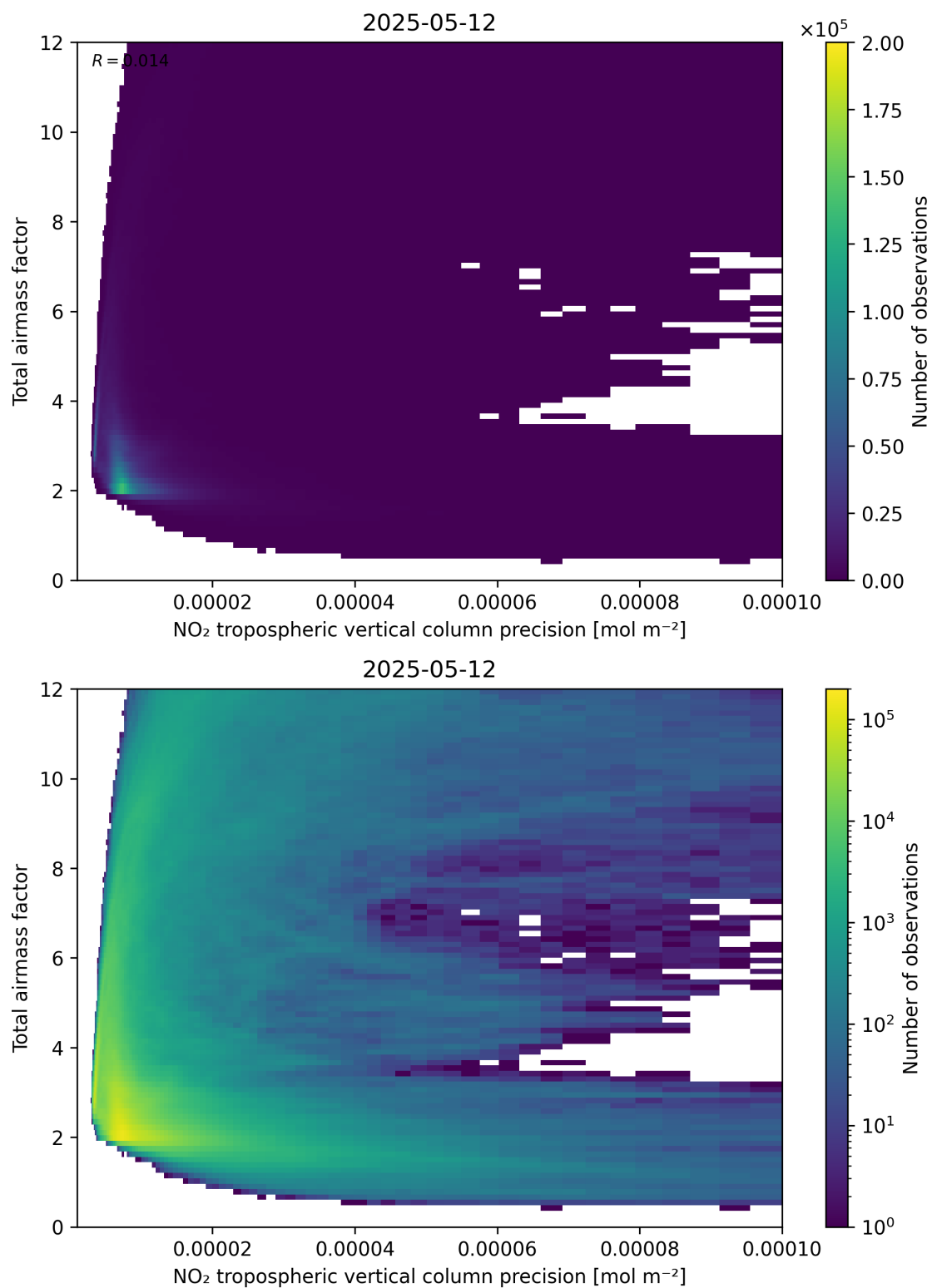
Figure 132: Scatter density plot of “NO 2 tropospheric vertical column precision” against “Total air mass factor” for 2025-05-12 to 2025-05-13.
