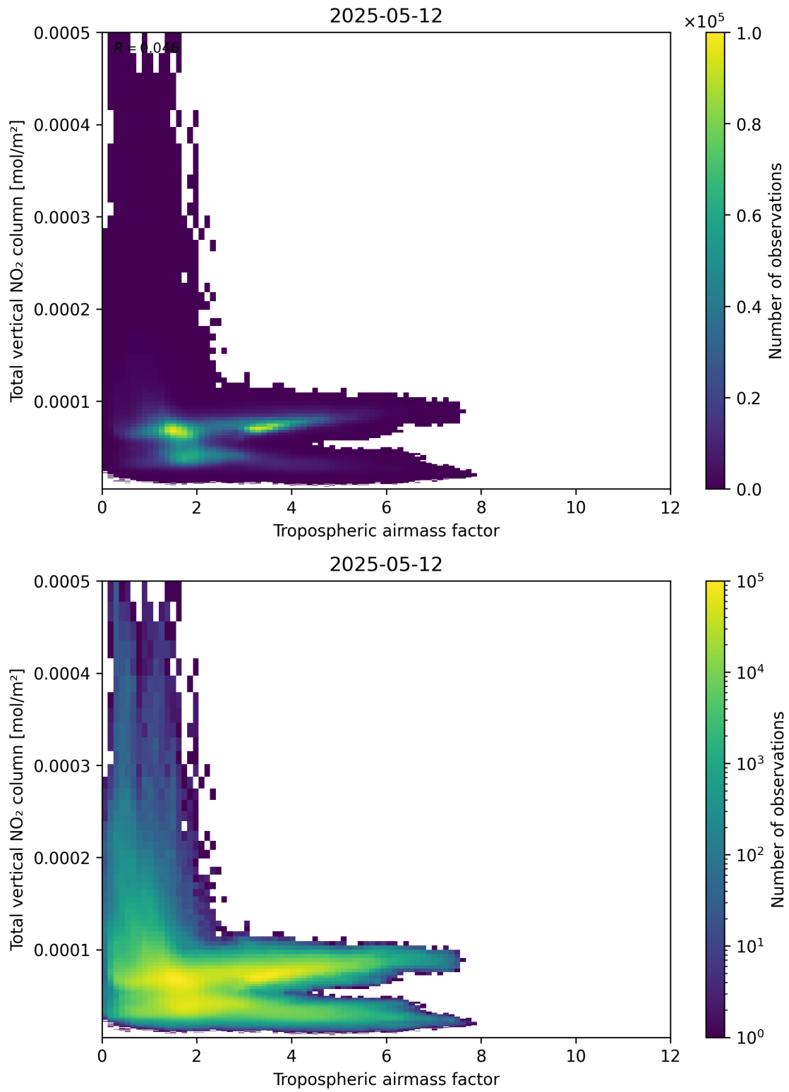
Figure 77: Scatter density plot of “Tropospheric airmass factor” against “Total vertical NO 2 column” for 2025-05-12 to 2025-05-13.
