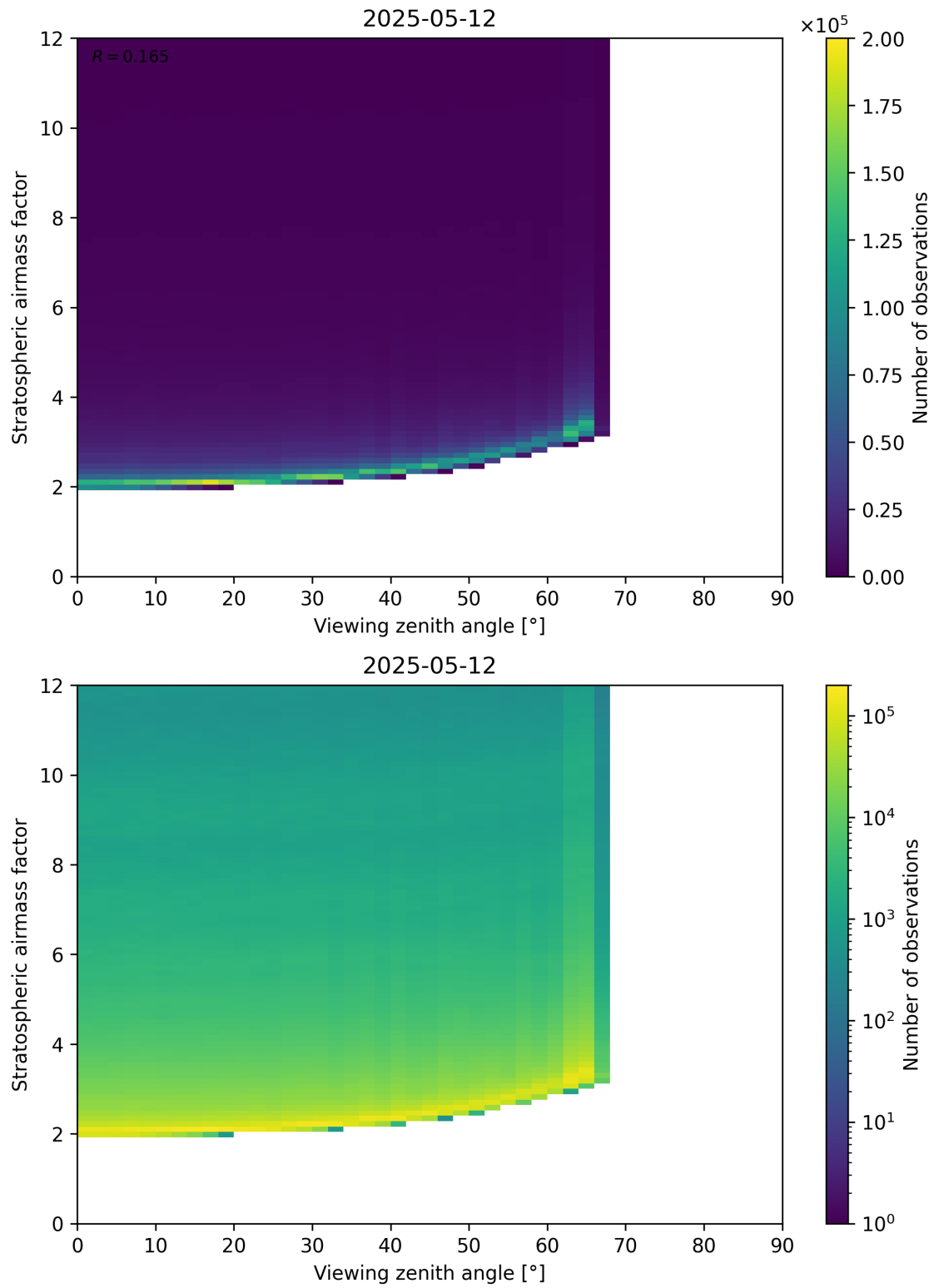
Figure 159: Scatter density plot of “Viewing zenith angle” against “Stratospheric airmass factor” for 2025-05-12 to 2025-05-13.
