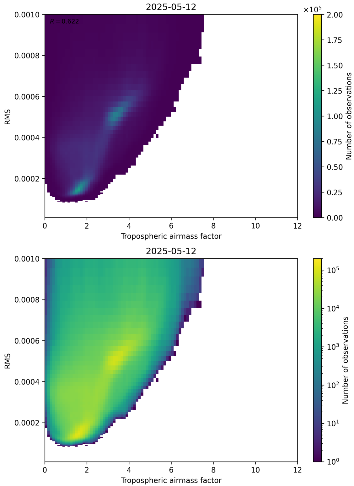
Figure 79: Scatter density plot of “Tropospheric airmass factor” against “RMS” for 2025-05-12 to 2025-05-13.
