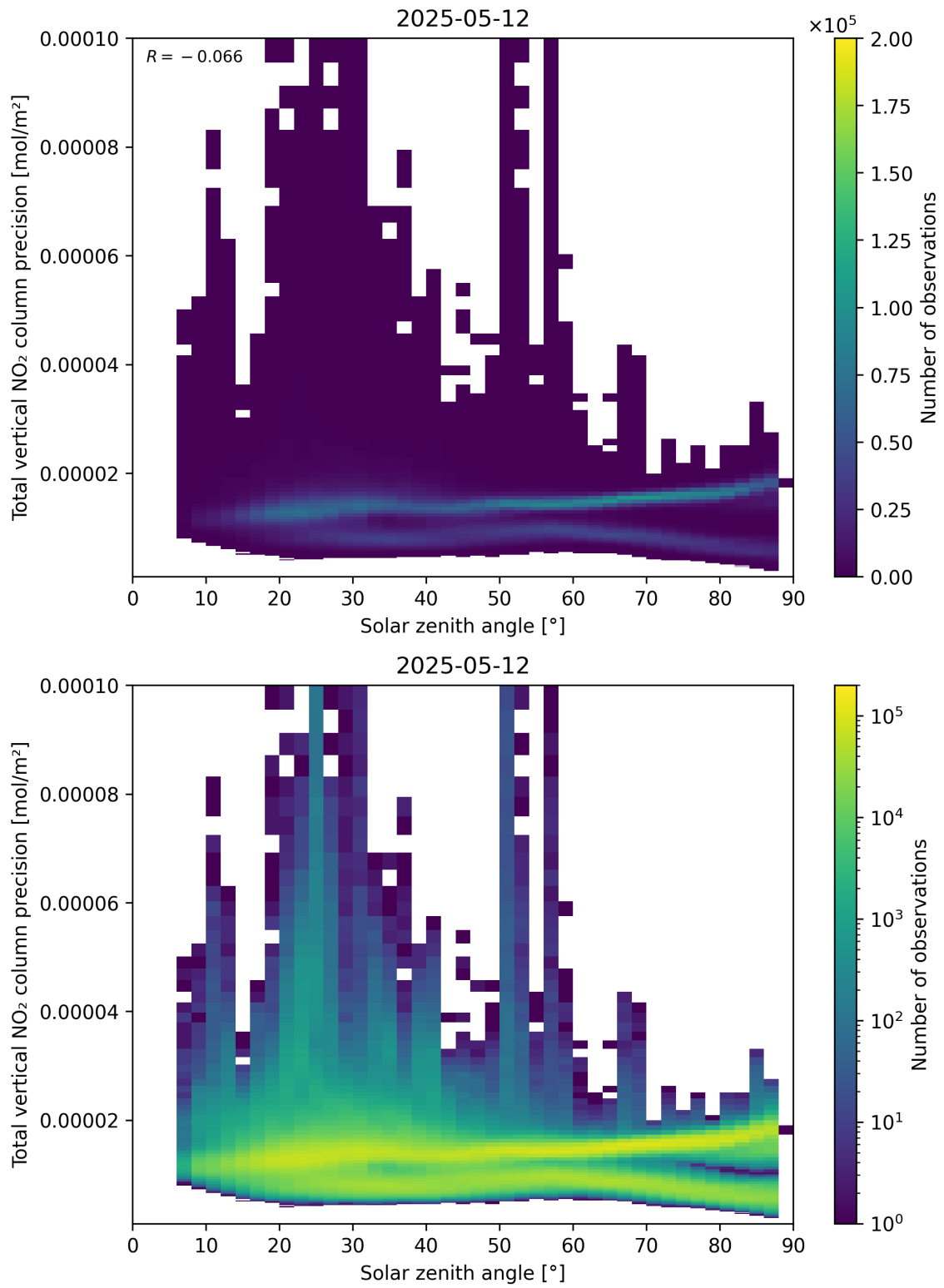
Figure 154: Scatter density plot of “Solar zenith angle” against “Total vertical NO 2 column precision” for 2025-05-12 to 2025-05-13.
