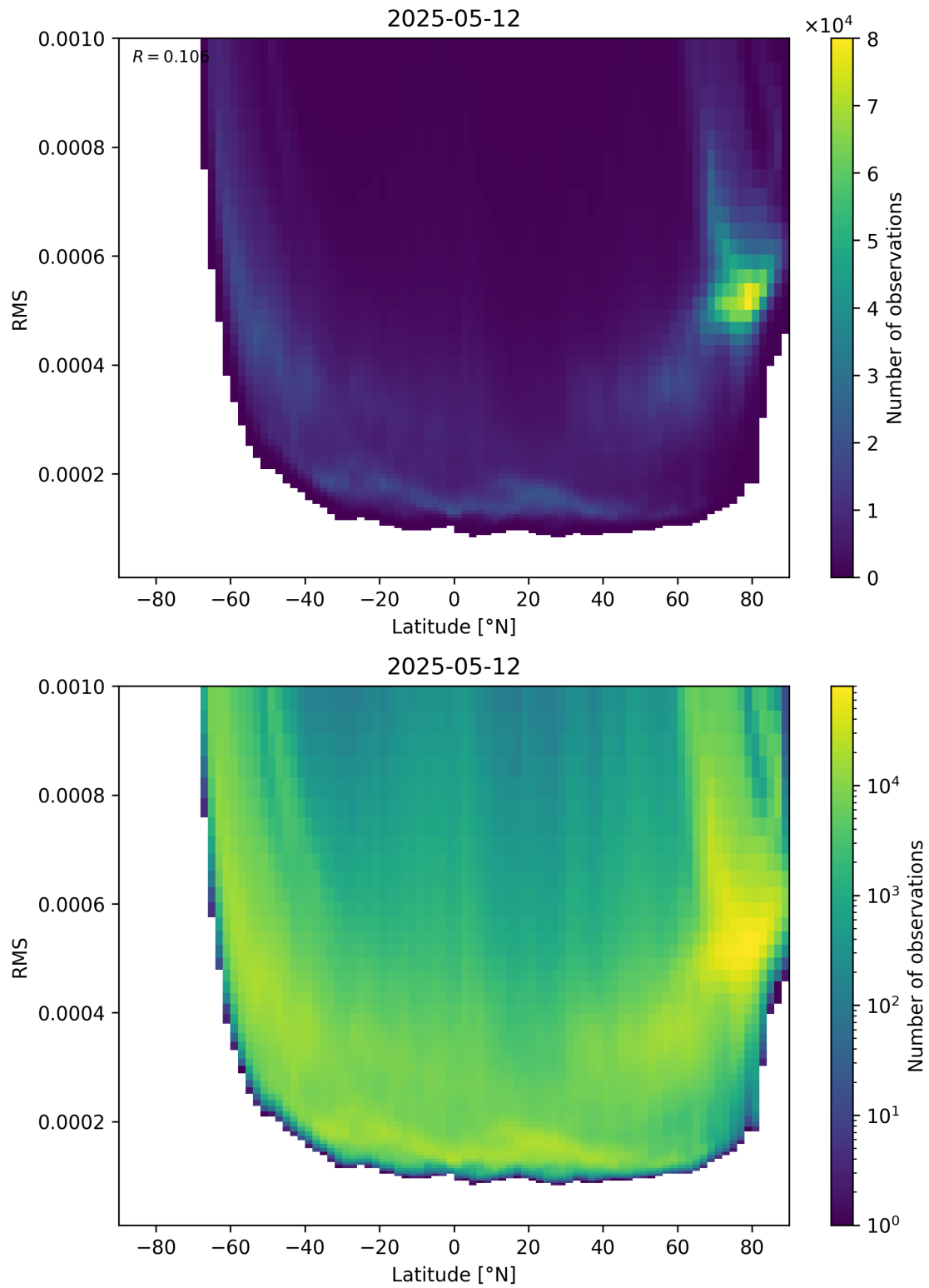
Figure 94: Scatter density plot of “Latitude” against “RMS” for 2025-05-12 to 2025-05-13.
