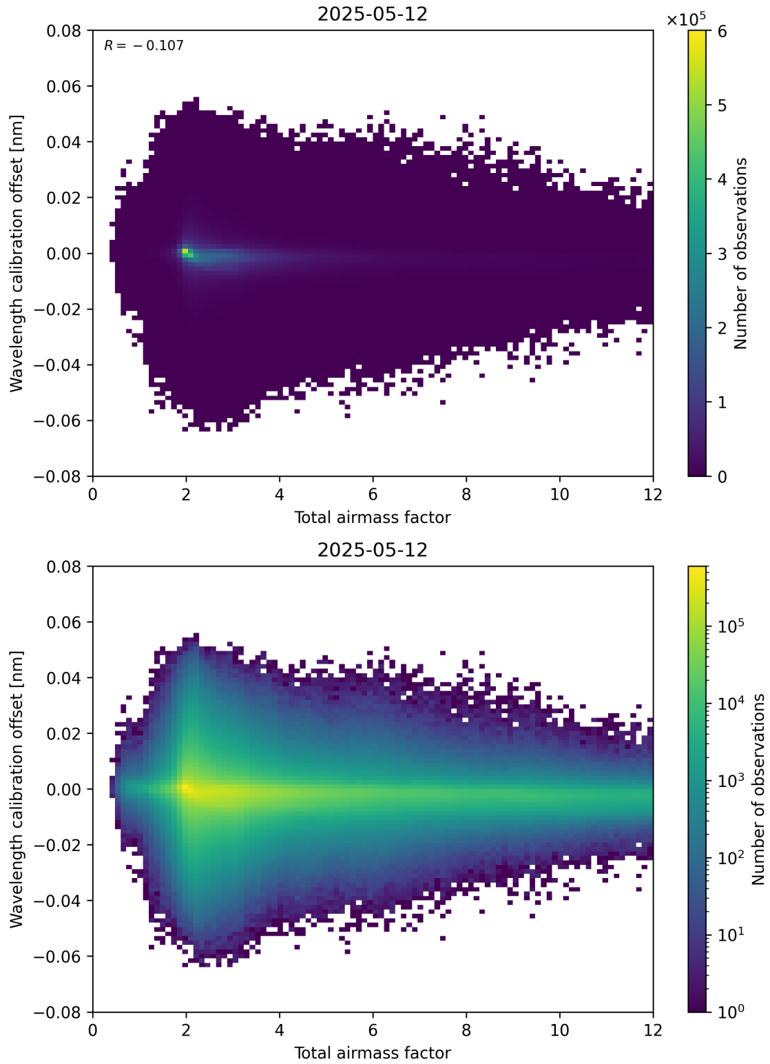
Figure 70: Scatter density plot of “Total airmass factor” against “Wavelength calibration offset” for 2025-05-12 to 2025-05-13.
