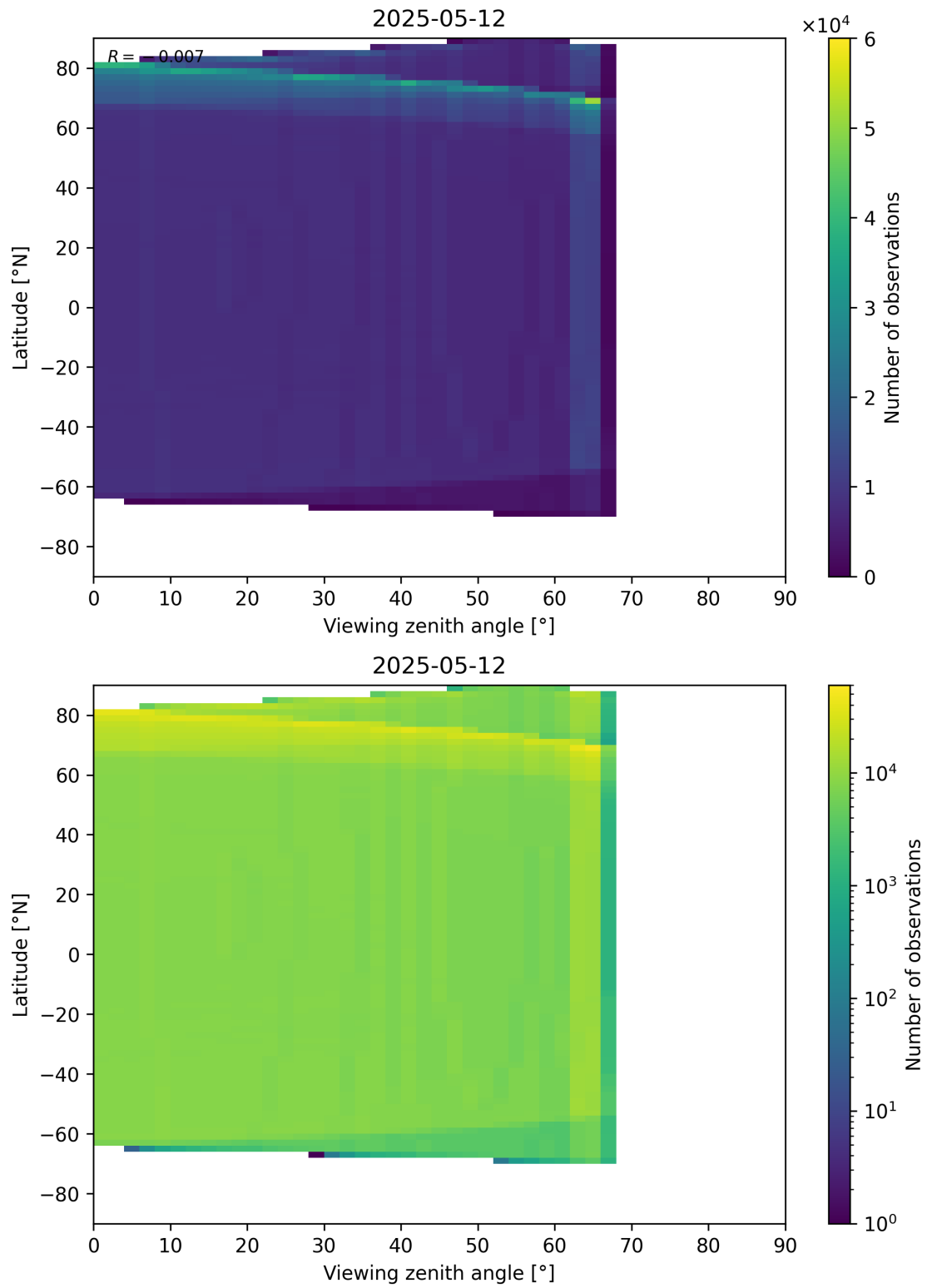
Figure 163: Scatter density plot of “Viewing zenith angle” against “Latitude” for 2025-05-12 to 2025-05-13.
