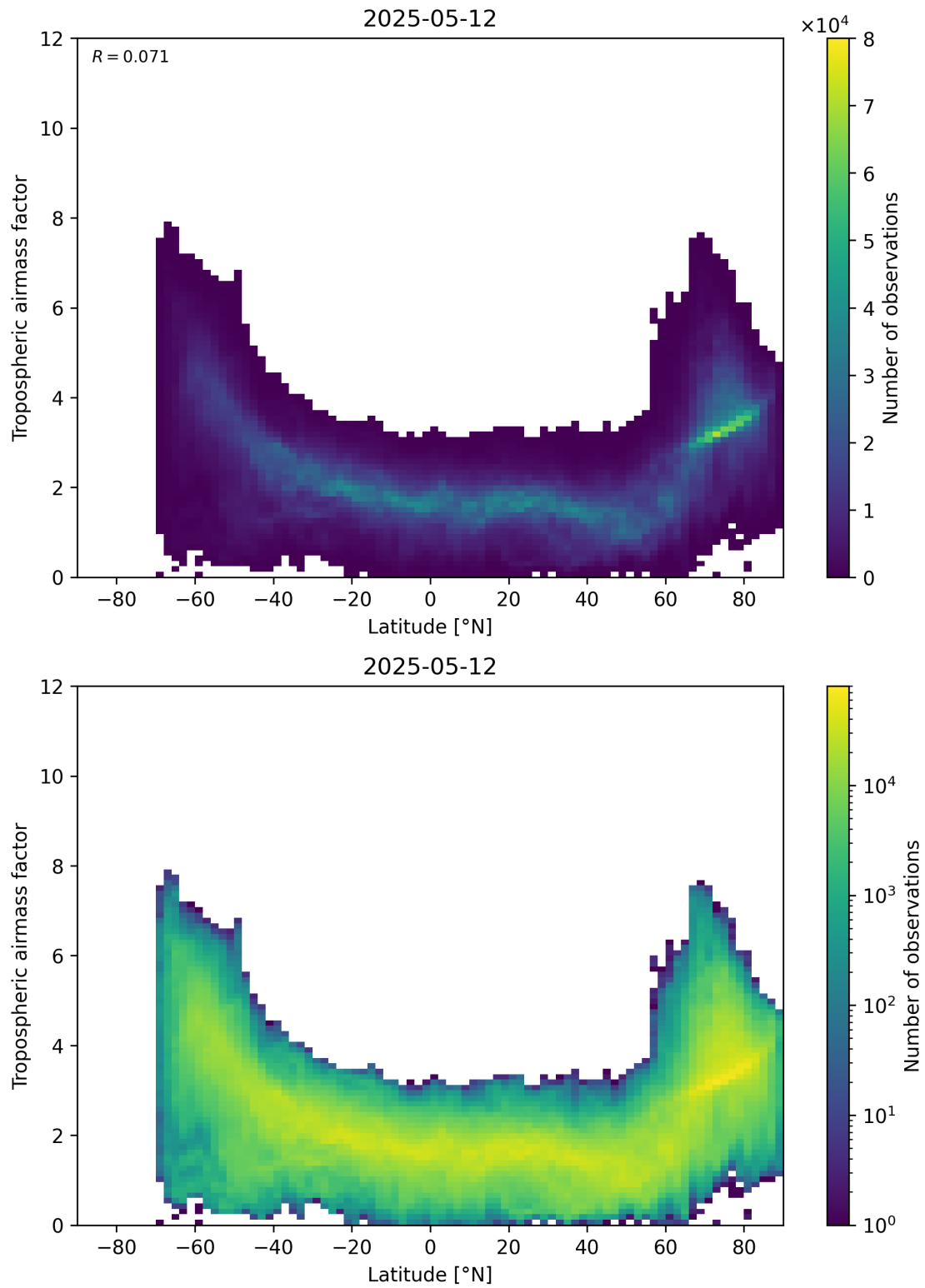
Figure 85: Scatter density plot of “Latitude” against “Tropospheric airmass factor” for 2025-05-12 to 2025-05-13.
