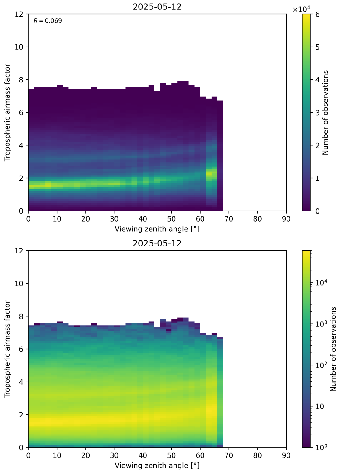
Figure 161: Scatter density plot of “Viewing zenith angle” against “Tropospheric airmass factor” for 2025-05-12 to 2025-05-13.
