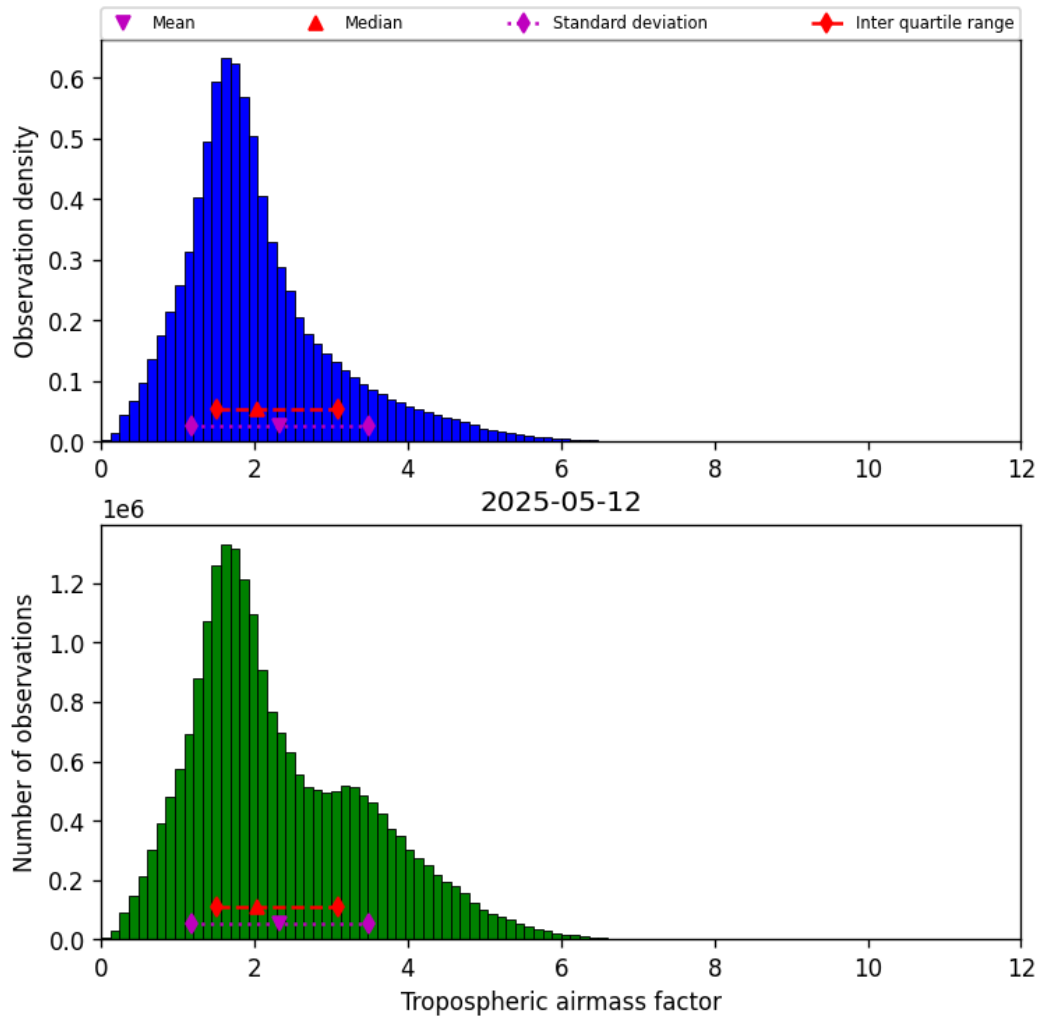
Figure 31: Histogram of “Tropospheric airmass factor” for 2025-05-12 to 2025-05-13
