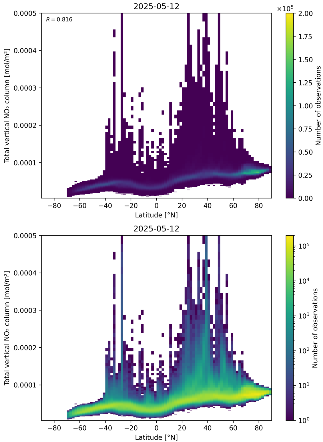
Figure 90: Scatter density plot of “Latitude” against “Total vertical NO 2 column” for 2025-05-12 to 2025-05-13.
