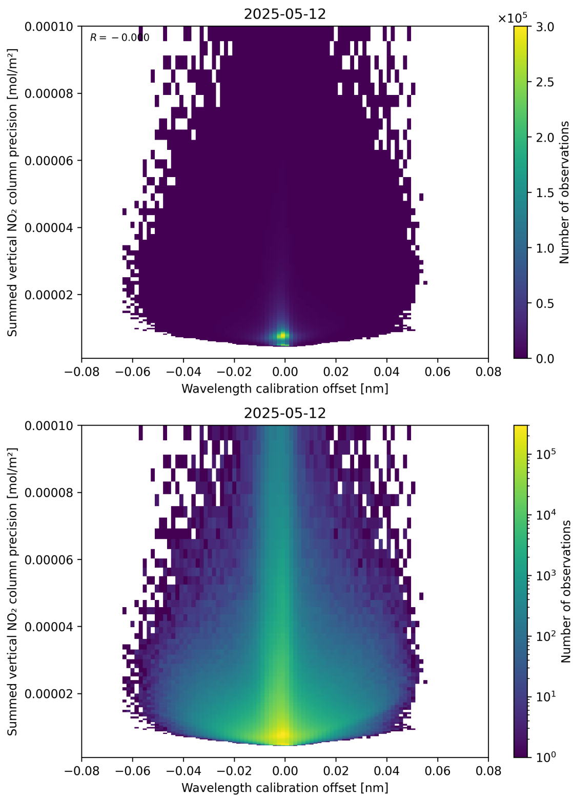
Figure 178: Scatter density plot of “Wavelength calibration offset” against “Summed vertical NO 2 column precision” for 2025-05-12 to 2025-05-13.
