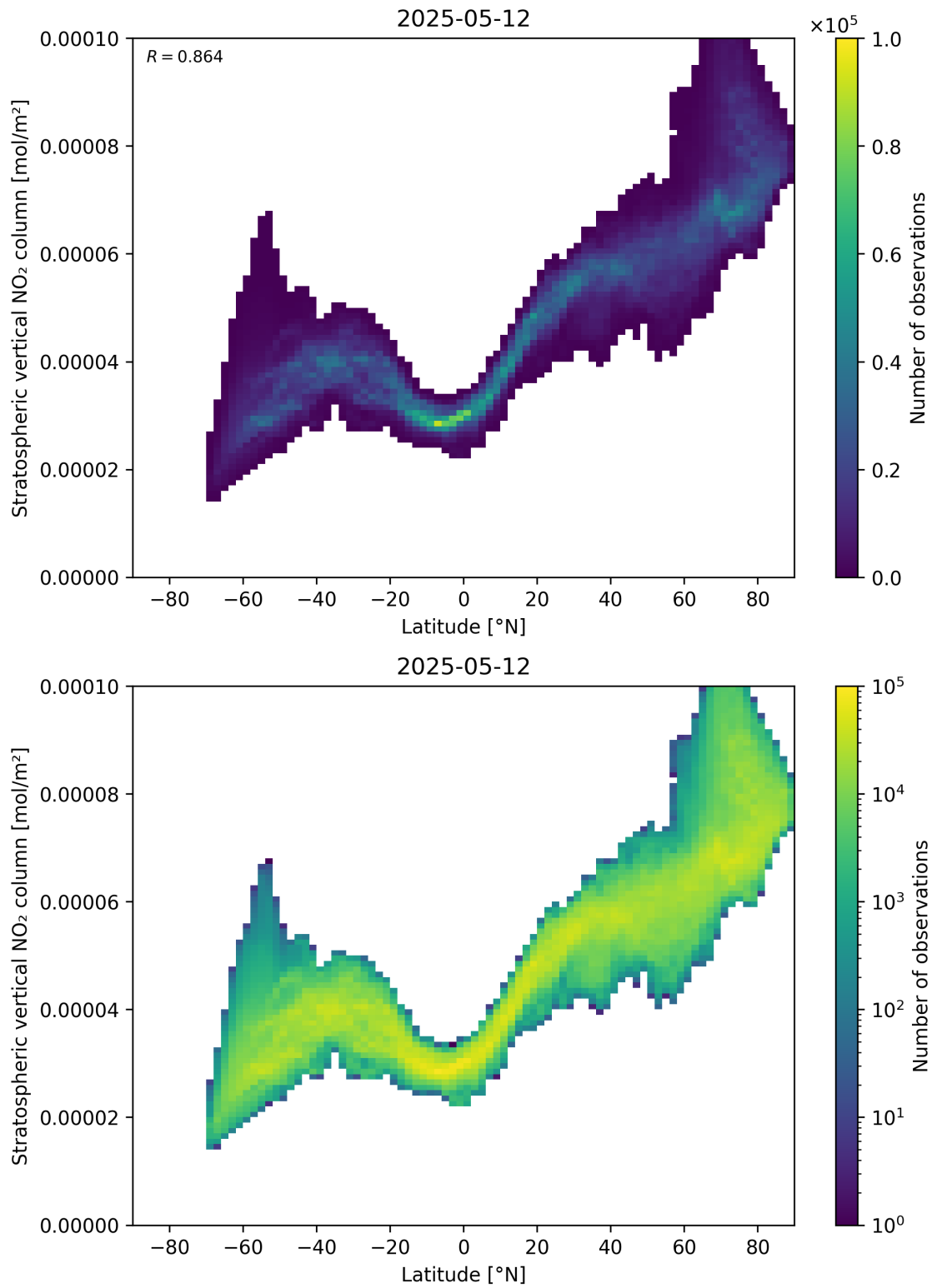
Figure 87: Scatter density plot of “Latitude” against “Stratospheric vertical \text{NO}_2 column” for 2025-05-12 to 2025-05-13.
