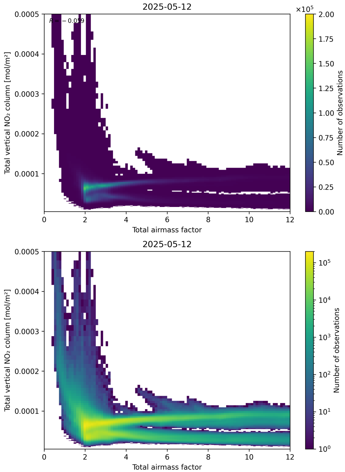
Figure 67: Scatter density plot of “Total airmass factor” against “Total vertical NO 2 column” for 2025-05-12 to 2025-05-13.
