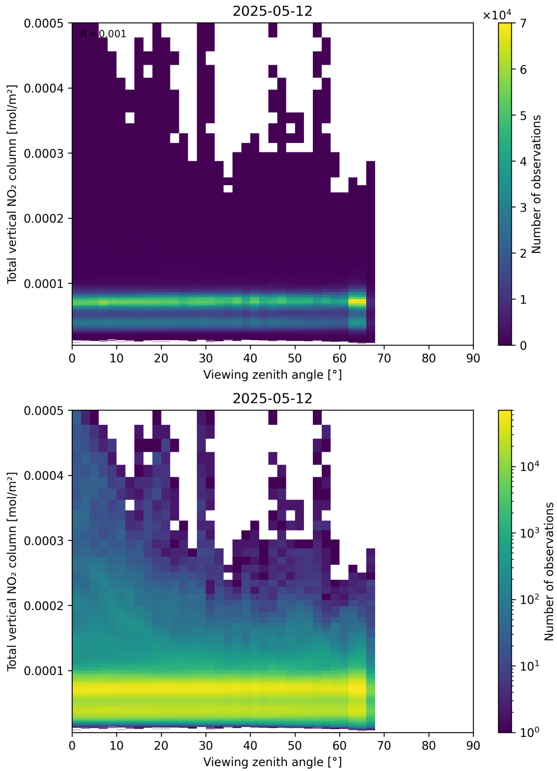
Figure 167: Scatter density plot of “Viewing zenith angle” against “Total vertical NO 2 column” for 2025-05-12 to 2025-05-13.
