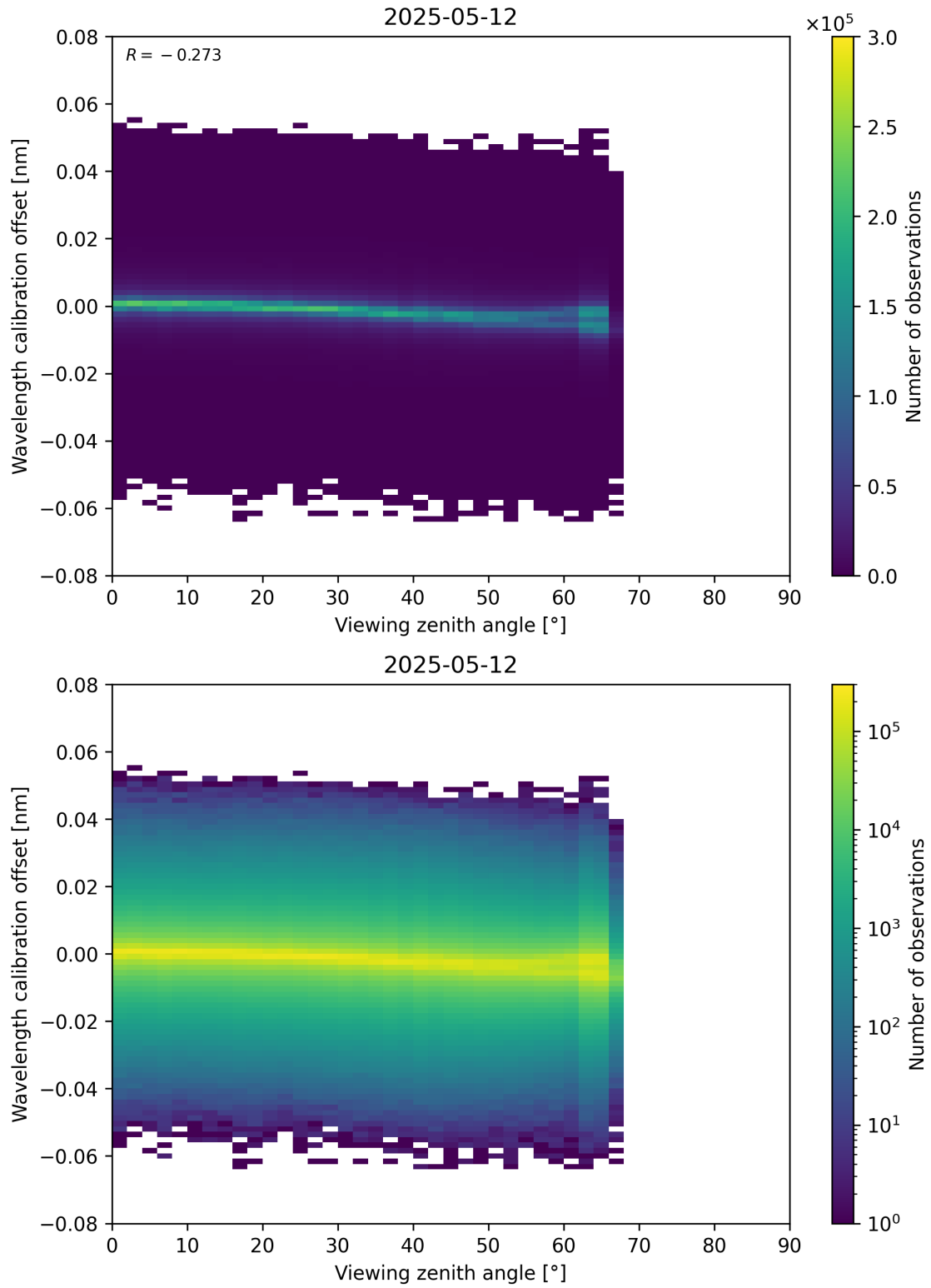
Figure 173: Scatter density plot of “Viewing zenith angle” against “Wavelength calibration offset” for 2025-05-12 to 2025-05-13.
