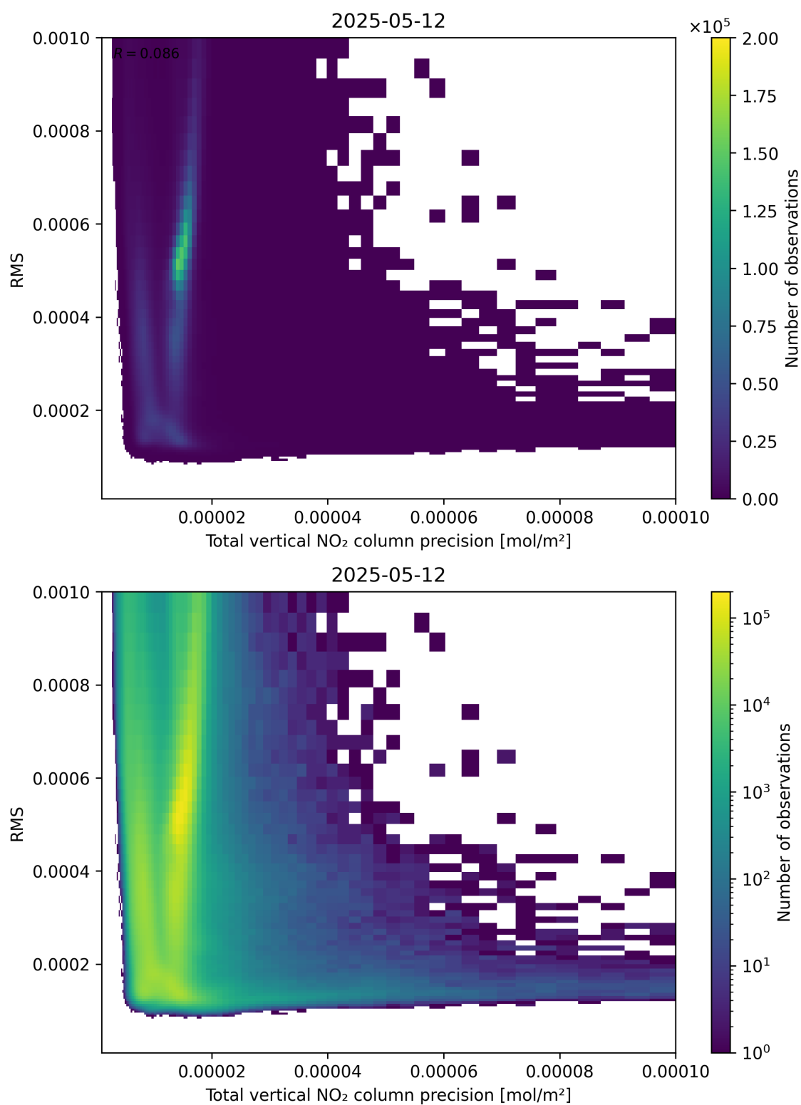
Figure 119: Scatter density plot of “Total vertical NO 2 column precision” against “RMS” for 2025-05-12 to 2025-05-13.
