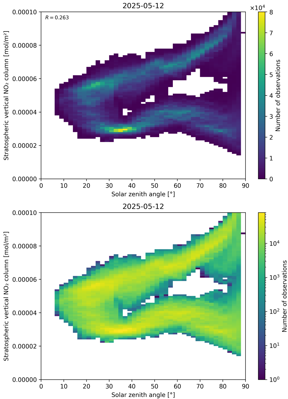
Figure 150: Scatter density plot of “Solar zenith angle” against “Stratospheric vertical NO 2 column” for 2025-05-12 to 2025-05-13.
