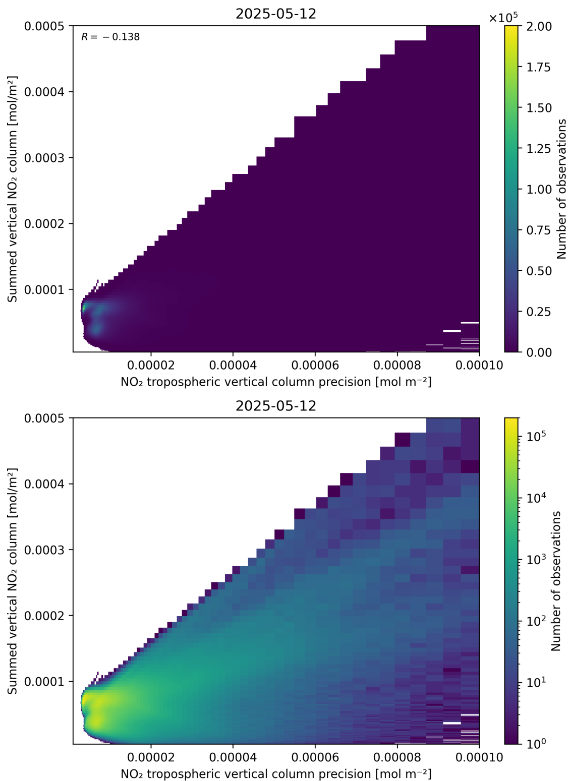
Figure 136: Scatter density plot of “NO 2 tropospheric vertical column precision” against “Summed vertical NO 2 column” for 2025-05-12 to 2025-05-13.
