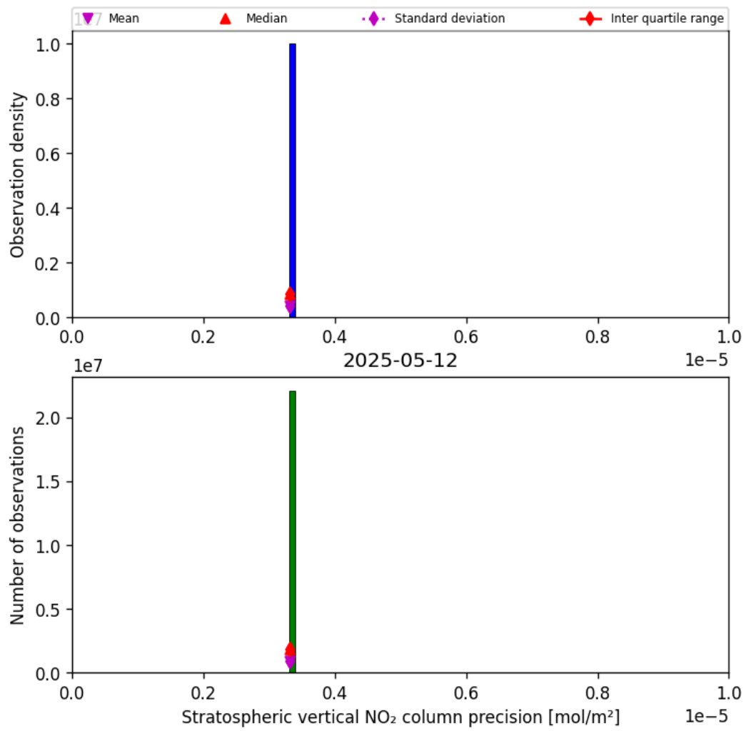
Figure 37: Histogram of “Stratospheric vertical NO 2 column precision” for 2025-05-12 to 2025-05-13
