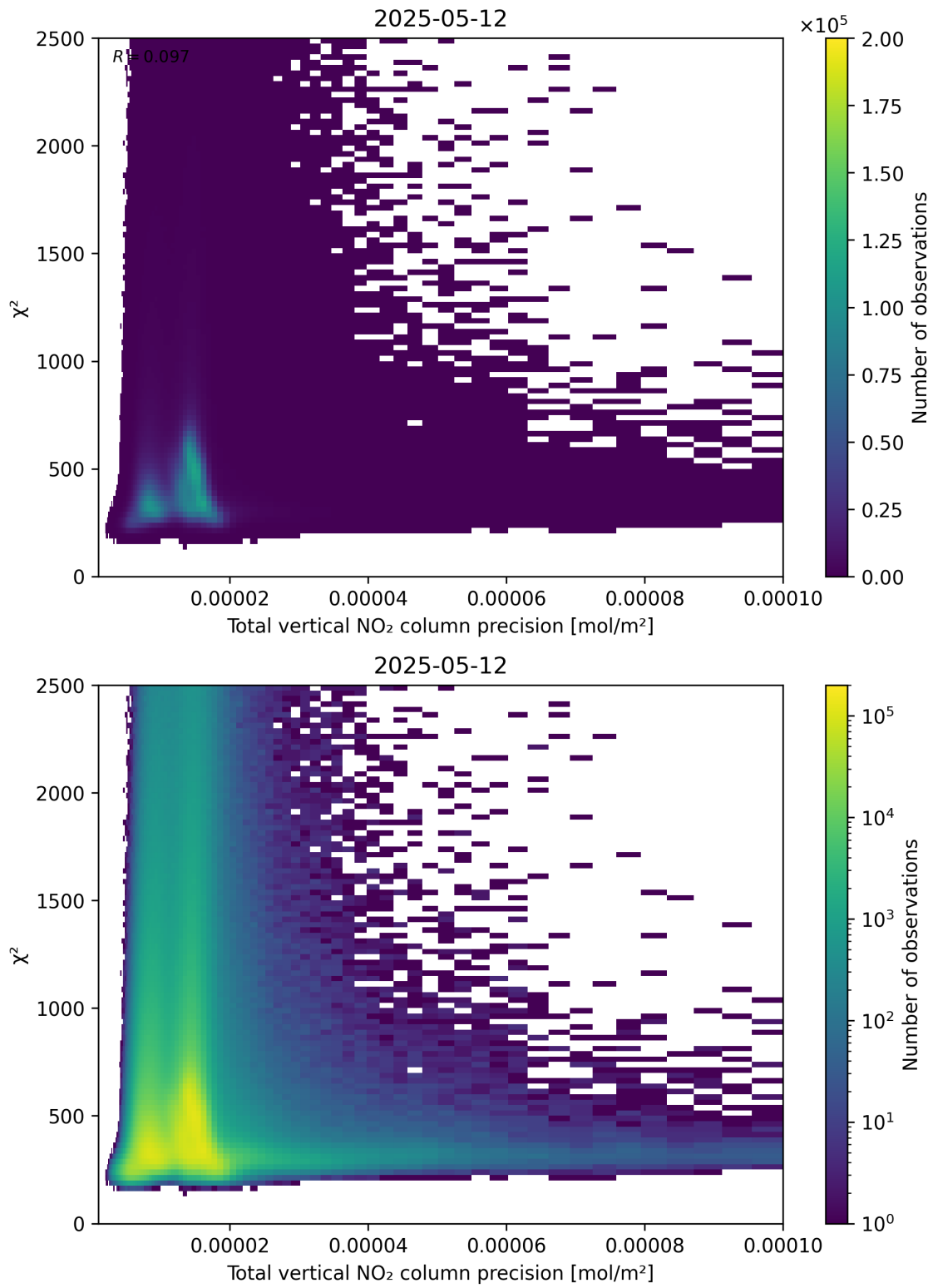
Figure 116: Scatter density plot of “Total vertical NO 2 column precision” against “ \chi^2 ” for 2025-05-12 to 2025-05-13.
