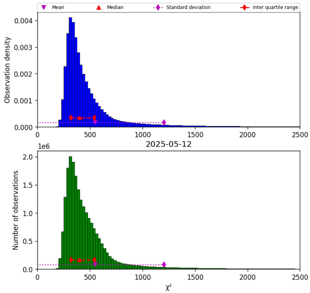
Figure 42: Histogram of “ \chi^2 ” for 2025-05-12 to 2025-05-13
