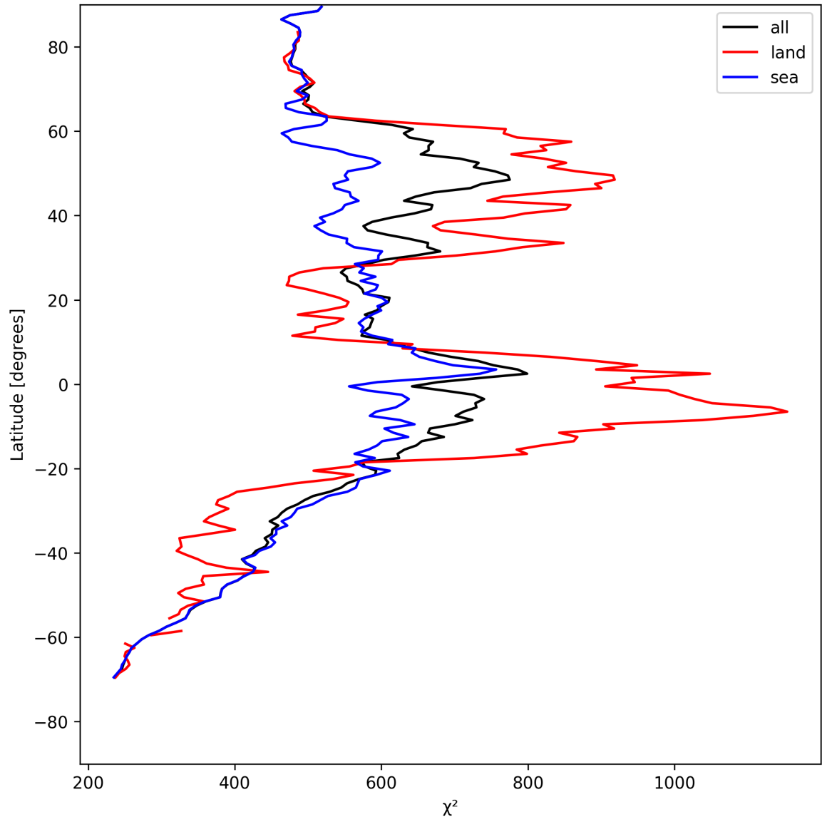
Figure 25: Zonal average of “ \chi^2 ” for 2025-05-12 to 2025-05-13.
