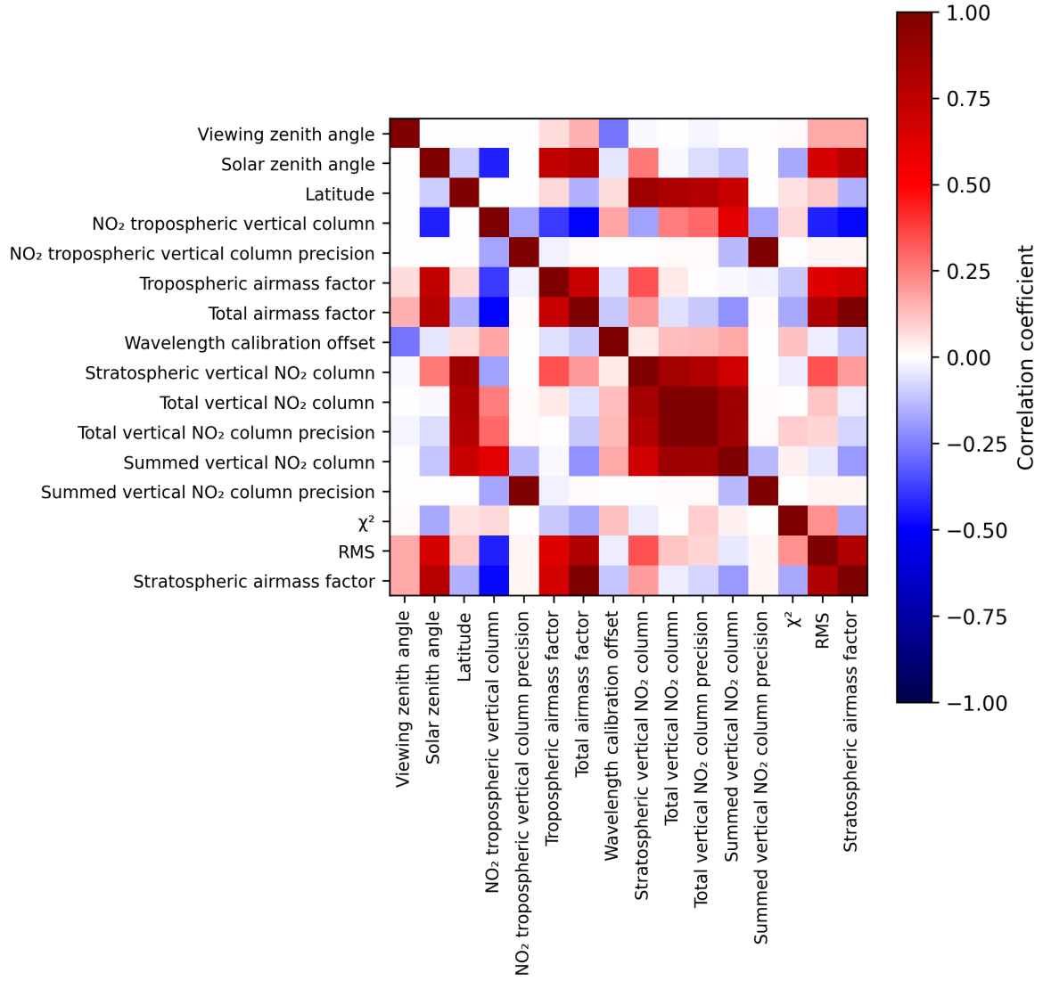
Figure 2: Map of correlation matrix for 2025-05-12 to 2025-05-13.
