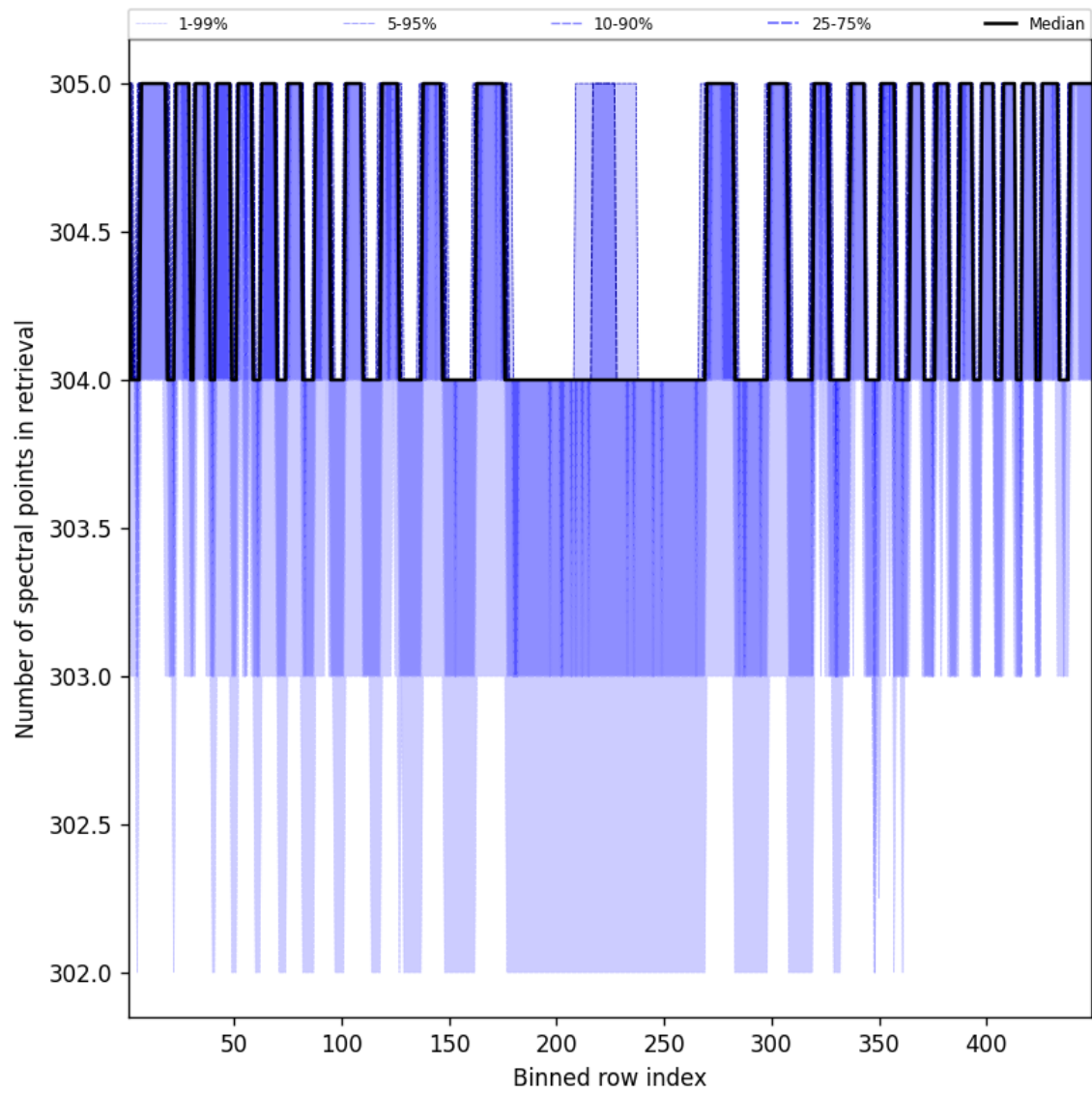
Figure 50: Along track statistics of “Number of spectral points in retrieval” for 2025-05-12 to 2025-05-13
