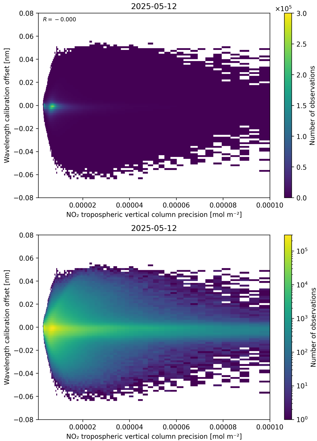
Figure 141: Scatter density plot of “NO 2 tropospheric vertical column precision” against “Wavelength calibration offset” for 2025-05-12 to 2025-05-13.
