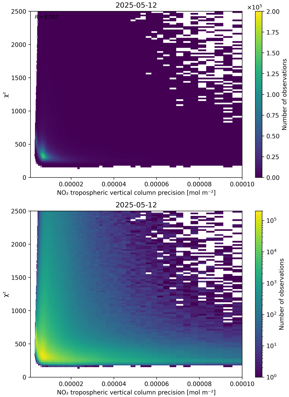
Figure 134: Scatter density plot of “NO 2 tropospheric vertical column precision” against “ \chi^2 ” for 2025-05-12 to 2025-05-13.
