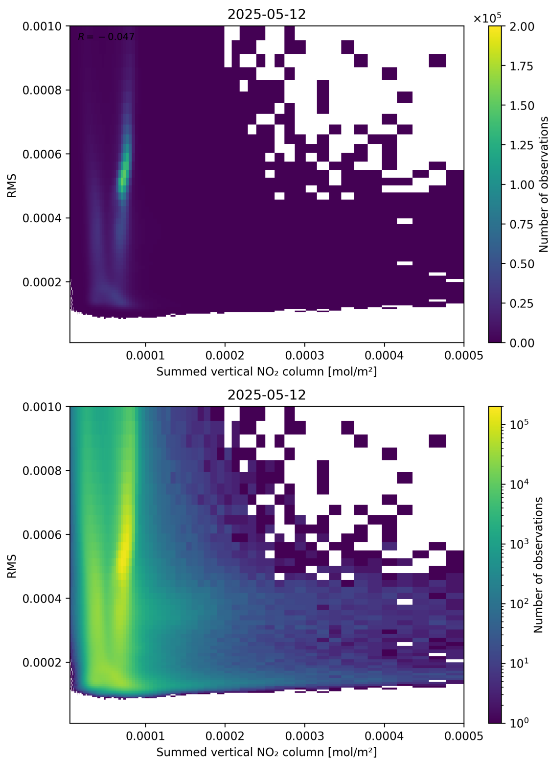
Figure 109: Scatter density plot of “Summed vertical NO 2 column” against “RMS” for 2025-05-12 to 2025-05-13.
