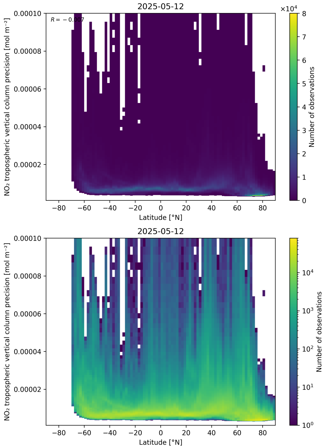
Figure 93: Scatter density plot of “Latitude” against “NO 2 tropospheric vertical column precision” for 2025-05-12 to 2025-05-13.
