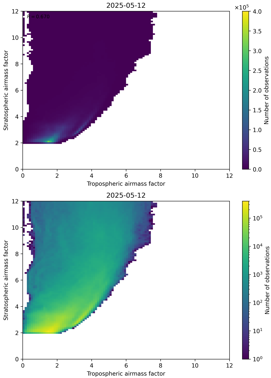
Figure 71: Scatter density plot of “Tropospheric airmass factor” against “Stratospheric airmass factor” for 2025-05-12 to 2025-05-13.
