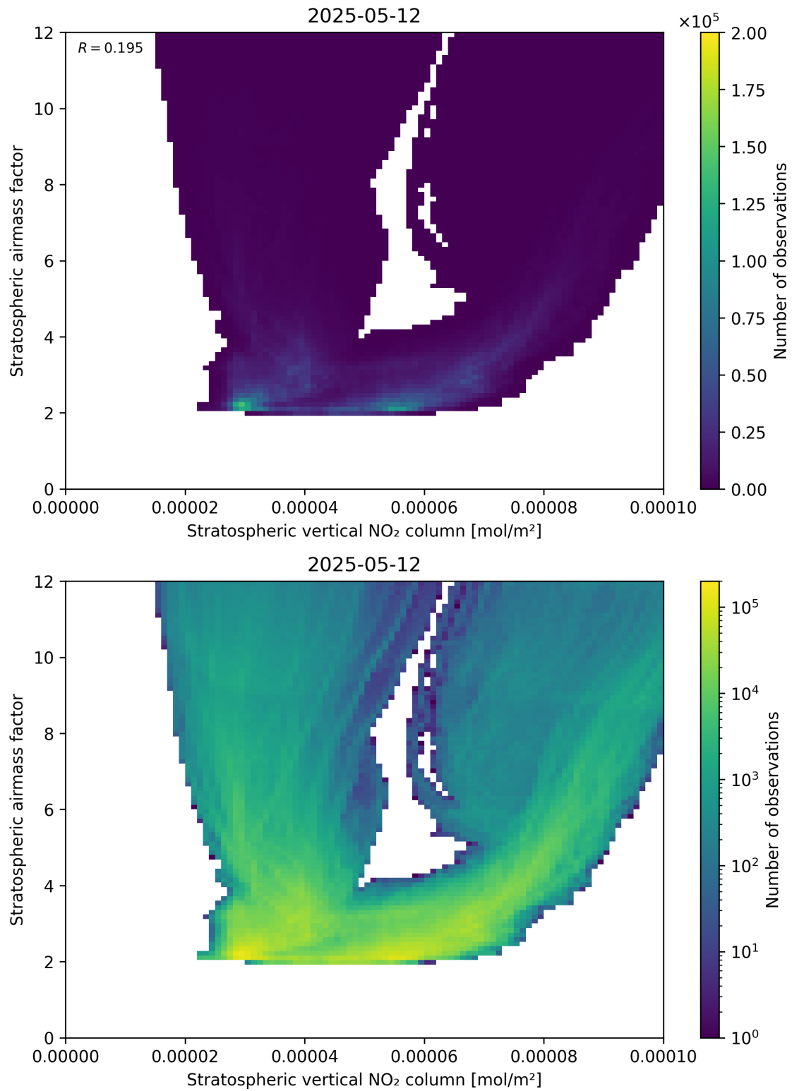
Figure 96: Scatter density plot of “Stratospheric vertical NO 2 column” against “Stratospheric airmass factor” for 2025-05-12 to 2025-05-13.
