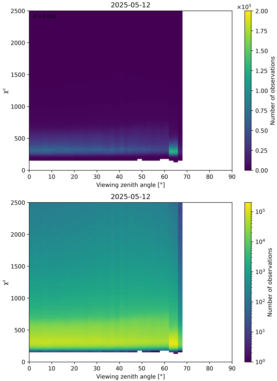
Figure 162: Scatter density plot of “Viewing zenith angle” against “ \chi^2 ” for 2025-05-12 to 2025-05-13.
