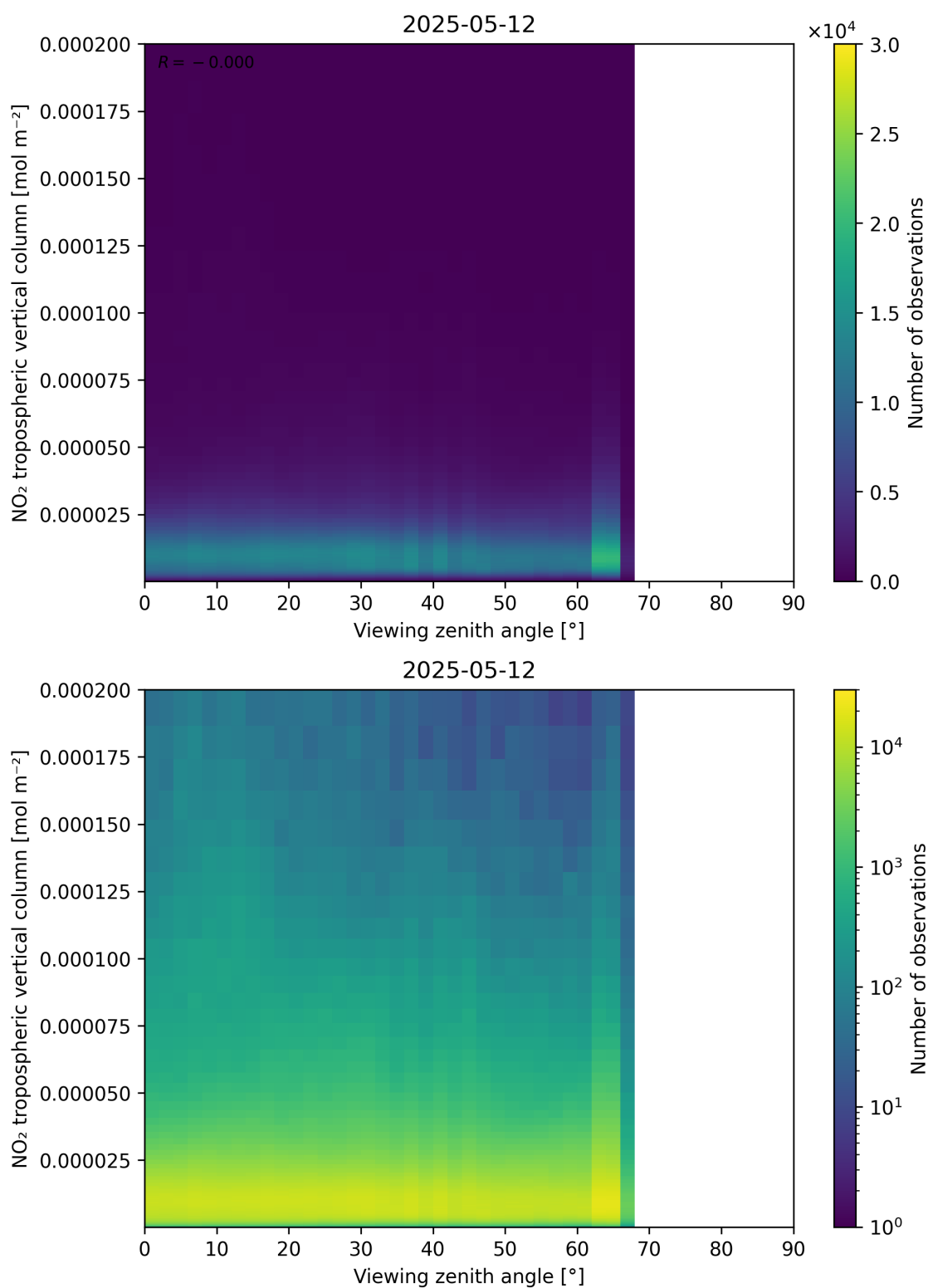
Figure 169: Scatter density plot of “Viewing zenith angle” against “NO 2 tropospheric vertical column” for 2025-05-12 to 2025-05-13.
