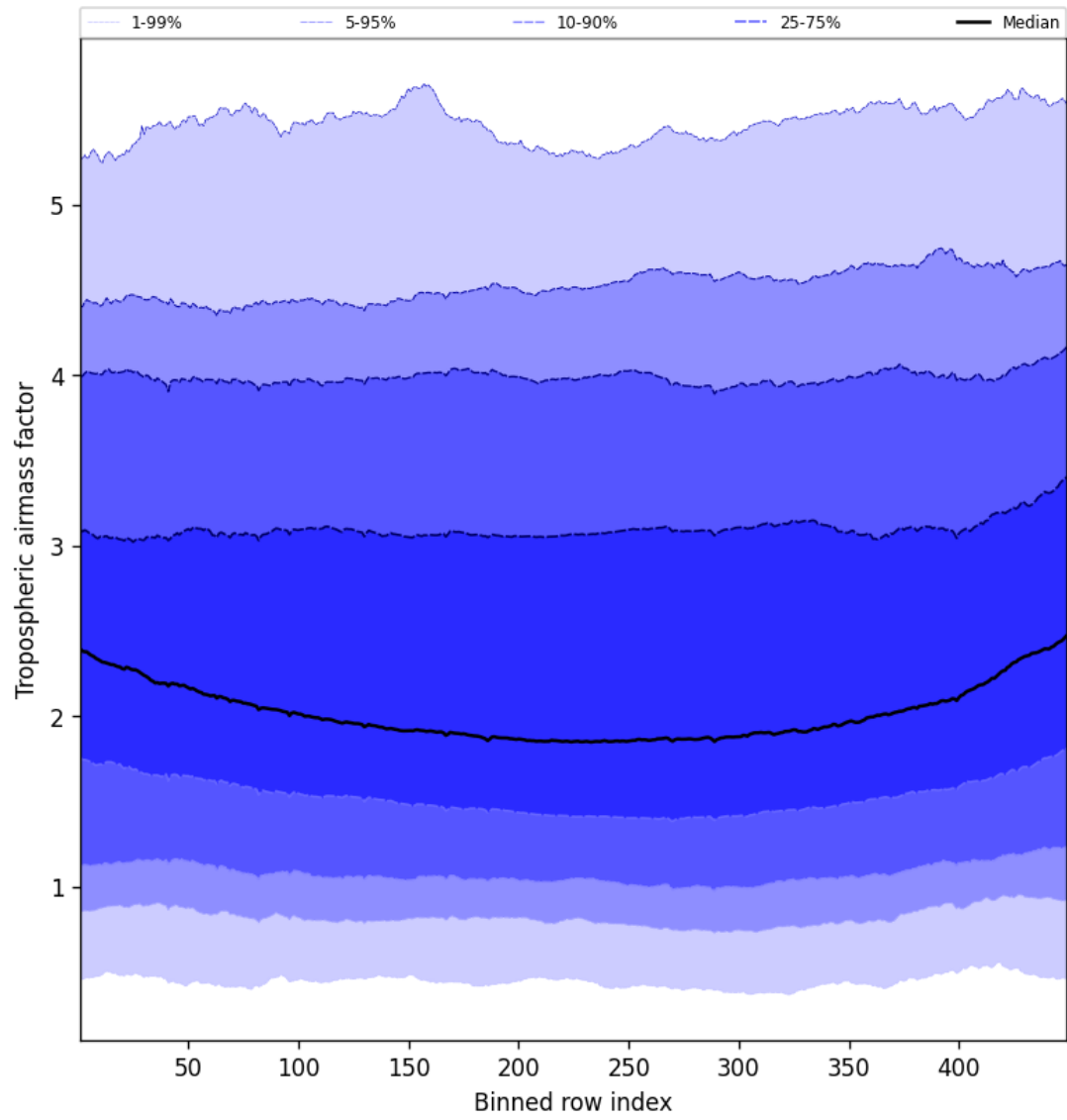
Figure 48: Along track statistics of “Tropospheric airmass factor” for 2025-05-12 to 2025-05-13
