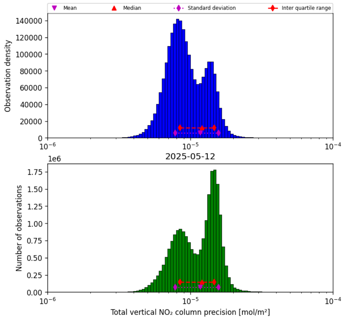
Figure 39: Histogram of “Total vertical NO 2 column precision” for 2025-05-12 to 2025-05-13
