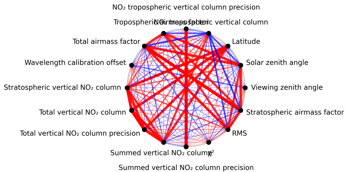
Figure 1: Map of correlation graph for 2025-05-12 to 2025-05-13.
