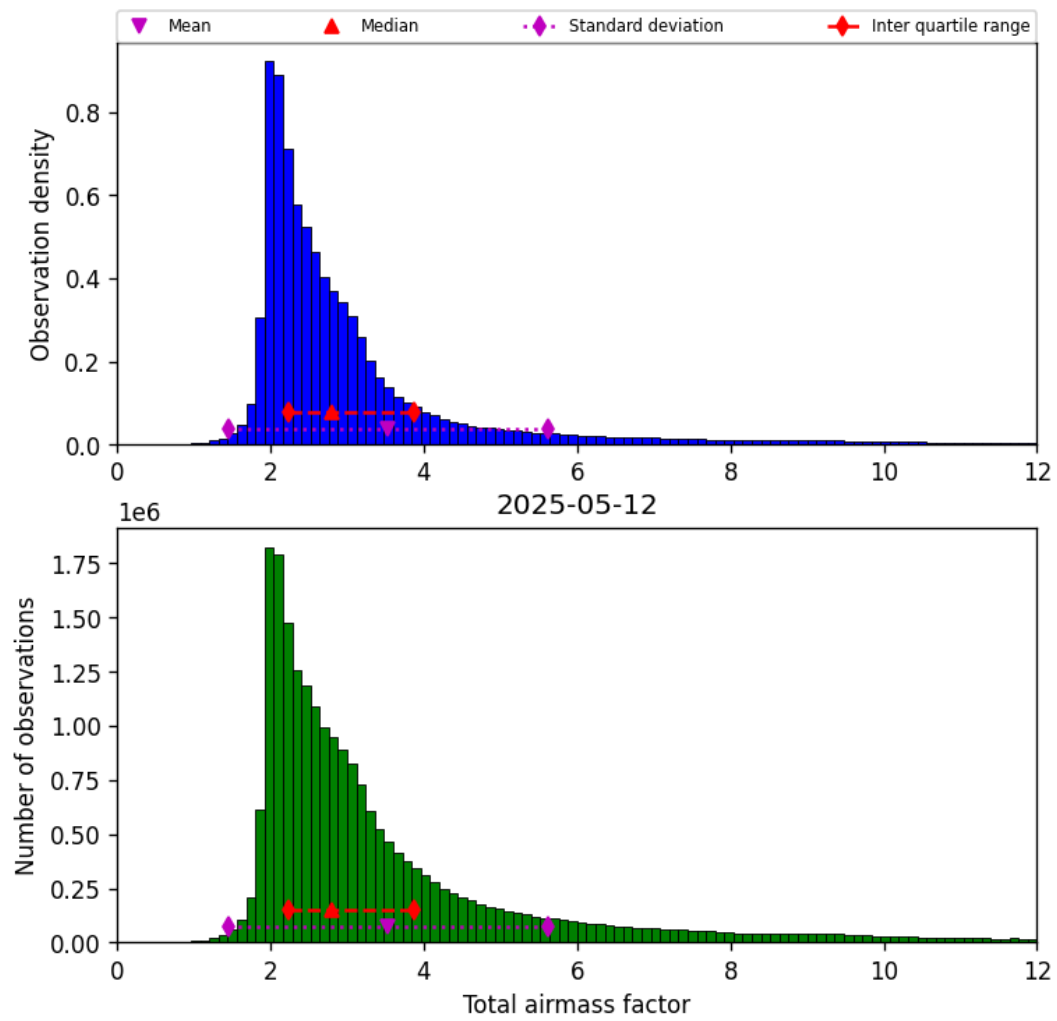
Figure 32: Histogram of “Total airmass factor” for 2025-05-12 to 2025-05-13
