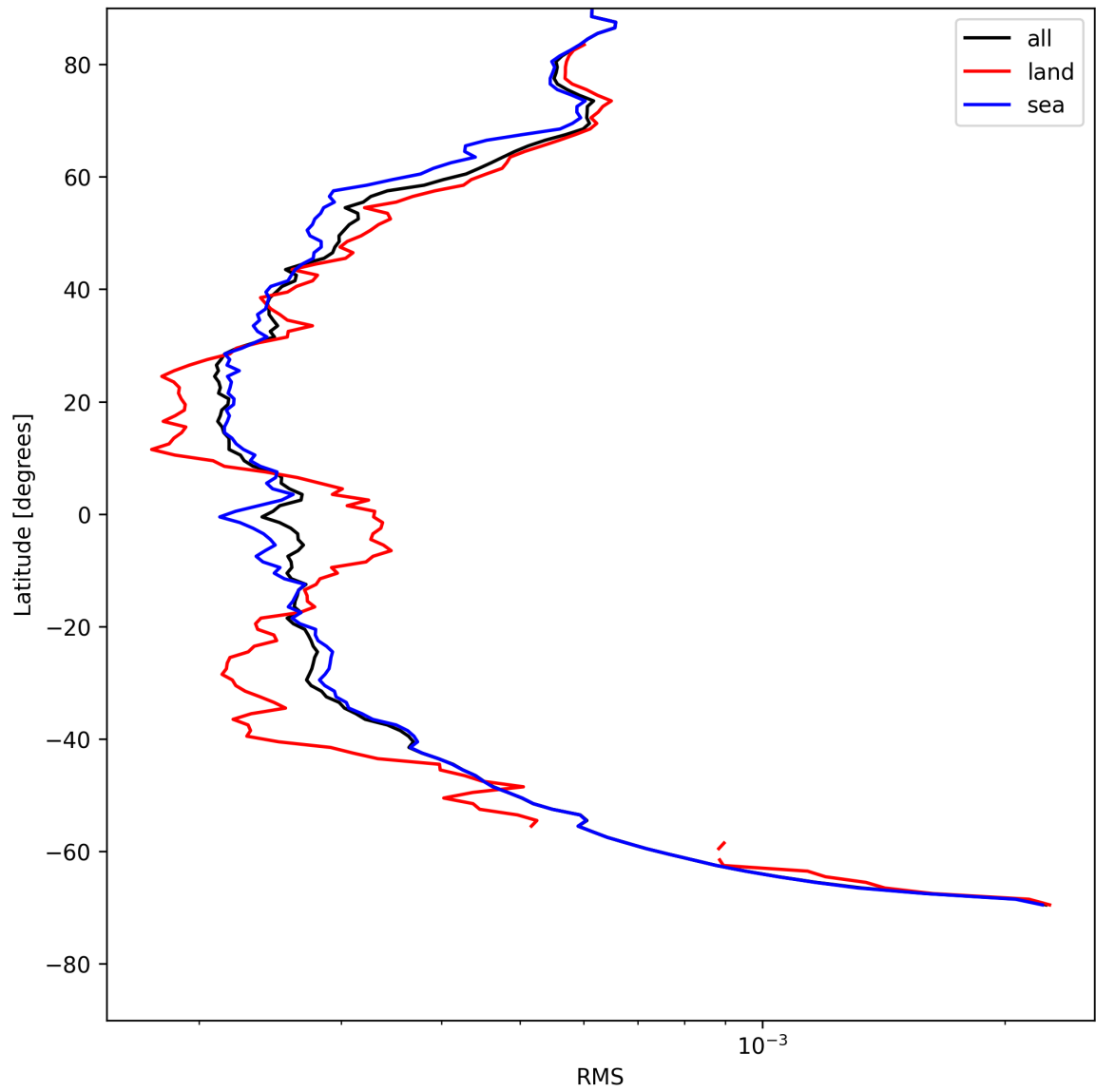
Figure 26: Zonal average of “RMS” for 2025-05-12 to 2025-05-13.
