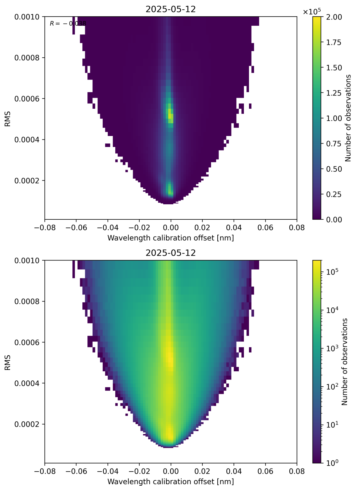
Figure 181: Scatter density plot of “Wavelength calibration offset” against “RMS” for 2025-05-12 to 2025-05-13.
