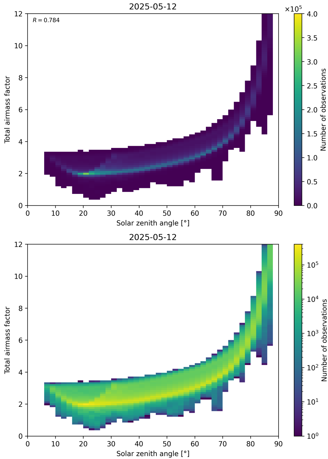
Figure 146: Scatter density plot of “Solar zenith angle” against “Total air mass factor” for 2025-05-12 to 2025-05-13.
