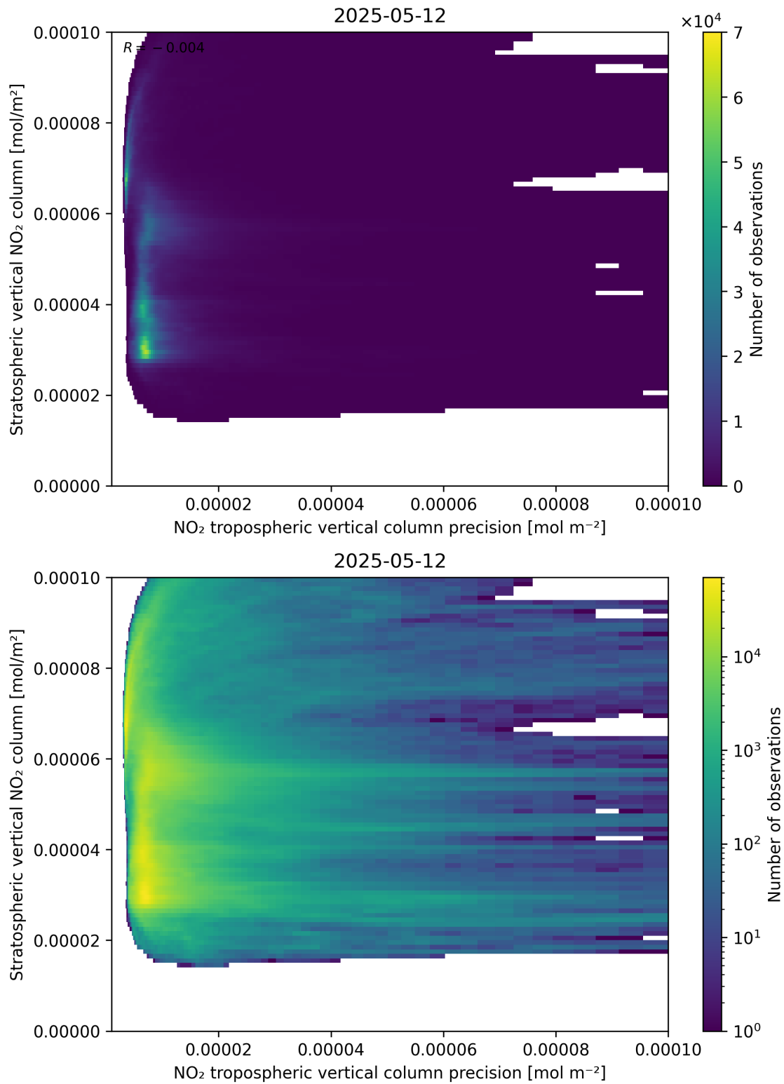
Figure 135: Scatter density plot of “NO 2 tropospheric vertical column precision” against “Stratospheric vertical NO 2 column” for 2025-05-12 to 2025-05-13.
