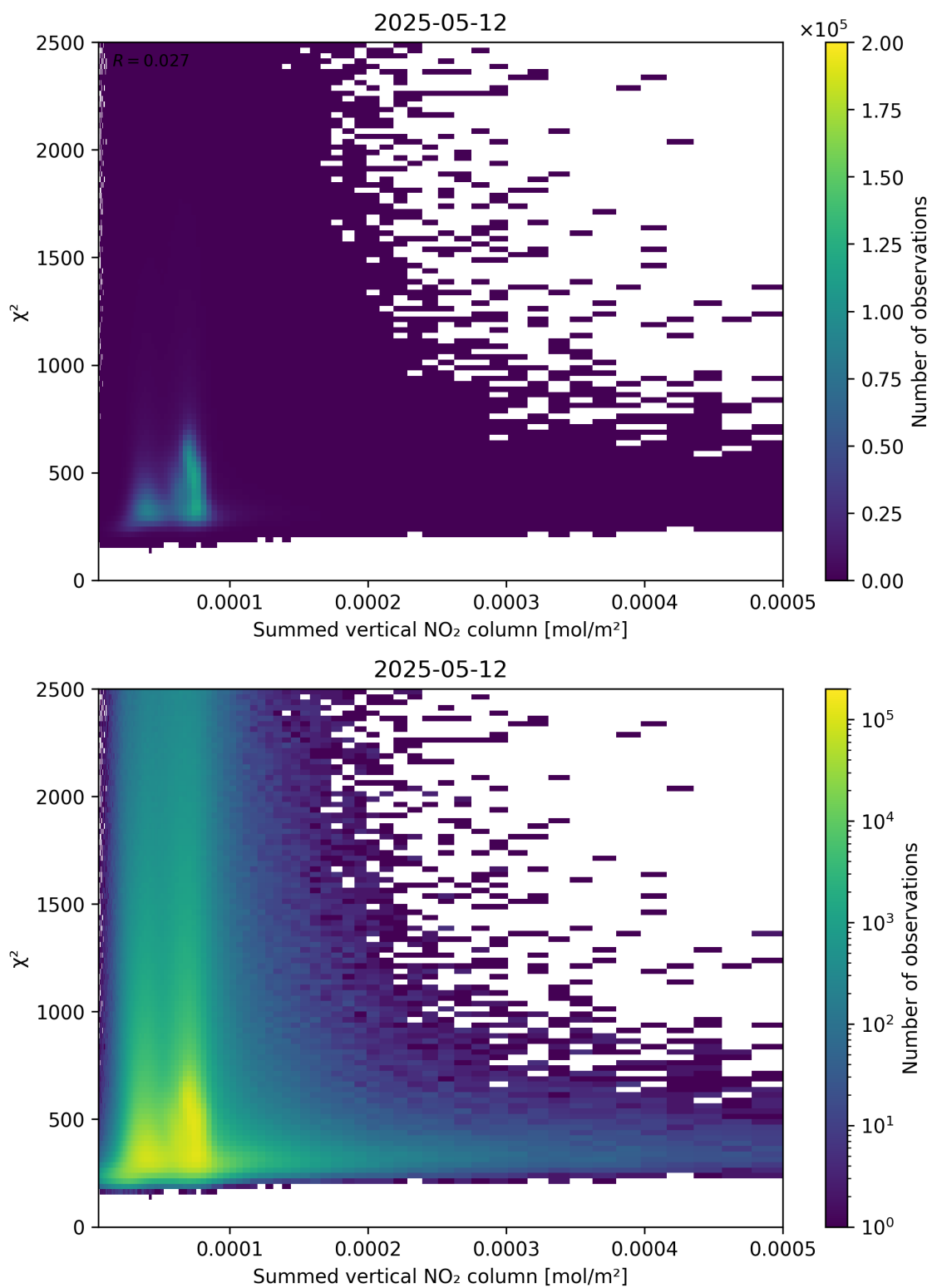
Figure 104: Scatter density plot of “Summed vertical NO 2 column” against “ \chi^2 ” for 2025-05-12 to 2025-05-13.
