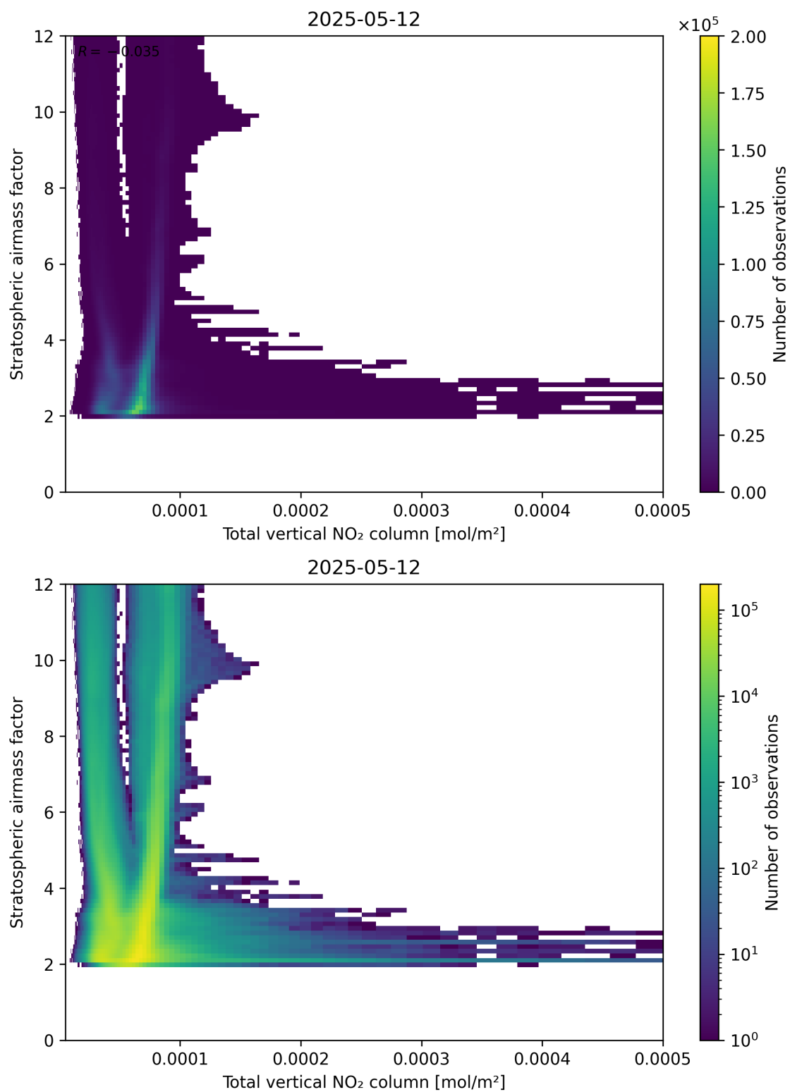
Figure 110: Scatter density plot of “Total vertical NO 2 column” against “Stratospheric airmass factor” for 2025-05-12 to 2025-05-13.
