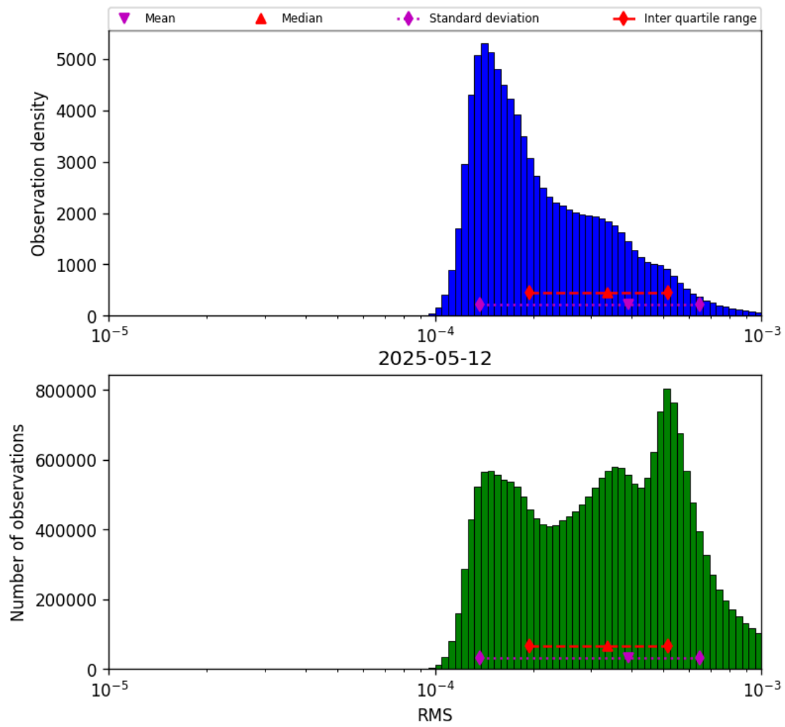
Figure 43: Histogram of “RMS” for 2025-05-12 to 2025-05-13
