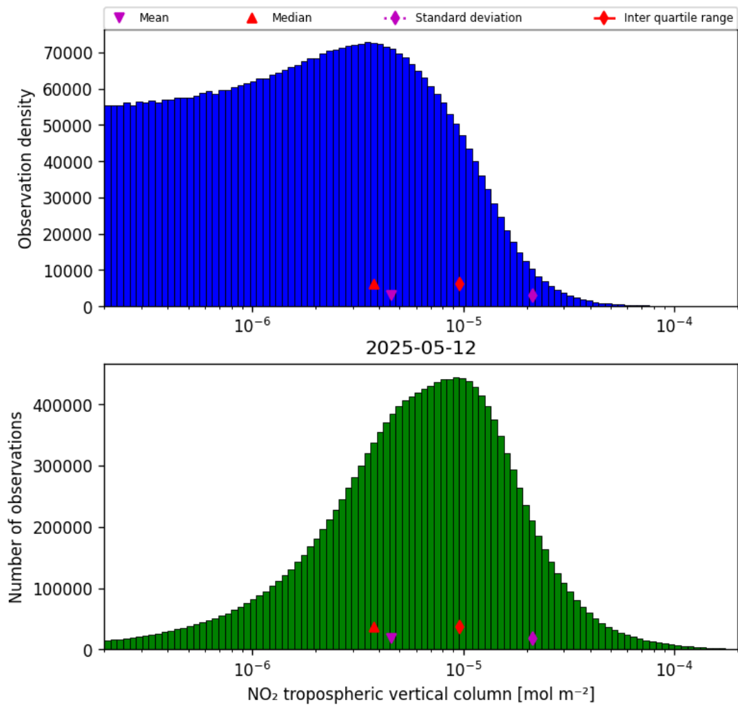
Figure 29: Histogram of “NO 2 tropospheric vertical column” for 2025-05-12 to 2025-05-13
