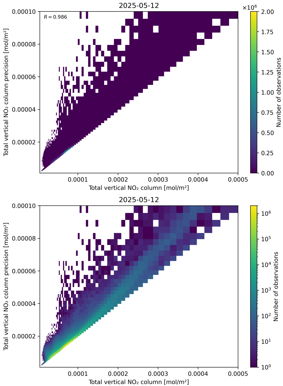
Figure 114: Scatter density plot of “Total vertical NO 2 column” against “Total vertical NO 2 column precision” for 2025-05-12 to 2025-05-13.
