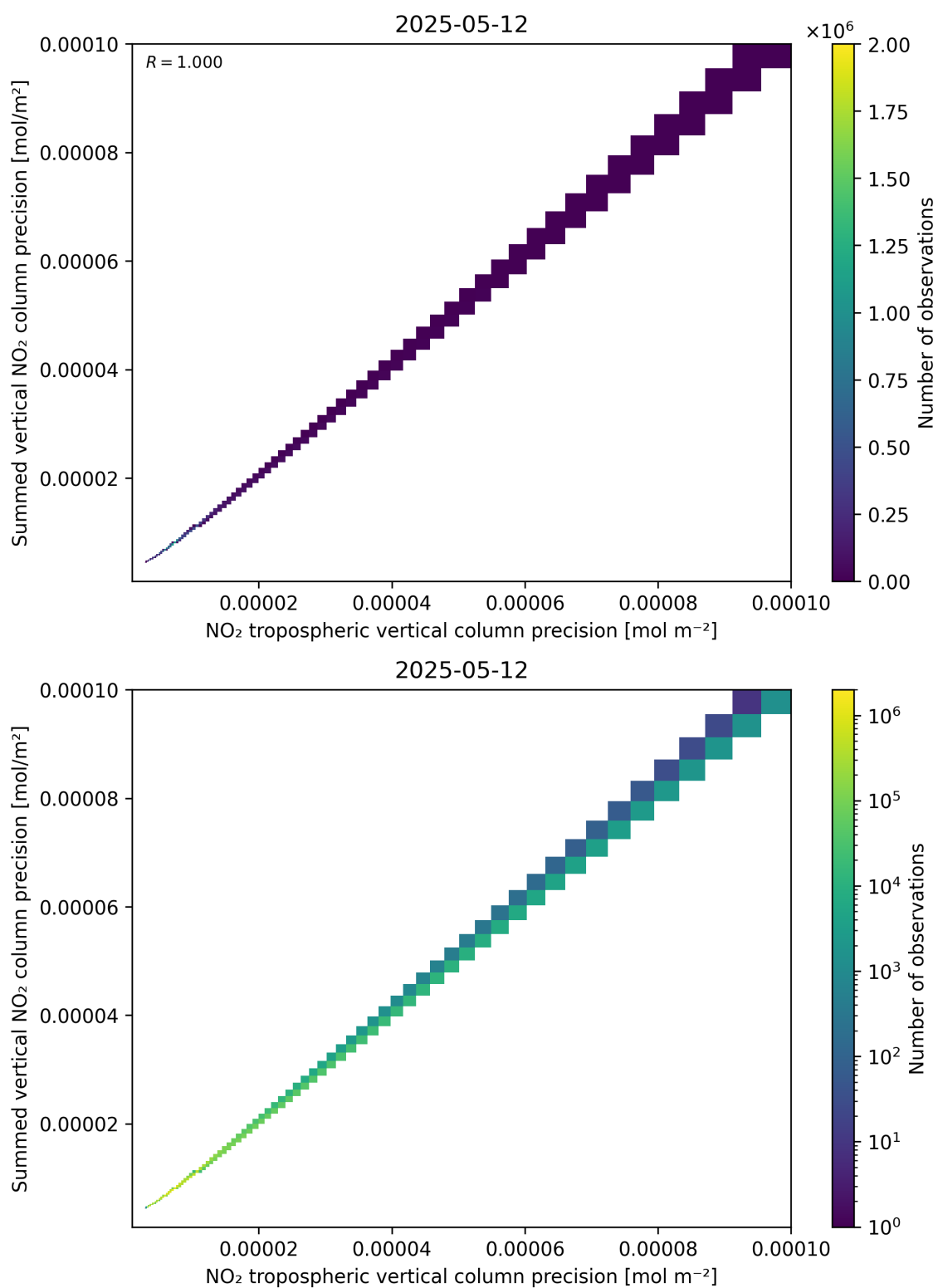
Figure 137: Scatter density plot of “NO 2 tropospheric vertical column precision” against “Summed vertical NO 2 column precision” for 2025-05-12 to 2025-05-13.
