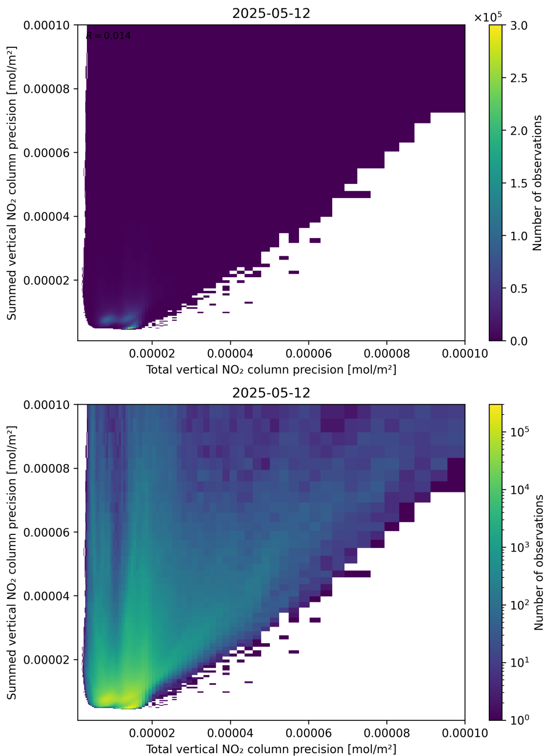
Figure 118: Scatter density plot of “Total vertical NO 2 column precision” against “Summed vertical NO 2 column precision” for 2025-05-12 to 2025-05-13.
