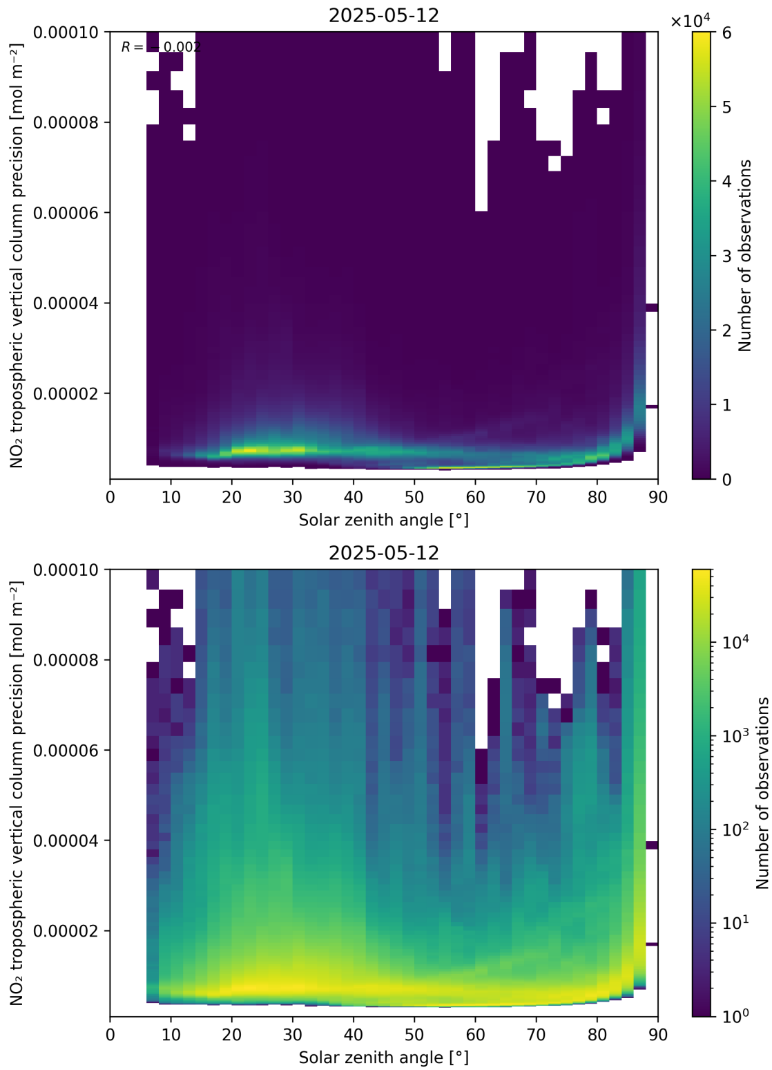
Figure 156: Scatter density plot of “Solar zenith angle” against “NO 2 tropospheric vertical column precision” for 2025-05-12 to 2025-05-13.
