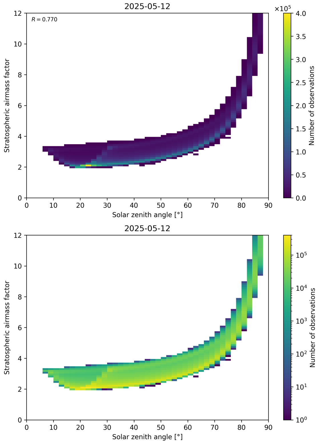
Figure 145: Scatter density plot of “Solar zenith angle” against “Stratospheric airmass factor” for 2025-05-12 to 2025-05-13.
