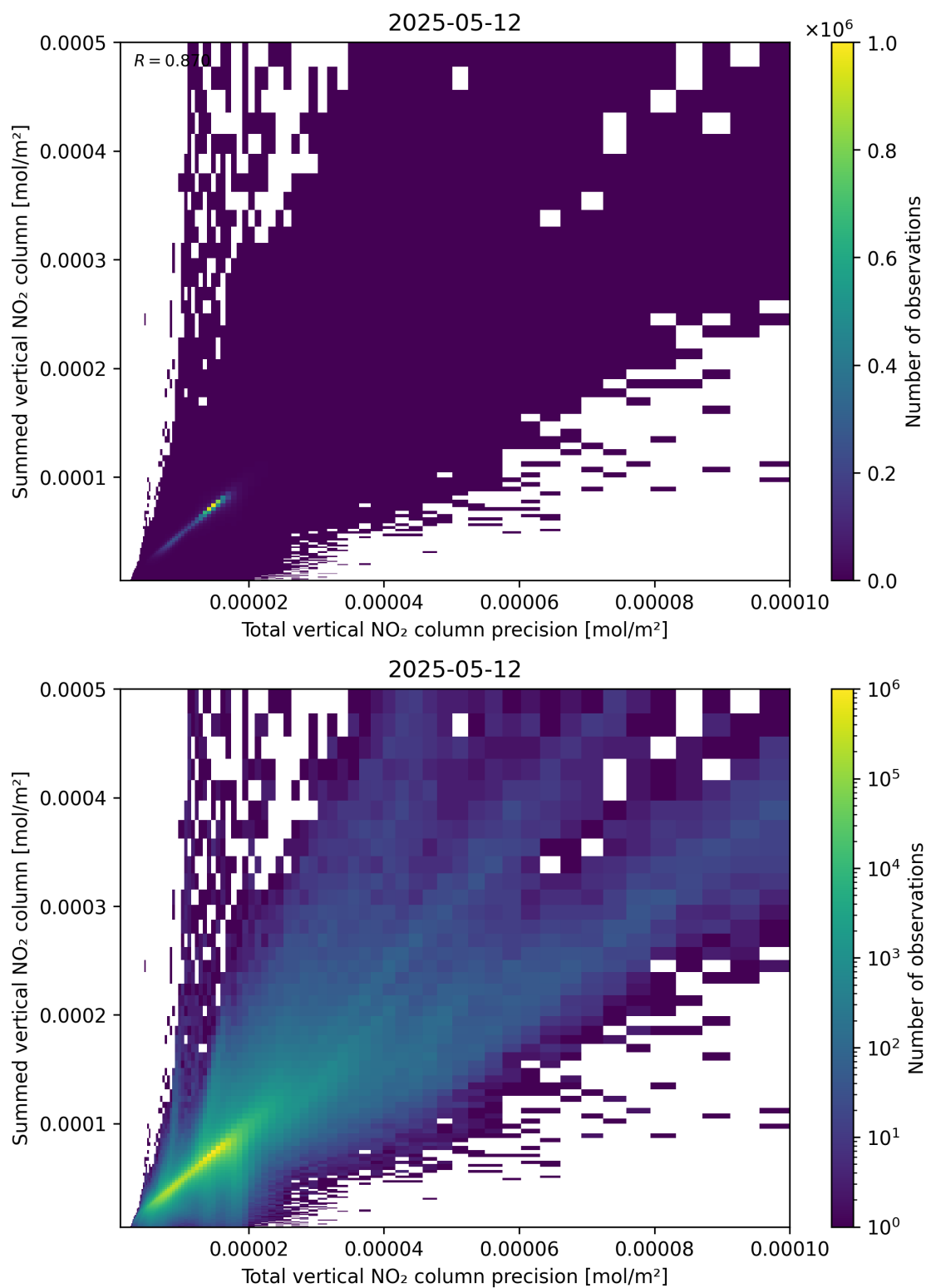
Figure 117: Scatter density plot of “Total vertical NO 2 column precision” against “Summed vertical NO 2 column” for 2025-05-12 to 2025-05-13.
