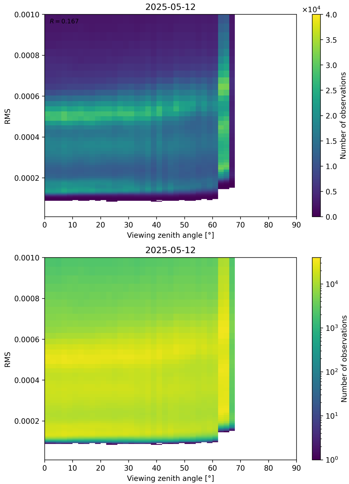
Figure 171: Scatter density plot of “Viewing zenith angle” against “RMS” for 2025-05-12 to 2025-05-13.
