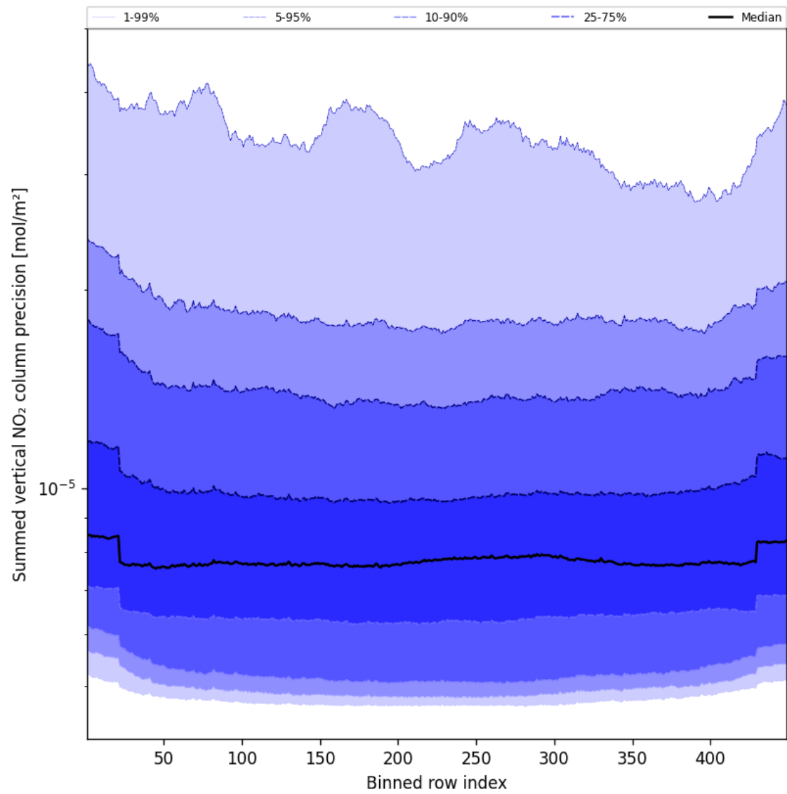
Figure 58: Along track statistics of “Summed vertical NO 2 column precision” for 2025-05-12 to 2025-05-13
