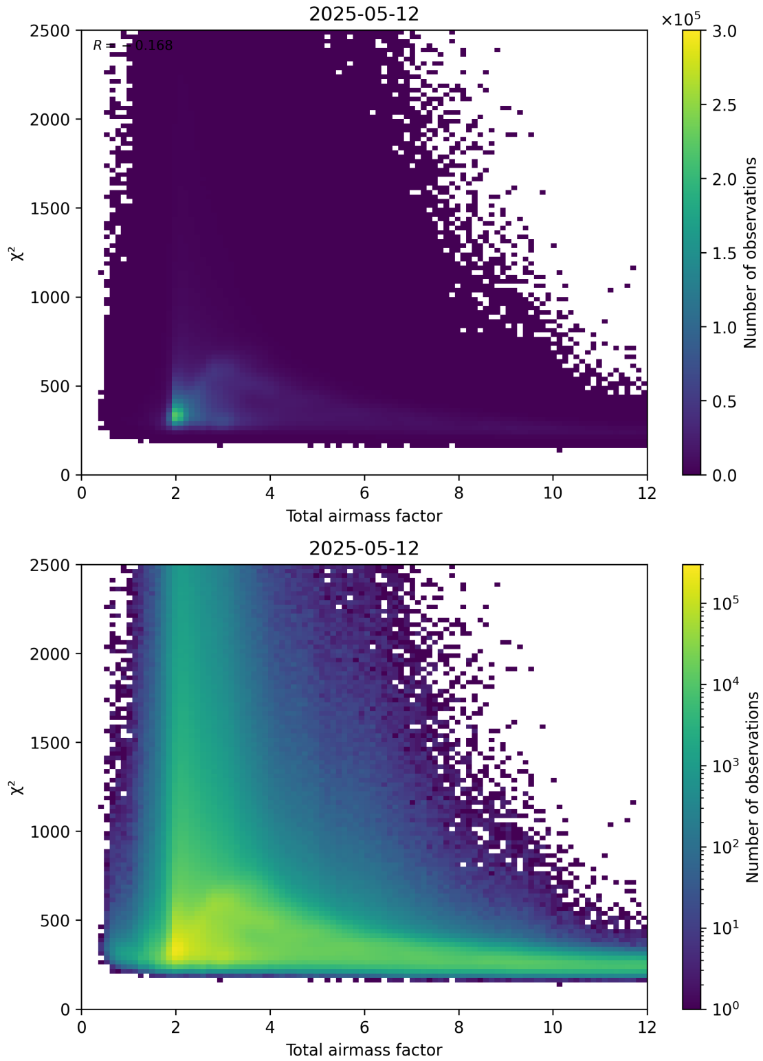
Figure 63: Scatter density plot of “Total airmass factor” against “ \chi^2 ” for 2025-05-12 to 2025-05-13.
