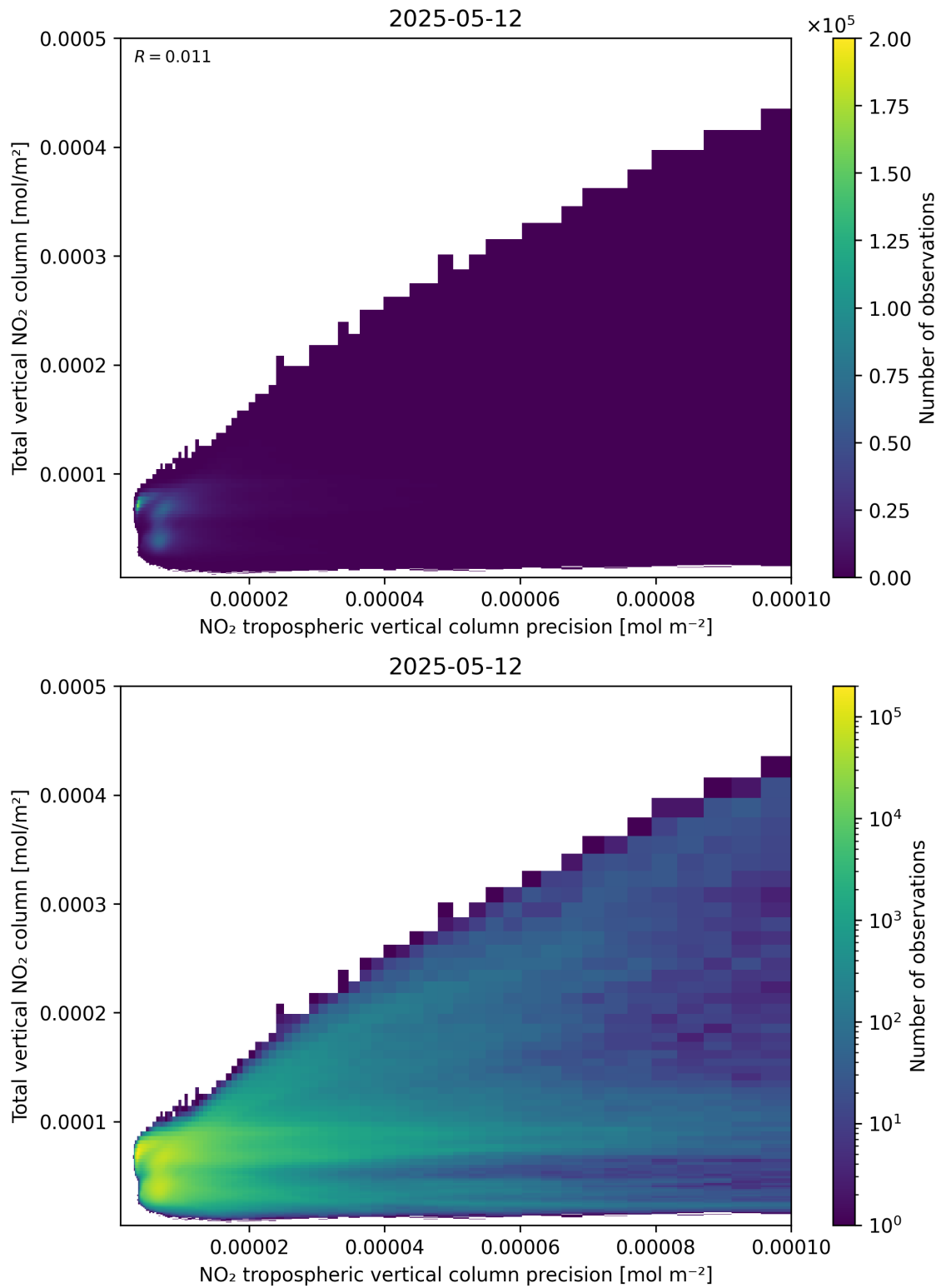
Figure 138: Scatter density plot of “NO 2 tropospheric vertical column precision” against “Total vertical NO 2 column” for 2025-05-12 to 2025-05-13.
