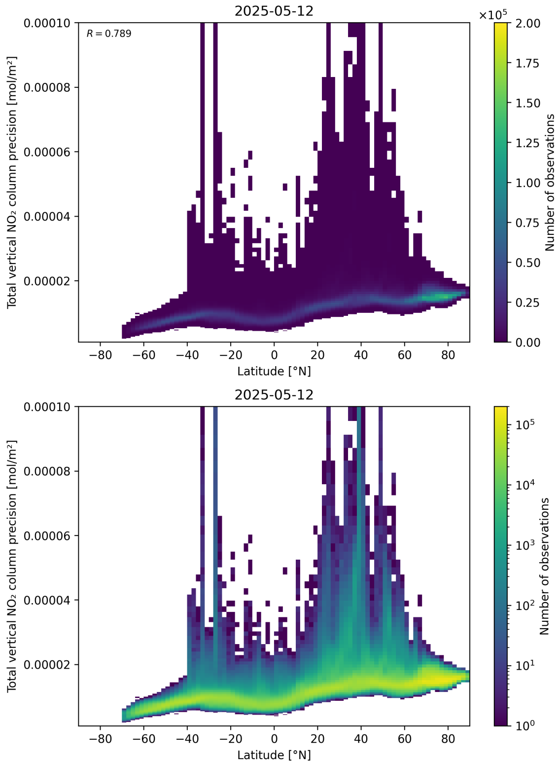
Figure 91: Scatter density plot of “Latitude” against “Total vertical NO 2 column precision” for 2025-05-12 to 2025-05-13.
