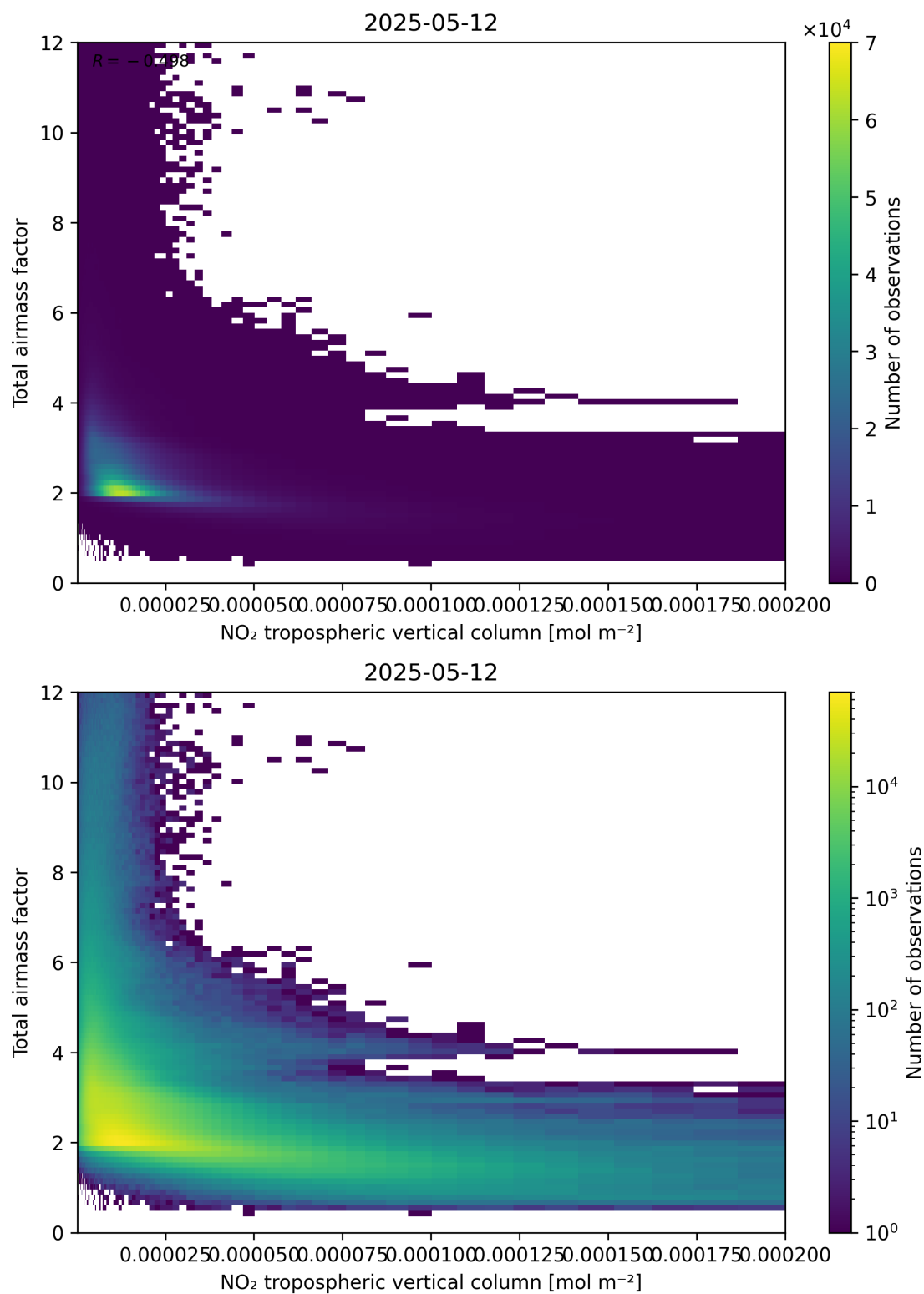
Figure 122: Scatter density plot of “NO 2 tropospheric vertical column” against “Total air mass factor” for 2025-05-12 to 2025-05-13.
