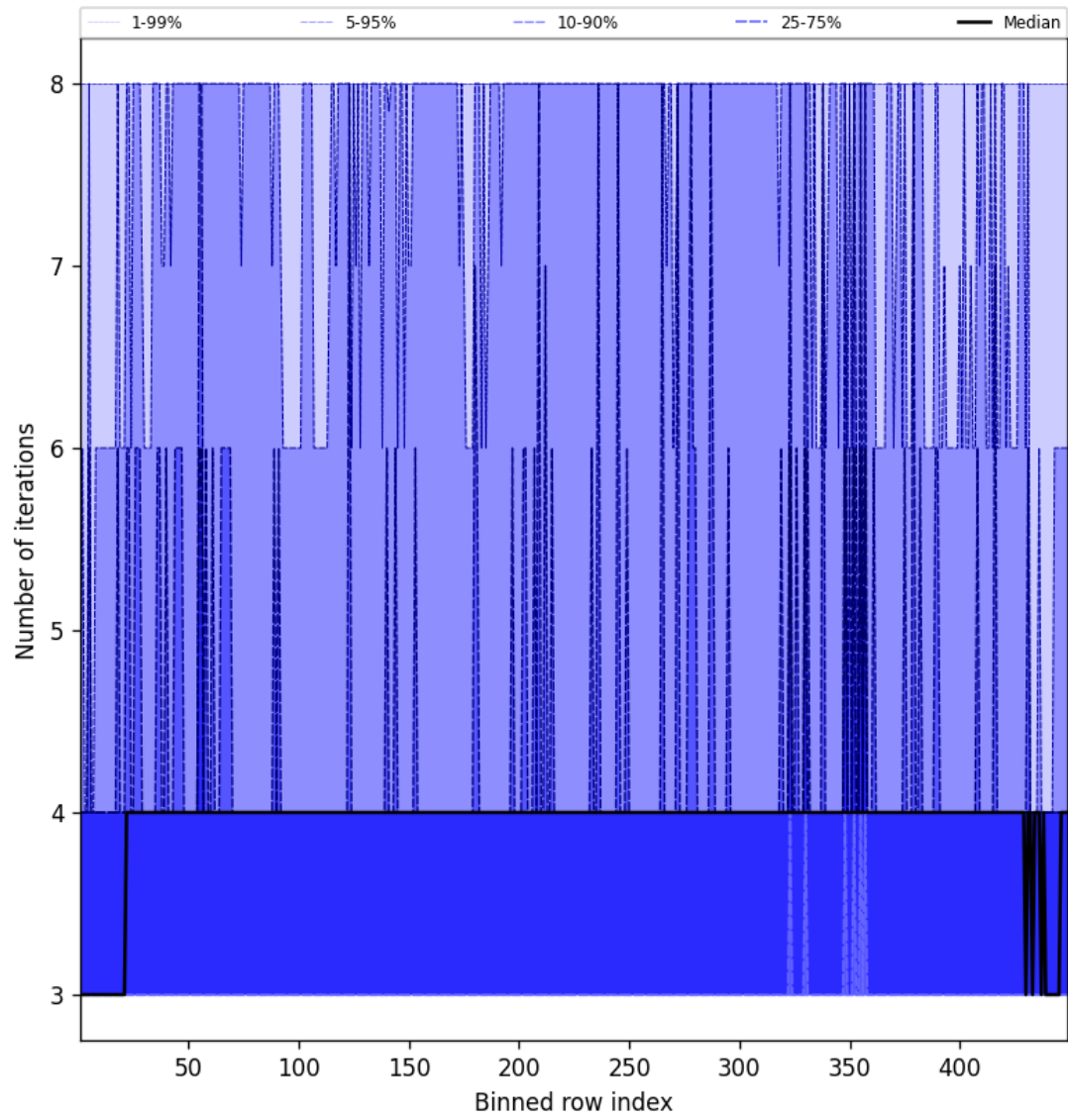
Figure 51: Along track statistics of “Number of iterations” for 2025-05-12 to 2025-05-13
