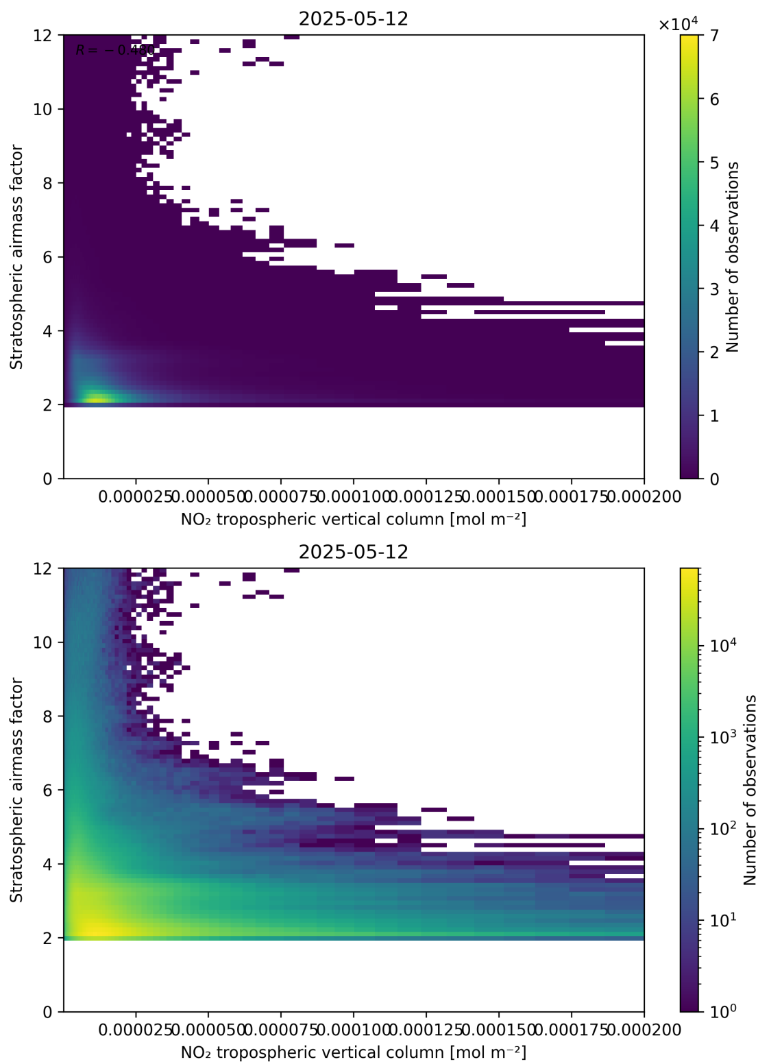
Figure 121: Scatter density plot of “NO 2 tropospheric vertical column” against “Stratospheric airmass factor” for 2025-05-12 to 2025-05-13.
