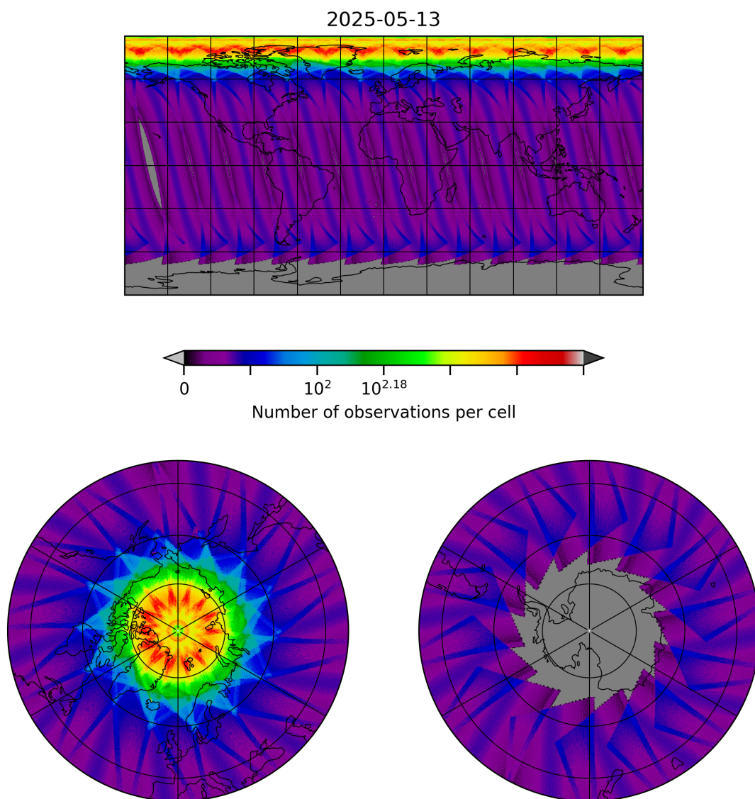
Figure 10: Map of the number of observations for 2025-05-13 to 2025-05-13
