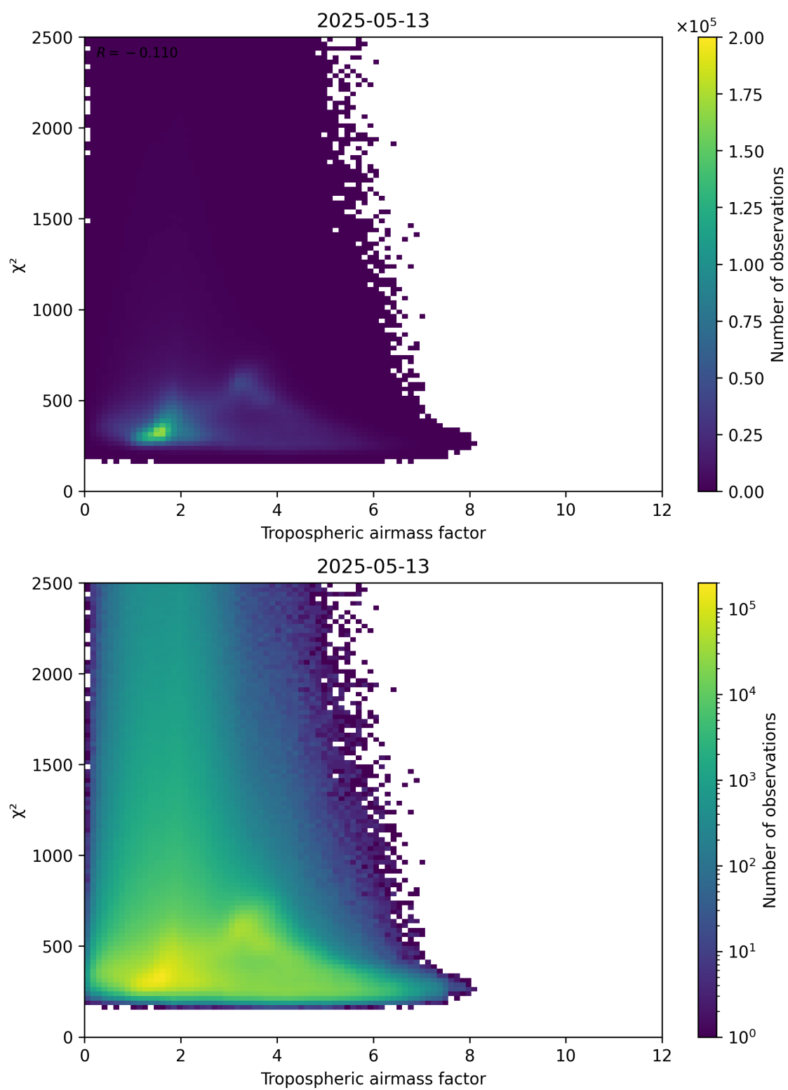
Figure 73: Scatter density plot of “Tropospheric airmass factor” against “ \chi^2 ” for 2025-05-13 to 2025-05-13.
