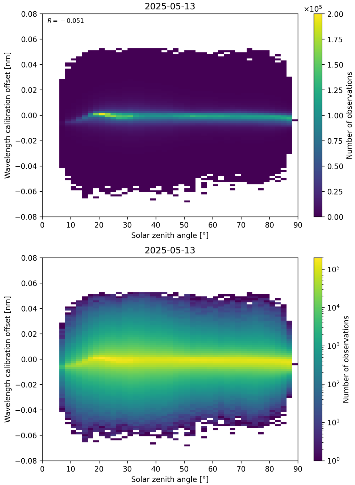
Figure 158: Scatter density plot of “Solar zenith angle” against “Wavelength calibration offset” for 2025-05-13 to 2025-05-13.
