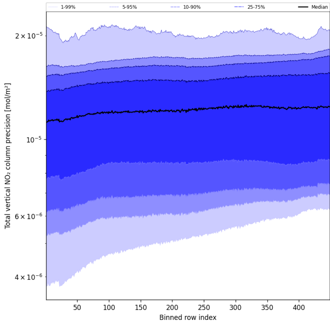
Figure 56: Along track statistics of “Total vertical NO 2 column precision” for 2025-05-13 to 2025-05-13
