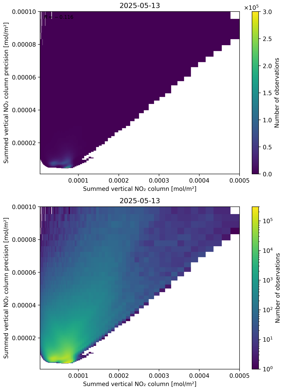
Figure 105: Scatter density plot of “Summed vertical NO 2 column” against “Summed vertical NO 2 column precision” for 2025-05-13 to 2025-05-13.
