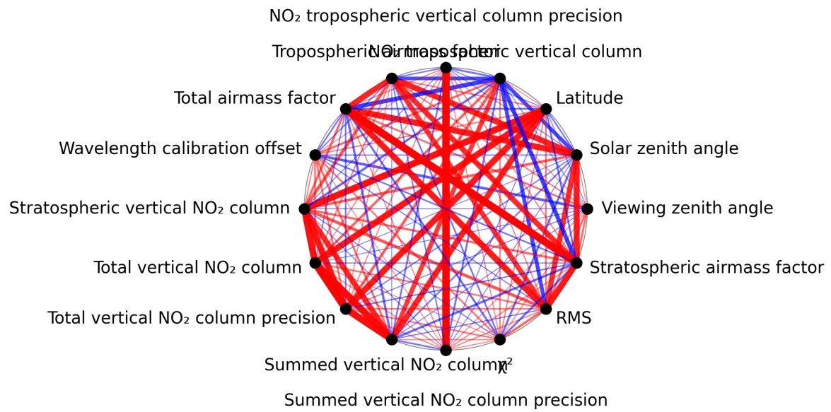
Figure 1: Map of correlation graph for 2025-05-13 to 2025-05-13.
