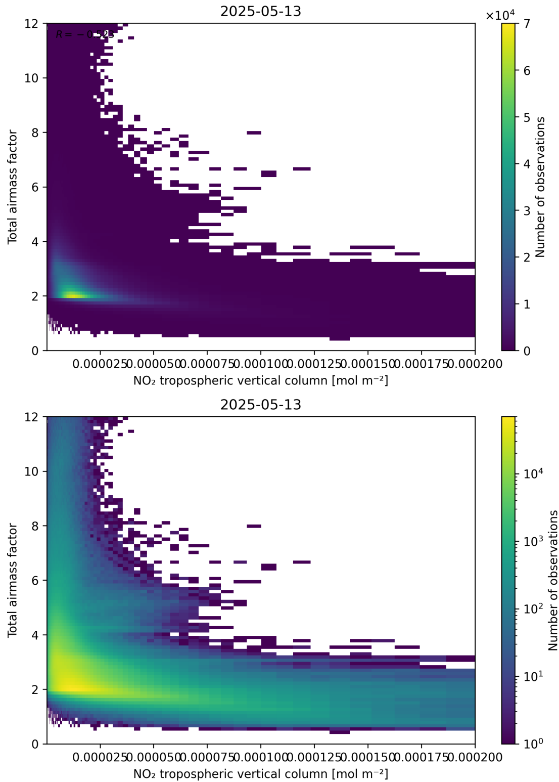
Figure 122: Scatter density plot of “NO 2 tropospheric vertical column” against “Total air mass factor” for 2025-05-13 to 2025-05-13.
