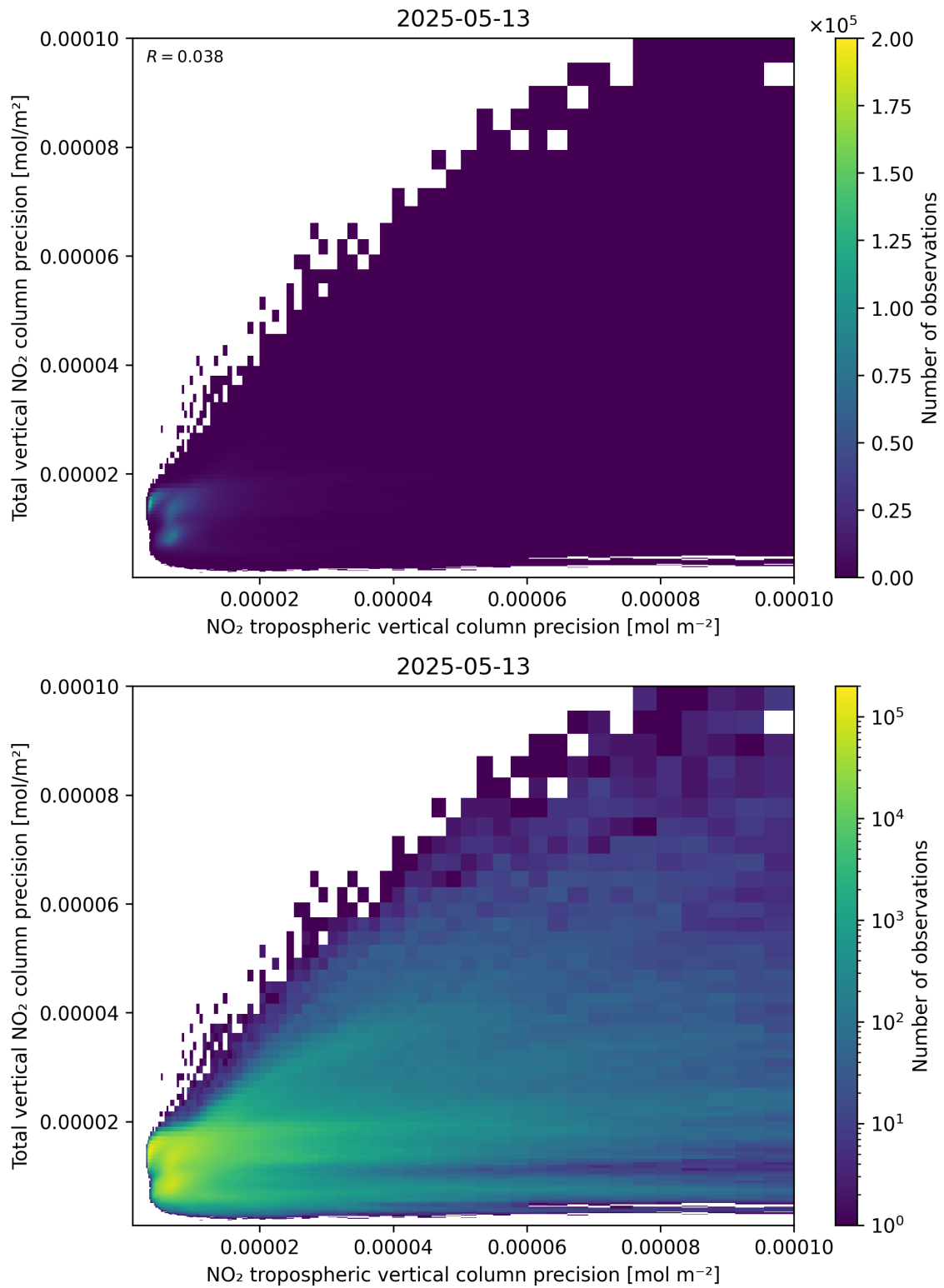
Figure 139: Scatter density plot of “NO 2 tropospheric vertical column precision” against “Total vertical NO 2 column precision” for 2025-05-13 to 2025-05-13.
