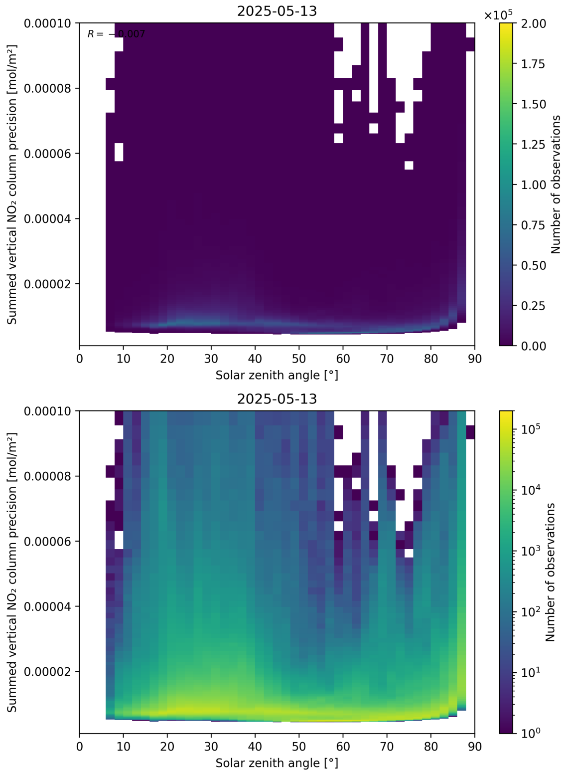
Figure 152: Scatter density plot of “Solar zenith angle” against “Summed vertical NO 2 column precision” for 2025-05-13 to 2025-05-13.
