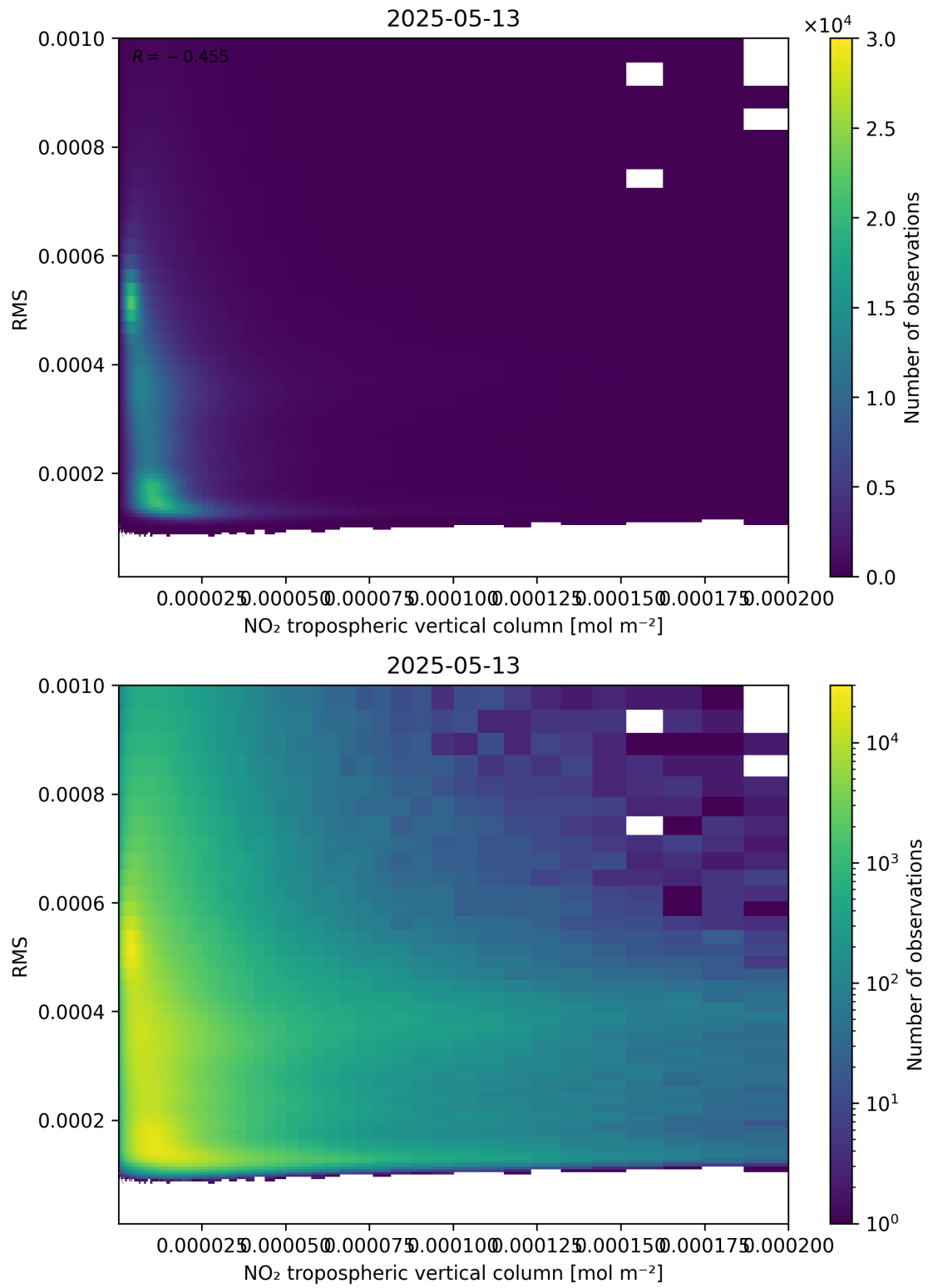
Figure 142: Scatter density plot of “NO 2 tropospheric vertical column” against “RMS” for 2025-05-13 to 2025-05-13.
