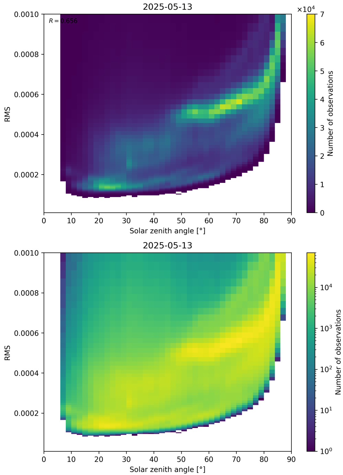
Figure 157: Scatter density plot of “Solar zenith angle” against “RMS” for 2025-05-13 to 2025-05-13.
