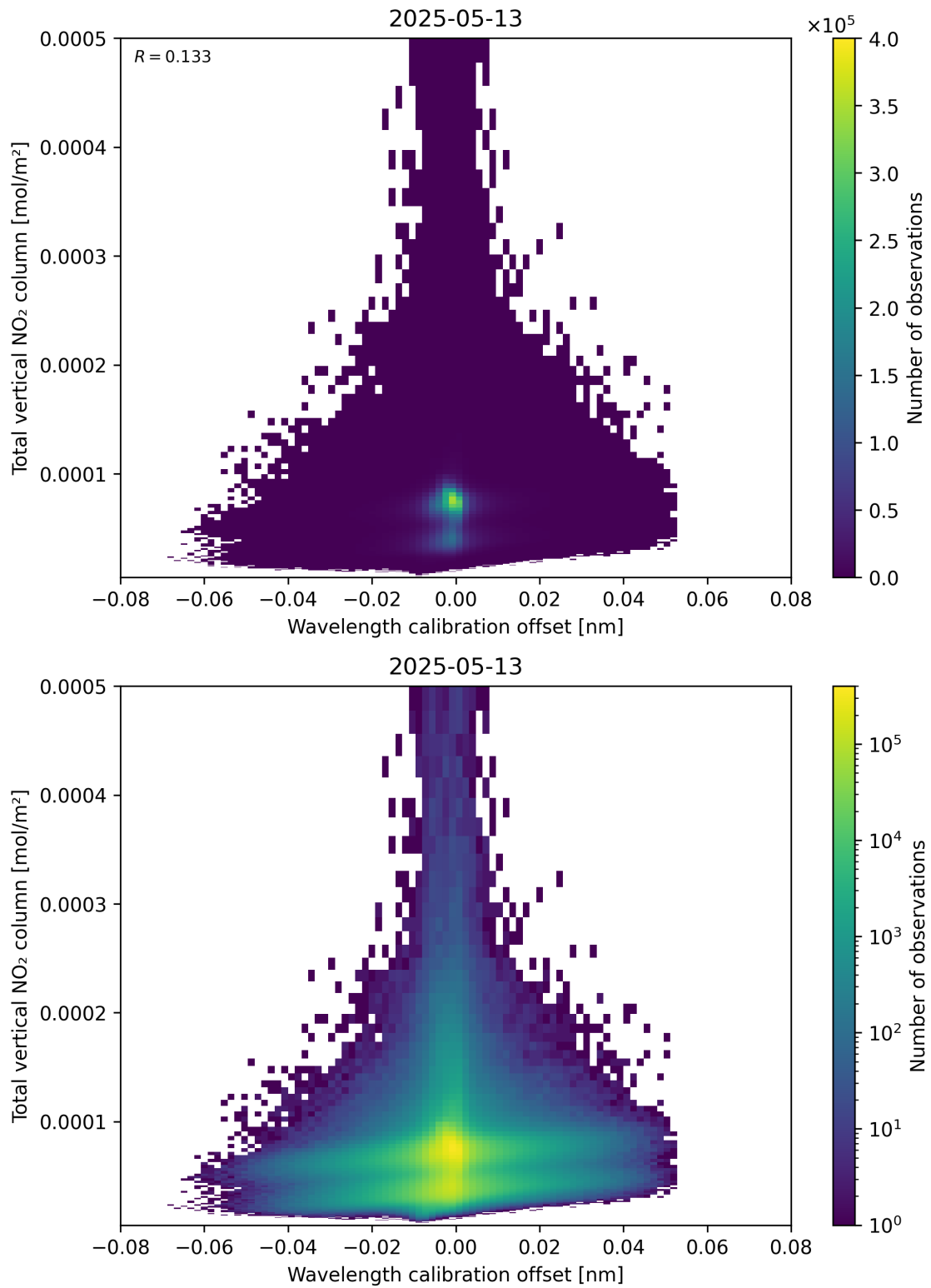
Figure 179: Scatter density plot of “Wavelength calibration offset” against “Total vertical NO 2 column” for 2025-05-13 to 2025-05-13.
