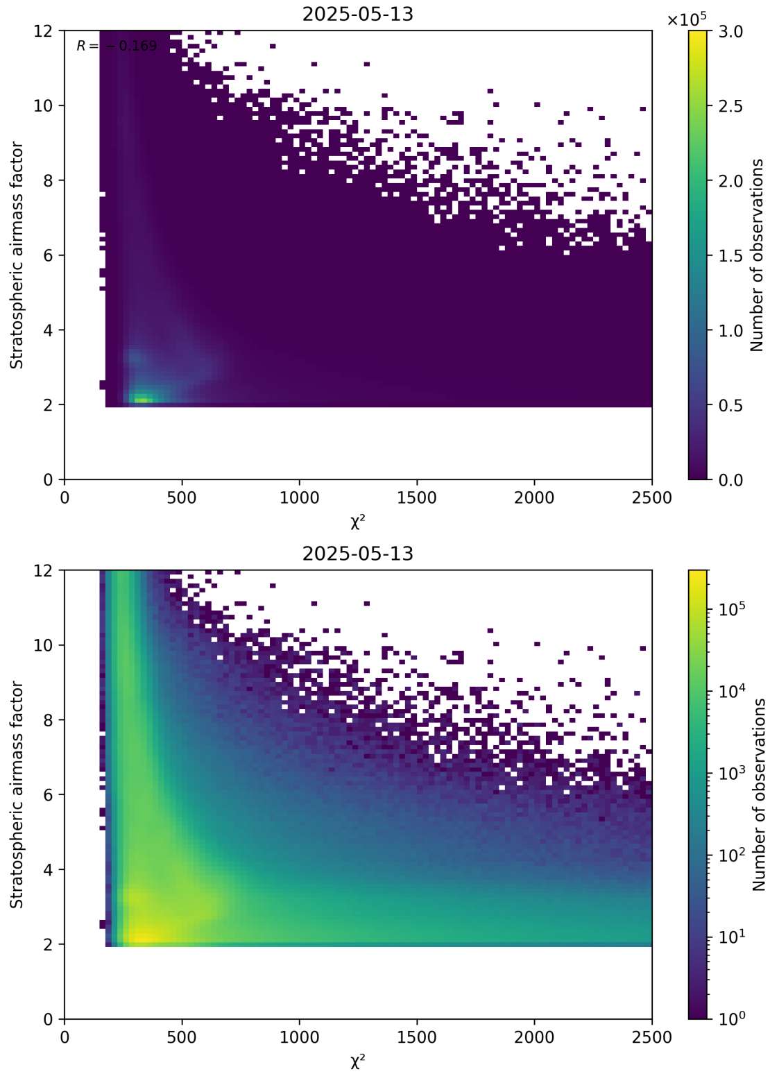
Figure 81: Scatter density plot of “ \chi^2 ” against “Stratospheric airmass factor” for 2025-05-13 to 2025-05-13.
