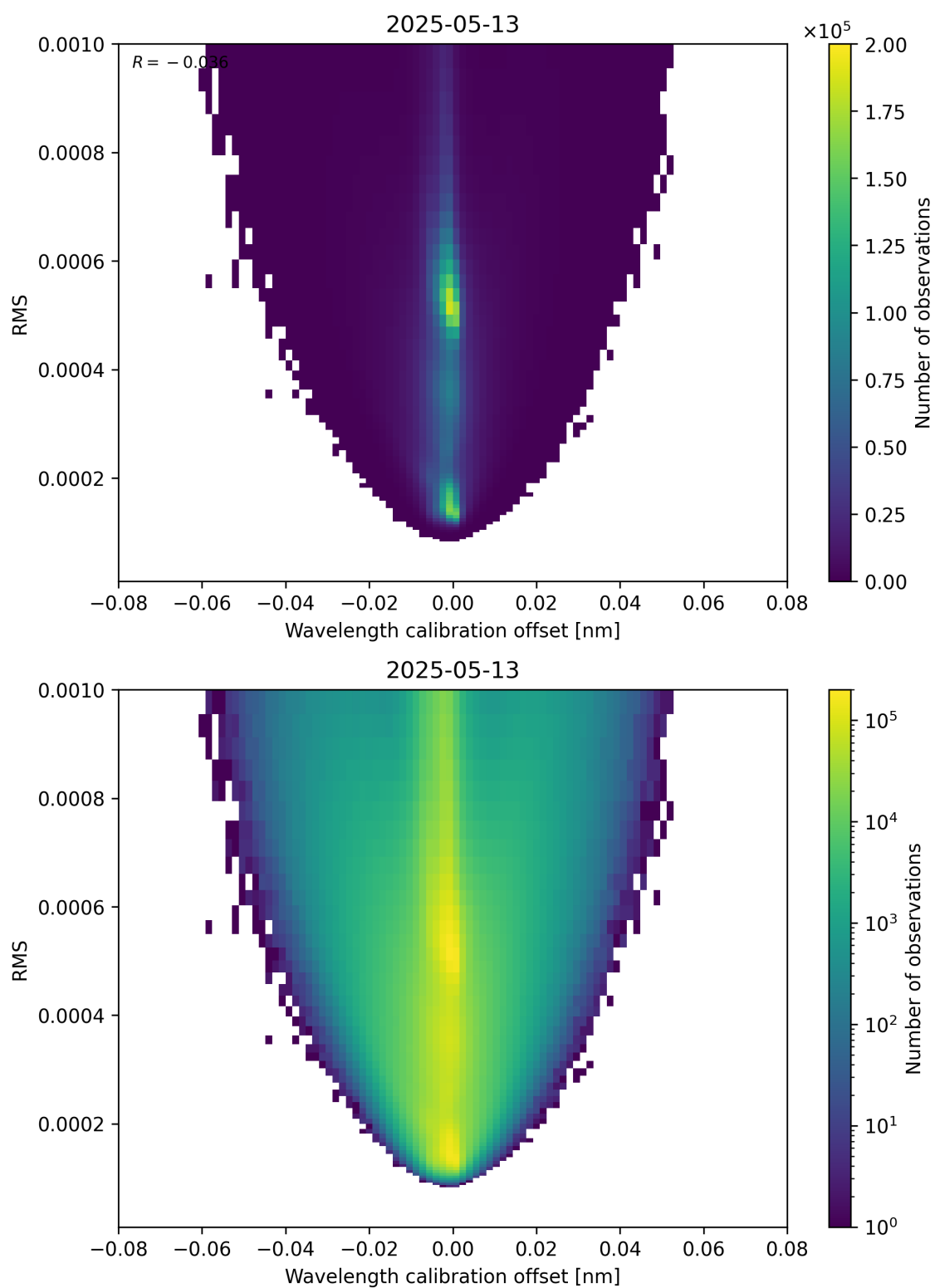
Figure 181: Scatter density plot of “Wavelength calibration offset” against “RMS” for 2025-05-13 to 2025-05-13.
