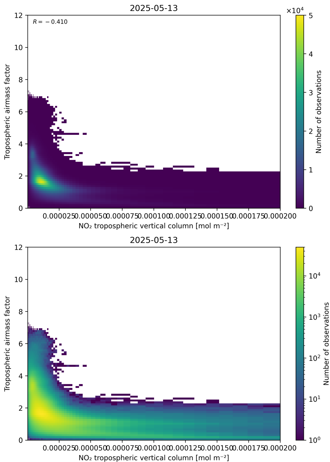
Figure 123: Scatter density plot of “NO 2 tropospheric vertical column” against “Tropospheric airmass factor” for 2025-05-13 to 2025-05-13.
