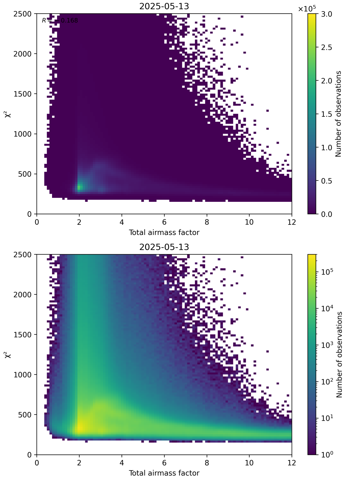
Figure 63: Scatter density plot of “Total airmass factor” against “ \chi^2 ” for 2025-05-13 to 2025-05-13.
