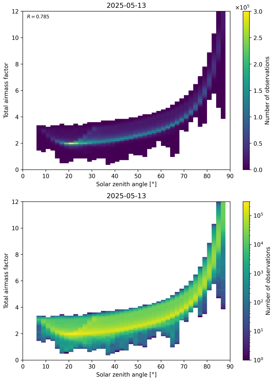
Figure 146: Scatter density plot of “Solar zenith angle” against “Total air mass factor” for 2025-05-13 to 2025-05-13.
