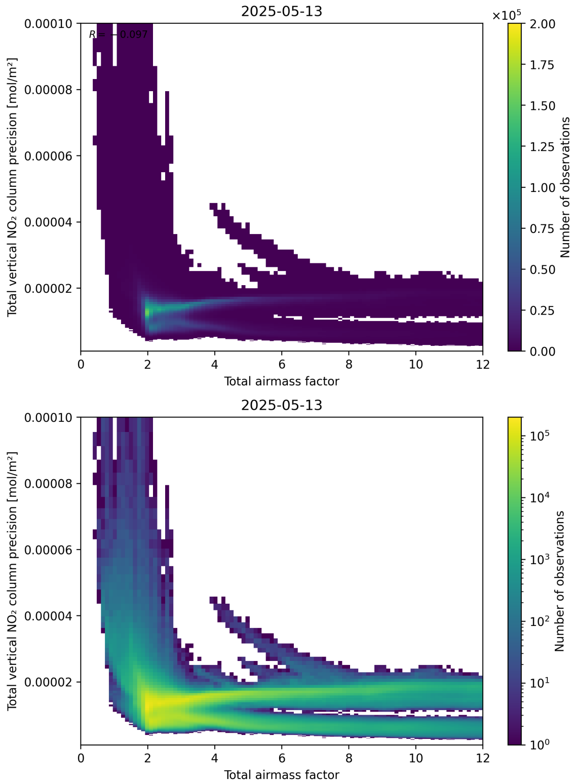
Figure 68: Scatter density plot of “Total airmass factor” against “Total vertical NO 2 column precision” for 2025-05-13 to 2025-05-13.
