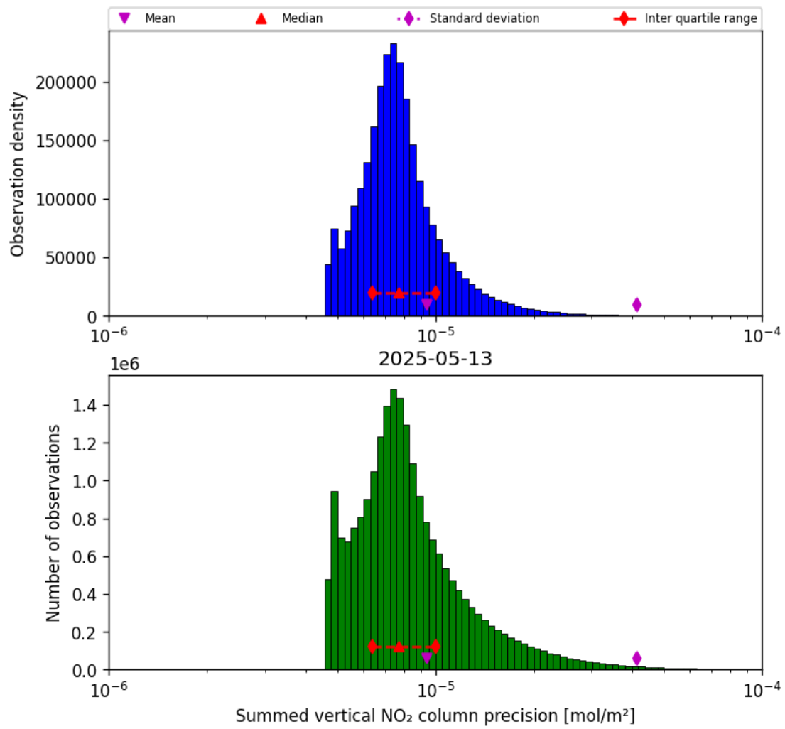
Figure 41: Histogram of "Summed vertical NO 2 column precision" for 2025-05-13 to 2025-05-13
