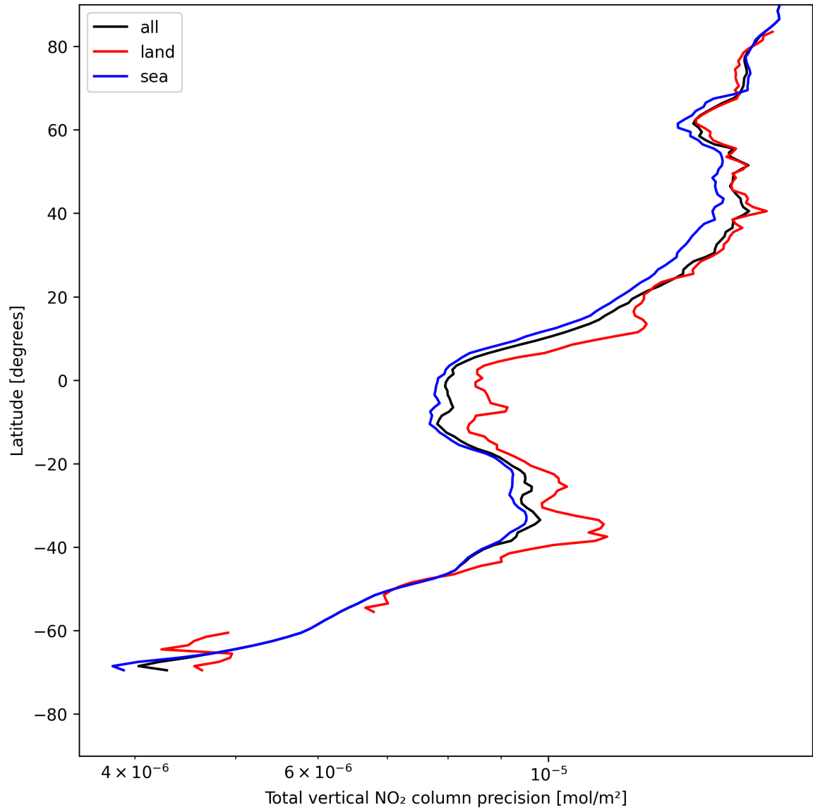
Figure 22: Zonal average of “Total vertical NO 2 column precision” for 2025-05-13 to 2025-05-13.
