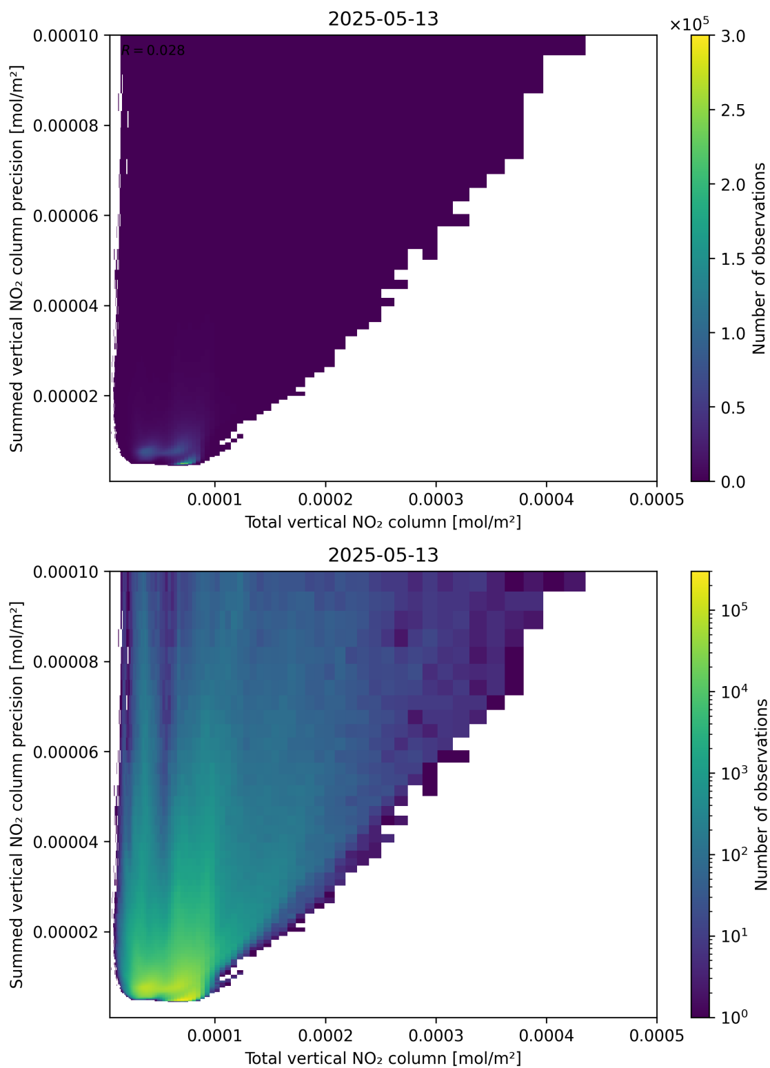
Figure 113: Scatter density plot of “Total vertical NO 2 column” against “Summed vertical NO 2 column precision” for 2025-05-13 to 2025-05-13.
