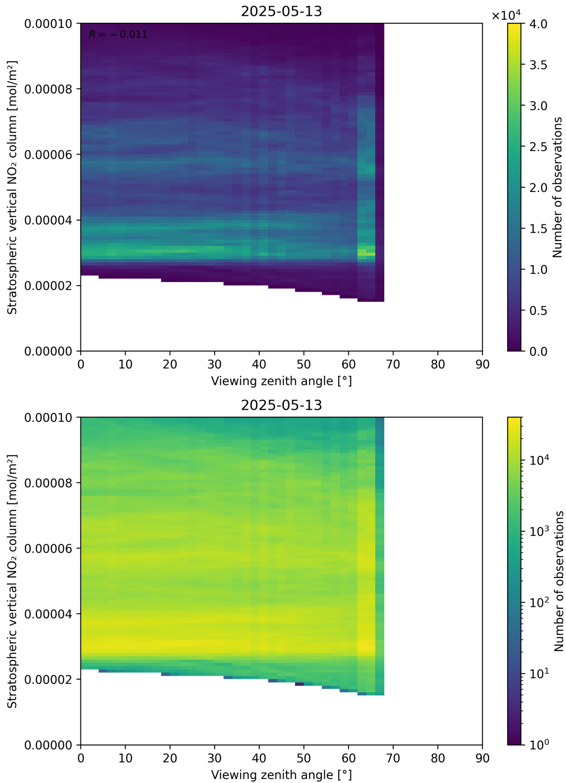
Figure 164: Scatter density plot of “Viewing zenith angle” against “Stratospheric vertical NO 2 column” for 2025-05-13 to 2025-05-13.
