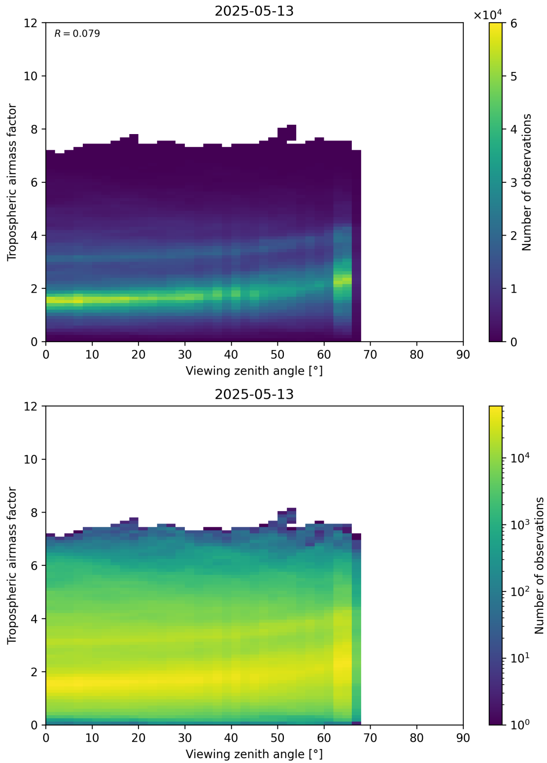
Figure 161: Scatter density plot of “Viewing zenith angle” against “Tropospheric airmass factor” for 2025-05-13 to 2025-05-13.
