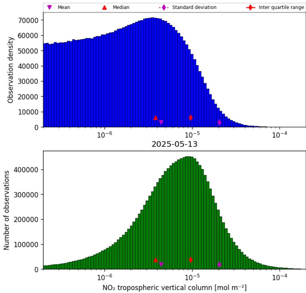
Figure 29: Histogram of “NO 2 tropospheric vertical column” for 2025-05-13 to 2025-05-13
