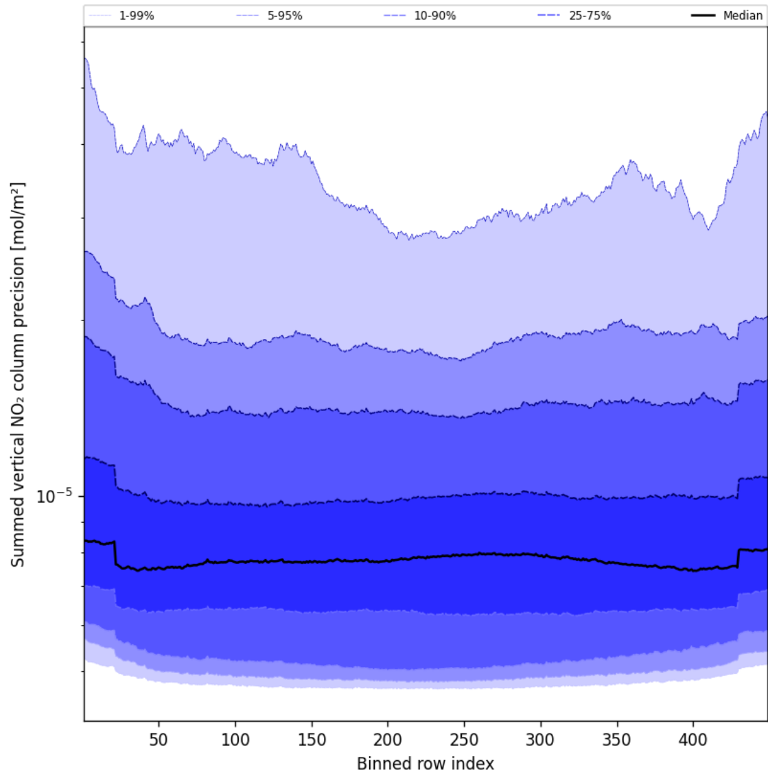
Figure 58: Along track statistics of “Summed vertical NO 2 column precision” for 2025-05-13 to 2025-05-13
