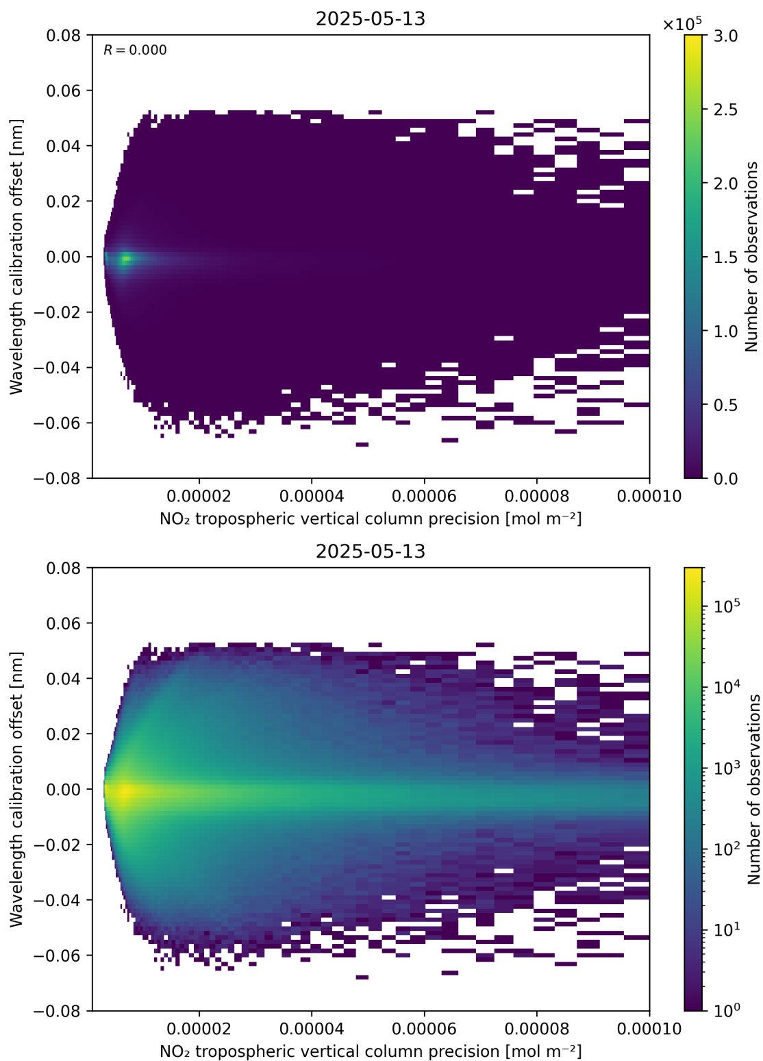
Figure 141: Scatter density plot of “NO 2 tropospheric vertical column precision” against “Wavelength calibration offset” for 2025-05-13 to 2025-05-13.
