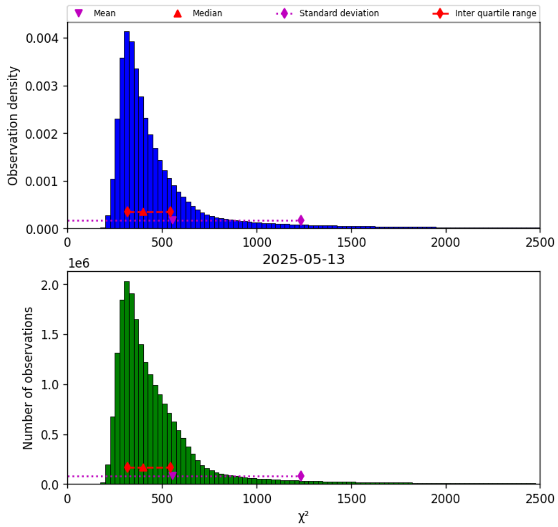
Figure 42: Histogram of “ \chi^2 ” for 2025-05-13 to 2025-05-13
