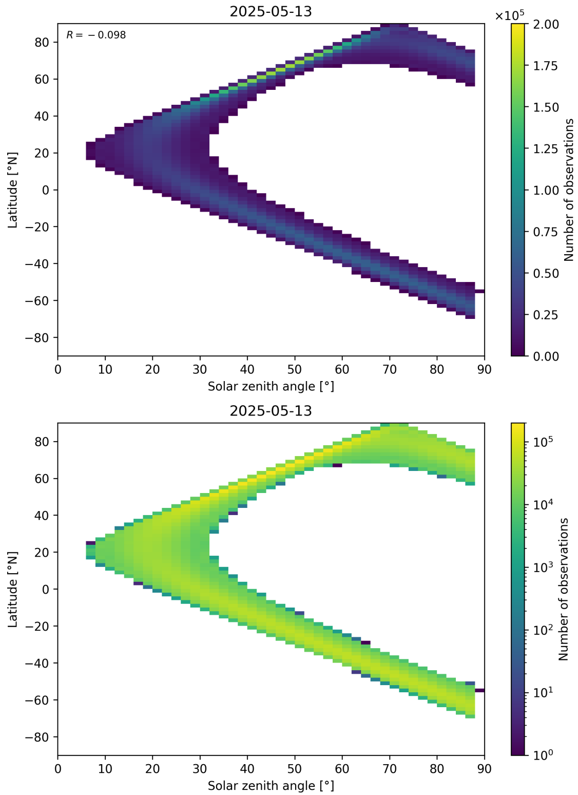
Figure 149: Scatter density plot of “Solar zenith angle” against “Latitude” for 2025-05-13 to 2025-05-13.
