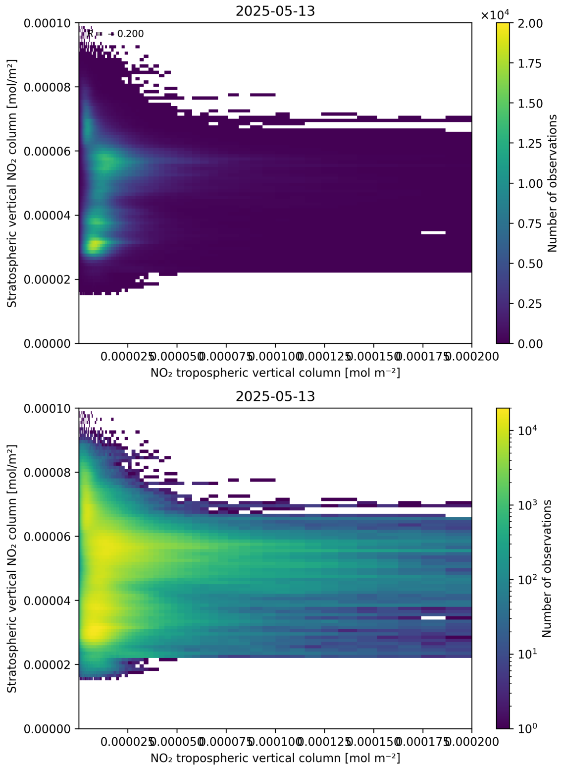
Figure 125: Scatter density plot of “NO 2 tropospheric vertical column” against “Stratospheric vertical NO 2 column” for 2025-05-13 to 2025-05-13.
