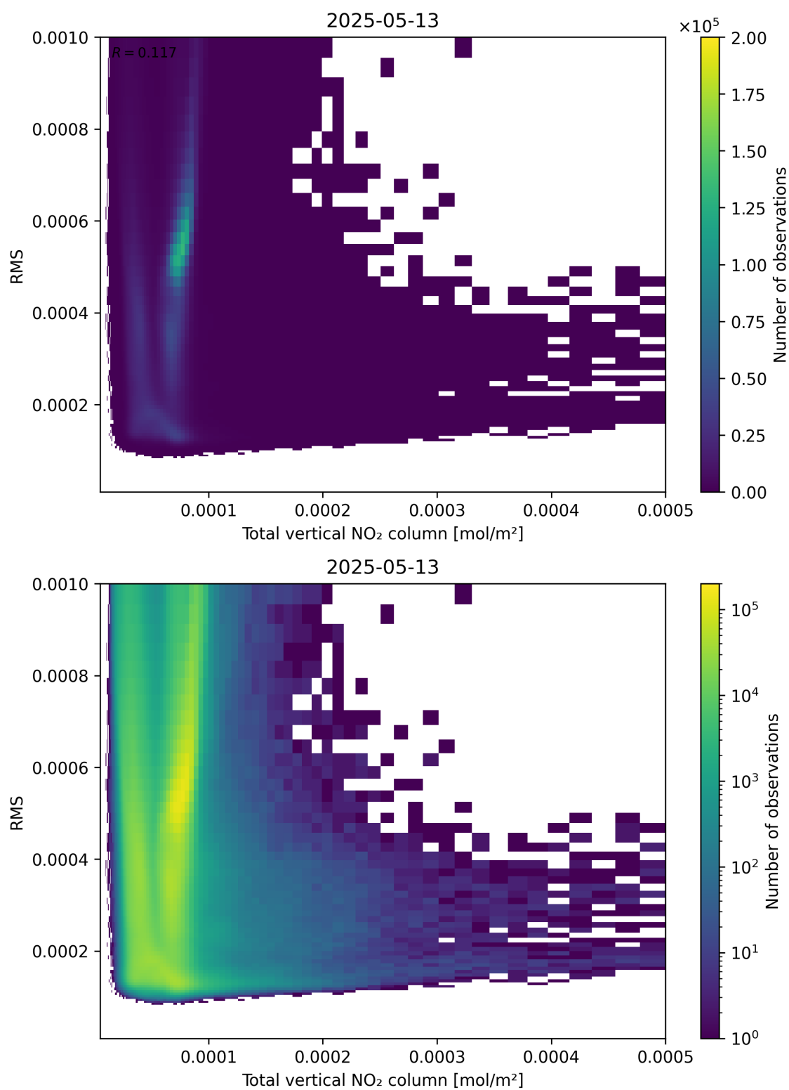
Figure 120: Scatter density plot of “Total vertical NO 2 column” against “RMS” for 2025-05-13 to 2025-05-13.
