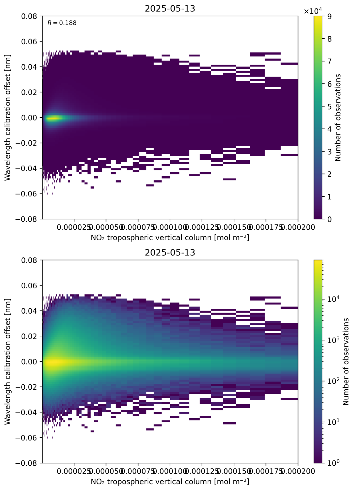
Figure 143: Scatter density plot of “NO 2 tropospheric vertical column” against “Wavelength calibration offset” for 2025-05-13 to 2025-05-13.
