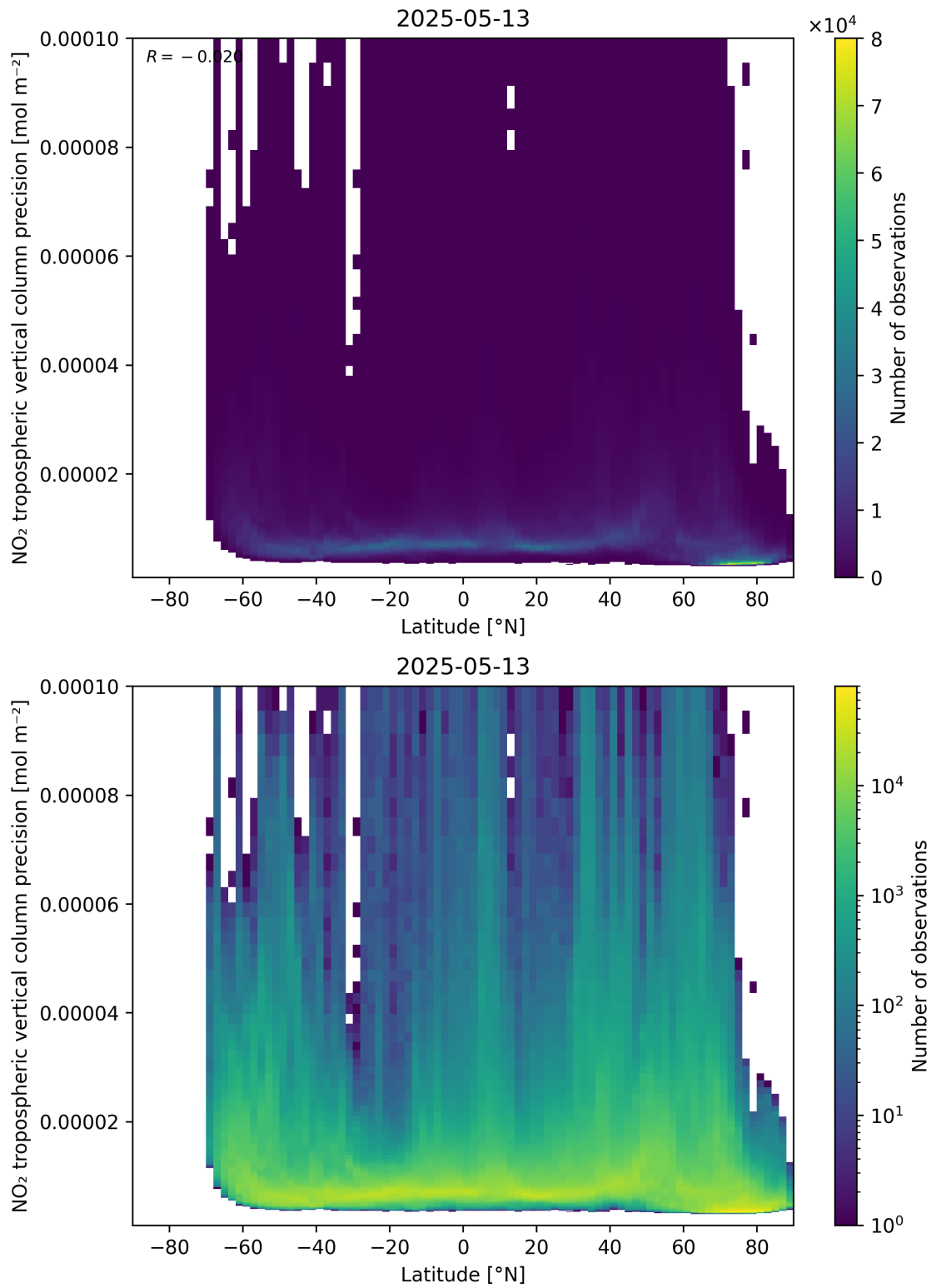
Figure 93: Scatter density plot of “Latitude” against “NO 2 tropospheric vertical column precision” for 2025-05-13 to 2025-05-13.
