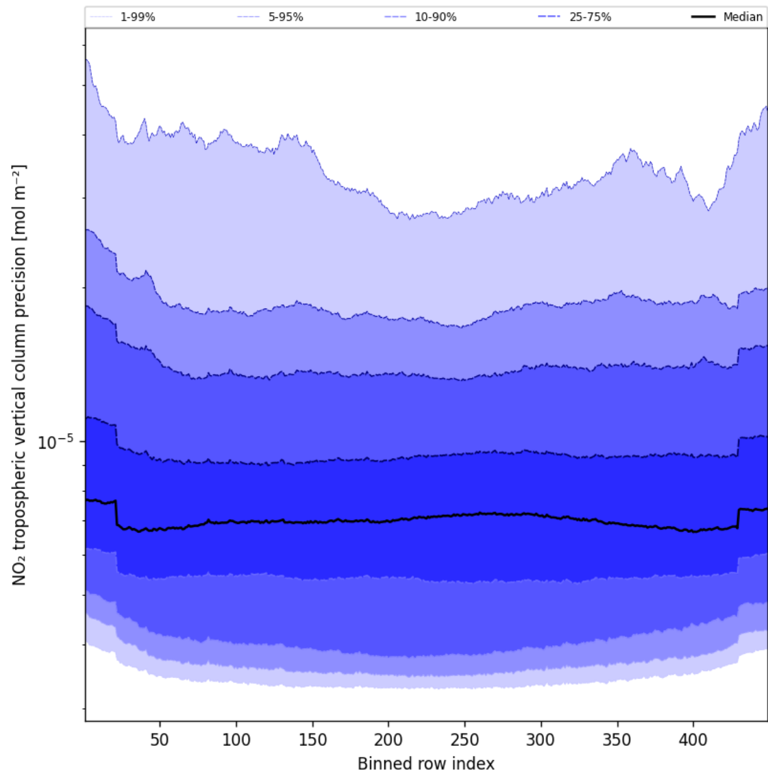
Figure 47: Along track statistics of “NO 2 tropospheric vertical column precision” for 2025-05-13 to 2025-05-13
