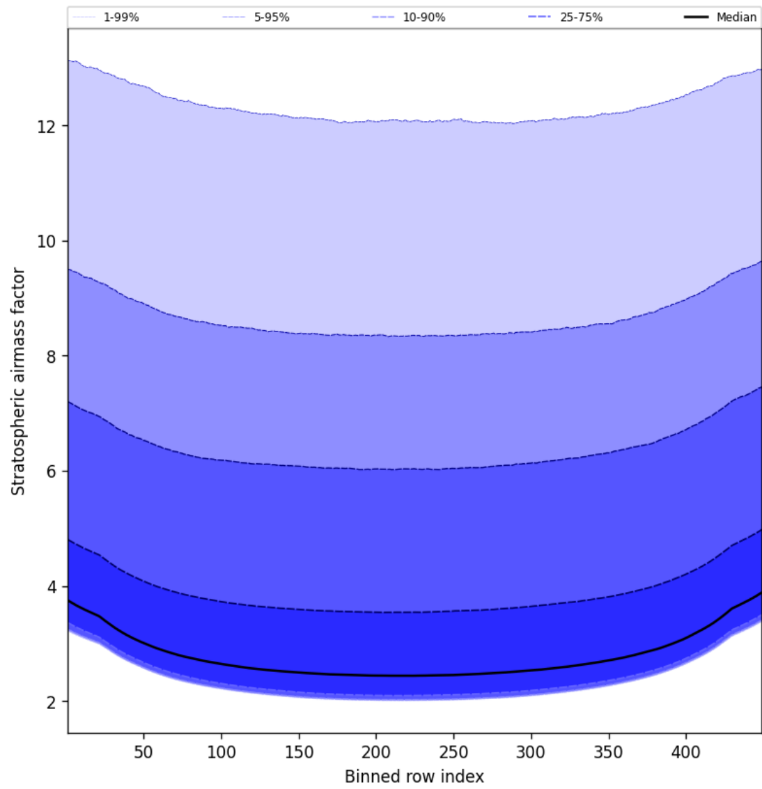
Figure 61: Along track statistics of “Stratospheric airmass factor” for 2025-05-13 to 2025-05-13
