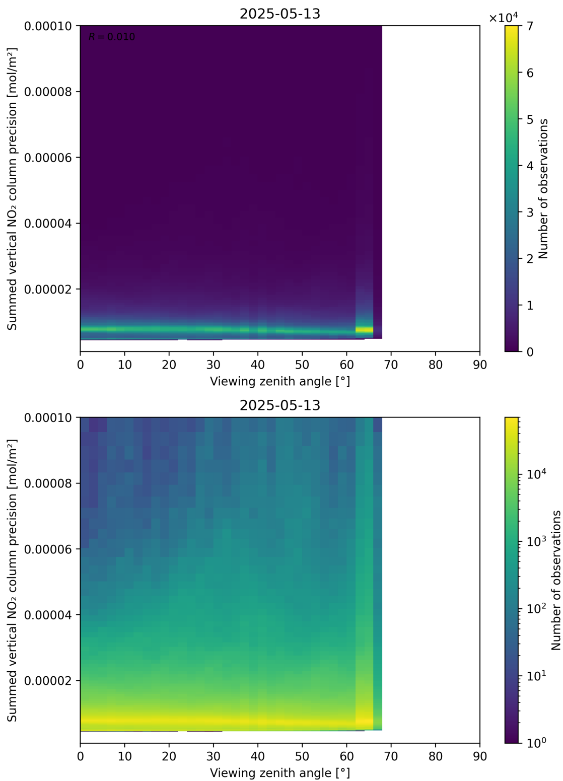
Figure 166: Scatter density plot of “Viewing zenith angle” against “Summed vertical NO 2 column precision” for 2025-05-13 to 2025-05-13.
