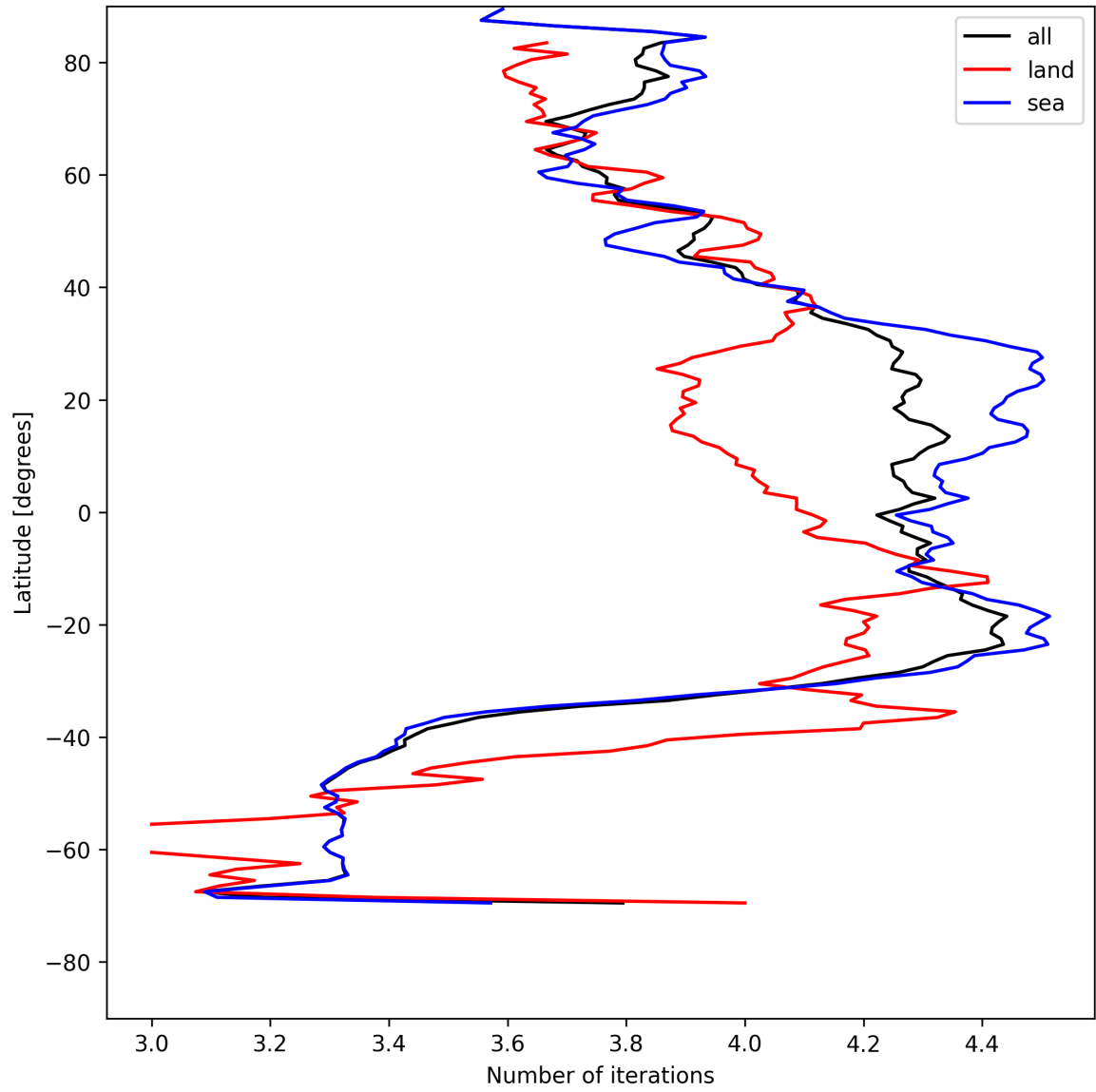
Figure 17: Zonal average of “Number of iterations” for 2025-05-13 to 2025-05-13.
