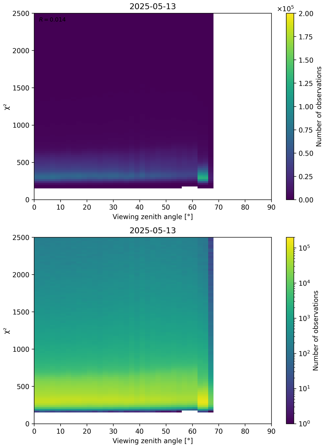
Figure 162: Scatter density plot of “Viewing zenith angle” against “ \chi^2 ” for 2025-05-13 to 2025-05-13.
