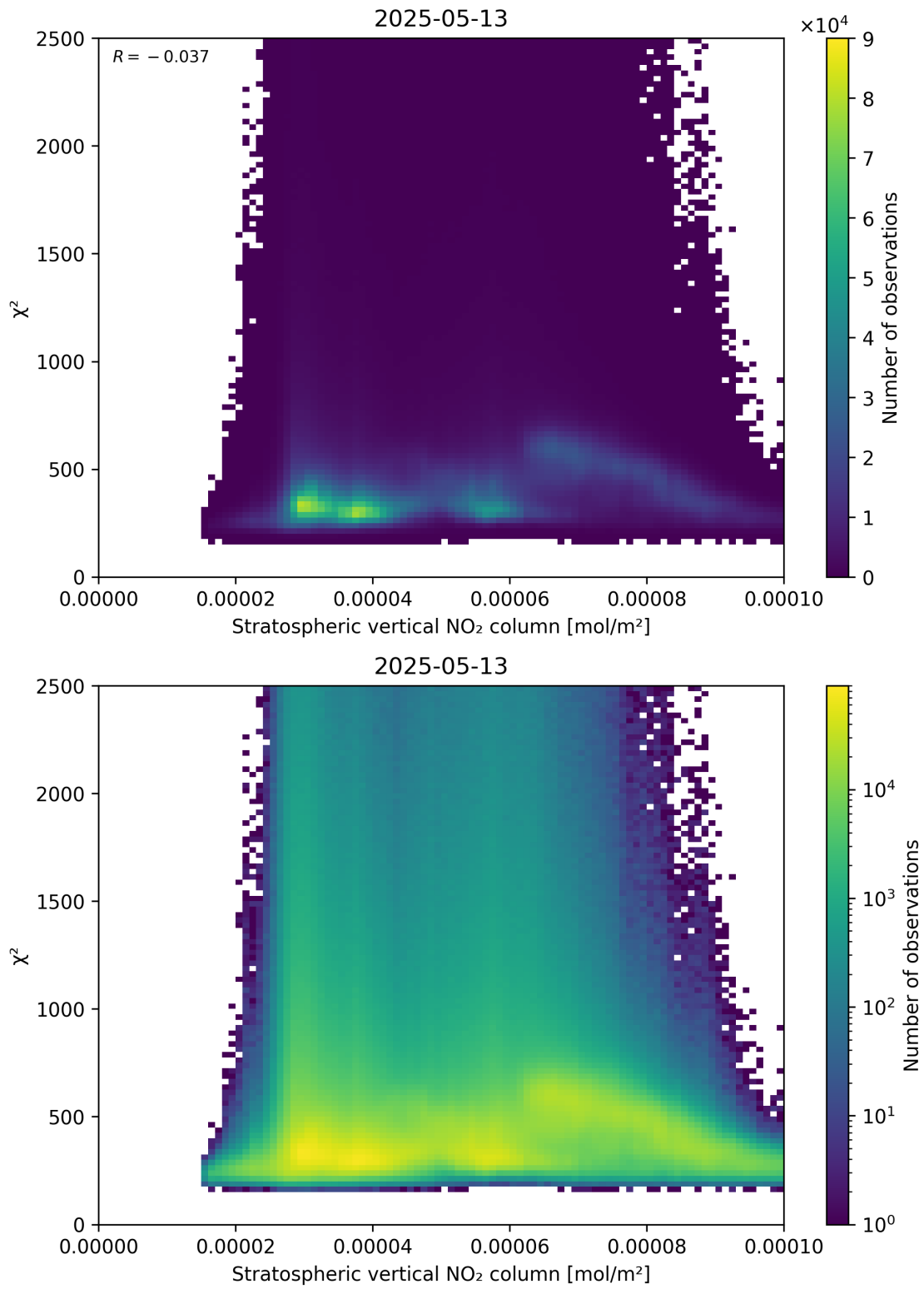
Figure 97: Scatter density plot of “Stratospheric vertical NO 2 column” against “ \chi^2 ” for 2025-05-13 to 2025-05-13.
