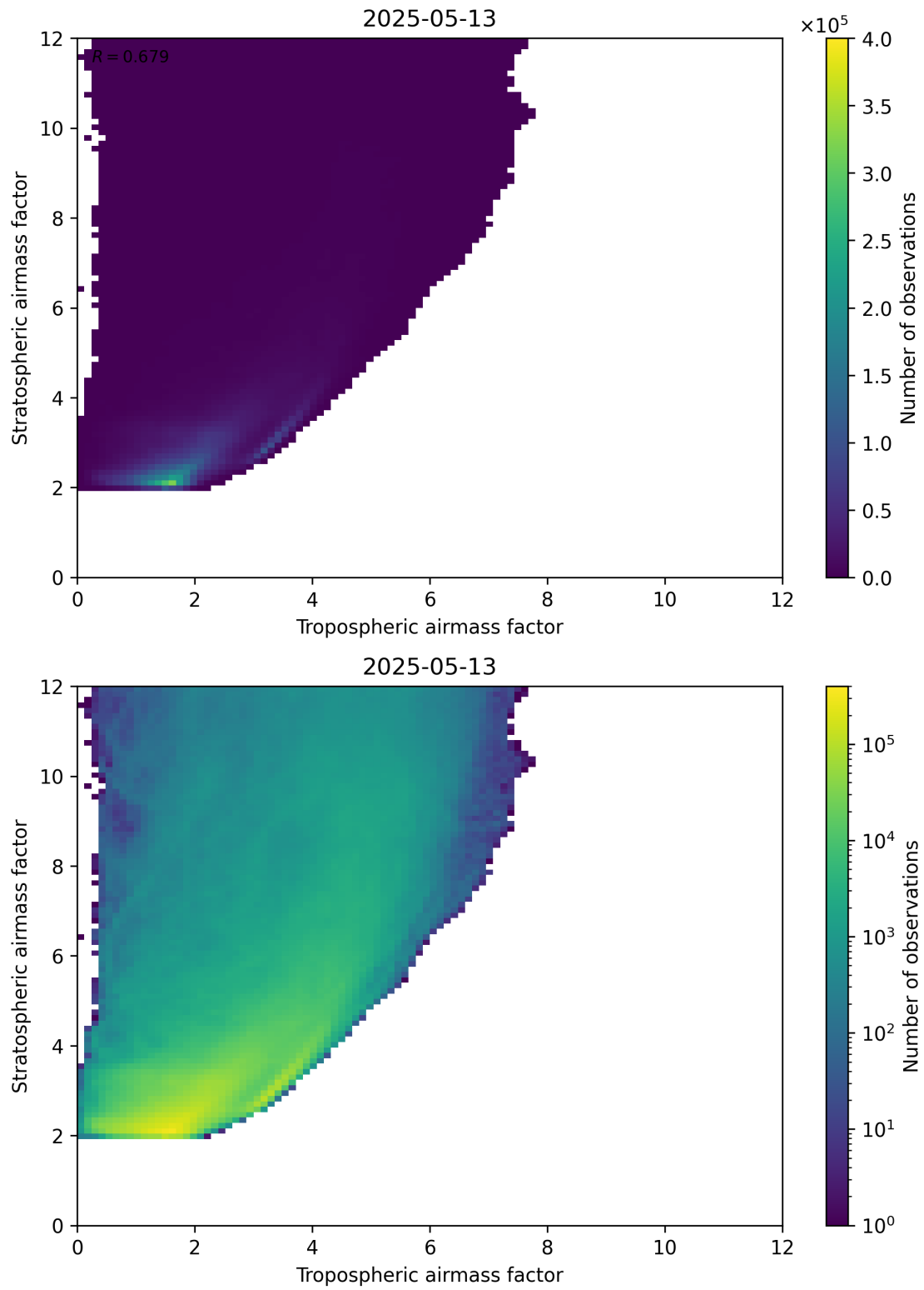
Figure 71: Scatter density plot of “Tropospheric airmass factor” against “Stratospheric airmass factor” for 2025-05-13 to 2025-05-13.
