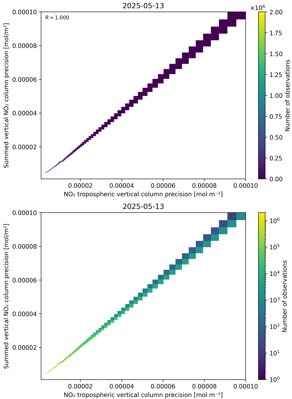
Figure 137: Scatter density plot of “NO 2 tropospheric vertical column precision” against “Summed vertical NO 2 column precision” for 2025-05-13 to 2025-05-13.
