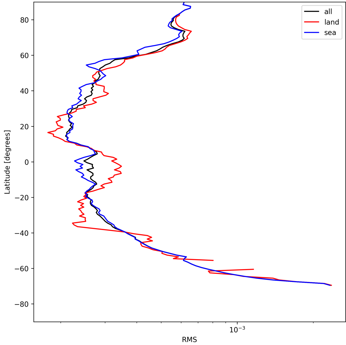
Figure 26: Zonal average of “RMS” for 2025-05-13 to 2025-05-13.
