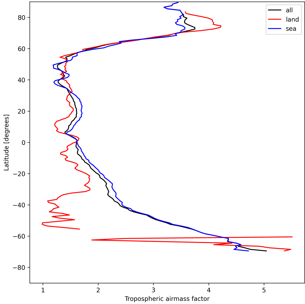
Figure 14: Zonal average of “Tropospheric air mass factor” for 2025-05-13 to 2025-05-13.
