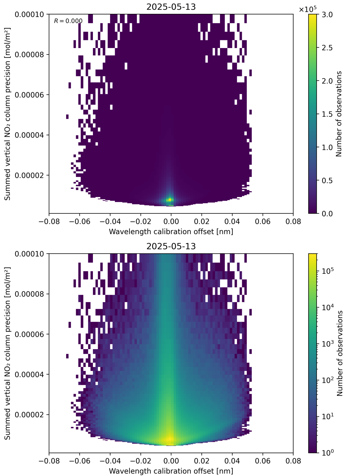
Figure 178: Scatter density plot of “Wavelength calibration offset” against “Summed vertical NO 2 column precision” for 2025-05-13 to 2025-05-13.
