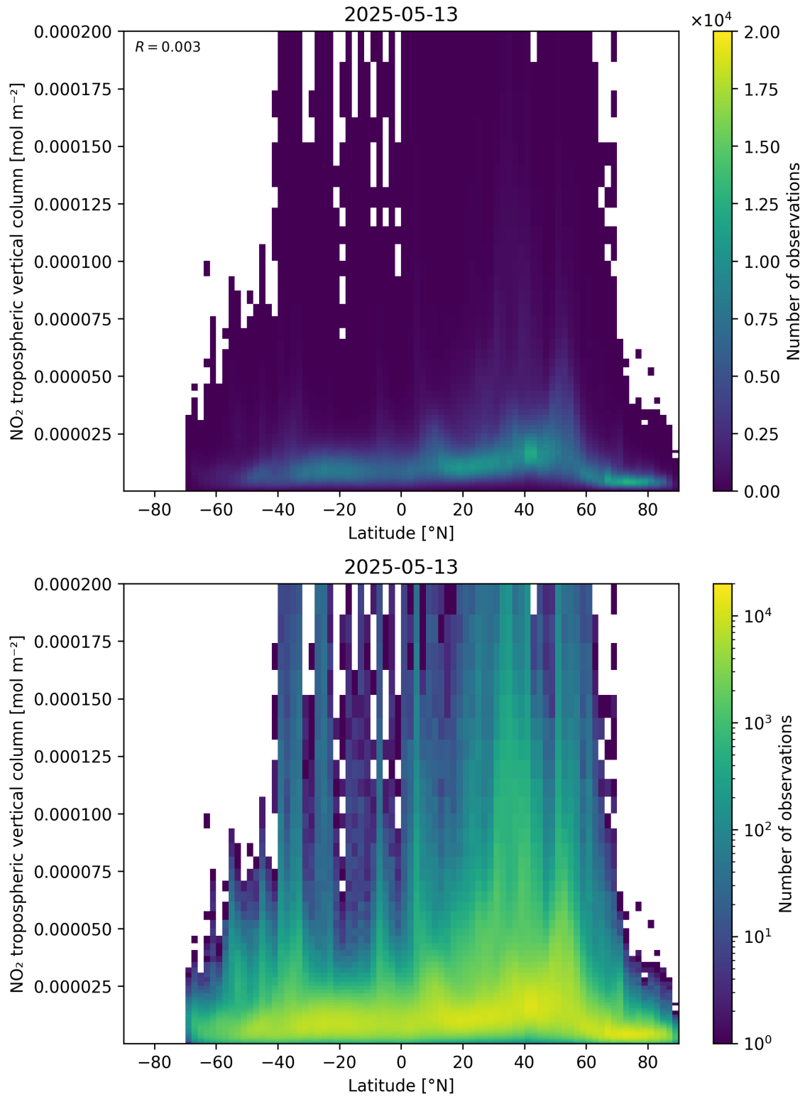
Figure 92: Scatter density plot of “Latitude” against “NO 2 tropospheric vertical column” for 2025-05-13 to 2025-05-13.
