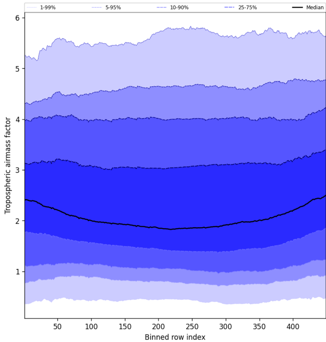
Figure 48: Along track statistics of "Tropospheric airmass factor" for 2025-05-13 to 2025-05-13
