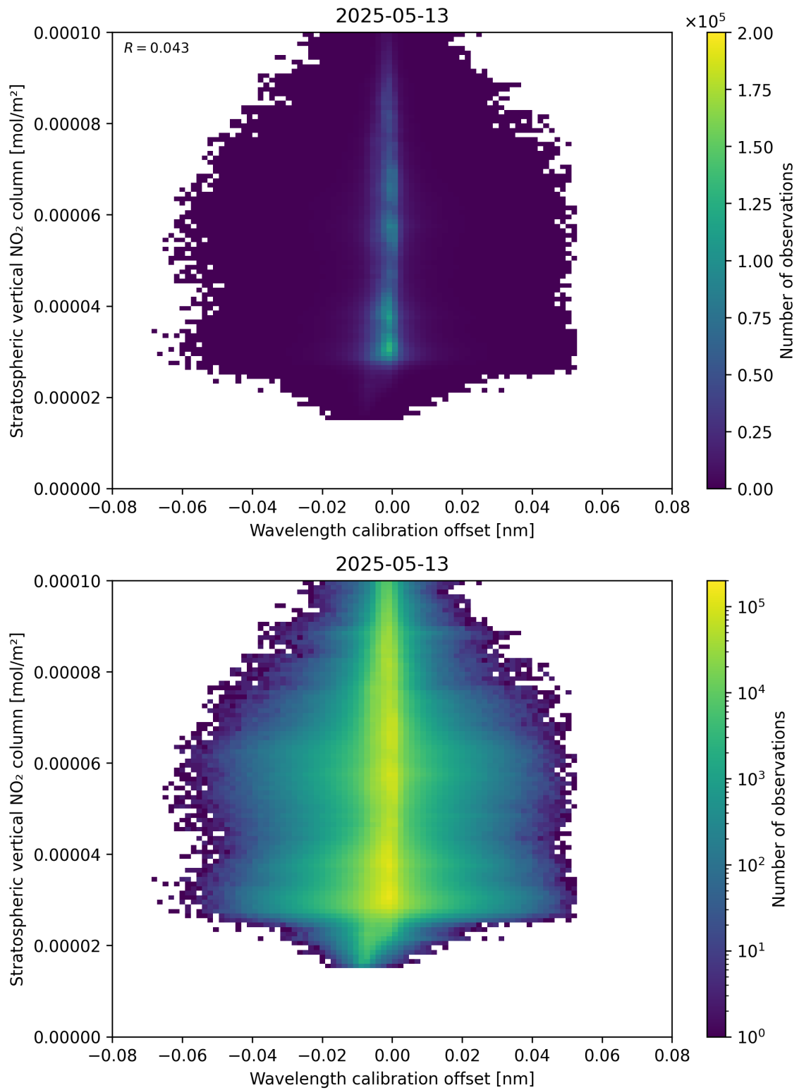
Figure 176: Scatter density plot of “Wavelength calibration offset” against “Stratospheric vertical NO 2 column” for 2025-05-13 to 2025-05-13.
