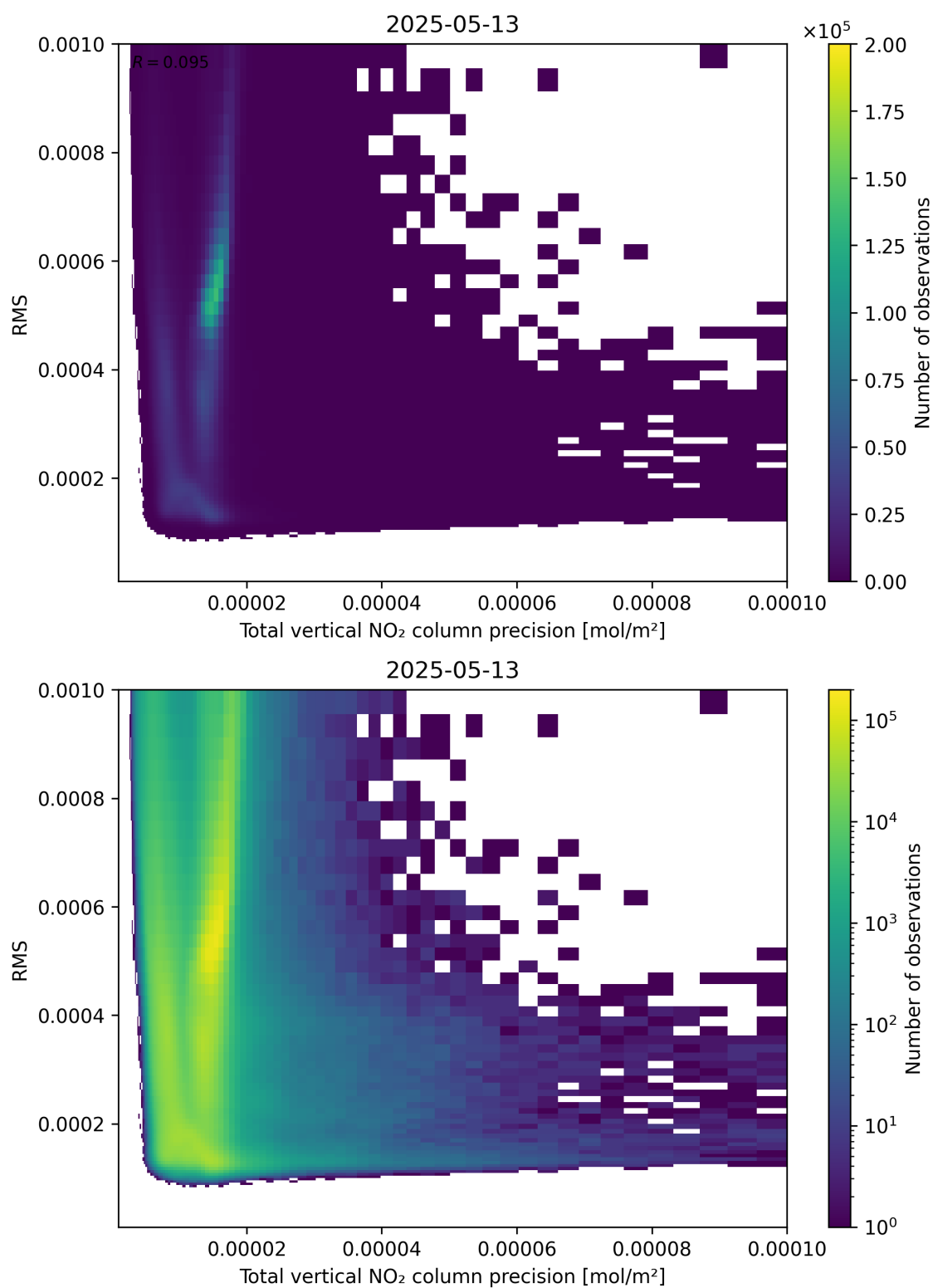
Figure 119: Scatter density plot of “Total vertical NO 2 column precision” against “RMS” for 2025-05-13 to 2025-05-13.
