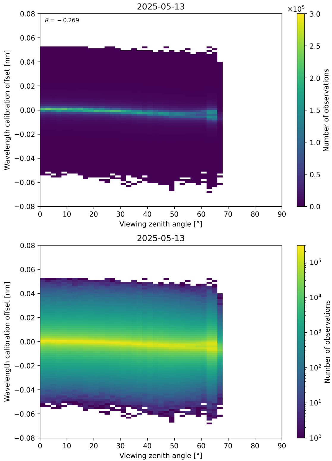
Figure 173: Scatter density plot of “Viewing zenith angle” against “Wavelength calibration offset” for 2025-05-13 to 2025-05-13.
