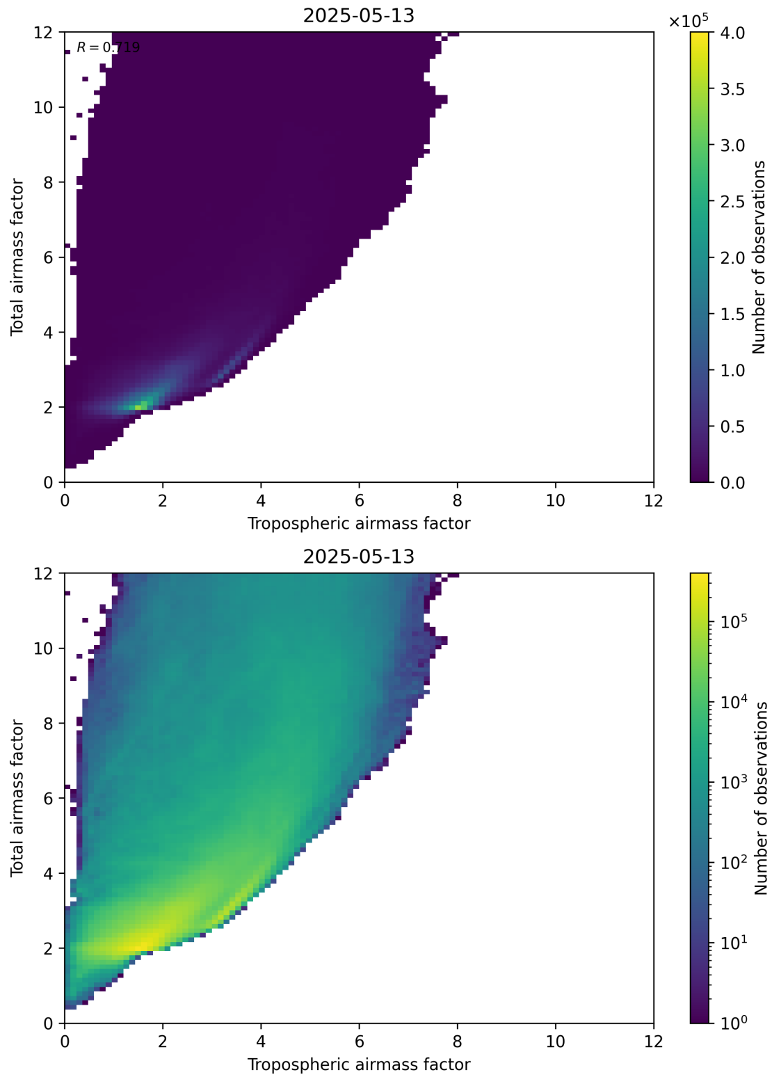
Figure 72: Scatter density plot of “Tropospheric airmass factor” against “Total airmass factor” for 2025-05-13 to 2025-05-13.
