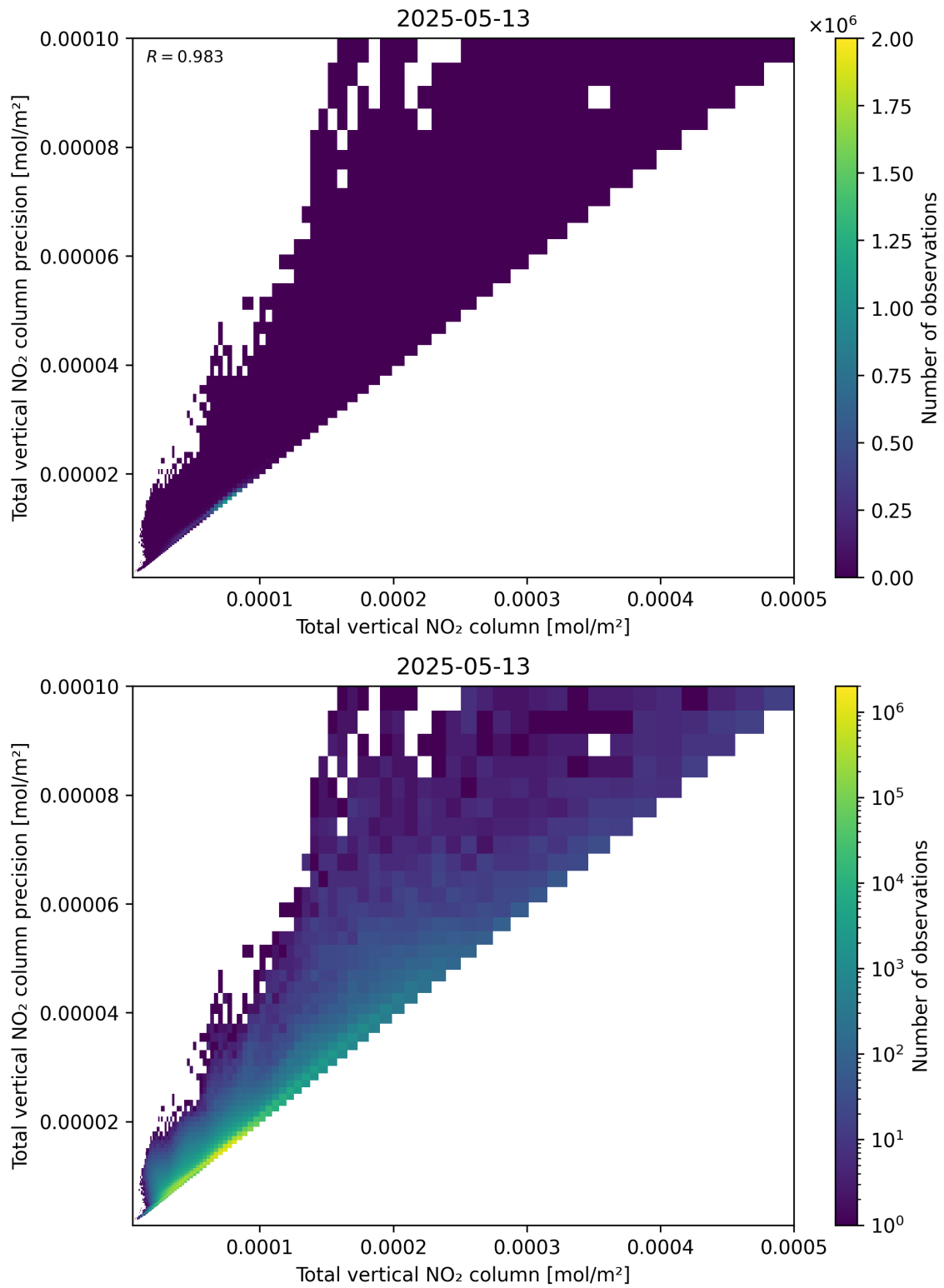
Figure 114: Scatter density plot of “Total vertical NO 2 column” against “Total vertical NO 2 column precision” for 2025-05-13 to 2025-05-13.
