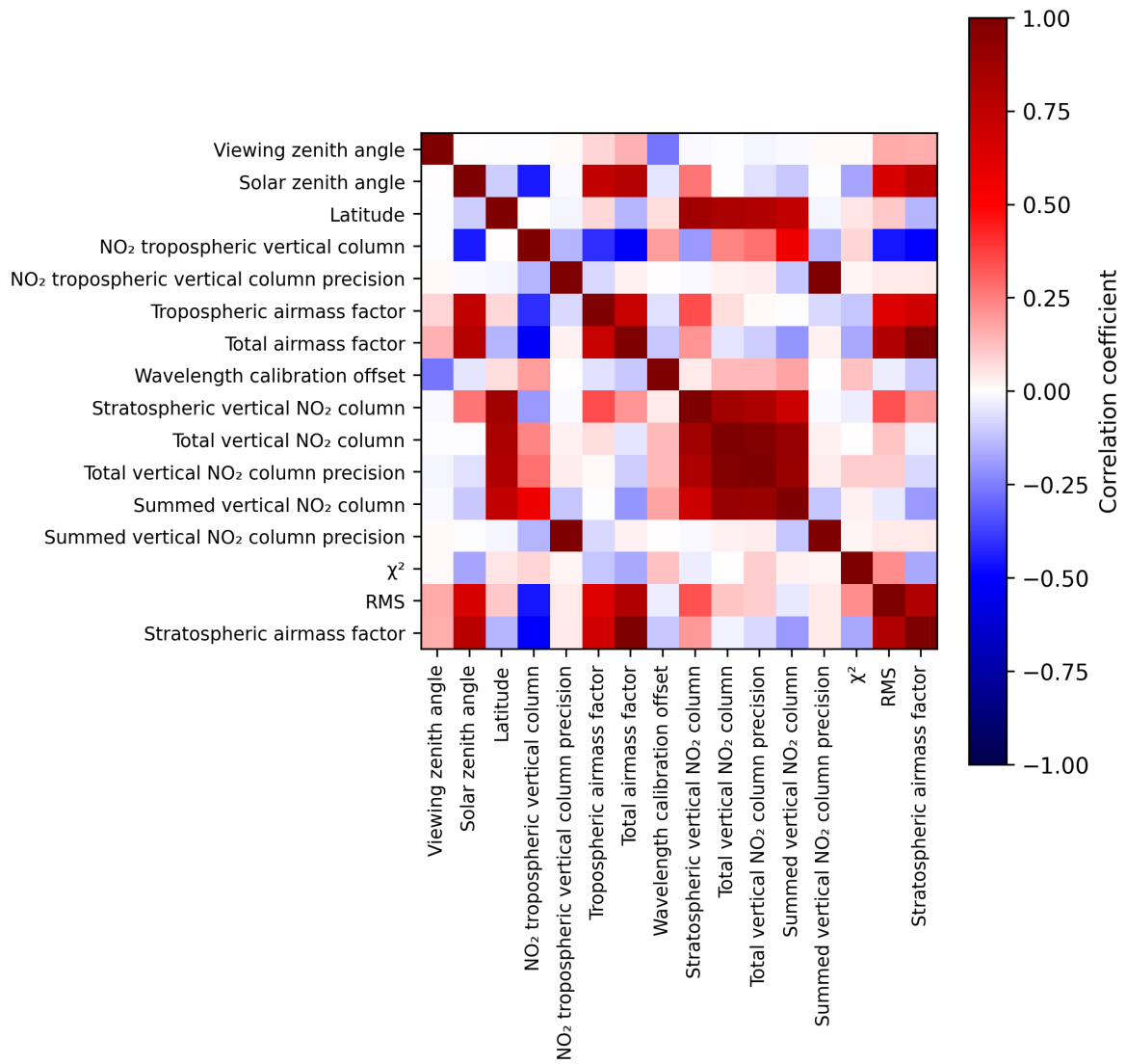
Figure 2: Map of correlation matrix for 2025-05-13 to 2025-05-13.
