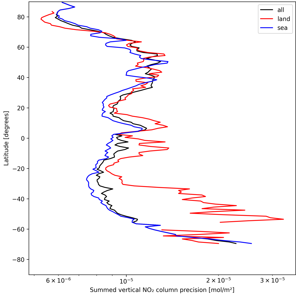
Figure 24: Zonal average of “Summed vertical NO 2 column precision” for 2025-05-13 to 2025-05-13.
