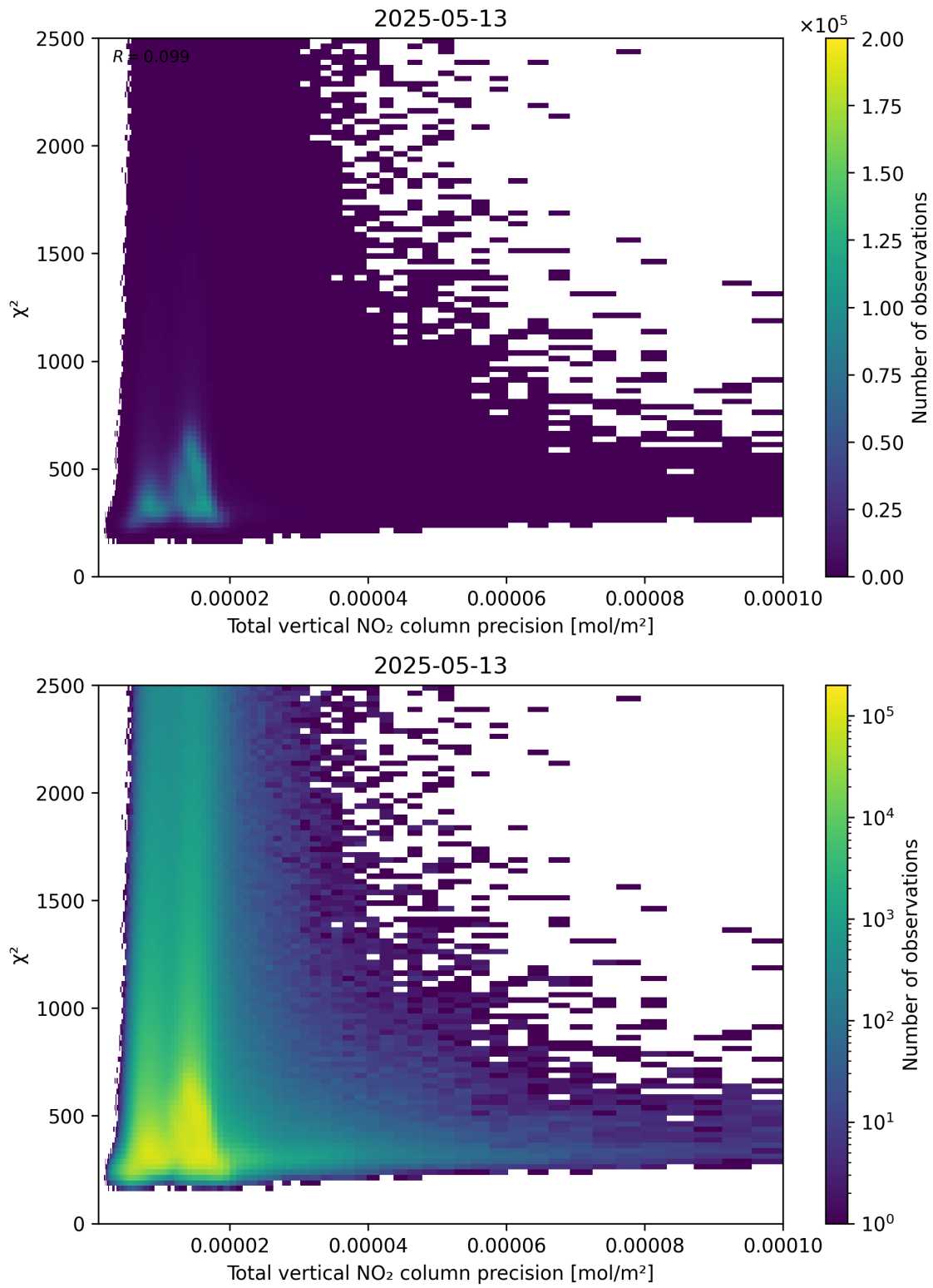
Figure 116: Scatter density plot of “Total vertical NO 2 column precision” against “ \chi^2 ” for 2025-05-13 to 2025-05-13.
