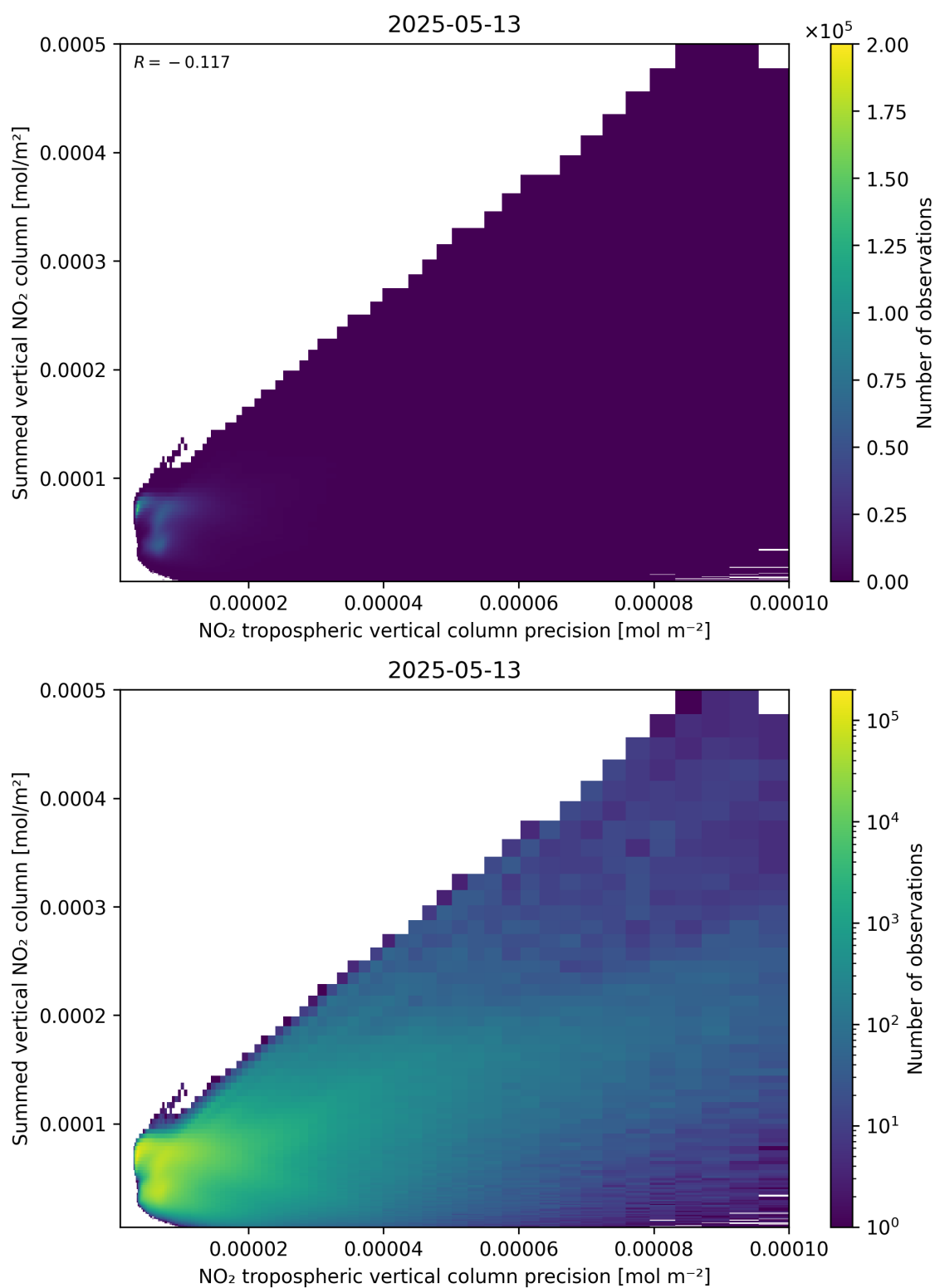
Figure 136: Scatter density plot of “NO 2 tropospheric vertical column precision” against “Summed vertical NO 2 column” for 2025-05-13 to 2025-05-13.
