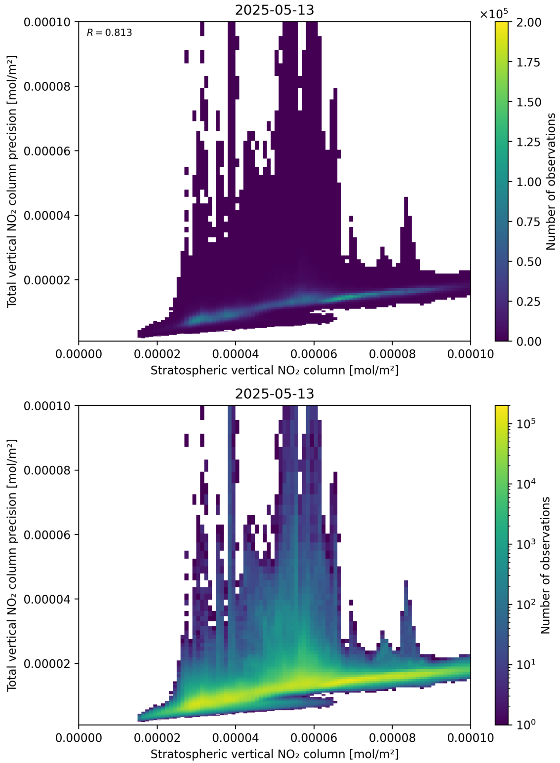
Figure 101: Scatter density plot of “Stratospheric vertical NO 2 column” against “Total vertical NO 2 column precision” for 2025-05-13 to 2025-05-13.
