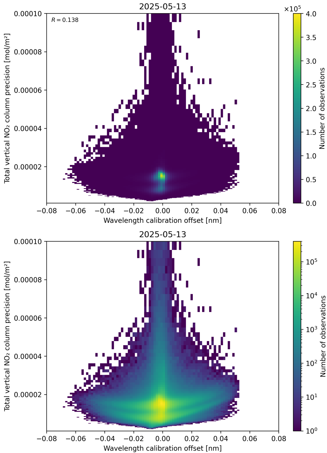
Figure 180: Scatter density plot of “Wavelength calibration offset” against “Total vertical NO 2 column precision” for 2025-05-13 to 2025-05-13.
