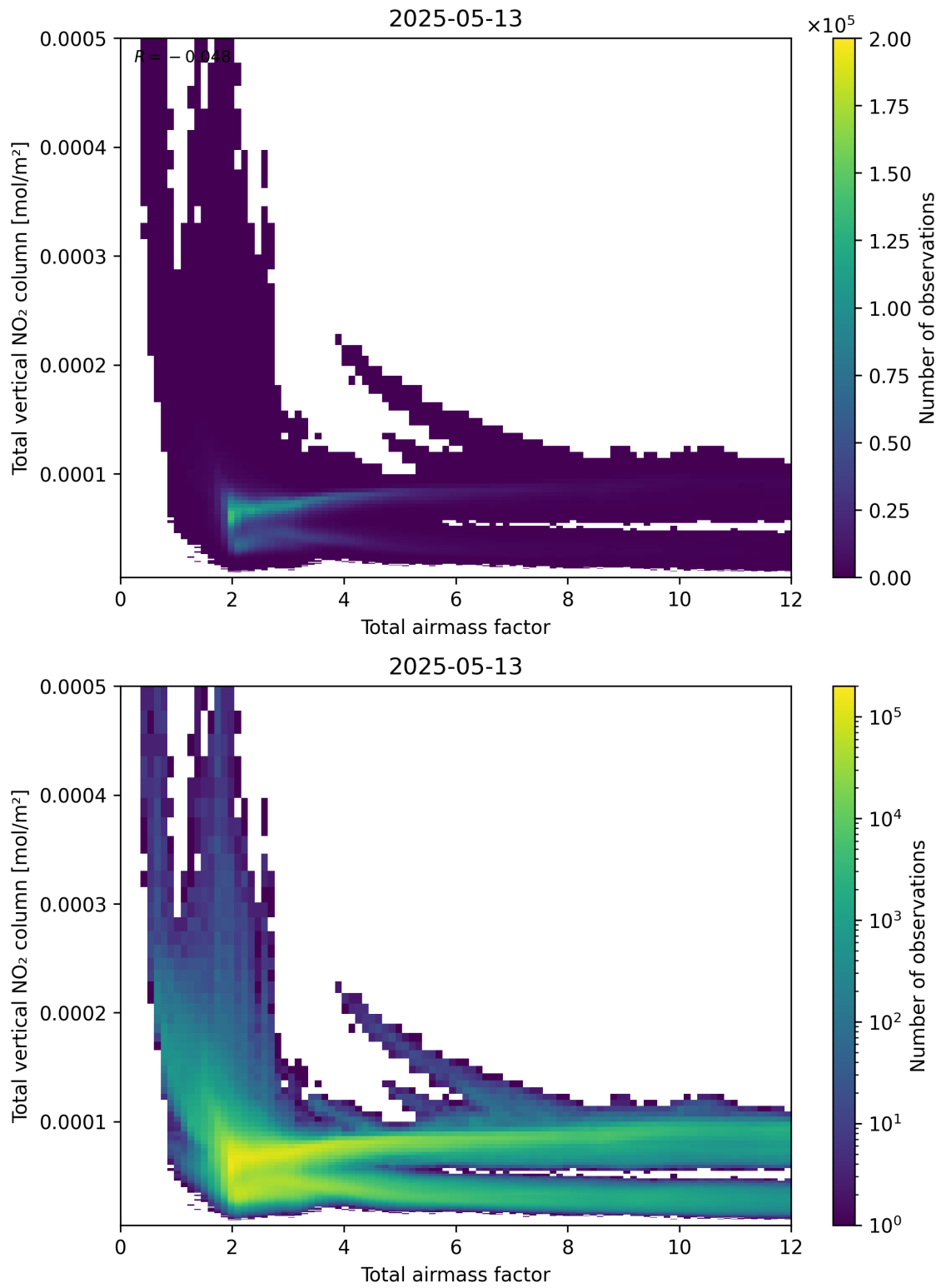
Figure 67: Scatter density plot of “Total airmass factor” against “Total vertical NO 2 column” for 2025-05-13 to 2025-05-13.
