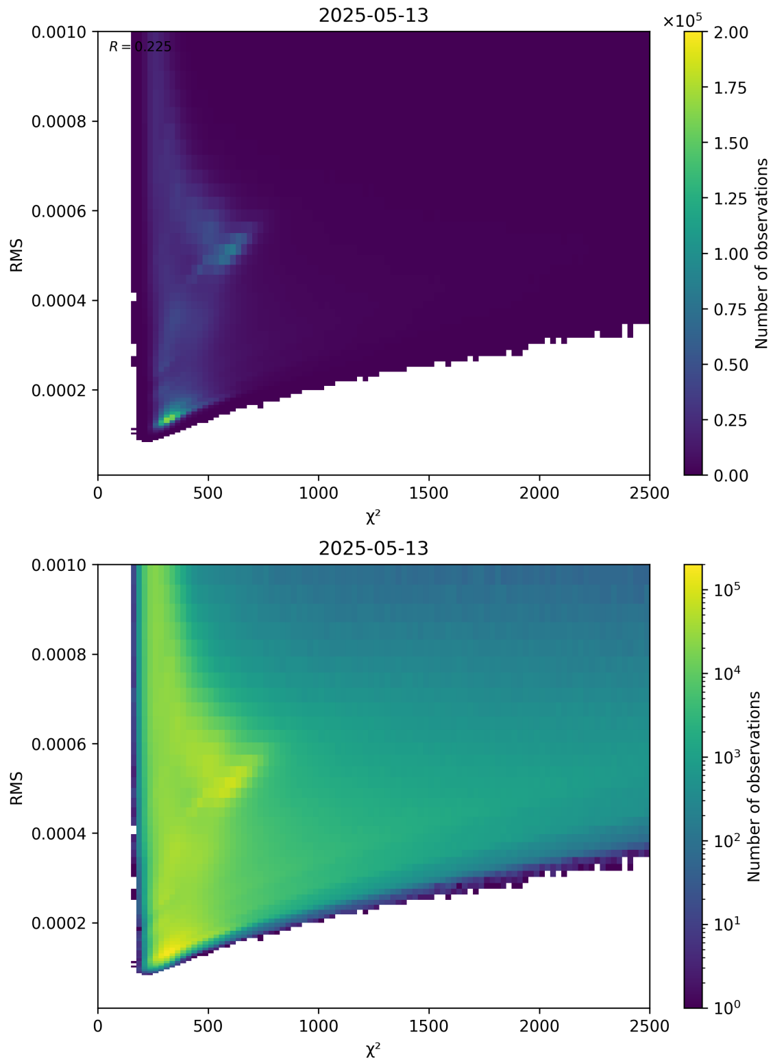
Figure 82: Scatter density plot of “ \chi^2 ” against “RMS” for 2025-05-13 to 2025-05-13.
