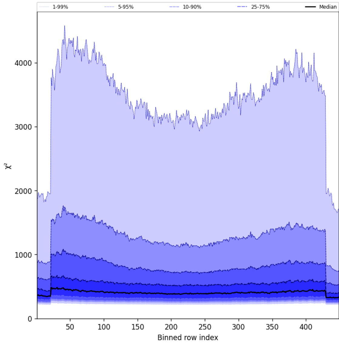
Figure 59: Along track statistics of “ \chi^2 ” for 2025-05-13 to 2025-05-13
