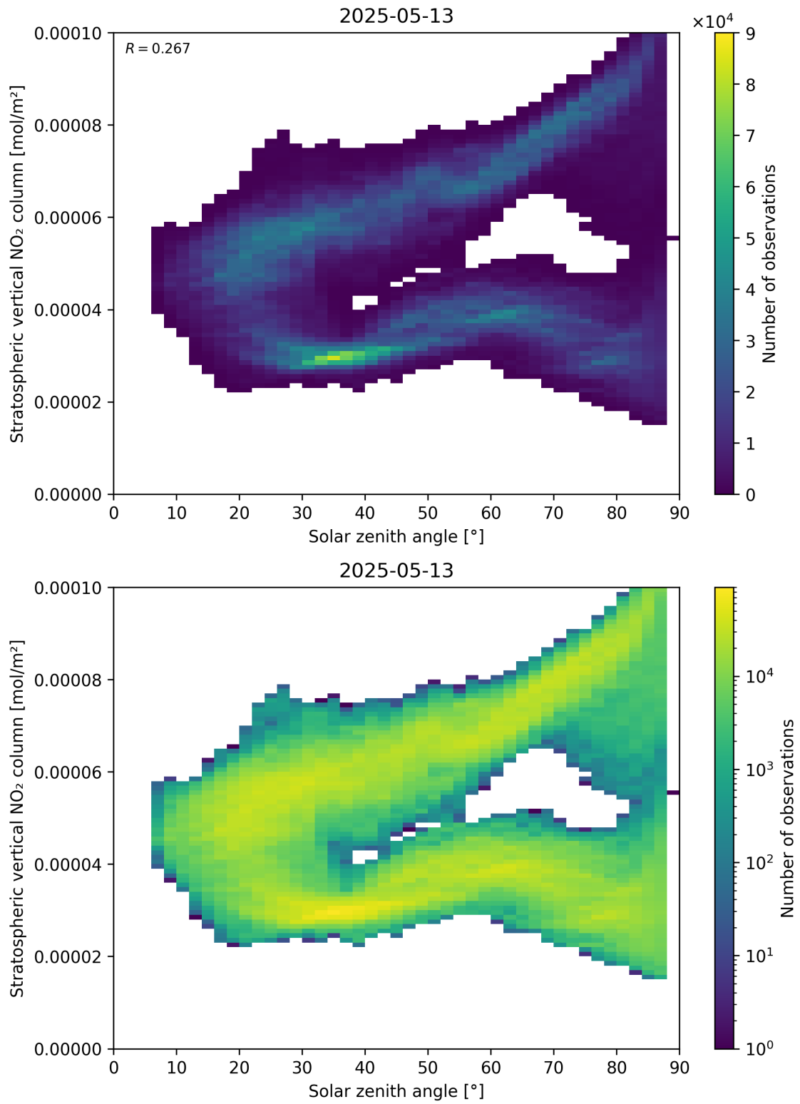
Figure 150: Scatter density plot of “Solar zenith angle” against “Stratospheric vertical NO 2 column” for 2025-05-13 to 2025-05-13.
