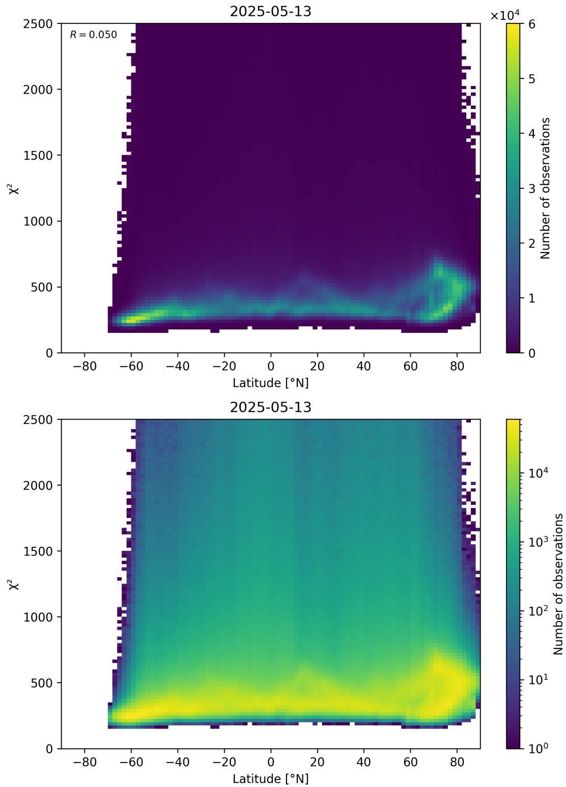
Figure 86: Scatter density plot of “Latitude” against “ \chi^2 ” for 2025-05-13 to 2025-05-13.
