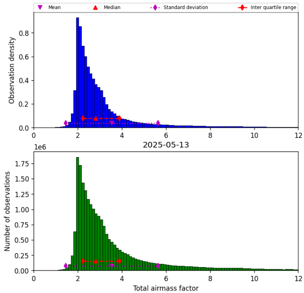
Figure 32: Histogram of “Total airmass factor” for 2025-05-13 to 2025-05-13
