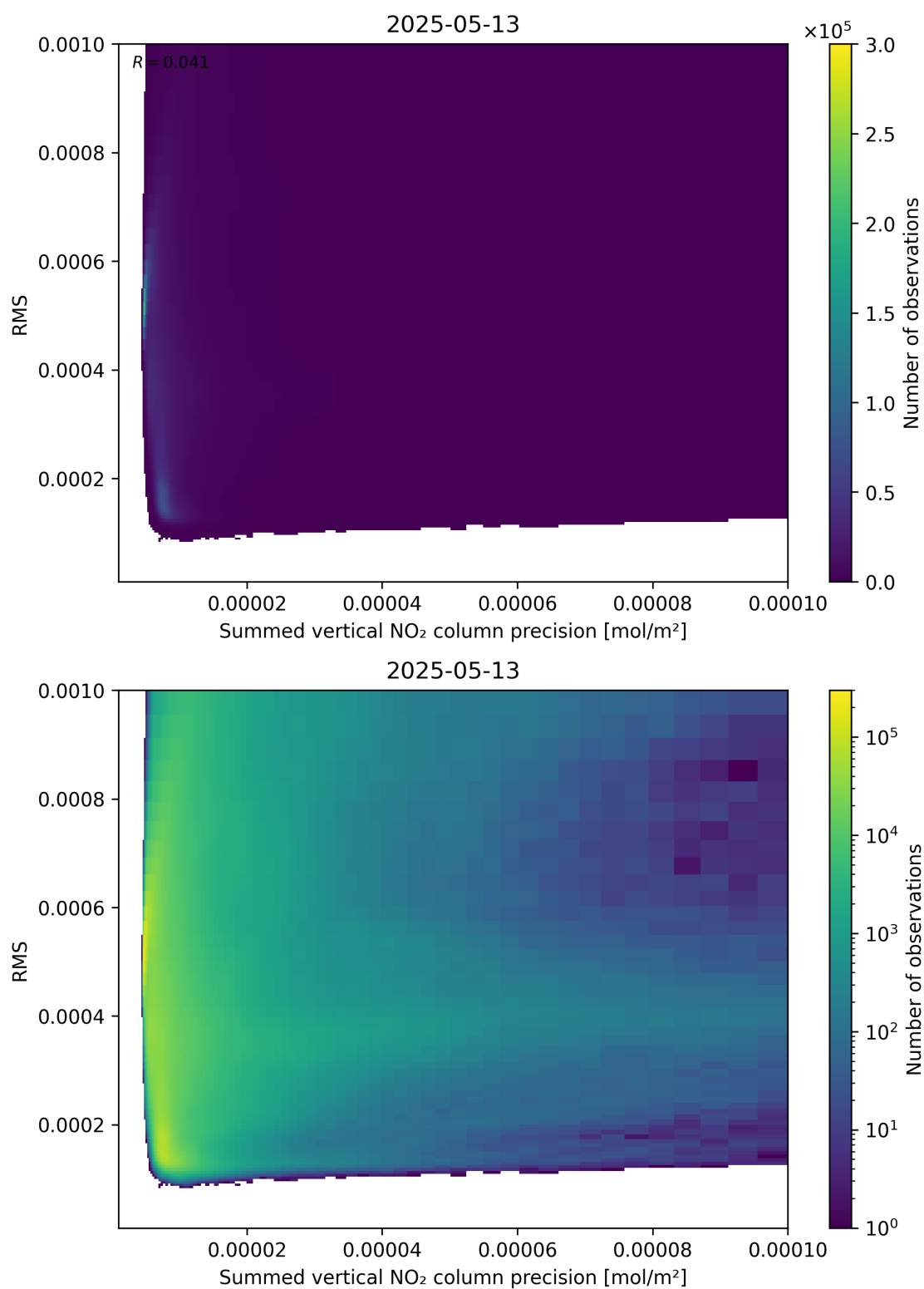
Figure 108: Scatter density plot of “Summed vertical NO 2 column precision” against “RMS” for 2025-05-13 to 2025-05-13.
