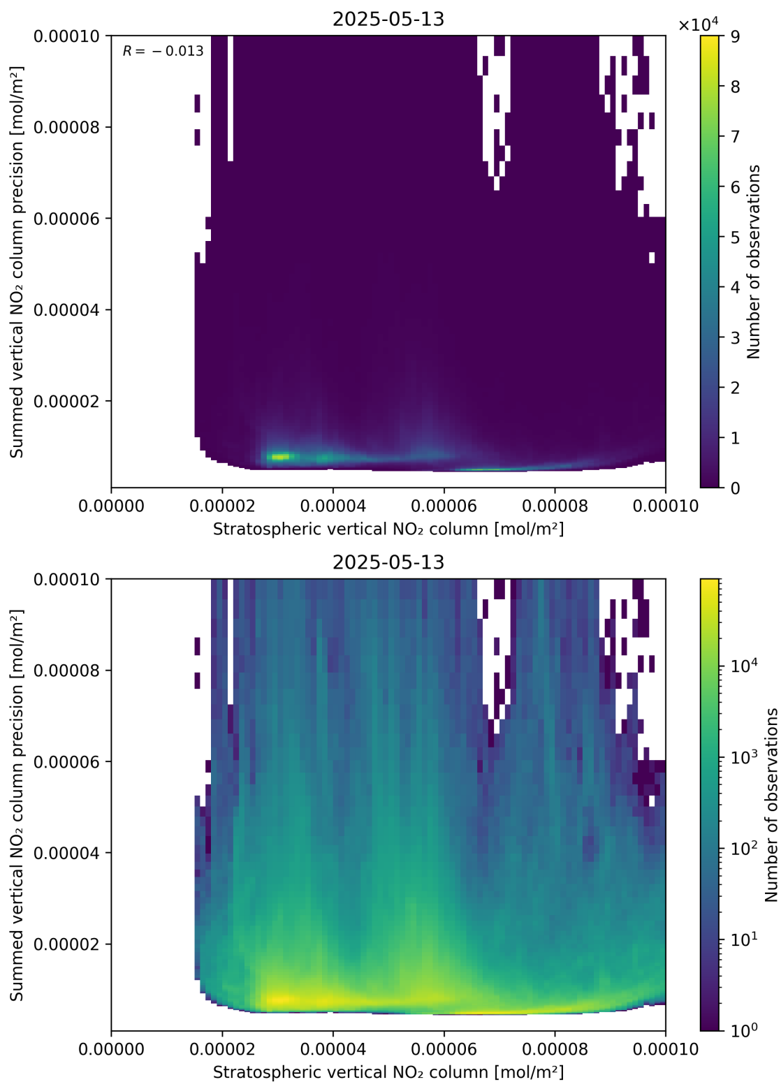
Figure 99: Scatter density plot of “Stratospheric vertical NO 2 column” against “Summed vertical NO 2 column precision” for 2025-05-13 to 2025-05-13.
