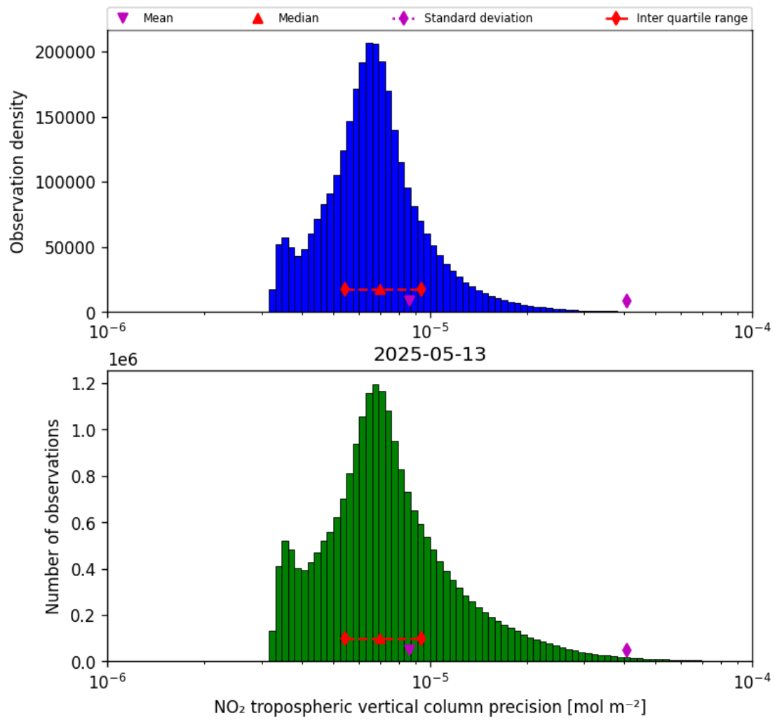
Figure 30: Histogram of “NO 2 tropospheric vertical column precision” for 2025-05-13 to 2025-05-13
