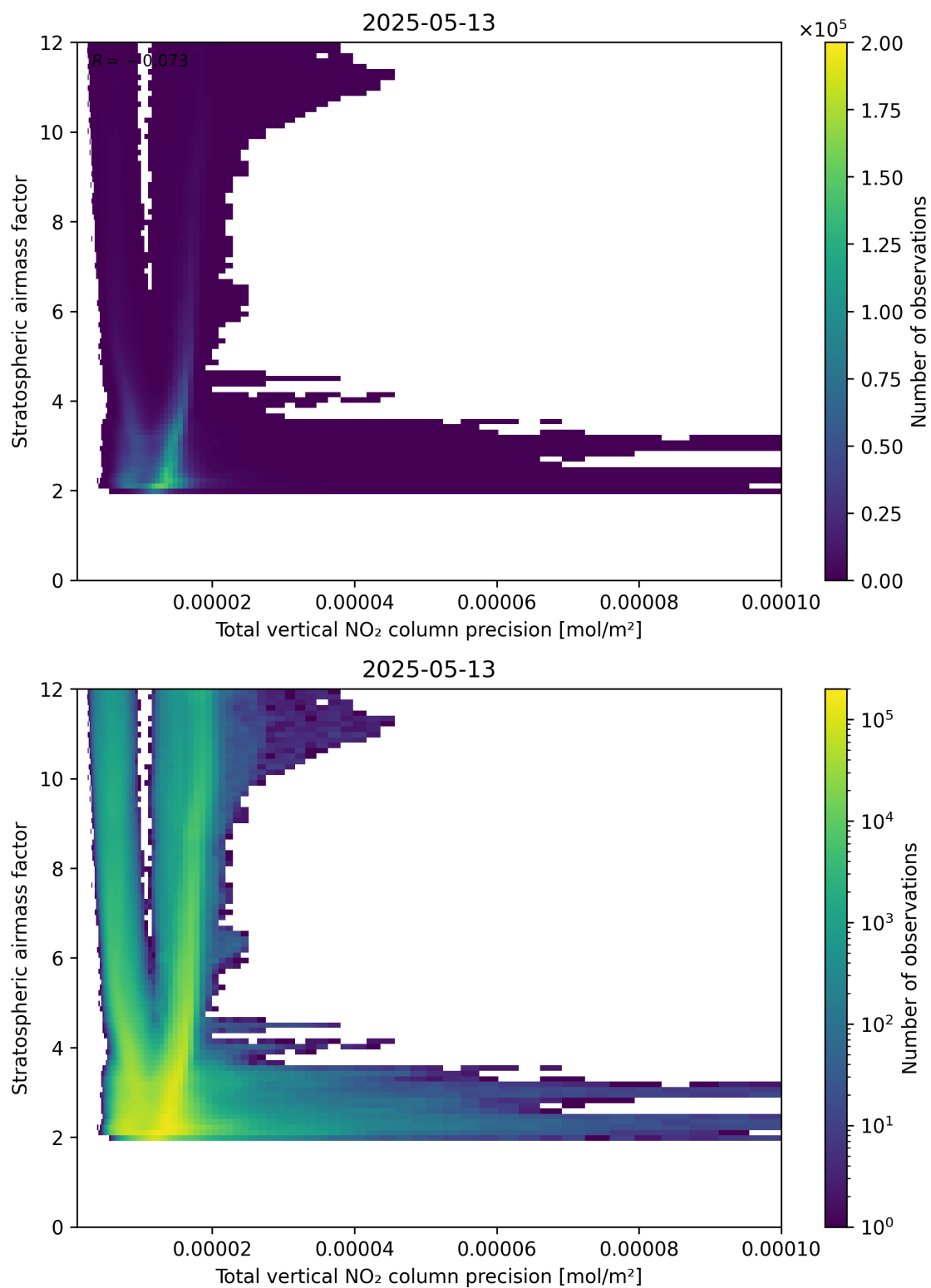
Figure 115: Scatter density plot of “Total vertical NO 2 column precision” against “Stratospheric air mass factor” for 2025-05-13 to 2025-05-13.
