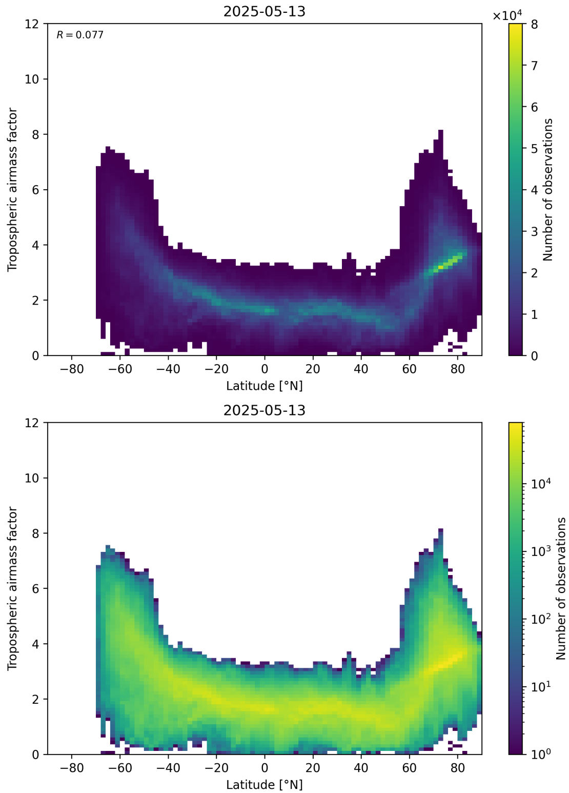
Figure 85: Scatter density plot of “Latitude” against “Tropospheric air mass factor” for 2025-05-13 to 2025-05-13.
