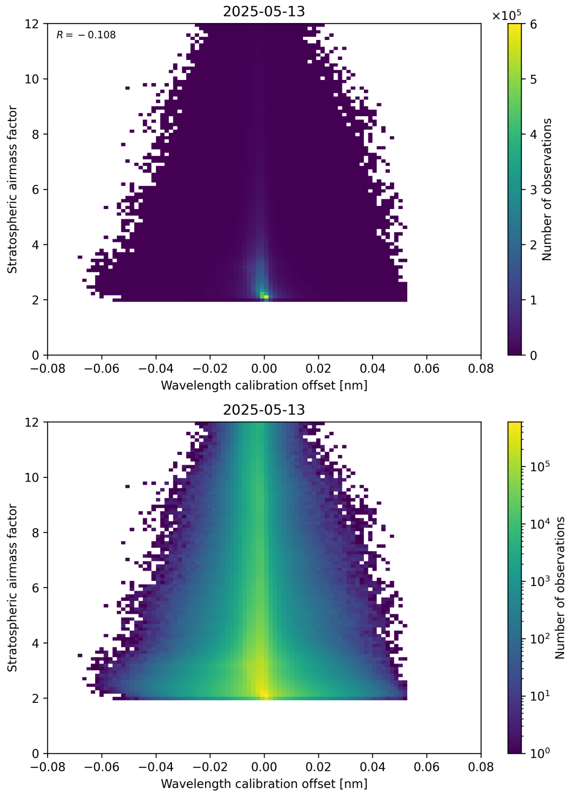
Figure 174: Scatter density plot of “Wavelength calibration offset” against “Stratospheric airmass factor” for 2025-05-13 to 2025-05-13.
