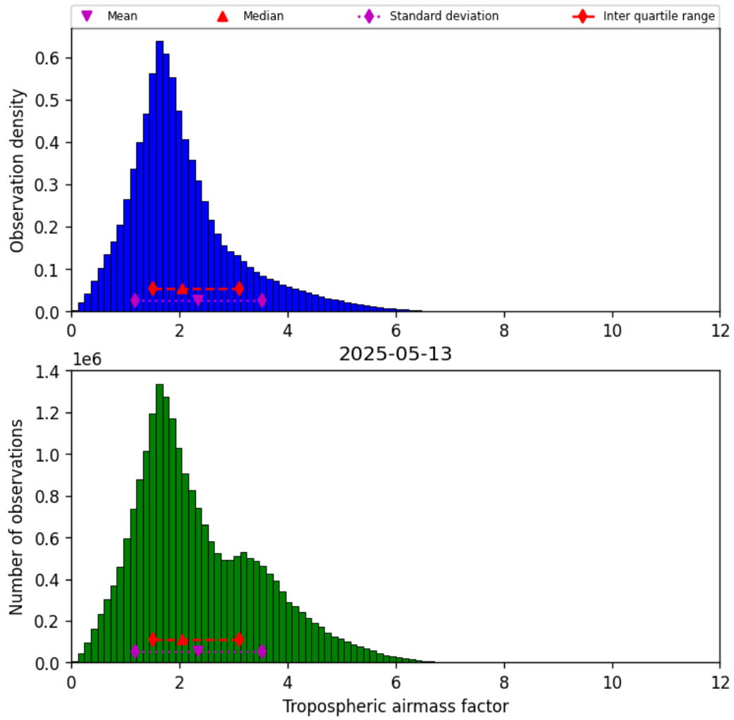
Figure 31: Histogram of “Tropospheric airmass factor” for 2025-05-13 to 2025-05-13
