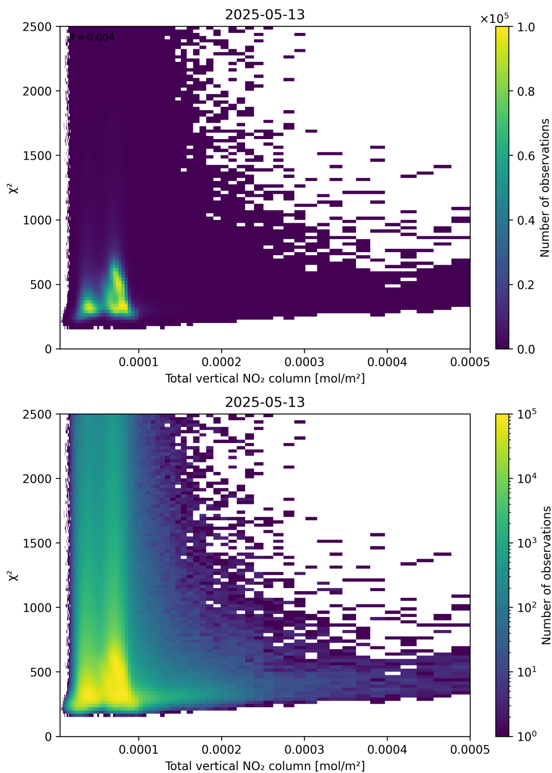
Figure 111: Scatter density plot of “Total vertical NO 2 column” against “ \chi^2 ” for 2025-05-13 to 2025-05-13.
