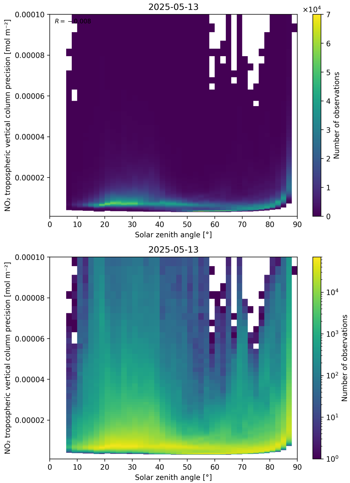
Figure 156: Scatter density plot of “Solar zenith angle” against “NO 2 tropospheric vertical column precision” for 2025-05-13 to 2025-05-13.
