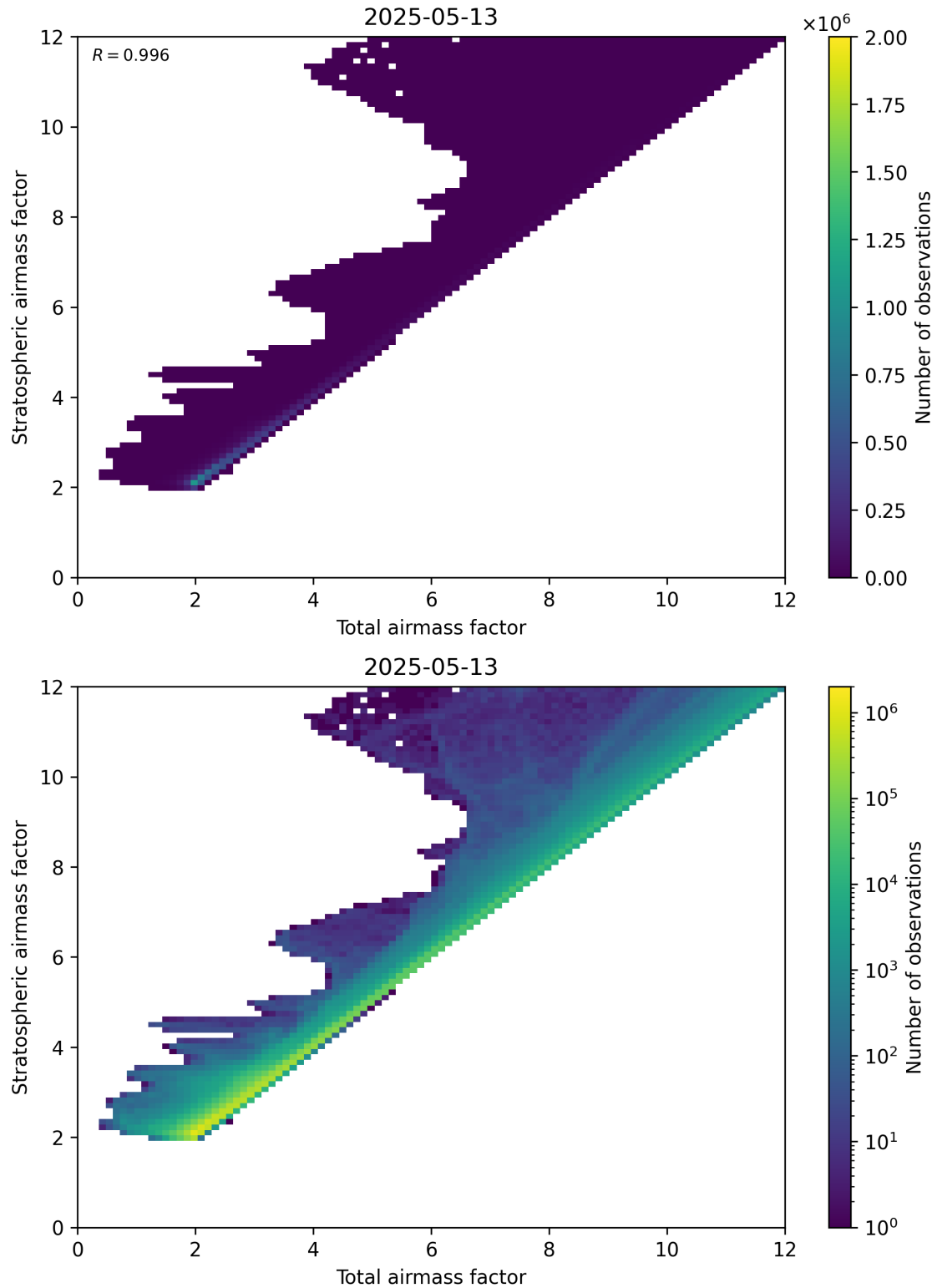
Figure 62: Scatter density plot of “Total airmass factor” against “Stratospheric airmass factor” for 2025-05-13 to 2025-05-13.
