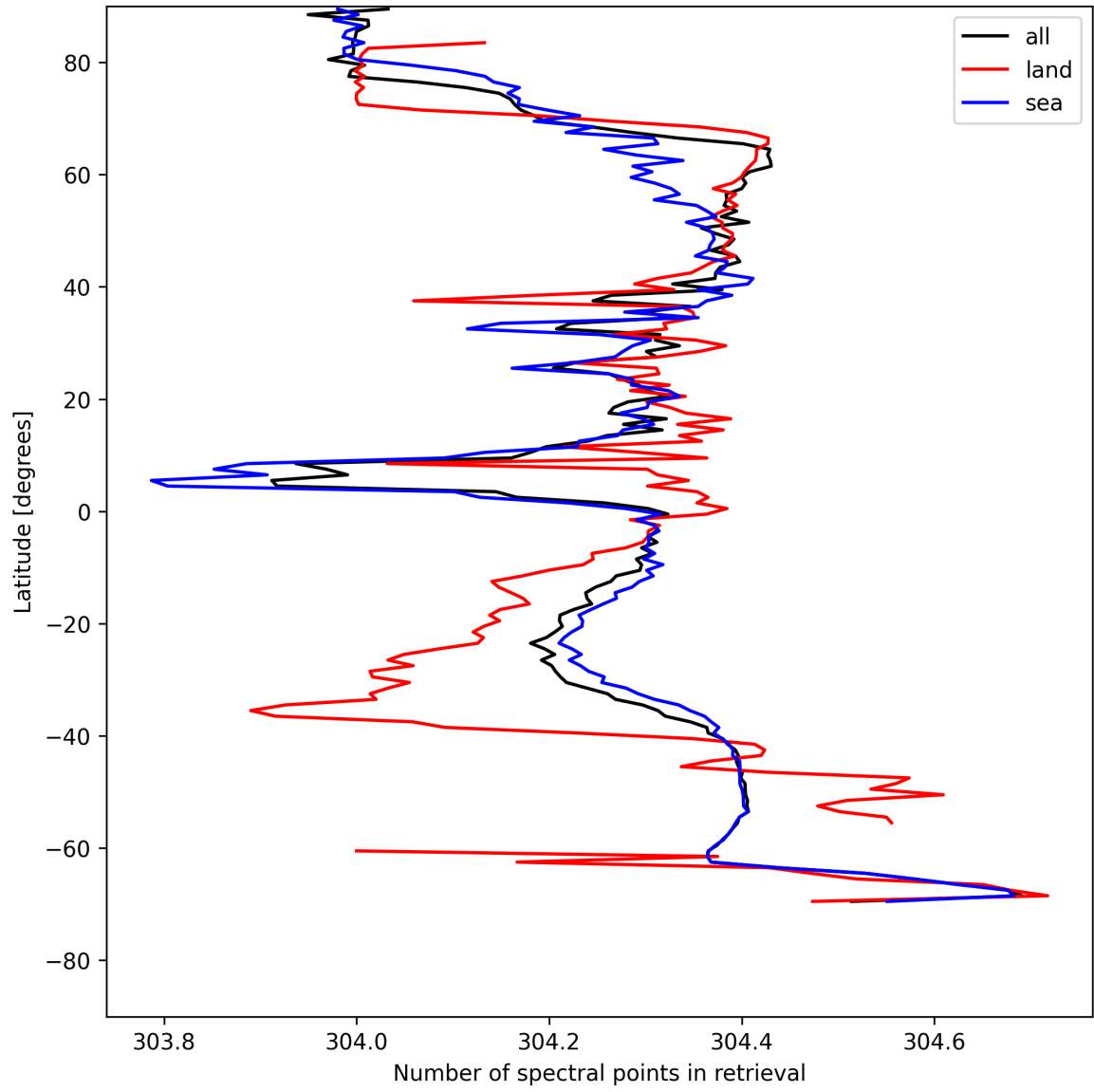
Figure 16: Zonal average of “Number of spectral points in retrieval” for 2025-05-13 to 2025-05-13.
