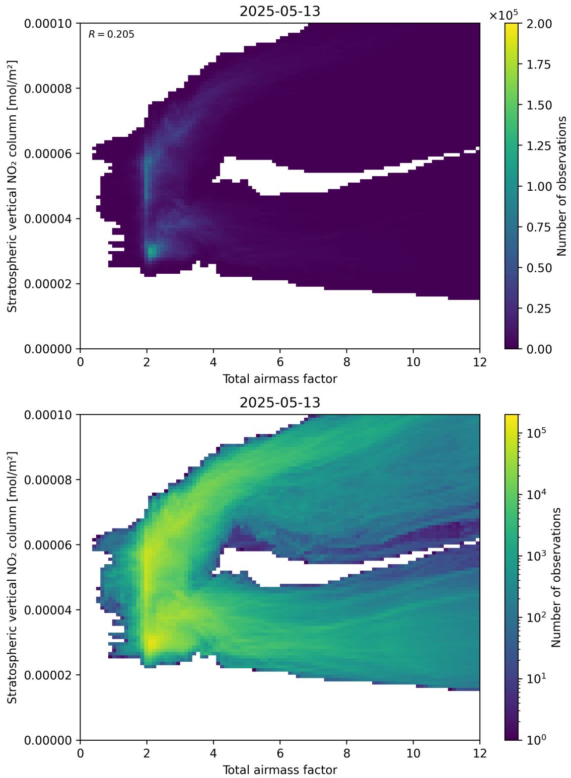
Figure 64: Scatter density plot of “Total airmass factor” against “Stratospheric vertical \text{NO}_2 column” for 2025-05-13 to 2025-05-13.
