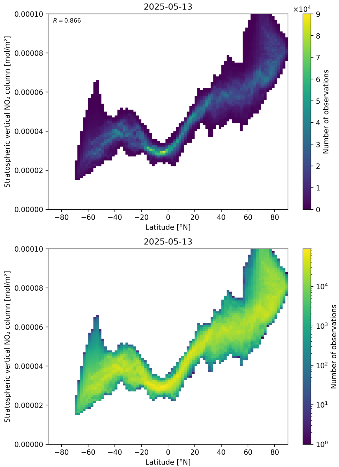
Figure 87: Scatter density plot of “Latitude” against “Stratospheric vertical \text{NO}_2 column” for 2025-05-13 to 2025-05-13.
