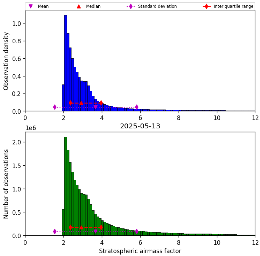
Figure 44: Histogram of “Stratospheric airmass factor” for 2025-05-13 to 2025-05-13
