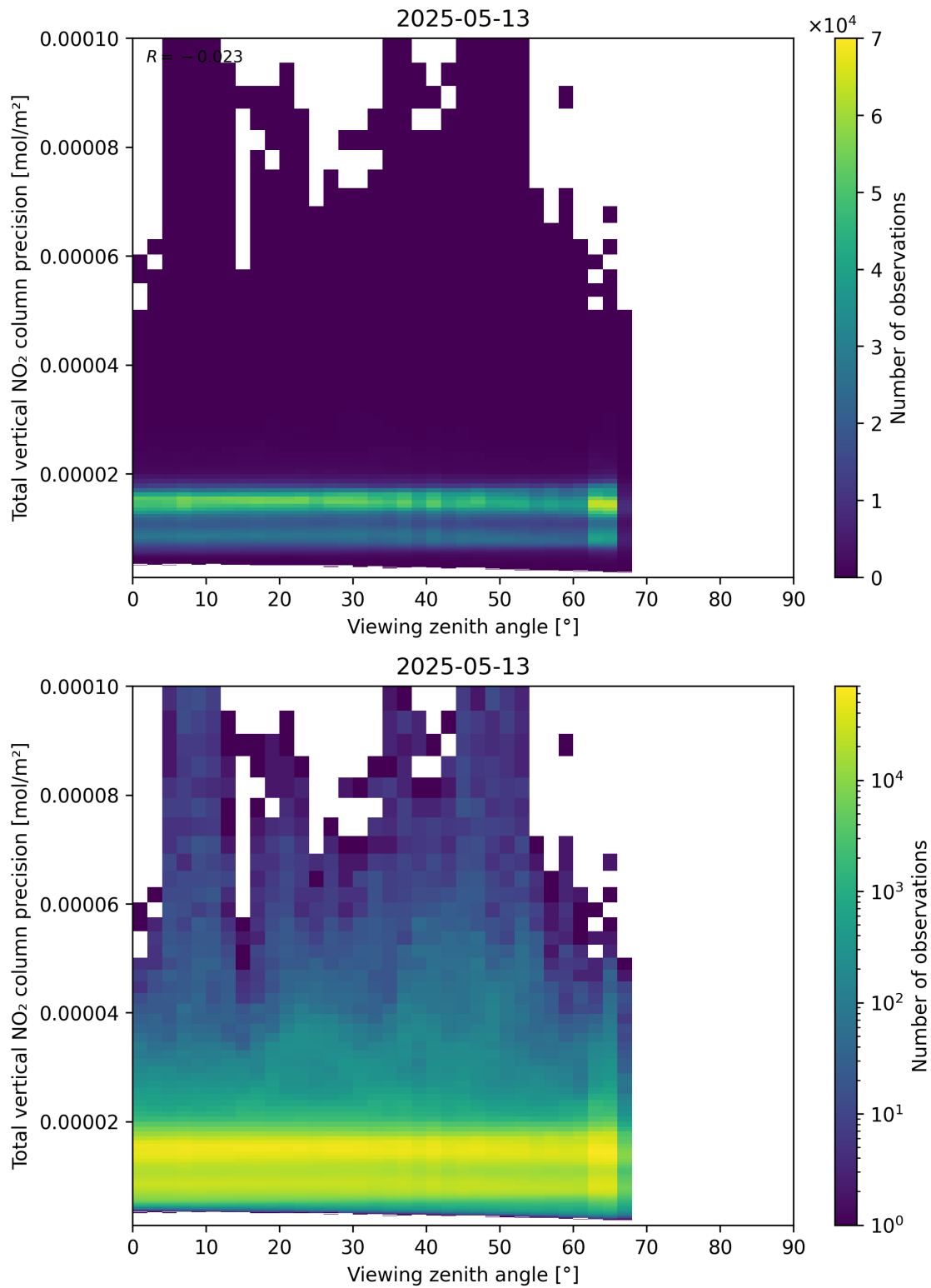
Figure 168: Scatter density plot of “Viewing zenith angle” against “Total vertical NO 2 column precision” for 2025-05-13 to 2025-05-13.
