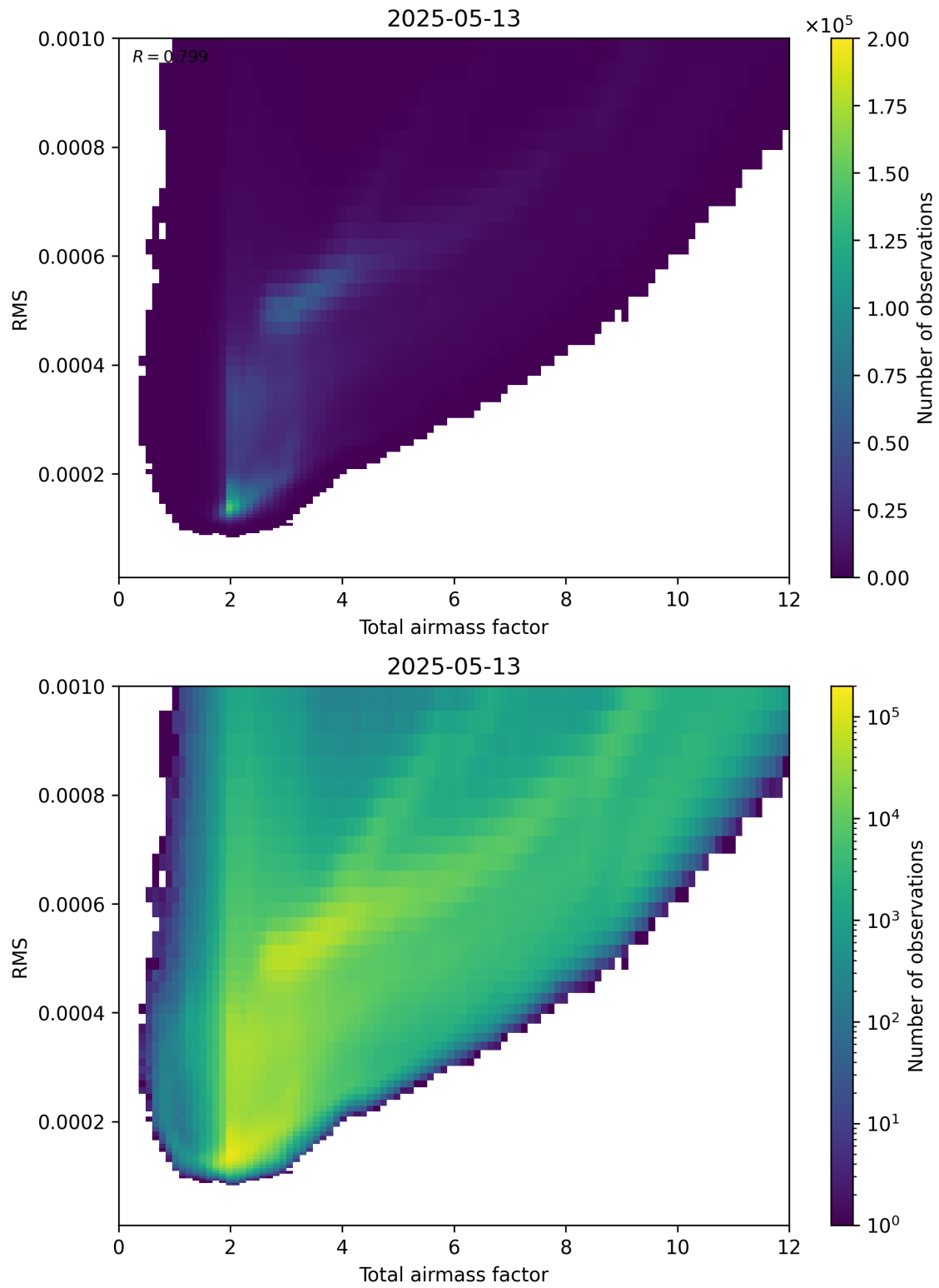
Figure 69: Scatter density plot of “Total airmass factor” against “RMS” for 2025-05-13 to 2025-05-13.
