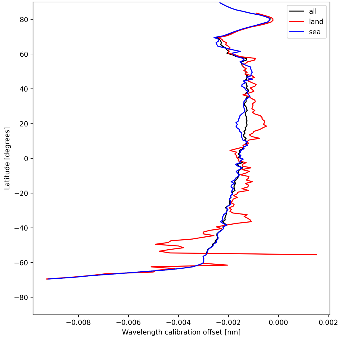
Figure 18: Zonal average of “Wavelength calibration offset” for 2025-05-13 to 2025-05-13.
