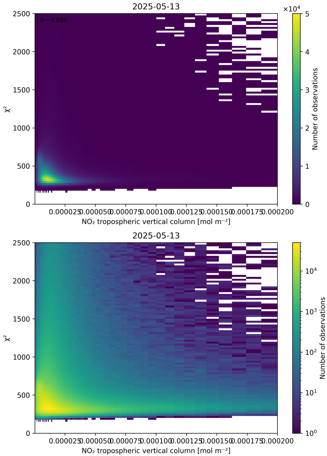
Figure 124: Scatter density plot of “NO 2 tropospheric vertical column” against “ \chi^2 ” for 2025-05-13 to 2025-05-13.
