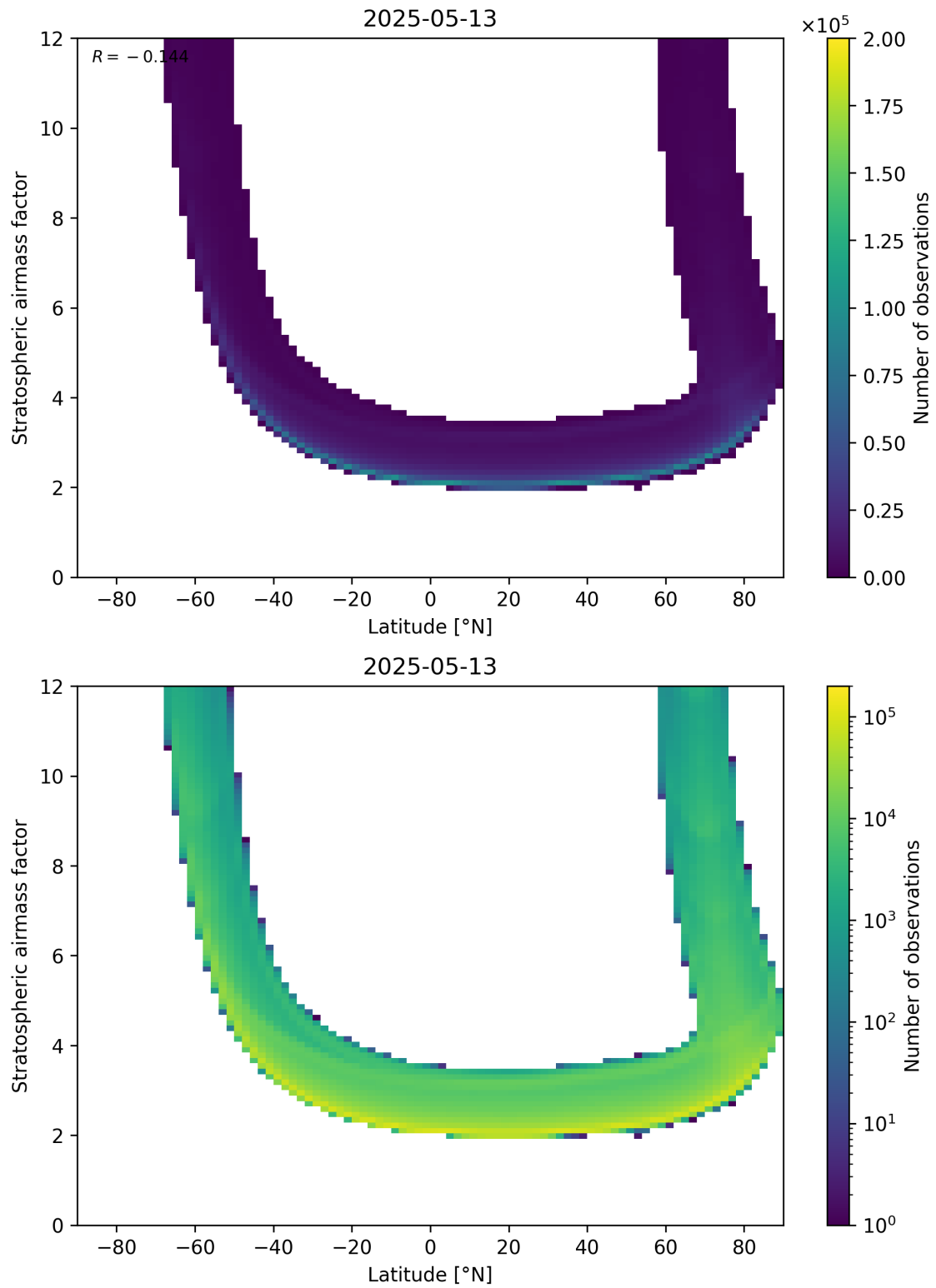
Figure 83: Scatter density plot of “Latitude” against “Stratospheric air mass factor” for 2025-05-13 to 2025-05-13.
