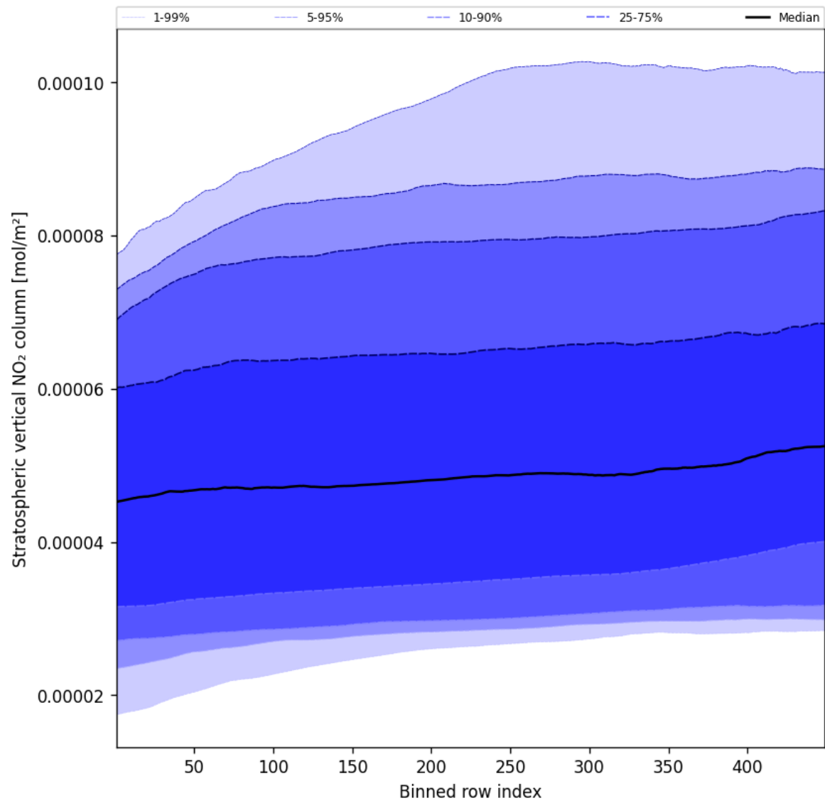
Figure 53: Along track statistics of “Stratospheric vertical NO 2 column” for 2025-05-13 to 2025-05-13
