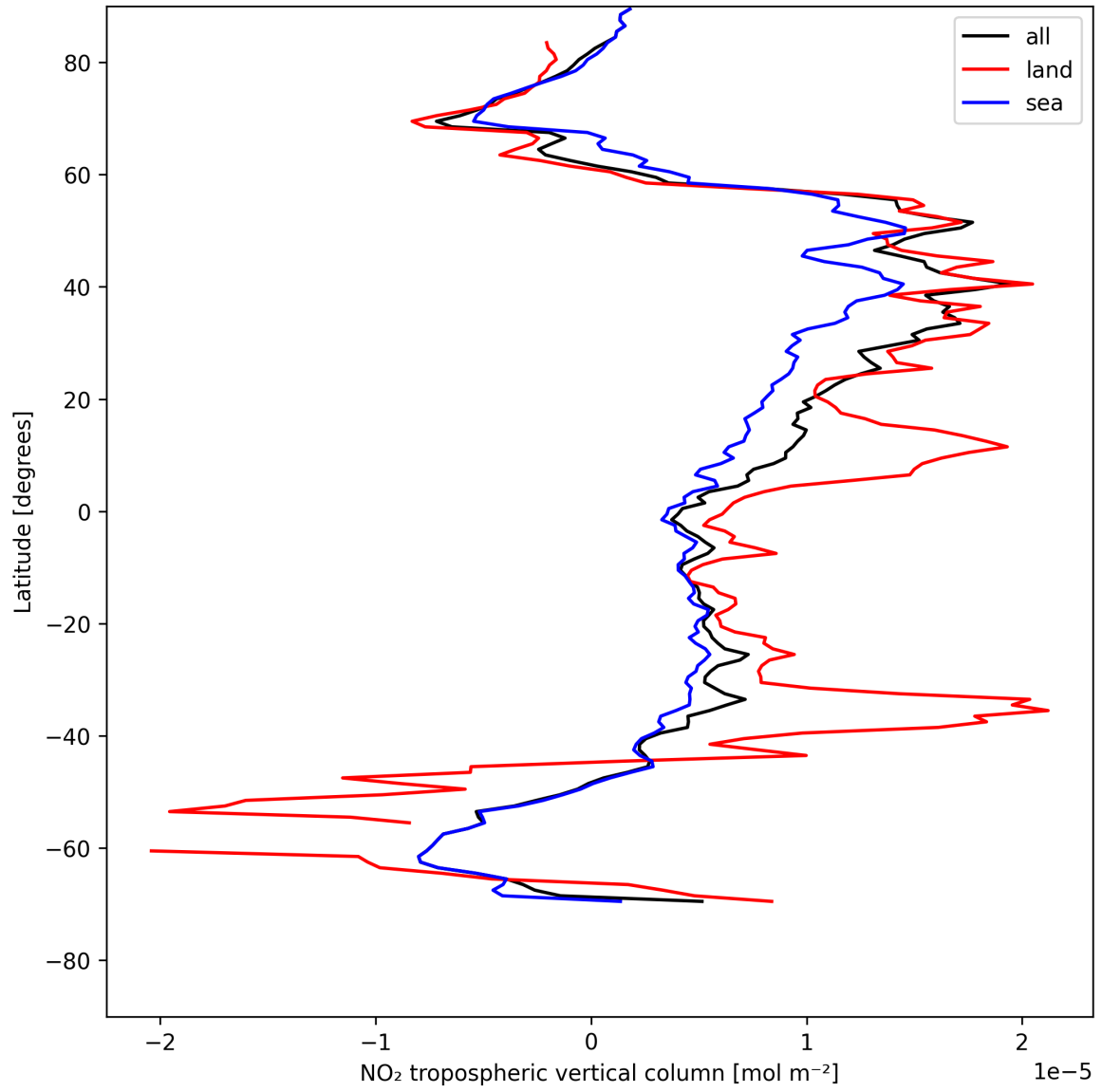
Figure 12: Zonal average of “NO 2 tropospheric vertical column” for 2025-05-13 to 2025-05-13.
