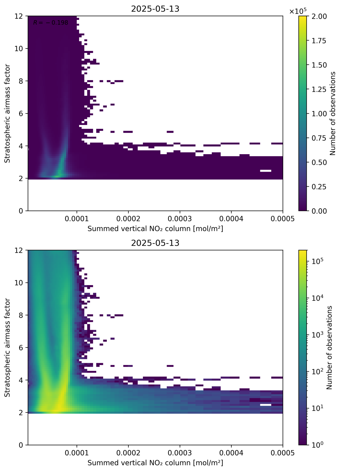
Figure 103: Scatter density plot of “Summed vertical NO 2 column” against “Stratospheric airmass factor” for 2025-05-13 to 2025-05-13.
