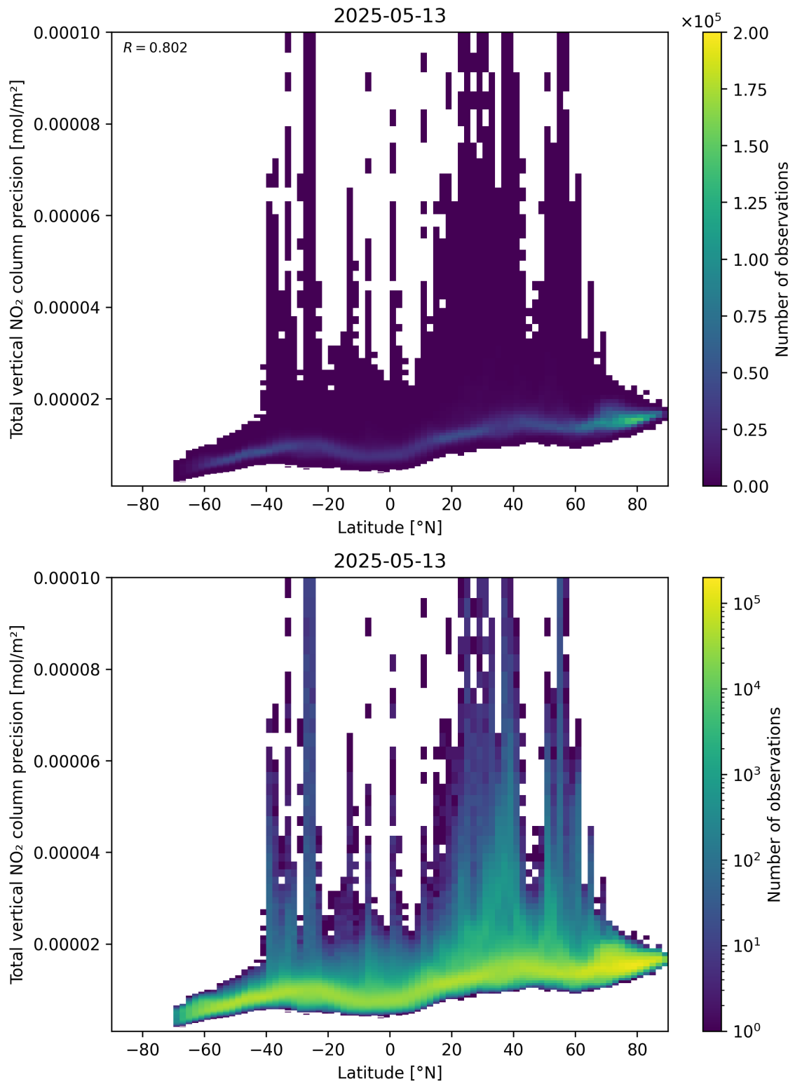
Figure 91: Scatter density plot of “Latitude” against “Total vertical NO 2 column precision” for 2025-05-13 to 2025-05-13.
