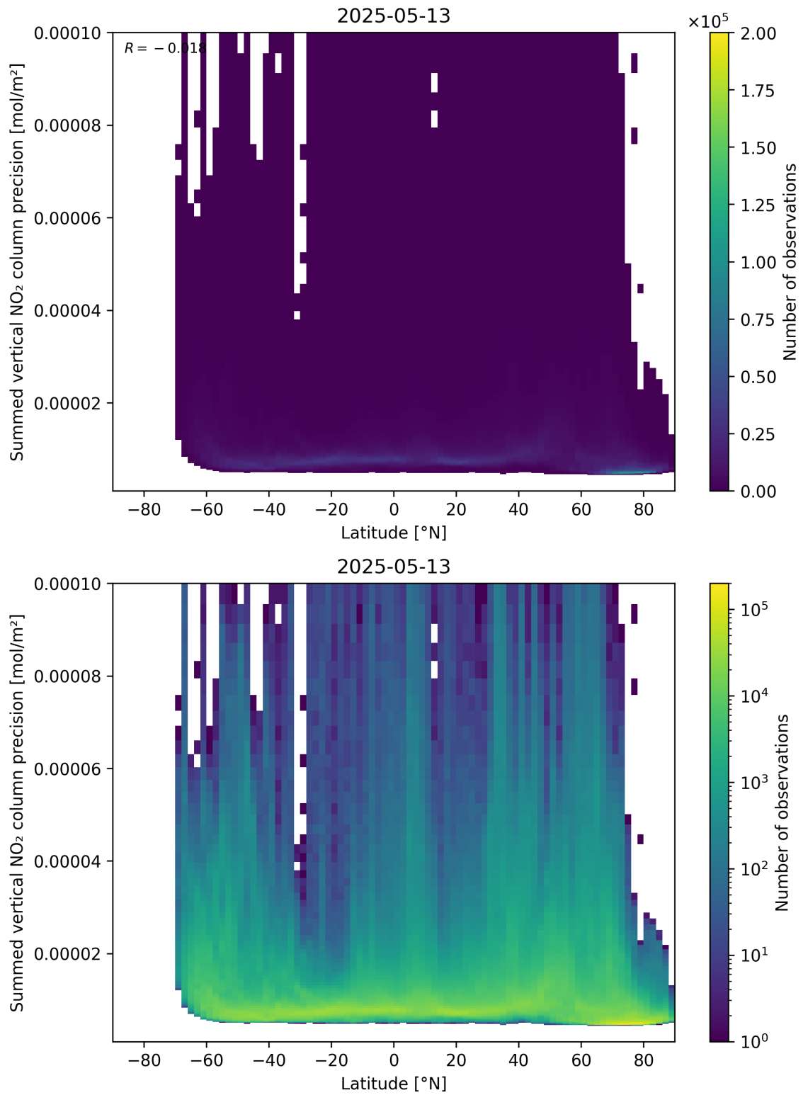
Figure 89: Scatter density plot of “Latitude” against “Summed vertical NO 2 column precision” for 2025-05-13 to 2025-05-13.
