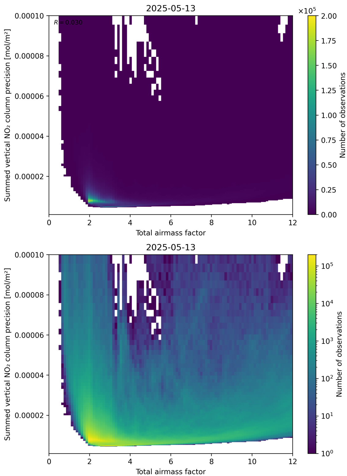
Figure 66: Scatter density plot of “Total airmass factor” against “Summed vertical NO 2 column precision” for 2025-05-13 to 2025-05-13.
