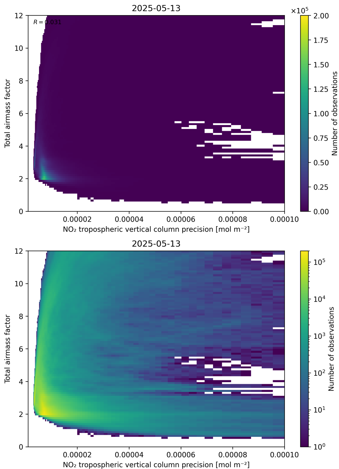
Figure 132: Scatter density plot of “NO 2 tropospheric vertical column precision” against “Total air mass factor” for 2025-05-13 to 2025-05-13.
