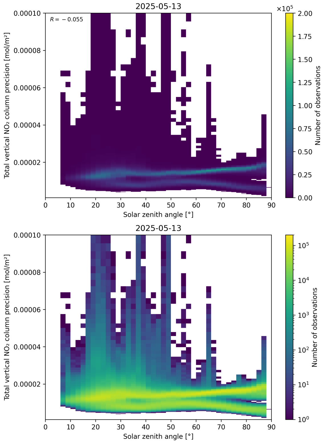
Figure 154: Scatter density plot of “Solar zenith angle” against “Total vertical NO 2 column precision” for 2025-05-13 to 2025-05-13.
