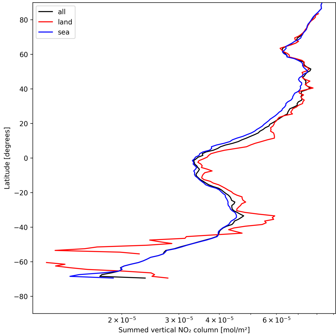
Figure 23: Zonal average of “Summed vertical NO 2 column” for 2025-05-13 to 2025-05-13.
