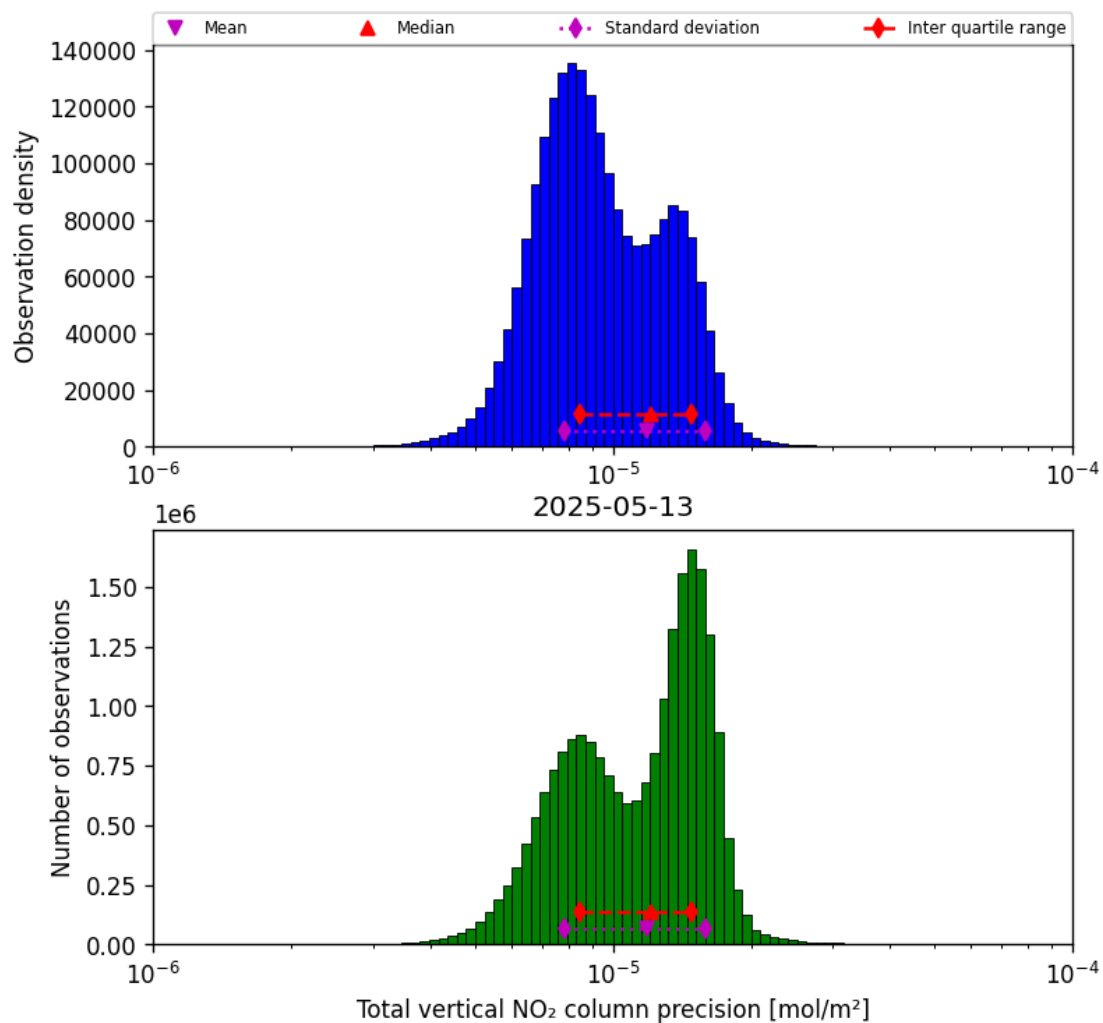
Figure 39: Histogram of “Total vertical NO 2 column precision” for 2025-05-13 to 2025-05-13
