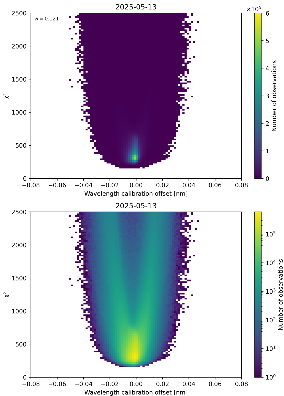
Figure 175: Scatter density plot of “Wavelength calibration offset” against “ \chi^2 ” for 2025-05-13 to 2025-05-13.
