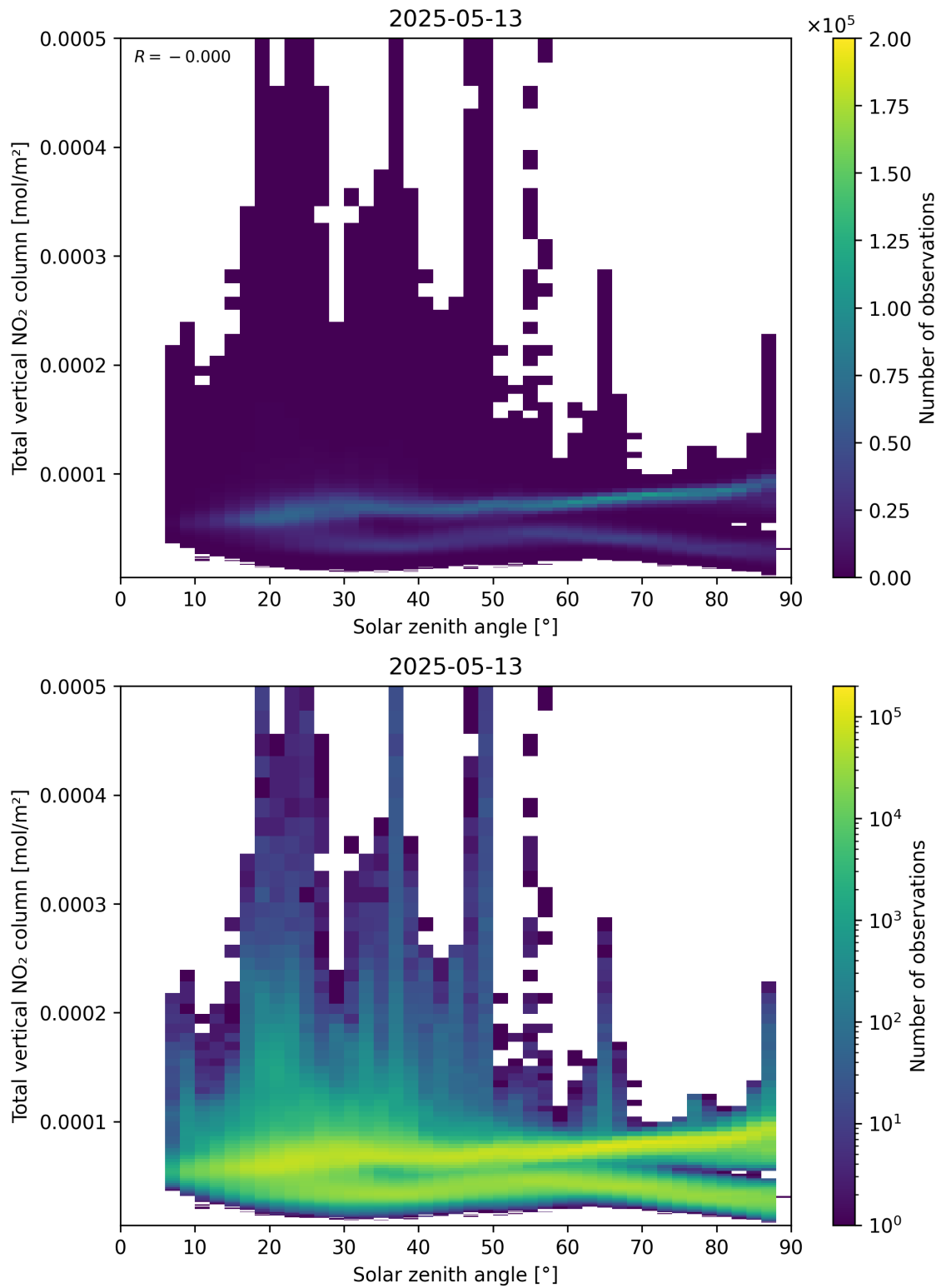
Figure 153: Scatter density plot of “Solar zenith angle” against “Total vertical NO 2 column” for 2025-05-13 to 2025-05-13.
