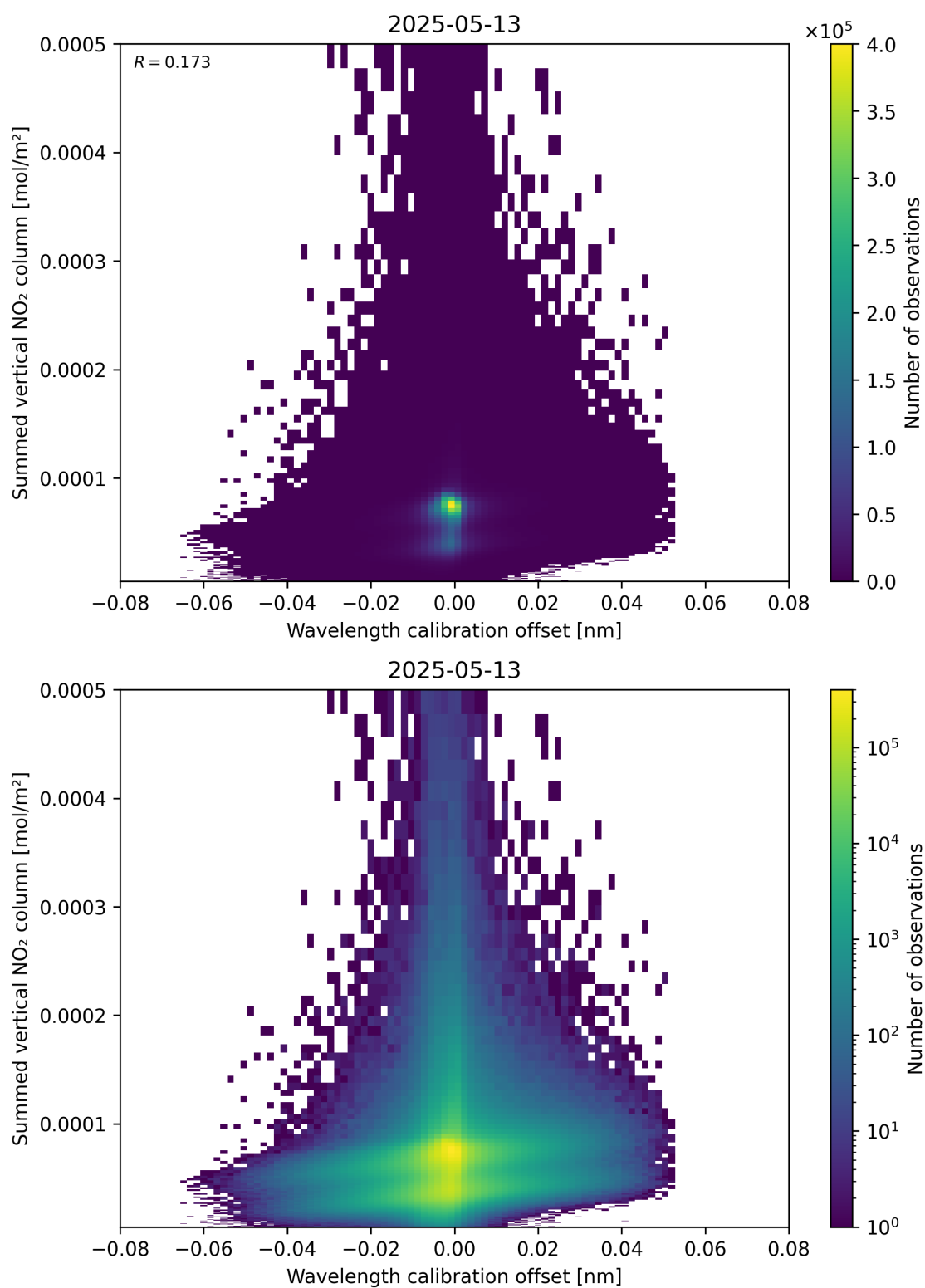
Figure 177: Scatter density plot of “Wavelength calibration offset” against “Summed vertical NO 2 column” for 2025-05-13 to 2025-05-13.
