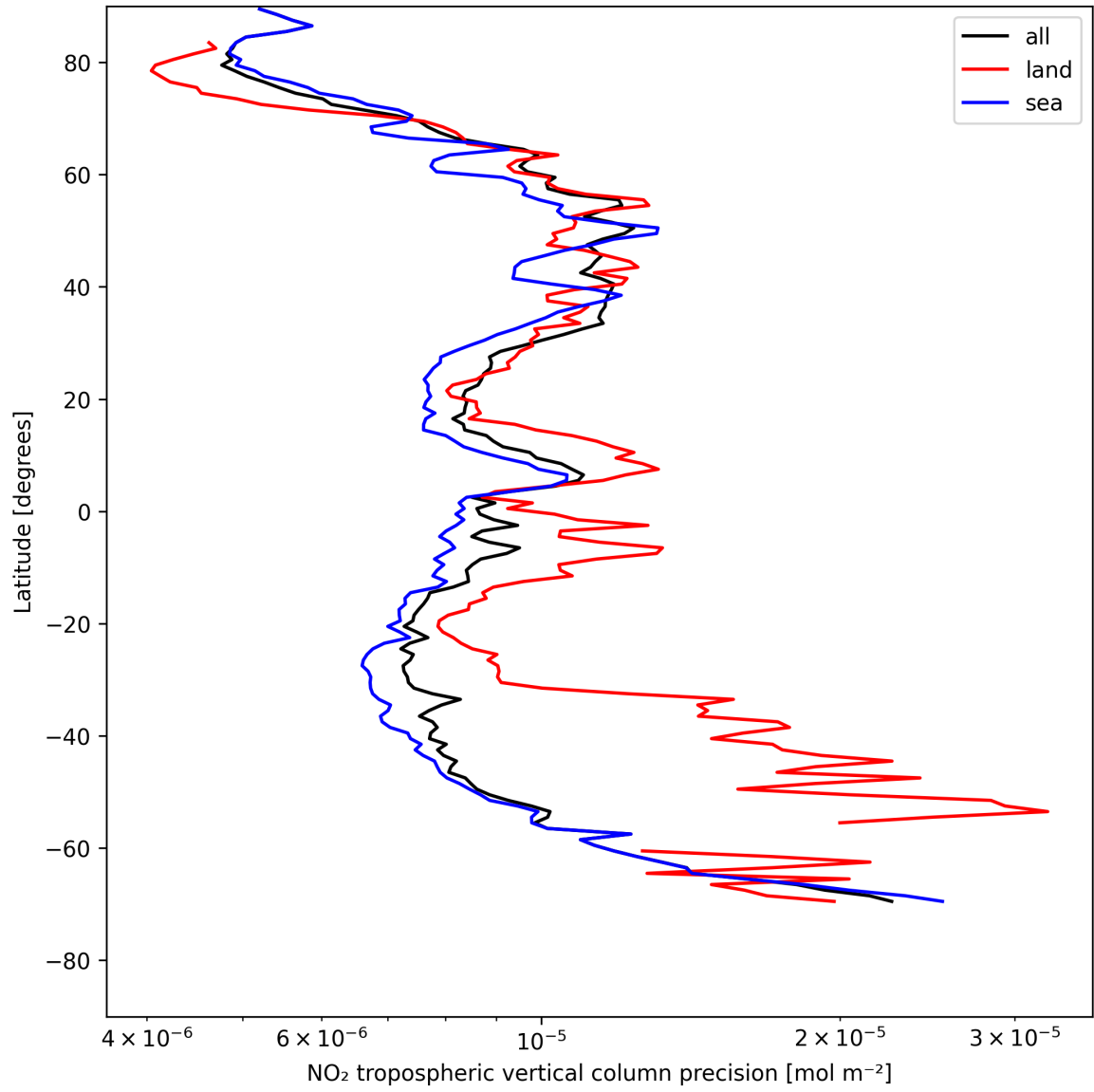
Figure 13: Zonal average of “NO 2 tropospheric vertical column precision” for 2025-05-13 to 2025-05-13.
