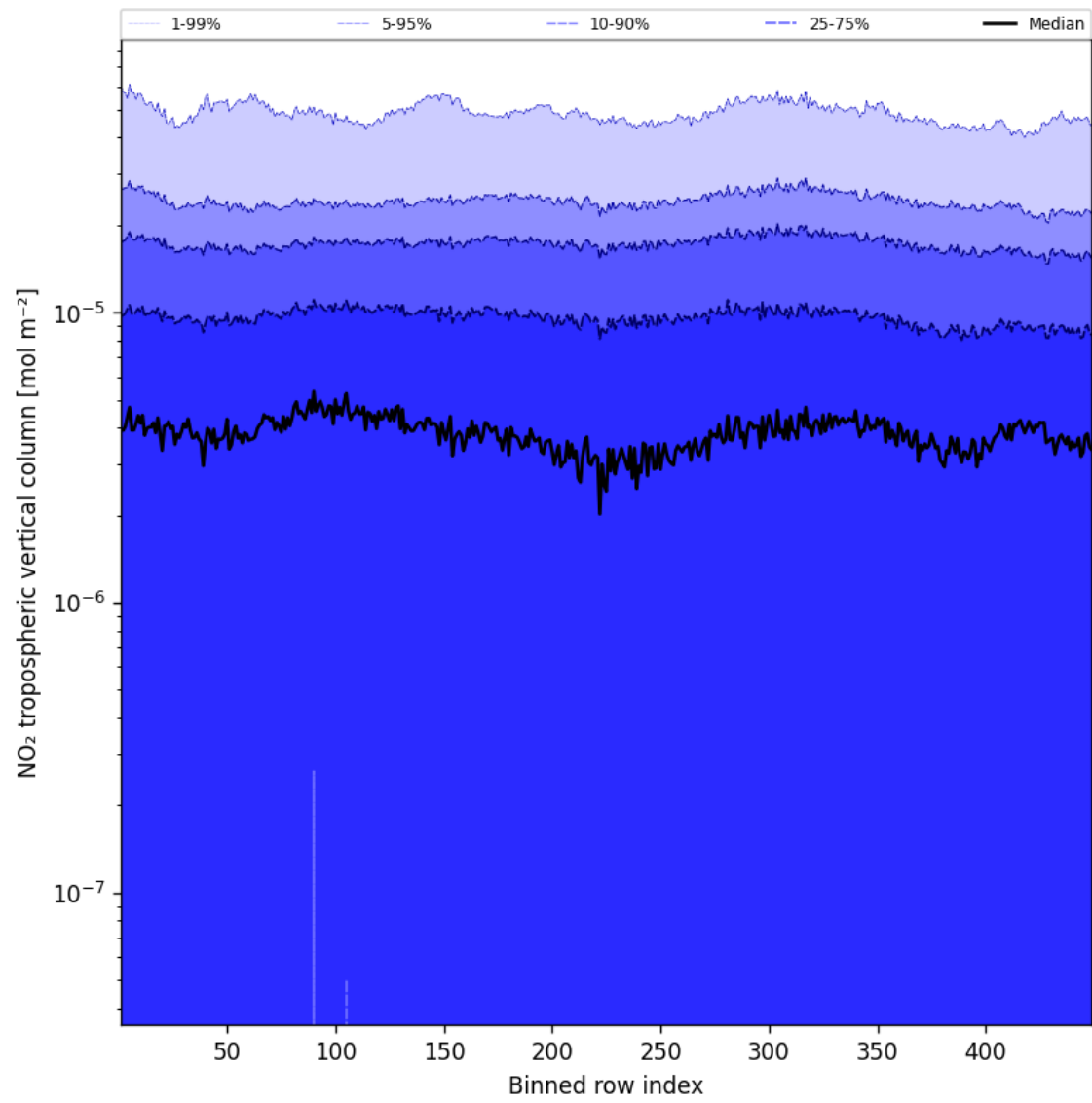
Figure 46: Along track statistics of “NO 2 tropospheric vertical column” for 2025-05-13 to 2025-05-13
