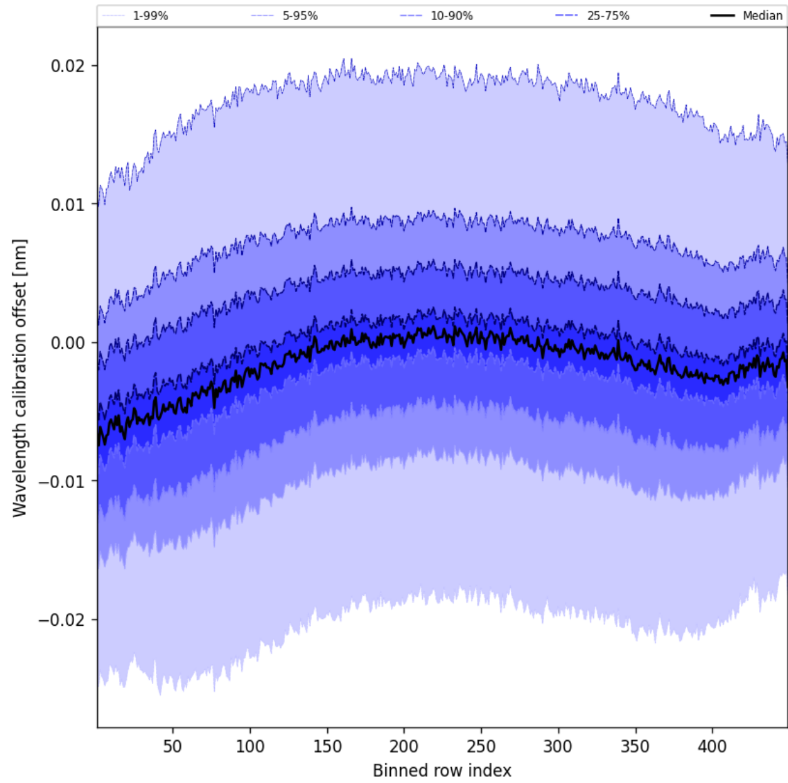
Figure 52: Along track statistics of “Wavelength calibration offset” for 2025-05-13 to 2025-05-13
