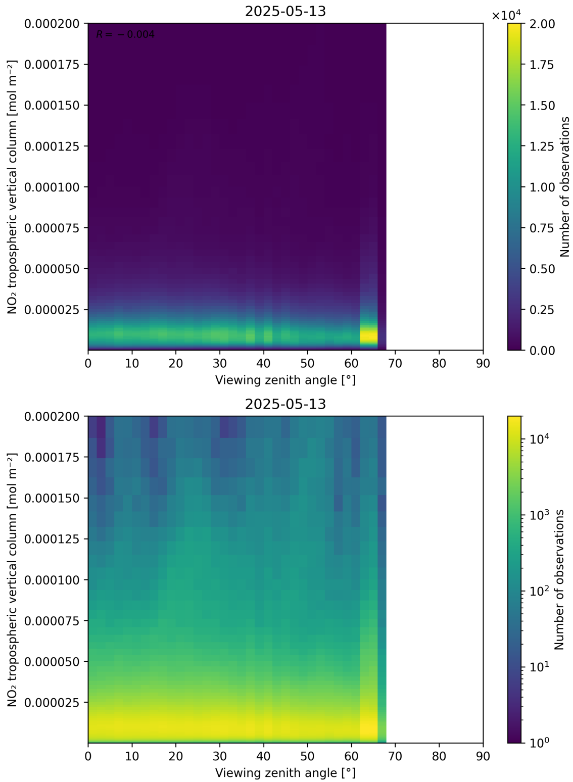
Figure 169: Scatter density plot of “Viewing zenith angle” against “NO 2 tropospheric vertical column” for 2025-05-13 to 2025-05-13.
