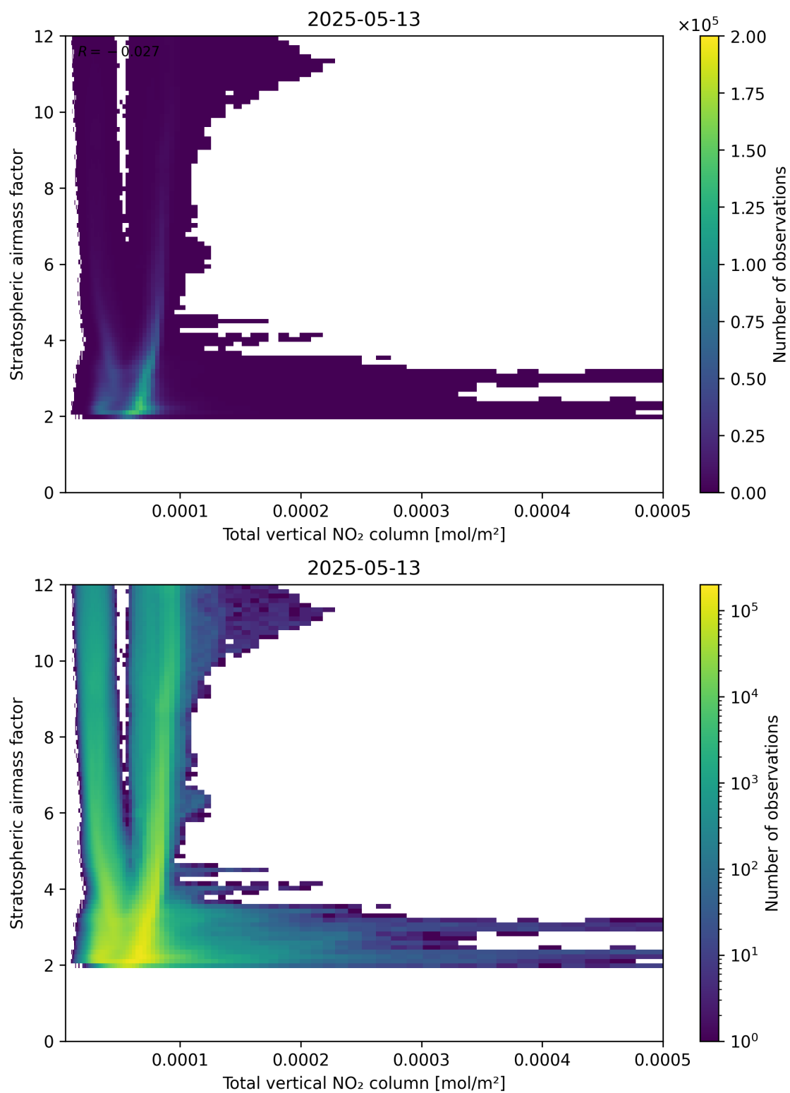
Figure 110: Scatter density plot of “Total vertical NO 2 column” against “Stratospheric airmass factor” for 2025-05-13 to 2025-05-13.
