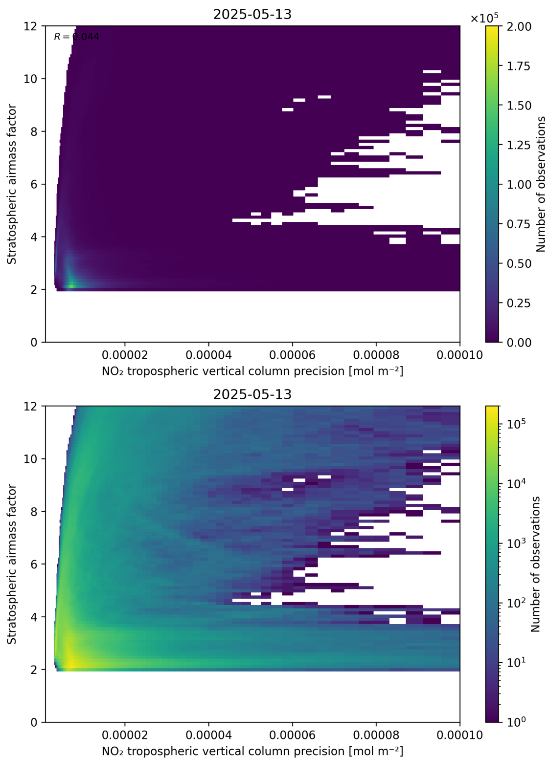
Figure 131: Scatter density plot of “NO 2 tropospheric vertical column precision” against “Stratospheric airmass factor” for 2025-05-13 to 2025-05-13.
