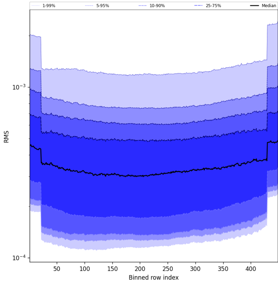
Figure 60: Along track statistics of “RMS” for 2025-05-13 to 2025-05-13
