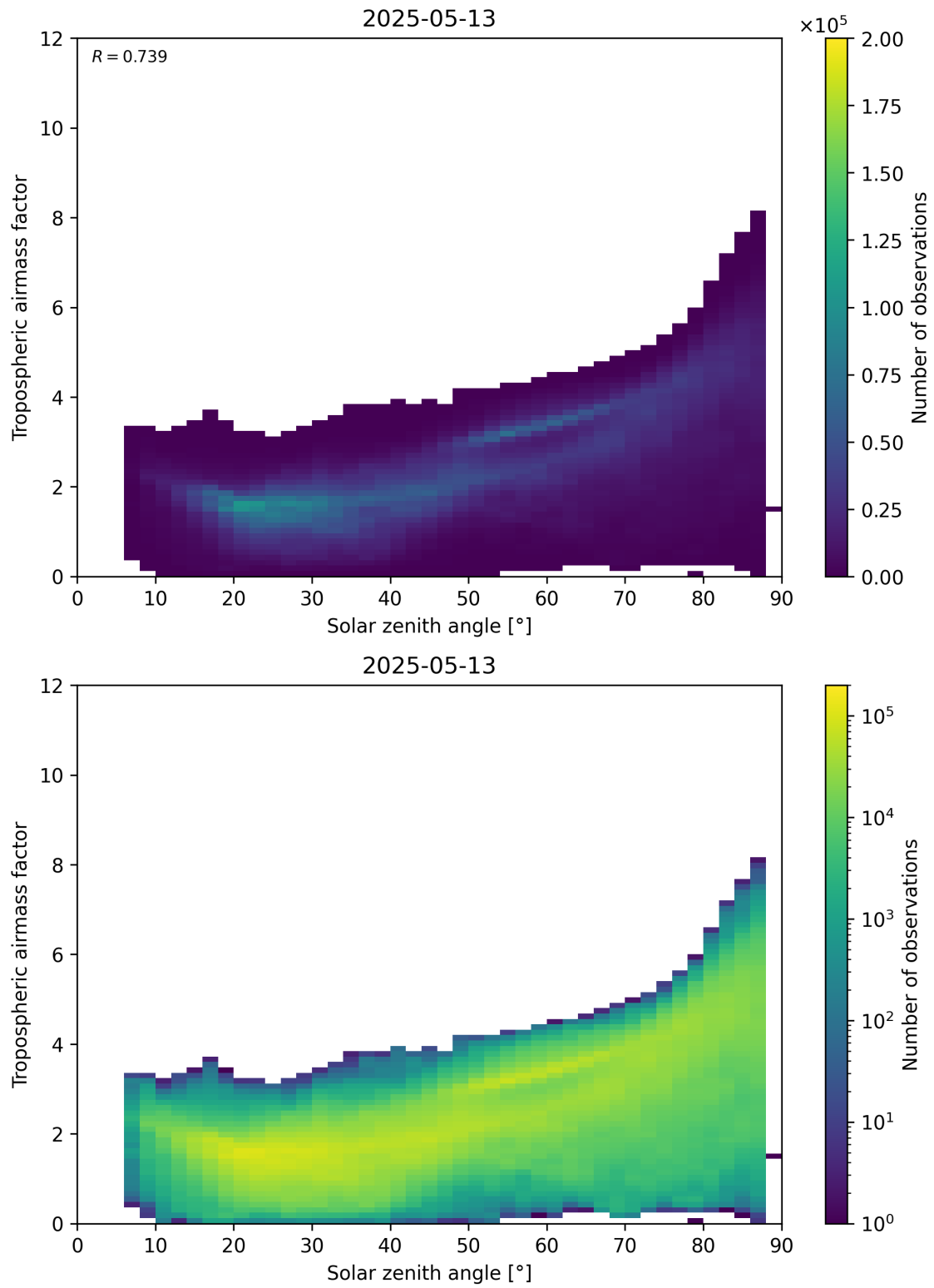
Figure 147: Scatter density plot of “Solar zenith angle” against “Tropospheric airmass factor” for 2025-05-13 to 2025-05-13.
