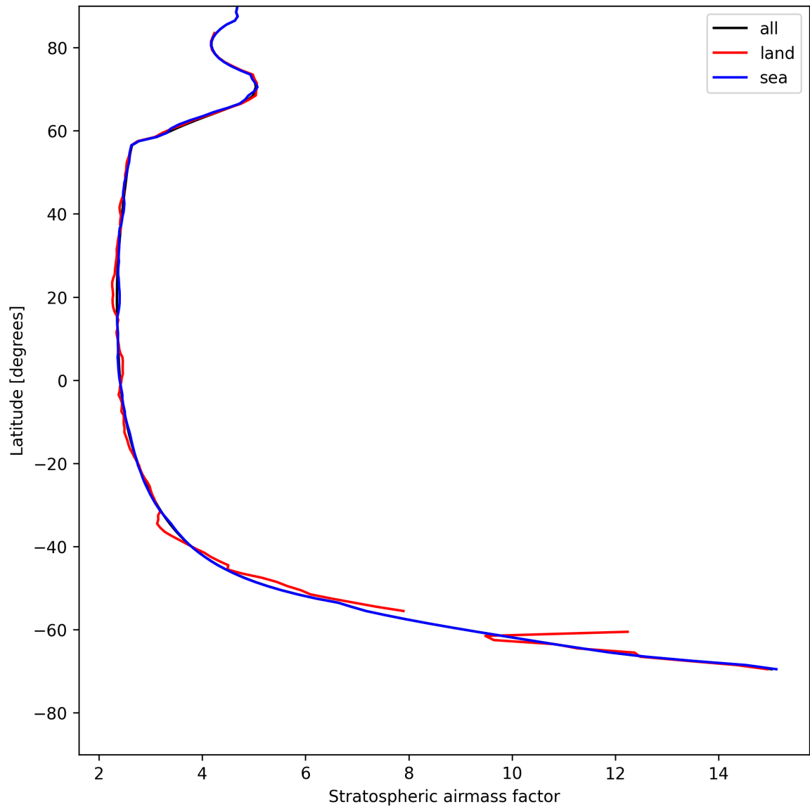
Figure 27: Zonal average of “Stratospheric airmass factor” for 2025-05-13 to 2025-05-13.
