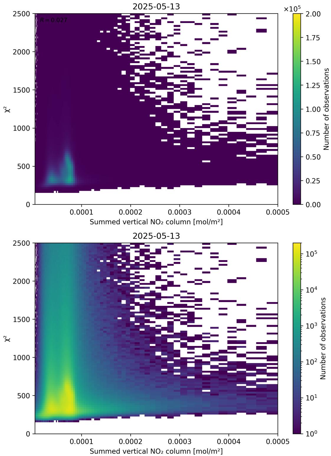
Figure 104: Scatter density plot of “Summed vertical NO 2 column” against “ \chi^2 ” for 2025-05-13 to 2025-05-13.
