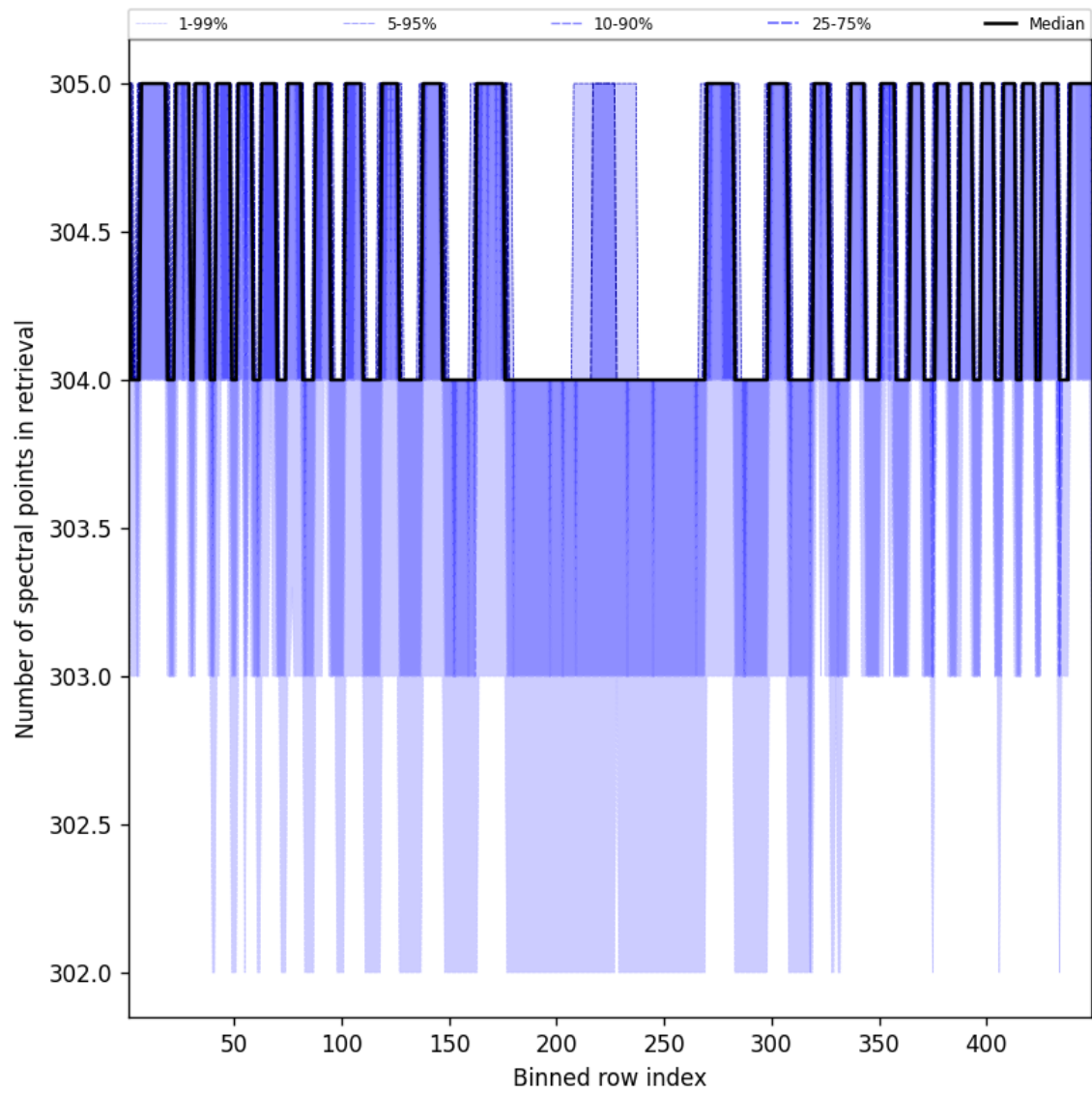
Figure 50: Along track statistics of “Number of spectral points in retrieval” for 2025-05-13 to 2025-05-13
