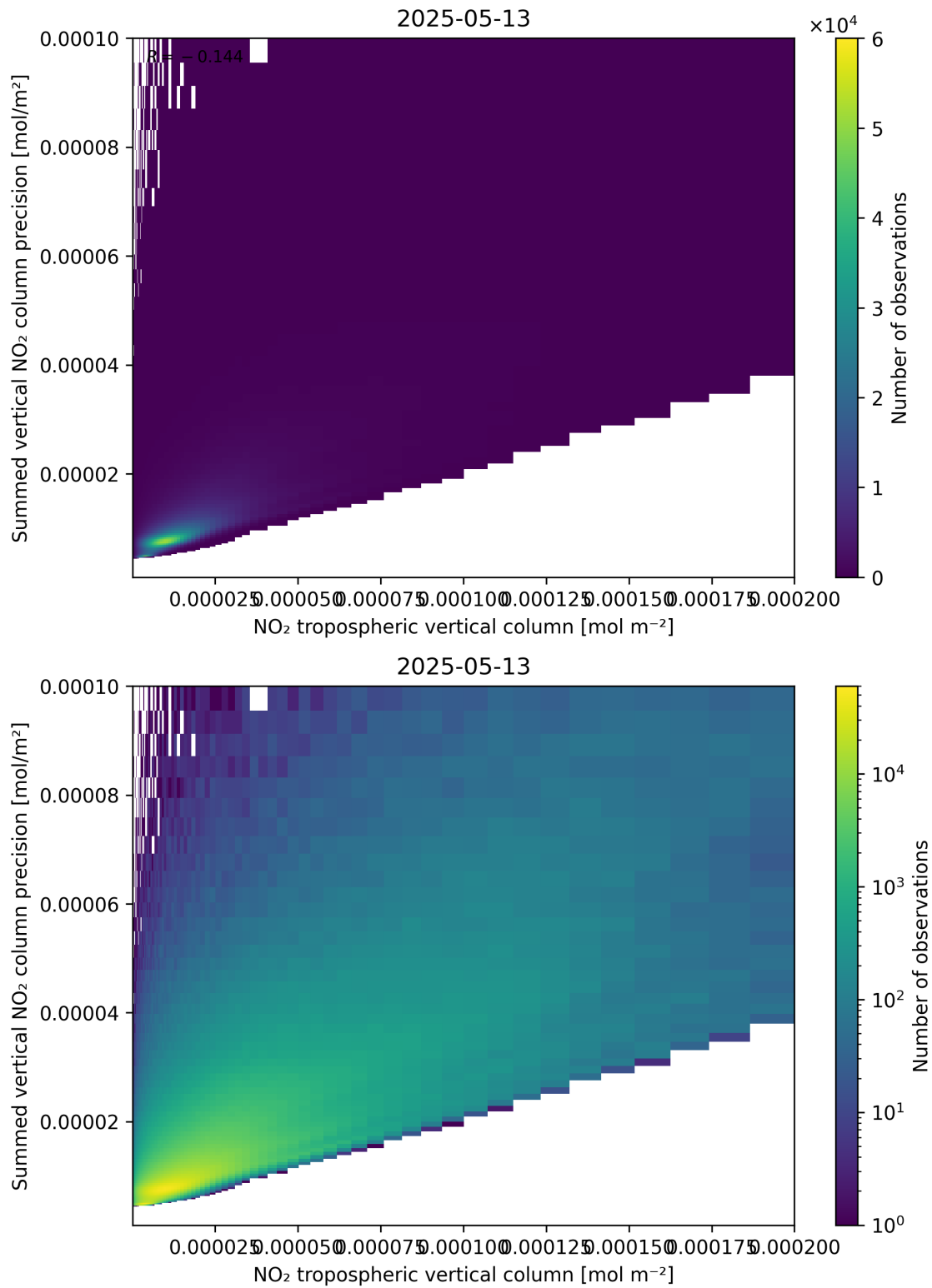
Figure 127: Scatter density plot of “NO 2 tropospheric vertical column” against “Summed vertical NO 2 column precision” for 2025-05-13 to 2025-05-13.
