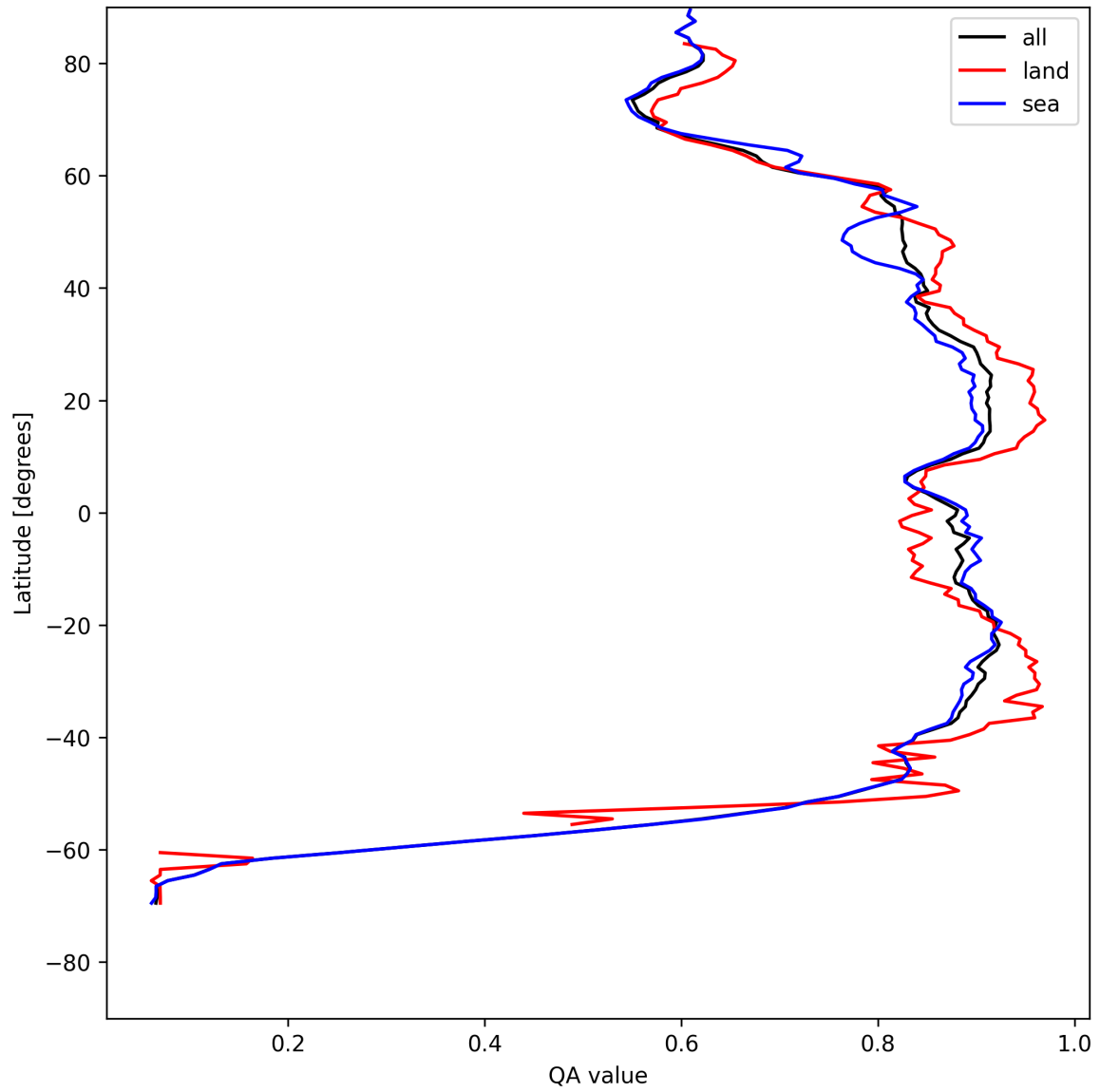
Figure 11: Zonal average of “QA value” for 2025-05-13 to 2025-05-13.
