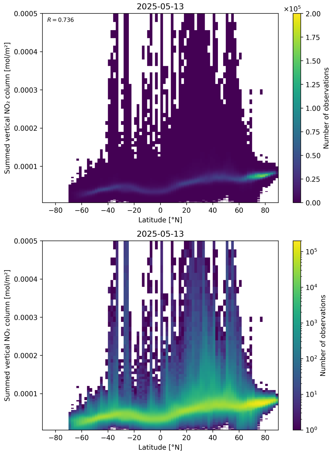
Figure 88: Scatter density plot of “Latitude” against “Summed vertical NO 2 column” for 2025-05-13 to 2025-05-13.
