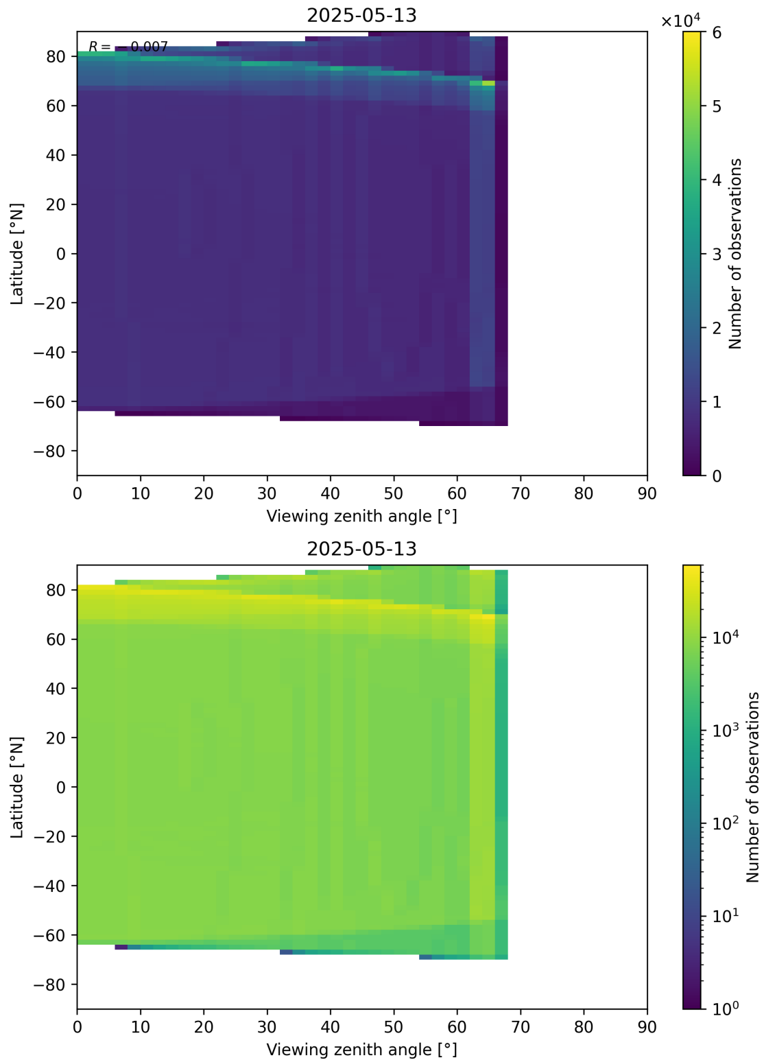
Figure 163: Scatter density plot of “Viewing zenith angle” against “Latitude” for 2025-05-13 to 2025-05-13.
