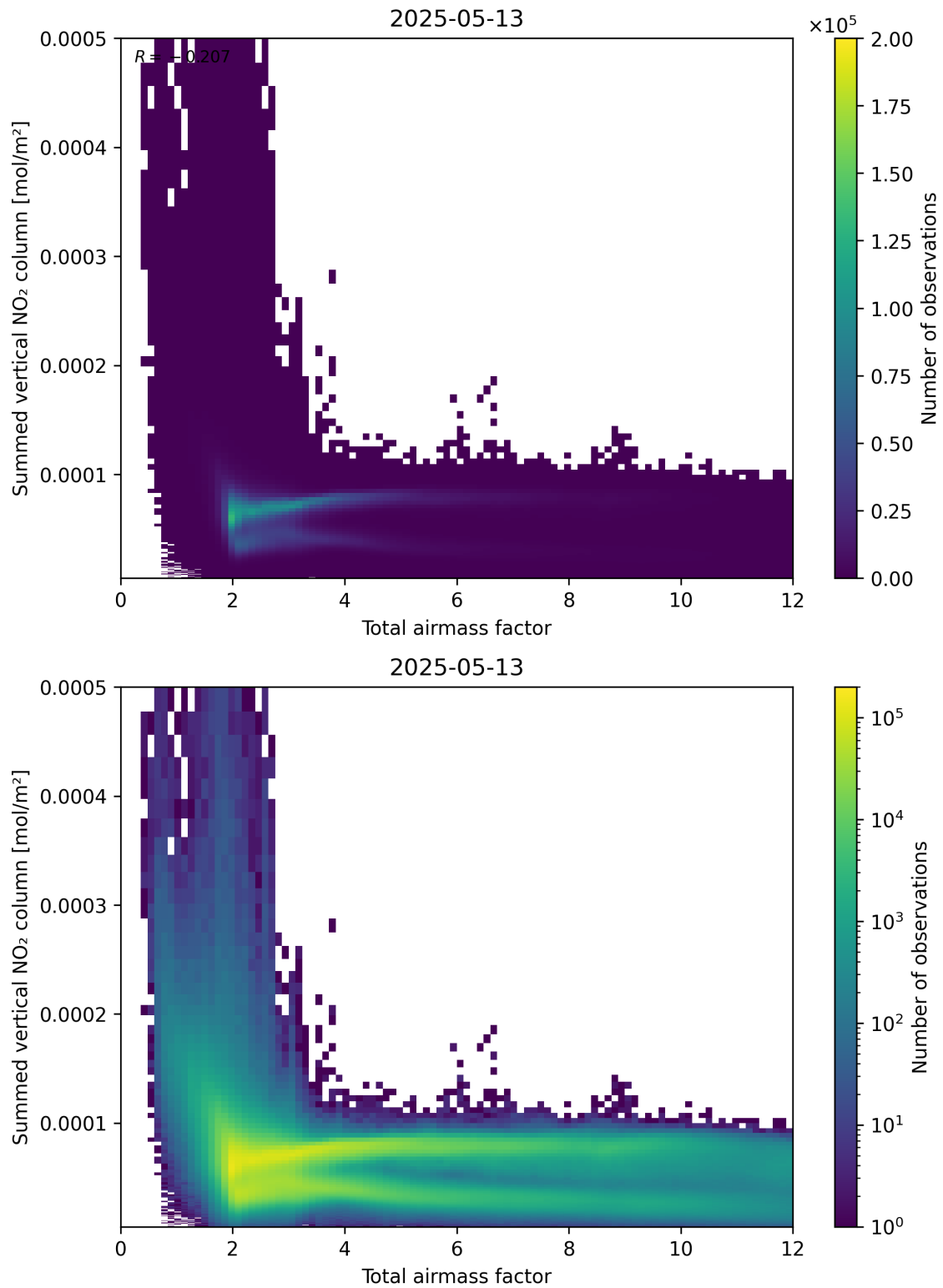
Figure 65: Scatter density plot of “Total airmass factor” against “Summed vertical NO 2 column” for 2025-05-13 to 2025-05-13.
