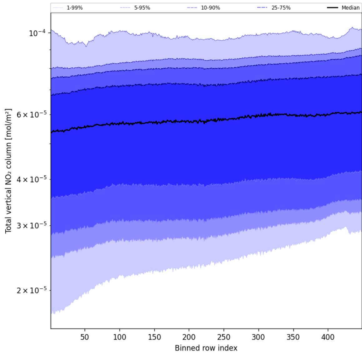
Figure 55: Along track statistics of “Total vertical NO 2 column” for 2025-05-13 to 2025-05-13
