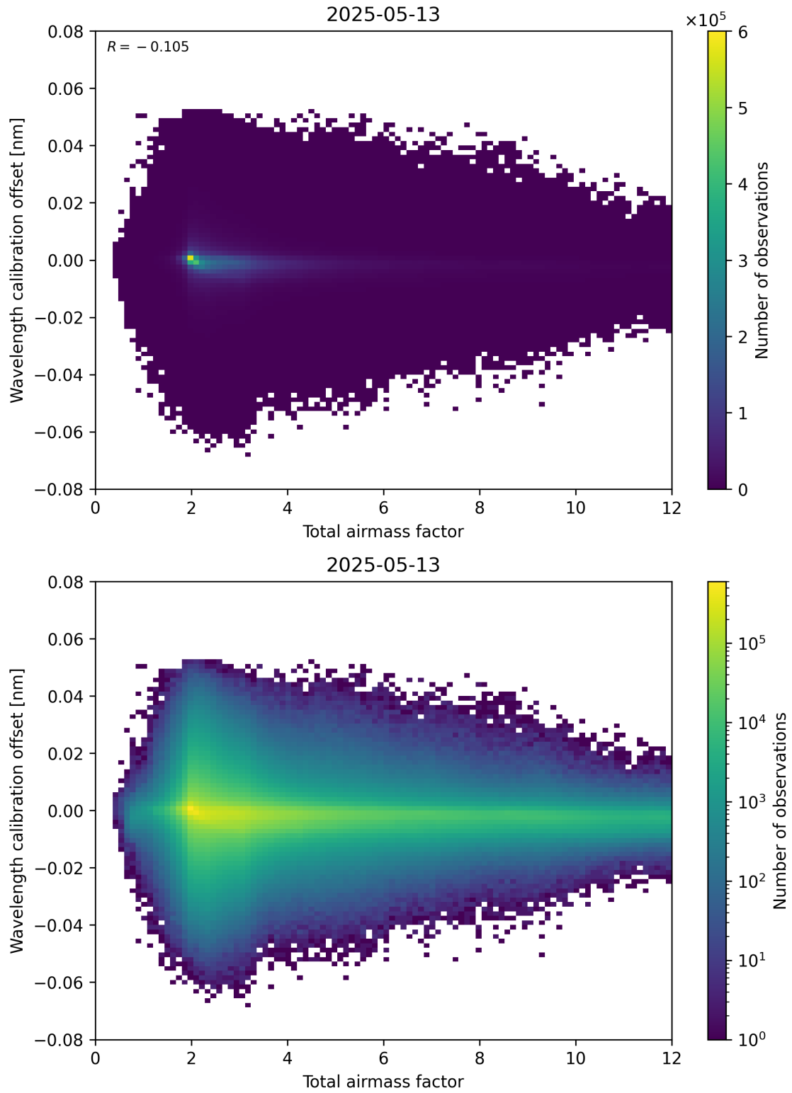
Figure 70: Scatter density plot of “Total airmass factor” against “Wavelength calibration offset” for 2025-05-13 to 2025-05-13.
