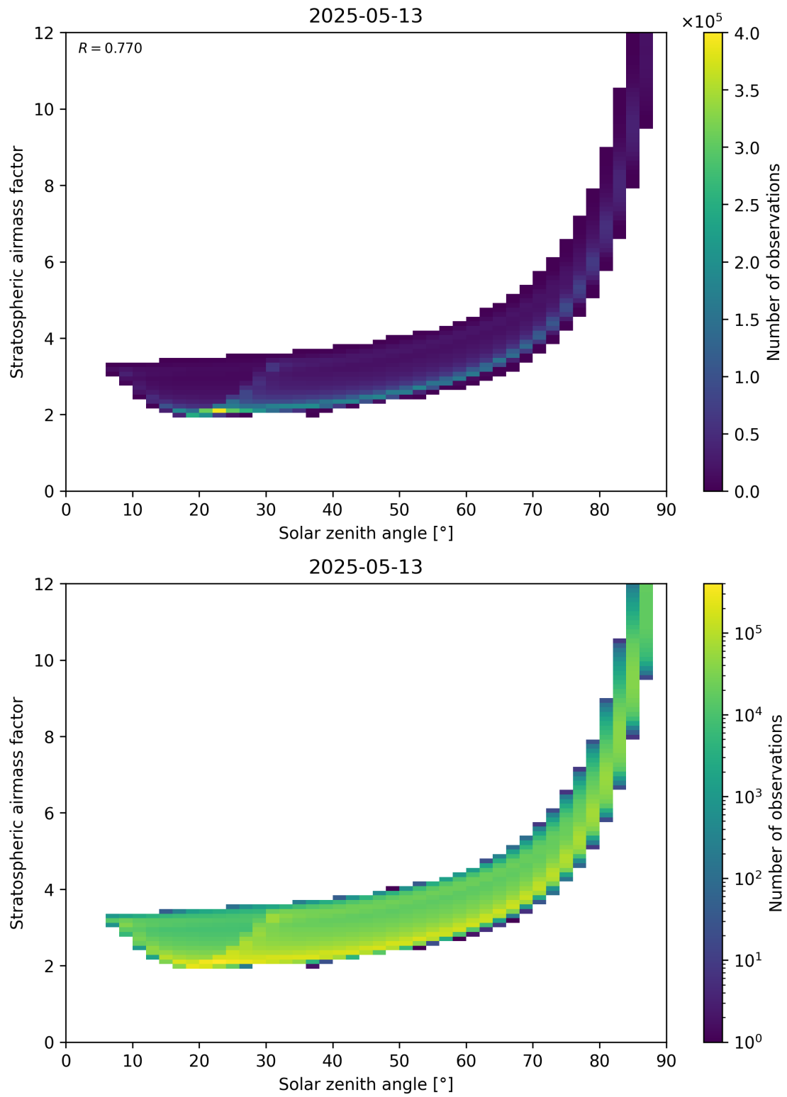
Figure 145: Scatter density plot of “Solar zenith angle” against “Stratospheric airmass factor” for 2025-05-13 to 2025-05-13.
