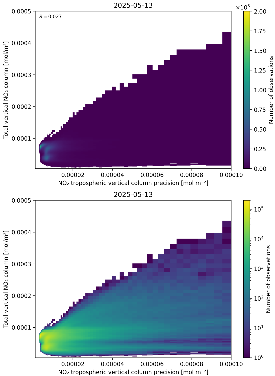
Figure 138: Scatter density plot of “NO 2 tropospheric vertical column precision” against “Total vertical NO 2 column” for 2025-05-13 to 2025-05-13.
