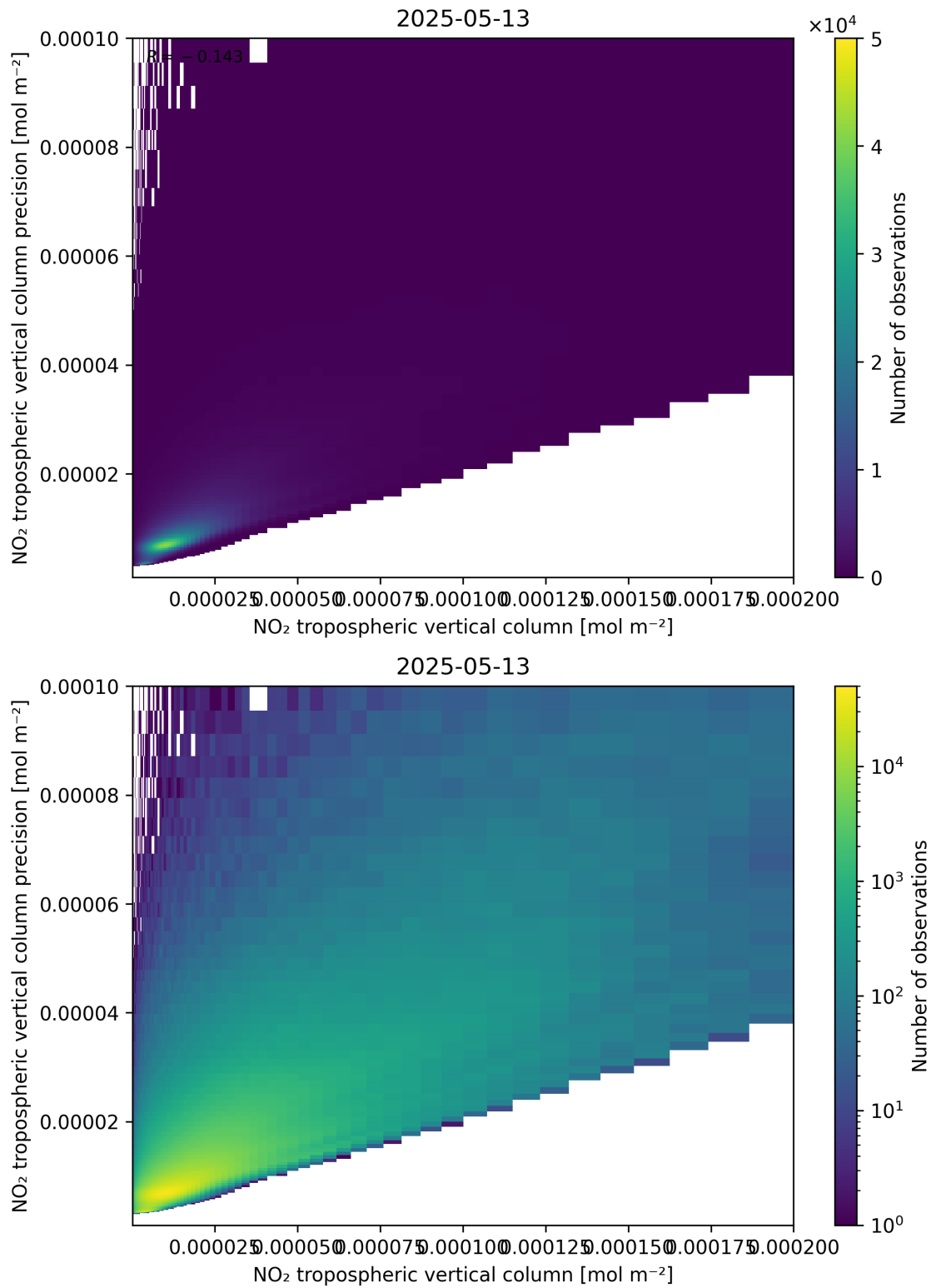
Figure 130: Scatter density plot of “NO 2 tropospheric vertical column” against “NO 2 tropospheric vertical column precision” for 2025-05-13 to 2025-05-13.
