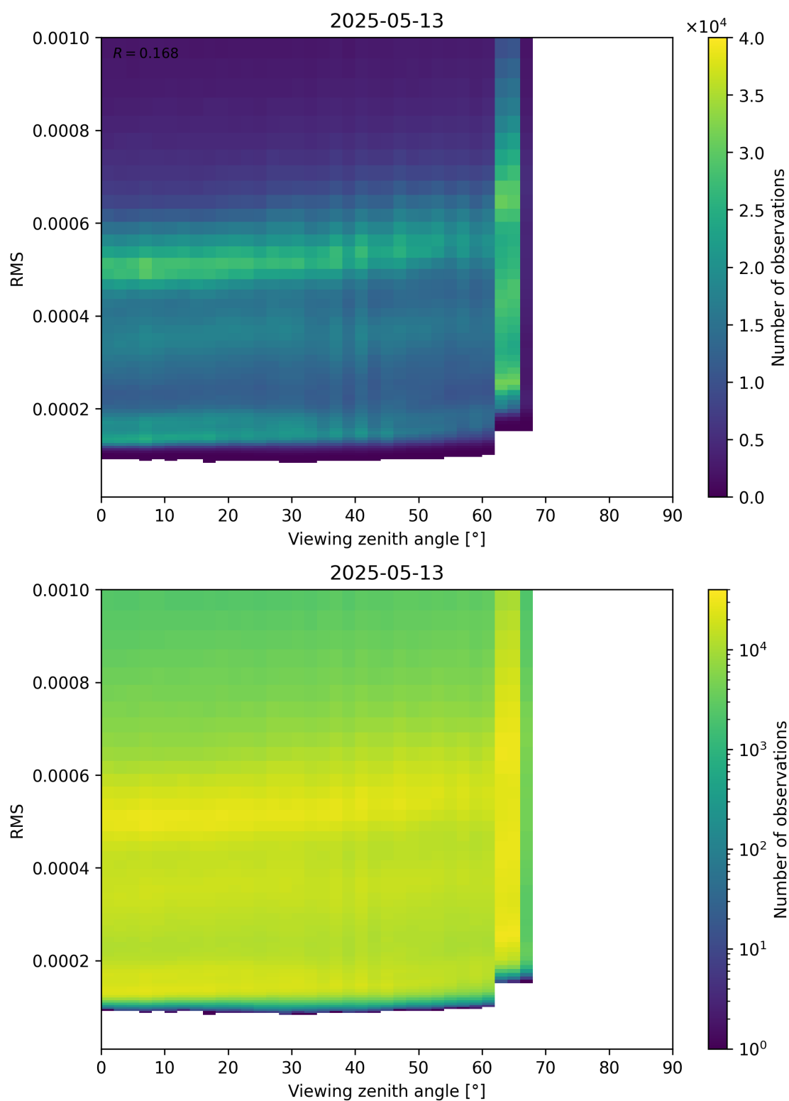
Figure 171: Scatter density plot of “Viewing zenith angle” against “RMS” for 2025-05-13 to 2025-05-13.
