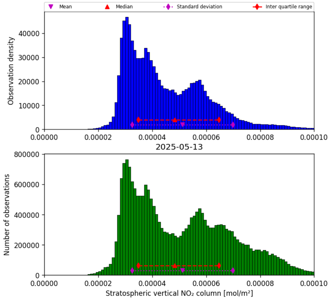
Figure 36: Histogram of “Stratospheric vertical NO 2 column” for 2025-05-13 to 2025-05-13
