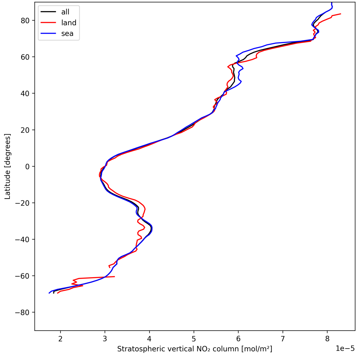
Figure 19: Zonal average of “Stratospheric vertical NO 2 column” for 2025-05-13 to 2025-05-13.
