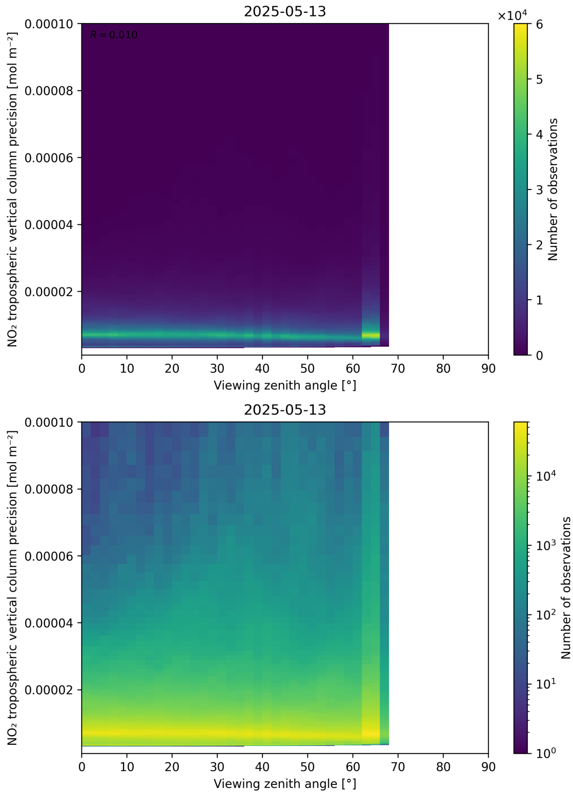
Figure 170: Scatter density plot of “Viewing zenith angle” against “NO 2 tropospheric vertical column precision” for 2025-05-13 to 2025-05-13.
