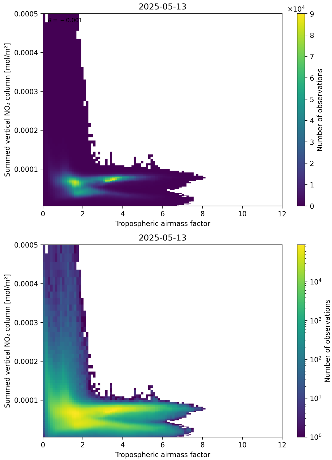
Figure 75: Scatter density plot of “Tropospheric air mass factor” against “Summed vertical NO 2 column” for 2025-05-13 to 2025-05-13.
