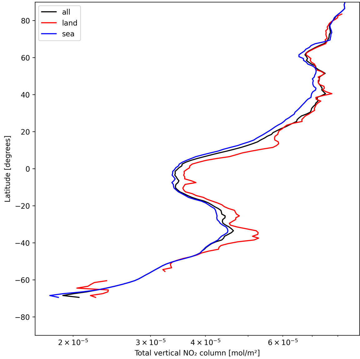
Figure 21: Zonal average of “Total vertical NO 2 column” for 2025-05-13 to 2025-05-13.
