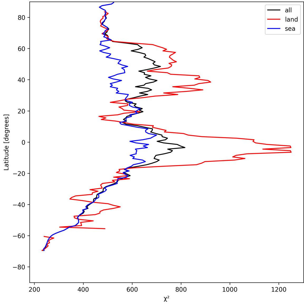
Figure 25: Zonal average of “ \chi^2 ” for 2025-05-13 to 2025-05-13.
