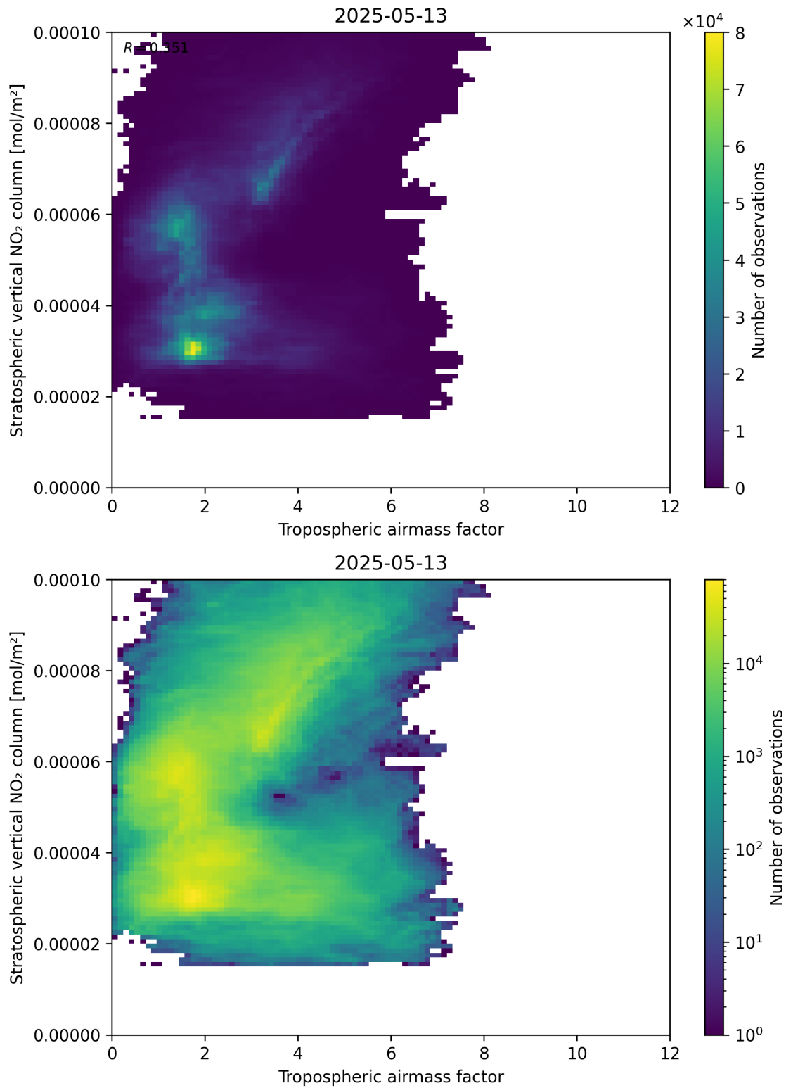
Figure 74: Scatter density plot of “Tropospheric air mass factor” against “Stratospheric vertical NO 2 column” for 2025-05-13 to 2025-05-13.
