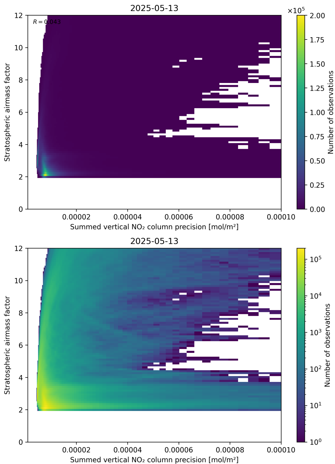
Figure 106: Scatter density plot of “Summed vertical NO 2 column precision” against “Stratospheric airmass factor” for 2025-05-13 to 2025-05-13.
