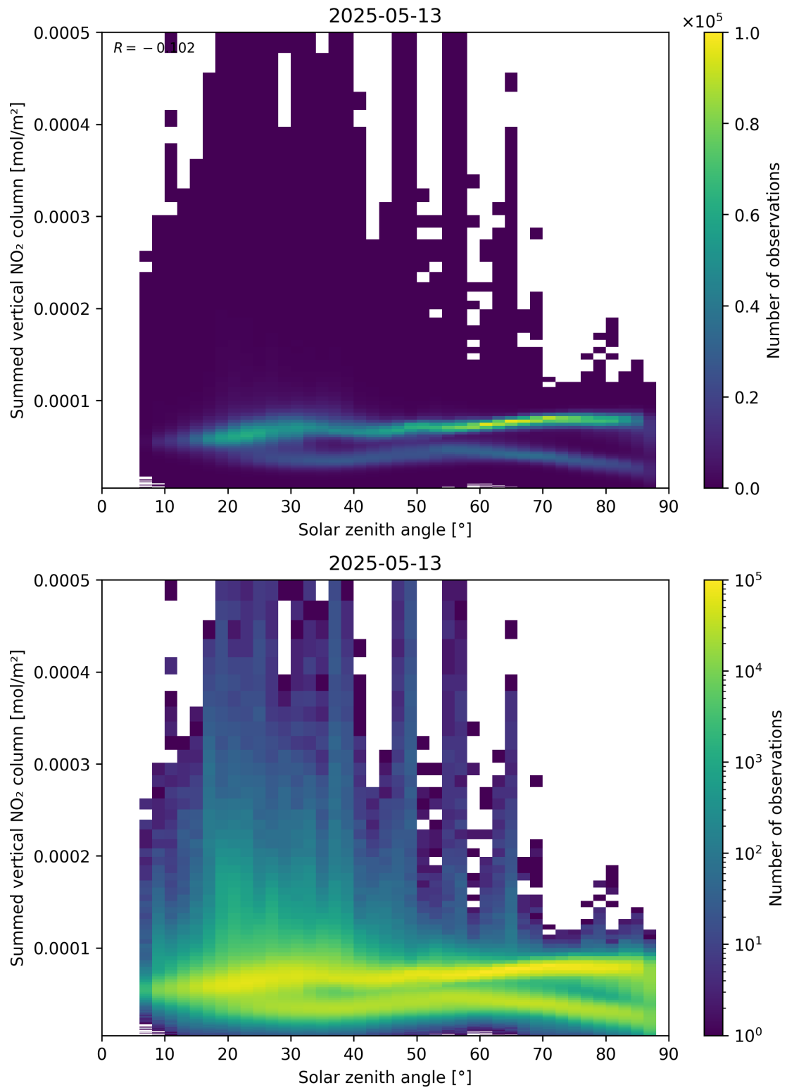
Figure 151: Scatter density plot of “Solar zenith angle” against “Summed vertical NO 2 column” for 2025-05-13 to 2025-05-13.
