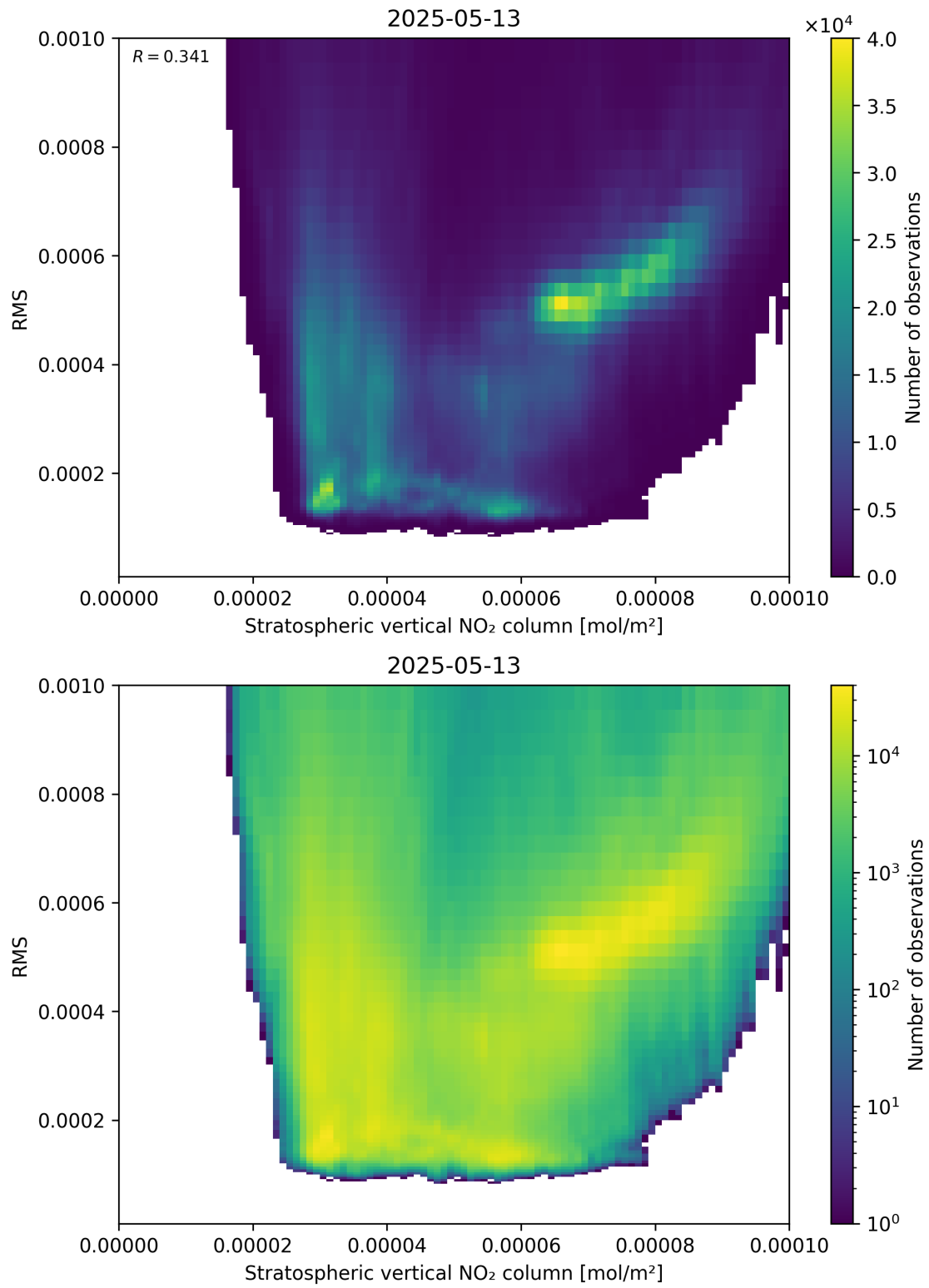
Figure 102: Scatter density plot of “Stratospheric vertical NO 2 column” against “RMS” for 2025-05-13 to 2025-05-13.
