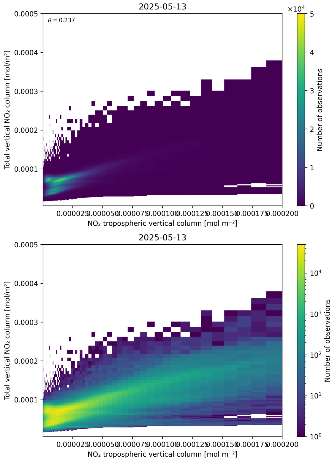
Figure 128: Scatter density plot of “NO 2 tropospheric vertical column” against “Total vertical NO 2 column” for 2025-05-13 to 2025-05-13.
