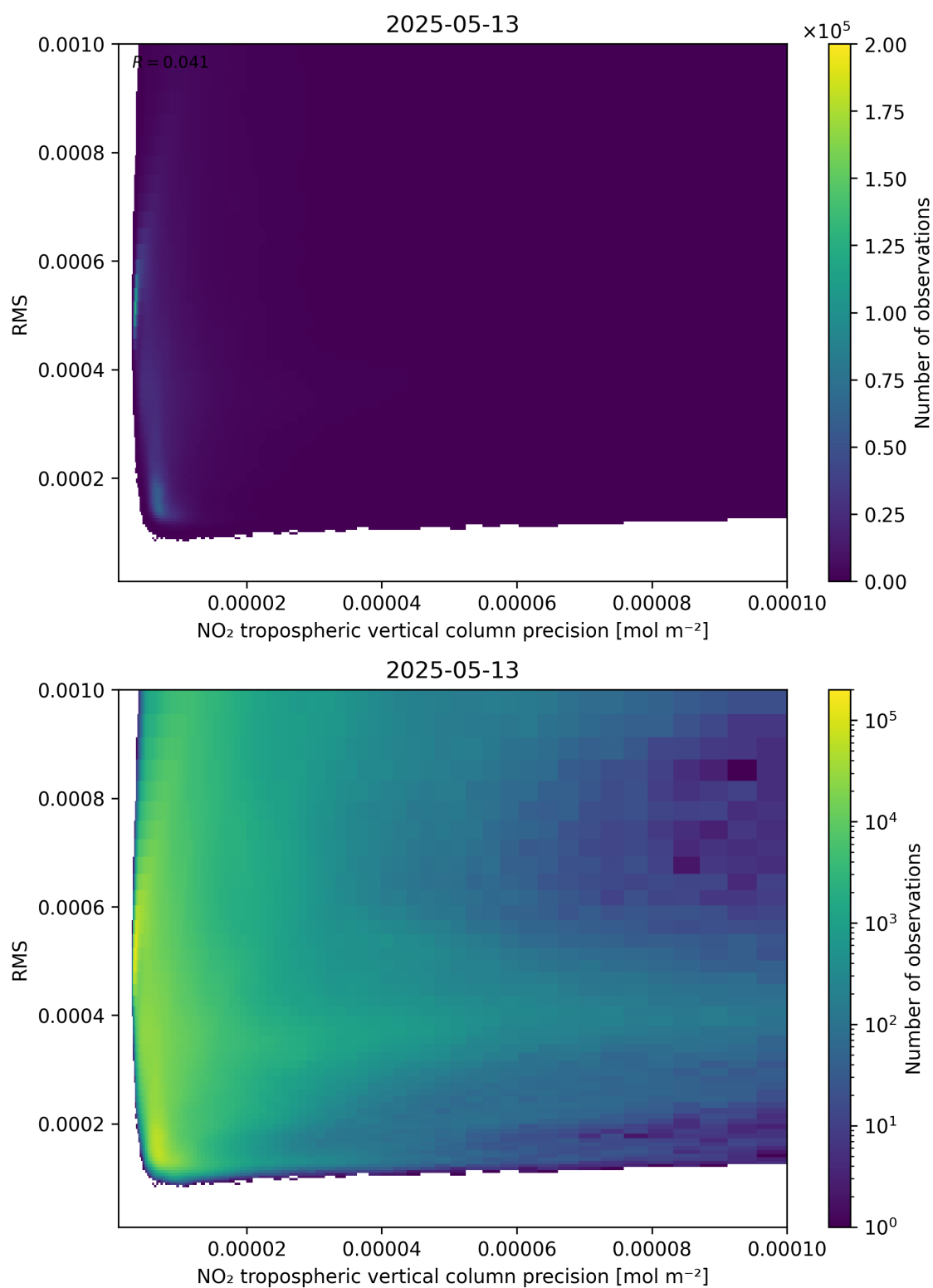
Figure 140: Scatter density plot of “NO 2 tropospheric vertical column precision” against “RMS” for 2025-05-13 to 2025-05-13.
