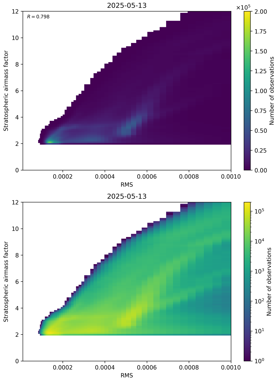
Figure 144: Scatter density plot of “RMS” against “Stratospheric airmass factor” for 2025-05-13 to 2025-05-13.
