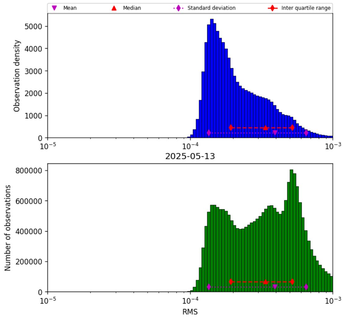
Figure 43: Histogram of “RMS” for 2025-05-13 to 2025-05-13
