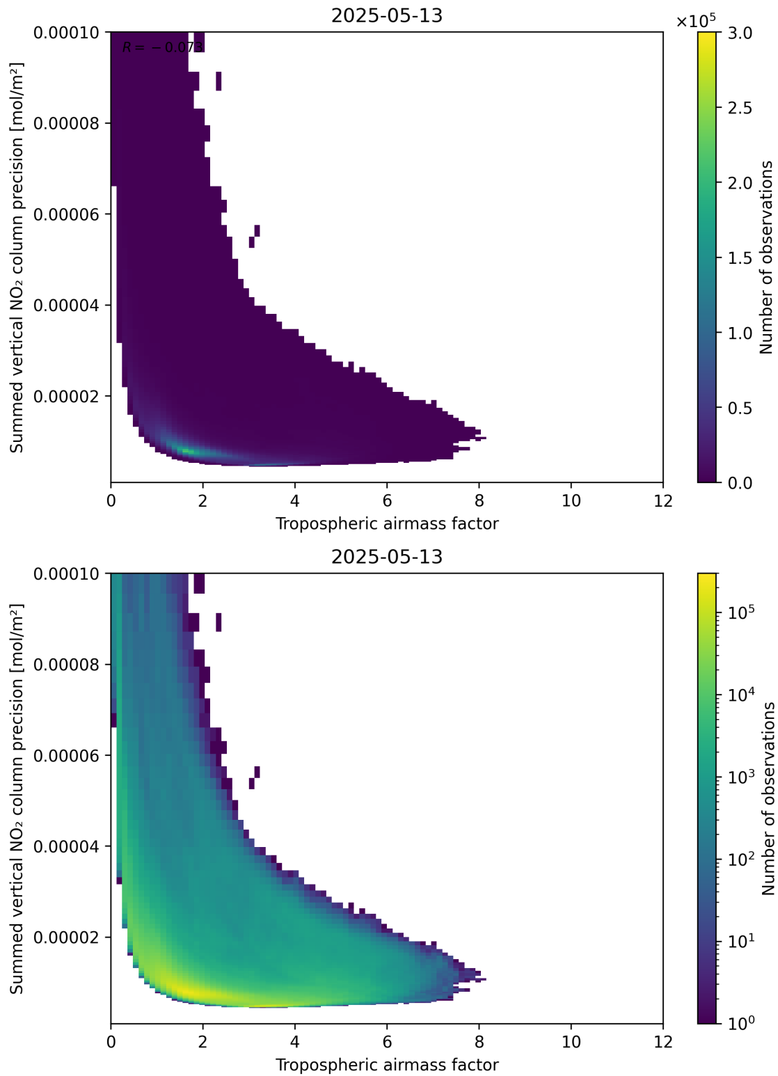
Figure 76: Scatter density plot of “Tropospheric air mass factor” against “Summed vertical NO 2 column precision” for 2025-05-13 to 2025-05-13.
