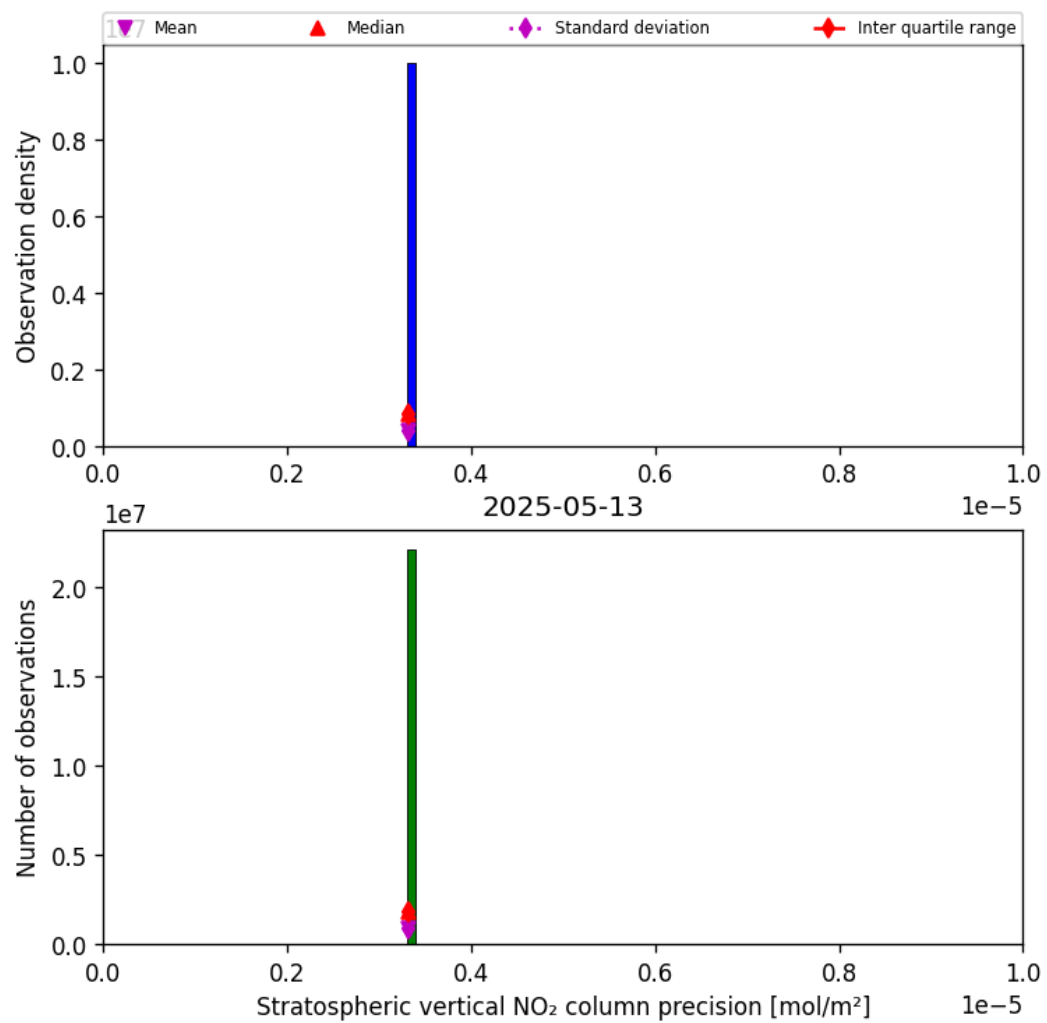
Figure 37: Histogram of “Stratospheric vertical NO 2 column precision” for 2025-05-13 to 2025-05-13
