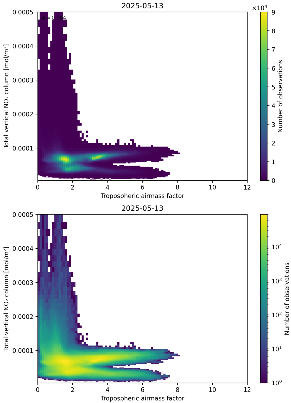
Figure 77: Scatter density plot of “Tropospheric airmass factor” against “Total vertical NO 2 column” for 2025-05-13 to 2025-05-13.
