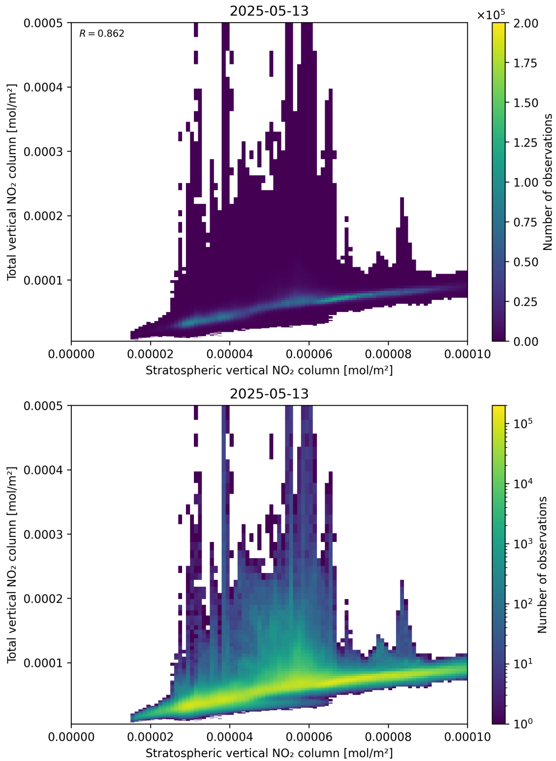
Figure 100: Scatter density plot of “Stratospheric vertical NO 2 column” against “Total vertical NO 2 column” for 2025-05-13 to 2025-05-13.
