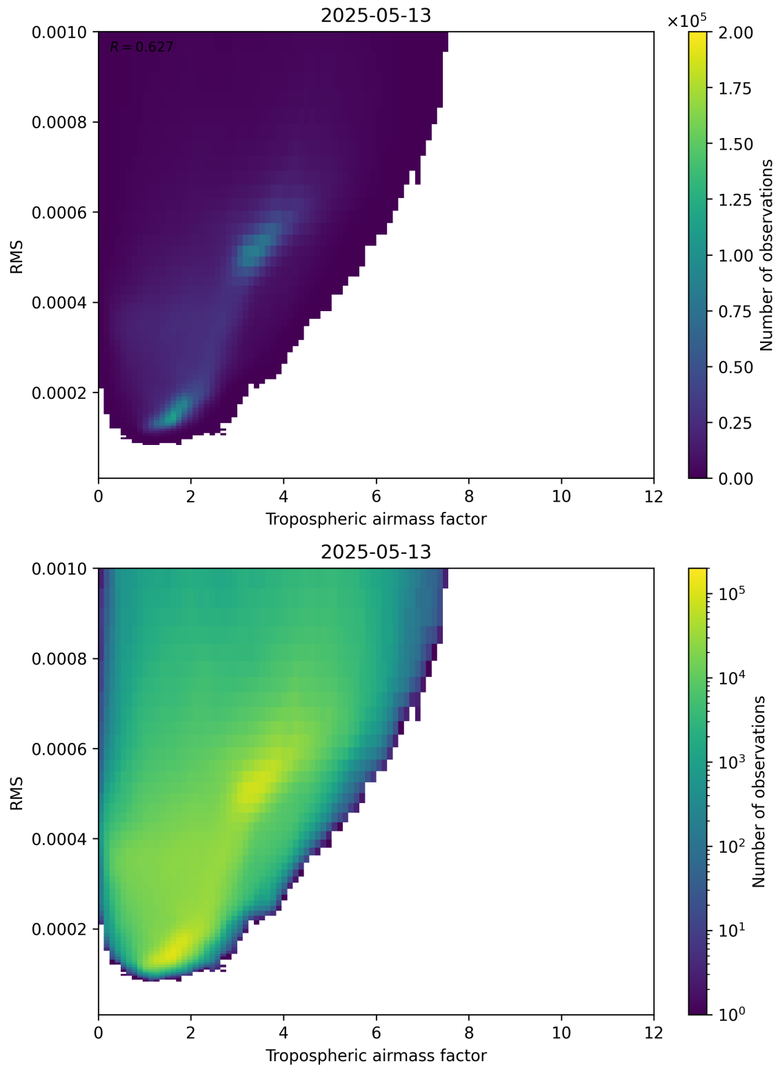
Figure 79: Scatter density plot of “Tropospheric airmass factor” against “RMS” for 2025-05-13 to 2025-05-13.
