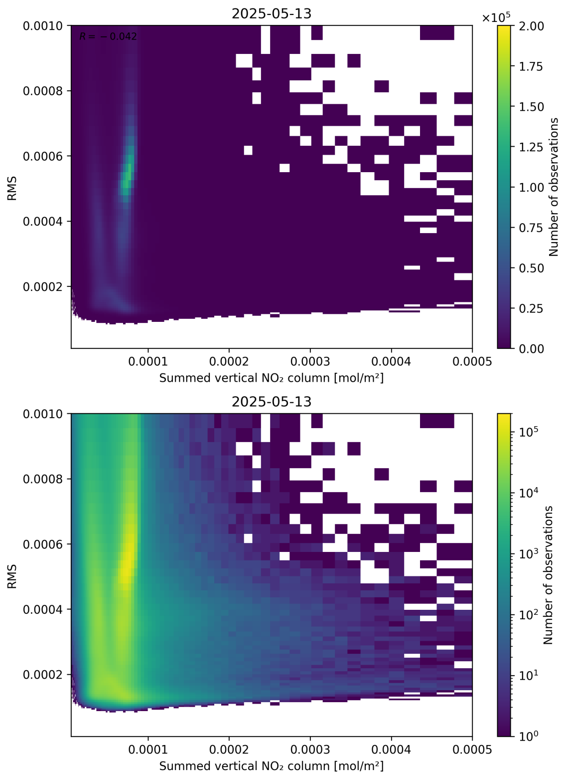
Figure 109: Scatter density plot of “Summed vertical NO 2 column” against “RMS” for 2025-05-13 to 2025-05-13.
