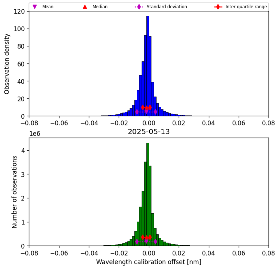
Figure 35: Histogram of “Wavelength calibration offset” for 2025-05-13 to 2025-05-13
