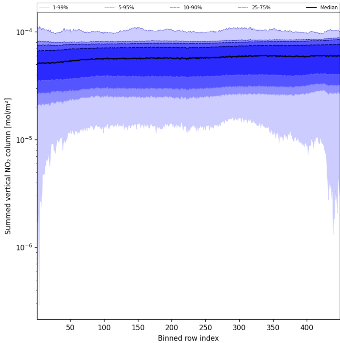
Figure 57: Along track statistics of “Summed vertical NO 2 column” for 2025-05-13 to 2025-05-13
