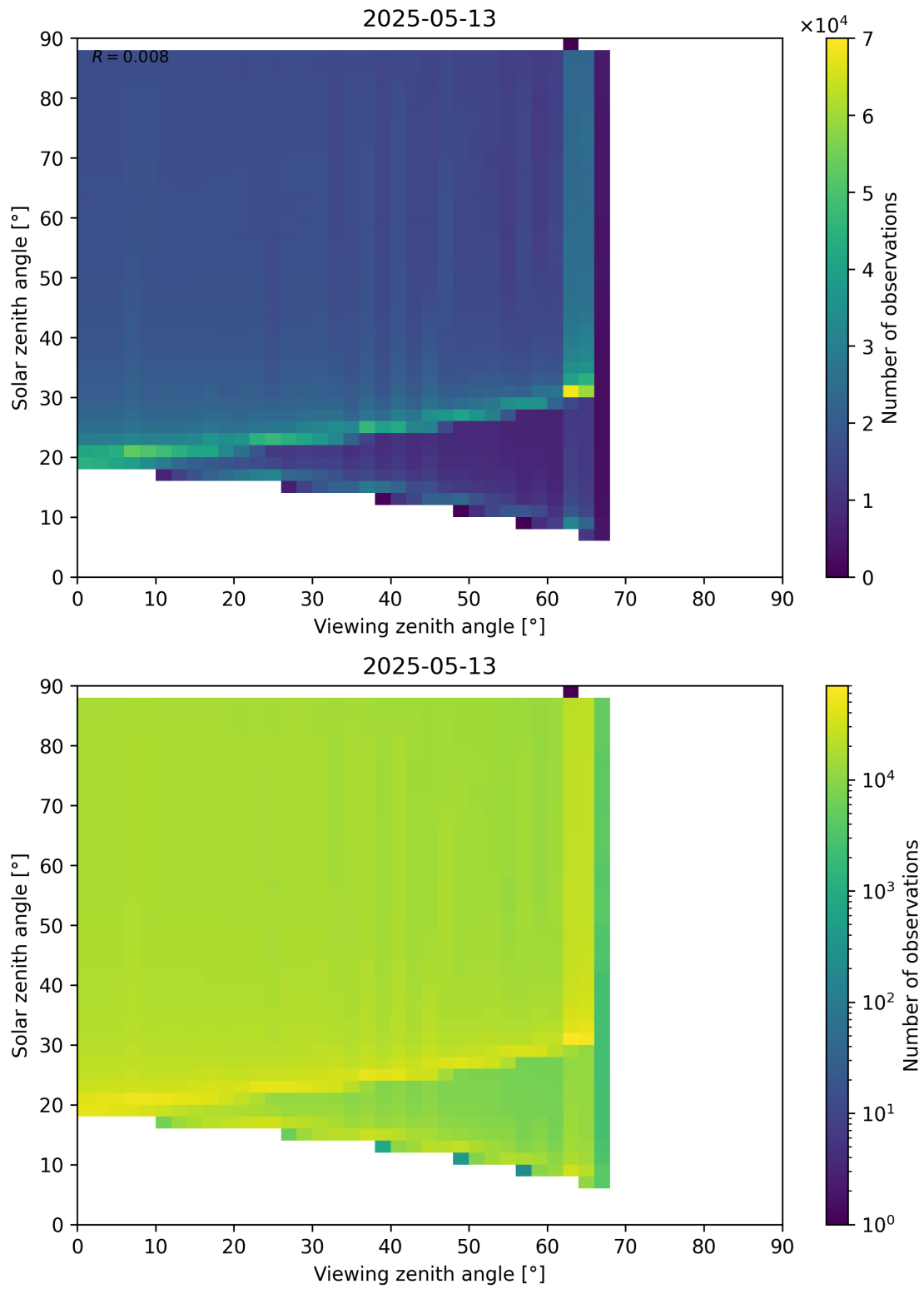
Figure 172: Scatter density plot of “Viewing zenith angle” against “Solar zenith angle” for 2025-05-13 to 2025-05-13.
