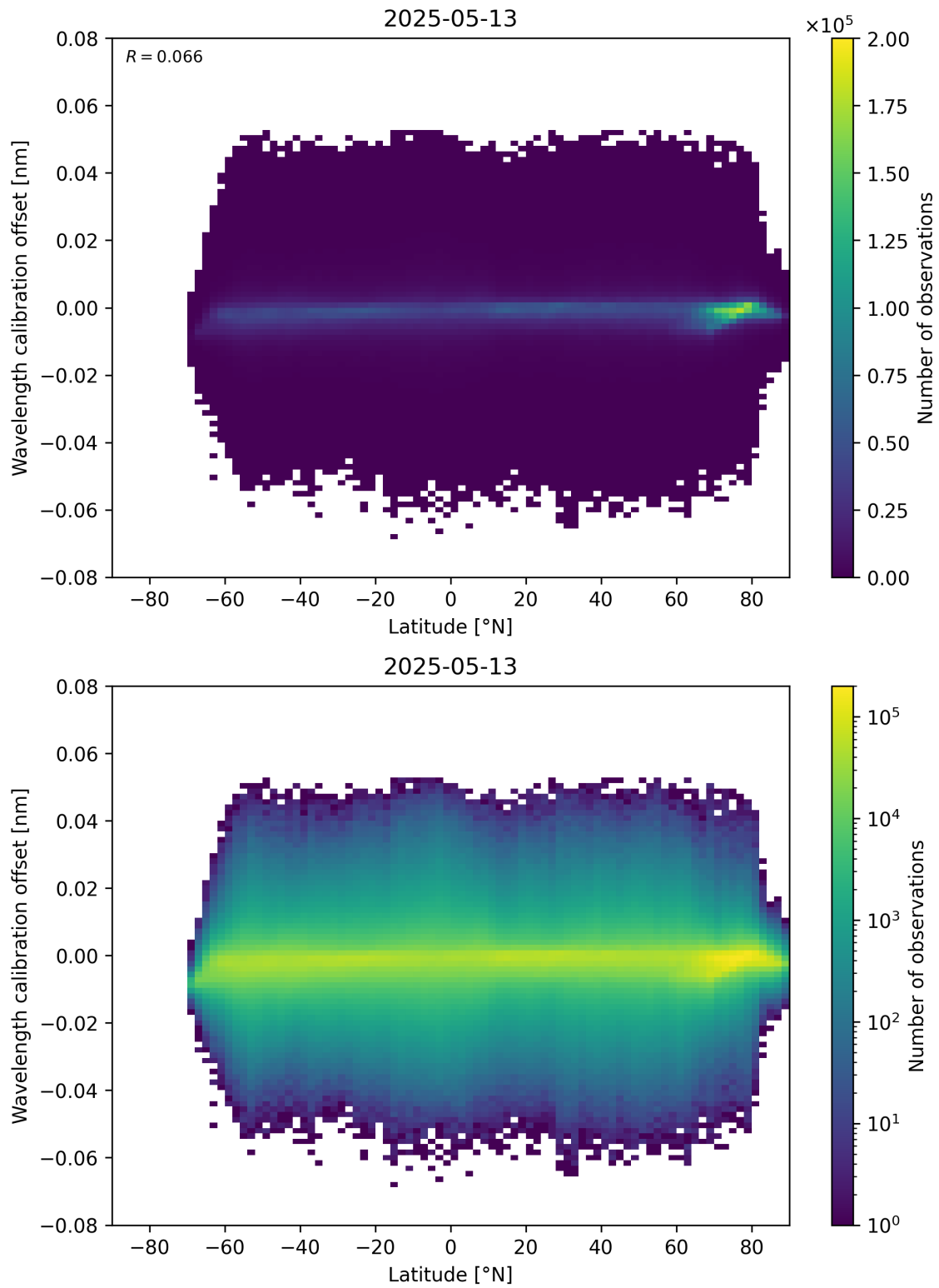
Figure 95: Scatter density plot of “Latitude” against “Wavelength calibration offset” for 2025-05-13 to 2025-05-13.
