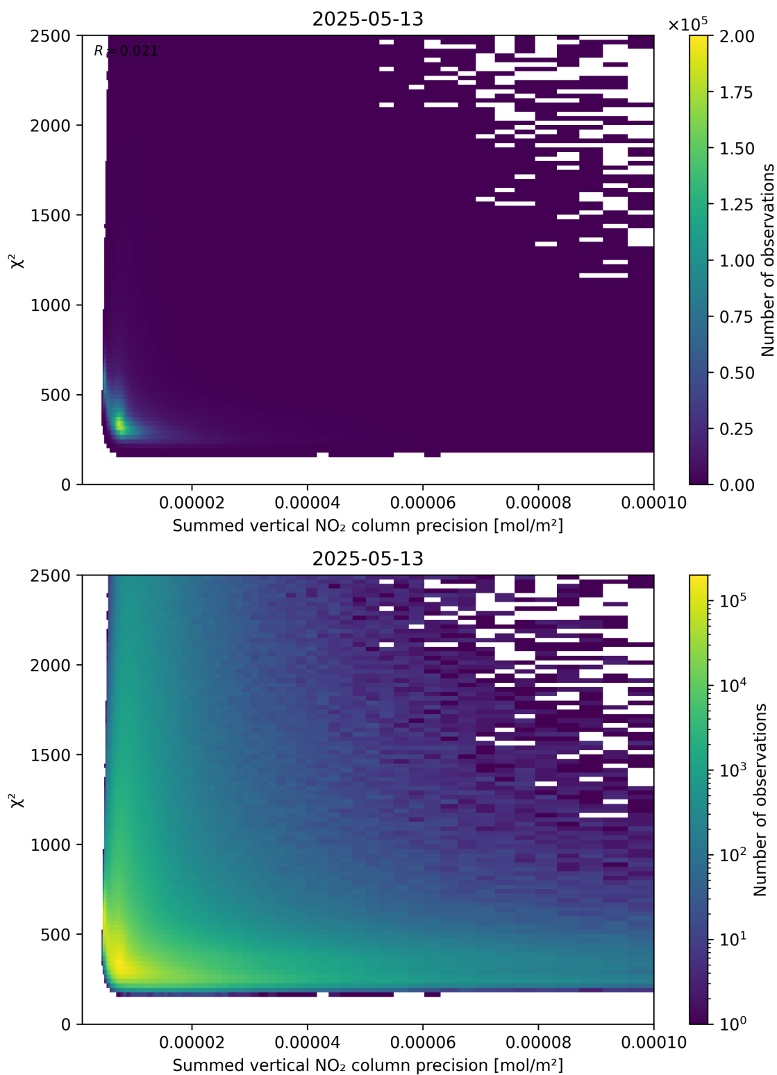
Figure 107: Scatter density plot of “Summed vertical NO 2 column precision” against “ \chi^2 ” for 2025-05-13 to 2025-05-13.
