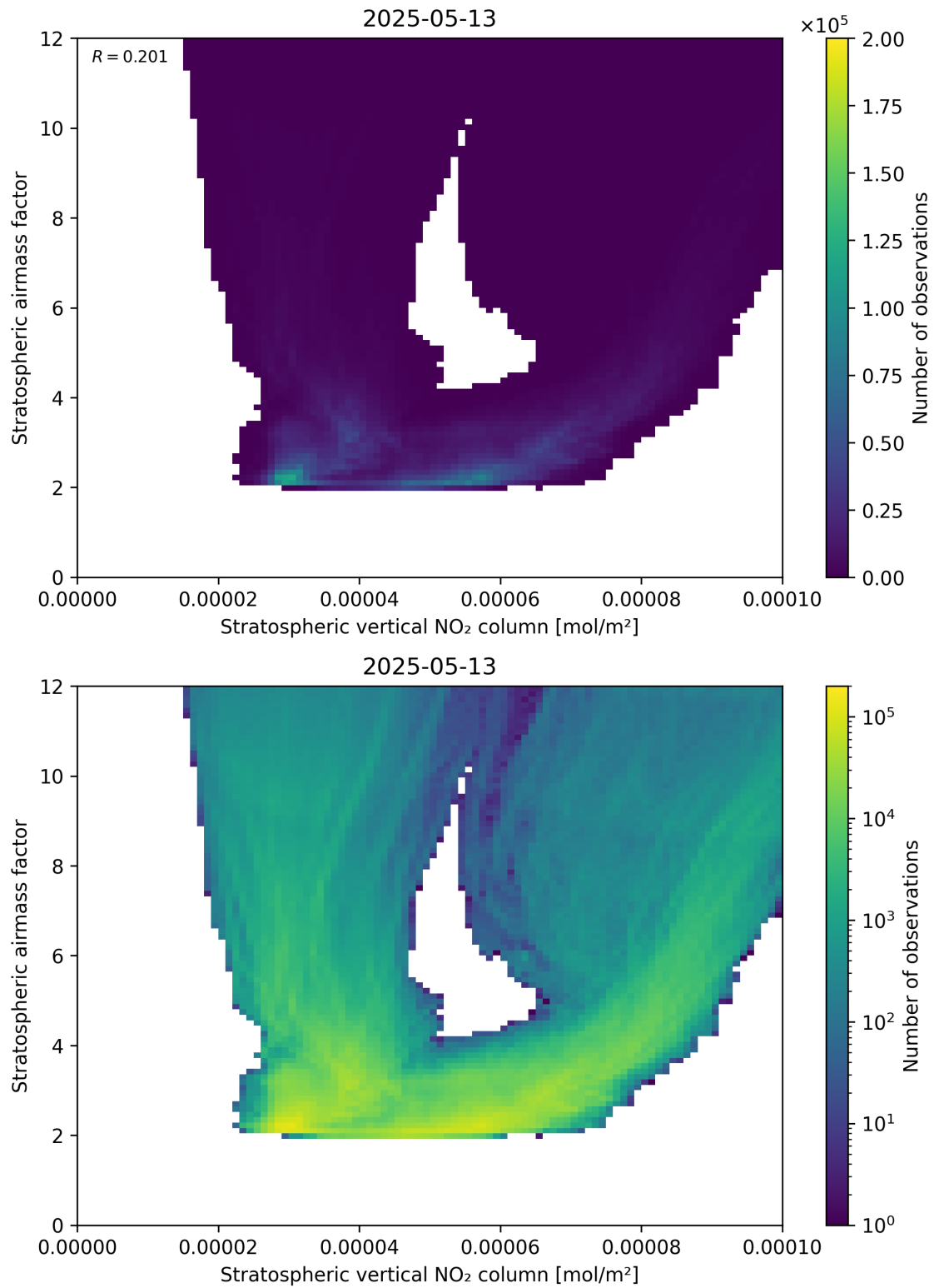
Figure 96: Scatter density plot of “Stratospheric vertical NO 2 column” against “Stratospheric airmass factor” for 2025-05-13 to 2025-05-13.
