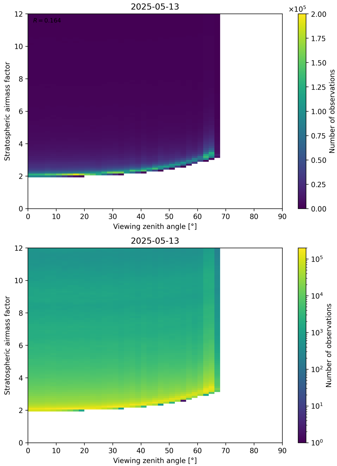
Figure 159: Scatter density plot of “Viewing zenith angle” against “Stratospheric airmass factor” for 2025-05-13 to 2025-05-13.
