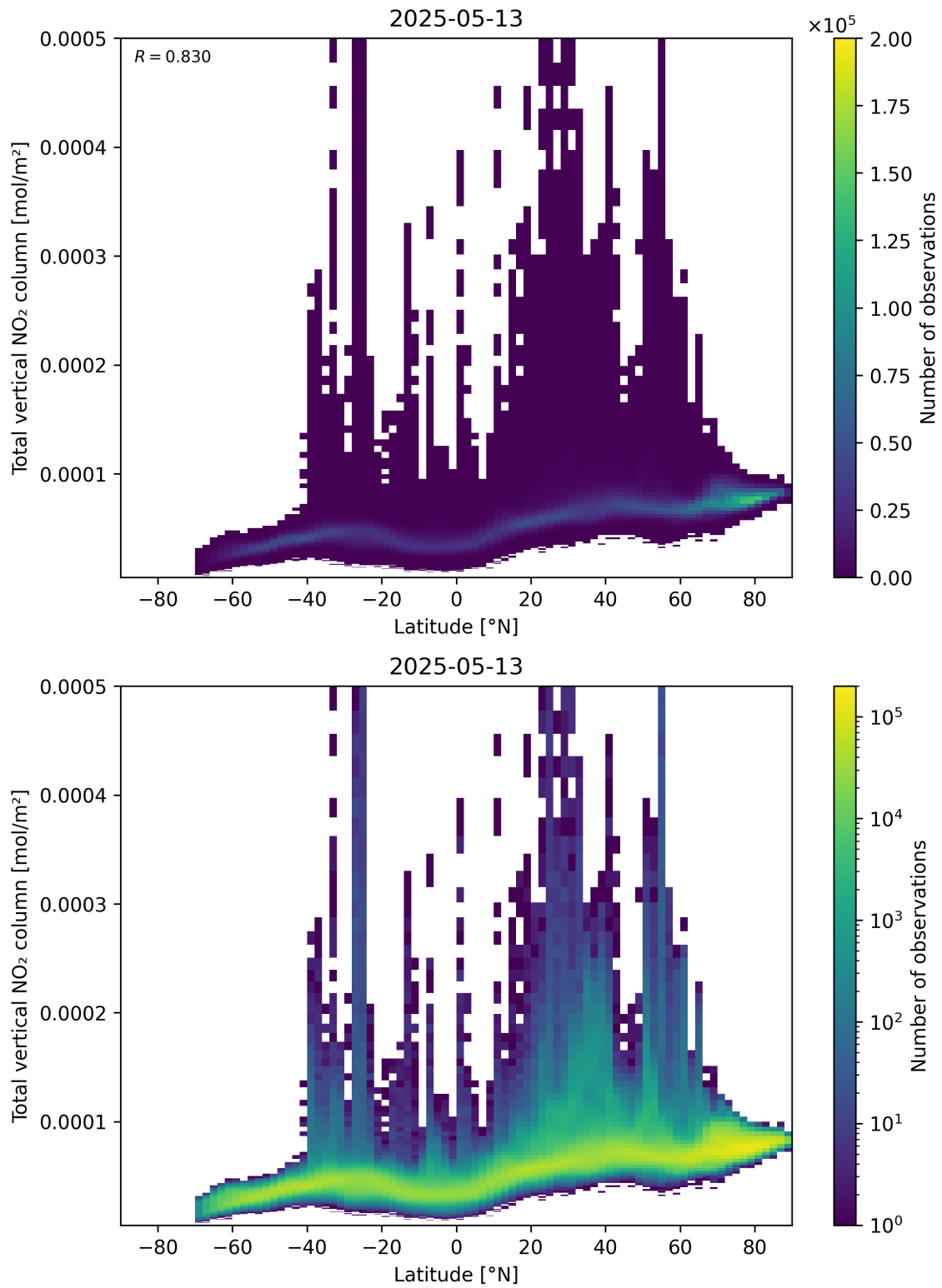
Figure 90: Scatter density plot of “Latitude” against “Total vertical NO 2 column” for 2025-05-13 to 2025-05-13.
