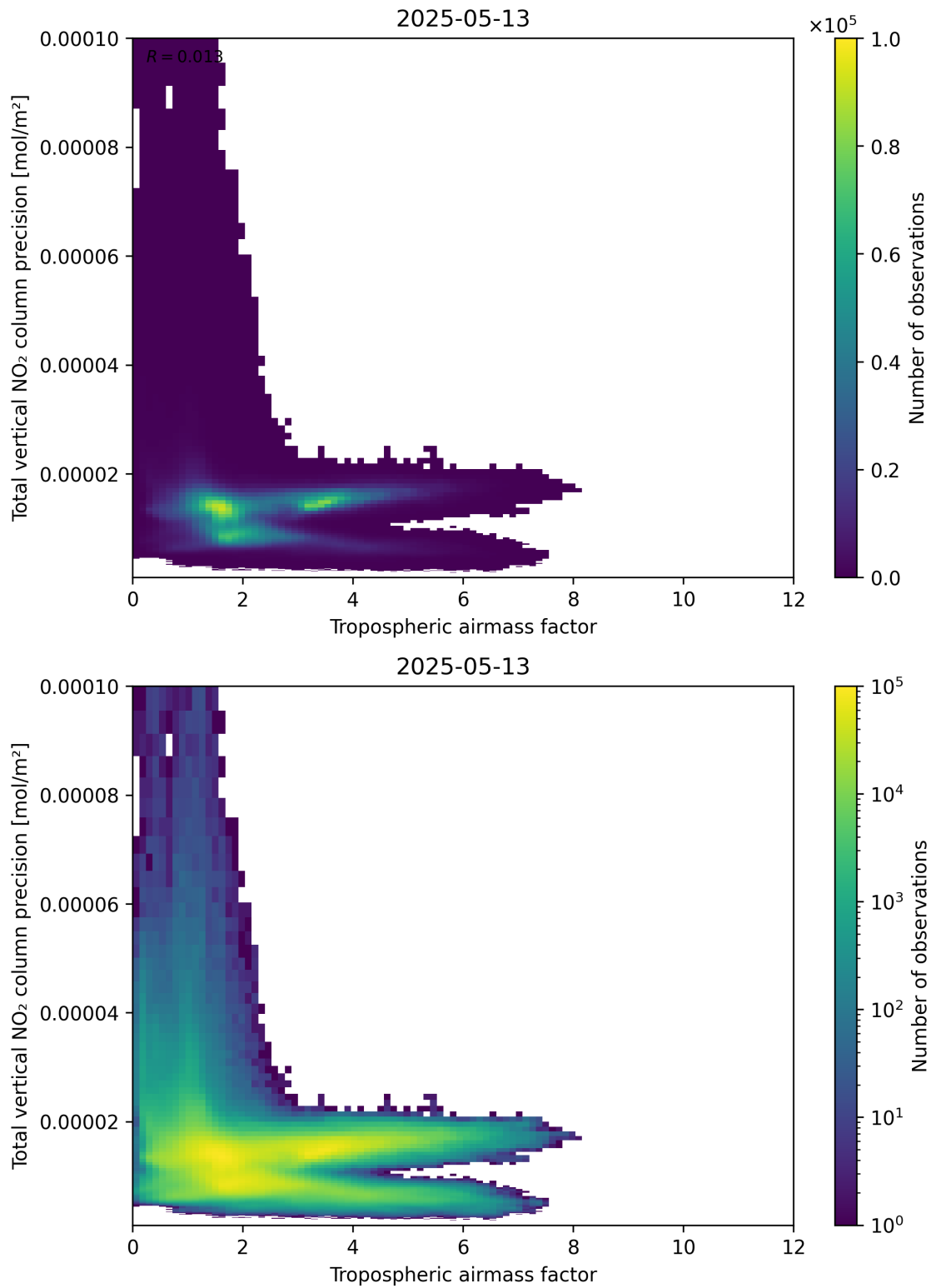
Figure 78: Scatter density plot of “Tropospheric air mass factor” against “Total vertical NO 2 column precision” for 2025-05-13 to 2025-05-13.
