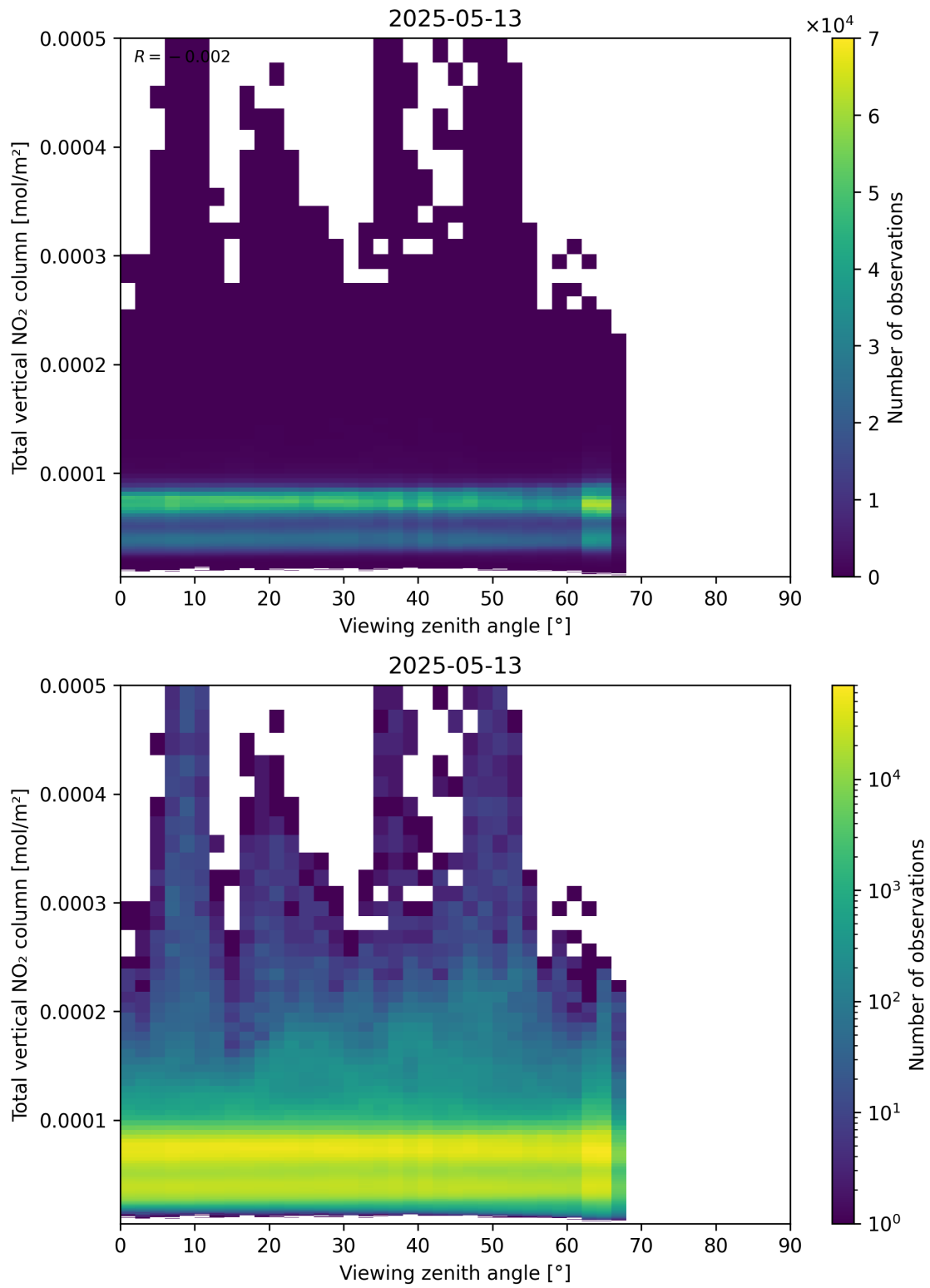
Figure 167: Scatter density plot of “Viewing zenith angle” against “Total vertical NO 2 column” for 2025-05-13 to 2025-05-13.
