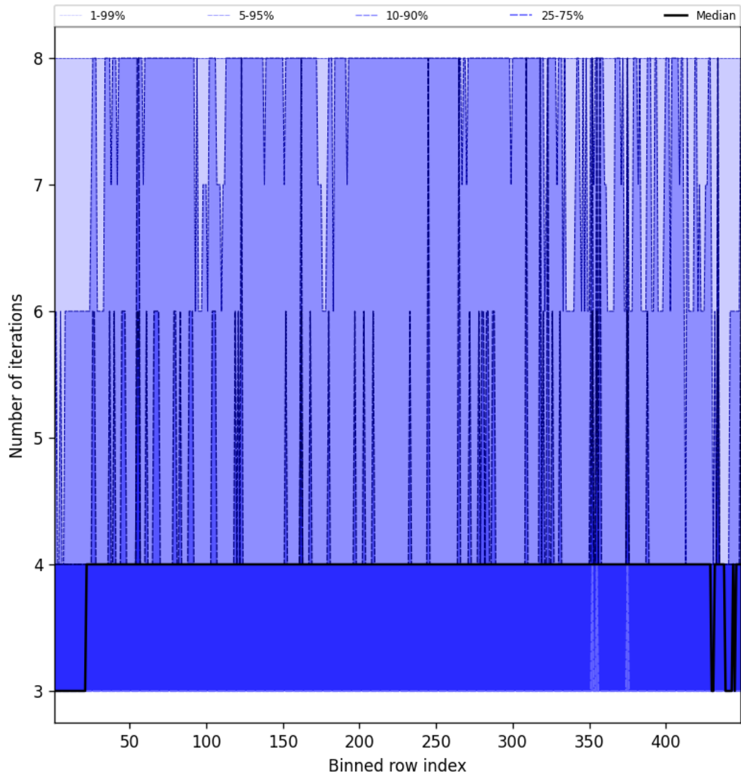
Figure 51: Along track statistics of “Number of iterations” for 2025-05-13 to 2025-05-13
