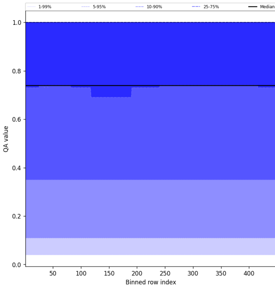
Figure 45: Along track statistics of “QA value” for 2025-05-13 to 2025-05-13
