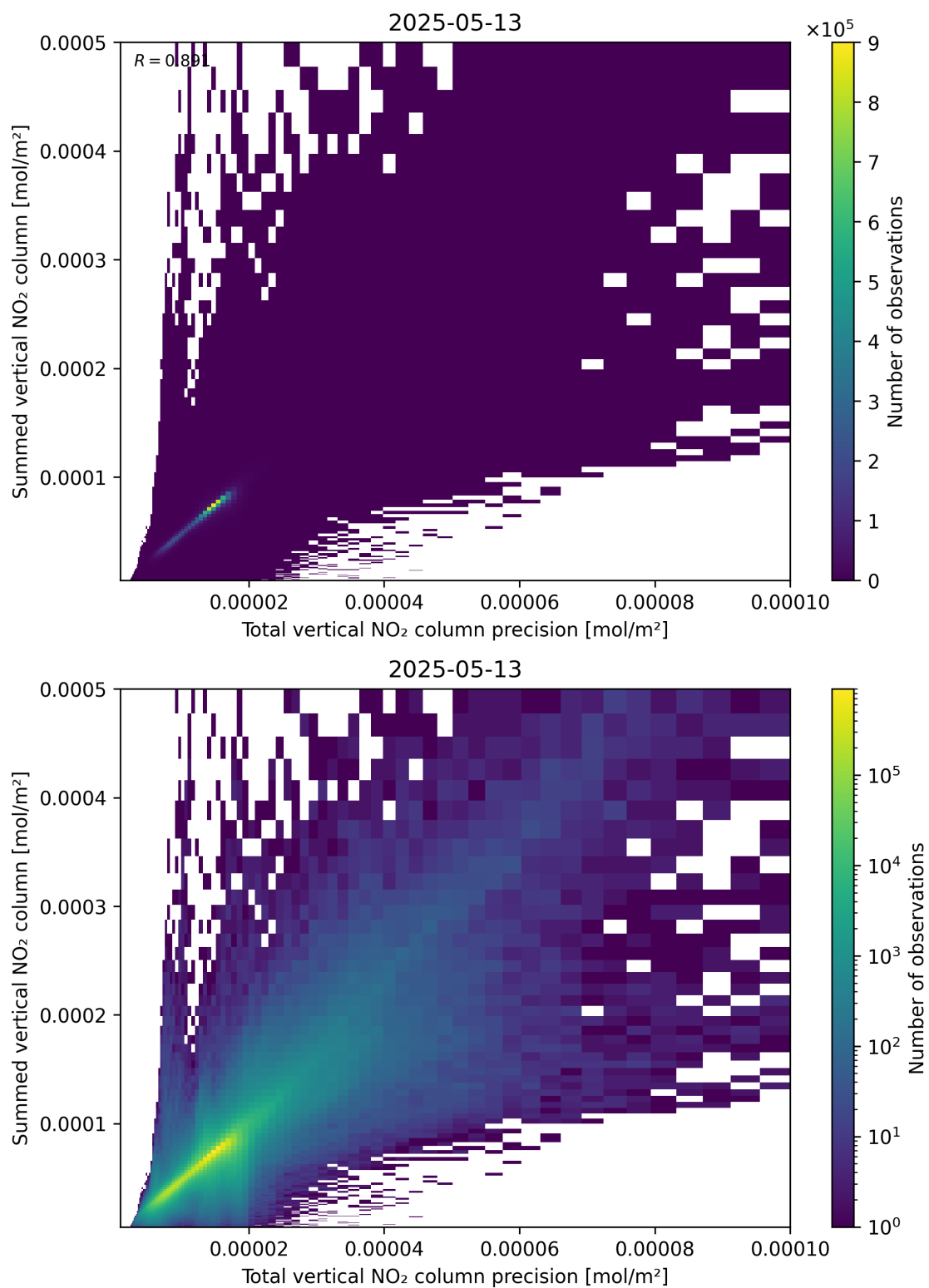
Figure 117: Scatter density plot of “Total vertical NO 2 column precision” against “Summed vertical NO 2 column” for 2025-05-13 to 2025-05-13.
