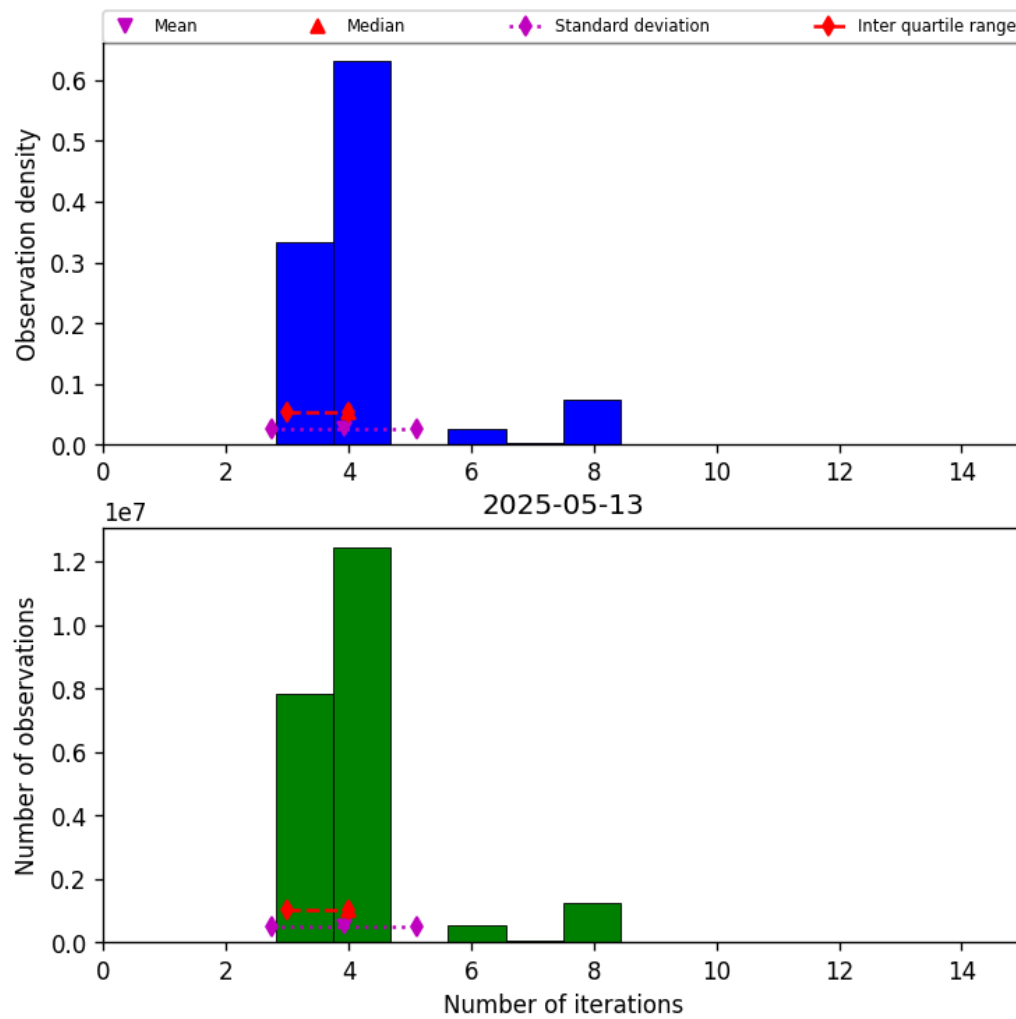
Figure 34: Histogram of “Number of iterations” for 2025-05-13 to 2025-05-13
