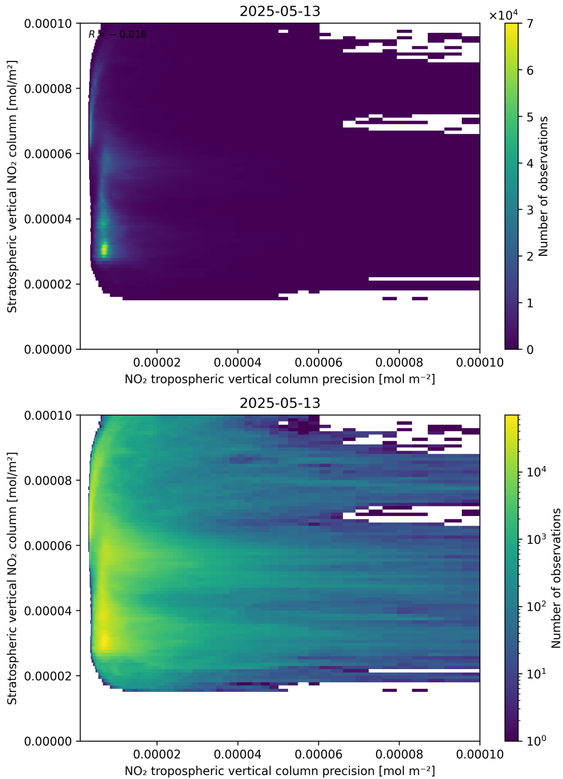
Figure 135: Scatter density plot of “NO 2 tropospheric vertical column precision” against “Stratospheric vertical NO 2 column” for 2025-05-13 to 2025-05-13.
