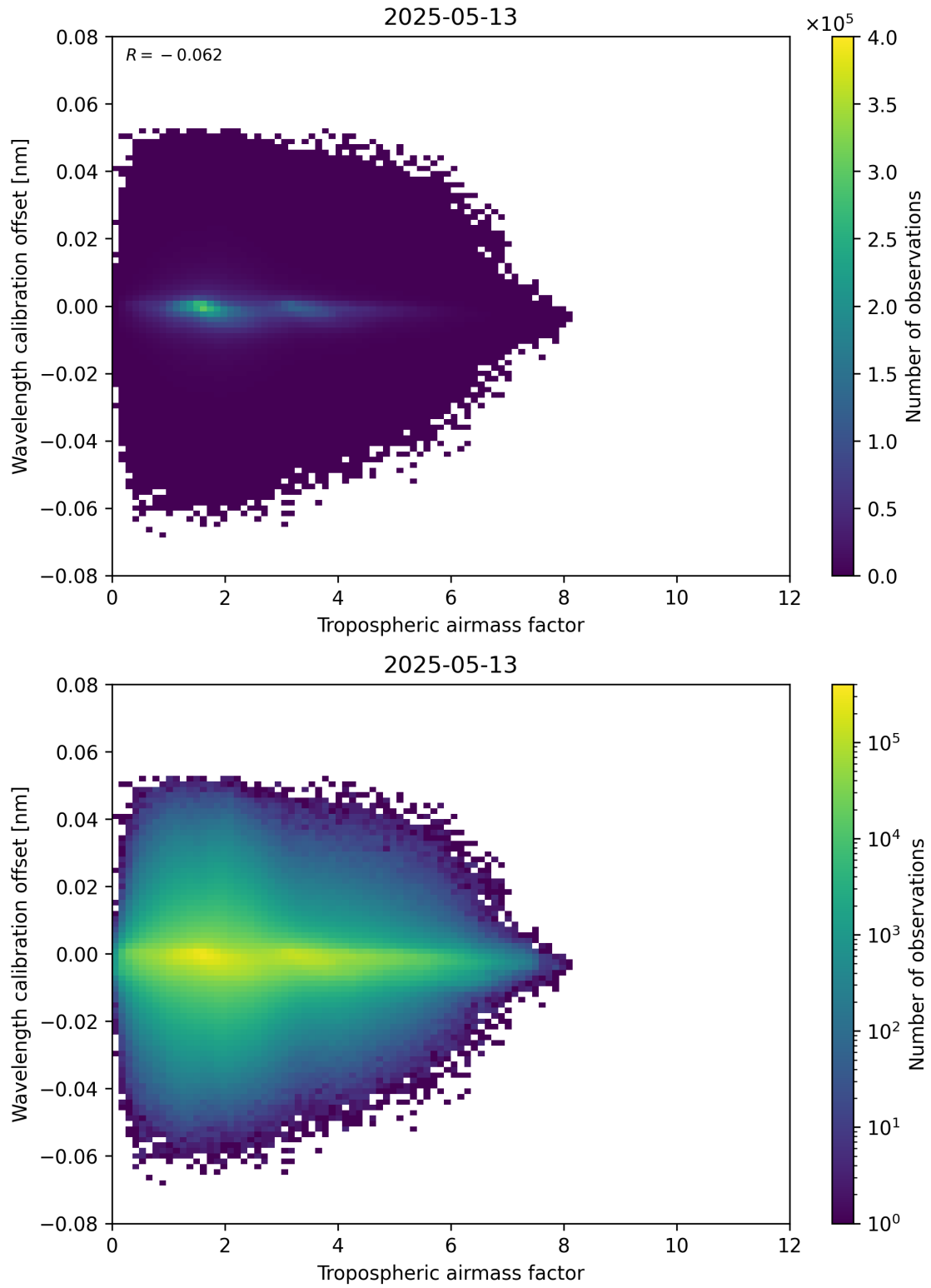
Figure 80: Scatter density plot of “Tropospheric airmass factor” against “Wavelength calibration offset” for 2025-05-13 to 2025-05-13.
