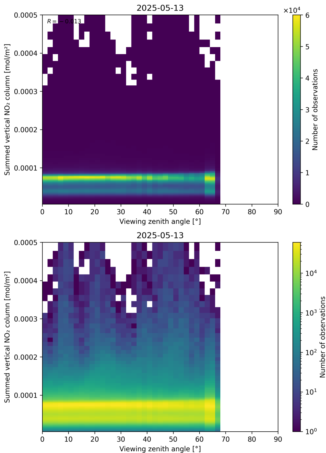
Figure 165: Scatter density plot of “Viewing zenith angle” against “Summed vertical NO 2 column” for 2025-05-13 to 2025-05-13.
