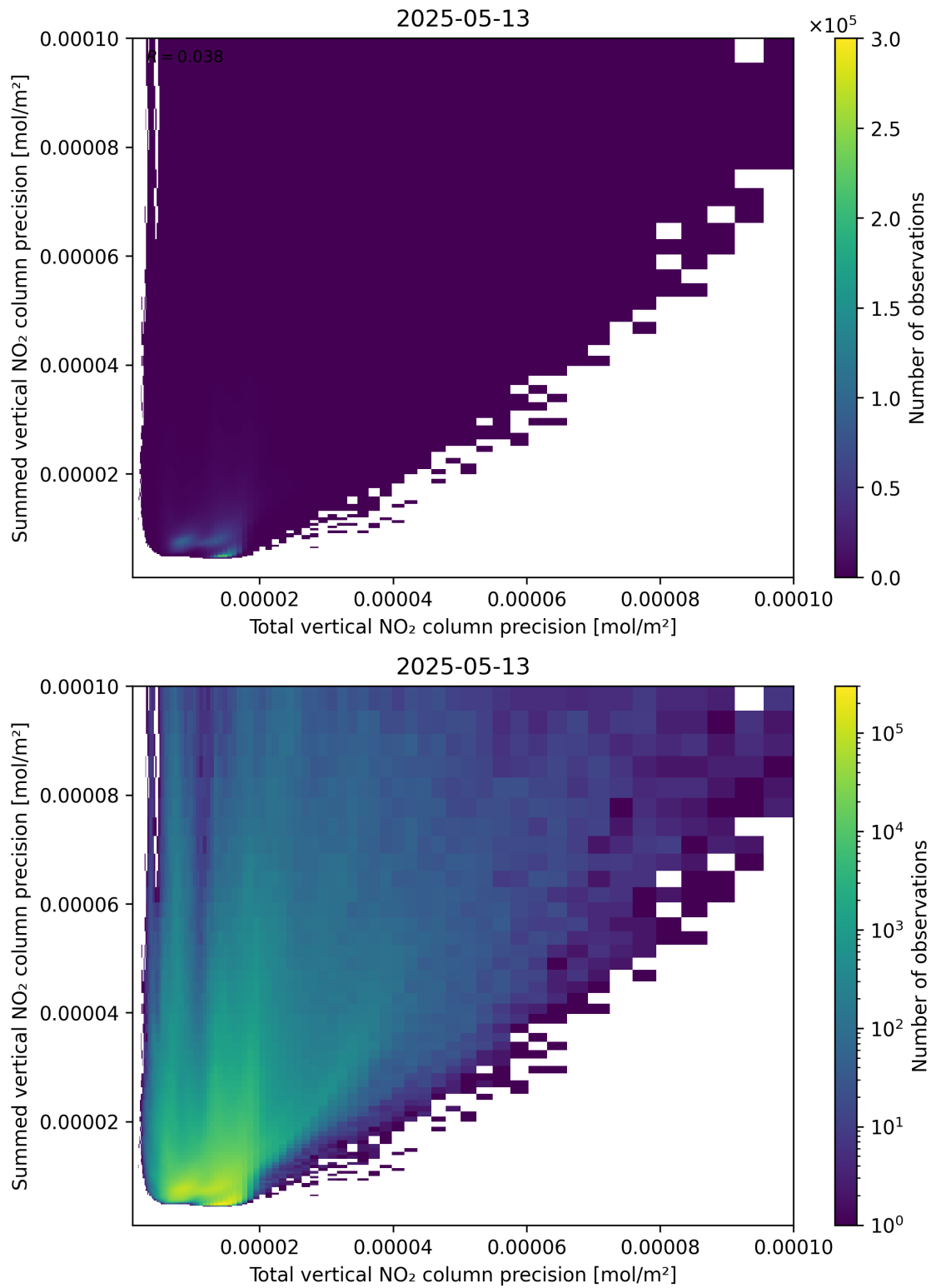
Figure 118: Scatter density plot of “Total vertical NO 2 column precision” against “Summed vertical NO 2 column precision” for 2025-05-13 to 2025-05-13.
