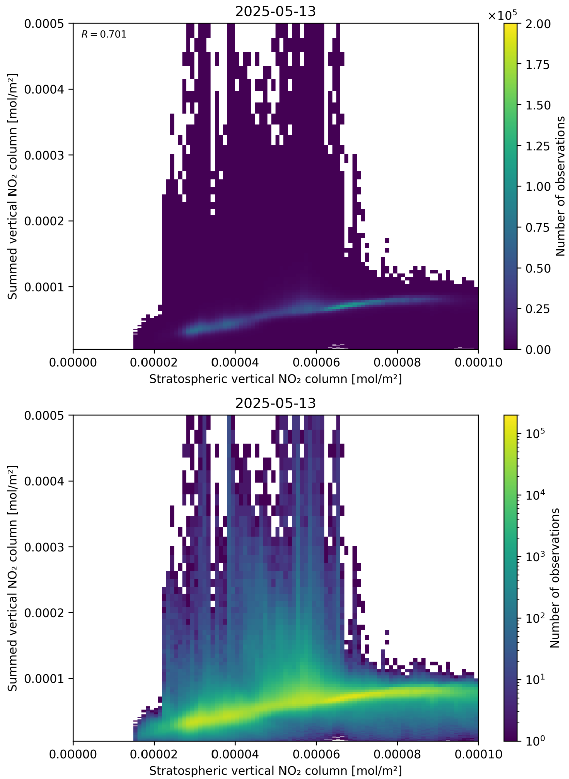
Figure 98: Scatter density plot of “Stratospheric vertical NO 2 column” against “Summed vertical NO 2 column” for 2025-05-13 to 2025-05-13.
