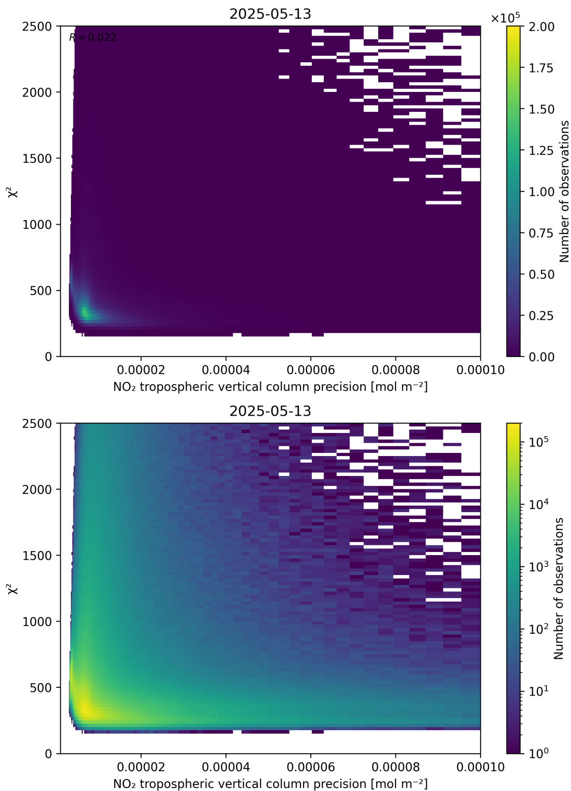
Figure 134: Scatter density plot of “NO 2 tropospheric vertical column precision” against “ \chi^2 ” for 2025-05-13 to 2025-05-13.
