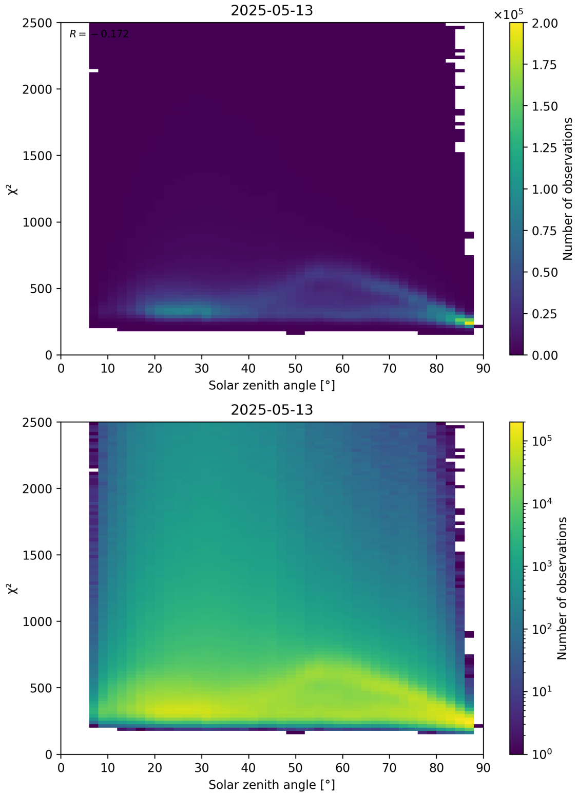
Figure 148: Scatter density plot of “Solar zenith angle” against “ \chi^2 ” for 2025-05-13 to 2025-05-13.
