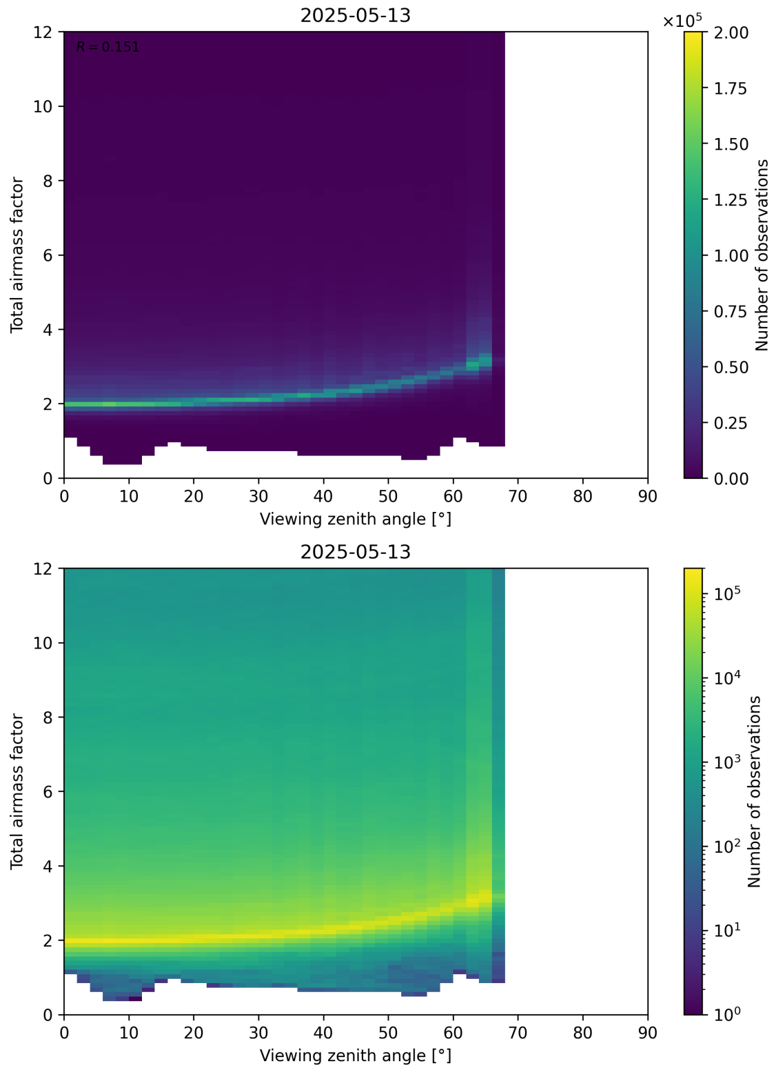
Figure 160: Scatter density plot of “Viewing zenith angle” against “Total airmass factor” for 2025-05-13 to 2025-05-13.
