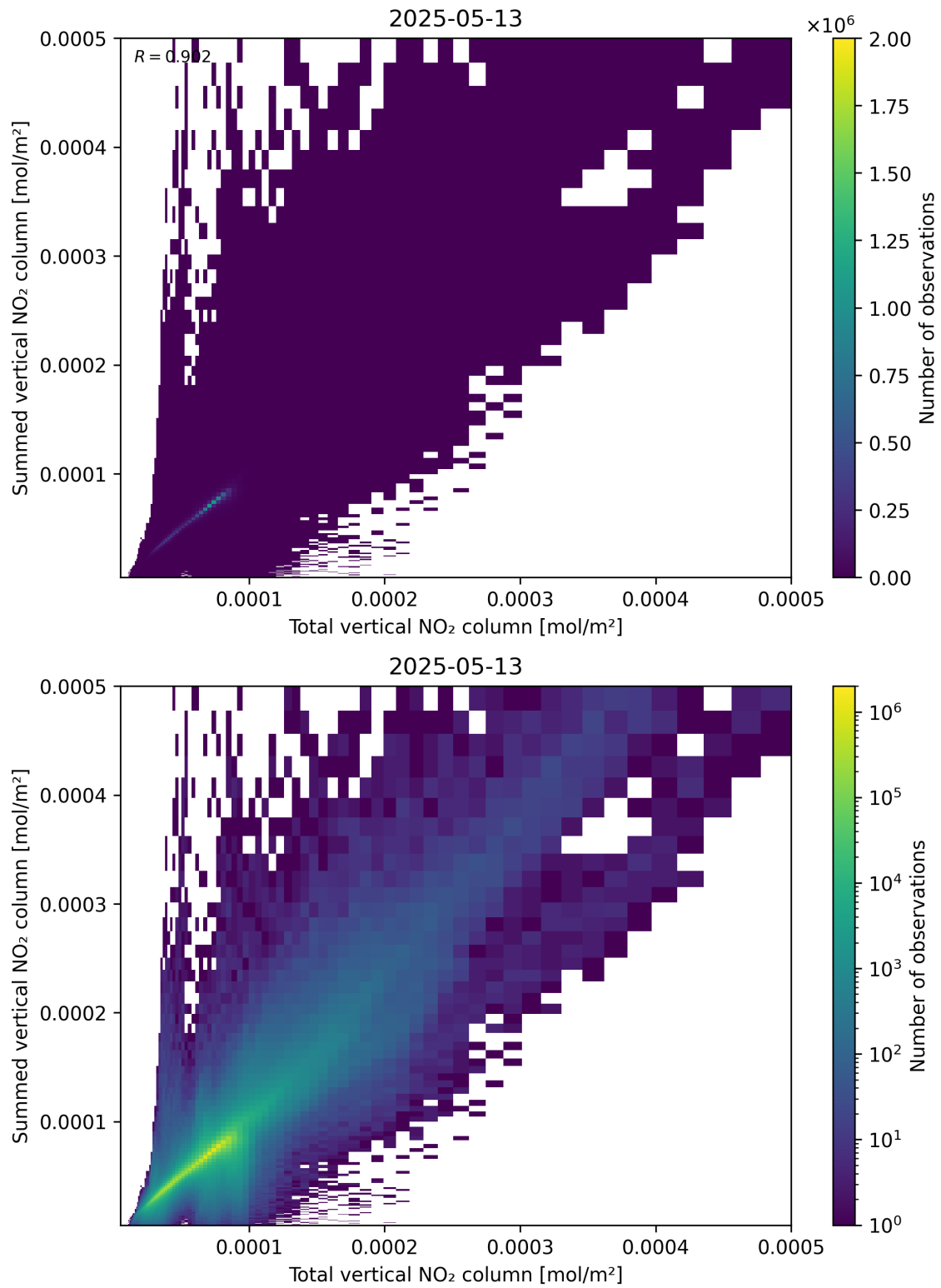
Figure 112: Scatter density plot of “Total vertical NO 2 column” against “Summed vertical NO 2 column” for 2025-05-13 to 2025-05-13.
