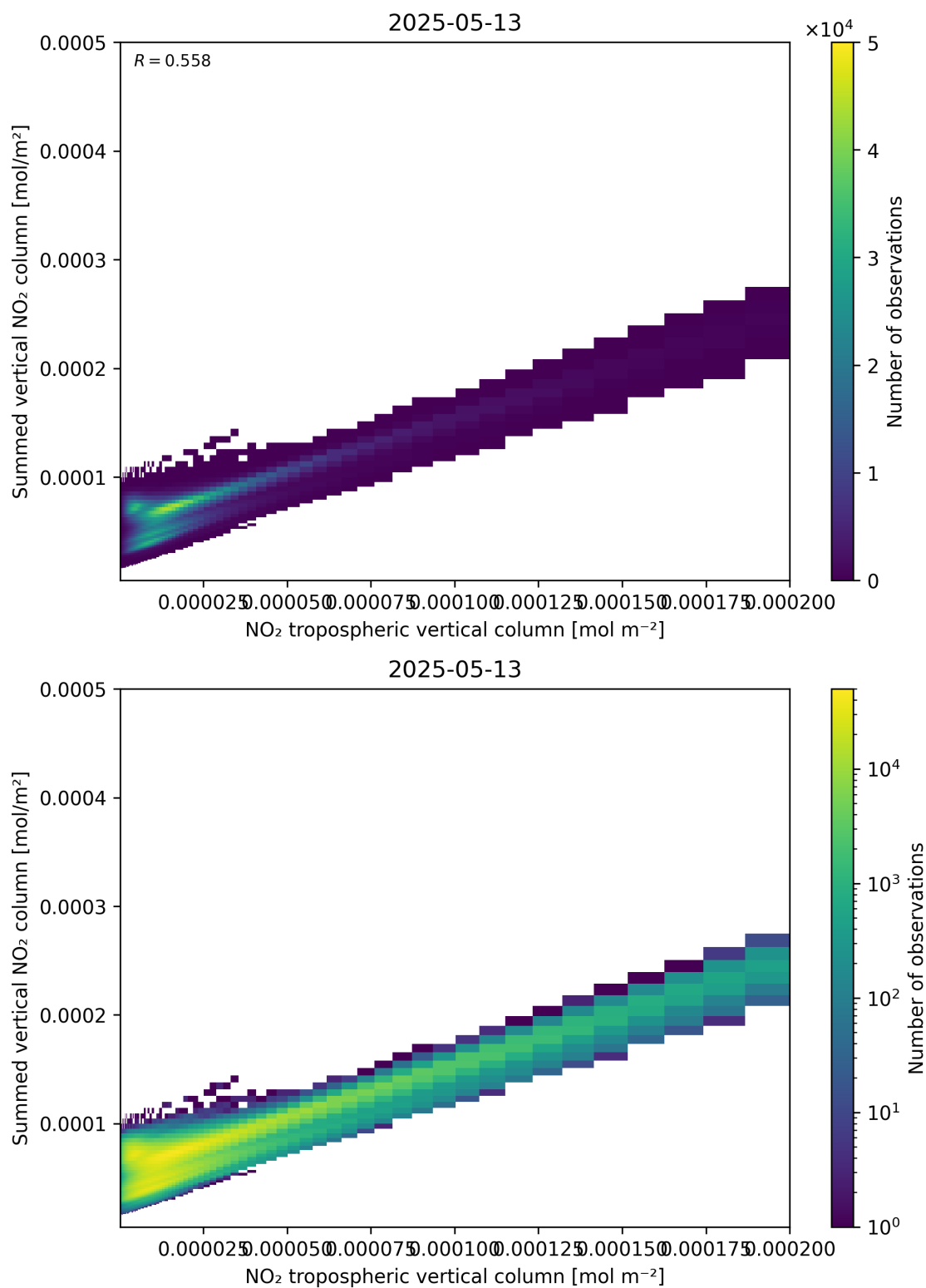
Figure 126: Scatter density plot of “NO 2 tropospheric vertical column” against “Summed vertical NO 2 column” for 2025-05-13 to 2025-05-13.
