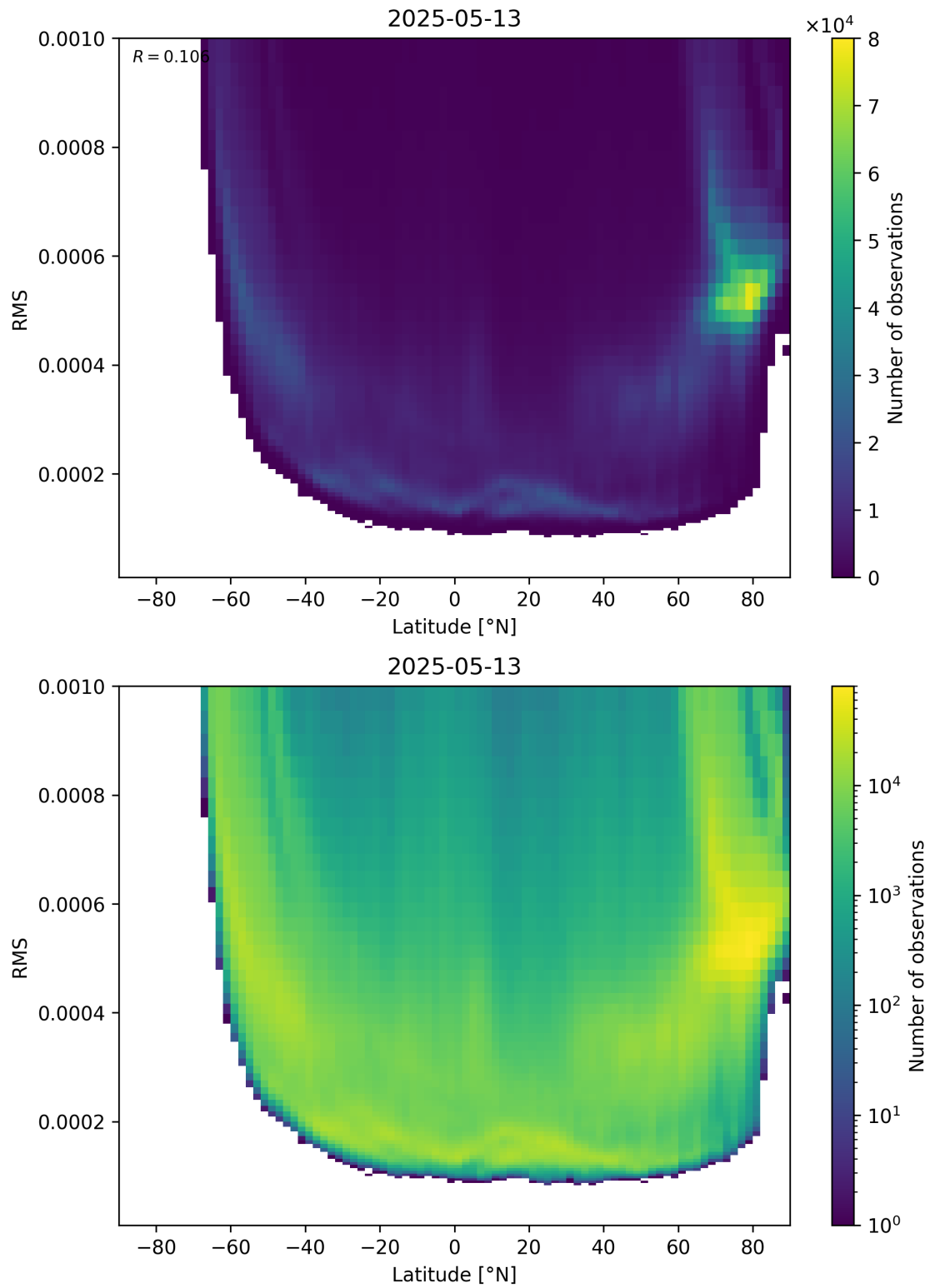
Figure 94: Scatter density plot of “Latitude” against “RMS” for 2025-05-13 to 2025-05-13.
