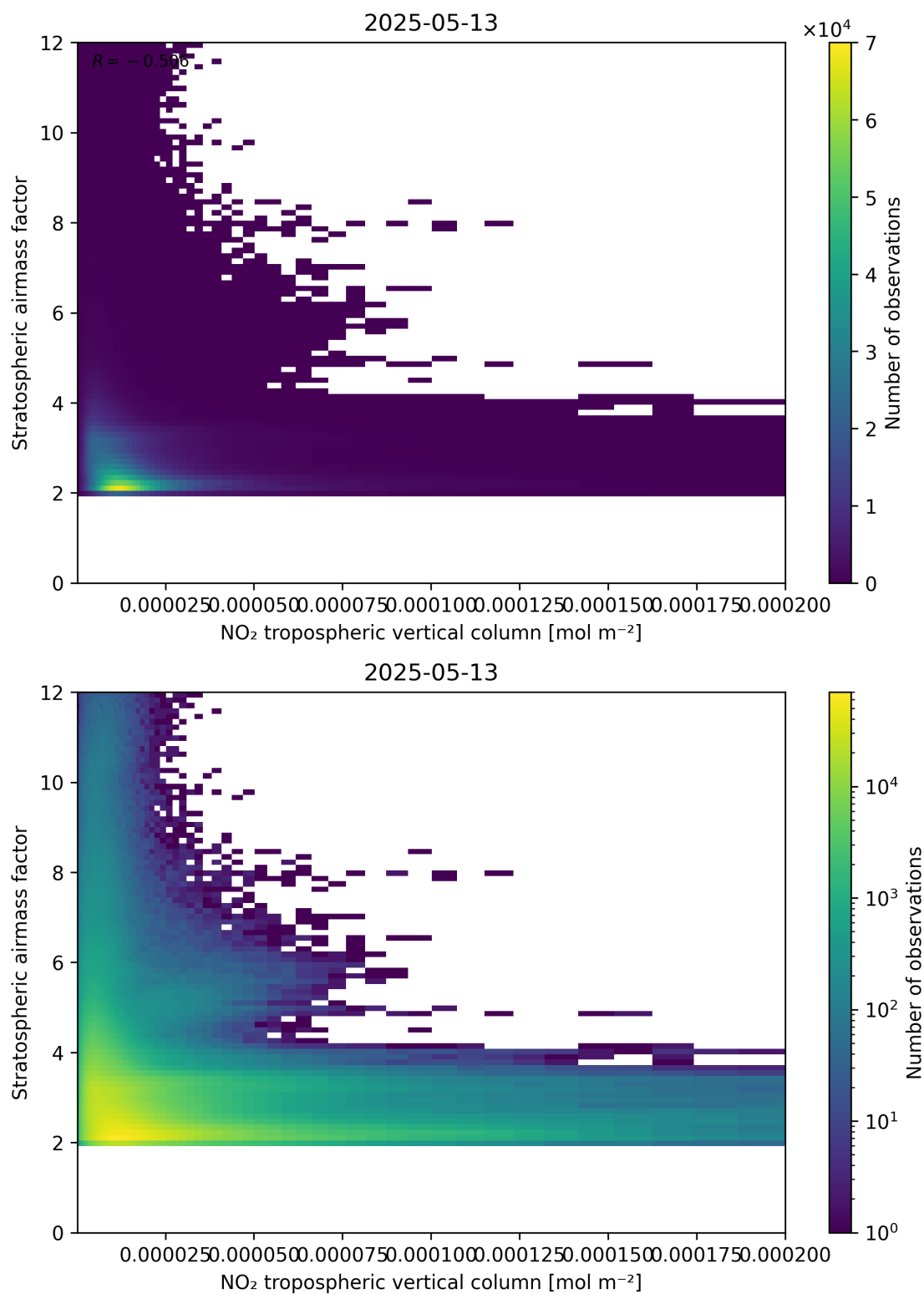
Figure 121: Scatter density plot of “NO 2 tropospheric vertical column” against “Stratospheric air mass factor” for 2025-05-13 to 2025-05-13.
