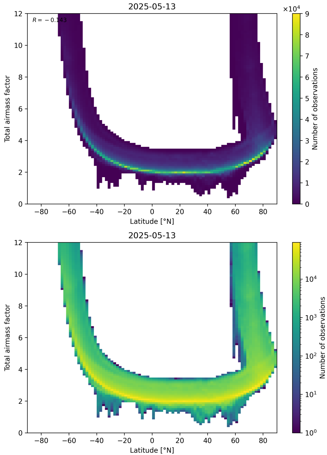
Figure 84: Scatter density plot of “Latitude” against “Total air mass factor” for 2025-05-13 to 2025-05-13.
