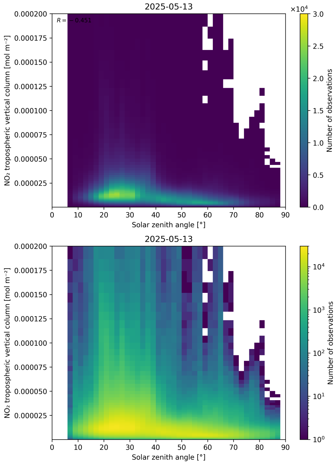
Figure 155: Scatter density plot of “Solar zenith angle” against “NO 2 tropospheric vertical column” for 2025-05-13 to 2025-05-13.
