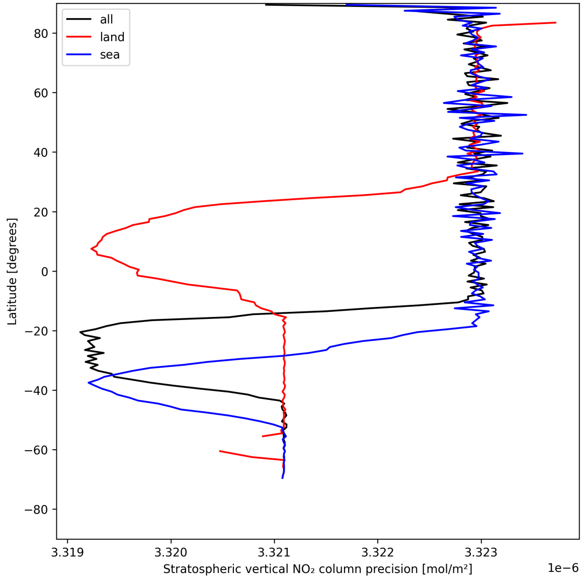
Figure 20: Zonal average of “Stratospheric vertical NO 2 column precision” for 2025-05-13 to 2025-05-13.
