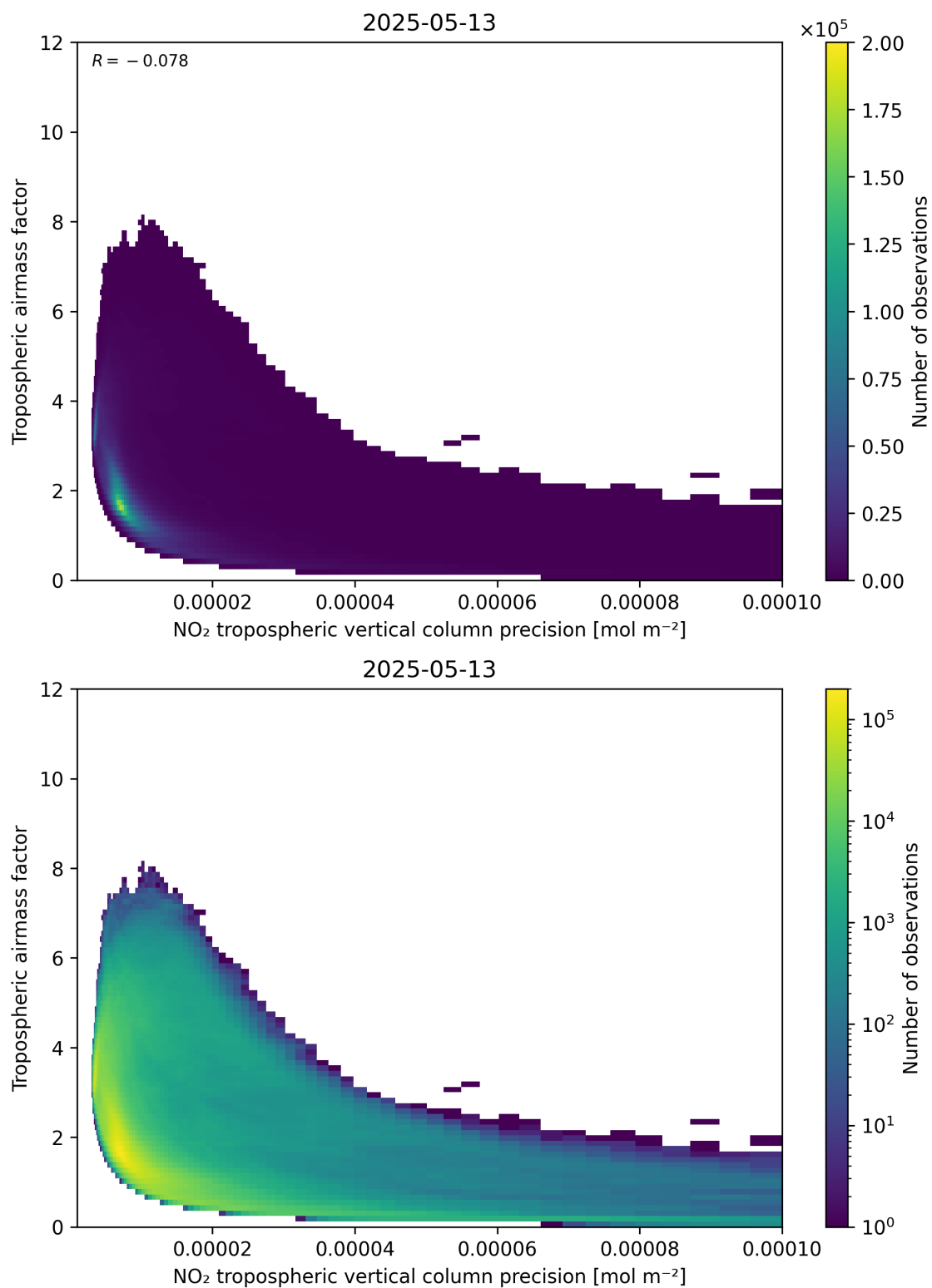
Figure 133: Scatter density plot of “NO 2 tropospheric vertical column precision” against “Tropospheric air mass factor” for 2025-05-13 to 2025-05-13.
