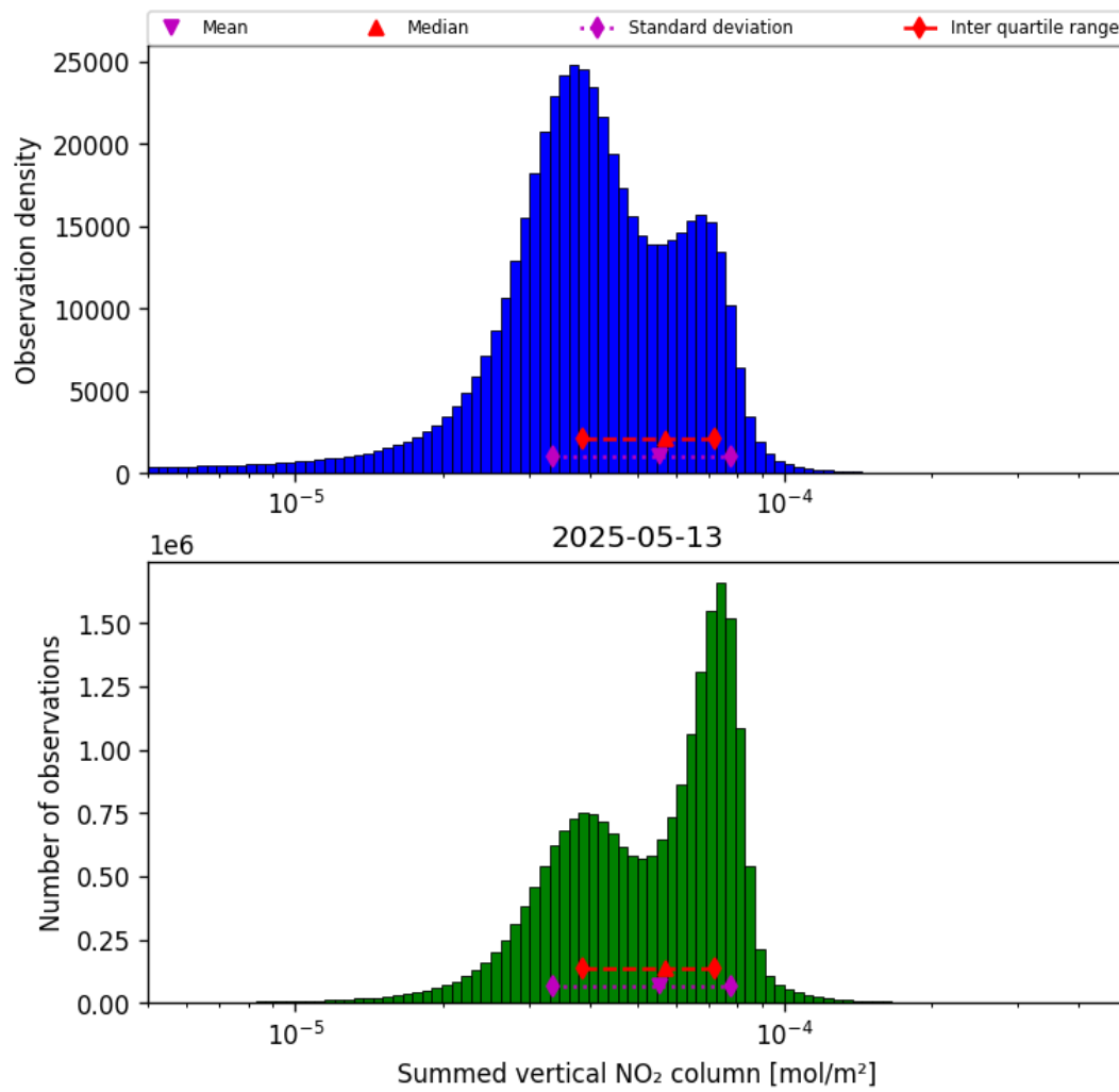
Figure 40: Histogram of "Summed vertical NO 2 column" for 2025-05-13 to 2025-05-13
