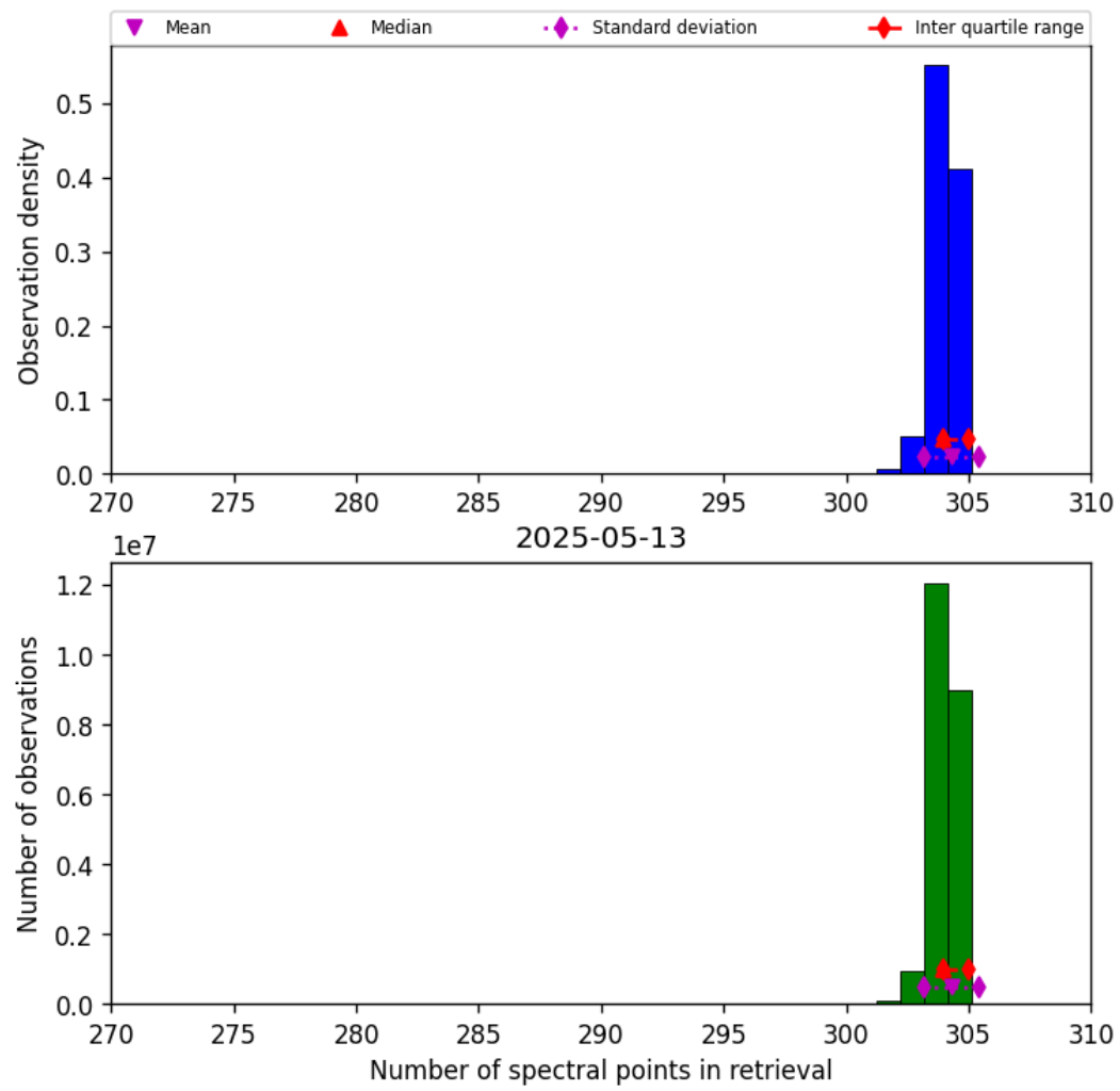
Figure 33: Histogram of “Number of spectral points in retrieval” for 2025-05-13 to 2025-05-13
