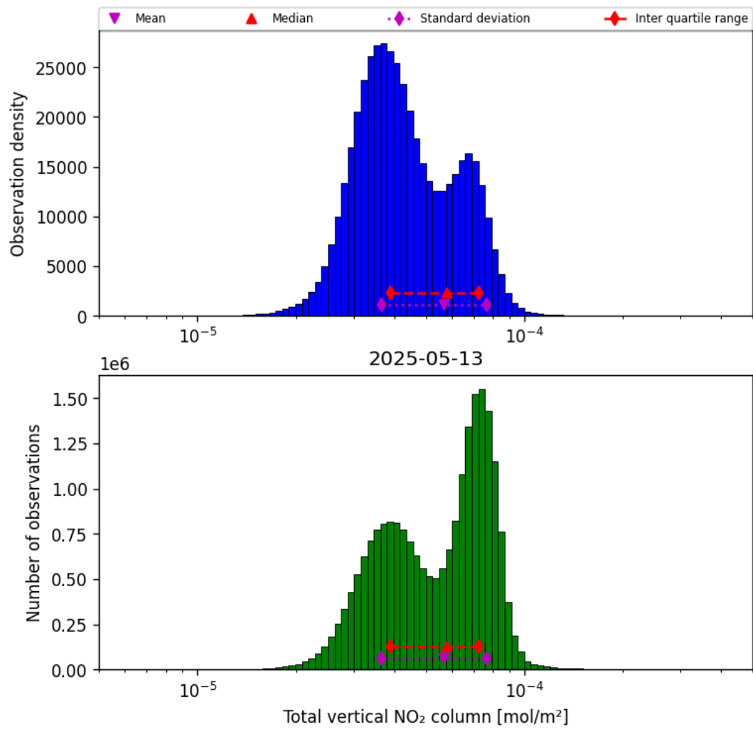
Figure 38: Histogram of "Total vertical NO 2 column" for 2025-05-13 to 2025-05-13
