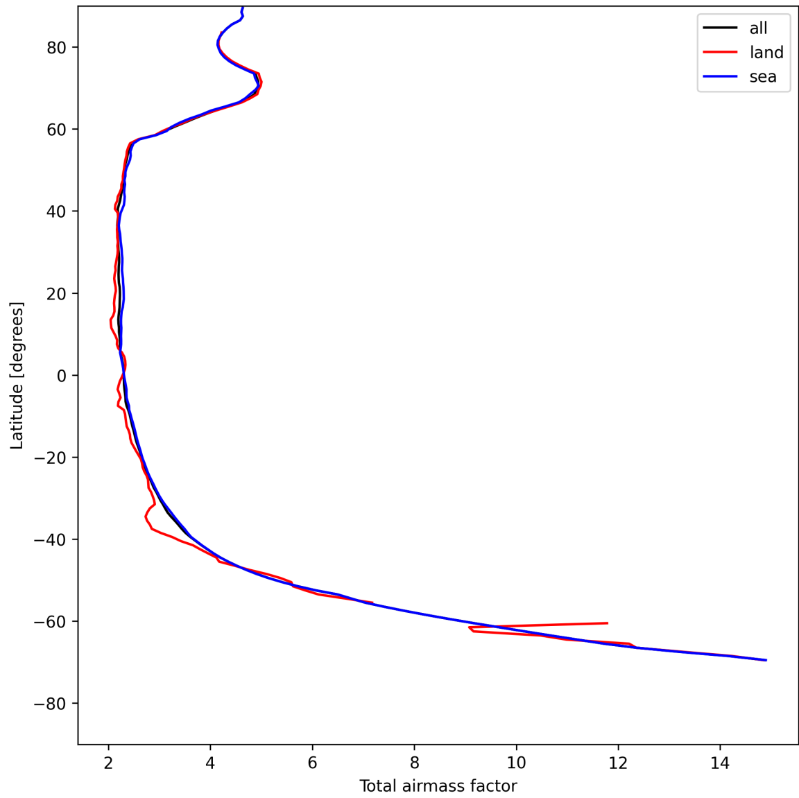
Figure 15: Zonal average of “Total airmass factor” for 2025-05-13 to 2025-05-13.
