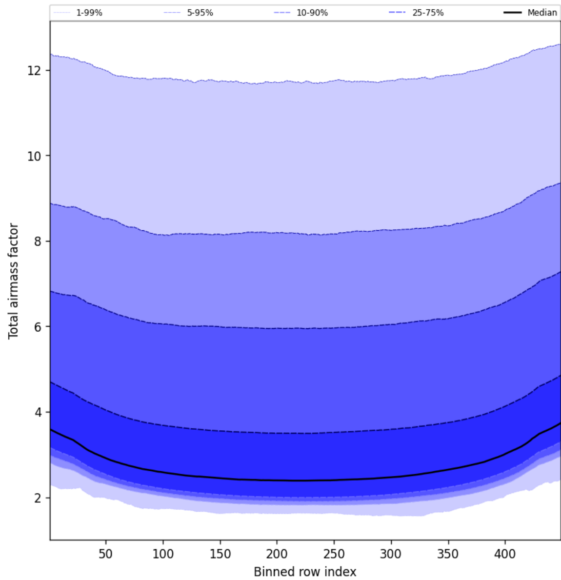
Figure 49: Along track statistics of “Total airmass factor” for 2025-05-13 to 2025-05-13
