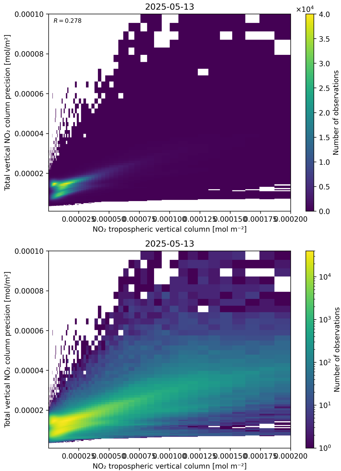
Figure 129: Scatter density plot of “NO 2 tropospheric vertical column” against “Total vertical NO 2 column precision” for 2025-05-13 to 2025-05-13.
