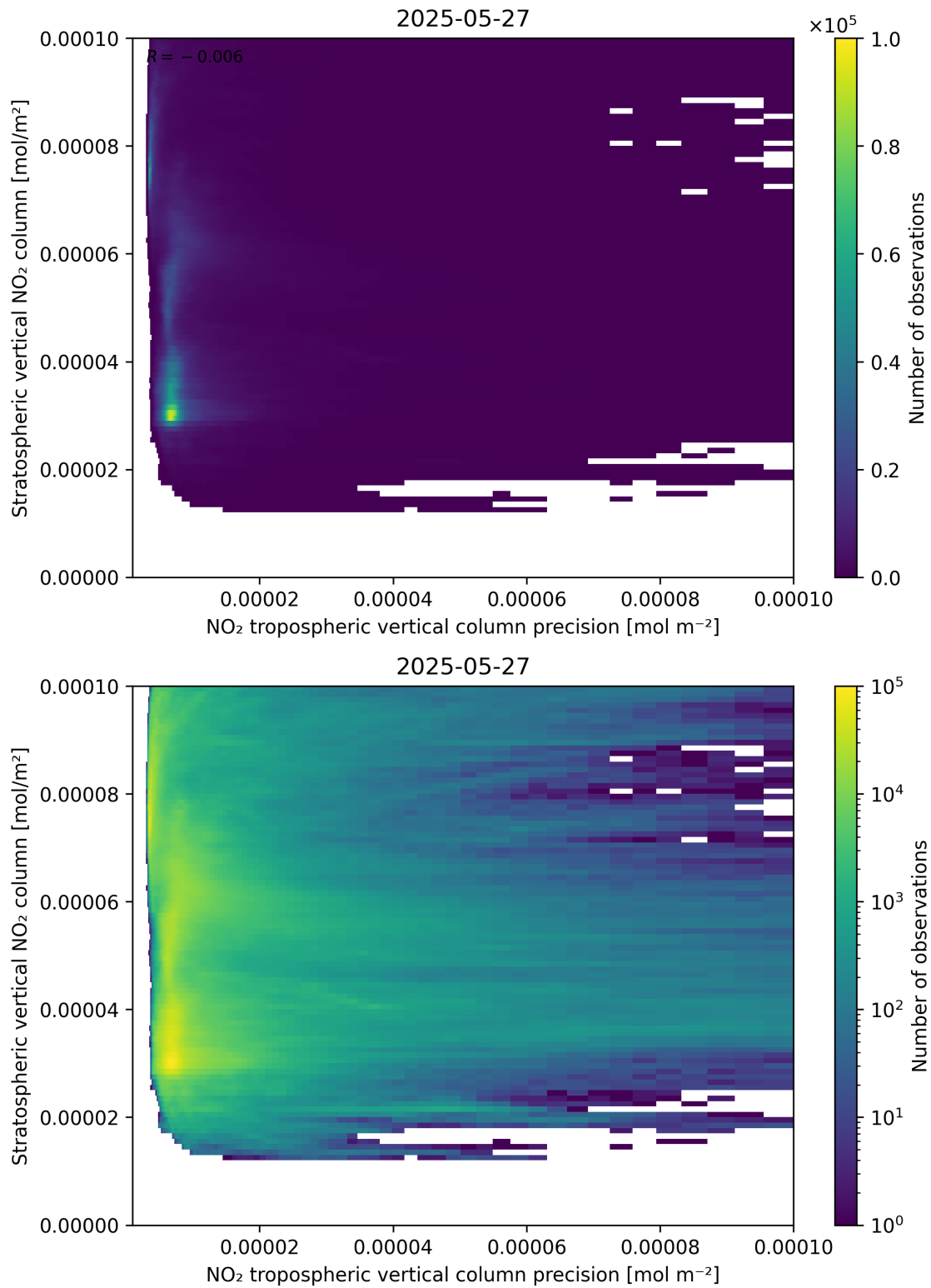
Figure 135: Scatter density plot of “NO 2 tropospheric vertical column precision” against “Stratospheric vertical NO 2 column” for 2025-05-26 to 2025-05-28.
