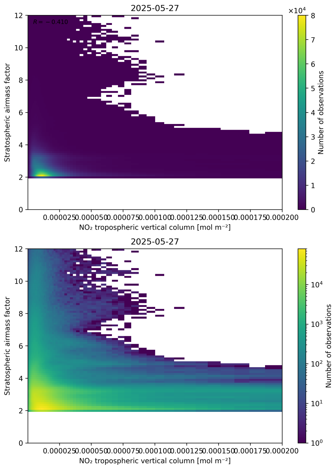
Figure 121: Scatter density plot of “NO 2 tropospheric vertical column” against “Stratospheric air mass factor” for 2025-05-26 to 2025-05-28.
