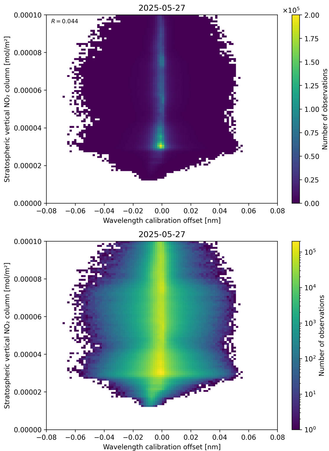
Figure 176: Scatter density plot of “Wavelength calibration offset” against “Stratospheric vertical NO 2 column” for 2025-05-26 to 2025-05-28.
