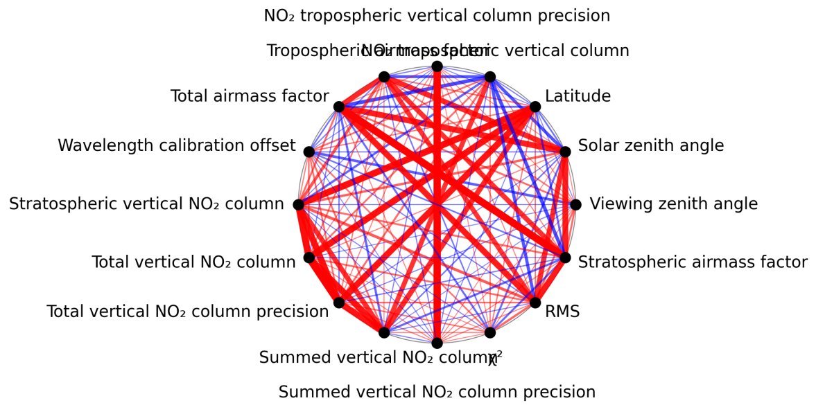
Figure 1: Map of correlation graph for 2025-05-26 to 2025-05-28.
