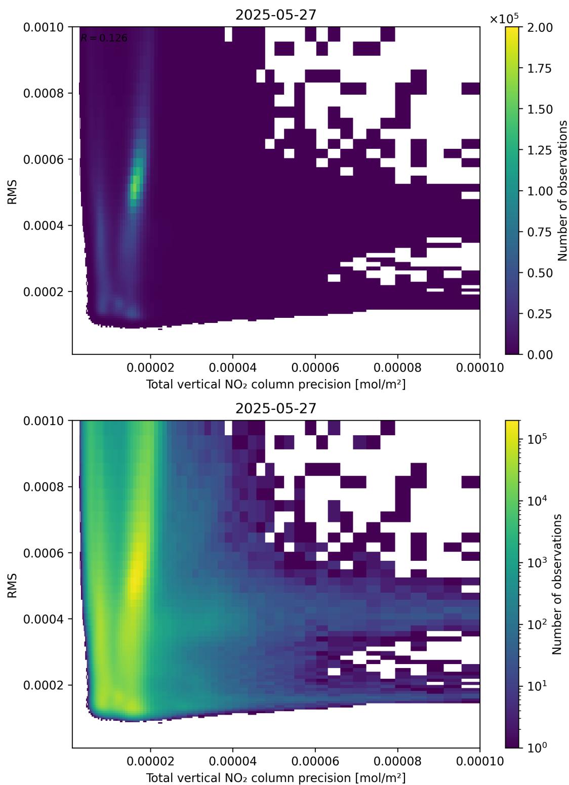
Figure 119: Scatter density plot of “Total vertical NO 2 column precision” against “RMS” for 2025-05-26 to 2025-05-28.
