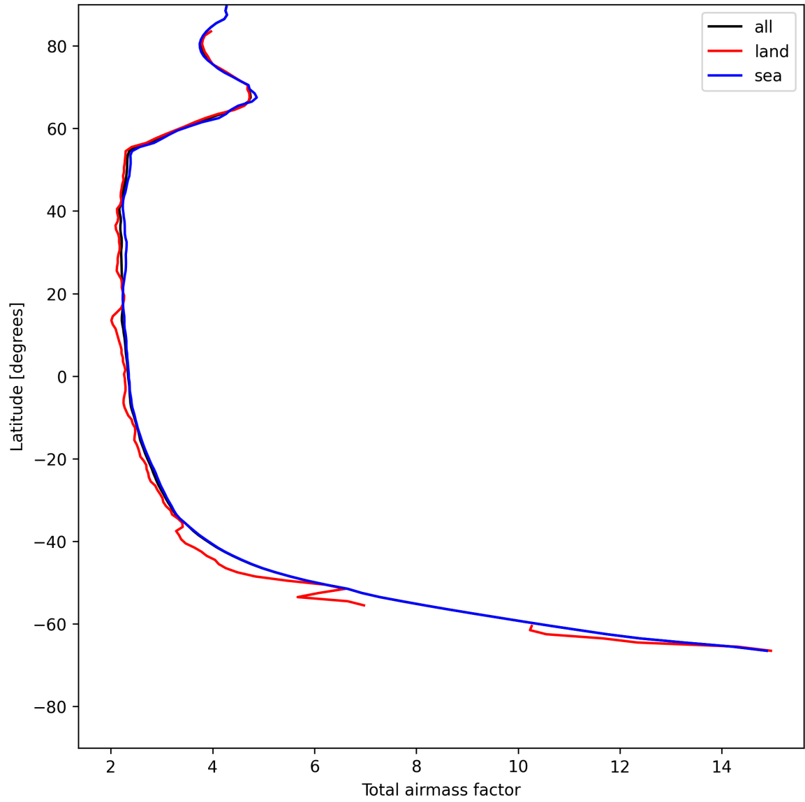
Figure 15: Zonal average of “Total airmass factor” for 2025-05-26 to 2025-05-28.
