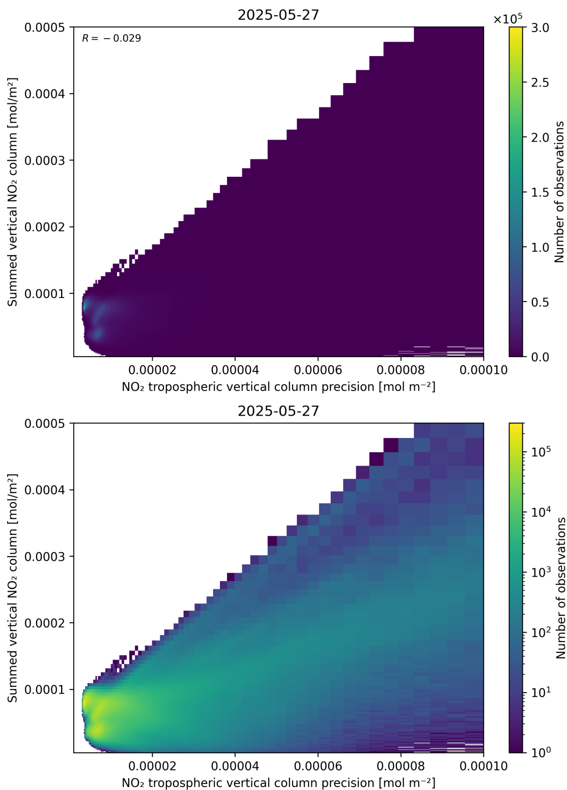
Figure 136: Scatter density plot of “NO 2 tropospheric vertical column precision” against “Summed vertical NO 2 column” for 2025-05-26 to 2025-05-28.
