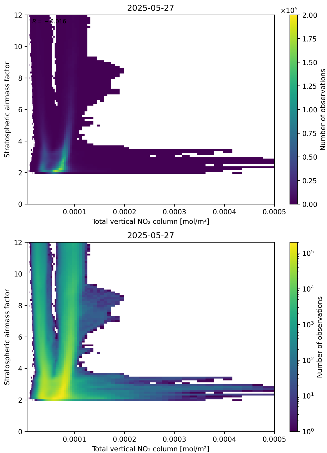
Figure 110: Scatter density plot of “Total vertical NO 2 column” against “Stratospheric airmass factor” for 2025-05-26 to 2025-05-28.
