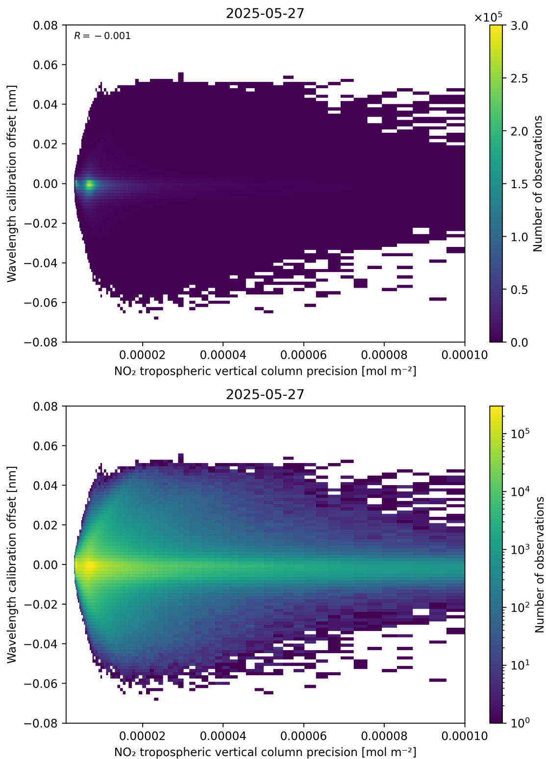
Figure 141: Scatter density plot of “NO 2 tropospheric vertical column precision” against “Wavelength calibration offset” for 2025-05-26 to 2025-05-28.
