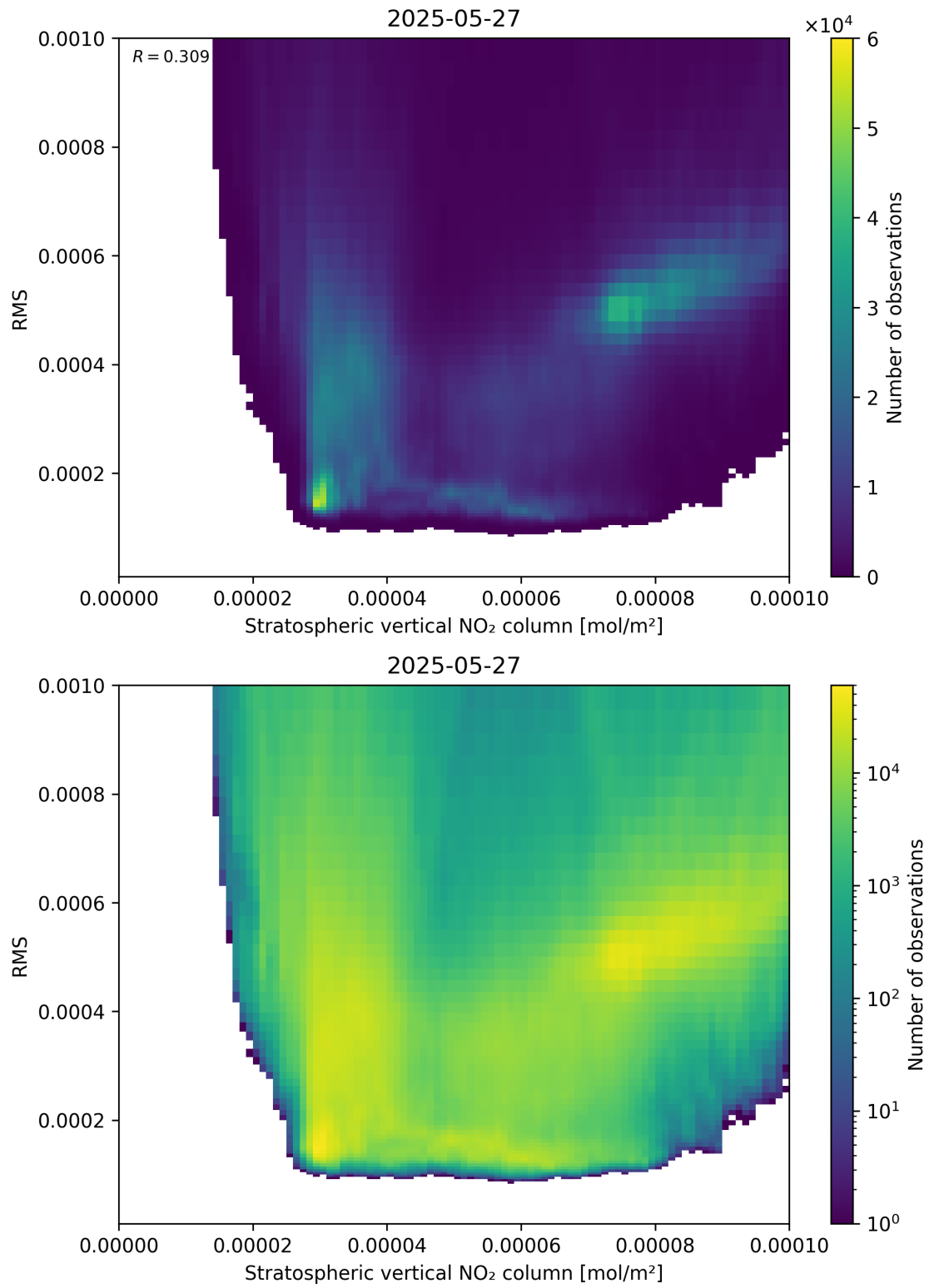
Figure 102: Scatter density plot of “Stratospheric vertical NO 2 column” against “RMS” for 2025-05-26 to 2025-05-28.
