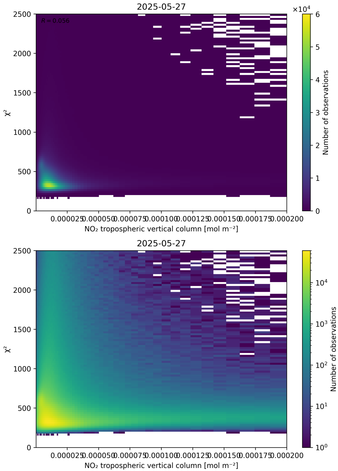
Figure 124: Scatter density plot of “NO 2 tropospheric vertical column” against “ \chi^2 ” for 2025-05-26 to 2025-05-28.
