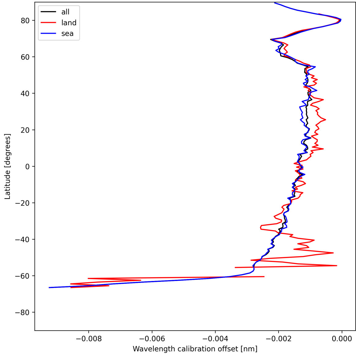
Figure 18: Zonal average of “Wavelength calibration offset” for 2025-05-26 to 2025-05-28.
