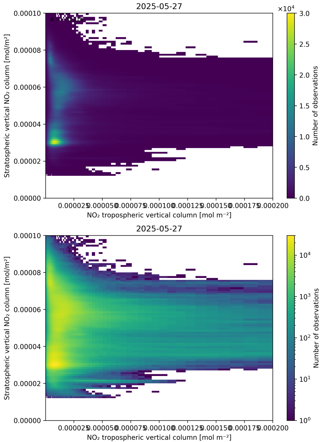
Figure 125: Scatter density plot of “NO 2 tropospheric vertical column” against “Stratospheric vertical NO 2 column” for 2025-05-26 to 2025-05-28.
