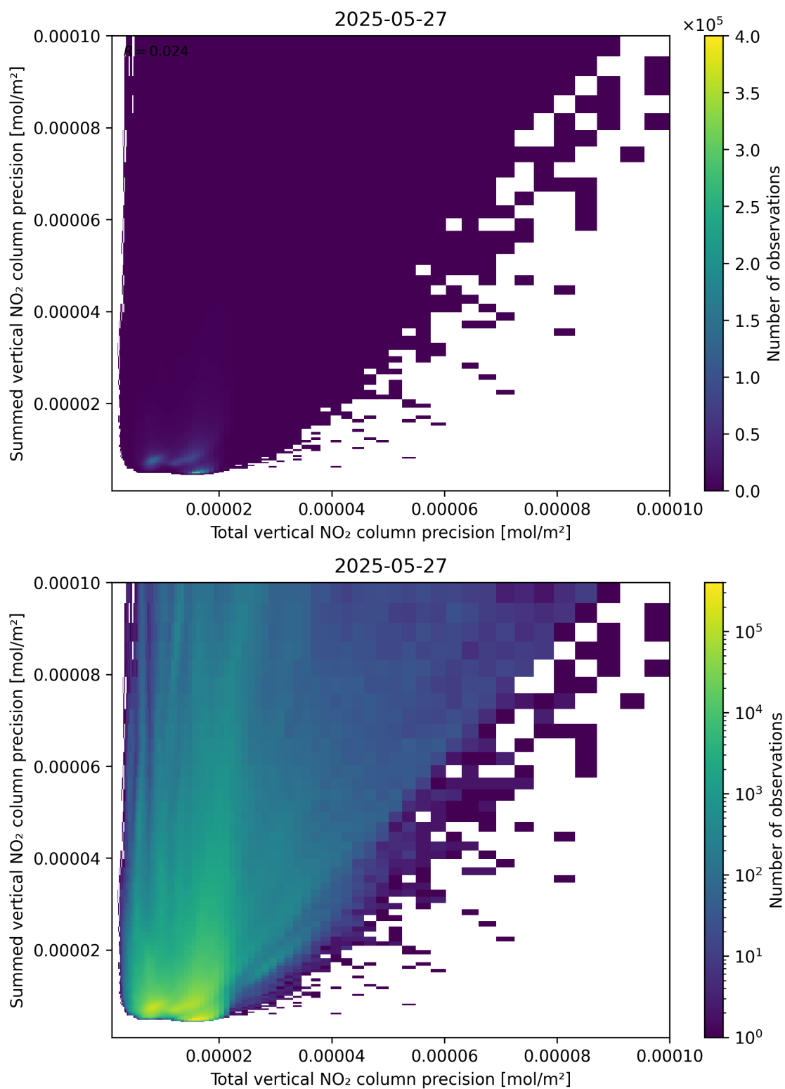
Figure 118: Scatter density plot of “Total vertical NO 2 column precision” against “Summed vertical NO 2 column precision” for 2025-05-26 to 2025-05-28.
