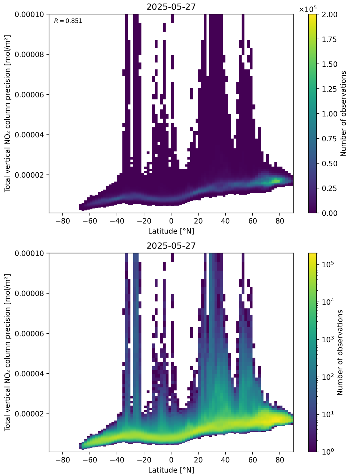
Figure 91: Scatter density plot of “Latitude” against “Total vertical NO 2 column precision” for 2025-05-26 to 2025-05-28.
