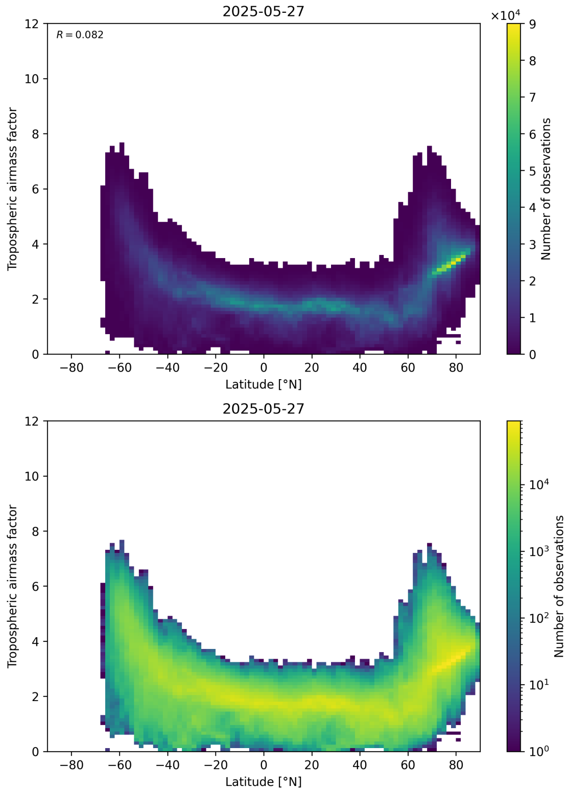
Figure 85: Scatter density plot of “Latitude” against “Tropospheric air mass factor” for 2025-05-26 to 2025-05-28.
