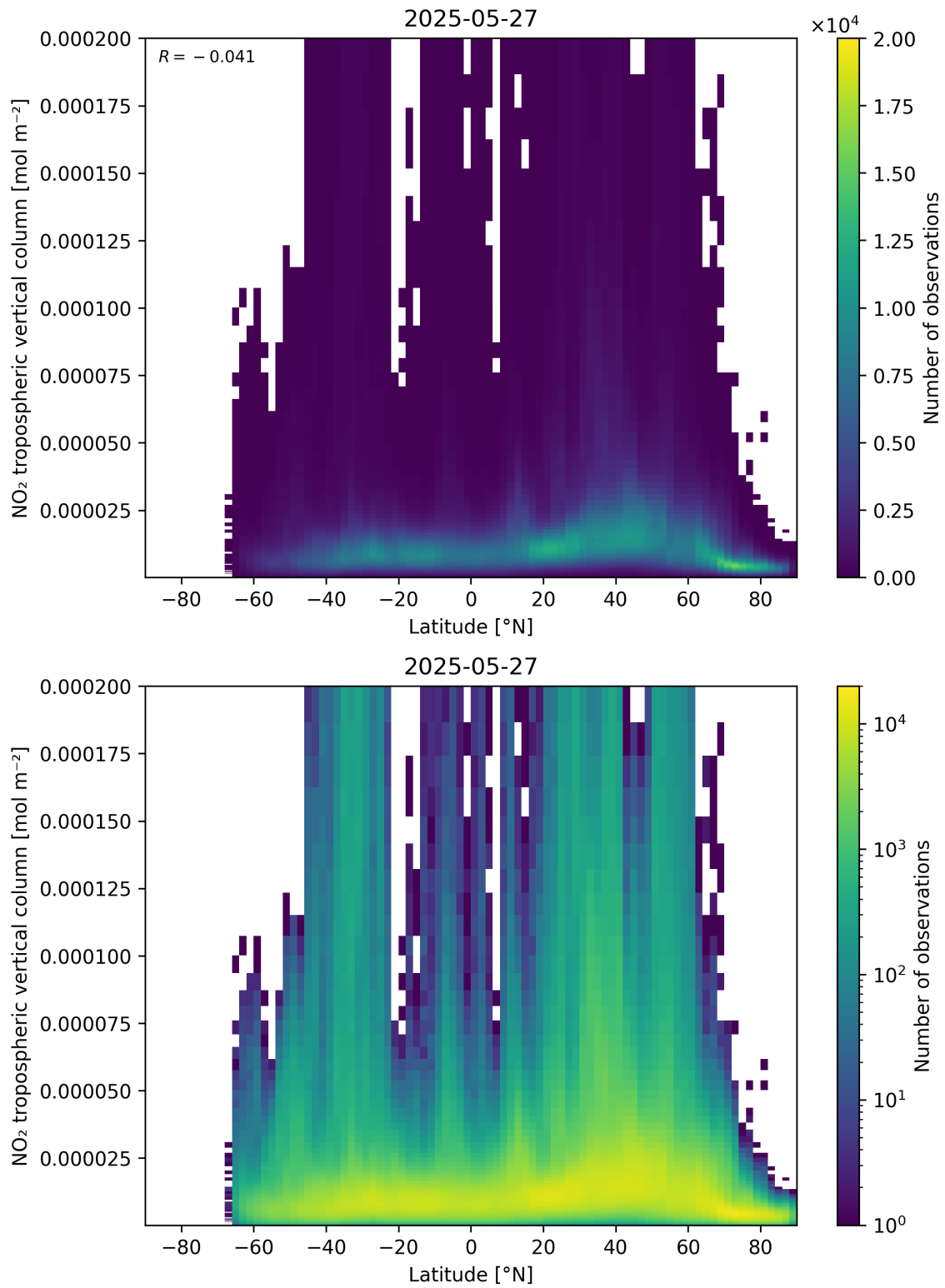
Figure 92: Scatter density plot of “Latitude” against “NO 2 tropospheric vertical column” for 2025-05-26 to 2025-05-28.
