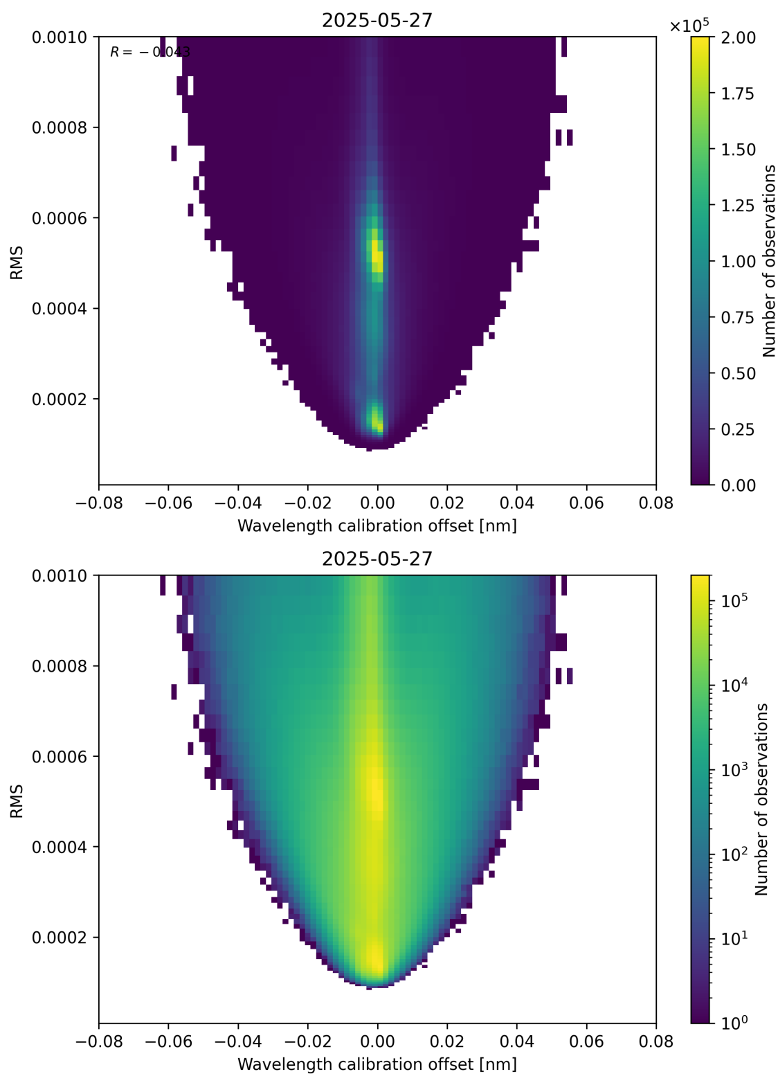
Figure 181: Scatter density plot of “Wavelength calibration offset” against “RMS” for 2025-05-26 to 2025-05-28.
