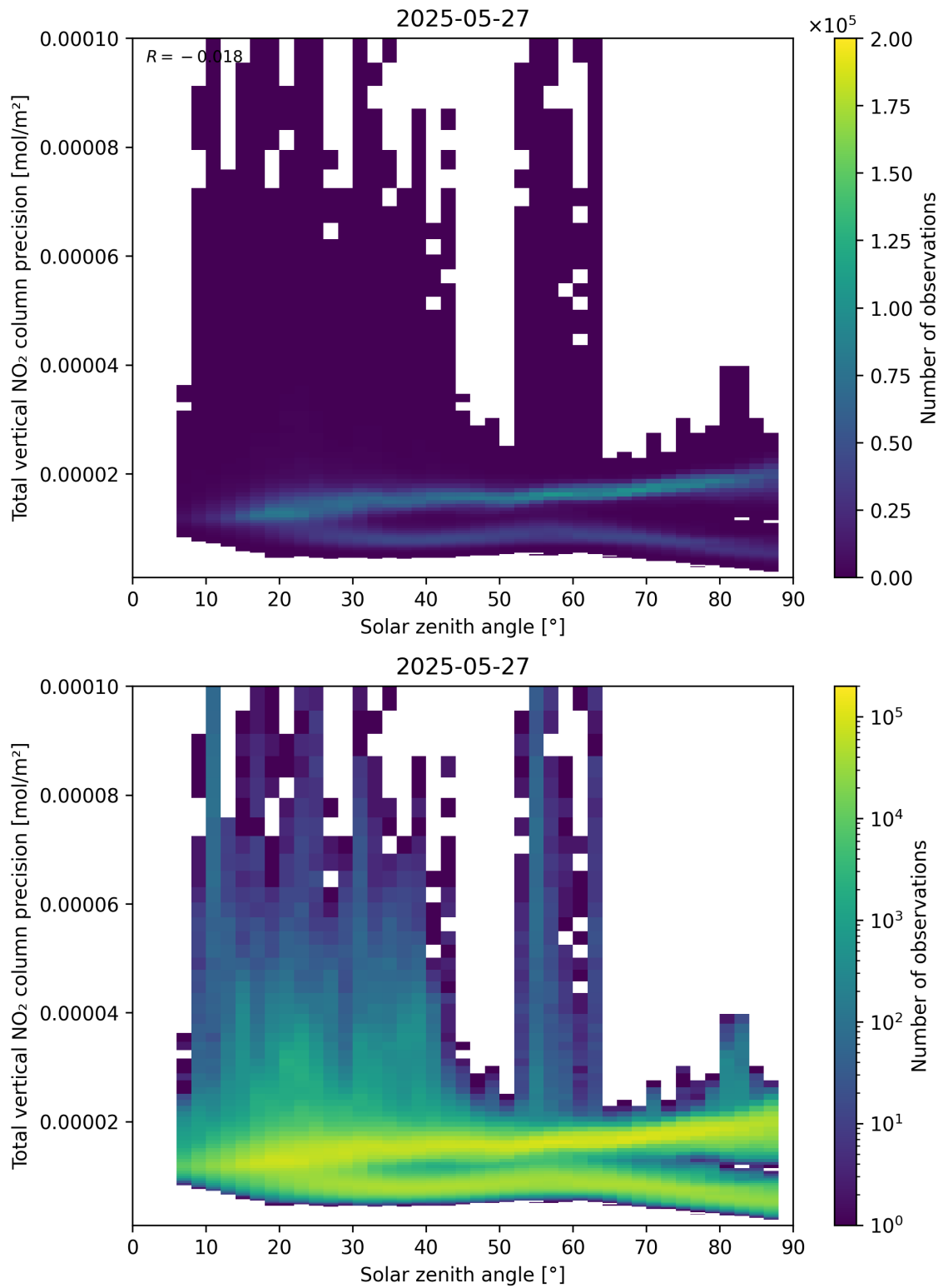
Figure 154: Scatter density plot of “Solar zenith angle” against “Total vertical NO 2 column precision” for 2025-05-26 to 2025-05-28.
