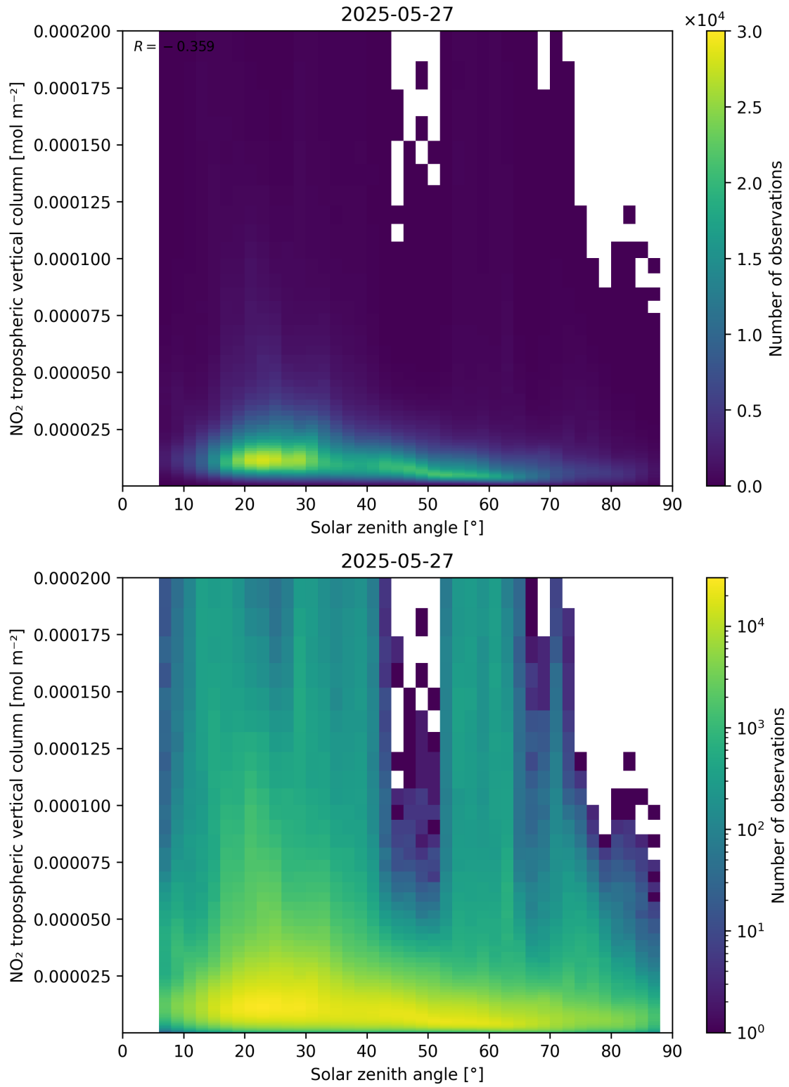
Figure 155: Scatter density plot of “Solar zenith angle” against “NO 2 tropospheric vertical column” for 2025-05-26 to 2025-05-28.
