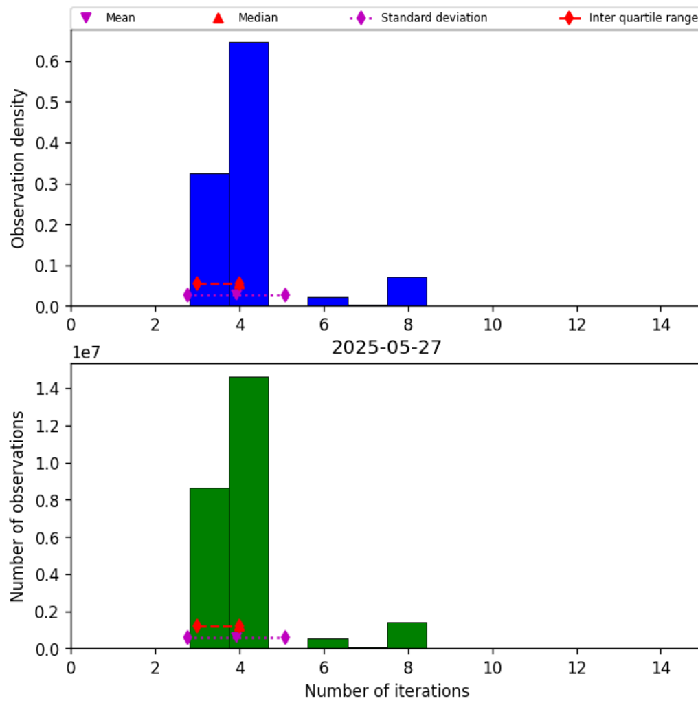
Figure 34: Histogram of “Number of iterations” for 2025-05-26 to 2025-05-28
