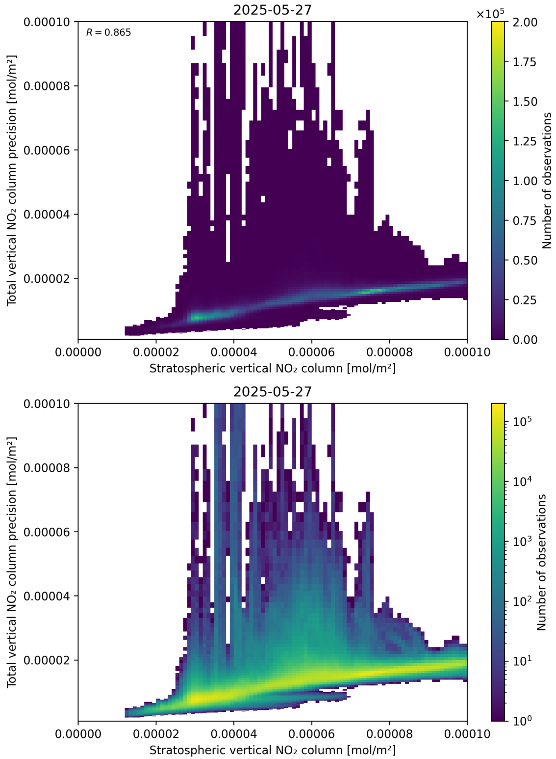
Figure 101: Scatter density plot of “Stratospheric vertical NO 2 column” against “Total vertical NO 2 column precision” for 2025-05-26 to 2025-05-28.
