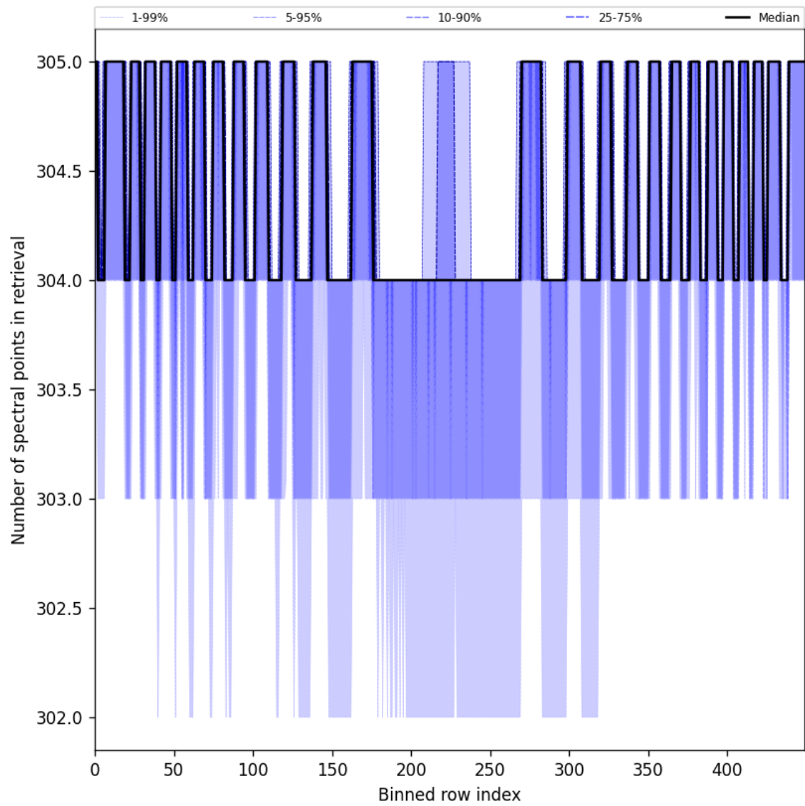
Figure 50: Along track statistics of “Number of spectral points in retrieval” for 2025-05-26 to 2025-05-28
