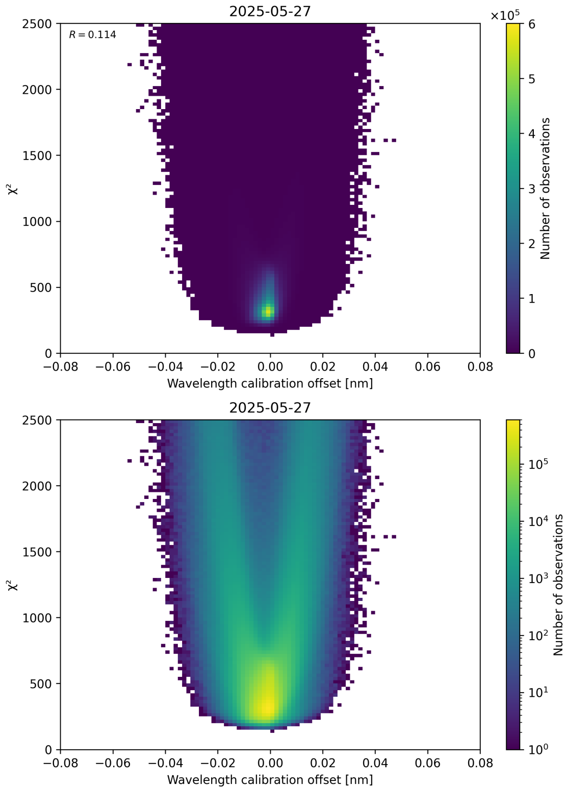
Figure 175: Scatter density plot of “Wavelength calibration offset” against “ \chi^2 ” for 2025-05-26 to 2025-05-28.
