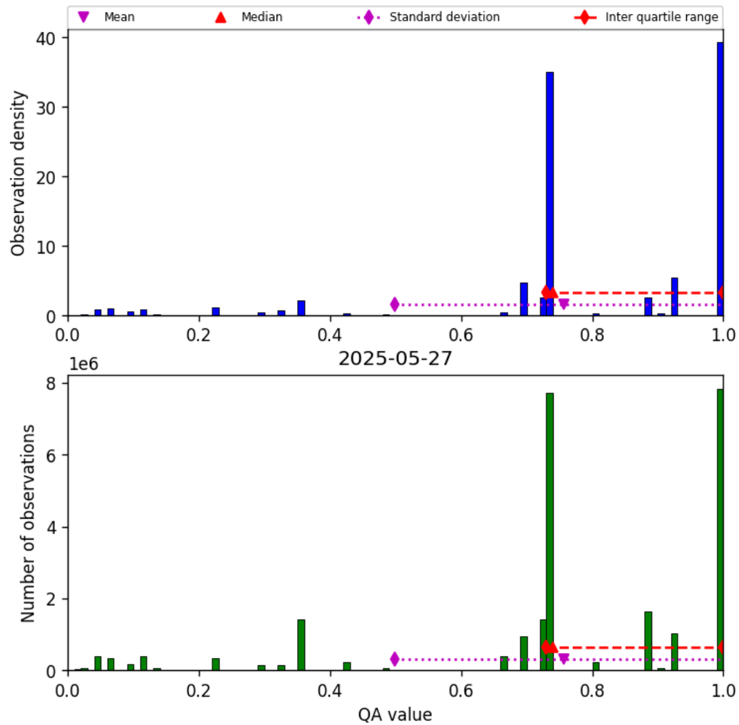
Figure 28: Histogram of “QA value” for 2025-05-26 to 2025-05-28
