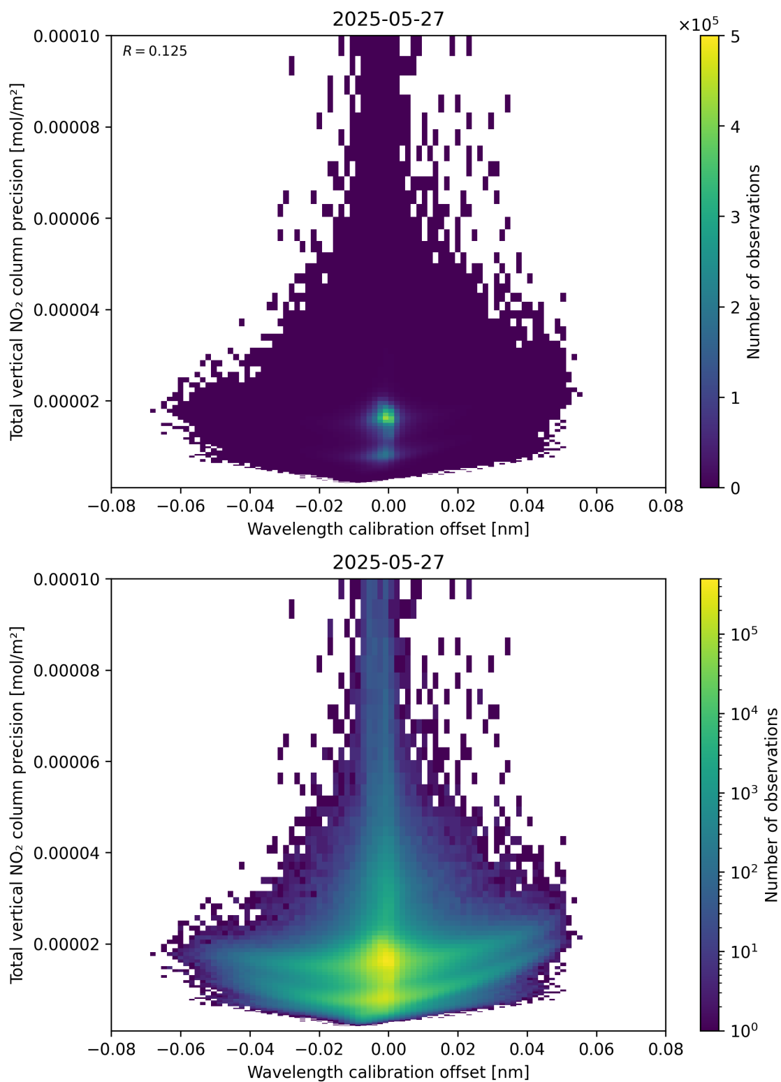
Figure 180: Scatter density plot of “Wavelength calibration offset” against “Total vertical NO 2 column precision” for 2025-05-26 to 2025-05-28.
