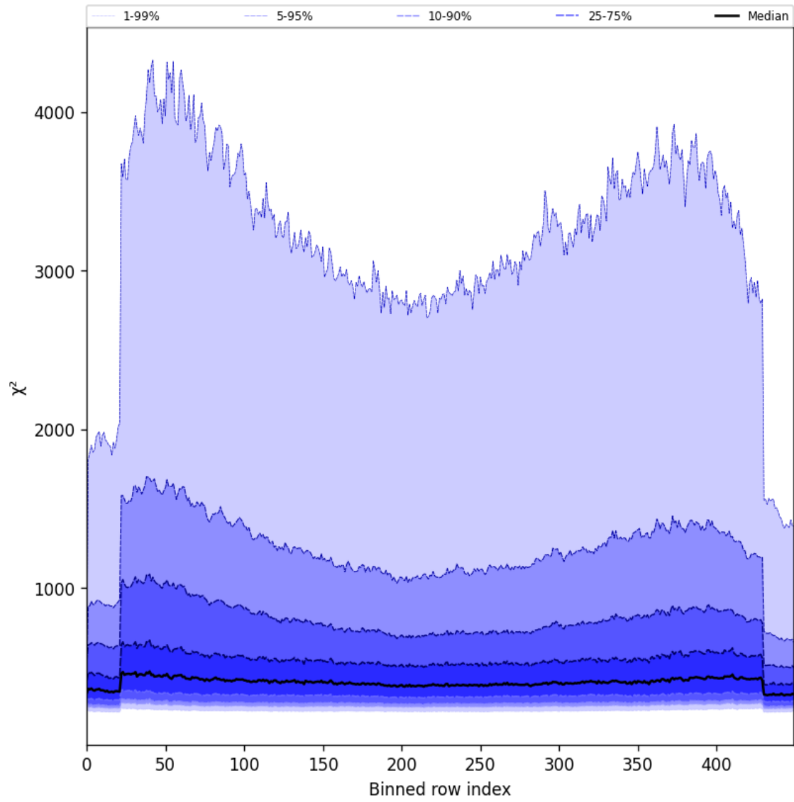
Figure 59: Along track statistics of “ \chi^2 ” for 2025-05-26 to 2025-05-28
