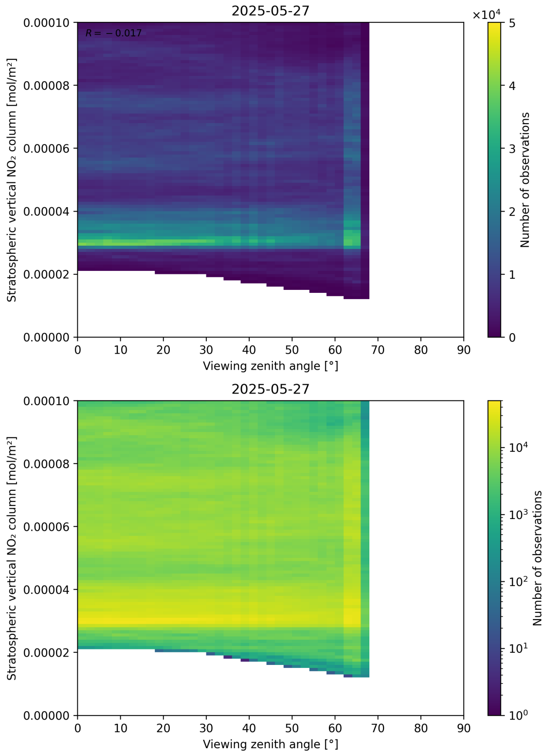
Figure 164: Scatter density plot of “Viewing zenith angle” against “Stratospheric vertical NO 2 column” for 2025-05-26 to 2025-05-28.
