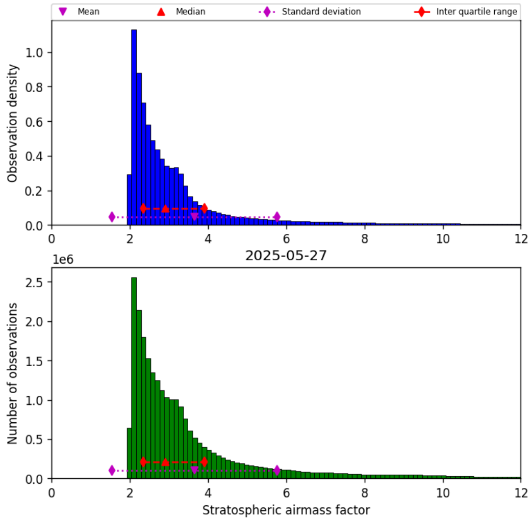
Figure 44: Histogram of “Stratospheric airmass factor” for 2025-05-26 to 2025-05-28
