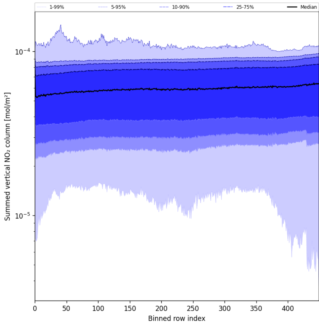
Figure 57: Along track statistics of “Summed vertical NO 2 column” for 2025-05-26 to 2025-05-28
