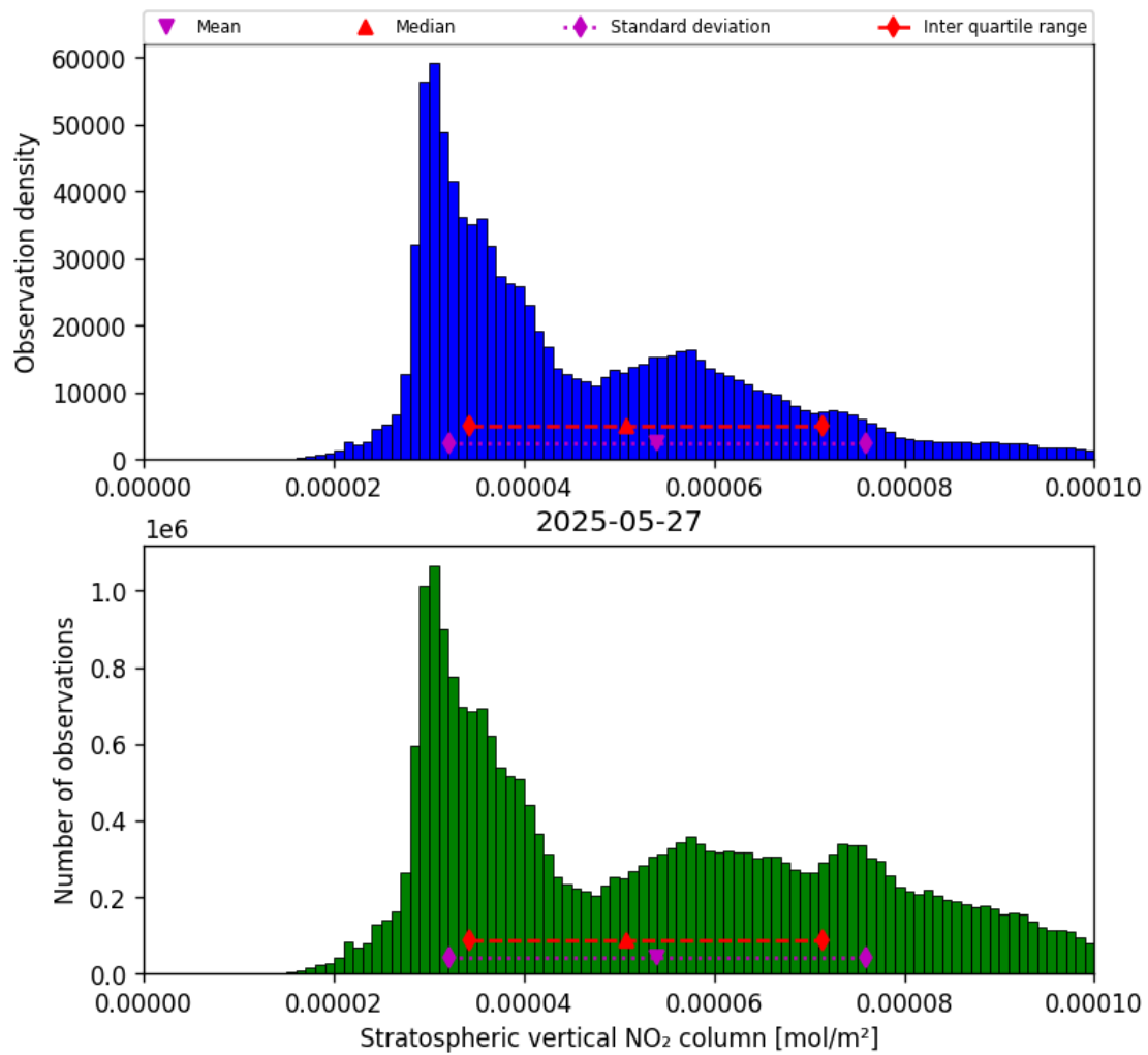
Figure 36: Histogram of “Stratospheric vertical NO 2 column” for 2025-05-26 to 2025-05-28
