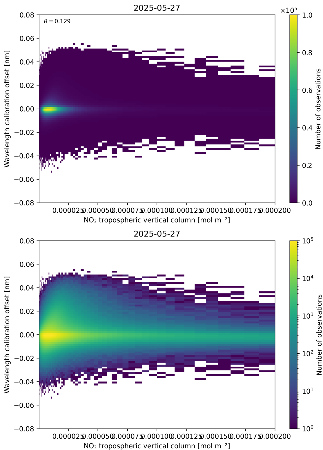
Figure 143: Scatter density plot of “NO 2 tropospheric vertical column” against “Wavelength calibration offset” for 2025-05-26 to 2025-05-28.
