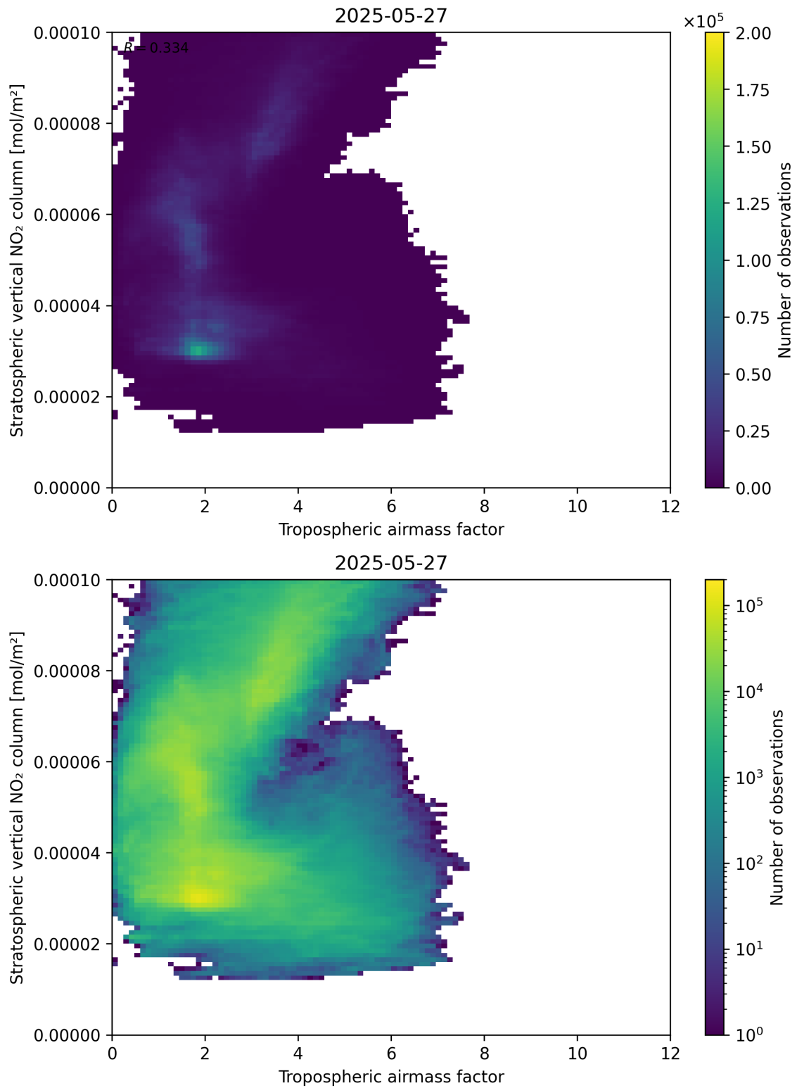
Figure 74: Scatter density plot of “Tropospheric air mass factor” against “Stratospheric vertical NO 2 column” for 2025-05-26 to 2025-05-28.
