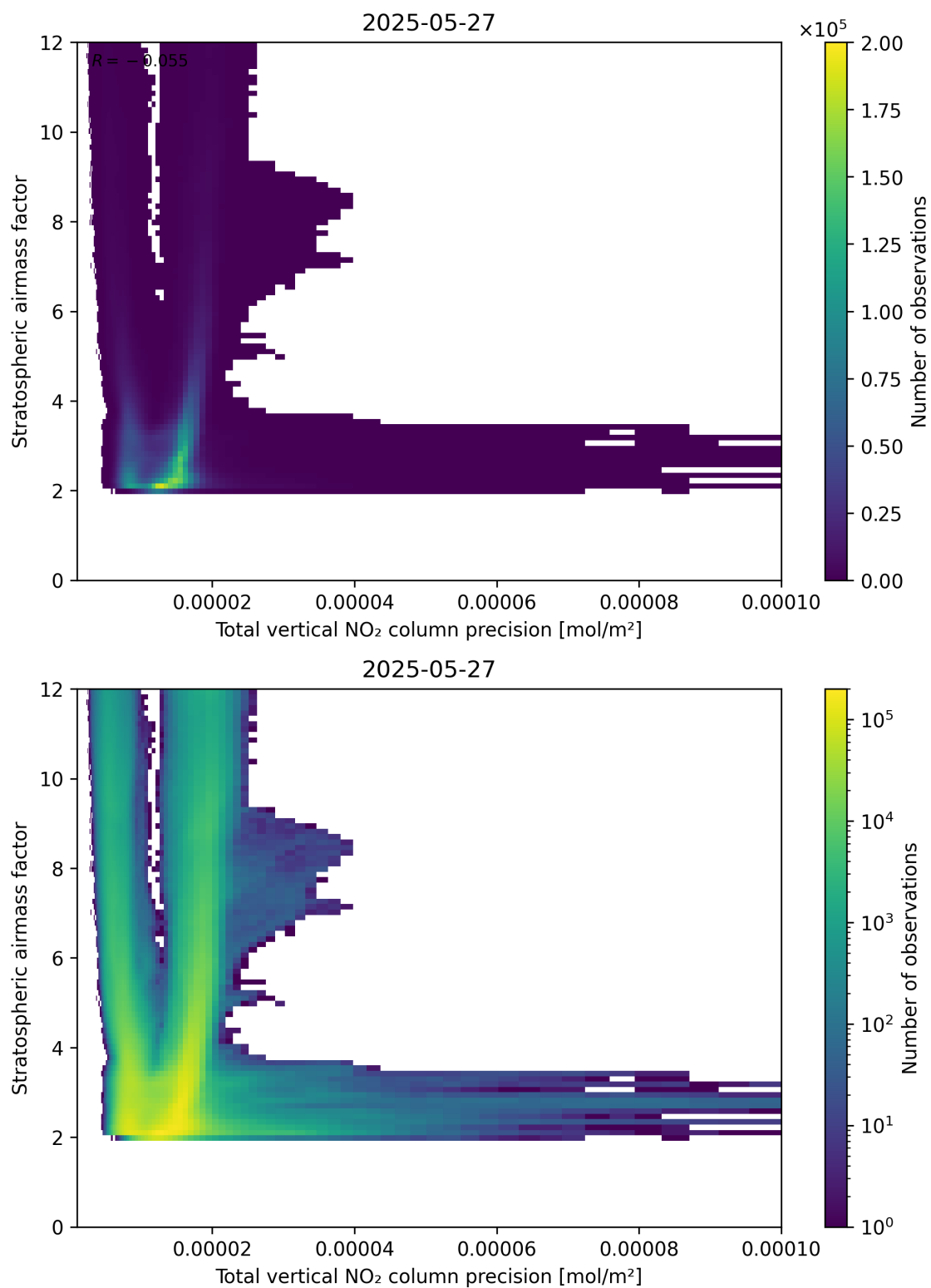
Figure 115: Scatter density plot of “Total vertical NO 2 column precision” against “Stratospheric airmass factor” for 2025-05-26 to 2025-05-28.
