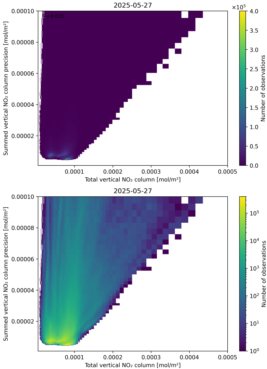
Figure 113: Scatter density plot of “Total vertical NO 2 column” against “Summed vertical NO 2 column precision” for 2025-05-26 to 2025-05-28.
