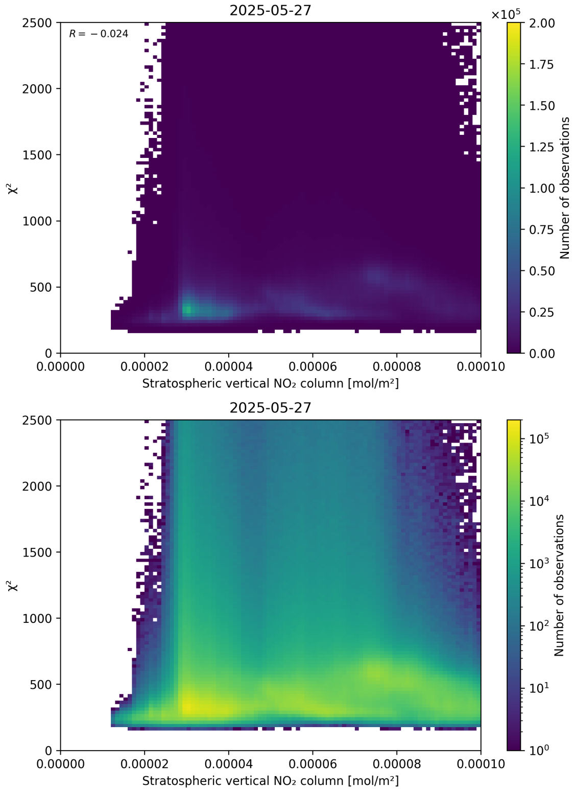
Figure 97: Scatter density plot of “Stratospheric vertical NO 2 column” against “ \chi^2 ” for 2025-05-26 to 2025-05-28.
