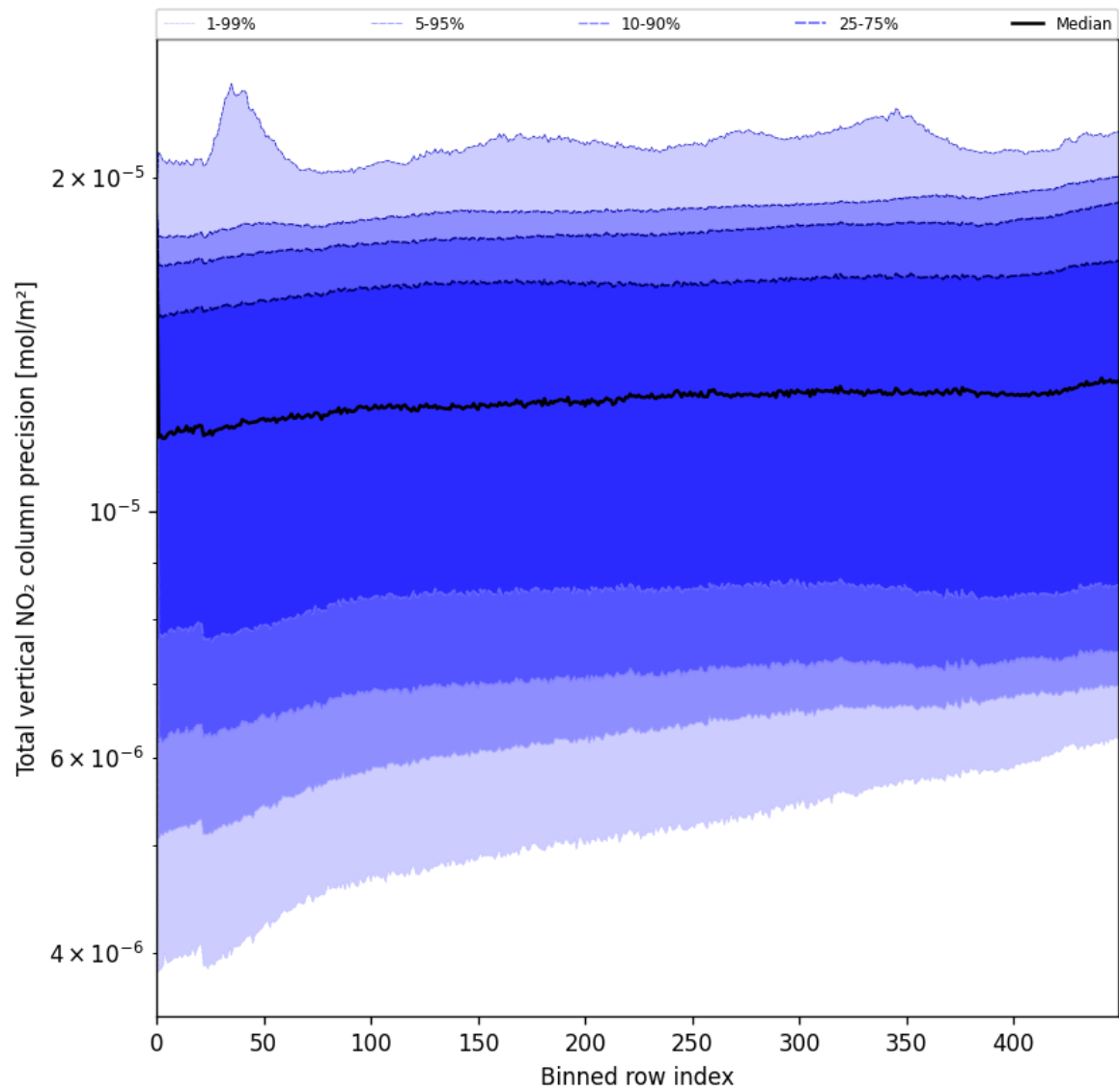
Figure 56: Along track statistics of “Total vertical NO 2 column precision” for 2025-05-26 to 2025-05-28
