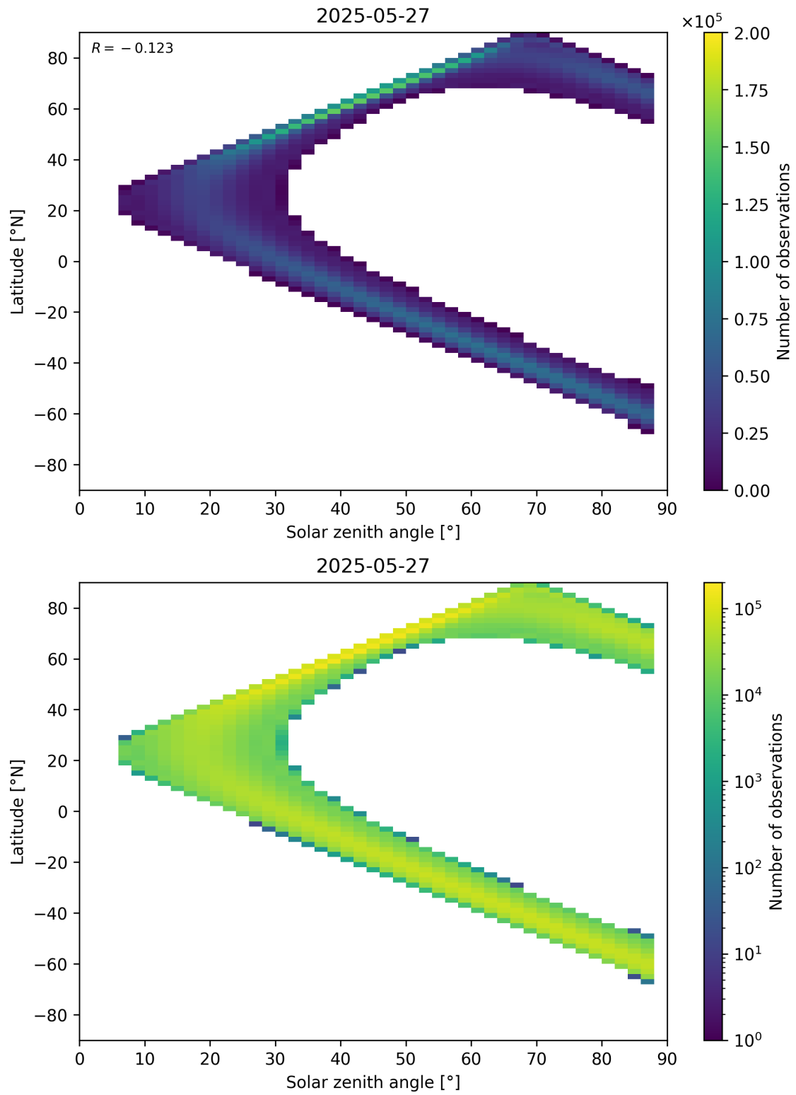
Figure 149: Scatter density plot of “Solar zenith angle” against “Latitude” for 2025-05-26 to 2025-05-28.
