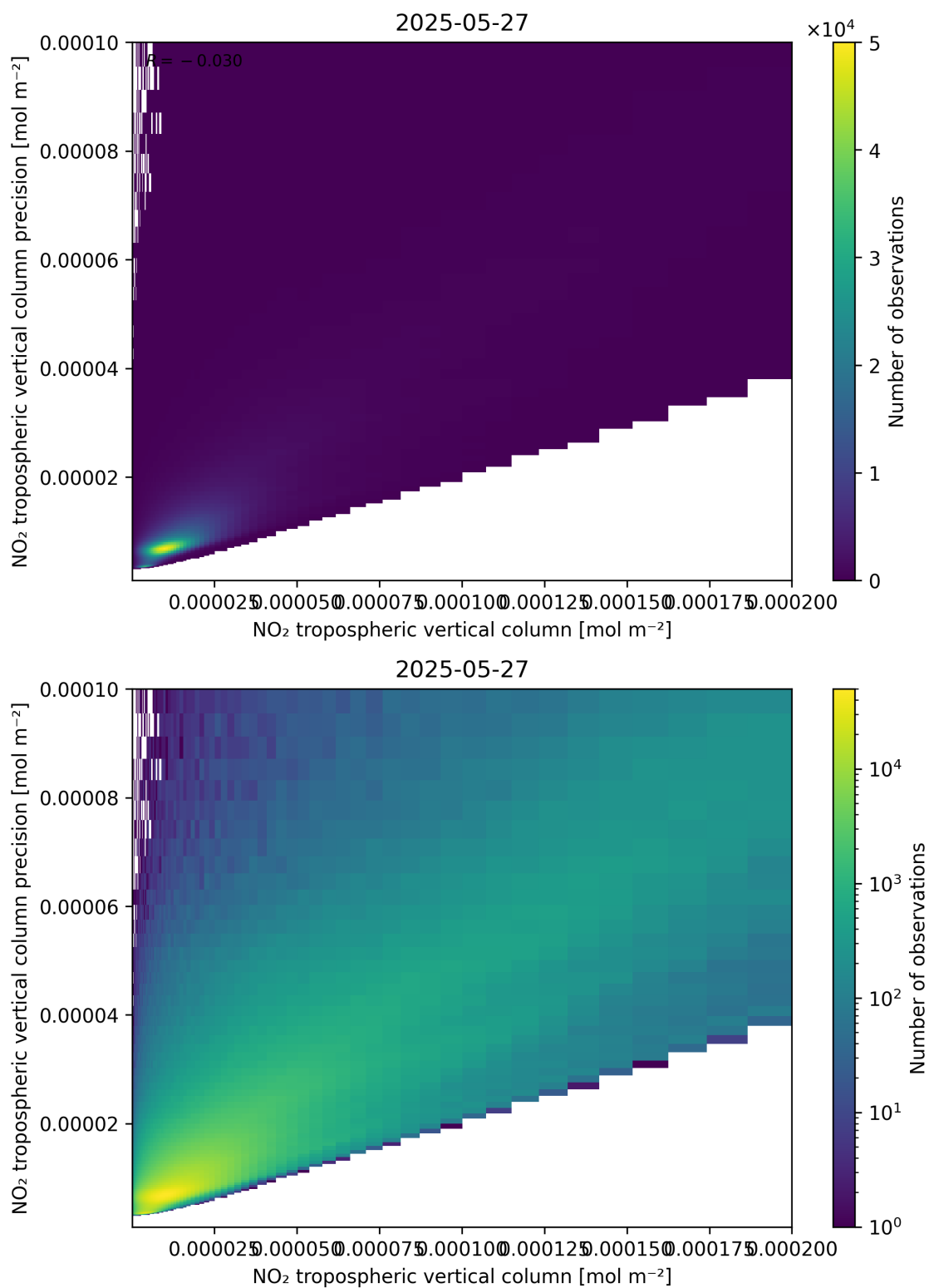
Figure 130: Scatter density plot of “NO 2 tropospheric vertical column” against “NO 2 tropospheric vertical column precision” for 2025-05-26 to 2025-05-28.
