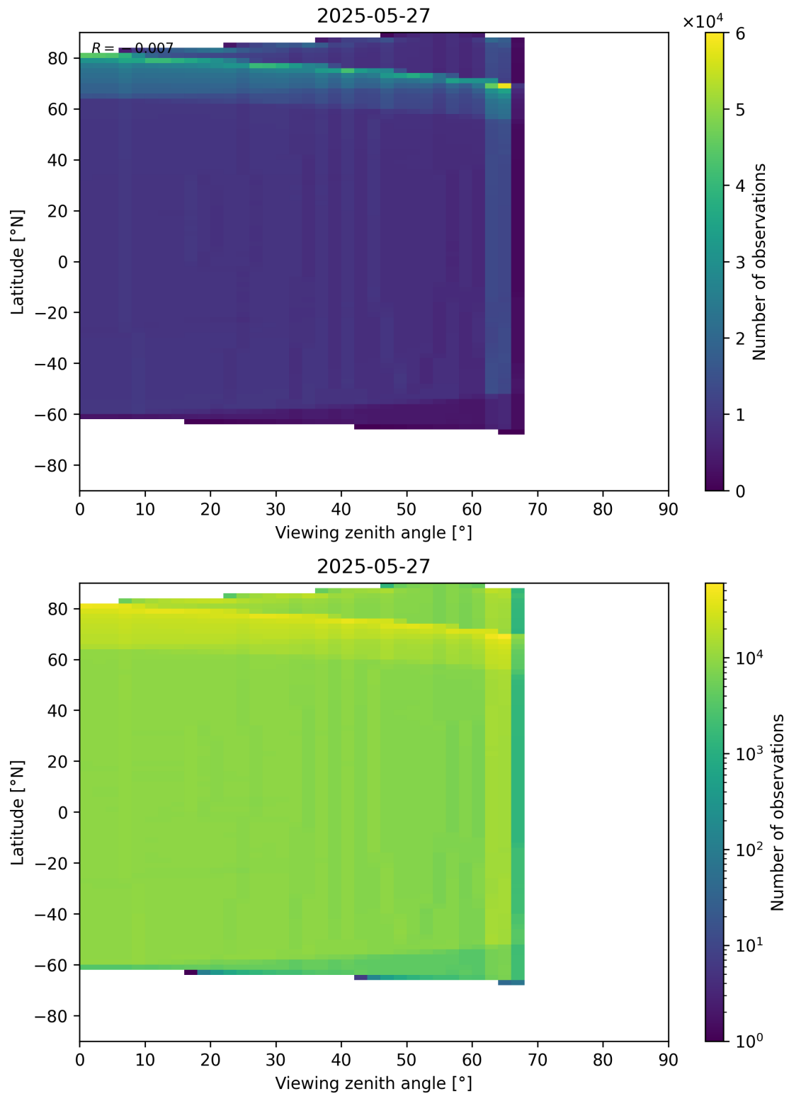
Figure 163: Scatter density plot of “Viewing zenith angle” against “Latitude” for 2025-05-26 to 2025-05-28.
