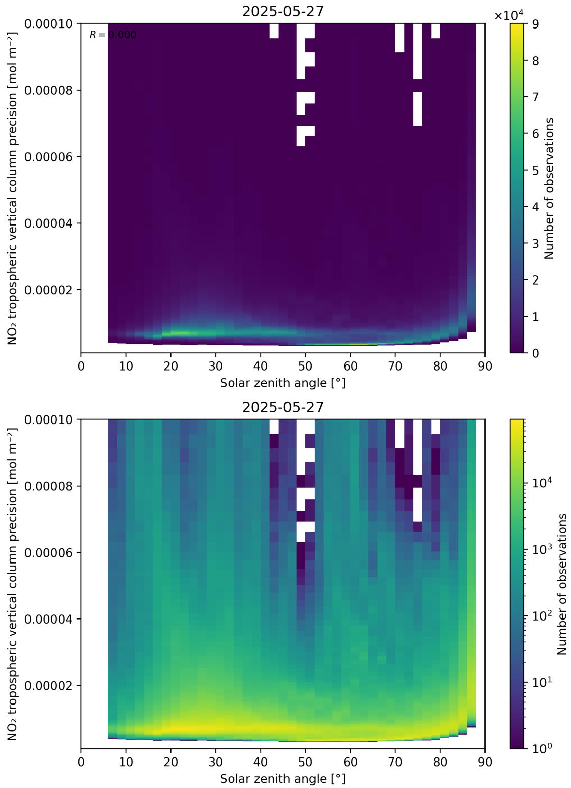
Figure 156: Scatter density plot of “Solar zenith angle” against “NO 2 tropospheric vertical column precision” for 2025-05-26 to 2025-05-28.
