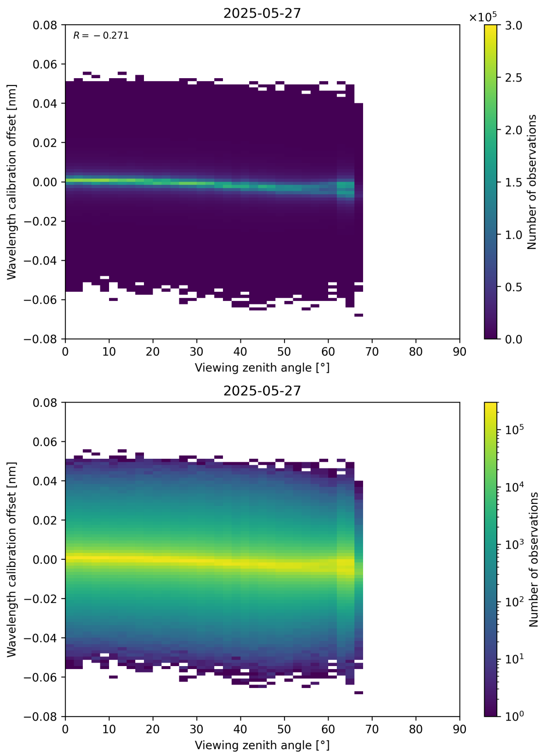
Figure 173: Scatter density plot of “Viewing zenith angle” against “Wavelength calibration offset” for 2025-05-26 to 2025-05-28.
