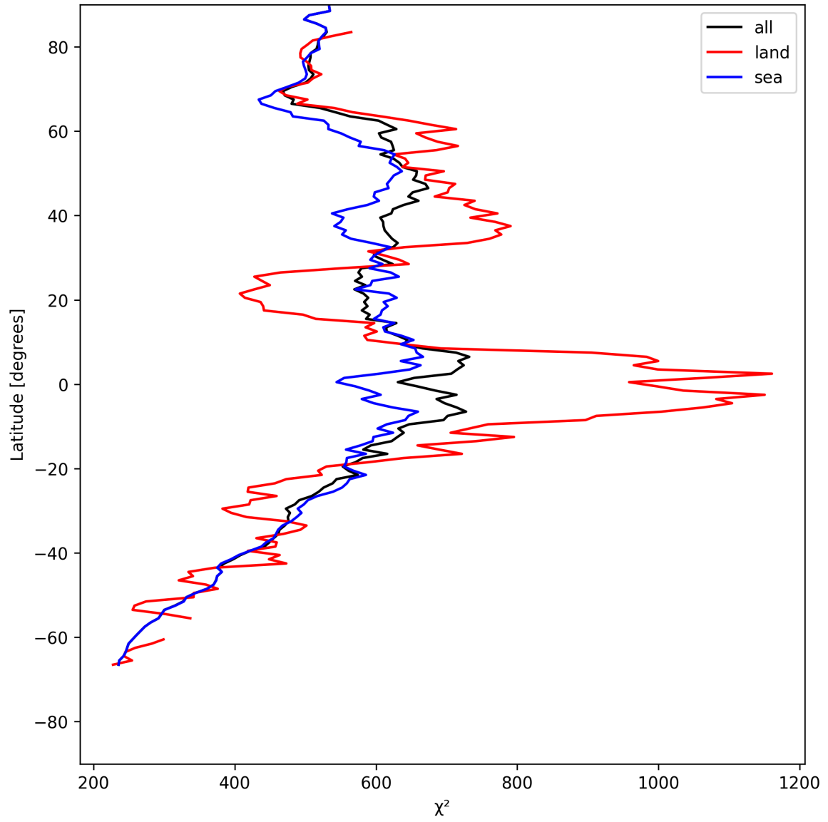
Figure 25: Zonal average of “ \chi^2 ” for 2025-05-26 to 2025-05-28.
