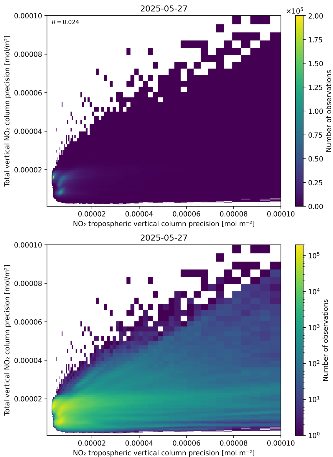
Figure 139: Scatter density plot of “NO 2 tropospheric vertical column precision” against “Total vertical NO 2 column precision” for 2025-05-26 to 2025-05-28.
