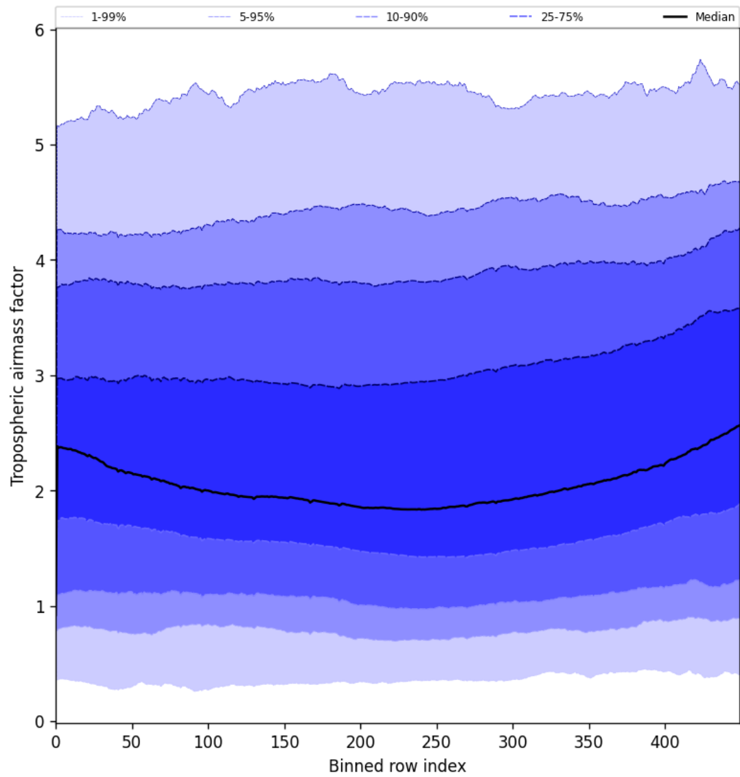
Figure 48: Along track statistics of “Tropospheric air mass factor” for 2025-05-26 to 2025-05-28
