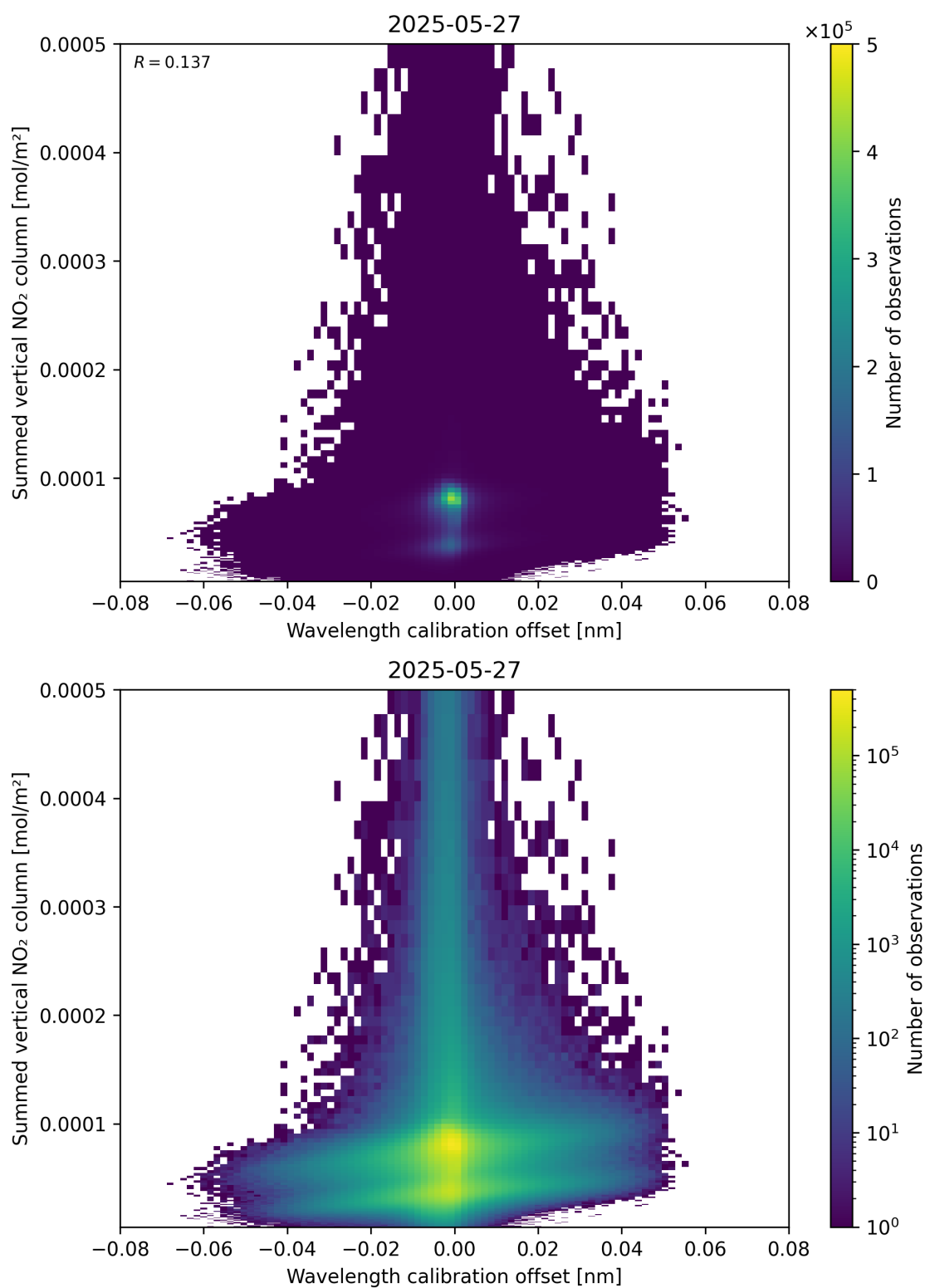
Figure 177: Scatter density plot of “Wavelength calibration offset” against “Summed vertical NO 2 column” for 2025-05-26 to 2025-05-28.
