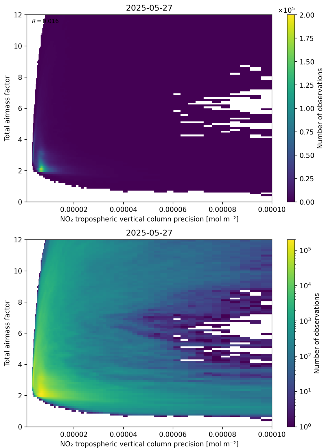
Figure 132: Scatter density plot of “NO 2 tropospheric vertical column precision” against “Total air mass factor” for 2025-05-26 to 2025-05-28.
