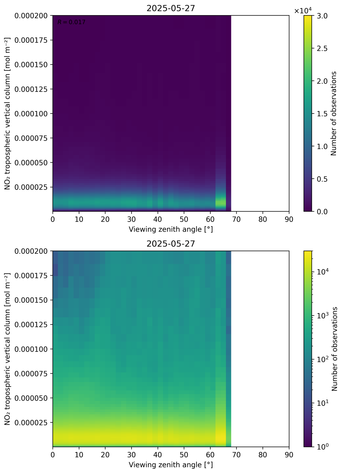
Figure 169: Scatter density plot of “Viewing zenith angle” against “NO 2 tropospheric vertical column” for 2025-05-26 to 2025-05-28.
