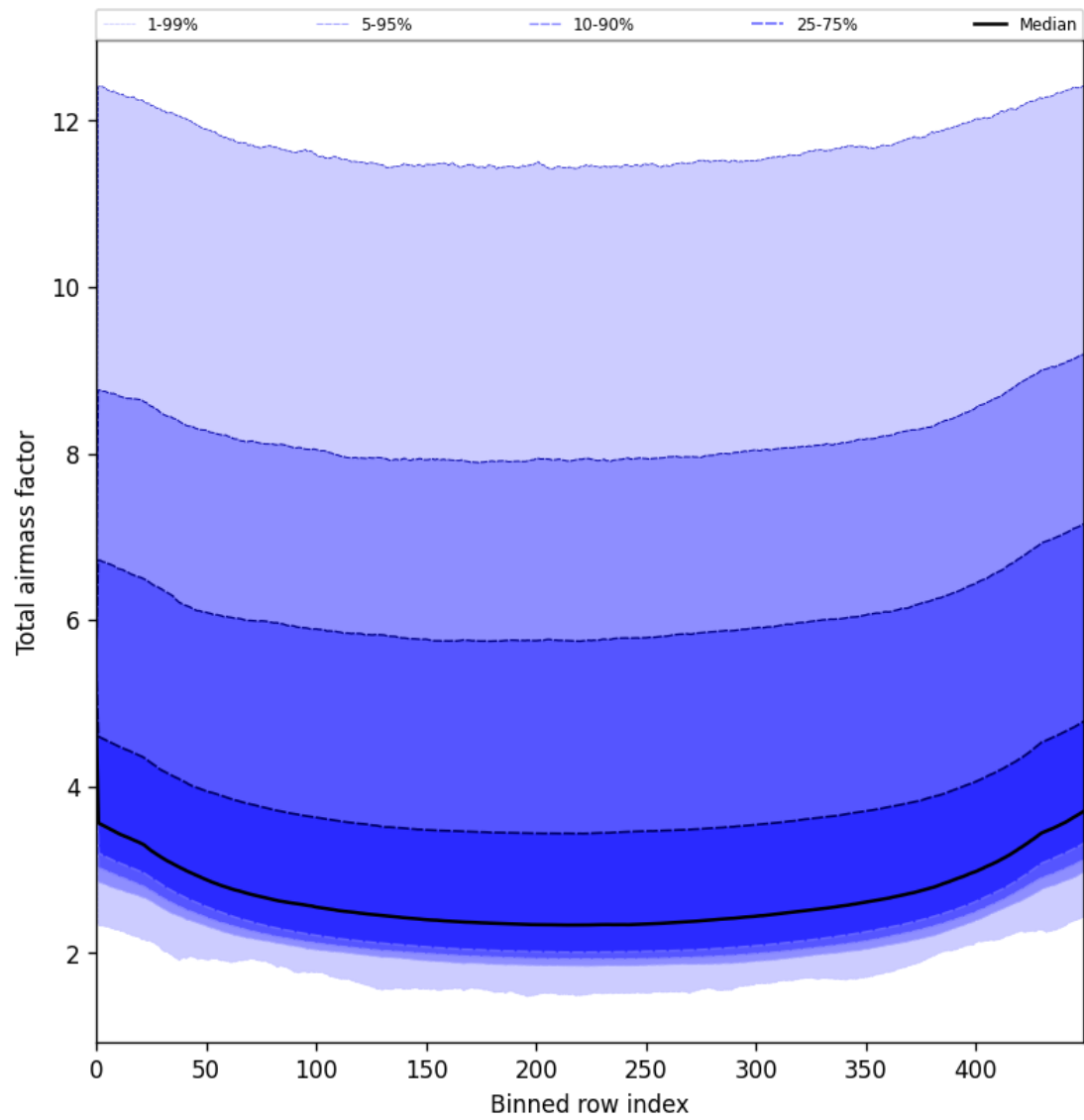
Figure 49: Along track statistics of “Total airmass factor” for 2025-05-26 to 2025-05-28
