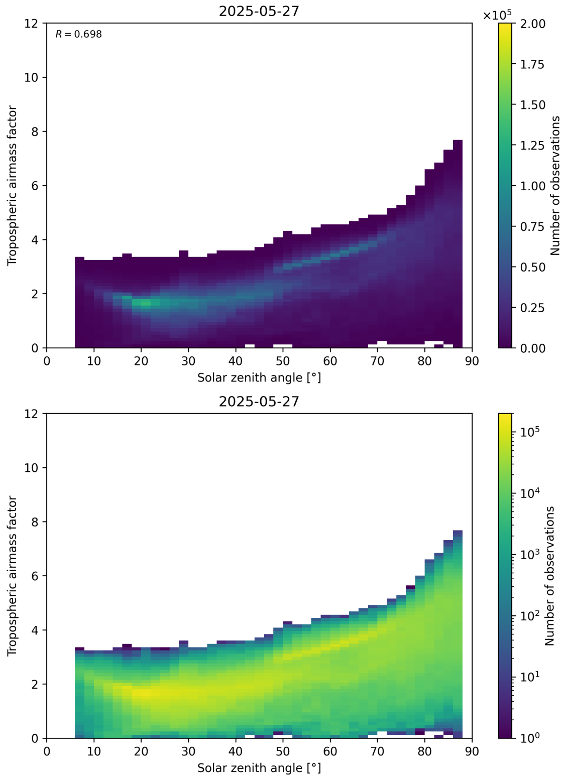
Figure 147: Scatter density plot of “Solar zenith angle” against “Tropospheric airmass factor” for 2025-05-26 to 2025-05-28.
