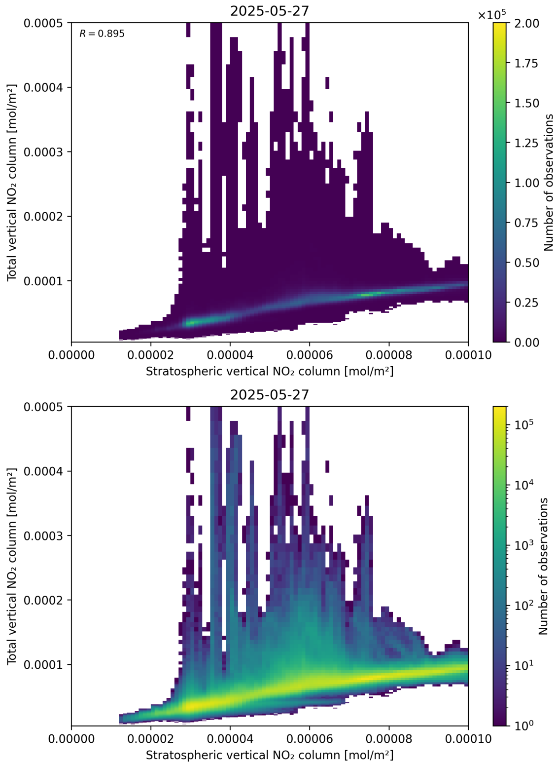
Figure 100: Scatter density plot of “Stratospheric vertical NO 2 column” against “Total vertical NO 2 column” for 2025-05-26 to 2025-05-28.
