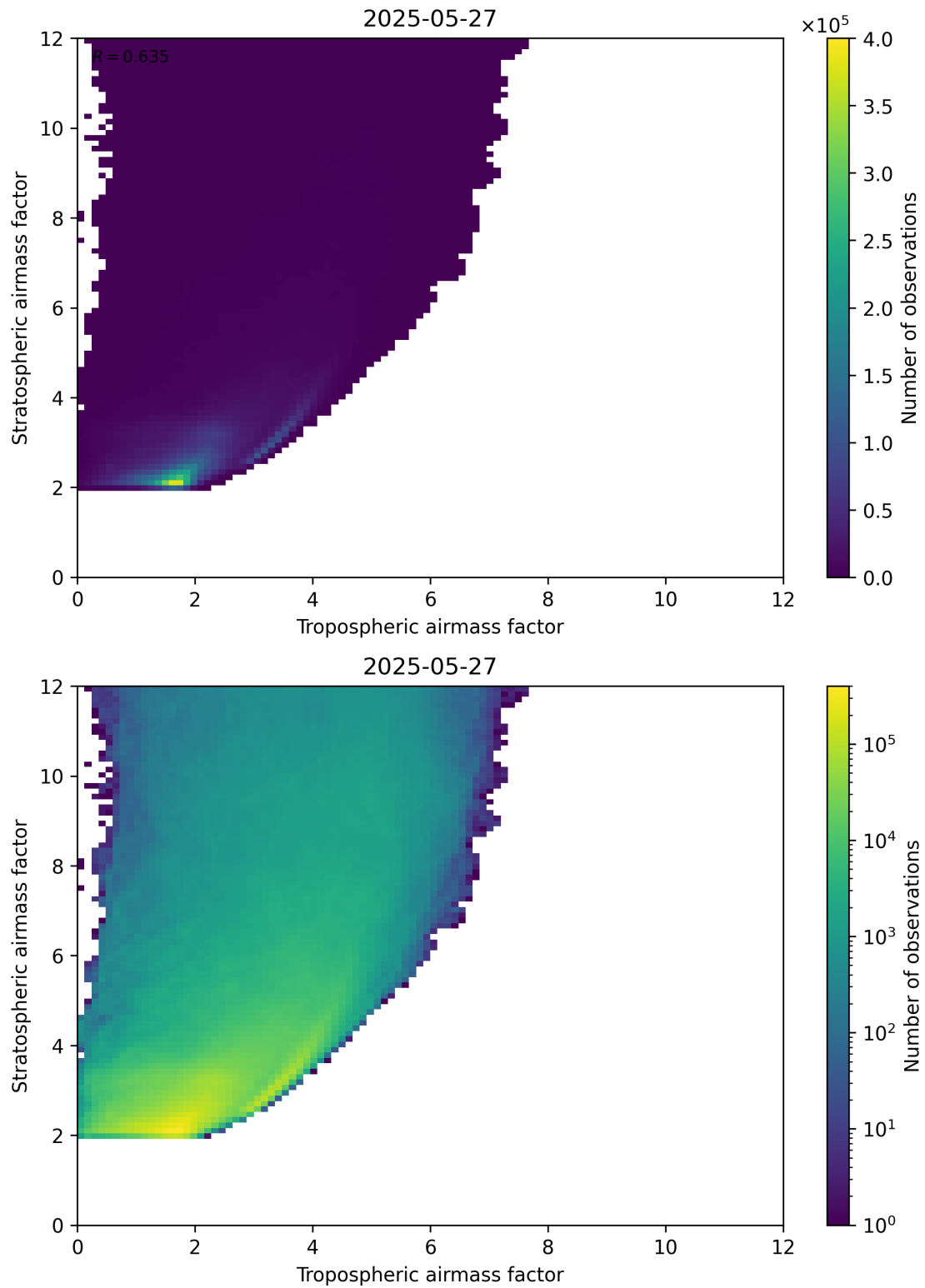
Figure 71: Scatter density plot of “Tropospheric airmass factor” against “Stratospheric airmass factor” for 2025-05-26 to 2025-05-28.
