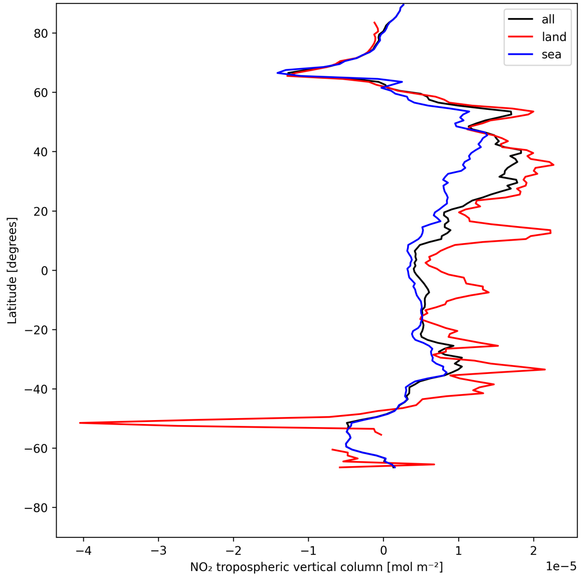
Figure 12: Zonal average of “NO 2 tropospheric vertical column” for 2025-05-26 to 2025-05-28.
