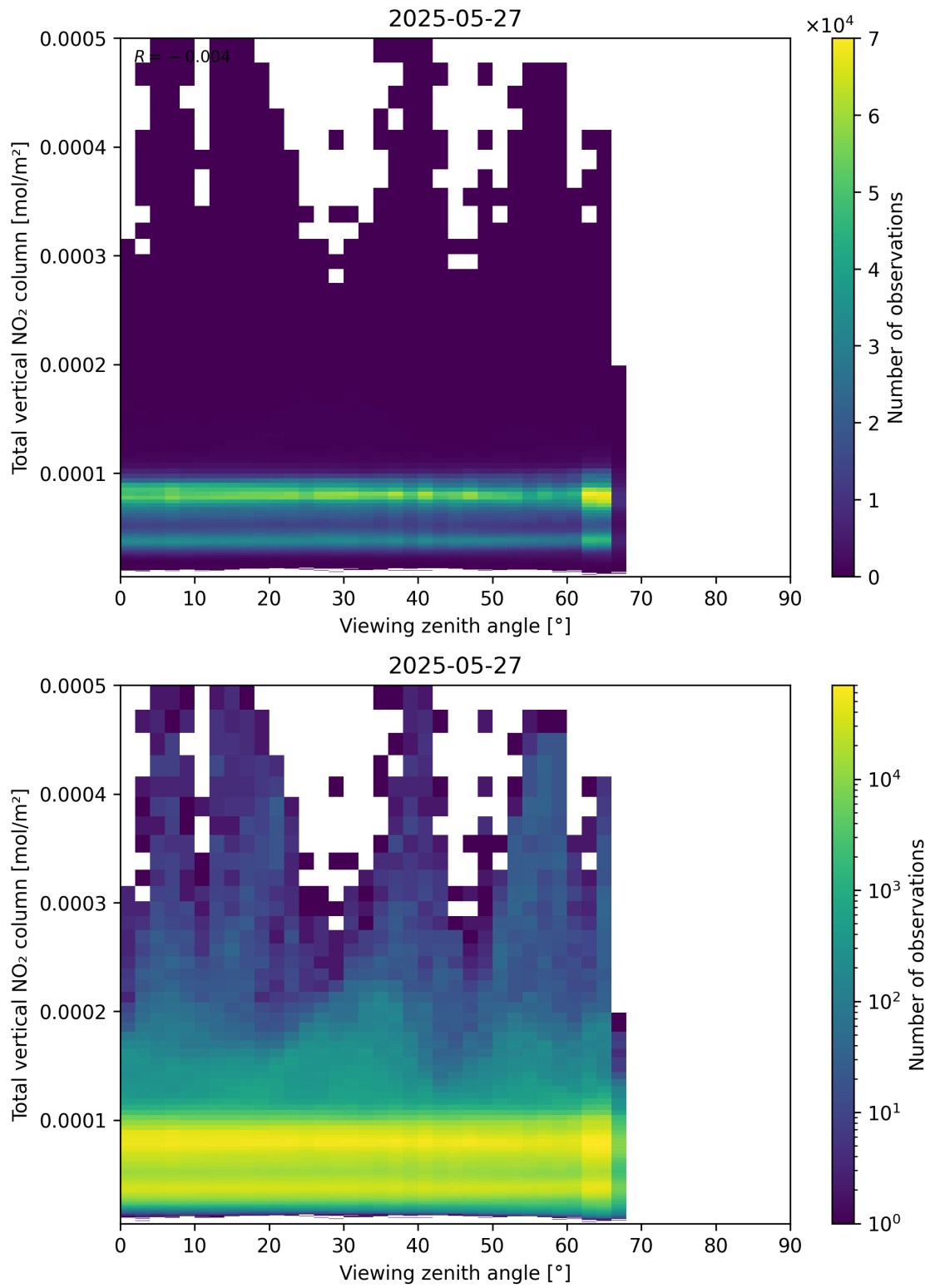
Figure 167: Scatter density plot of “Viewing zenith angle” against “Total vertical NO 2 column” for 2025-05-26 to 2025-05-28.
