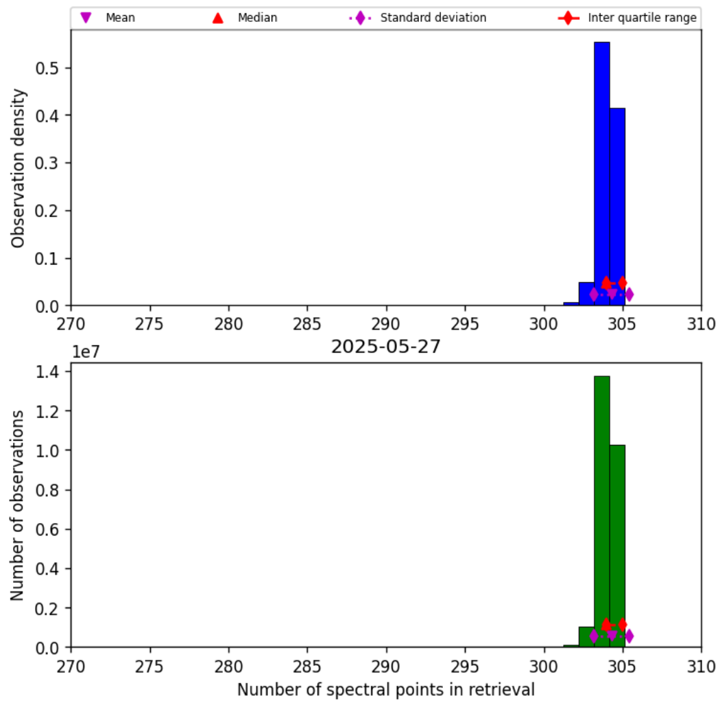
Figure 33: Histogram of “Number of spectral points in retrieval” for 2025-05-26 to 2025-05-28
