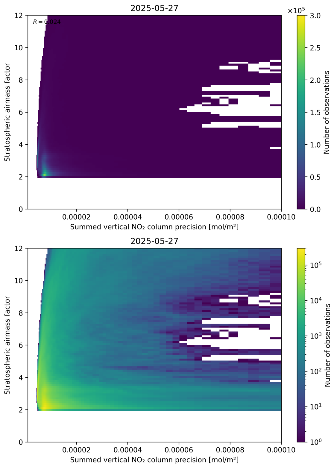
Figure 106: Scatter density plot of “Summed vertical NO 2 column precision” against “Stratospheric airmass factor” for 2025-05-26 to 2025-05-28.
