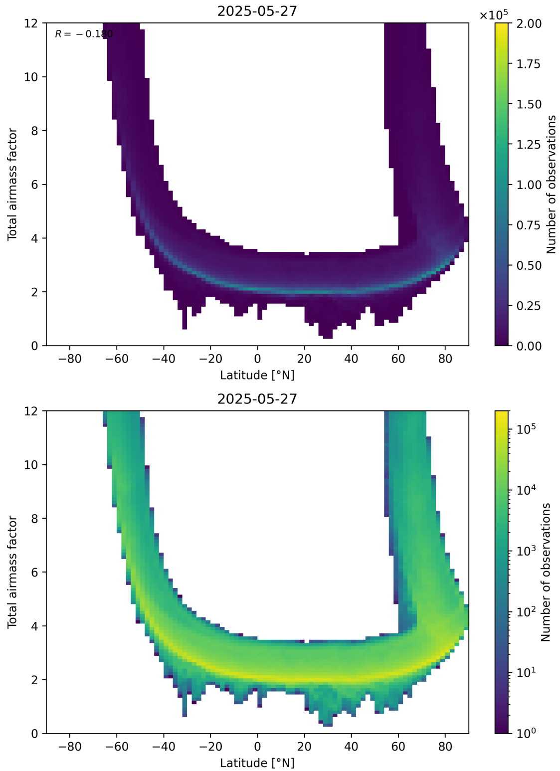
Figure 84: Scatter density plot of “Latitude” against “Total airmass factor” for 2025-05-26 to 2025-05-28.
