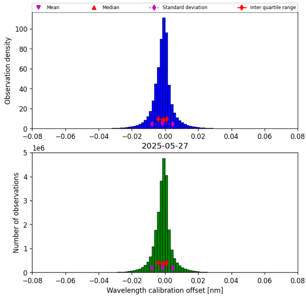
Figure 35: Histogram of “Wavelength calibration offset” for 2025-05-26 to 2025-05-28
