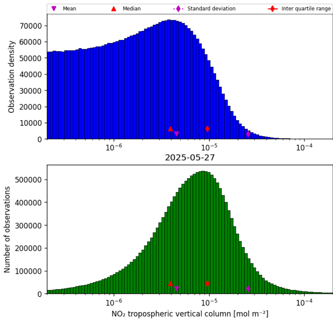
Figure 29: Histogram of “NO 2 tropospheric vertical column” for 2025-05-26 to 2025-05-28
