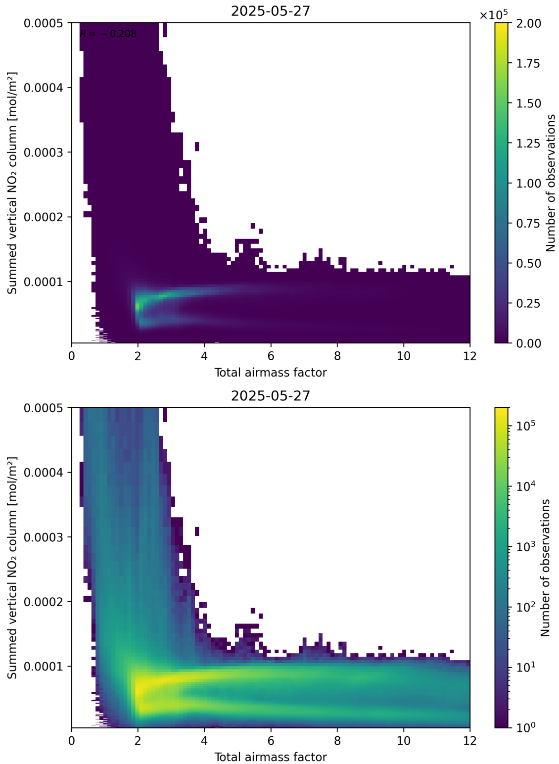
Figure 65: Scatter density plot of “Total airmass factor” against “Summed vertical NO 2 column” for 2025-05-26 to 2025-05-28.
