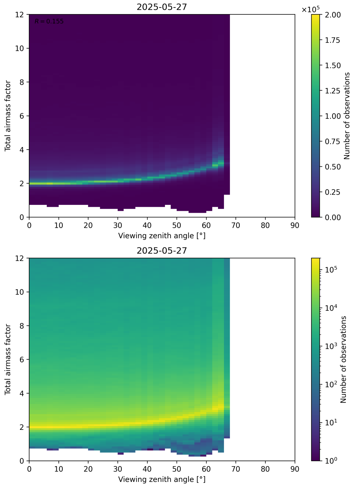
Figure 160: Scatter density plot of “Viewing zenith angle” against “Total airmass factor” for 2025-05-26 to 2025-05-28.
