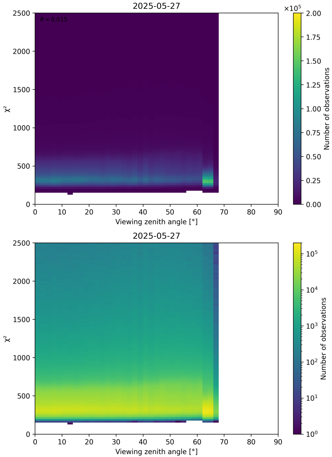
Figure 162: Scatter density plot of “Viewing zenith angle” against “ \chi^2 ” for 2025-05-26 to 2025-05-28.
