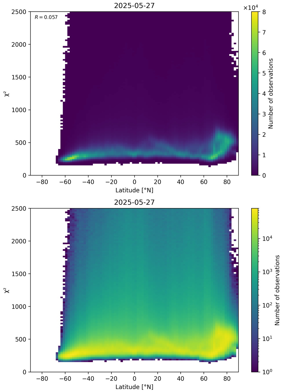
Figure 86: Scatter density plot of “Latitude” against “ \chi^2 ” for 2025-05-26 to 2025-05-28.
