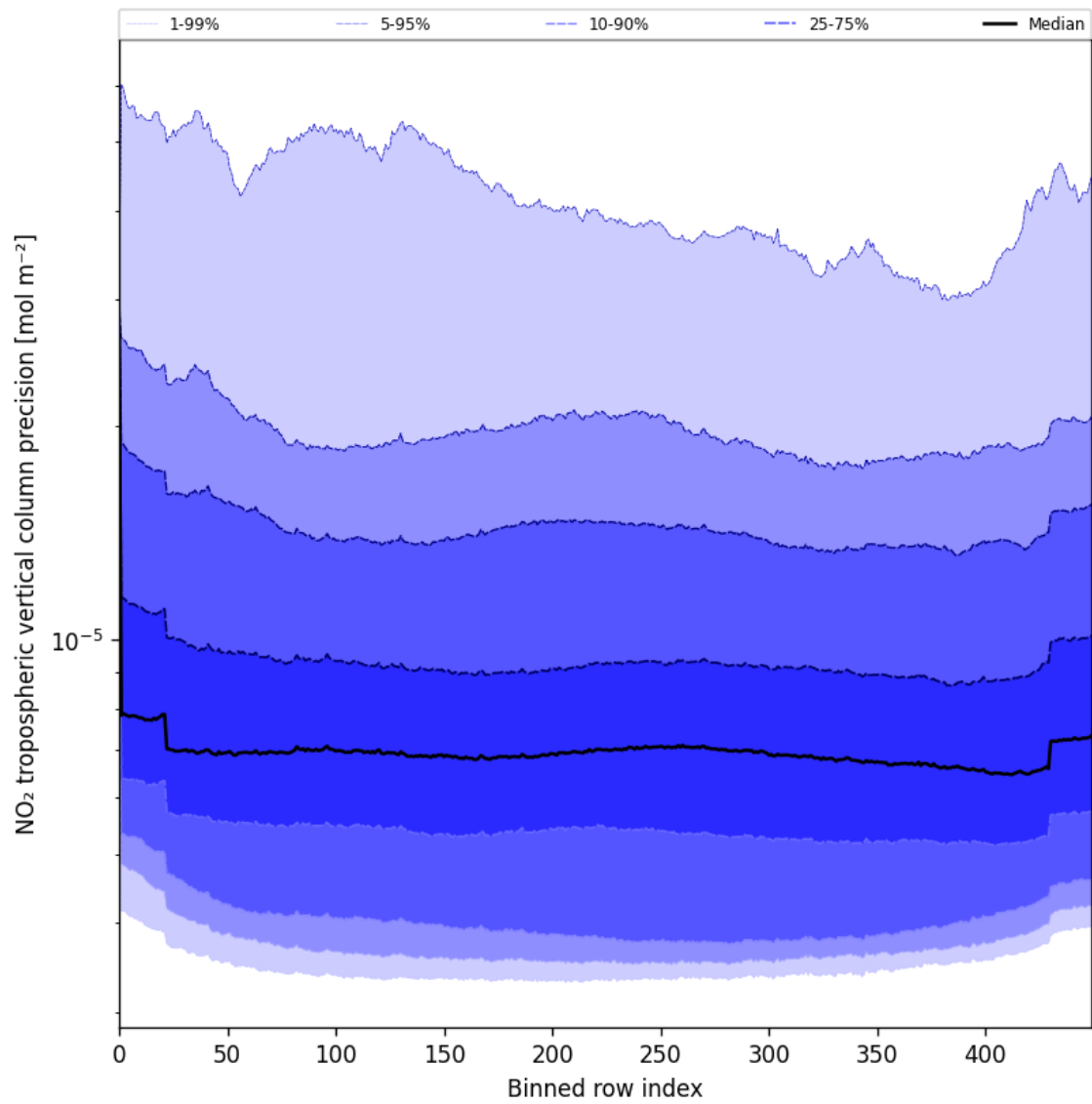
Figure 47: Along track statistics of “NO 2 tropospheric vertical column precision” for 2025-05-26 to 2025-05-28
