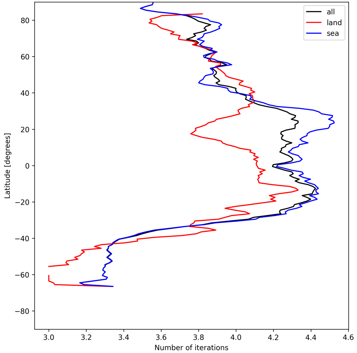
Figure 17: Zonal average of “Number of iterations” for 2025-05-26 to 2025-05-28.
