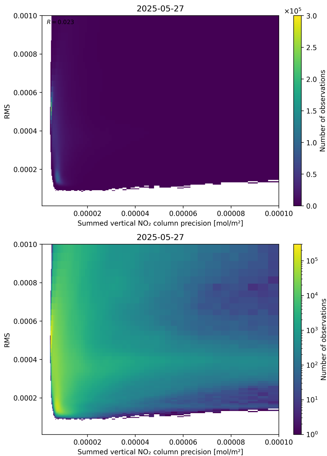
Figure 108: Scatter density plot of “Summed vertical NO 2 column precision” against “RMS” for 2025-05-26 to 2025-05-28.
