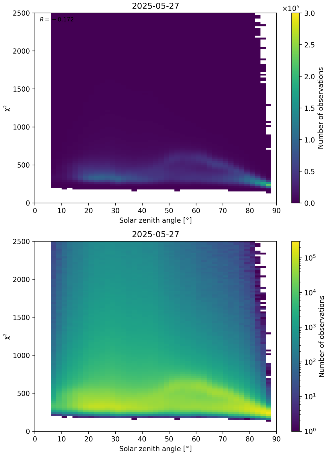
Figure 148: Scatter density plot of “Solar zenith angle” against “ \chi^2 ” for 2025-05-26 to 2025-05-28.
