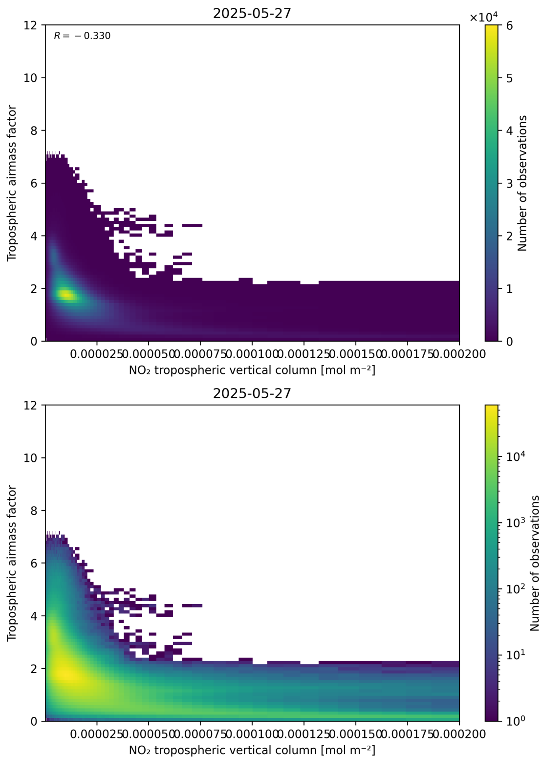
Figure 123: Scatter density plot of “NO 2 tropospheric vertical column” against “Tropospheric air mass factor” for 2025-05-26 to 2025-05-28.
