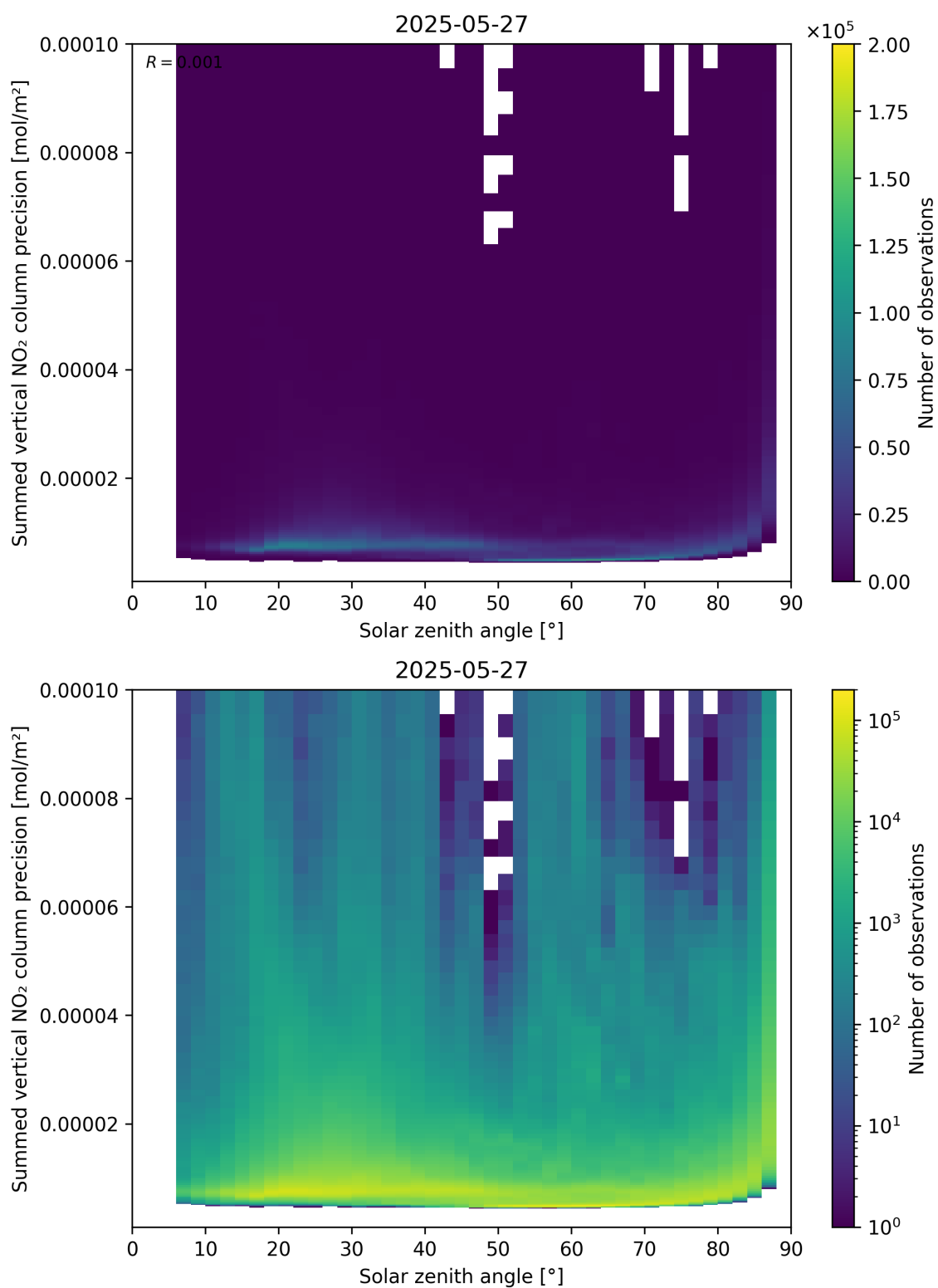
Figure 152: Scatter density plot of “Solar zenith angle” against “Summed vertical NO 2 column precision” for 2025-05-26 to 2025-05-28.
