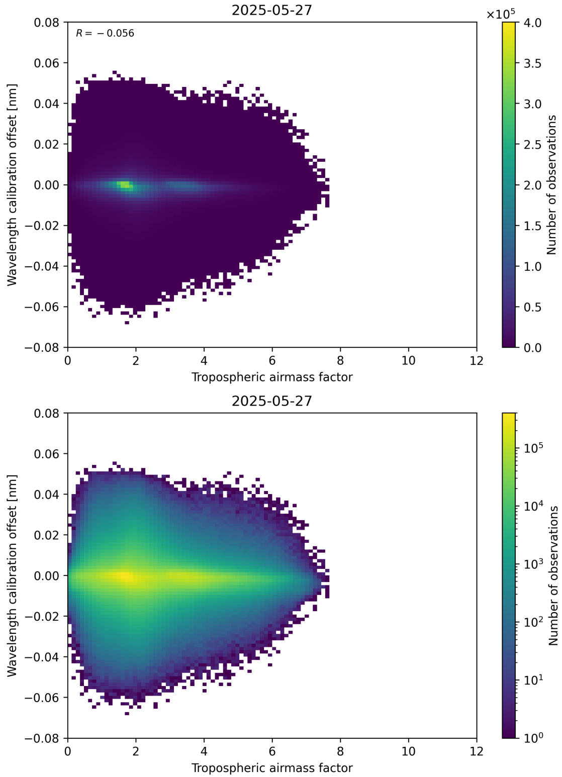
Figure 80: Scatter density plot of “Tropospheric airmass factor” against “Wavelength calibration offset” for 2025-05-26 to 2025-05-28.
