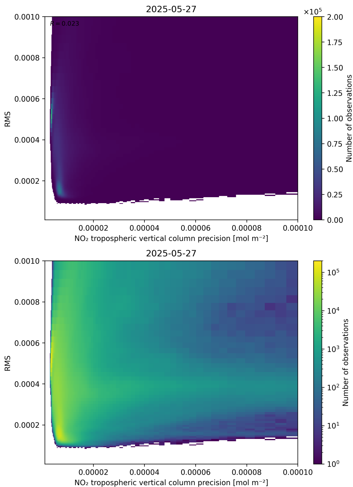
Figure 140: Scatter density plot of “NO 2 tropospheric vertical column precision” against “RMS” for 2025-05-26 to 2025-05-28.
