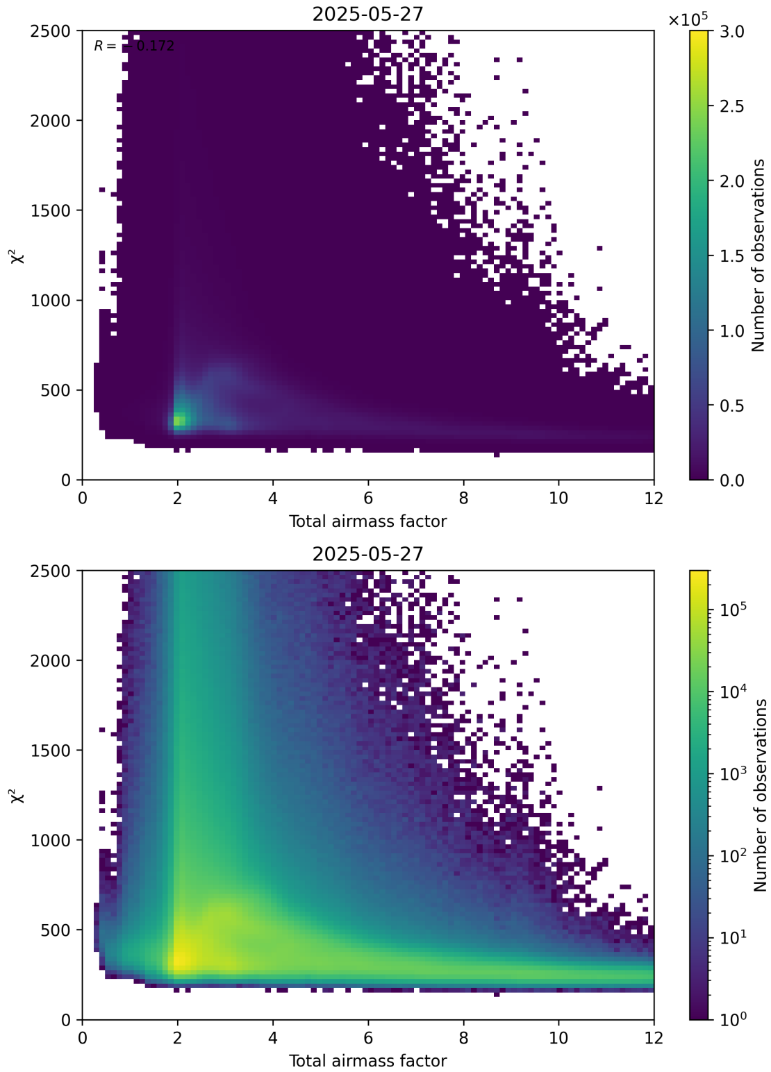
Figure 63: Scatter density plot of “Total airmass factor” against “ \chi^2 ” for 2025-05-26 to 2025-05-28.
