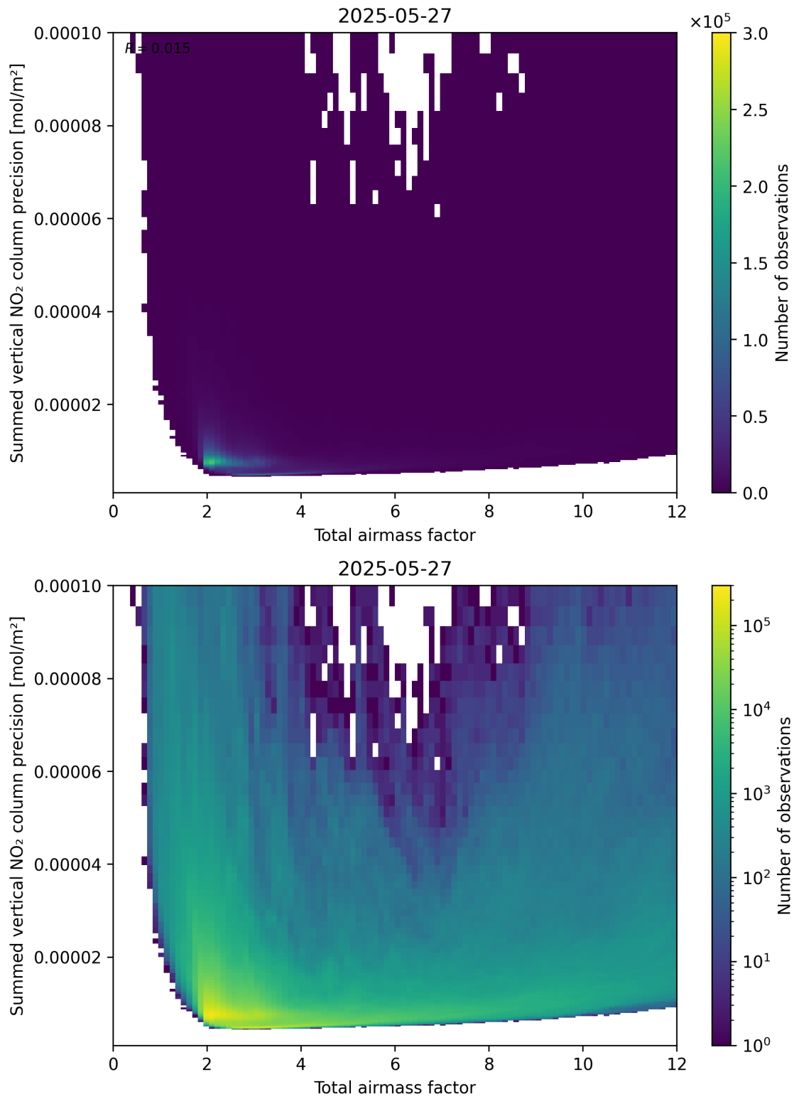
Figure 66: Scatter density plot of “Total airmass factor” against “Summed vertical NO 2 column precision” for 2025-05-26 to 2025-05-28.
