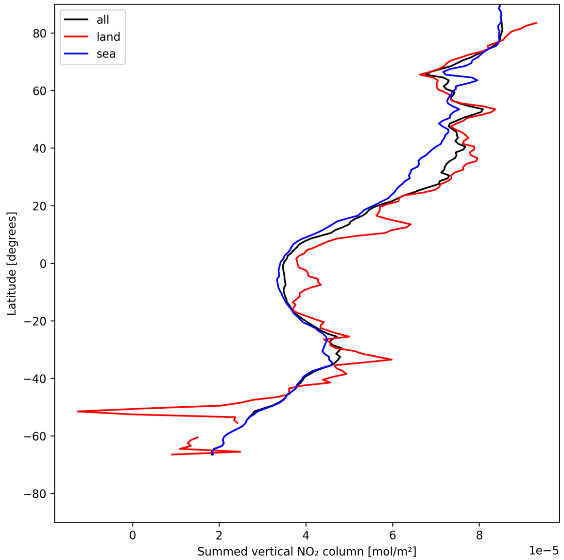
Figure 23: Zonal average of “Summed vertical NO 2 column” for 2025-05-26 to 2025-05-28.
