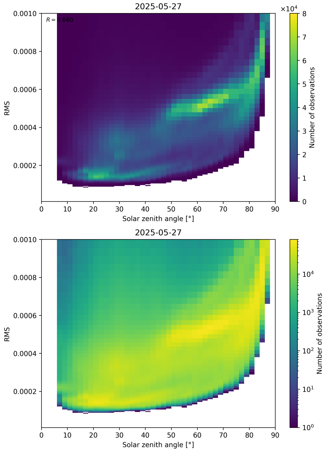
Figure 157: Scatter density plot of “Solar zenith angle” against “RMS” for 2025-05-26 to 2025-05-28.
