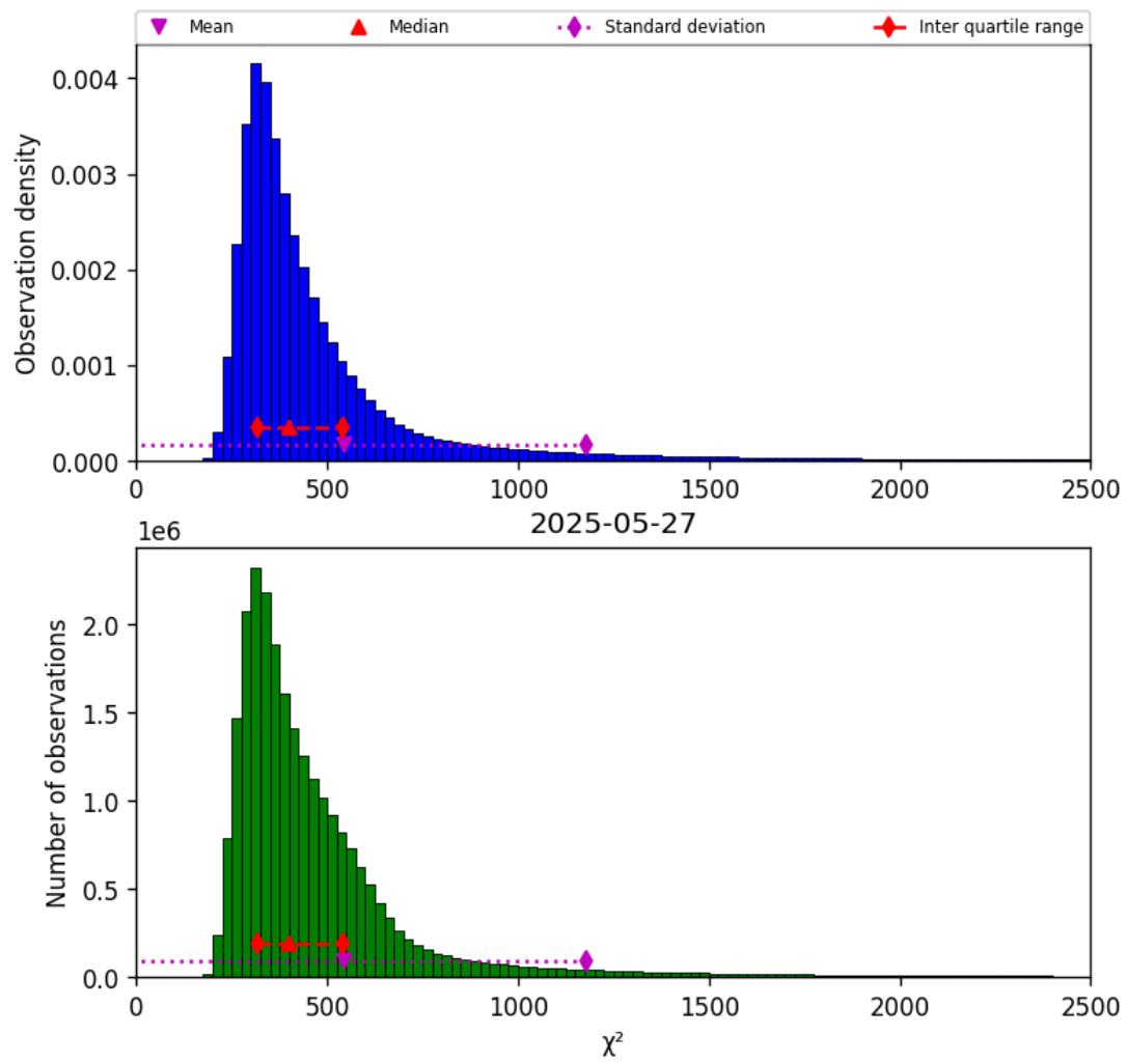
Figure 42: Histogram of “ \chi^2 ” for 2025-05-26 to 2025-05-28
