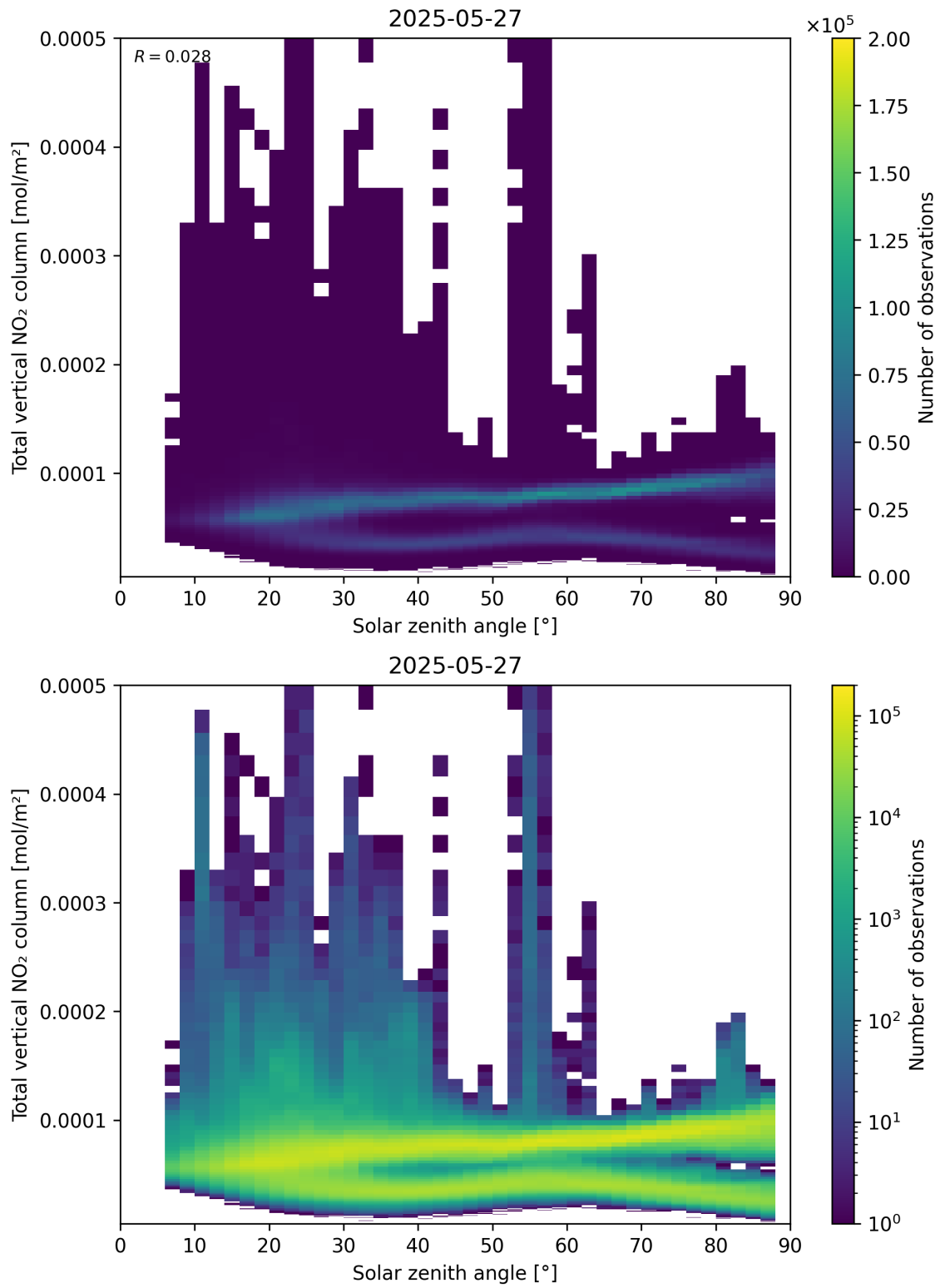
Figure 153: Scatter density plot of “Solar zenith angle” against “Total vertical NO 2 column” for 2025-05-26 to 2025-05-28.
