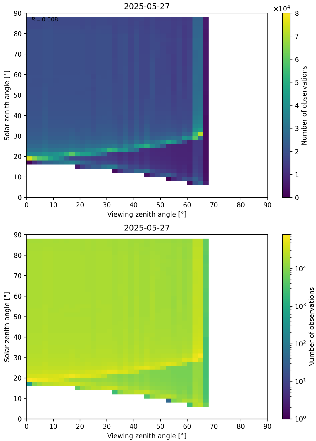
Figure 172: Scatter density plot of “Viewing zenith angle” against “Solar zenith angle” for 2025-05-26 to 2025-05-28.
