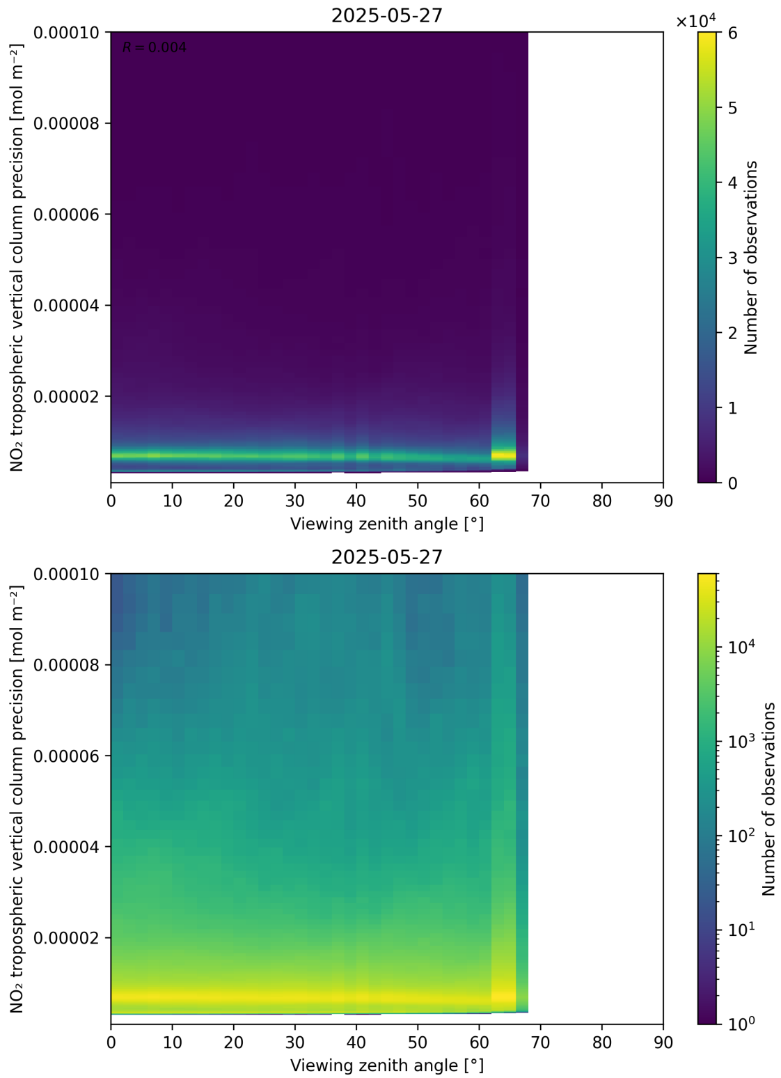
Figure 170: Scatter density plot of “Viewing zenith angle” against “NO 2 tropospheric vertical column precision” for 2025-05-26 to 2025-05-28.
