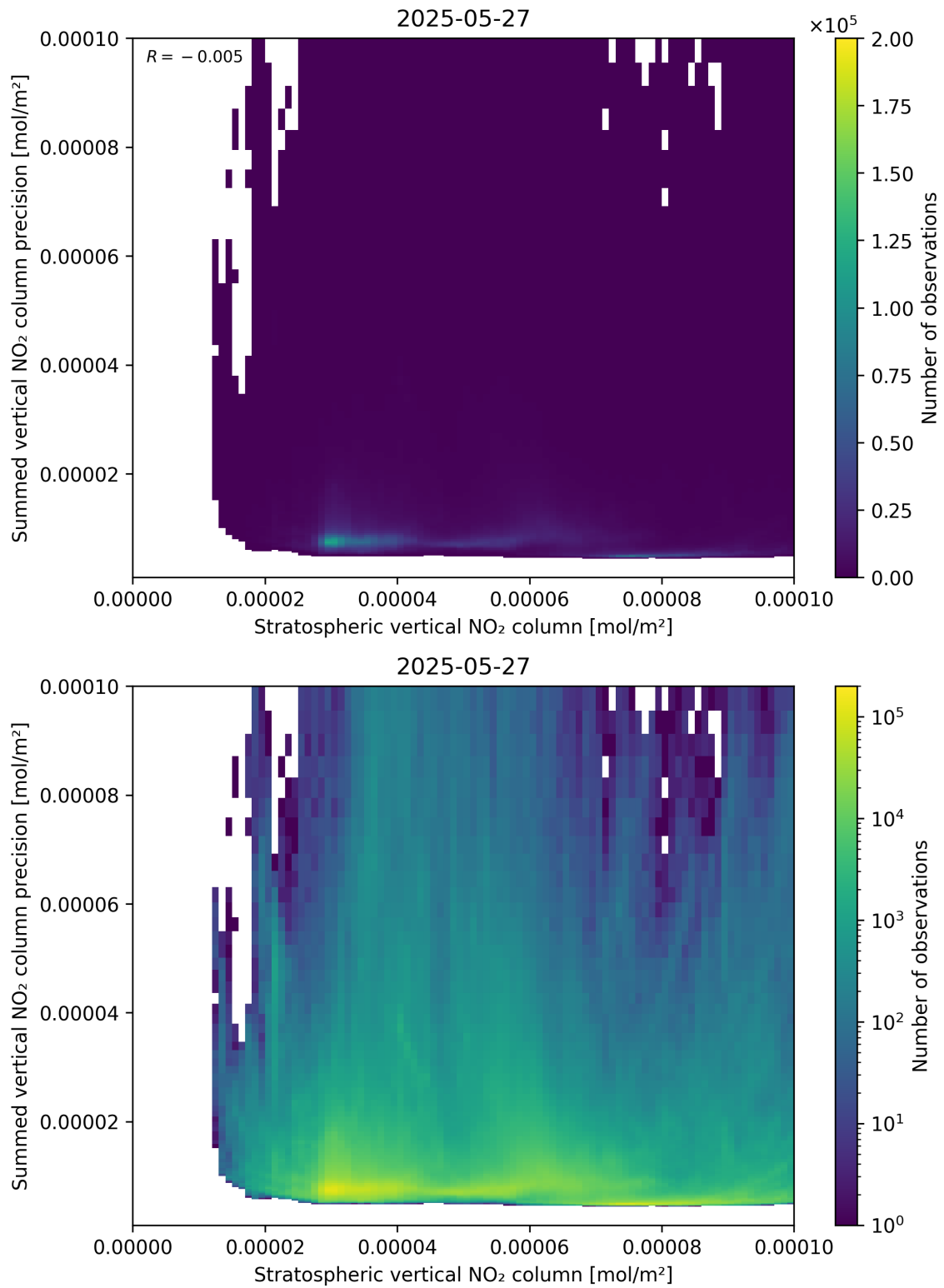
Figure 99: Scatter density plot of “Stratospheric vertical NO 2 column” against “Summed vertical NO 2 column precision” for 2025-05-26 to 2025-05-28.
