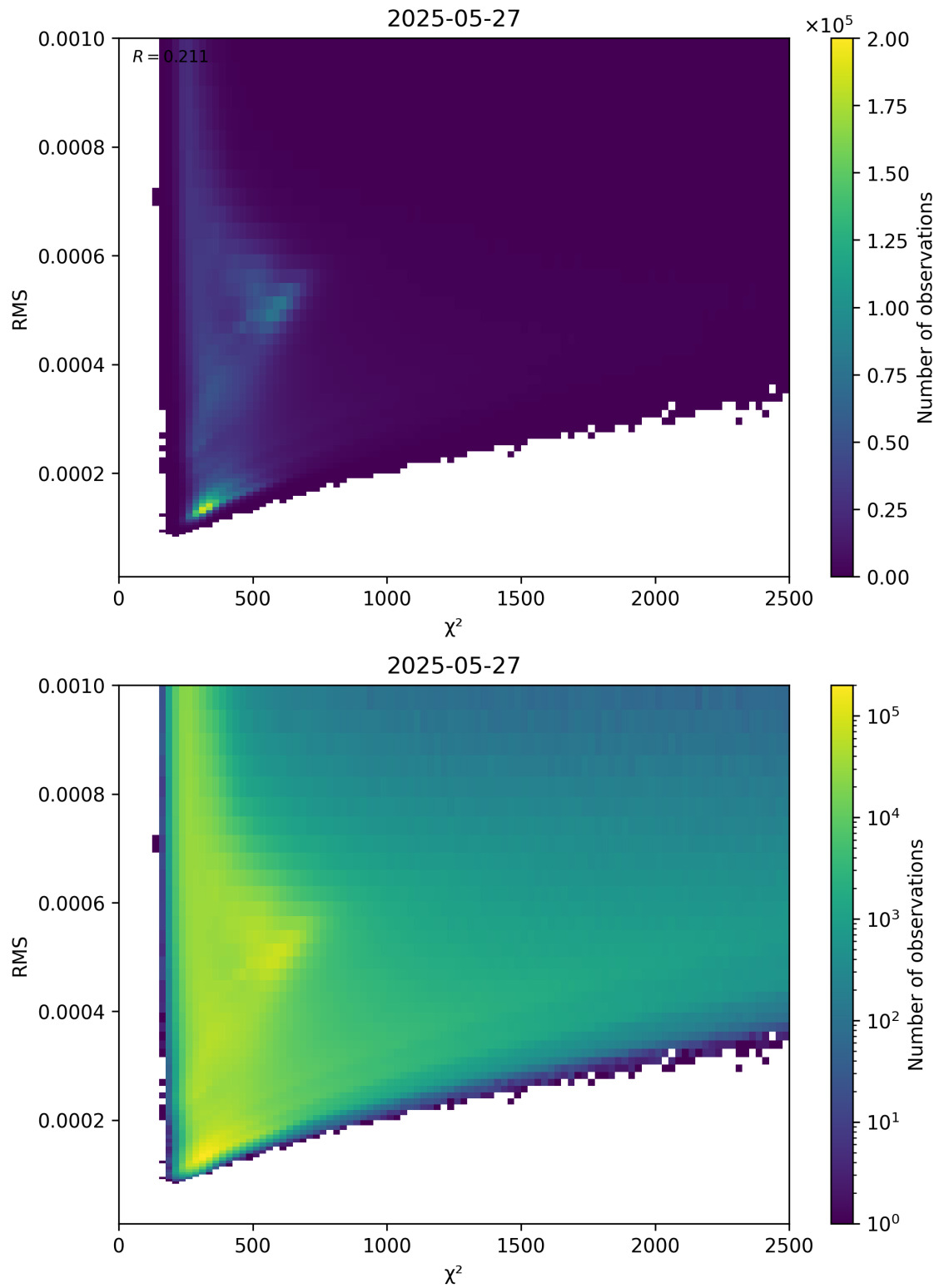
Figure 82: Scatter density plot of “ \chi^2 ” against “RMS” for 2025-05-26 to 2025-05-28.
