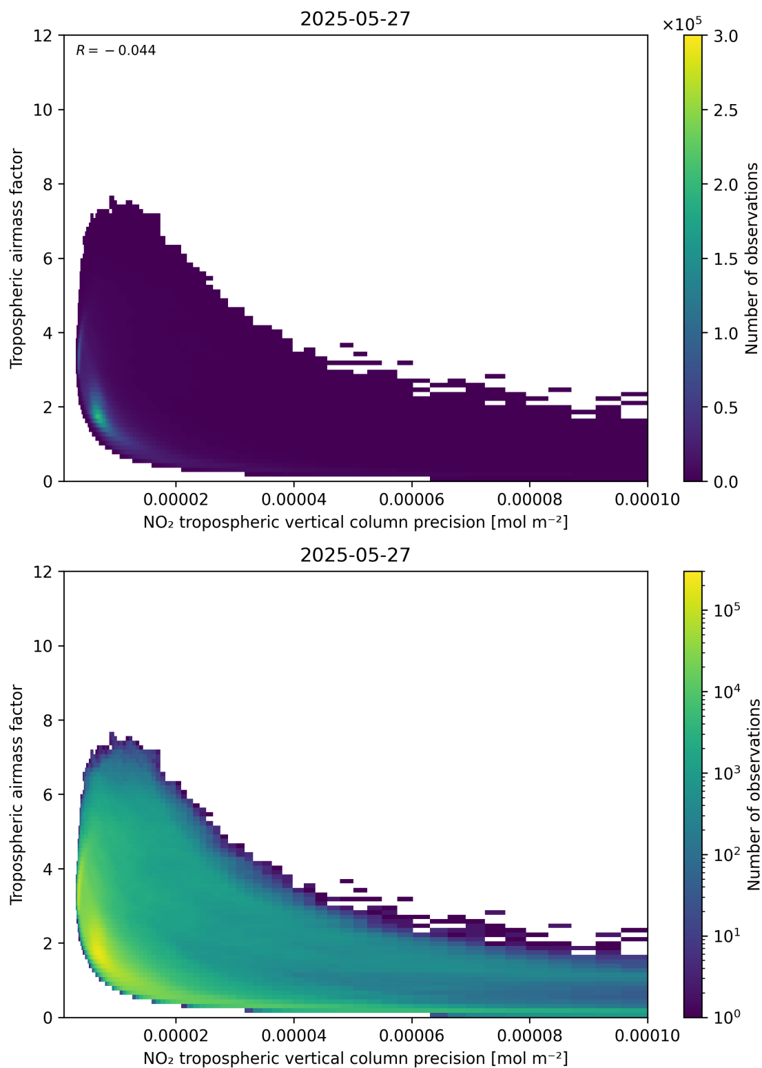
Figure 133: Scatter density plot of “NO 2 tropospheric vertical column precision” against “Tropospheric air mass factor” for 2025-05-26 to 2025-05-28.
