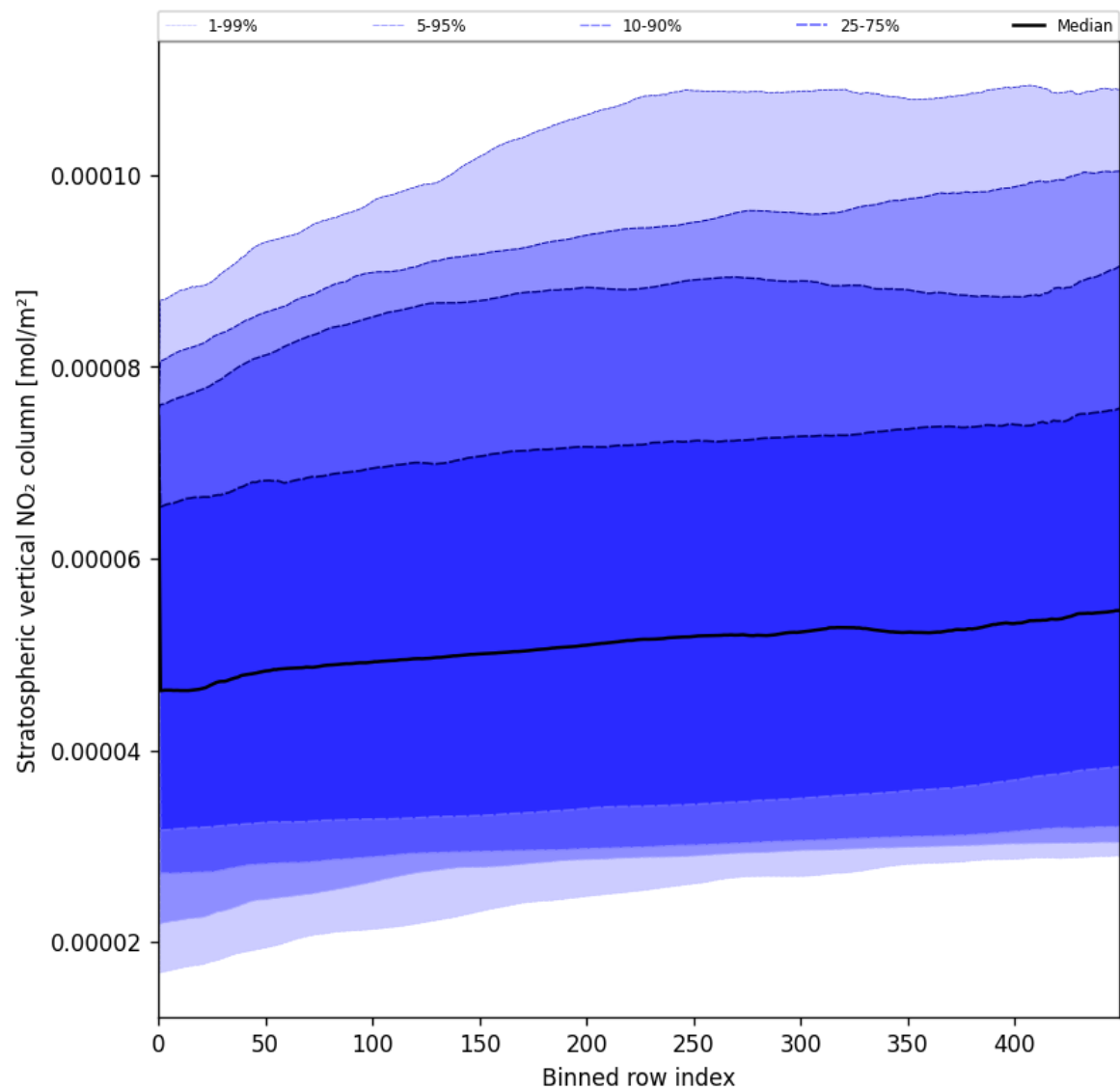
Figure 53: Along track statistics of “Stratospheric vertical NO 2 column” for 2025-05-26 to 2025-05-28
