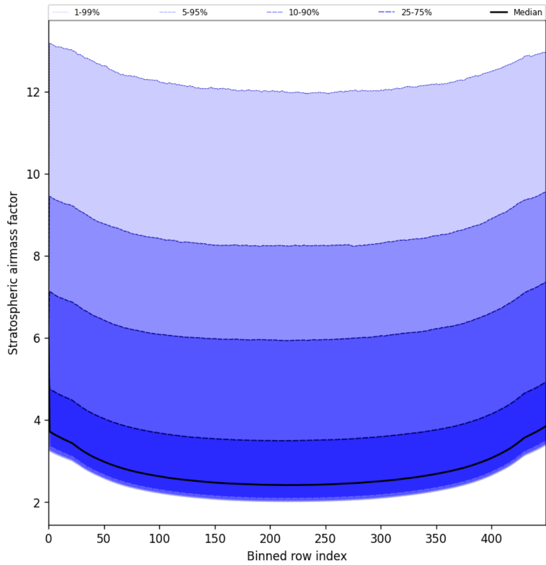
Figure 61: Along track statistics of “Stratospheric airmass factor” for 2025-05-26 to 2025-05-28
