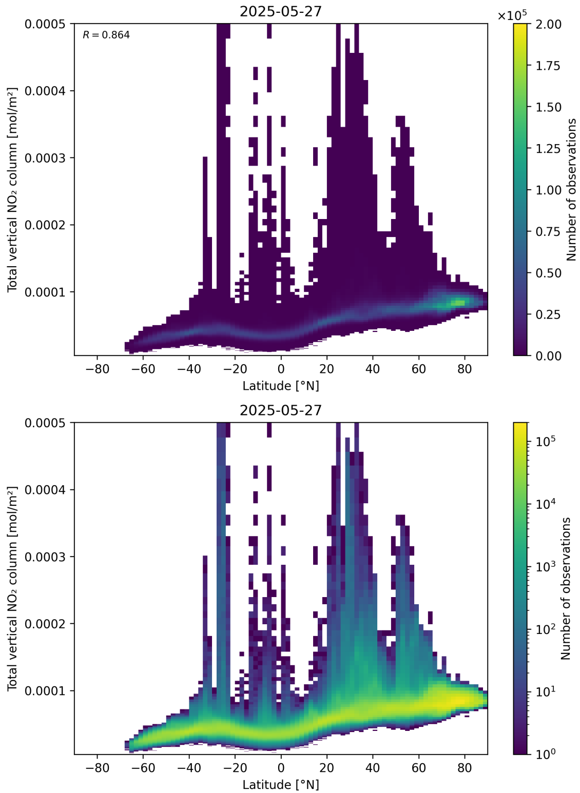
Figure 90: Scatter density plot of “Latitude” against “Total vertical NO 2 column” for 2025-05-26 to 2025-05-28.
