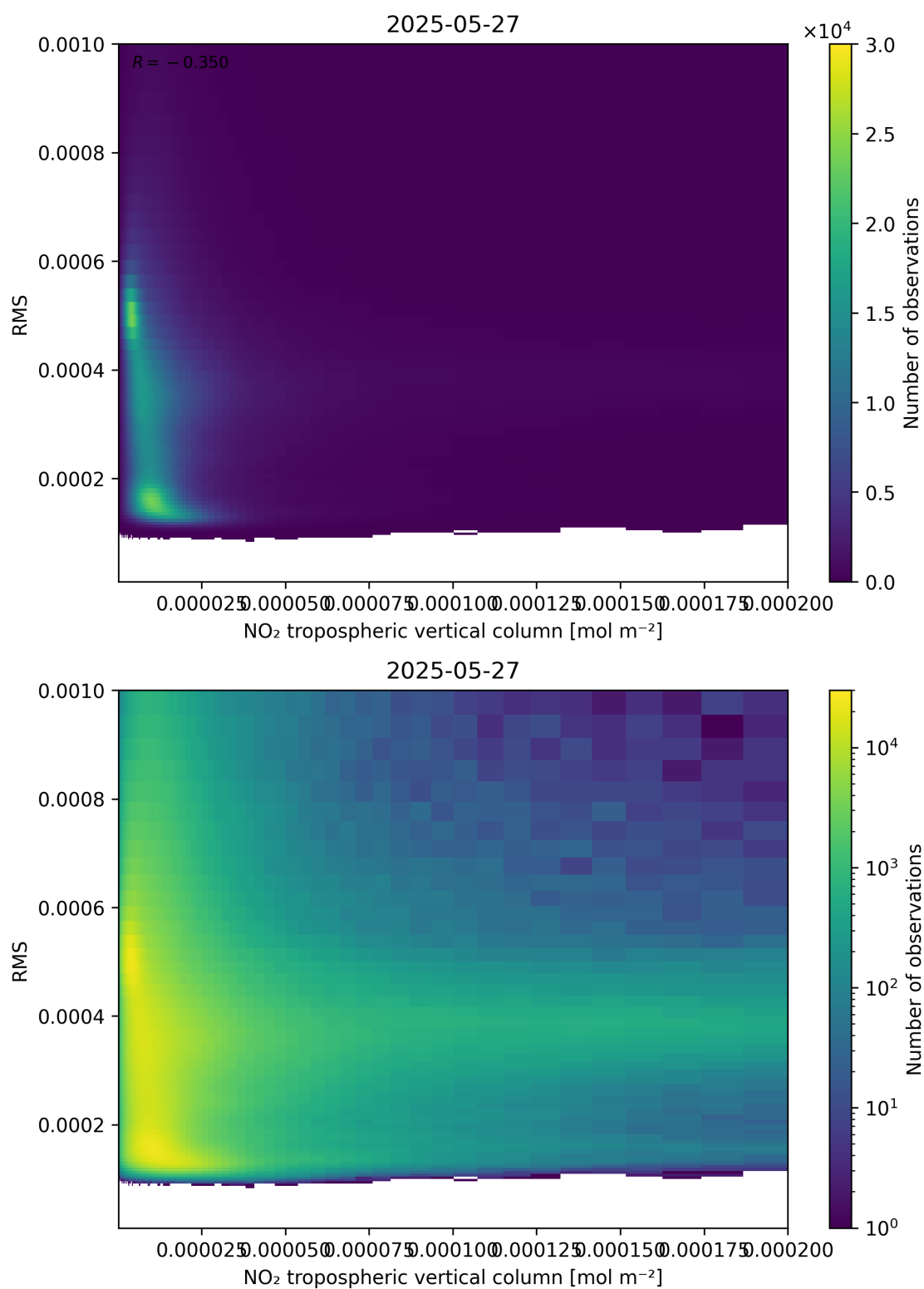
Figure 142: Scatter density plot of “NO 2 tropospheric vertical column” against “RMS” for 2025-05-26 to 2025-05-28.
