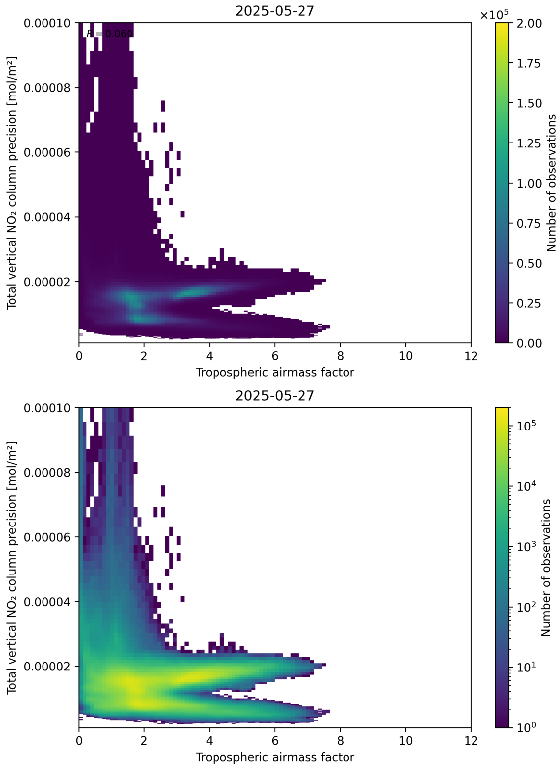
Figure 78: Scatter density plot of “Tropospheric air mass factor” against “Total vertical NO 2 column precision” for 2025-05-26 to 2025-05-28.
