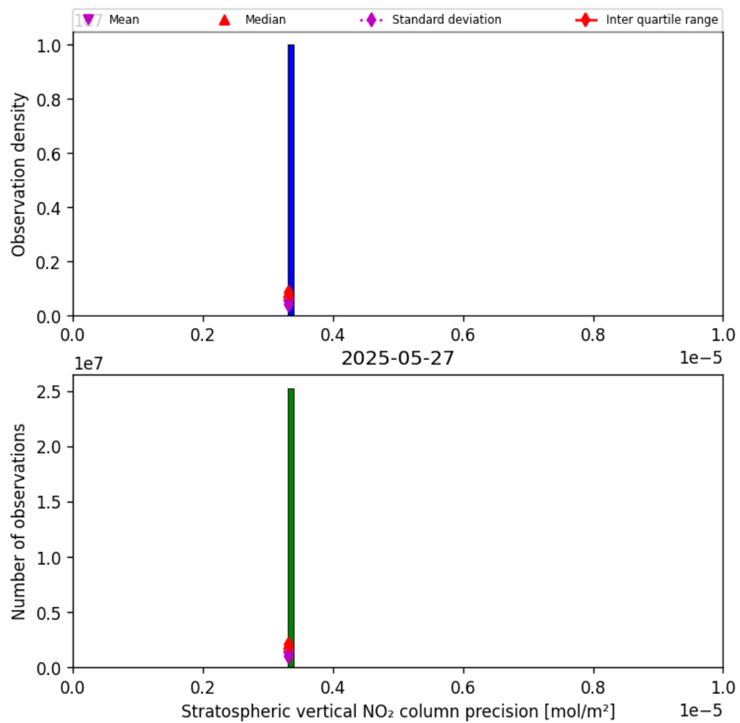
Figure 37: Histogram of “Stratospheric vertical NO 2 column precision” for 2025-05-26 to 2025-05-28
