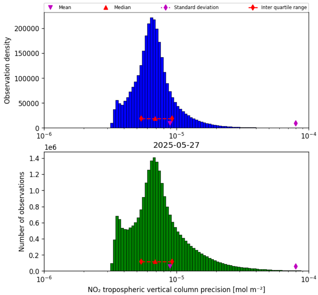
Figure 30: Histogram of “NO 2 tropospheric vertical column precision” for 2025-05-26 to 2025-05-28
