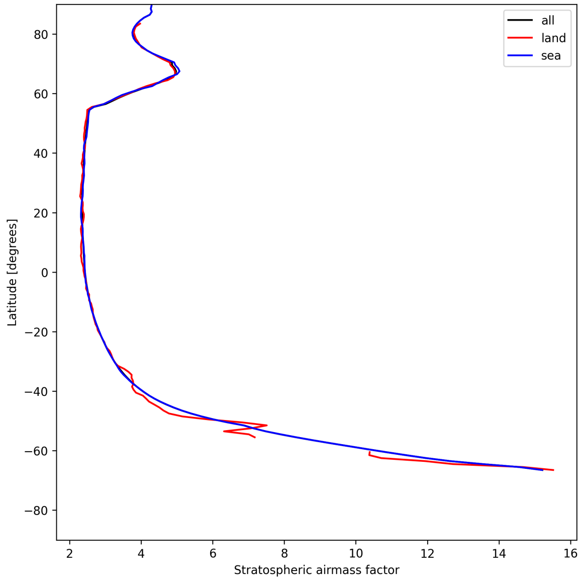
Figure 27: Zonal average of “Stratospheric airmass factor” for 2025-05-26 to 2025-05-28.
