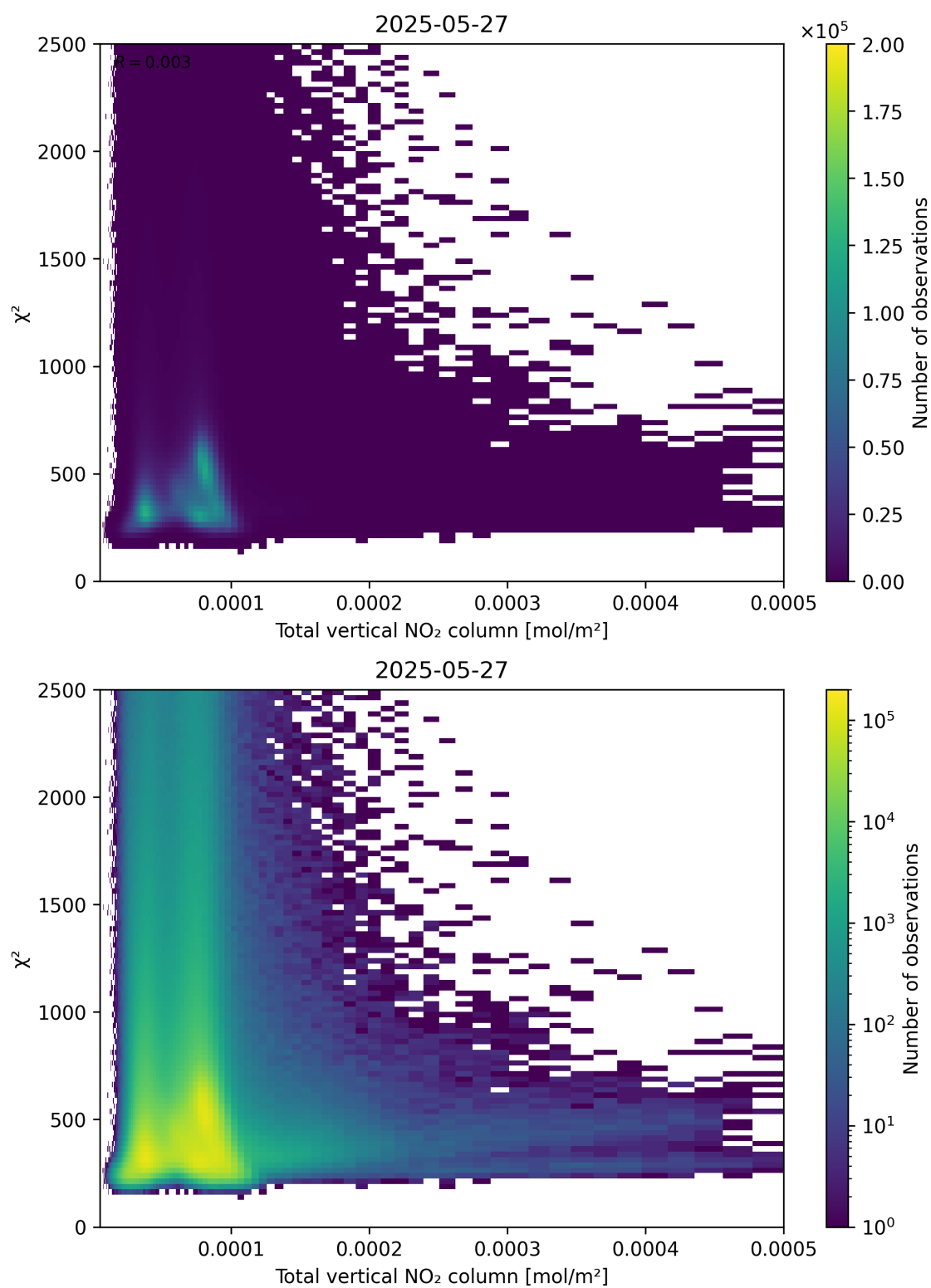
Figure 111: Scatter density plot of “Total vertical NO 2 column” against “ \chi^2 ” for 2025-05-26 to 2025-05-28.
