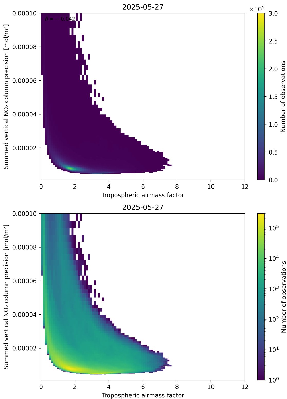
Figure 76: Scatter density plot of “Tropospheric air mass factor” against “Summed vertical NO 2 column precision” for 2025-05-26 to 2025-05-28.
