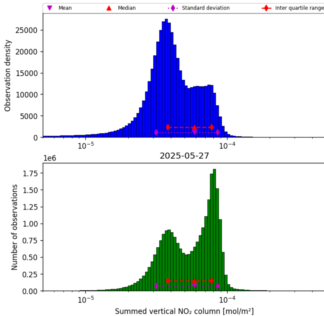
Figure 40: Histogram of “Summed vertical NO 2 column” for 2025-05-26 to 2025-05-28
