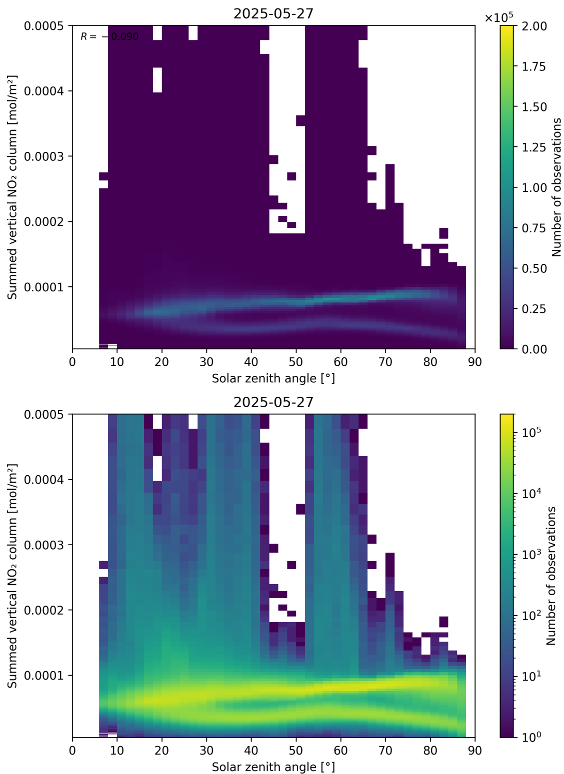
Figure 151: Scatter density plot of “Solar zenith angle” against “Summed vertical NO 2 column” for 2025-05-26 to 2025-05-28.
