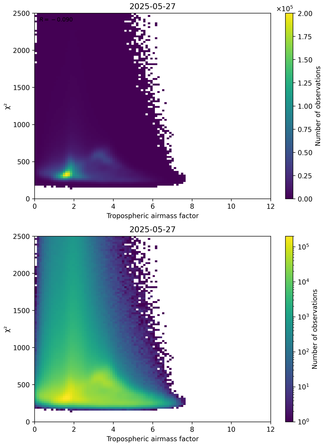
Figure 73: Scatter density plot of “Tropospheric airmass factor” against “ \chi^2 ” for 2025-05-26 to 2025-05-28.
