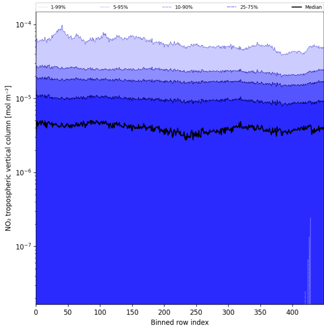
Figure 46: Along track statistics of “NO 2 tropospheric vertical column” for 2025-05-26 to 2025-05-28
