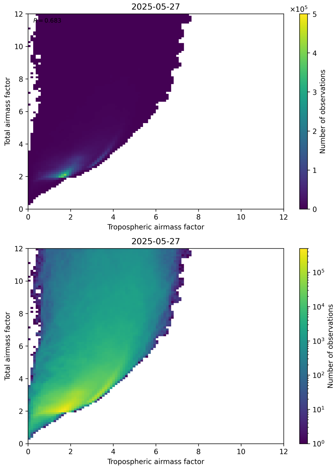
Figure 72: Scatter density plot of “Tropospheric airmass factor” against “Total airmass factor” for 2025-05-26 to 2025-05-28.
