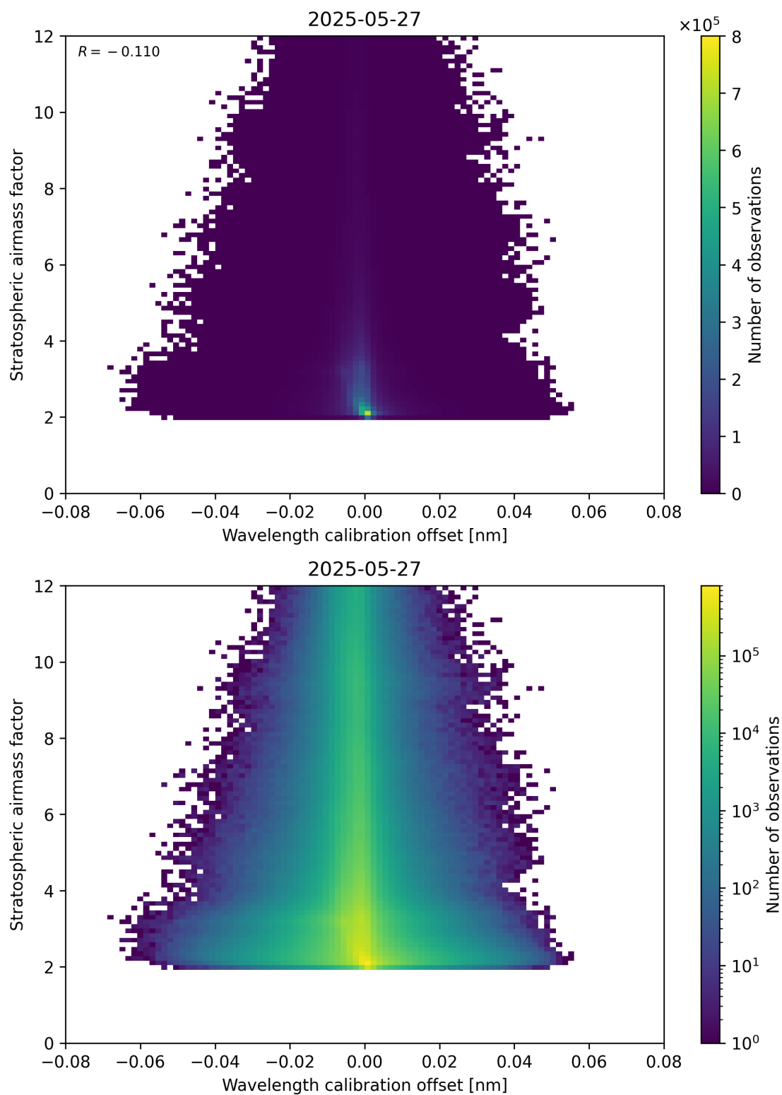
Figure 174: Scatter density plot of “Wavelength calibration offset” against “Stratospheric airmass factor” for 2025-05-26 to 2025-05-28.
