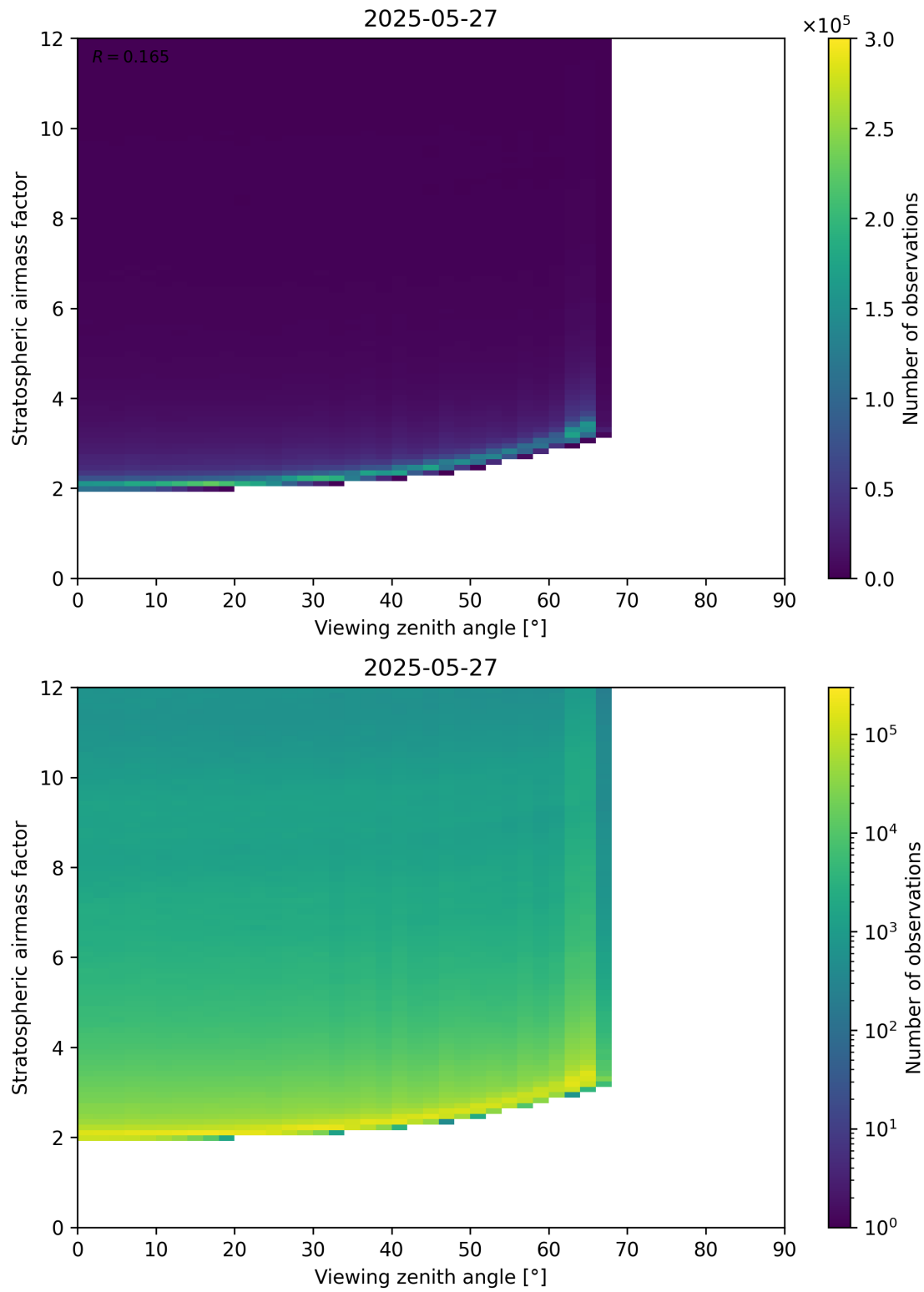
Figure 159: Scatter density plot of “Viewing zenith angle” against “Stratospheric airmass factor” for 2025-05-26 to 2025-05-28.
