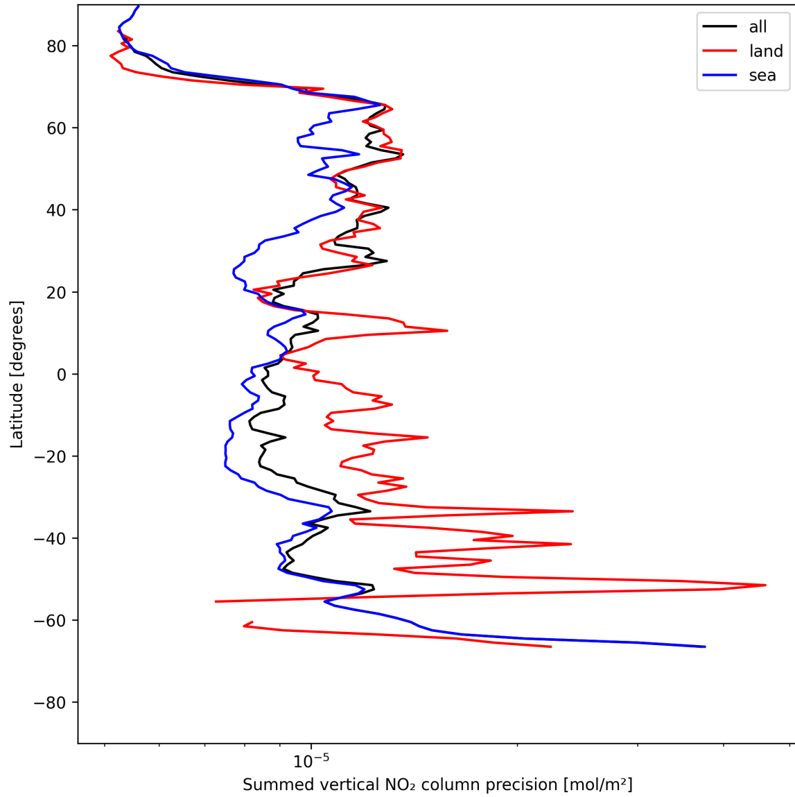
Figure 24: Zonal average of “Summed vertical NO 2 column precision” for 2025-05-26 to 2025-05-28.
