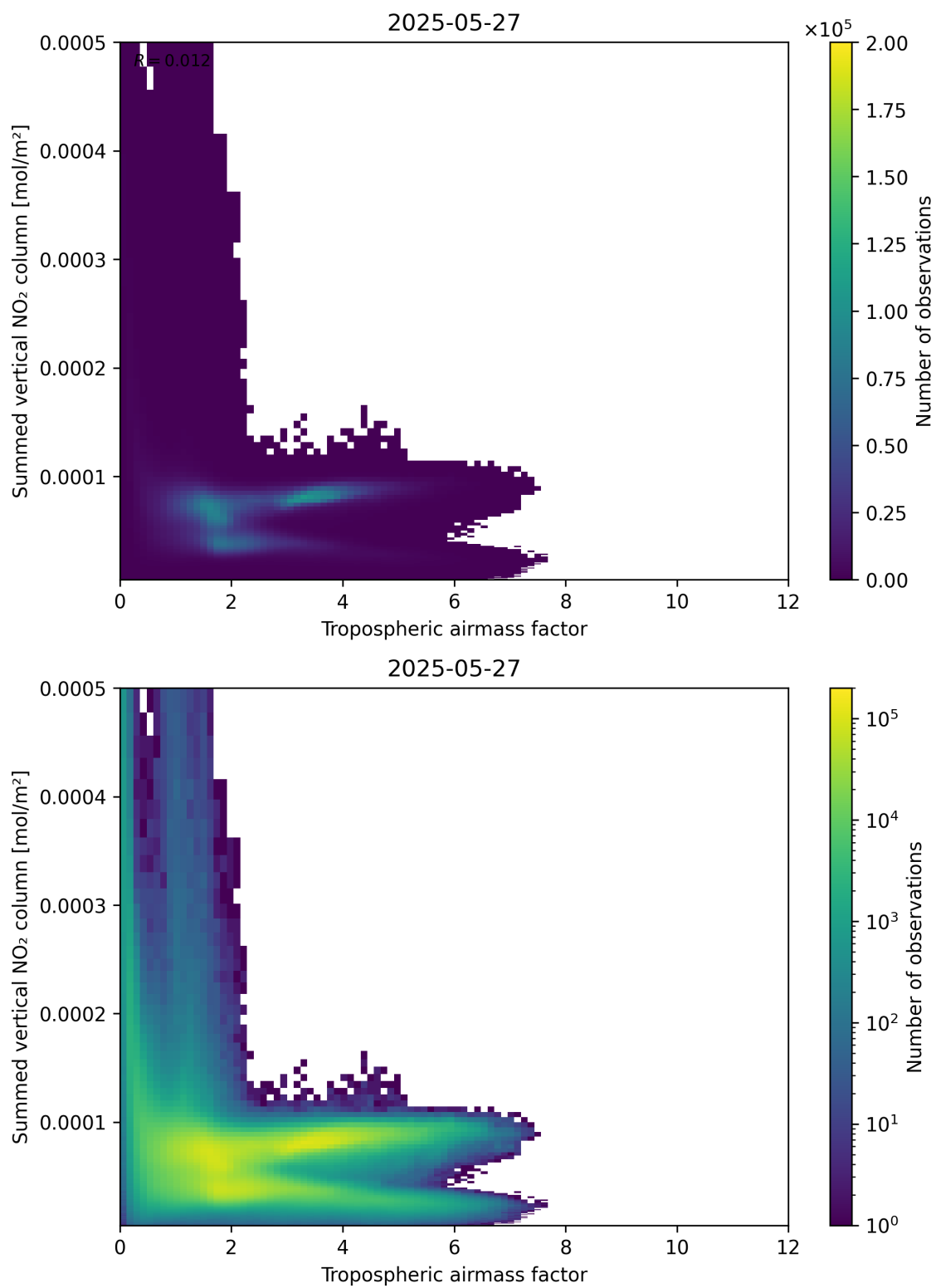
Figure 75: Scatter density plot of “Tropospheric air mass factor” against “Summed vertical NO 2 column” for 2025-05-26 to 2025-05-28.
