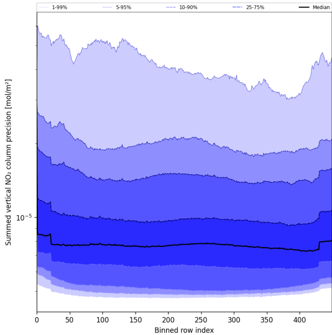
Figure 58: Along track statistics of “Summed vertical NO 2 column precision” for 2025-05-26 to 2025-05-28
