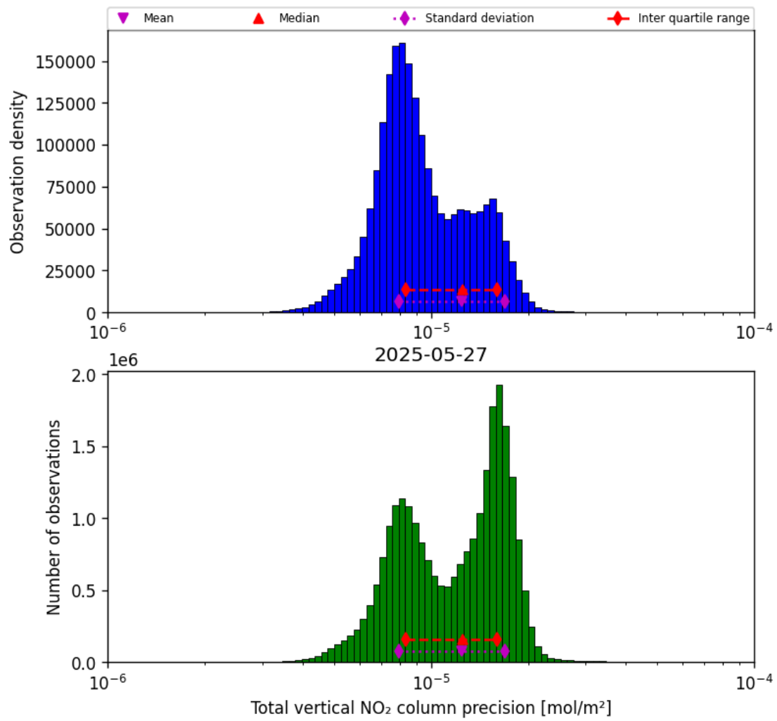
Figure 39: Histogram of “Total vertical NO 2 column precision” for 2025-05-26 to 2025-05-28
