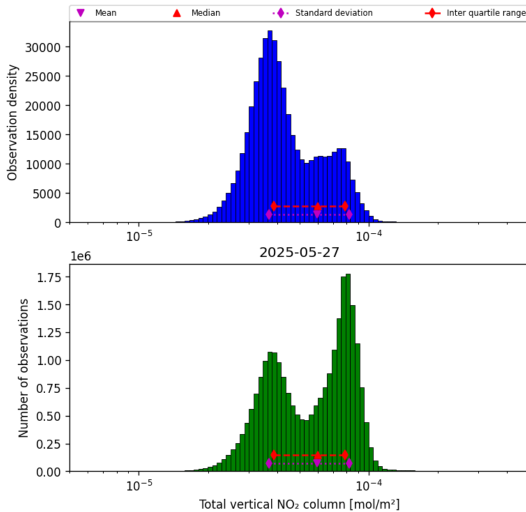
Figure 38: Histogram of “Total vertical NO 2 column” for 2025-05-26 to 2025-05-28
