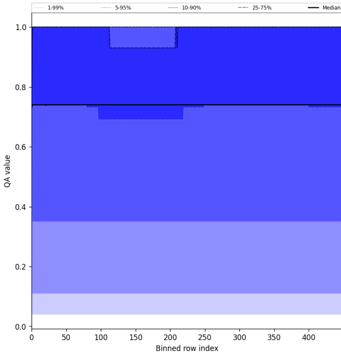
Figure 45: Along track statistics of “QA value” for 2025-05-26 to 2025-05-28
