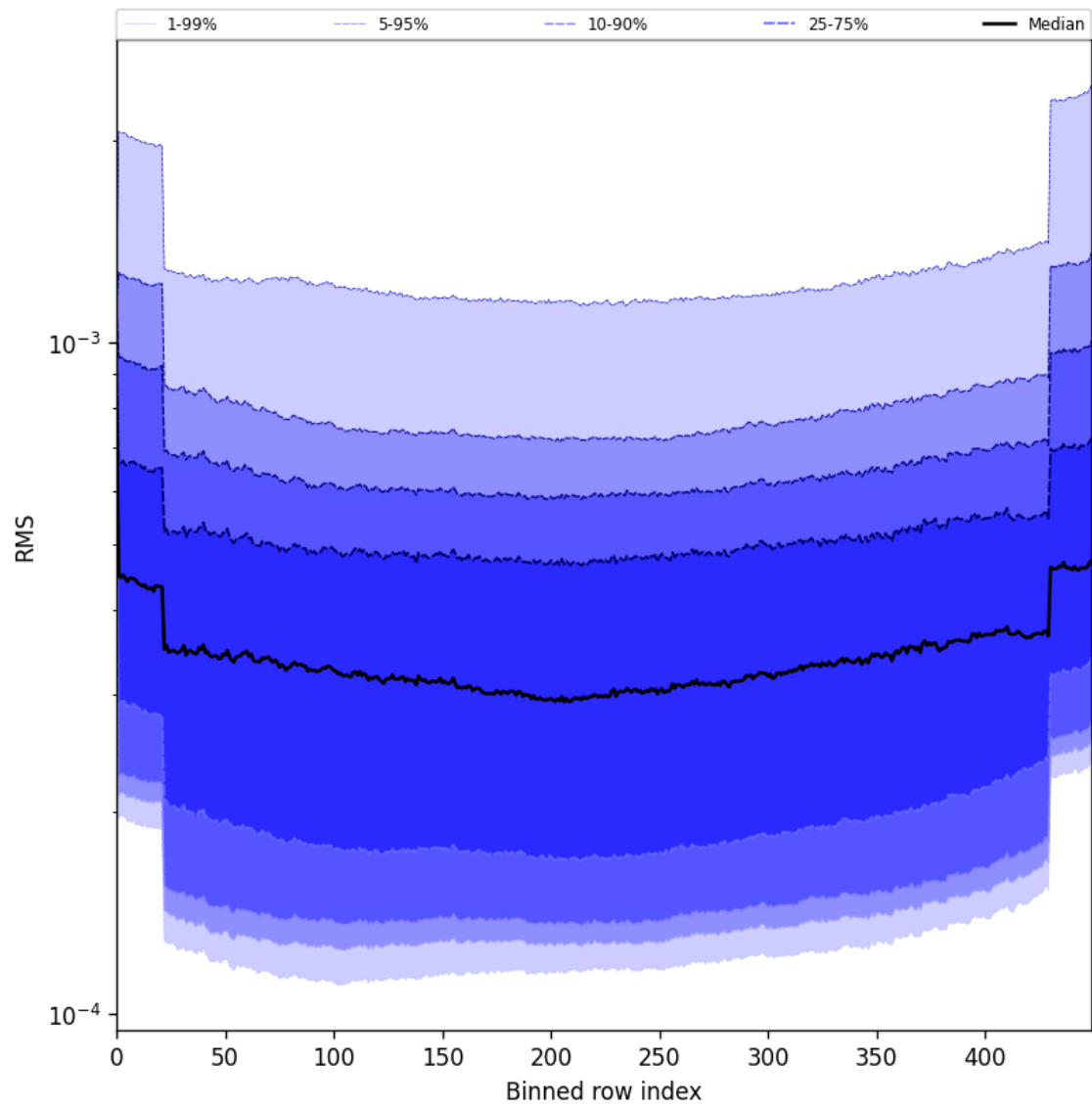
Figure 60: Along track statistics of “RMS” for 2025-05-26 to 2025-05-28
