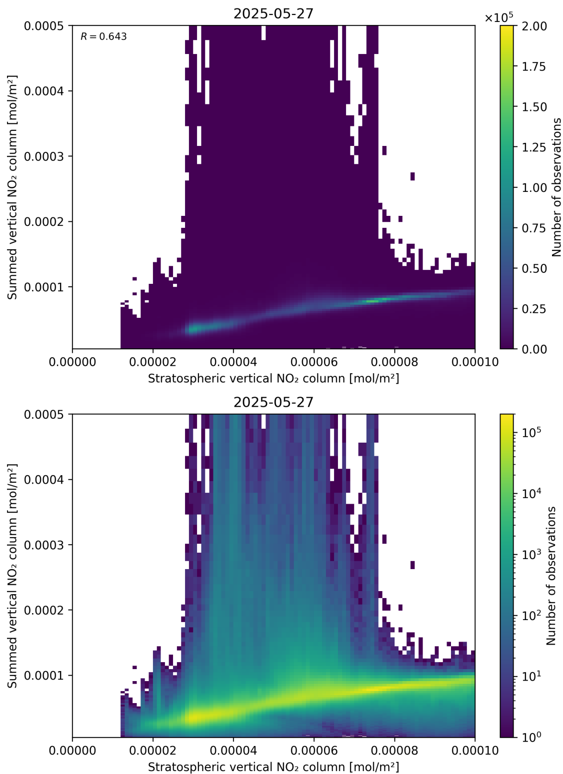
Figure 98: Scatter density plot of “Stratospheric vertical NO 2 column” against “Summed vertical NO 2 column” for 2025-05-26 to 2025-05-28.
