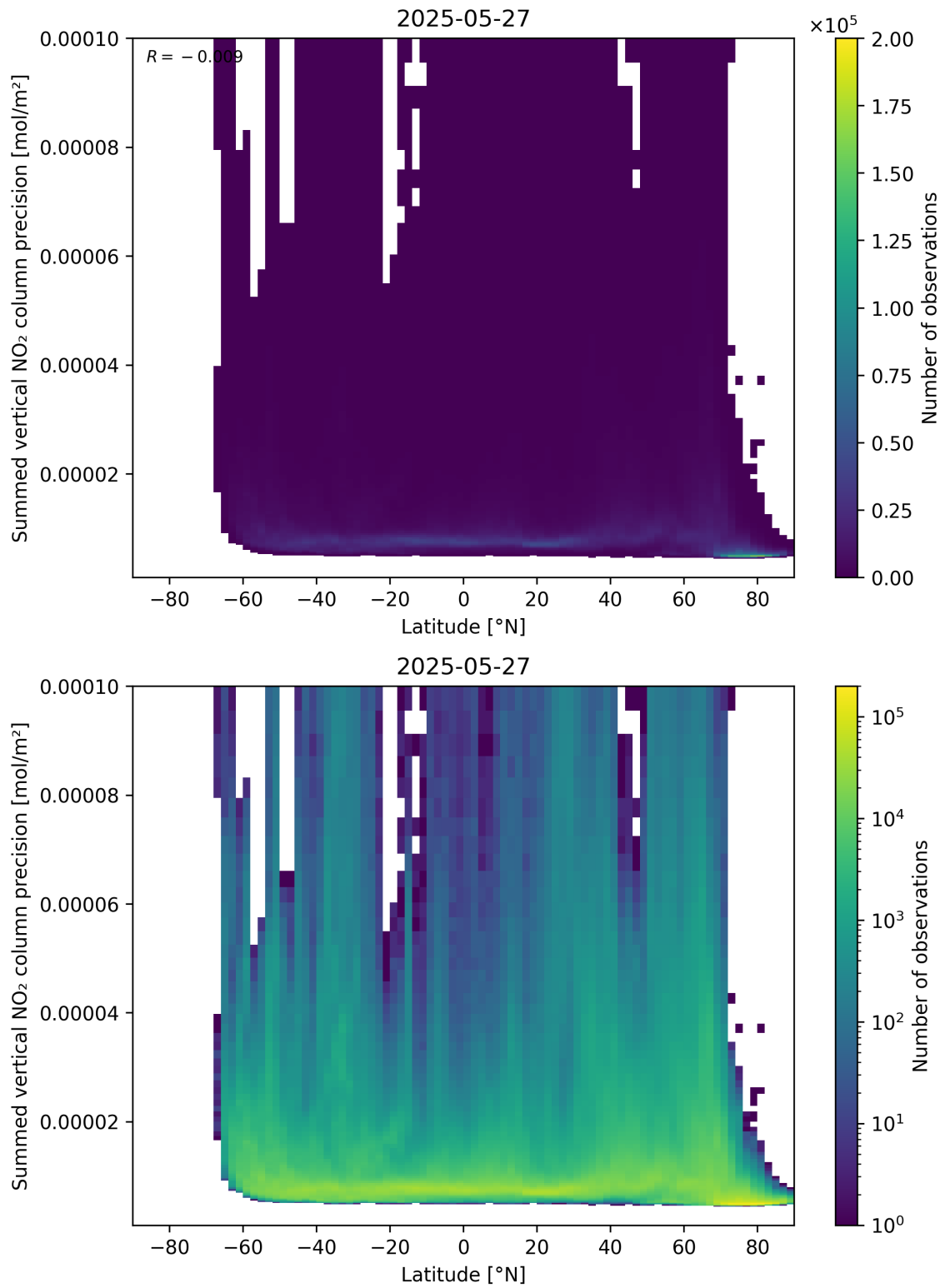
Figure 89: Scatter density plot of “Latitude” against “Summed vertical NO 2 column precision” for 2025-05-26 to 2025-05-28.
