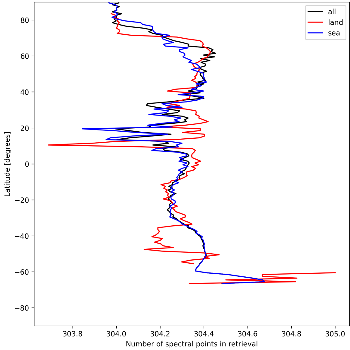
Figure 16: Zonal average of “Number of spectral points in retrieval” for 2025-05-26 to 2025-05-28.
