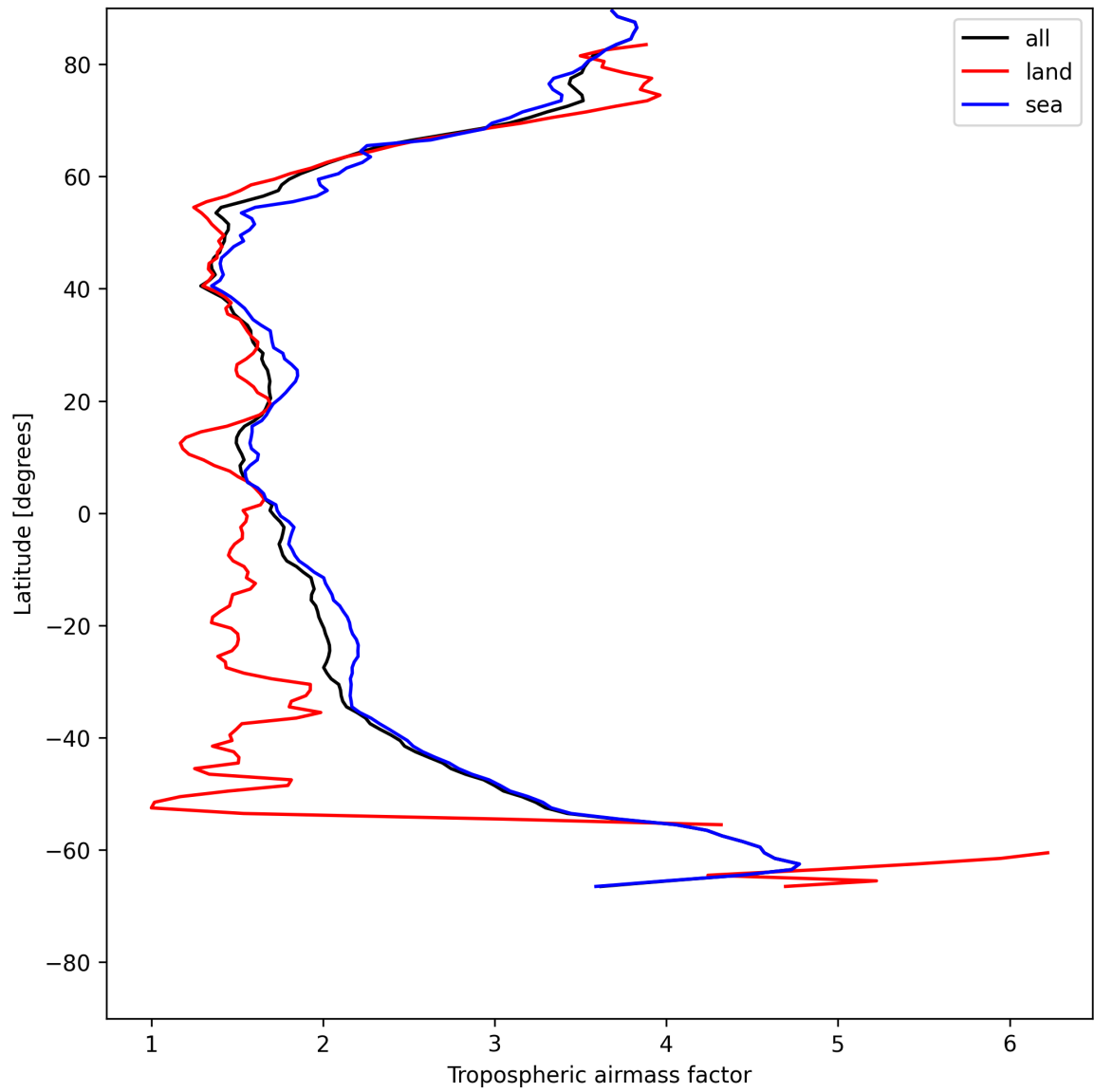
Figure 14: Zonal average of “Tropospheric airmass factor” for 2025-05-26 to 2025-05-28.
