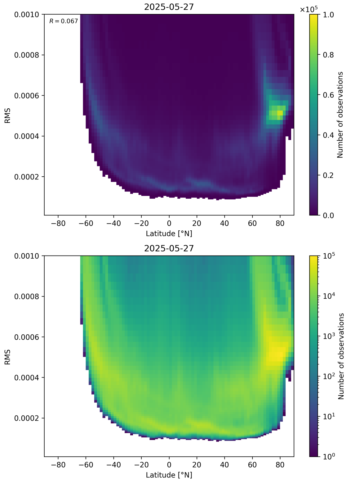
Figure 94: Scatter density plot of “Latitude” against “RMS” for 2025-05-26 to 2025-05-28.
