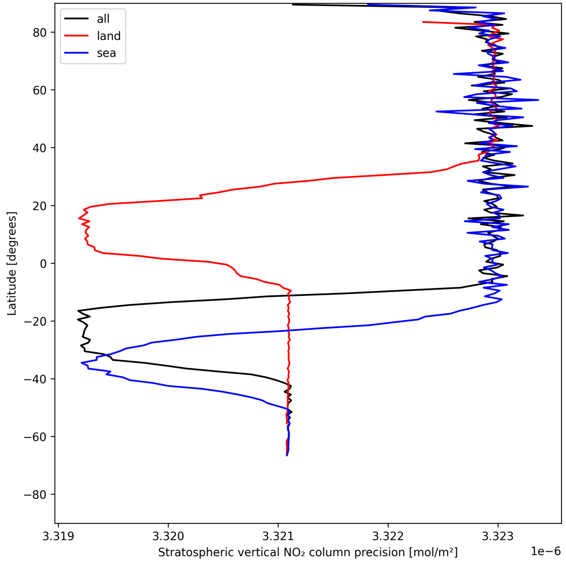
Figure 20: Zonal average of “Stratospheric vertical NO 2 column precision” for 2025-05-26 to 2025-05-28.
