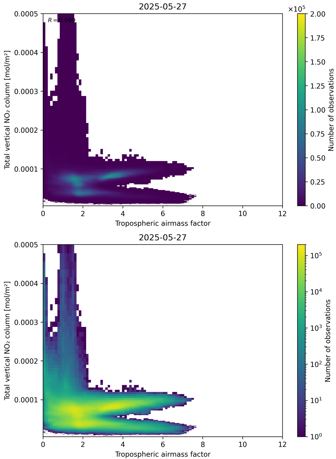
Figure 77: Scatter density plot of “Tropospheric airmass factor” against “Total vertical NO 2 column” for 2025-05-26 to 2025-05-28.
