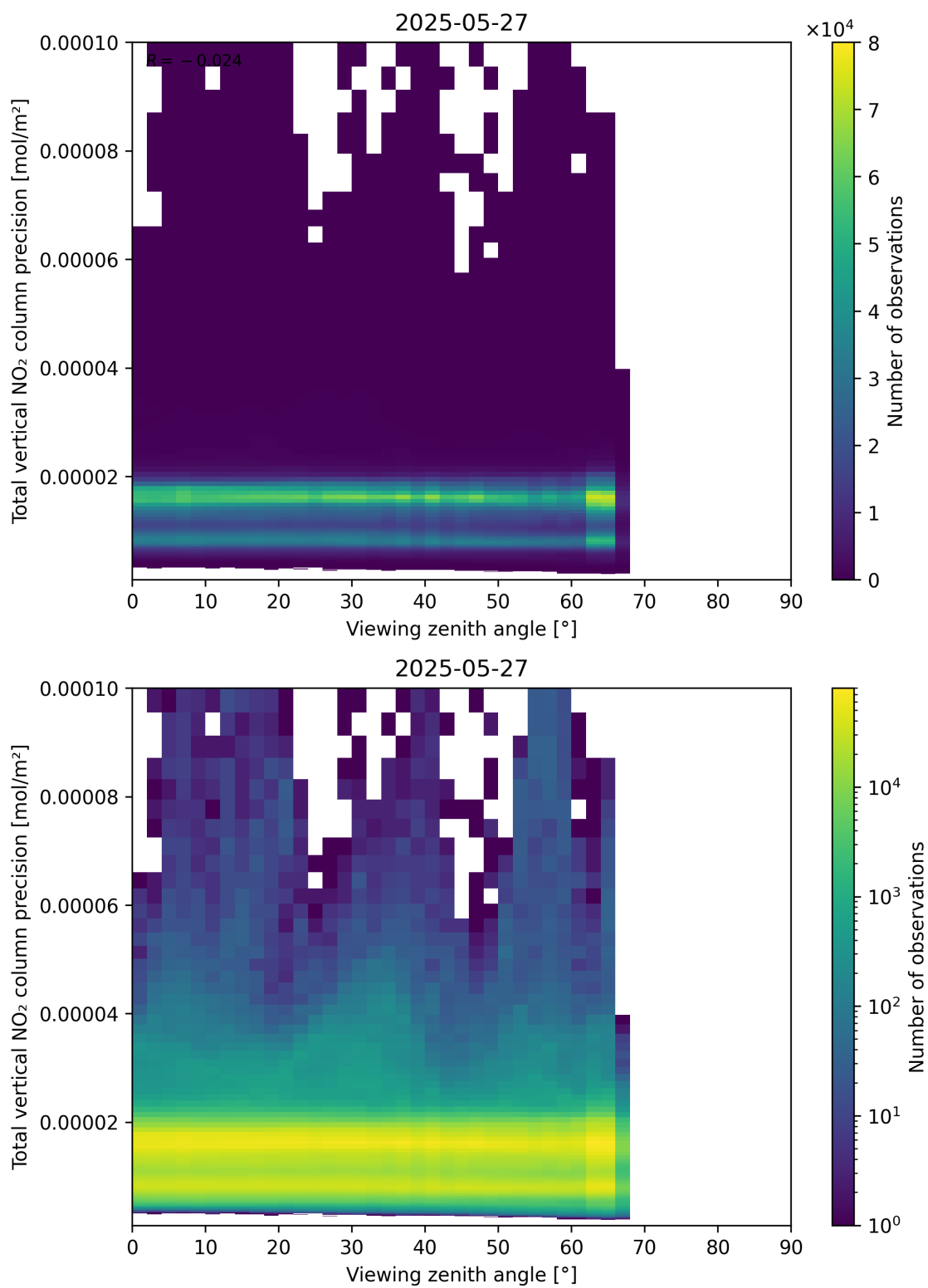
Figure 168: Scatter density plot of “Viewing zenith angle” against “Total vertical NO 2 column precision” for 2025-05-26 to 2025-05-28.
