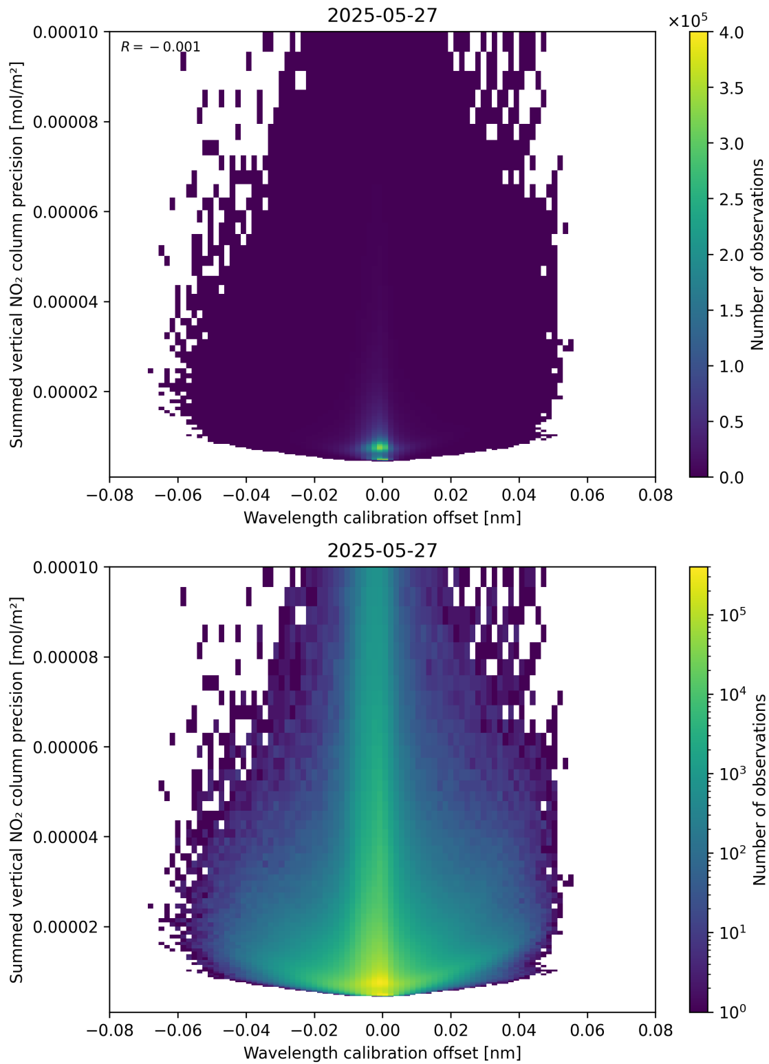
Figure 178: Scatter density plot of “Wavelength calibration offset” against “Summed vertical NO 2 column precision” for 2025-05-26 to 2025-05-28.
