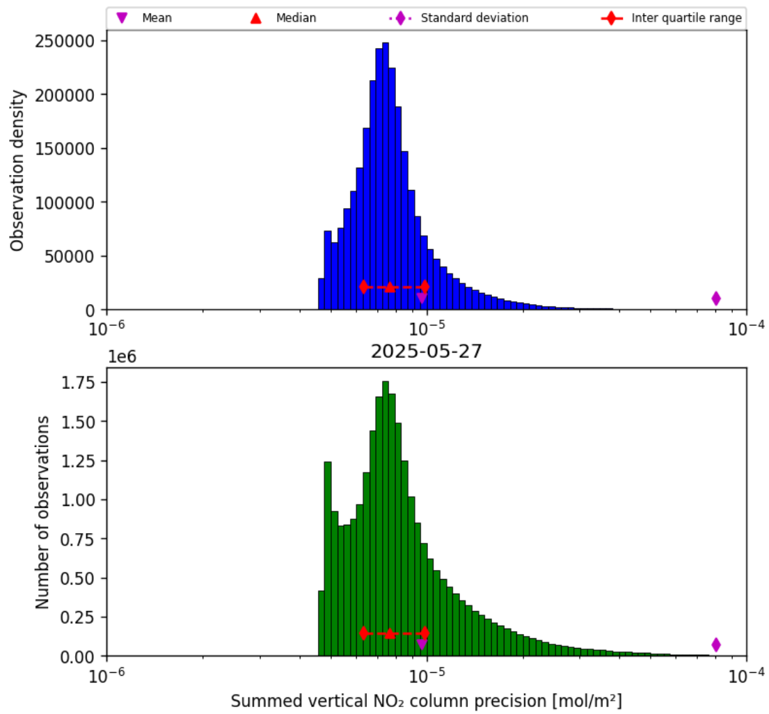
Figure 41: Histogram of “Summed vertical NO 2 column precision” for 2025-05-26 to 2025-05-28
