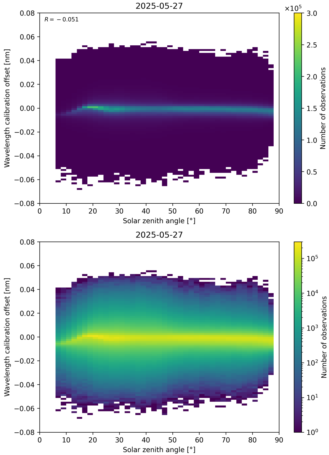
Figure 158: Scatter density plot of “Solar zenith angle” against “Wavelength calibration offset” for 2025-05-26 to 2025-05-28.
