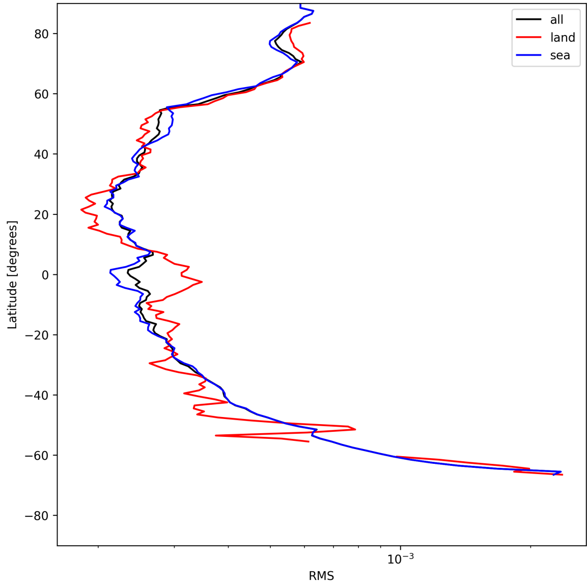
Figure 26: Zonal average of “RMS” for 2025-05-26 to 2025-05-28.
