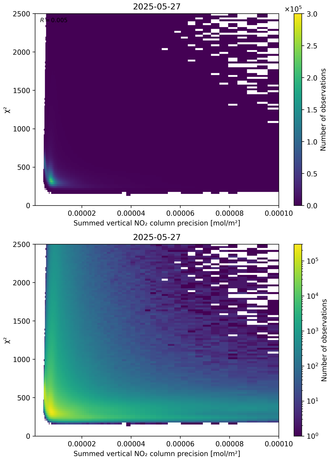
Figure 107: Scatter density plot of “Summed vertical NO 2 column precision” against “ \chi^2 ” for 2025-05-26 to 2025-05-28.
