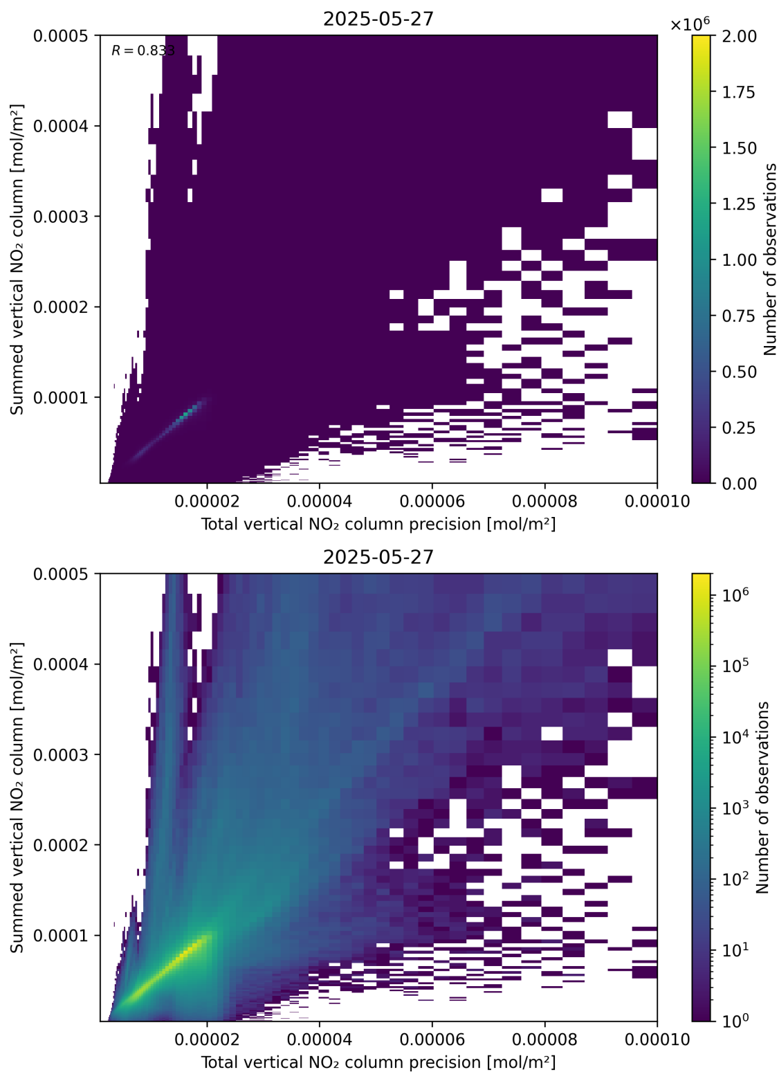
Figure 117: Scatter density plot of “Total vertical NO 2 column precision” against “Summed vertical NO 2 column” for 2025-05-26 to 2025-05-28.
