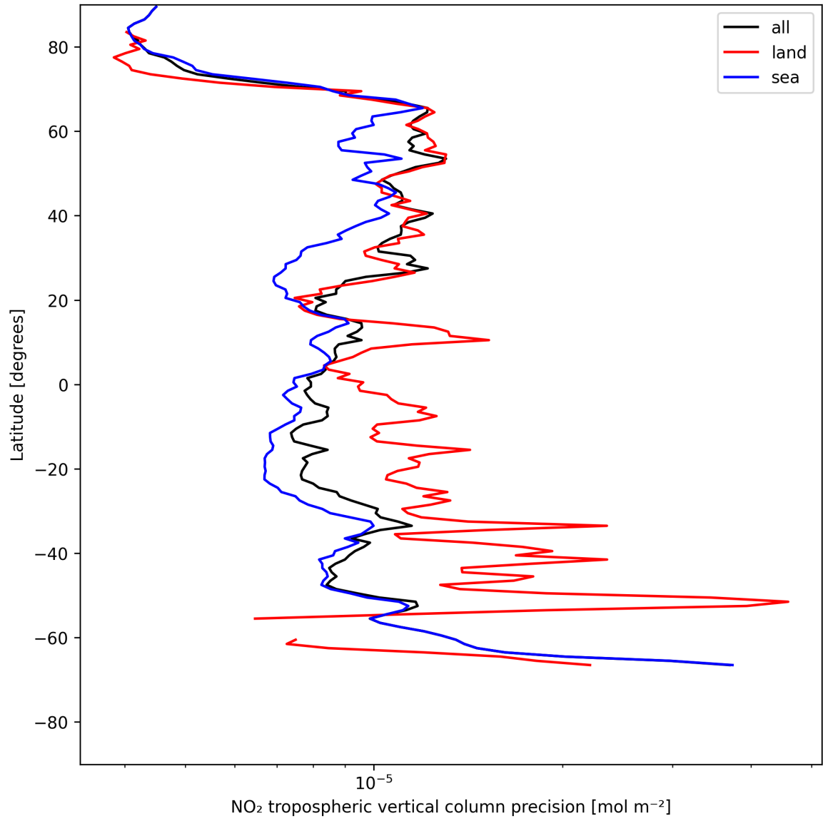
Figure 13: Zonal average of “NO 2 tropospheric vertical column precision” for 2025-05-26 to 2025-05-28.
