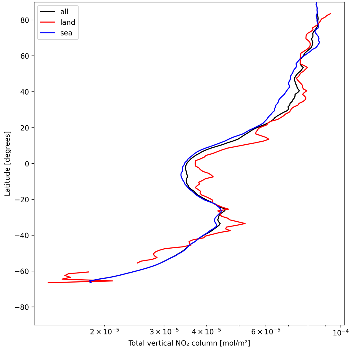
Figure 21: Zonal average of “Total vertical NO 2 column” for 2025-05-26 to 2025-05-28.
