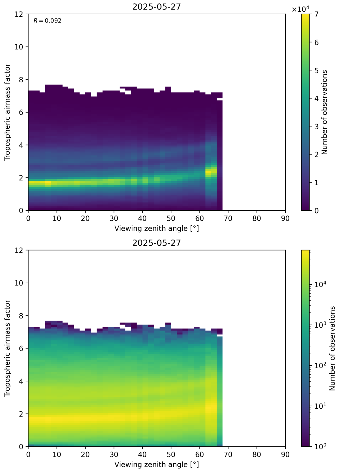
Figure 161: Scatter density plot of “Viewing zenith angle” against “Tropospheric airmass factor” for 2025-05-26 to 2025-05-28.
