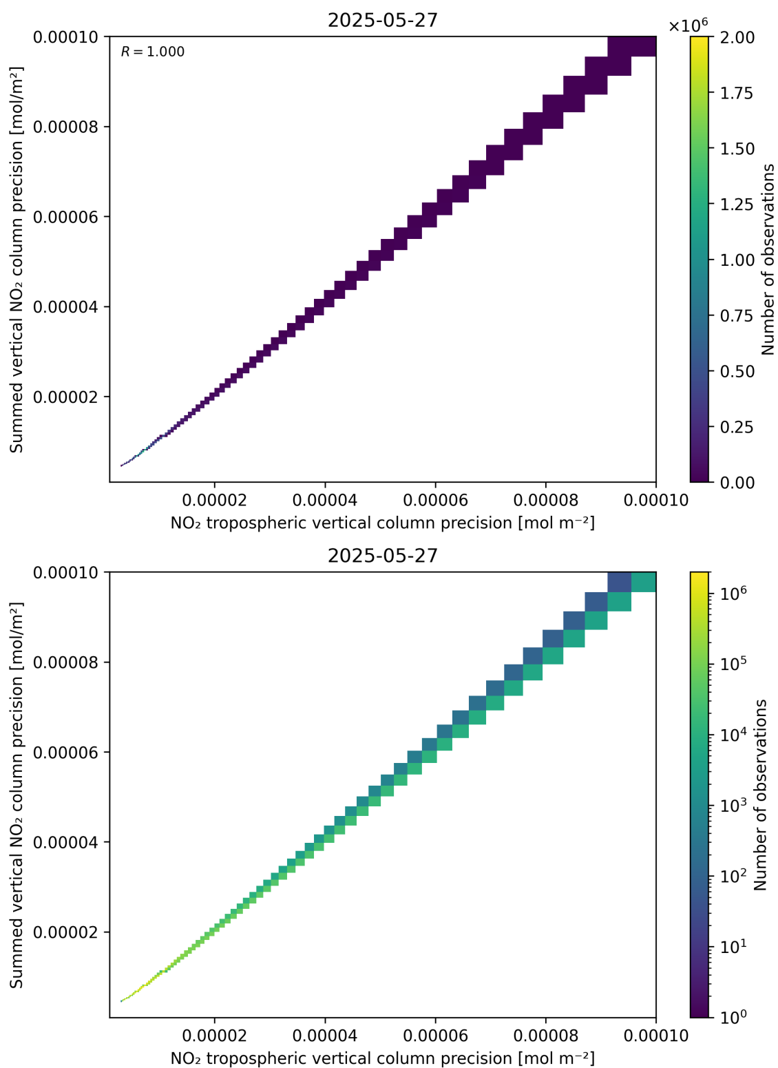
Figure 137: Scatter density plot of “NO 2 tropospheric vertical column precision” against “Summed vertical NO 2 column precision” for 2025-05-26 to 2025-05-28.
