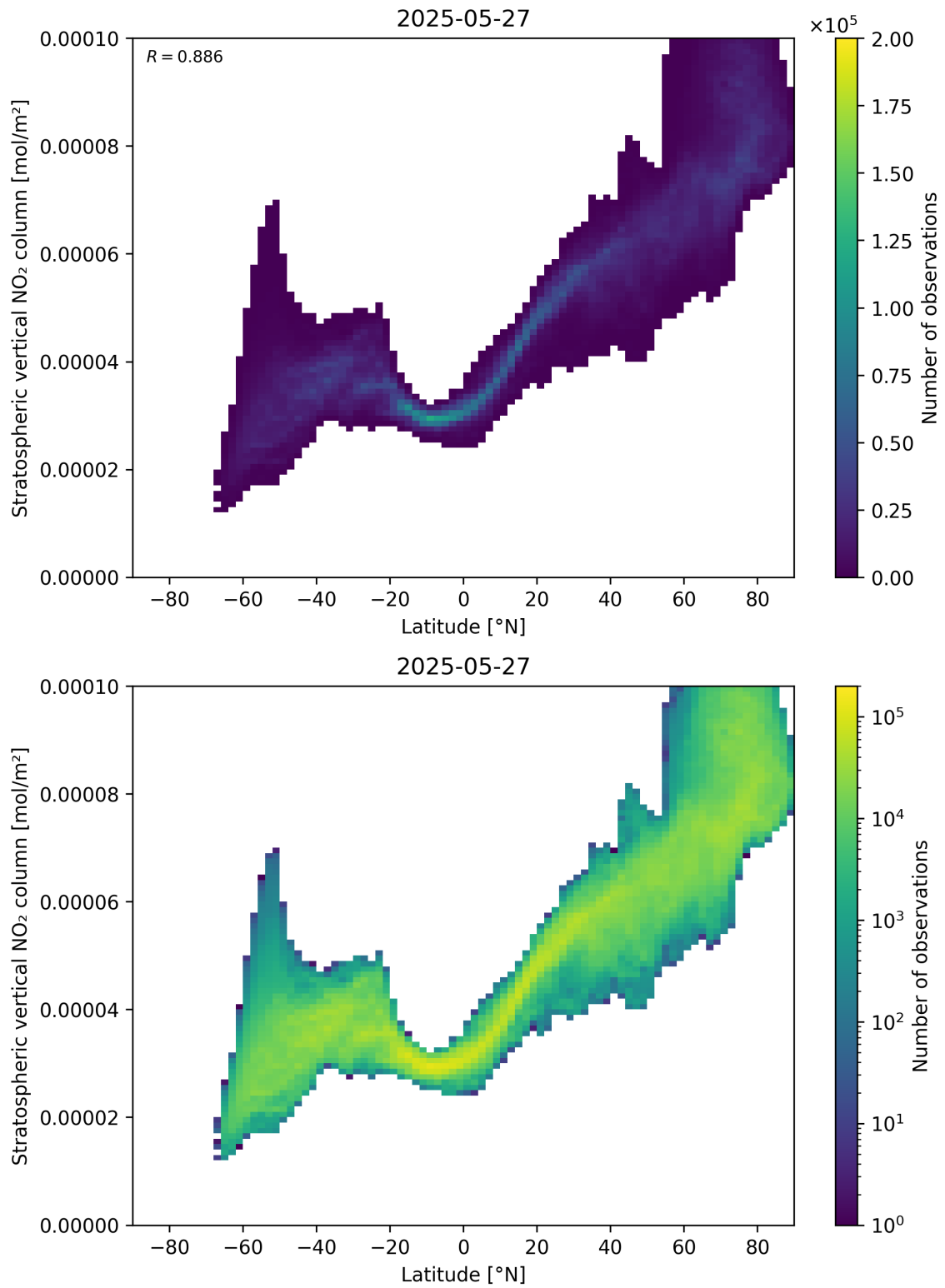
Figure 87: Scatter density plot of “Latitude” against “Stratospheric vertical \text{NO}_2 column” for 2025-05-26 to 2025-05-28.
