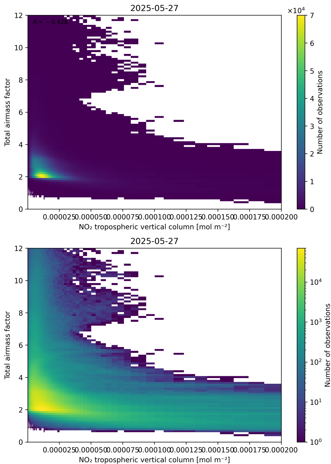
Figure 122: Scatter density plot of “NO 2 tropospheric vertical column” against “Total air mass factor” for 2025-05-26 to 2025-05-28.
