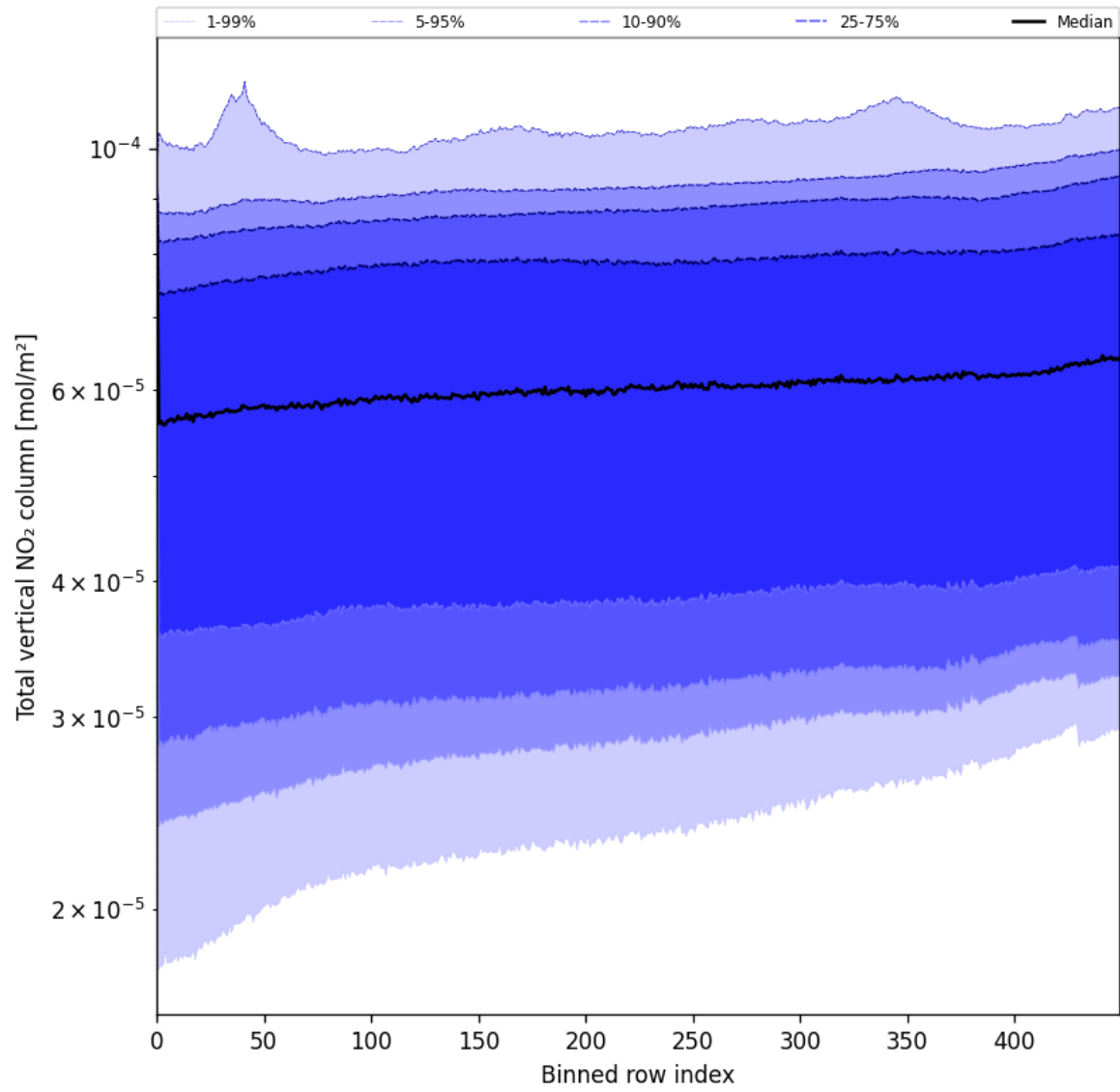
Figure 55: Along track statistics of “Total vertical NO 2 column” for 2025-05-26 to 2025-05-28
