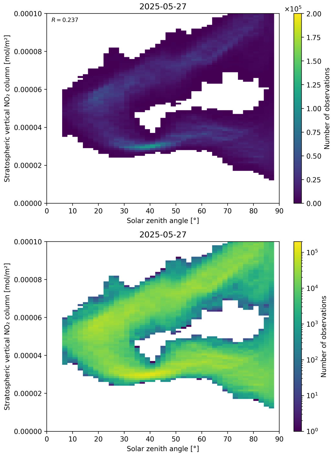
Figure 150: Scatter density plot of “Solar zenith angle” against “Stratospheric vertical NO 2 column” for 2025-05-26 to 2025-05-28.
