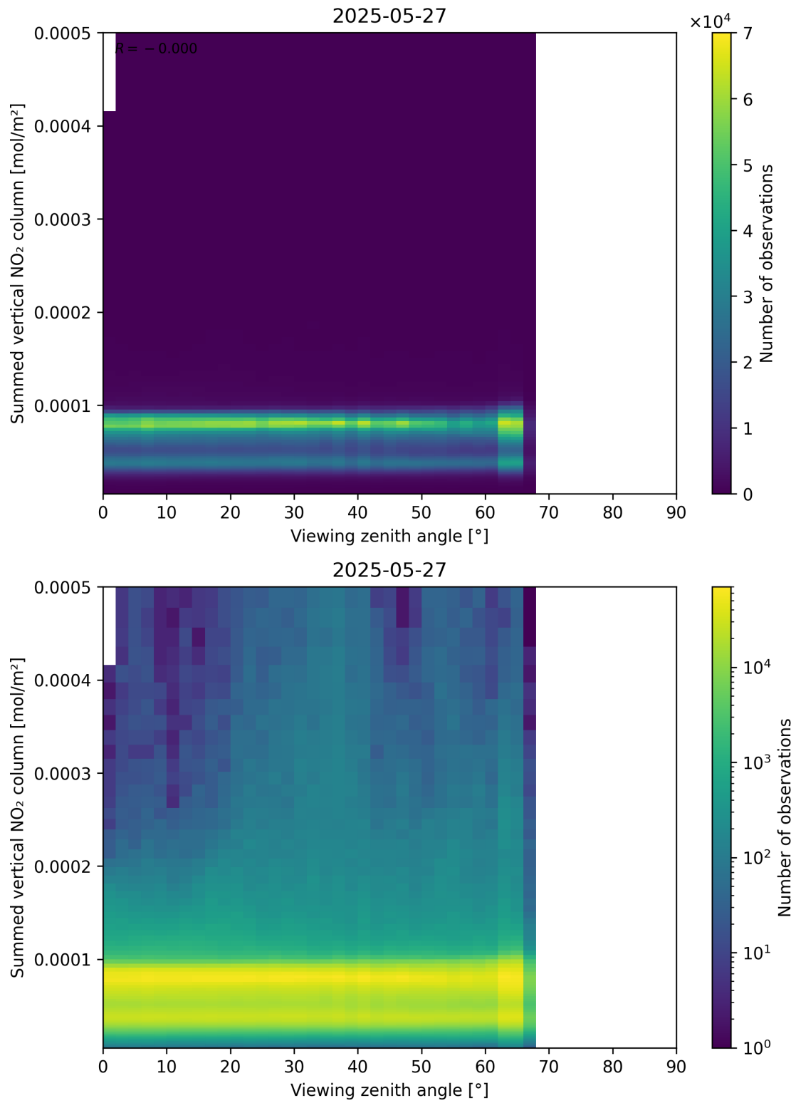
Figure 165: Scatter density plot of “Viewing zenith angle” against “Summed vertical NO 2 column” for 2025-05-26 to 2025-05-28.
