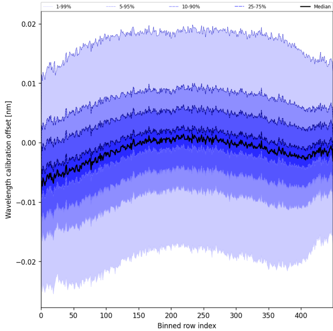
Figure 52: Along track statistics of “Wavelength calibration offset” for 2025-05-26 to 2025-05-28
