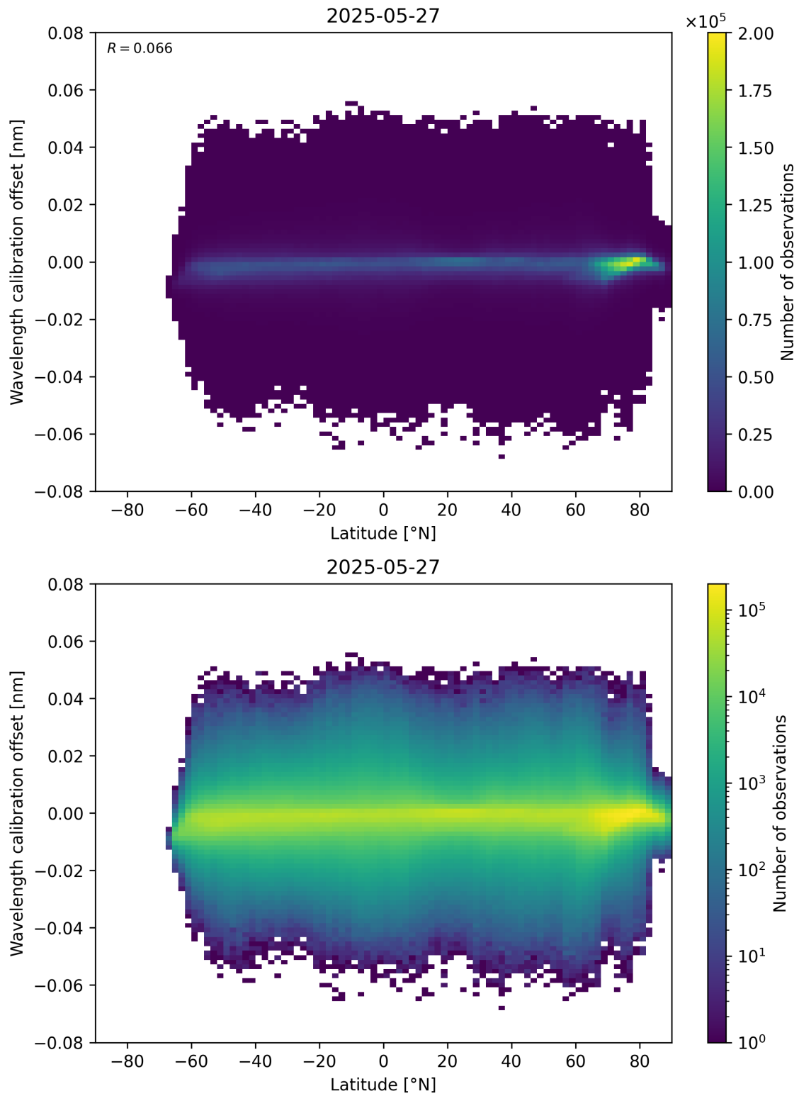
Figure 95: Scatter density plot of “Latitude” against “Wavelength calibration offset” for 2025-05-26 to 2025-05-28.
