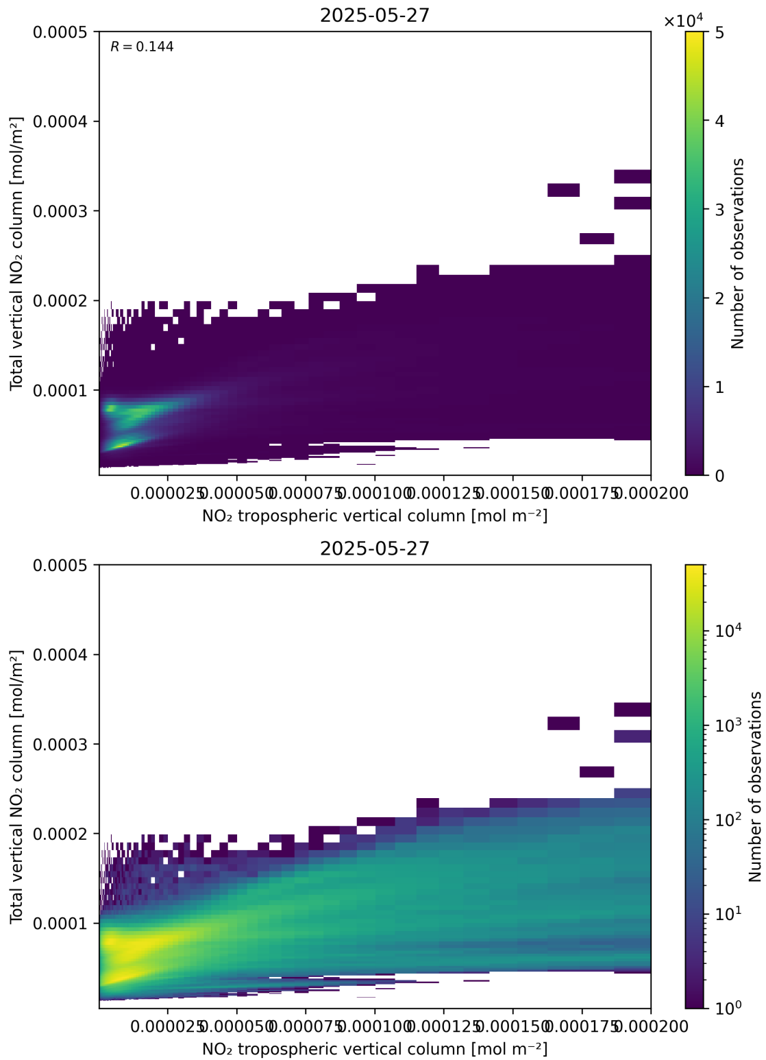
Figure 128: Scatter density plot of “NO 2 tropospheric vertical column” against “Total vertical NO 2 column” for 2025-05-26 to 2025-05-28.
