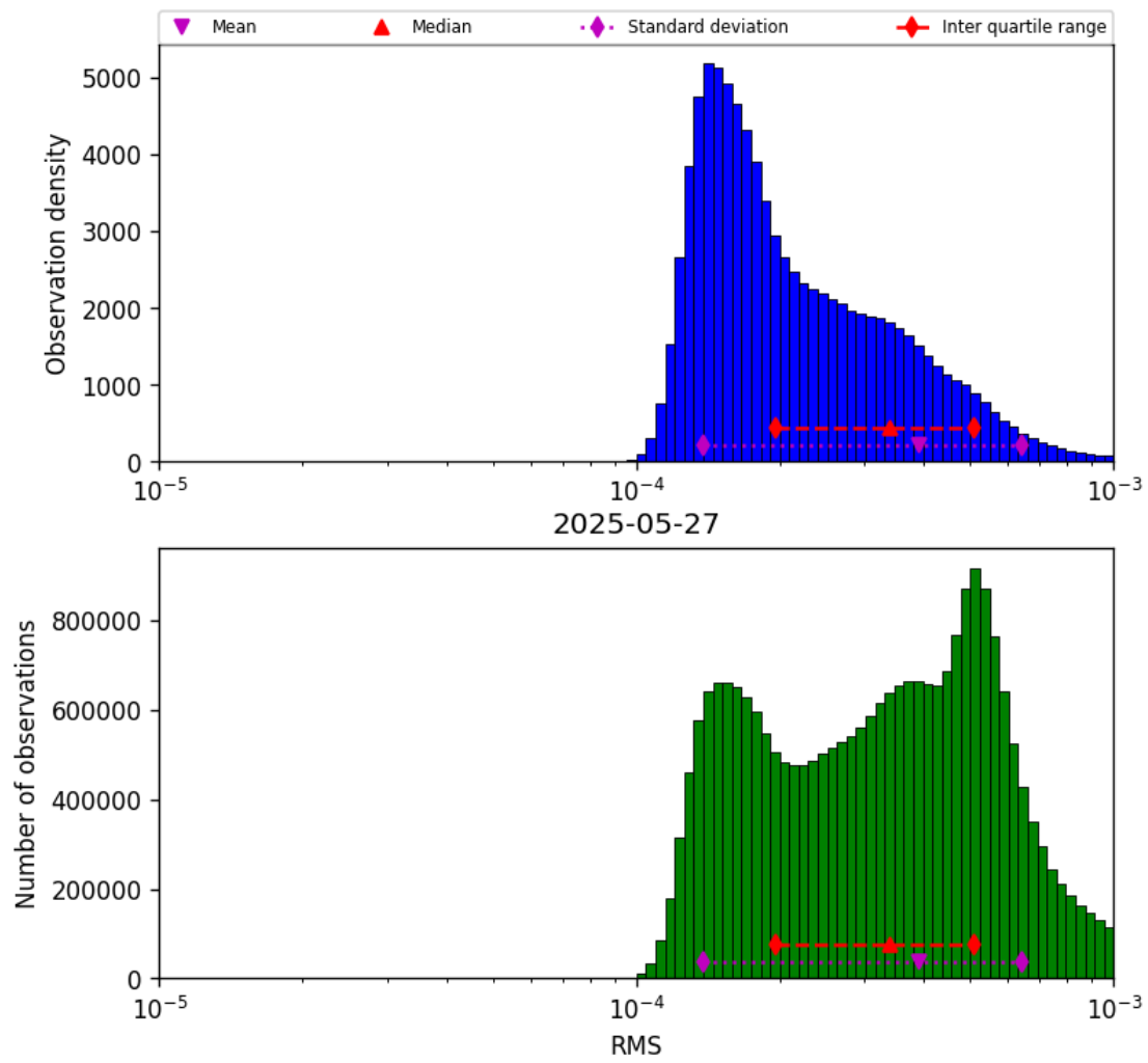
Figure 43: Histogram of “RMS” for 2025-05-26 to 2025-05-28
