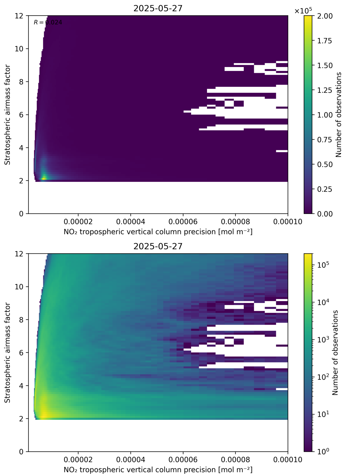
Figure 131: Scatter density plot of “NO 2 tropospheric vertical column precision” against “Stratospheric airmass factor” for 2025-05-26 to 2025-05-28.
