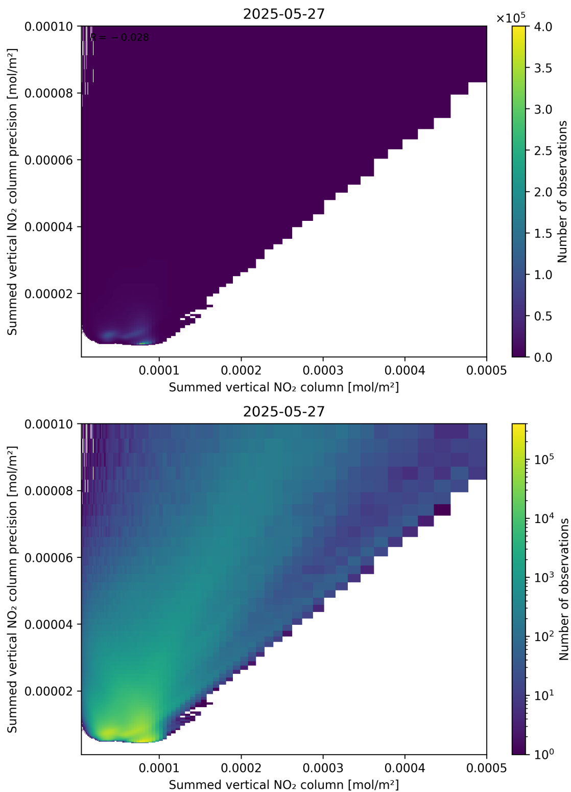
Figure 105: Scatter density plot of “Summed vertical NO 2 column” against “Summed vertical NO 2 column precision” for 2025-05-26 to 2025-05-28.
