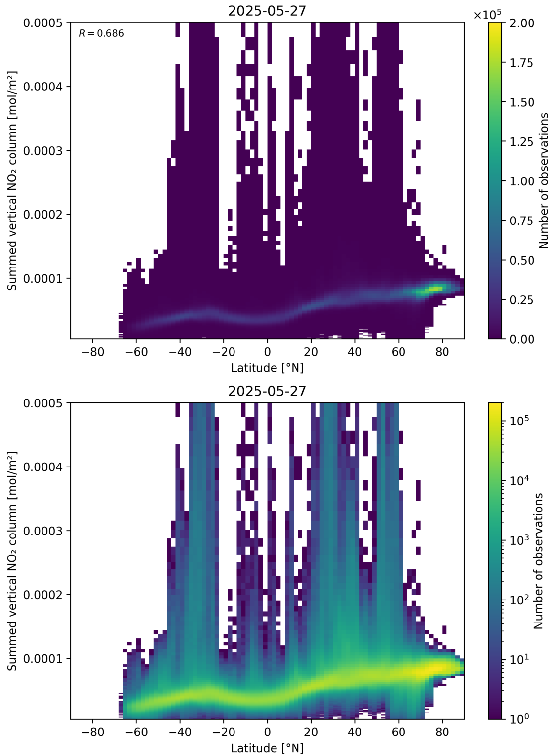
Figure 88: Scatter density plot of “Latitude” against “Summed vertical NO 2 column” for 2025-05-26 to 2025-05-28.
