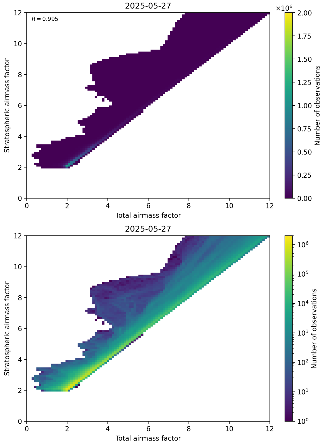
Figure 62: Scatter density plot of “Total airmass factor” against “Stratospheric airmass factor” for 2025-05-26 to 2025-05-28.
