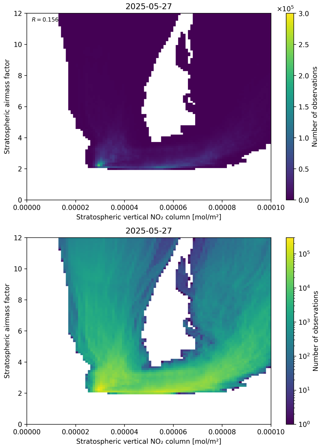
Figure 96: Scatter density plot of “Stratospheric vertical NO 2 column” against “Stratospheric airmass factor” for 2025-05-26 to 2025-05-28.
