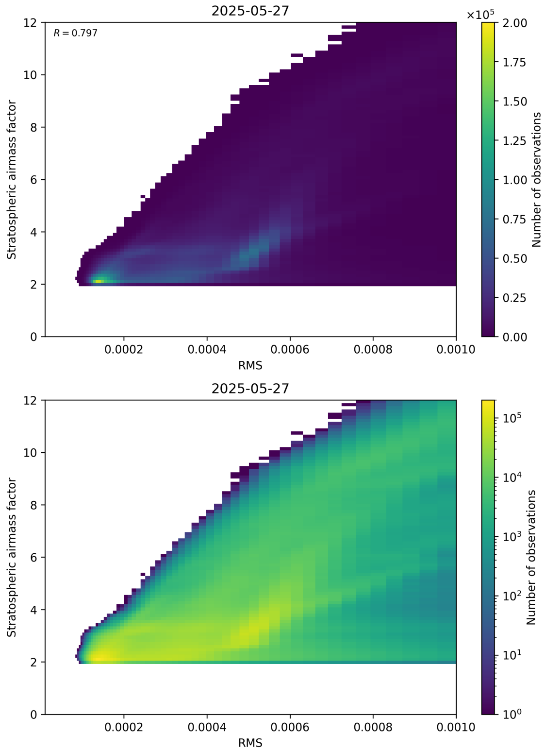
Figure 144: Scatter density plot of “RMS” against “Stratospheric airmass factor” for 2025-05-26 to 2025-05-28.
