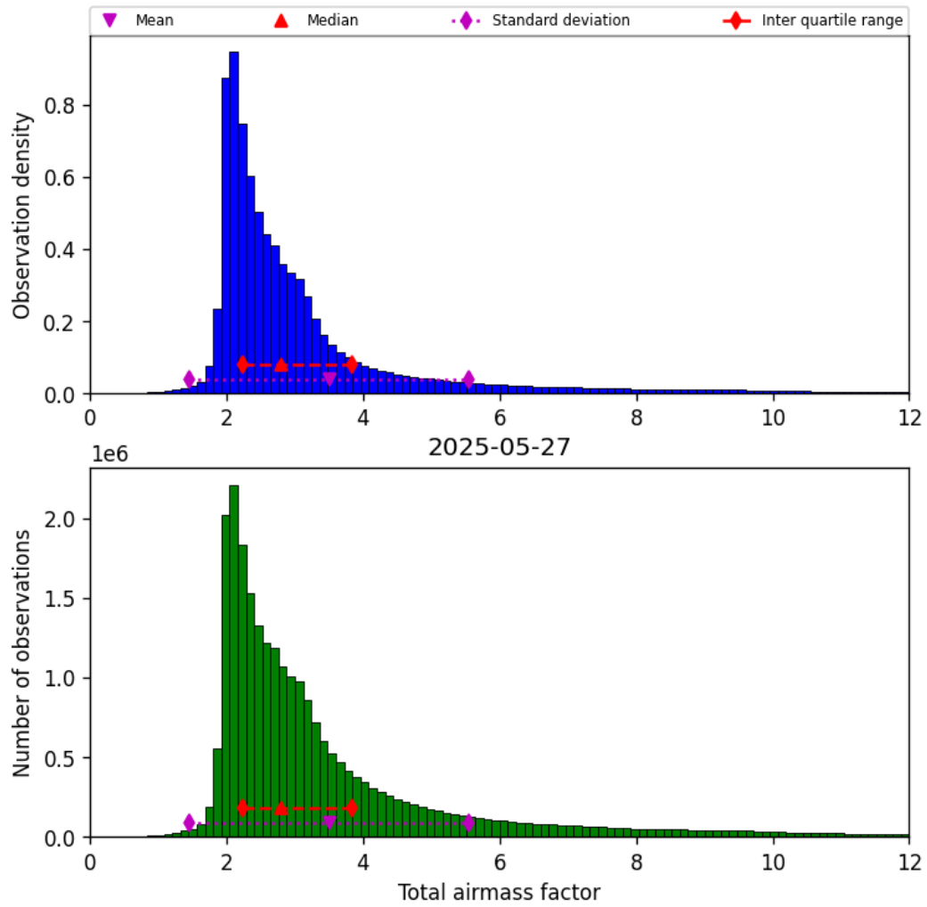
Figure 32: Histogram of “Total airmass factor” for 2025-05-26 to 2025-05-28
