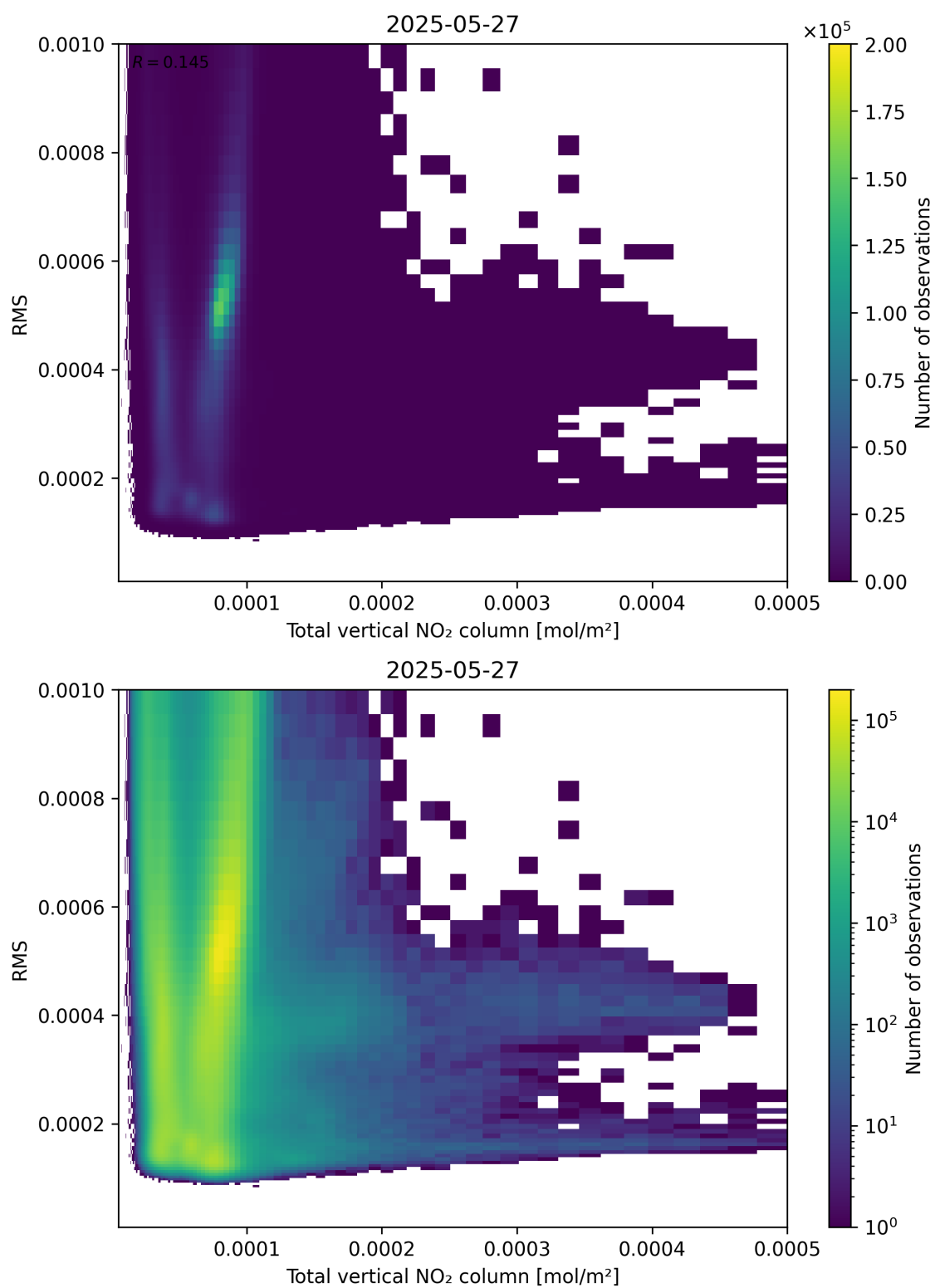
Figure 120: Scatter density plot of “Total vertical NO 2 column” against “RMS” for 2025-05-26 to 2025-05-28.
