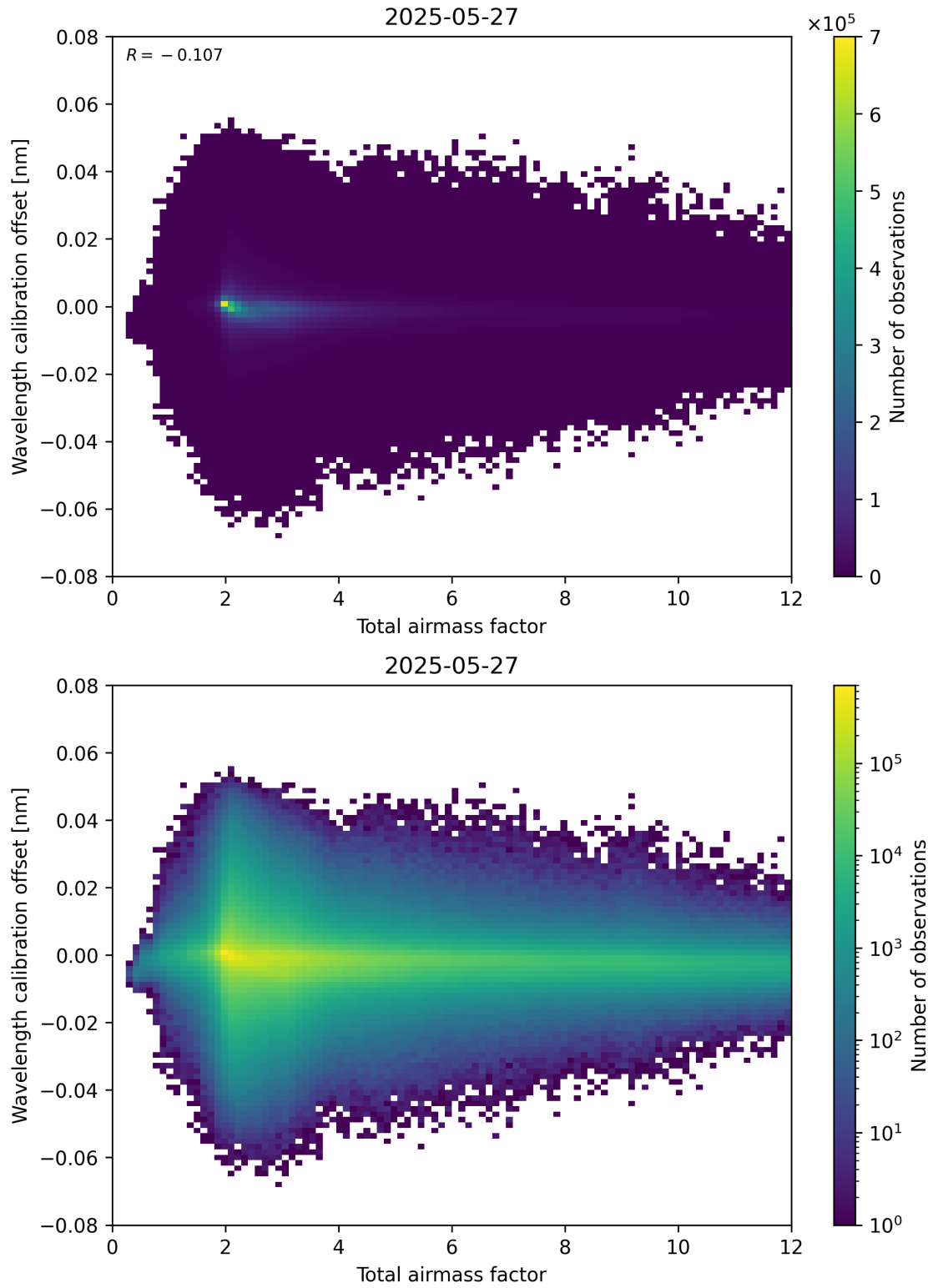
Figure 70: Scatter density plot of “Total airmass factor” against “Wavelength calibration offset” for 2025-05-26 to 2025-05-28.
