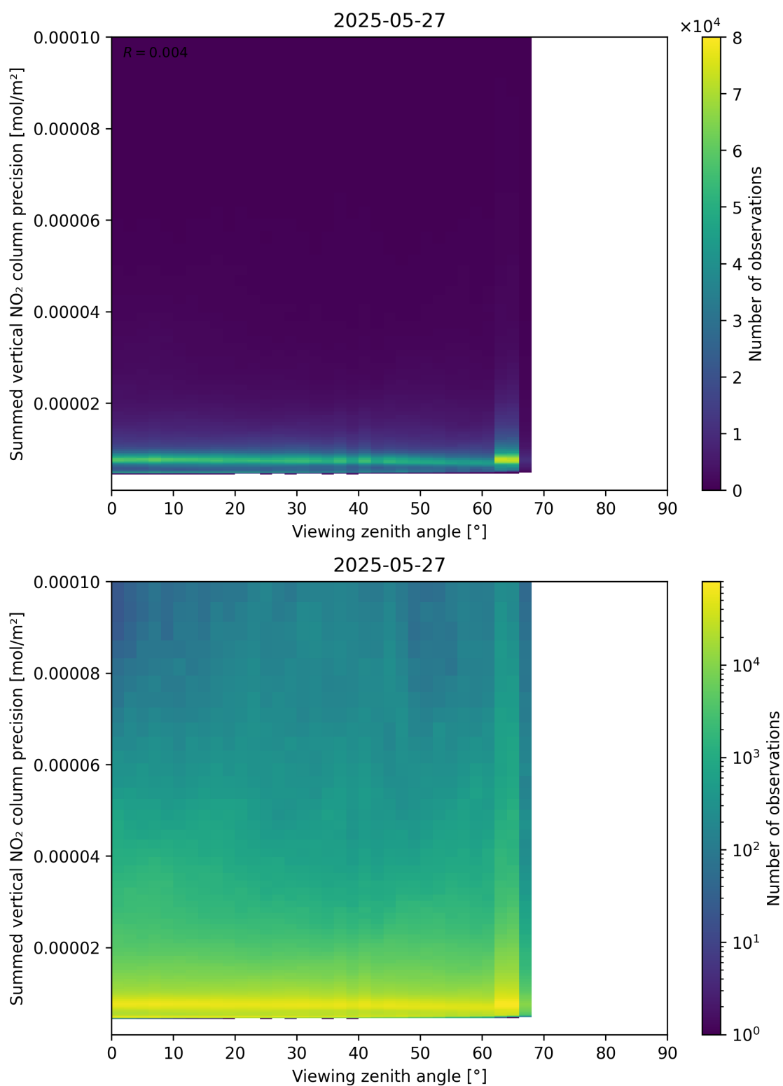
Figure 166: Scatter density plot of “Viewing zenith angle” against “Summed vertical NO 2 column precision” for 2025-05-26 to 2025-05-28.
