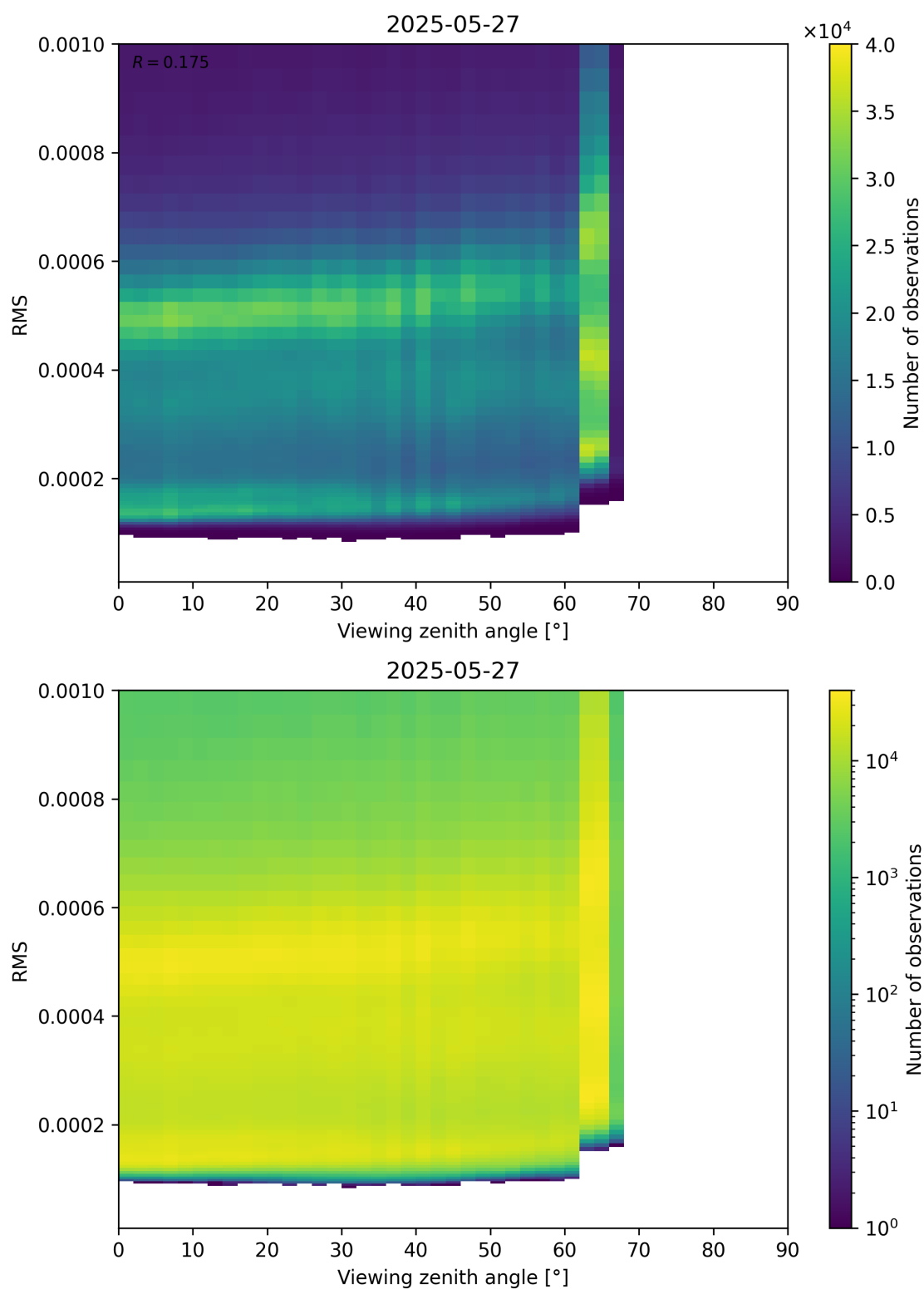
Figure 171: Scatter density plot of “Viewing zenith angle” against “RMS” for 2025-05-26 to 2025-05-28.
