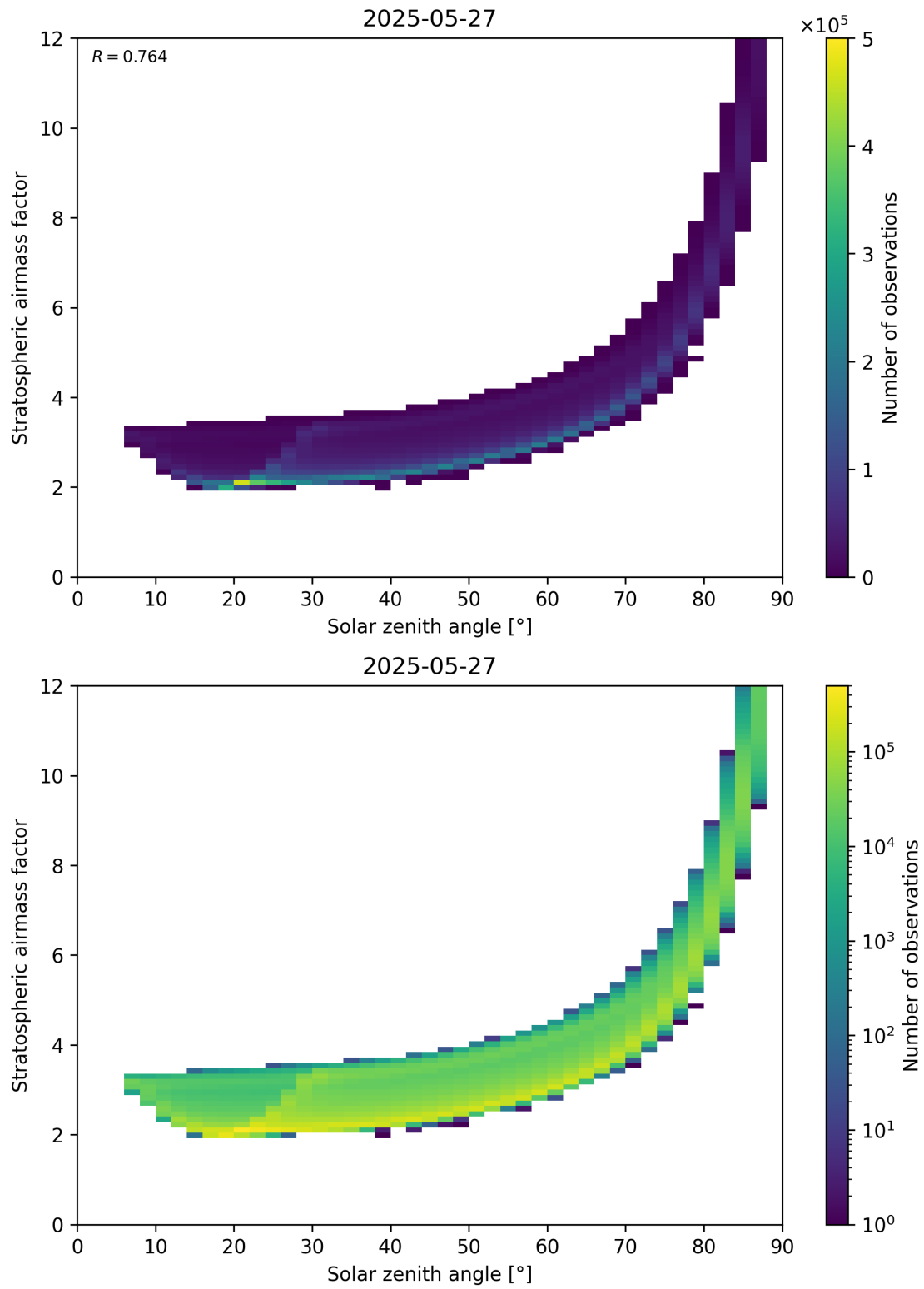
Figure 145: Scatter density plot of “Solar zenith angle” against “Stratospheric airmass factor” for 2025-05-26 to 2025-05-28.
