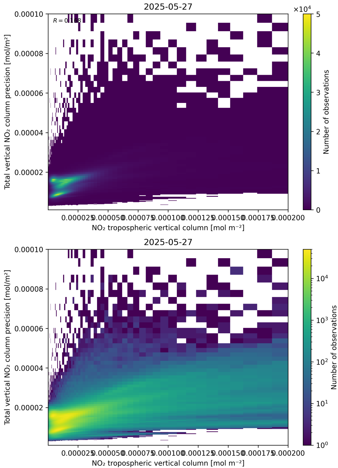
Figure 129: Scatter density plot of “NO 2 tropospheric vertical column” against “Total vertical NO 2 column precision” for 2025-05-26 to 2025-05-28.
