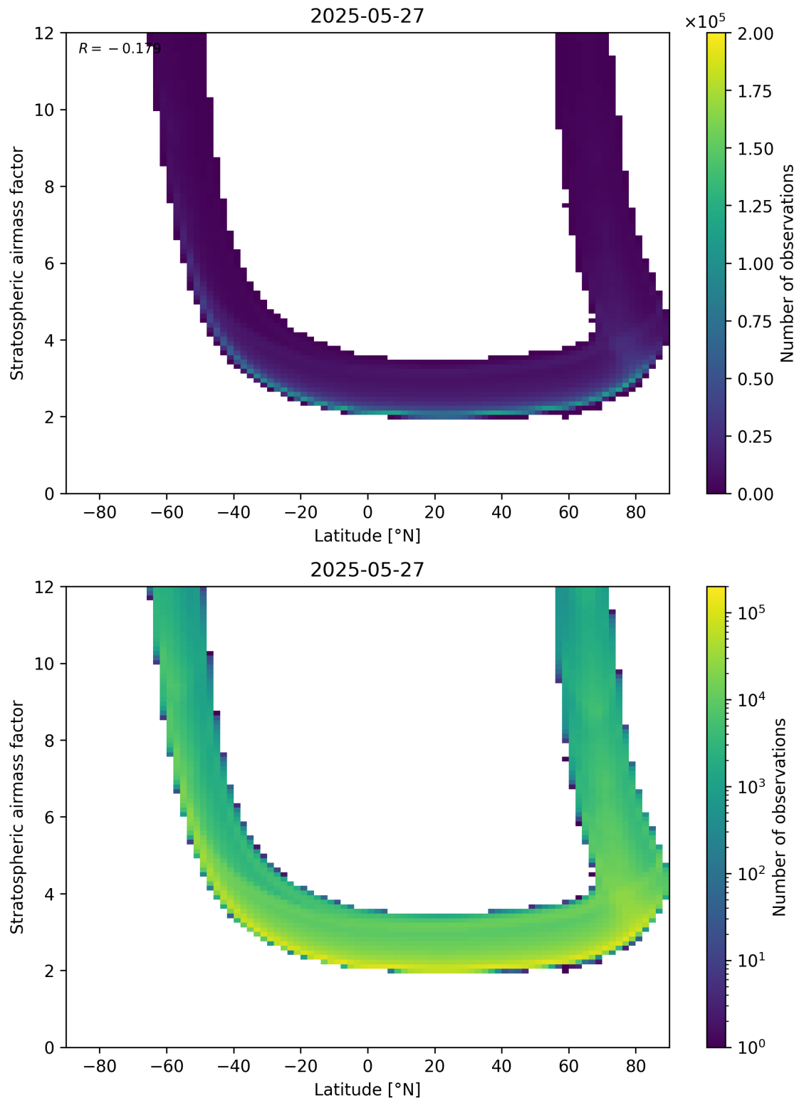
Figure 83: Scatter density plot of “Latitude” against “Stratospheric air mass factor” for 2025-05-26 to 2025-05-28.
