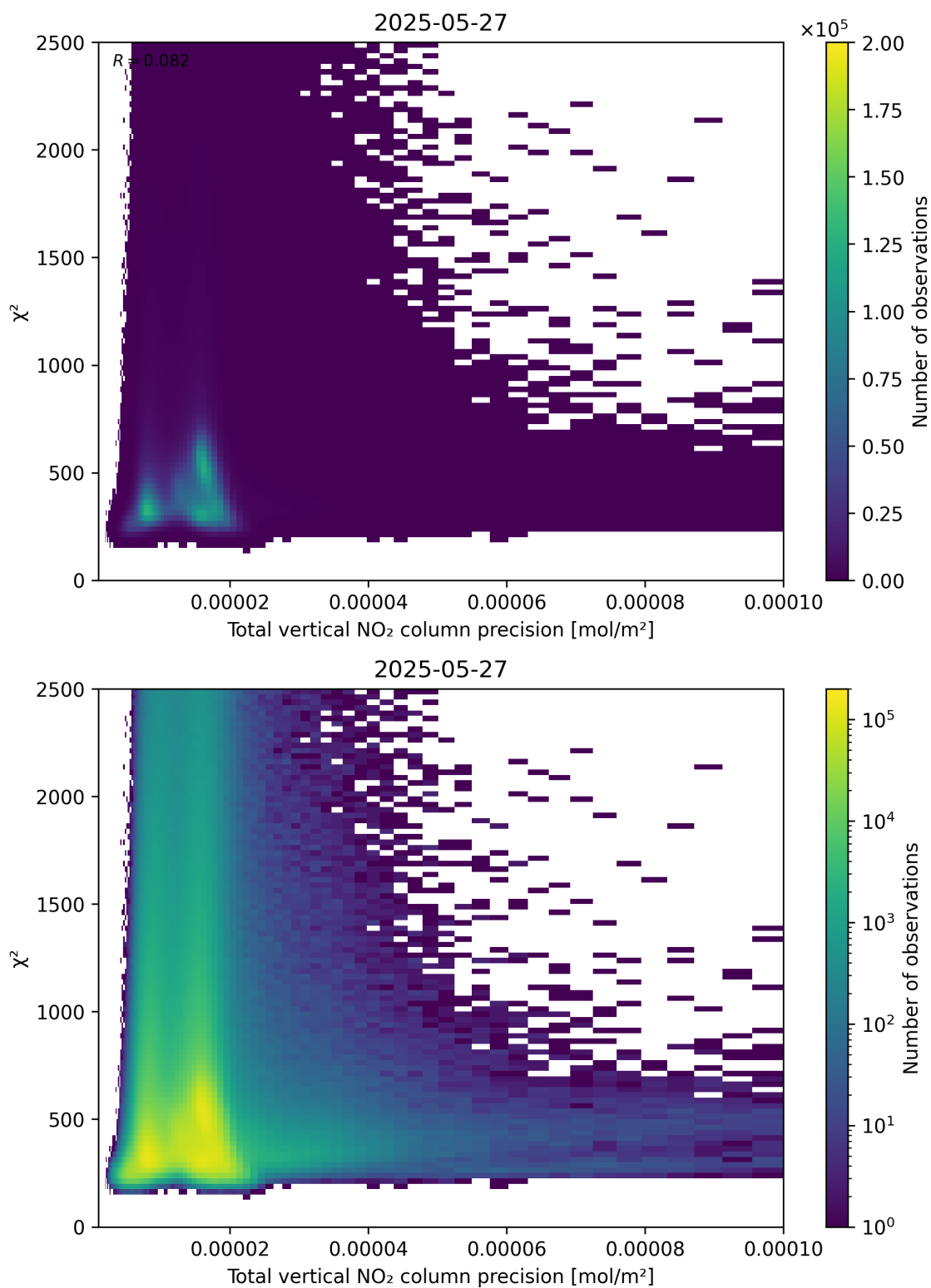
Figure 116: Scatter density plot of “Total vertical NO 2 column precision” against “ \chi^2 ” for 2025-05-26 to 2025-05-28.
