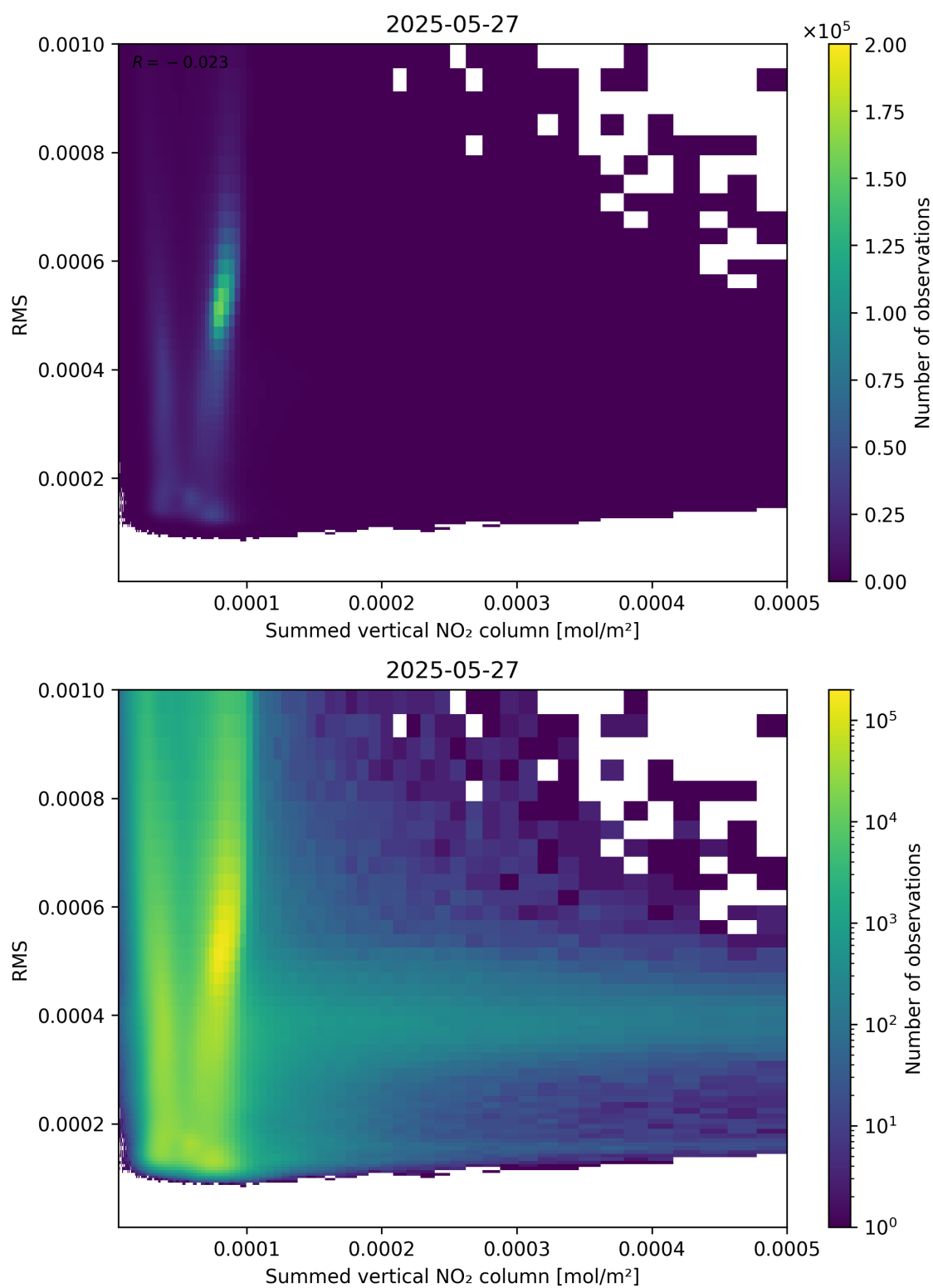
Figure 109: Scatter density plot of “Summed vertical NO 2 column” against “RMS” for 2025-05-26 to 2025-05-28.
