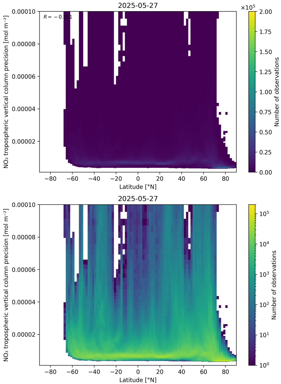
Figure 93: Scatter density plot of “Latitude” against “NO 2 tropospheric vertical column precision” for 2025-05-26 to 2025-05-28.
