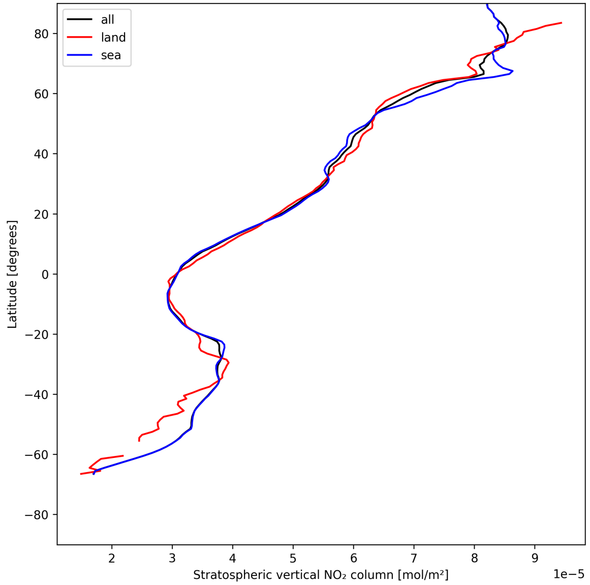
Figure 19: Zonal average of “Stratospheric vertical NO 2 column” for 2025-05-26 to 2025-05-28.
