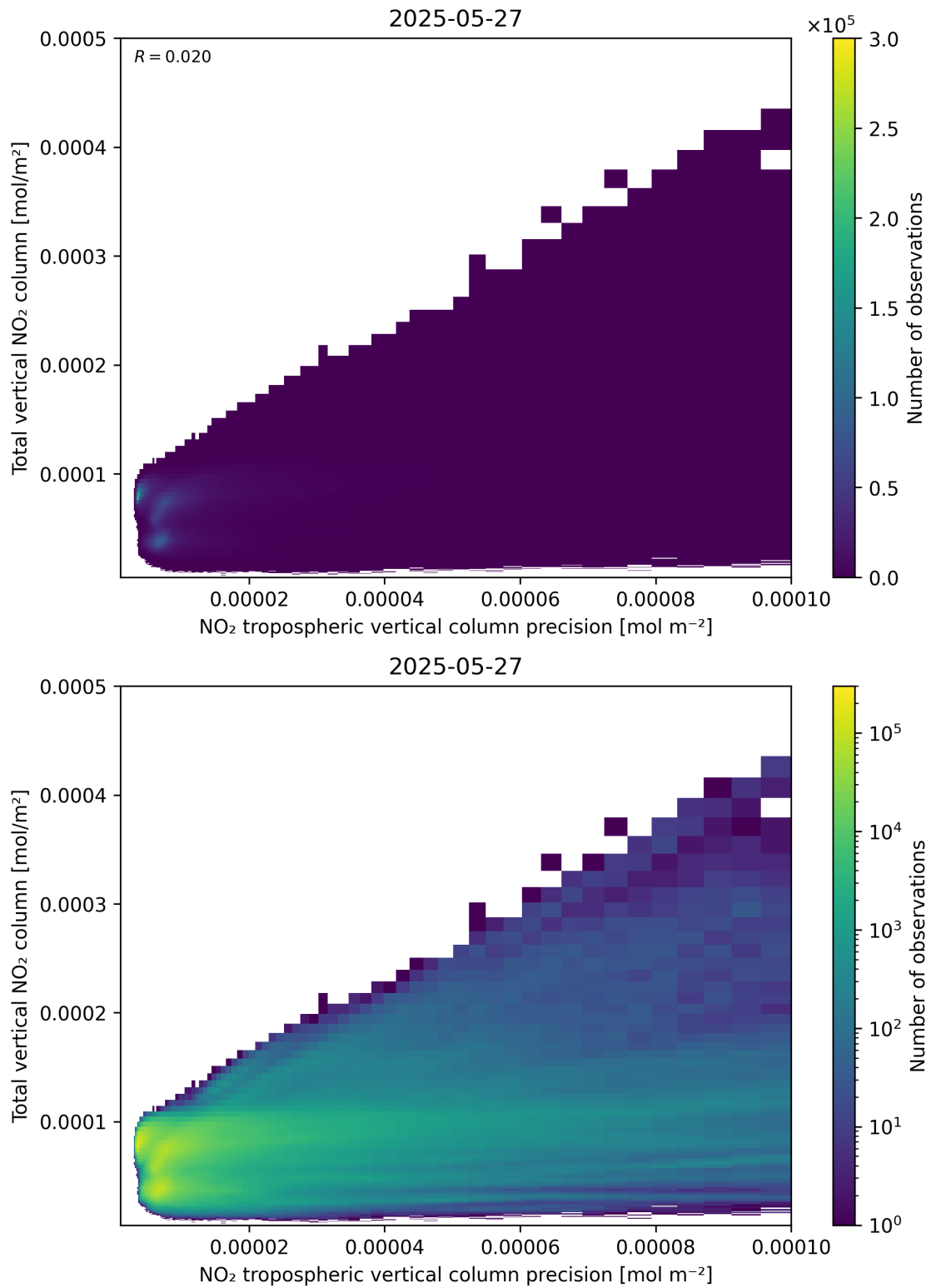
Figure 138: Scatter density plot of “NO 2 tropospheric vertical column precision” against “Total vertical NO 2 column” for 2025-05-26 to 2025-05-28.
