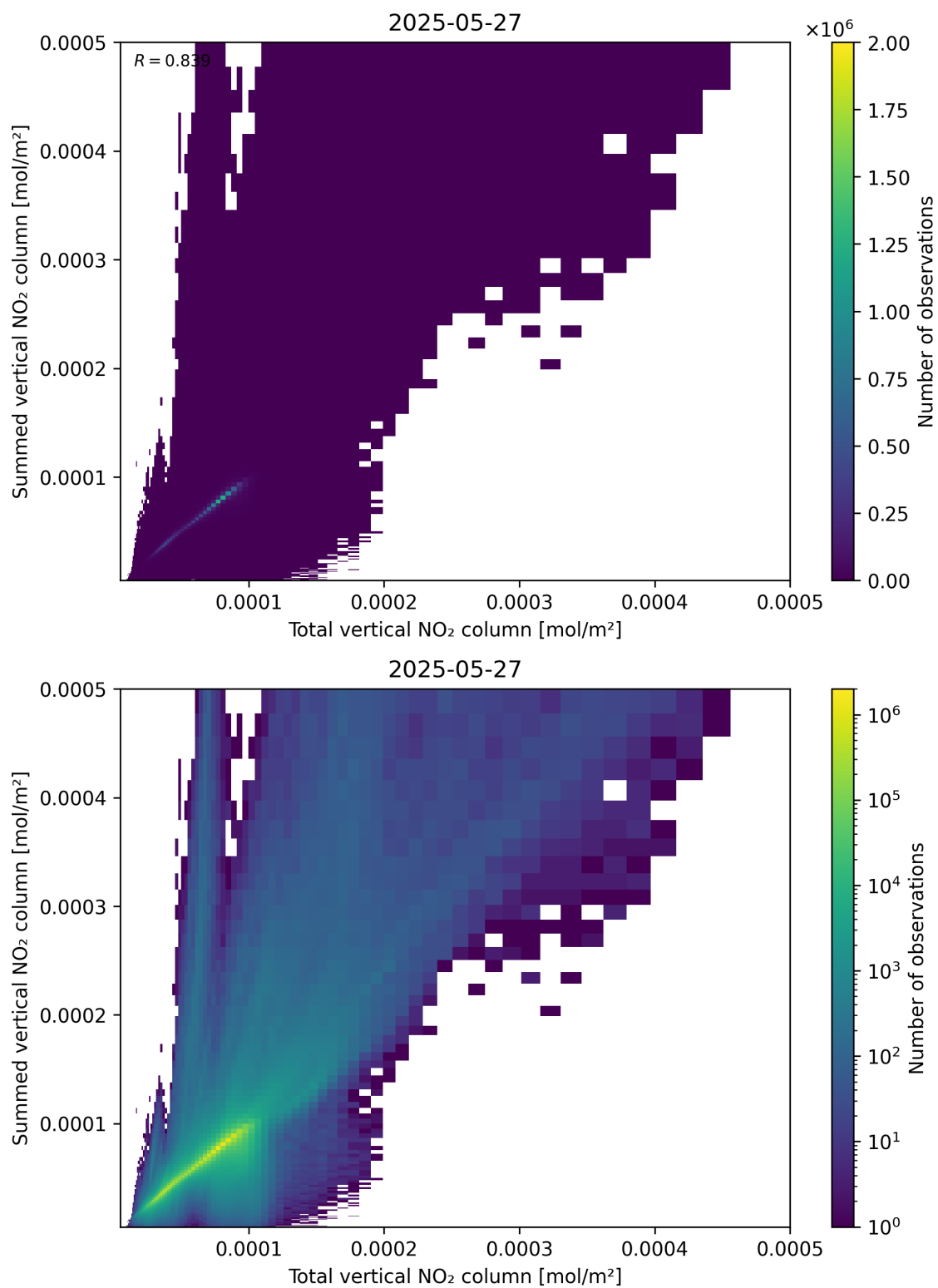
Figure 112: Scatter density plot of “Total vertical NO 2 column” against “Summed vertical NO 2 column” for 2025-05-26 to 2025-05-28.
