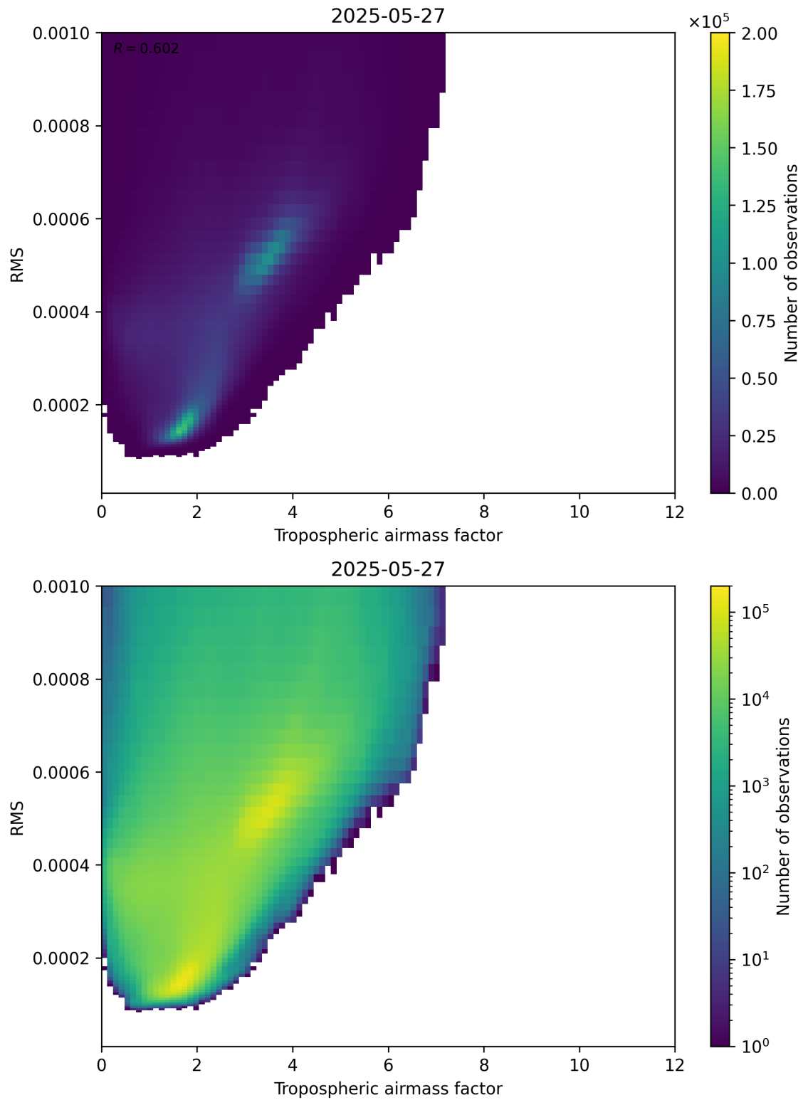
Figure 79: Scatter density plot of “Tropospheric airmass factor” against “RMS” for 2025-05-26 to 2025-05-28.
