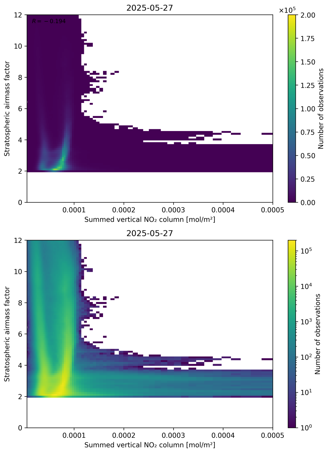
Figure 103: Scatter density plot of “Summed vertical NO 2 column” against “Stratospheric airmass factor” for 2025-05-26 to 2025-05-28.
