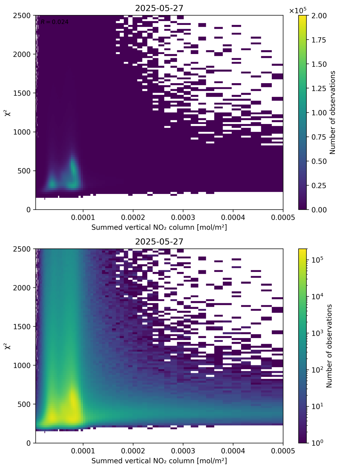
Figure 104: Scatter density plot of “Summed vertical NO 2 column” against “ \chi^2 ” for 2025-05-26 to 2025-05-28.
