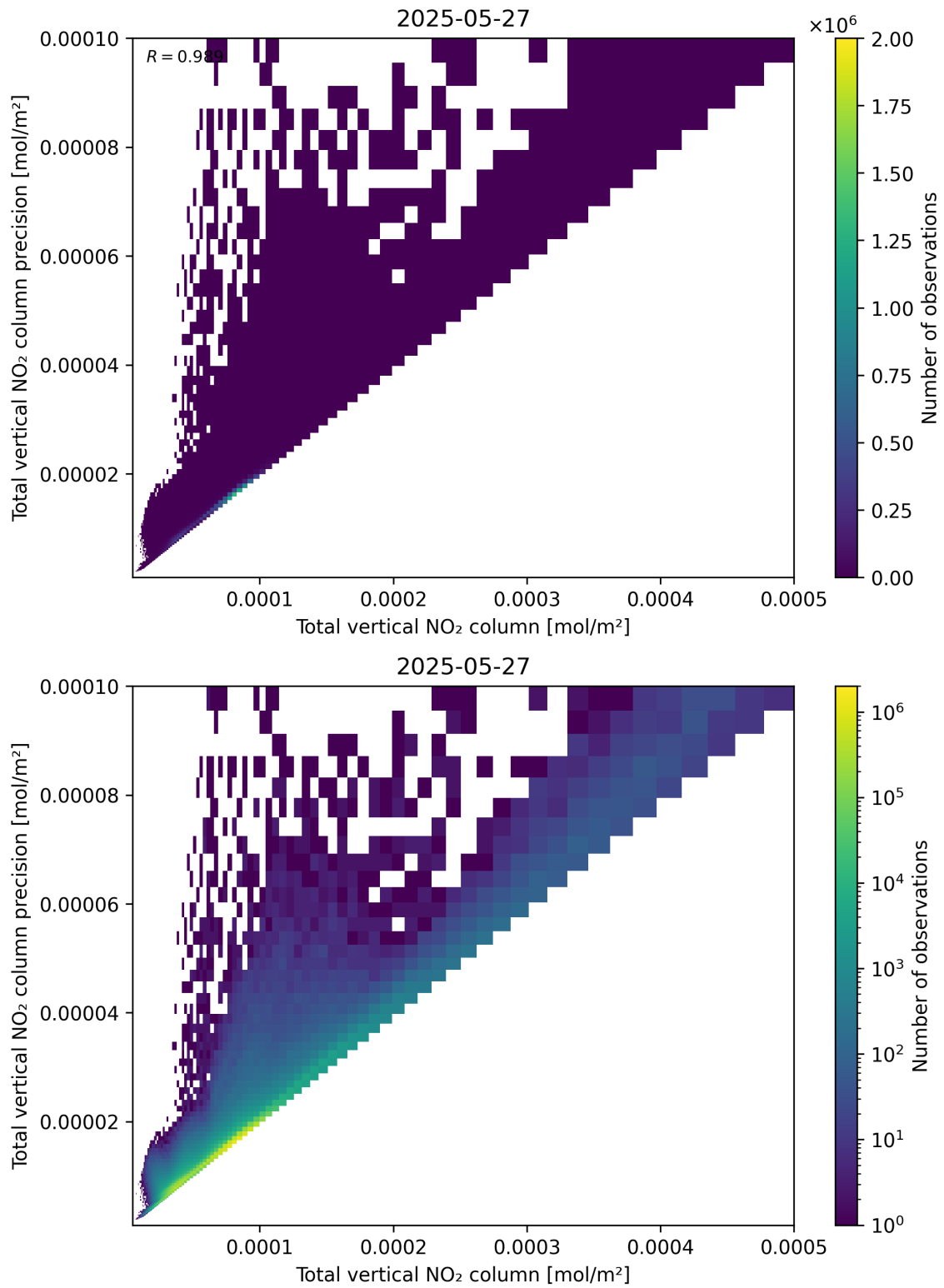
Figure 114: Scatter density plot of “Total vertical NO 2 column” against “Total vertical NO 2 column precision” for 2025-05-26 to 2025-05-28.
