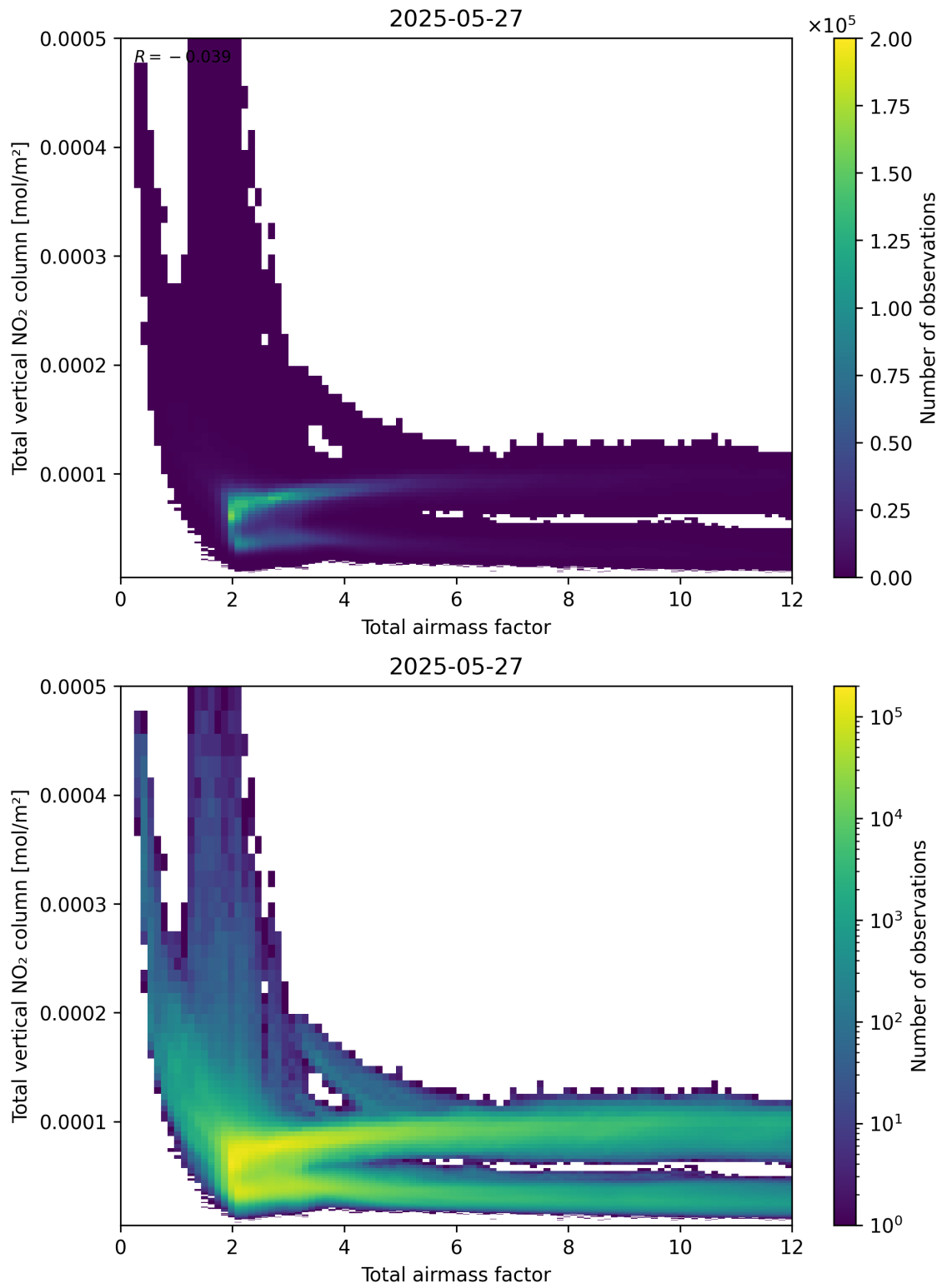
Figure 67: Scatter density plot of “Total airmass factor” against “Total vertical NO 2 column” for 2025-05-26 to 2025-05-28.
