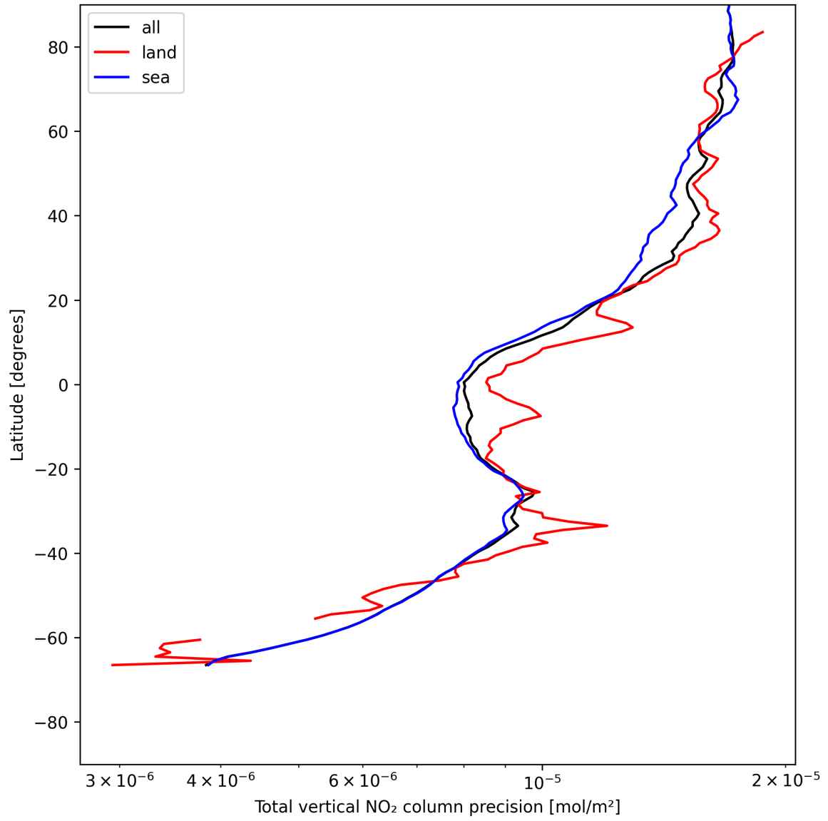
Figure 22: Zonal average of “Total vertical NO 2 column precision” for 2025-05-26 to 2025-05-28.
