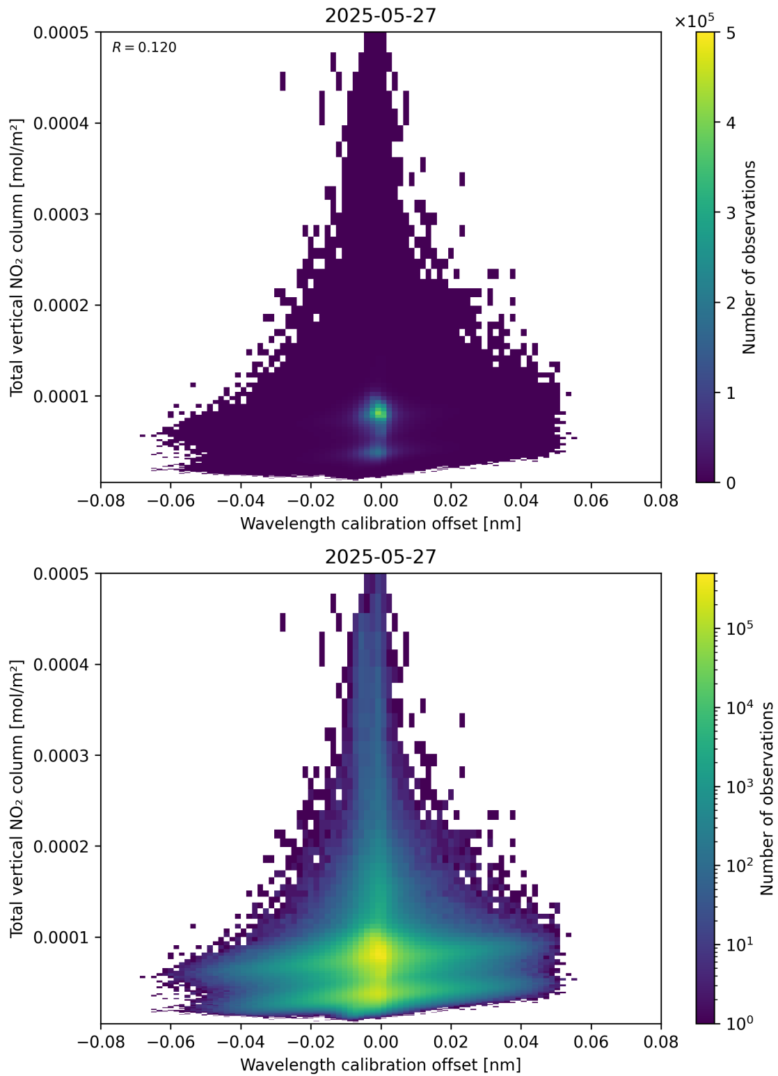
Figure 179: Scatter density plot of “Wavelength calibration offset” against “Total vertical NO 2 column” for 2025-05-26 to 2025-05-28.
