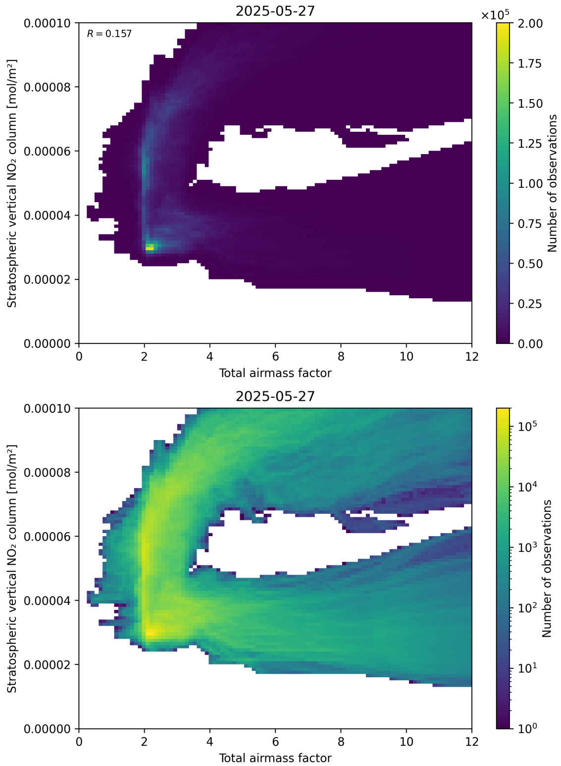
Figure 64: Scatter density plot of “Total airmass factor” against “Stratospheric vertical NO 2 column” for 2025-05-26 to 2025-05-28.
