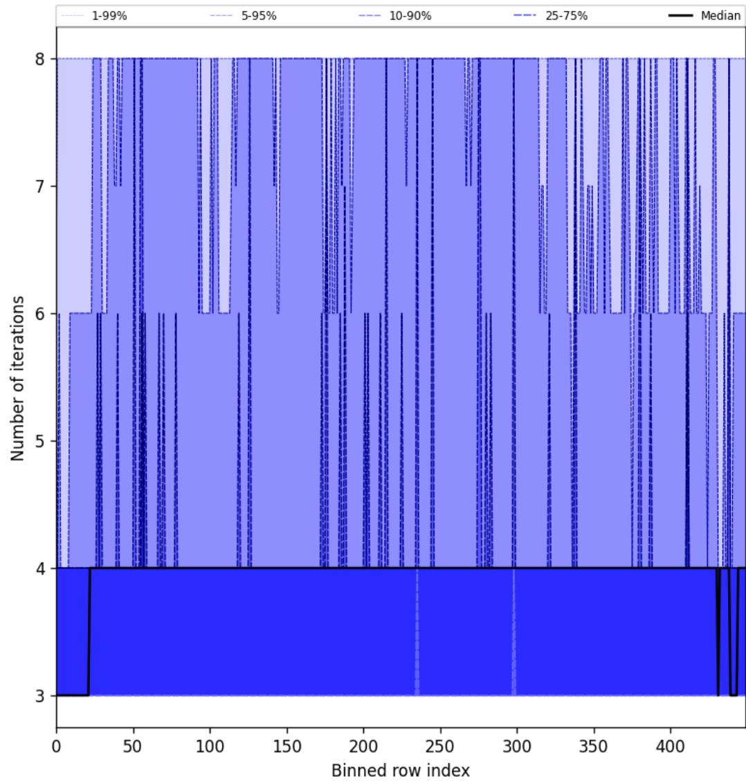
Figure 51: Along track statistics of “Number of iterations” for 2025-05-26 to 2025-05-28
