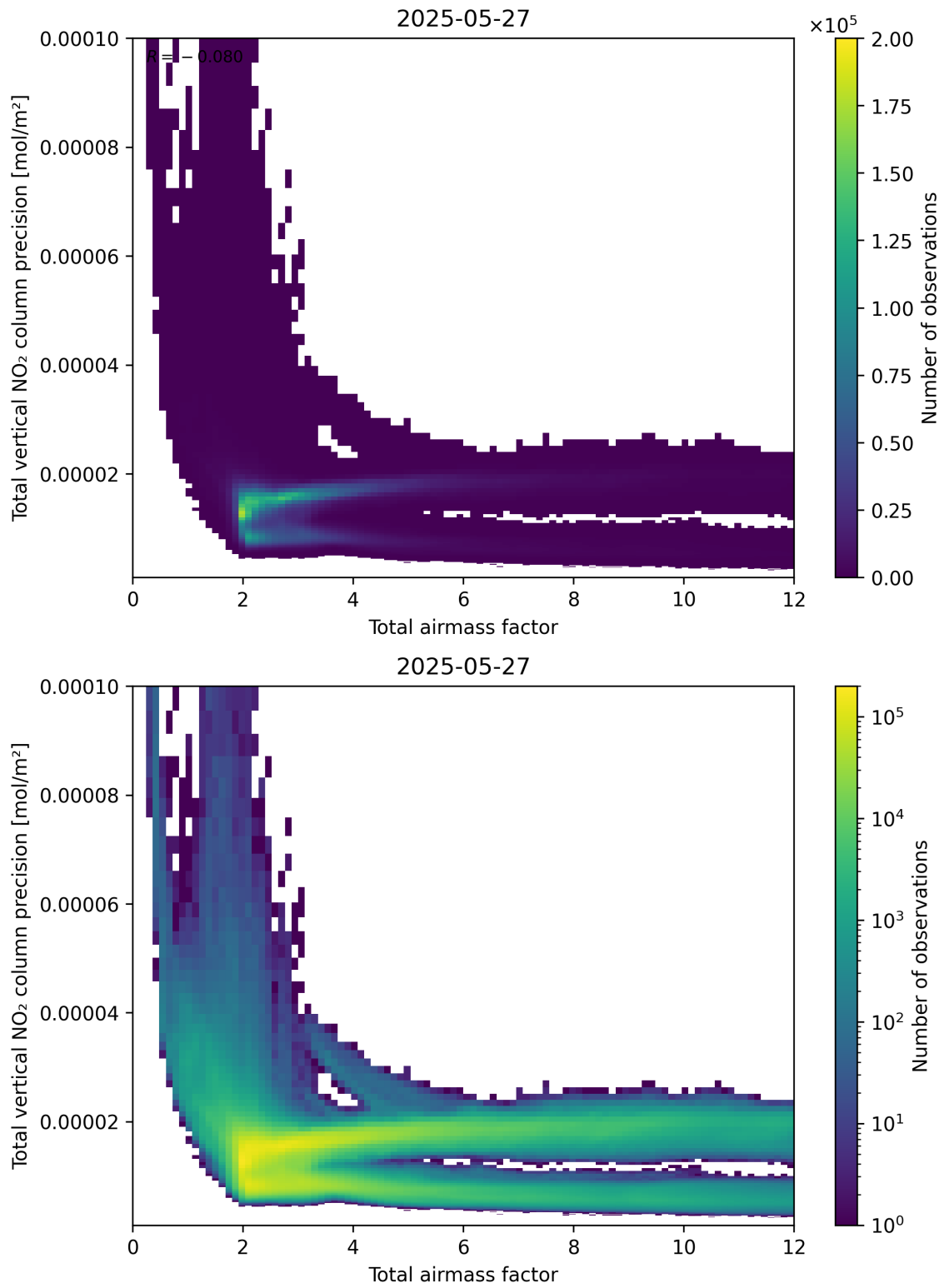
Figure 68: Scatter density plot of “Total airmass factor” against “Total vertical NO 2 column precision” for 2025-05-26 to 2025-05-28.
