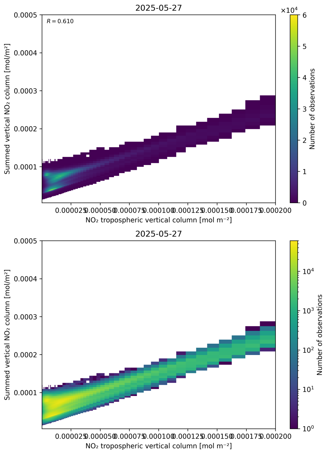
Figure 126: Scatter density plot of “NO 2 tropospheric vertical column” against “Summed vertical NO 2 column” for 2025-05-26 to 2025-05-28.
