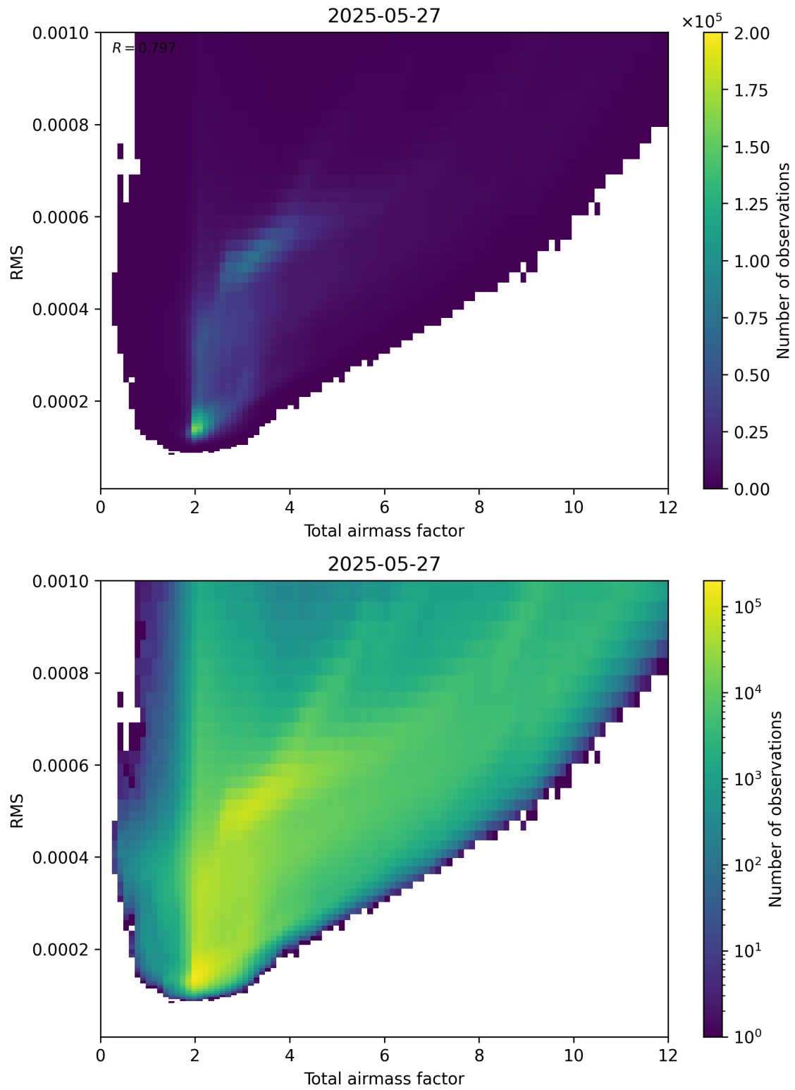
Figure 69: Scatter density plot of “Total airmass factor” against “RMS” for 2025-05-26 to 2025-05-28.
