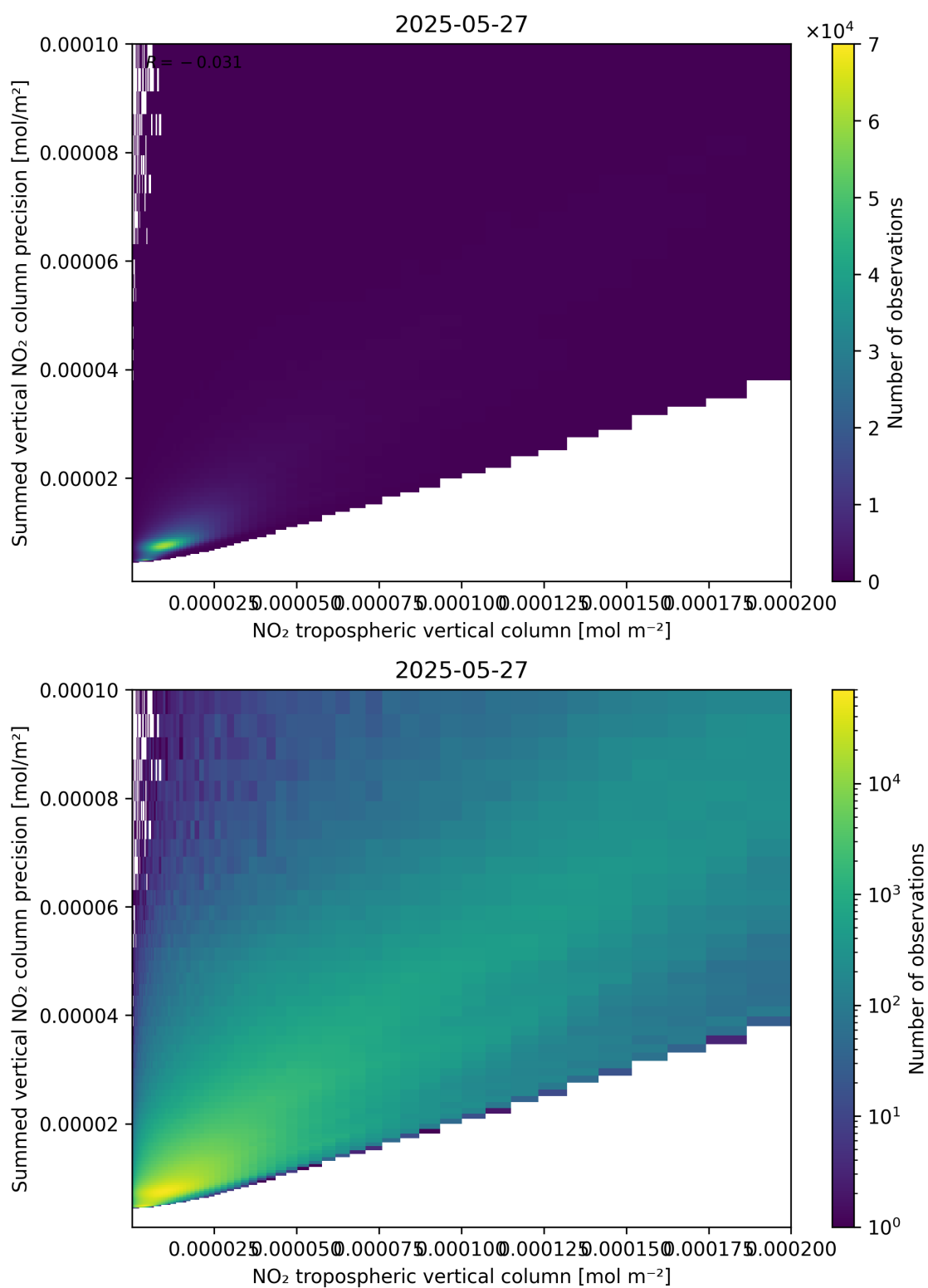
Figure 127: Scatter density plot of “NO 2 tropospheric vertical column” against “Summed vertical NO 2 column precision” for 2025-05-26 to 2025-05-28.
