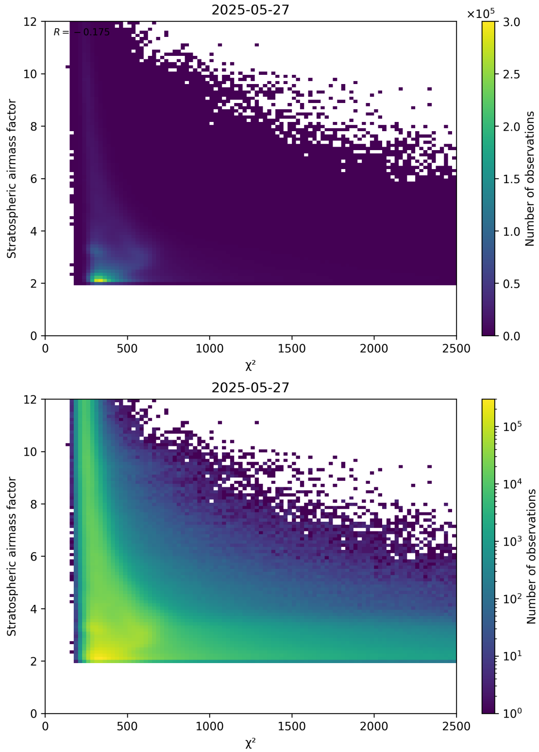
Figure 81: Scatter density plot of “ \chi^2 ” against “Stratospheric airmass factor” for 2025-05-26 to 2025-05-28.
