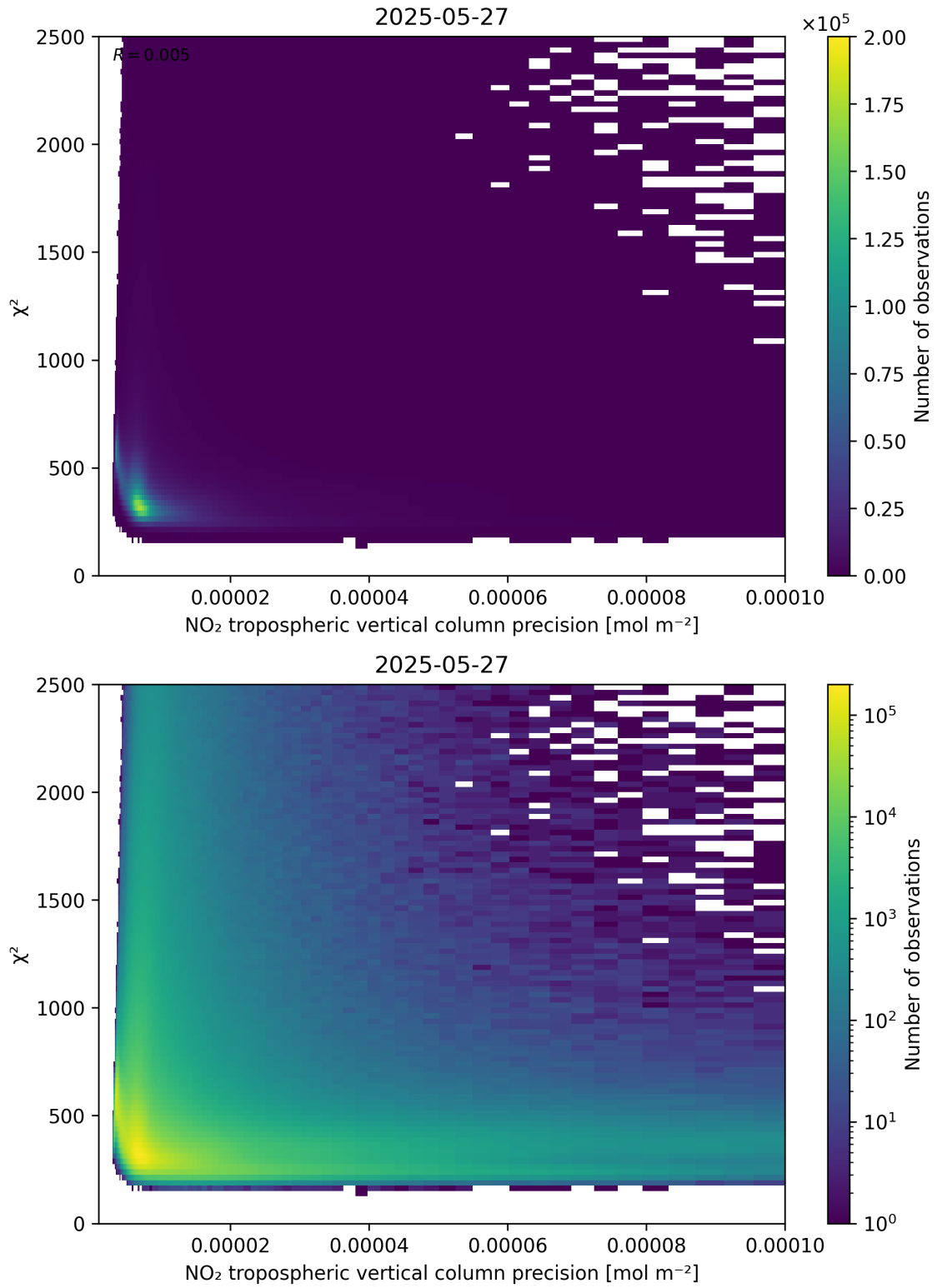
Figure 134: Scatter density plot of “NO 2 tropospheric vertical column precision” against “ \chi^2 ” for 2025-05-26 to 2025-05-28.
