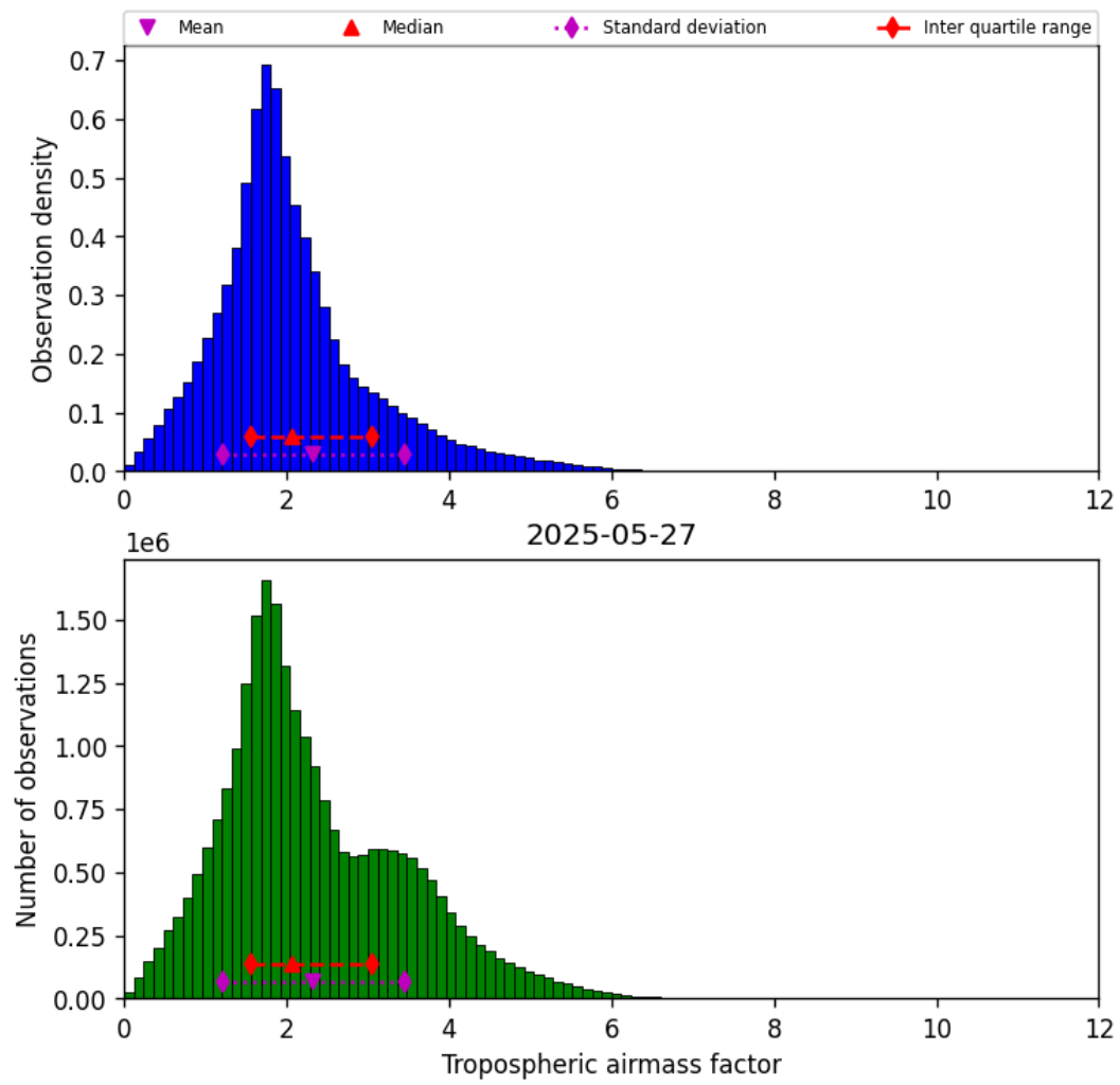
Figure 31: Histogram of “Tropospheric airmass factor” for 2025-05-26 to 2025-05-28
