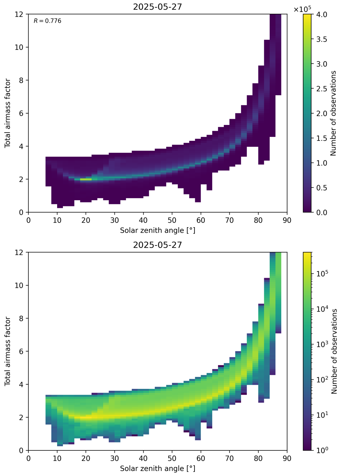
Figure 146: Scatter density plot of “Solar zenith angle” against “Total air mass factor” for 2025-05-26 to 2025-05-28.
