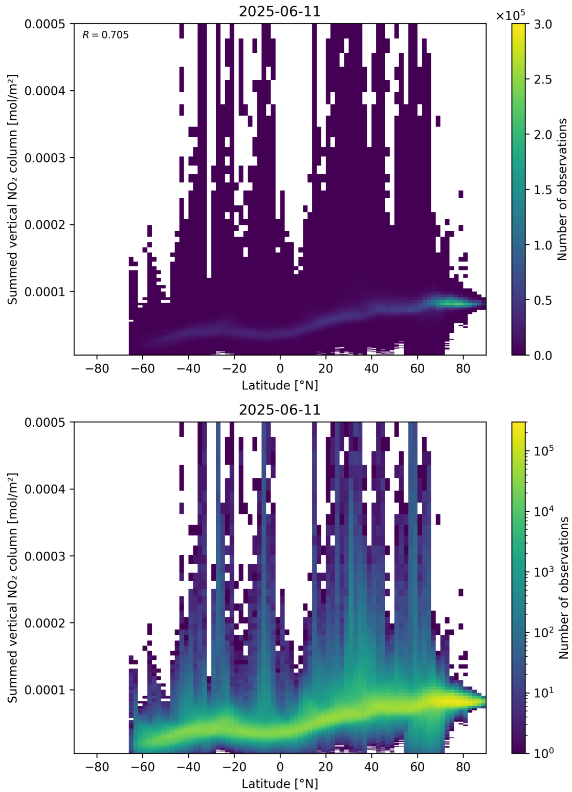
Figure 88: Scatter density plot of “Latitude” against “Summed vertical NO 2 column” for 2025-06-11 to 2025-06-12.
