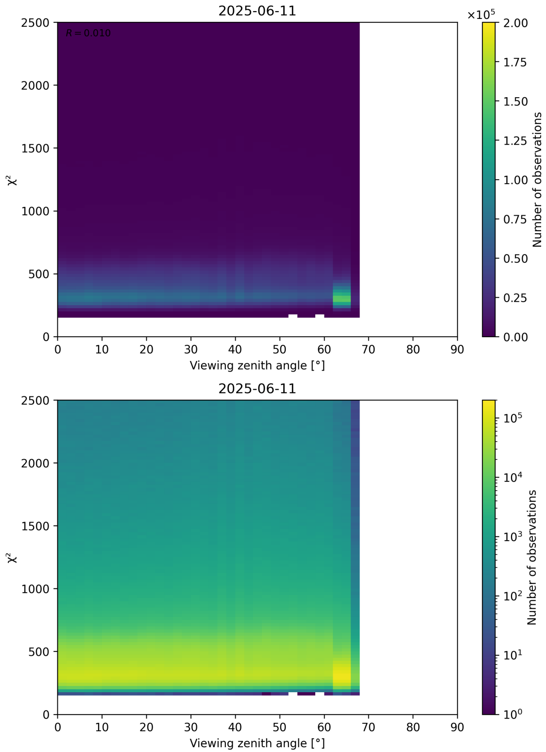
Figure 162: Scatter density plot of “Viewing zenith angle” against “ \chi^2 ” for 2025-06-11 to 2025-06-12.
