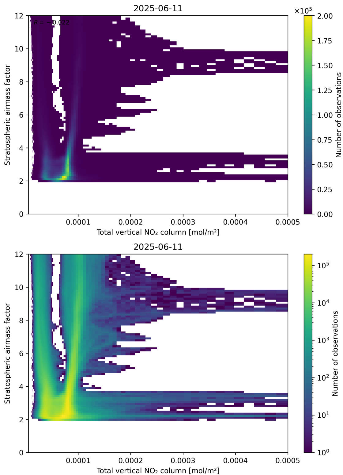
Figure 110: Scatter density plot of “Total vertical NO 2 column” against “Stratospheric air mass factor” for 2025-06-11 to 2025-06-12.
