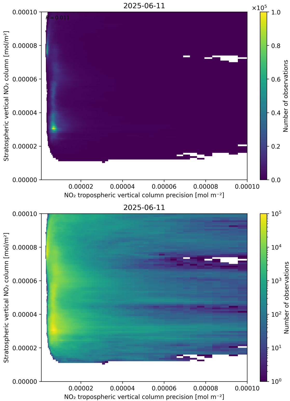
Figure 135: Scatter density plot of “NO 2 tropospheric vertical column precision” against “Stratospheric vertical NO 2 column” for 2025-06-11 to 2025-06-12.
