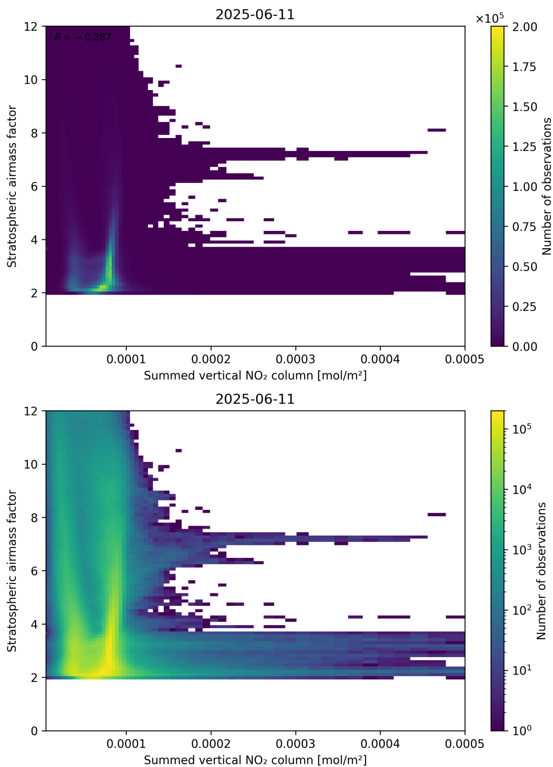
Figure 103: Scatter density plot of “Summed vertical NO 2 column” against “Stratospheric airmass factor” for 2025-06-11 to 2025-06-12.
