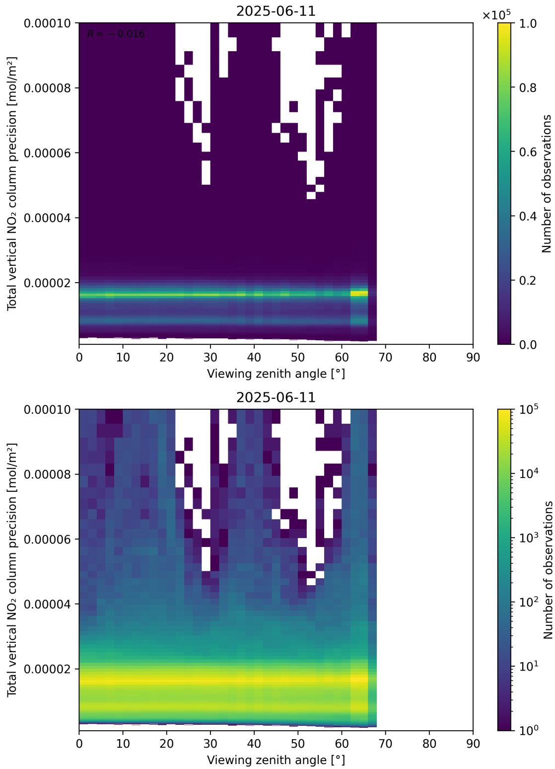
Figure 168: Scatter density plot of “Viewing zenith angle” against “Total vertical NO 2 column precision” for 2025-06-11 to 2025-06-12.
