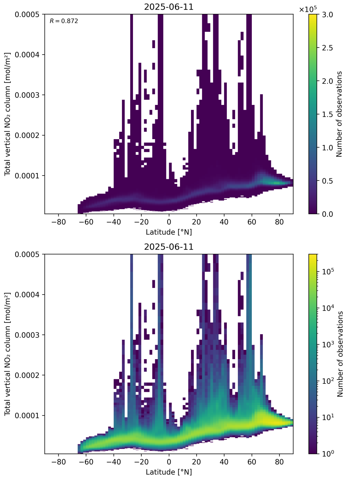
Figure 90: Scatter density plot of “Latitude” against “Total vertical NO 2 column” for 2025-06-11 to 2025-06-12.
