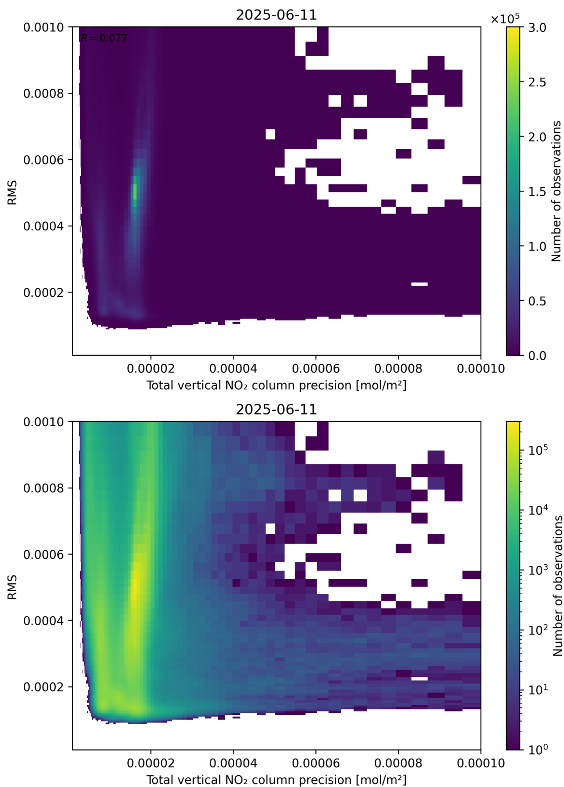
Figure 119: Scatter density plot of “Total vertical NO 2 column precision” against “RMS” for 2025-06-11 to 2025-06-12.
