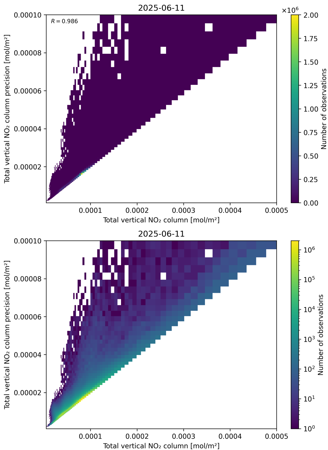
Figure 114: Scatter density plot of “Total vertical NO 2 column” against “Total vertical NO 2 column precision” for 2025-06-11 to 2025-06-12.
