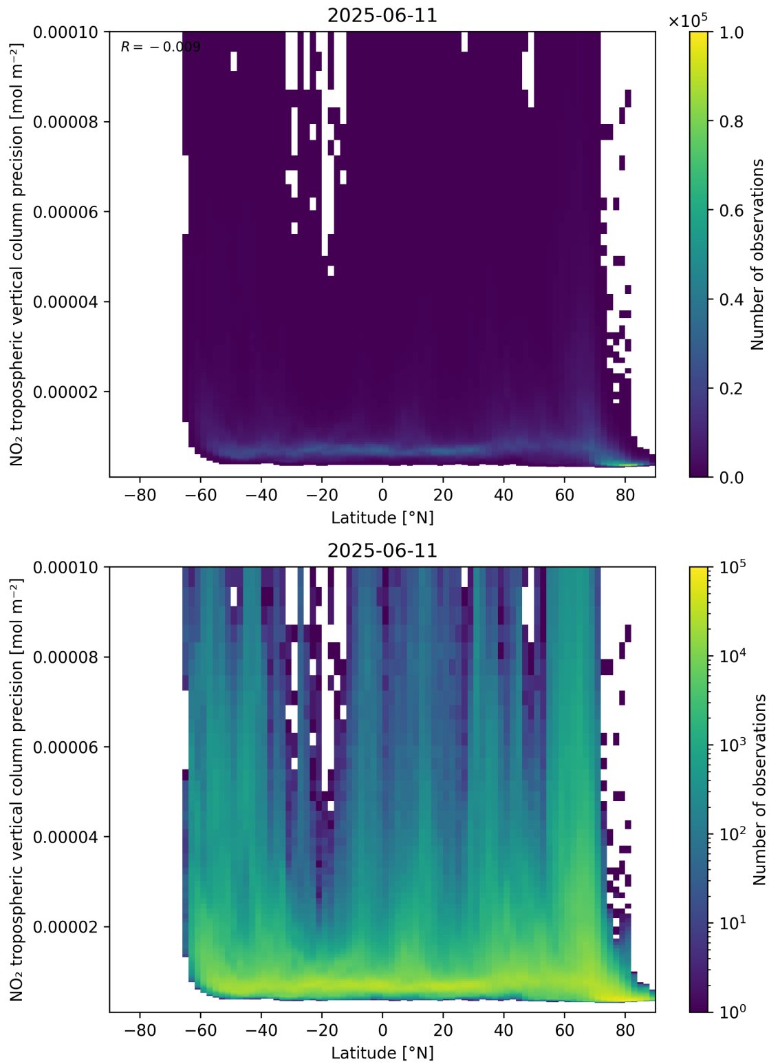
Figure 93: Scatter density plot of “Latitude” against “NO 2 tropospheric vertical column precision” for 2025-06-11 to 2025-06-12.
