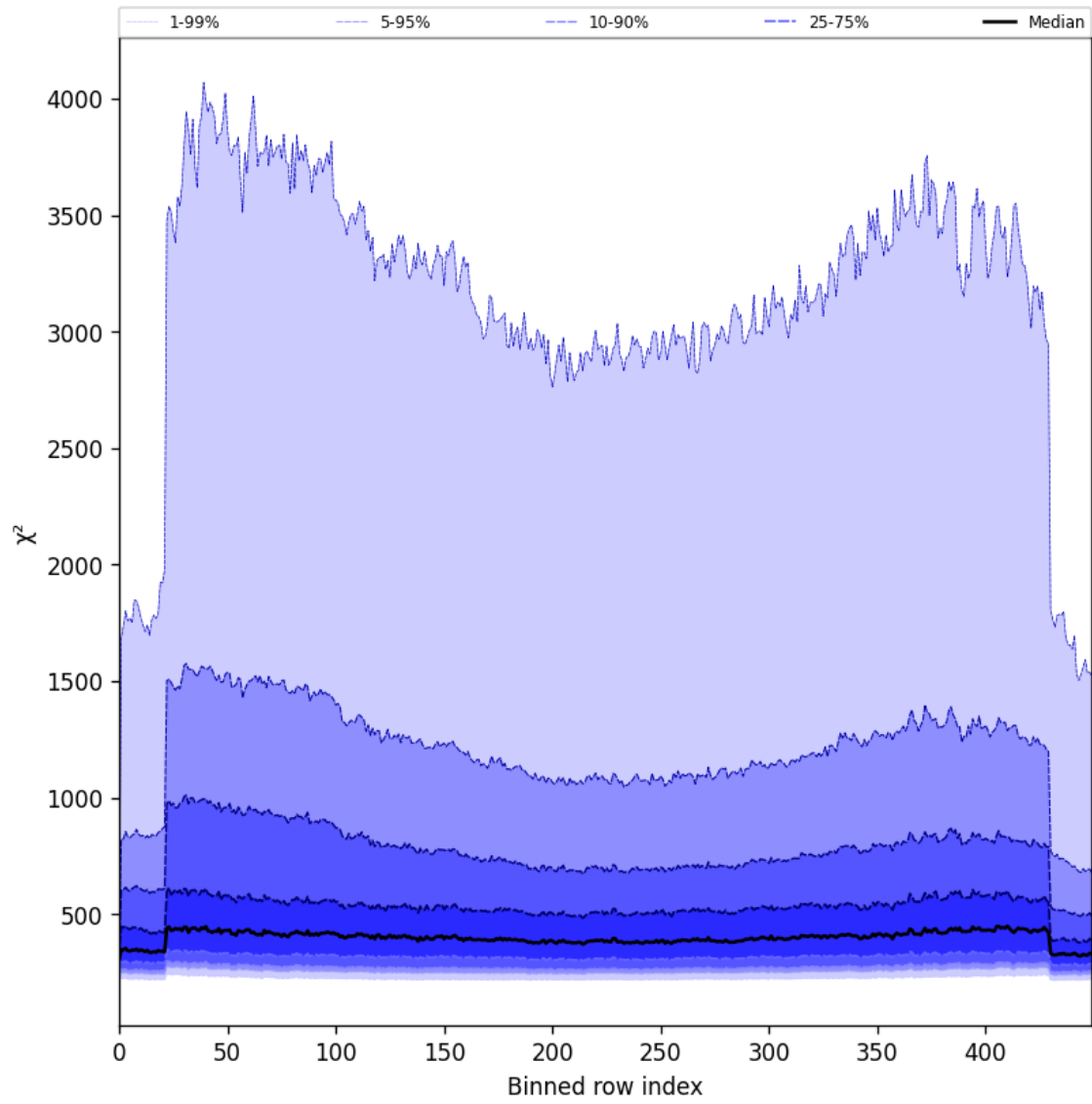
Figure 59: Along track statistics of “ \chi^2 ” for 2025-06-11 to 2025-06-12
