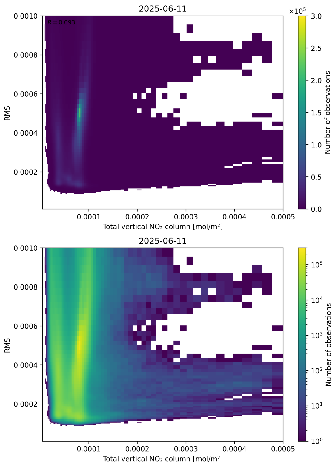
Figure 120: Scatter density plot of “Total vertical NO 2 column” against “RMS” for 2025-06-11 to 2025-06-12.
