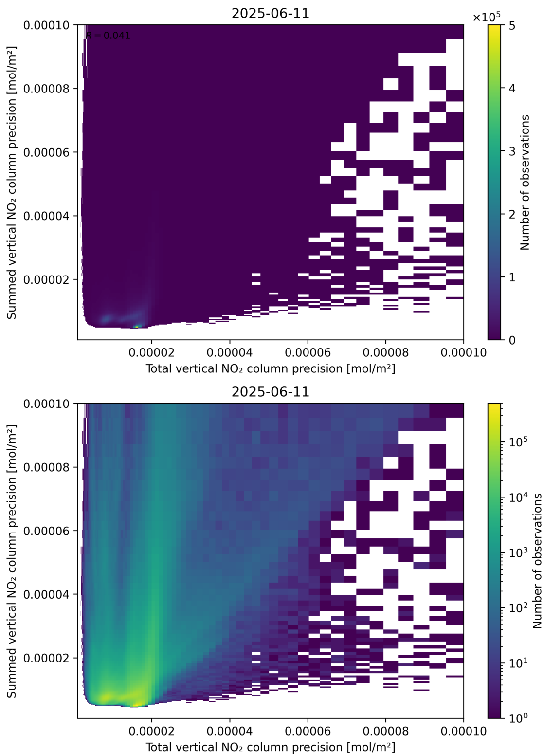
Figure 118: Scatter density plot of “Total vertical NO 2 column precision” against “Summed vertical NO 2 column precision” for 2025-06-11 to 2025-06-12.
