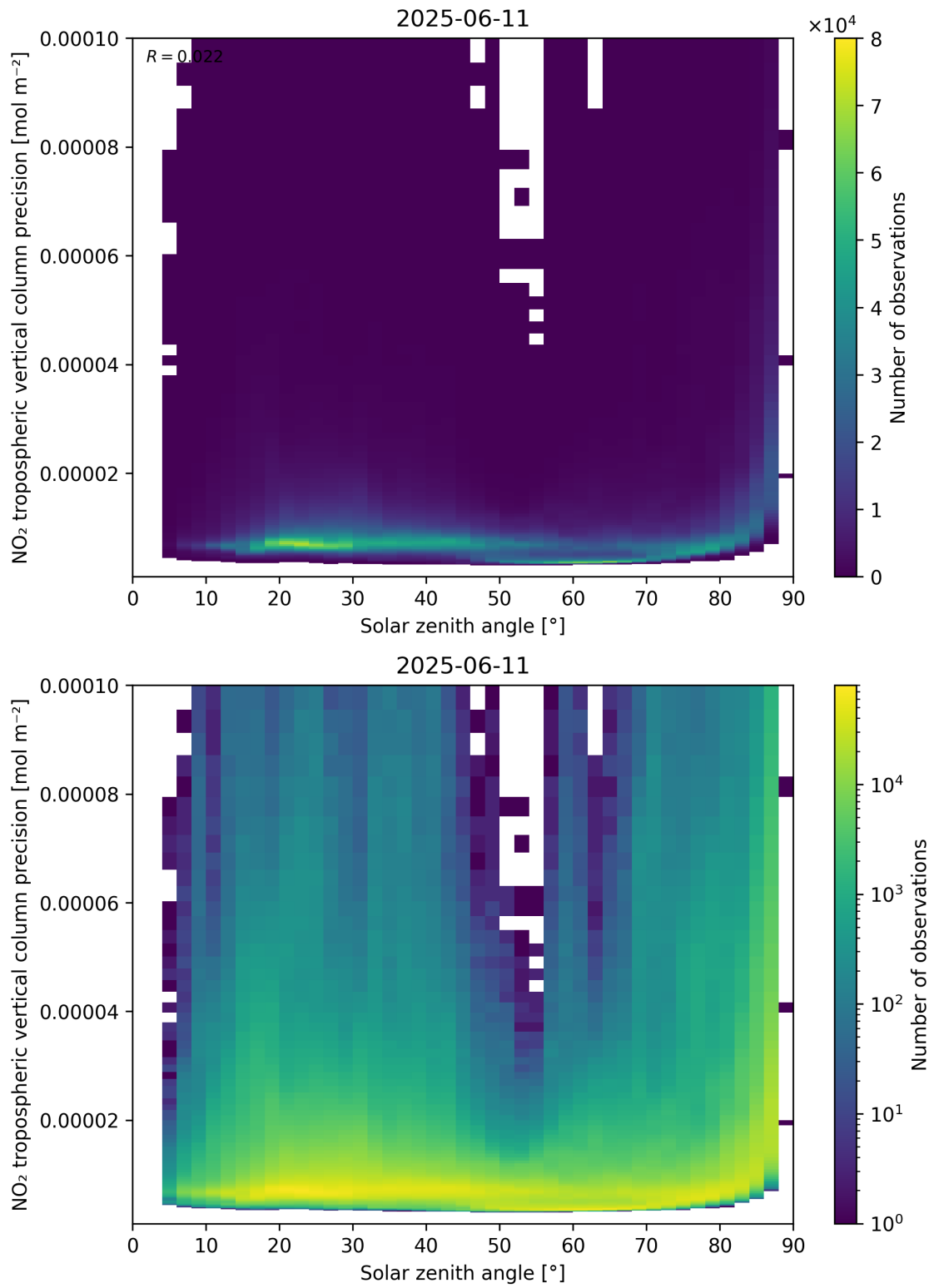
Figure 156: Scatter density plot of “Solar zenith angle” against “NO 2 tropospheric vertical column precision” for 2025-06-11 to 2025-06-12.
