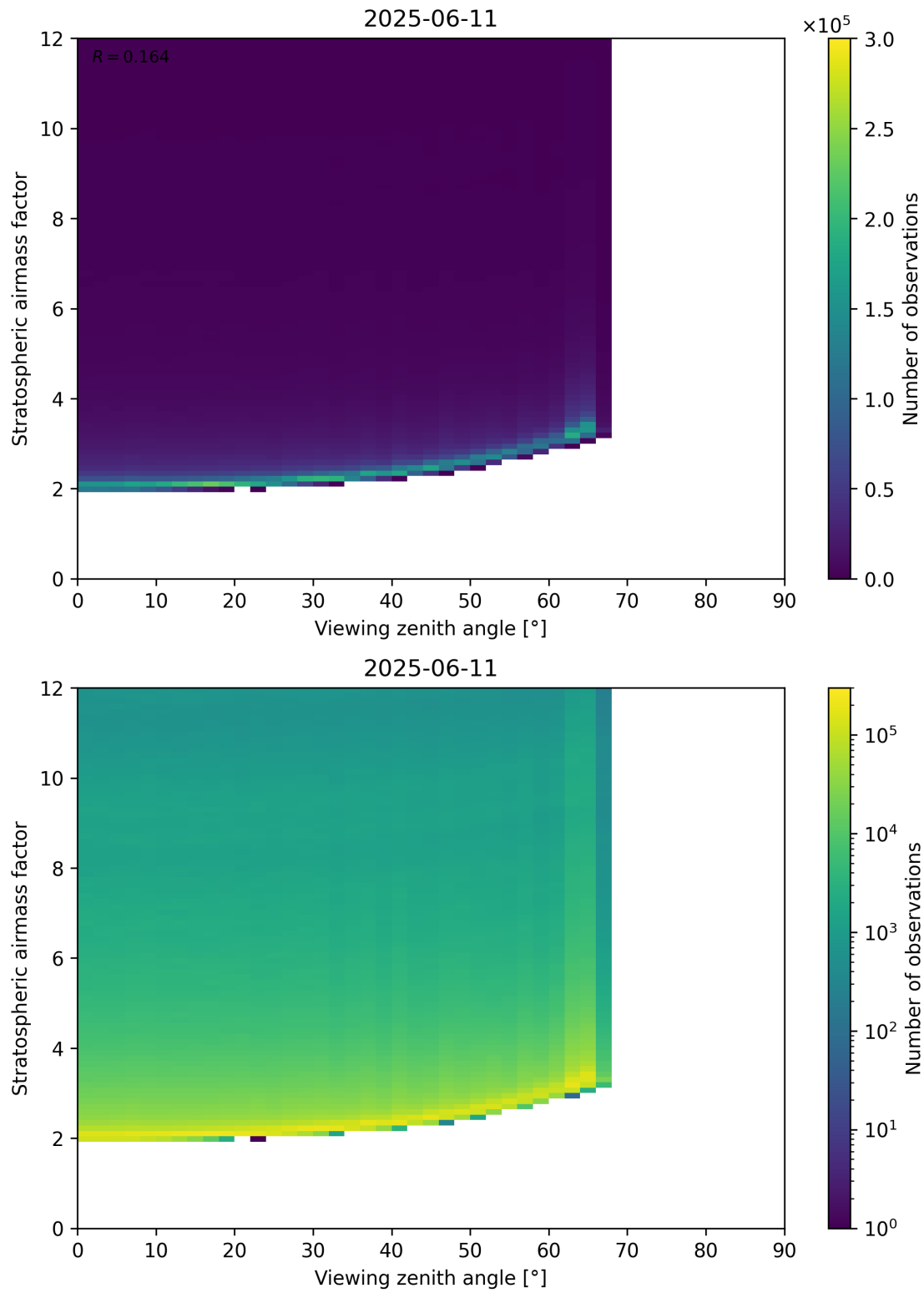
Figure 159: Scatter density plot of “Viewing zenith angle” against “Stratospheric airmass factor” for 2025-06-11 to 2025-06-12.
