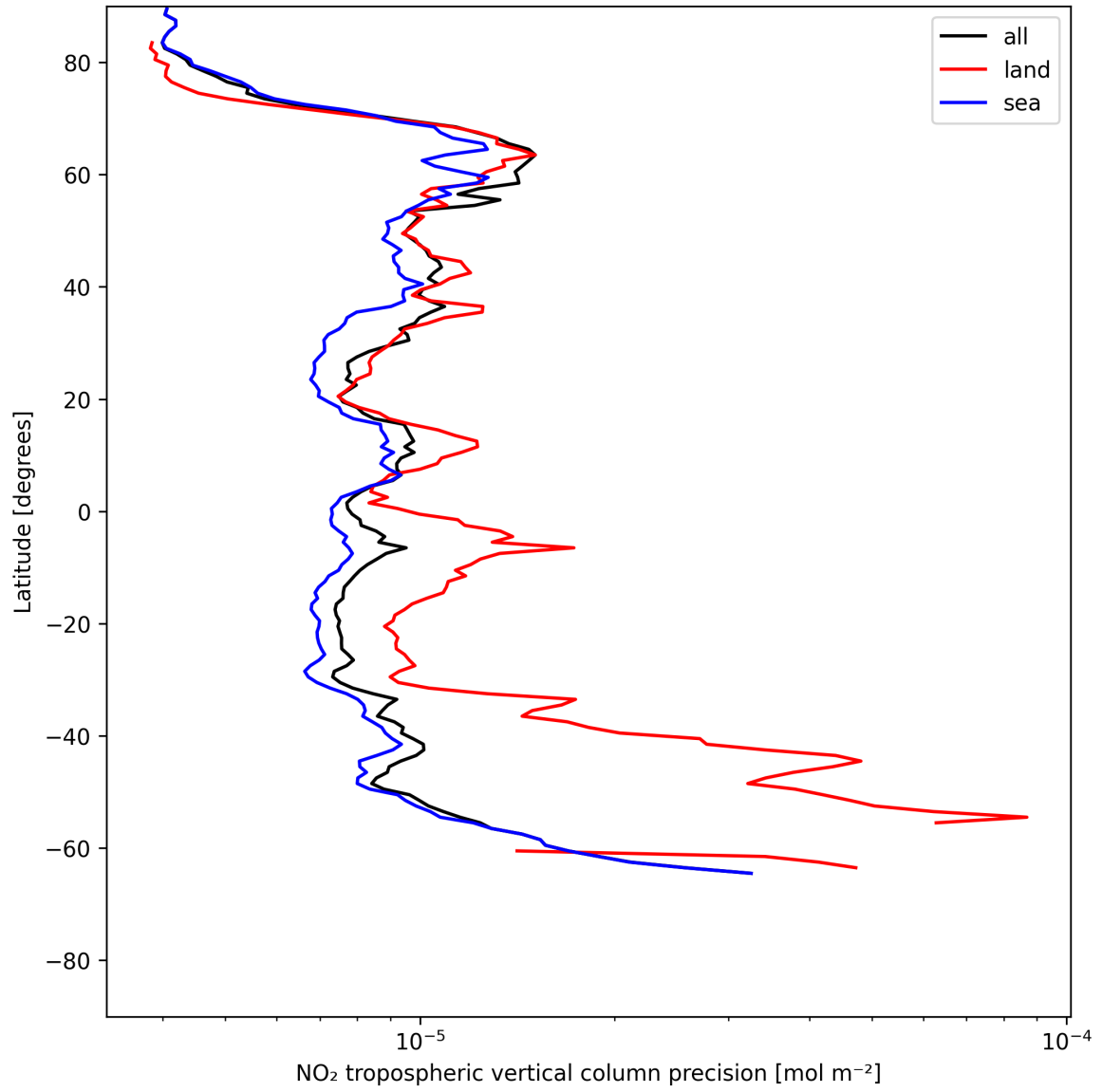
Figure 13: Zonal average of “NO 2 tropospheric vertical column precision” for 2025-06-11 to 2025-06-12.
