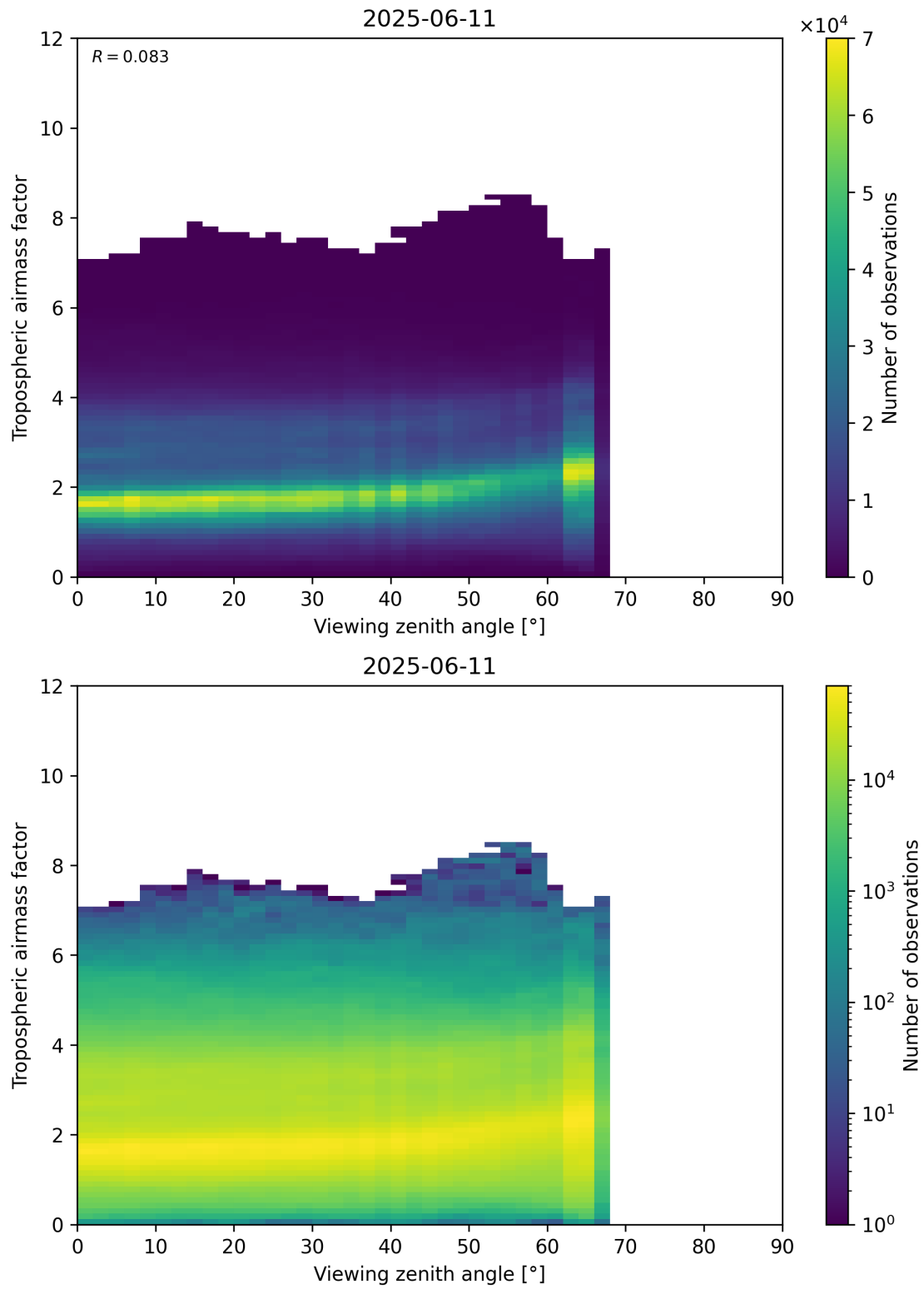
Figure 161: Scatter density plot of “Viewing zenith angle” against “Tropospheric airmass factor” for 2025-06-11 to 2025-06-12.
