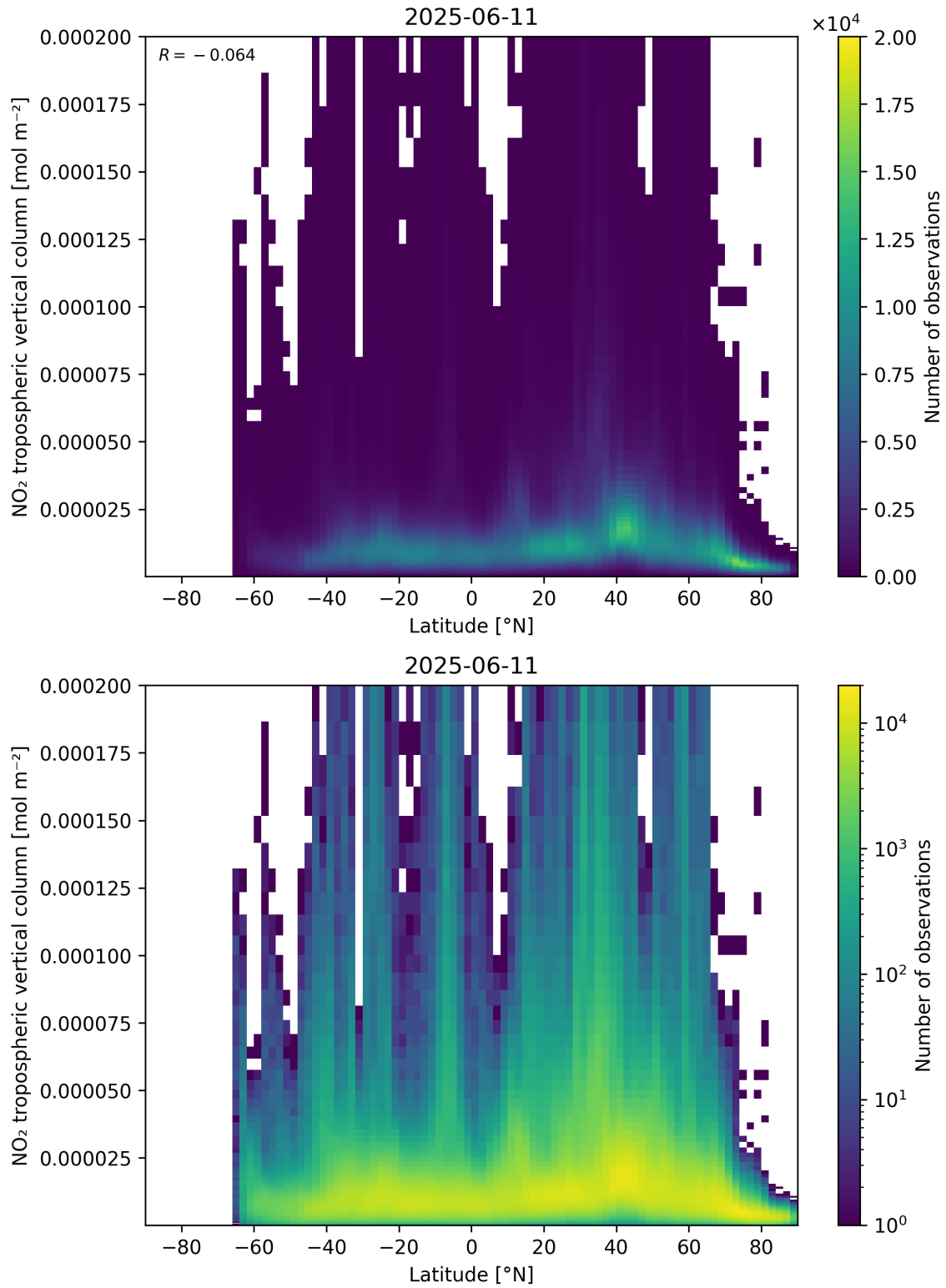
Figure 92: Scatter density plot of “Latitude” against “NO 2 tropospheric vertical column” for 2025-06-11 to 2025-06-12.
