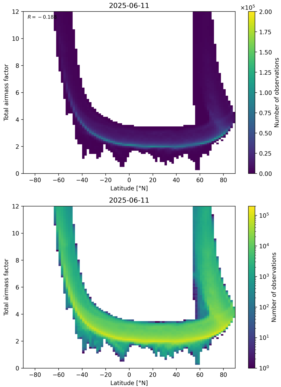
Figure 84: Scatter density plot of “Latitude” against “Total airmass factor” for 2025-06-11 to 2025-06-12.
