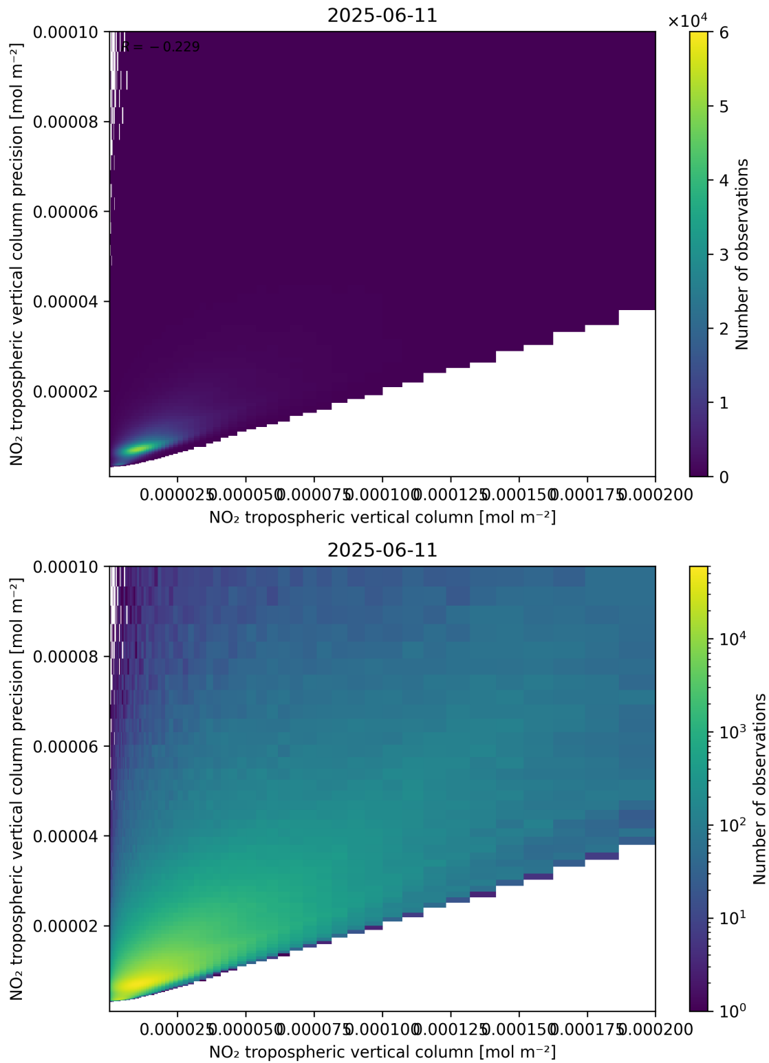
Figure 130: Scatter density plot of “NO 2 tropospheric vertical column” against “NO 2 tropospheric vertical column precision” for 2025-06-11 to 2025-06-12.
