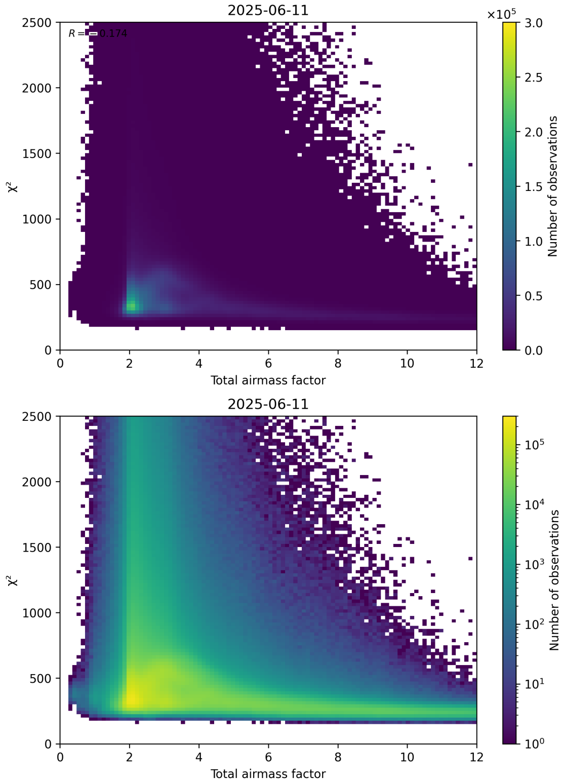
Figure 63: Scatter density plot of “Total airmass factor” against “ \chi^2 ” for 2025-06-11 to 2025-06-12.
