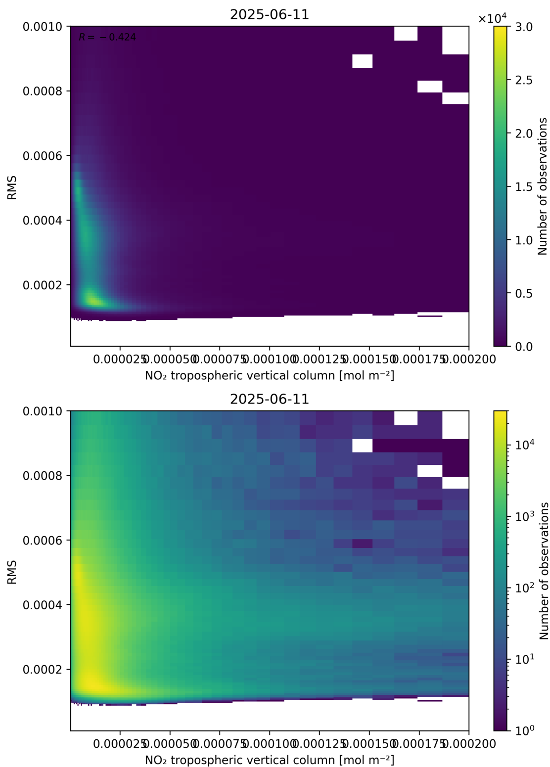
Figure 142: Scatter density plot of “NO 2 tropospheric vertical column” against “RMS” for 2025-06-11 to 2025-06-12.
