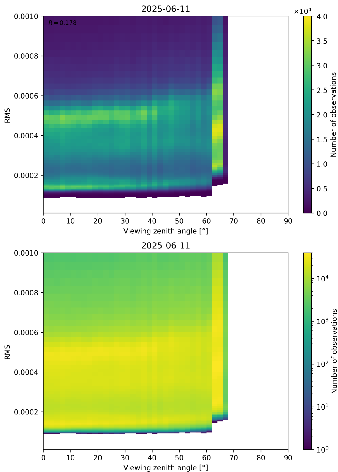
Figure 171: Scatter density plot of “Viewing zenith angle” against “RMS” for 2025-06-11 to 2025-06-12.
