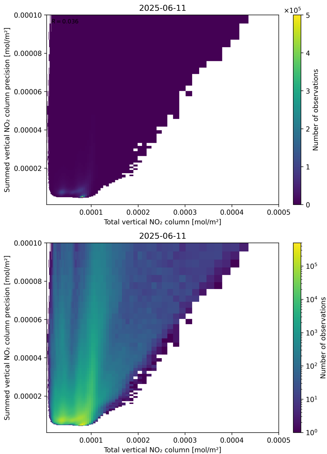
Figure 113: Scatter density plot of “Total vertical NO 2 column” against “Summed vertical NO 2 column precision” for 2025-06-11 to 2025-06-12.
