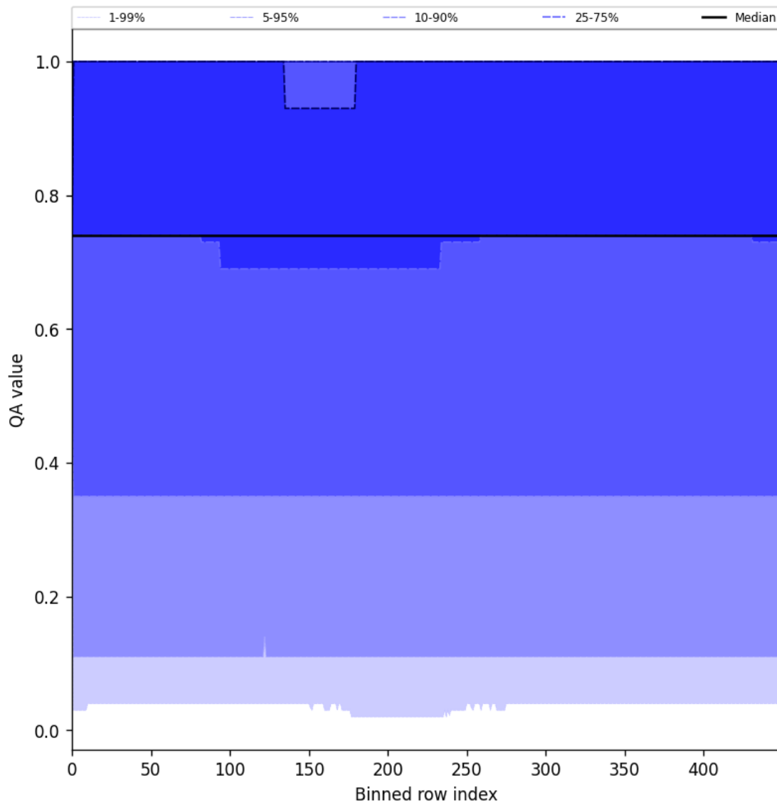
Figure 45: Along track statistics of “QA value” for 2025-06-11 to 2025-06-12
