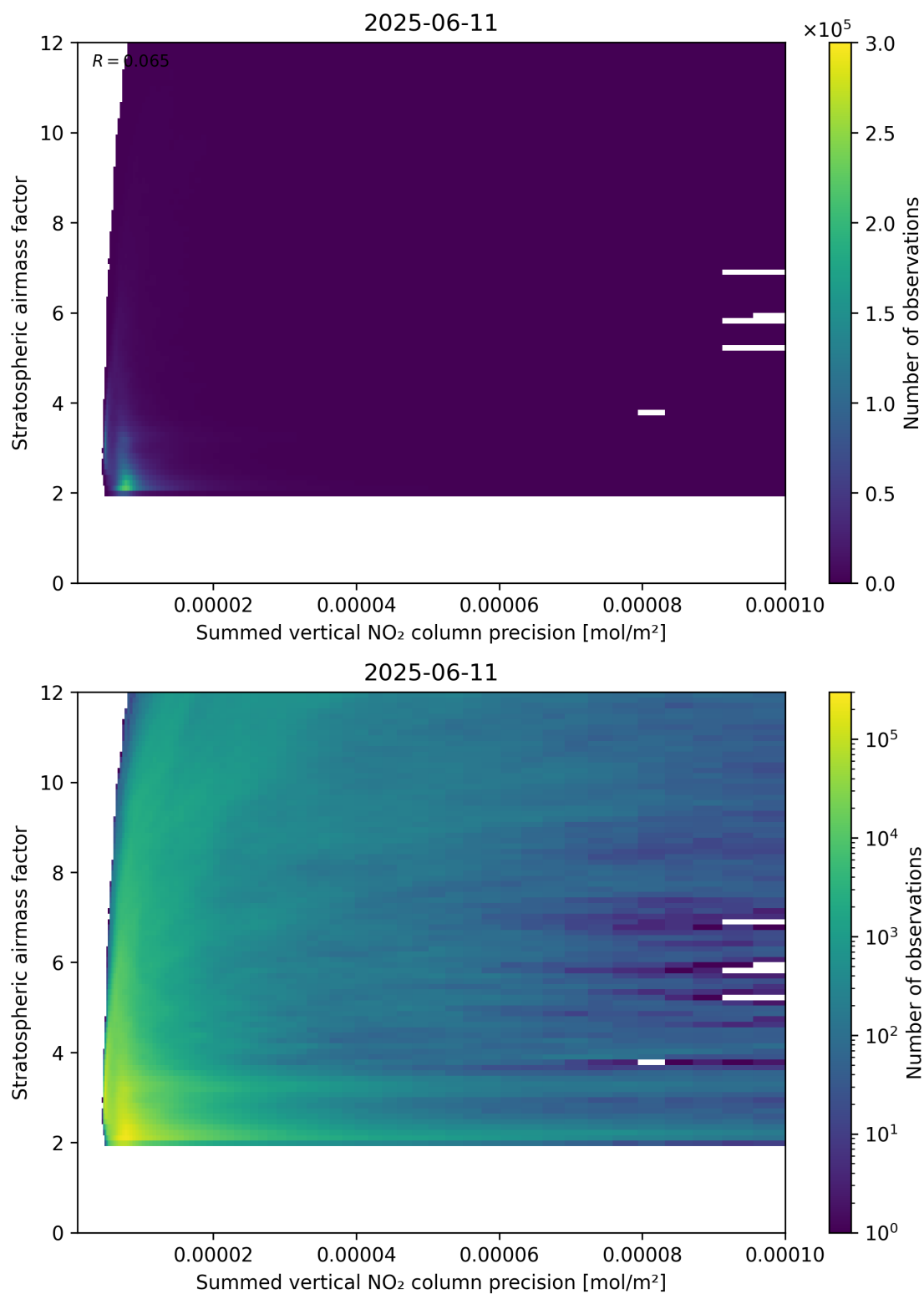
Figure 106: Scatter density plot of “Summed vertical NO 2 column precision” against “Stratospheric airmass factor” for 2025-06-11 to 2025-06-12.
