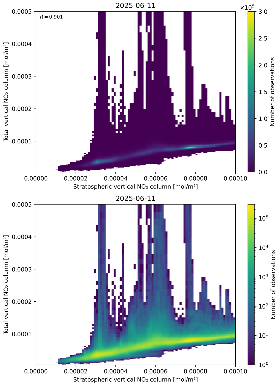
Figure 100: Scatter density plot of “Stratospheric vertical NO 2 column” against “Total vertical NO 2 column” for 2025-06-11 to 2025-06-12.
