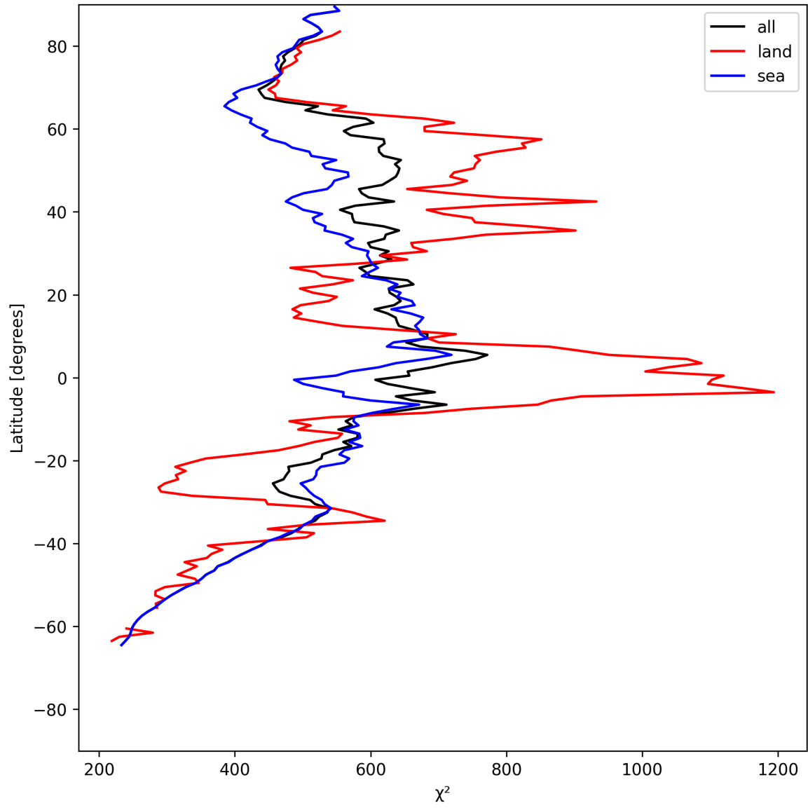
Figure 25: Zonal average of “ \chi^2 ” for 2025-06-11 to 2025-06-12.
