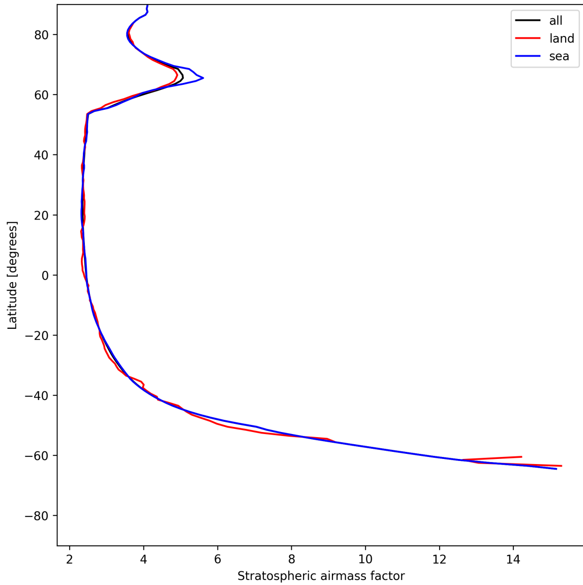
Figure 27: Zonal average of “Stratospheric air mass factor” for 2025-06-11 to 2025-06-12.
