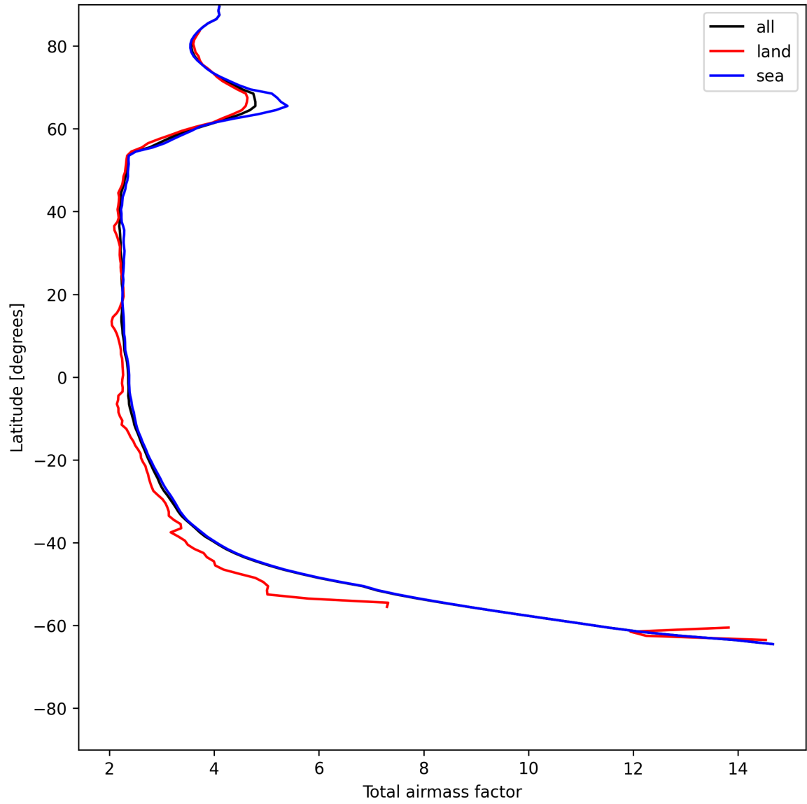
Figure 15: Zonal average of “Total airmass factor” for 2025-06-11 to 2025-06-12.
