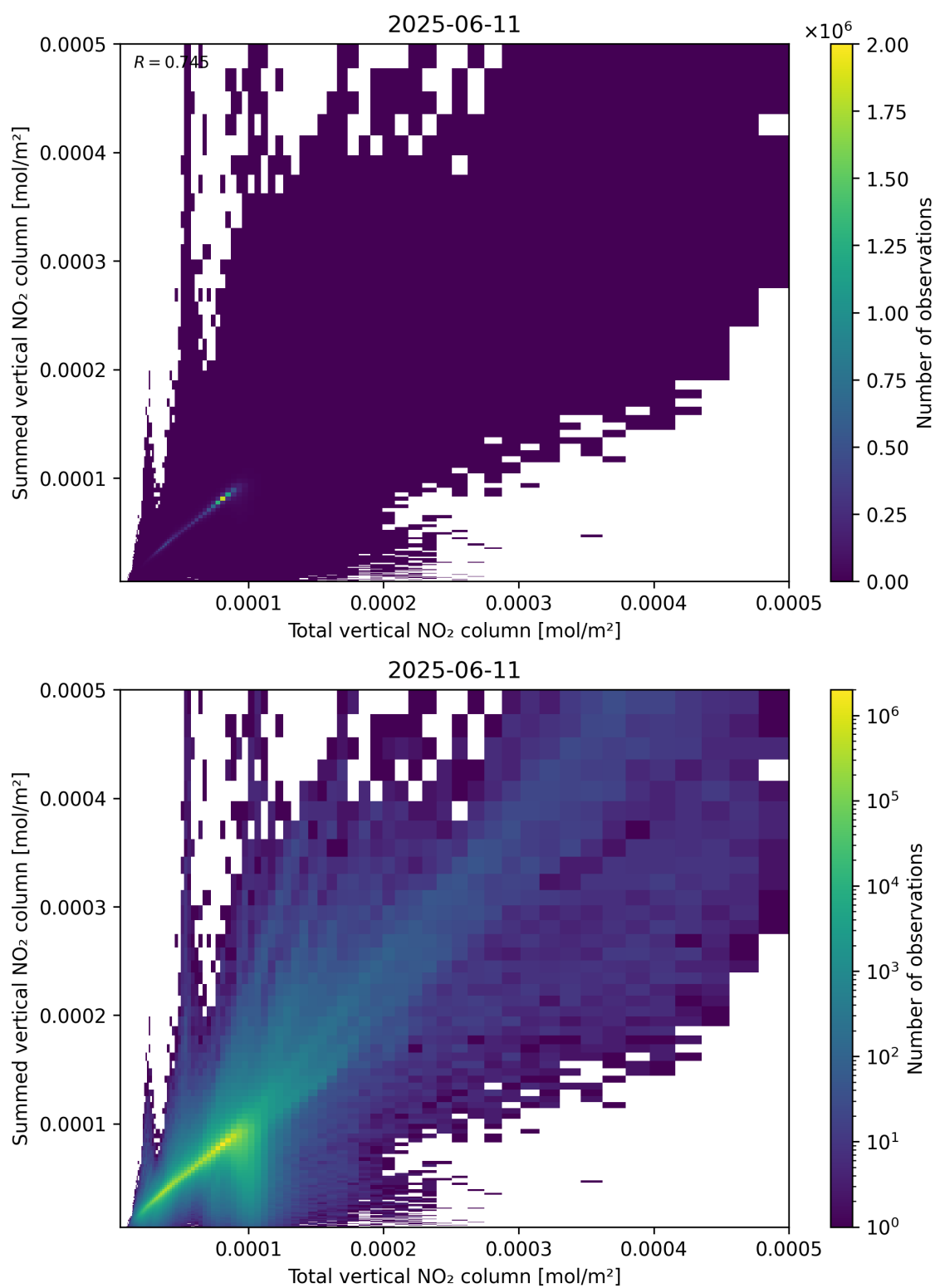
Figure 112: Scatter density plot of “Total vertical NO 2 column” against “Summed vertical NO 2 column” for 2025-06-11 to 2025-06-12.
