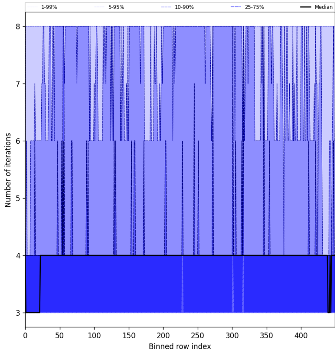
Figure 51: Along track statistics of “Number of iterations” for 2025-06-11 to 2025-06-12
