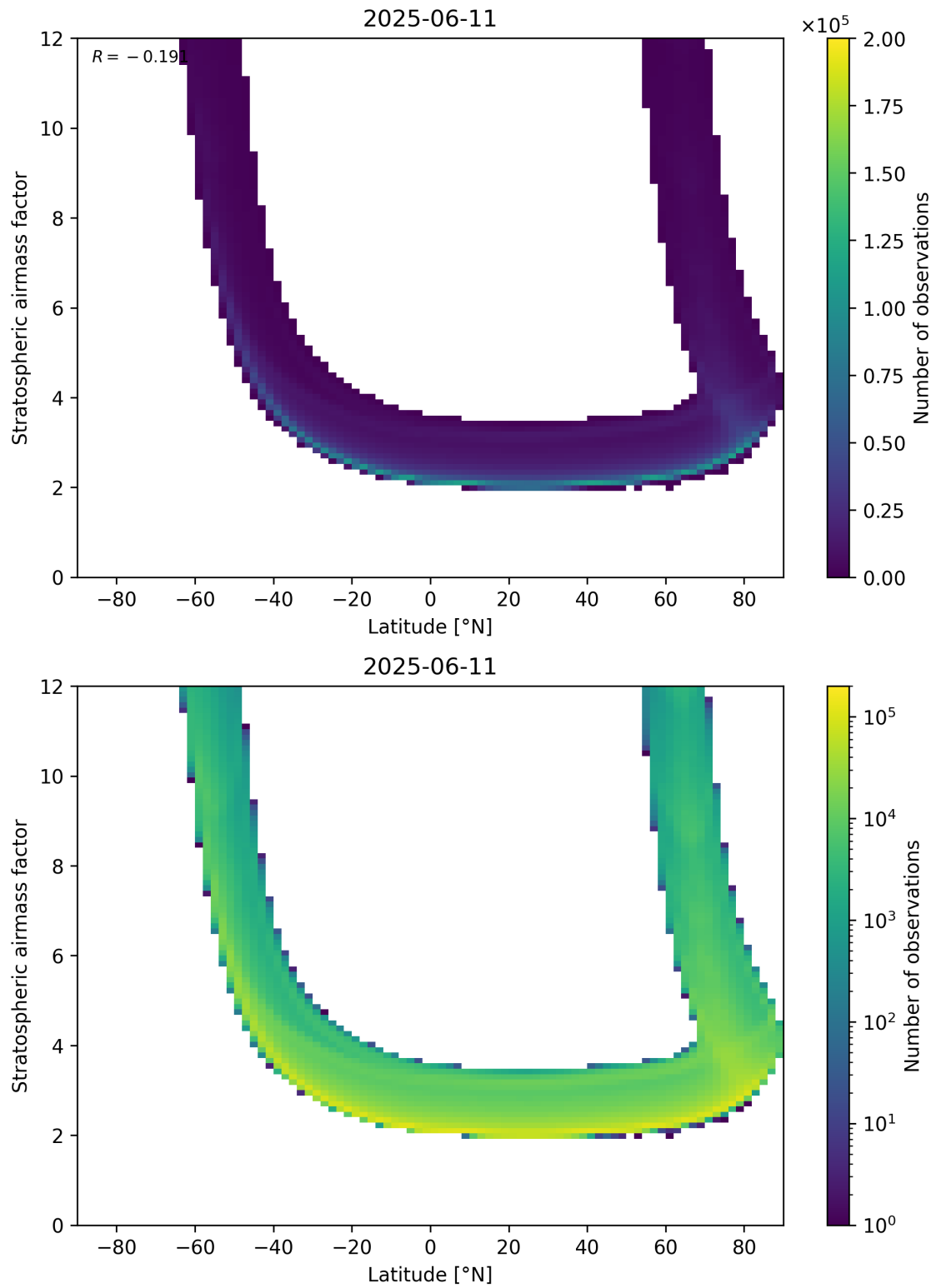
Figure 83: Scatter density plot of “Latitude” against “Stratospheric air mass factor” for 2025-06-11 to 2025-06-12.
