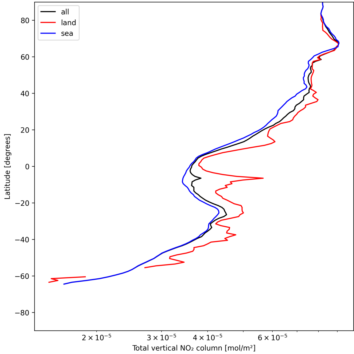
Figure 21: Zonal average of “Total vertical NO 2 column” for 2025-06-11 to 2025-06-12.
