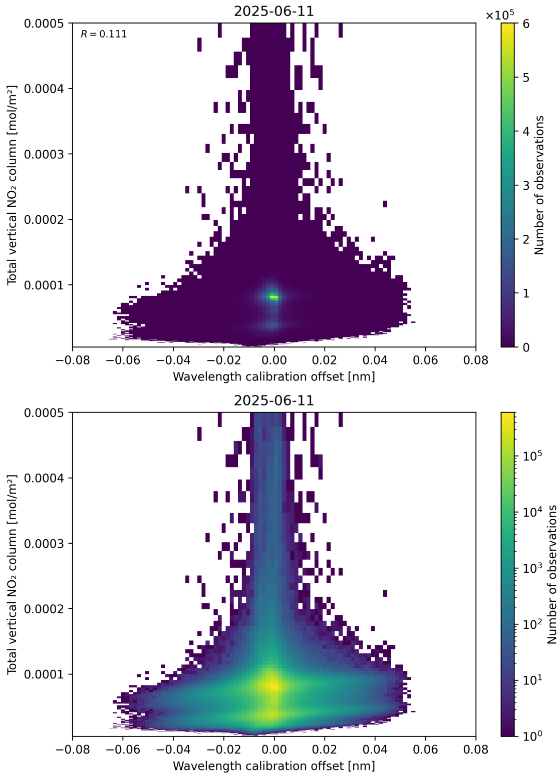
Figure 179: Scatter density plot of “Wavelength calibration offset” against “Total vertical NO 2 column” for 2025-06-11 to 2025-06-12.
