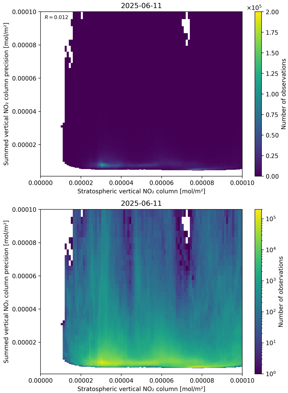
Figure 99: Scatter density plot of “Stratospheric vertical NO 2 column” against “Summed vertical NO 2 column precision” for 2025-06-11 to 2025-06-12.
