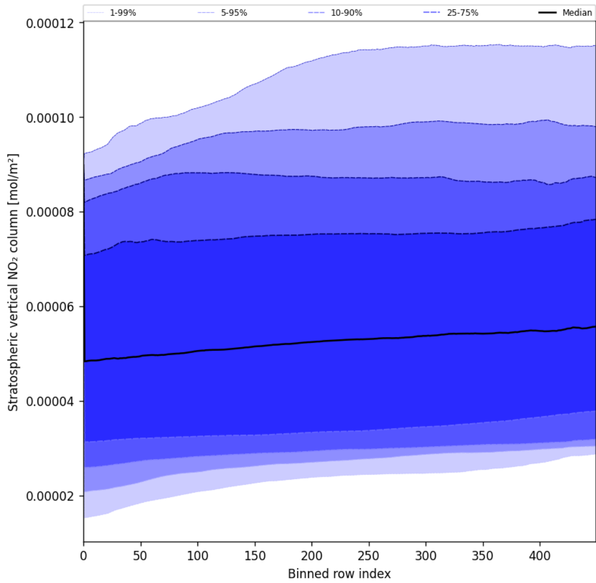
Figure 53: Along track statistics of “Stratospheric vertical NO 2 column” for 2025-06-11 to 2025-06-12
