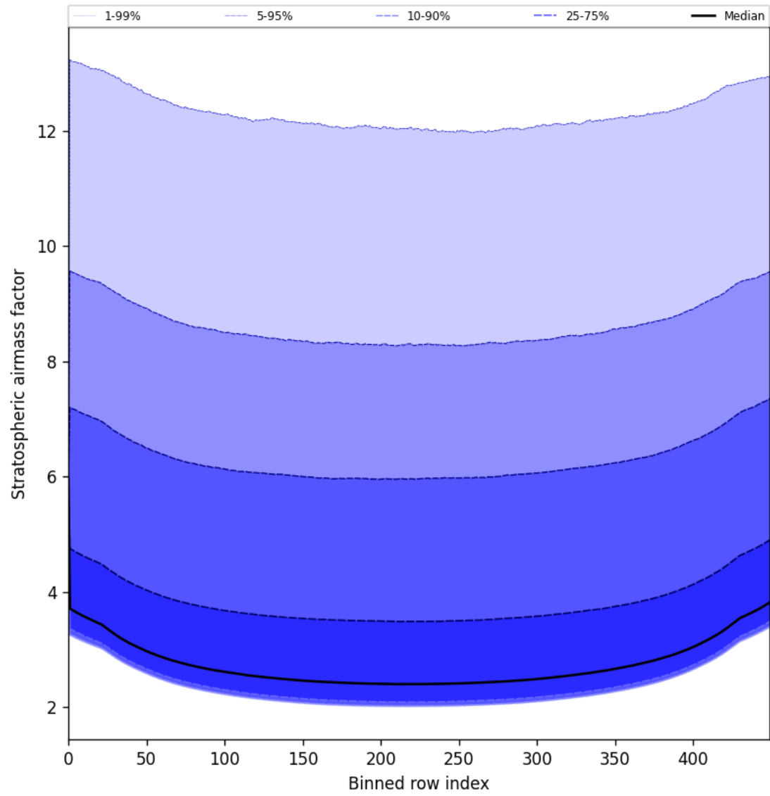
Figure 61: Along track statistics of “Stratospheric airmass factor” for 2025-06-11 to 2025-06-12
