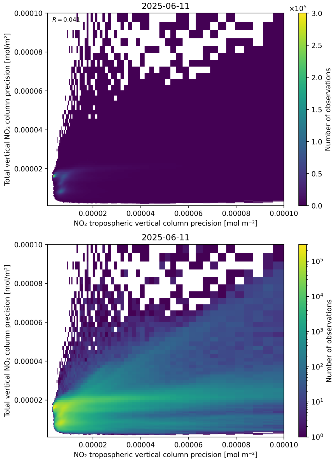
Figure 139: Scatter density plot of “NO 2 tropospheric vertical column precision” against “Total vertical NO 2 column precision” for 2025-06-11 to 2025-06-12.
