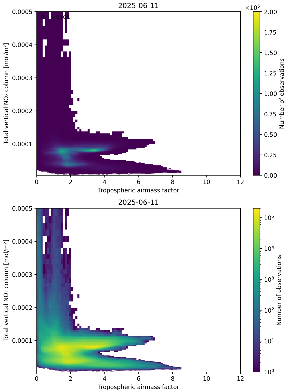
Figure 77: Scatter density plot of “Tropospheric airmass factor” against “Total vertical NO 2 column” for 2025-06-11 to 2025-06-12.
