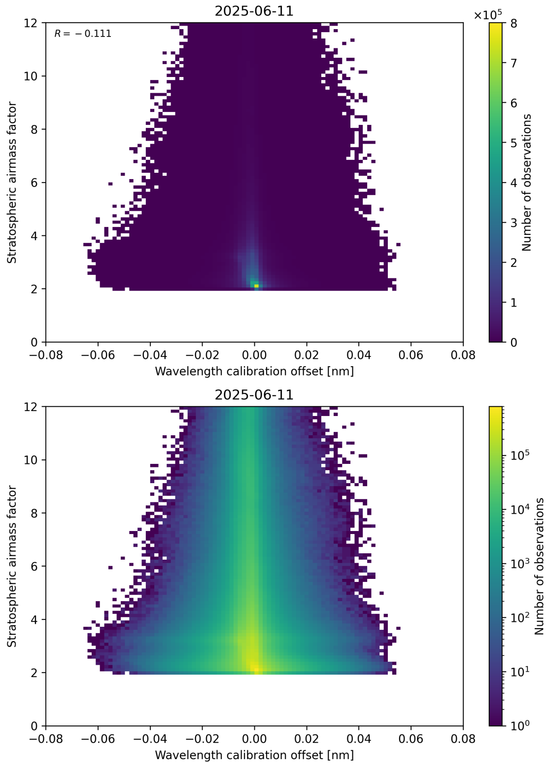
Figure 174: Scatter density plot of “Wavelength calibration offset” against “Stratospheric air mass factor” for 2025-06-11 to 2025-06-12.
