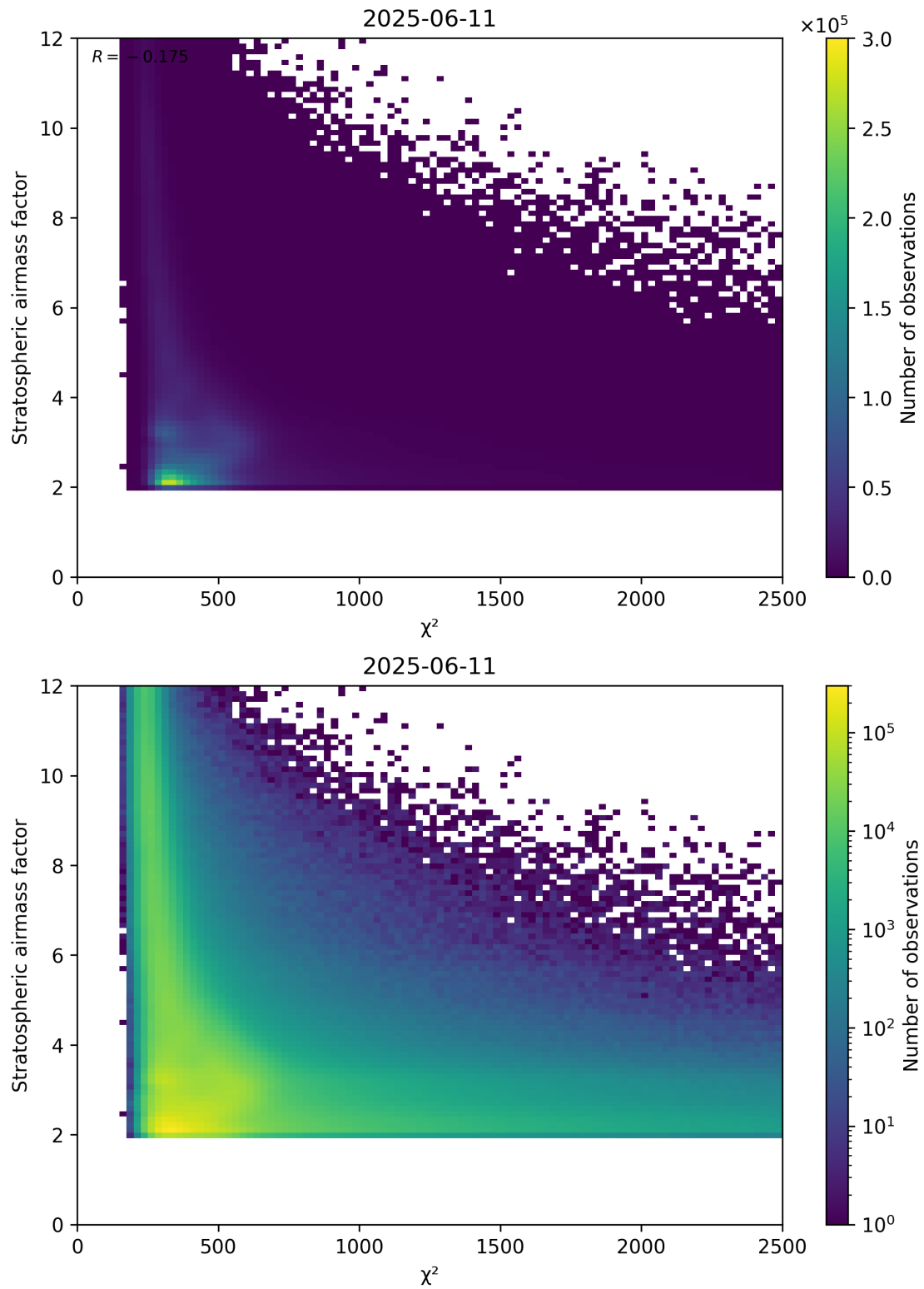
Figure 81: Scatter density plot of “ \chi^2 ” against “Stratospheric airmass factor” for 2025-06-11 to 2025-06-12.
