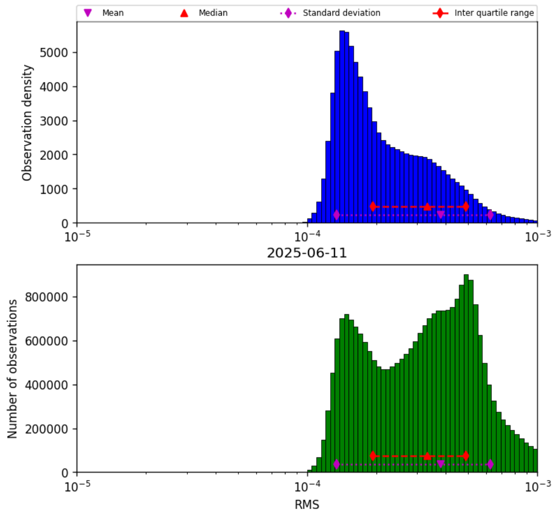
Figure 43: Histogram of “RMS” for 2025-06-11 to 2025-06-12
