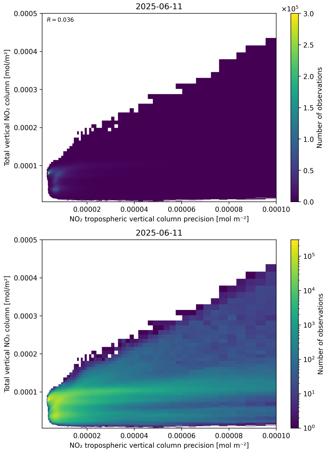
Figure 138: Scatter density plot of “NO 2 tropospheric vertical column precision” against “Total vertical NO 2 column” for 2025-06-11 to 2025-06-12.
