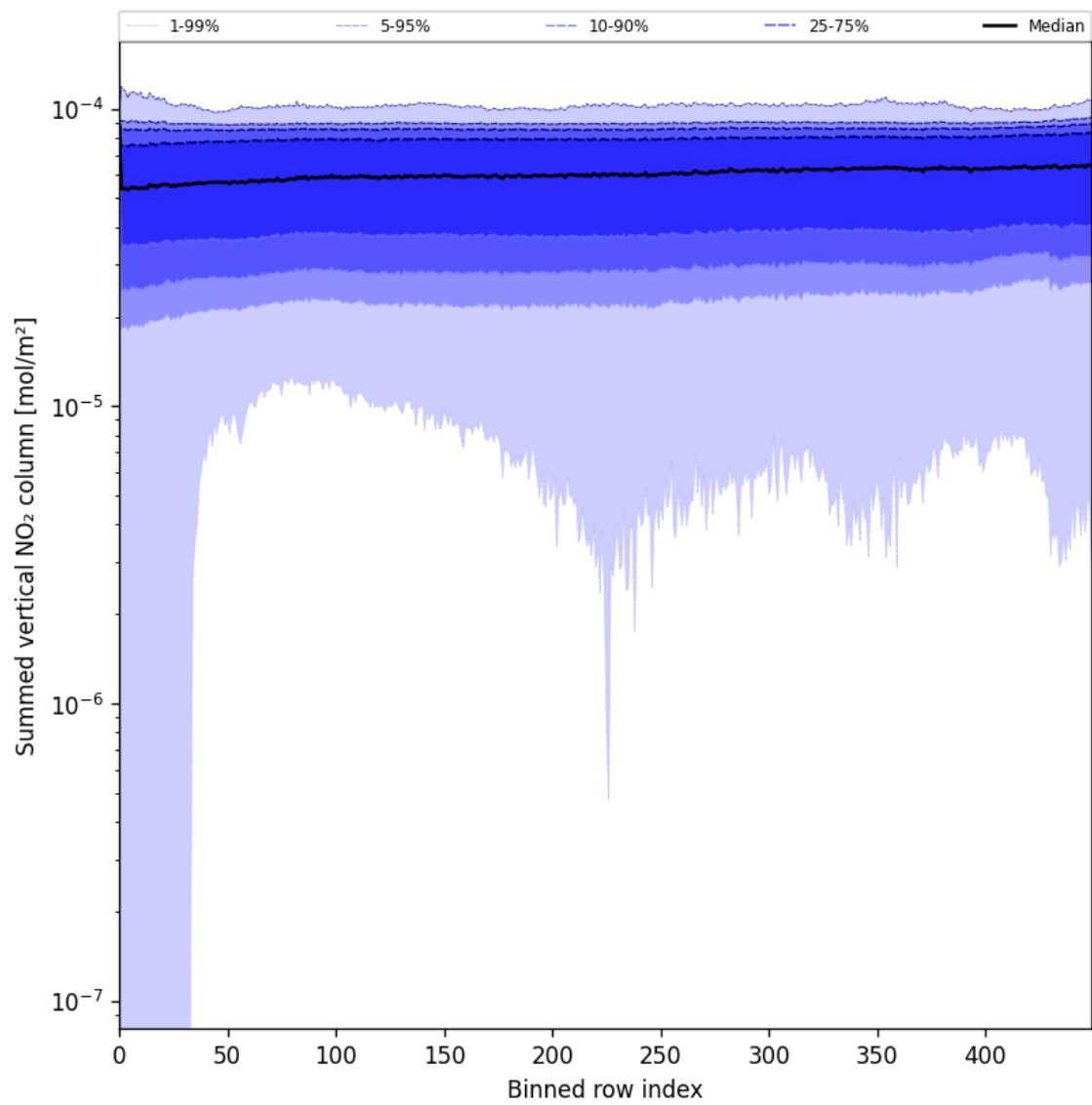
Figure 57: Along track statistics of “Summed vertical NO 2 column” for 2025-06-11 to 2025-06-12
