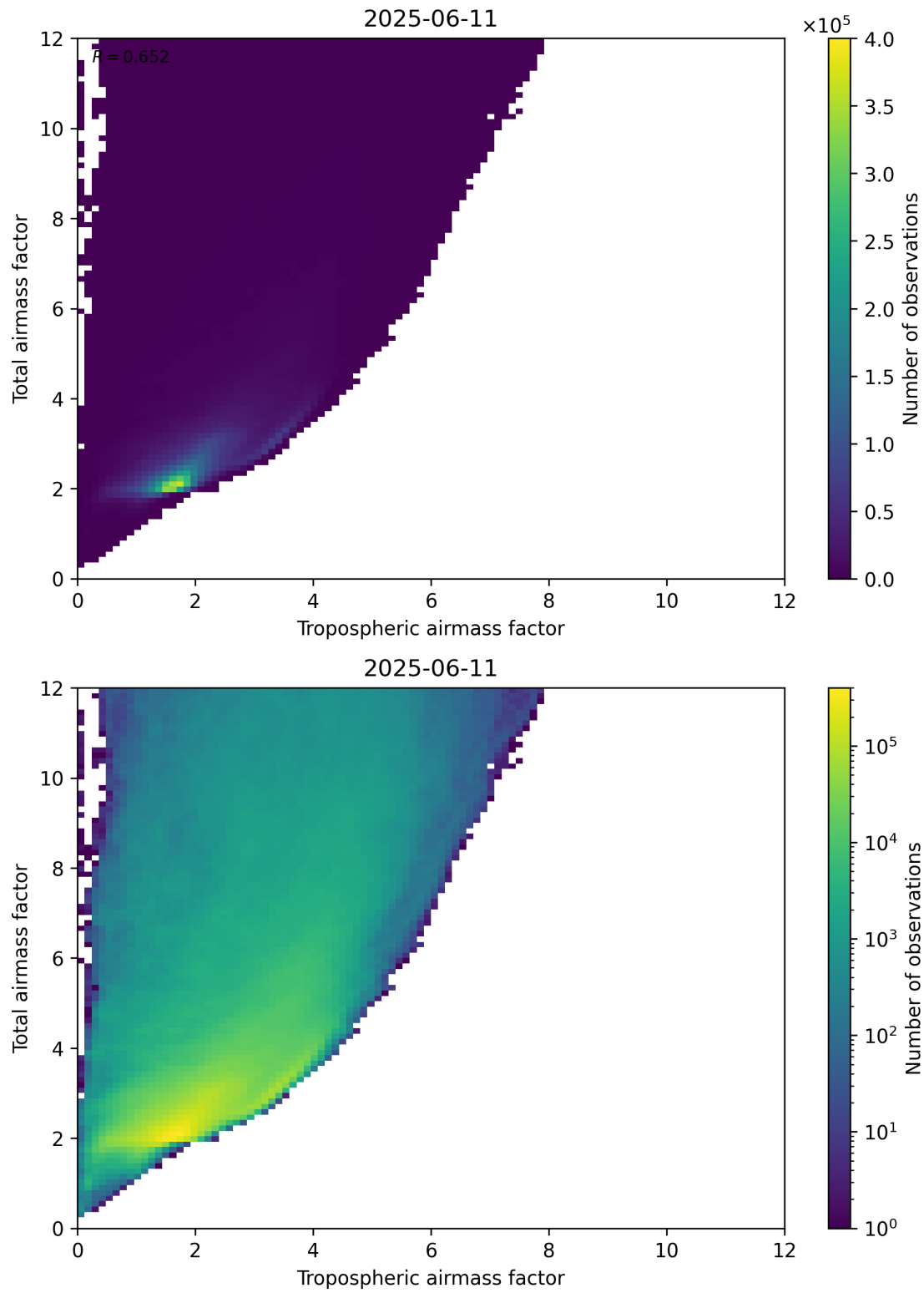
Figure 72: Scatter density plot of “Tropospheric airmass factor” against “Total airmass factor” for 2025-06-11 to 2025-06-12.
