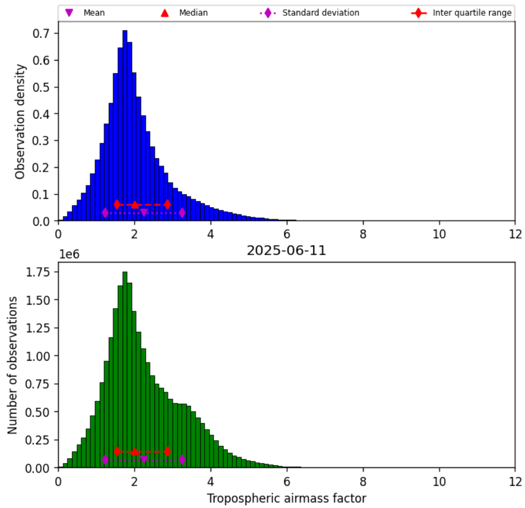
Figure 31: Histogram of “Tropospheric airmass factor” for 2025-06-11 to 2025-06-12
