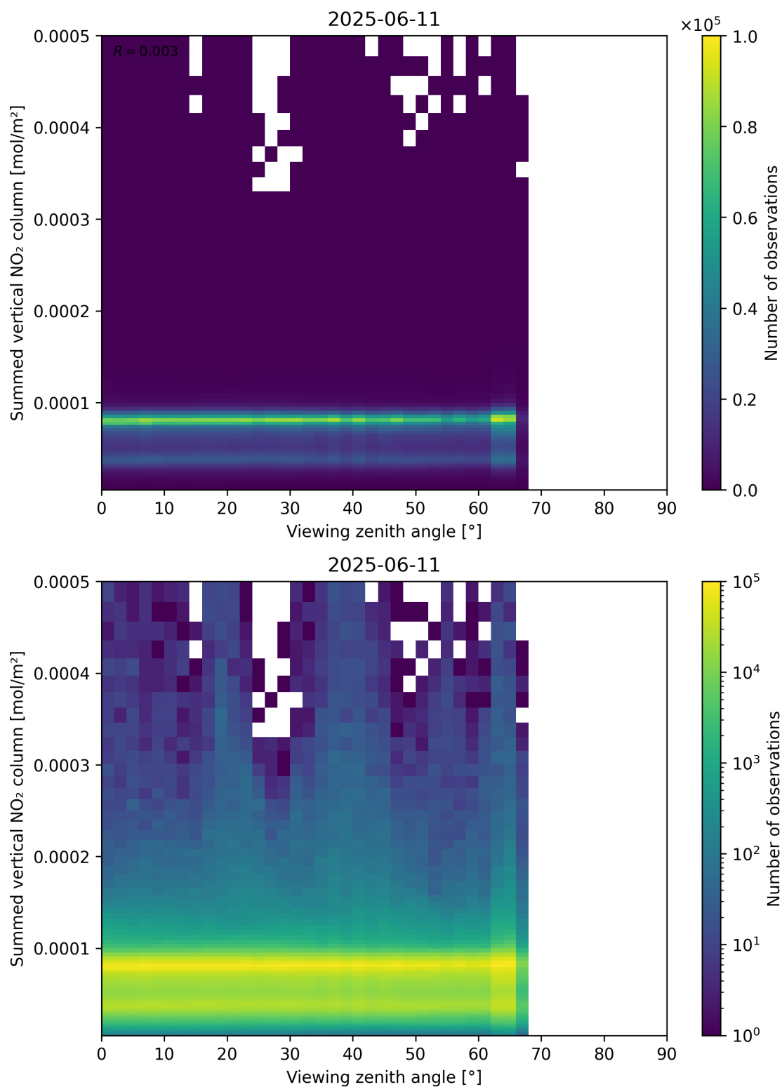
Figure 165: Scatter density plot of “Viewing zenith angle” against “Summed vertical NO 2 column” for 2025-06-11 to 2025-06-12.
