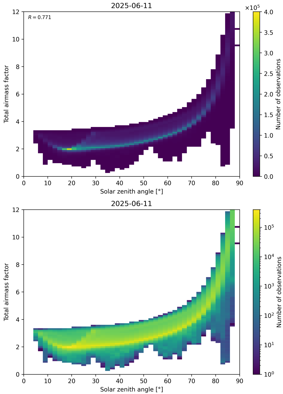
Figure 146: Scatter density plot of “Solar zenith angle” against “Total air mass factor” for 2025-06-11 to 2025-06-12.
