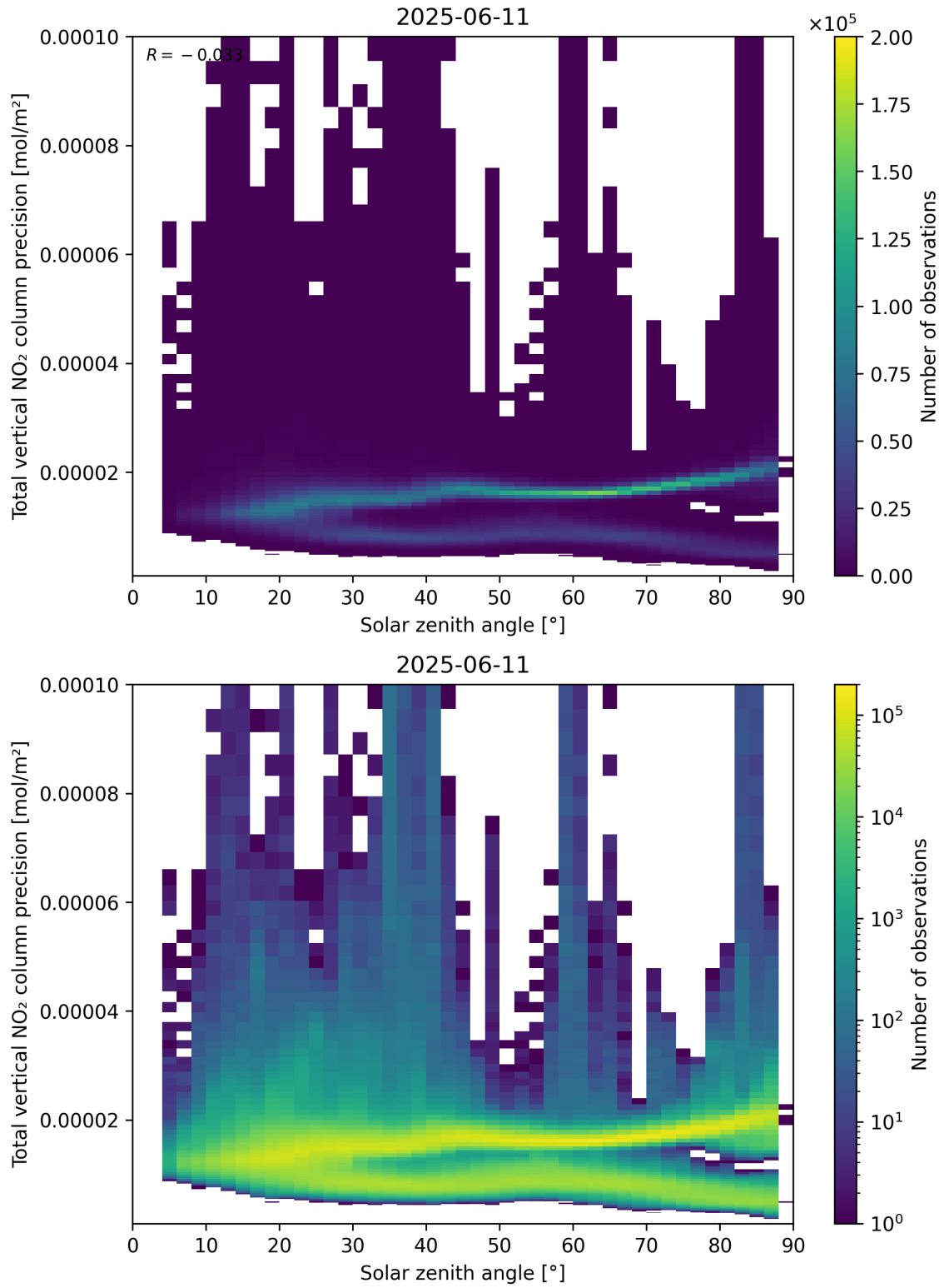
Figure 154: Scatter density plot of “Solar zenith angle” against “Total vertical NO 2 column precision” for 2025-06-11 to 2025-06-12.
