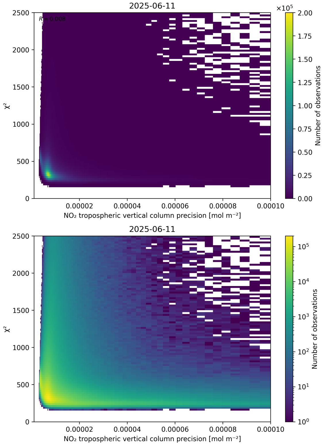
Figure 134: Scatter density plot of “NO 2 tropospheric vertical column precision” against “ \chi^2 ” for 2025-06-11 to 2025-06-12.
