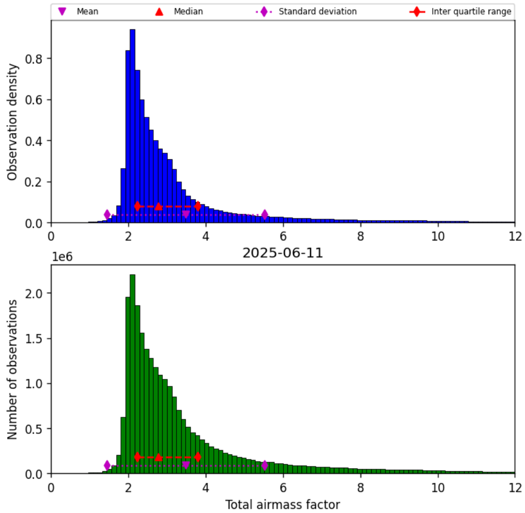
Figure 32: Histogram of “Total airmass factor” for 2025-06-11 to 2025-06-12
