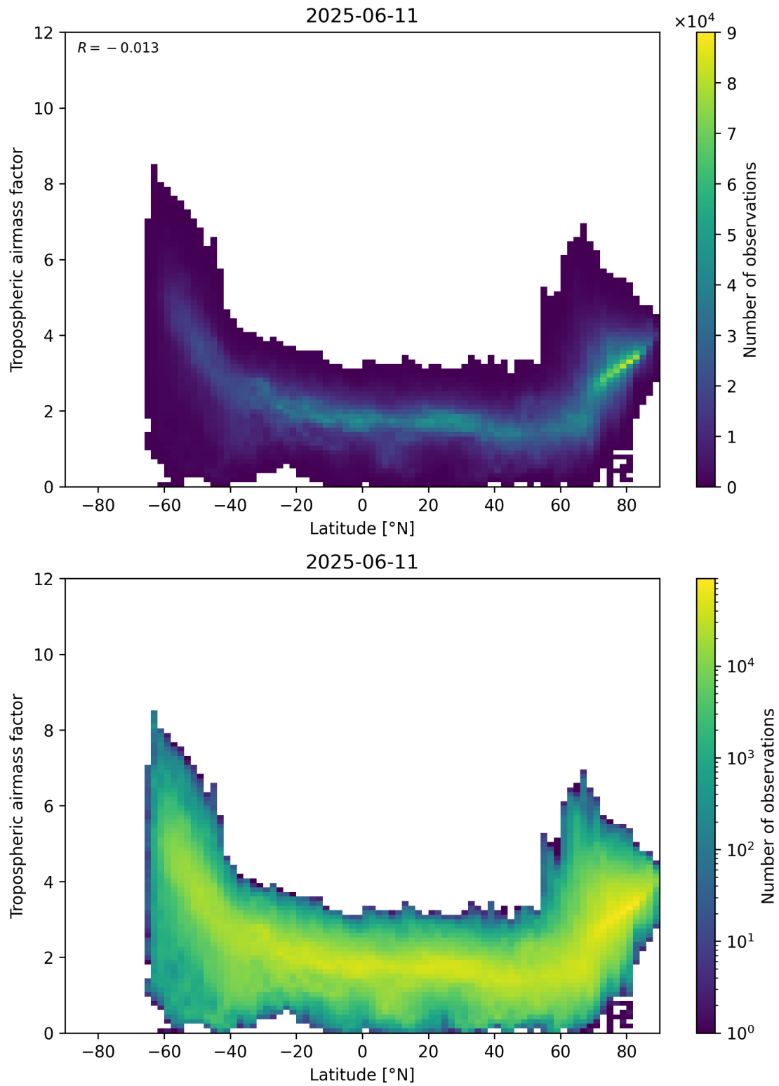
Figure 85: Scatter density plot of “Latitude” against “Tropospheric airmass factor” for 2025-06-11 to 2025-06-12.
