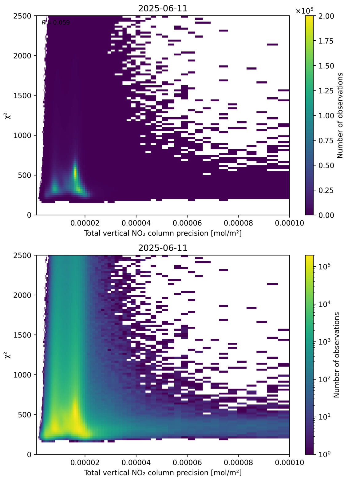
Figure 116: Scatter density plot of “Total vertical NO 2 column precision” against “ \chi^2 ” for 2025-06-11 to 2025-06-12.
