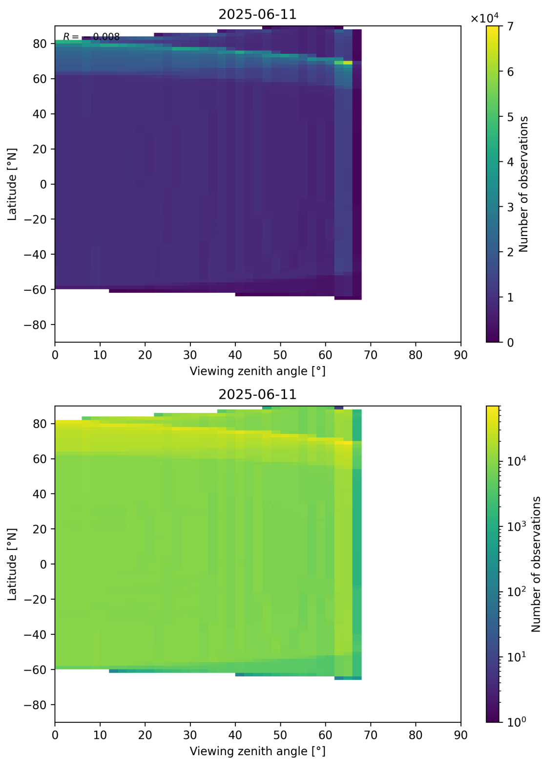
Figure 163: Scatter density plot of “Viewing zenith angle” against “Latitude” for 2025-06-11 to 2025-06-12.
