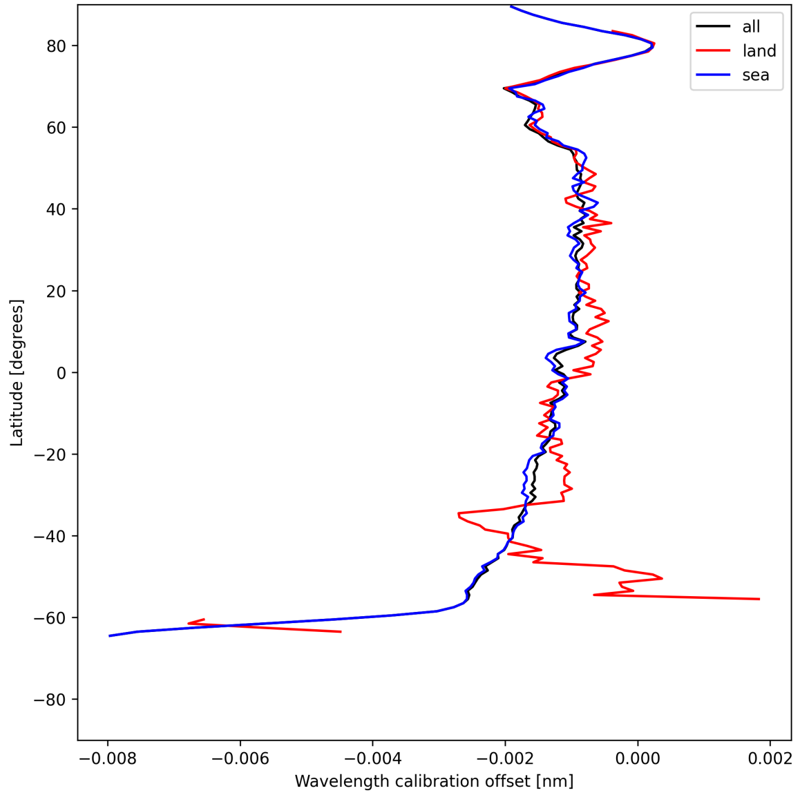
Figure 18: Zonal average of “Wavelength calibration offset” for 2025-06-11 to 2025-06-12.
