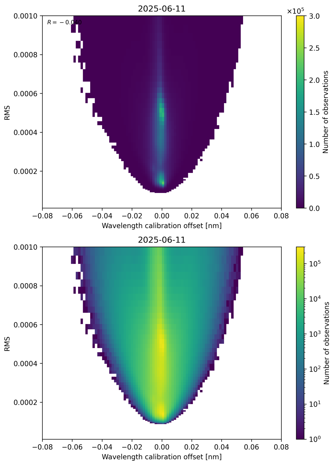
Figure 181: Scatter density plot of “Wavelength calibration offset” against “RMS” for 2025-06-11 to 2025-06-12.
