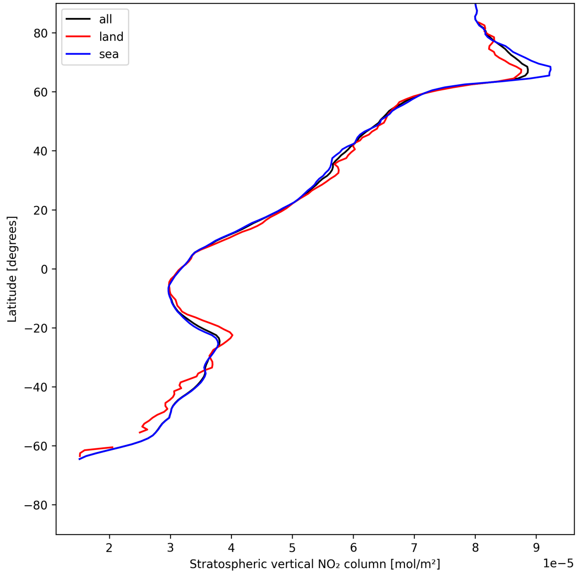
Figure 19: Zonal average of “Stratospheric vertical NO 2 column” for 2025-06-11 to 2025-06-12.
