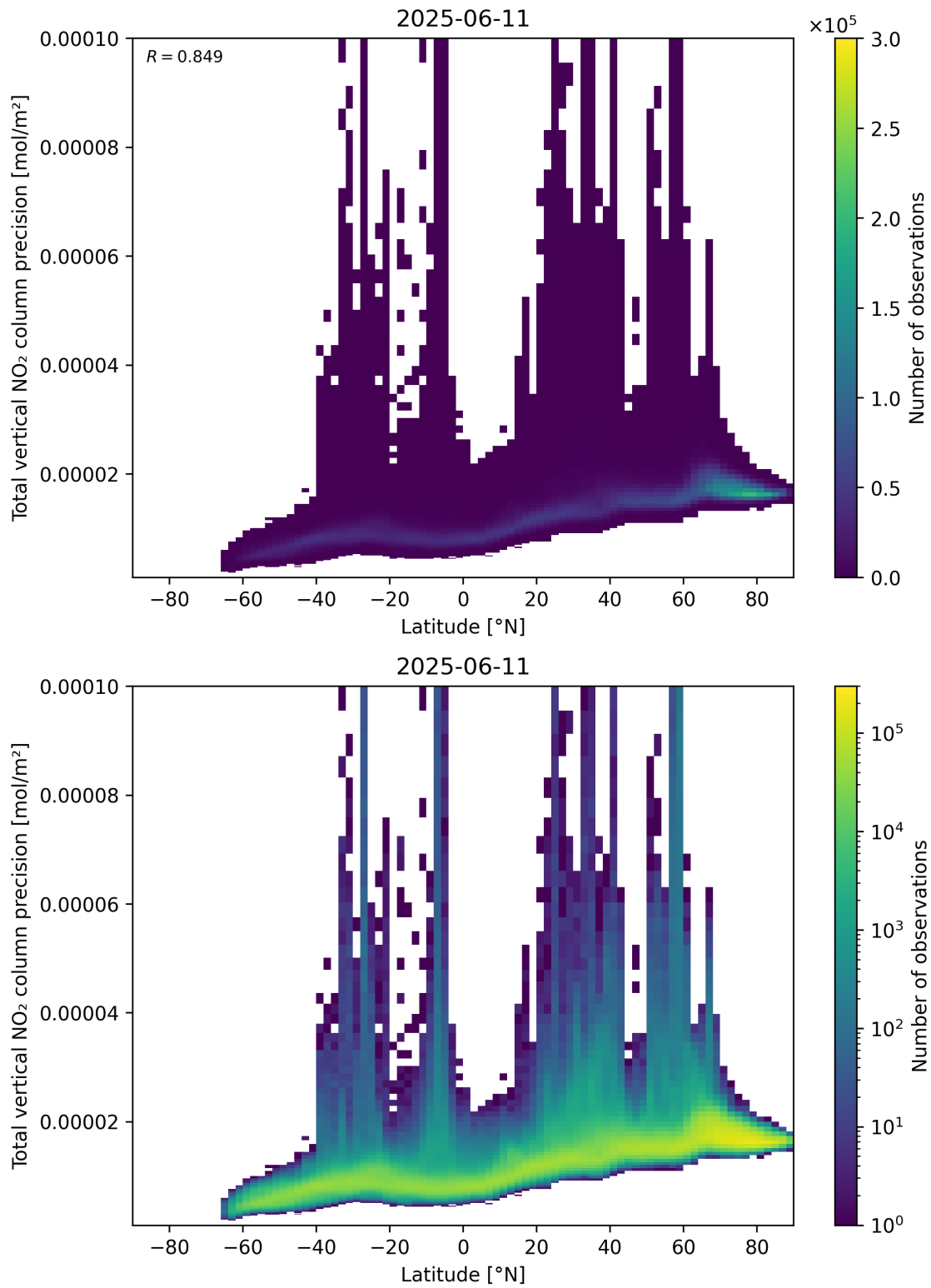
Figure 91: Scatter density plot of “Latitude” against “Total vertical NO 2 column precision” for 2025-06-11 to 2025-06-12.
