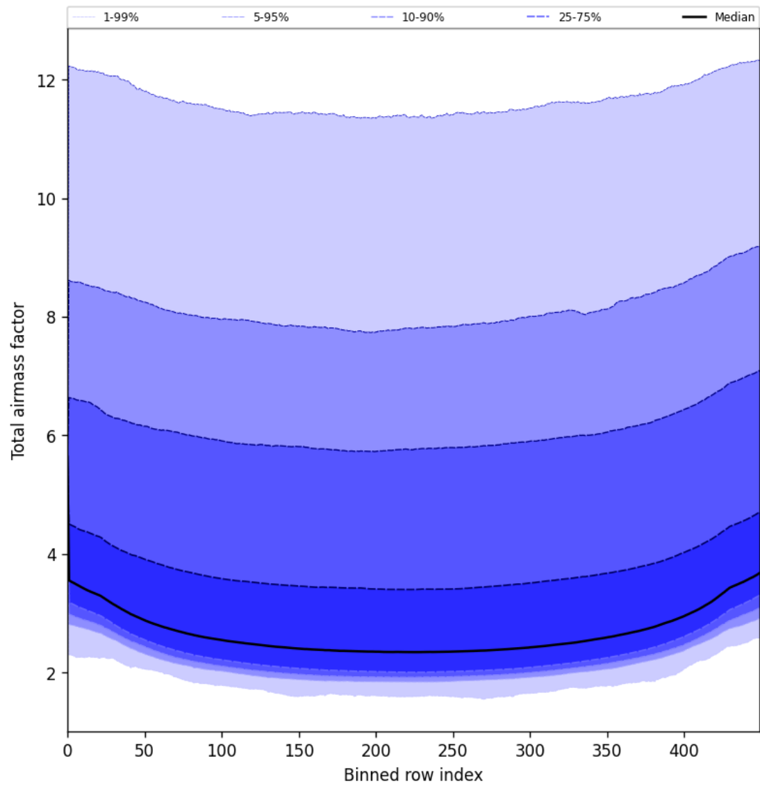
Figure 49: Along track statistics of “Total airmass factor” for 2025-06-11 to 2025-06-12
