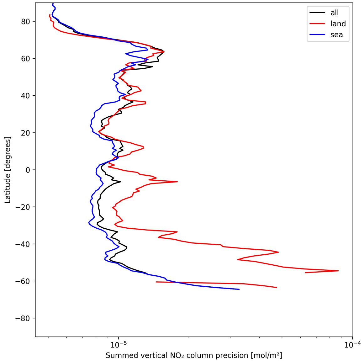
Figure 24: Zonal average of “Summed vertical NO 2 column precision” for 2025-06-11 to 2025-06-12.
