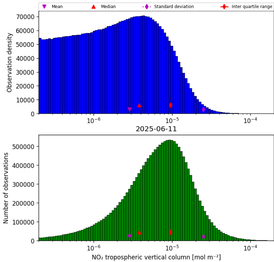
Figure 29: Histogram of “NO 2 tropospheric vertical column” for 2025-06-11 to 2025-06-12
