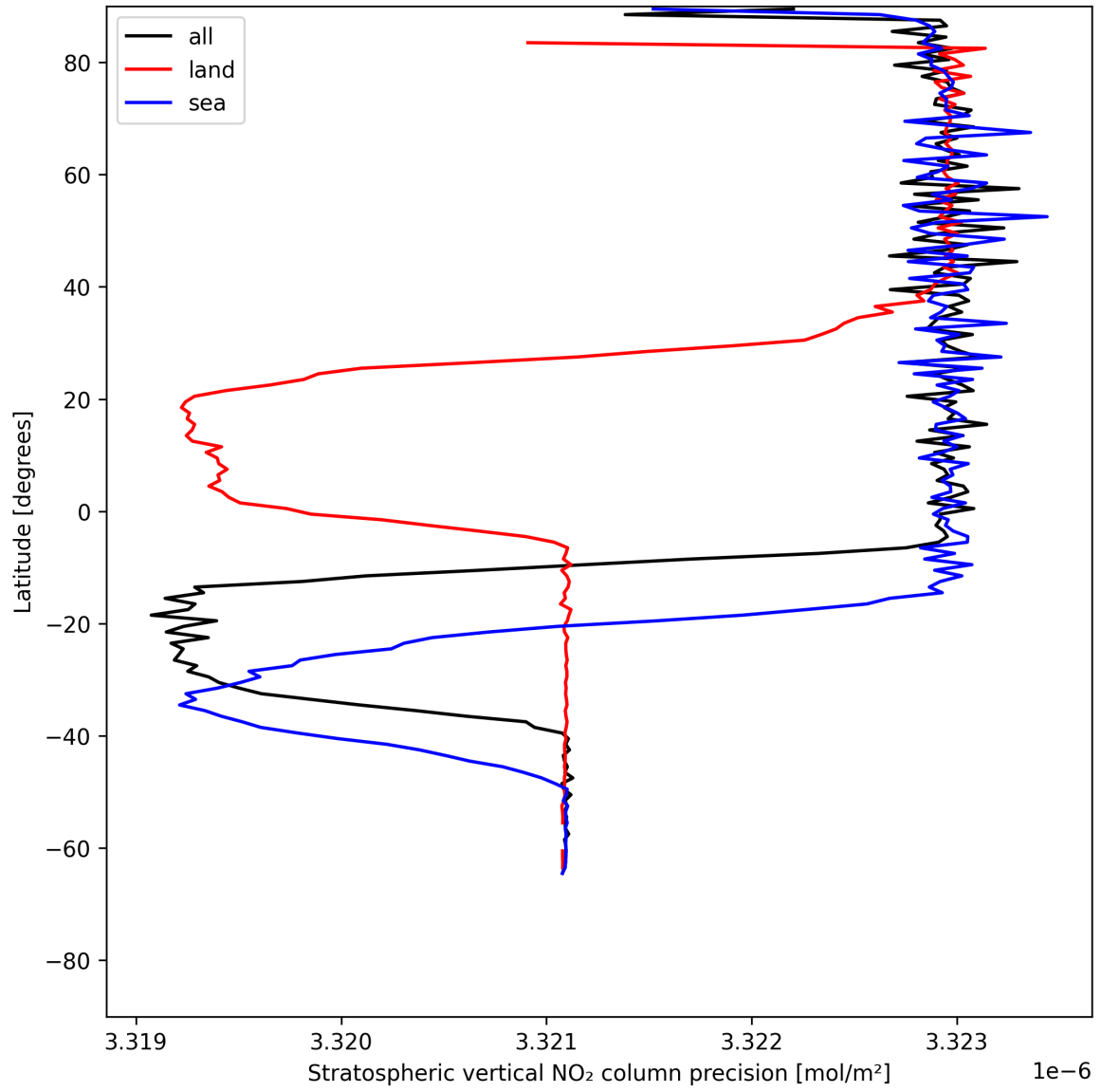
Figure 20: Zonal average of “Stratospheric vertical NO 2 column precision” for 2025-06-11 to 2025-06-12.
