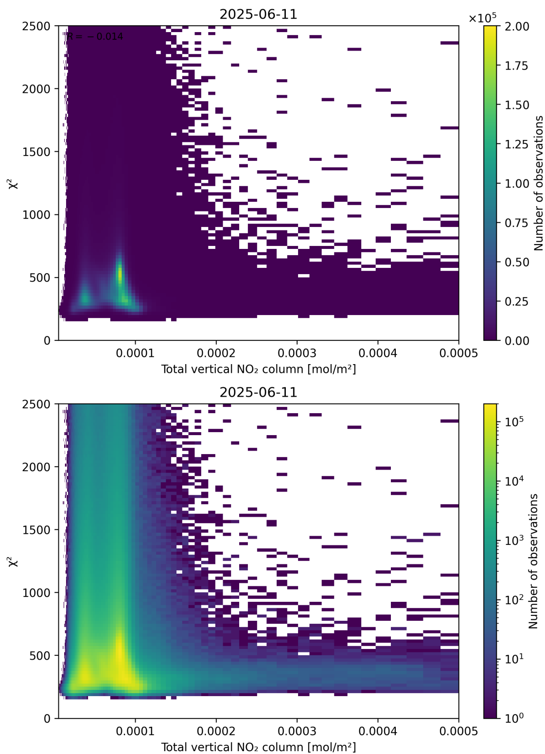
Figure 111: Scatter density plot of “Total vertical NO 2 column” against “ \chi^2 ” for 2025-06-11 to 2025-06-12.
