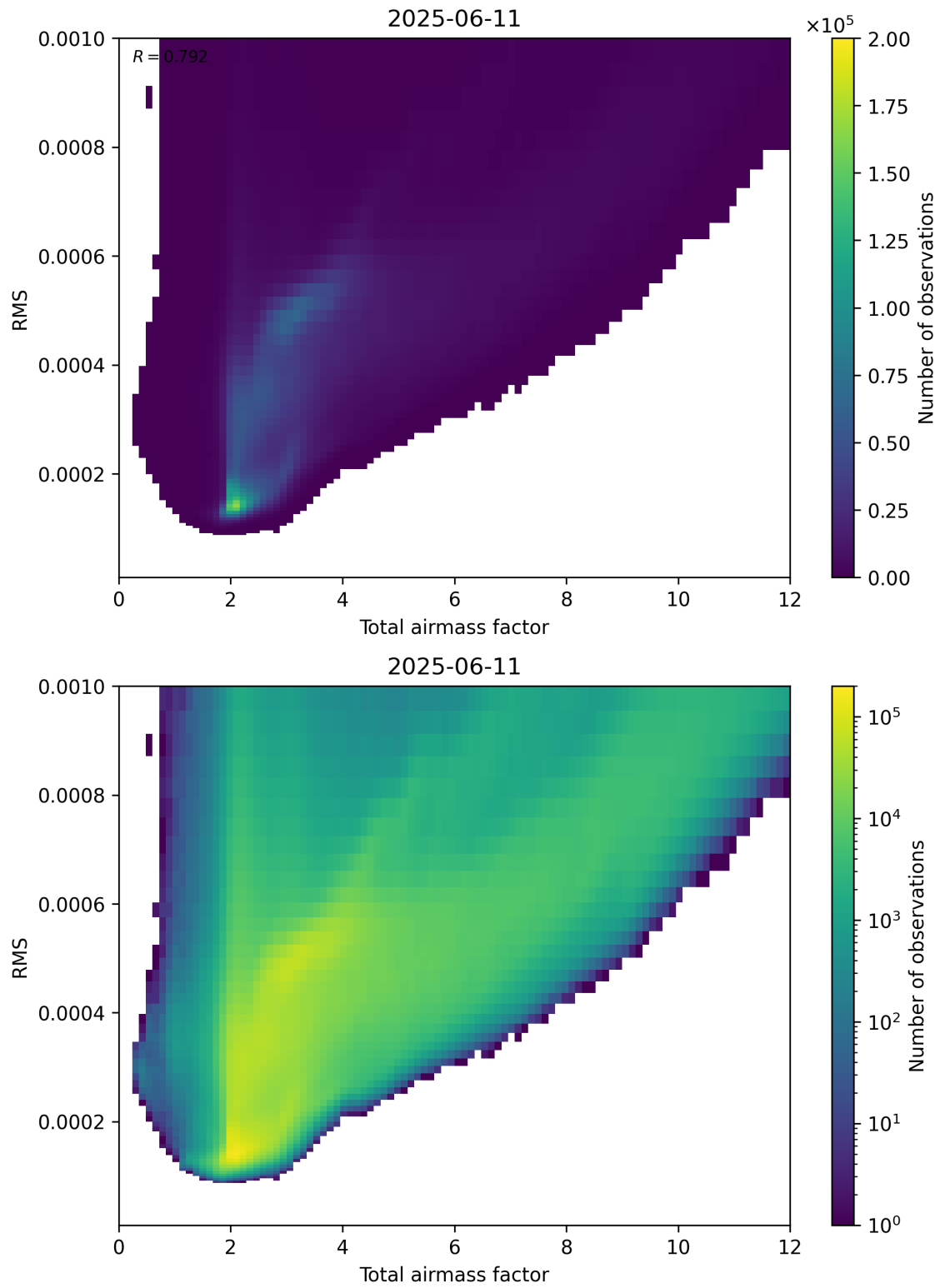
Figure 69: Scatter density plot of “Total airmass factor” against “RMS” for 2025-06-11 to 2025-06-12.
