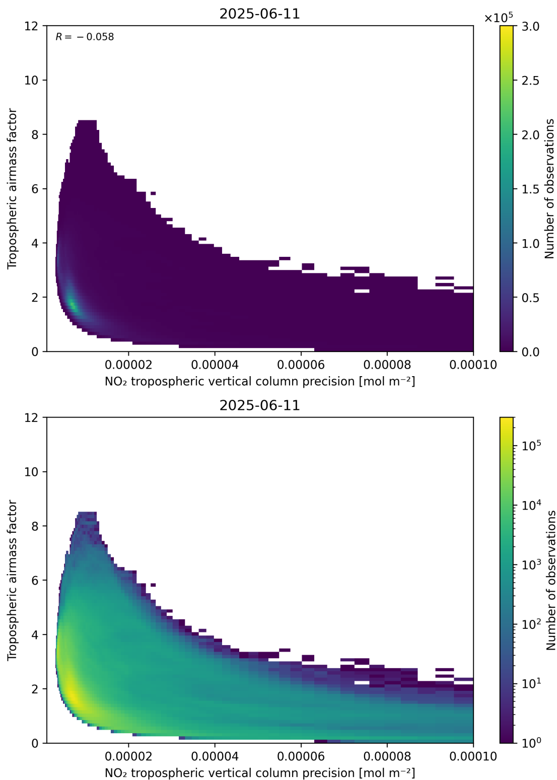
Figure 133: Scatter density plot of “NO 2 tropospheric vertical column precision” against “Tropospheric air mass factor” for 2025-06-11 to 2025-06-12.
