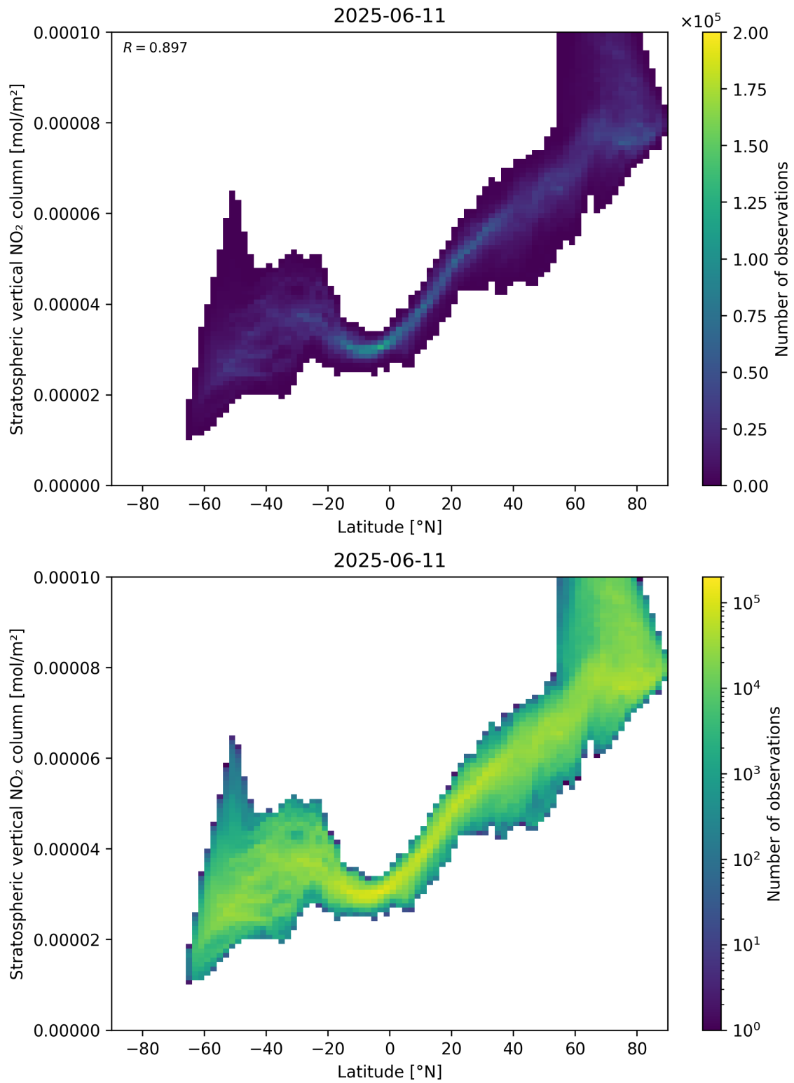
Figure 87: Scatter density plot of “Latitude” against “Stratospheric vertical \text{NO}_2 column” for 2025-06-11 to 2025-06-12.
