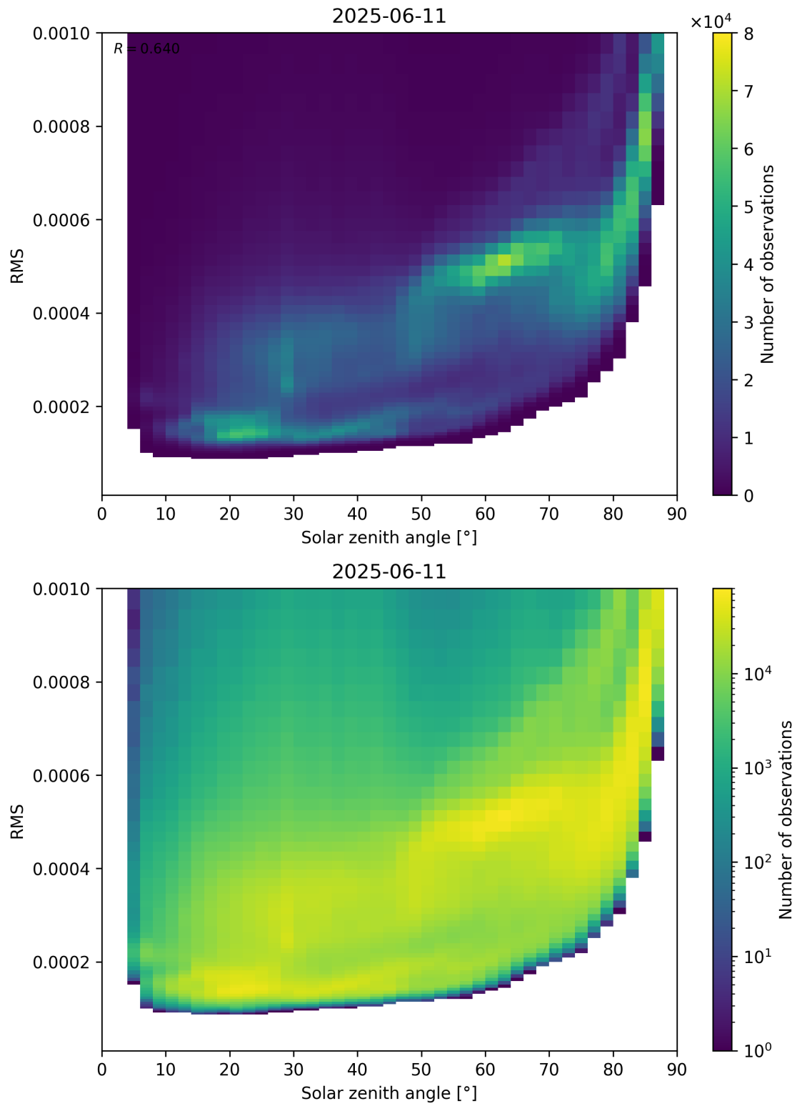
Figure 157: Scatter density plot of “Solar zenith angle” against “RMS” for 2025-06-11 to 2025-06-12.
