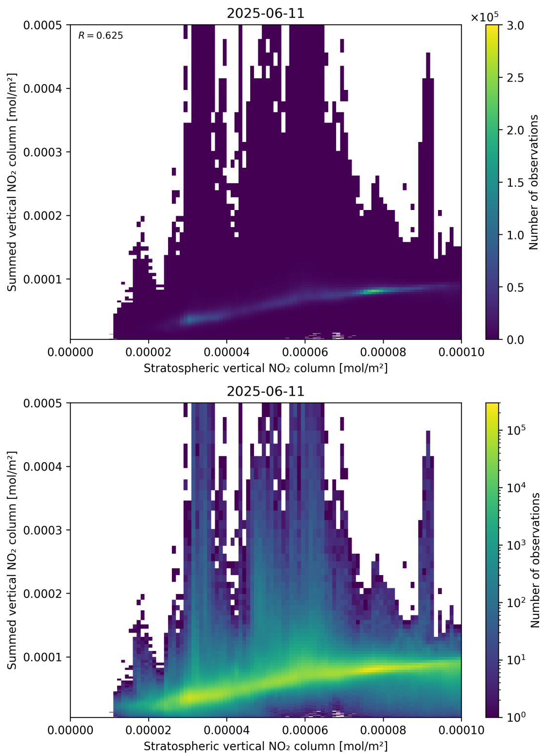
Figure 98: Scatter density plot of “Stratospheric vertical NO 2 column” against “Summed vertical NO 2 column” for 2025-06-11 to 2025-06-12.
