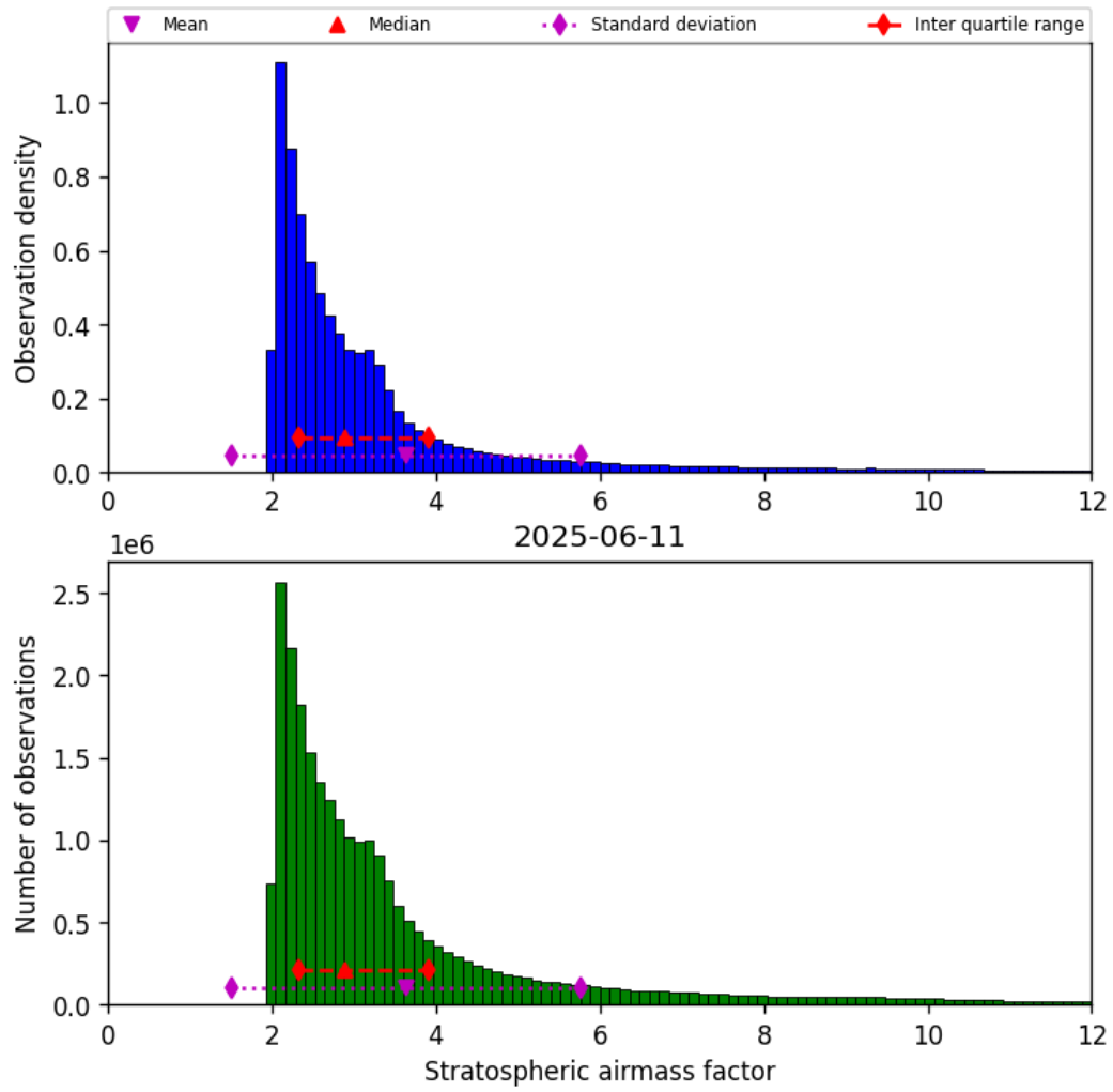
Figure 44: Histogram of “Stratospheric airmass factor” for 2025-06-11 to 2025-06-12
