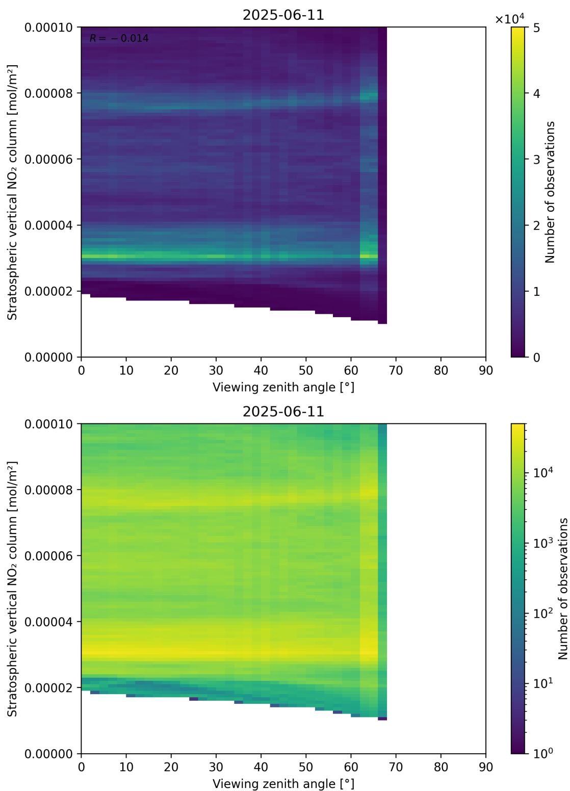
Figure 164: Scatter density plot of “Viewing zenith angle” against “Stratospheric vertical NO 2 column” for 2025-06-11 to 2025-06-12.
