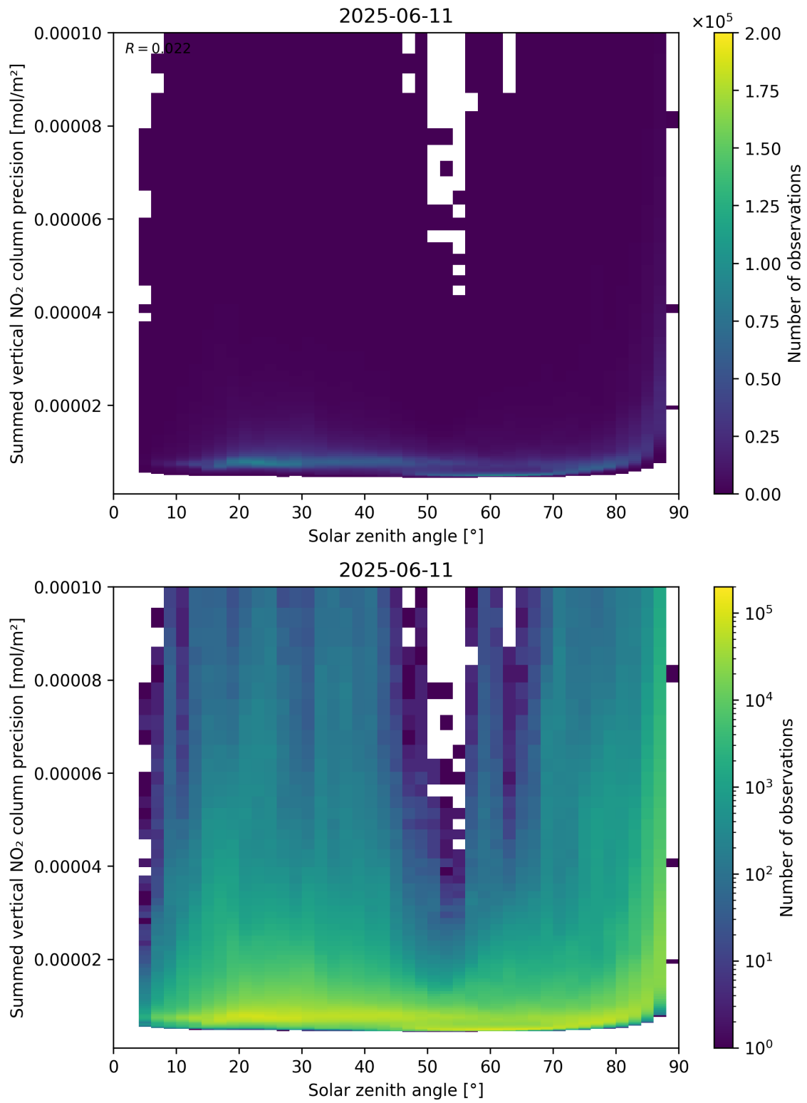
Figure 152: Scatter density plot of “Solar zenith angle” against “Summed vertical NO 2 column precision” for 2025-06-11 to 2025-06-12.
