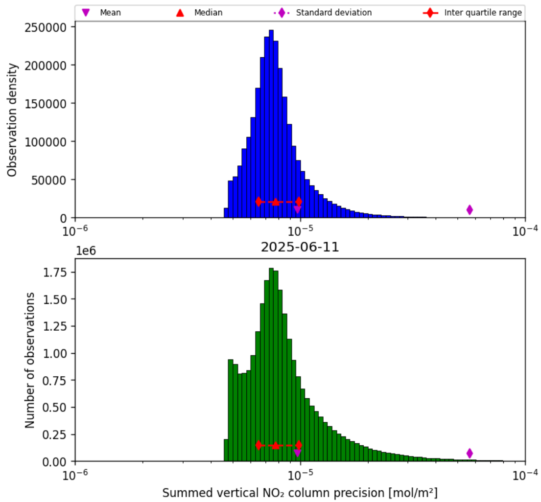
Figure 41: Histogram of “Summed vertical NO 2 column precision” for 2025-06-11 to 2025-06-12
