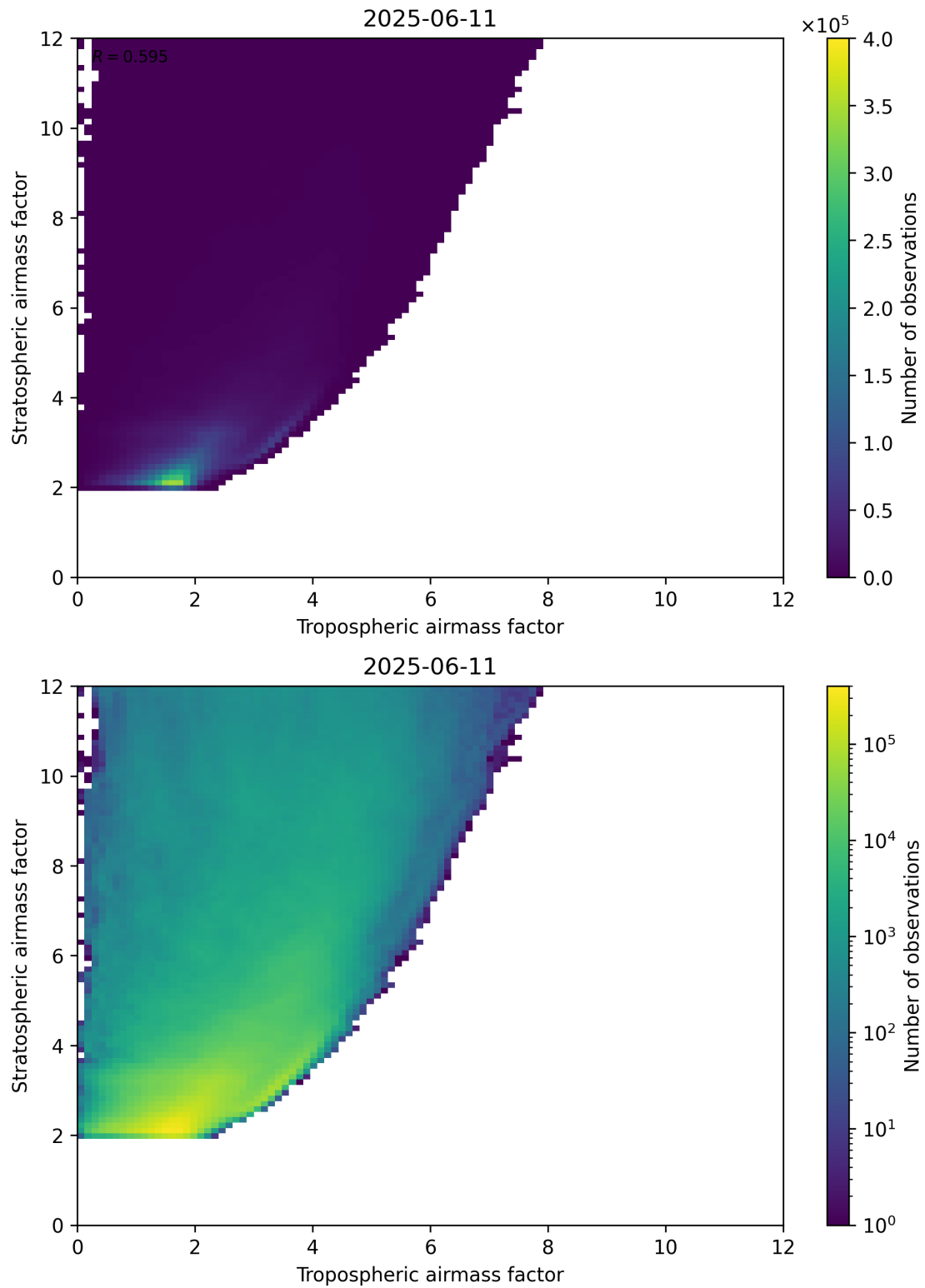
Figure 71: Scatter density plot of “Tropospheric airmass factor” against “Stratospheric airmass factor” for 2025-06-11 to 2025-06-12.
