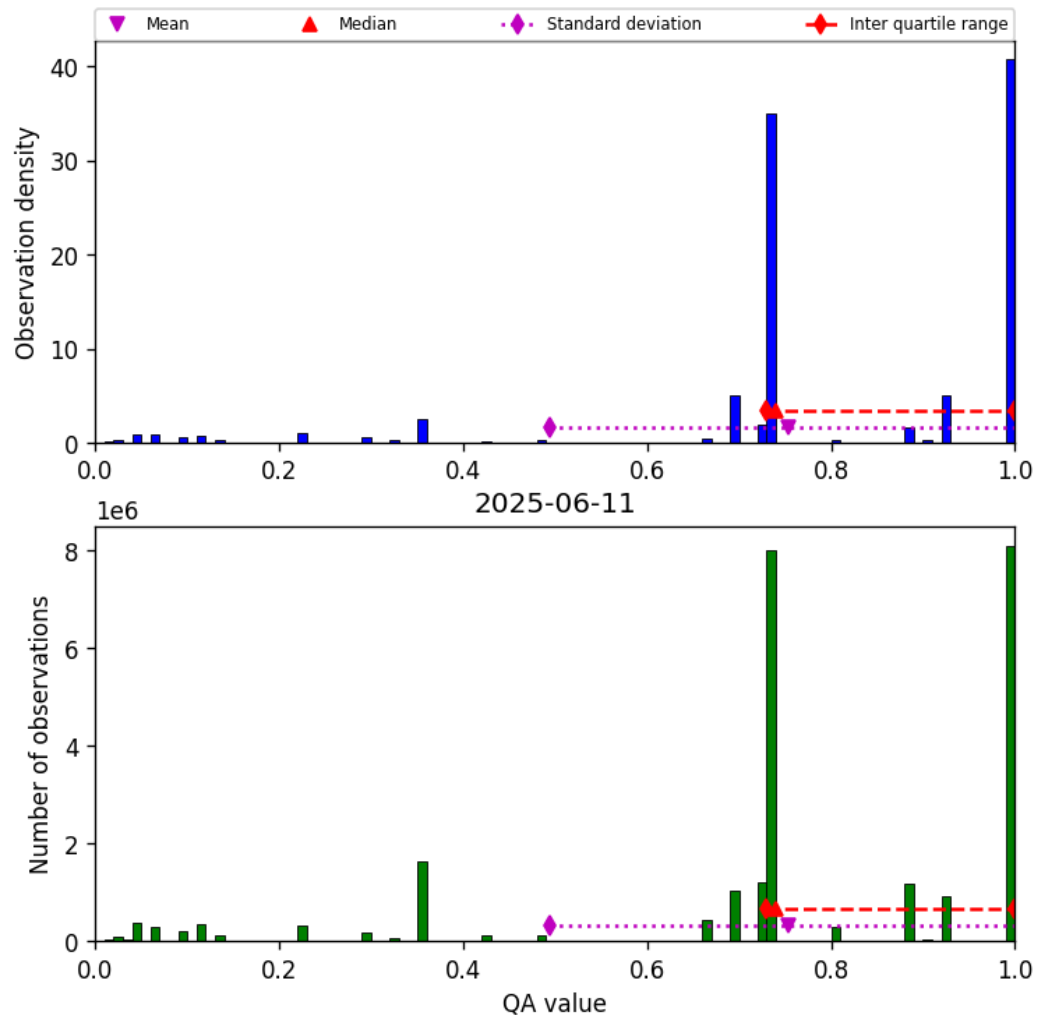
Figure 28: Histogram of “QA value” for 2025-06-11 to 2025-06-12
