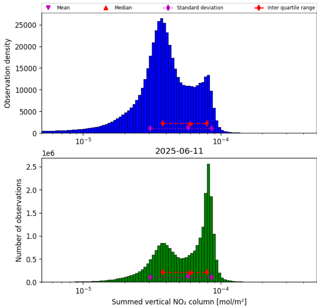
Figure 40: Histogram of "Summed vertical NO 2 column" for 2025-06-11 to 2025-06-12
