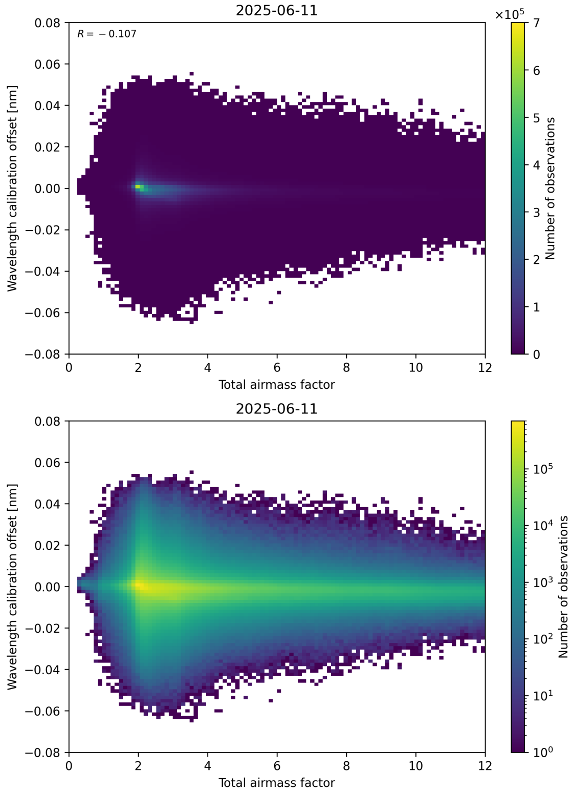
Figure 70: Scatter density plot of “Total airmass factor” against “Wavelength calibration offset” for 2025-06-11 to 2025-06-12.
