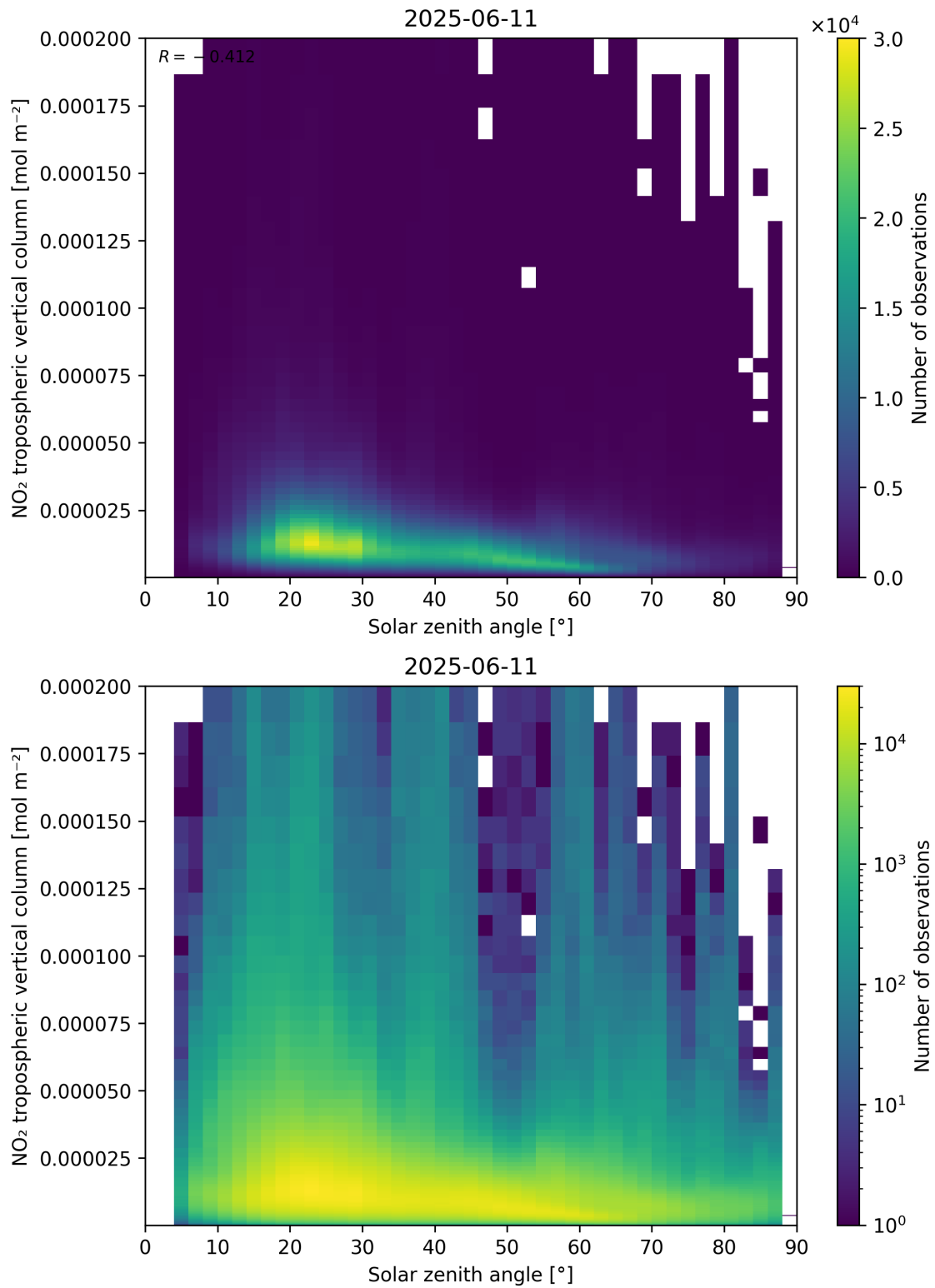
Figure 155: Scatter density plot of “Solar zenith angle” against “NO 2 tropospheric vertical column” for 2025-06-11 to 2025-06-12.
