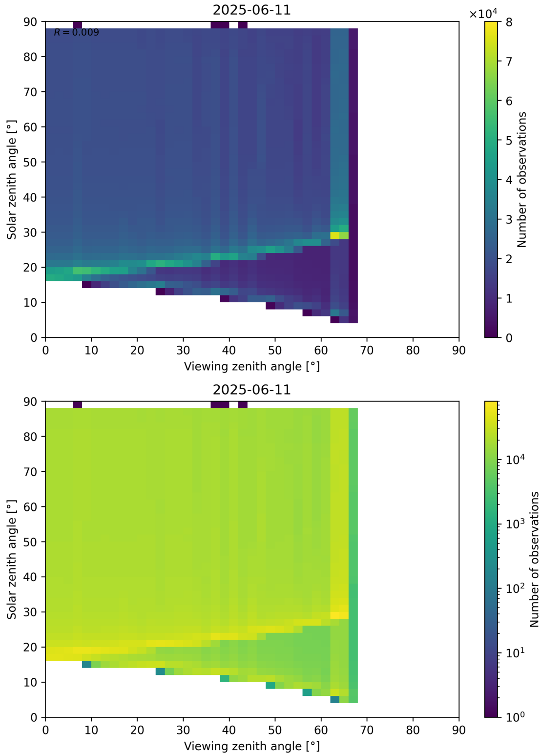
Figure 172: Scatter density plot of “Viewing zenith angle” against “Solar zenith angle” for 2025-06-11 to 2025-06-12.
