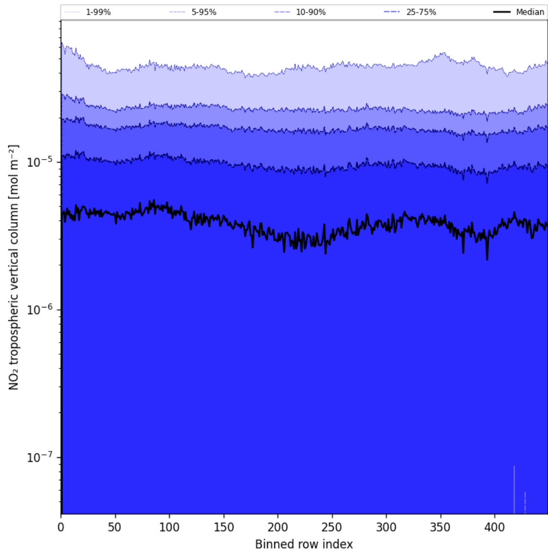
Figure 46: Along track statistics of “NO 2 tropospheric vertical column” for 2025-06-11 to 2025-06-12
