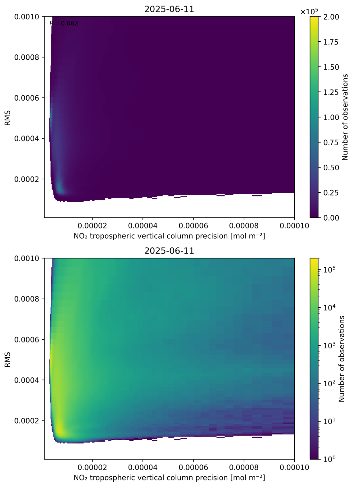
Figure 140: Scatter density plot of “NO 2 tropospheric vertical column precision” against “RMS” for 2025-06-11 to 2025-06-12.
