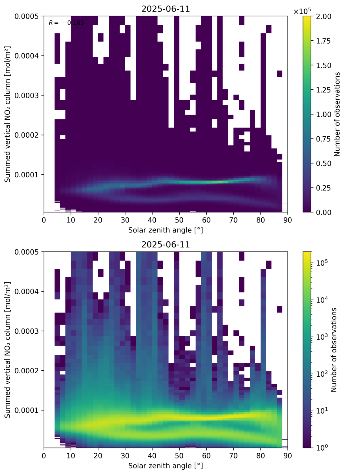
Figure 151: Scatter density plot of “Solar zenith angle” against “Summed vertical NO 2 column” for 2025-06-11 to 2025-06-12.
