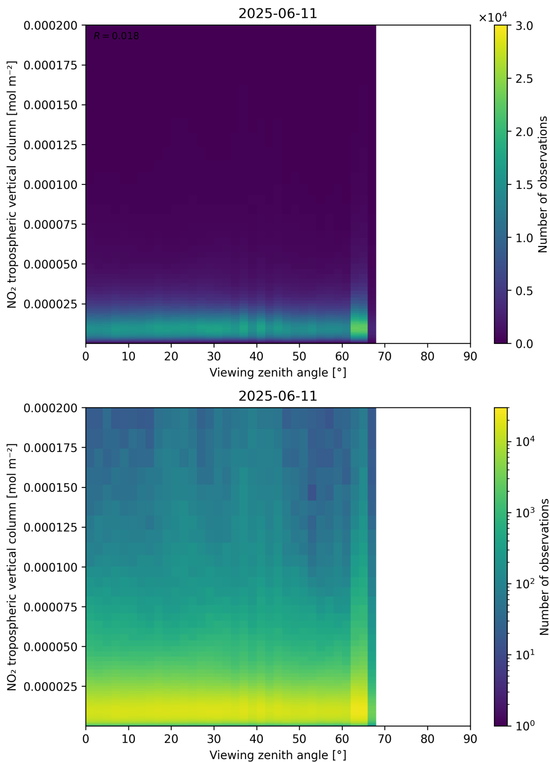
Figure 169: Scatter density plot of “Viewing zenith angle” against “NO 2 tropospheric vertical column” for 2025-06-11 to 2025-06-12.
