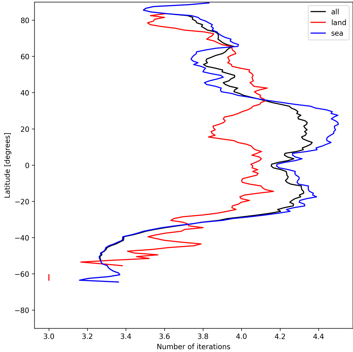
Figure 17: Zonal average of “Number of iterations” for 2025-06-11 to 2025-06-12.
