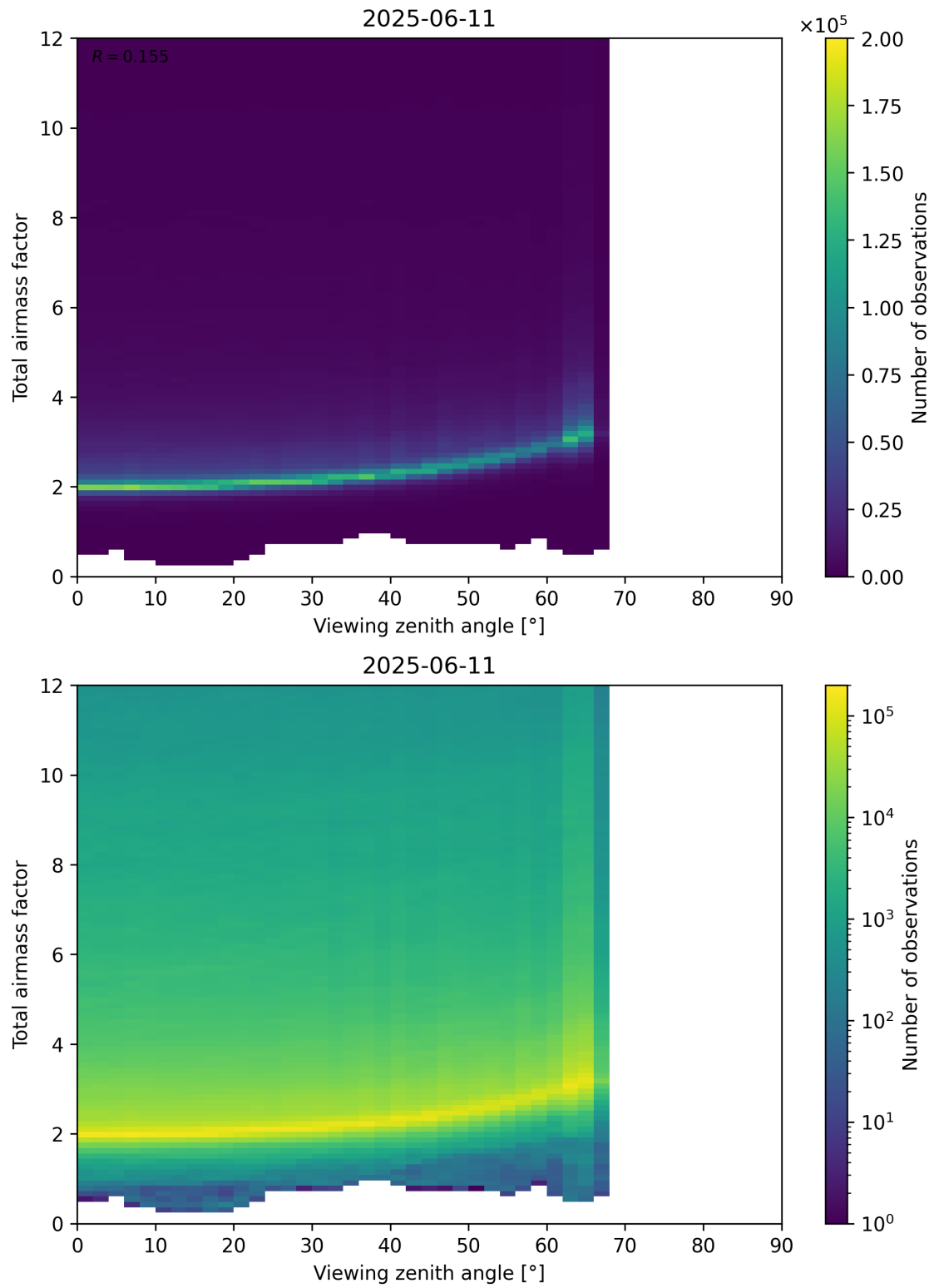
Figure 160: Scatter density plot of “Viewing zenith angle” against “Total airmass factor” for 2025-06-11 to 2025-06-12.
