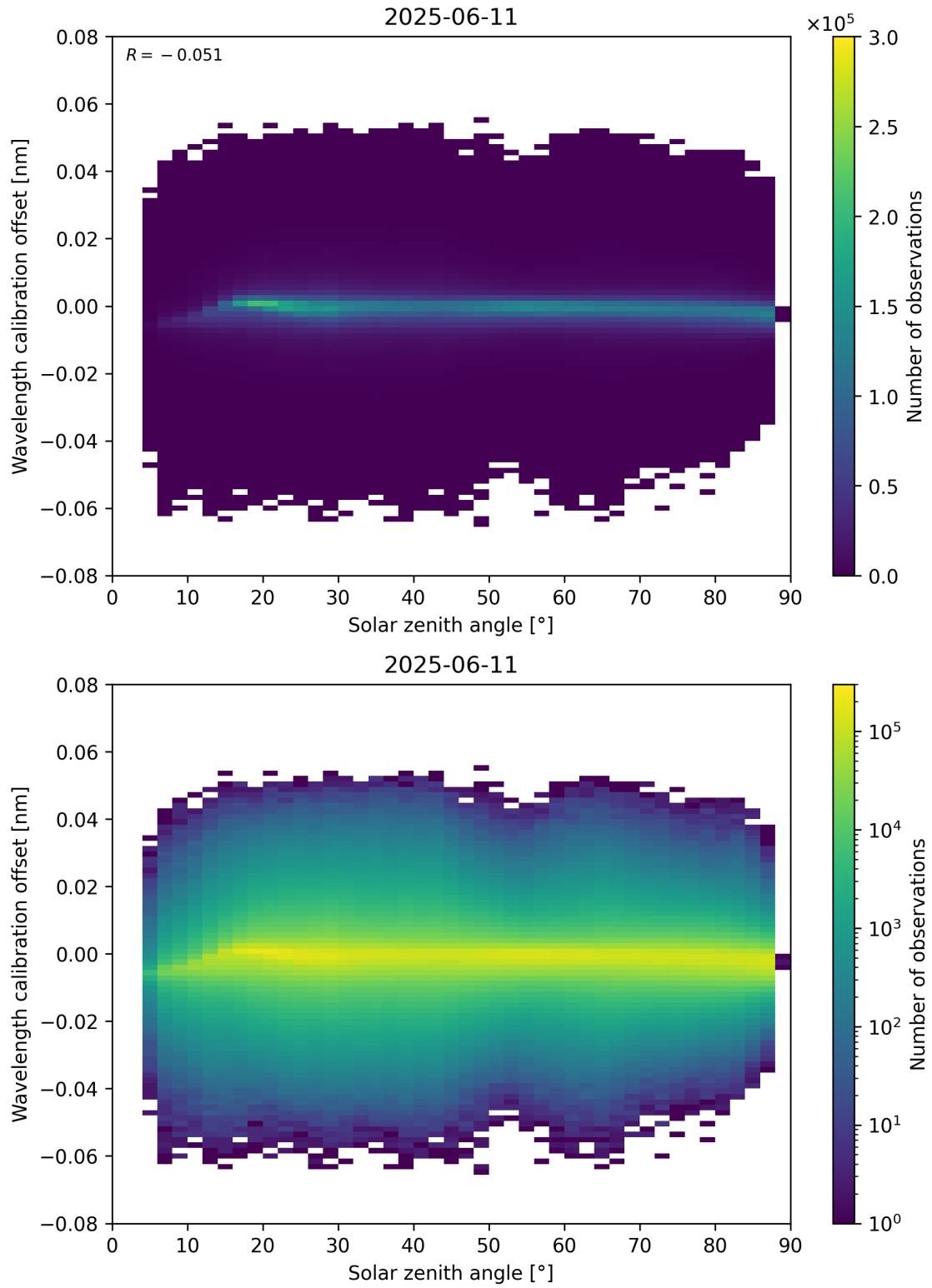
Figure 158: Scatter density plot of “Solar zenith angle” against “Wavelength calibration offset” for 2025-06-11 to 2025-06-12.
