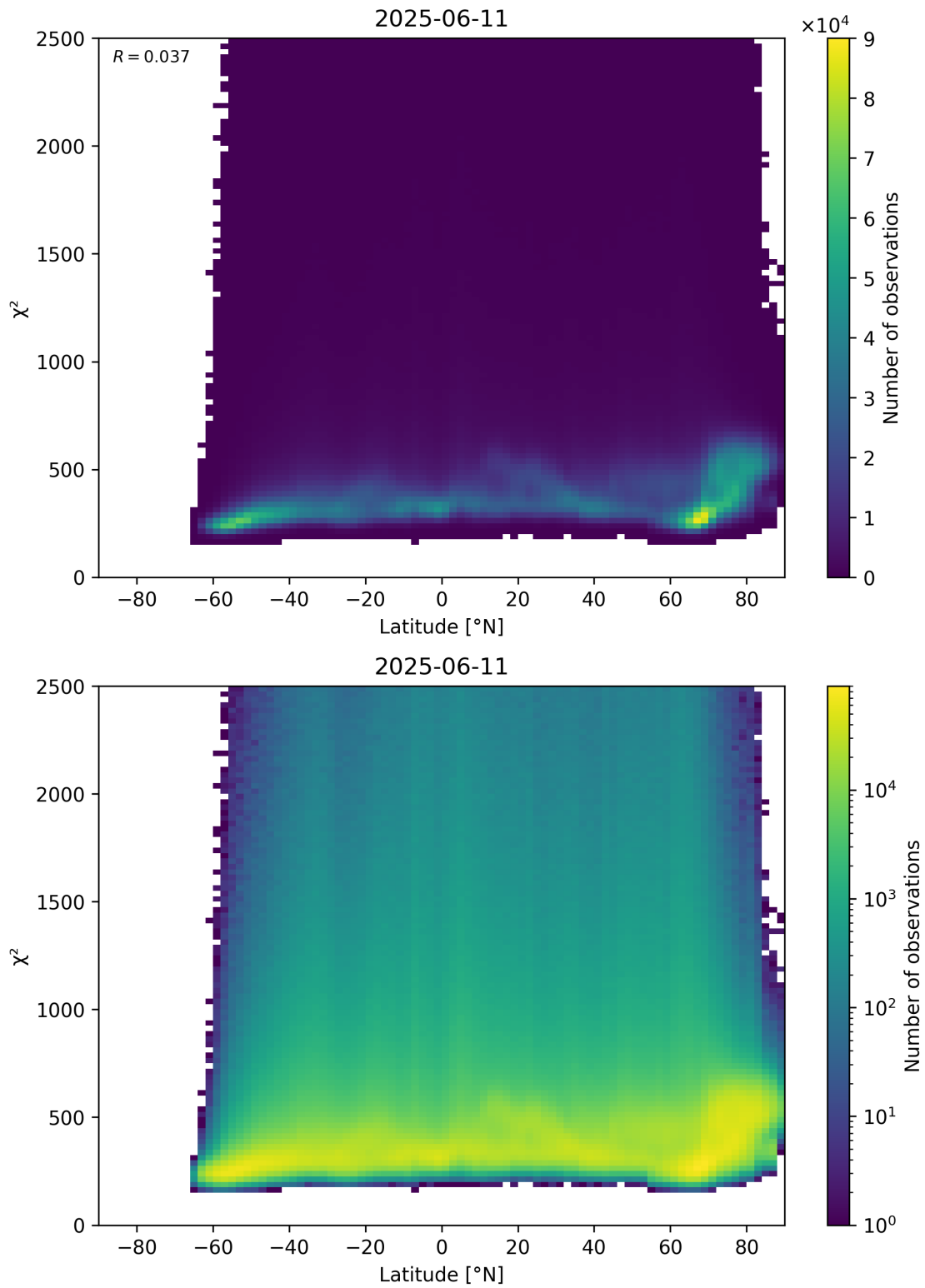
Figure 86: Scatter density plot of “Latitude” against “ \chi^2 ” for 2025-06-11 to 2025-06-12.
