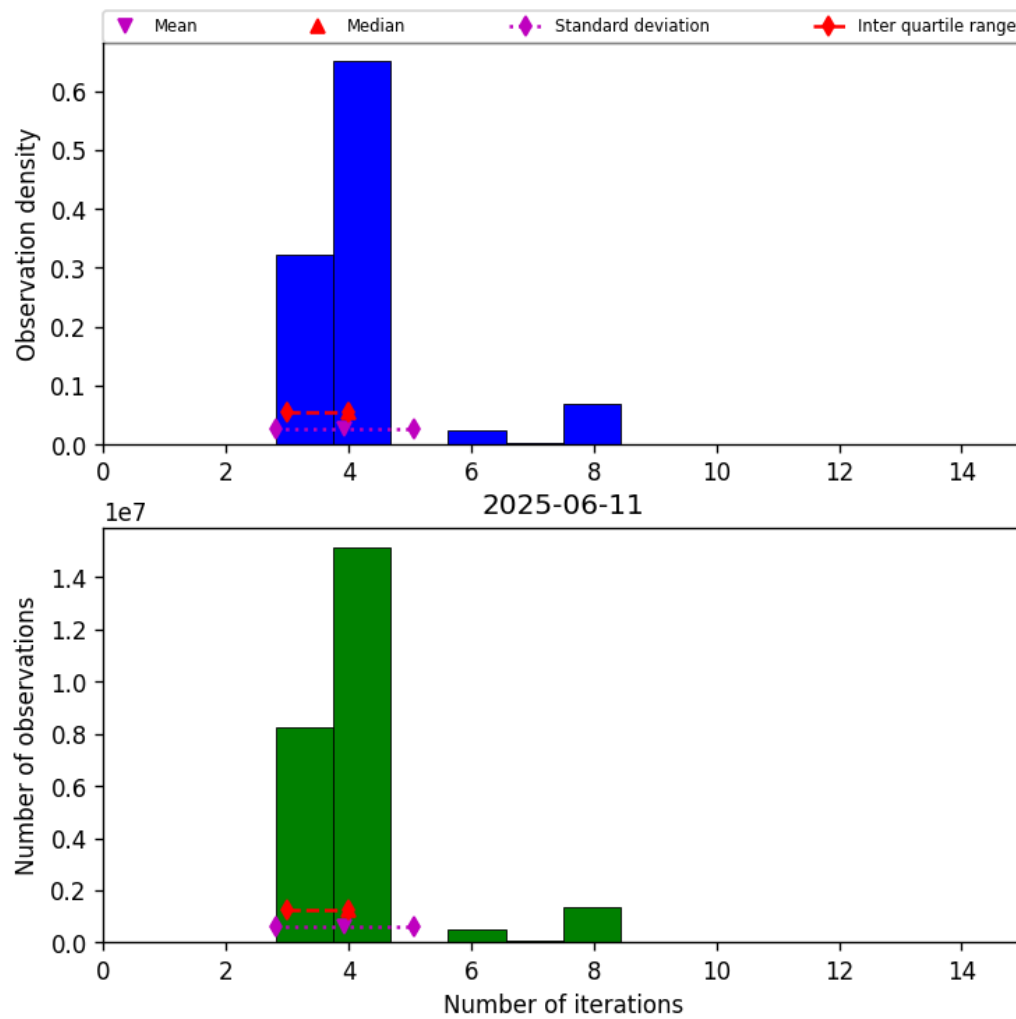
Figure 34: Histogram of “Number of iterations” for 2025-06-11 to 2025-06-12
