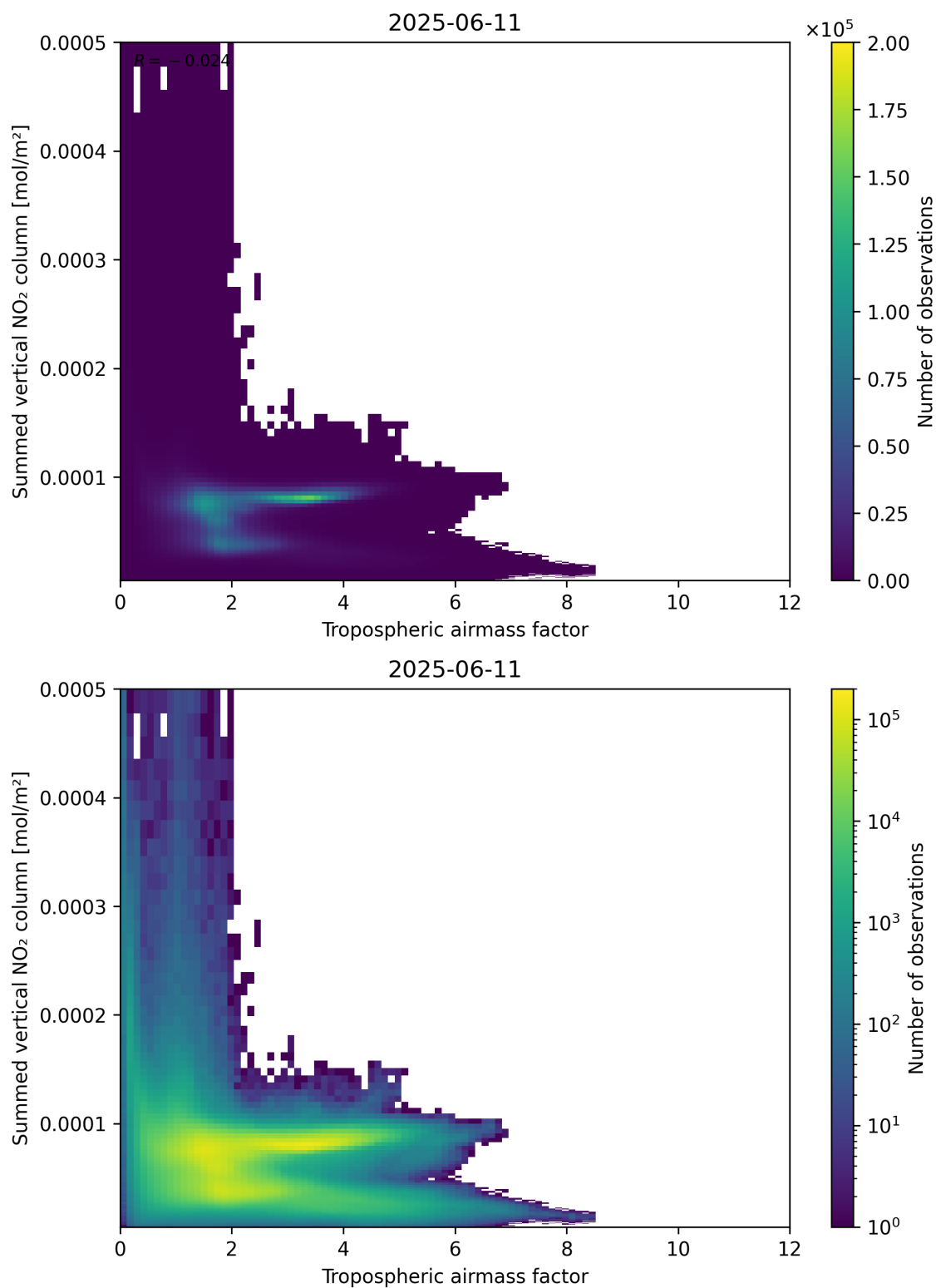
Figure 75: Scatter density plot of “Tropospheric airmass factor” against “Summed vertical NO 2 column” for 2025-06-11 to 2025-06-12.
