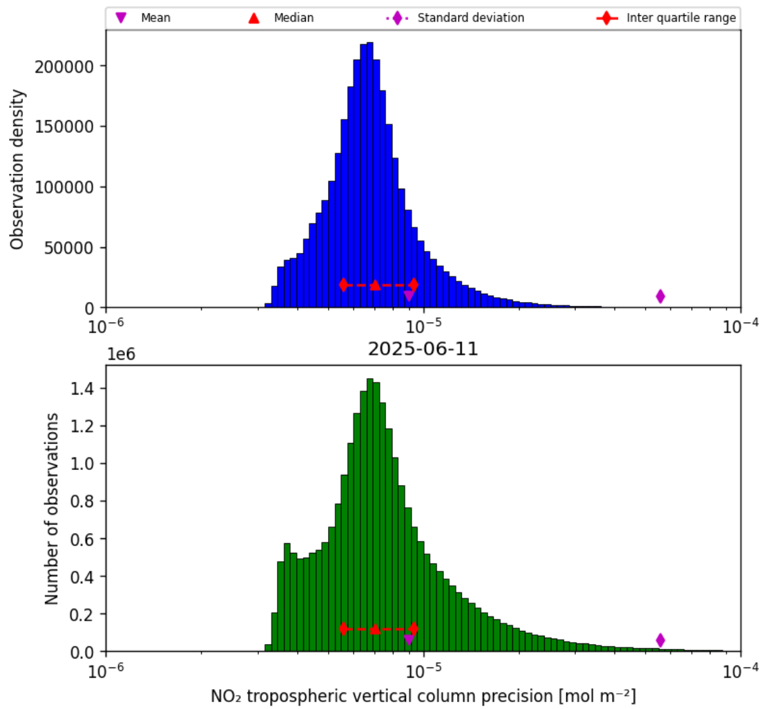
Figure 30: Histogram of “NO 2 tropospheric vertical column precision” for 2025-06-11 to 2025-06-12
