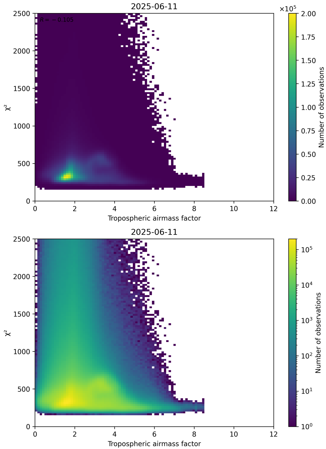
Figure 73: Scatter density plot of “Tropospheric airmass factor” against “ \chi^2 ” for 2025-06-11 to 2025-06-12.
