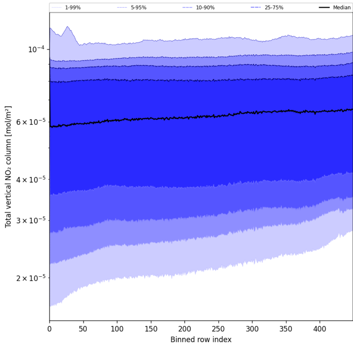
Figure 55: Along track statistics of “Total vertical NO 2 column” for 2025-06-11 to 2025-06-12
