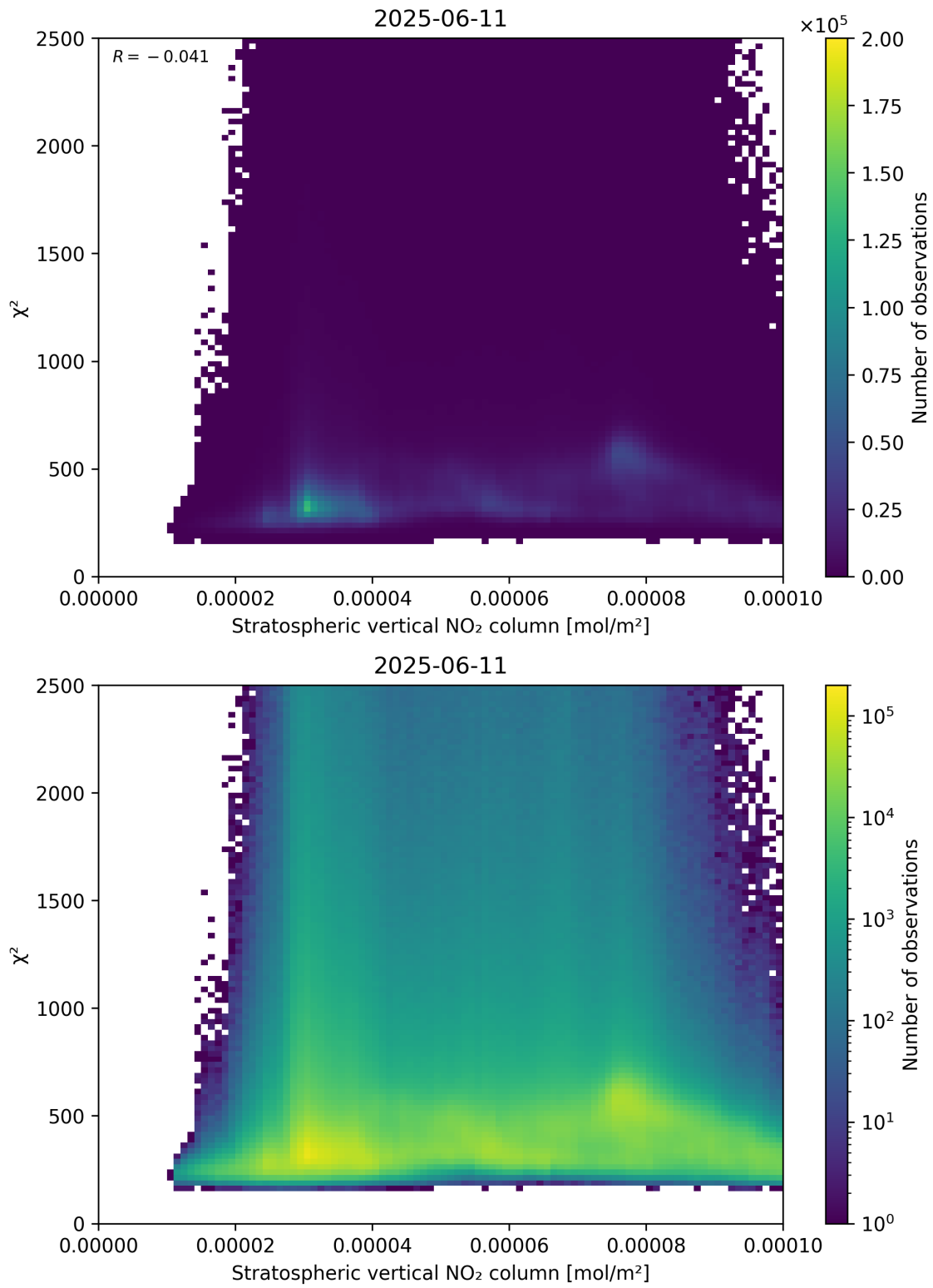
Figure 97: Scatter density plot of “Stratospheric vertical NO 2 column” against “ \chi^2 ” for 2025-06-11 to 2025-06-12.
