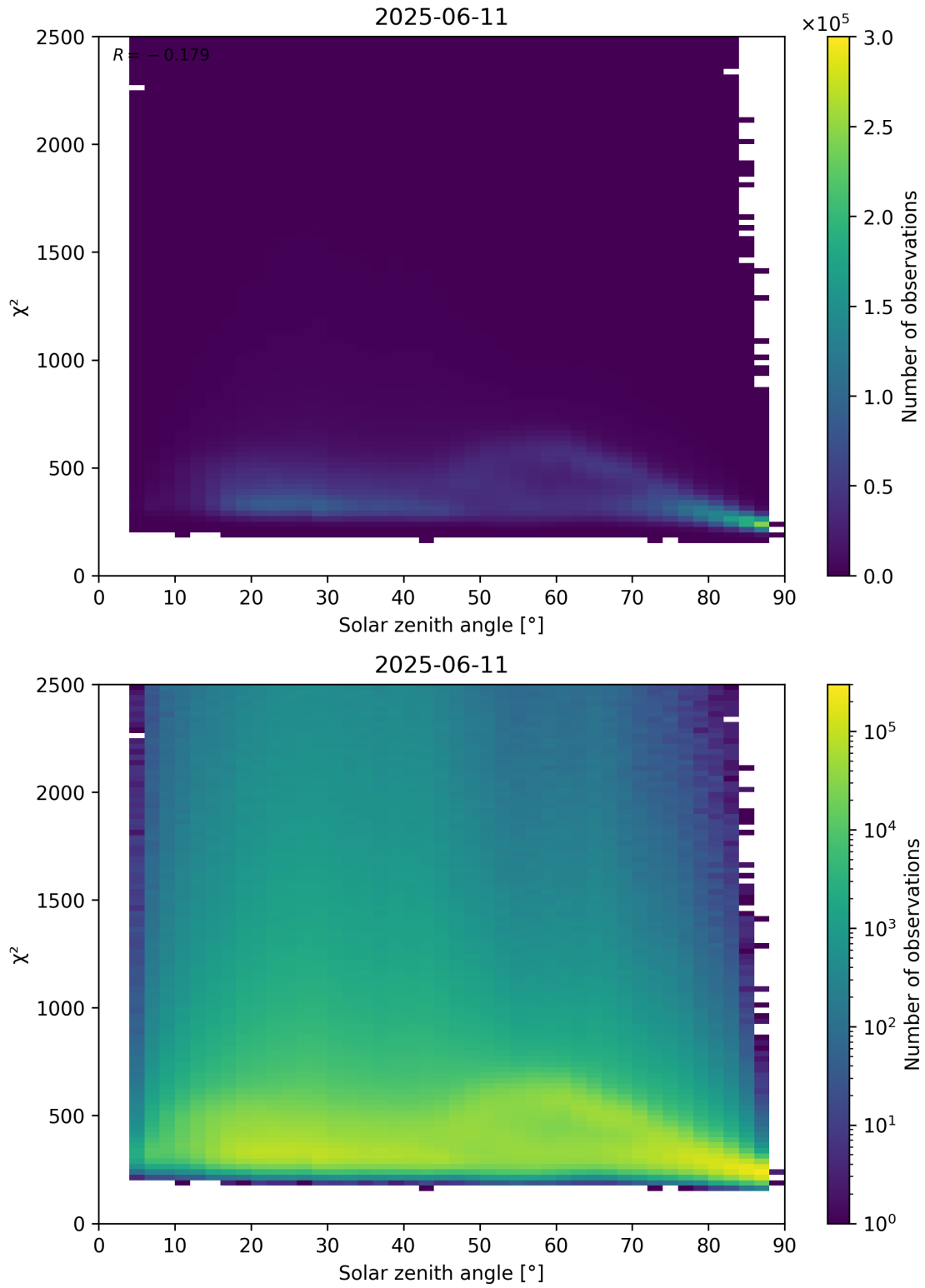
Figure 148: Scatter density plot of “Solar zenith angle” against “ \chi^2 ” for 2025-06-11 to 2025-06-12.
