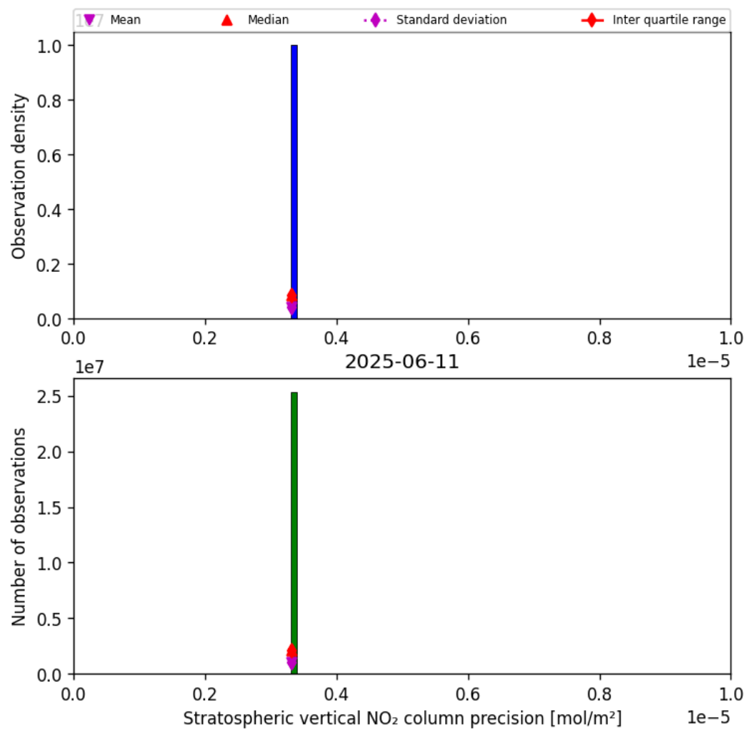
Figure 37: Histogram of “Stratospheric vertical NO 2 column precision” for 2025-06-11 to 2025-06-12
