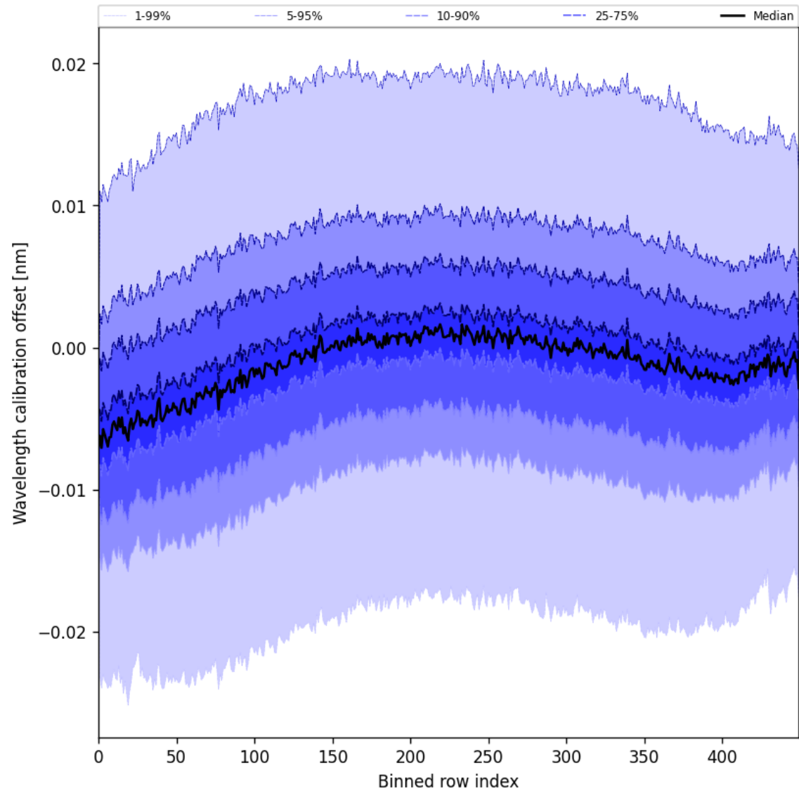
Figure 52: Along track statistics of “Wavelength calibration offset” for 2025-06-11 to 2025-06-12
