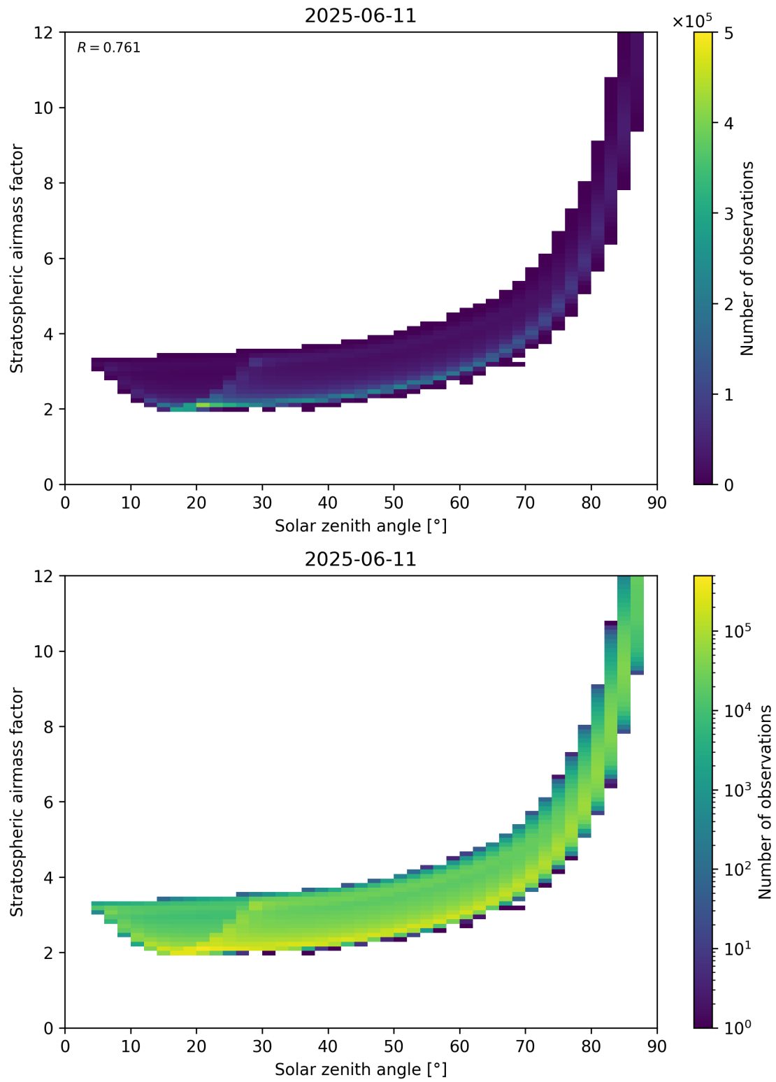
Figure 145: Scatter density plot of “Solar zenith angle” against “Stratospheric airmass factor” for 2025-06-11 to 2025-06-12.
