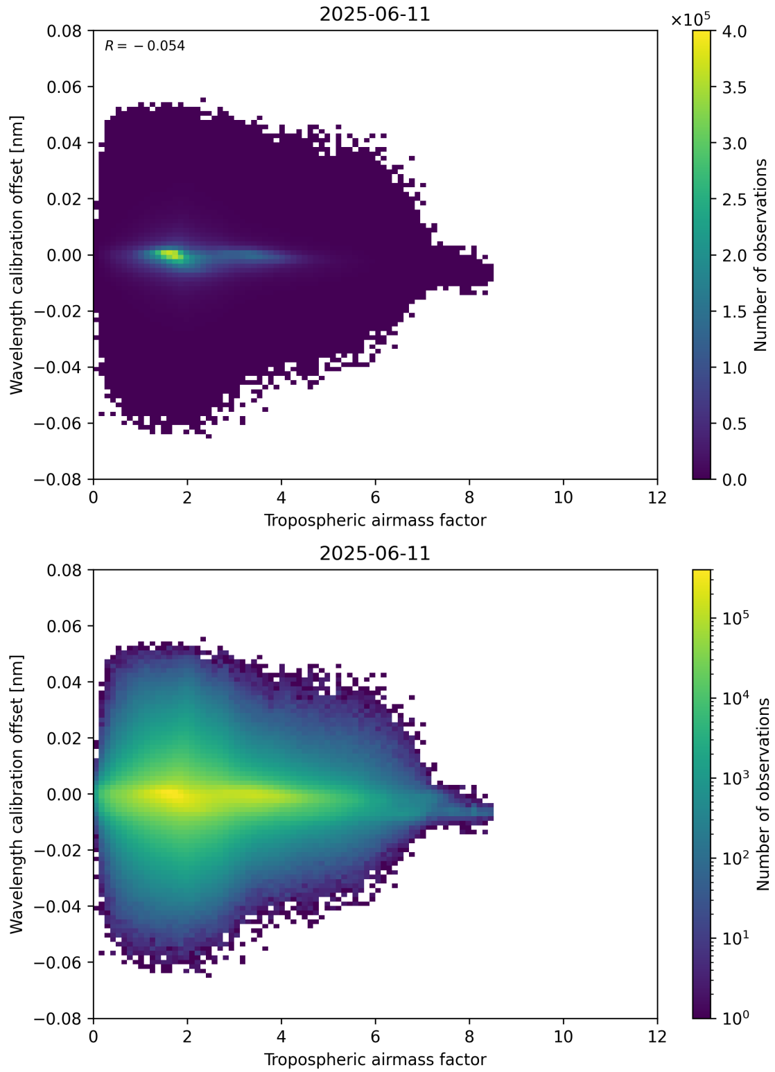
Figure 80: Scatter density plot of “Tropospheric airmass factor” against “Wavelength calibration offset” for 2025-06-11 to 2025-06-12.
