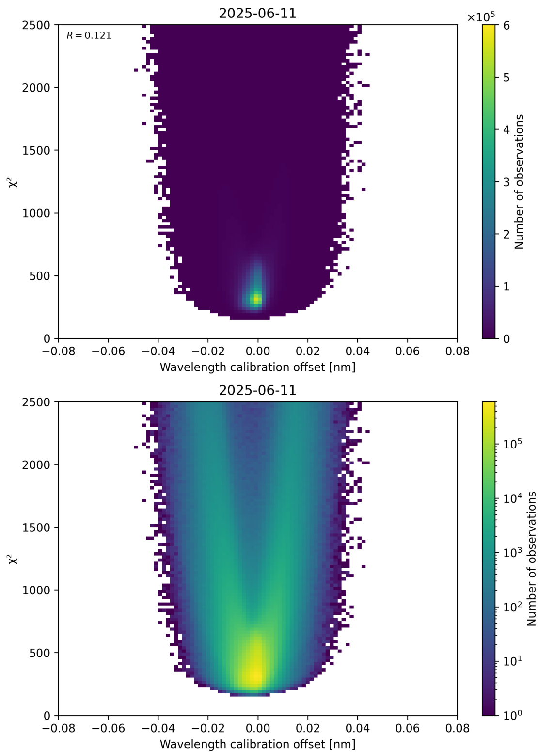
Figure 175: Scatter density plot of “Wavelength calibration offset” against “ \chi^2 ” for 2025-06-11 to 2025-06-12.
