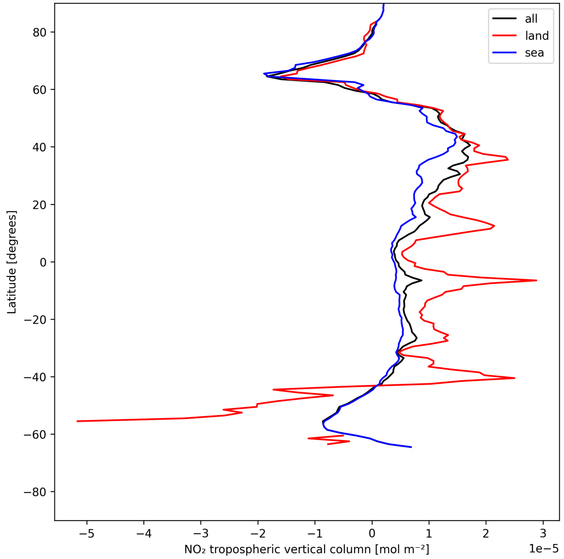
Figure 12: Zonal average of “NO 2 tropospheric vertical column” for 2025-06-11 to 2025-06-12.
