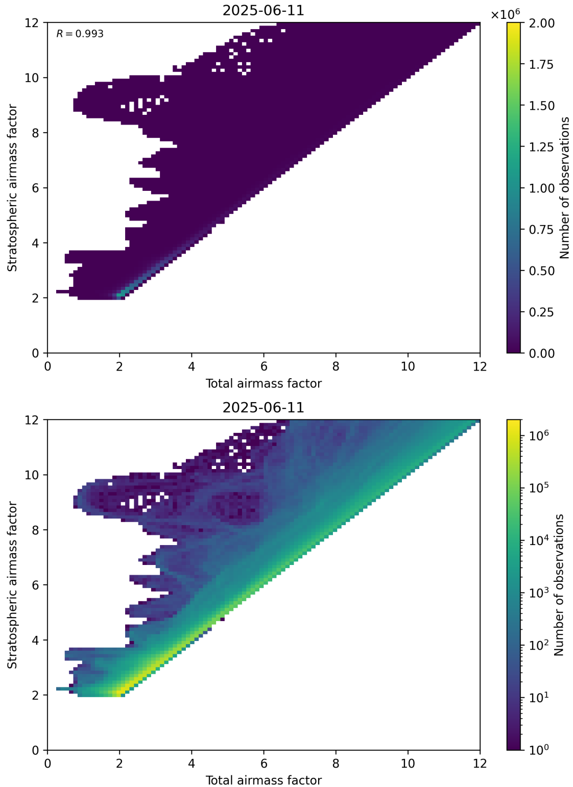
Figure 62: Scatter density plot of “Total airmass factor” against “Stratospheric airmass factor” for 2025-06-11 to 2025-06-12.
