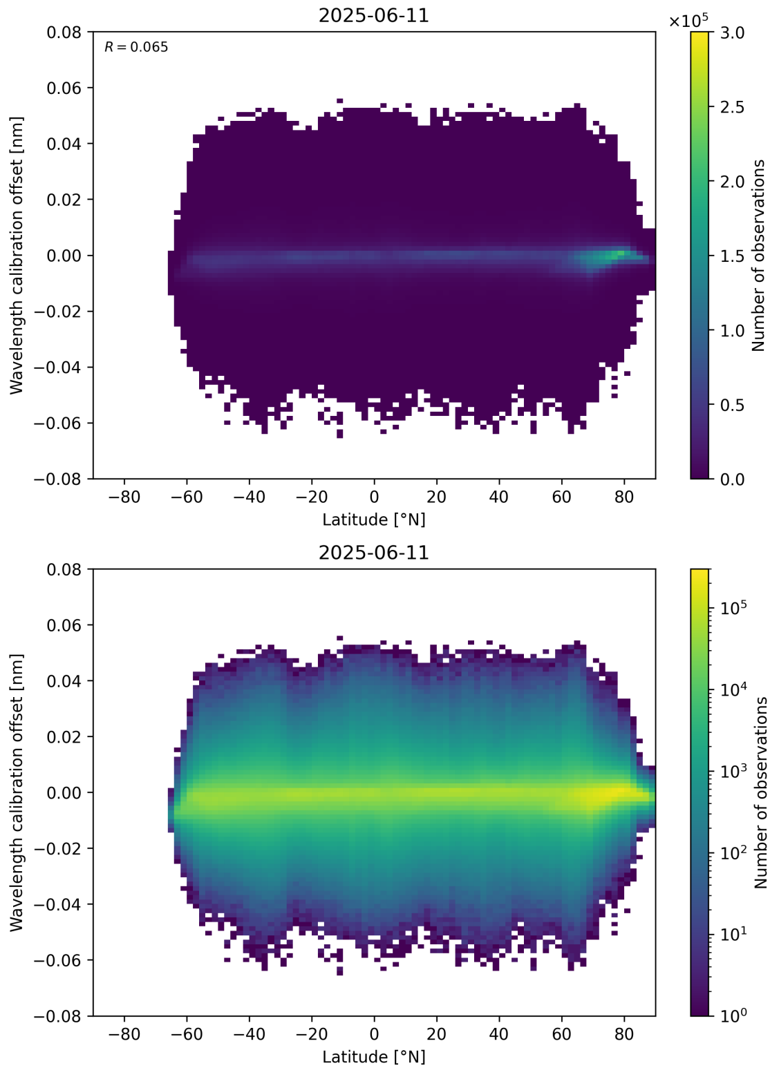
Figure 95: Scatter density plot of “Latitude” against “Wavelength calibration offset” for 2025-06-11 to 2025-06-12.
