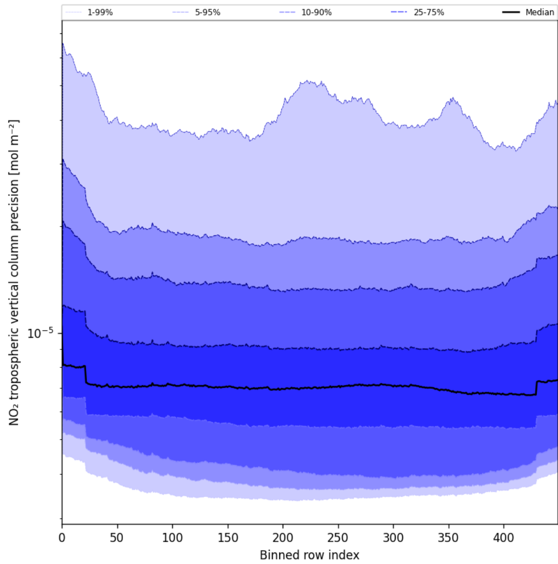
Figure 47: Along track statistics of “NO 2 tropospheric vertical column precision” for 2025-06-11 to 2025-06-12
