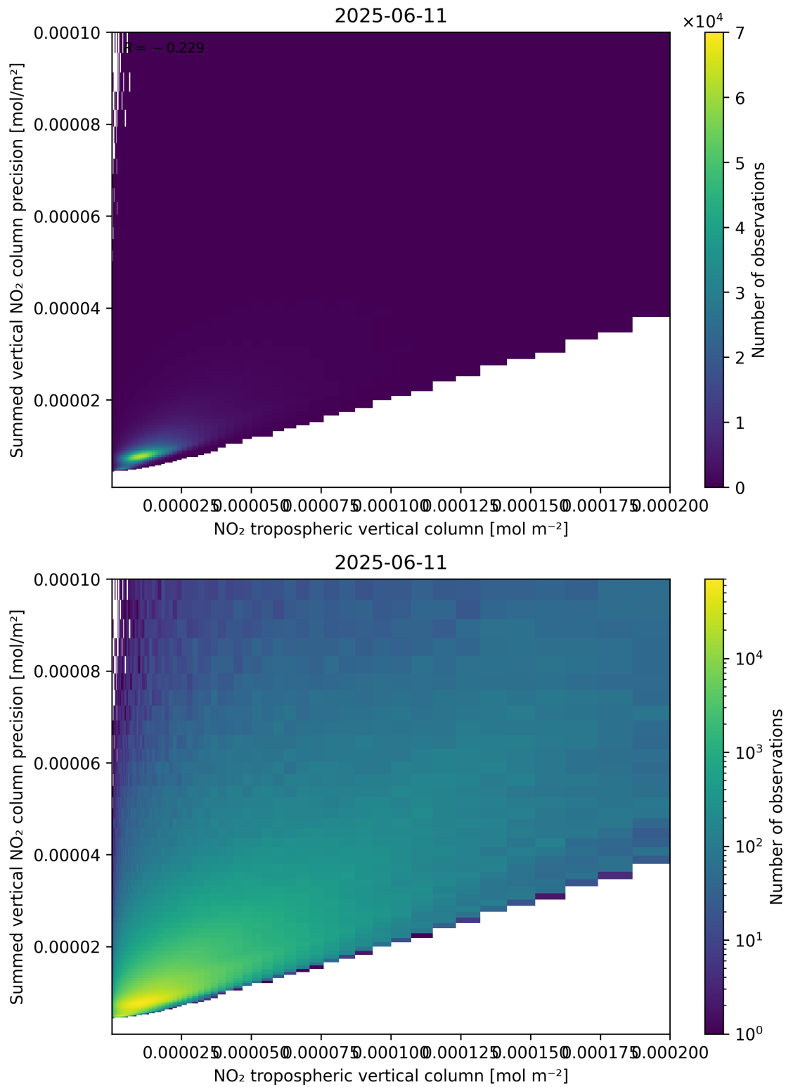
Figure 127: Scatter density plot of “NO 2 tropospheric vertical column” against “Summed vertical NO 2 column precision” for 2025-06-11 to 2025-06-12.
