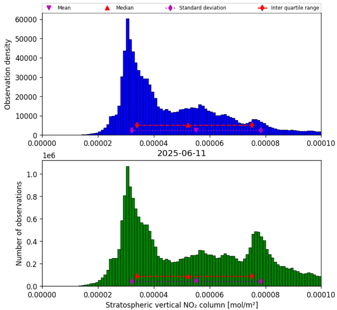
Figure 36: Histogram of “Stratospheric vertical NO 2 column” for 2025-06-11 to 2025-06-12
