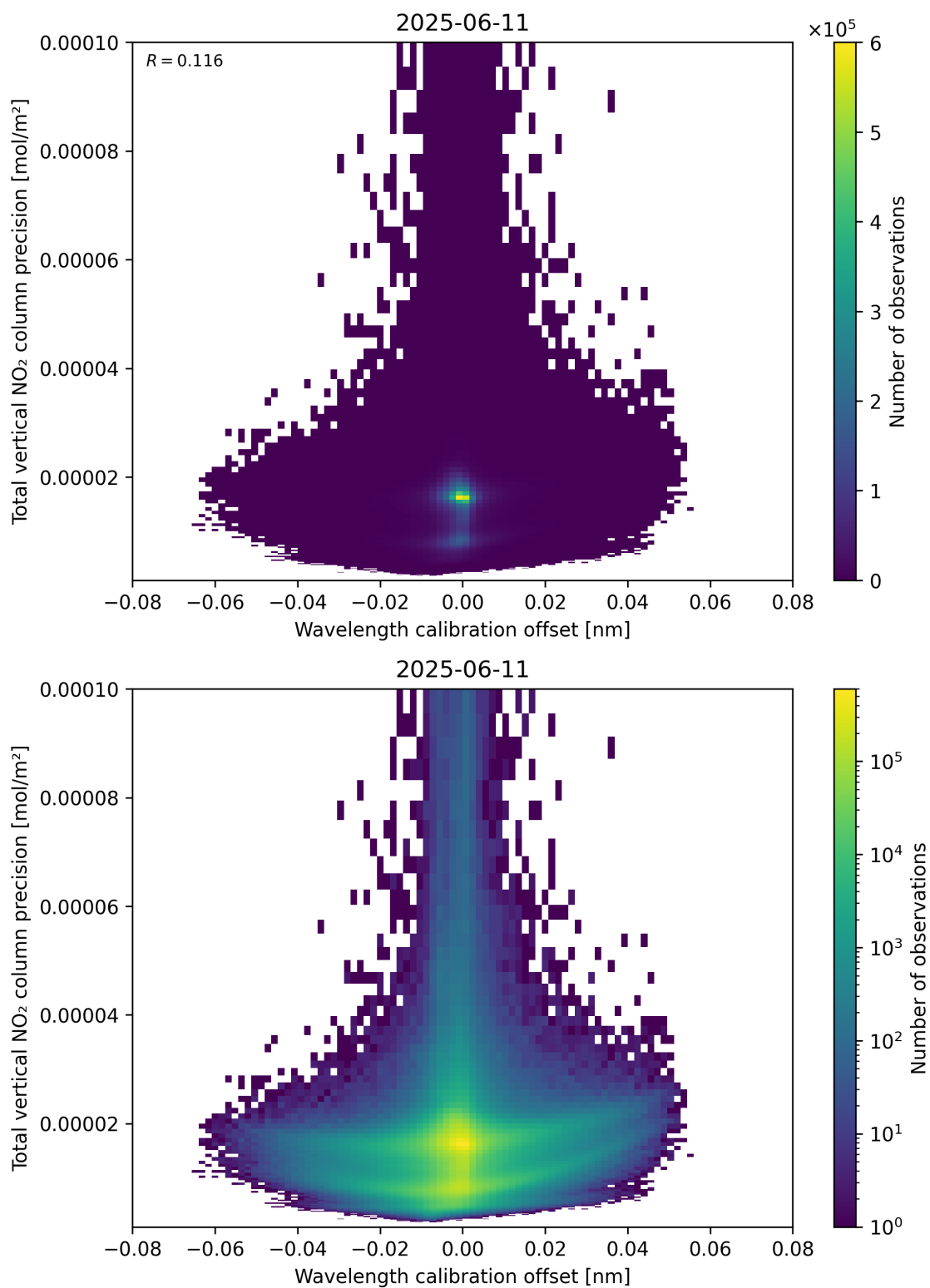
Figure 180: Scatter density plot of “Wavelength calibration offset” against “Total vertical NO 2 column precision” for 2025-06-11 to 2025-06-12.
