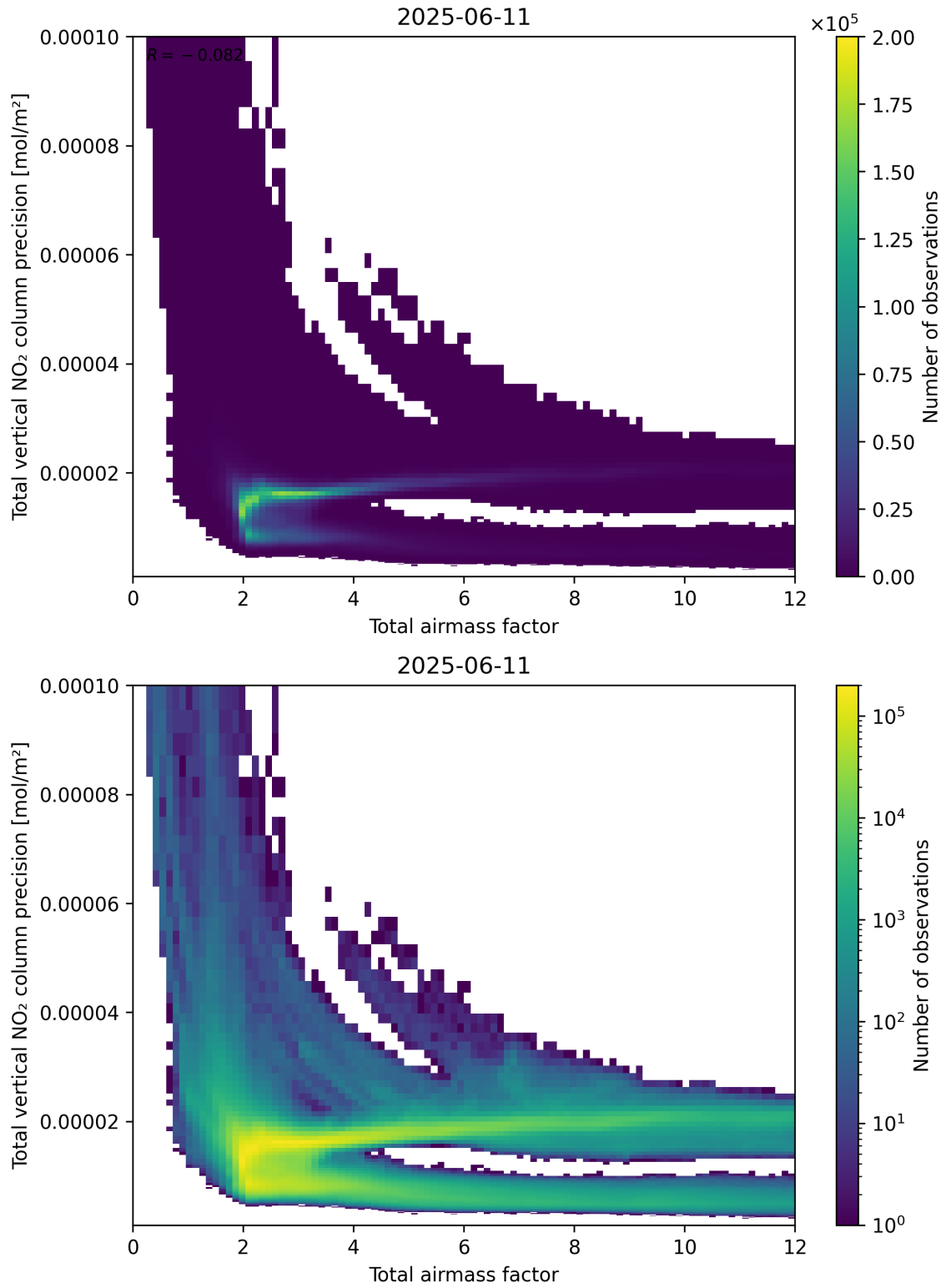
Figure 68: Scatter density plot of “Total airmass factor” against “Total vertical NO 2 column precision” for 2025-06-11 to 2025-06-12.
