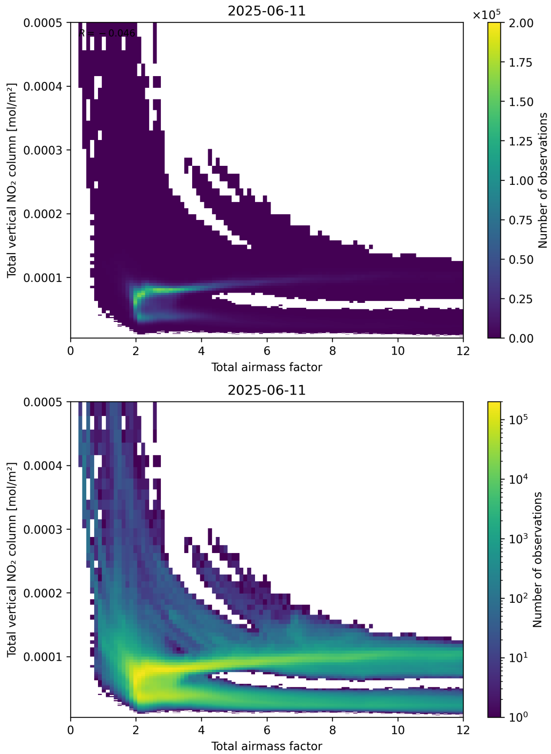
Figure 67: Scatter density plot of “Total airmass factor” against “Total vertical NO 2 column” for 2025-06-11 to 2025-06-12.
