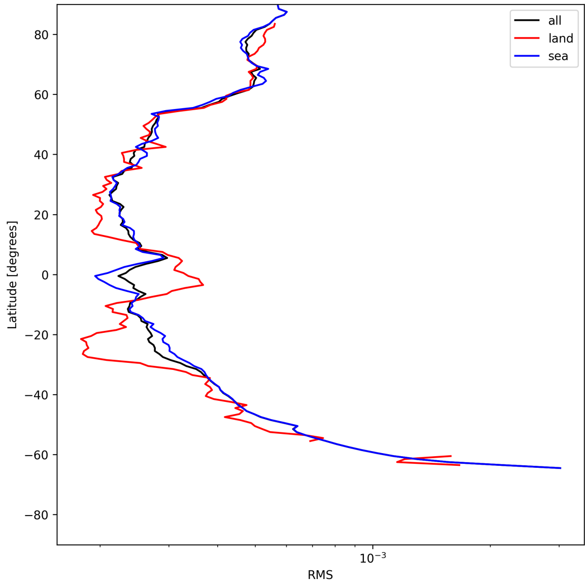
Figure 26: Zonal average of “RMS” for 2025-06-11 to 2025-06-12.
