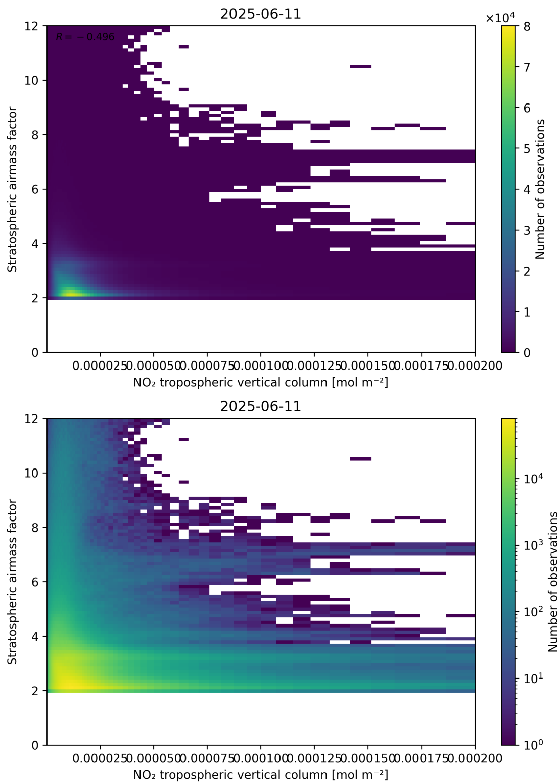
Figure 121: Scatter density plot of “NO 2 tropospheric vertical column” against “Stratospheric air mass factor” for 2025-06-11 to 2025-06-12.
