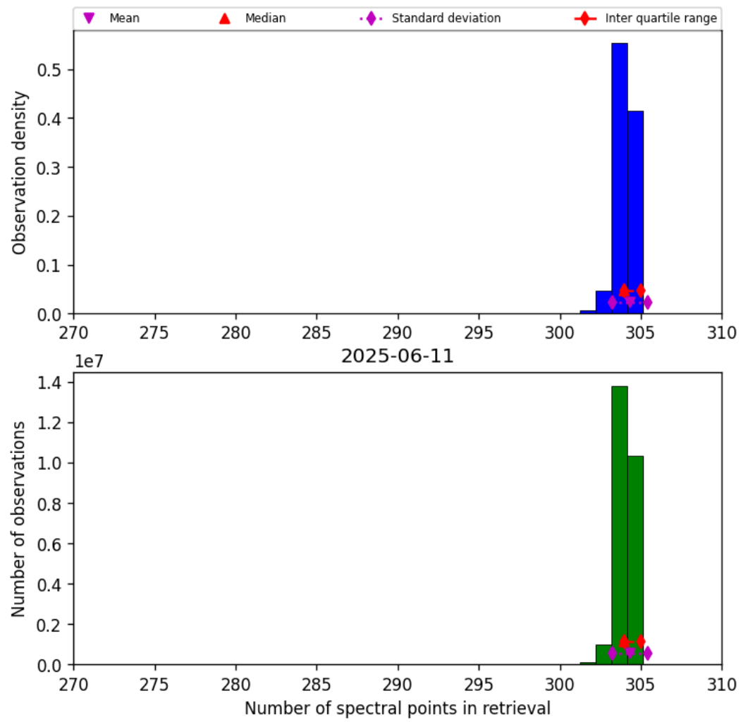
Figure 33: Histogram of “Number of spectral points in retrieval” for 2025-06-11 to 2025-06-12
