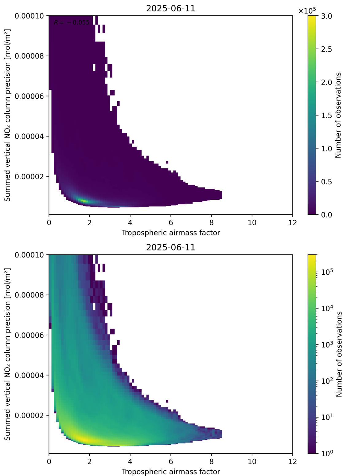
Figure 76: Scatter density plot of “Tropospheric air mass factor” against “Summed vertical NO 2 column precision” for 2025-06-11 to 2025-06-12.
