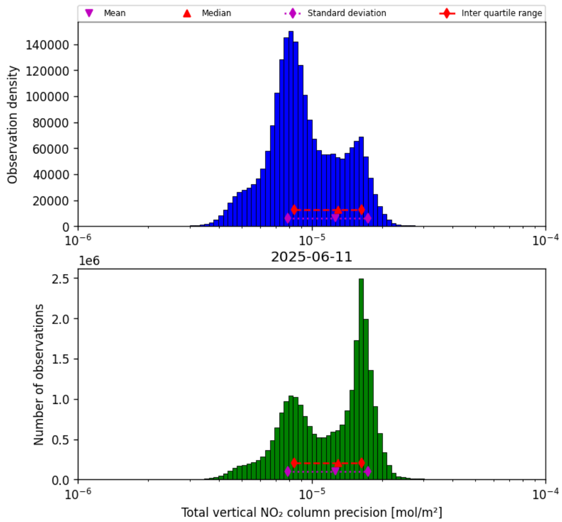
Figure 39: Histogram of “Total vertical NO 2 column precision” for 2025-06-11 to 2025-06-12
