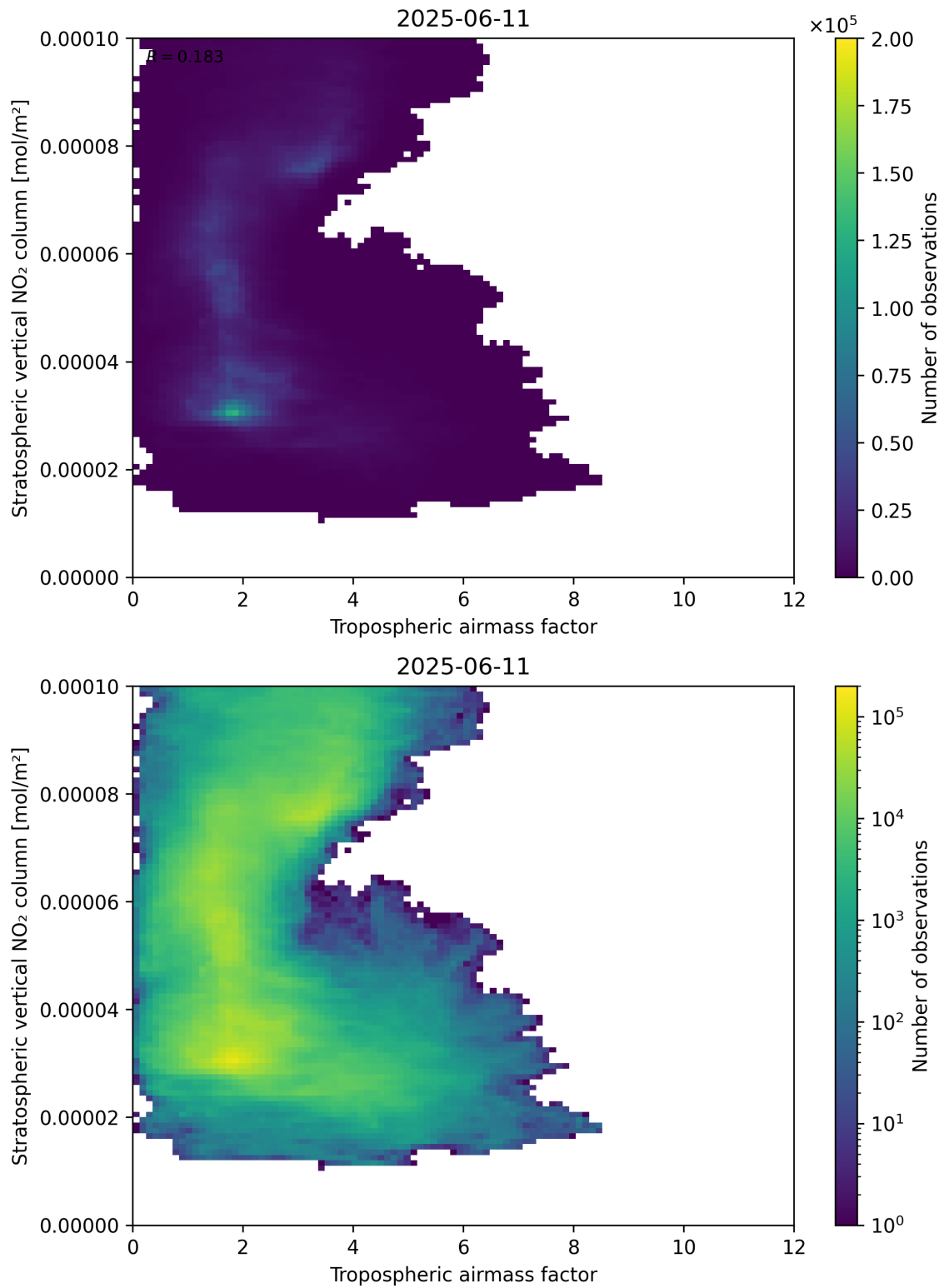
Figure 74: Scatter density plot of “Tropospheric air mass factor” against “Stratospheric vertical NO 2 column” for 2025-06-11 to 2025-06-12.
