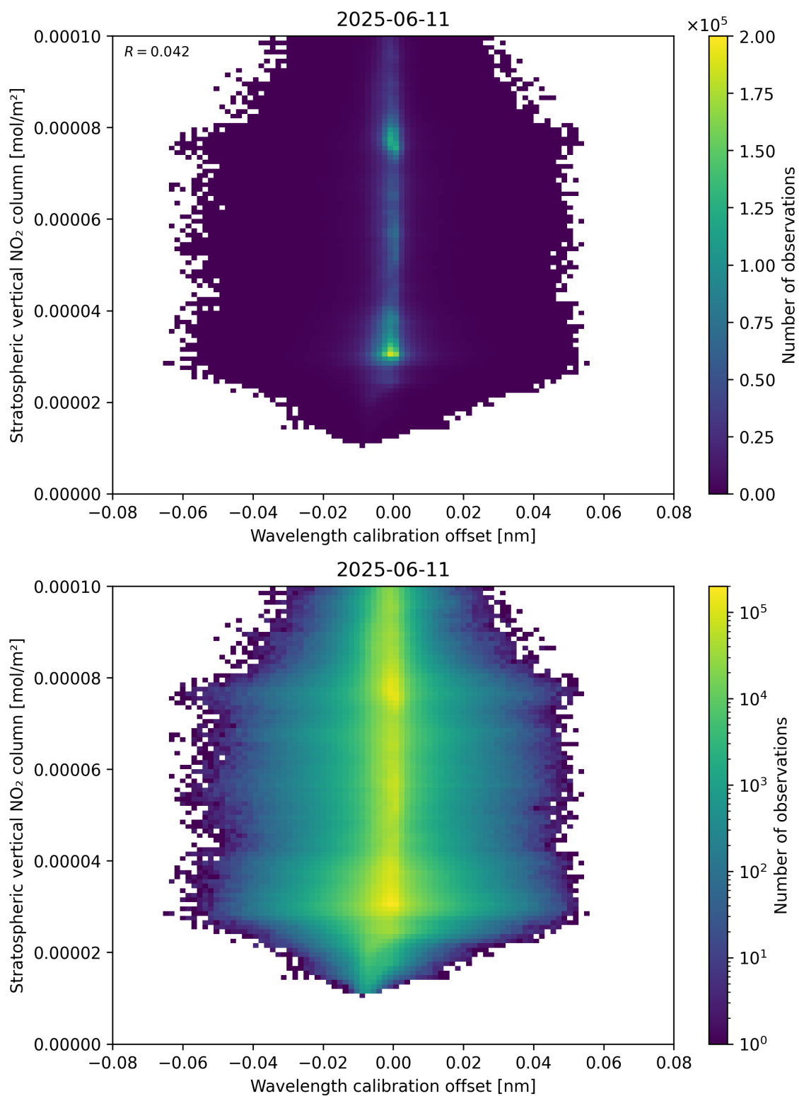
Figure 176: Scatter density plot of “Wavelength calibration offset” against “Stratospheric vertical NO 2 column” for 2025-06-11 to 2025-06-12.
