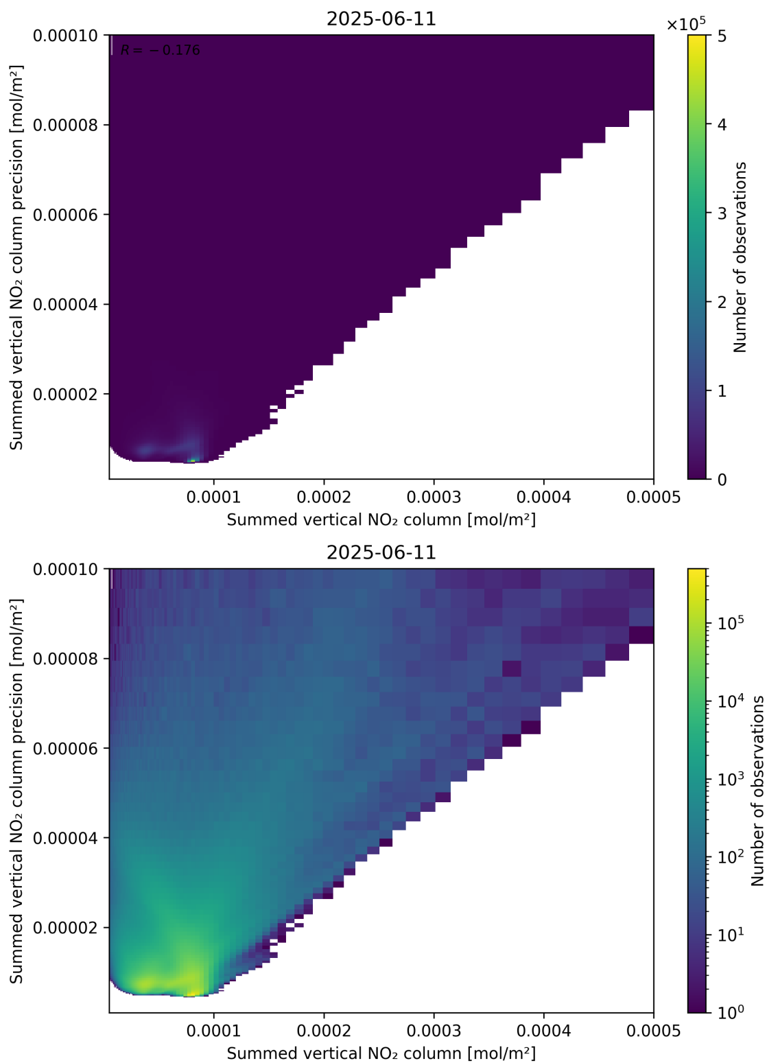
Figure 105: Scatter density plot of “Summed vertical NO 2 column” against “Summed vertical NO 2 column precision” for 2025-06-11 to 2025-06-12.
