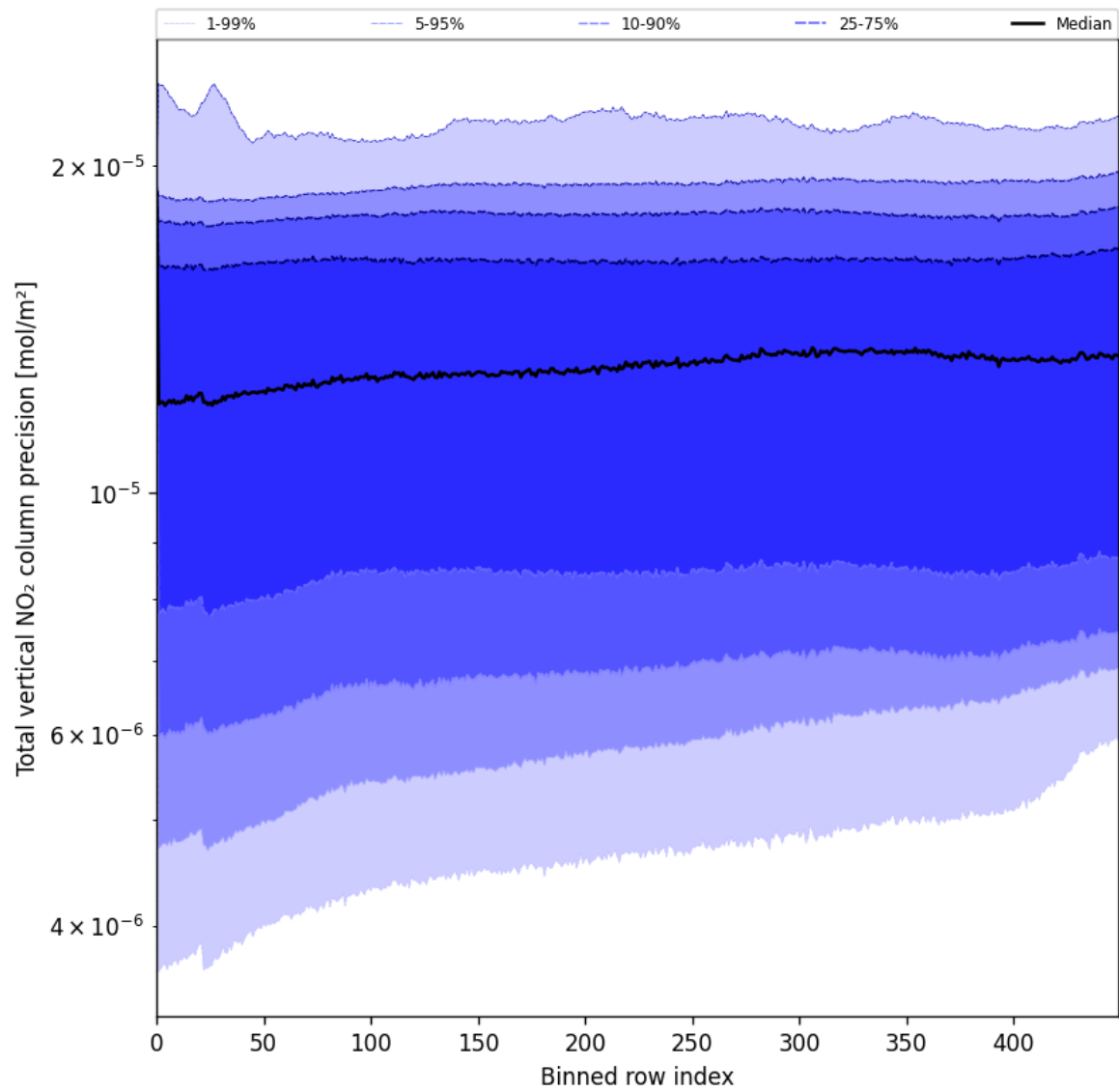
Figure 56: Along track statistics of "Total vertical NO 2 column precision" for 2025-06-11 to 2025-06-12
