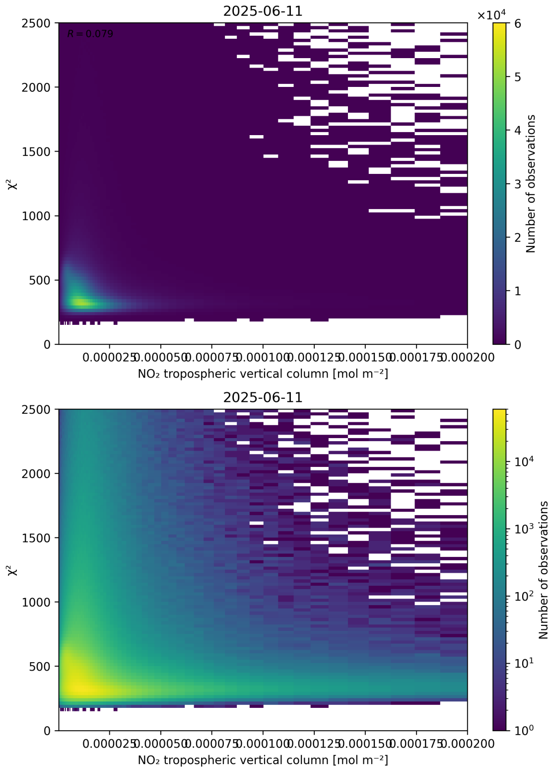
Figure 124: Scatter density plot of “NO 2 tropospheric vertical column” against “ \chi^2 ” for 2025-06-11 to 2025-06-12.
