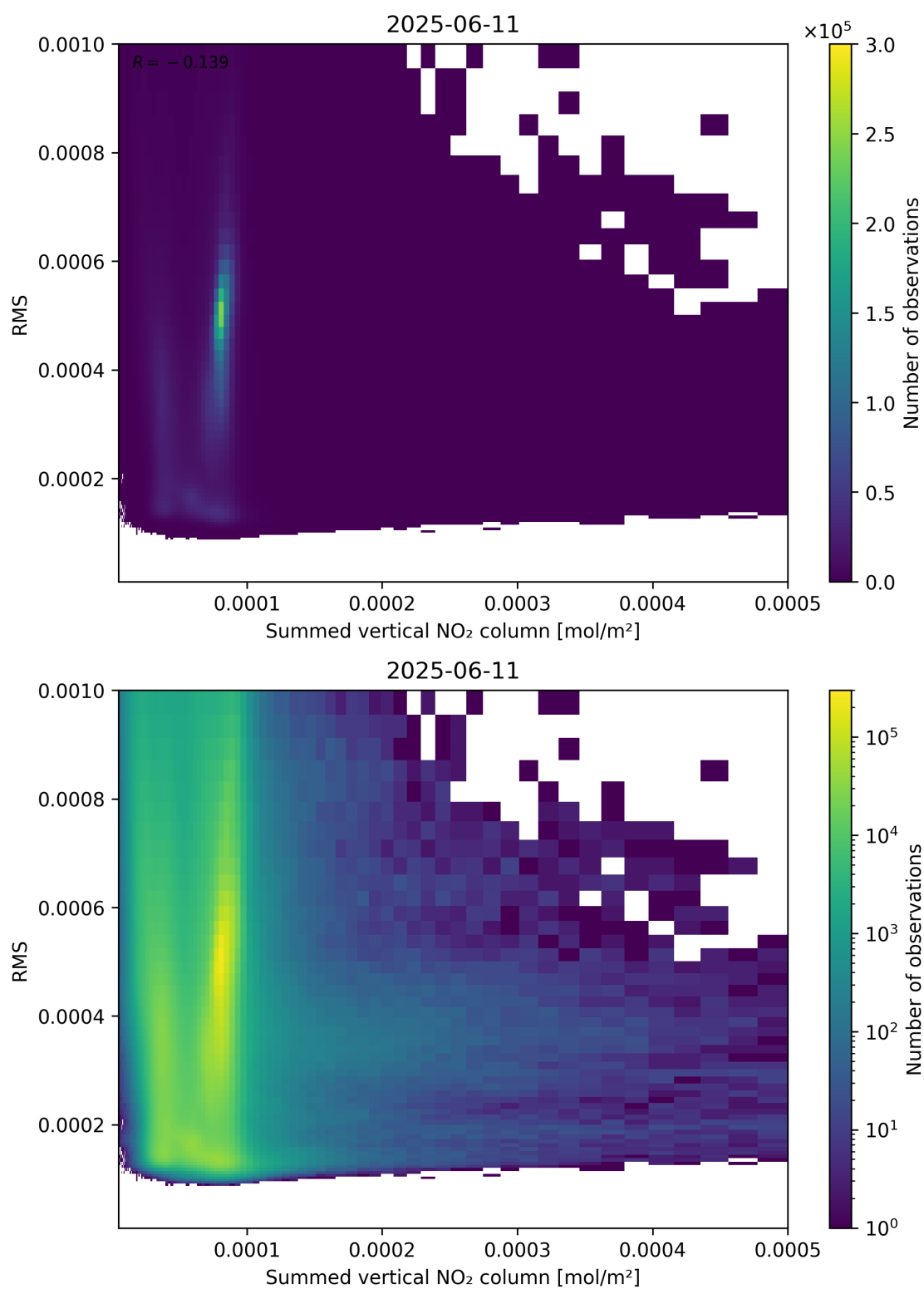
Figure 109: Scatter density plot of “Summed vertical NO 2 column” against “RMS” for 2025-06-11 to 2025-06-12.
