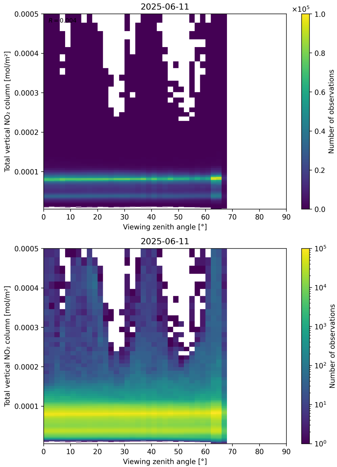
Figure 167: Scatter density plot of “Viewing zenith angle” against “Total vertical NO 2 column” for 2025-06-11 to 2025-06-12.
