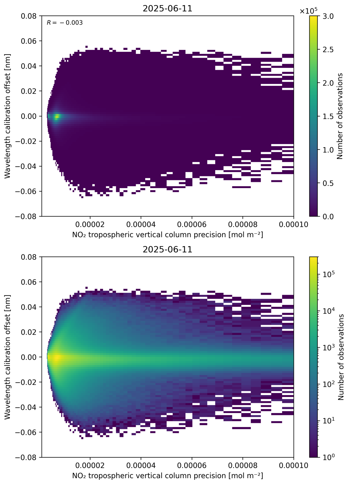
Figure 141: Scatter density plot of “NO 2 tropospheric vertical column precision” against “Wavelength calibration offset” for 2025-06-11 to 2025-06-12.
