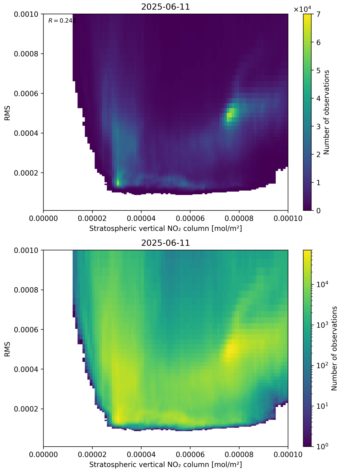
Figure 102: Scatter density plot of “Stratospheric vertical NO 2 column” against “RMS” for 2025-06-11 to 2025-06-12.
