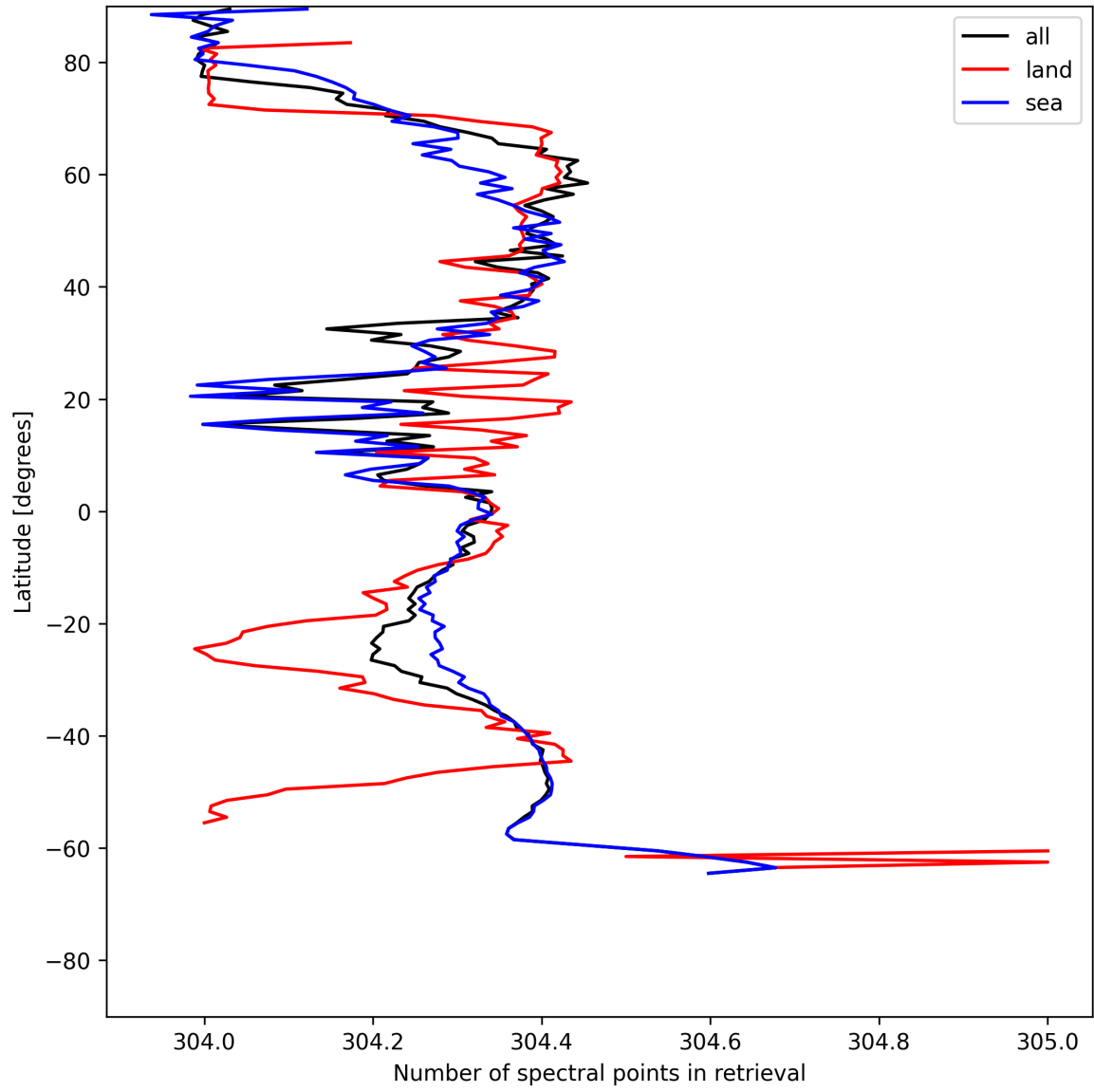
Figure 16: Zonal average of “Number of spectral points in retrieval” for 2025-06-11 to 2025-06-12.
