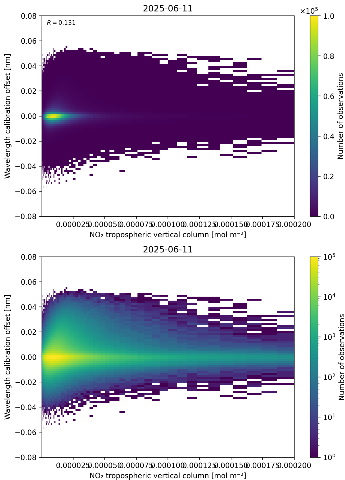
Figure 143: Scatter density plot of “NO 2 tropospheric vertical column” against “Wavelength calibration offset” for 2025-06-11 to 2025-06-12.
