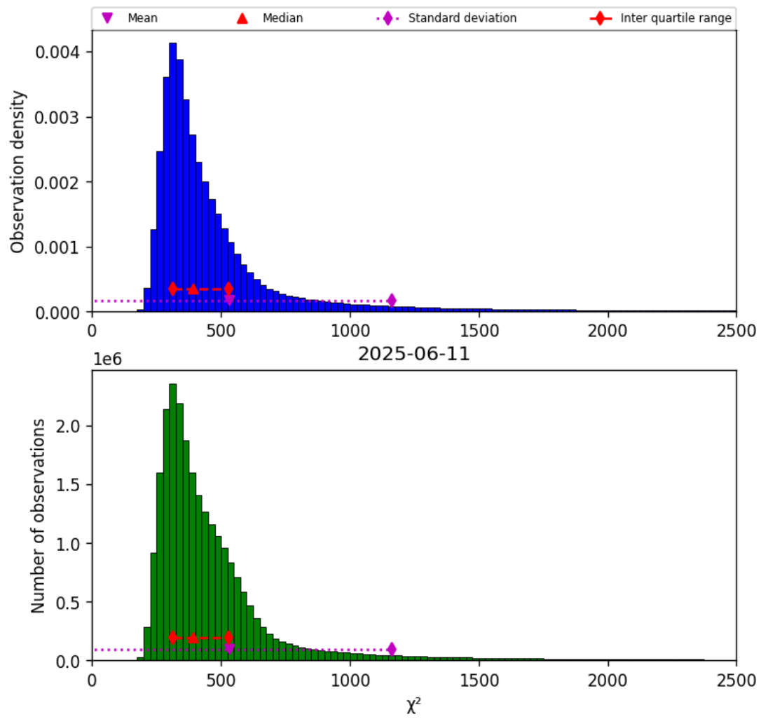
Figure 42: Histogram of “ \chi^2 ” for 2025-06-11 to 2025-06-12
