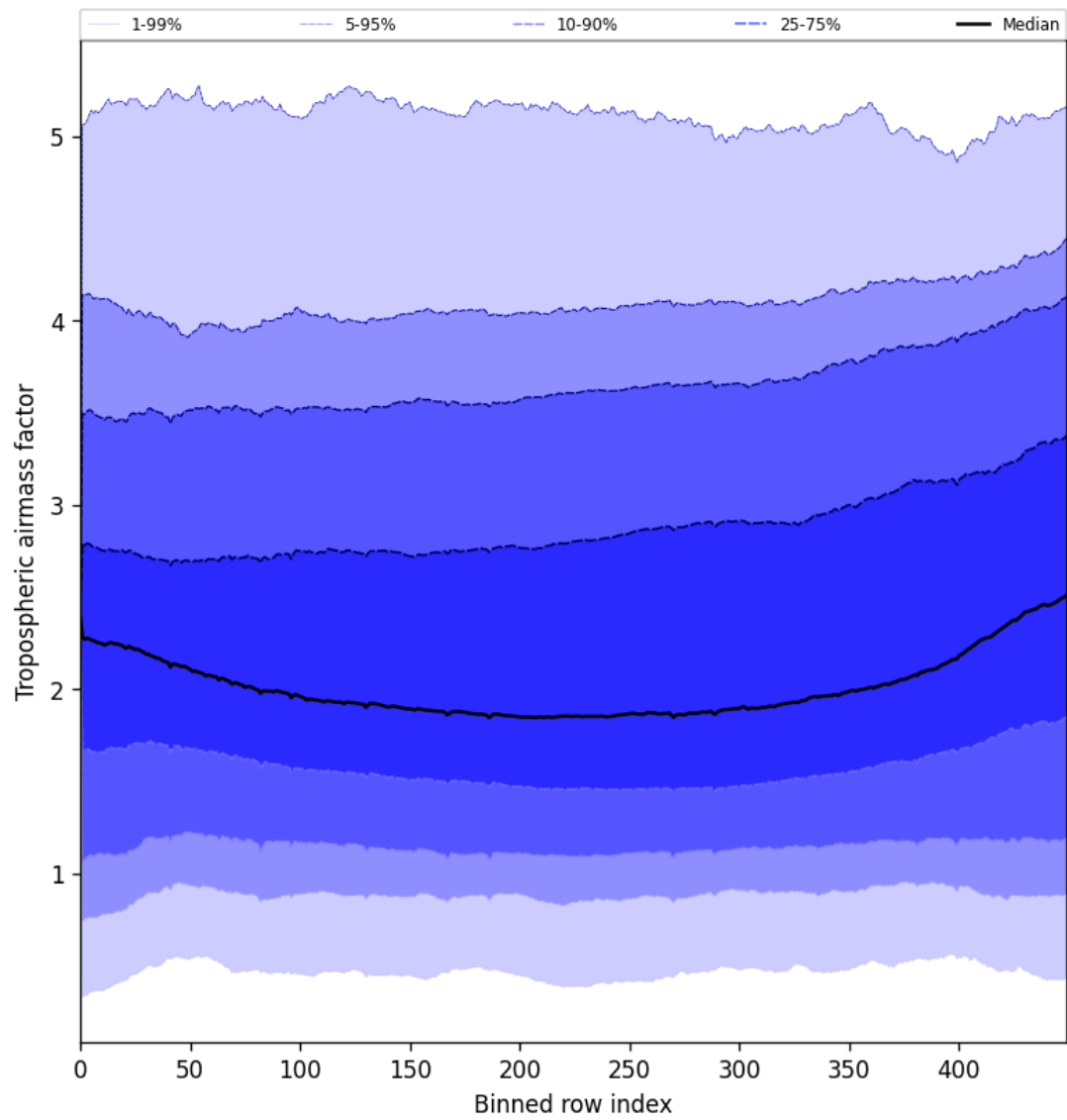
Figure 48: Along track statistics of “Tropospheric airmass factor” for 2025-06-11 to 2025-06-12
