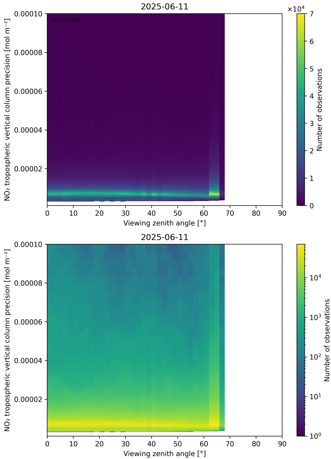
Figure 170: Scatter density plot of “Viewing zenith angle” against “NO 2 tropospheric vertical column precision” for 2025-06-11 to 2025-06-12.
