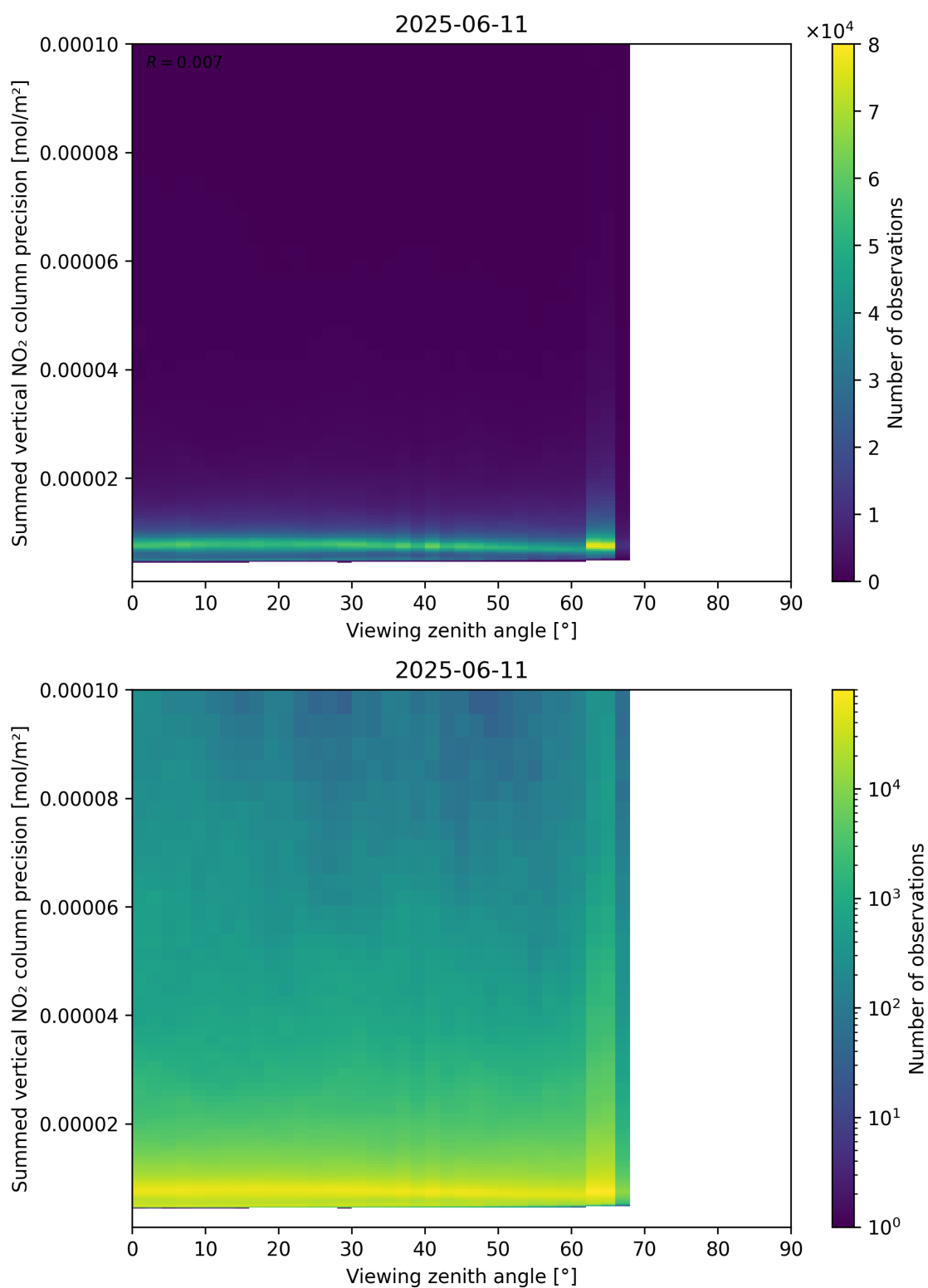
Figure 166: Scatter density plot of “Viewing zenith angle” against “Summed vertical NO 2 column precision” for 2025-06-11 to 2025-06-12.
