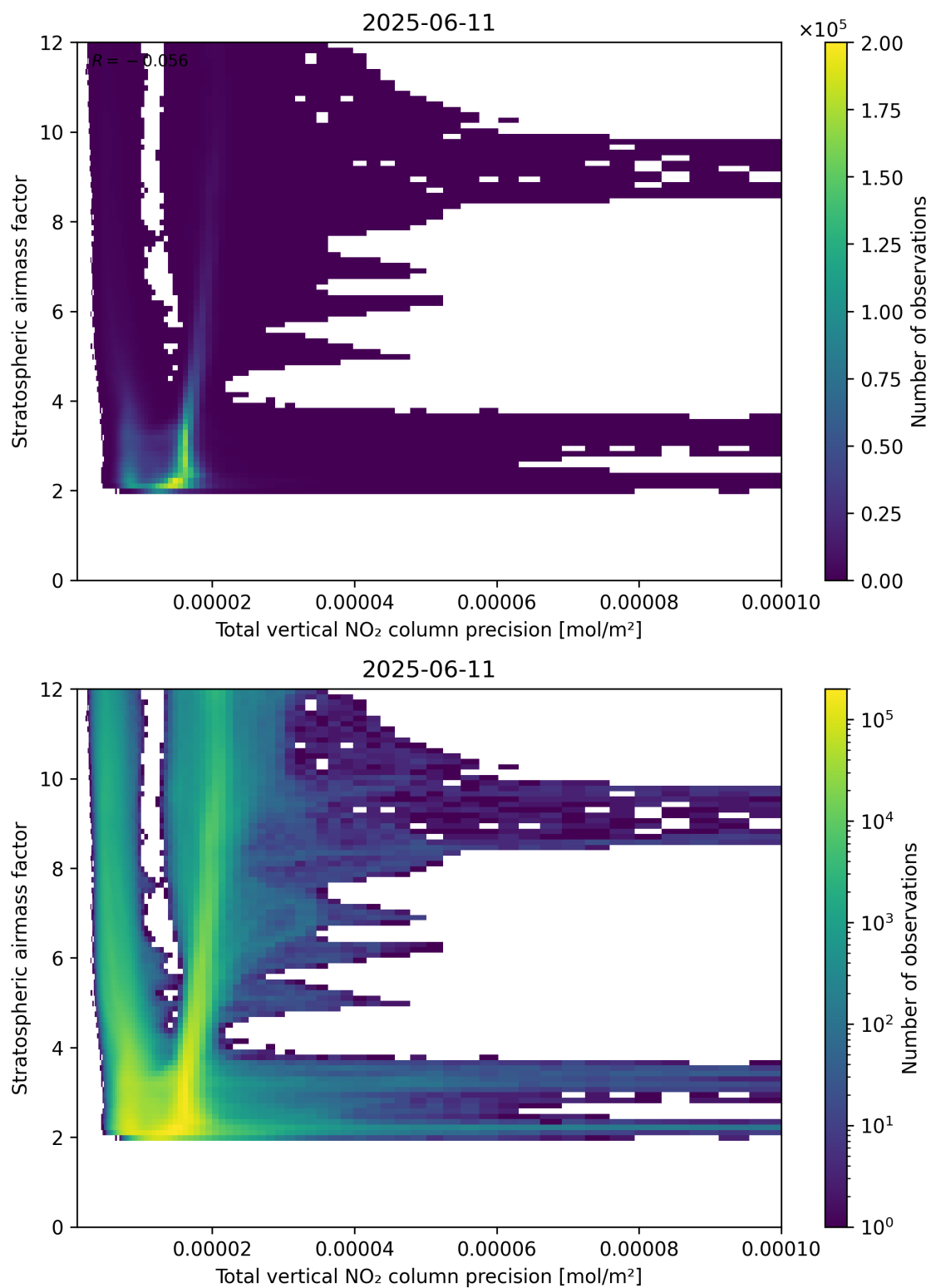
Figure 115: Scatter density plot of “Total vertical NO 2 column precision” against “Stratospheric air mass factor” for 2025-06-11 to 2025-06-12.
