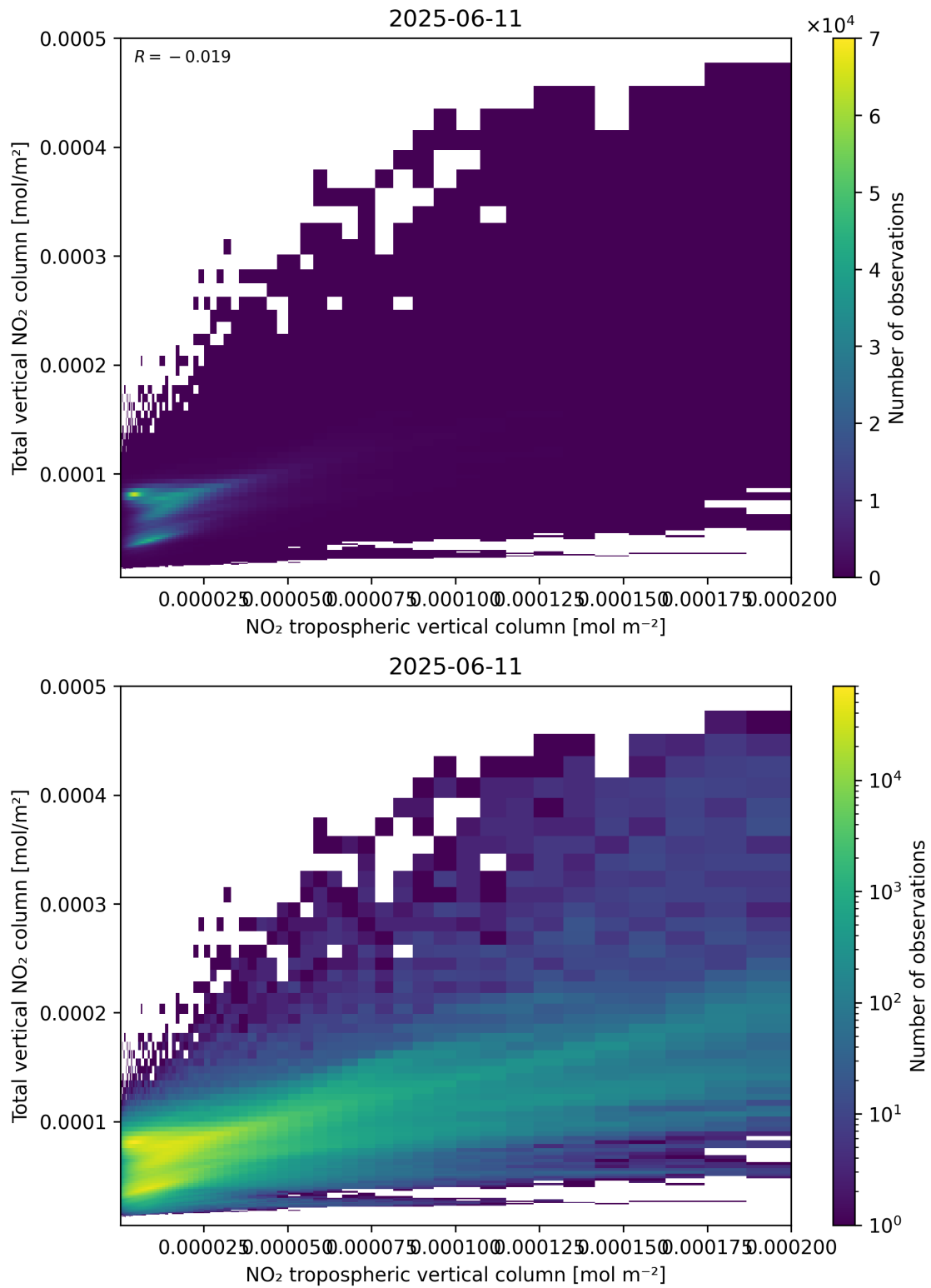
Figure 128: Scatter density plot of “NO 2 tropospheric vertical column” against “Total vertical NO 2 column” for 2025-06-11 to 2025-06-12.
