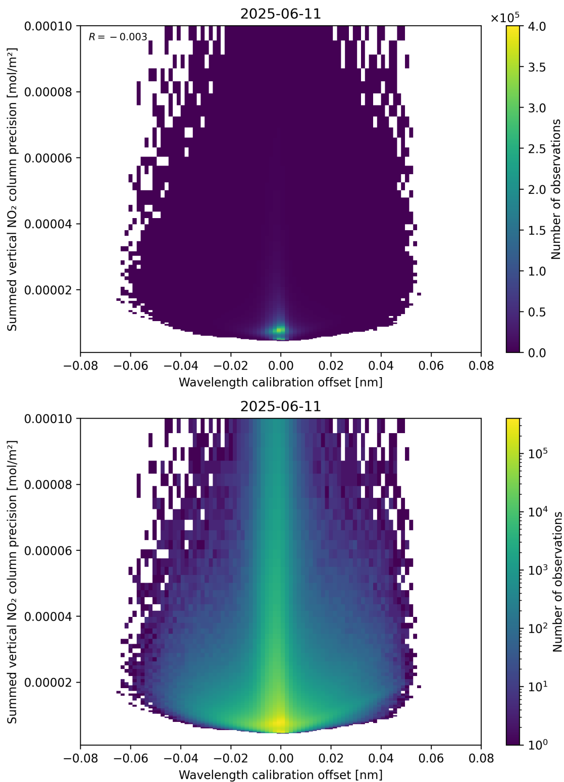
Figure 178: Scatter density plot of “Wavelength calibration offset” against “Summed vertical NO 2 column precision” for 2025-06-11 to 2025-06-12.
