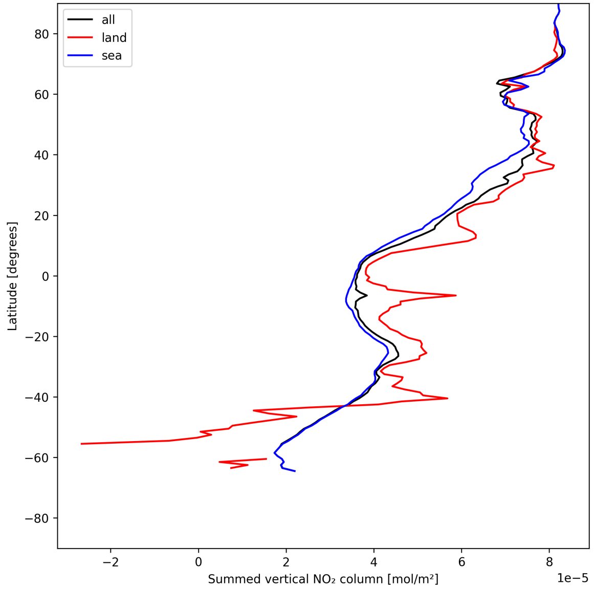
Figure 23: Zonal average of “Summed vertical NO 2 column” for 2025-06-11 to 2025-06-12.
