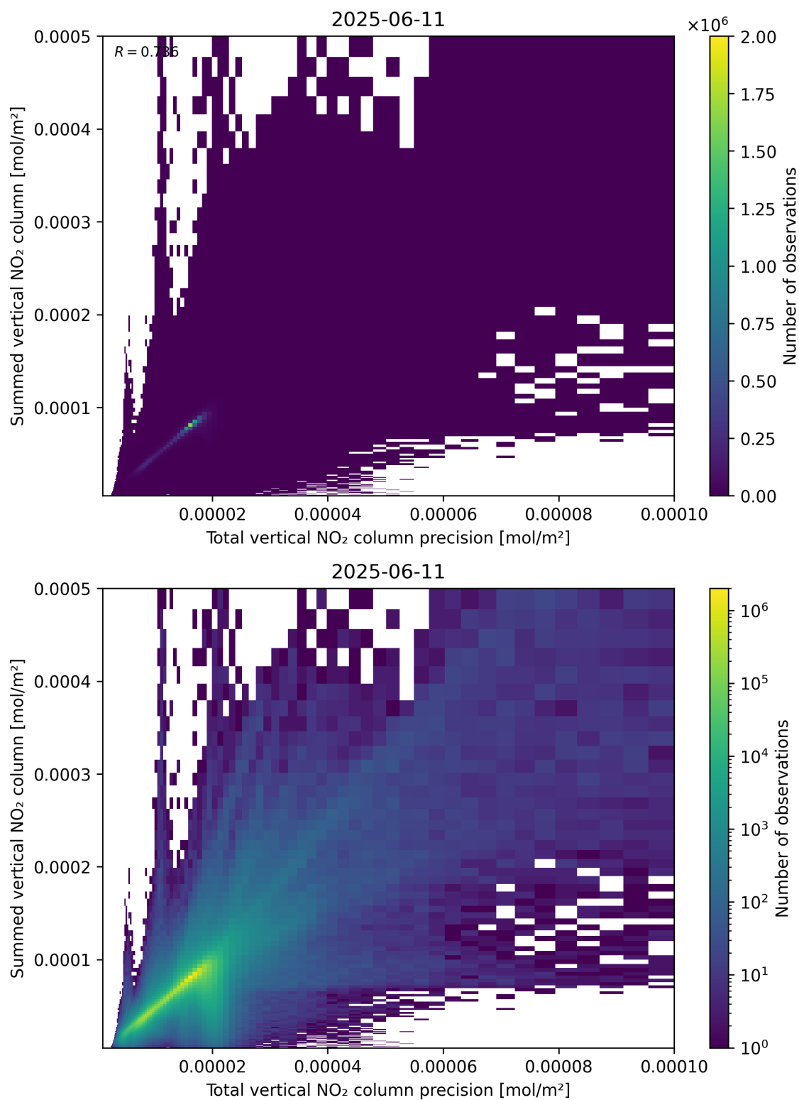
Figure 117: Scatter density plot of “Total vertical NO 2 column precision” against “Summed vertical NO 2 column” for 2025-06-11 to 2025-06-12.
