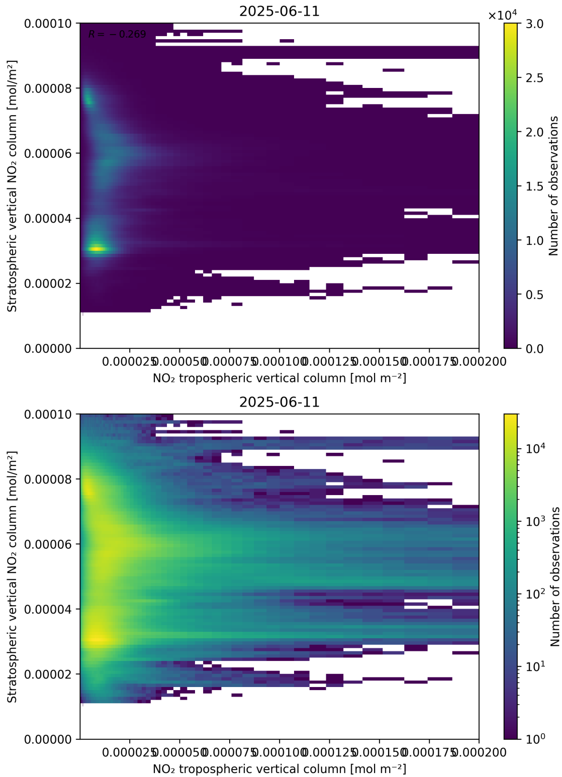
Figure 125: Scatter density plot of “NO 2 tropospheric vertical column” against “Stratospheric vertical NO 2 column” for 2025-06-11 to 2025-06-12.
