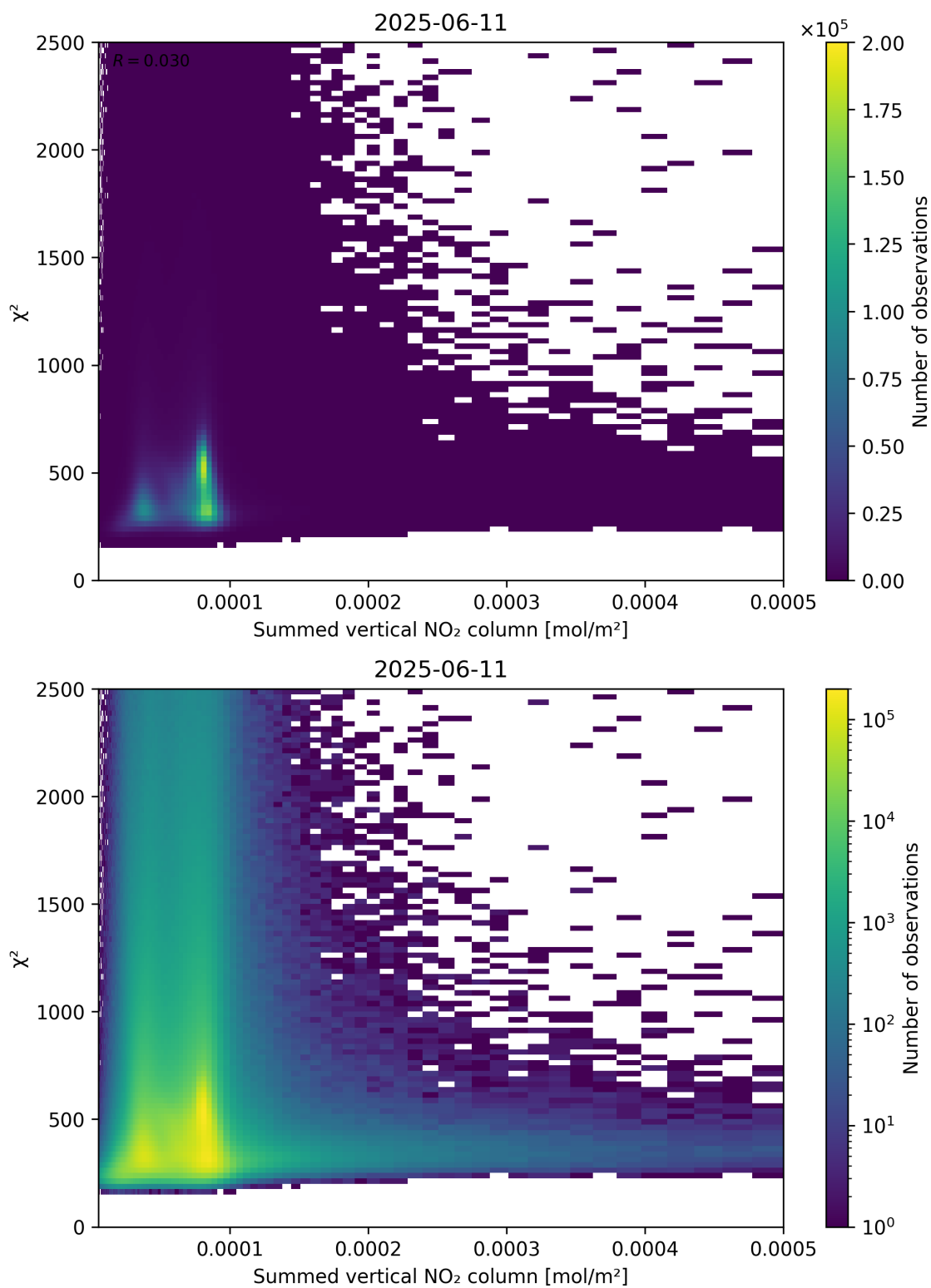
Figure 104: Scatter density plot of “Summed vertical NO 2 column” against “ \chi^2 ” for 2025-06-11 to 2025-06-12.
