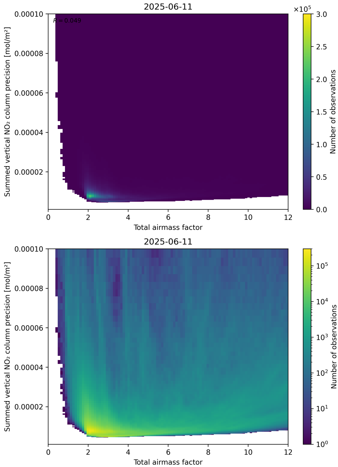
Figure 66: Scatter density plot of “Total airmass factor” against “Summed vertical NO 2 column precision” for 2025-06-11 to 2025-06-12.
