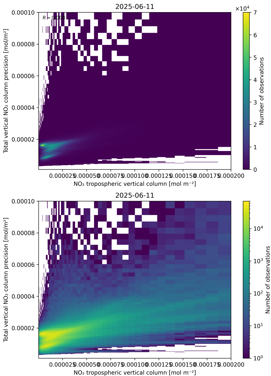
Figure 129: Scatter density plot of “NO 2 tropospheric vertical column” against “Total vertical NO 2 column precision” for 2025-06-11 to 2025-06-12.
