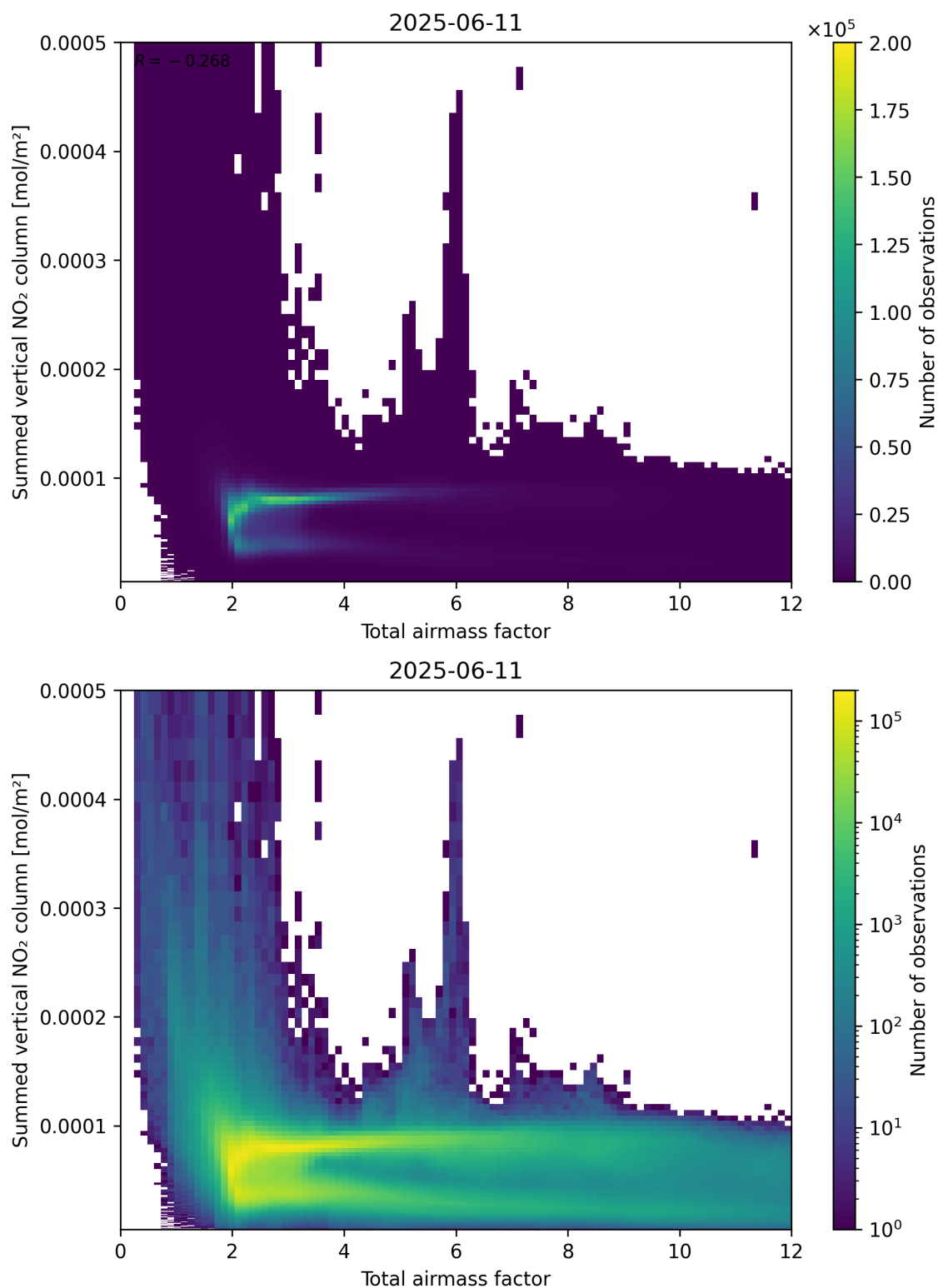
Figure 65: Scatter density plot of “Total airmass factor” against “Summed vertical NO 2 column” for 2025-06-11 to 2025-06-12.
