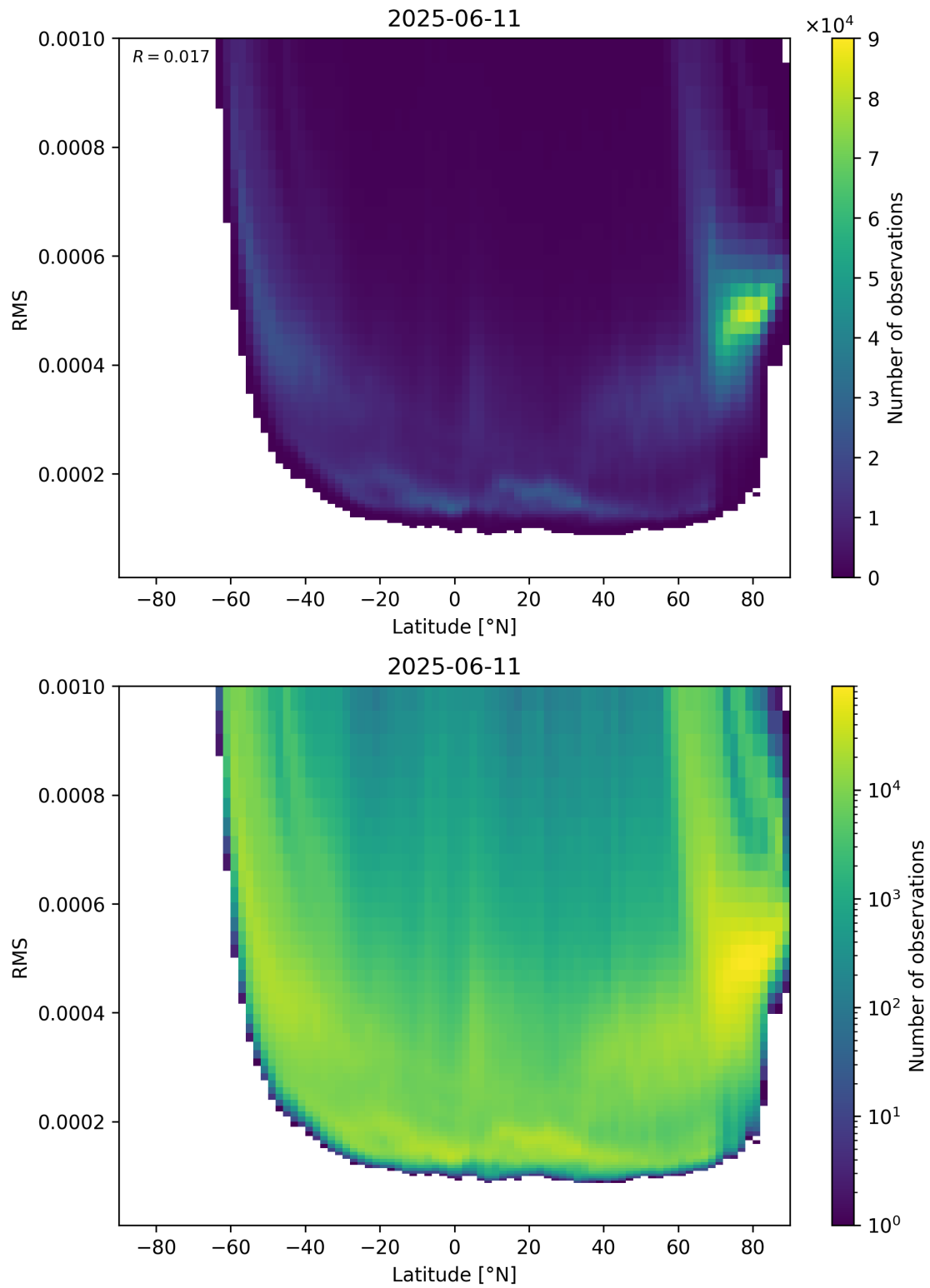
Figure 94: Scatter density plot of “Latitude” against “RMS” for 2025-06-11 to 2025-06-12.
