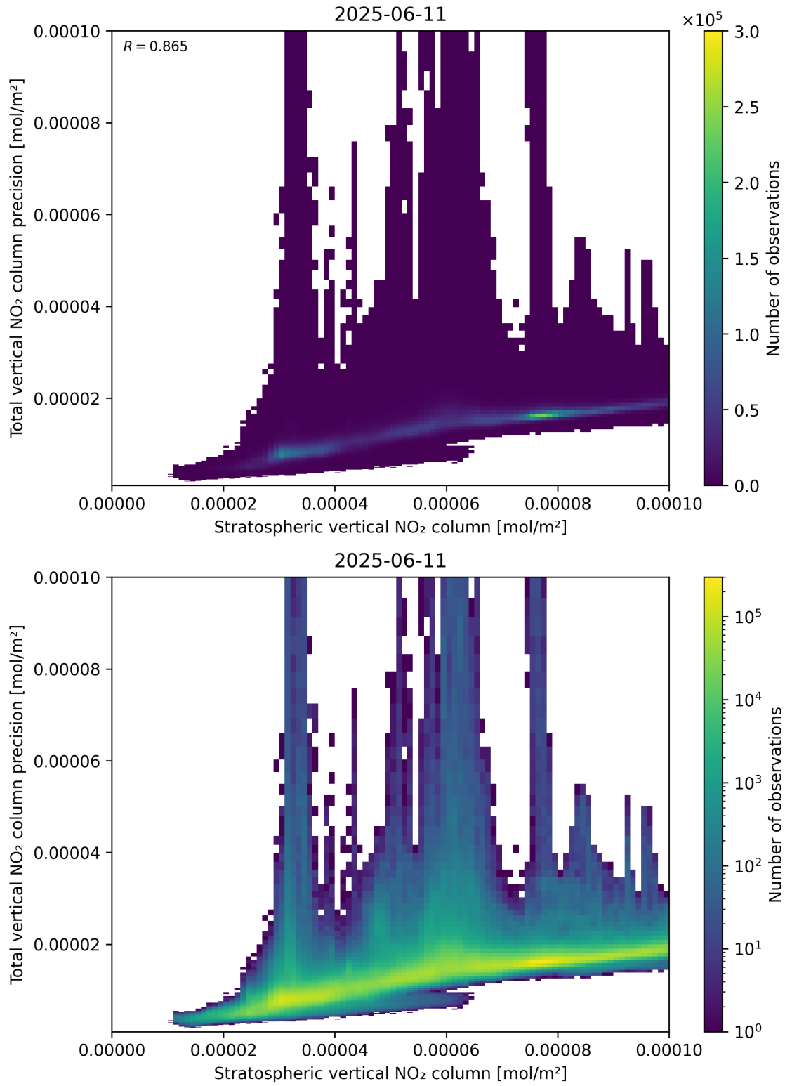
Figure 101: Scatter density plot of “Stratospheric vertical NO 2 column” against “Total vertical NO 2 column precision” for 2025-06-11 to 2025-06-12.
