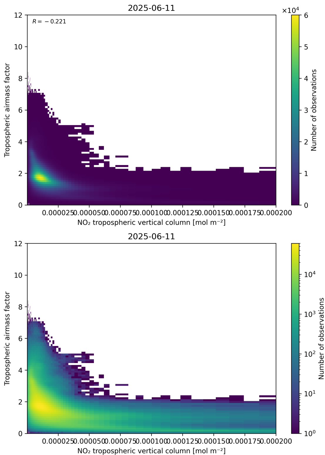
Figure 123: Scatter density plot of “NO 2 tropospheric vertical column” against “Tropospheric air mass factor” for 2025-06-11 to 2025-06-12.
