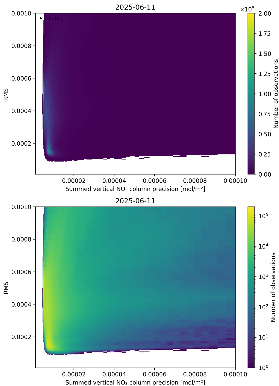
Figure 108: Scatter density plot of “Summed vertical NO 2 column precision” against “RMS” for 2025-06-11 to 2025-06-12.
