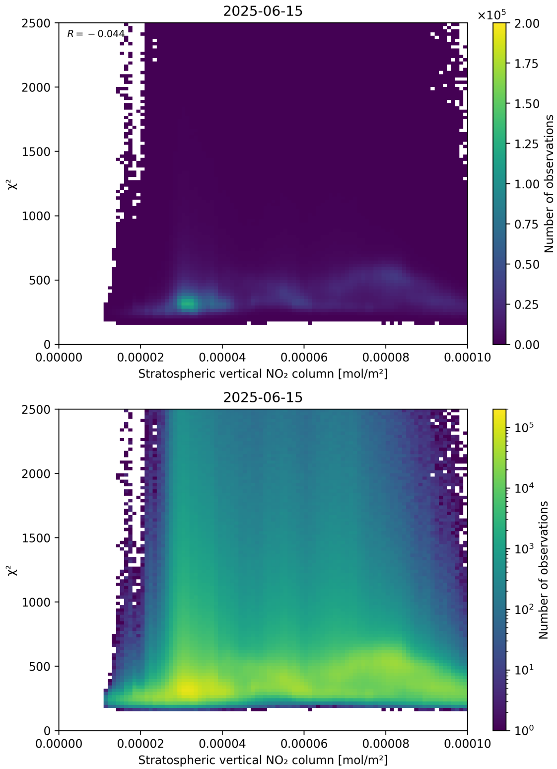
Figure 97: Scatter density plot of “Stratospheric vertical NO 2 column” against “ \chi^2 ” for 2025-06-14 to 2025-06-16.
