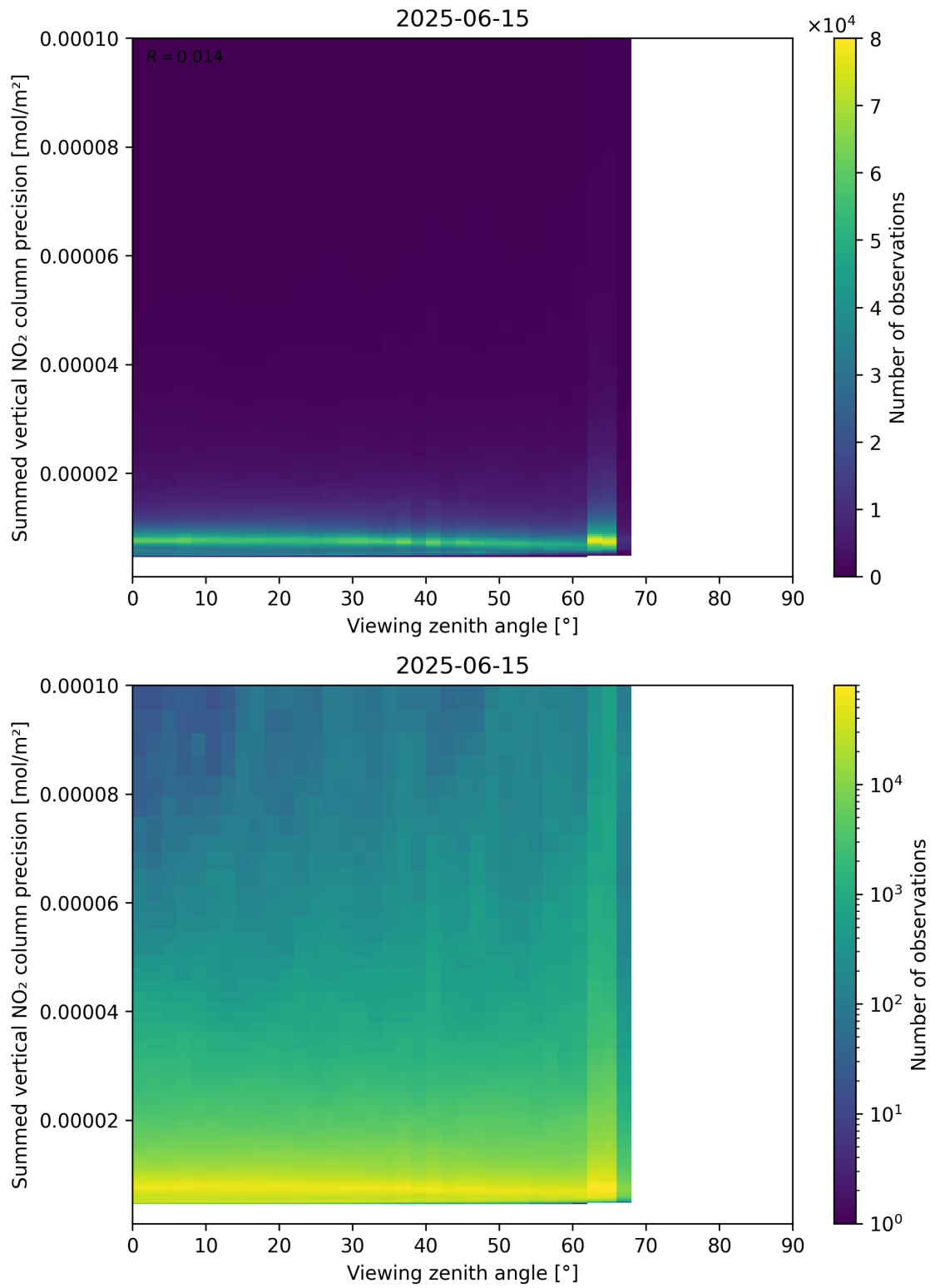
Figure 166: Scatter density plot of “Viewing zenith angle” against “Summed vertical NO 2 column precision” for 2025-06-14 to 2025-06-16.
