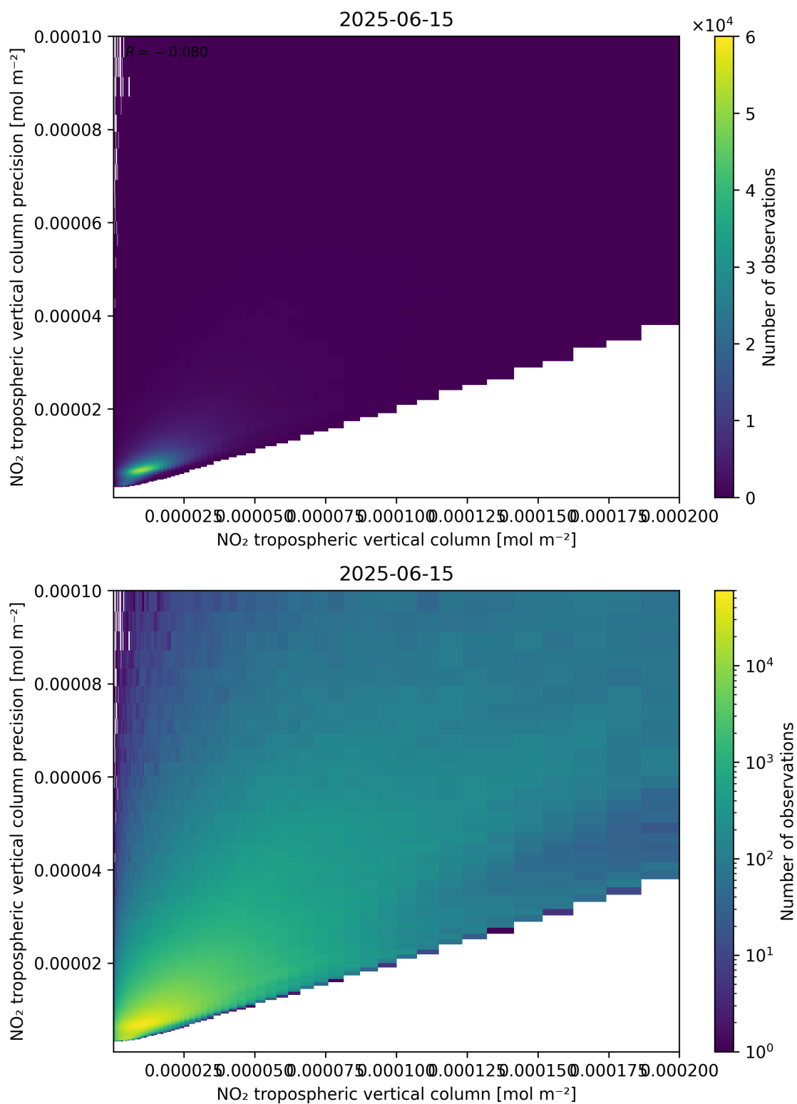
Figure 130: Scatter density plot of “NO 2 tropospheric vertical column” against “NO 2 tropospheric vertical column precision” for 2025-06-14 to 2025-06-16.
