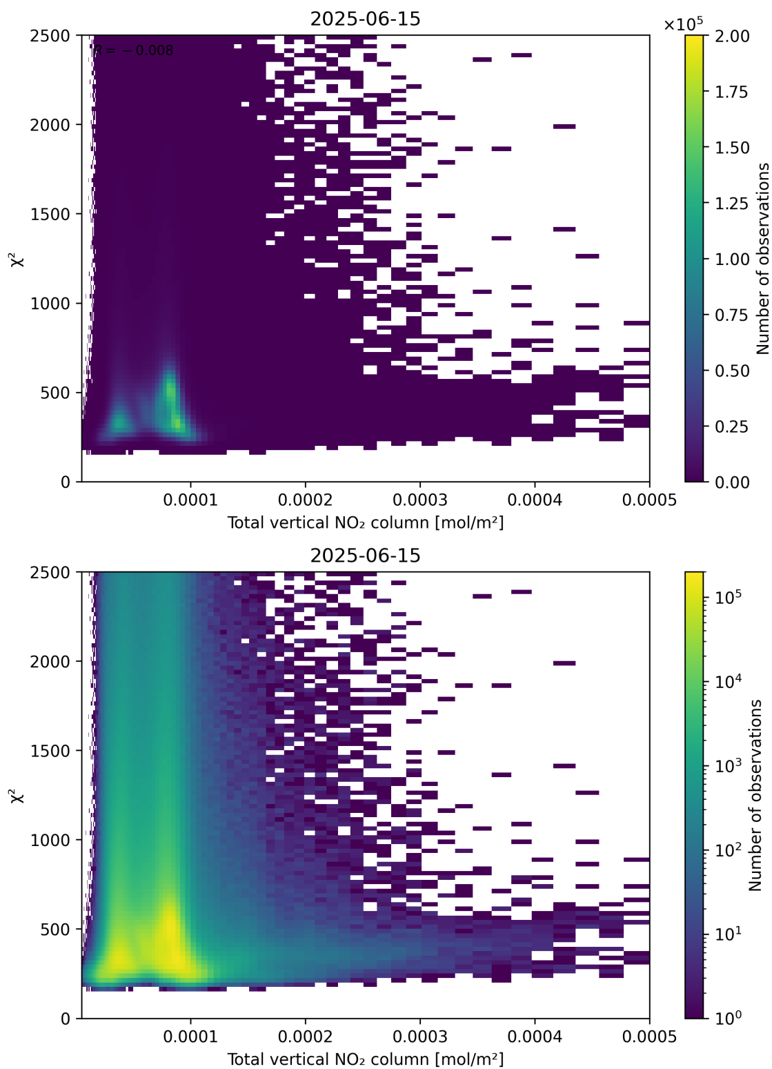
Figure 111: Scatter density plot of “Total vertical NO 2 column” against “ \chi^2 ” for 2025-06-14 to 2025-06-16.
