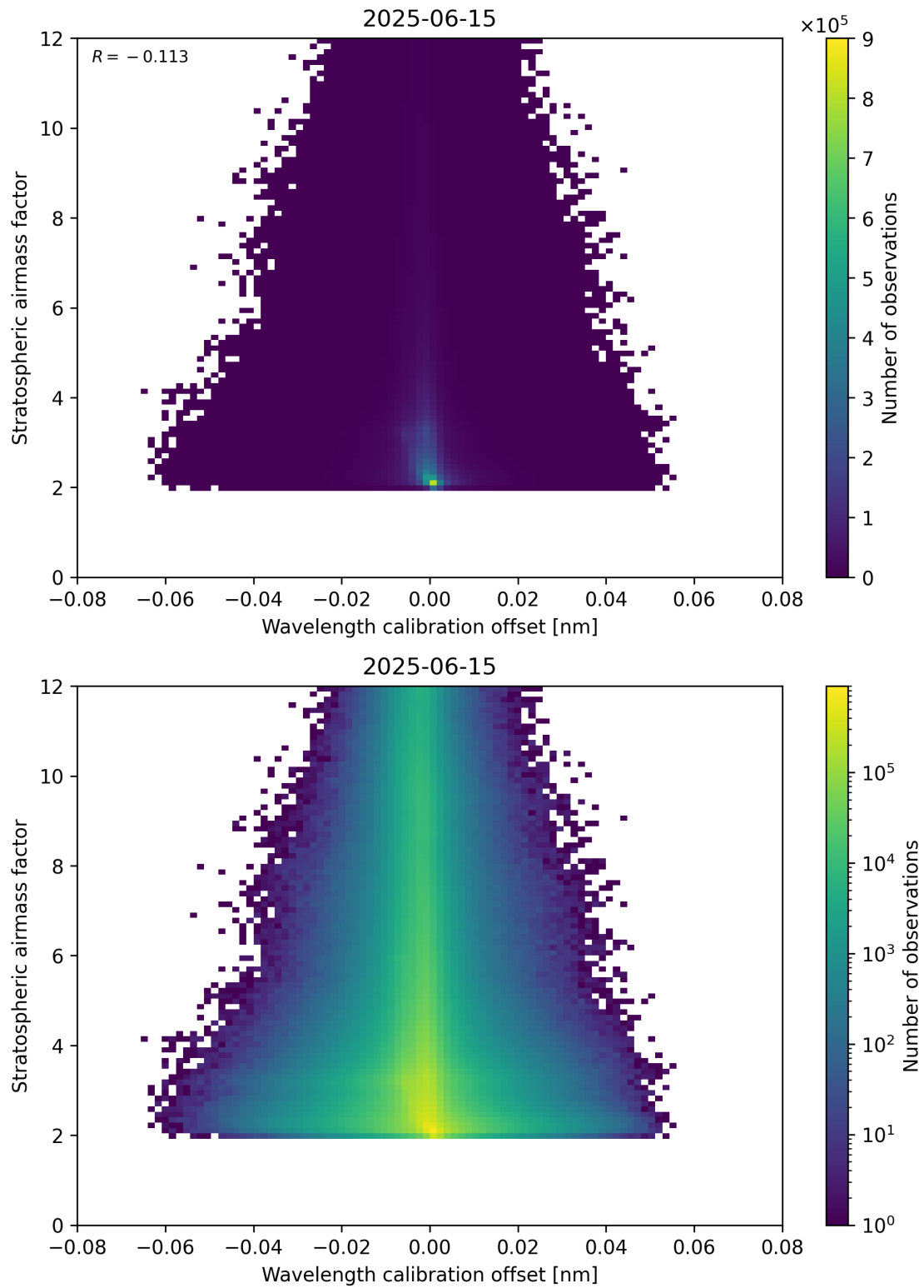
Figure 174: Scatter density plot of “Wavelength calibration offset” against “Stratospheric airmass factor” for 2025-06-14 to 2025-06-16.
