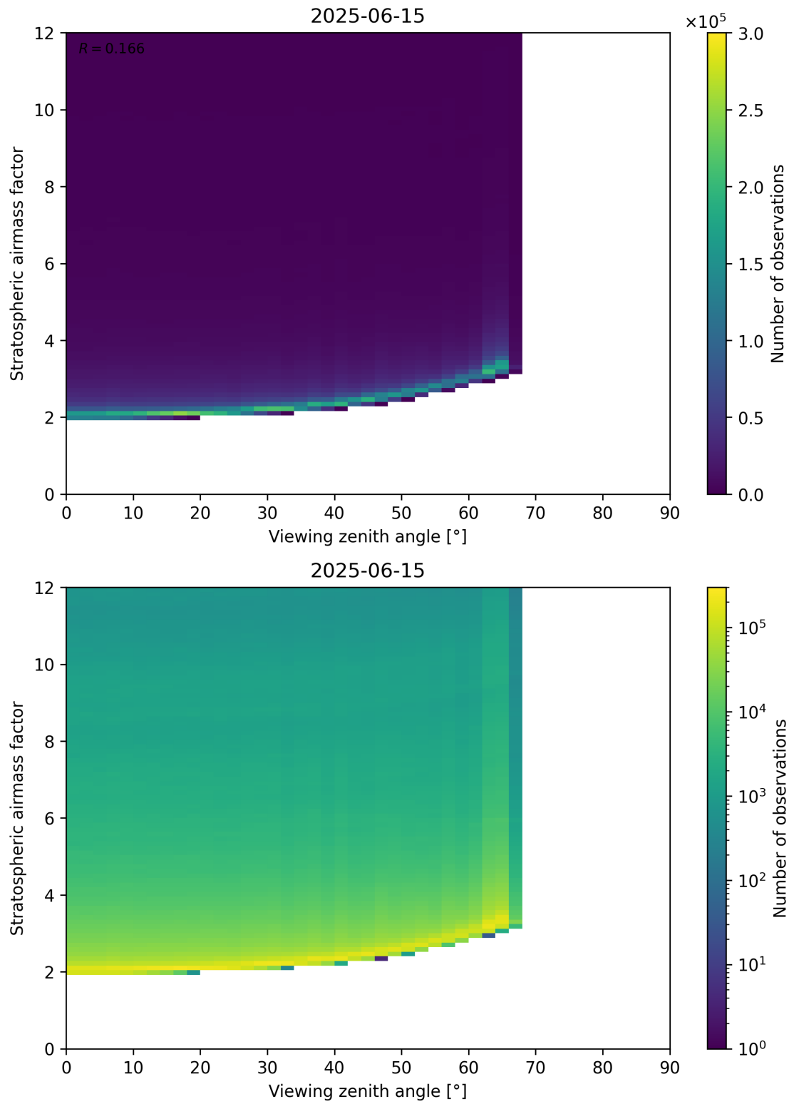
Figure 159: Scatter density plot of “Viewing zenith angle” against “Stratospheric airmass factor” for 2025-06-14 to 2025-06-16.
