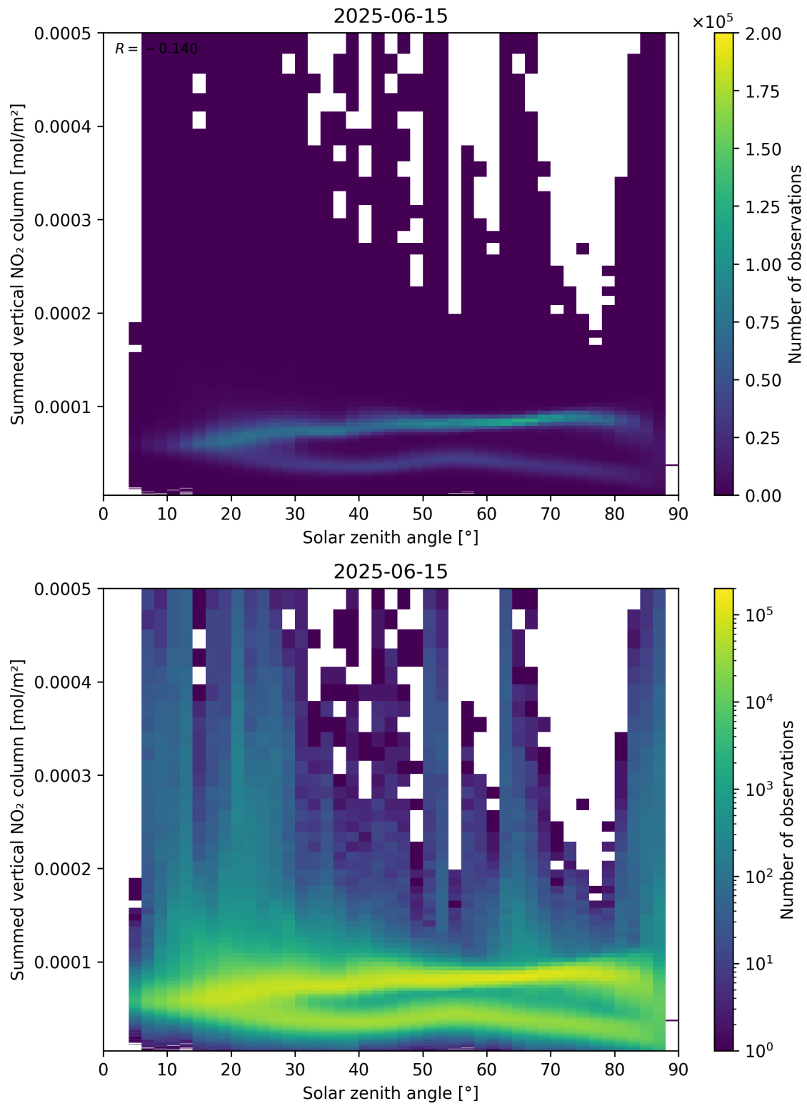
Figure 151: Scatter density plot of “Solar zenith angle” against “Summed vertical NO 2 column” for 2025-06-14 to 2025-06-16.
