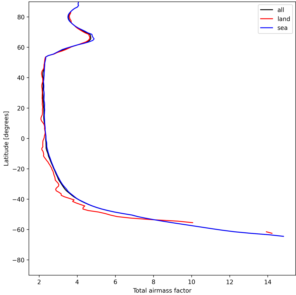
Figure 15: Zonal average of “Total airmass factor” for 2025-06-14 to 2025-06-16.
