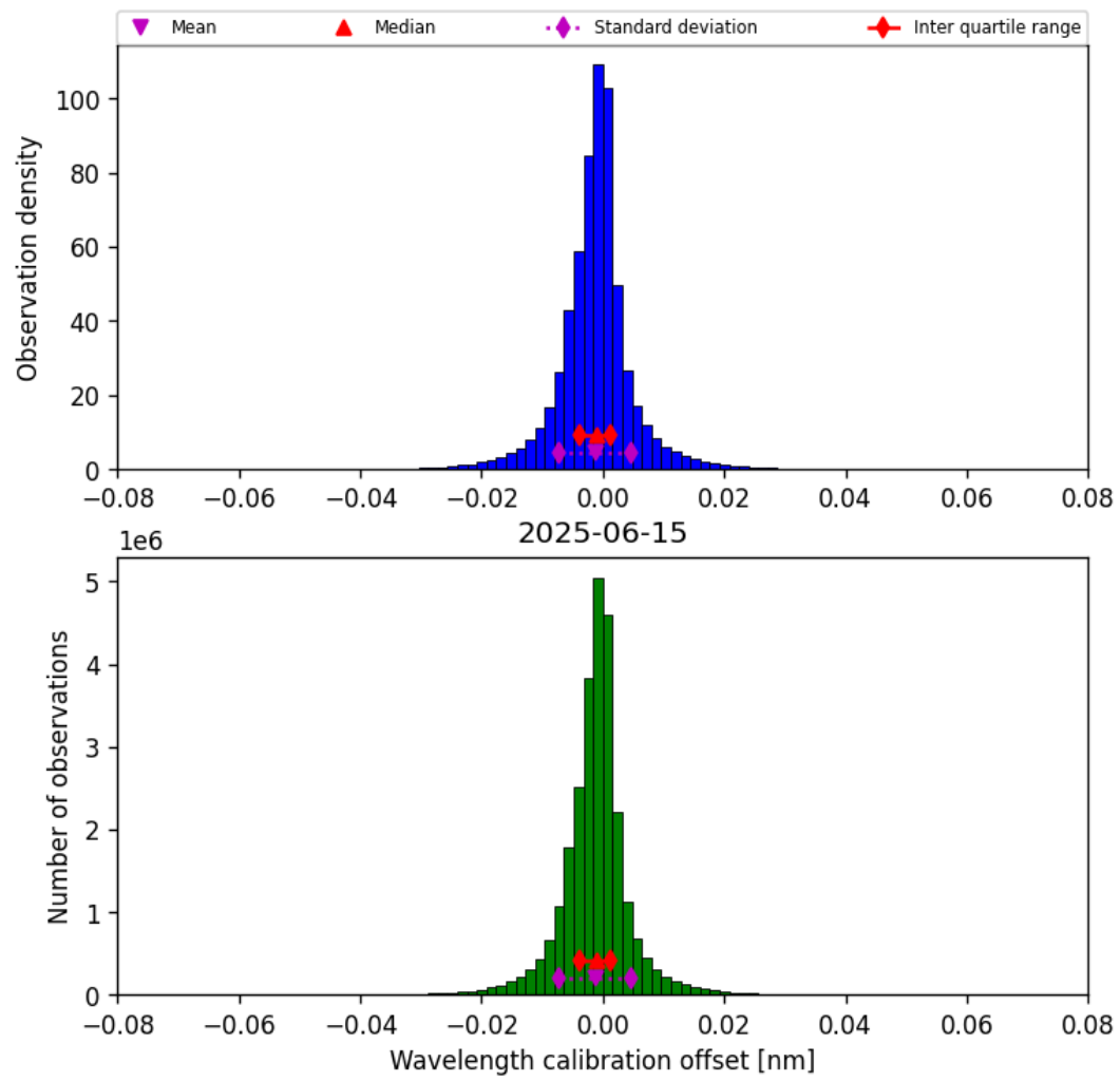
Figure 35: Histogram of “Wavelength calibration offset” for 2025-06-14 to 2025-06-16
