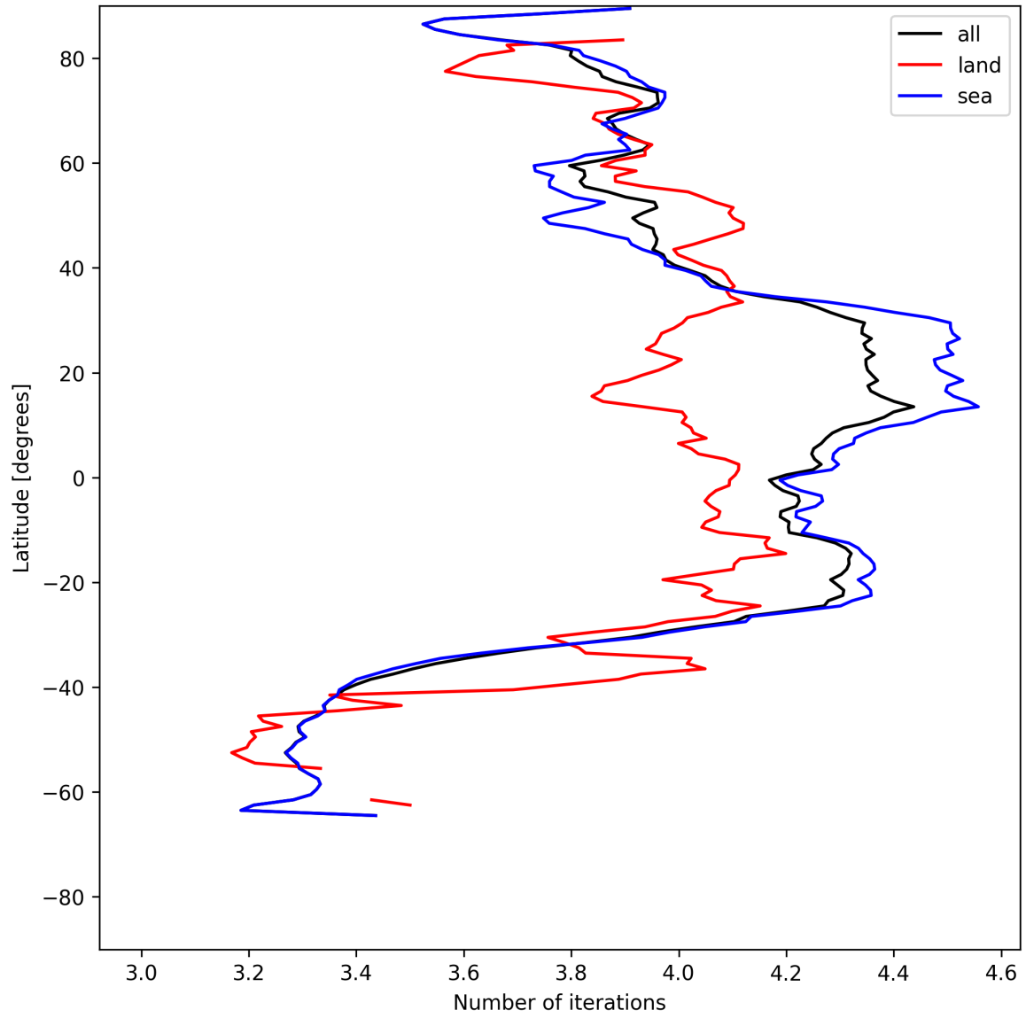
Figure 17: Zonal average of “Number of iterations” for 2025-06-14 to 2025-06-16.
