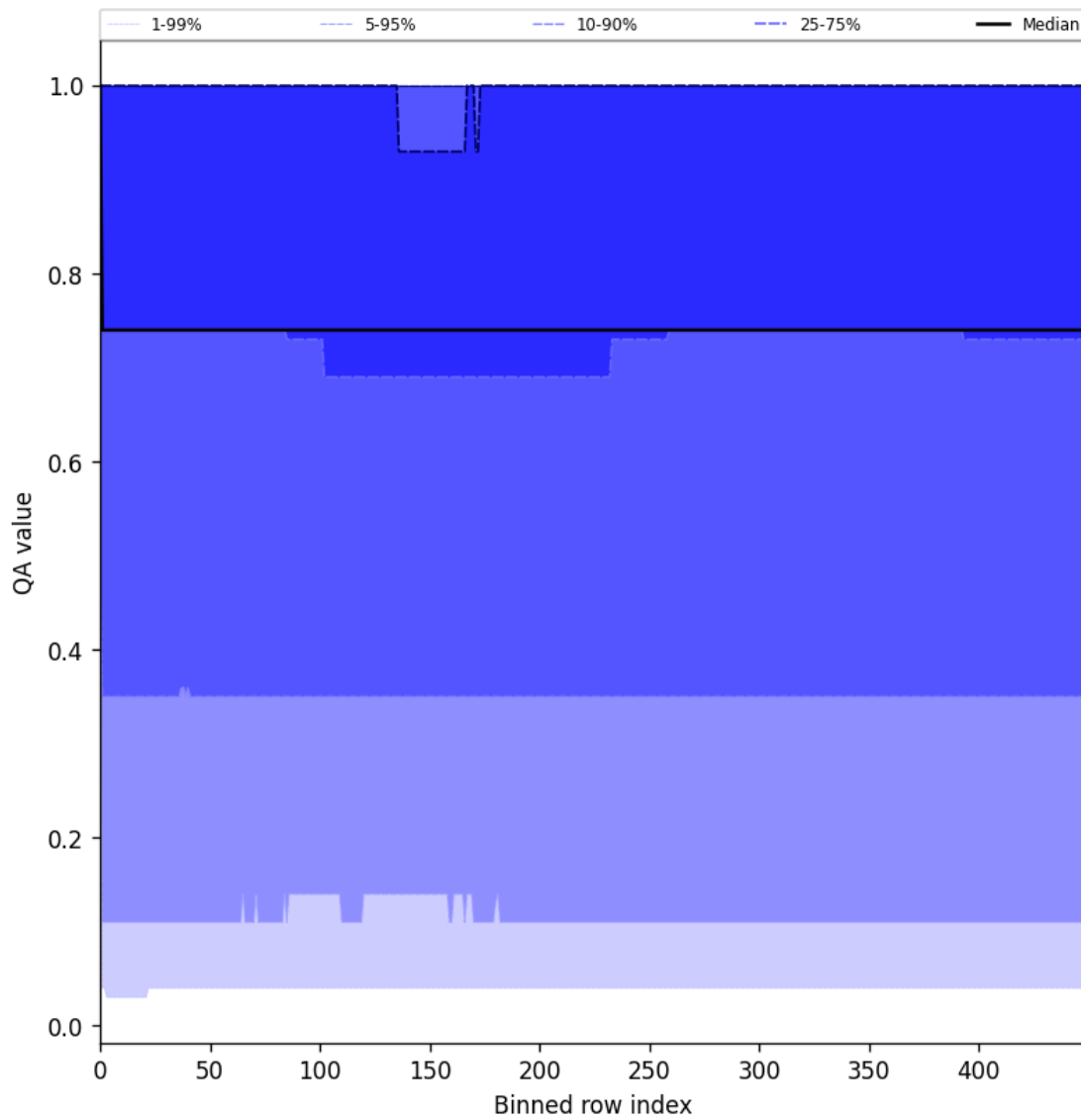
Figure 45: Along track statistics of “QA value” for 2025-06-14 to 2025-06-16
