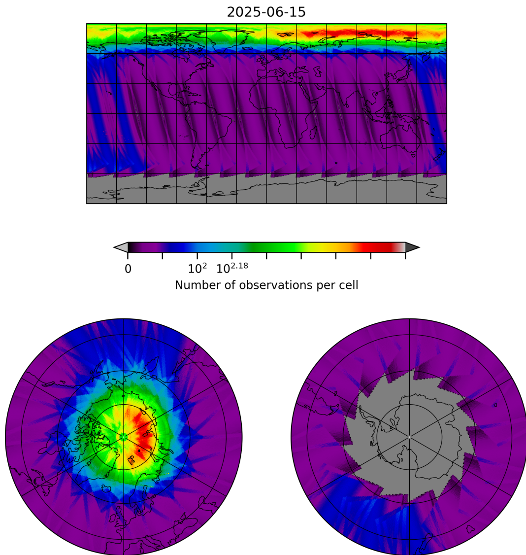
Figure 10: Map of the number of observations for 2025-06-14 to 2025-06-16
