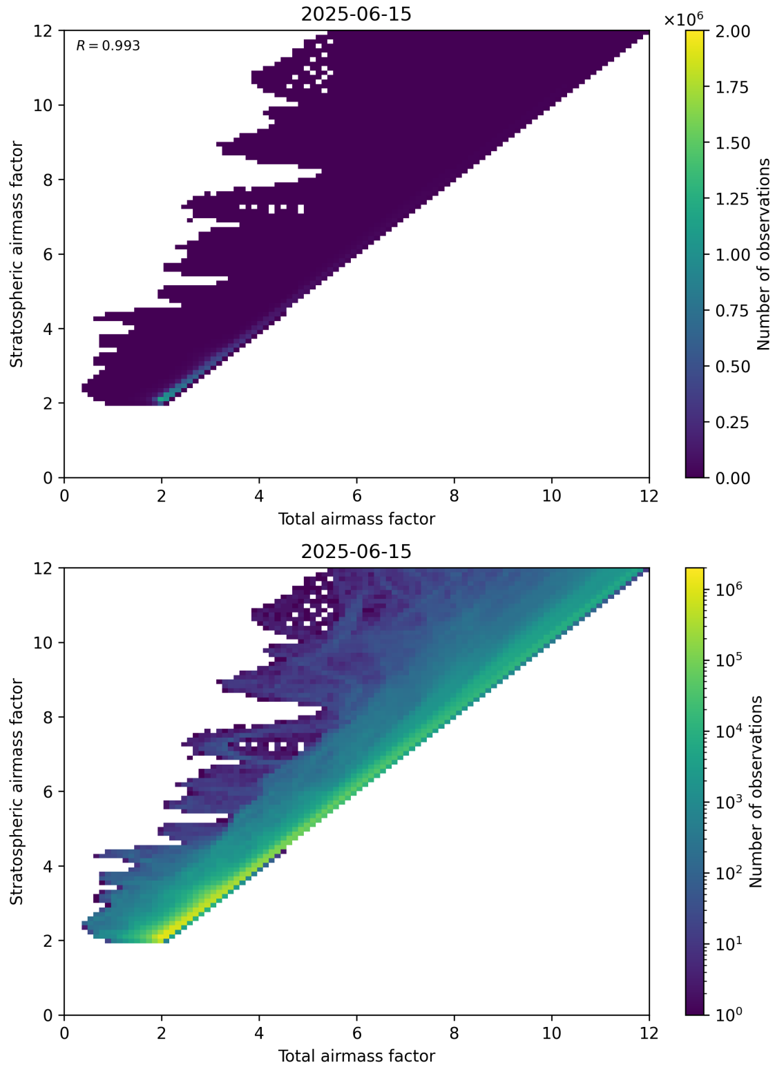
Figure 62: Scatter density plot of “Total airmass factor” against “Stratospheric airmass factor” for 2025-06-14 to 2025-06-16.
