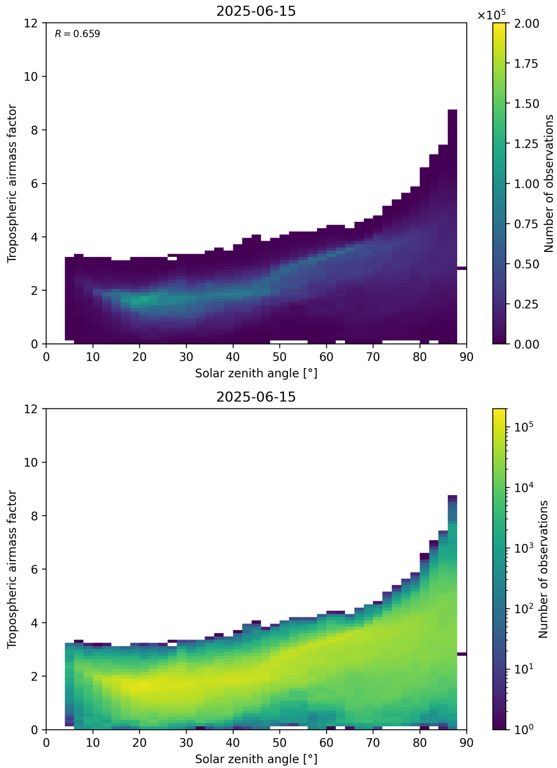
Figure 147: Scatter density plot of “Solar zenith angle” against “Tropospheric airmass factor” for 2025-06-14 to 2025-06-16.
