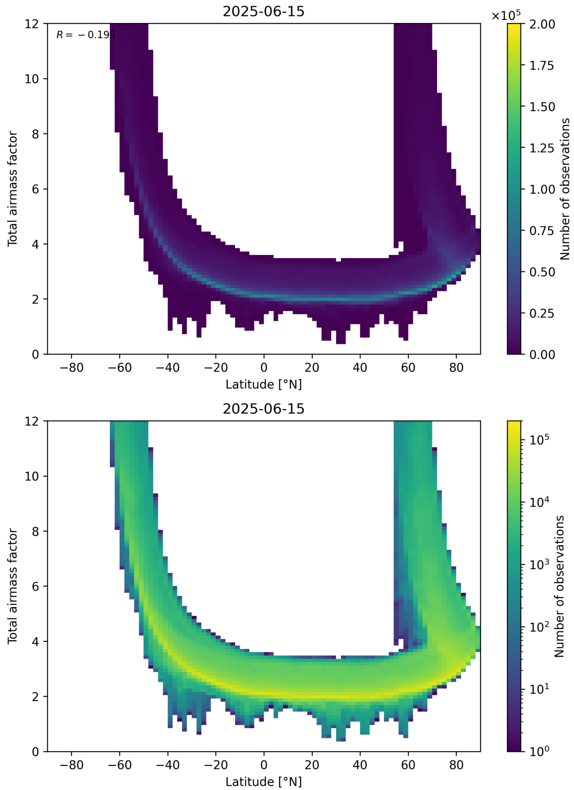
Figure 84: Scatter density plot of “Latitude” against “Total airmass factor” for 2025-06-14 to 2025-06-16.
