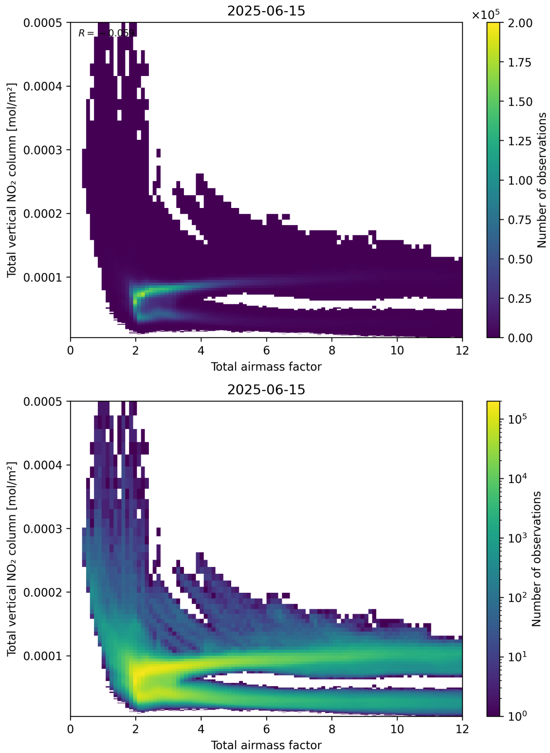
Figure 67: Scatter density plot of “Total airmass factor” against “Total vertical NO 2 column” for 2025-06-14 to 2025-06-16.
