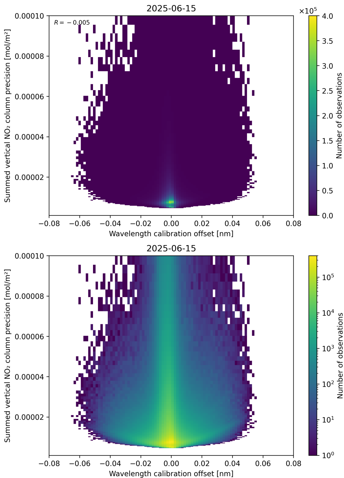
Figure 178: Scatter density plot of “Wavelength calibration offset” against “Summed vertical NO 2 column precision” for 2025-06-14 to 2025-06-16.
