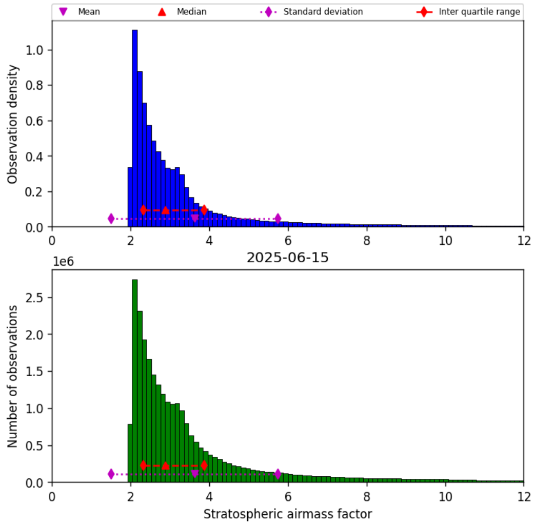
Figure 44: Histogram of “Stratospheric airmass factor” for 2025-06-14 to 2025-06-16
