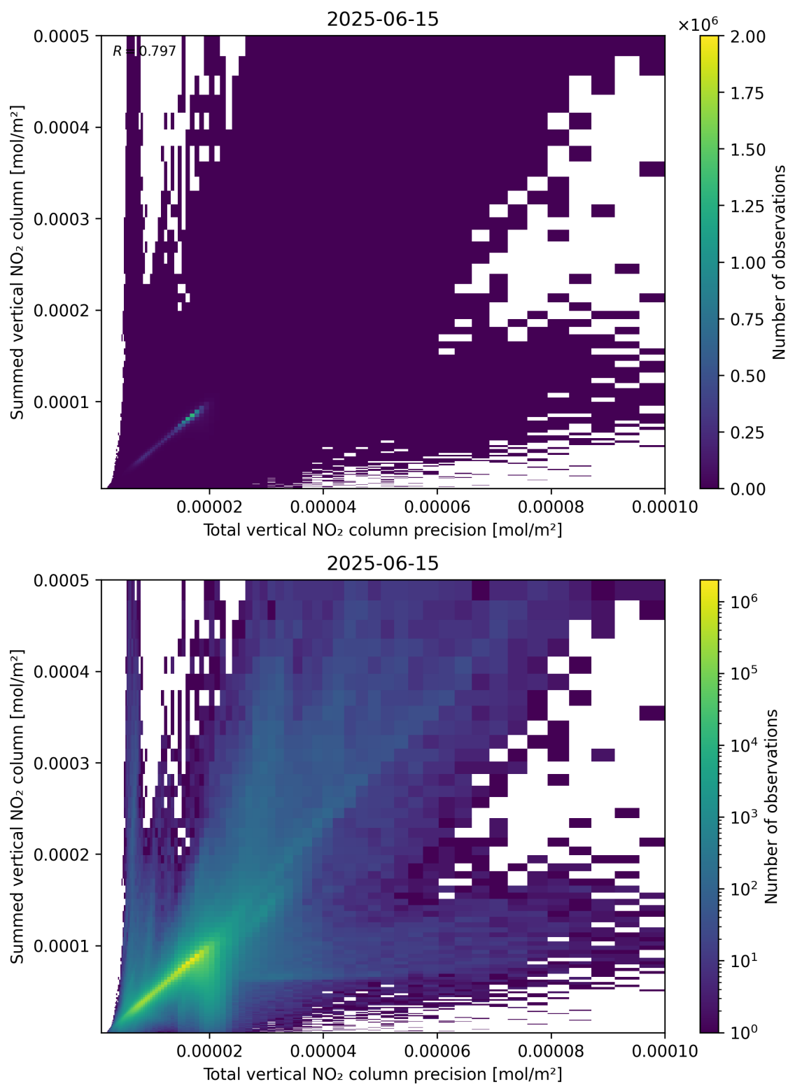
Figure 117: Scatter density plot of “Total vertical NO 2 column precision” against “Summed vertical NO 2 column” for 2025-06-14 to 2025-06-16.
