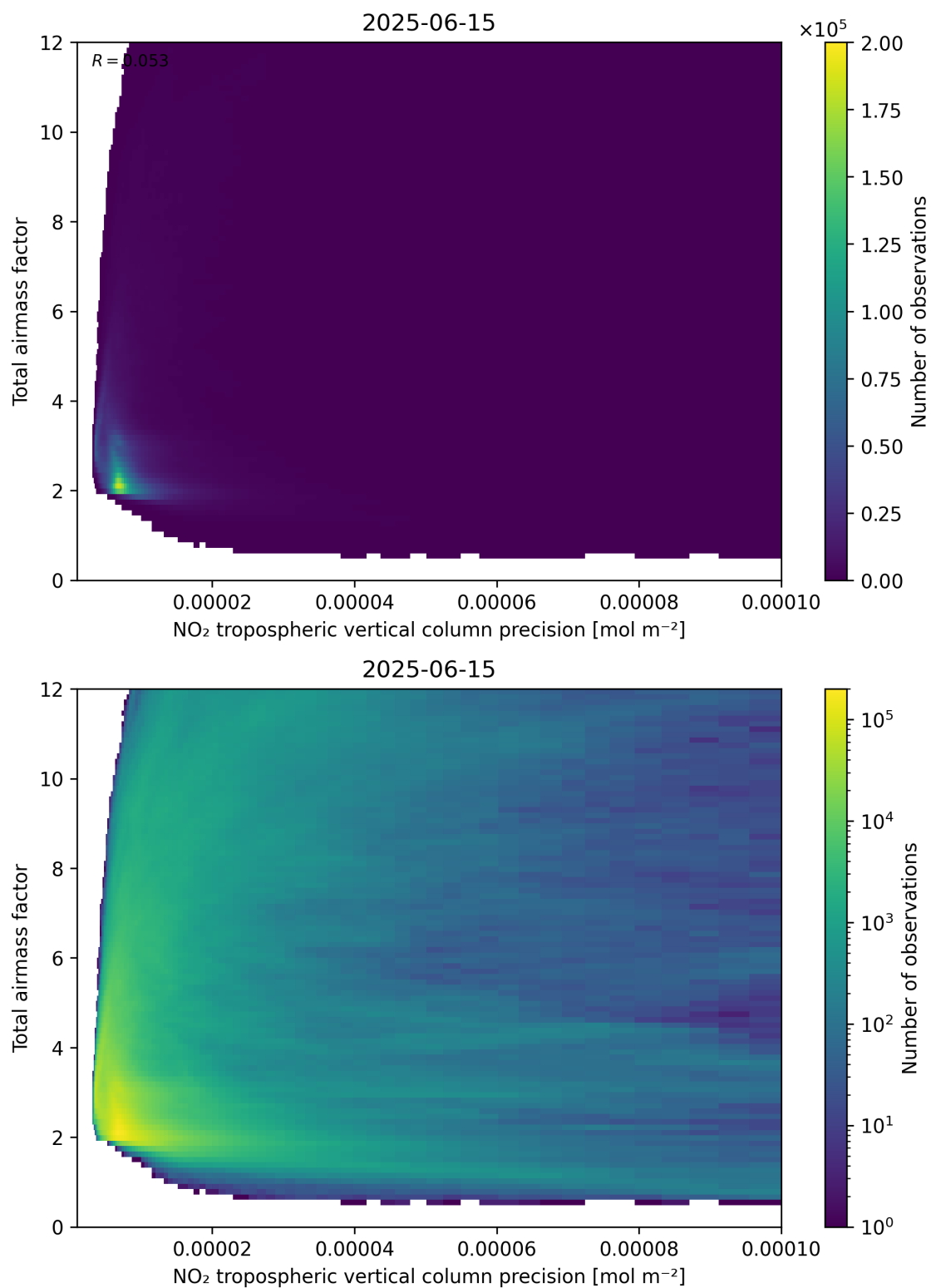
Figure 132: Scatter density plot of “NO 2 tropospheric vertical column precision” against “Total air mass factor” for 2025-06-14 to 2025-06-16.
