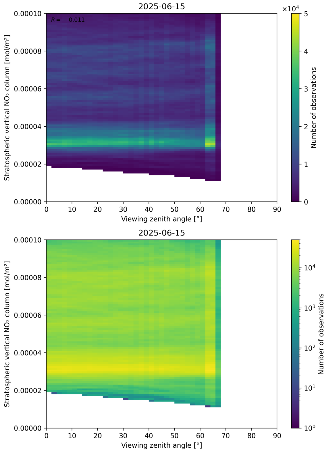
Figure 164: Scatter density plot of “Viewing zenith angle” against “Stratospheric vertical NO 2 column” for 2025-06-14 to 2025-06-16.
