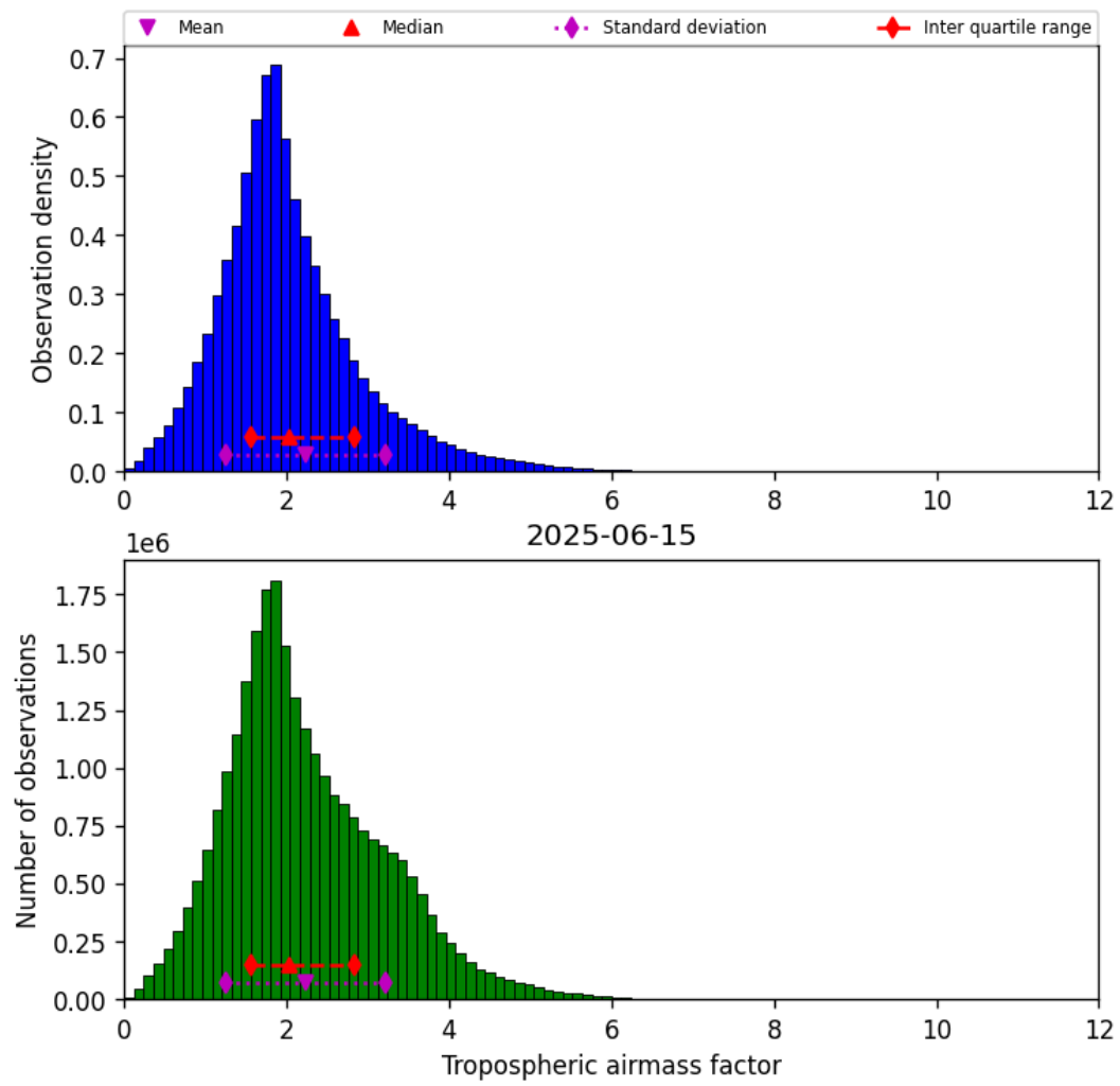
Figure 31: Histogram of “Tropospheric airmass factor” for 2025-06-14 to 2025-06-16
