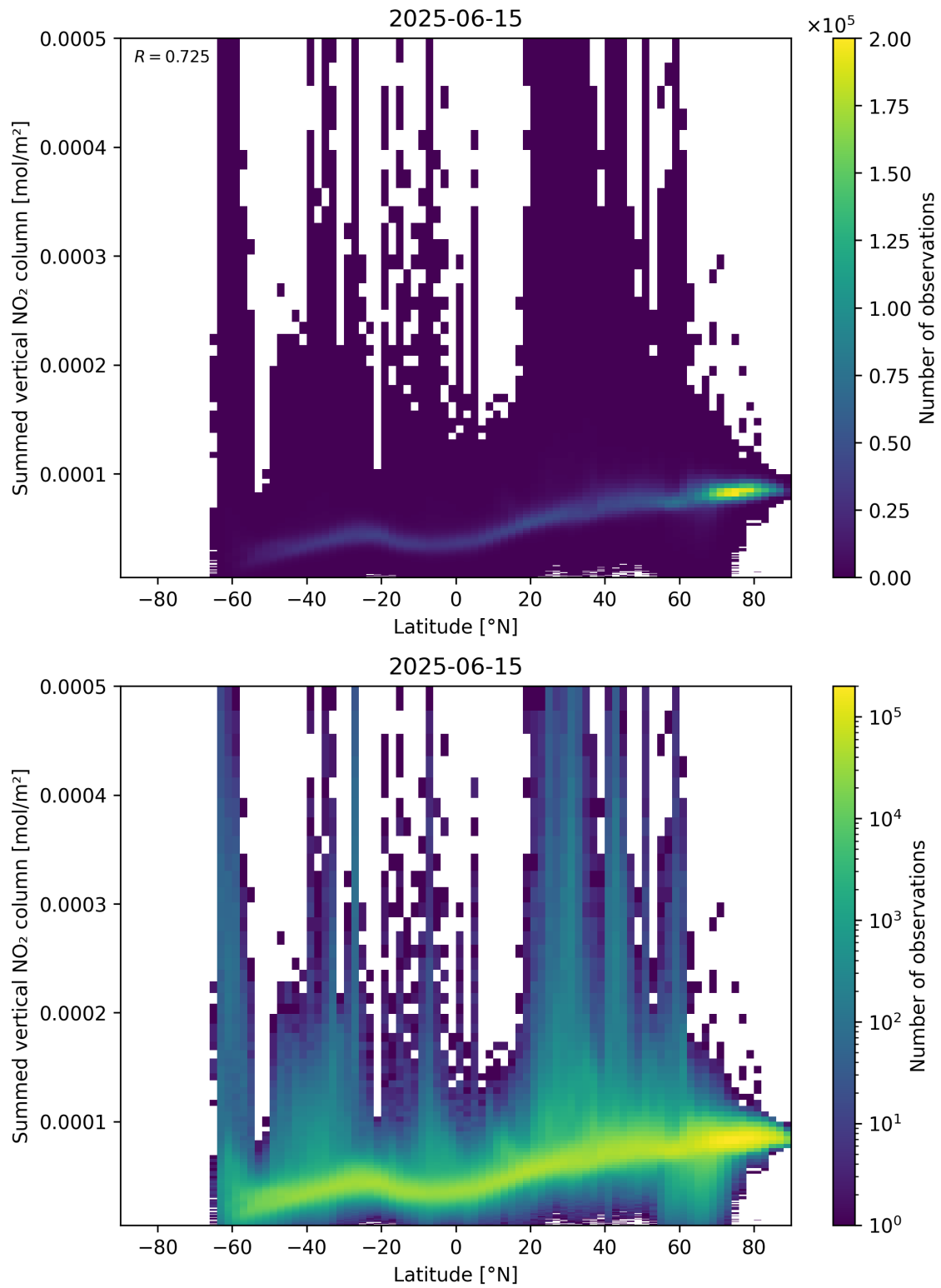
Figure 88: Scatter density plot of “Latitude” against “Summed vertical NO 2 column” for 2025-06-14 to 2025-06-16.
