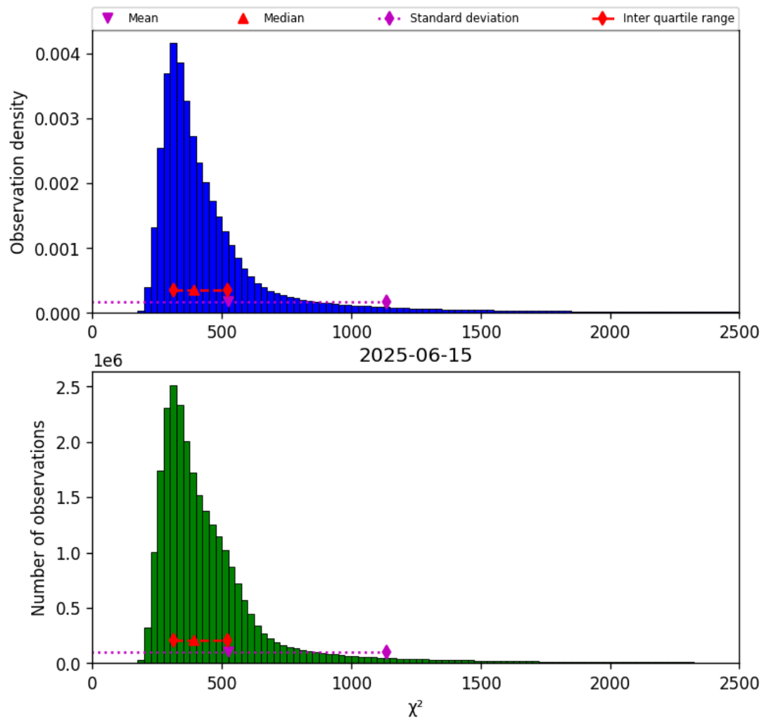
Figure 42: Histogram of " \chi^2 " for 2025-06-14 to 2025-06-16
