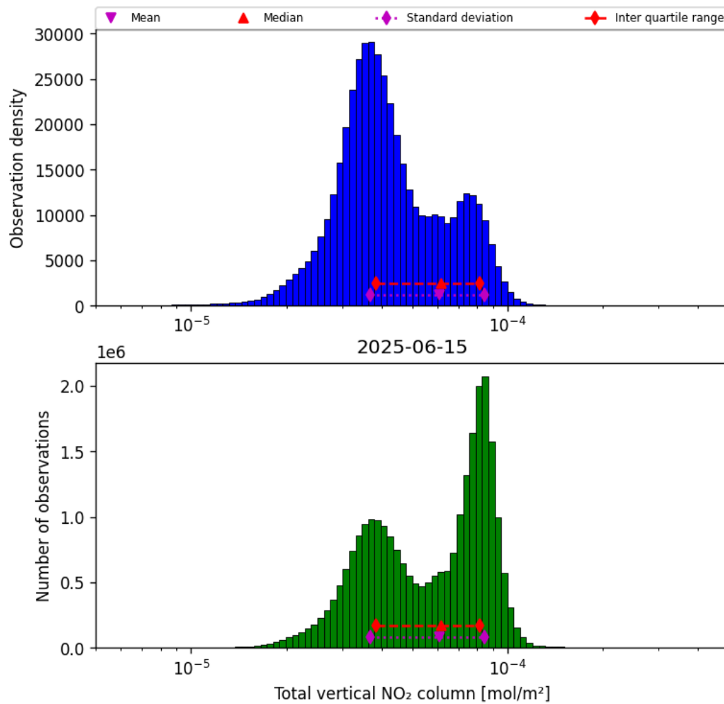
Figure 38: Histogram of “Total vertical NO 2 column” for 2025-06-14 to 2025-06-16
