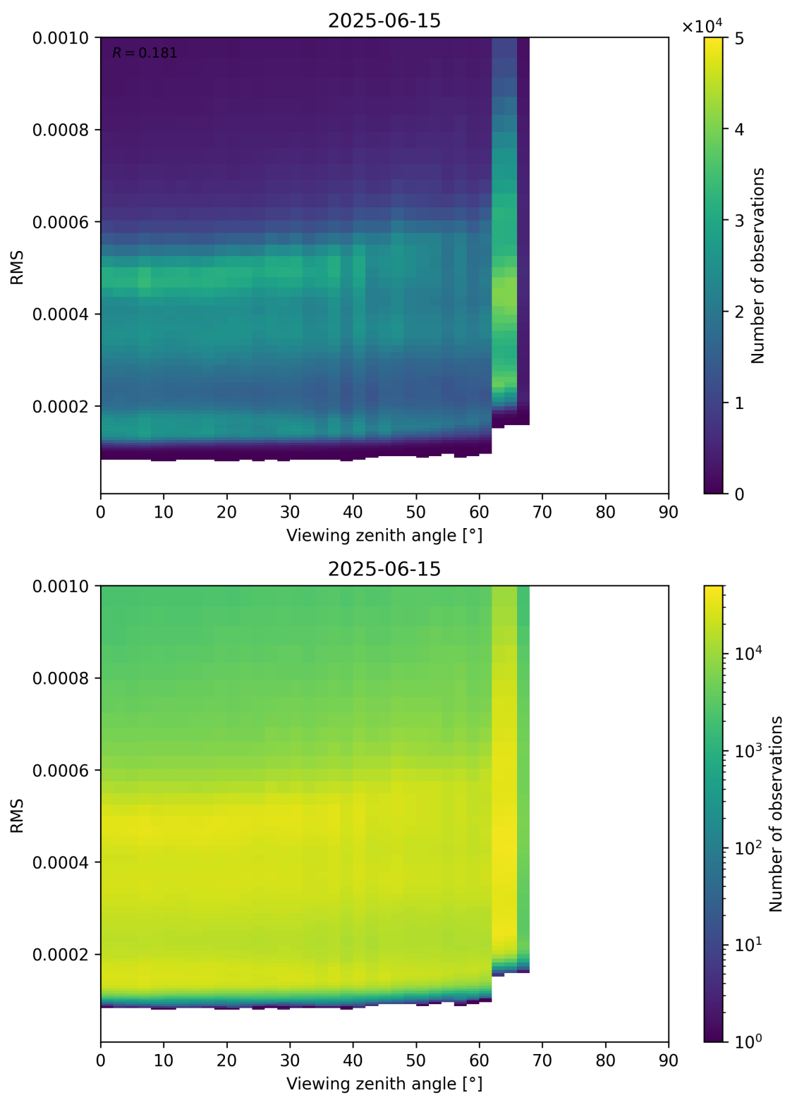
Figure 171: Scatter density plot of “Viewing zenith angle” against “RMS” for 2025-06-14 to 2025-06-16.
