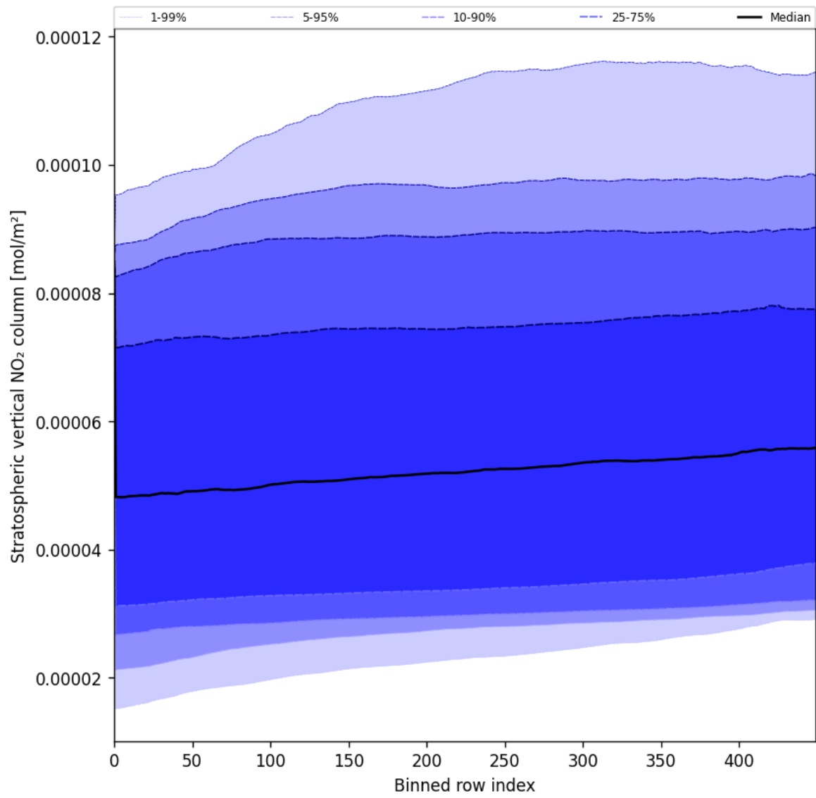
Figure 53: Along track statistics of “Stratospheric vertical NO 2 column” for 2025-06-14 to 2025-06-16
