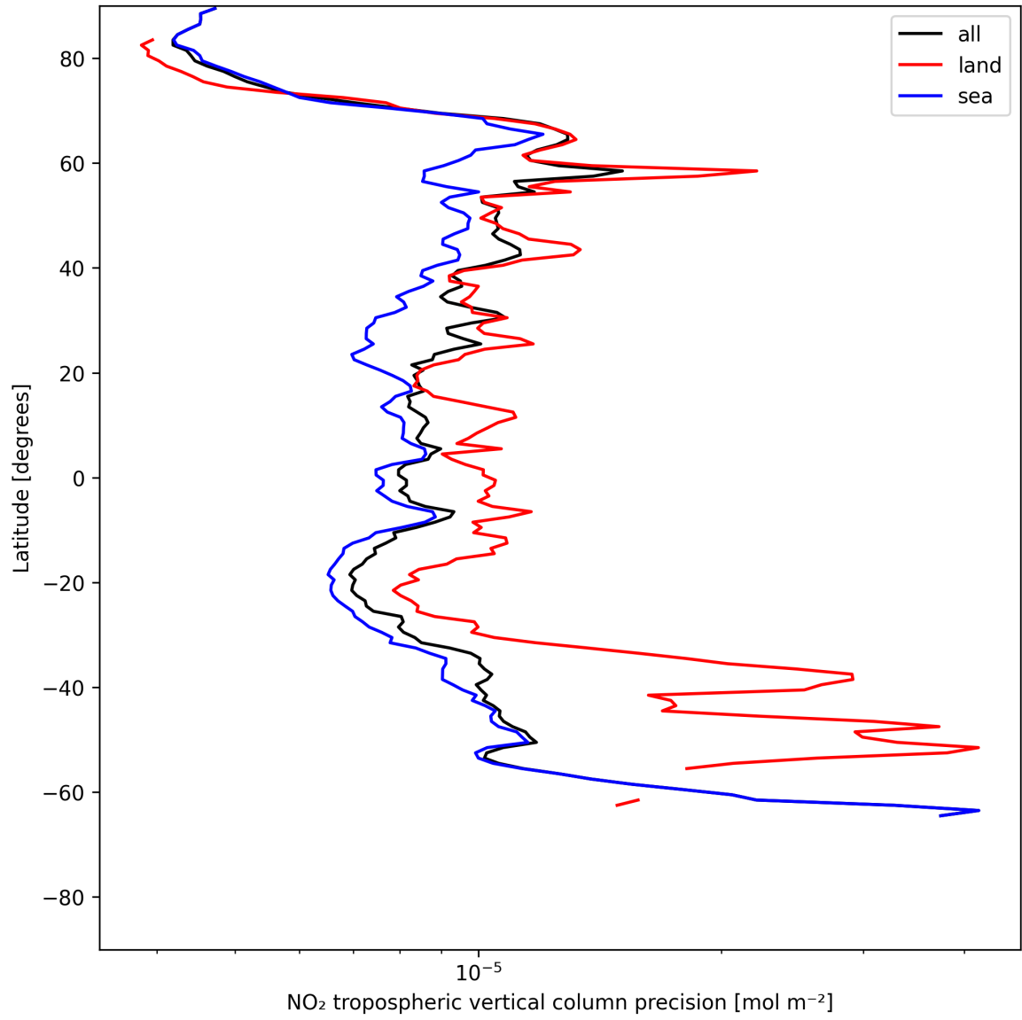
Figure 13: Zonal average of “NO 2 tropospheric vertical column precision” for 2025-06-14 to 2025-06-16.
