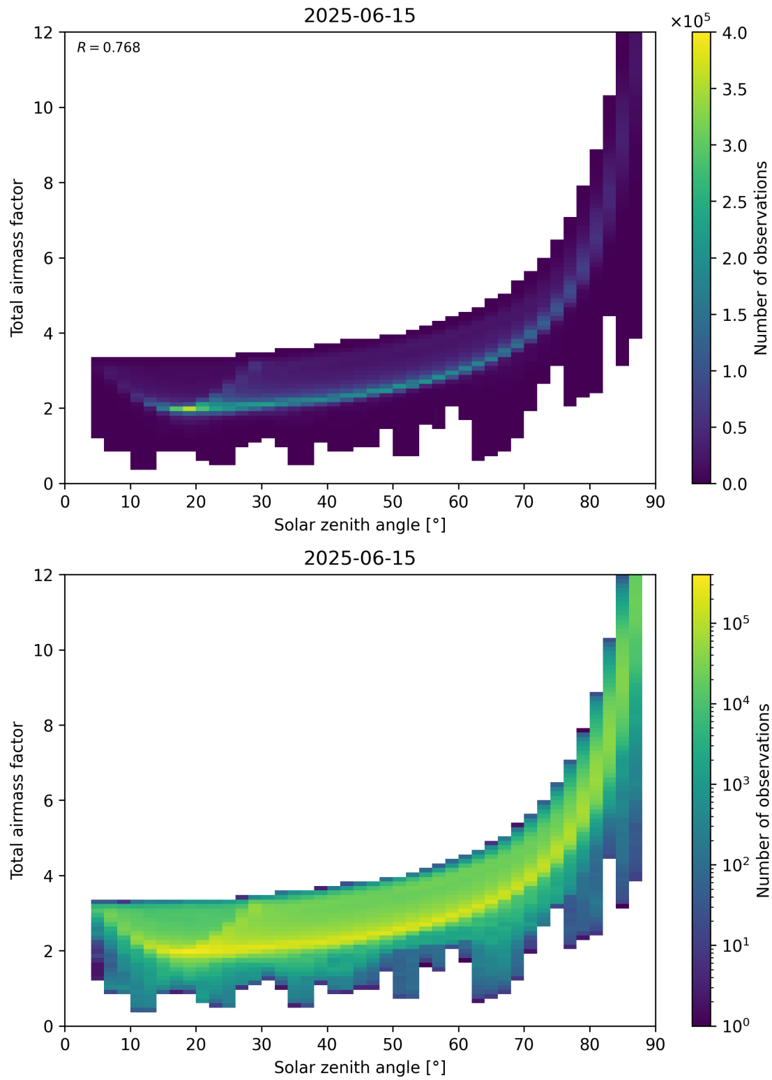
Figure 146: Scatter density plot of “Solar zenith angle” against “Total air mass factor” for 2025-06-14 to 2025-06-16.
