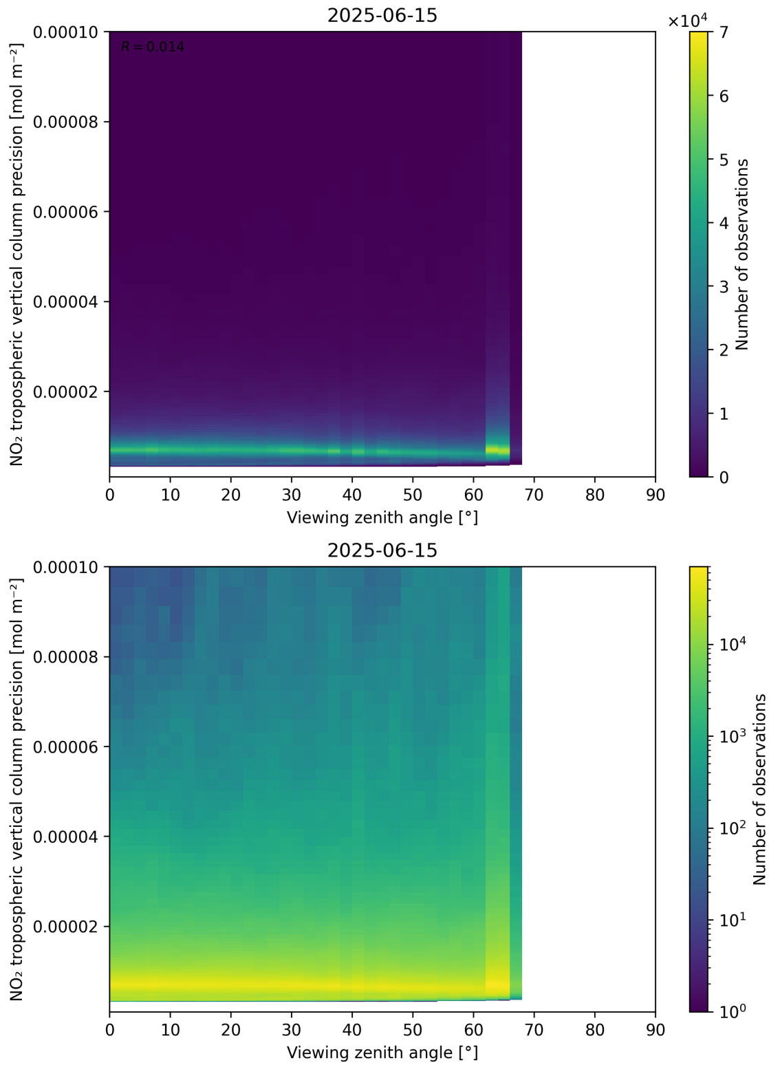
Figure 170: Scatter density plot of “Viewing zenith angle” against “NO 2 tropospheric vertical column precision” for 2025-06-14 to 2025-06-16.
