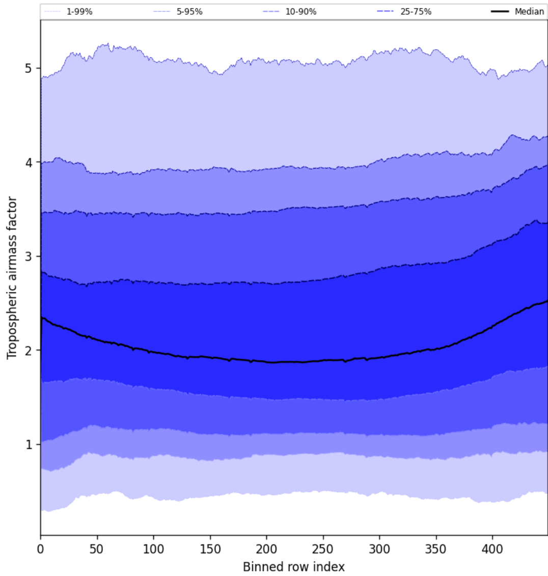
Figure 48: Along track statistics of “Tropospheric airmass factor” for 2025-06-14 to 2025-06-16
