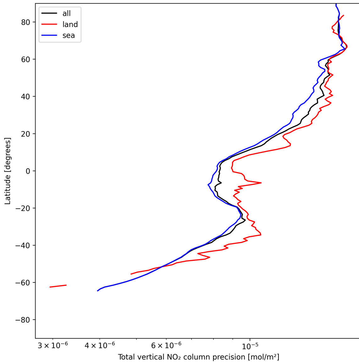
Figure 22: Zonal average of “Total vertical NO 2 column precision” for 2025-06-14 to 2025-06-16.
