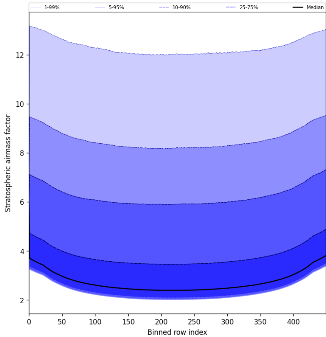
Figure 61: Along track statistics of “Stratospheric air mass factor” for 2025-06-14 to 2025-06-16
