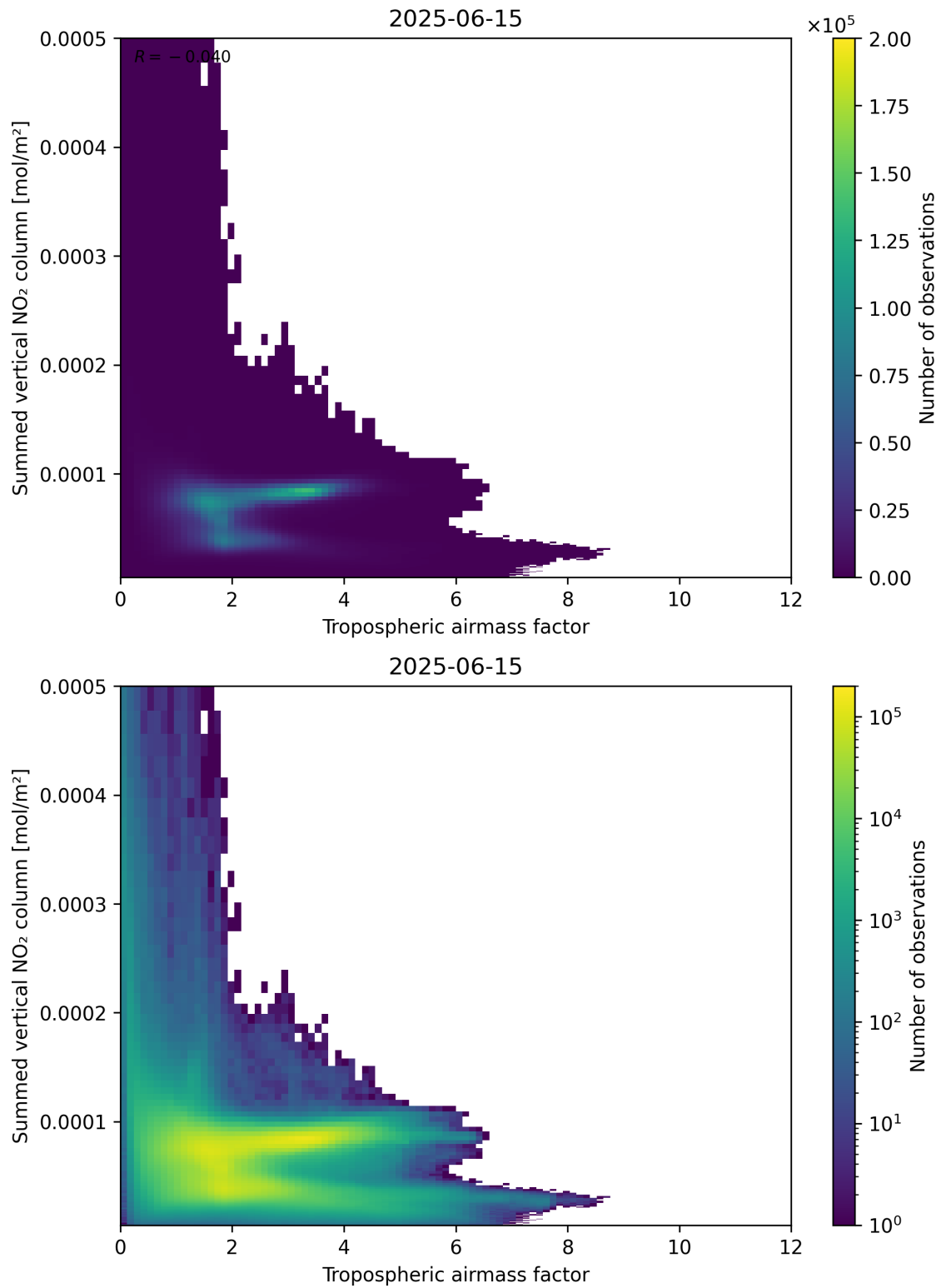
Figure 75: Scatter density plot of “Tropospheric airmass factor” against “Summed vertical NO 2 column” for 2025-06-14 to 2025-06-16.
