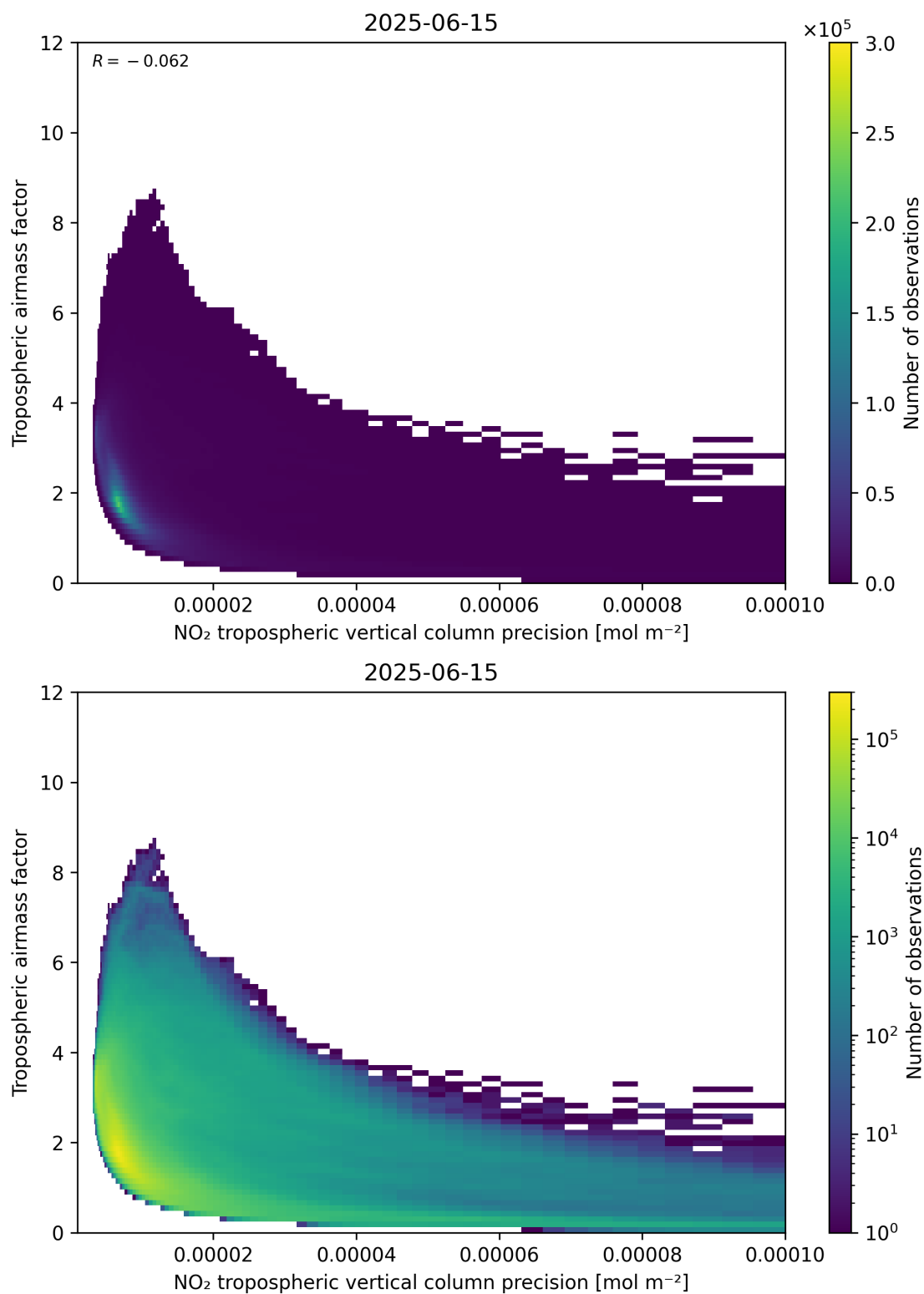
Figure 133: Scatter density plot of “NO 2 tropospheric vertical column precision” against “Tropospheric airmass factor” for 2025-06-14 to 2025-06-16.
