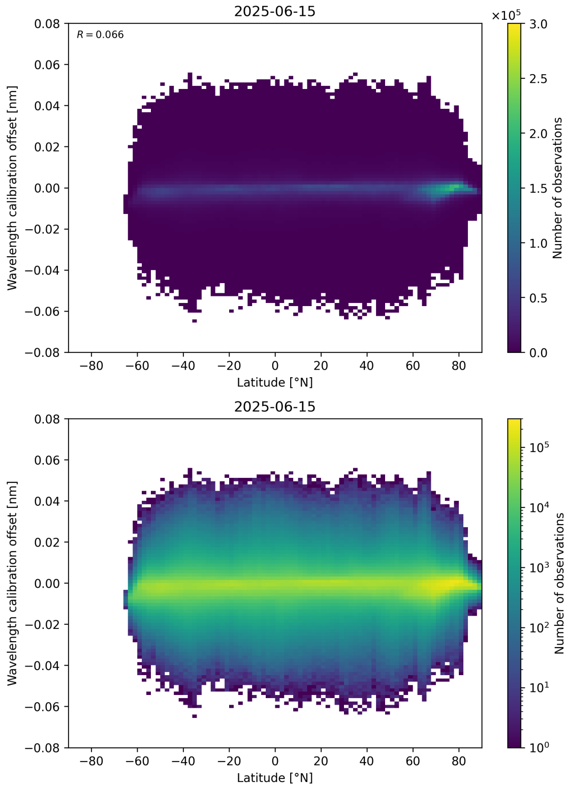
Figure 95: Scatter density plot of “Latitude” against “Wavelength calibration offset” for 2025-06-14 to 2025-06-16.
