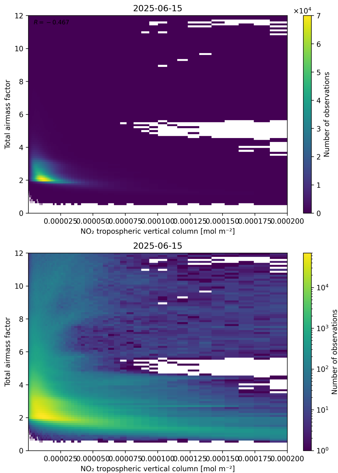
Figure 122: Scatter density plot of “NO 2 tropospheric vertical column” against “Total air mass factor” for 2025-06-14 to 2025-06-16.
