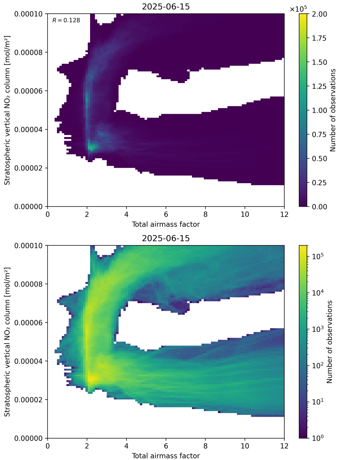
Figure 64: Scatter density plot of “Total airmass factor” against “Stratospheric vertical NO 2 column” for 2025-06-14 to 2025-06-16.
