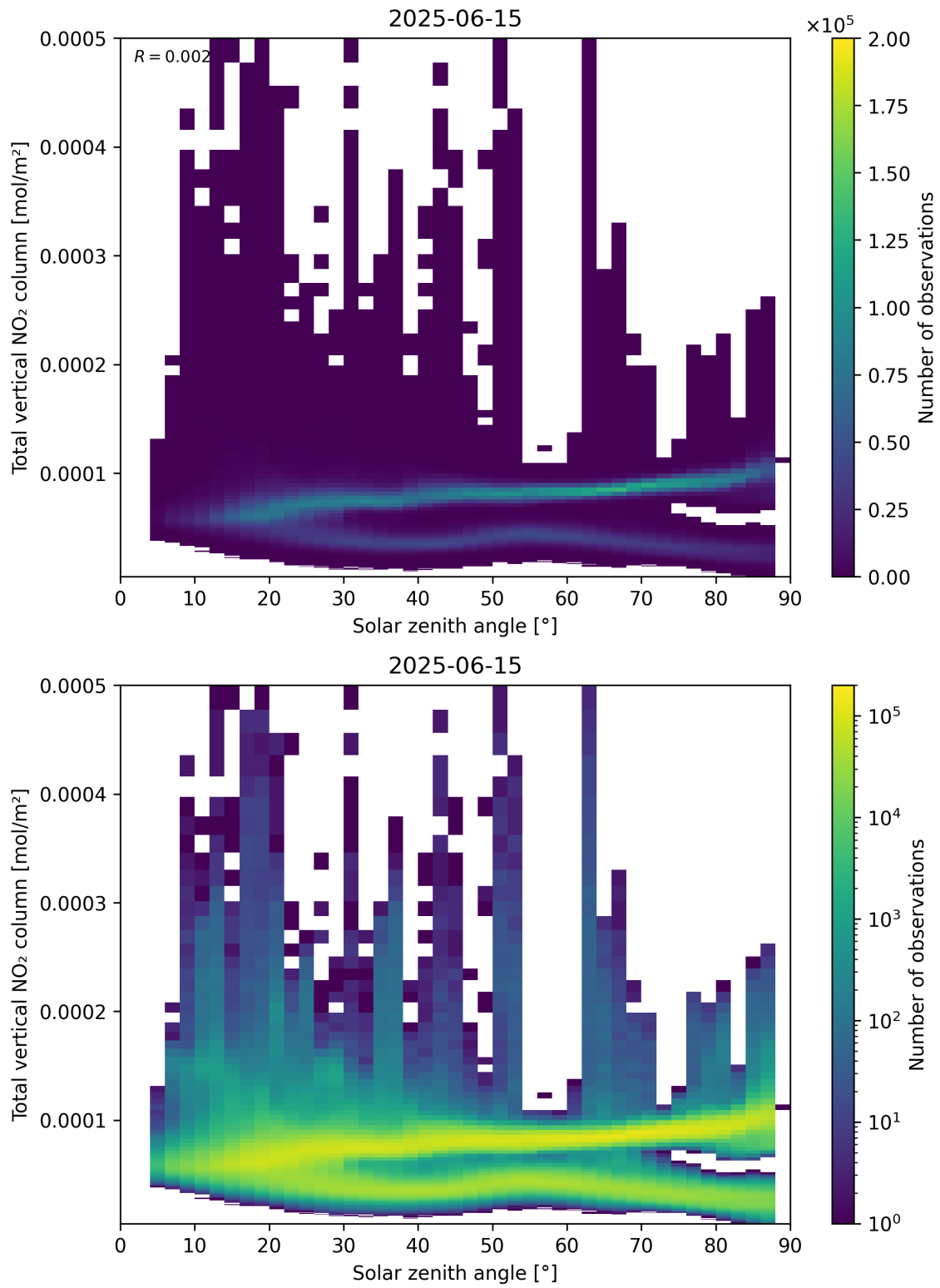
Figure 153: Scatter density plot of “Solar zenith angle” against “Total vertical NO 2 column” for 2025-06-14 to 2025-06-16.
