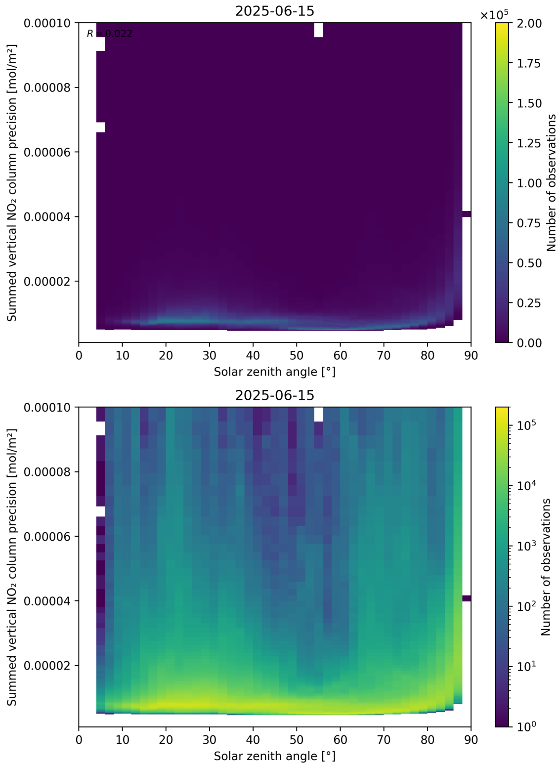
Figure 152: Scatter density plot of “Solar zenith angle” against “Summed vertical NO 2 column precision” for 2025-06-14 to 2025-06-16.
