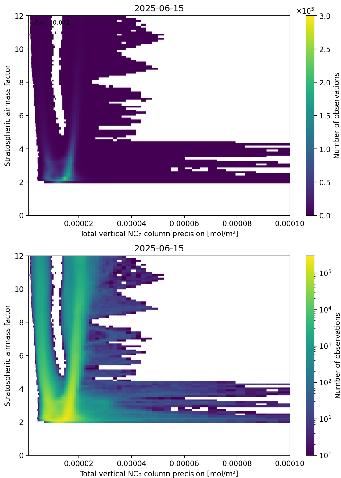
Figure 115: Scatter density plot of “Total vertical NO 2 column precision” against “Stratospheric air mass factor” for 2025-06-14 to 2025-06-16.
