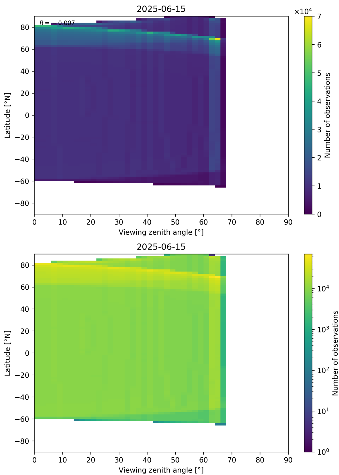
Figure 163: Scatter density plot of “Viewing zenith angle” against “Latitude” for 2025-06-14 to 2025-06-16.
