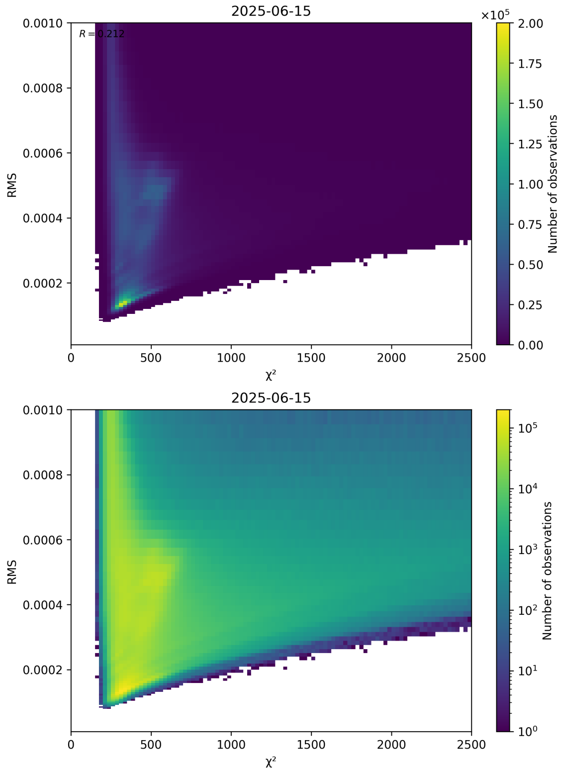
Figure 82: Scatter density plot of “ \chi^2 ” against “RMS” for 2025-06-14 to 2025-06-16.
