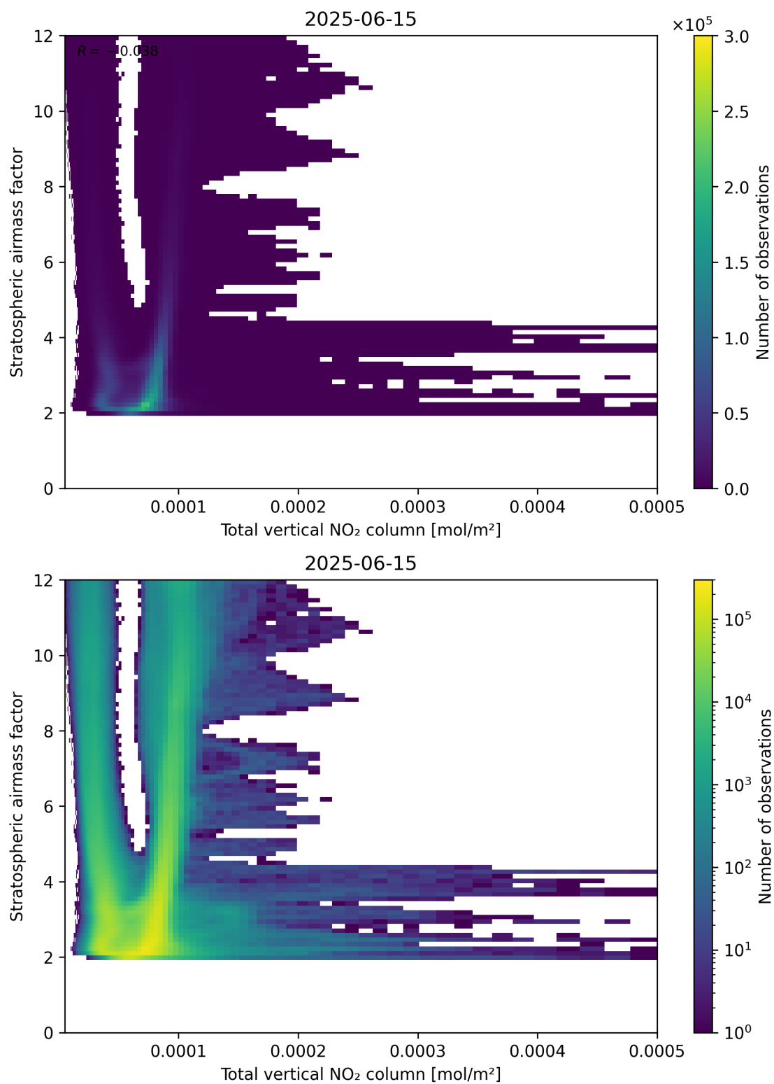
Figure 110: Scatter density plot of “Total vertical NO 2 column” against “Stratospheric air mass factor” for 2025-06-14 to 2025-06-16.
