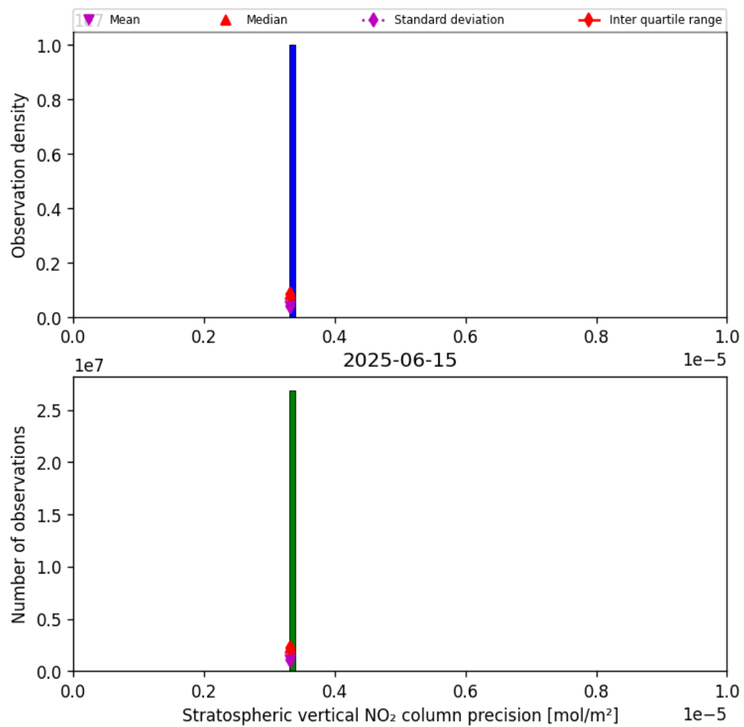
Figure 37: Histogram of “Stratospheric vertical NO 2 column precision” for 2025-06-14 to 2025-06-16
