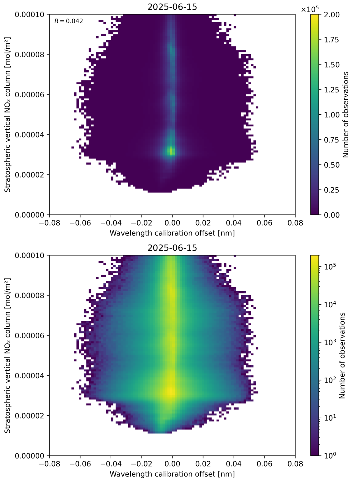
Figure 176: Scatter density plot of “Wavelength calibration offset” against “Stratospheric vertical NO 2 column” for 2025-06-14 to 2025-06-16.
