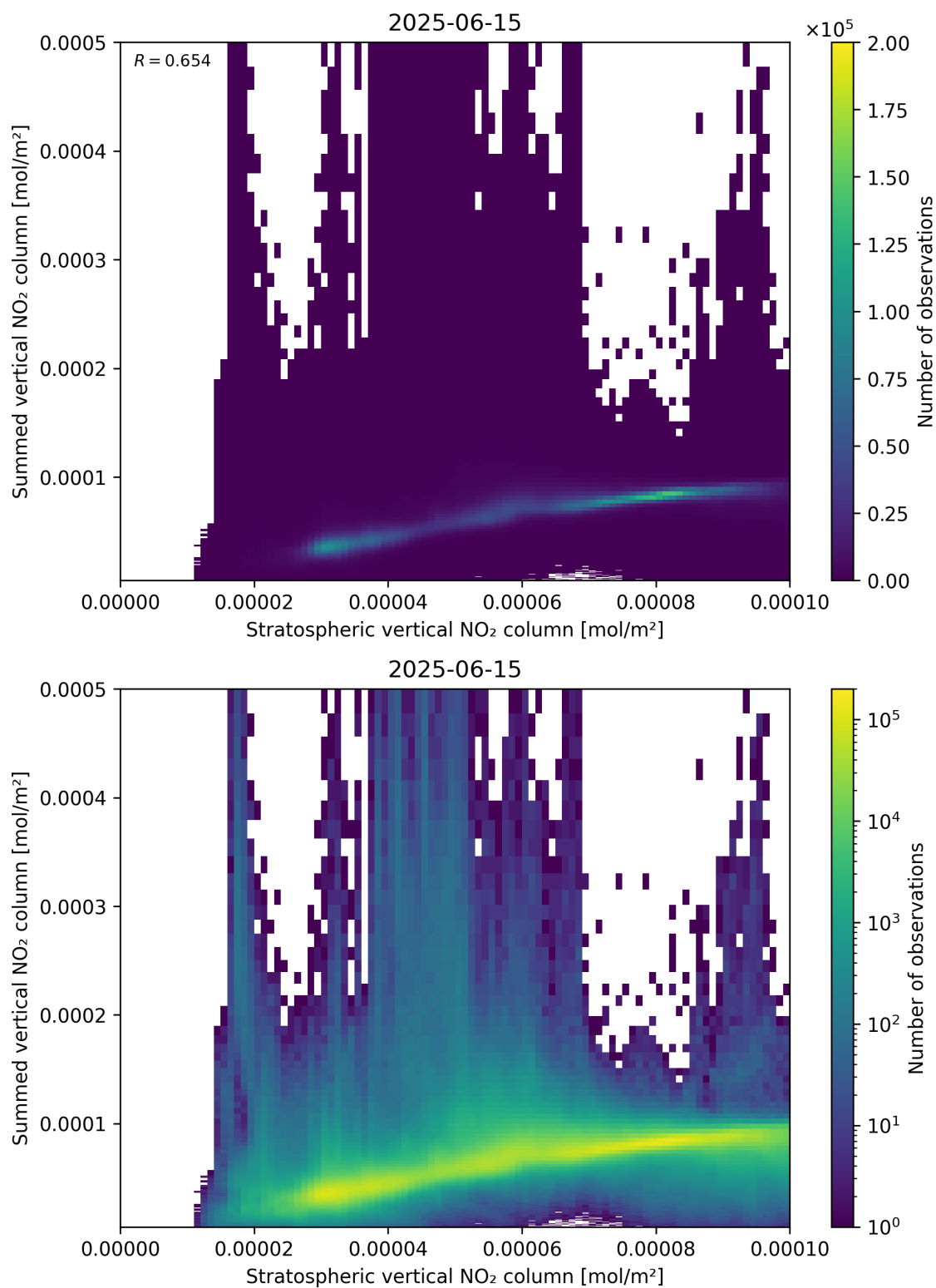
Figure 98: Scatter density plot of “Stratospheric vertical NO 2 column” against “Summed vertical NO 2 column” for 2025-06-14 to 2025-06-16.
