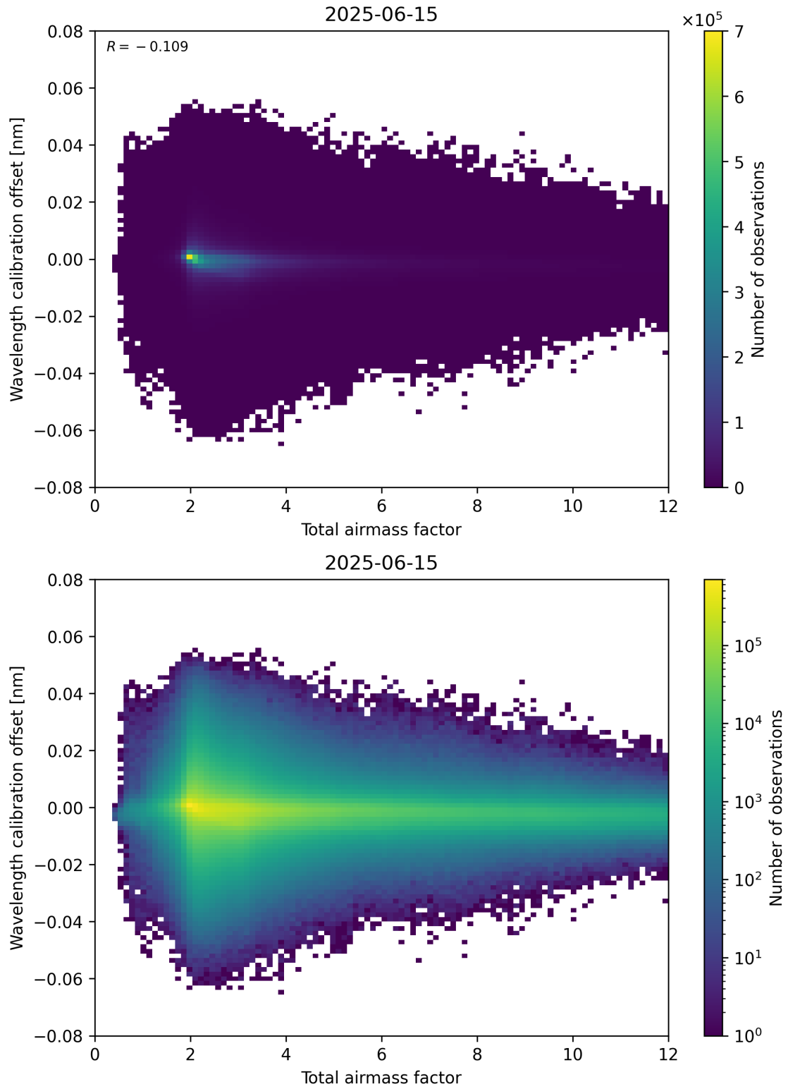
Figure 70: Scatter density plot of “Total airmass factor” against “Wavelength calibration offset” for 2025-06-14 to 2025-06-16.
