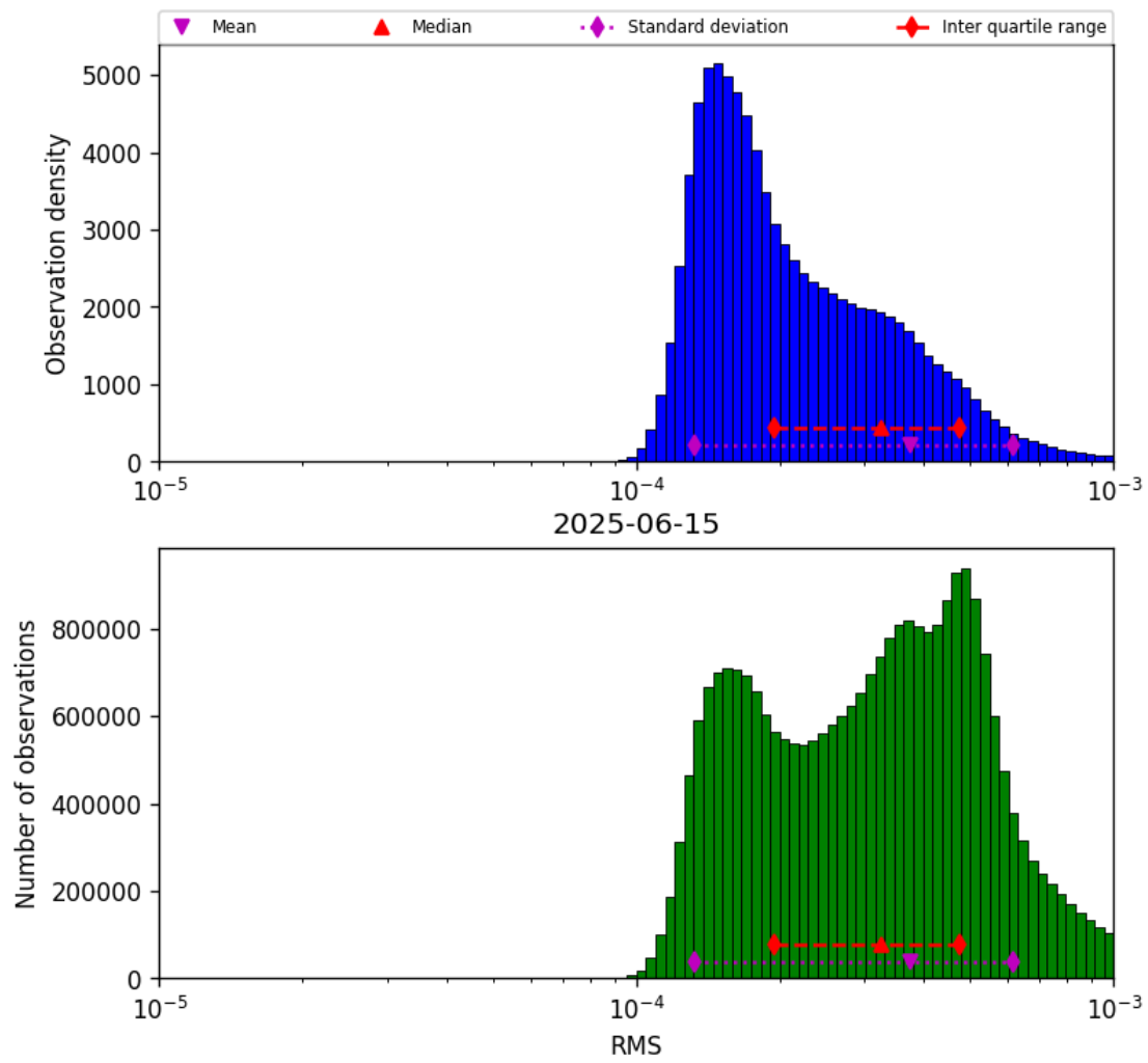
Figure 43: Histogram of “RMS” for 2025-06-14 to 2025-06-16
