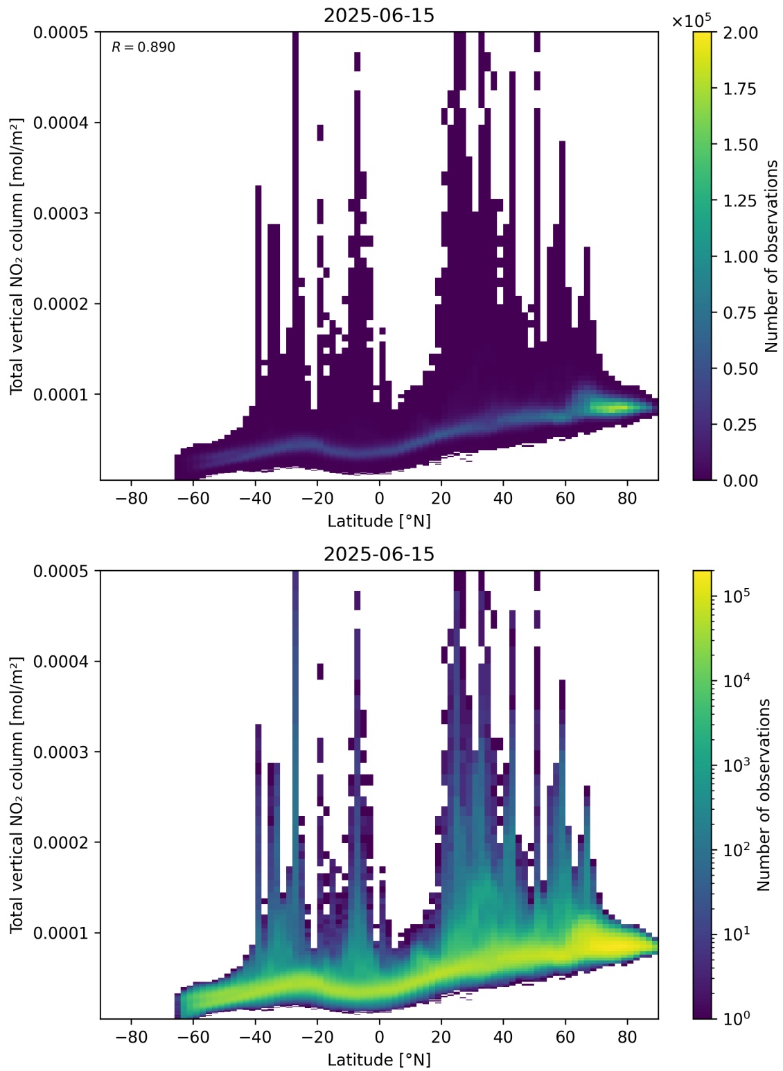
Figure 90: Scatter density plot of “Latitude” against “Total vertical NO 2 column” for 2025-06-14 to 2025-06-16.
