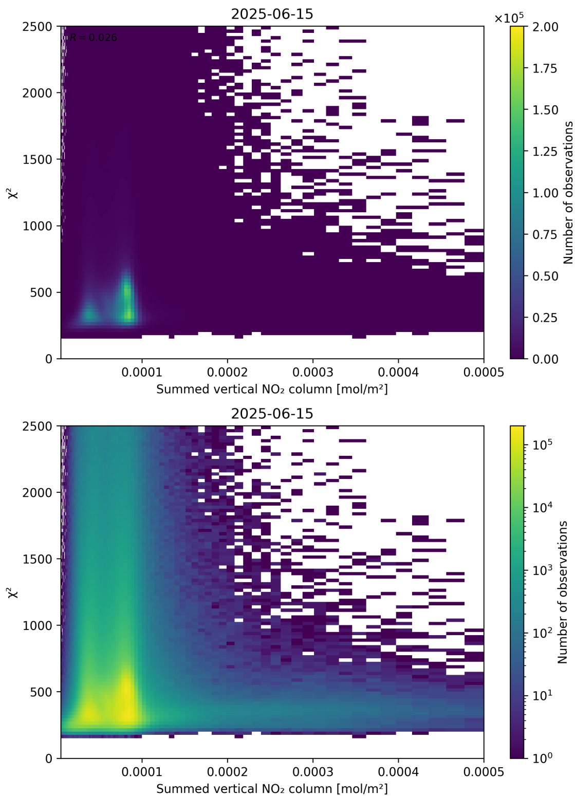
Figure 104: Scatter density plot of “Summed vertical NO 2 column” against “ \chi^2 ” for 2025-06-14 to 2025-06-16.
