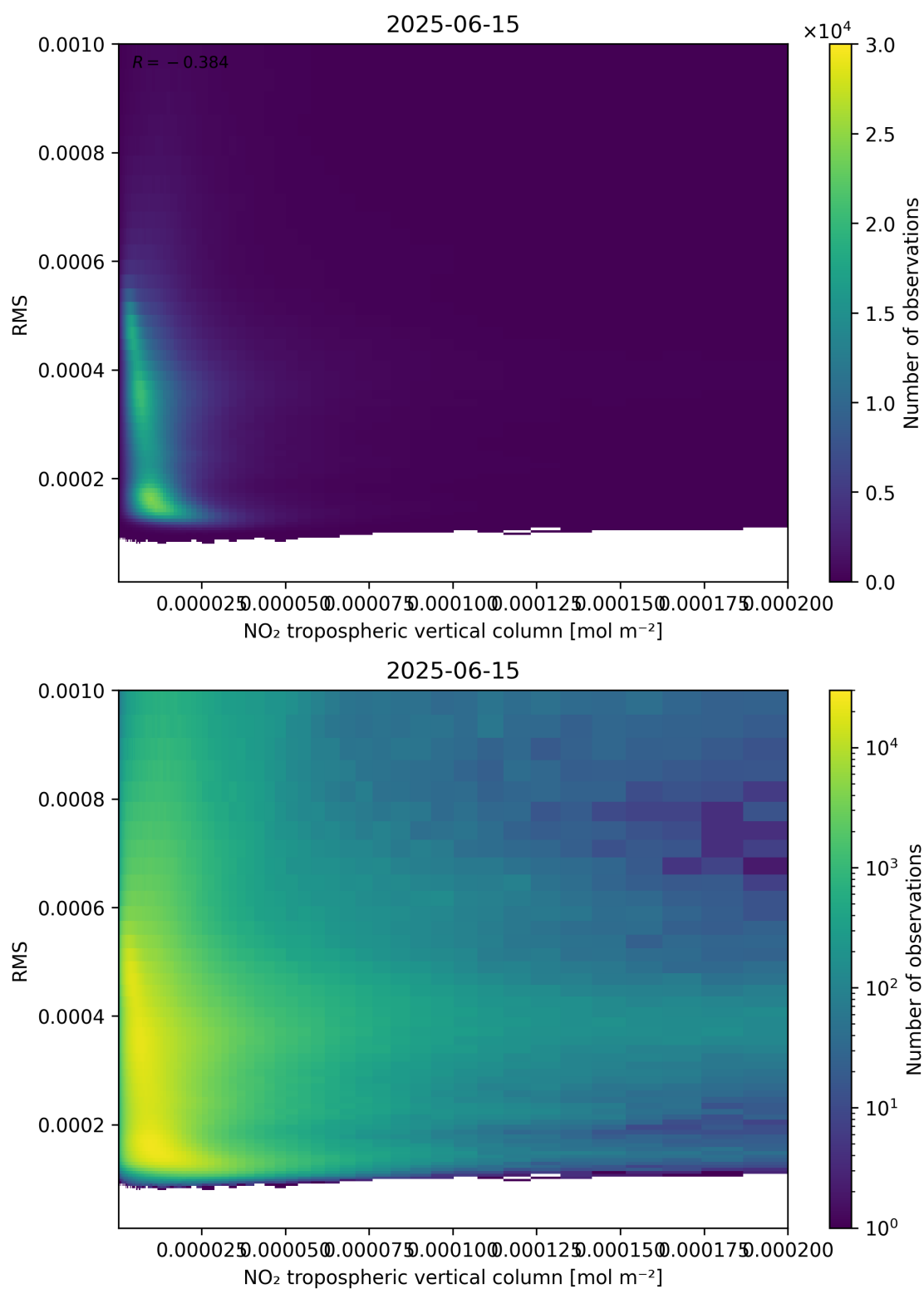
Figure 142: Scatter density plot of “NO 2 tropospheric vertical column” against “RMS” for 2025-06-14 to 2025-06-16.
