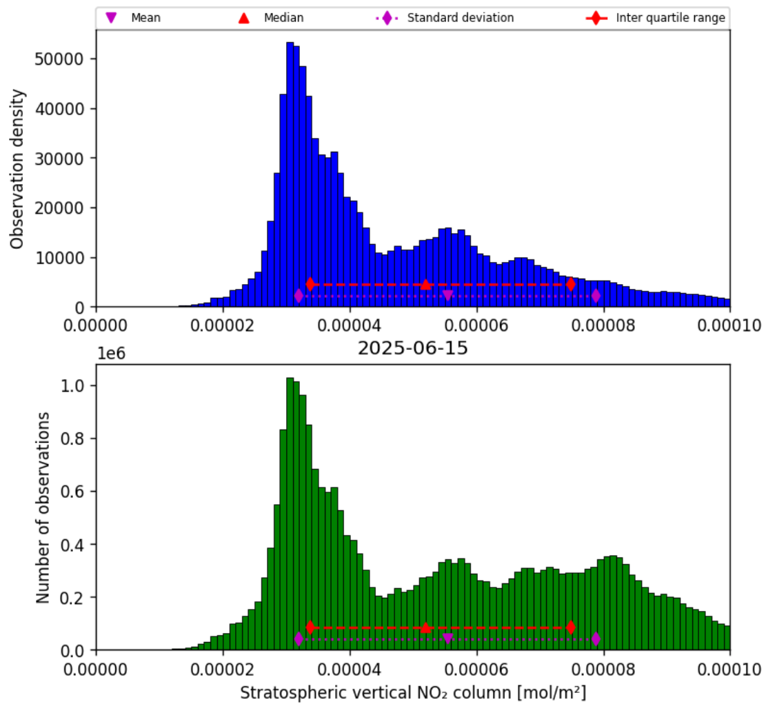
Figure 36: Histogram of “Stratospheric vertical NO 2 column” for 2025-06-14 to 2025-06-16
