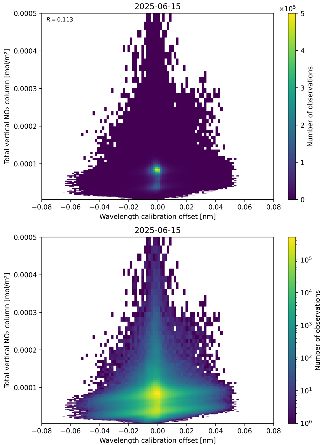
Figure 179: Scatter density plot of “Wavelength calibration offset” against “Total vertical NO 2 column” for 2025-06-14 to 2025-06-16.
