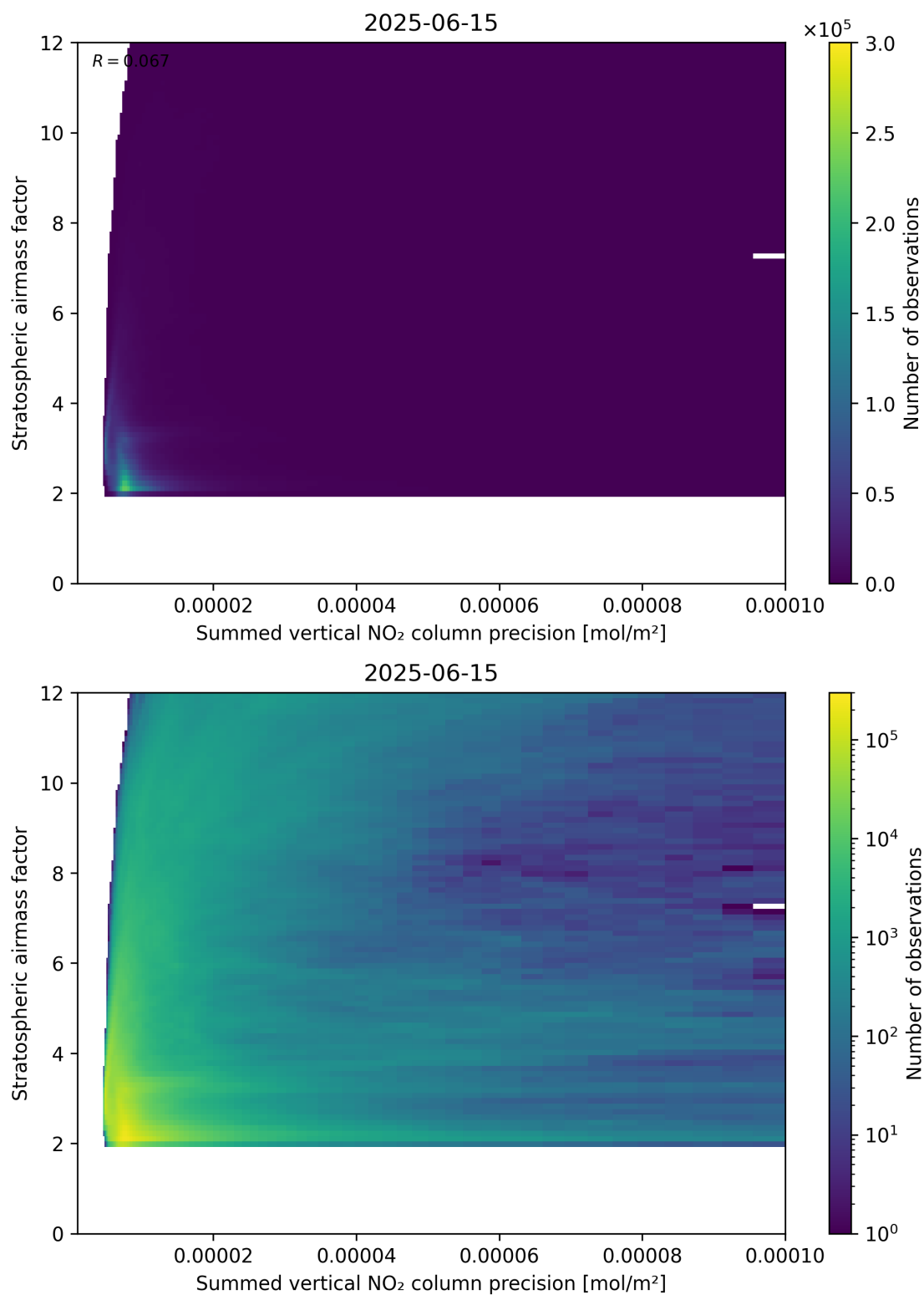
Figure 106: Scatter density plot of “Summed vertical NO 2 column precision” against “Stratospheric airmass factor” for 2025-06-14 to 2025-06-16.
