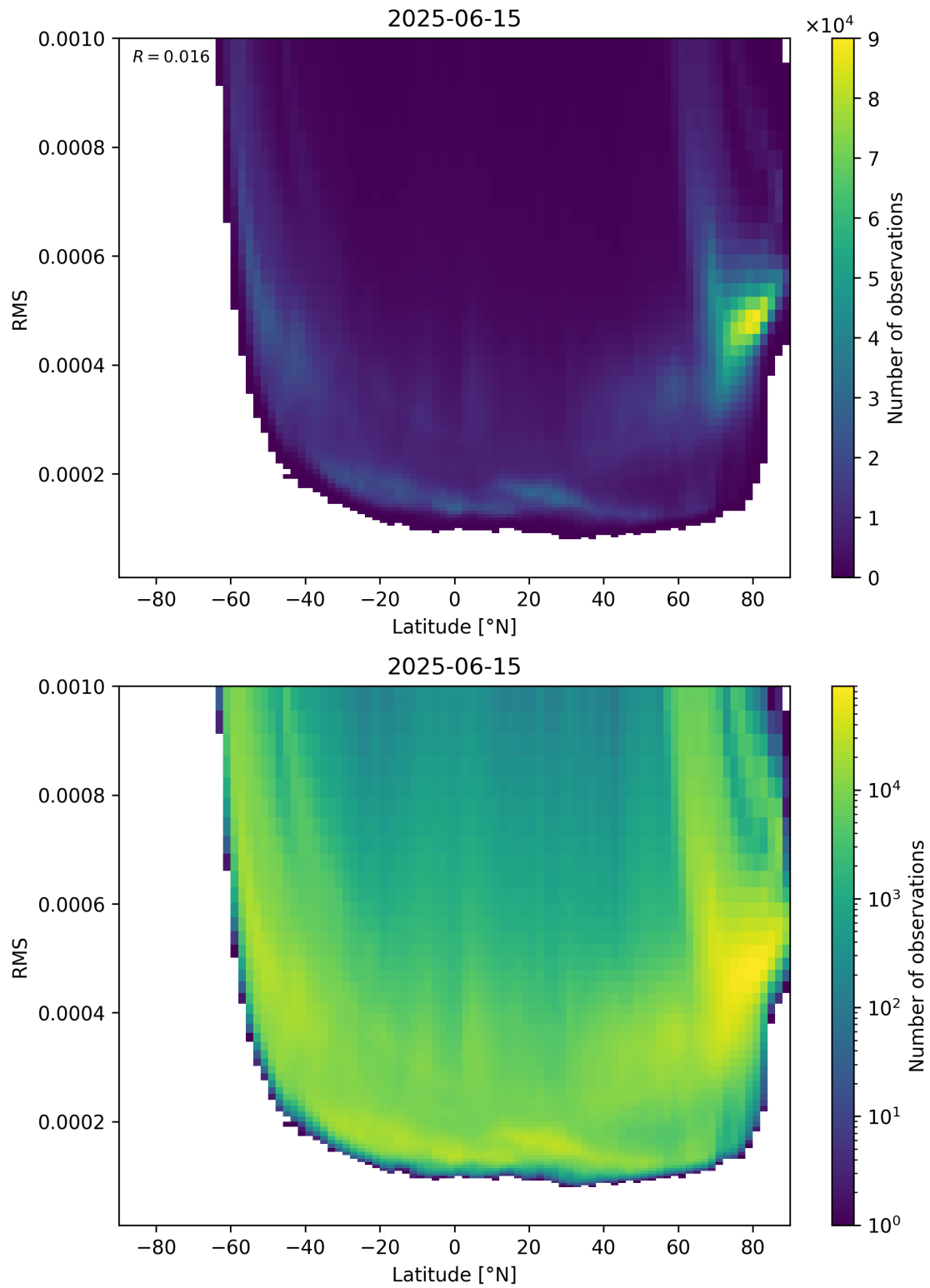
Figure 94: Scatter density plot of “Latitude” against “RMS” for 2025-06-14 to 2025-06-16.
