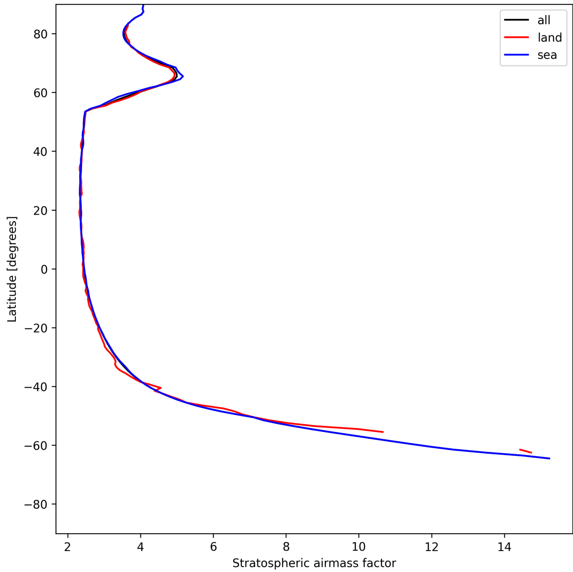
Figure 27: Zonal average of “Stratospheric airmass factor” for 2025-06-14 to 2025-06-16.
