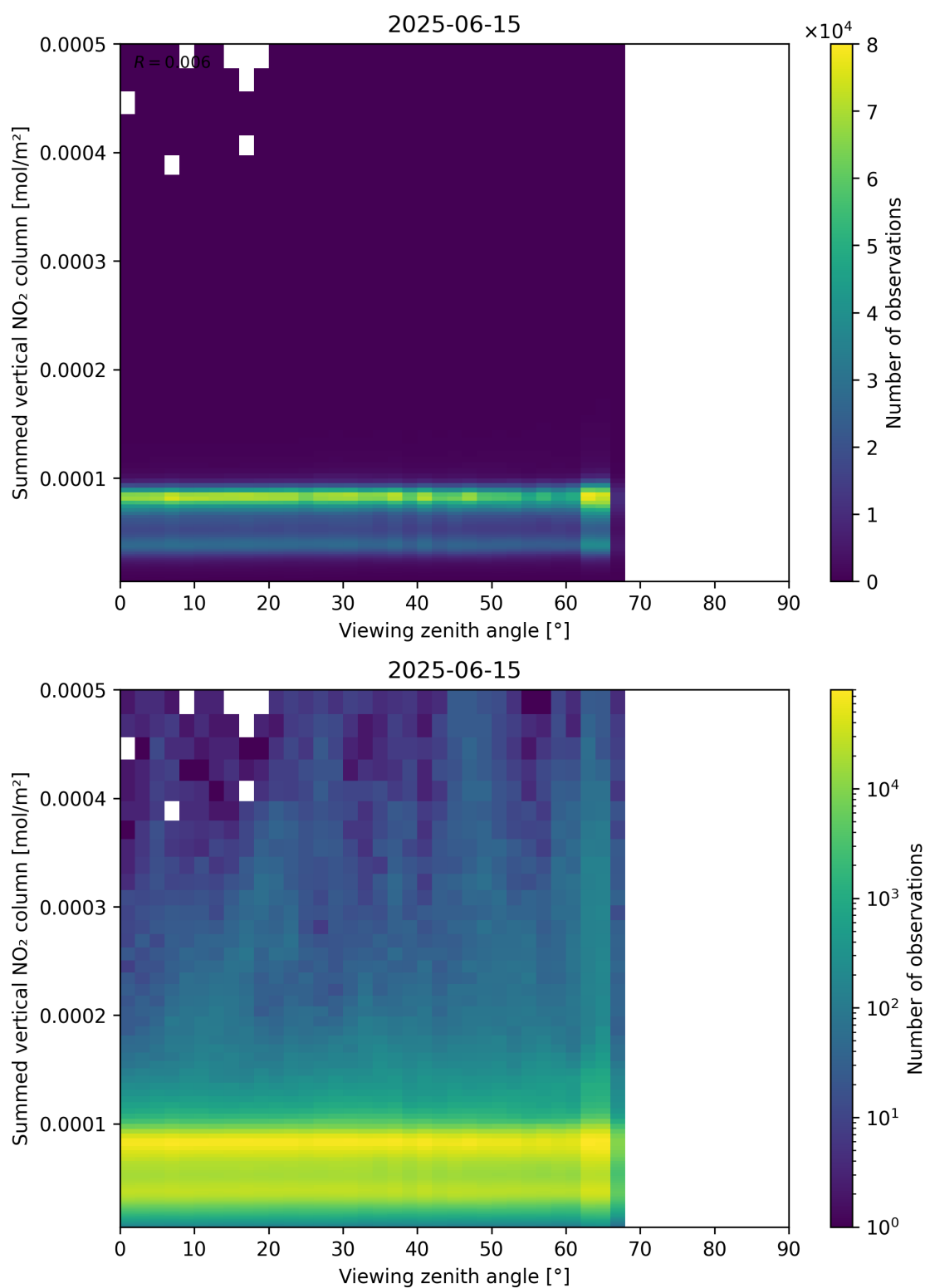
Figure 165: Scatter density plot of “Viewing zenith angle” against “Summed vertical NO 2 column” for 2025-06-14 to 2025-06-16.
