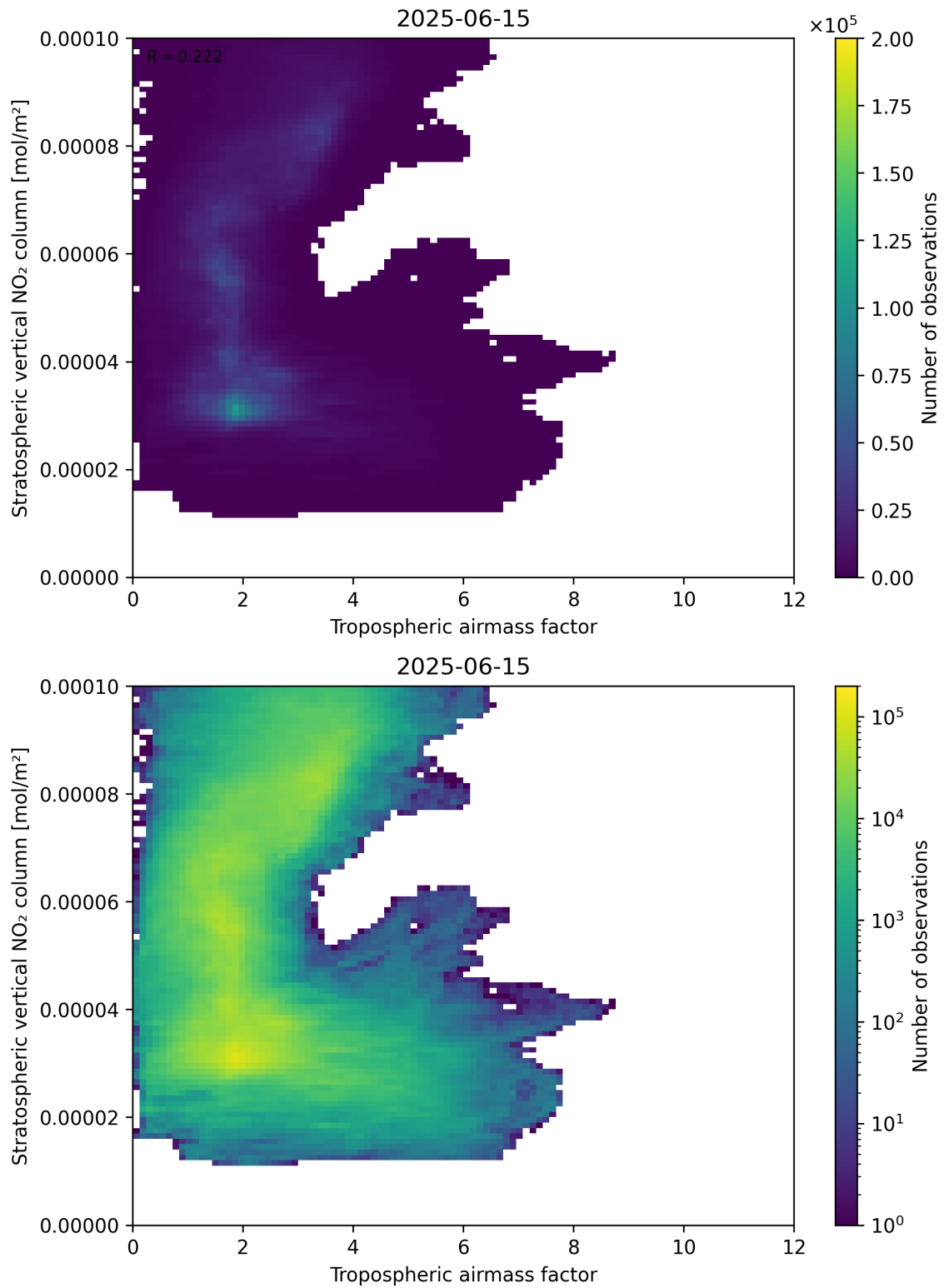
Figure 74: Scatter density plot of “Tropospheric air mass factor” against “Stratospheric vertical NO 2 column” for 2025-06-14 to 2025-06-16.
