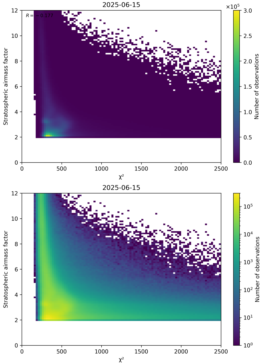
Figure 81: Scatter density plot of “ \chi^2 ” against “Stratospheric airmass factor” for 2025-06-14 to 2025-06-16.
