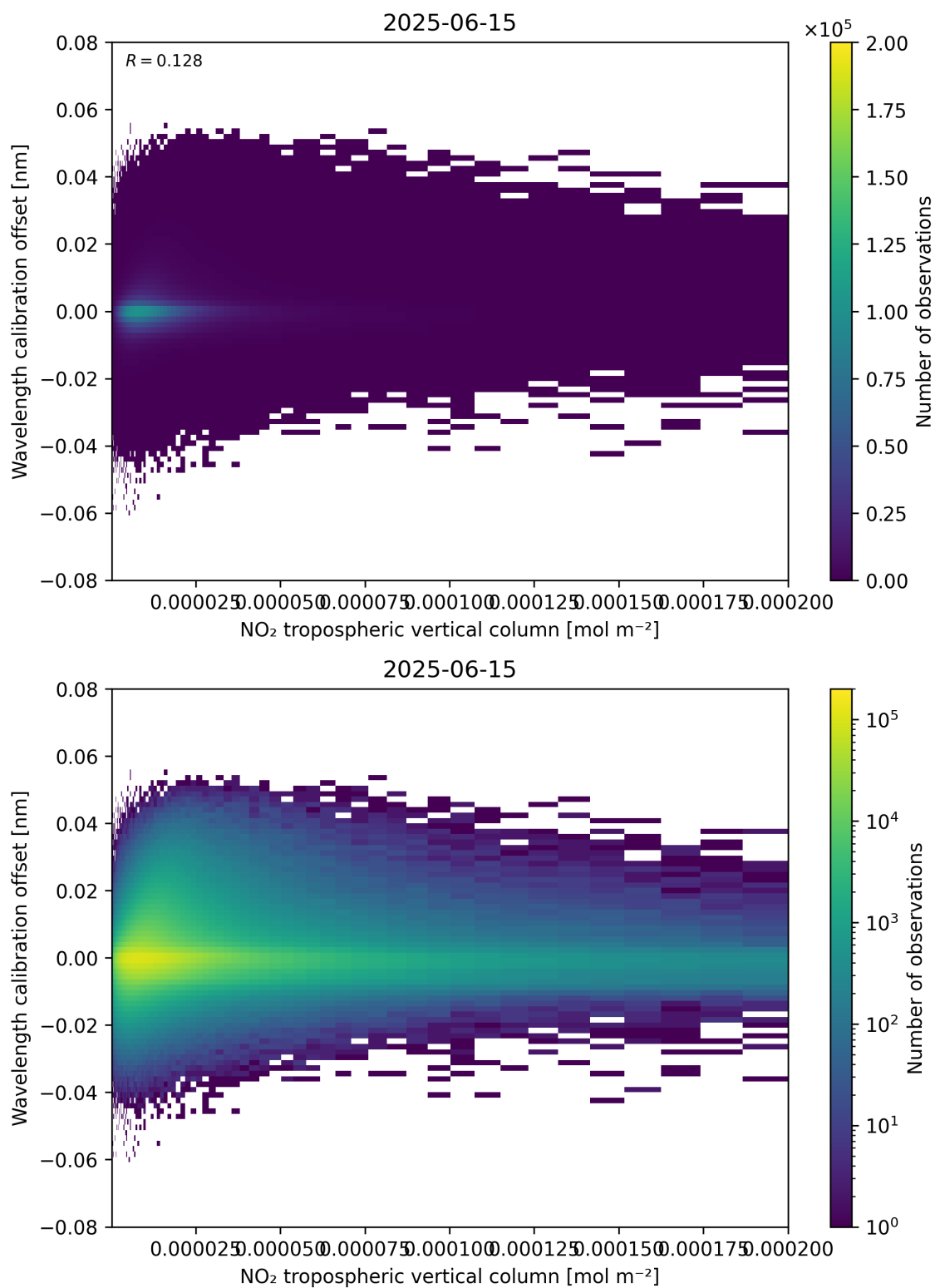
Figure 143: Scatter density plot of “NO 2 tropospheric vertical column” against “Wavelength calibration offset” for 2025-06-14 to 2025-06-16.
