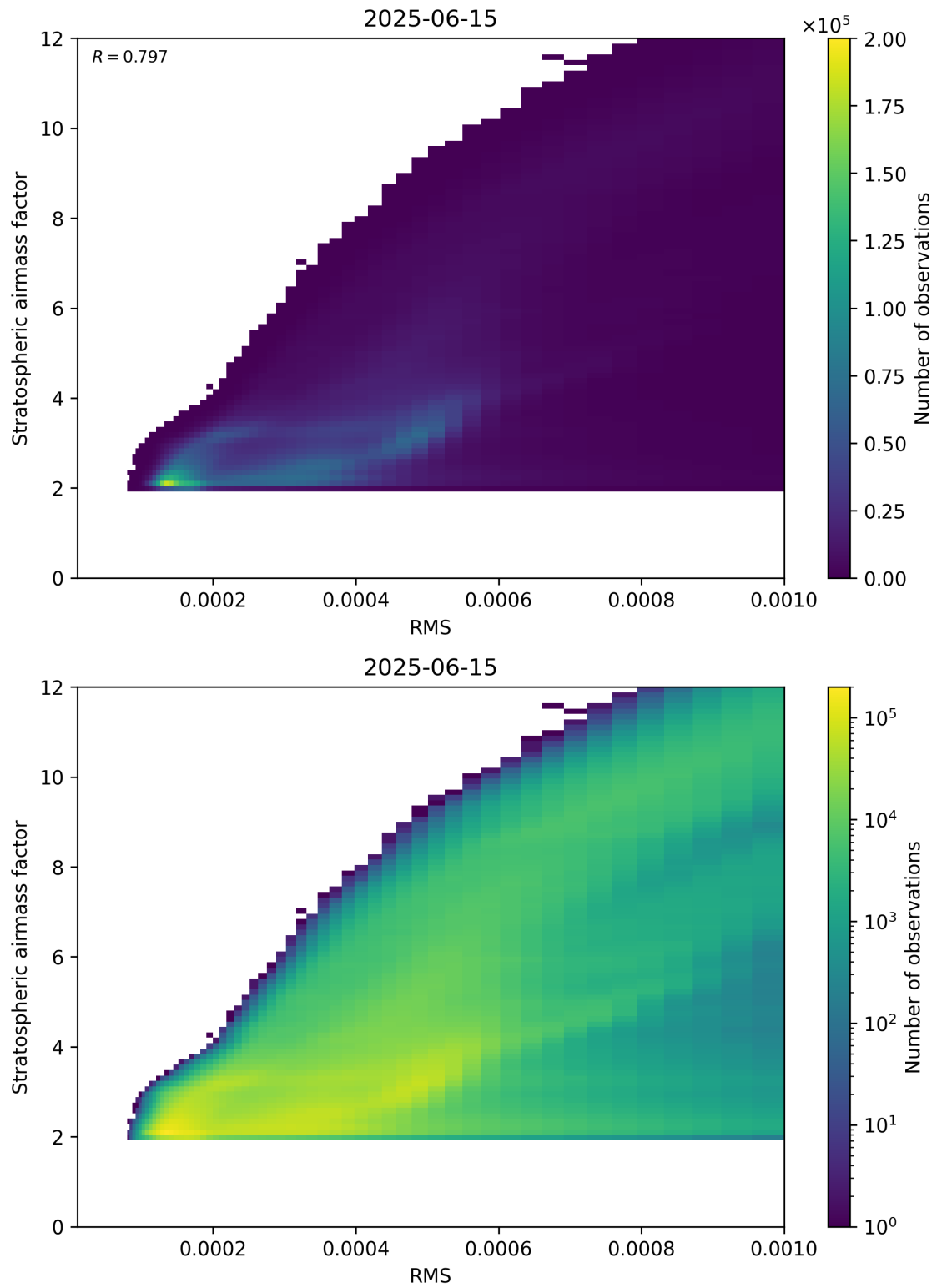
Figure 144: Scatter density plot of “RMS” against “Stratospheric airmass factor” for 2025-06-14 to 2025-06-16.
