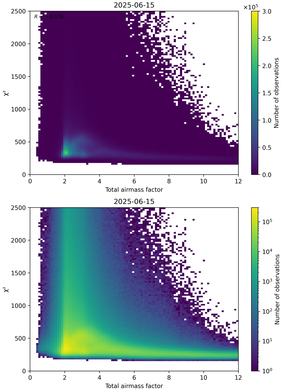
Figure 63: Scatter density plot of “Total airmass factor” against “ \chi^2 ” for 2025-06-14 to 2025-06-16.
