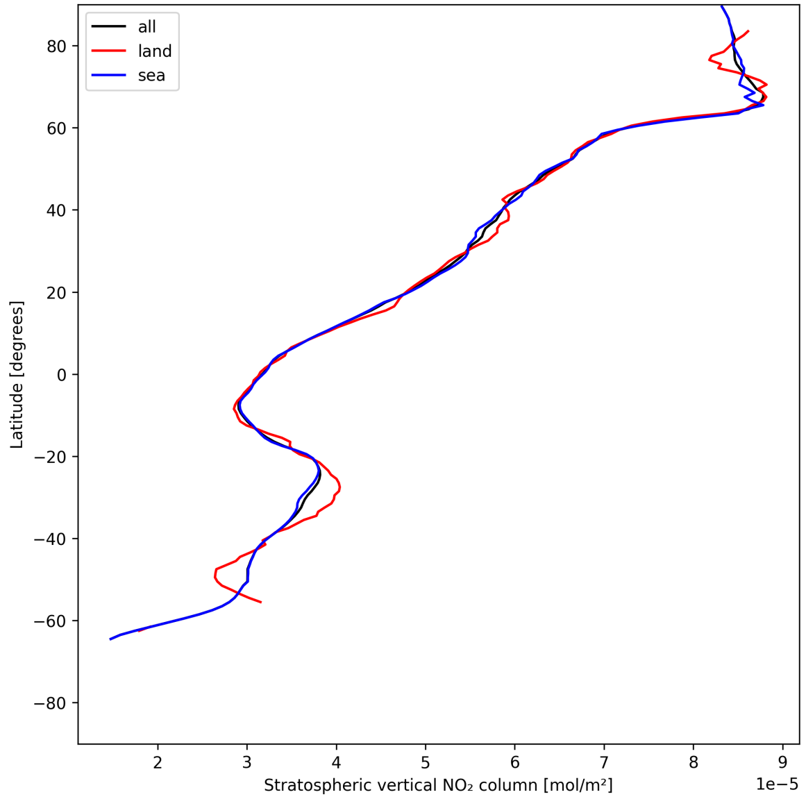
Figure 19: Zonal average of “Stratospheric vertical NO 2 column” for 2025-06-14 to 2025-06-16.
