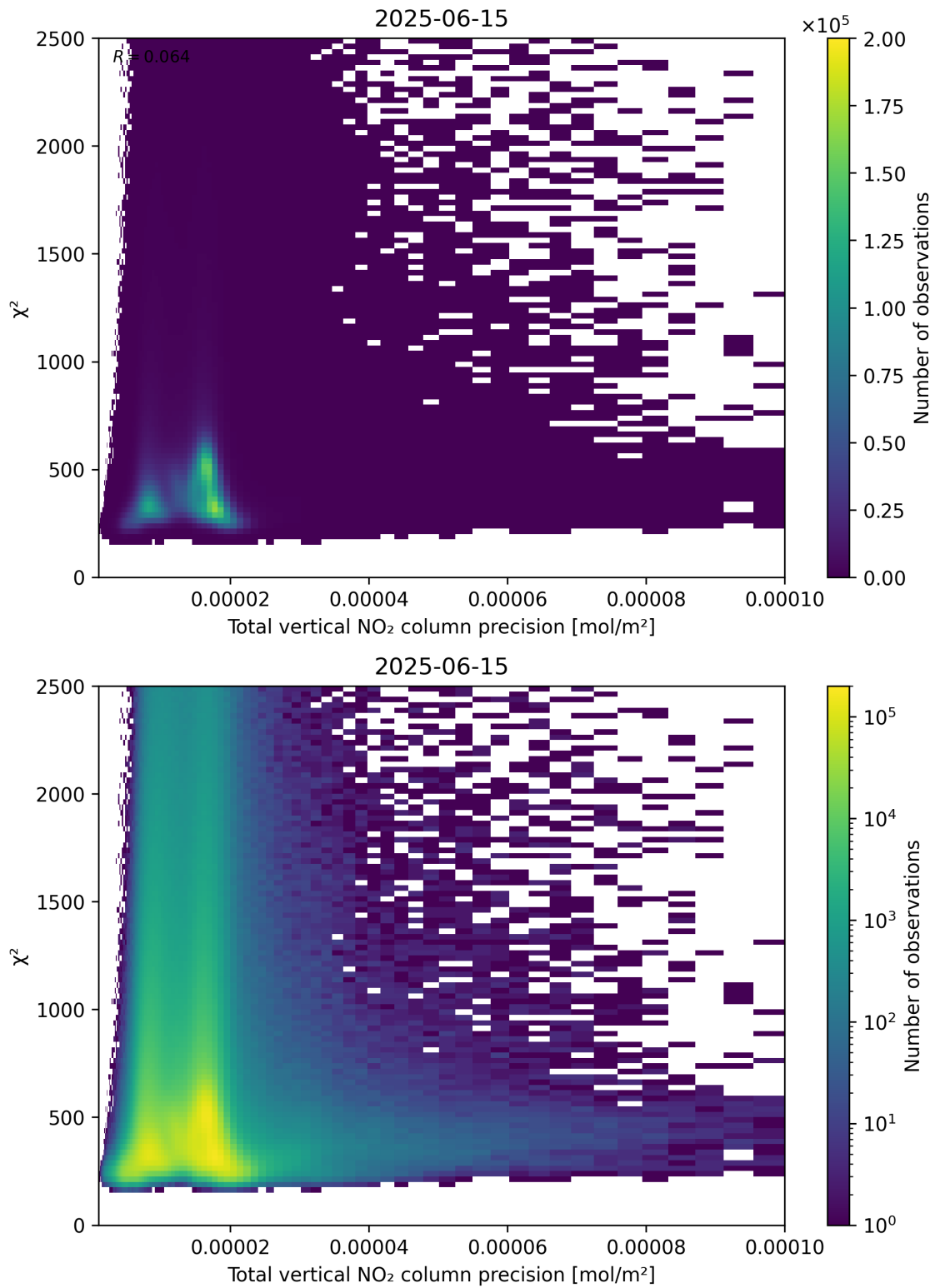
Figure 116: Scatter density plot of “Total vertical NO 2 column precision” against “ \chi^2 ” for 2025-06-14 to 2025-06-16.
