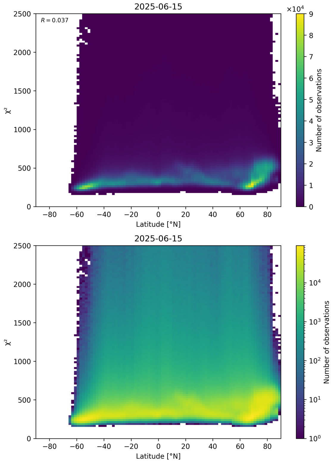
Figure 86: Scatter density plot of “Latitude” against “ \chi^2 ” for 2025-06-14 to 2025-06-16.
