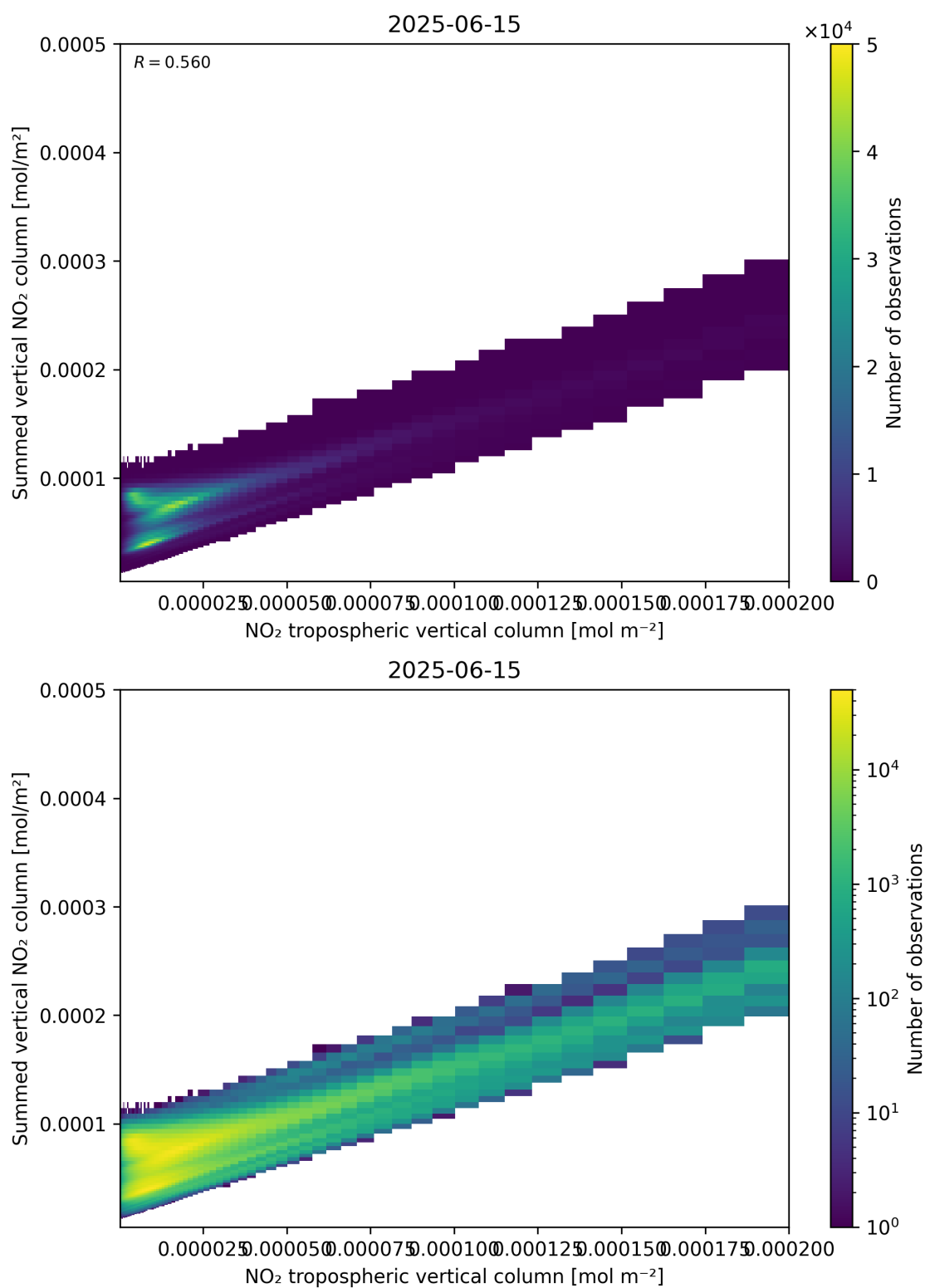
Figure 126: Scatter density plot of “NO 2 tropospheric vertical column” against “Summed vertical NO 2 column” for 2025-06-14 to 2025-06-16.
