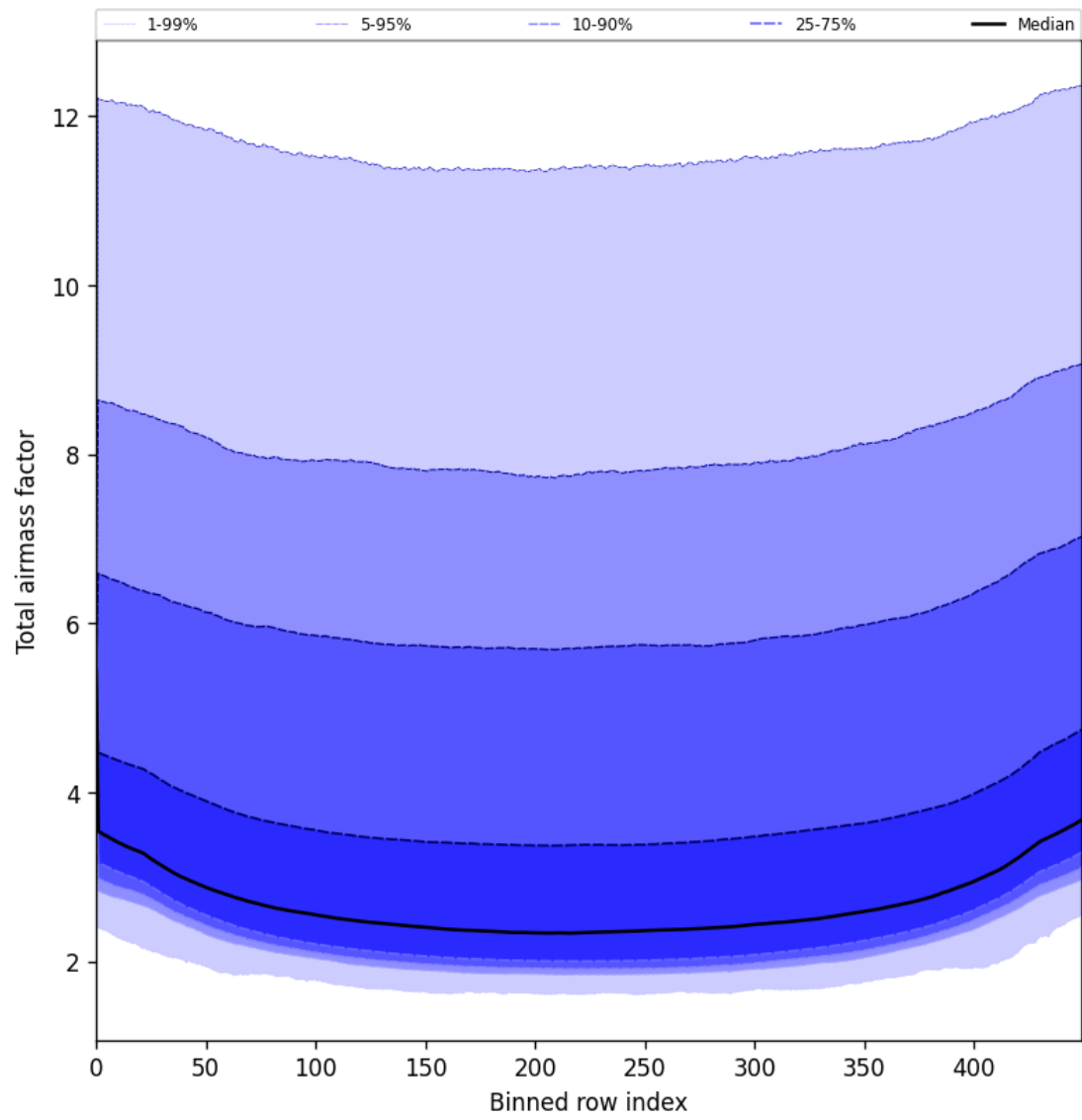
Figure 49: Along track statistics of “Total airmass factor” for 2025-06-14 to 2025-06-16
