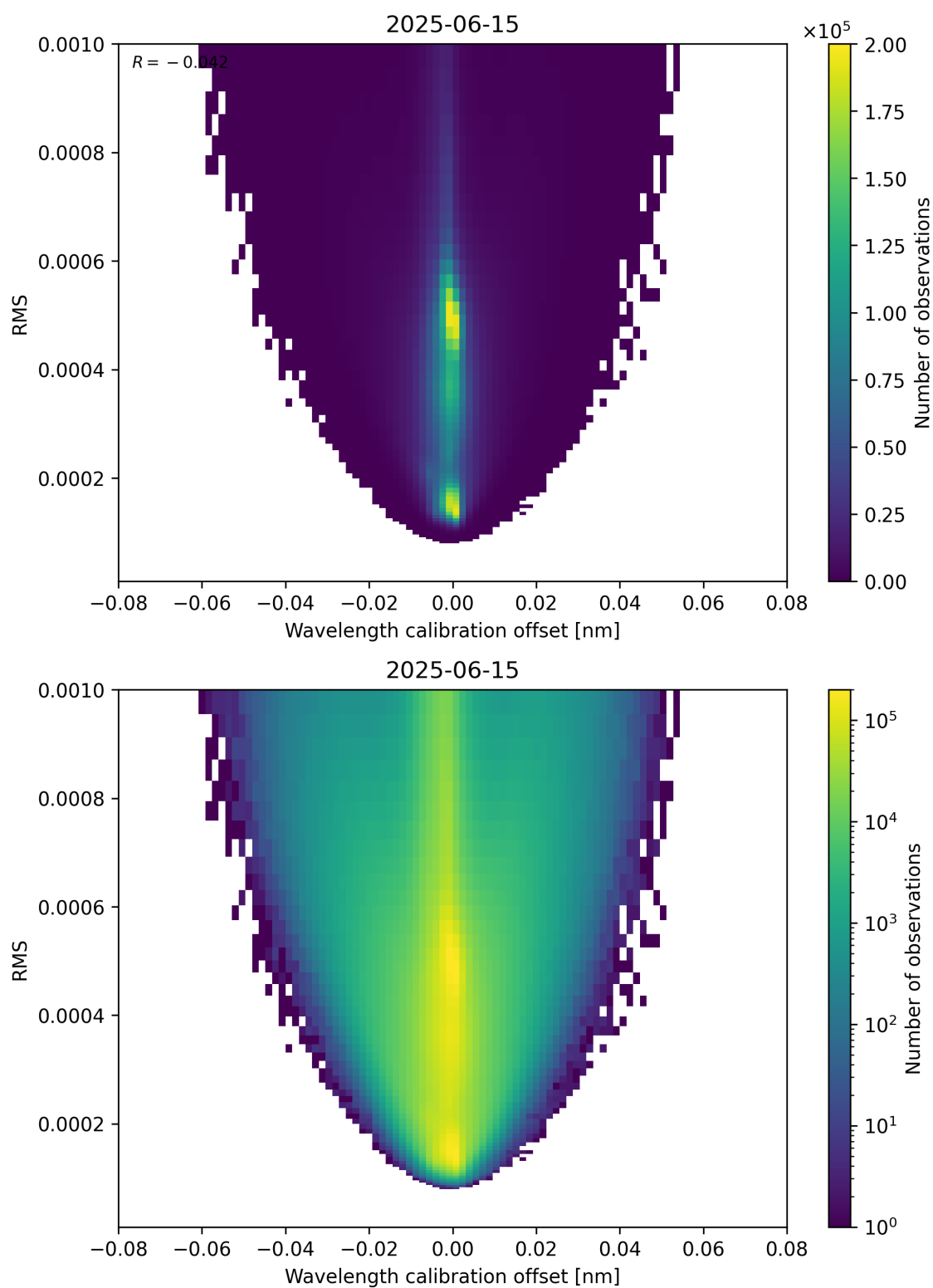
Figure 181: Scatter density plot of “Wavelength calibration offset” against “RMS” for 2025-06-14 to 2025-06-16.
