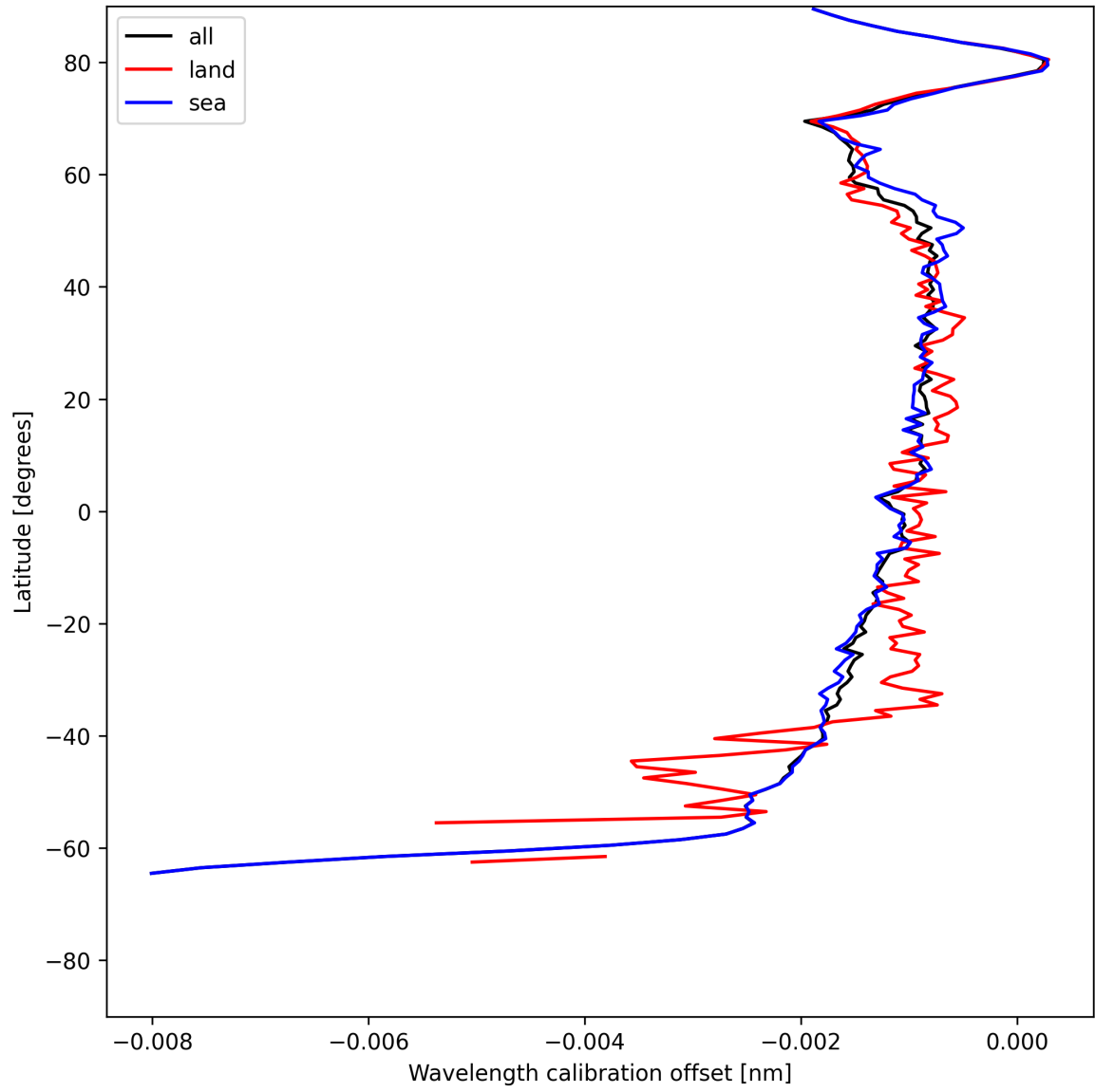
Figure 18: Zonal average of “Wavelength calibration offset” for 2025-06-14 to 2025-06-16.
