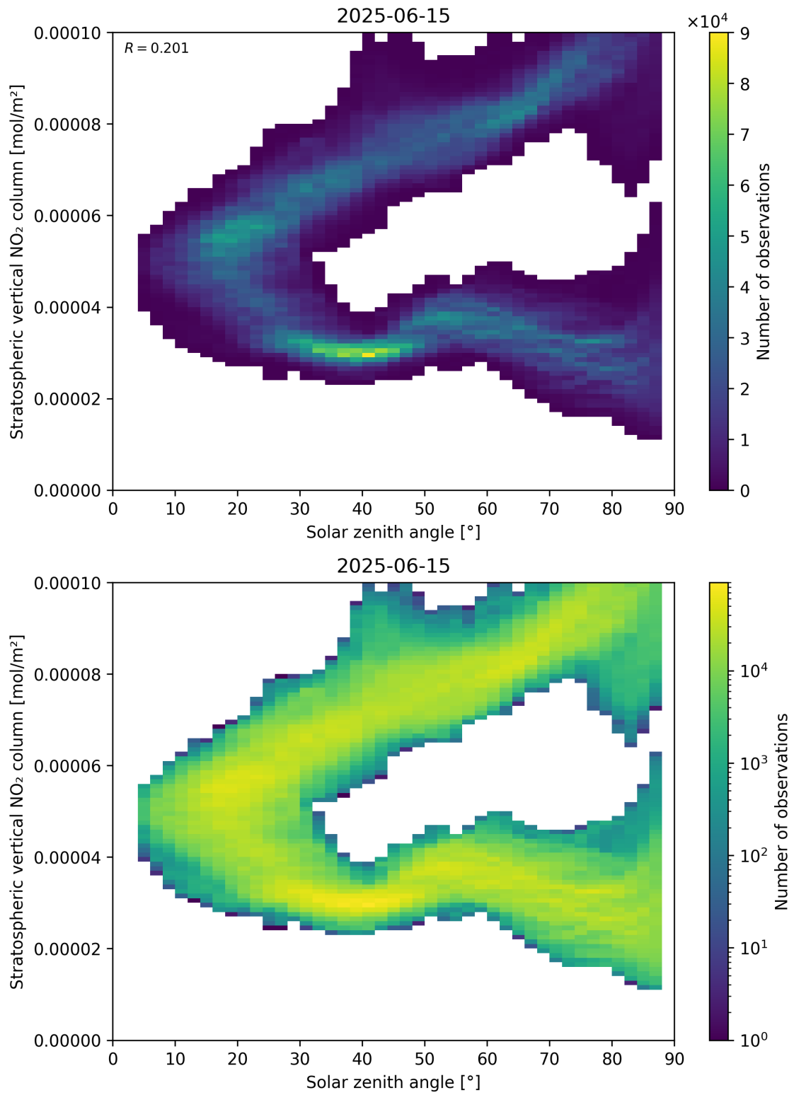
Figure 150: Scatter density plot of “Solar zenith angle” against “Stratospheric vertical NO 2 column” for 2025-06-14 to 2025-06-16.
