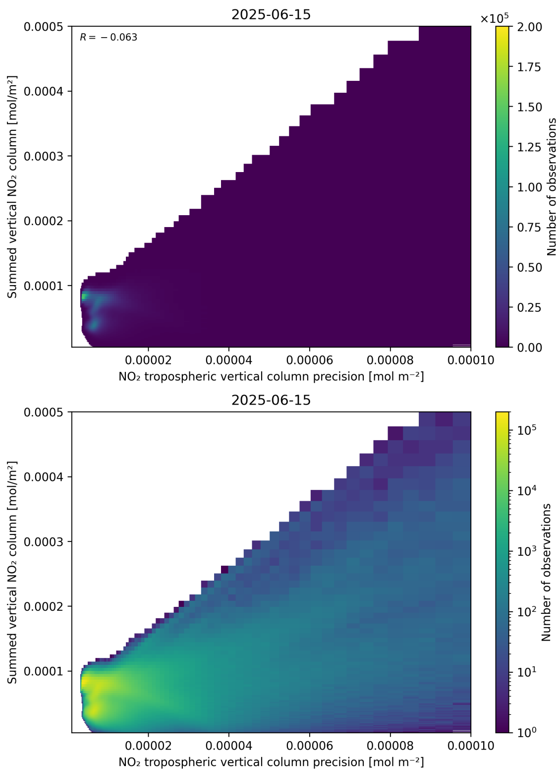
Figure 136: Scatter density plot of “NO 2 tropospheric vertical column precision” against “Summed vertical NO 2 column” for 2025-06-14 to 2025-06-16.
