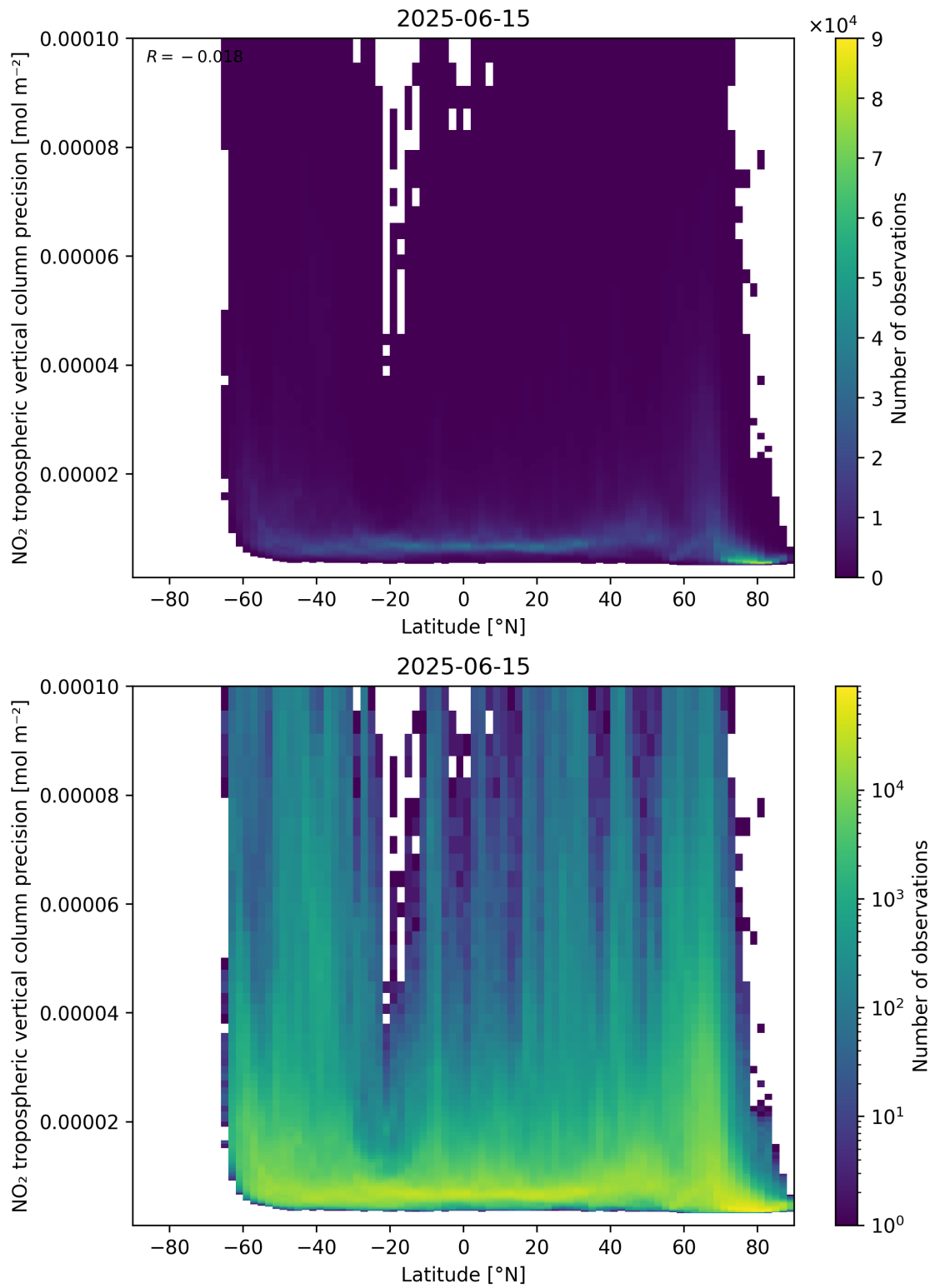
Figure 93: Scatter density plot of “Latitude” against “NO 2 tropospheric vertical column precision” for 2025-06-14 to 2025-06-16.
