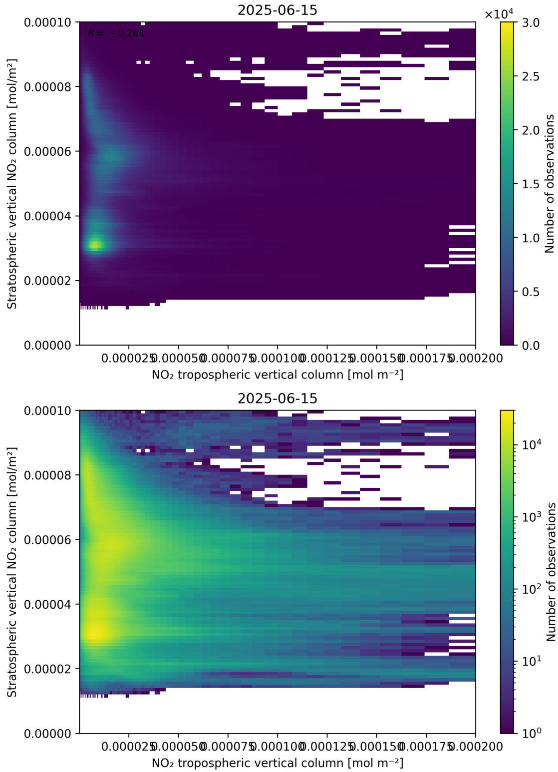
Figure 125: Scatter density plot of “NO 2 tropospheric vertical column” against “Stratospheric vertical NO 2 column” for 2025-06-14 to 2025-06-16.
