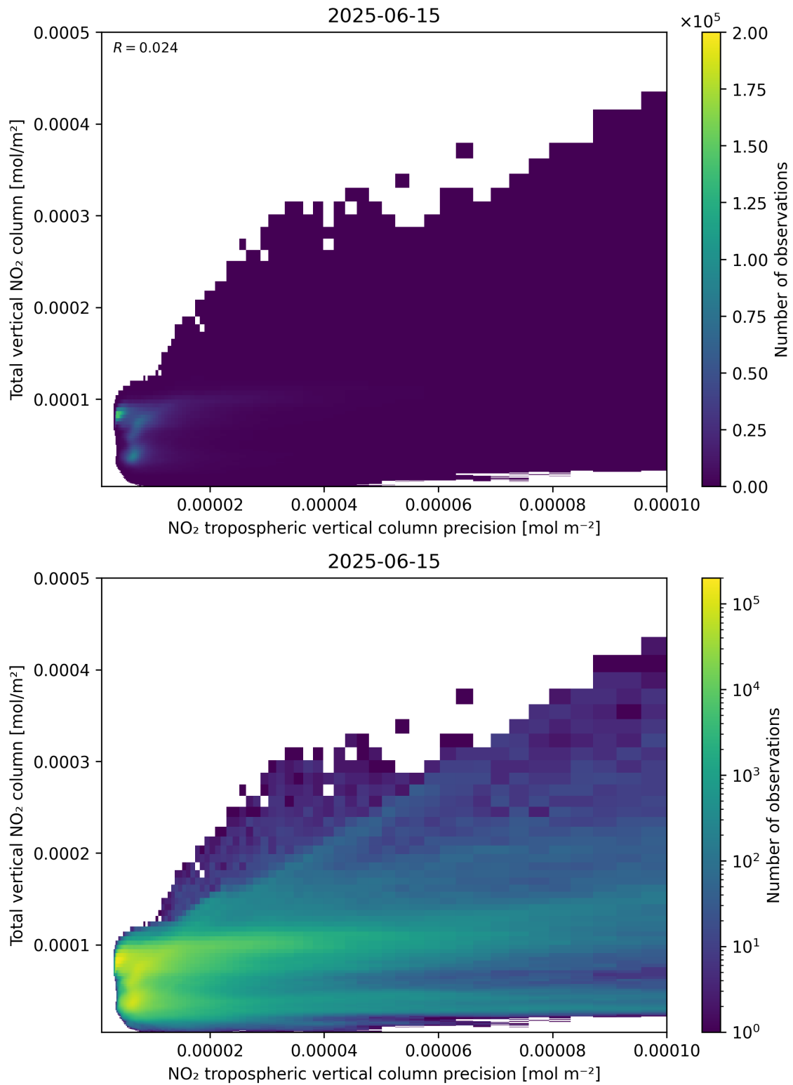
Figure 138: Scatter density plot of “NO 2 tropospheric vertical column precision” against “Total vertical NO 2 column” for 2025-06-14 to 2025-06-16.
