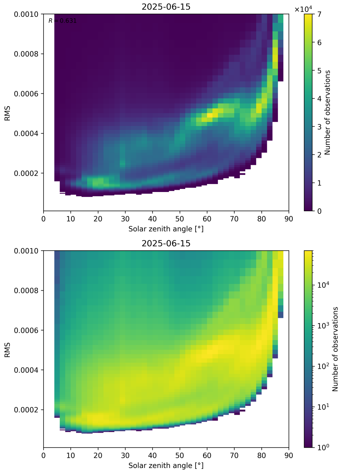
Figure 157: Scatter density plot of “Solar zenith angle” against “RMS” for 2025-06-14 to 2025-06-16.
