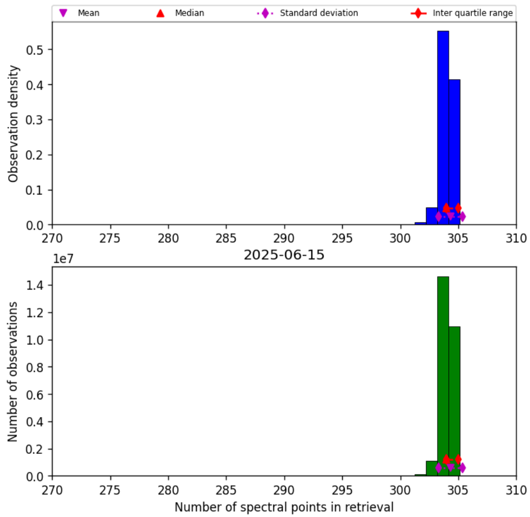
Figure 33: Histogram of “Number of spectral points in retrieval” for 2025-06-14 to 2025-06-16
