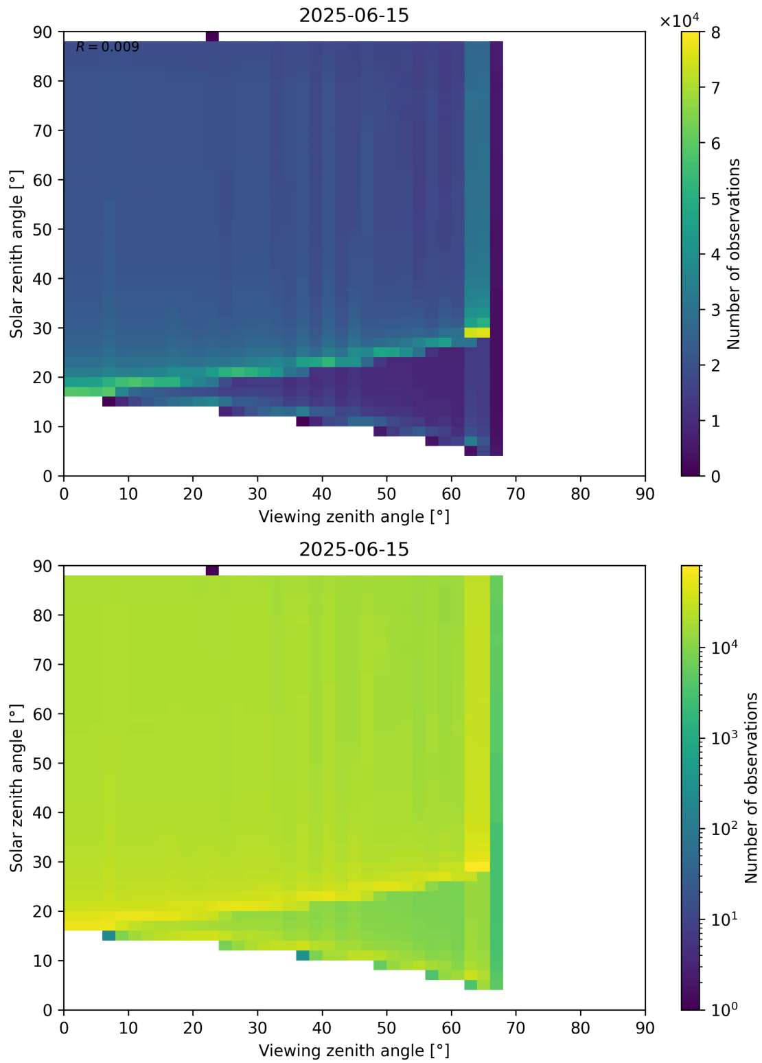
Figure 172: Scatter density plot of “Viewing zenith angle” against “Solar zenith angle” for 2025-06-14 to 2025-06-16.
