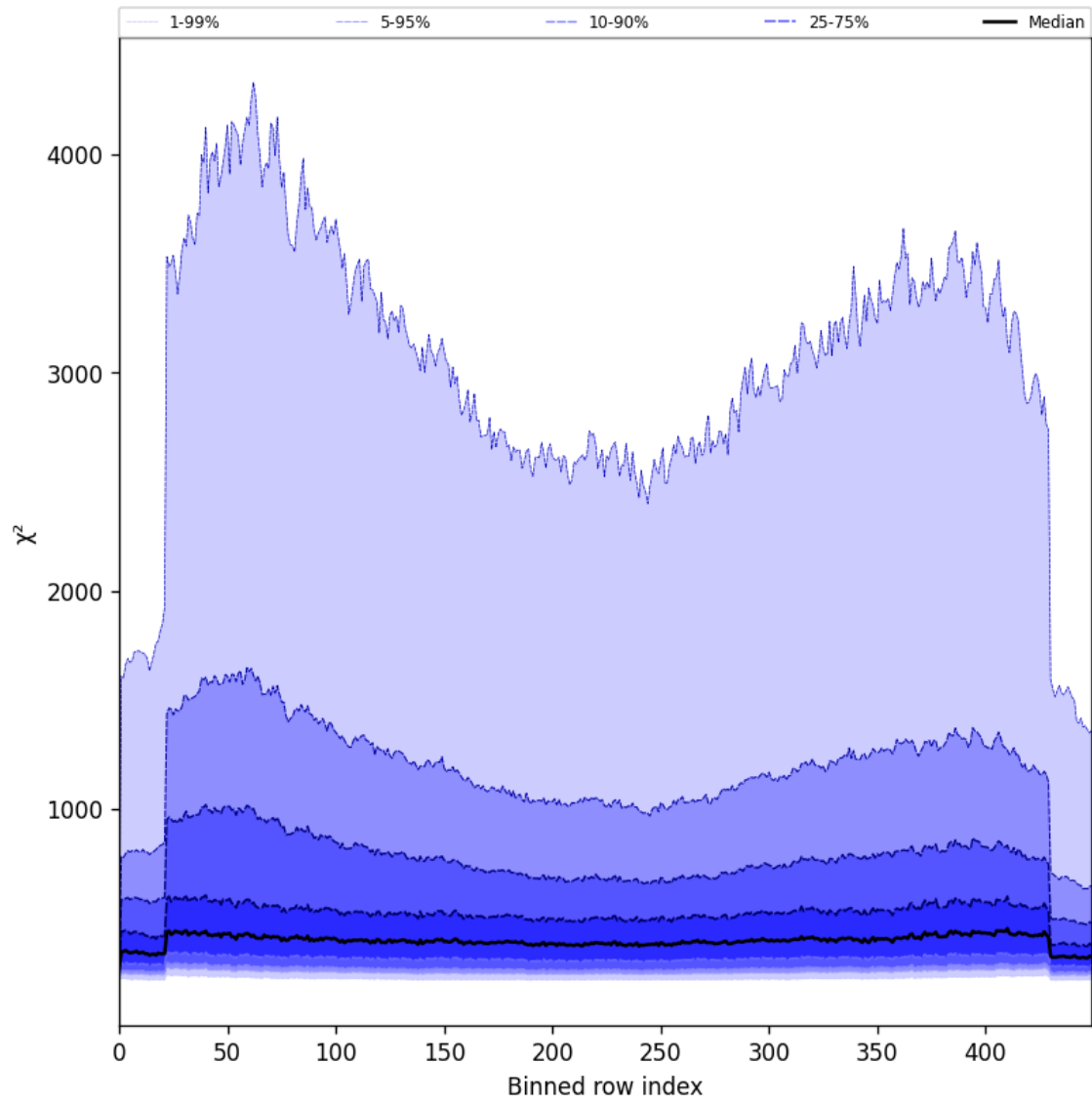
Figure 59: Along track statistics of “ \chi^2 ” for 2025-06-14 to 2025-06-16
