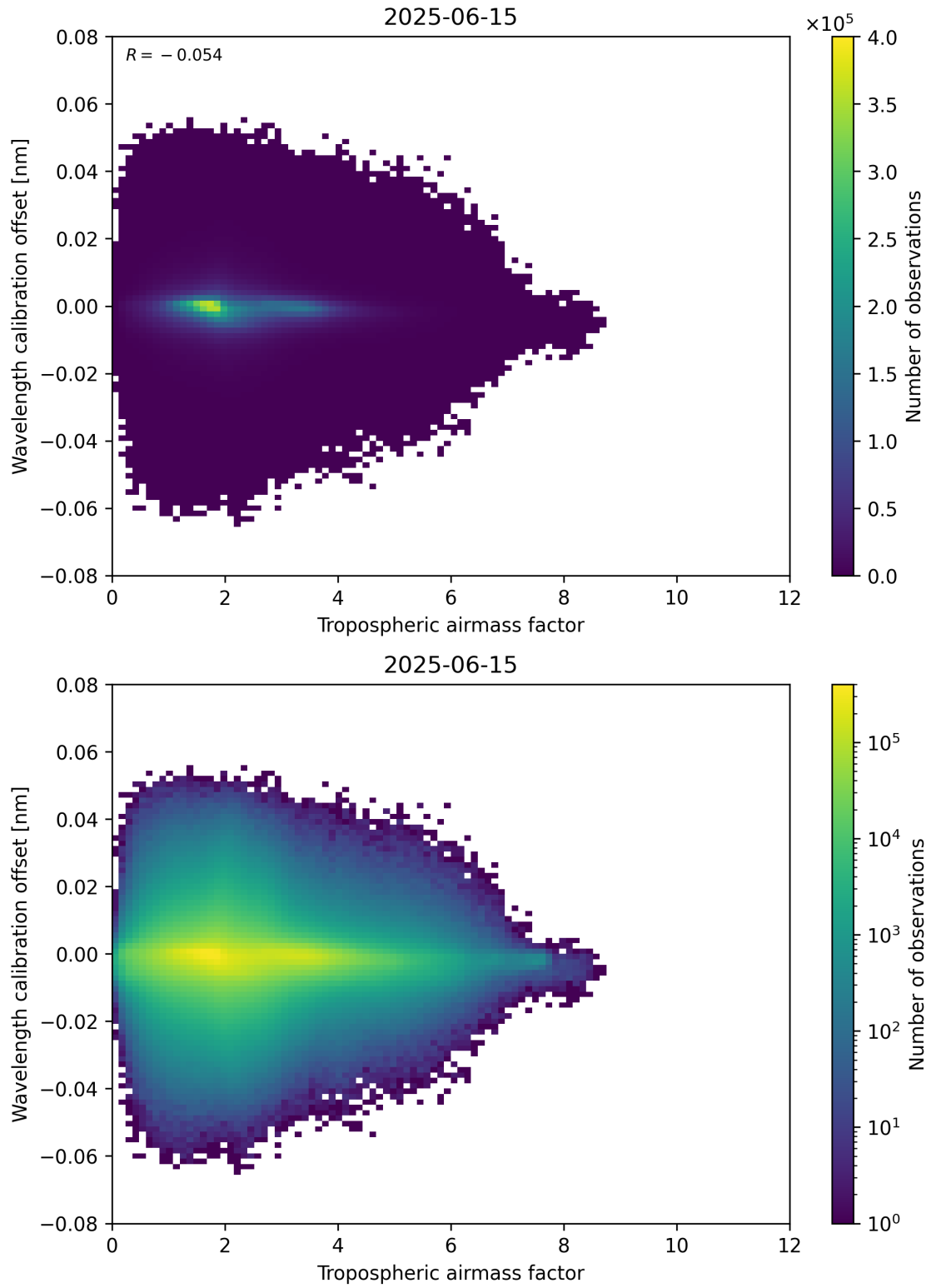
Figure 80: Scatter density plot of “Tropospheric airmass factor” against “Wavelength calibration offset” for 2025-06-14 to 2025-06-16.
