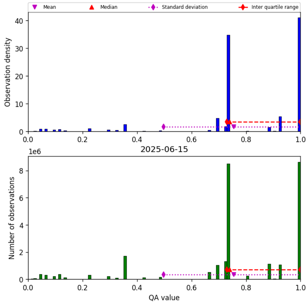
Figure 28: Histogram of “QA value” for 2025-06-14 to 2025-06-16
