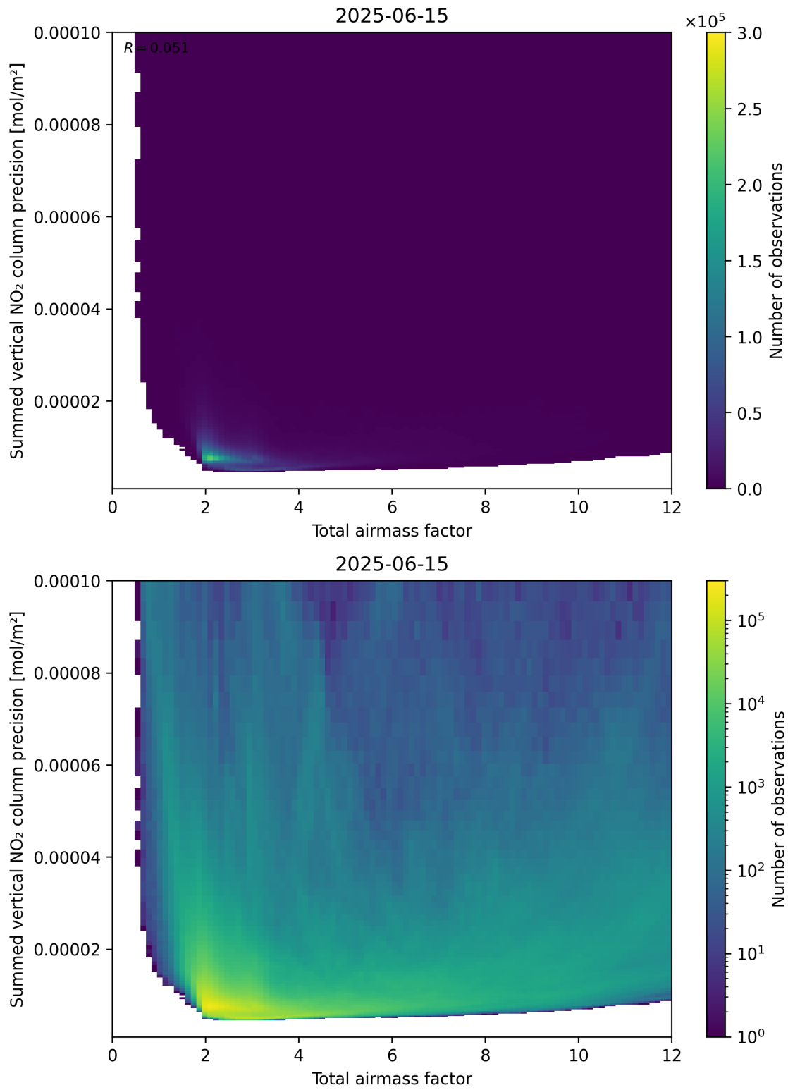
Figure 66: Scatter density plot of “Total airmass factor” against “Summed vertical NO 2 column precision” for 2025-06-14 to 2025-06-16.
