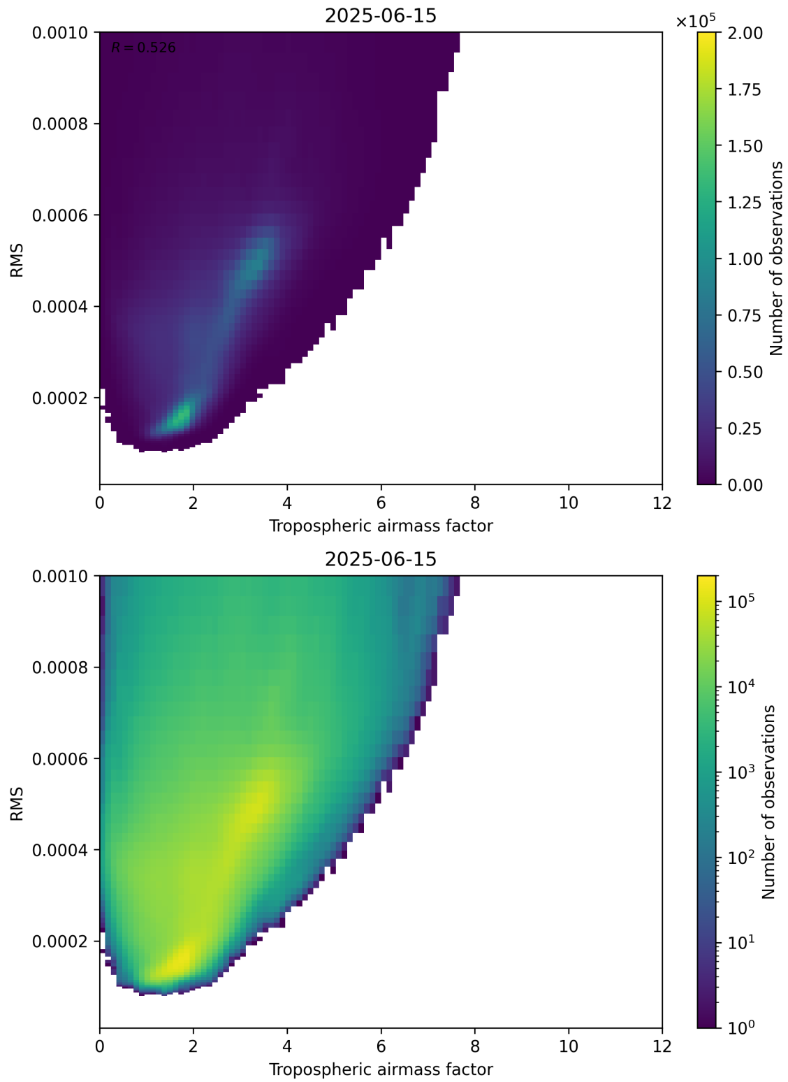
Figure 79: Scatter density plot of “Tropospheric airmass factor” against “RMS” for 2025-06-14 to 2025-06-16.
