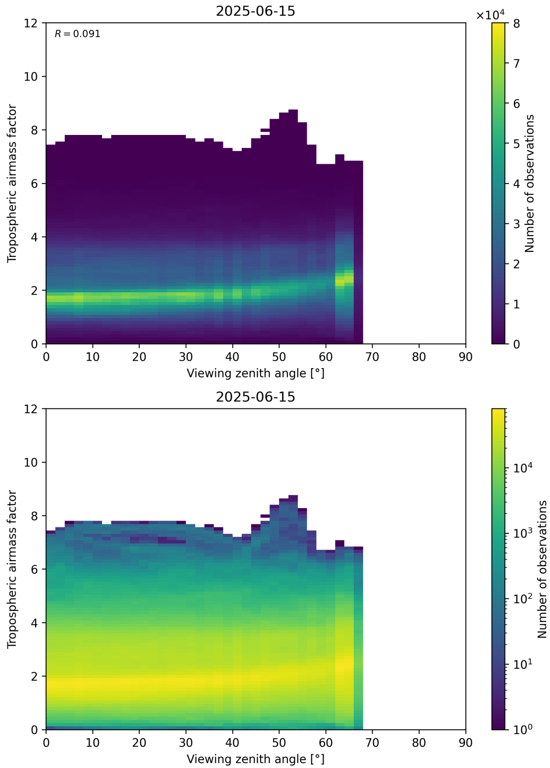
Figure 161: Scatter density plot of “Viewing zenith angle” against “Tropospheric airmass factor” for 2025-06-14 to 2025-06-16.
