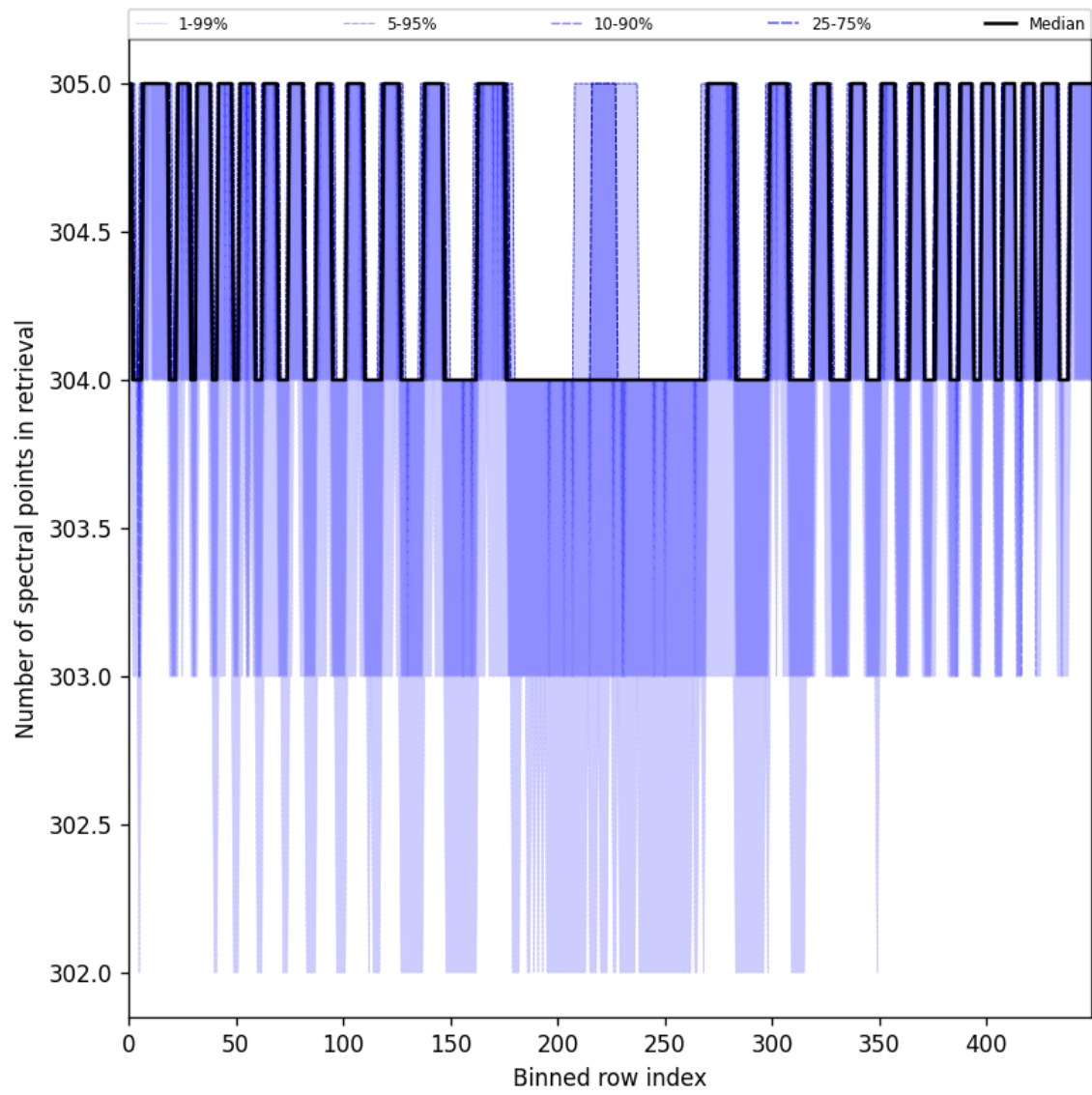
Figure 50: Along track statistics of “Number of spectral points in retrieval” for 2025-06-14 to 2025-06-16
