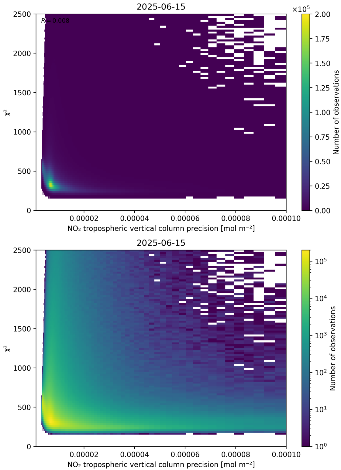
Figure 134: Scatter density plot of “NO 2 tropospheric vertical column precision” against “ \chi^2 ” for 2025-06-14 to 2025-06-16.
