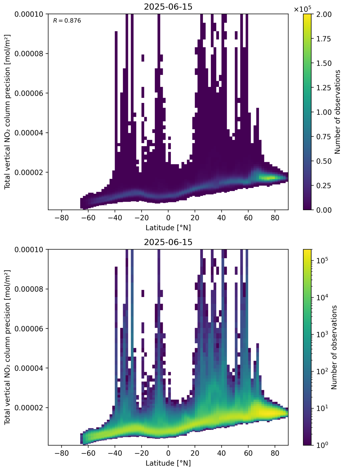
Figure 91: Scatter density plot of “Latitude” against “Total vertical NO 2 column precision” for 2025-06-14 to 2025-06-16.
