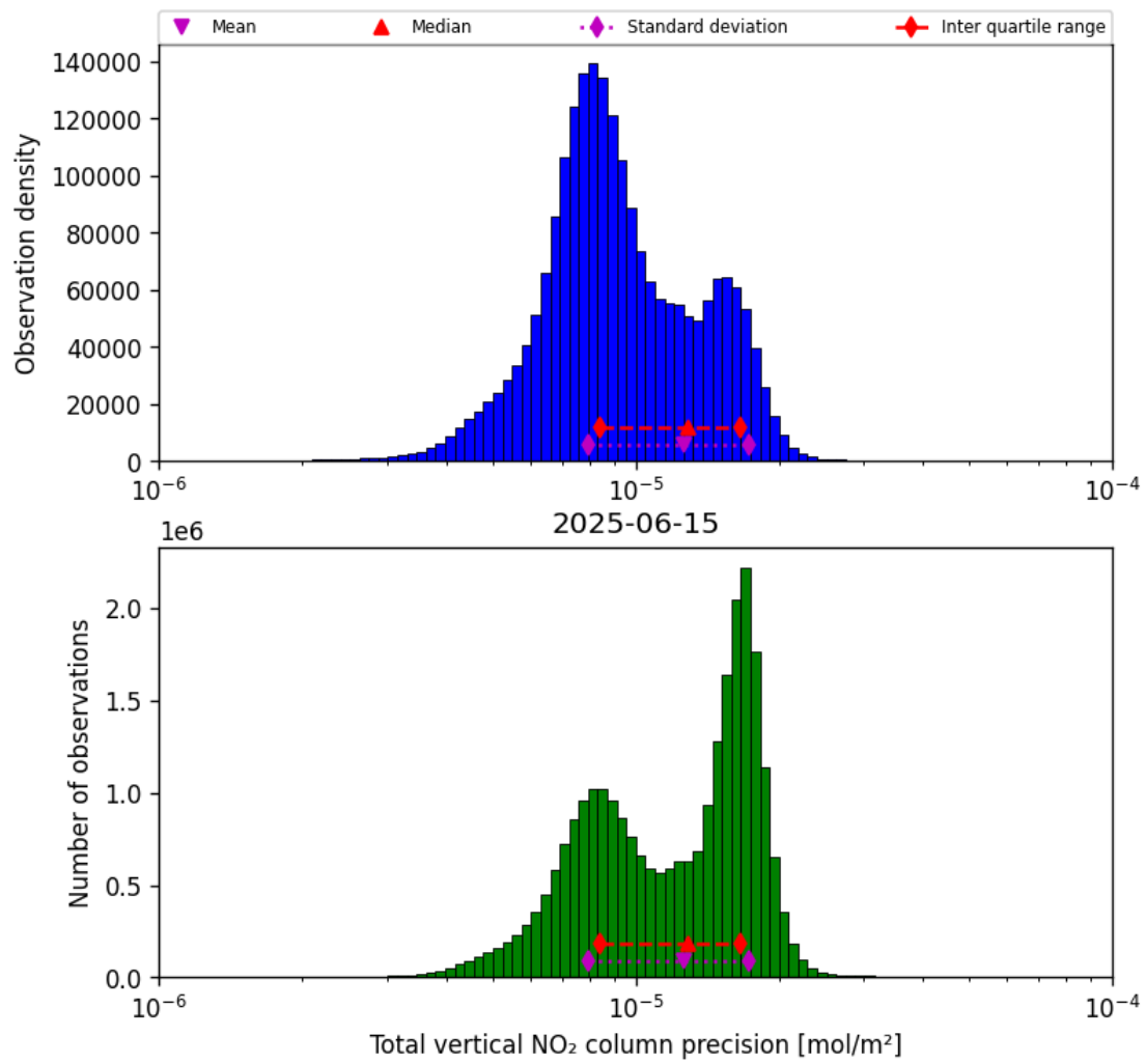
Figure 39: Histogram of “Total vertical NO 2 column precision” for 2025-06-14 to 2025-06-16
