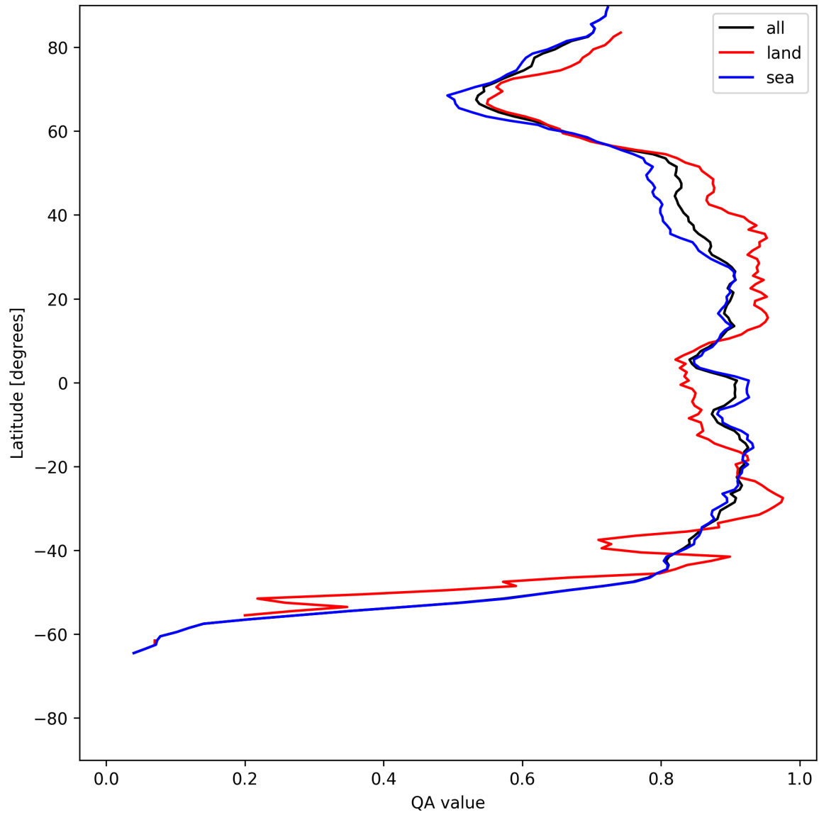
Figure 11: Zonal average of “QA value” for 2025-06-14 to 2025-06-16.
