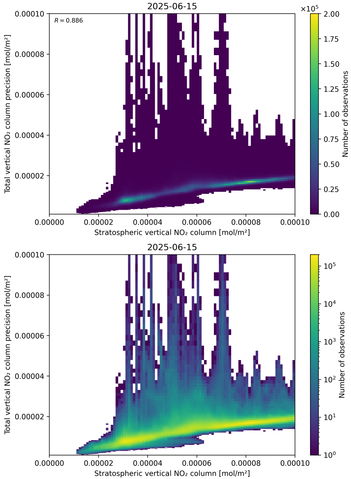
Figure 101: Scatter density plot of “Stratospheric vertical NO 2 column” against “Total vertical NO 2 column precision” for 2025-06-14 to 2025-06-16.
