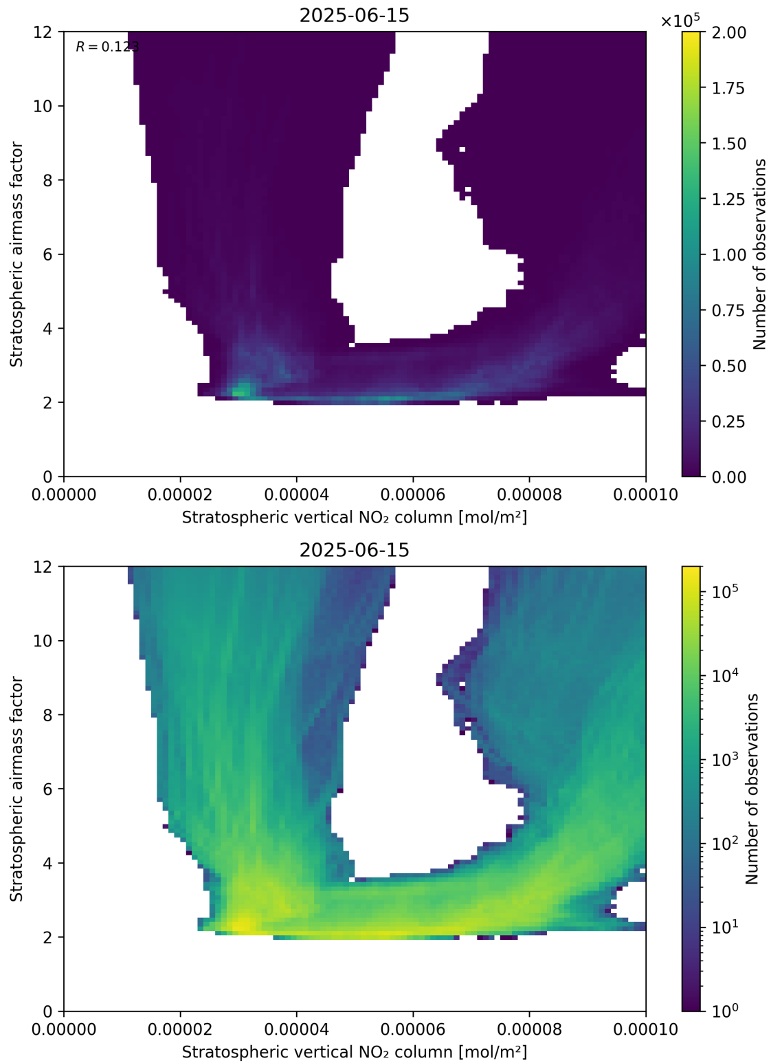
Figure 96: Scatter density plot of “Stratospheric vertical NO 2 column” against “Stratospheric airmass factor” for 2025-06-14 to 2025-06-16.
