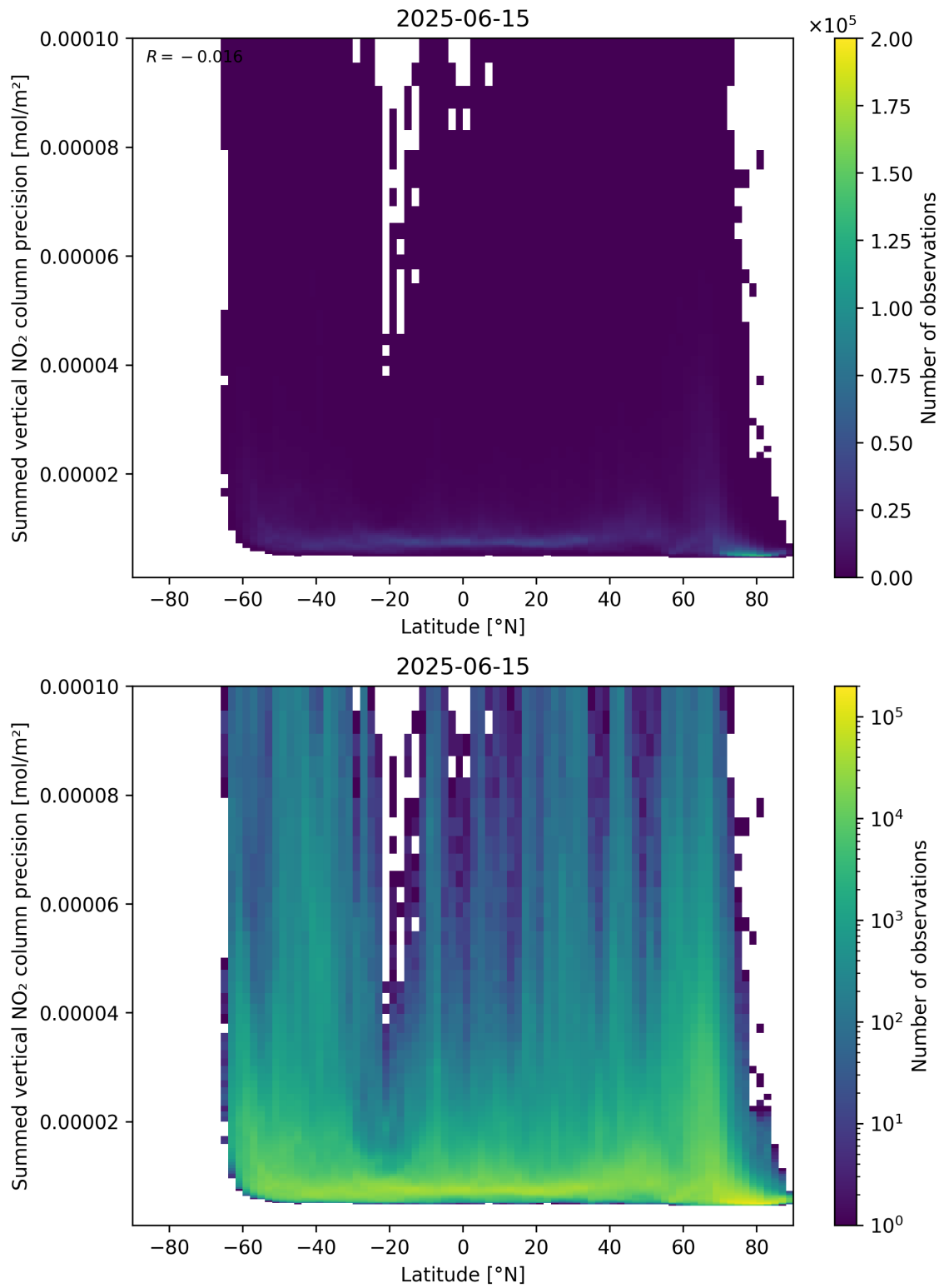
Figure 89: Scatter density plot of “Latitude” against “Summed vertical NO 2 column precision” for 2025-06-14 to 2025-06-16.
