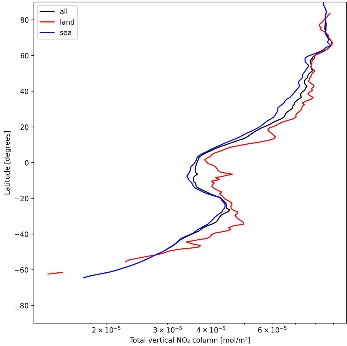
Figure 21: Zonal average of “Total vertical NO 2 column” for 2025-06-14 to 2025-06-16.
