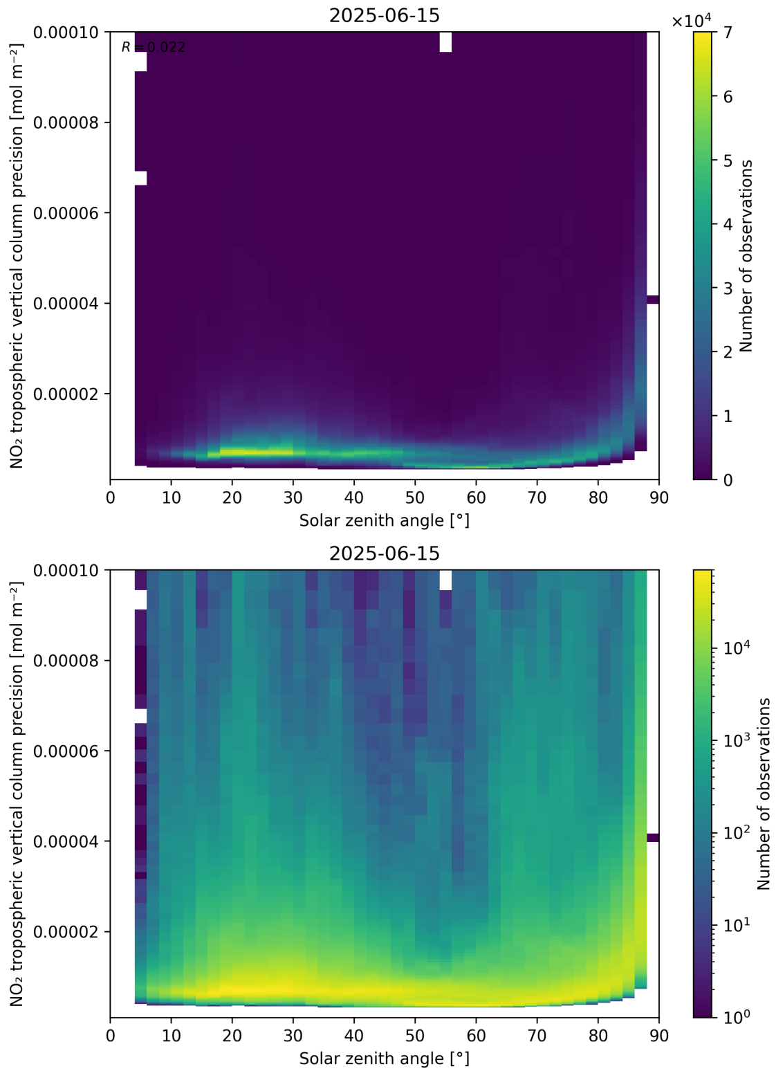
Figure 156: Scatter density plot of “Solar zenith angle” against “NO 2 tropospheric vertical column precision” for 2025-06-14 to 2025-06-16.
