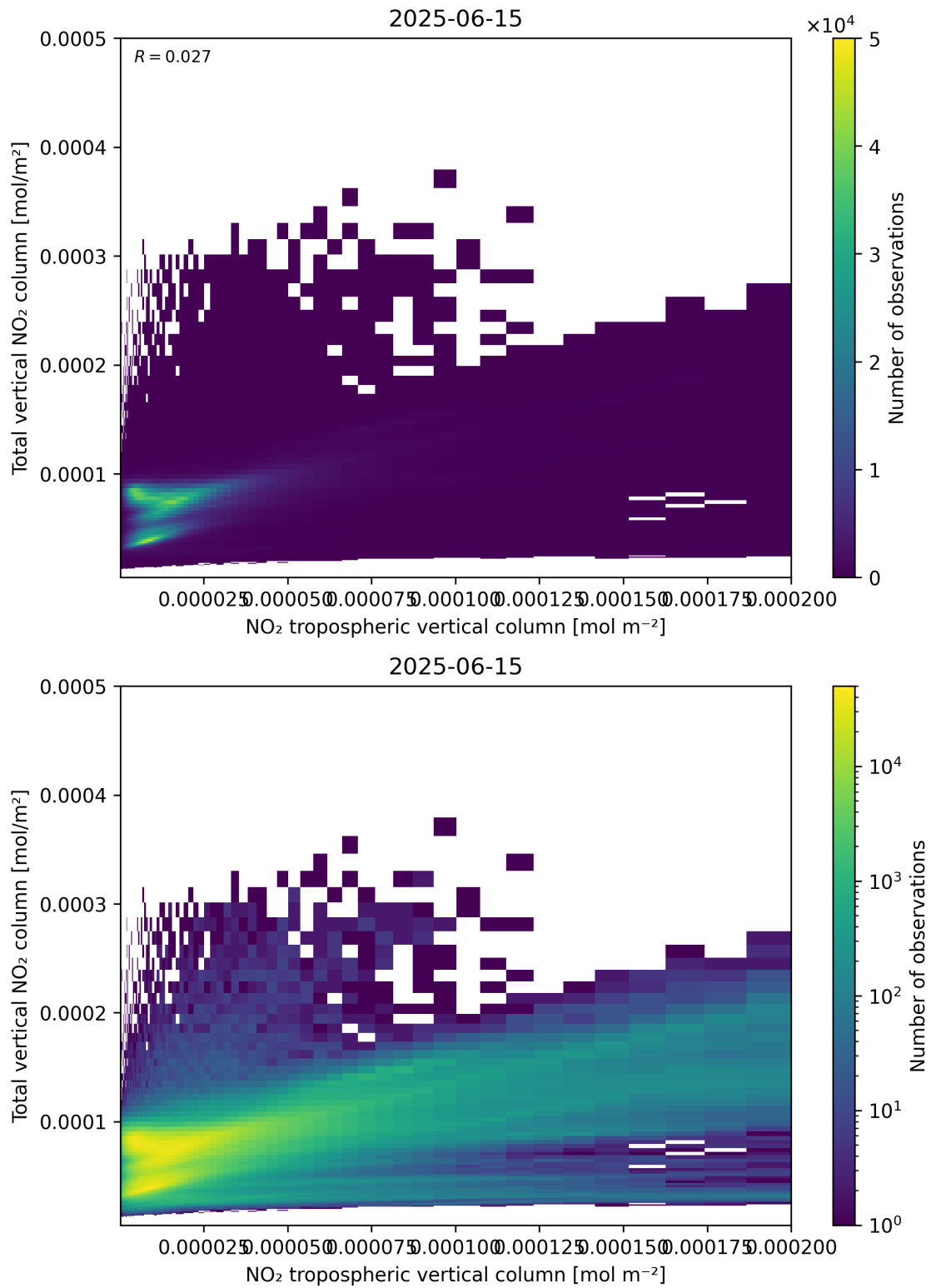
Figure 128: Scatter density plot of “NO 2 tropospheric vertical column” against “Total vertical NO 2 column” for 2025-06-14 to 2025-06-16.
