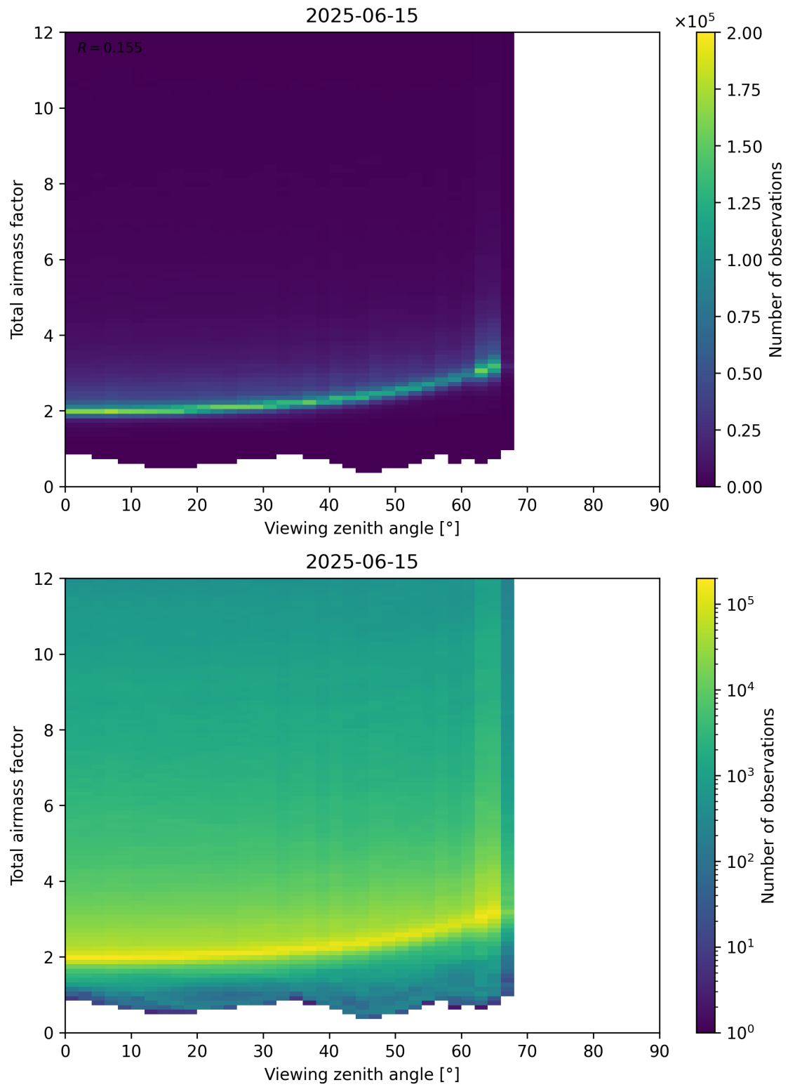
Figure 160: Scatter density plot of “Viewing zenith angle” against “Total airmass factor” for 2025-06-14 to 2025-06-16.
