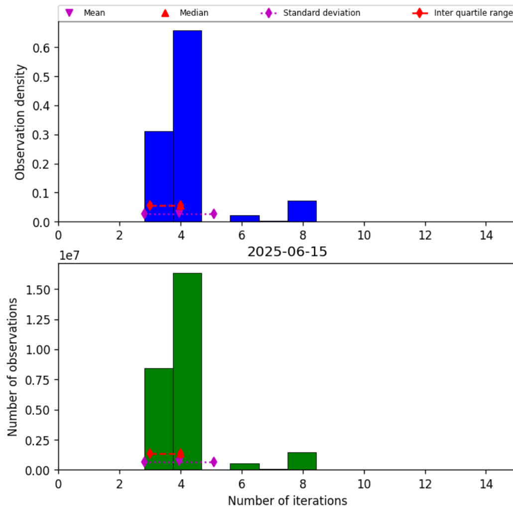
Figure 34: Histogram of “Number of iterations” for 2025-06-14 to 2025-06-16
