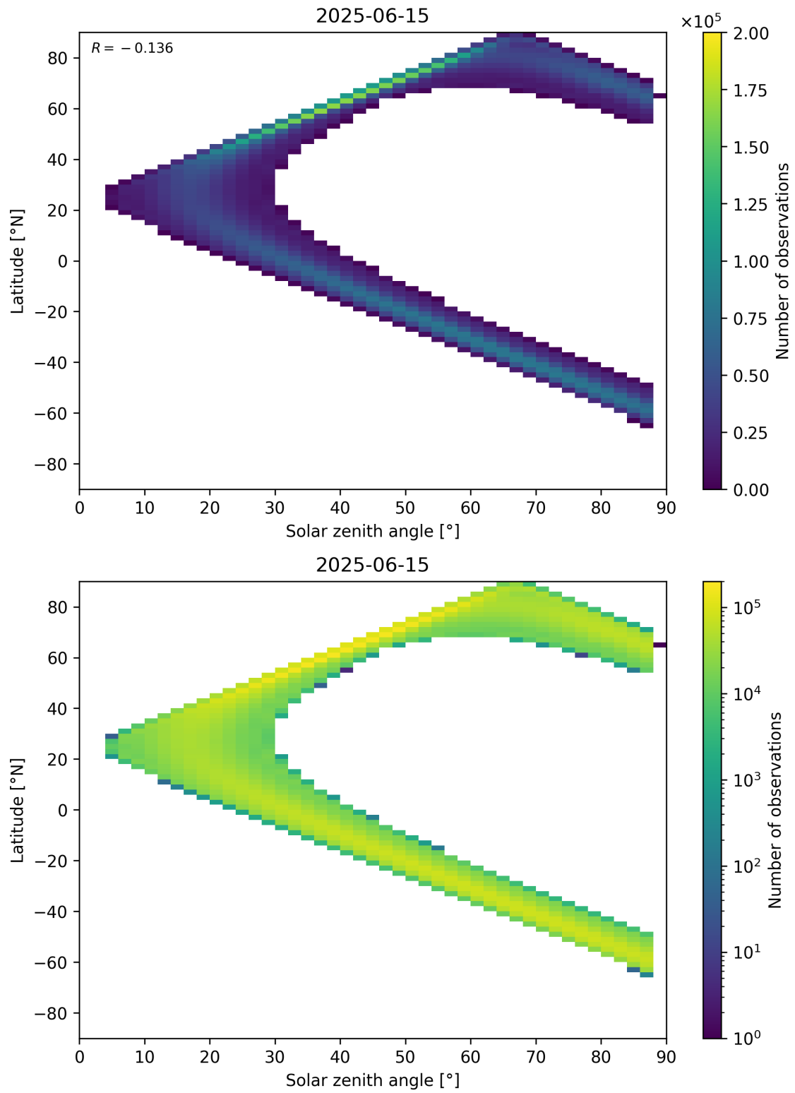
Figure 149: Scatter density plot of “Solar zenith angle” against “Latitude” for 2025-06-14 to 2025-06-16.
