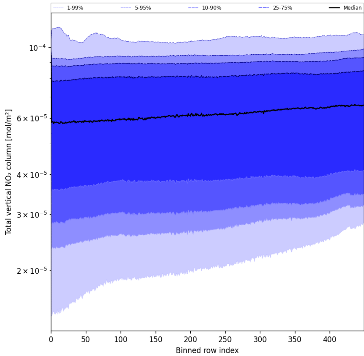
Figure 55: Along track statistics of “Total vertical NO 2 column” for 2025-06-14 to 2025-06-16
