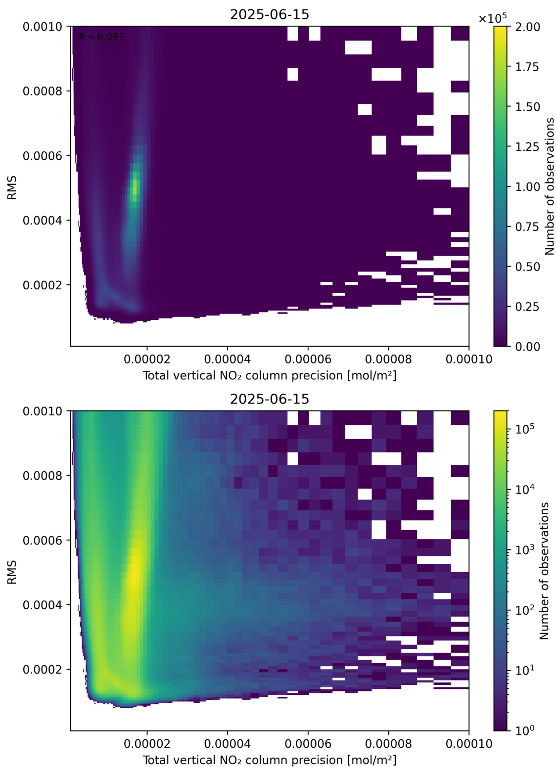
Figure 119: Scatter density plot of “Total vertical NO 2 column precision” against “RMS” for 2025-06-14 to 2025-06-16.
