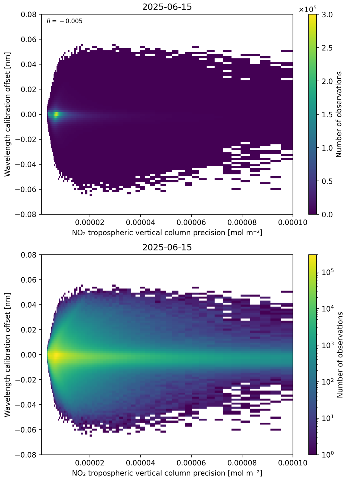
Figure 141: Scatter density plot of “NO 2 tropospheric vertical column precision” against “Wavelength calibration offset” for 2025-06-14 to 2025-06-16.
