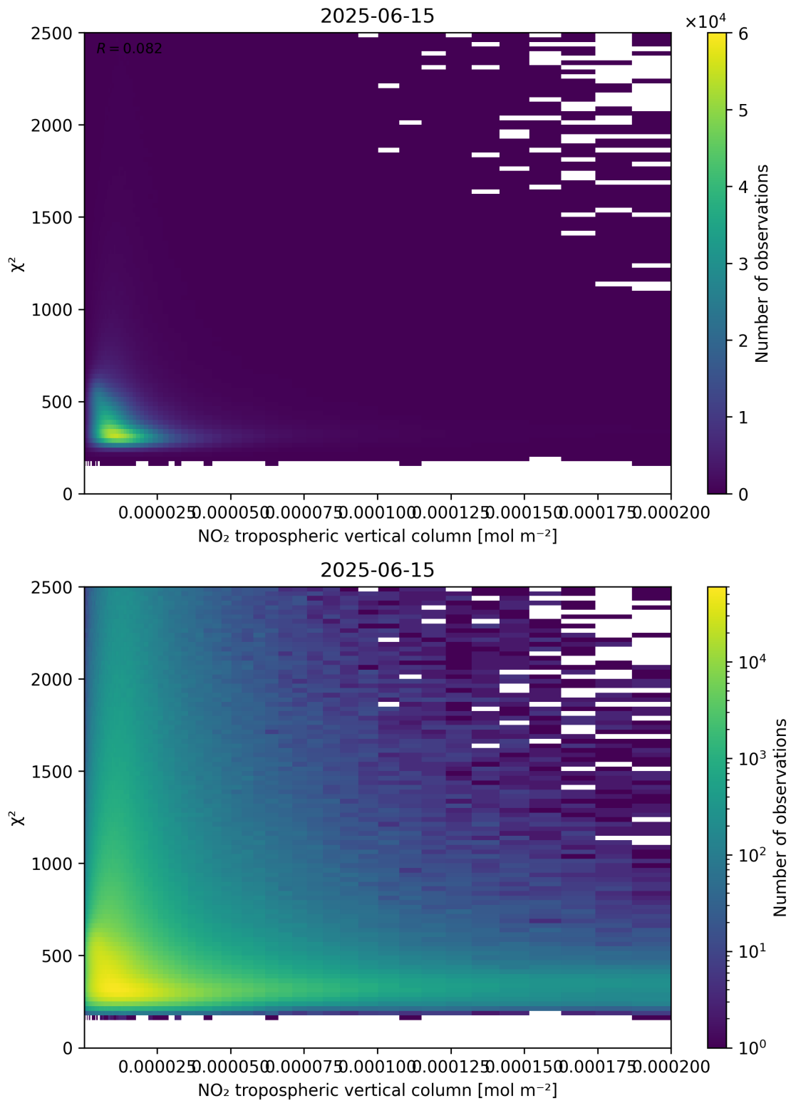
Figure 124: Scatter density plot of “NO 2 tropospheric vertical column” against “ \chi^2 ” for 2025-06-14 to 2025-06-16.
