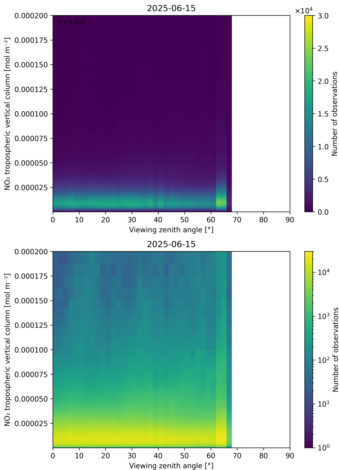
Figure 169: Scatter density plot of “Viewing zenith angle” against “NO 2 tropospheric vertical column” for 2025-06-14 to 2025-06-16.
