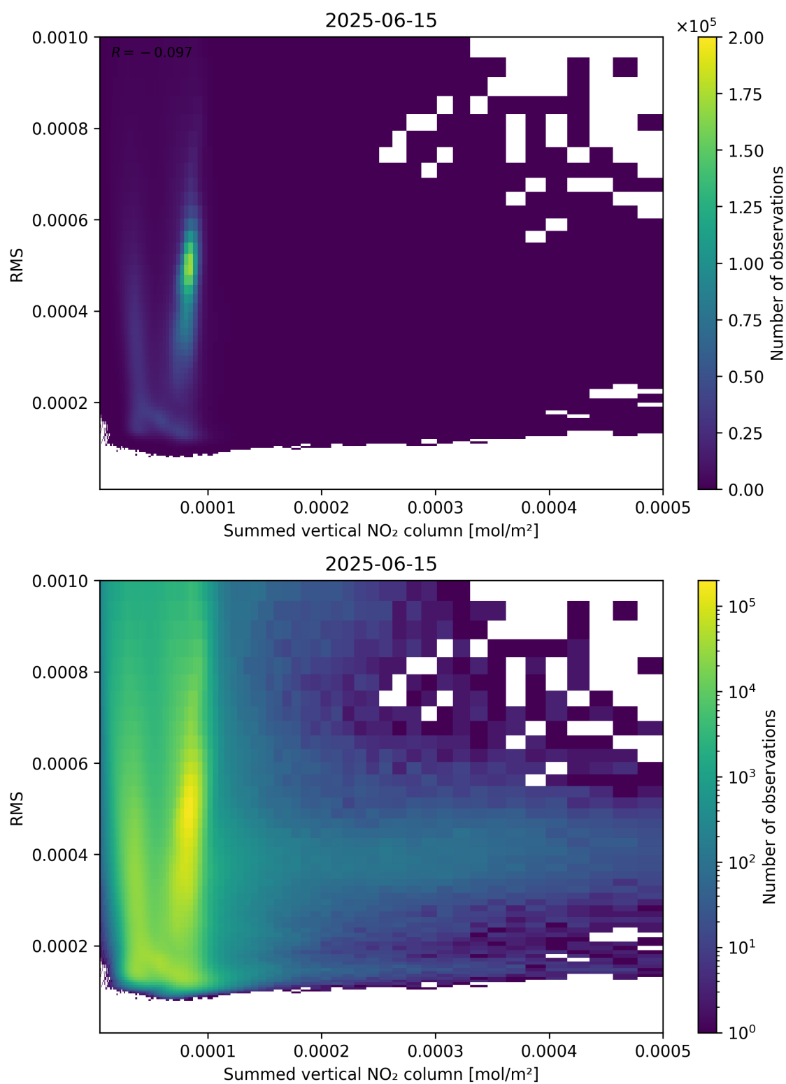
Figure 109: Scatter density plot of “Summed vertical NO 2 column” against “RMS” for 2025-06-14 to 2025-06-16.
