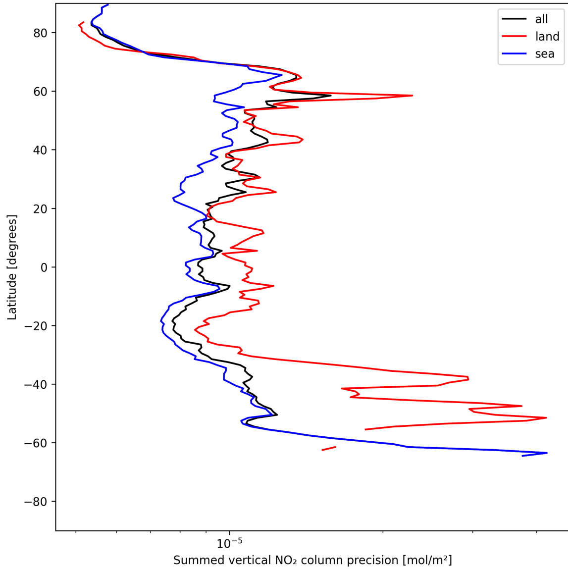
Figure 24: Zonal average of “Summed vertical NO 2 column precision” for 2025-06-14 to 2025-06-16.
