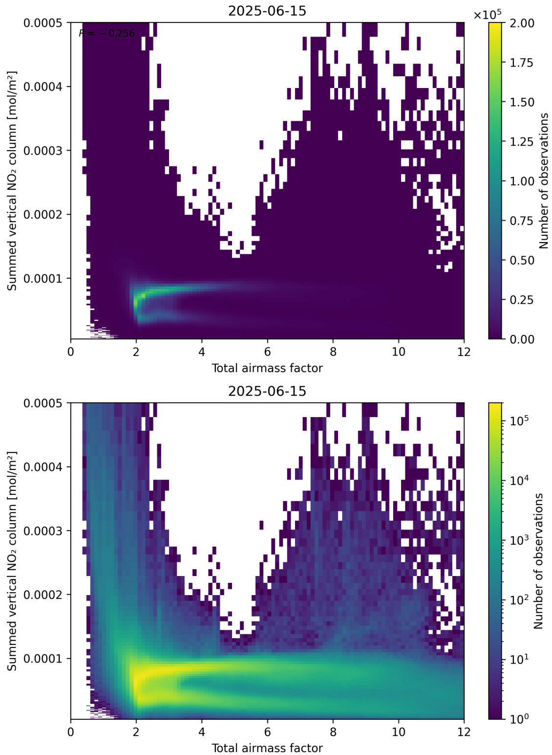
Figure 65: Scatter density plot of “Total airmass factor” against “Summed vertical NO 2 column” for 2025-06-14 to 2025-06-16.
