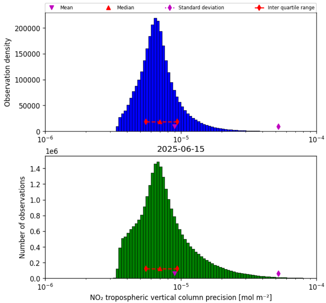
Figure 30: Histogram of “NO 2 tropospheric vertical column precision” for 2025-06-14 to 2025-06-16
