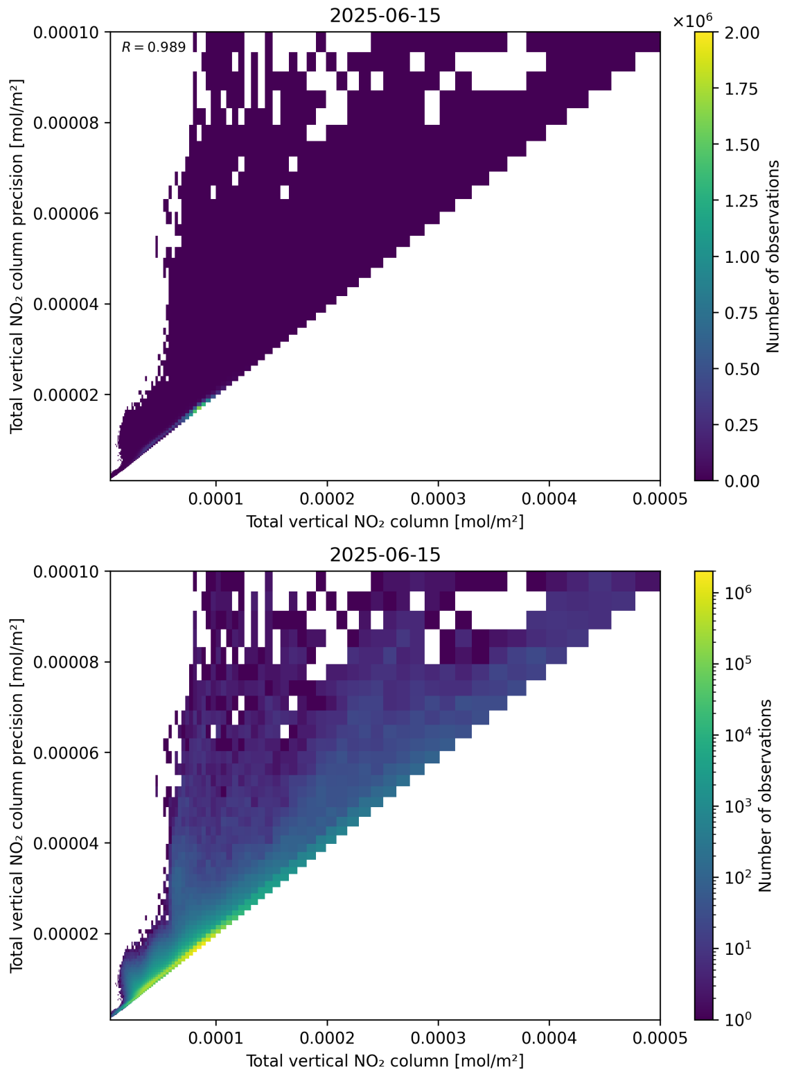
Figure 114: Scatter density plot of “Total vertical NO 2 column” against “Total vertical NO 2 column precision” for 2025-06-14 to 2025-06-16.
