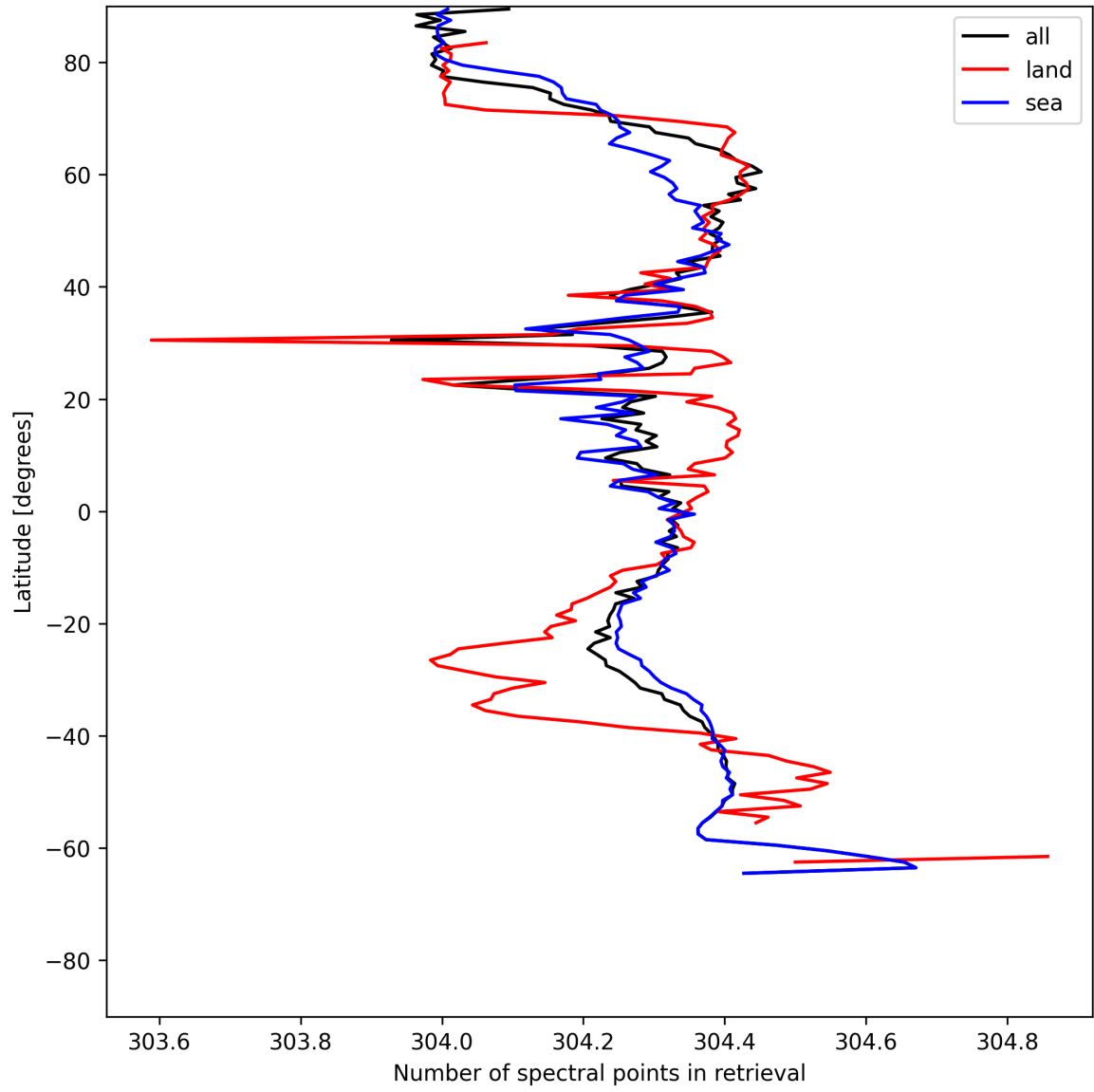
Figure 16: Zonal average of “Number of spectral points in retrieval” for 2025-06-14 to 2025-06-16.
