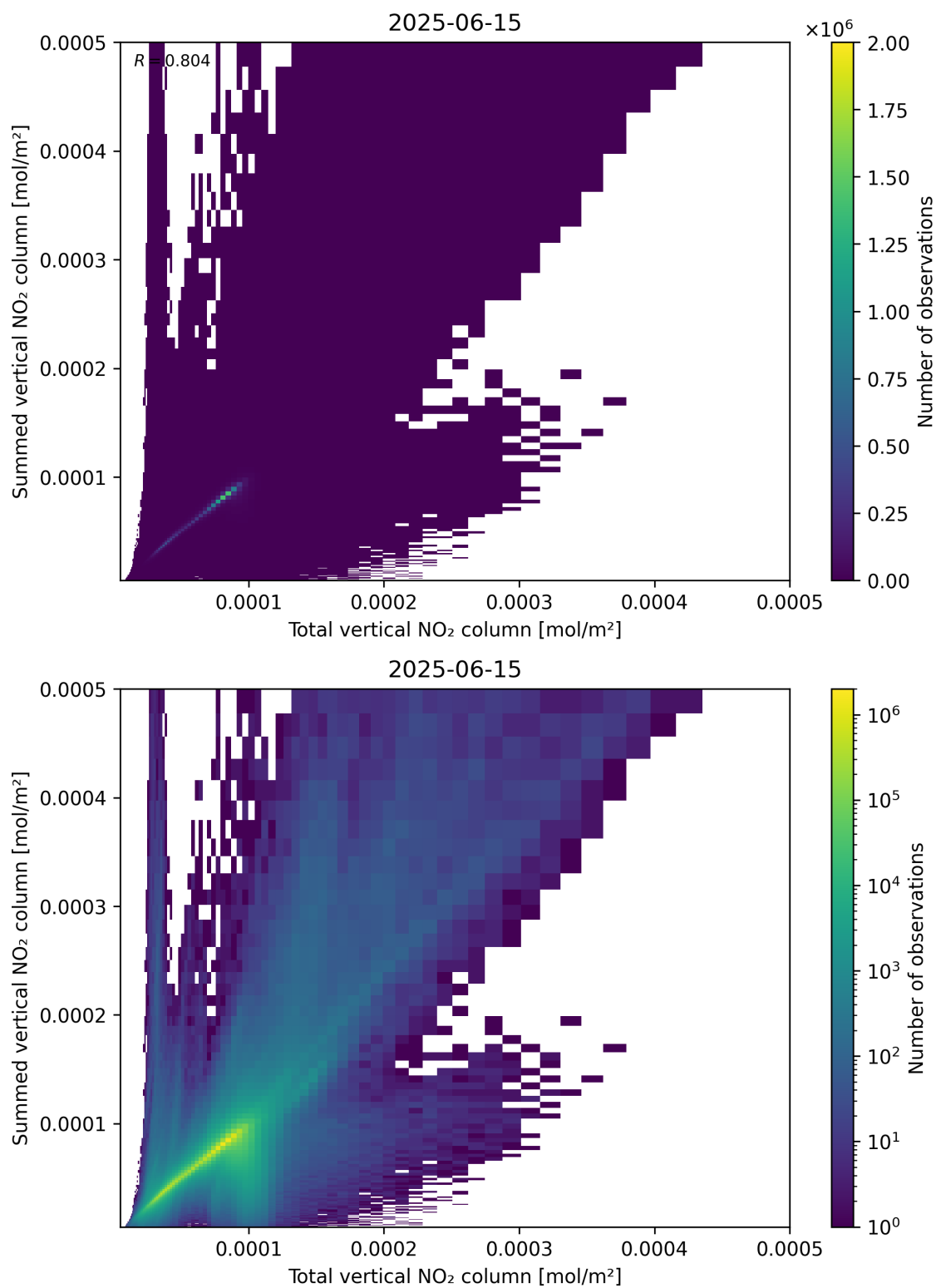
Figure 112: Scatter density plot of “Total vertical NO 2 column” against “Summed vertical NO 2 column” for 2025-06-14 to 2025-06-16.
