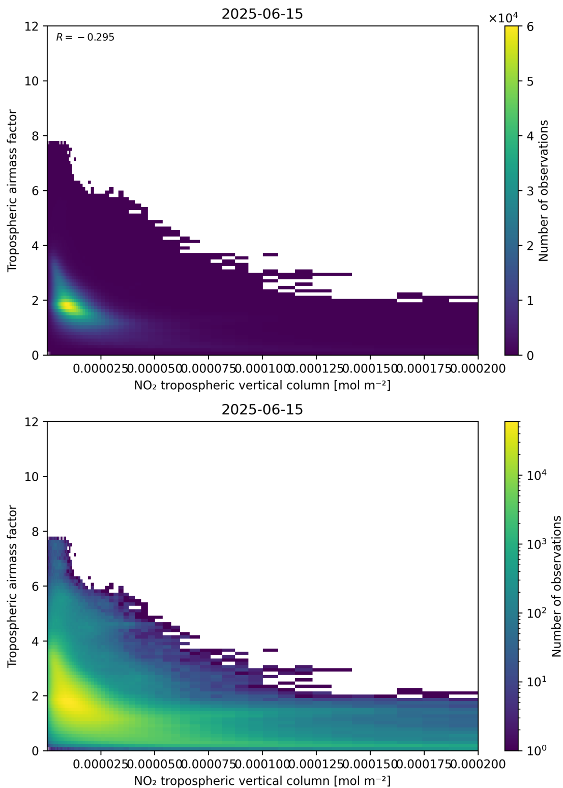
Figure 123: Scatter density plot of “NO 2 tropospheric vertical column” against “Tropospheric air mass factor” for 2025-06-14 to 2025-06-16.
