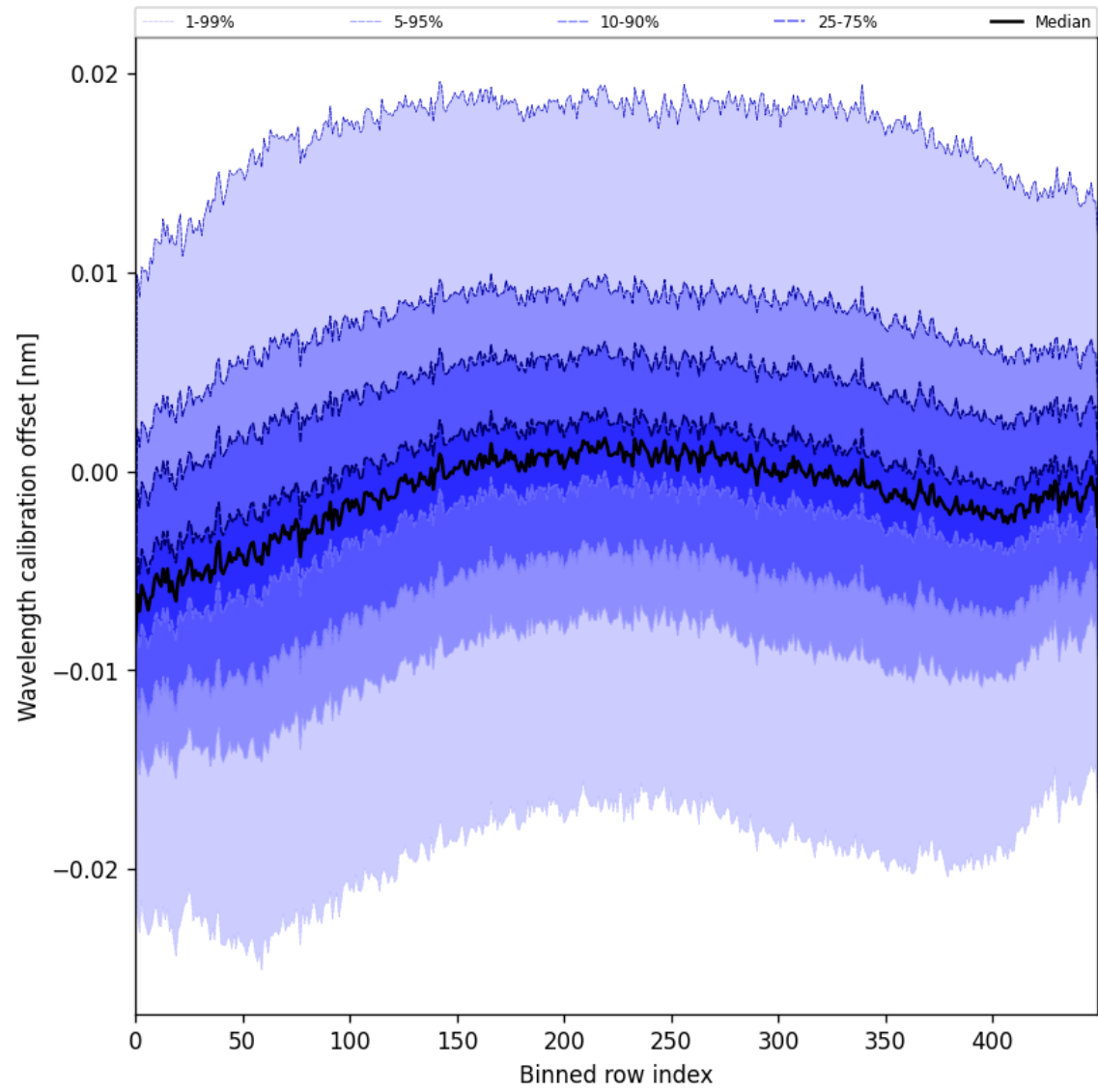
Figure 52: Along track statistics of “Wavelength calibration offset” for 2025-06-14 to 2025-06-16
