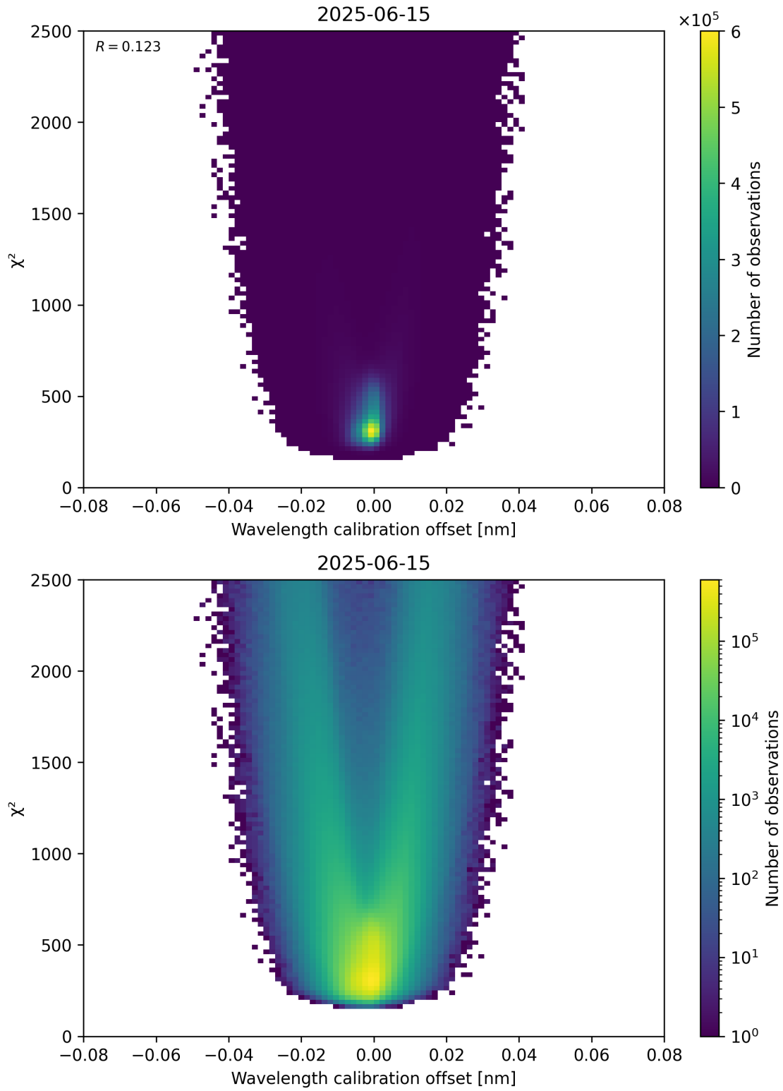
Figure 175: Scatter density plot of “Wavelength calibration offset” against “ \chi^2 ” for 2025-06-14 to 2025-06-16.
