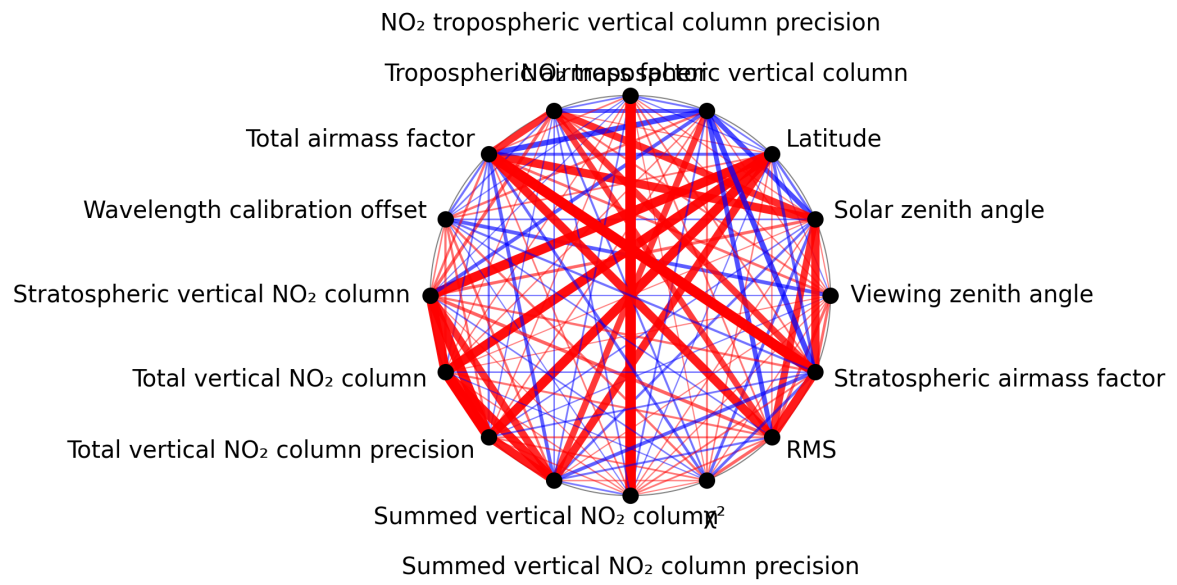
Figure 1: Map of correlation graph for 2025-06-14 to 2025-06-16.
