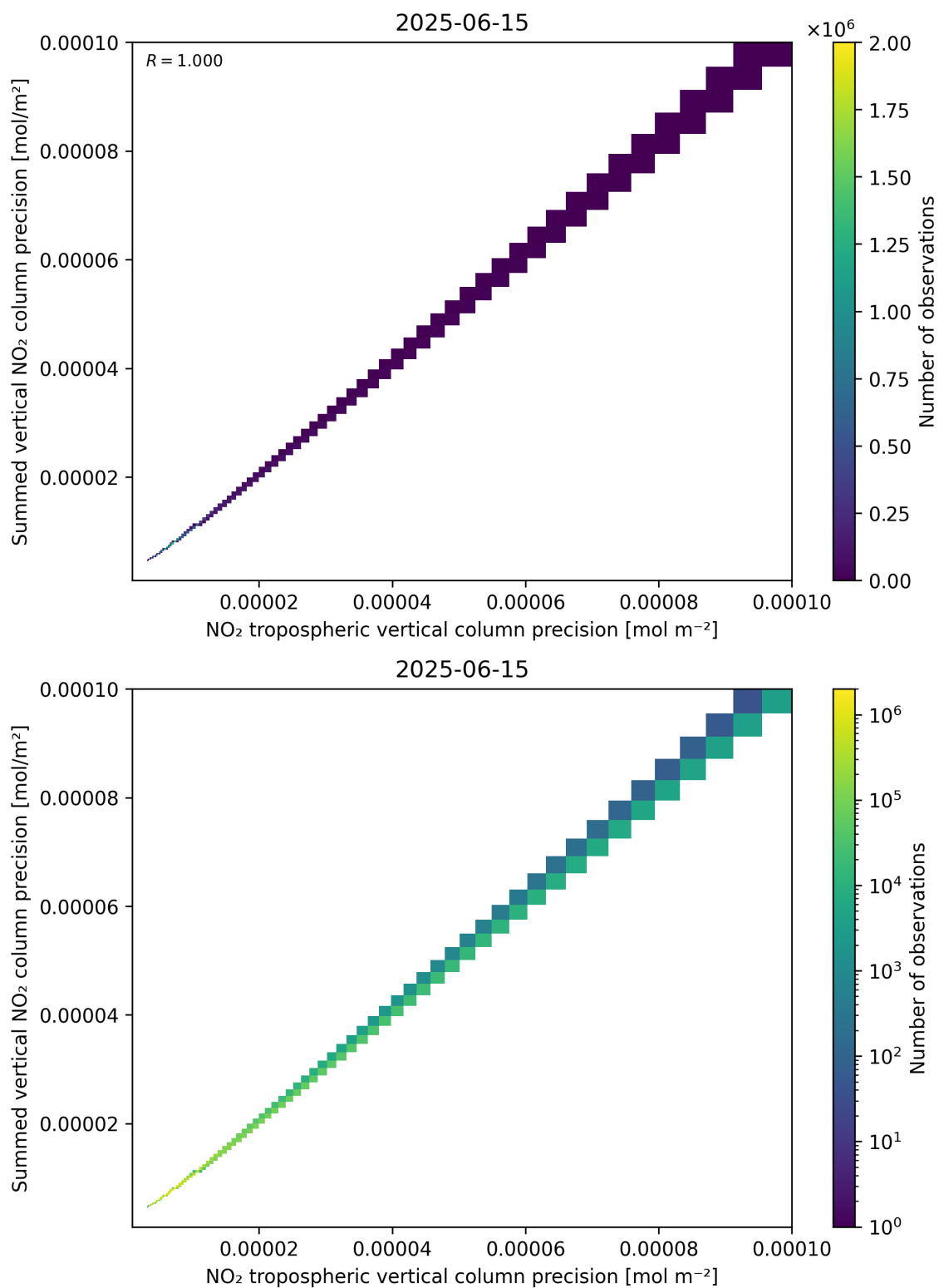
Figure 137: Scatter density plot of “NO 2 tropospheric vertical column precision” against “Summed vertical NO 2 column precision” for 2025-06-14 to 2025-06-16.
