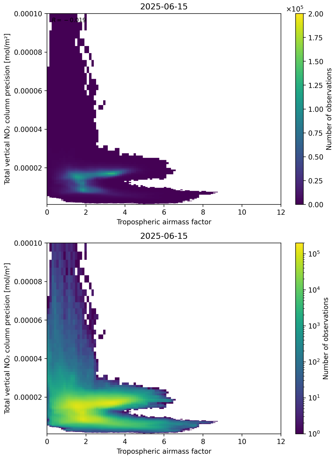
Figure 78: Scatter density plot of “Tropospheric air mass factor” against “Total vertical NO 2 column precision” for 2025-06-14 to 2025-06-16.
