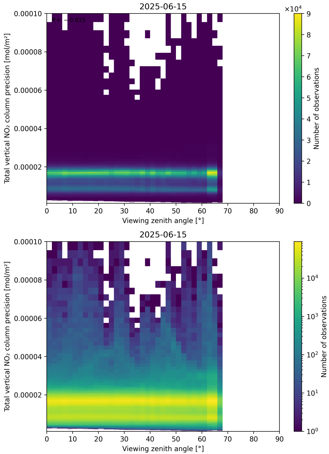
Figure 168: Scatter density plot of “Viewing zenith angle” against “Total vertical NO 2 column precision” for 2025-06-14 to 2025-06-16.
