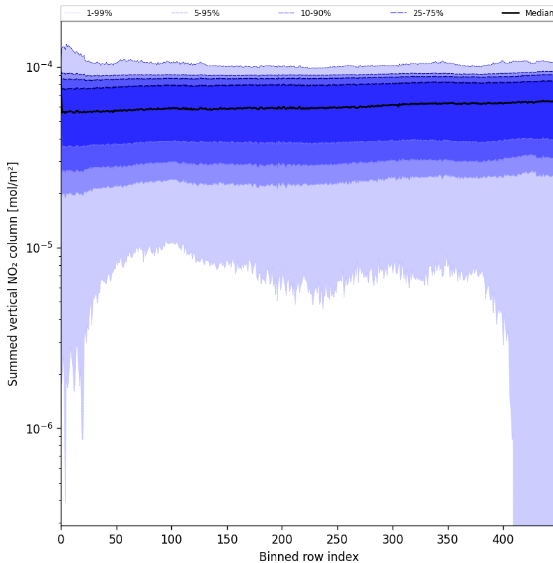
Figure 57: Along track statistics of “Summed vertical NO 2 column” for 2025-06-14 to 2025-06-16
