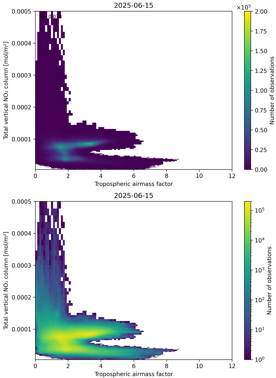
Figure 77: Scatter density plot of “Tropospheric airmass factor” against “Total vertical NO 2 column” for 2025-06-14 to 2025-06-16.
