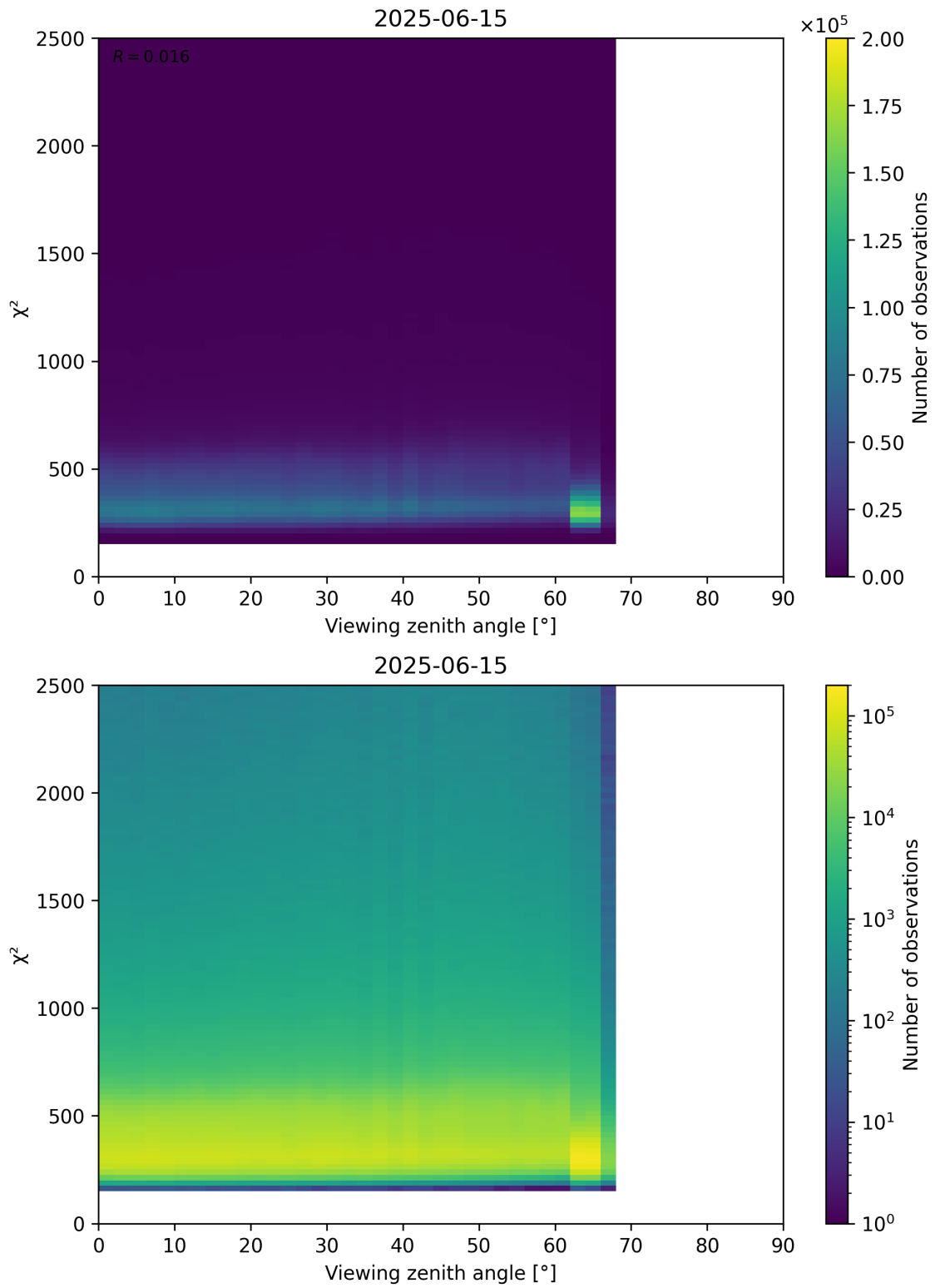
Figure 162: Scatter density plot of “Viewing zenith angle” against “ \chi^2 ” for 2025-06-14 to 2025-06-16.
