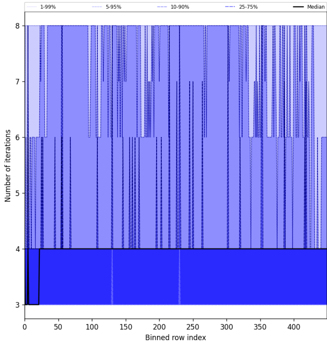
Figure 51: Along track statistics of “Number of iterations” for 2025-06-14 to 2025-06-16
