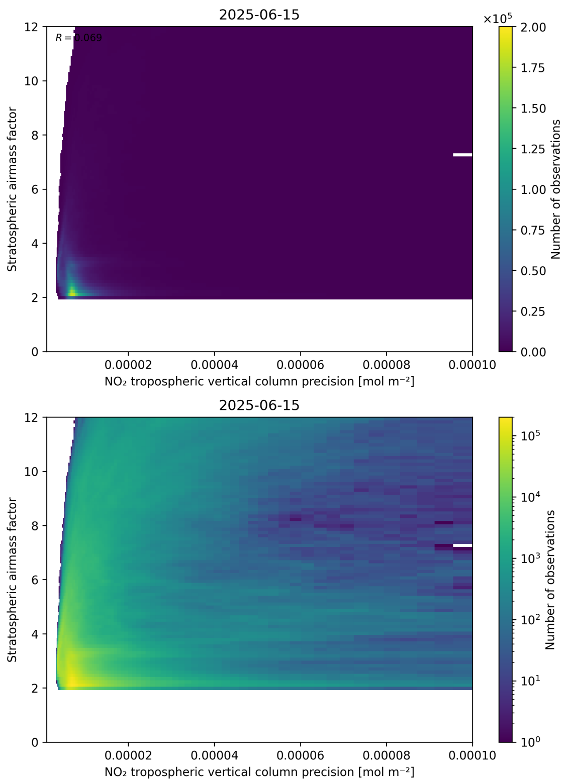
Figure 131: Scatter density plot of “NO 2 tropospheric vertical column precision” against “Stratospheric airmass factor” for 2025-06-14 to 2025-06-16.
