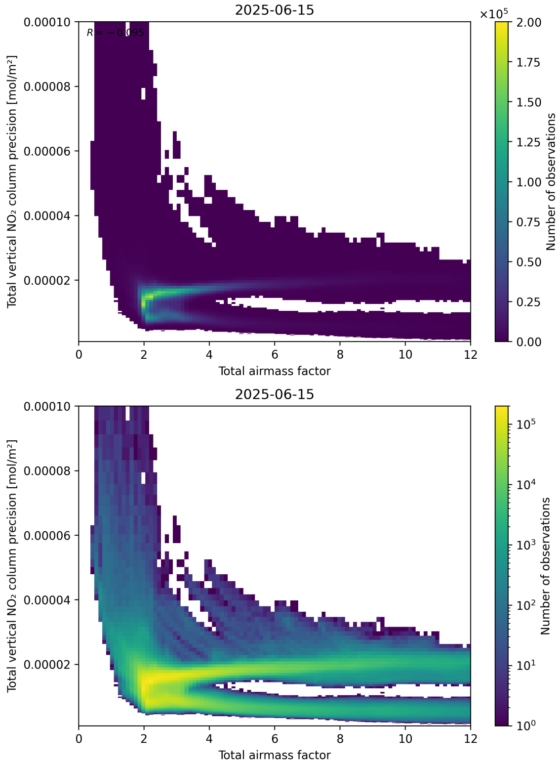
Figure 68: Scatter density plot of “Total airmass factor” against “Total vertical NO 2 column precision” for 2025-06-14 to 2025-06-16.
