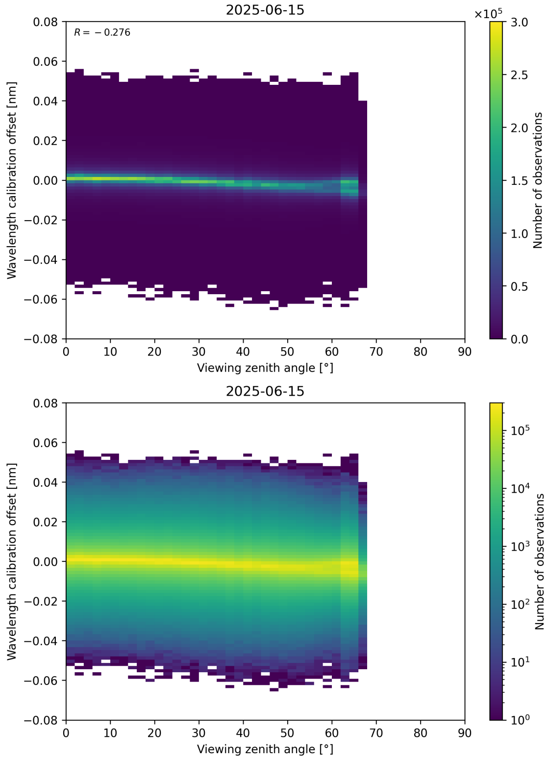
Figure 173: Scatter density plot of “Viewing zenith angle” against “Wavelength calibration offset” for 2025-06-14 to 2025-06-16.
