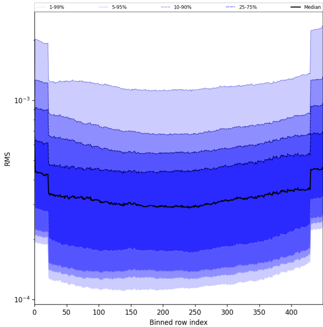
Figure 60: Along track statistics of “RMS” for 2025-06-14 to 2025-06-16
