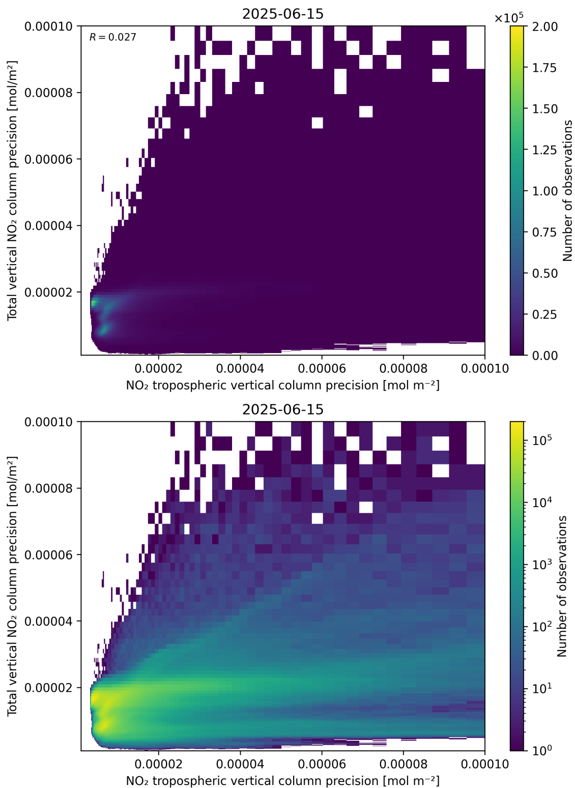
Figure 139: Scatter density plot of “NO 2 tropospheric vertical column precision” against “Total vertical NO 2 column precision” for 2025-06-14 to 2025-06-16.
