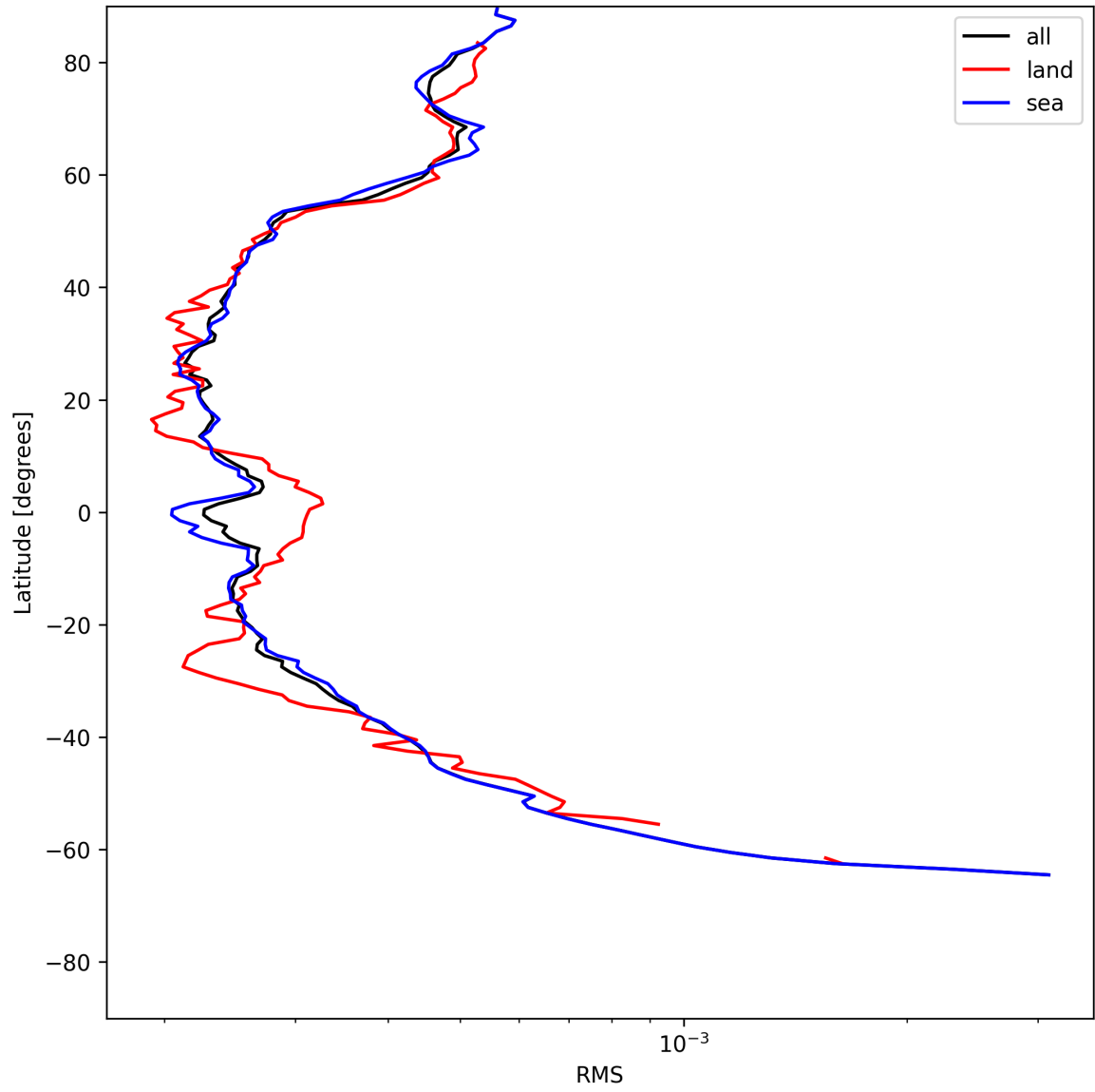
Figure 26: Zonal average of “RMS” for 2025-06-14 to 2025-06-16.
