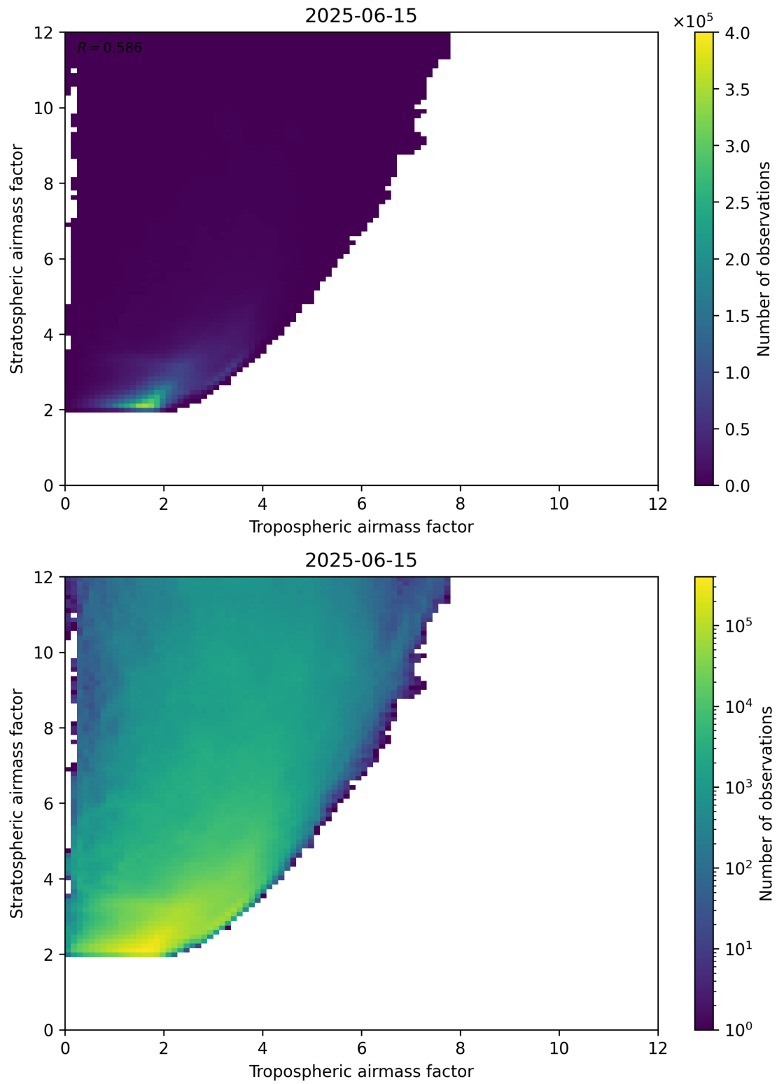
Figure 71: Scatter density plot of “Tropospheric airmass factor” against “Stratospheric airmass factor” for 2025-06-14 to 2025-06-16.
