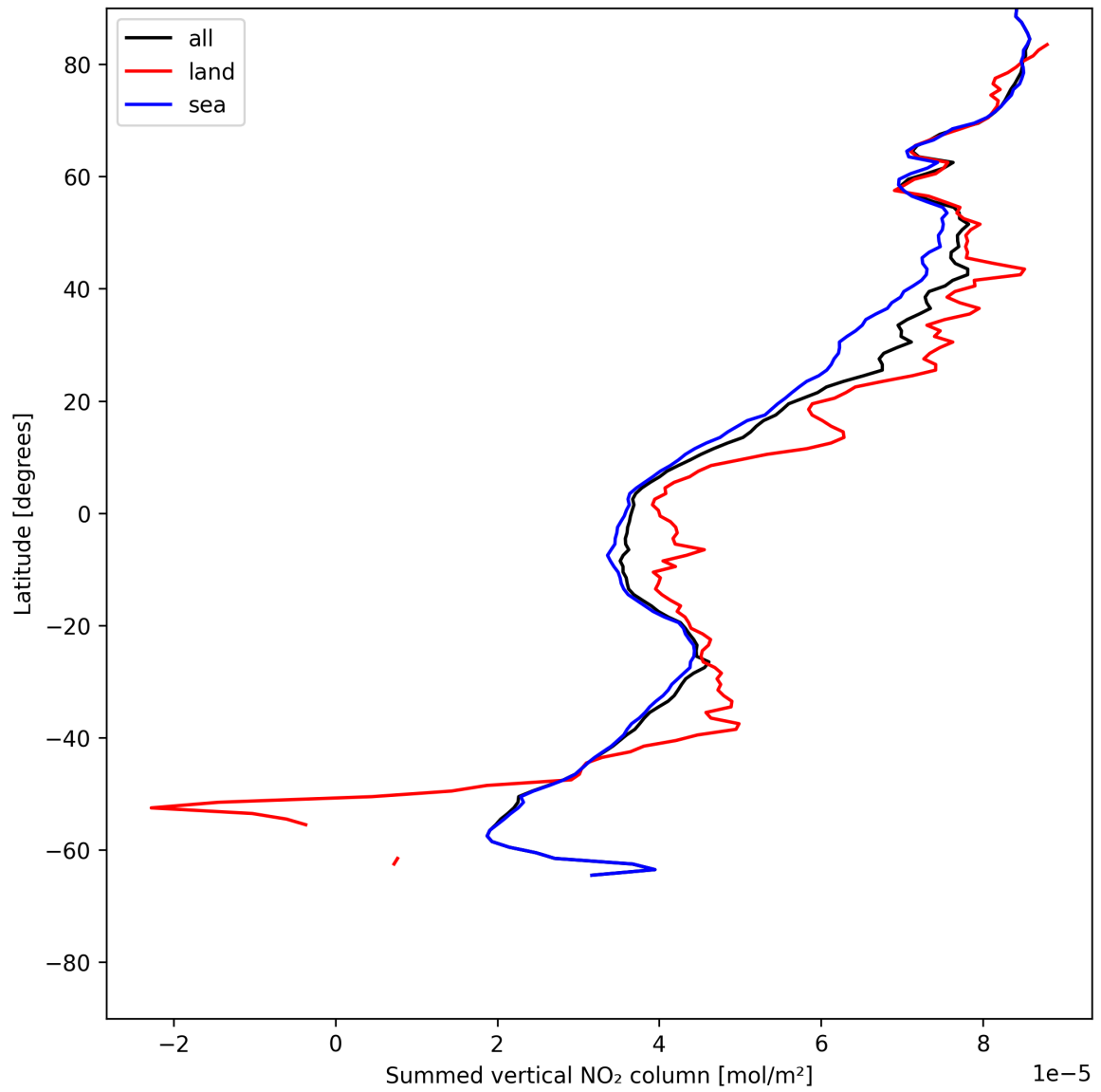
Figure 23: Zonal average of “Summed vertical NO 2 column” for 2025-06-14 to 2025-06-16.
