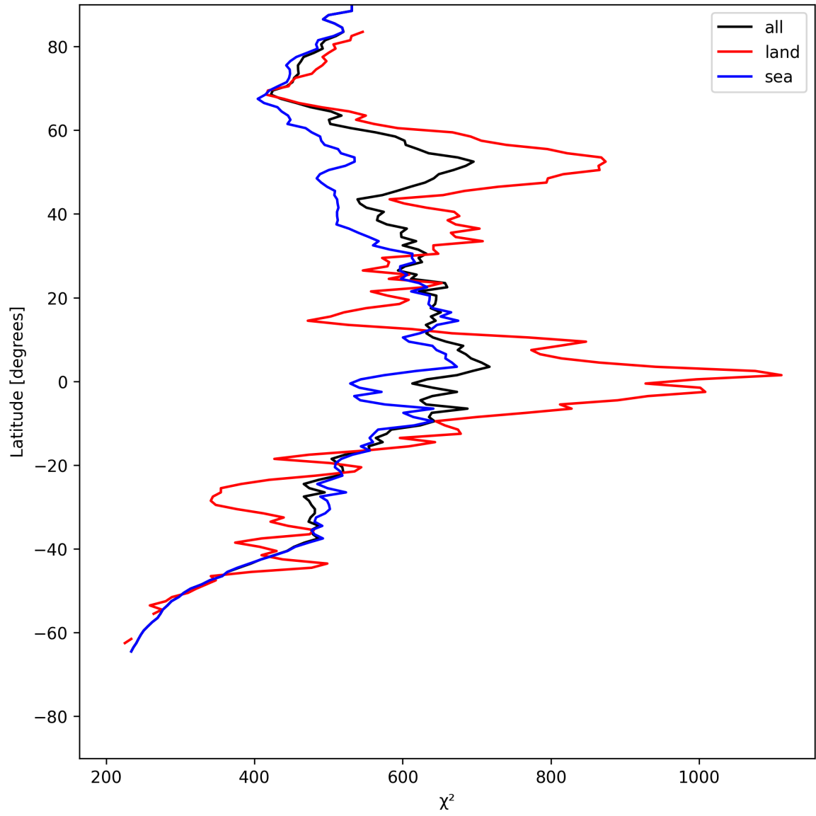
Figure 25: Zonal average of “ \chi^2 ” for 2025-06-14 to 2025-06-16.
