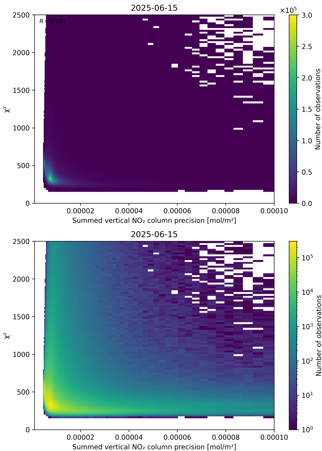
Figure 107: Scatter density plot of “Summed vertical NO 2 column precision” against “ \chi^2 ” for 2025-06-14 to 2025-06-16.
