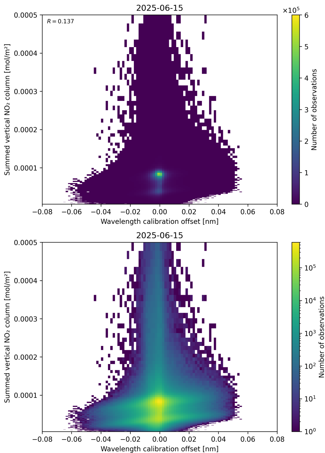
Figure 177: Scatter density plot of “Wavelength calibration offset” against “Summed vertical NO 2 column” for 2025-06-14 to 2025-06-16.
