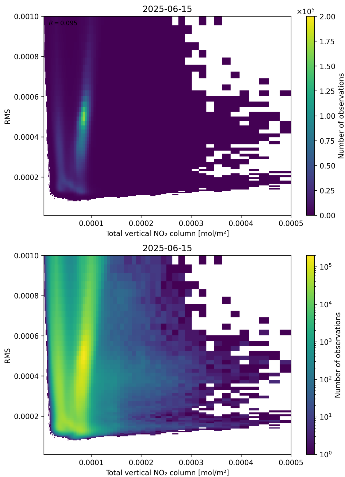
Figure 120: Scatter density plot of “Total vertical NO 2 column” against “RMS” for 2025-06-14 to 2025-06-16.
