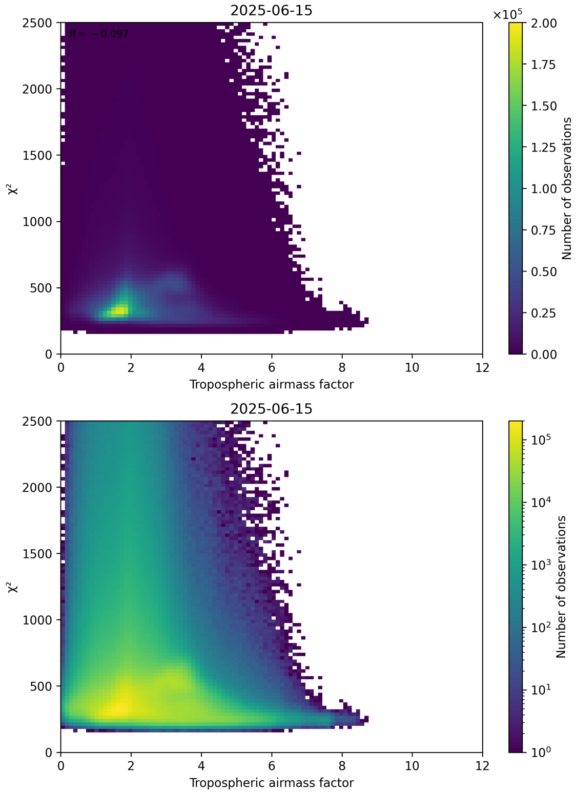
Figure 73: Scatter density plot of “Tropospheric airmass factor” against “ \chi^2 ” for 2025-06-14 to 2025-06-16.
