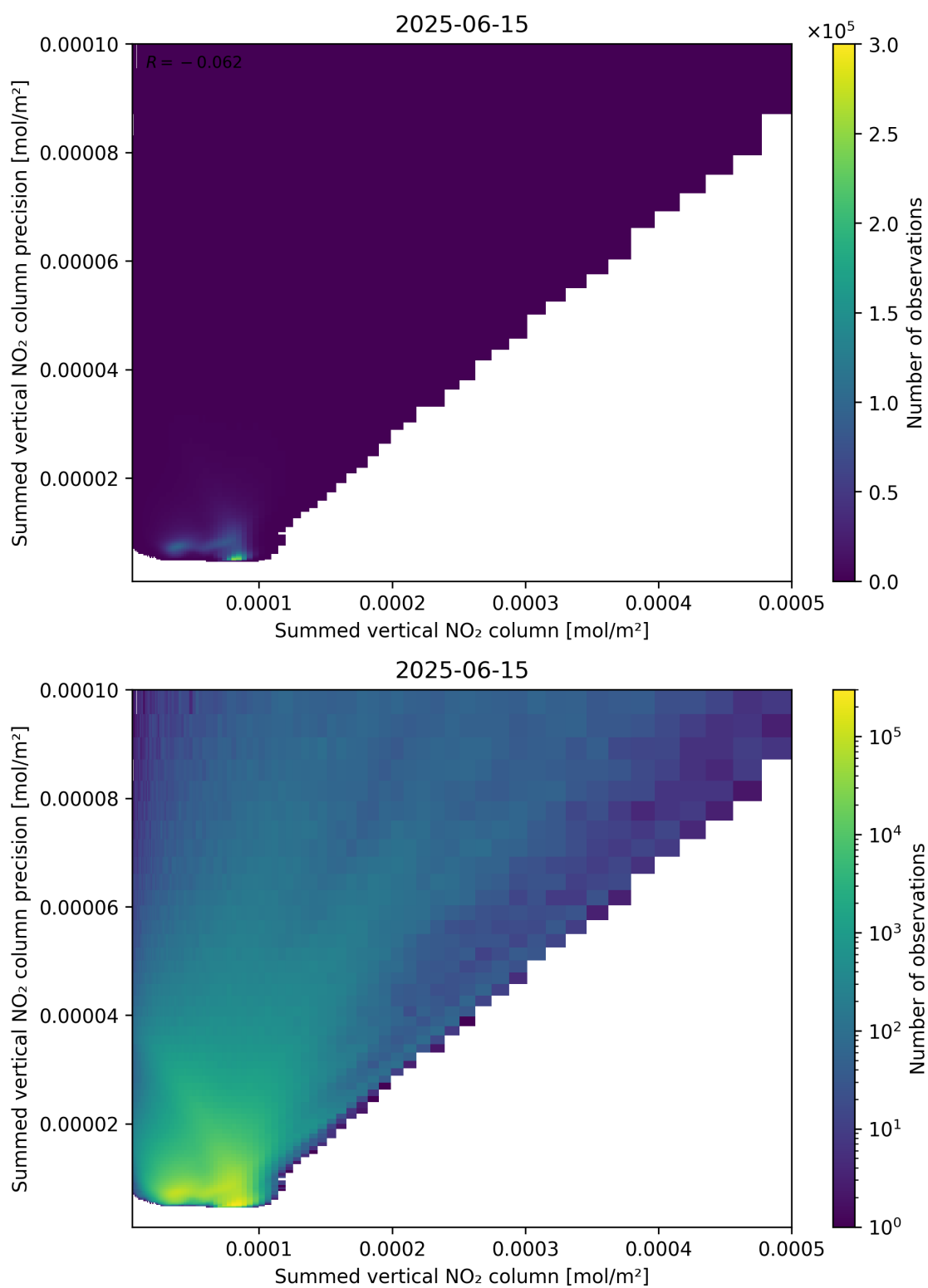
Figure 105: Scatter density plot of “Summed vertical NO 2 column” against “Summed vertical NO 2 column precision” for 2025-06-14 to 2025-06-16.
