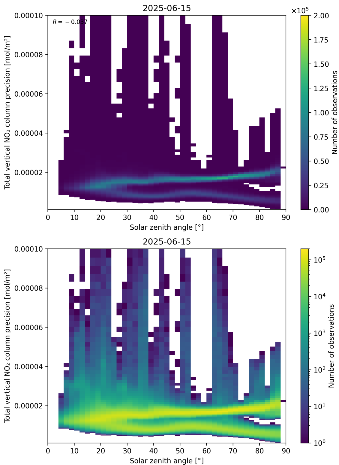
Figure 154: Scatter density plot of “Solar zenith angle” against “Total vertical NO 2 column precision” for 2025-06-14 to 2025-06-16.
