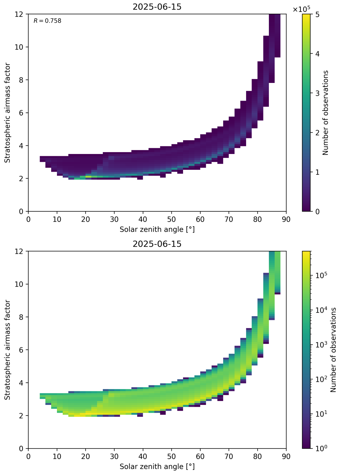
Figure 145: Scatter density plot of “Solar zenith angle” against “Stratospheric airmass factor” for 2025-06-14 to 2025-06-16.
