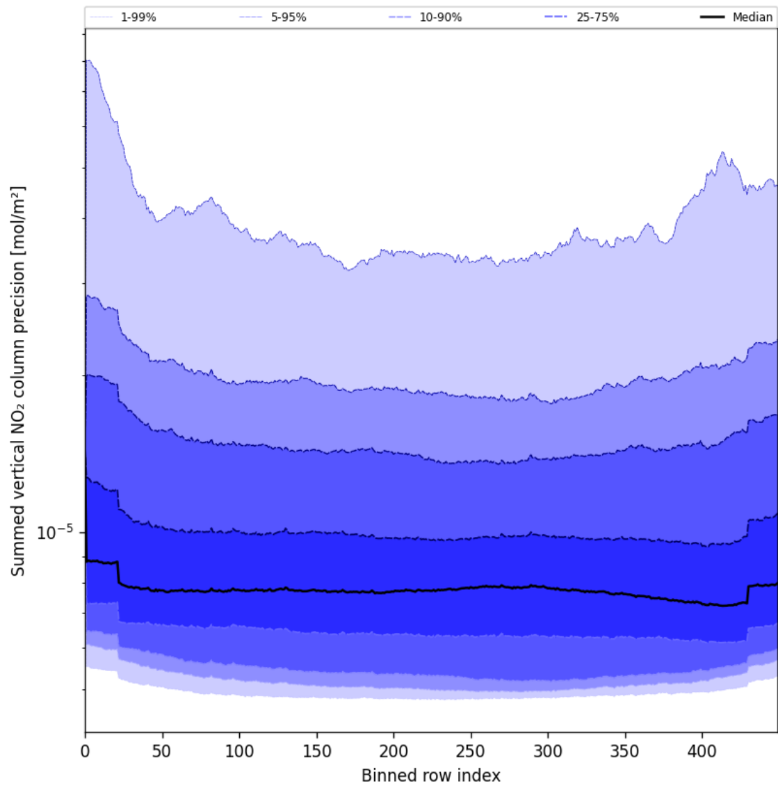
Figure 58: Along track statistics of “Summed vertical NO 2 column precision” for 2025-06-14 to 2025-06-16
