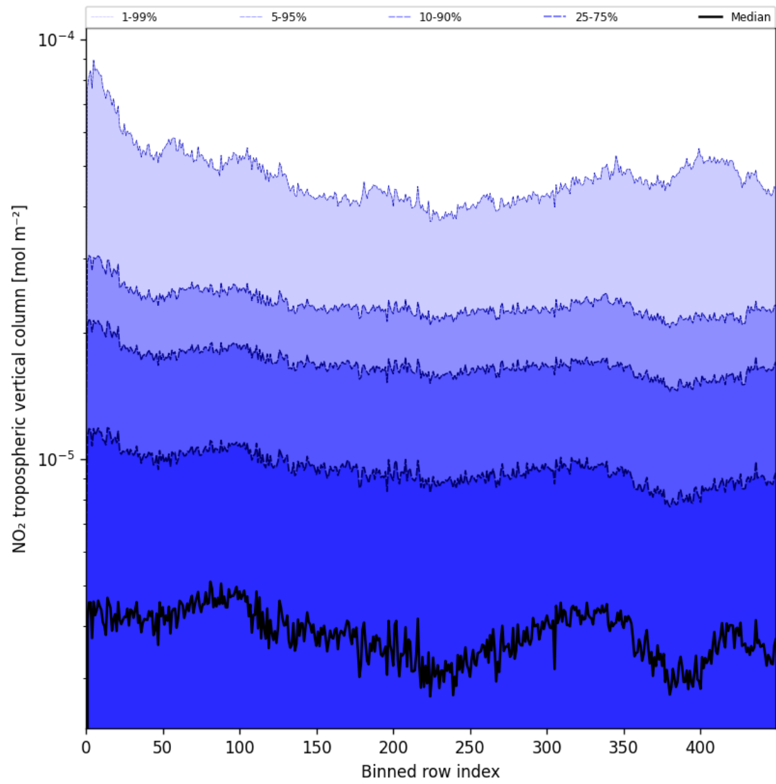
Figure 46: Along track statistics of “NO 2 tropospheric vertical column” for 2025-06-14 to 2025-06-16
