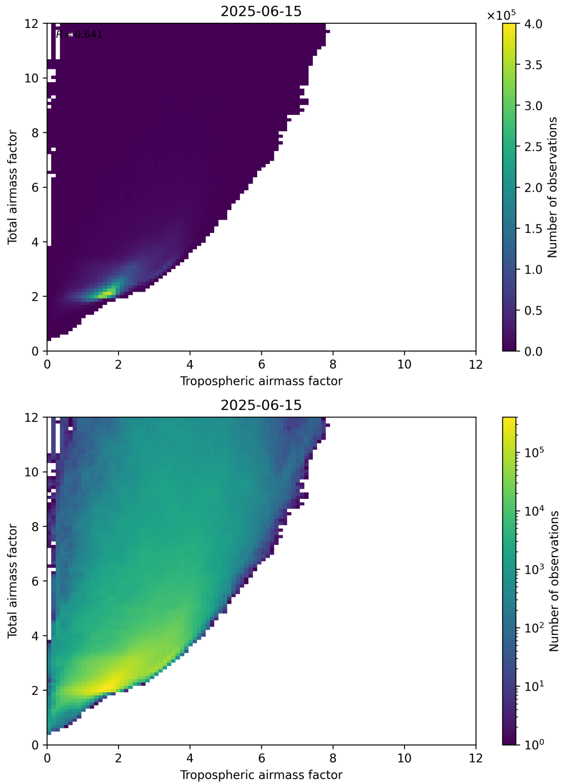
Figure 72: Scatter density plot of “Tropospheric airmass factor” against “Total airmass factor” for 2025-06-14 to 2025-06-16.
