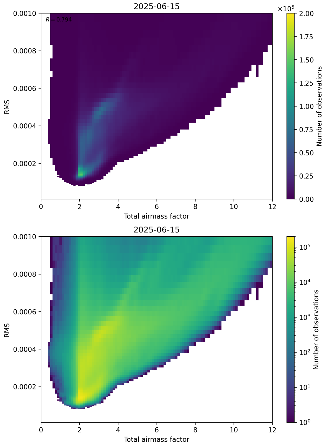
Figure 69: Scatter density plot of “Total airmass factor” against “RMS” for 2025-06-14 to 2025-06-16.
