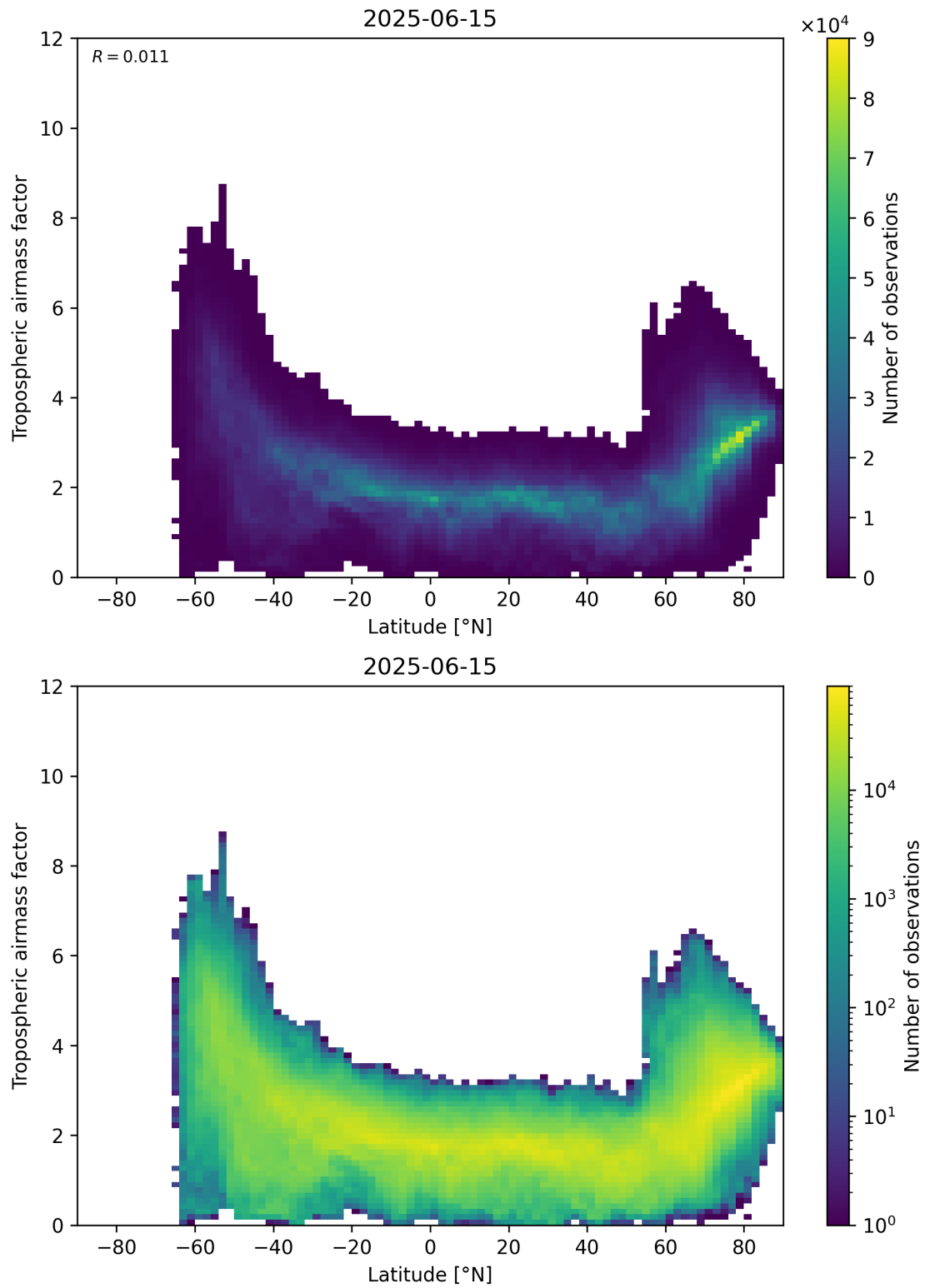
Figure 85: Scatter density plot of “Latitude” against “Tropospheric airmass factor” for 2025-06-14 to 2025-06-16.
