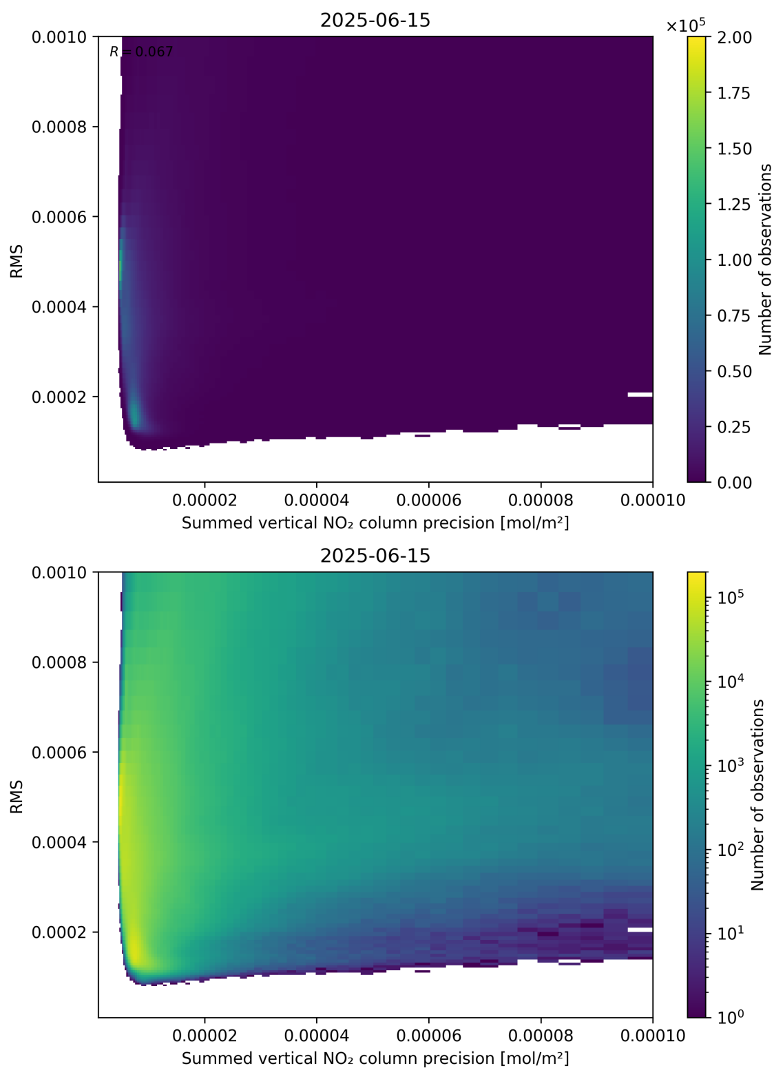
Figure 108: Scatter density plot of “Summed vertical NO 2 column precision” against “RMS” for 2025-06-14 to 2025-06-16.
