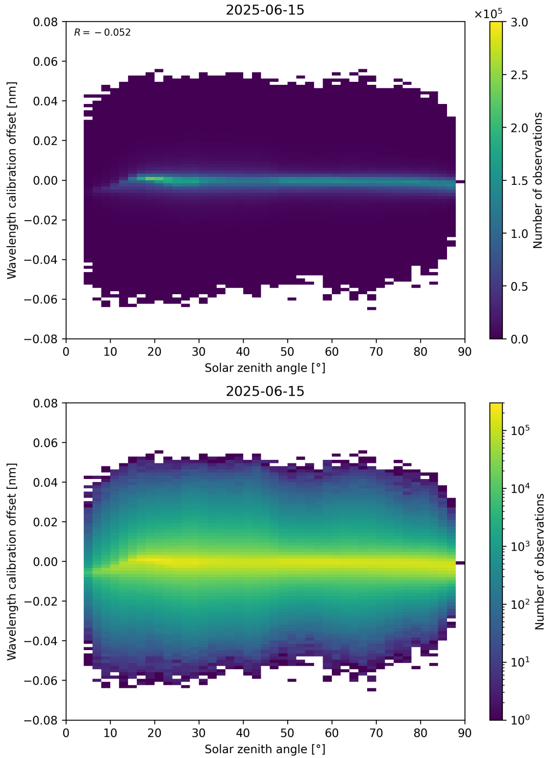
Figure 158: Scatter density plot of “Solar zenith angle” against “Wavelength calibration offset” for 2025-06-14 to 2025-06-16.
