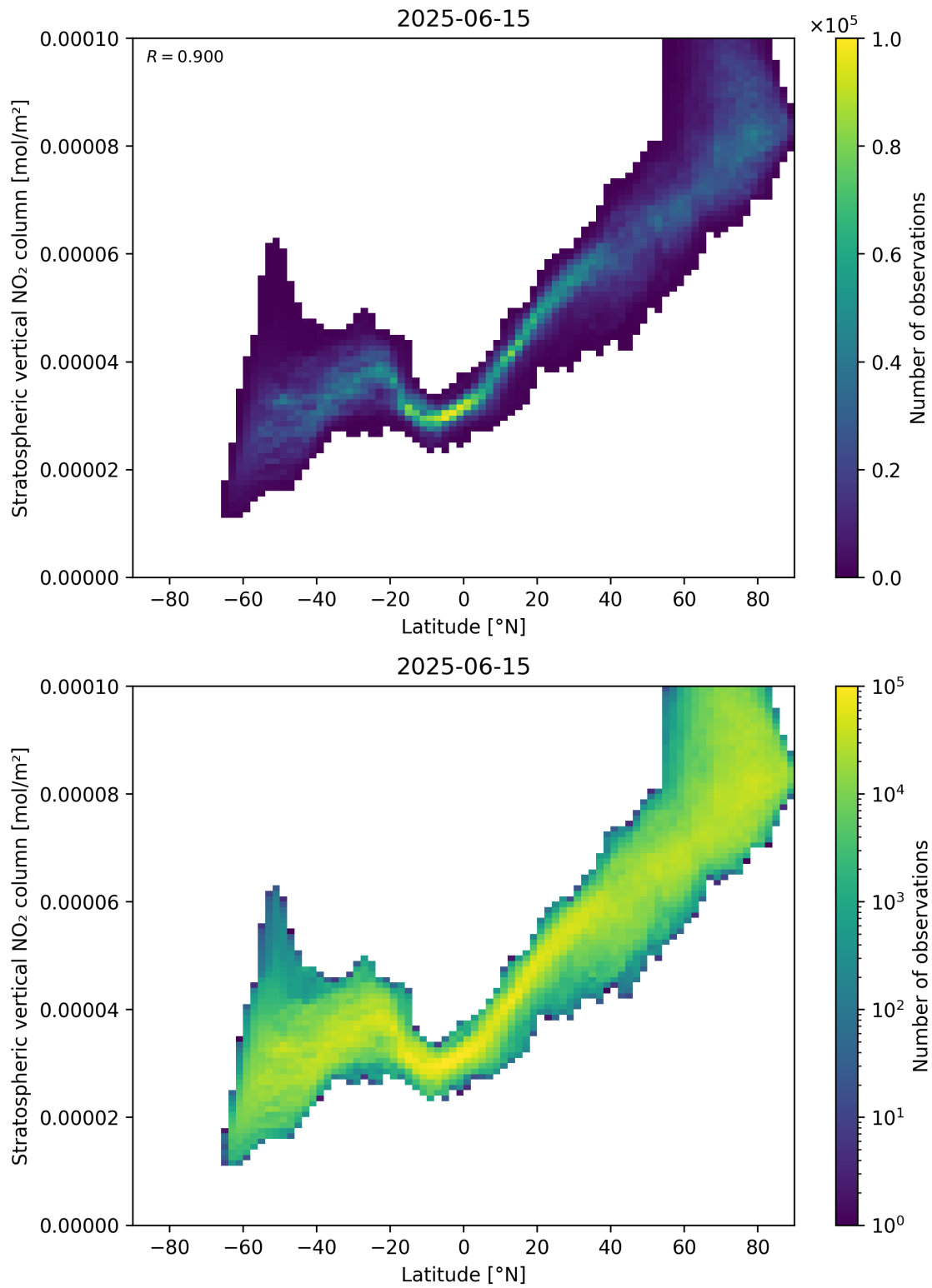
Figure 87: Scatter density plot of “Latitude” against “Stratospheric vertical \text{NO}_2 column” for 2025-06-14 to 2025-06-16.
