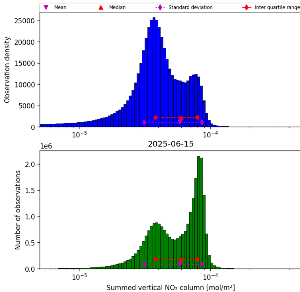
Figure 40: Histogram of “Summed vertical NO 2 column” for 2025-06-14 to 2025-06-16
