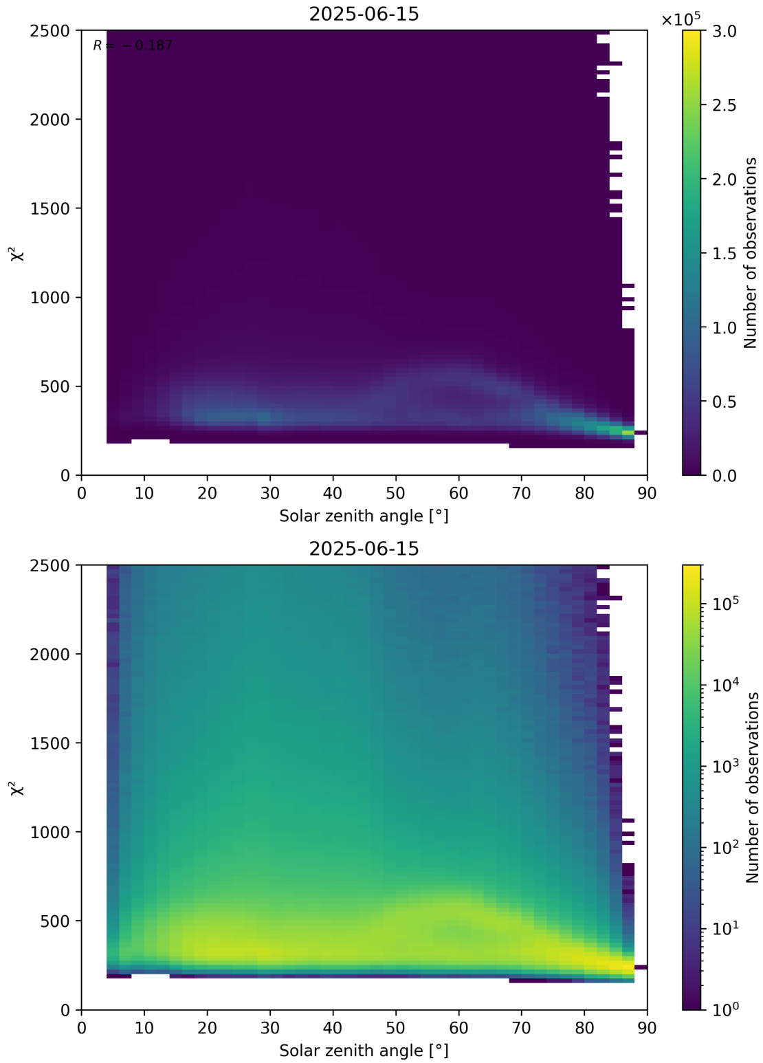
Figure 148: Scatter density plot of “Solar zenith angle” against “ \chi^2 ” for 2025-06-14 to 2025-06-16.
