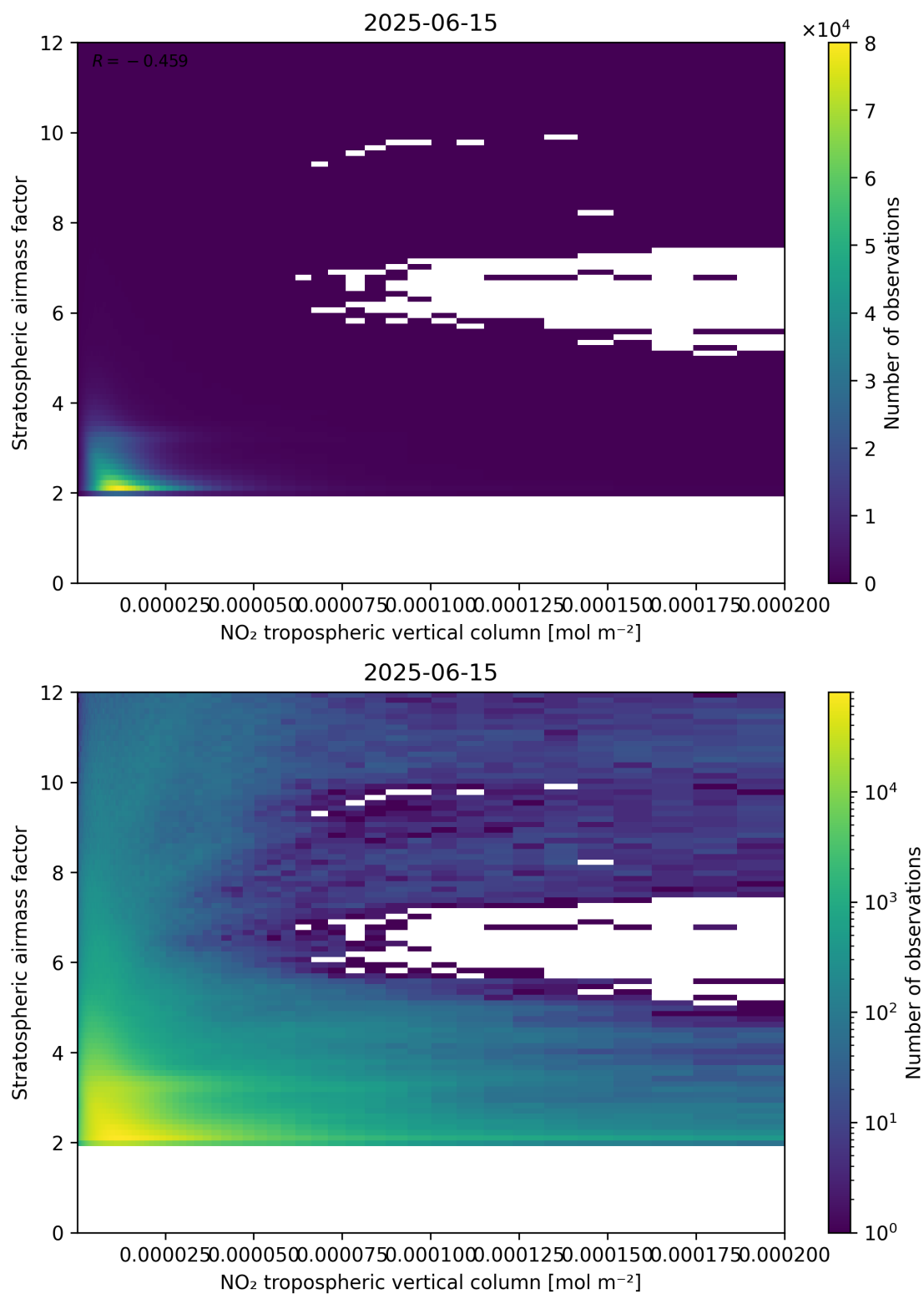
Figure 121: Scatter density plot of “NO 2 tropospheric vertical column” against “Stratospheric air mass factor” for 2025-06-14 to 2025-06-16.
