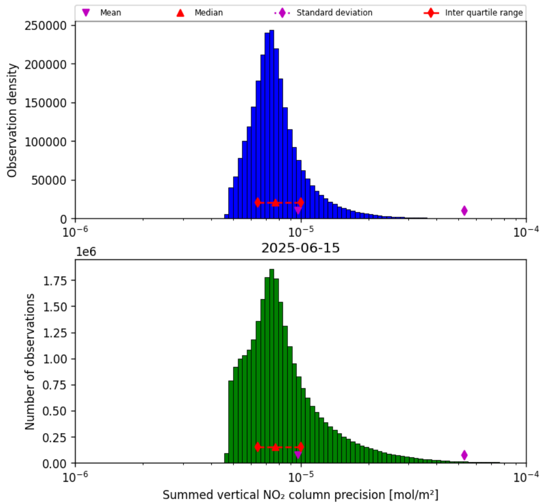
Figure 41: Histogram of “Summed vertical NO 2 column precision” for 2025-06-14 to 2025-06-16
