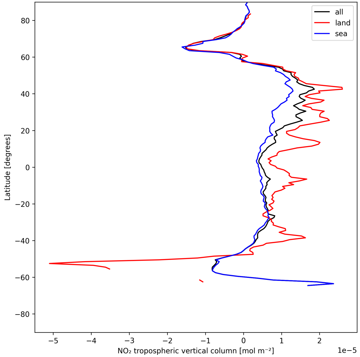
Figure 12: Zonal average of “NO 2 tropospheric vertical column” for 2025-06-14 to 2025-06-16.
