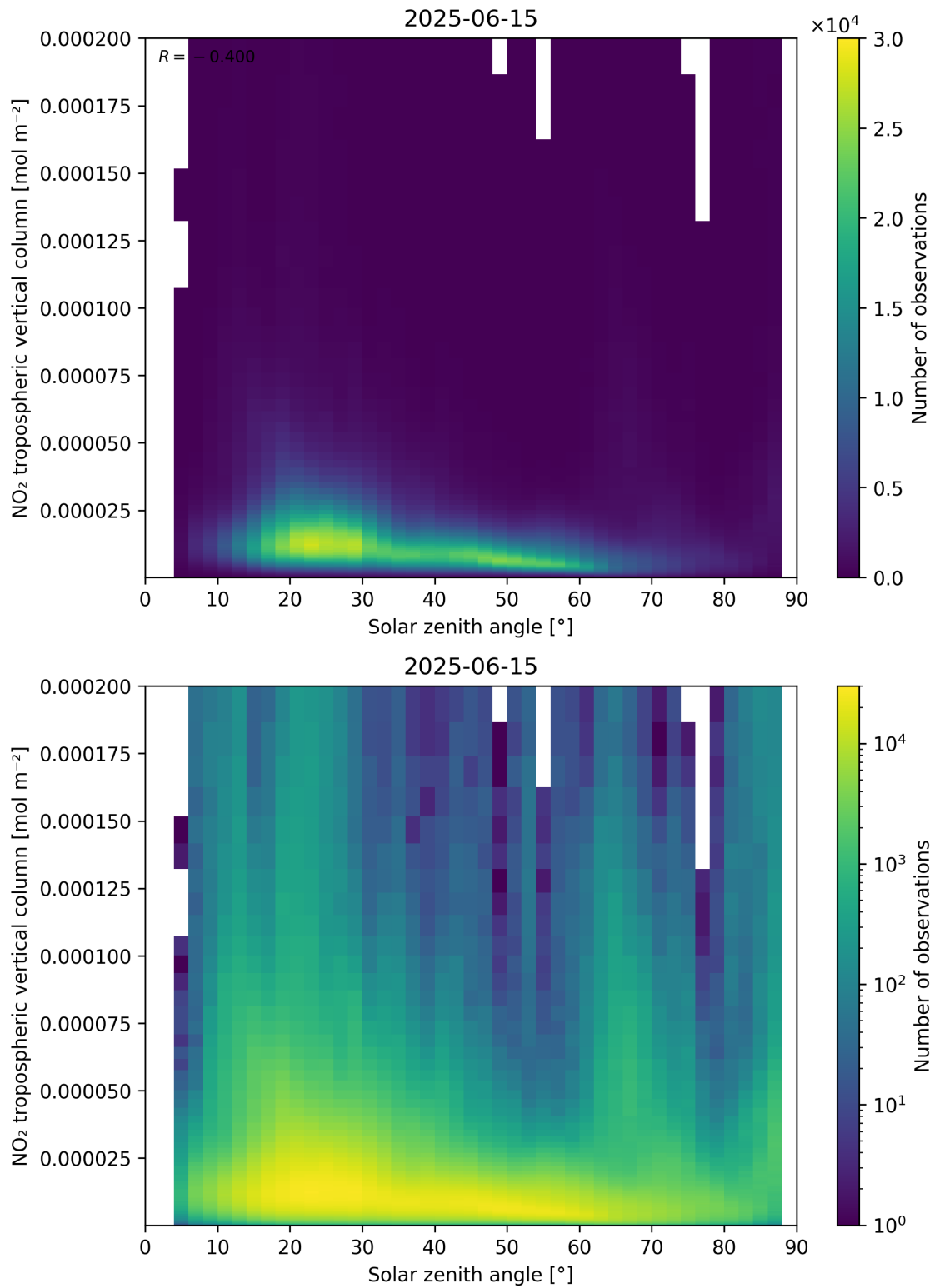
Figure 155: Scatter density plot of “Solar zenith angle” against “NO 2 tropospheric vertical column” for 2025-06-14 to 2025-06-16.
