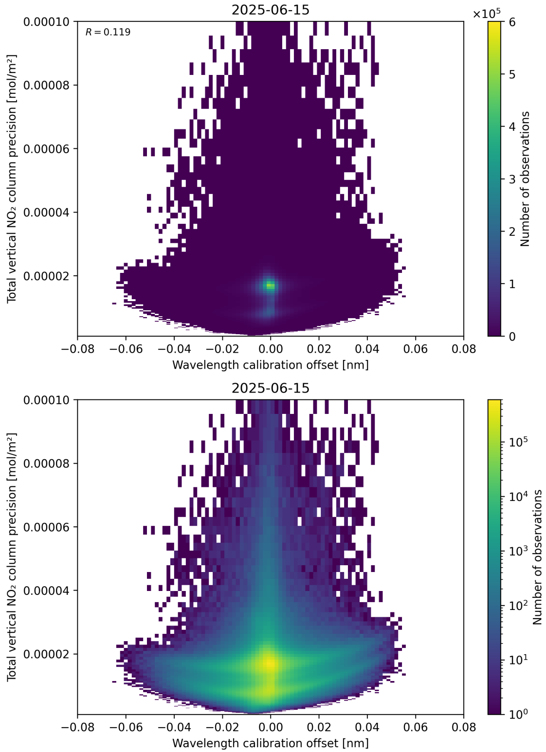
Figure 180: Scatter density plot of “Wavelength calibration offset” against “Total vertical NO 2 column precision” for 2025-06-14 to 2025-06-16.
