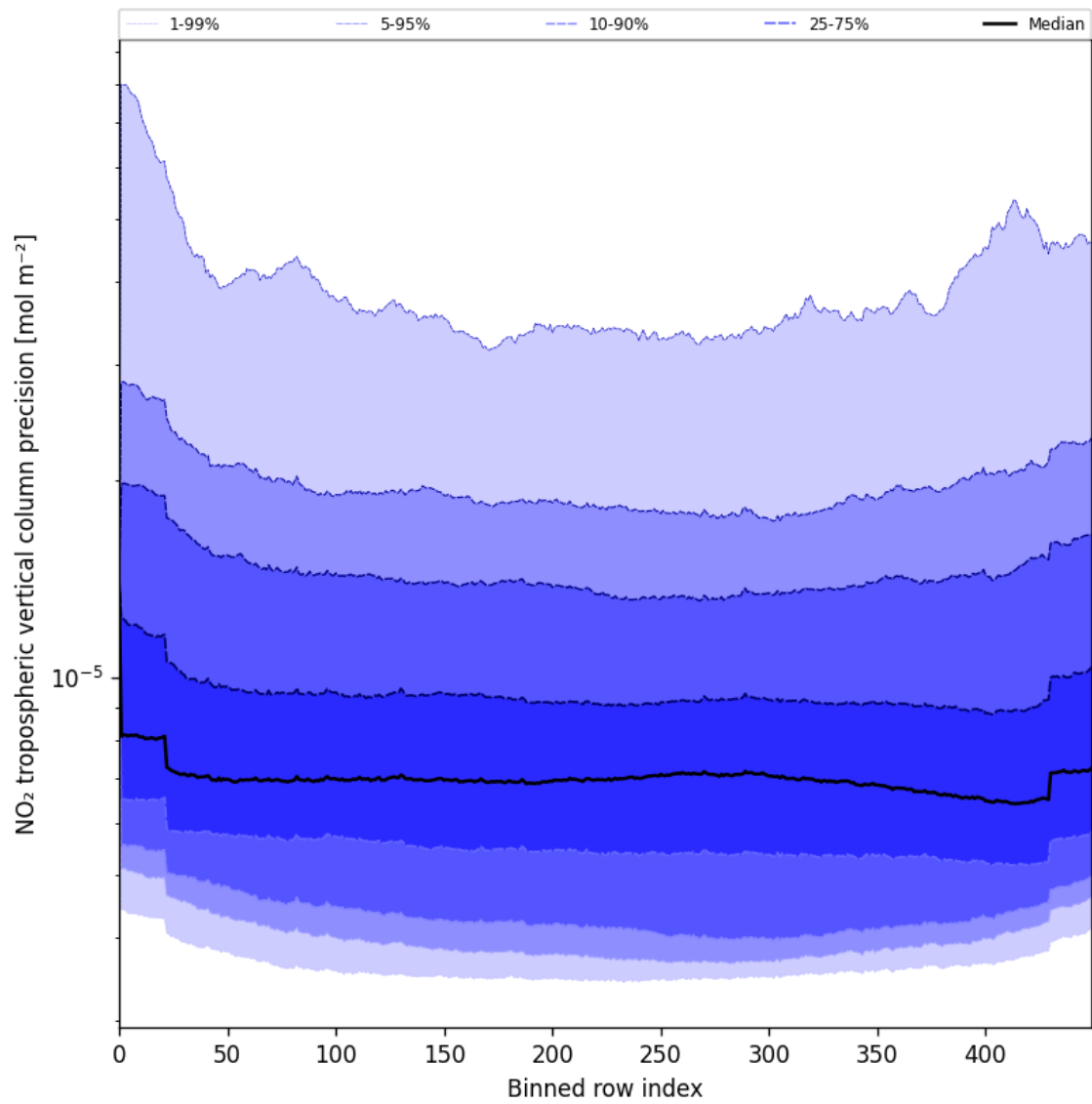
Figure 47: Along track statistics of “NO 2 tropospheric vertical column precision” for 2025-06-14 to 2025-06-16
