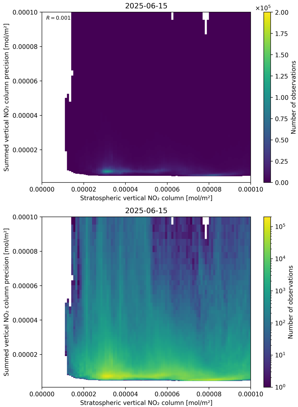
Figure 99: Scatter density plot of “Stratospheric vertical NO 2 column” against “Summed vertical NO 2 column precision” for 2025-06-14 to 2025-06-16.
