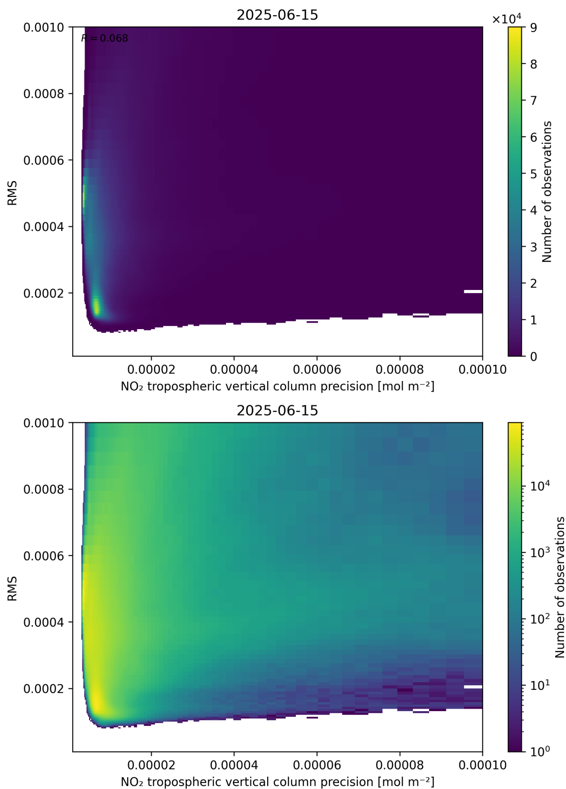
Figure 140: Scatter density plot of “NO 2 tropospheric vertical column precision” against “RMS” for 2025-06-14 to 2025-06-16.
