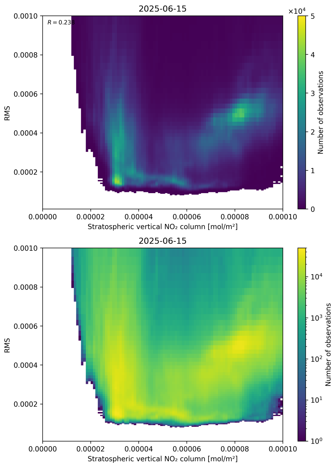
Figure 102: Scatter density plot of “Stratospheric vertical NO 2 column” against “RMS” for 2025-06-14 to 2025-06-16.
