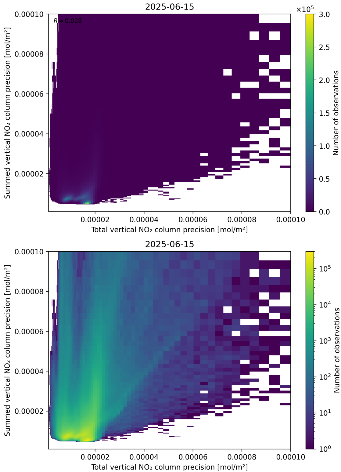
Figure 118: Scatter density plot of “Total vertical NO 2 column precision” against “Summed vertical NO 2 column precision” for 2025-06-14 to 2025-06-16.
