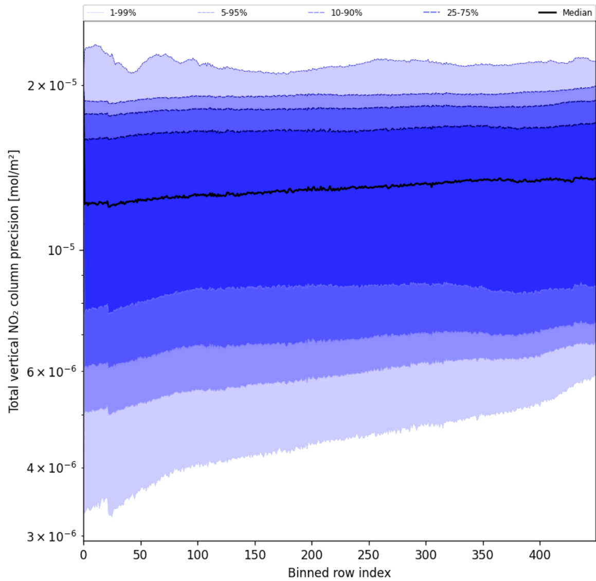
Figure 56: Along track statistics of “Total vertical NO 2 column precision” for 2025-06-14 to 2025-06-16
