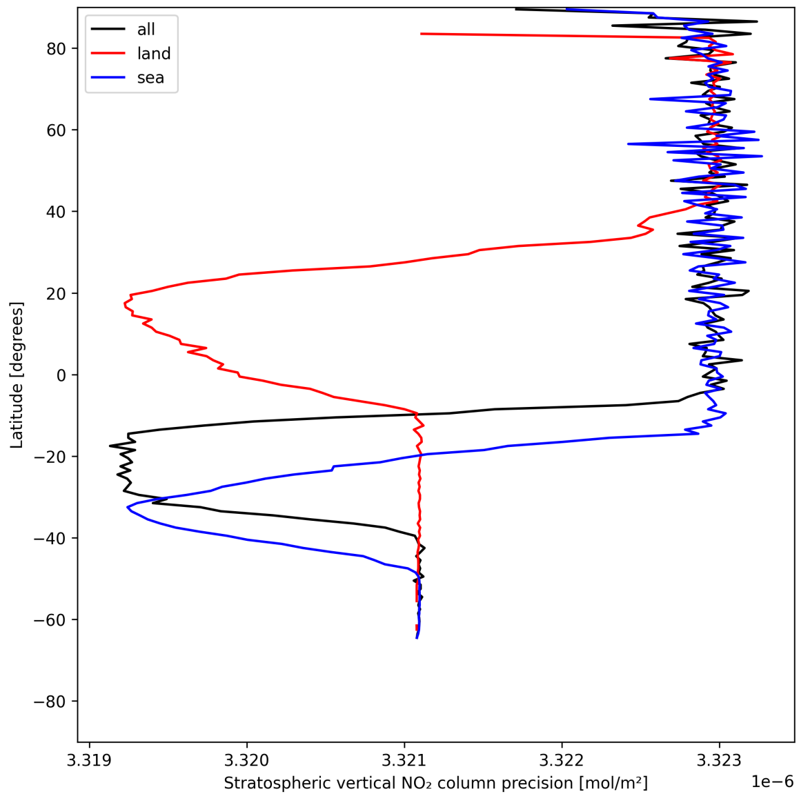
Figure 20: Zonal average of “Stratospheric vertical NO 2 column precision” for 2025-06-14 to 2025-06-16.
