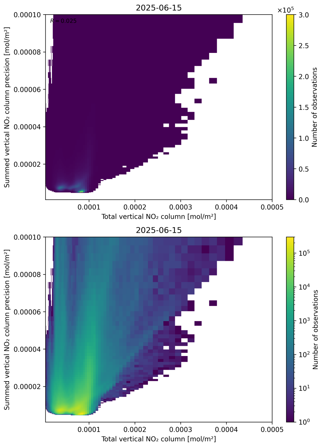
Figure 113: Scatter density plot of “Total vertical NO 2 column” against “Summed vertical NO 2 column precision” for 2025-06-14 to 2025-06-16.
