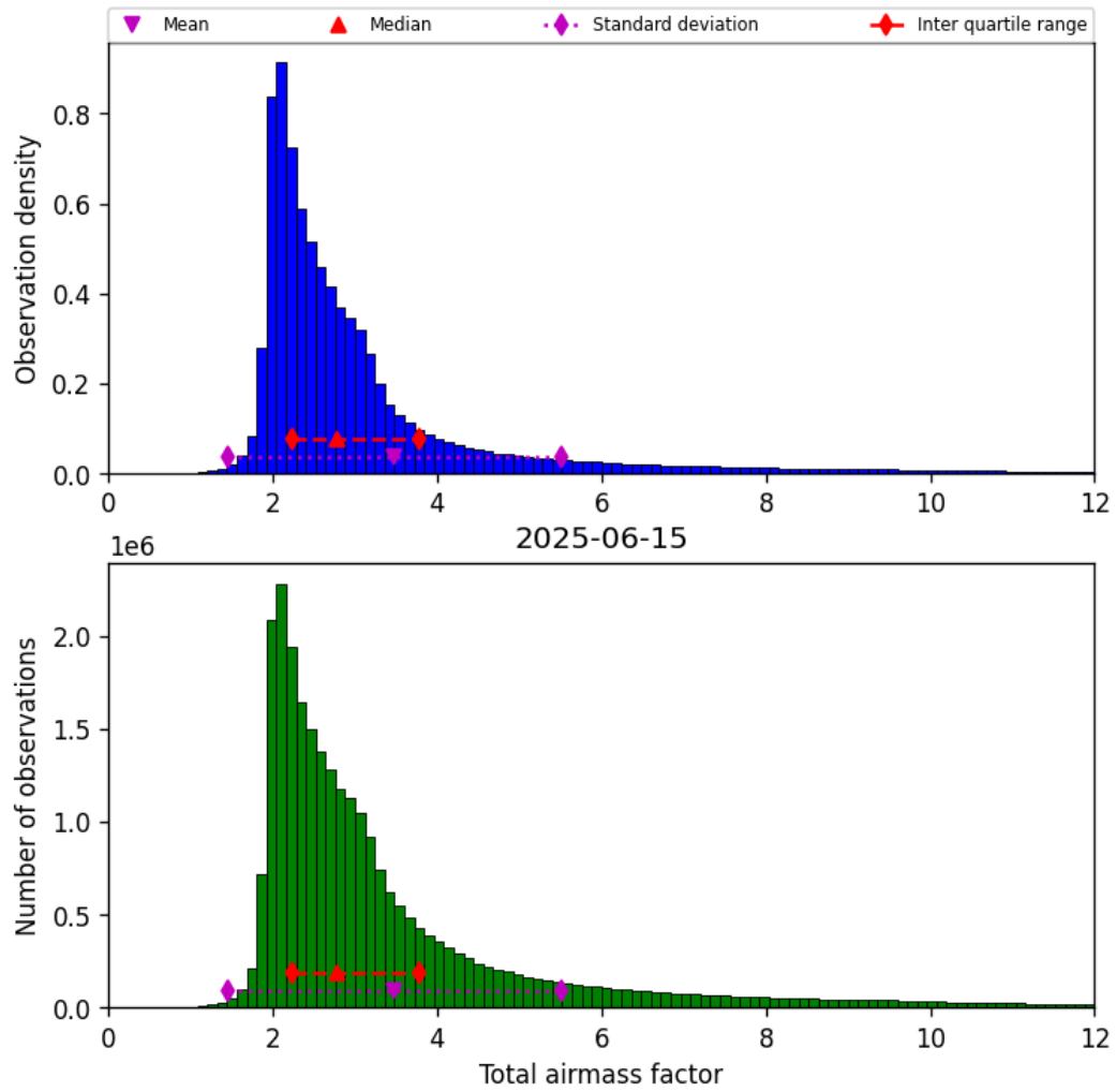
Figure 32: Histogram of “Total airmass factor” for 2025-06-14 to 2025-06-16
