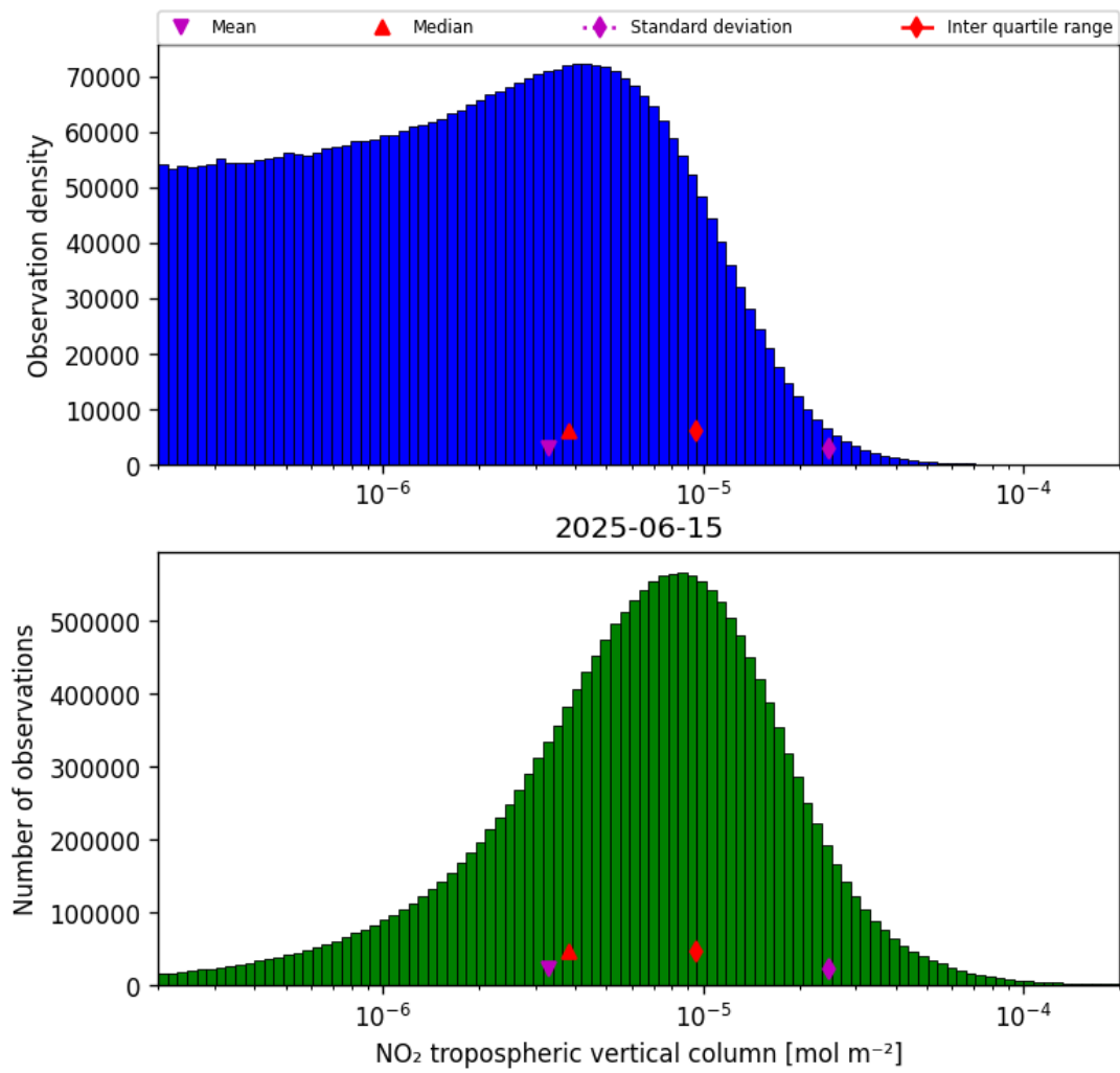
Figure 29: Histogram of “NO 2 tropospheric vertical column” for 2025-06-14 to 2025-06-16
