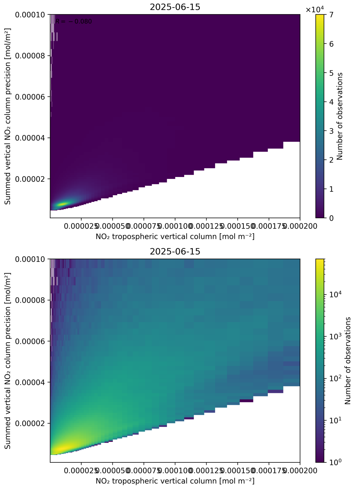
Figure 127: Scatter density plot of “NO 2 tropospheric vertical column” against “Summed vertical NO 2 column precision” for 2025-06-14 to 2025-06-16.
