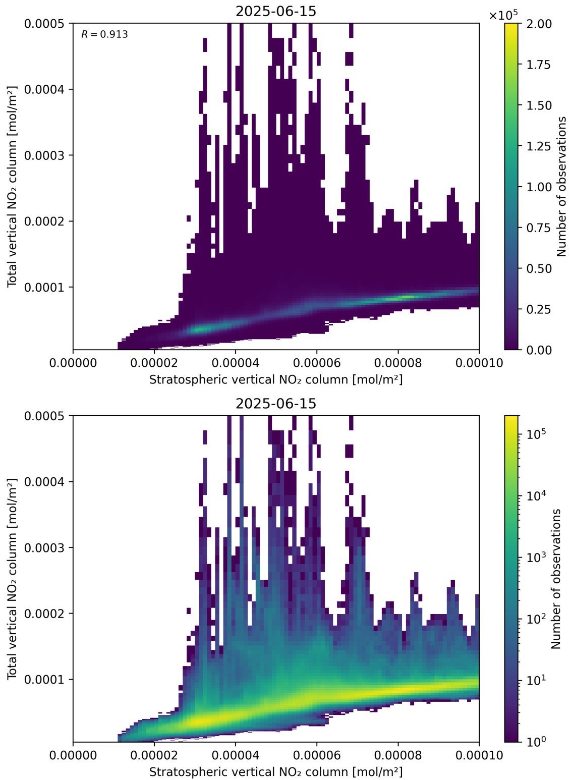
Figure 100: Scatter density plot of “Stratospheric vertical NO 2 column” against “Total vertical NO 2 column” for 2025-06-14 to 2025-06-16.
