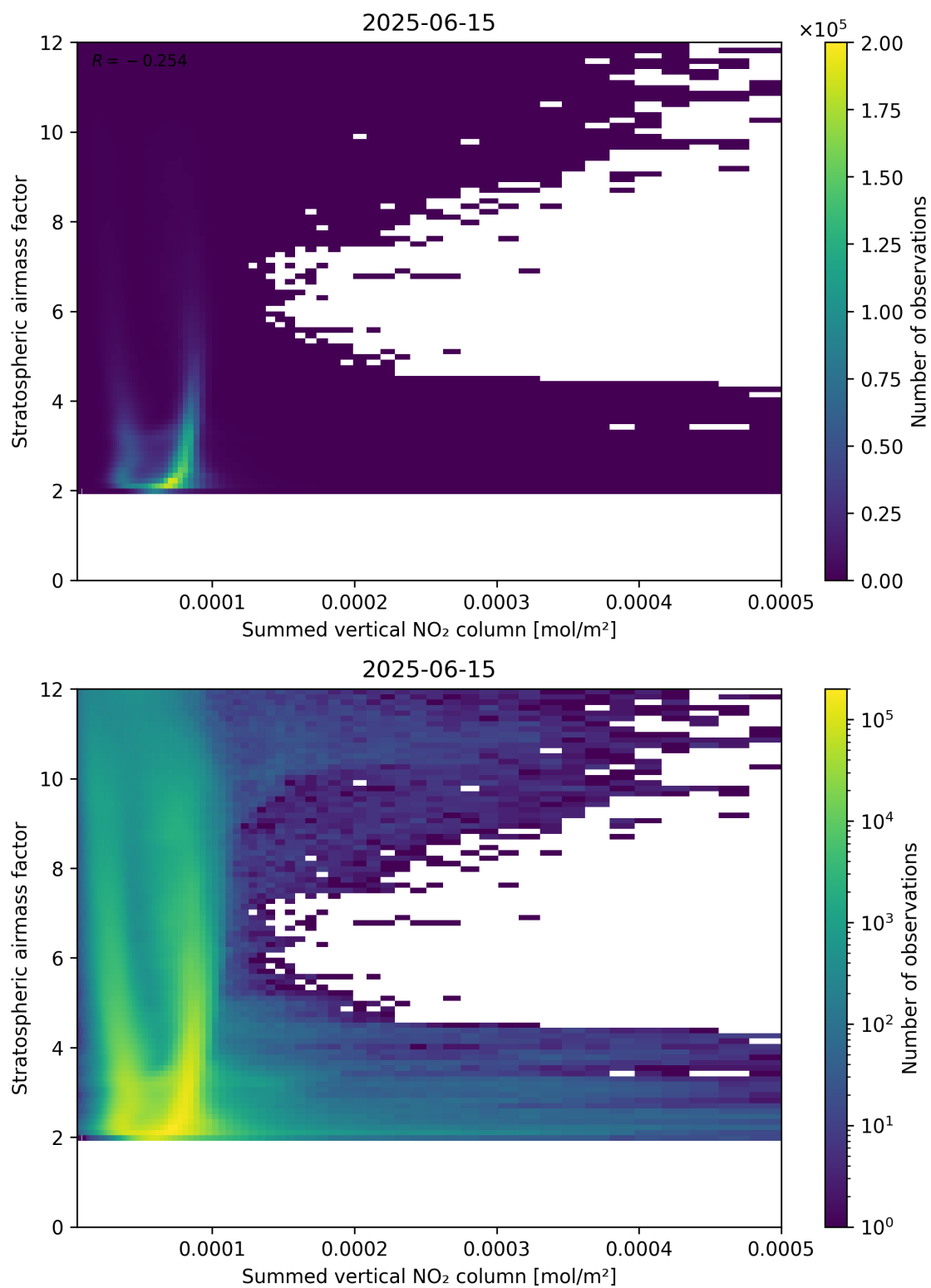
Figure 103: Scatter density plot of “Summed vertical NO 2 column” against “Stratospheric airmass factor” for 2025-06-14 to 2025-06-16.
