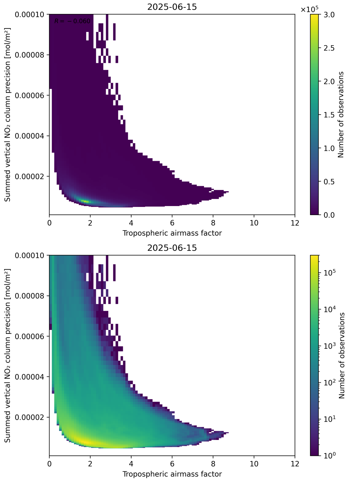
Figure 76: Scatter density plot of “Tropospheric air mass factor” against “Summed vertical NO 2 column precision” for 2025-06-14 to 2025-06-16.
