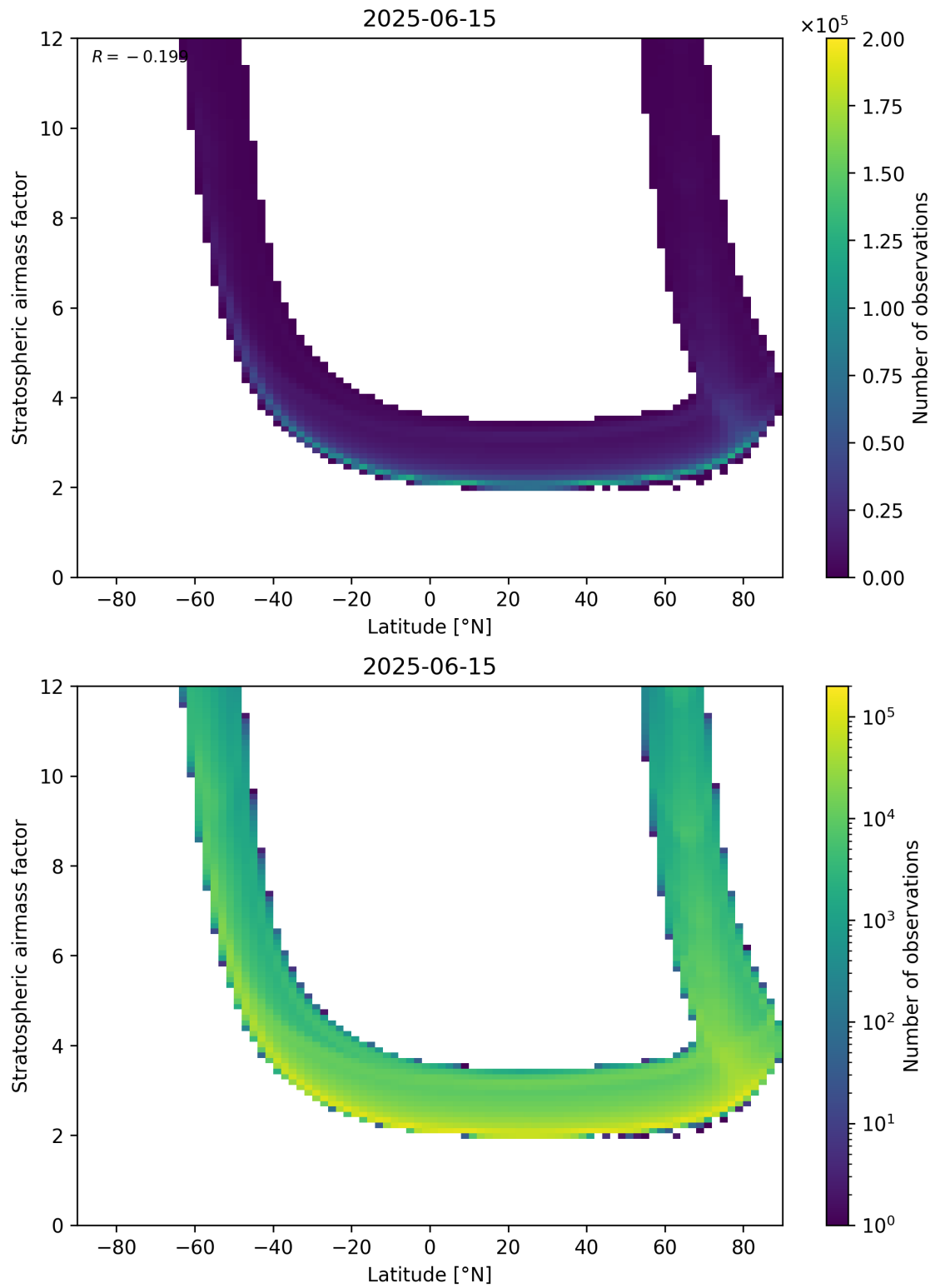
Figure 83: Scatter density plot of “Latitude” against “Stratospheric air mass factor” for 2025-06-14 to 2025-06-16.
