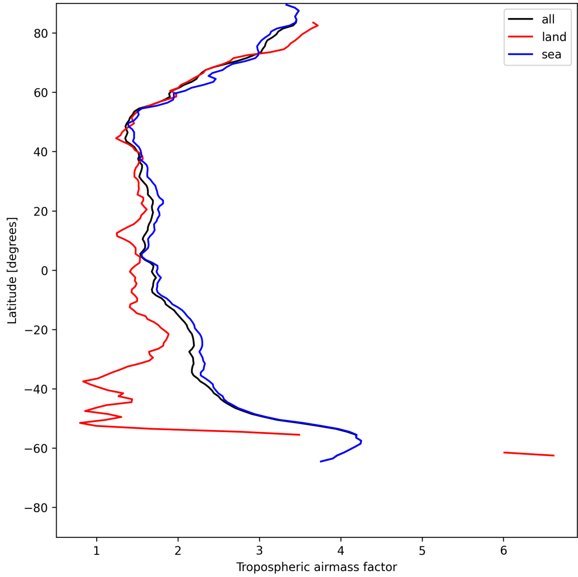
Figure 14: Zonal average of “Tropospheric airmass factor” for 2025-06-14 to 2025-06-16.
