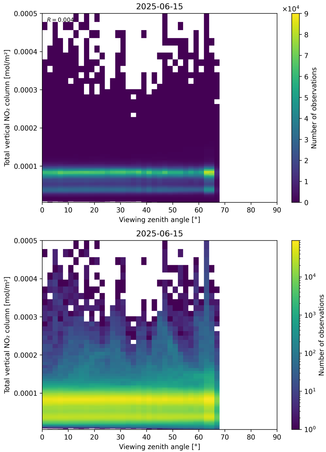
Figure 167: Scatter density plot of “Viewing zenith angle” against “Total vertical NO 2 column” for 2025-06-14 to 2025-06-16.
