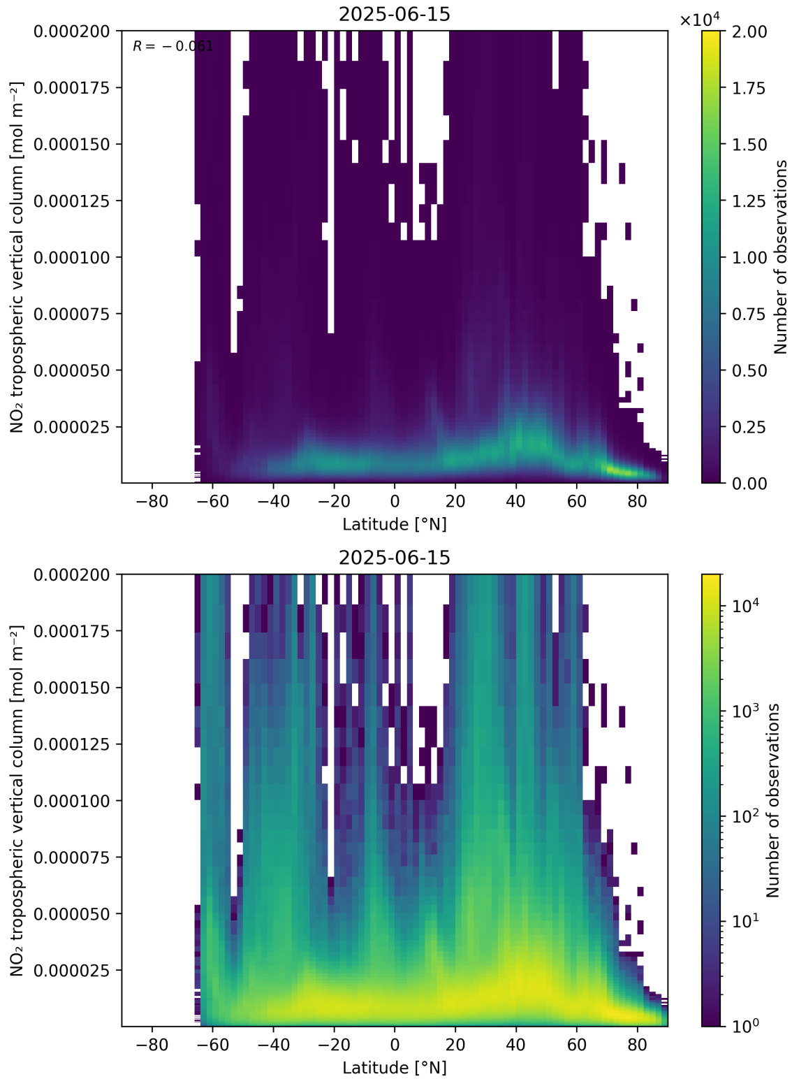
Figure 92: Scatter density plot of “Latitude” against “NO 2 tropospheric vertical column” for 2025-06-14 to 2025-06-16.
