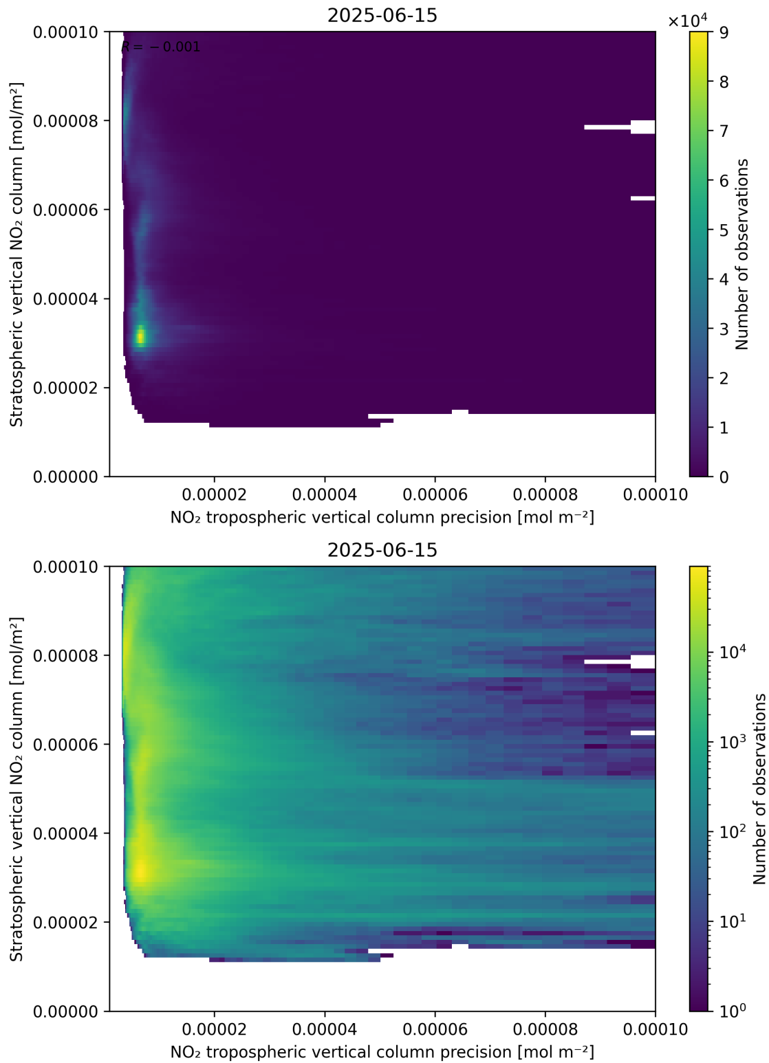
Figure 135: Scatter density plot of “NO 2 tropospheric vertical column precision” against “Stratospheric vertical NO 2 column” for 2025-06-14 to 2025-06-16.
