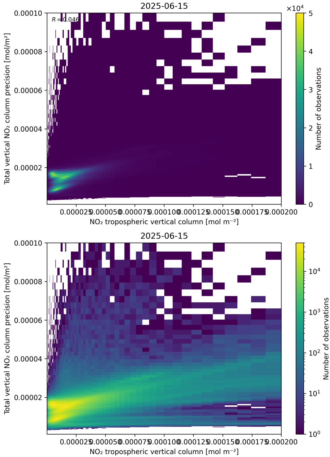
Figure 129: Scatter density plot of “NO 2 tropospheric vertical column” against “Total vertical NO 2 column precision” for 2025-06-14 to 2025-06-16.
