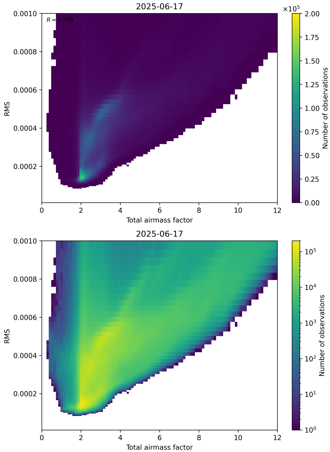
Figure 69: Scatter density plot of “Total airmass factor” against “RMS” for 2025-06-17 to 2025-06-18.
