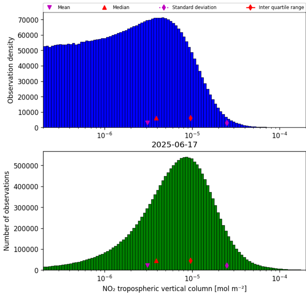
Figure 29: Histogram of “NO 2 tropospheric vertical column” for 2025-06-17 to 2025-06-18
