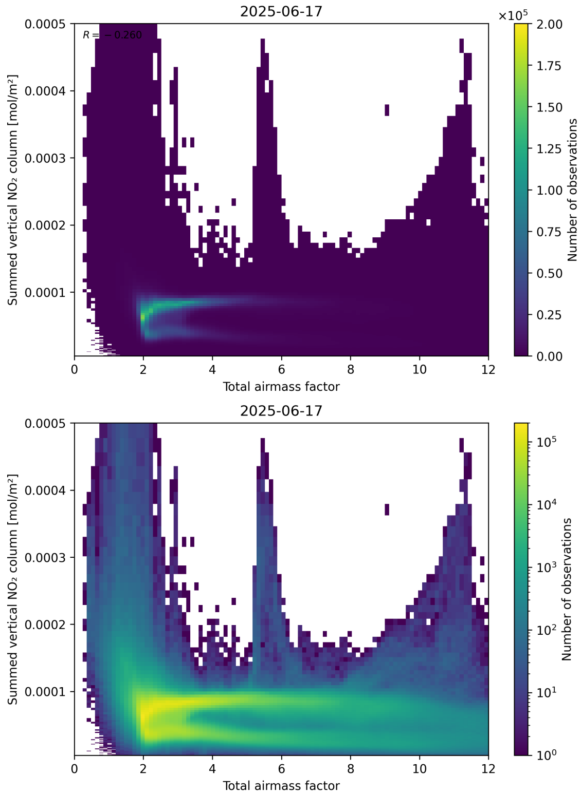
Figure 65: Scatter density plot of “Total airmass factor” against “Summed vertical NO 2 column” for 2025-06-17 to 2025-06-18.
