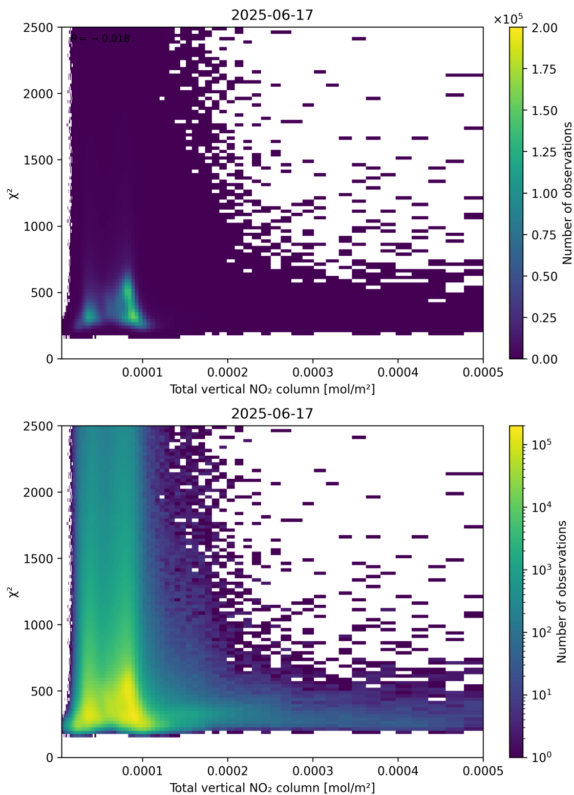
Figure 111: Scatter density plot of “Total vertical NO 2 column” against “ \chi^2 ” for 2025-06-17 to 2025-06-18.
