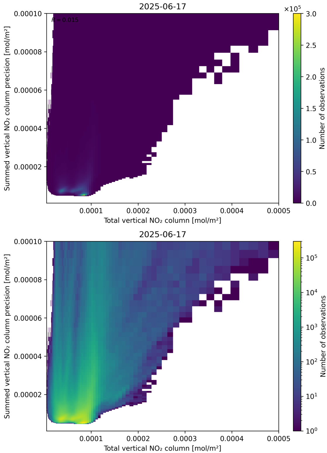
Figure 113: Scatter density plot of “Total vertical NO 2 column” against “Summed vertical NO 2 column precision” for 2025-06-17 to 2025-06-18.
