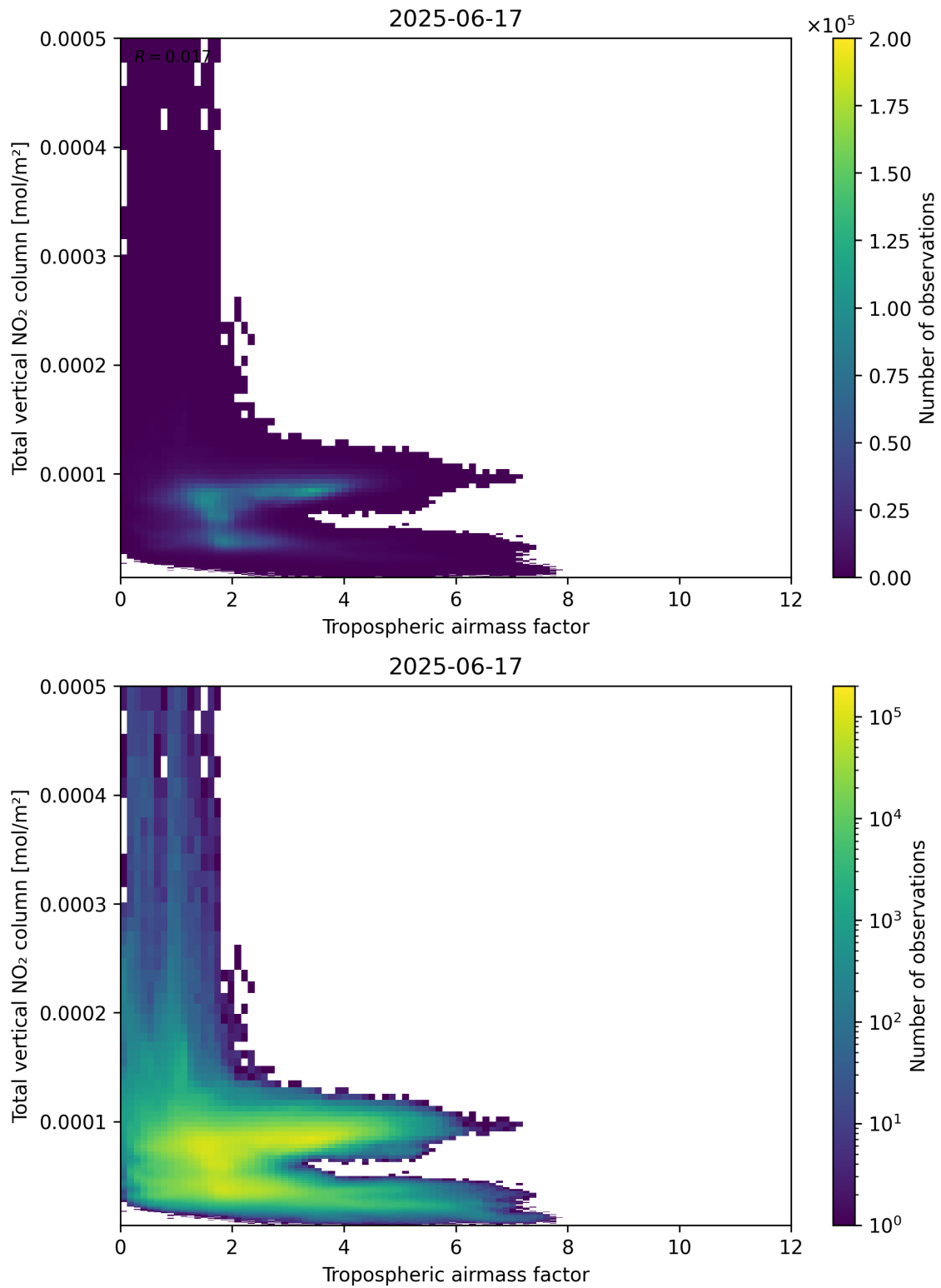
Figure 77: Scatter density plot of “Tropospheric airmass factor” against “Total vertical NO 2 column” for 2025-06-17 to 2025-06-18.
