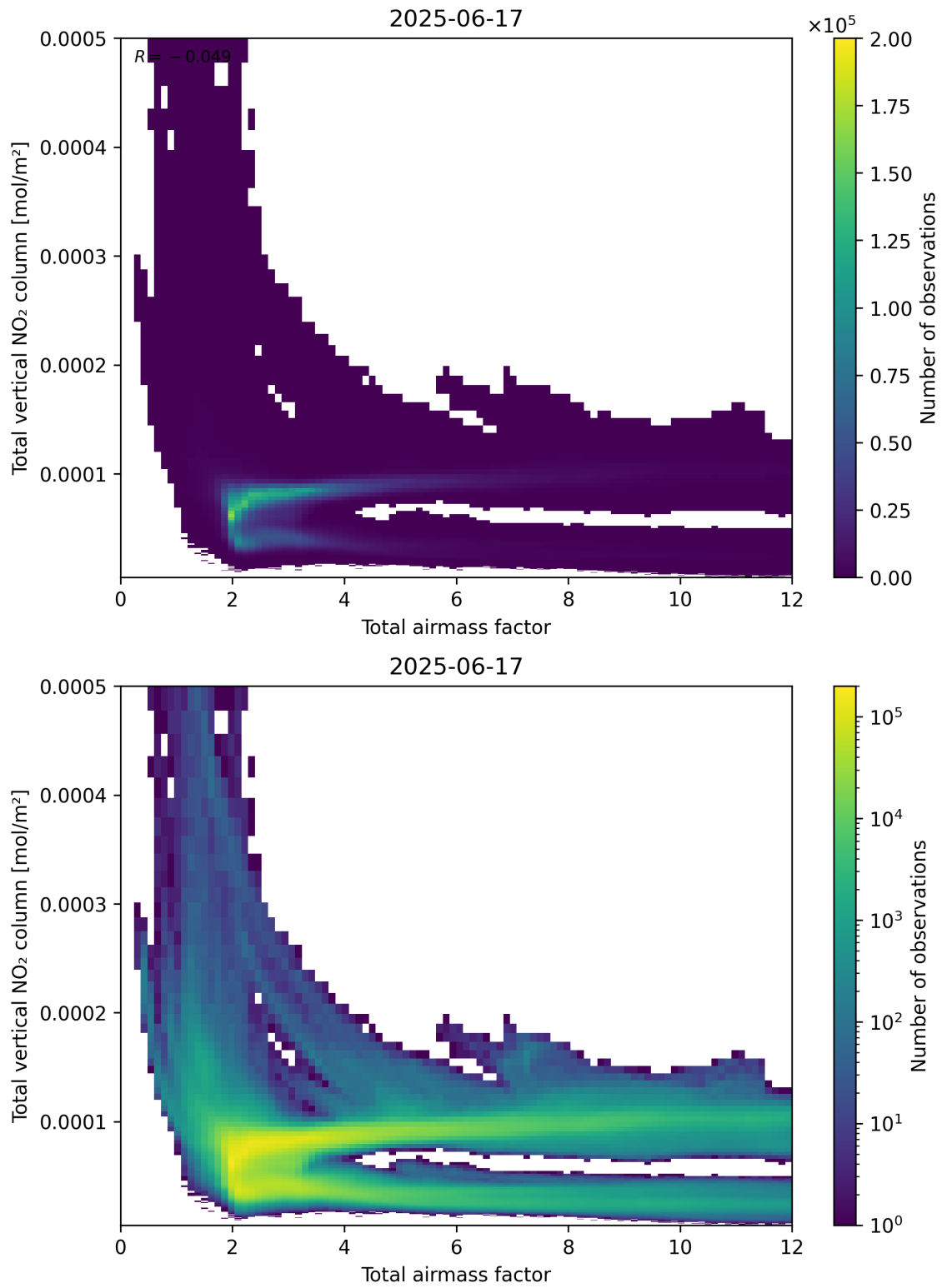
Figure 67: Scatter density plot of “Total airmass factor” against “Total vertical NO 2 column” for 2025-06-17 to 2025-06-18.
