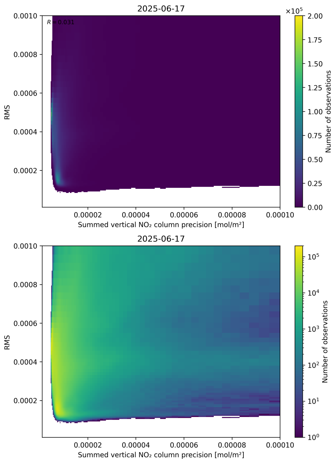
Figure 108: Scatter density plot of “Summed vertical NO 2 column precision” against “RMS” for 2025-06-17 to 2025-06-18.
