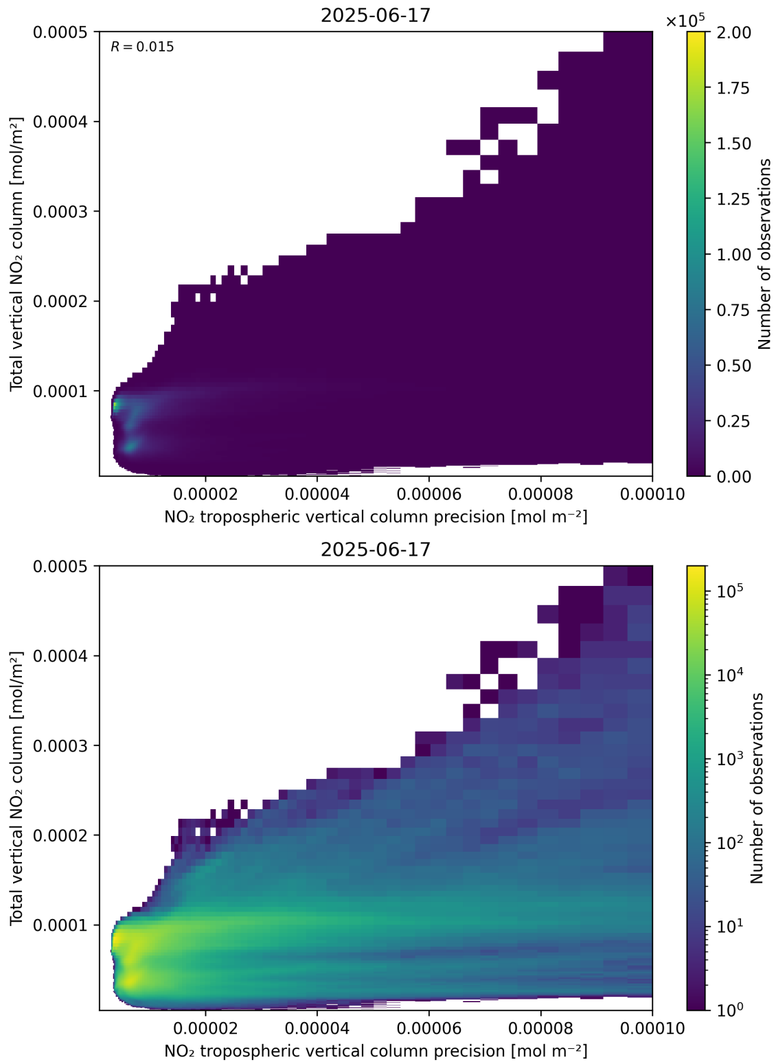
Figure 138: Scatter density plot of “NO 2 tropospheric vertical column precision” against “Total vertical NO 2 column” for 2025-06-17 to 2025-06-18.
