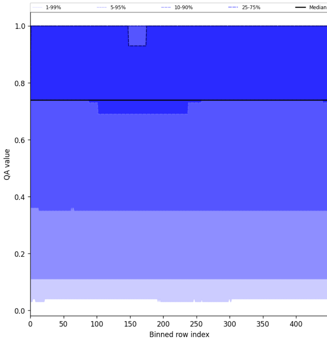
Figure 45: Along track statistics of “QA value” for 2025-06-17 to 2025-06-18
