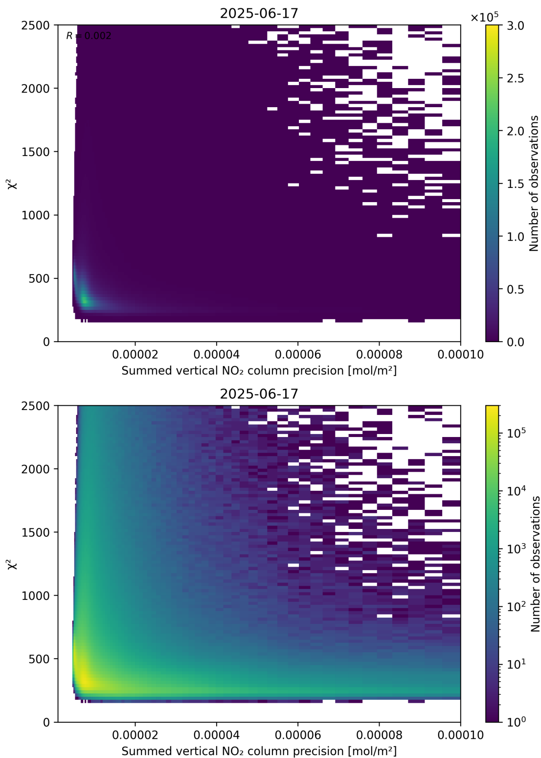
Figure 107: Scatter density plot of “Summed vertical NO 2 column precision” against “ \chi^2 ” for 2025-06-17 to 2025-06-18.
