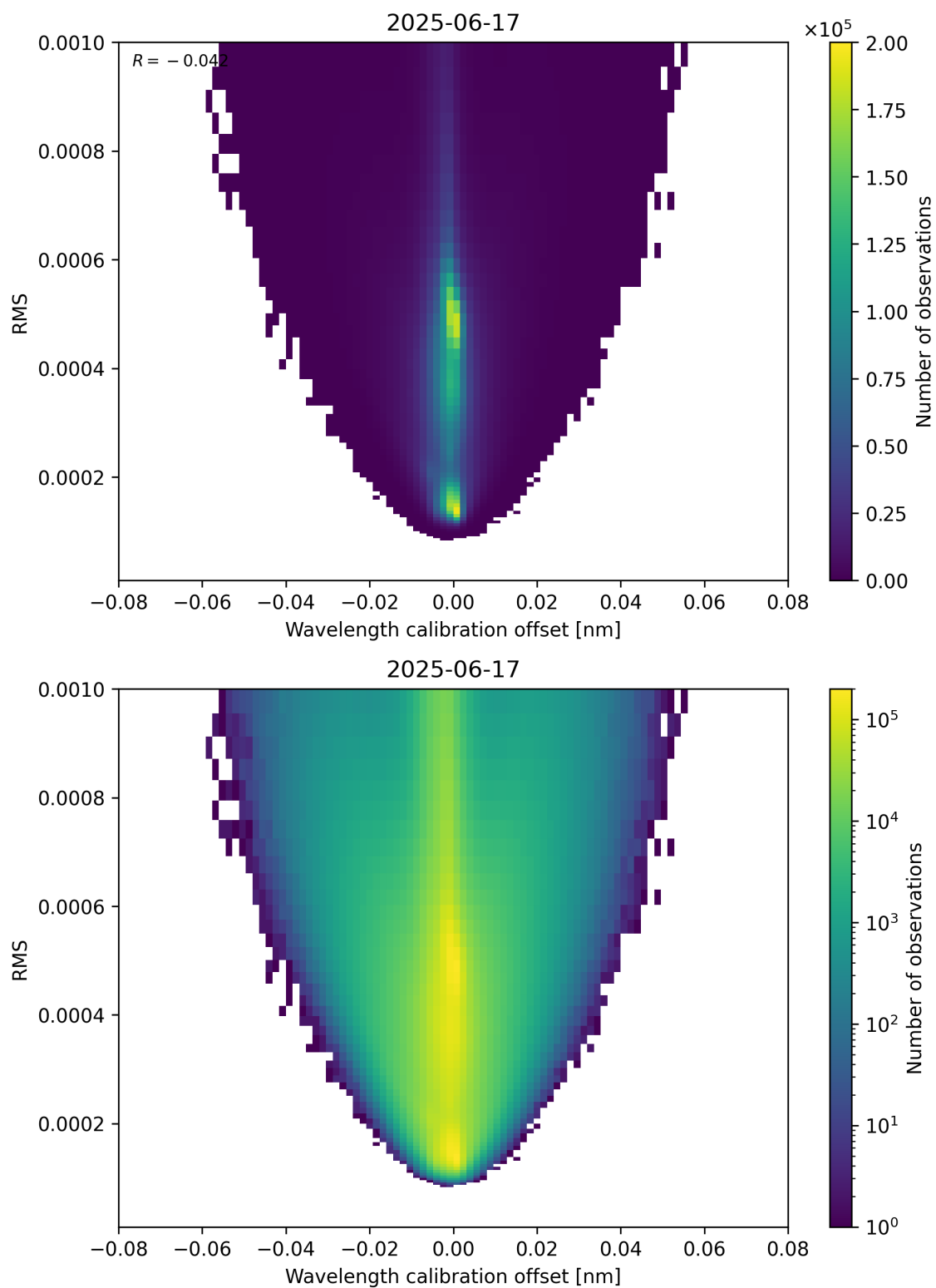
Figure 181: Scatter density plot of “Wavelength calibration offset” against “RMS” for 2025-06-17 to 2025-06-18.
