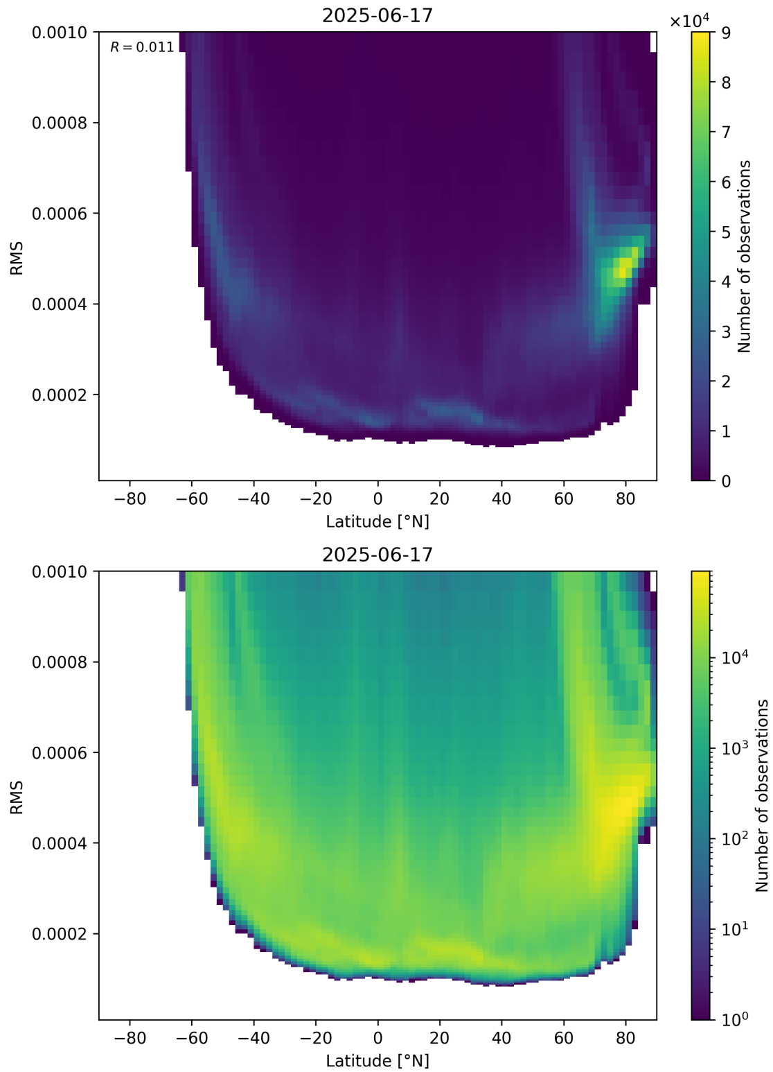
Figure 94: Scatter density plot of “Latitude” against “RMS” for 2025-06-17 to 2025-06-18.
