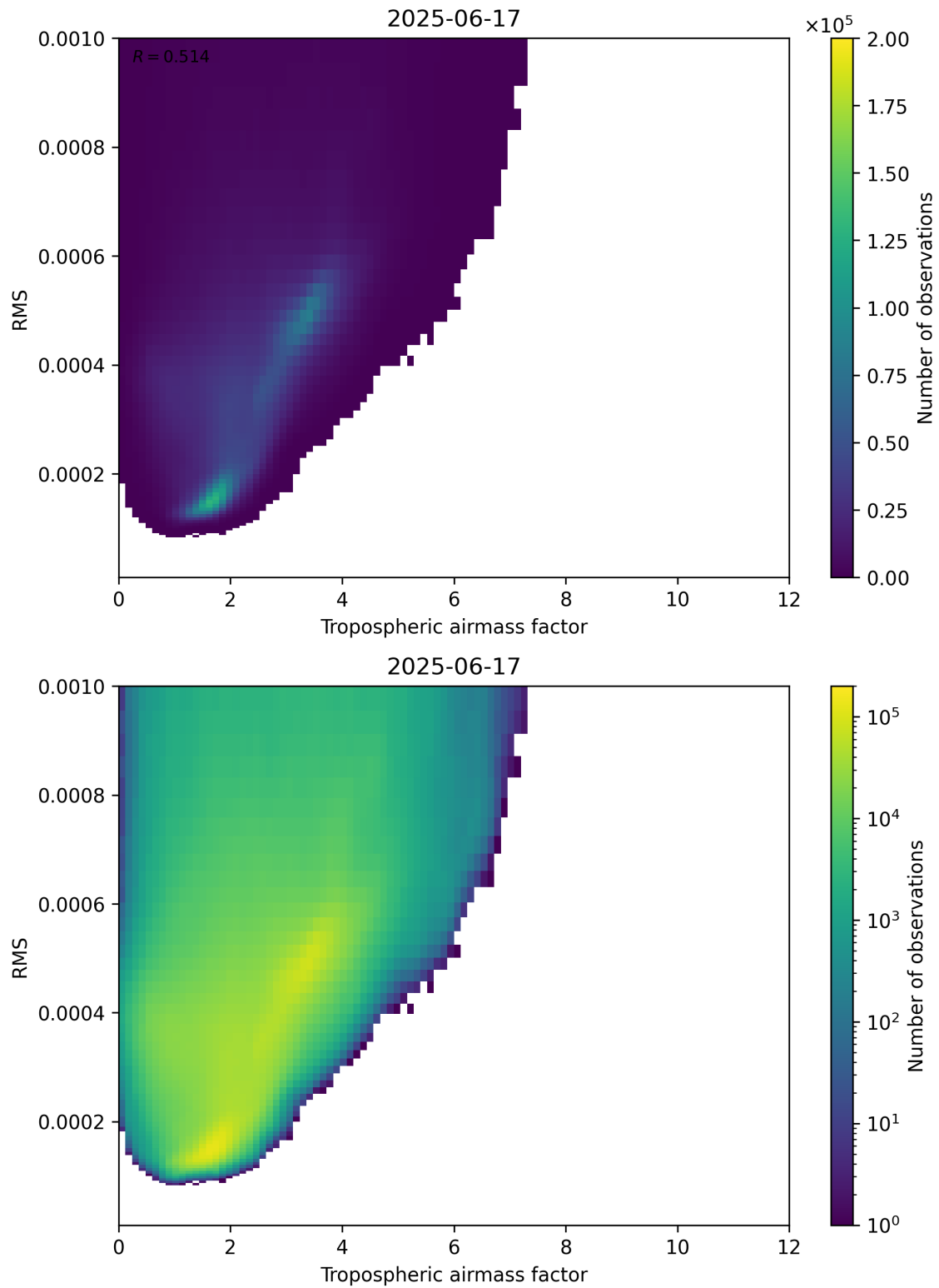
Figure 79: Scatter density plot of “Tropospheric airmass factor” against “RMS” for 2025-06-17 to 2025-06-18.
