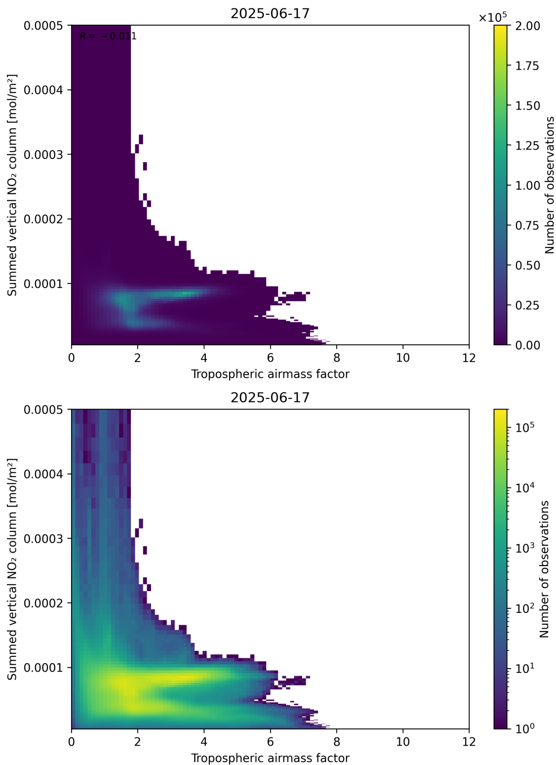
Figure 75: Scatter density plot of “Tropospheric airmass factor” against “Summed vertical NO 2 column” for 2025-06-17 to 2025-06-18.
