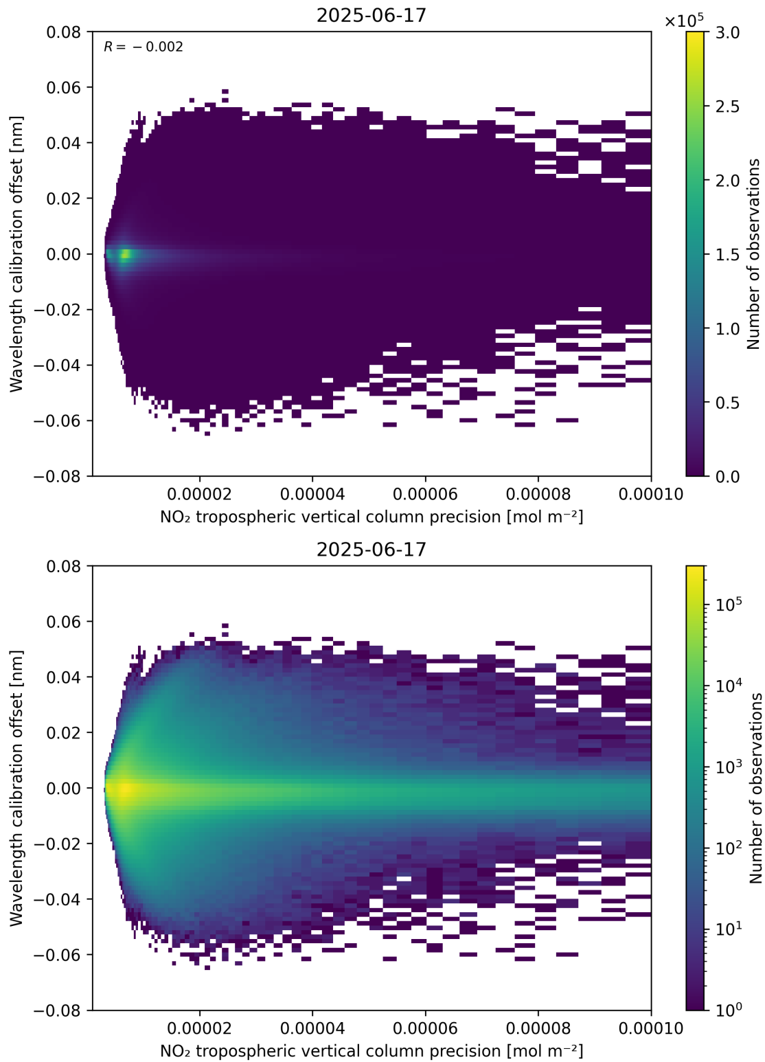
Figure 141: Scatter density plot of “NO 2 tropospheric vertical column precision” against “Wavelength calibration offset” for 2025-06-17 to 2025-06-18.
