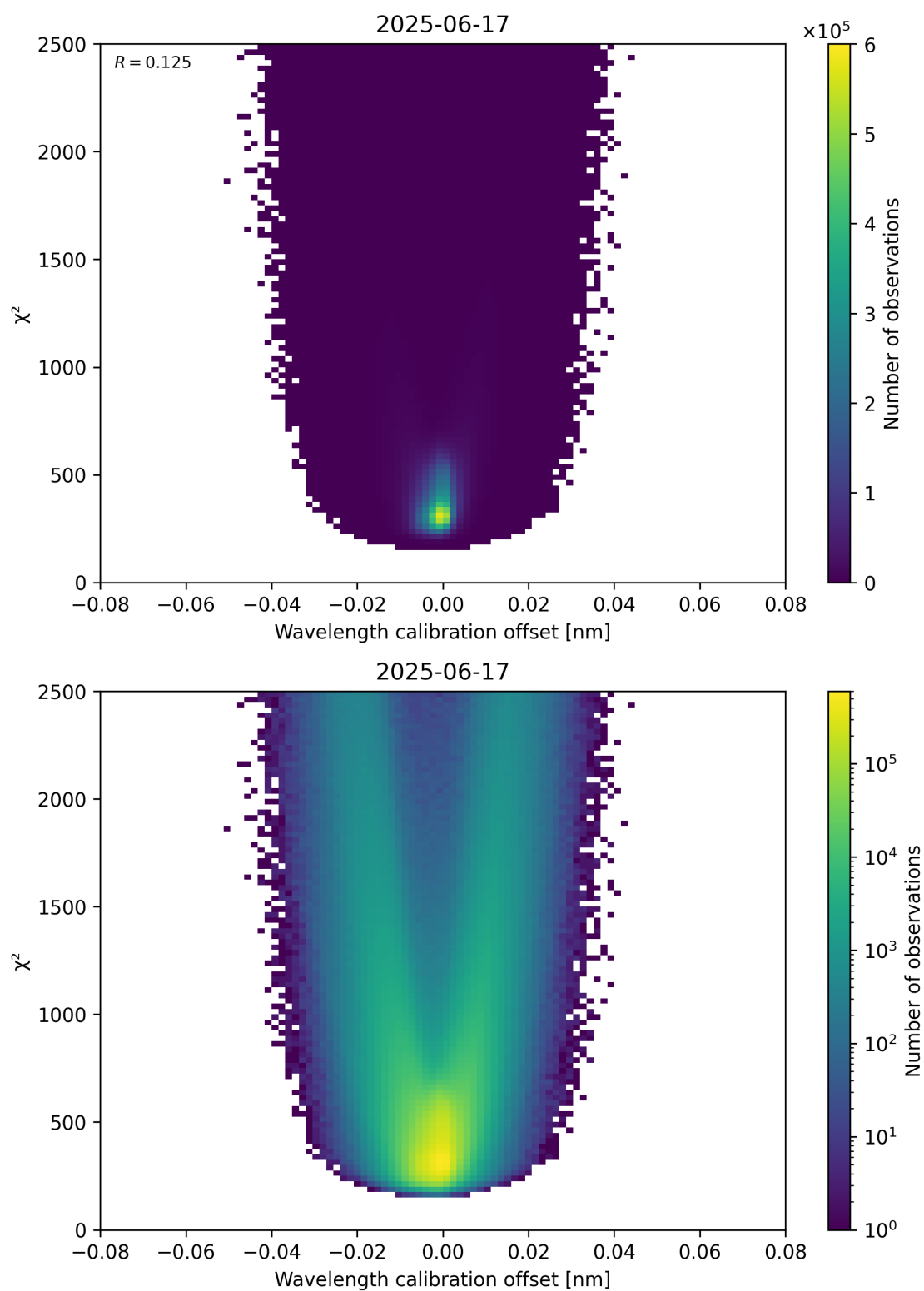
Figure 175: Scatter density plot of “Wavelength calibration offset” against “ \chi^2 ” for 2025-06-17 to 2025-06-18.
