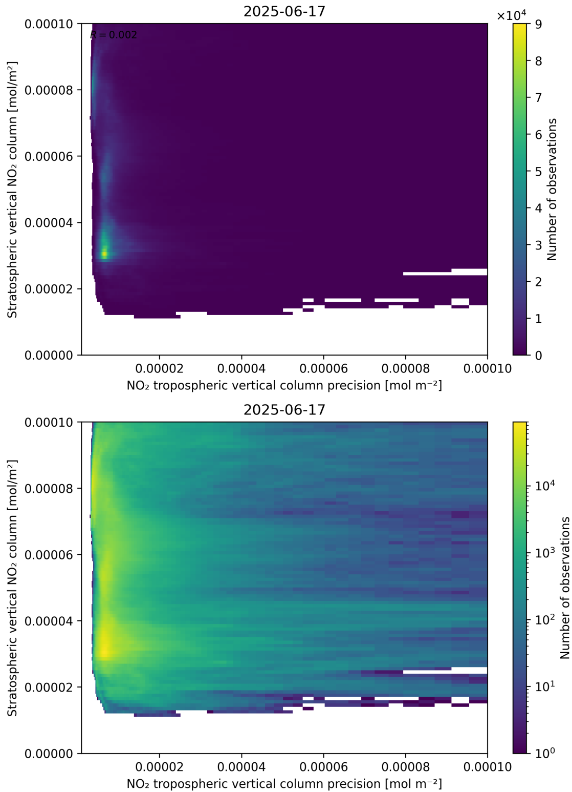
Figure 135: Scatter density plot of “NO 2 tropospheric vertical column precision” against “Stratospheric vertical NO 2 column” for 2025-06-17 to 2025-06-18.
