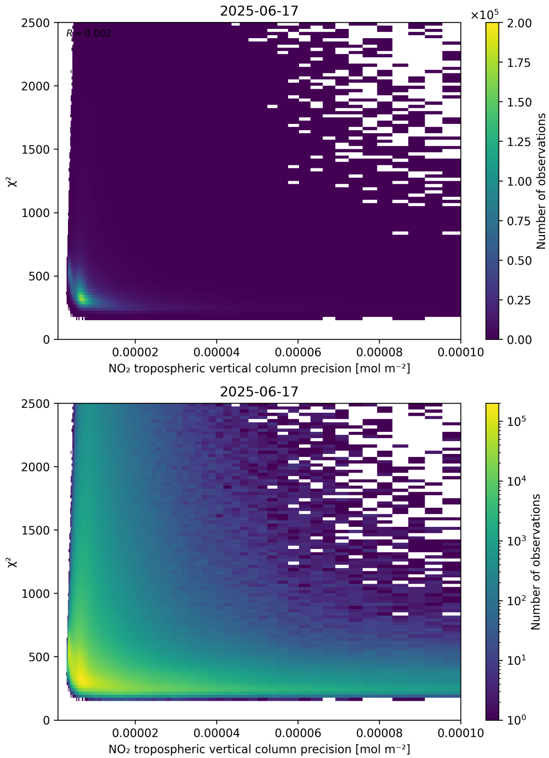
Figure 134: Scatter density plot of “NO 2 tropospheric vertical column precision” against “ \chi^2 ” for 2025-06-17 to 2025-06-18.
