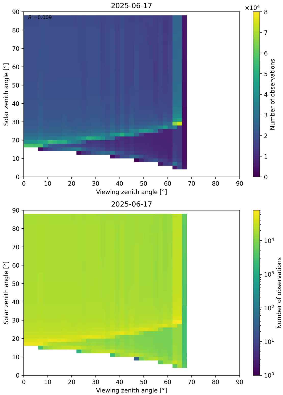
Figure 172: Scatter density plot of “Viewing zenith angle” against “Solar zenith angle” for 2025-06-17 to 2025-06-18.
