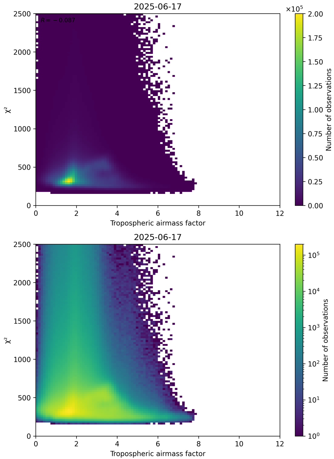
Figure 73: Scatter density plot of “Tropospheric airmass factor” against “ \chi^2 ” for 2025-06-17 to 2025-06-18.
