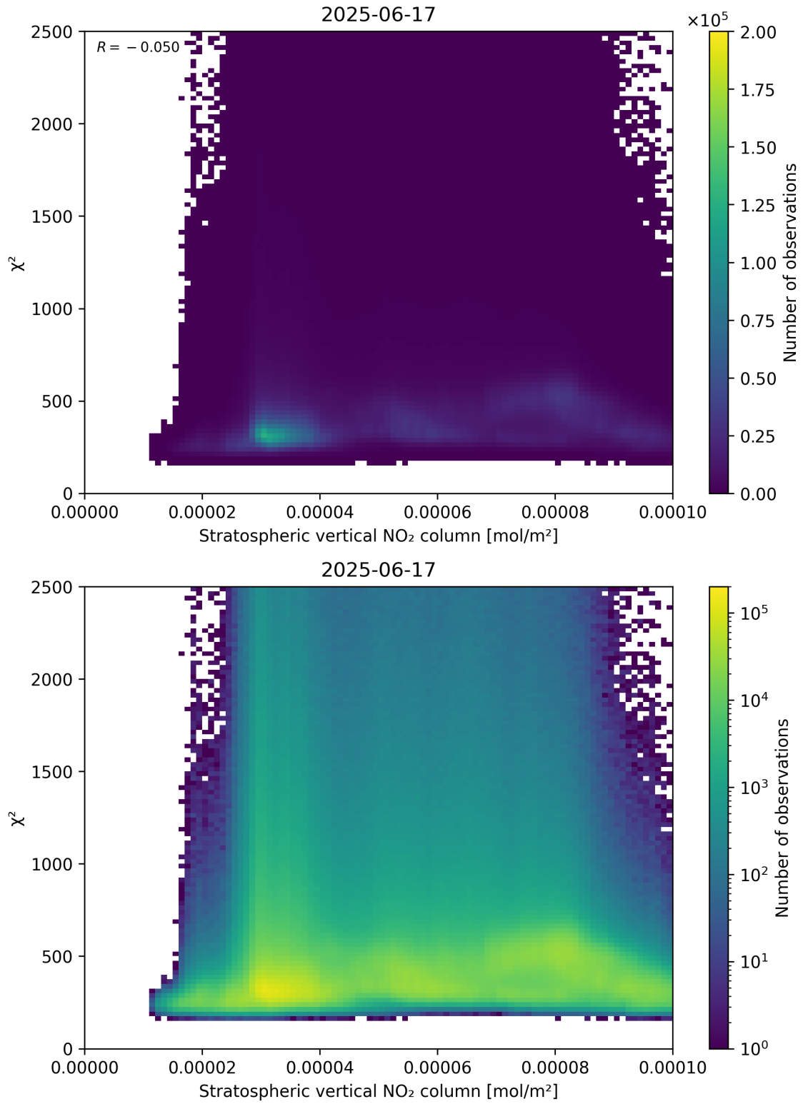
Figure 97: Scatter density plot of “Stratospheric vertical NO 2 column” against “ \chi^2 ” for 2025-06-17 to 2025-06-18.
