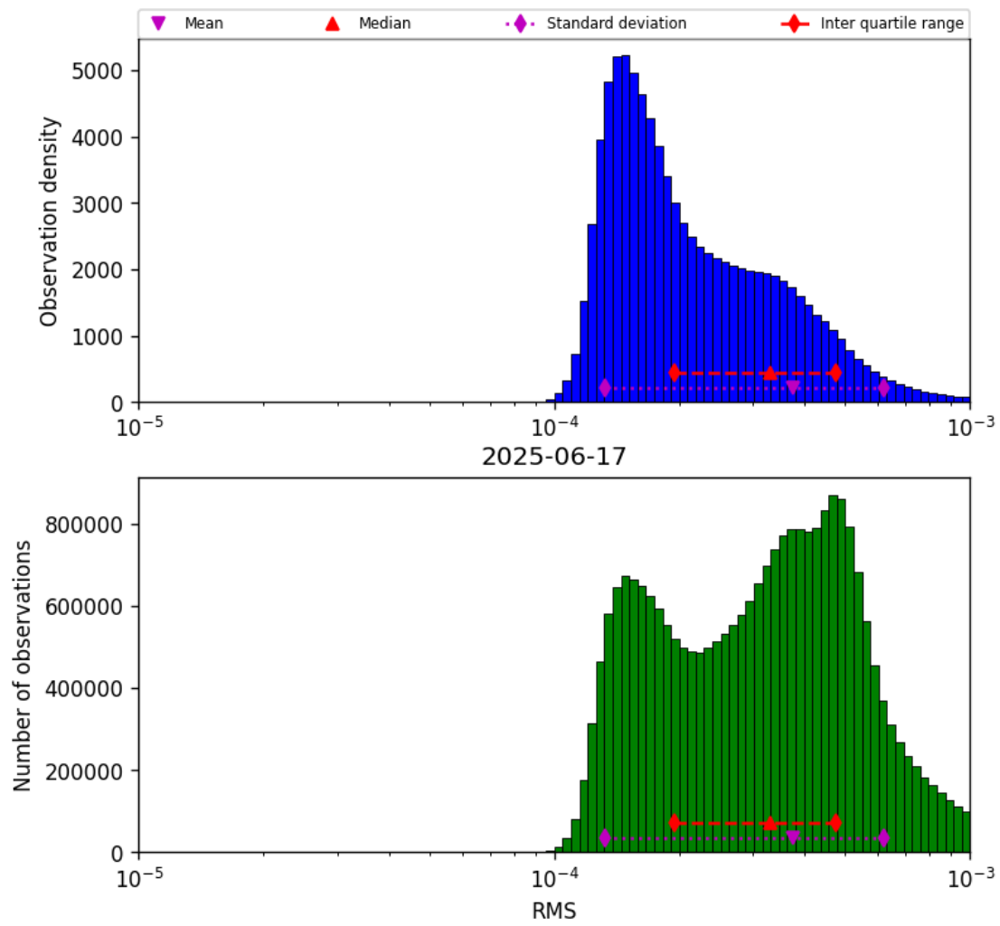
Figure 43: Histogram of “RMS” for 2025-06-17 to 2025-06-18
