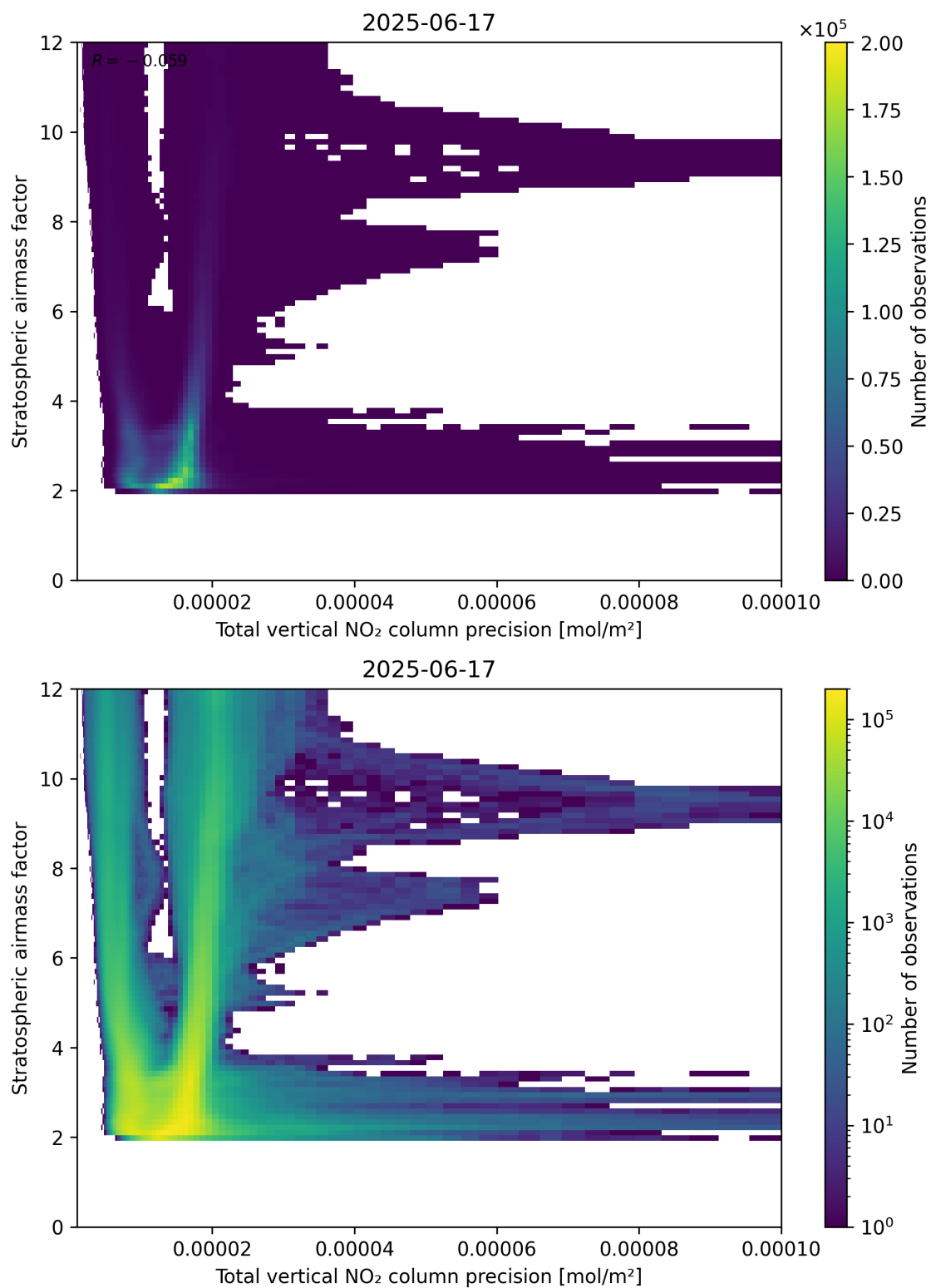
Figure 115: Scatter density plot of “Total vertical NO 2 column precision” against “Stratospheric air mass factor” for 2025-06-17 to 2025-06-18.
