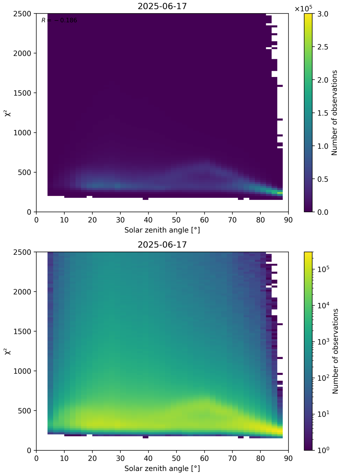
Figure 148: Scatter density plot of “Solar zenith angle” against “ \chi^2 ” for 2025-06-17 to 2025-06-18.
