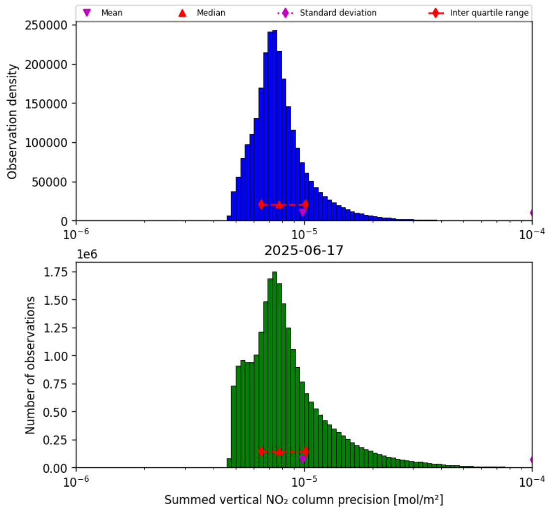
Figure 41: Histogram of "Summed vertical NO 2 column precision" for 2025-06-17 to 2025-06-18
