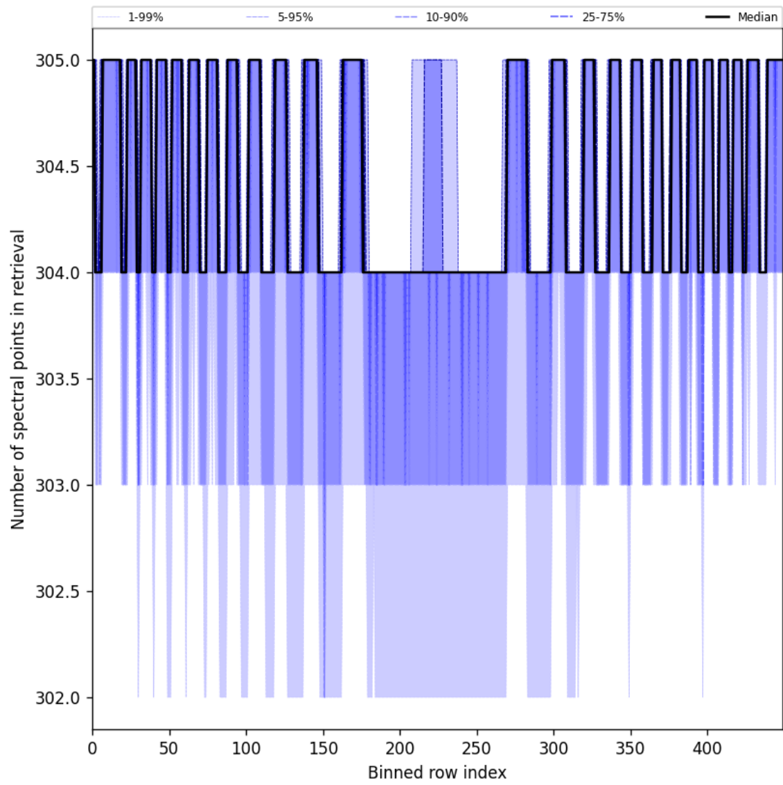
Figure 50: Along track statistics of “Number of spectral points in retrieval” for 2025-06-17 to 2025-06-18
