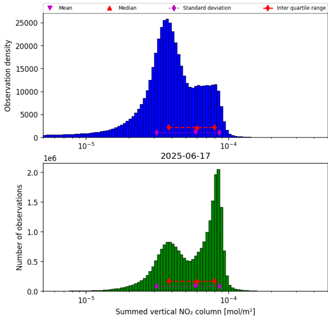
Figure 40: Histogram of “Summed vertical NO 2 column” for 2025-06-17 to 2025-06-18
