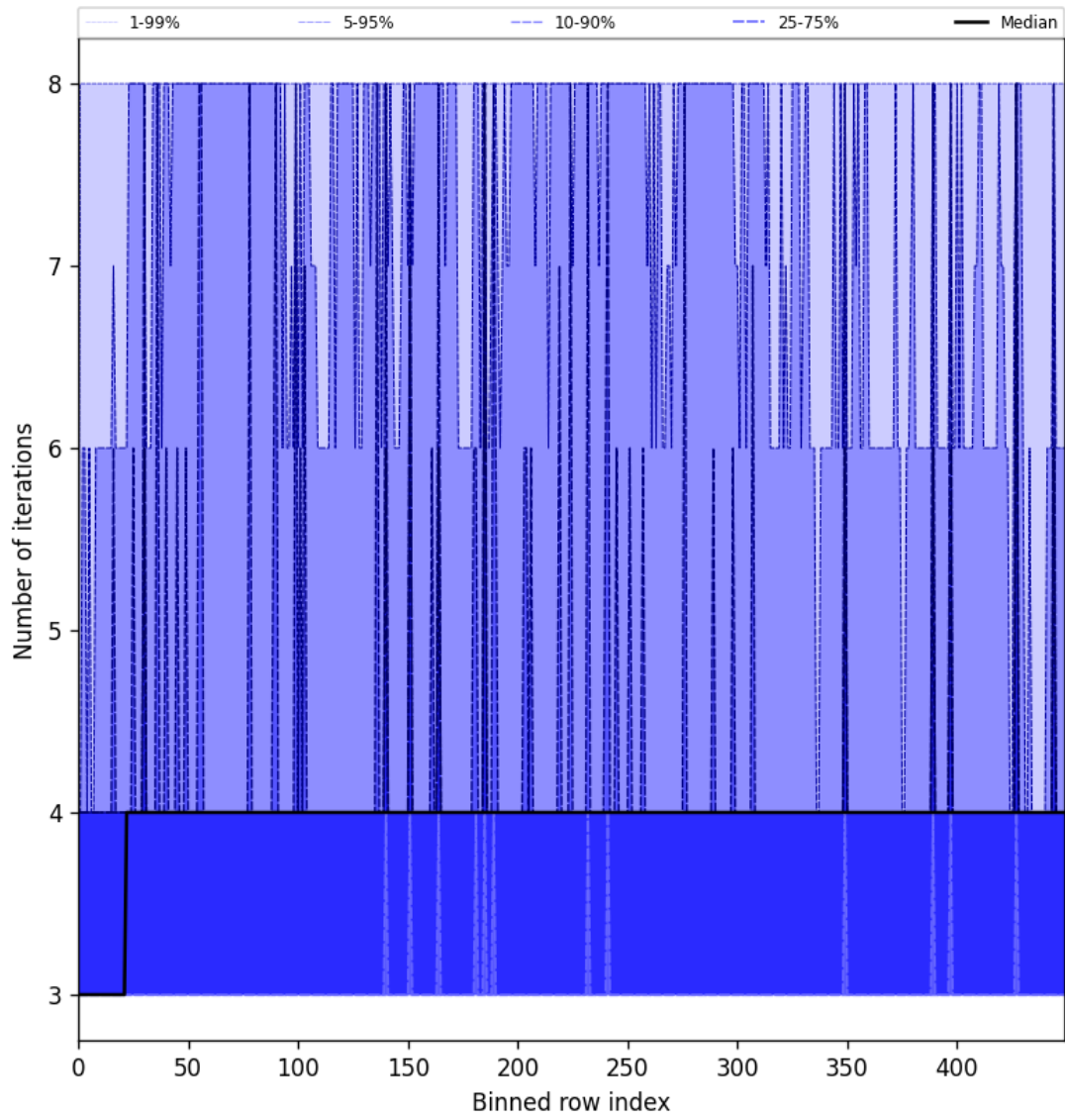
Figure 51: Along track statistics of “Number of iterations” for 2025-06-17 to 2025-06-18
