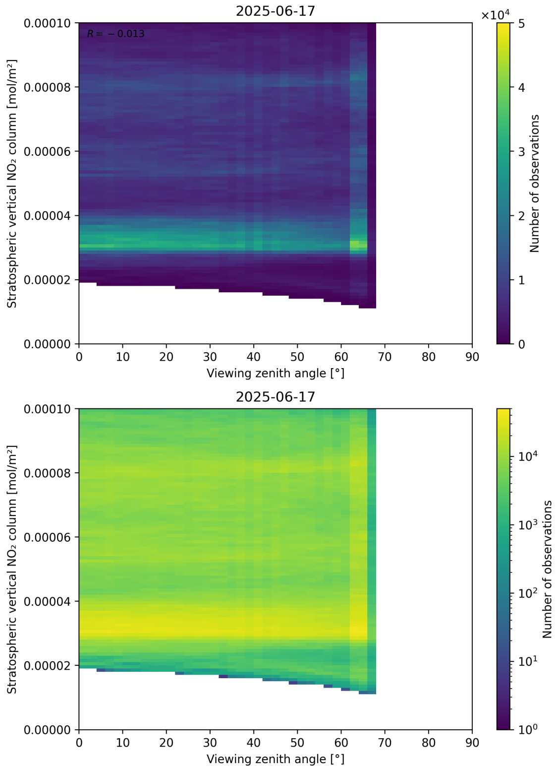
Figure 164: Scatter density plot of “Viewing zenith angle” against “Stratospheric vertical NO 2 column” for 2025-06-17 to 2025-06-18.
