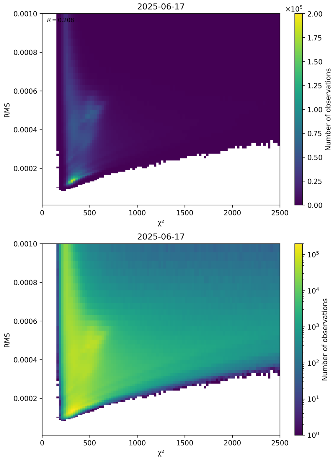
Figure 82: Scatter density plot of “ \chi^2 ” against “RMS” for 2025-06-17 to 2025-06-18.
