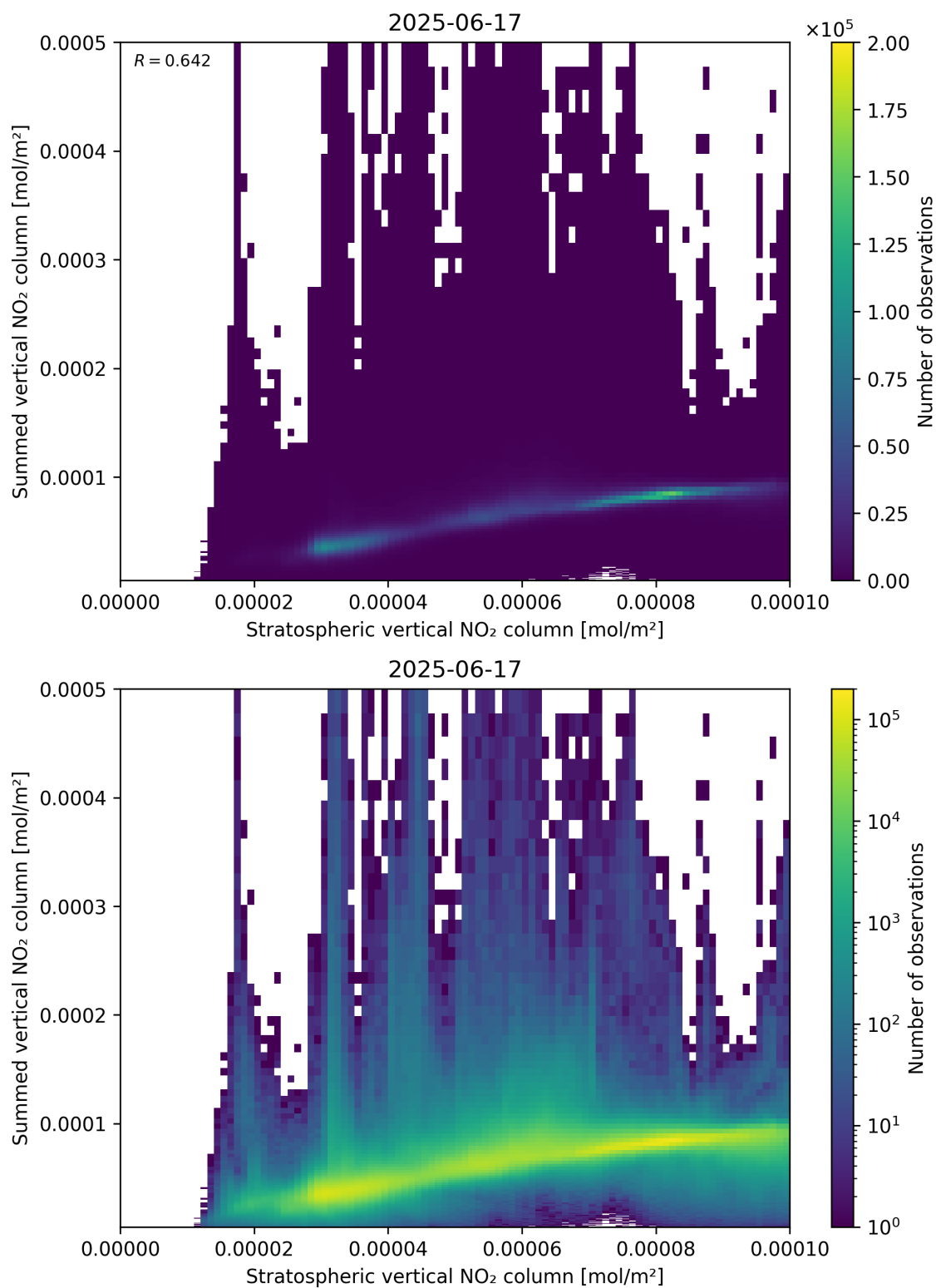
Figure 98: Scatter density plot of “Stratospheric vertical NO 2 column” against “Summed vertical NO 2 column” for 2025-06-17 to 2025-06-18.
