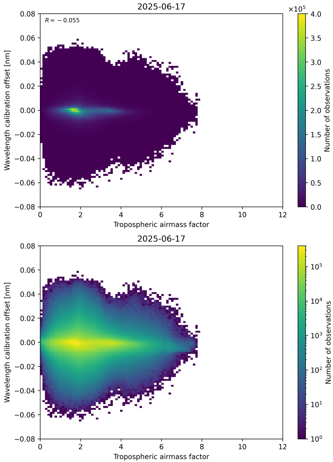
Figure 80: Scatter density plot of “Tropospheric airmass factor” against “Wavelength calibration offset” for 2025-06-17 to 2025-06-18.
