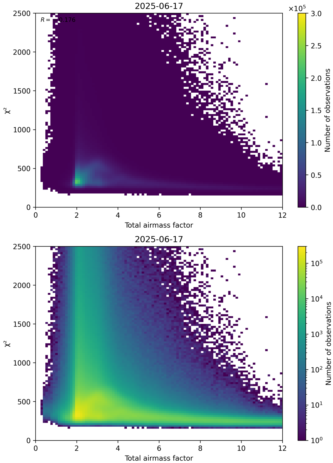
Figure 63: Scatter density plot of “Total airmass factor” against “ \chi^2 ” for 2025-06-17 to 2025-06-18.
