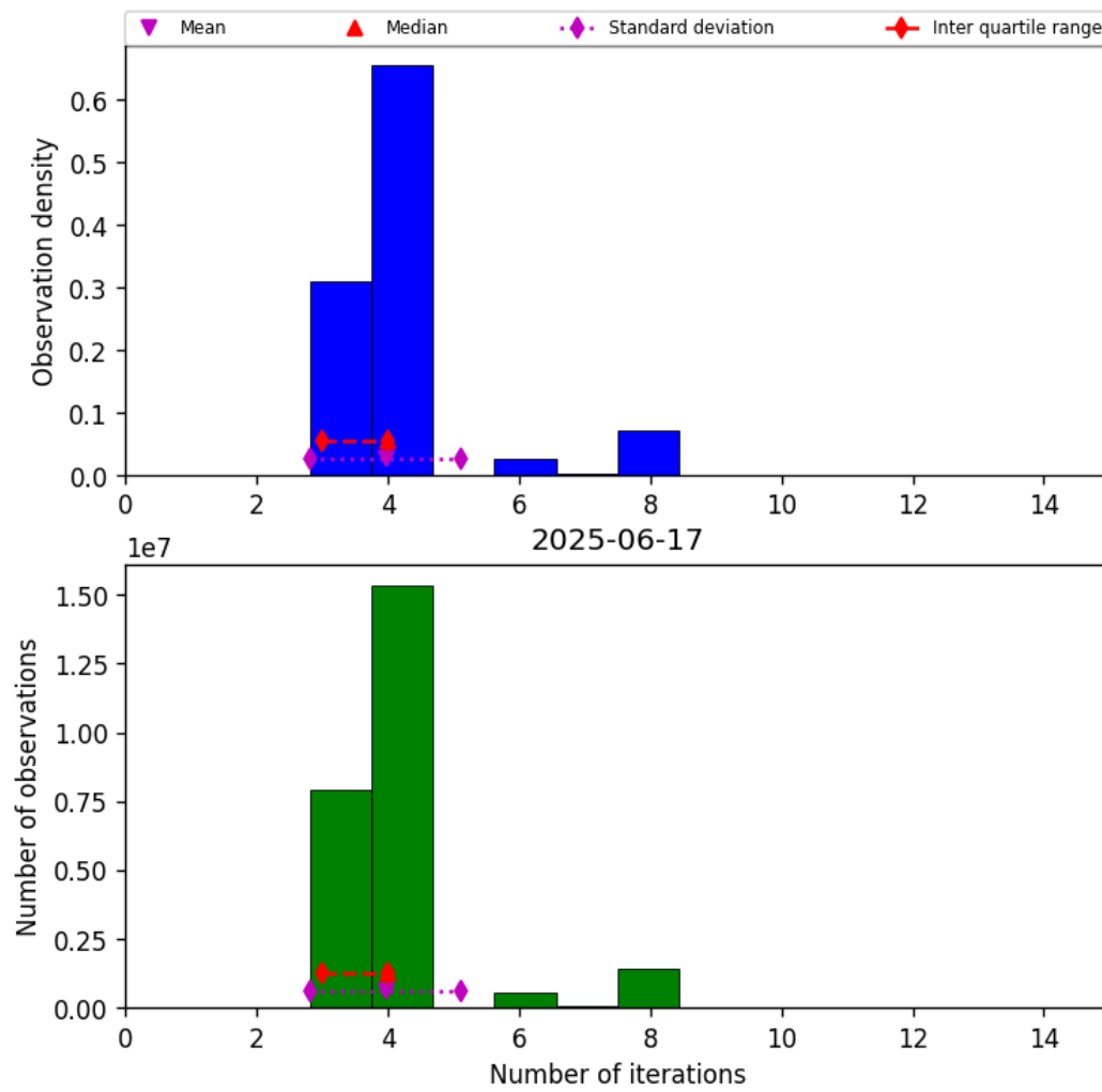
Figure 34: Histogram of “Number of iterations” for 2025-06-17 to 2025-06-18
