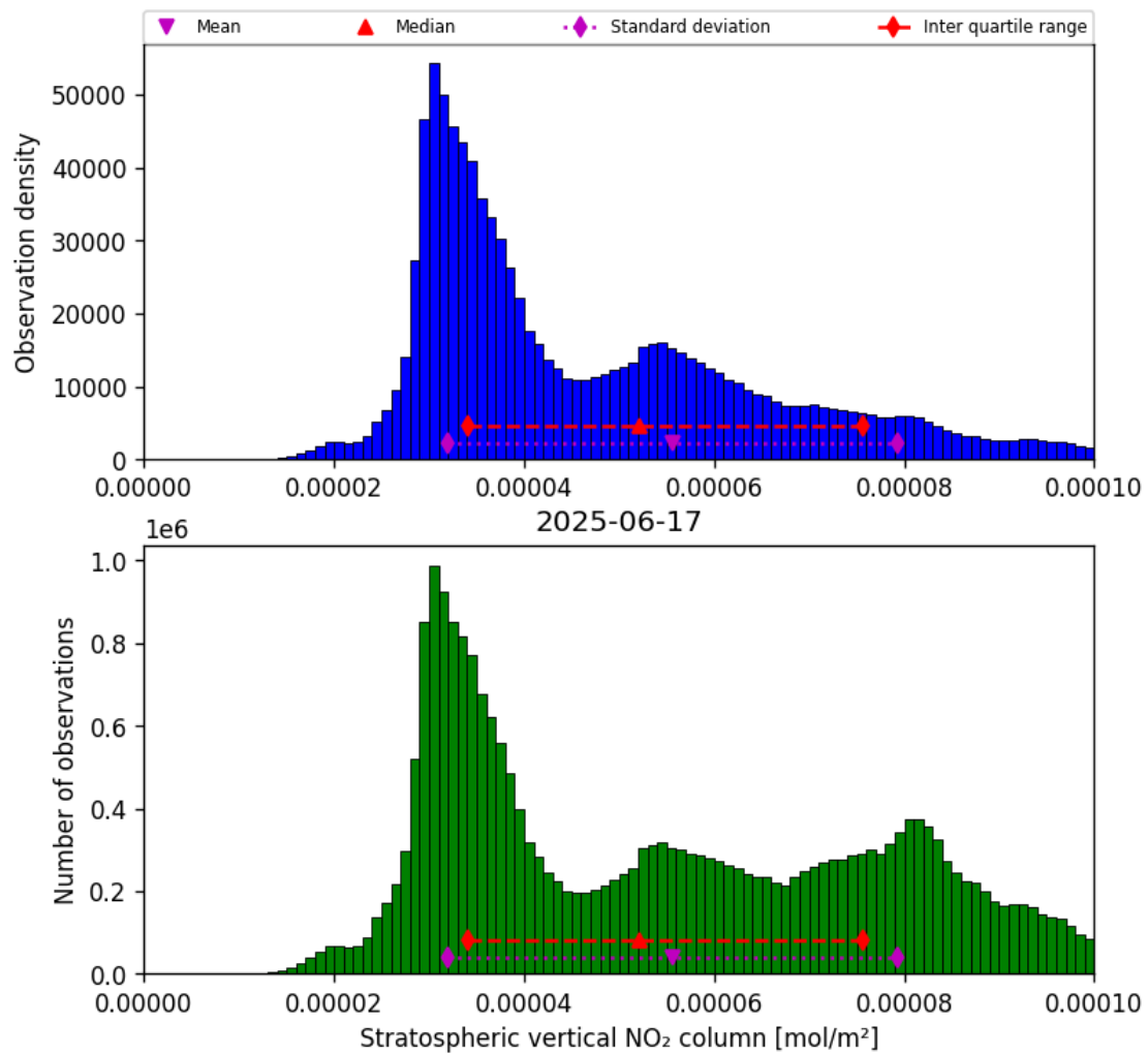
Figure 36: Histogram of “Stratospheric vertical NO 2 column” for 2025-06-17 to 2025-06-18
