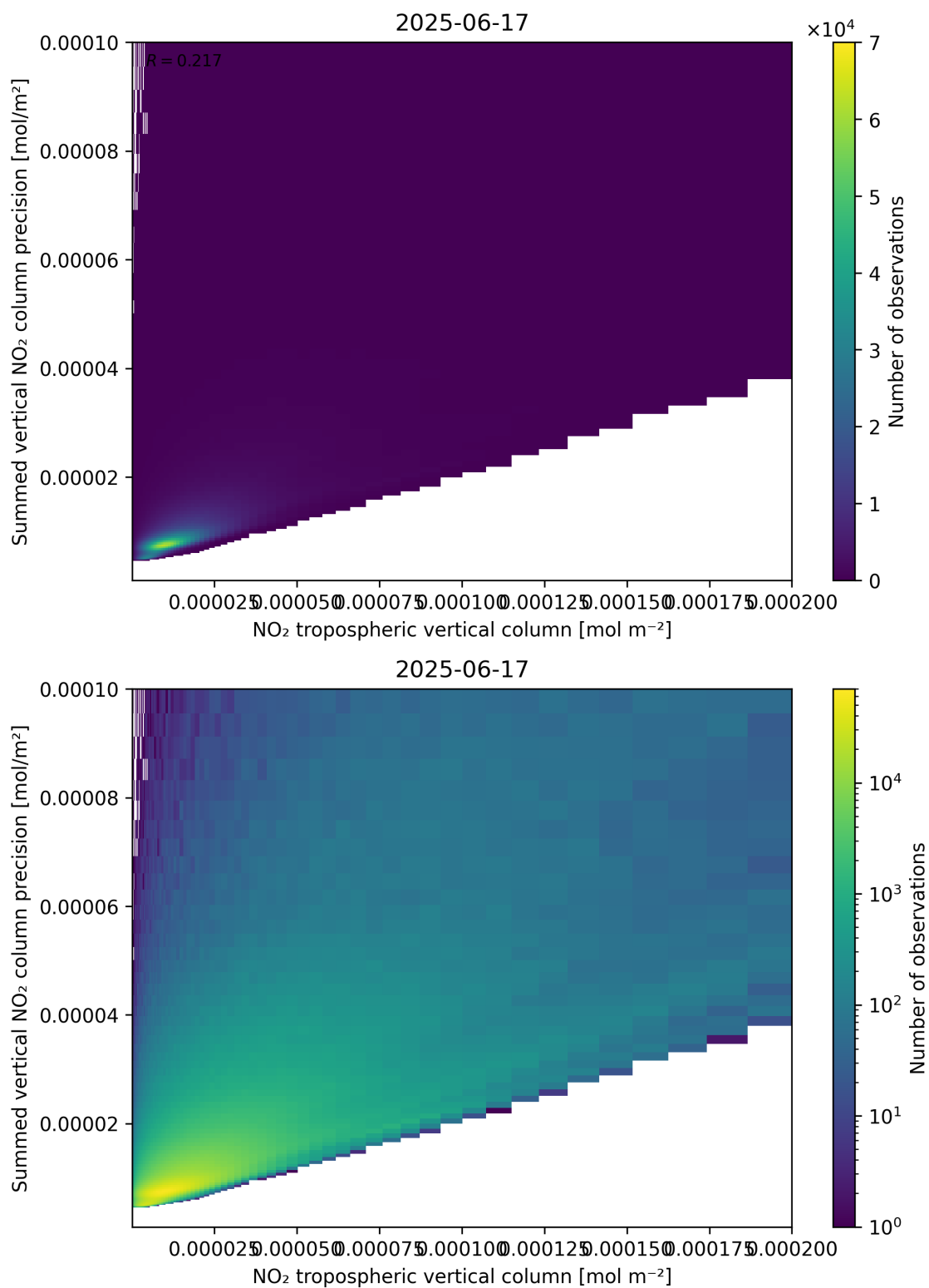
Figure 127: Scatter density plot of “NO 2 tropospheric vertical column” against “Summed vertical NO 2 column precision” for 2025-06-17 to 2025-06-18.
