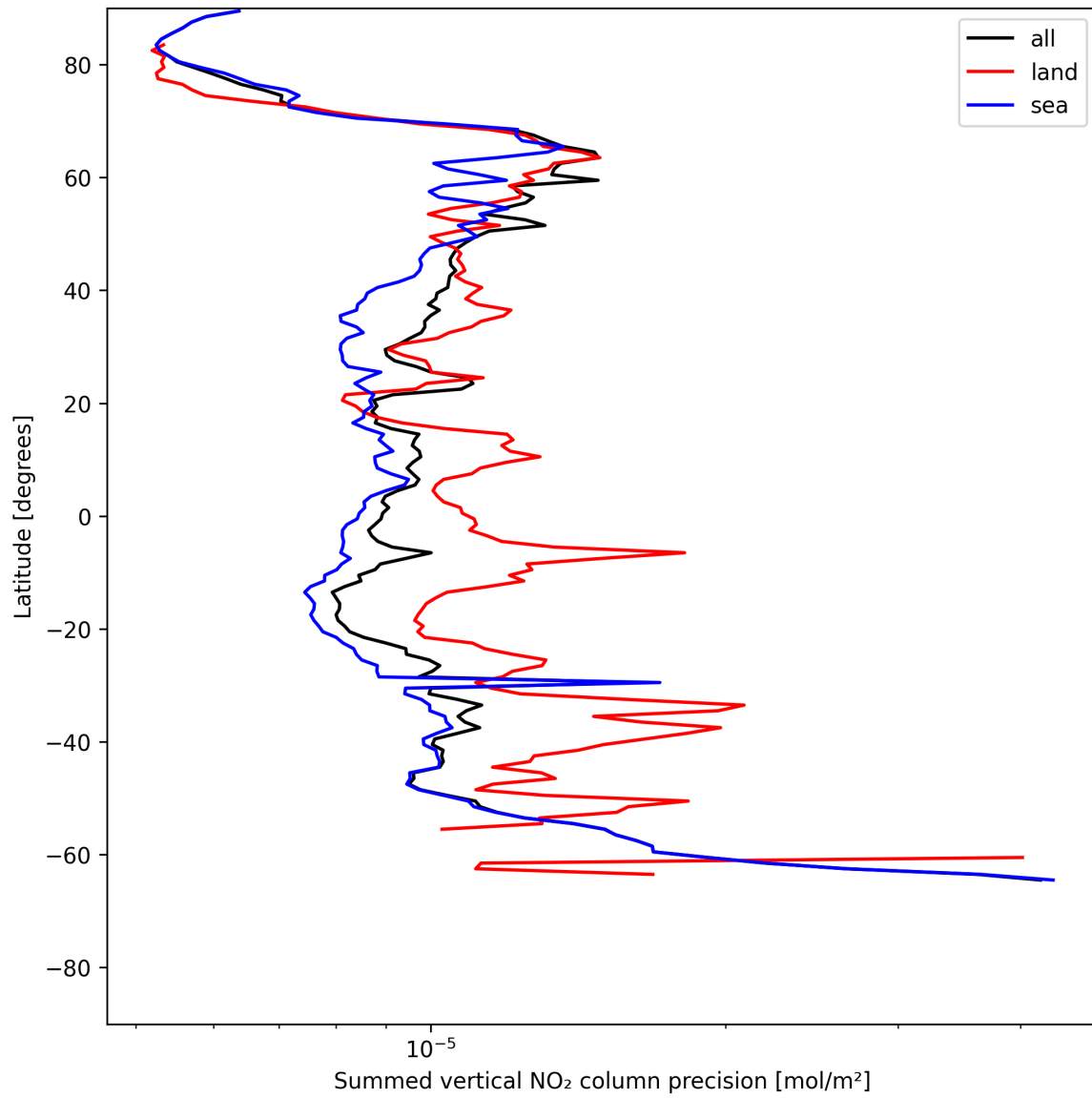
Figure 24: Zonal average of “Summed vertical NO 2 column precision” for 2025-06-17 to 2025-06-18.
