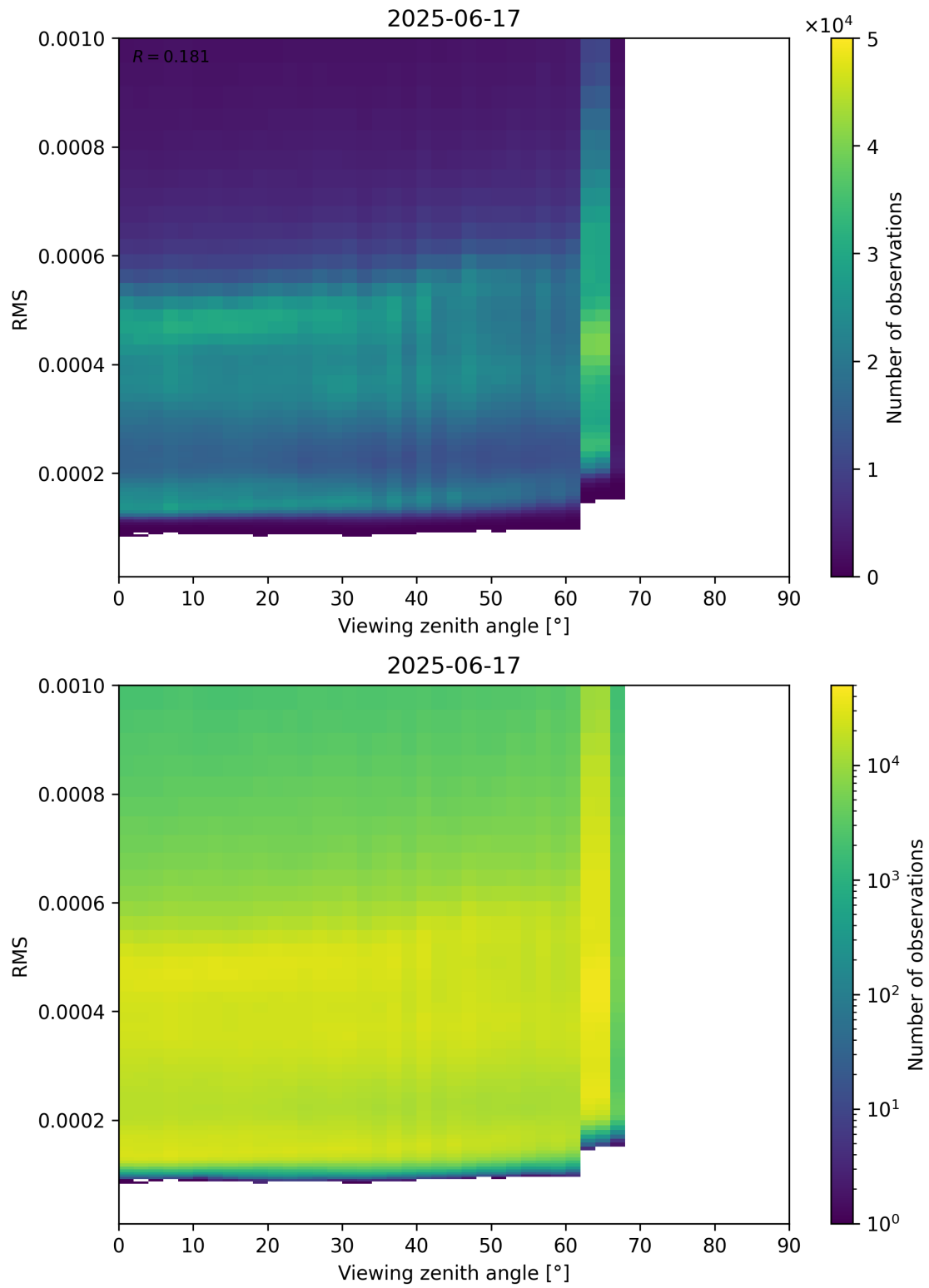
Figure 171: Scatter density plot of “Viewing zenith angle” against “RMS” for 2025-06-17 to 2025-06-18.
