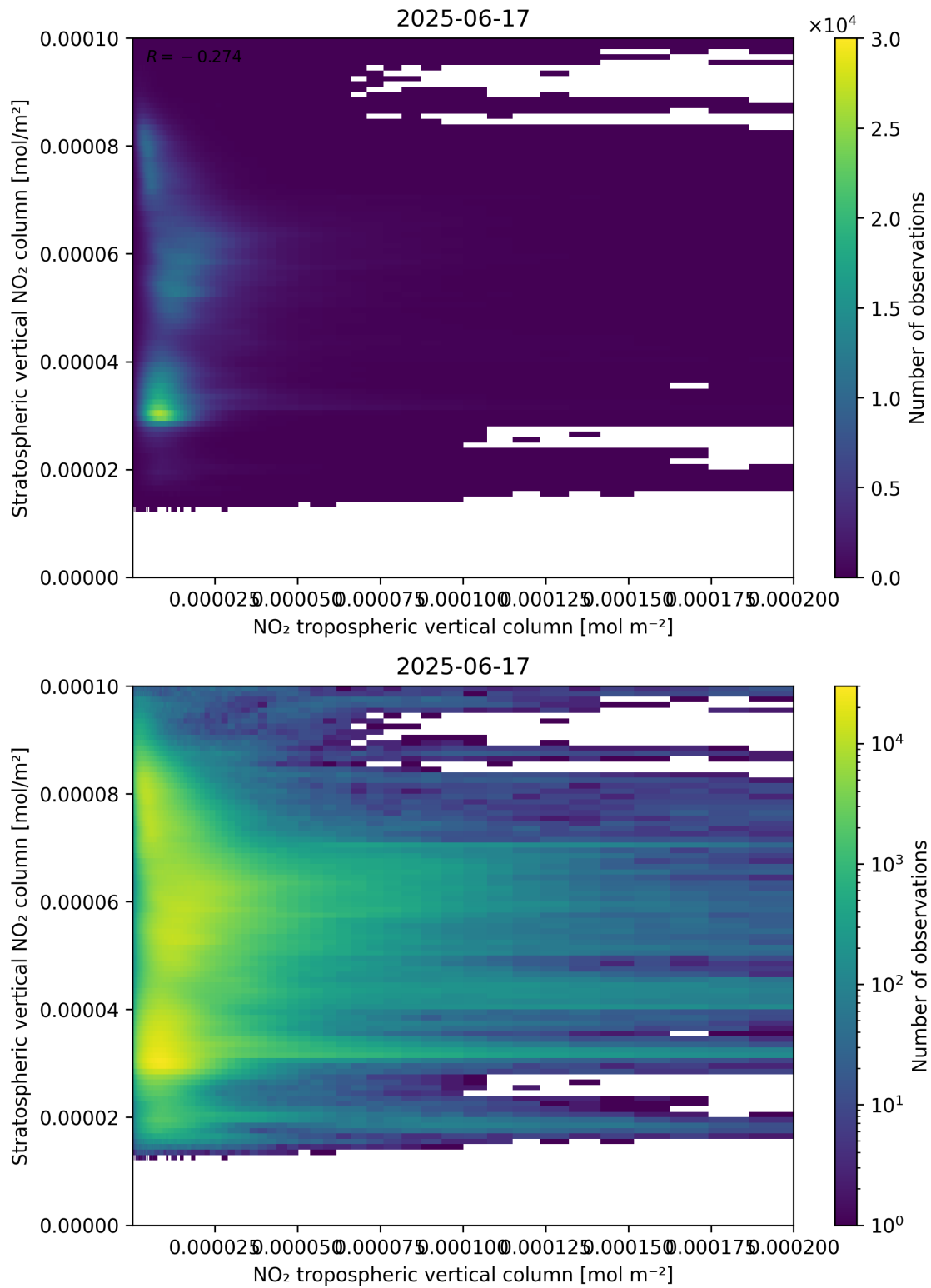
Figure 125: Scatter density plot of “NO 2 tropospheric vertical column” against “Stratospheric vertical NO 2 column” for 2025-06-17 to 2025-06-18.
