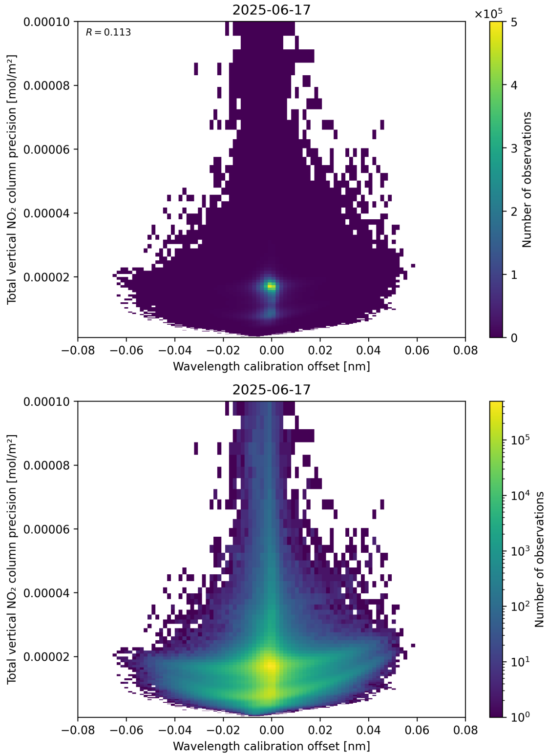
Figure 180: Scatter density plot of “Wavelength calibration offset” against “Total vertical NO 2 column precision” for 2025-06-17 to 2025-06-18.
