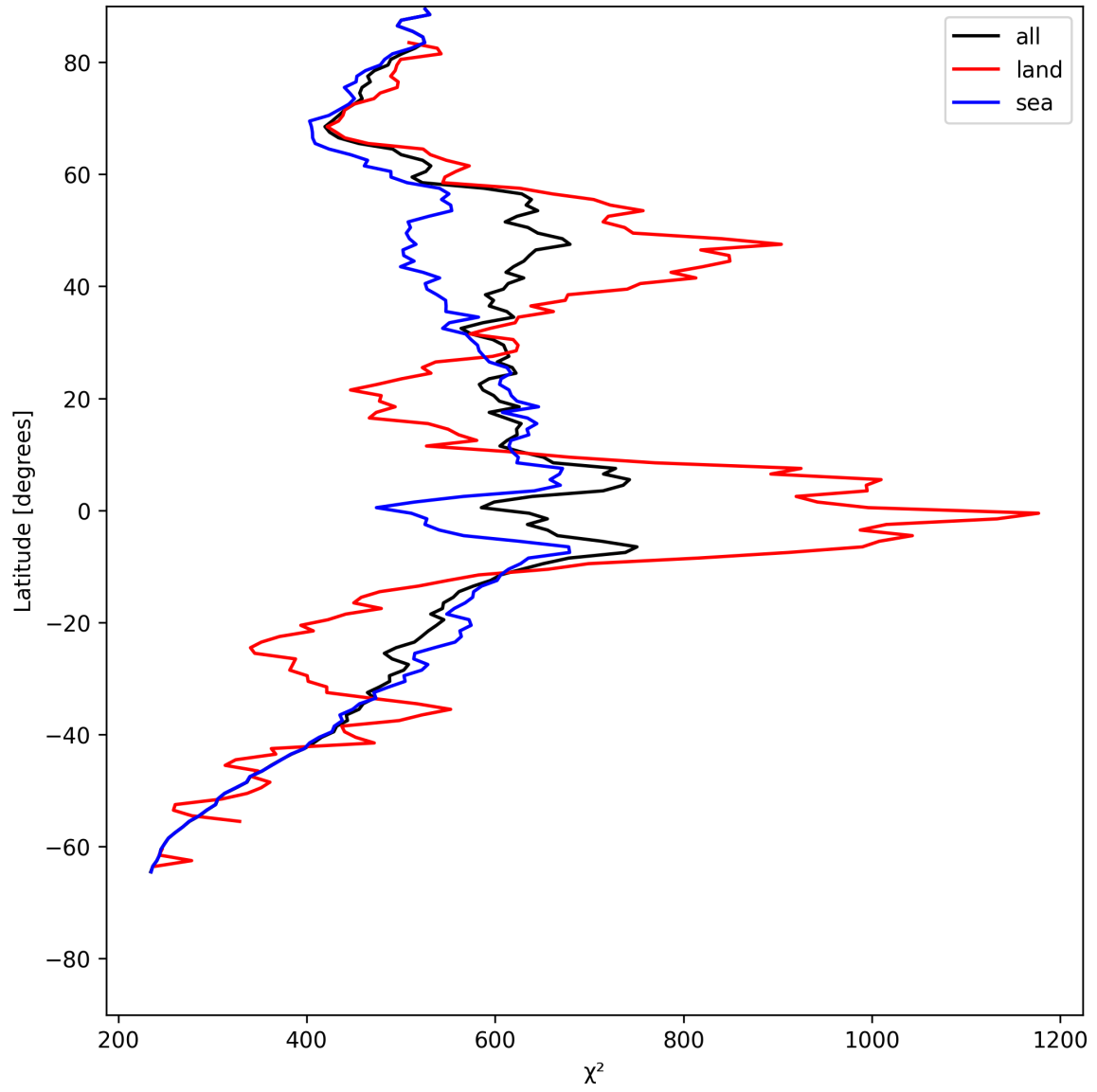
Figure 25: Zonal average of “ \chi^2 ” for 2025-06-17 to 2025-06-18.
