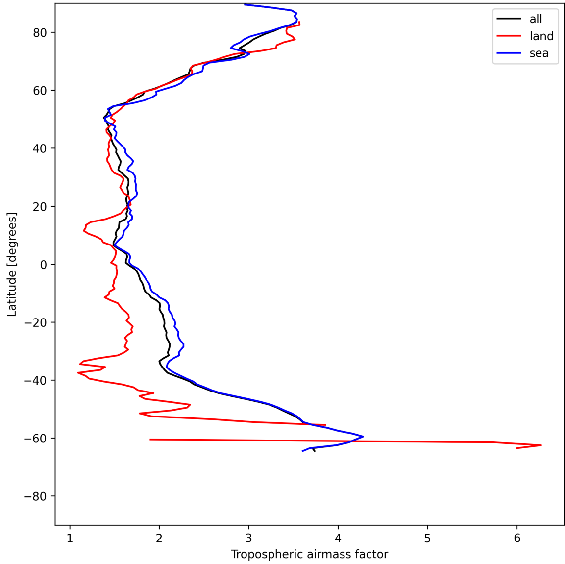
Figure 14: Zonal average of “Tropospheric airmass factor” for 2025-06-17 to 2025-06-18.
