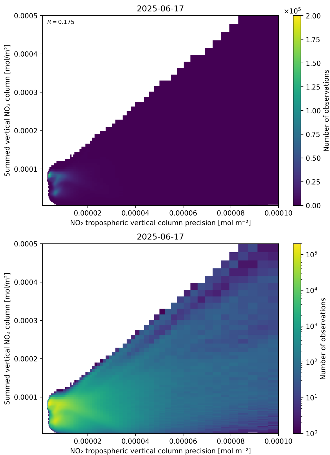
Figure 136: Scatter density plot of “NO 2 tropospheric vertical column precision” against “Summed vertical NO 2 column” for 2025-06-17 to 2025-06-18.
