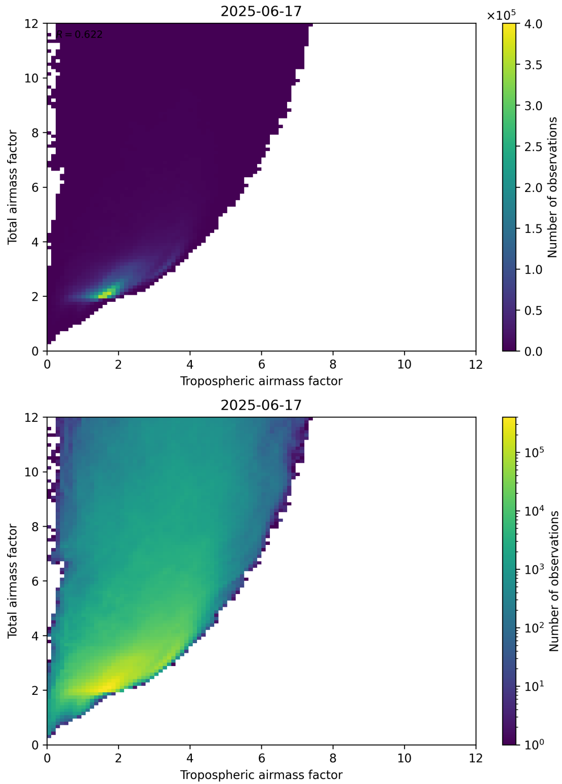
Figure 72: Scatter density plot of “Tropospheric airmass factor” against “Total airmass factor” for 2025-06-17 to 2025-06-18.
