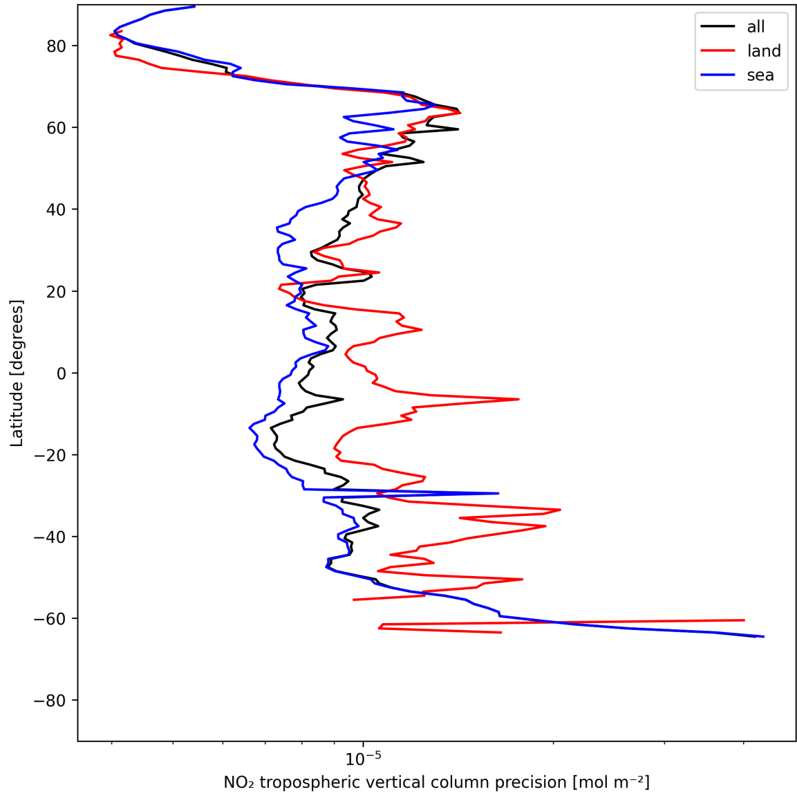
Figure 13: Zonal average of “NO 2 tropospheric vertical column precision” for 2025-06-17 to 2025-06-18.
