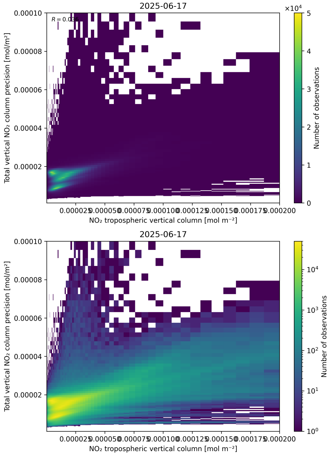
Figure 129: Scatter density plot of “NO 2 tropospheric vertical column” against “Total vertical NO 2 column precision” for 2025-06-17 to 2025-06-18.
