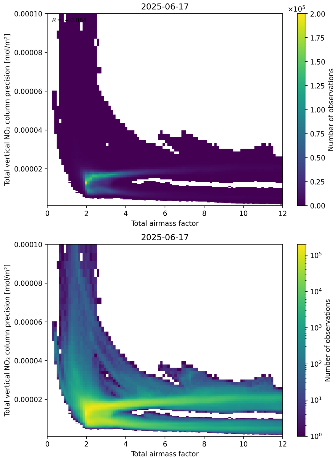
Figure 68: Scatter density plot of “Total airmass factor” against “Total vertical NO 2 column precision” for 2025-06-17 to 2025-06-18.
