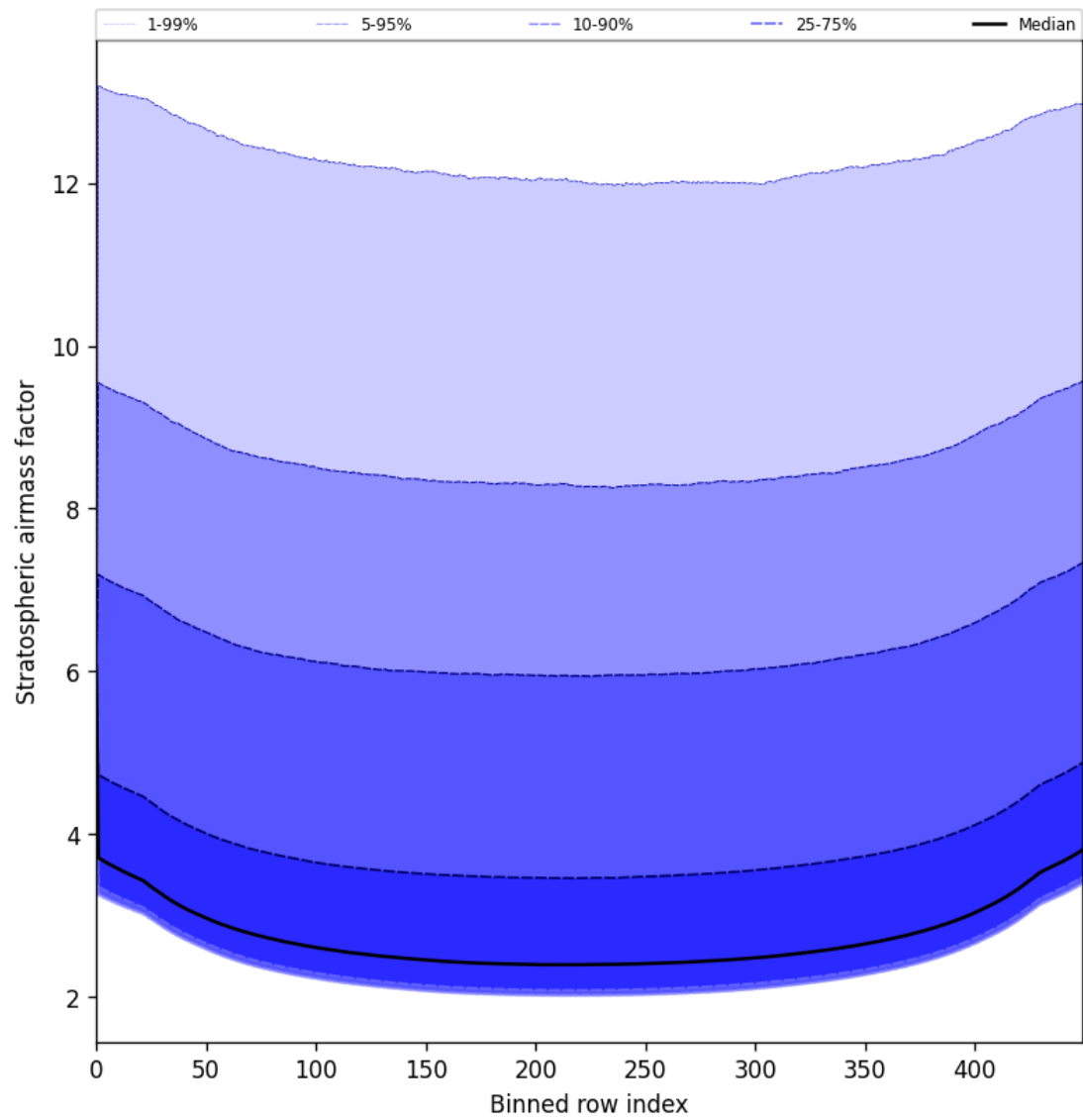
Figure 61: Along track statistics of “Stratospheric airmass factor” for 2025-06-17 to 2025-06-18
