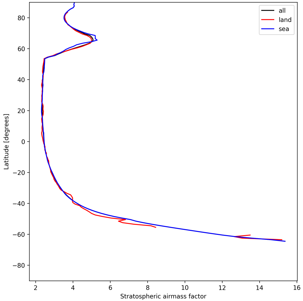
Figure 27: Zonal average of “Stratospheric airmass factor” for 2025-06-17 to 2025-06-18.
