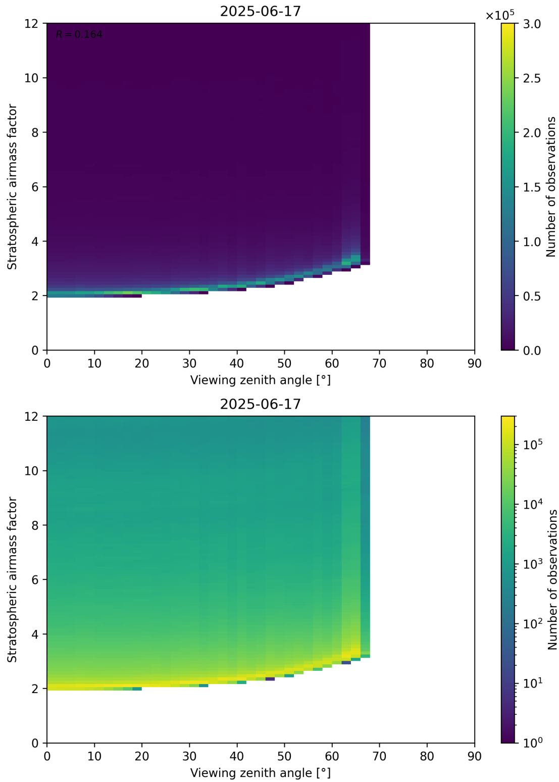
Figure 159: Scatter density plot of “Viewing zenith angle” against “Stratospheric airmass factor” for 2025-06-17 to 2025-06-18.
