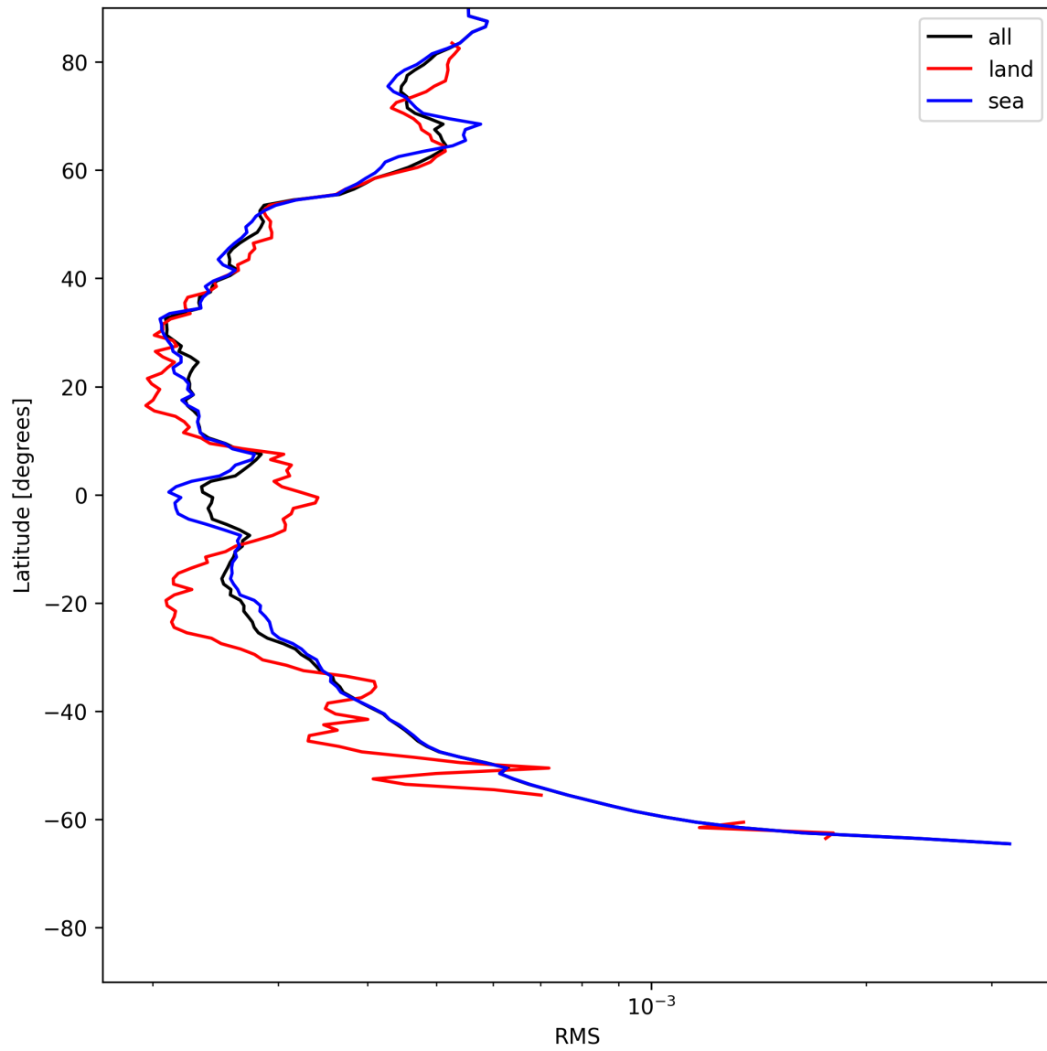
Figure 26: Zonal average of “RMS” for 2025-06-17 to 2025-06-18.
