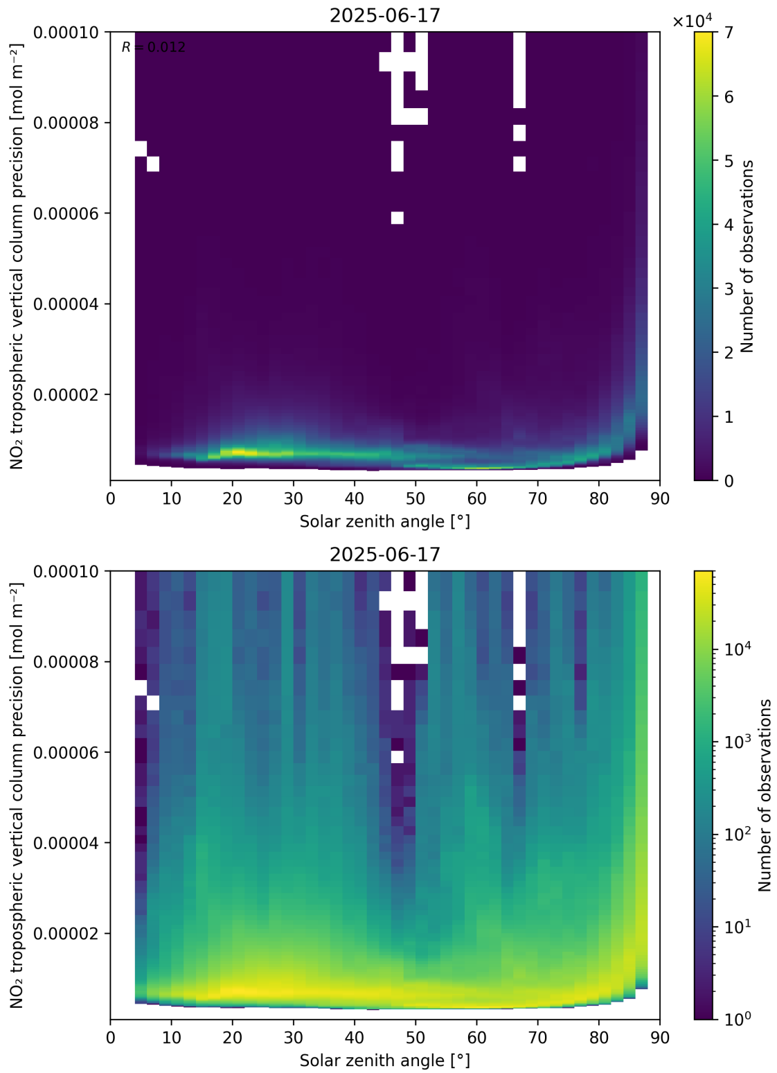
Figure 156: Scatter density plot of “Solar zenith angle” against “NO 2 tropospheric vertical column precision” for 2025-06-17 to 2025-06-18.
