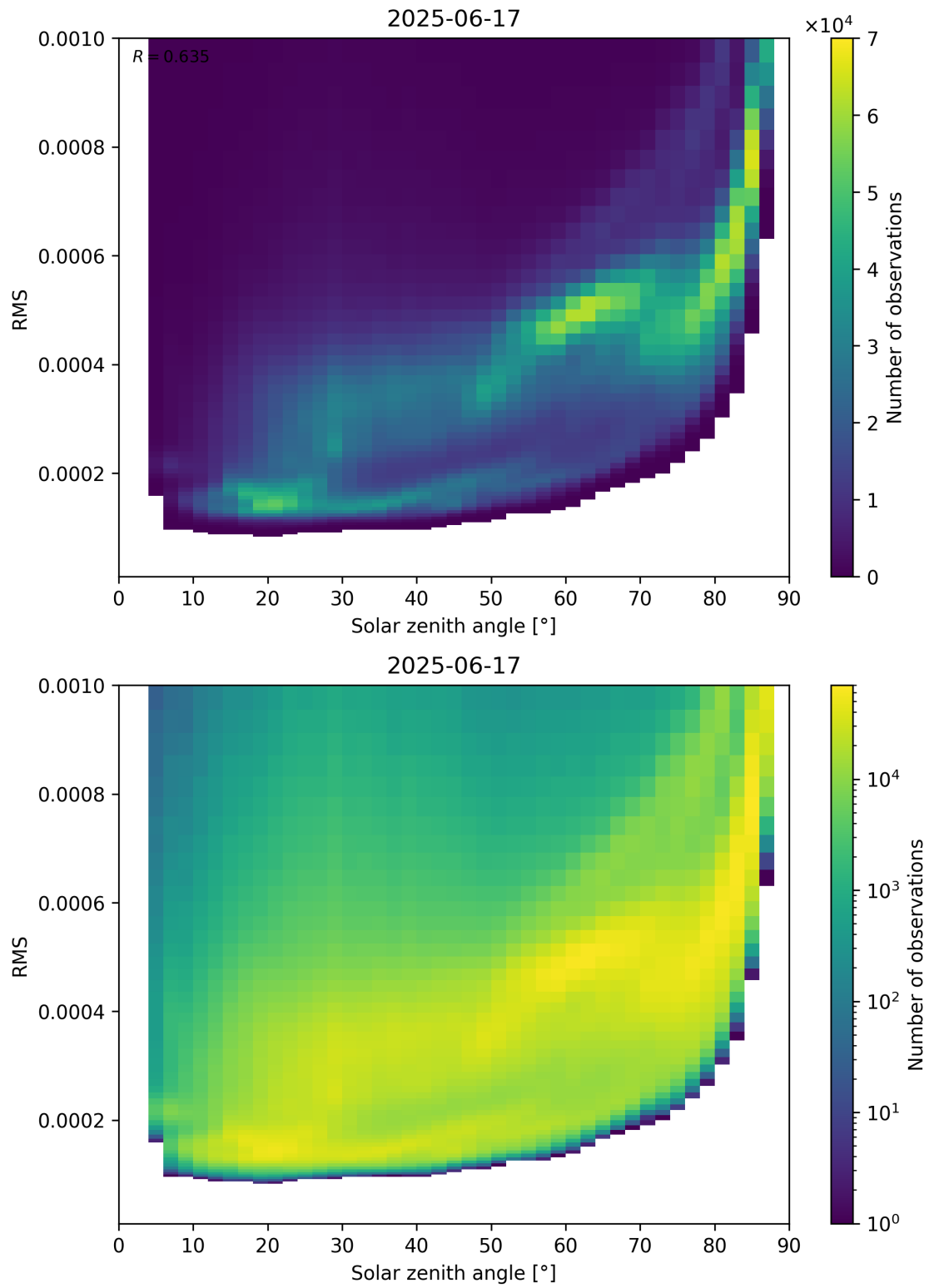
Figure 157: Scatter density plot of “Solar zenith angle” against “RMS” for 2025-06-17 to 2025-06-18.
