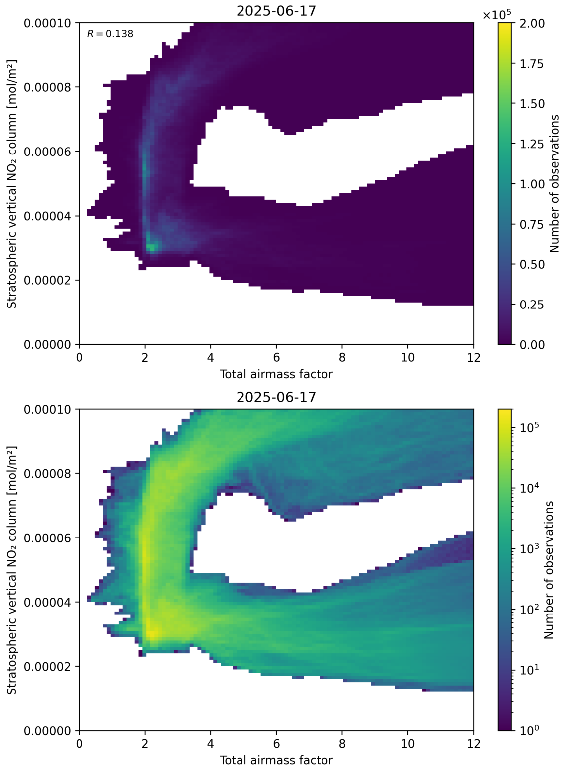
Figure 64: Scatter density plot of “Total airmass factor” against “Stratospheric vertical NO 2 column” for 2025-06-17 to 2025-06-18.
