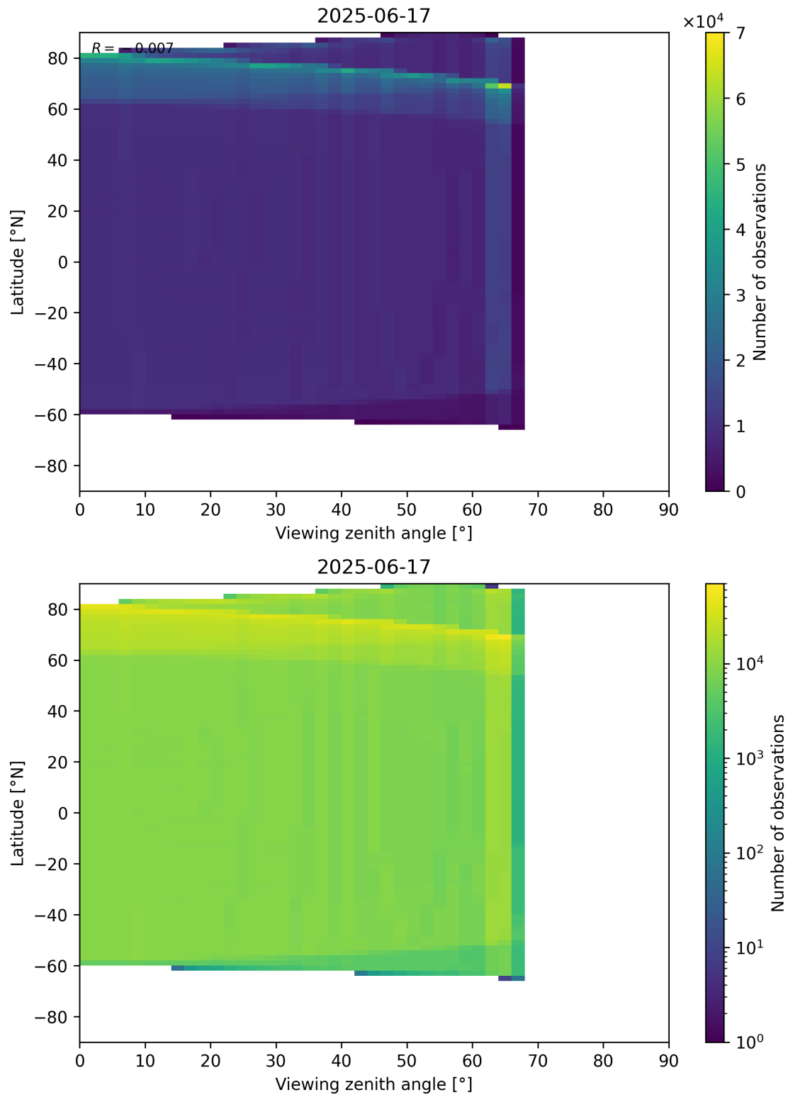
Figure 163: Scatter density plot of “Viewing zenith angle” against “Latitude” for 2025-06-17 to 2025-06-18.
