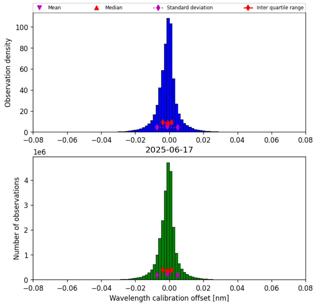
Figure 35: Histogram of “Wavelength calibration offset” for 2025-06-17 to 2025-06-18
