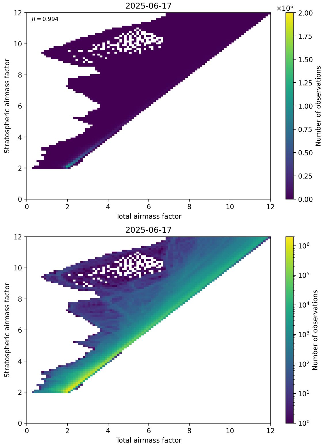
Figure 62: Scatter density plot of “Total airmass factor” against “Stratospheric airmass factor” for 2025-06-17 to 2025-06-18.
