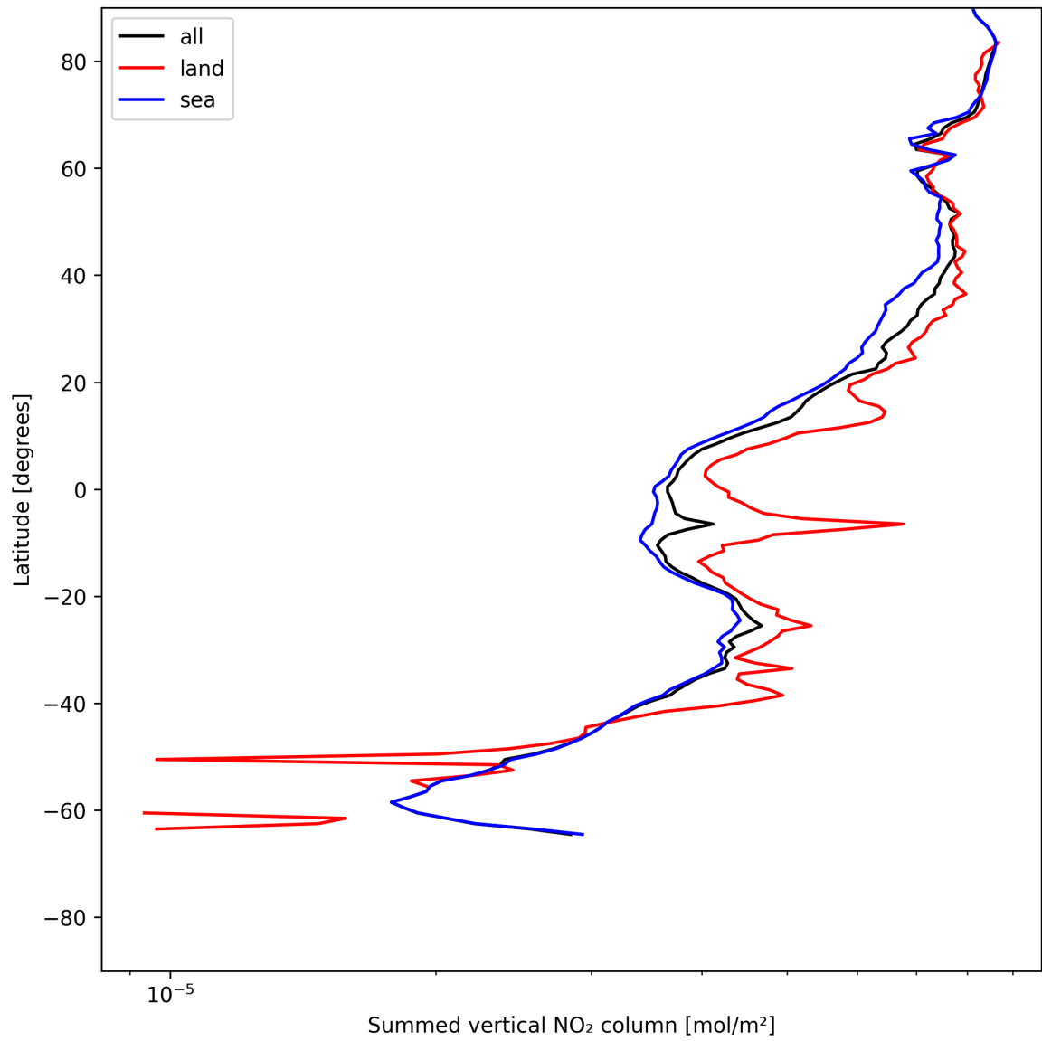
Figure 23: Zonal average of “Summed vertical NO 2 column” for 2025-06-17 to 2025-06-18.
