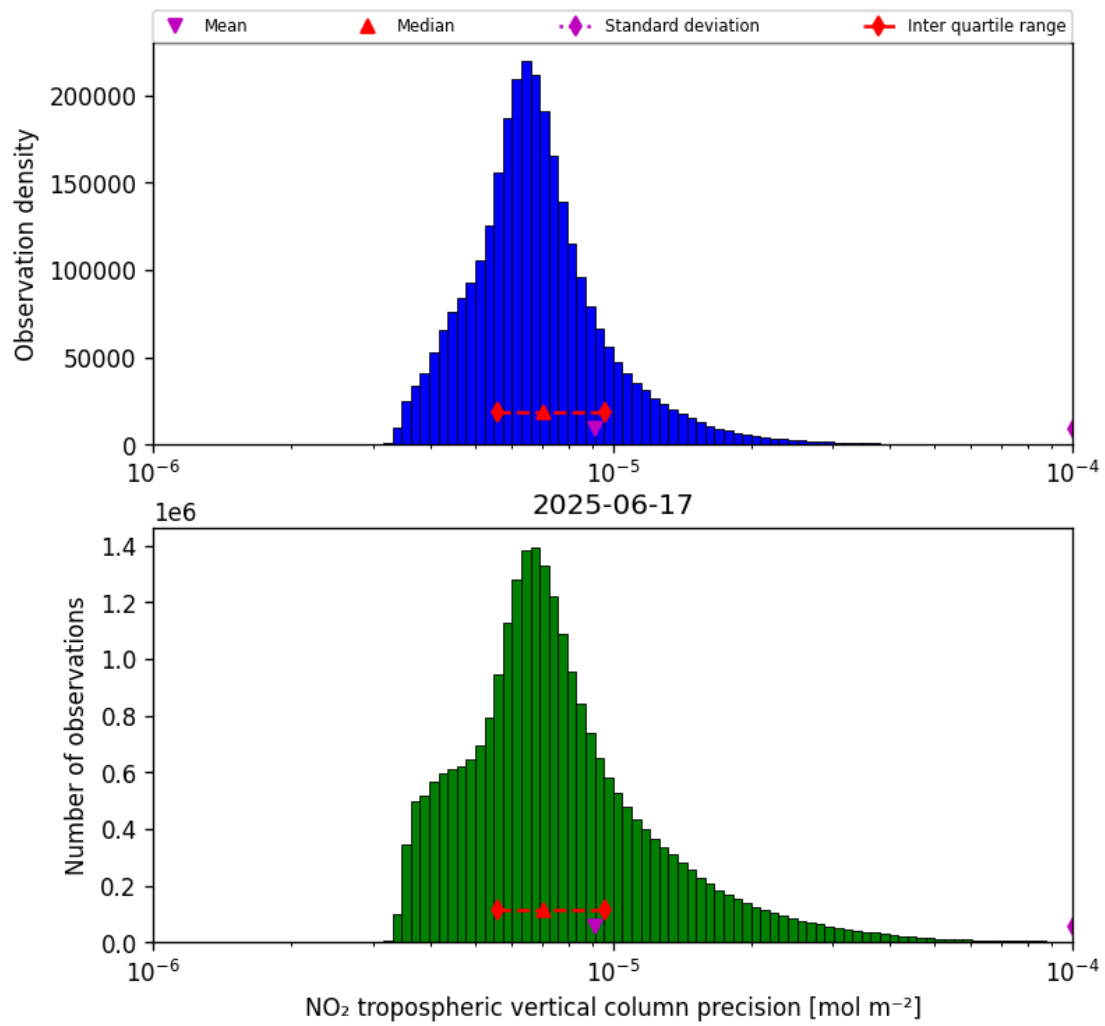
Figure 30: Histogram of “NO 2 tropospheric vertical column precision” for 2025-06-17 to 2025-06-18
