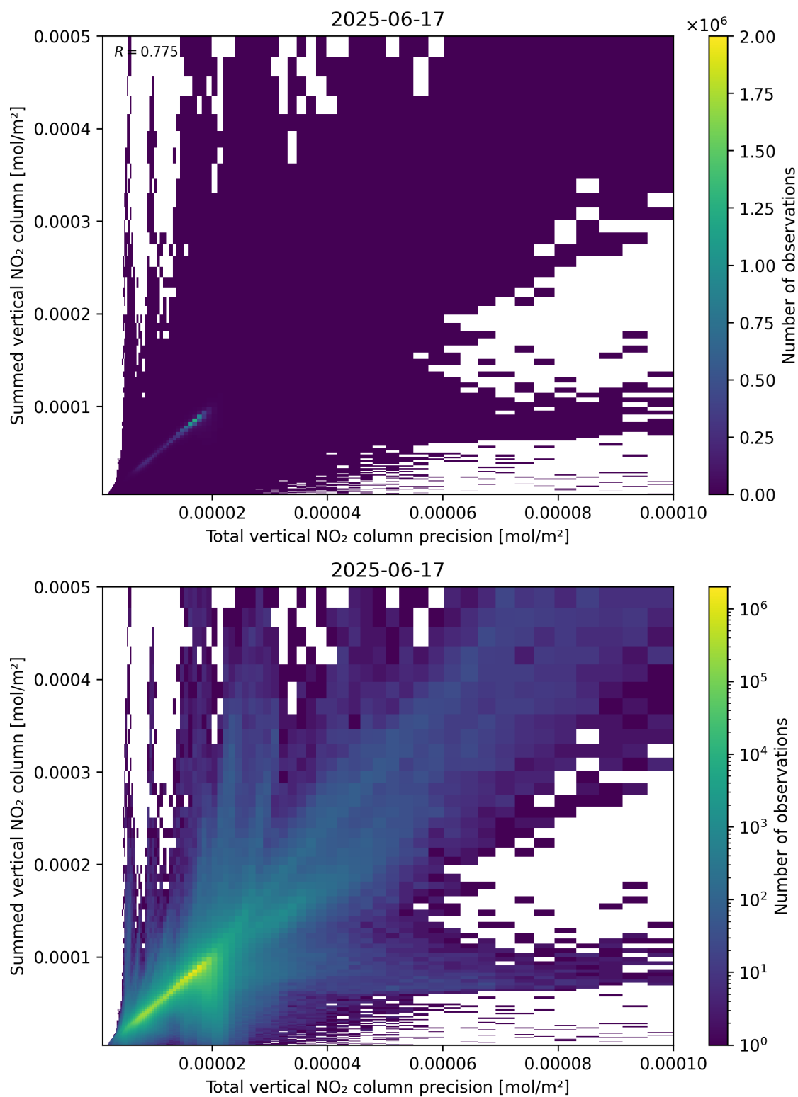
Figure 117: Scatter density plot of “Total vertical NO 2 column precision” against “Summed vertical NO 2 column” for 2025-06-17 to 2025-06-18.
