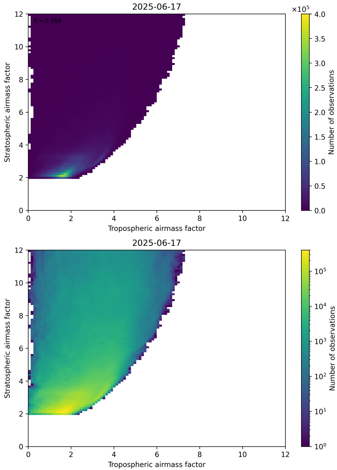
Figure 71: Scatter density plot of “Tropospheric airmass factor” against “Stratospheric airmass factor” for 2025-06-17 to 2025-06-18.
