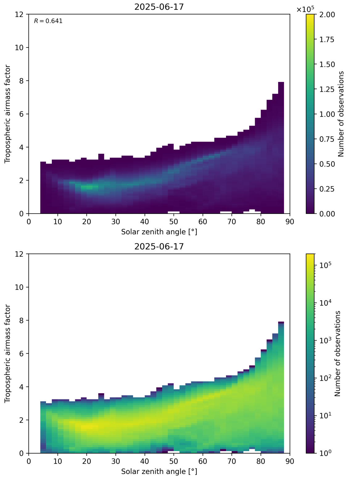
Figure 147: Scatter density plot of “Solar zenith angle” against “Tropospheric airmass factor” for 2025-06-17 to 2025-06-18.
