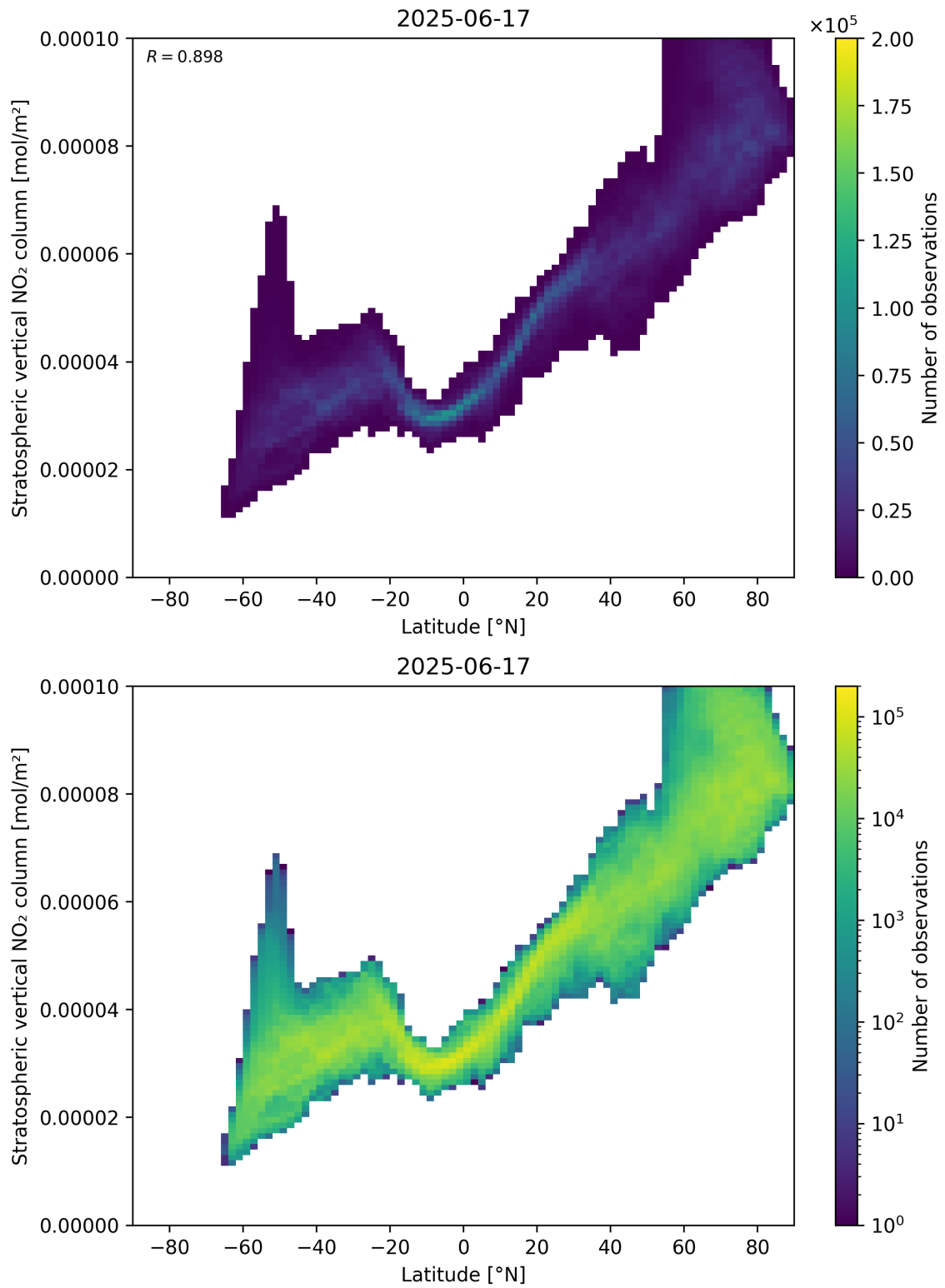
Figure 87: Scatter density plot of “Latitude” against “Stratospheric vertical \text{NO}_2 column” for 2025-06-17 to 2025-06-18.
