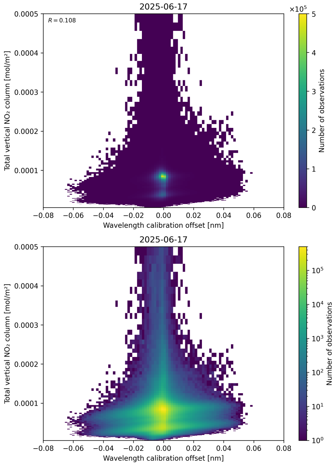
Figure 179: Scatter density plot of “Wavelength calibration offset” against “Total vertical NO 2 column” for 2025-06-17 to 2025-06-18.
