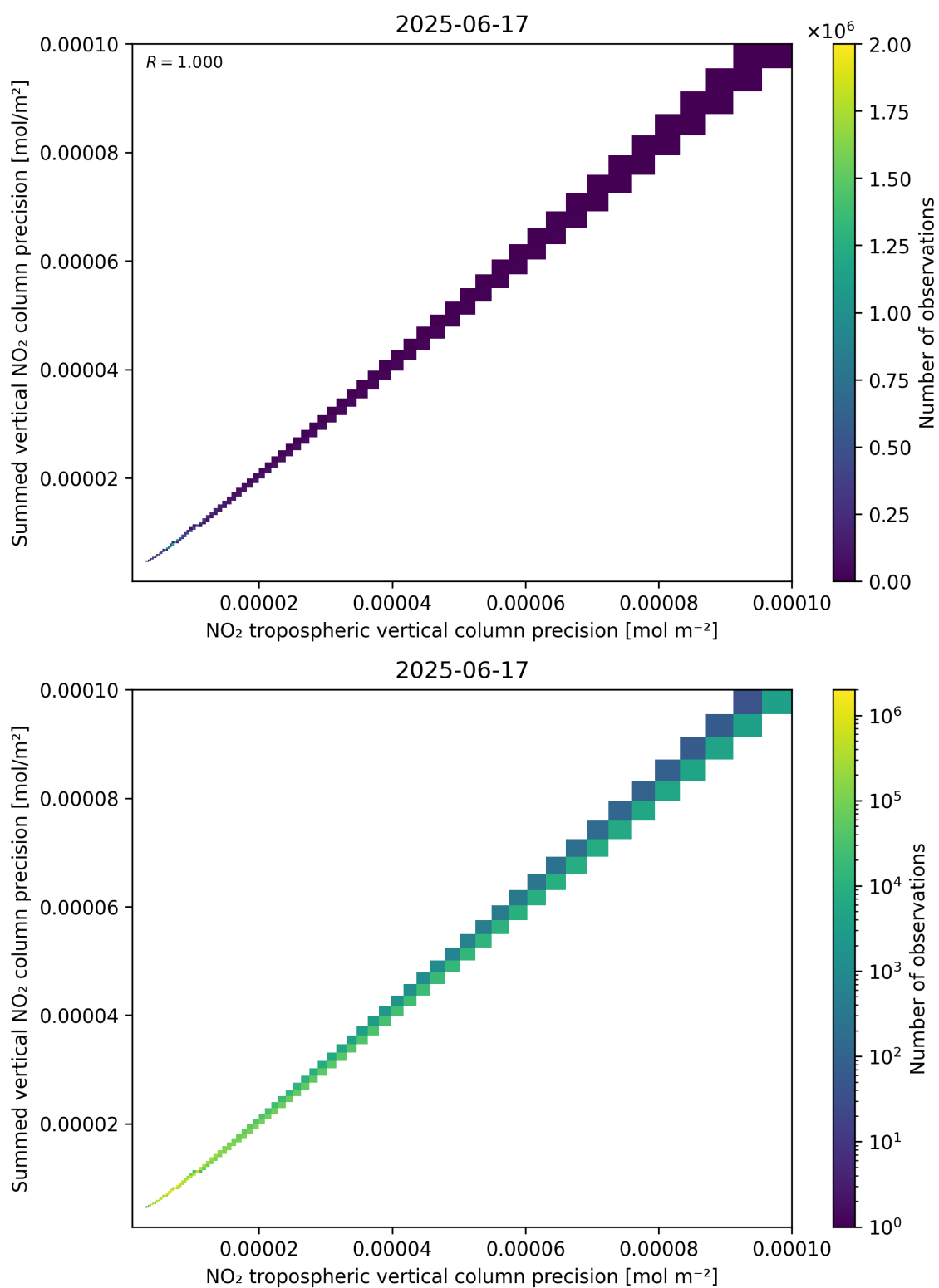
Figure 137: Scatter density plot of “NO 2 tropospheric vertical column precision” against “Summed vertical NO 2 column precision” for 2025-06-17 to 2025-06-18.
