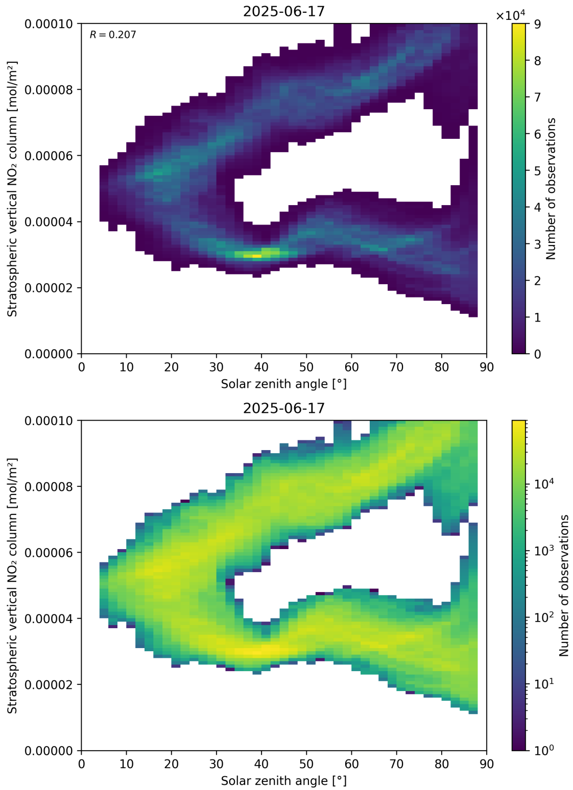
Figure 150: Scatter density plot of “Solar zenith angle” against “Stratospheric vertical NO 2 column” for 2025-06-17 to 2025-06-18.
