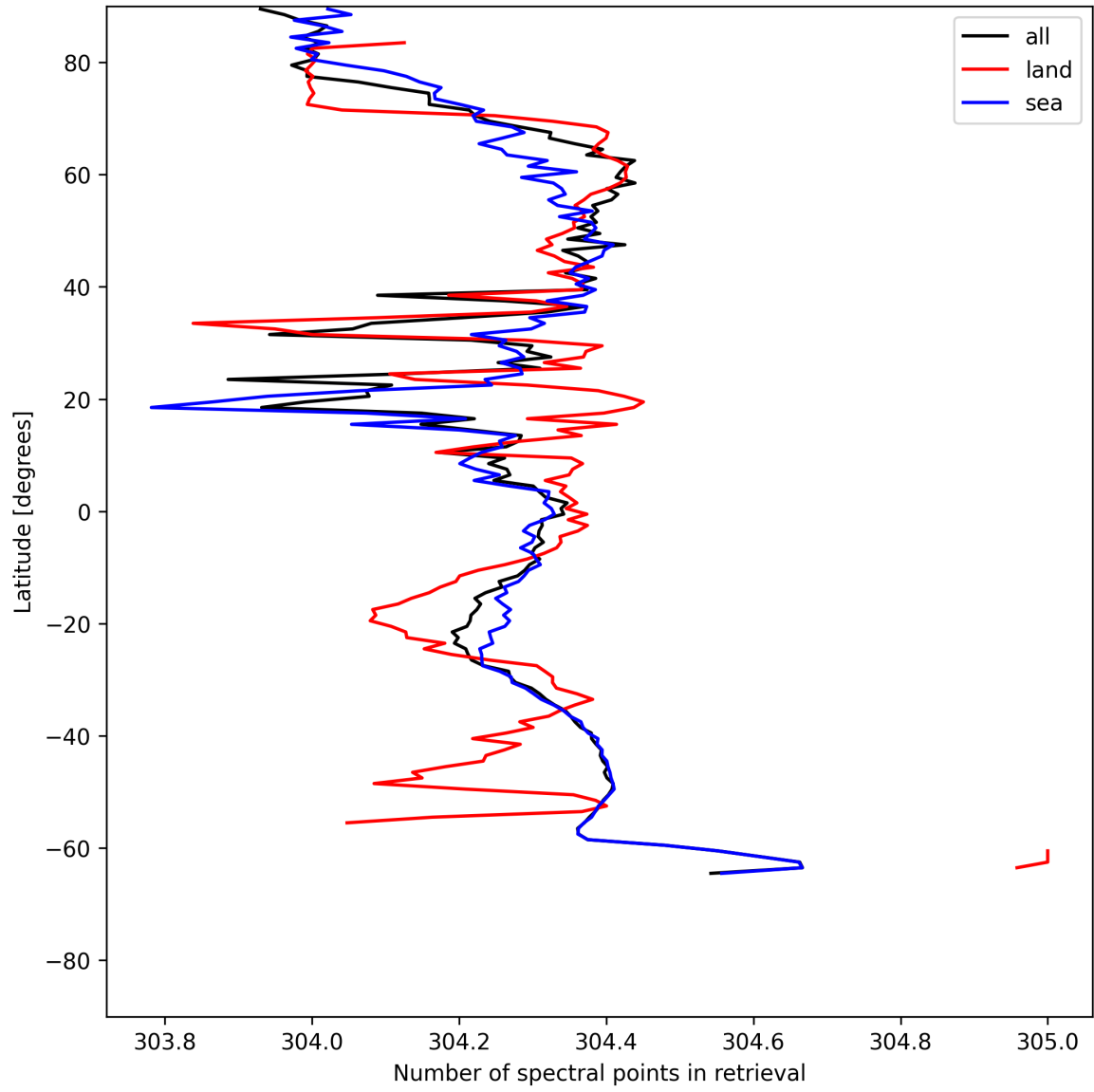
Figure 16: Zonal average of “Number of spectral points in retrieval” for 2025-06-17 to 2025-06-18.
