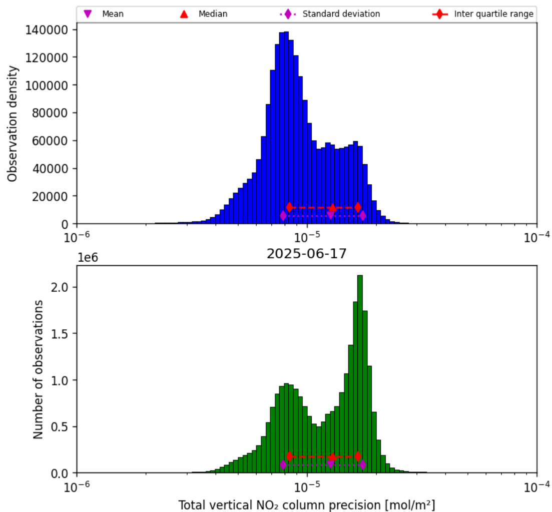
Figure 39: Histogram of “Total vertical NO 2 column precision” for 2025-06-17 to 2025-06-18
