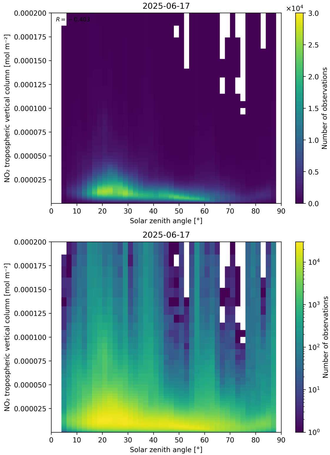
Figure 155: Scatter density plot of “Solar zenith angle” against “NO 2 tropospheric vertical column” for 2025-06-17 to 2025-06-18.
