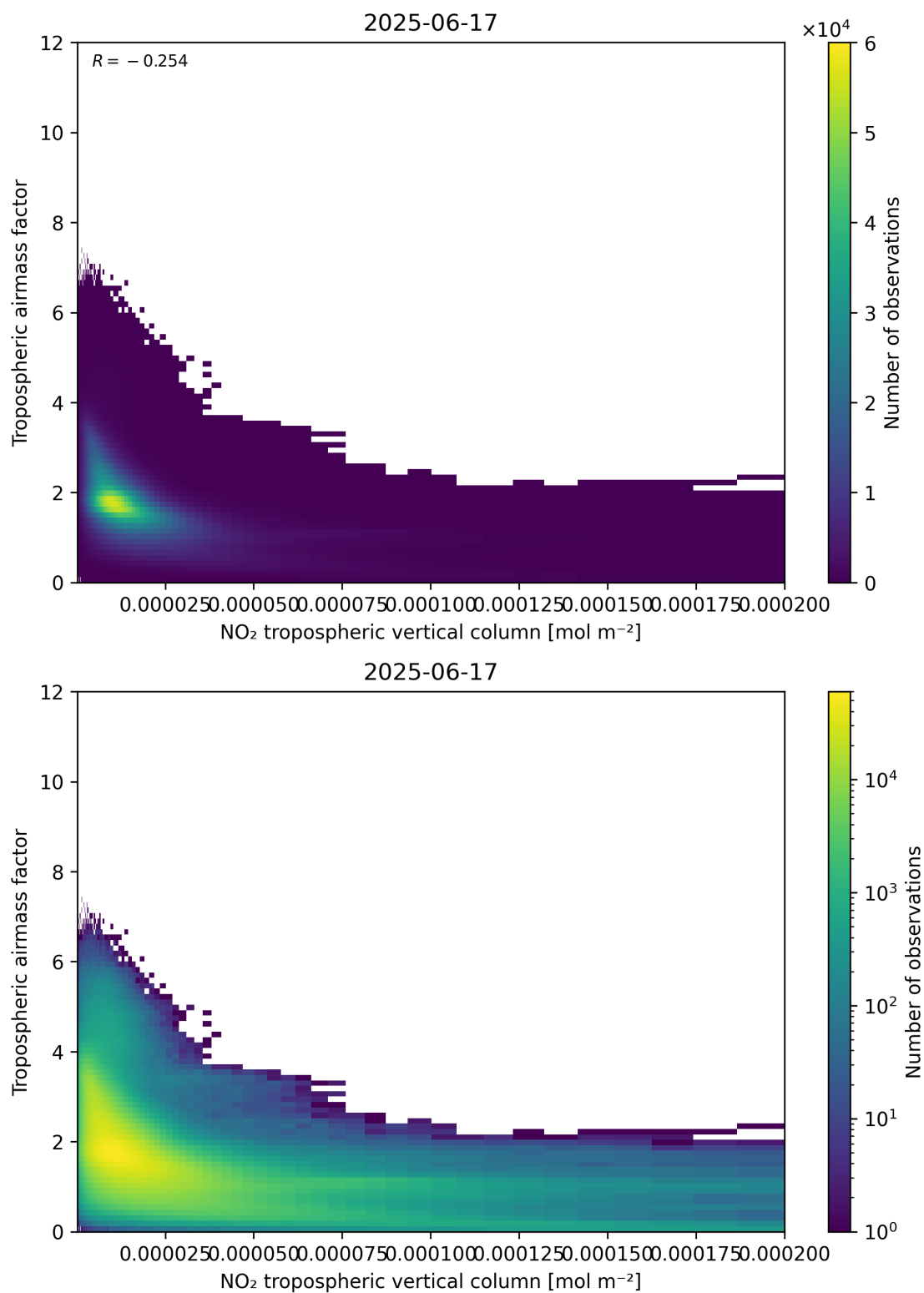
Figure 123: Scatter density plot of “NO 2 tropospheric vertical column” against “Tropospheric air mass factor” for 2025-06-17 to 2025-06-18.
