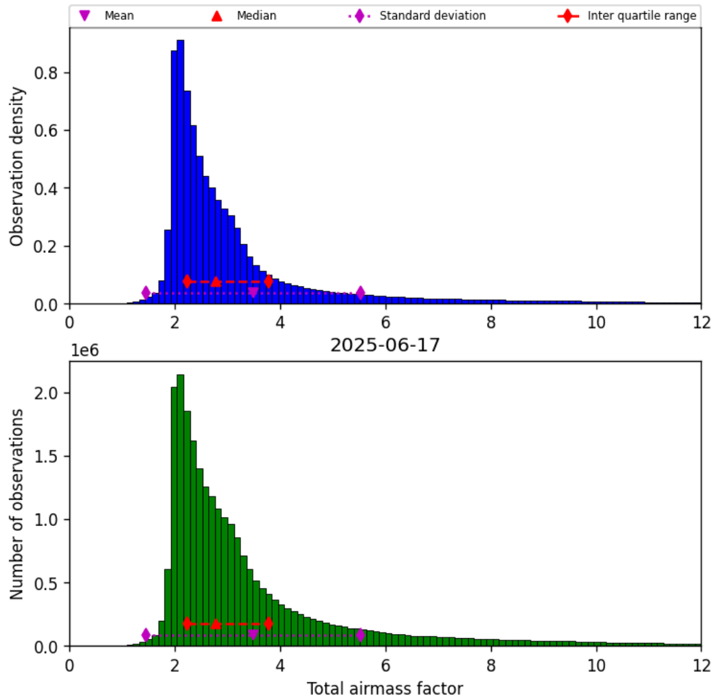
Figure 32: Histogram of “Total airmass factor” for 2025-06-17 to 2025-06-18
