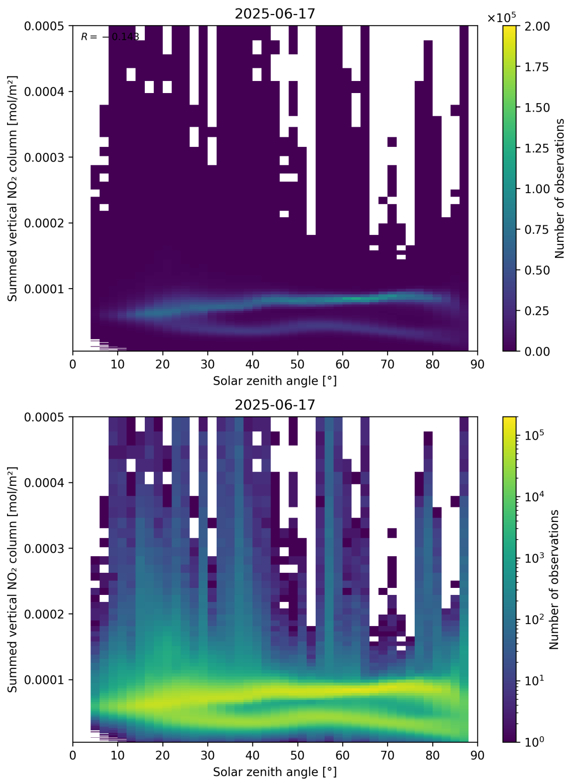
Figure 151: Scatter density plot of “Solar zenith angle” against “Summed vertical NO 2 column” for 2025-06-17 to 2025-06-18.
