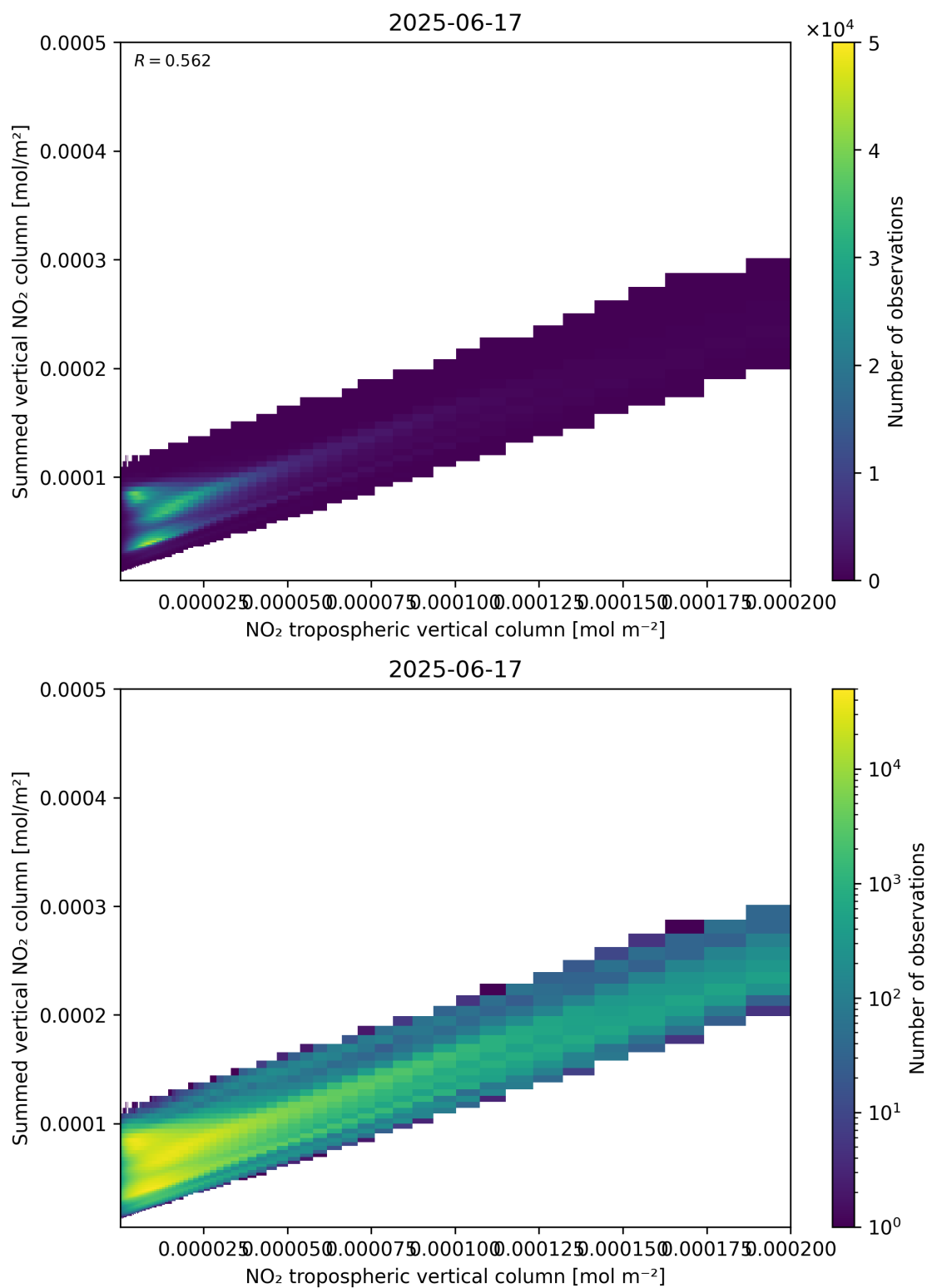
Figure 126: Scatter density plot of “NO 2 tropospheric vertical column” against “Summed vertical NO 2 column” for 2025-06-17 to 2025-06-18.
