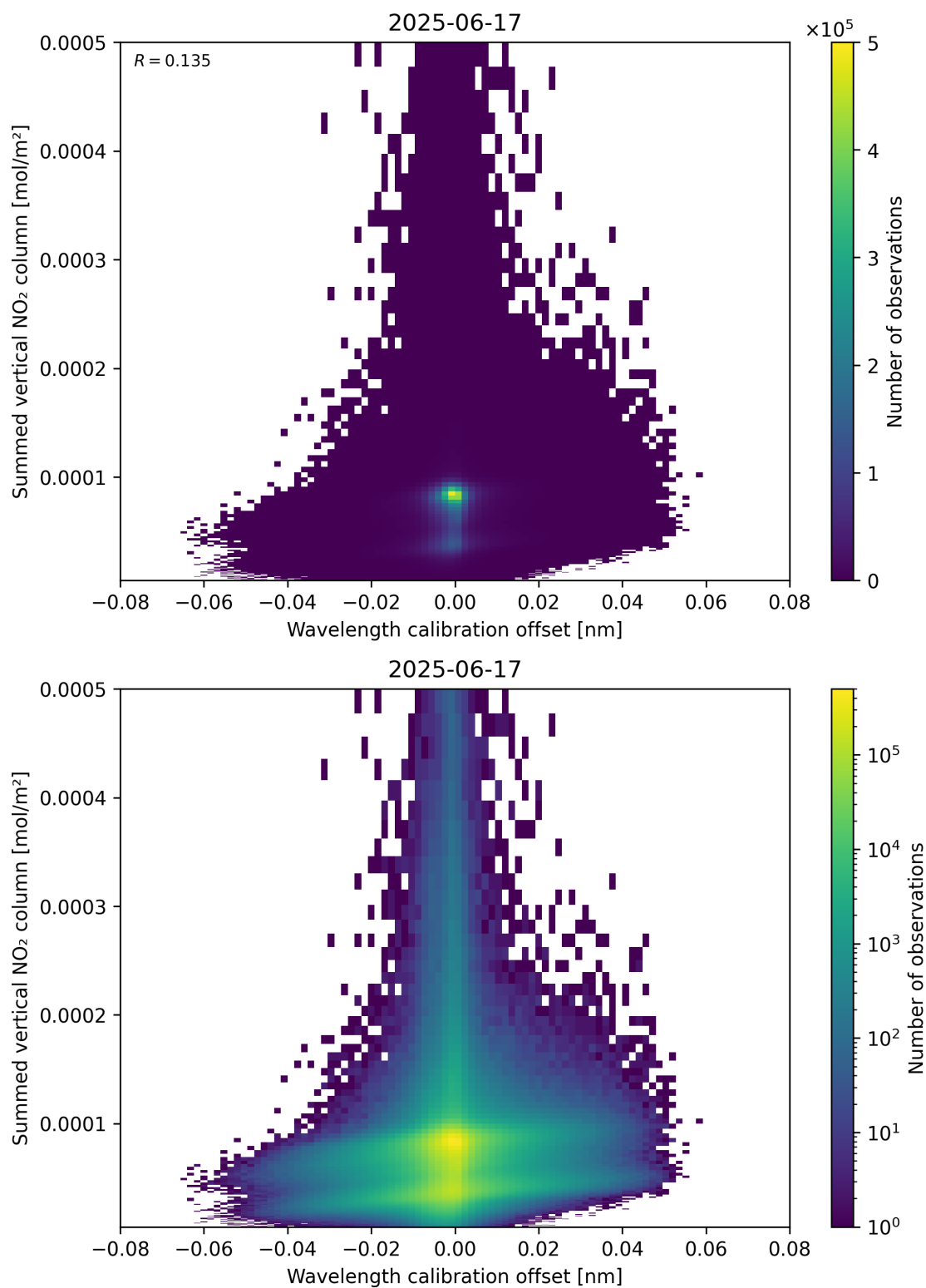
Figure 177: Scatter density plot of “Wavelength calibration offset” against “Summed vertical NO 2 column” for 2025-06-17 to 2025-06-18.
