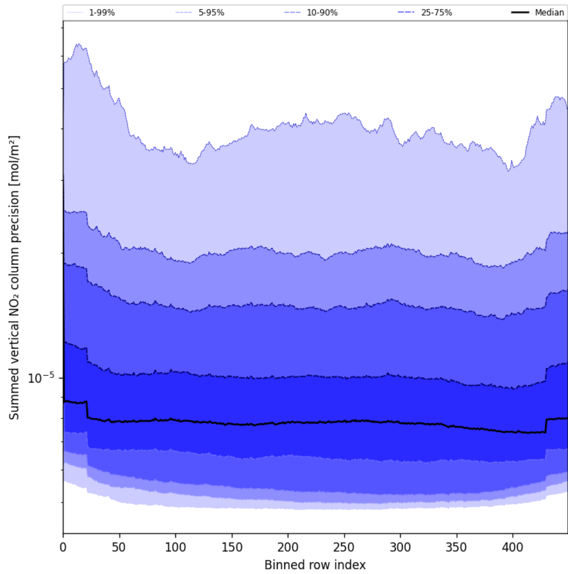
Figure 58: Along track statistics of “Summed vertical NO 2 column precision” for 2025-06-17 to 2025-06-18
