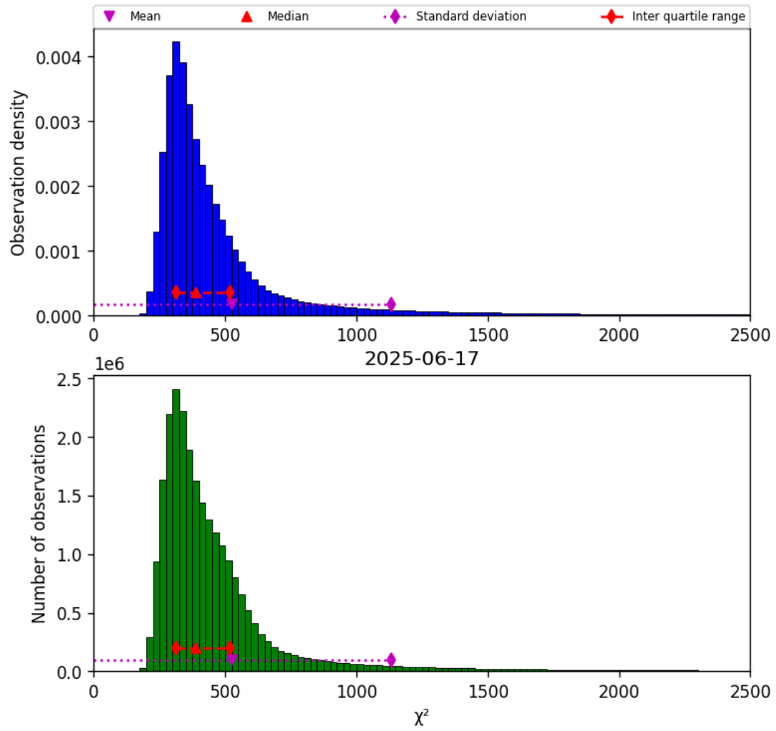
Figure 42: Histogram of “ \chi^2 ” for 2025-06-17 to 2025-06-18
