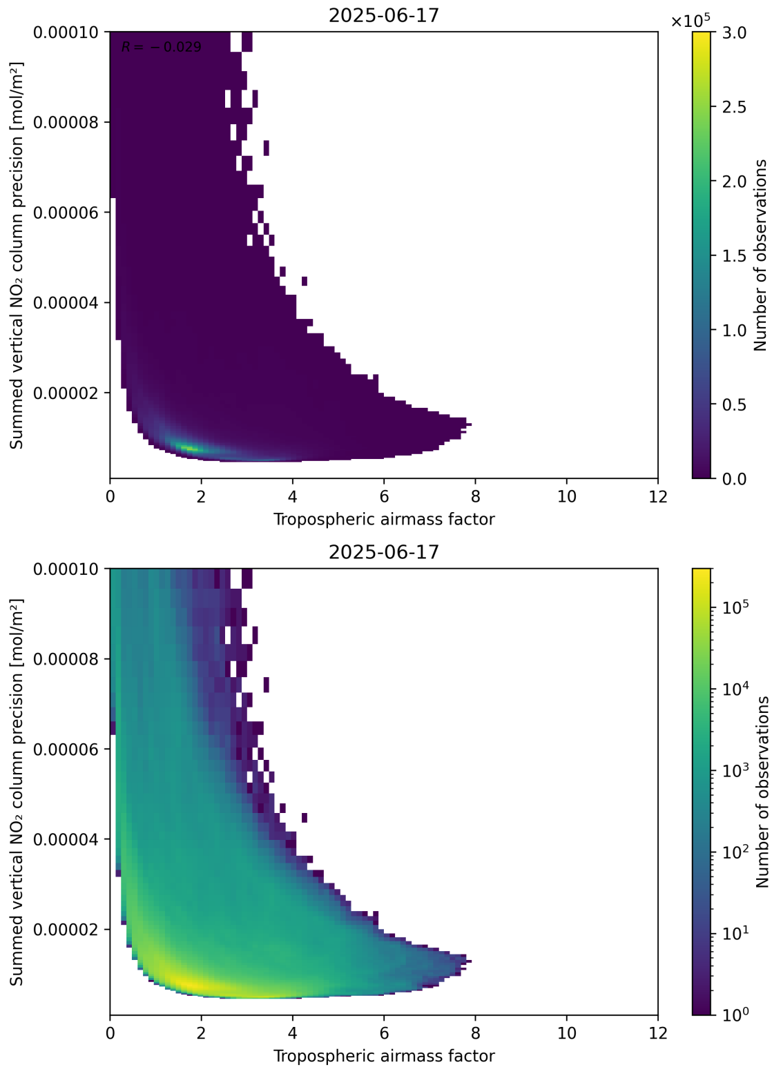
Figure 76: Scatter density plot of “Tropospheric air mass factor” against “Summed vertical NO 2 column precision” for 2025-06-17 to 2025-06-18.
