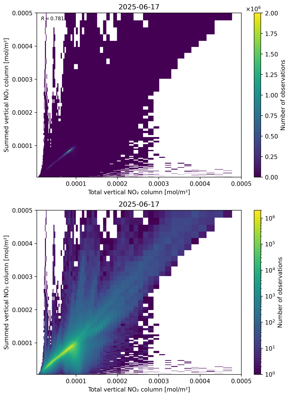
Figure 112: Scatter density plot of “Total vertical NO 2 column” against “Summed vertical NO 2 column” for 2025-06-17 to 2025-06-18.
