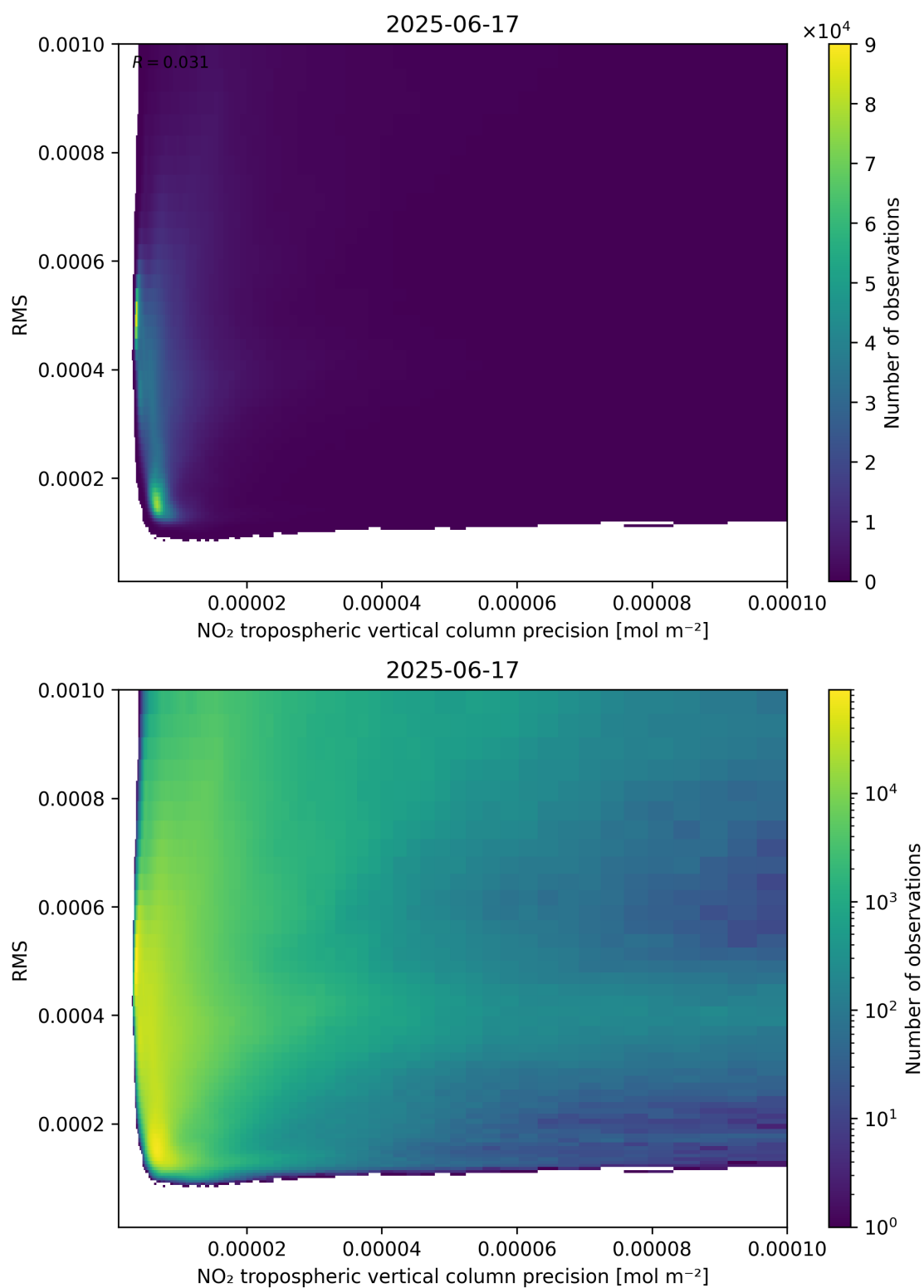
Figure 140: Scatter density plot of “NO 2 tropospheric vertical column precision” against “RMS” for 2025-06-17 to 2025-06-18.
