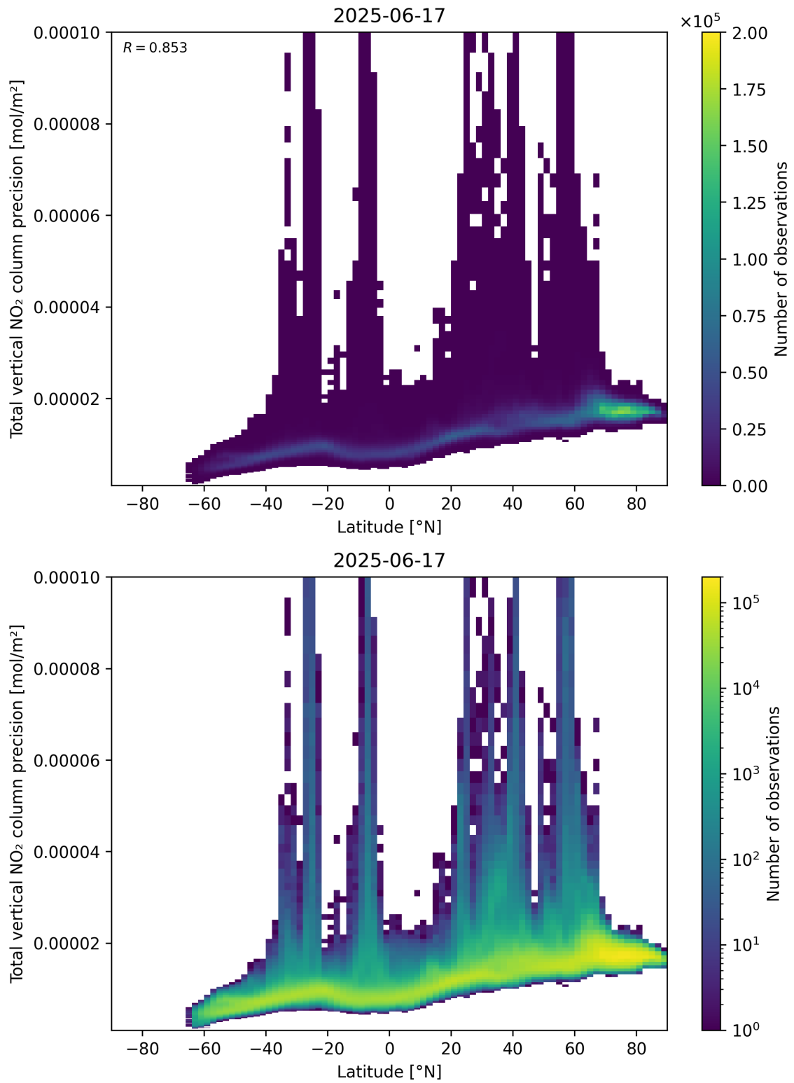
Figure 91: Scatter density plot of “Latitude” against “Total vertical NO 2 column precision” for 2025-06-17 to 2025-06-18.
