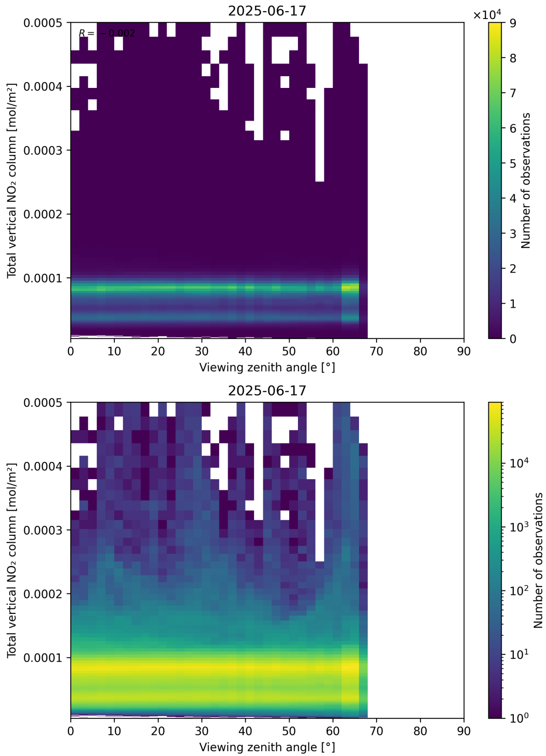
Figure 167: Scatter density plot of “Viewing zenith angle” against “Total vertical NO 2 column” for 2025-06-17 to 2025-06-18.
