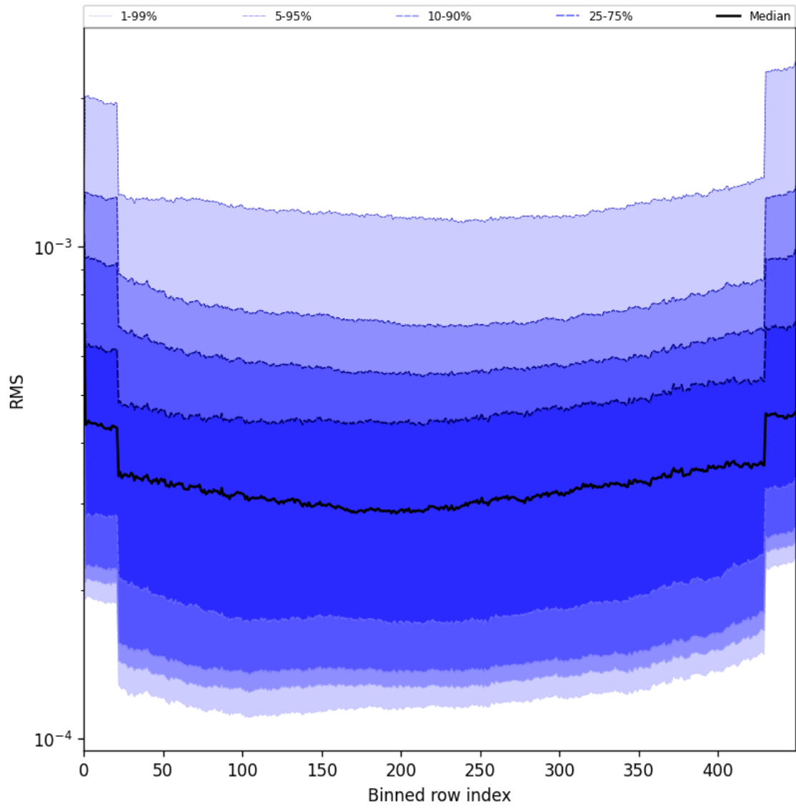
Figure 60: Along track statistics of “RMS” for 2025-06-17 to 2025-06-18
