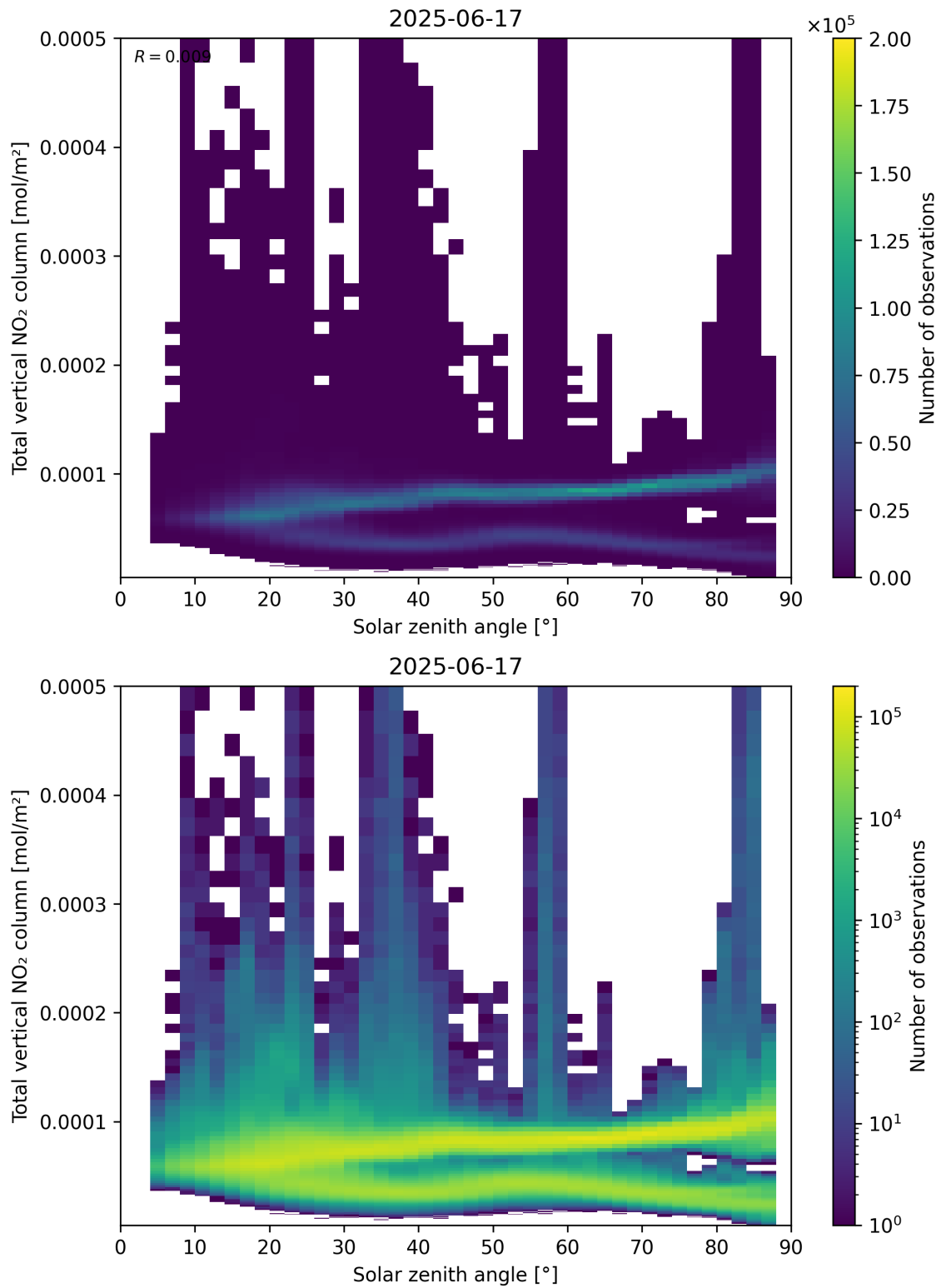
Figure 153: Scatter density plot of “Solar zenith angle” against “Total vertical NO 2 column” for 2025-06-17 to 2025-06-18.
