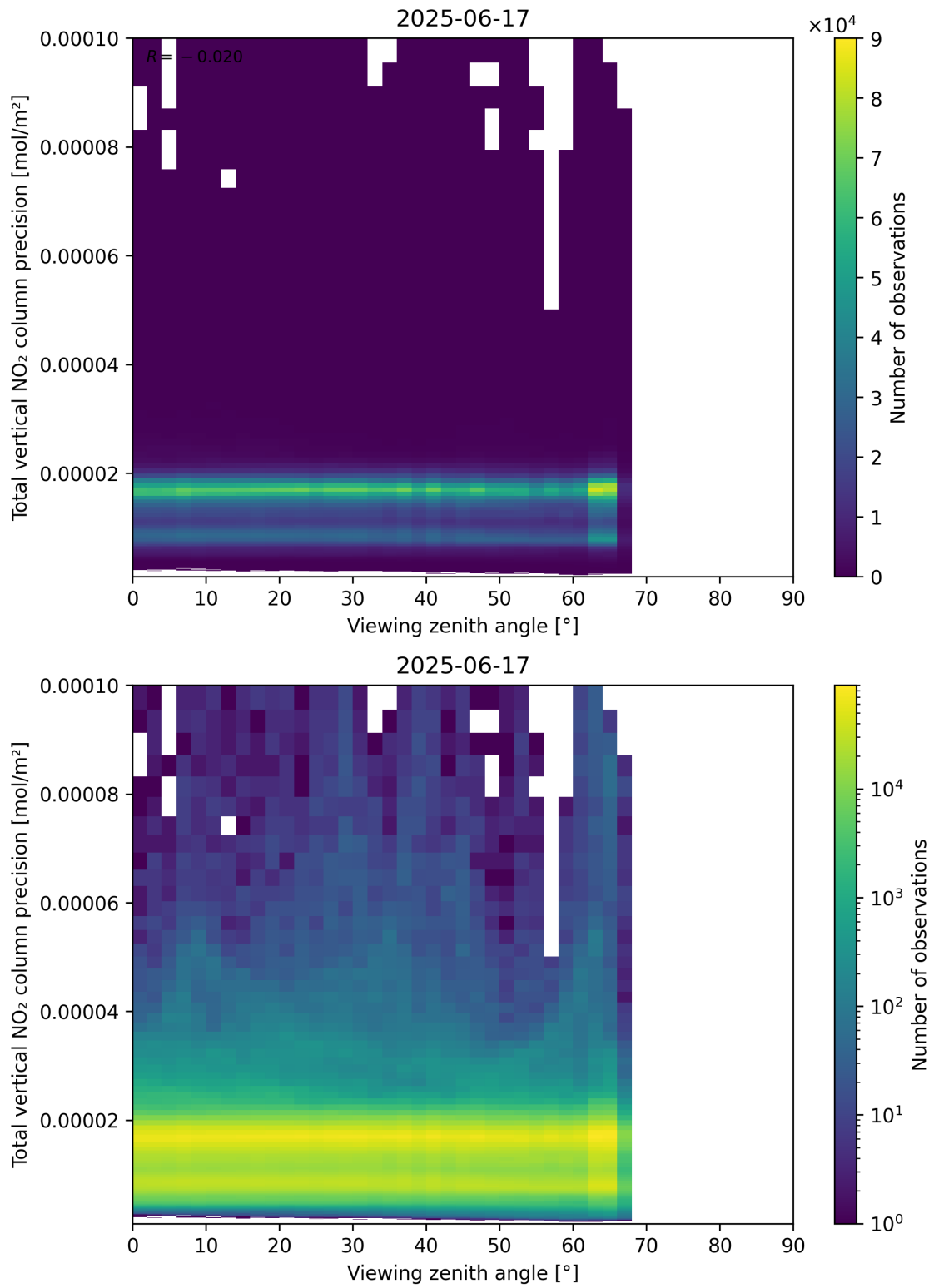
Figure 168: Scatter density plot of “Viewing zenith angle” against “Total vertical NO 2 column precision” for 2025-06-17 to 2025-06-18.
