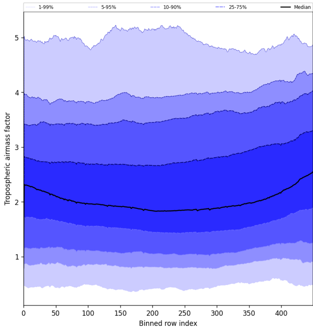
Figure 48: Along track statistics of “Tropospheric airmass factor” for 2025-06-17 to 2025-06-18
