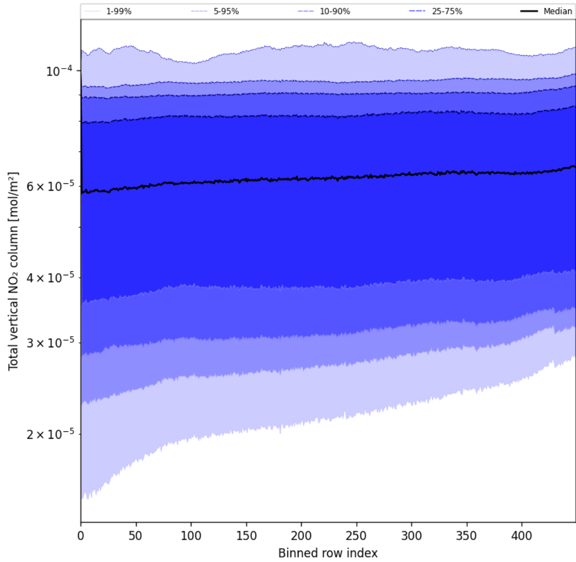
Figure 55: Along track statistics of “Total vertical NO 2 column” for 2025-06-17 to 2025-06-18
