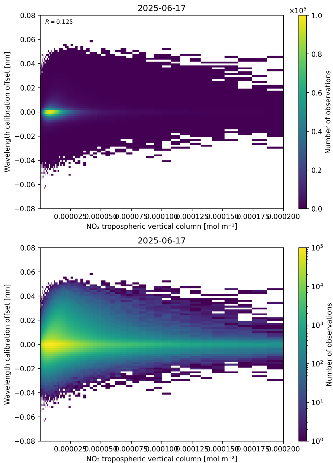
Figure 143: Scatter density plot of “NO 2 tropospheric vertical column” against “Wavelength calibration offset” for 2025-06-17 to 2025-06-18.
