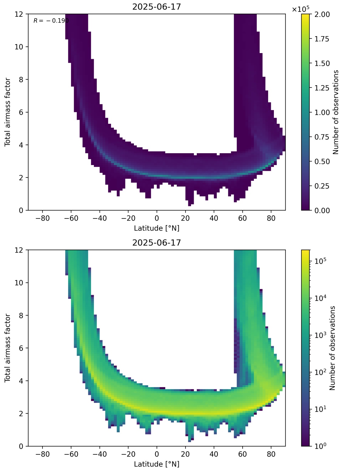
Figure 84: Scatter density plot of “Latitude” against “Total airmass factor” for 2025-06-17 to 2025-06-18.
