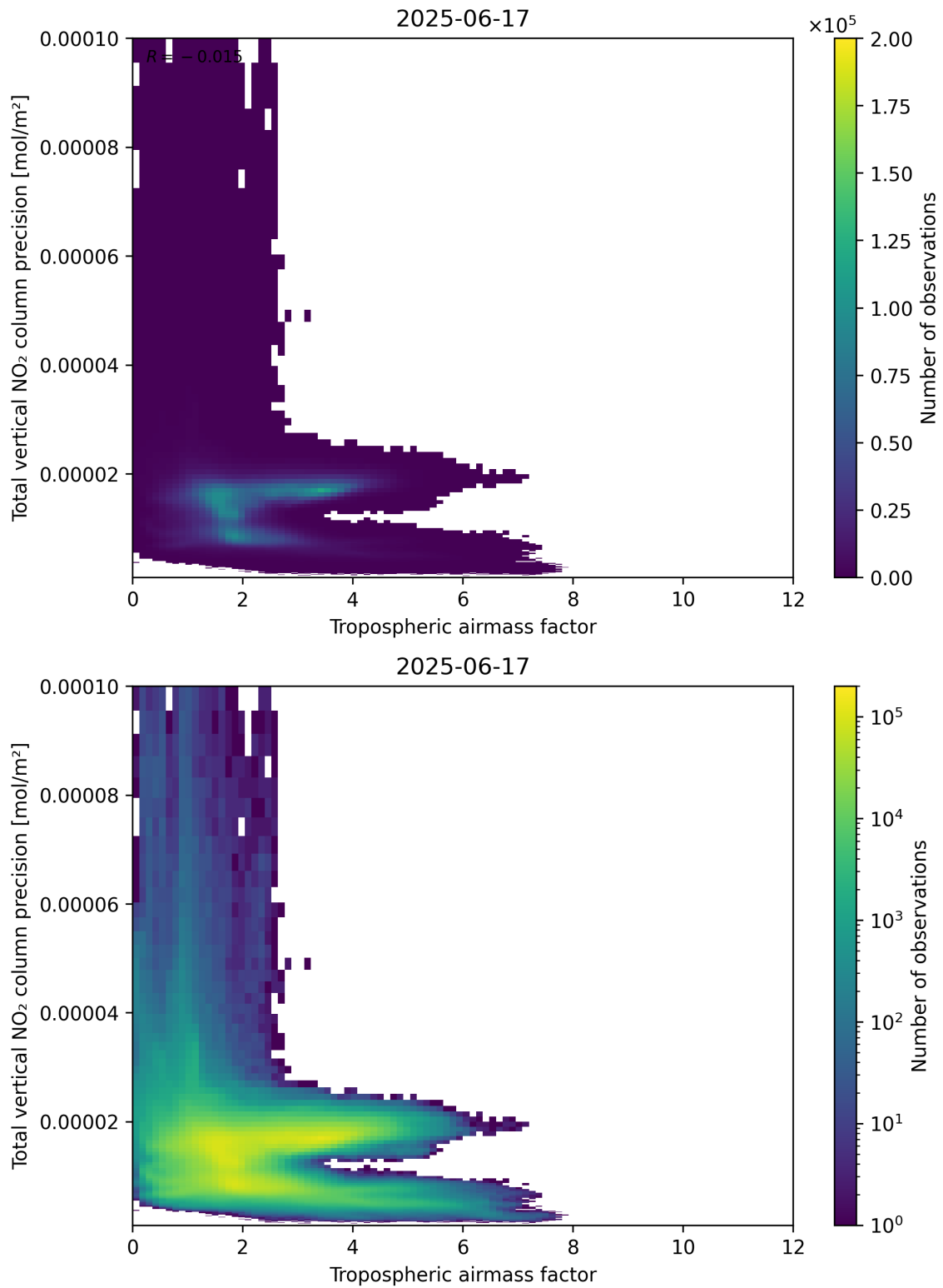
Figure 78: Scatter density plot of “Tropospheric air mass factor” against “Total vertical NO 2 column precision” for 2025-06-17 to 2025-06-18.
