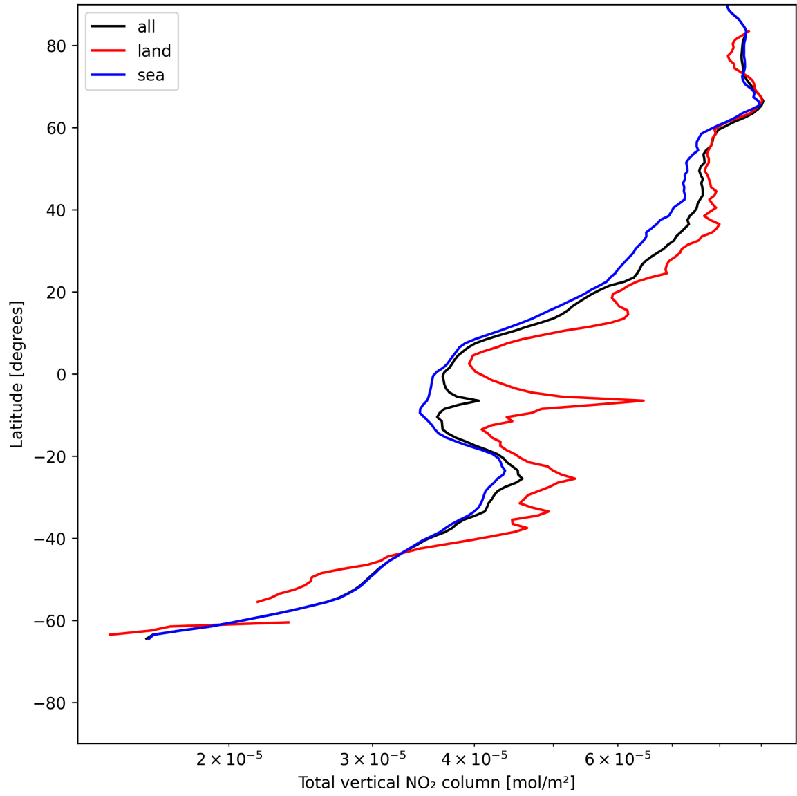
Figure 21: Zonal average of “Total vertical NO 2 column” for 2025-06-17 to 2025-06-18.
