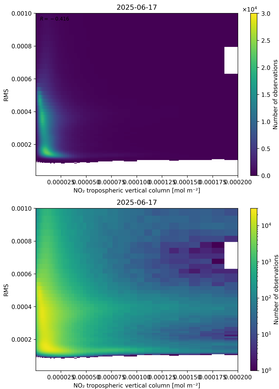
Figure 142: Scatter density plot of “NO 2 tropospheric vertical column” against “RMS” for 2025-06-17 to 2025-06-18.
