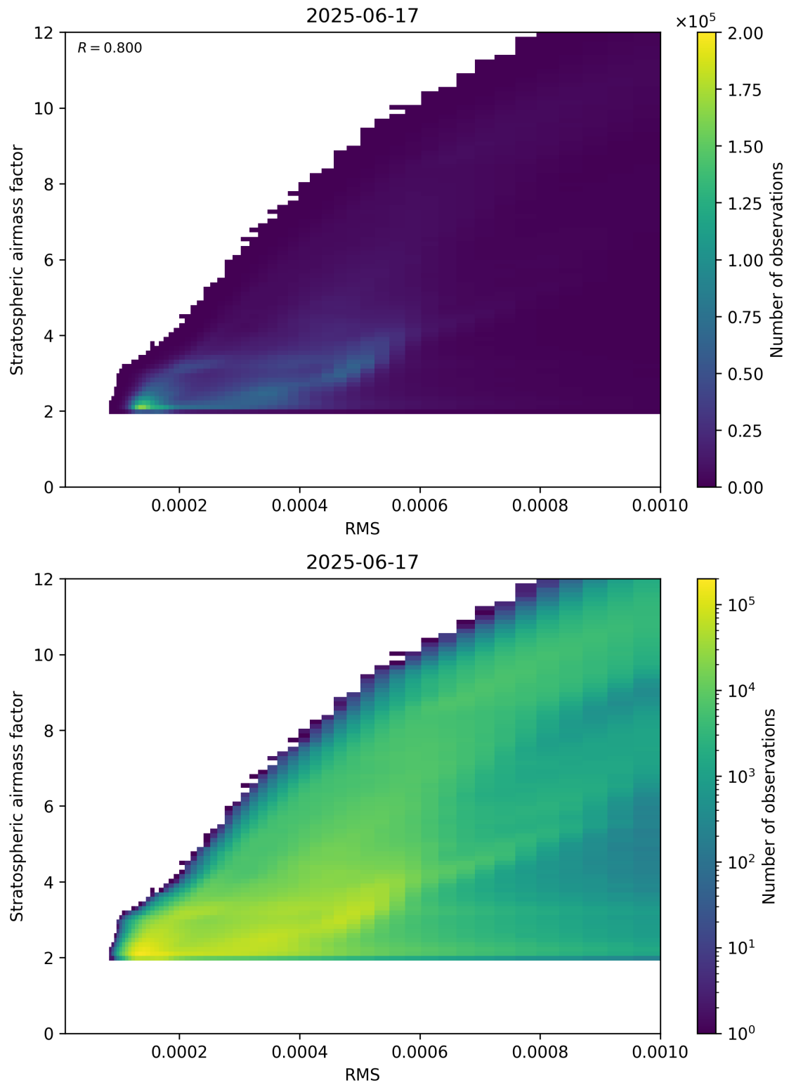
Figure 144: Scatter density plot of “RMS” against “Stratospheric airmass factor” for 2025-06-17 to 2025-06-18.
