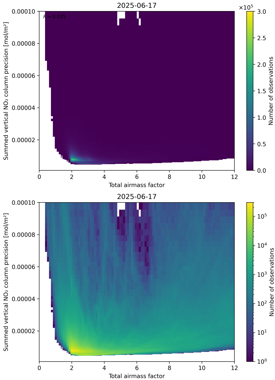
Figure 66: Scatter density plot of “Total airmass factor” against “Summed vertical NO 2 column precision” for 2025-06-17 to 2025-06-18.
