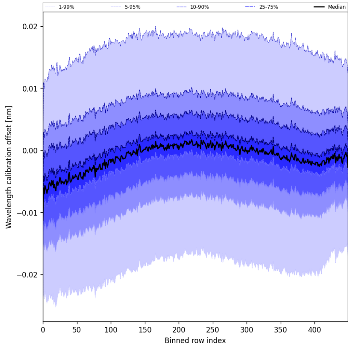
Figure 52: Along track statistics of “Wavelength calibration offset” for 2025-06-17 to 2025-06-18
