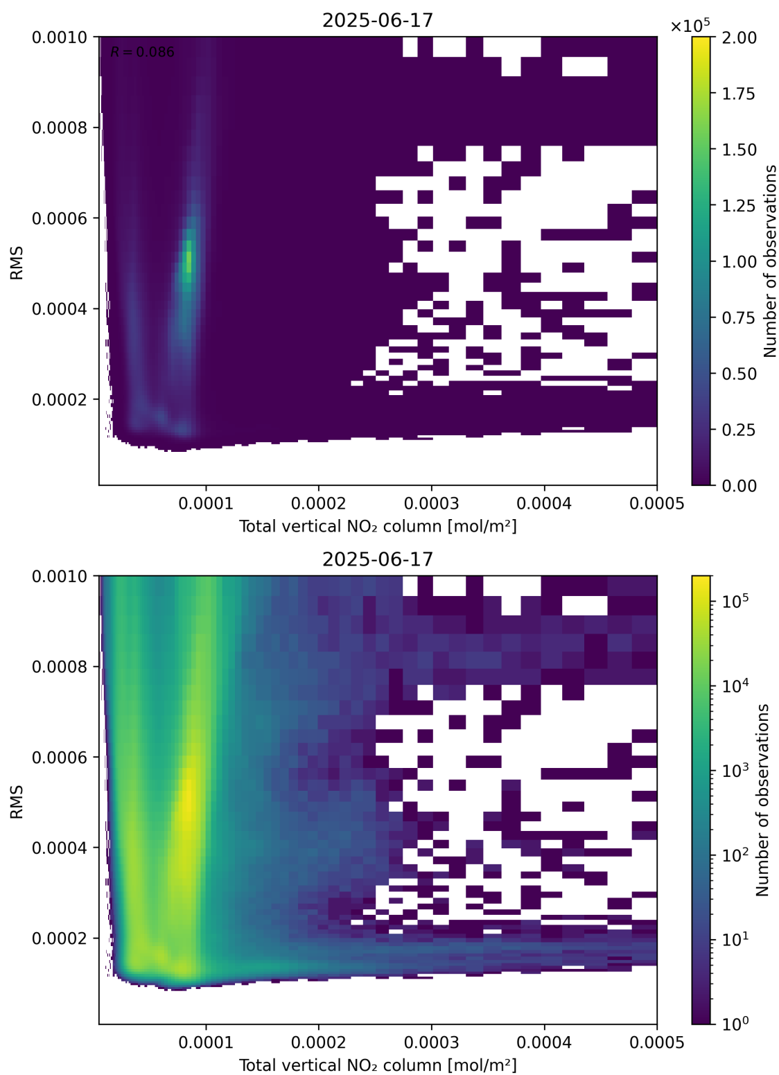
Figure 120: Scatter density plot of “Total vertical NO 2 column” against “RMS” for 2025-06-17 to 2025-06-18.
