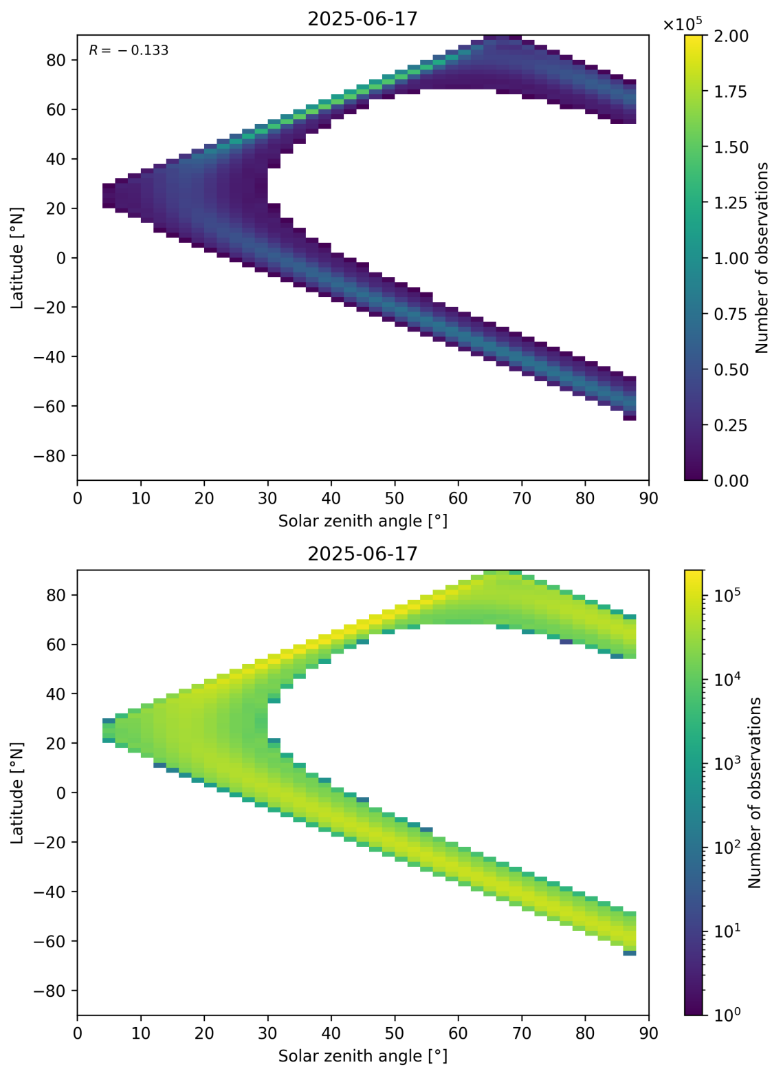
Figure 149: Scatter density plot of “Solar zenith angle” against “Latitude” for 2025-06-17 to 2025-06-18.
