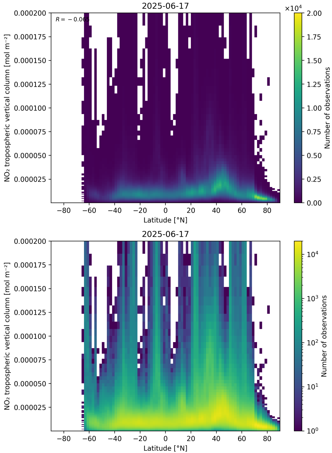
Figure 92: Scatter density plot of “Latitude” against “NO 2 tropospheric vertical column” for 2025-06-17 to 2025-06-18.
