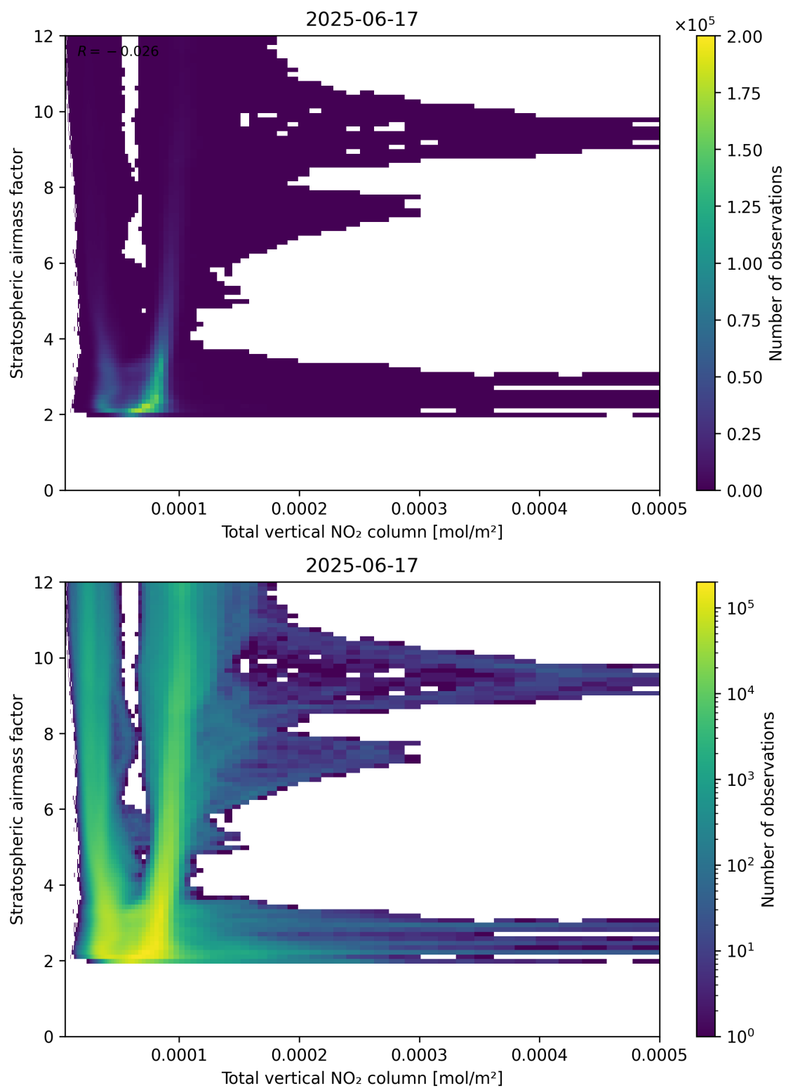
Figure 110: Scatter density plot of “Total vertical NO 2 column” against “Stratospheric airmass factor” for 2025-06-17 to 2025-06-18.
