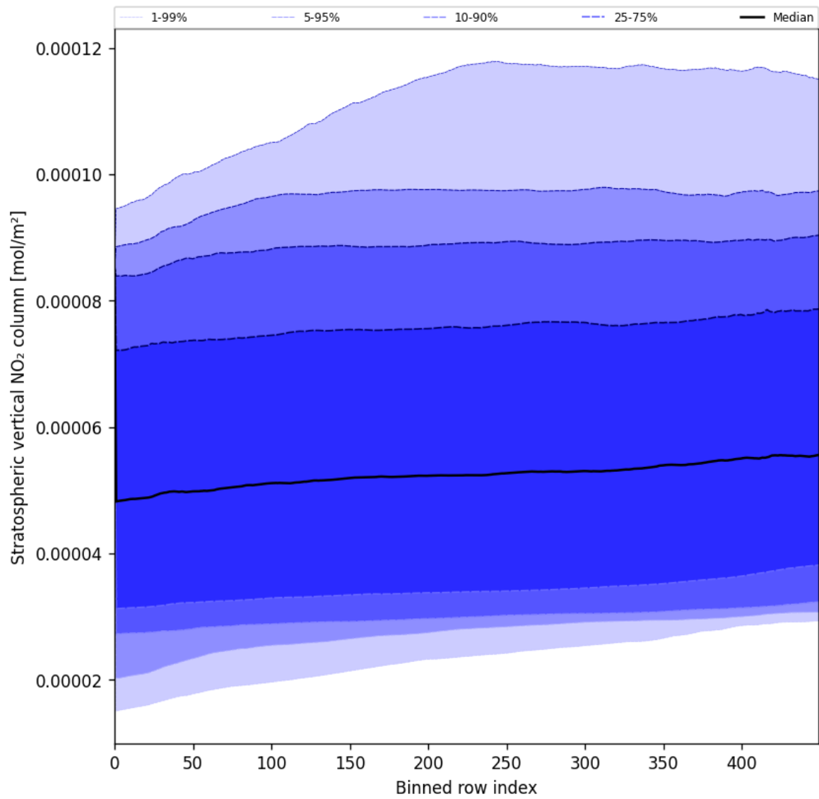
Figure 53: Along track statistics of “Stratospheric vertical NO 2 column” for 2025-06-17 to 2025-06-18
