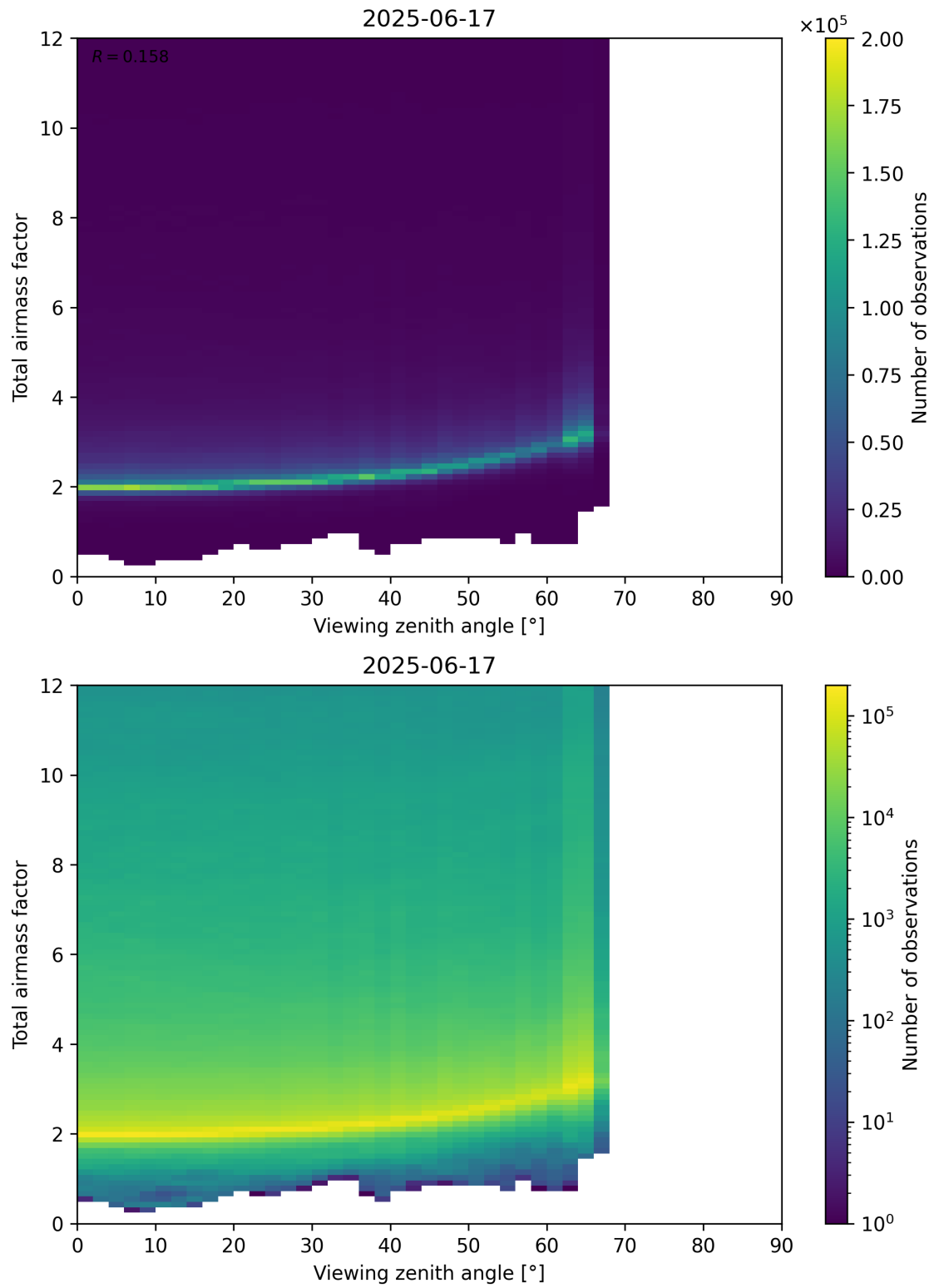
Figure 160: Scatter density plot of “Viewing zenith angle” against “Total airmass factor” for 2025-06-17 to 2025-06-18.
