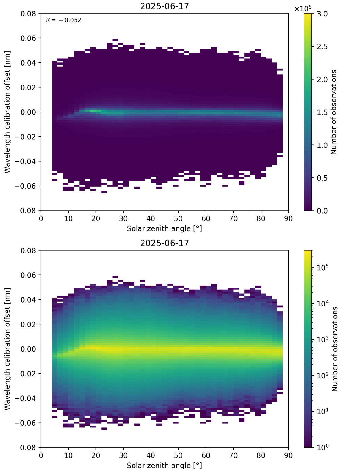
Figure 158: Scatter density plot of “Solar zenith angle” against “Wavelength calibration offset” for 2025-06-17 to 2025-06-18.
