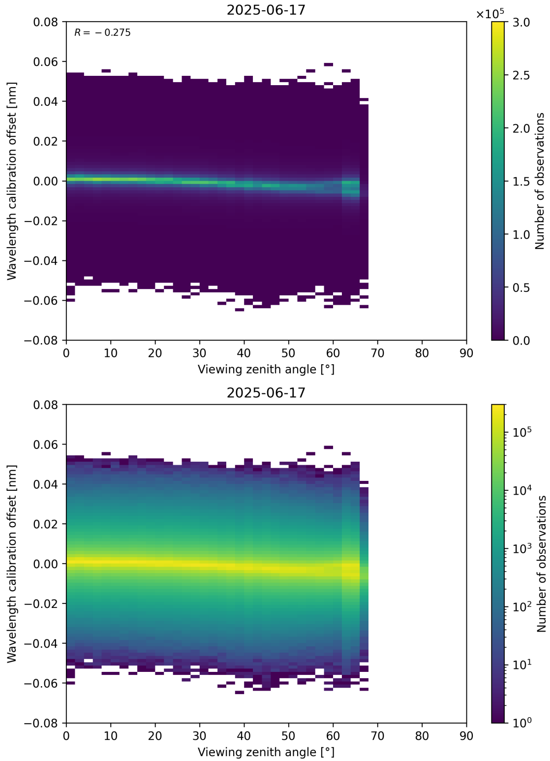
Figure 173: Scatter density plot of “Viewing zenith angle” against “Wavelength calibration offset” for 2025-06-17 to 2025-06-18.
