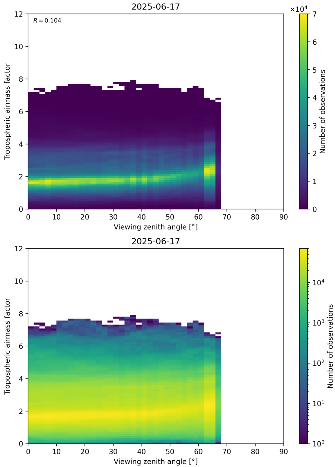
Figure 161: Scatter density plot of “Viewing zenith angle” against “Tropospheric airmass factor” for 2025-06-17 to 2025-06-18.
