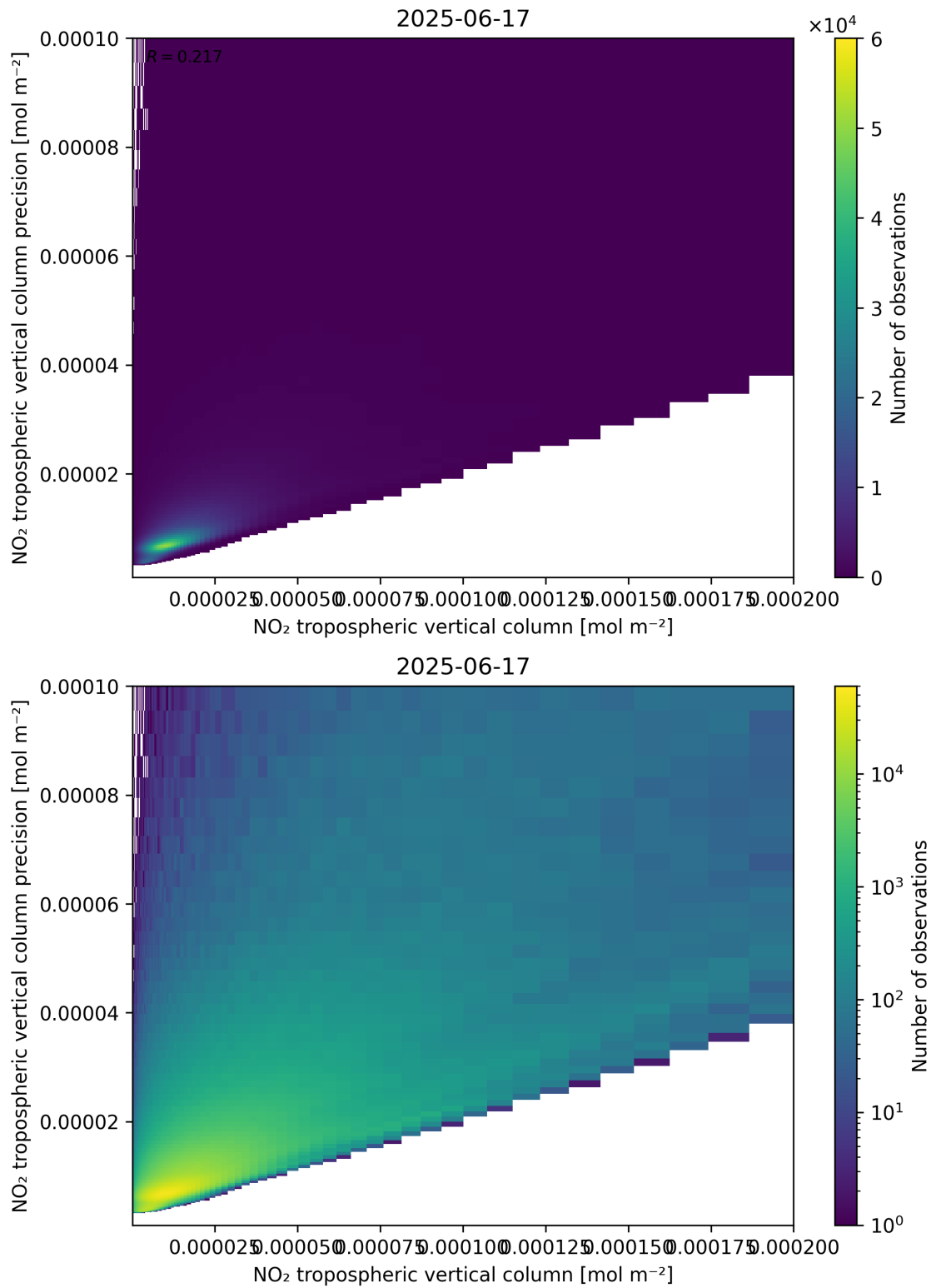
Figure 130: Scatter density plot of “NO 2 tropospheric vertical column” against “NO 2 tropospheric vertical column precision” for 2025-06-17 to 2025-06-18.
