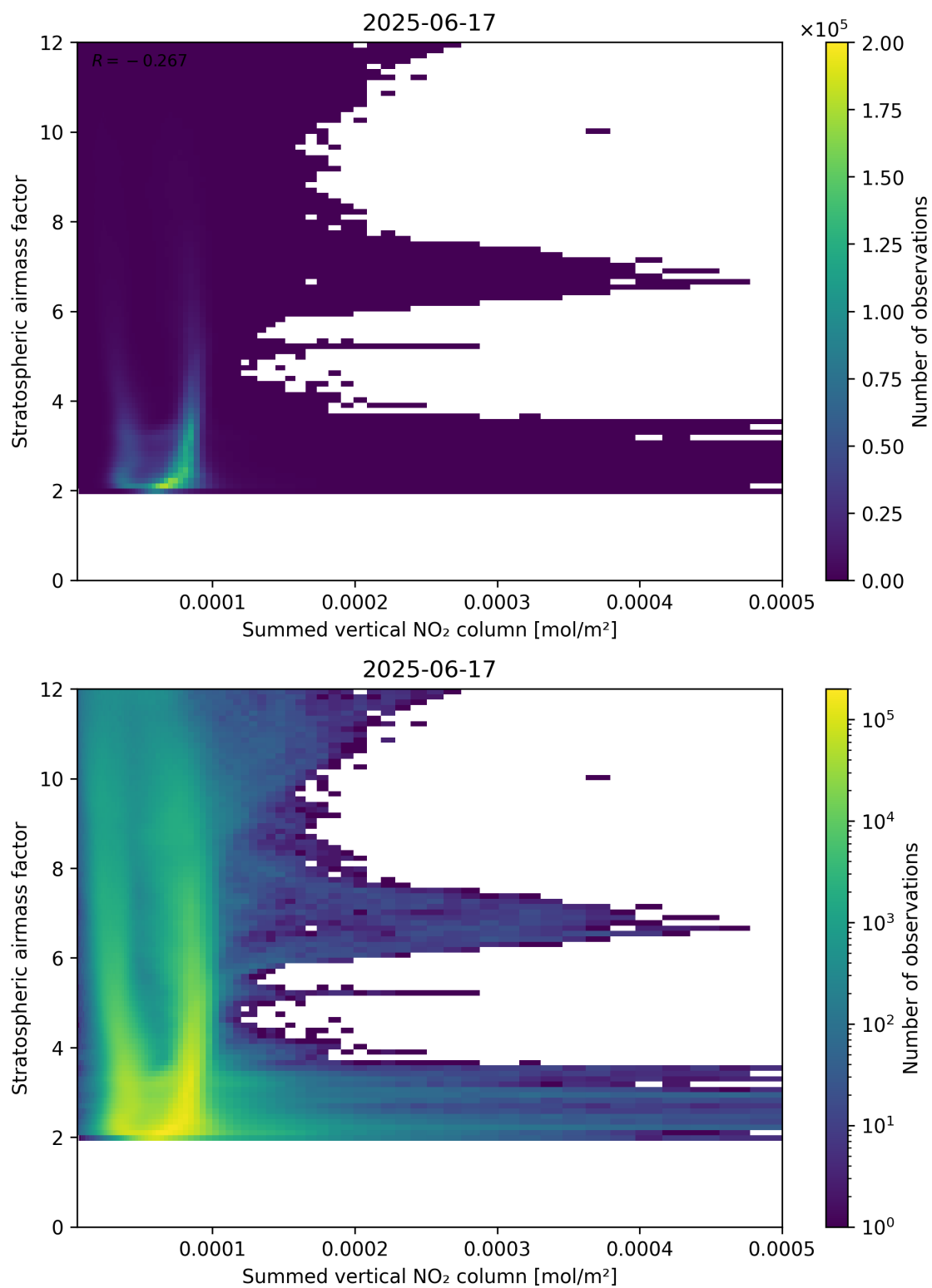
Figure 103: Scatter density plot of “Summed vertical NO 2 column” against “Stratospheric air mass factor” for 2025-06-17 to 2025-06-18.
