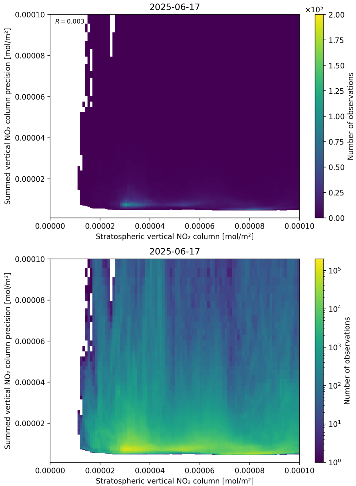
Figure 99: Scatter density plot of “Stratospheric vertical NO 2 column” against “Summed vertical NO 2 column precision” for 2025-06-17 to 2025-06-18.
