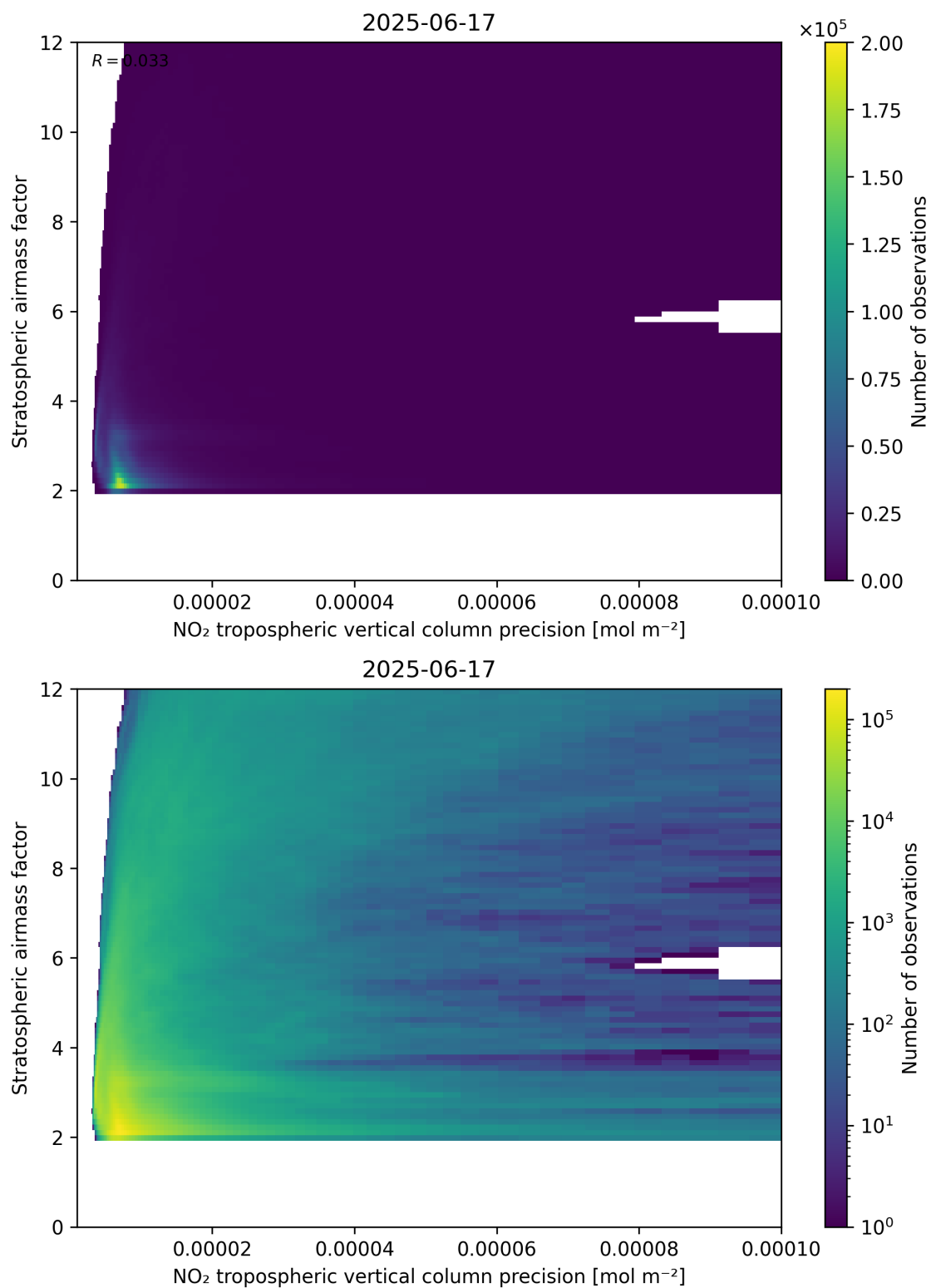
Figure 131: Scatter density plot of “NO 2 tropospheric vertical column precision” against “Stratospheric airmass factor” for 2025-06-17 to 2025-06-18.
