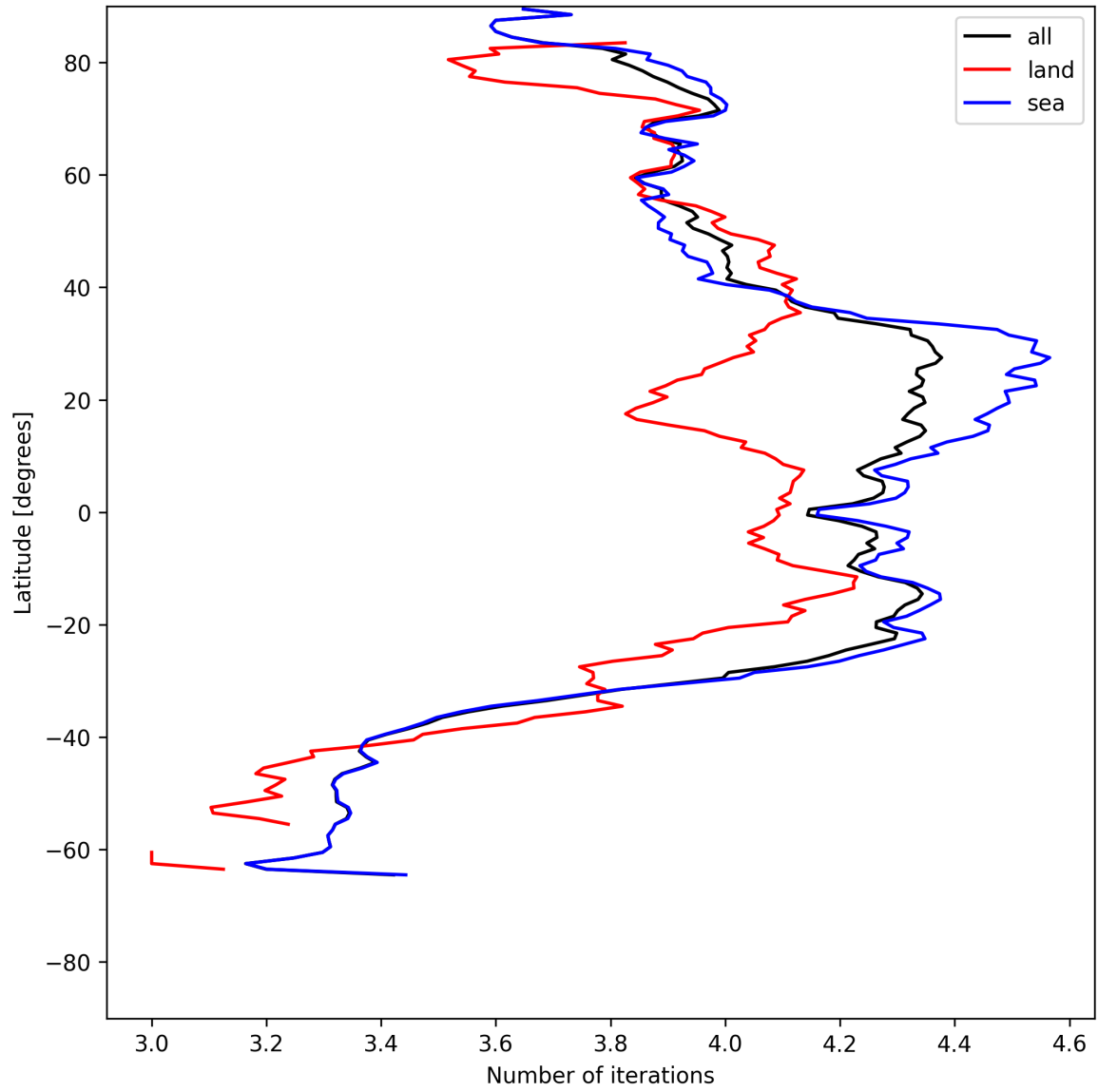
Figure 17: Zonal average of “Number of iterations” for 2025-06-17 to 2025-06-18.
