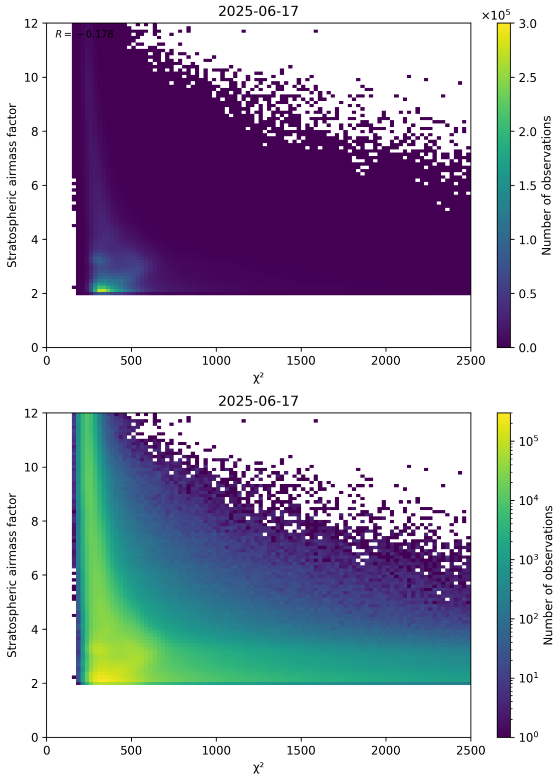
Figure 81: Scatter density plot of “ \chi^2 ” against “Stratospheric airmass factor” for 2025-06-17 to 2025-06-18.
