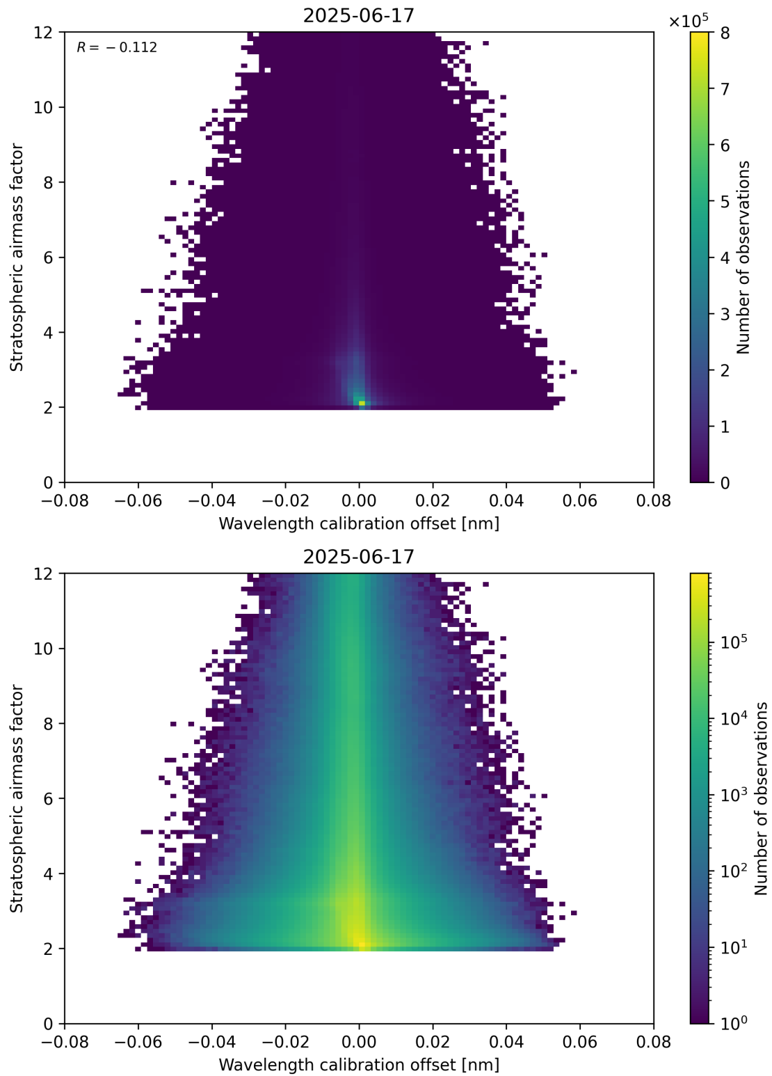
Figure 174: Scatter density plot of “Wavelength calibration offset” against “Stratospheric airmass factor” for 2025-06-17 to 2025-06-18.
