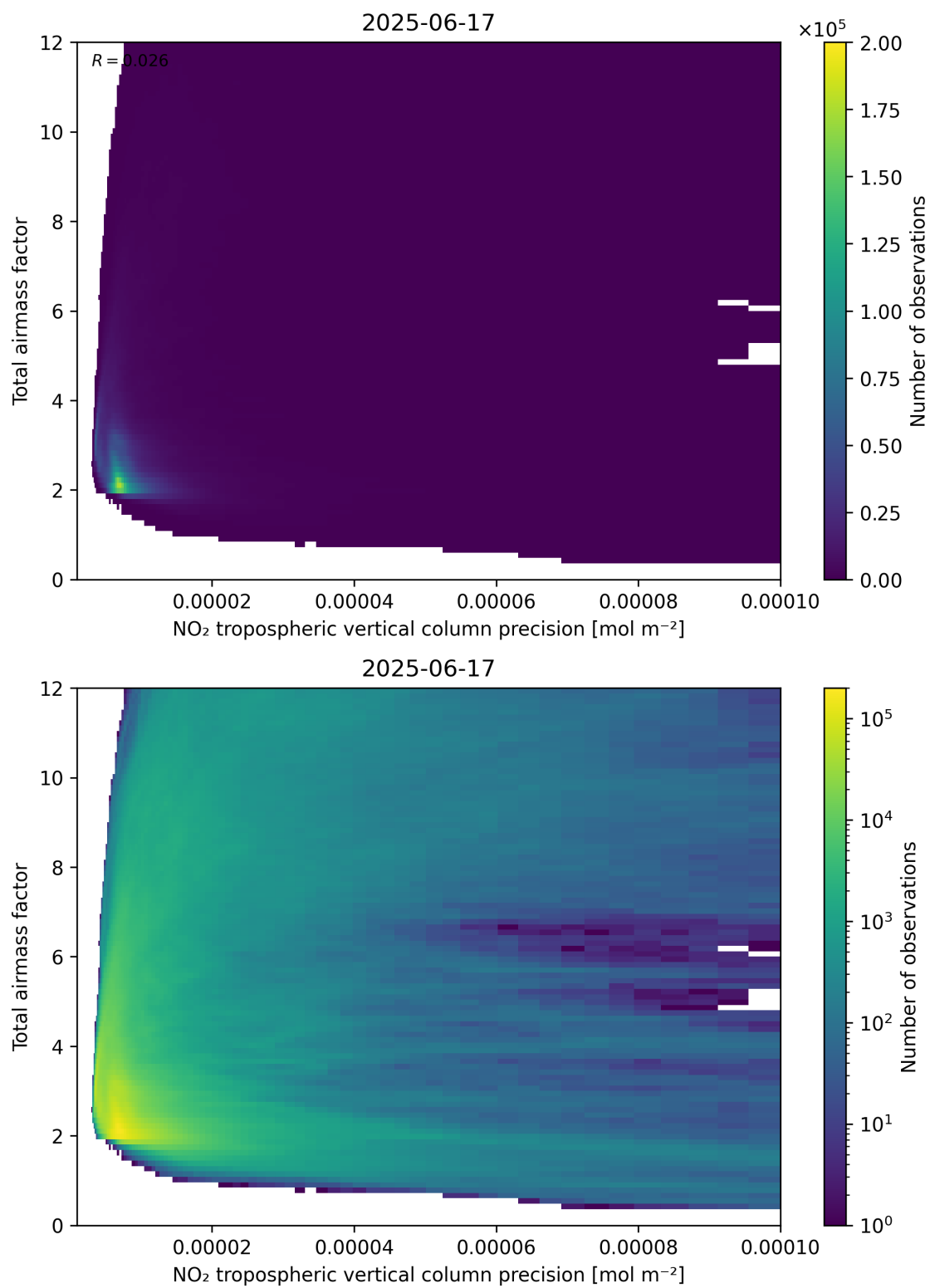
Figure 132: Scatter density plot of “NO 2 tropospheric vertical column precision” against “Total air mass factor” for 2025-06-17 to 2025-06-18.
