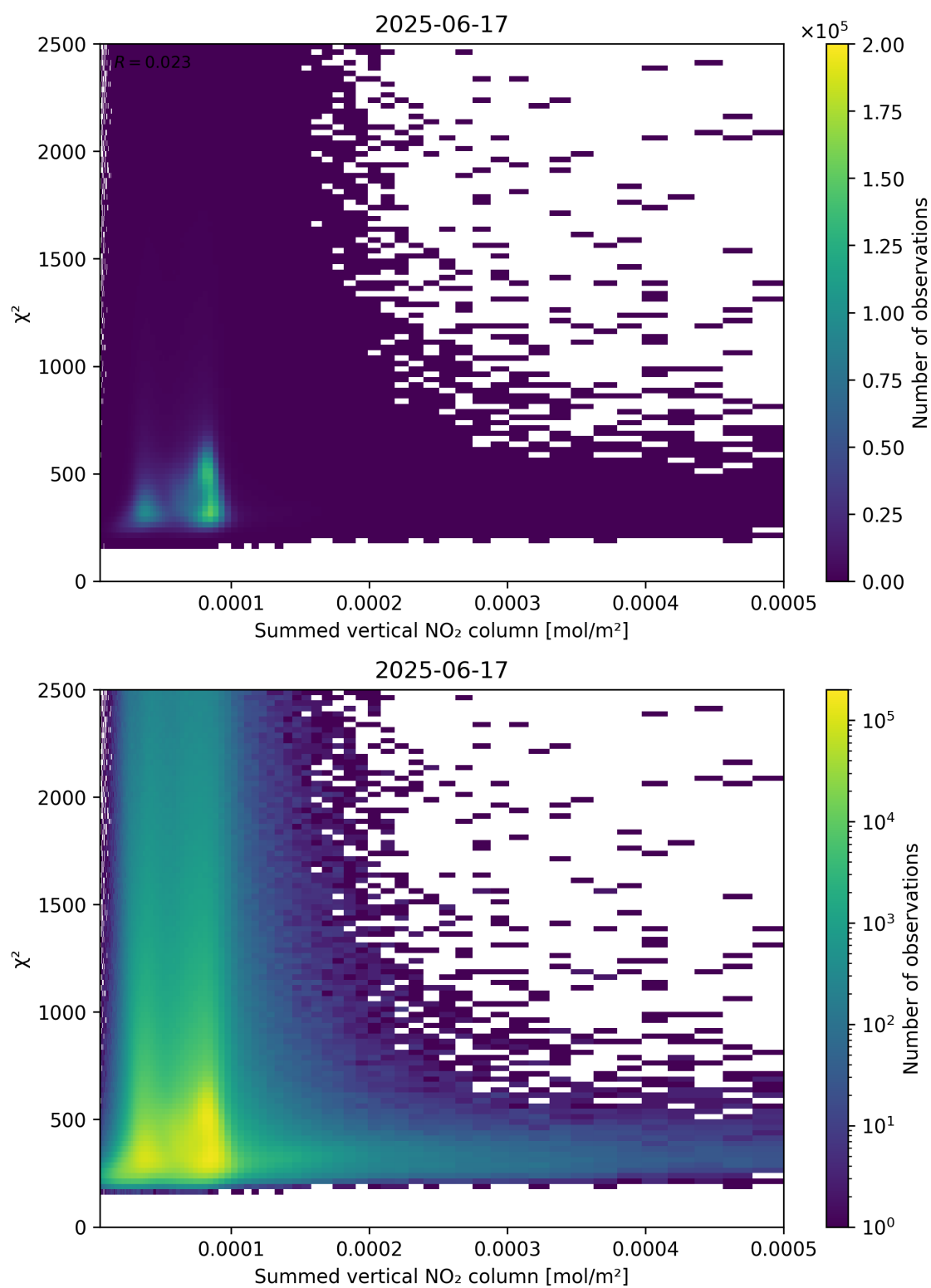
Figure 104: Scatter density plot of “Summed vertical NO 2 column” against “ \chi^2 ” for 2025-06-17 to 2025-06-18.
