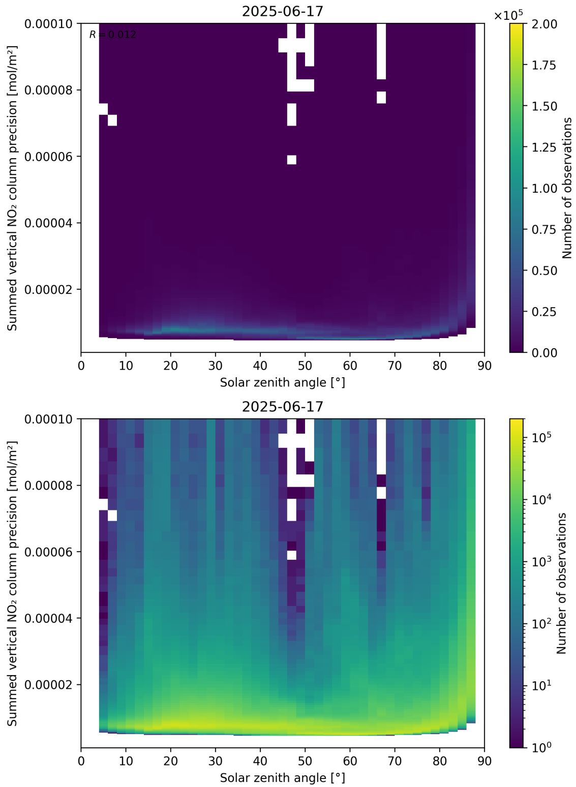
Figure 152: Scatter density plot of “Solar zenith angle” against “Summed vertical NO 2 column precision” for 2025-06-17 to 2025-06-18.
