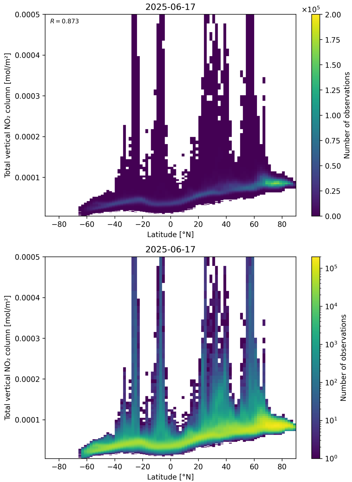
Figure 90: Scatter density plot of “Latitude” against “Total vertical NO 2 column” for 2025-06-17 to 2025-06-18.
