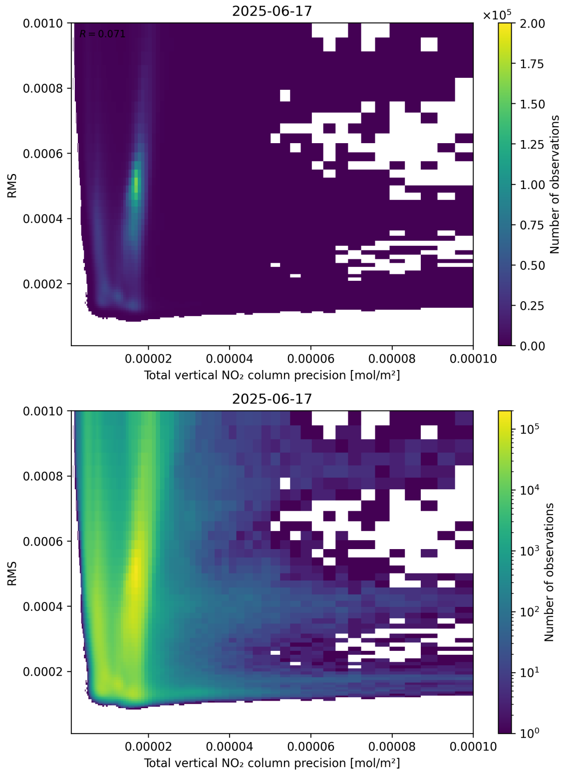
Figure 119: Scatter density plot of “Total vertical NO 2 column precision” against “RMS” for 2025-06-17 to 2025-06-18.
