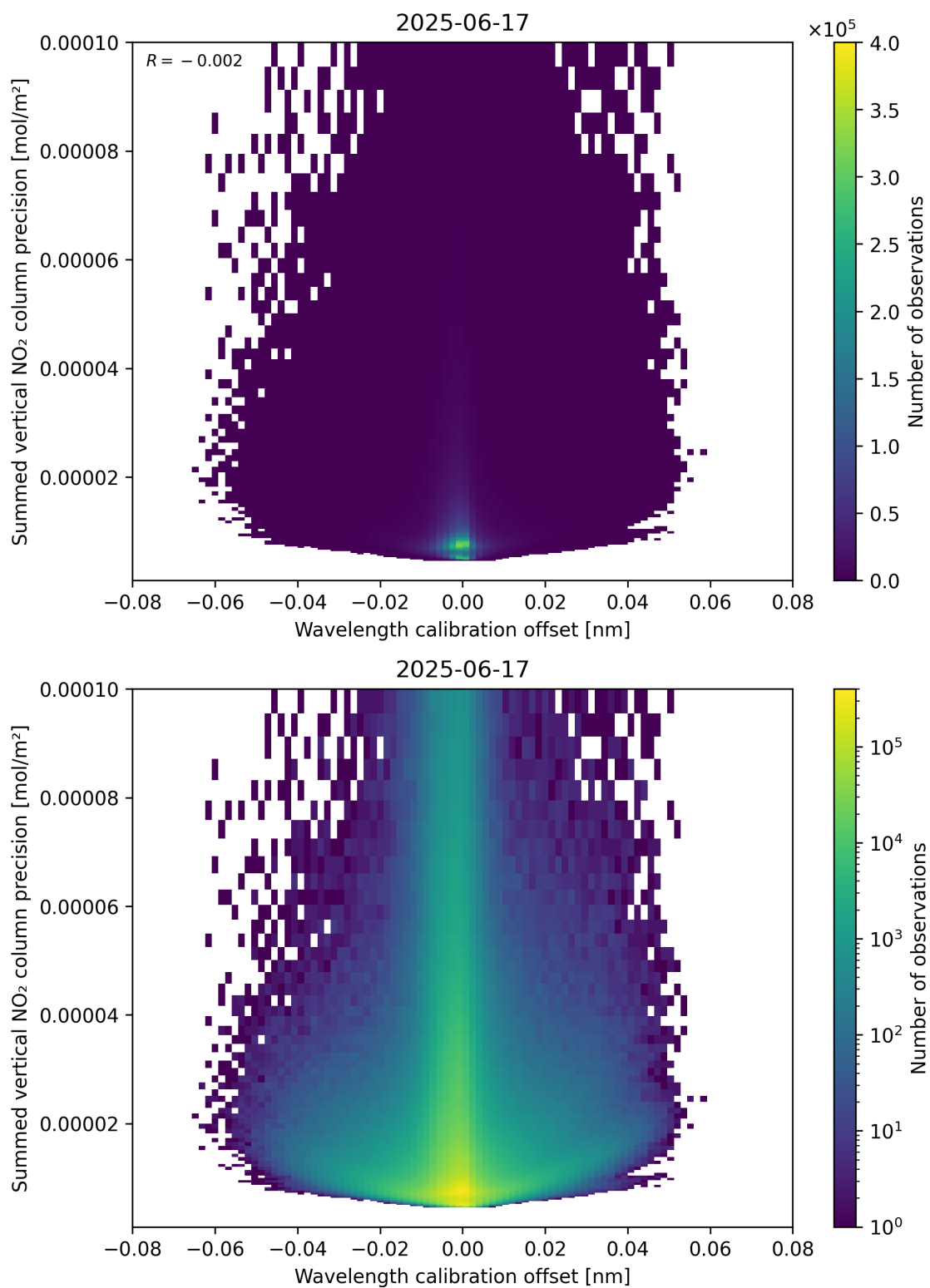
Figure 178: Scatter density plot of “Wavelength calibration offset” against “Summed vertical NO 2 column precision” for 2025-06-17 to 2025-06-18.
