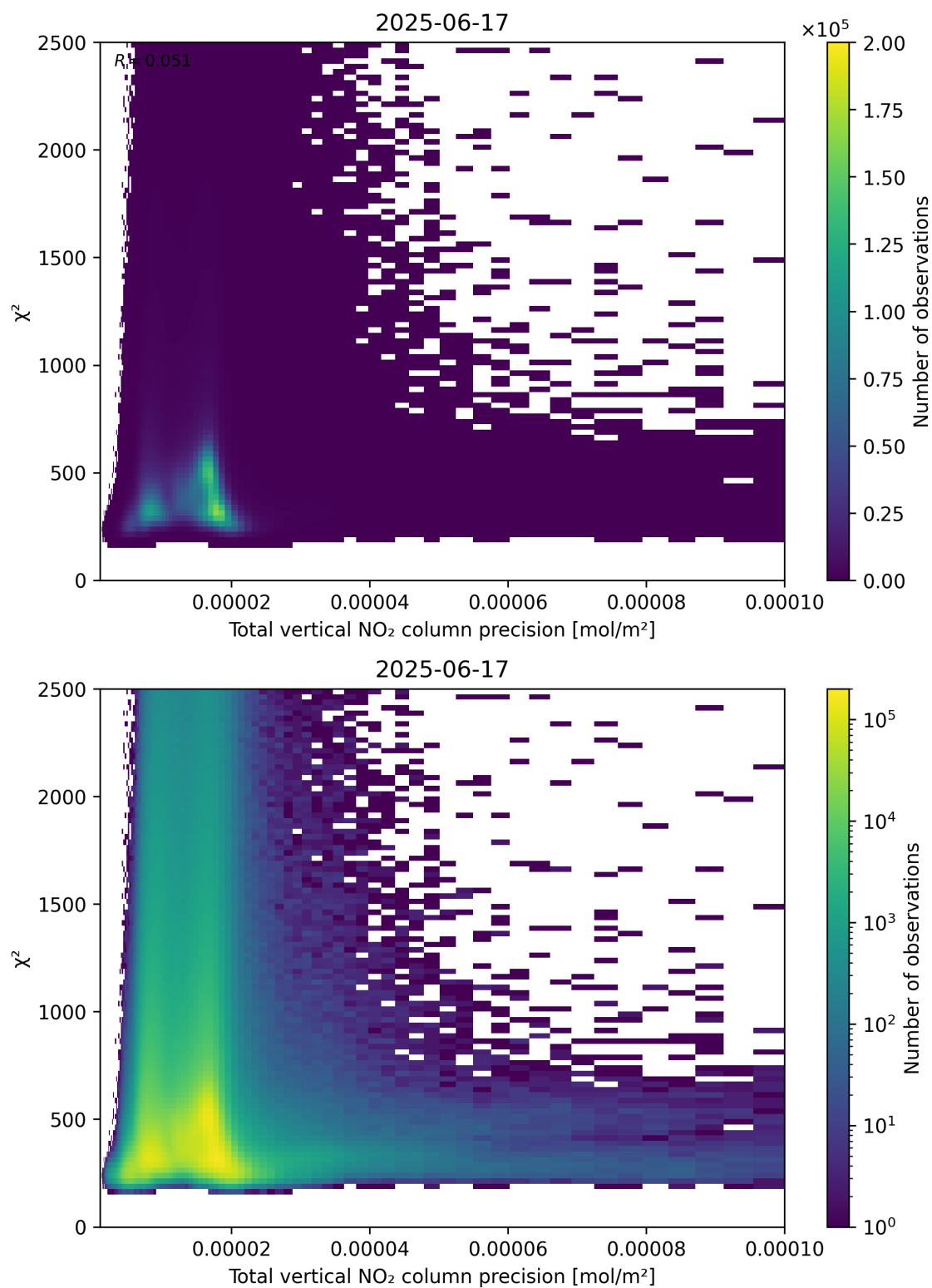
Figure 116: Scatter density plot of “Total vertical NO 2 column precision” against “ \chi^2 ” for 2025-06-17 to 2025-06-18.
