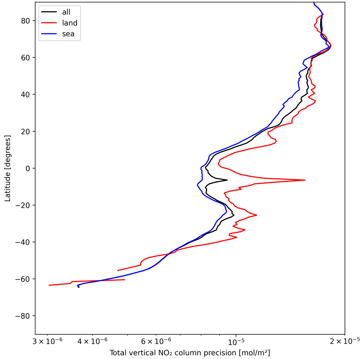
Figure 22: Zonal average of “Total vertical NO 2 column precision” for 2025-06-17 to 2025-06-18.
