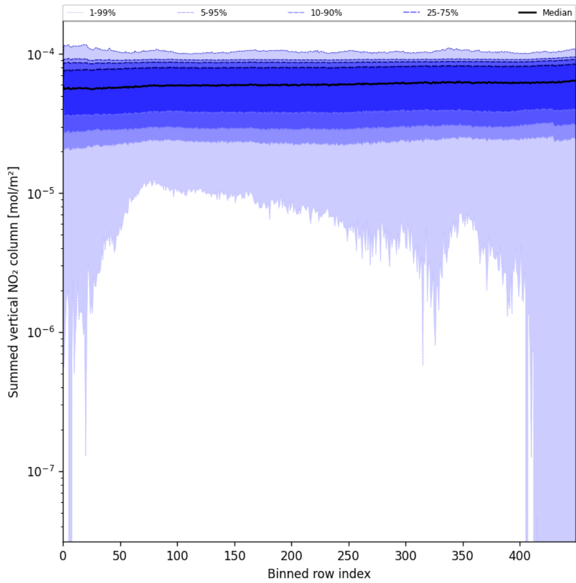
Figure 57: Along track statistics of “Summed vertical NO 2 column” for 2025-06-17 to 2025-06-18
