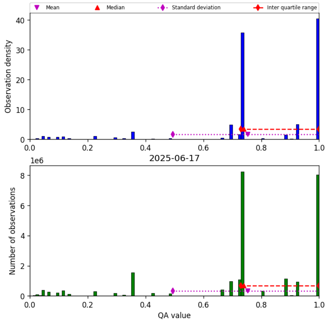
Figure 28: Histogram of “QA value” for 2025-06-17 to 2025-06-18
