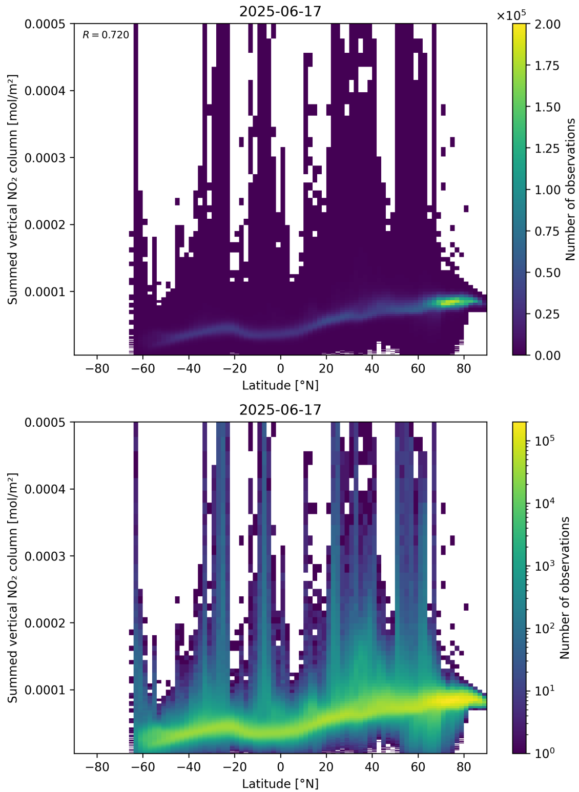
Figure 88: Scatter density plot of “Latitude” against “Summed vertical NO 2 column” for 2025-06-17 to 2025-06-18.
