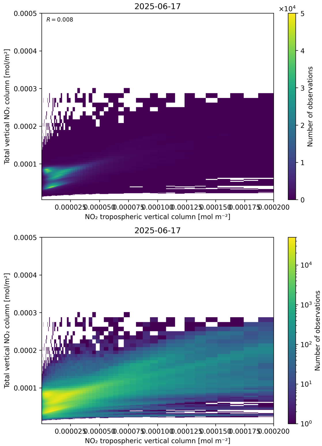
Figure 128: Scatter density plot of “NO 2 tropospheric vertical column” against “Total vertical NO 2 column” for 2025-06-17 to 2025-06-18.
