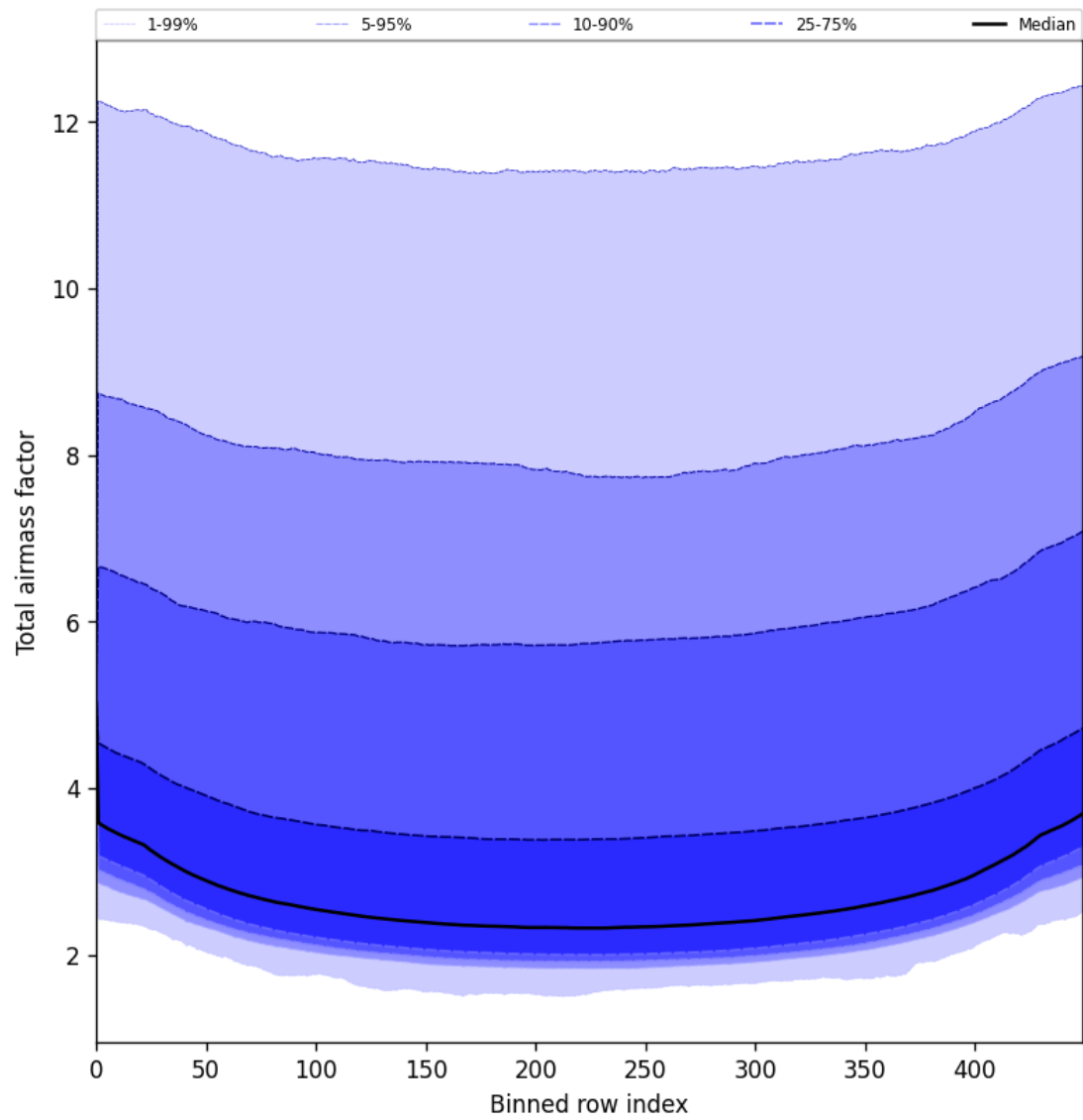
Figure 49: Along track statistics of “Total airmass factor” for 2025-06-17 to 2025-06-18
