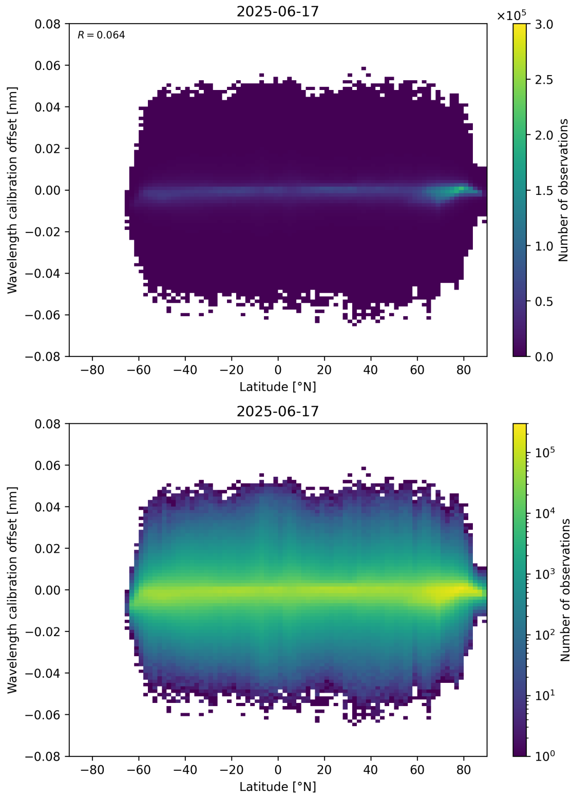
Figure 95: Scatter density plot of “Latitude” against “Wavelength calibration offset” for 2025-06-17 to 2025-06-18.
