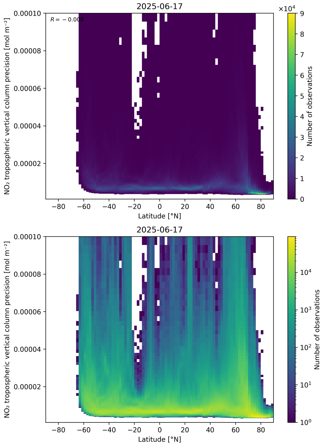
Figure 93: Scatter density plot of “Latitude” against “NO 2 tropospheric vertical column precision” for 2025-06-17 to 2025-06-18.
