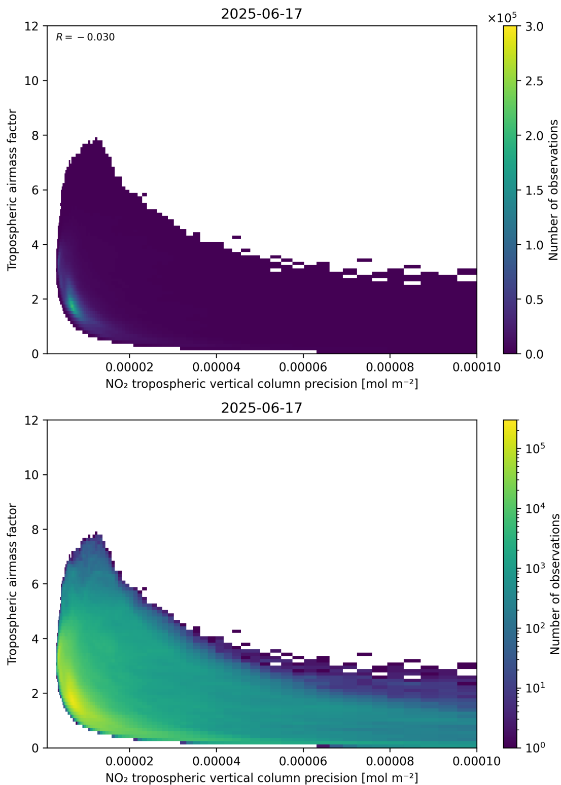
Figure 133: Scatter density plot of “NO 2 tropospheric vertical column precision” against “Tropospheric airmass factor” for 2025-06-17 to 2025-06-18.
