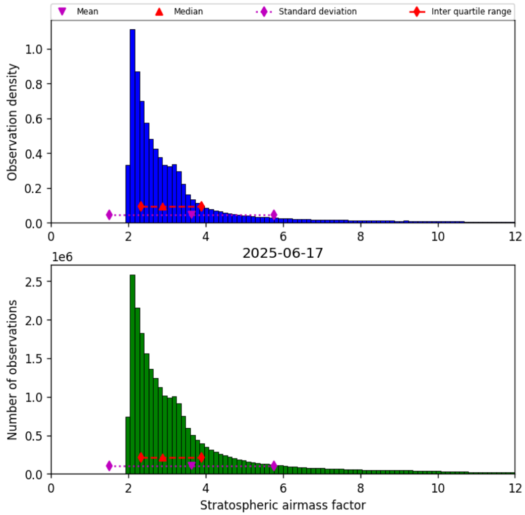
Figure 44: Histogram of “Stratospheric airmass factor” for 2025-06-17 to 2025-06-18
