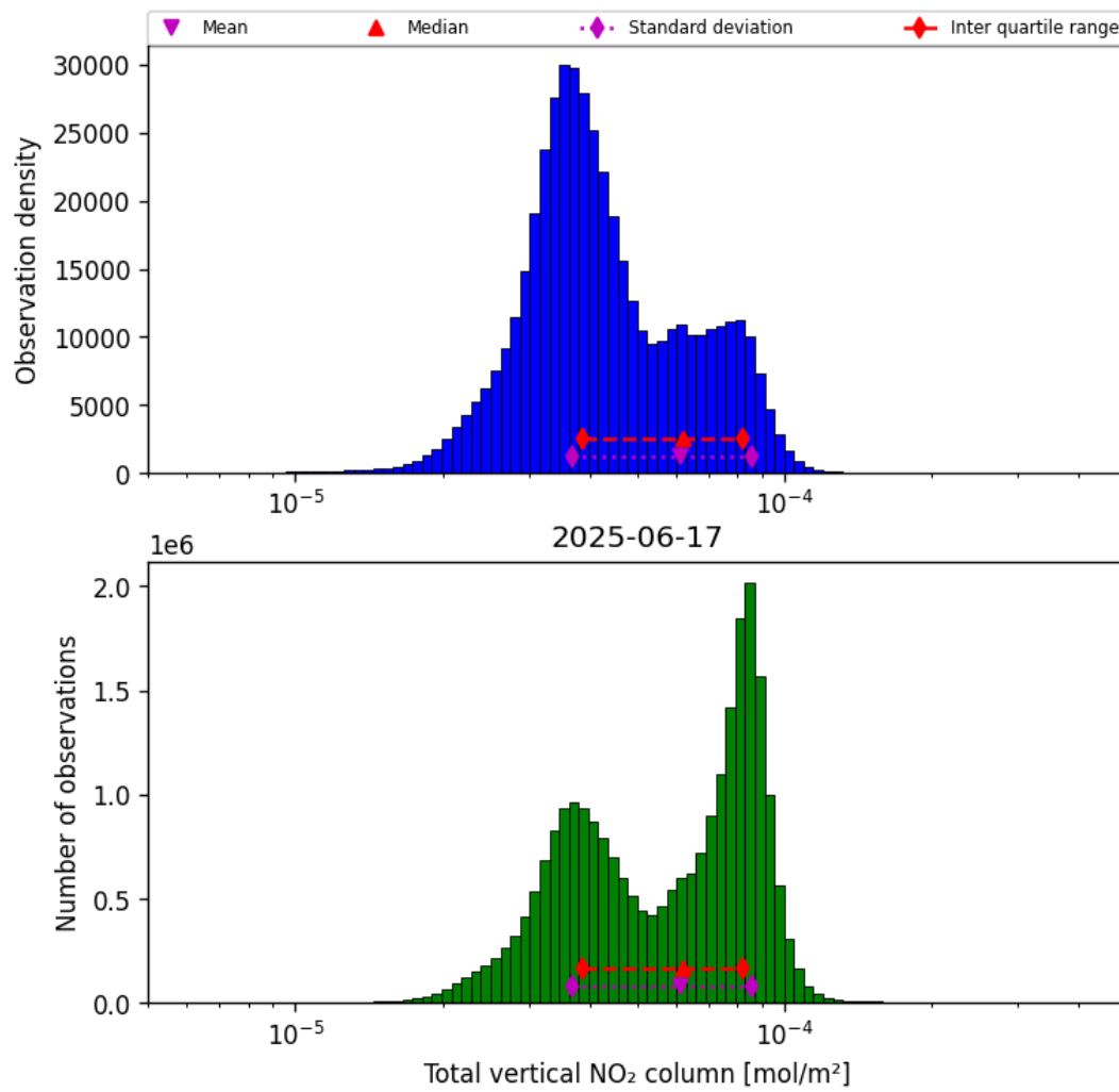
Figure 38: Histogram of “Total vertical NO 2 column” for 2025-06-17 to 2025-06-18
