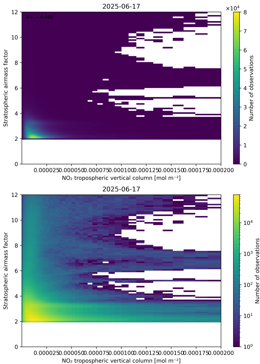
Figure 121: Scatter density plot of “NO 2 tropospheric vertical column” against “Stratospheric air mass factor” for 2025-06-17 to 2025-06-18.
