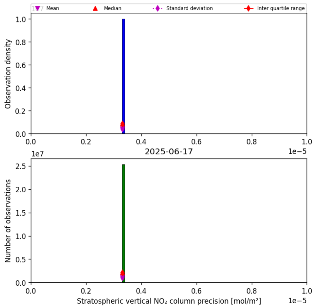
Figure 37: Histogram of “Stratospheric vertical NO 2 column precision” for 2025-06-17 to 2025-06-18
