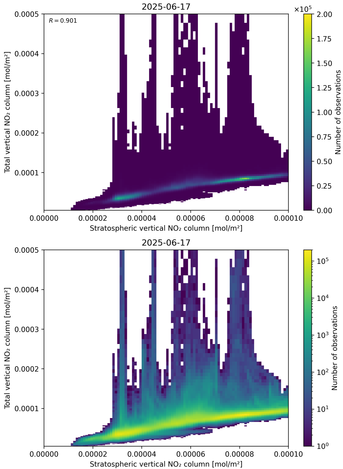
Figure 100: Scatter density plot of “Stratospheric vertical NO 2 column” against “Total vertical NO 2 column” for 2025-06-17 to 2025-06-18.
