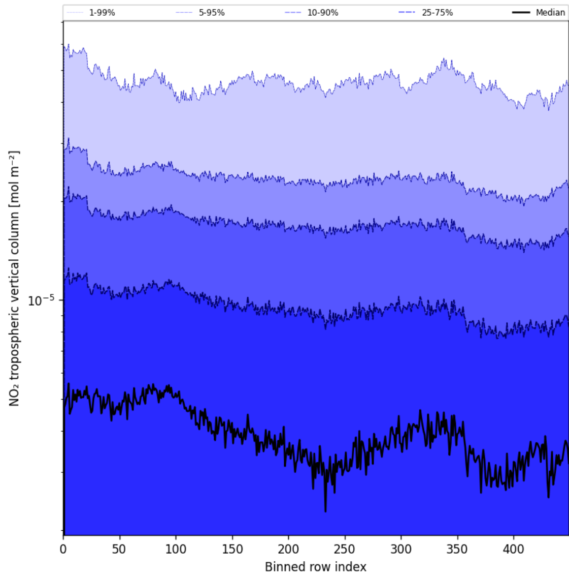
Figure 46: Along track statistics of “NO 2 tropospheric vertical column” for 2025-06-17 to 2025-06-18
