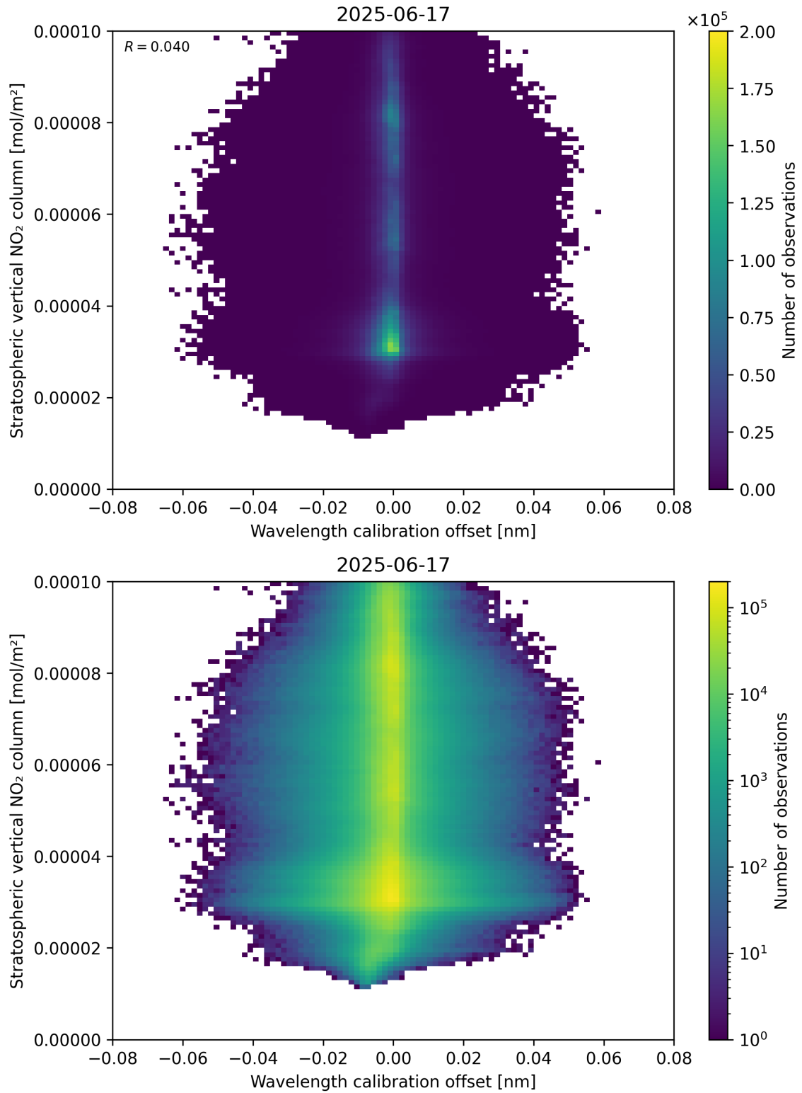
Figure 176: Scatter density plot of “Wavelength calibration offset” against “Stratospheric vertical NO 2 column” for 2025-06-17 to 2025-06-18.
