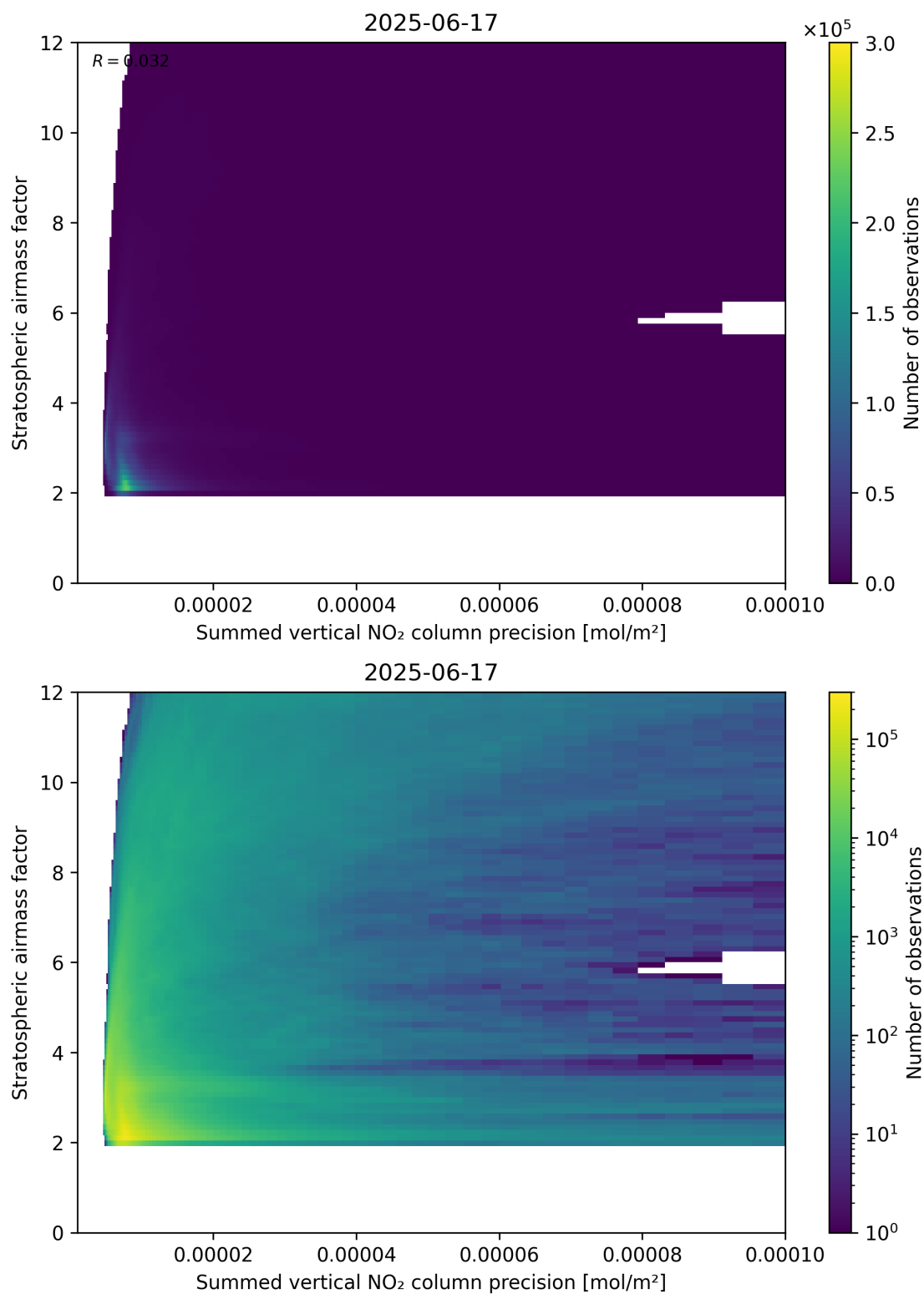
Figure 106: Scatter density plot of “Summed vertical NO 2 column precision” against “Stratospheric airmass factor” for 2025-06-17 to 2025-06-18.
