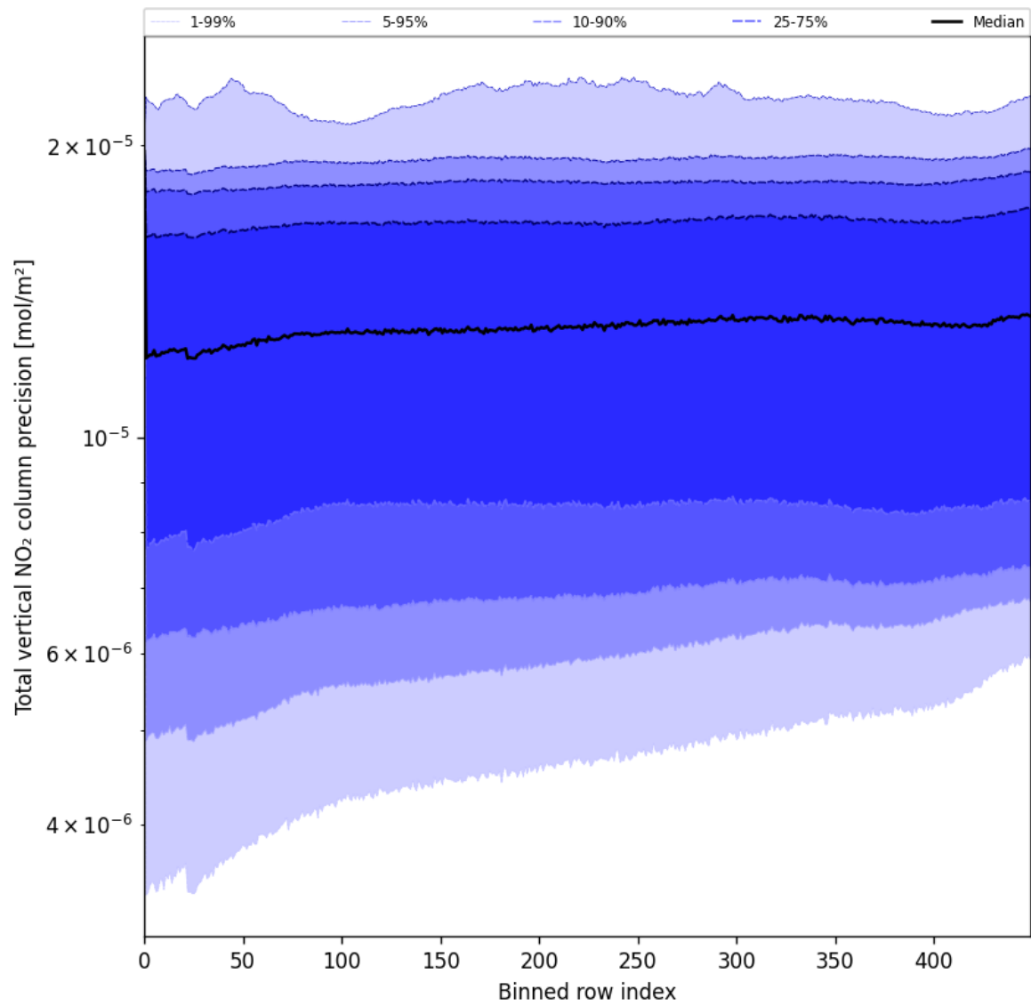
Figure 56: Along track statistics of “Total vertical NO 2 column precision” for 2025-06-17 to 2025-06-18
