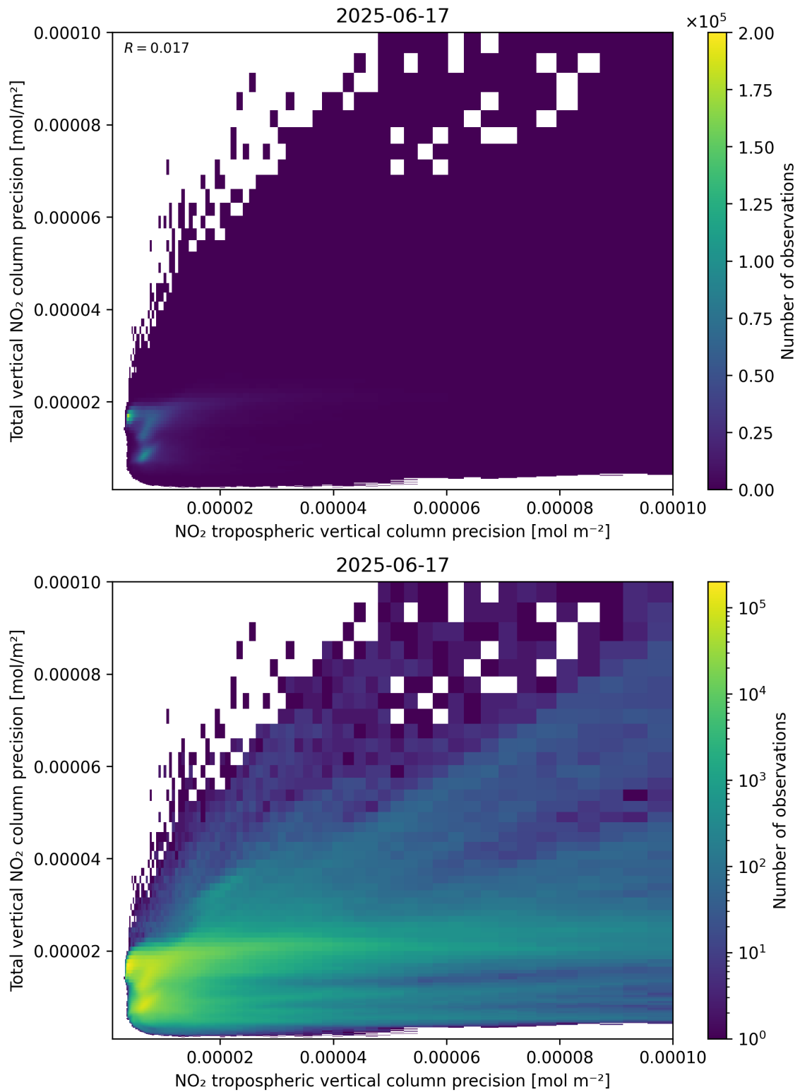
Figure 139: Scatter density plot of “NO 2 tropospheric vertical column precision” against “Total vertical NO 2 column precision” for 2025-06-17 to 2025-06-18.
