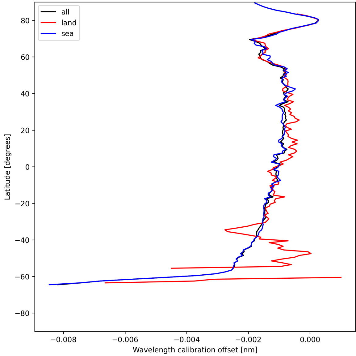
Figure 18: Zonal average of “Wavelength calibration offset” for 2025-06-17 to 2025-06-18.
