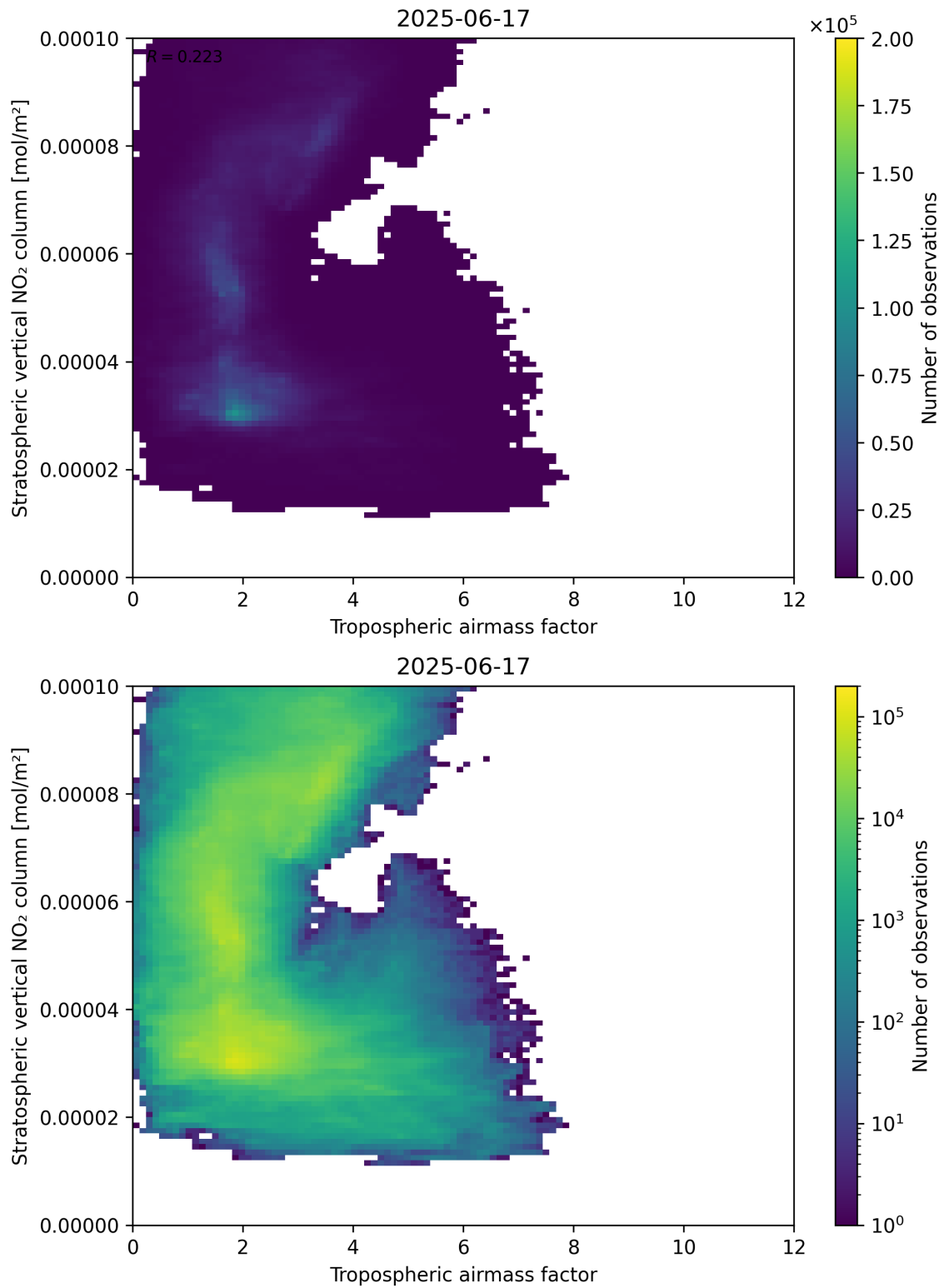
Figure 74: Scatter density plot of “Tropospheric air mass factor” against “Stratospheric vertical NO 2 column” for 2025-06-17 to 2025-06-18.
