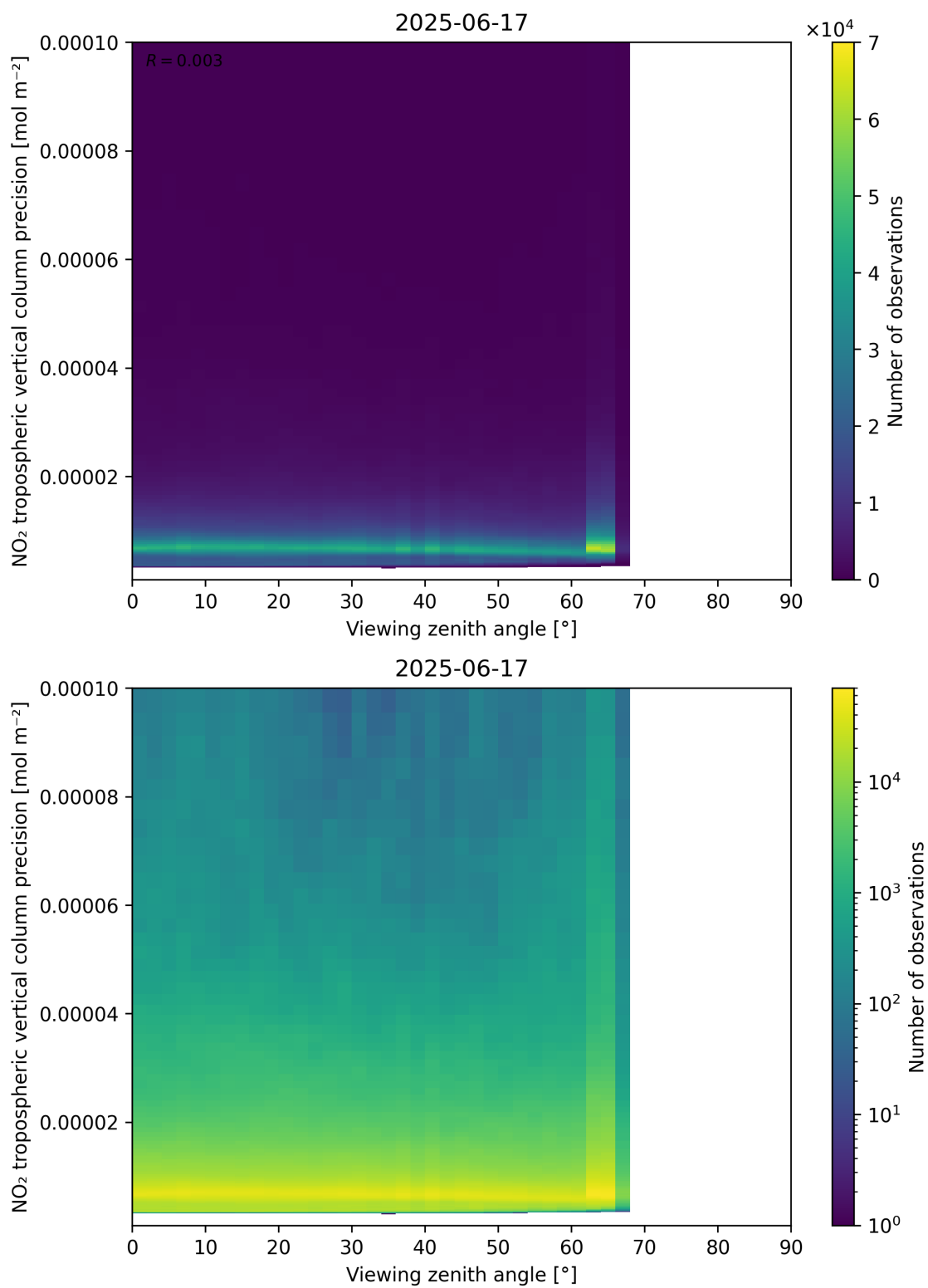
Figure 170: Scatter density plot of “Viewing zenith angle” against “NO 2 tropospheric vertical column precision” for 2025-06-17 to 2025-06-18.
