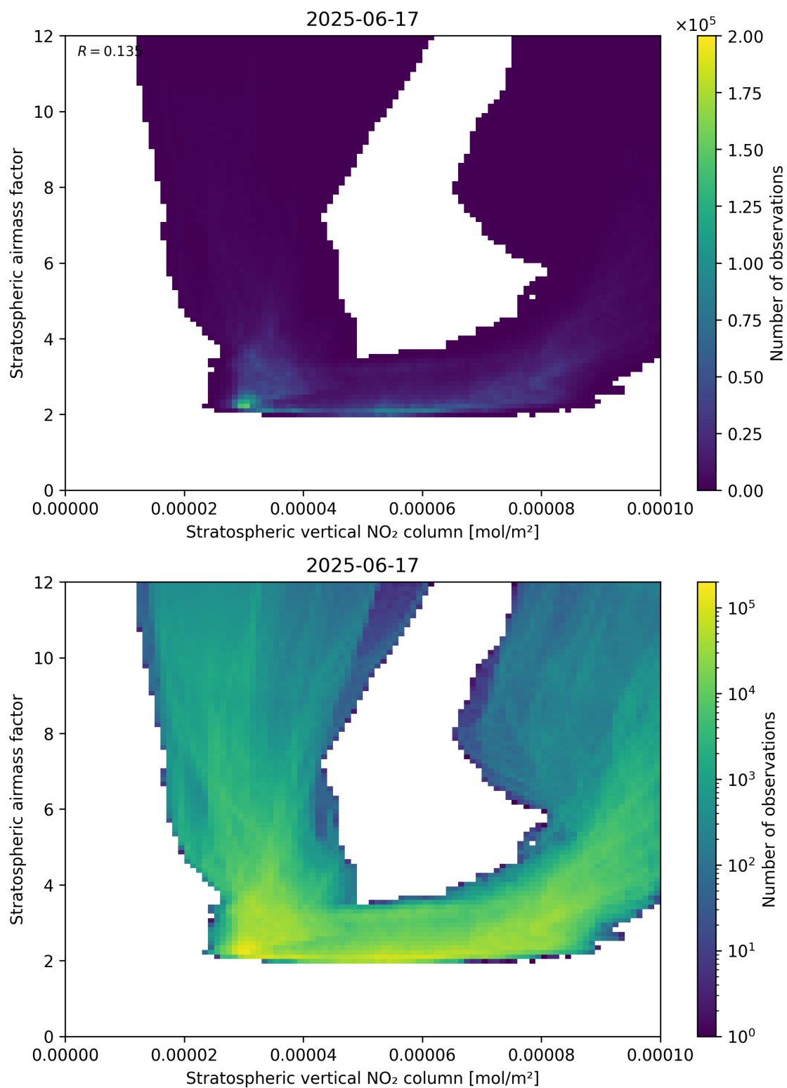
Figure 96: Scatter density plot of “Stratospheric vertical NO 2 column” against “Stratospheric airmass factor” for 2025-06-17 to 2025-06-18.
