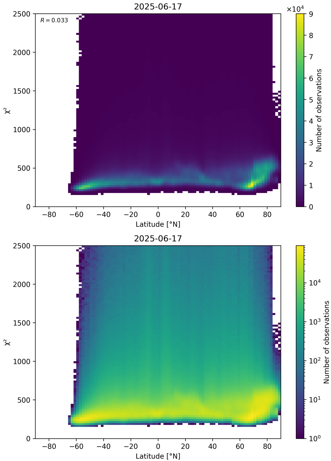
Figure 86: Scatter density plot of “Latitude” against “ \chi^2 ” for 2025-06-17 to 2025-06-18.
