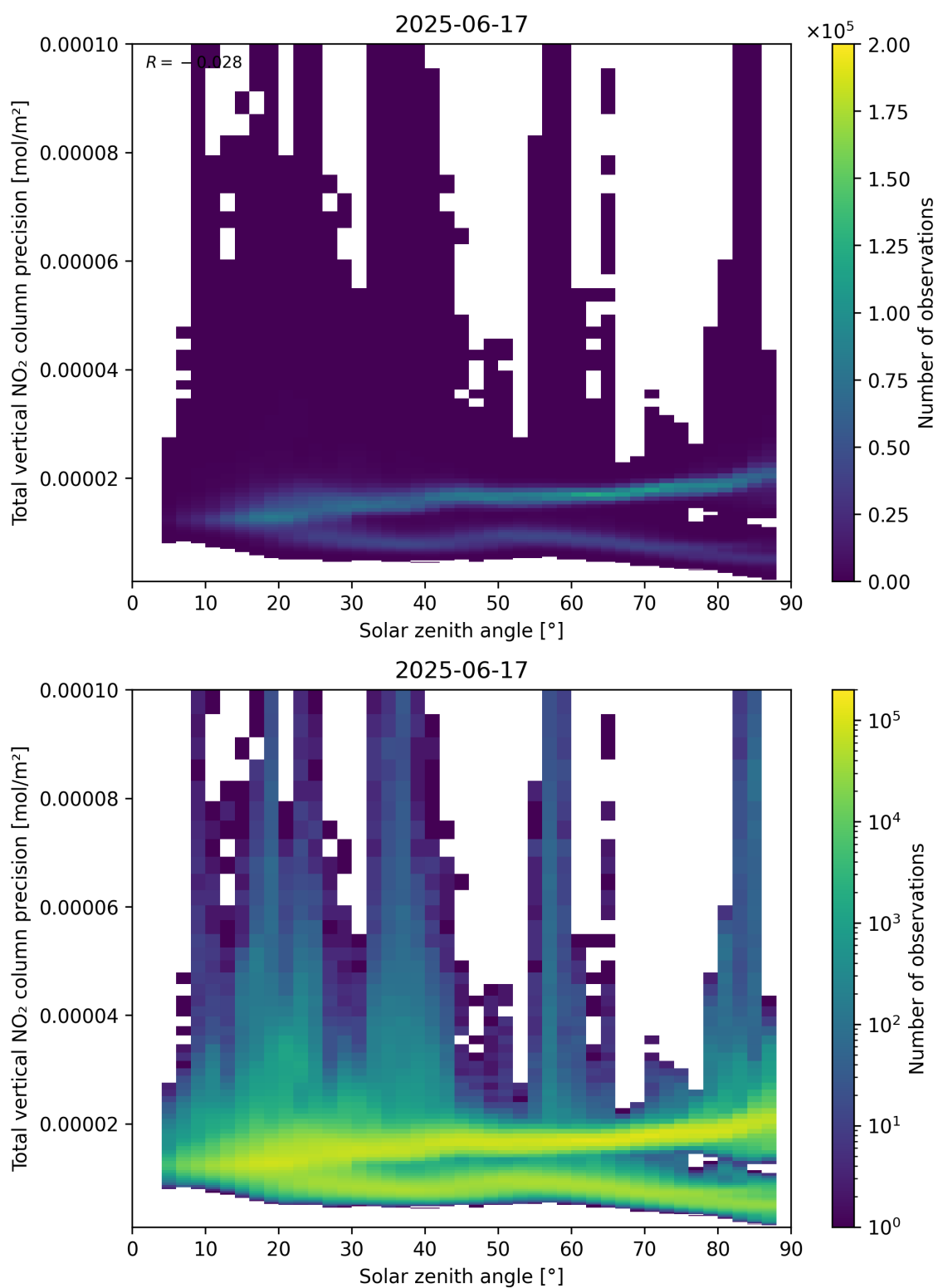
Figure 154: Scatter density plot of “Solar zenith angle” against “Total vertical NO 2 column precision” for 2025-06-17 to 2025-06-18.
