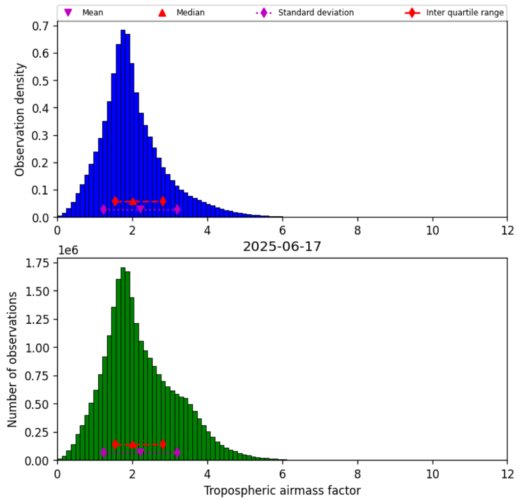
Figure 31: Histogram of “Tropospheric airmass factor” for 2025-06-17 to 2025-06-18
