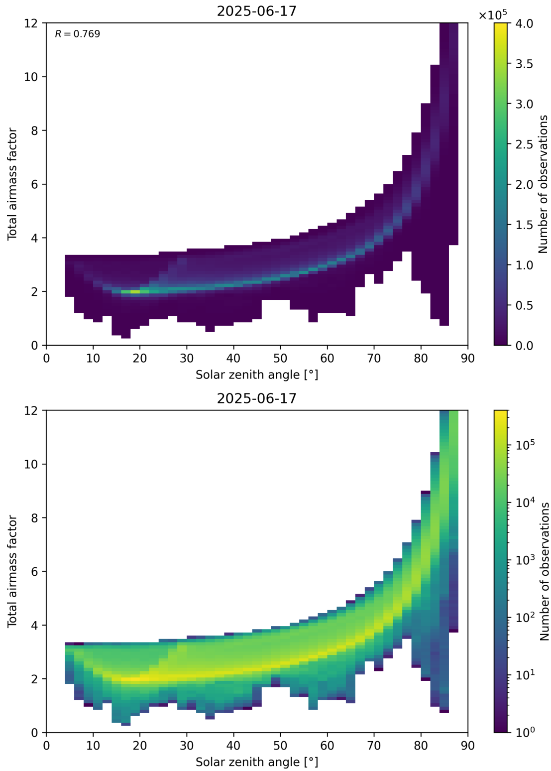
Figure 146: Scatter density plot of “Solar zenith angle” against “Total air mass factor” for 2025-06-17 to 2025-06-18.
