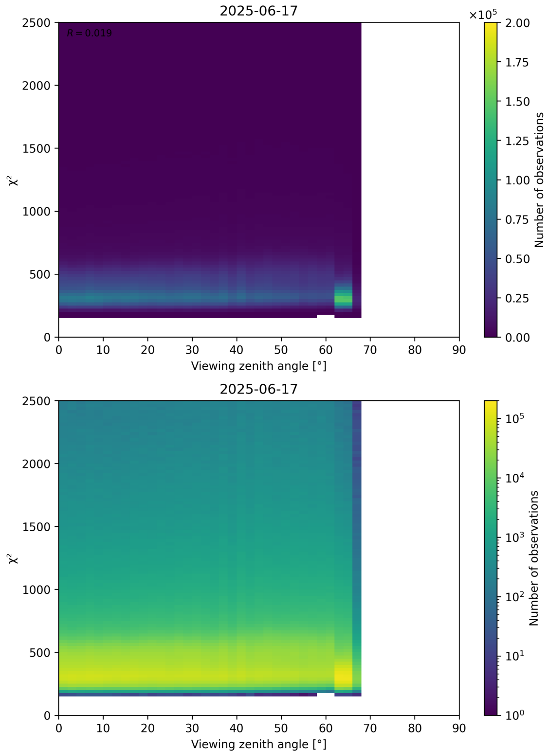
Figure 162: Scatter density plot of “Viewing zenith angle” against “ \chi^2 ” for 2025-06-17 to 2025-06-18.
