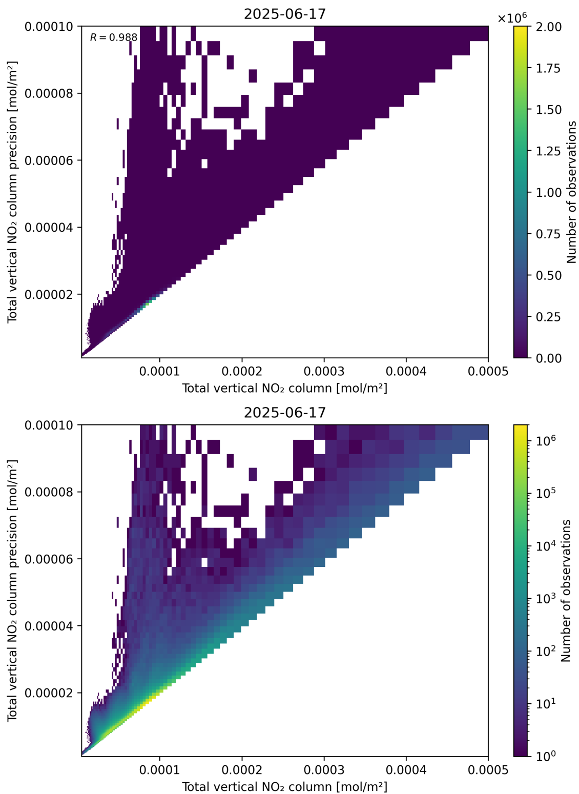
Figure 114: Scatter density plot of “Total vertical NO 2 column” against “Total vertical NO 2 column precision” for 2025-06-17 to 2025-06-18.
