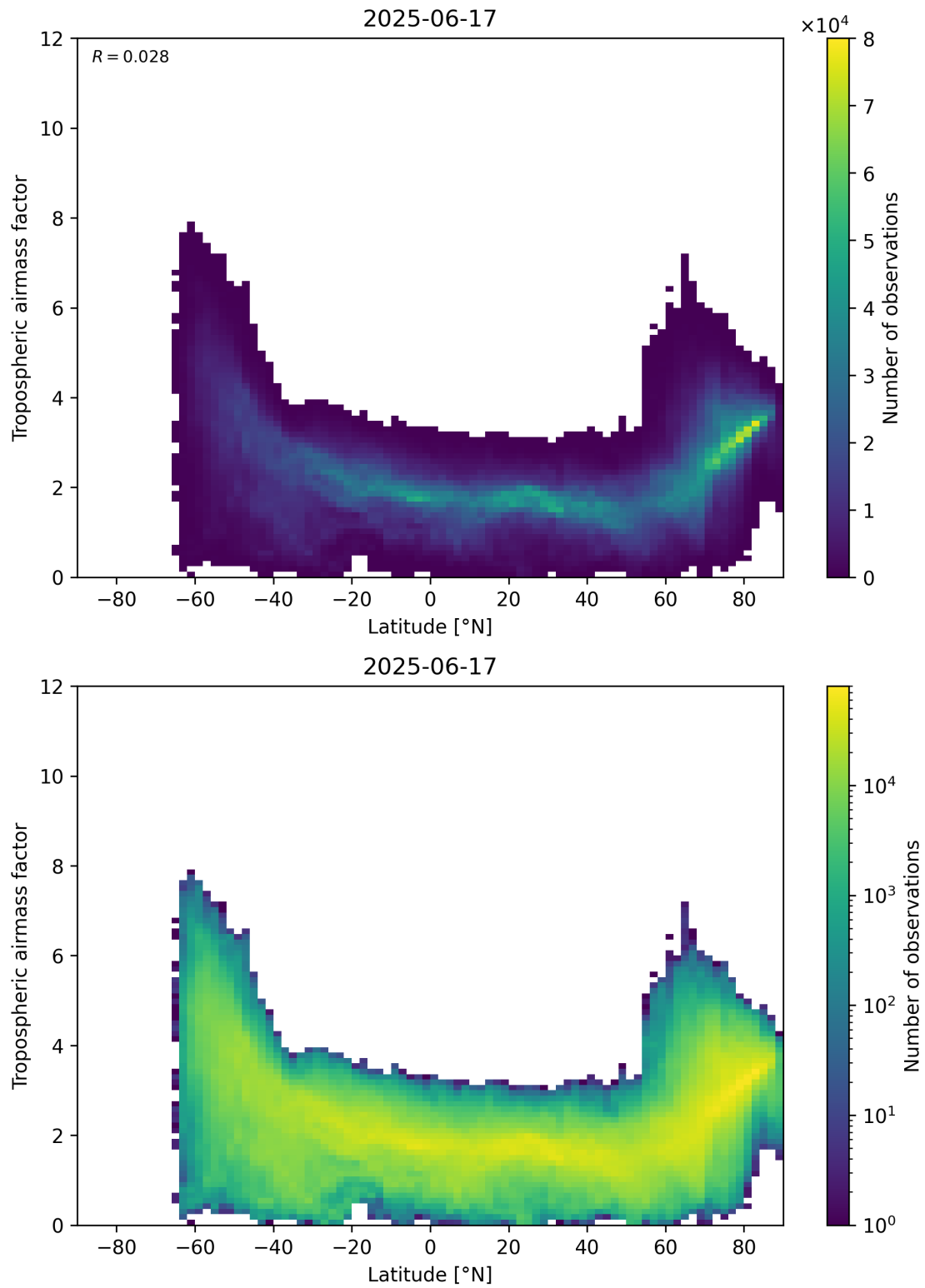
Figure 85: Scatter density plot of “Latitude” against “Tropospheric airmass factor” for 2025-06-17 to 2025-06-18.
