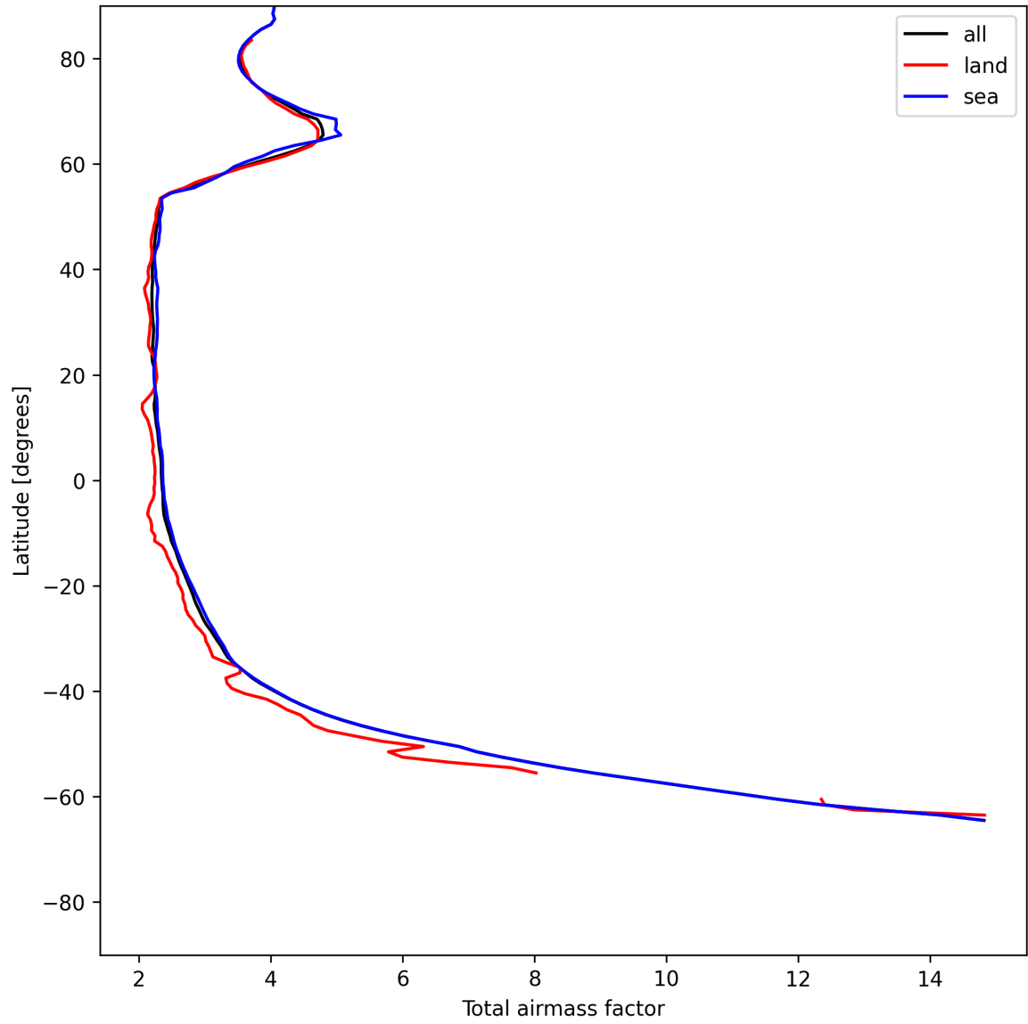
Figure 15: Zonal average of “Total airmass factor” for 2025-06-17 to 2025-06-18.
