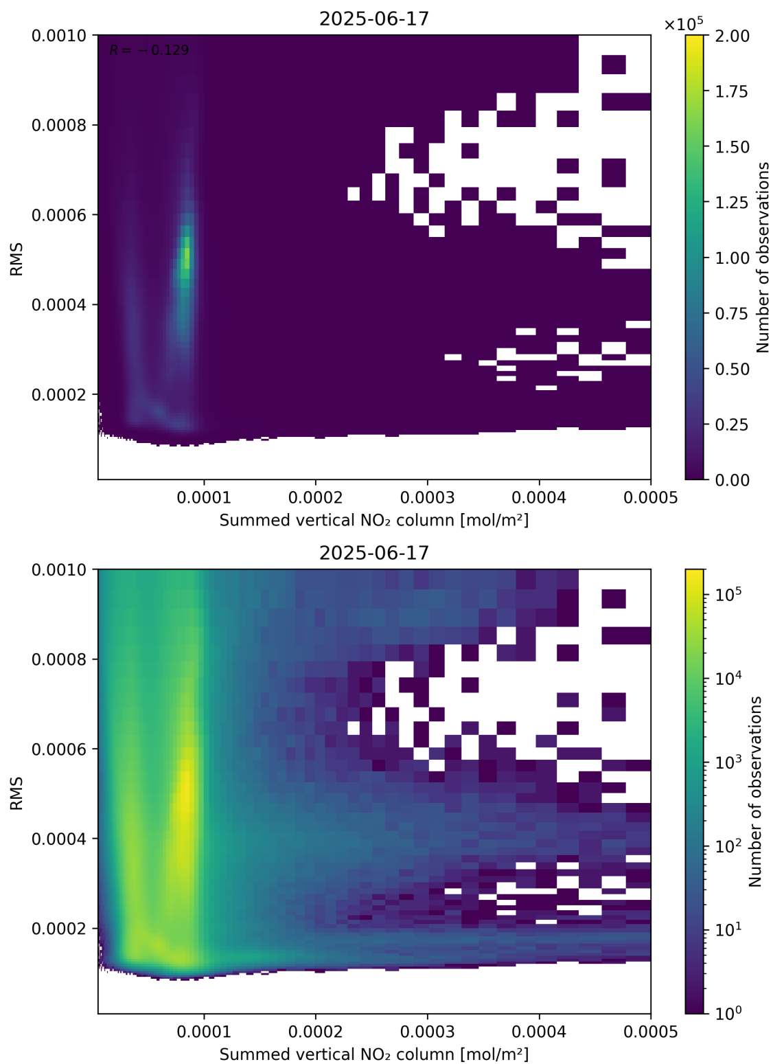
Figure 109: Scatter density plot of “Summed vertical NO 2 column” against “RMS” for 2025-06-17 to 2025-06-18.
