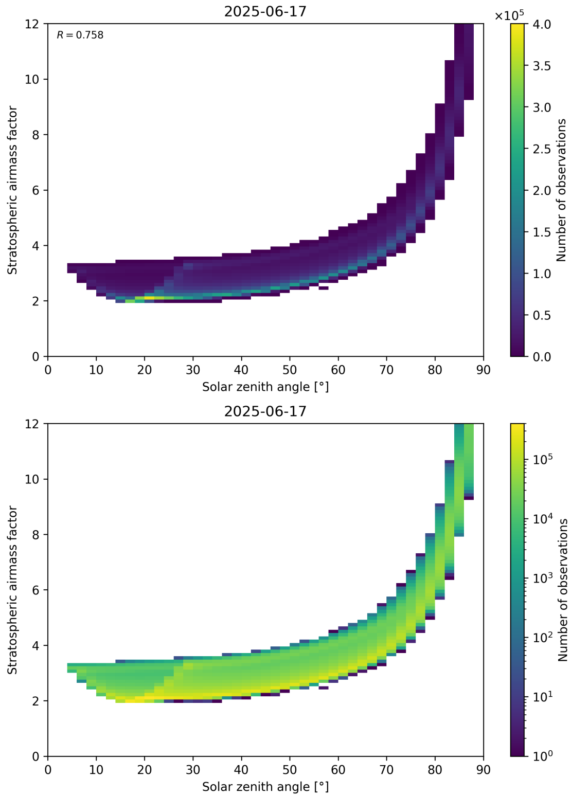
Figure 145: Scatter density plot of “Solar zenith angle” against “Stratospheric airmass factor” for 2025-06-17 to 2025-06-18.
