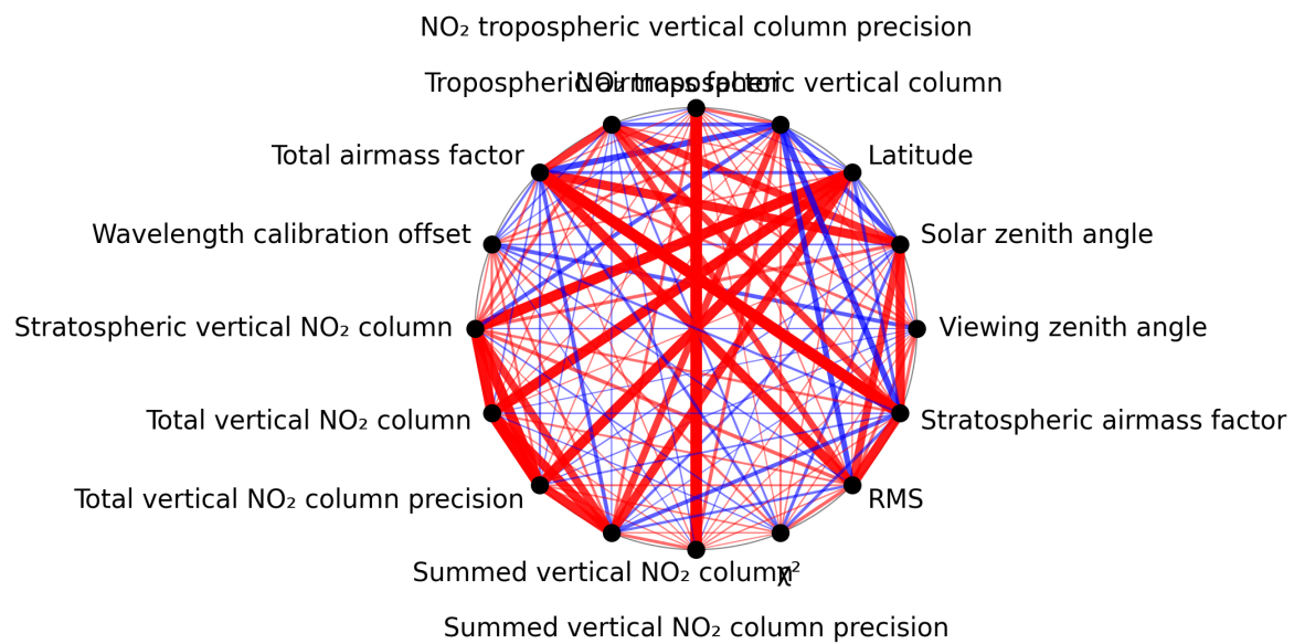
Figure 1: Map of correlation graph for 2025-06-17 to 2025-06-18.
