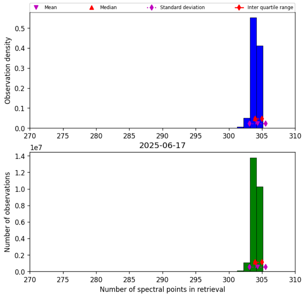
Figure 33: Histogram of “Number of spectral points in retrieval” for 2025-06-17 to 2025-06-18
