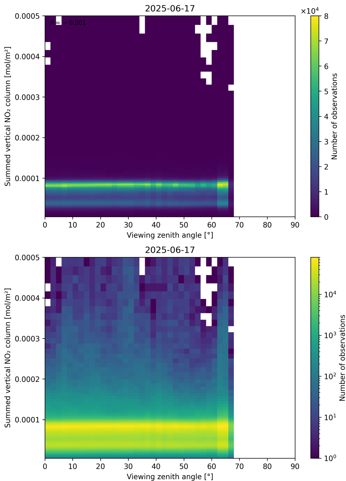
Figure 165: Scatter density plot of “Viewing zenith angle” against “Summed vertical NO 2 column” for 2025-06-17 to 2025-06-18.
