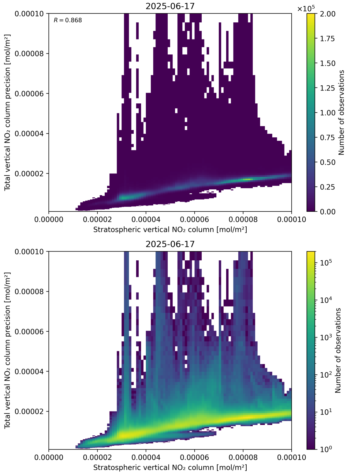
Figure 101: Scatter density plot of “Stratospheric vertical NO 2 column” against “Total vertical NO 2 column precision” for 2025-06-17 to 2025-06-18.
