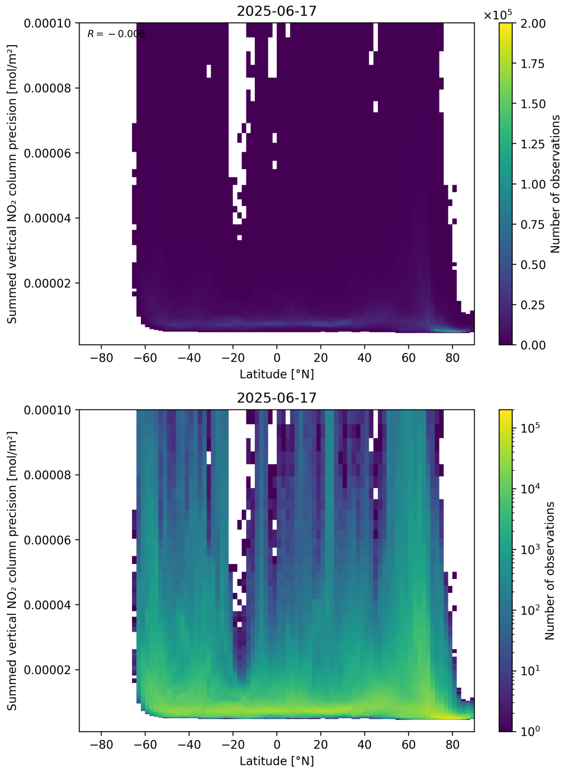
Figure 89: Scatter density plot of “Latitude” against “Summed vertical NO 2 column precision” for 2025-06-17 to 2025-06-18.
