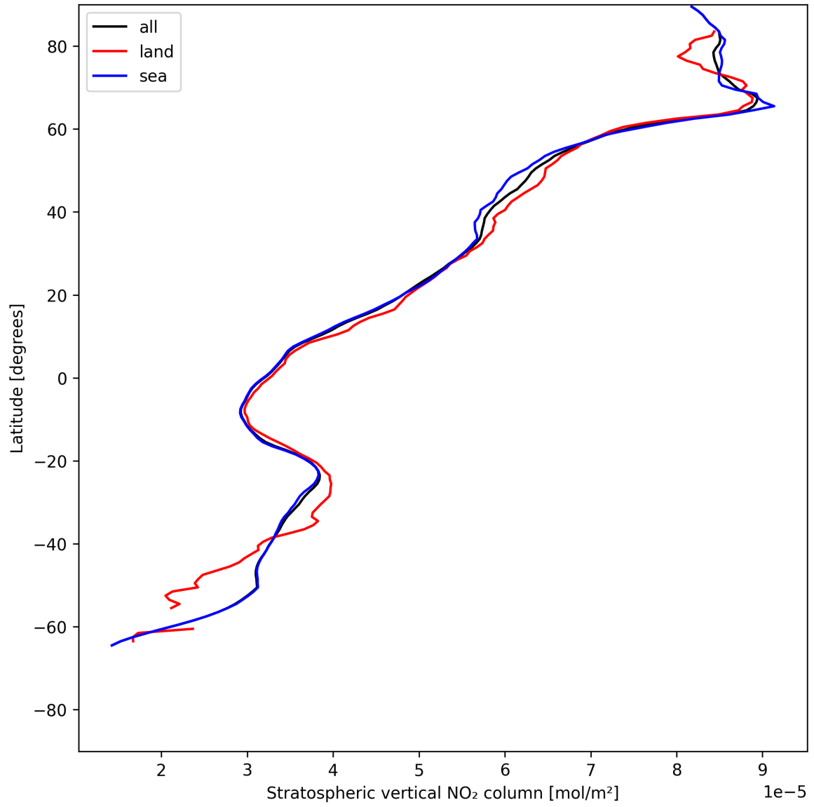
Figure 19: Zonal average of “Stratospheric vertical NO 2 column” for 2025-06-17 to 2025-06-18.
