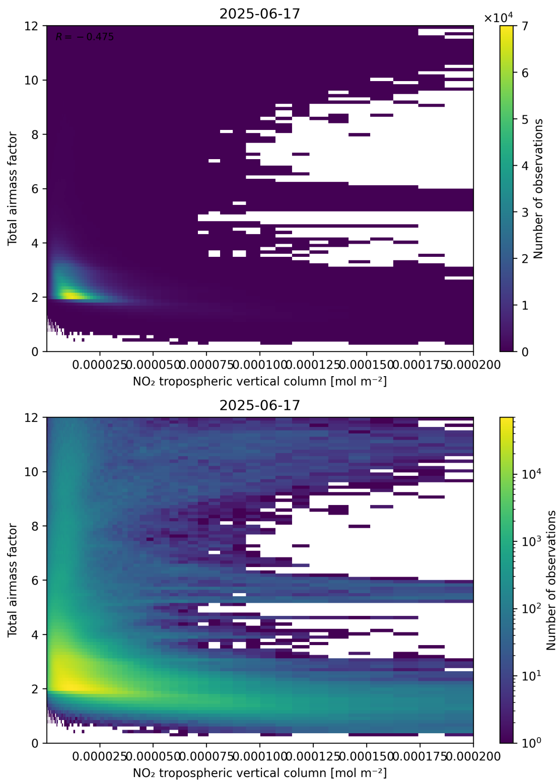
Figure 122: Scatter density plot of “NO 2 tropospheric vertical column” against “Total air mass factor” for 2025-06-17 to 2025-06-18.
