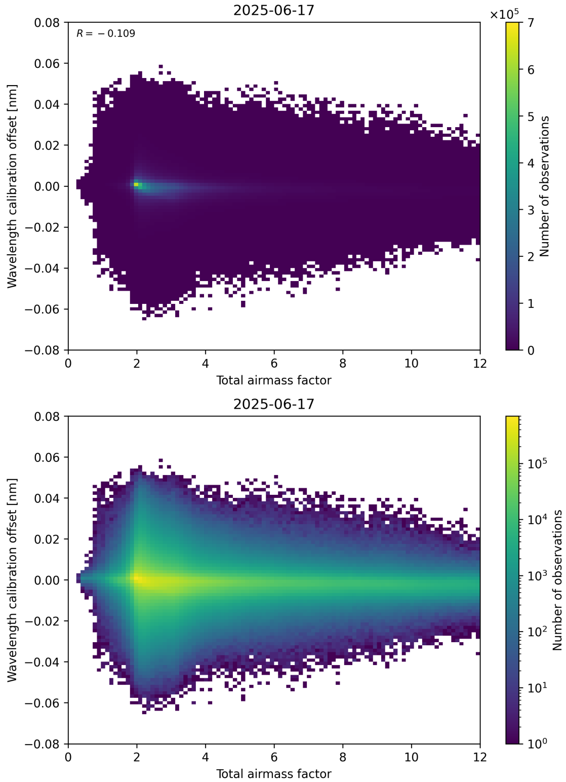
Figure 70: Scatter density plot of “Total airmass factor” against “Wavelength calibration offset” for 2025-06-17 to 2025-06-18.
