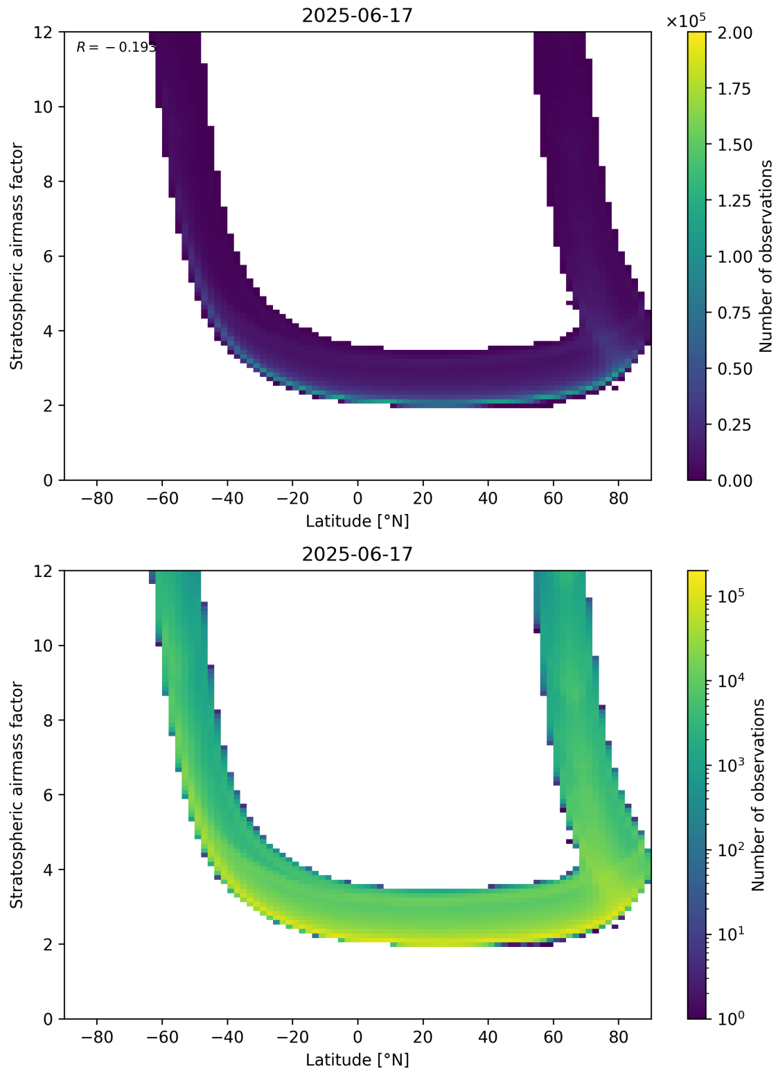
Figure 83: Scatter density plot of “Latitude” against “Stratospheric air mass factor” for 2025-06-17 to 2025-06-18.
