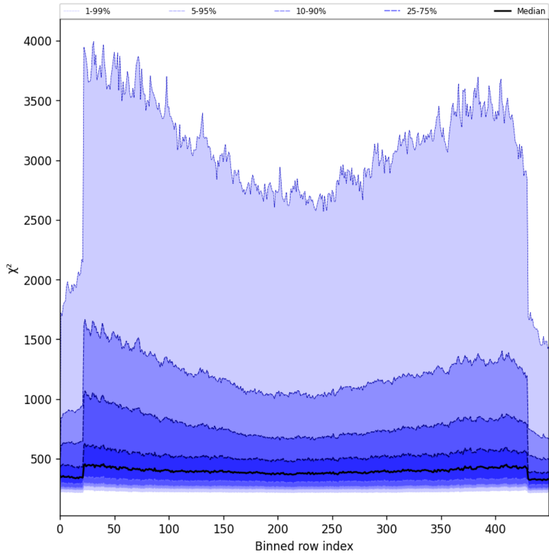
Figure 59: Along track statistics of “ \chi^2 ” for 2025-06-17 to 2025-06-18
