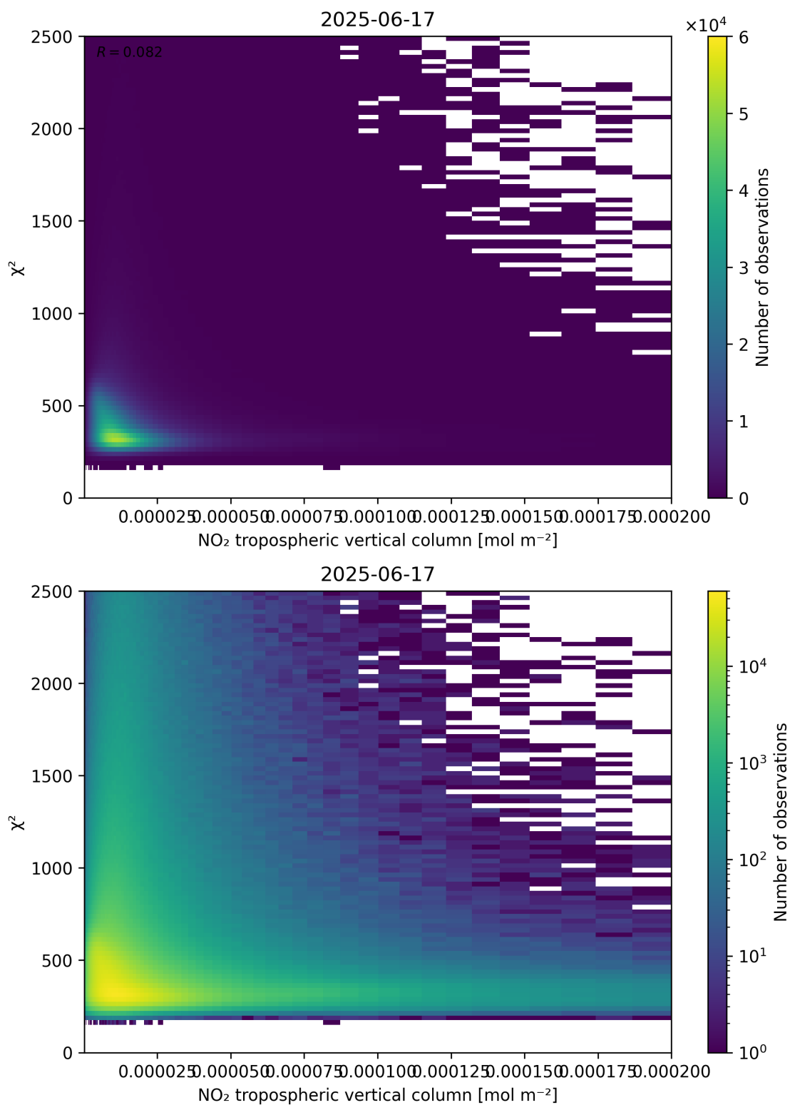
Figure 124: Scatter density plot of “NO 2 tropospheric vertical column” against “ \chi^2 ” for 2025-06-17 to 2025-06-18.
