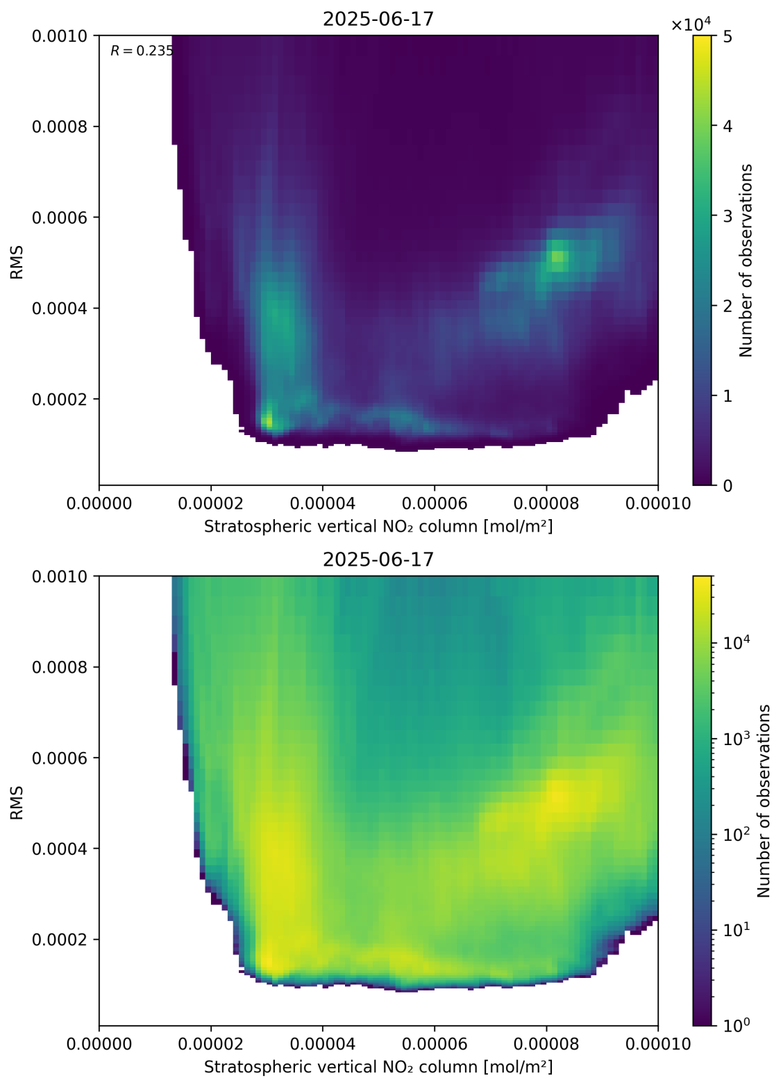
Figure 102: Scatter density plot of “Stratospheric vertical NO 2 column” against “RMS” for 2025-06-17 to 2025-06-18.
