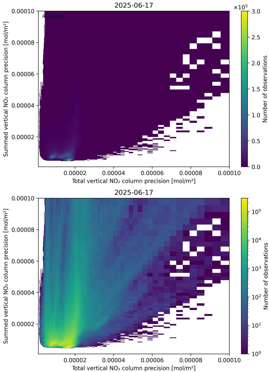
Figure 118: Scatter density plot of “Total vertical NO 2 column precision” against “Summed vertical NO 2 column precision” for 2025-06-17 to 2025-06-18.
