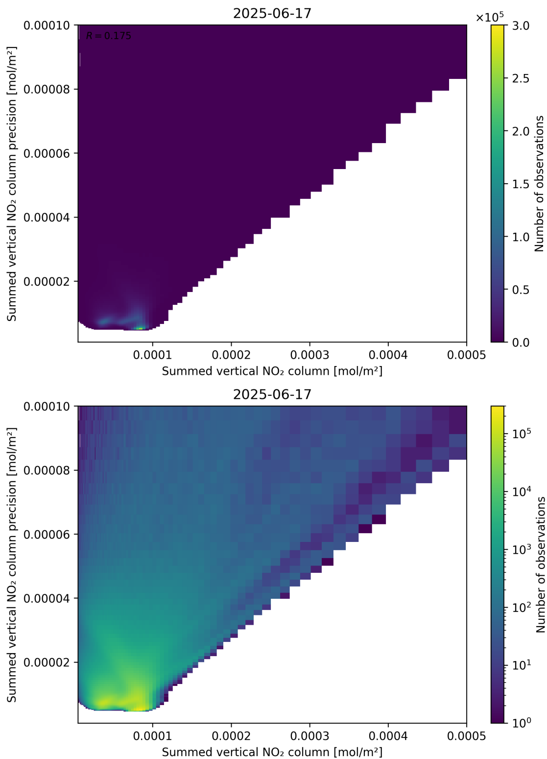
Figure 105: Scatter density plot of “Summed vertical NO 2 column” against “Summed vertical NO 2 column precision” for 2025-06-17 to 2025-06-18.
