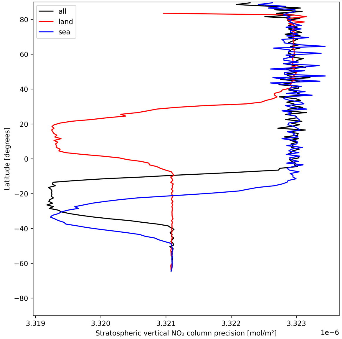
Figure 20: Zonal average of “Stratospheric vertical NO 2 column precision” for 2025-06-17 to 2025-06-18.
