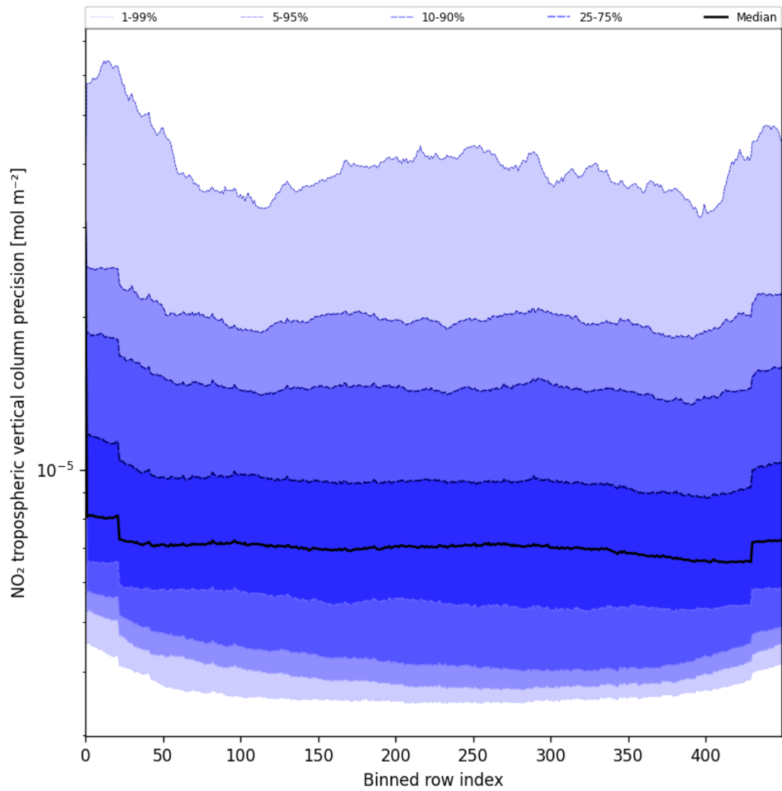
Figure 47: Along track statistics of “NO 2 tropospheric vertical column precision” for 2025-06-17 to 2025-06-18
