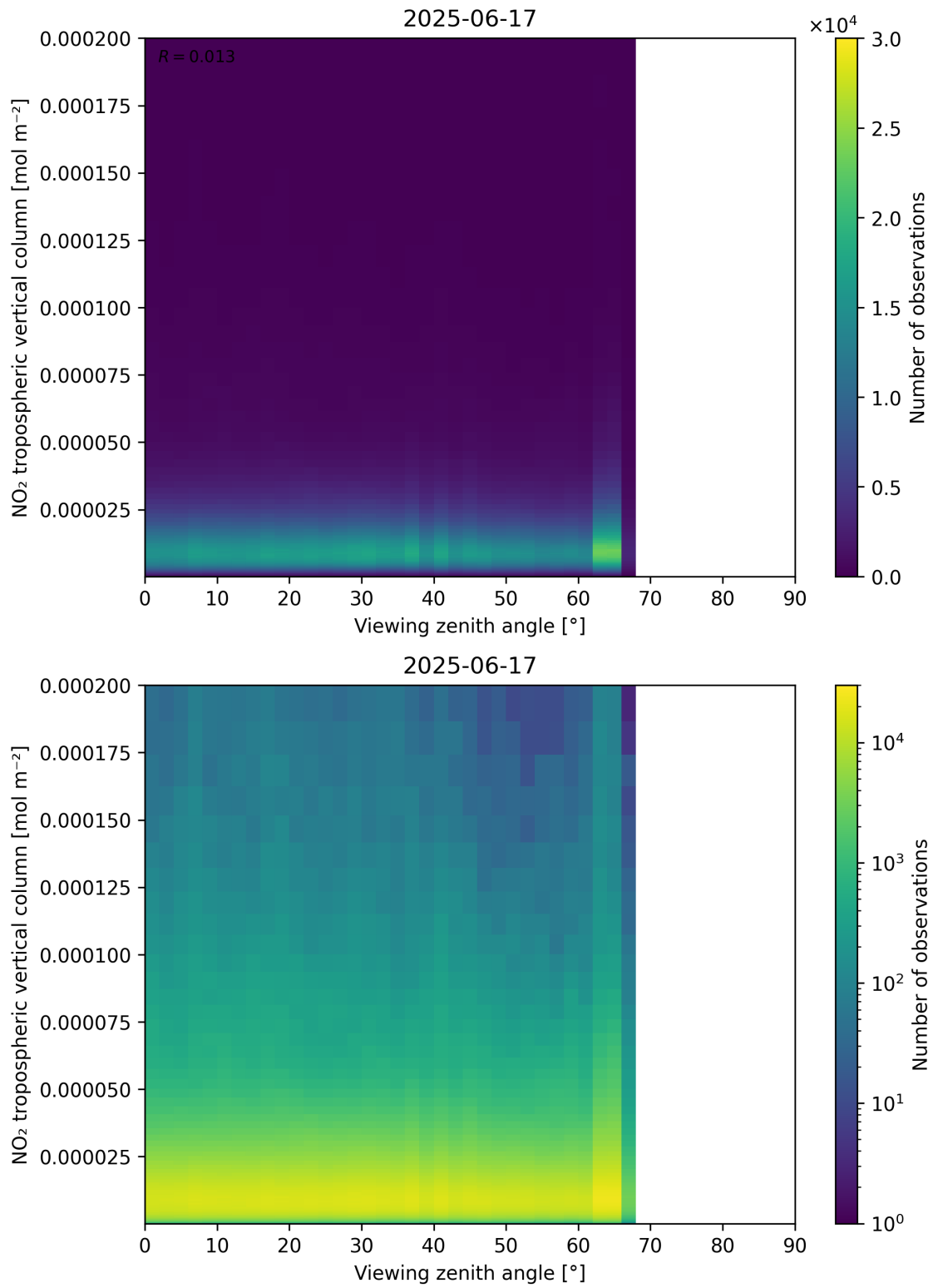
Figure 169: Scatter density plot of “Viewing zenith angle” against “NO 2 tropospheric vertical column” for 2025-06-17 to 2025-06-18.
