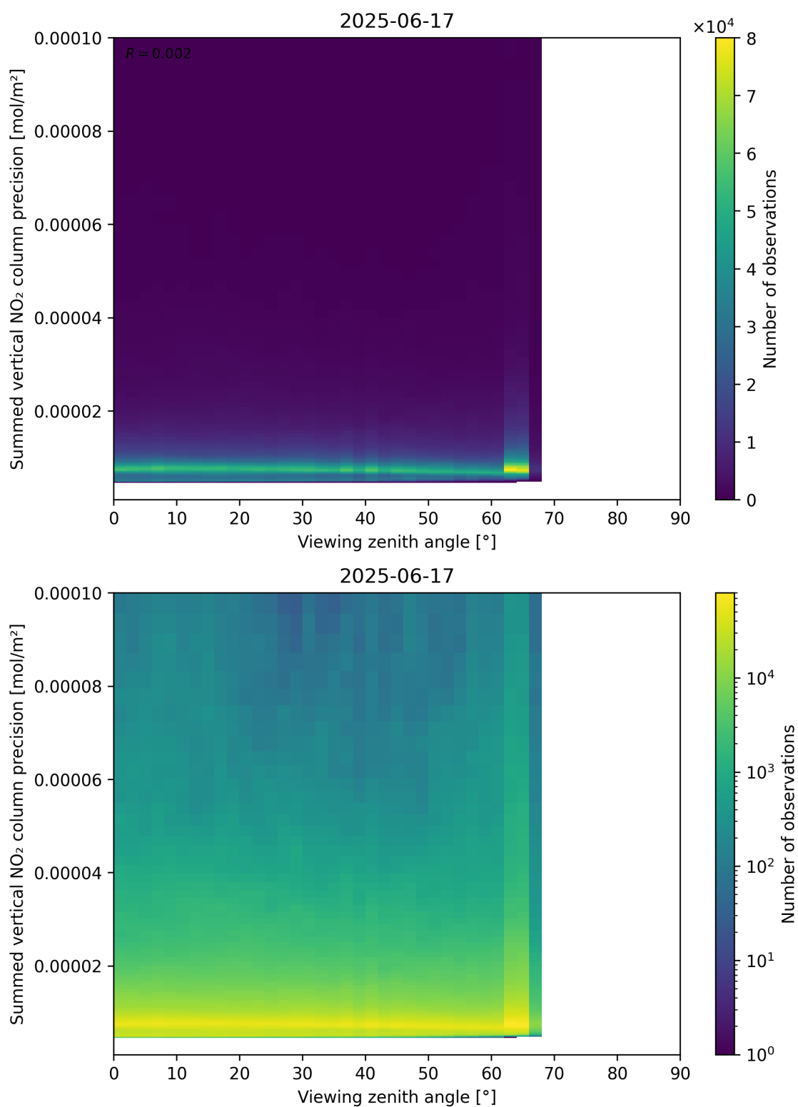
Figure 166: Scatter density plot of “Viewing zenith angle” against “Summed vertical NO 2 column precision” for 2025-06-17 to 2025-06-18.
