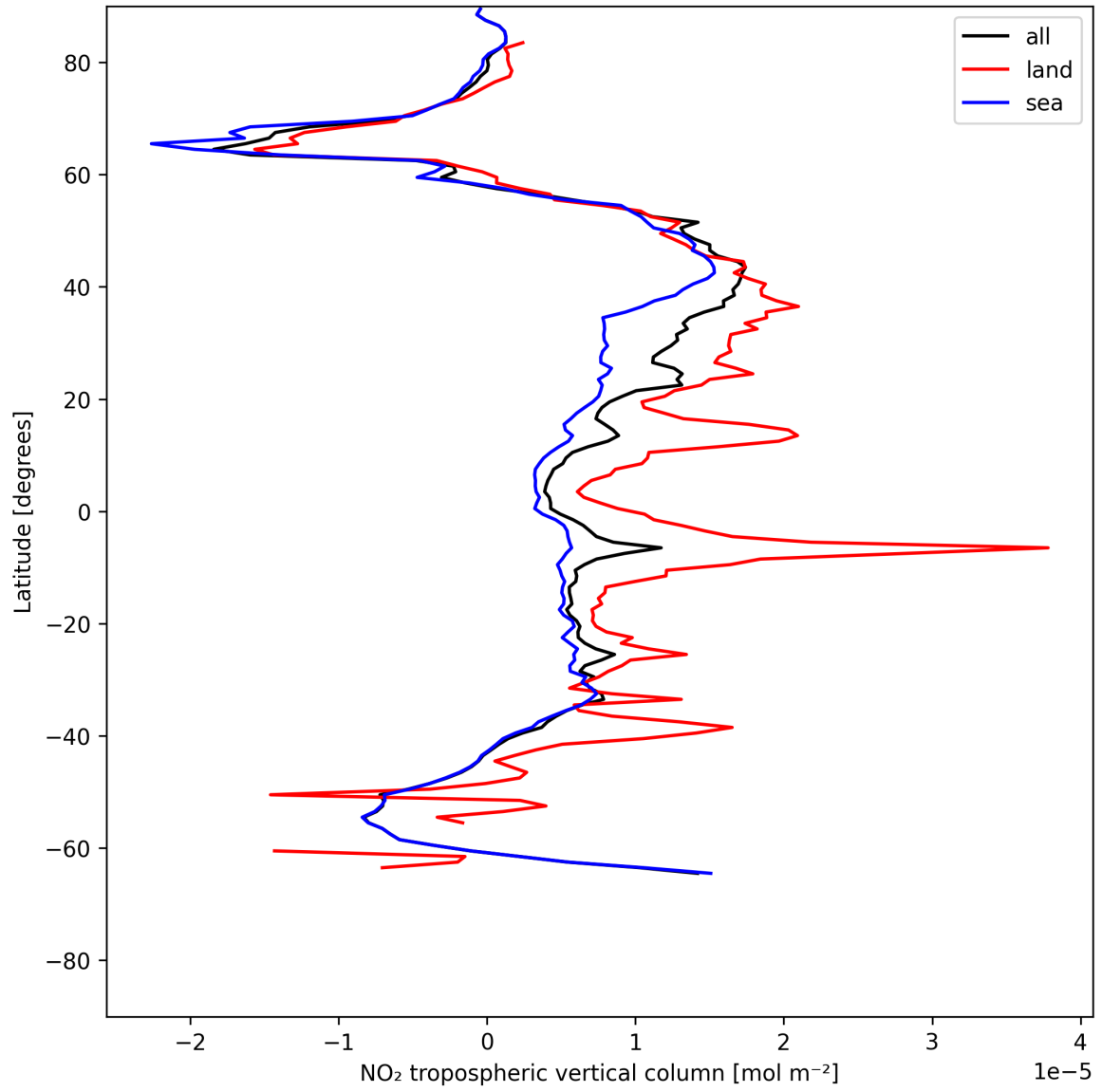
Figure 12: Zonal average of “NO 2 tropospheric vertical column” for 2025-06-17 to 2025-06-18.
