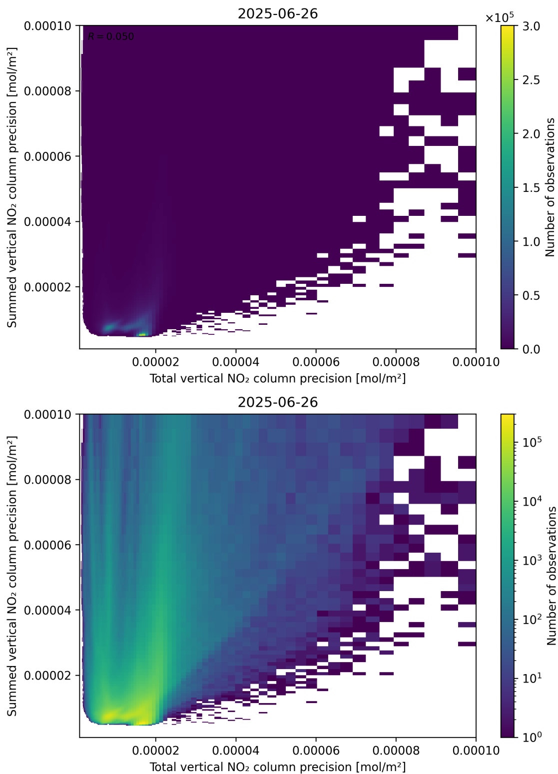
Figure 118: Scatter density plot of “Total vertical NO 2 column precision” against “Summed vertical NO 2 column precision” for 2025-06-25 to 2025-06-27.
