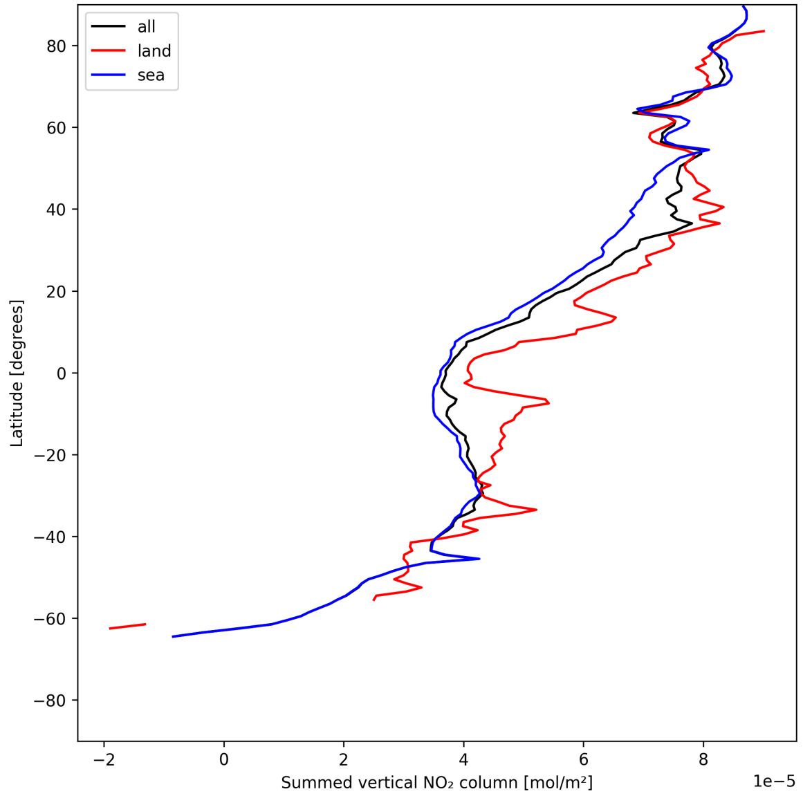
Figure 23: Zonal average of “Summed vertical NO 2 column” for 2025-06-25 to 2025-06-27.
