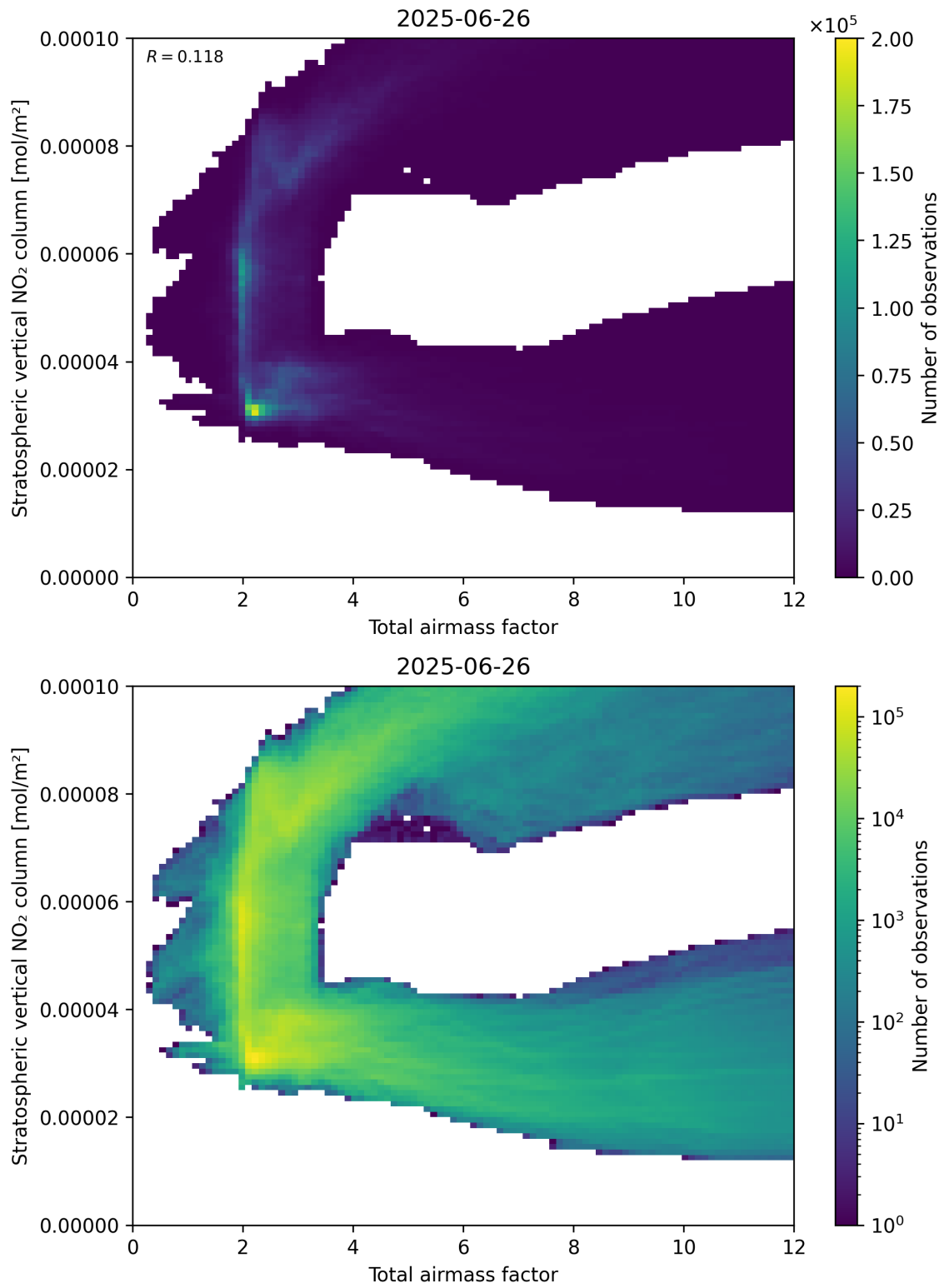
Figure 64: Scatter density plot of “Total airmass factor” against “Stratospheric vertical \text{NO}_2 column” for 2025-06-25 to 2025-06-27.
