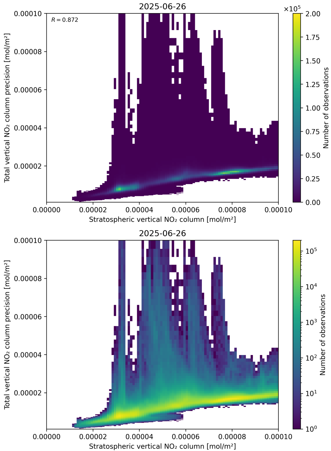
Figure 101: Scatter density plot of “Stratospheric vertical NO 2 column” against “Total vertical NO 2 column precision” for 2025-06-25 to 2025-06-27.
