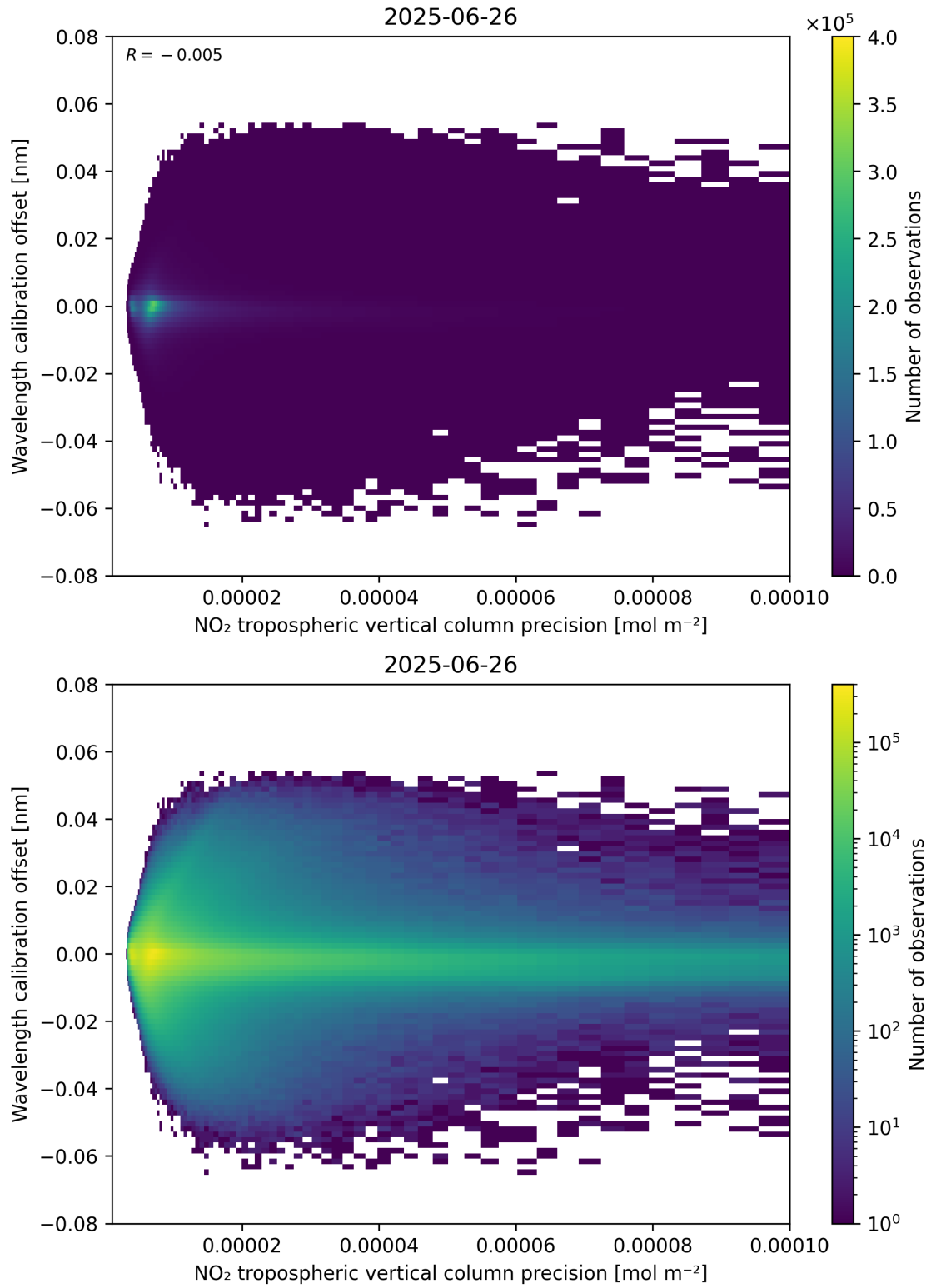
Figure 141: Scatter density plot of “NO 2 tropospheric vertical column precision” against “Wavelength calibration offset” for 2025-06-25 to 2025-06-27.
