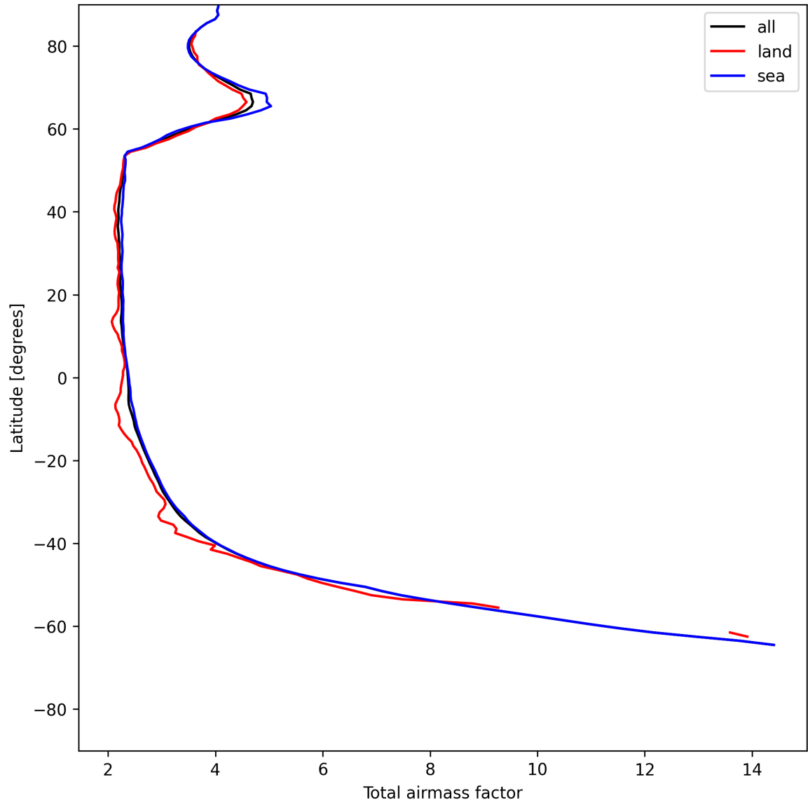
Figure 15: Zonal average of “Total airmass factor” for 2025-06-25 to 2025-06-27.
