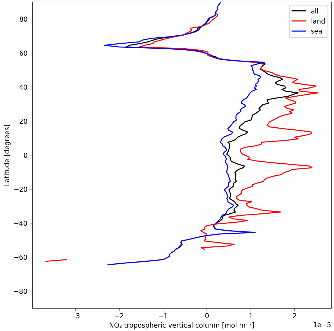
Figure 12: Zonal average of “NO 2 tropospheric vertical column” for 2025-06-25 to 2025-06-27.
