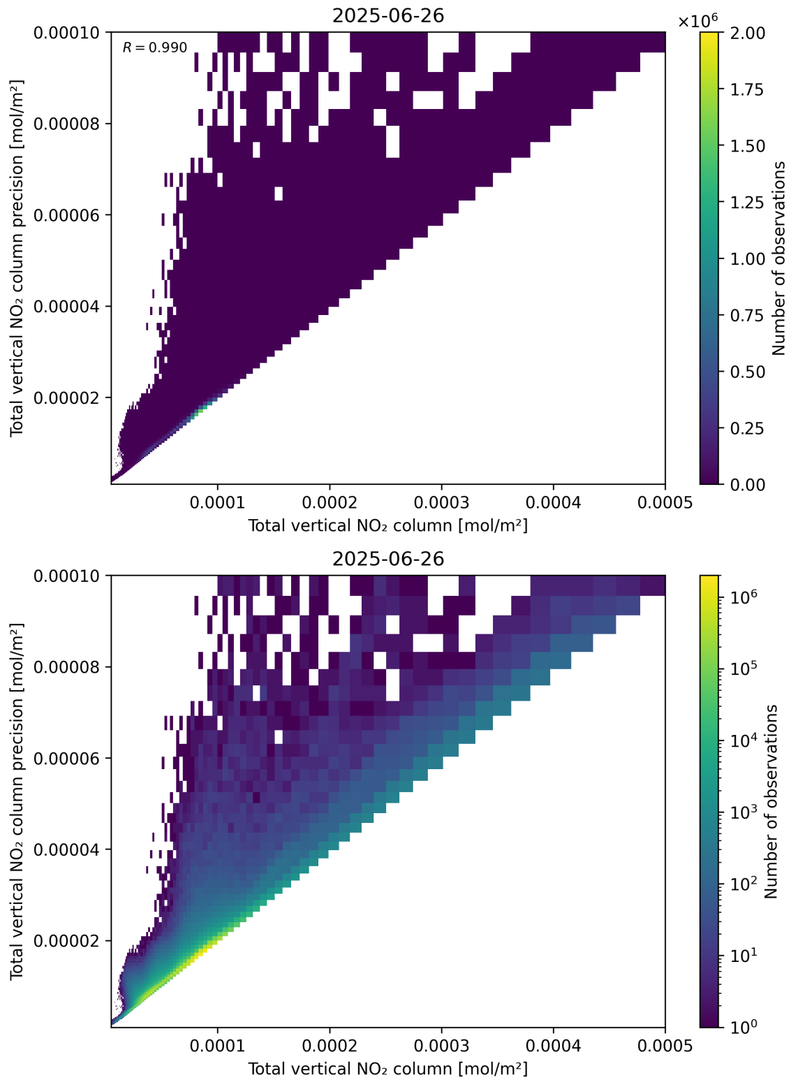
Figure 114: Scatter density plot of “Total vertical NO 2 column” against “Total vertical NO 2 column precision” for 2025-06-25 to 2025-06-27.
