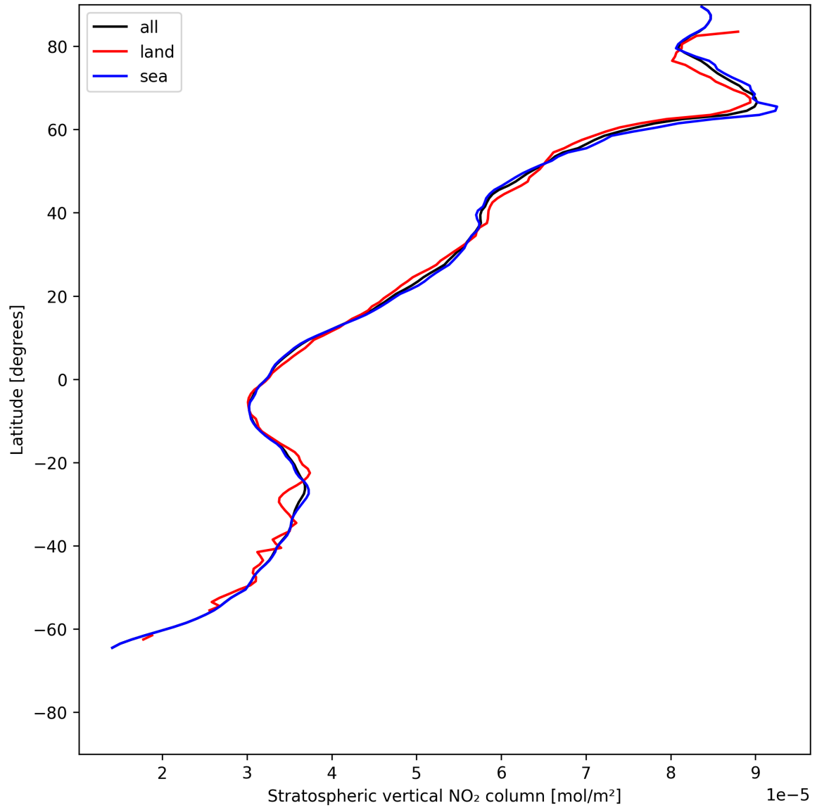
Figure 19: Zonal average of “Stratospheric vertical NO 2 column” for 2025-06-25 to 2025-06-27.
