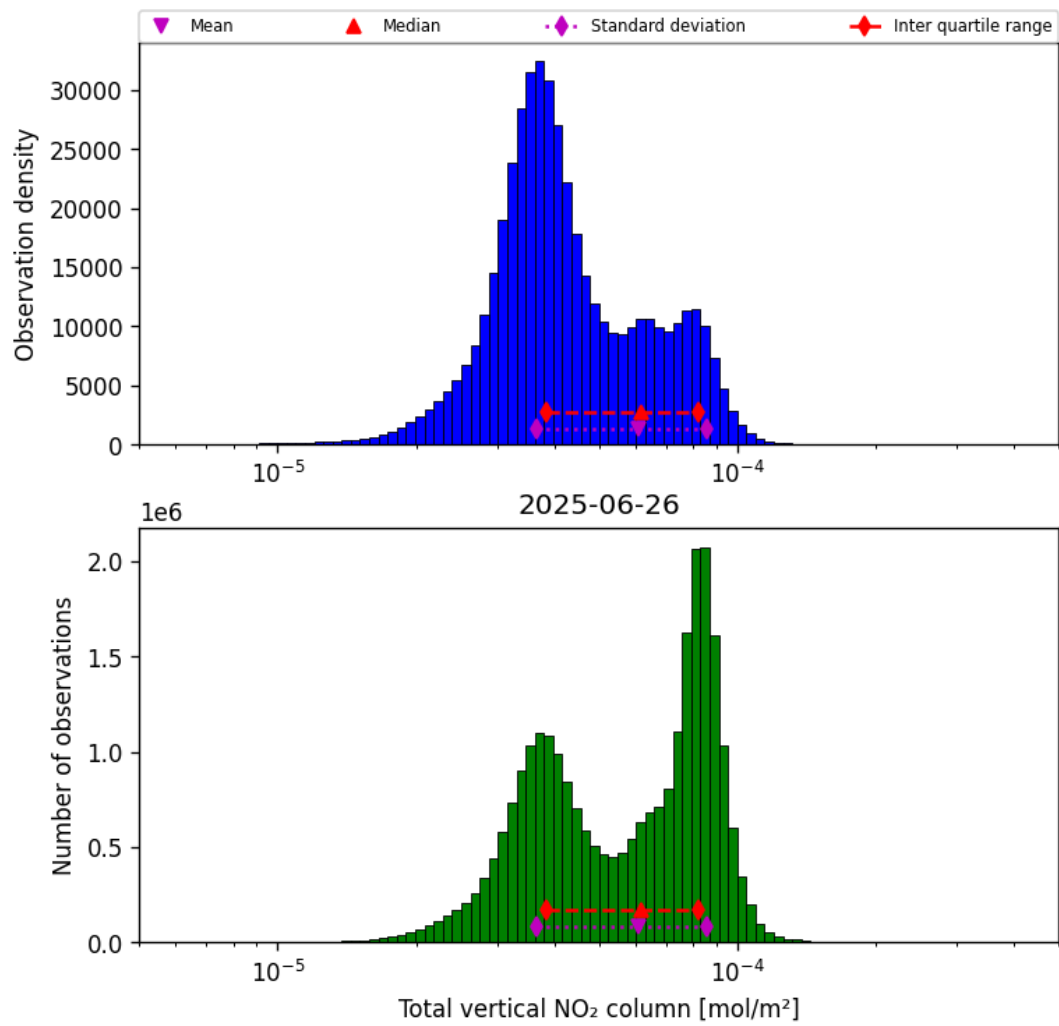
Figure 38: Histogram of “Total vertical NO 2 column” for 2025-06-25 to 2025-06-27
