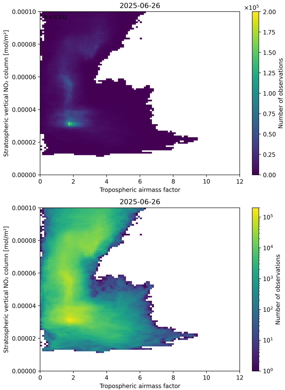
Figure 74: Scatter density plot of “Tropospheric air mass factor” against “Stratospheric vertical NO 2 column” for 2025-06-25 to 2025-06-27.
