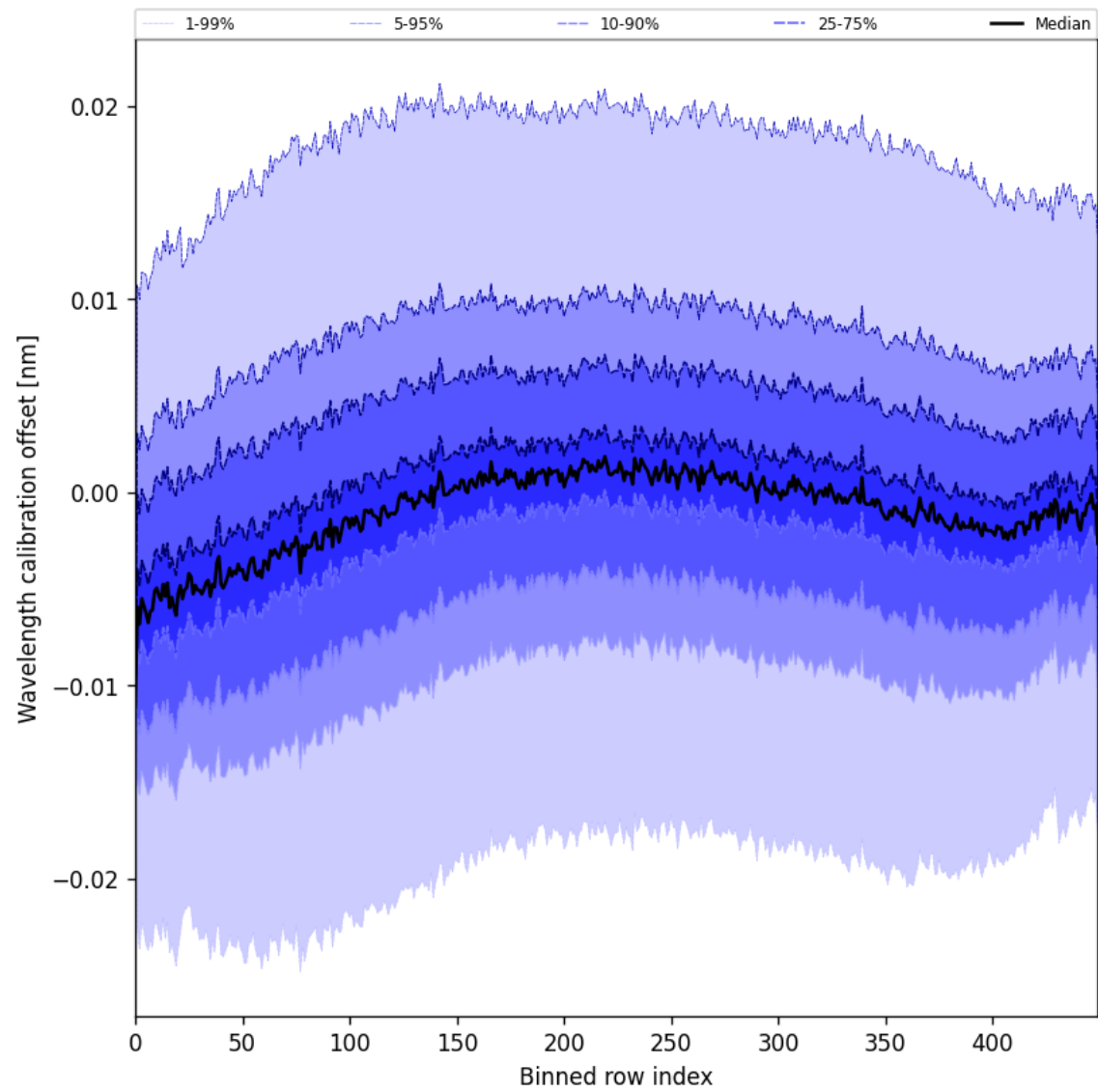
Figure 52: Along track statistics of “Wavelength calibration offset” for 2025-06-25 to 2025-06-27
