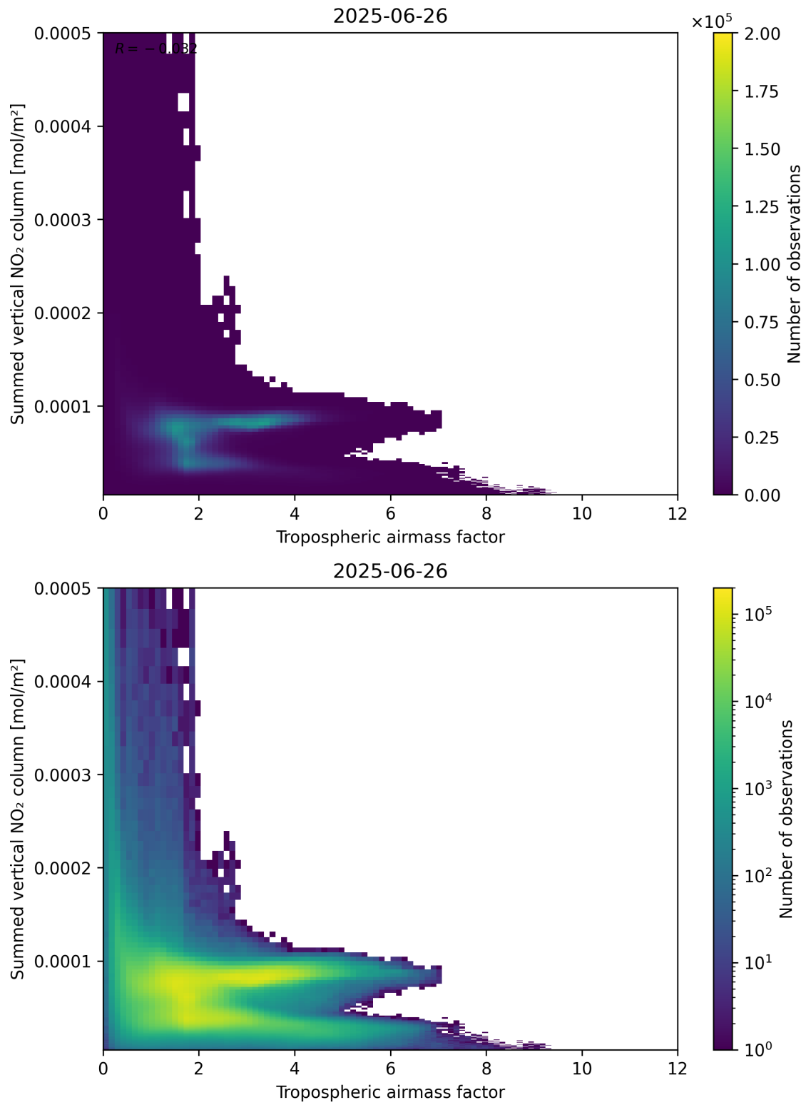
Figure 75: Scatter density plot of “Tropospheric air mass factor” against “Summed vertical NO 2 column” for 2025-06-25 to 2025-06-27.
