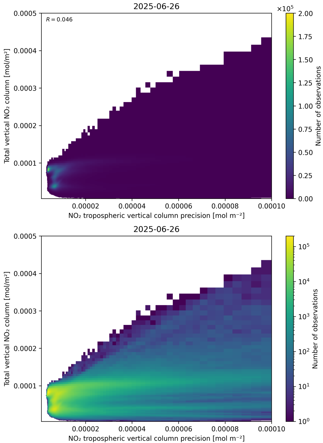
Figure 138: Scatter density plot of “NO 2 tropospheric vertical column precision” against “Total vertical NO 2 column” for 2025-06-25 to 2025-06-27.
