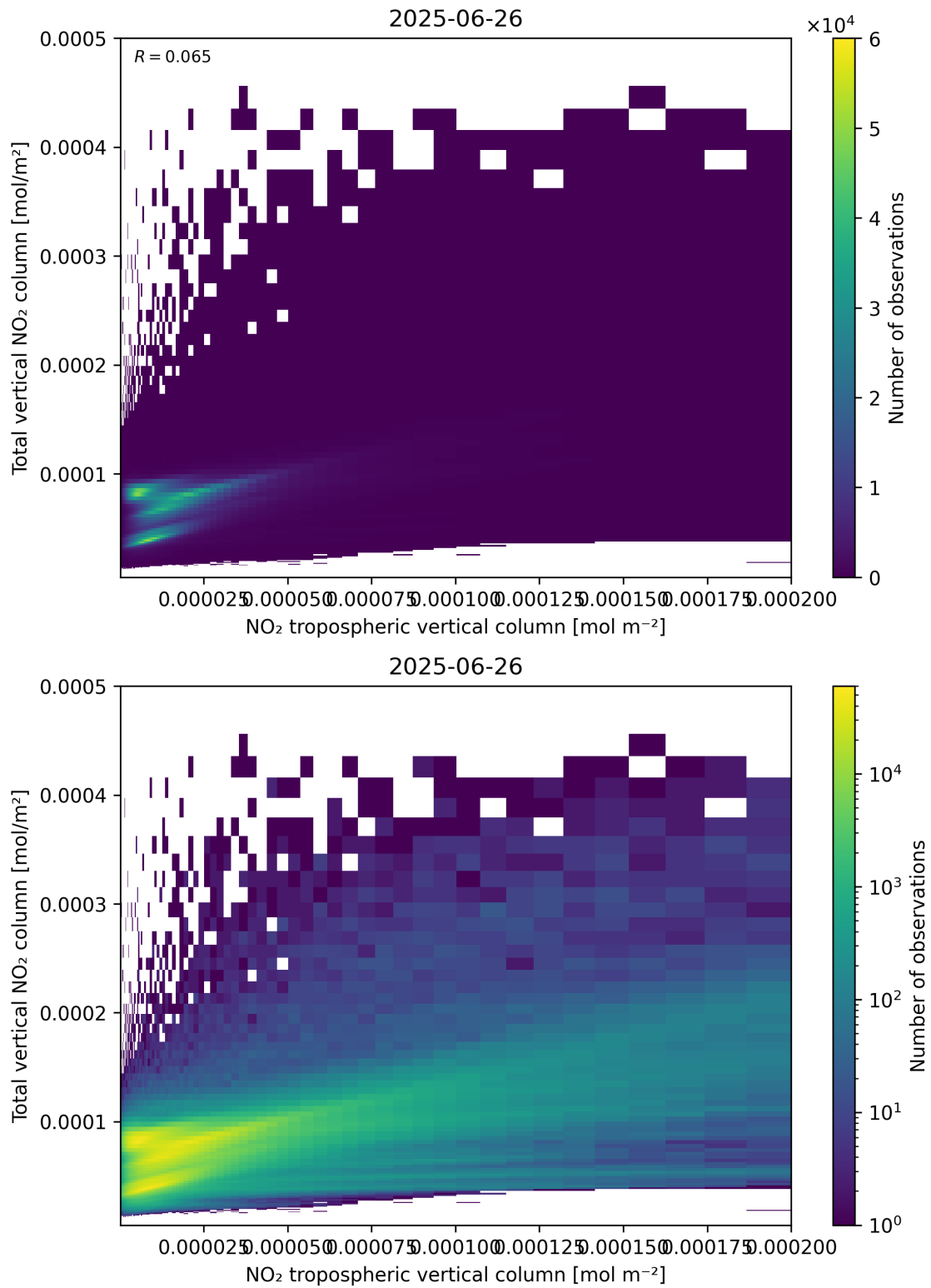
Figure 128: Scatter density plot of “NO 2 tropospheric vertical column” against “Total vertical NO 2 column” for 2025-06-25 to 2025-06-27.
