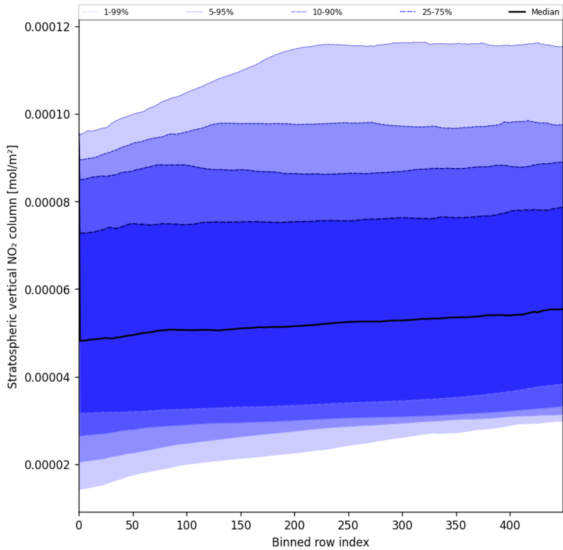
Figure 53: Along track statistics of “Stratospheric vertical NO 2 column” for 2025-06-25 to 2025-06-27
