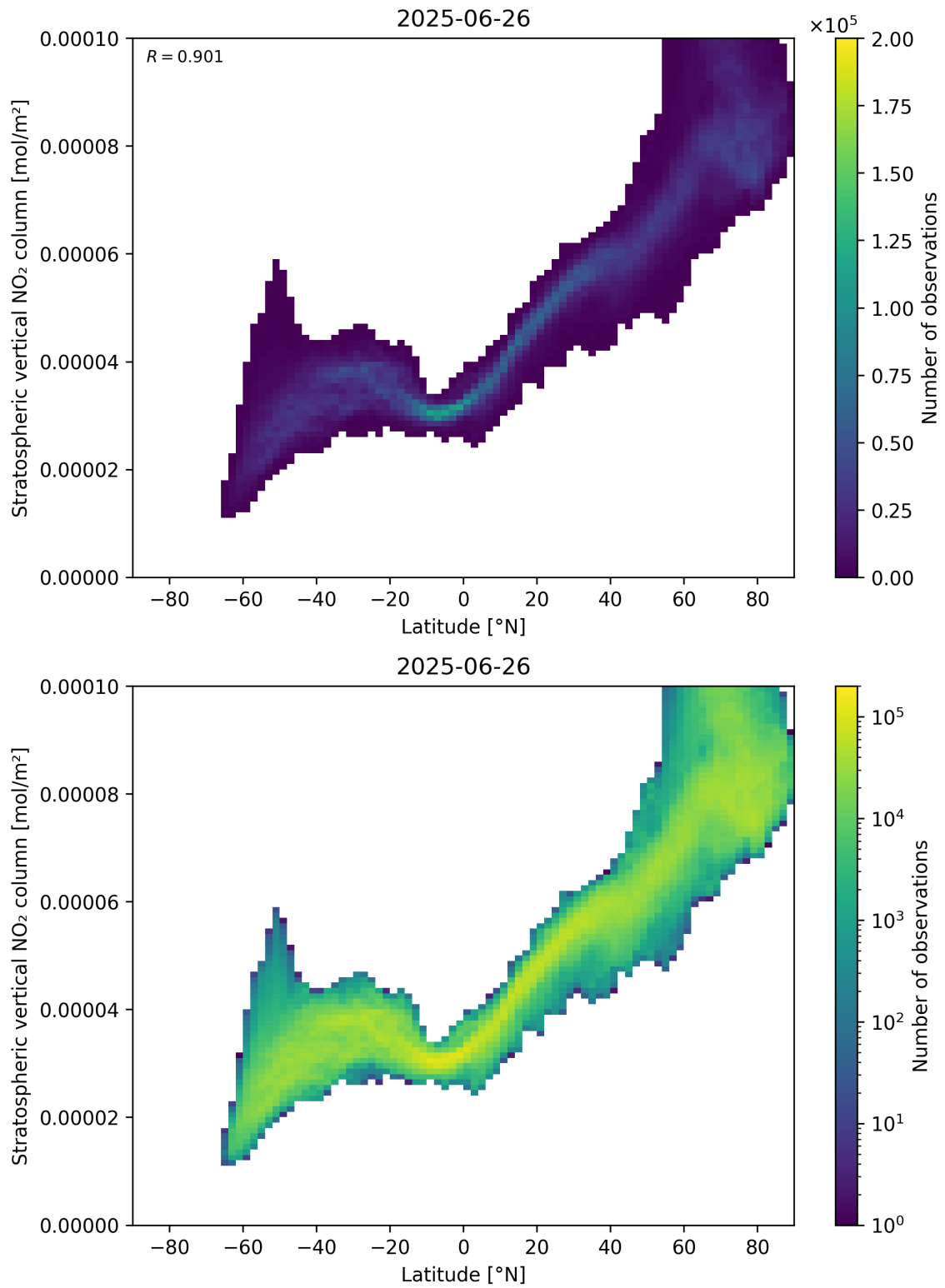
Figure 87: Scatter density plot of “Latitude” against “Stratospheric vertical \text{NO}_2 column” for 2025-06-25 to 2025-06-27.
