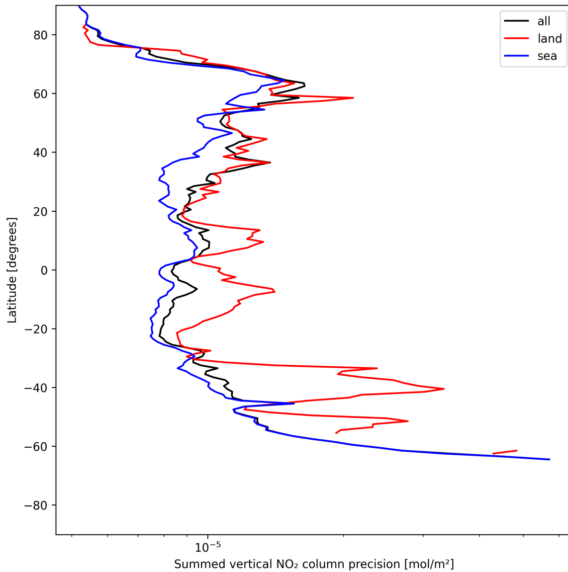
Figure 24: Zonal average of “Summed vertical NO 2 column precision” for 2025-06-25 to 2025-06-27.
