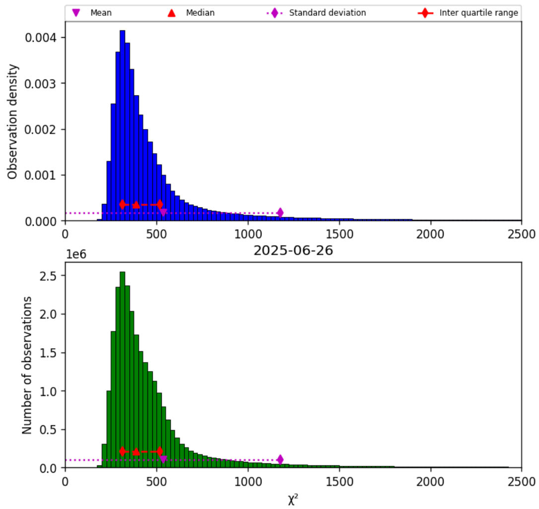
Figure 42: Histogram of " \chi^2 " for 2025-06-25 to 2025-06-27
