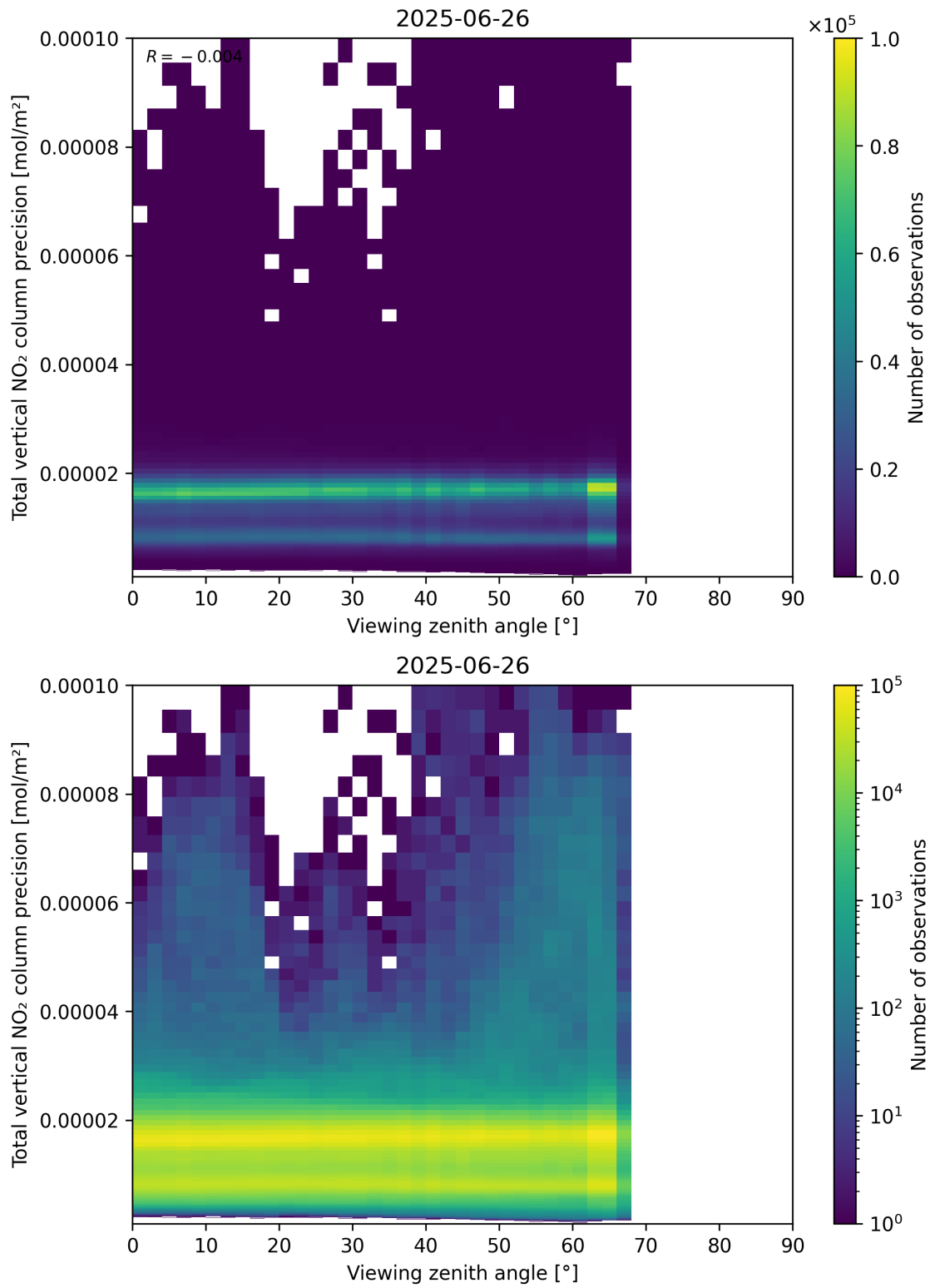
Figure 168: Scatter density plot of “Viewing zenith angle” against “Total vertical NO 2 column precision” for 2025-06-25 to 2025-06-27.
