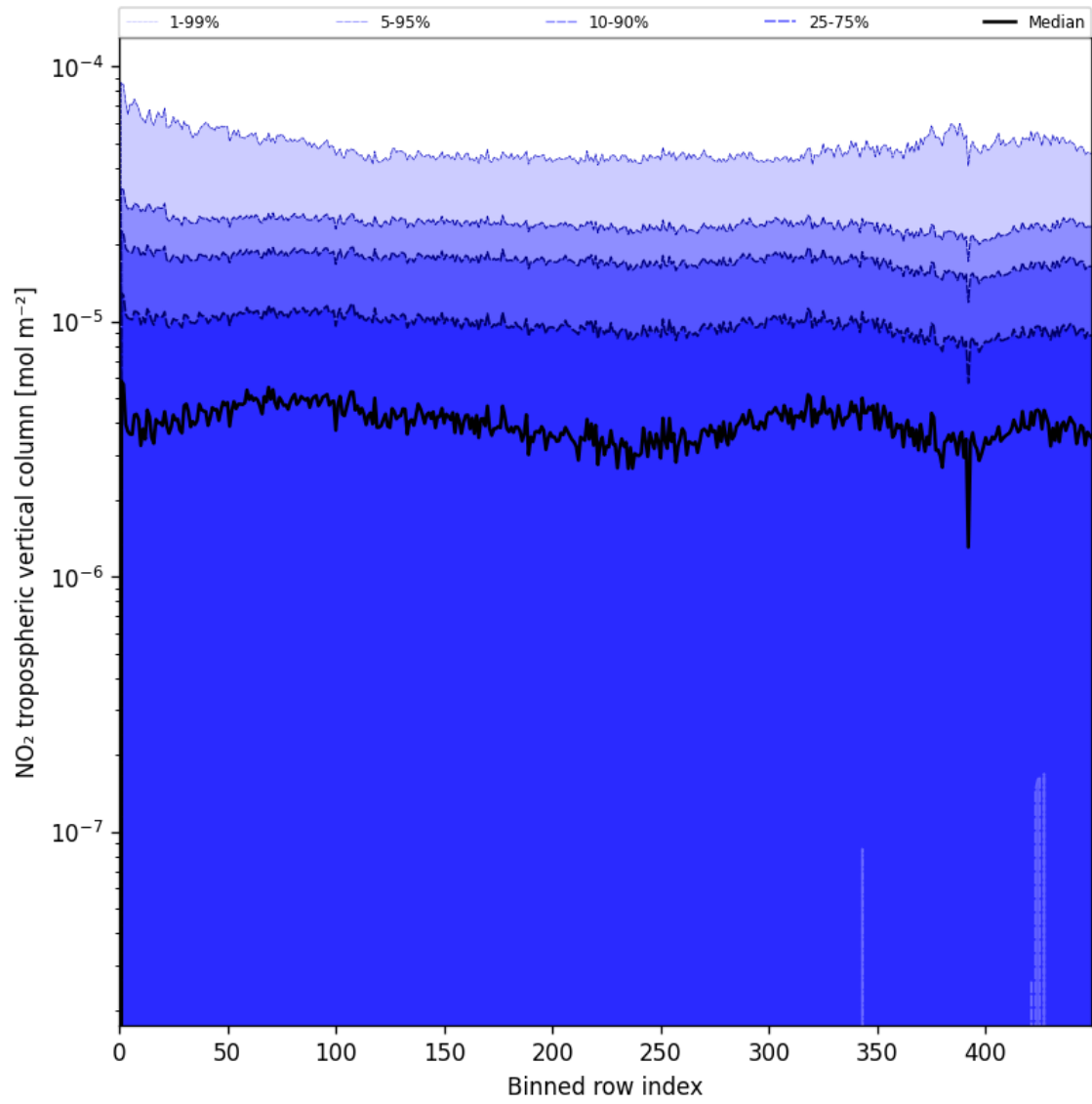
Figure 46: Along track statistics of “NO 2 tropospheric vertical column” for 2025-06-25 to 2025-06-27
