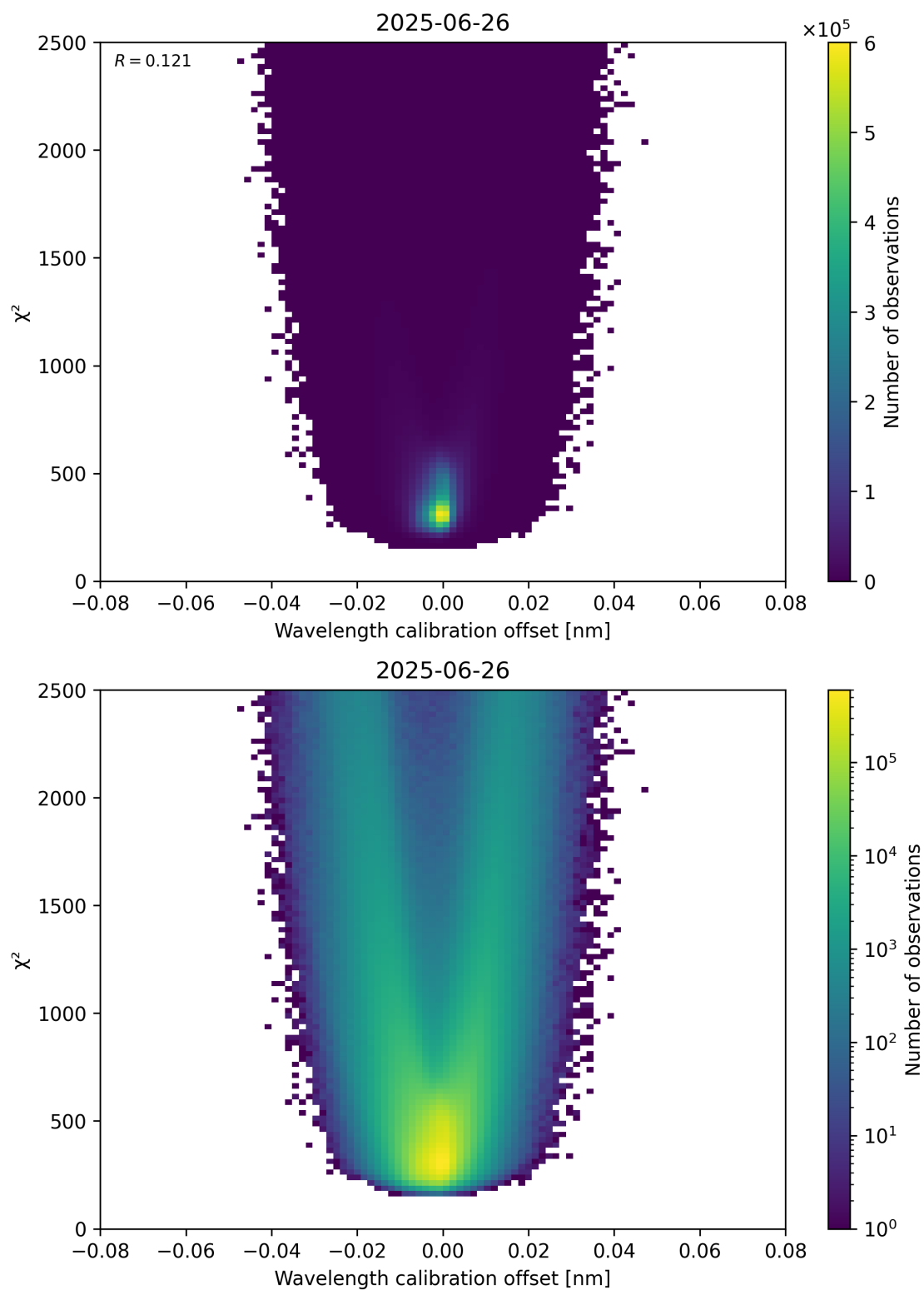
Figure 175: Scatter density plot of “Wavelength calibration offset” against “ \chi^2 ” for 2025-06-25 to 2025-06-27.
