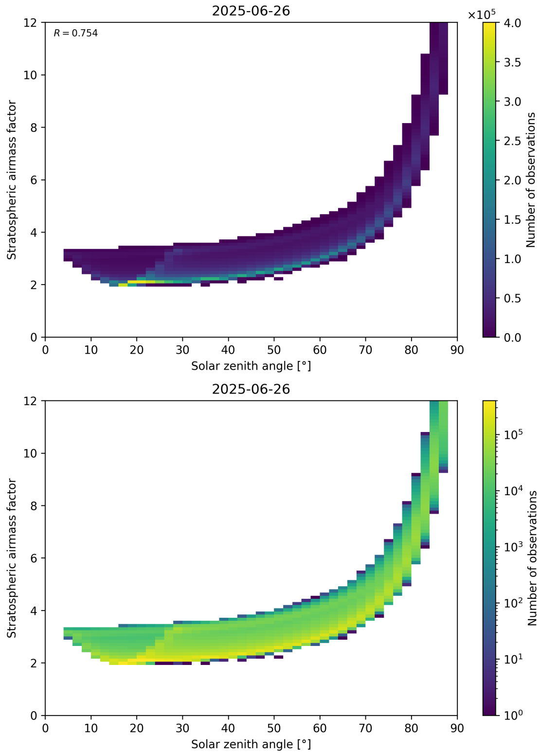
Figure 145: Scatter density plot of “Solar zenith angle” against “Stratospheric airmass factor” for 2025-06-25 to 2025-06-27.
