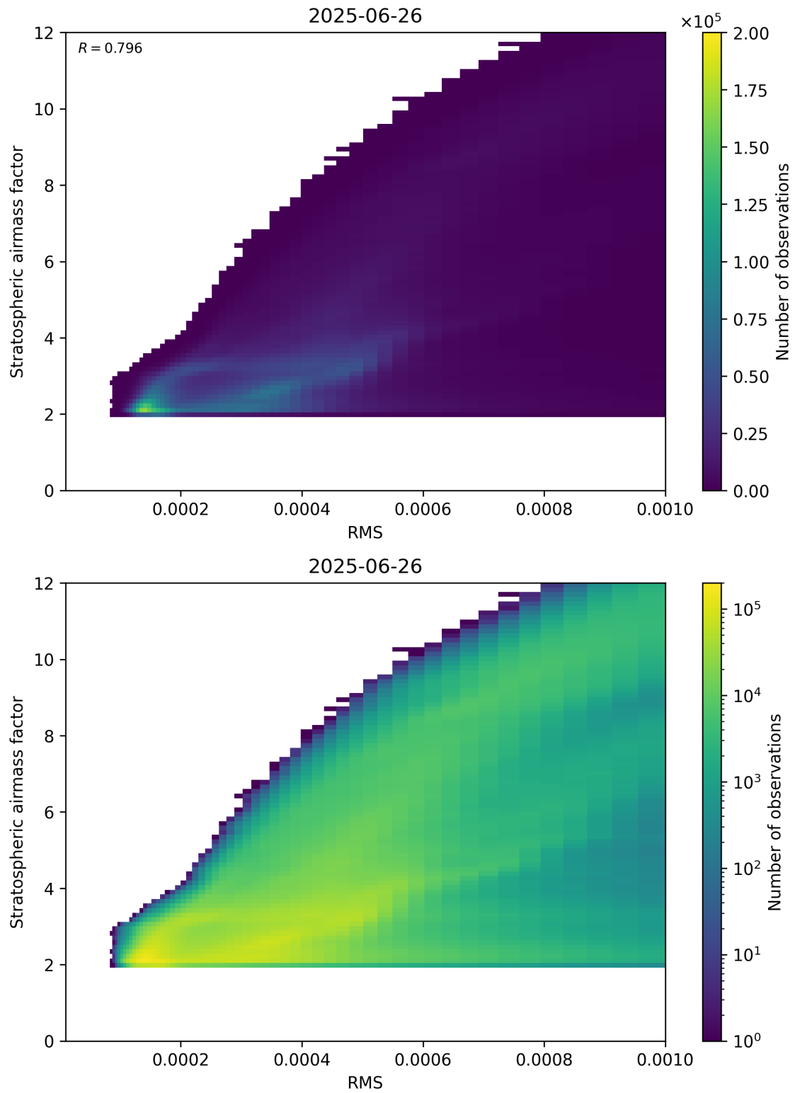
Figure 144: Scatter density plot of “RMS” against “Stratospheric airmass factor” for 2025-06-25 to 2025-06-27.
