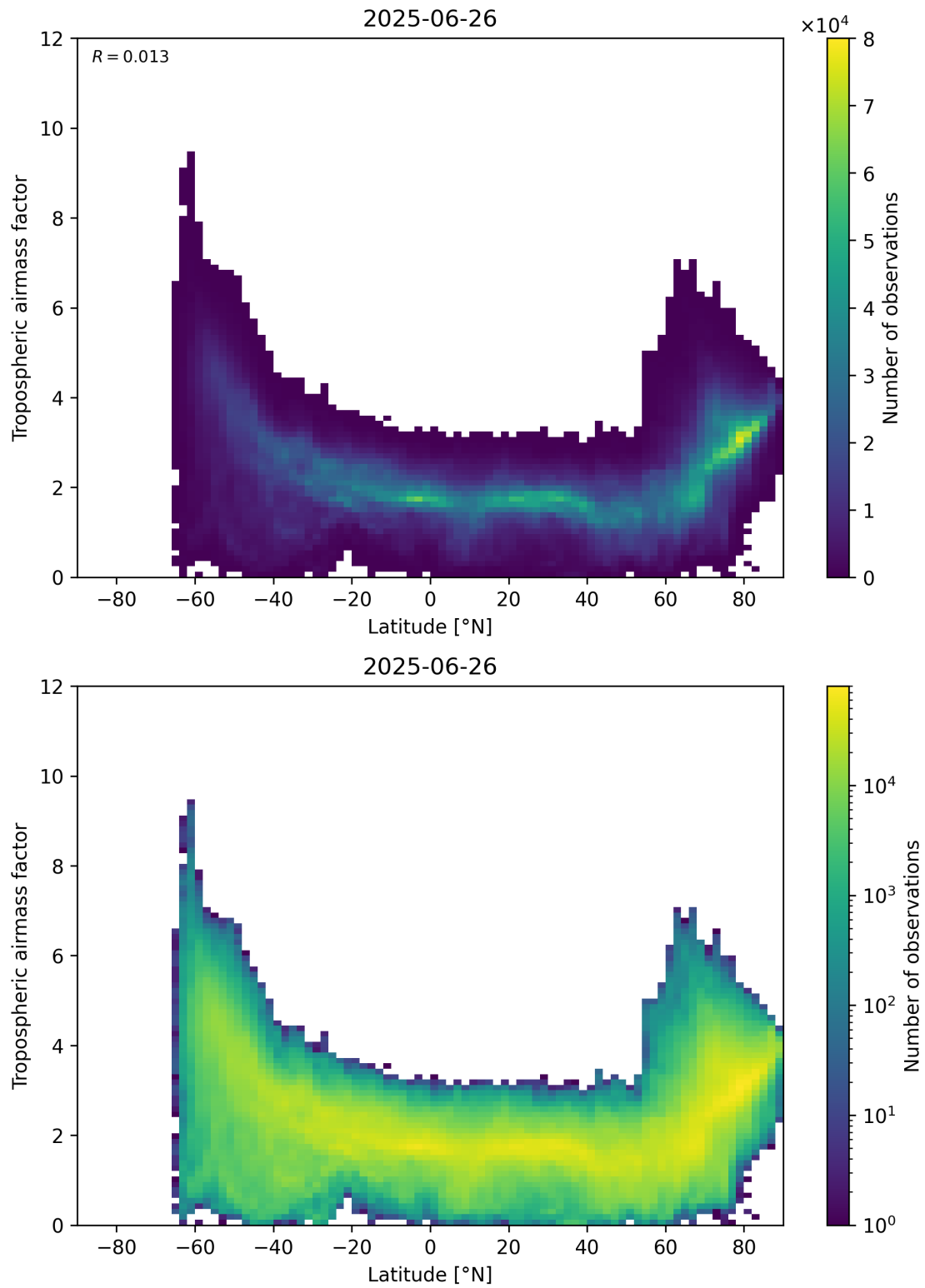
Figure 85: Scatter density plot of “Latitude” against “Tropospheric air mass factor” for 2025-06-25 to 2025-06-27.
