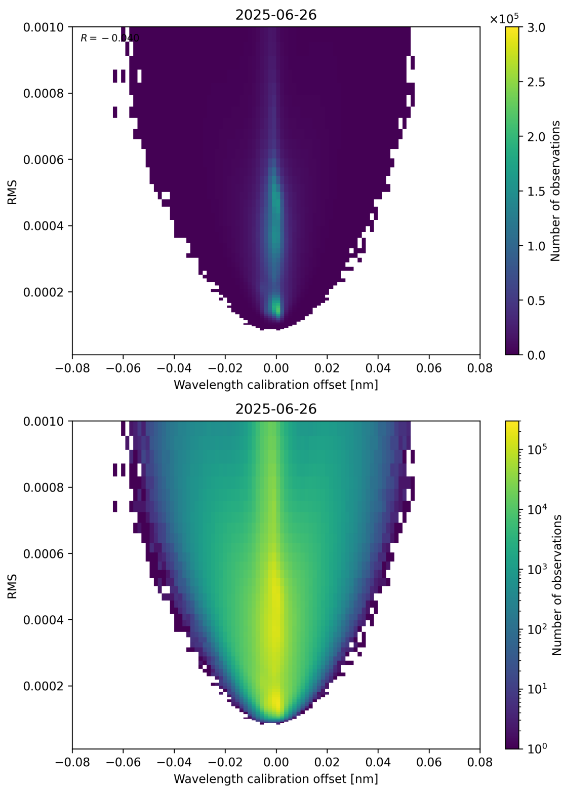
Figure 181: Scatter density plot of “Wavelength calibration offset” against “RMS” for 2025-06-25 to 2025-06-27.
