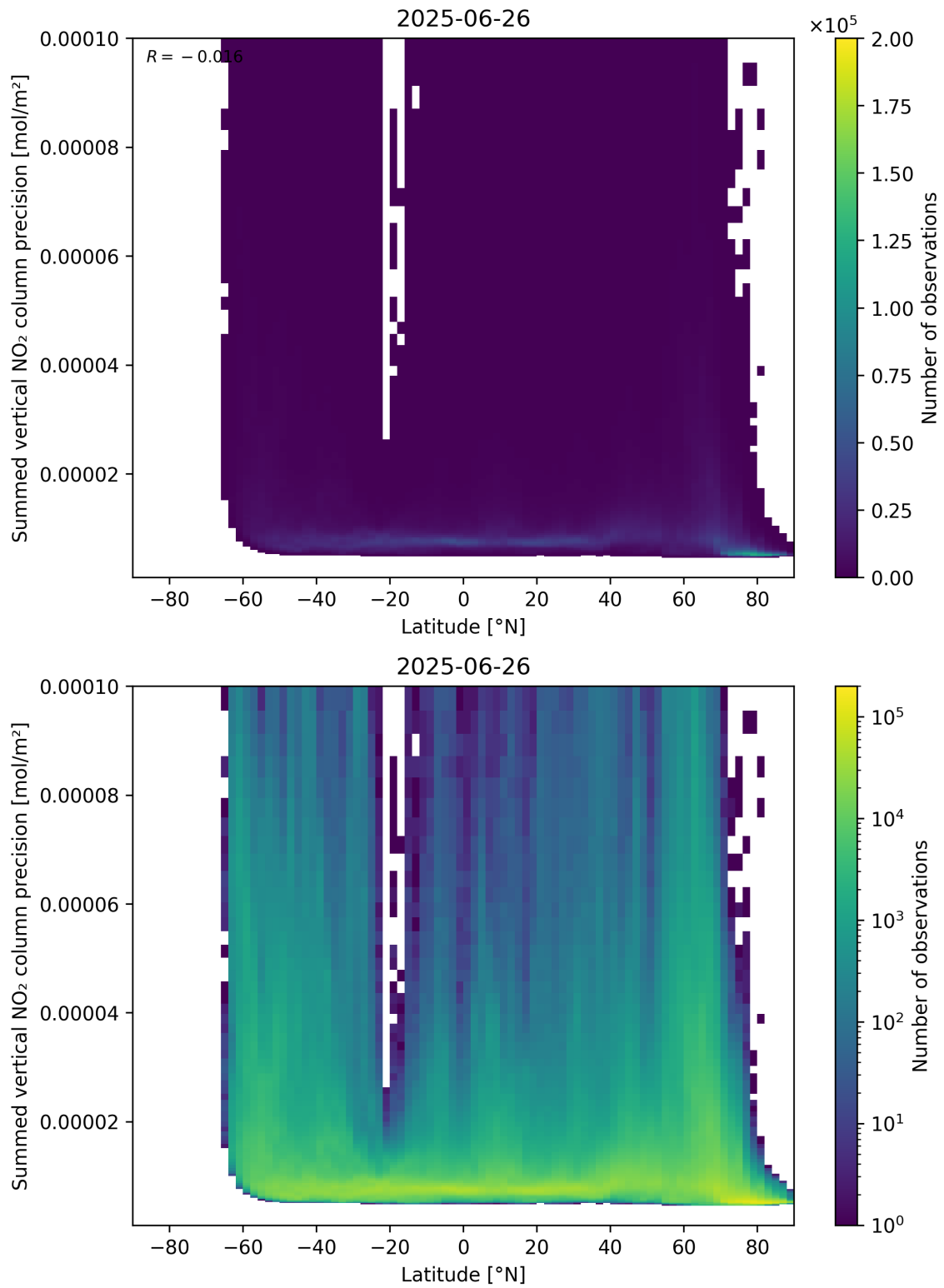
Figure 89: Scatter density plot of “Latitude” against “Summed vertical NO 2 column precision” for 2025-06-25 to 2025-06-27.
