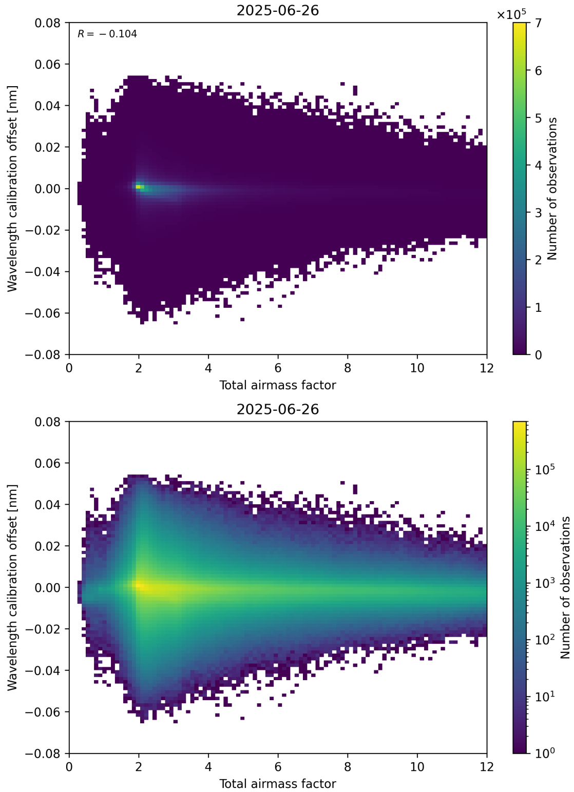
Figure 70: Scatter density plot of “Total airmass factor” against “Wavelength calibration offset” for 2025-06-25 to 2025-06-27.
