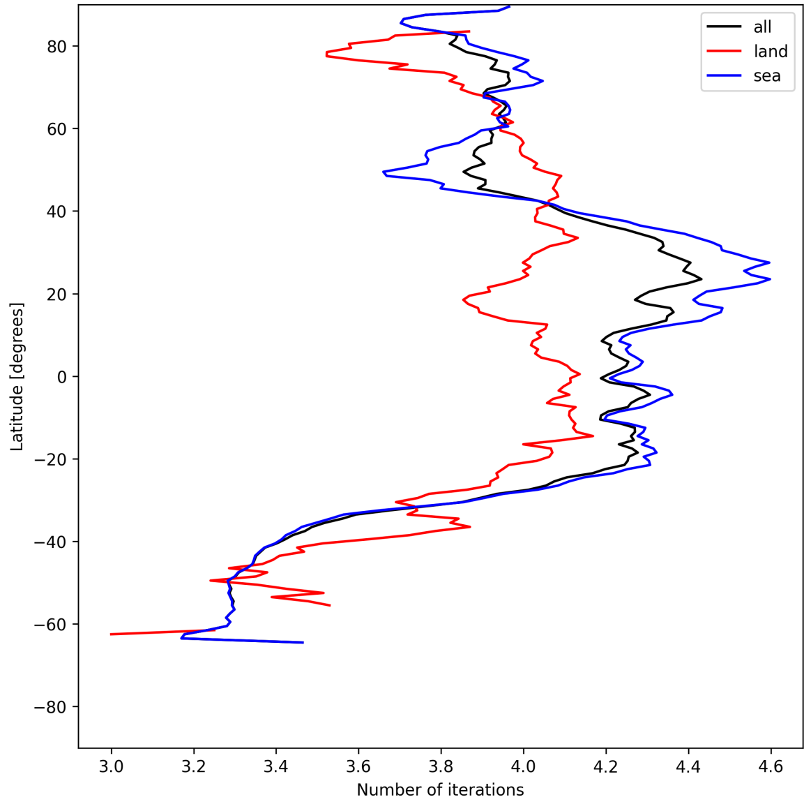
Figure 17: Zonal average of “Number of iterations” for 2025-06-25 to 2025-06-27.
