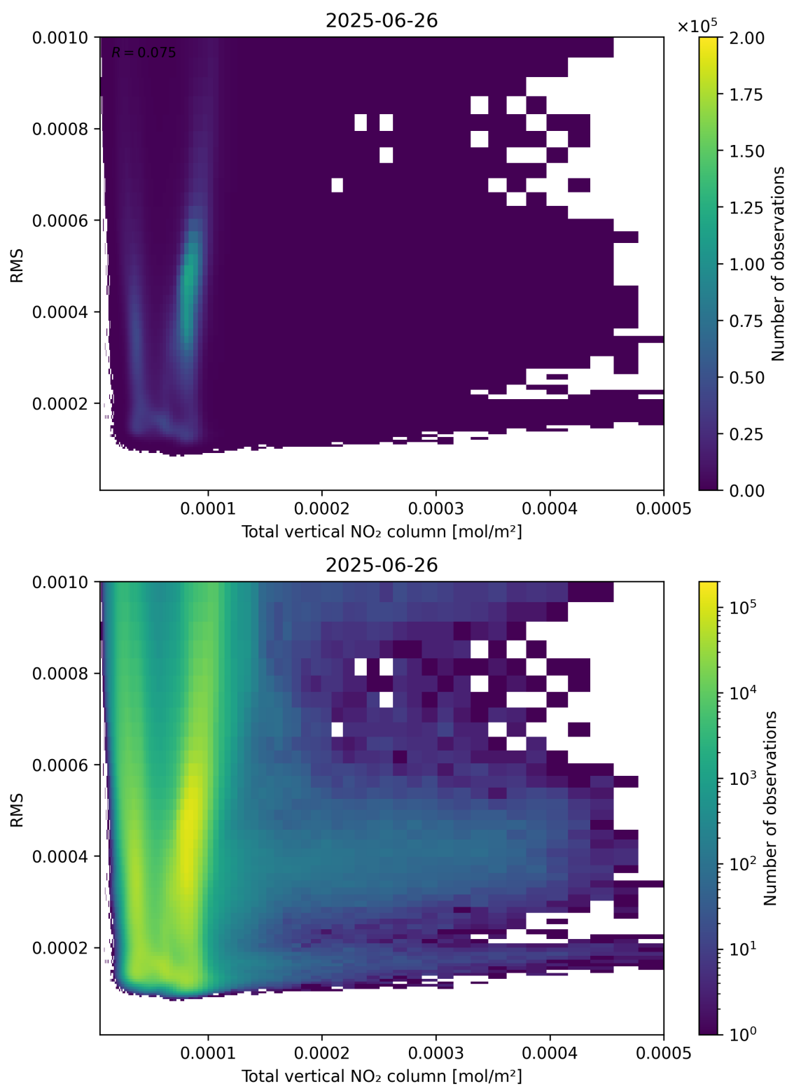
Figure 120: Scatter density plot of “Total vertical NO 2 column” against “RMS” for 2025-06-25 to 2025-06-27.
