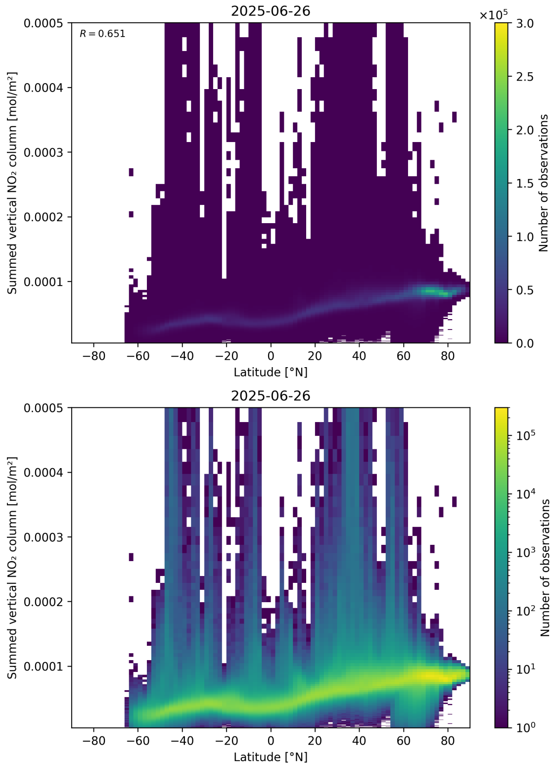
Figure 88: Scatter density plot of “Latitude” against “Summed vertical NO 2 column” for 2025-06-25 to 2025-06-27.
