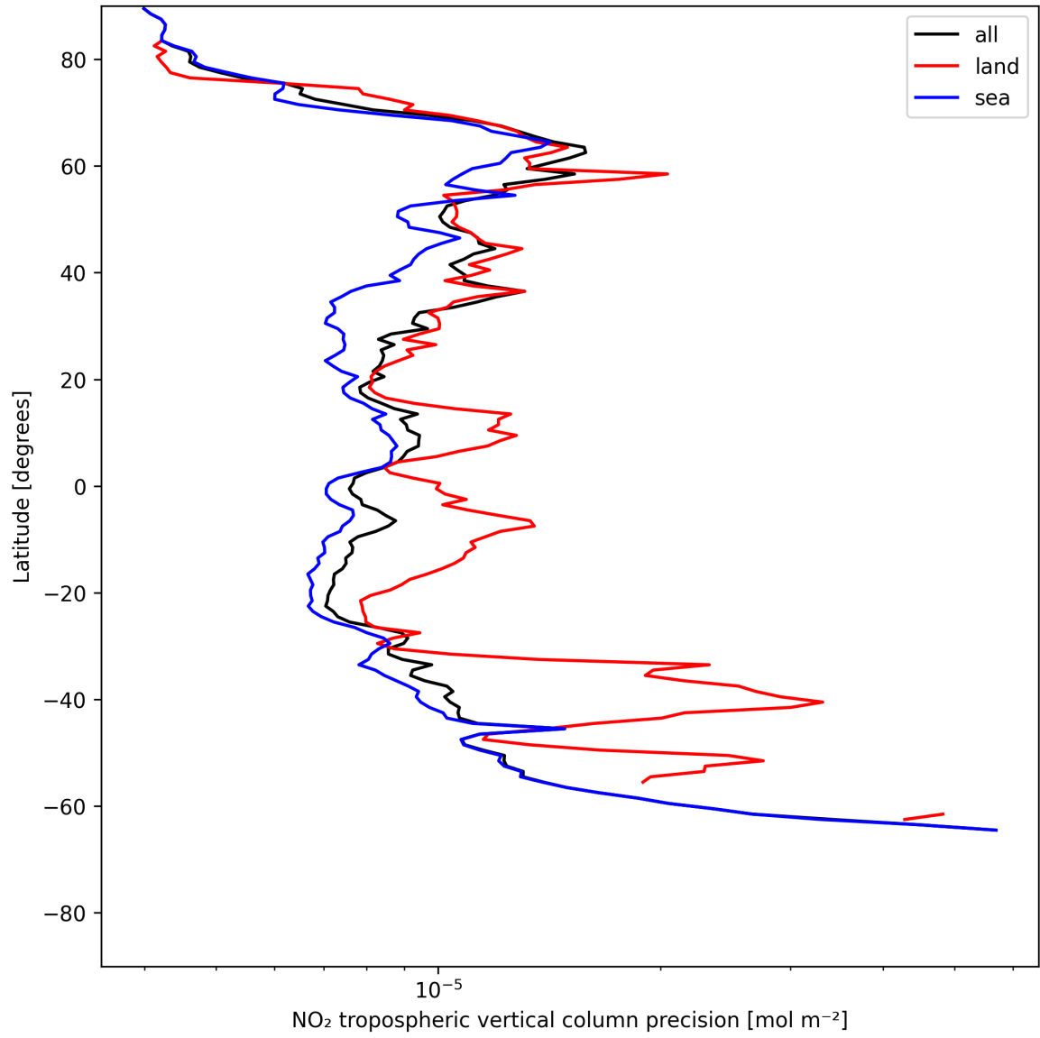
Figure 13: Zonal average of “NO 2 tropospheric vertical column precision” for 2025-06-25 to 2025-06-27.
