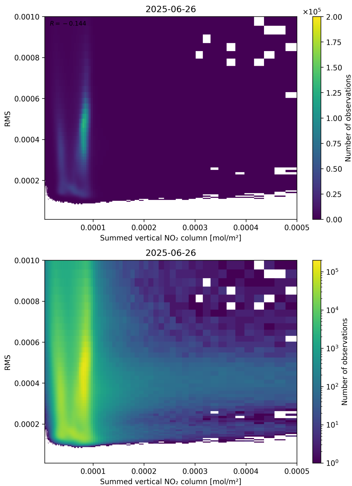
Figure 109: Scatter density plot of “Summed vertical NO 2 column” against “RMS” for 2025-06-25 to 2025-06-27.
