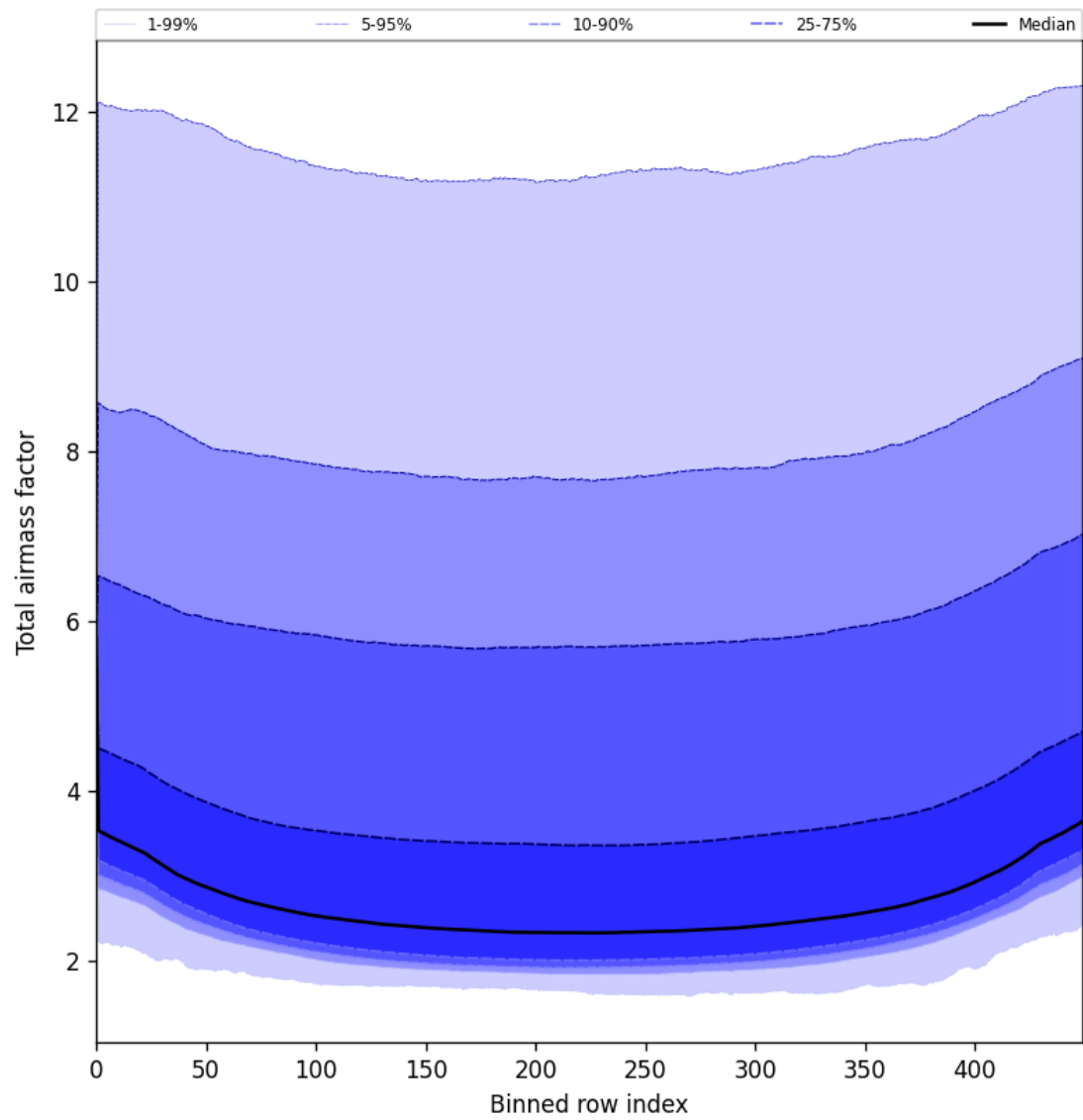
Figure 49: Along track statistics of “Total airmass factor” for 2025-06-25 to 2025-06-27
