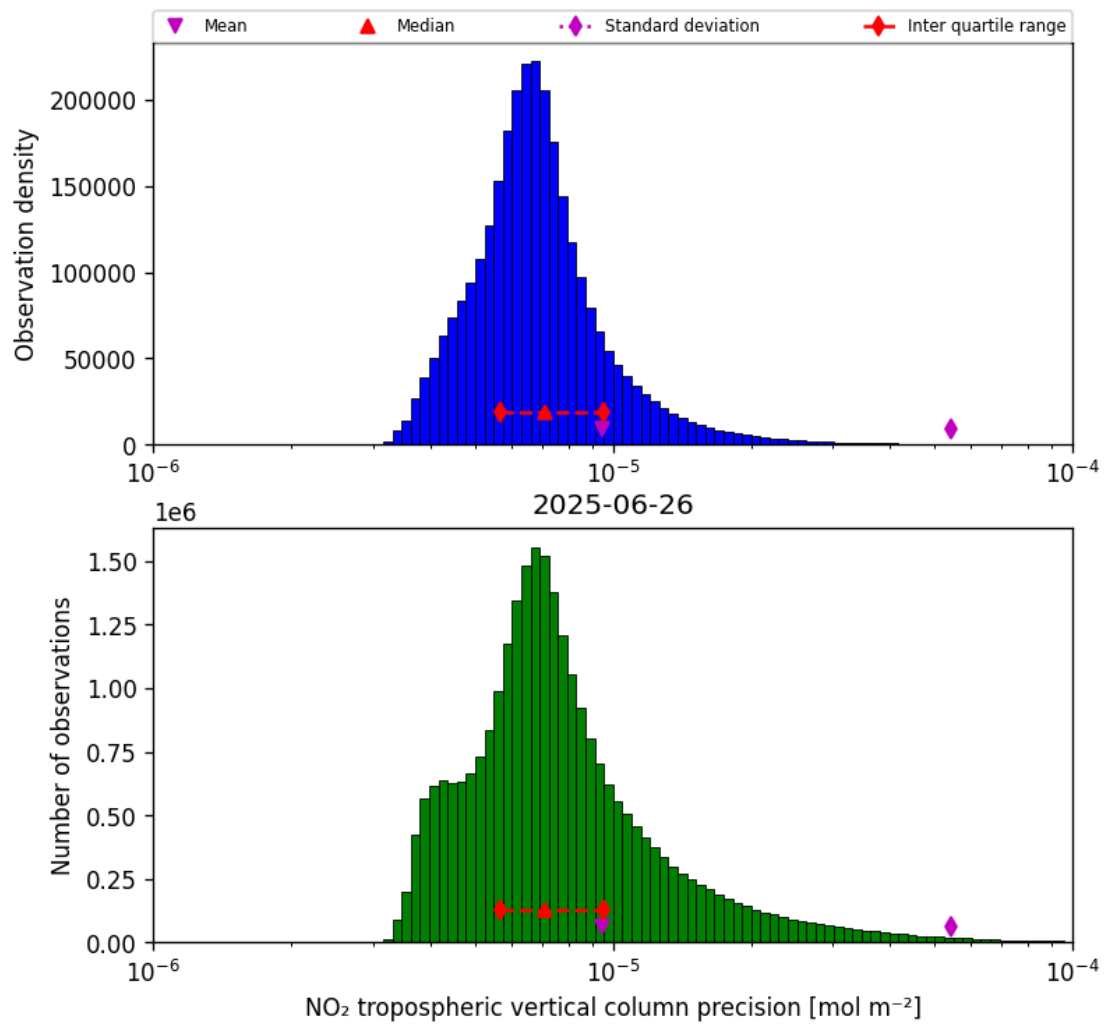
Figure 30: Histogram of “NO 2 tropospheric vertical column precision” for 2025-06-25 to 2025-06-27
