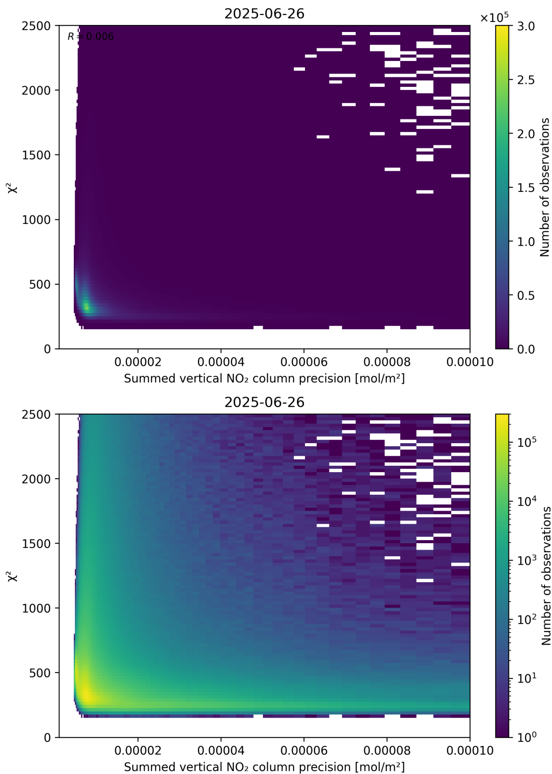
Figure 107: Scatter density plot of “Summed vertical NO 2 column precision” against “ \chi^2 ” for 2025-06-25 to 2025-06-27.
