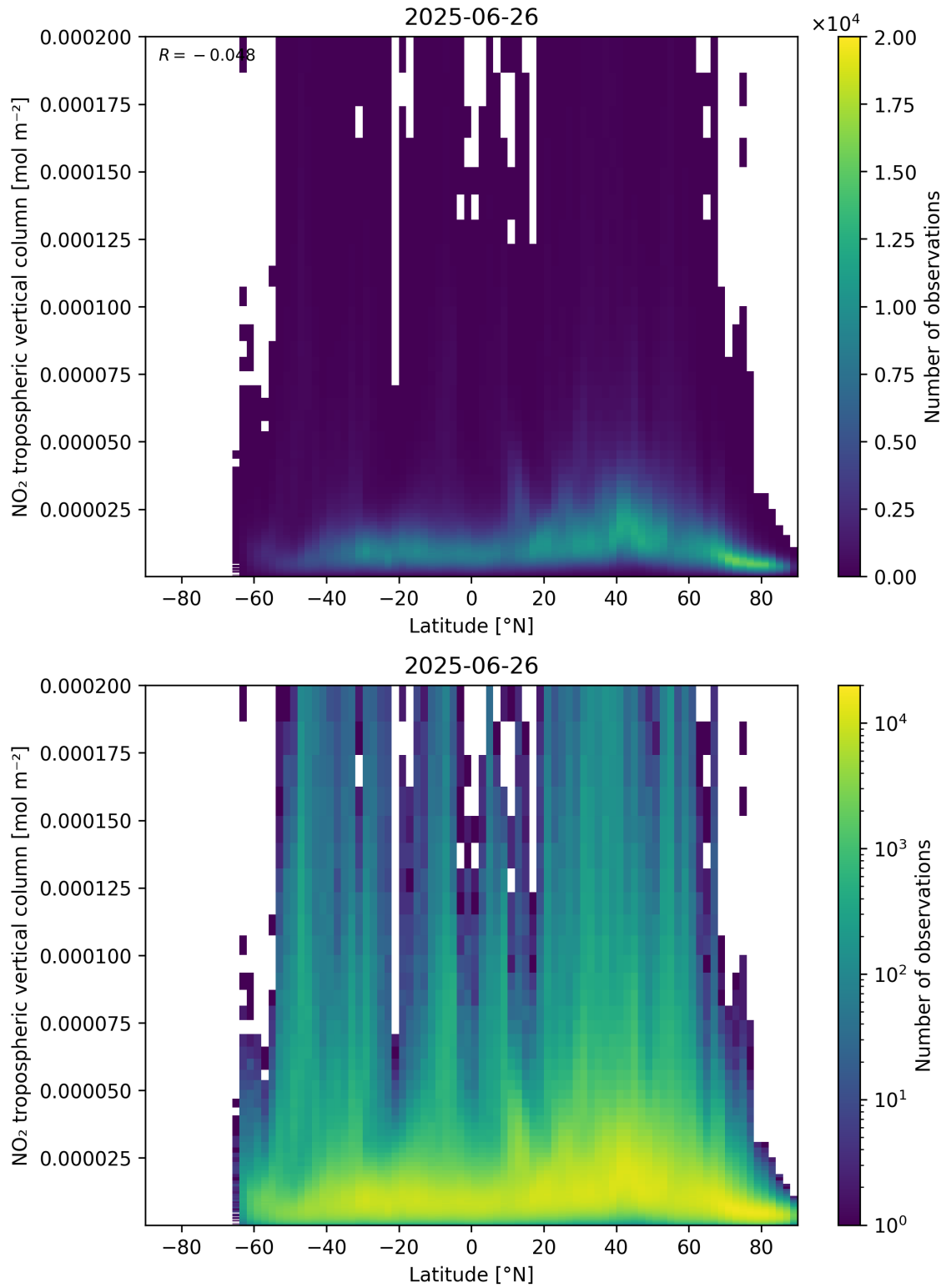
Figure 92: Scatter density plot of “Latitude” against “NO 2 tropospheric vertical column” for 2025-06-25 to 2025-06-27.
