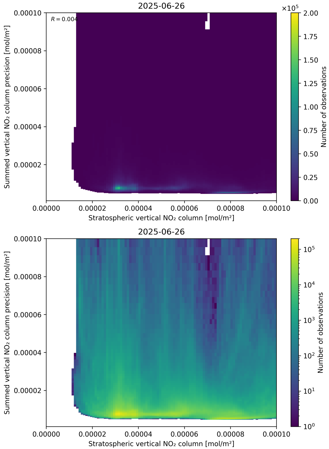
Figure 99: Scatter density plot of “Stratospheric vertical NO 2 column” against “Summed vertical NO 2 column precision” for 2025-06-25 to 2025-06-27.
