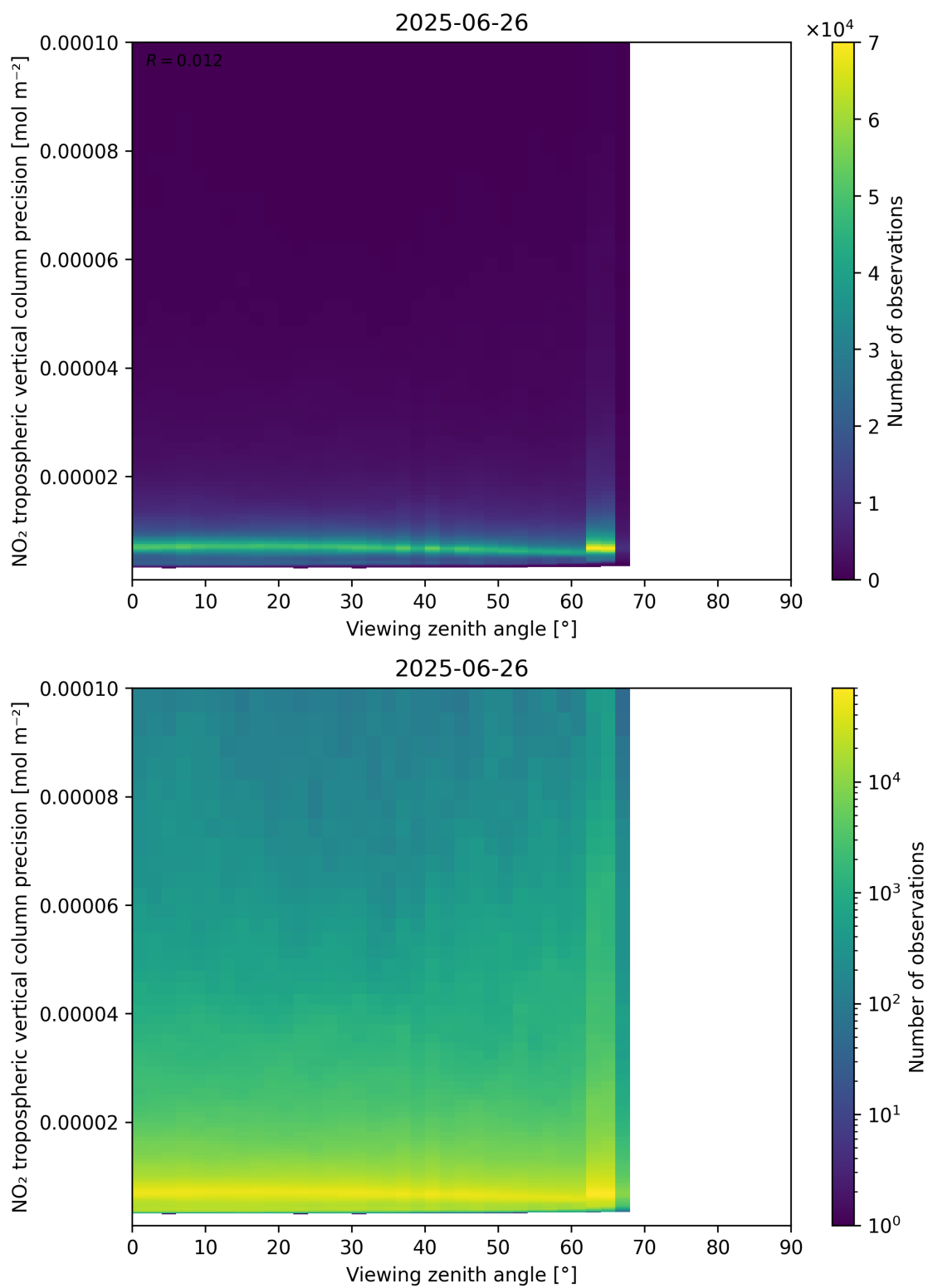
Figure 170: Scatter density plot of “Viewing zenith angle” against “NO 2 tropospheric vertical column precision” for 2025-06-25 to 2025-06-27.
