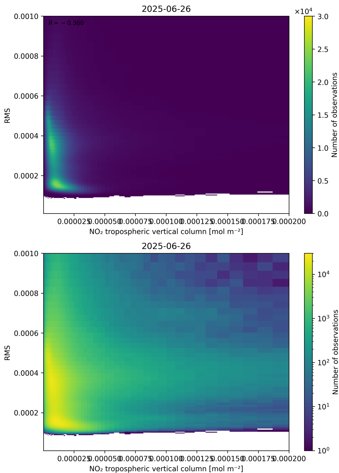
Figure 142: Scatter density plot of “NO 2 tropospheric vertical column” against “RMS” for 2025-06-25 to 2025-06-27.
