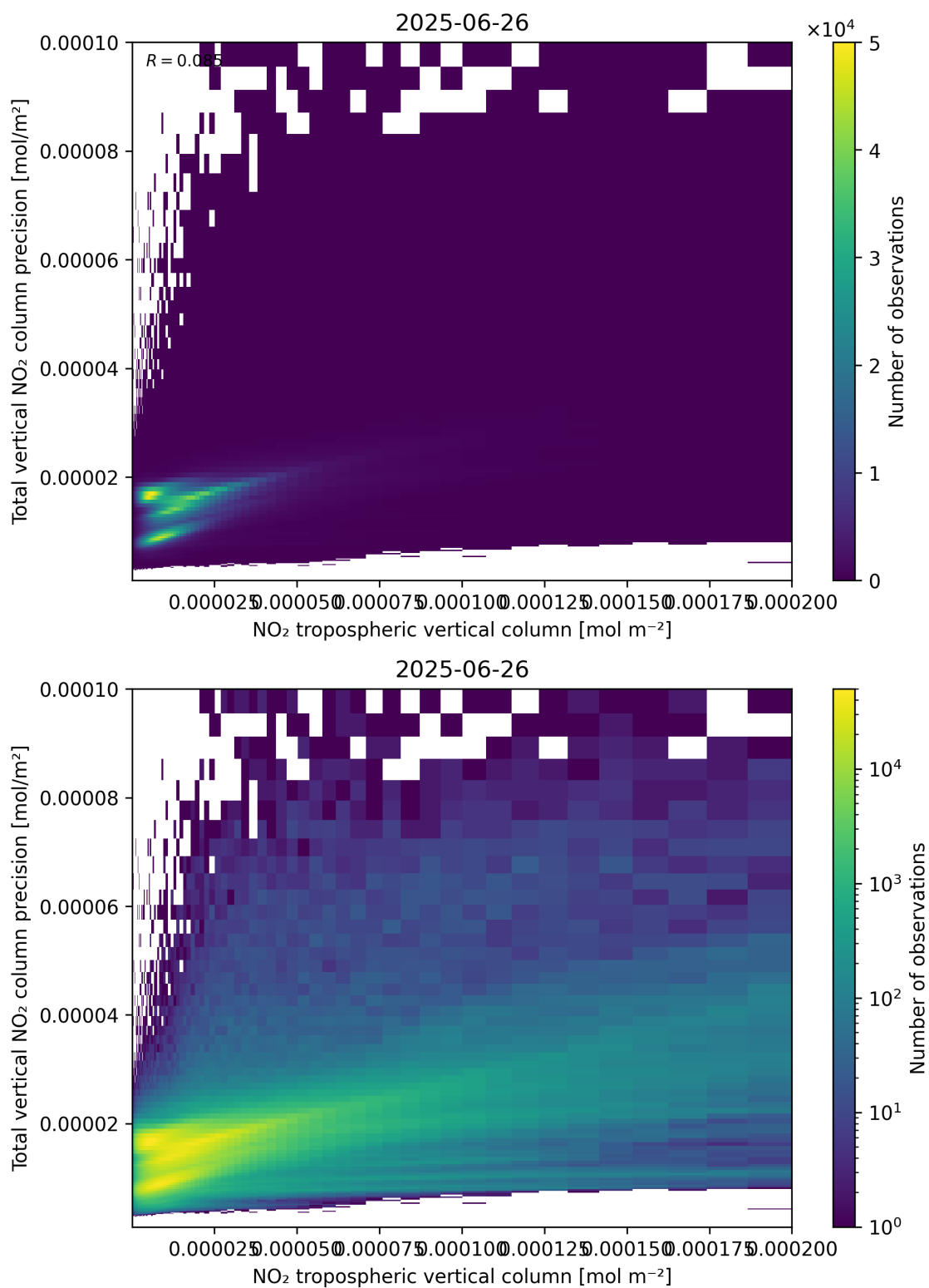
Figure 129: Scatter density plot of “NO 2 tropospheric vertical column” against “Total vertical NO 2 column precision” for 2025-06-25 to 2025-06-27.
