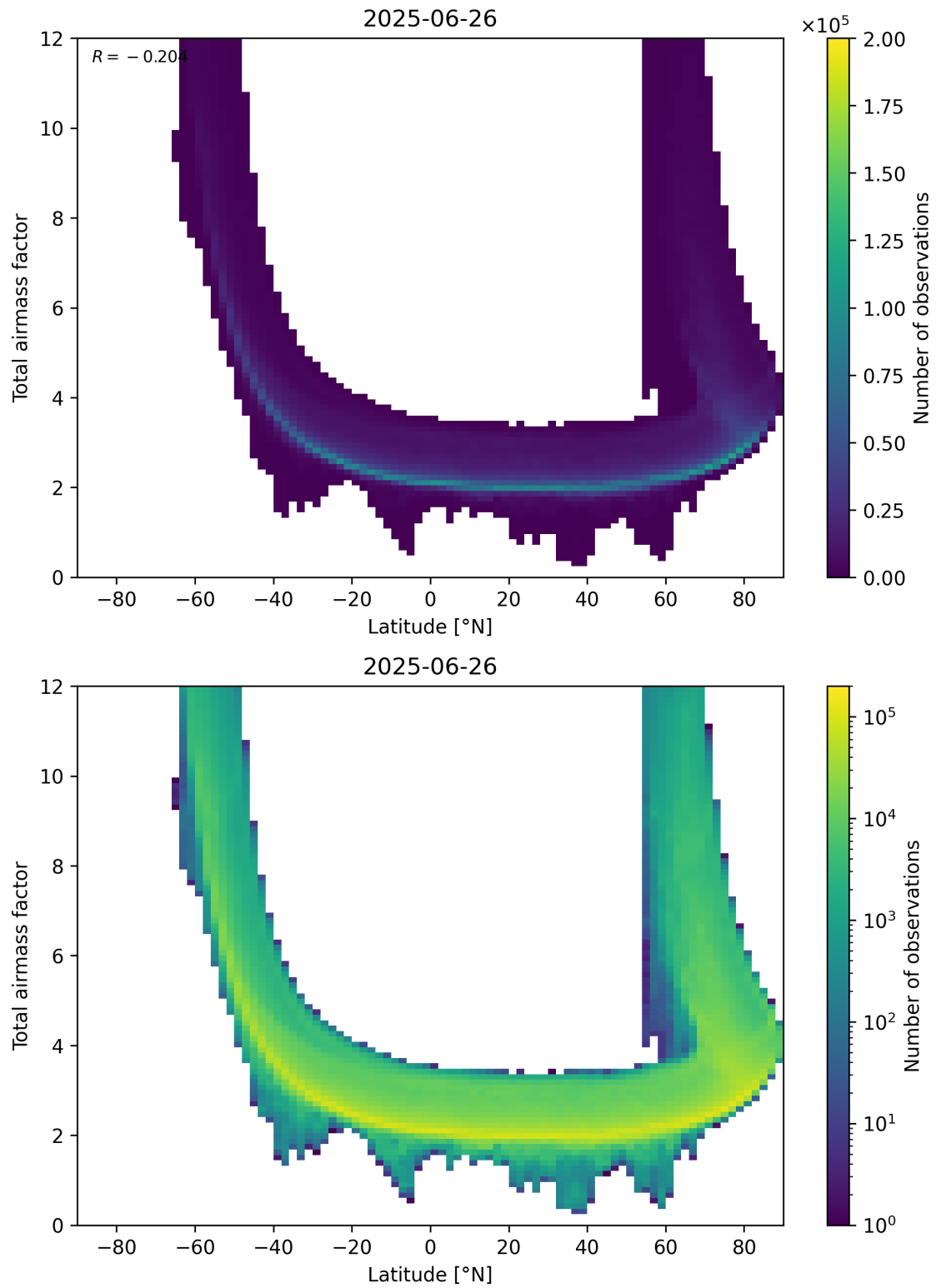
Figure 84: Scatter density plot of “Latitude” against “Total airmass factor” for 2025-06-25 to 2025-06-27.
