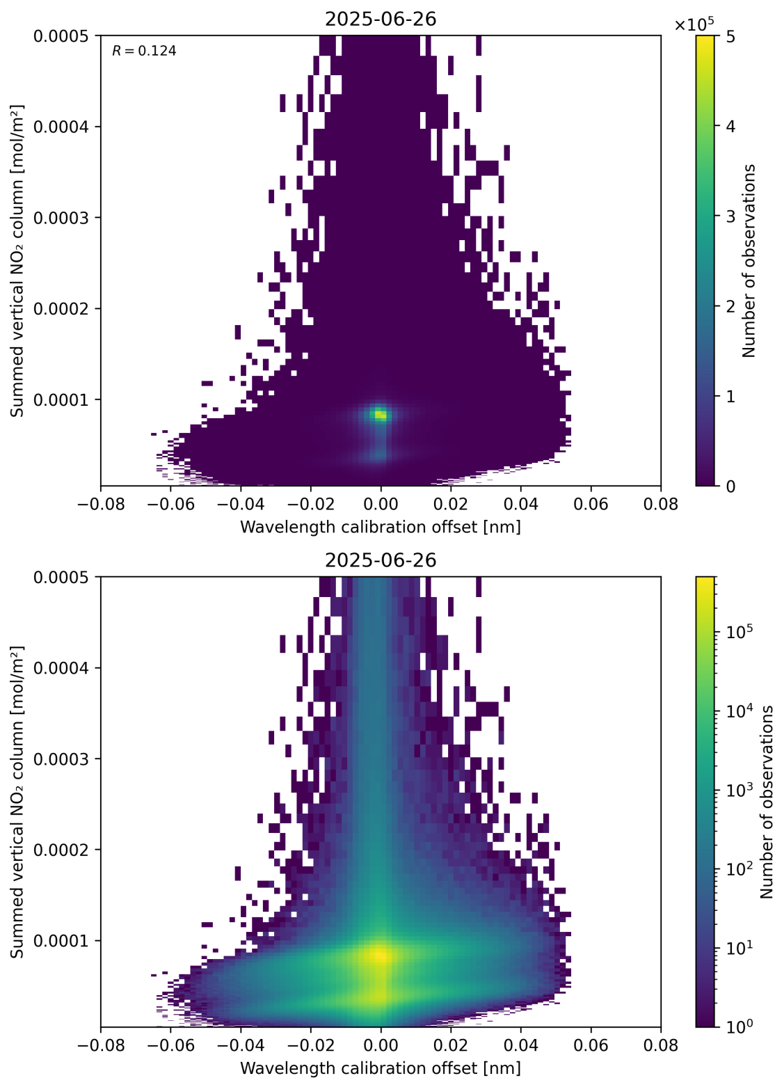
Figure 177: Scatter density plot of “Wavelength calibration offset” against “Summed vertical NO 2 column” for 2025-06-25 to 2025-06-27.
