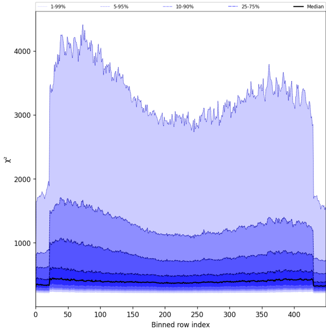
Figure 59: Along track statistics of “ \chi^2 ” for 2025-06-25 to 2025-06-27
