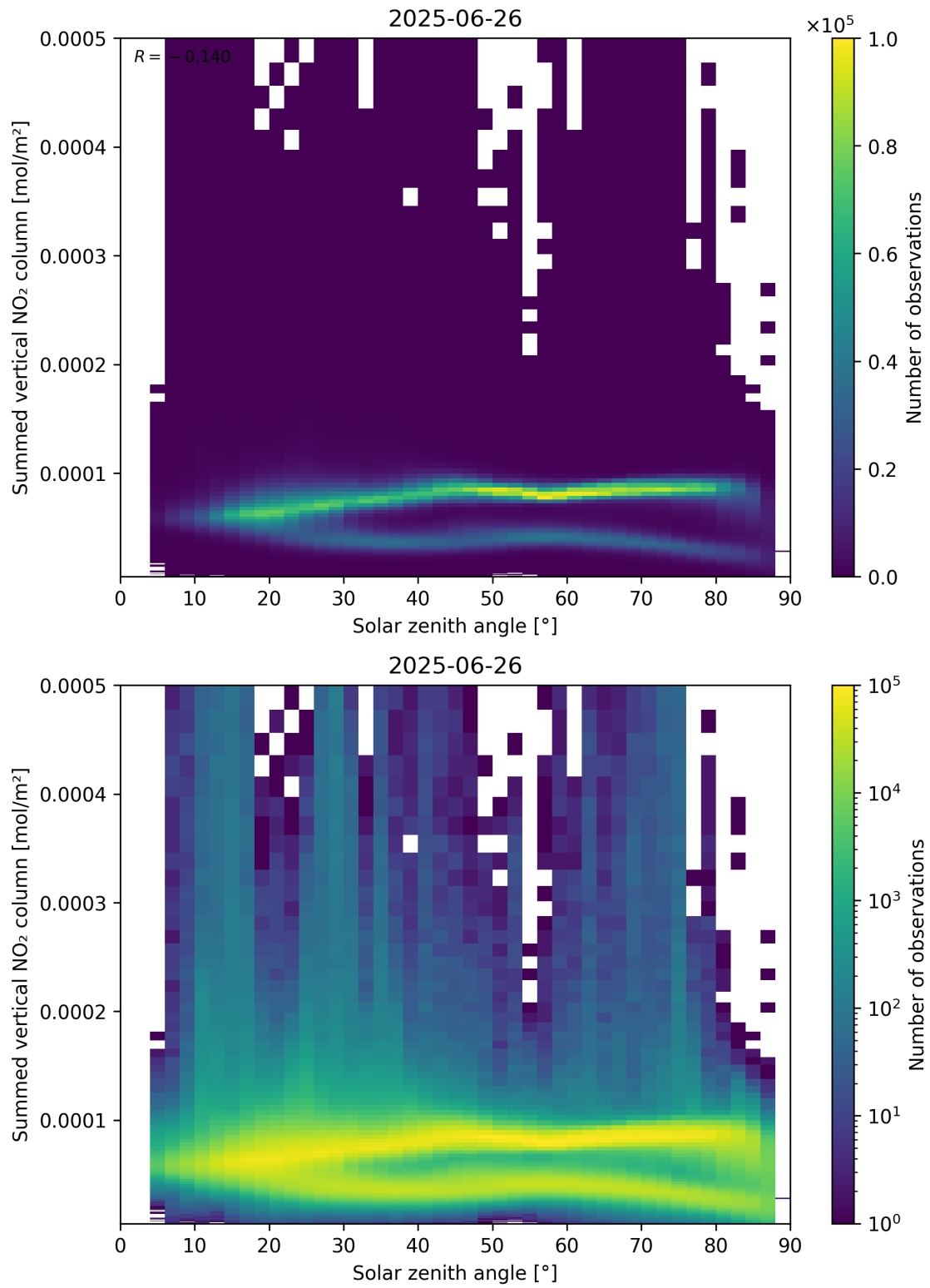
Figure 151: Scatter density plot of “Solar zenith angle” against “Summed vertical NO 2 column” for 2025-06-25 to 2025-06-27.
