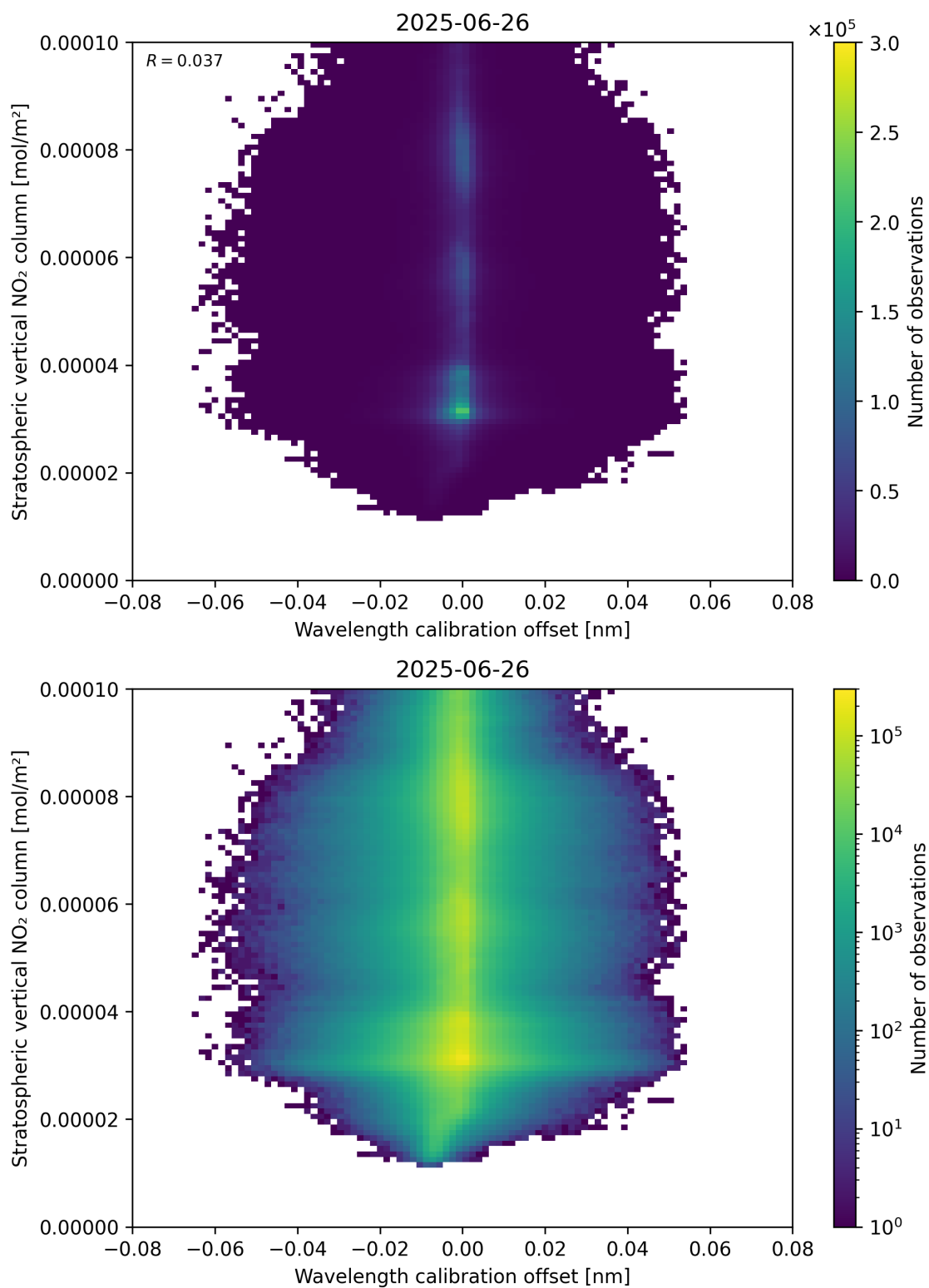
Figure 176: Scatter density plot of “Wavelength calibration offset” against “Stratospheric vertical NO 2 column” for 2025-06-25 to 2025-06-27.
