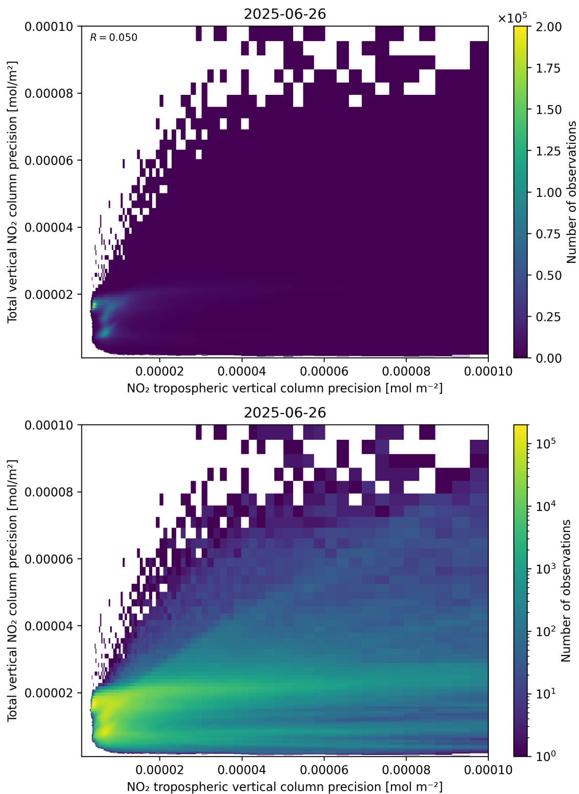
Figure 139: Scatter density plot of “NO 2 tropospheric vertical column precision” against “Total vertical NO 2 column precision” for 2025-06-25 to 2025-06-27.
