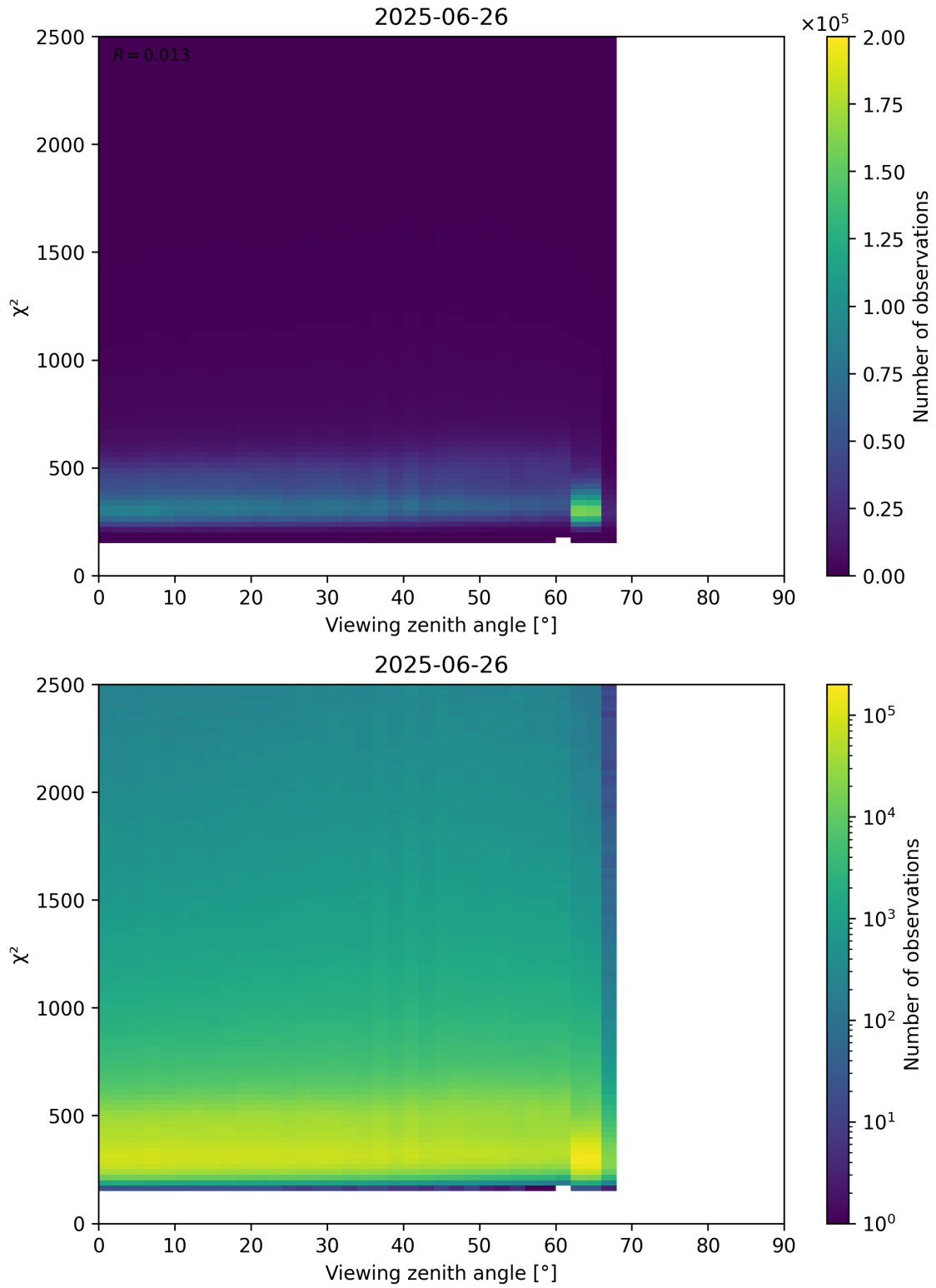
Figure 162: Scatter density plot of “Viewing zenith angle” against “ \chi^2 ” for 2025-06-25 to 2025-06-27.
