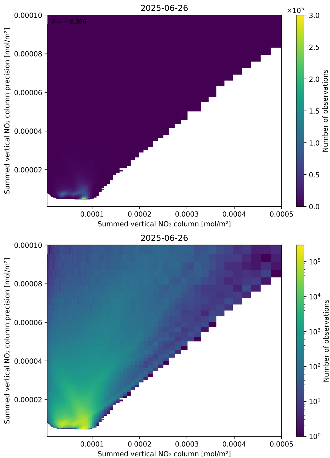
Figure 105: Scatter density plot of “Summed vertical NO 2 column” against “Summed vertical NO 2 column precision” for 2025-06-25 to 2025-06-27.
