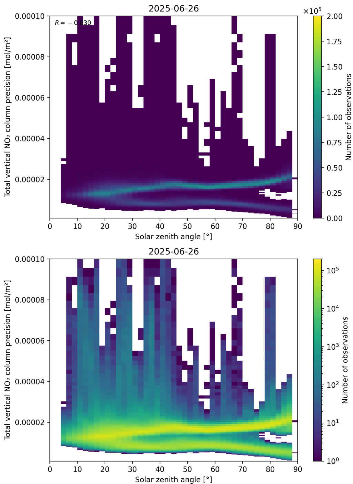
Figure 154: Scatter density plot of “Solar zenith angle” against “Total vertical NO 2 column precision” for 2025-06-25 to 2025-06-27.
