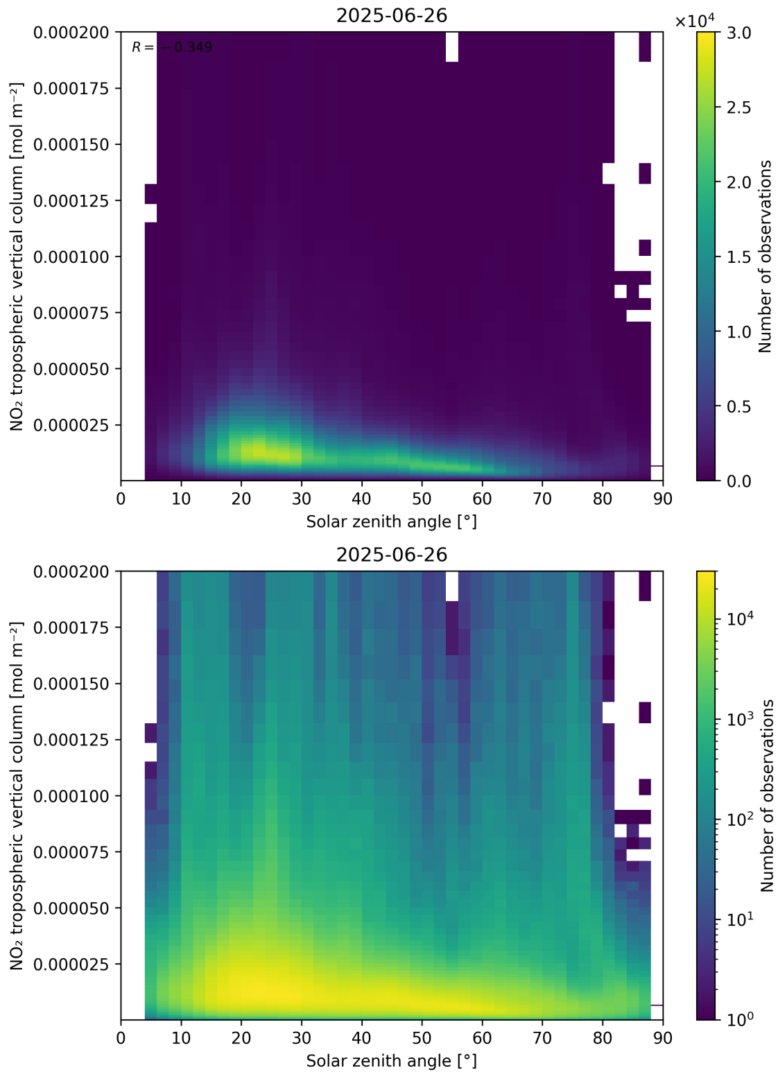
Figure 155: Scatter density plot of “Solar zenith angle” against “NO 2 tropospheric vertical column” for 2025-06-25 to 2025-06-27.
