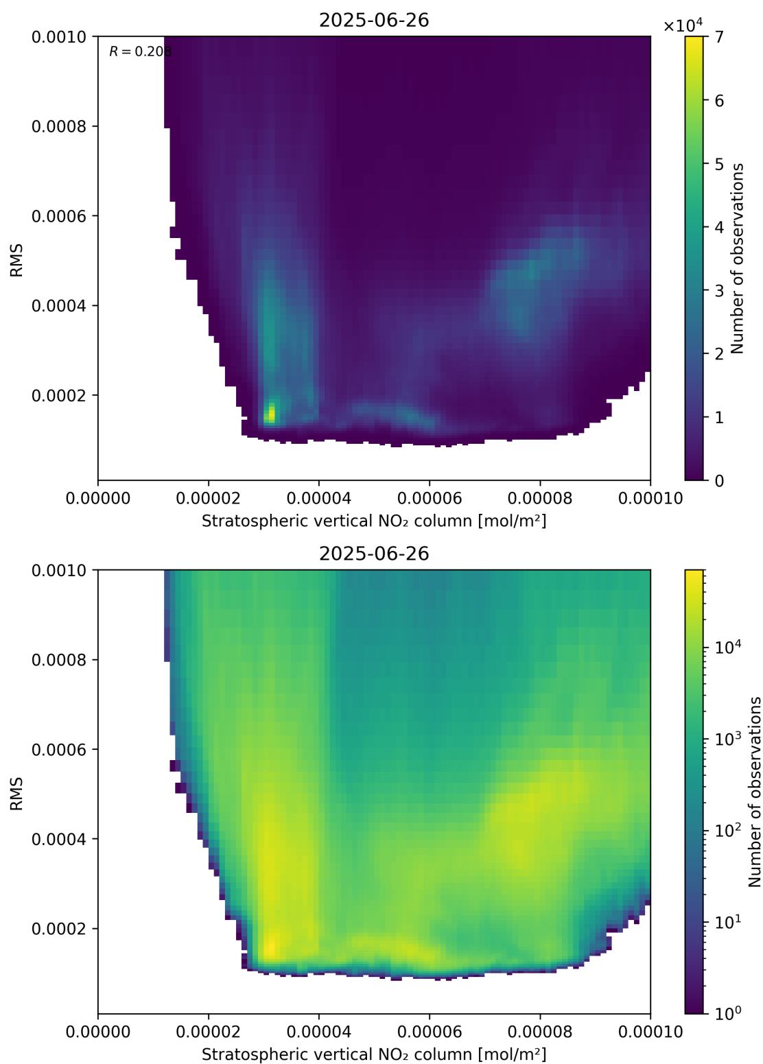
Figure 102: Scatter density plot of “Stratospheric vertical NO 2 column” against “RMS” for 2025-06-25 to 2025-06-27.
