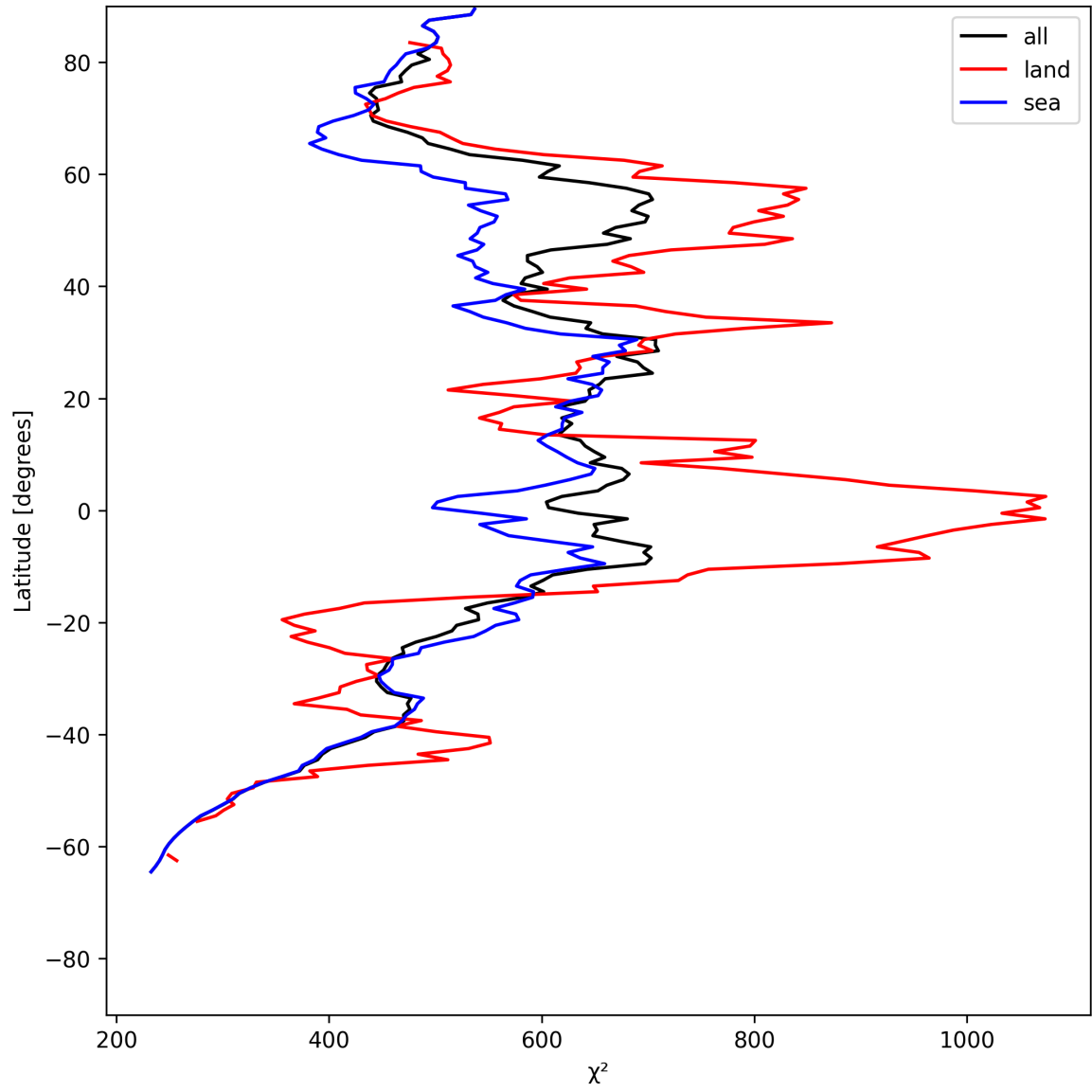
Figure 25: Zonal average of “ \chi^2 ” for 2025-06-25 to 2025-06-27.
