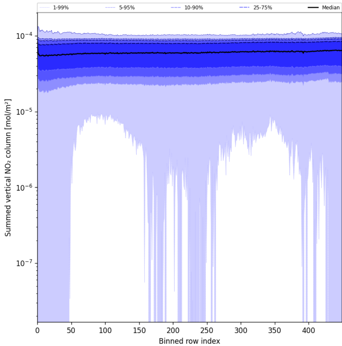
Figure 57: Along track statistics of “Summed vertical NO 2 column” for 2025-06-25 to 2025-06-27
