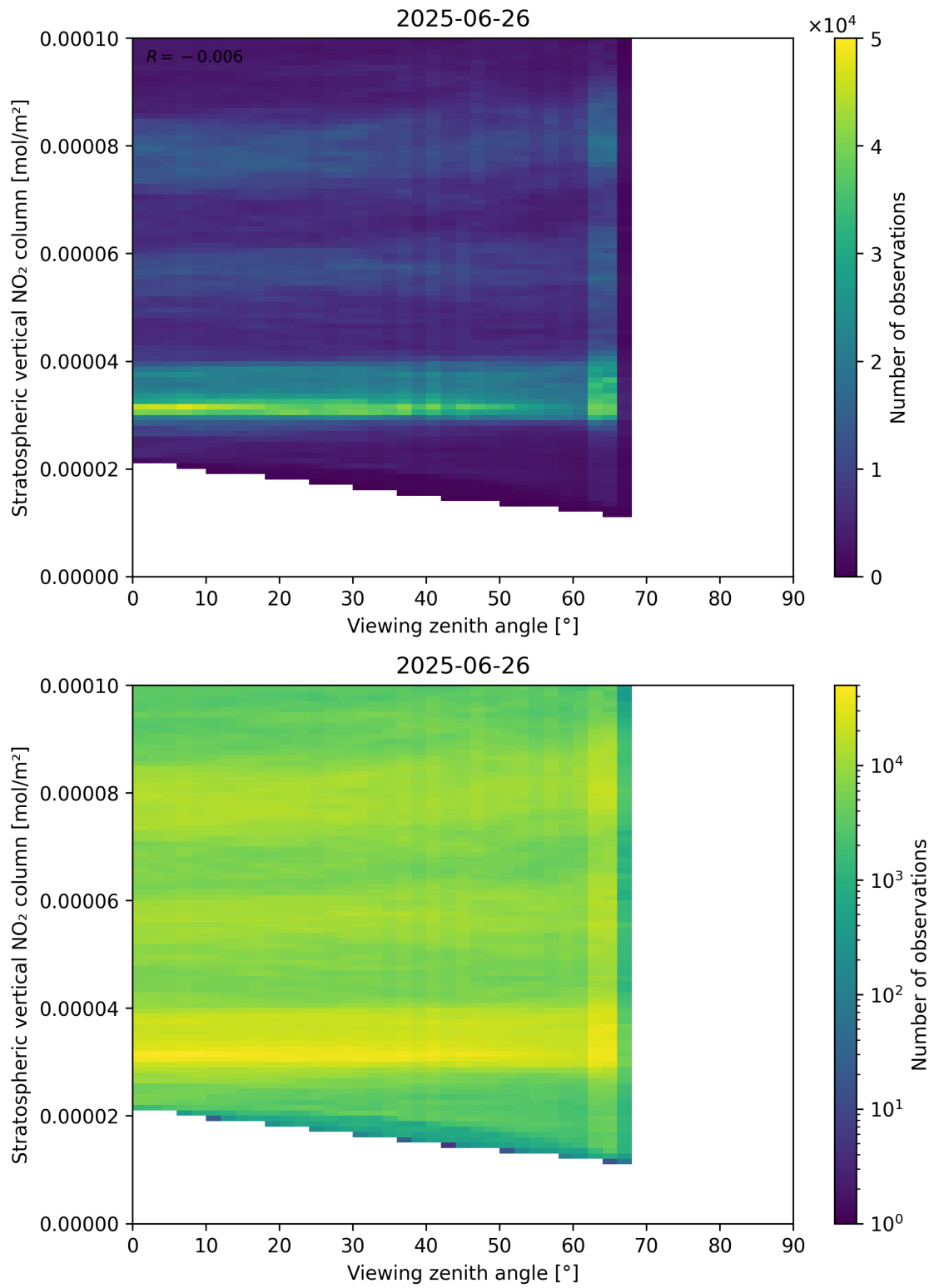
Figure 164: Scatter density plot of “Viewing zenith angle” against “Stratospheric vertical NO 2 column” for 2025-06-25 to 2025-06-27.
