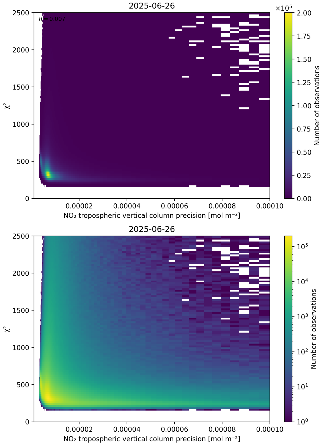
Figure 134: Scatter density plot of “NO 2 tropospheric vertical column precision” against “ \chi^2 ” for 2025-06-25 to 2025-06-27.
