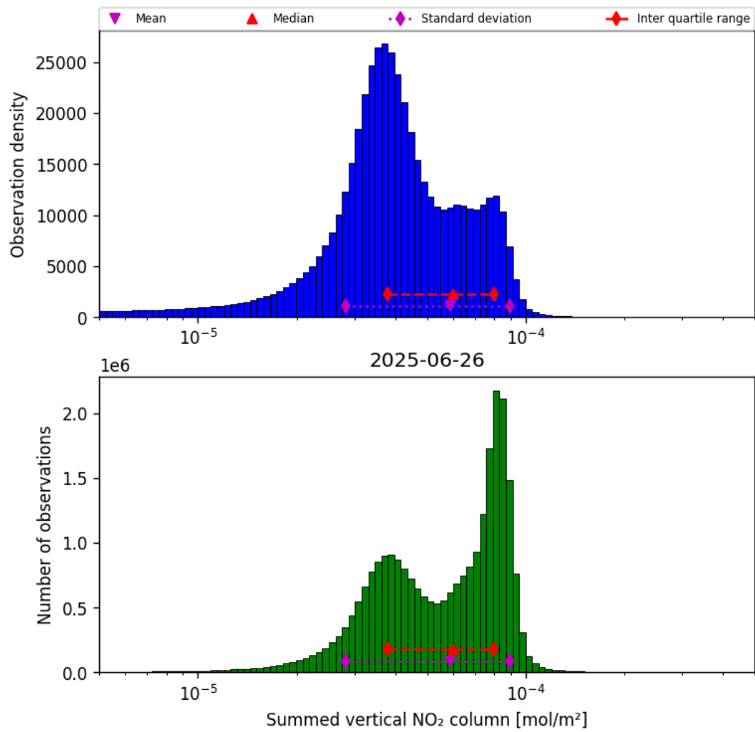
Figure 40: Histogram of “Summed vertical NO 2 column” for 2025-06-25 to 2025-06-27
