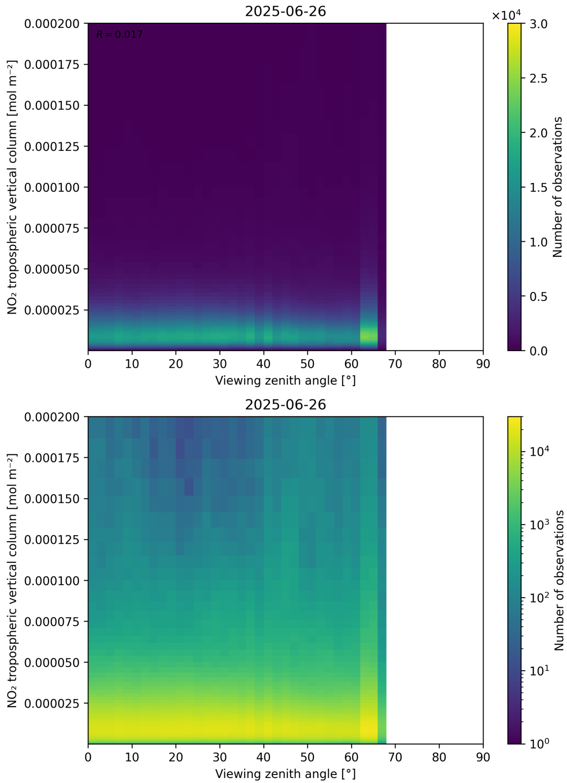
Figure 169: Scatter density plot of “Viewing zenith angle” against “NO 2 tropospheric vertical column” for 2025-06-25 to 2025-06-27.
