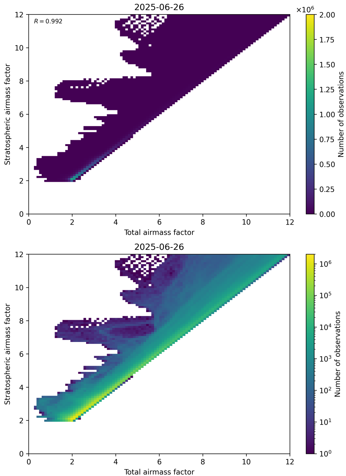
Figure 62: Scatter density plot of “Total airmass factor” against “Stratospheric airmass factor” for 2025-06-25 to 2025-06-27.
