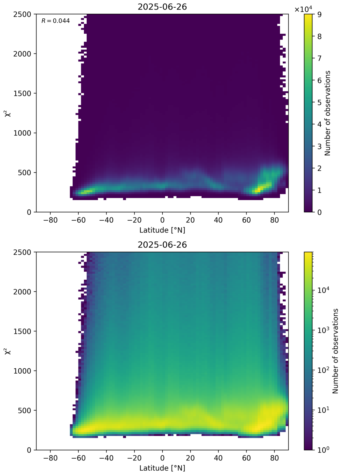
Figure 86: Scatter density plot of “Latitude” against “ \chi^2 ” for 2025-06-25 to 2025-06-27.
