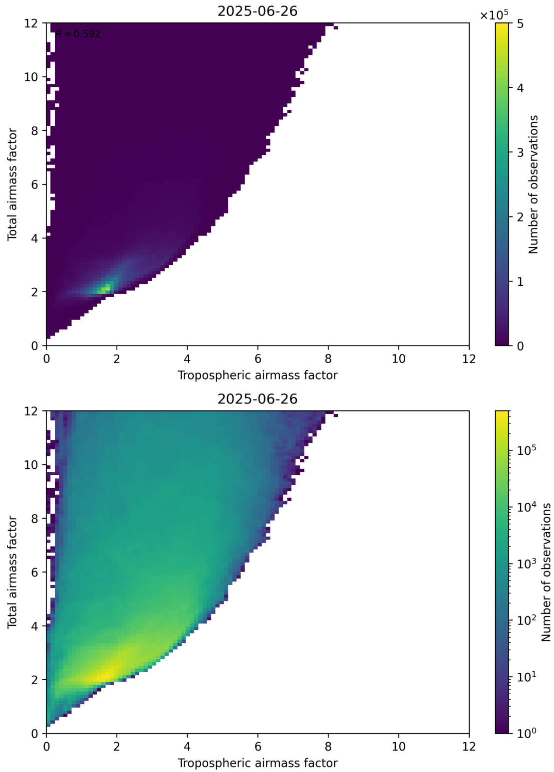
Figure 72: Scatter density plot of “Tropospheric airmass factor” against “Total airmass factor” for 2025-06-25 to 2025-06-27.
