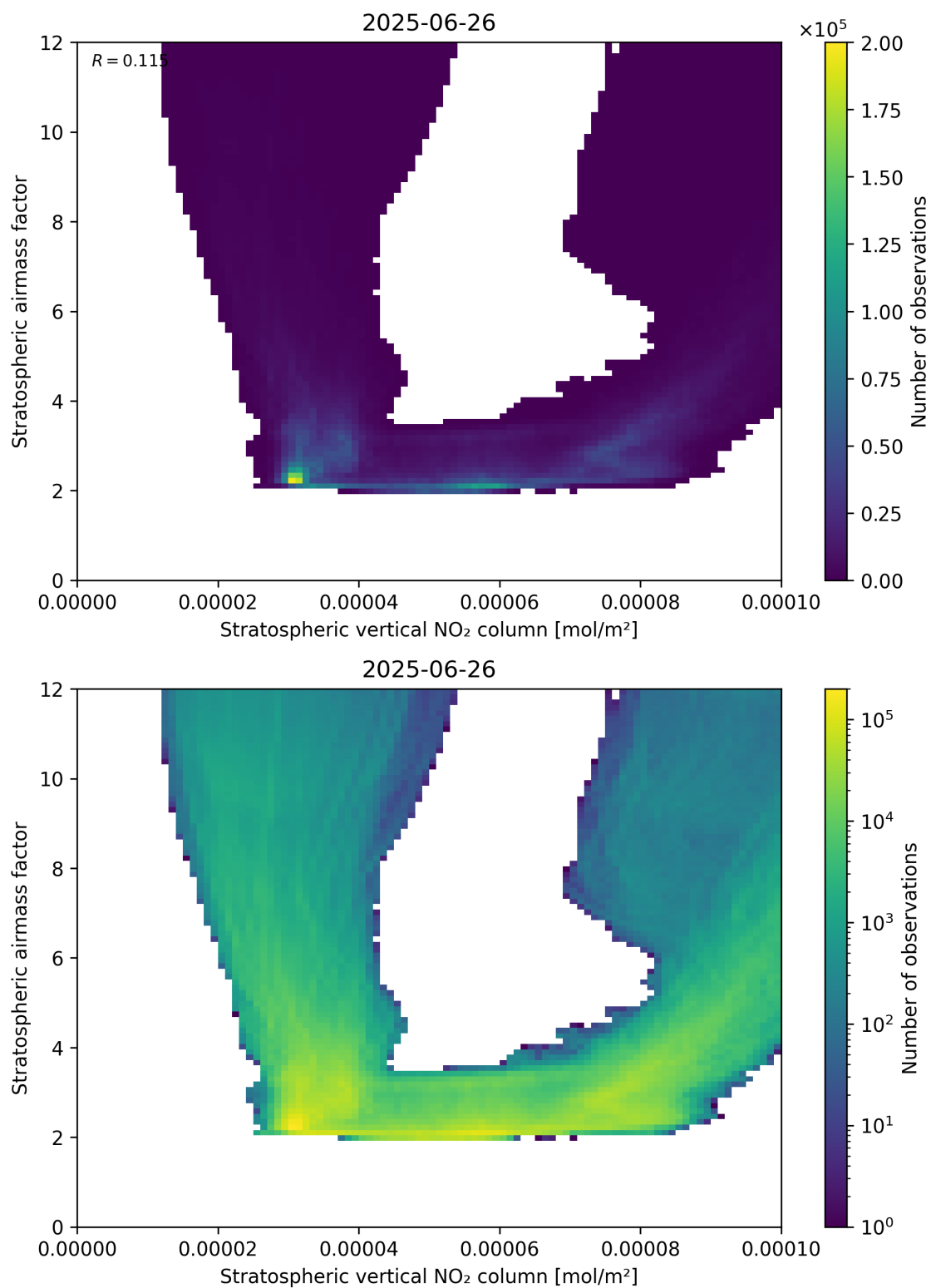
Figure 96: Scatter density plot of “Stratospheric vertical NO 2 column” against “Stratospheric airmass factor” for 2025-06-25 to 2025-06-27.
