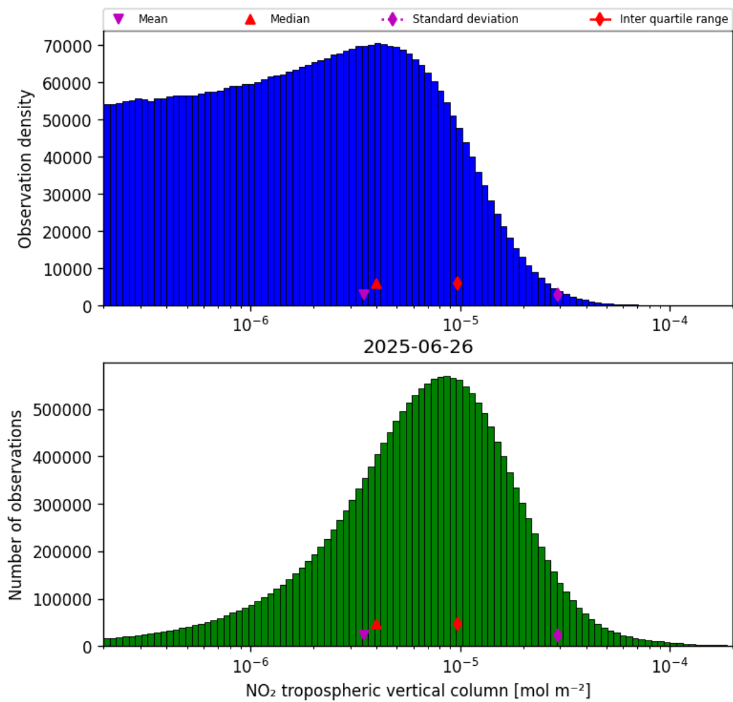
Figure 29: Histogram of “NO 2 tropospheric vertical column” for 2025-06-25 to 2025-06-27
