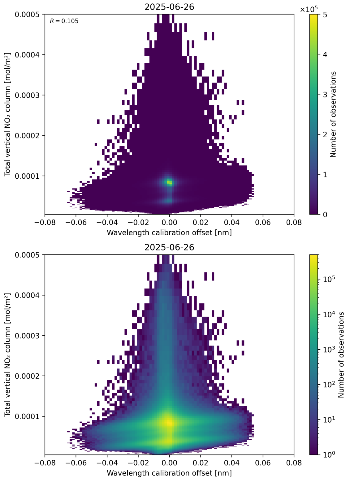
Figure 179: Scatter density plot of “Wavelength calibration offset” against “Total vertical NO 2 column” for 2025-06-25 to 2025-06-27.
