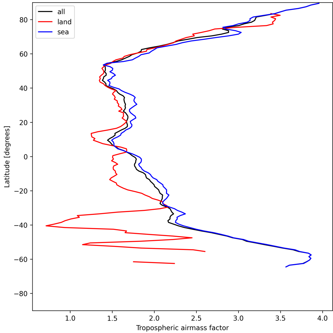
Figure 14: Zonal average of “Tropospheric air mass factor” for 2025-06-25 to 2025-06-27.
