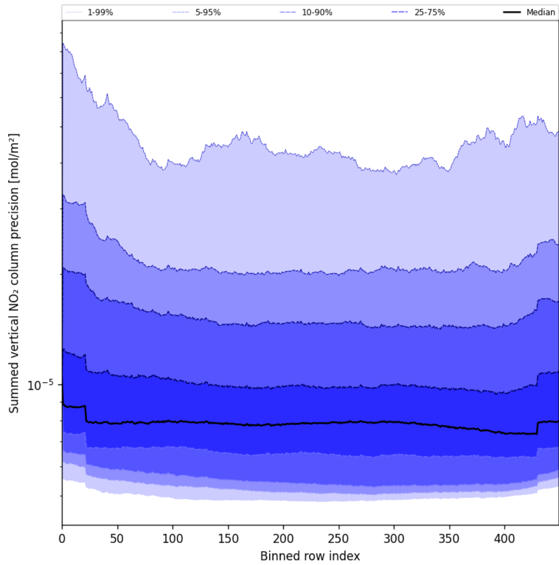
Figure 58: Along track statistics of “Summed vertical NO 2 column precision” for 2025-06-25 to 2025-06-27
