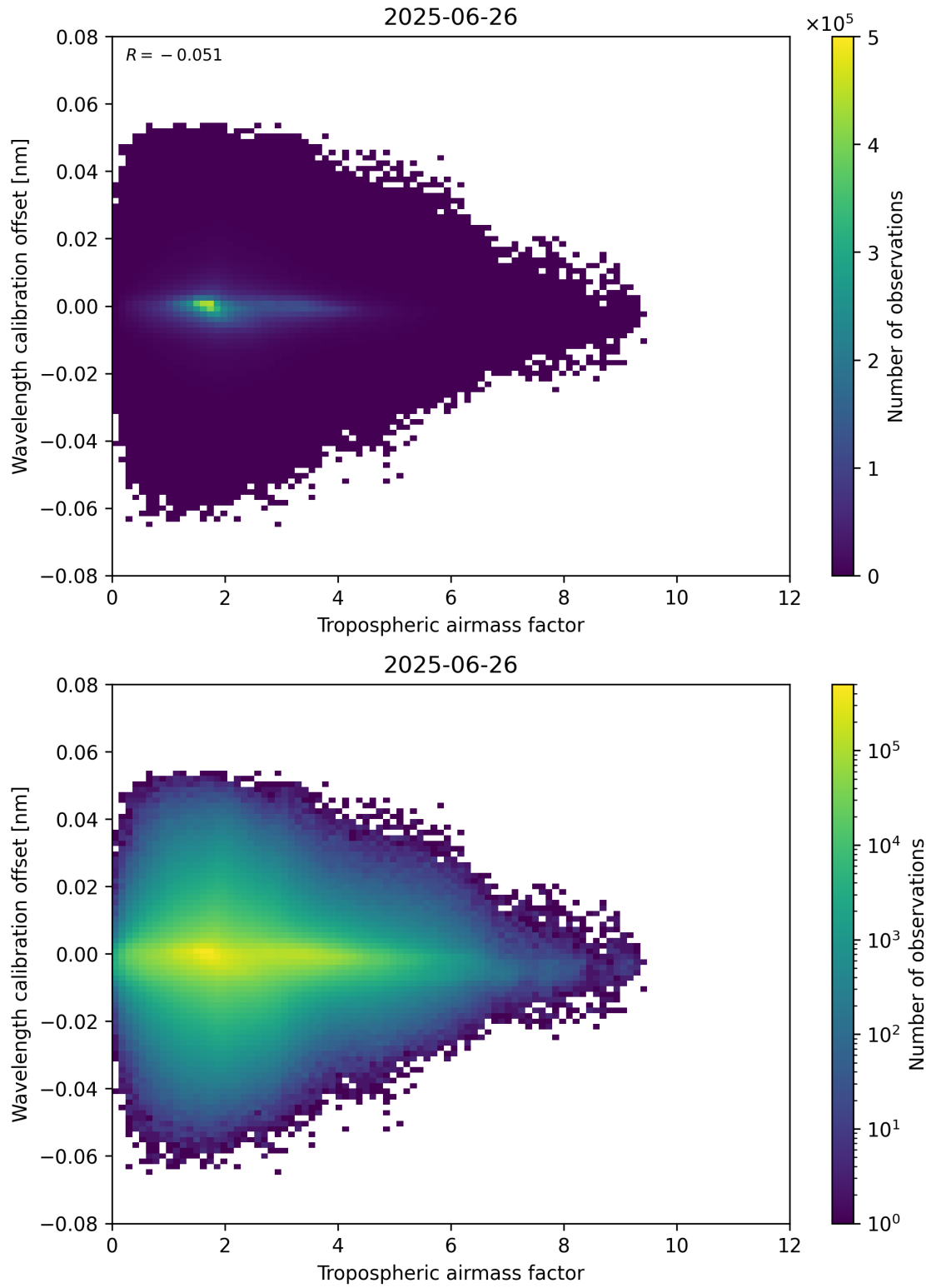
Figure 80: Scatter density plot of “Tropospheric airmass factor” against “Wavelength calibration offset” for 2025-06-25 to 2025-06-27.
