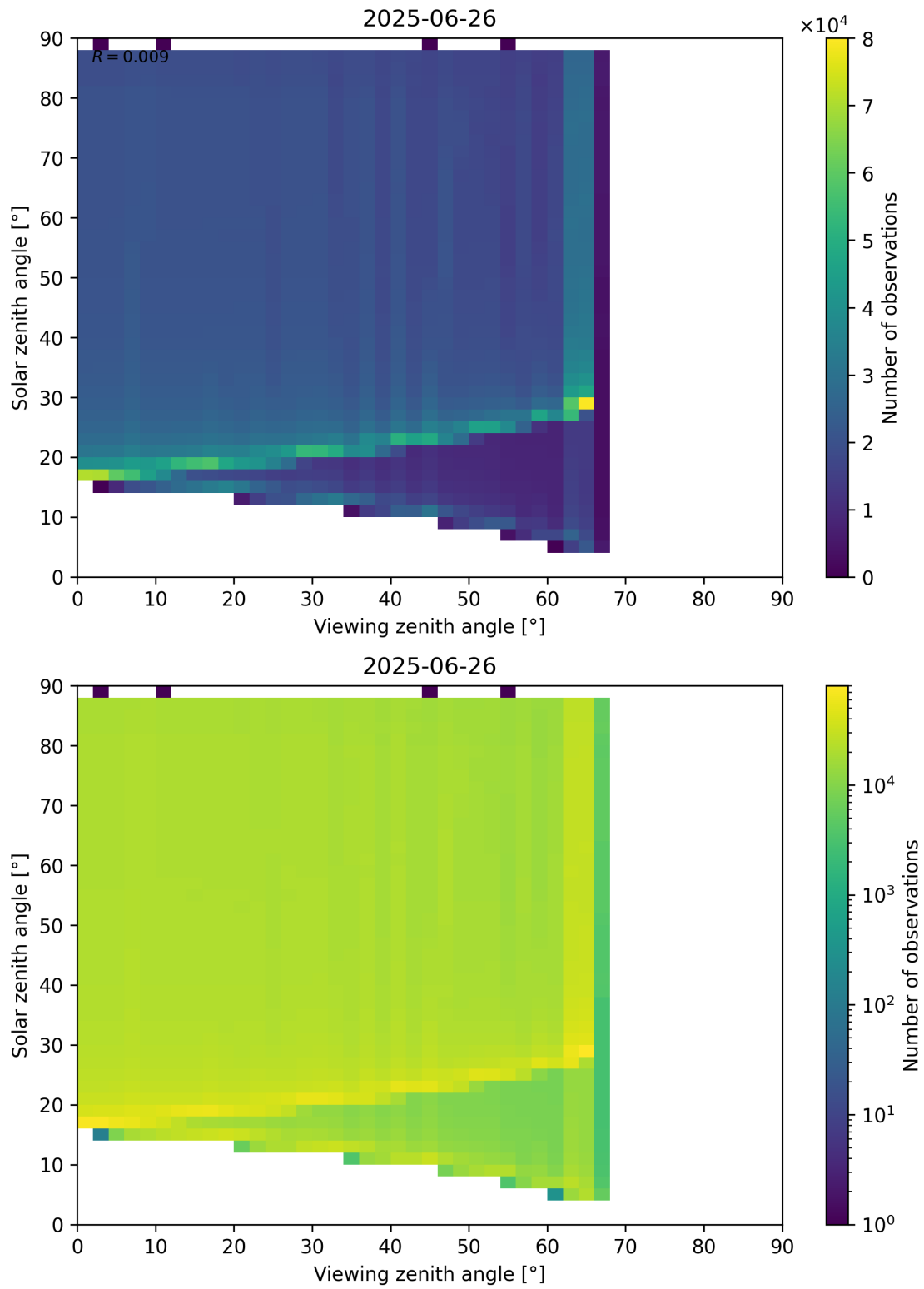
Figure 172: Scatter density plot of “Viewing zenith angle” against “Solar zenith angle” for 2025-06-25 to 2025-06-27.
