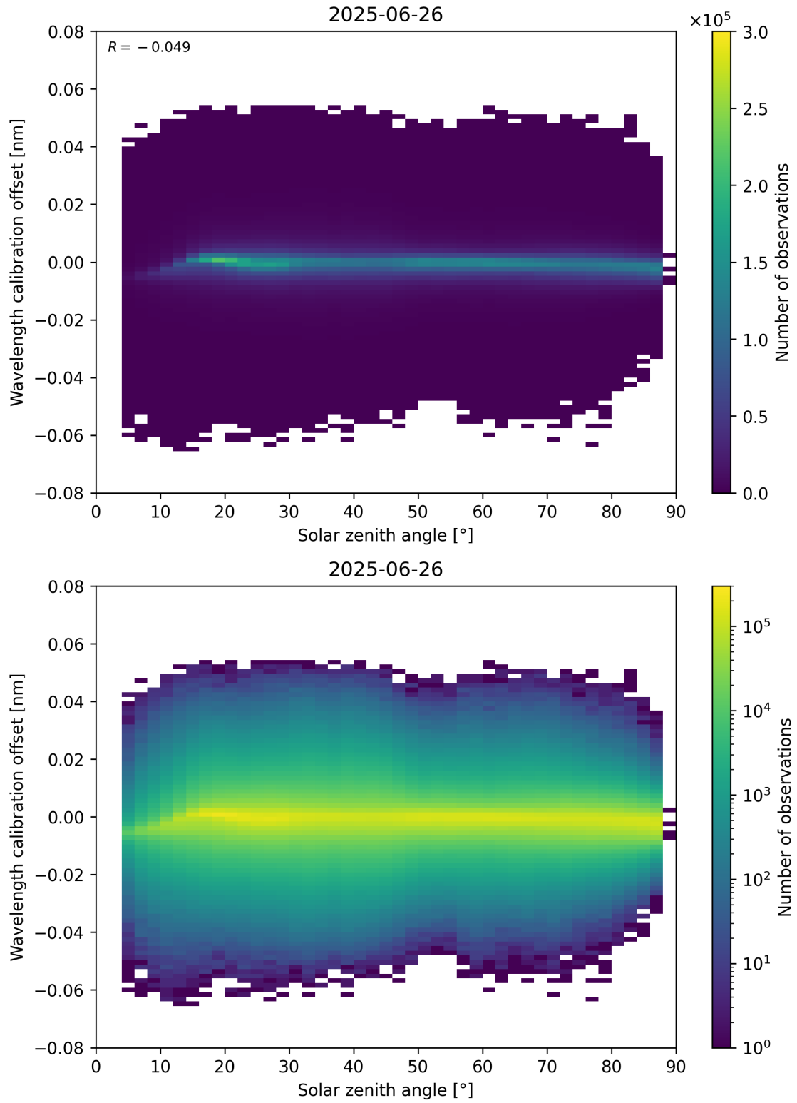
Figure 158: Scatter density plot of “Solar zenith angle” against “Wavelength calibration offset” for 2025-06-25 to 2025-06-27.
