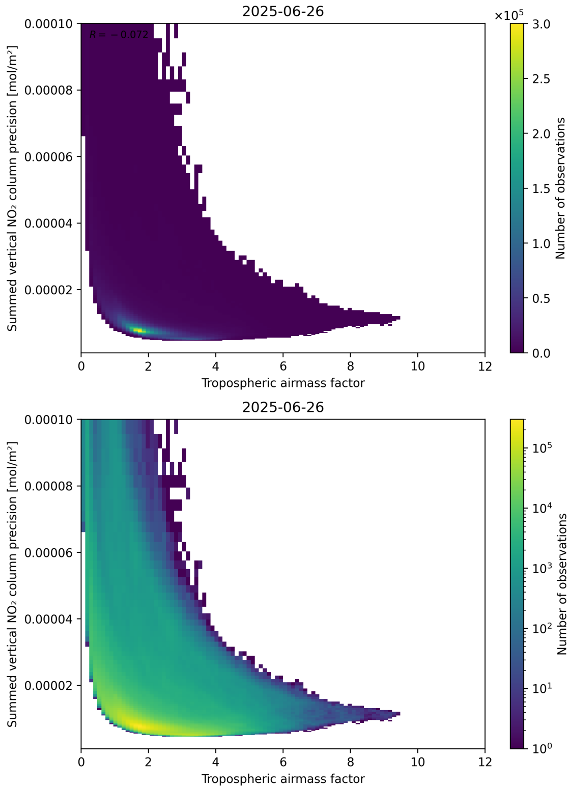
Figure 76: Scatter density plot of “Tropospheric air mass factor” against “Summed vertical NO 2 column precision” for 2025-06-25 to 2025-06-27.
