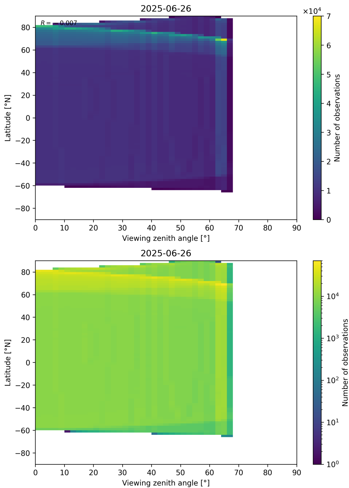
Figure 163: Scatter density plot of “Viewing zenith angle” against “Latitude” for 2025-06-25 to 2025-06-27.
