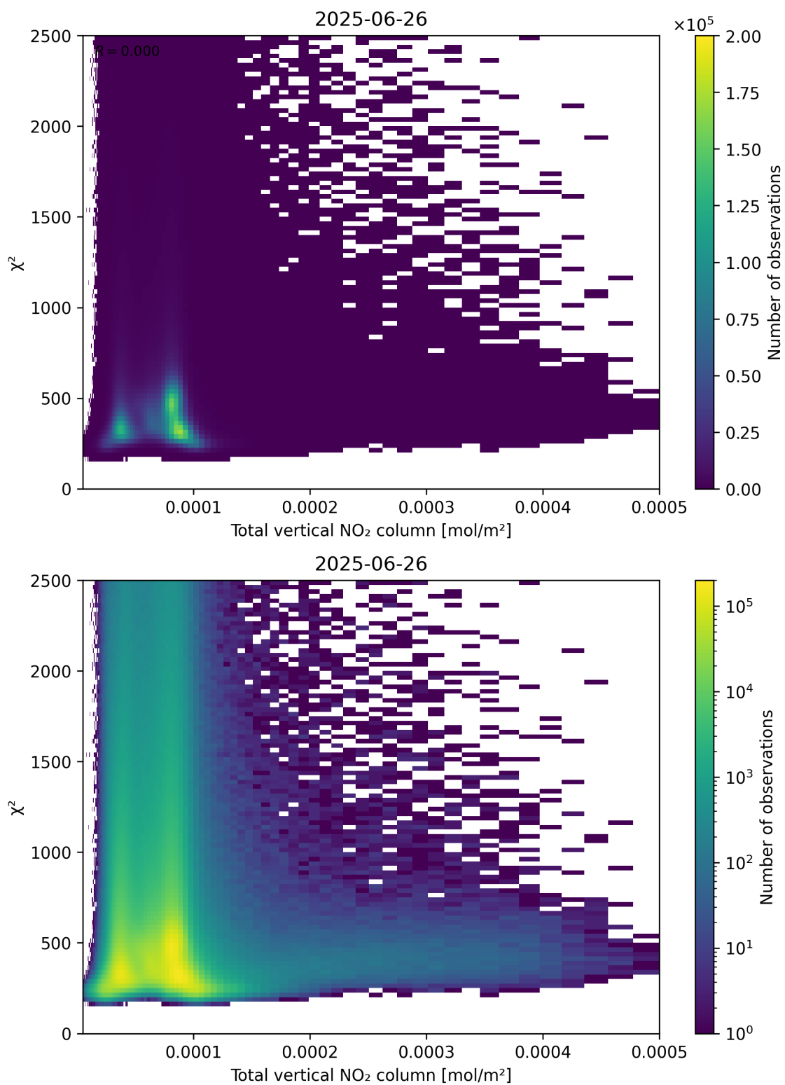
Figure 111: Scatter density plot of “Total vertical NO 2 column” against “ \chi^2 ” for 2025-06-25 to 2025-06-27.
