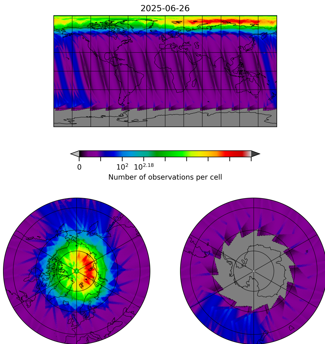
Figure 10: Map of the number of observations for 2025-06-25 to 2025-06-27
