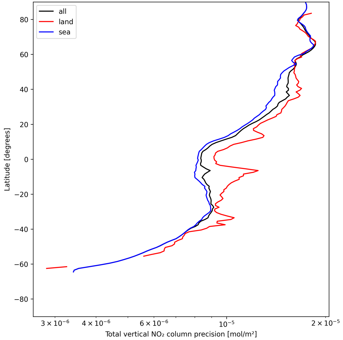
Figure 22: Zonal average of “Total vertical NO 2 column precision” for 2025-06-25 to 2025-06-27.
