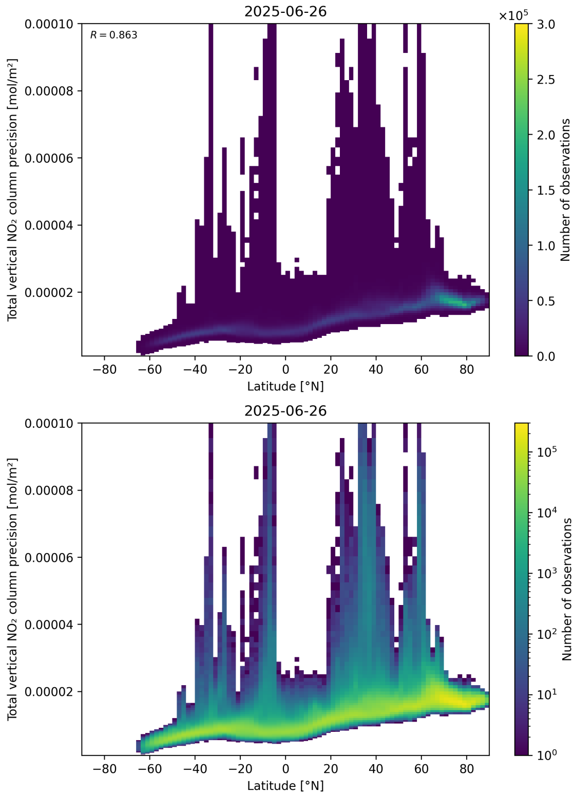
Figure 91: Scatter density plot of “Latitude” against “Total vertical NO 2 column precision” for 2025-06-25 to 2025-06-27.
