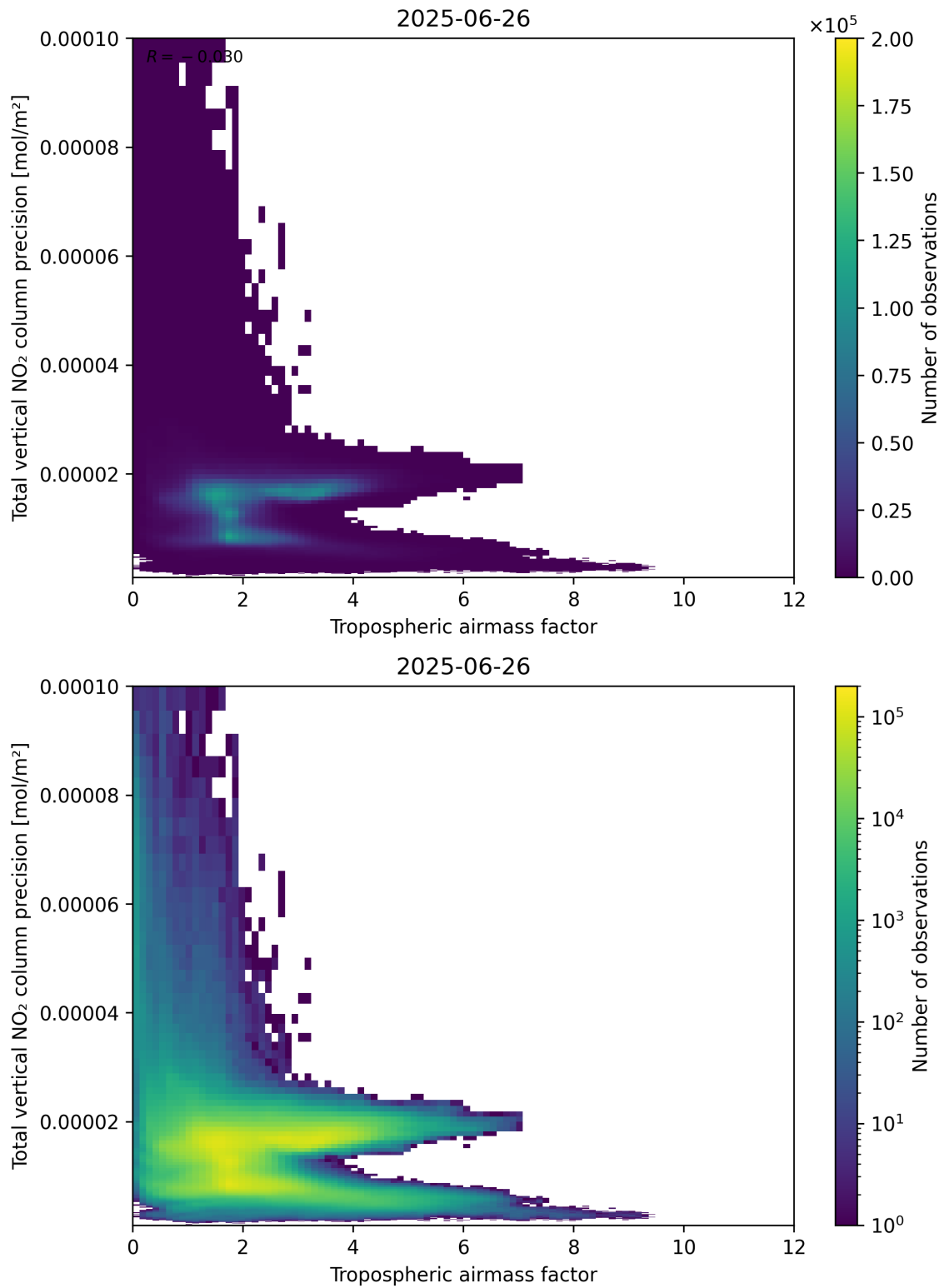
Figure 78: Scatter density plot of “Tropospheric air mass factor” against “Total vertical NO 2 column precision” for 2025-06-25 to 2025-06-27.
