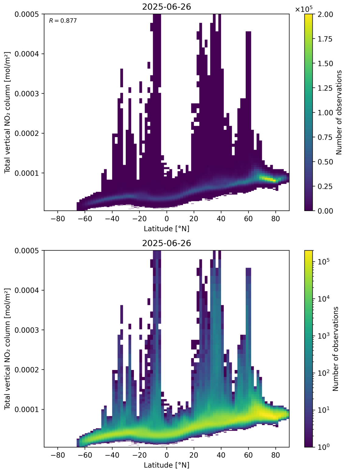
Figure 90: Scatter density plot of “Latitude” against “Total vertical NO 2 column” for 2025-06-25 to 2025-06-27.
