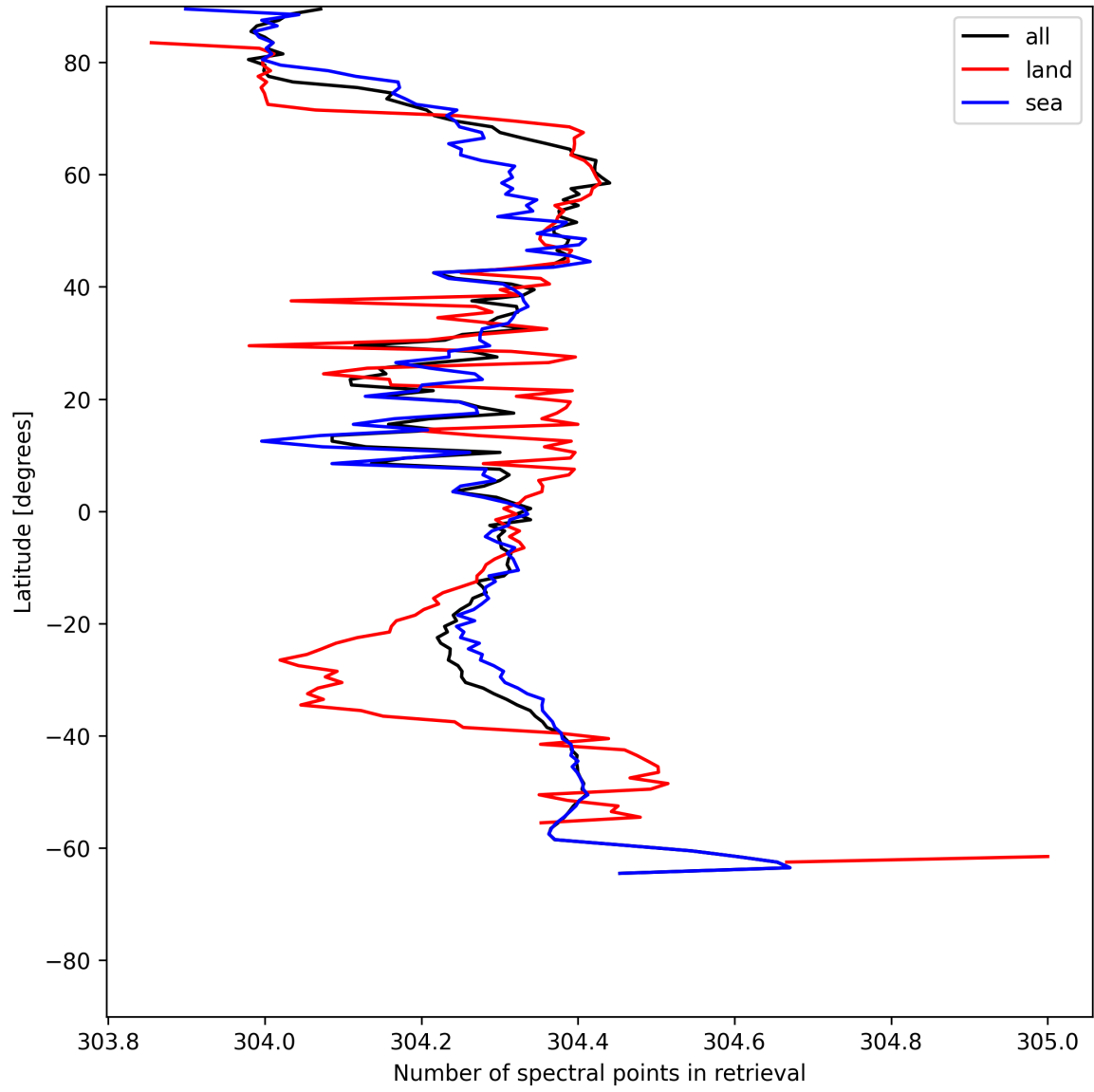
Figure 16: Zonal average of “Number of spectral points in retrieval” for 2025-06-25 to 2025-06-27.
