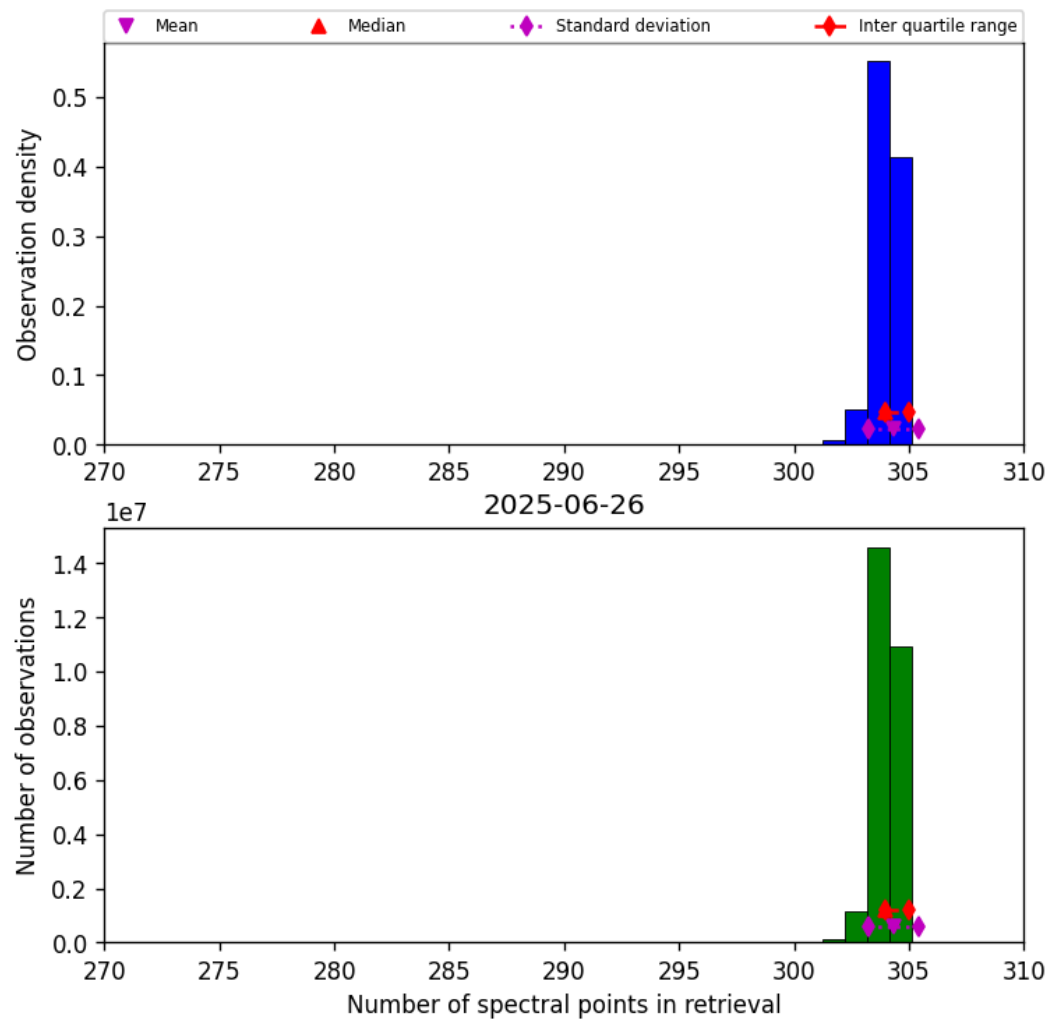
Figure 33: Histogram of “Number of spectral points in retrieval” for 2025-06-25 to 2025-06-27
