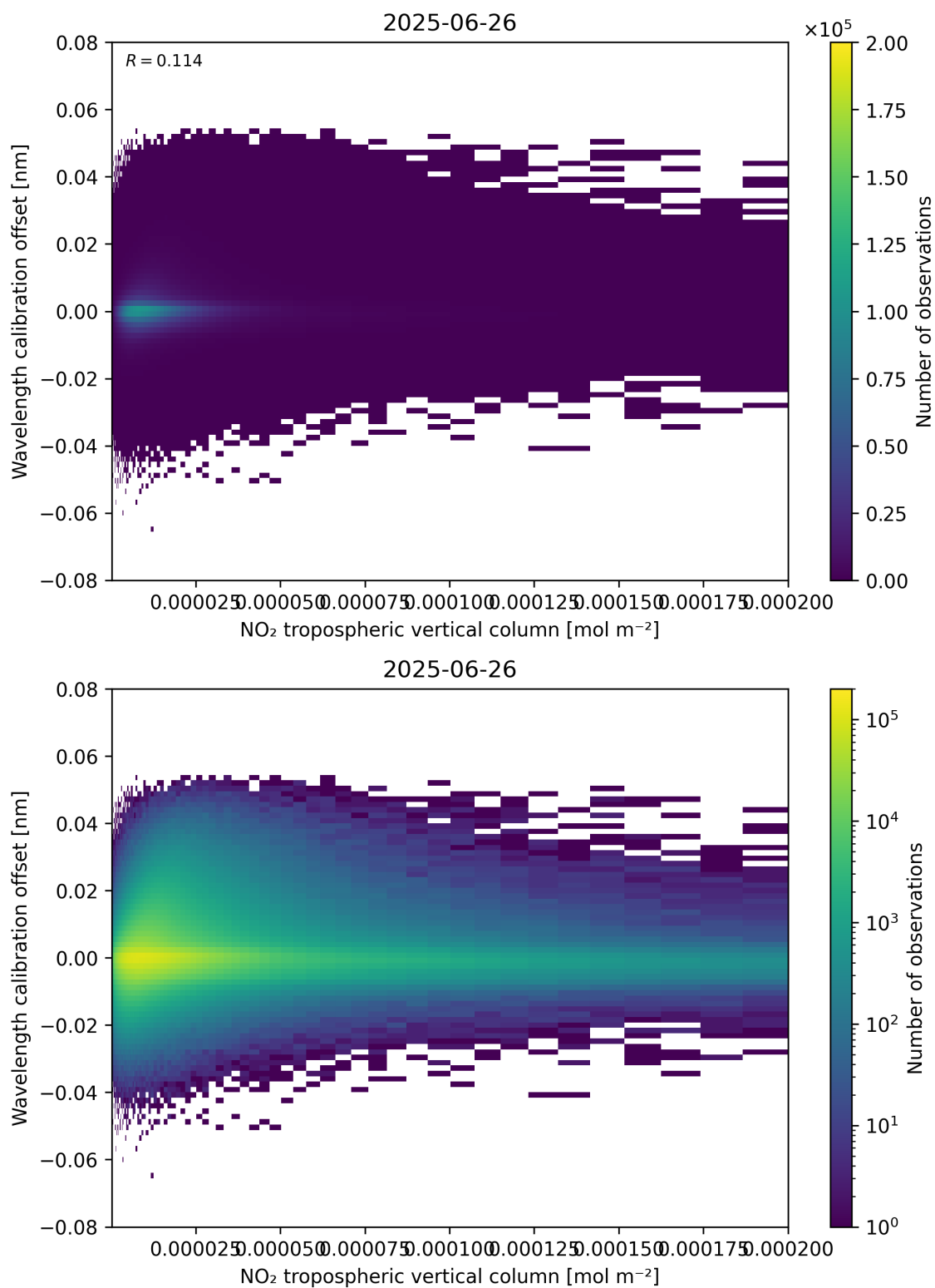
Figure 143: Scatter density plot of “NO 2 tropospheric vertical column” against “Wavelength calibration offset” for 2025-06-25 to 2025-06-27.
