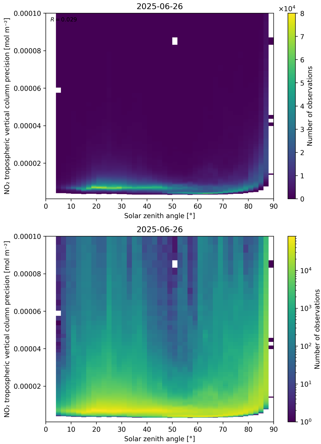
Figure 156: Scatter density plot of “Solar zenith angle” against “NO 2 tropospheric vertical column precision” for 2025-06-25 to 2025-06-27.
