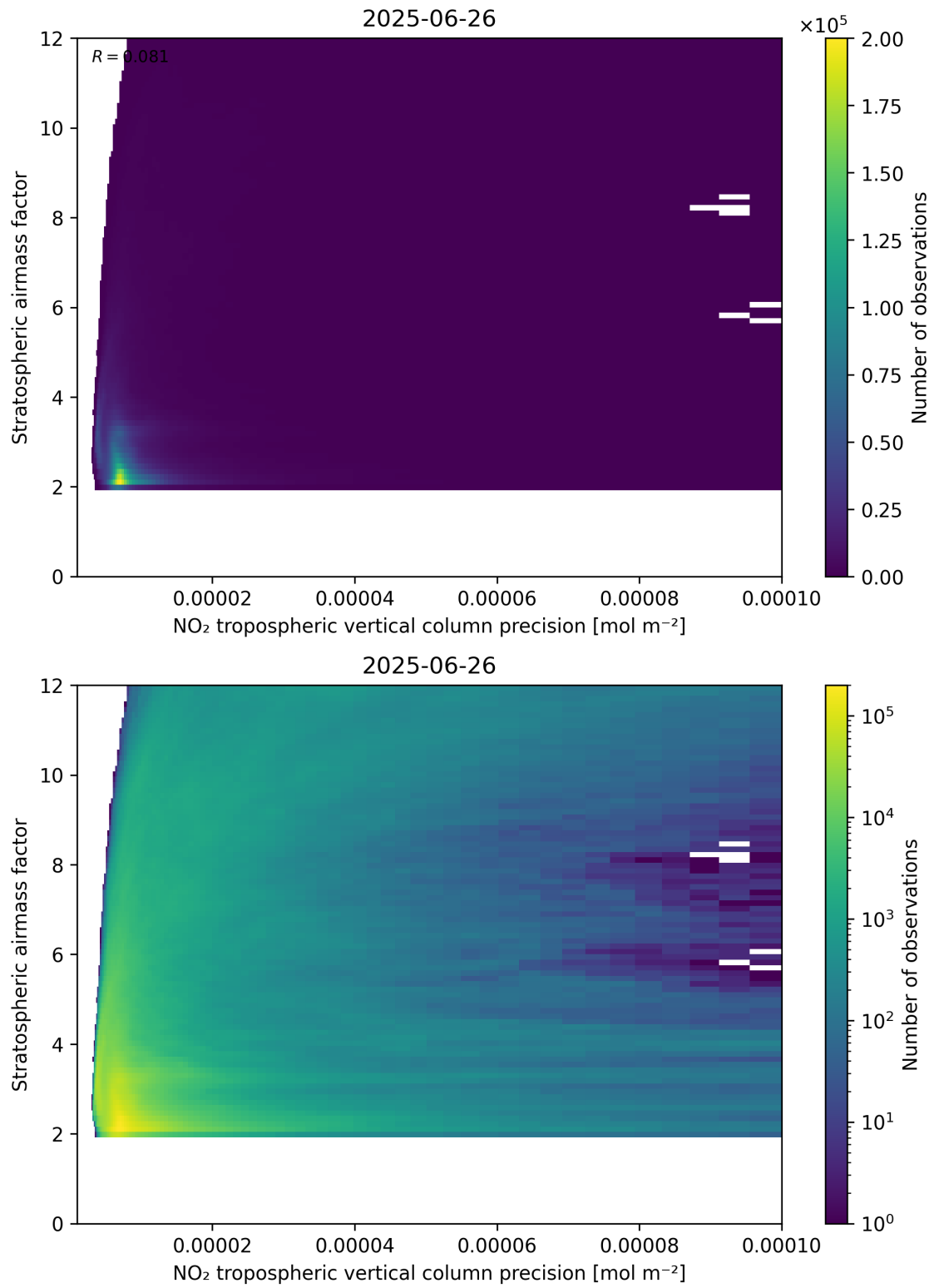
Figure 131: Scatter density plot of “NO 2 tropospheric vertical column precision” against “Stratospheric airmass factor” for 2025-06-25 to 2025-06-27.
