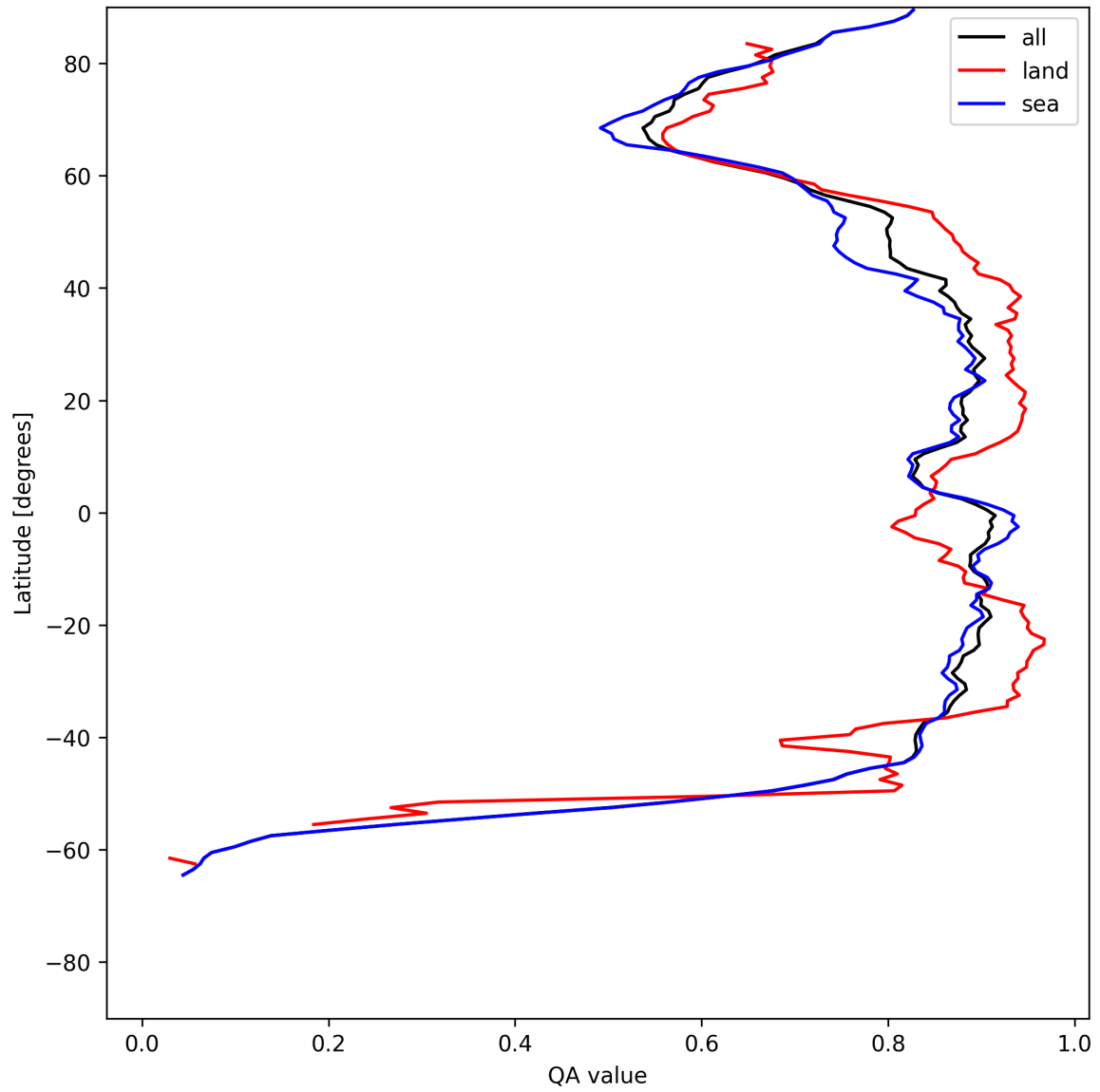
Figure 11: Zonal average of “QA value” for 2025-06-25 to 2025-06-27.
