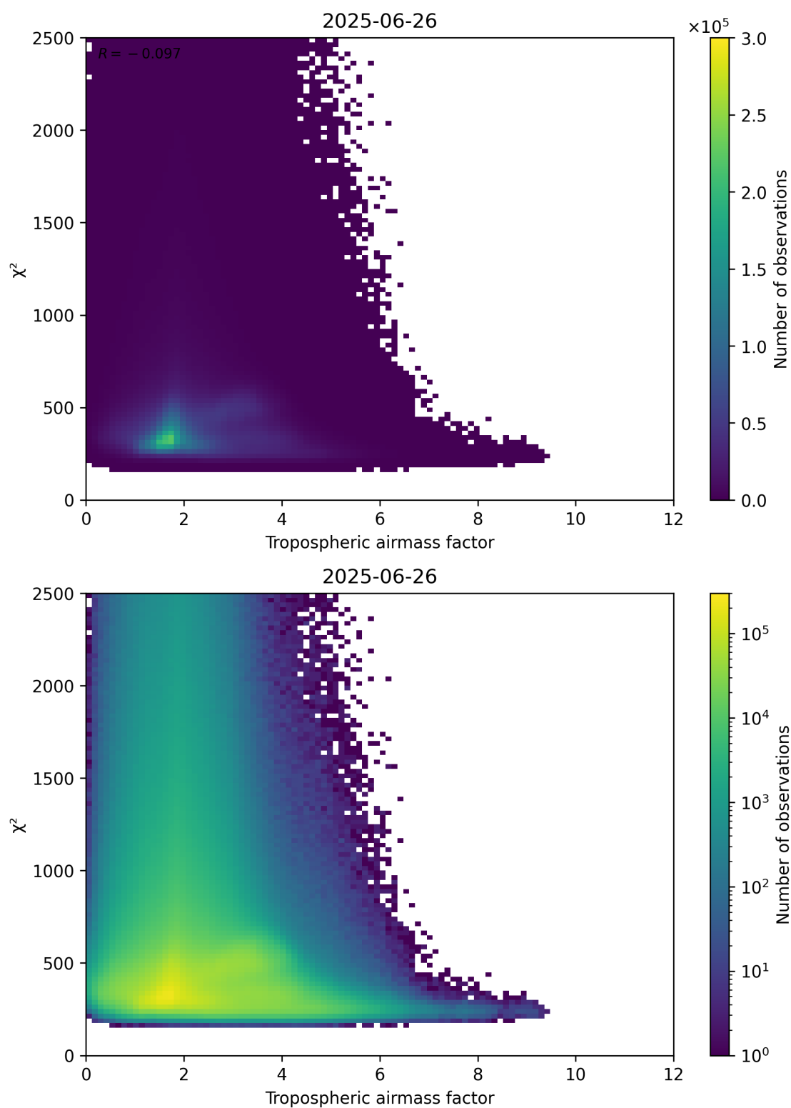
Figure 73: Scatter density plot of “Tropospheric airmass factor” against “ \chi^2 ” for 2025-06-25 to 2025-06-27.
