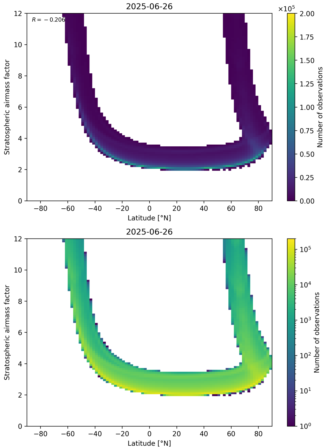
Figure 83: Scatter density plot of “Latitude” against “Stratospheric air mass factor” for 2025-06-25 to 2025-06-27.
