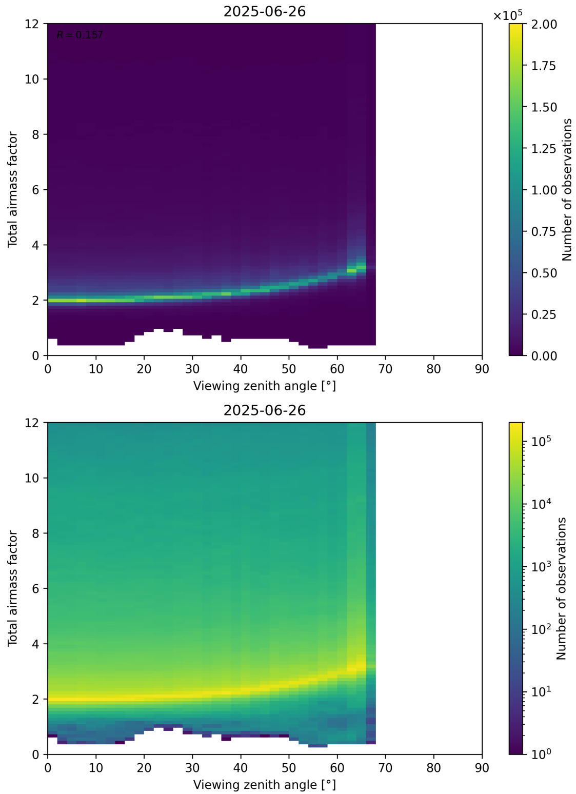
Figure 160: Scatter density plot of “Viewing zenith angle” against “Total airmass factor” for 2025-06-25 to 2025-06-27.
