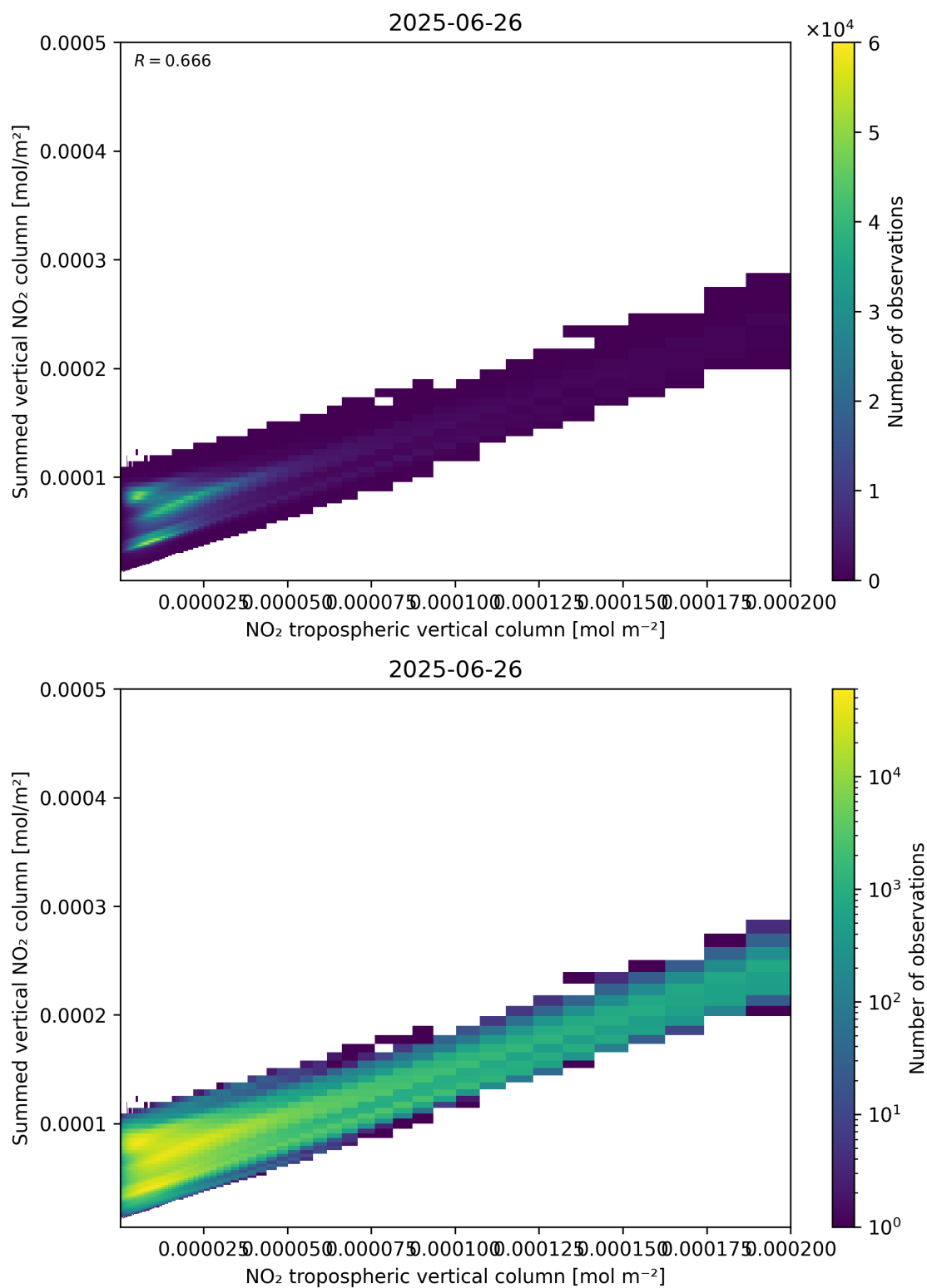
Figure 126: Scatter density plot of “NO 2 tropospheric vertical column” against “Summed vertical NO 2 column” for 2025-06-25 to 2025-06-27.
