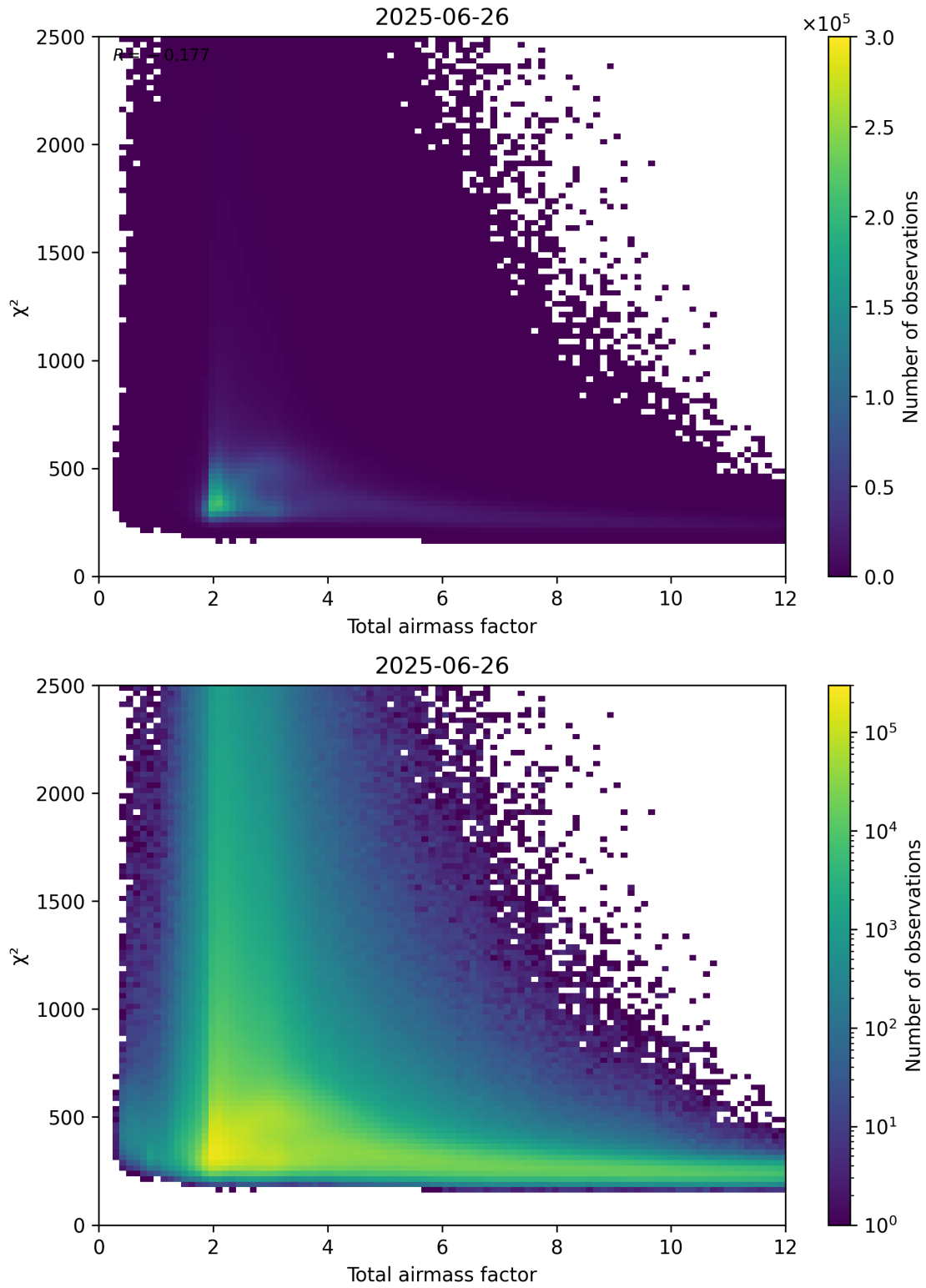
Figure 63: Scatter density plot of “Total airmass factor” against “ \chi^2 ” for 2025-06-25 to 2025-06-27.
