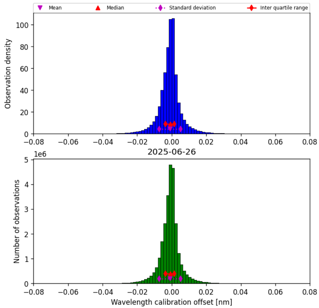
Figure 35: Histogram of “Wavelength calibration offset” for 2025-06-25 to 2025-06-27
