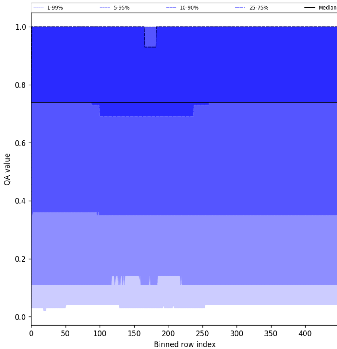
Figure 45: Along track statistics of “QA value” for 2025-06-25 to 2025-06-27
