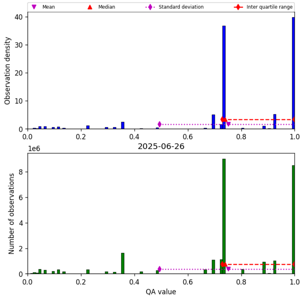
Figure 28: Histogram of “QA value” for 2025-06-25 to 2025-06-27
