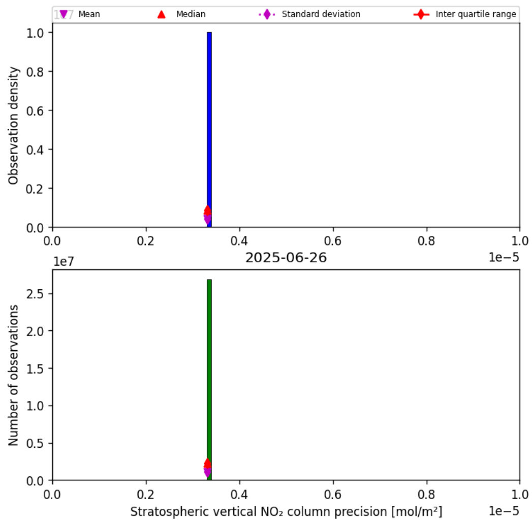
Figure 37: Histogram of “Stratospheric vertical NO 2 column precision” for 2025-06-25 to 2025-06-27
