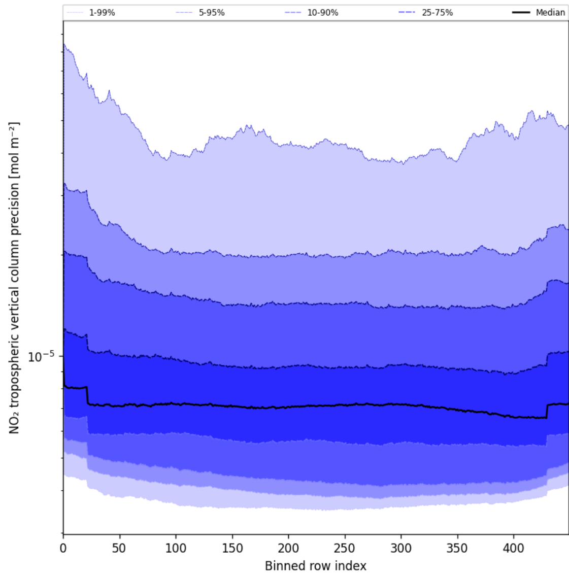
Figure 47: Along track statistics of “NO 2 tropospheric vertical column precision” for 2025-06-25 to 2025-06-27
