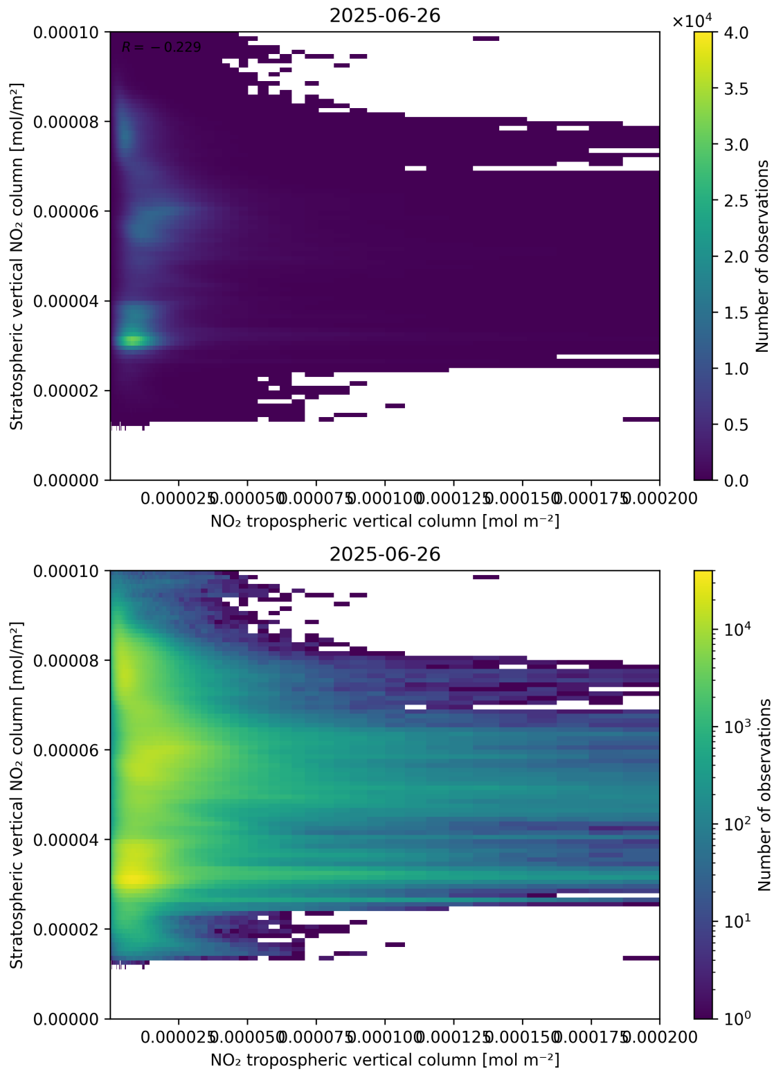
Figure 125: Scatter density plot of “NO 2 tropospheric vertical column” against “Stratospheric vertical NO 2 column” for 2025-06-25 to 2025-06-27.
