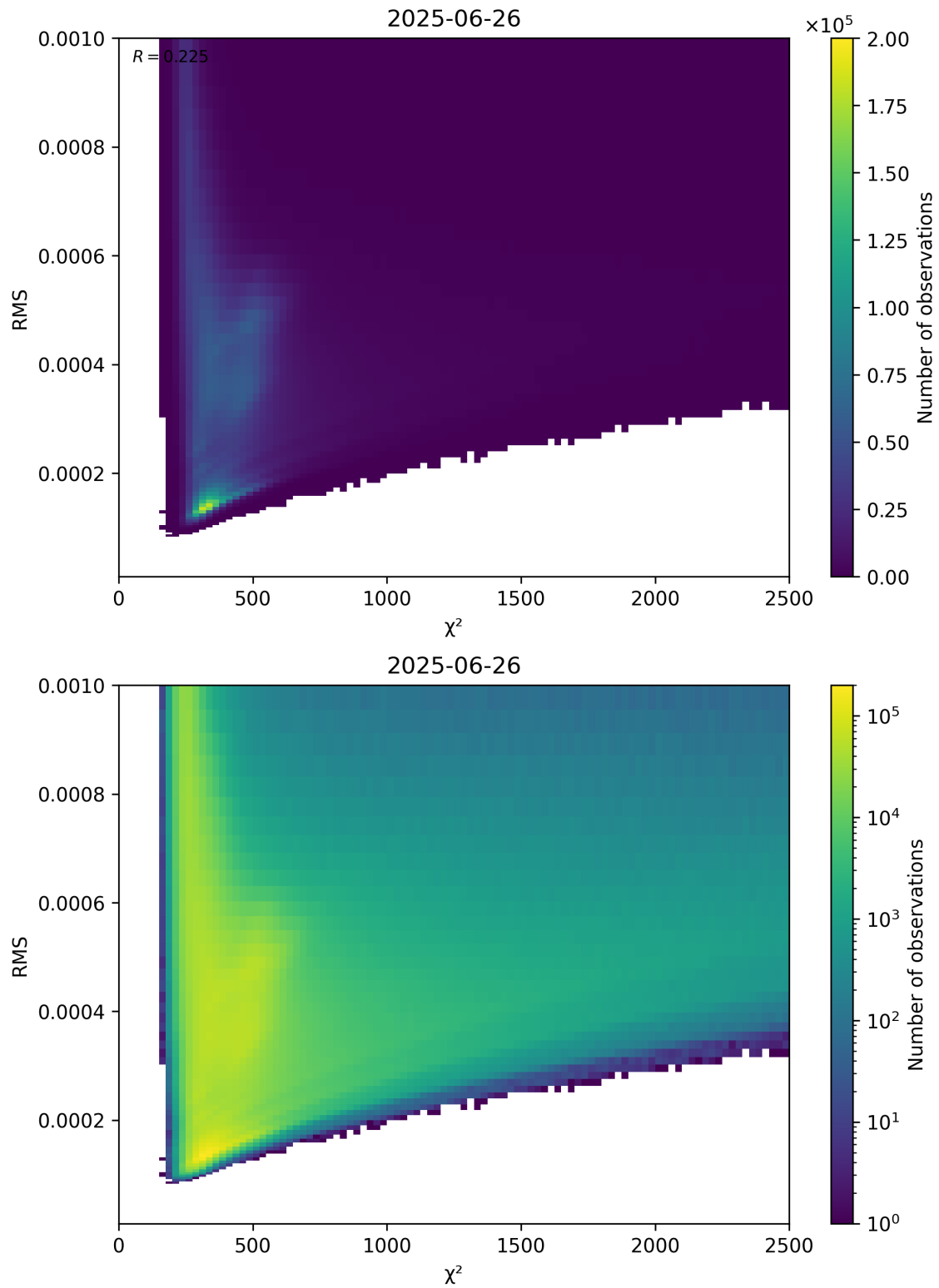
Figure 82: Scatter density plot of “ \chi^2 ” against “RMS” for 2025-06-25 to 2025-06-27.
