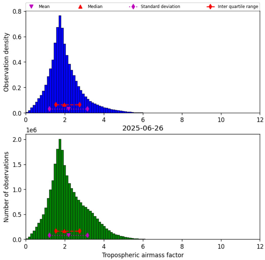
Figure 31: Histogram of “Tropospheric airmass factor” for 2025-06-25 to 2025-06-27
