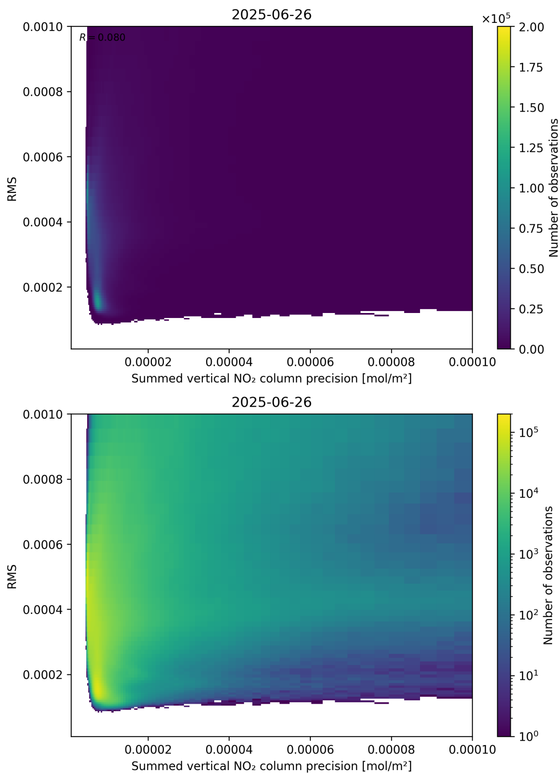
Figure 108: Scatter density plot of “Summed vertical NO 2 column precision” against “RMS” for 2025-06-25 to 2025-06-27.
