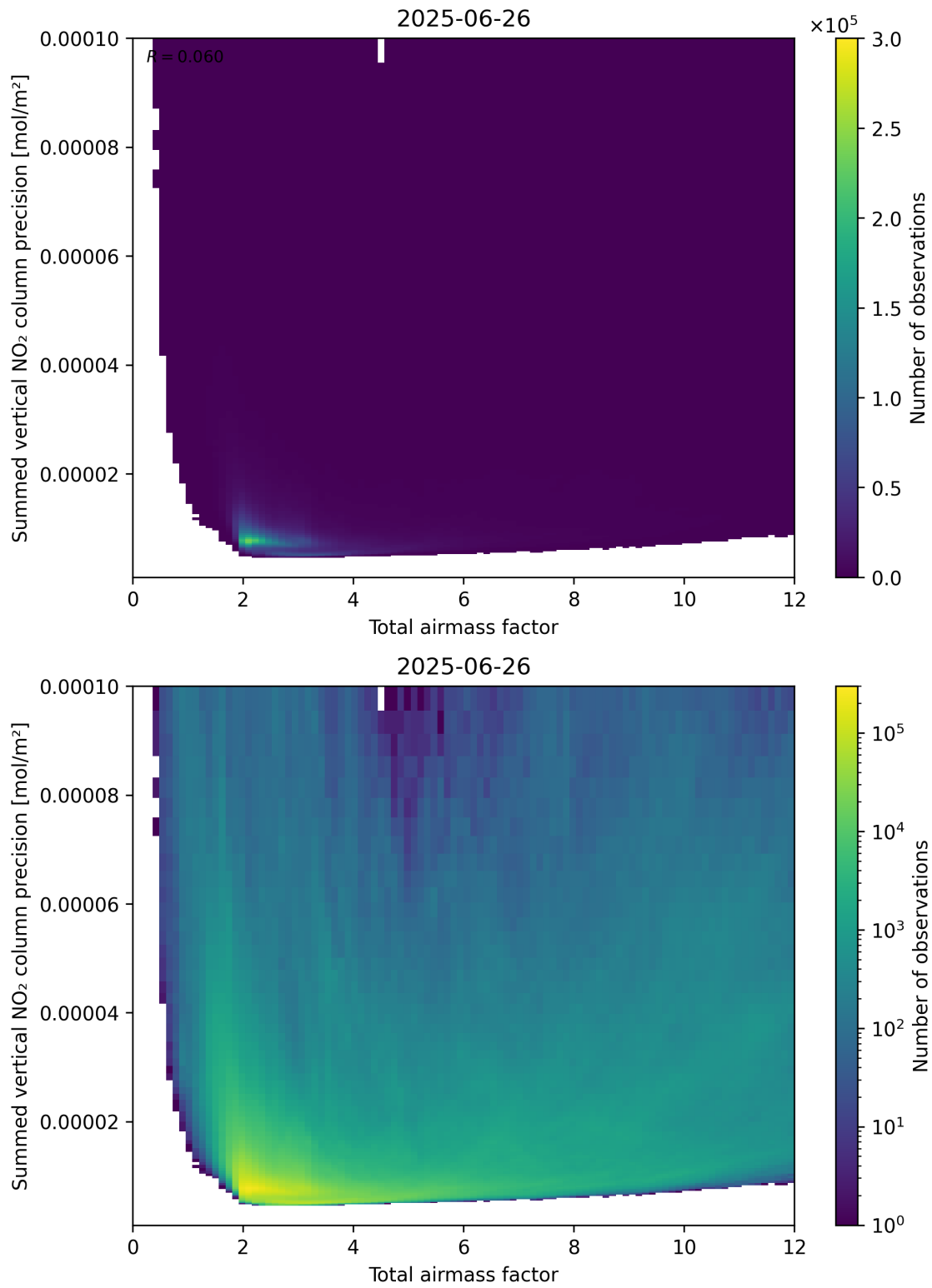
Figure 66: Scatter density plot of “Total airmass factor” against “Summed vertical NO 2 column precision” for 2025-06-25 to 2025-06-27.
