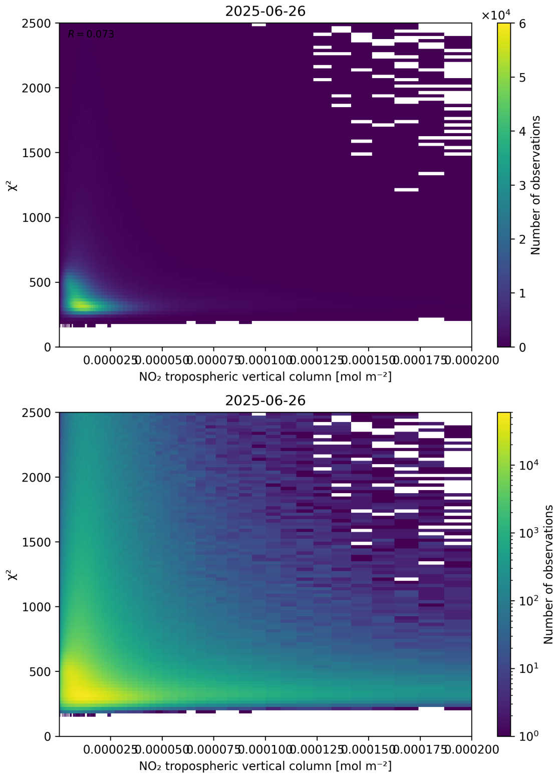
Figure 124: Scatter density plot of “NO 2 tropospheric vertical column” against “ \chi^2 ” for 2025-06-25 to 2025-06-27.
