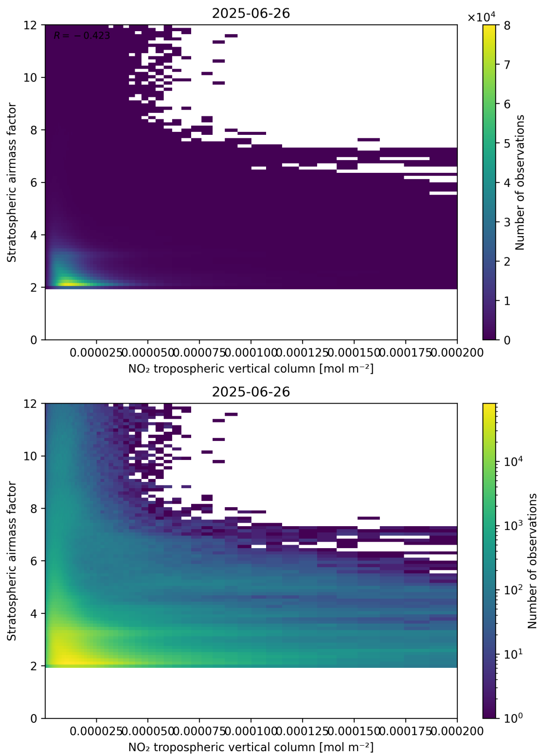
Figure 121: Scatter density plot of “NO 2 tropospheric vertical column” against “Stratospheric air mass factor” for 2025-06-25 to 2025-06-27.
