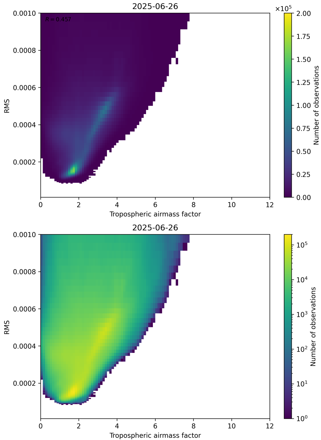
Figure 79: Scatter density plot of “Tropospheric airmass factor” against “RMS” for 2025-06-25 to 2025-06-27.
