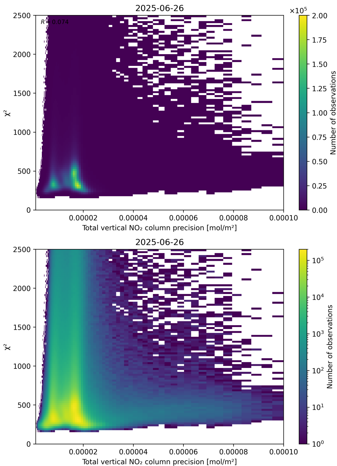
Figure 116: Scatter density plot of “Total vertical NO 2 column precision” against “ \chi^2 ” for 2025-06-25 to 2025-06-27.
