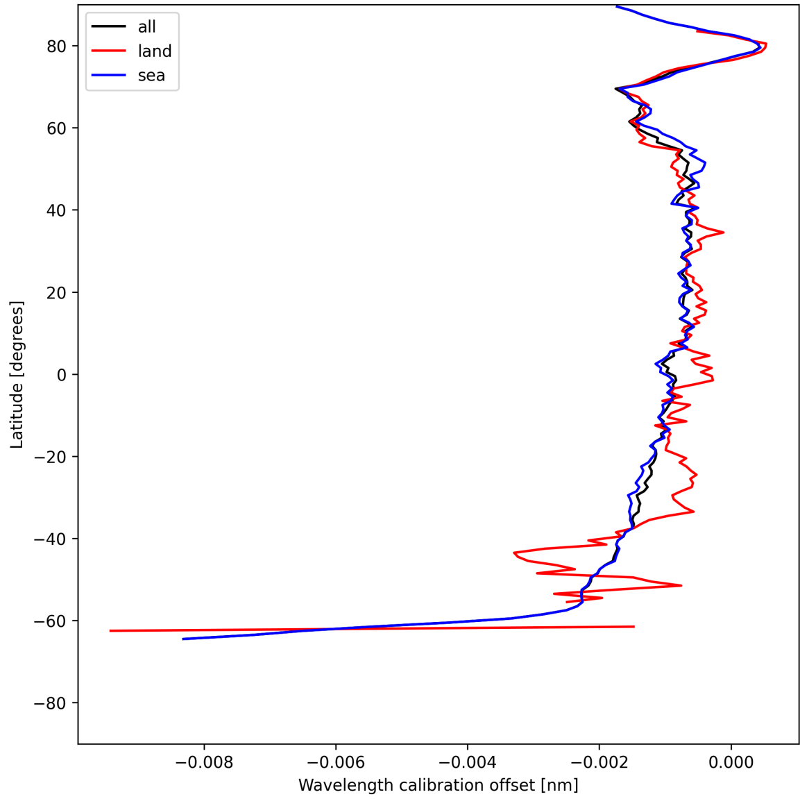
Figure 18: Zonal average of “Wavelength calibration offset” for 2025-06-25 to 2025-06-27.
