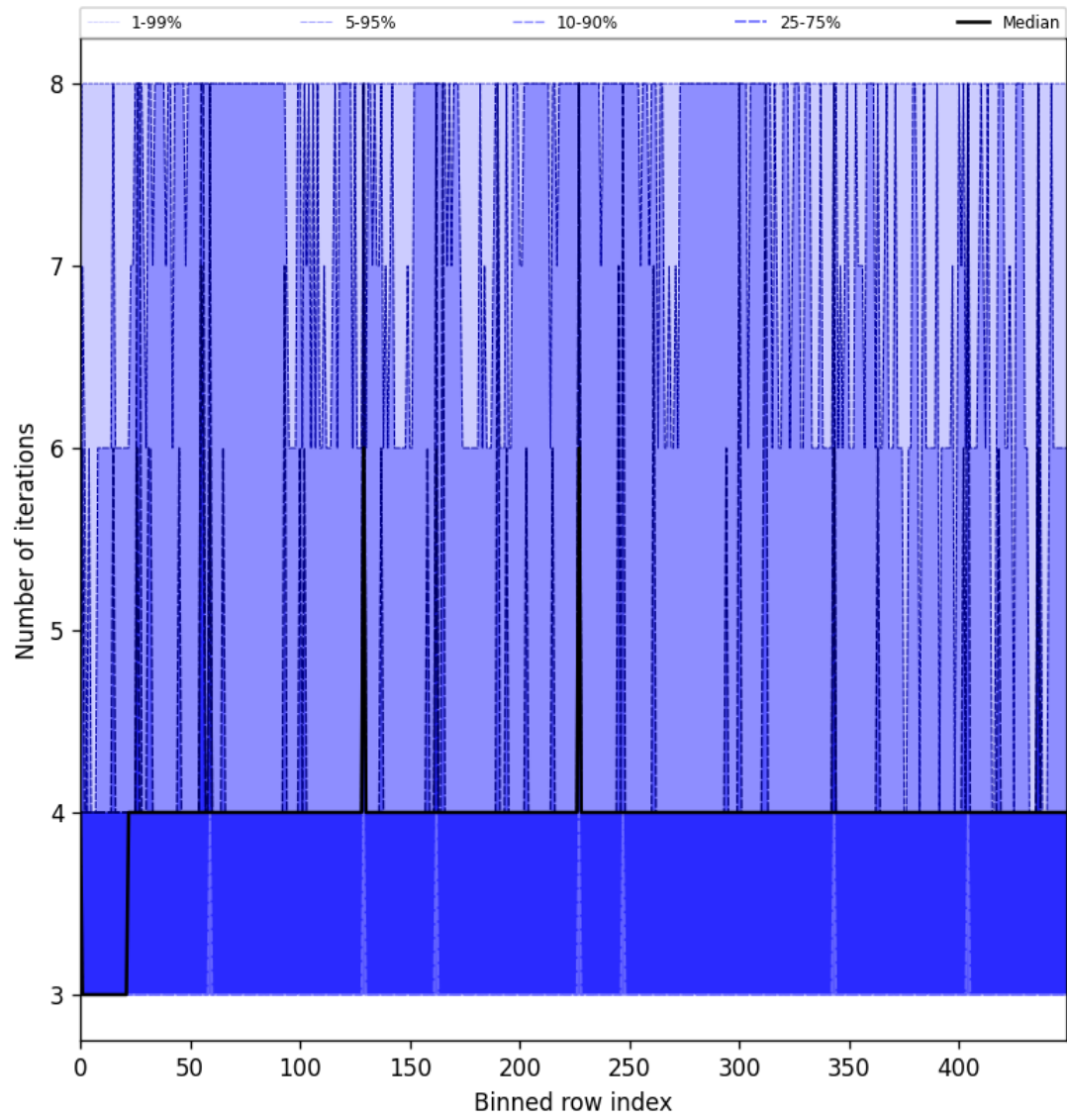
Figure 51: Along track statistics of “Number of iterations” for 2025-06-25 to 2025-06-27
