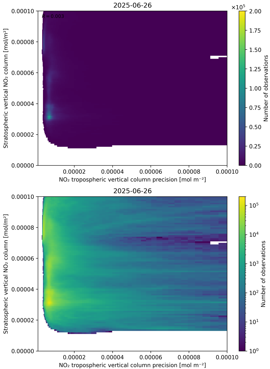
Figure 135: Scatter density plot of “NO 2 tropospheric vertical column precision” against “Stratospheric vertical NO 2 column” for 2025-06-25 to 2025-06-27.
