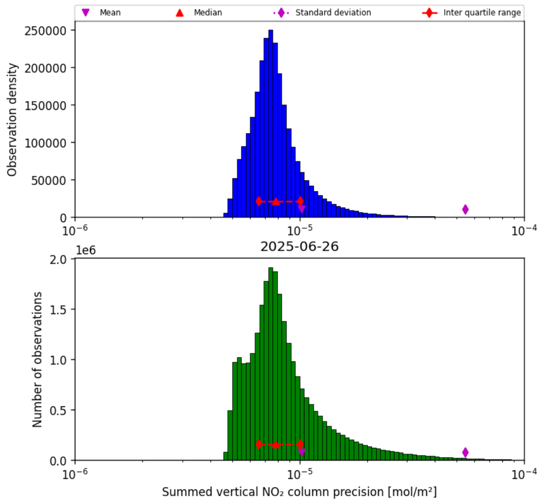
Figure 41: Histogram of “Summed vertical NO 2 column precision” for 2025-06-25 to 2025-06-27
