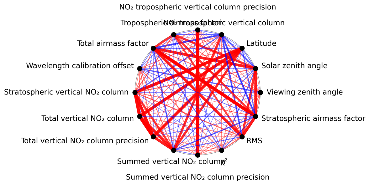
Figure 1: Map of correlation graph for 2025-06-25 to 2025-06-27.
