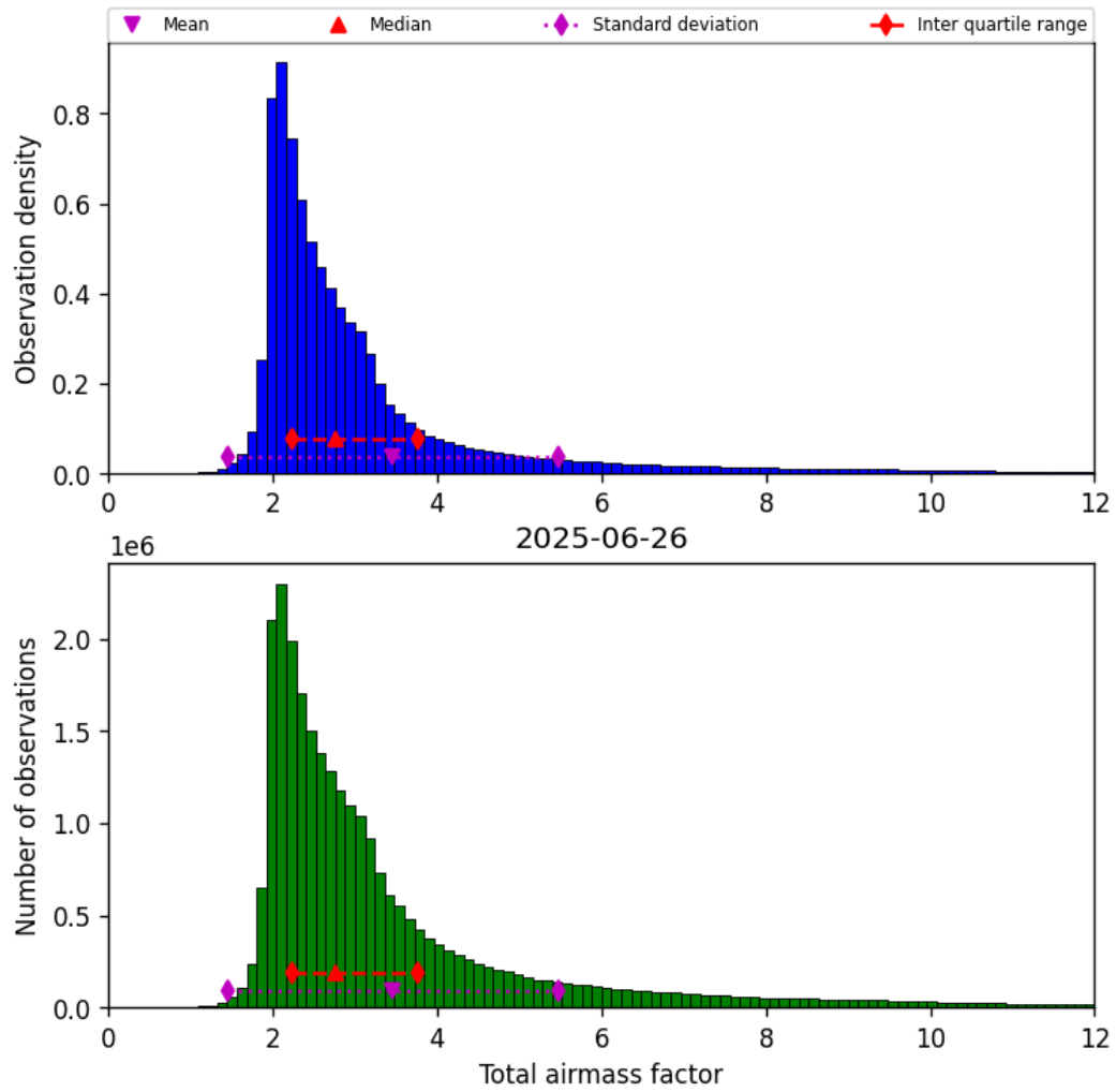
Figure 32: Histogram of “Total airmass factor” for 2025-06-25 to 2025-06-27
