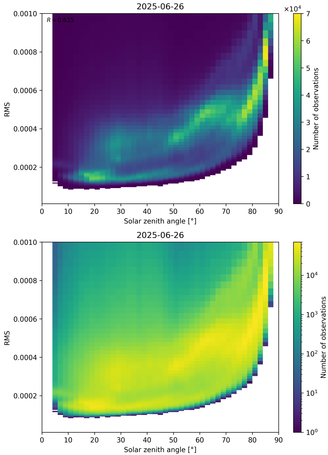
Figure 157: Scatter density plot of “Solar zenith angle” against “RMS” for 2025-06-25 to 2025-06-27.
