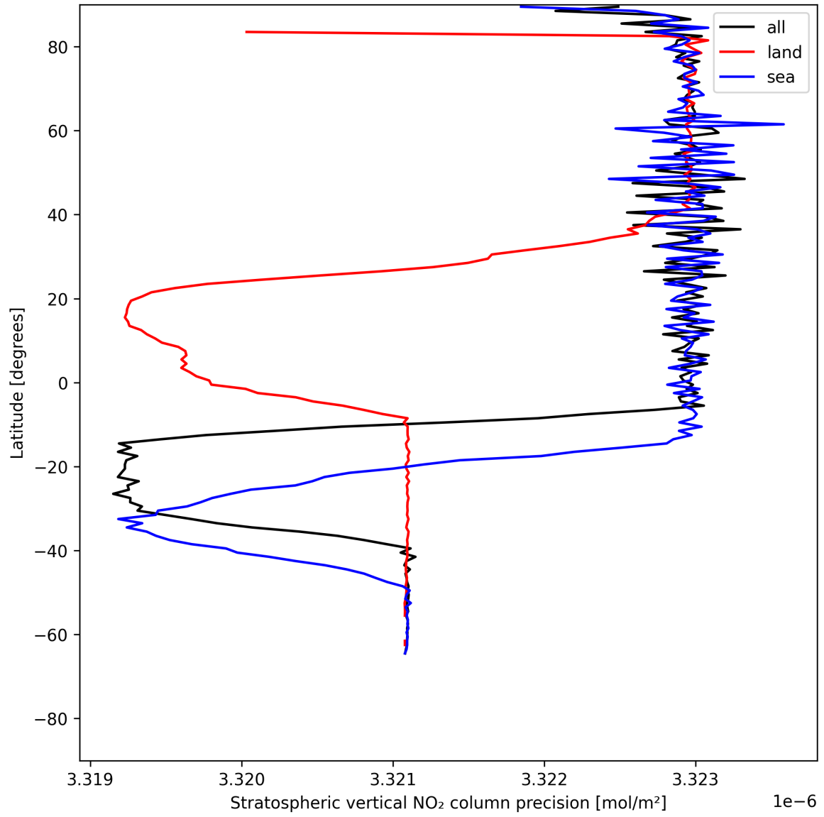
Figure 20: Zonal average of “Stratospheric vertical NO 2 column precision” for 2025-06-25 to 2025-06-27.
