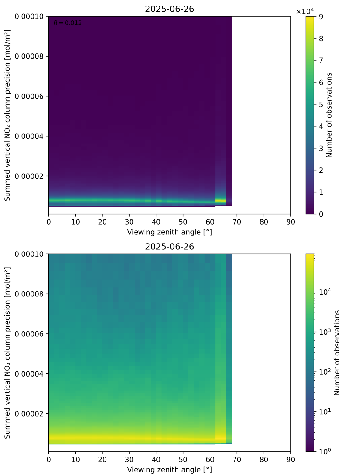
Figure 166: Scatter density plot of “Viewing zenith angle” against “Summed vertical NO 2 column precision” for 2025-06-25 to 2025-06-27.
