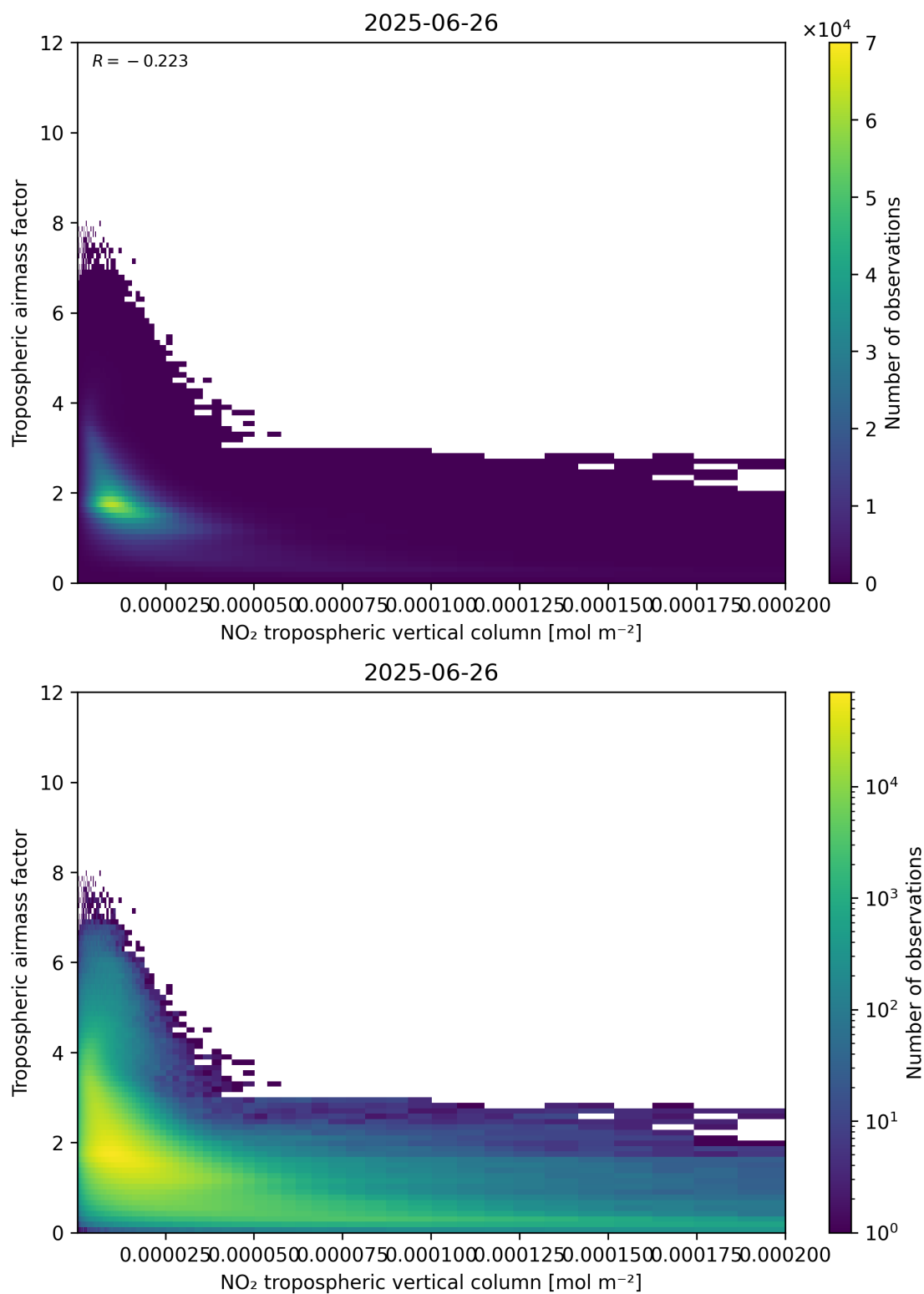
Figure 123: Scatter density plot of “NO 2 tropospheric vertical column” against “Tropospheric air mass factor” for 2025-06-25 to 2025-06-27.
