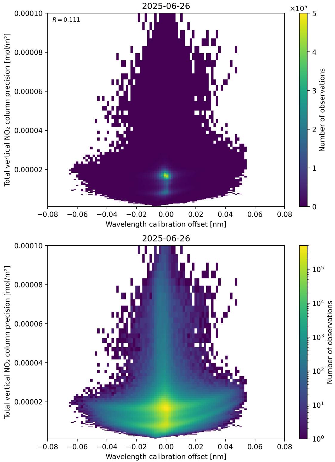
Figure 180: Scatter density plot of “Wavelength calibration offset” against “Total vertical NO 2 column precision” for 2025-06-25 to 2025-06-27.
