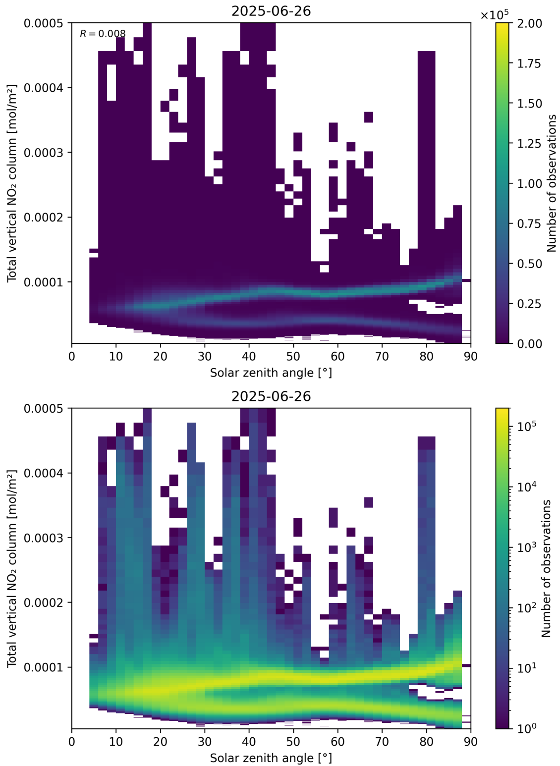
Figure 153: Scatter density plot of “Solar zenith angle” against “Total vertical NO 2 column” for 2025-06-25 to 2025-06-27.
