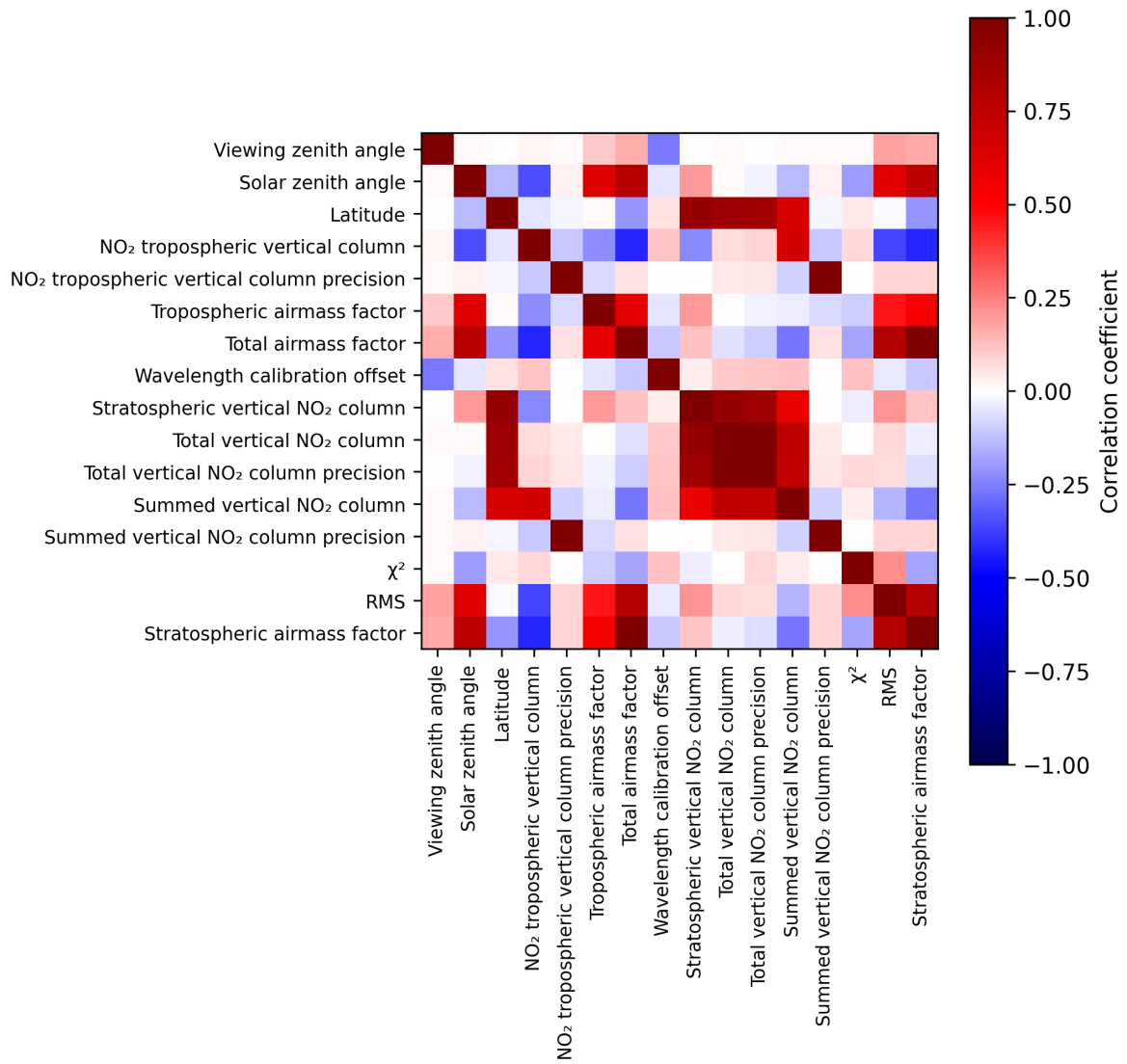
Figure 2: Map of correlation matrix for 2025-06-25 to 2025-06-27.
