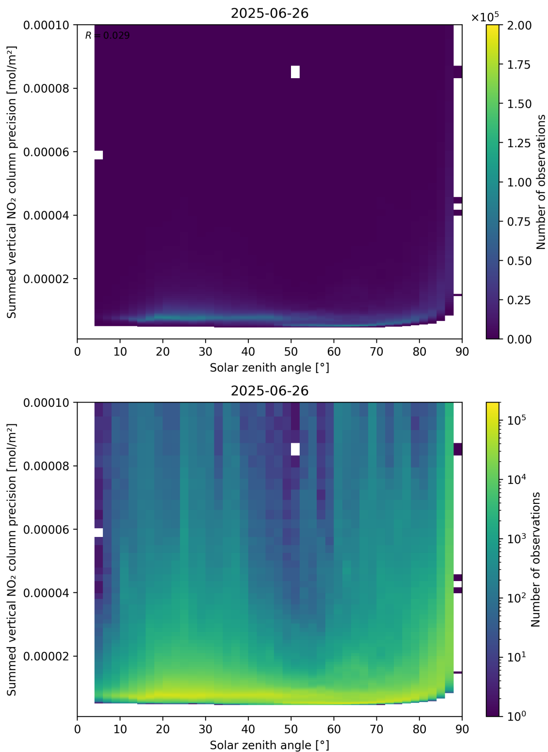
Figure 152: Scatter density plot of “Solar zenith angle” against “Summed vertical NO 2 column precision” for 2025-06-25 to 2025-06-27.
