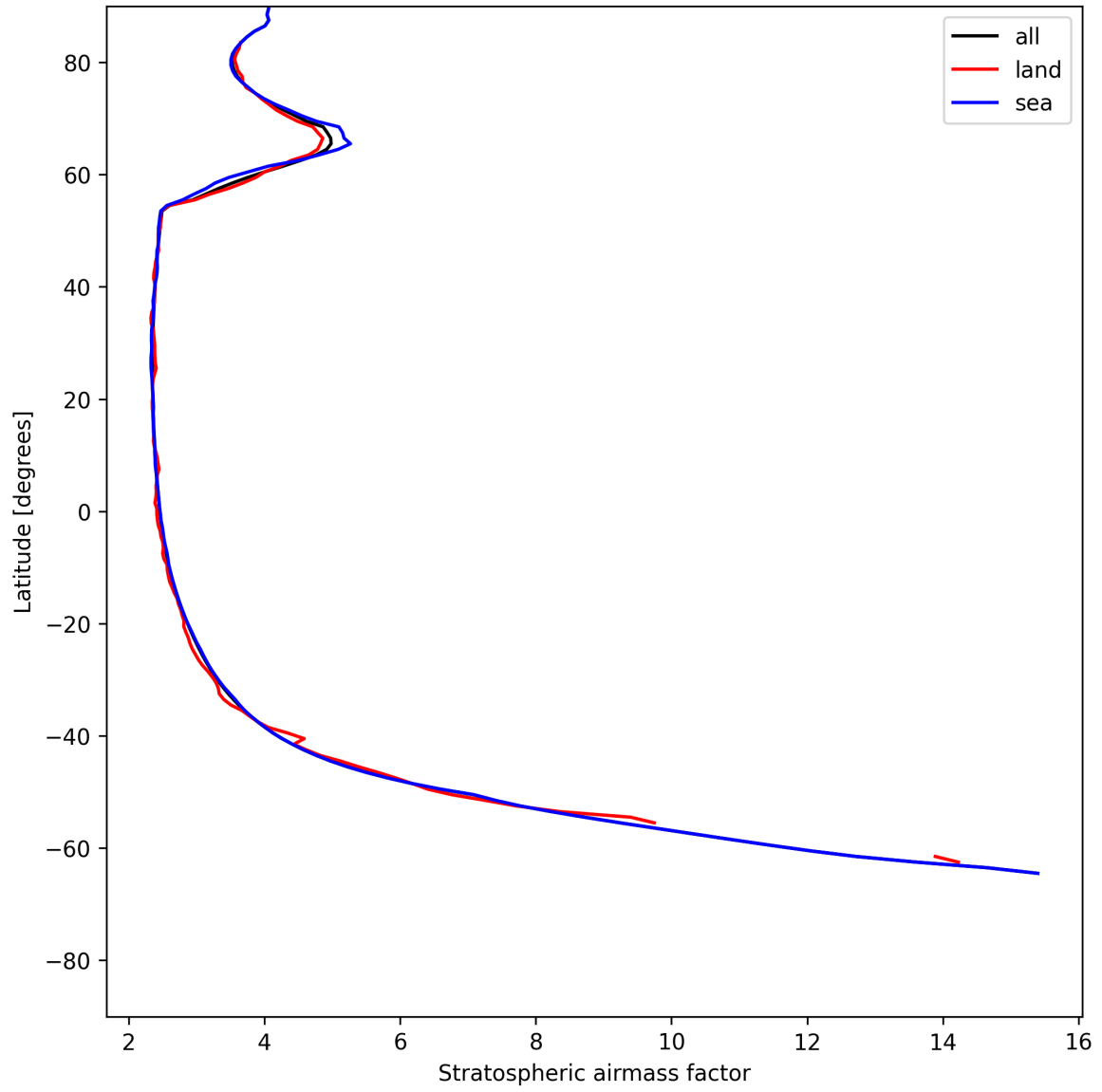
Figure 27: Zonal average of “Stratospheric airmass factor” for 2025-06-25 to 2025-06-27.
