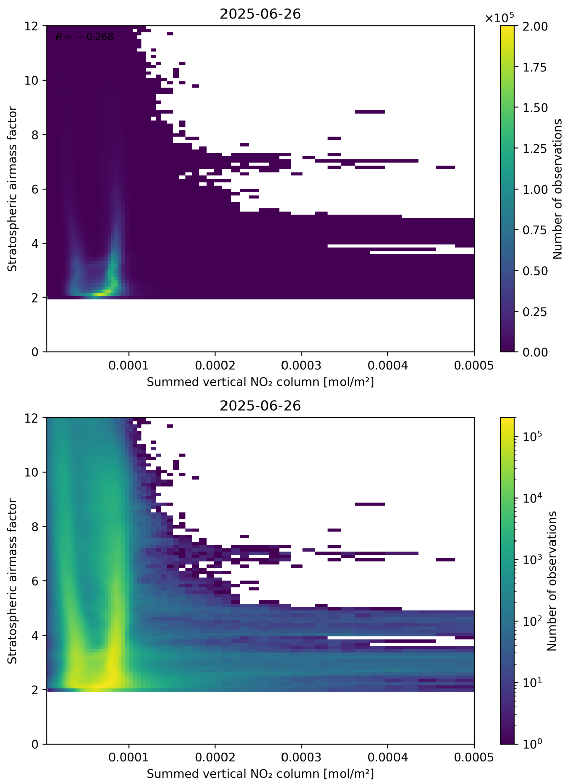
Figure 103: Scatter density plot of “Summed vertical NO 2 column” against “Stratospheric air mass factor” for 2025-06-25 to 2025-06-27.
