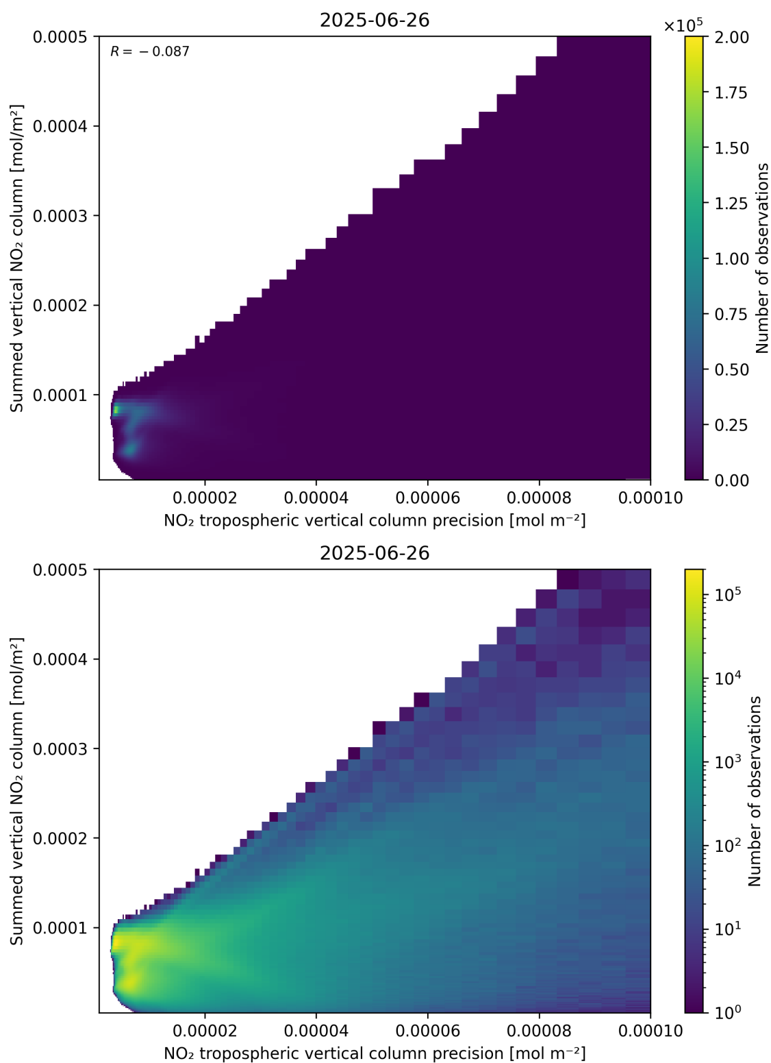
Figure 136: Scatter density plot of “NO 2 tropospheric vertical column precision” against “Summed vertical NO 2 column” for 2025-06-25 to 2025-06-27.
