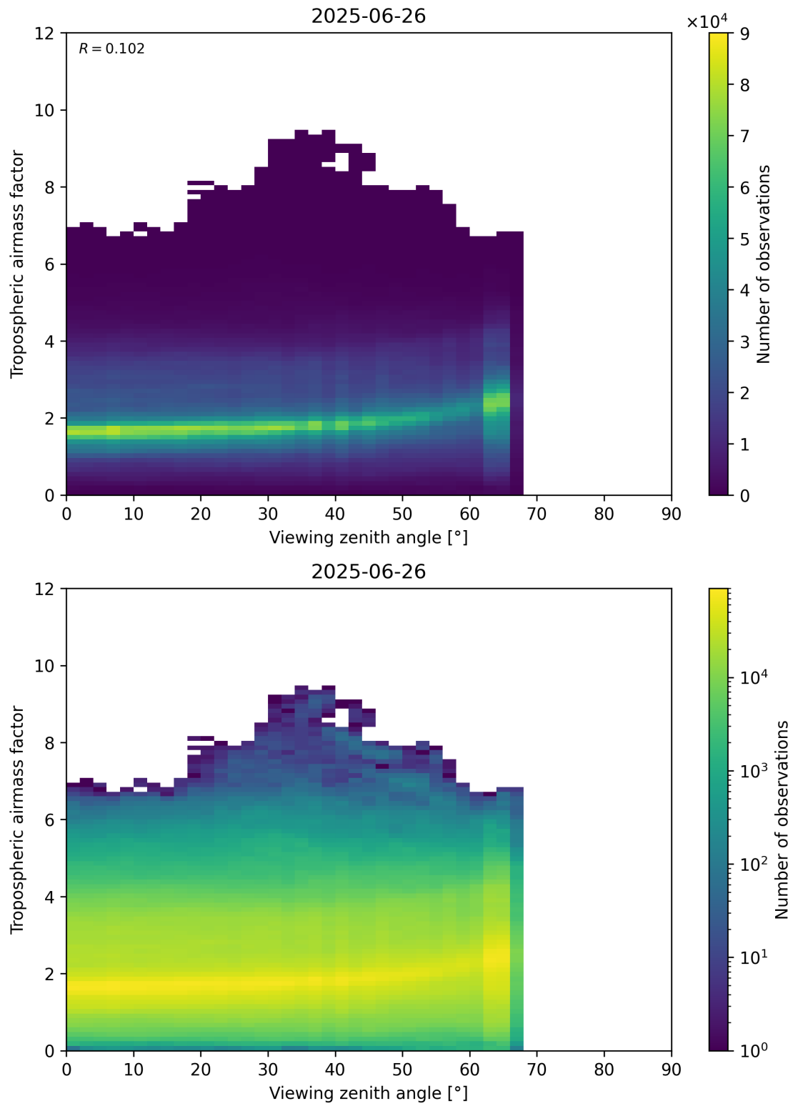
Figure 161: Scatter density plot of “Viewing zenith angle” against “Tropospheric airmass factor” for 2025-06-25 to 2025-06-27.
