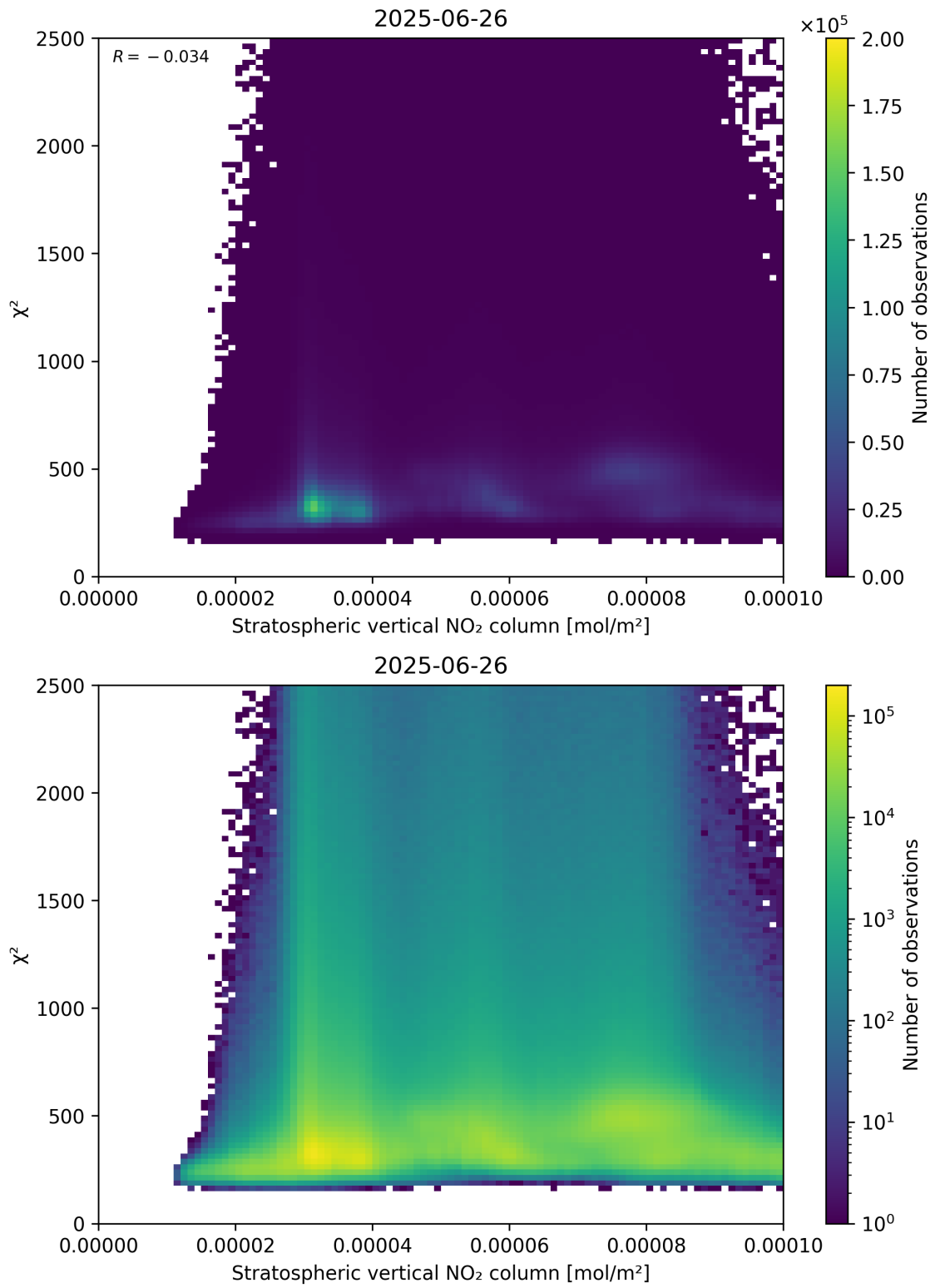
Figure 97: Scatter density plot of “Stratospheric vertical NO 2 column” against “ \chi^2 ” for 2025-06-25 to 2025-06-27.
