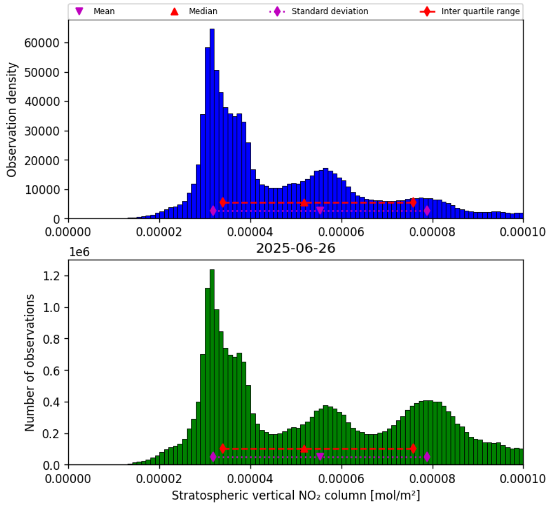
Figure 36: Histogram of “Stratospheric vertical NO 2 column” for 2025-06-25 to 2025-06-27
