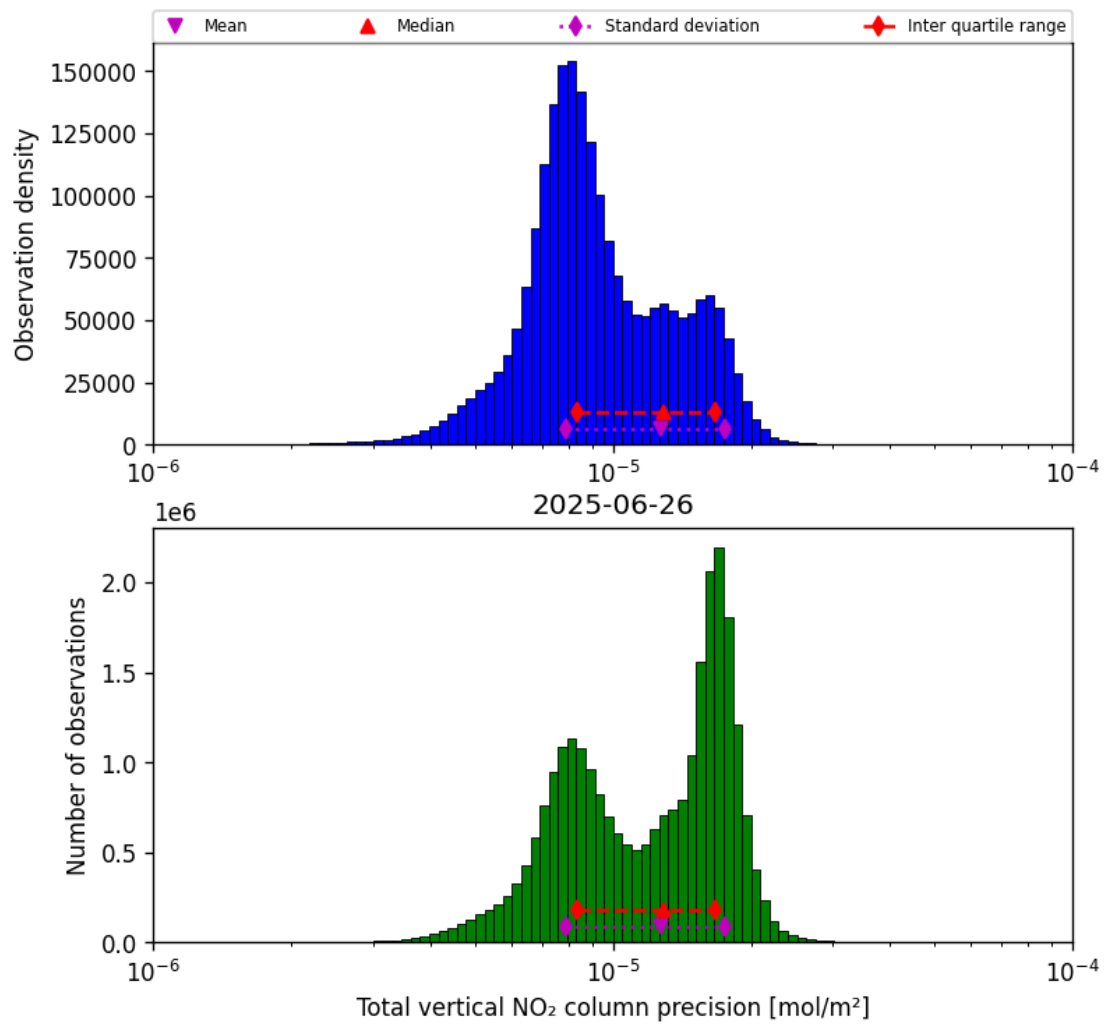
Figure 39: Histogram of “Total vertical NO 2 column precision” for 2025-06-25 to 2025-06-27
