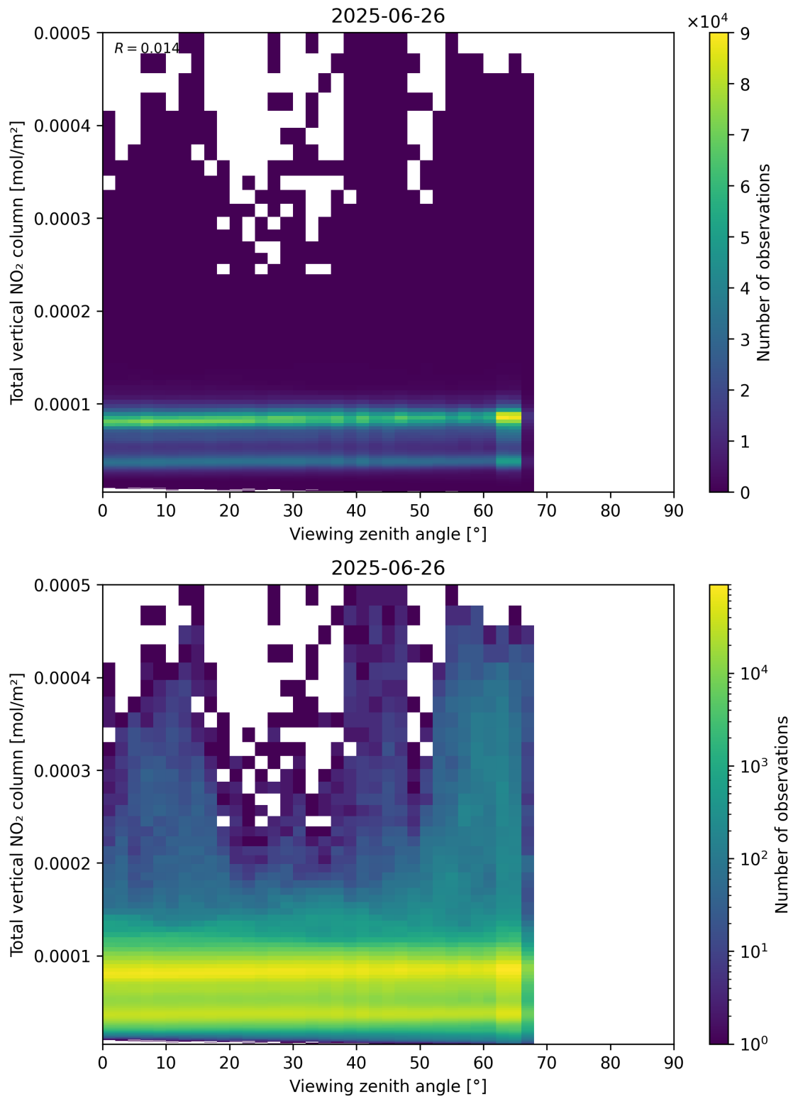
Figure 167: Scatter density plot of “Viewing zenith angle” against “Total vertical NO 2 column” for 2025-06-25 to 2025-06-27.
