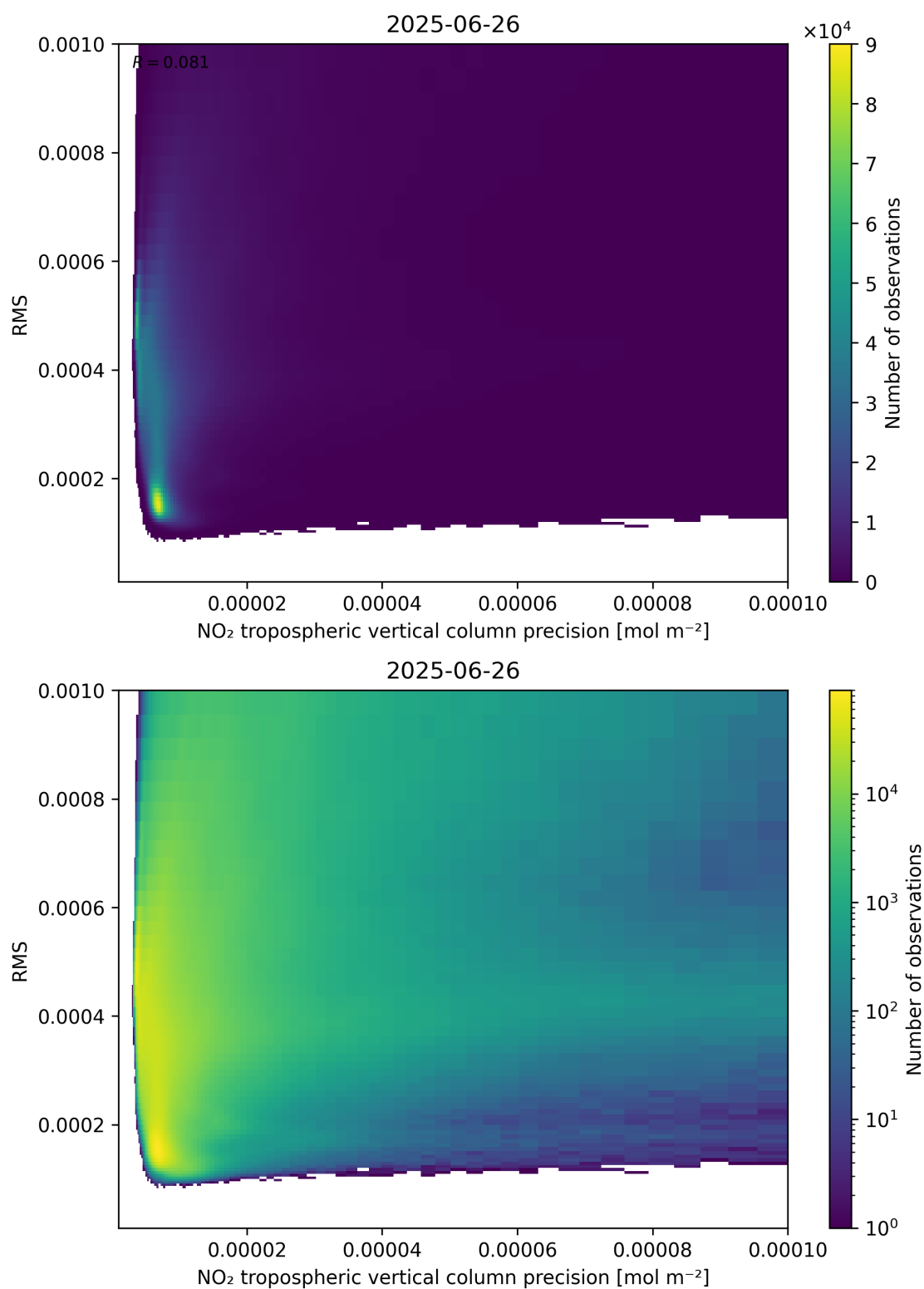
Figure 140: Scatter density plot of “NO 2 tropospheric vertical column precision” against “RMS” for 2025-06-25 to 2025-06-27.
