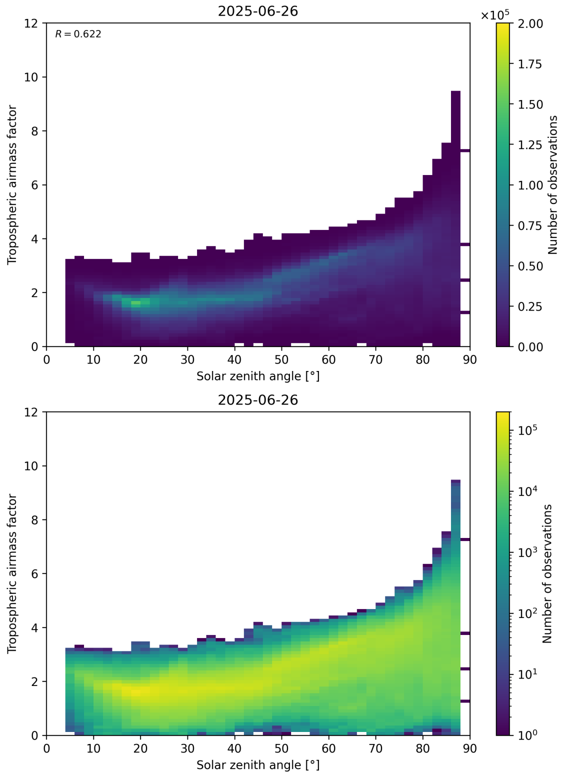
Figure 147: Scatter density plot of “Solar zenith angle” against “Tropospheric airmass factor” for 2025-06-25 to 2025-06-27.
