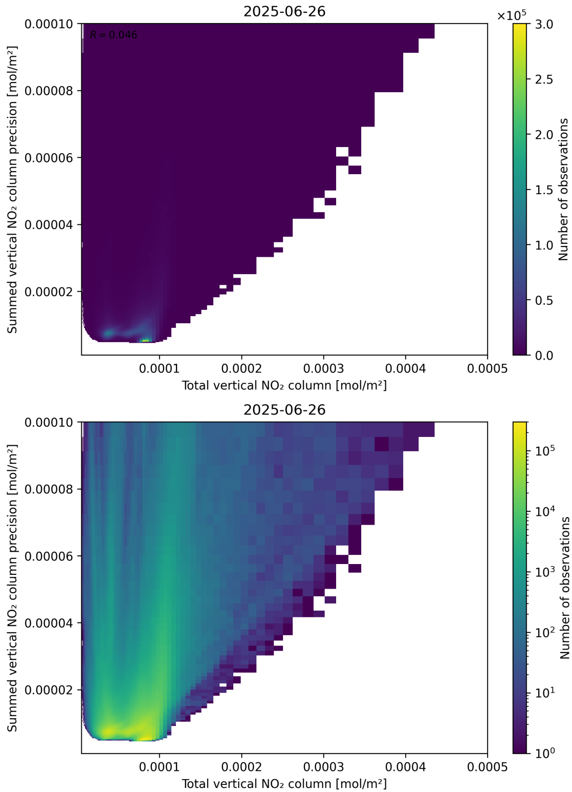
Figure 113: Scatter density plot of “Total vertical NO 2 column” against “Summed vertical NO 2 column precision” for 2025-06-25 to 2025-06-27.
