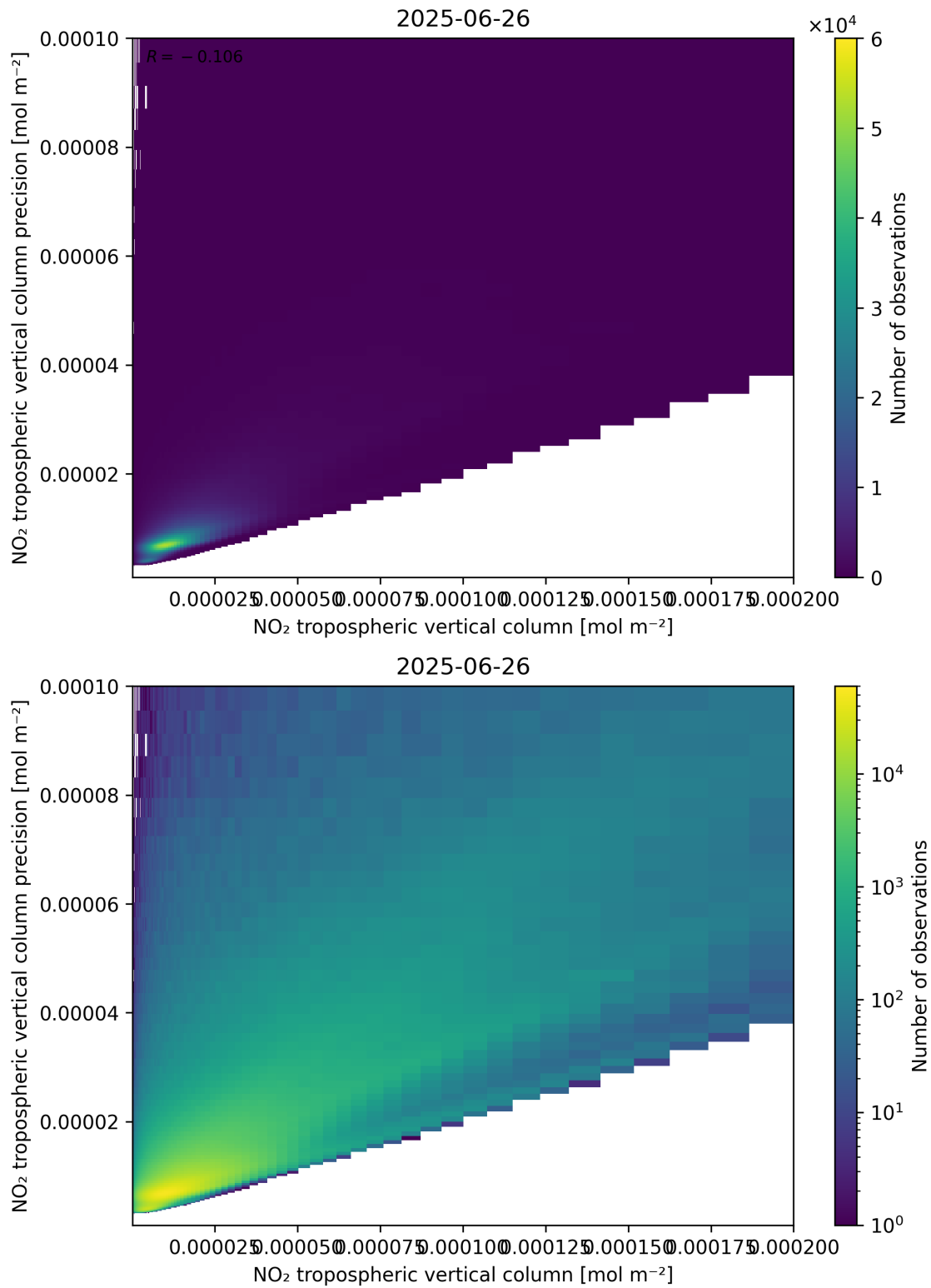
Figure 130: Scatter density plot of “NO 2 tropospheric vertical column” against “NO 2 tropospheric vertical column precision” for 2025-06-25 to 2025-06-27.
