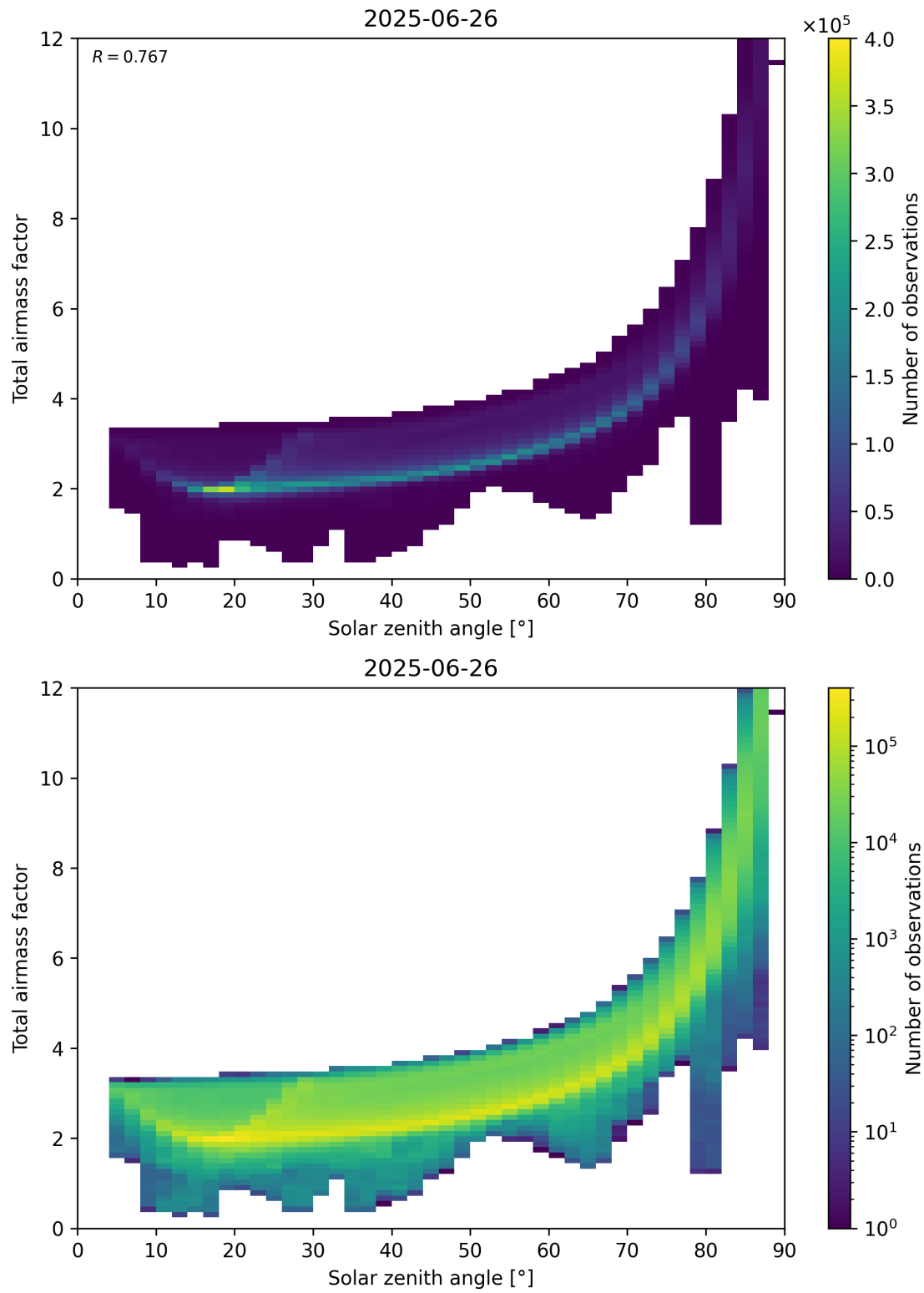
Figure 146: Scatter density plot of “Solar zenith angle” against “Total air mass factor” for 2025-06-25 to 2025-06-27.
