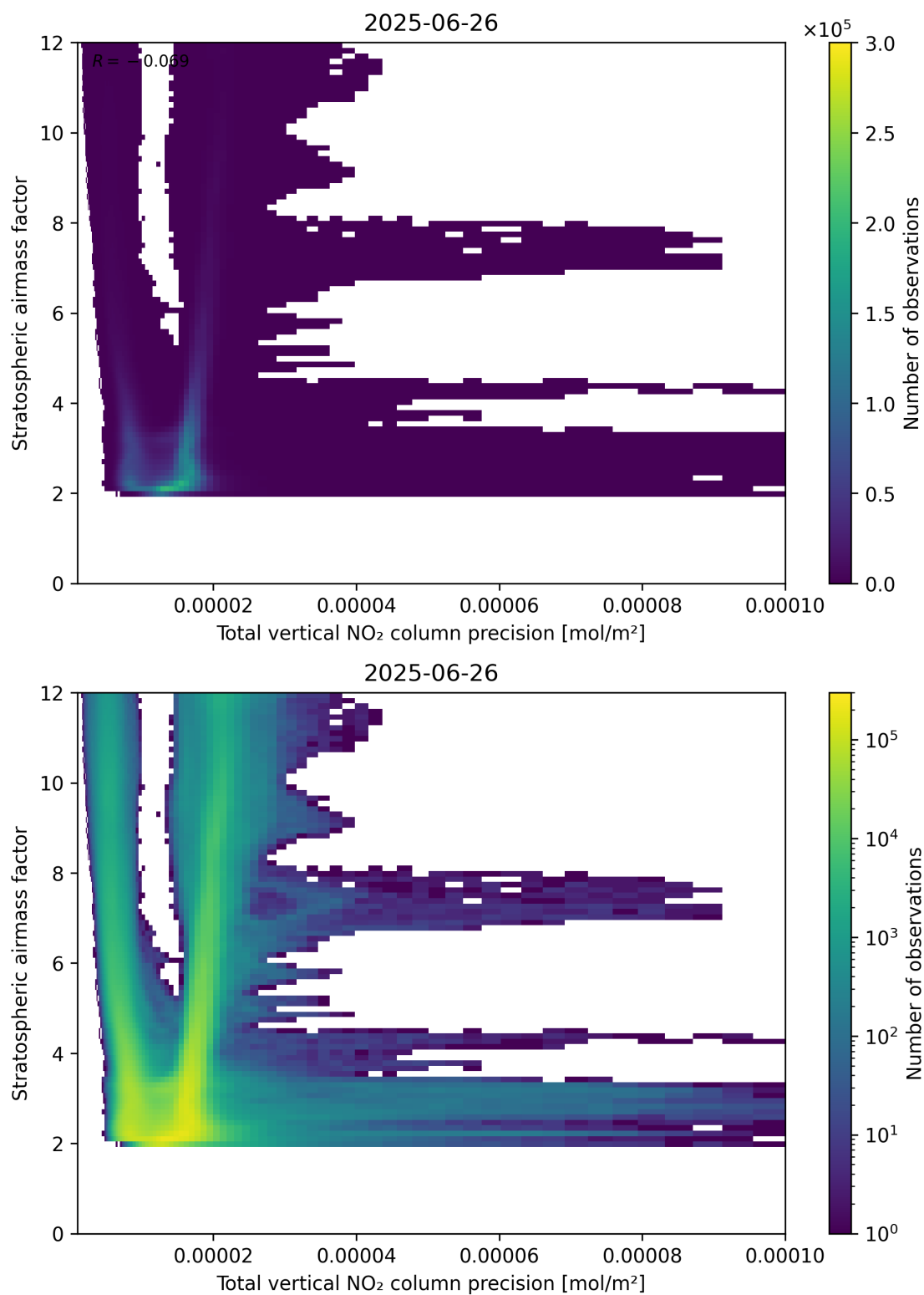
Figure 115: Scatter density plot of “Total vertical NO 2 column precision” against “Stratospheric air mass factor” for 2025-06-25 to 2025-06-27.
