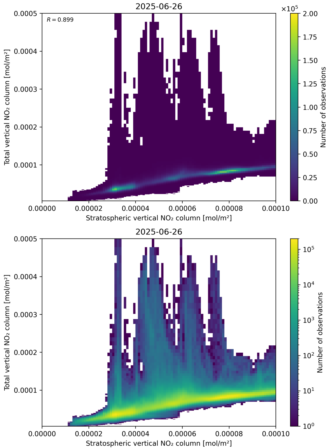
Figure 100: Scatter density plot of “Stratospheric vertical NO 2 column” against “Total vertical NO 2 column” for 2025-06-25 to 2025-06-27.
