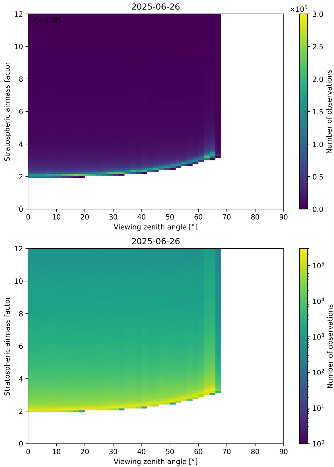
Figure 159: Scatter density plot of “Viewing zenith angle” against “Stratospheric airmass factor” for 2025-06-25 to 2025-06-27.
