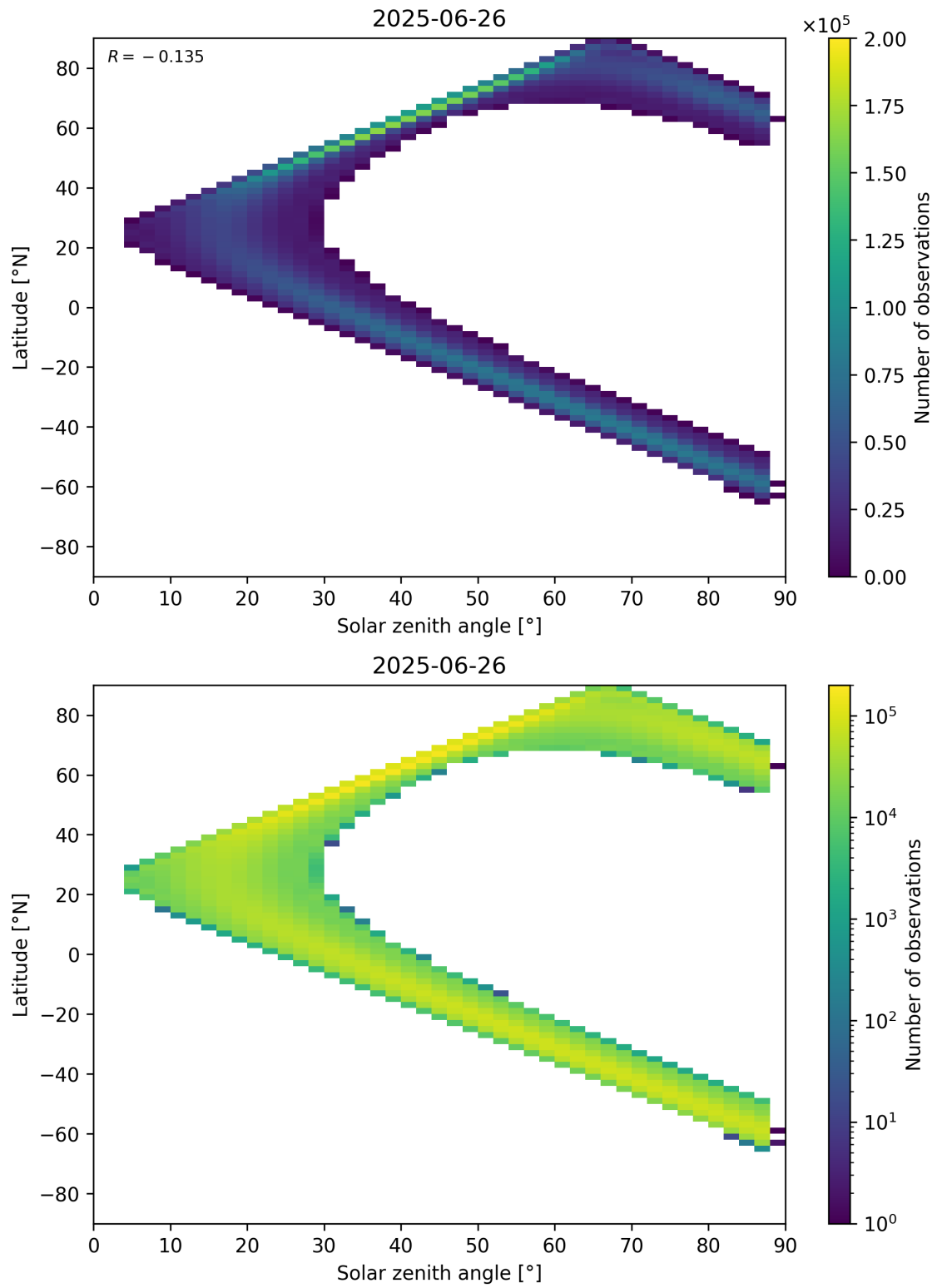
Figure 149: Scatter density plot of “Solar zenith angle” against “Latitude” for 2025-06-25 to 2025-06-27.
