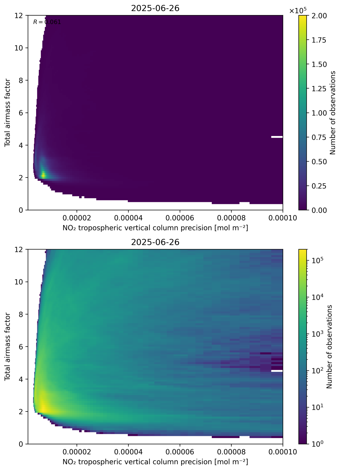
Figure 132: Scatter density plot of “NO 2 tropospheric vertical column precision” against “Total air mass factor” for 2025-06-25 to 2025-06-27.
