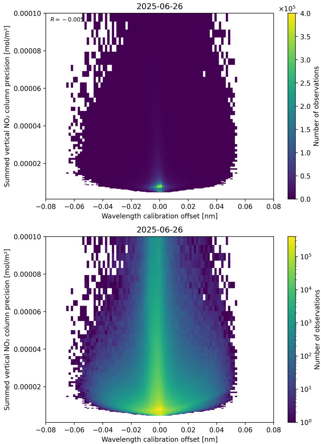
Figure 178: Scatter density plot of “Wavelength calibration offset” against “Summed vertical NO 2 column precision” for 2025-06-25 to 2025-06-27.
