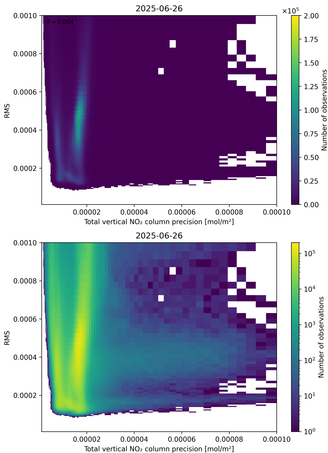
Figure 119: Scatter density plot of “Total vertical NO 2 column precision” against “RMS” for 2025-06-25 to 2025-06-27.
