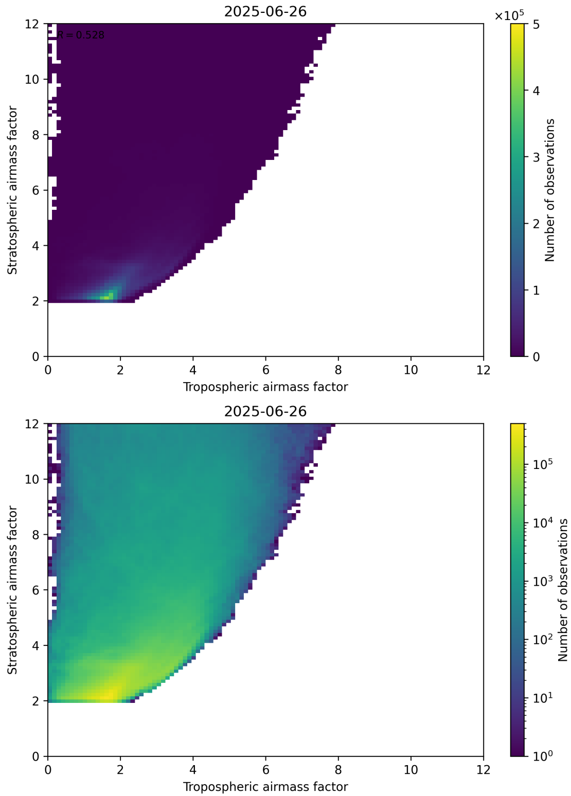
Figure 71: Scatter density plot of “Tropospheric airmass factor” against “Stratospheric airmass factor” for 2025-06-25 to 2025-06-27.
