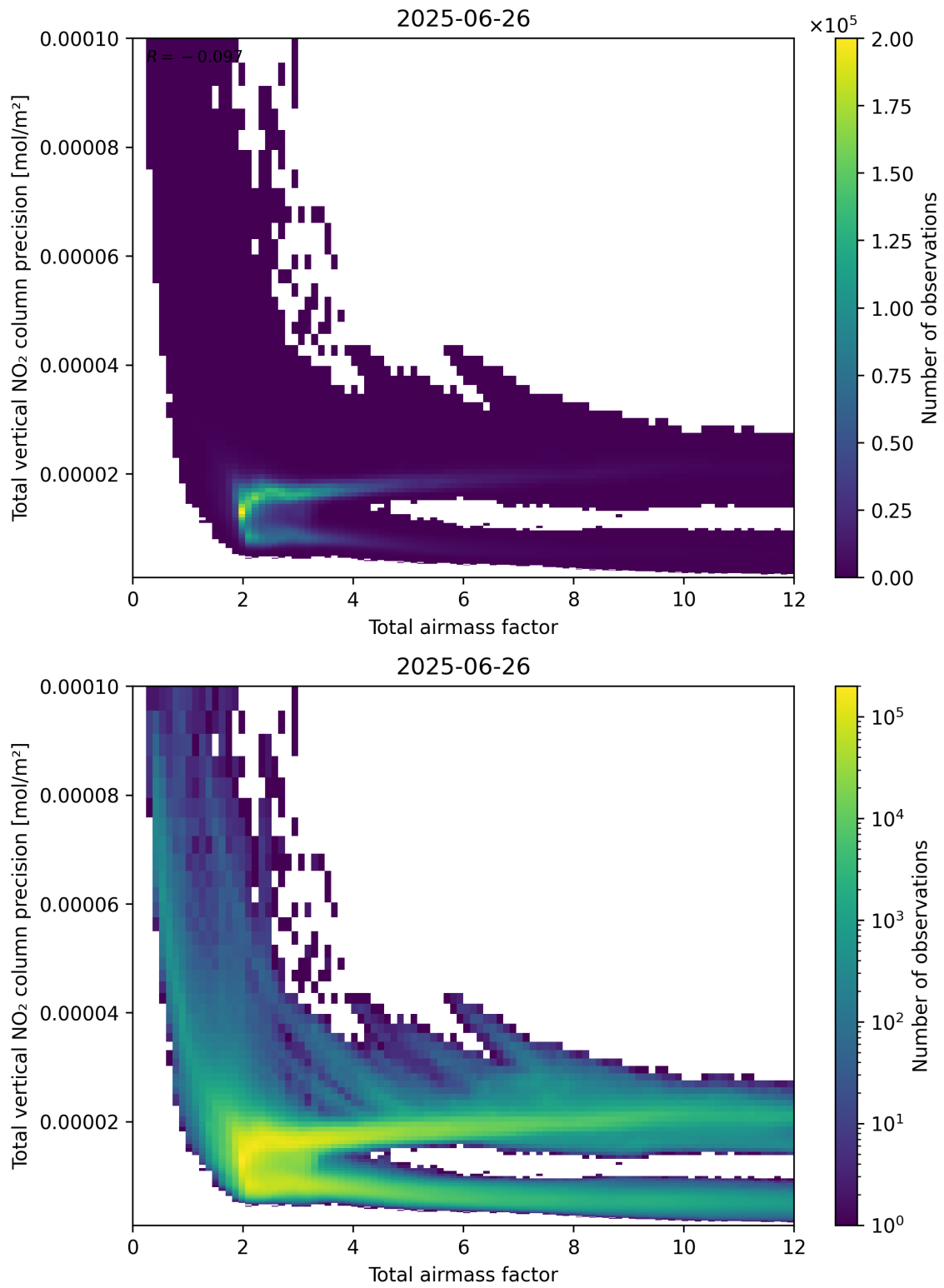
Figure 68: Scatter density plot of “Total airmass factor” against “Total vertical NO 2 column precision” for 2025-06-25 to 2025-06-27.
