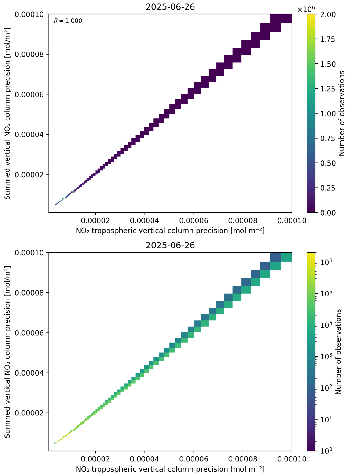
Figure 137: Scatter density plot of “NO 2 tropospheric vertical column precision” against “Summed vertical NO 2 column precision” for 2025-06-25 to 2025-06-27.
