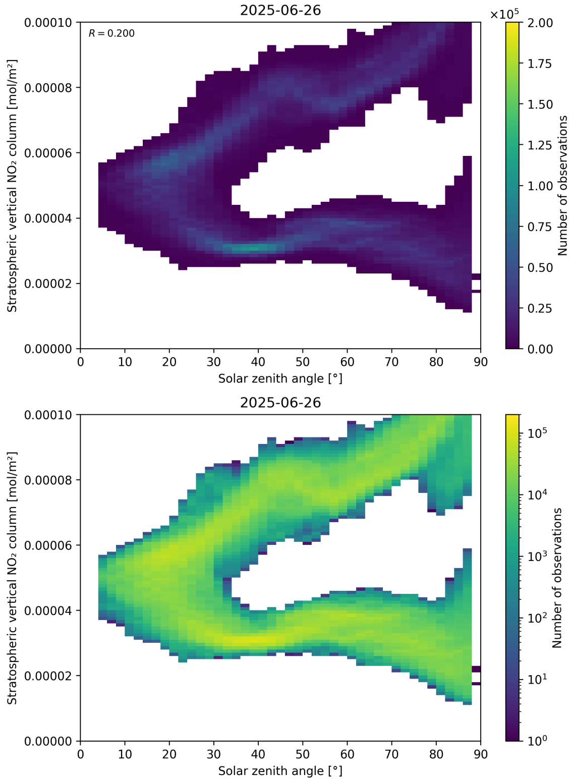
Figure 150: Scatter density plot of “Solar zenith angle” against “Stratospheric vertical NO 2 column” for 2025-06-25 to 2025-06-27.
