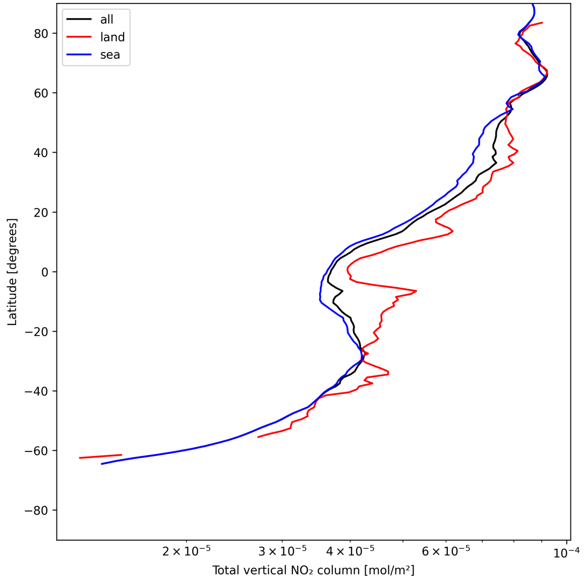
Figure 21: Zonal average of “Total vertical NO 2 column” for 2025-06-25 to 2025-06-27.
