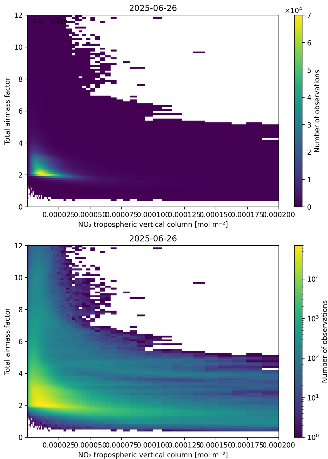
Figure 122: Scatter density plot of “NO 2 tropospheric vertical column” against “Total air mass factor” for 2025-06-25 to 2025-06-27.
