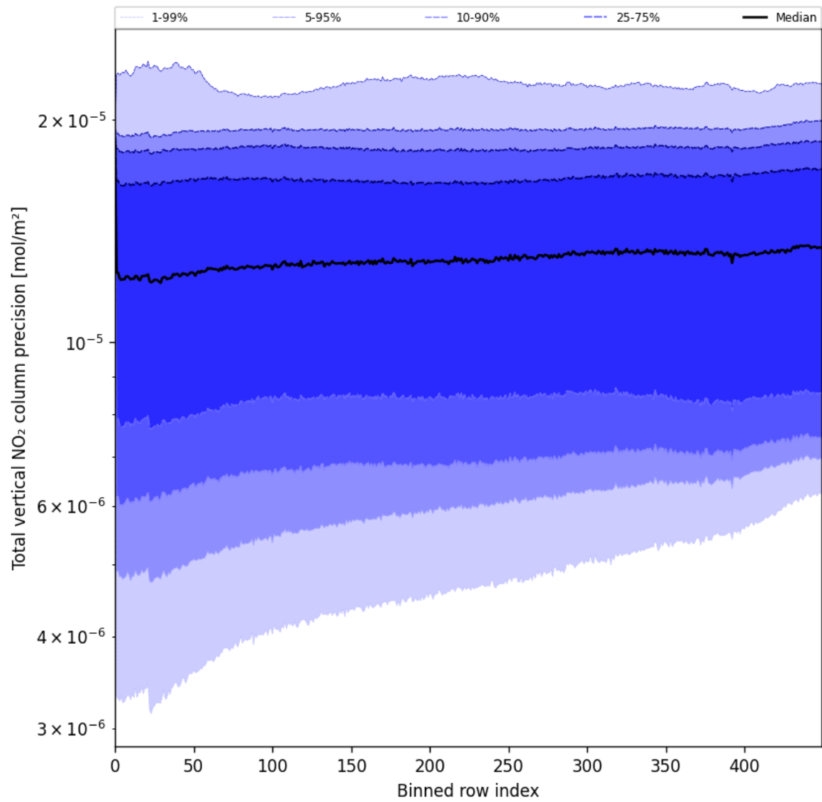
Figure 56: Along track statistics of “Total vertical NO 2 column precision” for 2025-06-25 to 2025-06-27
