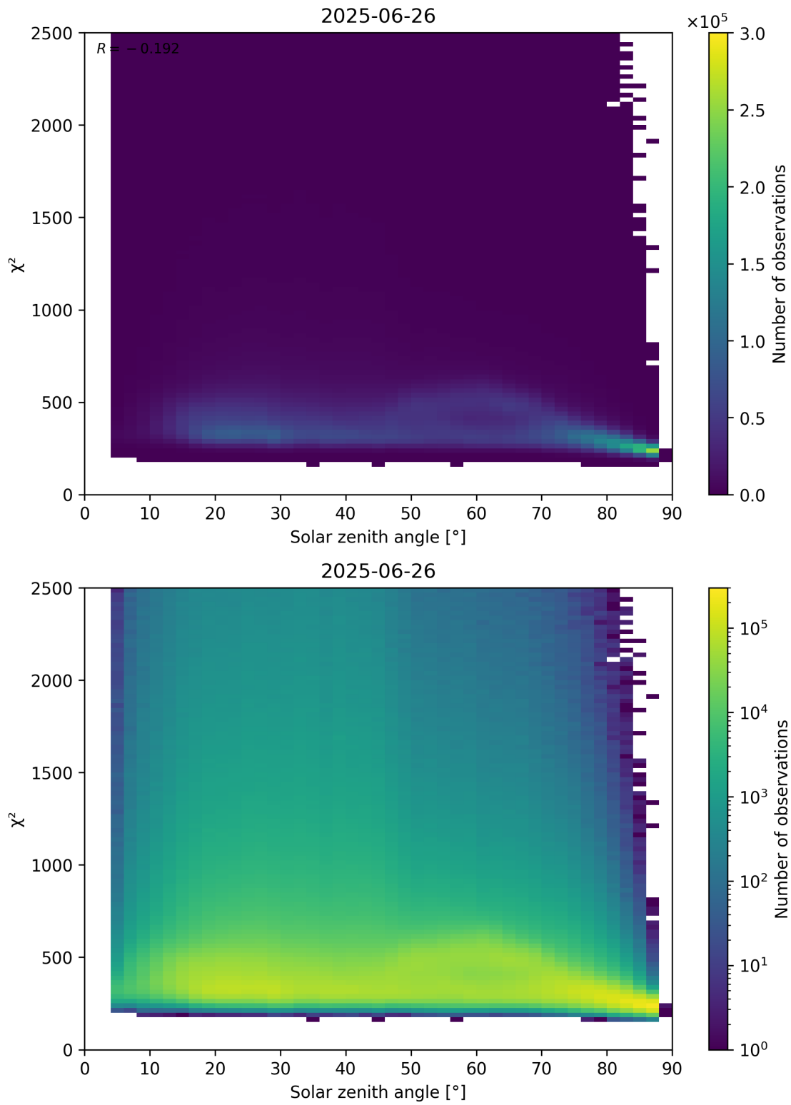
Figure 148: Scatter density plot of “Solar zenith angle” against “ \chi^2 ” for 2025-06-25 to 2025-06-27.
