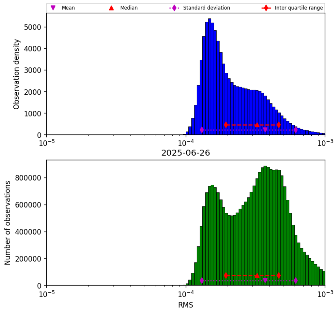
Figure 43: Histogram of “RMS” for 2025-06-25 to 2025-06-27
