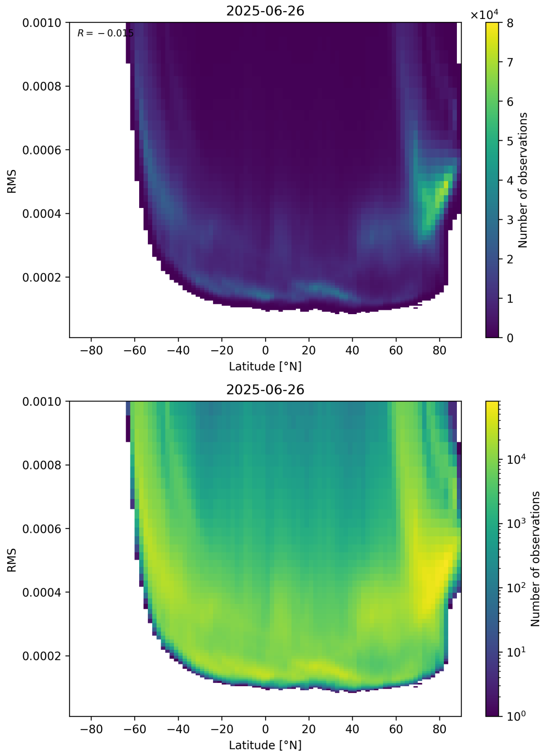
Figure 94: Scatter density plot of “Latitude” against “RMS” for 2025-06-25 to 2025-06-27.
