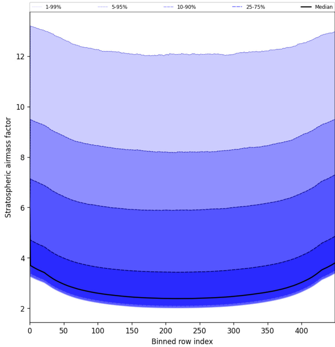
Figure 61: Along track statistics of “Stratospheric airmass factor” for 2025-06-25 to 2025-06-27
