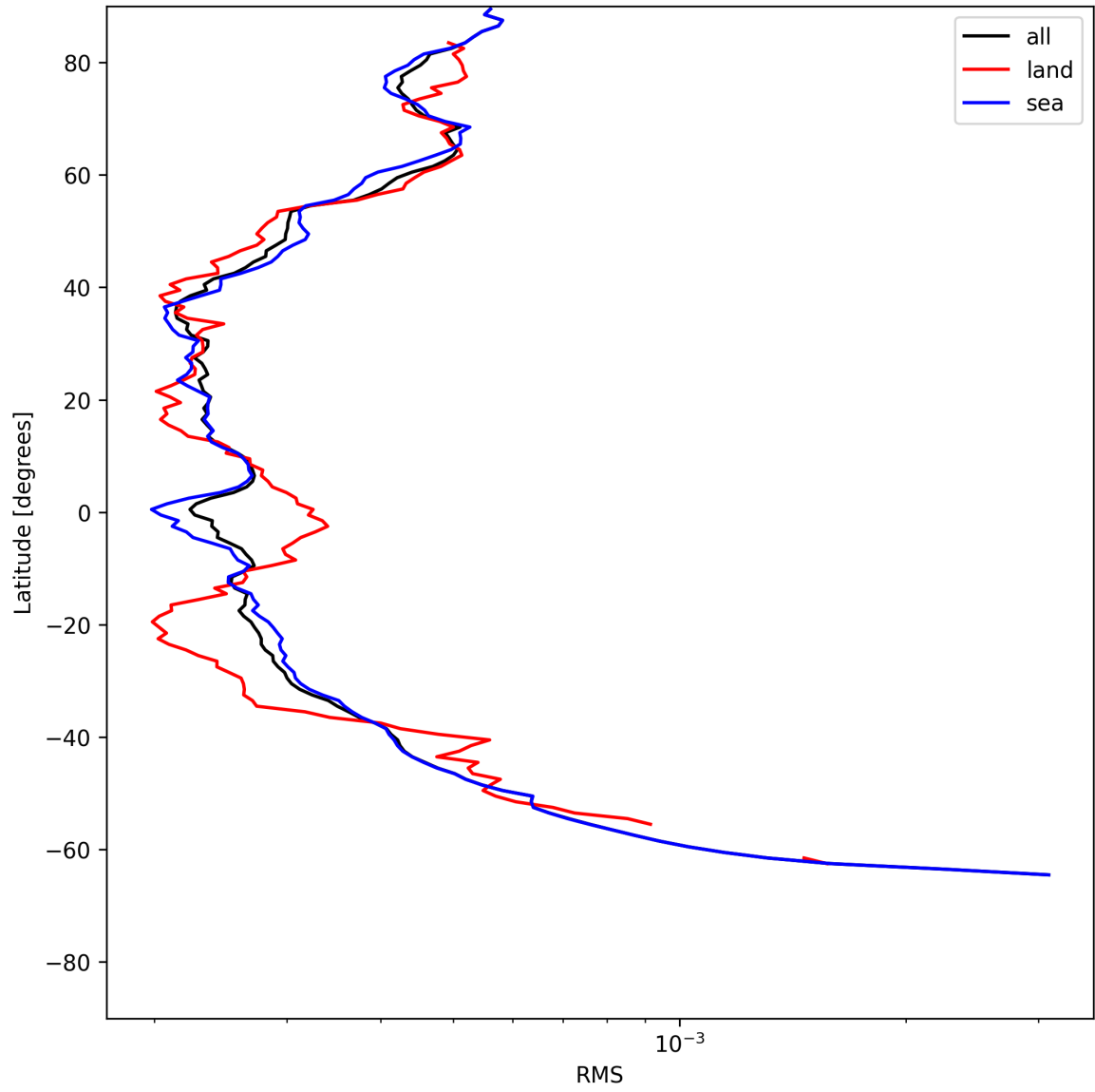
Figure 26: Zonal average of “RMS” for 2025-06-25 to 2025-06-27.
