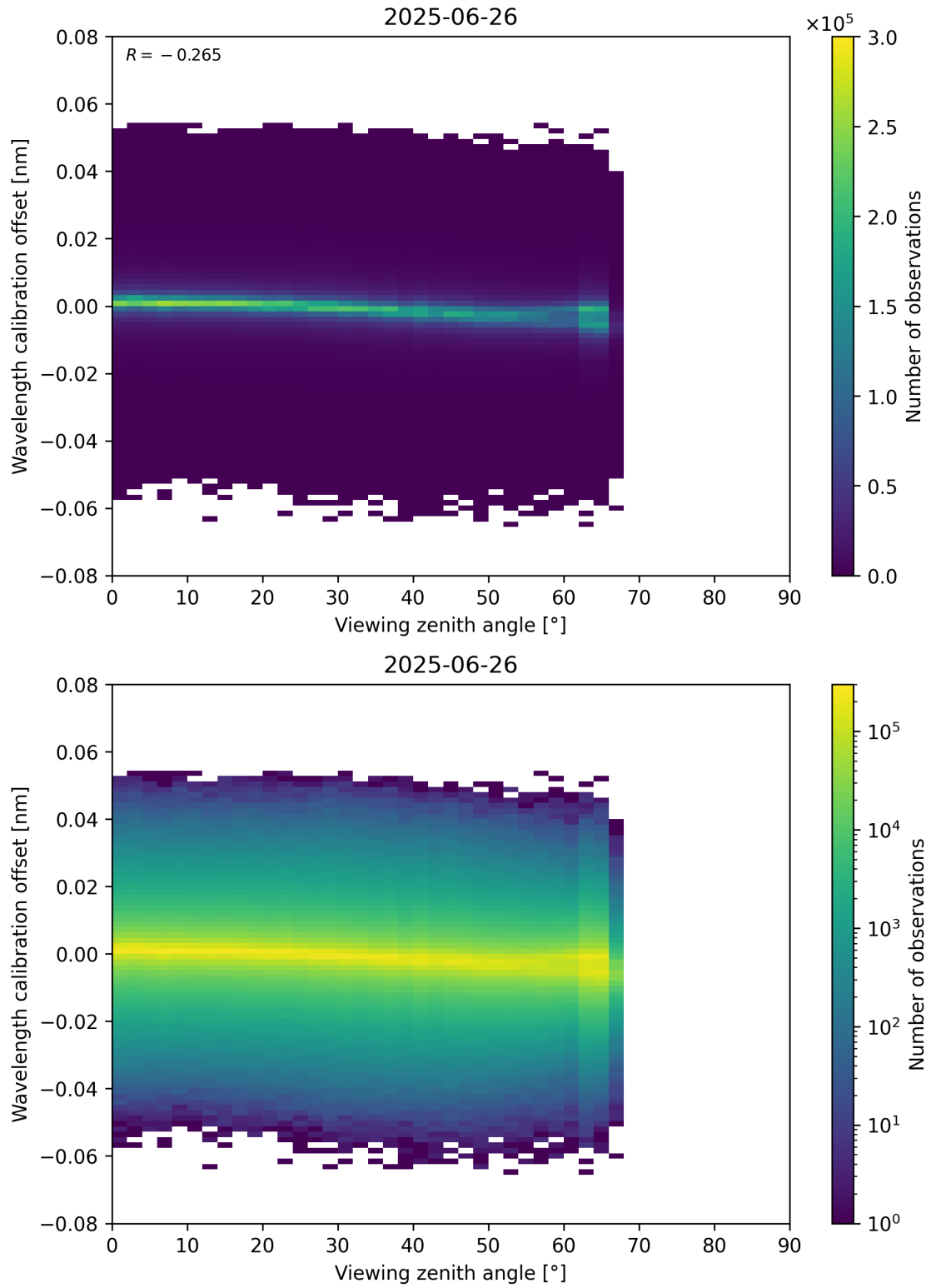
Figure 173: Scatter density plot of “Viewing zenith angle” against “Wavelength calibration offset” for 2025-06-25 to 2025-06-27.
