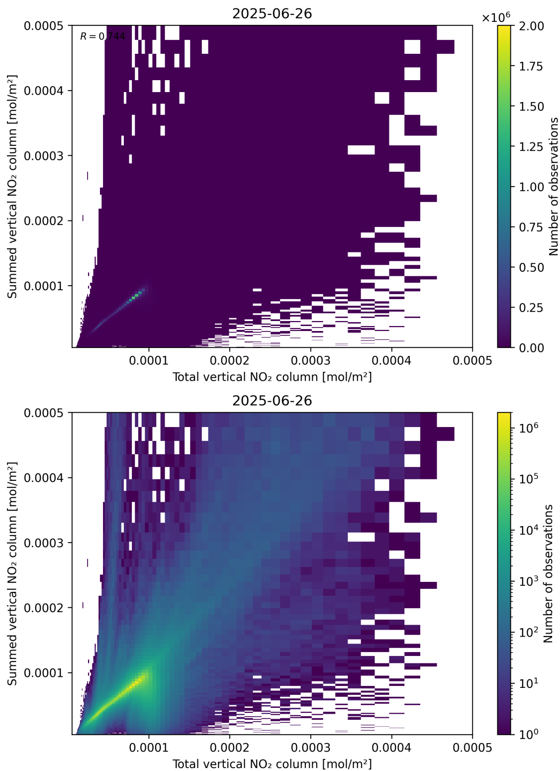
Figure 112: Scatter density plot of “Total vertical NO 2 column” against “Summed vertical NO 2 column” for 2025-06-25 to 2025-06-27.
