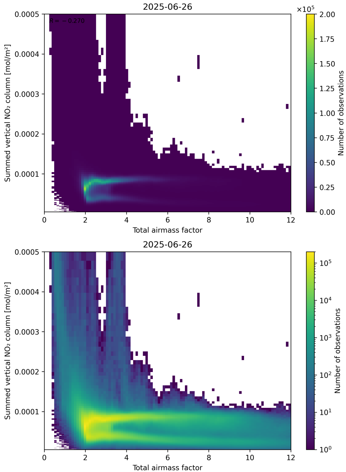
Figure 65: Scatter density plot of “Total airmass factor” against “Summed vertical NO 2 column” for 2025-06-25 to 2025-06-27.
