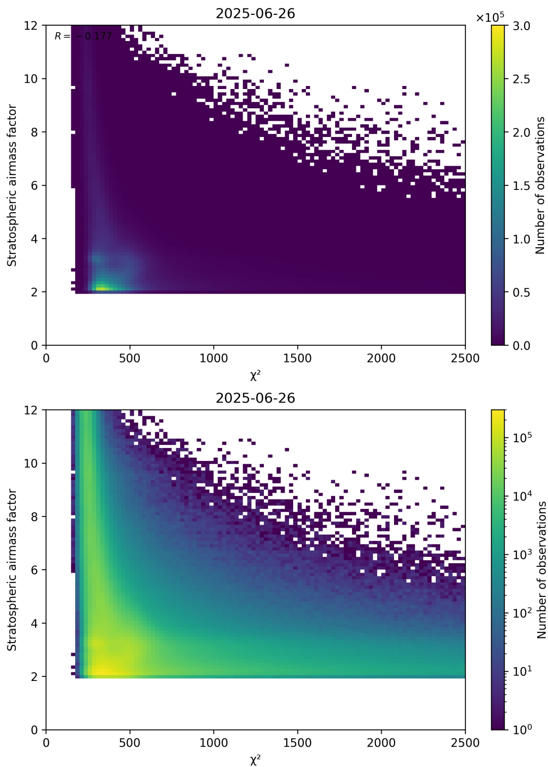
Figure 81: Scatter density plot of “ \chi^2 ” against “Stratospheric airmass factor” for 2025-06-25 to 2025-06-27.
