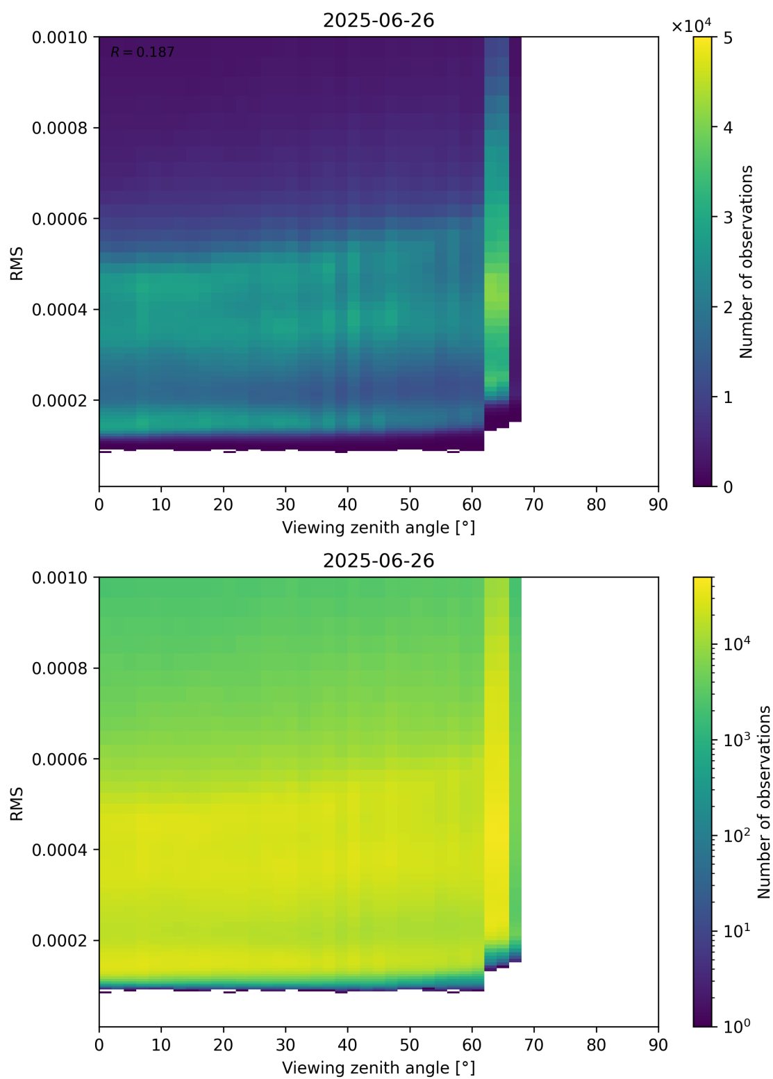
Figure 171: Scatter density plot of “Viewing zenith angle” against “RMS” for 2025-06-25 to 2025-06-27.
