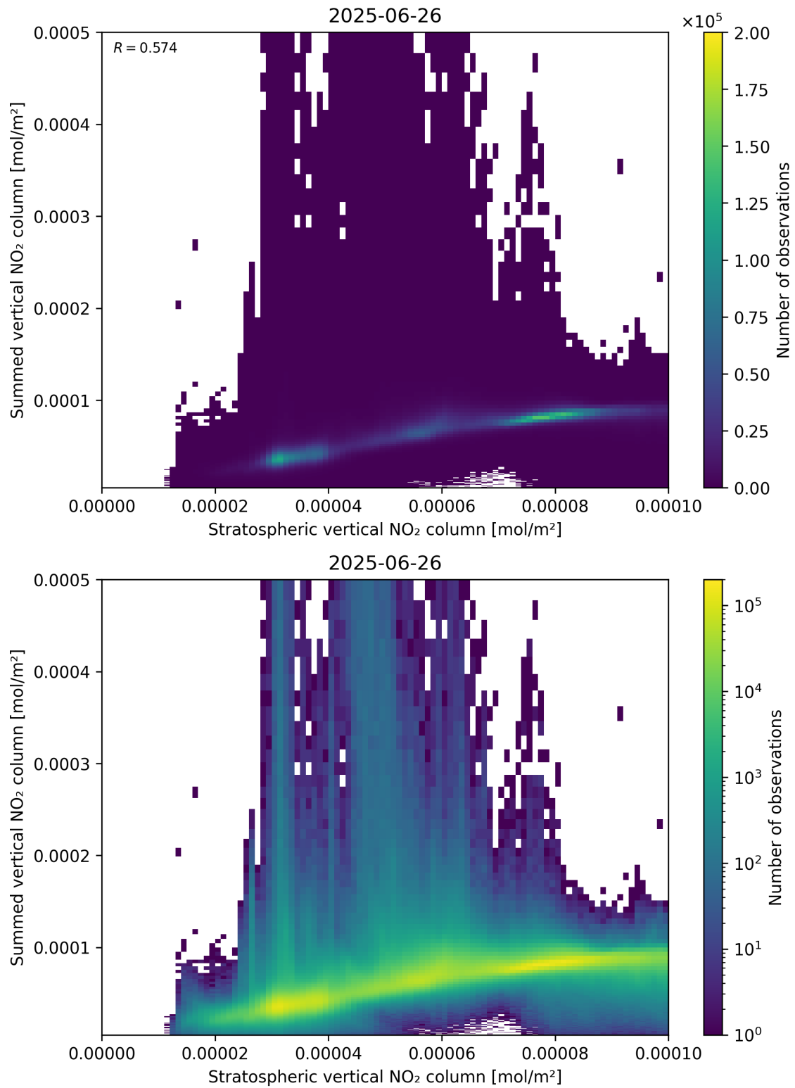
Figure 98: Scatter density plot of “Stratospheric vertical NO 2 column” against “Summed vertical NO 2 column” for 2025-06-25 to 2025-06-27.
