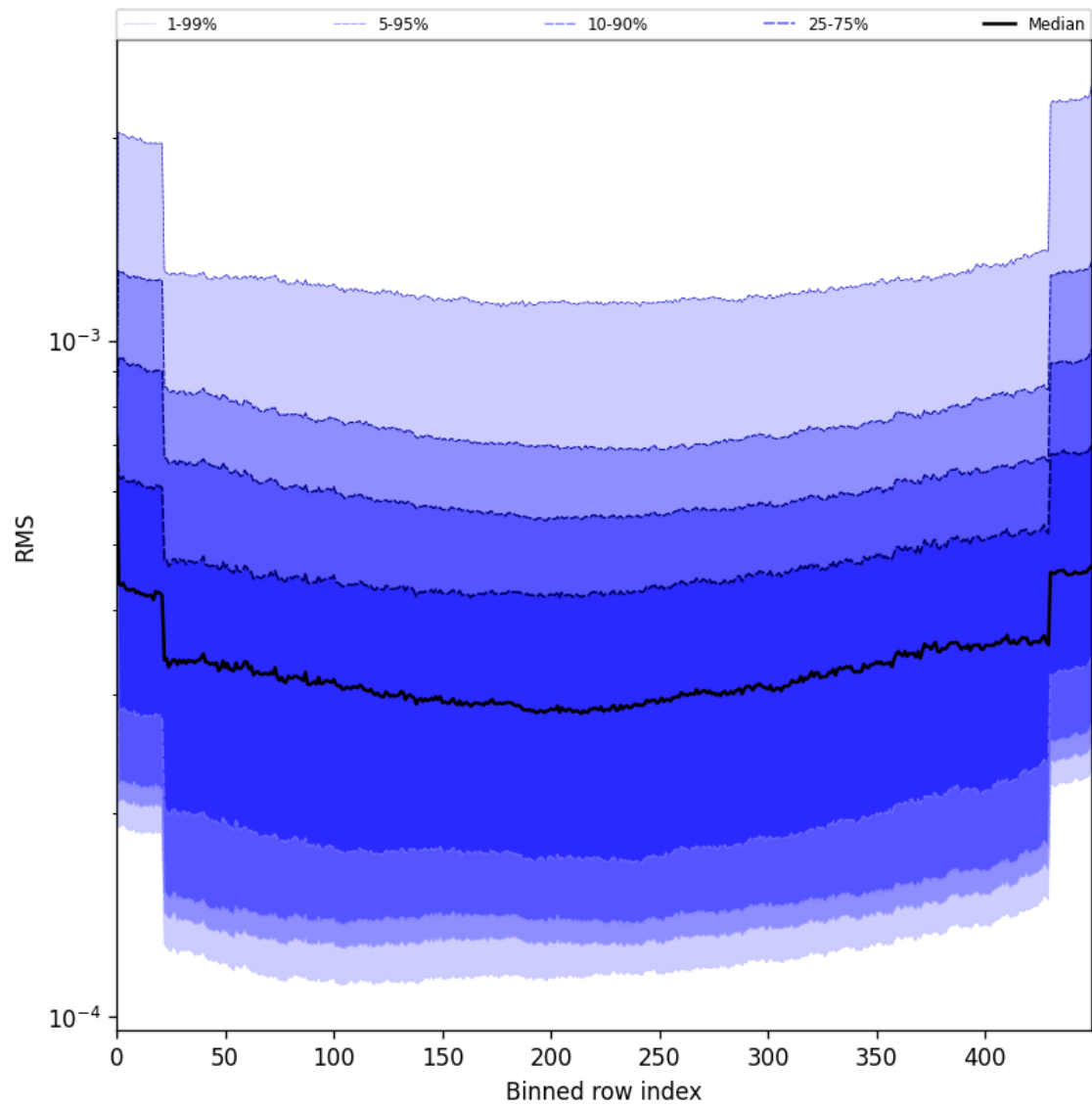
Figure 60: Along track statistics of “RMS” for 2025-06-25 to 2025-06-27
