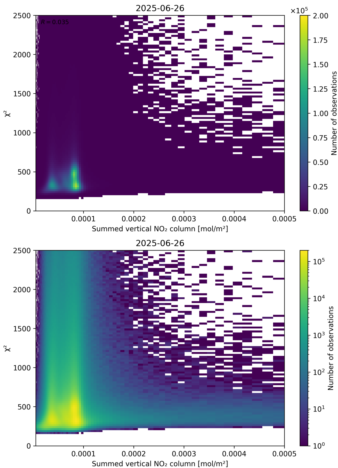
Figure 104: Scatter density plot of “Summed vertical NO 2 column” against “ \chi^2 ” for 2025-06-25 to 2025-06-27.
