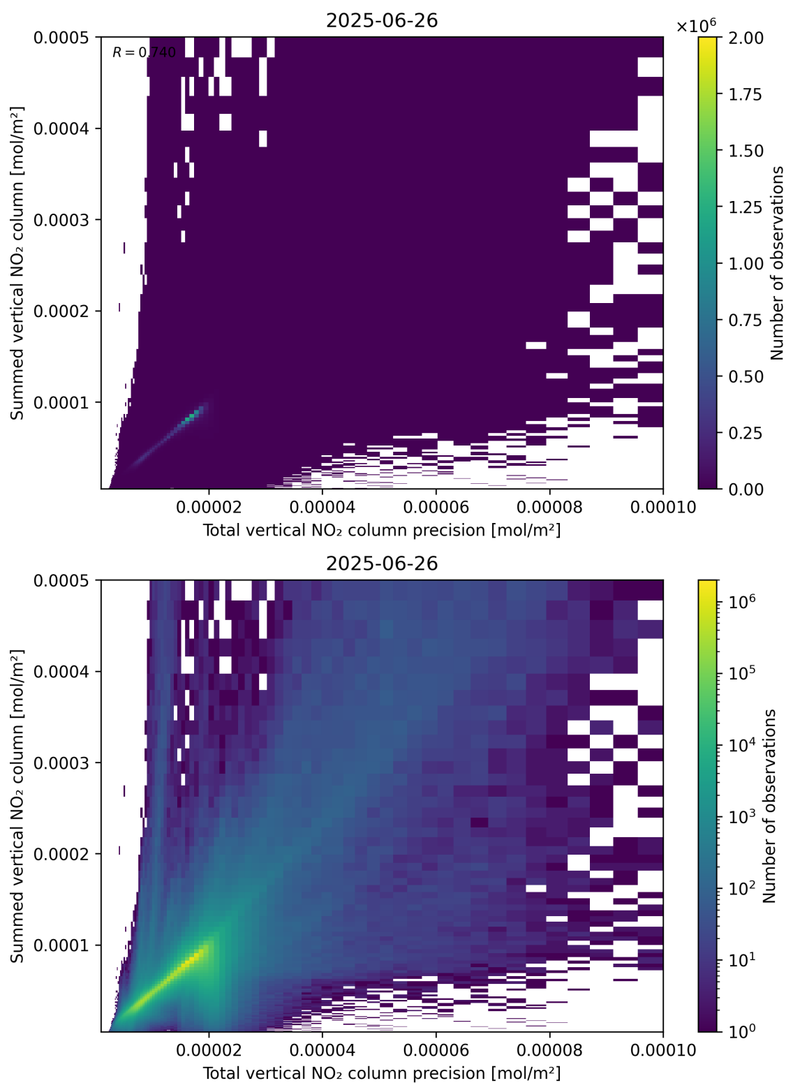
Figure 117: Scatter density plot of “Total vertical NO 2 column precision” against “Summed vertical NO 2 column” for 2025-06-25 to 2025-06-27.
