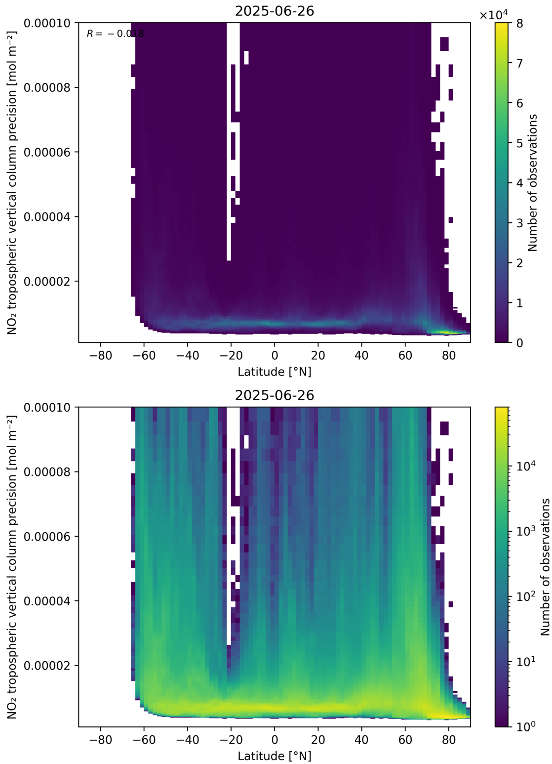
Figure 93: Scatter density plot of “Latitude” against “NO 2 tropospheric vertical column precision” for 2025-06-25 to 2025-06-27.
