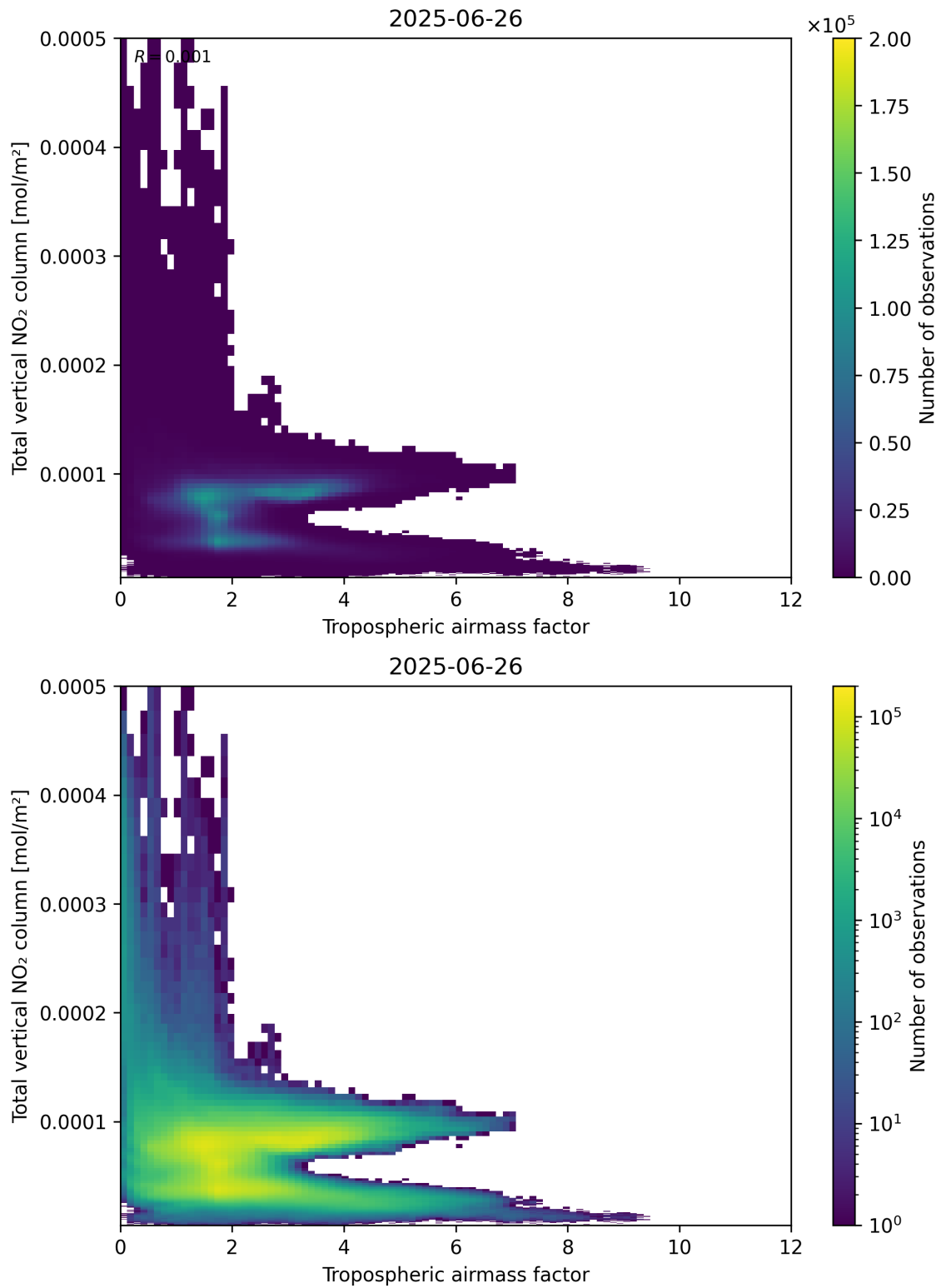
Figure 77: Scatter density plot of “Tropospheric airmass factor” against “Total vertical NO 2 column” for 2025-06-25 to 2025-06-27.
