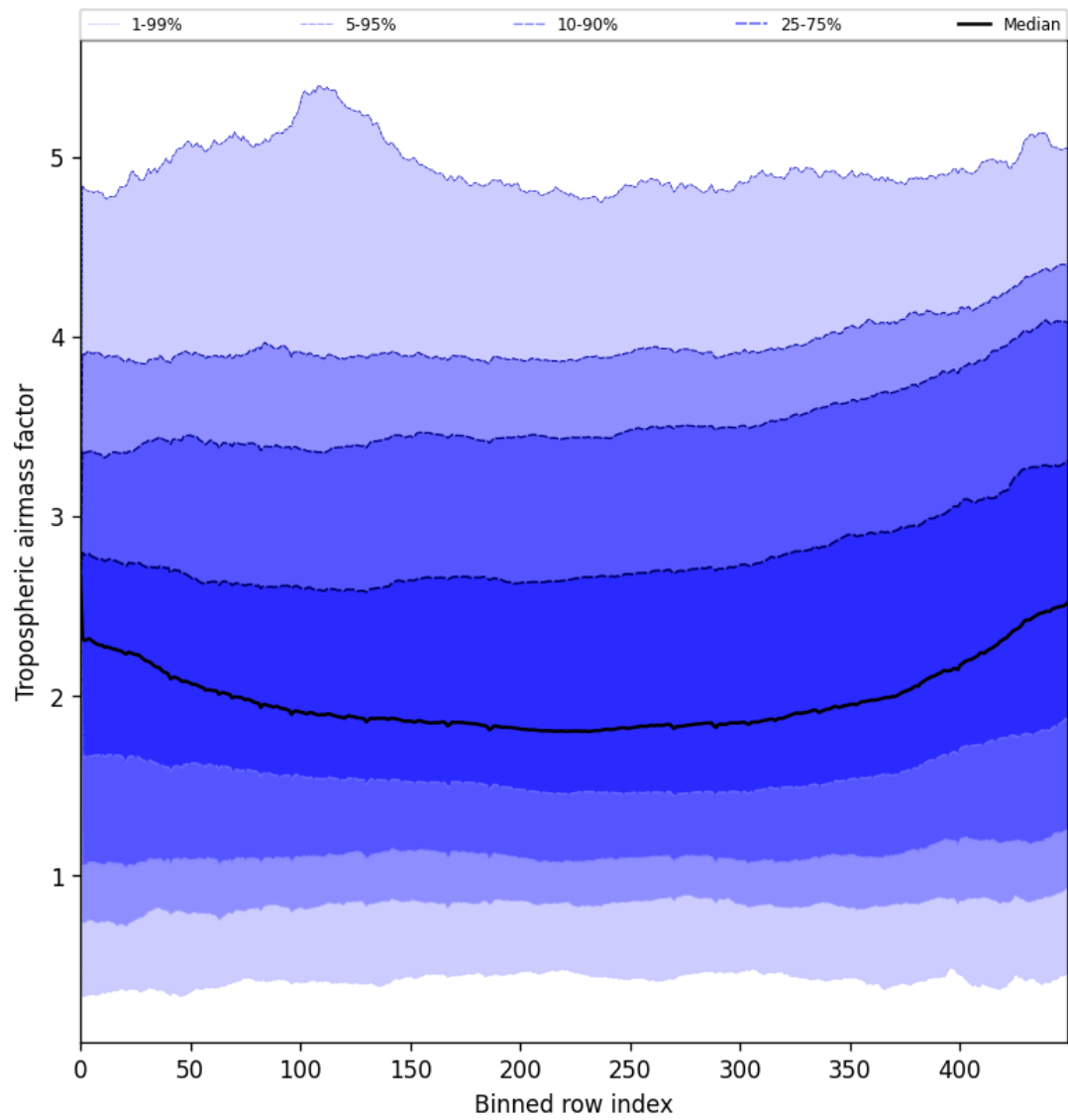
Figure 48: Along track statistics of “Tropospheric airmass factor” for 2025-06-25 to 2025-06-27
