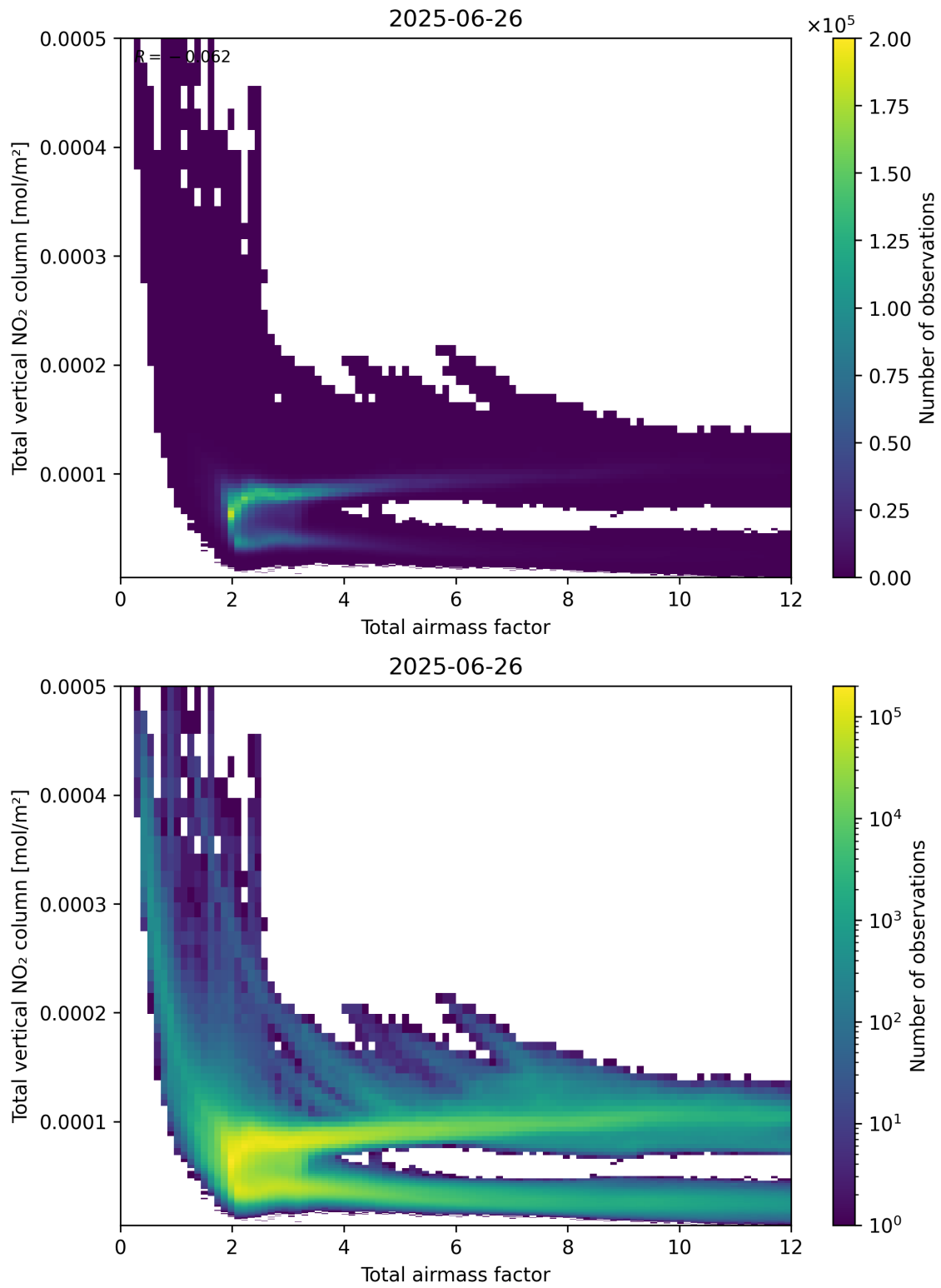
Figure 67: Scatter density plot of “Total airmass factor” against “Total vertical NO 2 column” for 2025-06-25 to 2025-06-27.
