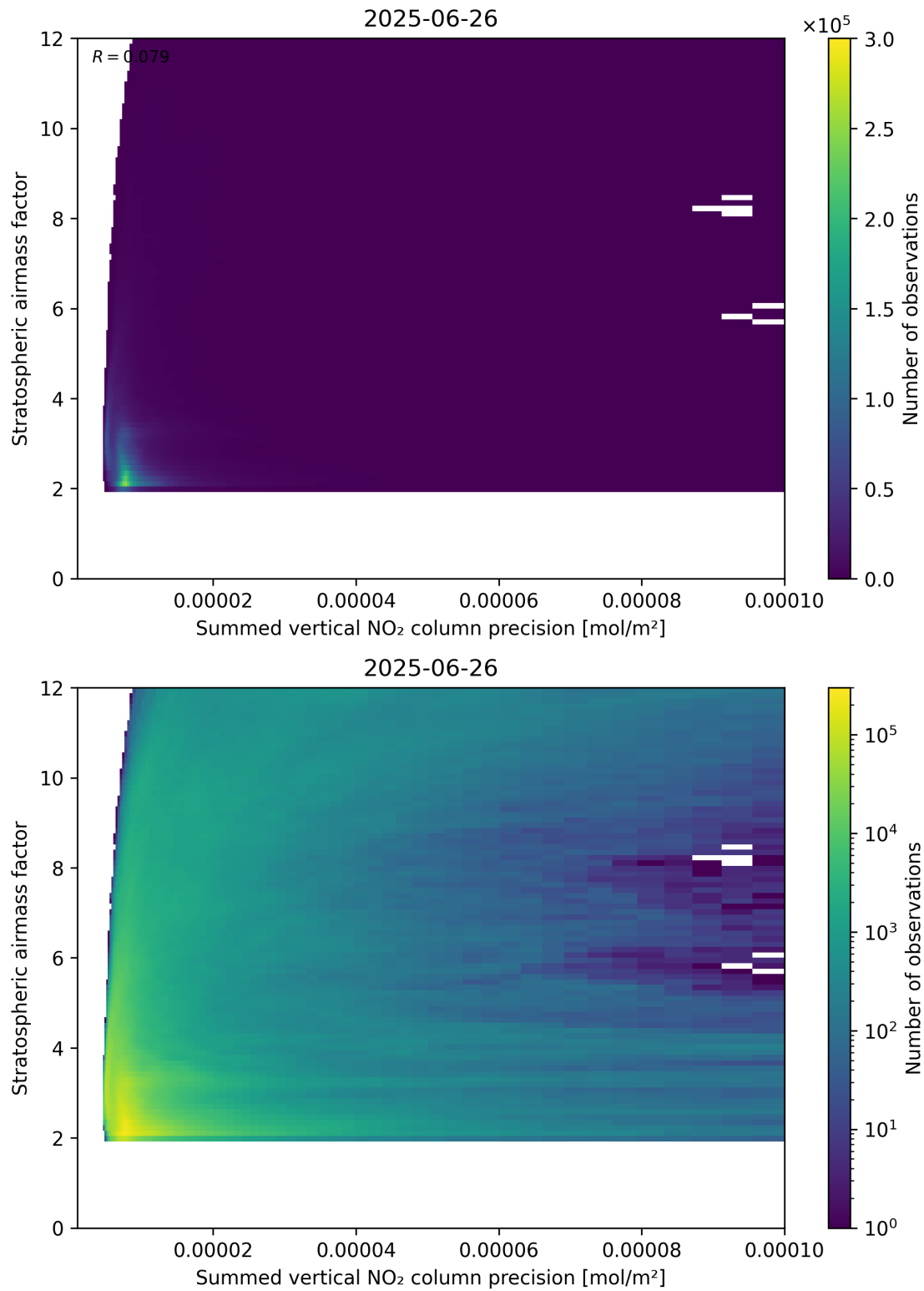
Figure 106: Scatter density plot of “Summed vertical NO 2 column precision” against “Stratospheric airmass factor” for 2025-06-25 to 2025-06-27.
