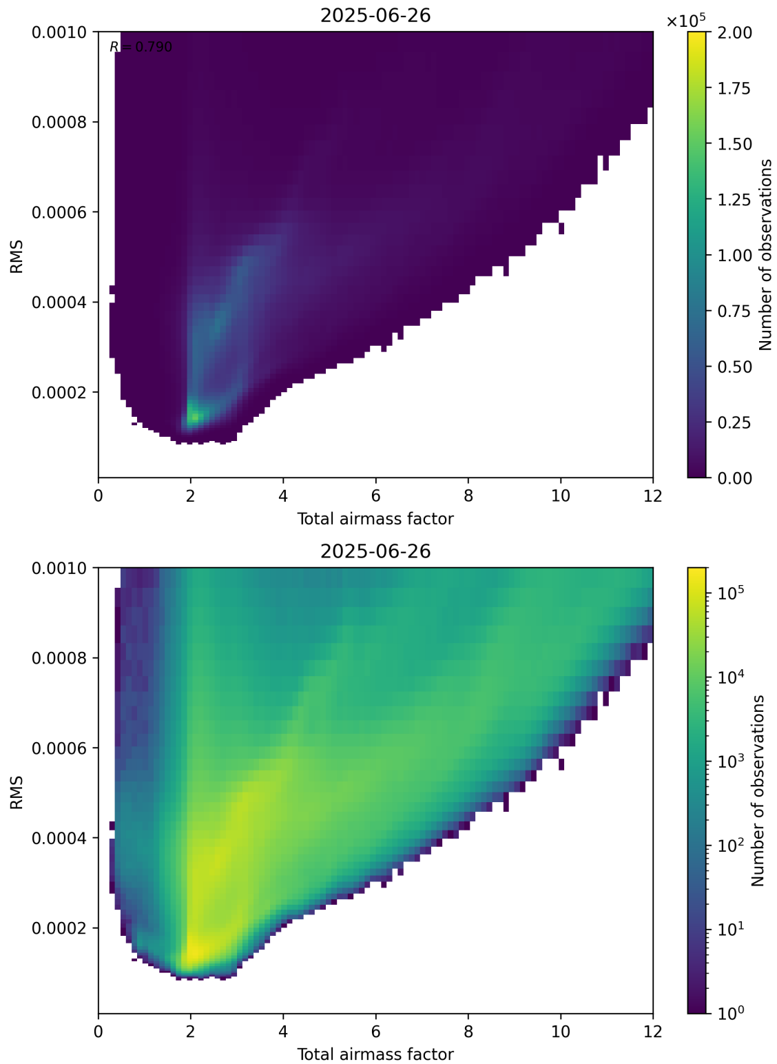
Figure 69: Scatter density plot of “Total airmass factor” against “RMS” for 2025-06-25 to 2025-06-27.
