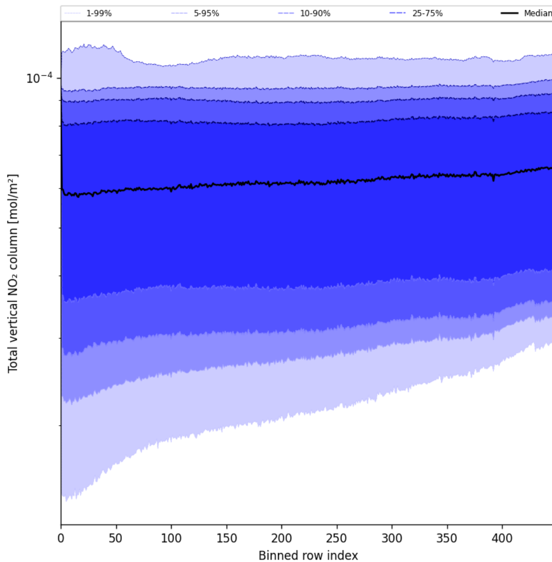
Figure 55: Along track statistics of “Total vertical NO 2 column” for 2025-06-25 to 2025-06-27
