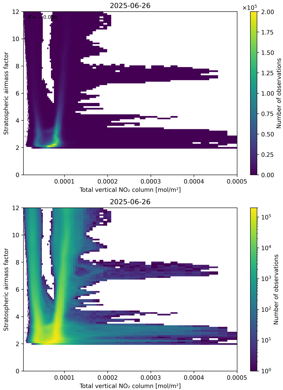
Figure 110: Scatter density plot of “Total vertical NO 2 column” against “Stratospheric airmass factor” for 2025-06-25 to 2025-06-27.
