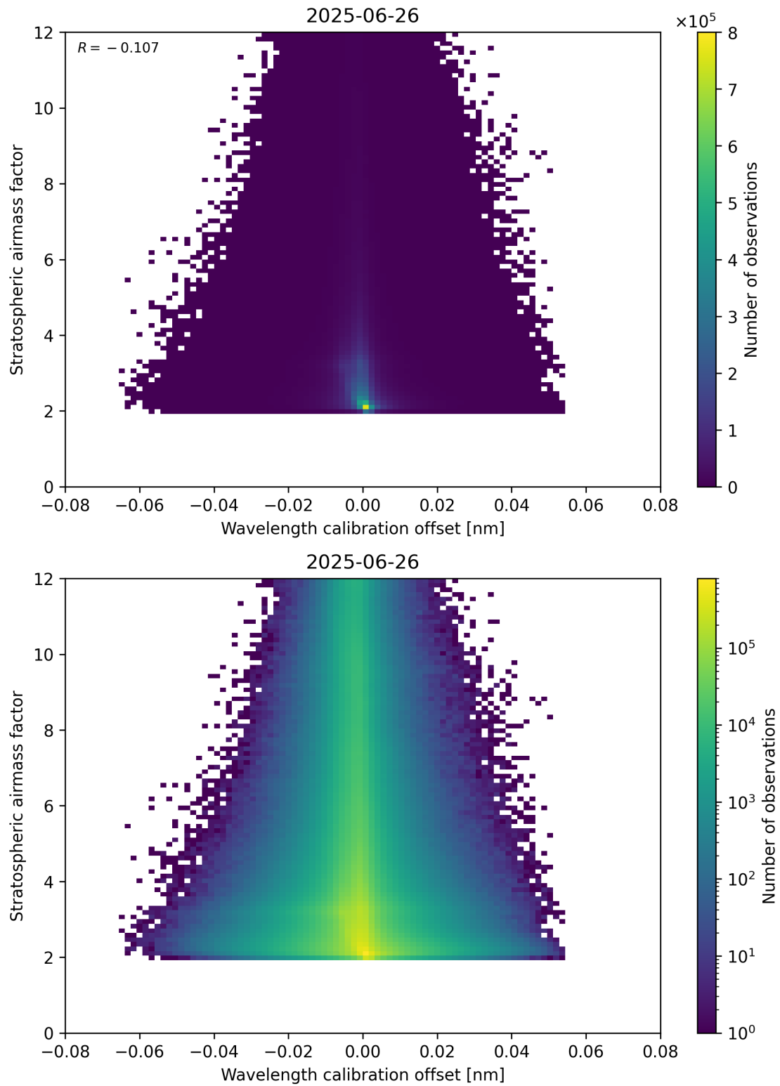
Figure 174: Scatter density plot of “Wavelength calibration offset” against “Stratospheric air mass factor” for 2025-06-25 to 2025-06-27.
