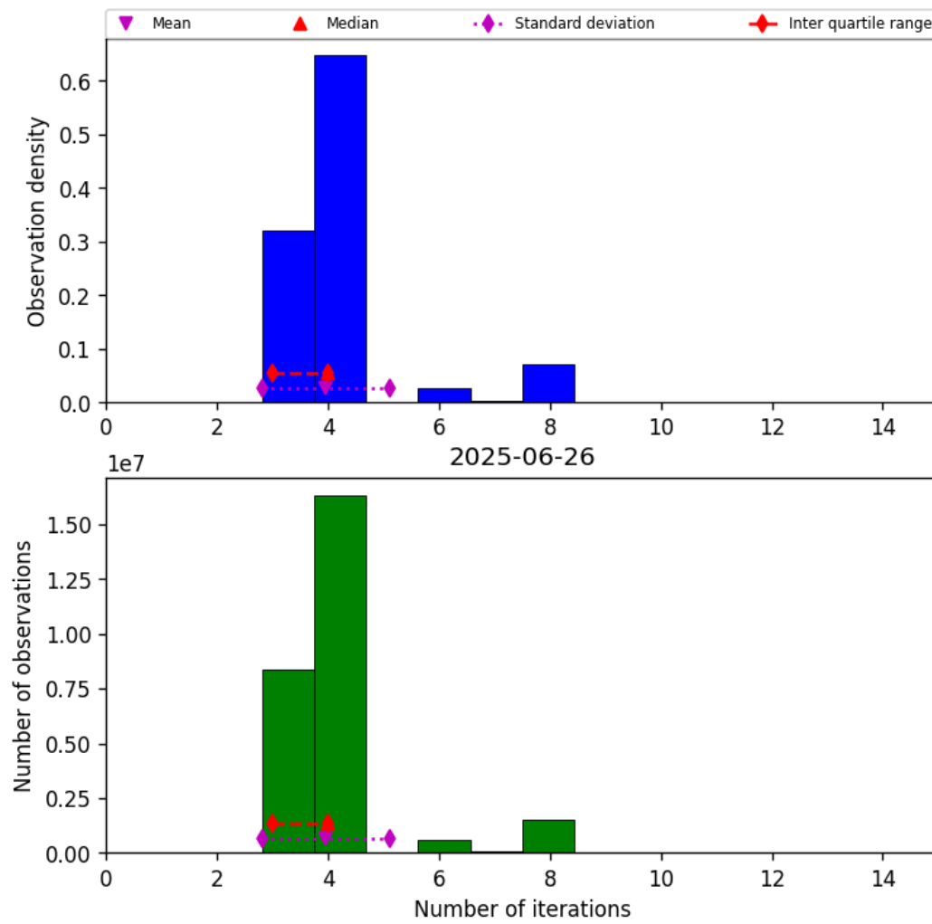
Figure 34: Histogram of “Number of iterations” for 2025-06-25 to 2025-06-27
