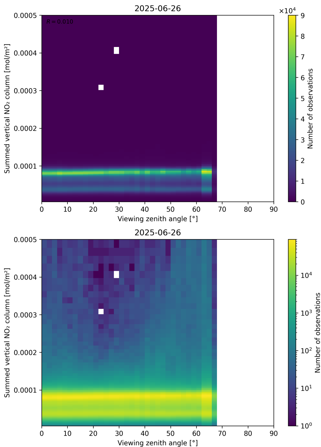
Figure 165: Scatter density plot of “Viewing zenith angle” against “Summed vertical NO 2 column” for 2025-06-25 to 2025-06-27.
