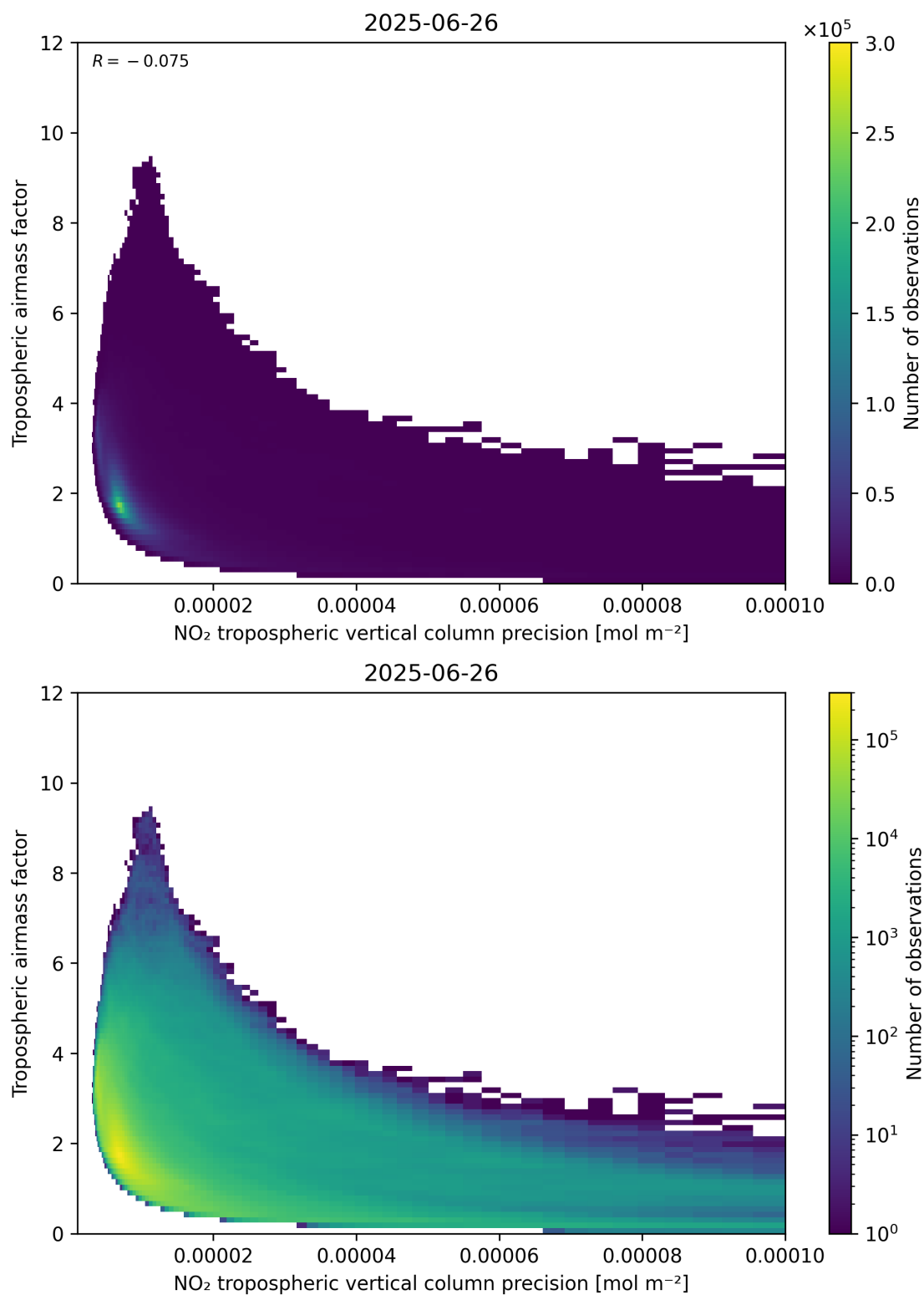
Figure 133: Scatter density plot of “NO 2 tropospheric vertical column precision” against “Tropospheric air mass factor” for 2025-06-25 to 2025-06-27.
