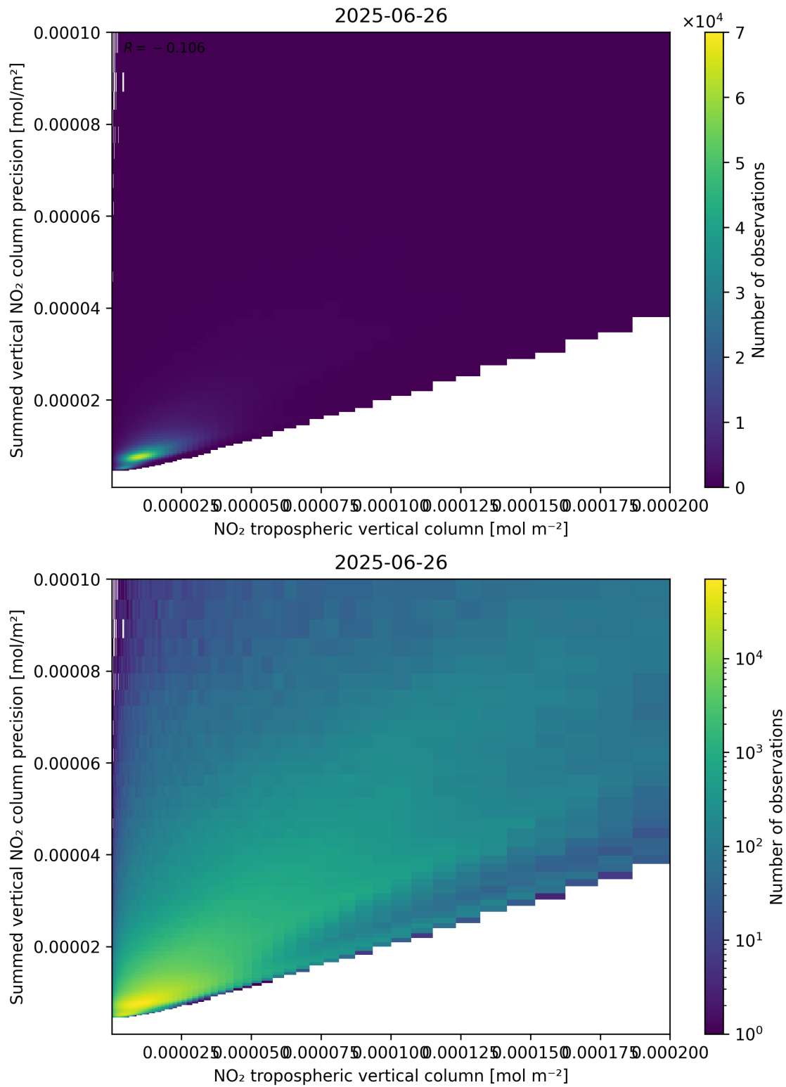
Figure 127: Scatter density plot of “NO 2 tropospheric vertical column” against “Summed vertical NO 2 column precision” for 2025-06-25 to 2025-06-27.
