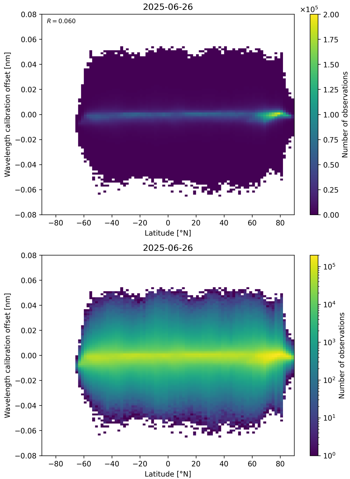
Figure 95: Scatter density plot of “Latitude” against “Wavelength calibration offset” for 2025-06-25 to 2025-06-27.
