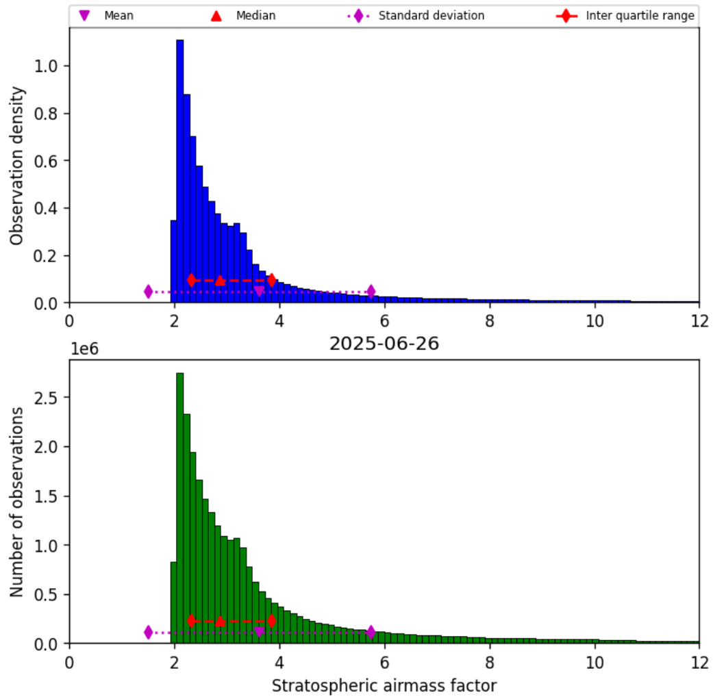
Figure 44: Histogram of “Stratospheric airmass factor” for 2025-06-25 to 2025-06-27
