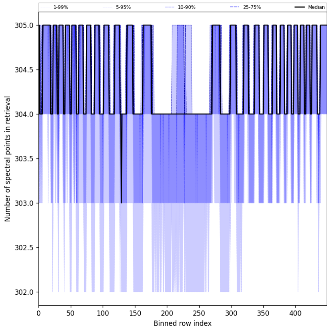
Figure 50: Along track statistics of “Number of spectral points in retrieval” for 2025-06-25 to 2025-06-27
