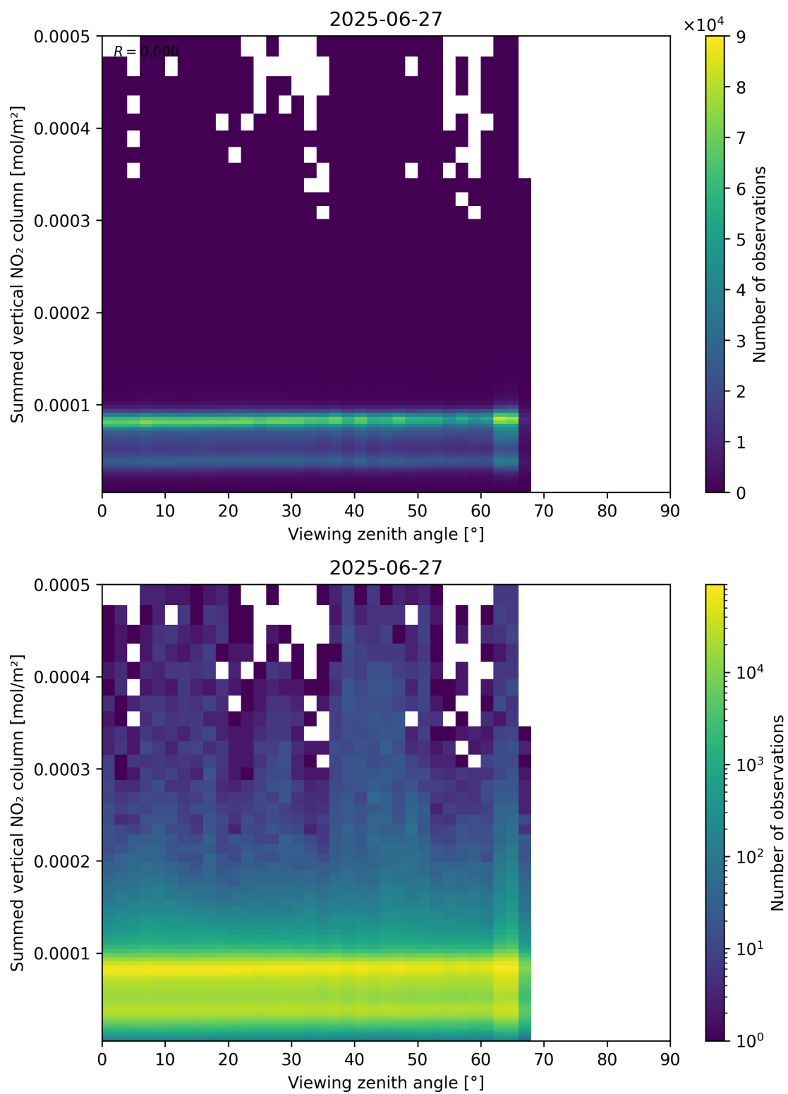
Figure 165: Scatter density plot of “Viewing zenith angle” against “Summed vertical NO 2 column” for 2025-06-27 to 2025-06-28.
