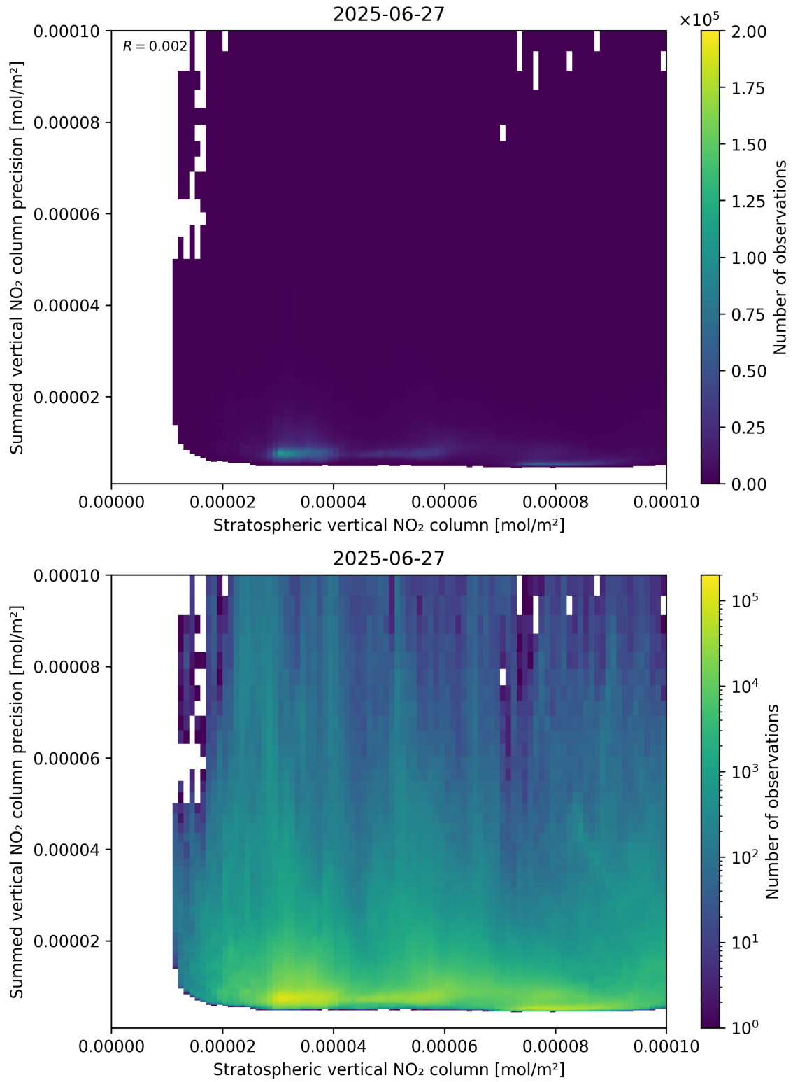
Figure 99: Scatter density plot of “Stratospheric vertical NO 2 column” against “Summed vertical NO 2 column precision” for 2025-06-27 to 2025-06-28.
