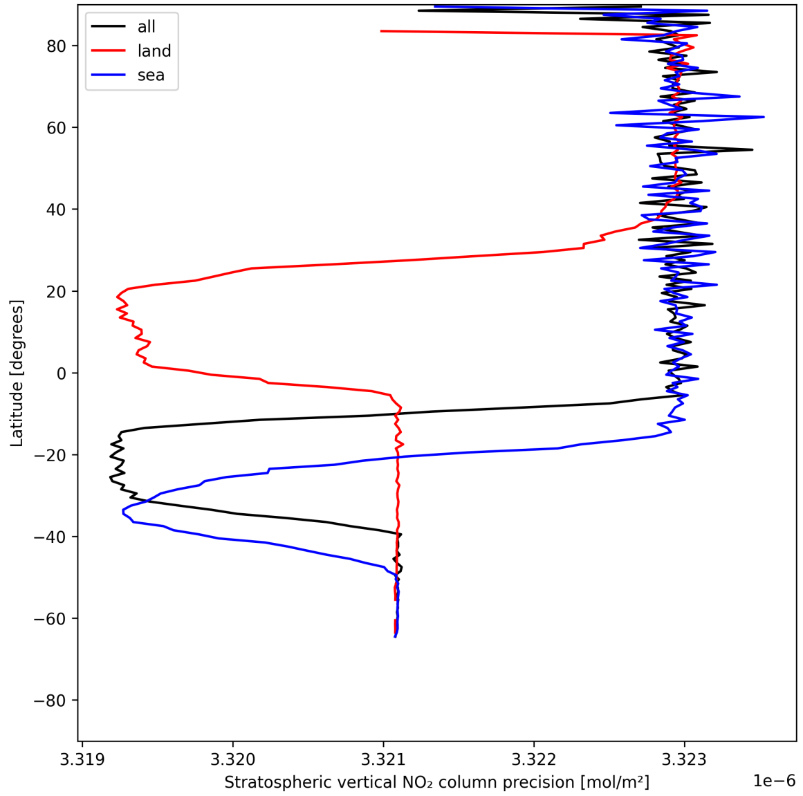
Figure 20: Zonal average of “Stratospheric vertical NO 2 column precision” for 2025-06-27 to 2025-06-28.
