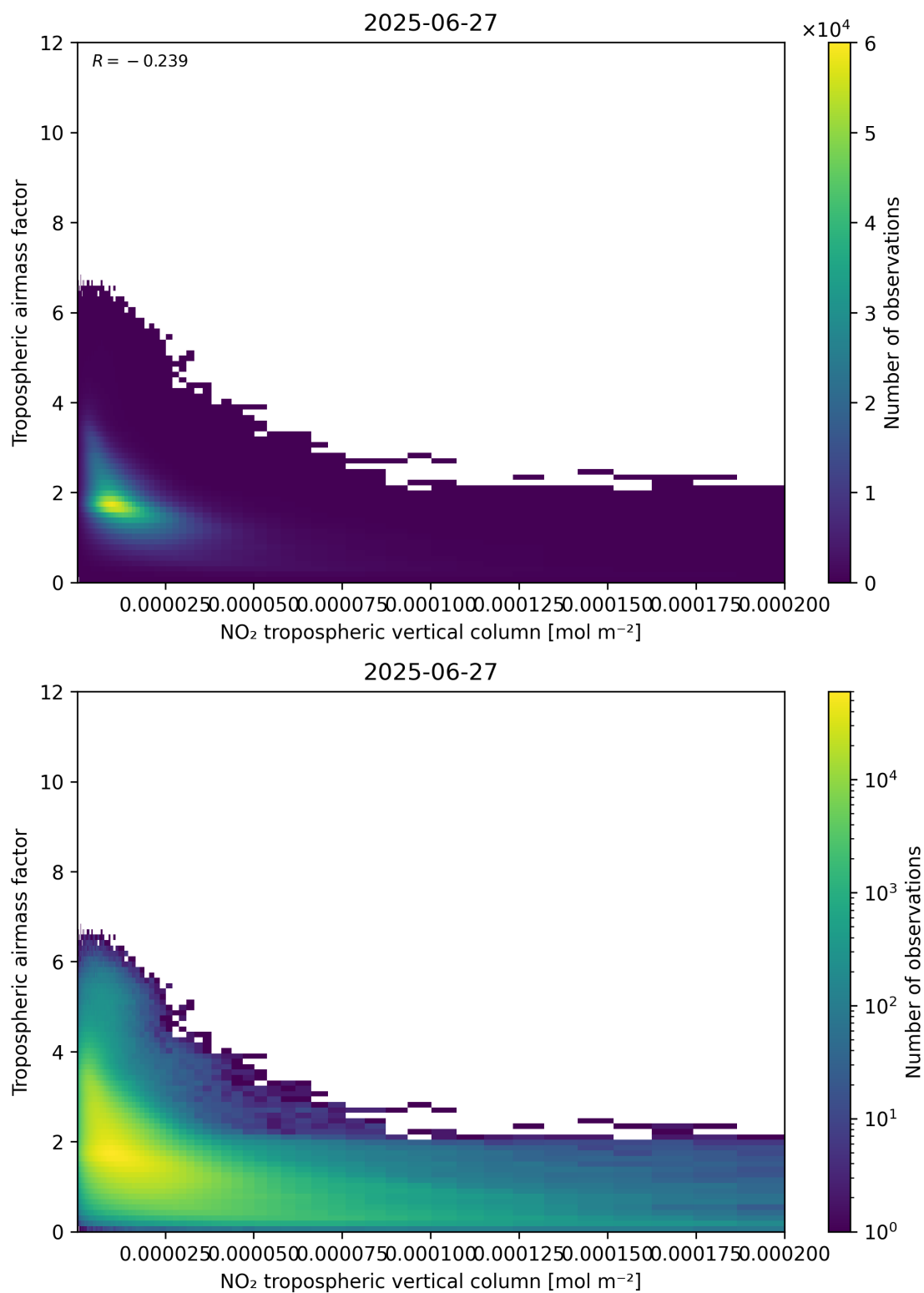
Figure 123: Scatter density plot of “NO 2 tropospheric vertical column” against “Tropospheric air mass factor” for 2025-06-27 to 2025-06-28.
