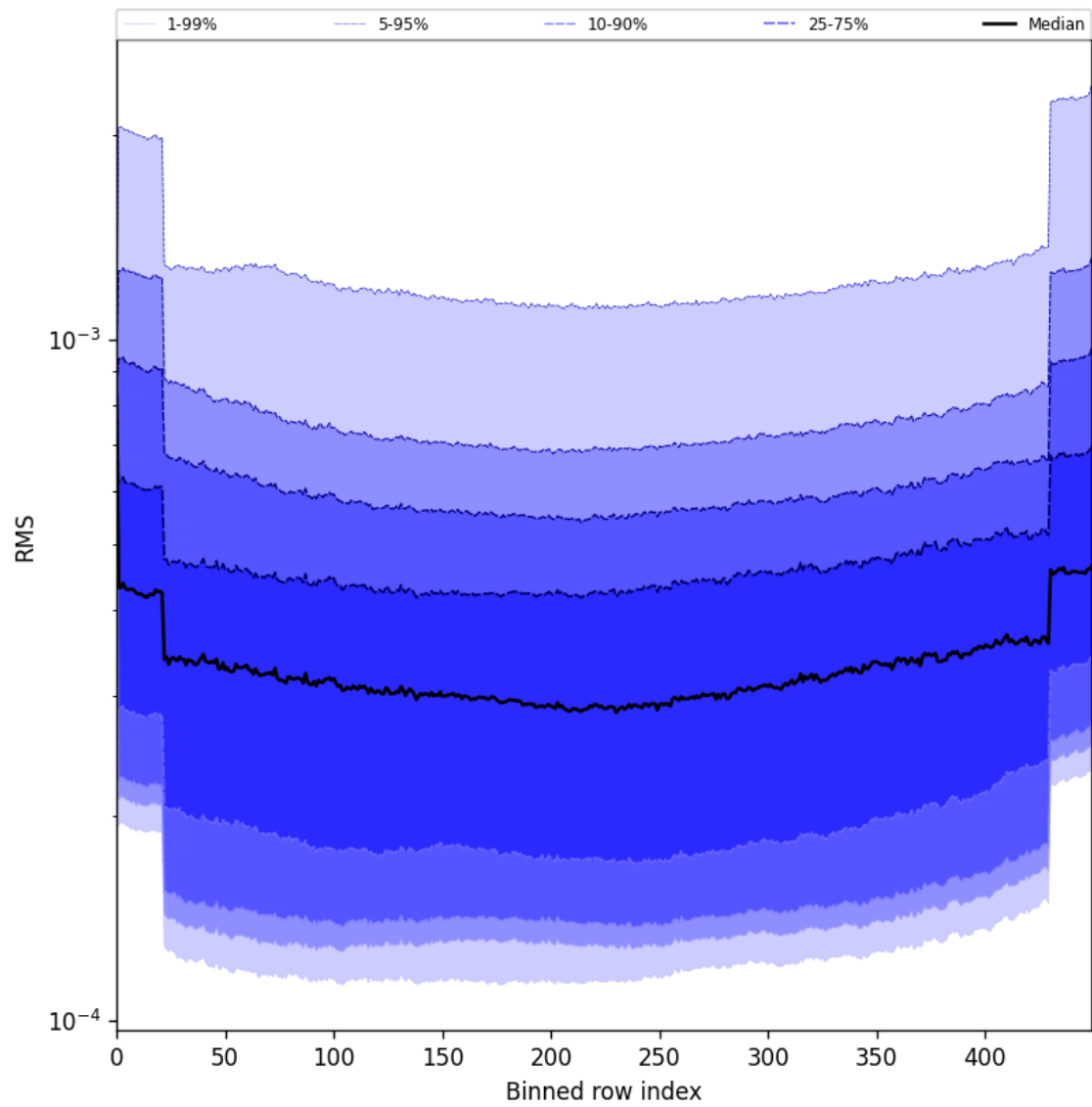
Figure 60: Along track statistics of “RMS” for 2025-06-27 to 2025-06-28
