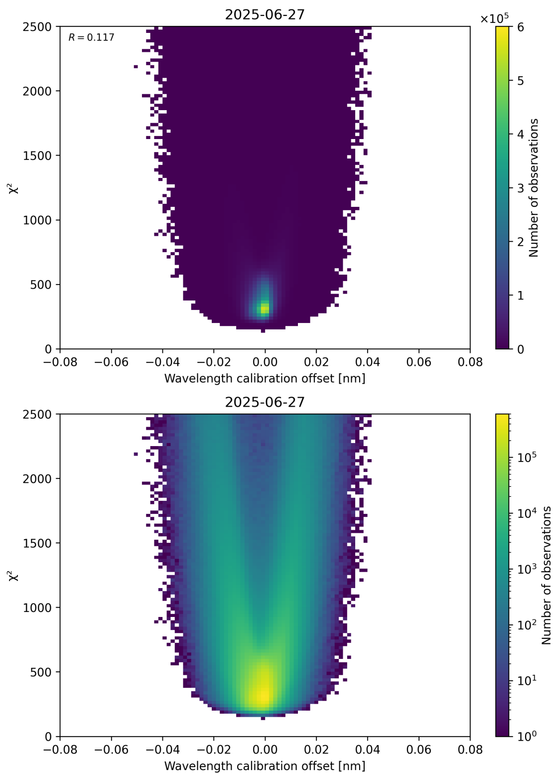
Figure 175: Scatter density plot of “Wavelength calibration offset” against “ \chi^2 ” for 2025-06-27 to 2025-06-28.
