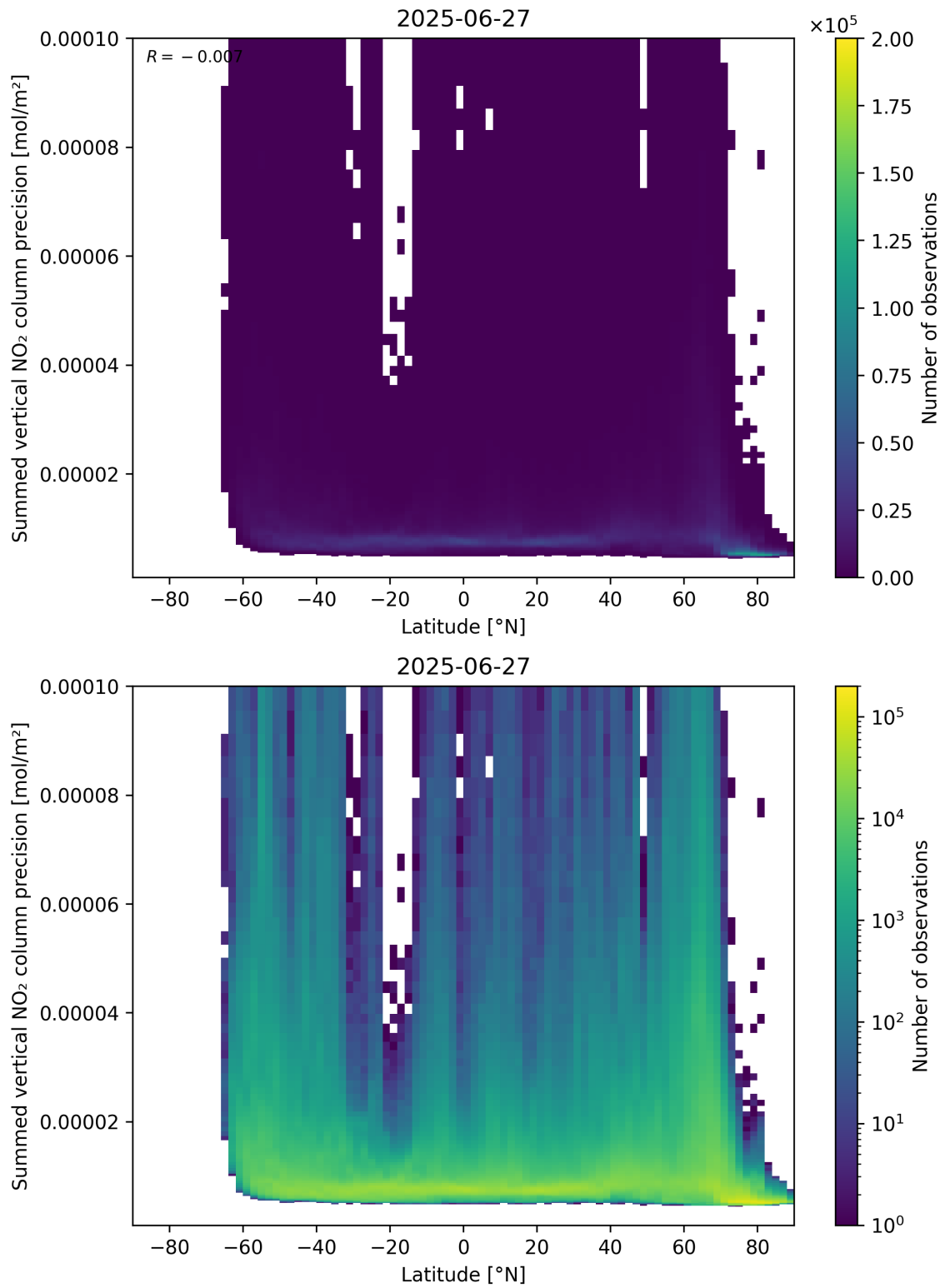
Figure 89: Scatter density plot of “Latitude” against “Summed vertical NO 2 column precision” for 2025-06-27 to 2025-06-28.
