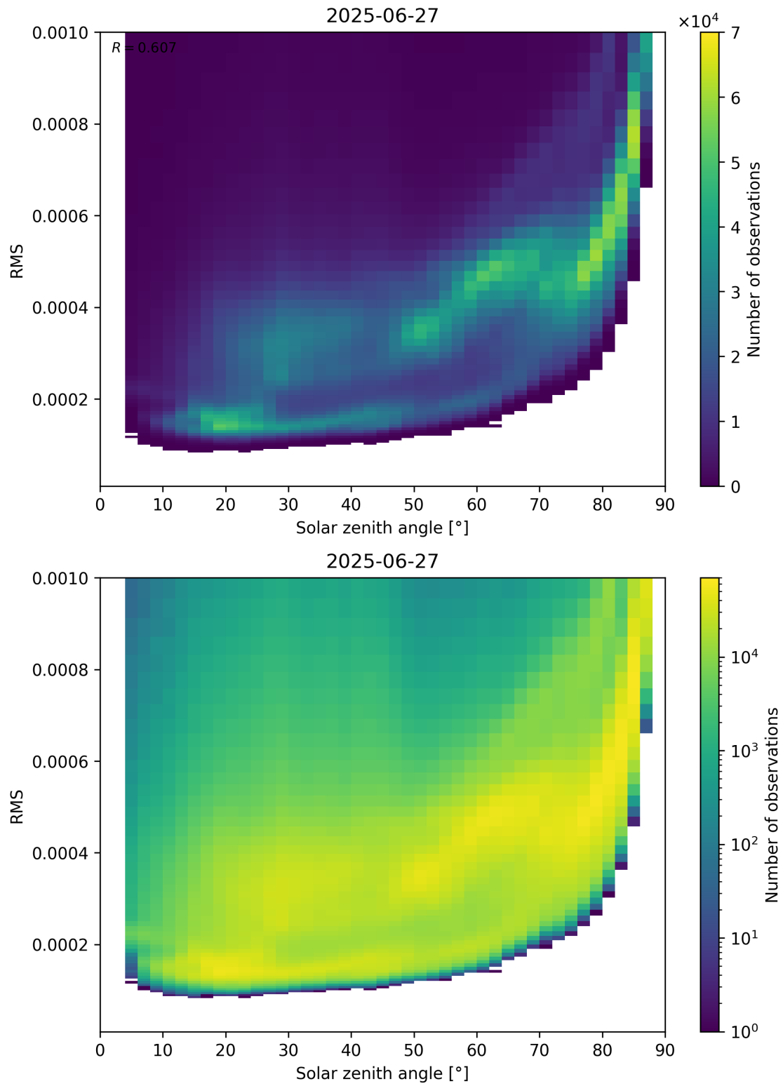
Figure 157: Scatter density plot of “Solar zenith angle” against “RMS” for 2025-06-27 to 2025-06-28.
