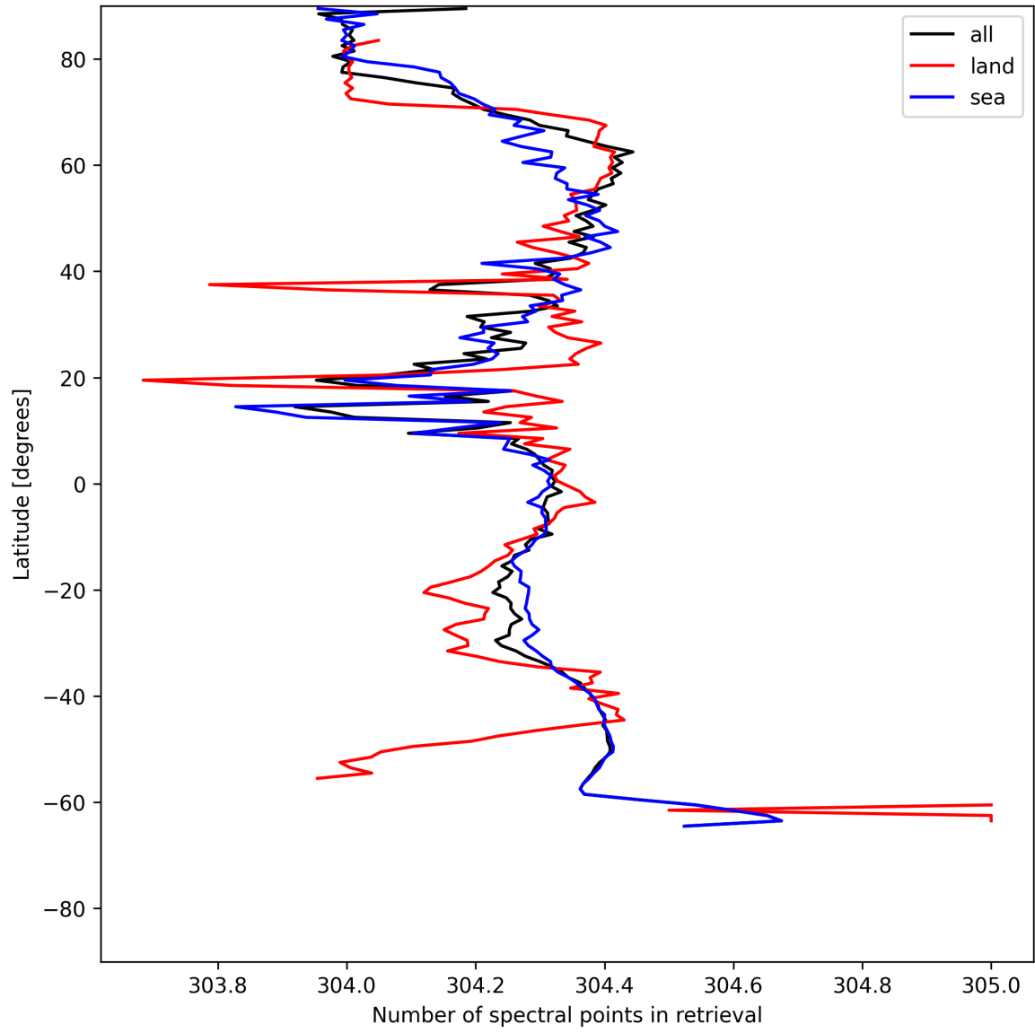
Figure 16: Zonal average of “Number of spectral points in retrieval” for 2025-06-27 to 2025-06-28.
