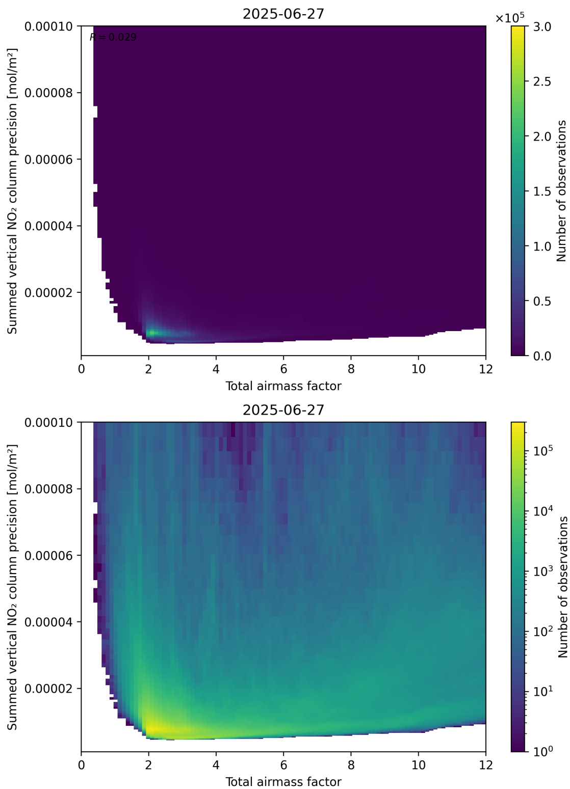
Figure 66: Scatter density plot of “Total airmass factor” against “Summed vertical NO 2 column precision” for 2025-06-27 to 2025-06-28.
