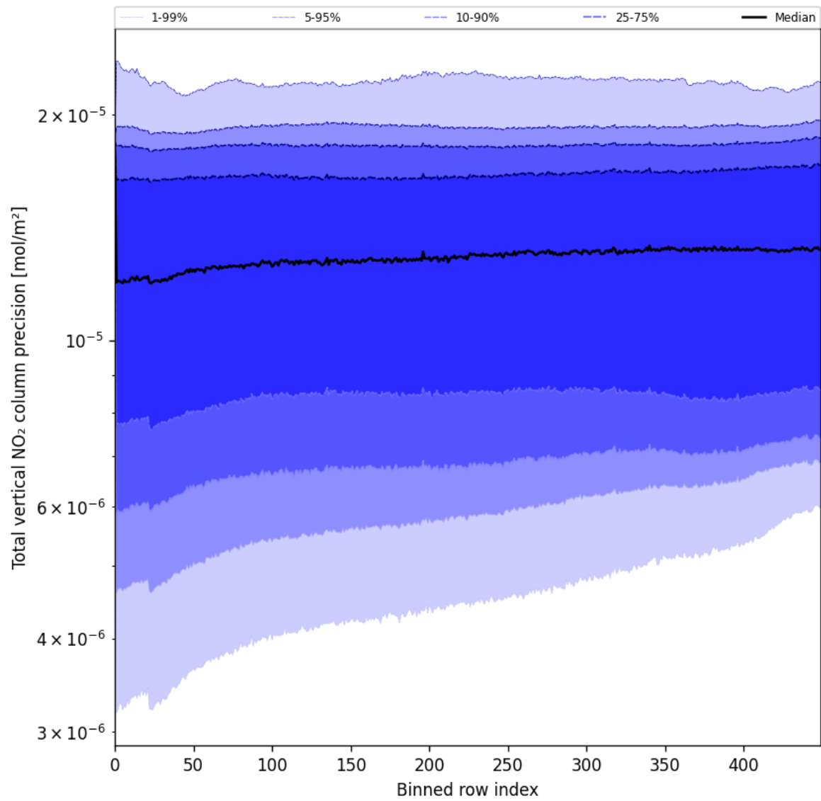
Figure 56: Along track statistics of “Total vertical NO 2 column precision” for 2025-06-27 to 2025-06-28
