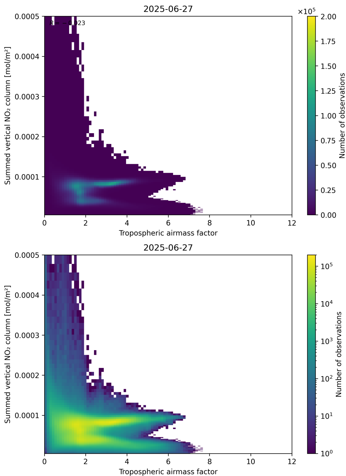
Figure 75: Scatter density plot of “Tropospheric airmass factor” against “Summed vertical NO 2 column” for 2025-06-27 to 2025-06-28.
