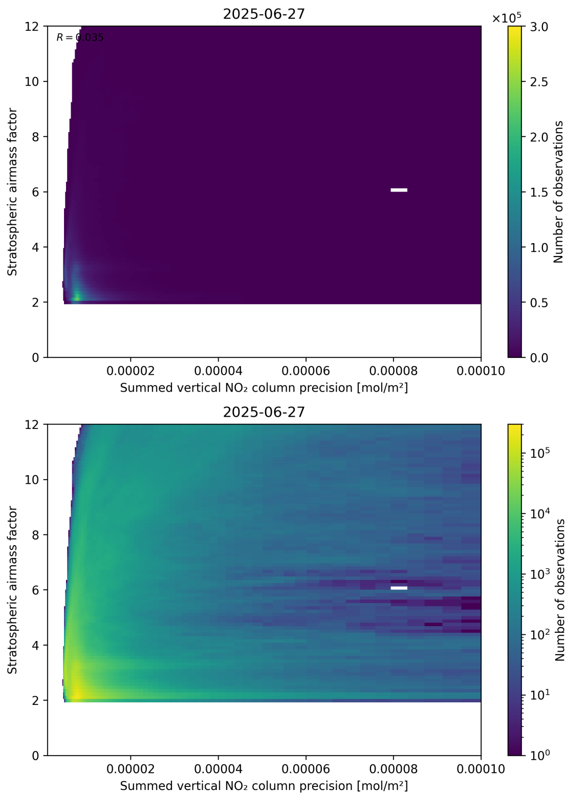
Figure 106: Scatter density plot of “Summed vertical NO 2 column precision” against “Stratospheric airmass factor” for 2025-06-27 to 2025-06-28.
