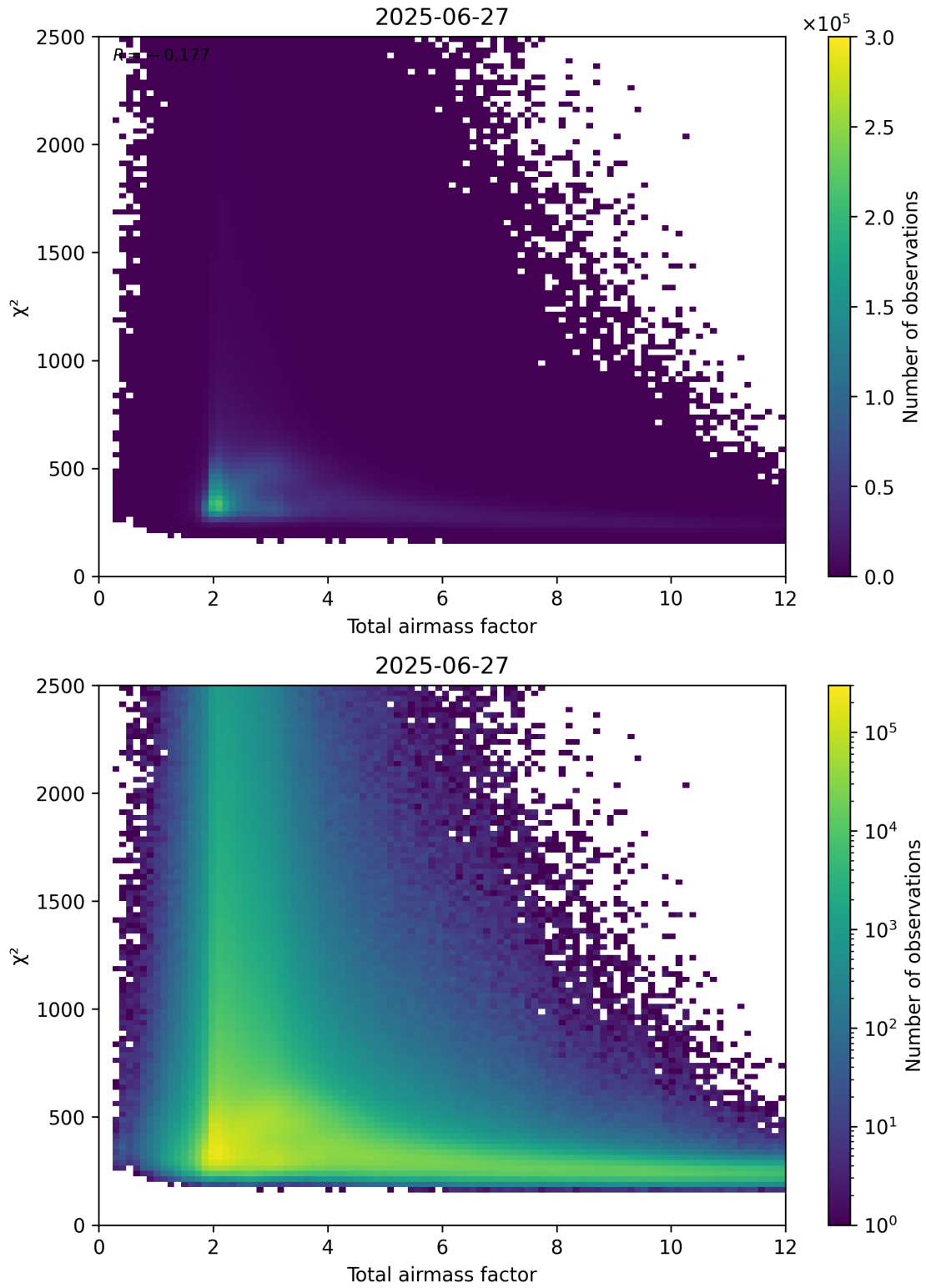
Figure 63: Scatter density plot of “Total airmass factor” against “ \chi^2 ” for 2025-06-27 to 2025-06-28.
