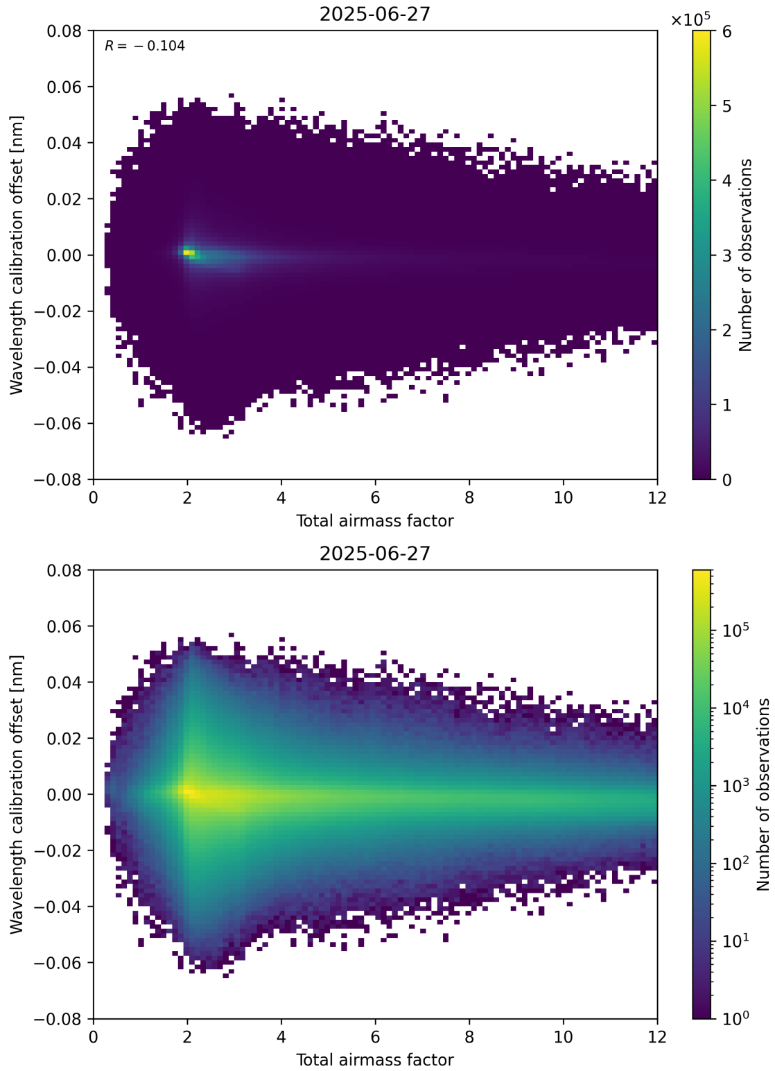
Figure 70: Scatter density plot of “Total airmass factor” against “Wavelength calibration offset” for 2025-06-27 to 2025-06-28.
