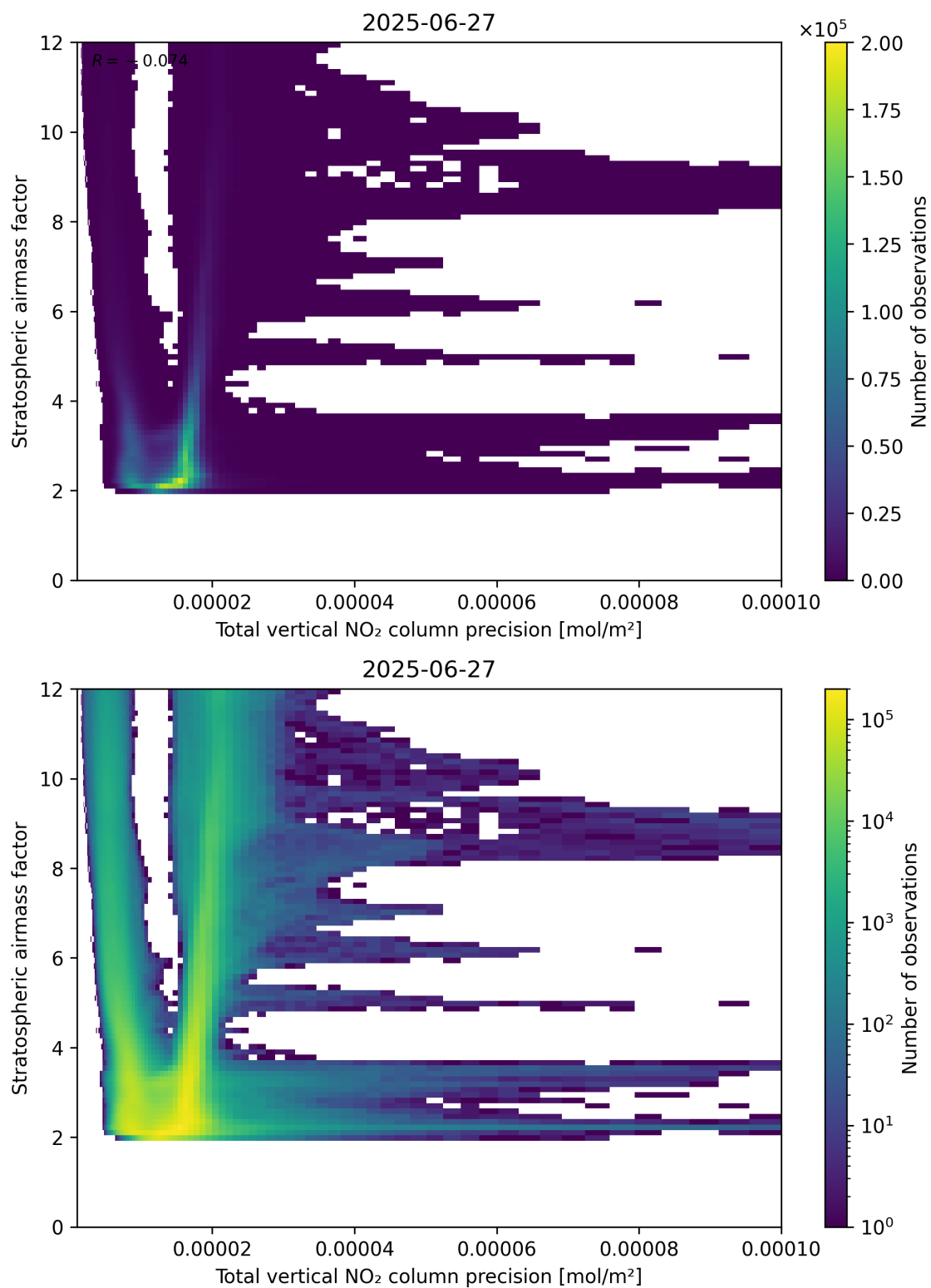
Figure 115: Scatter density plot of “Total vertical NO 2 column precision” against “Stratospheric air mass factor” for 2025-06-27 to 2025-06-28.
