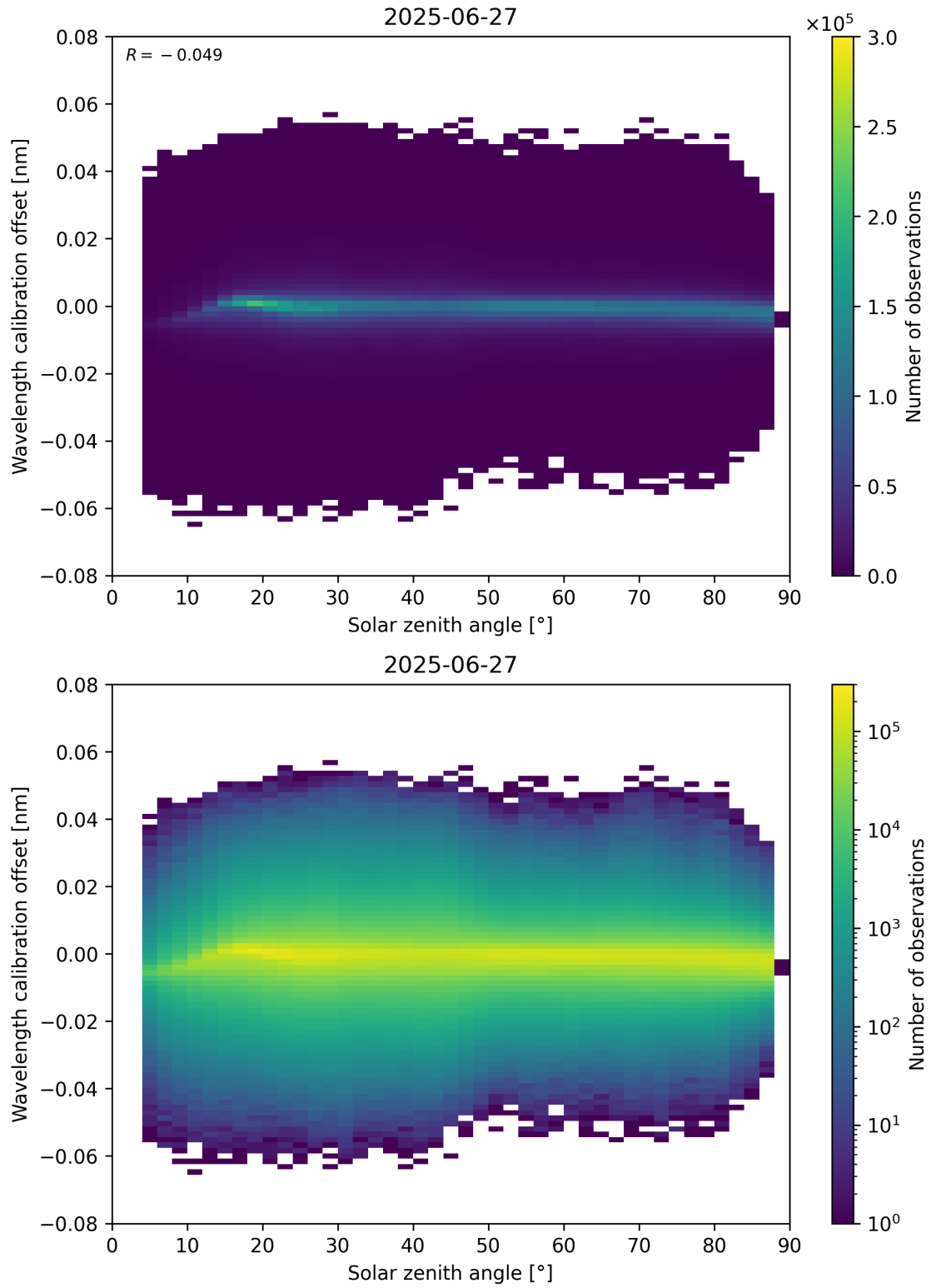
Figure 158: Scatter density plot of “Solar zenith angle” against “Wavelength calibration offset” for 2025-06-27 to 2025-06-28.
