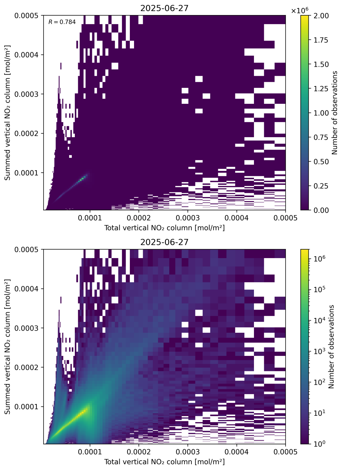
Figure 112: Scatter density plot of “Total vertical NO 2 column” against “Summed vertical NO 2 column” for 2025-06-27 to 2025-06-28.
