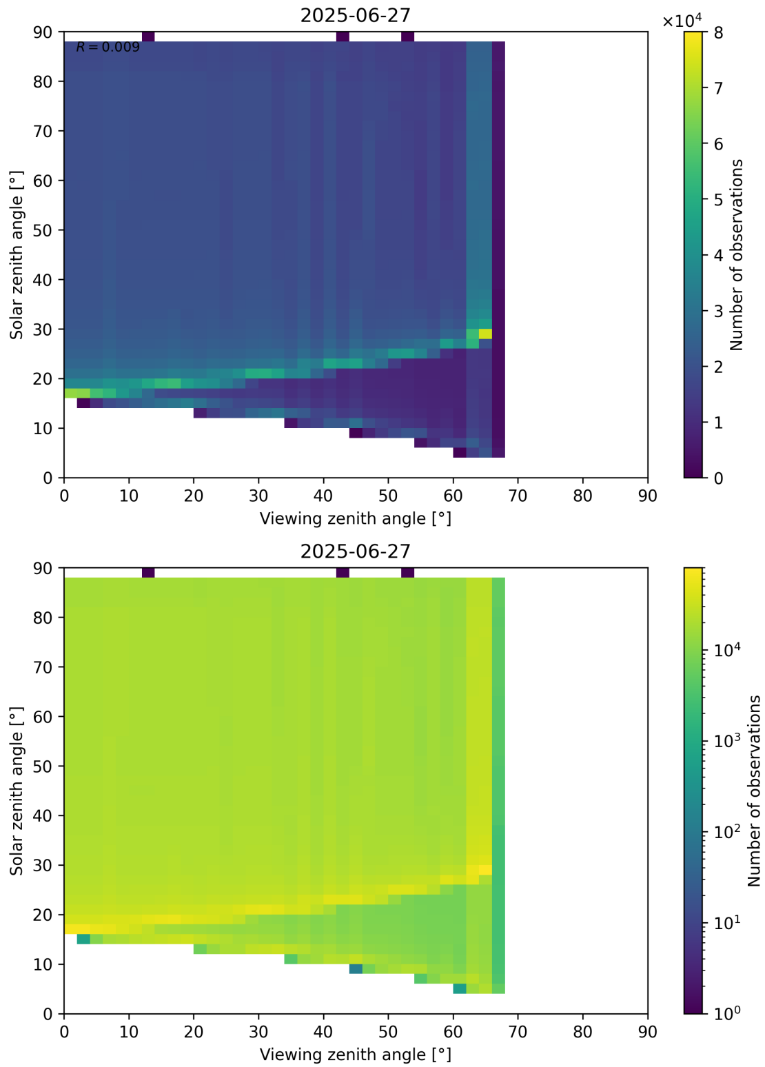
Figure 172: Scatter density plot of “Viewing zenith angle” against “Solar zenith angle” for 2025-06-27 to 2025-06-28.
