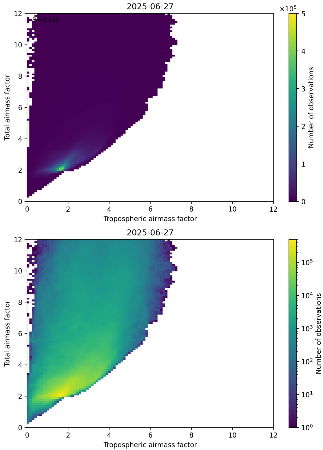
Figure 72: Scatter density plot of “Tropospheric airmass factor” against “Total airmass factor” for 2025-06-27 to 2025-06-28.
