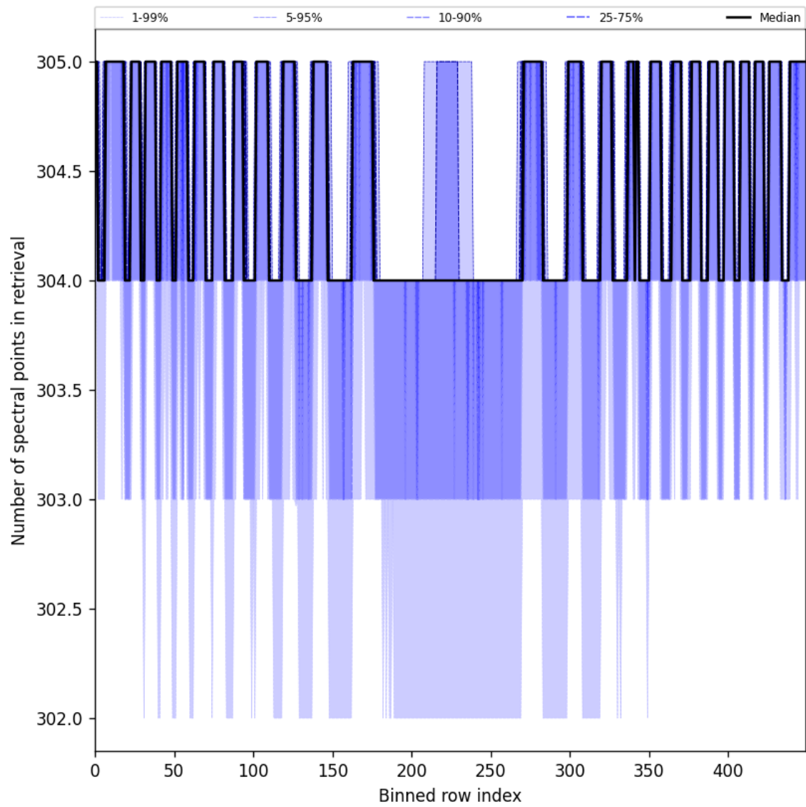
Figure 50: Along track statistics of “Number of spectral points in retrieval” for 2025-06-27 to 2025-06-28
