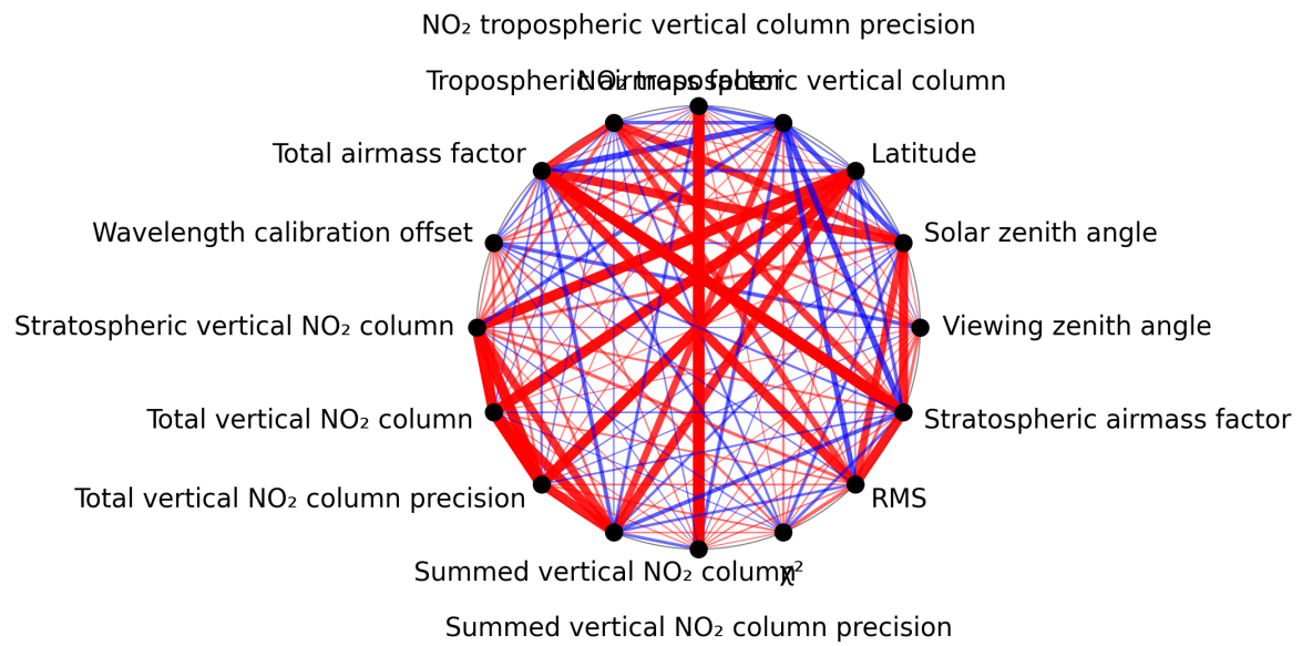
Figure 1: Map of correlation graph for 2025-06-27 to 2025-06-28.
