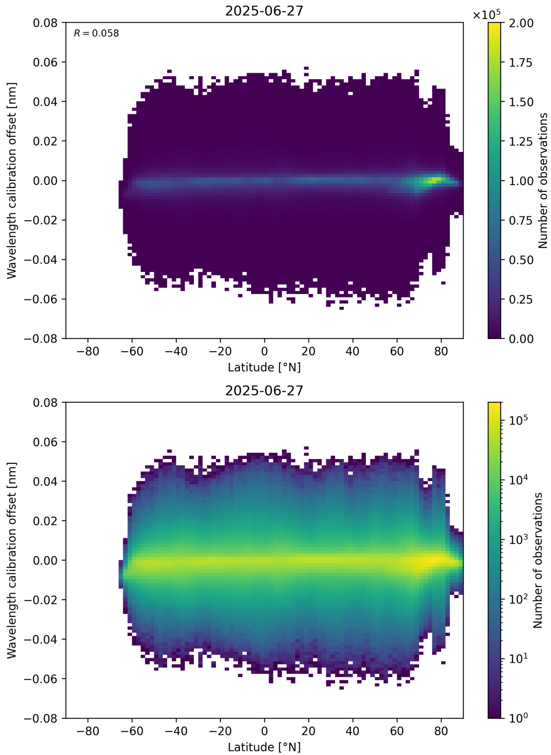
Figure 95: Scatter density plot of “Latitude” against “Wavelength calibration offset” for 2025-06-27 to 2025-06-28.
