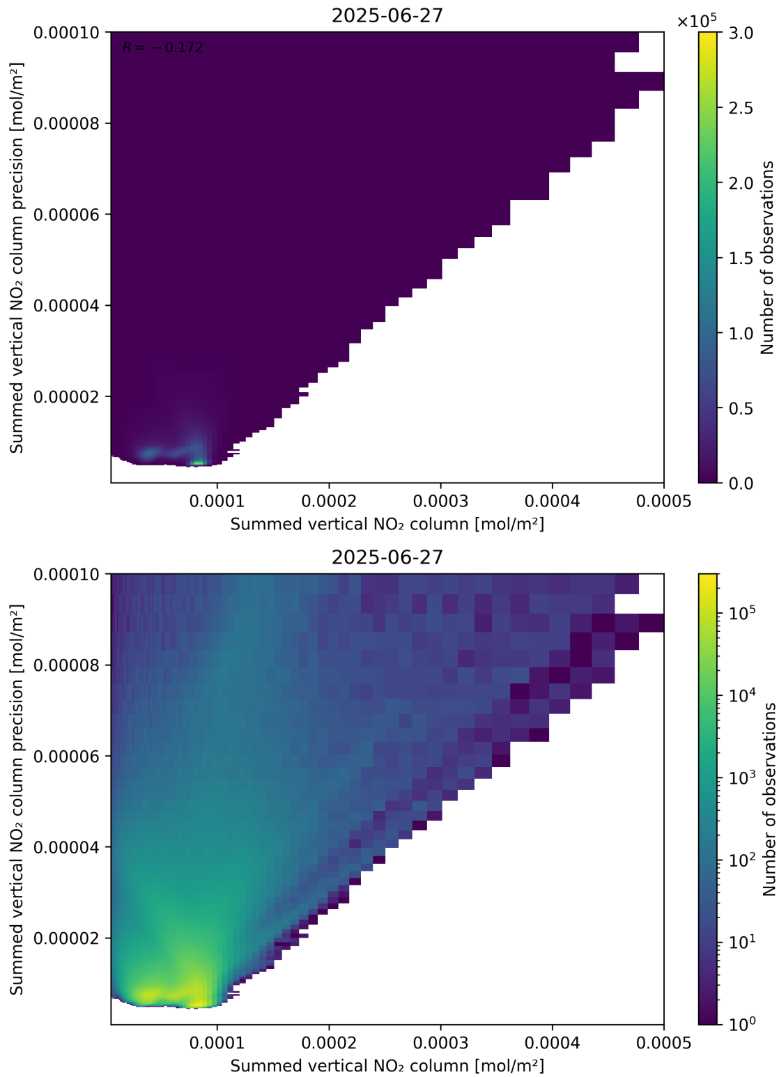
Figure 105: Scatter density plot of “Summed vertical NO 2 column” against “Summed vertical NO 2 column precision” for 2025-06-27 to 2025-06-28.
