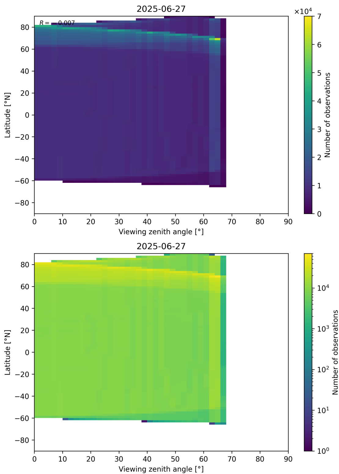
Figure 163: Scatter density plot of “Viewing zenith angle” against “Latitude” for 2025-06-27 to 2025-06-28.
