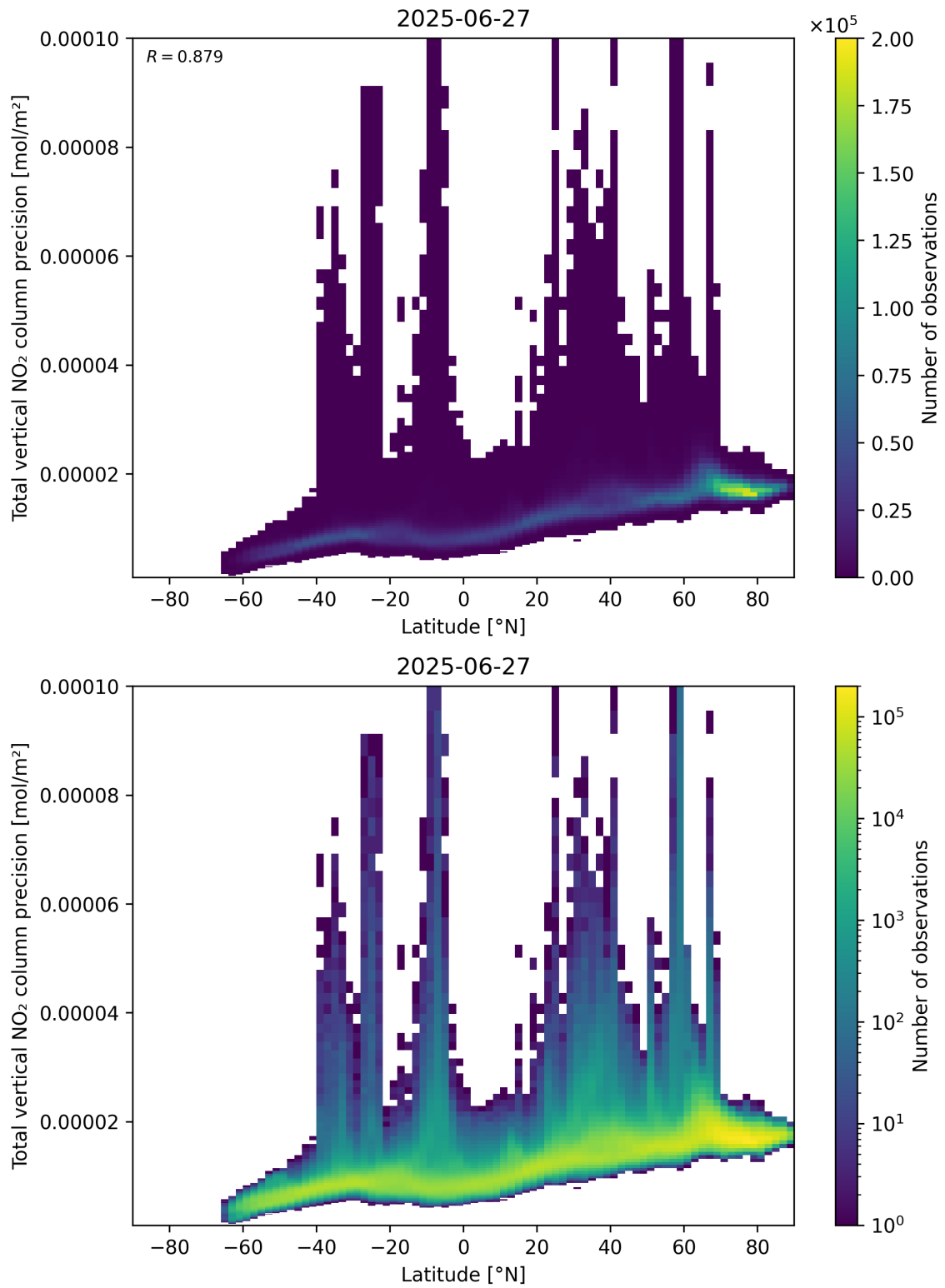
Figure 91: Scatter density plot of “Latitude” against “Total vertical NO 2 column precision” for 2025-06-27 to 2025-06-28.
