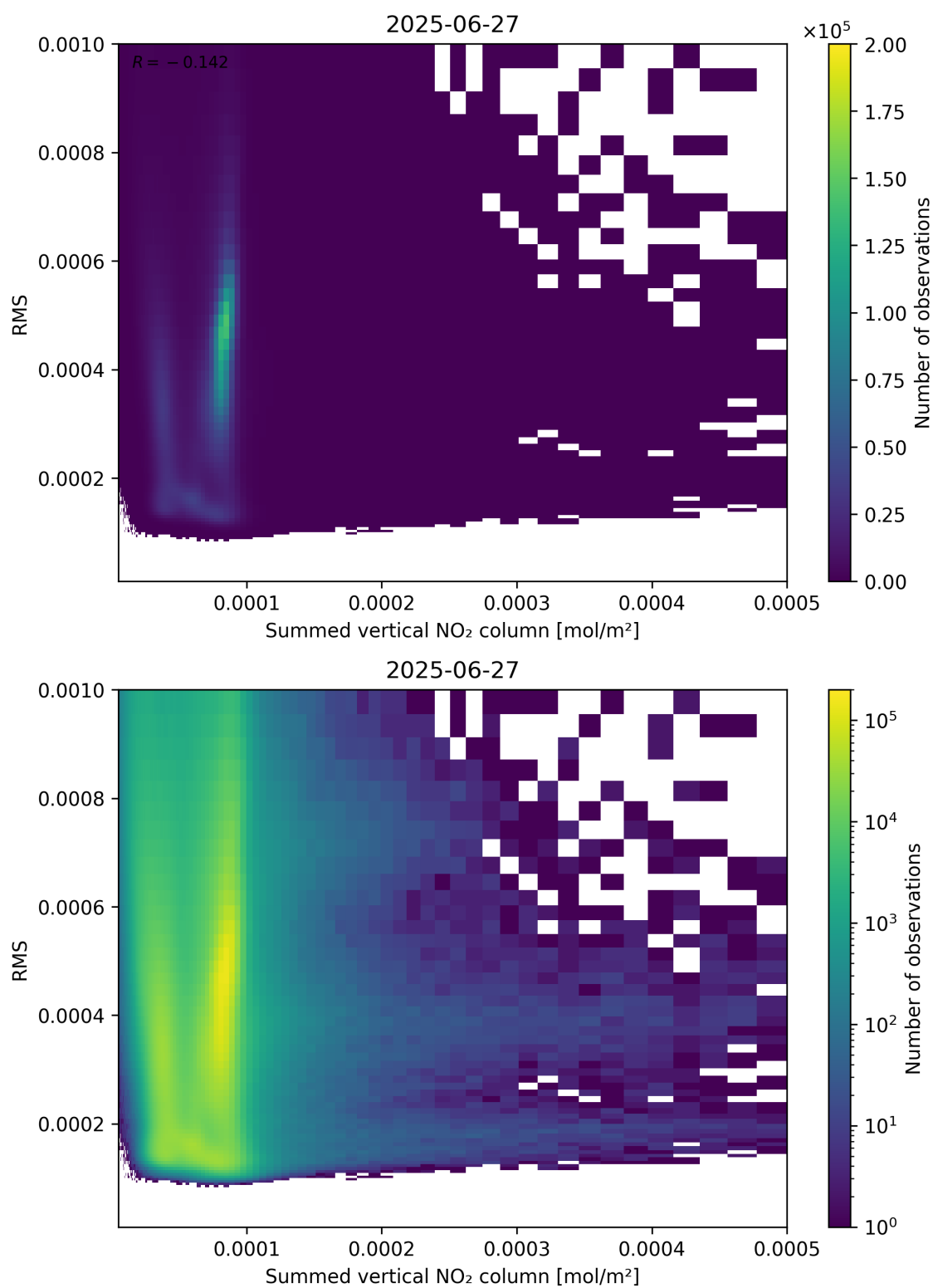
Figure 109: Scatter density plot of “Summed vertical NO 2 column” against “RMS” for 2025-06-27 to 2025-06-28.
