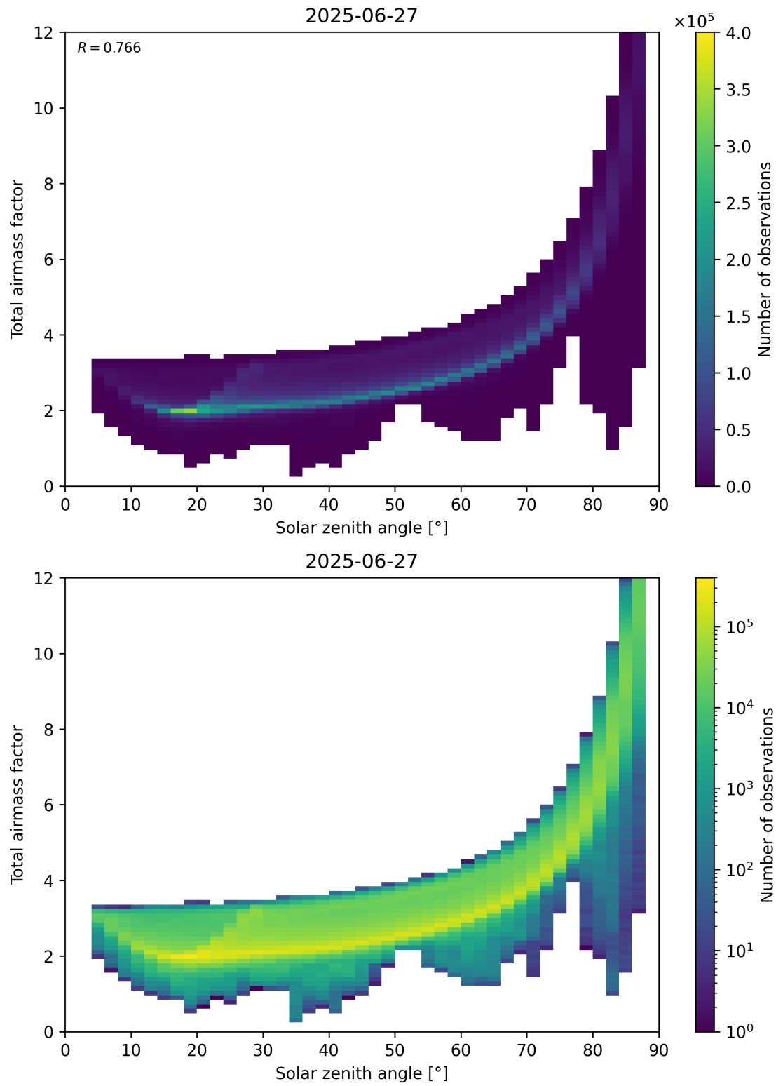
Figure 146: Scatter density plot of “Solar zenith angle” against “Total air mass factor” for 2025-06-27 to 2025-06-28.
