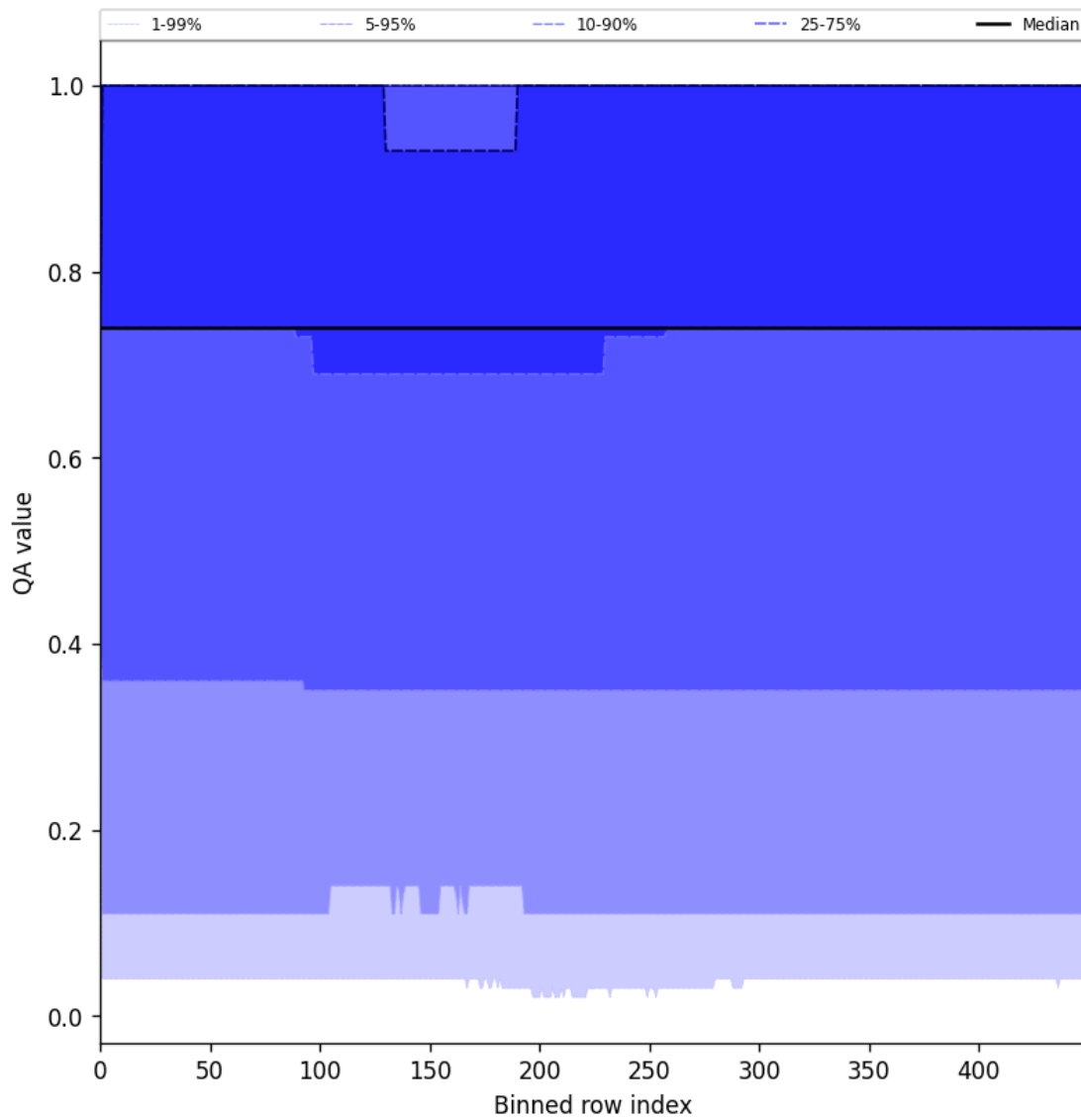
Figure 45: Along track statistics of “QA value” for 2025-06-27 to 2025-06-28
