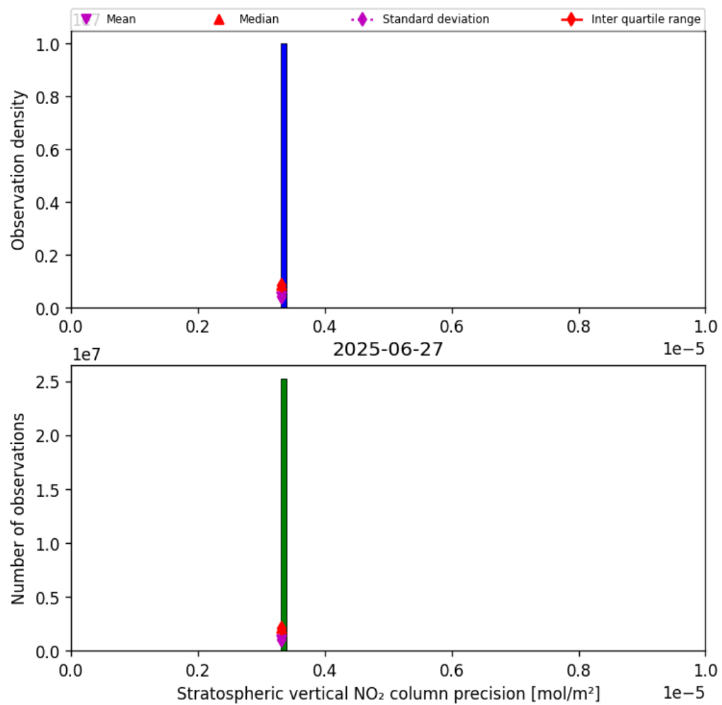
Figure 37: Histogram of “Stratospheric vertical NO 2 column precision” for 2025-06-27 to 2025-06-28
