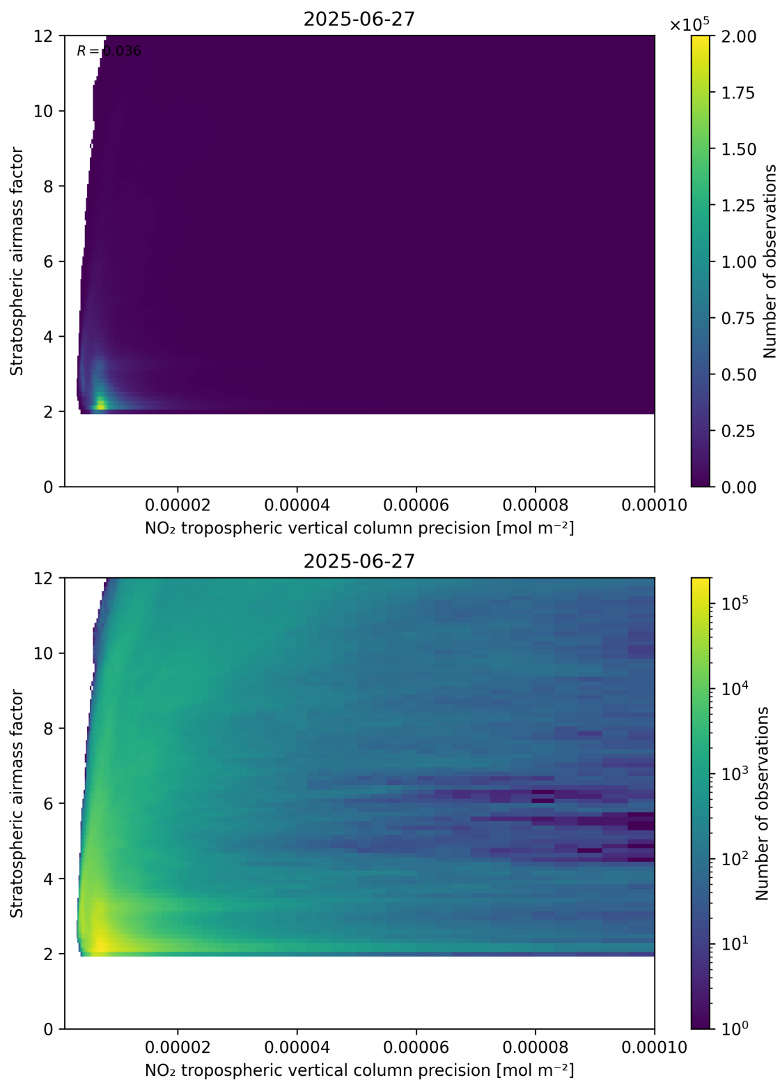
Figure 131: Scatter density plot of “NO 2 tropospheric vertical column precision” against “Stratospheric airmass factor” for 2025-06-27 to 2025-06-28.
