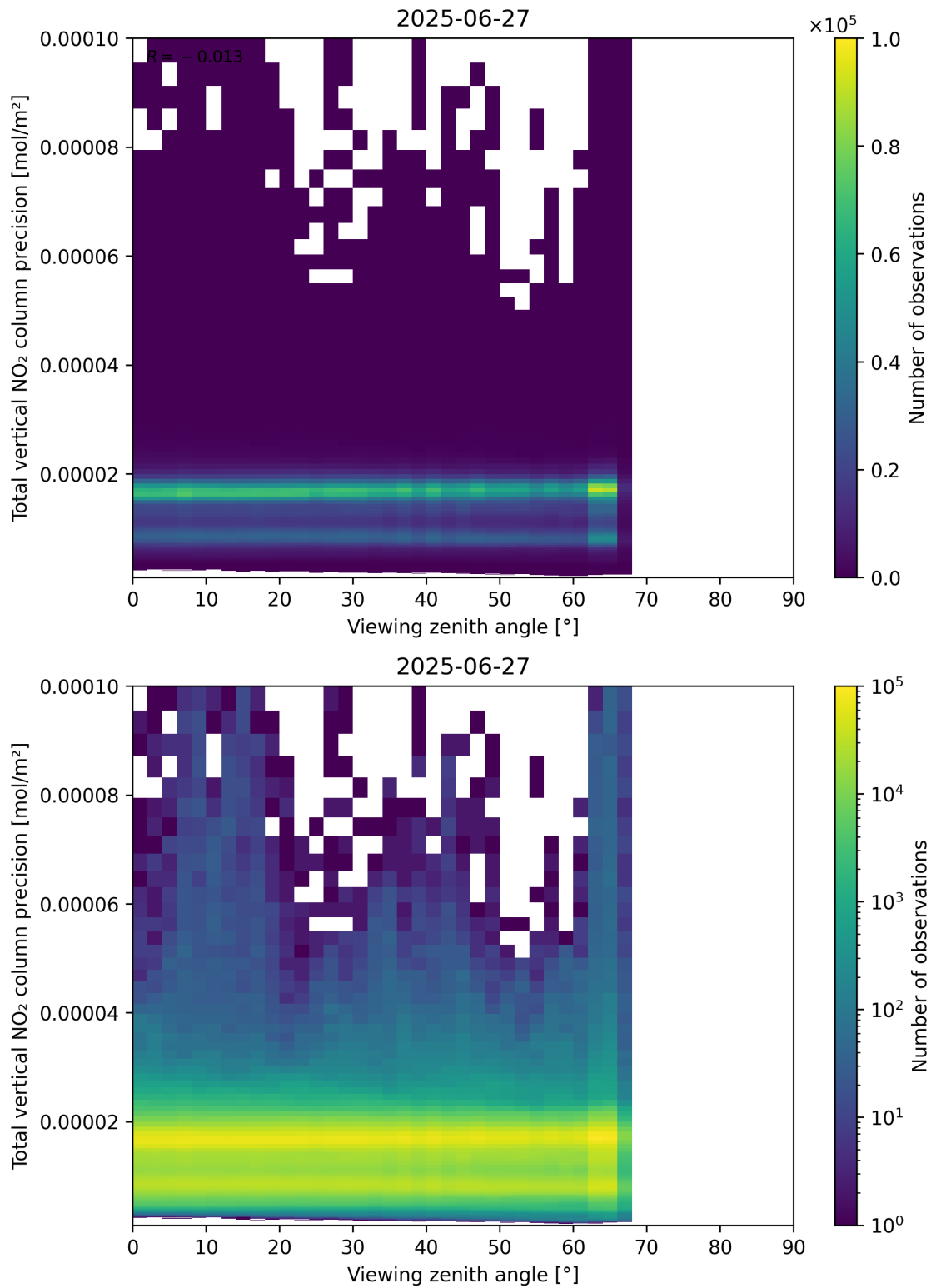
Figure 168: Scatter density plot of “Viewing zenith angle” against “Total vertical NO 2 column precision” for 2025-06-27 to 2025-06-28.
