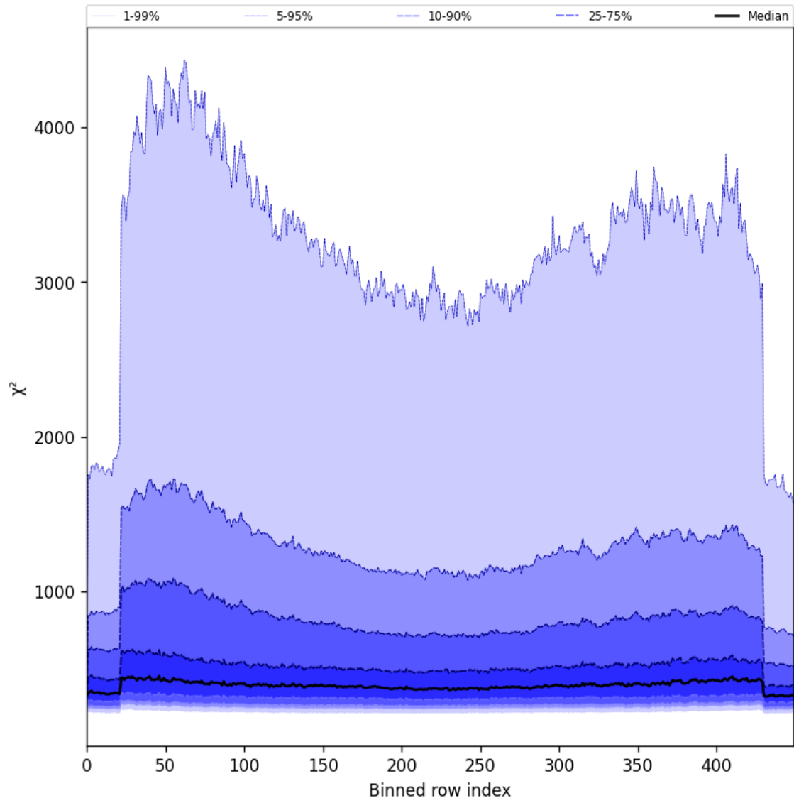
Figure 59: Along track statistics of “ \chi^2 ” for 2025-06-27 to 2025-06-28
