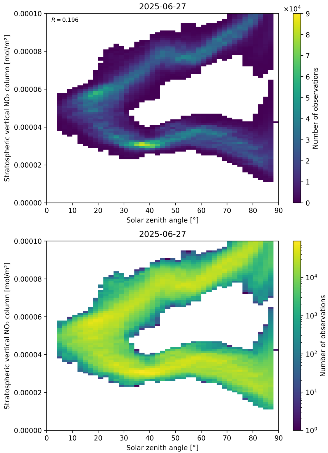
Figure 150: Scatter density plot of “Solar zenith angle” against “Stratospheric vertical NO 2 column” for 2025-06-27 to 2025-06-28.
