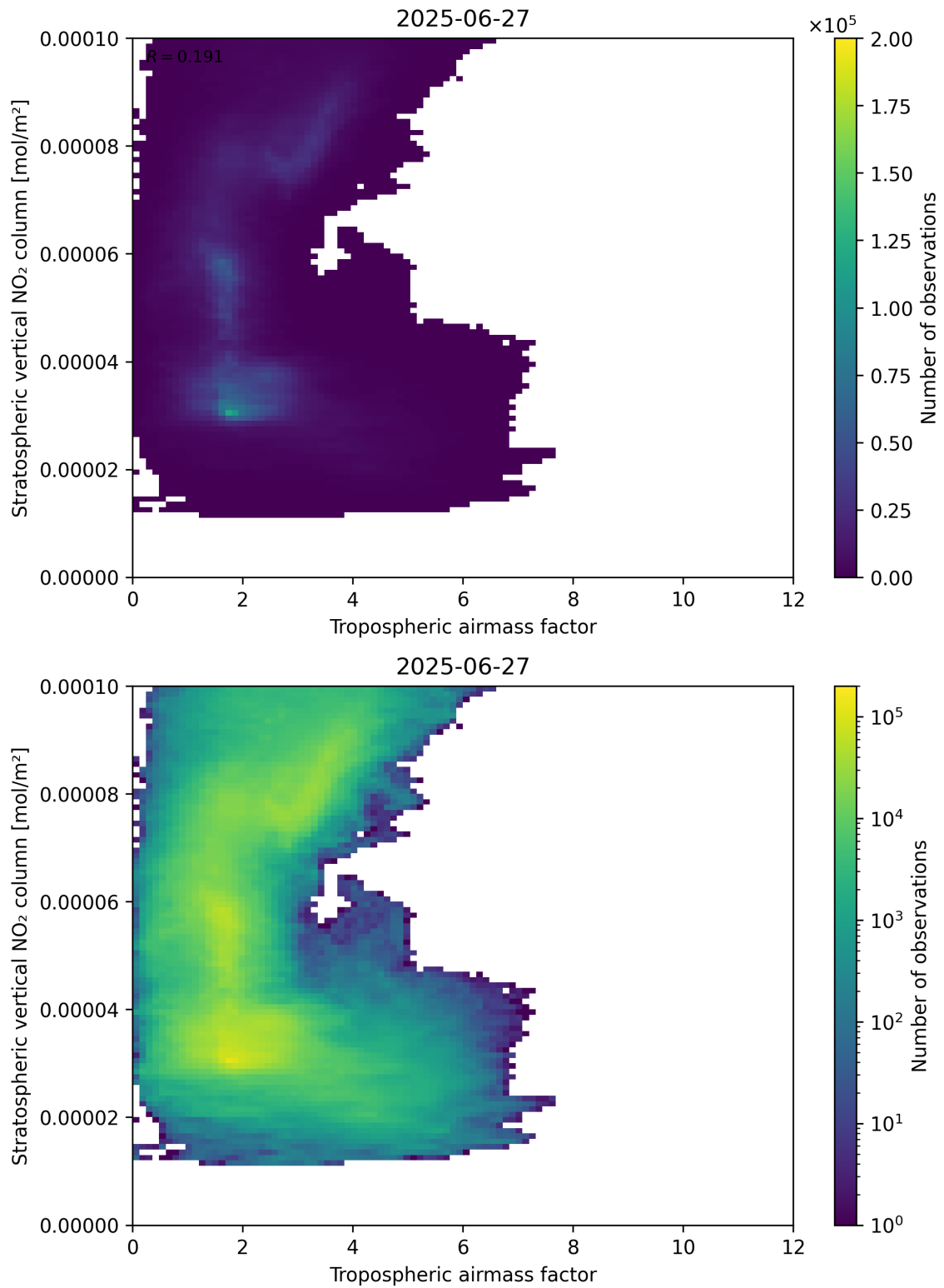
Figure 74: Scatter density plot of “Tropospheric air mass factor” against “Stratospheric vertical NO 2 column” for 2025-06-27 to 2025-06-28.
