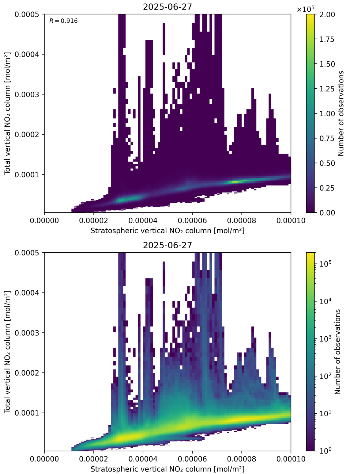
Figure 100: Scatter density plot of “Stratospheric vertical NO 2 column” against “Total vertical NO 2 column” for 2025-06-27 to 2025-06-28.
