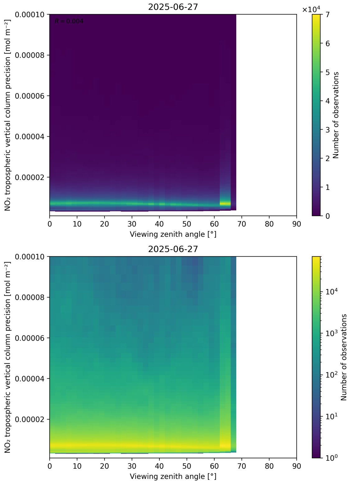
Figure 170: Scatter density plot of “Viewing zenith angle” against “NO 2 tropospheric vertical column precision” for 2025-06-27 to 2025-06-28.
