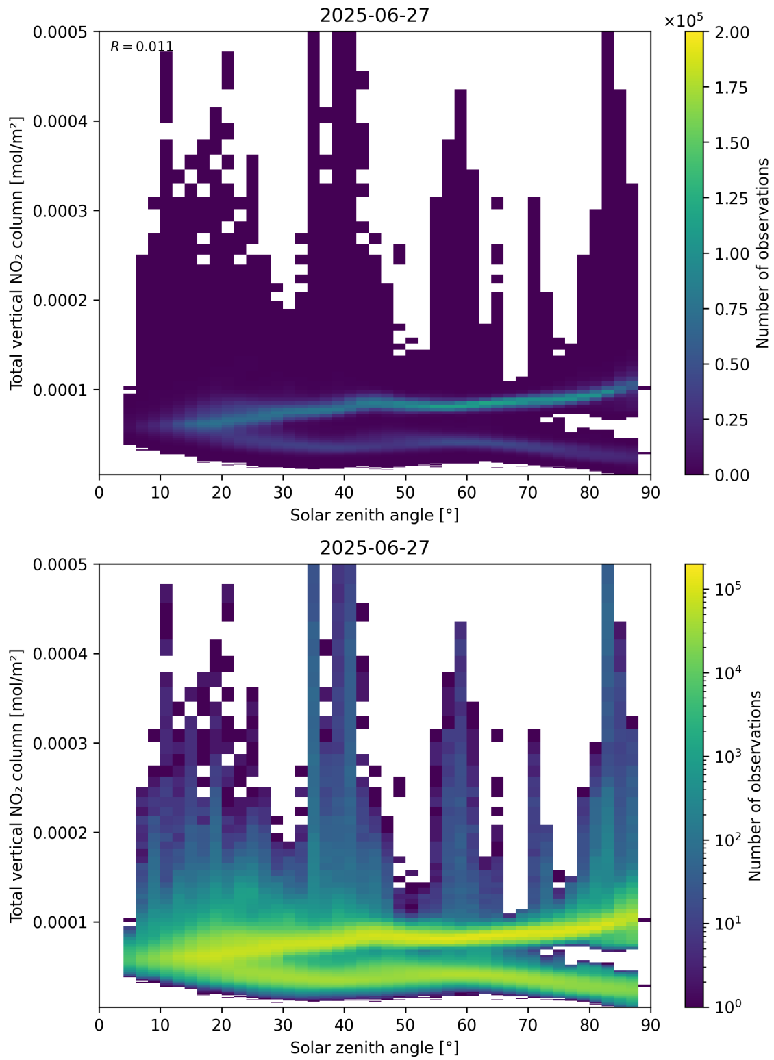
Figure 153: Scatter density plot of “Solar zenith angle” against “Total vertical NO 2 column” for 2025-06-27 to 2025-06-28.
