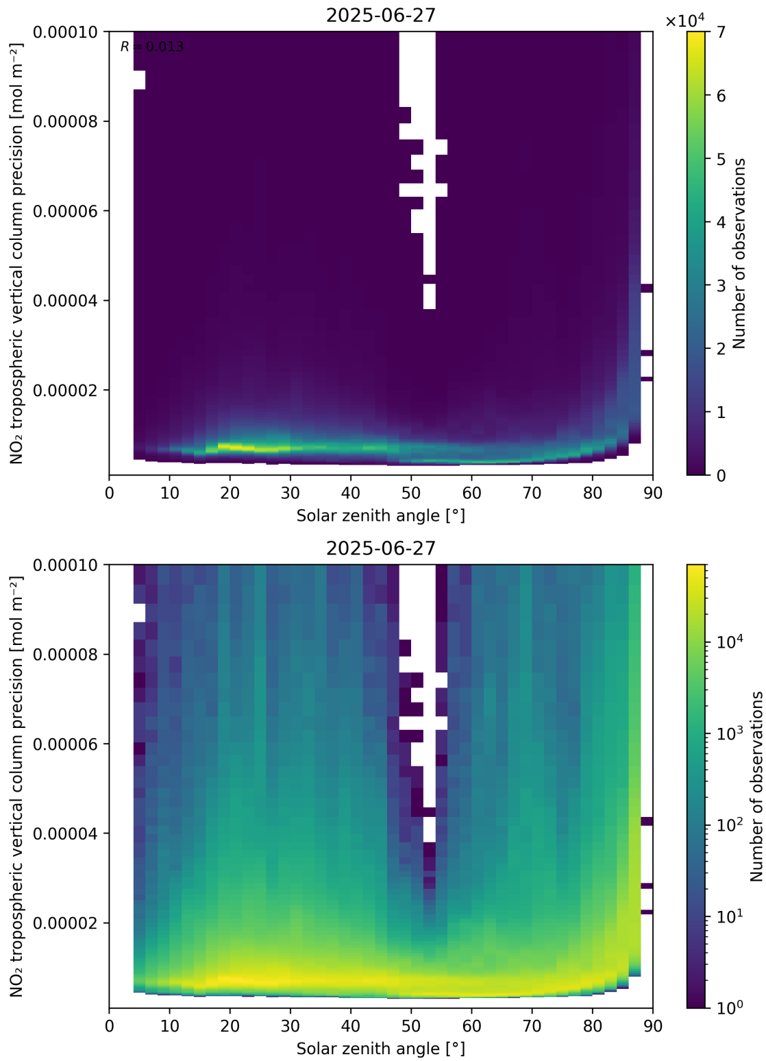
Figure 156: Scatter density plot of “Solar zenith angle” against “NO 2 tropospheric vertical column precision” for 2025-06-27 to 2025-06-28.
