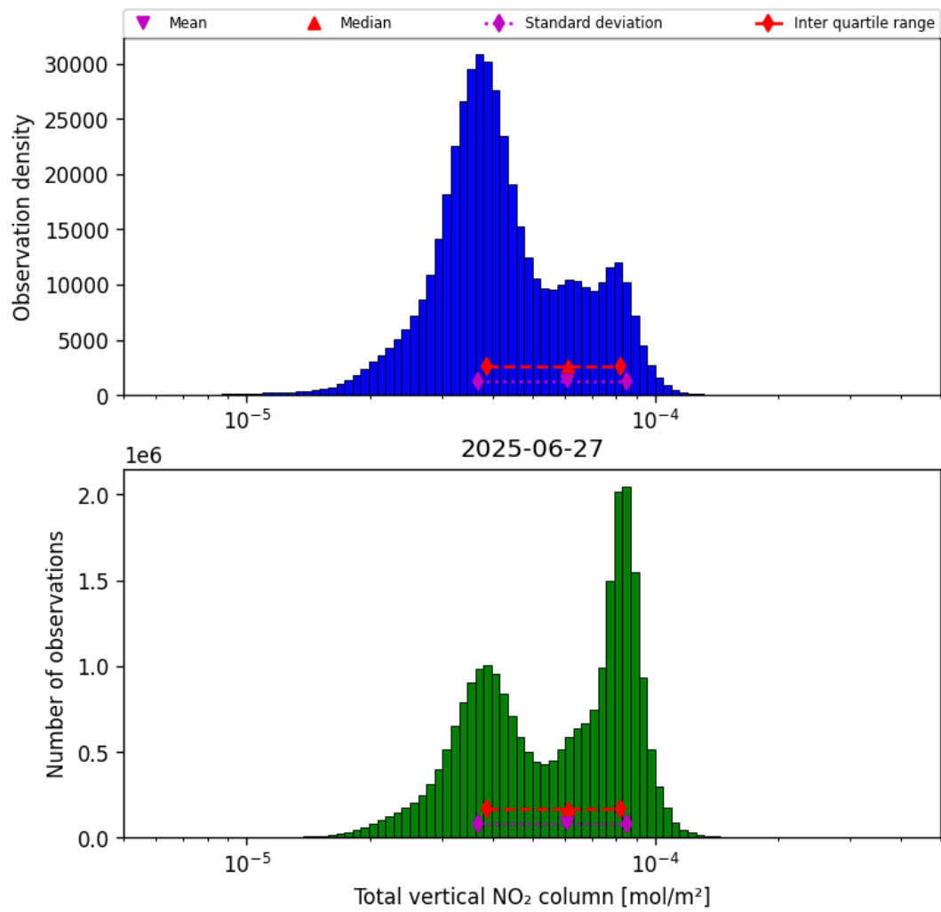
Figure 38: Histogram of “Total vertical NO 2 column” for 2025-06-27 to 2025-06-28
