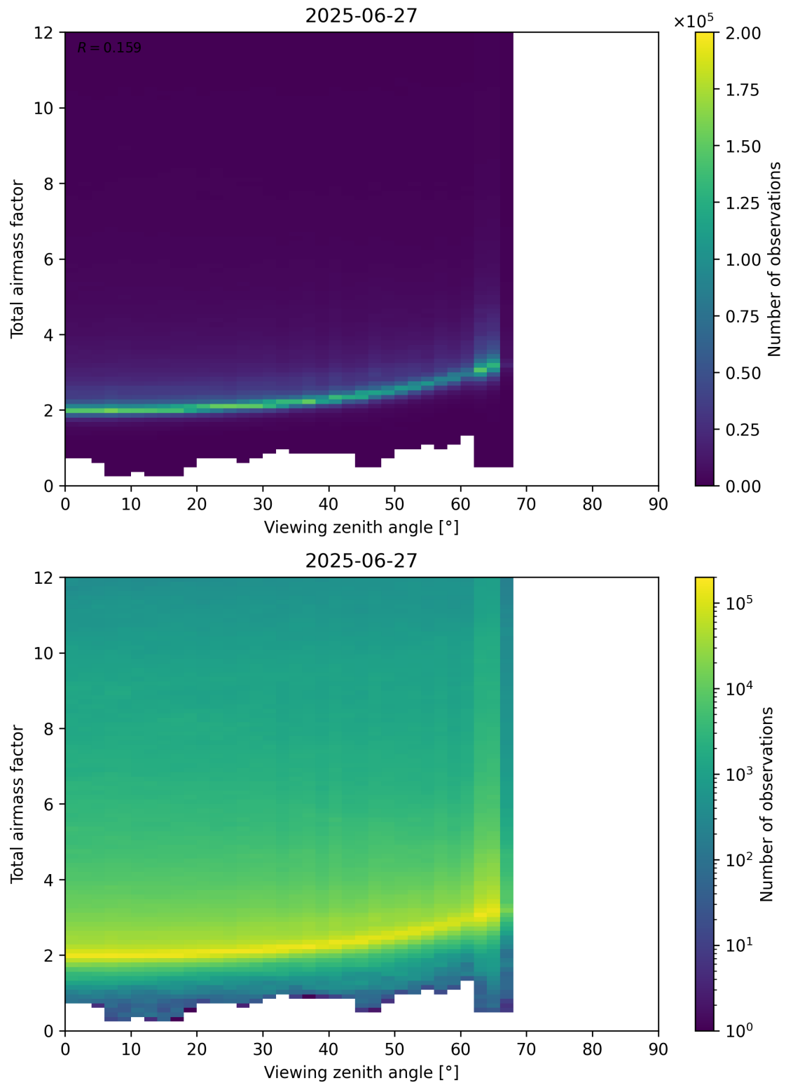
Figure 160: Scatter density plot of “Viewing zenith angle” against “Total airmass factor” for 2025-06-27 to 2025-06-28.
