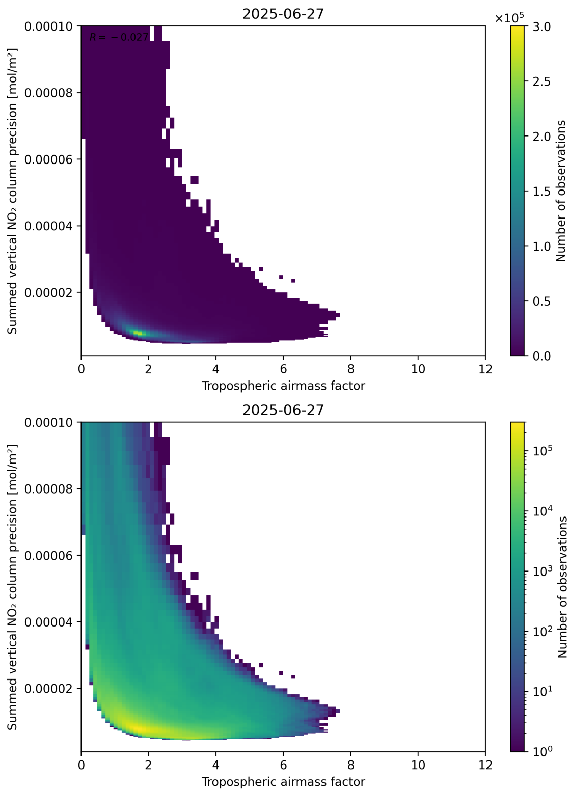
Figure 76: Scatter density plot of “Tropospheric air mass factor” against “Summed vertical NO 2 column precision” for 2025-06-27 to 2025-06-28.
