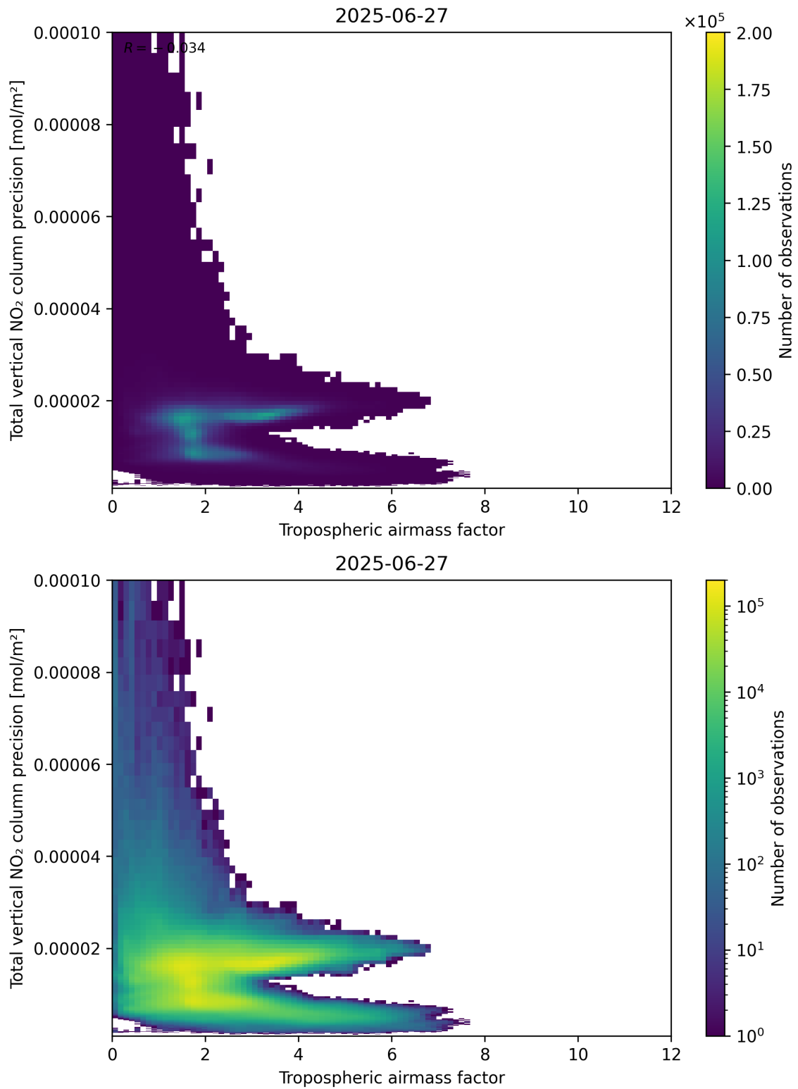
Figure 78: Scatter density plot of “Tropospheric airmass factor” against “Total vertical NO 2 column precision” for 2025-06-27 to 2025-06-28.
