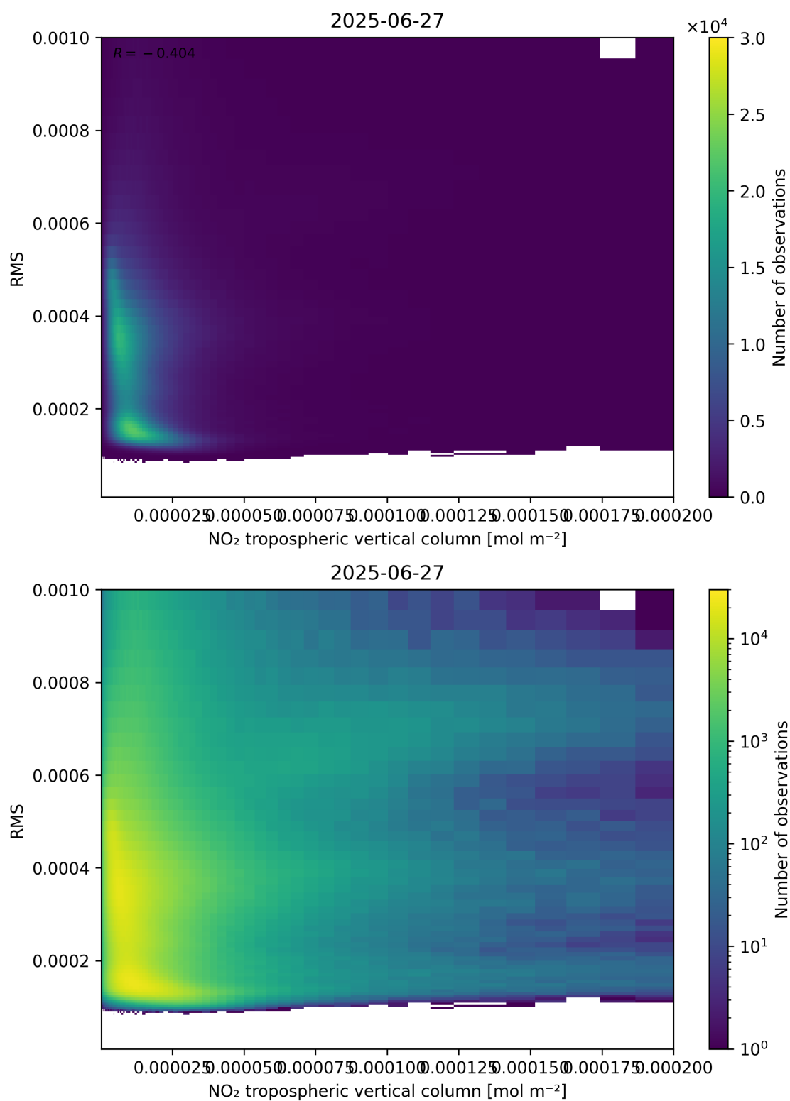
Figure 142: Scatter density plot of “NO 2 tropospheric vertical column” against “RMS” for 2025-06-27 to 2025-06-28.
