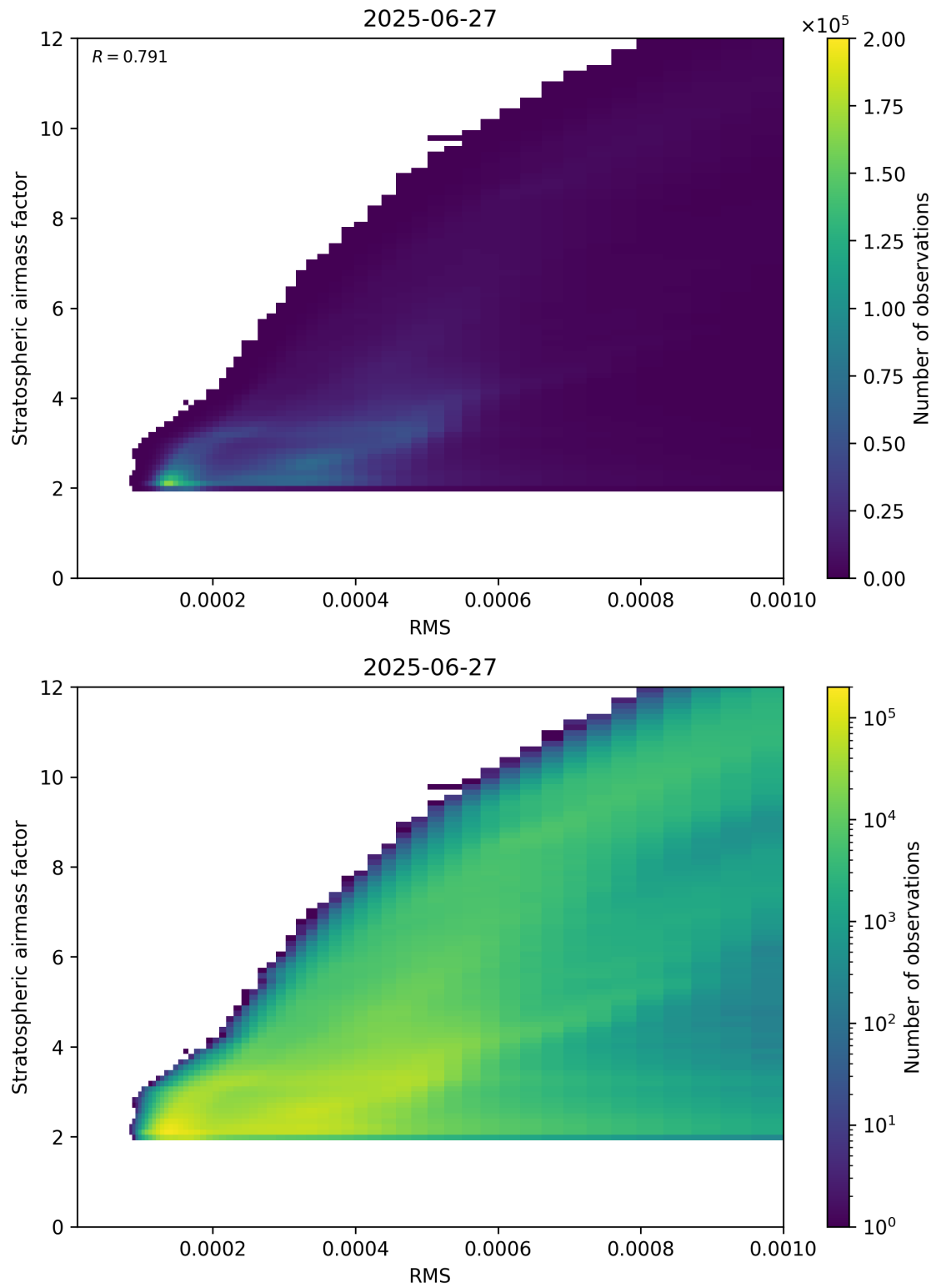
Figure 144: Scatter density plot of “RMS” against “Stratospheric airmass factor” for 2025-06-27 to 2025-06-28.
