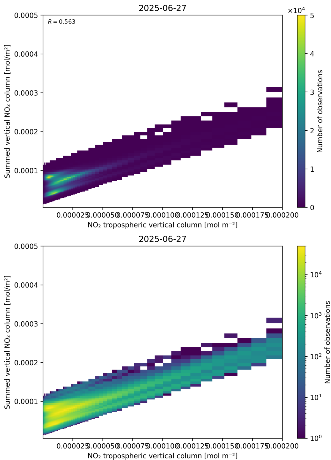
Figure 126: Scatter density plot of “NO 2 tropospheric vertical column” against “Summed vertical NO 2 column” for 2025-06-27 to 2025-06-28.
