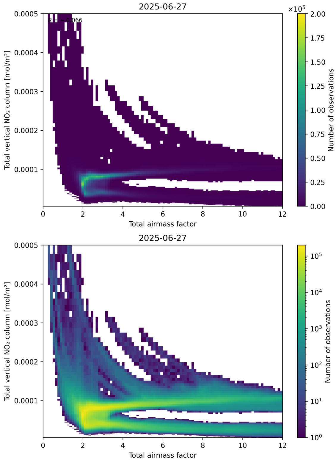
Figure 67: Scatter density plot of “Total air mass factor” against “Total vertical NO 2 column” for 2025-06-27 to 2025-06-28.
