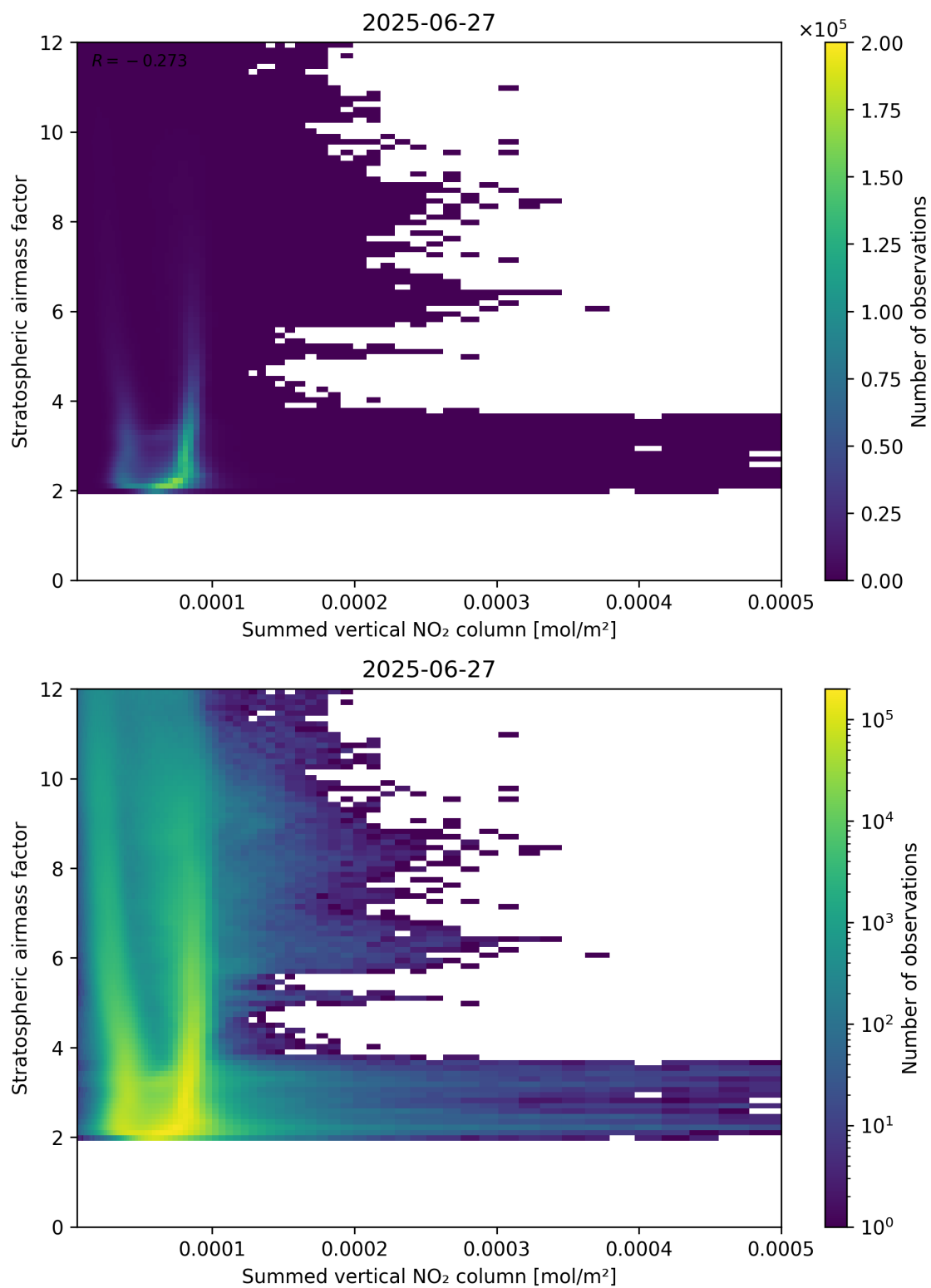
Figure 103: Scatter density plot of “Summed vertical NO 2 column” against “Stratospheric airmass factor” for 2025-06-27 to 2025-06-28.
