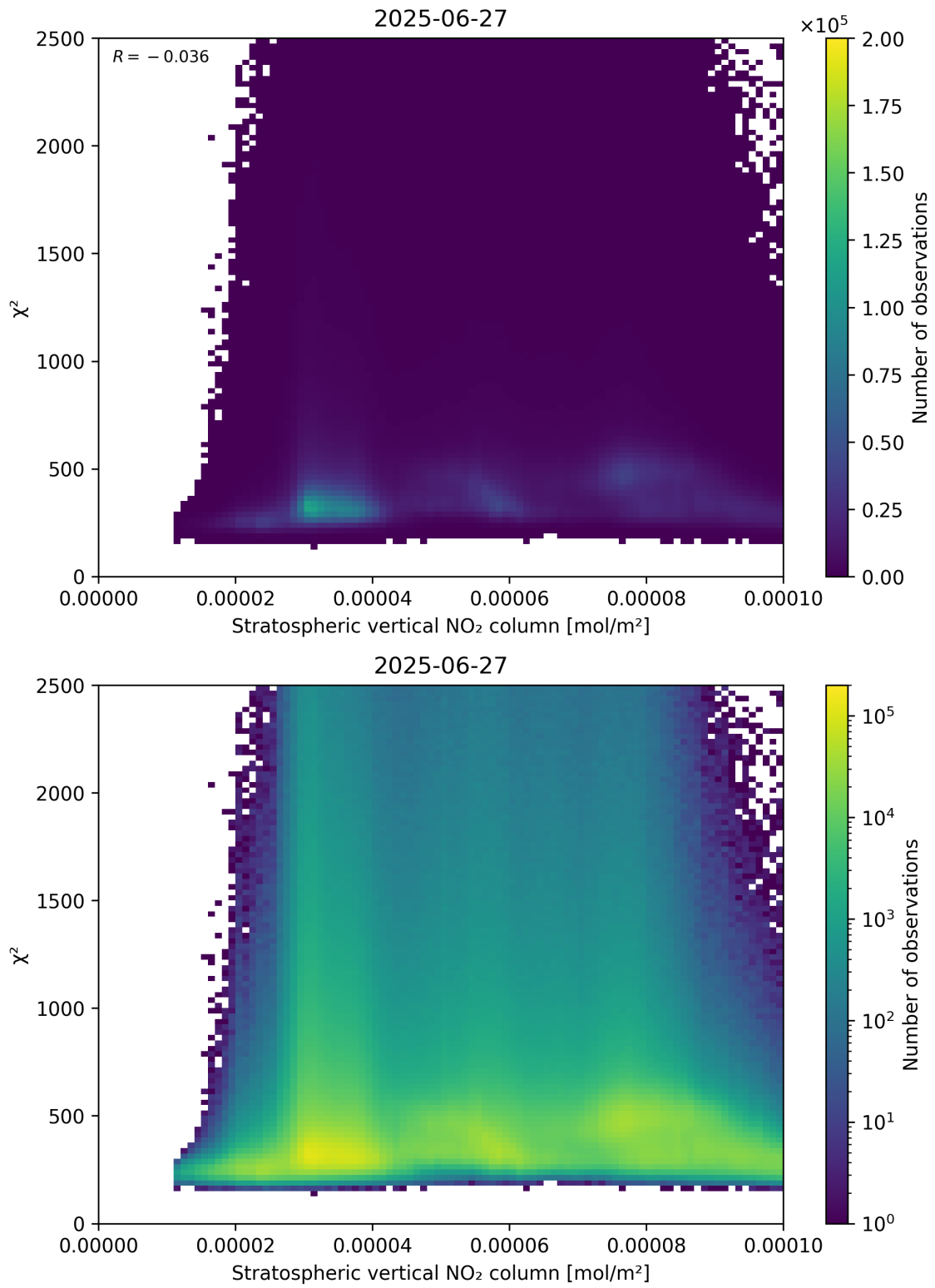
Figure 97: Scatter density plot of “Stratospheric vertical NO 2 column” against “ \chi^2 ” for 2025-06-27 to 2025-06-28.
