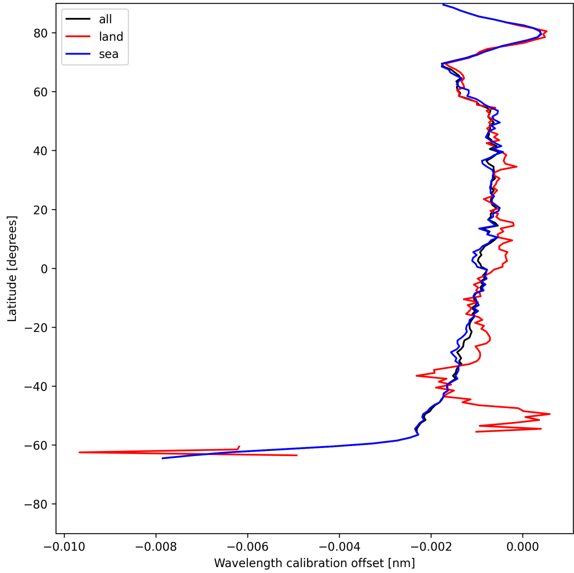
Figure 18: Zonal average of “Wavelength calibration offset” for 2025-06-27 to 2025-06-28.
