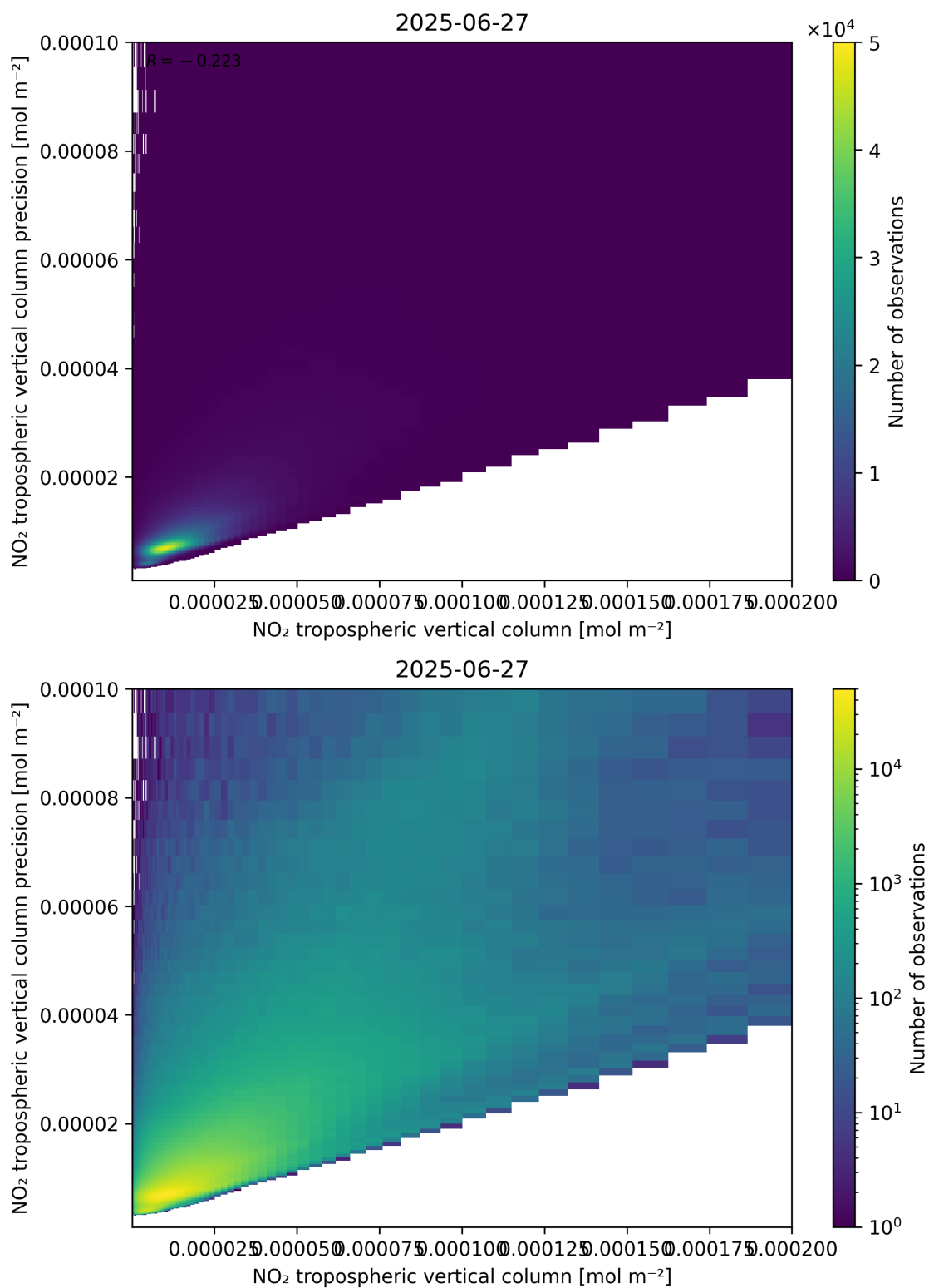
Figure 130: Scatter density plot of “NO 2 tropospheric vertical column” against “NO 2 tropospheric vertical column precision” for 2025-06-27 to 2025-06-28.
