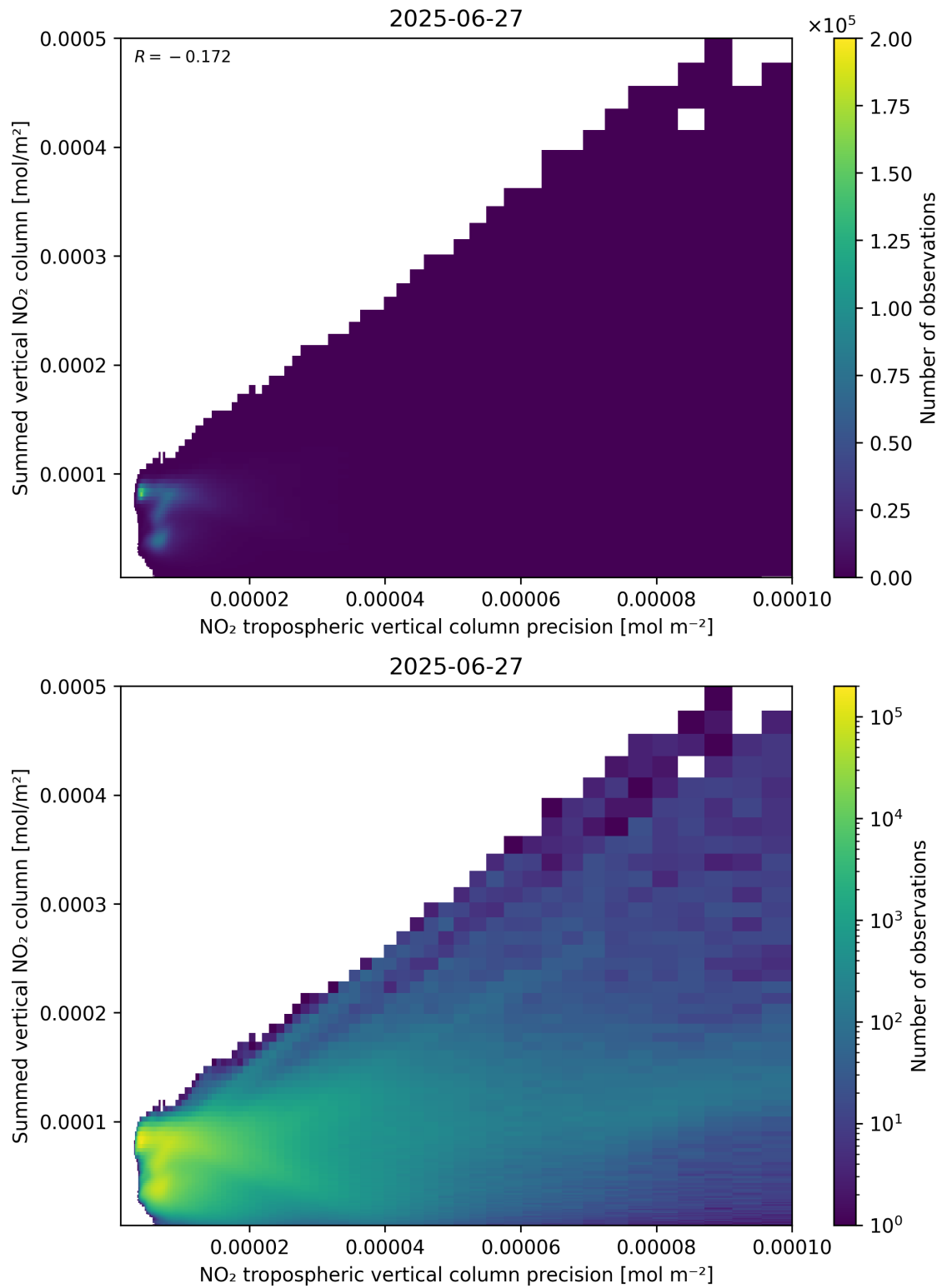
Figure 136: Scatter density plot of “NO 2 tropospheric vertical column precision” against “Summed vertical NO 2 column” for 2025-06-27 to 2025-06-28.
