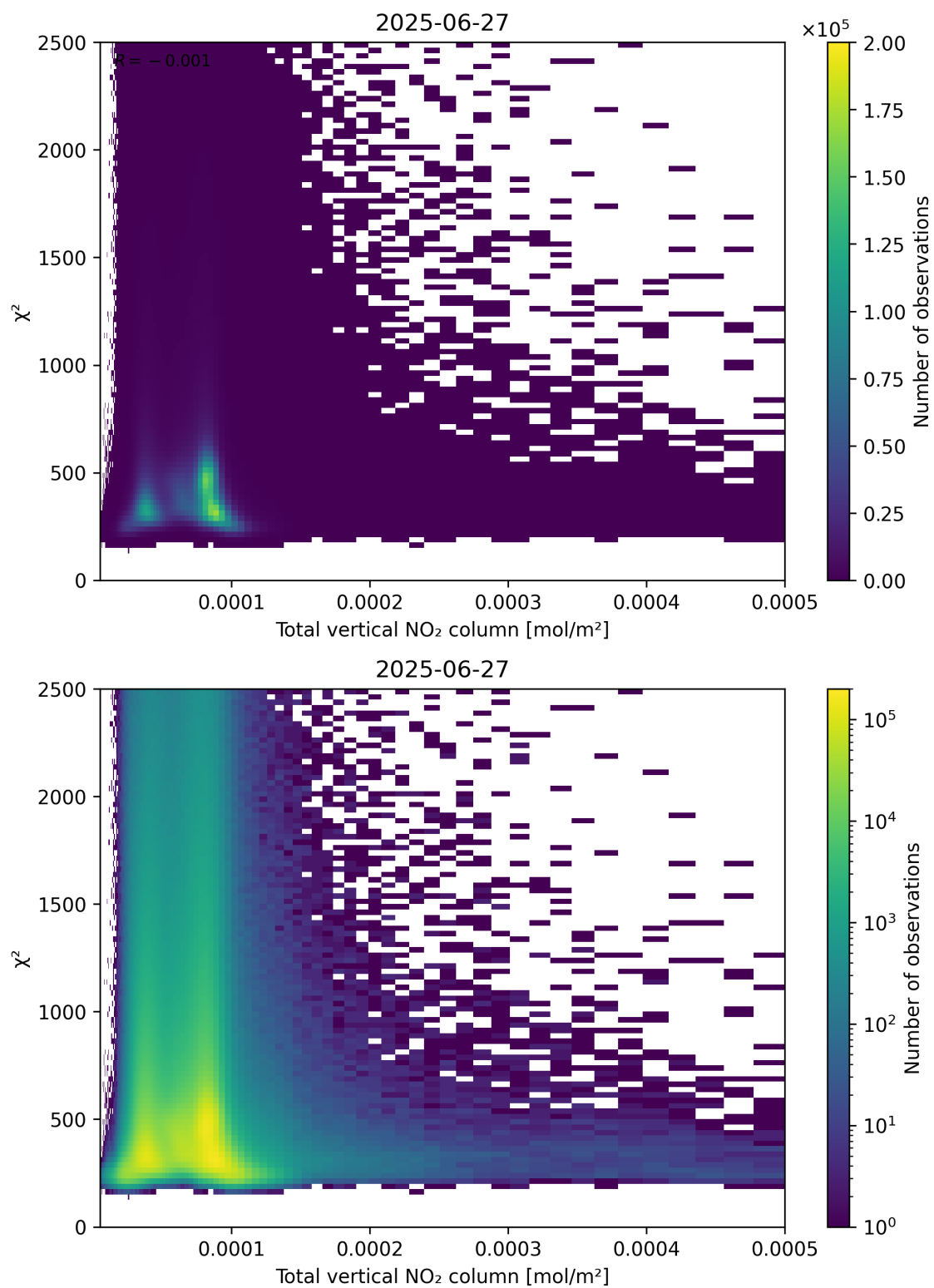
Figure 111: Scatter density plot of “Total vertical NO 2 column” against “ \chi^2 ” for 2025-06-27 to 2025-06-28.
