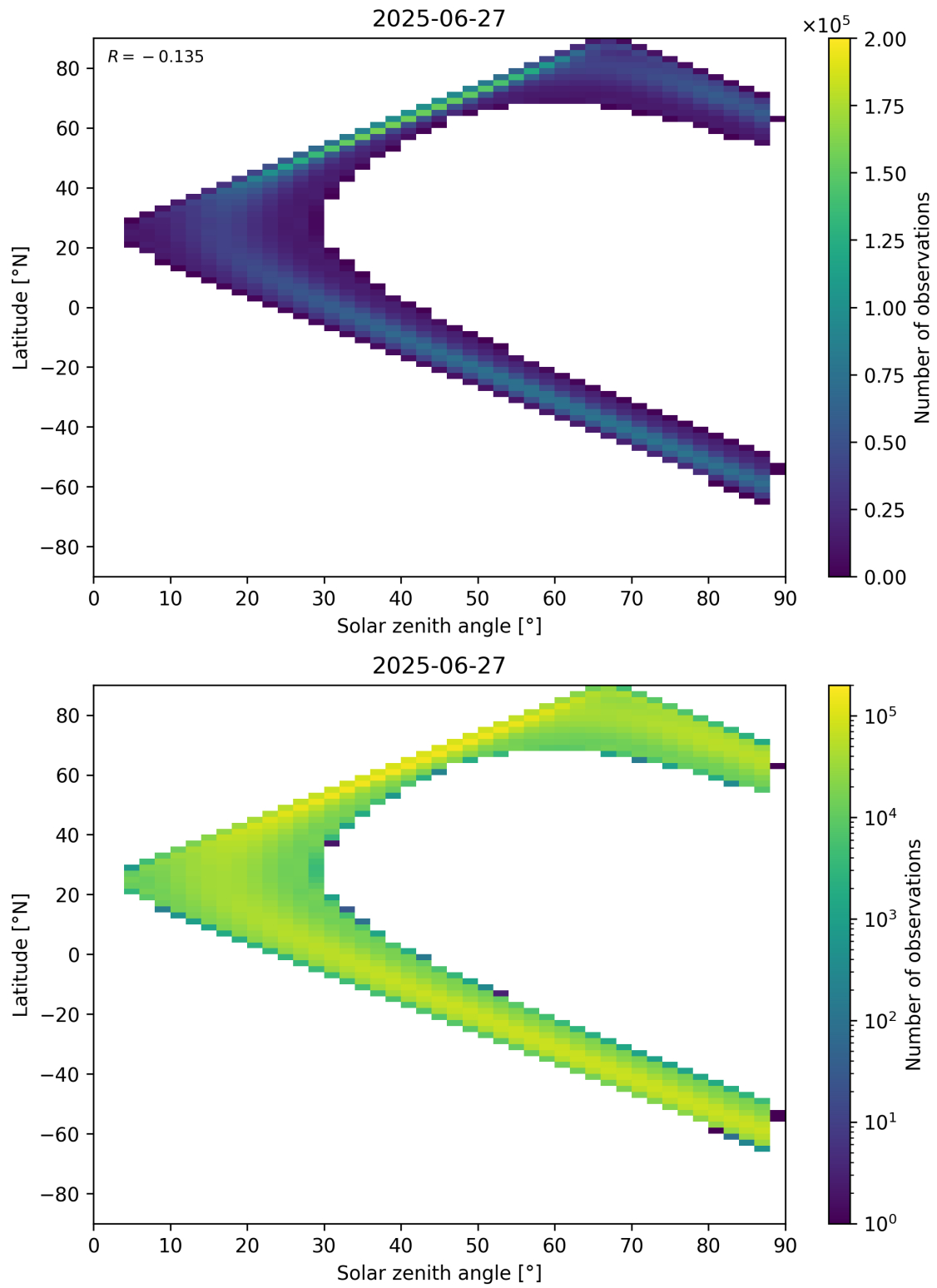
Figure 149: Scatter density plot of “Solar zenith angle” against “Latitude” for 2025-06-27 to 2025-06-28.
