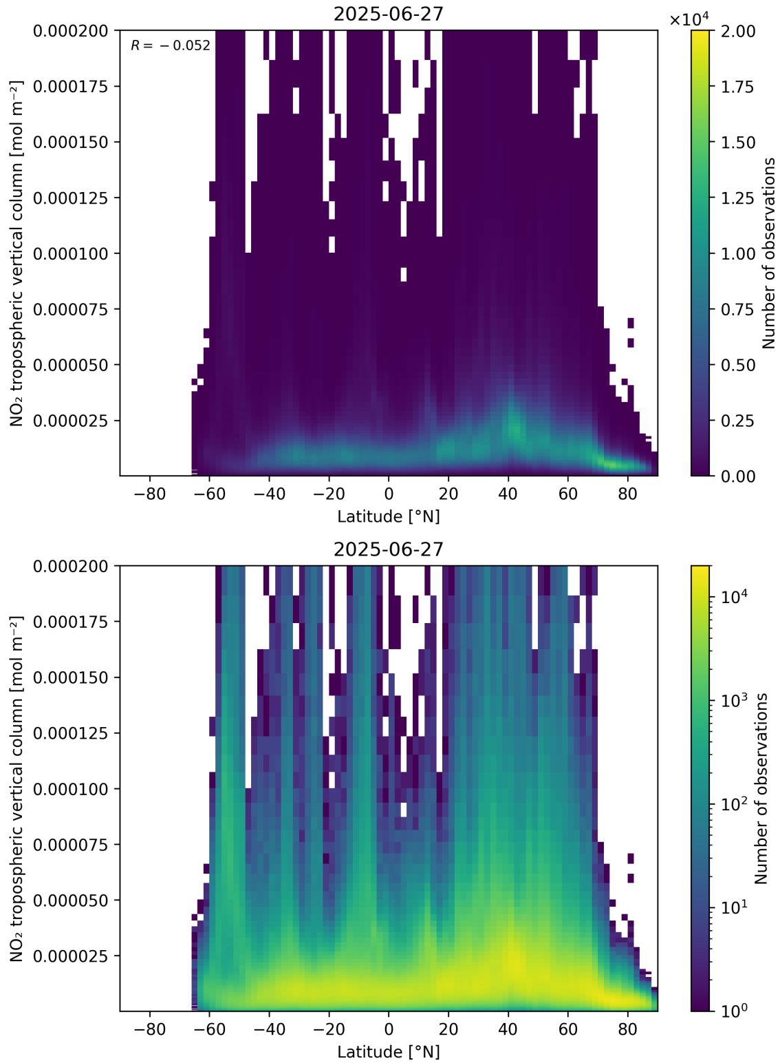
Figure 92: Scatter density plot of “Latitude” against “NO 2 tropospheric vertical column” for 2025-06-27 to 2025-06-28.
