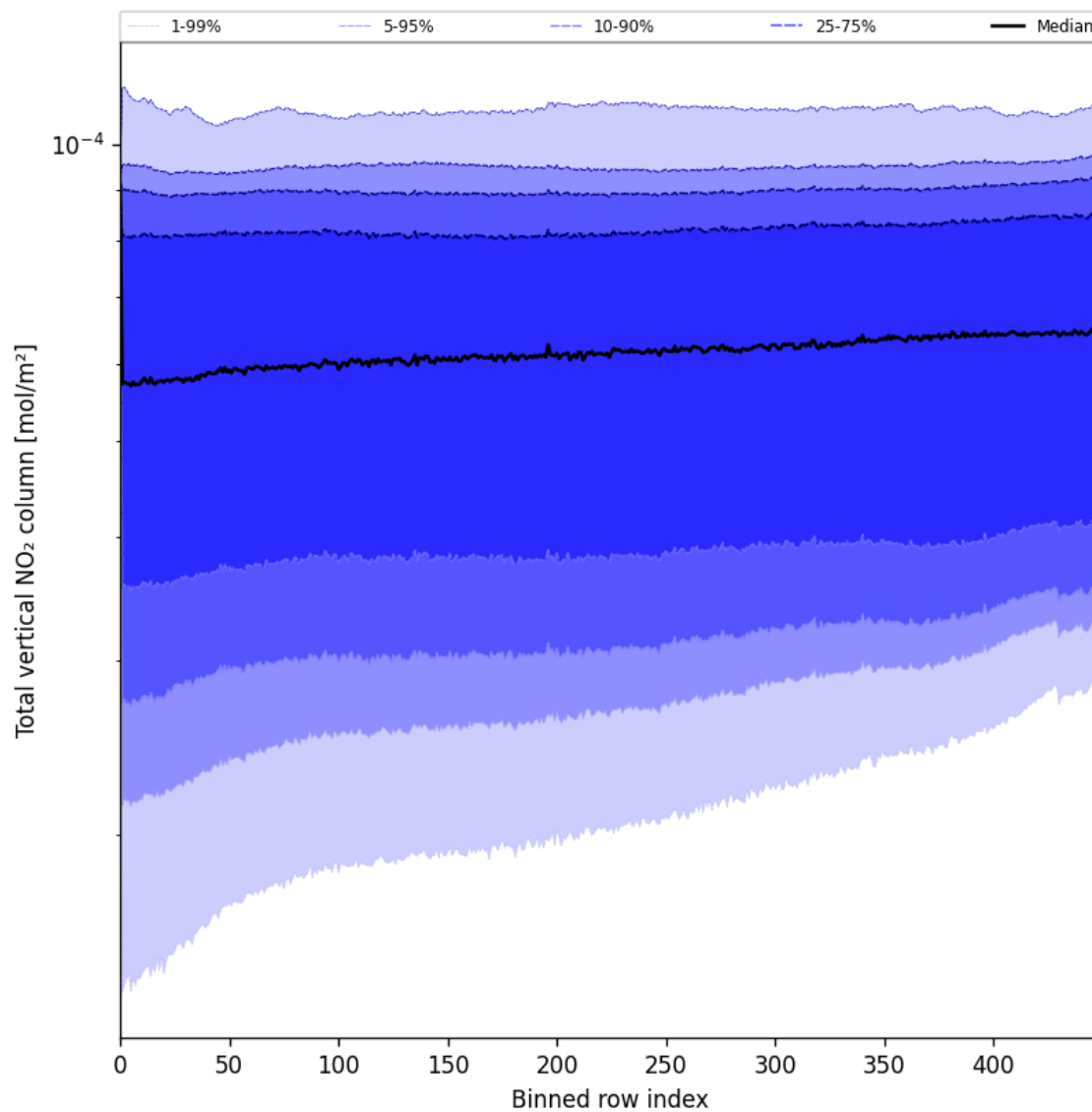
Figure 55: Along track statistics of “Total vertical NO 2 column” for 2025-06-27 to 2025-06-28
