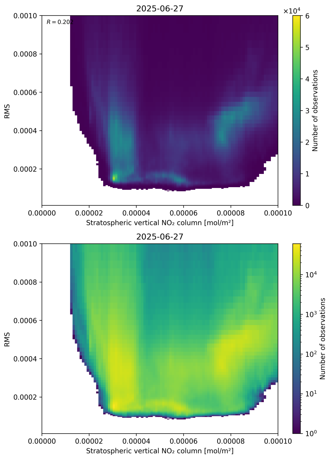
Figure 102: Scatter density plot of “Stratospheric vertical NO 2 column” against “RMS” for 2025-06-27 to 2025-06-28.
