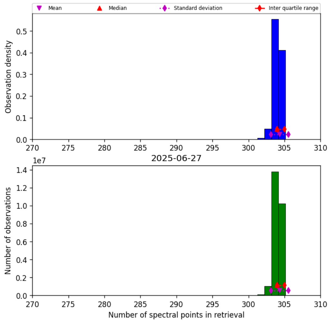
Figure 33: Histogram of “Number of spectral points in retrieval” for 2025-06-27 to 2025-06-28
