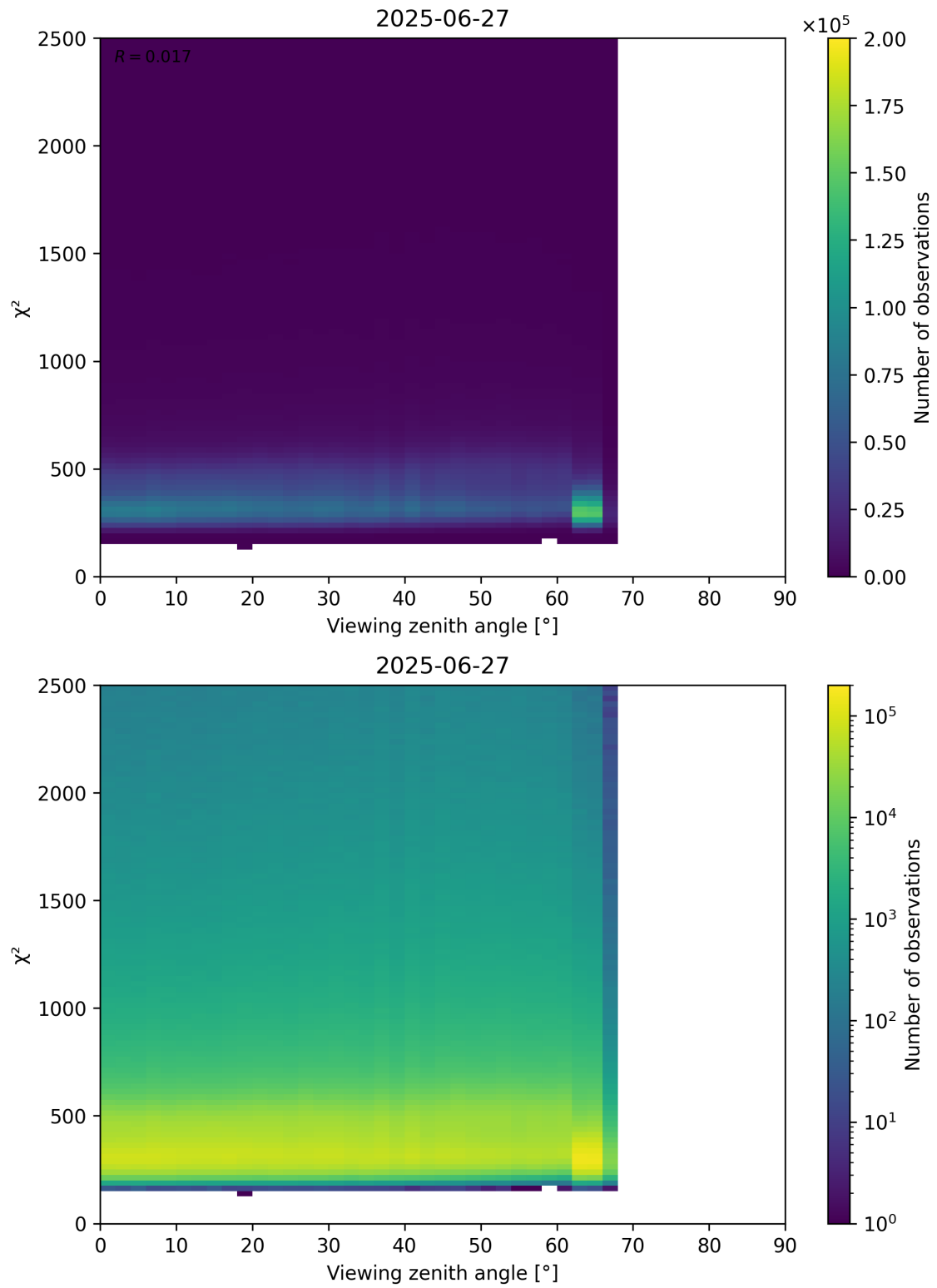
Figure 162: Scatter density plot of “Viewing zenith angle” against “ \chi^2 ” for 2025-06-27 to 2025-06-28.
