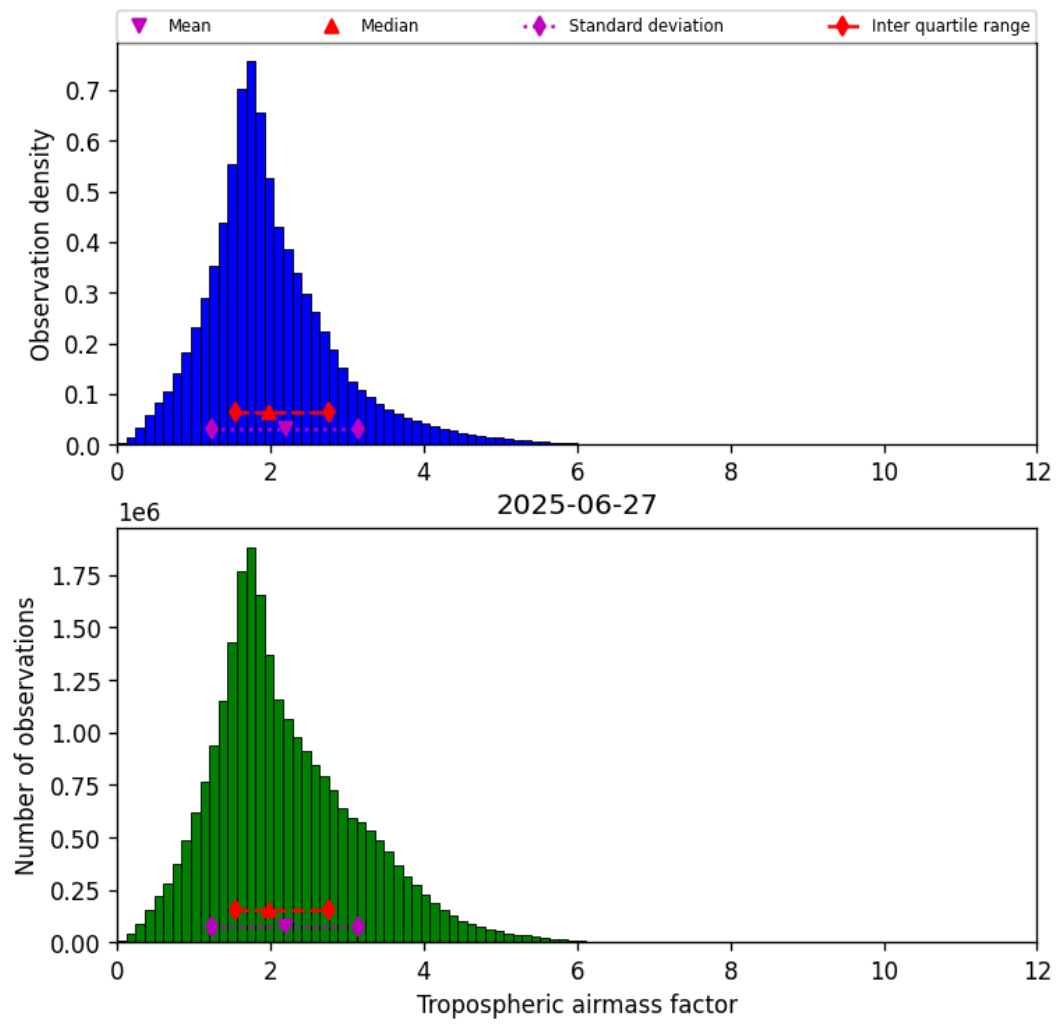
Figure 31: Histogram of “Tropospheric airmass factor” for 2025-06-27 to 2025-06-28
