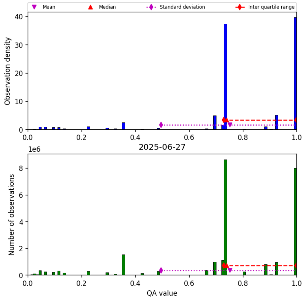
Figure 28: Histogram of “QA value” for 2025-06-27 to 2025-06-28
