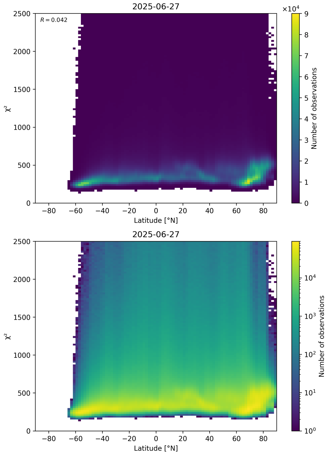
Figure 86: Scatter density plot of “Latitude” against “ \chi^2 ” for 2025-06-27 to 2025-06-28.
