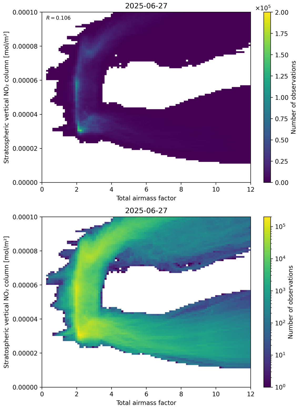
Figure 64: Scatter density plot of “Total airmass factor” against “Stratospheric vertical NO 2 column” for 2025-06-27 to 2025-06-28.
