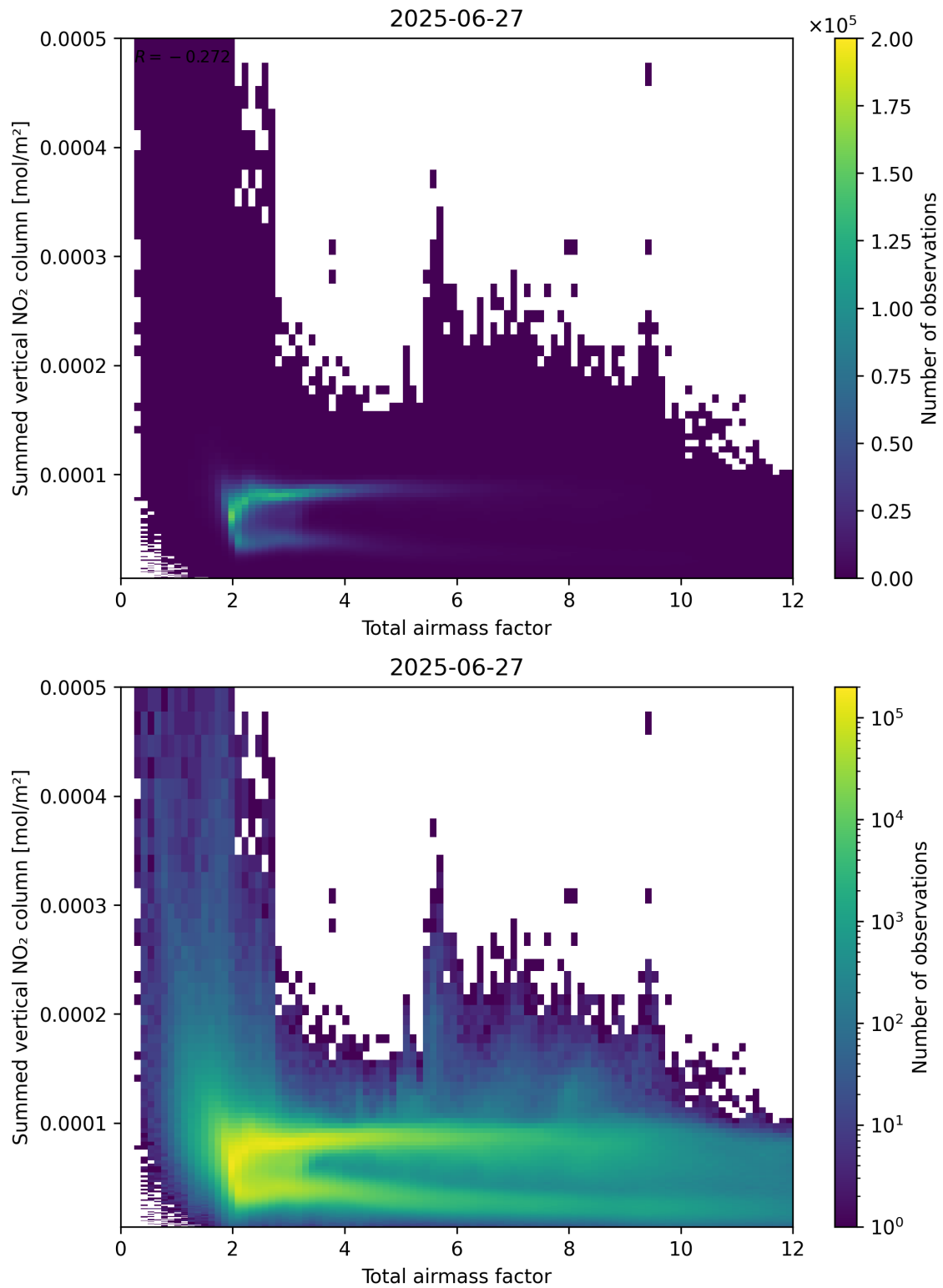
Figure 65: Scatter density plot of “Total airmass factor” against “Summed vertical NO 2 column” for 2025-06-27 to 2025-06-28.
