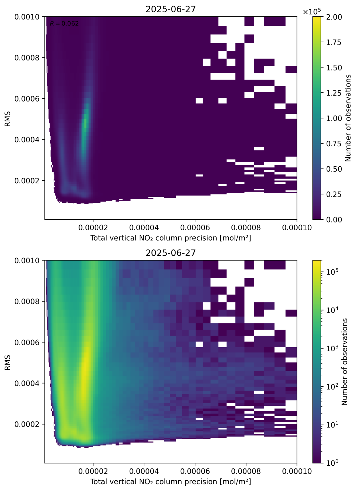
Figure 119: Scatter density plot of “Total vertical NO 2 column precision” against “RMS” for 2025-06-27 to 2025-06-28.
