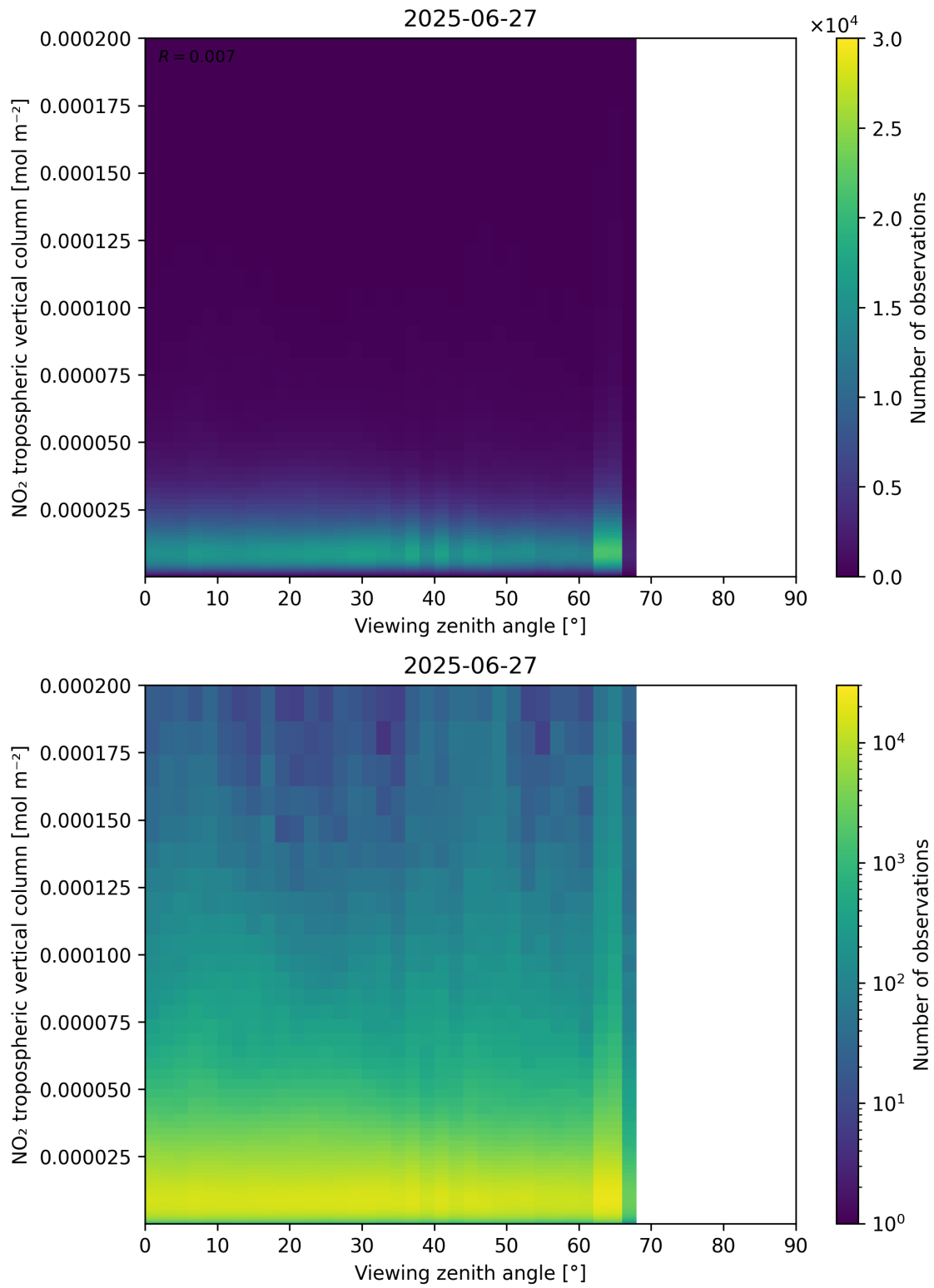
Figure 169: Scatter density plot of “Viewing zenith angle” against “NO 2 tropospheric vertical column” for 2025-06-27 to 2025-06-28.
