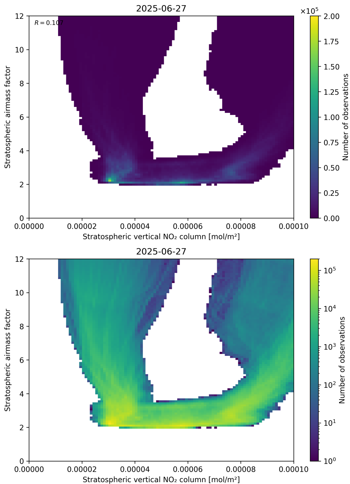
Figure 96: Scatter density plot of “Stratospheric vertical NO 2 column” against “Stratospheric airmass factor” for 2025-06-27 to 2025-06-28.
