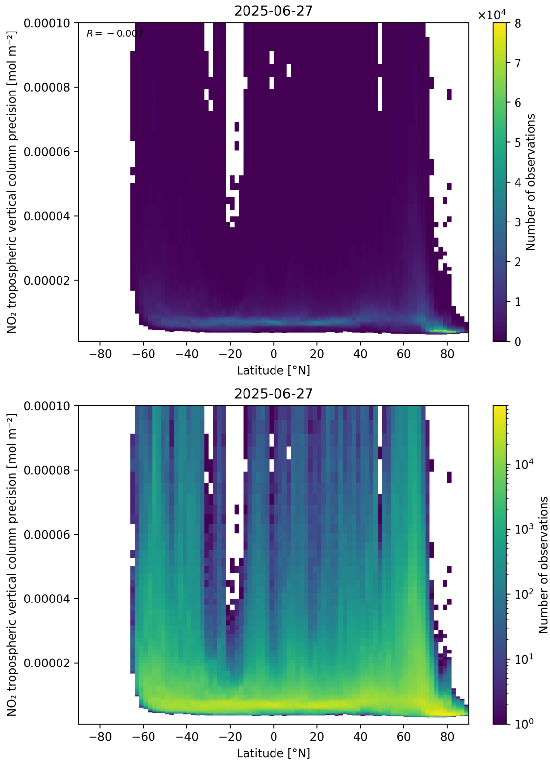
Figure 93: Scatter density plot of “Latitude” against “NO 2 tropospheric vertical column precision” for 2025-06-27 to 2025-06-28.
