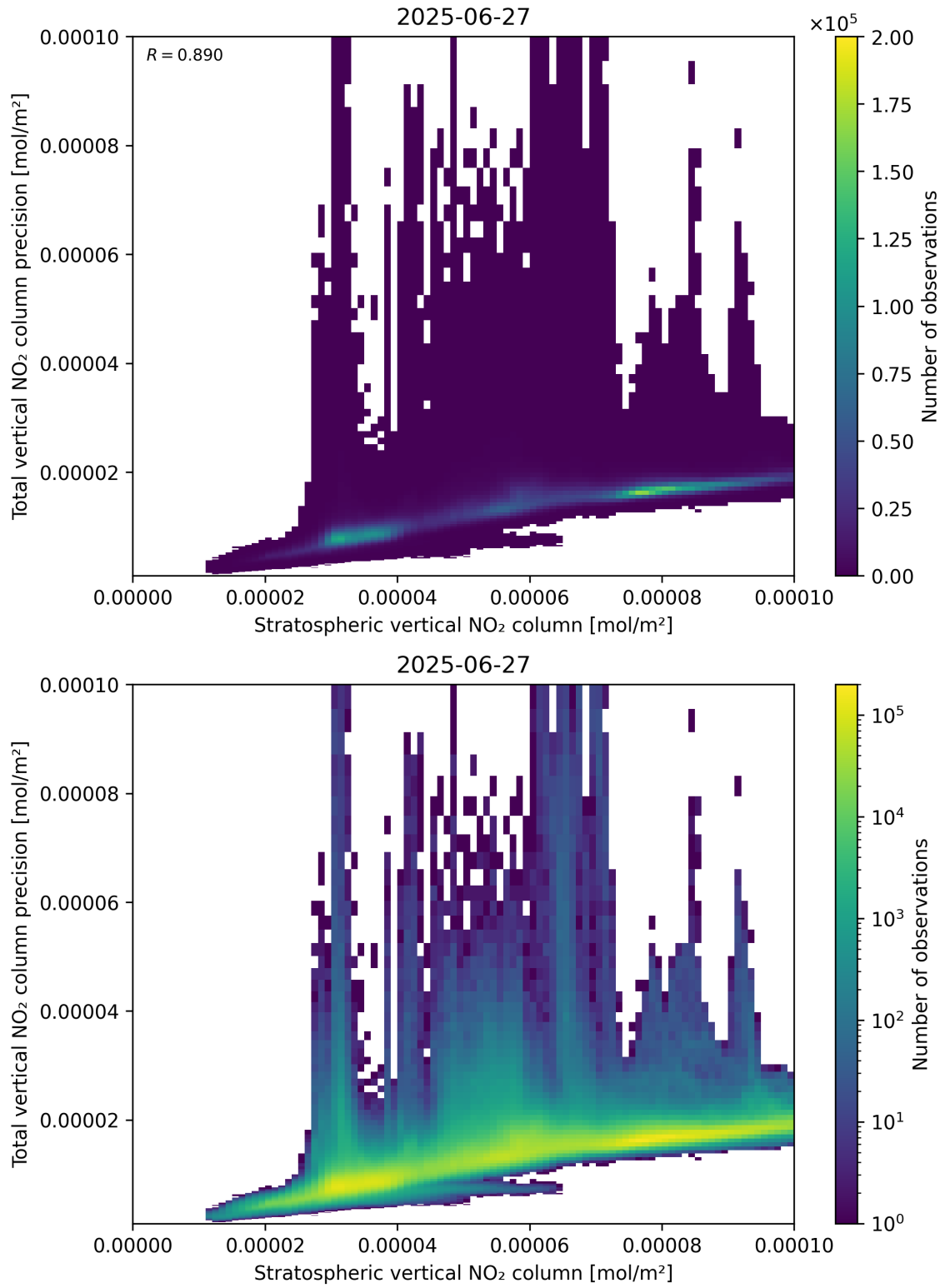
Figure 101: Scatter density plot of “Stratospheric vertical NO 2 column” against “Total vertical NO 2 column precision” for 2025-06-27 to 2025-06-28.
