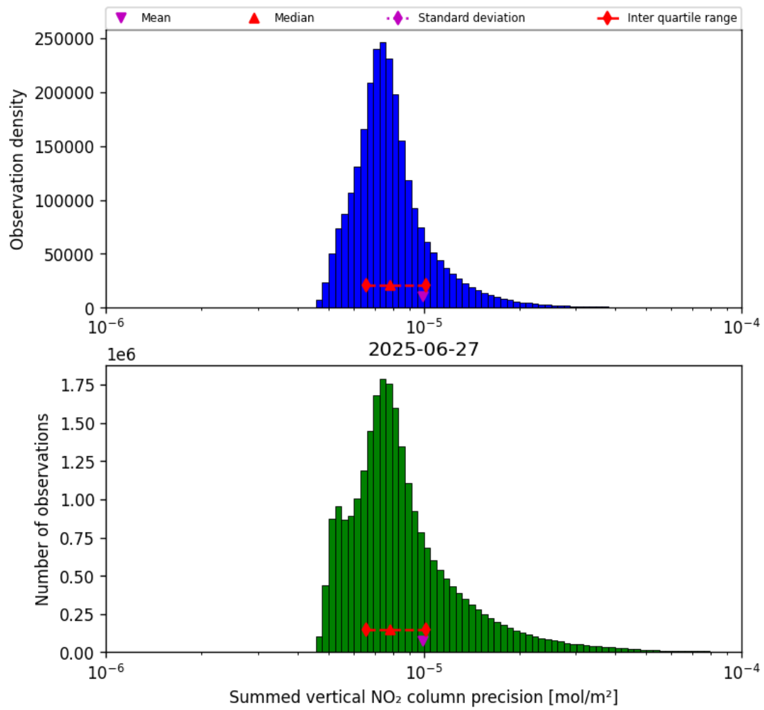
Figure 41: Histogram of “Summed vertical NO 2 column precision” for 2025-06-27 to 2025-06-28
