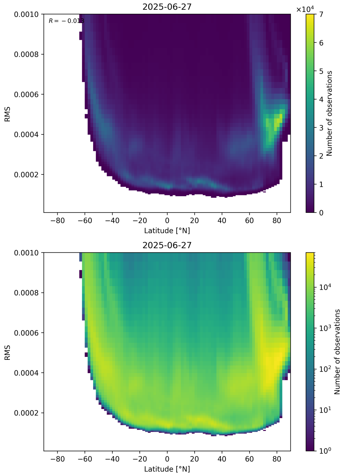
Figure 94: Scatter density plot of “Latitude” against “RMS” for 2025-06-27 to 2025-06-28.
