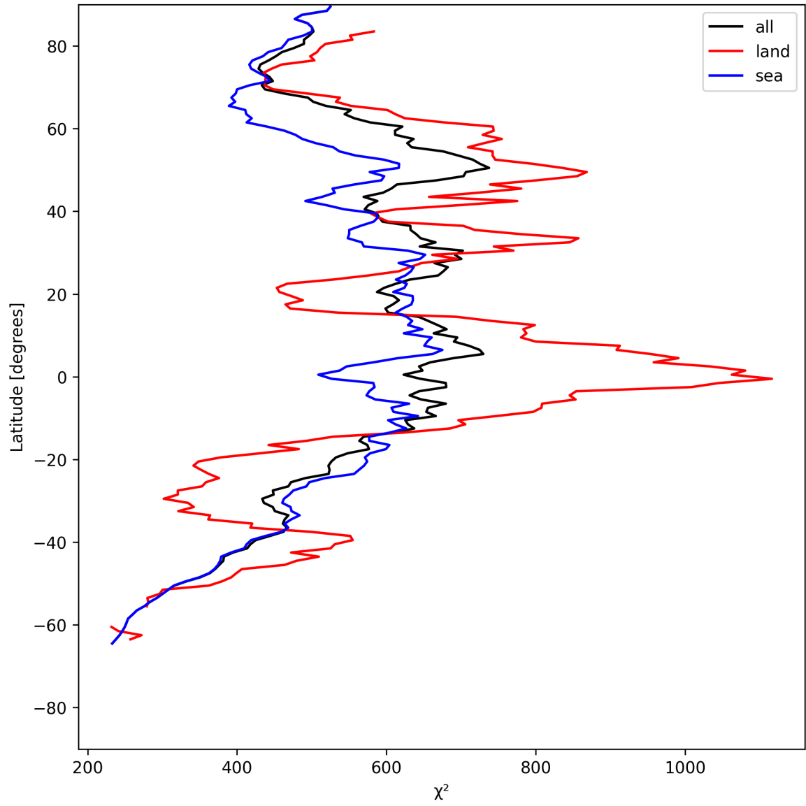
Figure 25: Zonal average of “ \chi^2 ” for 2025-06-27 to 2025-06-28.
