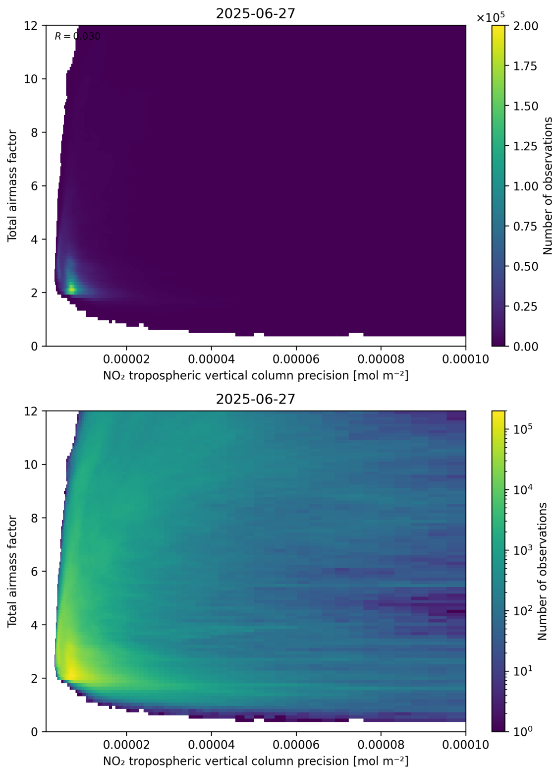
Figure 132: Scatter density plot of “NO 2 tropospheric vertical column precision” against “Total air mass factor” for 2025-06-27 to 2025-06-28.
