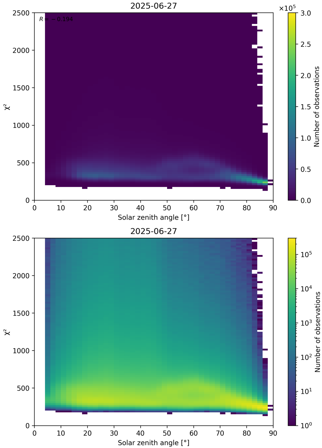
Figure 148: Scatter density plot of “Solar zenith angle” against “ \chi^2 ” for 2025-06-27 to 2025-06-28.
