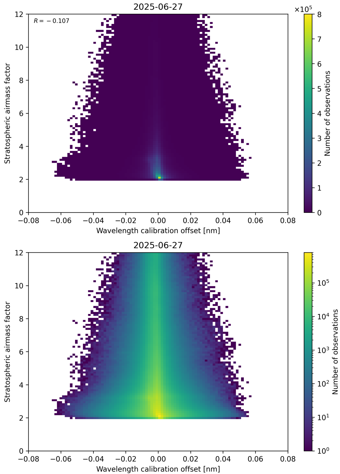
Figure 174: Scatter density plot of “Wavelength calibration offset” against “Stratospheric airmass factor” for 2025-06-27 to 2025-06-28.
