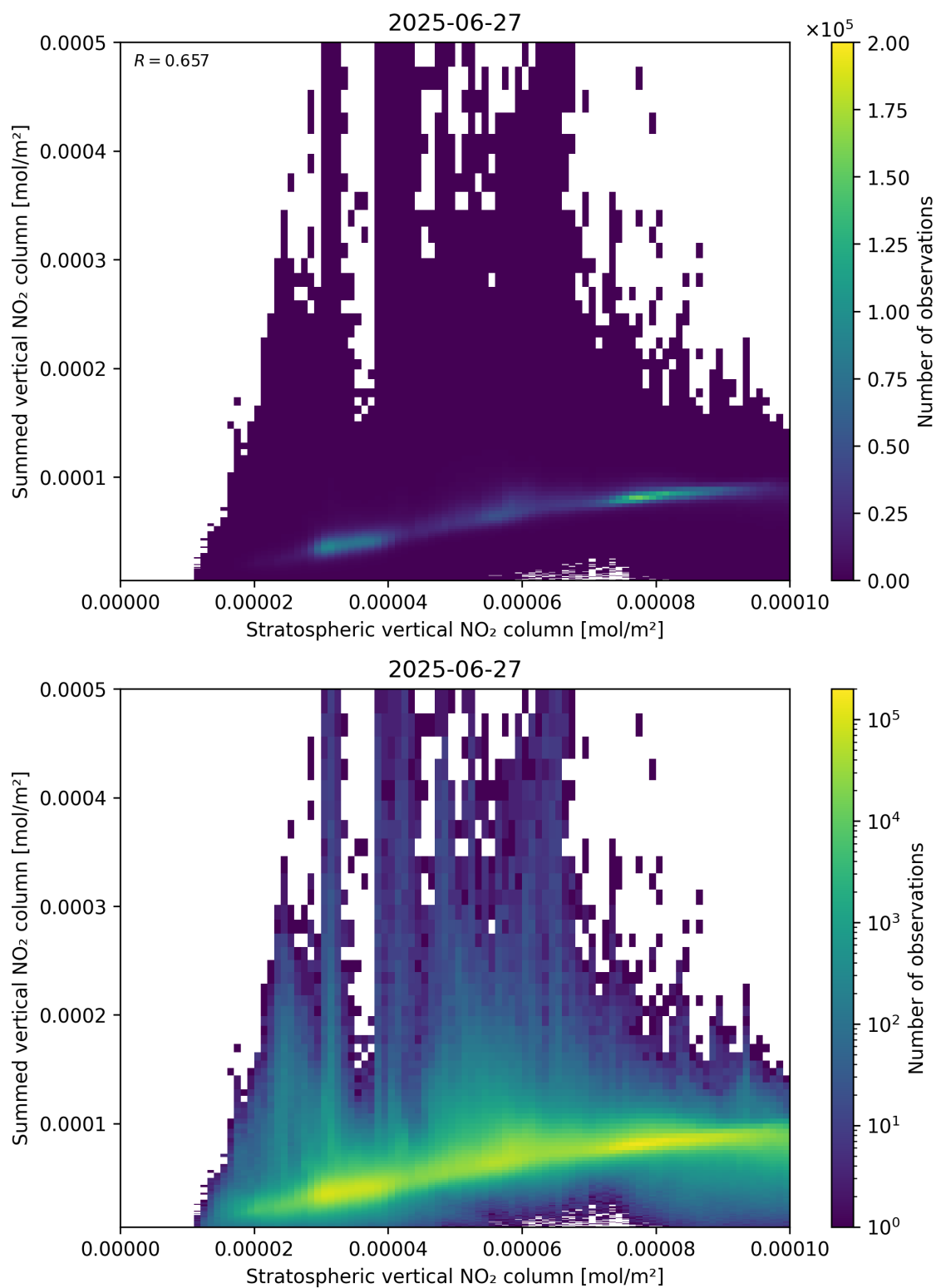
Figure 98: Scatter density plot of “Stratospheric vertical NO 2 column” against “Summed vertical NO 2 column” for 2025-06-27 to 2025-06-28.
