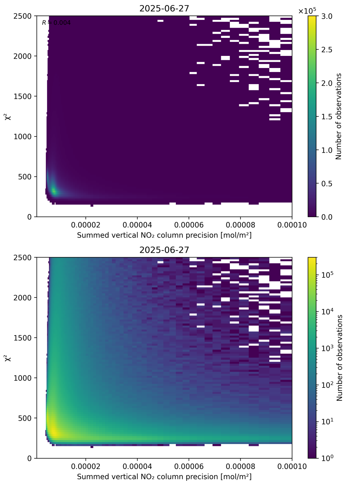
Figure 107: Scatter density plot of “Summed vertical NO 2 column precision” against “ \chi^2 ” for 2025-06-27 to 2025-06-28.
