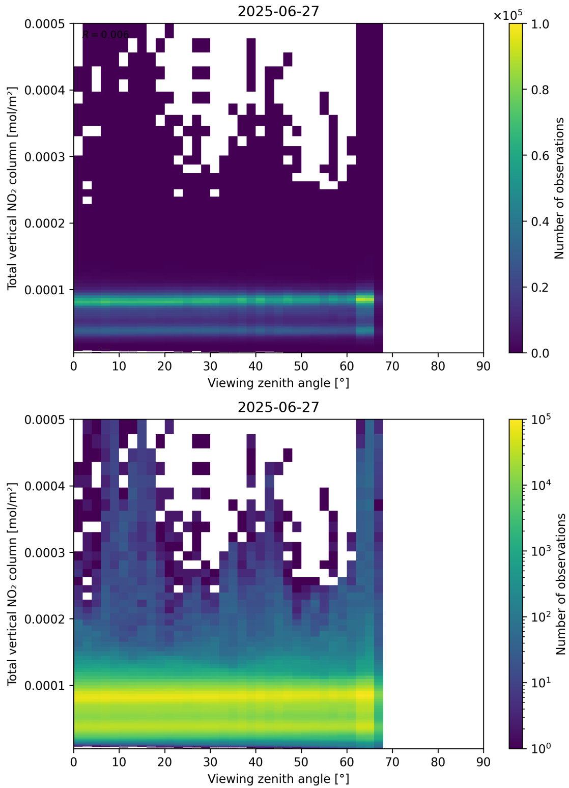
Figure 167: Scatter density plot of “Viewing zenith angle” against “Total vertical NO 2 column” for 2025-06-27 to 2025-06-28.
