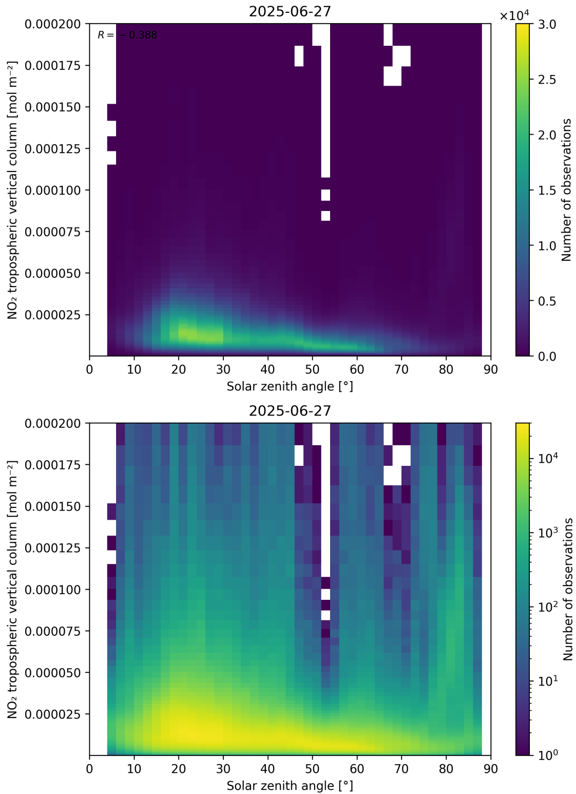
Figure 155: Scatter density plot of “Solar zenith angle” against “NO 2 tropospheric vertical column” for 2025-06-27 to 2025-06-28.
