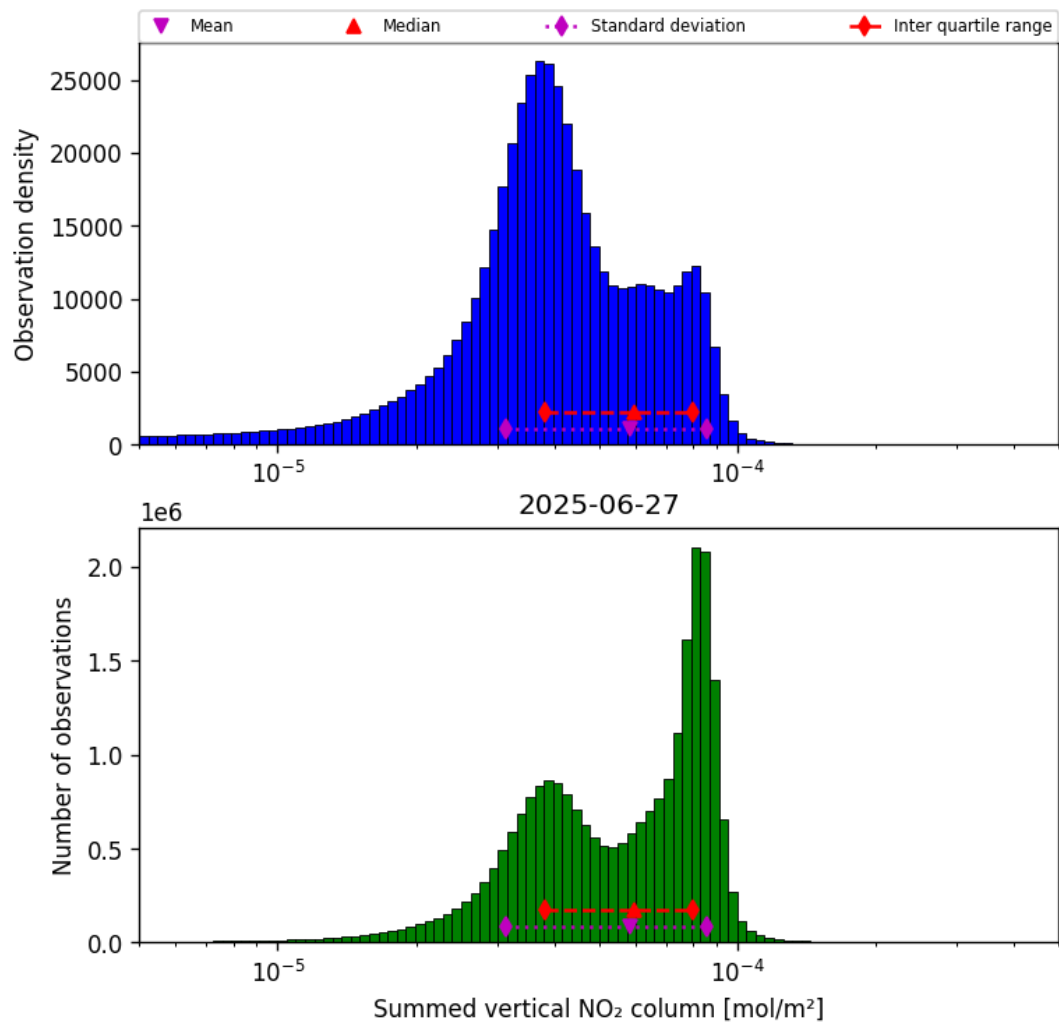
Figure 40: Histogram of “Summed vertical NO 2 column” for 2025-06-27 to 2025-06-28
