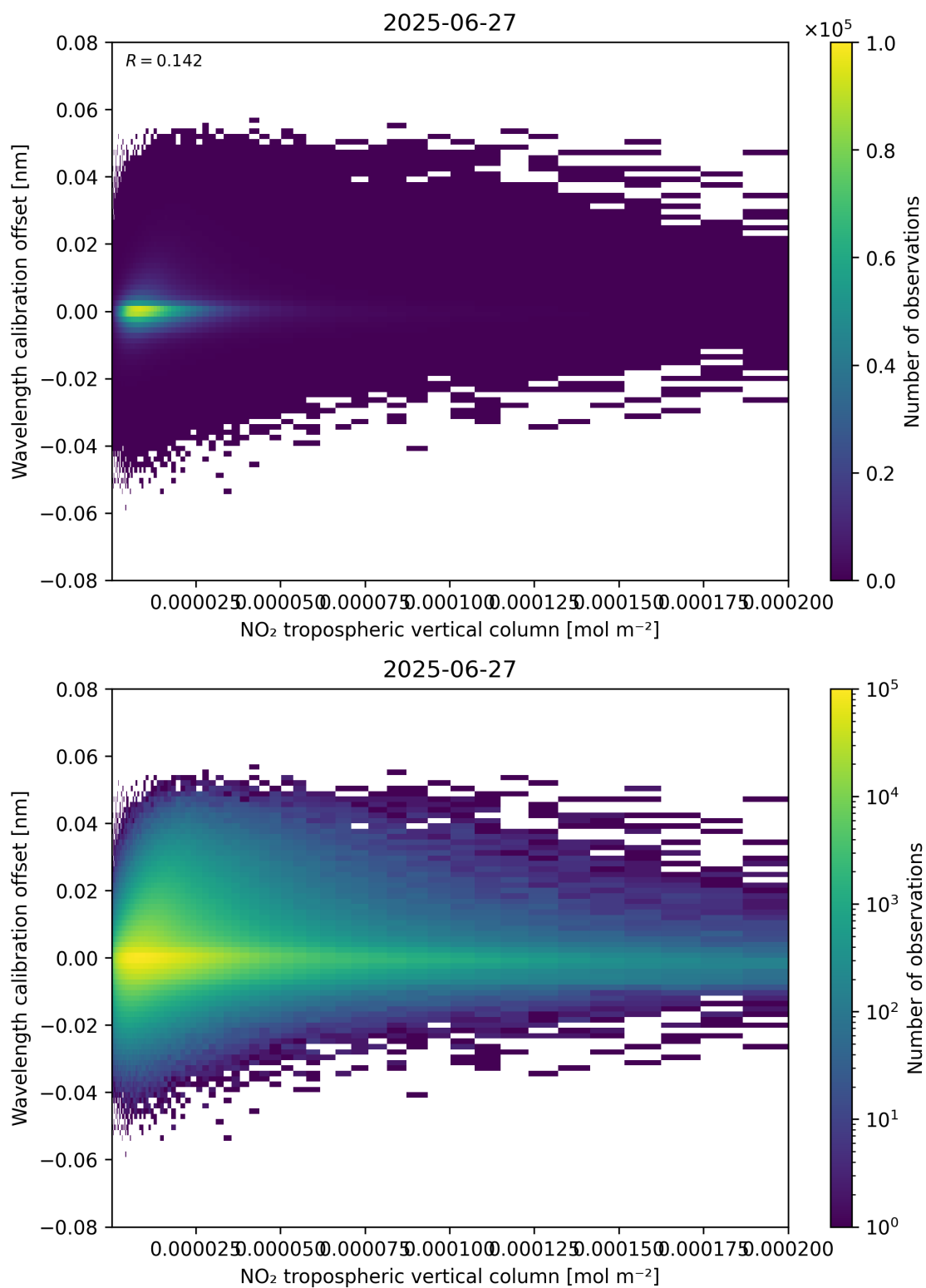
Figure 143: Scatter density plot of “NO 2 tropospheric vertical column” against “Wavelength calibration offset” for 2025-06-27 to 2025-06-28.
