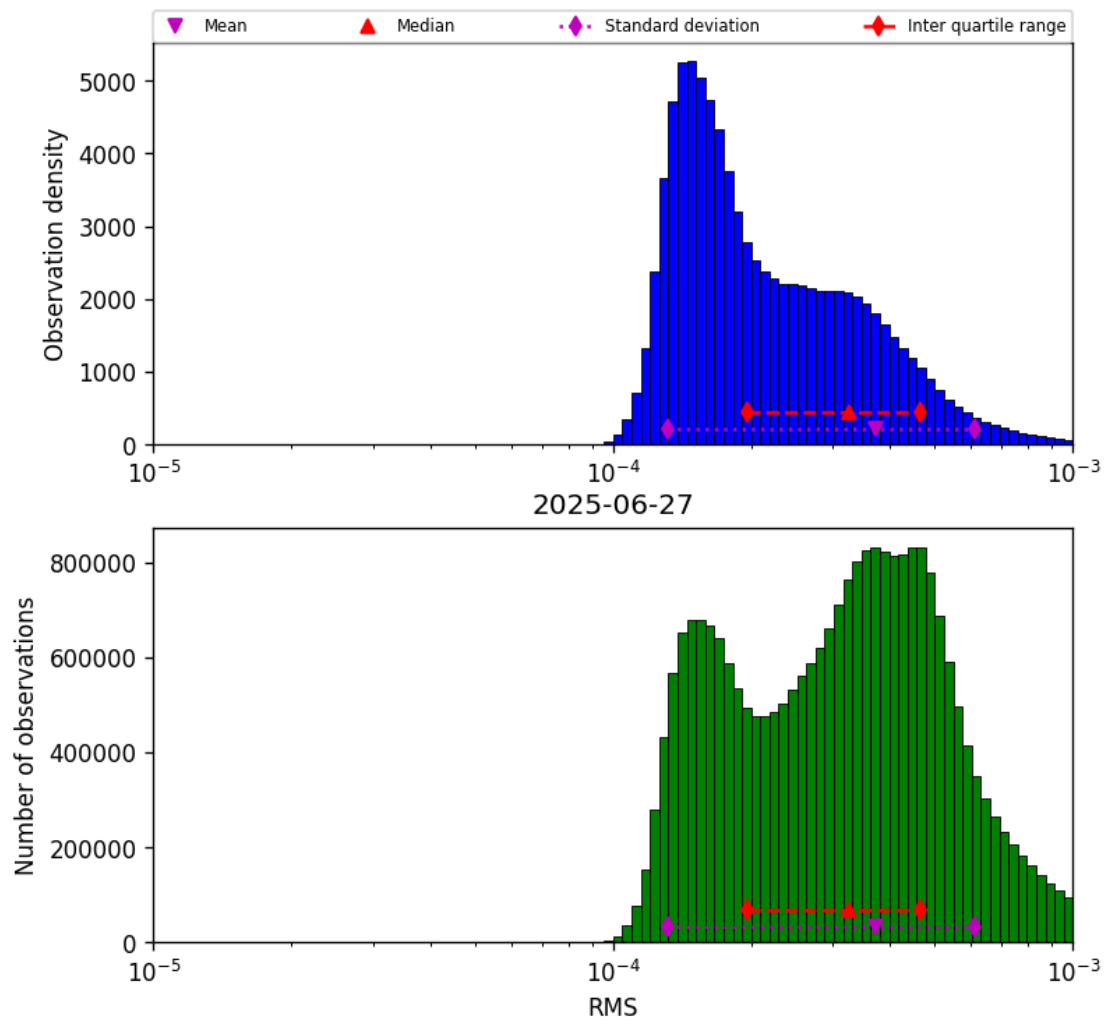
Figure 43: Histogram of “RMS” for 2025-06-27 to 2025-06-28
