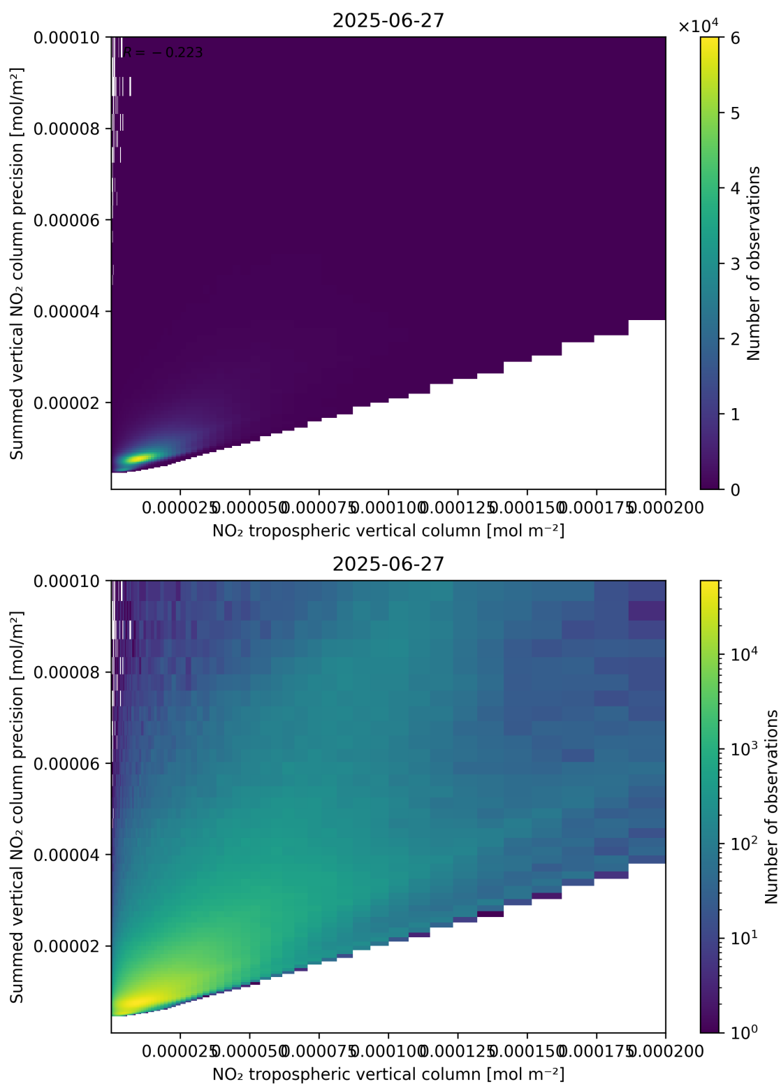
Figure 127: Scatter density plot of “NO 2 tropospheric vertical column” against “Summed vertical NO 2 column precision” for 2025-06-27 to 2025-06-28.
