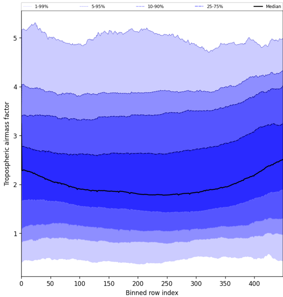
Figure 48: Along track statistics of “Tropospheric airmass factor” for 2025-06-27 to 2025-06-28
