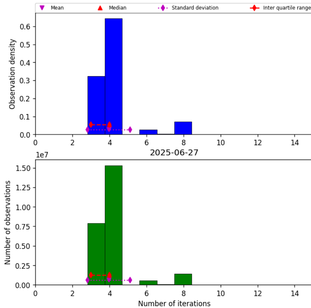
Figure 34: Histogram of “Number of iterations” for 2025-06-27 to 2025-06-28
