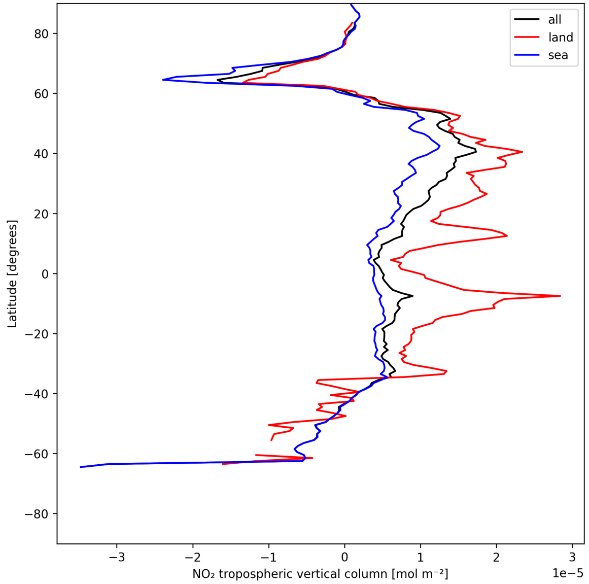
Figure 12: Zonal average of “NO 2 tropospheric vertical column” for 2025-06-27 to 2025-06-28.
