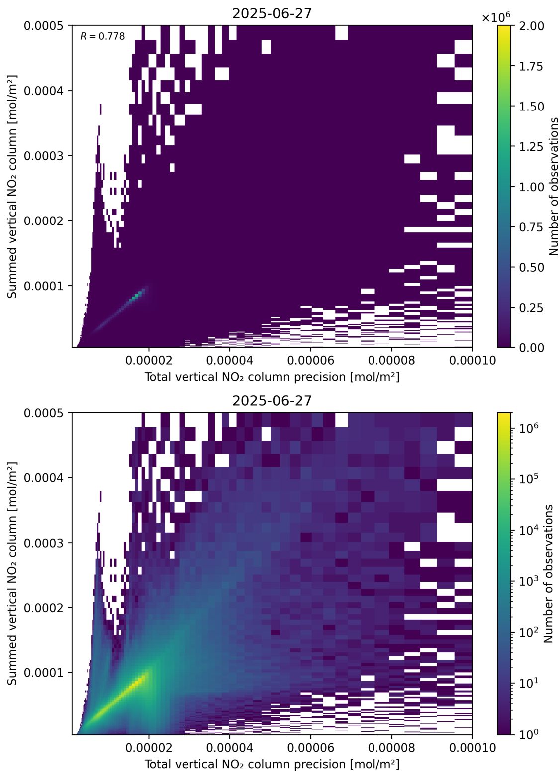
Figure 117: Scatter density plot of “Total vertical NO 2 column precision” against “Summed vertical NO 2 column” for 2025-06-27 to 2025-06-28.
