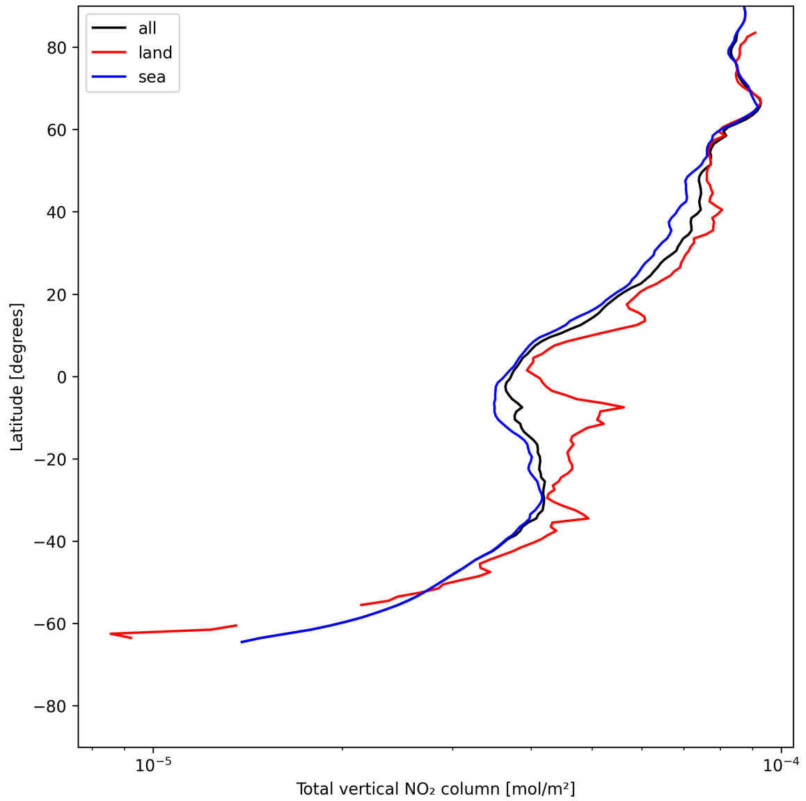
Figure 21: Zonal average of “Total vertical NO 2 column” for 2025-06-27 to 2025-06-28.
