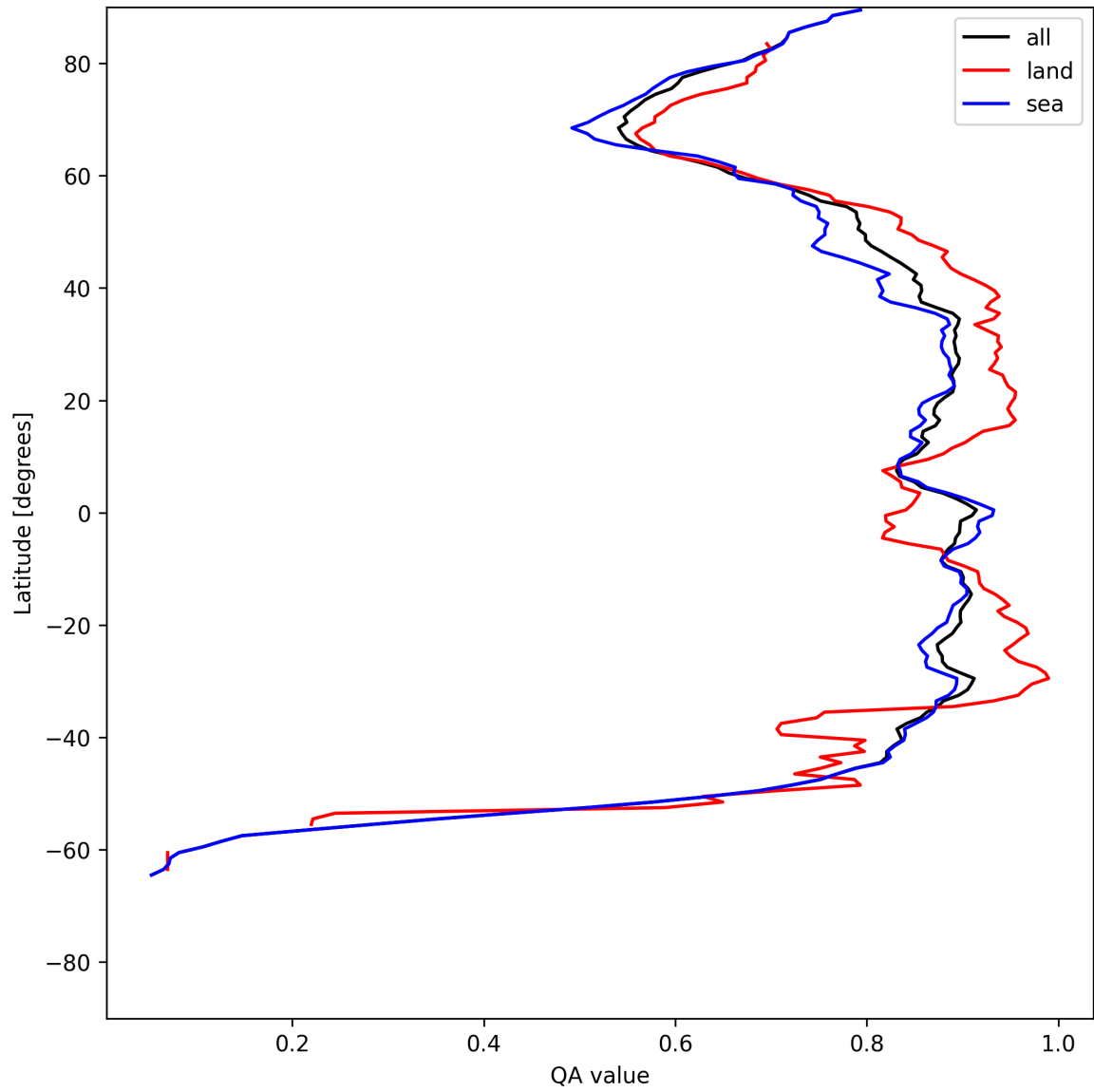
Figure 11: Zonal average of “QA value” for 2025-06-27 to 2025-06-28.
