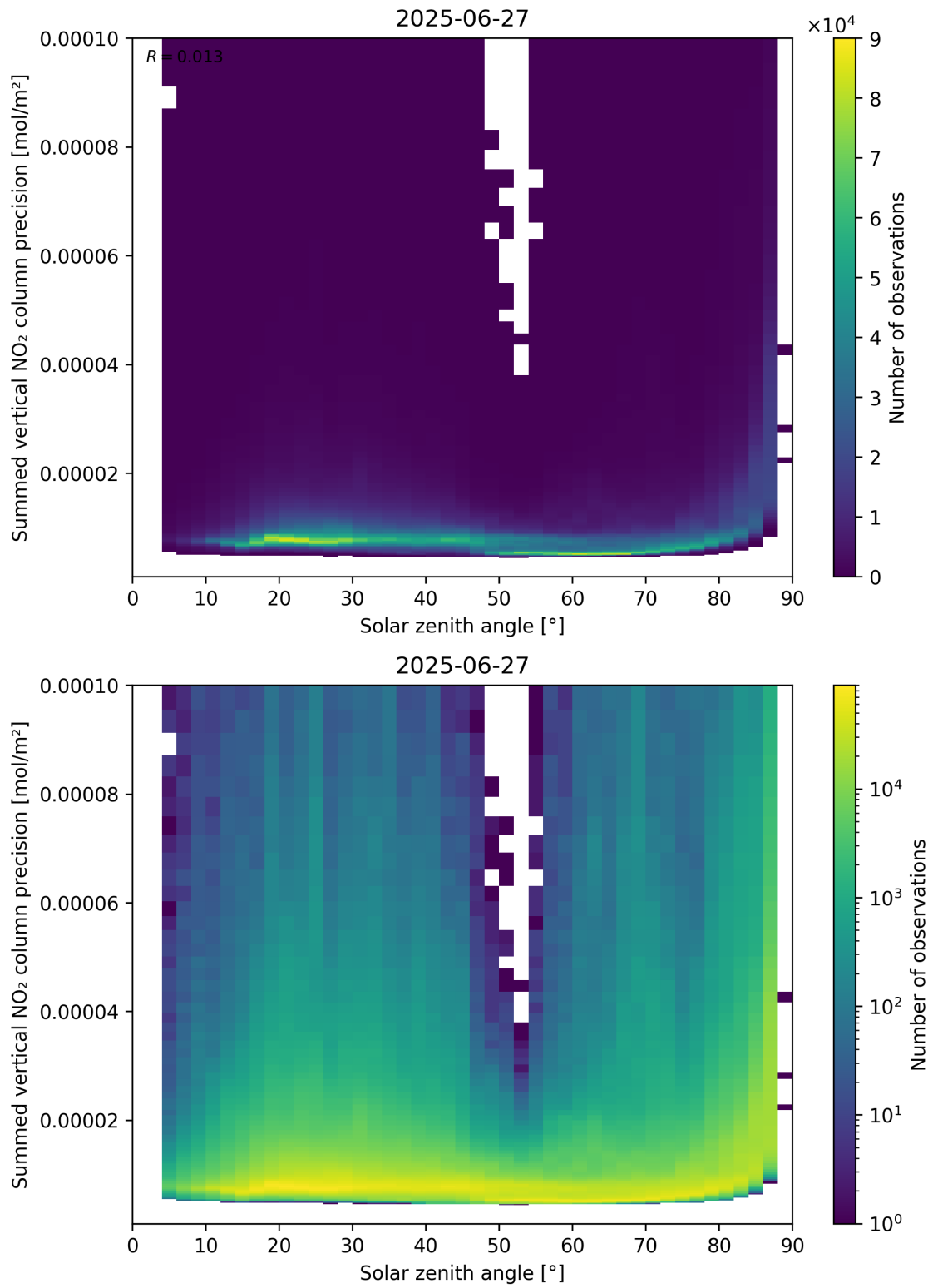
Figure 152: Scatter density plot of “Solar zenith angle” against “Summed vertical NO 2 column precision” for 2025-06-27 to 2025-06-28.
