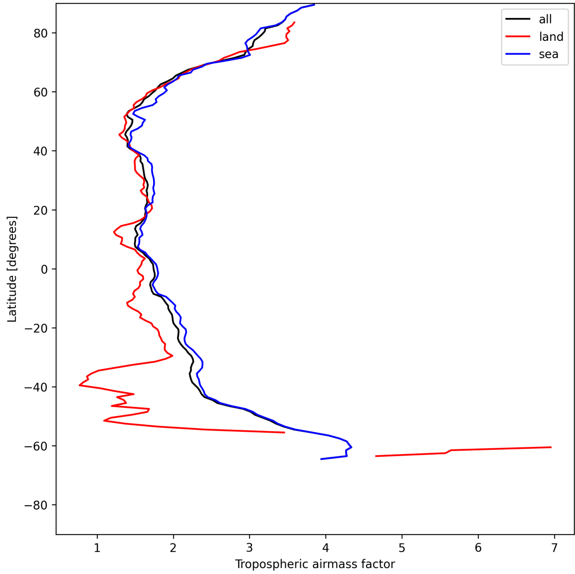
Figure 14: Zonal average of “Tropospheric airmass factor” for 2025-06-27 to 2025-06-28.
