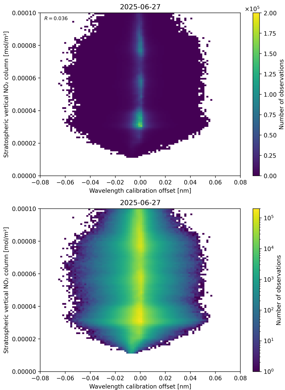
Figure 176: Scatter density plot of “Wavelength calibration offset” against “Stratospheric vertical NO 2 column” for 2025-06-27 to 2025-06-28.
