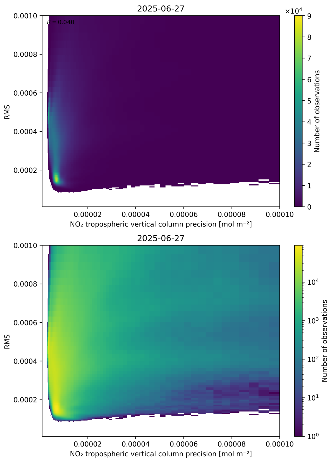
Figure 140: Scatter density plot of “NO 2 tropospheric vertical column precision” against “RMS” for 2025-06-27 to 2025-06-28.
