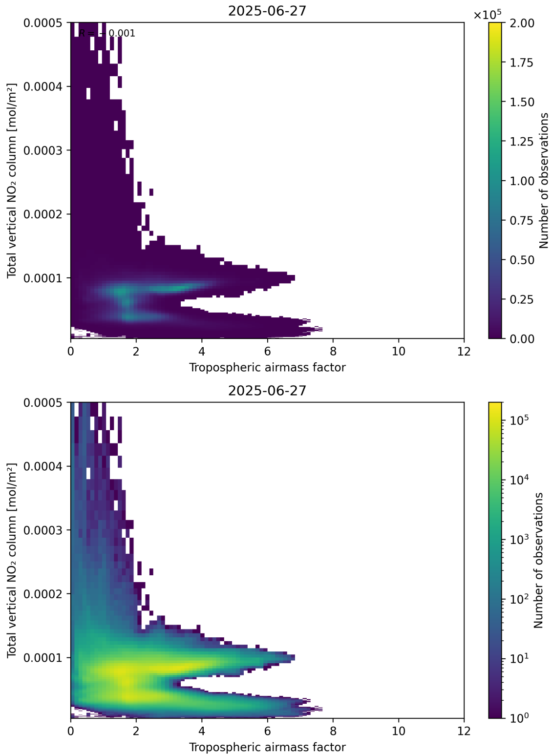
Figure 77: Scatter density plot of “Tropospheric airmass factor” against “Total vertical NO 2 column” for 2025-06-27 to 2025-06-28.
