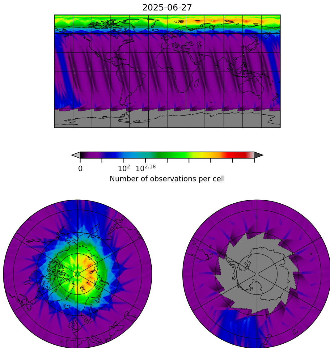
Figure 10: Map of the number of observations for 2025-06-27 to 2025-06-28
