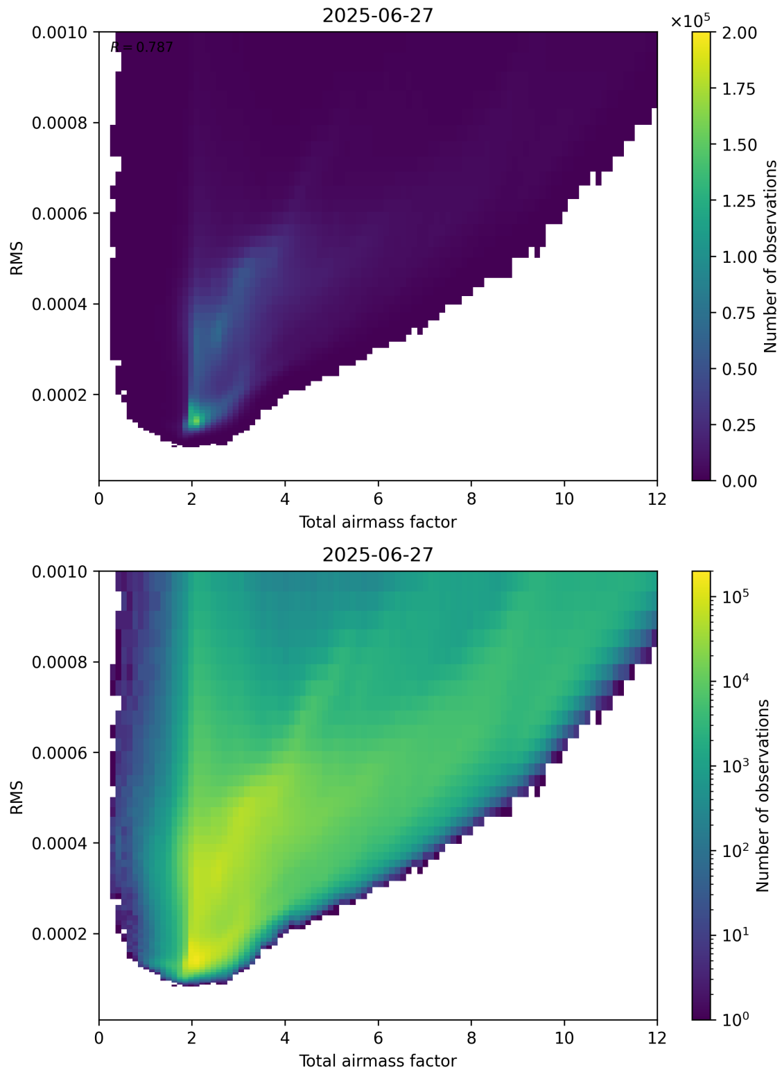
Figure 69: Scatter density plot of “Total airmass factor” against “RMS” for 2025-06-27 to 2025-06-28.
