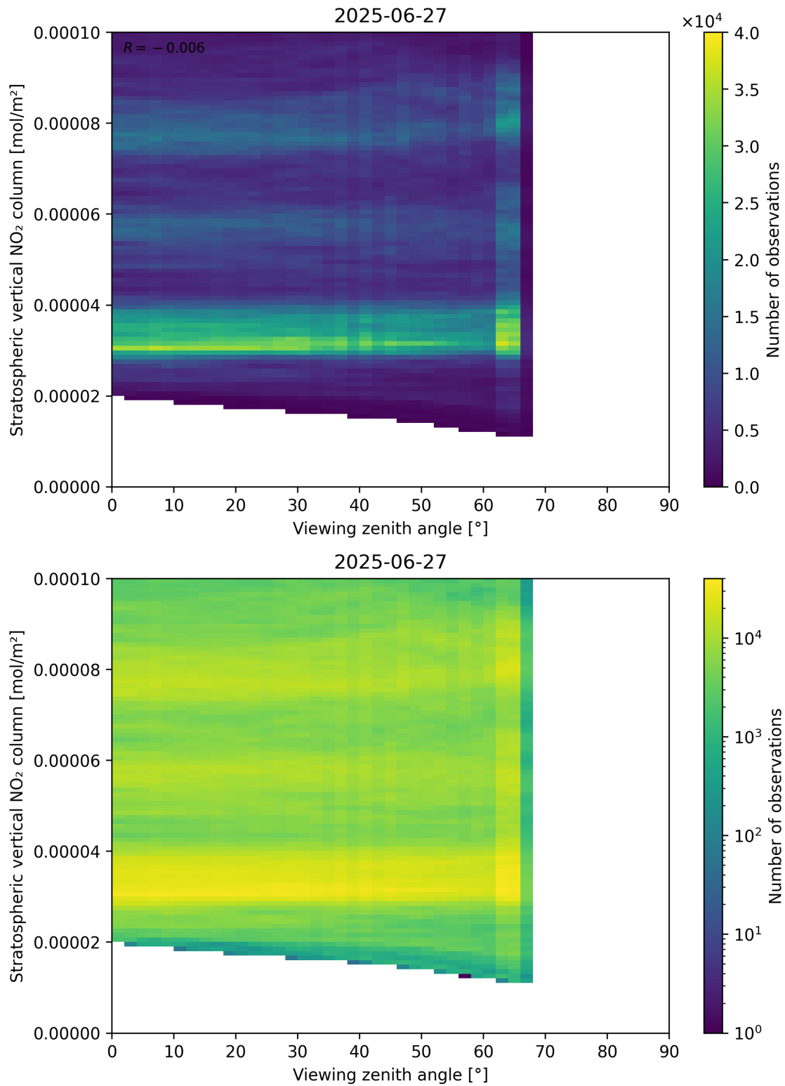
Figure 164: Scatter density plot of “Viewing zenith angle” against “Stratospheric vertical NO 2 column” for 2025-06-27 to 2025-06-28.
