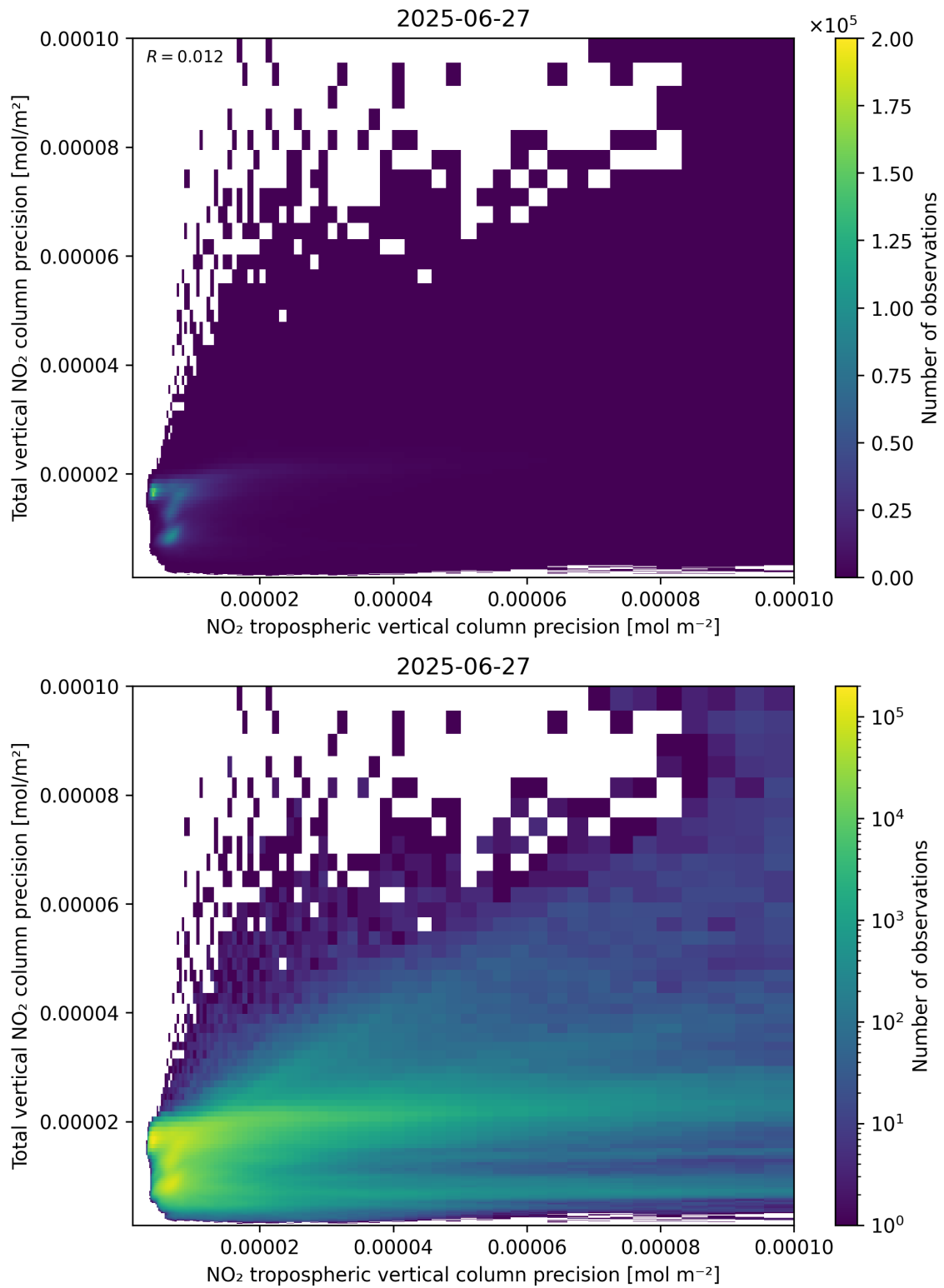
Figure 139: Scatter density plot of “NO 2 tropospheric vertical column precision” against “Total vertical NO 2 column precision” for 2025-06-27 to 2025-06-28.
