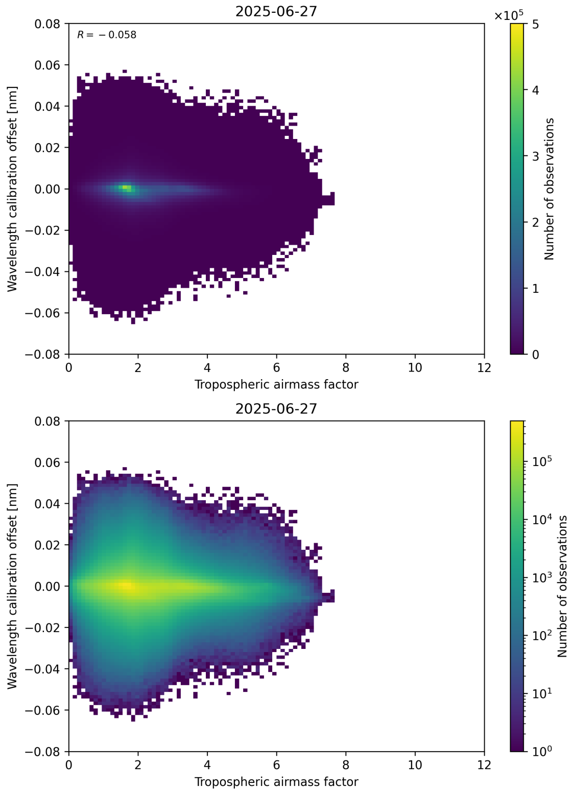
Figure 80: Scatter density plot of “Tropospheric airmass factor” against “Wavelength calibration offset” for 2025-06-27 to 2025-06-28.
