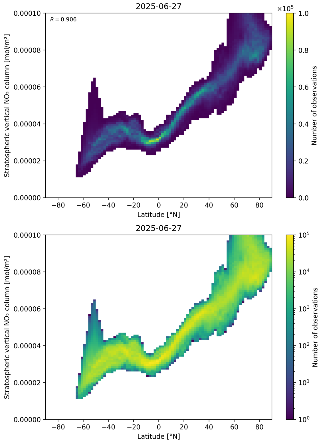
Figure 87: Scatter density plot of “Latitude” against “Stratospheric vertical \text{NO}_2 column” for 2025-06-27 to 2025-06-28.
