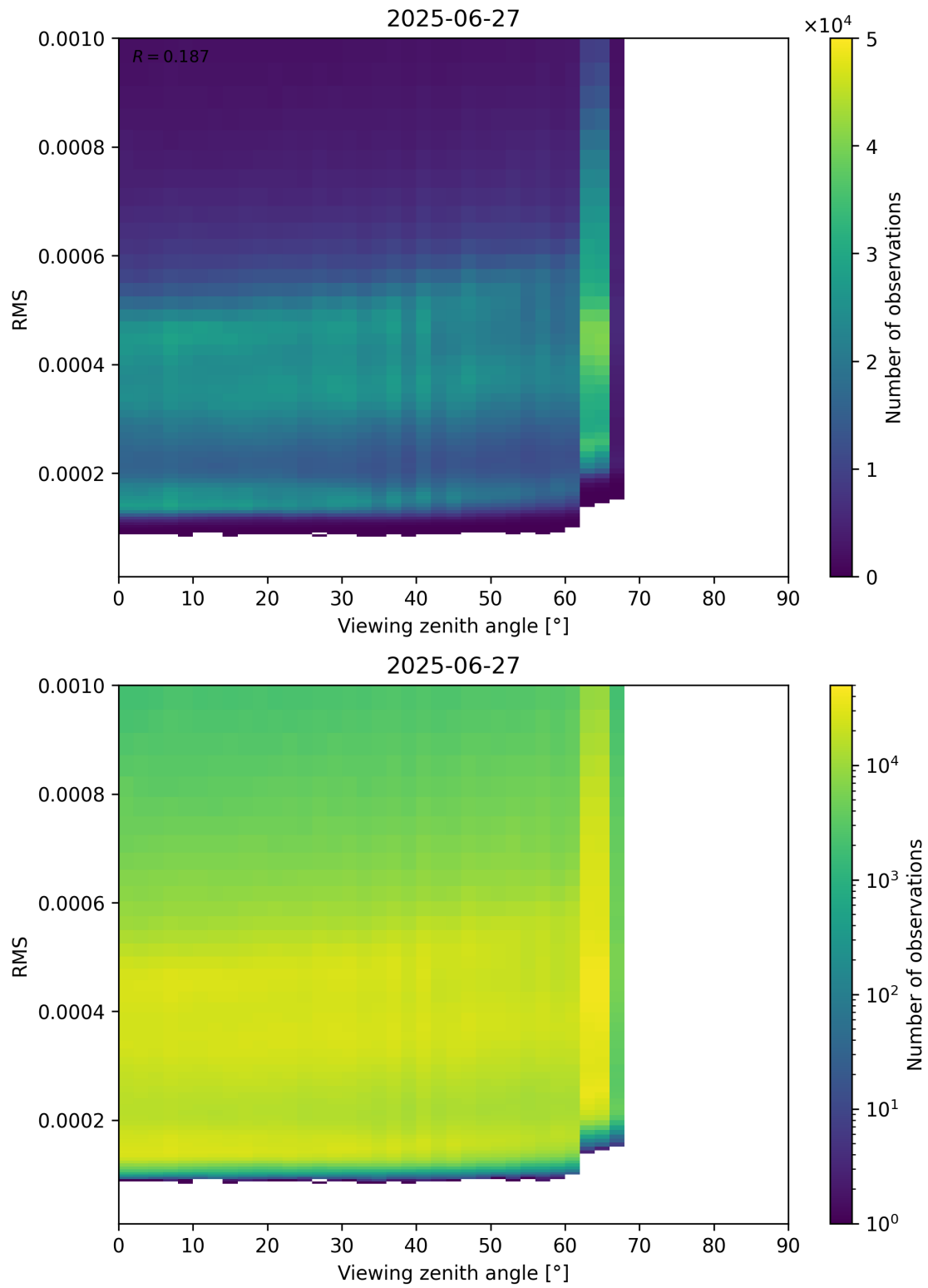
Figure 171: Scatter density plot of “Viewing zenith angle” against “RMS” for 2025-06-27 to 2025-06-28.
