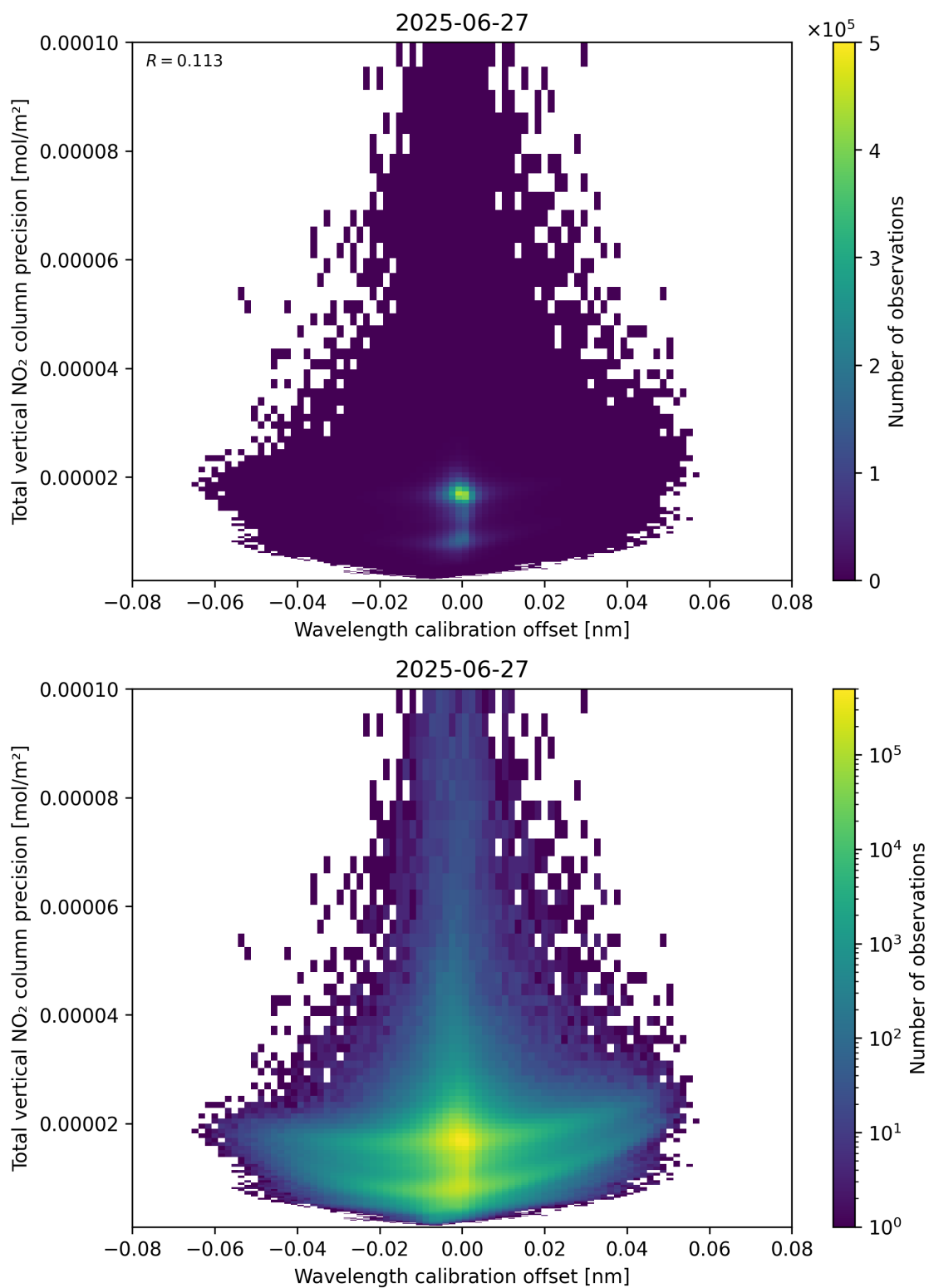
Figure 180: Scatter density plot of “Wavelength calibration offset” against “Total vertical NO 2 column precision” for 2025-06-27 to 2025-06-28.
