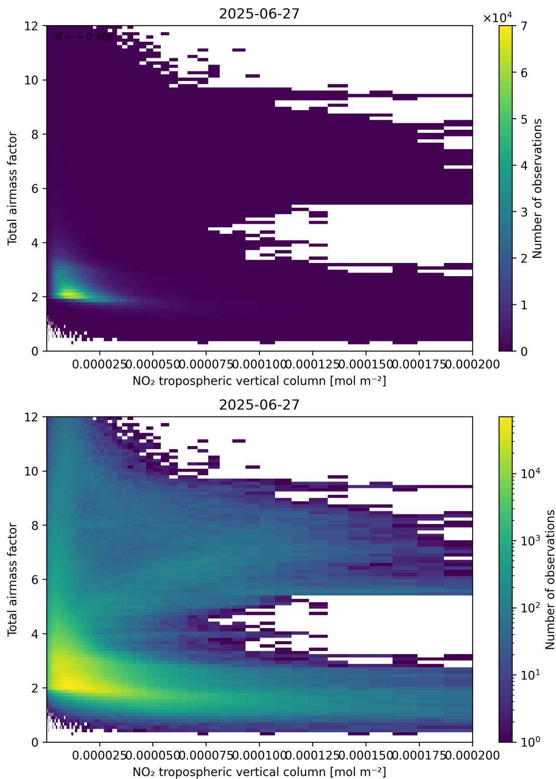
Figure 122: Scatter density plot of “NO 2 tropospheric vertical column” against “Total airmass factor” for 2025-06-27 to 2025-06-28.
