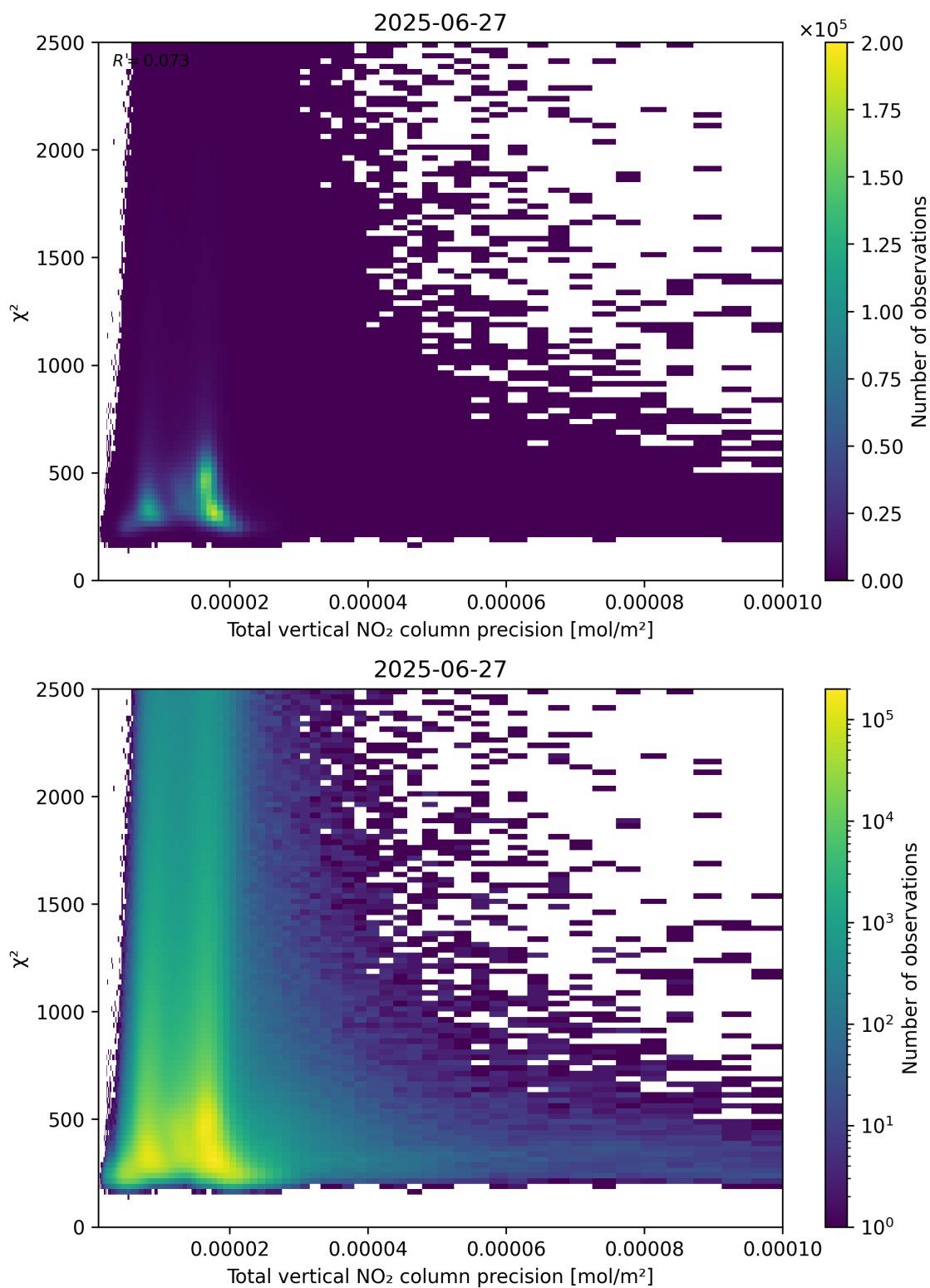
Figure 116: Scatter density plot of “Total vertical NO 2 column precision” against “ \chi^2 ” for 2025-06-27 to 2025-06-28.
