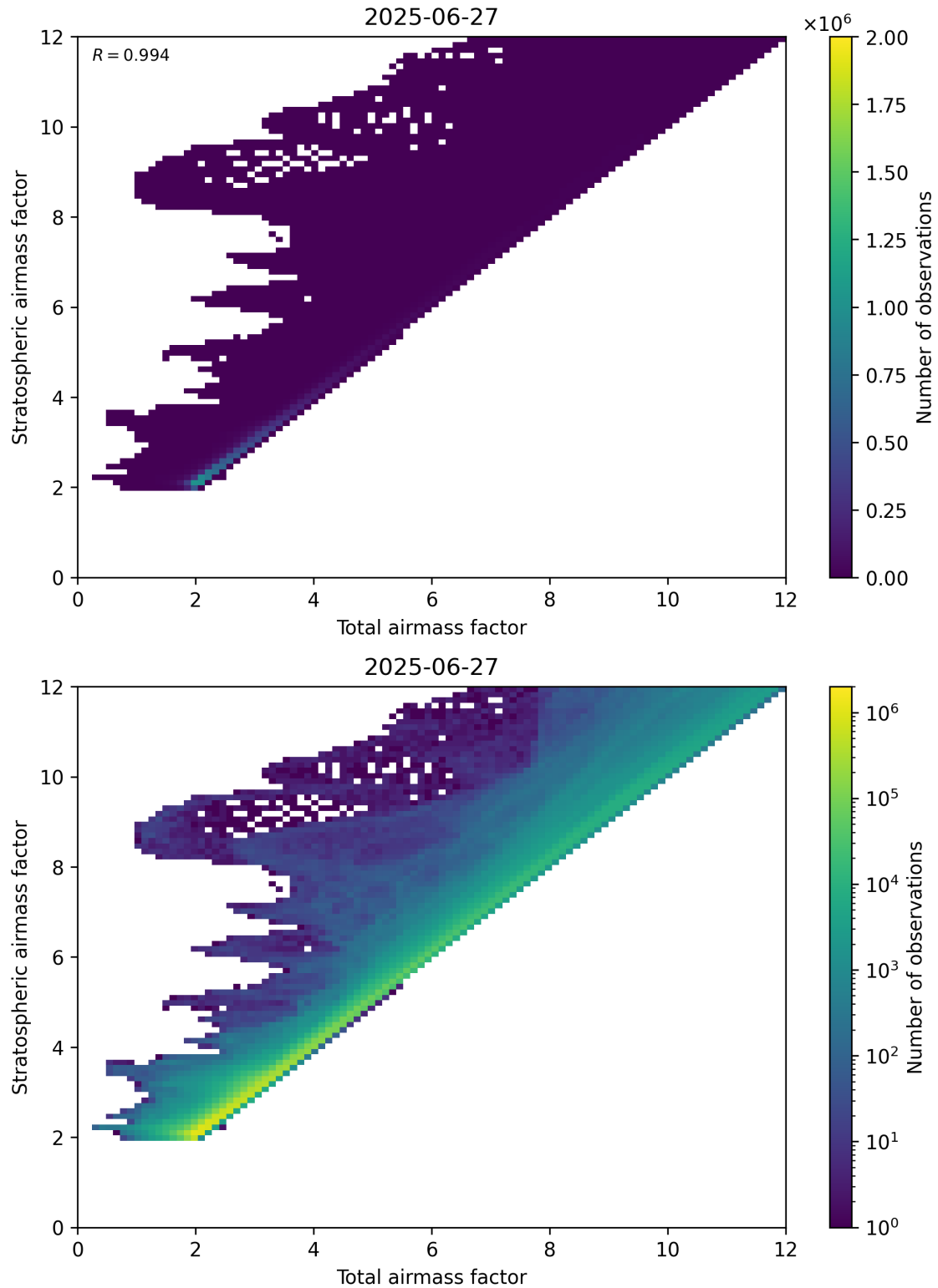
Figure 62: Scatter density plot of “Total airmass factor” against “Stratospheric airmass factor” for 2025-06-27 to 2025-06-28.
