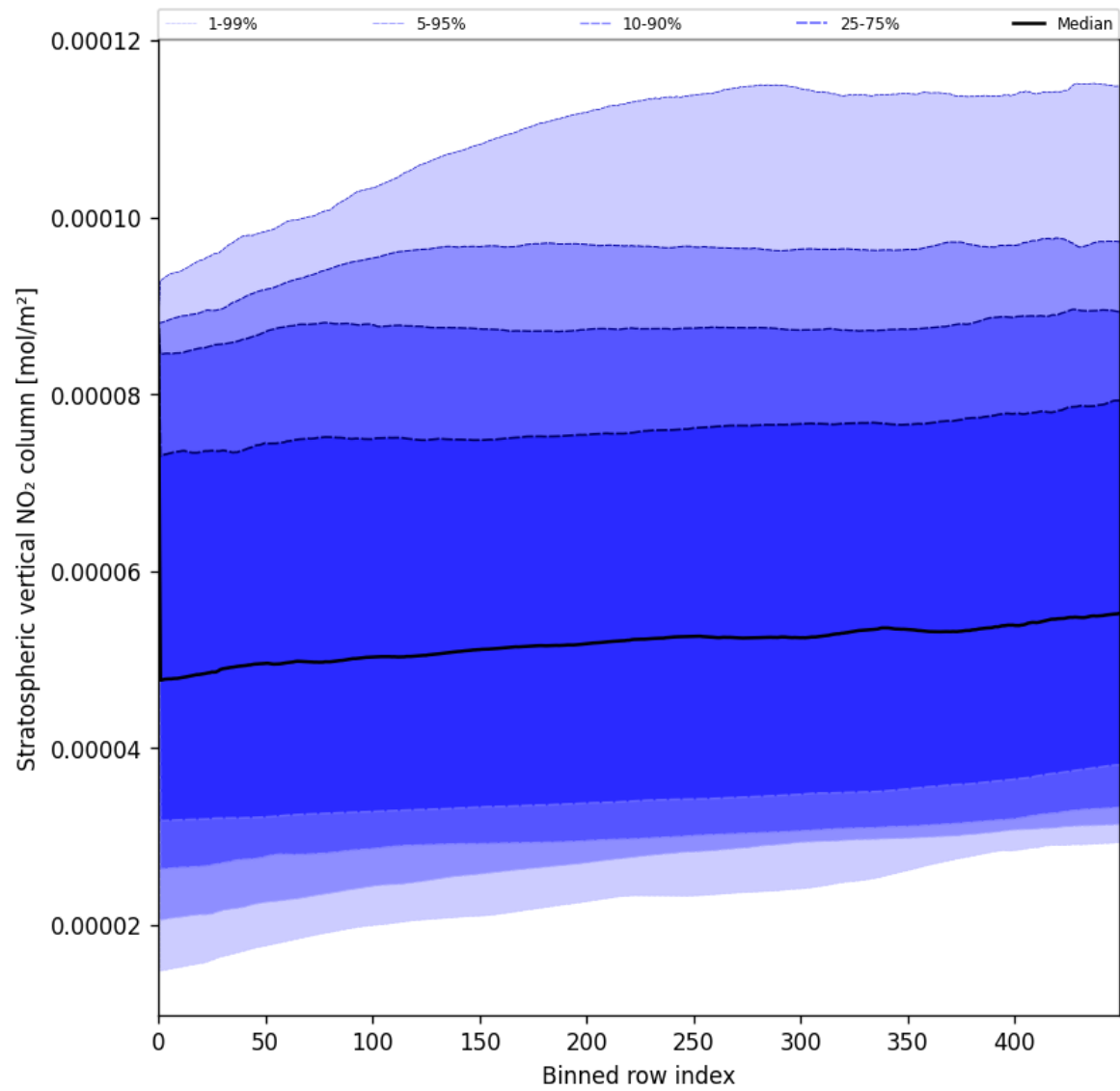
Figure 53: Along track statistics of “Stratospheric vertical NO 2 column” for 2025-06-27 to 2025-06-28
