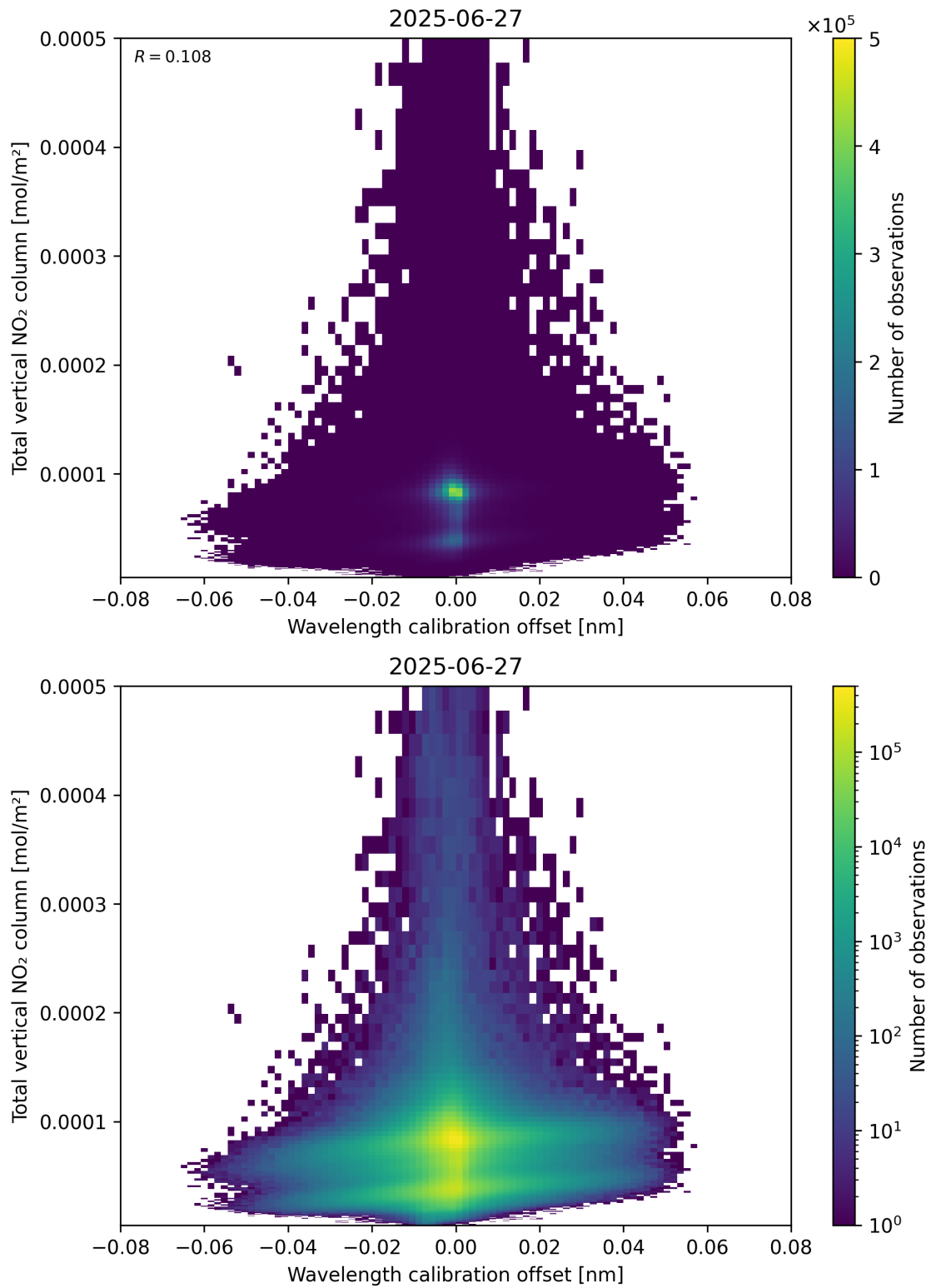
Figure 179: Scatter density plot of “Wavelength calibration offset” against “Total vertical NO 2 column” for 2025-06-27 to 2025-06-28.
