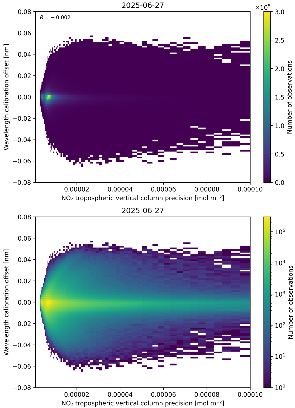
Figure 141: Scatter density plot of “NO 2 tropospheric vertical column precision” against “Wavelength calibration offset” for 2025-06-27 to 2025-06-28.
