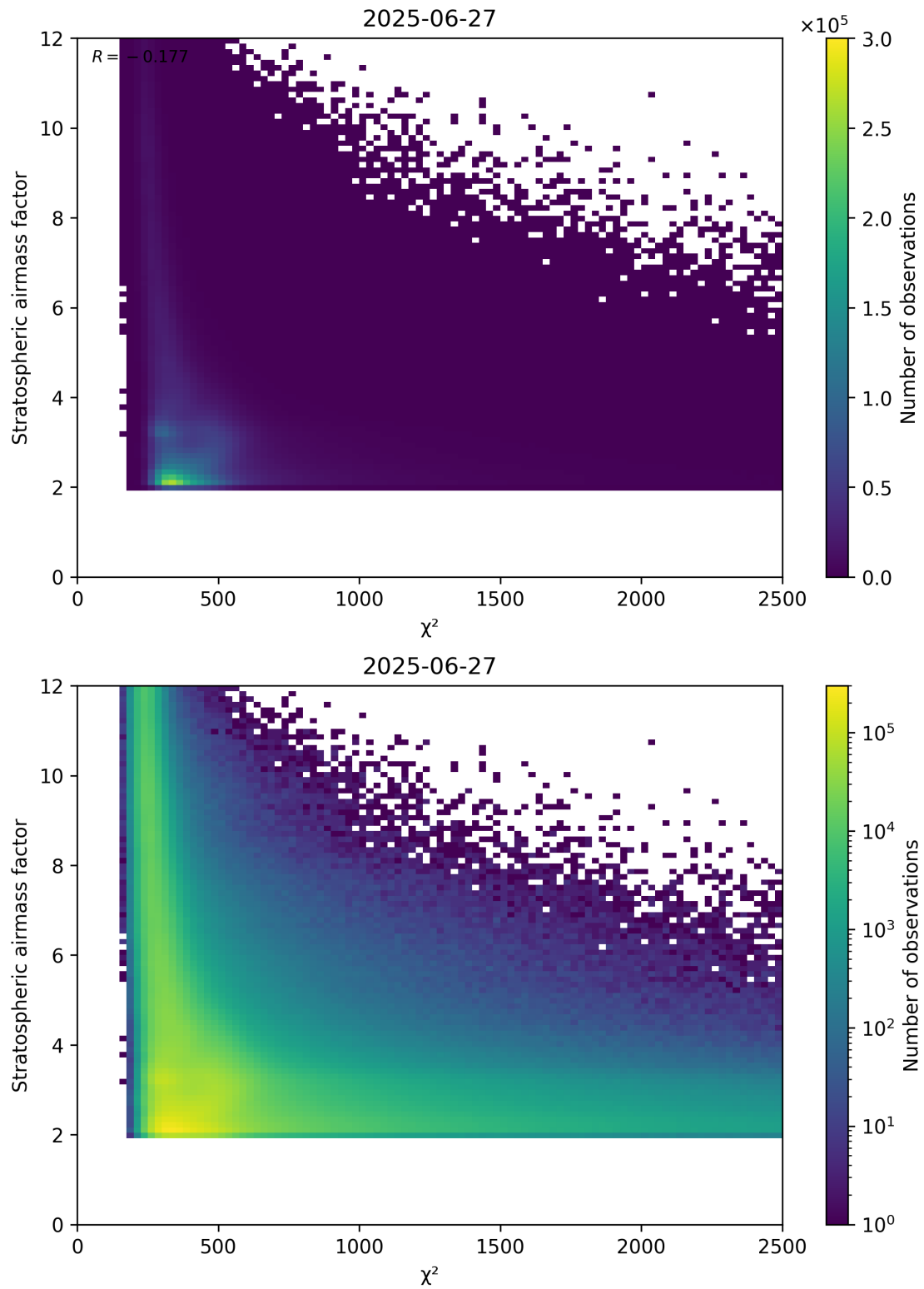
Figure 81: Scatter density plot of " \chi^2 " against "Stratospheric air mass factor" for 2025-06-27 to 2025-06-28.
