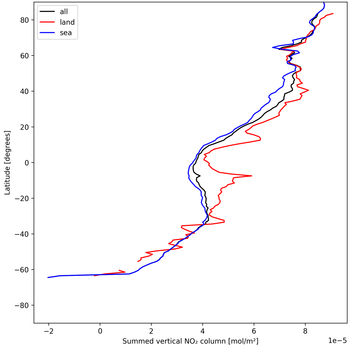
Figure 23: Zonal average of “Summed vertical NO 2 column” for 2025-06-27 to 2025-06-28.
