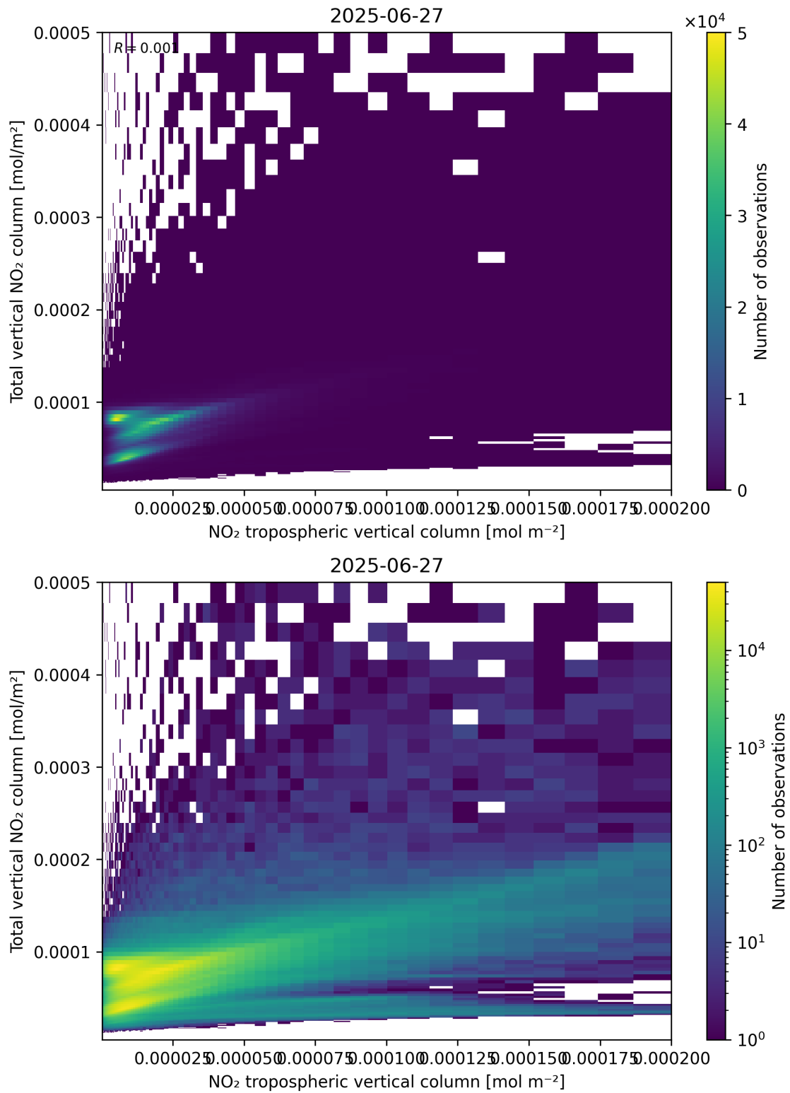
Figure 128: Scatter density plot of “NO 2 tropospheric vertical column” against “Total vertical NO 2 column” for 2025-06-27 to 2025-06-28.
