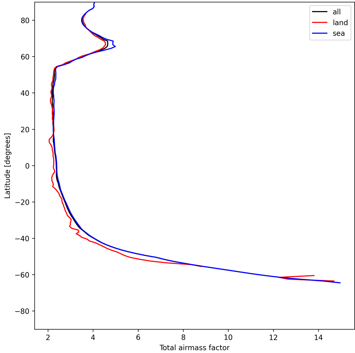
Figure 15: Zonal average of “Total airmass factor” for 2025-06-27 to 2025-06-28.
