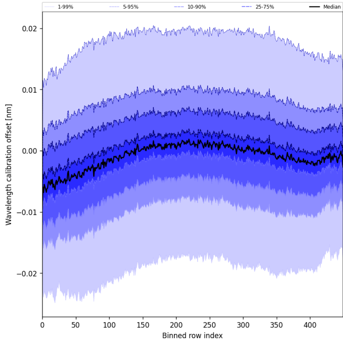
Figure 52: Along track statistics of “Wavelength calibration offset” for 2025-06-27 to 2025-06-28
