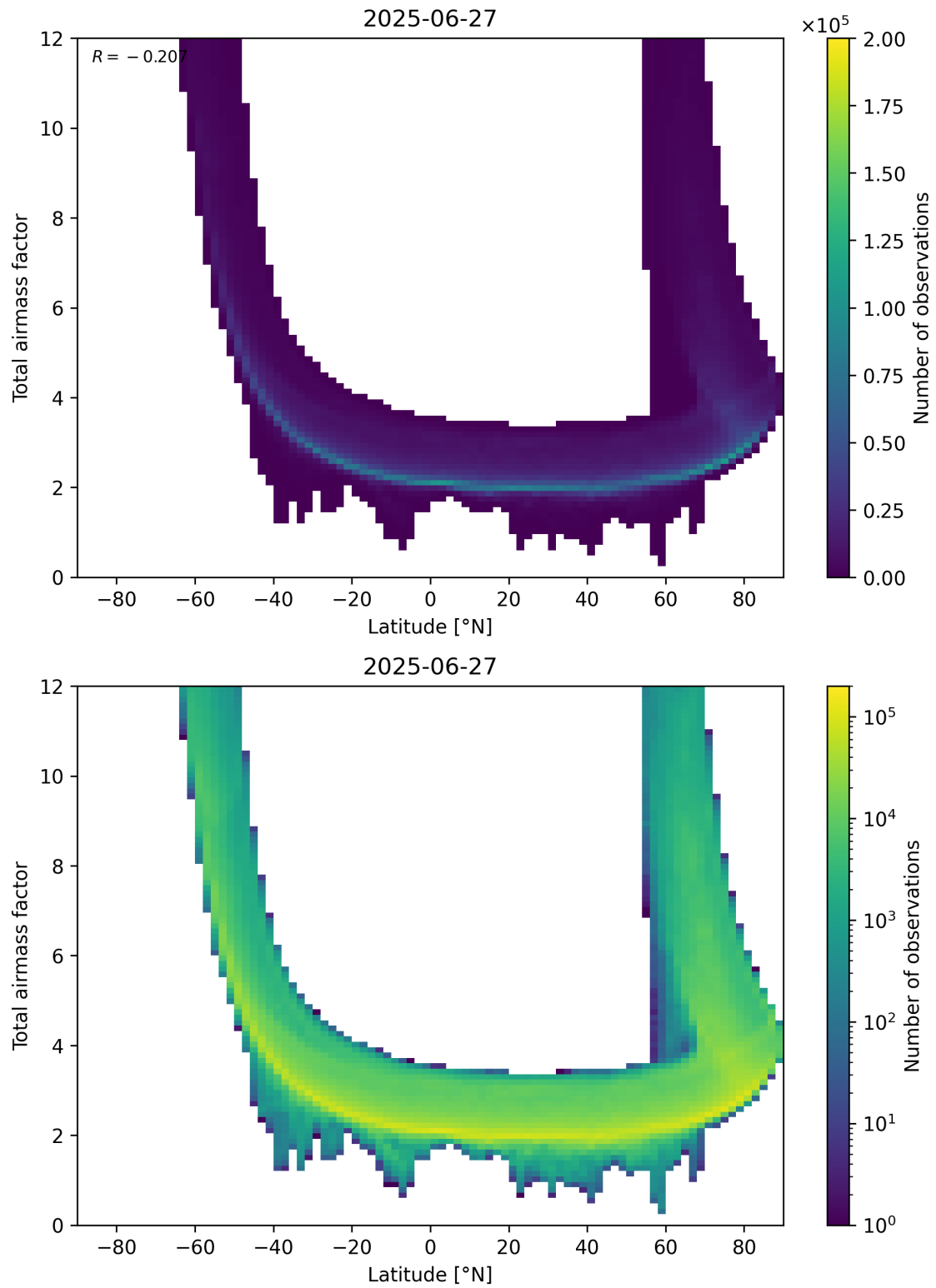
Figure 84: Scatter density plot of “Latitude” against “Total airmass factor” for 2025-06-27 to 2025-06-28.
