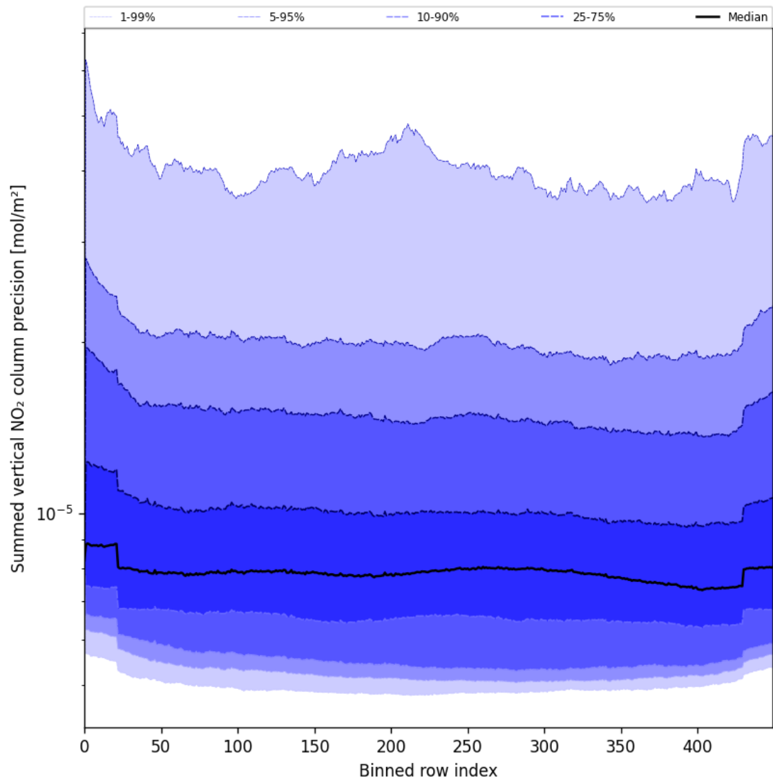
Figure 58: Along track statistics of “Summed vertical NO 2 column precision” for 2025-06-27 to 2025-06-28
