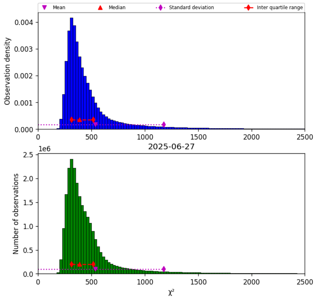
Figure 42: Histogram of " \chi^2 " for 2025-06-27 to 2025-06-28
