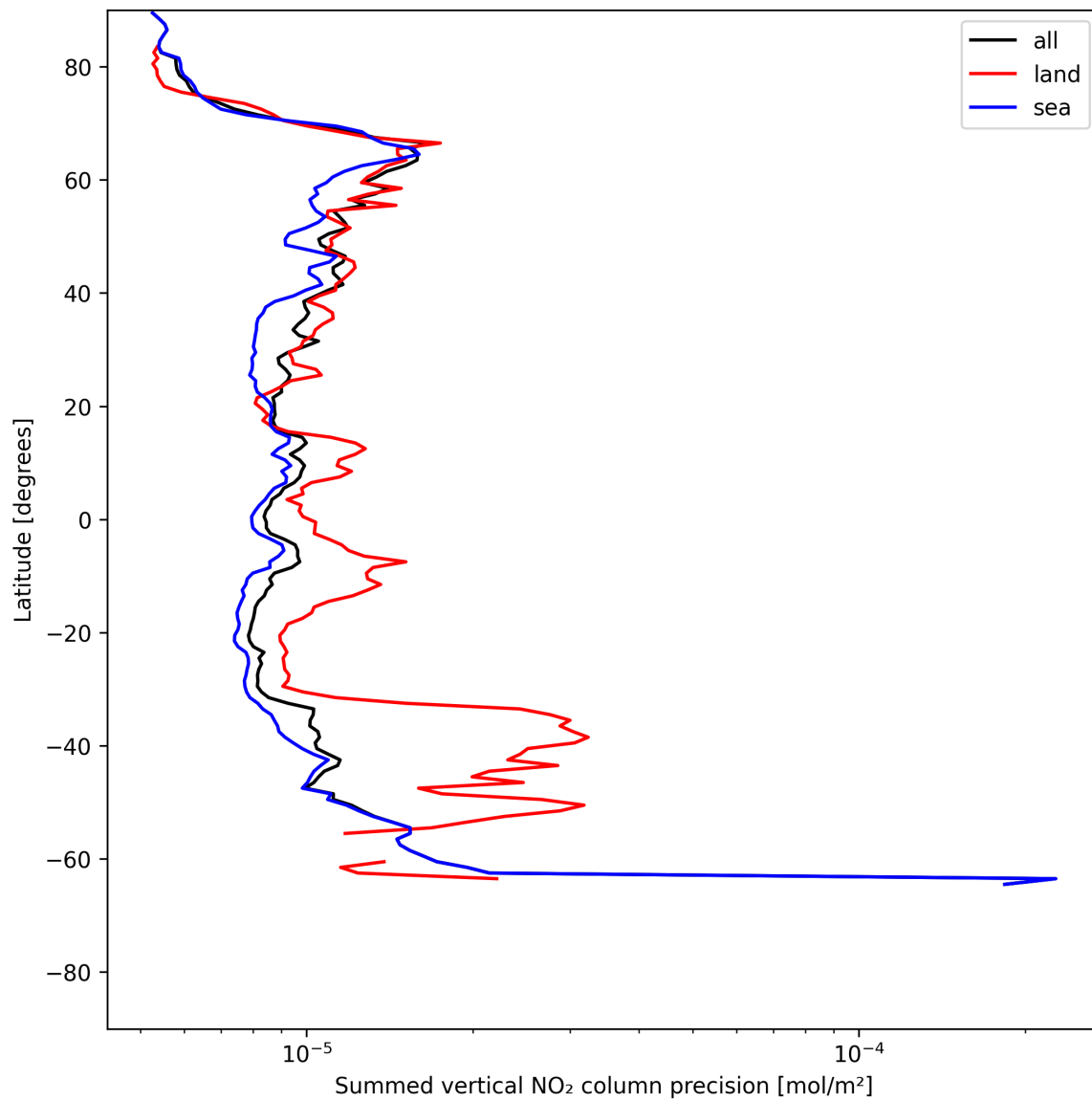
Figure 24: Zonal average of “Summed vertical NO 2 column precision” for 2025-06-27 to 2025-06-28.
