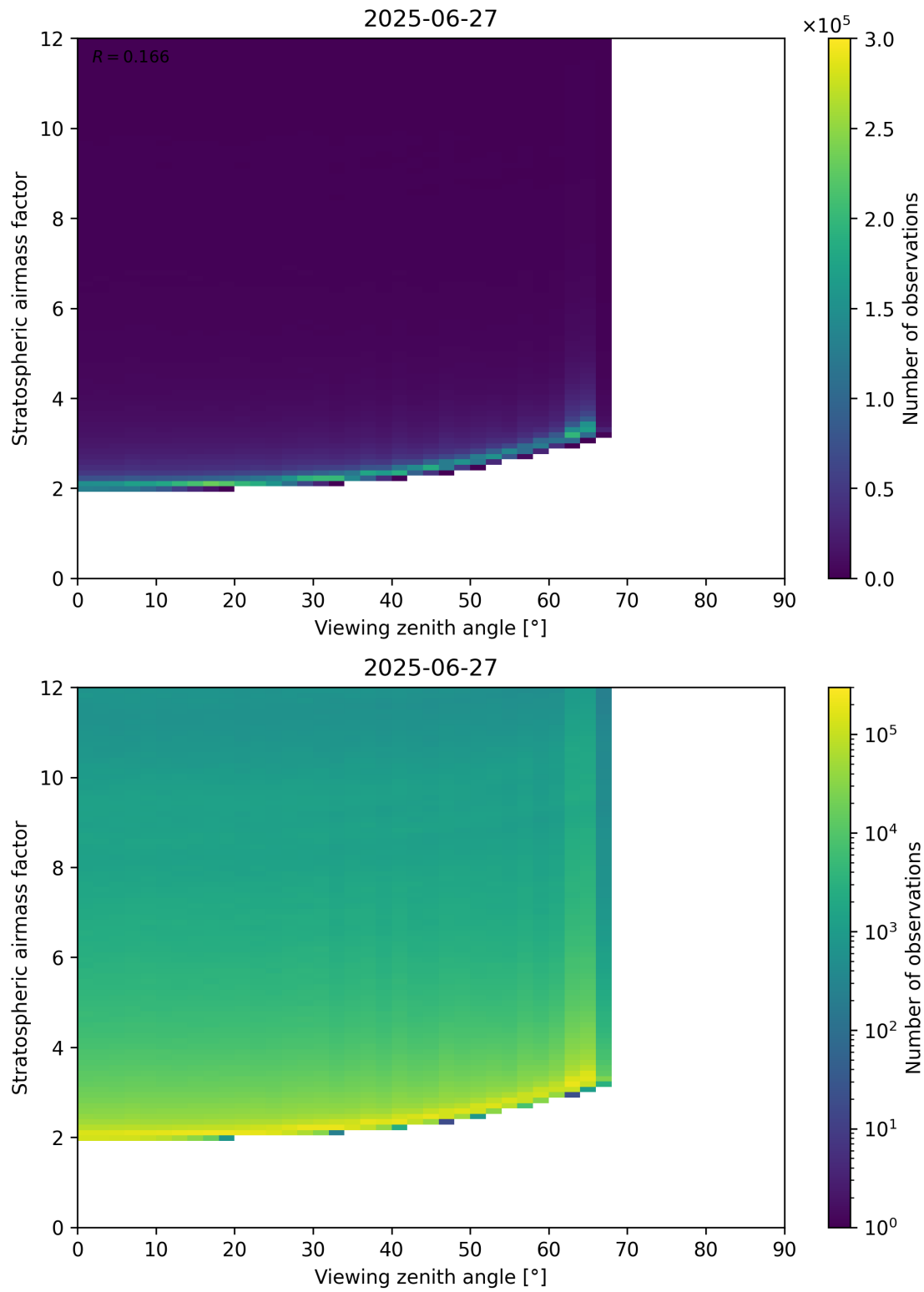
Figure 159: Scatter density plot of “Viewing zenith angle” against “Stratospheric airmass factor” for 2025-06-27 to 2025-06-28.
