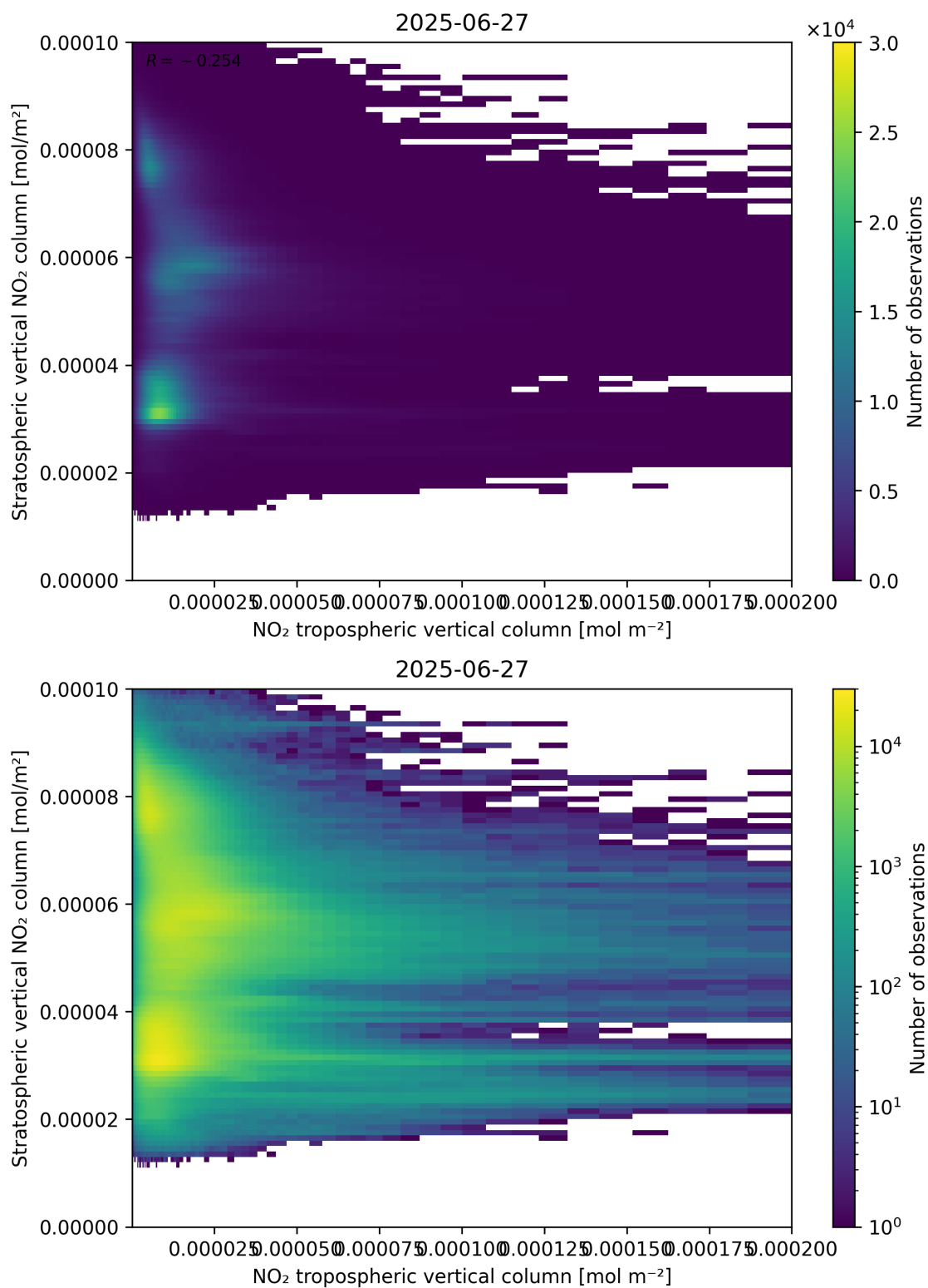
Figure 125: Scatter density plot of “NO 2 tropospheric vertical column” against “Stratospheric vertical NO 2 column” for 2025-06-27 to 2025-06-28.
