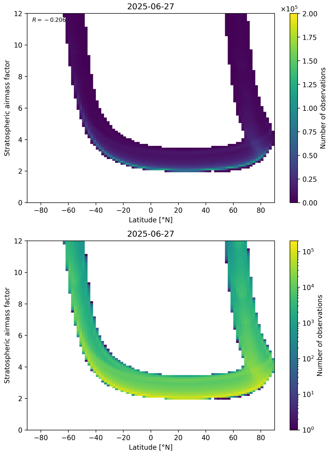
Figure 83: Scatter density plot of “Latitude” against “Stratospheric air mass factor” for 2025-06-27 to 2025-06-28.
