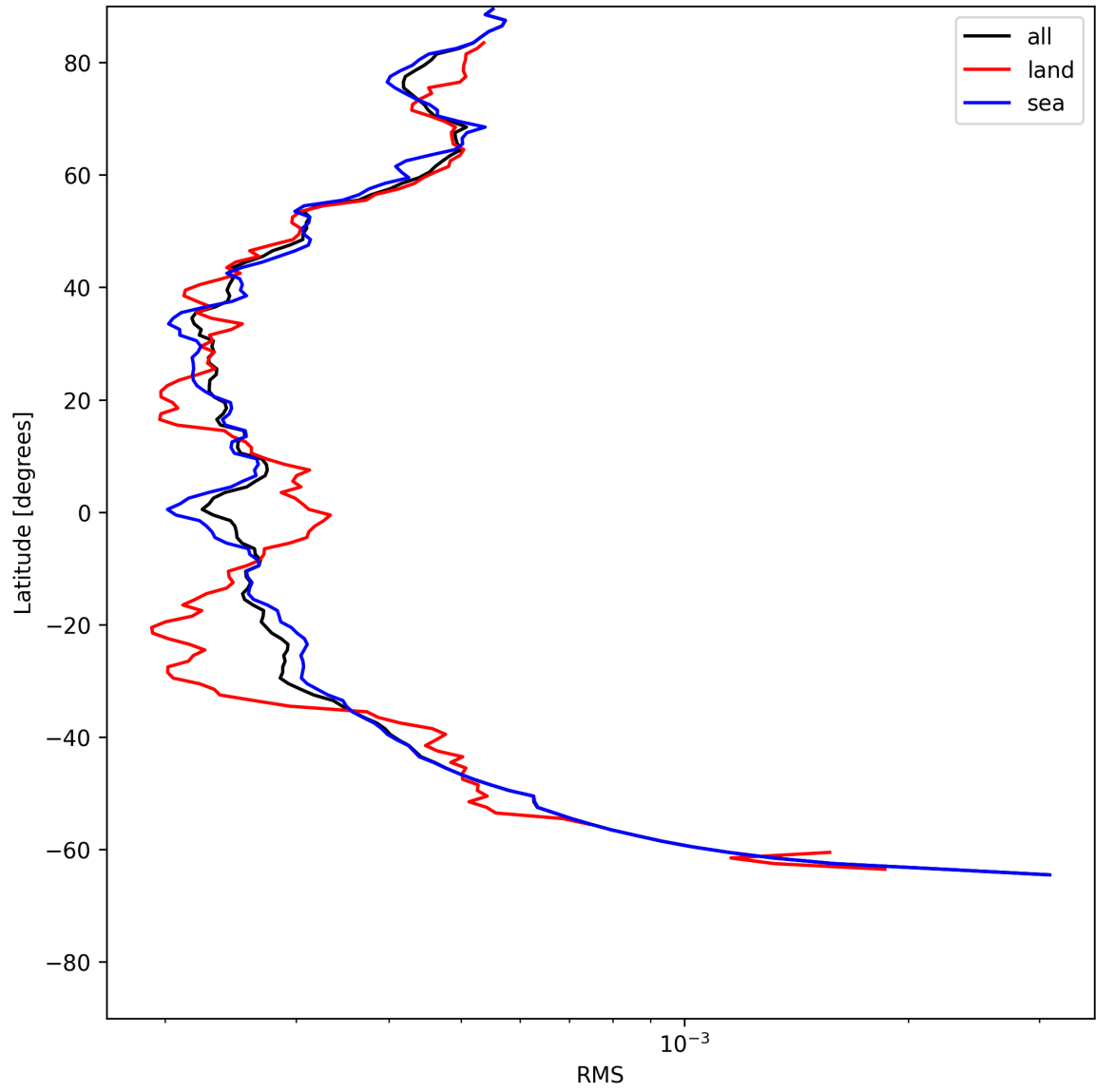
Figure 26: Zonal average of “RMS” for 2025-06-27 to 2025-06-28.
