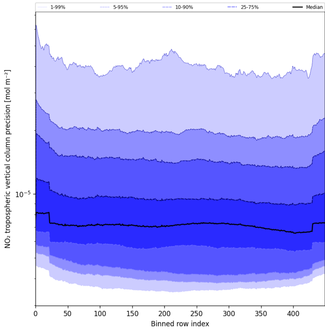
Figure 47: Along track statistics of “NO 2 tropospheric vertical column precision” for 2025-06-27 to 2025-06-28
