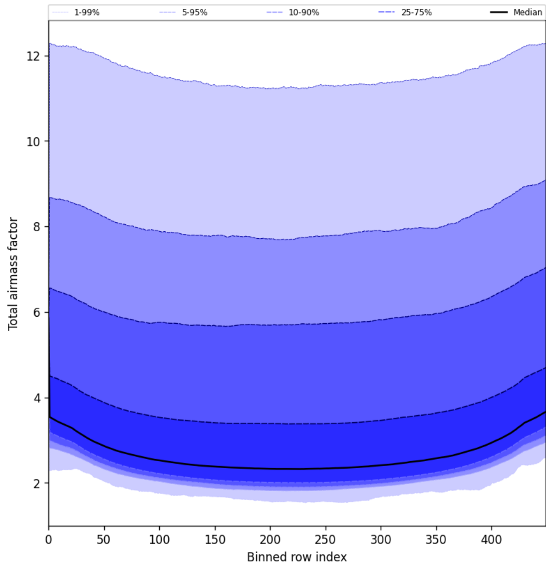
Figure 49: Along track statistics of “Total airmass factor” for 2025-06-27 to 2025-06-28
