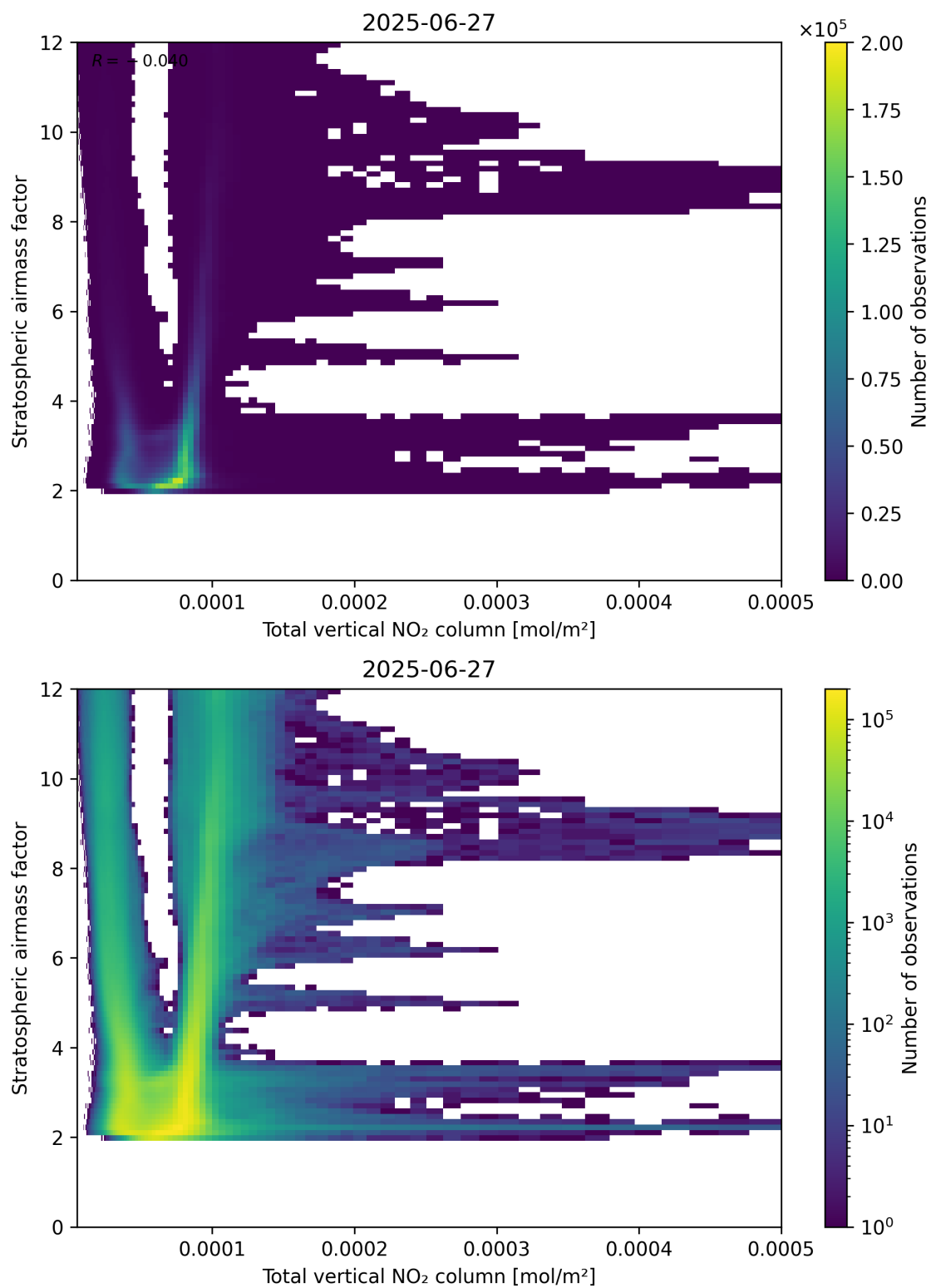
Figure 110: Scatter density plot of “Total vertical NO 2 column” against “Stratospheric airmass factor” for 2025-06-27 to 2025-06-28.
