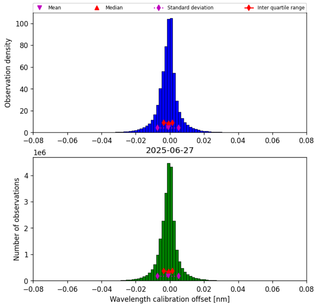
Figure 35: Histogram of “Wavelength calibration offset” for 2025-06-27 to 2025-06-28
