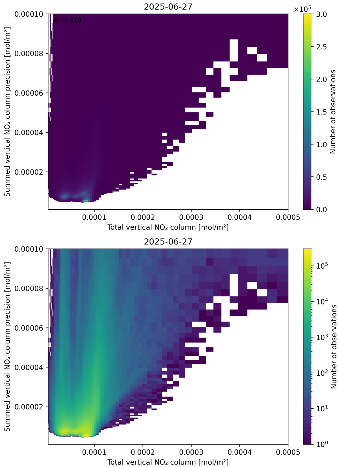
Figure 113: Scatter density plot of “Total vertical NO 2 column” against “Summed vertical NO 2 column precision” for 2025-06-27 to 2025-06-28.
