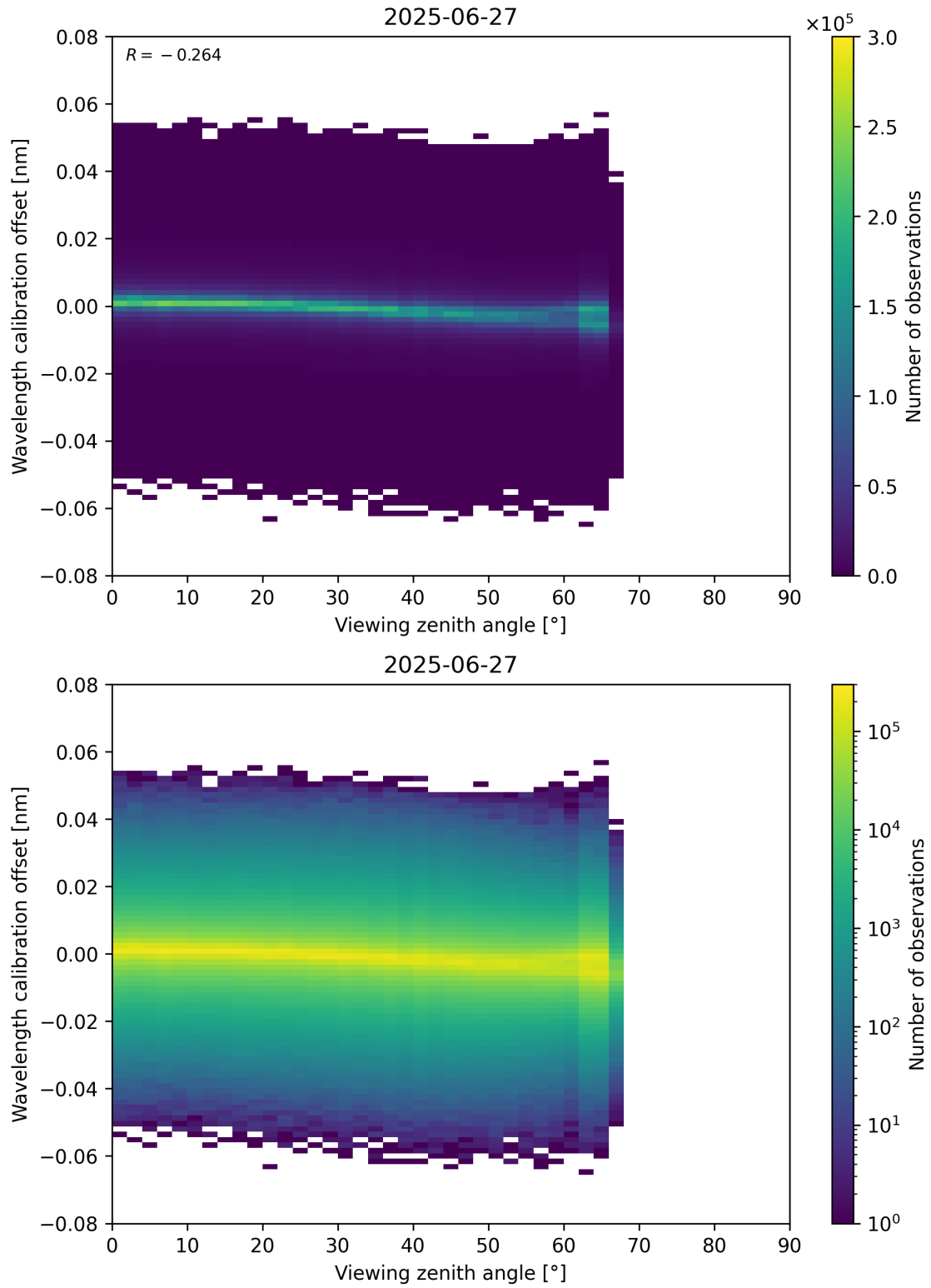
Figure 173: Scatter density plot of “Viewing zenith angle” against “Wavelength calibration offset” for 2025-06-27 to 2025-06-28.
