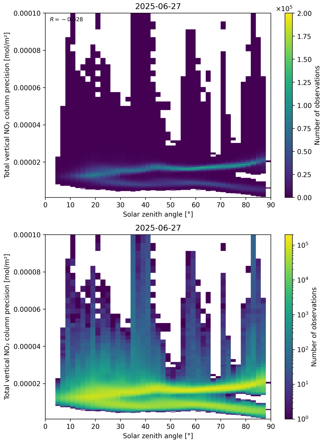
Figure 154: Scatter density plot of “Solar zenith angle” against “Total vertical NO 2 column precision” for 2025-06-27 to 2025-06-28.
