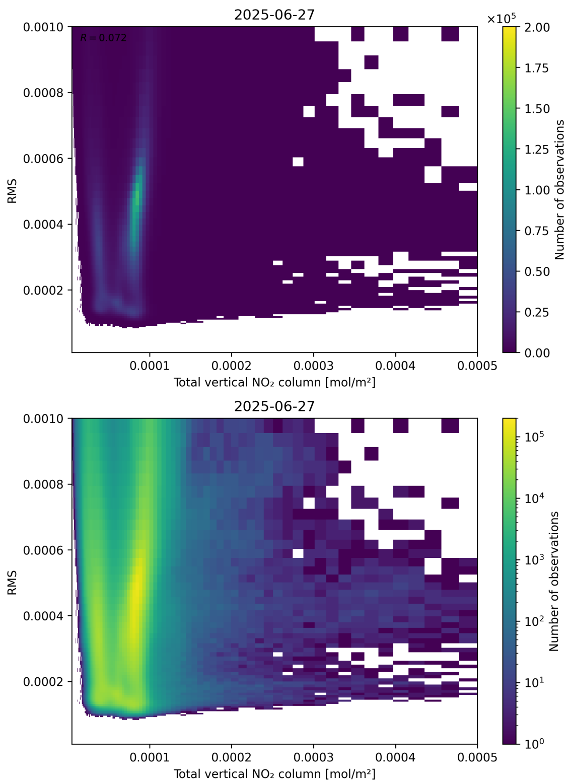
Figure 120: Scatter density plot of “Total vertical NO 2 column” against “RMS” for 2025-06-27 to 2025-06-28.
