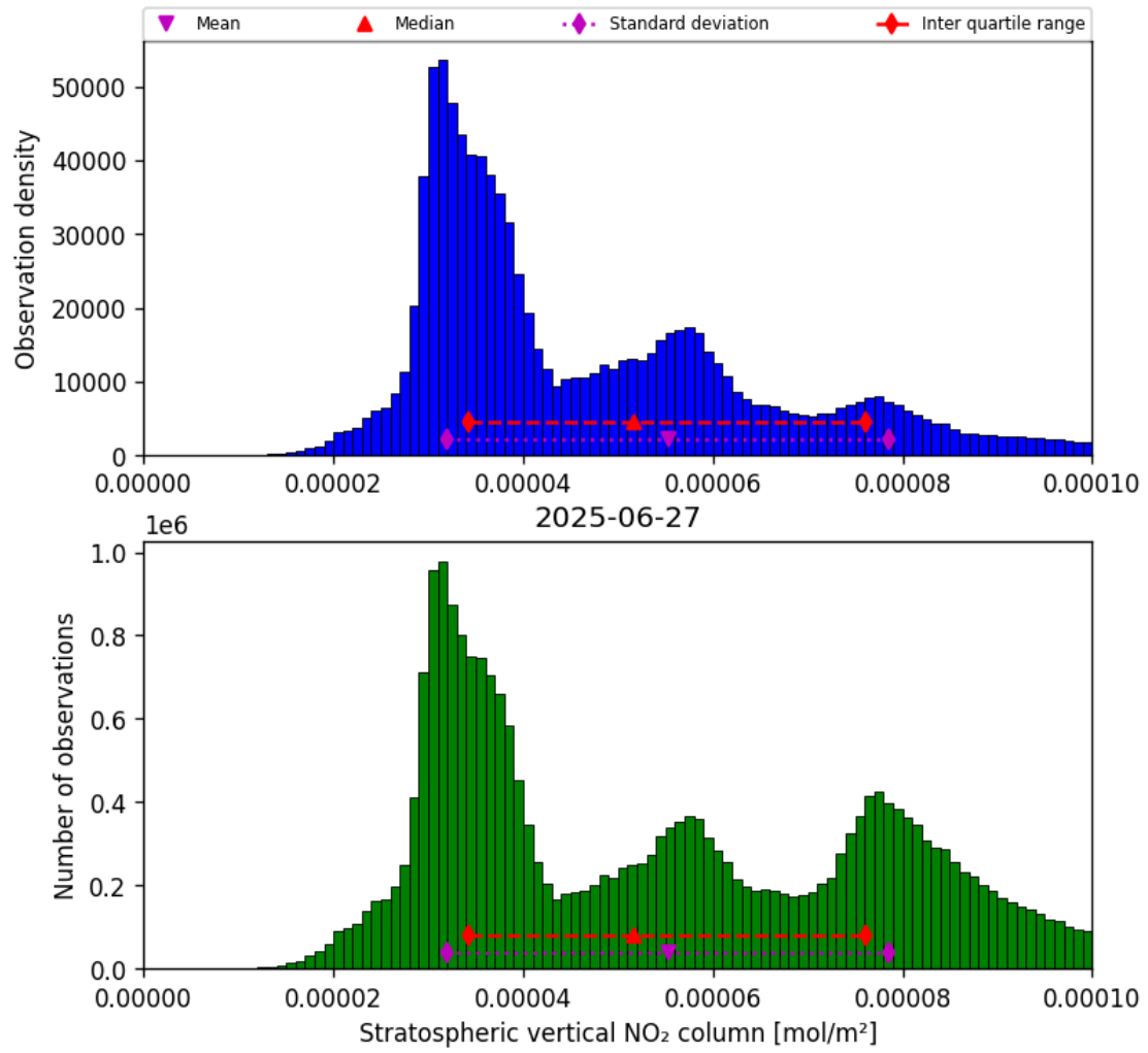
Figure 36: Histogram of “Stratospheric vertical NO 2 column” for 2025-06-27 to 2025-06-28
