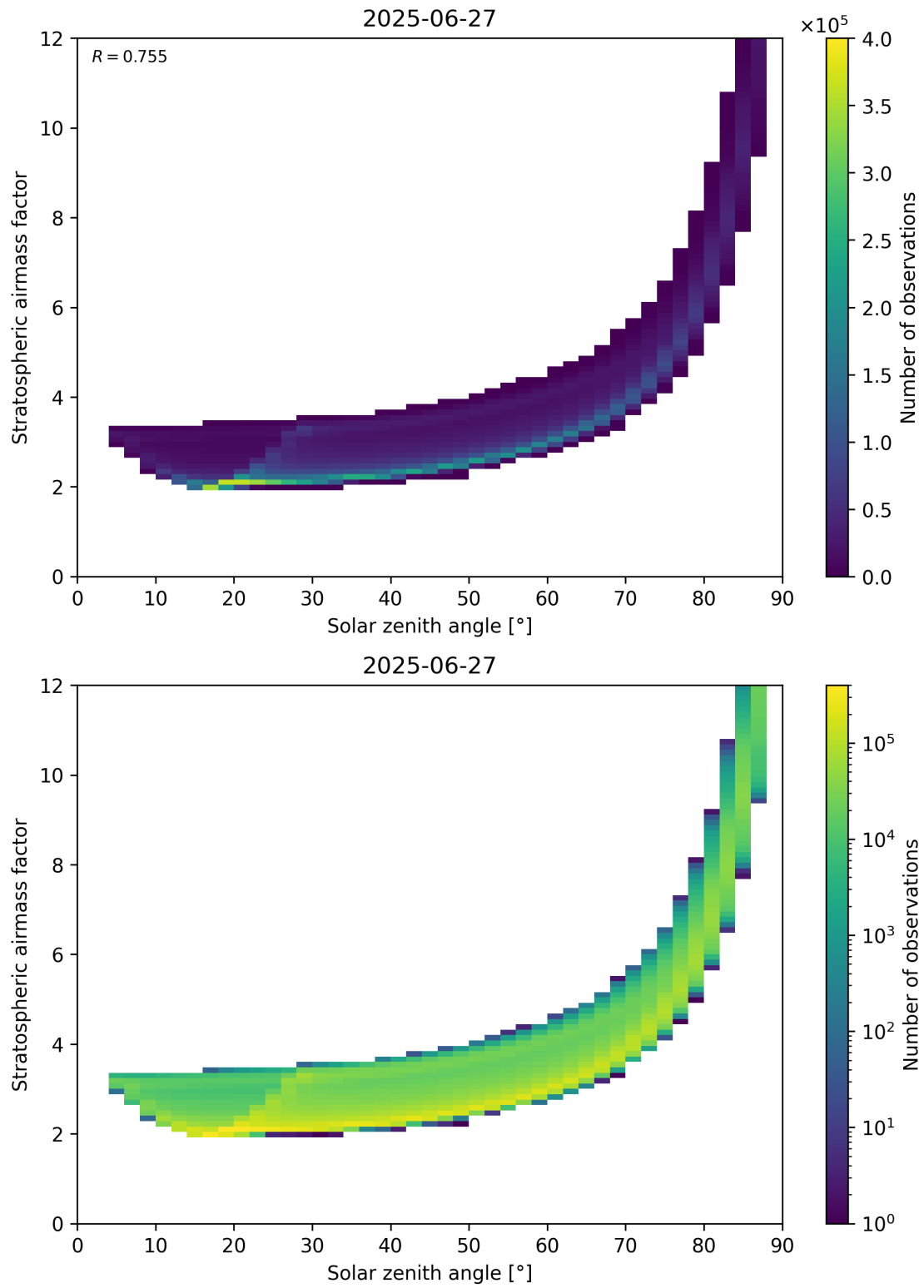
Figure 145: Scatter density plot of “Solar zenith angle” against “Stratospheric airmass factor” for 2025-06-27 to 2025-06-28.
