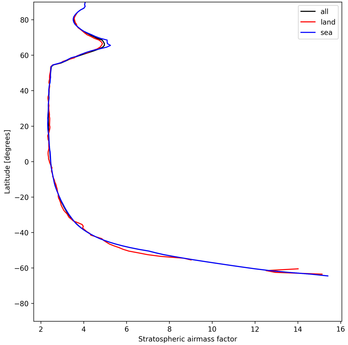
Figure 27: Zonal average of “Stratospheric airmass factor” for 2025-06-27 to 2025-06-28.
