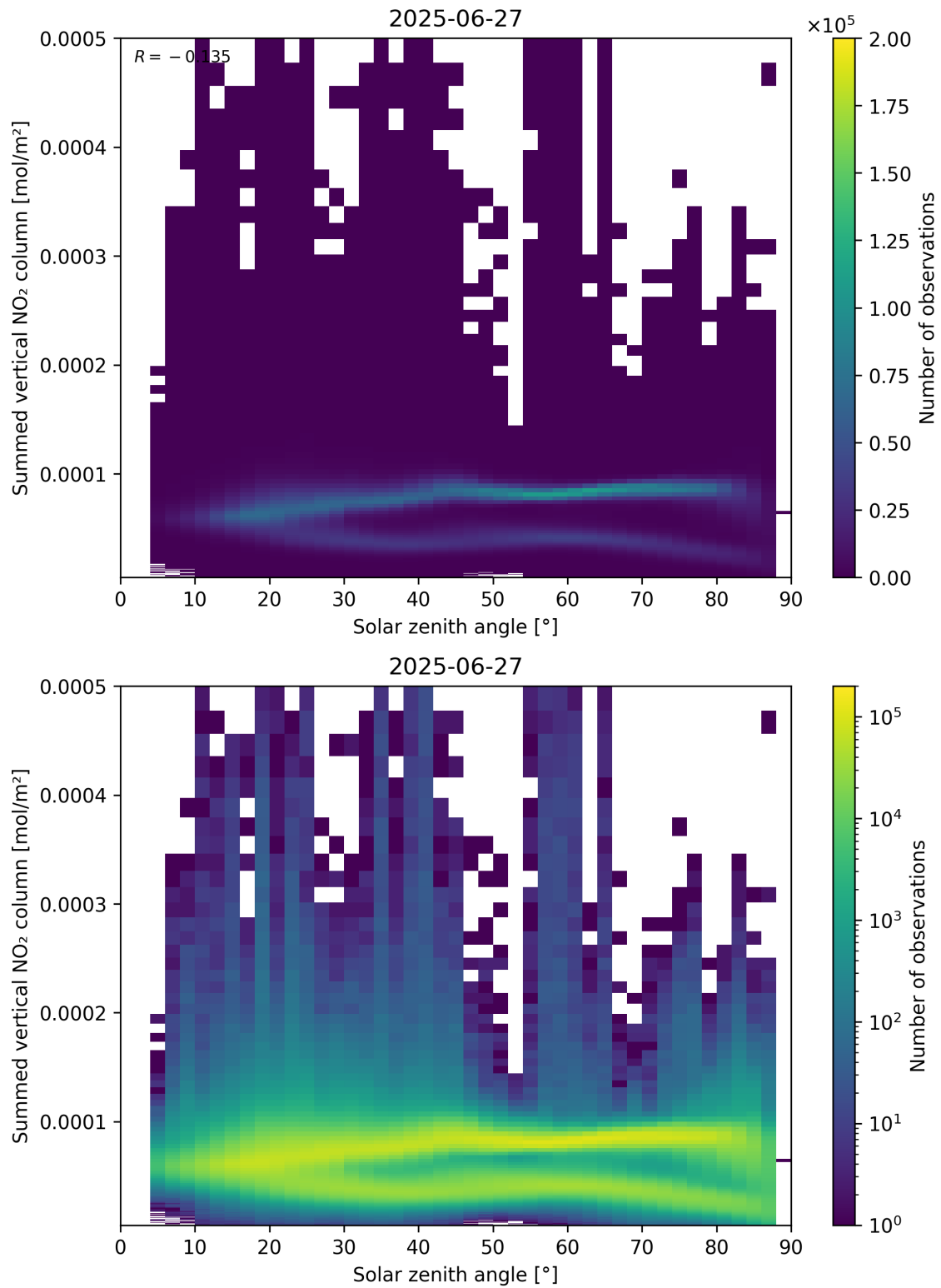
Figure 151: Scatter density plot of “Solar zenith angle” against “Summed vertical NO 2 column” for 2025-06-27 to 2025-06-28.
