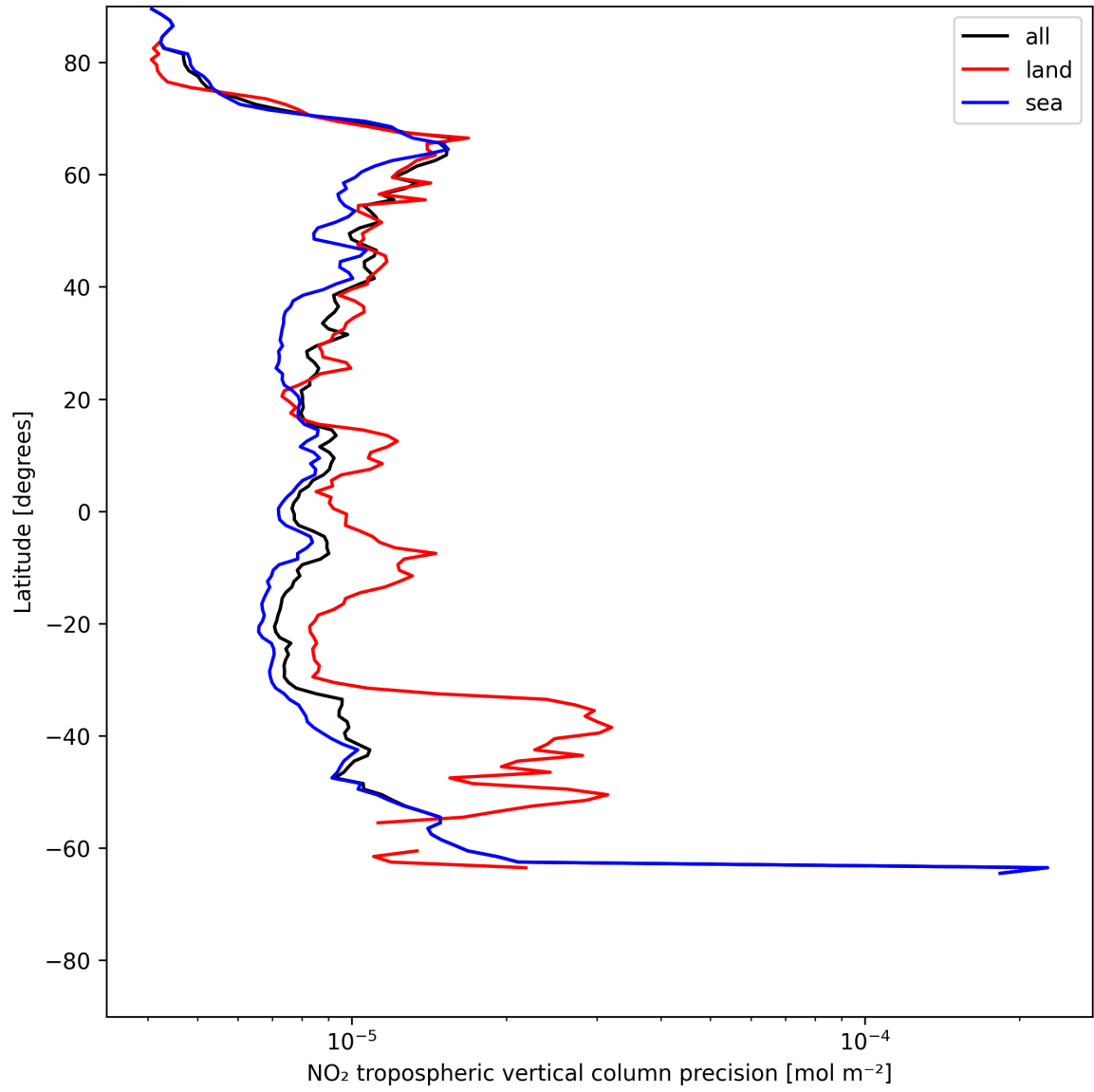
Figure 13: Zonal average of “NO 2 tropospheric vertical column precision” for 2025-06-27 to 2025-06-28.
