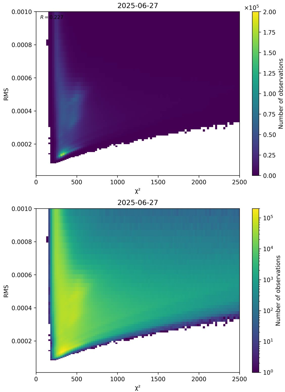
Figure 82: Scatter density plot of “ \chi^2 ” against “RMS” for 2025-06-27 to 2025-06-28.
