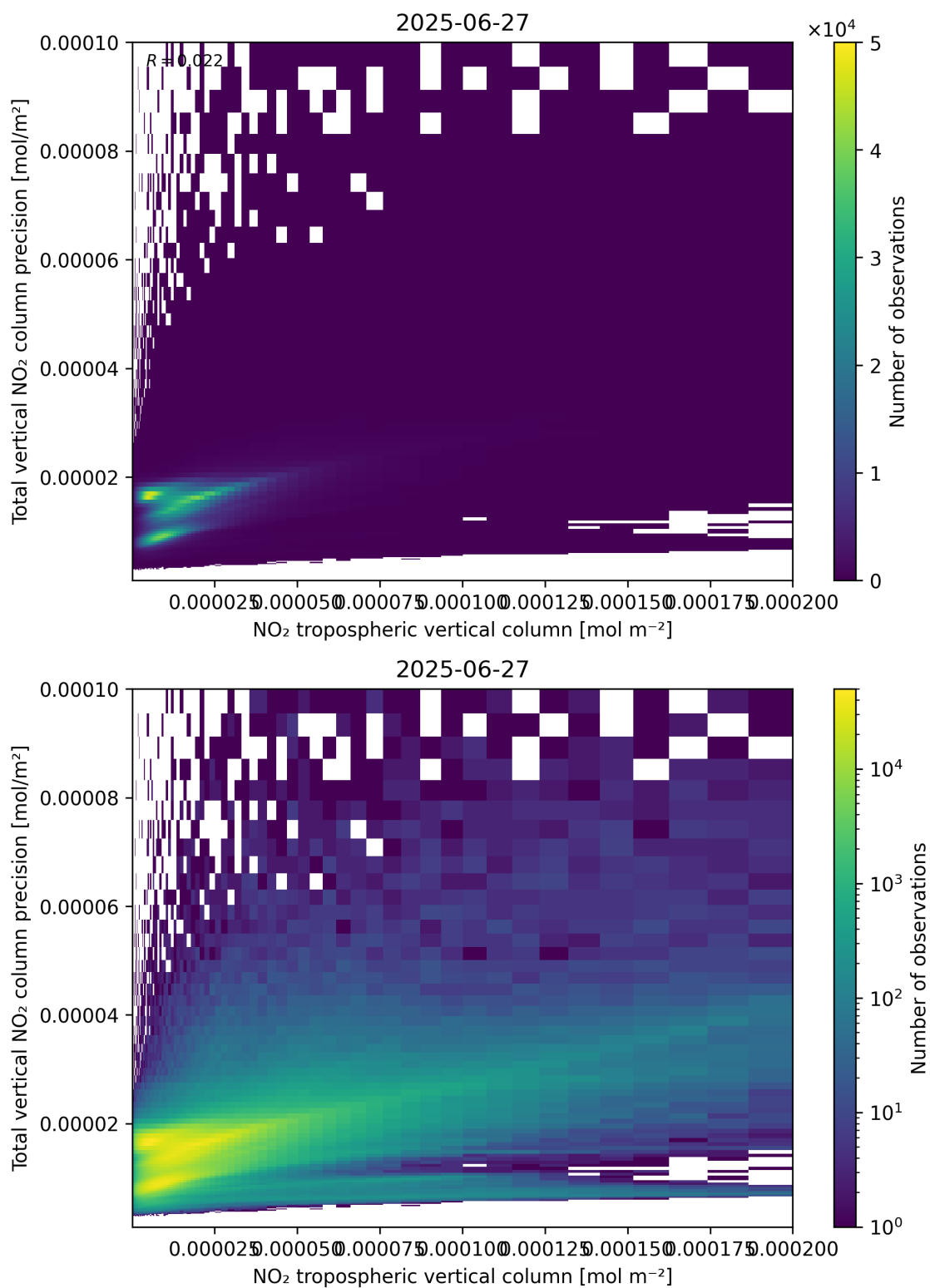
Figure 129: Scatter density plot of “NO 2 tropospheric vertical column” against “Total vertical NO 2 column precision” for 2025-06-27 to 2025-06-28.
