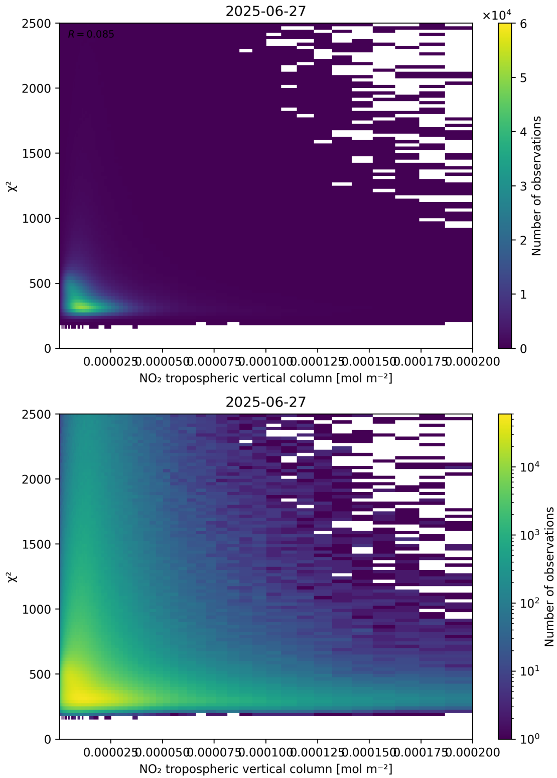
Figure 124: Scatter density plot of “NO 2 tropospheric vertical column” against “ \chi^2 ” for 2025-06-27 to 2025-06-28.
