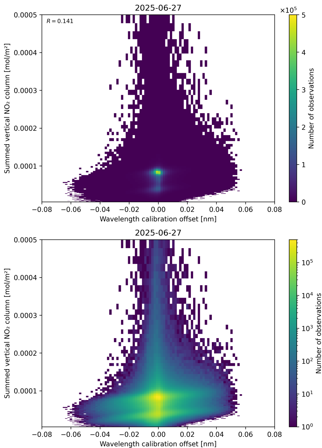
Figure 177: Scatter density plot of “Wavelength calibration offset” against “Summed vertical NO 2 column” for 2025-06-27 to 2025-06-28.
