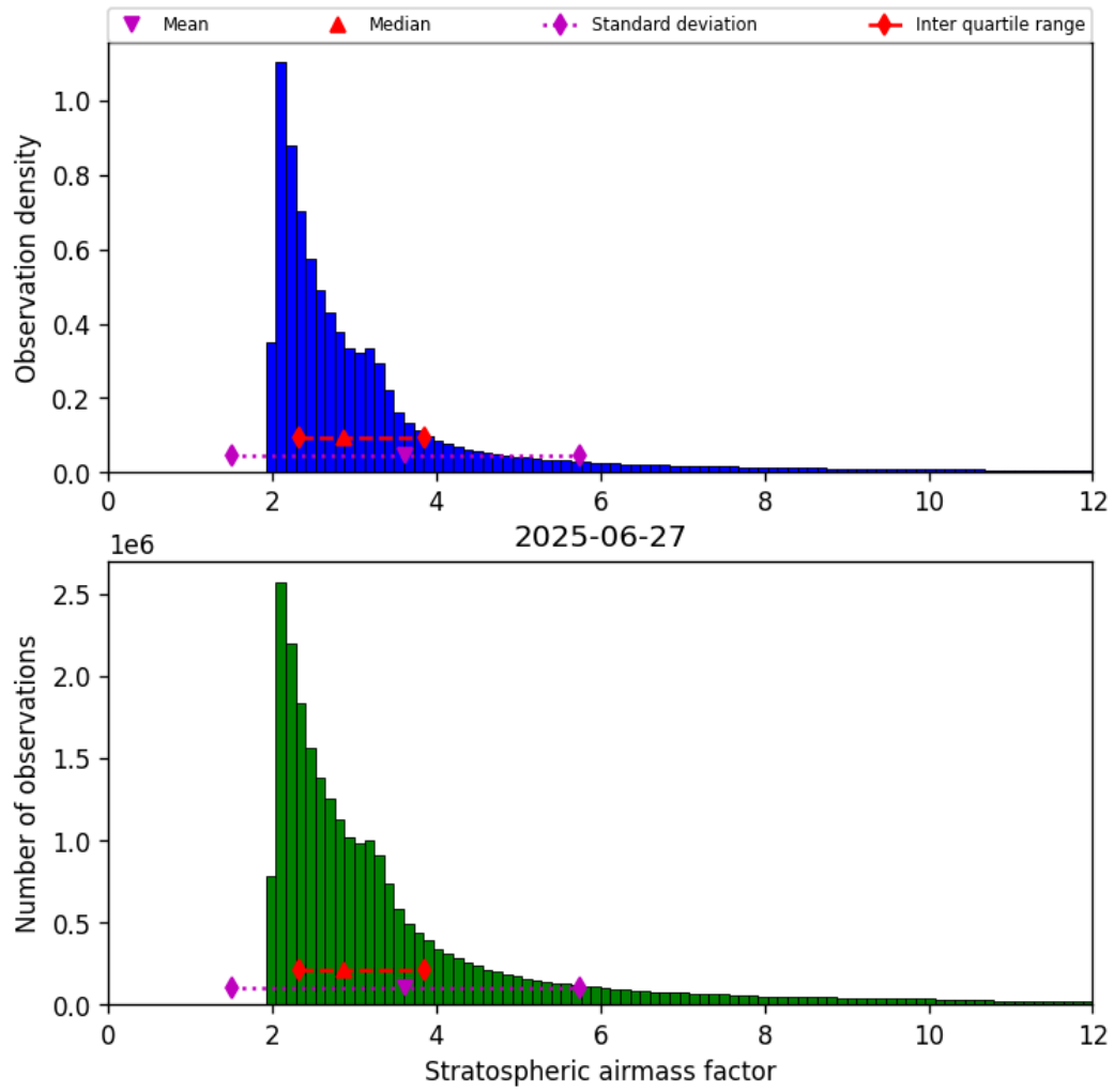
Figure 44: Histogram of “Stratospheric airmass factor” for 2025-06-27 to 2025-06-28
