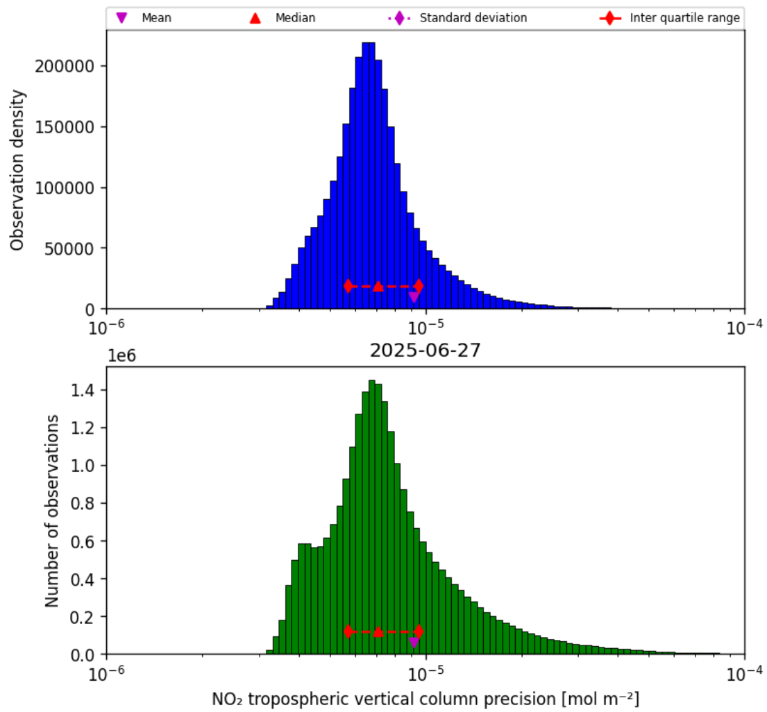
Figure 30: Histogram of “NO 2 tropospheric vertical column precision” for 2025-06-27 to 2025-06-28
