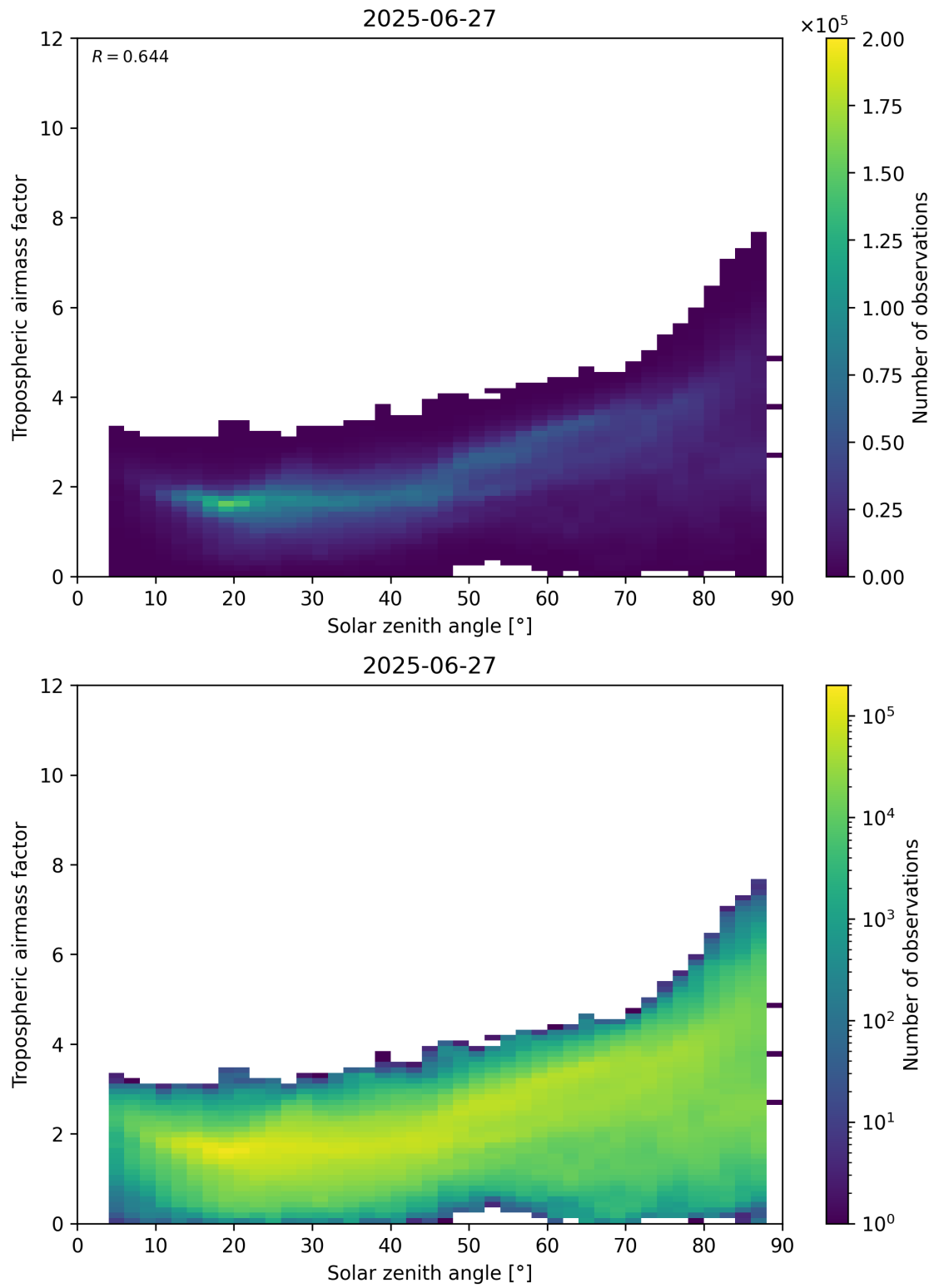
Figure 147: Scatter density plot of “Solar zenith angle” against “Tropospheric airmass factor” for 2025-06-27 to 2025-06-28.
