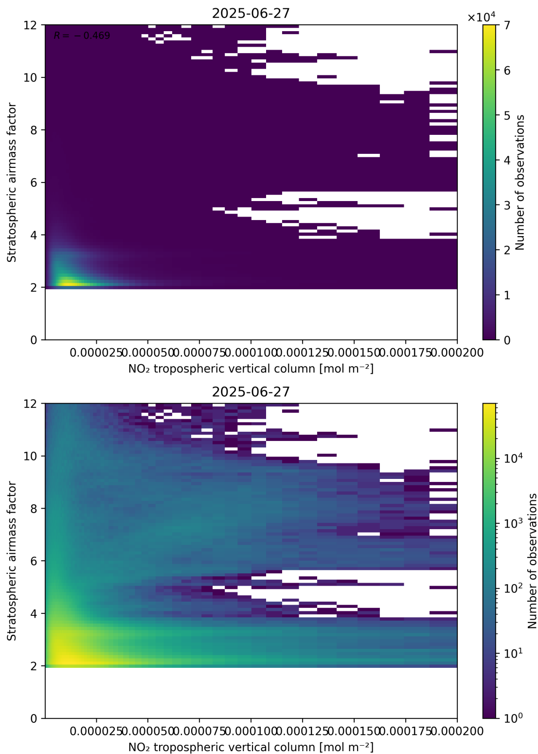
Figure 121: Scatter density plot of “NO 2 tropospheric vertical column” against “Stratospheric air mass factor” for 2025-06-27 to 2025-06-28.
