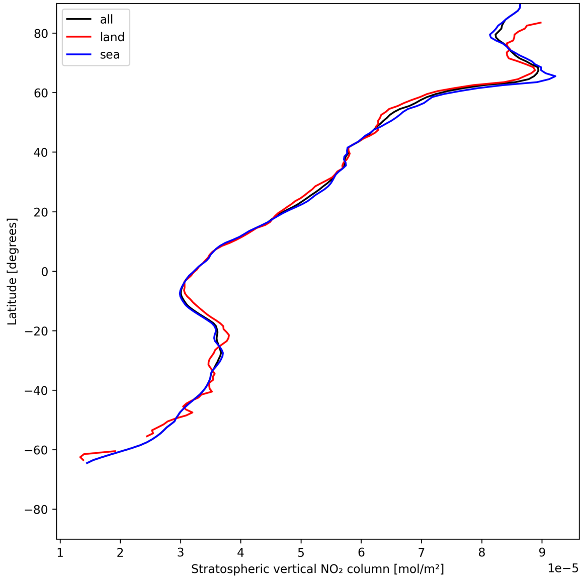
Figure 19: Zonal average of “Stratospheric vertical NO 2 column” for 2025-06-27 to 2025-06-28.
