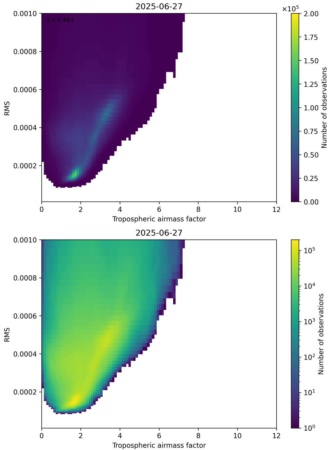
Figure 79: Scatter density plot of “Tropospheric airmass factor” against “RMS” for 2025-06-27 to 2025-06-28.
