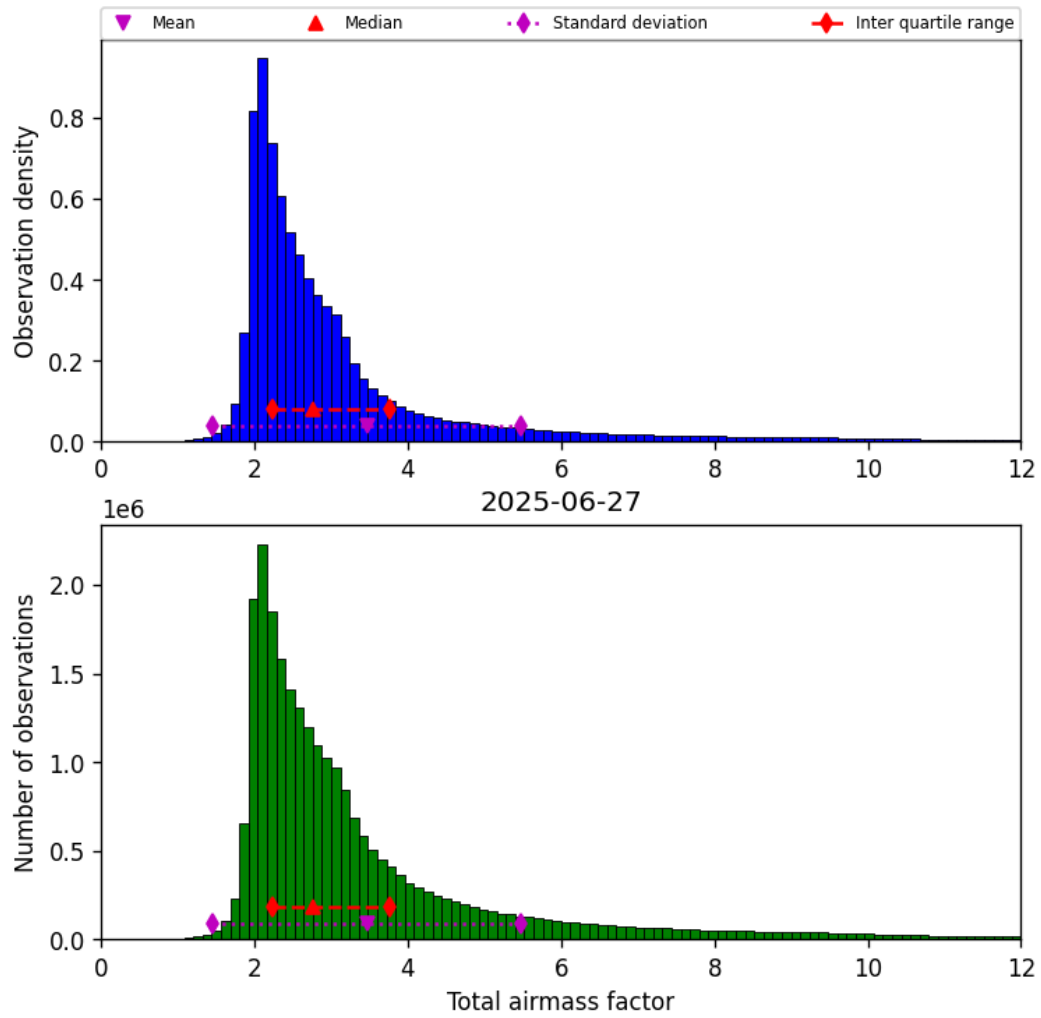
Figure 32: Histogram of “Total airmass factor” for 2025-06-27 to 2025-06-28
