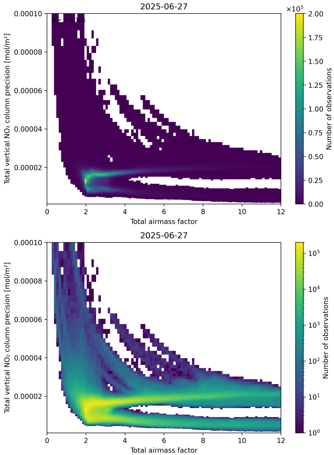
Figure 68: Scatter density plot of “Total airmass factor” against “Total vertical NO 2 column precision” for 2025-06-27 to 2025-06-28.
