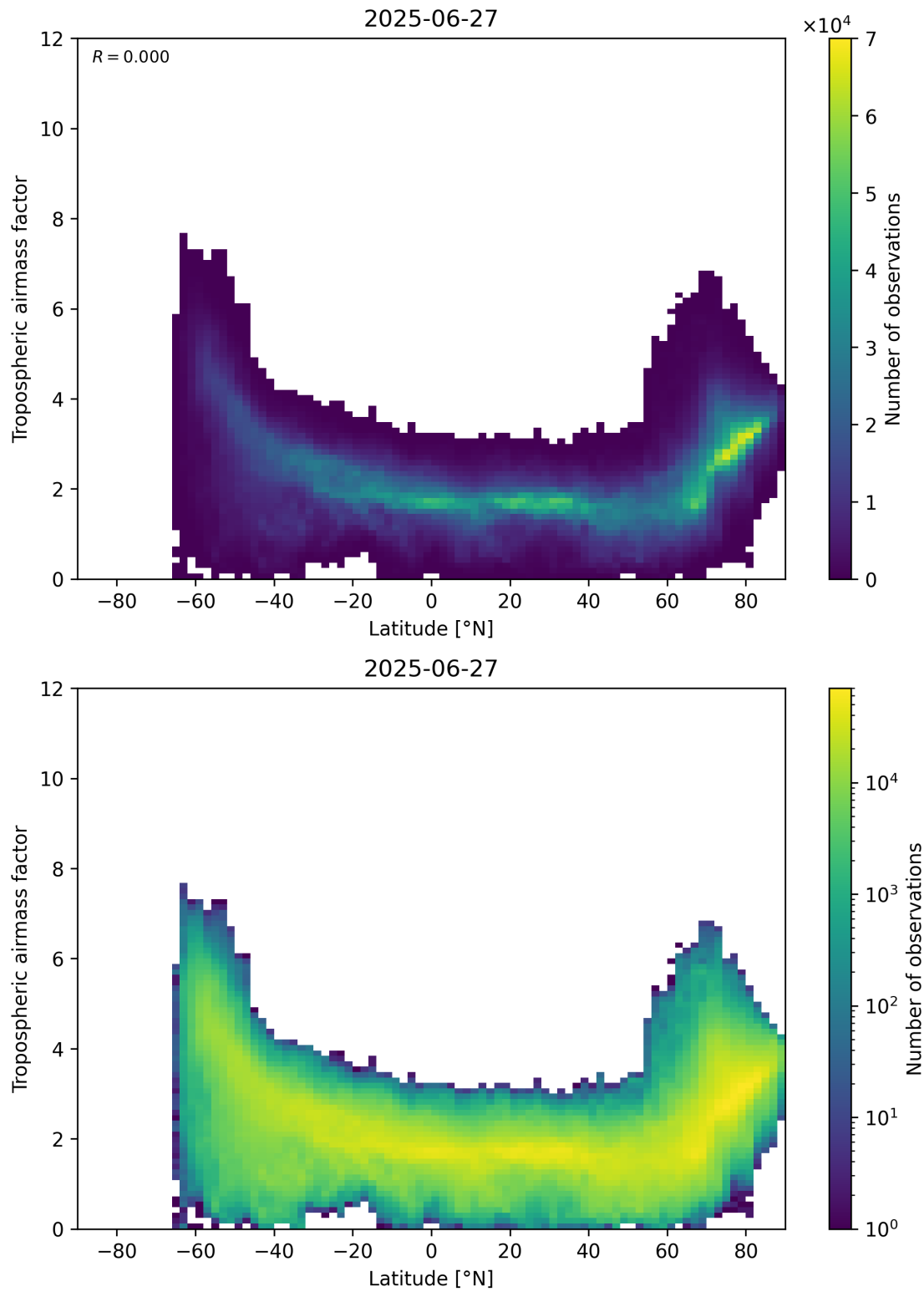
Figure 85: Scatter density plot of “Latitude” against “Tropospheric air mass factor” for 2025-06-27 to 2025-06-28.
