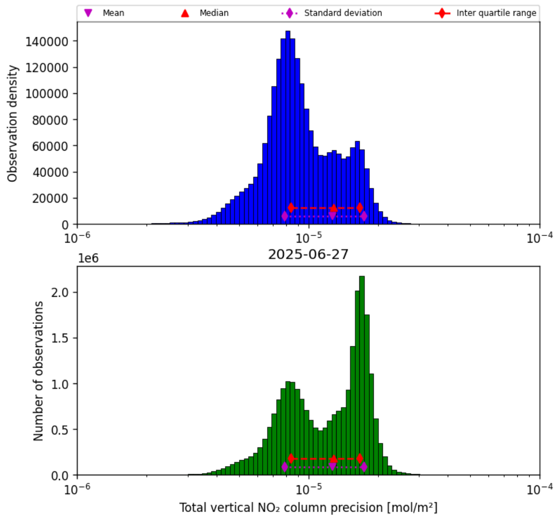
Figure 39: Histogram of “Total vertical NO 2 column precision” for 2025-06-27 to 2025-06-28
