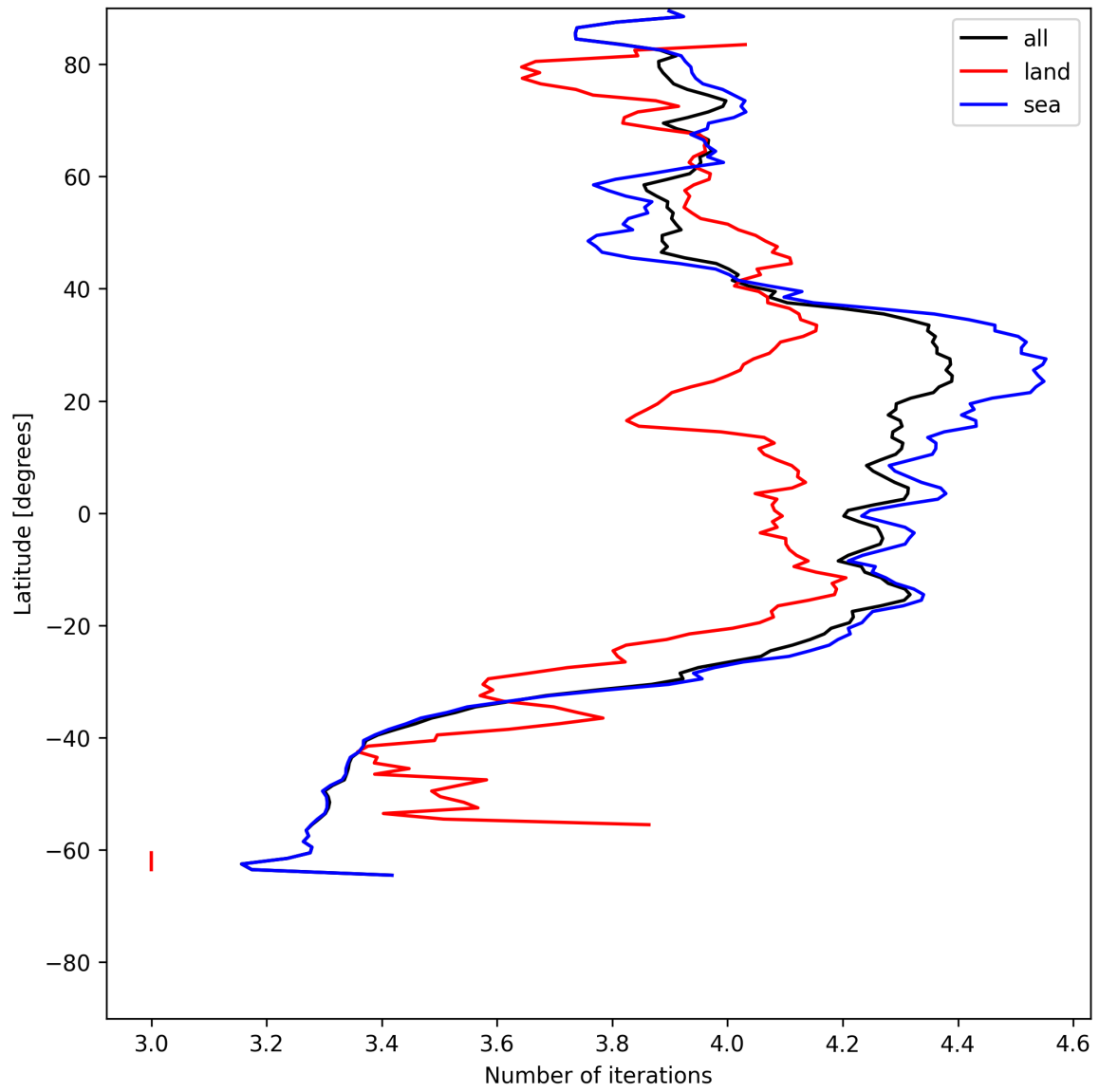
Figure 17: Zonal average of “Number of iterations” for 2025-06-27 to 2025-06-28.
