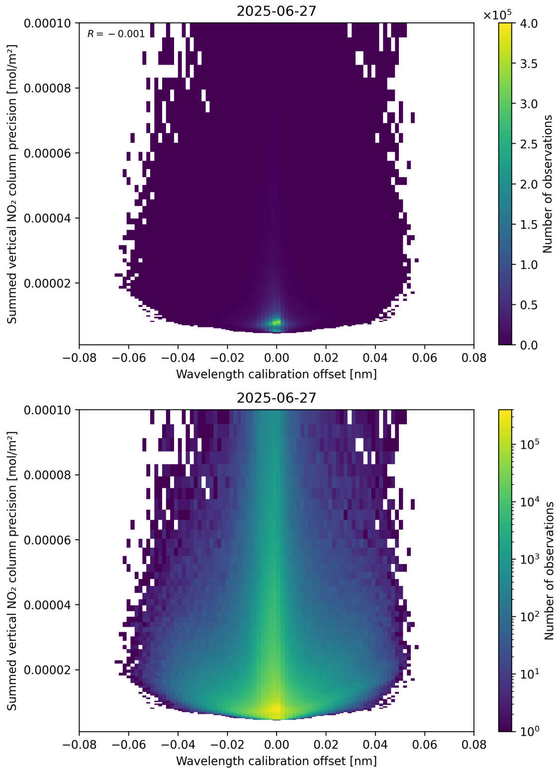
Figure 178: Scatter density plot of “Wavelength calibration offset” against “Summed vertical NO 2 column precision” for 2025-06-27 to 2025-06-28.
