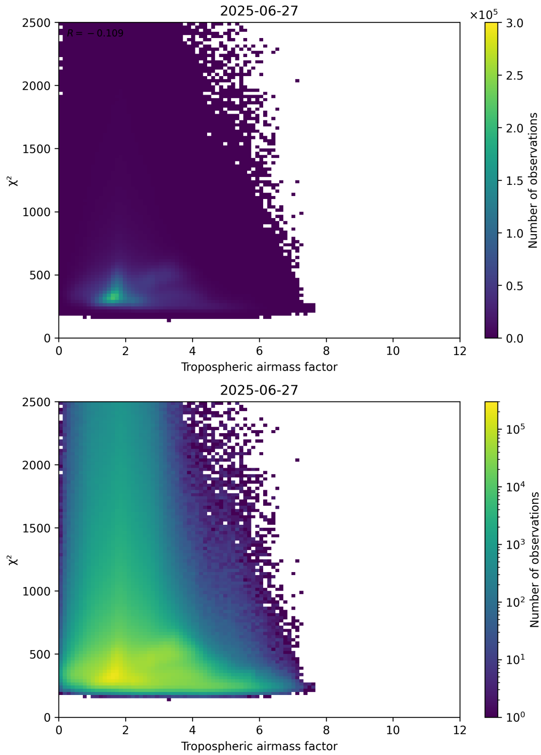
Figure 73: Scatter density plot of “Tropospheric airmass factor” against “ \chi^2 ” for 2025-06-27 to 2025-06-28.
