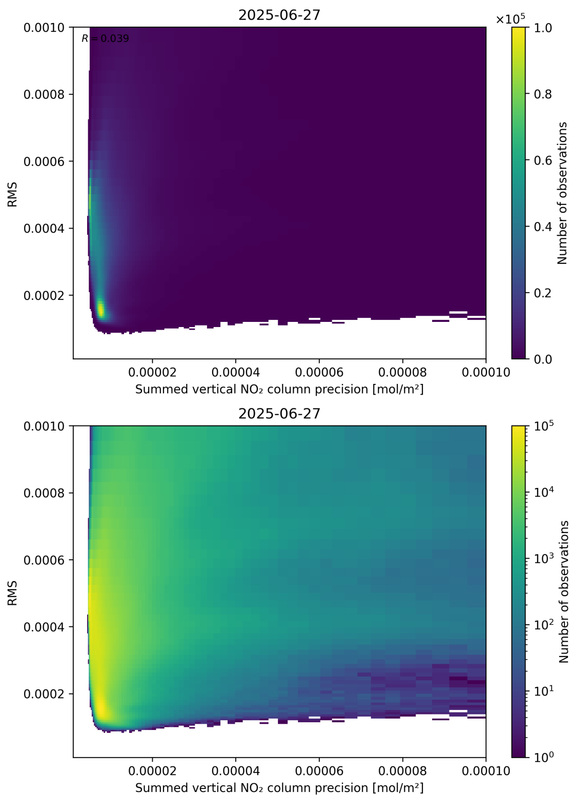
Figure 108: Scatter density plot of “Summed vertical NO 2 column precision” against “RMS” for 2025-06-27 to 2025-06-28.
