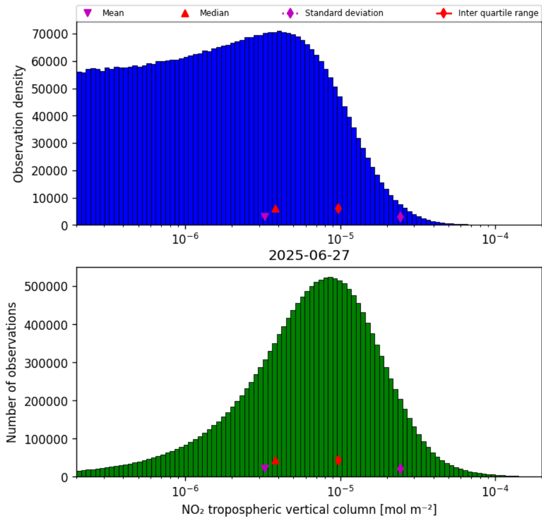
Figure 29: Histogram of “NO 2 tropospheric vertical column” for 2025-06-27 to 2025-06-28
