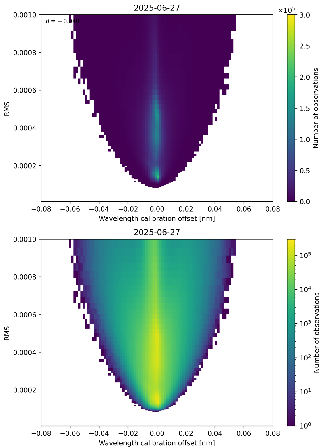
Figure 181: Scatter density plot of “Wavelength calibration offset” against “RMS” for 2025-06-27 to 2025-06-28.
