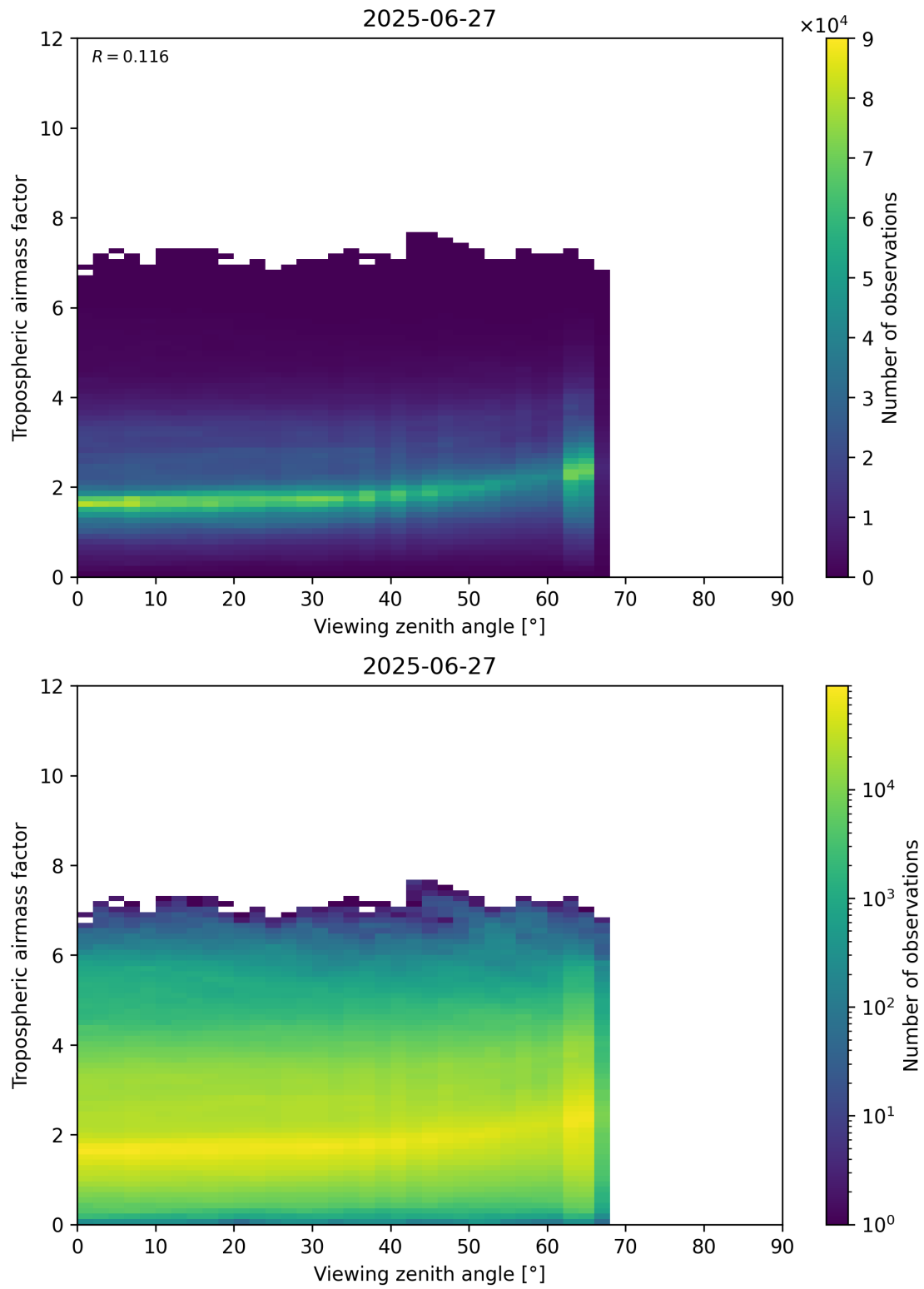
Figure 161: Scatter density plot of “Viewing zenith angle” against “Tropospheric airmass factor” for 2025-06-27 to 2025-06-28.
