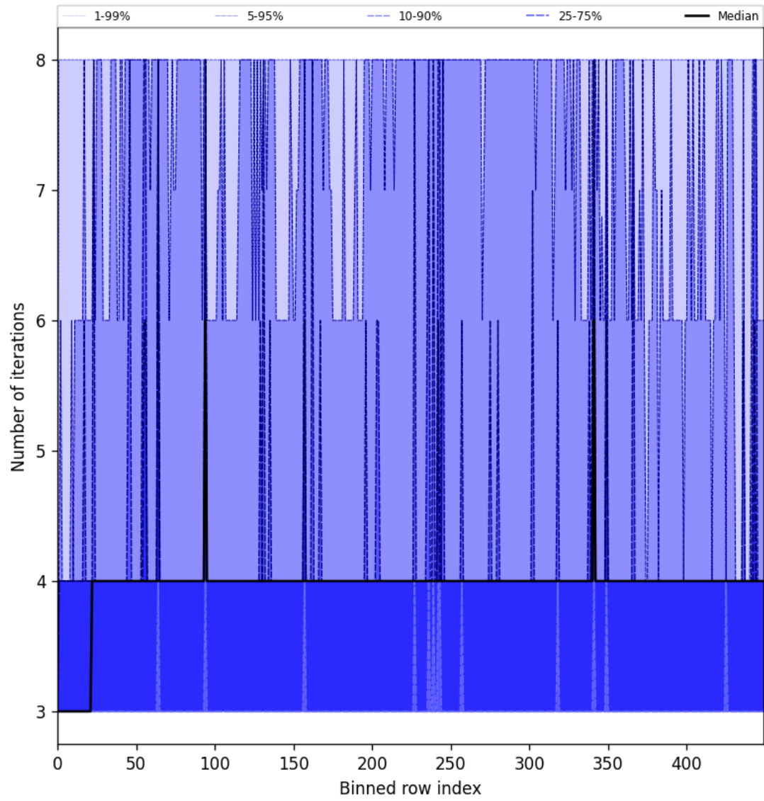
Figure 51: Along track statistics of “Number of iterations” for 2025-06-27 to 2025-06-28
