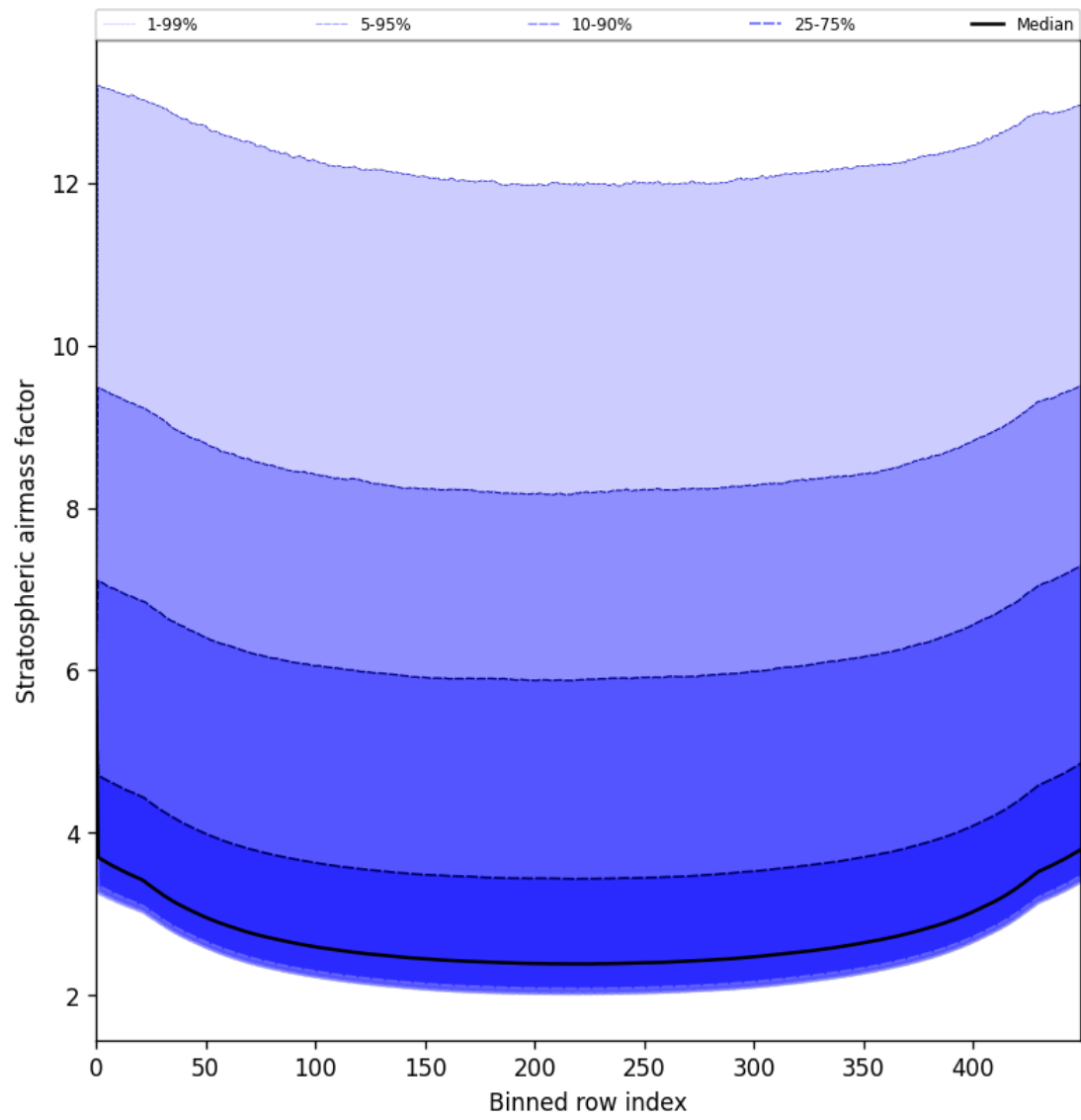
Figure 61: Along track statistics of “Stratospheric airmass factor” for 2025-06-27 to 2025-06-28
