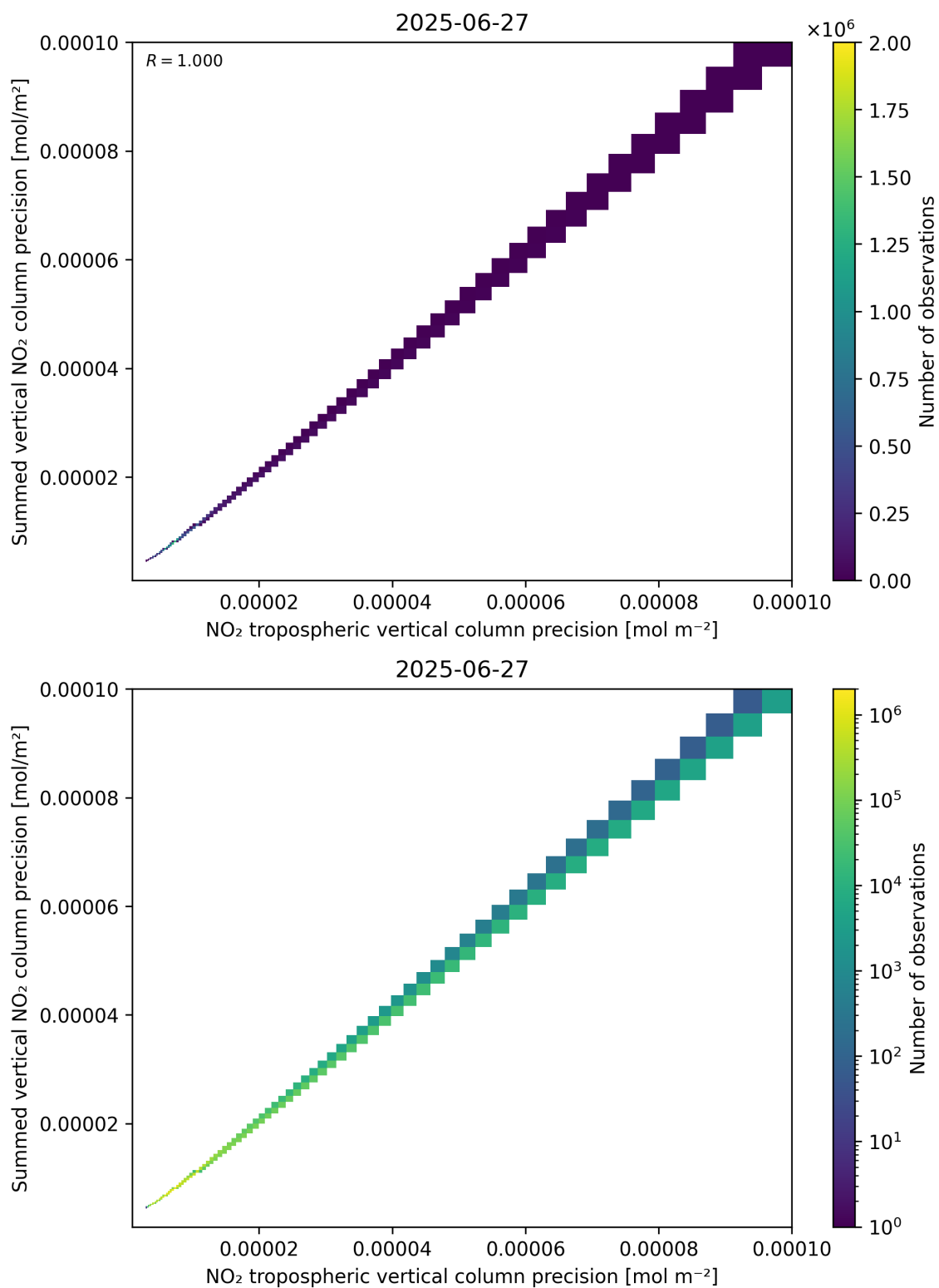
Figure 137: Scatter density plot of “NO 2 tropospheric vertical column precision” against “Summed vertical NO 2 column precision” for 2025-06-27 to 2025-06-28.
