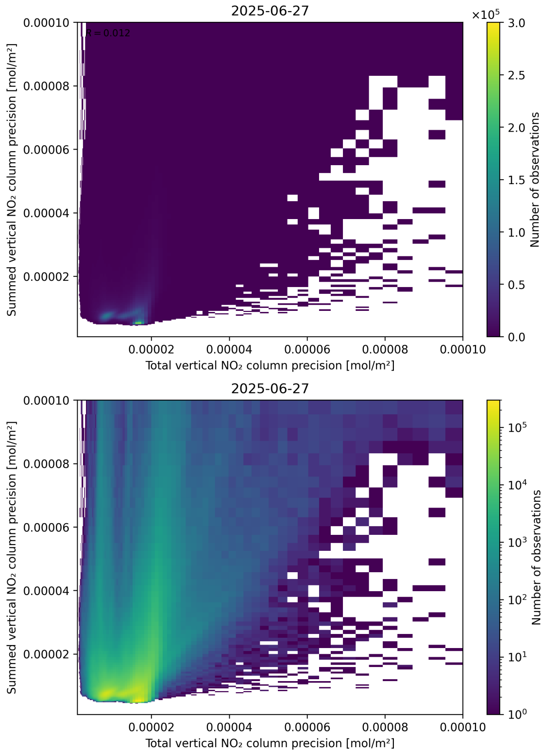
Figure 118: Scatter density plot of “Total vertical NO 2 column precision” against “Summed vertical NO 2 column precision” for 2025-06-27 to 2025-06-28.
