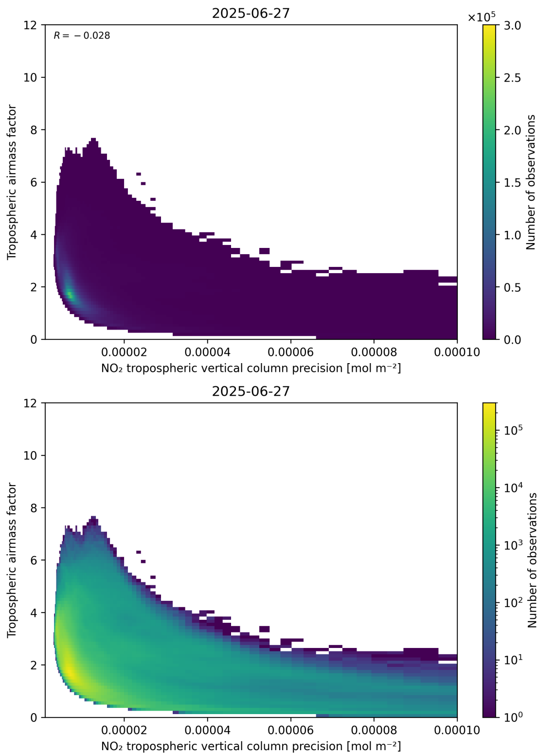
Figure 133: Scatter density plot of “NO 2 tropospheric vertical column precision” against “Tropospheric air mass factor” for 2025-06-27 to 2025-06-28.
