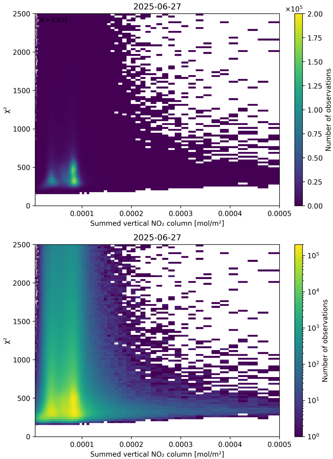
Figure 104: Scatter density plot of “Summed vertical NO 2 column” against “ \chi^2 ” for 2025-06-27 to 2025-06-28.
