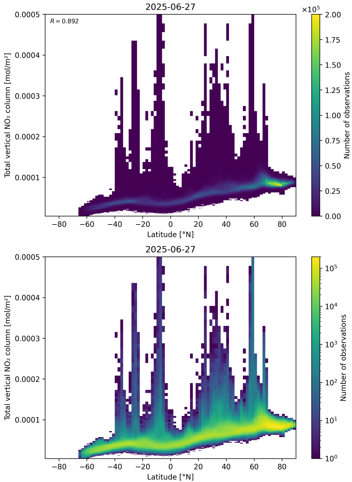
Figure 90: Scatter density plot of “Latitude” against “Total vertical NO 2 column” for 2025-06-27 to 2025-06-28.
