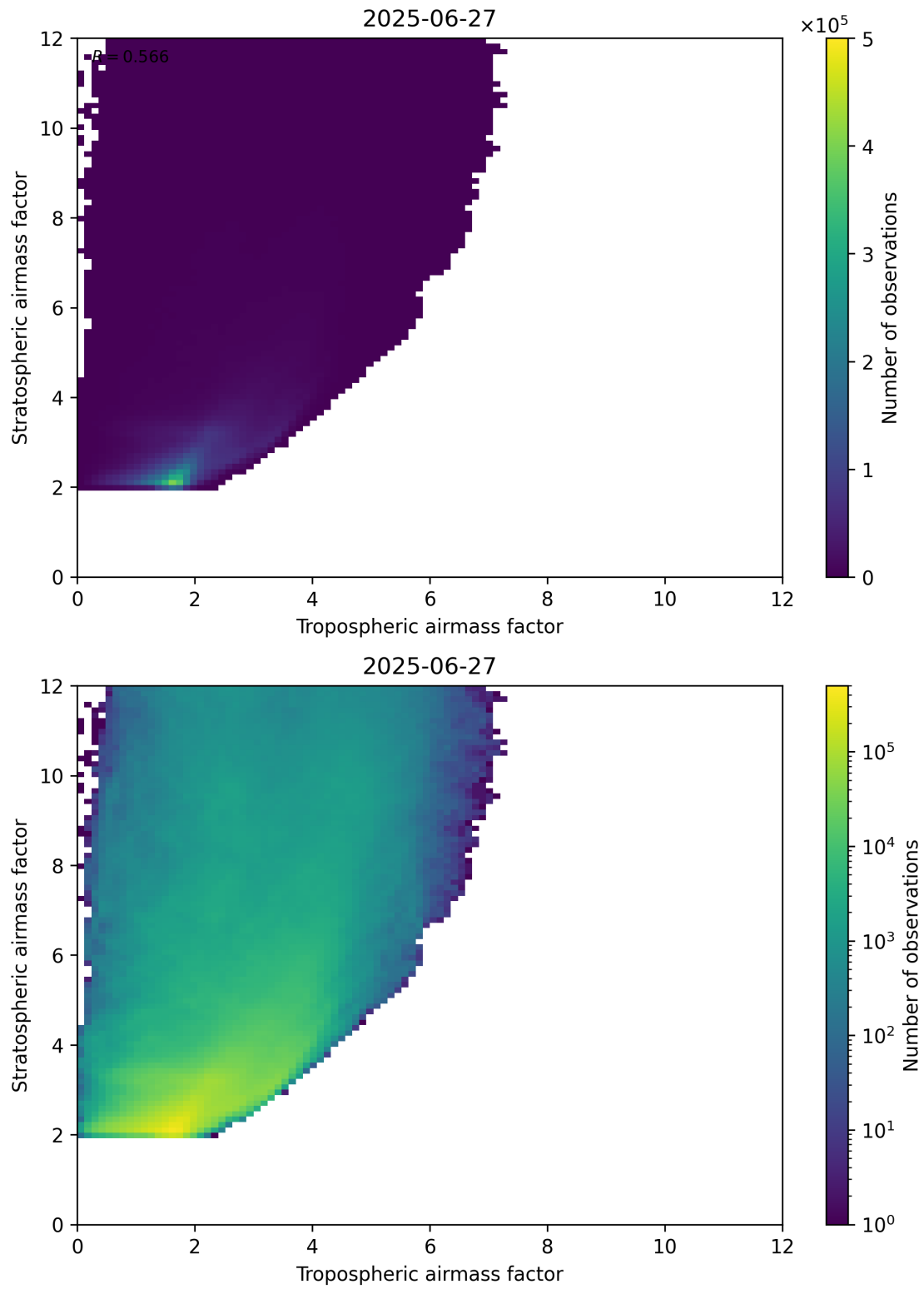
Figure 71: Scatter density plot of “Tropospheric airmass factor” against “Stratospheric airmass factor” for 2025-06-27 to 2025-06-28.
