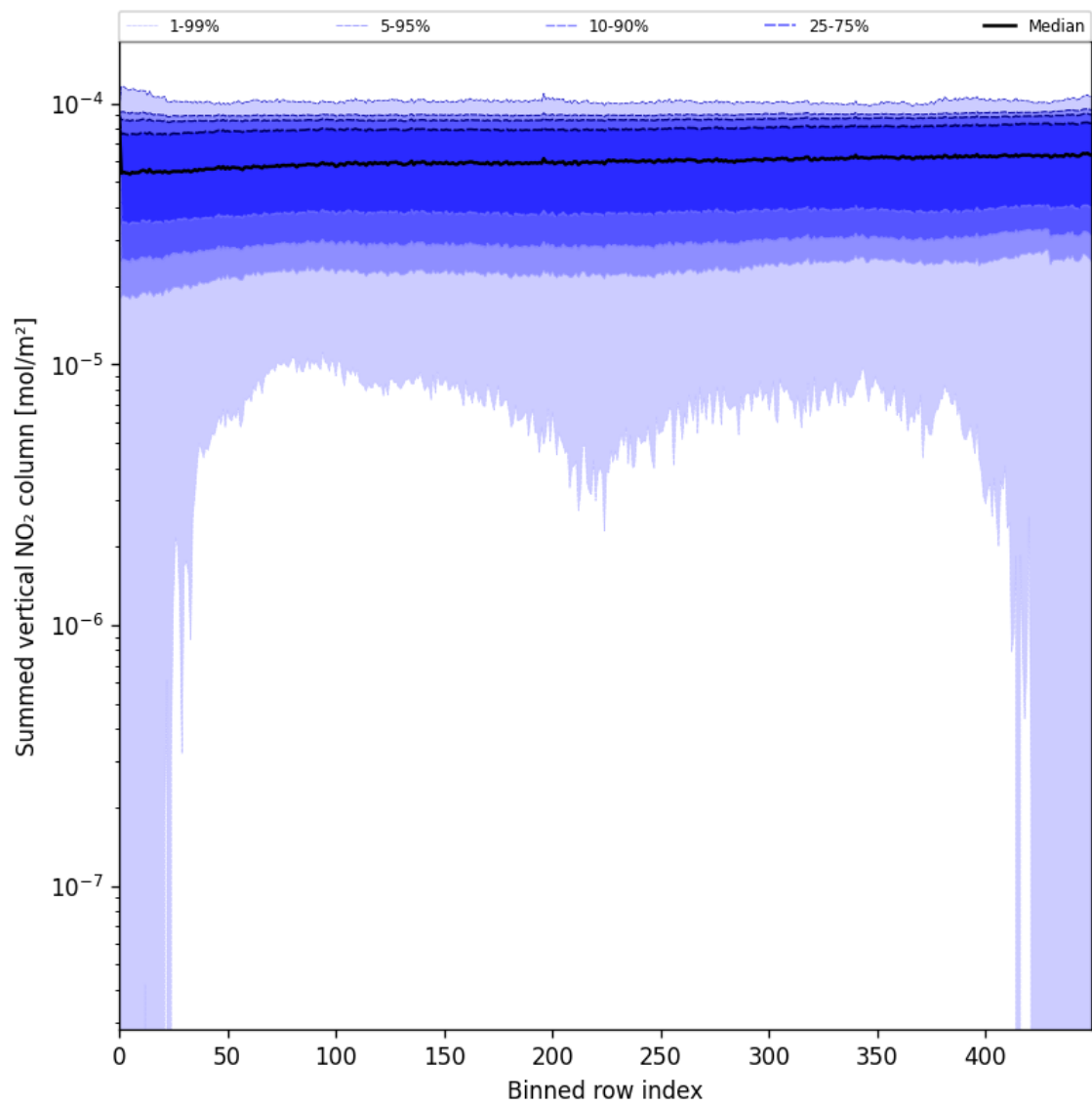
Figure 57: Along track statistics of “Summed vertical NO 2 column” for 2025-06-27 to 2025-06-28
