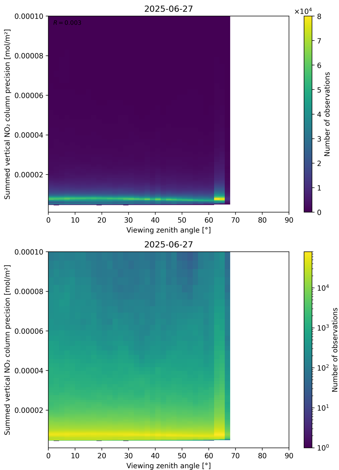
Figure 166: Scatter density plot of “Viewing zenith angle” against “Summed vertical NO 2 column precision” for 2025-06-27 to 2025-06-28.
