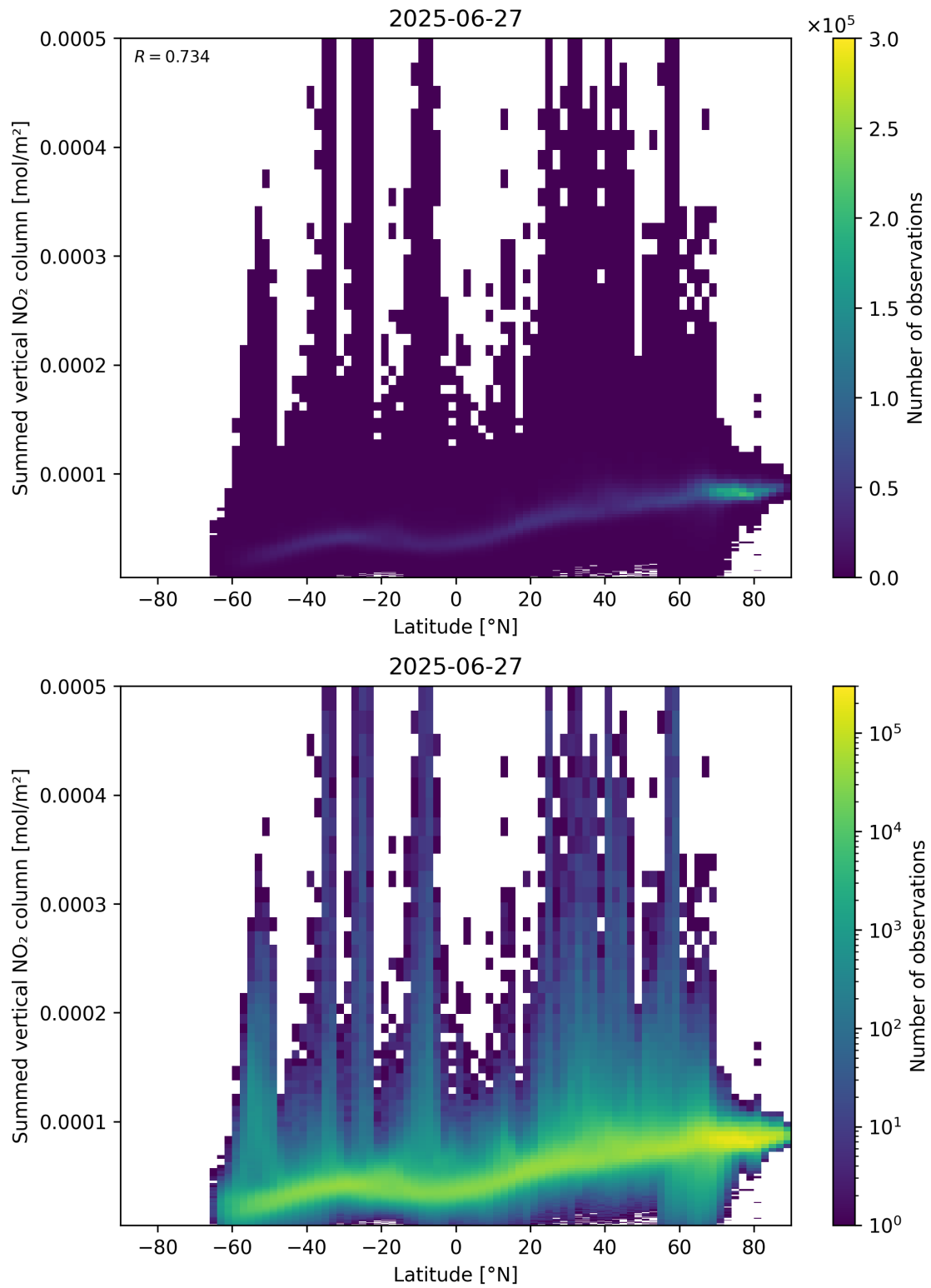
Figure 88: Scatter density plot of “Latitude” against “Summed vertical NO 2 column” for 2025-06-27 to 2025-06-28.
