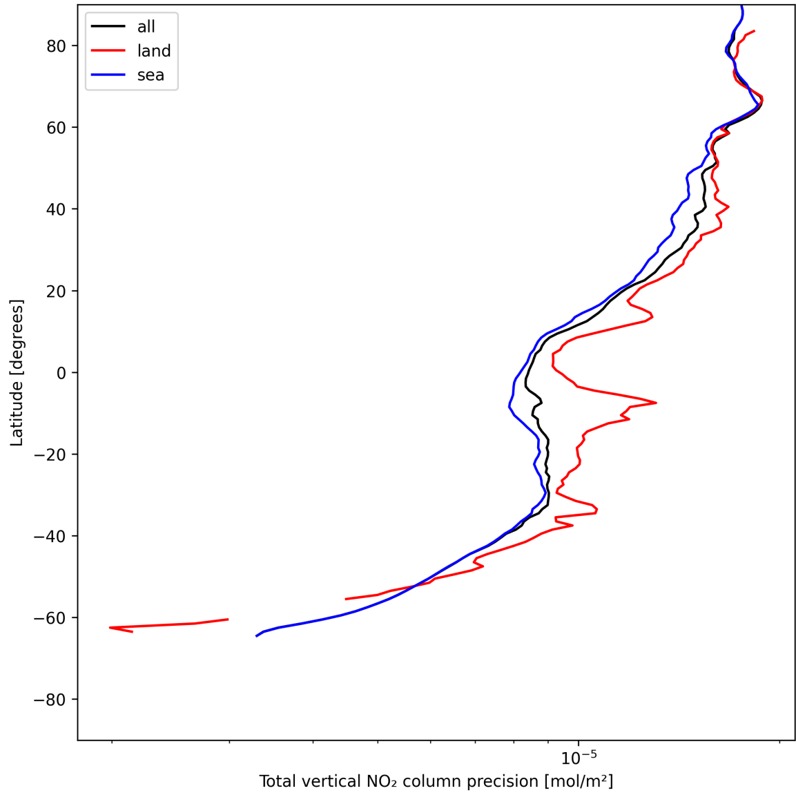
Figure 22: Zonal average of “Total vertical NO 2 column precision” for 2025-06-27 to 2025-06-28.
