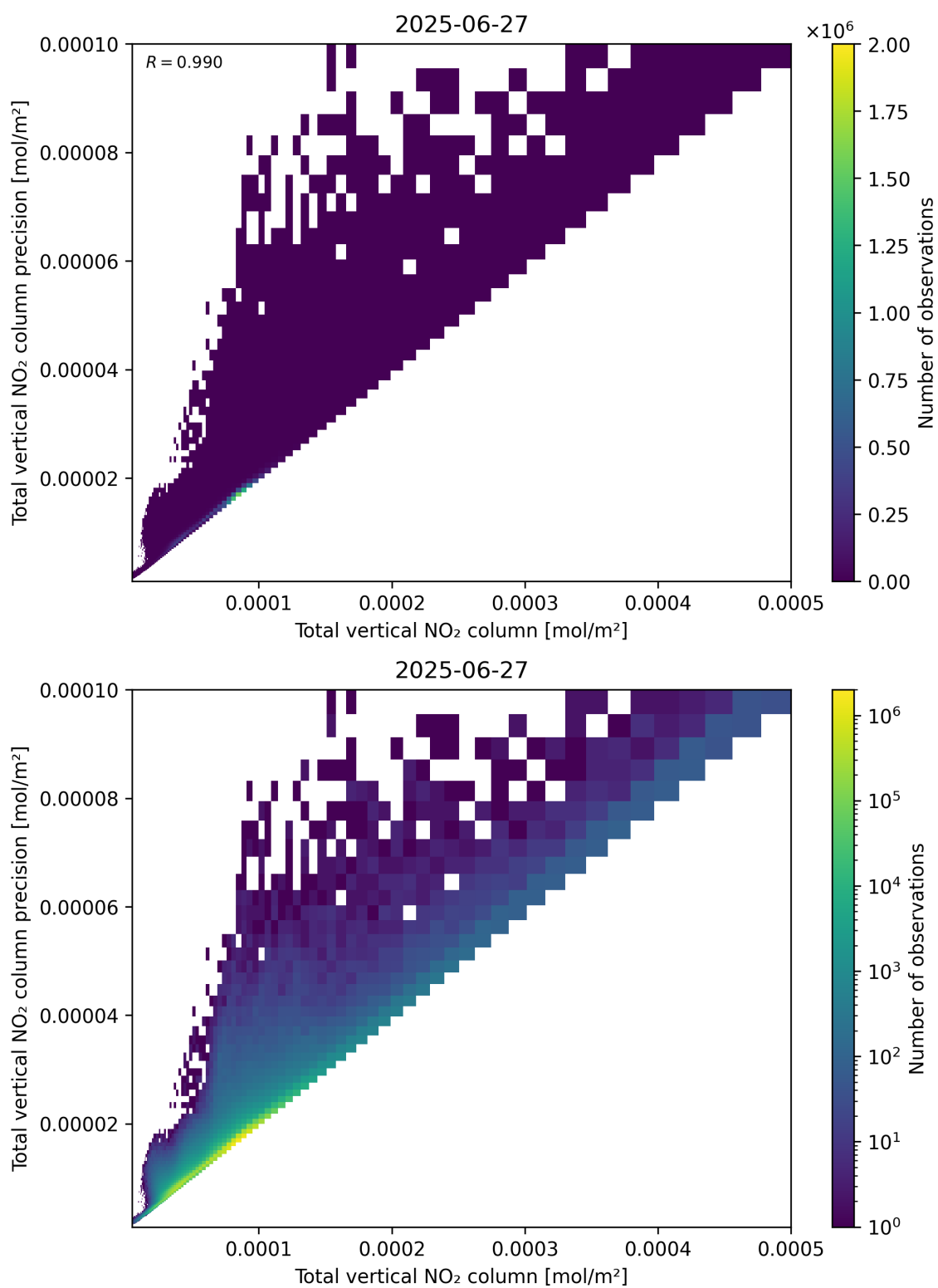
Figure 114: Scatter density plot of “Total vertical NO 2 column” against “Total vertical NO 2 column precision” for 2025-06-27 to 2025-06-28.
