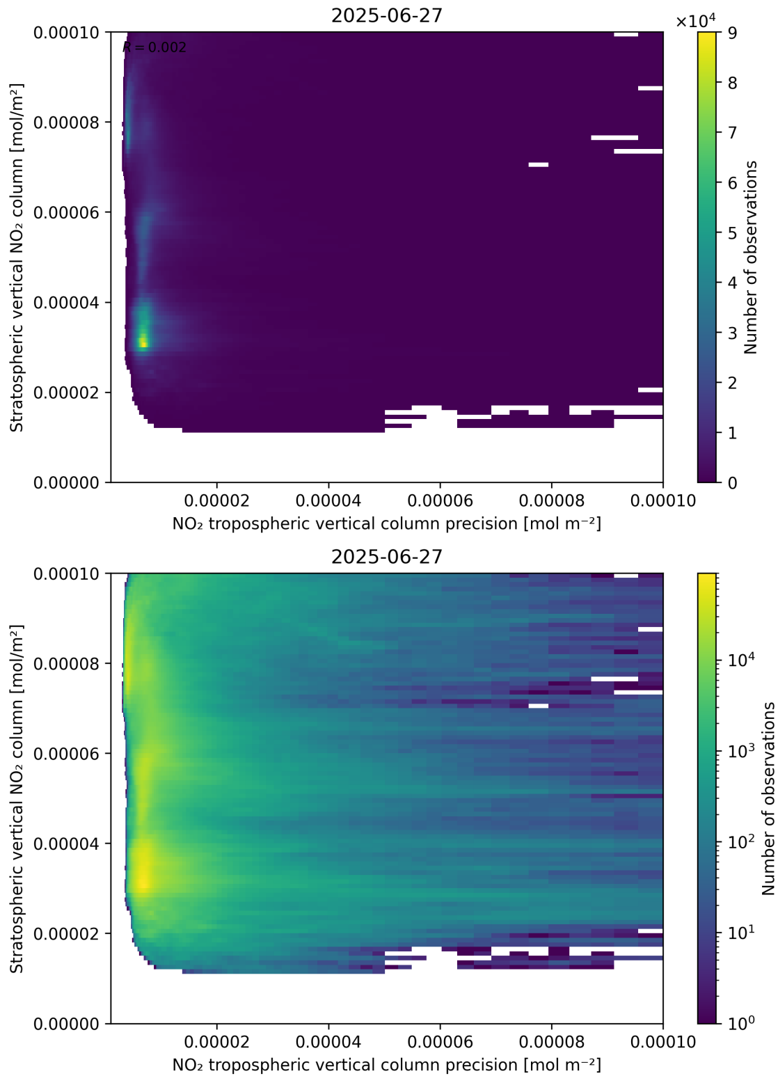
Figure 135: Scatter density plot of “NO 2 tropospheric vertical column precision” against “Stratospheric vertical NO 2 column” for 2025-06-27 to 2025-06-28.
