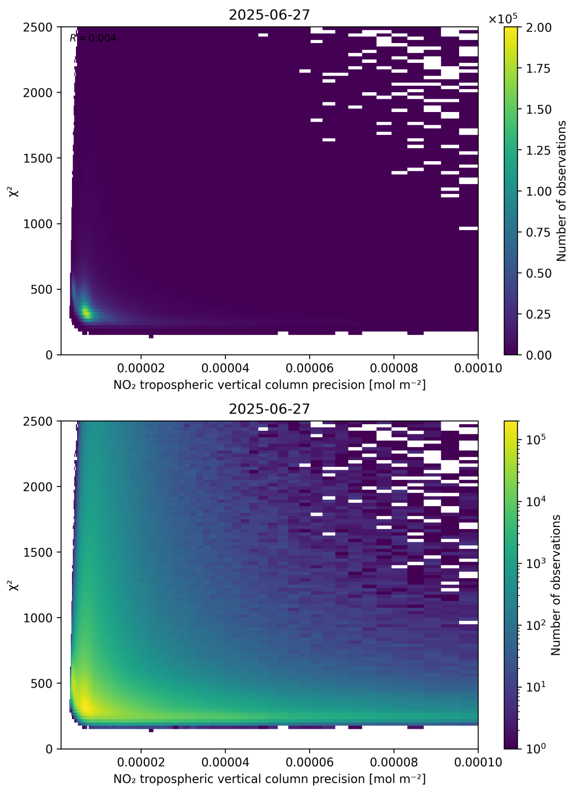
Figure 134: Scatter density plot of “NO 2 tropospheric vertical column precision” against “ \chi^2 ” for 2025-06-27 to 2025-06-28.
