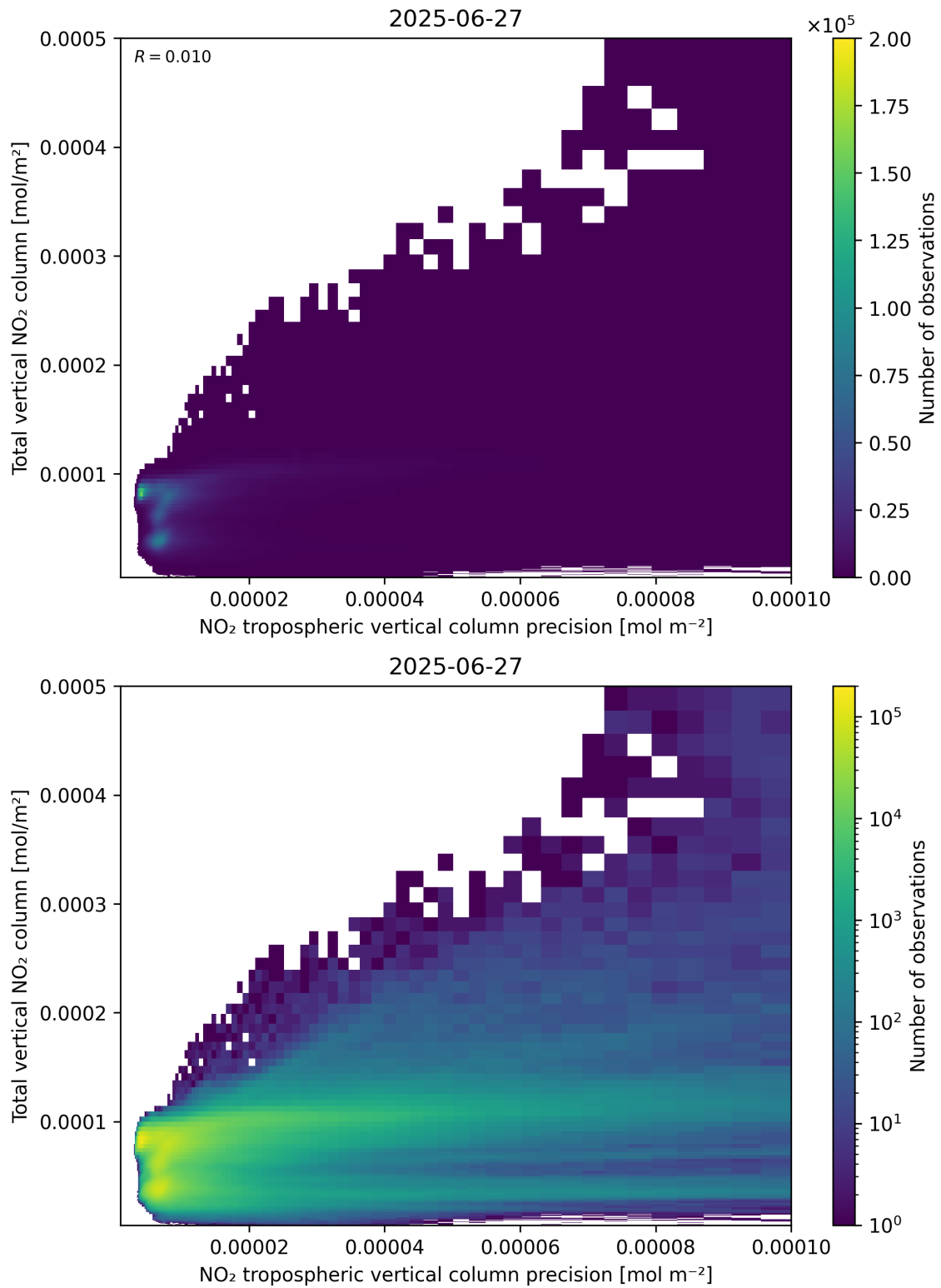
Figure 138: Scatter density plot of “NO 2 tropospheric vertical column precision” against “Total vertical NO 2 column” for 2025-06-27 to 2025-06-28.
