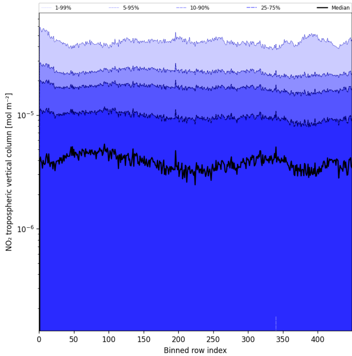
Figure 46: Along track statistics of “NO 2 tropospheric vertical column” for 2025-06-27 to 2025-06-28
