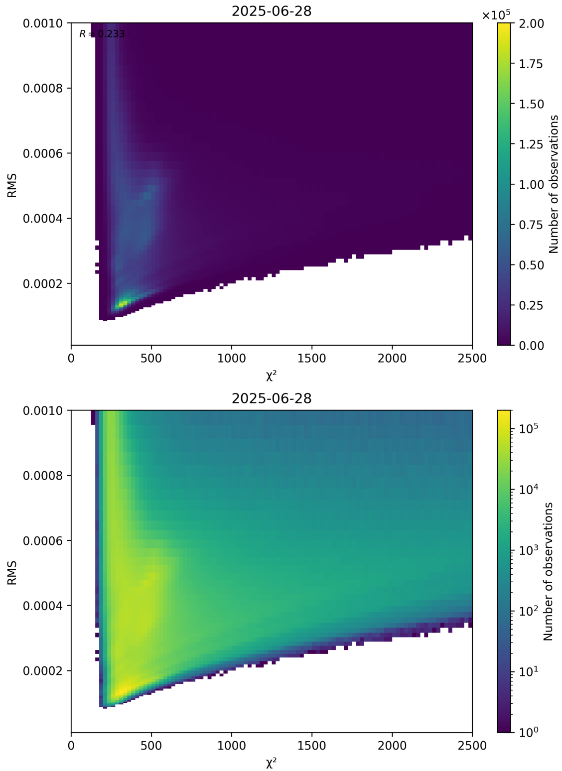
Figure 82: Scatter density plot of “ \chi^2 ” against “RMS” for 2025-06-27 to 2025-06-29.
