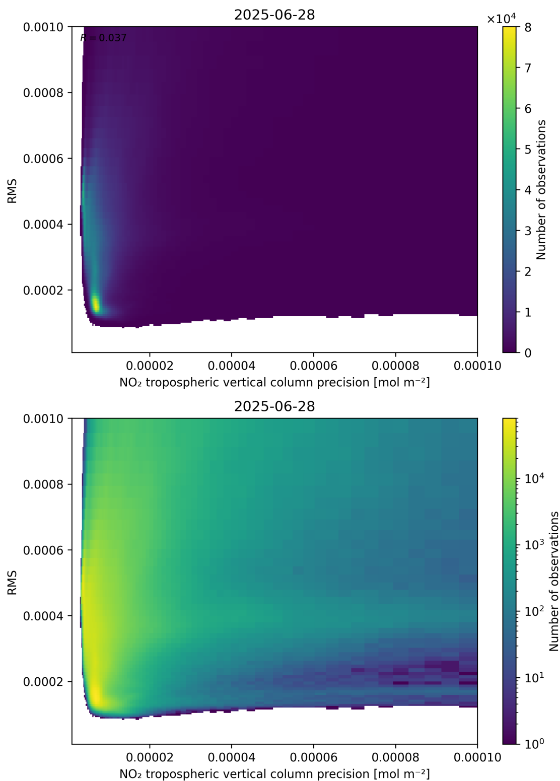
Figure 140: Scatter density plot of “NO 2 tropospheric vertical column precision” against “RMS” for 2025-06-27 to 2025-06-29.
