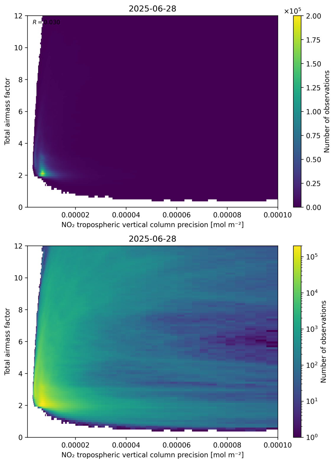
Figure 132: Scatter density plot of “NO 2 tropospheric vertical column precision” against “Total air mass factor” for 2025-06-27 to 2025-06-29.
