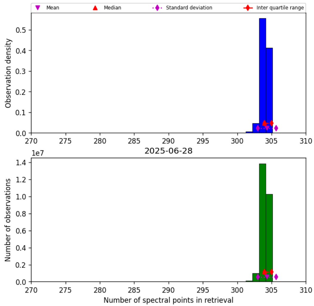
Figure 33: Histogram of “Number of spectral points in retrieval” for 2025-06-27 to 2025-06-29
