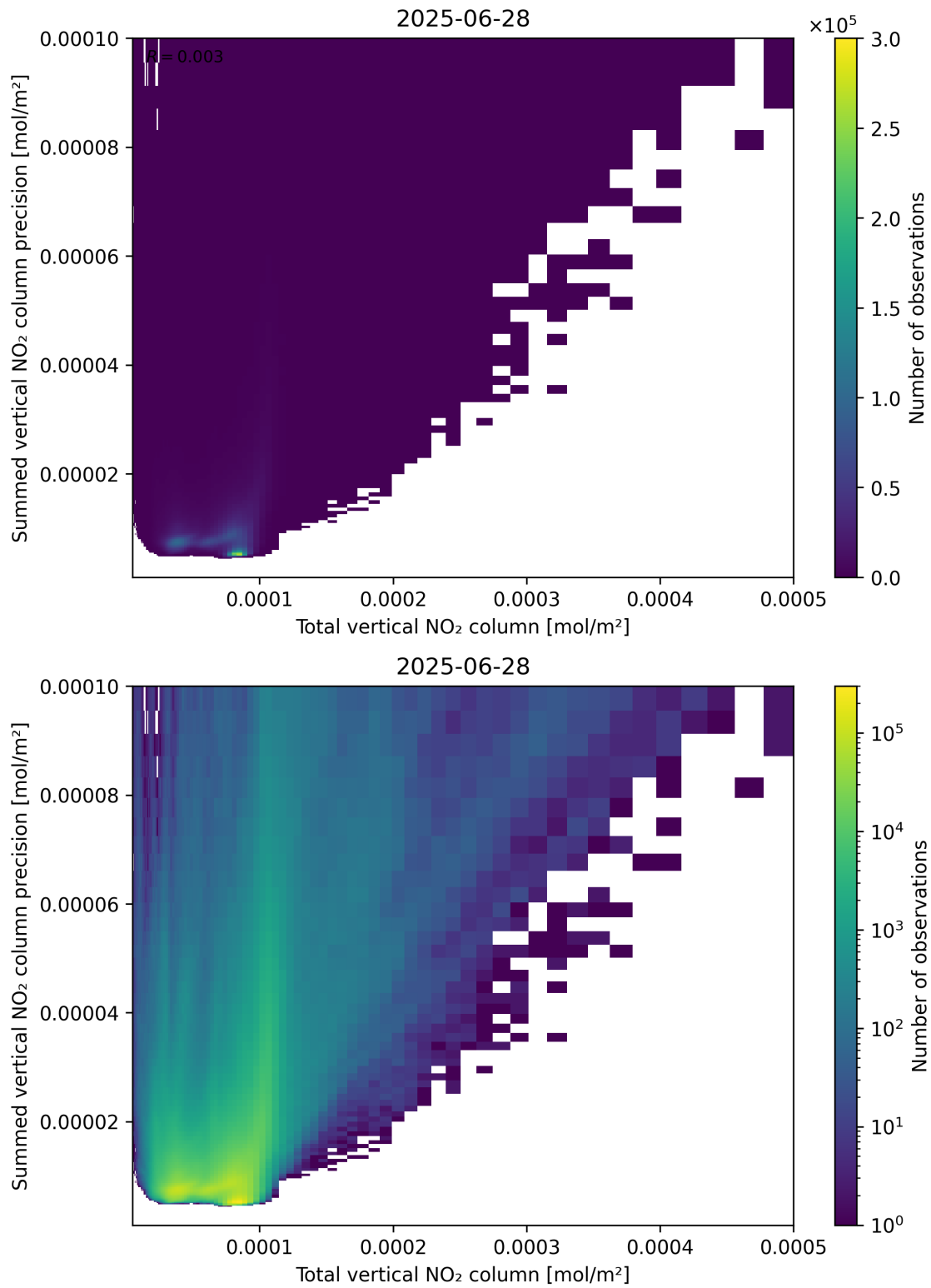
Figure 113: Scatter density plot of “Total vertical NO 2 column” against “Summed vertical NO 2 column precision” for 2025-06-27 to 2025-06-29.
