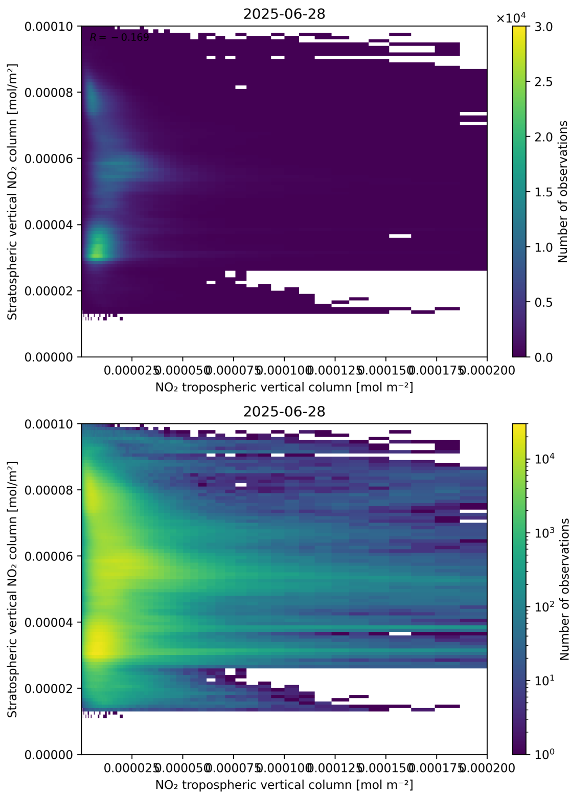
Figure 125: Scatter density plot of “NO 2 tropospheric vertical column” against “Stratospheric vertical NO 2 column” for 2025-06-27 to 2025-06-29.
