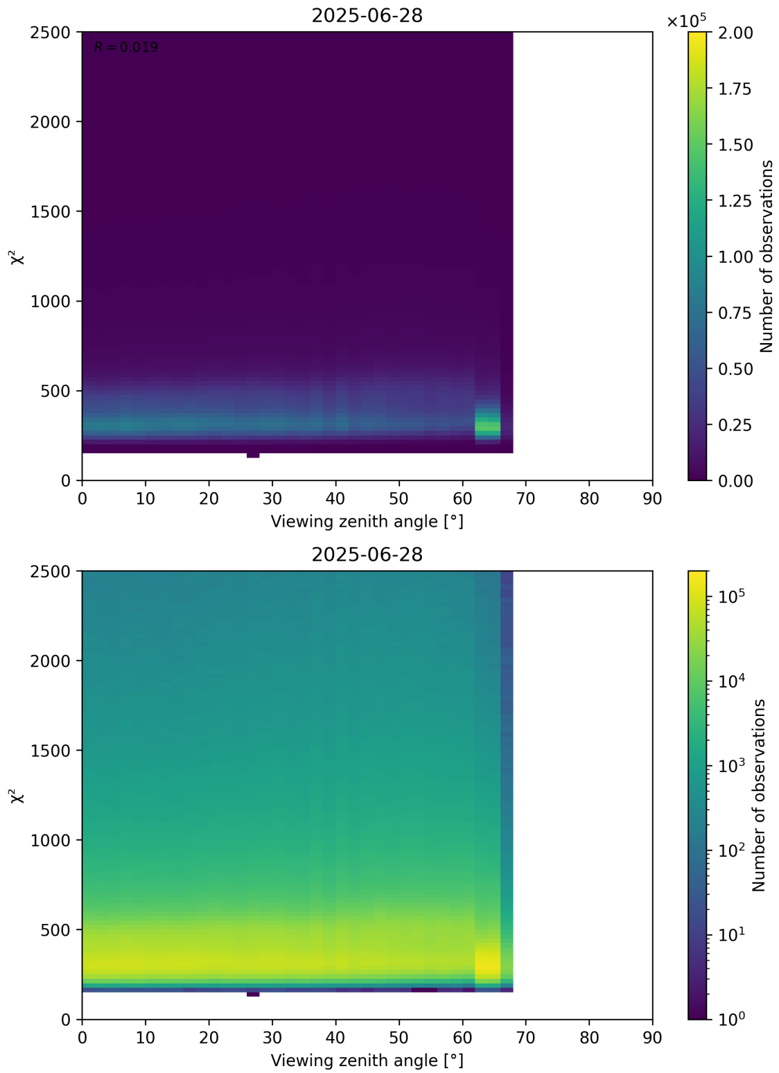
Figure 162: Scatter density plot of “Viewing zenith angle” against “ \chi^2 ” for 2025-06-27 to 2025-06-29.
