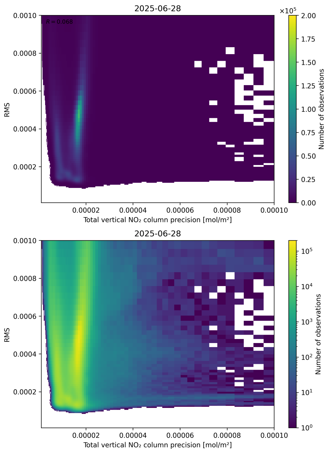
Figure 119: Scatter density plot of “Total vertical NO 2 column precision” against “RMS” for 2025-06-27 to 2025-06-29.
