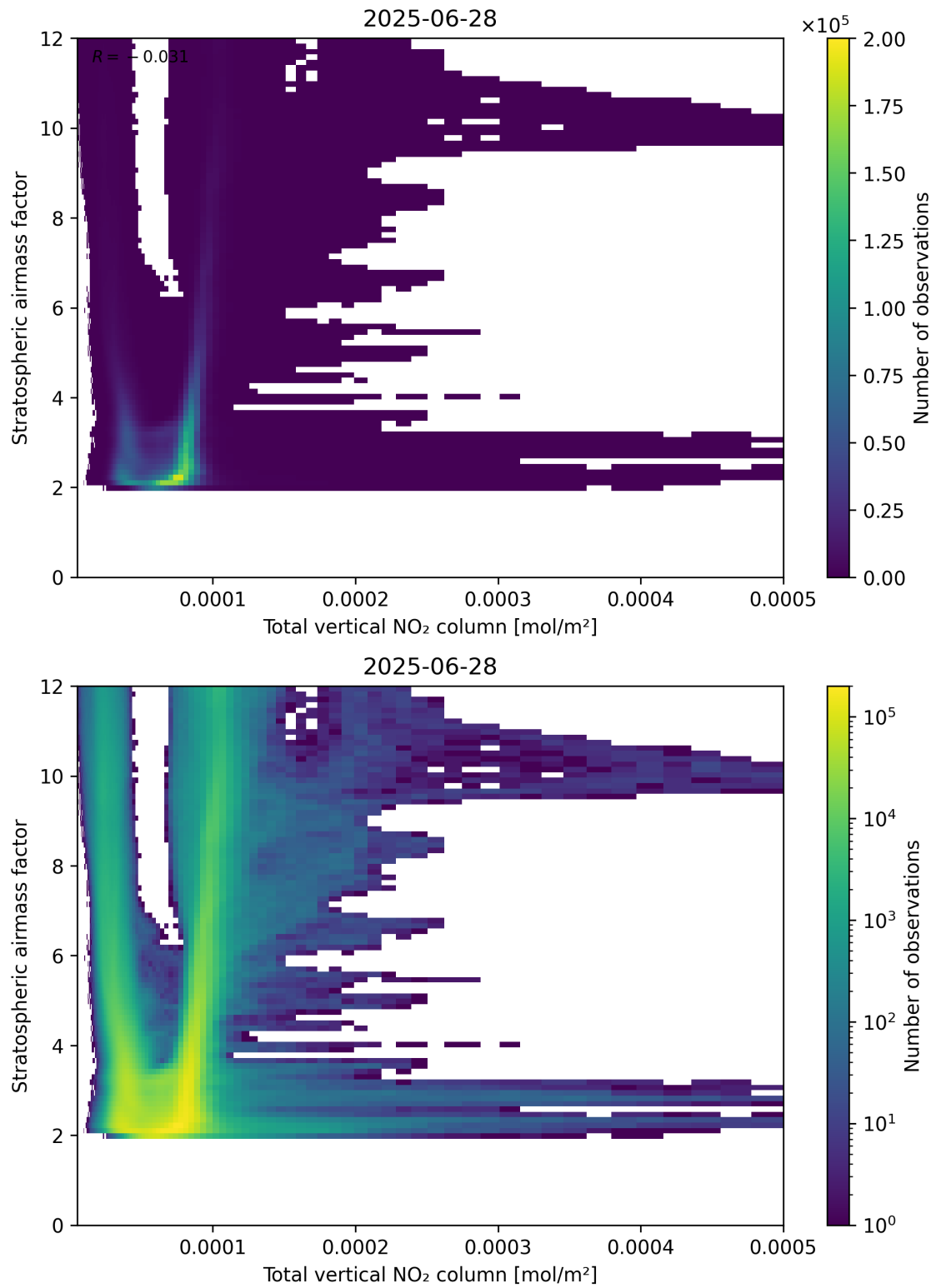
Figure 110: Scatter density plot of “Total vertical NO 2 column” against “Stratospheric air mass factor” for 2025-06-27 to 2025-06-29.
