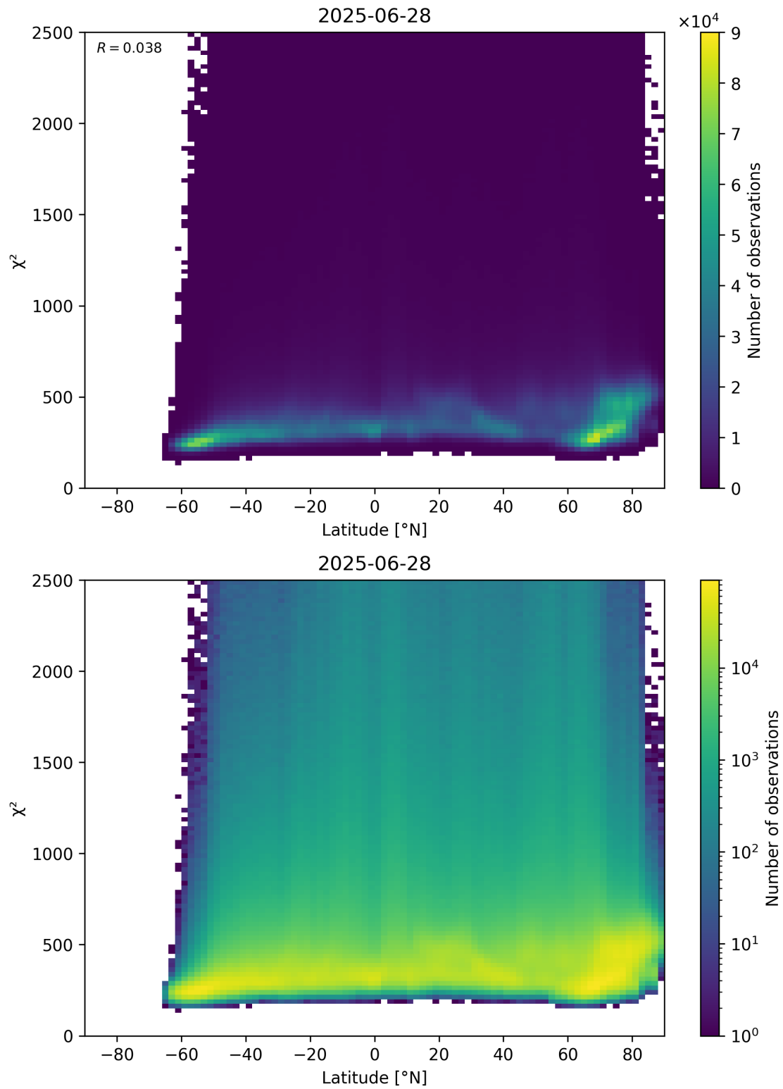
Figure 86: Scatter density plot of “Latitude” against “ \chi^2 ” for 2025-06-27 to 2025-06-29.
