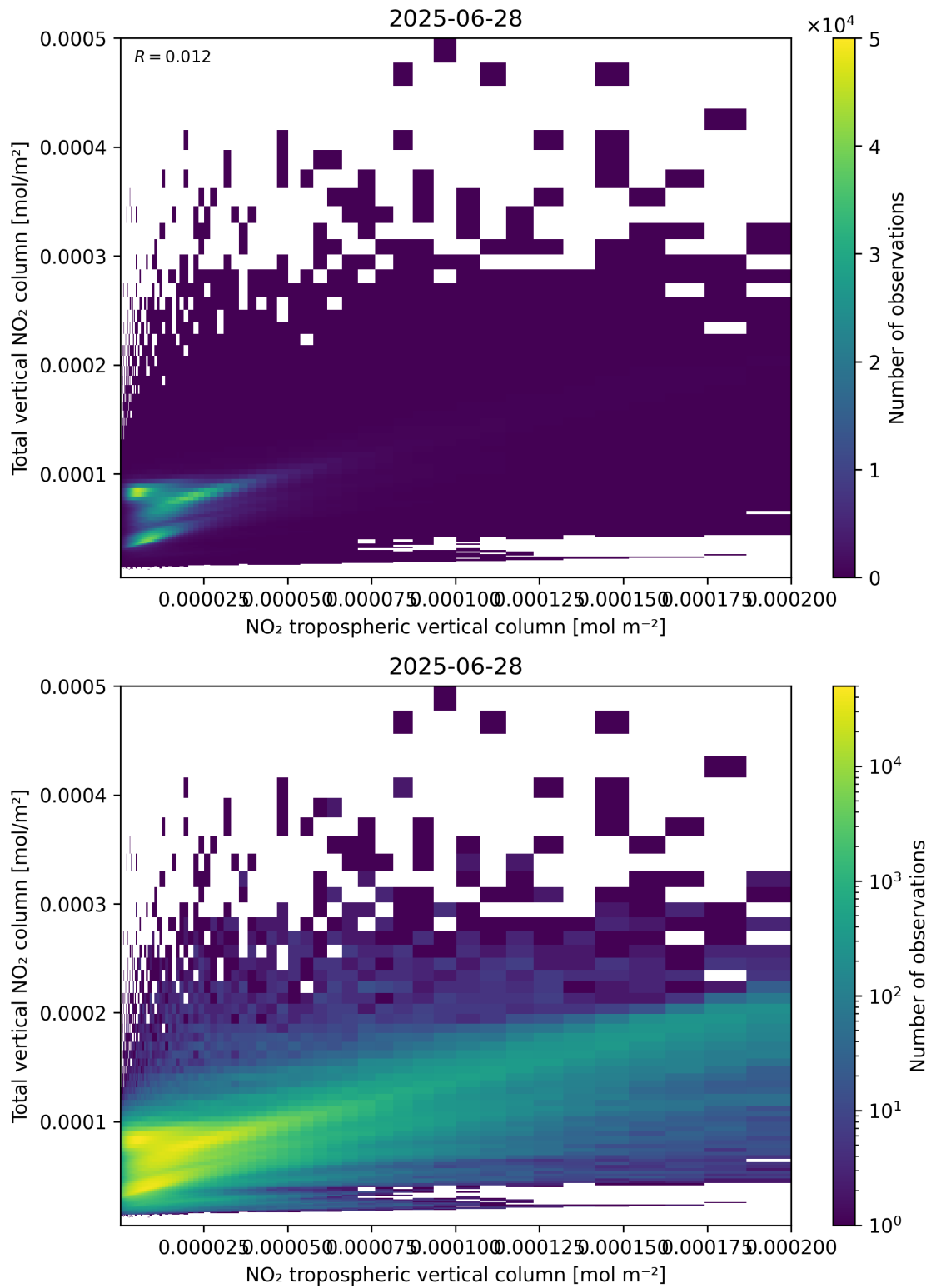
Figure 128: Scatter density plot of “NO 2 tropospheric vertical column” against “Total vertical NO 2 column” for 2025-06-27 to 2025-06-29.
