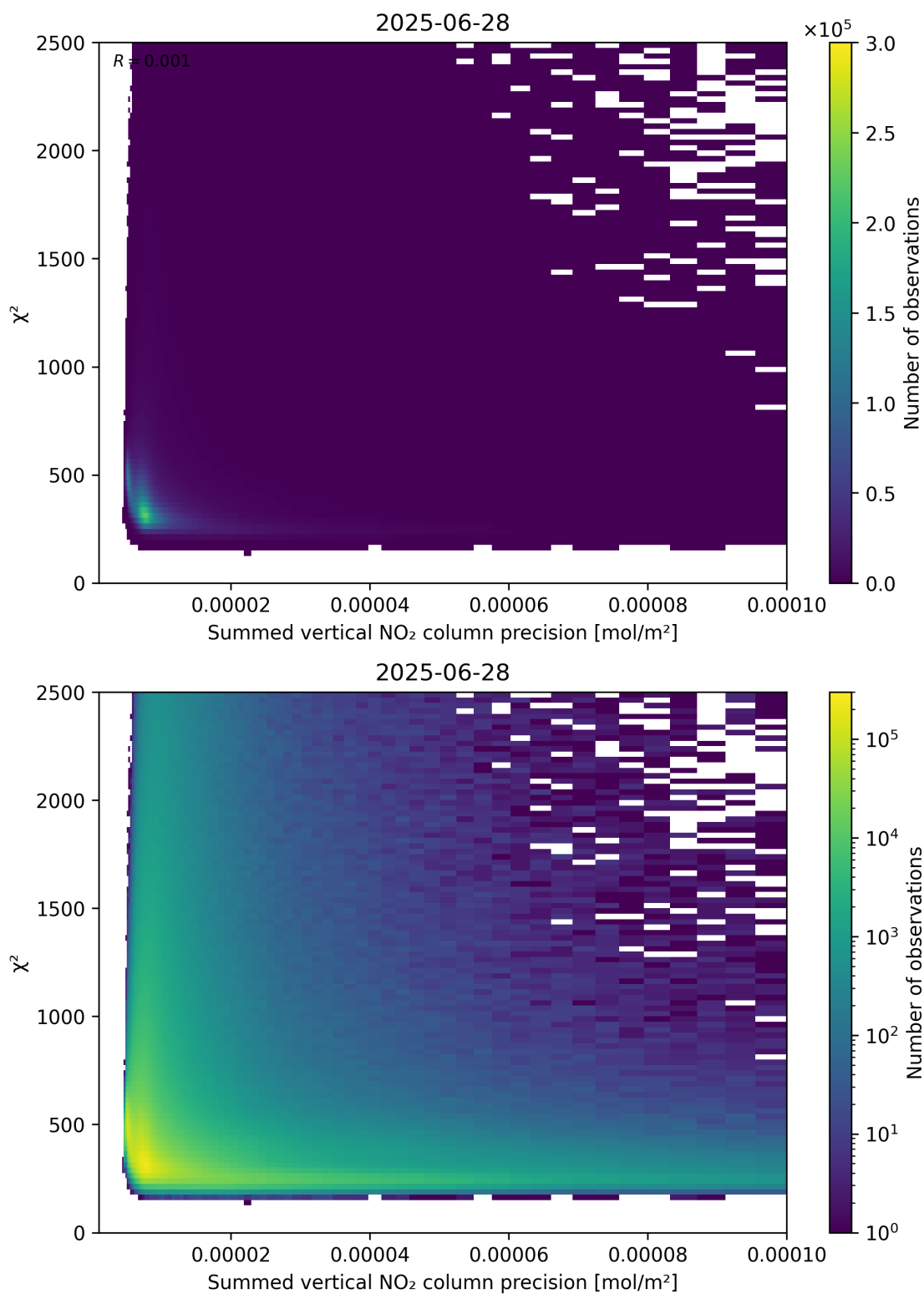
Figure 107: Scatter density plot of “Summed vertical NO 2 column precision” against “ \chi^2 ” for 2025-06-27 to 2025-06-29.
