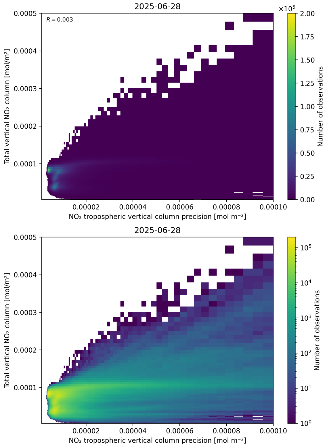
Figure 138: Scatter density plot of “NO 2 tropospheric vertical column precision” against “Total vertical NO 2 column” for 2025-06-27 to 2025-06-29.
