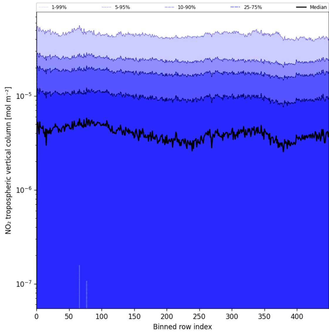
Figure 46: Along track statistics of “NO 2 tropospheric vertical column” for 2025-06-27 to 2025-06-29
