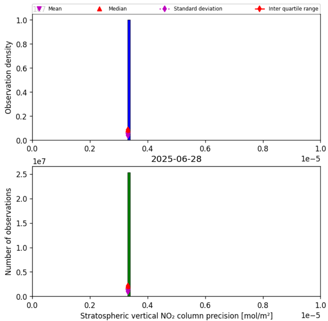
Figure 37: Histogram of “Stratospheric vertical NO 2 column precision” for 2025-06-27 to 2025-06-29
