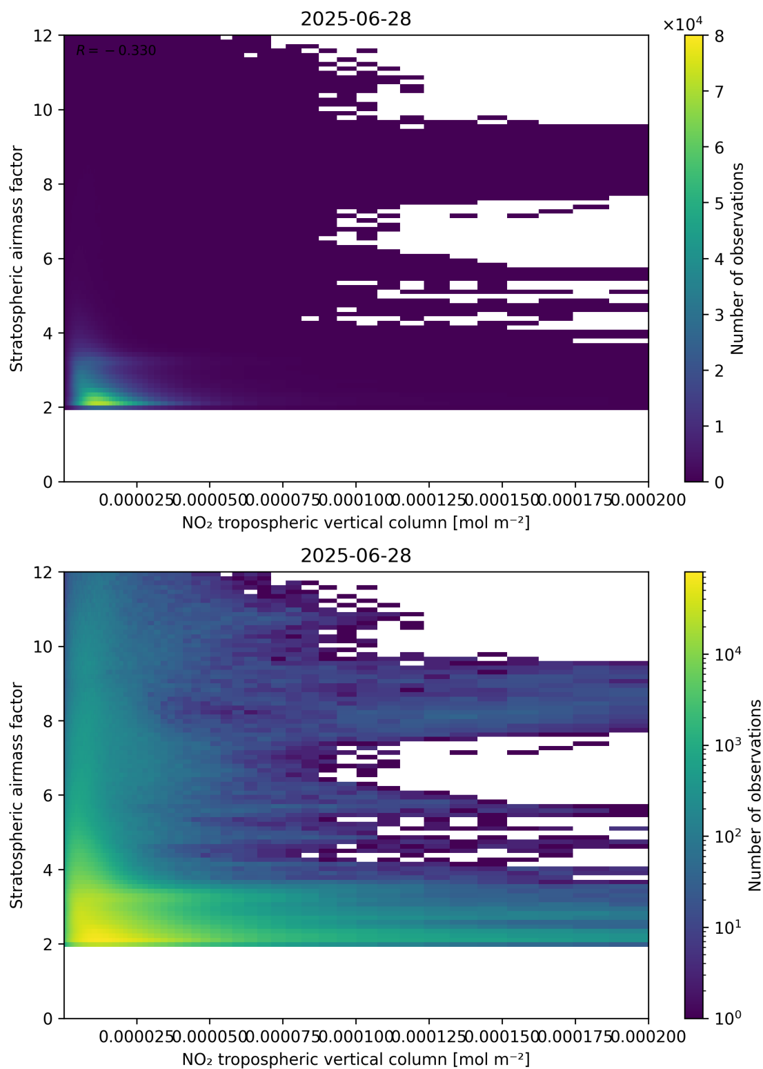
Figure 121: Scatter density plot of “NO 2 tropospheric vertical column” against “Stratospheric air mass factor” for 2025-06-27 to 2025-06-29.
