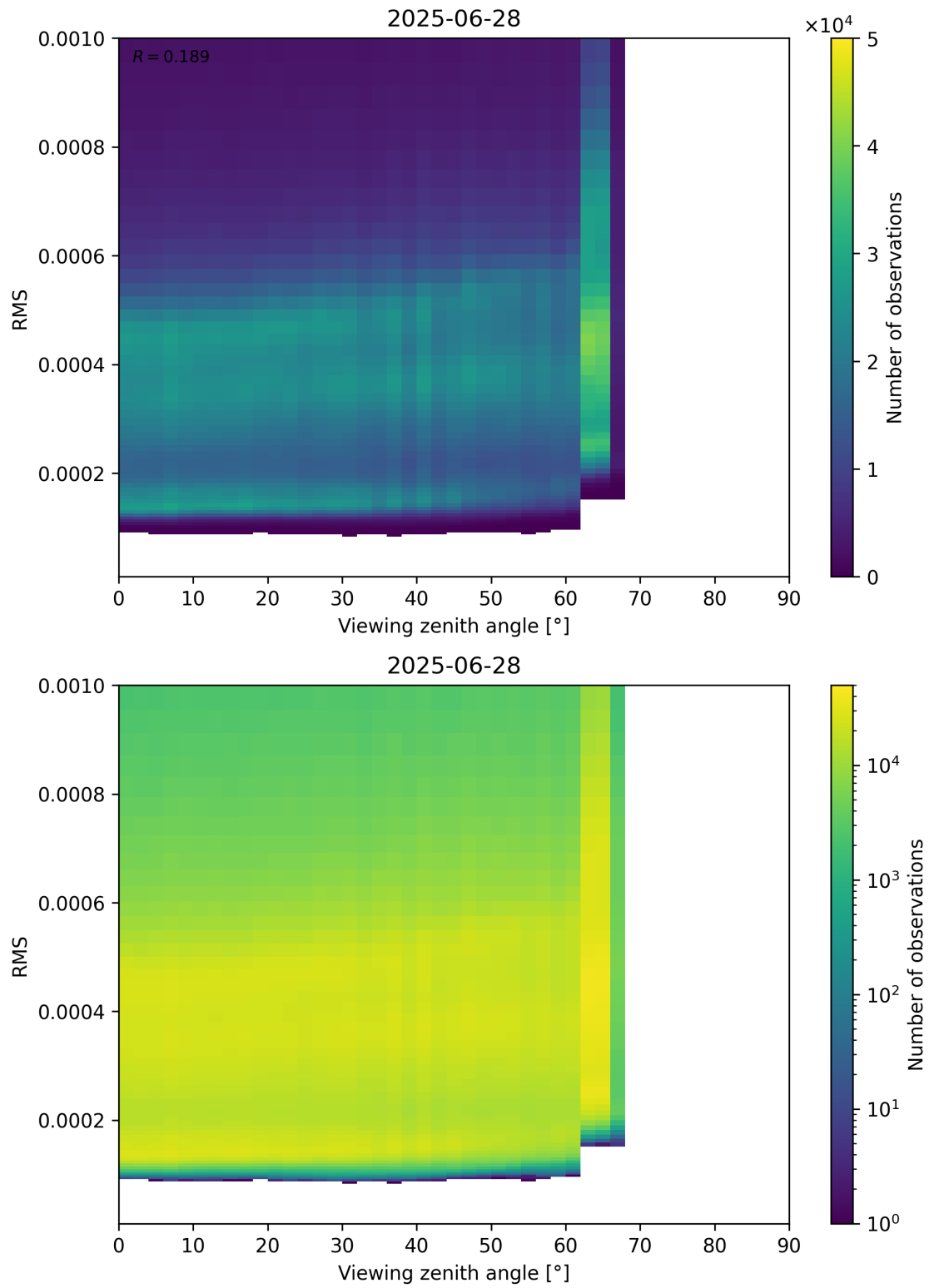
Figure 171: Scatter density plot of “Viewing zenith angle” against “RMS” for 2025-06-27 to 2025-06-29.
