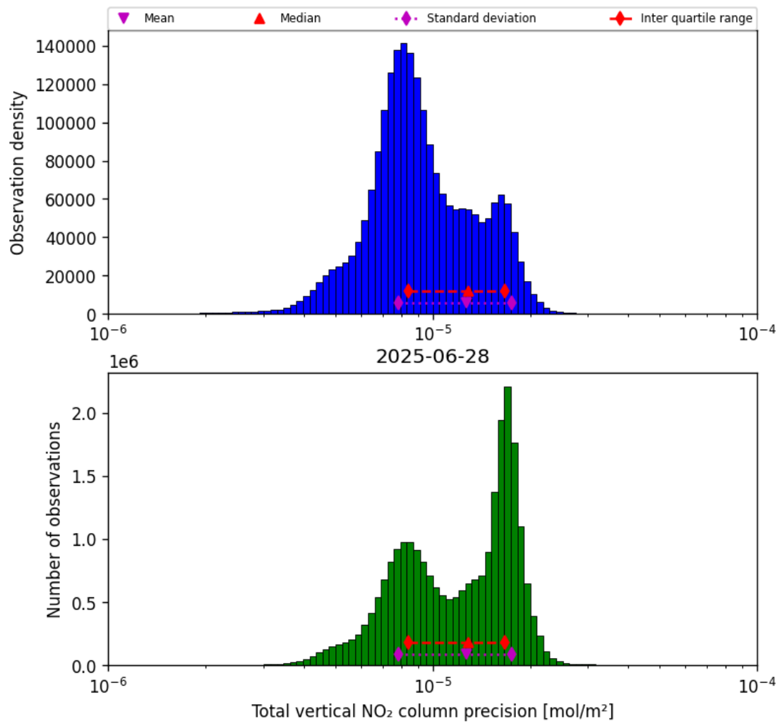
Figure 39: Histogram of “Total vertical NO 2 column precision” for 2025-06-27 to 2025-06-29
