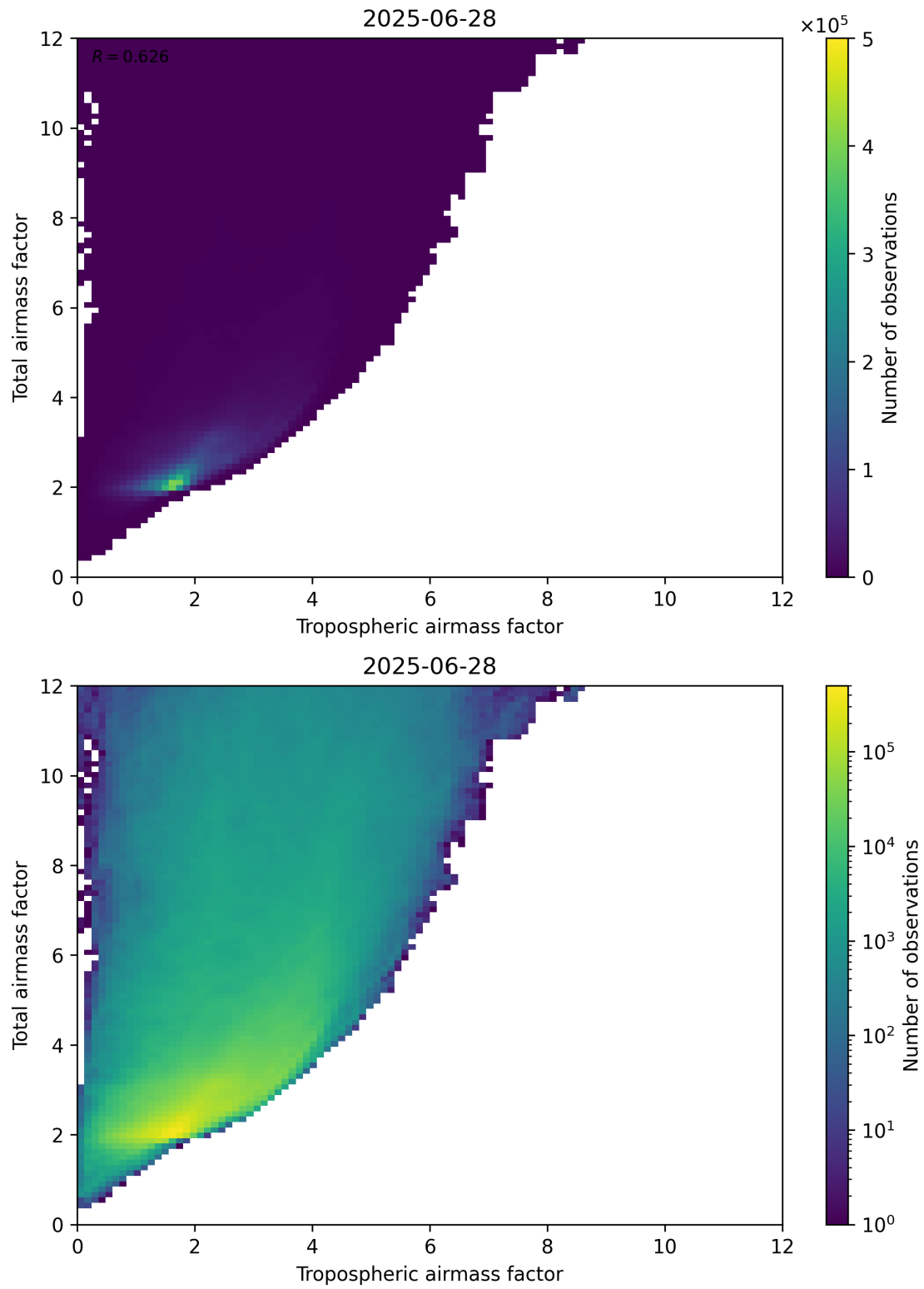
Figure 72: Scatter density plot of “Tropospheric airmass factor” against “Total airmass factor” for 2025-06-27 to 2025-06-29.
