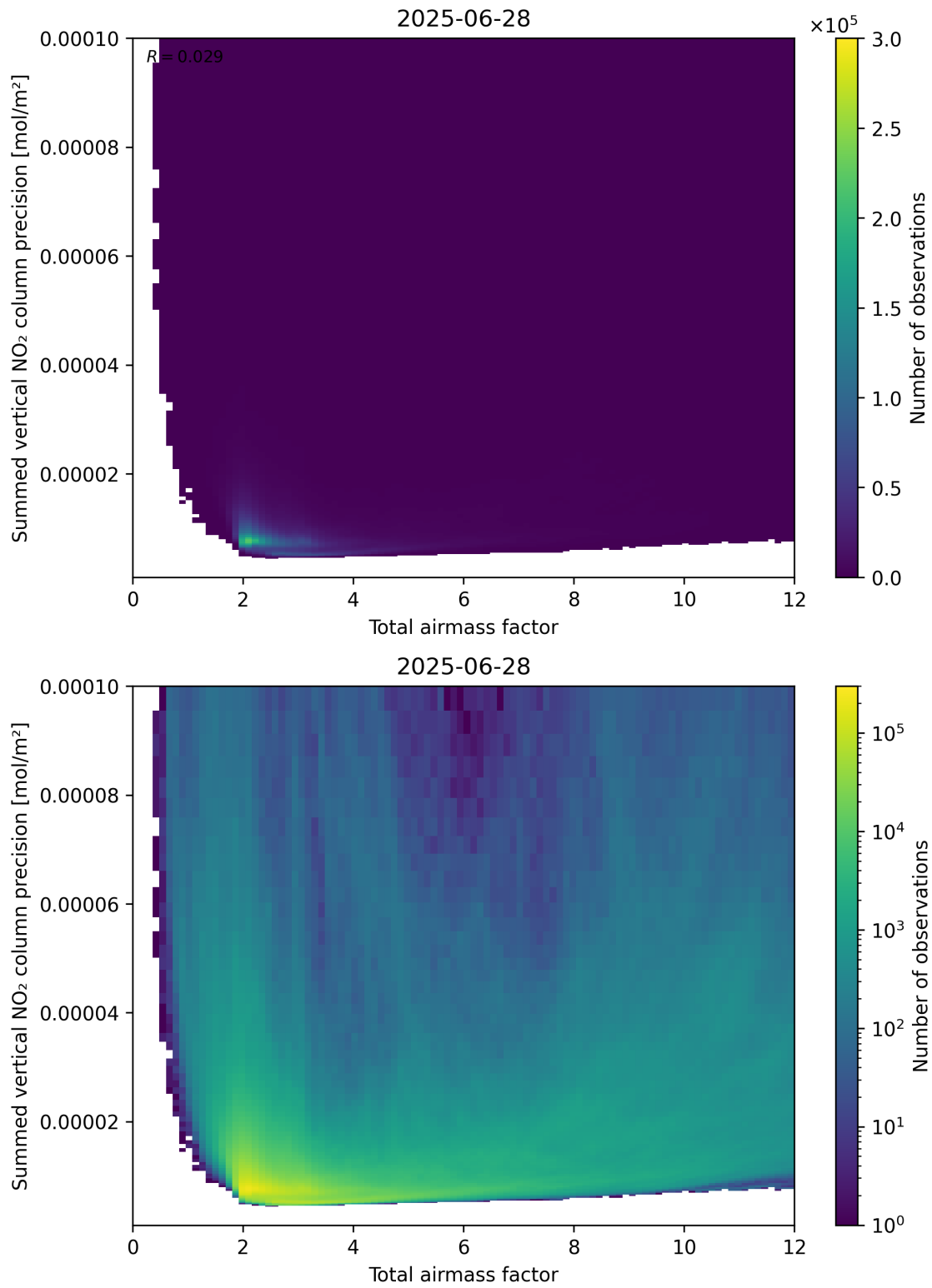
Figure 66: Scatter density plot of “Total airmass factor” against “Summed vertical NO 2 column precision” for 2025-06-27 to 2025-06-29.
