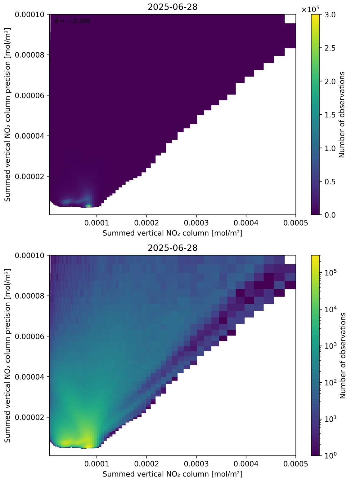
Figure 105: Scatter density plot of “Summed vertical NO 2 column” against “Summed vertical NO 2 column precision” for 2025-06-27 to 2025-06-29.
