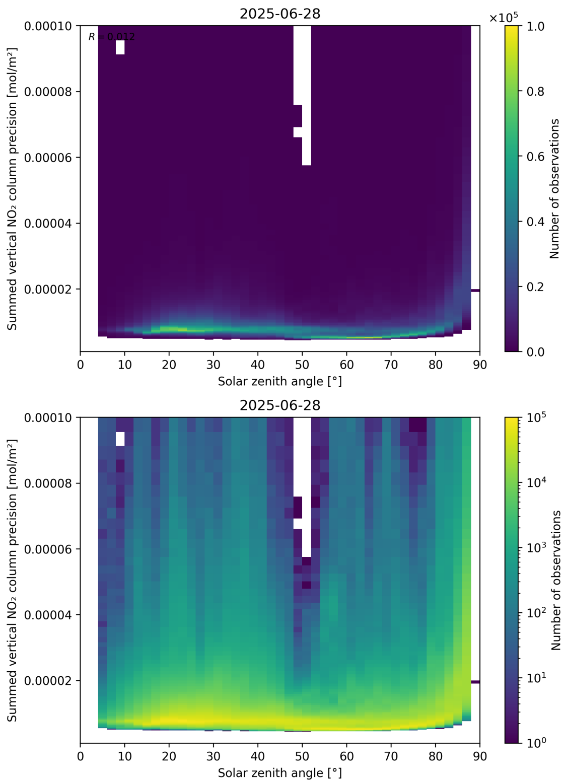
Figure 152: Scatter density plot of “Solar zenith angle” against “Summed vertical NO 2 column precision” for 2025-06-27 to 2025-06-29.
