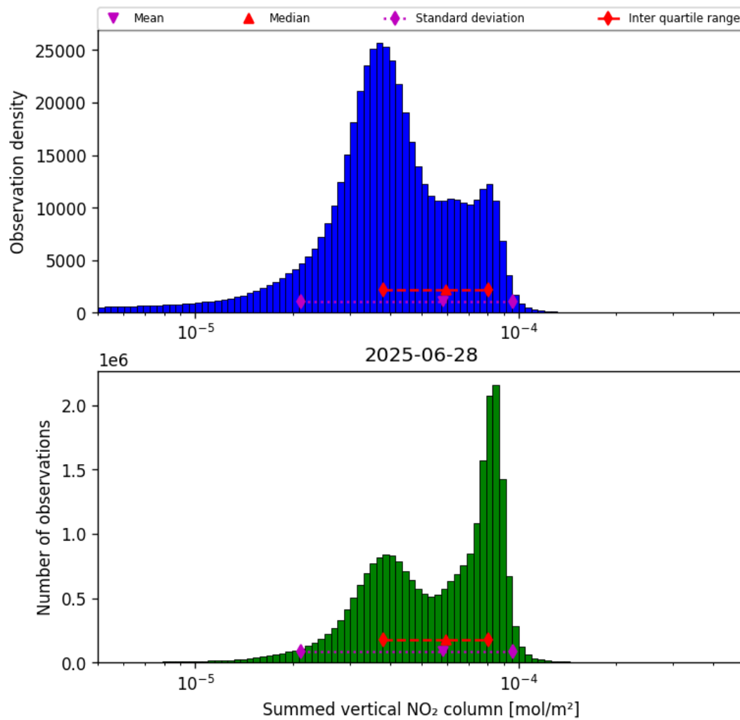
Figure 40: Histogram of “Summed vertical NO 2 column” for 2025-06-27 to 2025-06-29
