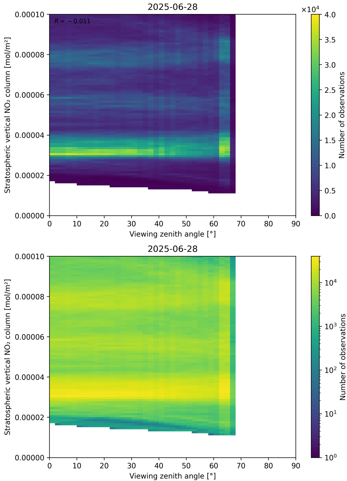
Figure 164: Scatter density plot of “Viewing zenith angle” against “Stratospheric vertical NO 2 column” for 2025-06-27 to 2025-06-29.
