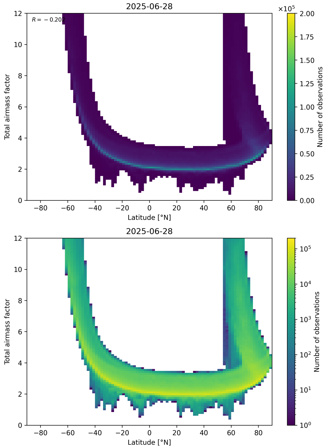
Figure 84: Scatter density plot of “Latitude” against “Total airmass factor” for 2025-06-27 to 2025-06-29.
