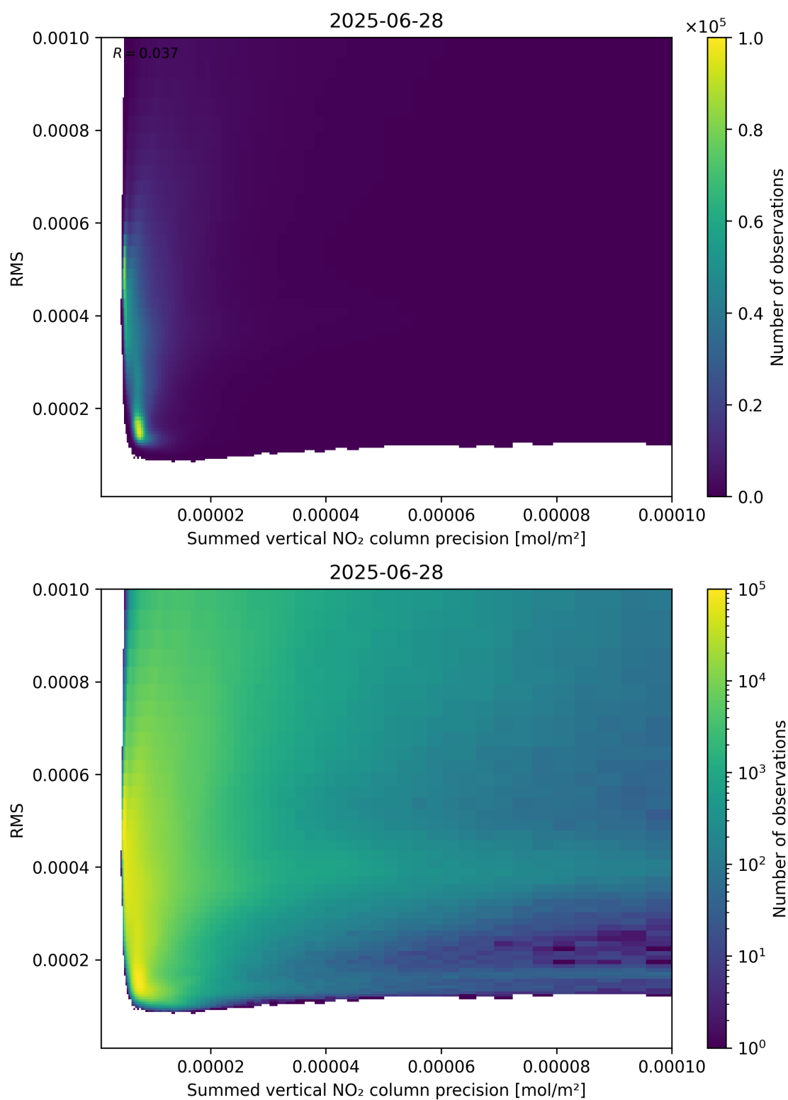
Figure 108: Scatter density plot of “Summed vertical NO 2 column precision” against “RMS” for 2025-06-27 to 2025-06-29.
