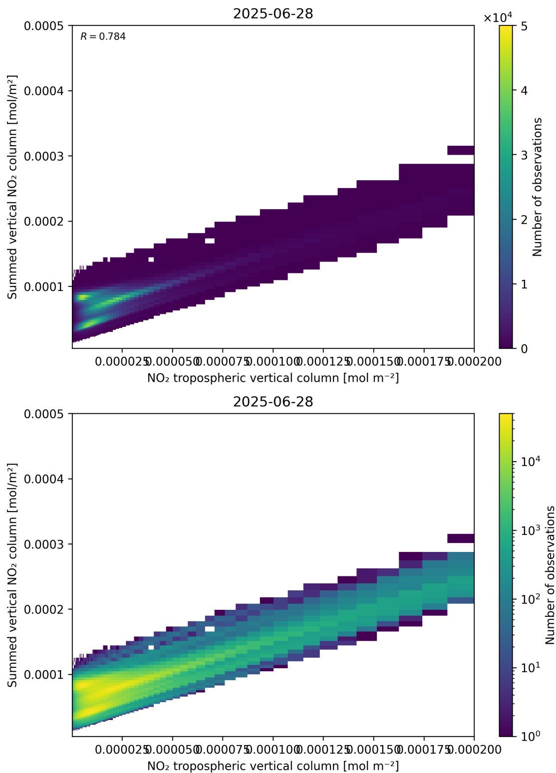
Figure 126: Scatter density plot of “NO 2 tropospheric vertical column” against “Summed vertical NO 2 column” for 2025-06-27 to 2025-06-29.
