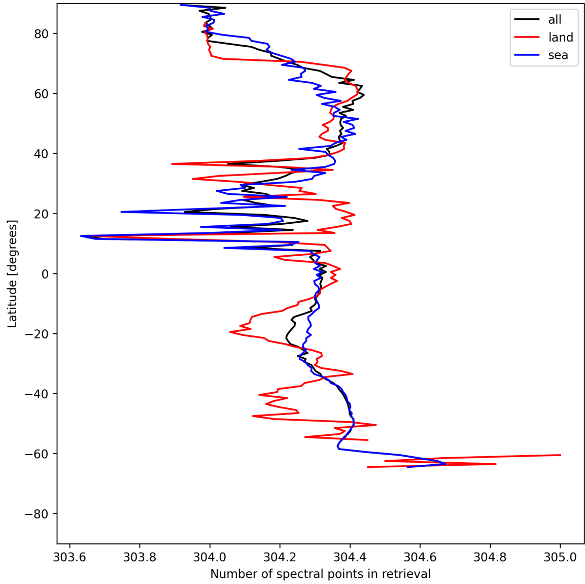
Figure 16: Zonal average of “Number of spectral points in retrieval” for 2025-06-27 to 2025-06-29.
