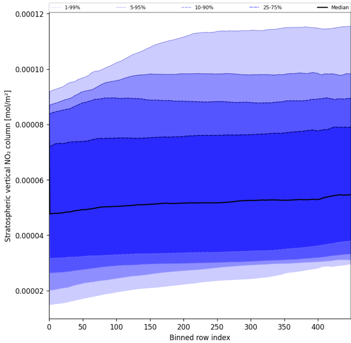
Figure 53: Along track statistics of “Stratospheric vertical NO 2 column” for 2025-06-27 to 2025-06-29
