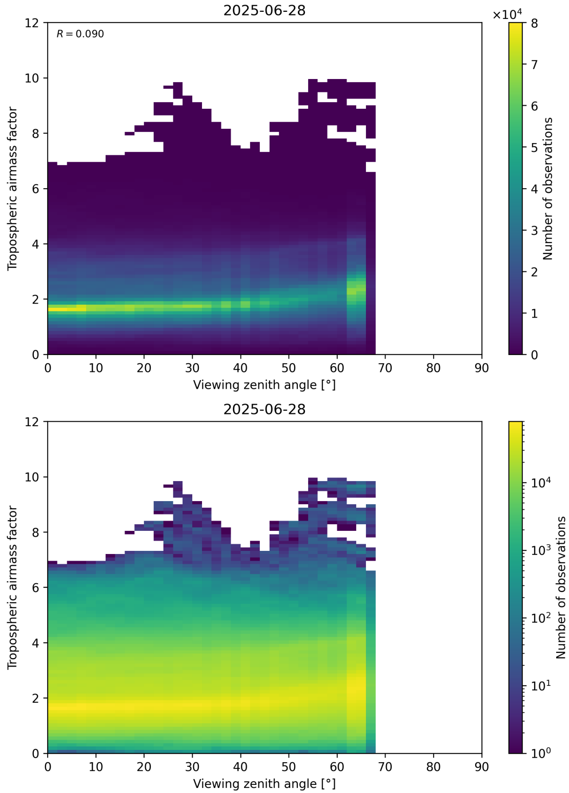
Figure 161: Scatter density plot of “Viewing zenith angle” against “Tropospheric airmass factor” for 2025-06-27 to 2025-06-29.
