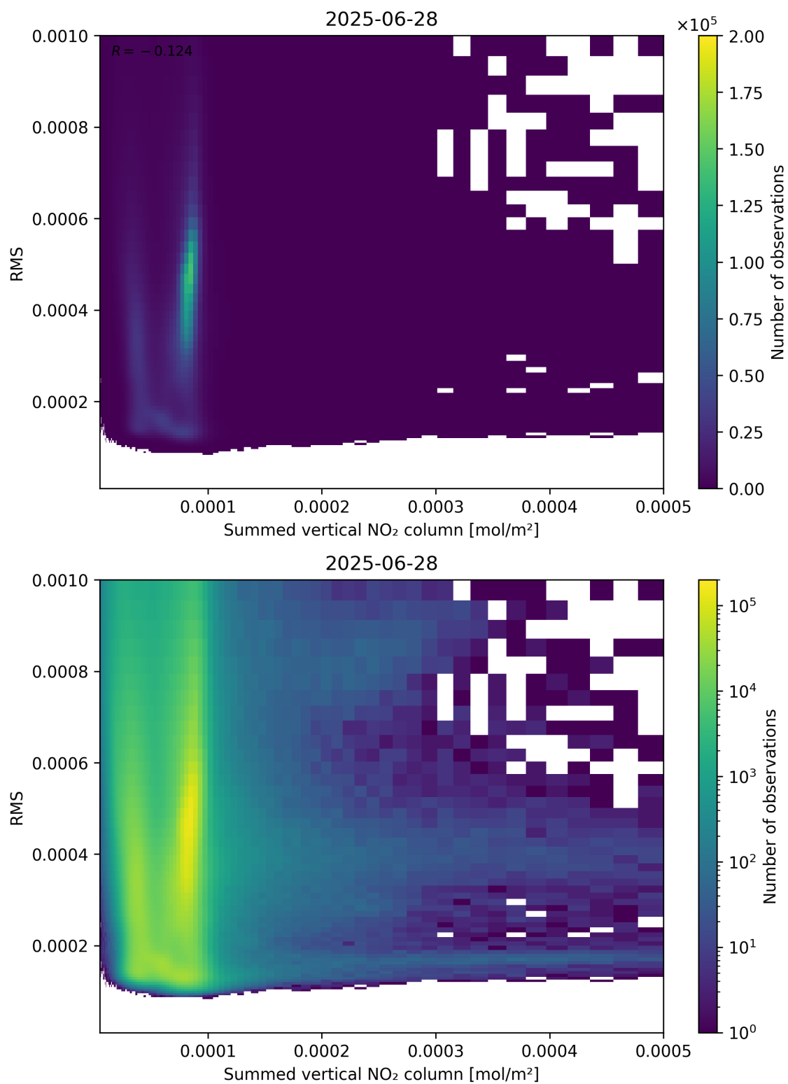
Figure 109: Scatter density plot of “Summed vertical NO 2 column” against “RMS” for 2025-06-27 to 2025-06-29.
