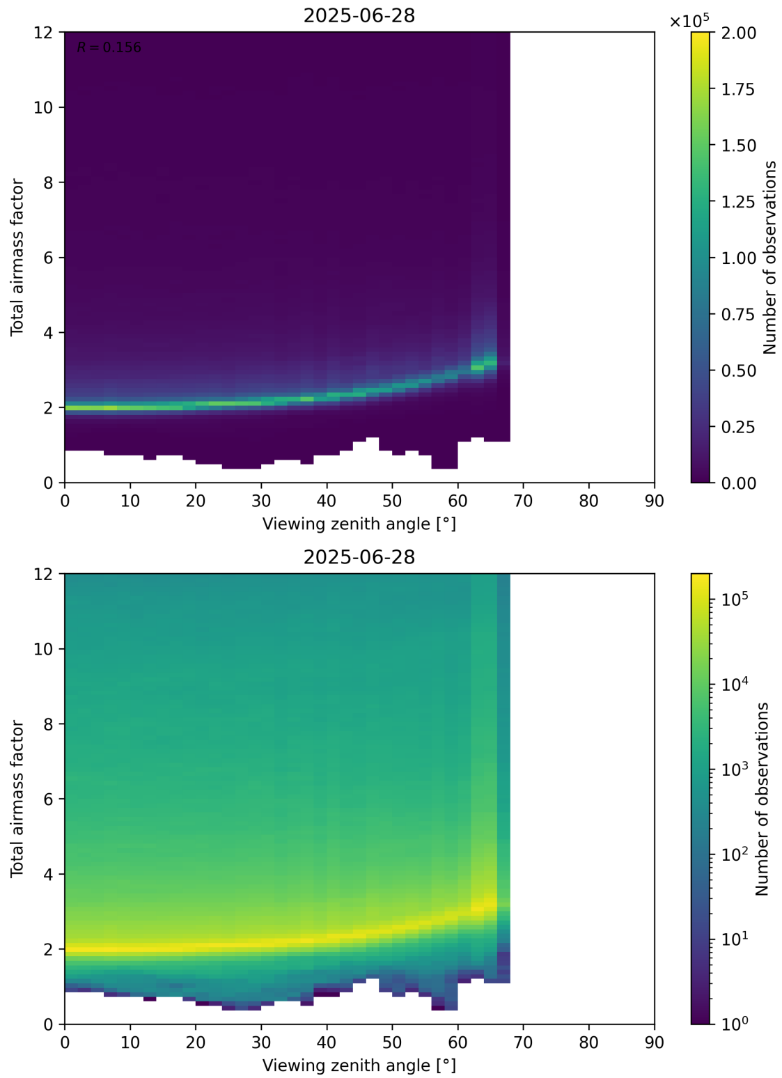
Figure 160: Scatter density plot of “Viewing zenith angle” against “Total airmass factor” for 2025-06-27 to 2025-06-29.
