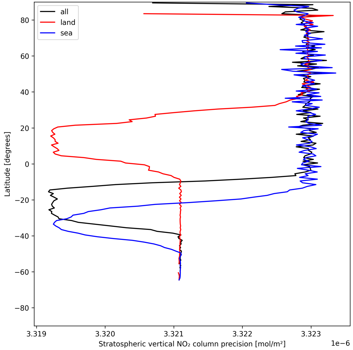
Figure 20: Zonal average of “Stratospheric vertical NO 2 column precision” for 2025-06-27 to 2025-06-29.
