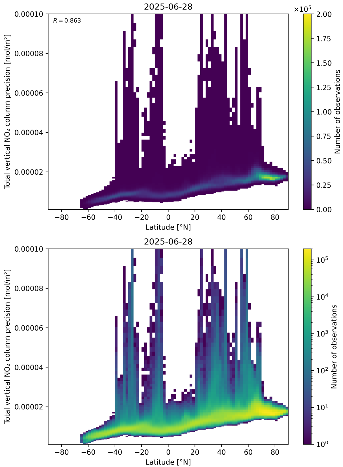
Figure 91: Scatter density plot of “Latitude” against “Total vertical NO 2 column precision” for 2025-06-27 to 2025-06-29.
