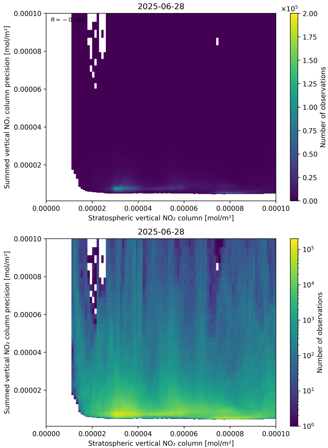
Figure 99: Scatter density plot of “Stratospheric vertical NO 2 column” against “Summed vertical NO 2 column precision” for 2025-06-27 to 2025-06-29.
