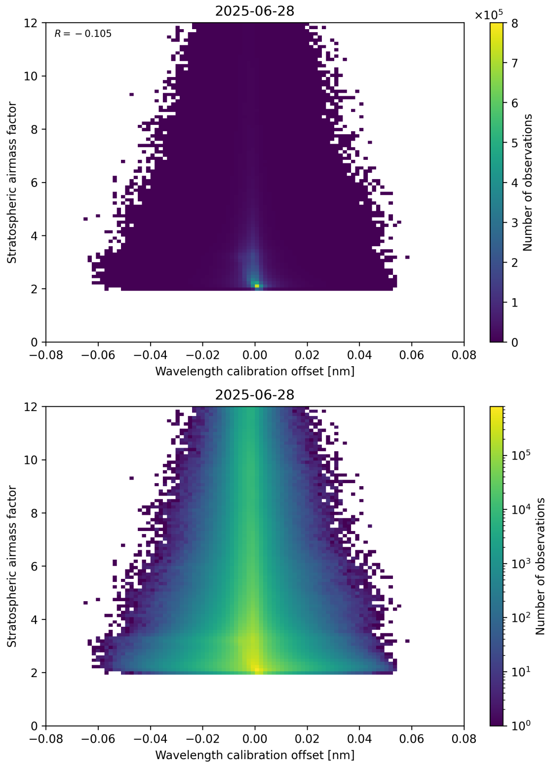
Figure 174: Scatter density plot of “Wavelength calibration offset” against “Stratospheric air mass factor” for 2025-06-27 to 2025-06-29.
