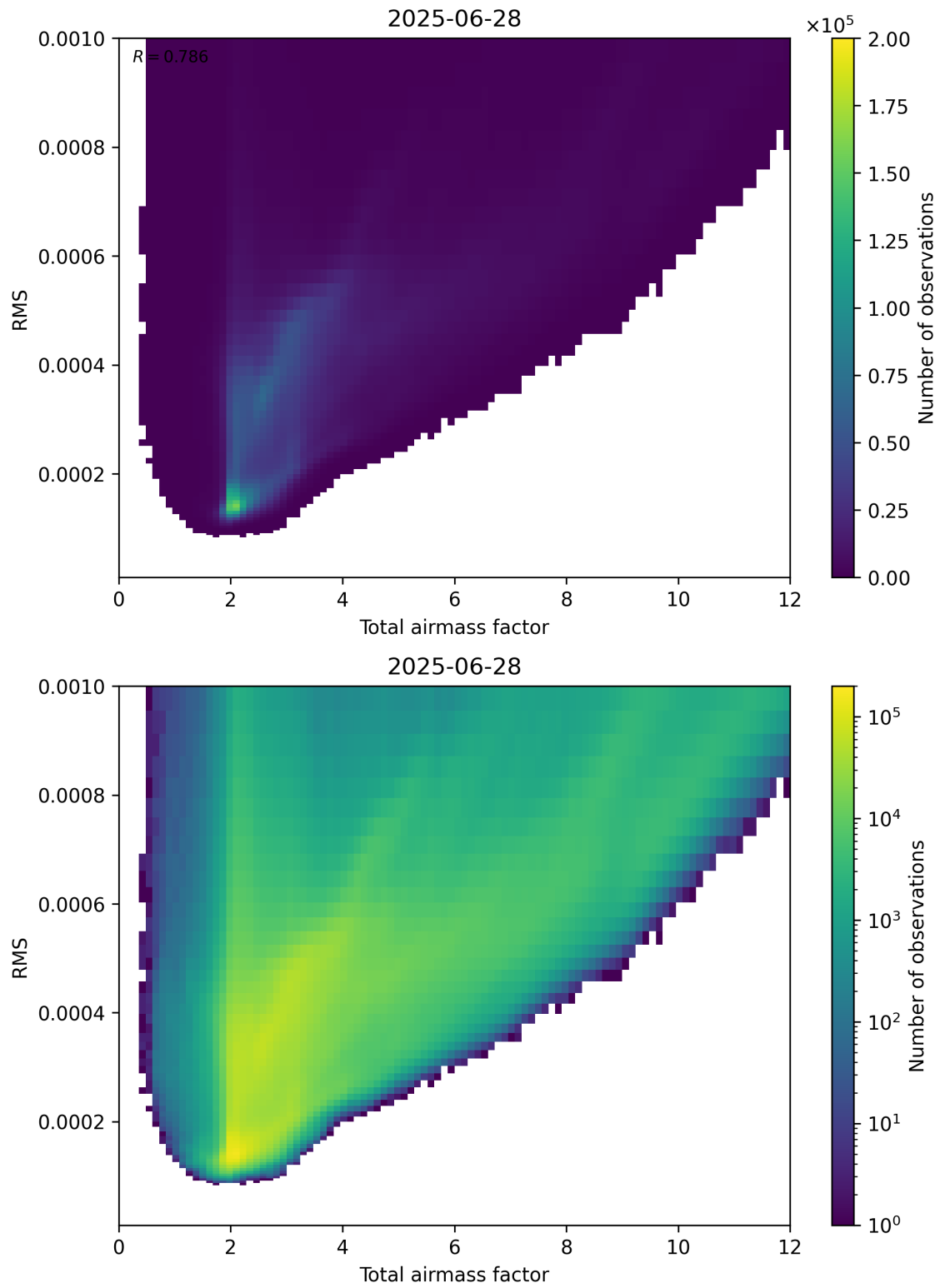
Figure 69: Scatter density plot of “Total airmass factor” against “RMS” for 2025-06-27 to 2025-06-29.
