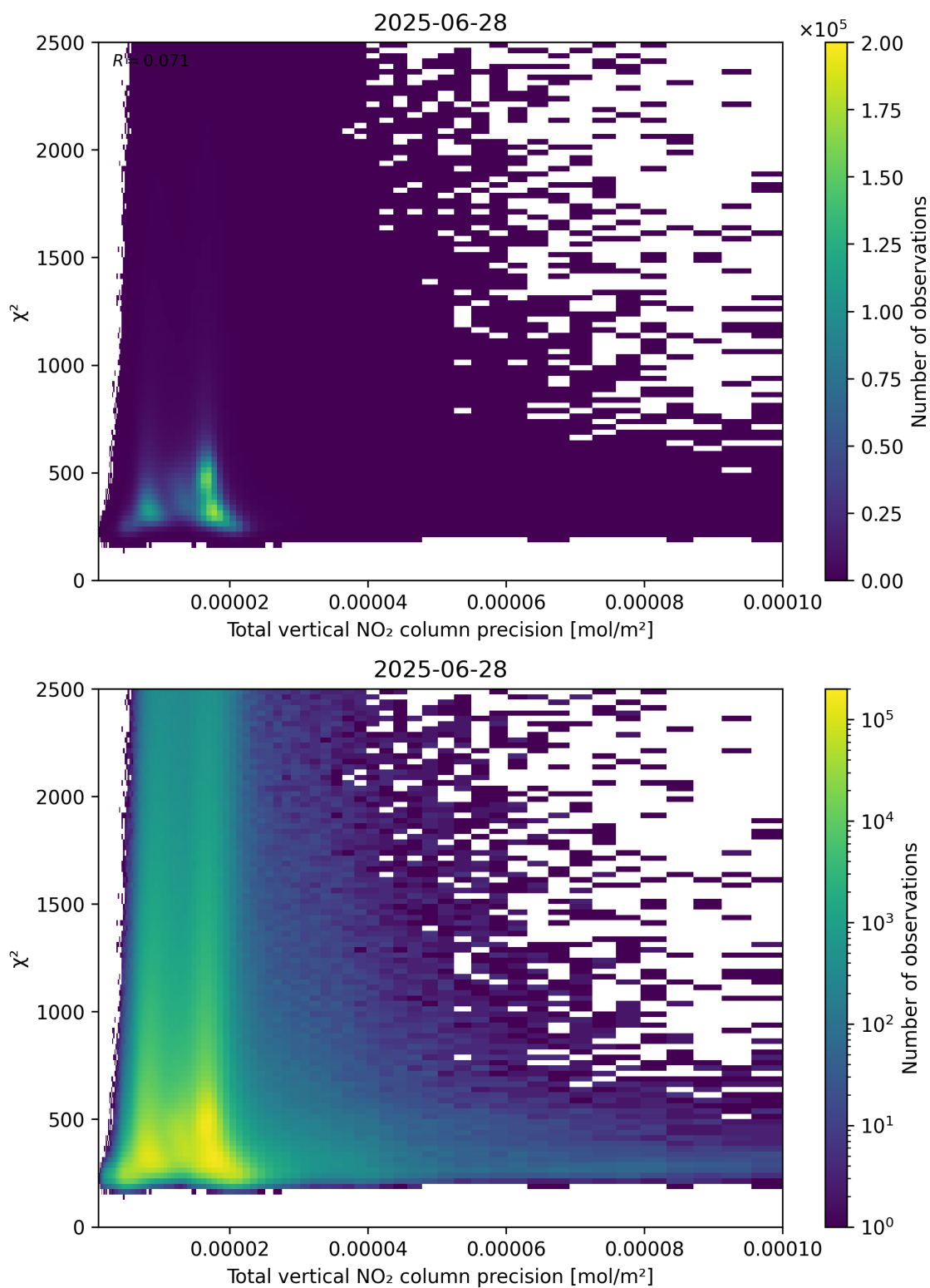
Figure 116: Scatter density plot of “Total vertical NO 2 column precision” against “ \chi^2 ” for 2025-06-27 to 2025-06-29.
