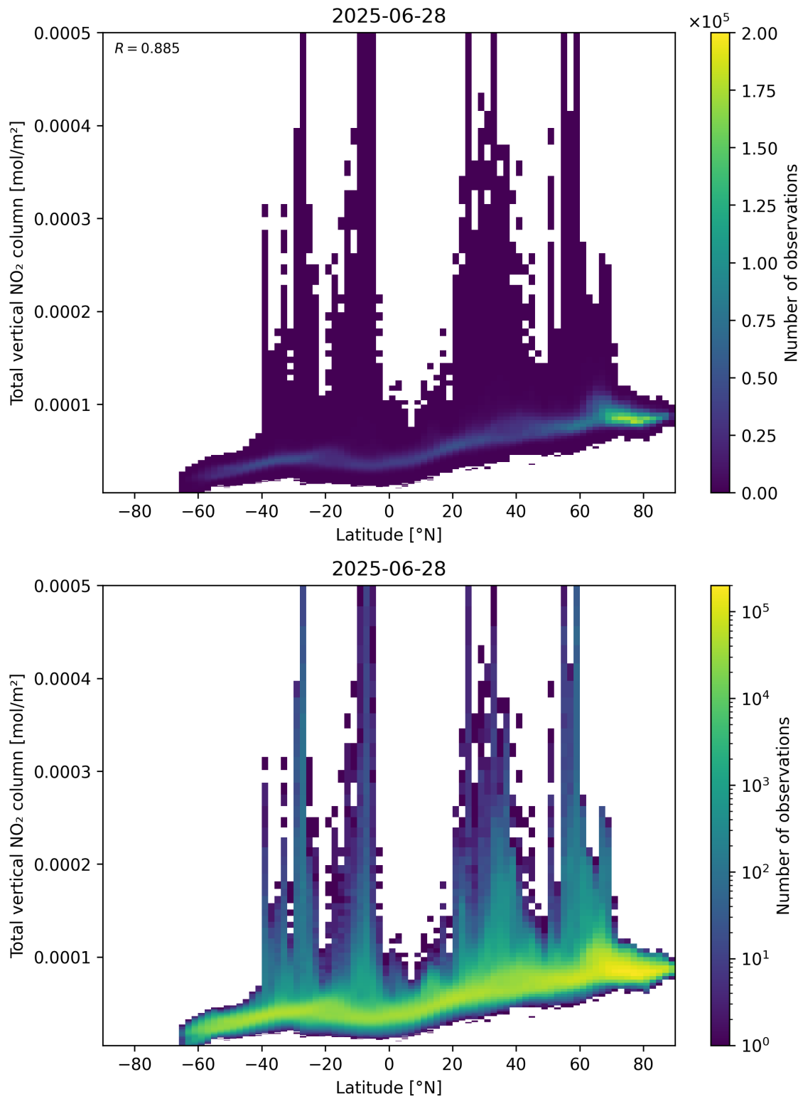
Figure 90: Scatter density plot of “Latitude” against “Total vertical NO 2 column” for 2025-06-27 to 2025-06-29.
