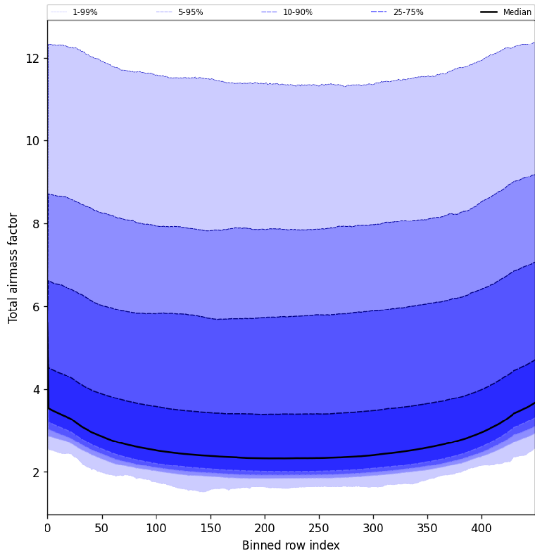
Figure 49: Along track statistics of “Total airmass factor” for 2025-06-27 to 2025-06-29
