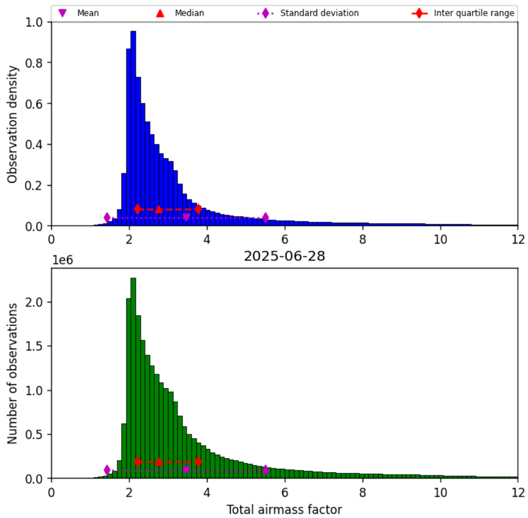
Figure 32: Histogram of “Total airmass factor” for 2025-06-27 to 2025-06-29
