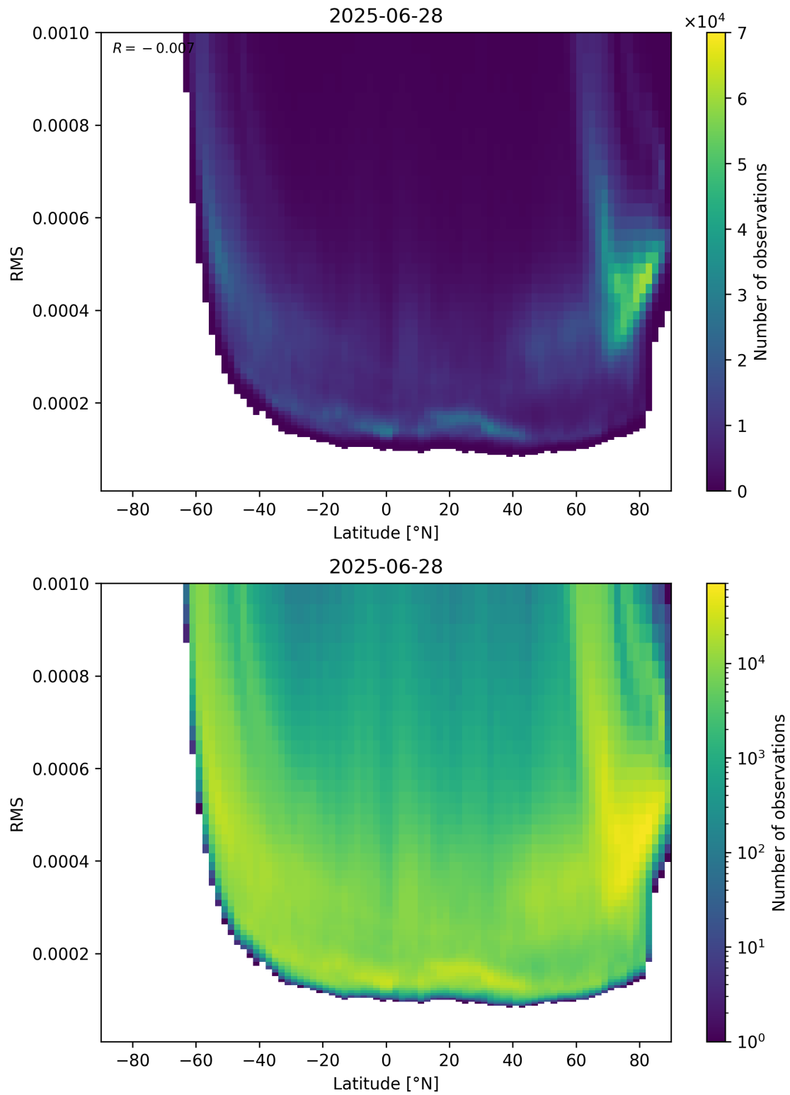
Figure 94: Scatter density plot of “Latitude” against “RMS” for 2025-06-27 to 2025-06-29.
