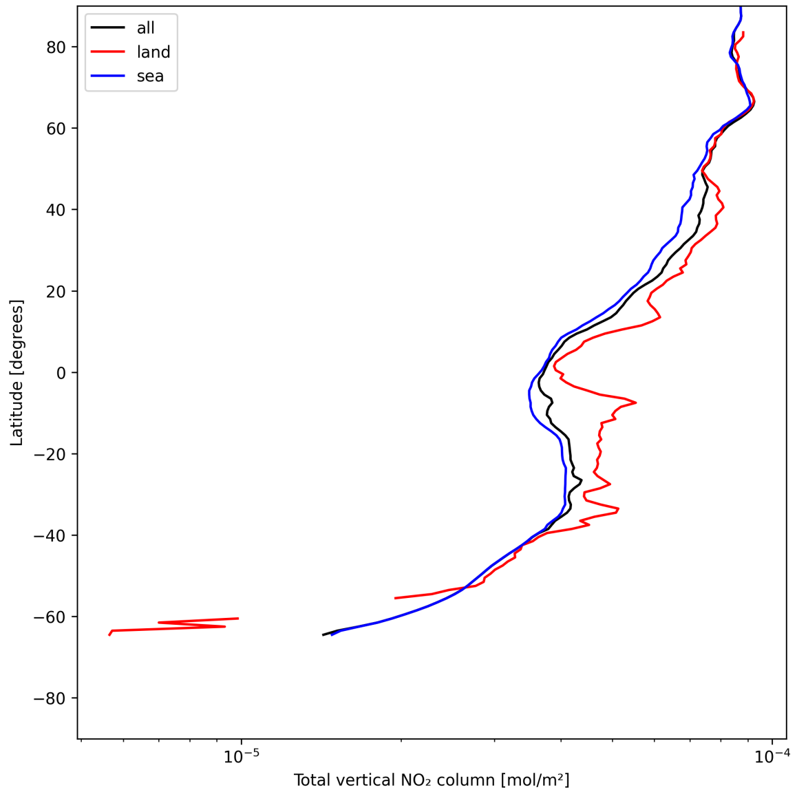
Figure 21: Zonal average of “Total vertical NO 2 column” for 2025-06-27 to 2025-06-29.
