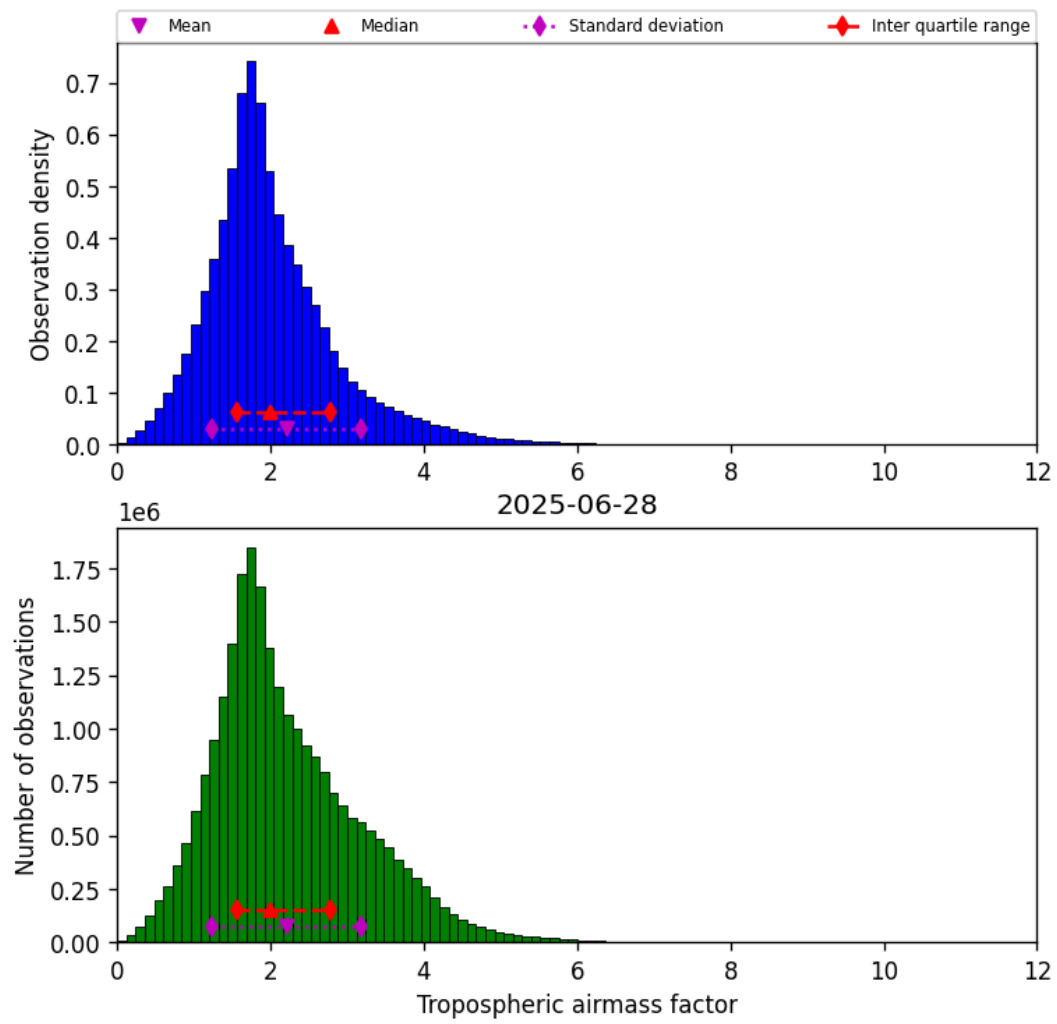
Figure 31: Histogram of “Tropospheric airmass factor” for 2025-06-27 to 2025-06-29
