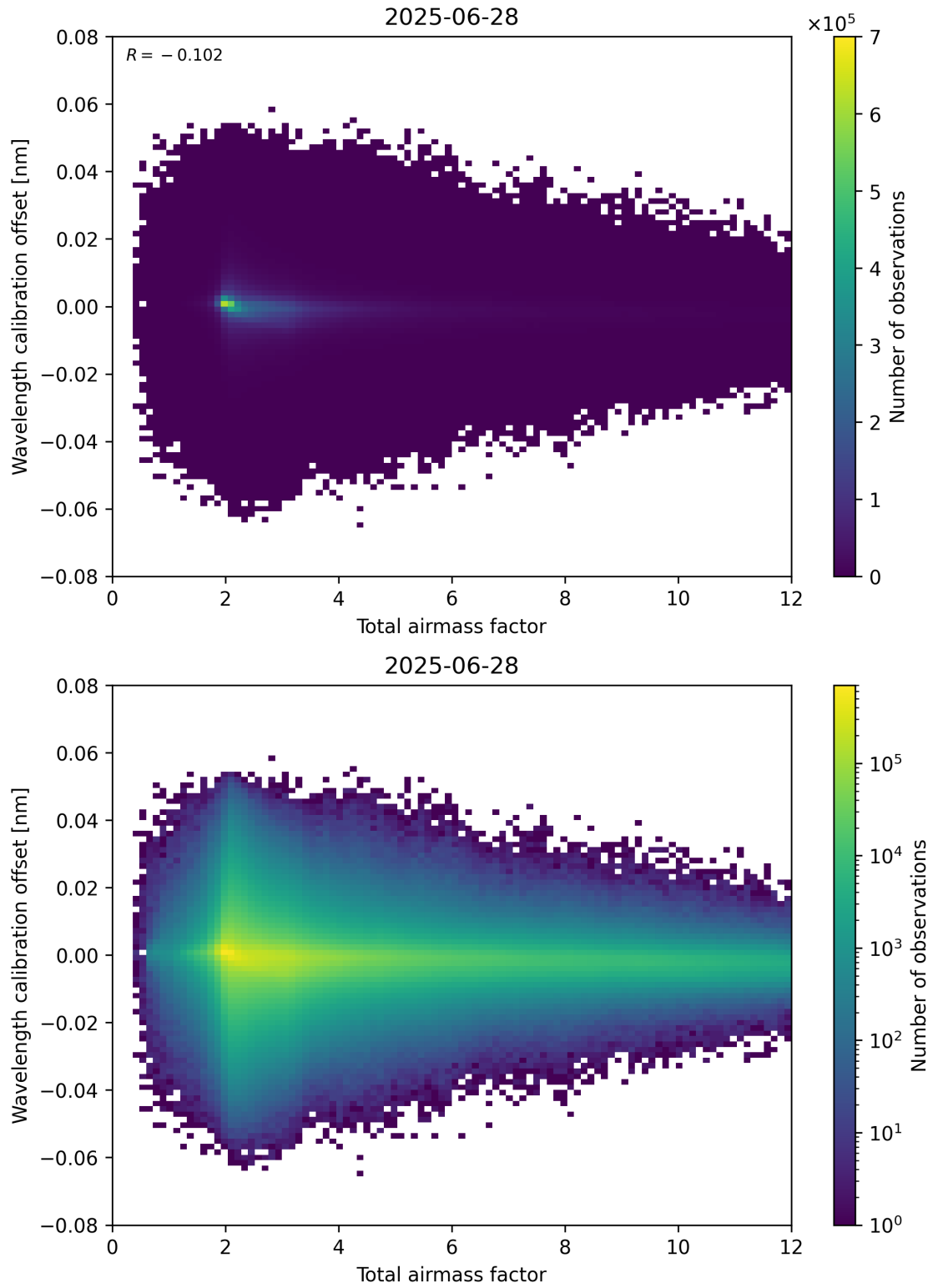
Figure 70: Scatter density plot of “Total airmass factor” against “Wavelength calibration offset” for 2025-06-27 to 2025-06-29.
