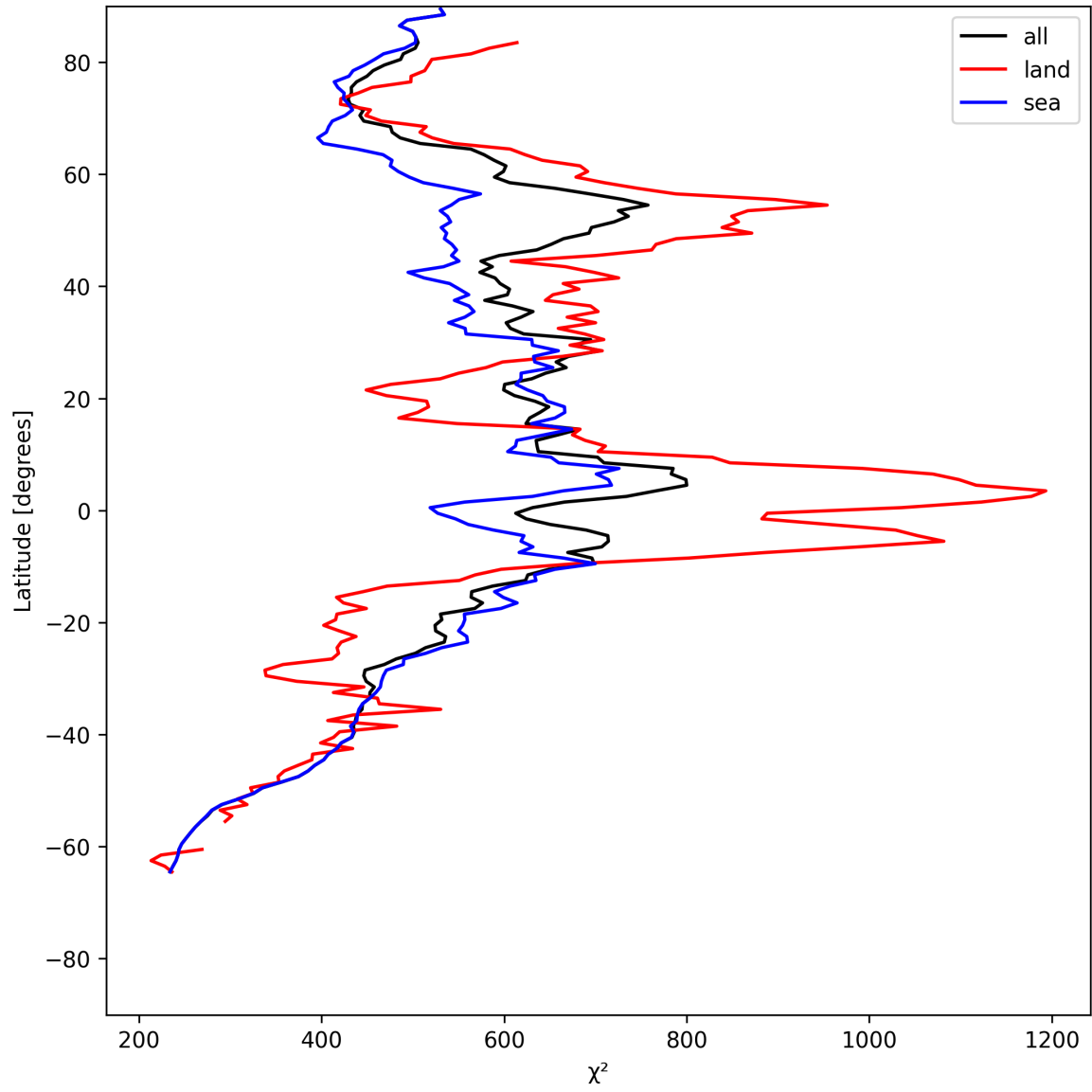
Figure 25: Zonal average of “ \chi^2 ” for 2025-06-27 to 2025-06-29.
