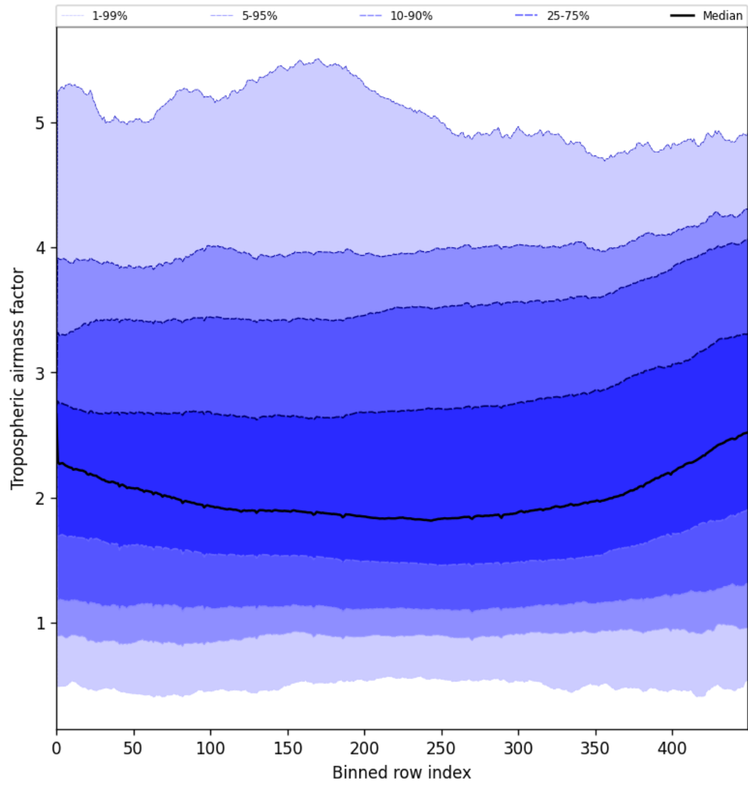
Figure 48: Along track statistics of “Tropospheric airmass factor” for 2025-06-27 to 2025-06-29
