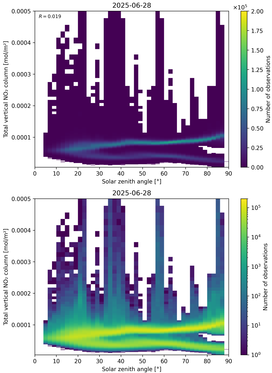
Figure 153: Scatter density plot of “Solar zenith angle” against “Total vertical NO 2 column” for 2025-06-27 to 2025-06-29.
