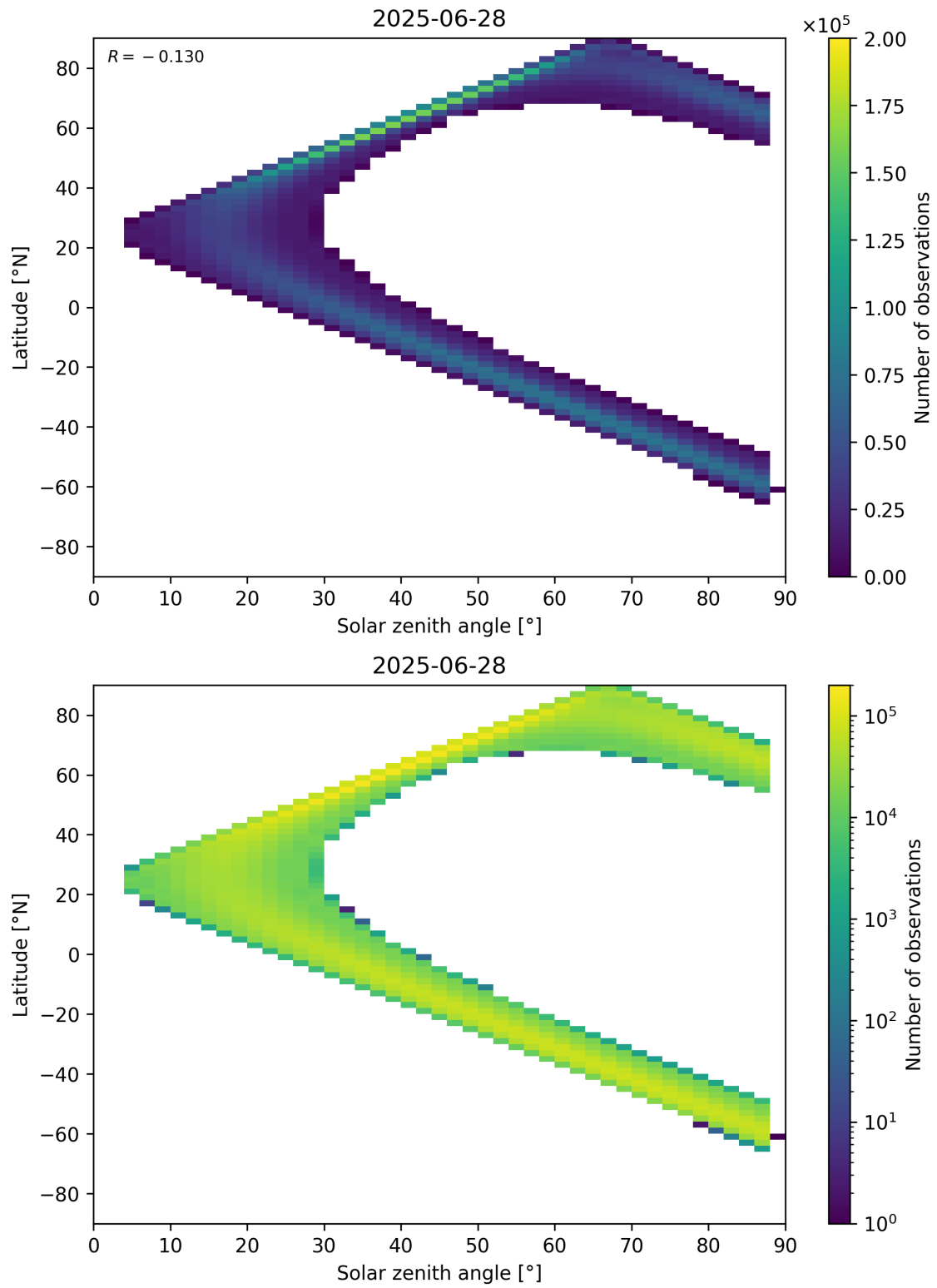
Figure 149: Scatter density plot of “Solar zenith angle” against “Latitude” for 2025-06-27 to 2025-06-29.
