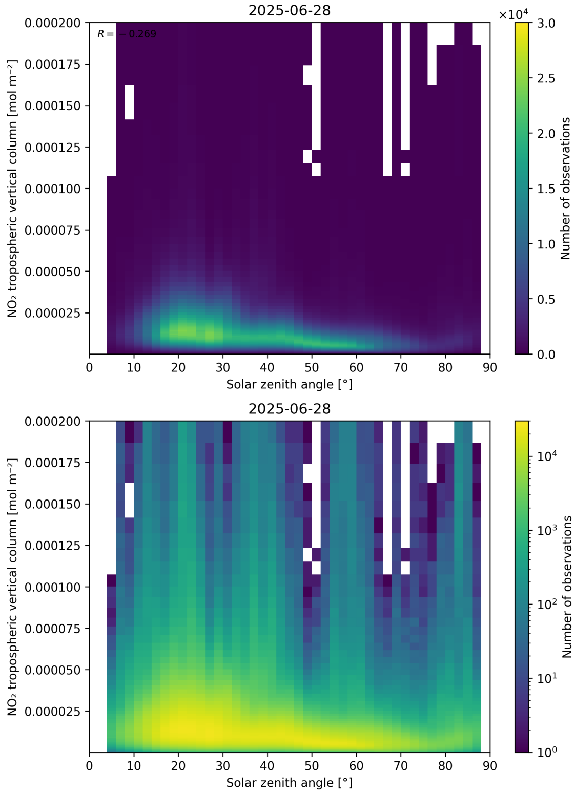
Figure 155: Scatter density plot of “Solar zenith angle” against “NO 2 tropospheric vertical column” for 2025-06-27 to 2025-06-29.
