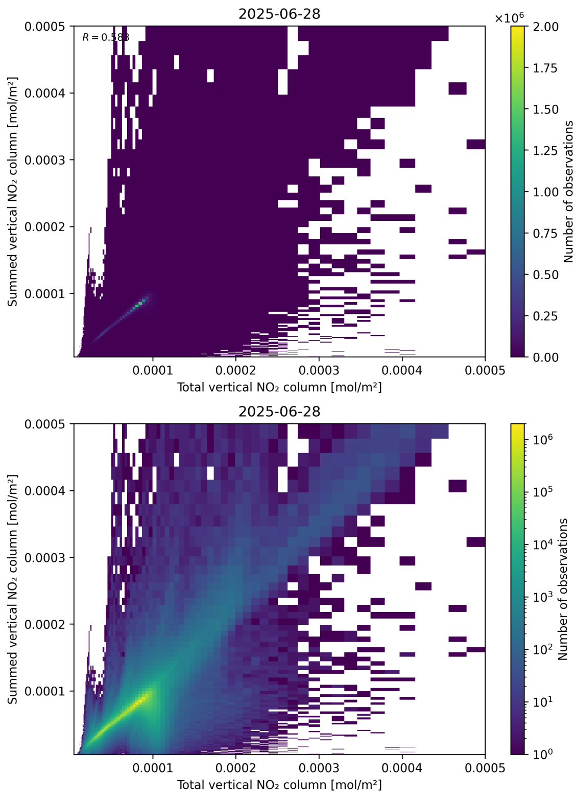
Figure 112: Scatter density plot of “Total vertical NO 2 column” against “Summed vertical NO 2 column” for 2025-06-27 to 2025-06-29.
