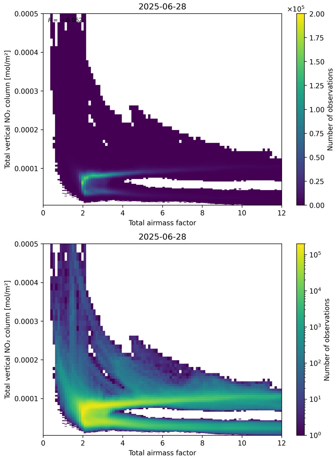
Figure 67: Scatter density plot of “Total airmass factor” against “Total vertical NO 2 column” for 2025-06-27 to 2025-06-29.
