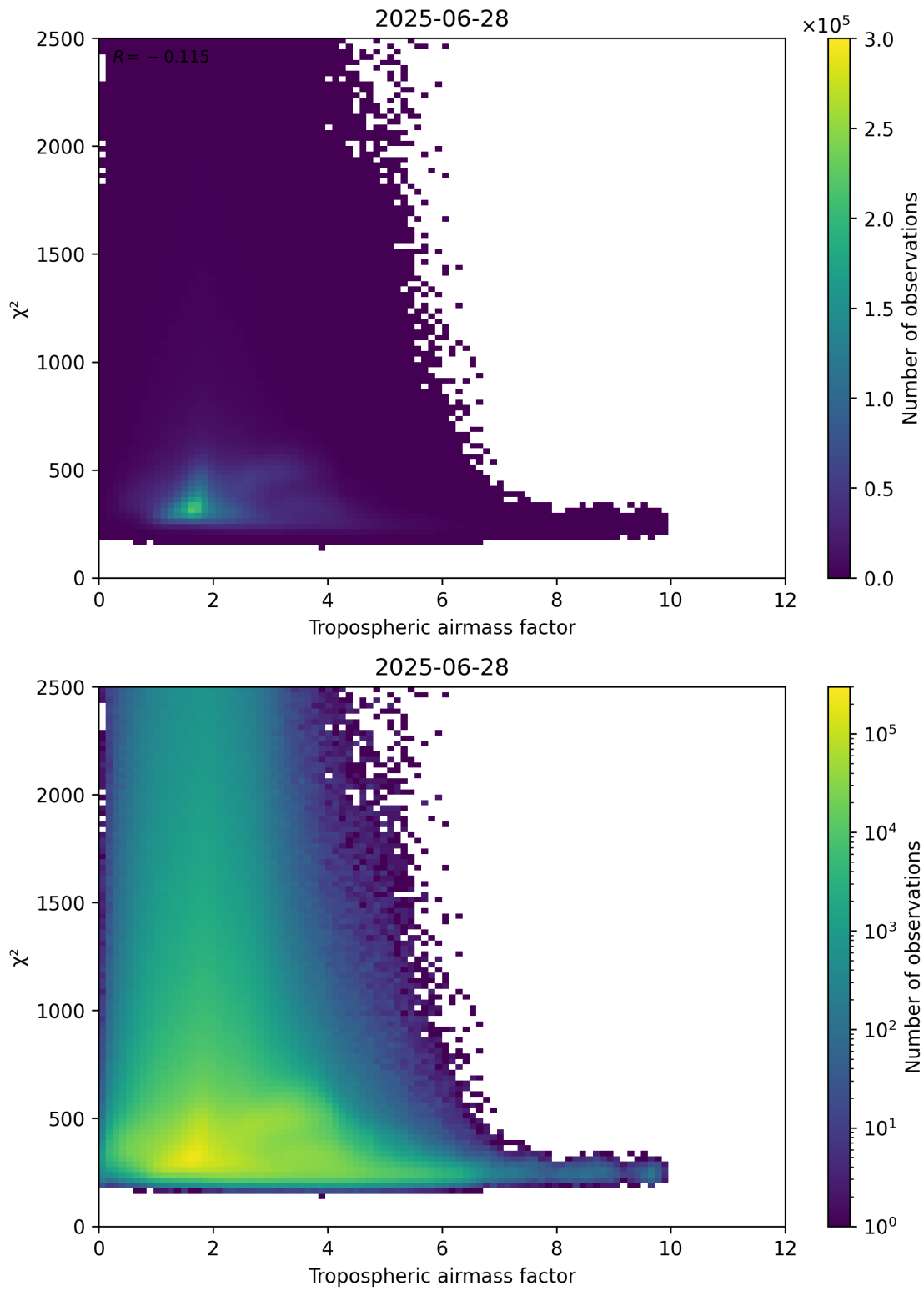
Figure 73: Scatter density plot of “Tropospheric airmass factor” against “ \chi^2 ” for 2025-06-27 to 2025-06-29.
