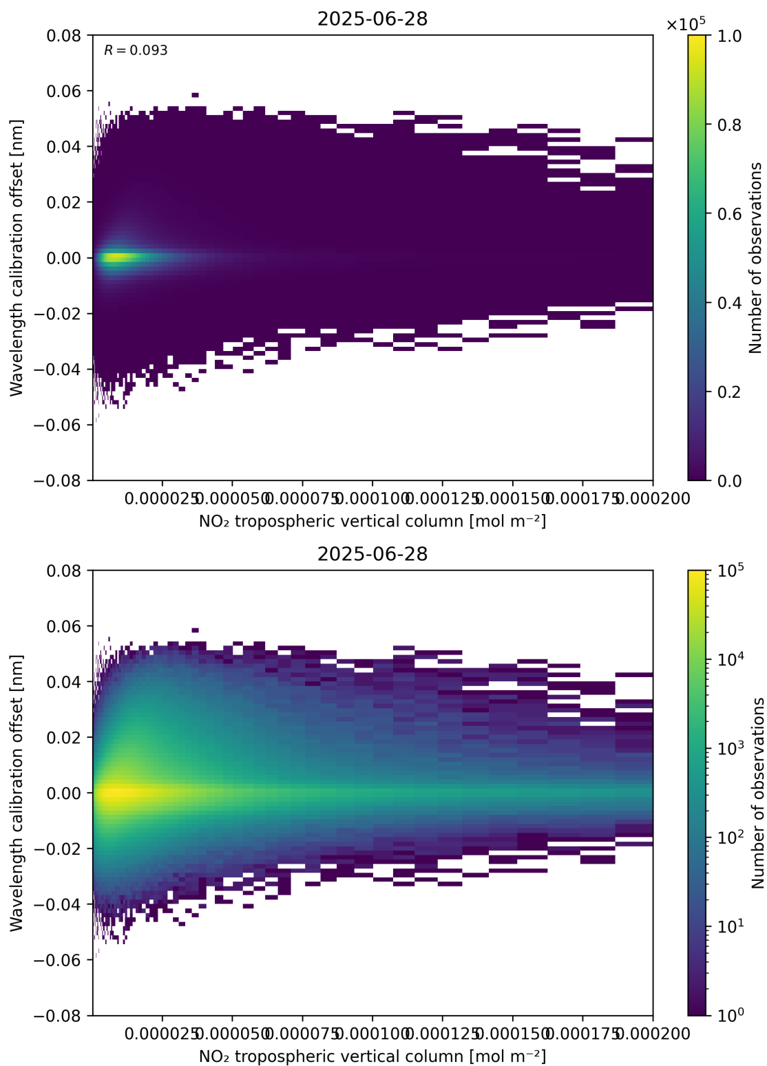
Figure 143: Scatter density plot of “NO 2 tropospheric vertical column” against “Wavelength calibration offset” for 2025-06-27 to 2025-06-29.
