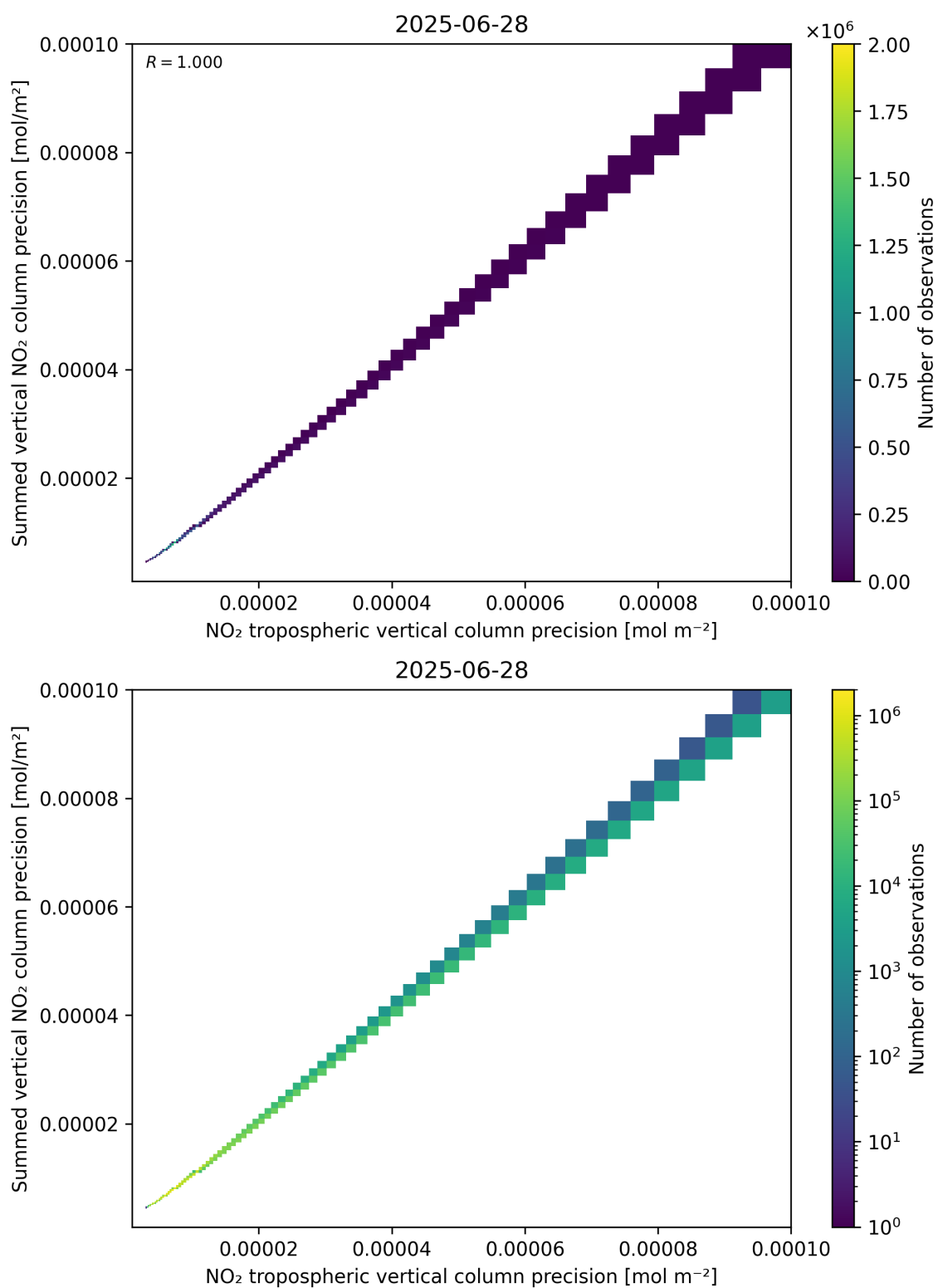
Figure 137: Scatter density plot of “NO 2 tropospheric vertical column precision” against “Summed vertical NO 2 column precision” for 2025-06-27 to 2025-06-29.
