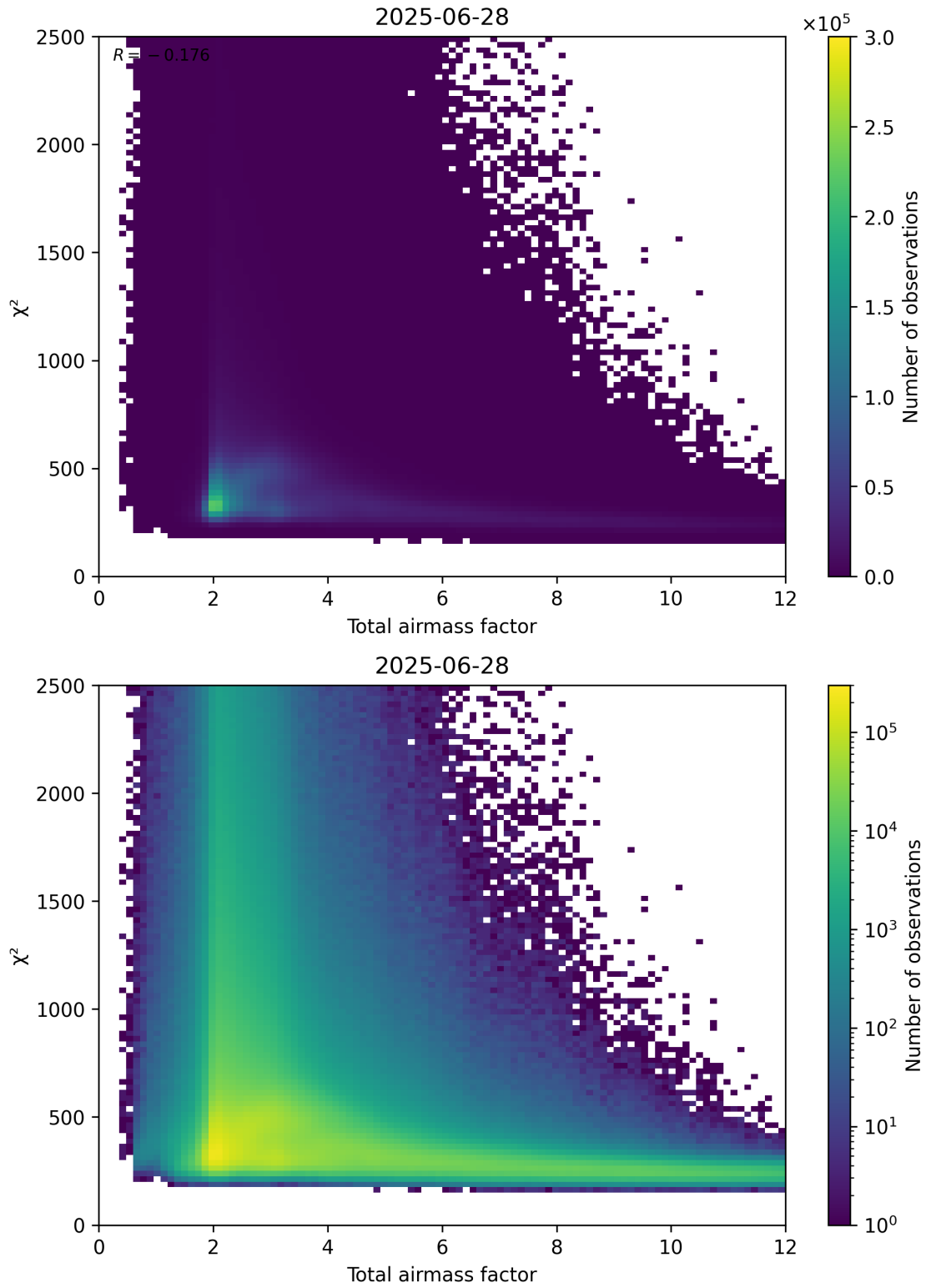
Figure 63: Scatter density plot of “Total airmass factor” against “ \chi^2 ” for 2025-06-27 to 2025-06-29.
