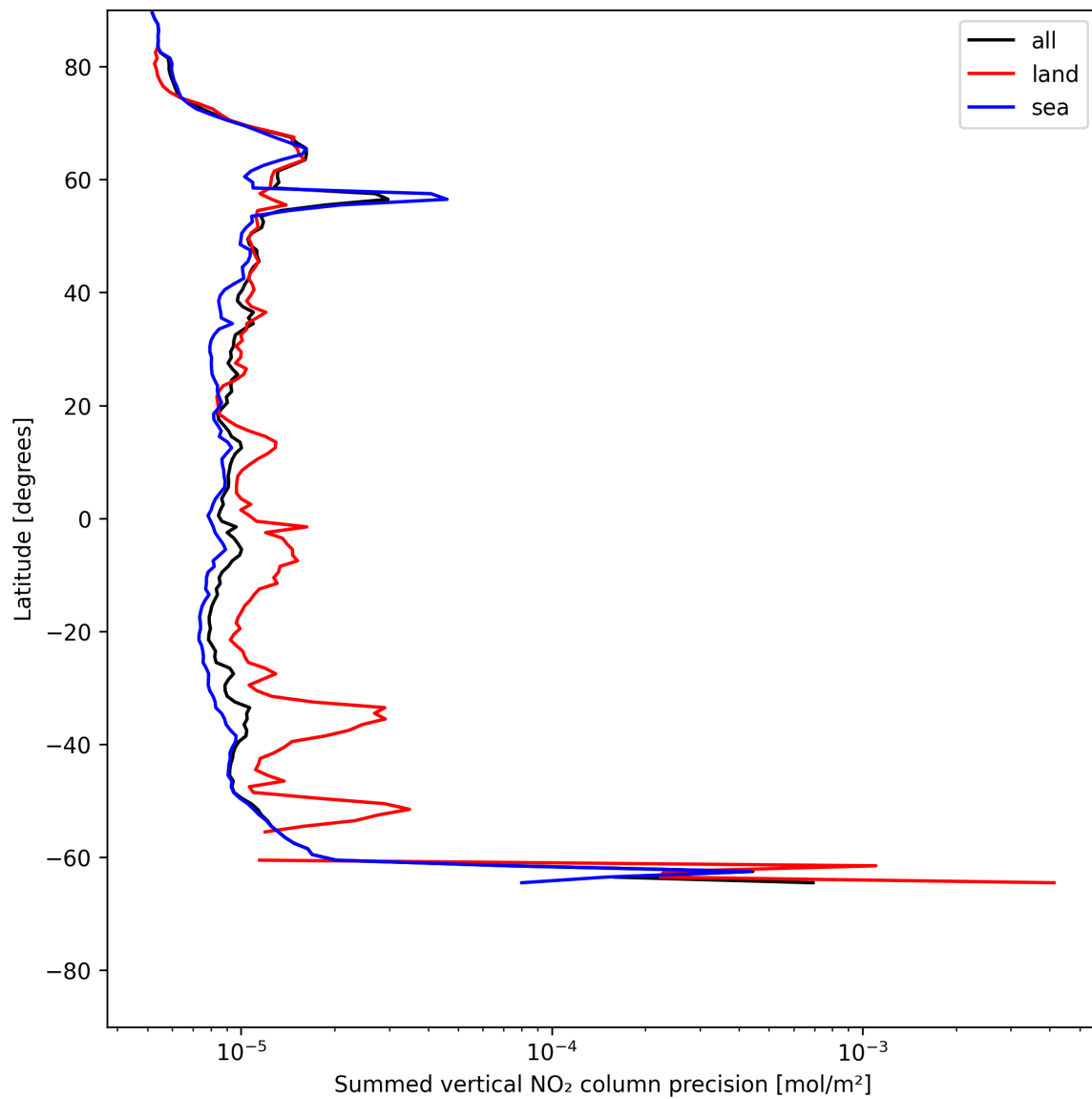
Figure 24: Zonal average of “Summed vertical NO 2 column precision” for 2025-06-27 to 2025-06-29.
