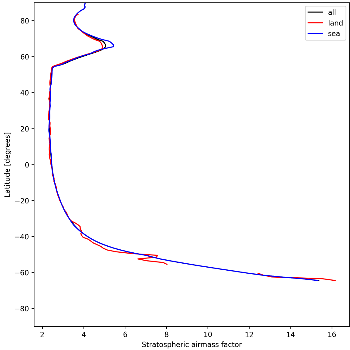
Figure 27: Zonal average of “Stratospheric airmass factor” for 2025-06-27 to 2025-06-29.
