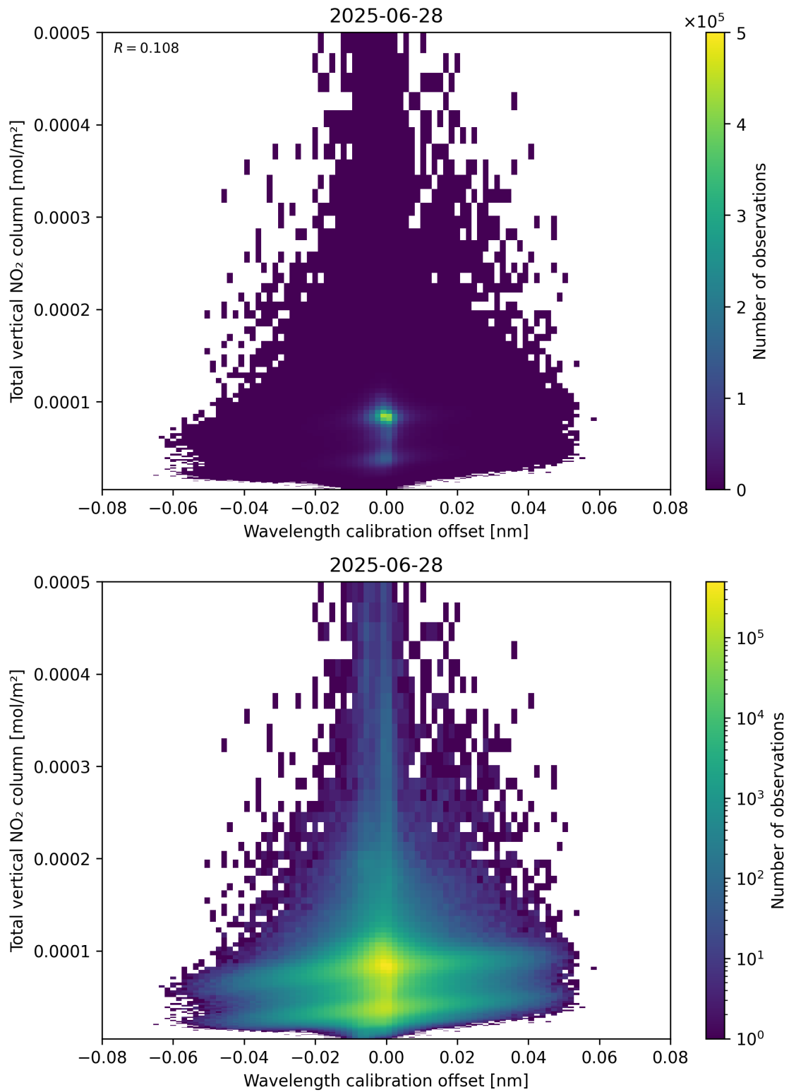
Figure 179: Scatter density plot of “Wavelength calibration offset” against “Total vertical NO 2 column” for 2025-06-27 to 2025-06-29.
