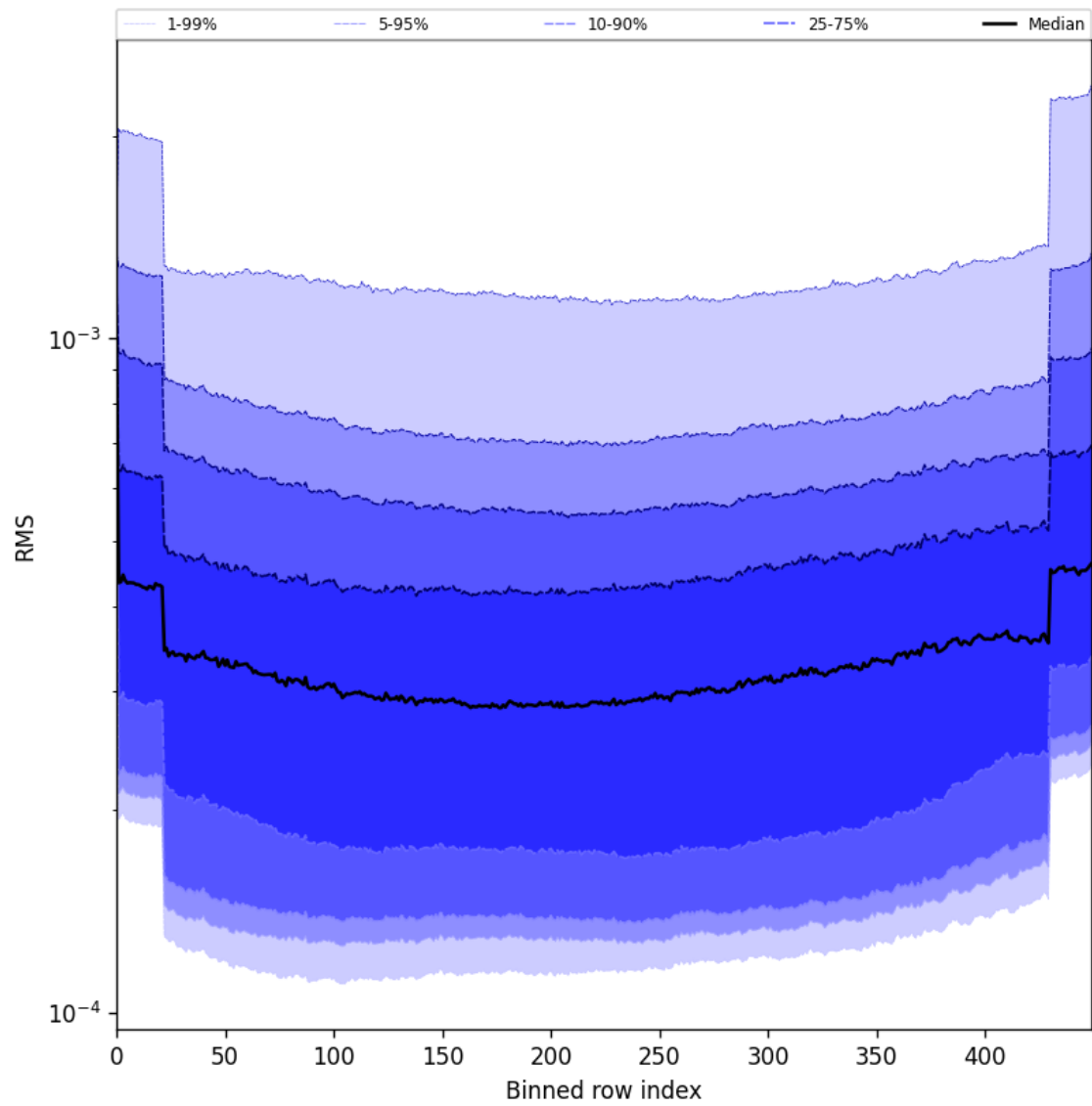
Figure 60: Along track statistics of “RMS” for 2025-06-27 to 2025-06-29
