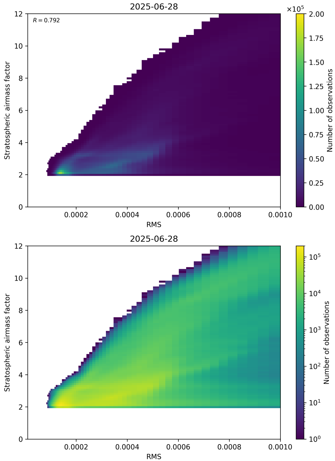
Figure 144: Scatter density plot of “RMS” against “Stratospheric airmass factor” for 2025-06-27 to 2025-06-29.
