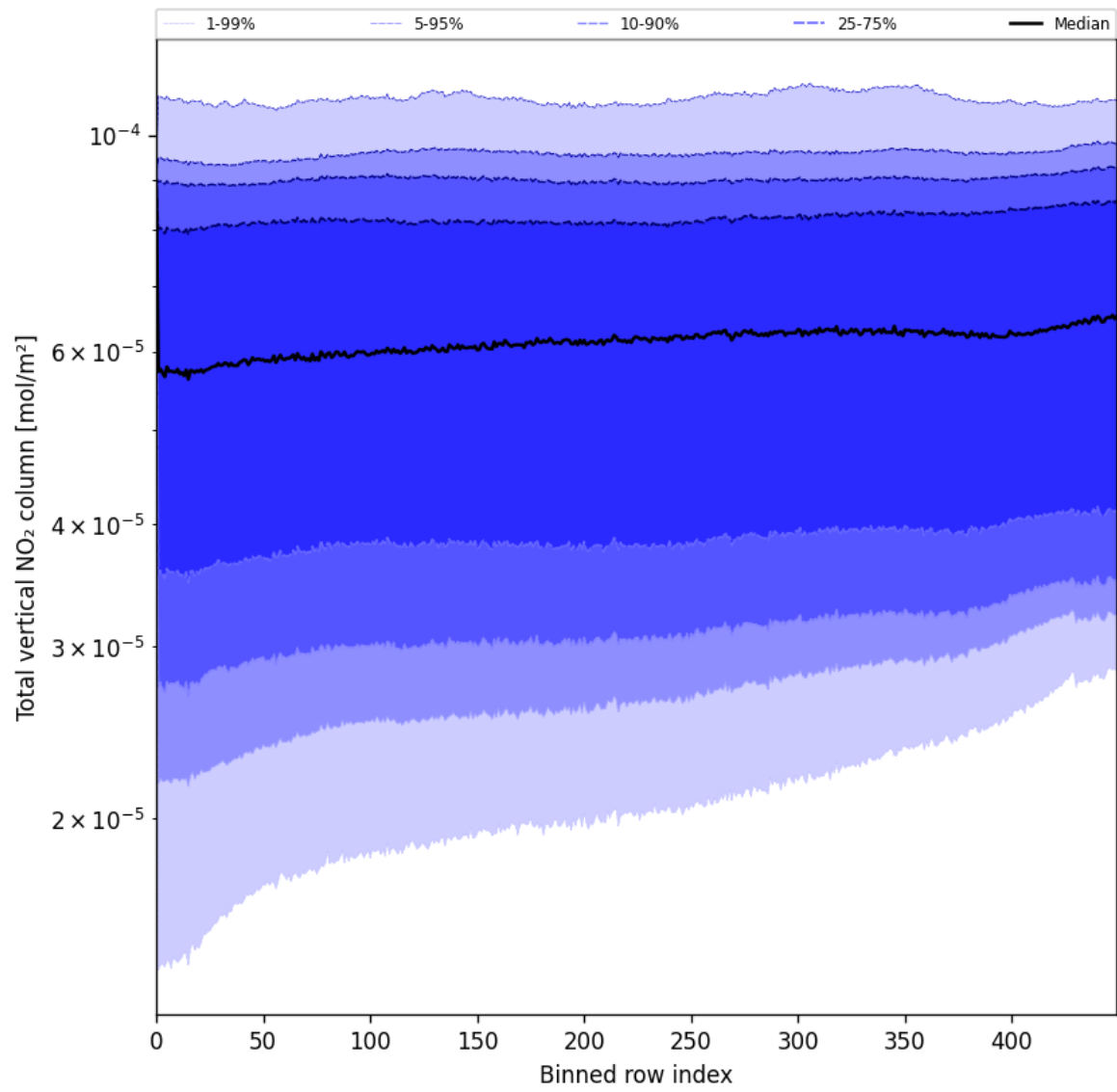
Figure 55: Along track statistics of “Total vertical NO 2 column” for 2025-06-27 to 2025-06-29
