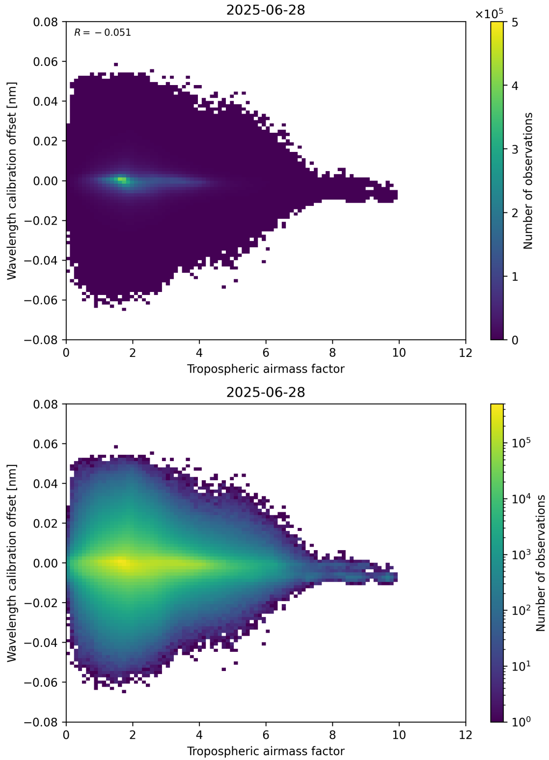
Figure 80: Scatter density plot of “Tropospheric airmass factor” against “Wavelength calibration offset” for 2025-06-27 to 2025-06-29.
