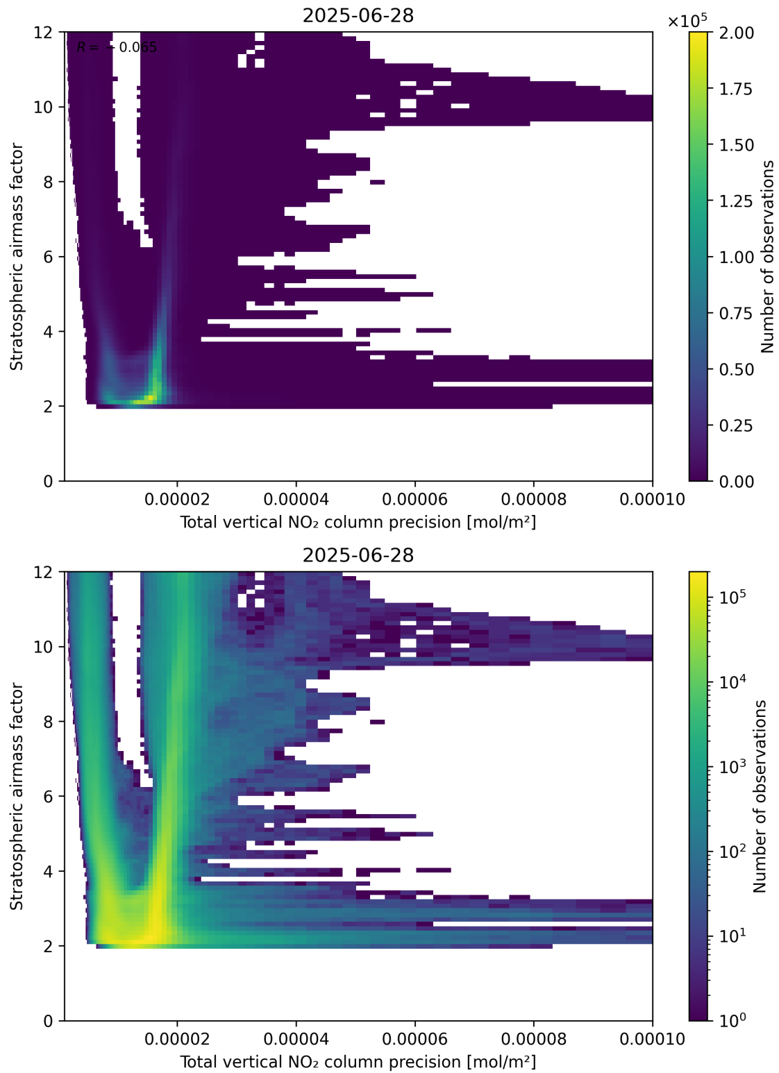
Figure 115: Scatter density plot of “Total vertical NO 2 column precision” against “Stratospheric air mass factor” for 2025-06-27 to 2025-06-29.
