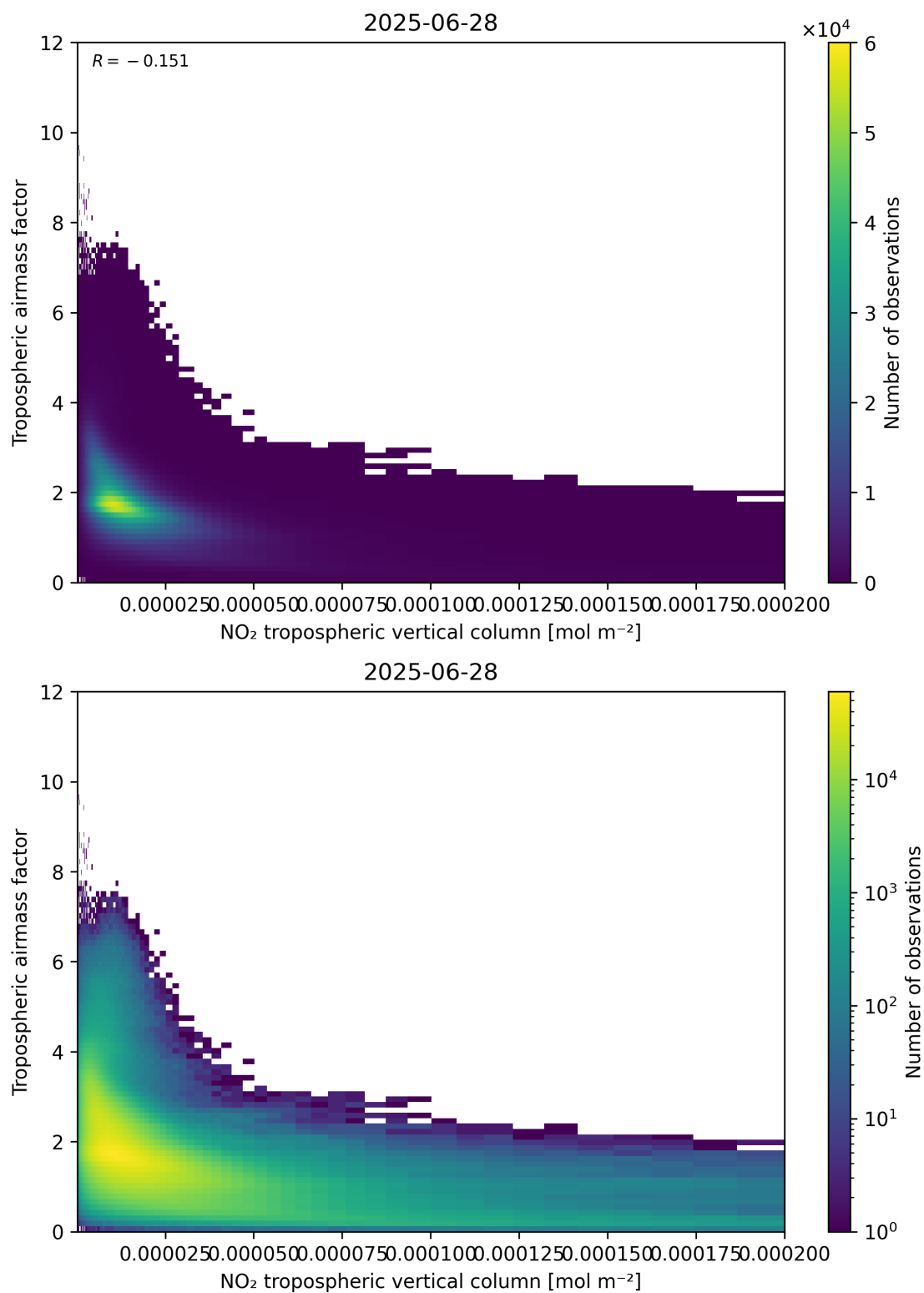
Figure 123: Scatter density plot of “NO 2 tropospheric vertical column” against “Tropospheric air mass factor” for 2025-06-27 to 2025-06-29.
