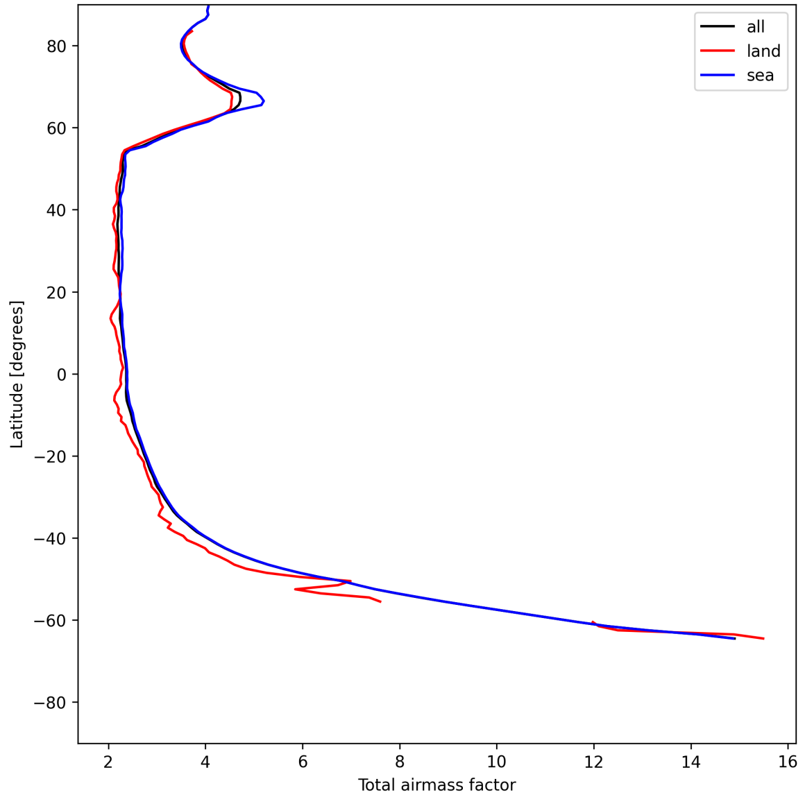
Figure 15: Zonal average of “Total airmass factor” for 2025-06-27 to 2025-06-29.
