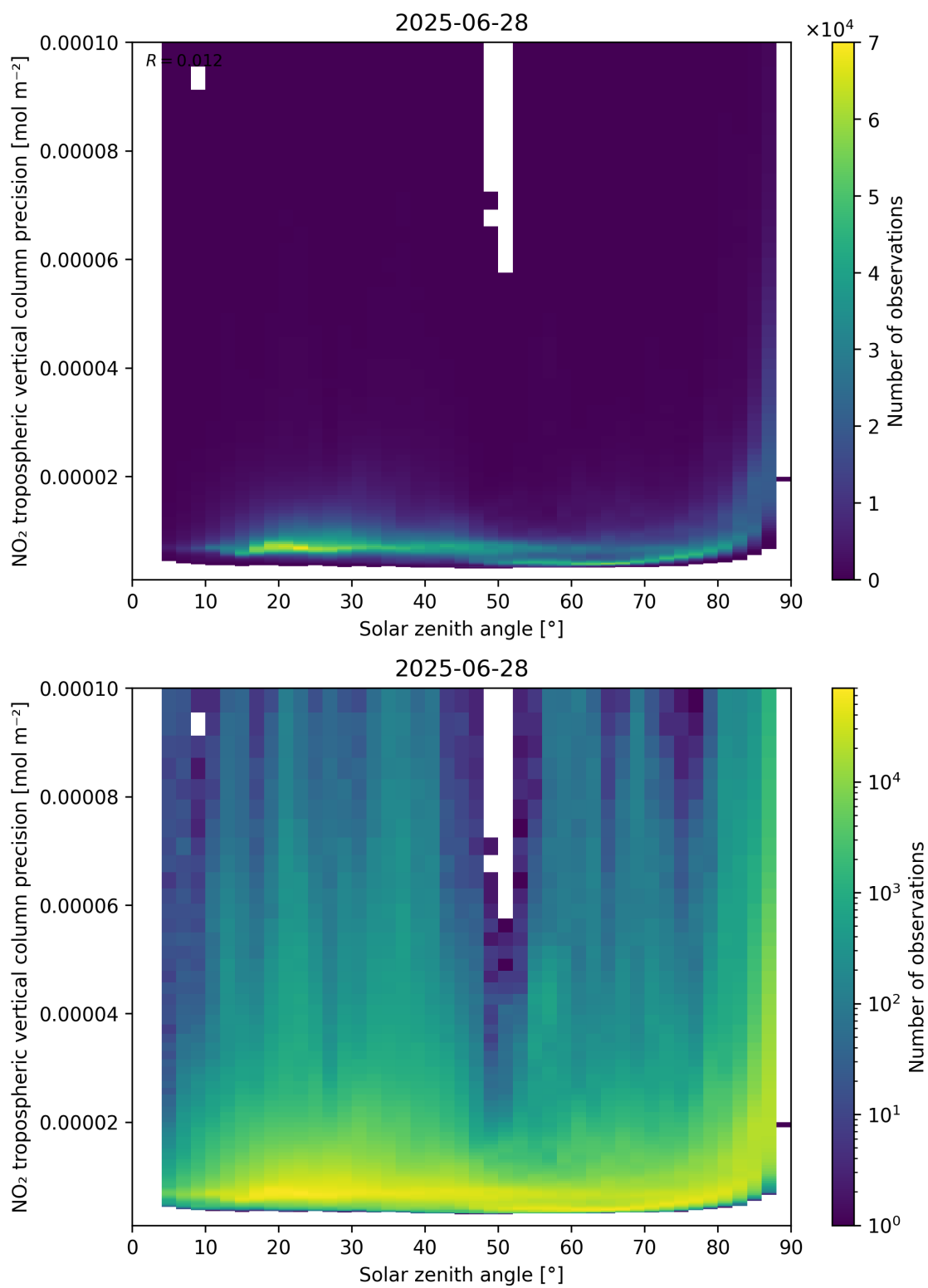
Figure 156: Scatter density plot of “Solar zenith angle” against “NO 2 tropospheric vertical column precision” for 2025-06-27 to 2025-06-29.
