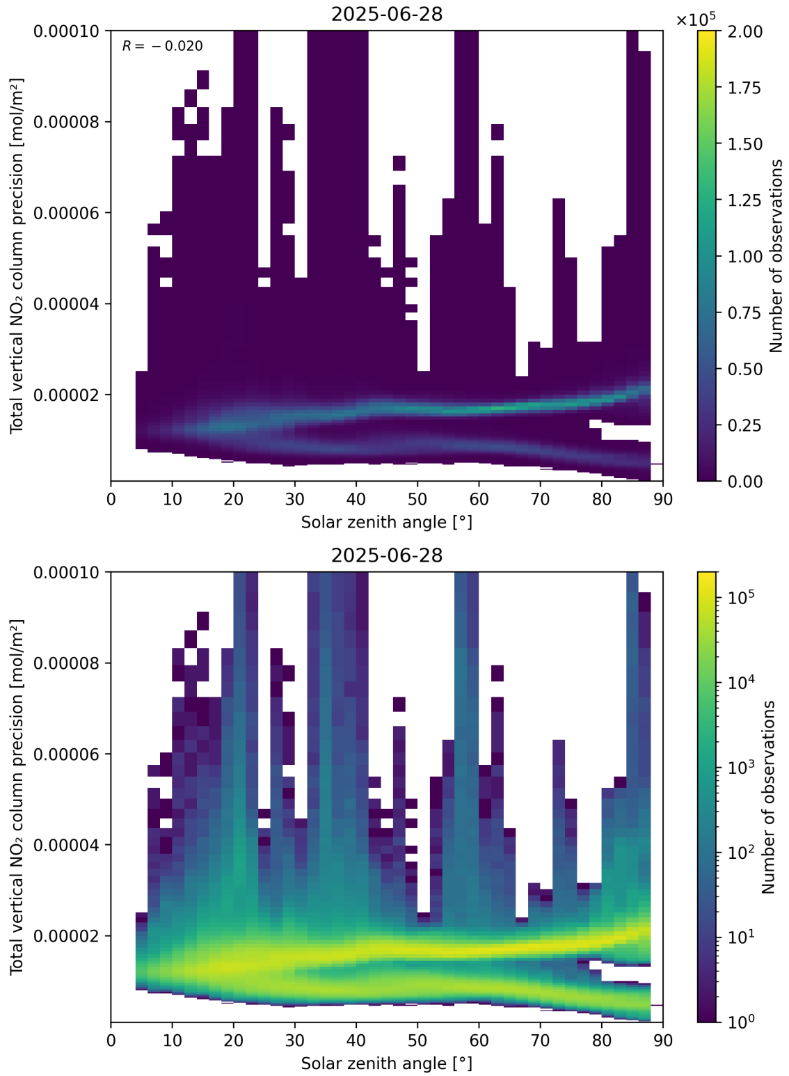
Figure 154: Scatter density plot of “Solar zenith angle” against “Total vertical NO 2 column precision” for 2025-06-27 to 2025-06-29.
