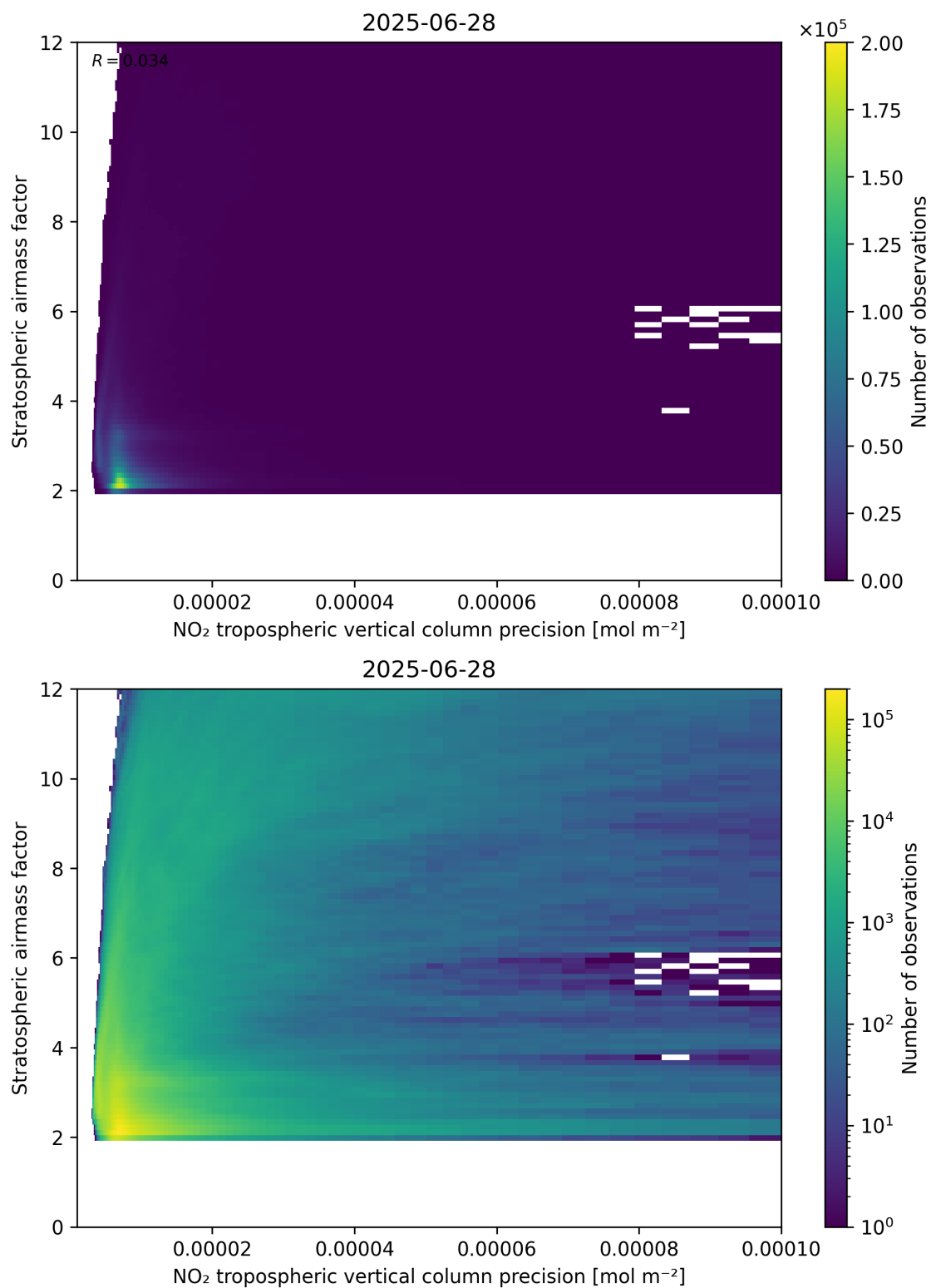
Figure 131: Scatter density plot of “NO 2 tropospheric vertical column precision” against “Stratospheric airmass factor” for 2025-06-27 to 2025-06-29.
