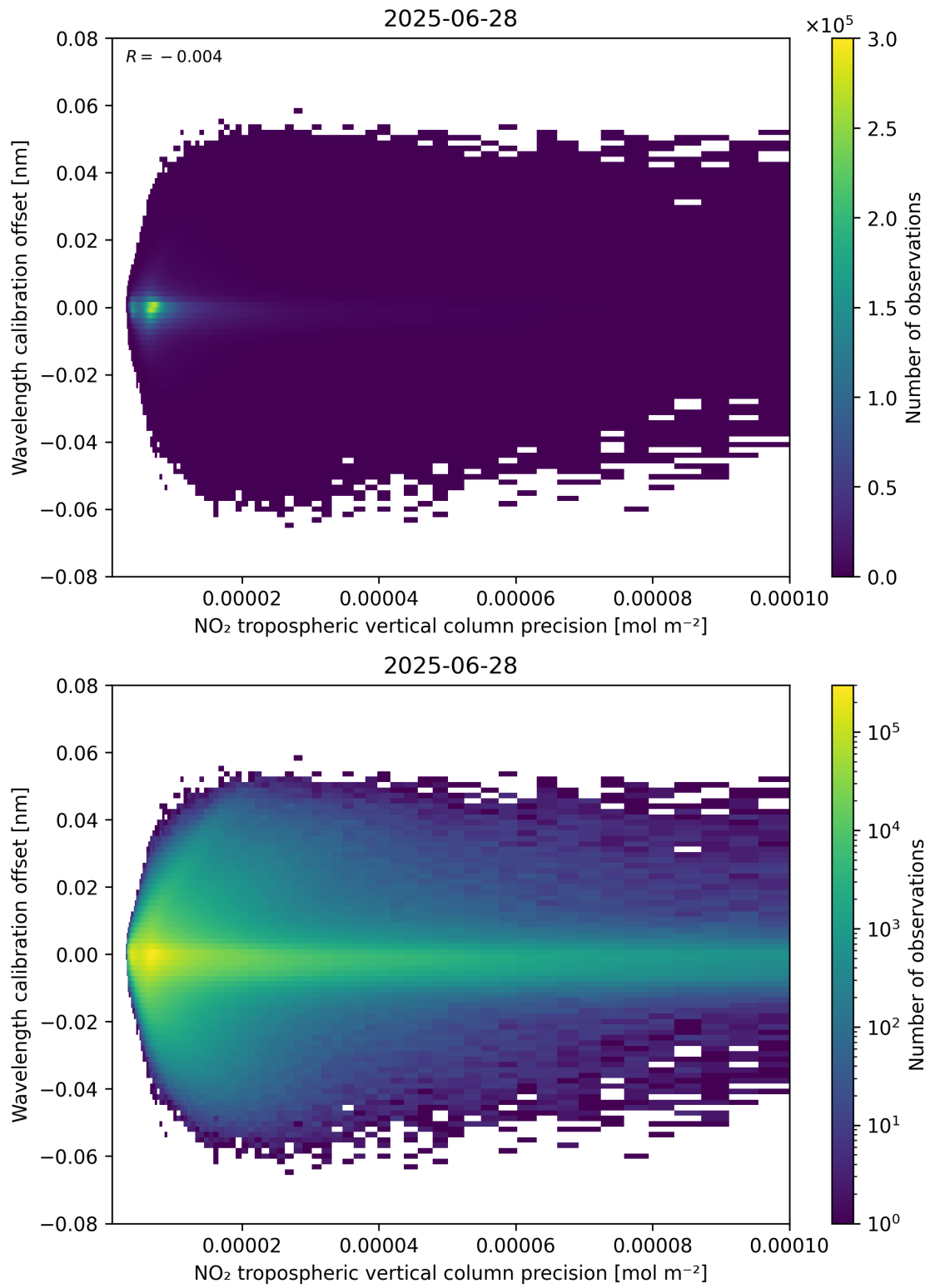
Figure 141: Scatter density plot of “NO 2 tropospheric vertical column precision” against “Wavelength calibration offset” for 2025-06-27 to 2025-06-29.
