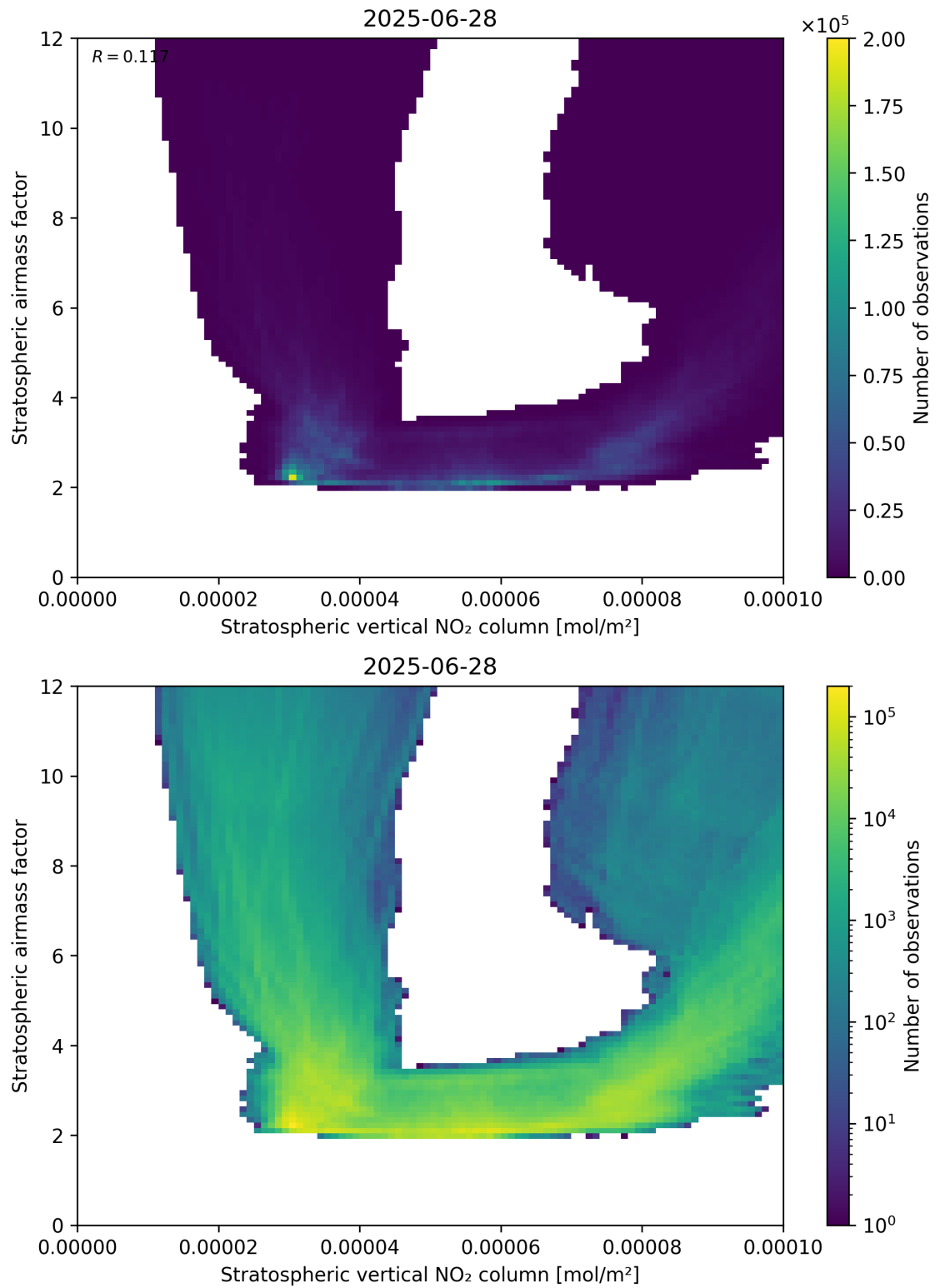
Figure 96: Scatter density plot of “Stratospheric vertical NO 2 column” against “Stratospheric airmass factor” for 2025-06-27 to 2025-06-29.
