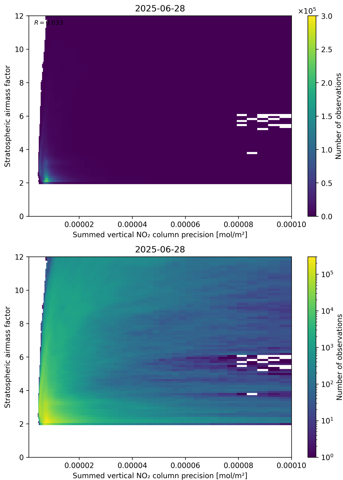
Figure 106: Scatter density plot of “Summed vertical NO 2 column precision” against “Stratospheric airmass factor” for 2025-06-27 to 2025-06-29.
