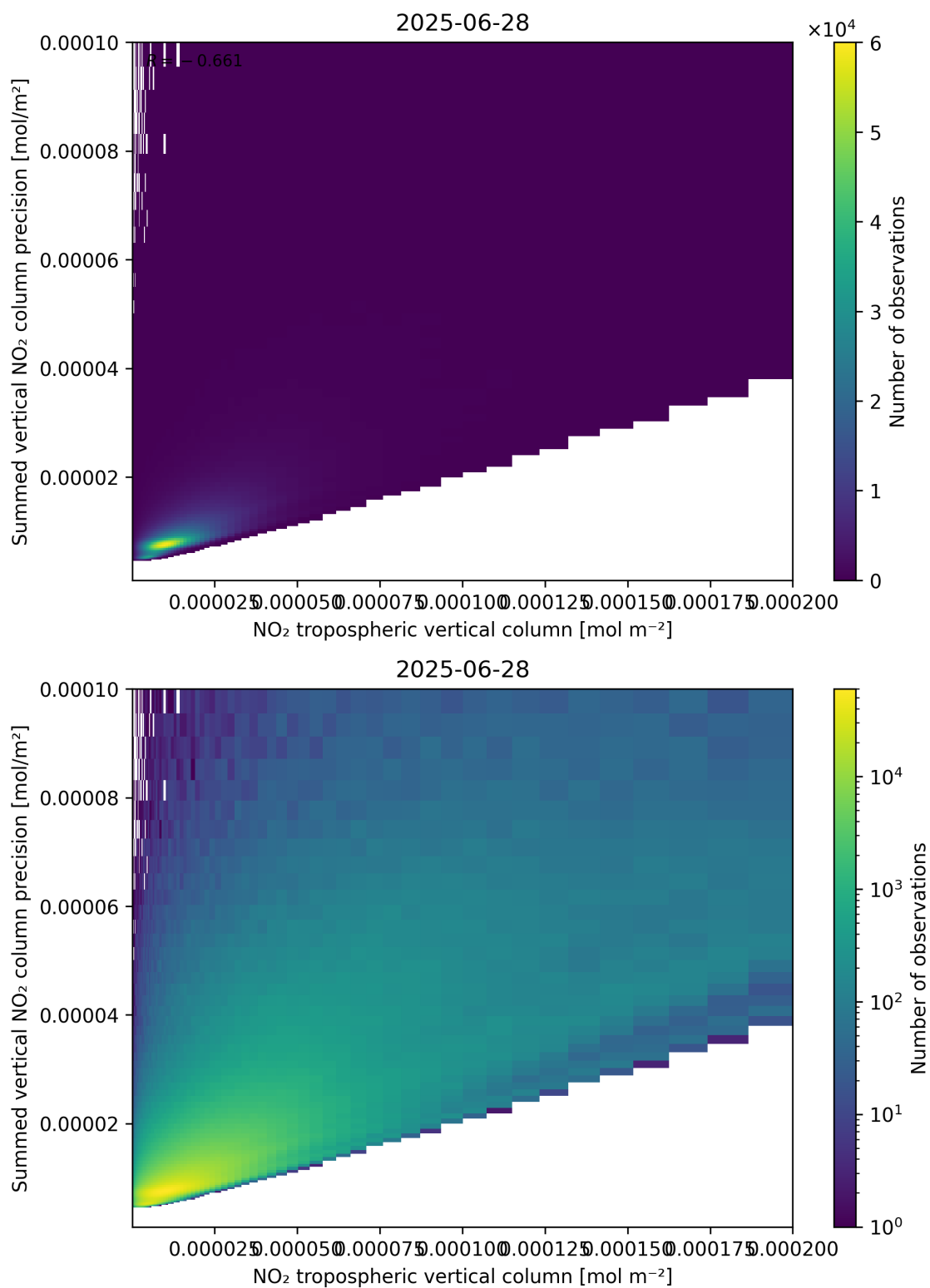
Figure 127: Scatter density plot of “NO 2 tropospheric vertical column” against “Summed vertical NO 2 column precision” for 2025-06-27 to 2025-06-29.
