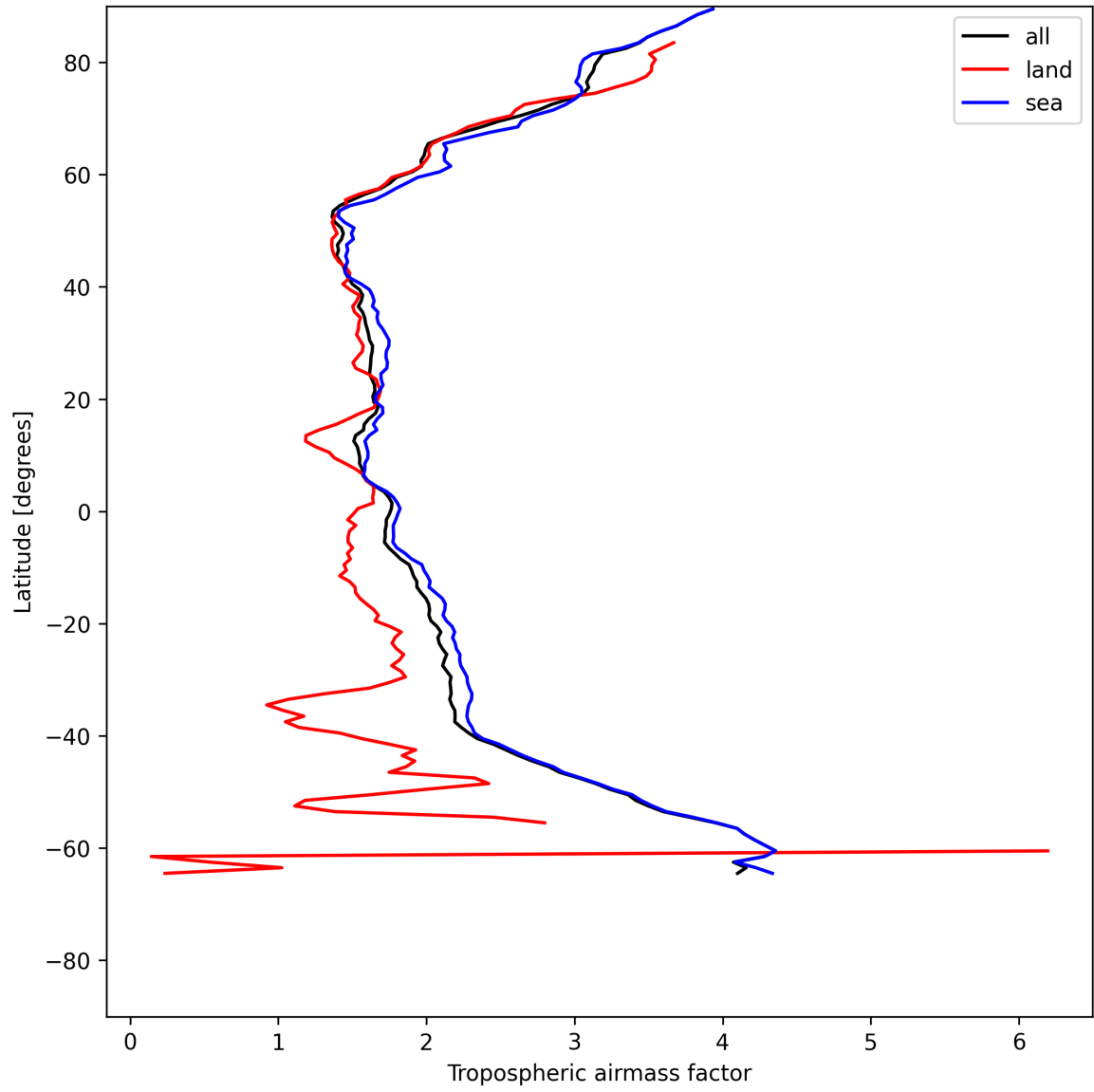
Figure 14: Zonal average of “Tropospheric airmass factor” for 2025-06-27 to 2025-06-29.
