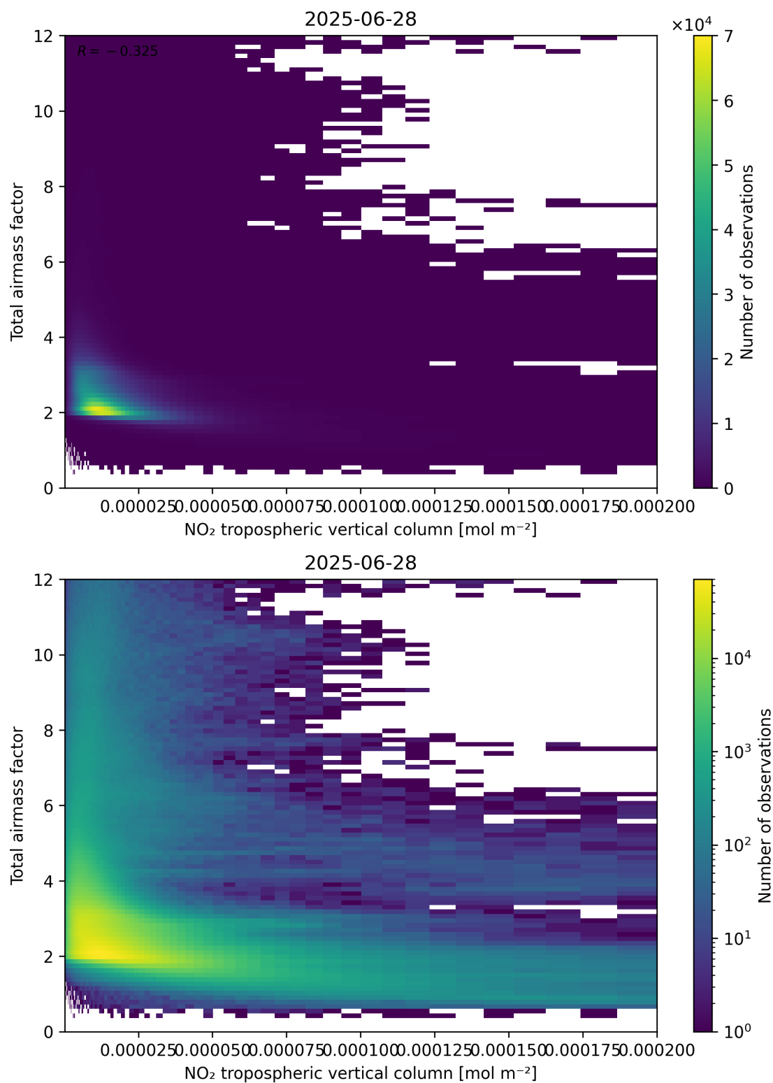
Figure 122: Scatter density plot of “NO 2 tropospheric vertical column” against “Total air mass factor” for 2025-06-27 to 2025-06-29.
