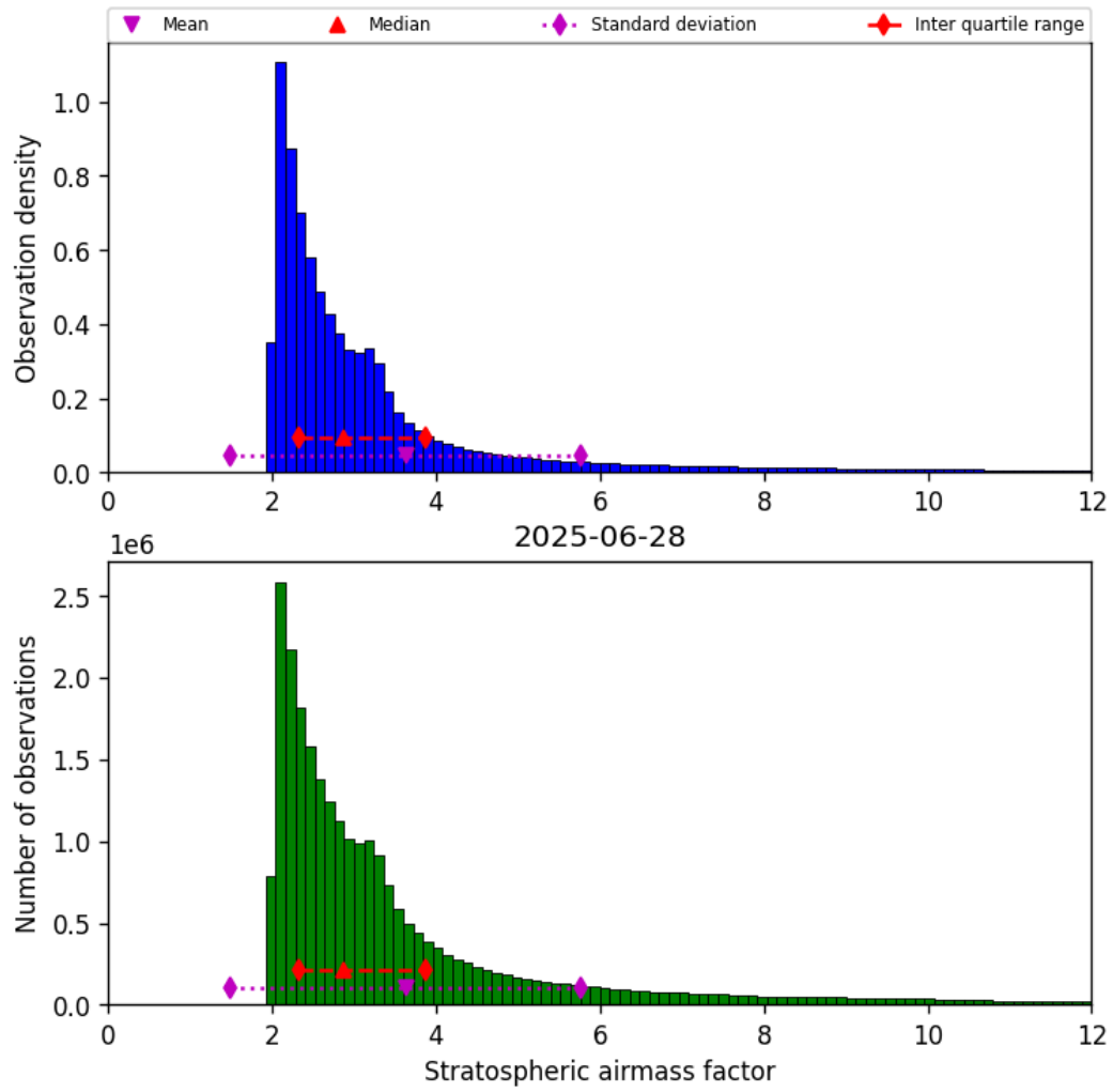
Figure 44: Histogram of “Stratospheric airmass factor” for 2025-06-27 to 2025-06-29
