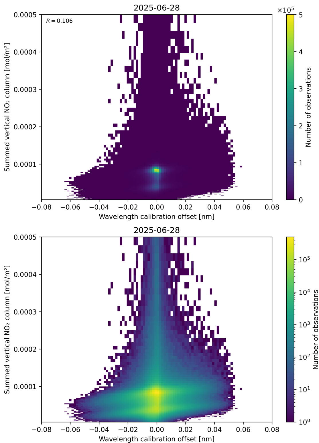
Figure 177: Scatter density plot of “Wavelength calibration offset” against “Summed vertical NO 2 column” for 2025-06-27 to 2025-06-29.
