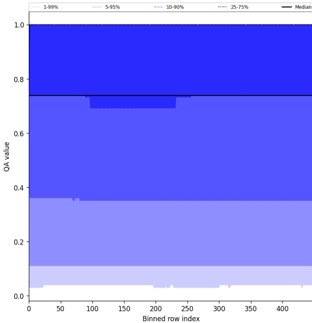
Figure 45: Along track statistics of “QA value” for 2025-06-27 to 2025-06-29
