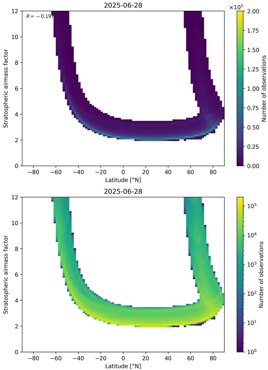
Figure 83: Scatter density plot of “Latitude” against “Stratospheric air mass factor” for 2025-06-27 to 2025-06-29.
