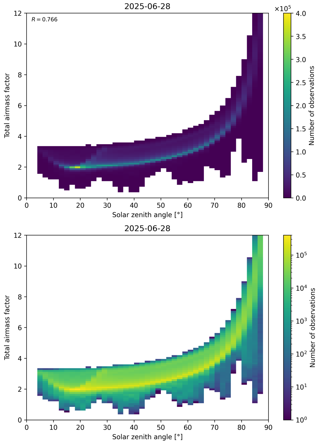
Figure 146: Scatter density plot of “Solar zenith angle” against “Total air mass factor” for 2025-06-27 to 2025-06-29.
