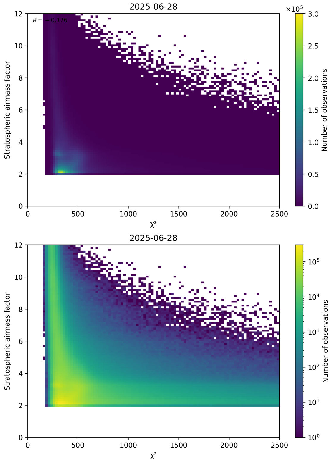
Figure 81: Scatter density plot of “ \chi^2 ” against “Stratospheric airmass factor” for 2025-06-27 to 2025-06-29.
