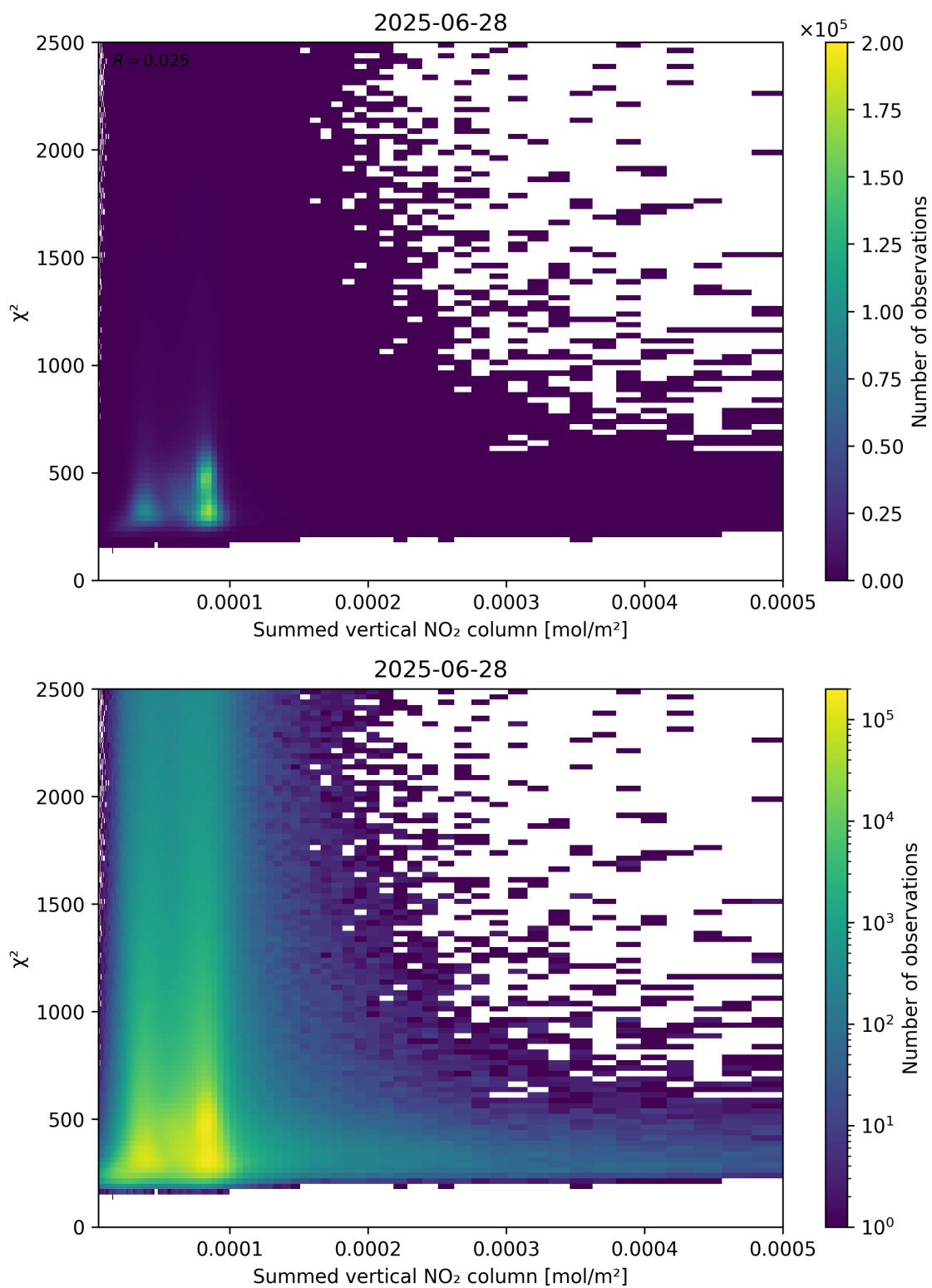
Figure 104: Scatter density plot of “Summed vertical NO 2 column” against “ \chi^2 ” for 2025-06-27 to 2025-06-29.
