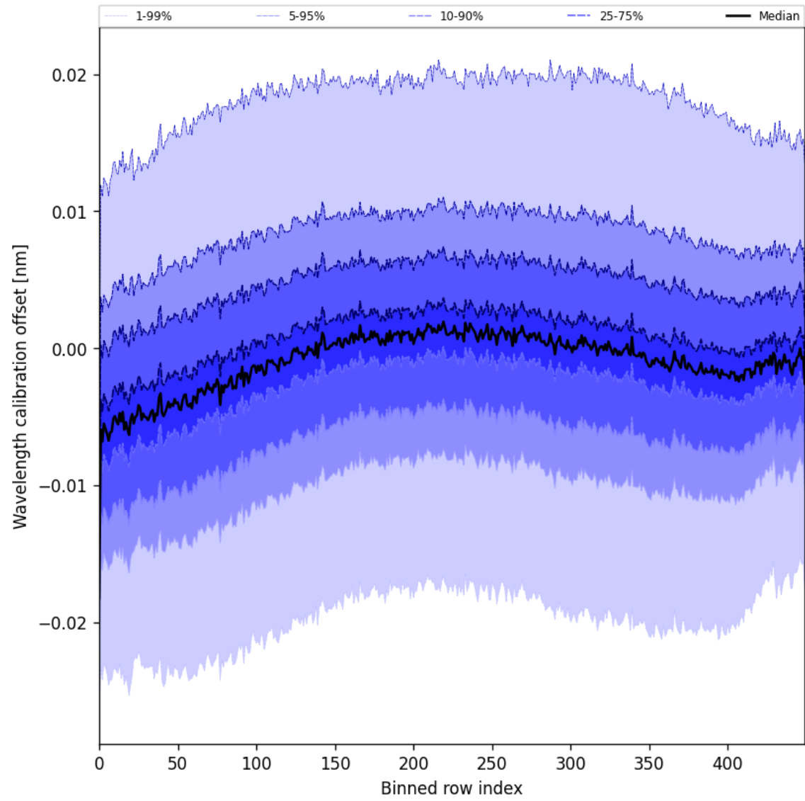
Figure 52: Along track statistics of “Wavelength calibration offset” for 2025-06-27 to 2025-06-29
