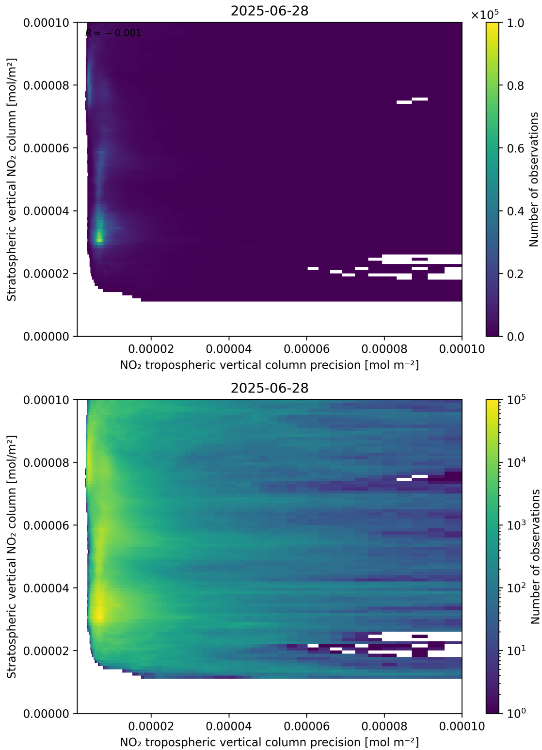
Figure 135: Scatter density plot of “NO 2 tropospheric vertical column precision” against “Stratospheric vertical NO 2 column” for 2025-06-27 to 2025-06-29.
