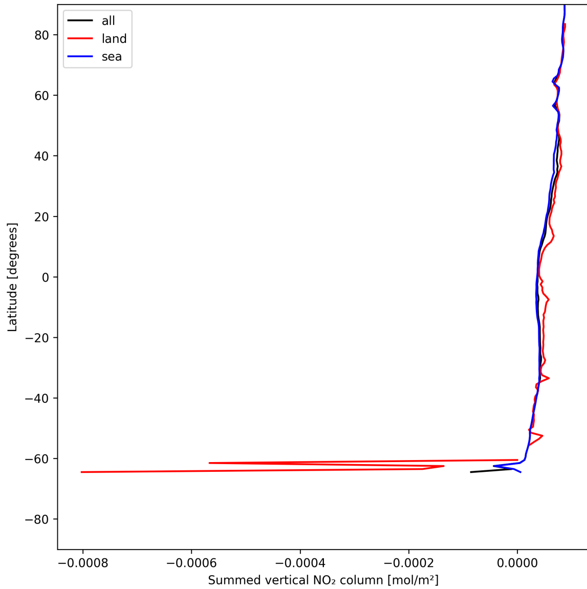
Figure 23: Zonal average of “Summed vertical NO 2 column” for 2025-06-27 to 2025-06-29.
