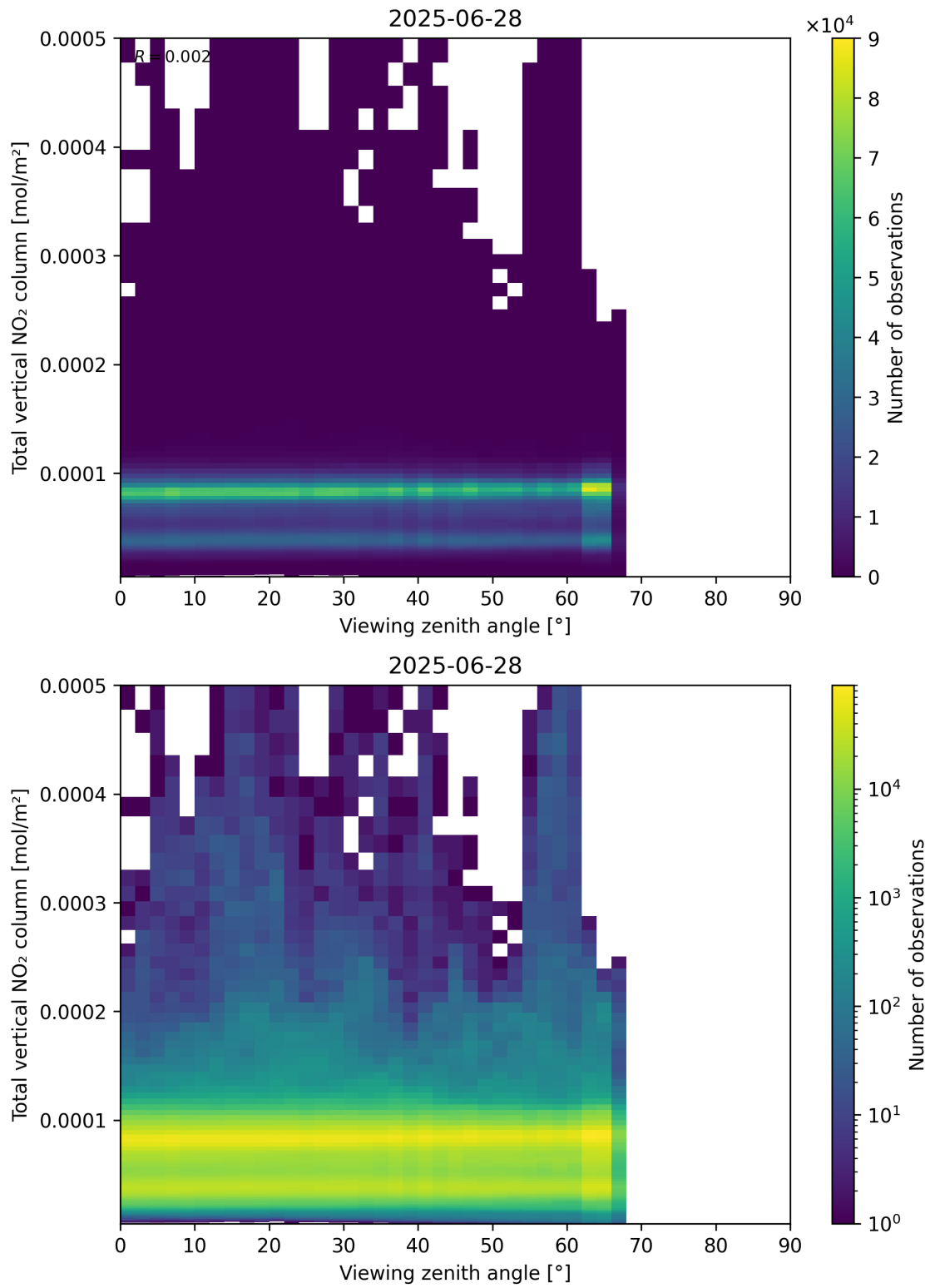
Figure 167: Scatter density plot of “Viewing zenith angle” against “Total vertical NO 2 column” for 2025-06-27 to 2025-06-29.
