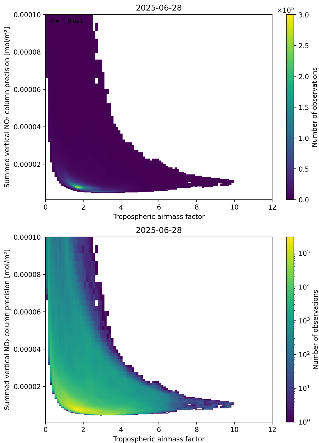
Figure 76: Scatter density plot of “Tropospheric airmass factor” against “Summed vertical NO 2 column precision” for 2025-06-27 to 2025-06-29.
