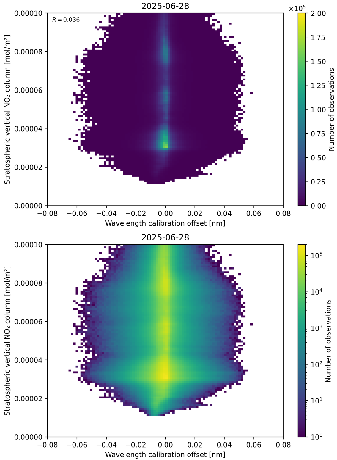
Figure 176: Scatter density plot of “Wavelength calibration offset” against “Stratospheric vertical NO 2 column” for 2025-06-27 to 2025-06-29.
