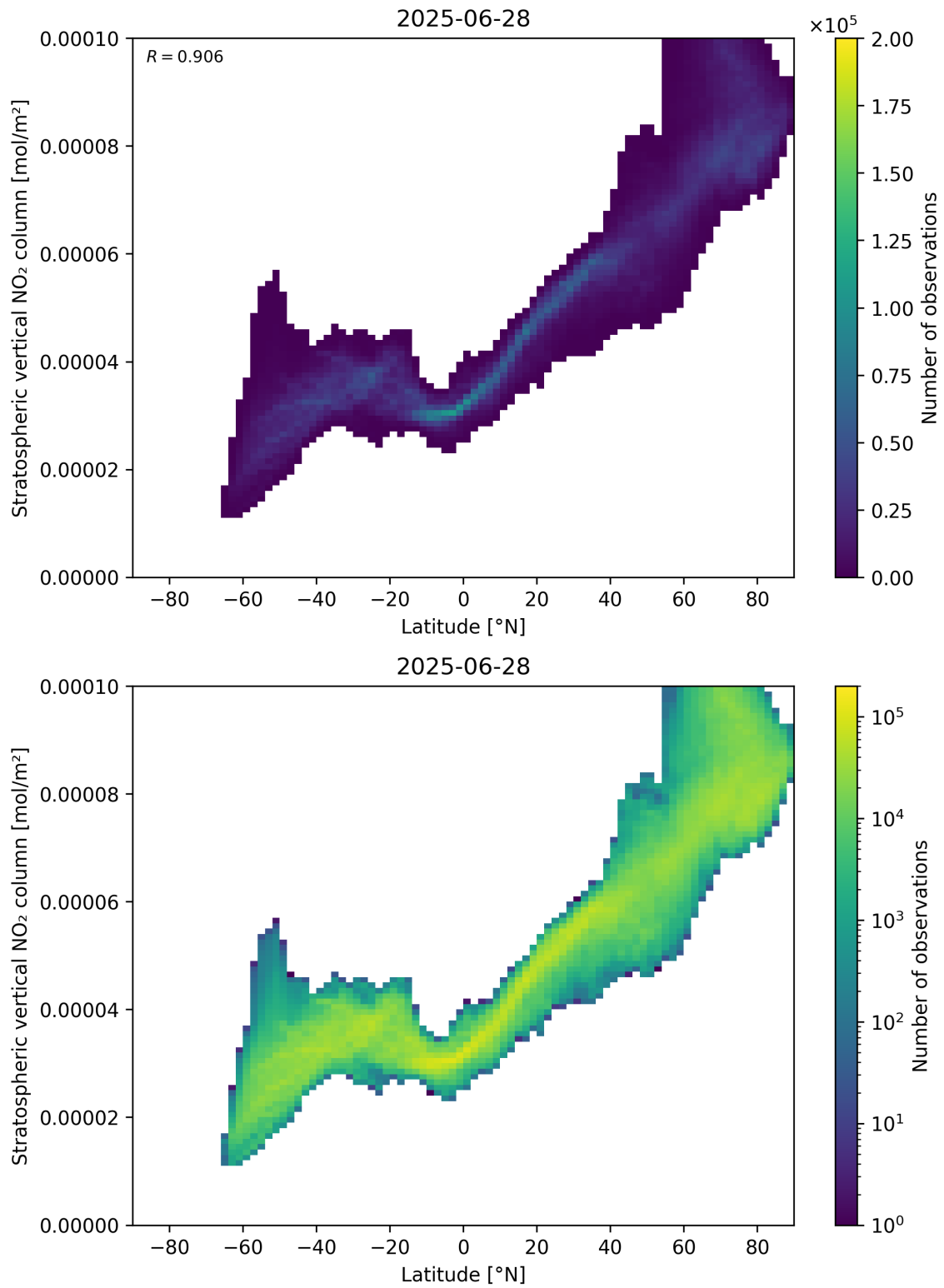
Figure 87: Scatter density plot of “Latitude” against “Stratospheric vertical \text{NO}_2 column” for 2025-06-27 to 2025-06-29.
