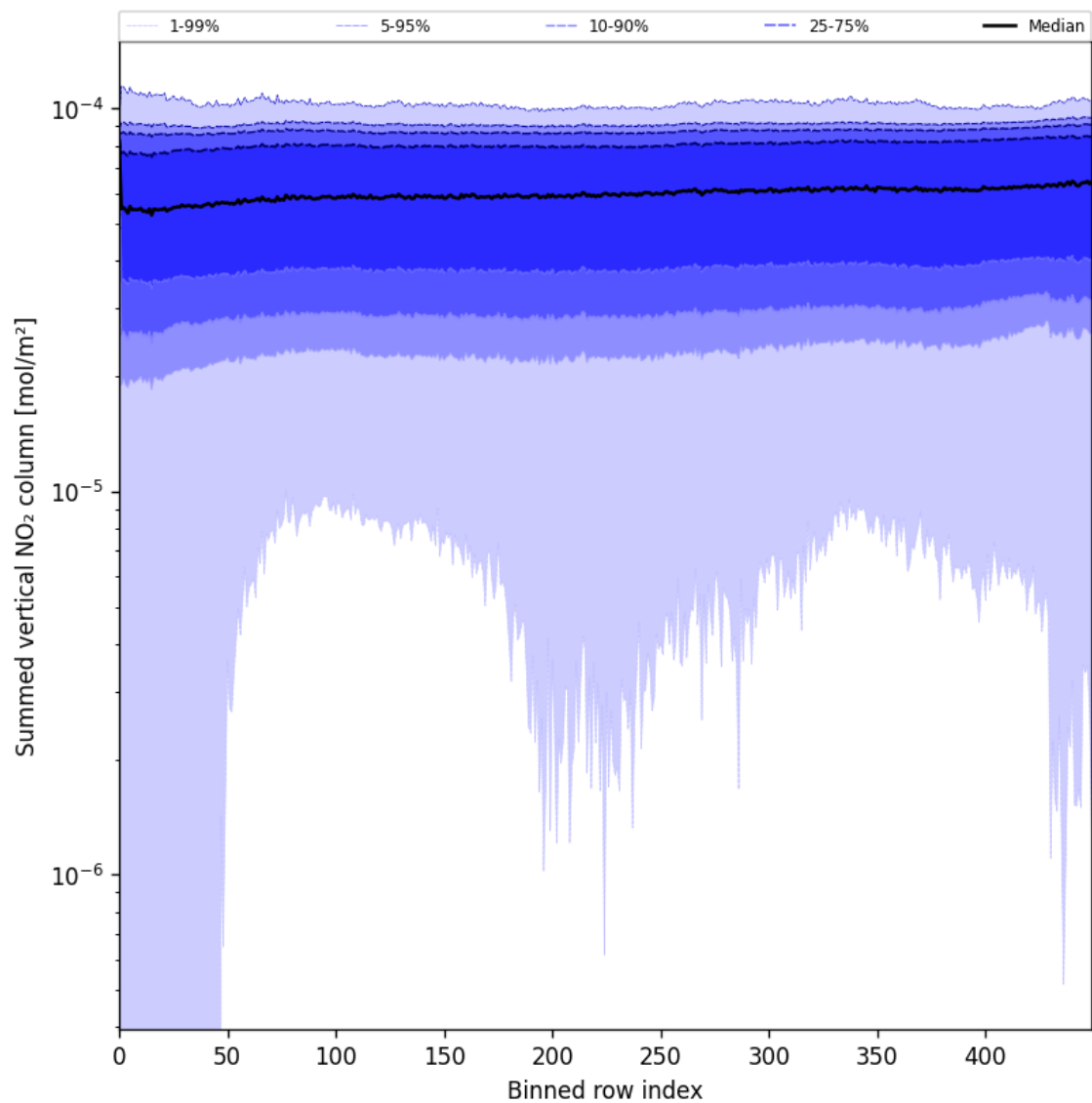
Figure 57: Along track statistics of “Summed vertical NO 2 column” for 2025-06-27 to 2025-06-29
