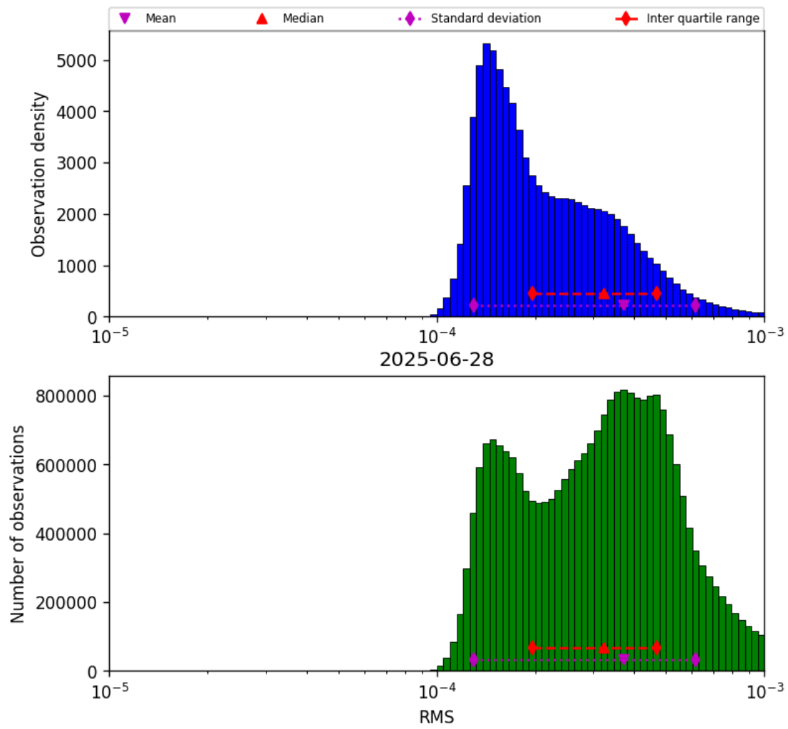
Figure 43: Histogram of “RMS” for 2025-06-27 to 2025-06-29
