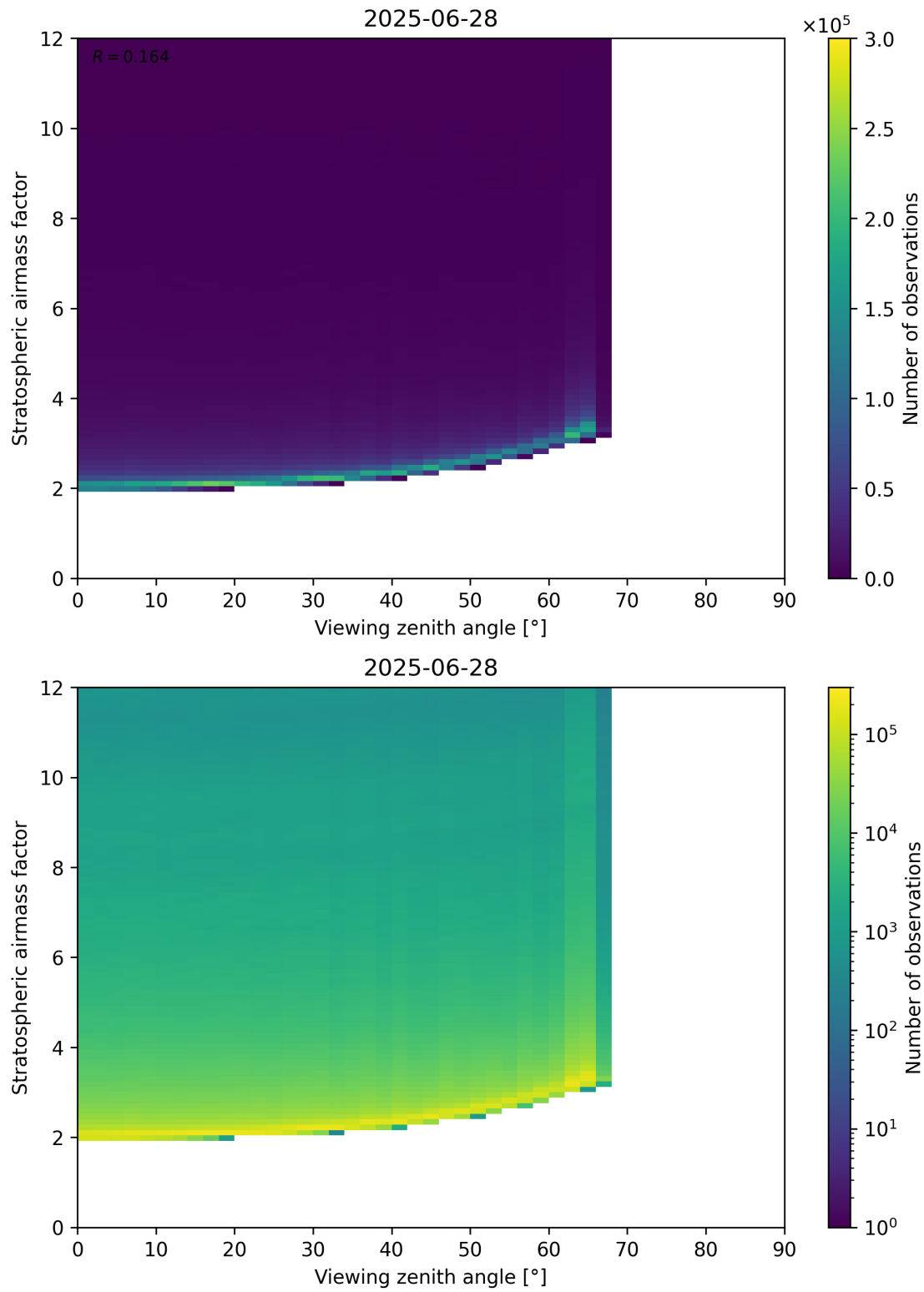
Figure 159: Scatter density plot of “Viewing zenith angle” against “Stratospheric airmass factor” for 2025-06-27 to 2025-06-29.
