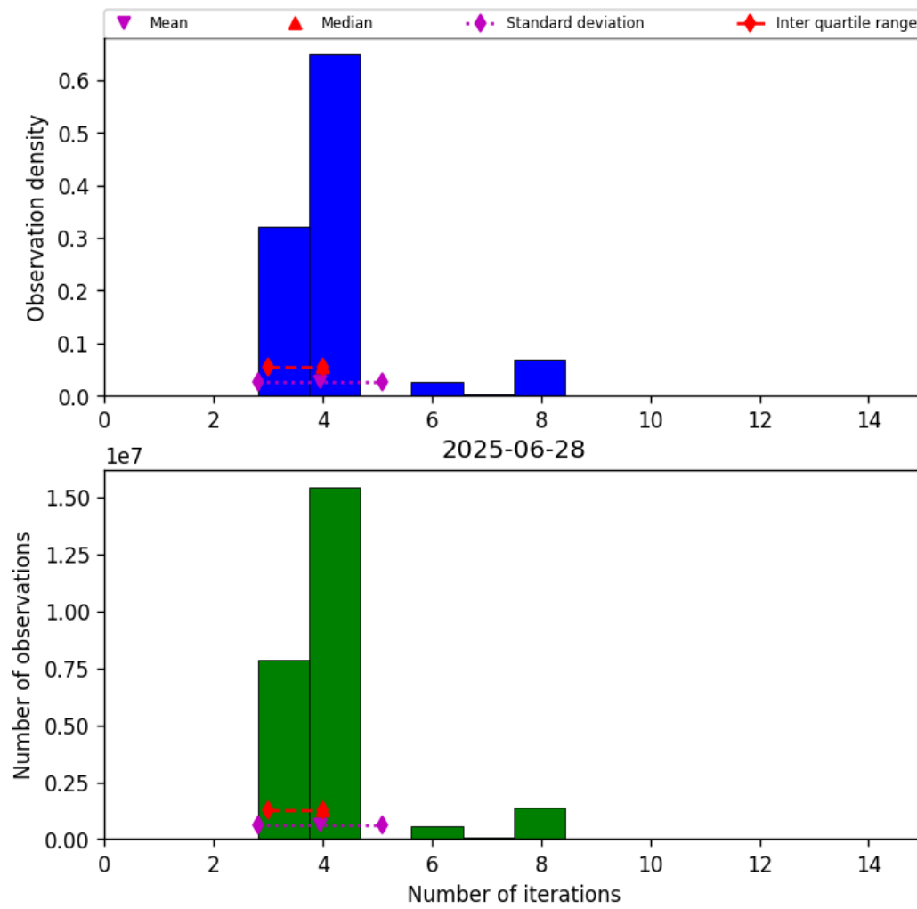
Figure 34: Histogram of “Number of iterations” for 2025-06-27 to 2025-06-29
