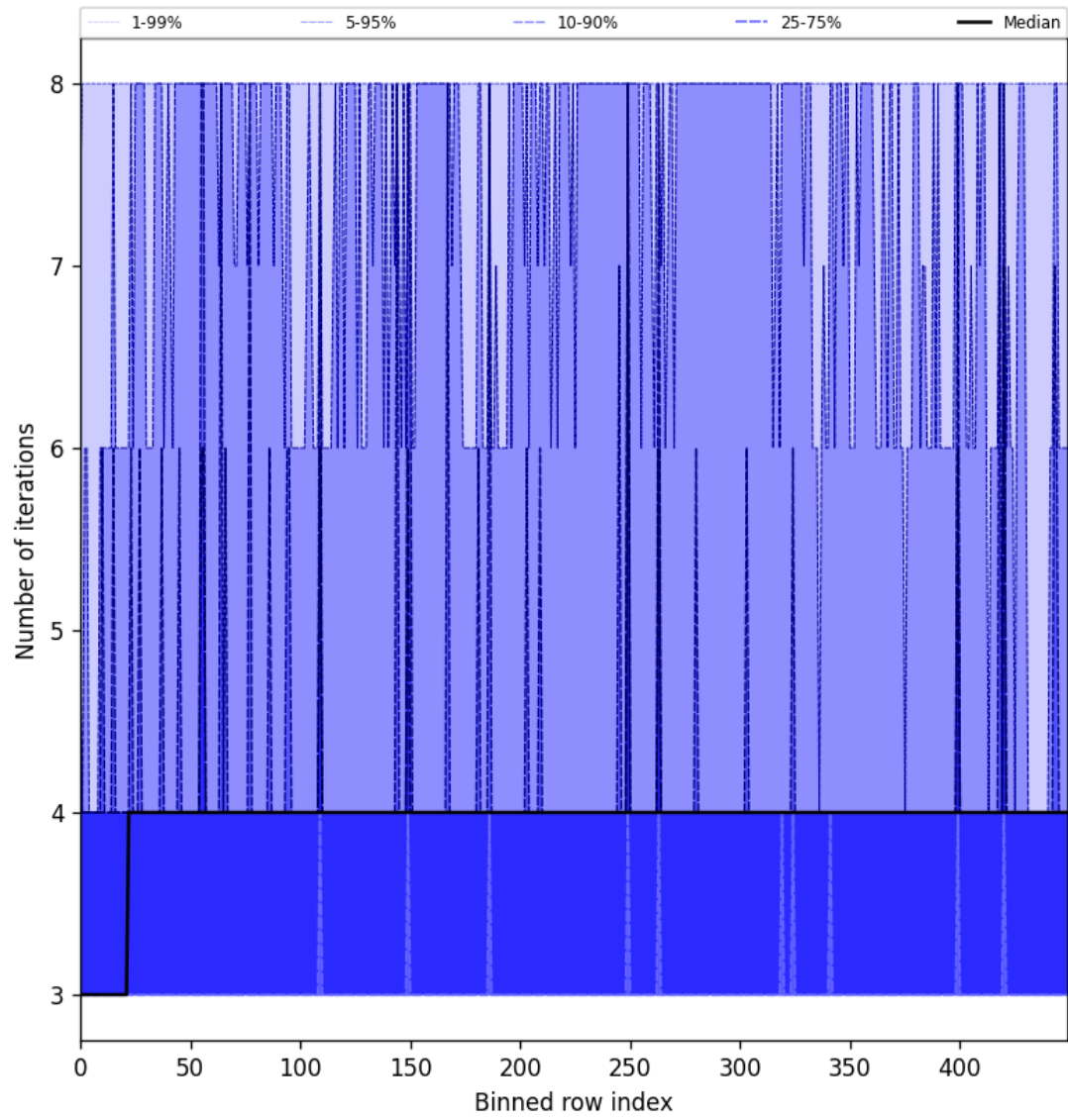
Figure 51: Along track statistics of “Number of iterations” for 2025-06-27 to 2025-06-29
