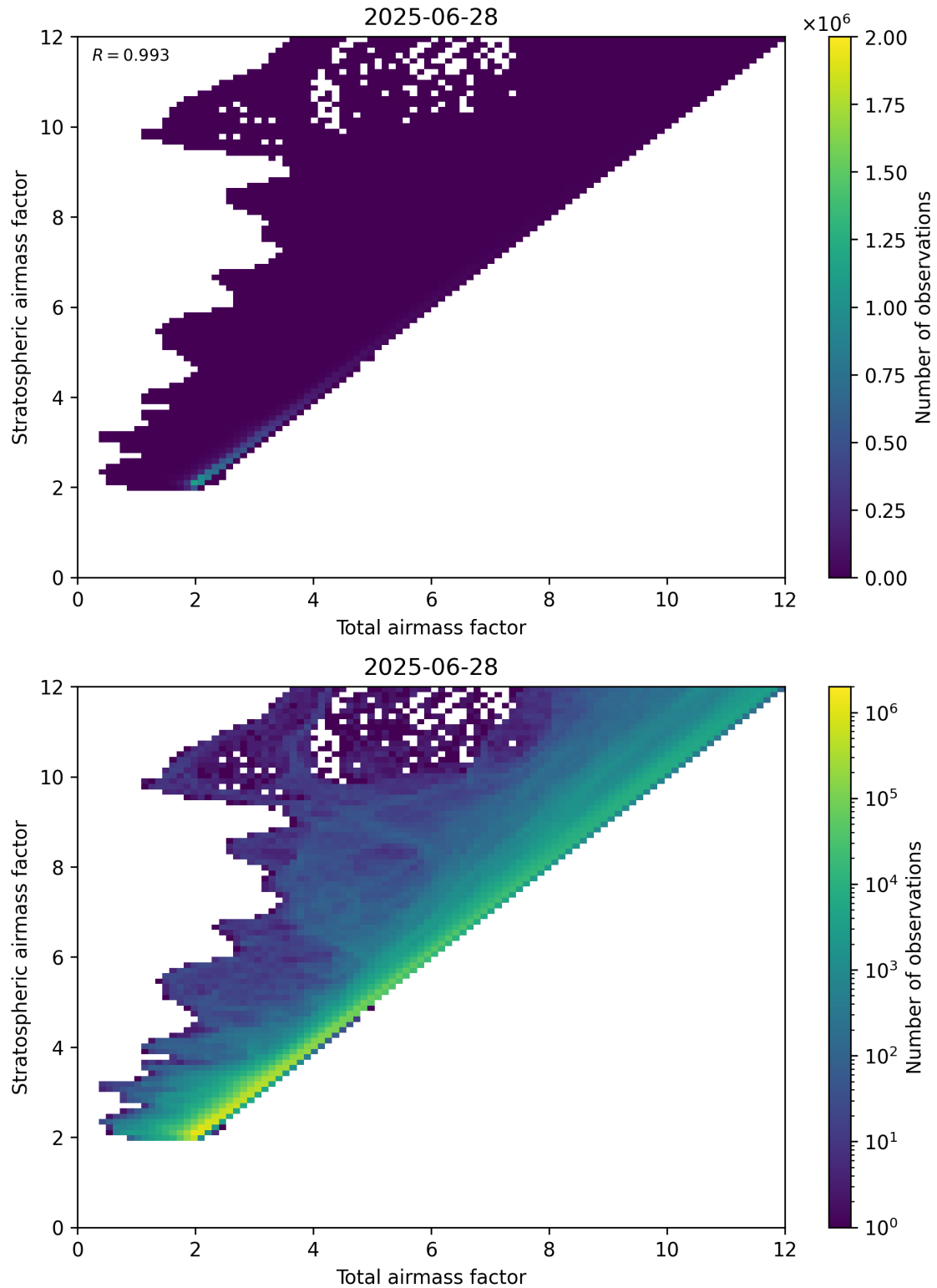
Figure 62: Scatter density plot of “Total airmass factor” against “Stratospheric airmass factor” for 2025-06-27 to 2025-06-29.
