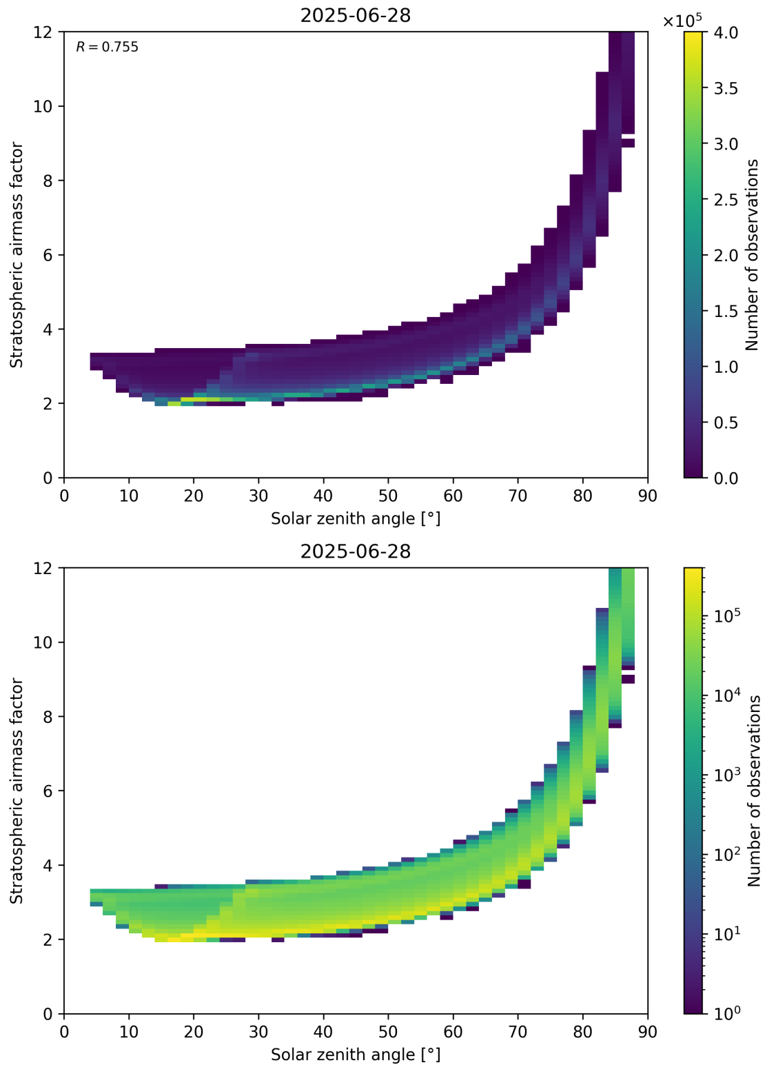
Figure 145: Scatter density plot of “Solar zenith angle” against “Stratospheric airmass factor” for 2025-06-27 to 2025-06-29.
