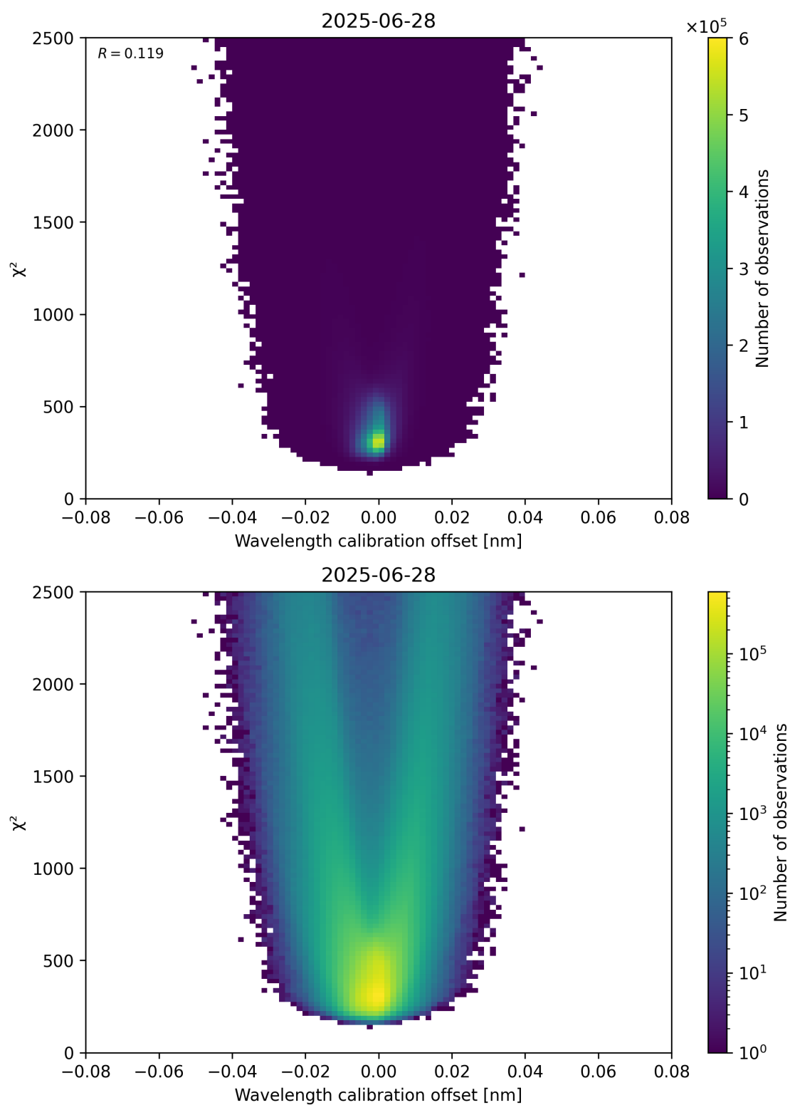
Figure 175: Scatter density plot of “Wavelength calibration offset” against “ \chi^2 ” for 2025-06-27 to 2025-06-29.
