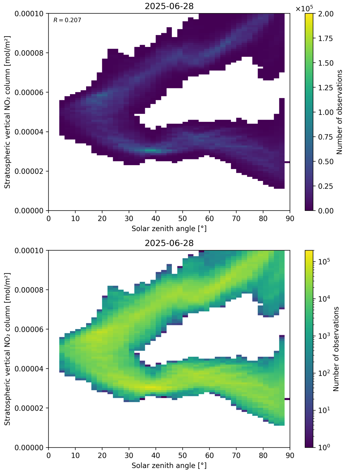
Figure 150: Scatter density plot of “Solar zenith angle” against “Stratospheric vertical NO 2 column” for 2025-06-27 to 2025-06-29.
