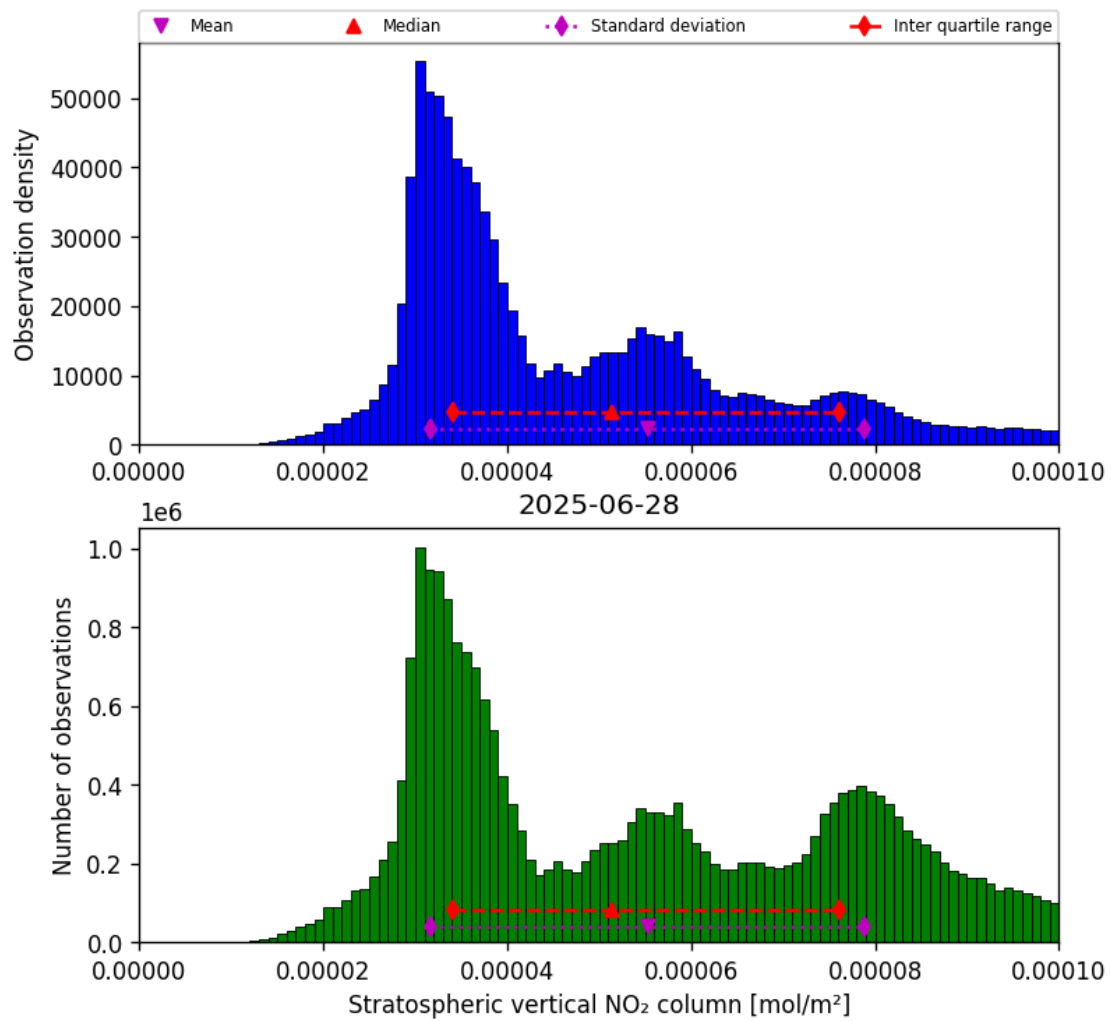
Figure 36: Histogram of “Stratospheric vertical NO 2 column” for 2025-06-27 to 2025-06-29
