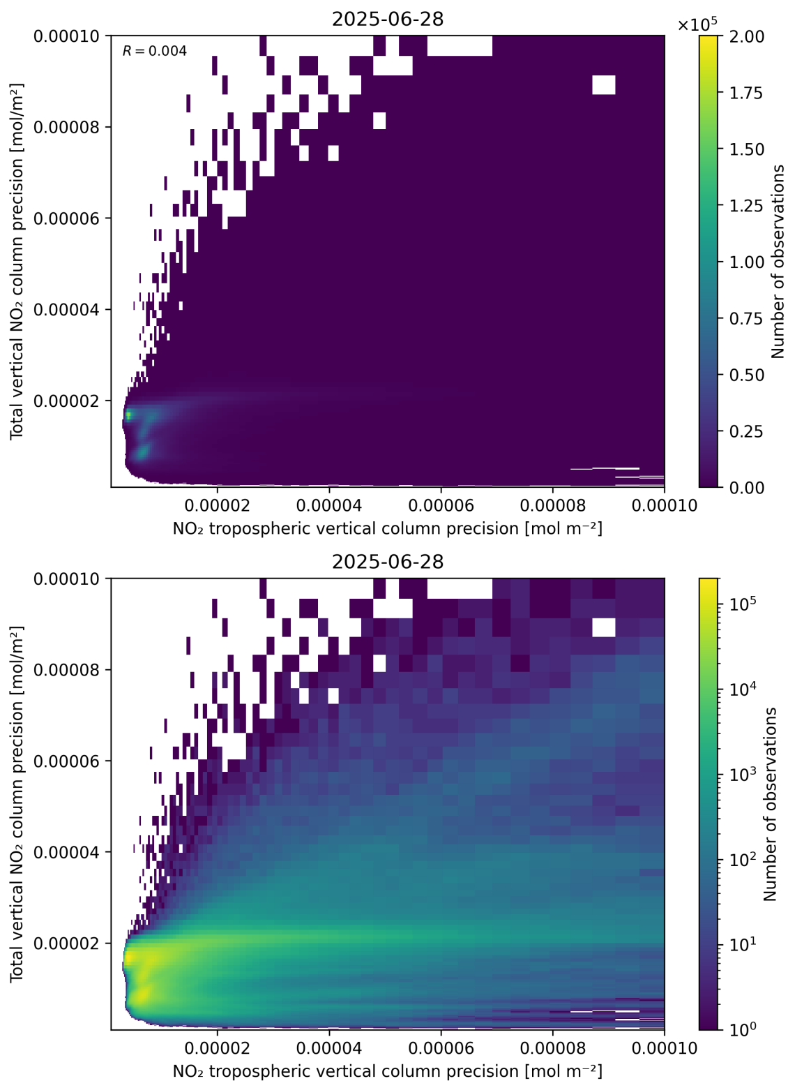
Figure 139: Scatter density plot of “NO 2 tropospheric vertical column precision” against “Total vertical NO 2 column precision” for 2025-06-27 to 2025-06-29.
