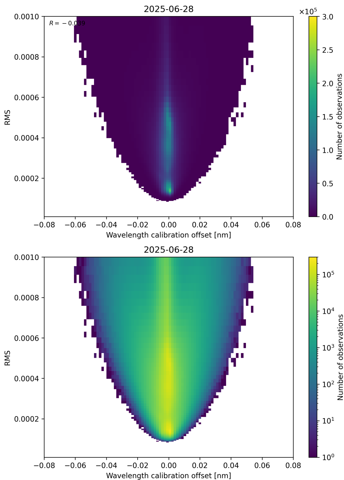
Figure 181: Scatter density plot of “Wavelength calibration offset” against “RMS” for 2025-06-27 to 2025-06-29.
