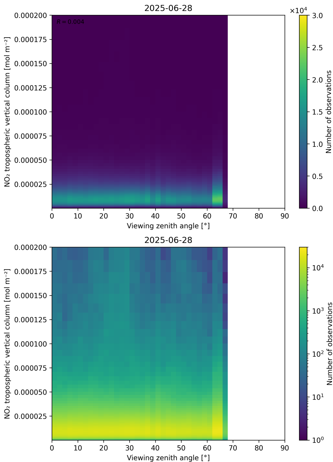
Figure 169: Scatter density plot of “Viewing zenith angle” against “NO 2 tropospheric vertical column” for 2025-06-27 to 2025-06-29.
