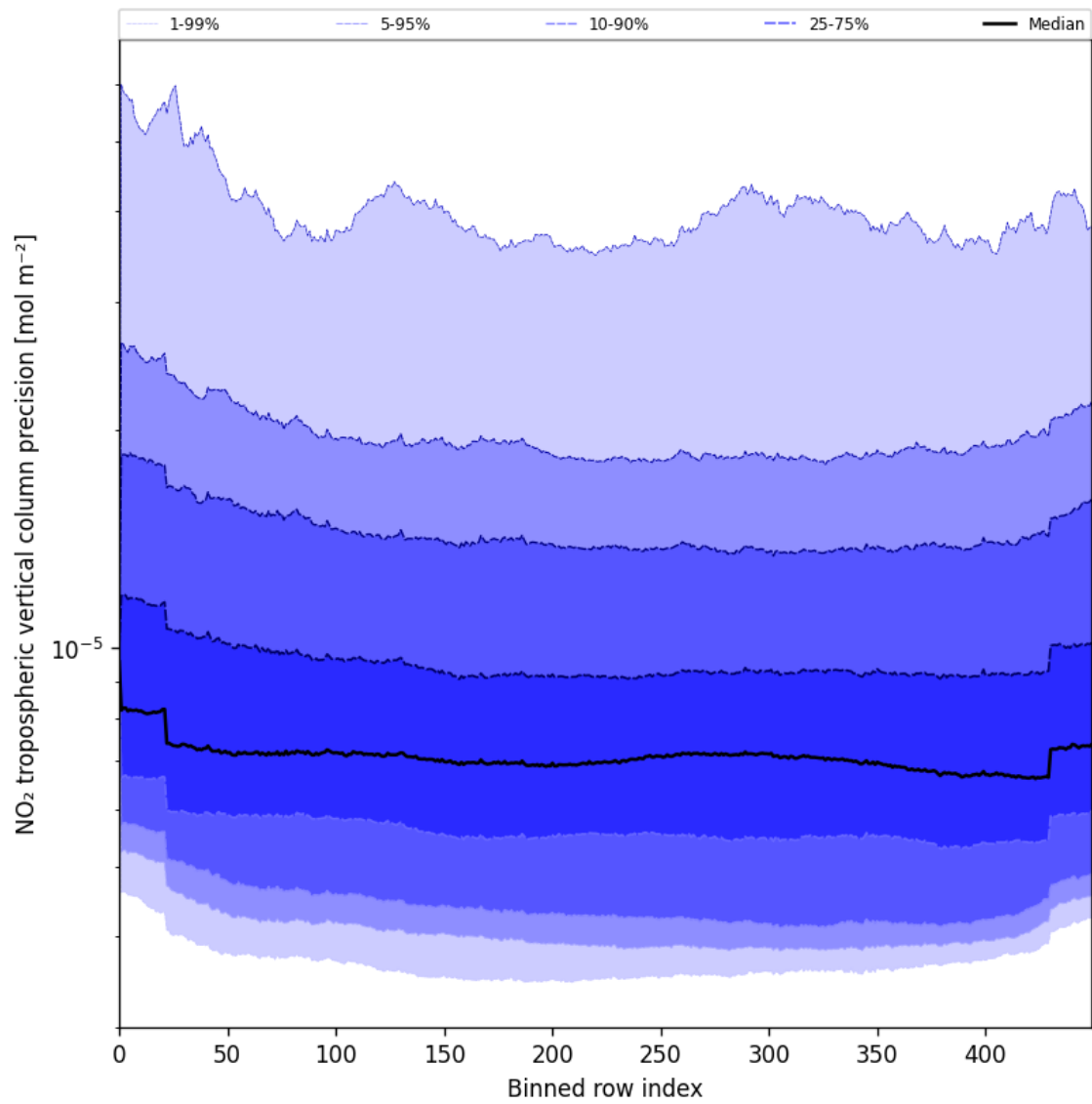
Figure 47: Along track statistics of “NO 2 tropospheric vertical column precision” for 2025-06-27 to 2025-06-29
