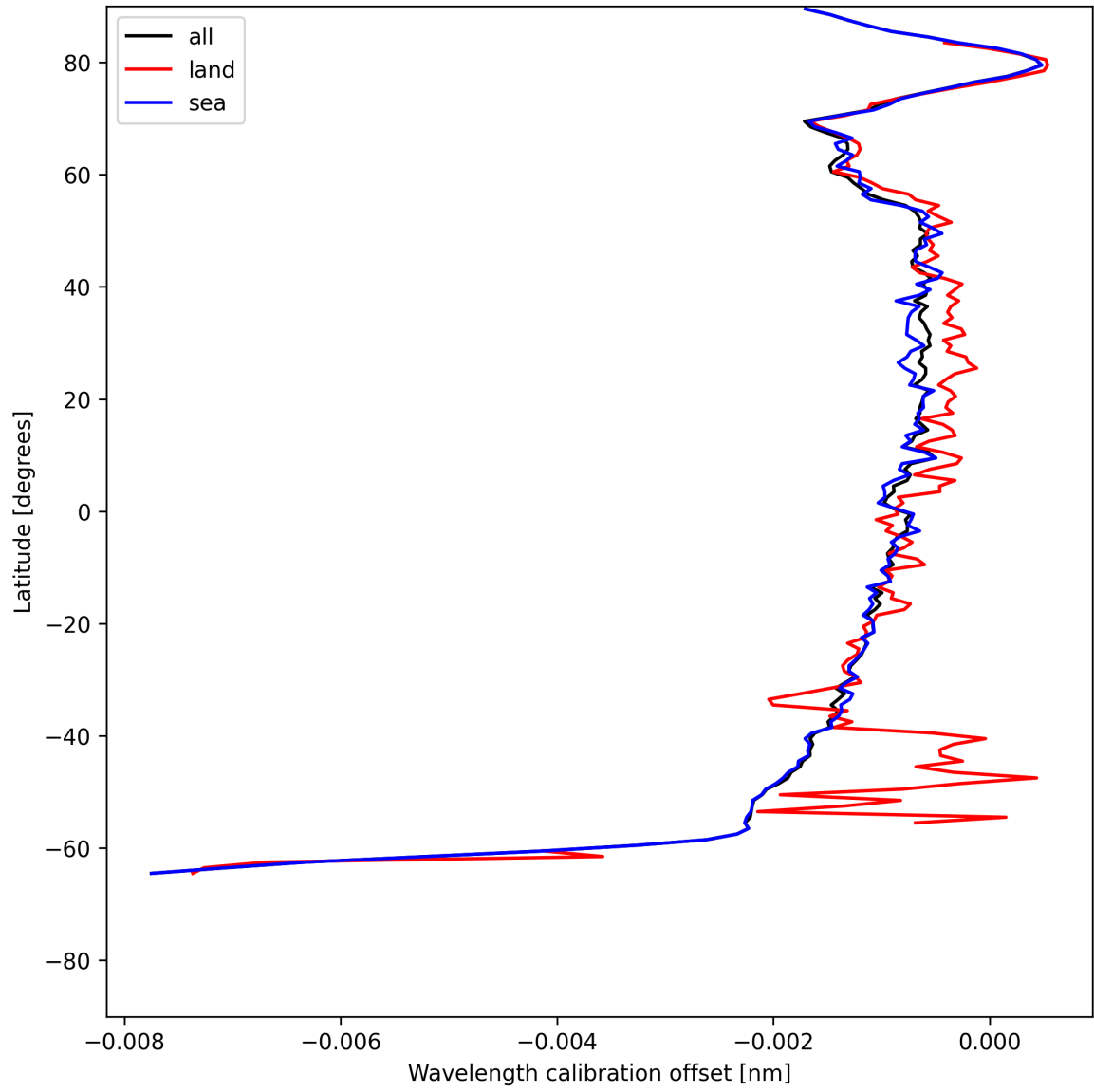
Figure 18: Zonal average of “Wavelength calibration offset” for 2025-06-27 to 2025-06-29.
