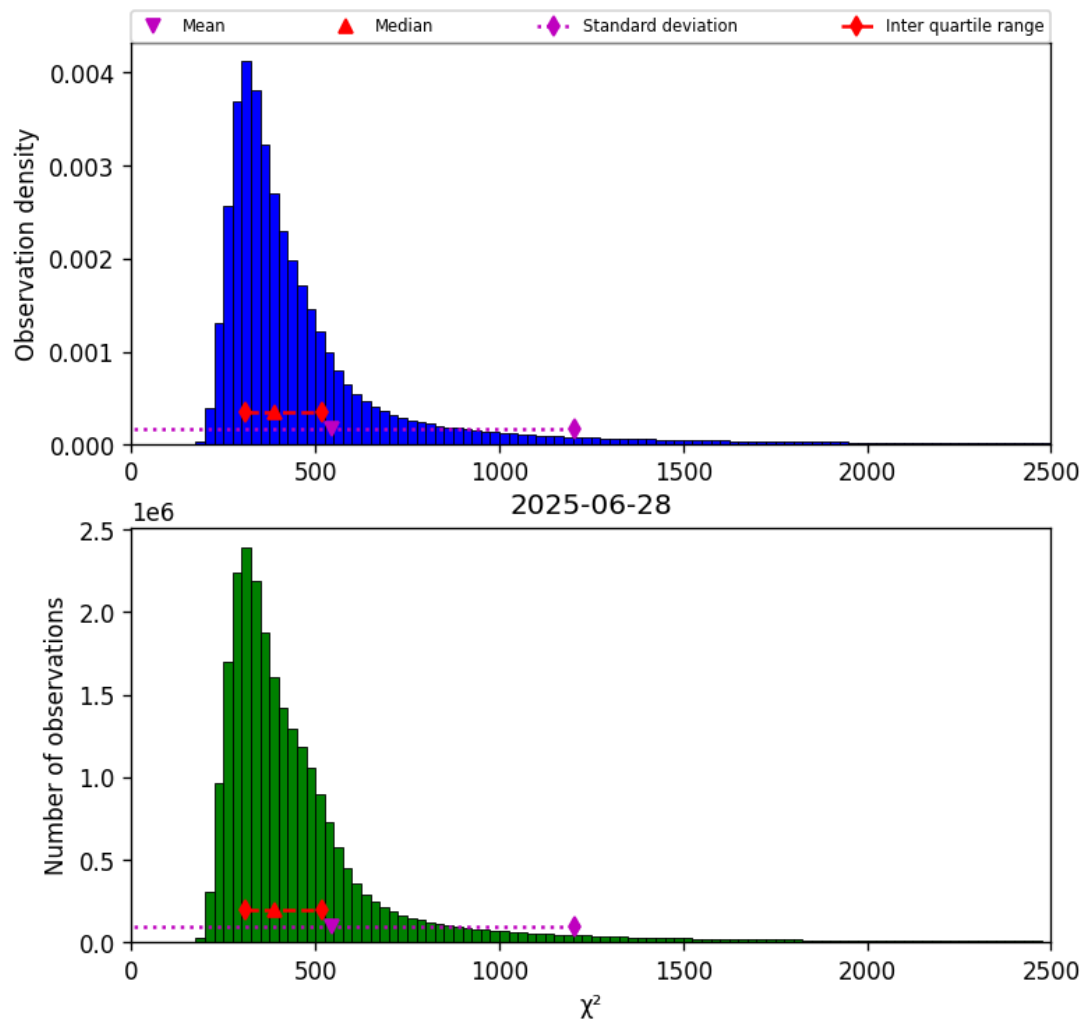
Figure 42: Histogram of “ \chi^2 ” for 2025-06-27 to 2025-06-29
