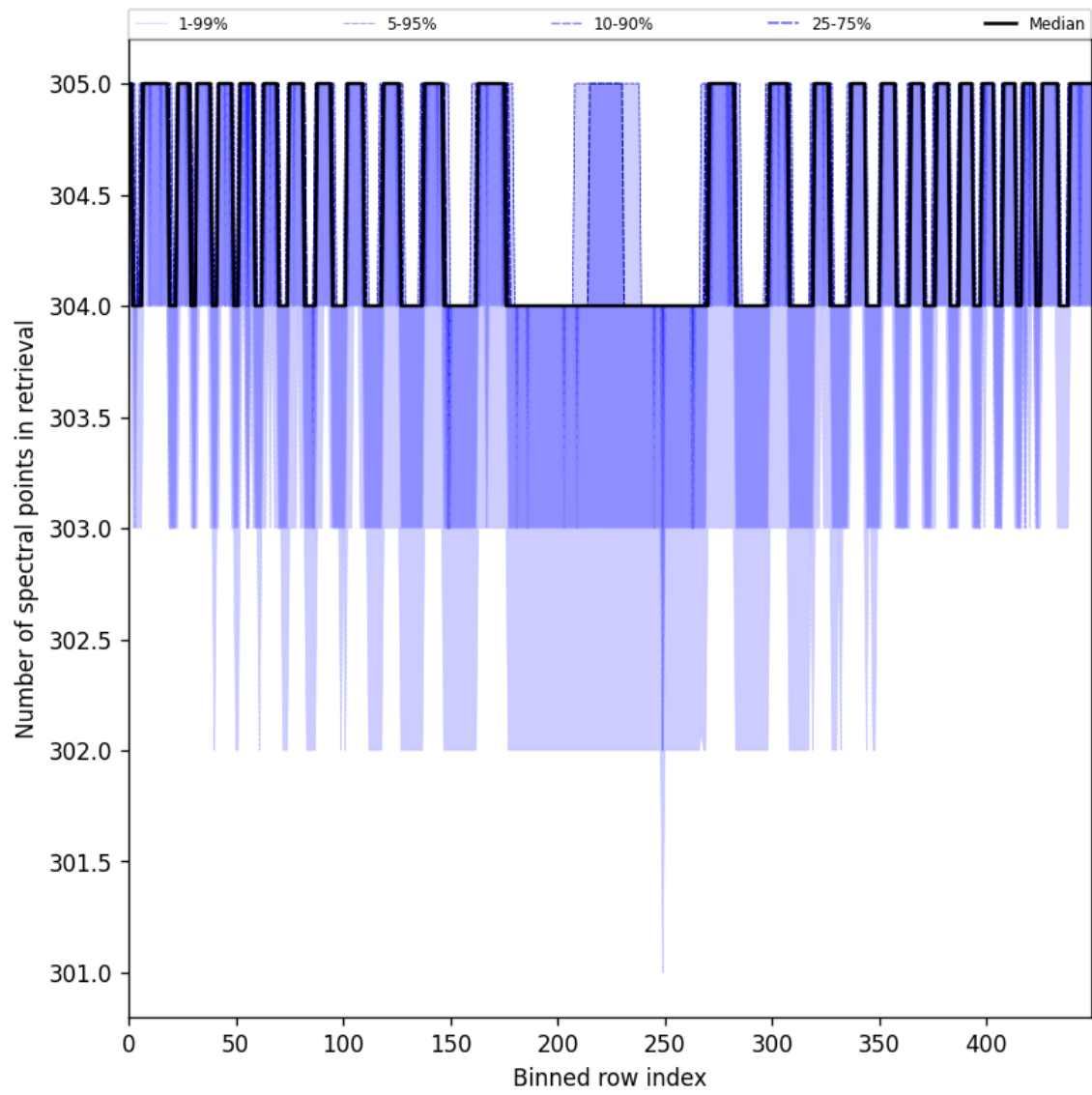
Figure 50: Along track statistics of “Number of spectral points in retrieval” for 2025-06-27 to 2025-06-29
