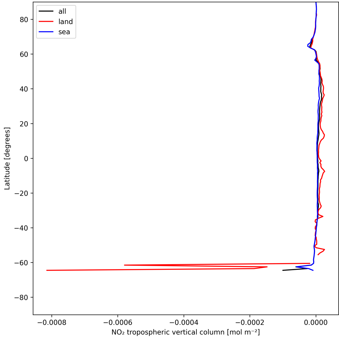
Figure 12: Zonal average of “NO 2 tropospheric vertical column” for 2025-06-27 to 2025-06-29.
