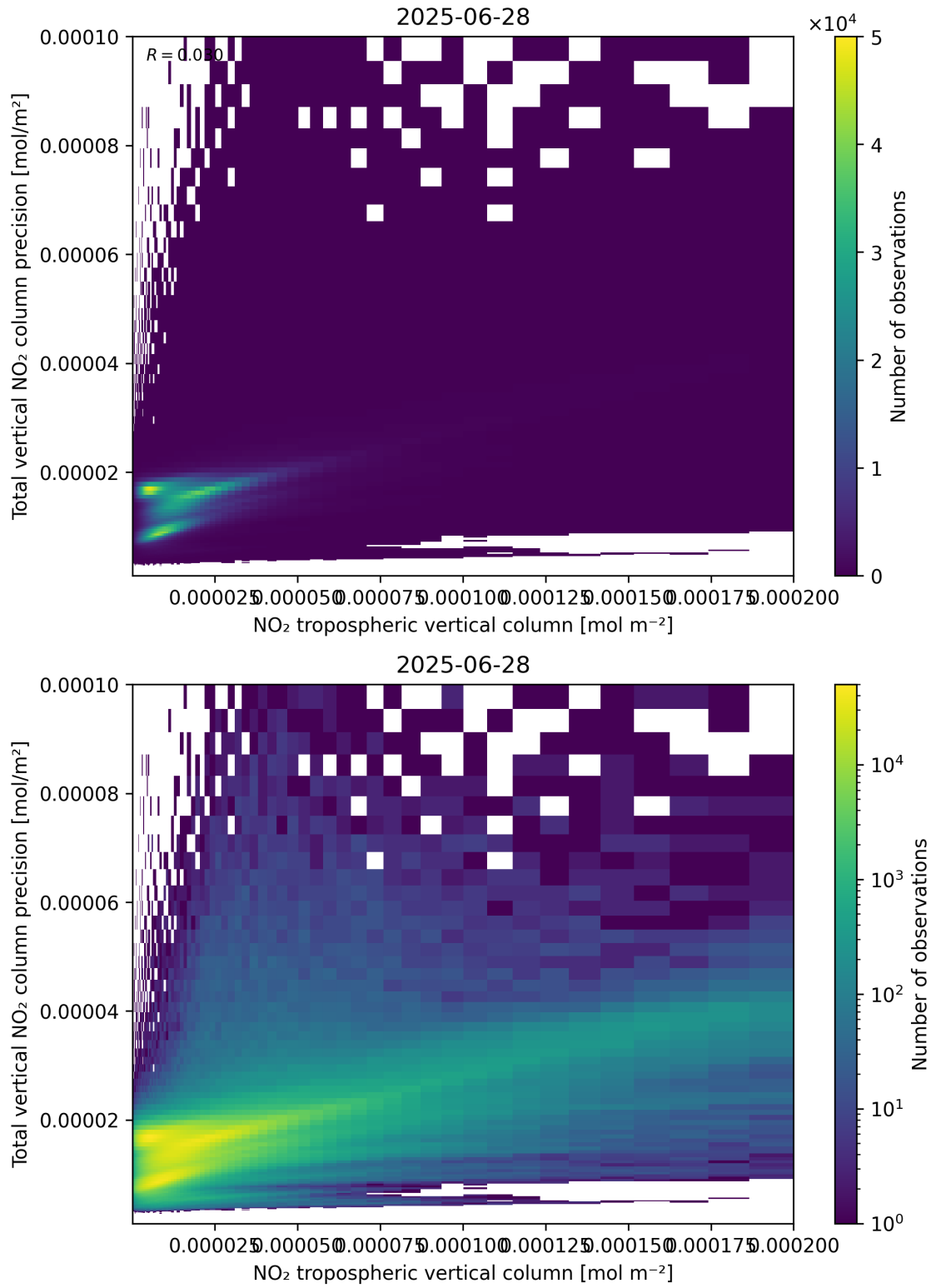
Figure 129: Scatter density plot of “NO 2 tropospheric vertical column” against “Total vertical NO 2 column precision” for 2025-06-27 to 2025-06-29.
