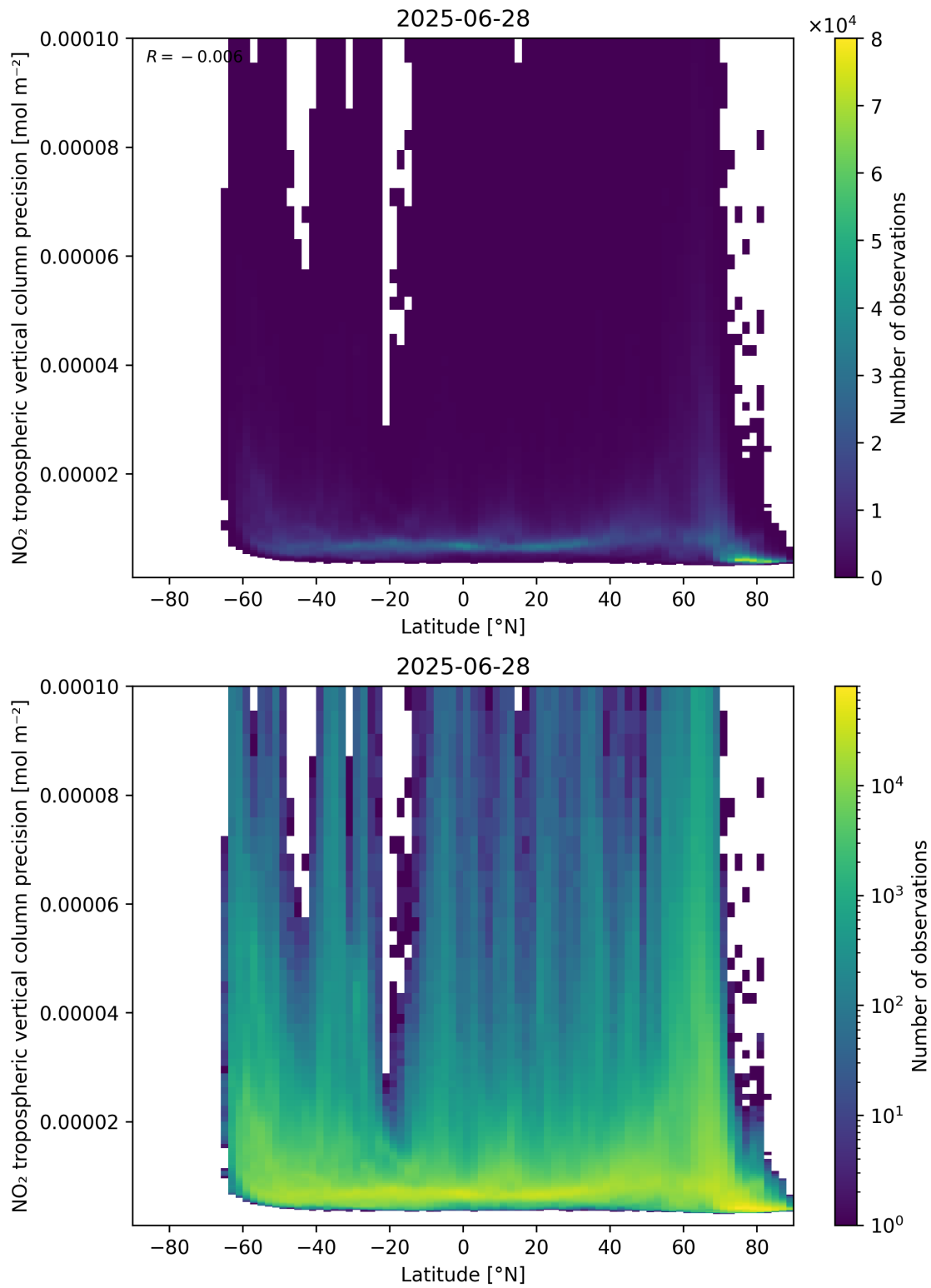
Figure 93: Scatter density plot of “Latitude” against “NO 2 tropospheric vertical column precision” for 2025-06-27 to 2025-06-29.
