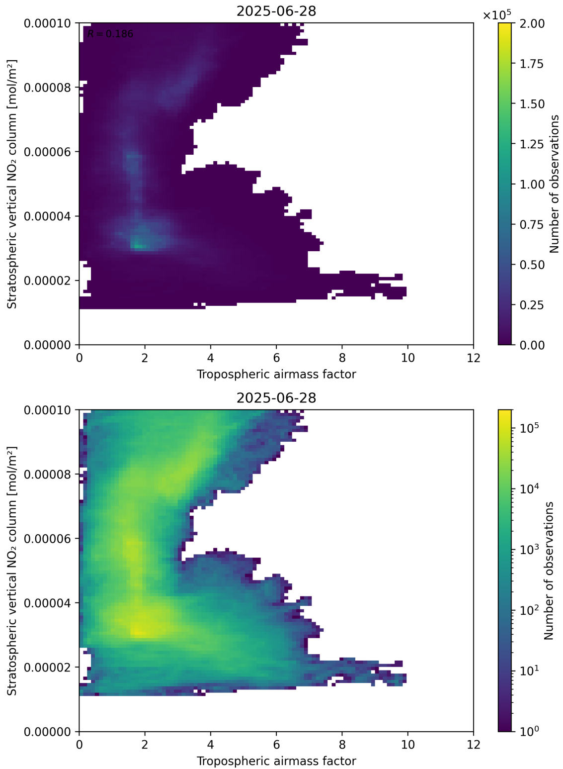
Figure 74: Scatter density plot of “Tropospheric airmass factor” against “Stratospheric vertical NO 2 column” for 2025-06-27 to 2025-06-29.
