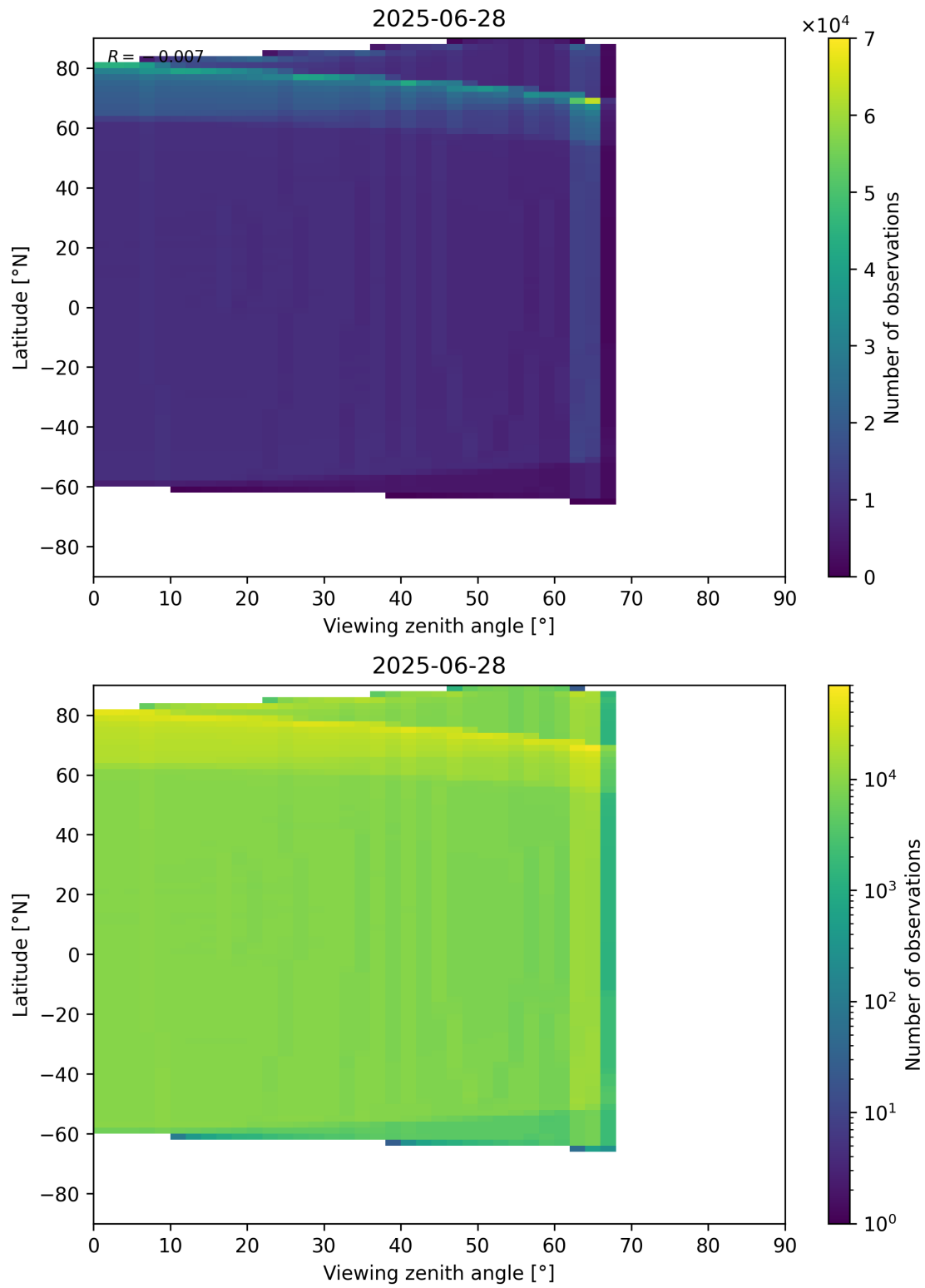
Figure 163: Scatter density plot of “Viewing zenith angle” against “Latitude” for 2025-06-27 to 2025-06-29.
