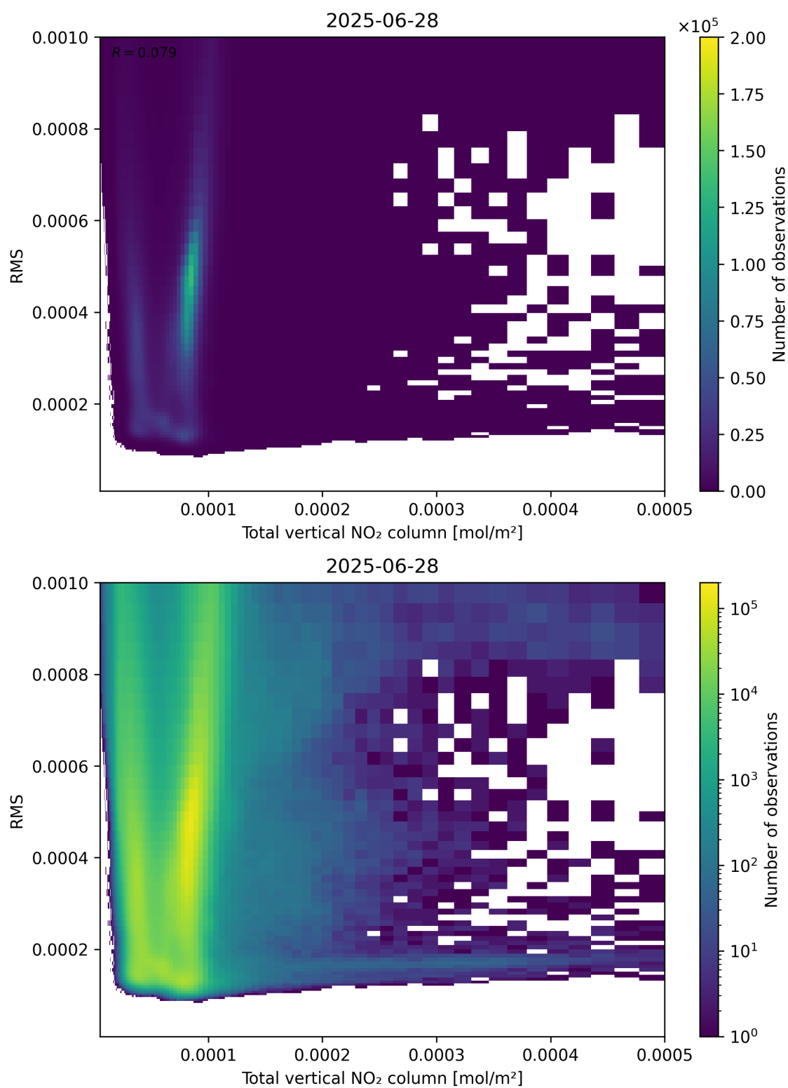
Figure 120: Scatter density plot of “Total vertical NO 2 column” against “RMS” for 2025-06-27 to 2025-06-29.
