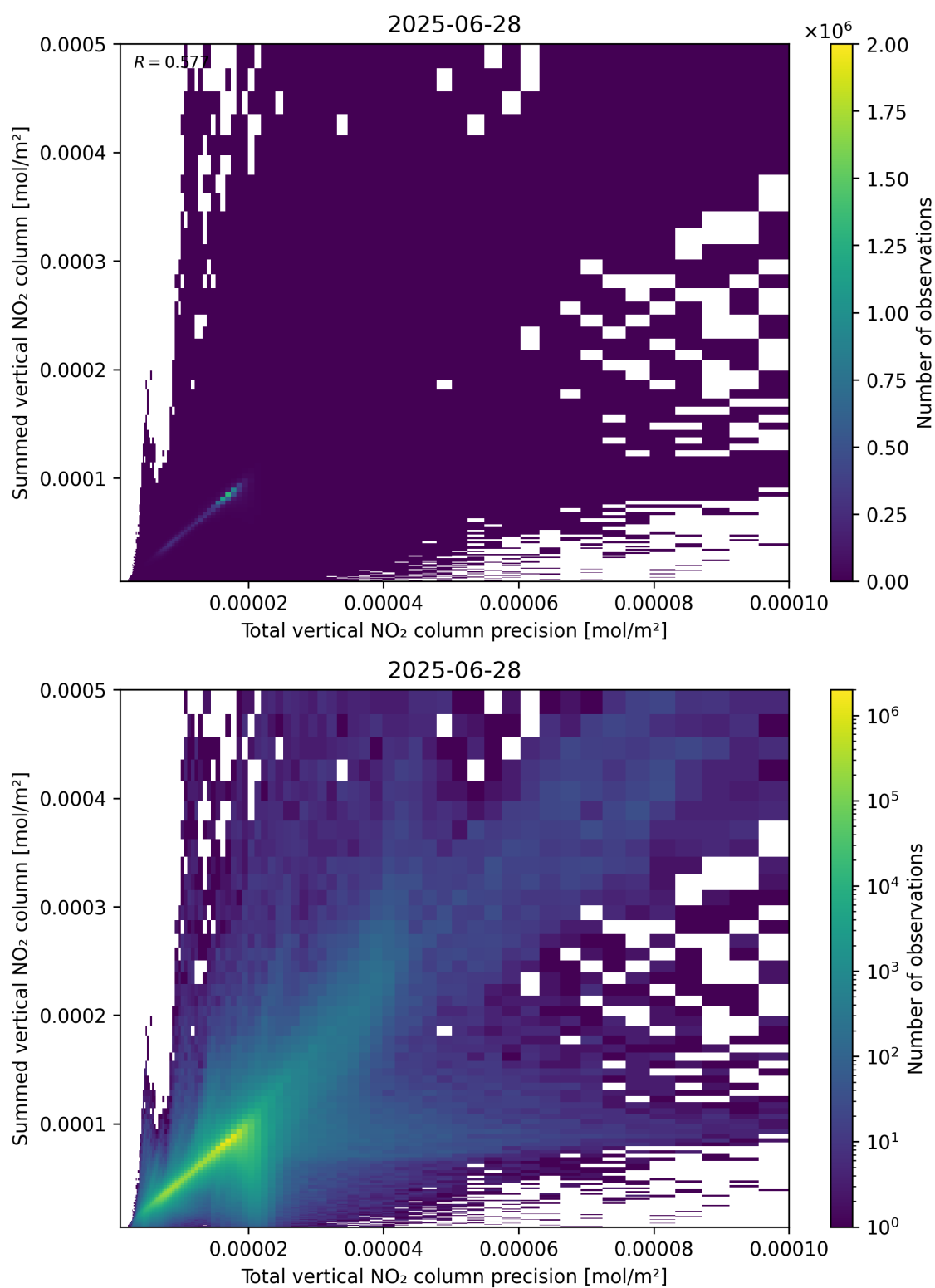
Figure 117: Scatter density plot of “Total vertical NO 2 column precision” against “Summed vertical NO 2 column” for 2025-06-27 to 2025-06-29.
