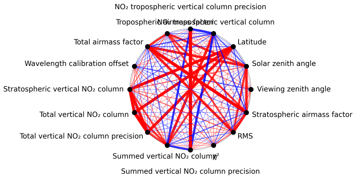
Figure 1: Map of correlation graph for 2025-06-27 to 2025-06-29.
