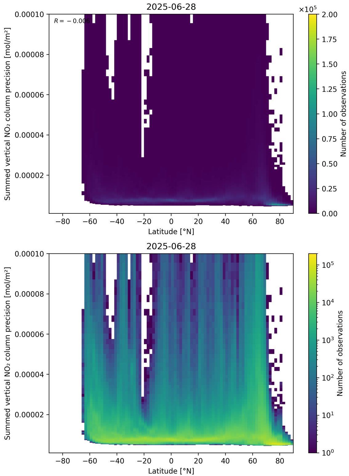
Figure 89: Scatter density plot of “Latitude” against “Summed vertical NO 2 column precision” for 2025-06-27 to 2025-06-29.
