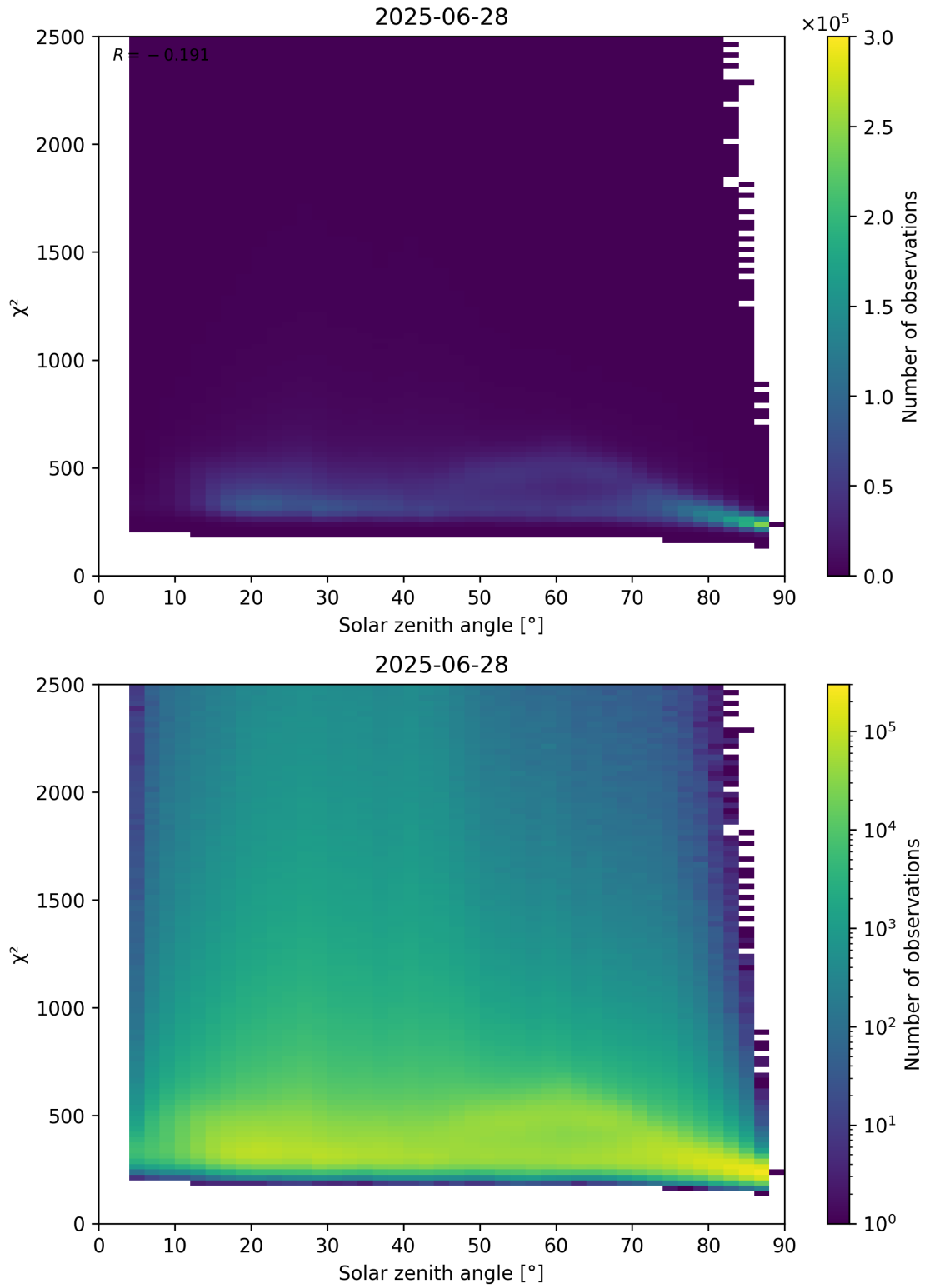
Figure 148: Scatter density plot of “Solar zenith angle” against “ \chi^2 ” for 2025-06-27 to 2025-06-29.
