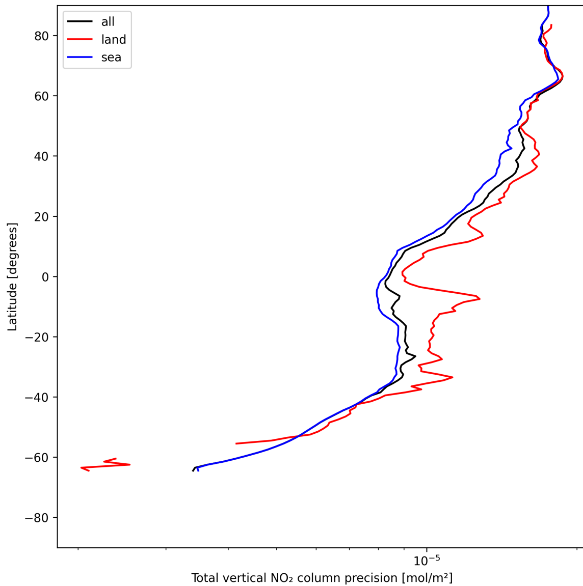
Figure 22: Zonal average of “Total vertical NO 2 column precision” for 2025-06-27 to 2025-06-29.
