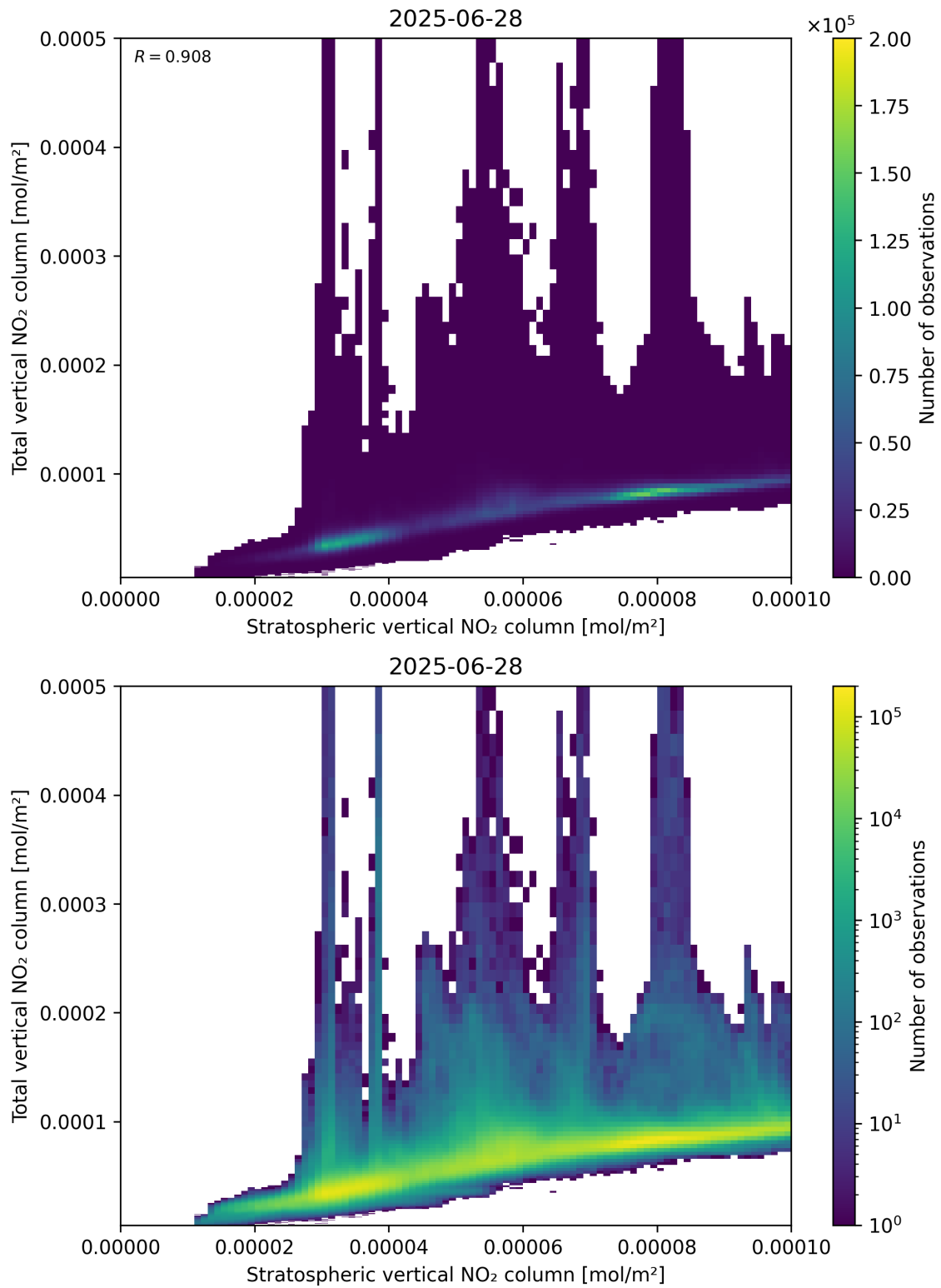
Figure 100: Scatter density plot of “Stratospheric vertical NO 2 column” against “Total vertical NO 2 column” for 2025-06-27 to 2025-06-29.
