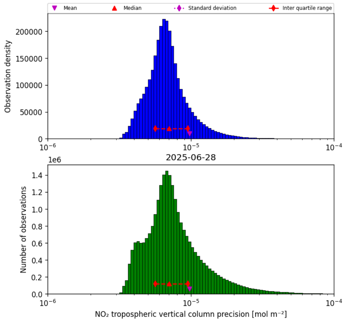
Figure 30: Histogram of “NO 2 tropospheric vertical column precision” for 2025-06-27 to 2025-06-29
