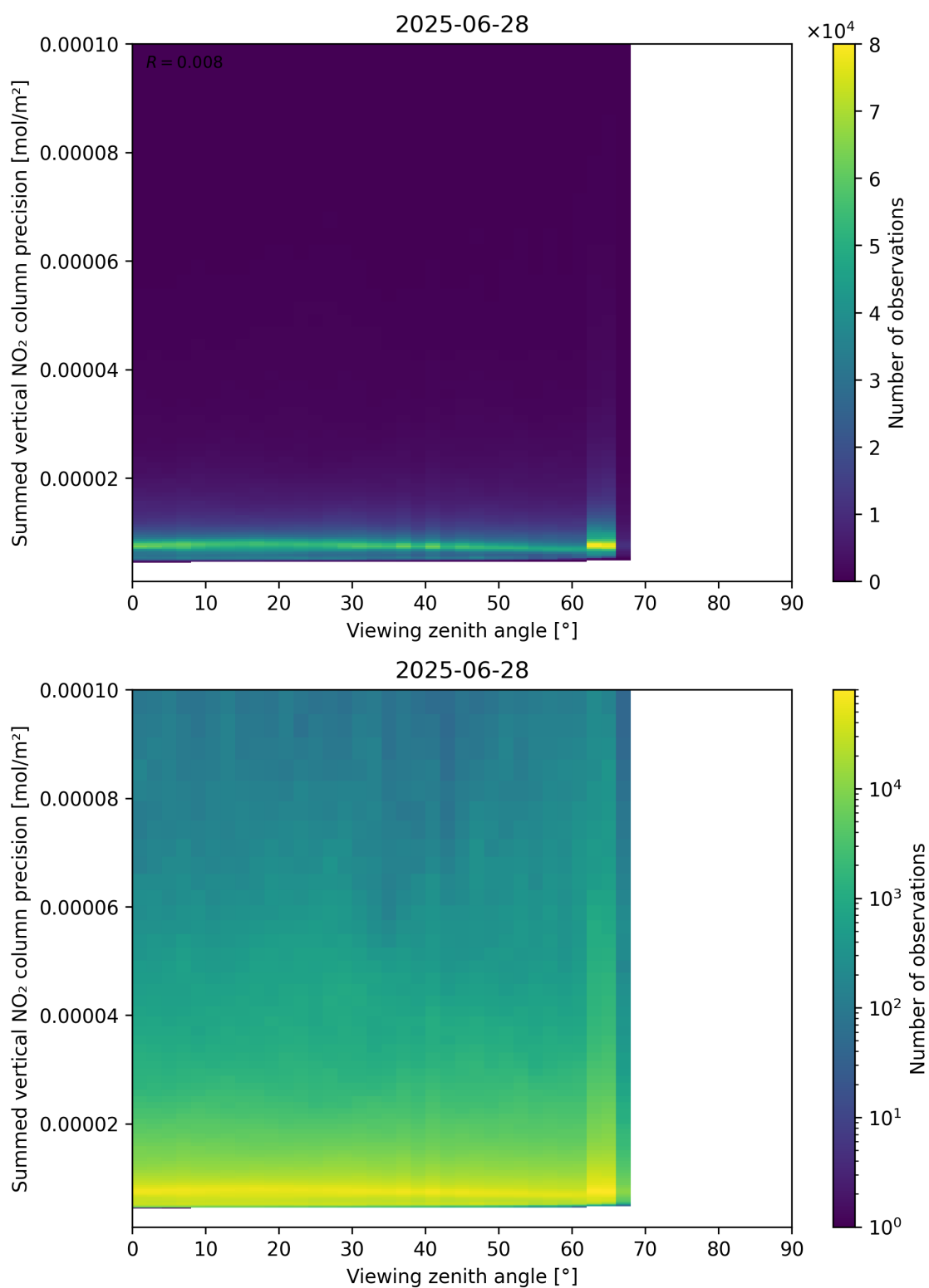
Figure 166: Scatter density plot of “Viewing zenith angle” against “Summed vertical NO 2 column precision” for 2025-06-27 to 2025-06-29.
