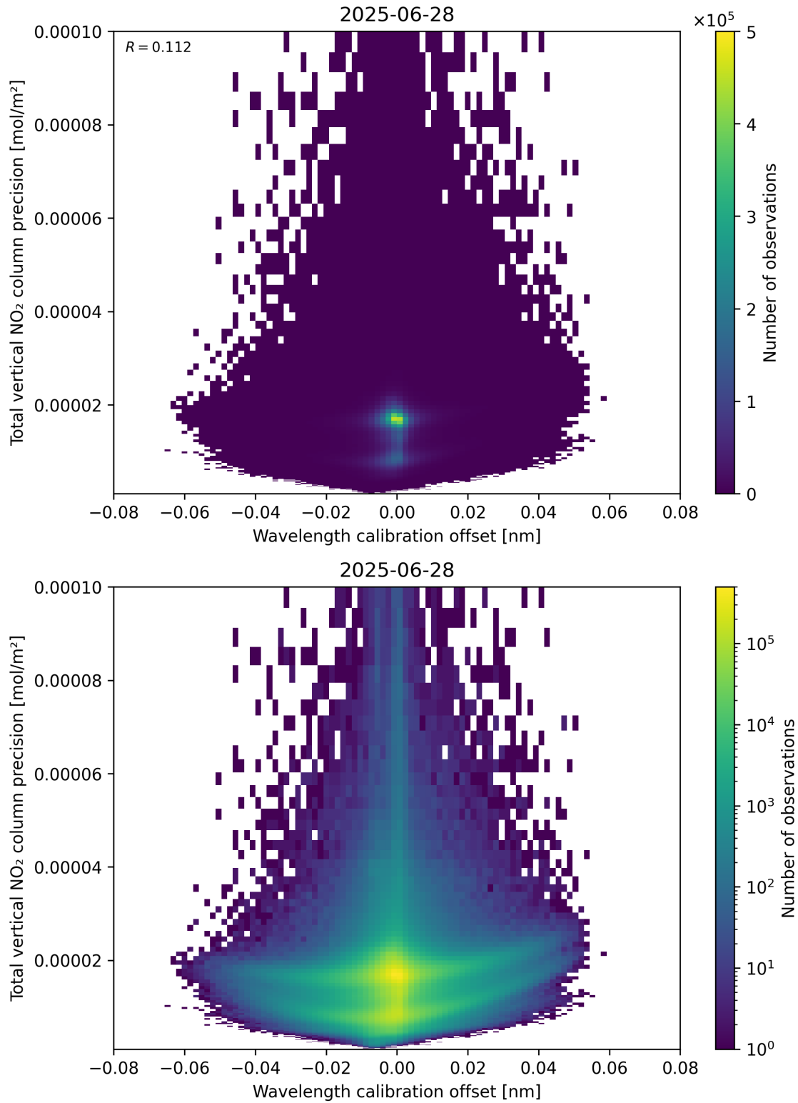
Figure 180: Scatter density plot of “Wavelength calibration offset” against “Total vertical NO 2 column precision” for 2025-06-27 to 2025-06-29.
