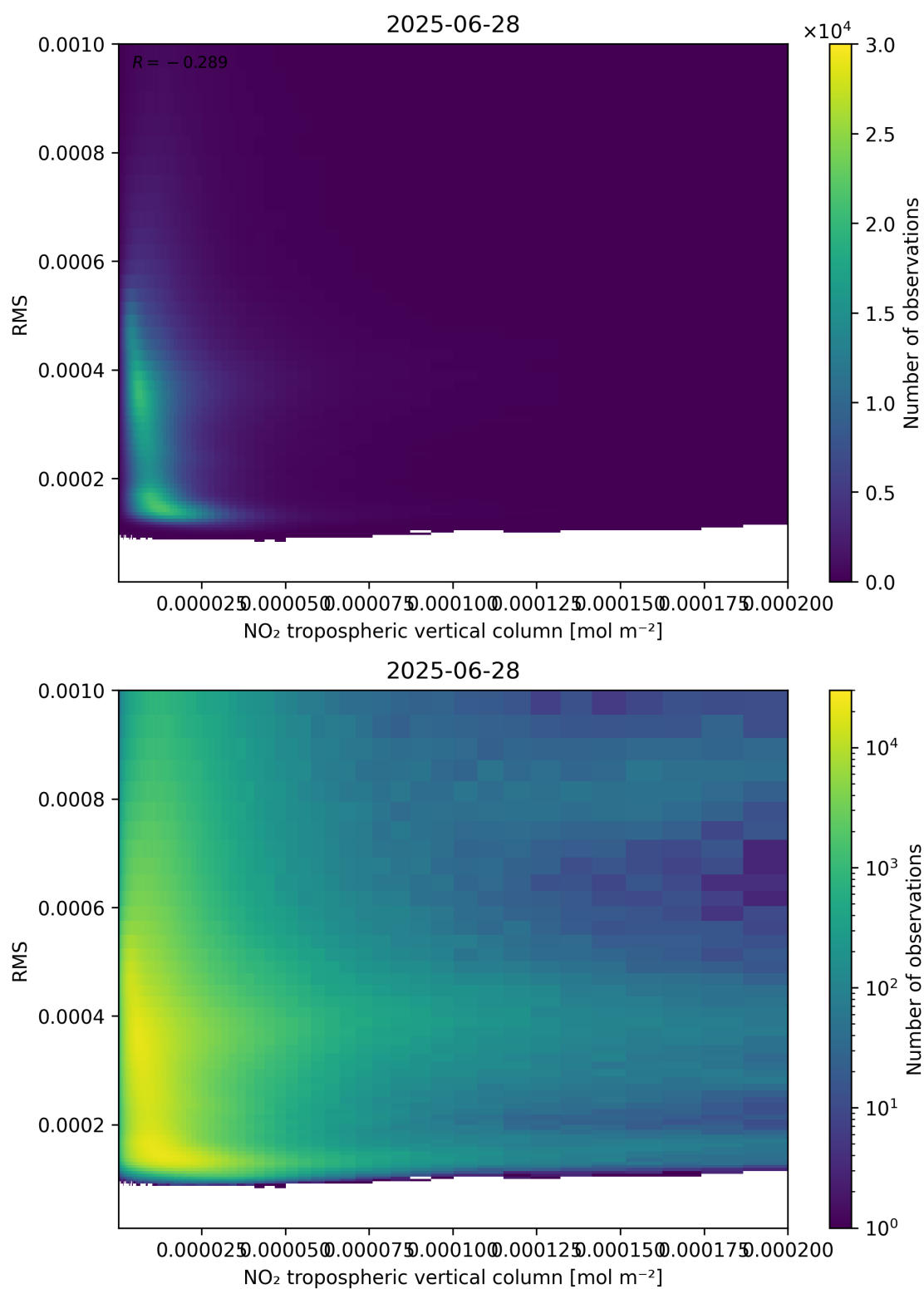
Figure 142: Scatter density plot of “NO 2 tropospheric vertical column” against “RMS” for 2025-06-27 to 2025-06-29.
