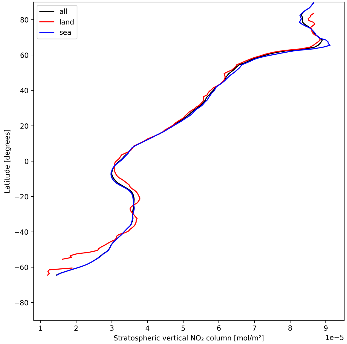
Figure 19: Zonal average of “Stratospheric vertical NO 2 column” for 2025-06-27 to 2025-06-29.
