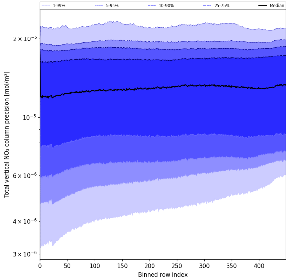
Figure 56: Along track statistics of “Total vertical NO 2 column precision” for 2025-06-27 to 2025-06-29
