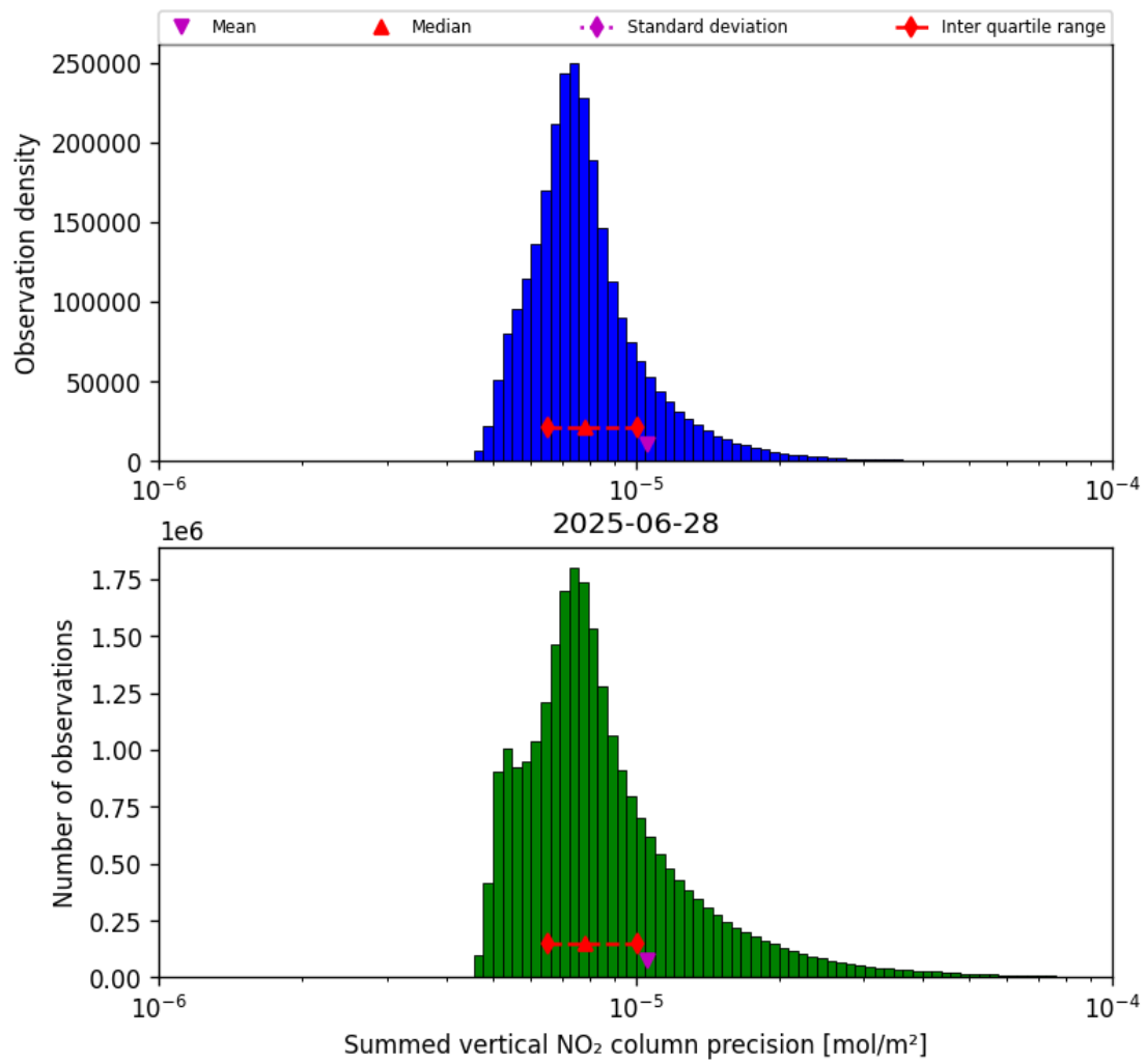
Figure 41: Histogram of "Summed vertical NO 2 column precision" for 2025-06-27 to 2025-06-29
