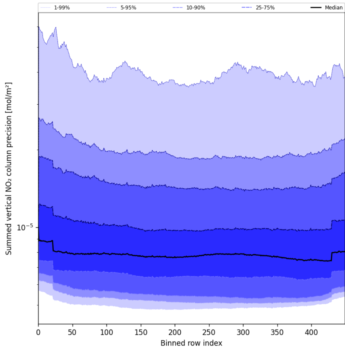
Figure 58: Along track statistics of “Summed vertical NO 2 column precision” for 2025-06-27 to 2025-06-29
