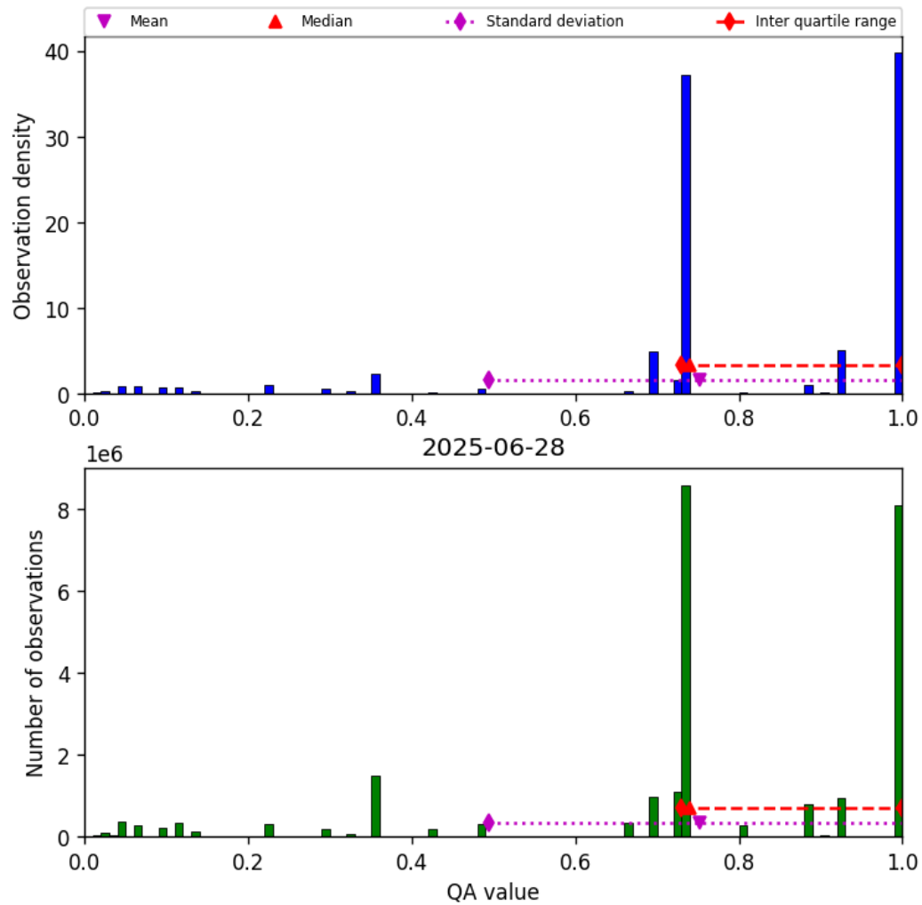
Figure 28: Histogram of “QA value” for 2025-06-27 to 2025-06-29
