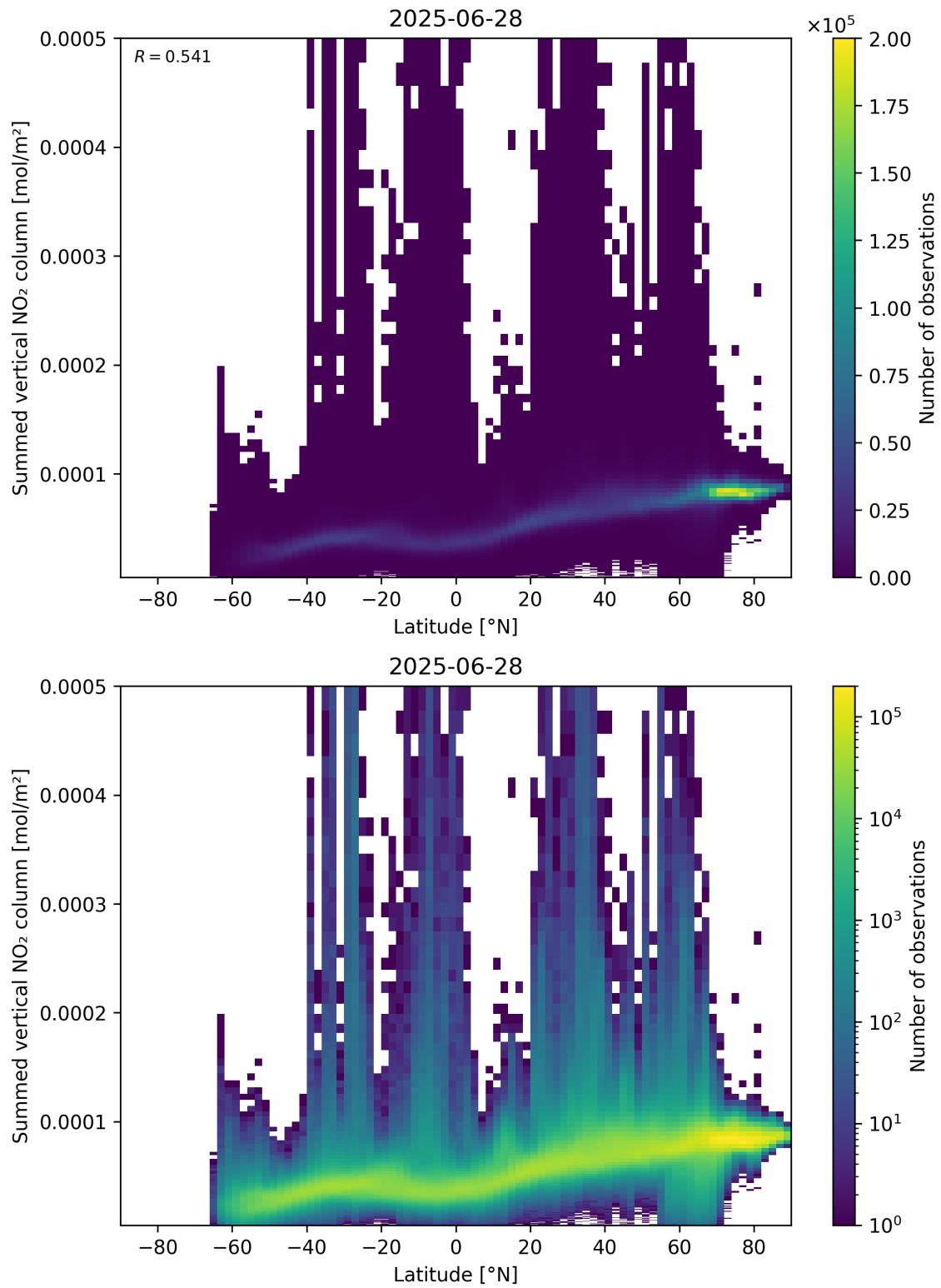
Figure 88: Scatter density plot of “Latitude” against “Summed vertical NO 2 column” for 2025-06-27 to 2025-06-29.
