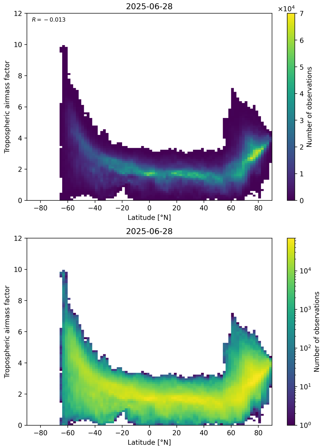
Figure 85: Scatter density plot of “Latitude” against “Tropospheric air mass factor” for 2025-06-27 to 2025-06-29.
