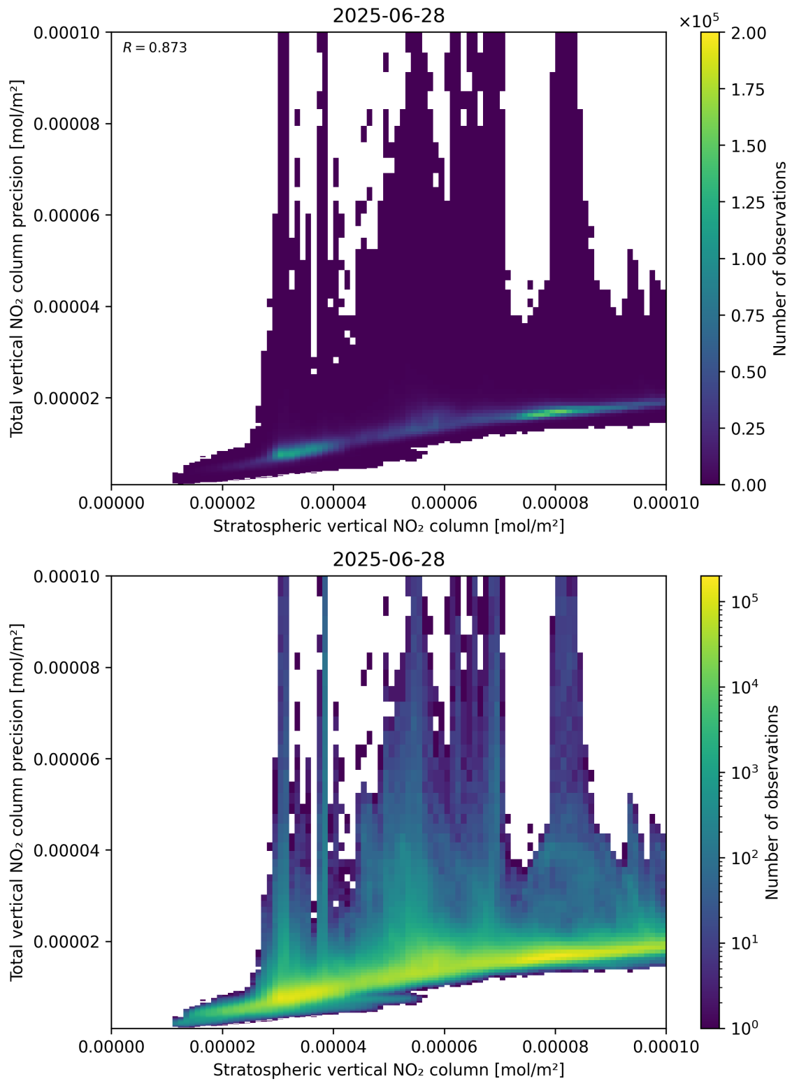
Figure 101: Scatter density plot of “Stratospheric vertical NO 2 column” against “Total vertical NO 2 column precision” for 2025-06-27 to 2025-06-29.
