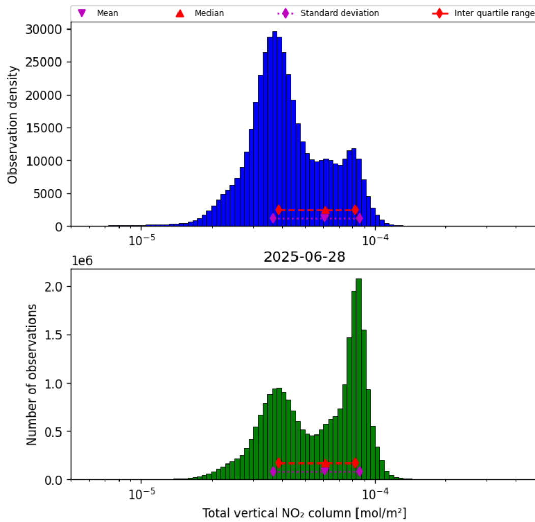
Figure 38: Histogram of “Total vertical NO 2 column” for 2025-06-27 to 2025-06-29
