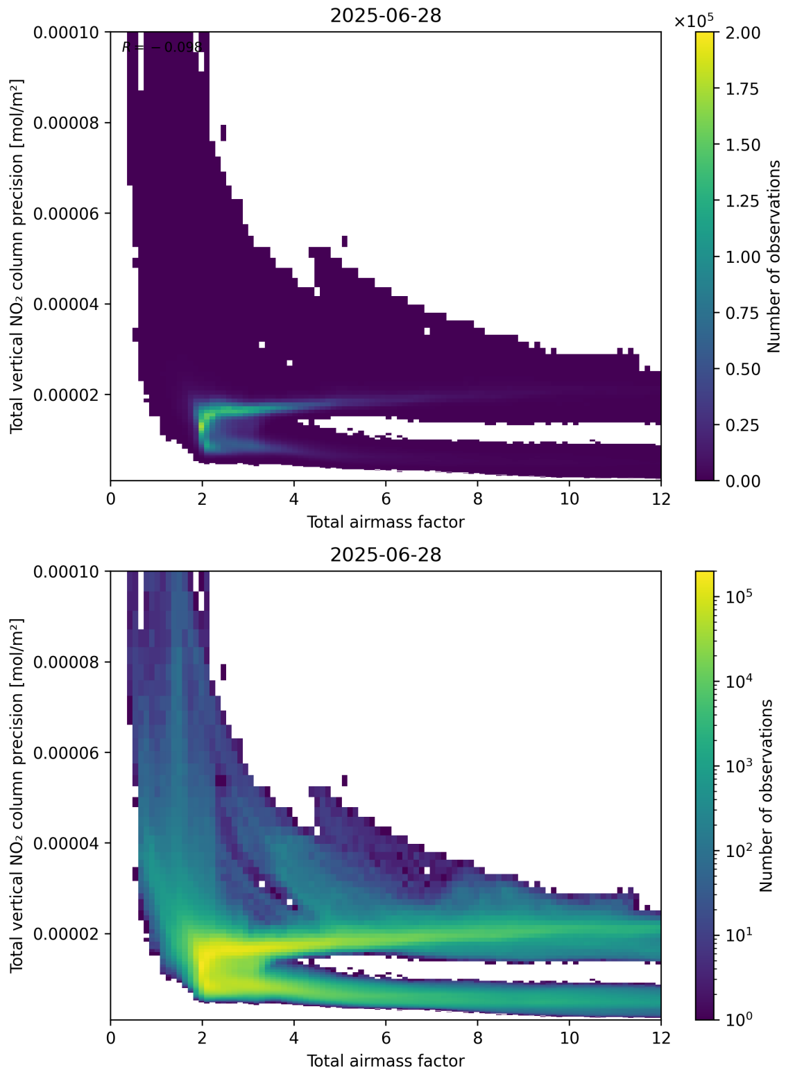
Figure 68: Scatter density plot of “Total airmass factor” against “Total vertical NO 2 column precision” for 2025-06-27 to 2025-06-29.
