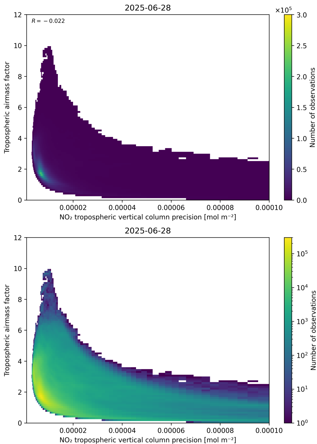
Figure 133: Scatter density plot of “NO 2 tropospheric vertical column precision” against “Tropospheric airmass factor” for 2025-06-27 to 2025-06-29.
