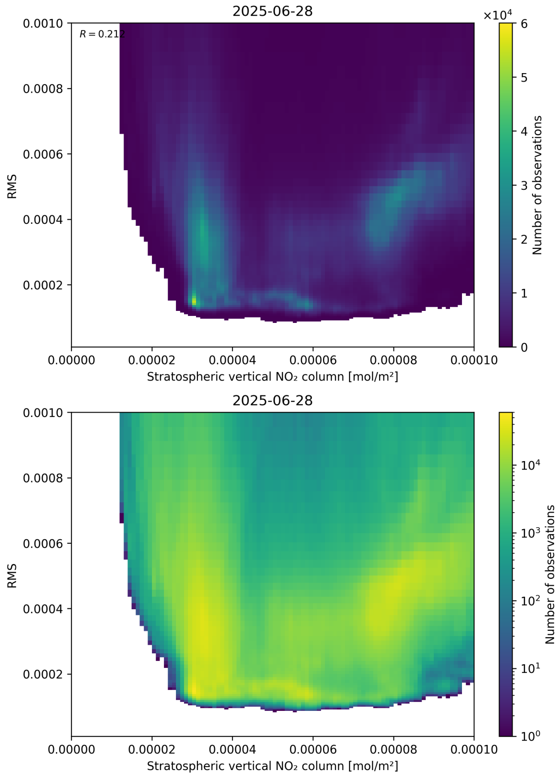
Figure 102: Scatter density plot of “Stratospheric vertical NO 2 column” against “RMS” for 2025-06-27 to 2025-06-29.
