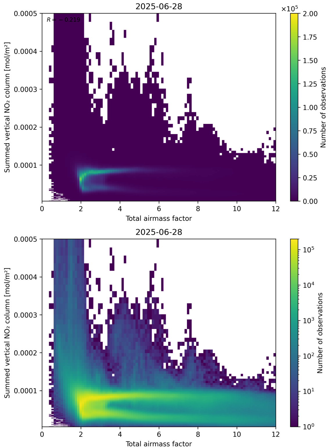
Figure 65: Scatter density plot of “Total airmass factor” against “Summed vertical NO 2 column” for 2025-06-27 to 2025-06-29.
