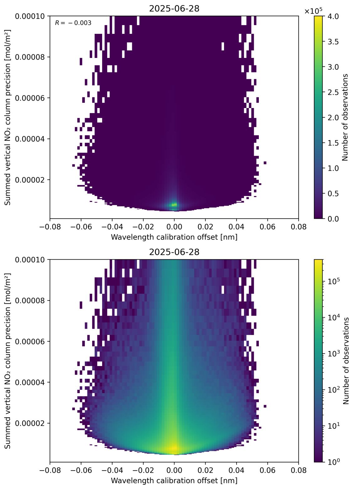
Figure 178: Scatter density plot of “Wavelength calibration offset” against “Summed vertical NO 2 column precision” for 2025-06-27 to 2025-06-29.
