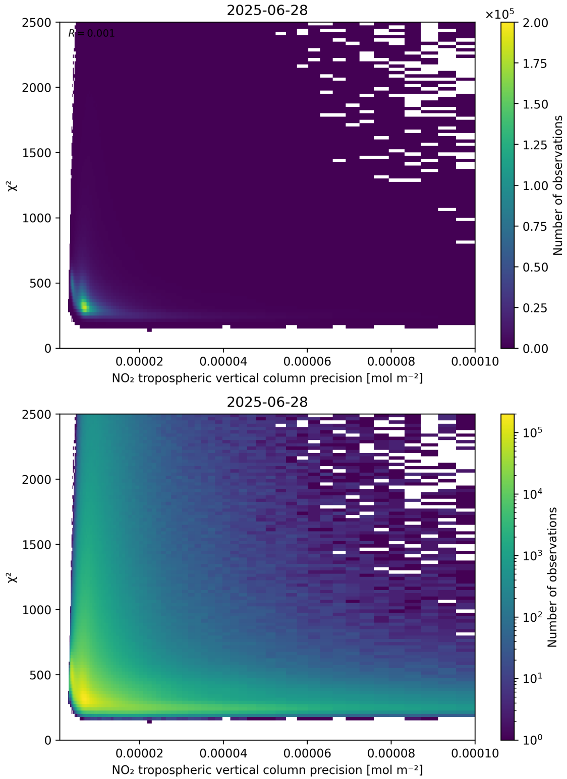
Figure 134: Scatter density plot of “NO 2 tropospheric vertical column precision” against “ \chi^2 ” for 2025-06-27 to 2025-06-29.
