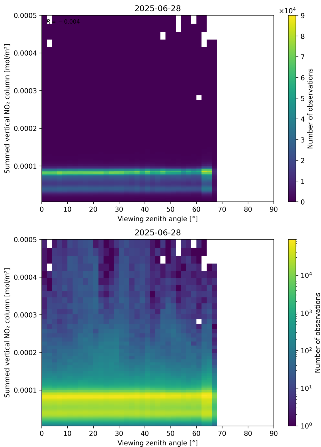
Figure 165: Scatter density plot of “Viewing zenith angle” against “Summed vertical NO 2 column” for 2025-06-27 to 2025-06-29.
