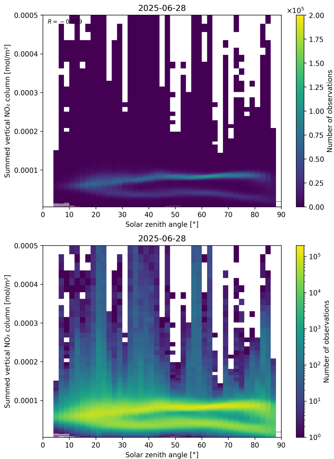
Figure 151: Scatter density plot of “Solar zenith angle” against “Summed vertical NO 2 column” for 2025-06-27 to 2025-06-29.
