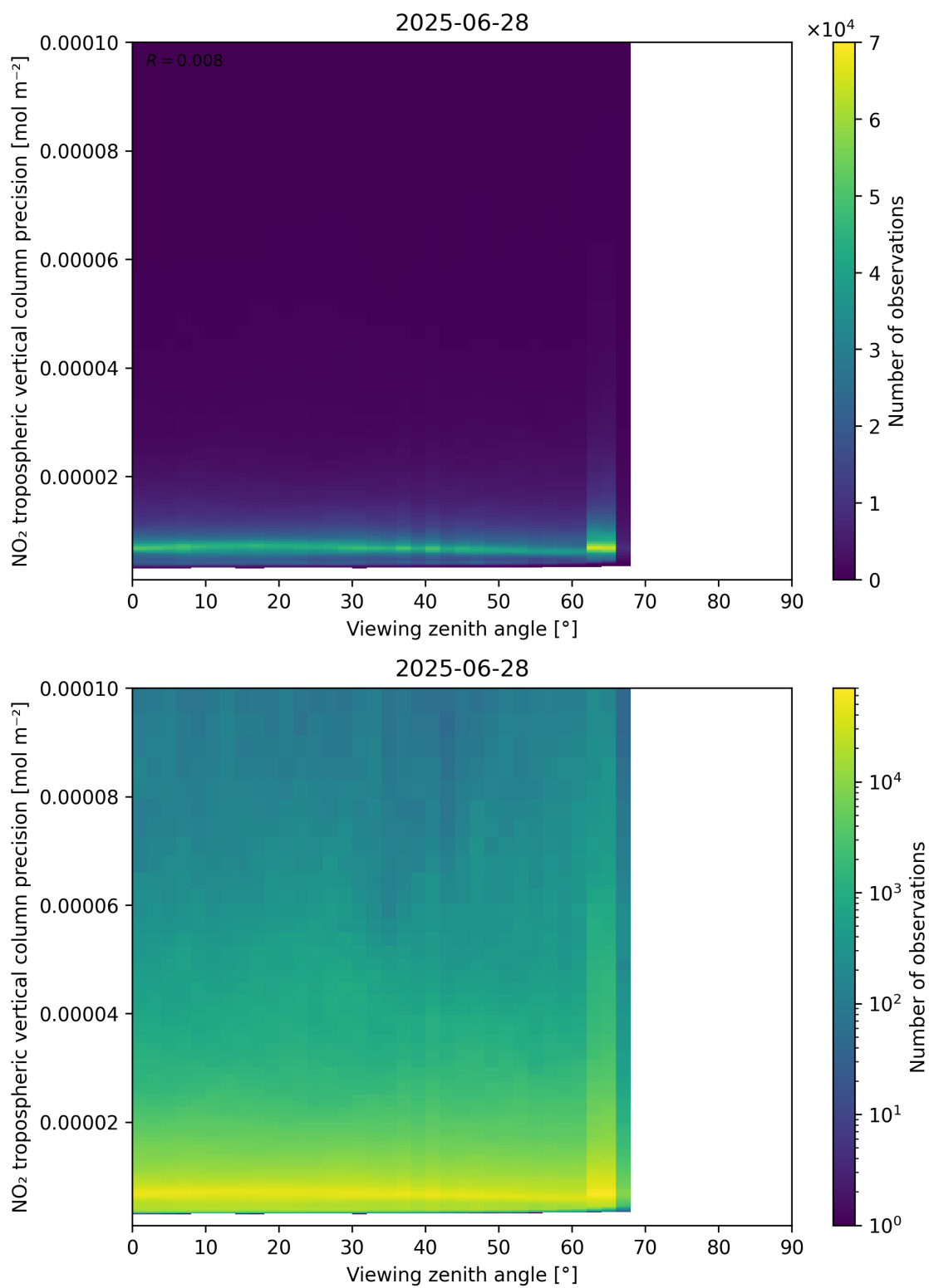
Figure 170: Scatter density plot of “Viewing zenith angle” against “NO 2 tropospheric vertical column precision” for 2025-06-27 to 2025-06-29.
