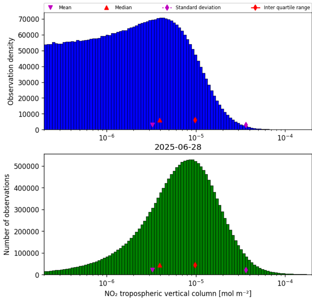
Figure 29: Histogram of “NO 2 tropospheric vertical column” for 2025-06-27 to 2025-06-29
