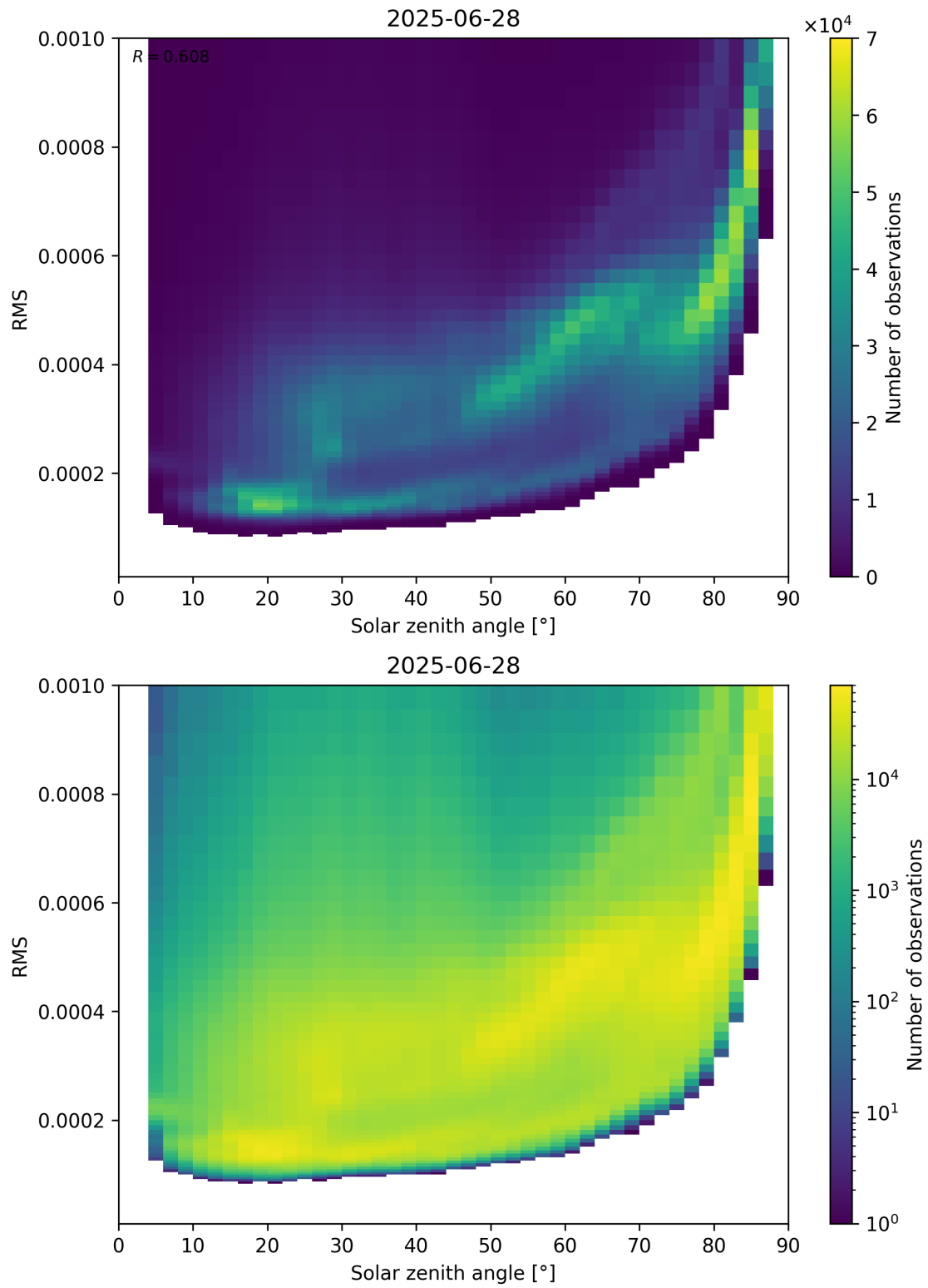
Figure 157: Scatter density plot of “Solar zenith angle” against “RMS” for 2025-06-27 to 2025-06-29.
