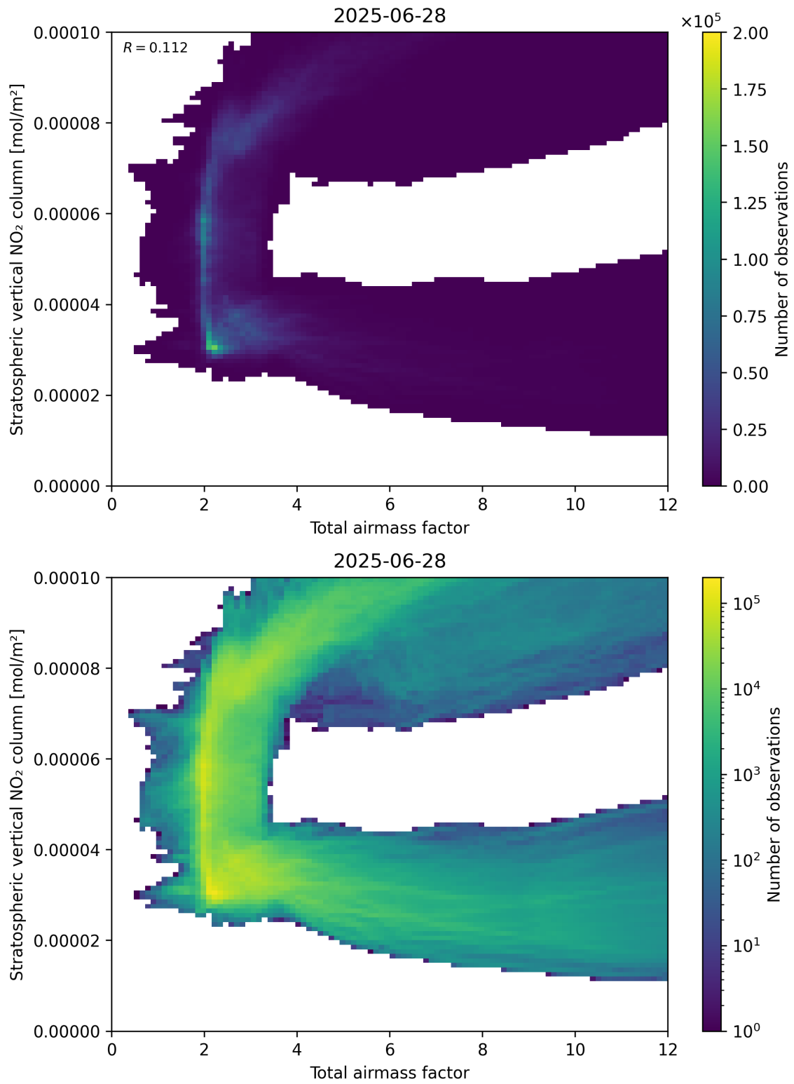
Figure 64: Scatter density plot of “Total airmass factor” against “Stratospheric vertical NO 2 column” for 2025-06-27 to 2025-06-29.
