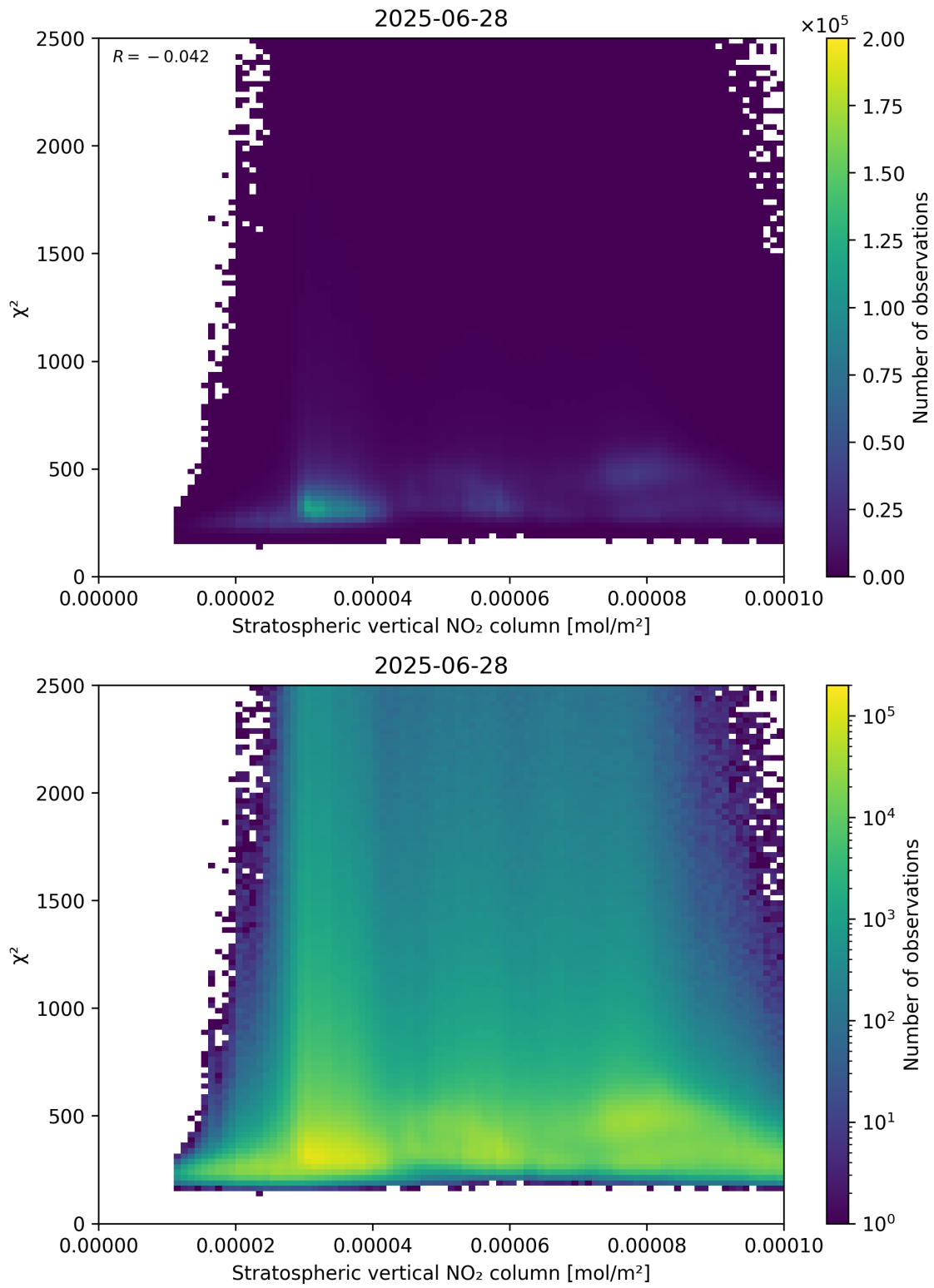
Figure 97: Scatter density plot of “Stratospheric vertical NO 2 column” against “ \chi^2 ” for 2025-06-27 to 2025-06-29.
