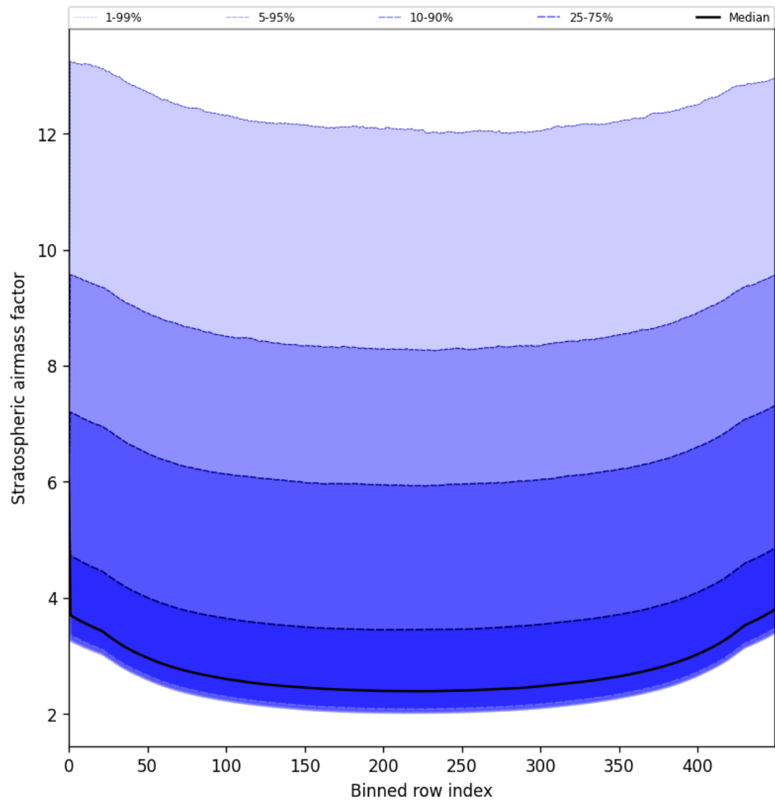
Figure 61: Along track statistics of “Stratospheric airmass factor” for 2025-06-27 to 2025-06-29
