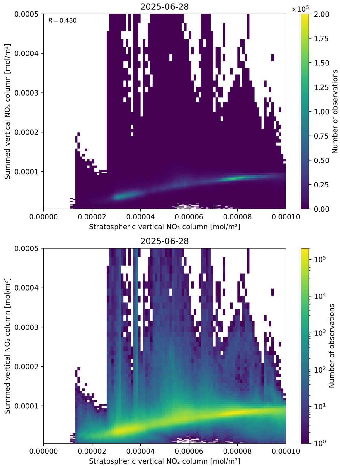
Figure 98: Scatter density plot of “Stratospheric vertical NO 2 column” against “Summed vertical NO 2 column” for 2025-06-27 to 2025-06-29.
