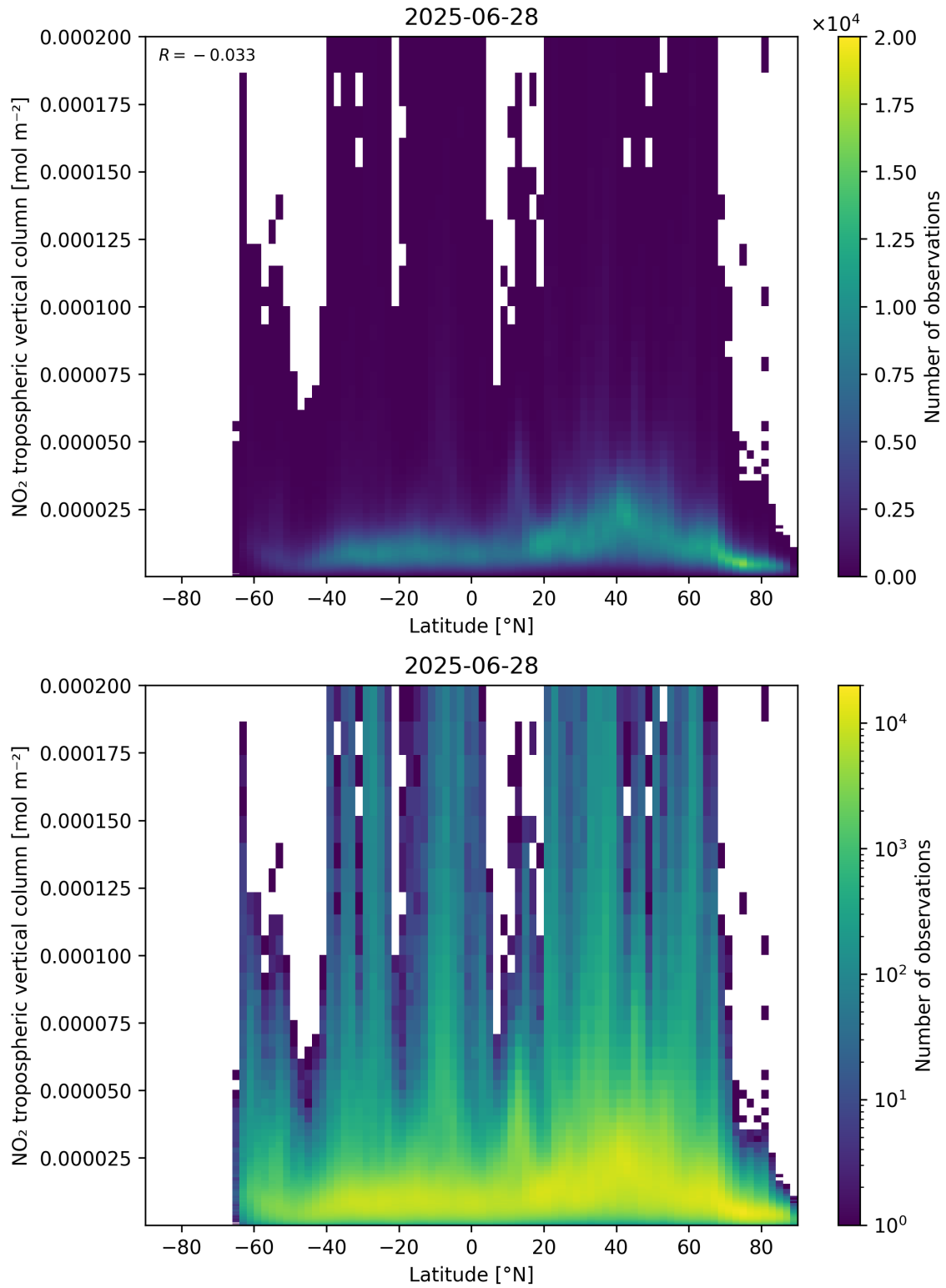
Figure 92: Scatter density plot of “Latitude” against “NO 2 tropospheric vertical column” for 2025-06-27 to 2025-06-29.
