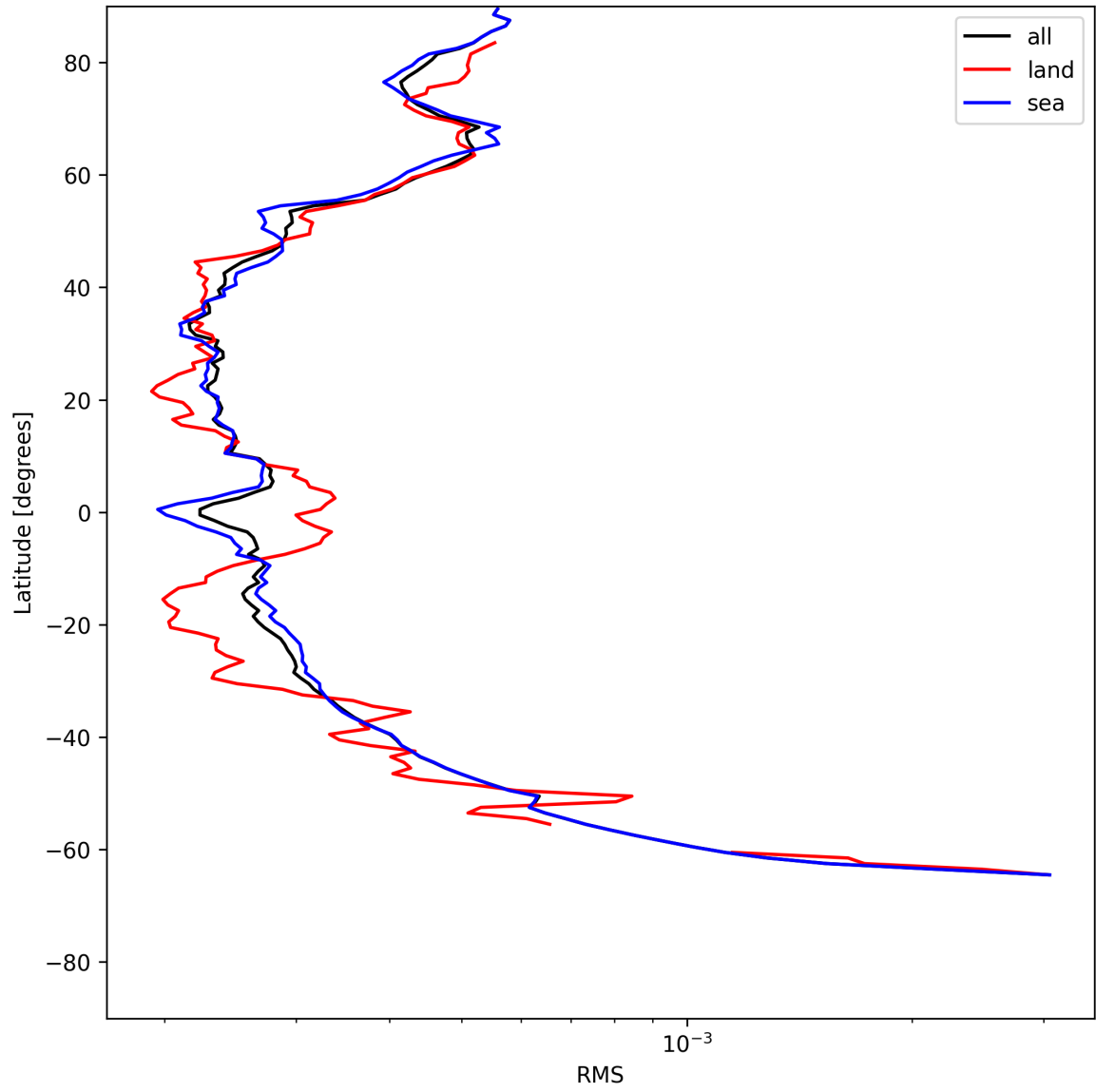
Figure 26: Zonal average of “RMS” for 2025-06-27 to 2025-06-29.
