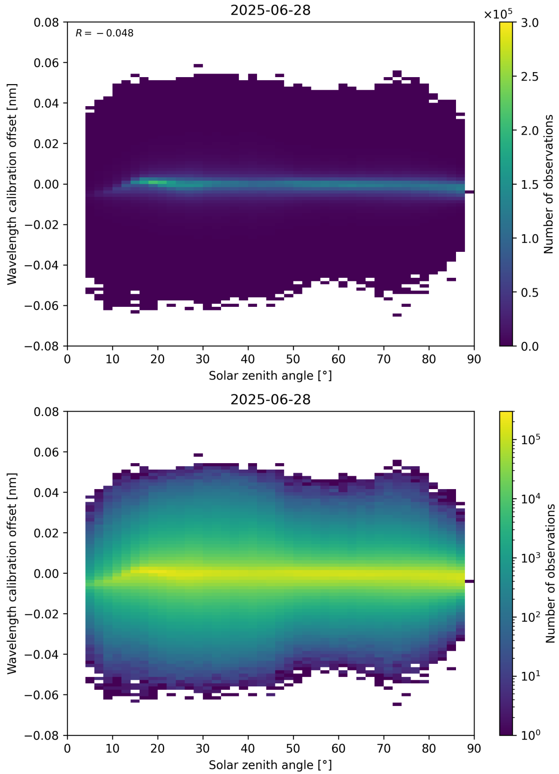
Figure 158: Scatter density plot of “Solar zenith angle” against “Wavelength calibration offset” for 2025-06-27 to 2025-06-29.
