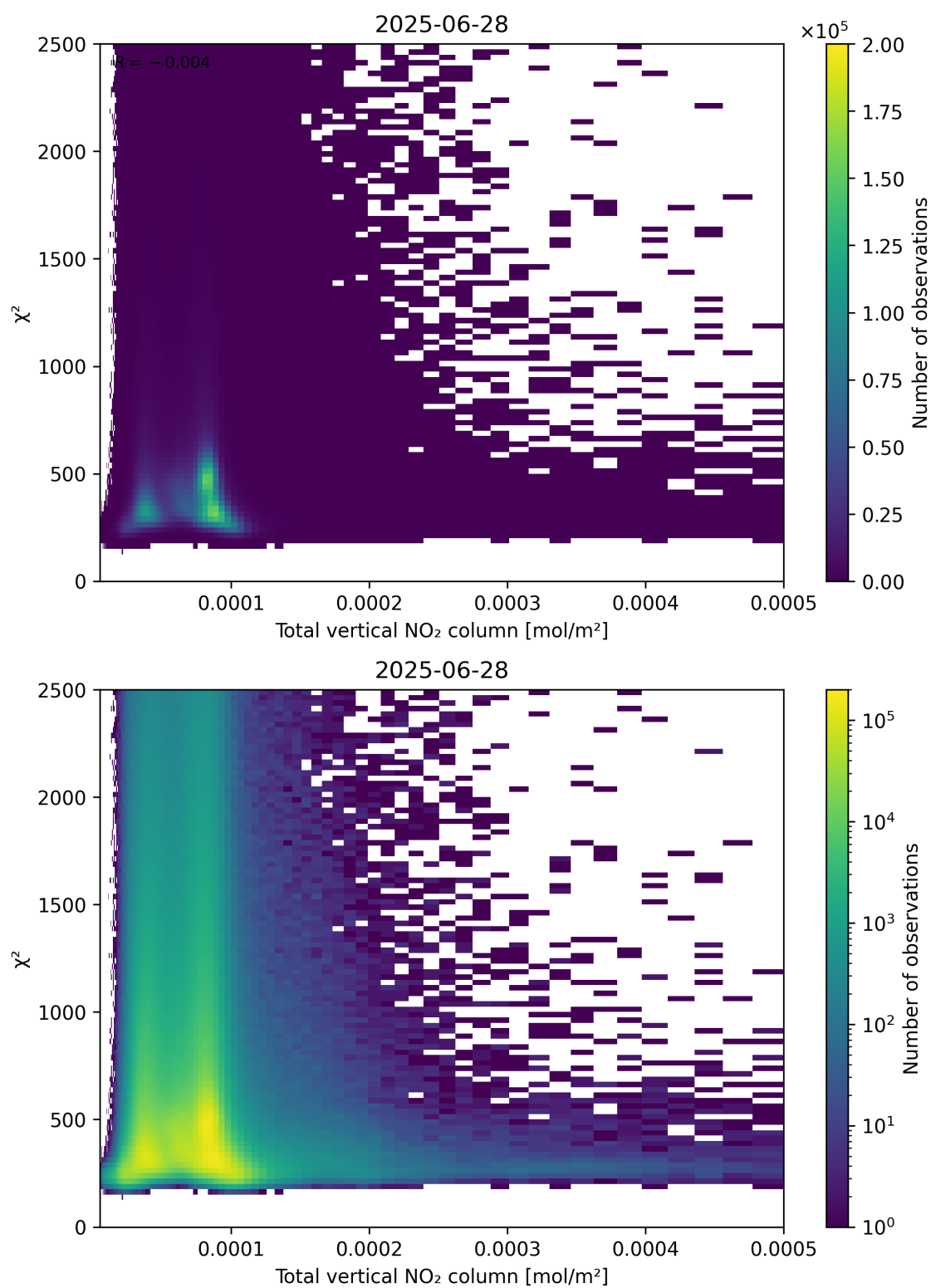
Figure 111: Scatter density plot of “Total vertical NO 2 column” against “ \chi^2 ” for 2025-06-27 to 2025-06-29.
