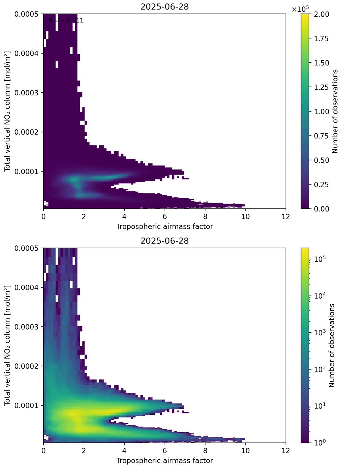
Figure 77: Scatter density plot of “Tropospheric airmass factor” against “Total vertical NO 2 column” for 2025-06-27 to 2025-06-29.
