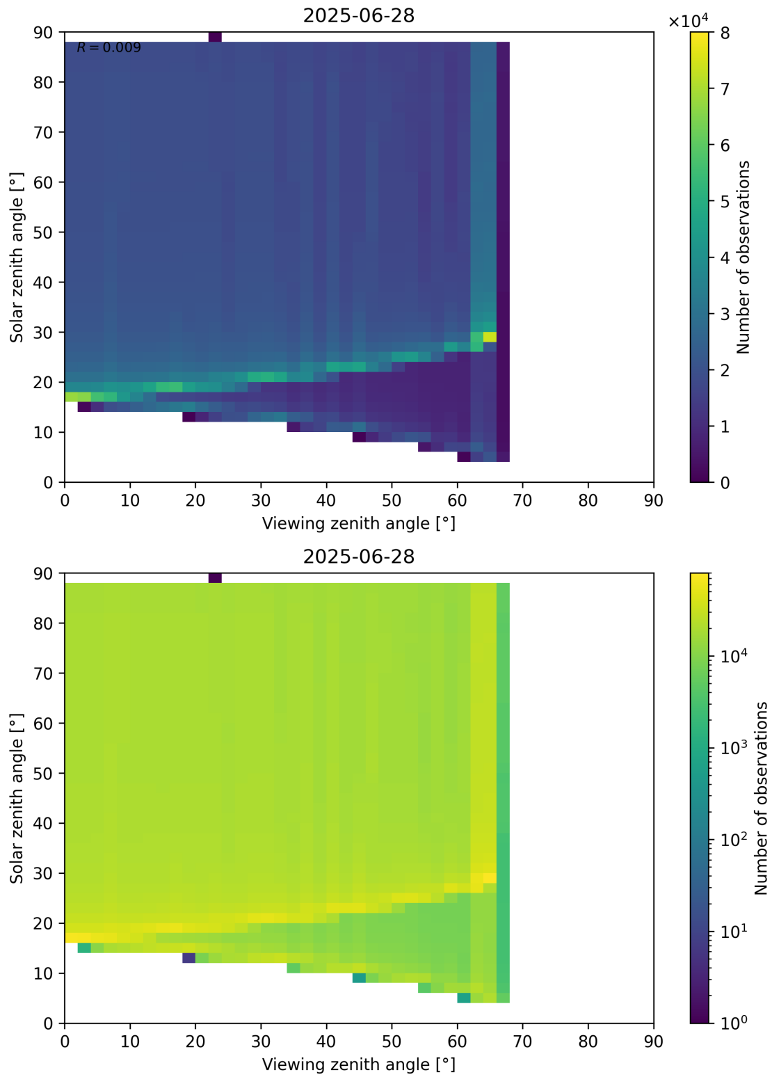
Figure 172: Scatter density plot of “Viewing zenith angle” against “Solar zenith angle” for 2025-06-27 to 2025-06-29.
